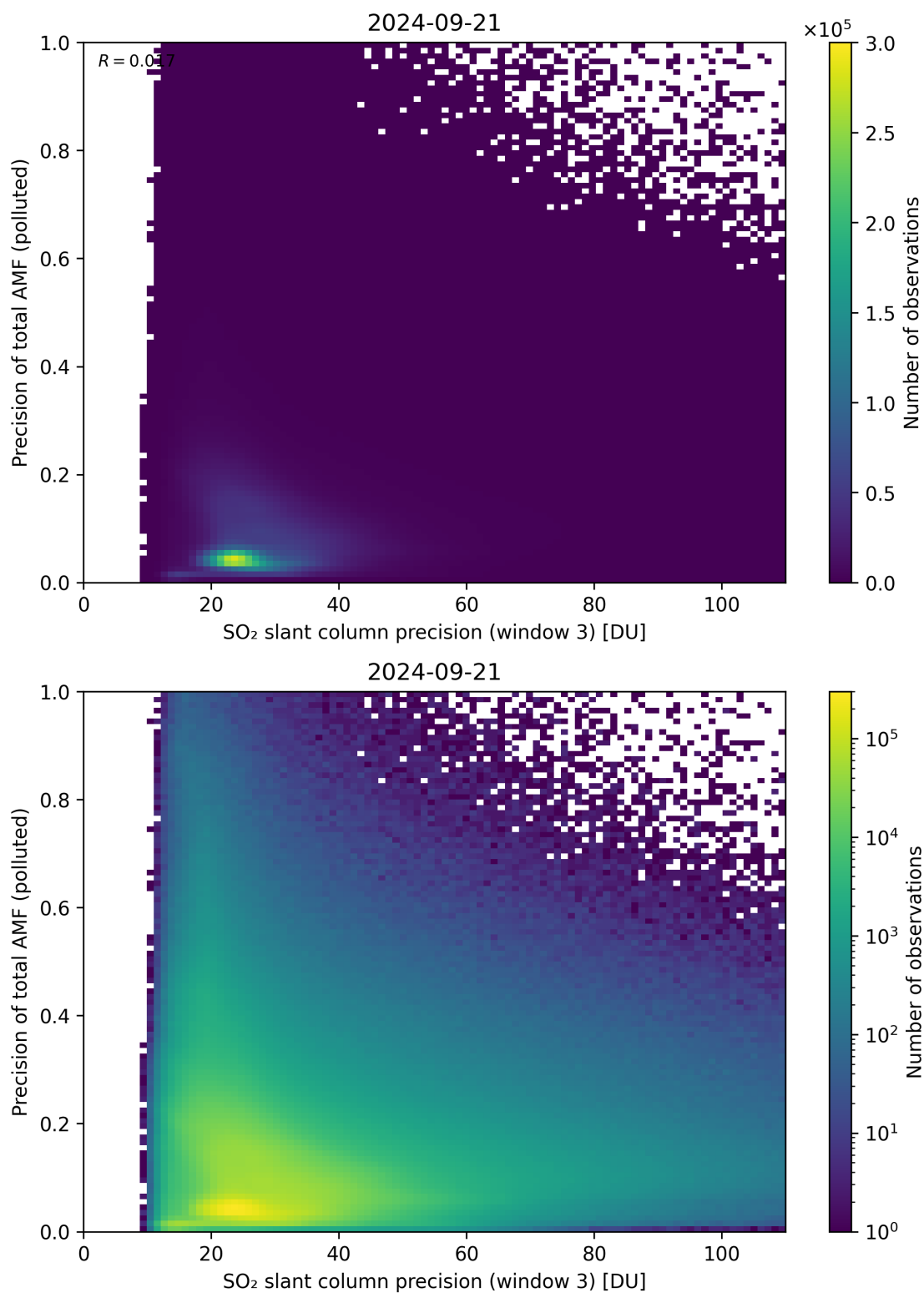
Figure 264: Scatter density plot of “SO 2 slant column precision (window 3)” against “Precision of total AMF (polluted)” for 2024-09-20 to 2024-09-22.
