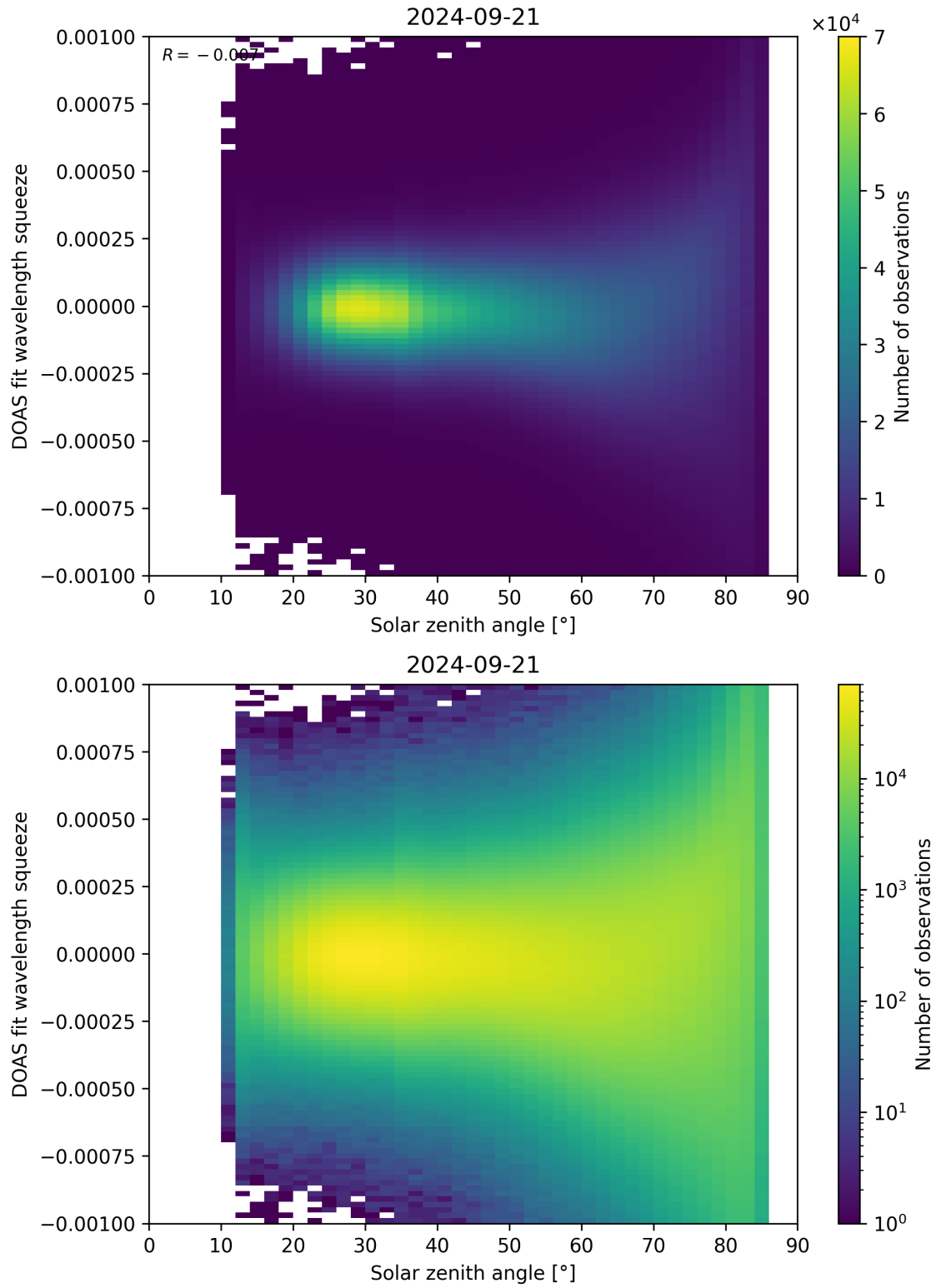
Figure 162: Scatter density plot of “Solar zenith angle” against “DOAS fit wavelength squeeze” for 2024-09-20 to 2024-09-22.
