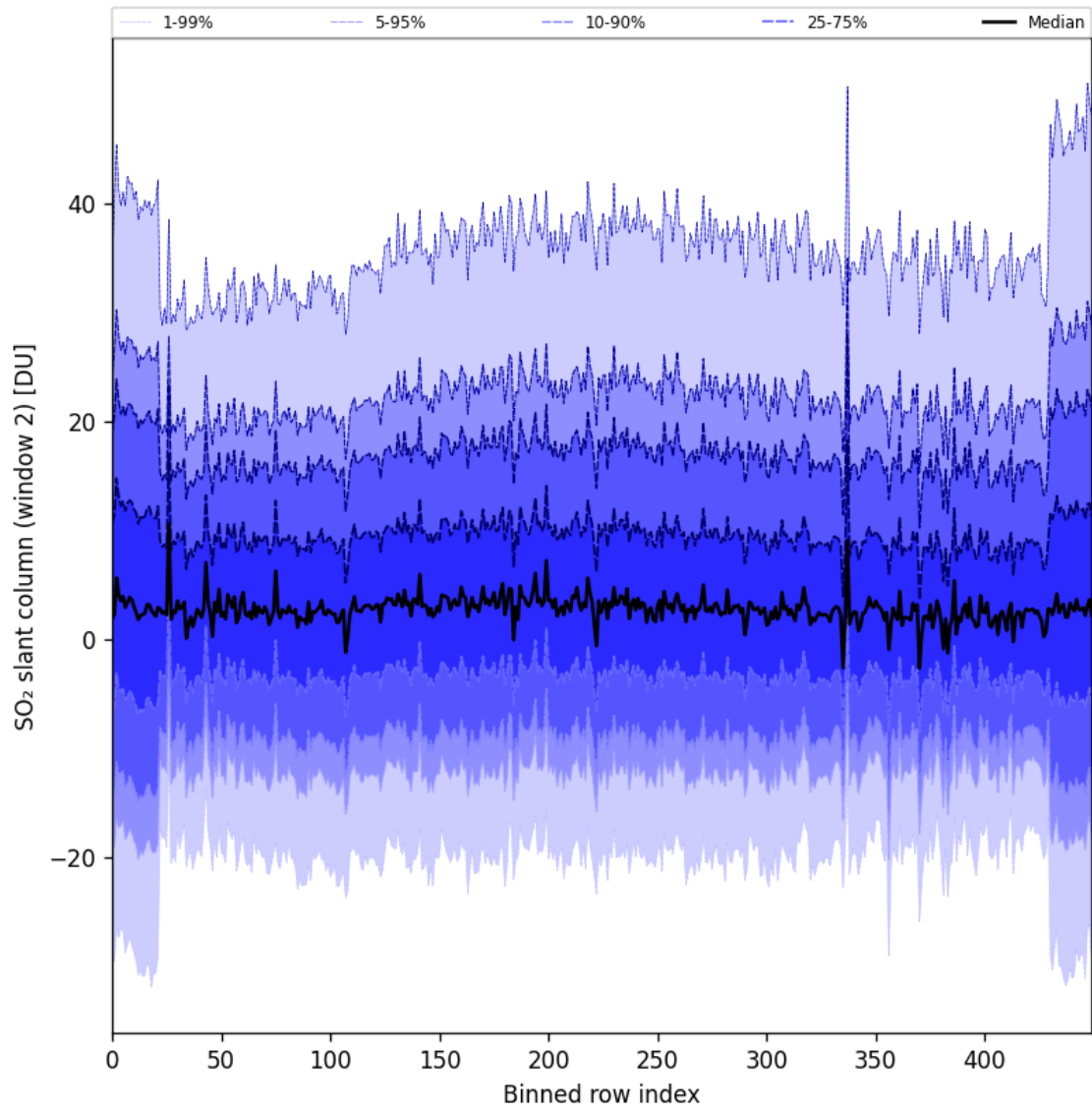
Figure 83: Along track statistics of “SO 2 slant column (window 2)” for 2024-09-20 to 2024-09-22
