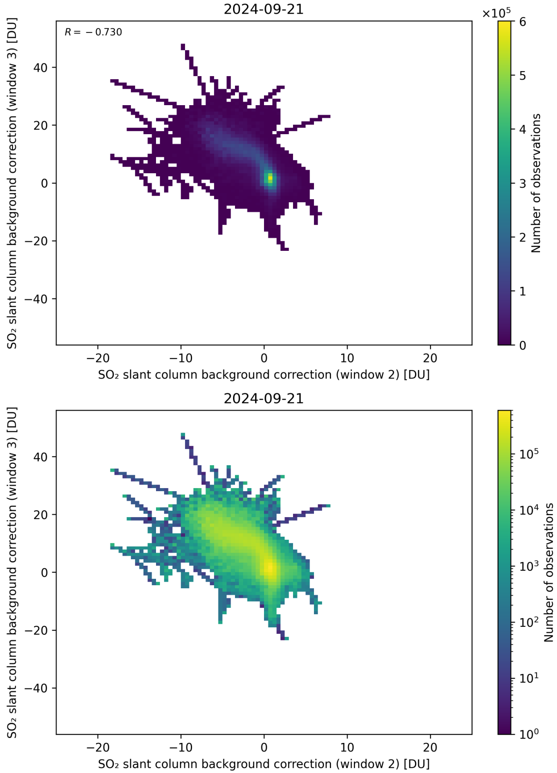
Figure 111: Scatter density plot of “SO 2 slant column background correction (window 2)” against “SO 2 slant column background correction (window 3)” for 2024-09-20 to 2024-09-22.
