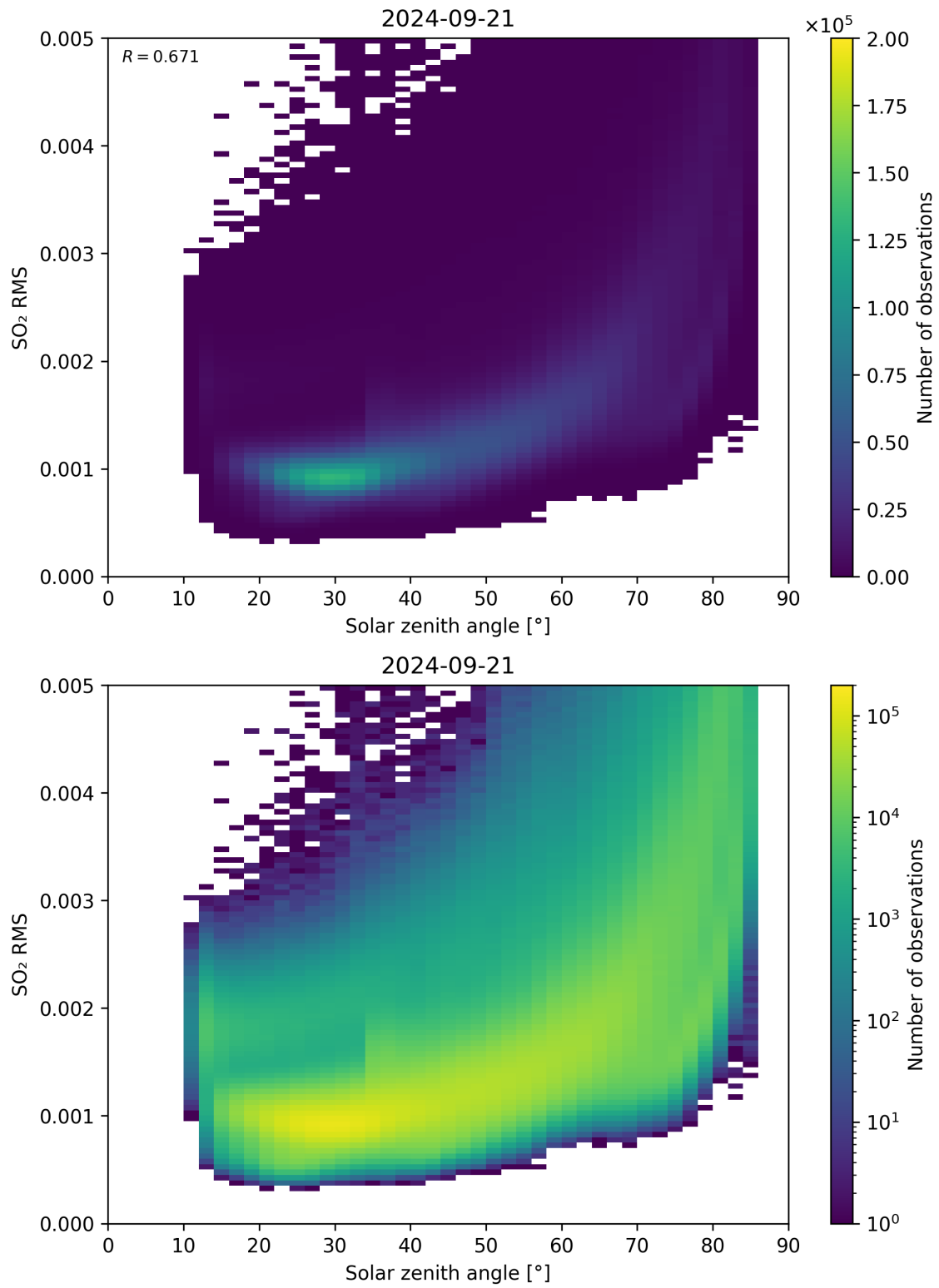
Figure 163: Scatter density plot of “Solar zenith angle” against “SO 2 RMS” for 2024-09-20 to 2024-09-22.
