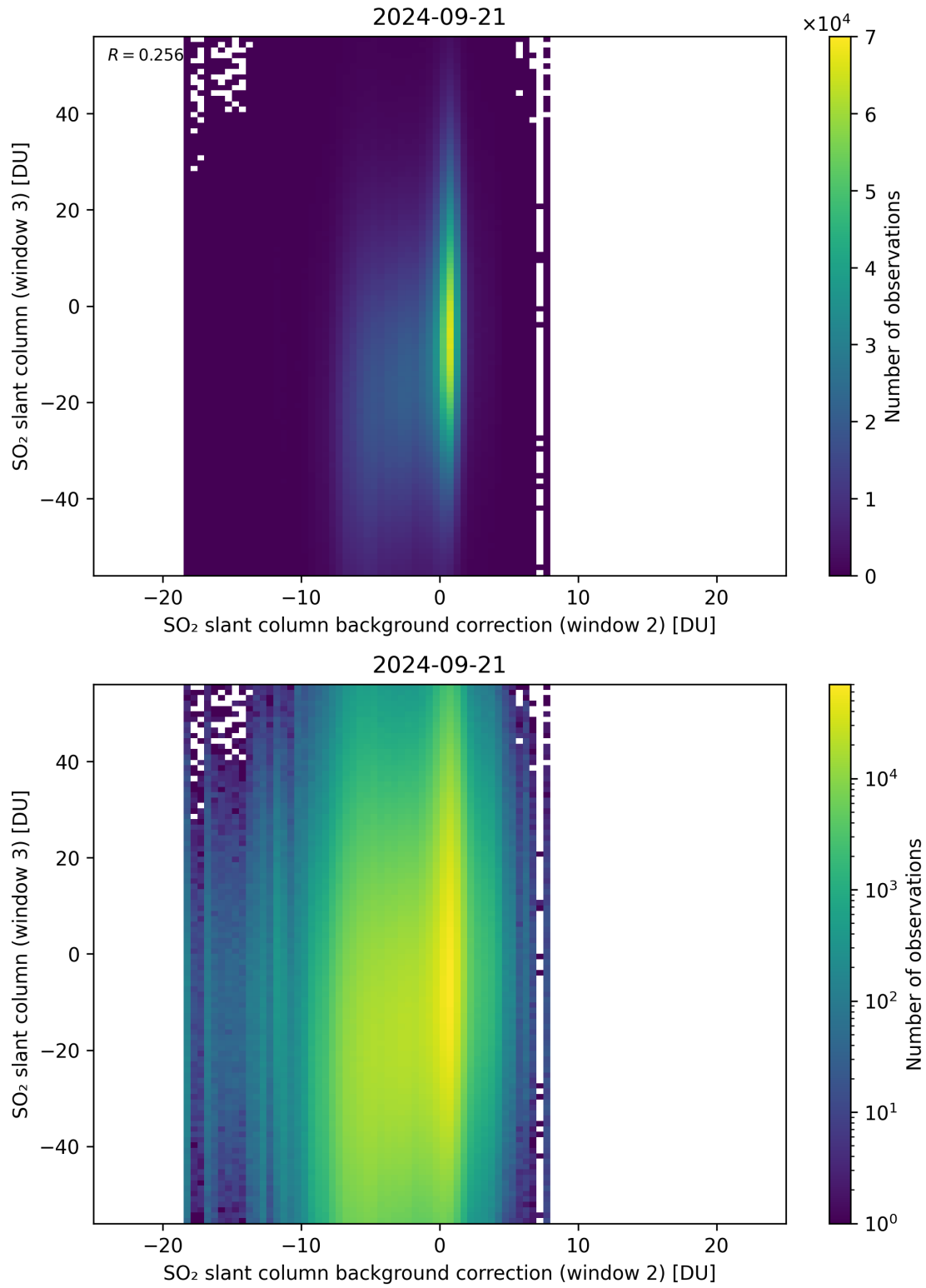
Figure 117: Scatter density plot of “SO 2 slant column background correction (window 2)” against “SO 2 slant column (window 3)” for 2024-09-20 to 2024-09-22.
