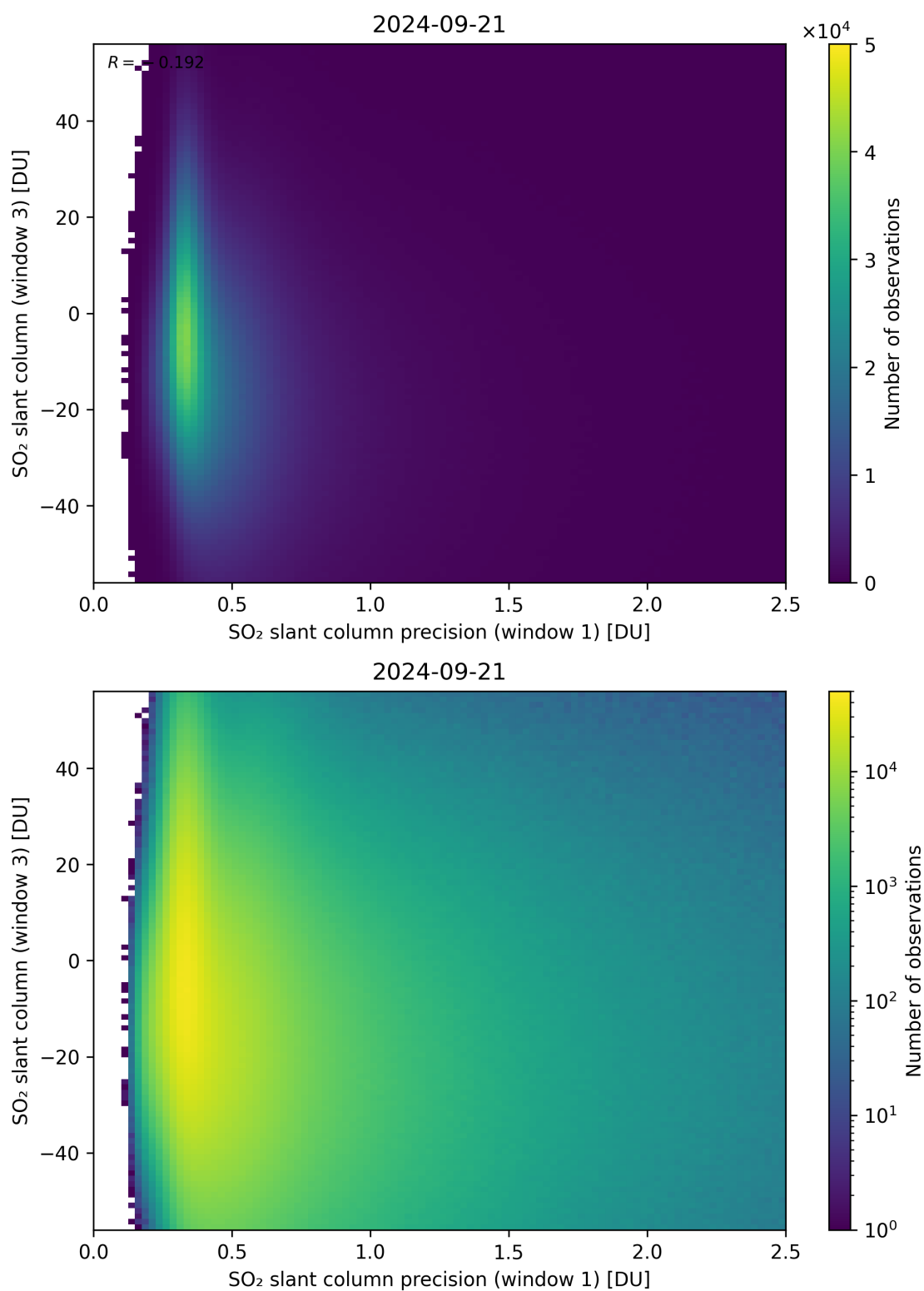
Figure 228: Scatter density plot of “SO 2 slant column precision (window 1)” against “SO 2 slant column (window 3)” for 2024-09-20 to 2024-09-22.
