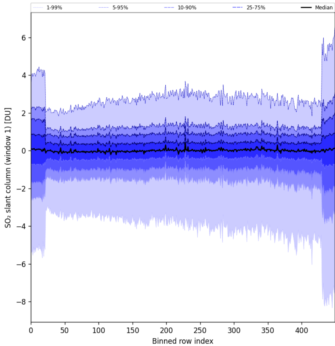
Figure 79: Along track statistics of “SO 2 slant column (window 1)” for 2024-09-20 to 2024-09-22
