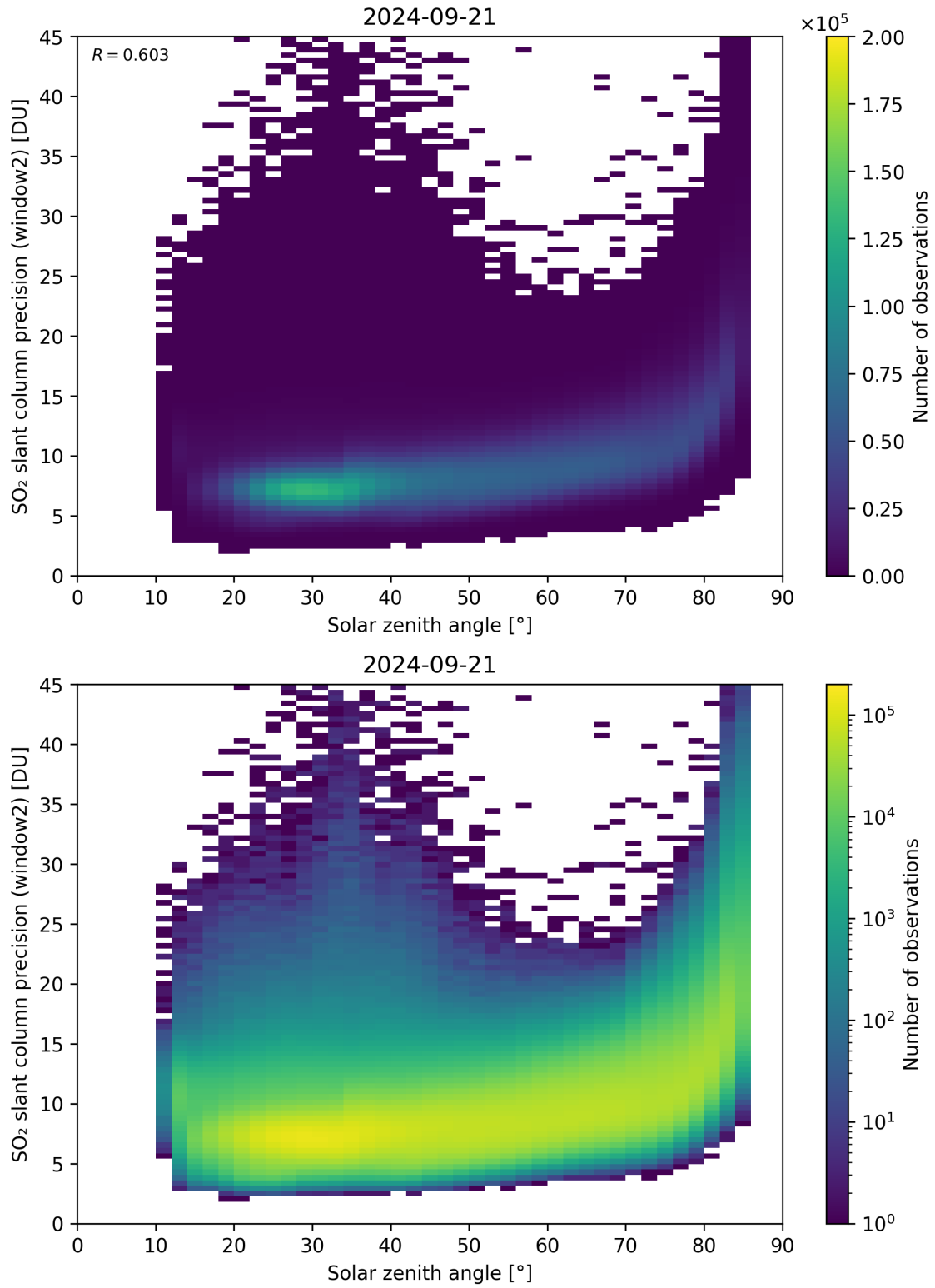
Figure 171: Scatter density plot of “Solar zenith angle” against “SO 2 slant column precision (window2)” for 2024-09-20 to 2024-09-22.
