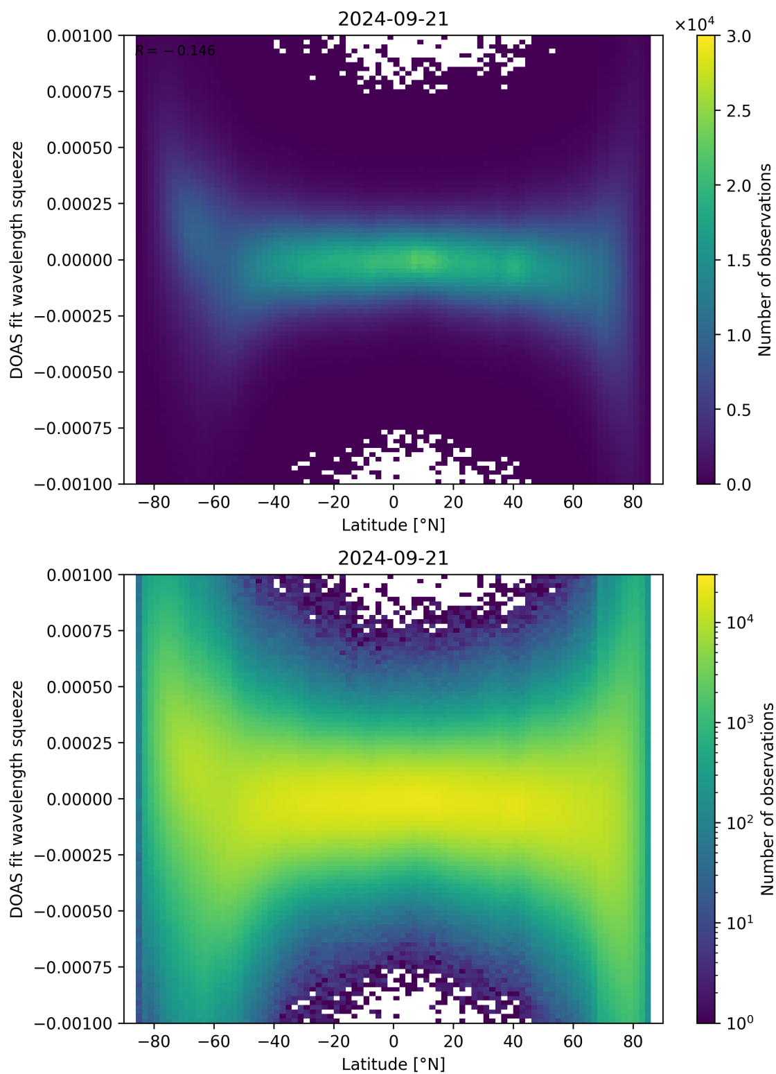
Figure 143: Scatter density plot of “Latitude” against “DOAS fit wavelength squeeze” for 2024-09-20 to 2024-09-22.
