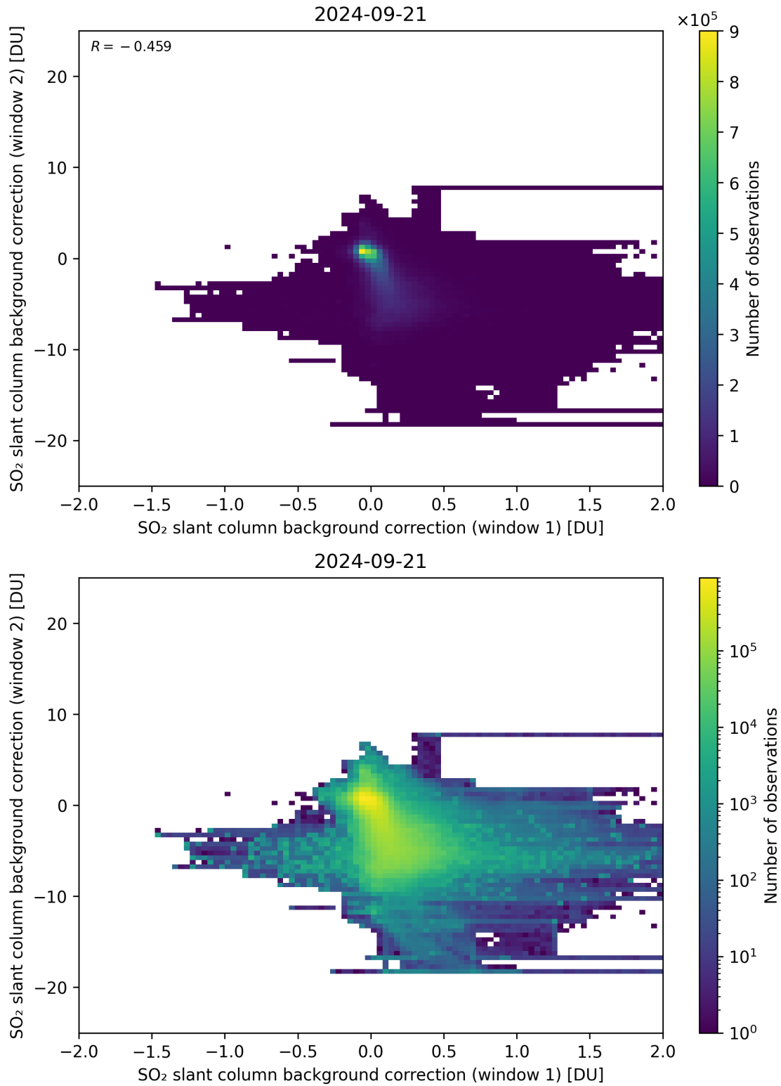
Figure 98: Scatter density plot of “SO 2 slant column background correction (window 1)” against “SO 2 slant column background correction (window 2)” for 2024-09-20 to 2024-09-22.
