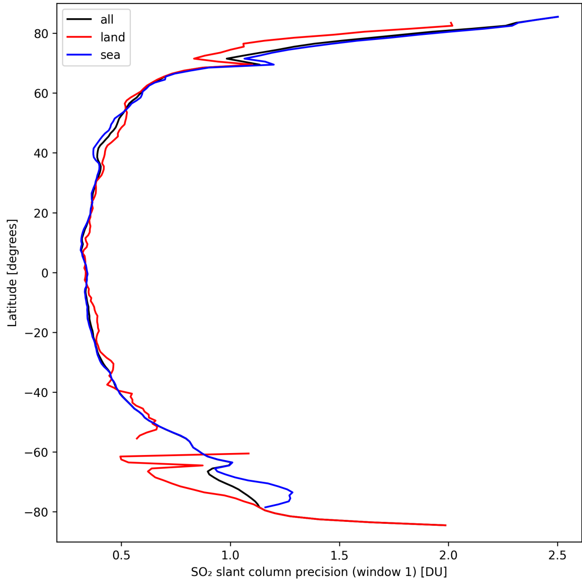
Figure 34: Zonal average of “SO 2 slant column precision (window 1)” for 2024-09-20 to 2024-09-22.
