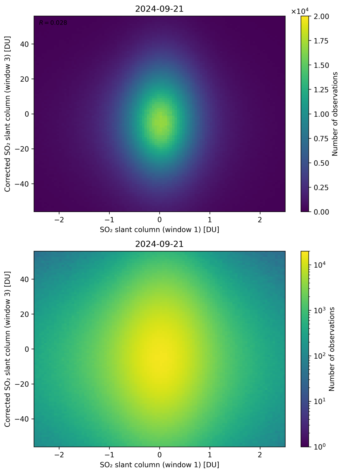
Figure 234: Scatter density plot of “SO 2 slant column (window 1)” against “Corrected SO 2 slant column (window 3)” for 2024-09-20 to 2024-09-22.
