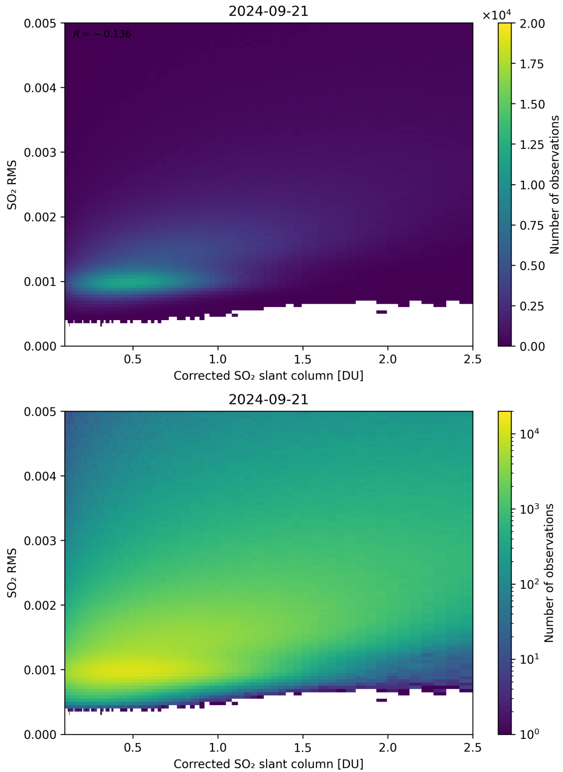
Figure 183: Scatter density plot of “Corrected SO 2 slant column” against “SO 2 RMS” for 2024-09-20 to 2024-09-22.
