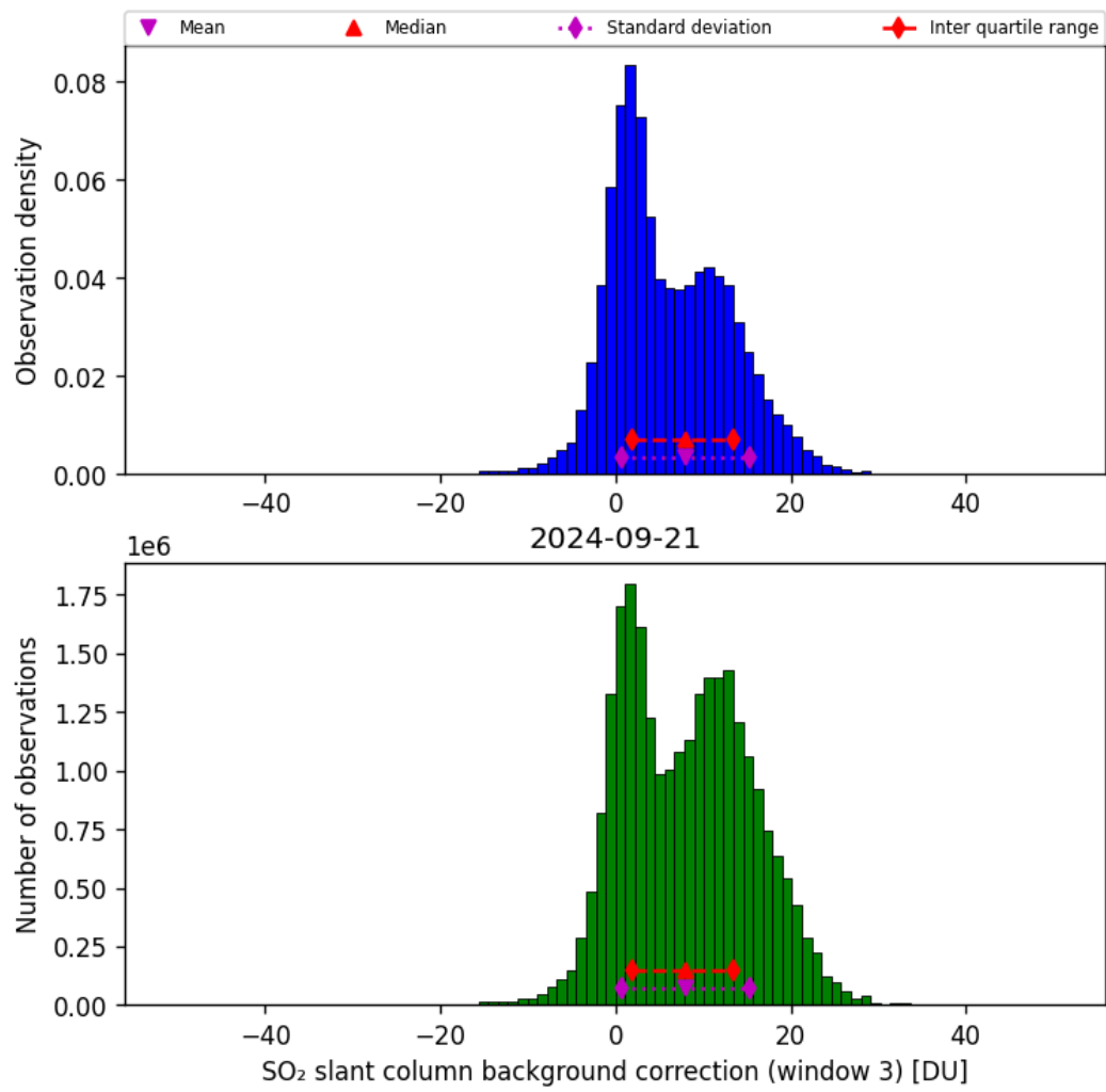
Figure 67: Histogram of “SO 2 slant column background correction (window 3)” for 2024-09-20 to 2024-09-22
