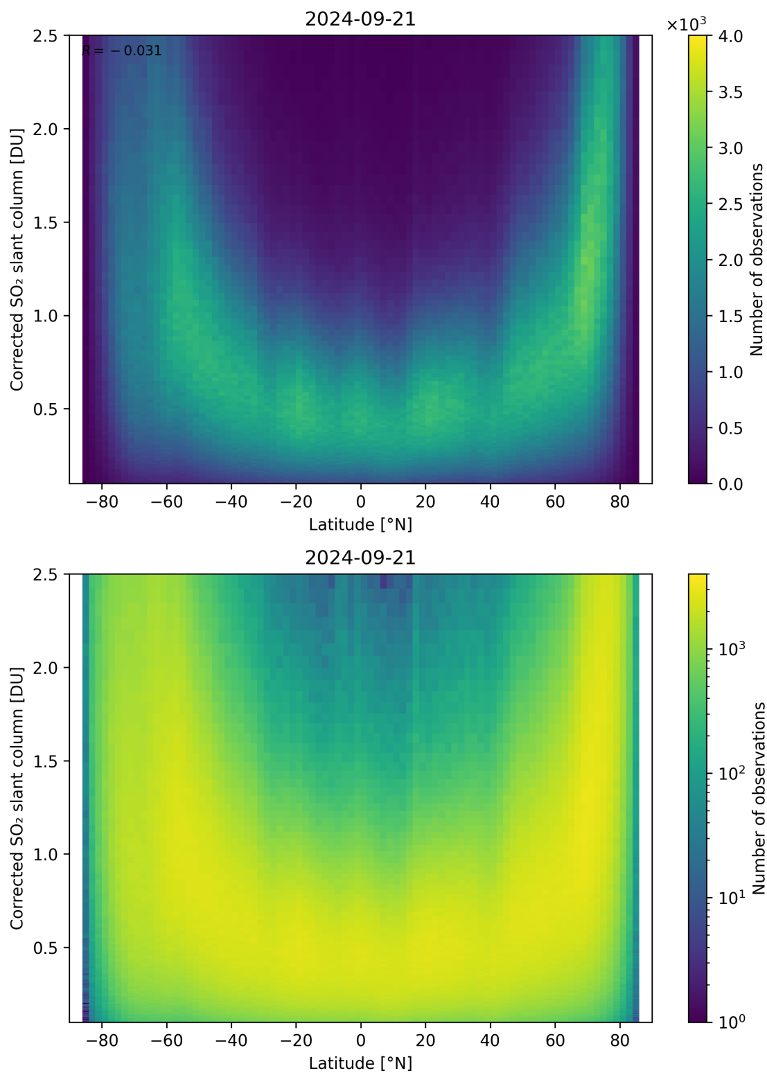
Figure 146: Scatter density plot of “Latitude” against “Corrected SO 2 slant column” for 2024-09-20 to 2024-09-22.
