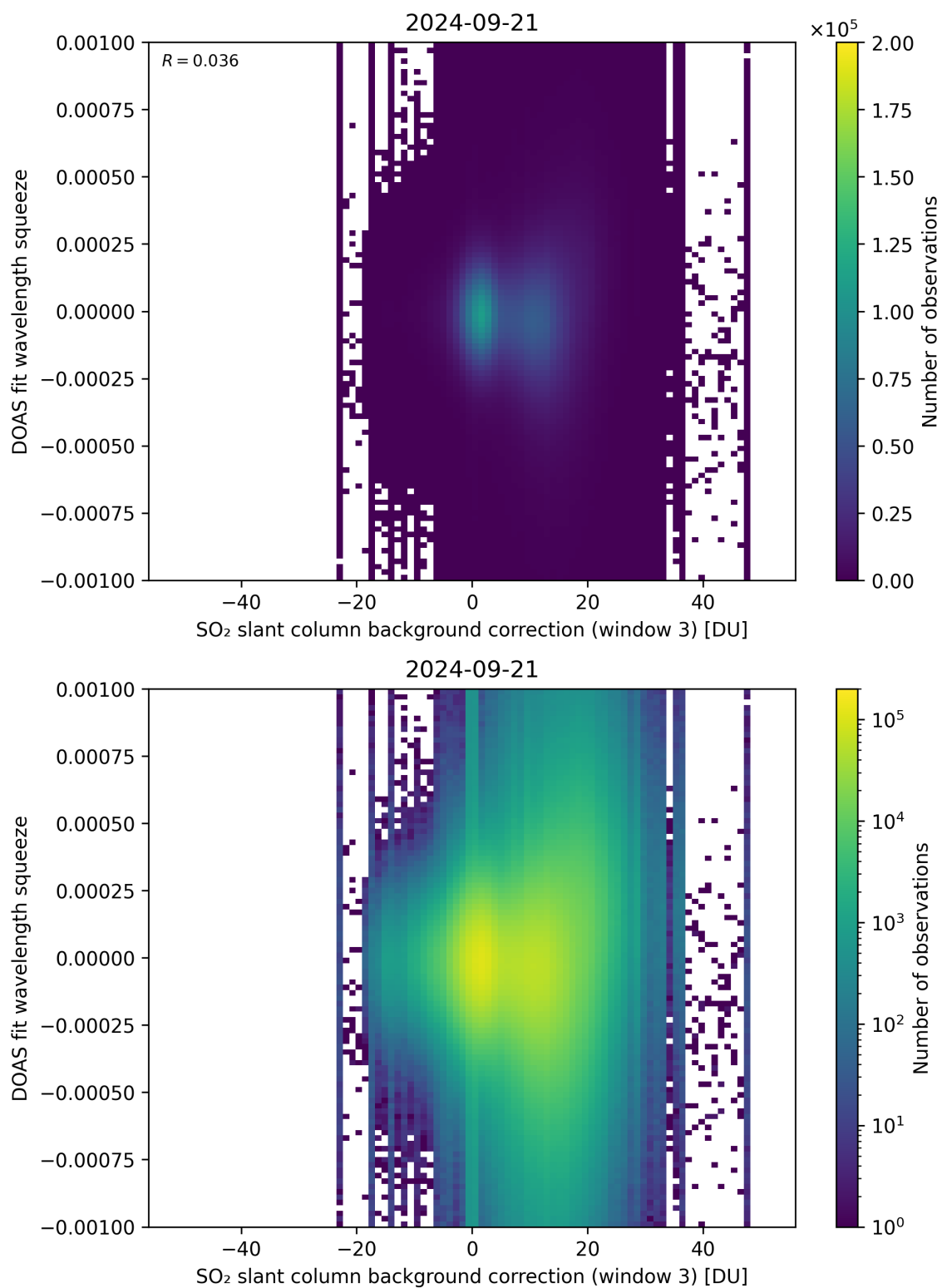
Figure 122: Scatter density plot of “SO 2 slant column background correction (window 3)” against “DOAS fit wavelength squeeze” for 2024-09-20 to 2024-09-22.
