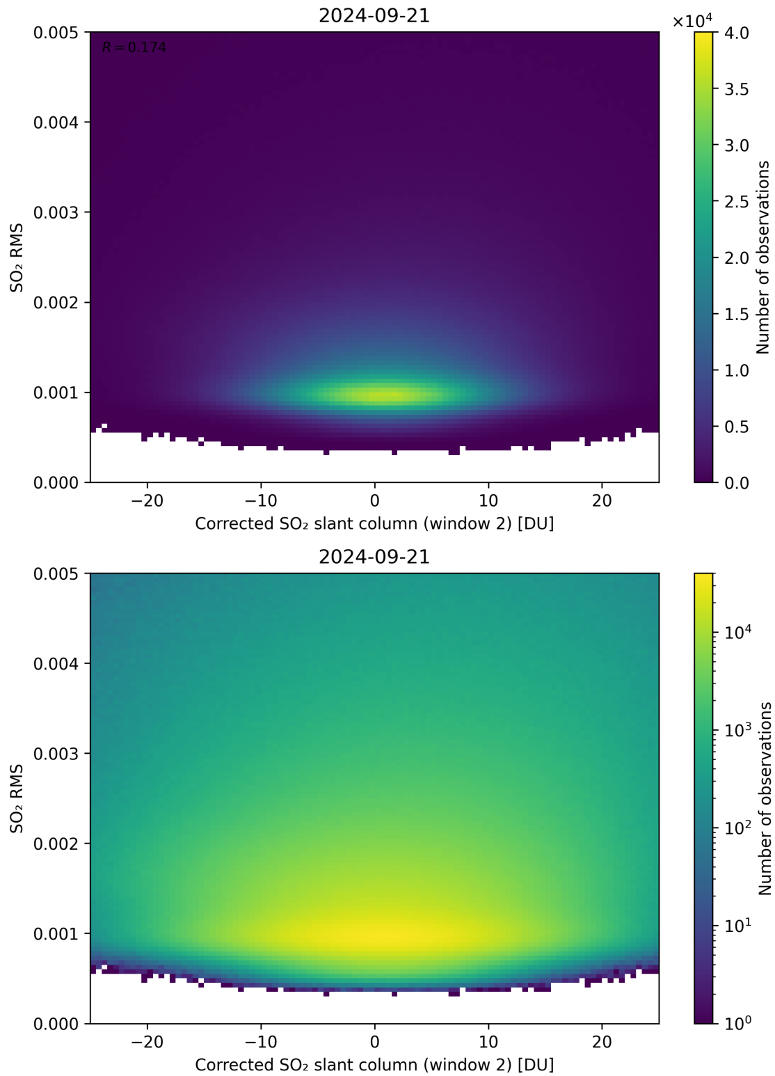
Figure 198: Scatter density plot of “Corrected SO 2 slant column (window 2)” against “SO 2 RMS” for 2024-09-20 to 2024-09-22.
