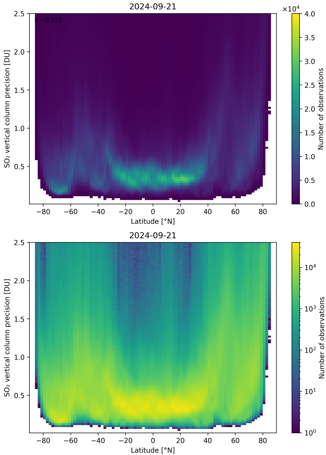
Figure 157: Scatter density plot of “Latitude” against “SO 2 vertical column precision” for 2024-09-20 to 2024-09-22.
