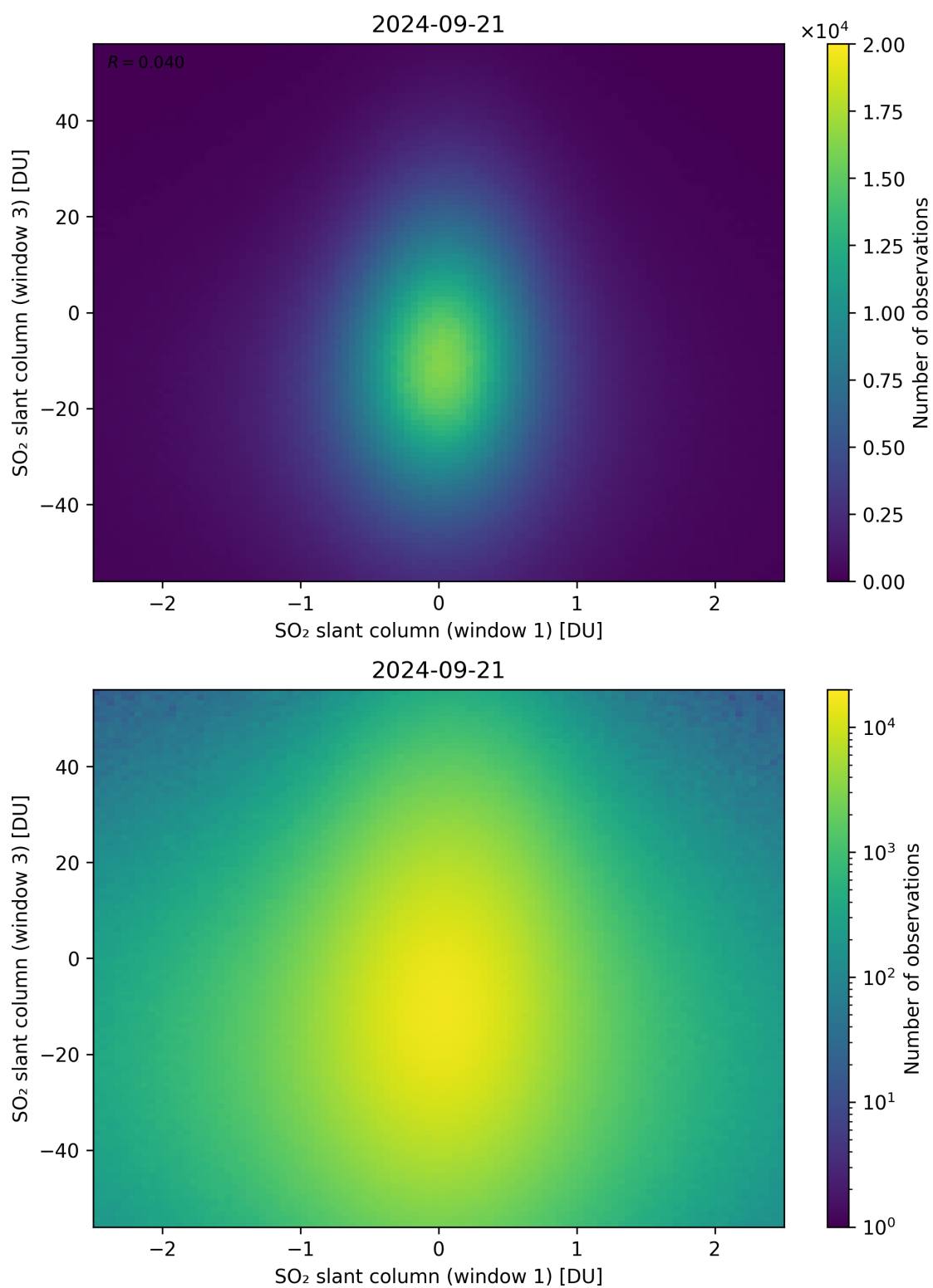
Figure 237: Scatter density plot of “SO 2 slant column (window 1)” against “SO 2 slant column (window 3)” for 2024-09-20 to 2024-09-22.
