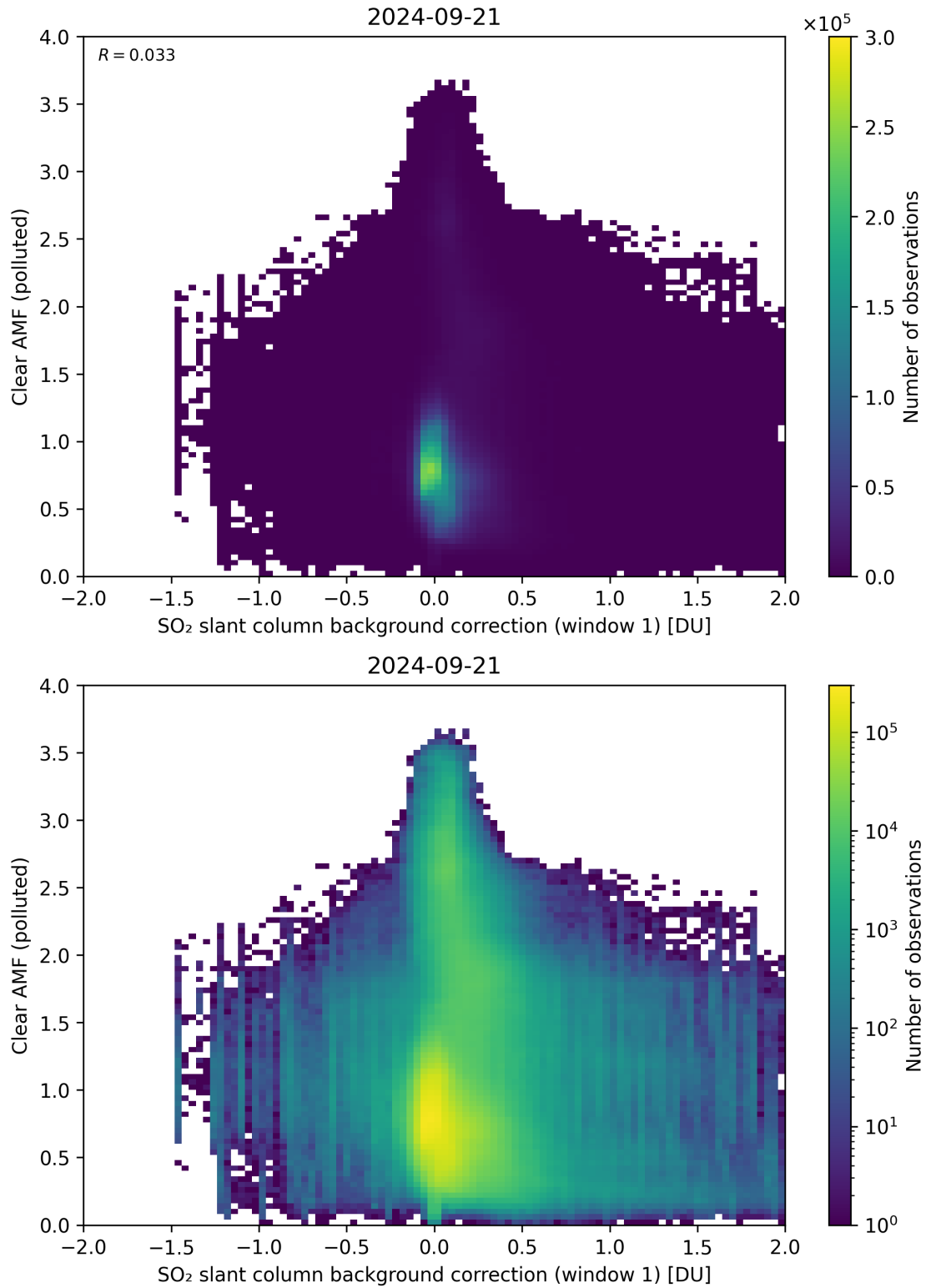
Figure 103: Scatter density plot of “SO 2 slant column background correction (window 1)” against “Clear AMF (polluted)” for 2024-09-20 to 2024-09-22.
