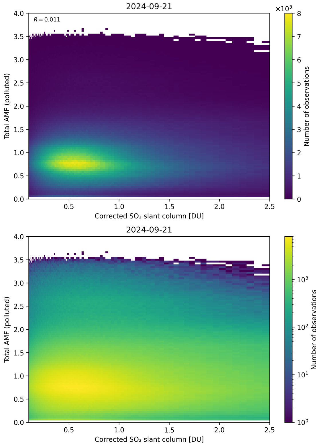
Figure 192: Scatter density plot of “Corrected SO 2 slant column” against “Total AMF (polluted)” for 2024-09-20 to 2024-09-22.
