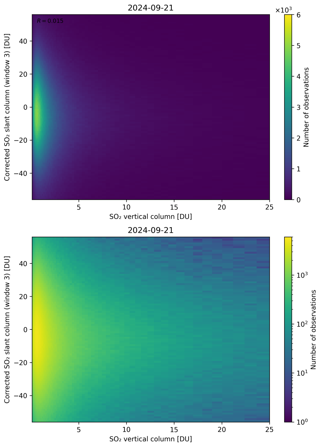
Figure 299: Scatter density plot of “SO 2 vertical column” against “Corrected SO 2 slant column (window 3)” for 2024-09-20 to 2024-09-22.
