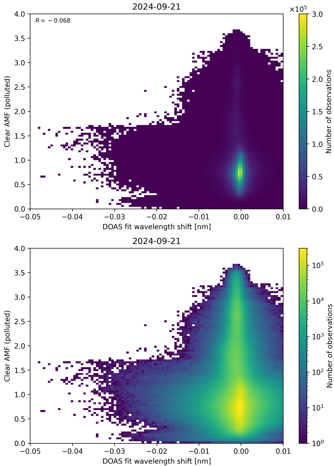
Figure 129: Scatter density plot of “DOAS fit wavelength shift” against “Clear AMF (polluted)” for 2024-09-20 to 2024-09-22.
