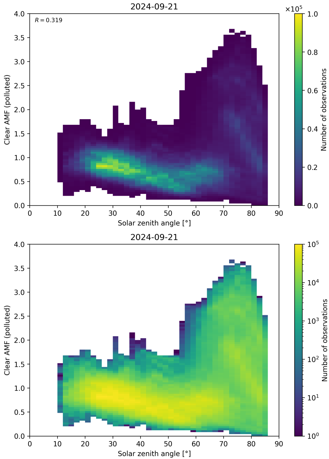
Figure 165: Scatter density plot of “Solar zenith angle” against “Clear AMF (polluted)” for 2024-09-20 to 2024-09-22.
