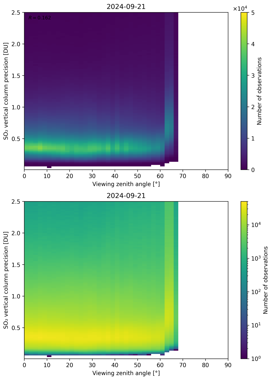
Figure 328: Scatter density plot of “Viewing zenith angle” against “SO 2 vertical column precision” for 2024-09-20 to 2024-09-22.
