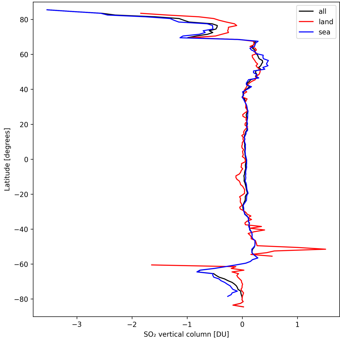
Figure 30: Zonal average of “SO 2 vertical column” for 2024-09-20 to 2024-09-22.
