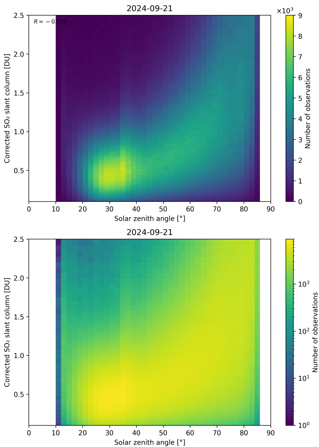
Figure 166: Scatter density plot of “Solar zenith angle” against “Corrected SO 2 slant column” for 2024-09-20 to 2024-09-22.
