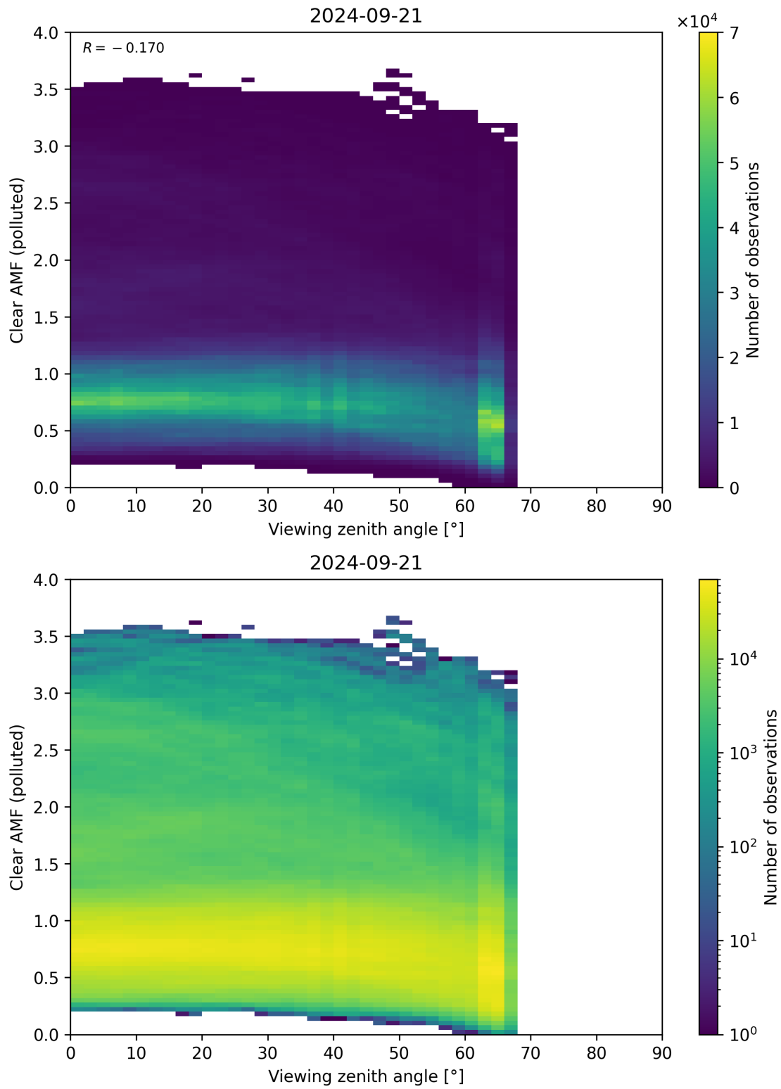
Figure 316: Scatter density plot of “Viewing zenith angle” against “Clear AMF (polluted)” for 2024-09-20 to 2024-09-22.
