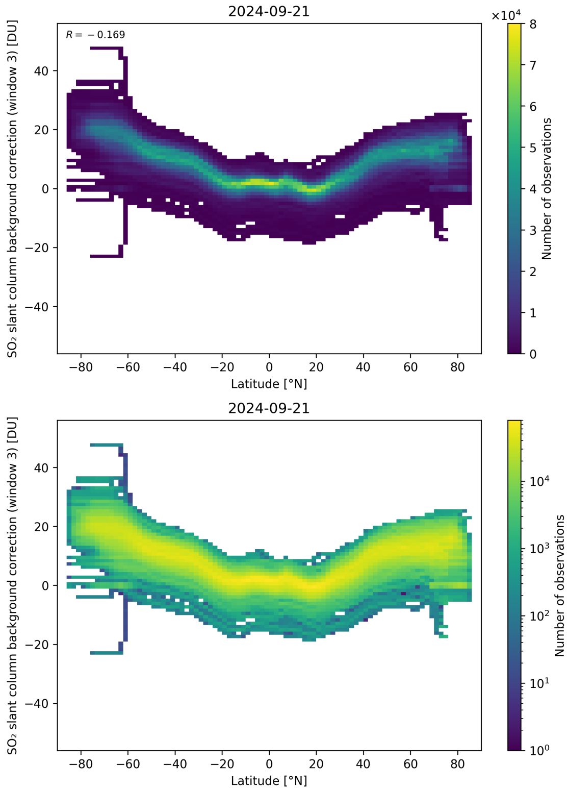
Figure 141: Scatter density plot of “Latitude” against “SO 2 slant column background correction (window 3)” for 2024-09-20 to 2024-09-22.
