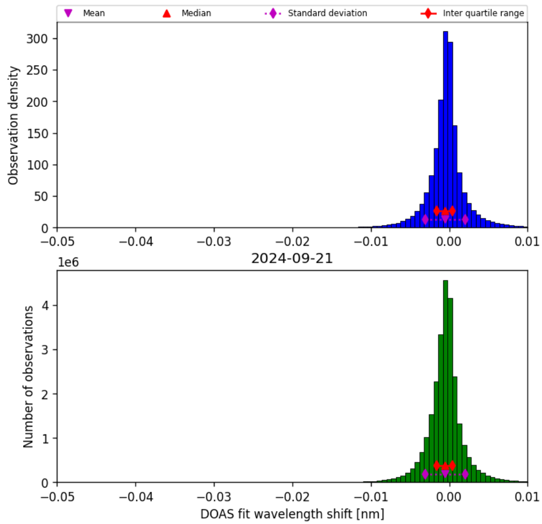
Figure 68: Histogram of “DOAS fit wavelength shift” for 2024-09-20 to 2024-09-22
