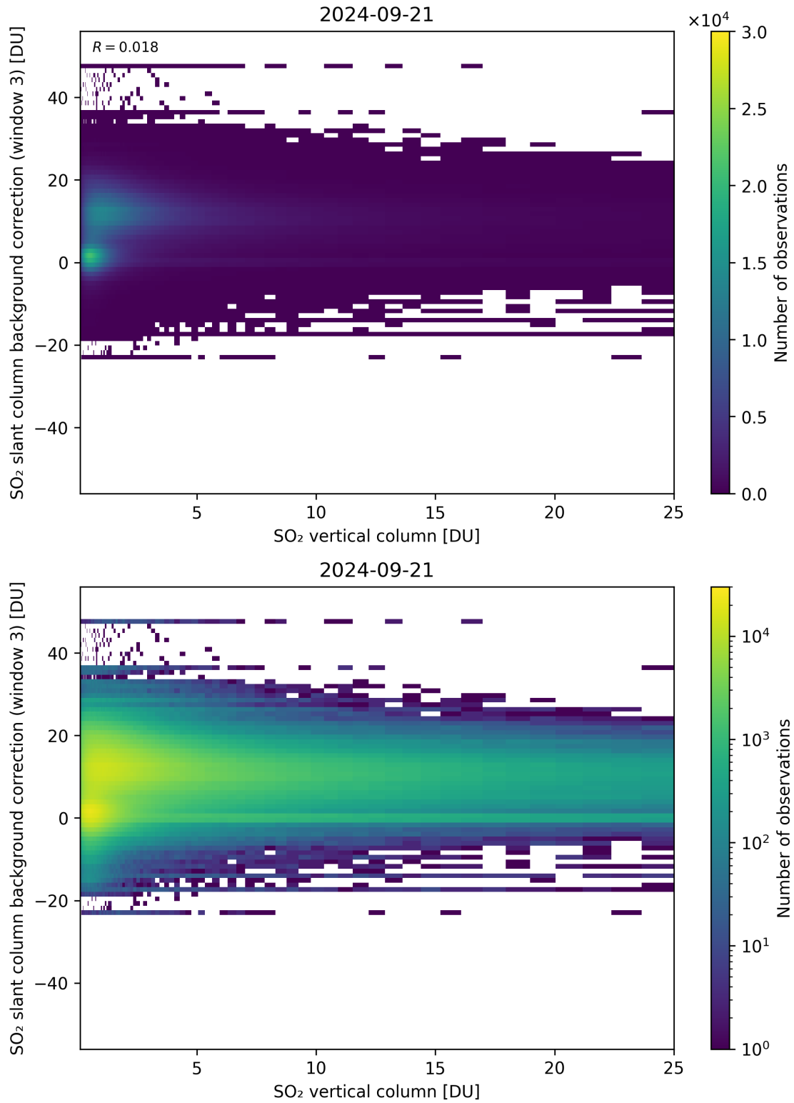
Figure 275: Scatter density plot of “SO 2 vertical column” against “SO 2 slant column background correction (window 3)” for 2024-09-20 to 2024-09-22.
