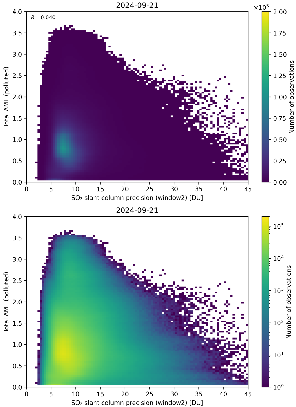
Figure 251: Scatter density plot of “SO 2 slant column precision (window2)” against “Total AMF (polluted)” for 2024-09-20 to 2024-09-22.
