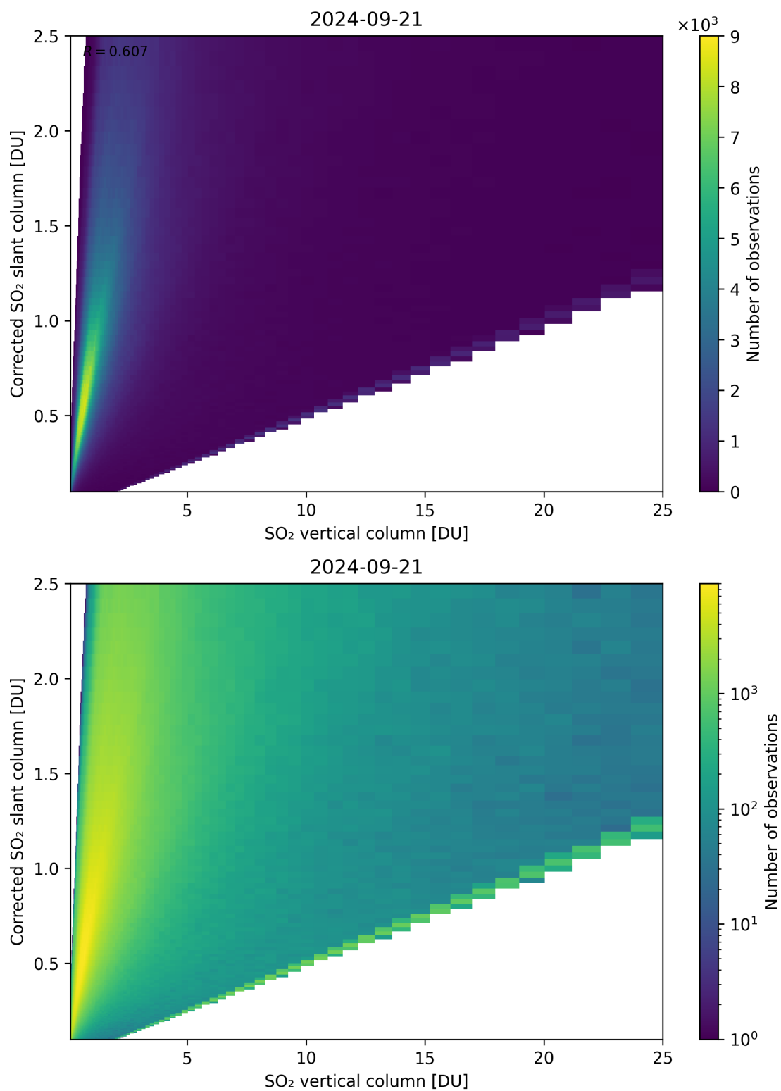
Figure 297: Scatter density plot of “SO 2 vertical column” against “Corrected SO 2 slant column” for 2024-09-20 to 2024-09-22.
