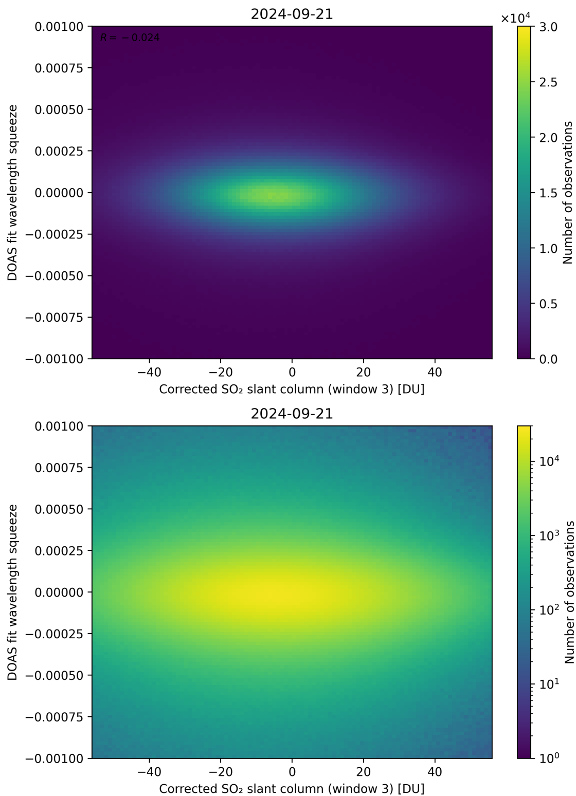
Figure 207: Scatter density plot of “Corrected SO 2 slant column (window 3)” against “DOAS fit wavelength squeeze” for 2024-09-20 to 2024-09-22.
