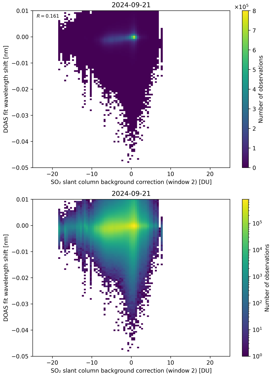
Figure 112: Scatter density plot of “SO 2 slant column background correction (window 2)” against “DOAS fit wavelength shift” for 2024-09-20 to 2024-09-22.
