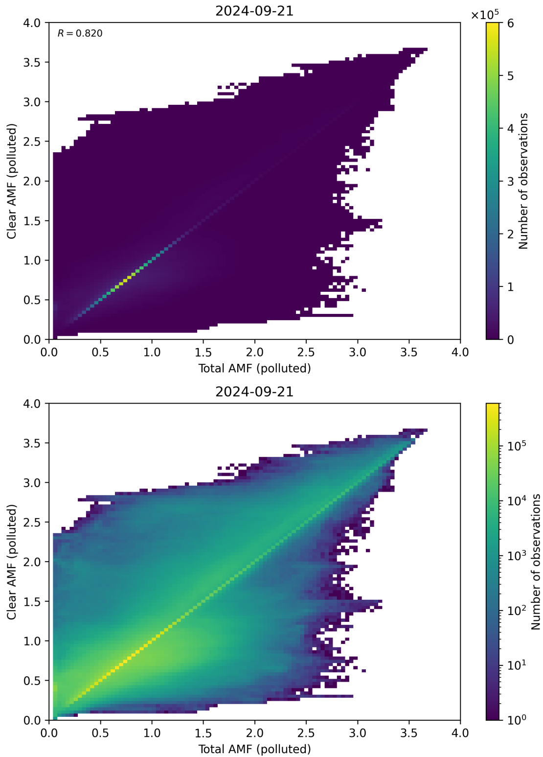
Figure 271: Scatter density plot of “Total AMF (polluted)” against “Clear AMF (polluted)” for 2024-09-20 to 2024-09-22.
