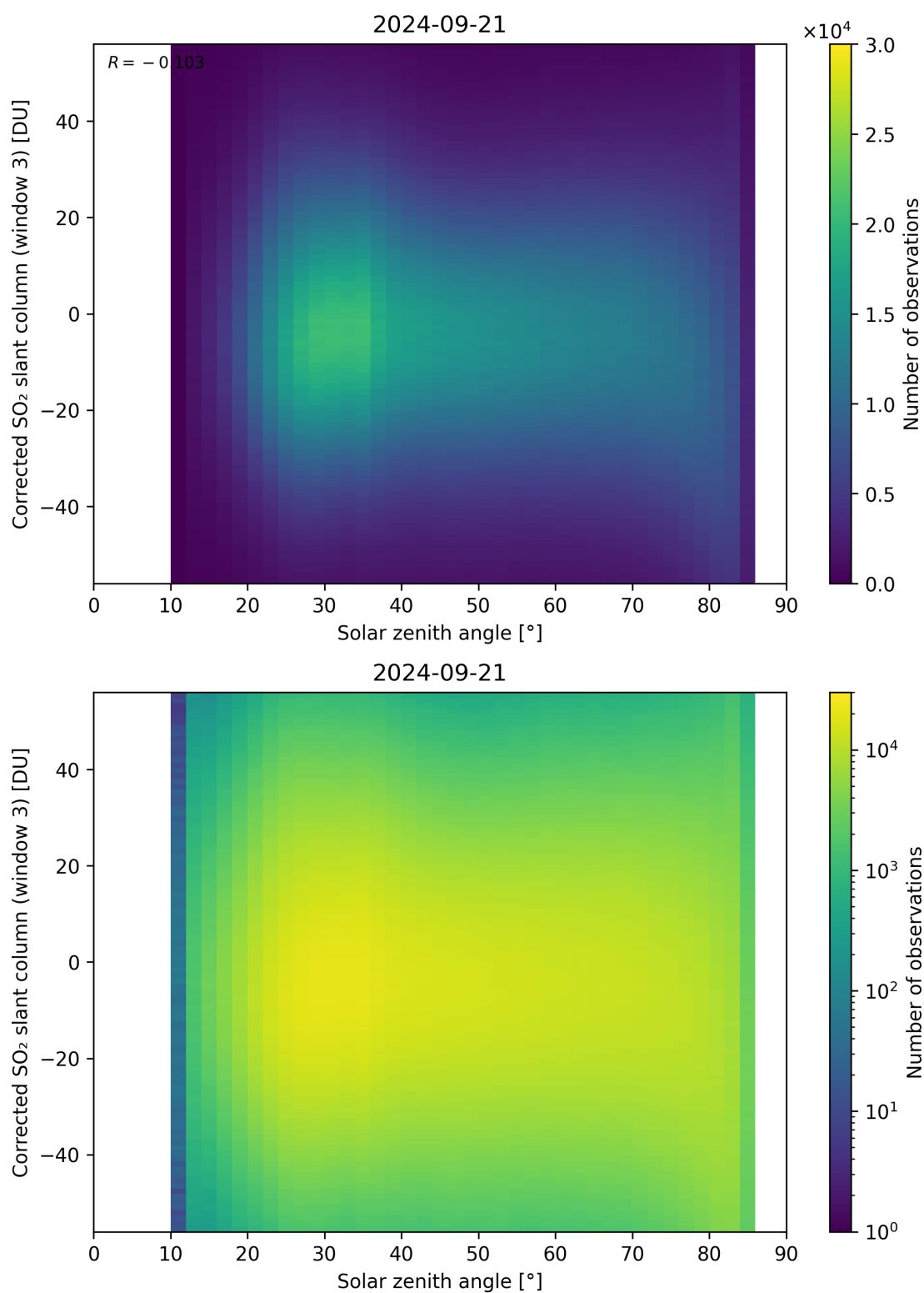
Figure 168: Scatter density plot of “Solar zenith angle” against “Corrected SO 2 slant column (window 3)” for 2024-09-20 to 2024-09-22.
