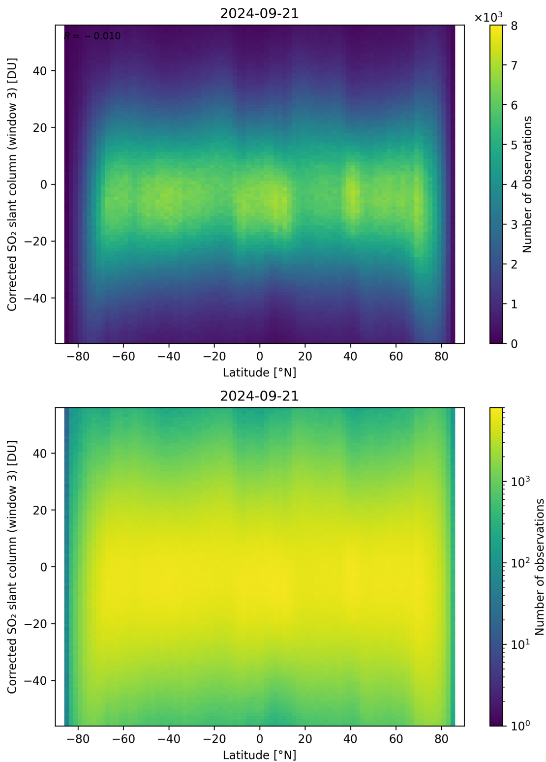
Figure 148: Scatter density plot of “Latitude” against “Corrected SO 2 slant column (window 3)” for 2024-09-20 to 2024-09-22.
