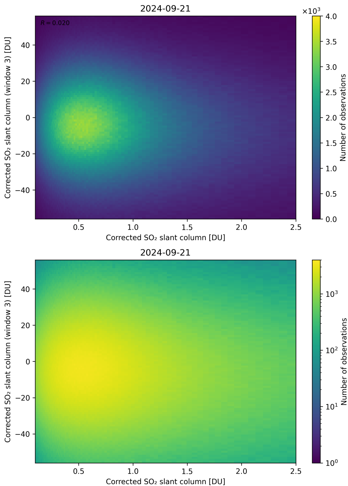
Figure 186: Scatter density plot of “Corrected SO 2 slant column” against “Corrected SO 2 slant column (window 3)” for 2024-09-20 to 2024-09-22.
