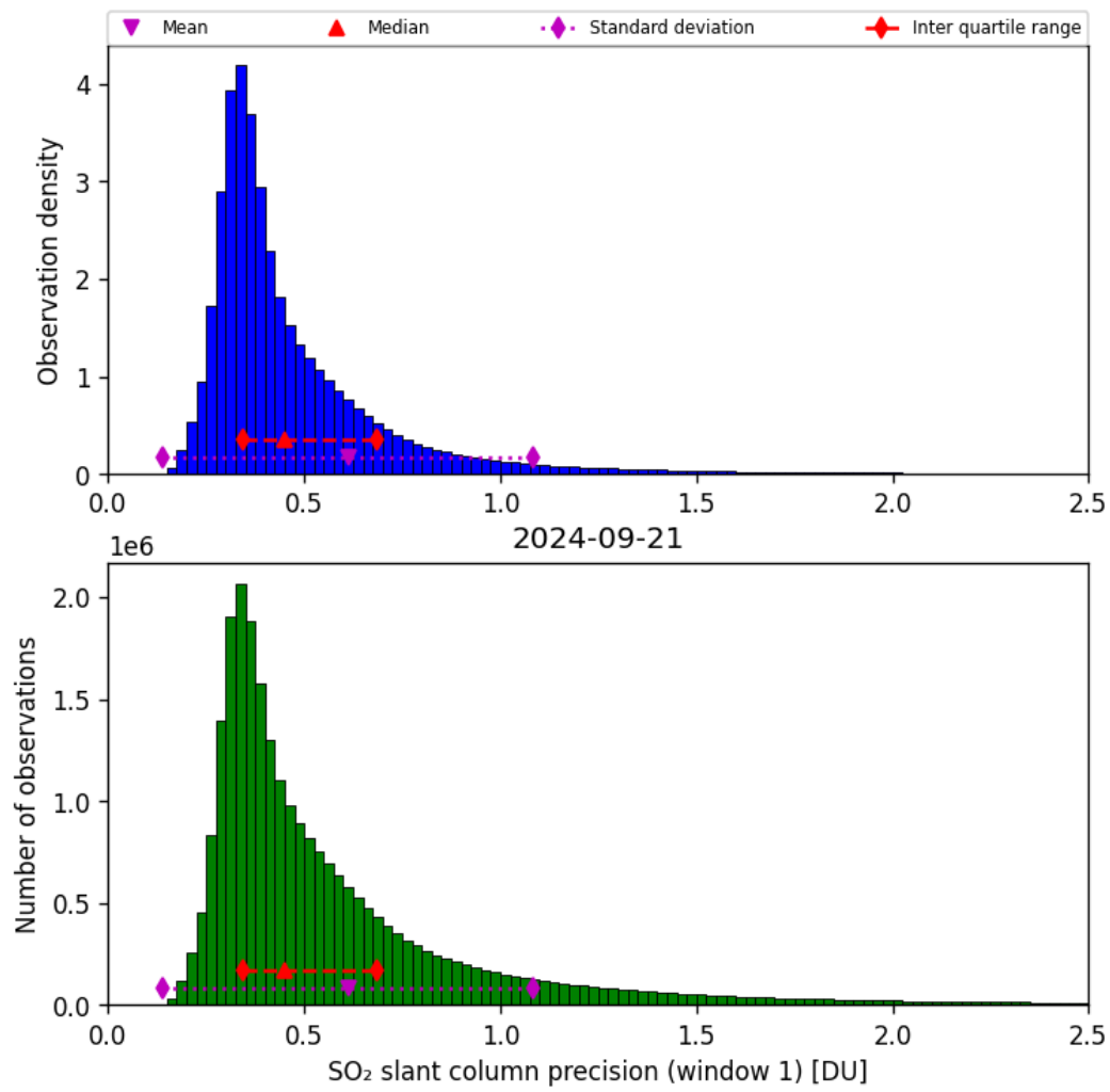
Figure 57: Histogram of “SO 2 slant column precision (window 1)” for 2024-09-20 to 2024-09-22
