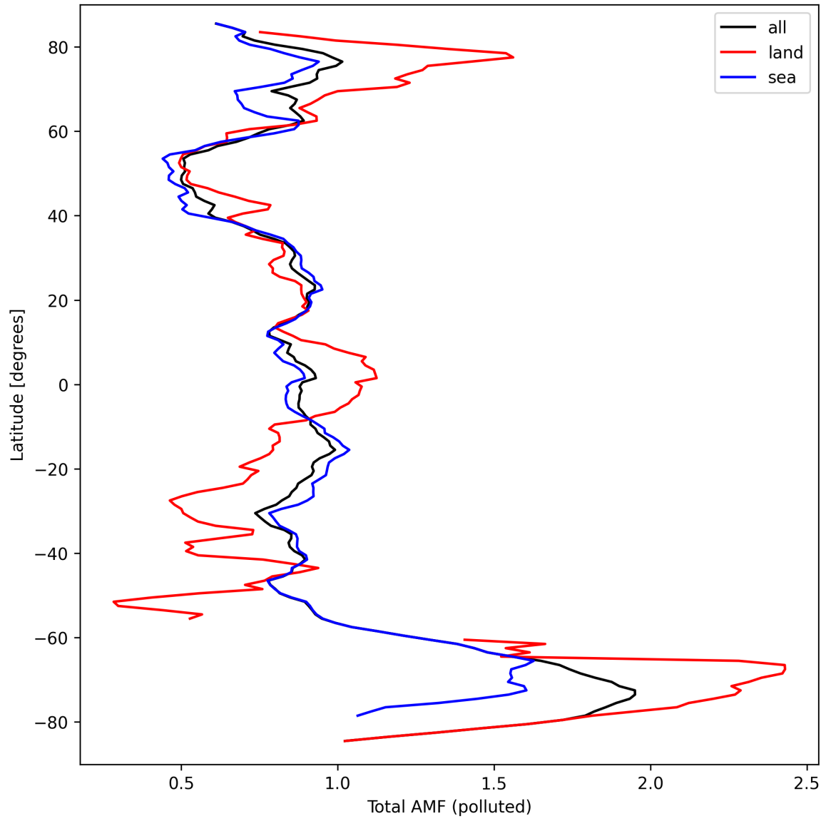
Figure 48: Zonal average of “Total AMF (polluted)” for 2024-09-20 to 2024-09-22.
