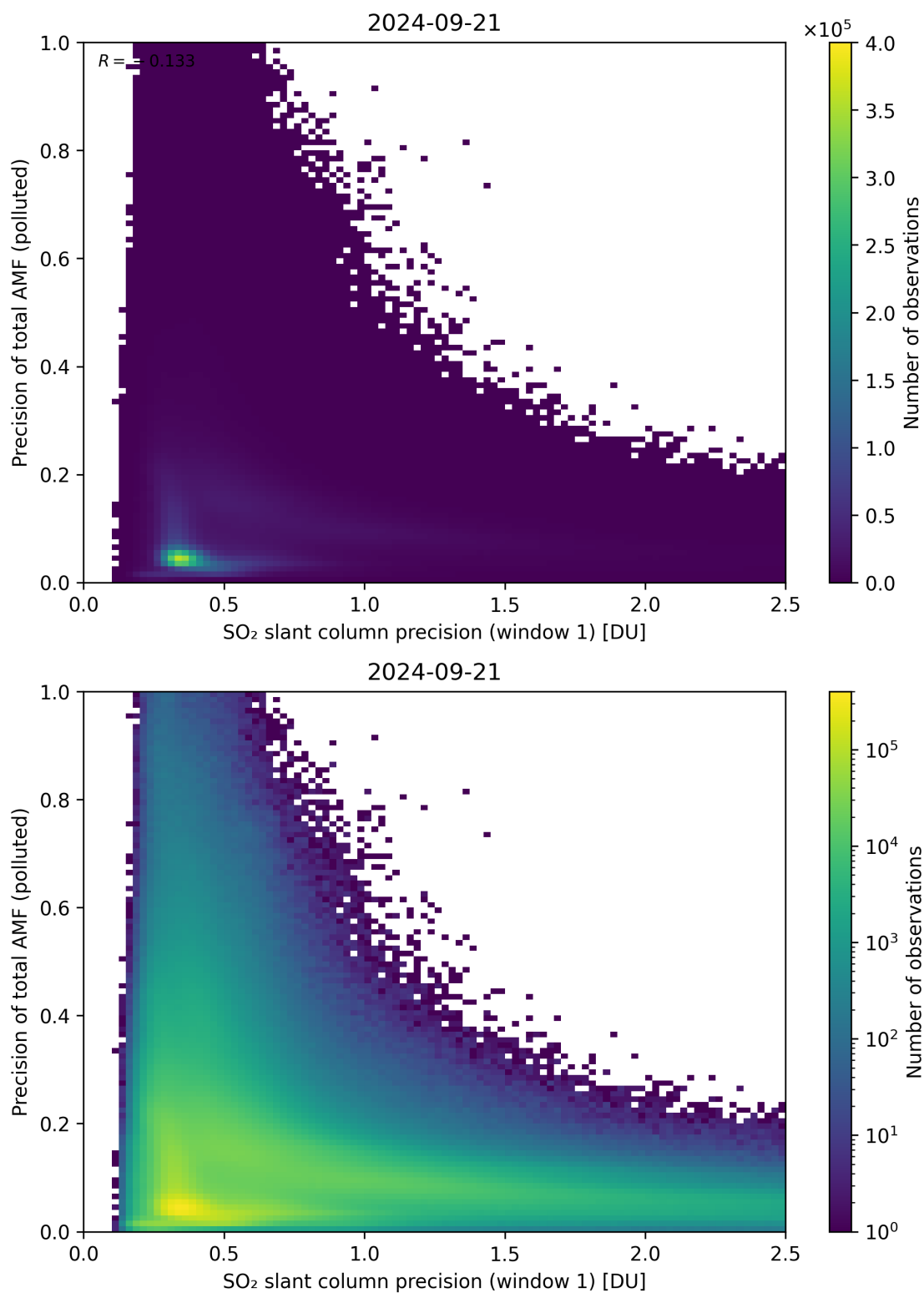
Figure 231: Scatter density plot of “SO 2 slant column precision (window 1)” against “Precision of total AMF (polluted)” for 2024-09-20 to 2024-09-22.
