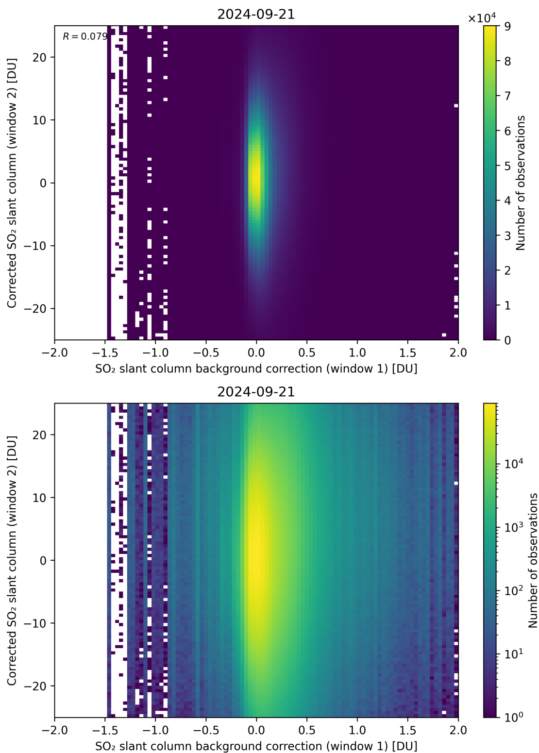
Figure 104: Scatter density plot of “SO 2 slant column background correction (window 1)” against “Corrected SO 2 slant column (window 2)” for 2024-09-20 to 2024-09-22.
