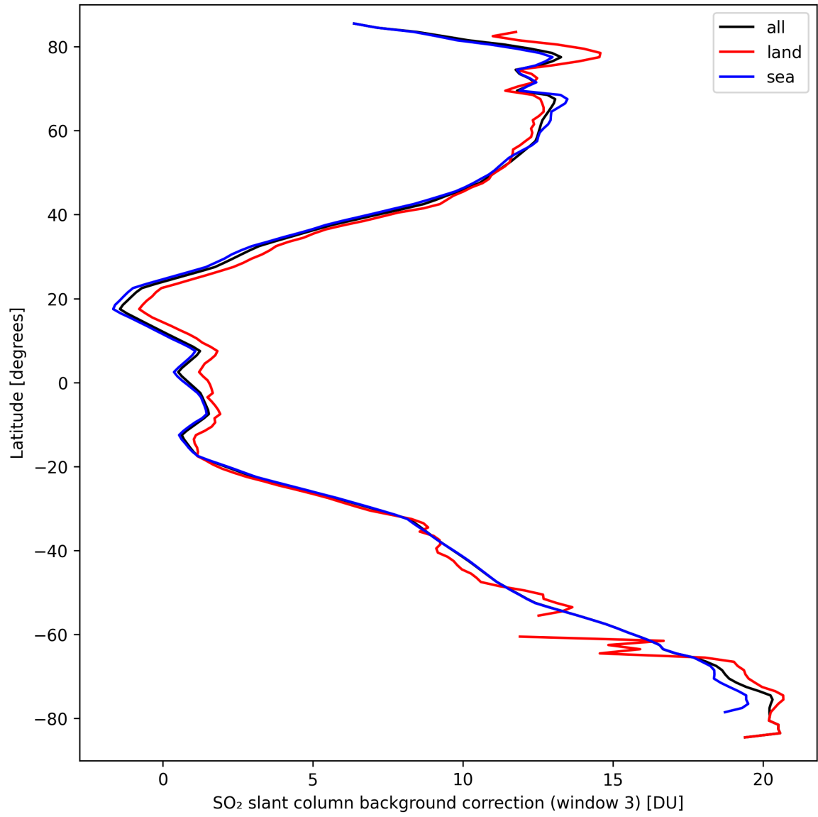
Figure 44: Zonal average of “SO 2 slant column background correction (window 3)” for 2024-09-20 to 2024-09-22.
