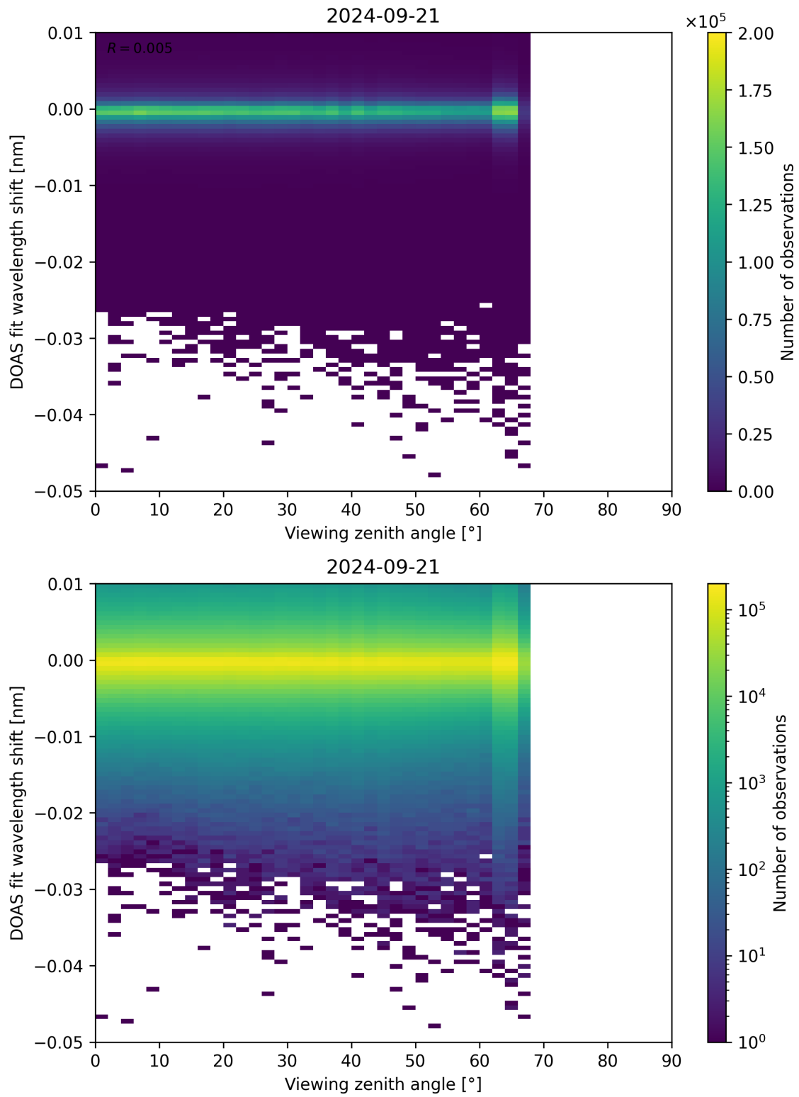
Figure 311: Scatter density plot of “Viewing zenith angle” against “DOAS fit wavelength shift” for 2024-09-20 to 2024-09-22.
