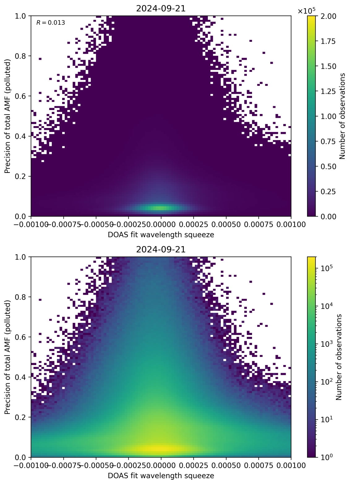
Figure 135: Scatter density plot of “DOAS fit wavelength squeeze” against “Precision of total AMF (polluted)” for 2024-09-20 to 2024-09-22.
