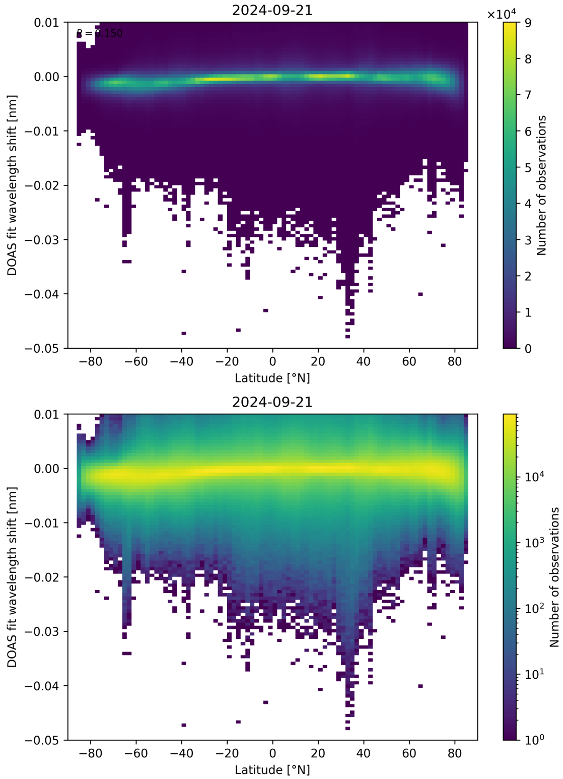
Figure 142: Scatter density plot of “Latitude” against “DOAS fit wavelength shift” for 2024-09-20 to 2024-09-22.
