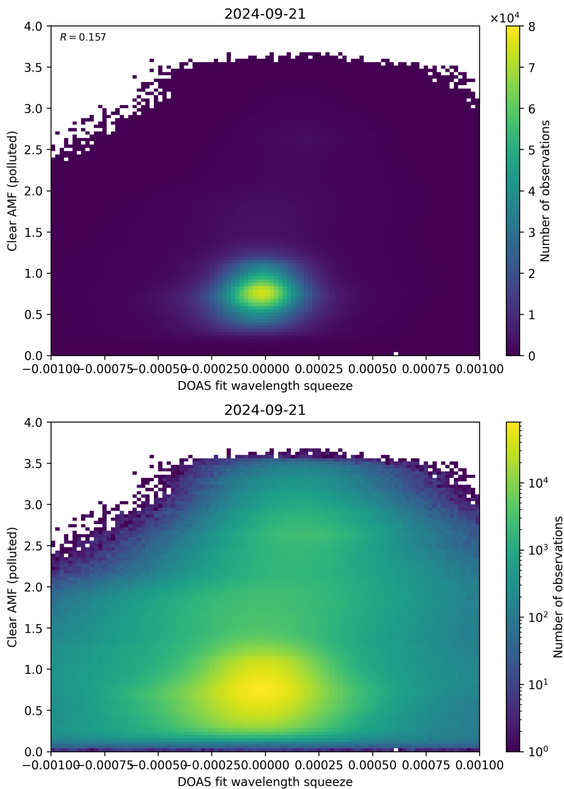
Figure 133: Scatter density plot of “DOAS fit wavelength squeeze” against “Clear AMF (polluted)” for 2024-09-20 to 2024-09-22.
