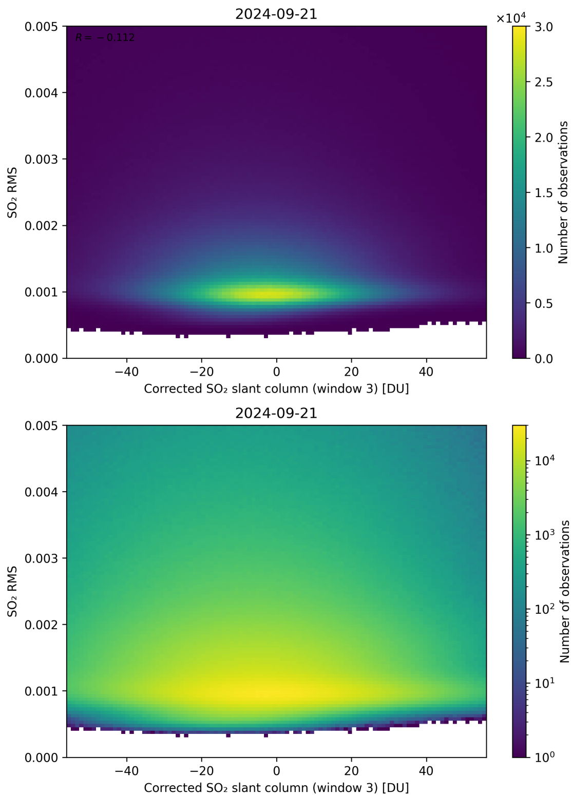
Figure 208: Scatter density plot of “Corrected SO 2 slant column (window 3)” against “SO 2 RMS” for 2024-09-20 to 2024-09-22.
