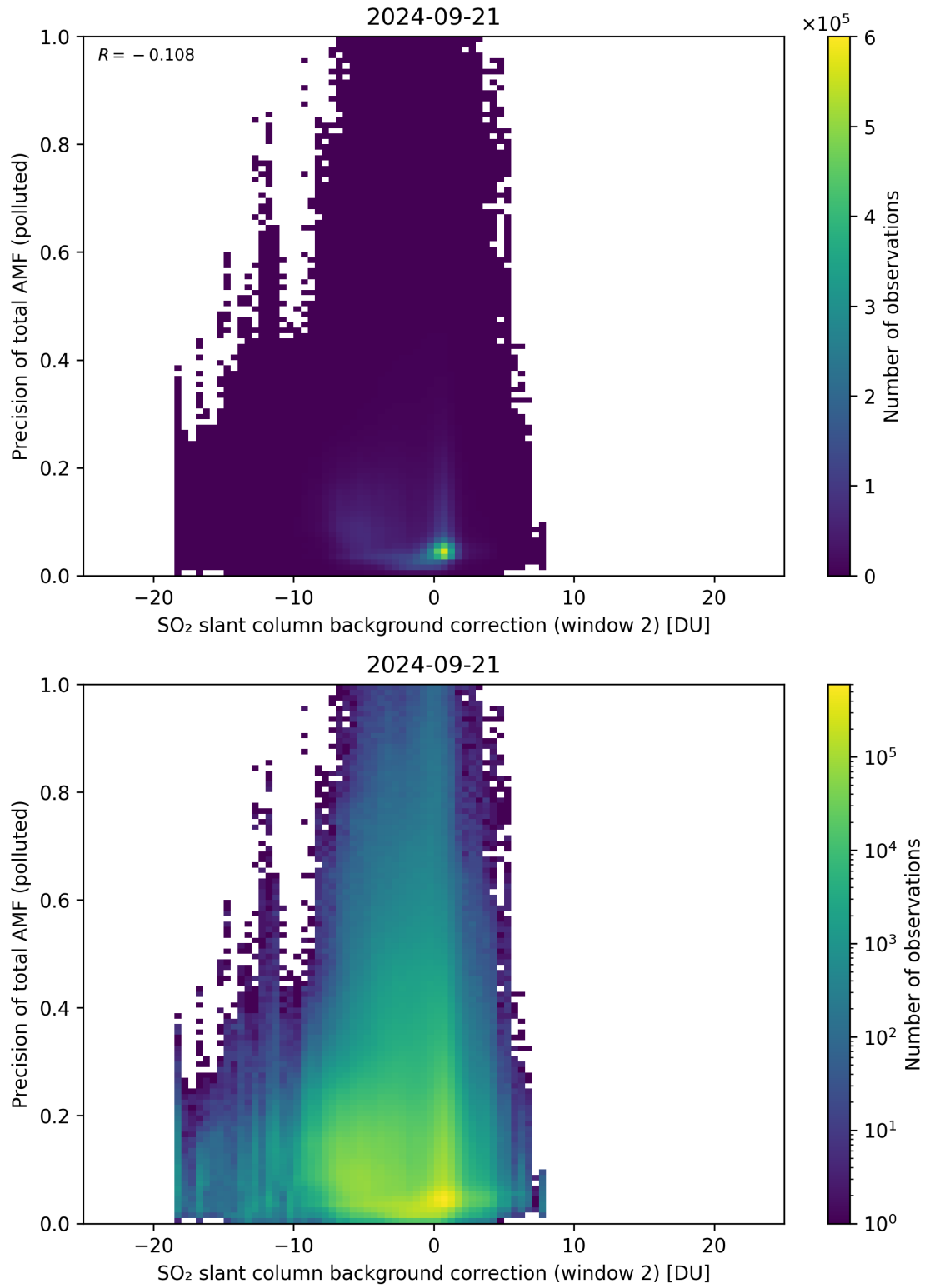
Figure 120: Scatter density plot of “SO 2 slant column background correction (window 2)” against “Precision of total AMF (polluted)” for 2024-09-20 to 2024-09-22.
