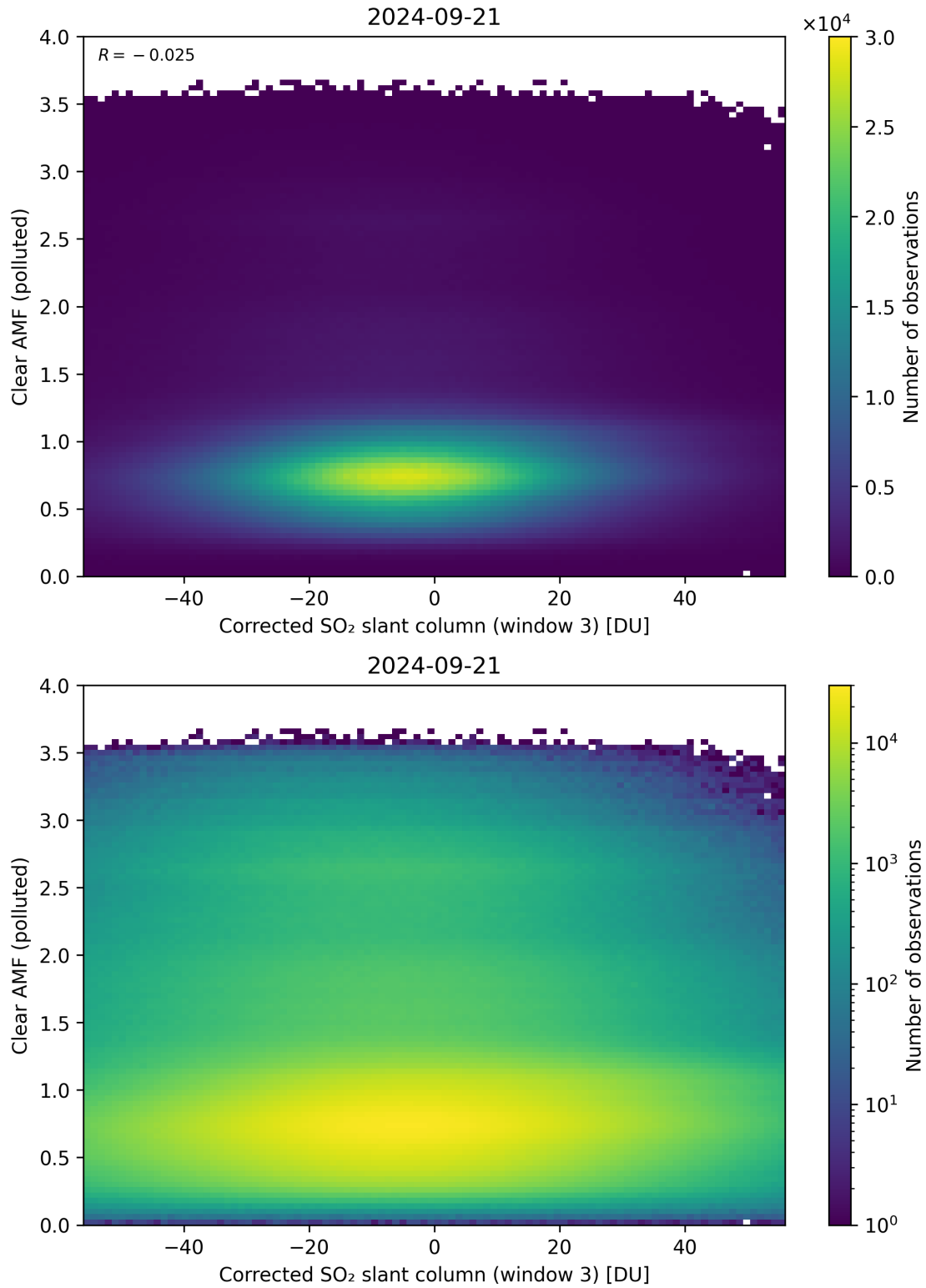
Figure 209: Scatter density plot of “Corrected SO 2 slant column (window 3)” against “Clear AMF (polluted)” for 2024-09-20 to 2024-09-22.
