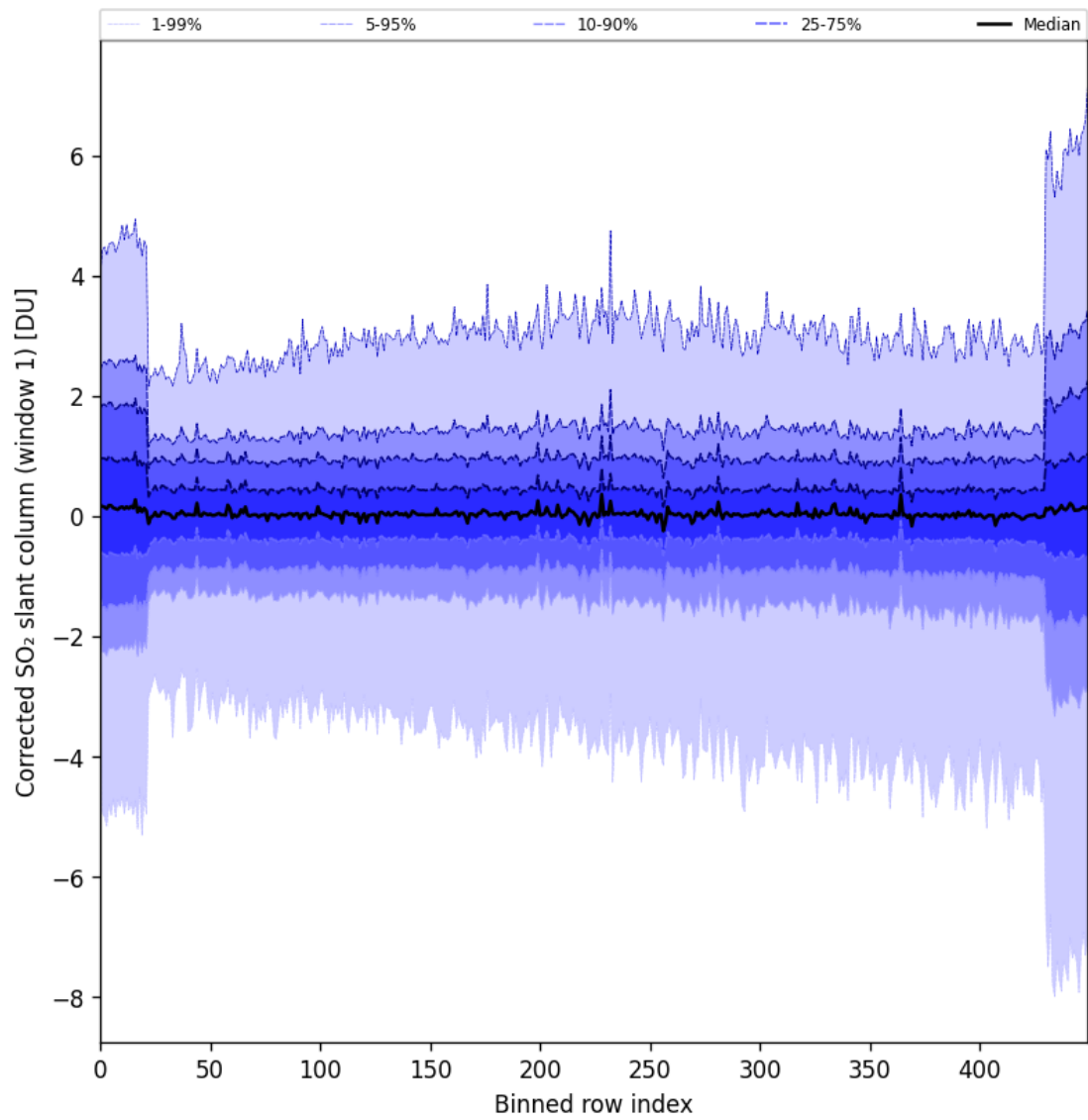
Figure 81: Along track statistics of “Corrected SO 2 slant column (window 1)” for 2024-09-20 to 2024-09-22
