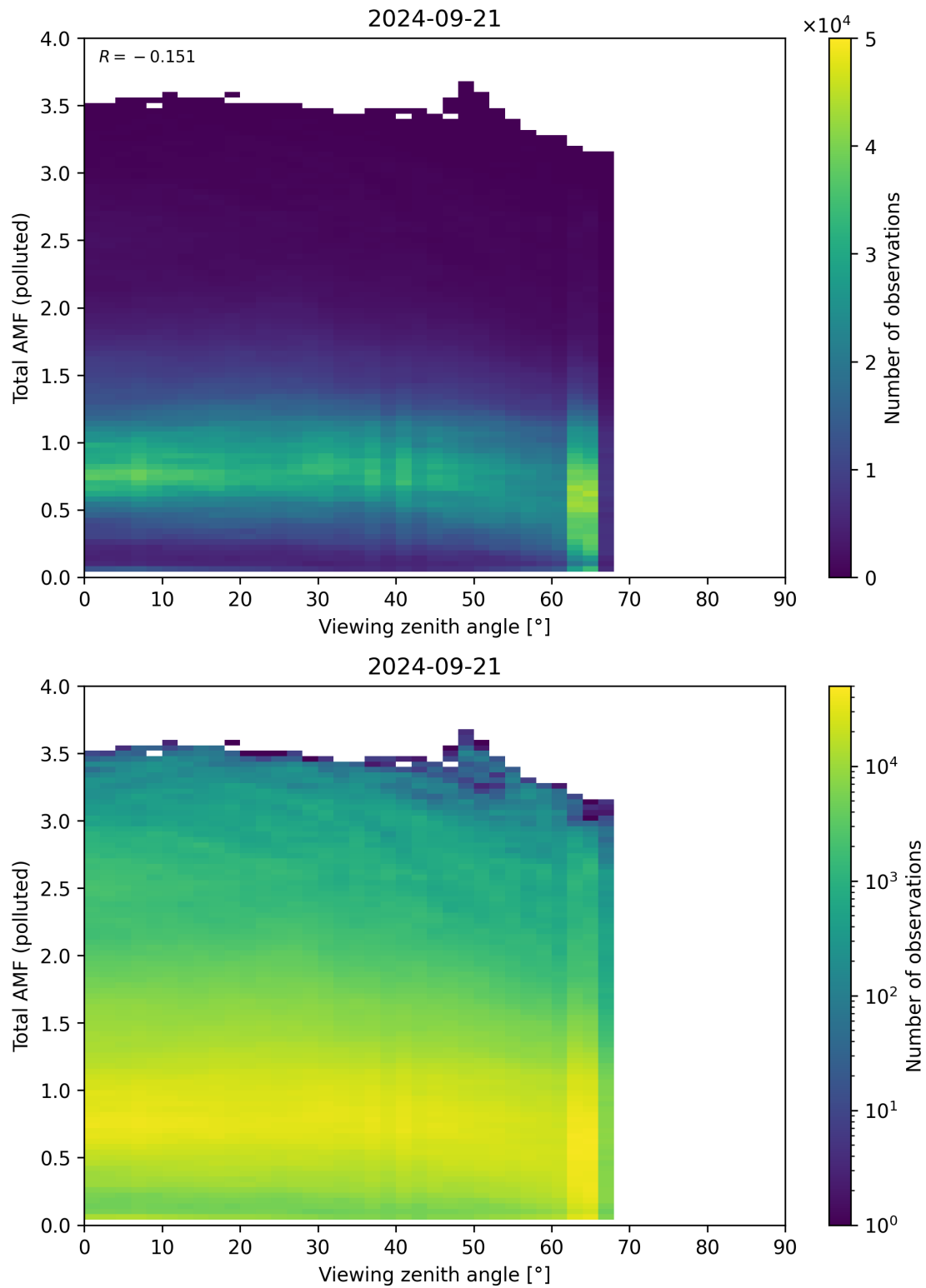
Figure 325: Scatter density plot of “Viewing zenith angle” against “Total AMF (polluted)” for 2024-09-20 to 2024-09-22.
