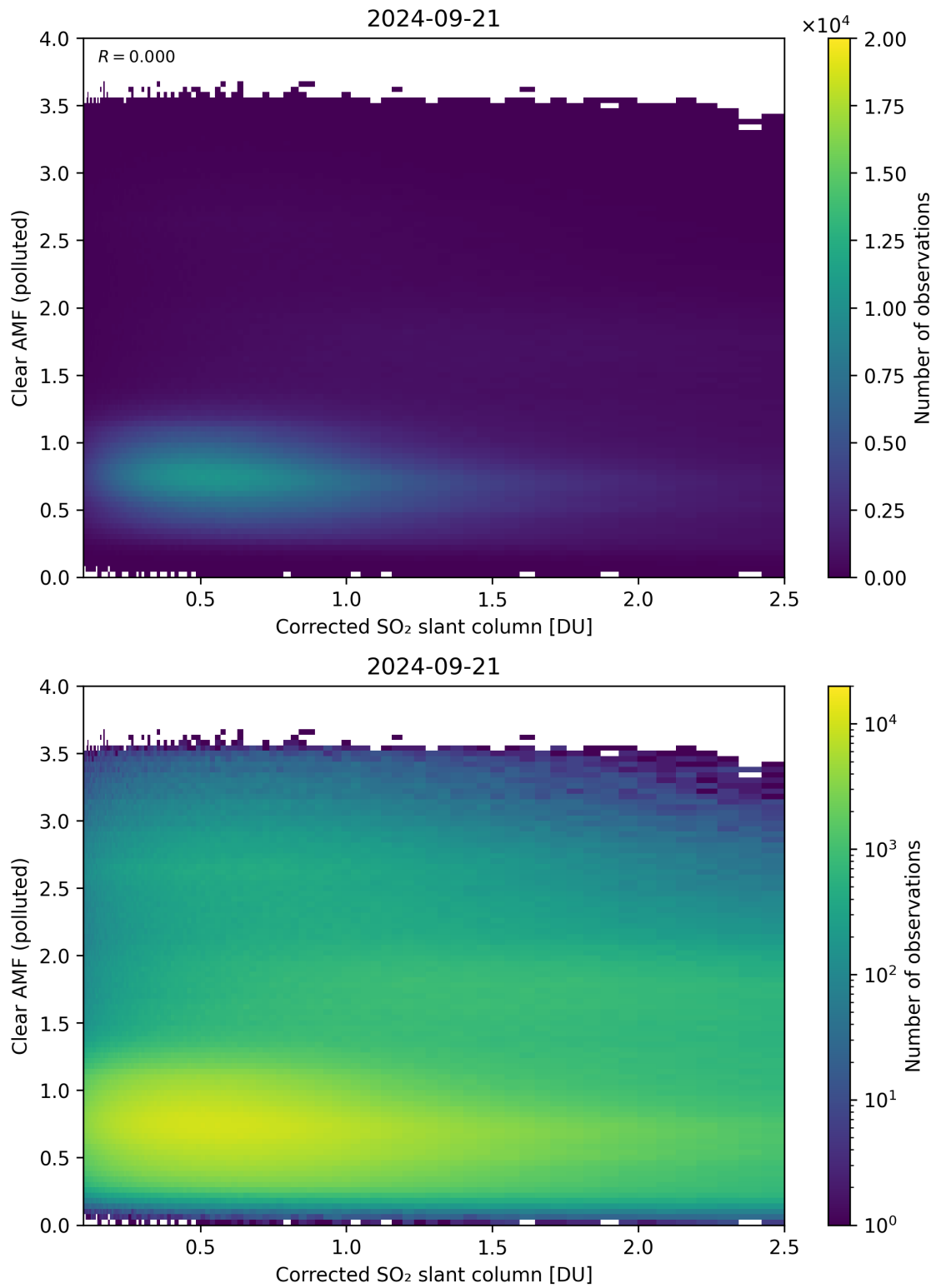
Figure 184: Scatter density plot of “Corrected SO 2 slant column” against “Clear AMF (polluted)” for 2024-09-20 to 2024-09-22.
