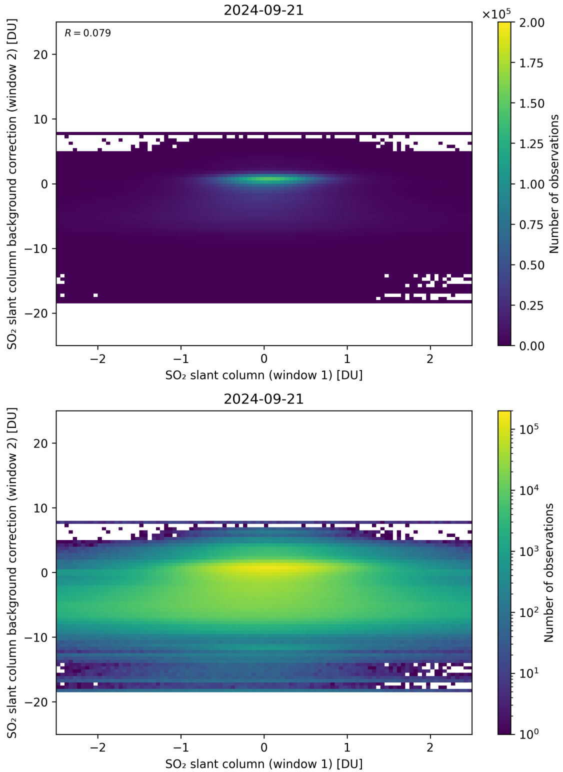
Figure 213: Scatter density plot of “SO 2 slant column (window 1)” against “SO 2 slant column background correction (window 2)” for 2024-09-20 to 2024-09-22.
