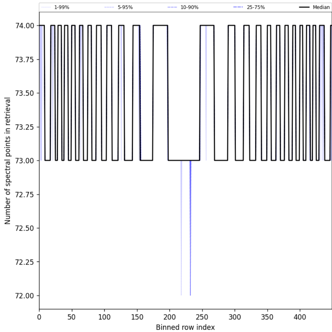
Figure 97: Along track statistics of “Number of spectral points in retrieval” for 2024-09-20 to 2024-09-22
