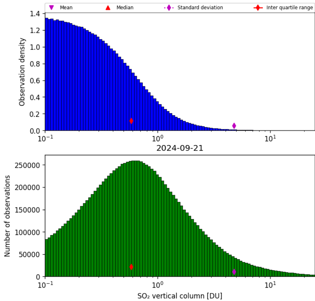
Figure 53: Histogram of “SO 2 vertical column” for 2024-09-20 to 2024-09-22
