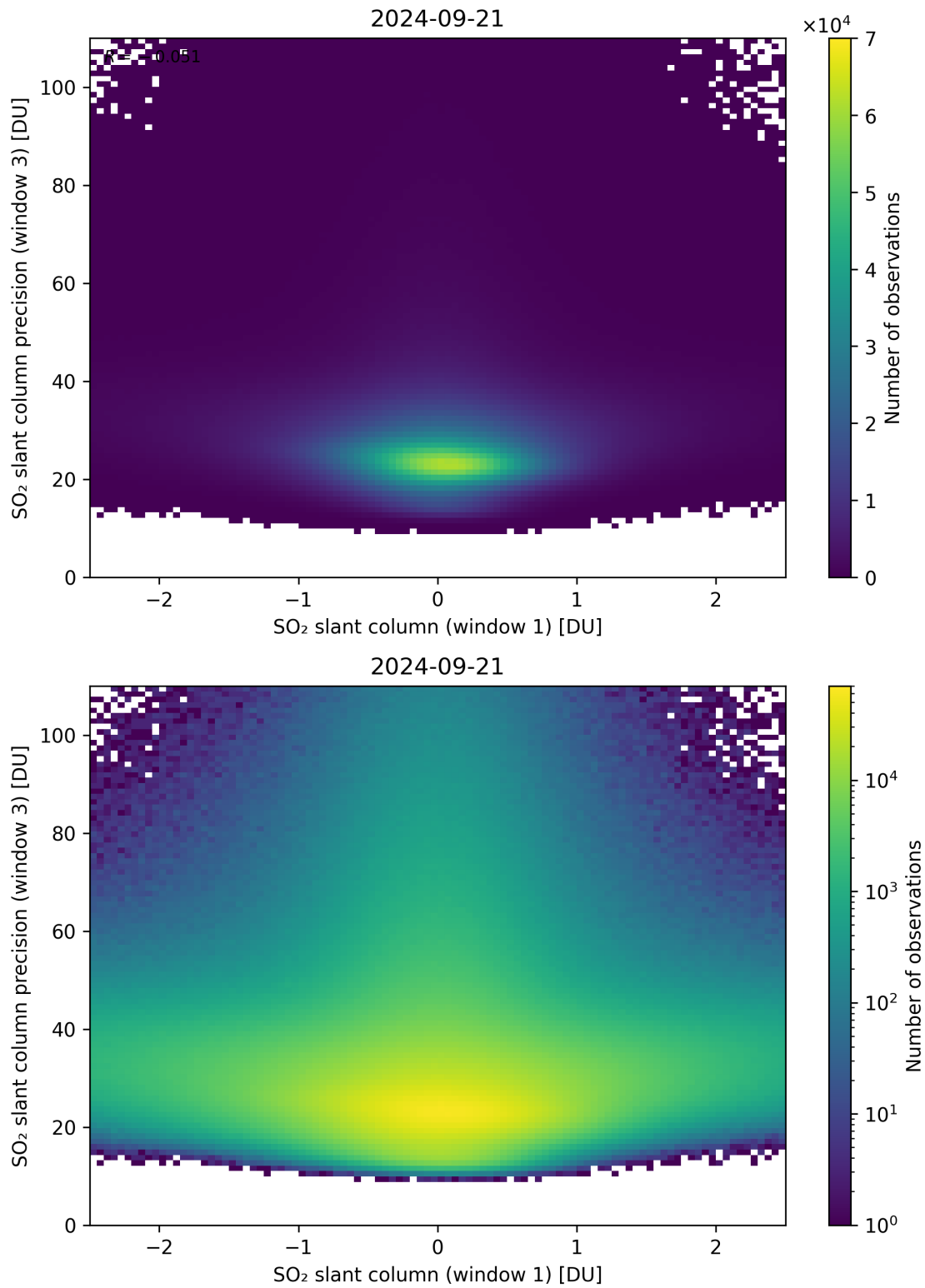
Figure 238: Scatter density plot of “SO 2 slant column (window 1)” against “SO 2 slant column precision (window 3)” for 2024-09-20 to 2024-09-22.
