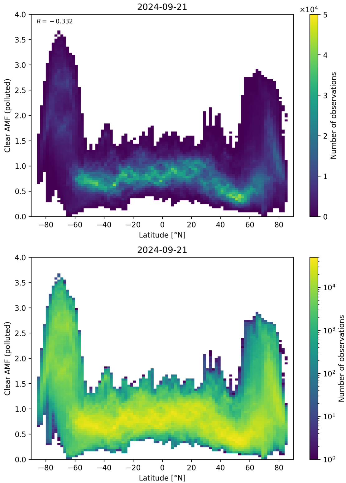
Figure 145: Scatter density plot of “Latitude” against “Clear AMF (polluted)” for 2024-09-20 to 2024-09-22.
