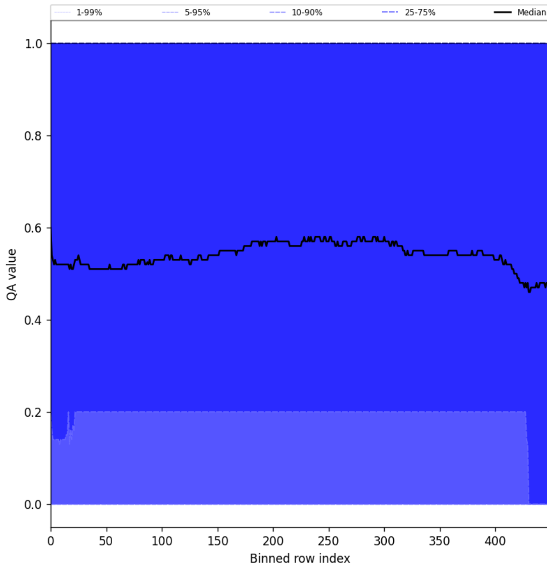
Figure 75: Along track statistics of “QA value” for 2024-09-20 to 2024-09-22
