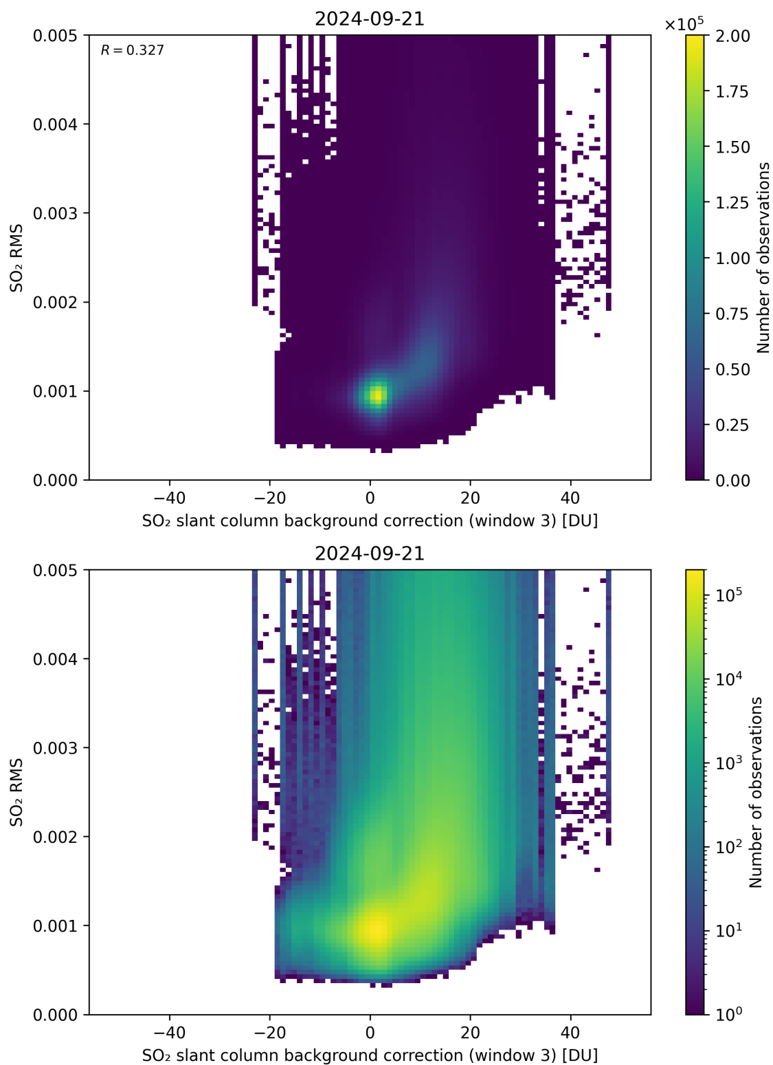
Figure 123: Scatter density plot of “SO 2 slant column background correction (window 3)” against “SO 2 RMS” for 2024-09-20 to 2024-09-22.
