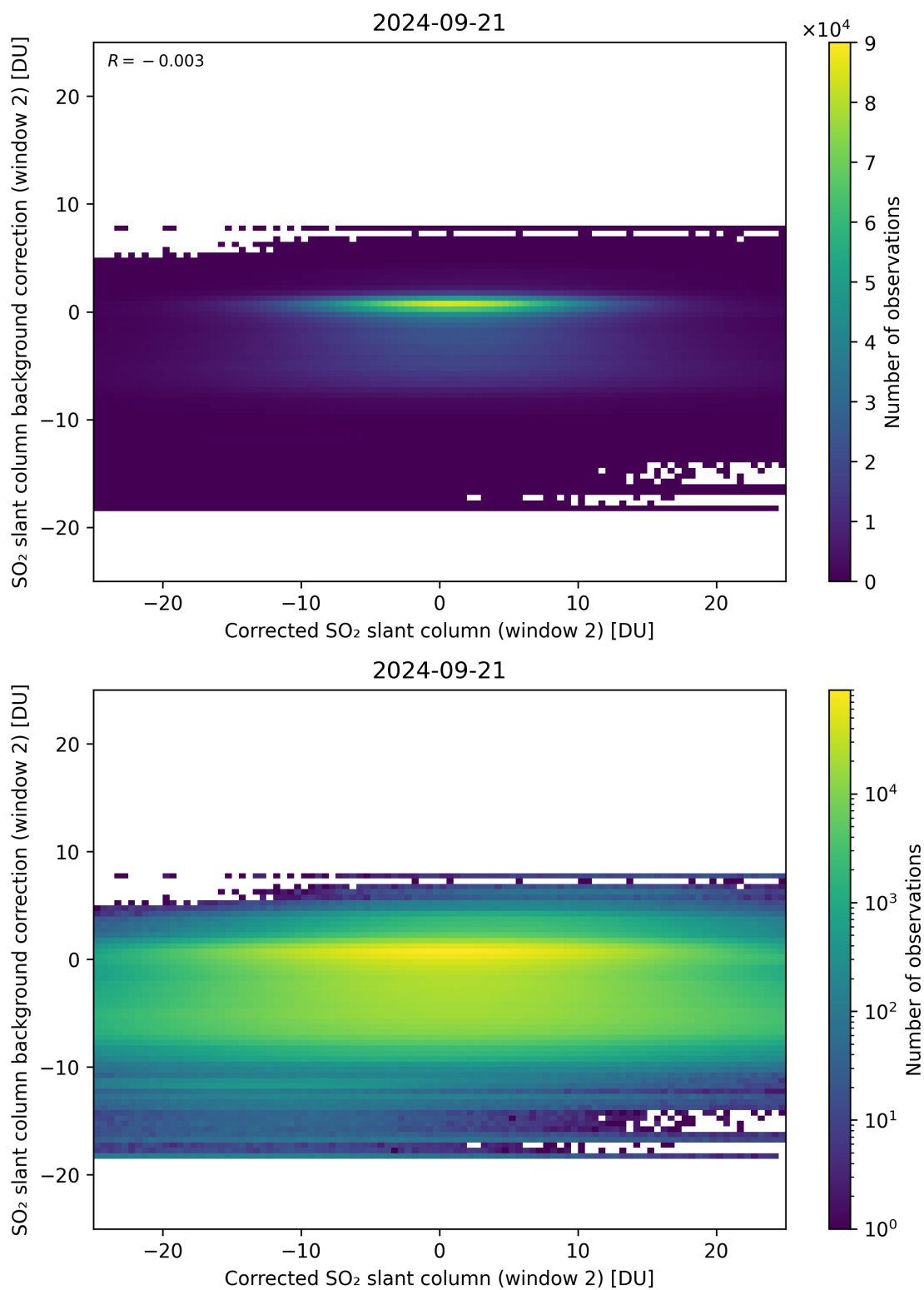
Figure 194: Scatter density plot of “Corrected SO 2 slant column (window 2)” against “SO 2 slant column background correction (window 2)” for 2024-09-20 to 2024-09-22.
