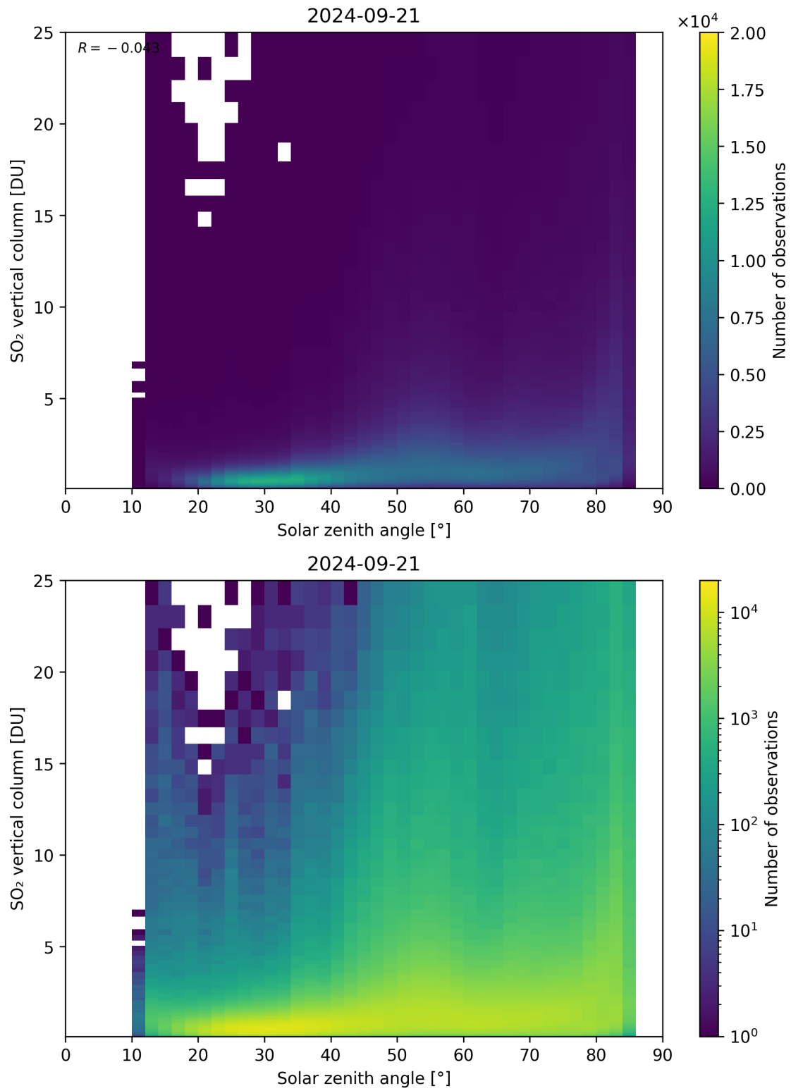
Figure 176: Scatter density plot of “Solar zenith angle” against “SO 2 vertical column” for 2024-09-20 to 2024-09-22.
