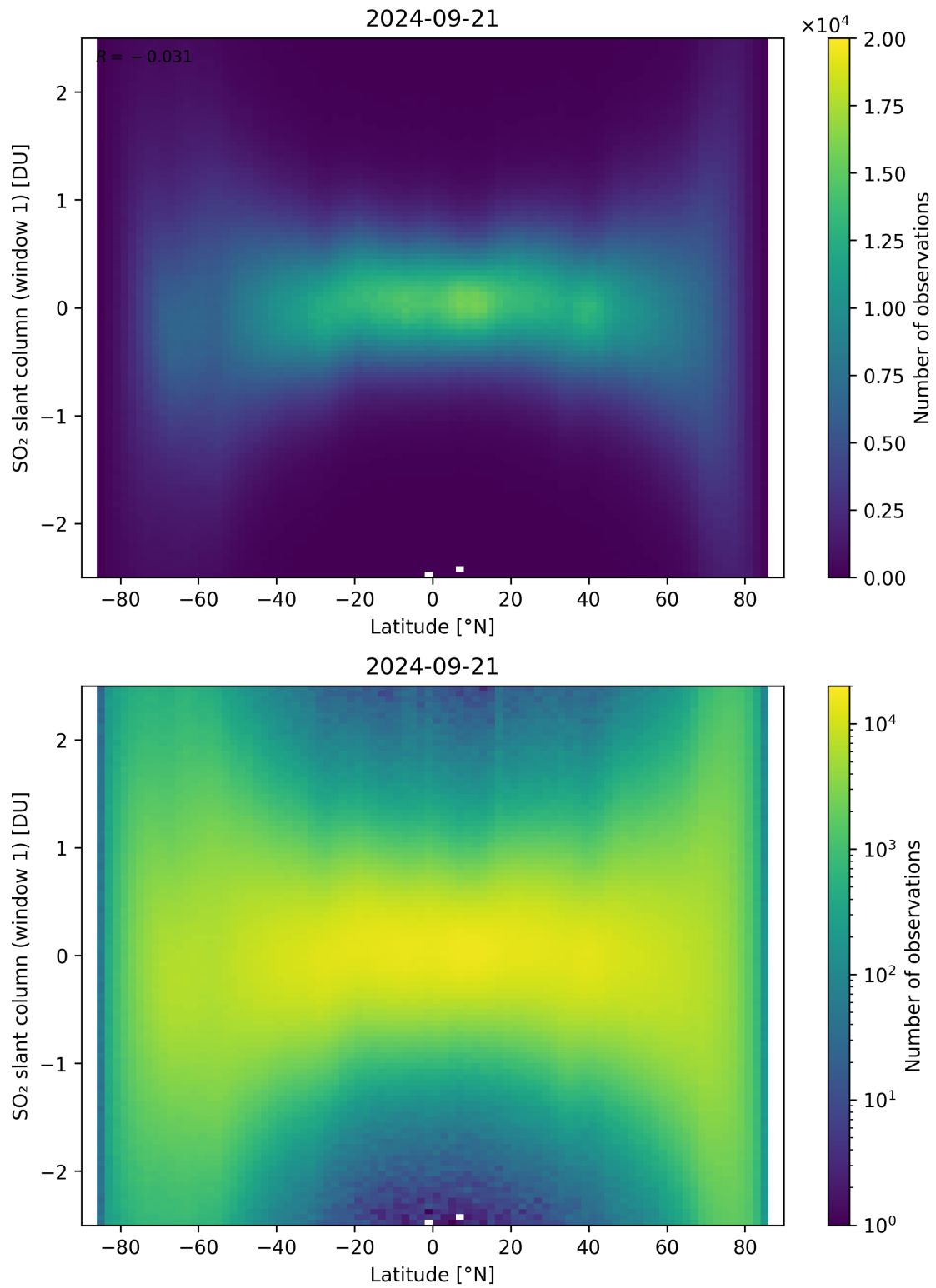
Figure 149: Scatter density plot of “Latitude” against “SO 2 slant column (window 1)” for 2024-09-20 to 2024-09-22.
