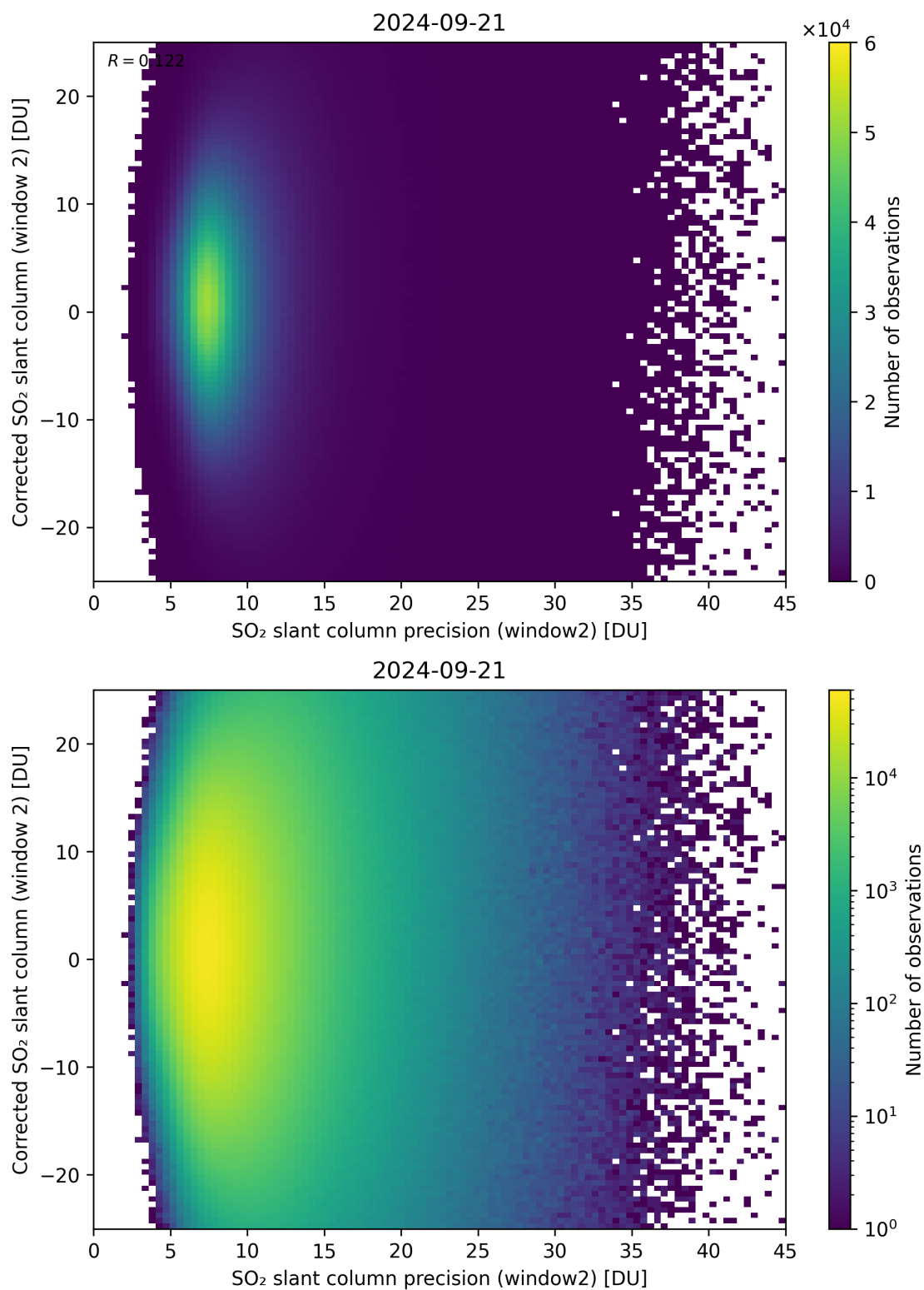
Figure 247: Scatter density plot of “SO 2 slant column precision (window2)” against “Corrected SO 2 slant column (window 2)” for 2024-09-20 to 2024-09-22.
