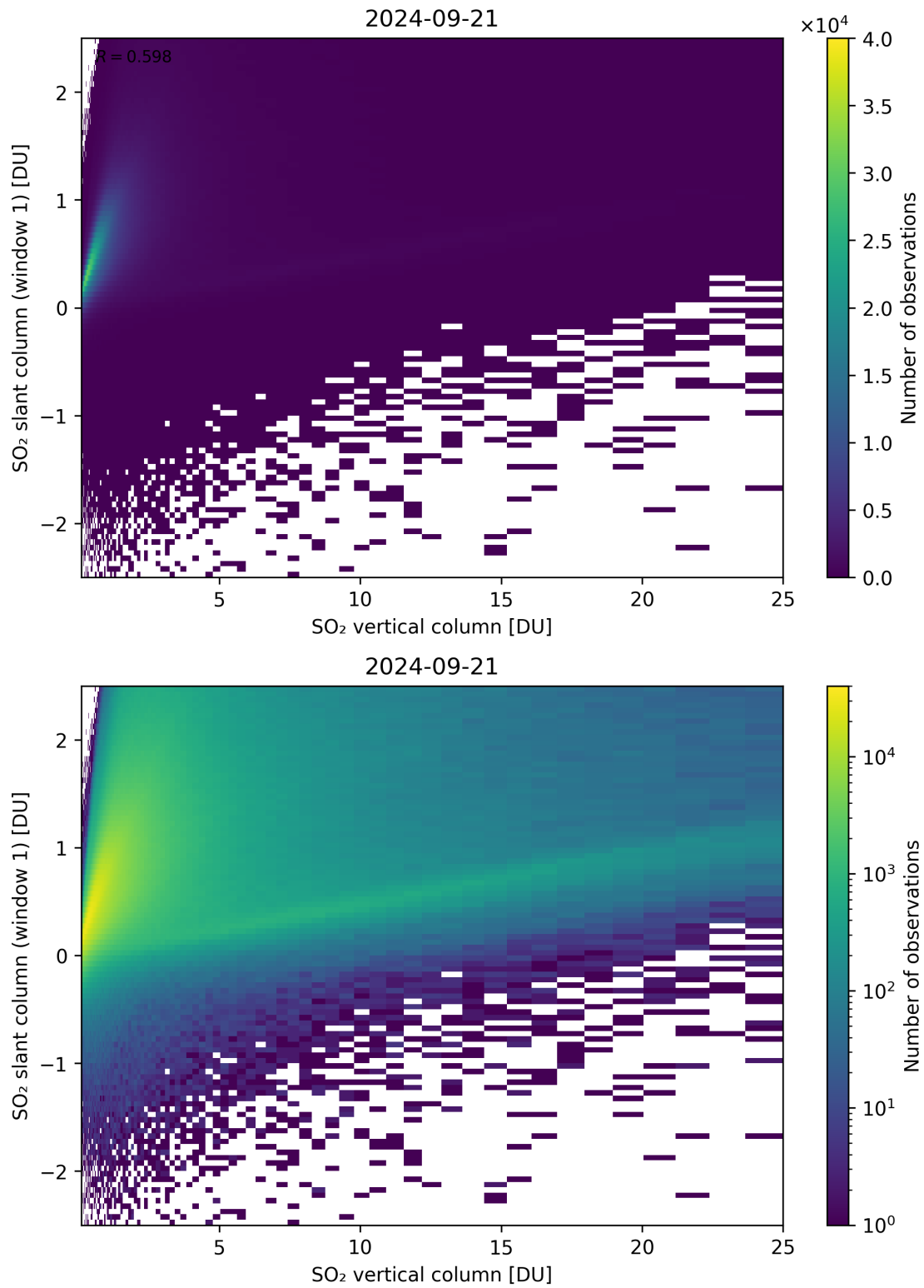
Figure 300: Scatter density plot of “SO 2 vertical column” against “SO 2 slant column (window 1)” for 2024-09-20 to 2024-09-22.
