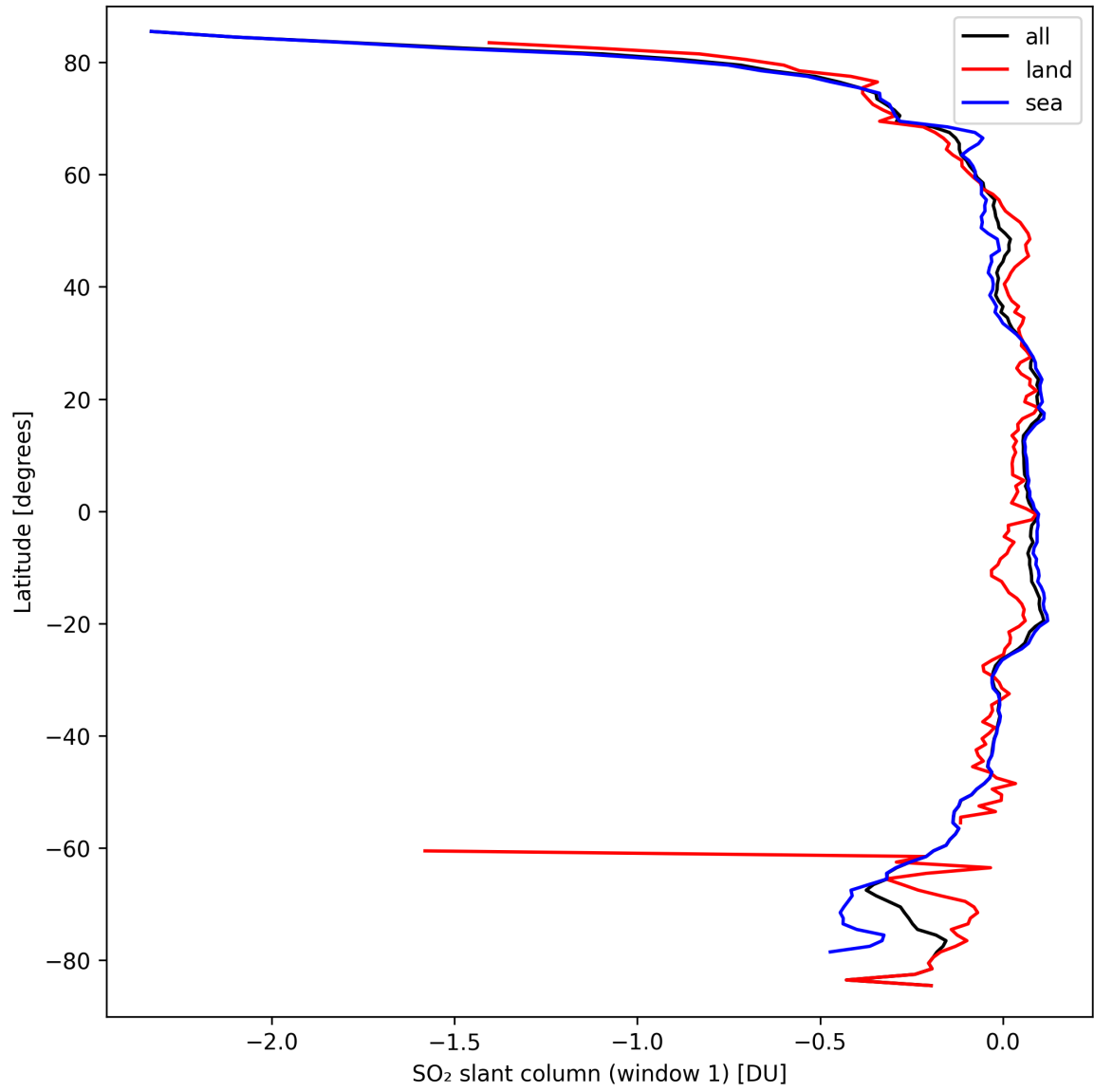
Figure 33: Zonal average of “SO 2 slant column (window 1)” for 2024-09-20 to 2024-09-22.
