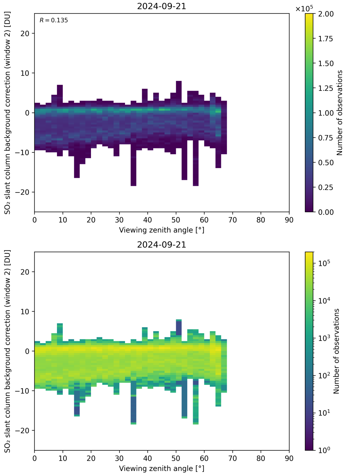
Figure 309: Scatter density plot of “Viewing zenith angle” against “SO 2 slant column background correction (window 2)” for 2024-09-20 to 2024-09-22.
