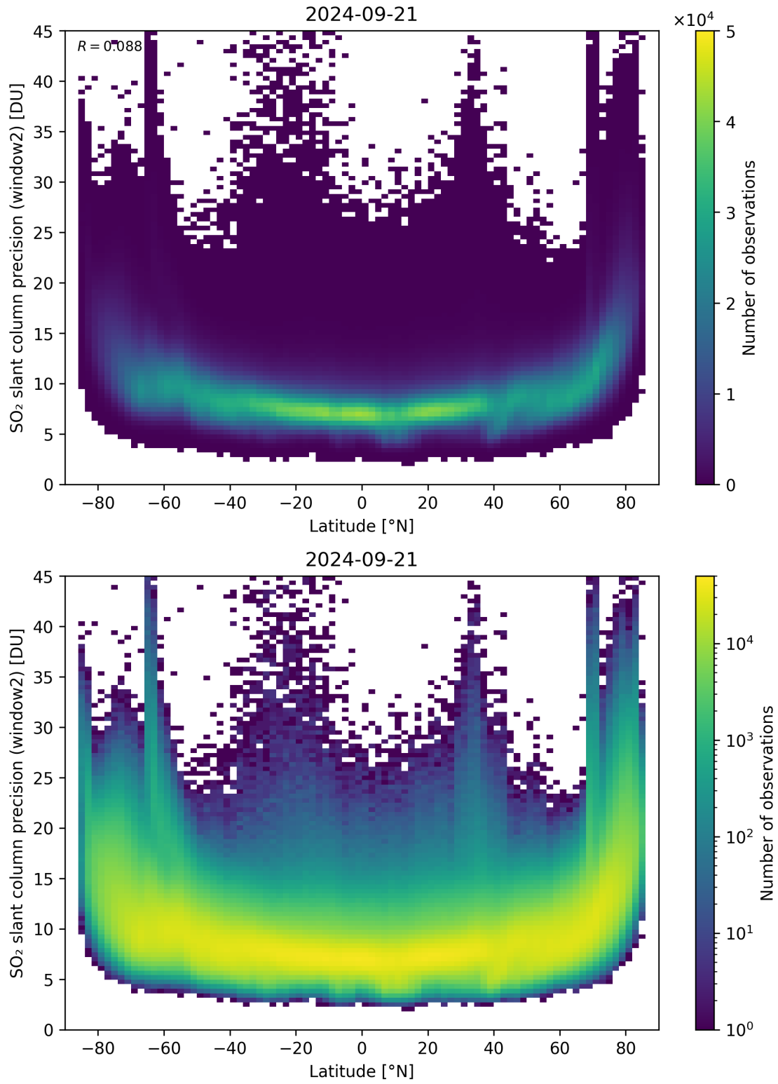
Figure 151: Scatter density plot of “Latitude” against “SO 2 slant column precision (window2)” for 2024-09-20 to 2024-09-22.
