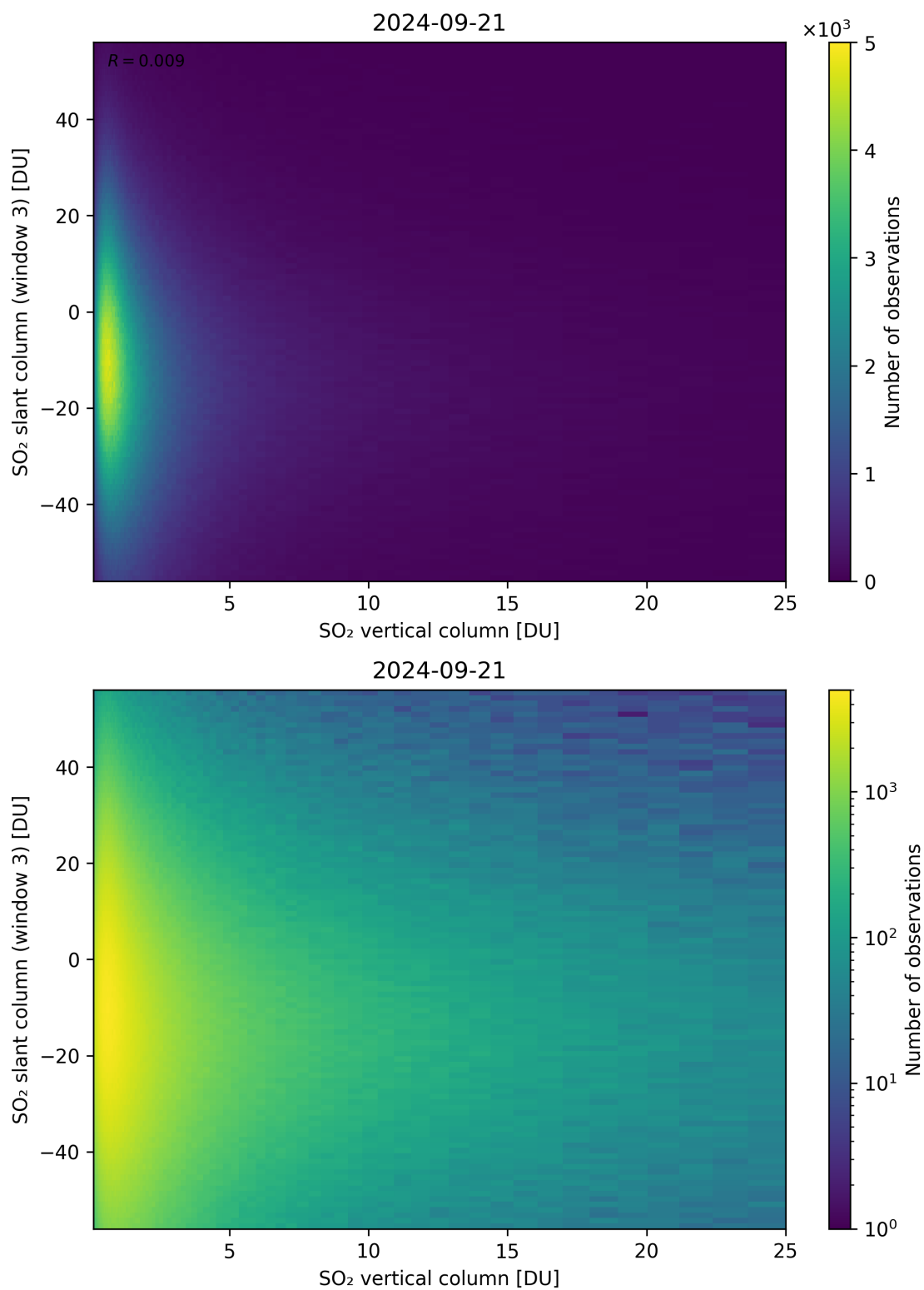
Figure 303: Scatter density plot of “SO 2 vertical column” against “SO 2 slant column (window 3)” for 2024-09-20 to 2024-09-22.
