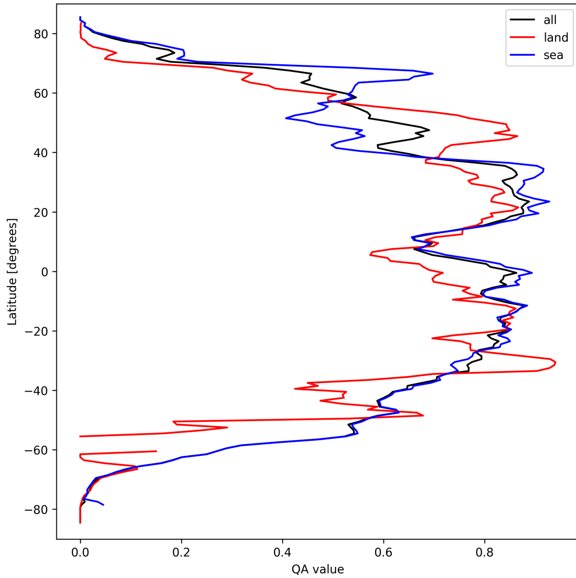
Figure 29: Zonal average of “QA value” for 2024-09-20 to 2024-09-22.
