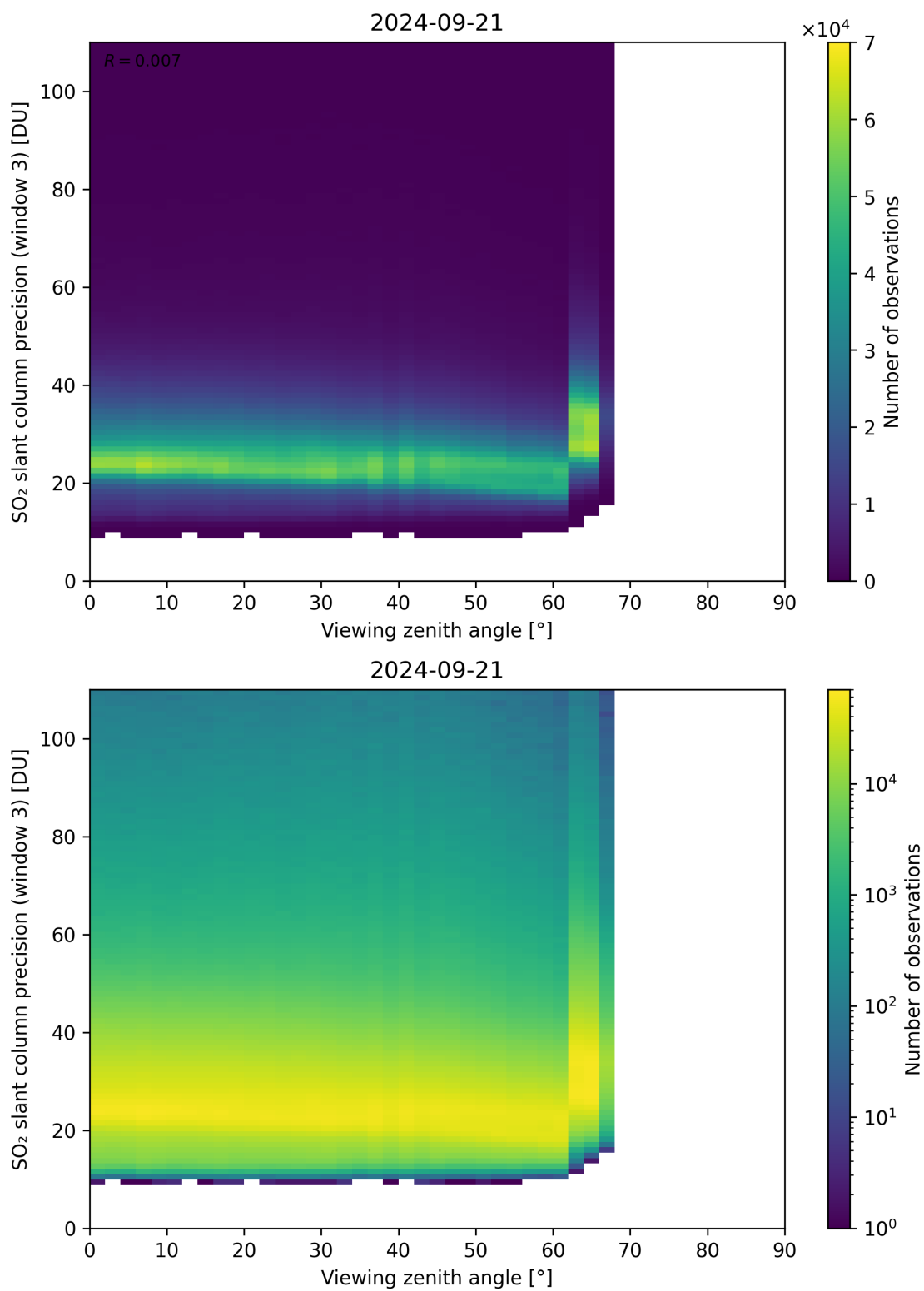
Figure 324: Scatter density plot of “Viewing zenith angle” against “SO 2 slant column precision (window 3)” for 2024-09-20 to 2024-09-22.
