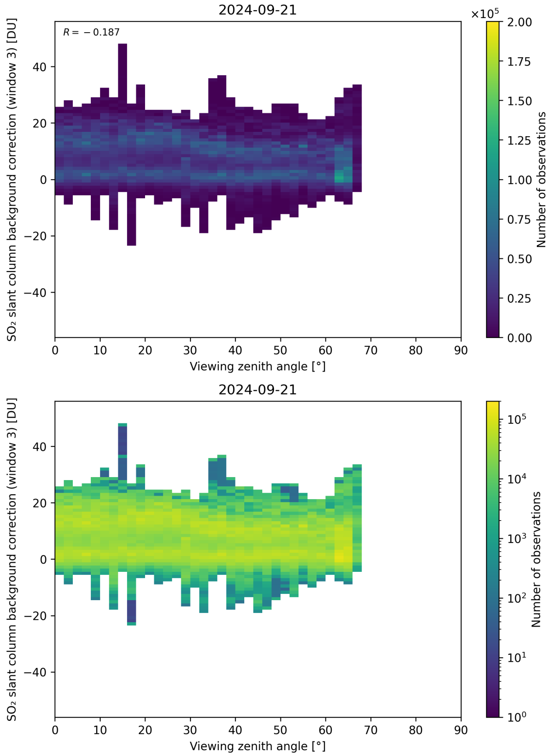
Figure 310: Scatter density plot of “Viewing zenith angle” against “SO 2 slant column background correction (window 3)” for 2024-09-20 to 2024-09-22.
