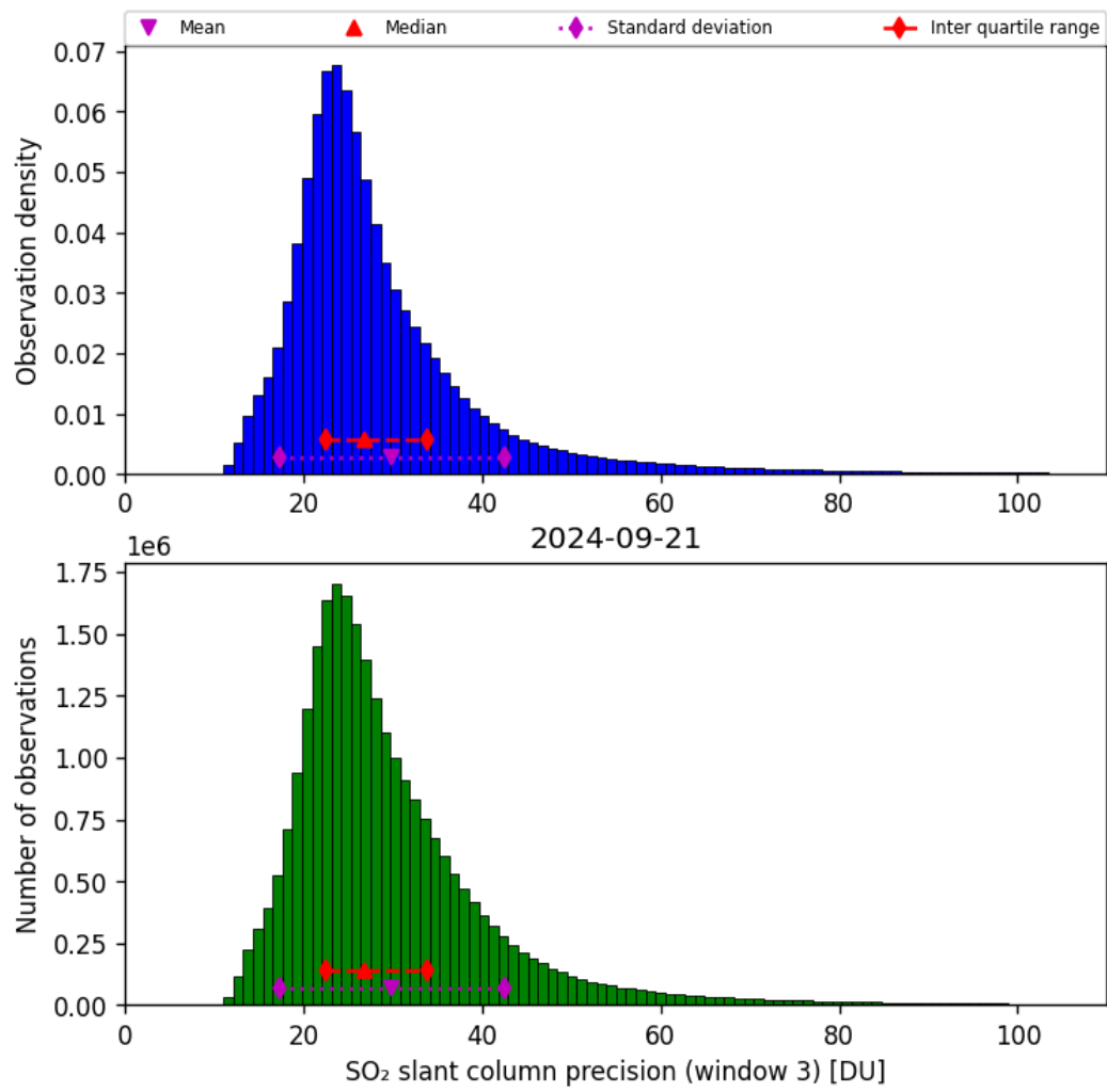
Figure 65: Histogram of “SO 2 slant column precision (window 3)” for 2024-09-20 to 2024-09-22
