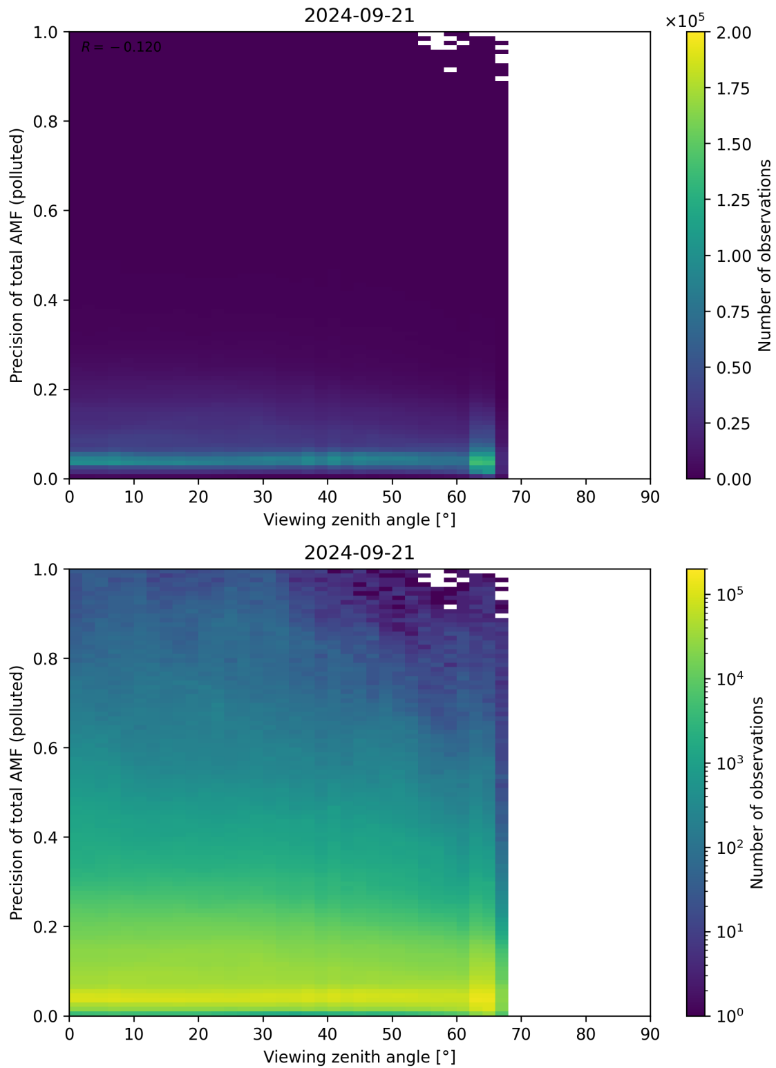
Figure 326: Scatter density plot of “Viewing zenith angle” against “Precision of total AMF (polluted)” for 2024-09-20 to 2024-09-22.
