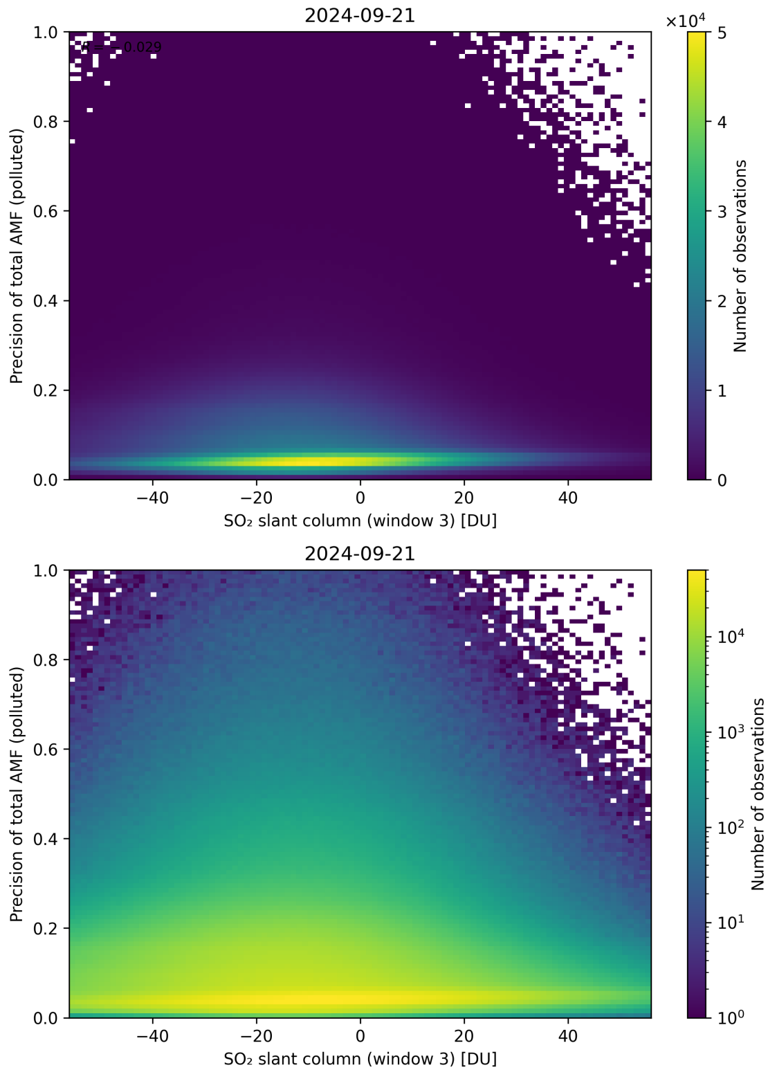
Figure 269: Scatter density plot of “SO 2 slant column (window 3)” against “Precision of total AMF (polluted)” for 2024-09-20 to 2024-09-22.
