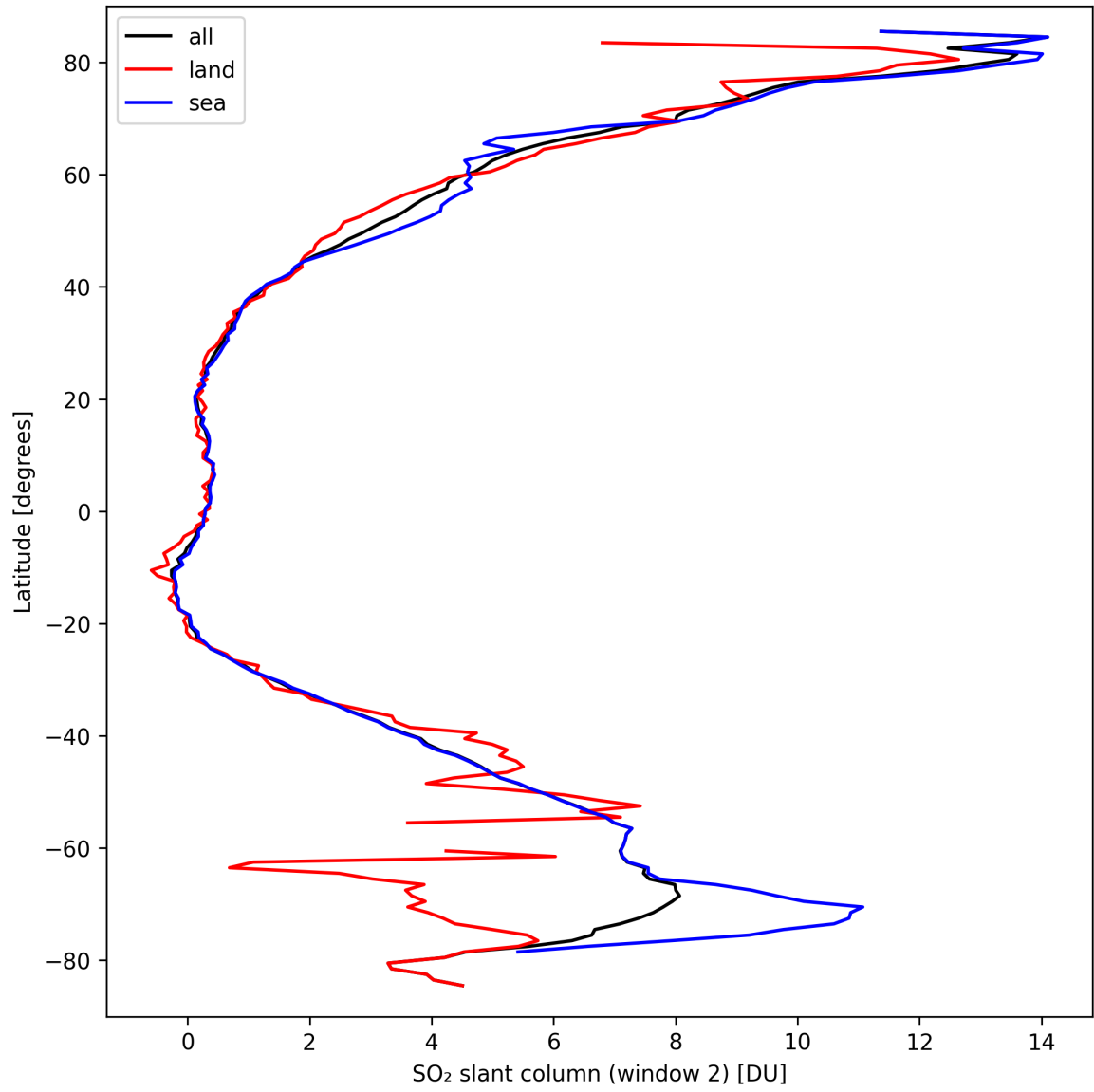
Figure 37: Zonal average of “SO 2 slant column (window 2)” for 2024-09-20 to 2024-09-22.
