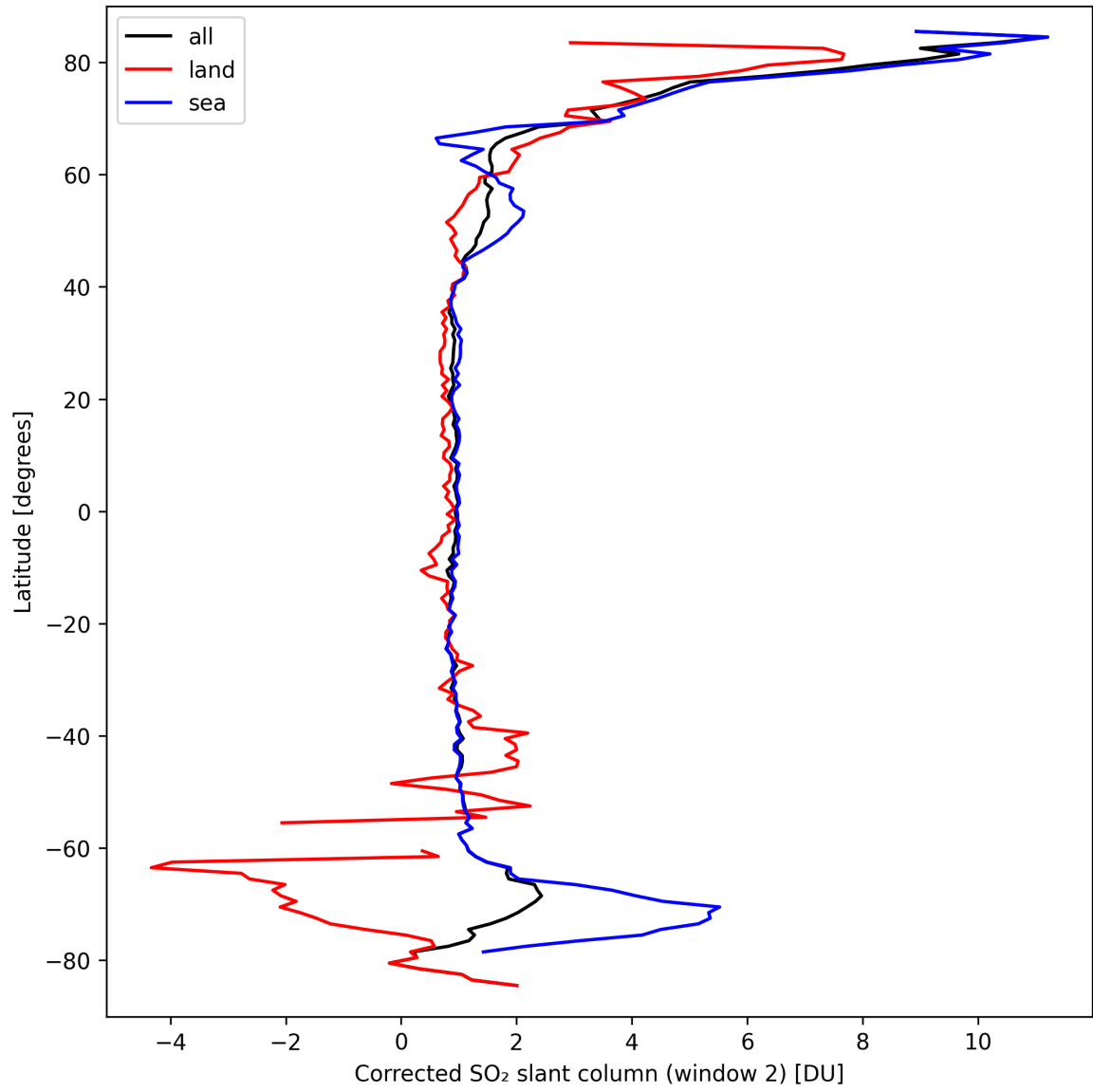
Figure 39: Zonal average of “Corrected SO 2 slant column (window 2)” for 2024-09-20 to 2024-09-22.
