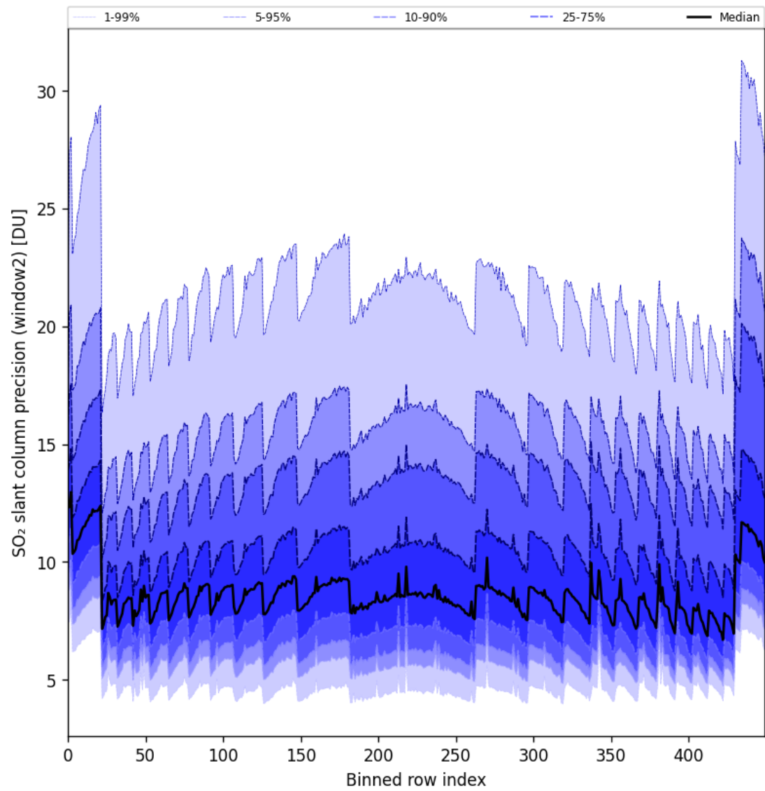
Figure 84: Along track statistics of “SO 2 slant column precision (window2)” for 2024-09-20 to 2024-09-22
