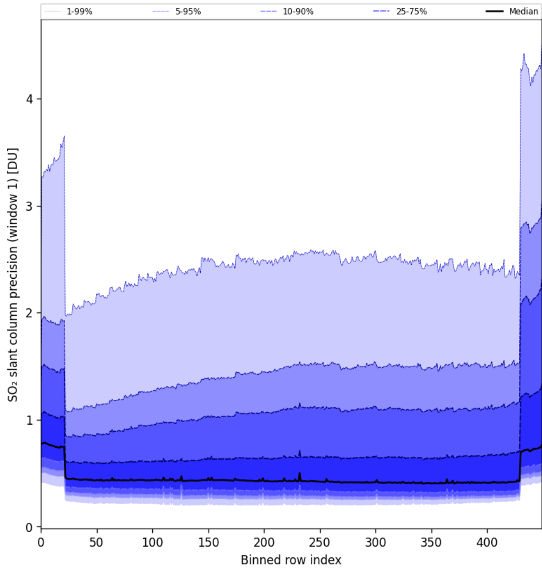
Figure 80: Along track statistics of “SO 2 slant column precision (window 1)” for 2024-09-20 to 2024-09-22
