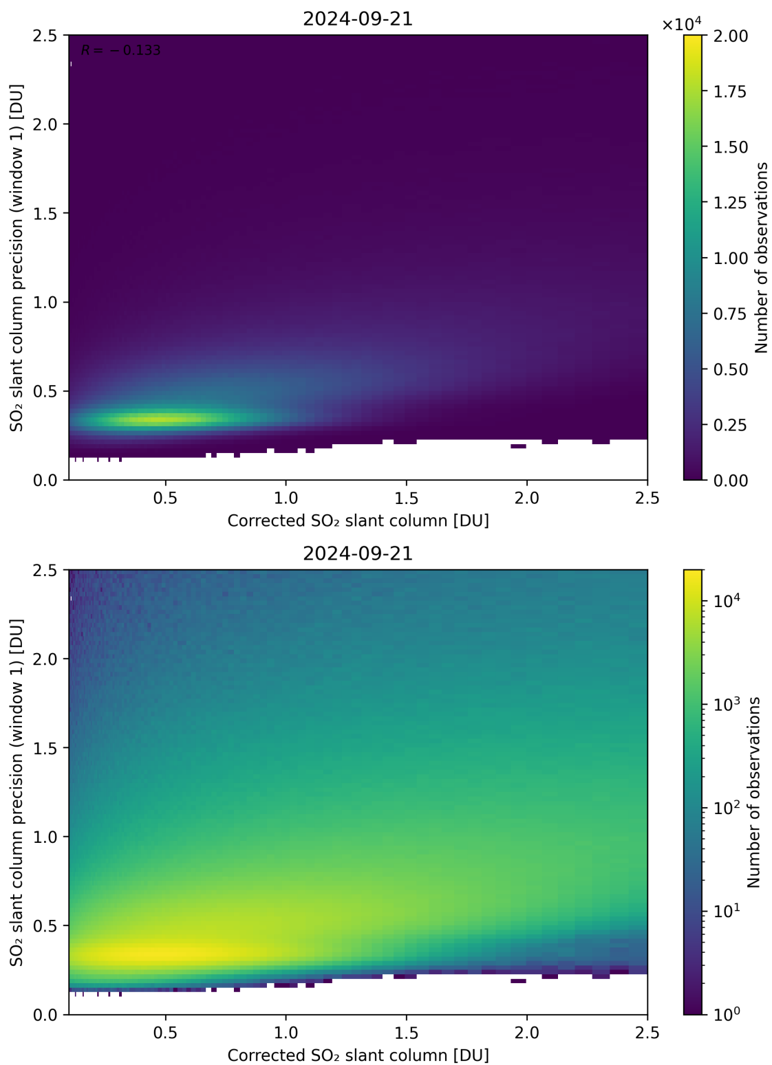
Figure 188: Scatter density plot of “Corrected SO 2 slant column” against “SO 2 slant column precision (window 1)” for 2024-09-20 to 2024-09-22.
