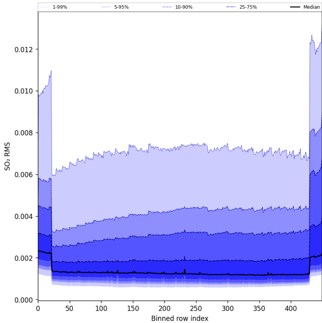
Figure 93: Along track statistics of “SO 2 RMS” for 2024-09-20 to 2024-09-22
