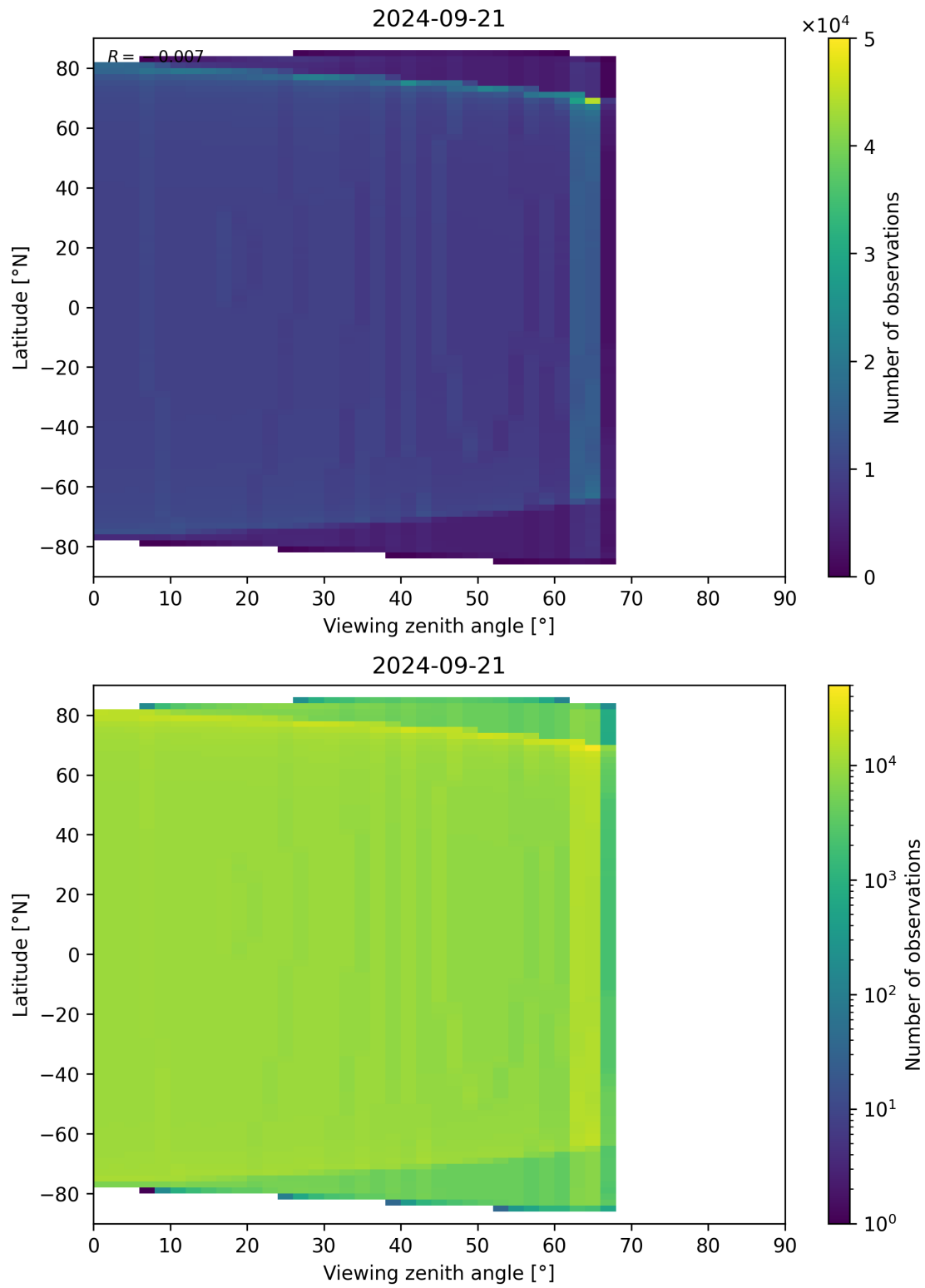
Figure 314: Scatter density plot of “Viewing zenith angle” against “Latitude” for 2024-09-20 to 2024-09-22.
