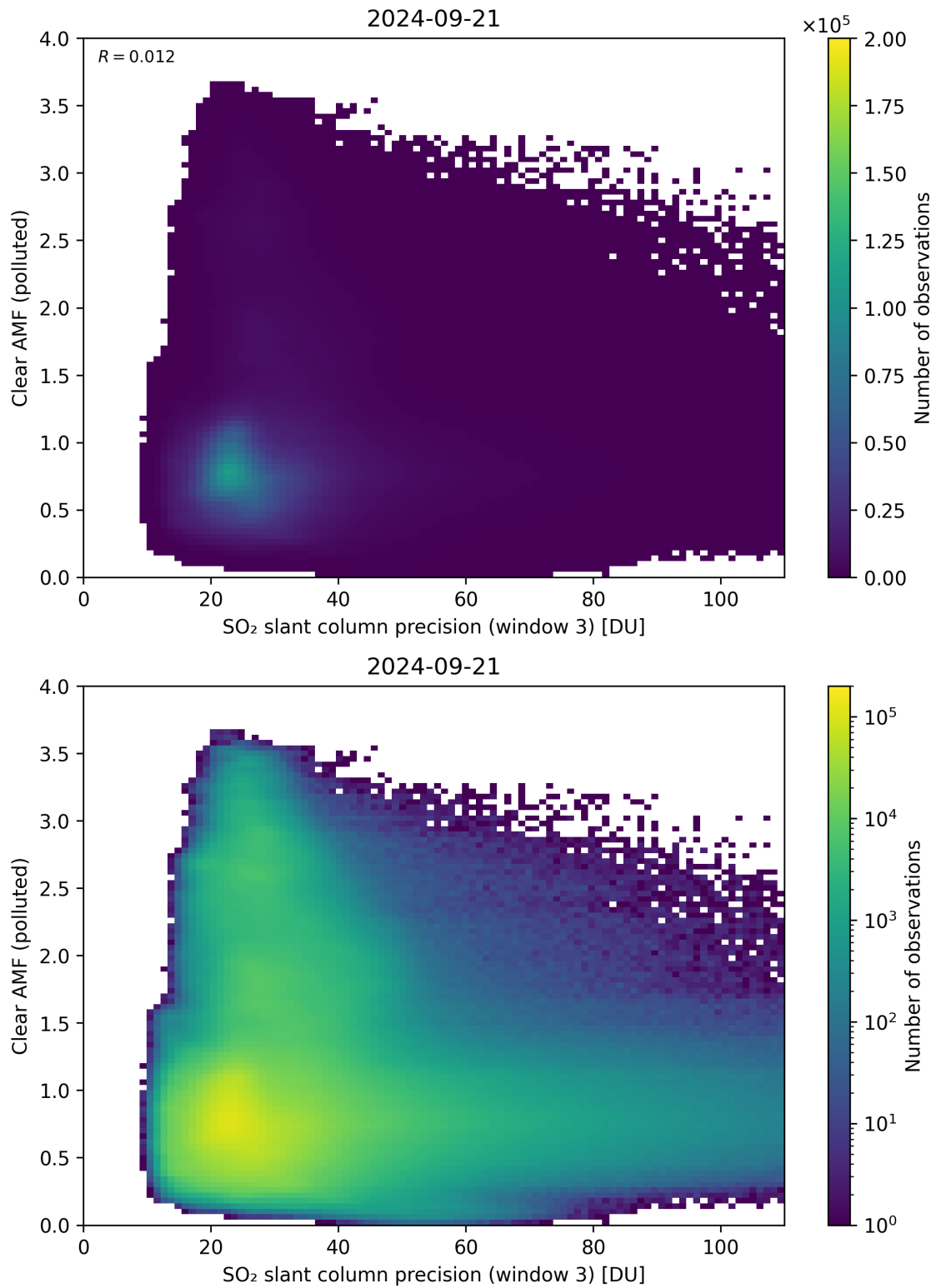
Figure 261: Scatter density plot of “SO 2 slant column precision (window 3)” against “Clear AMF (polluted)” for 2024-09-20 to 2024-09-22.
