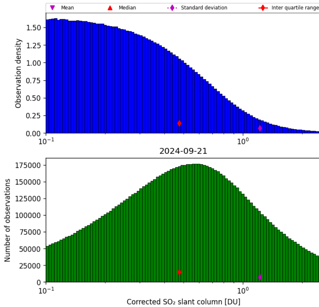
Figure 55: Histogram of “Corrected SO 2 slant column” for 2024-09-20 to 2024-09-22
