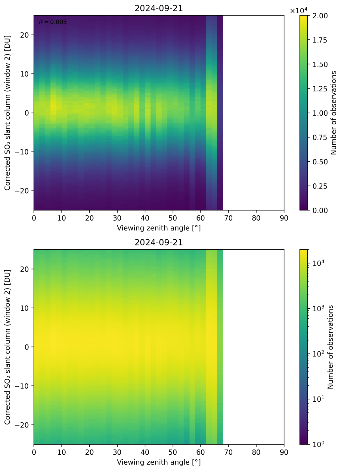
Figure 318: Scatter density plot of “Viewing zenith angle” against “Corrected SO 2 slant column (window 2)” for 2024-09-20 to 2024-09-22.
