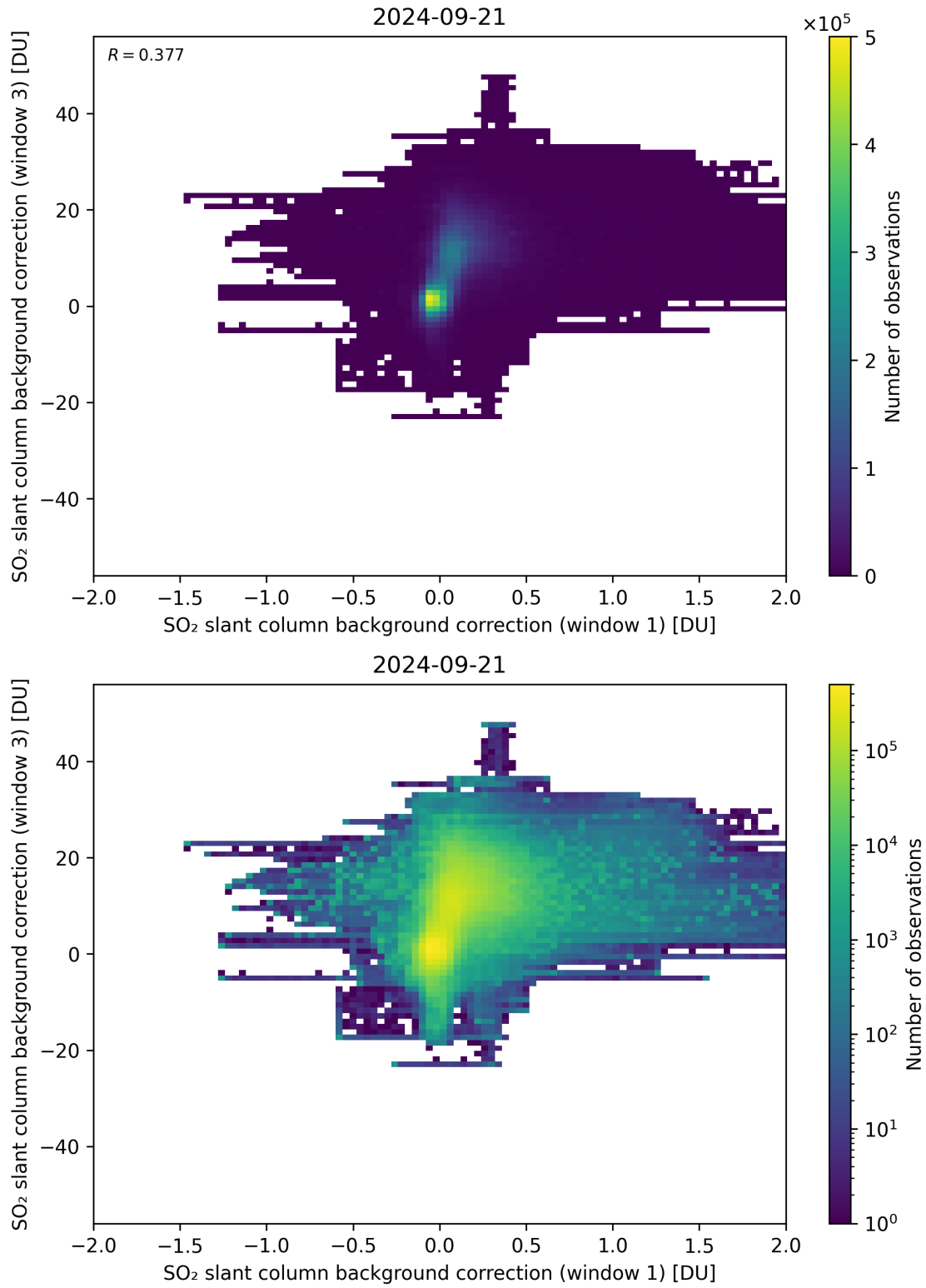
Figure 99: Scatter density plot of “SO 2 slant column background correction (window 1)” against “SO 2 slant column background correction (window 3)” for 2024-09-20 to 2024-09-22.
