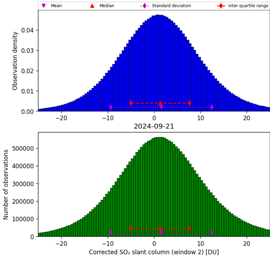
Figure 62: Histogram of “Corrected SO 2 slant column (window 2)” for 2024-09-20 to 2024-09-22
