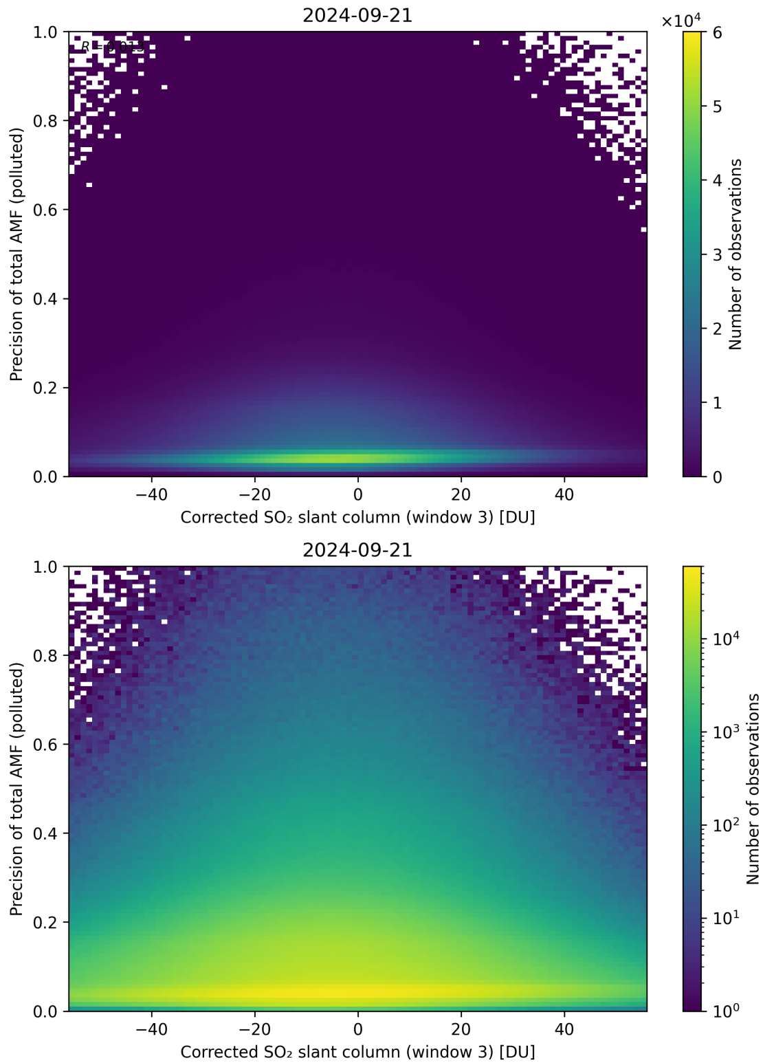
Figure 211: Scatter density plot of “Corrected SO 2 slant column (window 3)” against “Precision of total AMF (polluted)” for 2024-09-20 to 2024-09-22.
