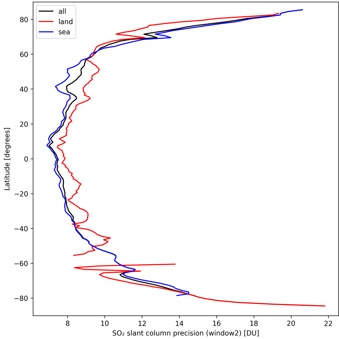
Figure 38: Zonal average of “SO 2 slant column precision (window2)” for 2024-09-20 to 2024-09-22.
