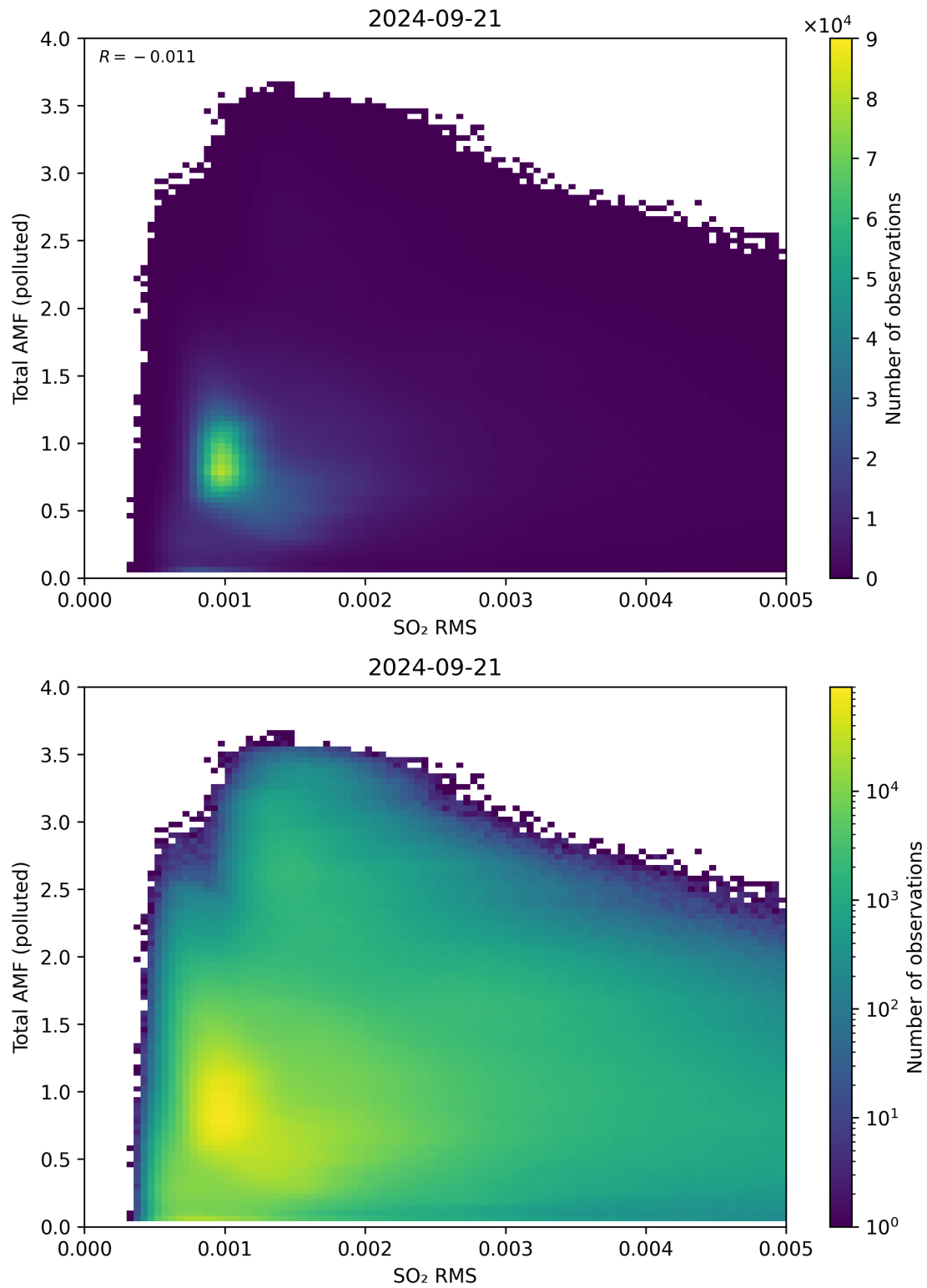
Figure 137: Scatter density plot of “SO 2 RMS” against “Total AMF (polluted)” for 2024-09-20 to 2024-09-22.
