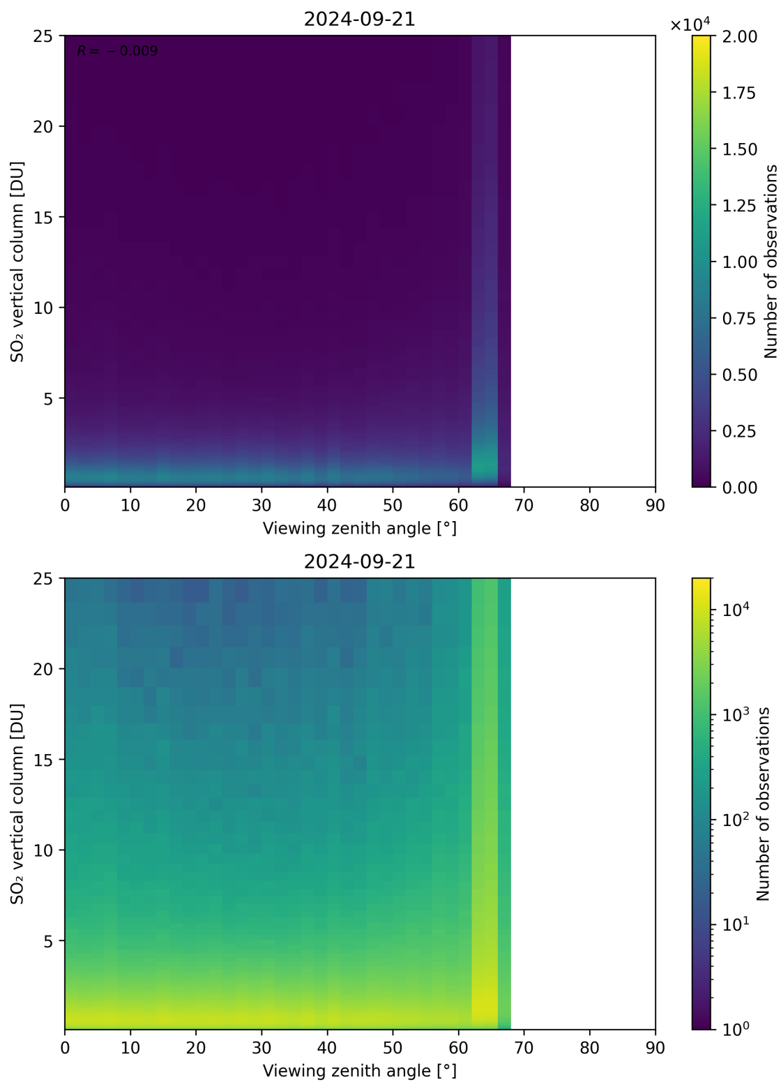
Figure 327: Scatter density plot of “Viewing zenith angle” against “SO 2 vertical column” for 2024-09-20 to 2024-09-22.
