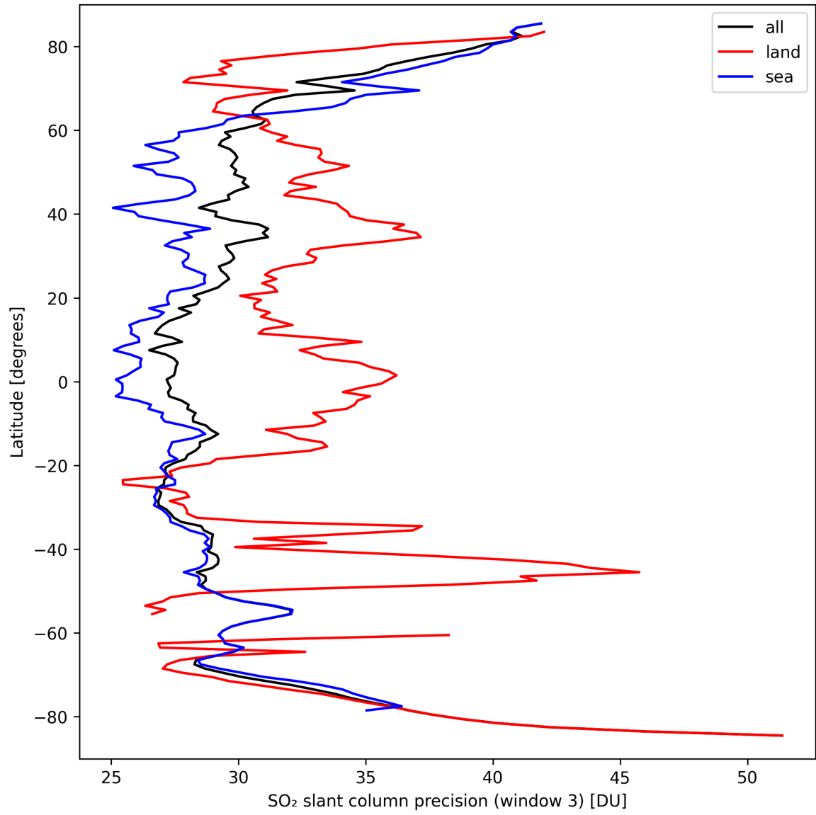
Figure 42: Zonal average of “SO 2 slant column precision (window 3)” for 2024-09-20 to 2024-09-22.
