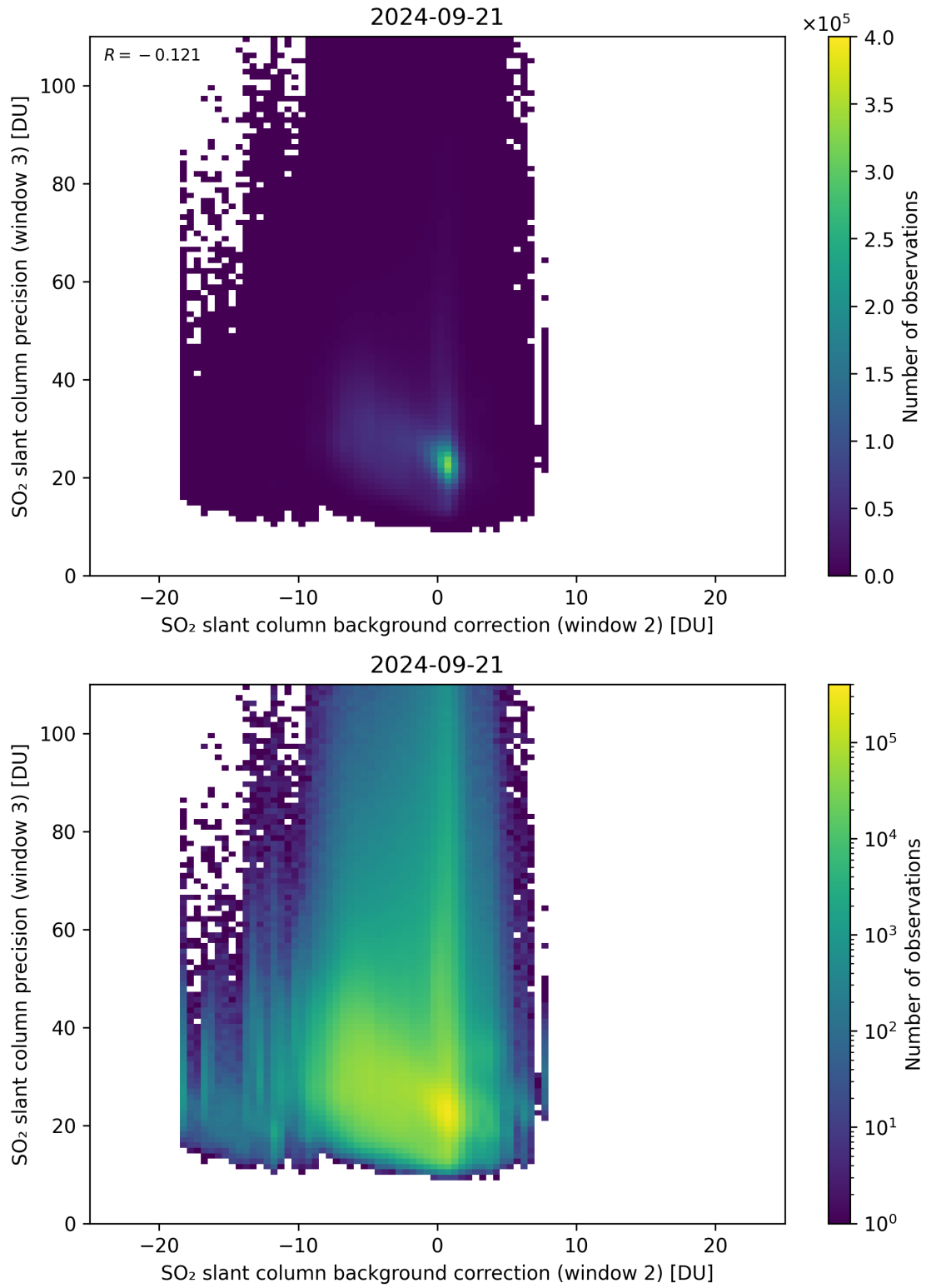
Figure 118: Scatter density plot of “SO 2 slant column background correction (window 2)” against “SO 2 slant column precision (window 3)” for 2024-09-20 to 2024-09-22.
