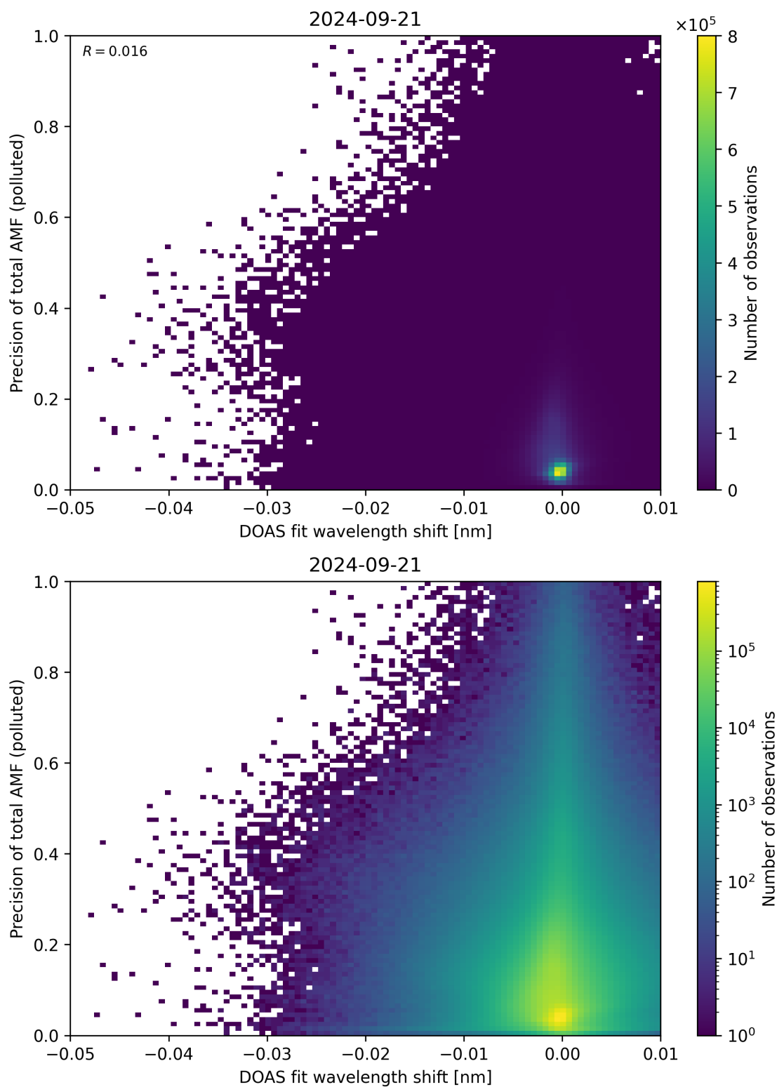
Figure 131: Scatter density plot of “DOAS fit wavelength shift” against “Precision of total AMF (polluted)” for 2024-09-20 to 2024-09-22.
