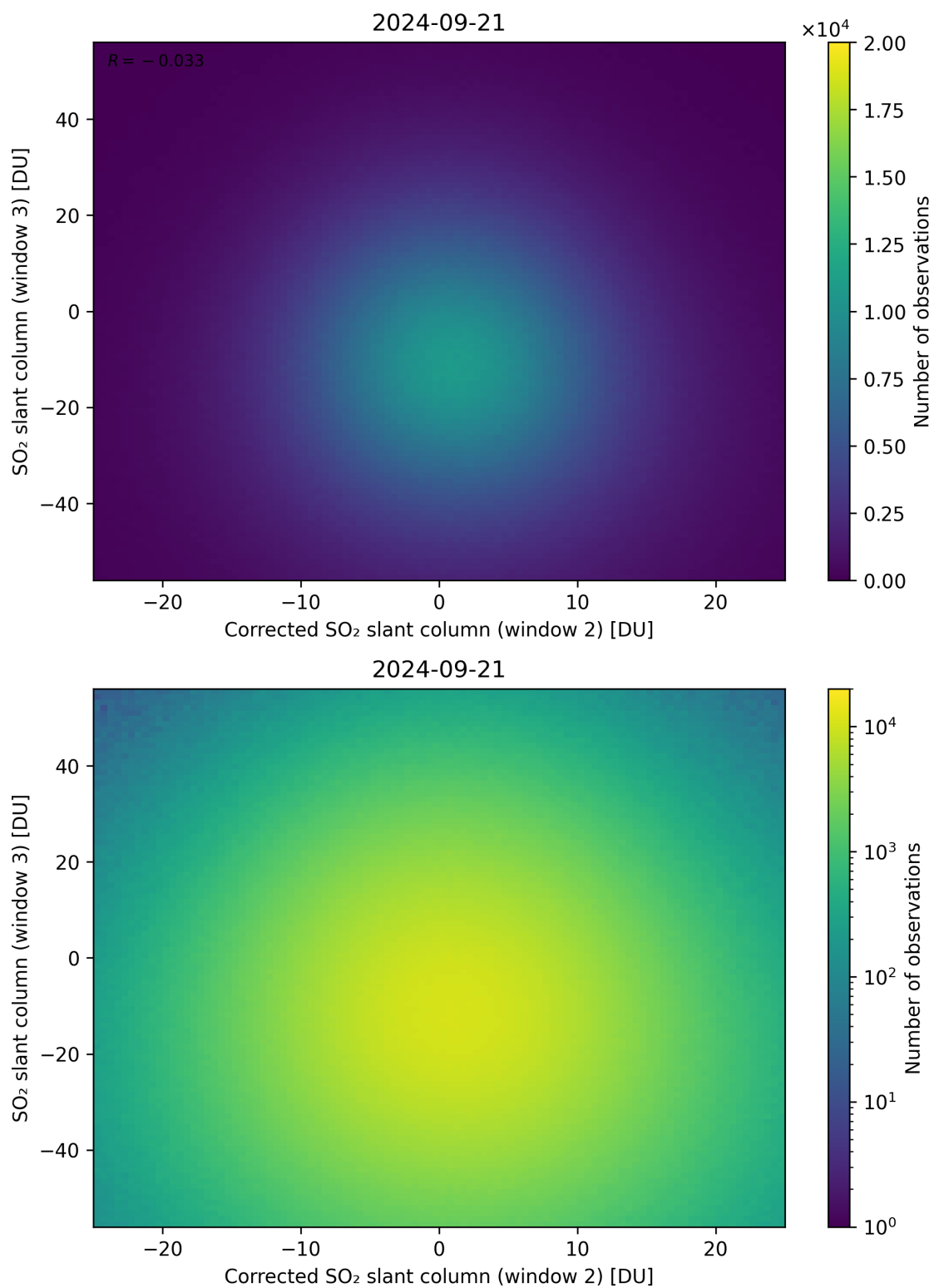
Figure 201: Scatter density plot of “Corrected SO 2 slant column (window 2)” against “SO 2 slant column (window 3)” for 2024-09-20 to 2024-09-22.
