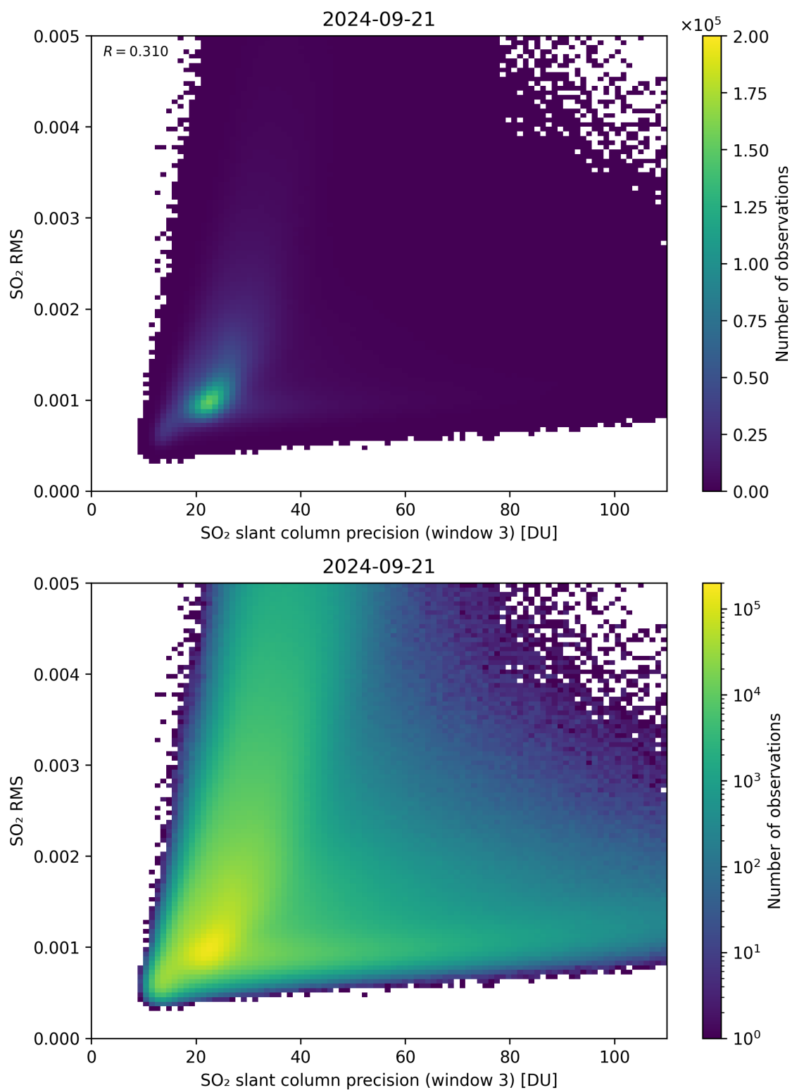
Figure 260: Scatter density plot of “SO 2 slant column precision (window 3)” against “SO 2 RMS” for 2024-09-20 to 2024-09-22.
