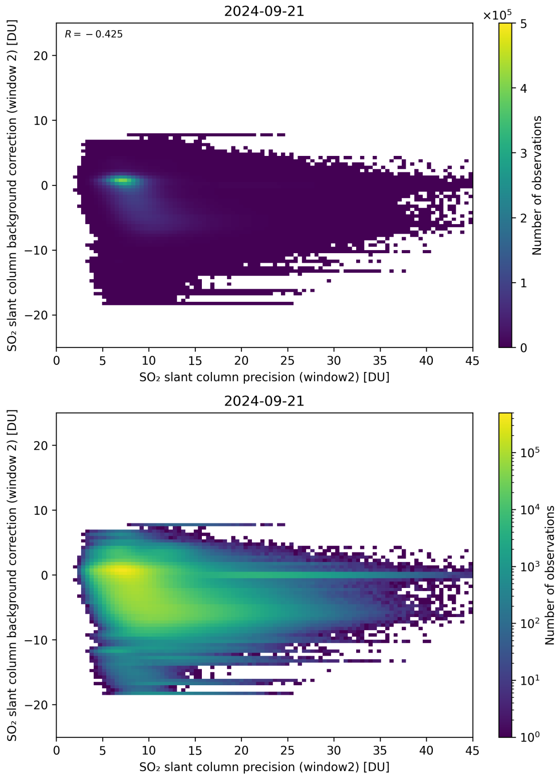
Figure 241: Scatter density plot of “SO 2 slant column precision (window2)” against “SO 2 slant column background correction (window 2)” for 2024-09-20 to 2024-09-22.
