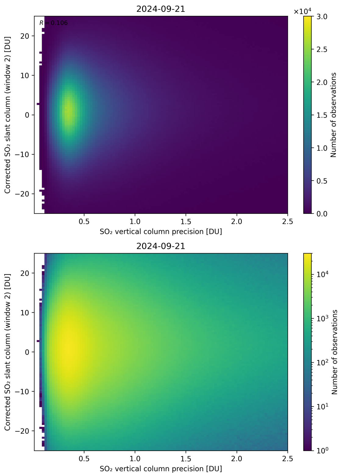
Figure 287: Scatter density plot of “SO 2 vertical column precision” against “Corrected SO 2 slant column (window 2)” for 2024-09-20 to 2024-09-22.
