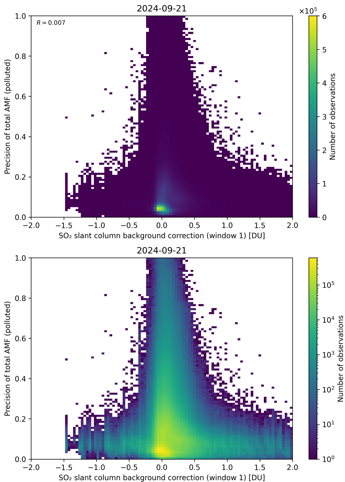
Figure 110: Scatter density plot of “SO 2 slant column background correction (window 1)” against “Precision of total AMF (polluted)” for 2024-09-20 to 2024-09-22.
