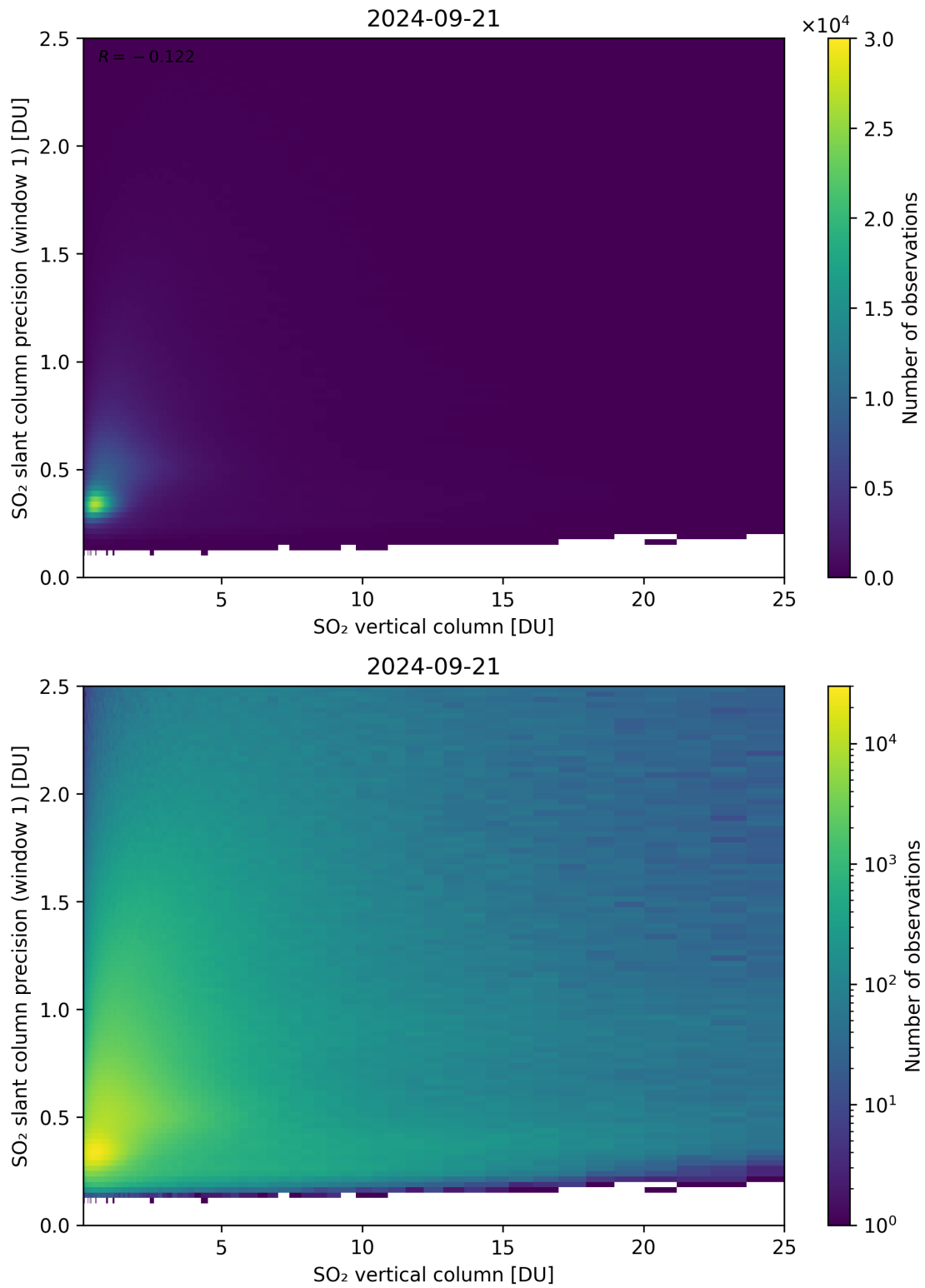
Figure 301: Scatter density plot of “SO 2 vertical column” against “SO 2 slant column precision (window 1)” for 2024-09-20 to 2024-09-22.
