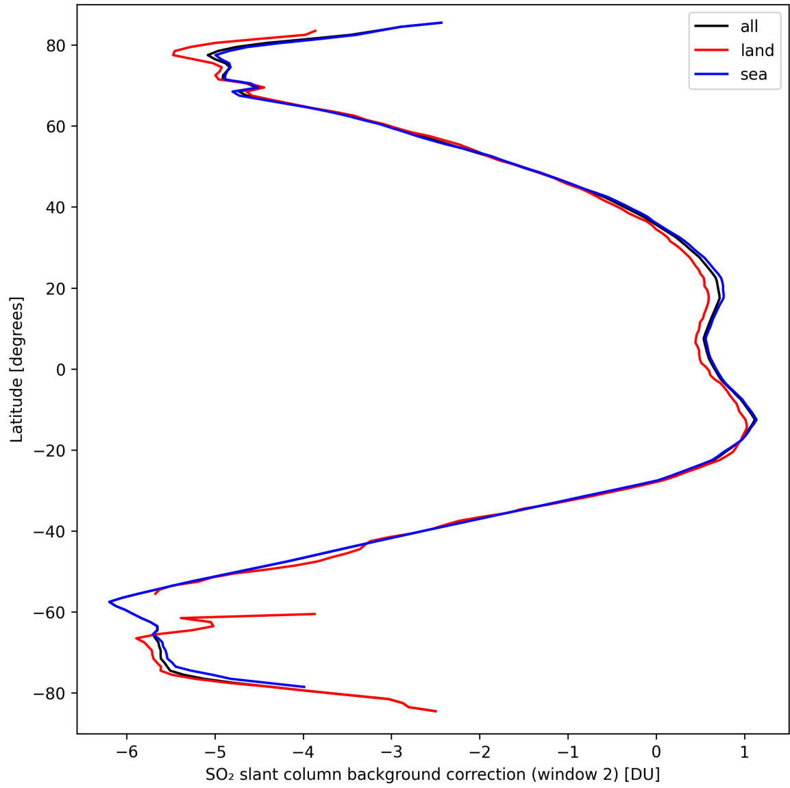
Figure 40: Zonal average of “SO 2 slant column background correction (window 2)” for 2024-09-20 to 2024-09-22.
