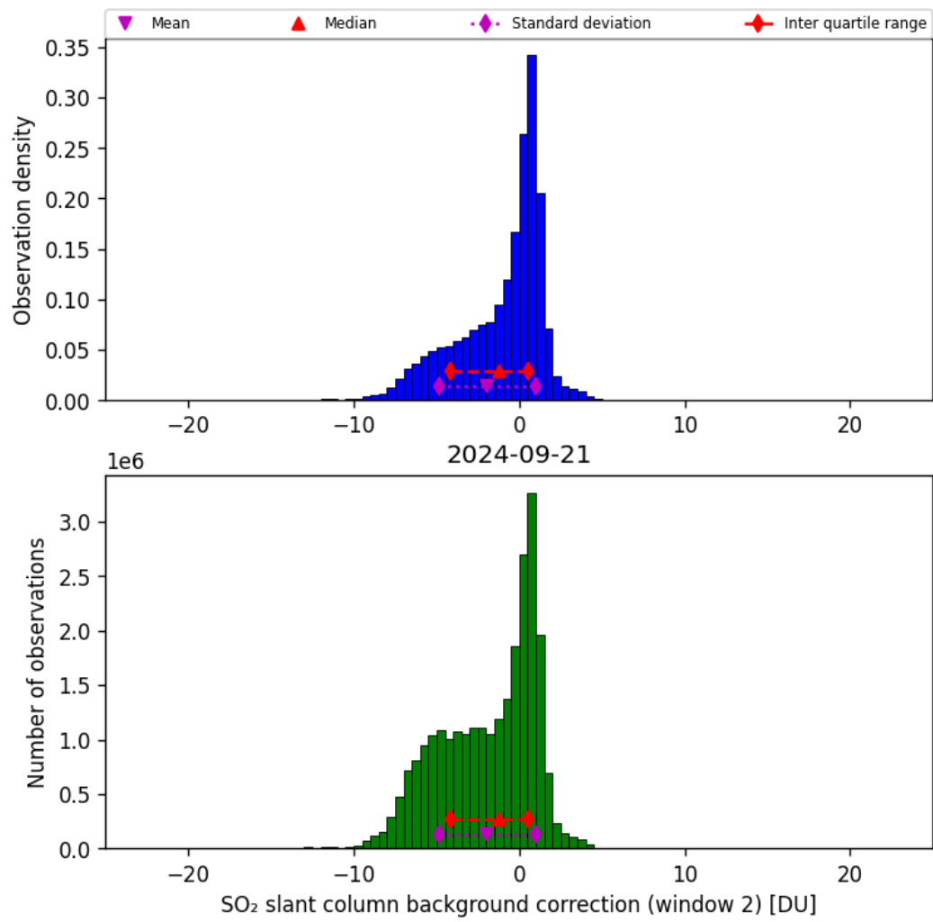
Figure 63: Histogram of “SO 2 slant column background correction (window 2)” for 2024-09-20 to 2024-09-22
