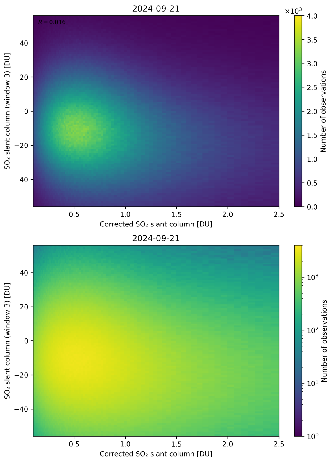
Figure 190: Scatter density plot of “Corrected SO 2 slant column” against “SO 2 slant column (window 3)” for 2024-09-20 to 2024-09-22.
