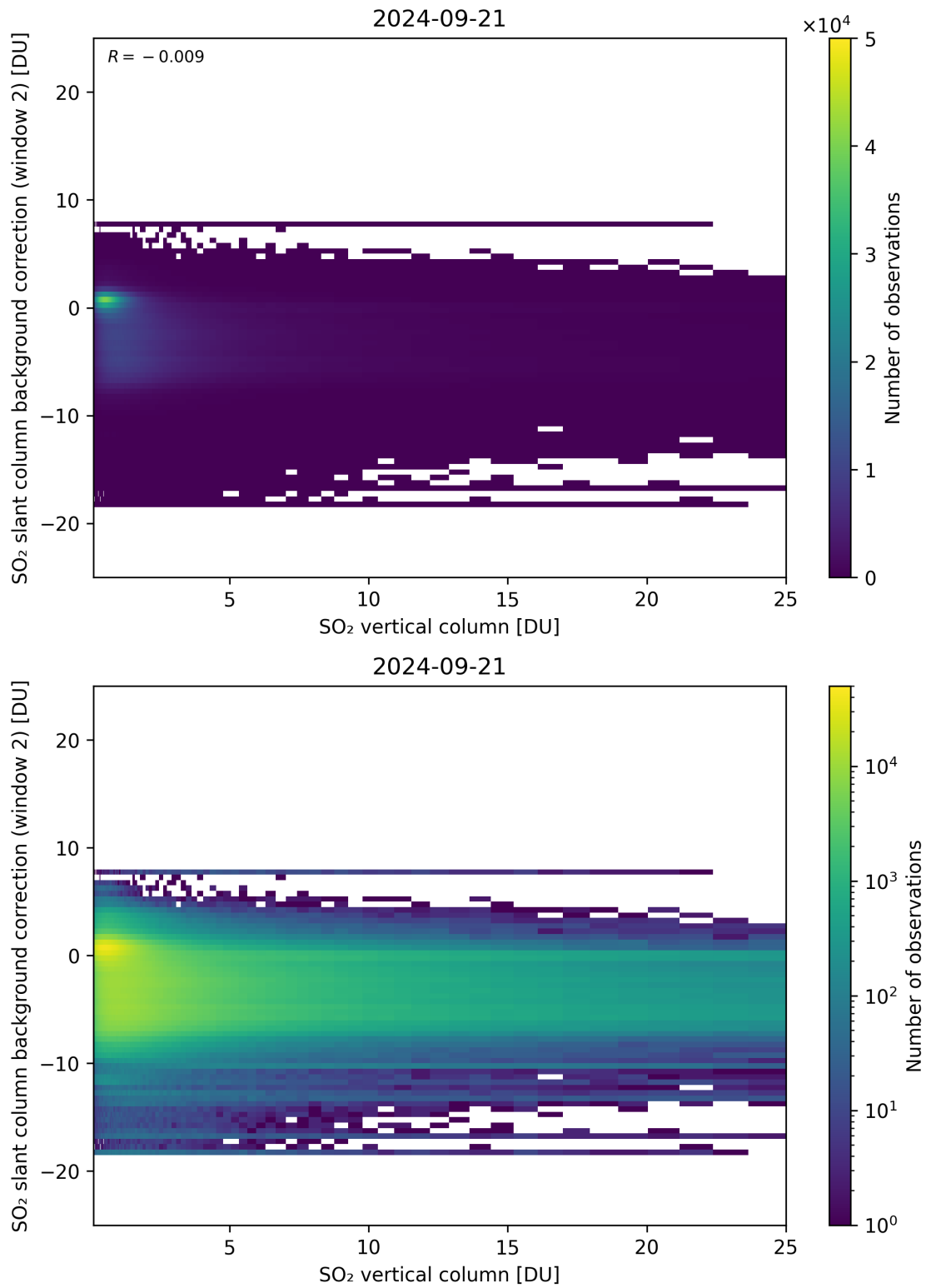
Figure 274: Scatter density plot of “SO 2 vertical column” against “SO 2 slant column background correction (window 2)” for 2024-09-20 to 2024-09-22.
