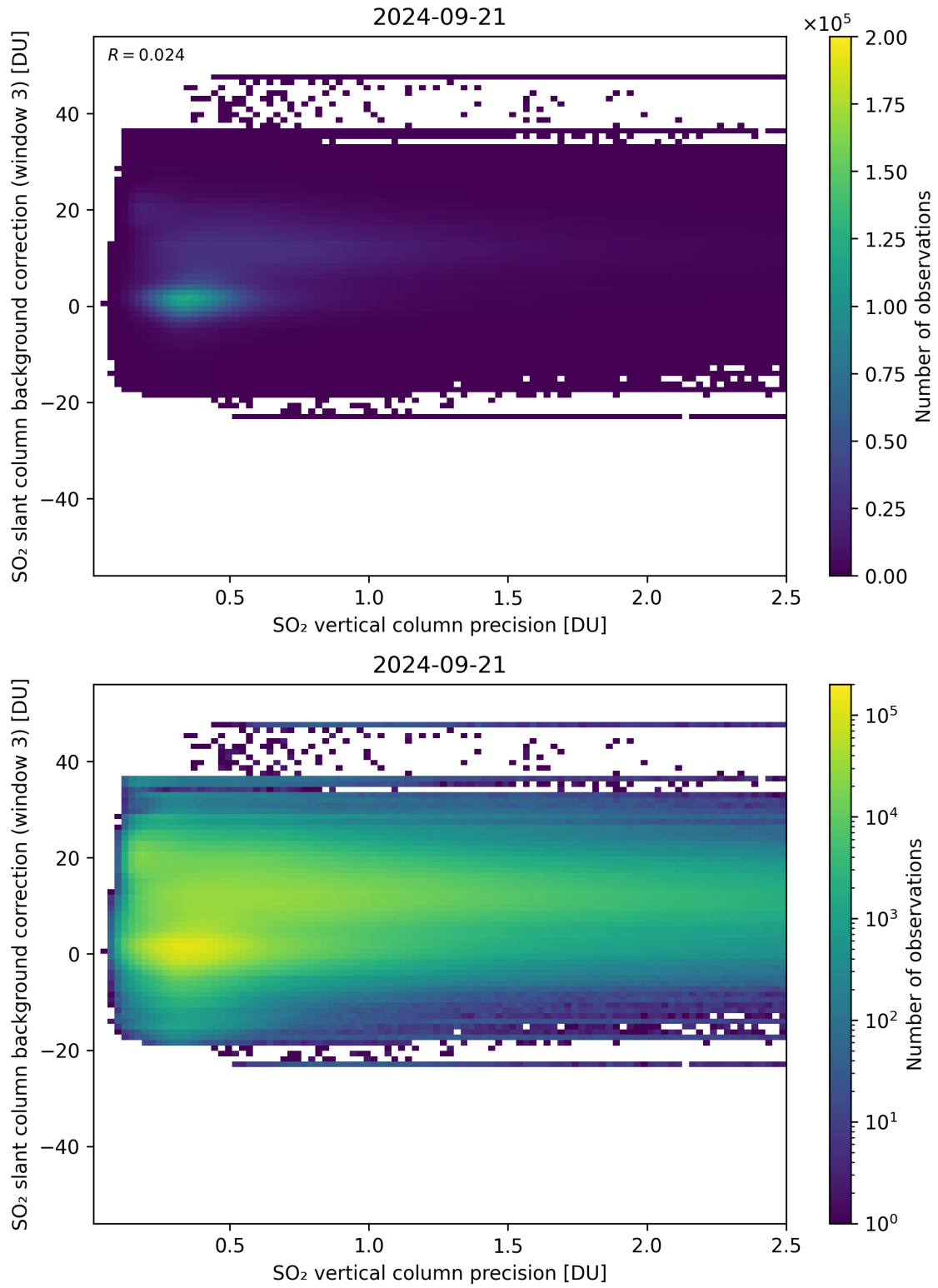
Figure 281: Scatter density plot of “SO 2 vertical column precision” against “SO 2 slant column background correction (window 3)” for 2024-09-20 to 2024-09-22.
