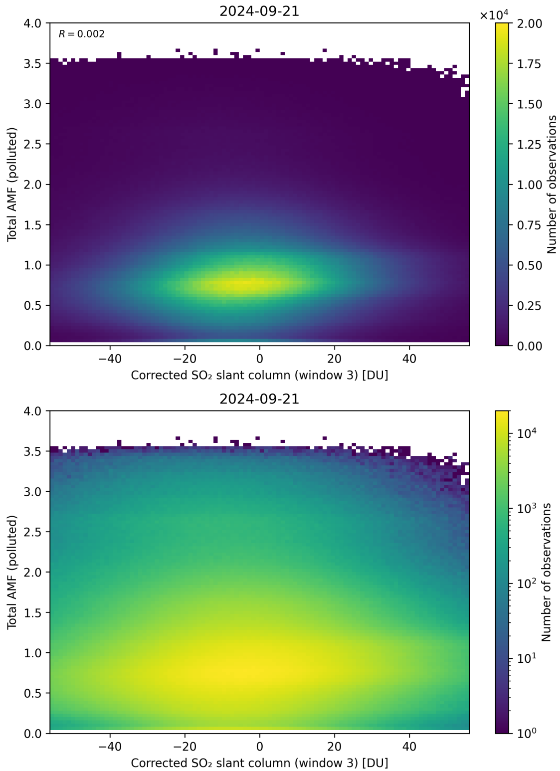
Figure 210: Scatter density plot of “Corrected SO 2 slant column (window 3)” against “Total AMF (polluted)” for 2024-09-20 to 2024-09-22.
