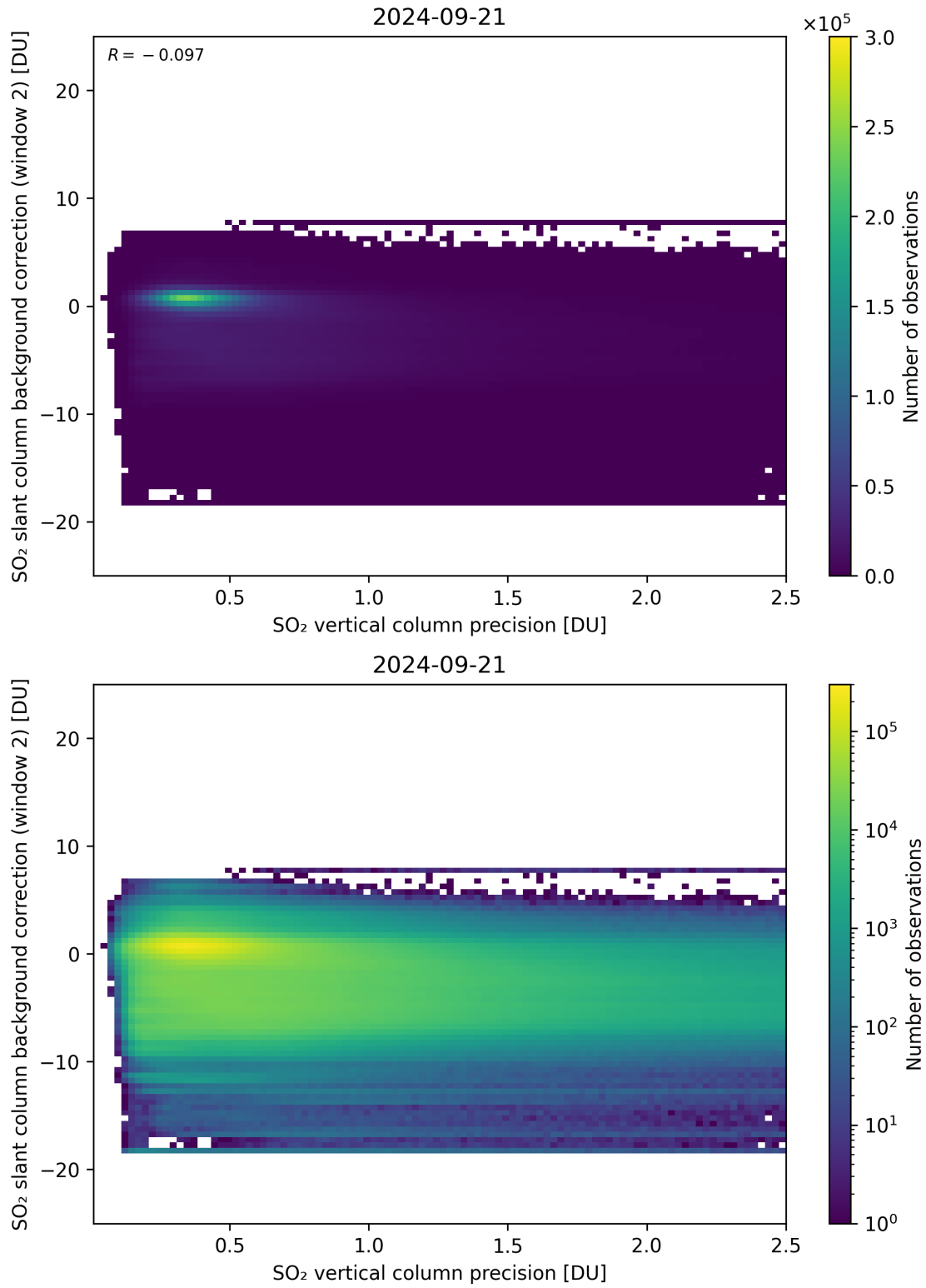
Figure 280: Scatter density plot of “SO 2 vertical column precision” against “SO 2 slant column background correction (window 2)” for 2024-09-20 to 2024-09-22.
