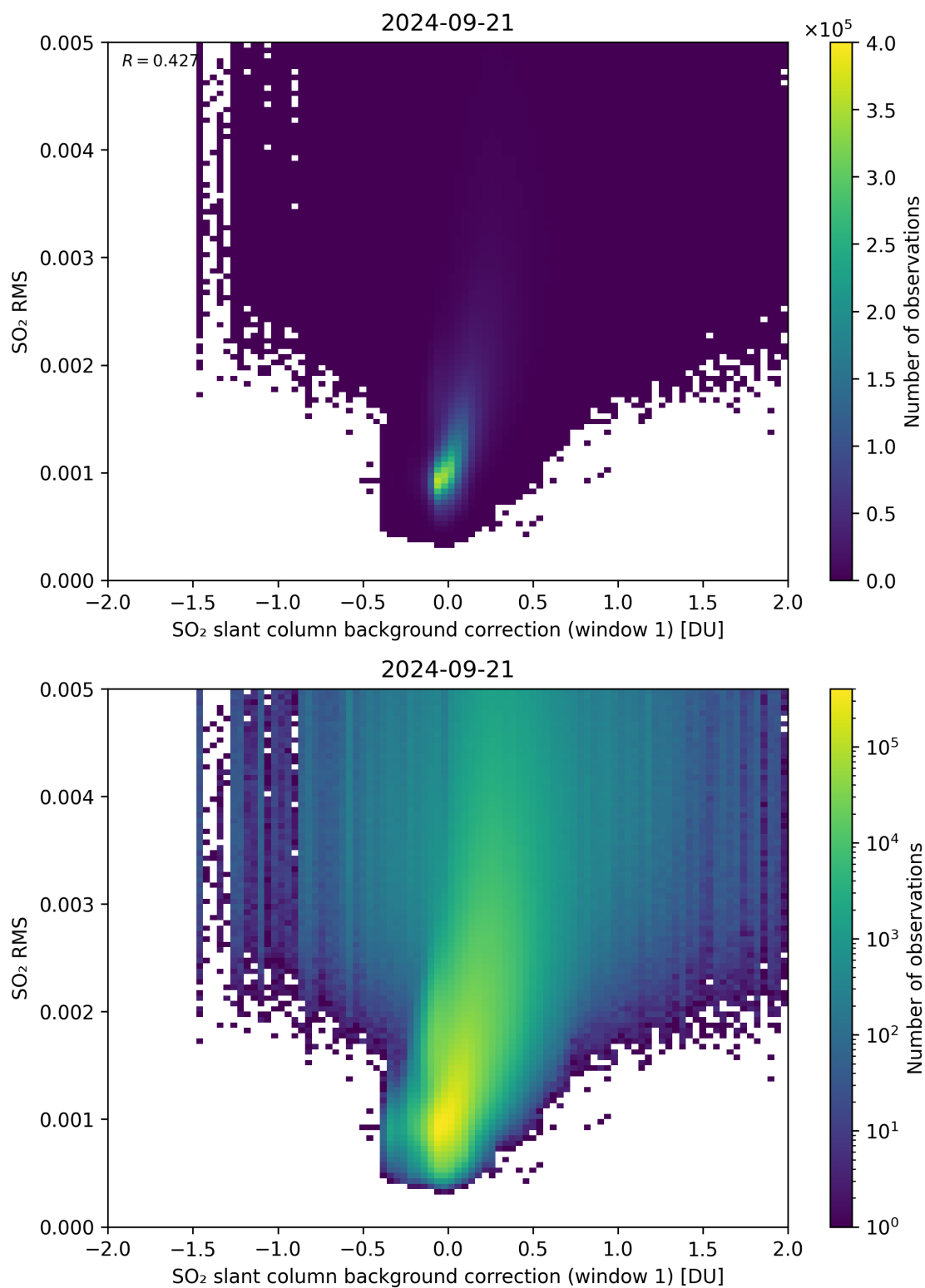
Figure 102: Scatter density plot of “SO 2 slant column background correction (window 1)” against “SO 2 RMS” for 2024-09-20 to 2024-09-22.
