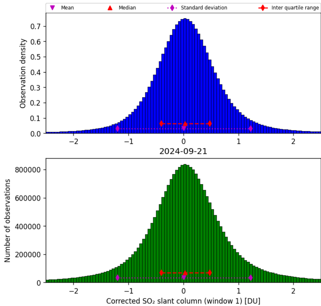
Figure 58: Histogram of “Corrected SO 2 slant column (window 1)” for 2024-09-20 to 2024-09-22
