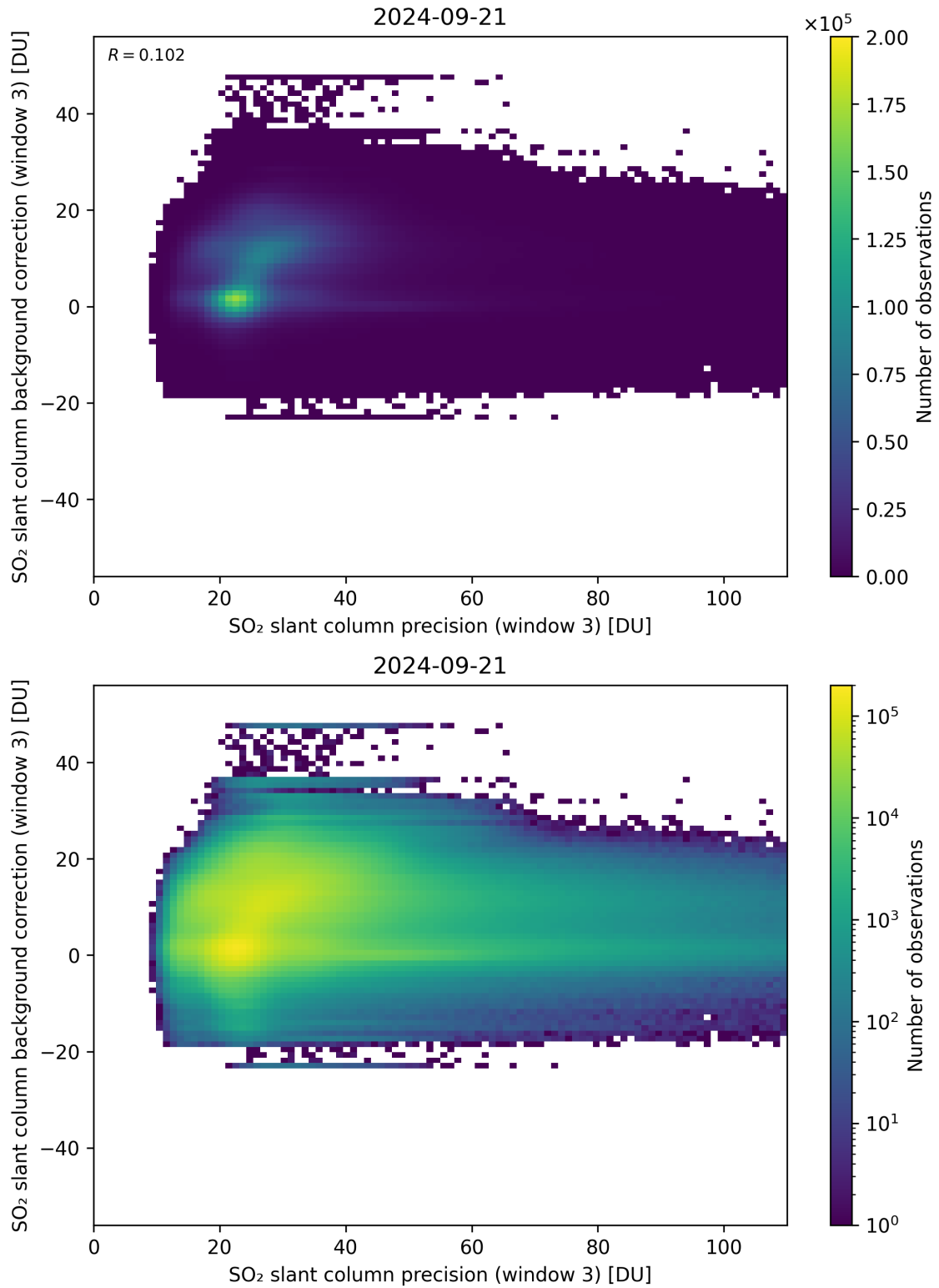
Figure 257: Scatter density plot of “SO 2 slant column precision (window 3)” against “SO 2 slant column background correction (window 3)” for 2024-09-20 to 2024-09-22.
