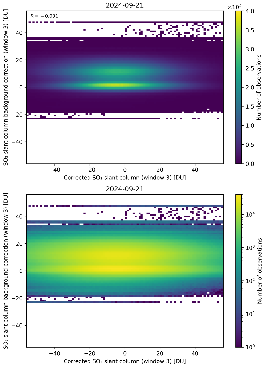
Figure 205: Scatter density plot of “Corrected SO 2 slant column (window 3)” against “SO 2 slant column background correction (window 3)” for 2024-09-20 to 2024-09-22.
