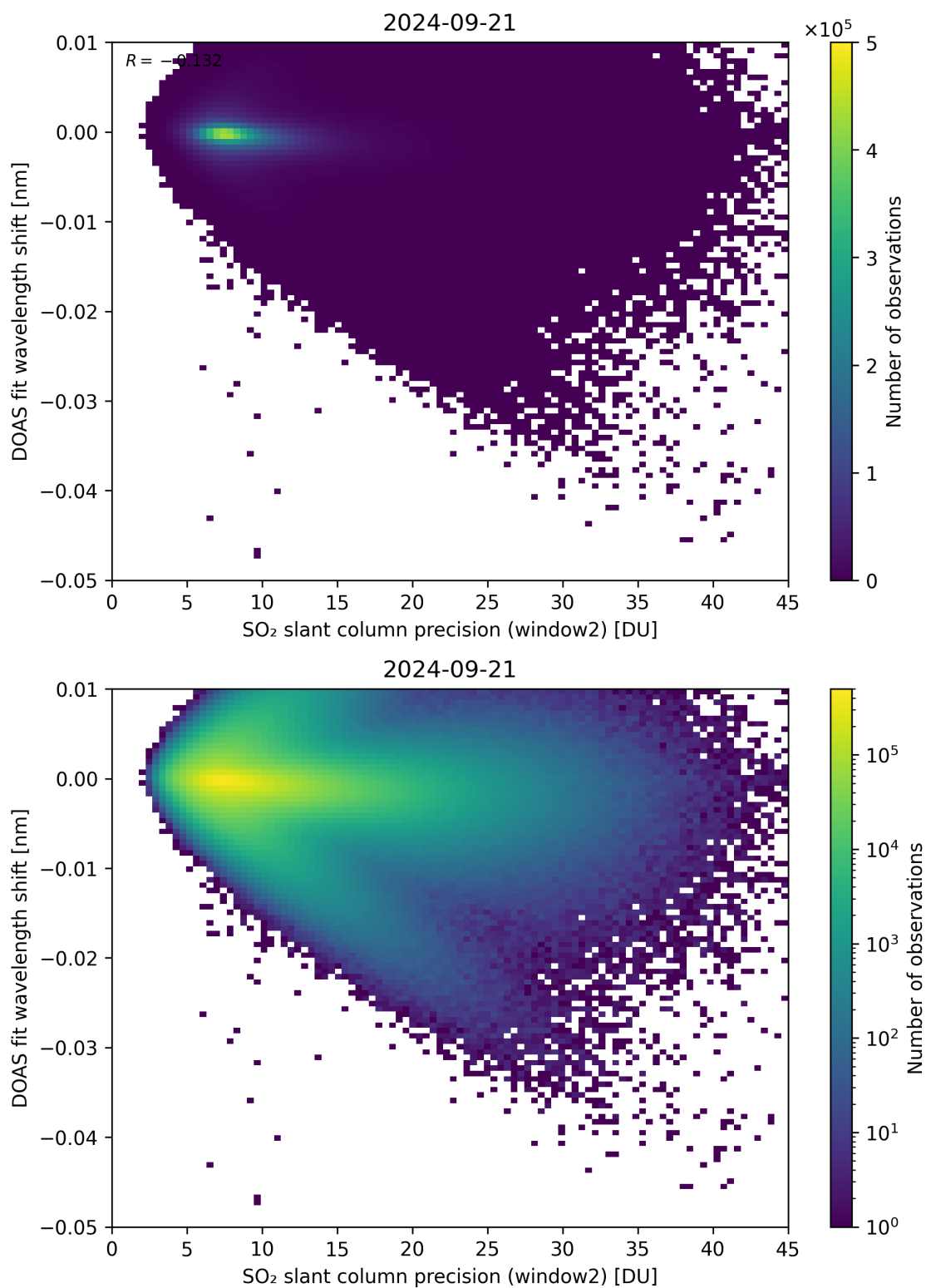
Figure 243: Scatter density plot of “SO 2 slant column precision (window2)” against “DOAS fit wavelength shift” for 2024-09-20 to 2024-09-22.
