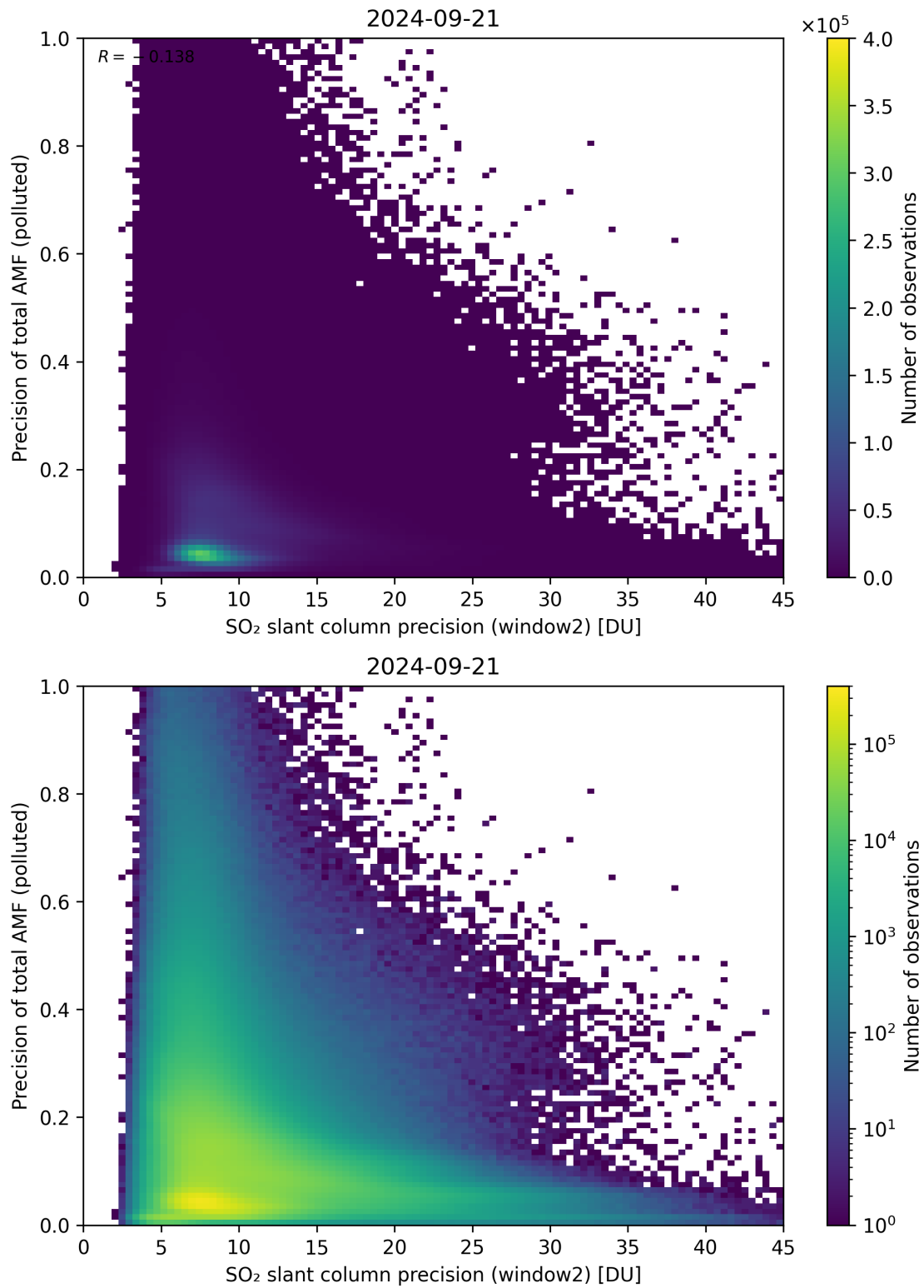
Figure 252: Scatter density plot of “SO 2 slant column precision (window2)” against “Precision of total AMF (polluted)” for 2024-09-20 to 2024-09-22.
