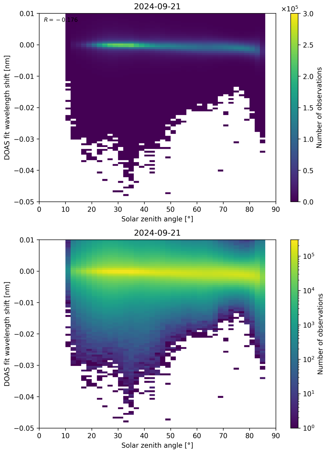
Figure 161: Scatter density plot of “Solar zenith angle” against “DOAS fit wavelength shift” for 2024-09-20 to 2024-09-22.
