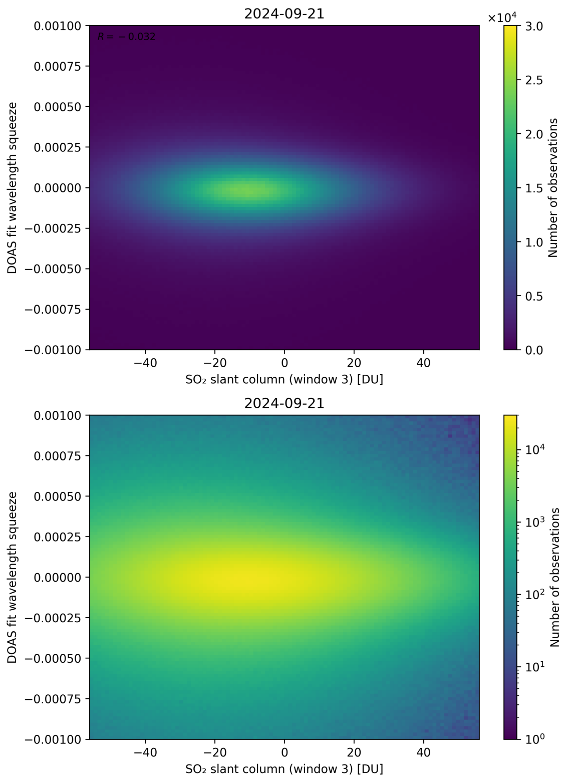
Figure 255: Scatter density plot of “SO 2 slant column (window 3)” against “DOAS fit wavelength squeeze” for 2024-09-20 to 2024-09-22.
