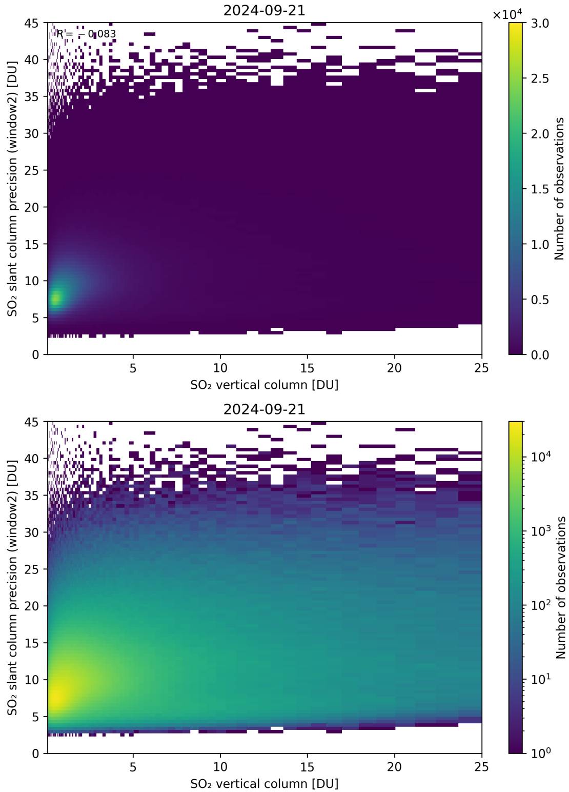
Figure 302: Scatter density plot of “SO 2 vertical column” against “SO 2 slant column precision (window2)” for 2024-09-20 to 2024-09-22.
