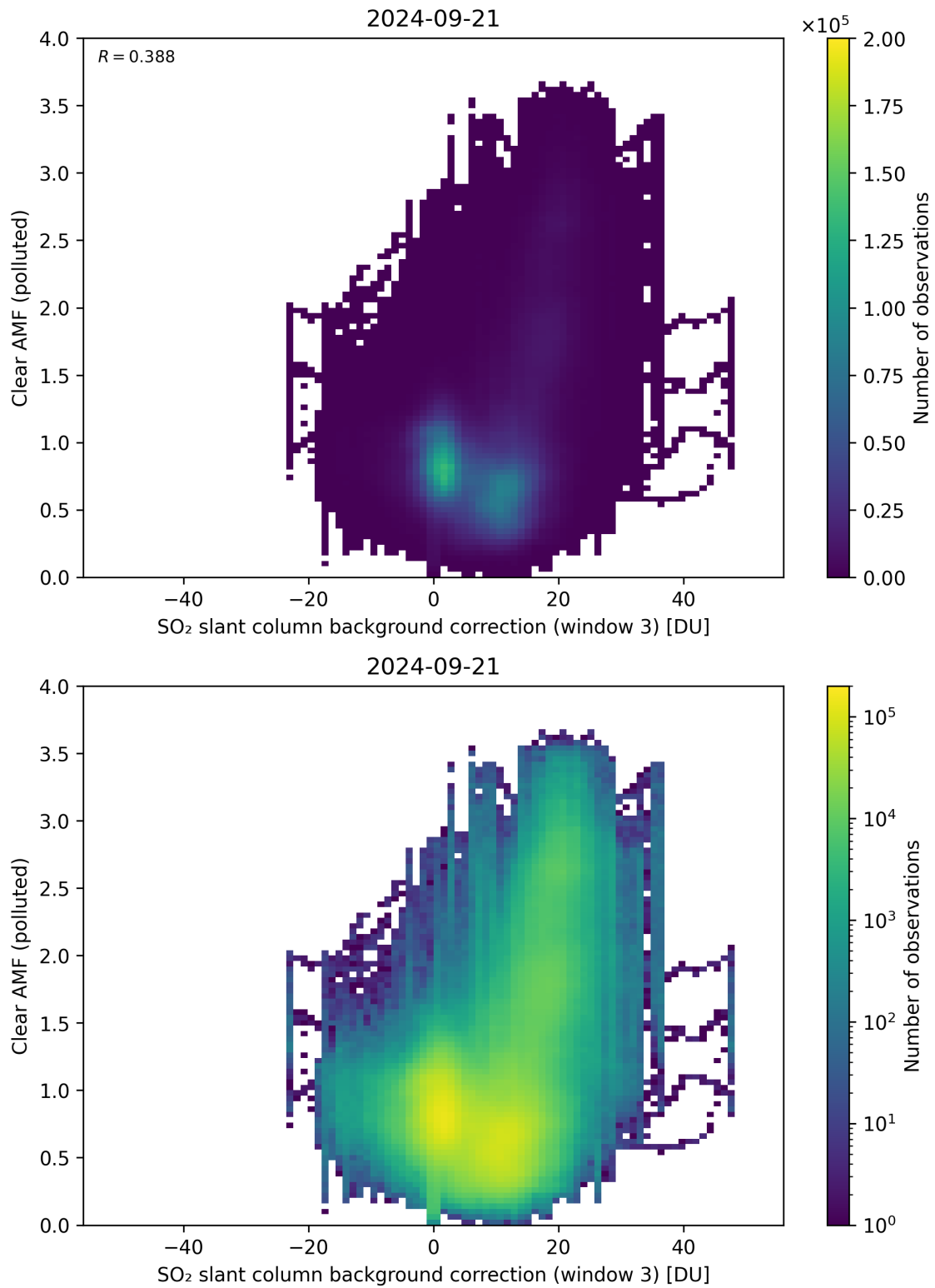
Figure 124: Scatter density plot of “SO 2 slant column background correction (window 3)” against “Clear AMF (polluted)” for 2024-09-20 to 2024-09-22.
