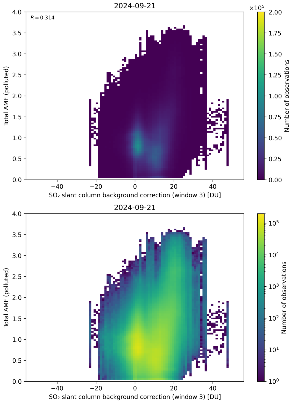
Figure 125: Scatter density plot of “SO 2 slant column background correction (window 3)” against “Total AMF (polluted)” for 2024-09-20 to 2024-09-22.
