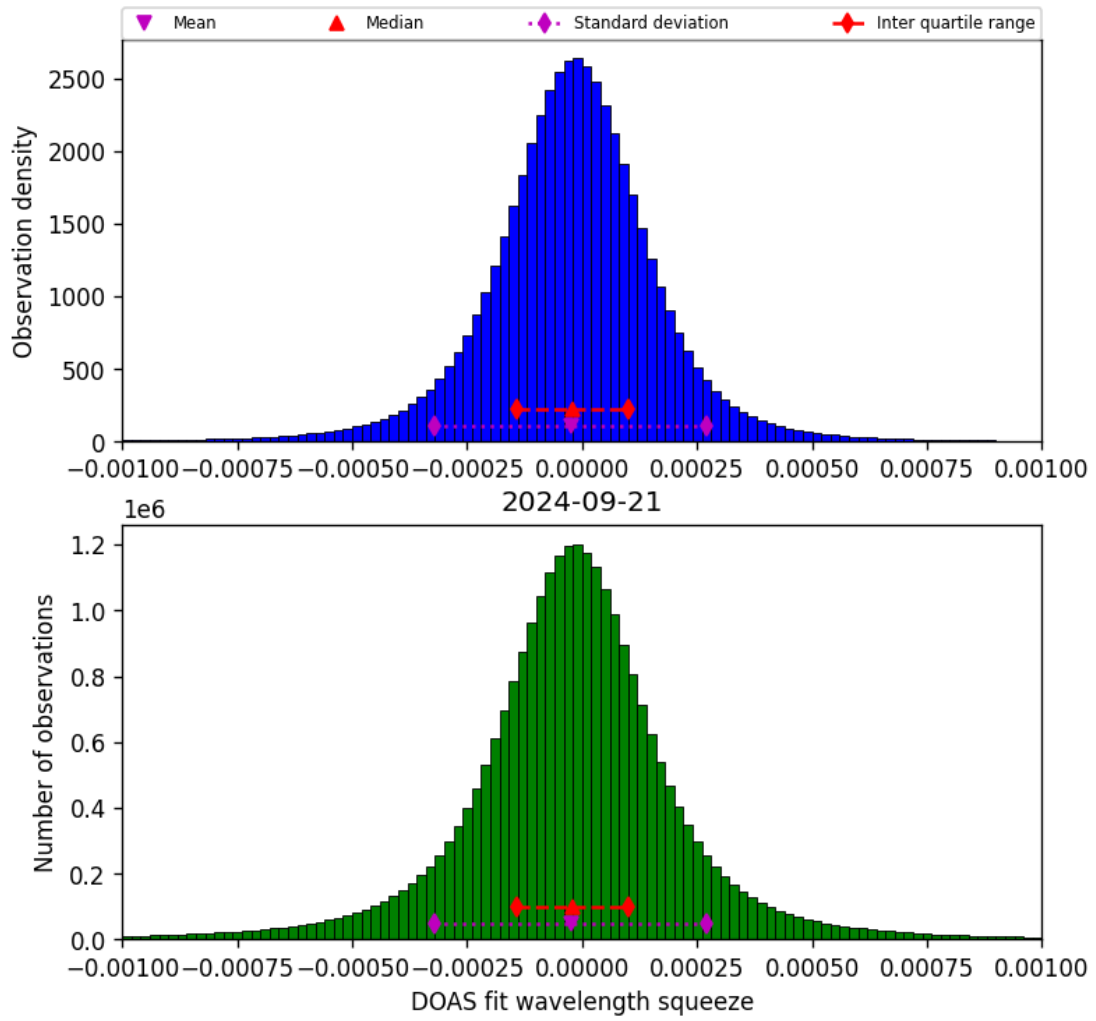
Figure 69: Histogram of “DOAS fit wavelength squeeze” for 2024-09-20 to 2024-09-22
