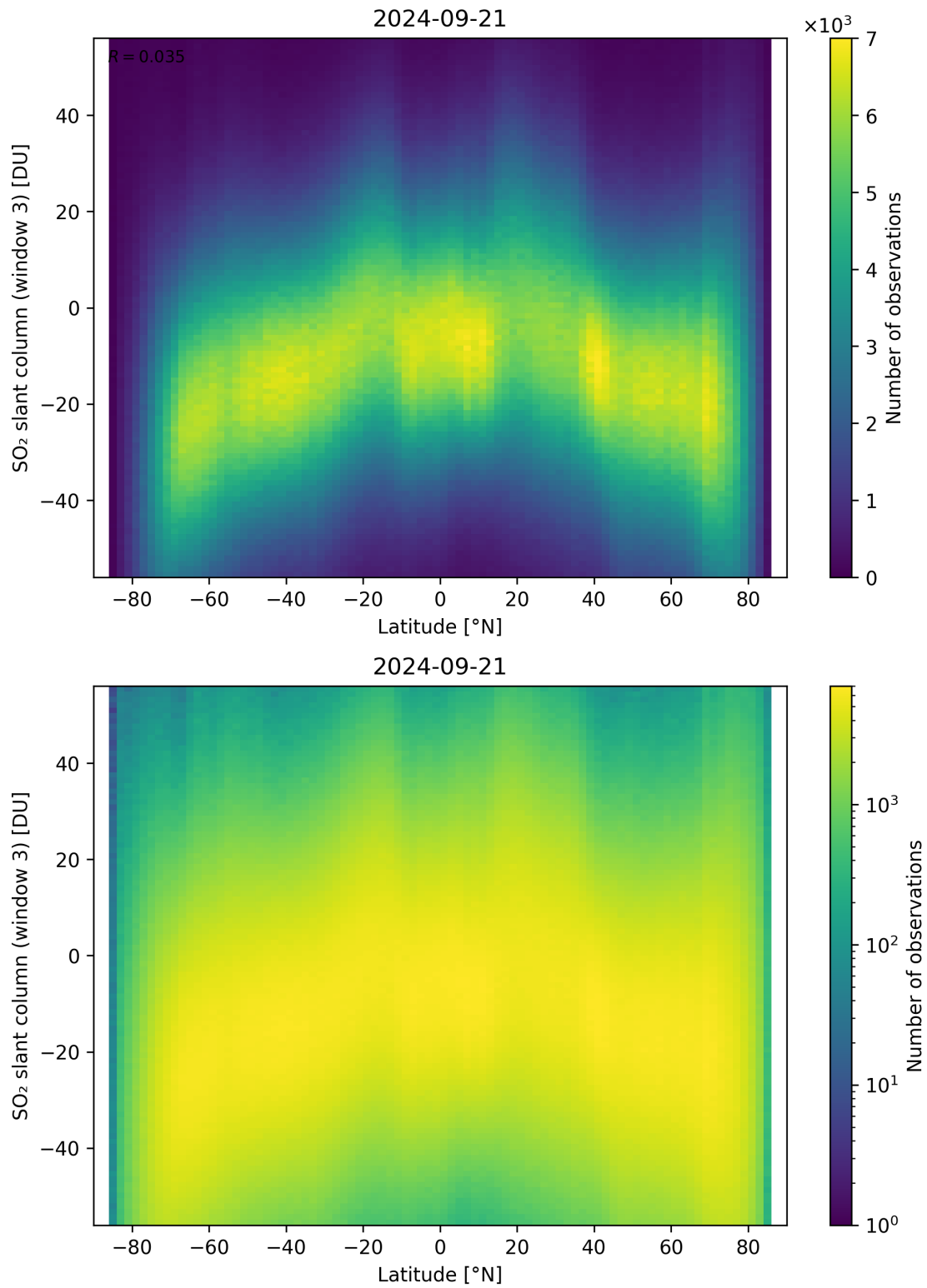
Figure 152: Scatter density plot of “Latitude” against “SO 2 slant column (window 3)” for 2024-09-20 to 2024-09-22.
