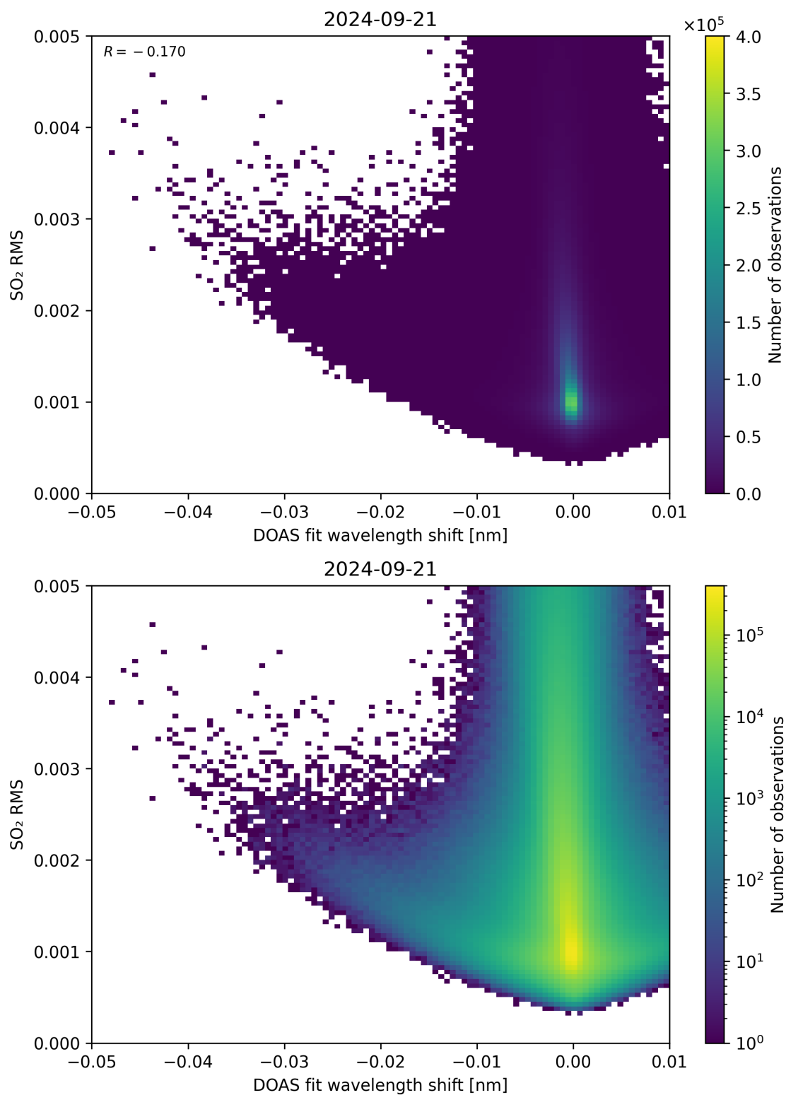
Figure 128: Scatter density plot of “DOAS fit wavelength shift” against “SO 2 RMS” for 2024-09-20 to 2024-09-22.
