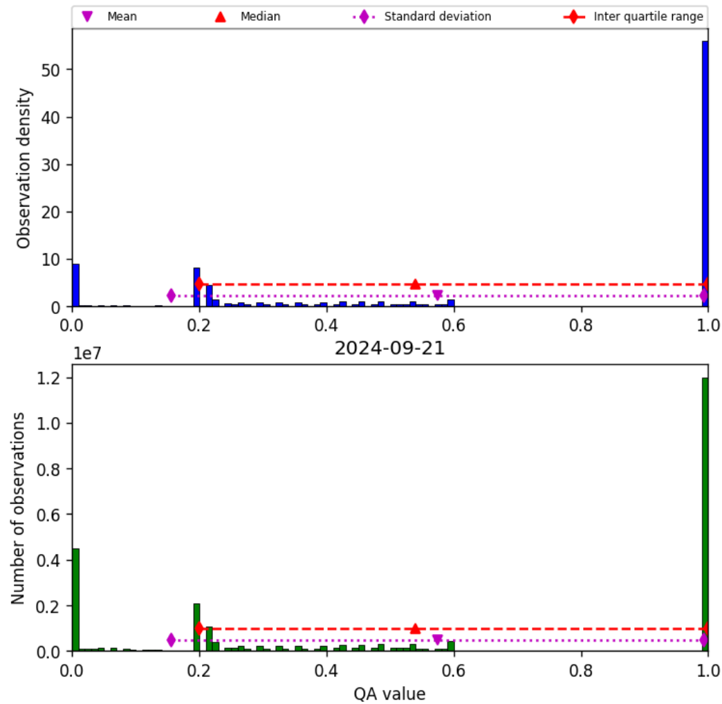
Figure 52: Histogram of “QA value” for 2024-09-20 to 2024-09-22
