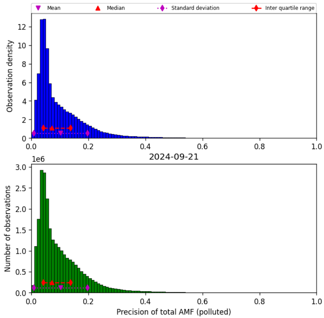
Figure 72: Histogram of “Precision of total AMF (polluted)” for 2024-09-20 to 2024-09-22
