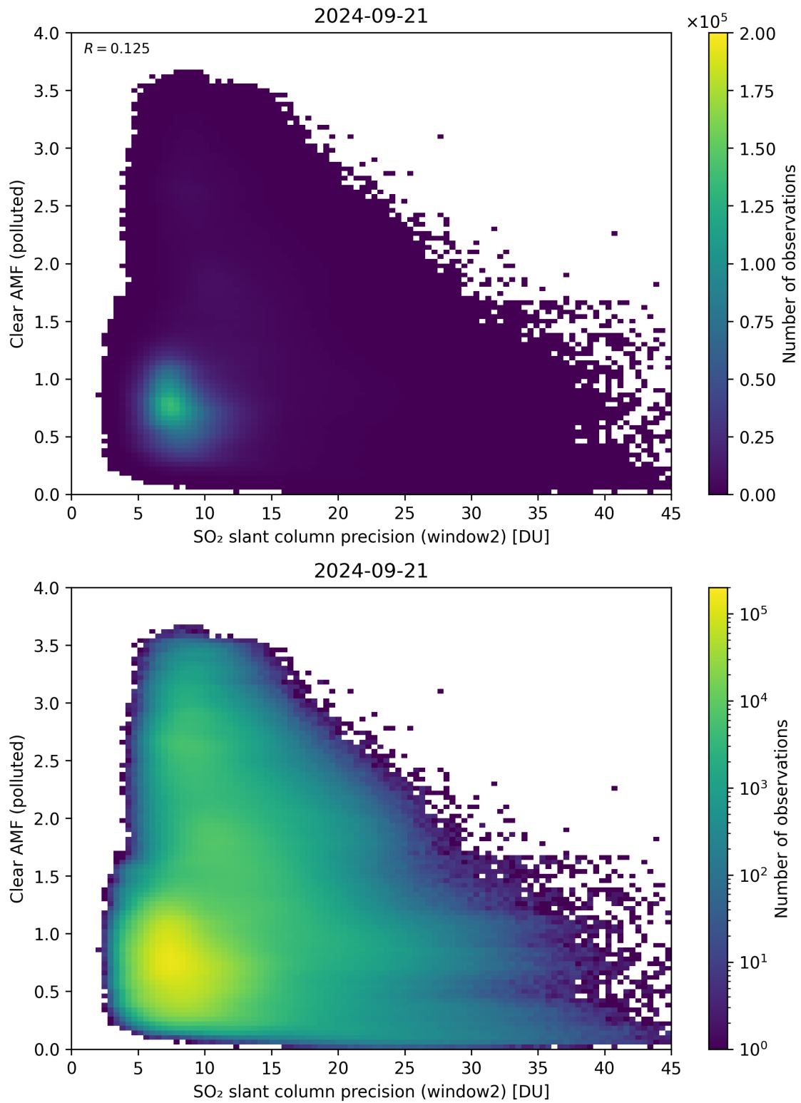
Figure 246: Scatter density plot of “SO 2 slant column precision (window2)” against “Clear AMF (polluted)” for 2024-09-20 to 2024-09-22.
