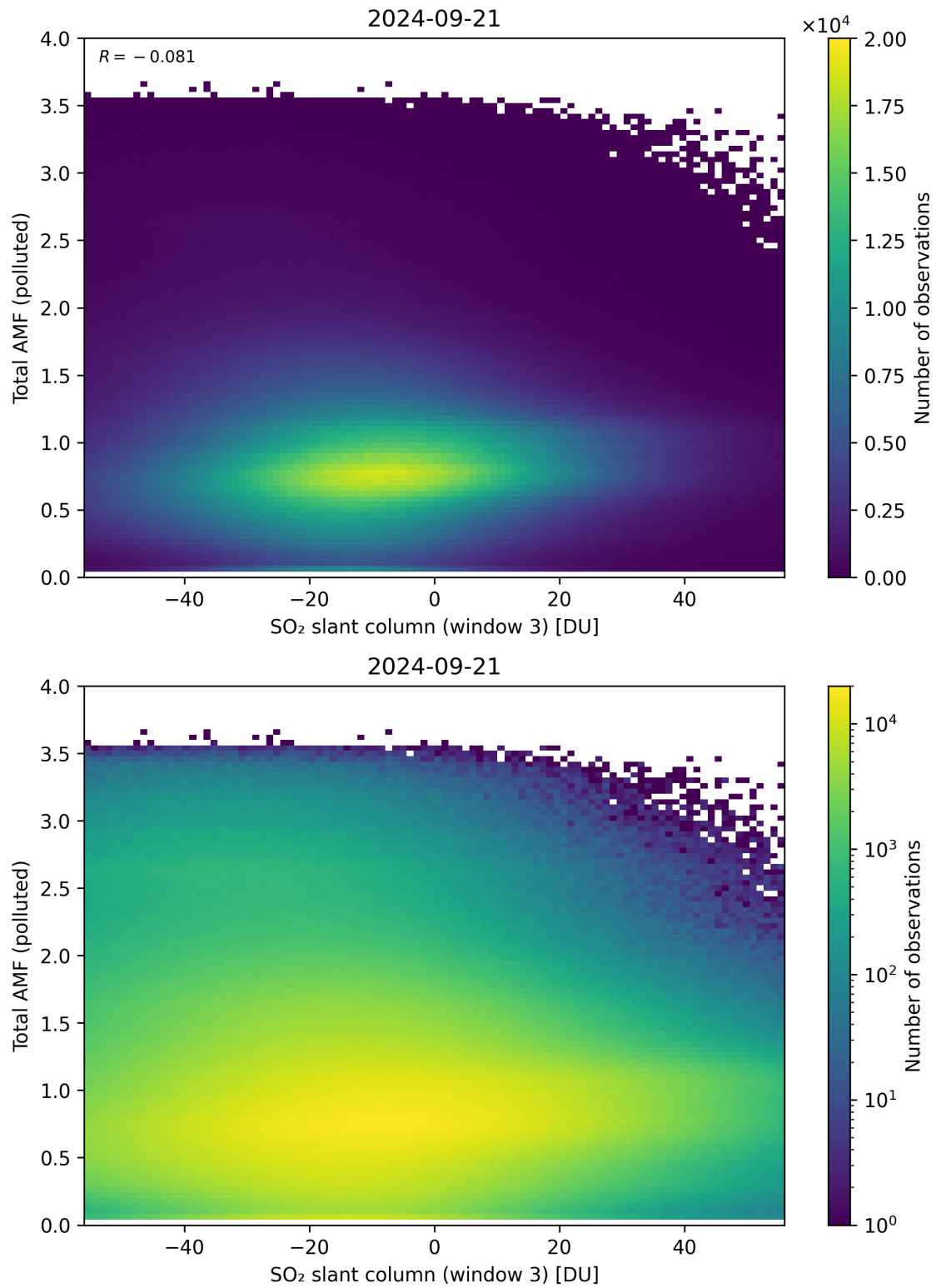
Figure 268: Scatter density plot of “SO 2 slant column (window 3)” against “Total AMF (polluted)” for 2024-09-20 to 2024-09-22.
