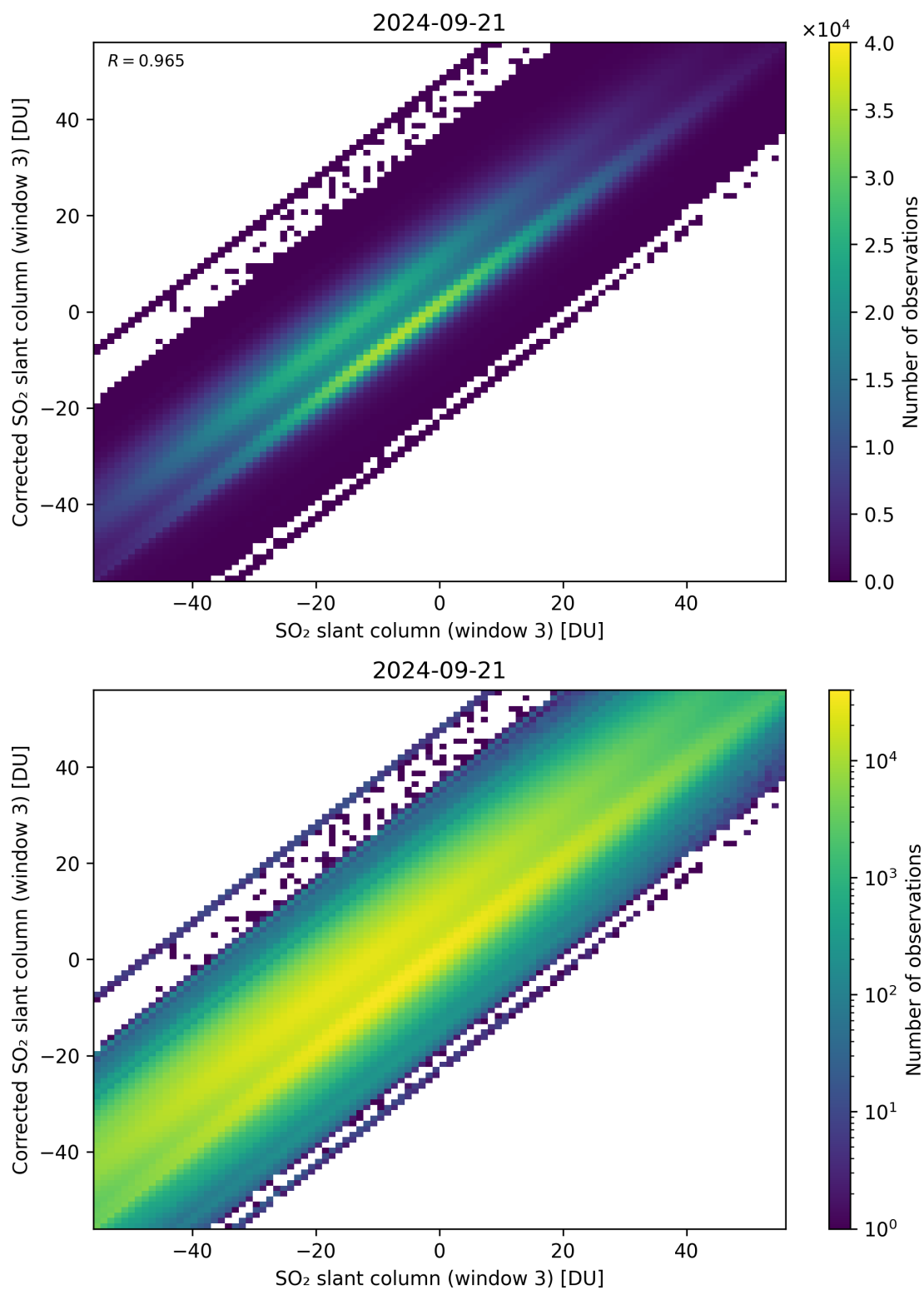
Figure 266: Scatter density plot of “SO 2 slant column (window 3)” against “Corrected SO 2 slant column (window 3)” for 2024-09-20 to 2024-09-22.
