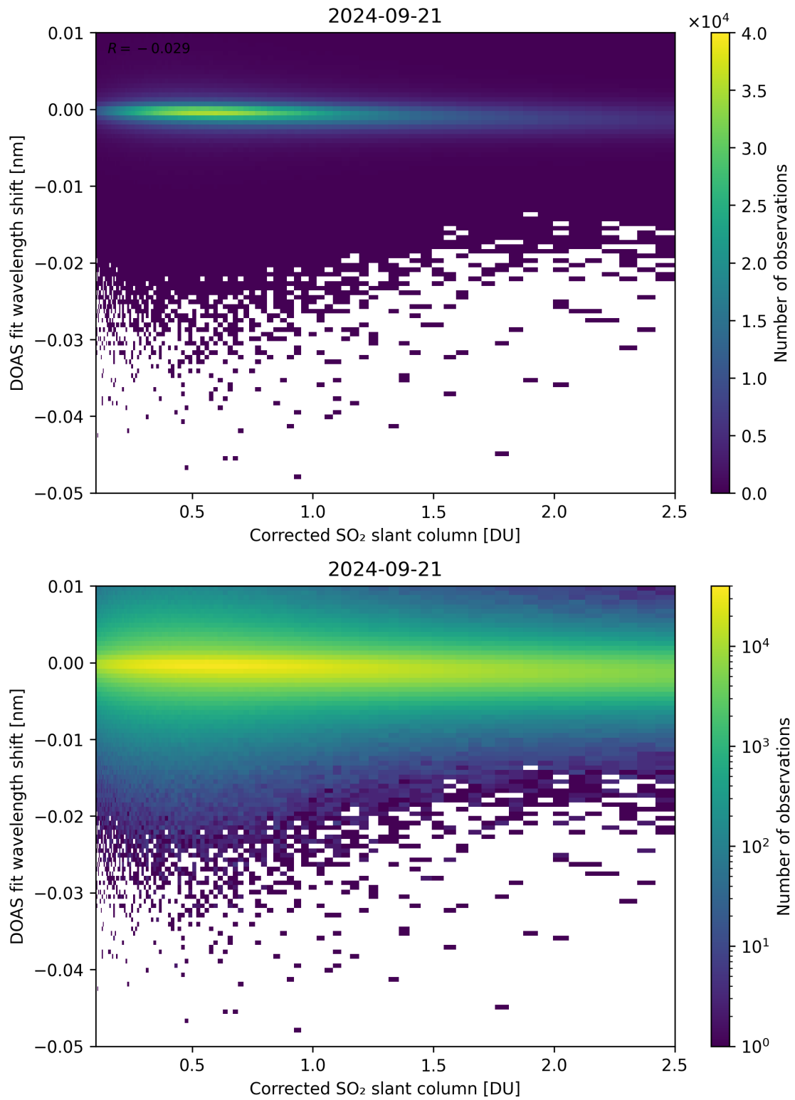
Figure 181: Scatter density plot of “Corrected SO 2 slant column” against “DOAS fit wavelength shift” for 2024-09-20 to 2024-09-22.
