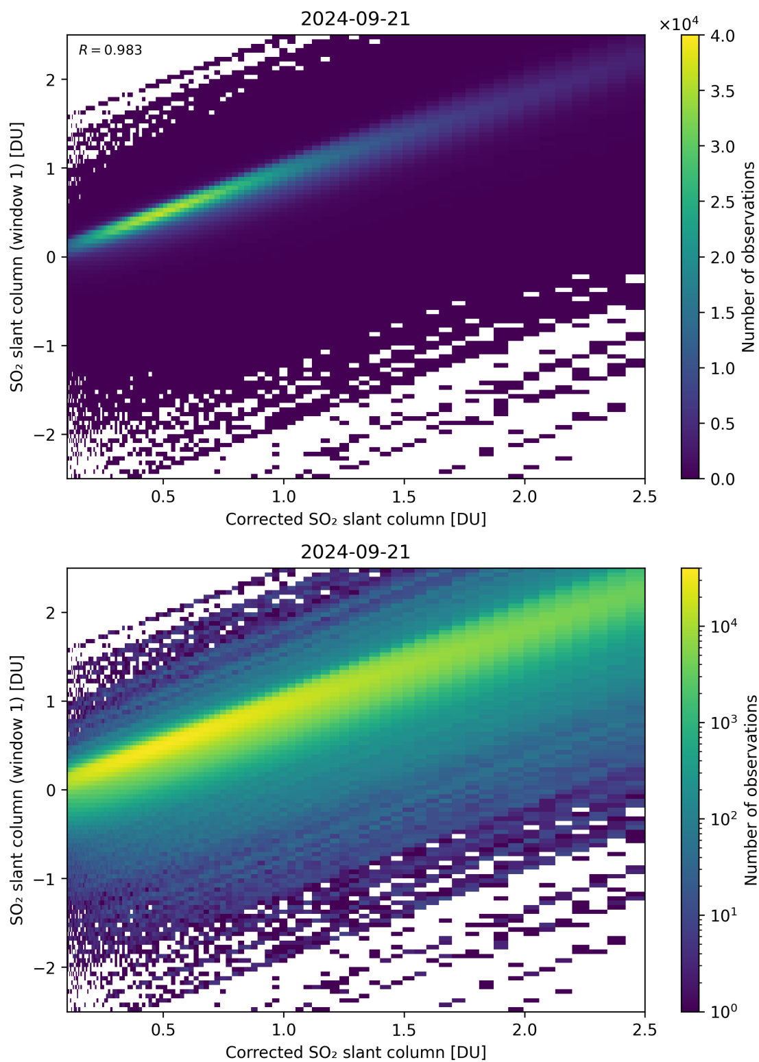
Figure 187: Scatter density plot of “Corrected SO 2 slant column” against “SO 2 slant column (window 1)” for 2024-09-20 to 2024-09-22.
