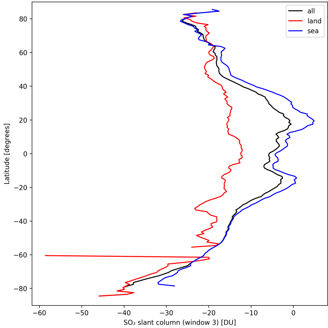
Figure 41: Zonal average of “SO 2 slant column (window 3)” for 2024-09-20 to 2024-09-22.
