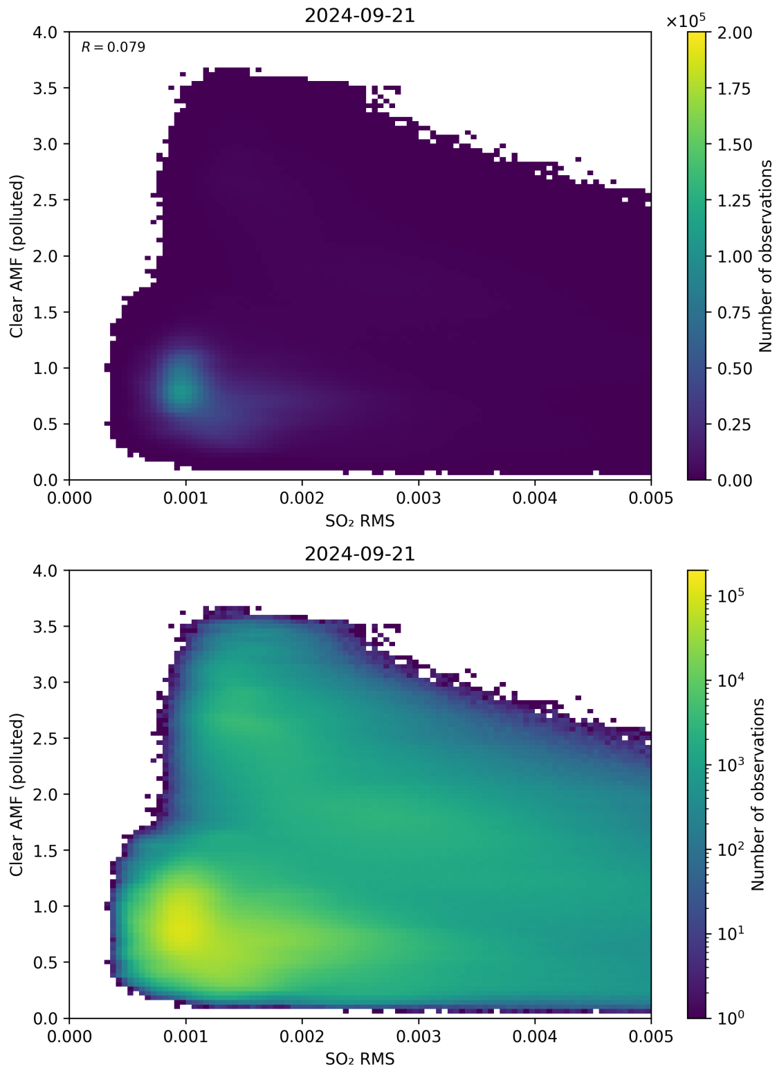
Figure 136: Scatter density plot of “SO 2 RMS” against “Clear AMF (polluted)” for 2024-09-20 to 2024-09-22.
