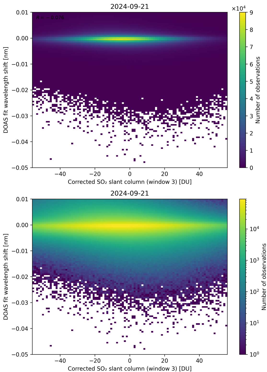
Figure 206: Scatter density plot of “Corrected SO 2 slant column (window 3)” against “DOAS fit wavelength shift” for 2024-09-20 to 2024-09-22.
