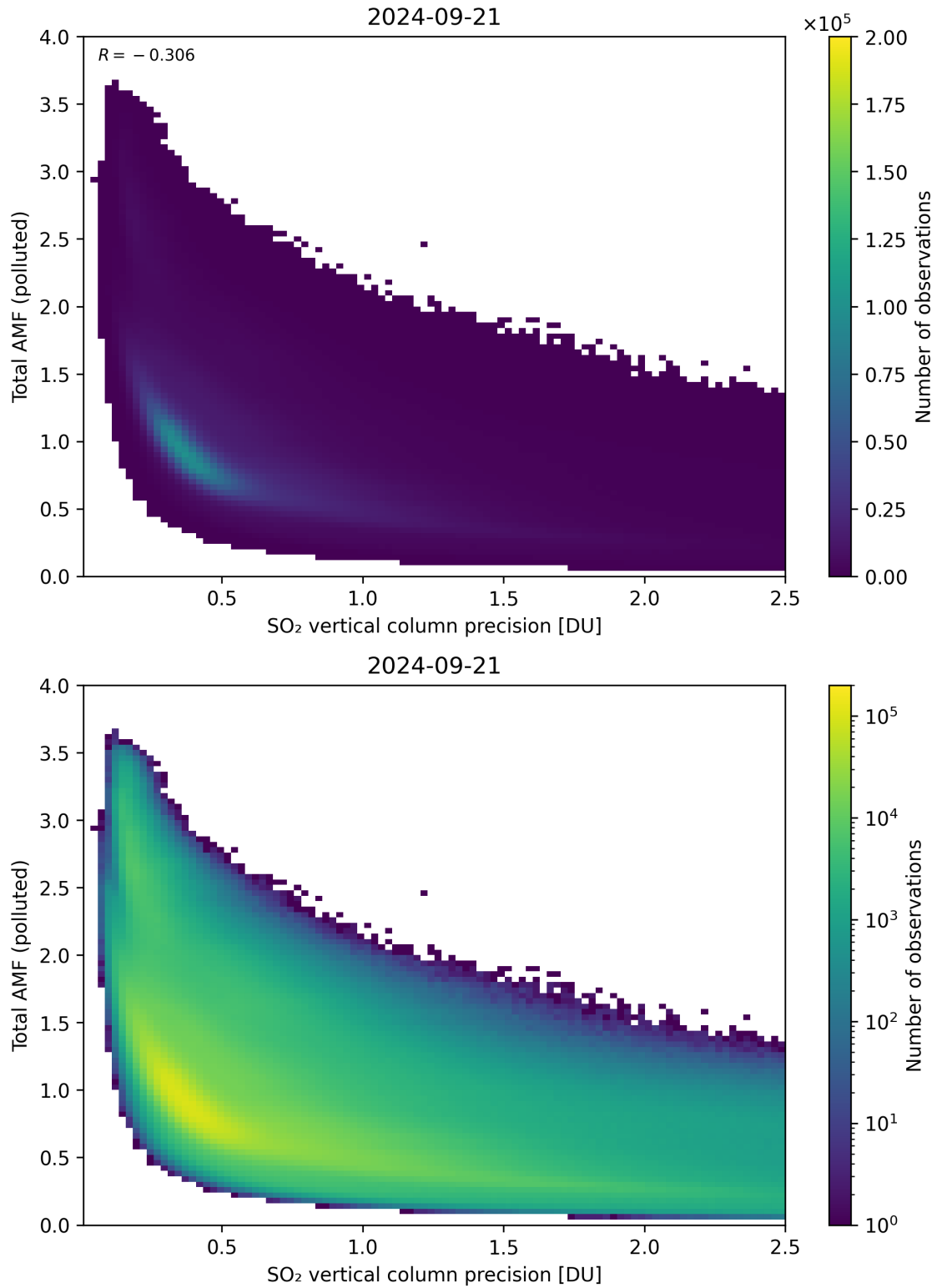
Figure 294: Scatter density plot of “SO 2 vertical column precision” against “Total AMF (polluted)” for 2024-09-20 to 2024-09-22.
