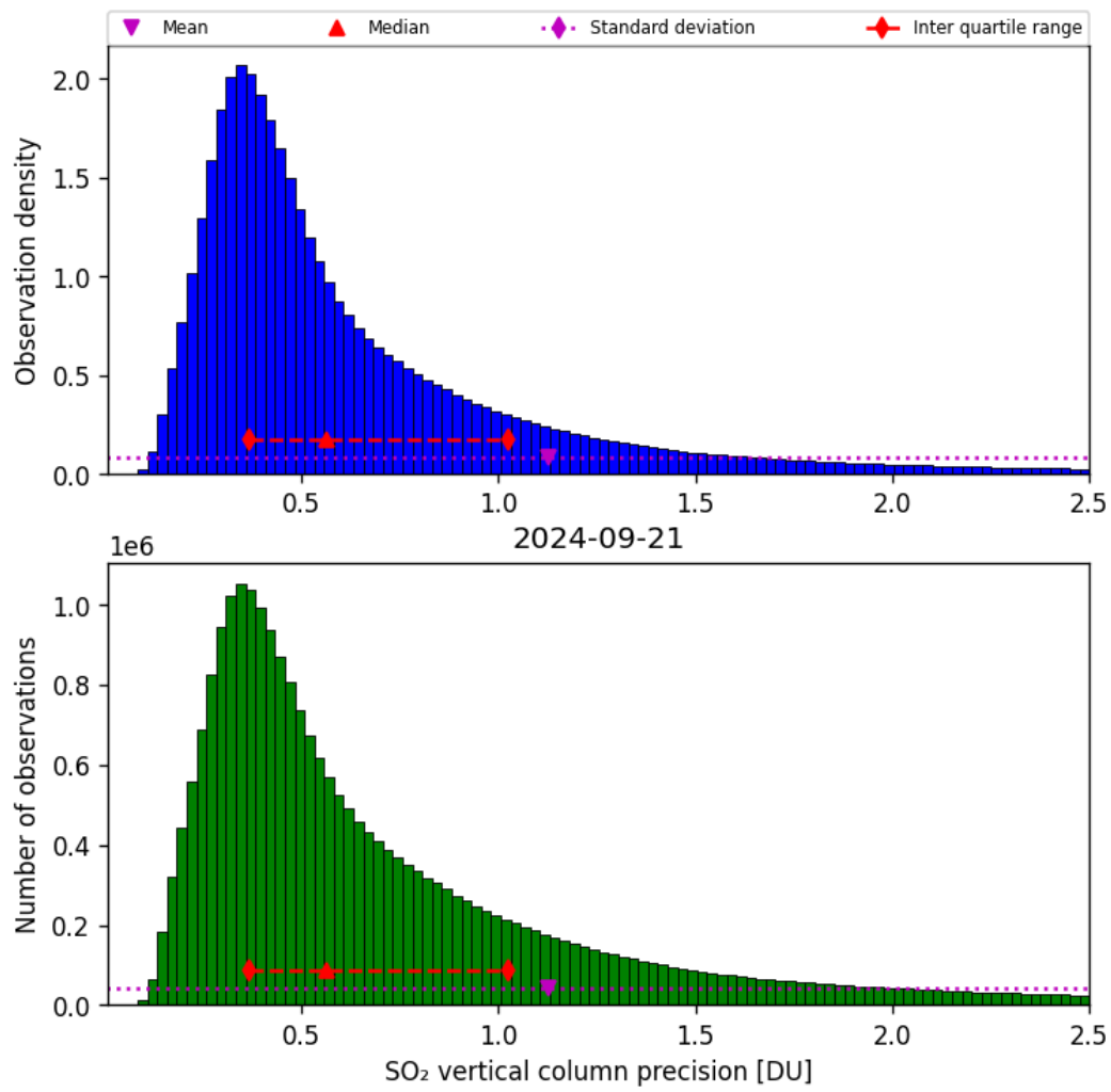
Figure 54: Histogram of “SO 2 vertical column precision” for 2024-09-20 to 2024-09-22
