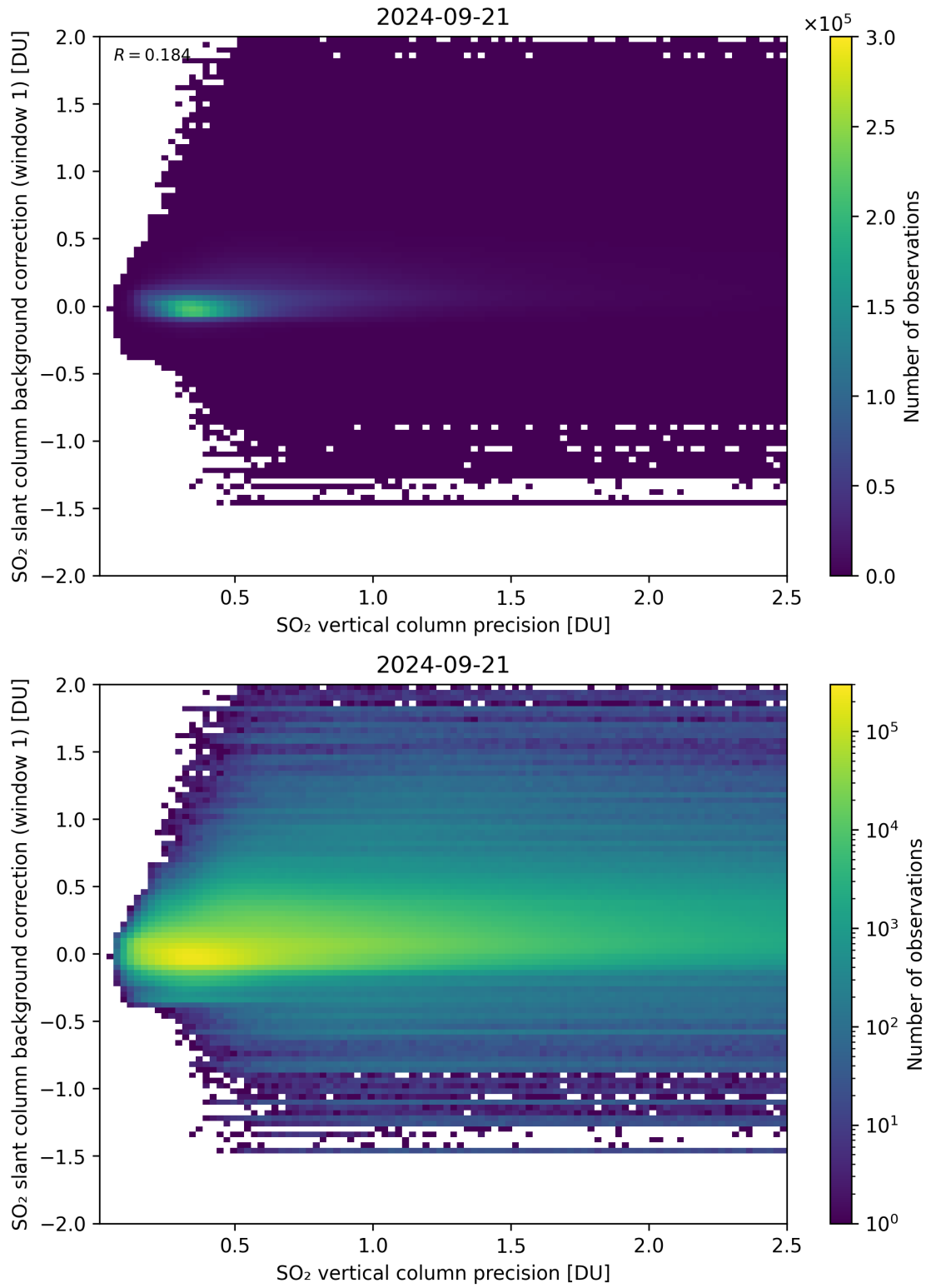
Figure 279: Scatter density plot of “SO 2 vertical column precision” against “SO 2 slant column background correction (window 1)” for 2024-09-20 to 2024-09-22.
