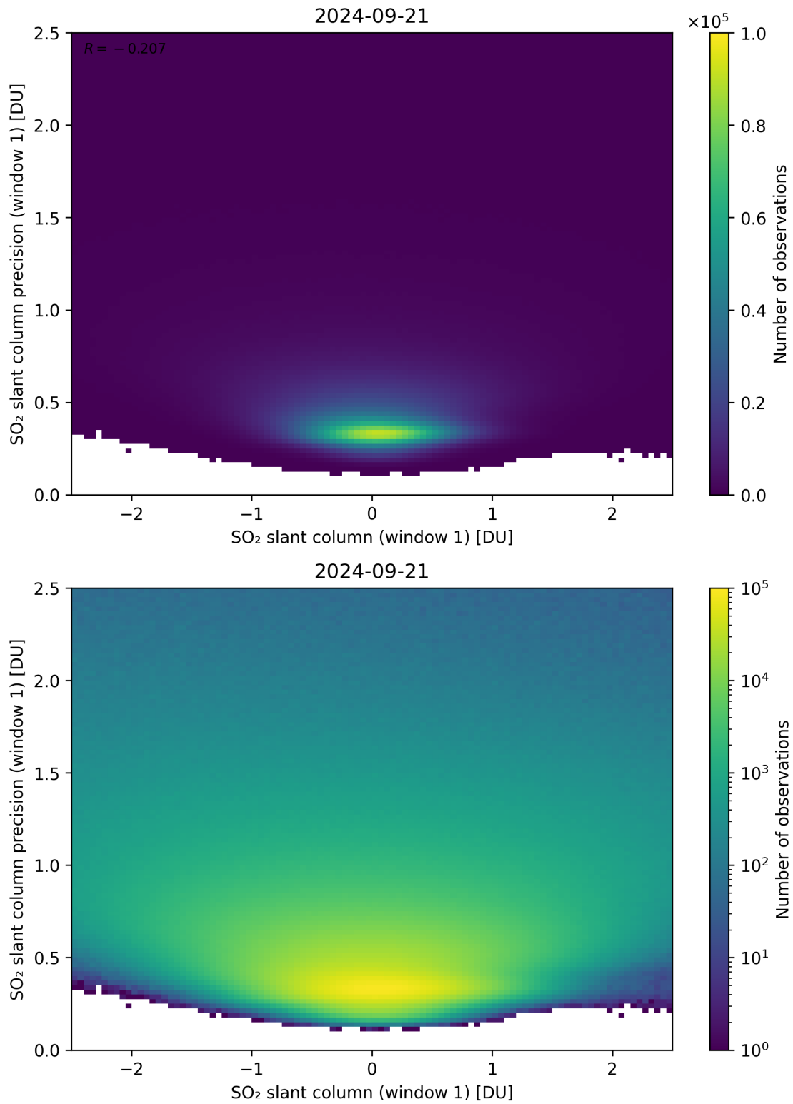
Figure 235: Scatter density plot of “SO 2 slant column (window 1)” against “SO 2 slant column precision (window 1)” for 2024-09-20 to 2024-09-22.
