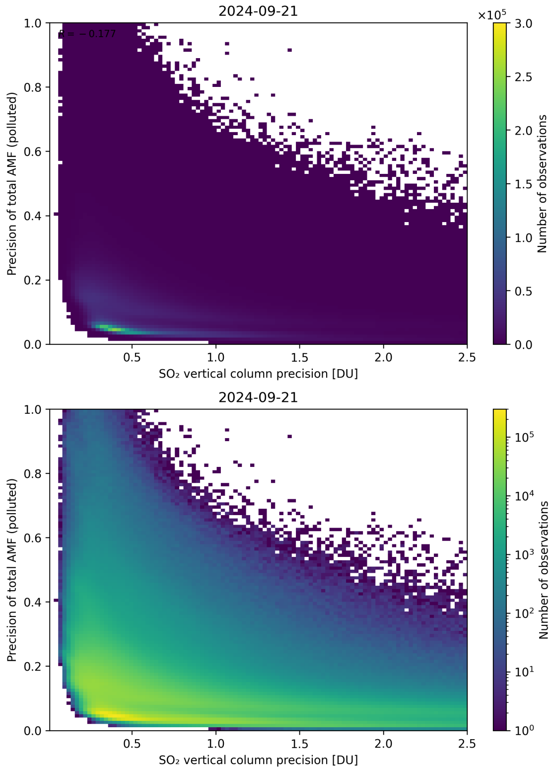
Figure 295: Scatter density plot of “SO 2 vertical column precision” against “Precision of total AMF (polluted)” for 2024-09-20 to 2024-09-22.
