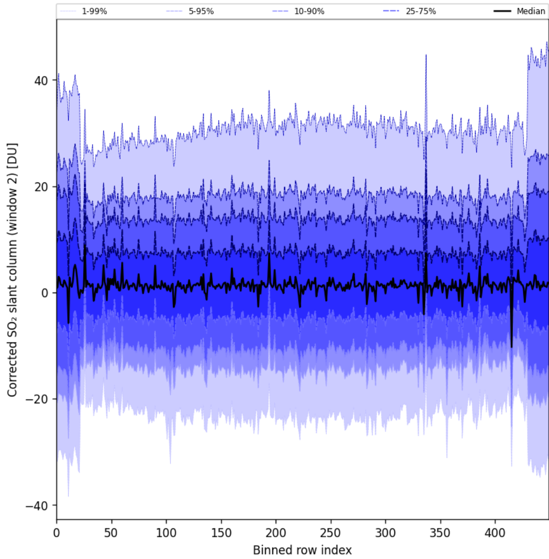
Figure 85: Along track statistics of “Corrected SO 2 slant column (window 2)” for 2024-09-20 to 2024-09-22
