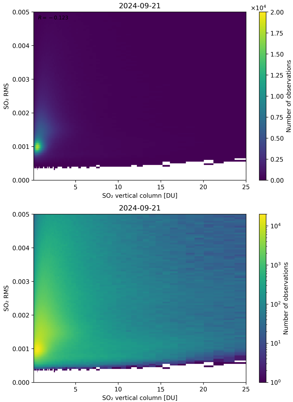
Figure 278: Scatter density plot of “SO 2 vertical column” against “SO 2 RMS” for 2024-09-20 to 2024-09-22.
