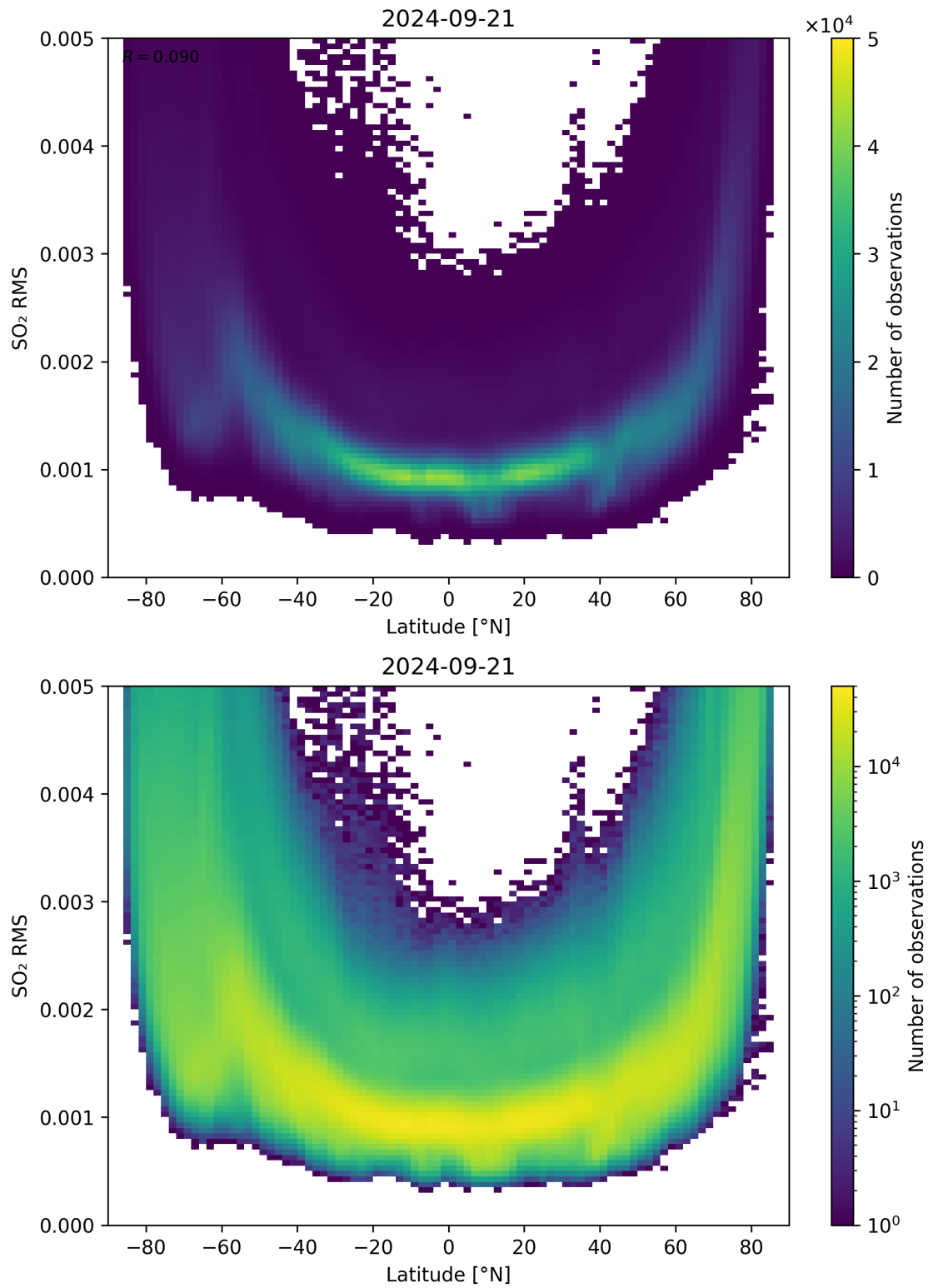
Figure 144: Scatter density plot of “Latitude” against “SO 2 RMS” for 2024-09-20 to 2024-09-22.
