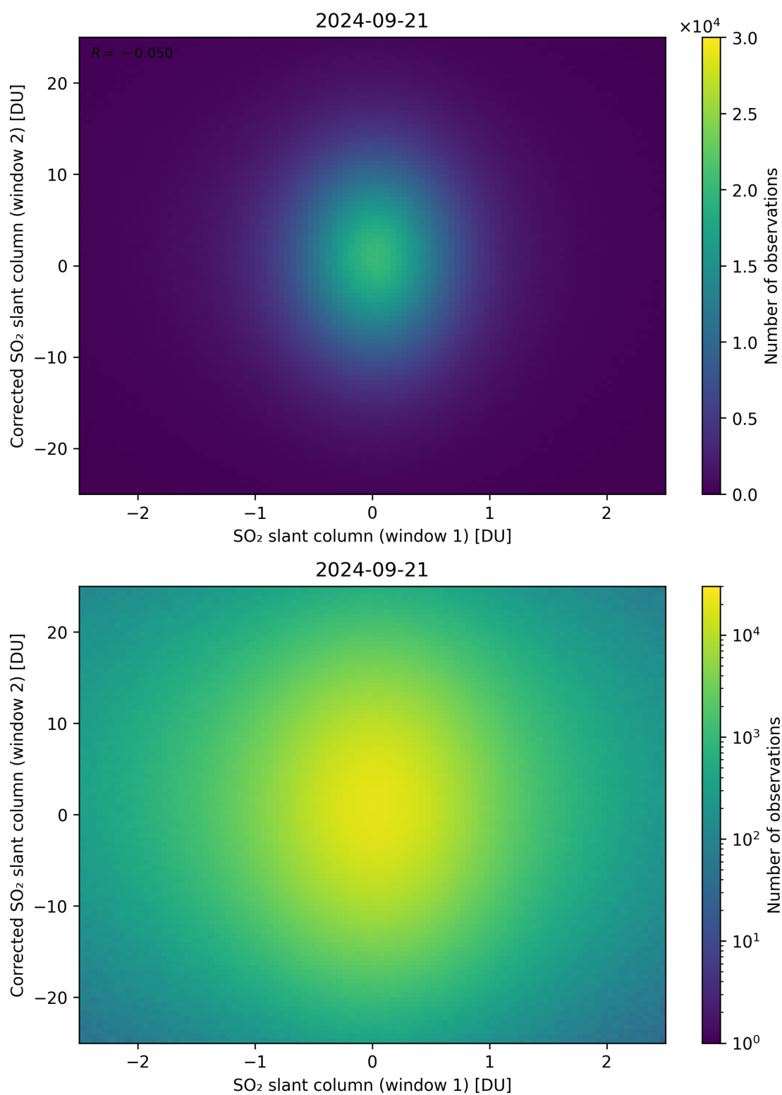
Figure 233: Scatter density plot of “SO 2 slant column (window 1)” against “Corrected SO 2 slant column (window 2)” for 2024-09-20 to 2024-09-22.
