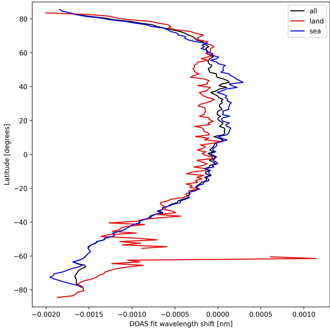
Figure 45: Zonal average of “DOAS fit wavelength shift” for 2024-09-20 to 2024-09-22.
