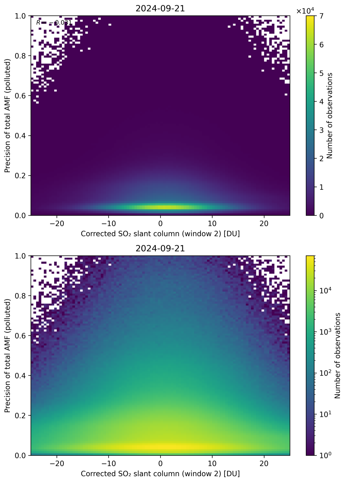
Figure 204: Scatter density plot of “Corrected SO 2 slant column (window 2)” against “Precision of total AMF (polluted)” for 2024-09-20 to 2024-09-22.
