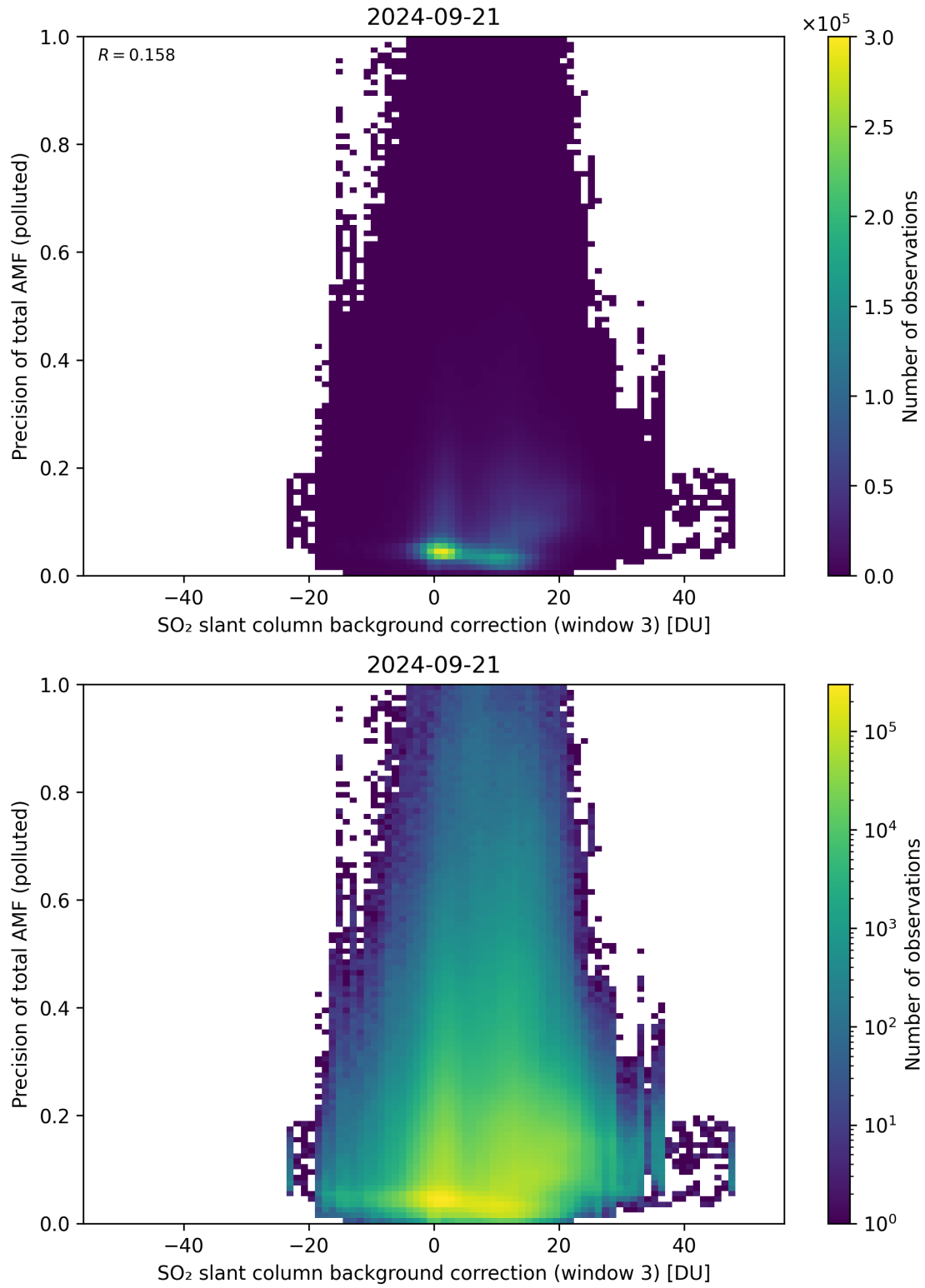
Figure 126: Scatter density plot of “SO 2 slant column background correction (window 3)” against “Precision of total AMF (polluted)” for 2024-09-20 to 2024-09-22.
