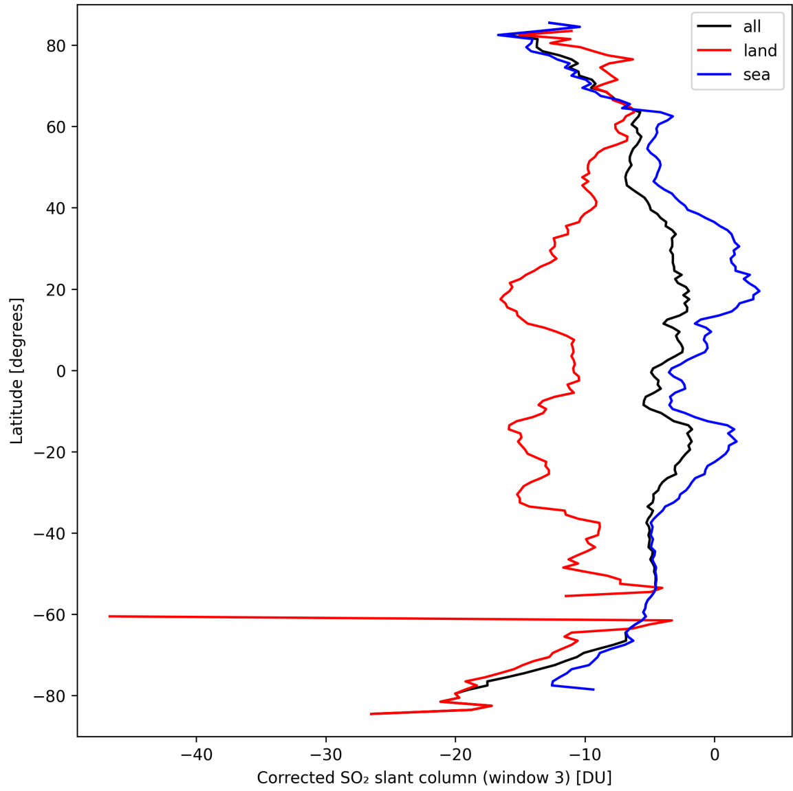
Figure 43: Zonal average of “Corrected SO 2 slant column (window 3)” for 2024-09-20 to 2024-09-22.
