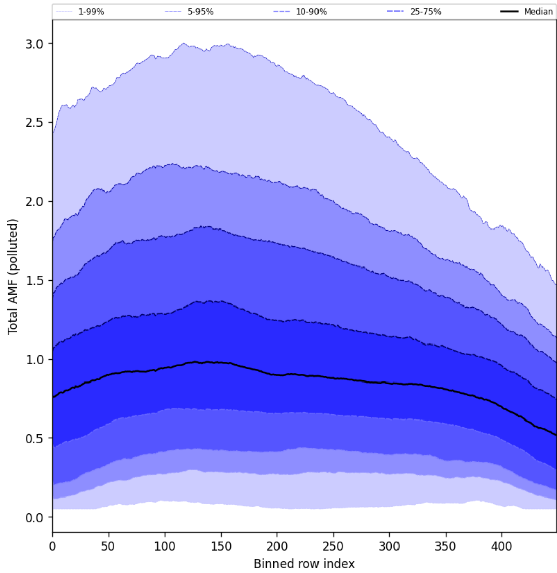
Figure 94: Along track statistics of “Total AMF (polluted)” for 2024-09-20 to 2024-09-22
