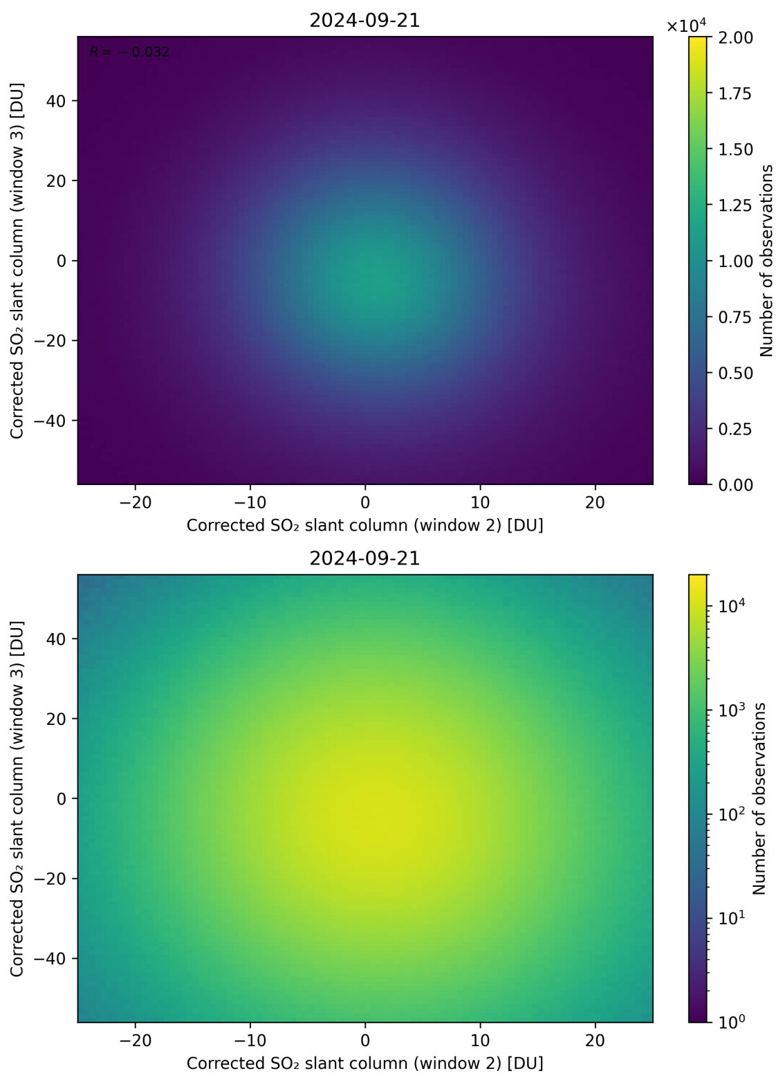
Figure 200: Scatter density plot of “Corrected SO 2 slant column (window 2)” against “Corrected SO 2 slant column (window 3)” for 2024-09-20 to 2024-09-22.
