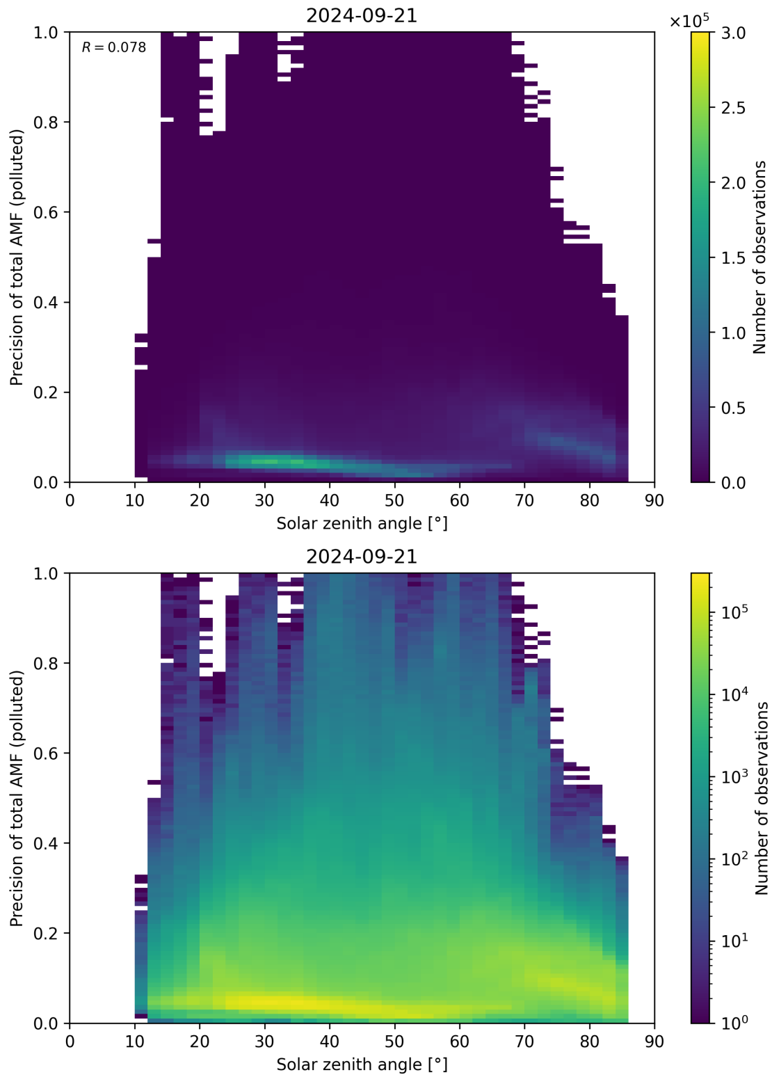
Figure 175: Scatter density plot of “Solar zenith angle” against “Precision of total AMF (polluted)” for 2024-09-20 to 2024-09-22.
