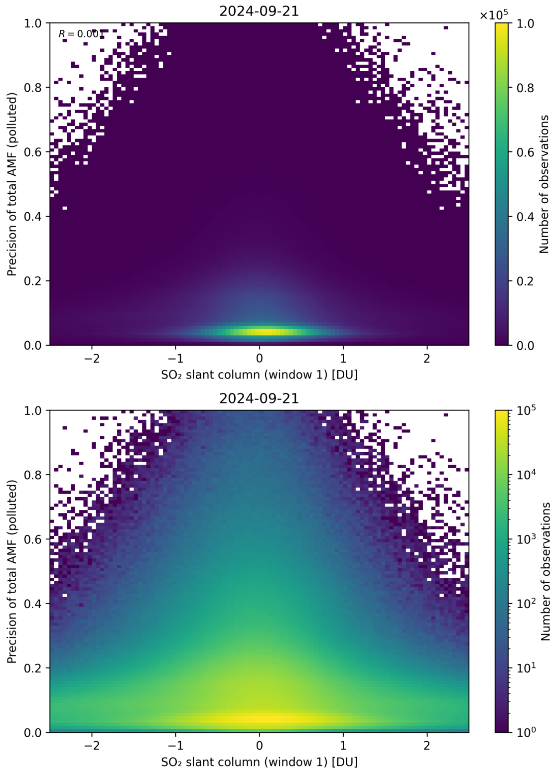
Figure 240: Scatter density plot of “SO 2 slant column (window 1)” against “Precision of total AMF (polluted)” for 2024-09-20 to 2024-09-22.
