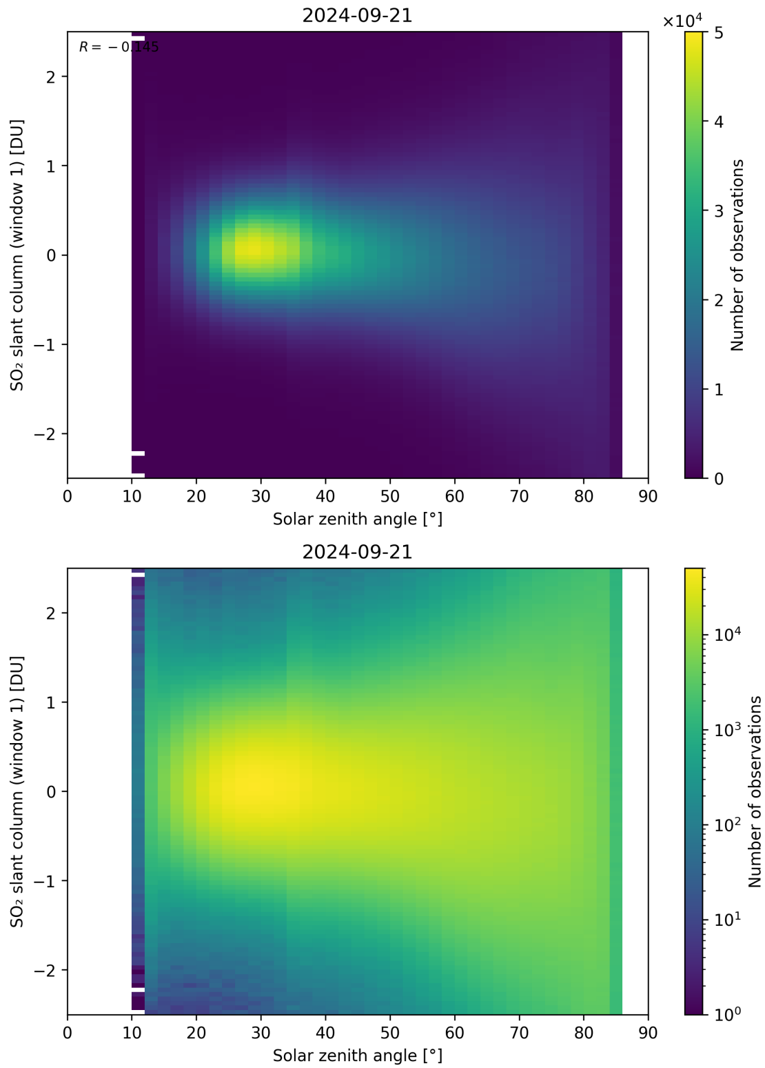
Figure 169: Scatter density plot of “Solar zenith angle” against “SO 2 slant column (window 1)” for 2024-09-20 to 2024-09-22.
