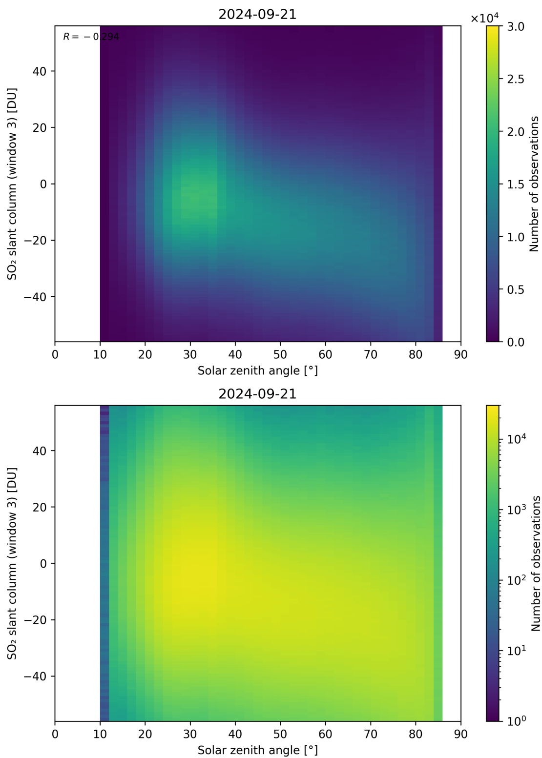
Figure 172: Scatter density plot of “Solar zenith angle” against “SO 2 slant column (window 3)” for 2024-09-20 to 2024-09-22.
