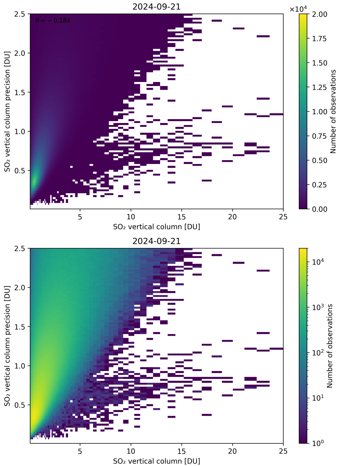
Figure 307: Scatter density plot of “SO 2 vertical column” against “SO 2 vertical column precision” for 2024-09-20 to 2024-09-22.
