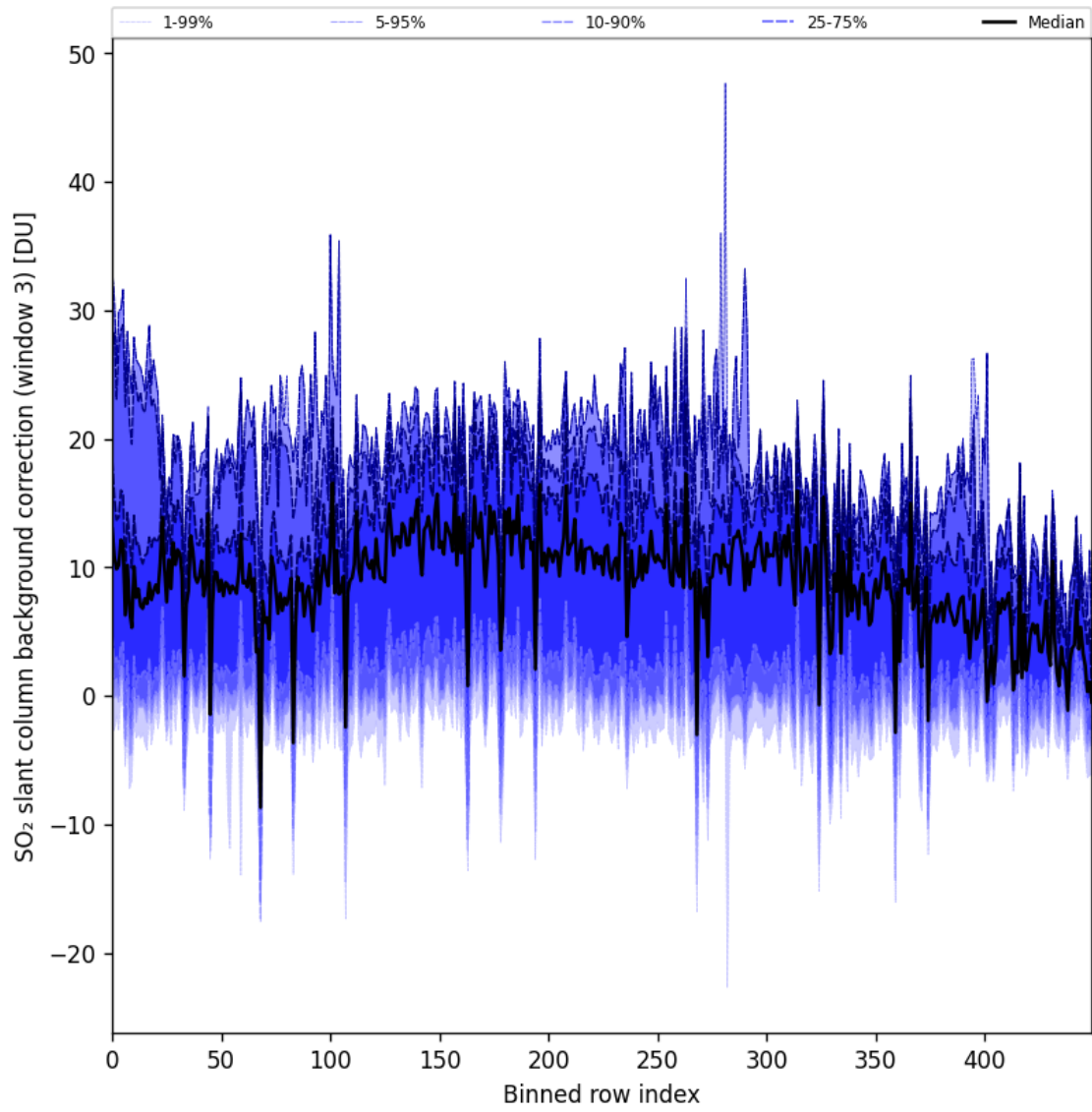
Figure 90: Along track statistics of “SO 2 slant column background correction (window 3)” for 2024-09-20 to 2024-09-22
