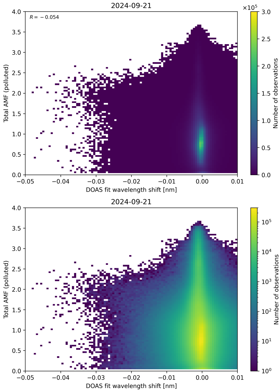
Figure 130: Scatter density plot of “DOAS fit wavelength shift” against “Total AMF (polluted)” for 2024-09-20 to 2024-09-22.
