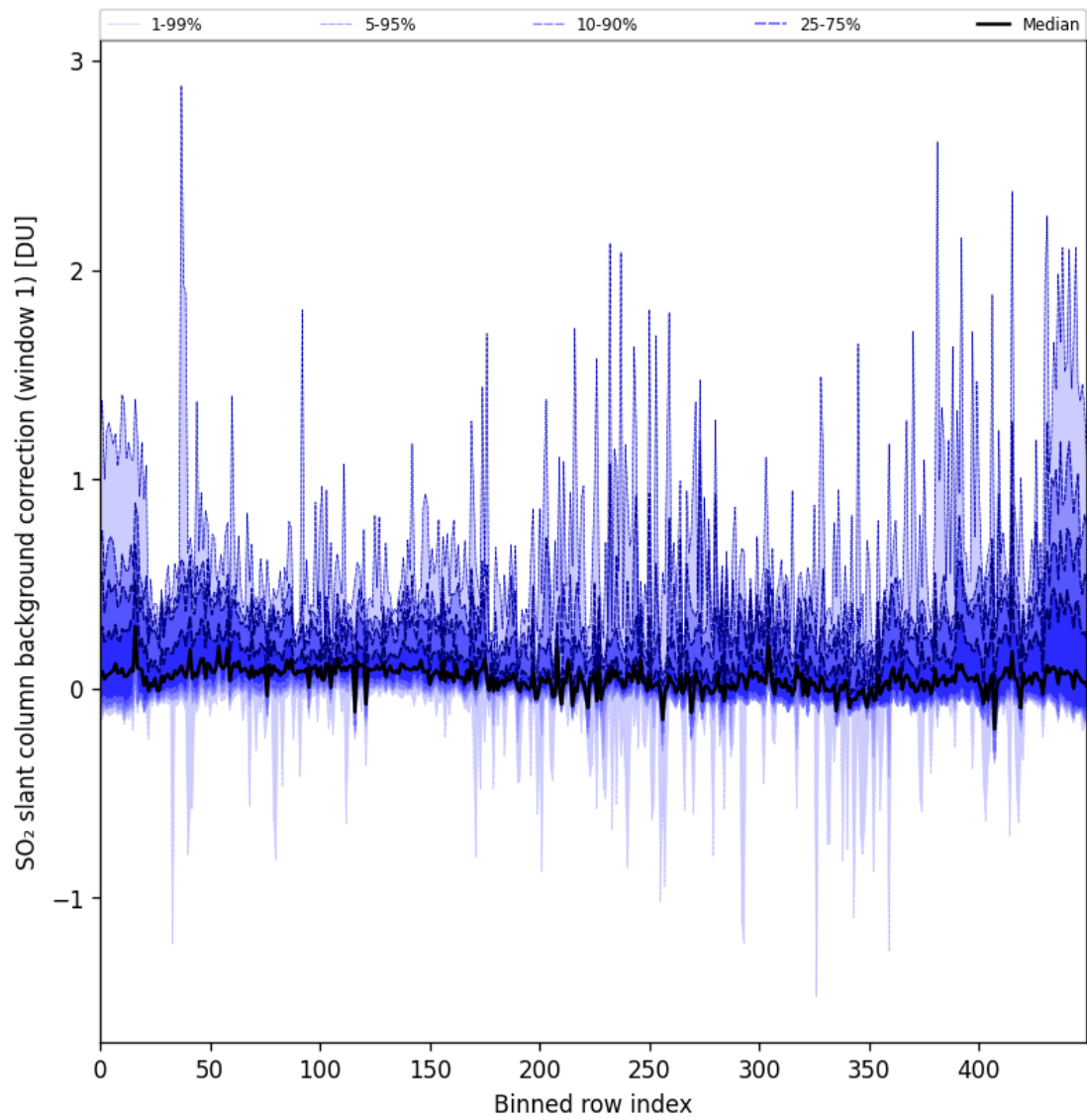
Figure 82: Along track statistics of “SO 2 slant column background correction (window 1)” for 2024-09-20 to 2024-09-22
