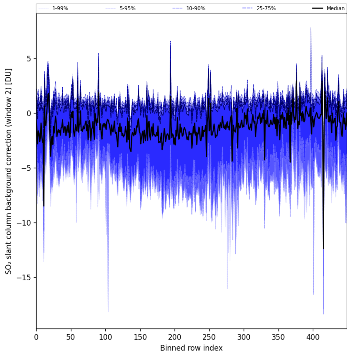
Figure 86: Along track statistics of “SO 2 slant column background correction (window 2)” for 2024-09-20 to 2024-09-22
