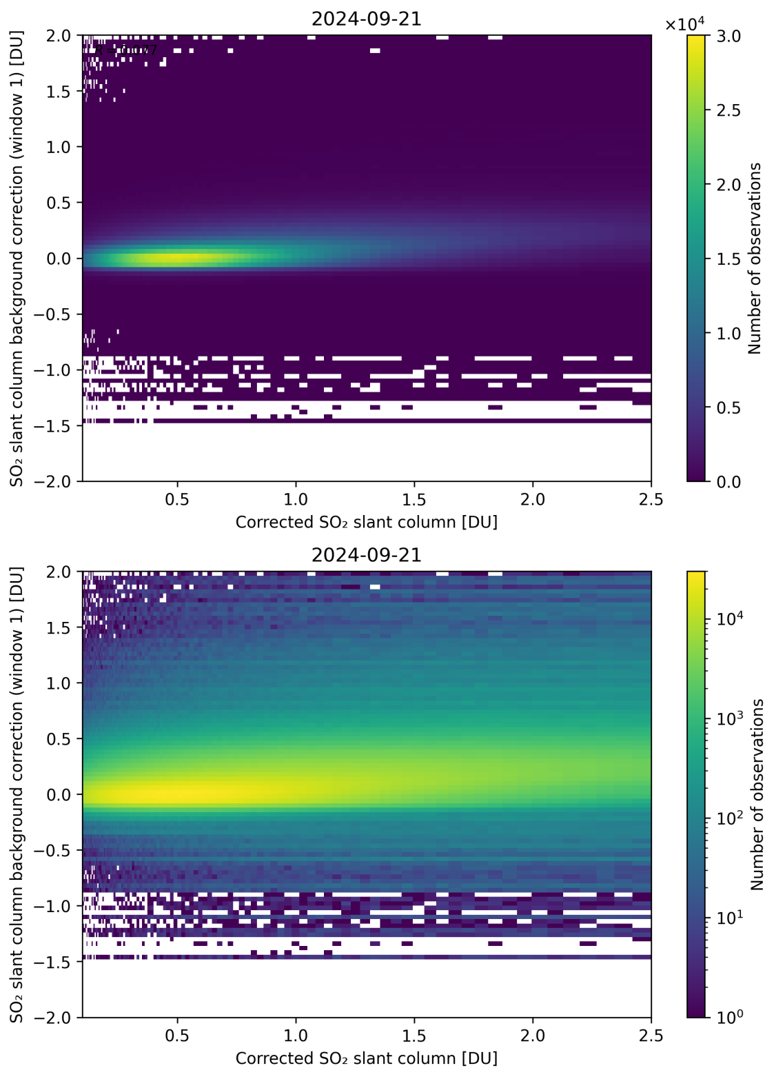
Figure 178: Scatter density plot of “Corrected SO 2 slant column” against “SO 2 slant column background correction (window 1)” for 2024-09-20 to 2024-09-22.
