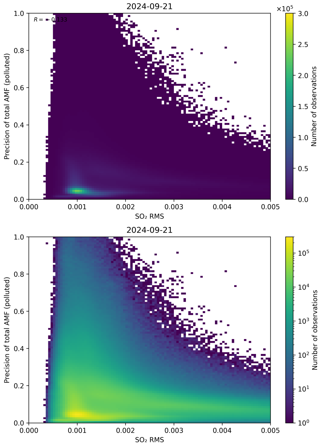
Figure 138: Scatter density plot of “SO 2 RMS” against “Precision of total AMF (polluted)” for 2024-09-20 to 2024-09-22.
