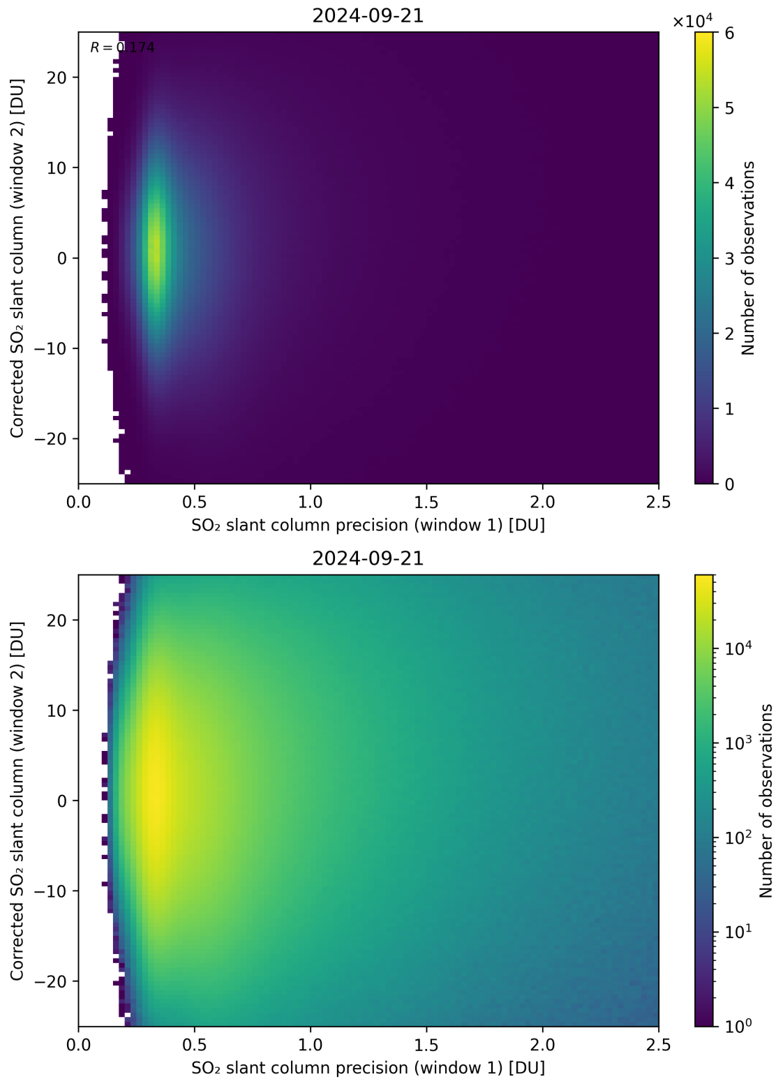
Figure 225: Scatter density plot of “SO 2 slant column precision (window 1)” against “Corrected SO 2 slant column (window 2)” for 2024-09-20 to 2024-09-22.
