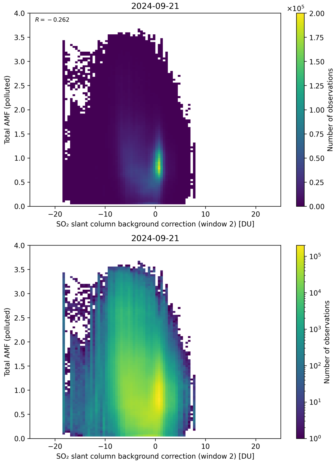
Figure 119: Scatter density plot of “SO 2 slant column background correction (window 2)” against “Total AMF (polluted)” for 2024-09-20 to 2024-09-22.
