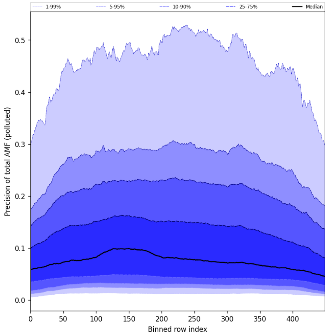
Figure 95: Along track statistics of “Precision of total AMF (polluted)” for 2024-09-20 to 2024-09-22
