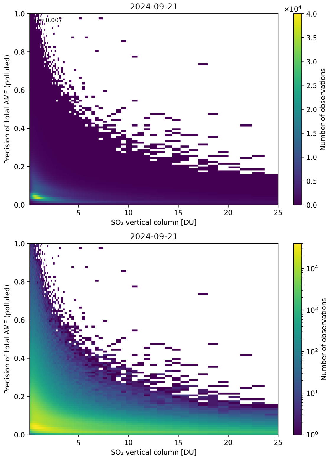
Figure 306: Scatter density plot of “SO 2 vertical column” against “Precision of total AMF (polluted)” for 2024-09-20 to 2024-09-22.
