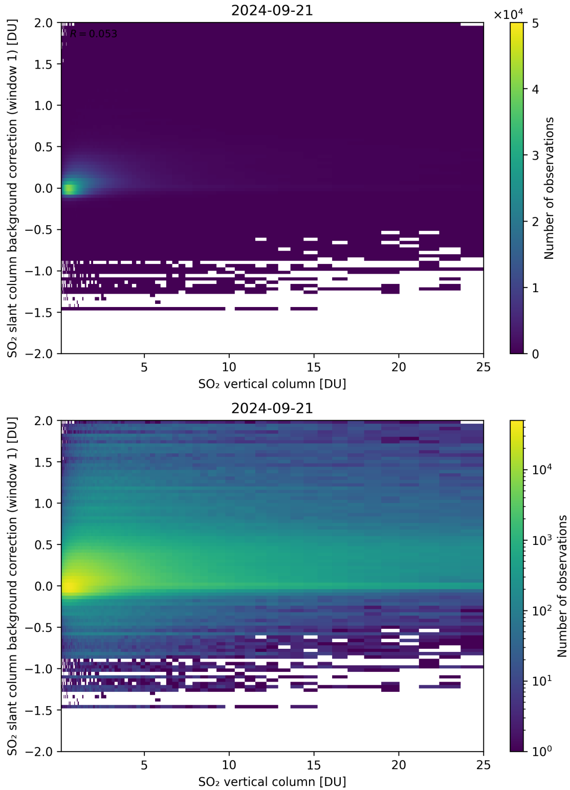
Figure 273: Scatter density plot of “SO 2 vertical column” against “SO 2 slant column background correction (window 1)” for 2024-09-20 to 2024-09-22.
