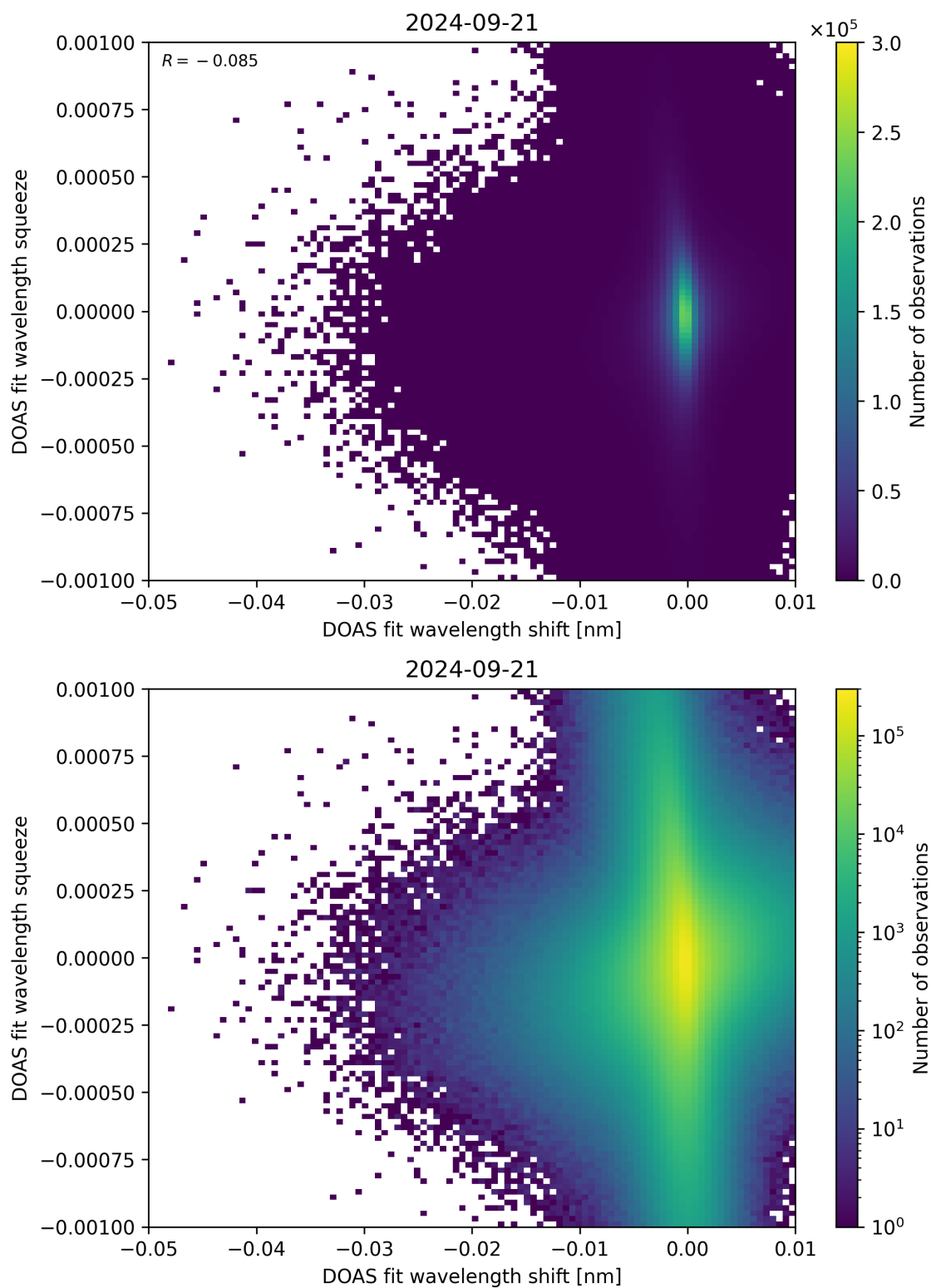
Figure 127: Scatter density plot of “DOAS fit wavelength shift” against “DOAS fit wavelength squeeze” for 2024-09-20 to 2024-09-22.
