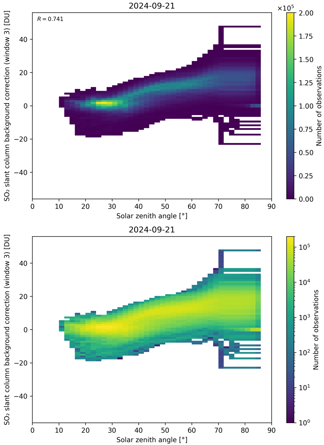
Figure 160: Scatter density plot of “Solar zenith angle” against “SO 2 slant column background correction (window 3)” for 2024-09-20 to 2024-09-22.
