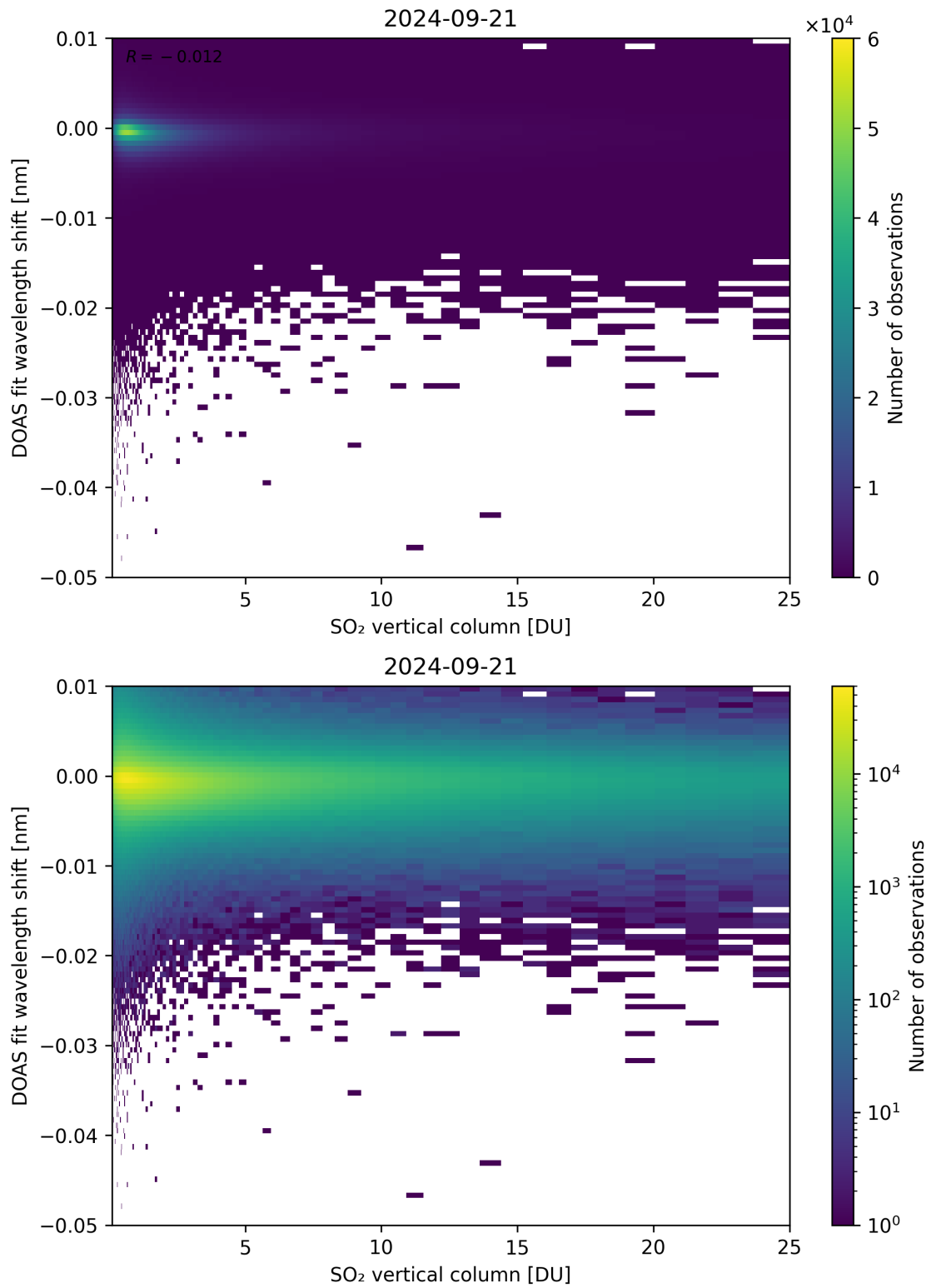
Figure 276: Scatter density plot of “SO 2 vertical column” against “DOAS fit wavelength shift” for 2024-09-20 to 2024-09-22.
