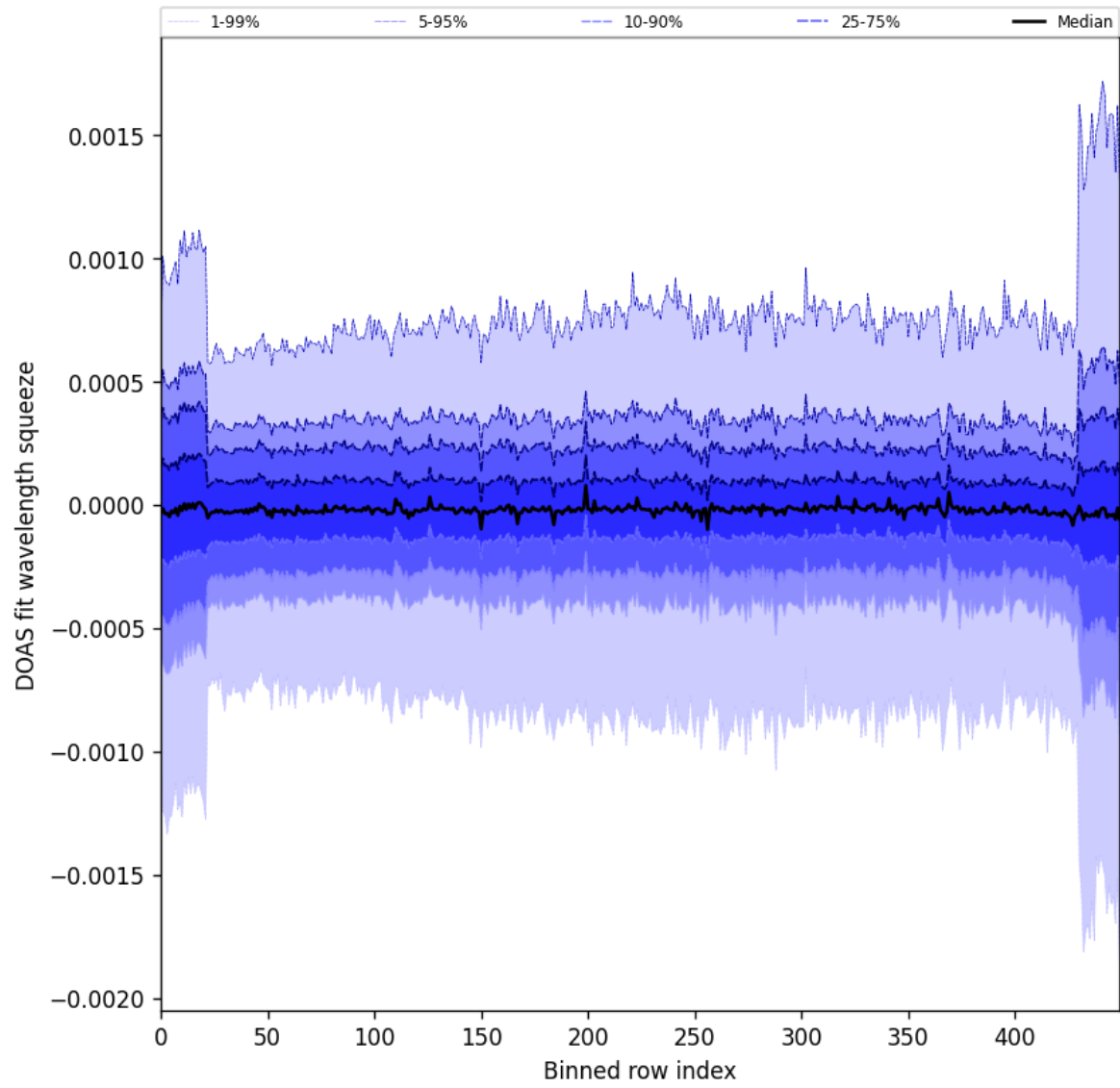
Figure 92: Along track statistics of “DOAS fit wavelength squeeze” for 2024-09-20 to 2024-09-22
