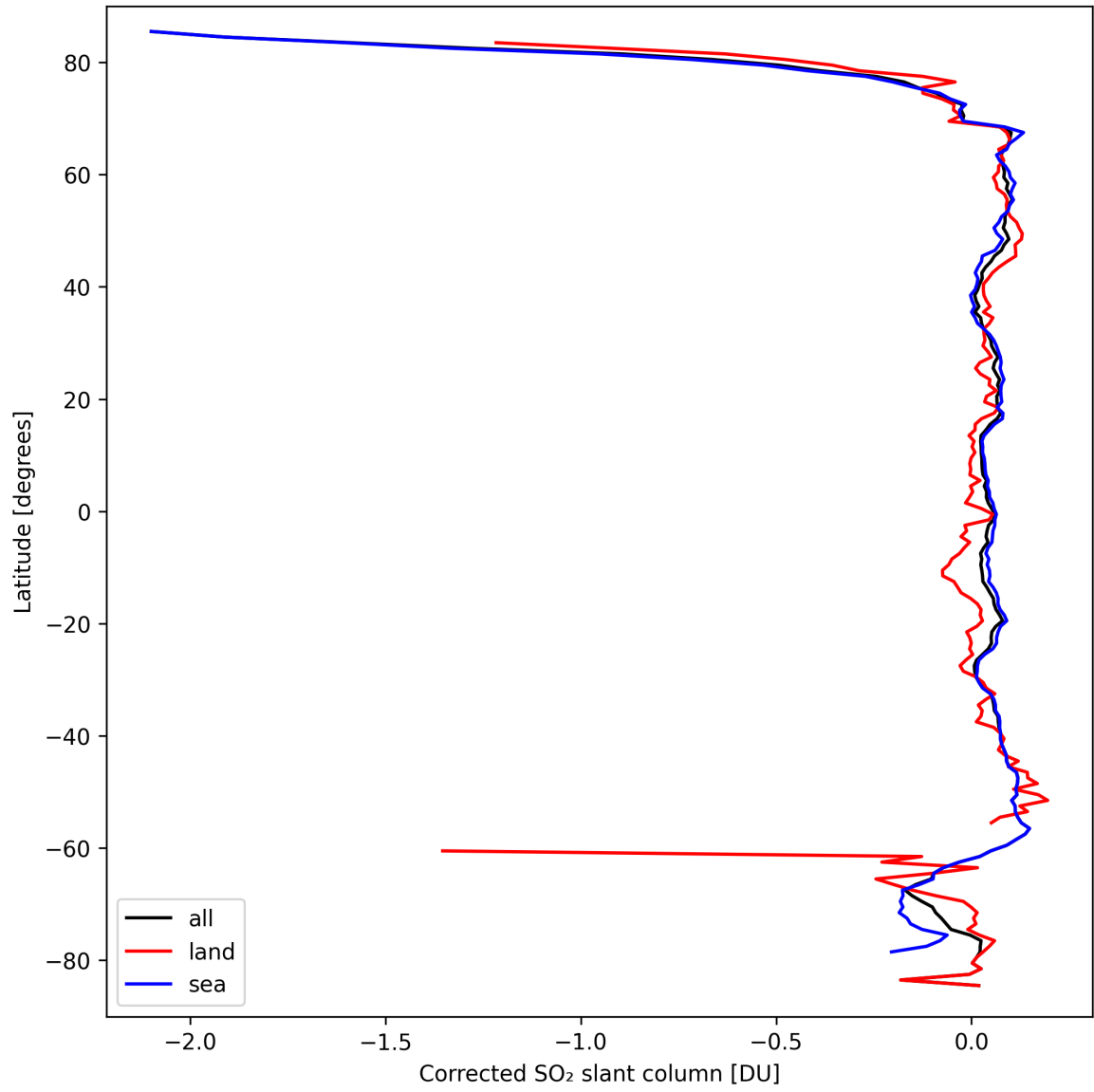
Figure 32: Zonal average of “Corrected SO 2 slant column” for 2024-09-20 to 2024-09-22.
