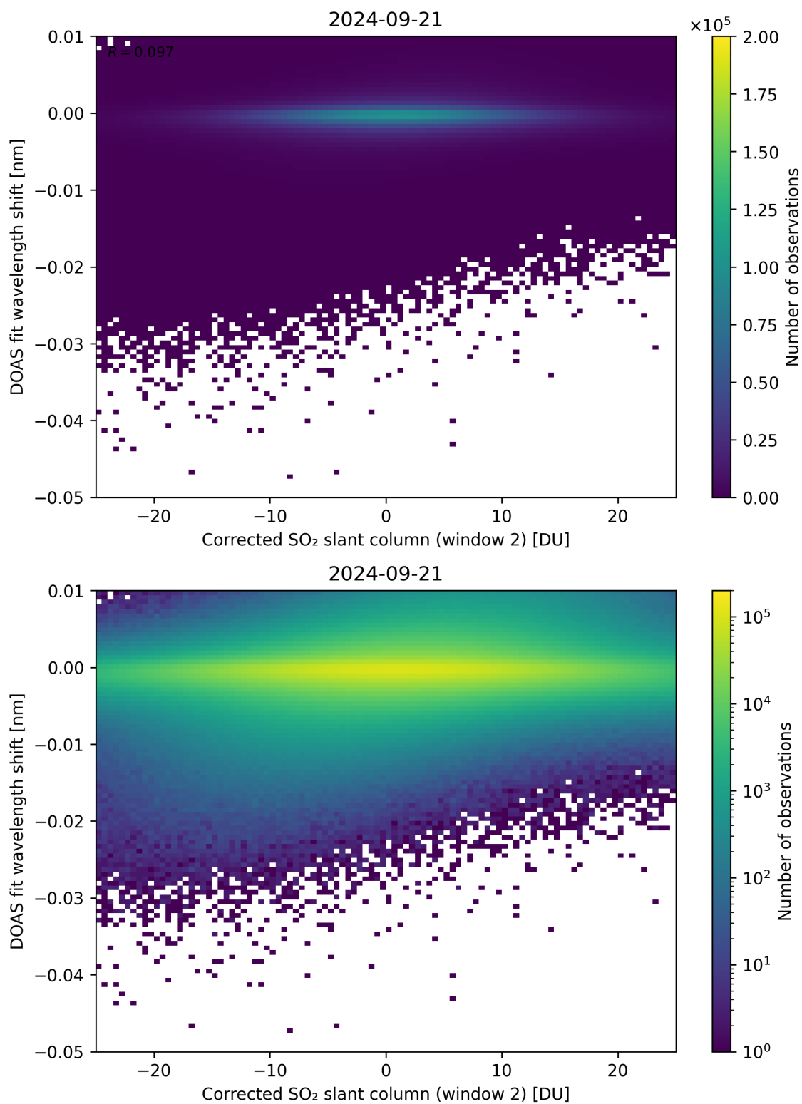
Figure 196: Scatter density plot of “Corrected SO 2 slant column (window 2)” against “DOAS fit wavelength shift” for 2024-09-20 to 2024-09-22.
