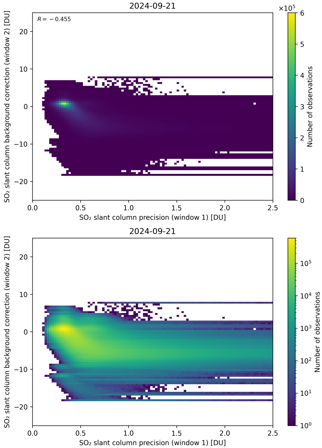
Figure 219: Scatter density plot of “SO 2 slant column precision (window 1)” against “SO 2 slant column background correction (window 2)” for 2024-09-20 to 2024-09-22.
