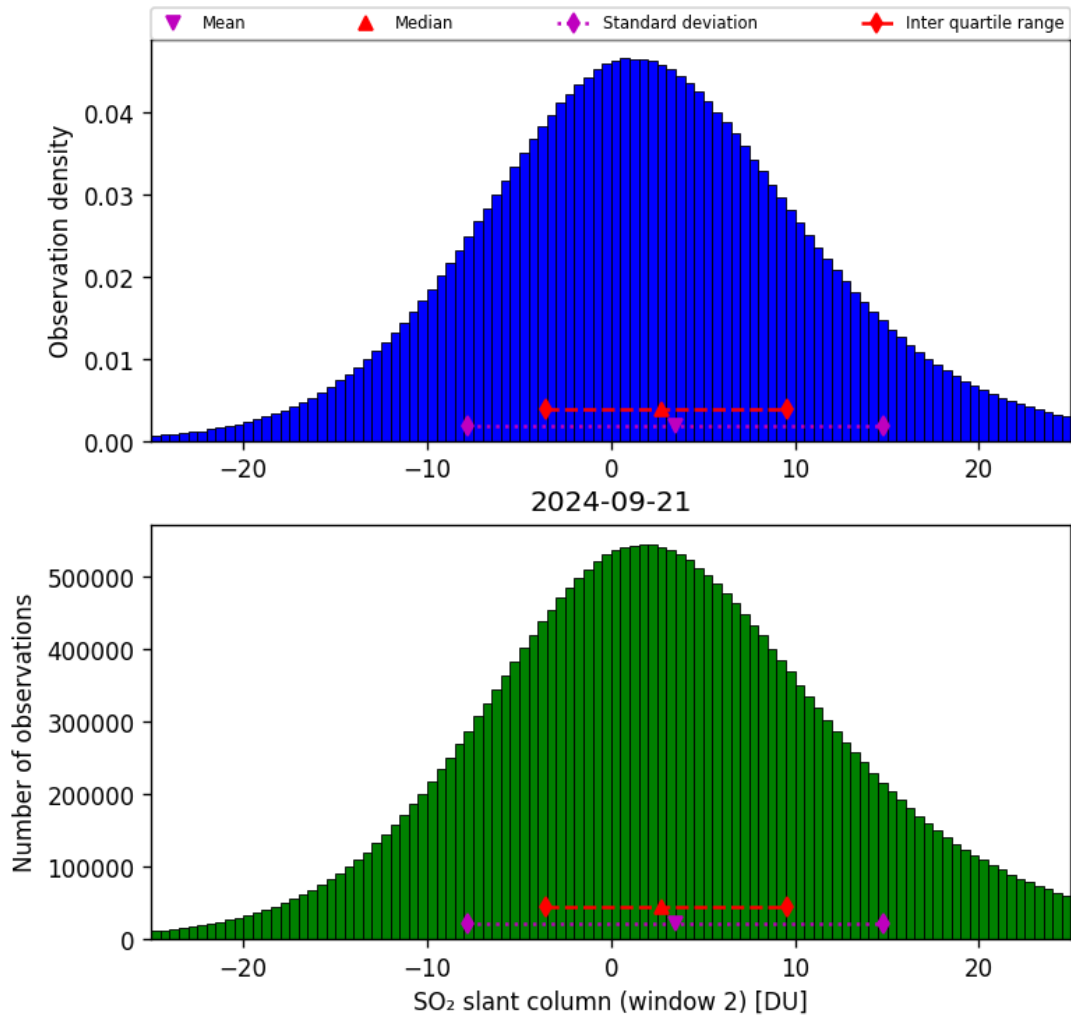
Figure 60: Histogram of “SO 2 slant column (window 2)” for 2024-09-20 to 2024-09-22
