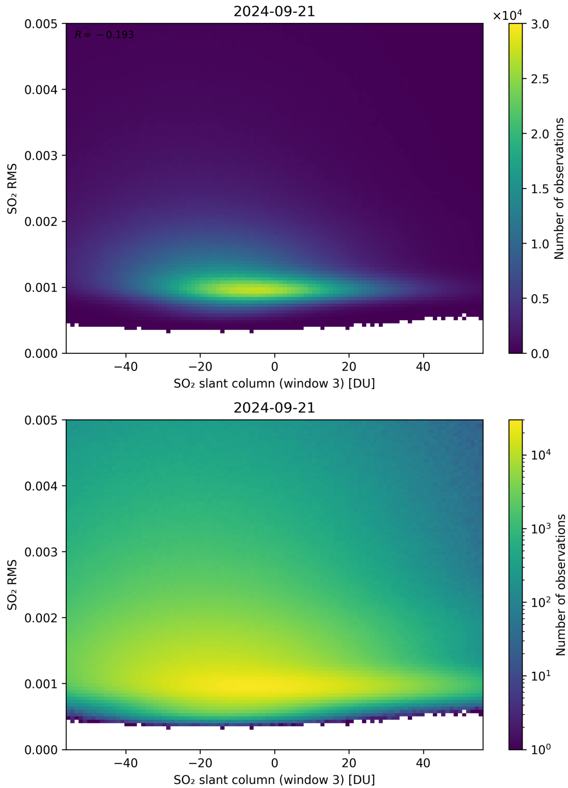
Figure 256: Scatter density plot of “SO 2 slant column (window 3)” against “SO 2 RMS” for 2024-09-20 to 2024-09-22.
