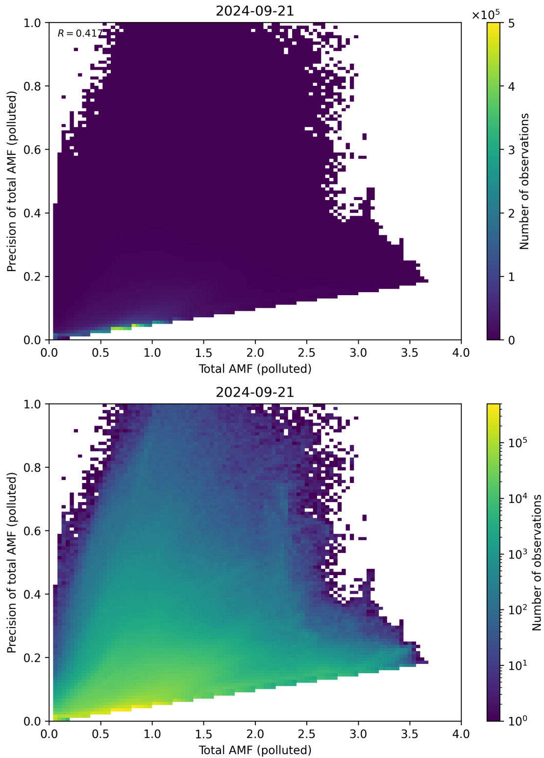
Figure 272: Scatter density plot of “Total AMF (polluted)” against “Precision of total AMF (polluted)” for 2024-09-20 to 2024-09-22.
