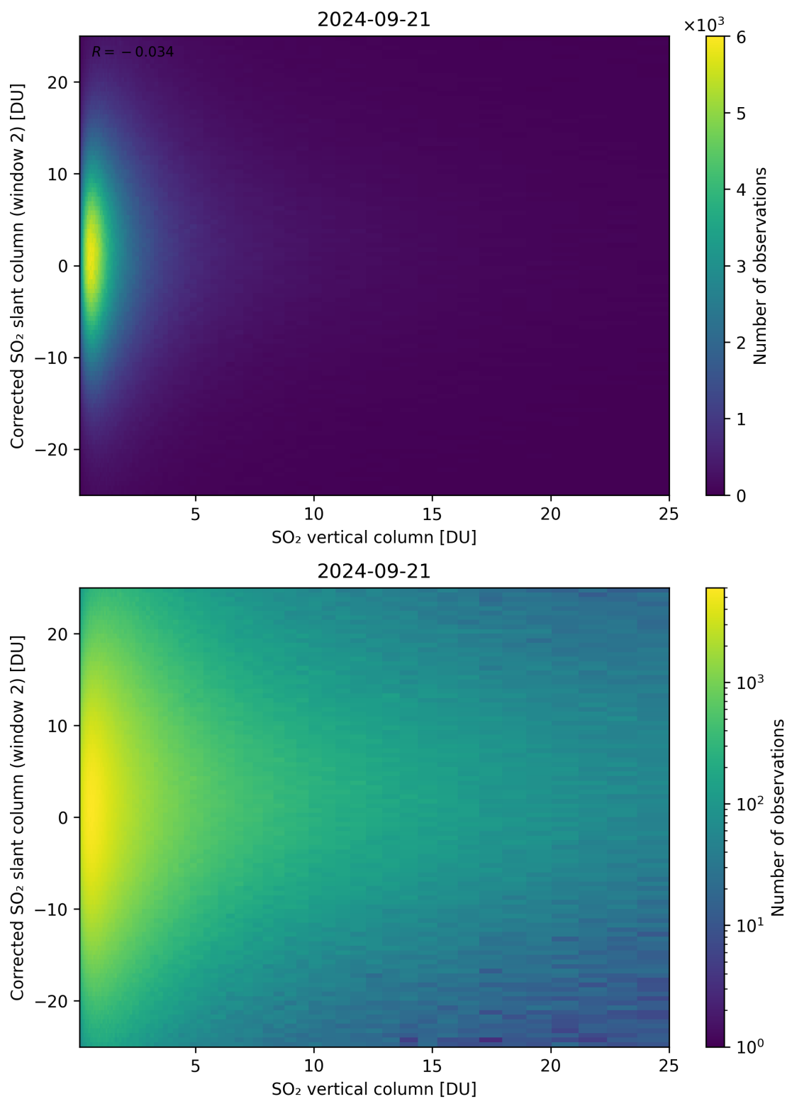
Figure 298: Scatter density plot of “SO 2 vertical column” against “Corrected SO 2 slant column (window 2)” for 2024-09-20 to 2024-09-22.
