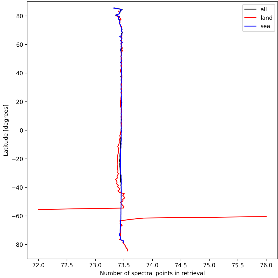
Figure 51: Zonal average of “Number of spectral points in retrieval” for 2024-09-20 to 2024-09-22.
