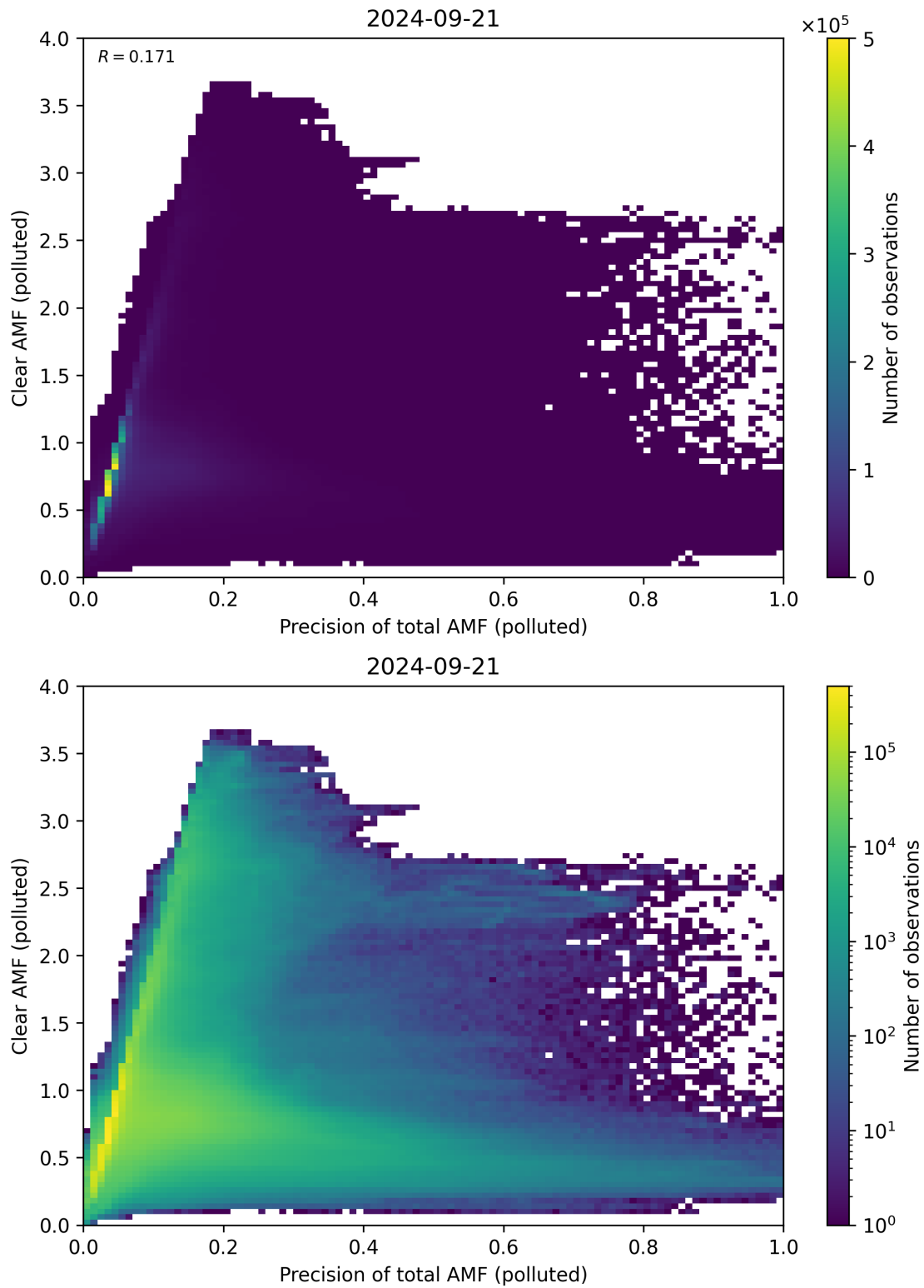
Figure 270: Scatter density plot of “Precision of total AMF (polluted)” against “Clear AMF (polluted)” for 2024-09-20 to 2024-09-22.
