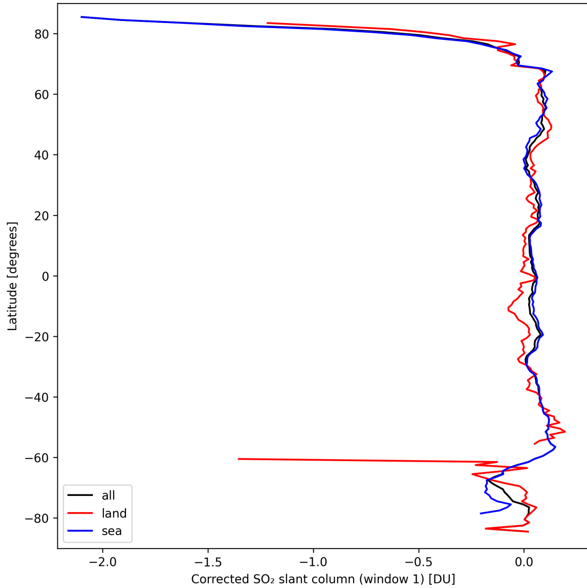
Figure 35: Zonal average of “Corrected SO 2 slant column (window 1)” for 2024-09-20 to 2024-09-22.
