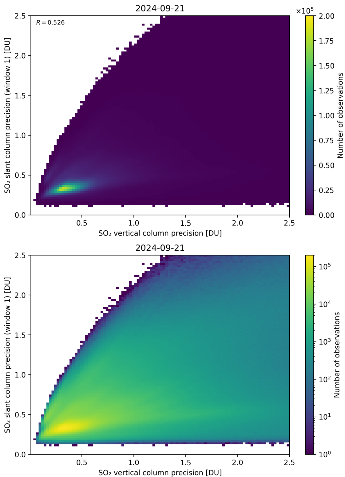
Figure 290: Scatter density plot of “SO 2 vertical column precision” against “SO 2 slant column precision (window 1)” for 2024-09-20 to 2024-09-22.
