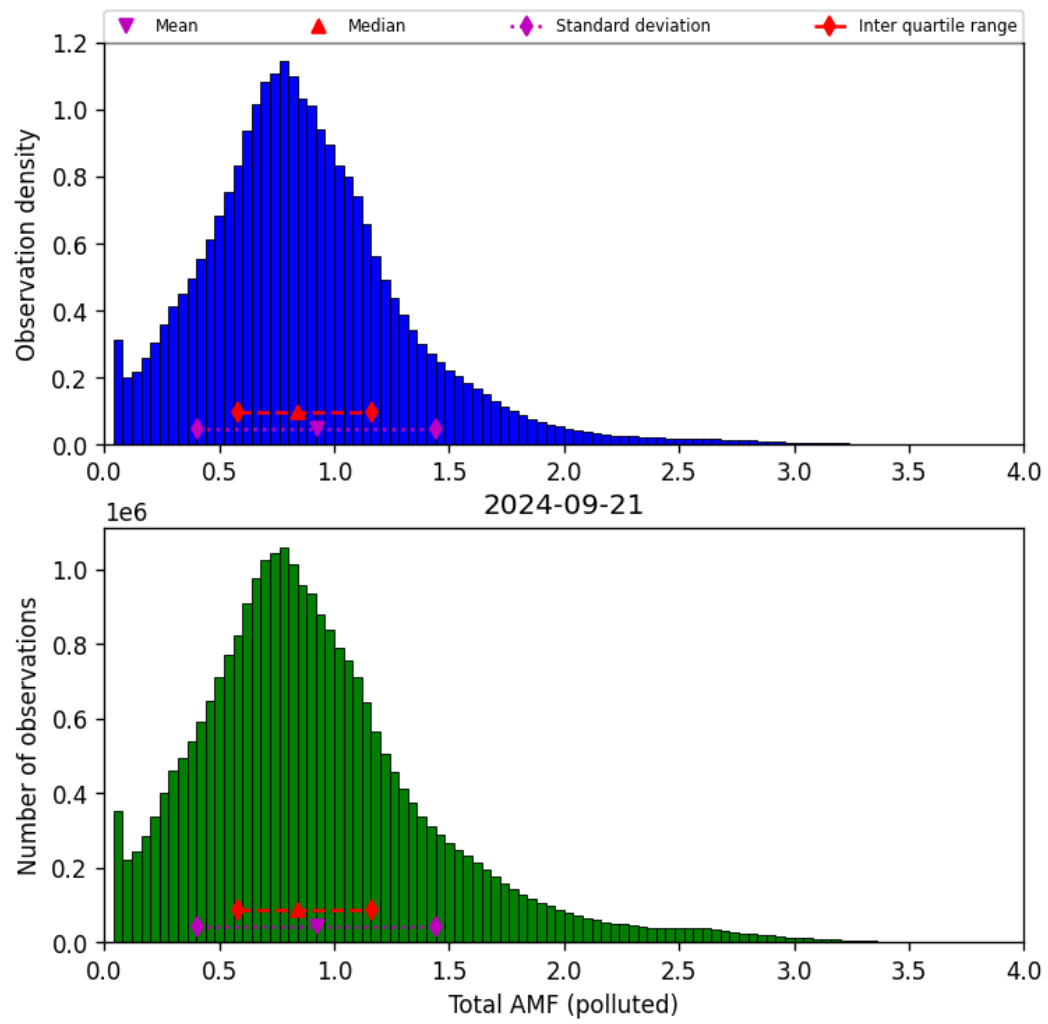
Figure 71: Histogram of “Total AMF (polluted)” for 2024-09-20 to 2024-09-22
