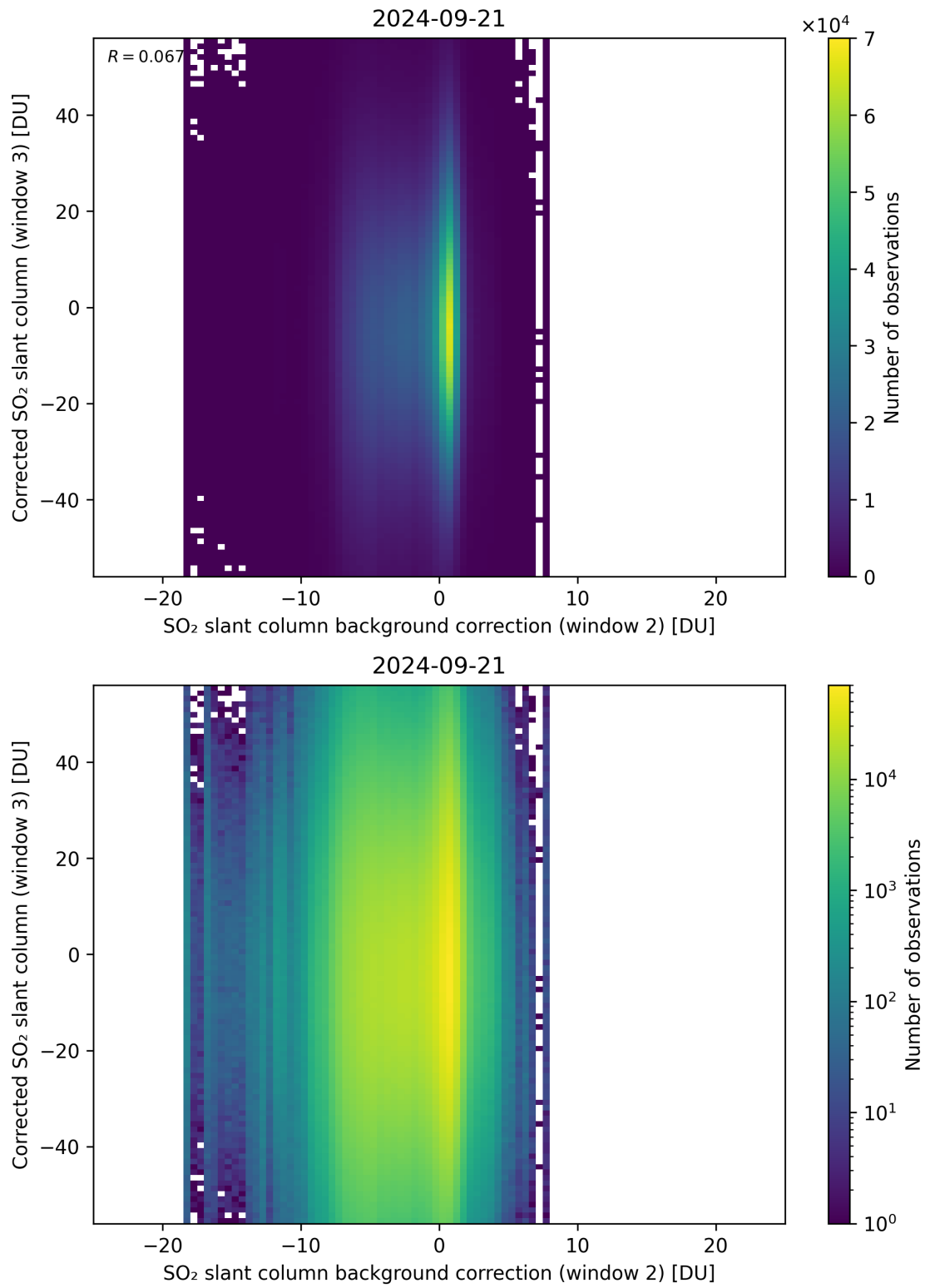
Figure 116: Scatter density plot of “SO 2 slant column background correction (window 2)” against “Corrected SO 2 slant column (window 3)” for 2024-09-20 to 2024-09-22.
