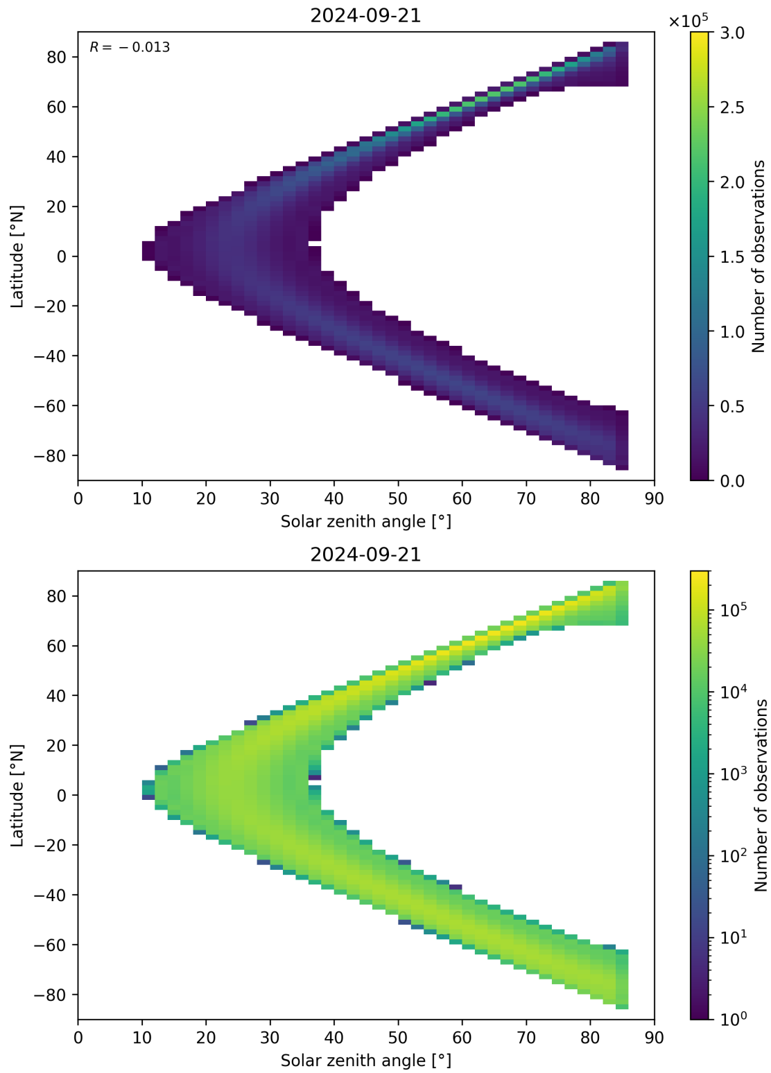
Figure 164: Scatter density plot of “Solar zenith angle” against “Latitude” for 2024-09-20 to 2024-09-22.
