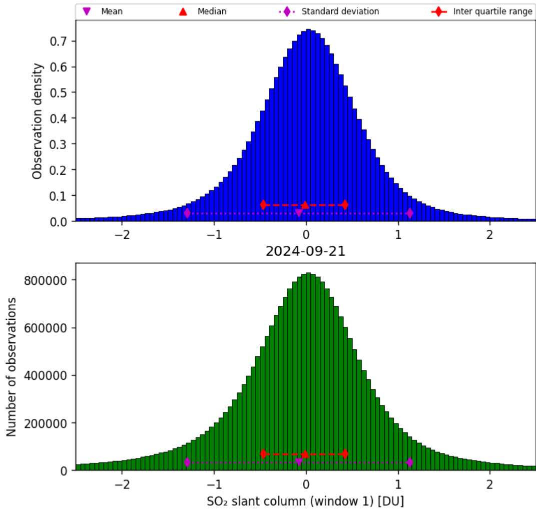
Figure 56: Histogram of “SO 2 slant column (window 1)” for 2024-09-20 to 2024-09-22
