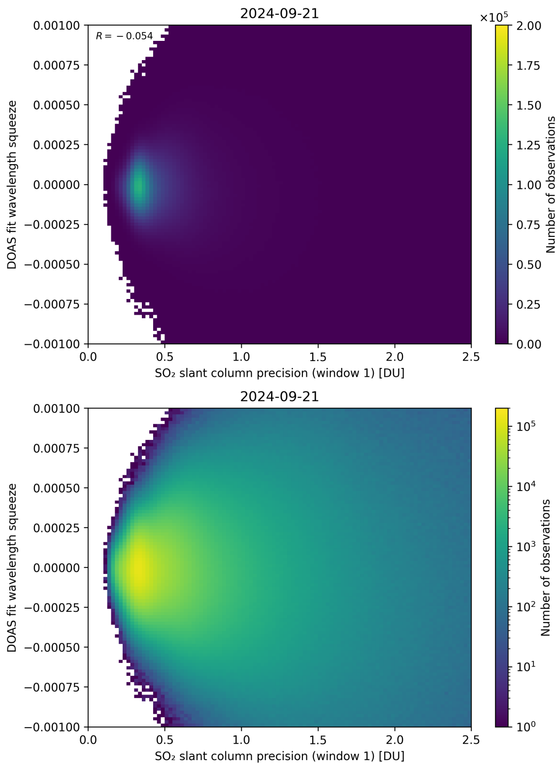
Figure 222: Scatter density plot of “SO 2 slant column precision (window 1)” against “DOAS fit wavelength squeeze” for 2024-09-20 to 2024-09-22.
