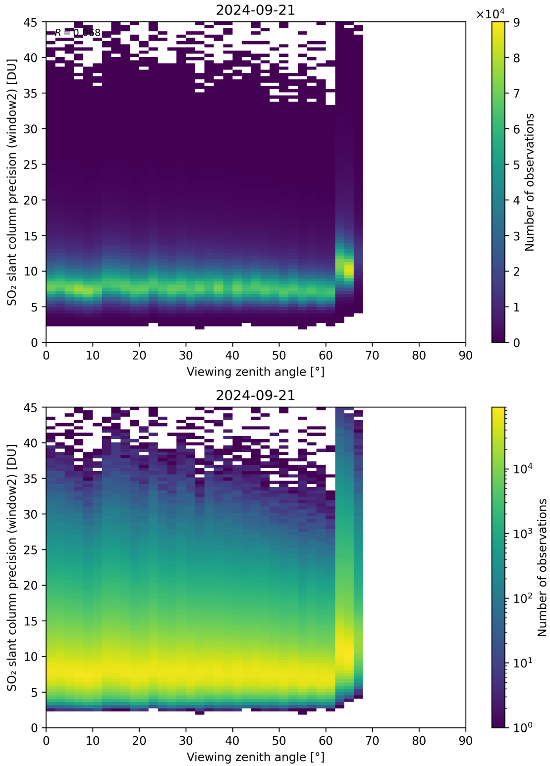
Figure 322: Scatter density plot of “Viewing zenith angle” against “SO 2 slant column precision (window2)” for 2024-09-20 to 2024-09-22.
