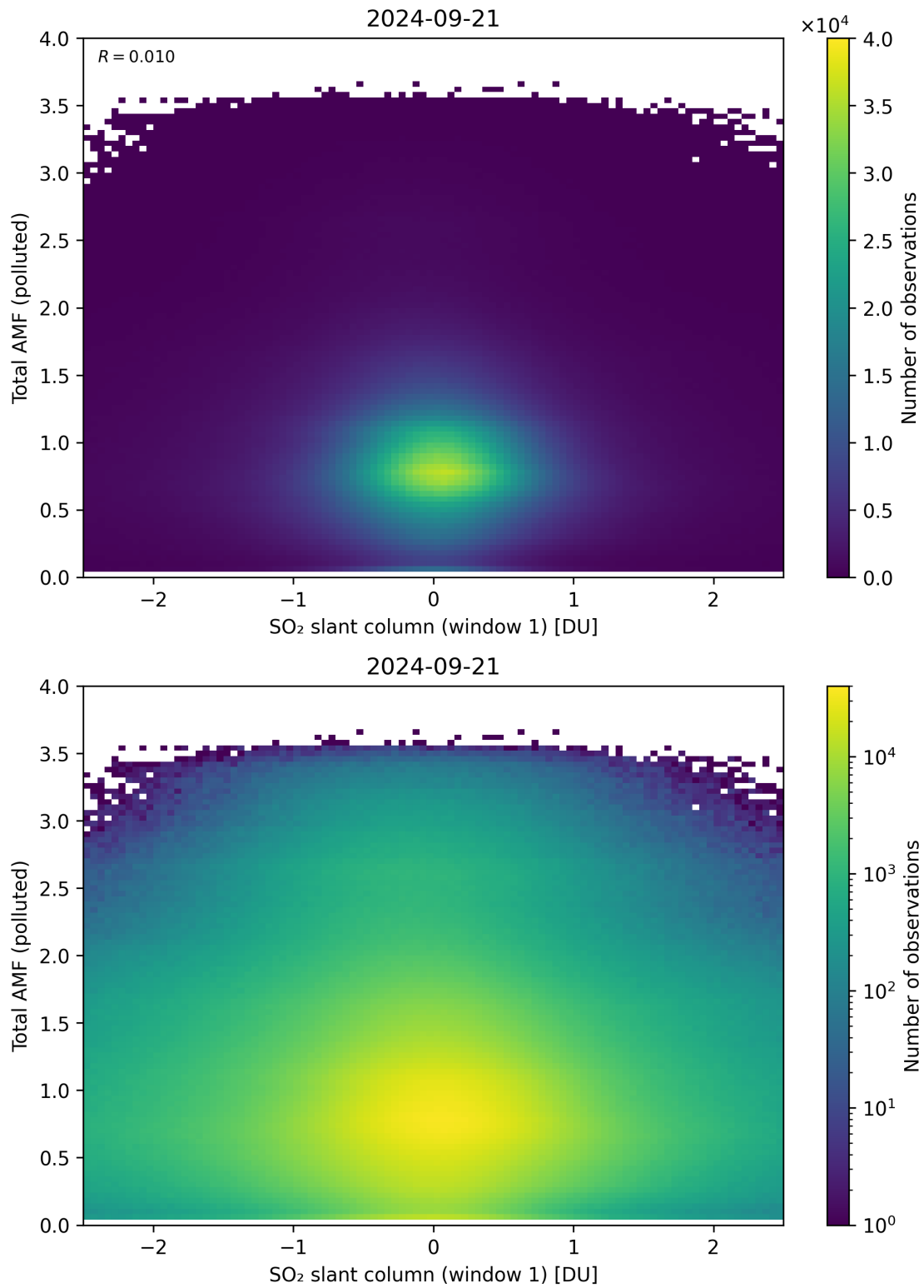
Figure 239: Scatter density plot of “SO 2 slant column (window 1)” against “Total AMF (polluted)” for 2024-09-20 to 2024-09-22.
