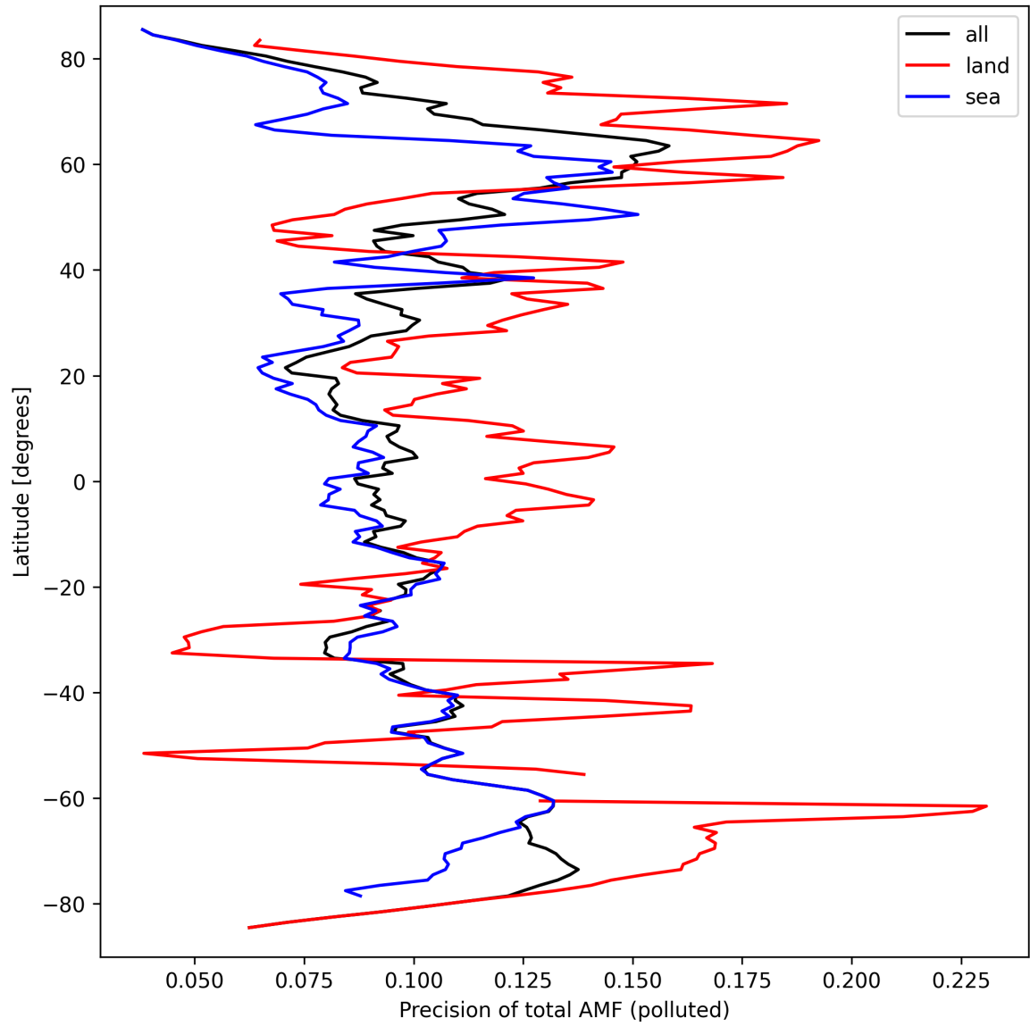
Figure 49: Zonal average of “Precision of total AMF (polluted)” for 2024-09-20 to 2024-09-22.
