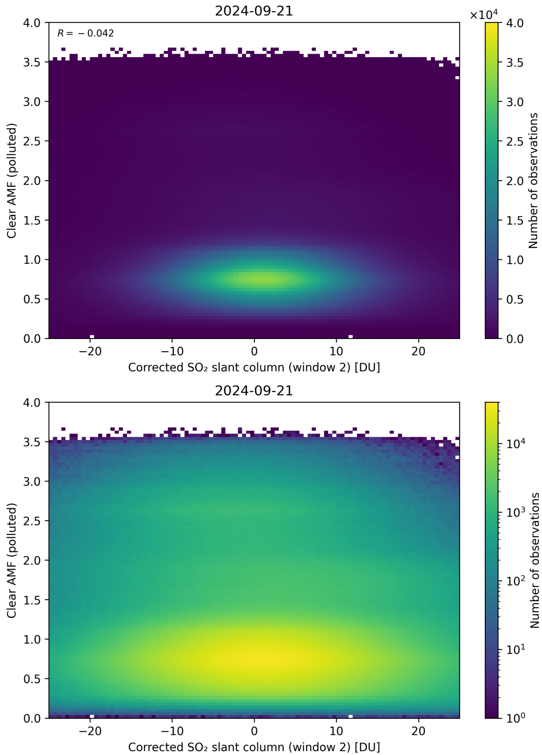
Figure 199: Scatter density plot of “Corrected SO 2 slant column (window 2)” against “Clear AMF (polluted)” for 2024-09-20 to 2024-09-22.
