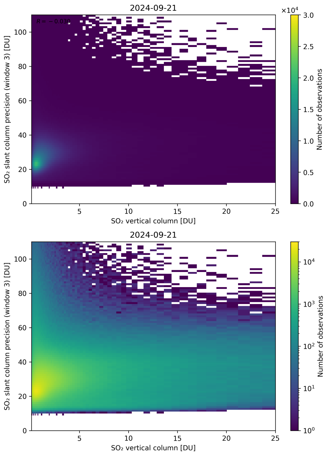
Figure 304: Scatter density plot of “SO 2 vertical column” against “SO 2 slant column precision (window 3)” for 2024-09-20 to 2024-09-22.
