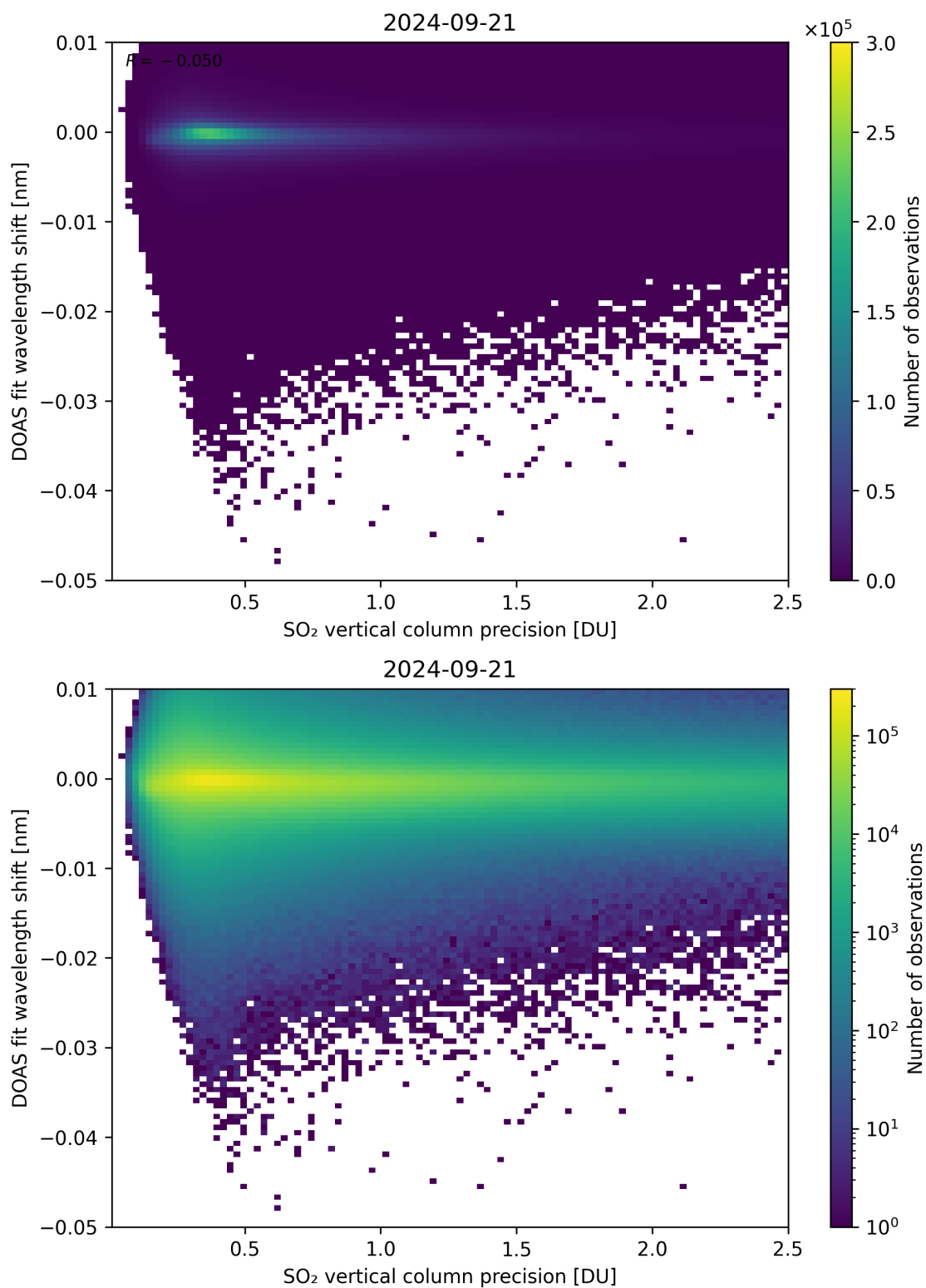
Figure 282: Scatter density plot of “SO 2 vertical column precision” against “DOAS fit wavelength shift” for 2024-09-20 to 2024-09-22.
