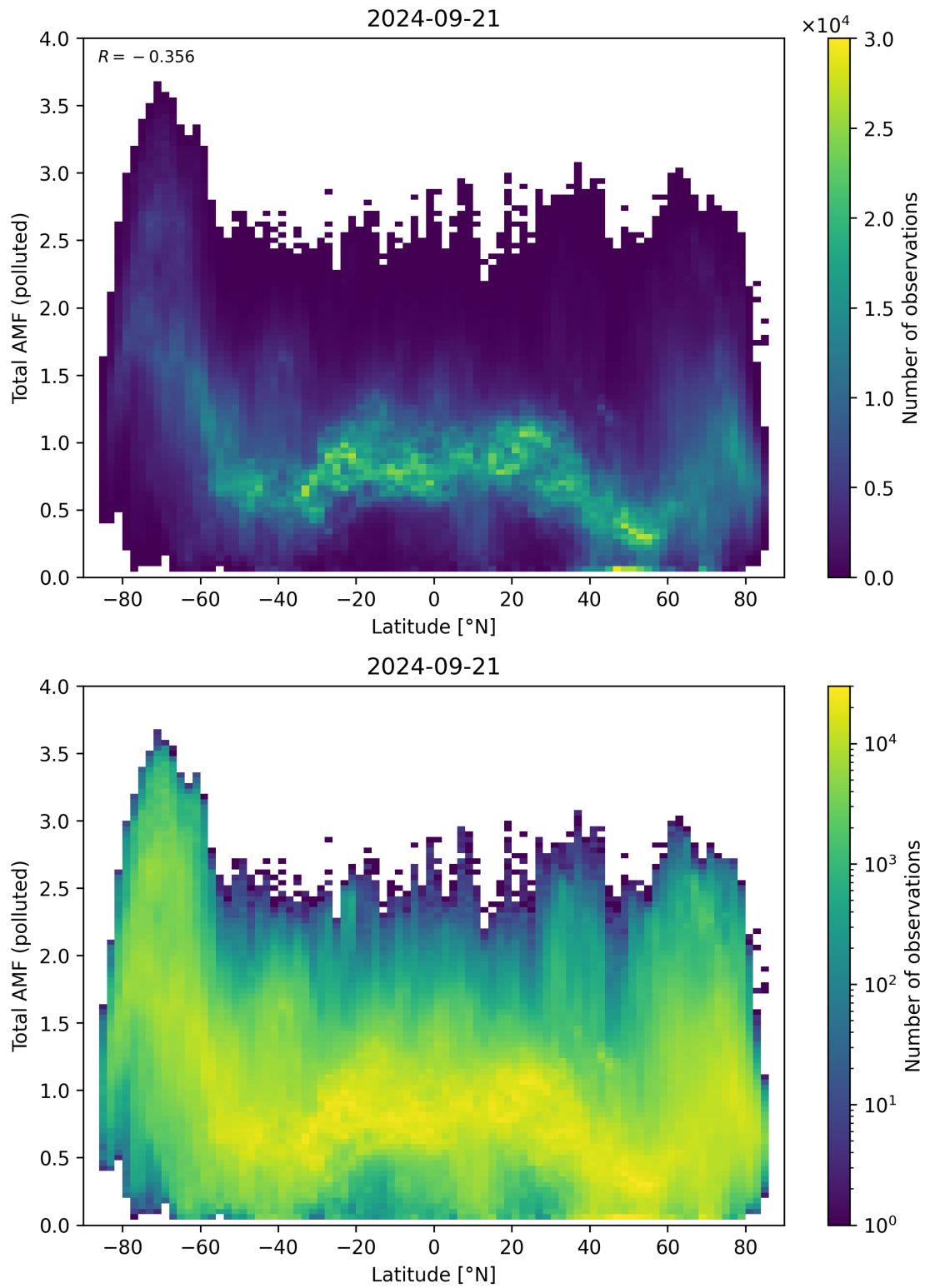
Figure 154: Scatter density plot of “Latitude” against “Total AMF (polluted)” for 2024-09-20 to 2024-09-22.
