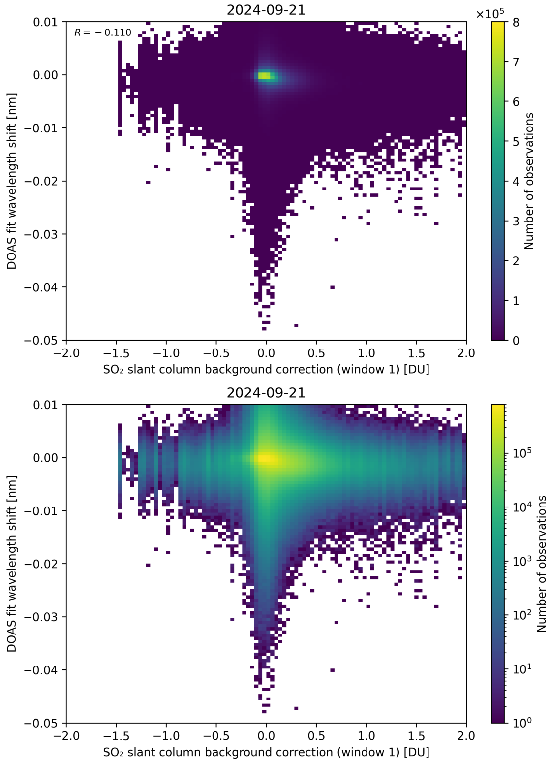
Figure 100: Scatter density plot of “SO 2 slant column background correction (window 1)” against “DOAS fit wavelength shift” for 2024-09-20 to 2024-09-22.
