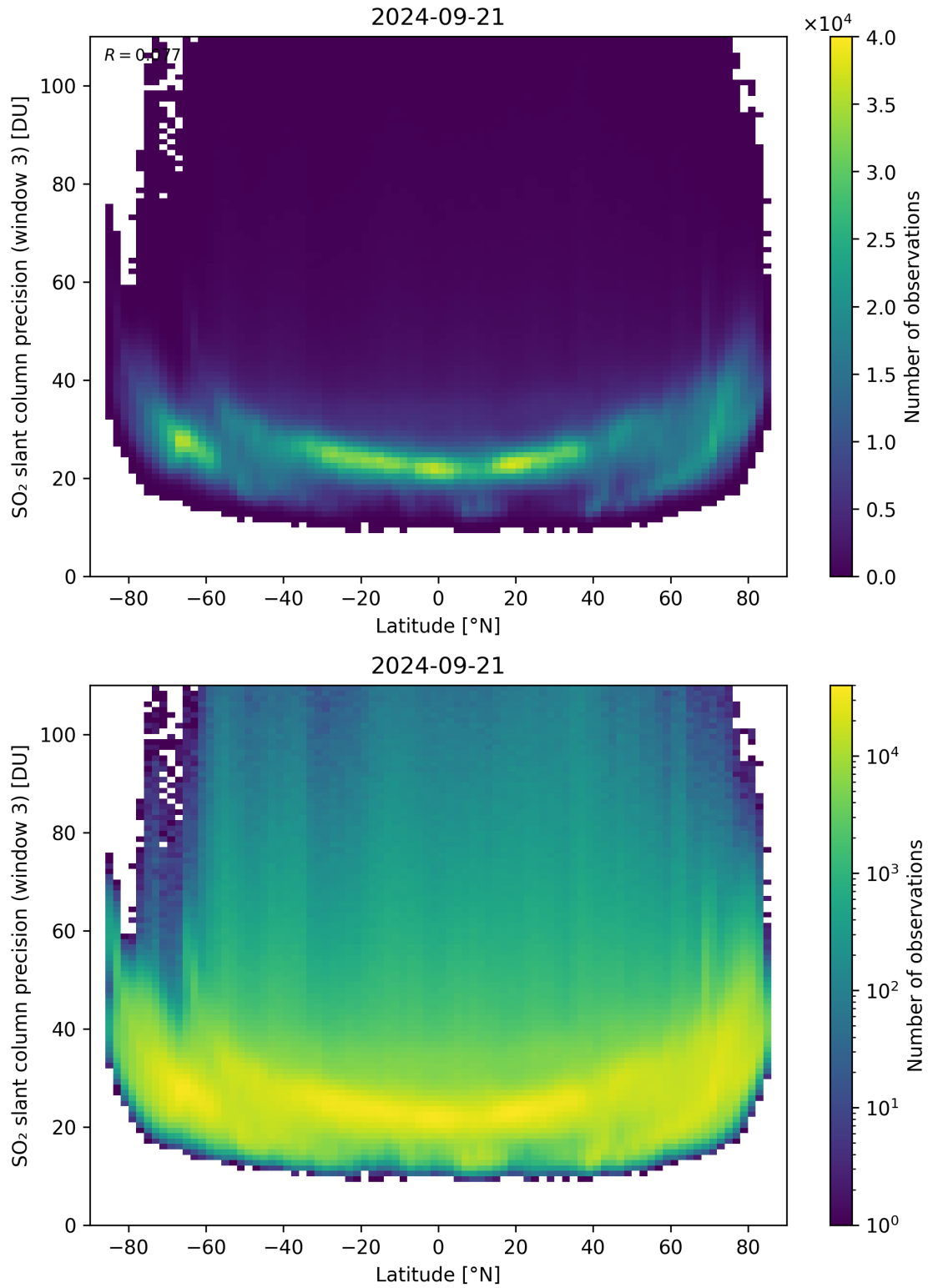
Figure 153: Scatter density plot of “Latitude” against “SO 2 slant column precision (window 3)” for 2024-09-20 to 2024-09-22.
