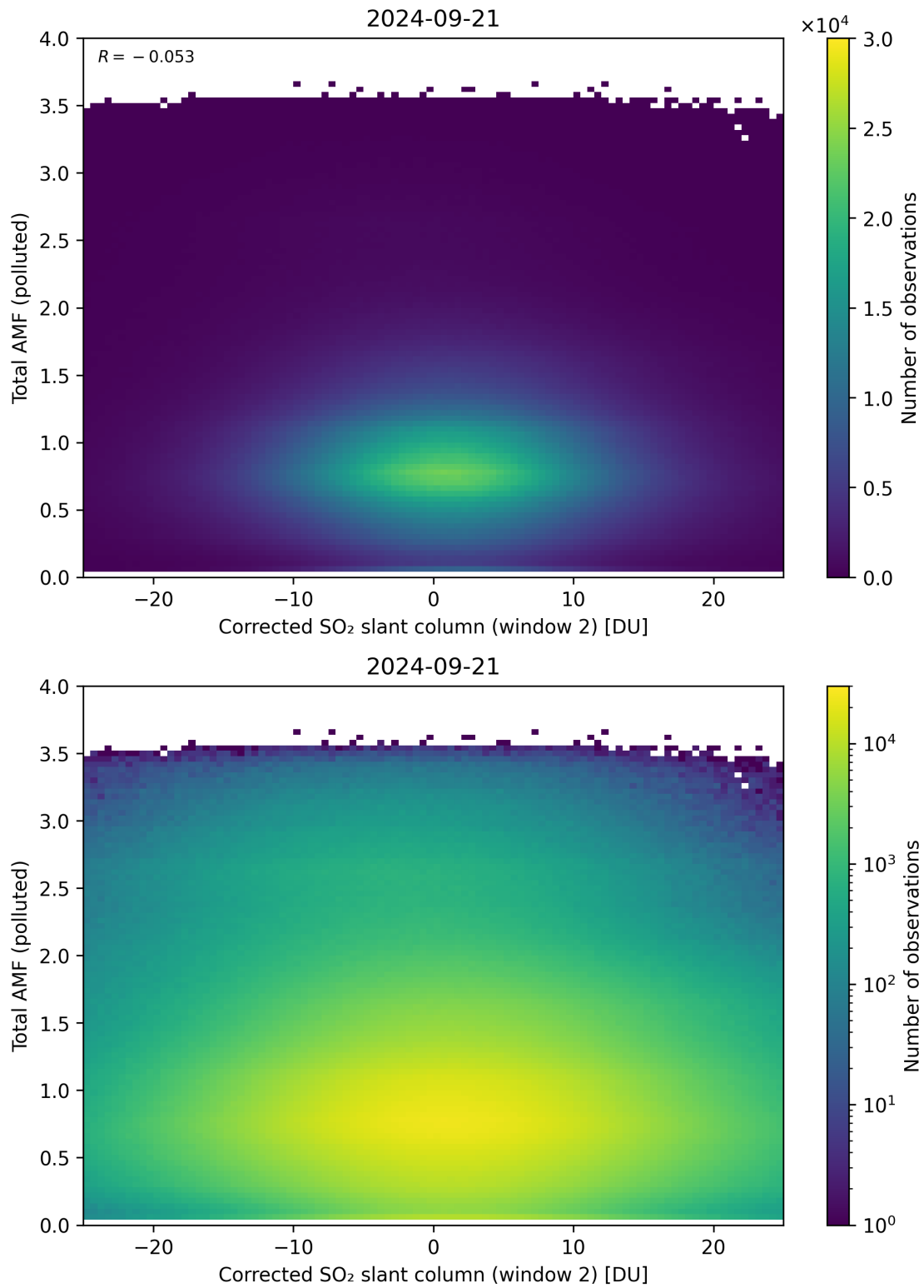
Figure 203: Scatter density plot of “Corrected SO 2 slant column (window 2)” against “Total AMF (polluted)” for 2024-09-20 to 2024-09-22.
