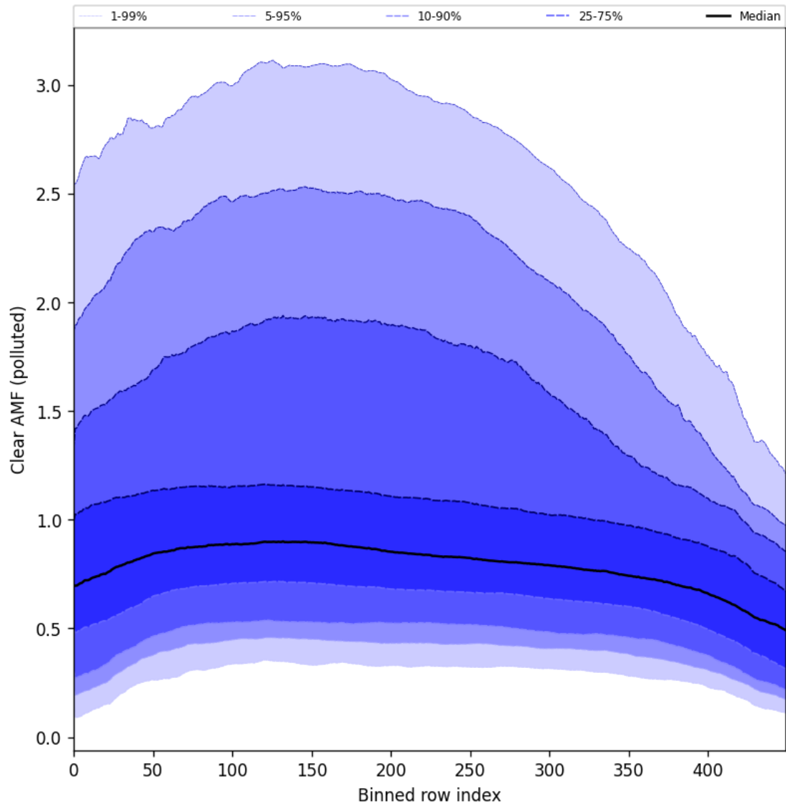
Figure 96: Along track statistics of “Clear AMF (polluted)” for 2024-09-20 to 2024-09-22
