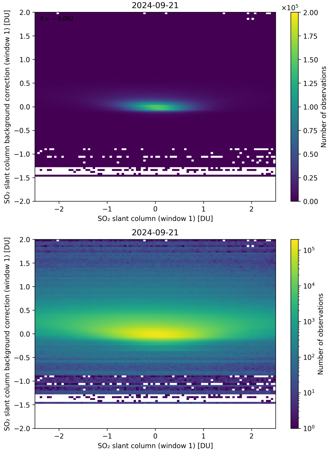
Figure 212: Scatter density plot of “SO 2 slant column (window 1)” against “SO 2 slant column background correction (window 1)” for 2024-09-20 to 2024-09-22.
