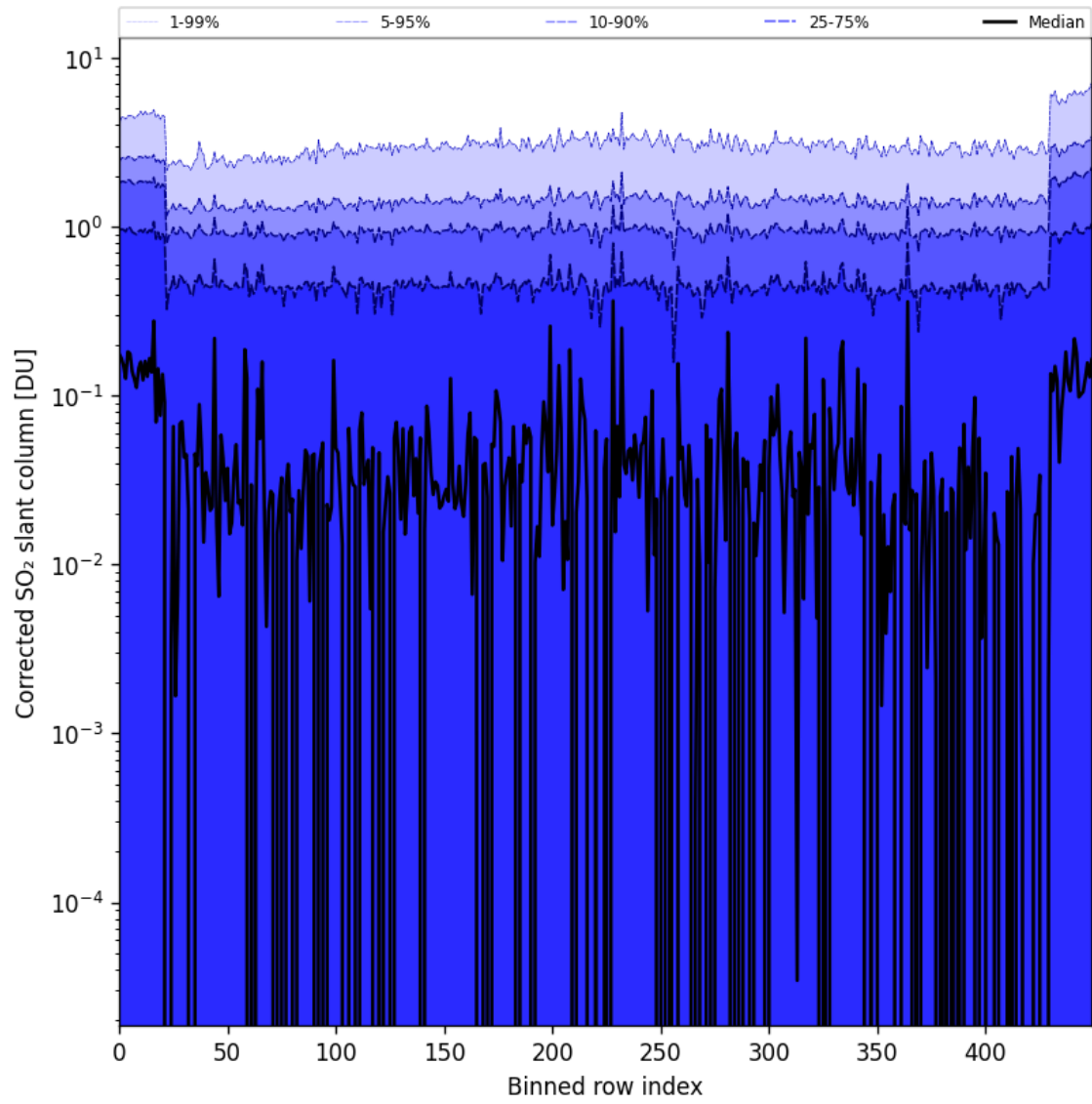
Figure 78: Along track statistics of “Corrected SO 2 slant column” for 2024-09-20 to 2024-09-22
