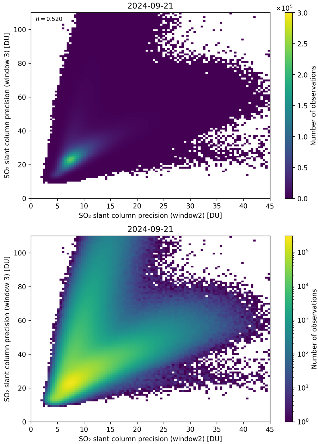
Figure 250: Scatter density plot of “SO 2 slant column precision (window2)” against “SO 2 slant column precision (window 3)” for 2024-09-20 to 2024-09-22.
