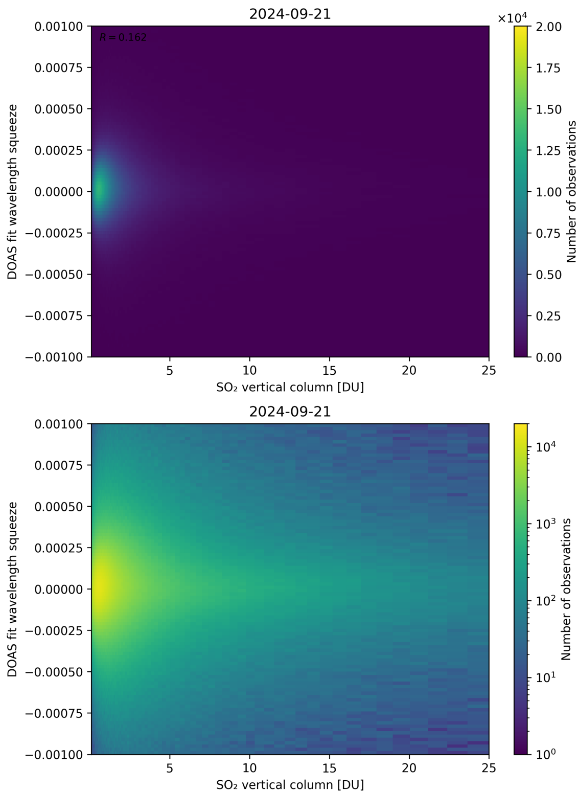
Figure 277: Scatter density plot of “SO 2 vertical column” against “DOAS fit wavelength squeeze” for 2024-09-20 to 2024-09-22.
