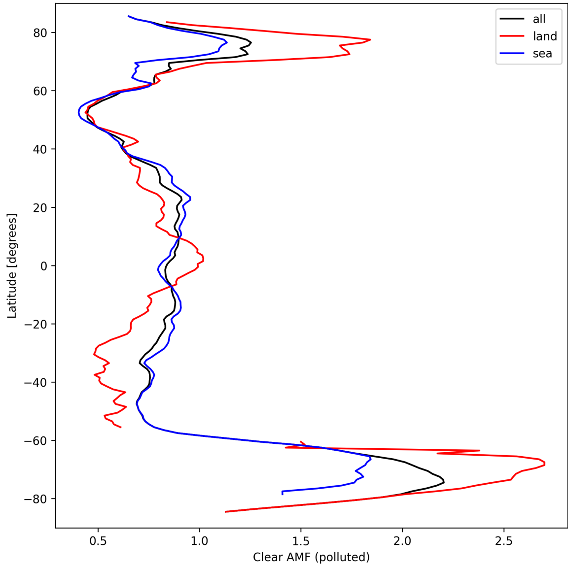
Figure 50: Zonal average of “Clear AMF (polluted)” for 2024-09-20 to 2024-09-22.
