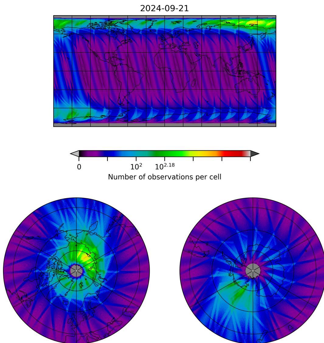
Figure 28: Map of the number of observations for 2024-09-20 to 2024-09-22
