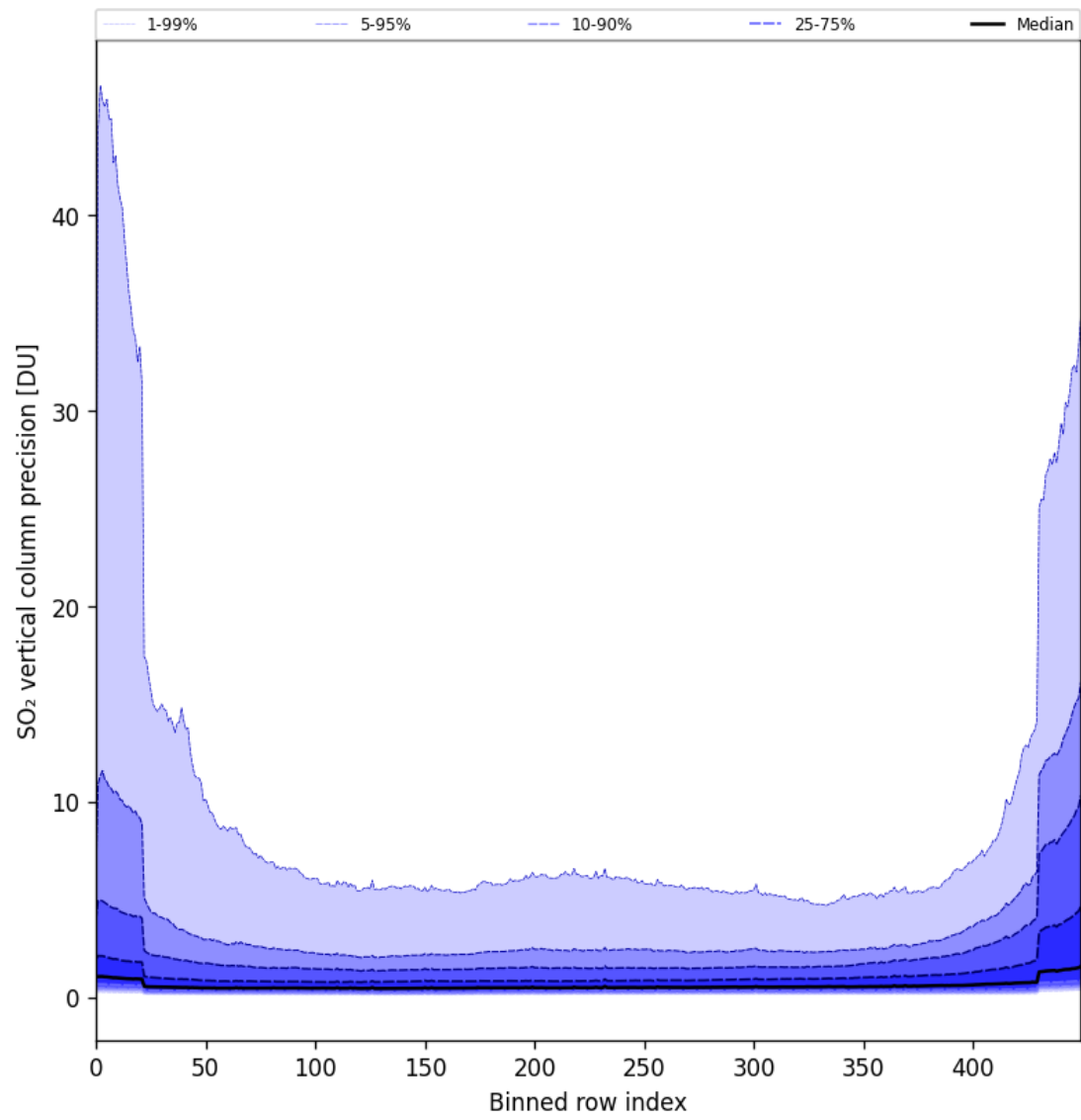
Figure 77: Along track statistics of “SO 2 vertical column precision” for 2024-09-20 to 2024-09-22
