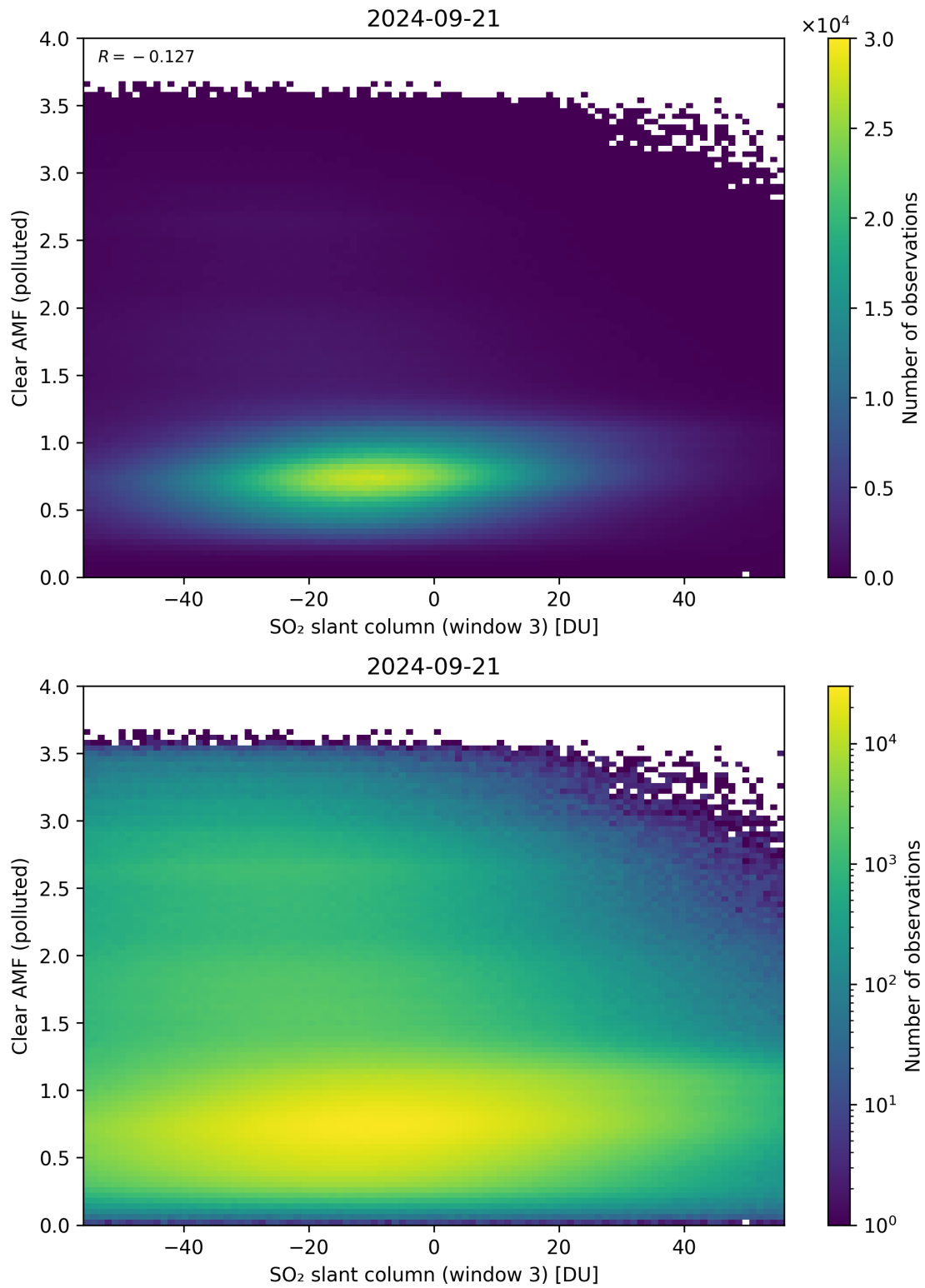
Figure 265: Scatter density plot of “SO 2 slant column (window 3)” against “Clear AMF (polluted)” for 2024-09-20 to 2024-09-22.
