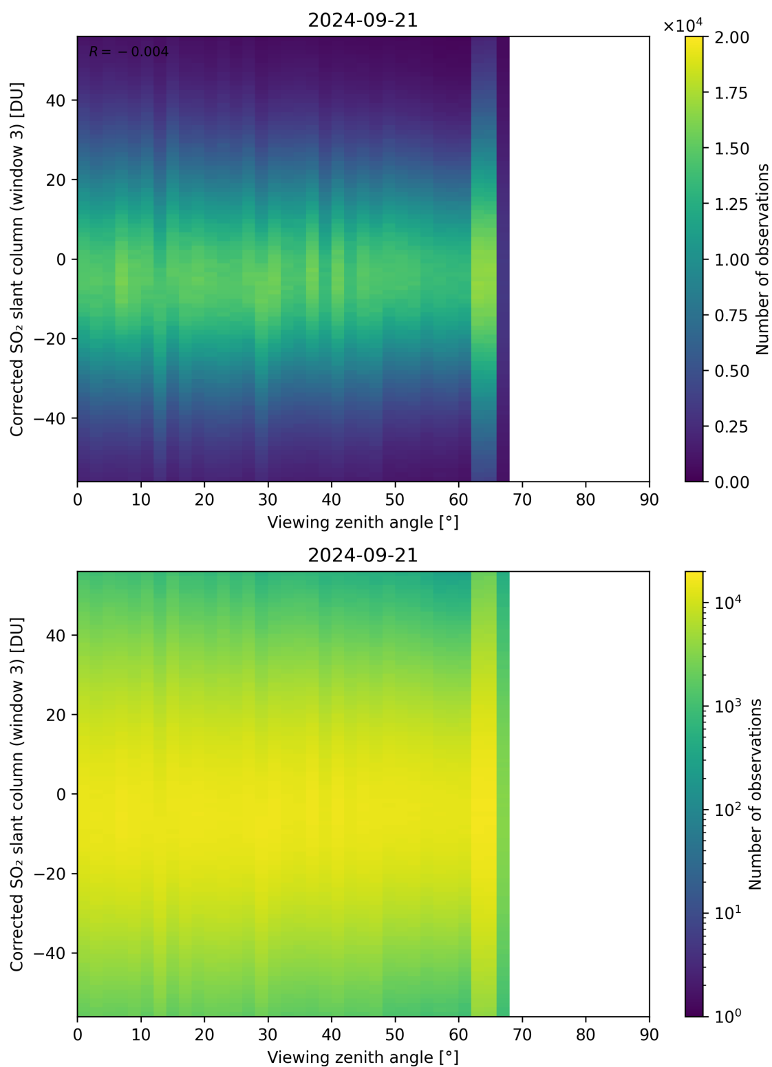
Figure 319: Scatter density plot of “Viewing zenith angle” against “Corrected SO 2 slant column (window 3)” for 2024-09-20 to 2024-09-22.
