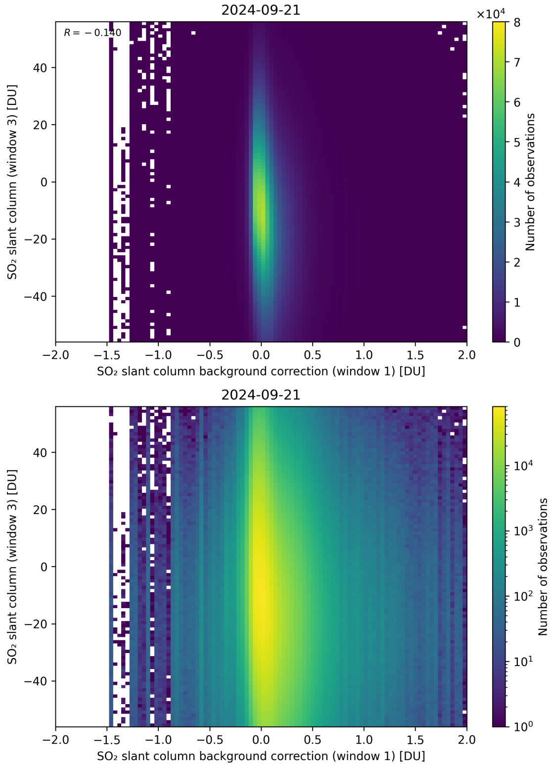
Figure 107: Scatter density plot of “SO 2 slant column background correction (window 1)” against “SO 2 slant column (window 3)” for 2024-09-20 to 2024-09-22.
