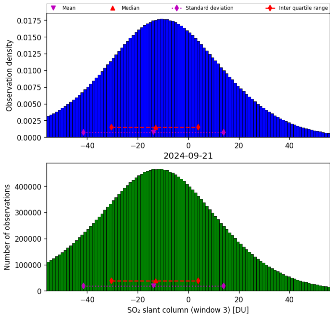
Figure 64: Histogram of “SO 2 slant column (window 3)” for 2024-09-20 to 2024-09-22
