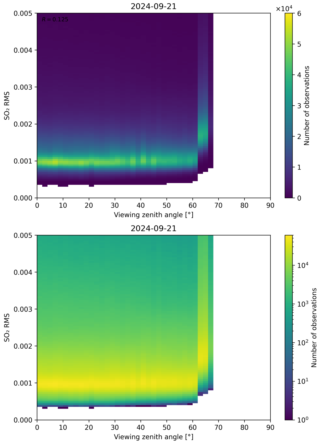
Figure 313: Scatter density plot of “Viewing zenith angle” against “SO 2 RMS” for 2024-09-20 to 2024-09-22.
