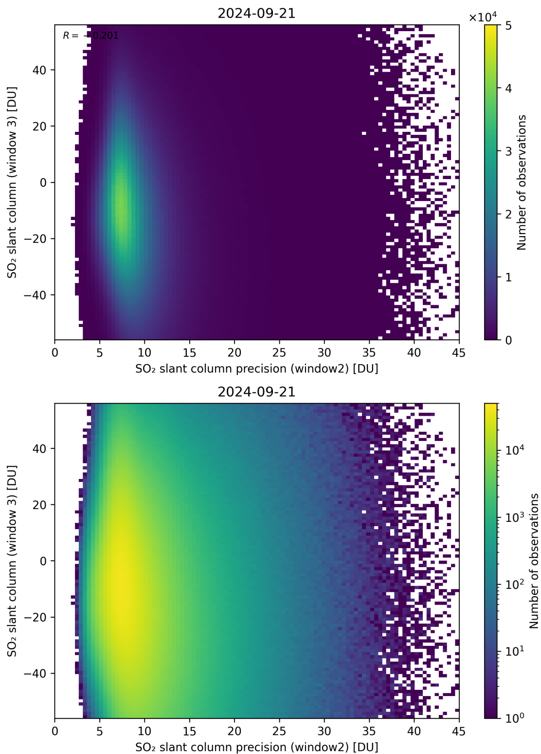
Figure 249: Scatter density plot of “SO 2 slant column precision (window2)” against “SO 2 slant column (window 3)” for 2024-09-20 to 2024-09-22.
