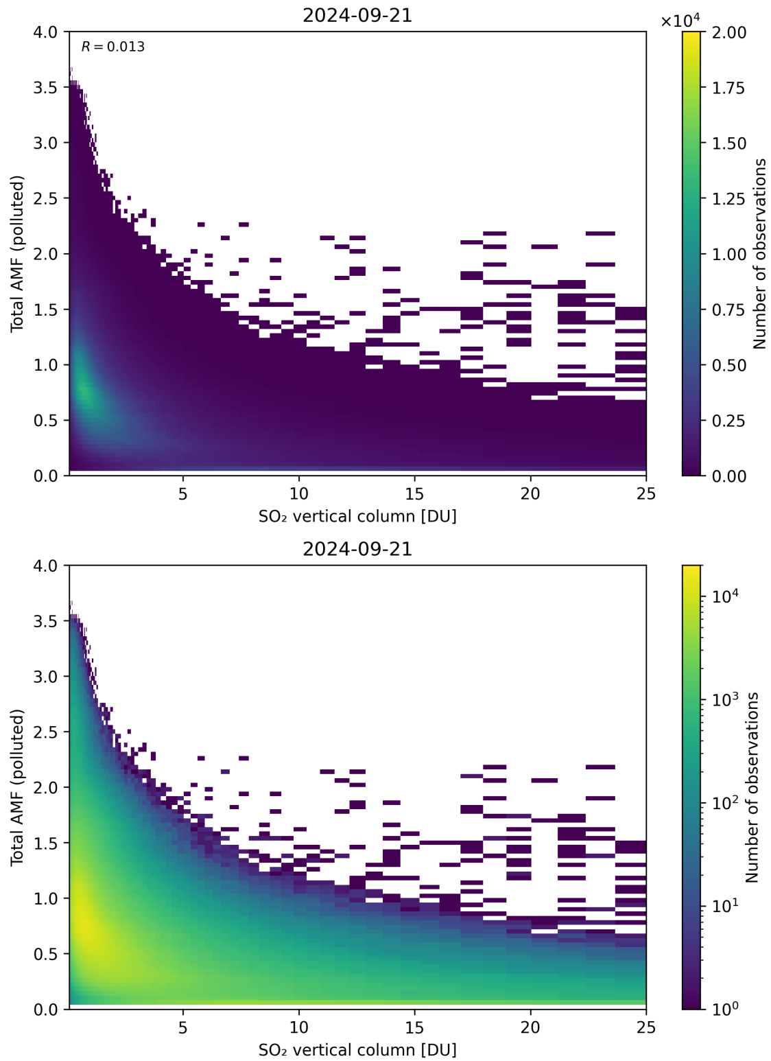
Figure 305: Scatter density plot of “SO 2 vertical column” against “Total AMF (polluted)” for 2024-09-20 to 2024-09-22.
