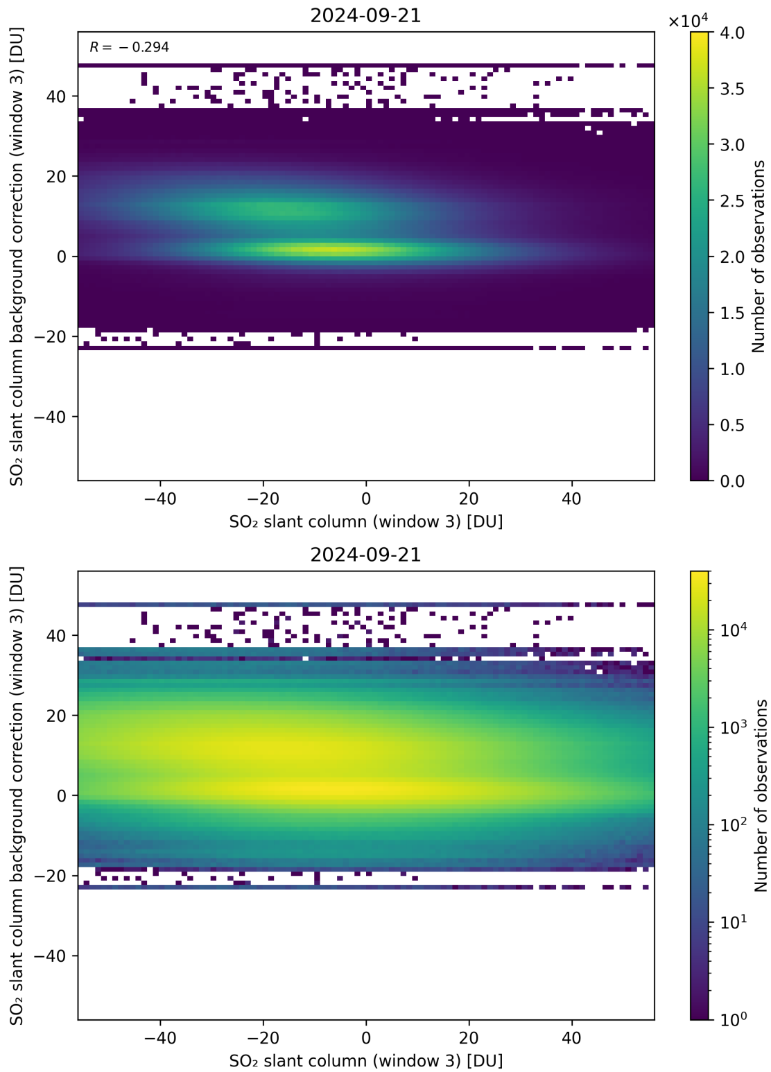
Figure 253: Scatter density plot of “SO 2 slant column (window 3)” against “SO 2 slant column background correction (window 3)” for 2024-09-20 to 2024-09-22.
