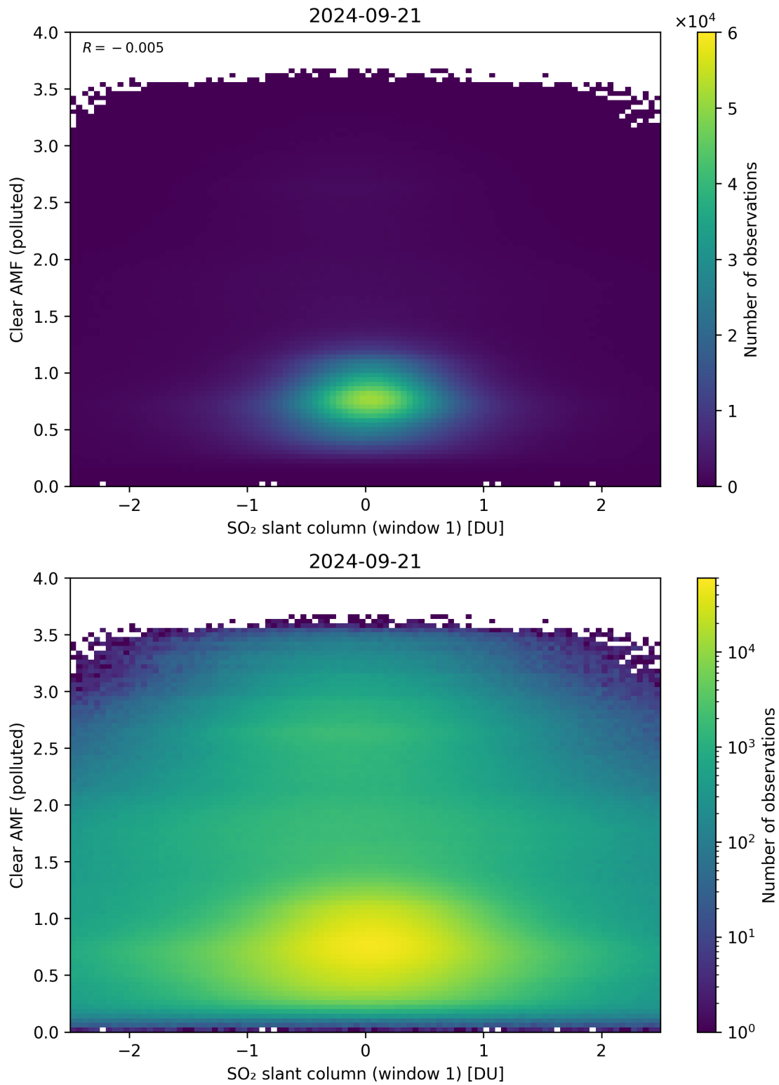
Figure 232: Scatter density plot of “SO 2 slant column (window 1)” against “Clear AMF (polluted)” for 2024-09-20 to 2024-09-22.
