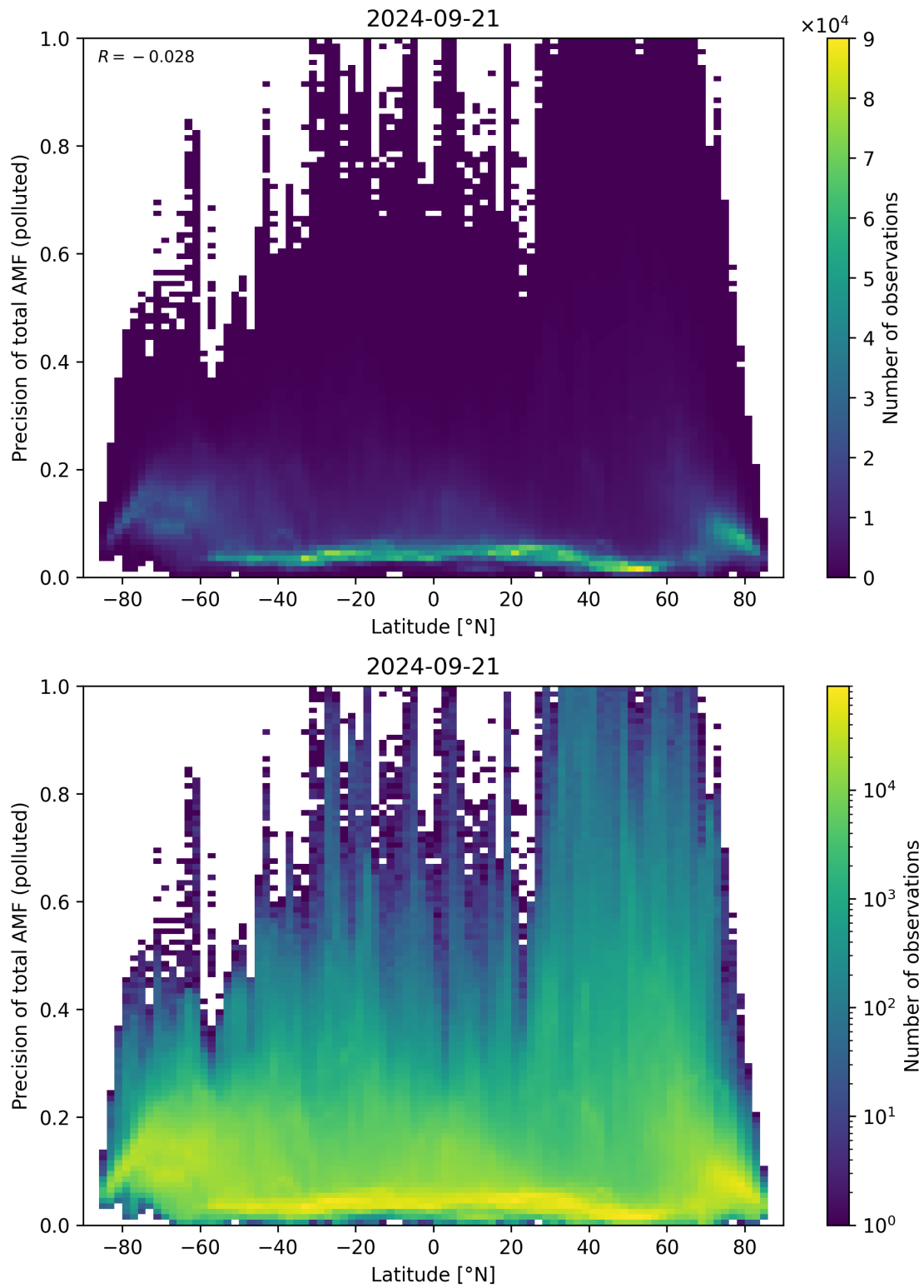
Figure 155: Scatter density plot of “Latitude” against “Precision of total AMF (polluted)” for 2024-09-20 to 2024-09-22.
