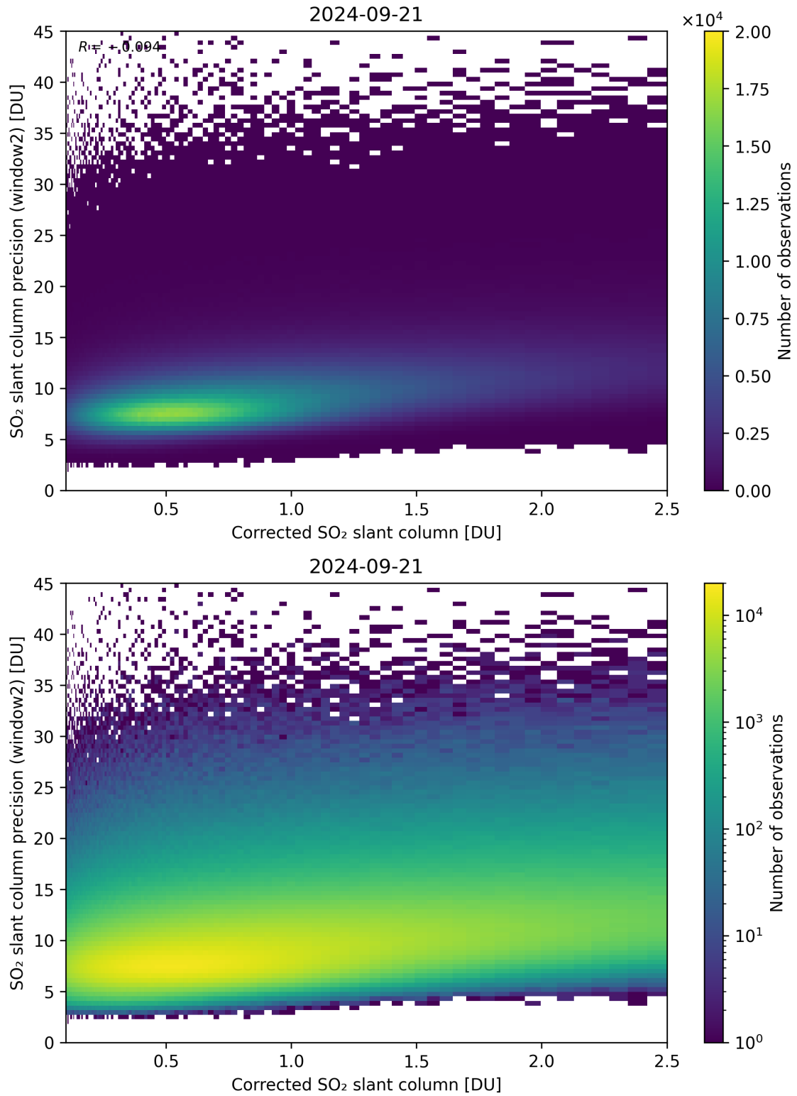
Figure 189: Scatter density plot of “Corrected SO 2 slant column” against “SO 2 slant column precision (window2)” for 2024-09-20 to 2024-09-22.
