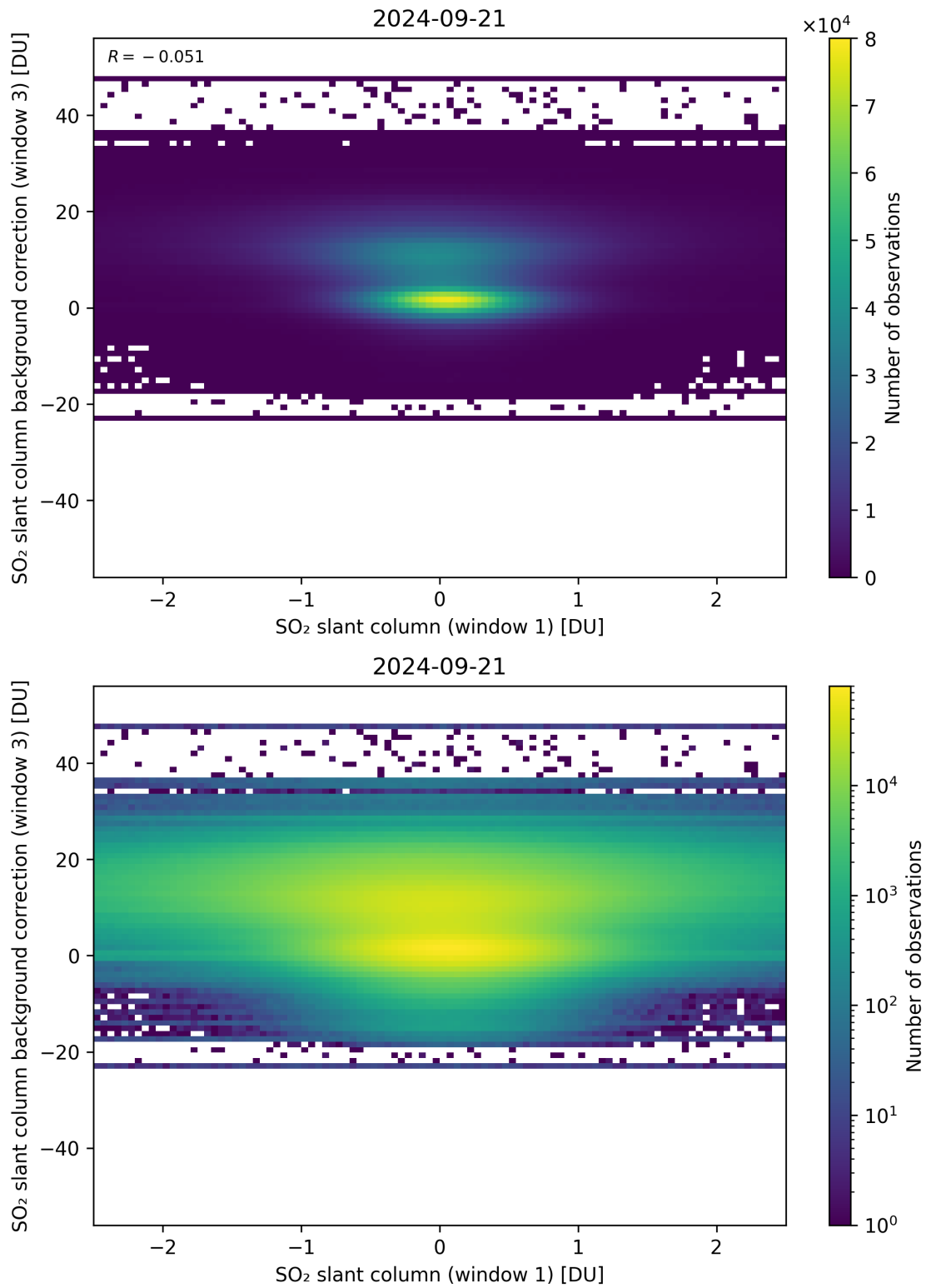
Figure 214: Scatter density plot of “SO 2 slant column (window 1)” against “SO 2 slant column background correction (window 3)” for 2024-09-20 to 2024-09-22.
