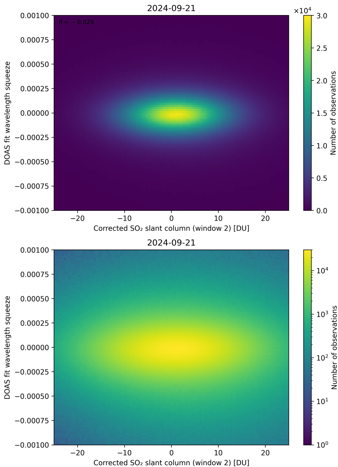
Figure 197: Scatter density plot of “Corrected SO 2 slant column (window 2)” against “DOAS fit wavelength squeeze” for 2024-09-20 to 2024-09-22.
