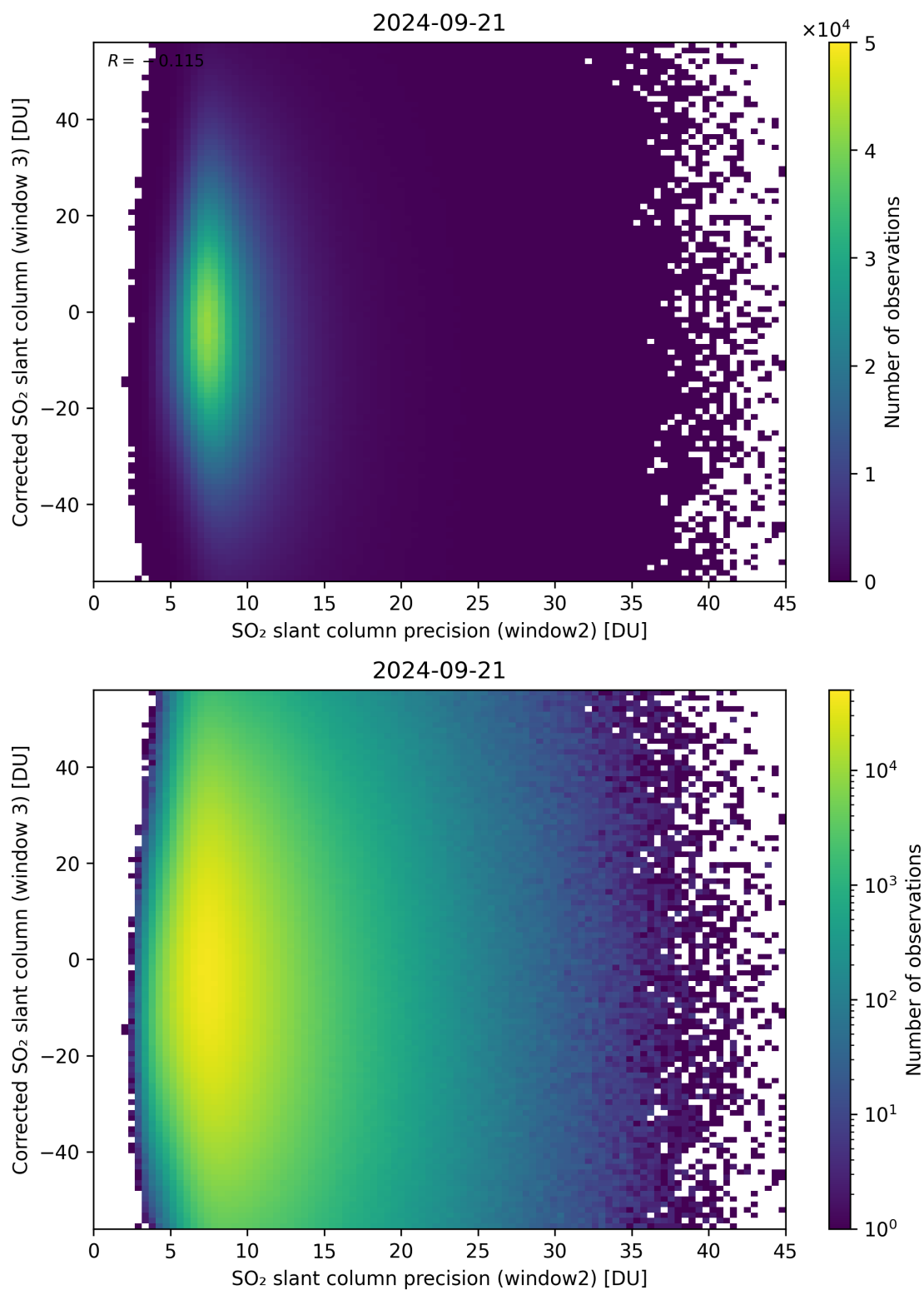
Figure 248: Scatter density plot of “SO 2 slant column precision (window2)” against “Corrected SO 2 slant column (window 3)” for 2024-09-20 to 2024-09-22.
