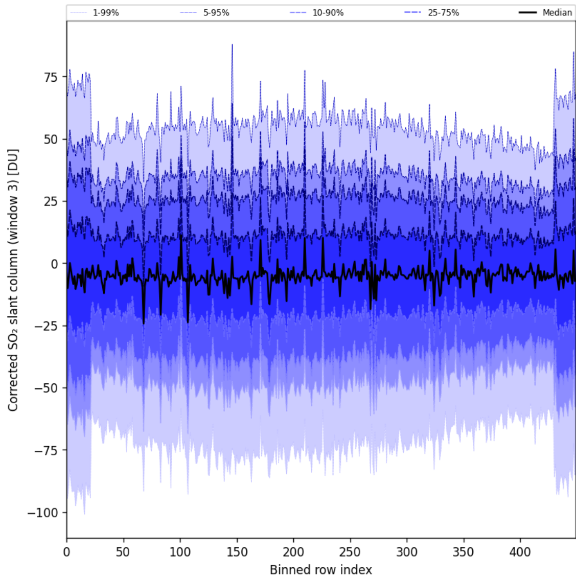
Figure 89: Along track statistics of “Corrected SO 2 slant column (window 3)” for 2024-09-20 to 2024-09-22
