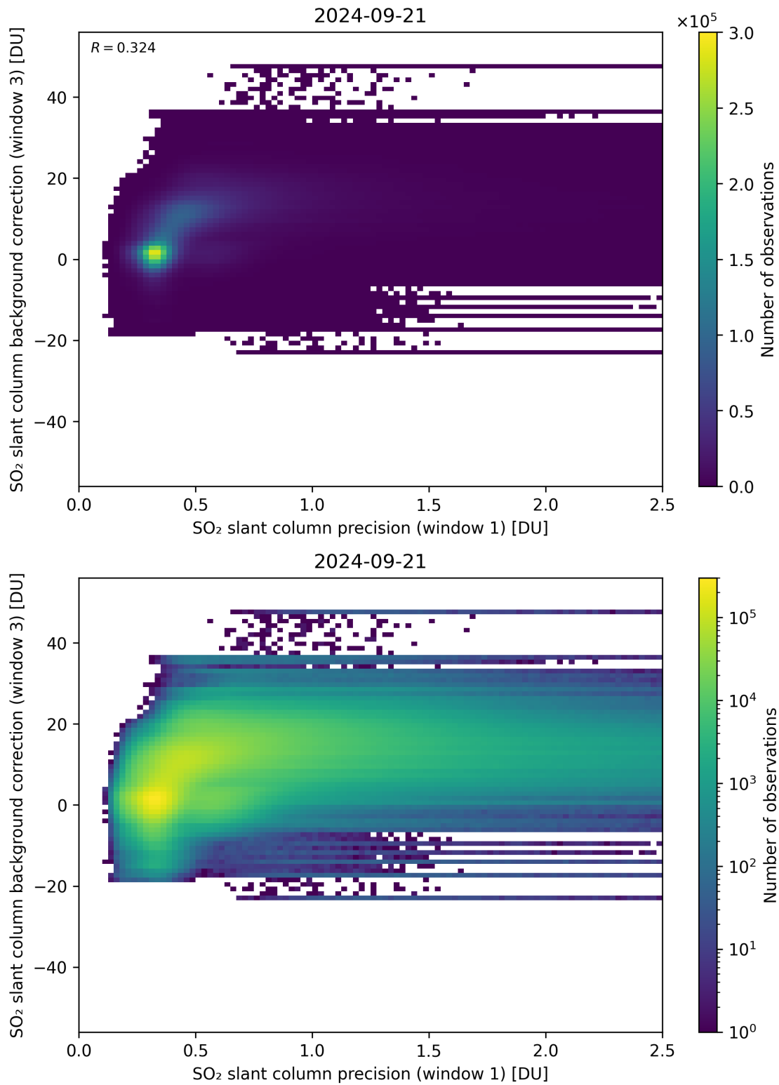
Figure 220: Scatter density plot of “SO 2 slant column precision (window 1)” against “SO 2 slant column background correction (window 3)” for 2024-09-20 to 2024-09-22.
