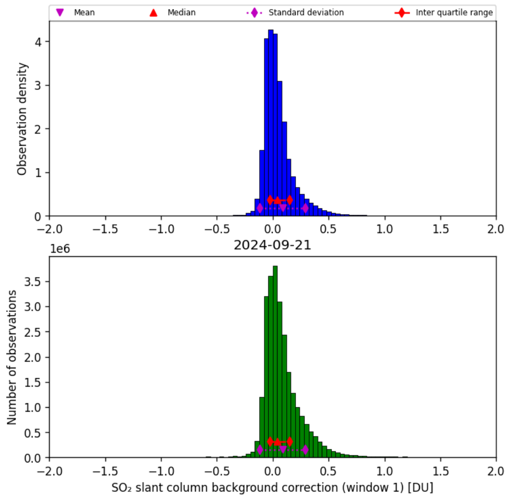
Figure 59: Histogram of “SO 2 slant column background correction (window 1)” for 2024-09-20 to 2024-09-22
