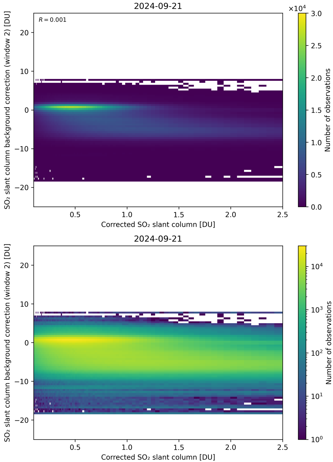
Figure 179: Scatter density plot of “Corrected SO 2 slant column” against “SO 2 slant column background correction (window 2)” for 2024-09-20 to 2024-09-22.
