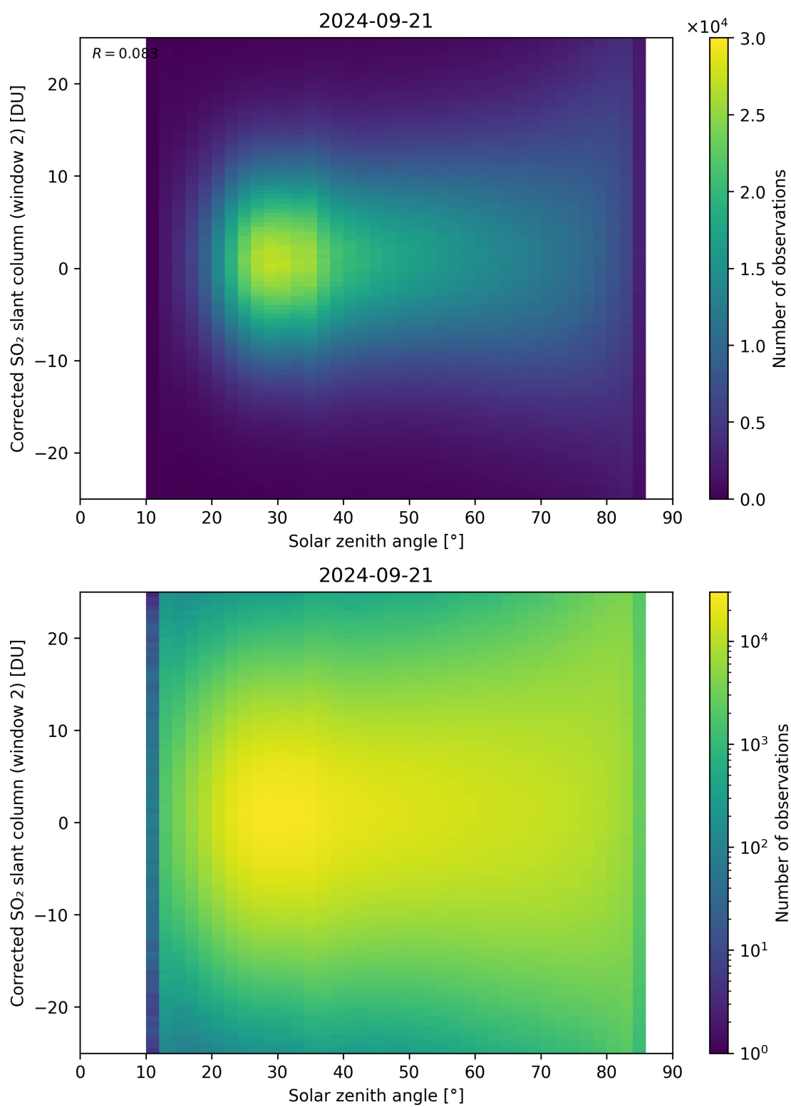
Figure 167: Scatter density plot of “Solar zenith angle” against “Corrected SO 2 slant column (window 2)” for 2024-09-20 to 2024-09-22.
