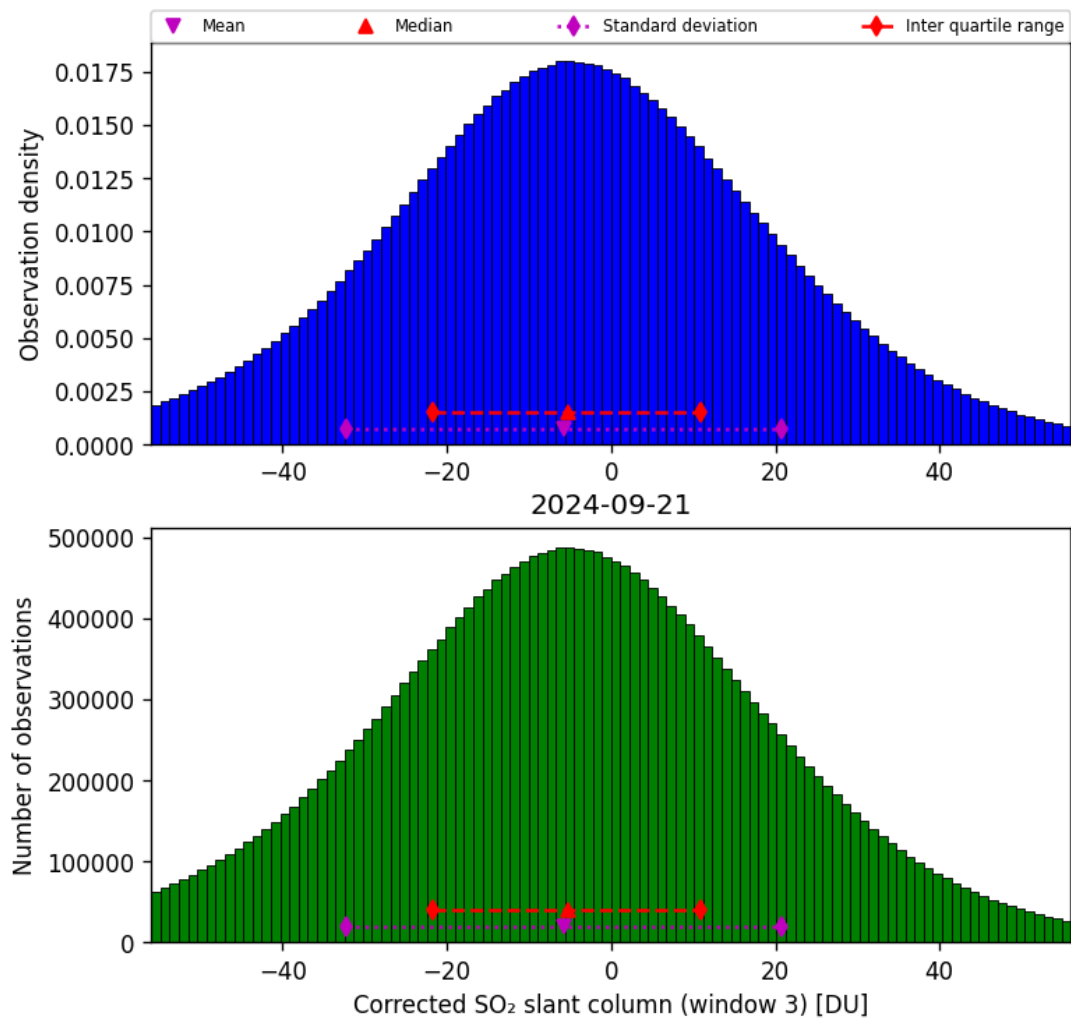
Figure 66: Histogram of “Corrected SO 2 slant column (window 3)” for 2024-09-20 to 2024-09-22
