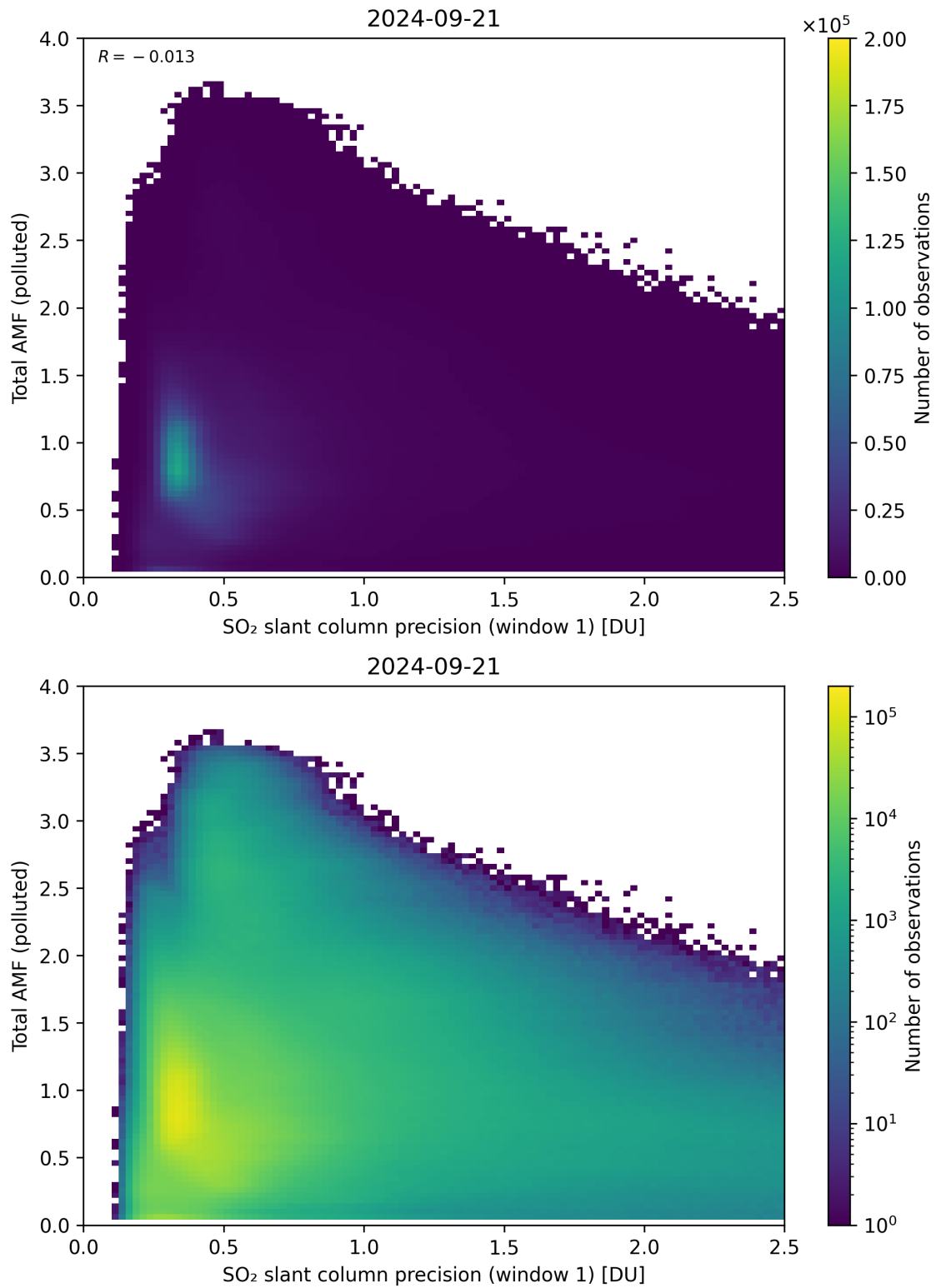
Figure 230: Scatter density plot of “SO 2 slant column precision (window 1)” against “Total AMF (polluted)” for 2024-09-20 to 2024-09-22.
