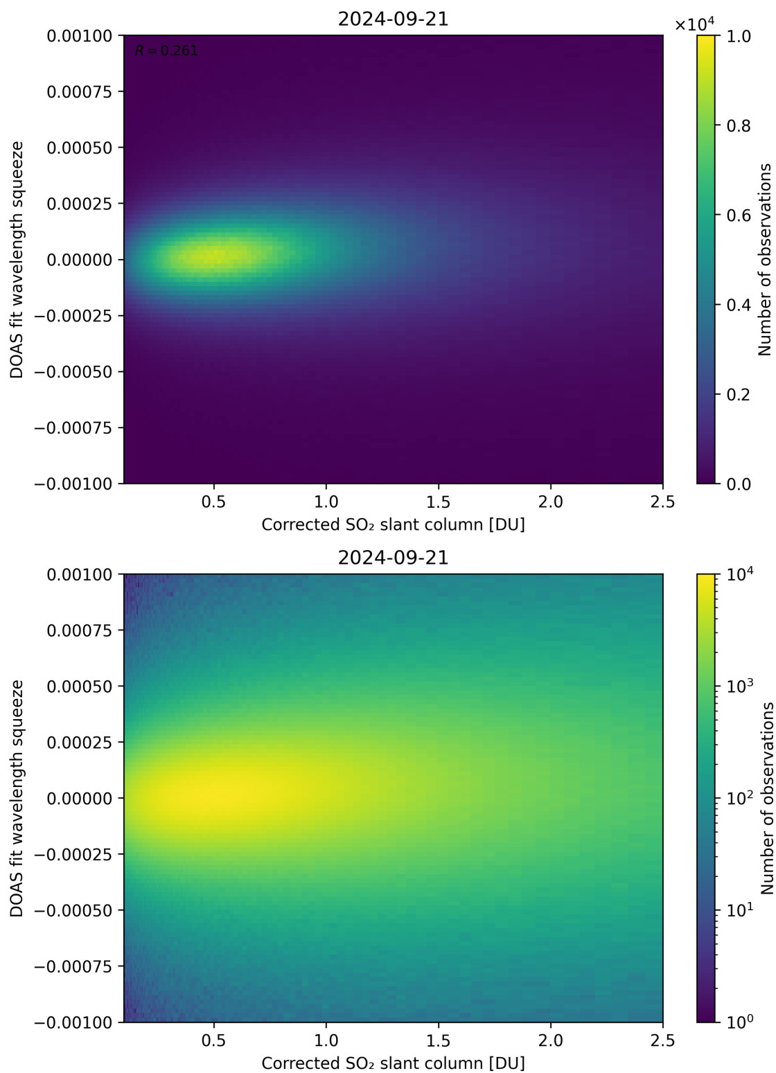
Figure 182: Scatter density plot of “Corrected SO 2 slant column” against “DOAS fit wavelength squeeze” for 2024-09-20 to 2024-09-22.
