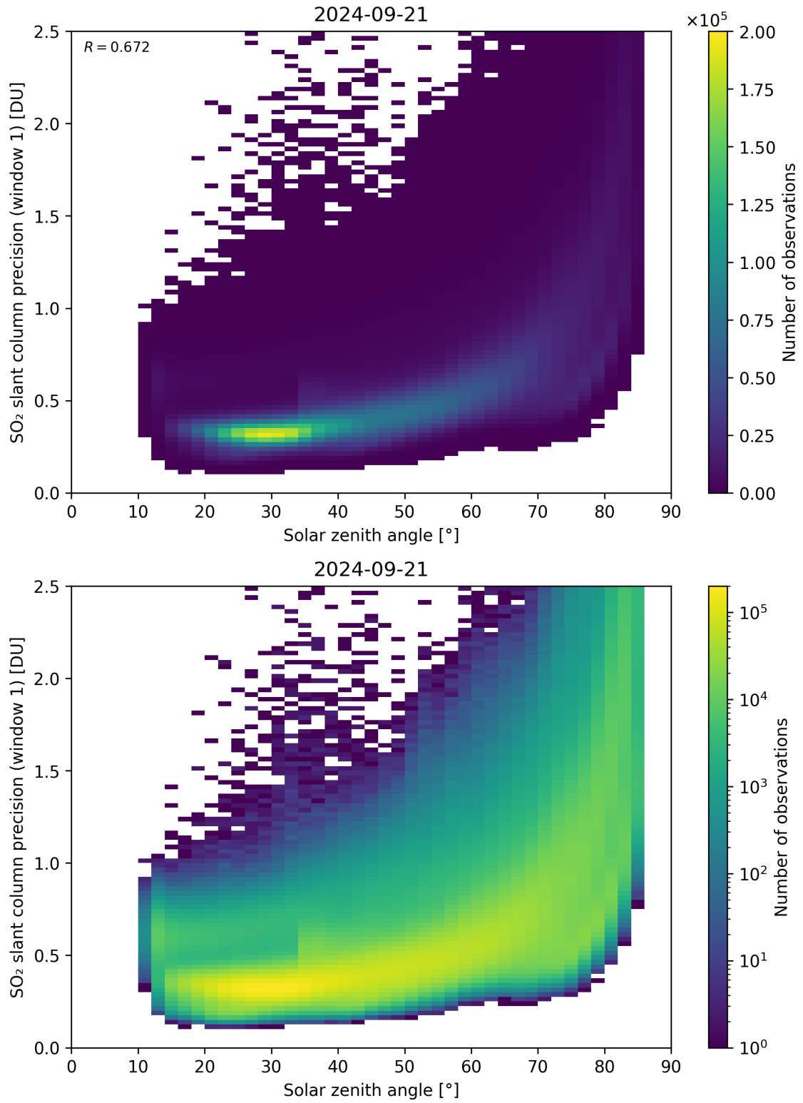
Figure 170: Scatter density plot of “Solar zenith angle” against “SO 2 slant column precision (window 1)” for 2024-09-20 to 2024-09-22.
