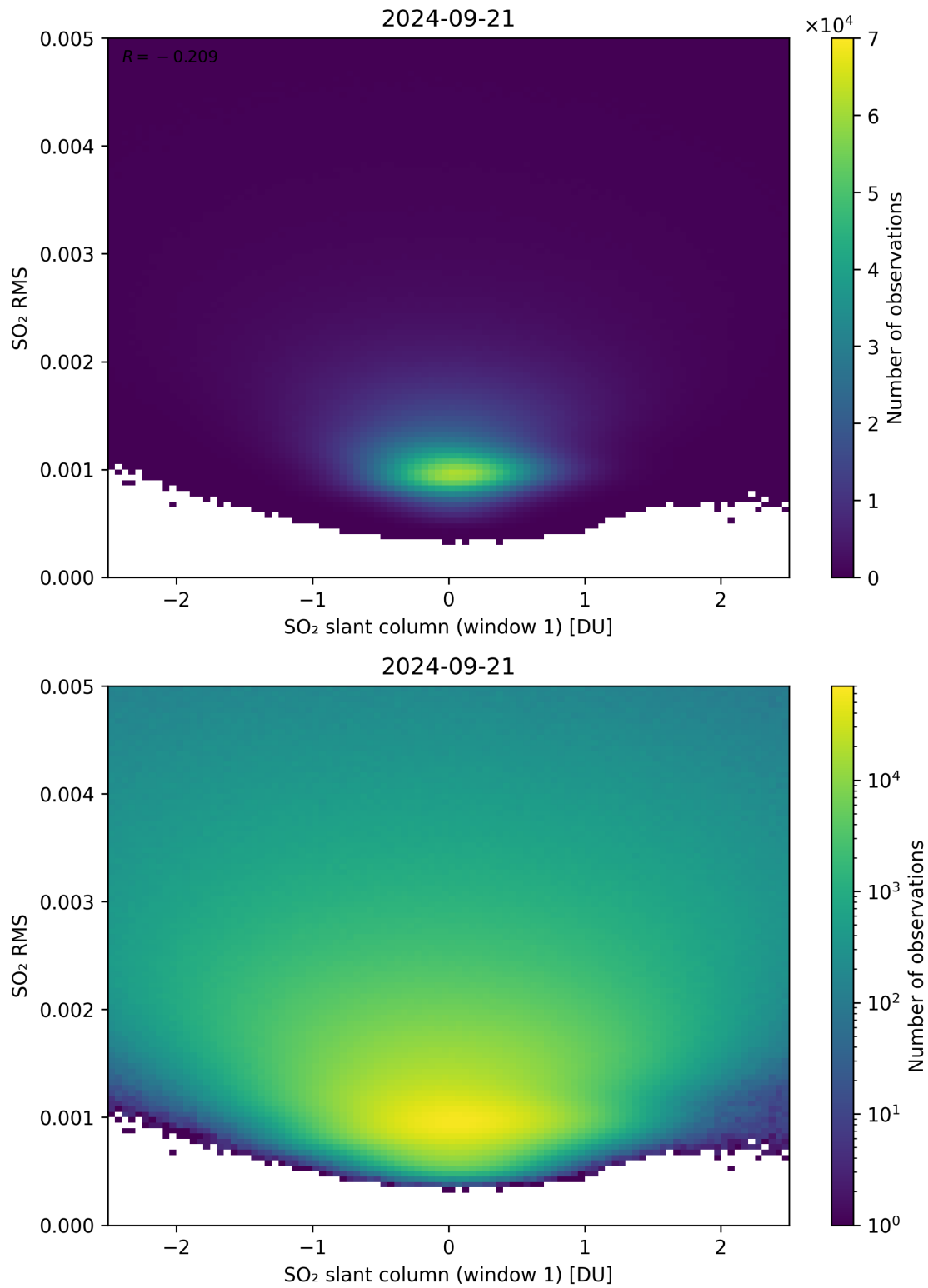
Figure 217: Scatter density plot of “SO 2 slant column (window 1)” against “SO 2 RMS” for 2024-09-20 to 2024-09-22.
