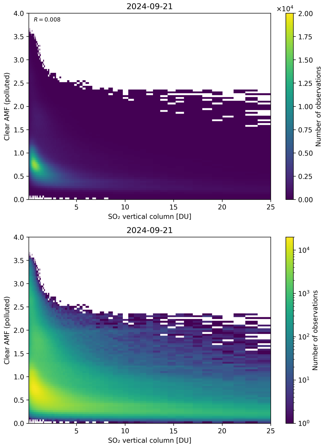
Figure 296: Scatter density plot of “SO 2 vertical column” against “Clear AMF (polluted)” for 2024-09-20 to 2024-09-22.
