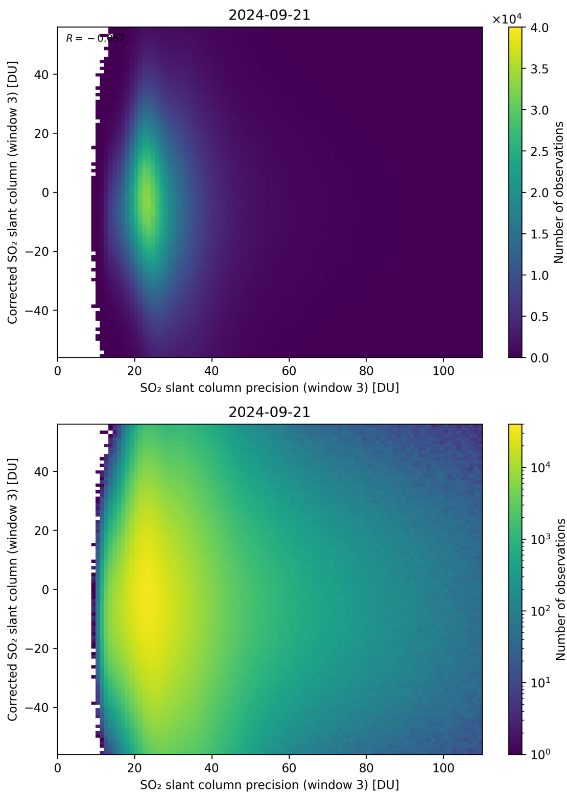
Figure 262: Scatter density plot of “SO 2 slant column precision (window 3)” against “Corrected SO 2 slant column (window 3)” for 2024-09-20 to 2024-09-22.
