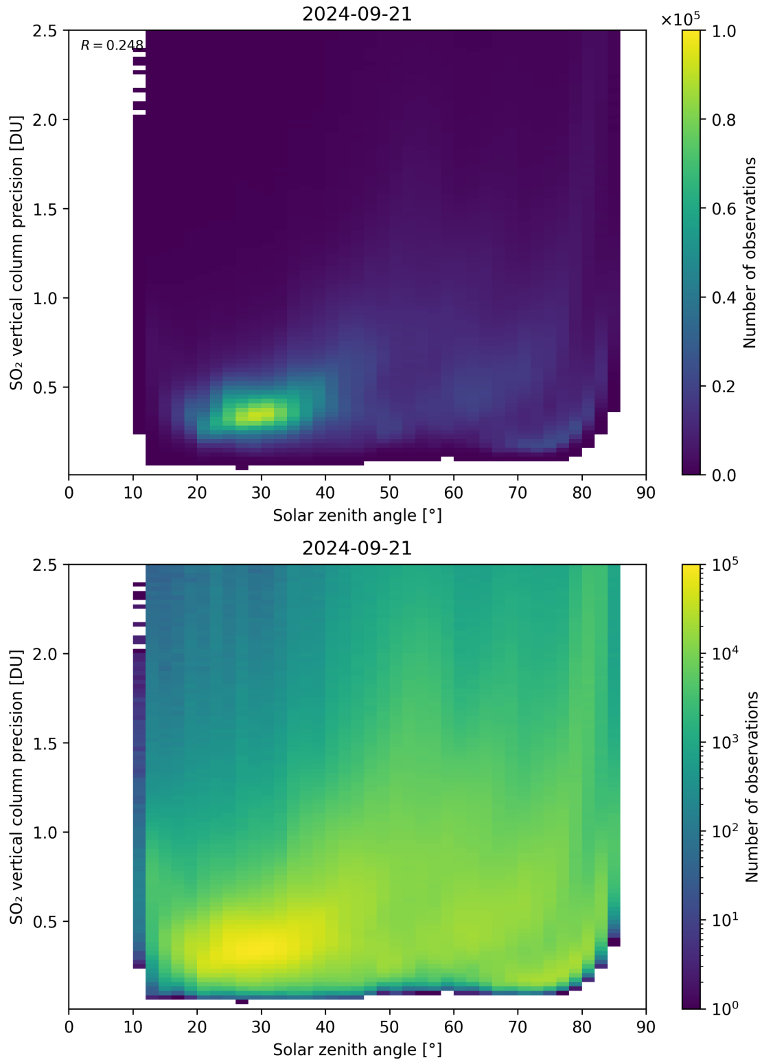
Figure 177: Scatter density plot of “Solar zenith angle” against “SO 2 vertical column precision” for 2024-09-20 to 2024-09-22.
