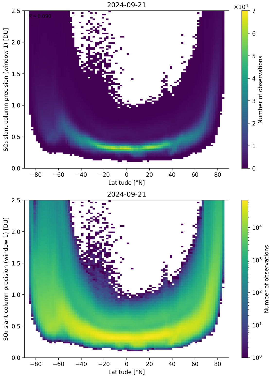
Figure 150: Scatter density plot of “Latitude” against “SO 2 slant column precision (window 1)” for 2024-09-20 to 2024-09-22.
