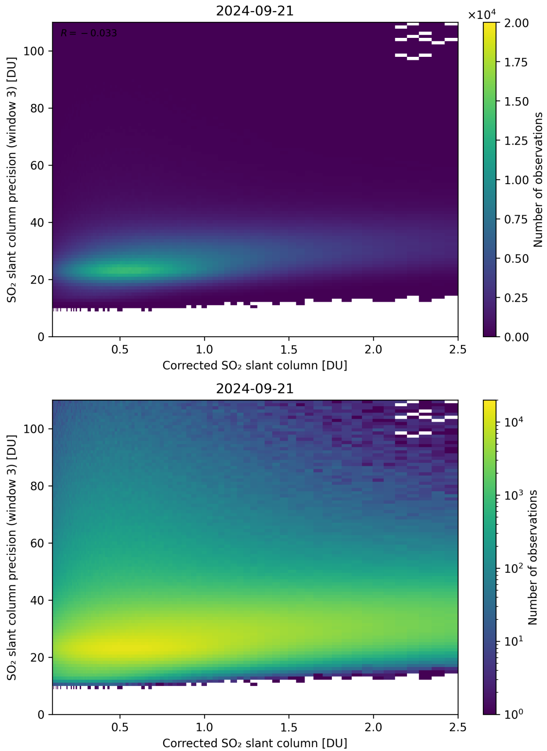
Figure 191: Scatter density plot of “Corrected SO 2 slant column” against “SO 2 slant column precision (window 3)” for 2024-09-20 to 2024-09-22.
