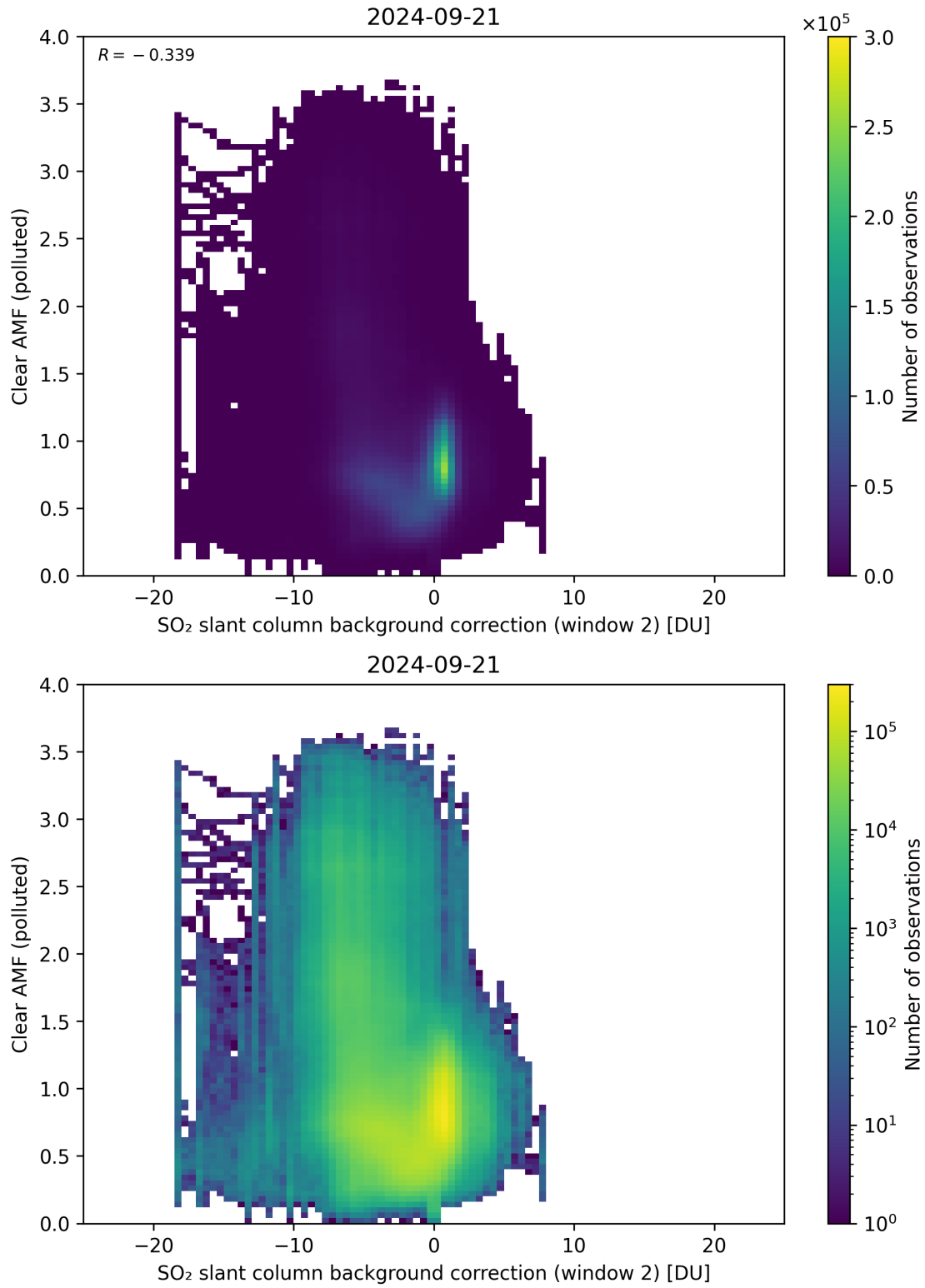
Figure 115: Scatter density plot of “SO 2 slant column background correction (window 2)” against “Clear AMF (polluted)” for 2024-09-20 to 2024-09-22.
