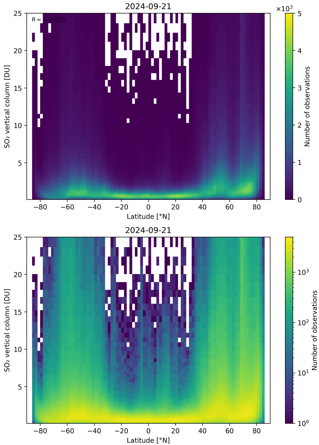
Figure 156: Scatter density plot of “Latitude” against “SO 2 vertical column” for 2024-09-20 to 2024-09-22.
