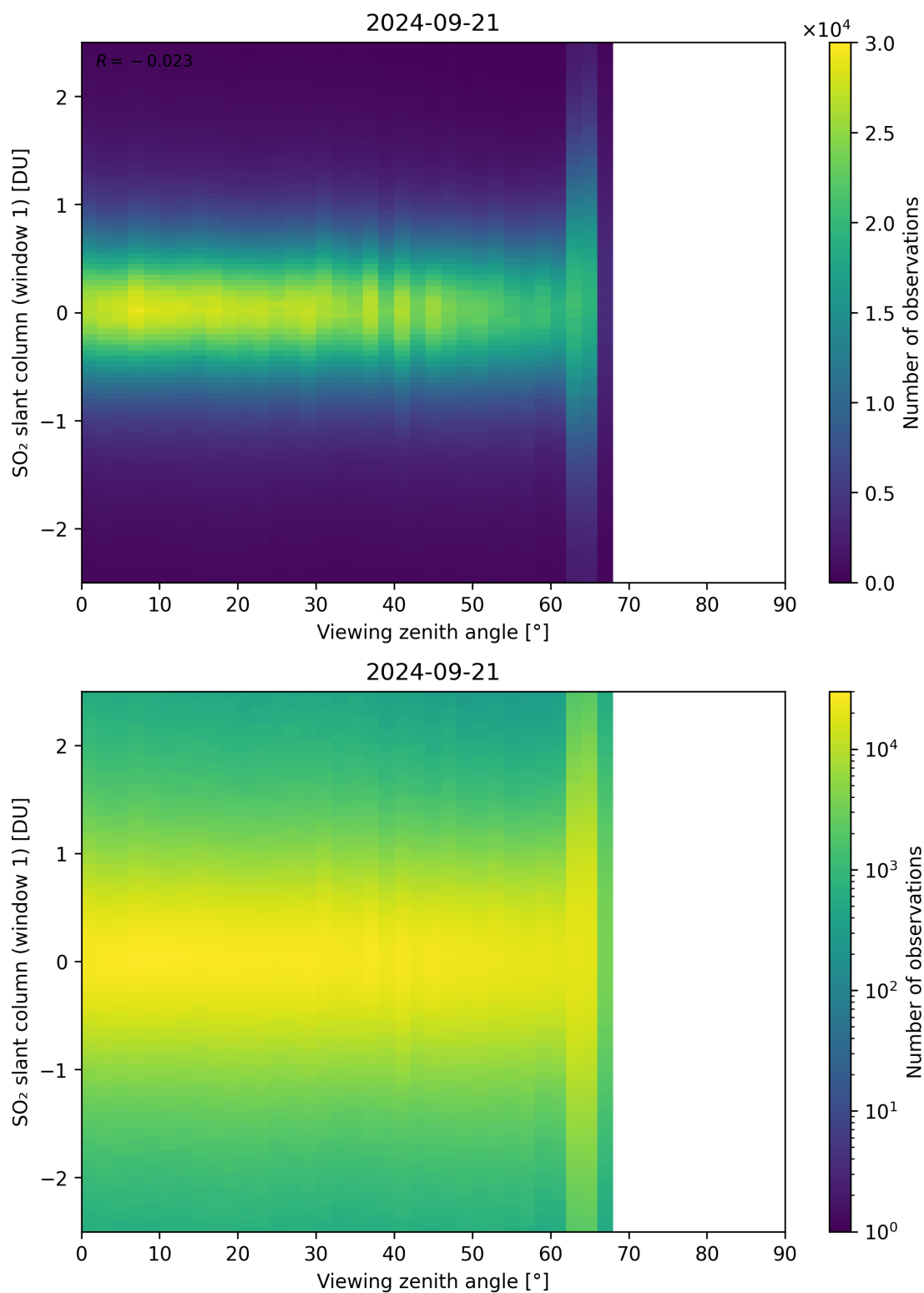
Figure 320: Scatter density plot of “Viewing zenith angle” against “SO 2 slant column (window 1)” for 2024-09-20 to 2024-09-22.
