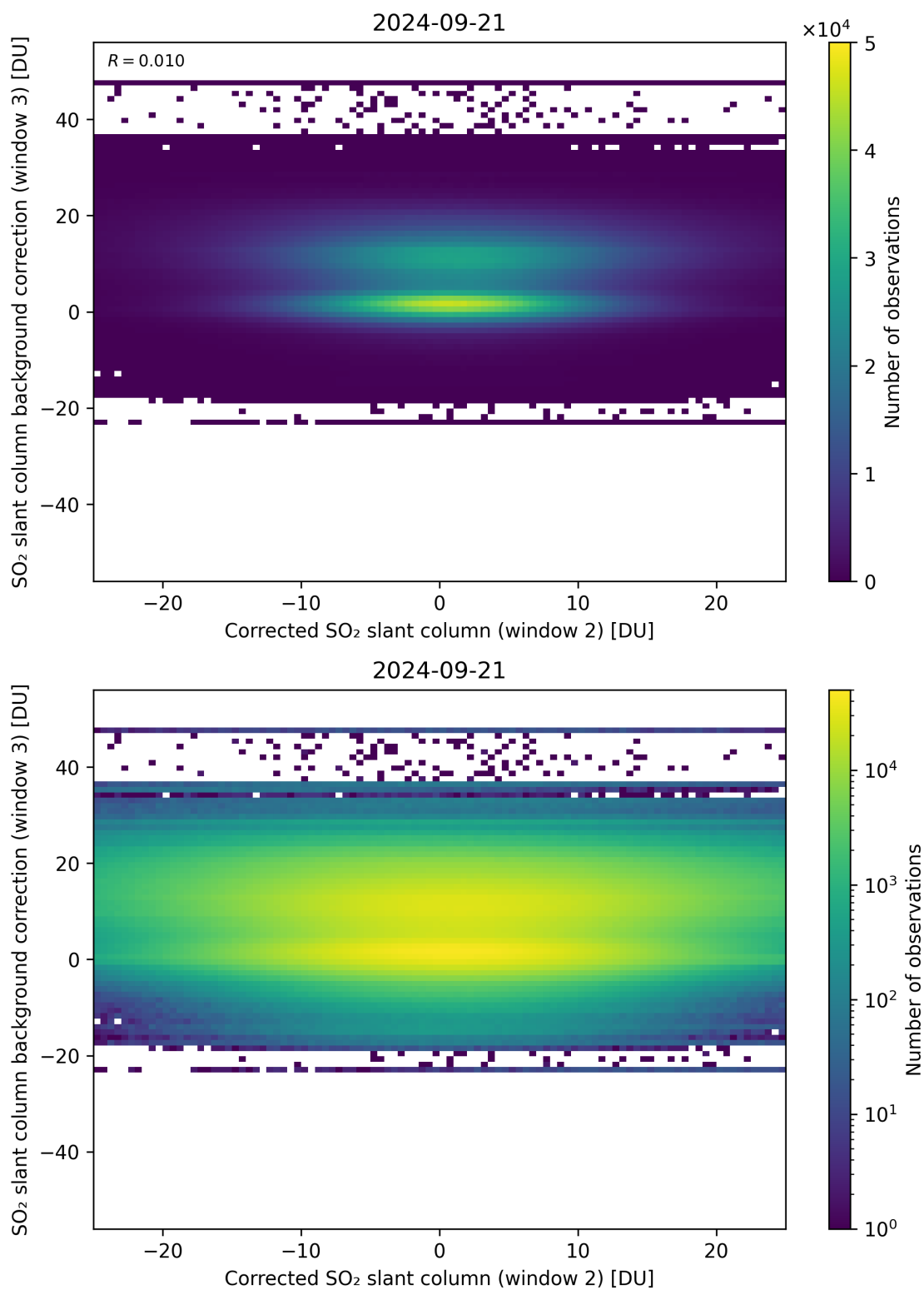
Figure 195: Scatter density plot of “Corrected SO 2 slant column (window 2)” against “SO 2 slant column background correction (window 3)” for 2024-09-20 to 2024-09-22.
