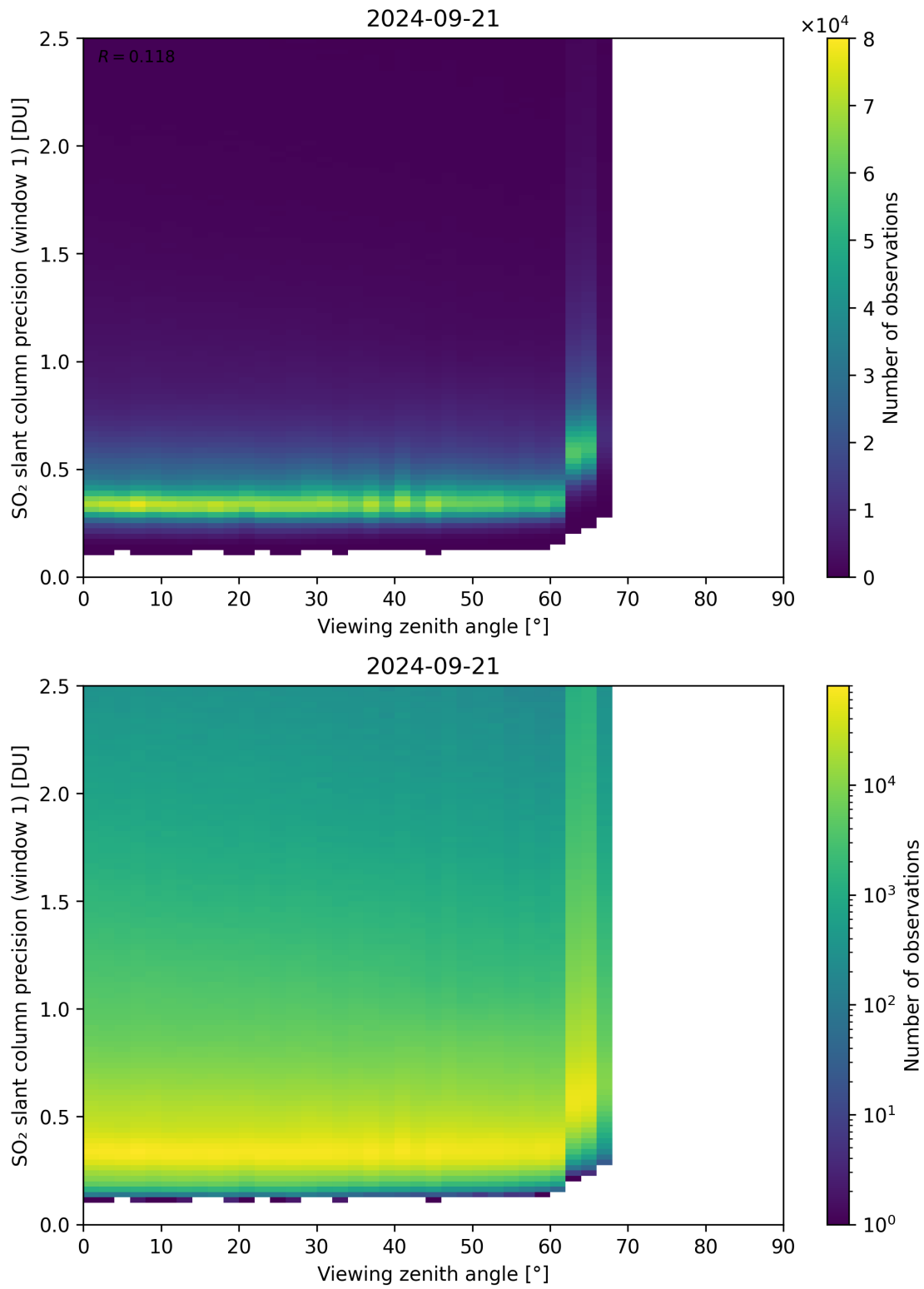
Figure 321: Scatter density plot of “Viewing zenith angle” against “SO 2 slant column precision (window 1)” for 2024-09-20 to 2024-09-22.
