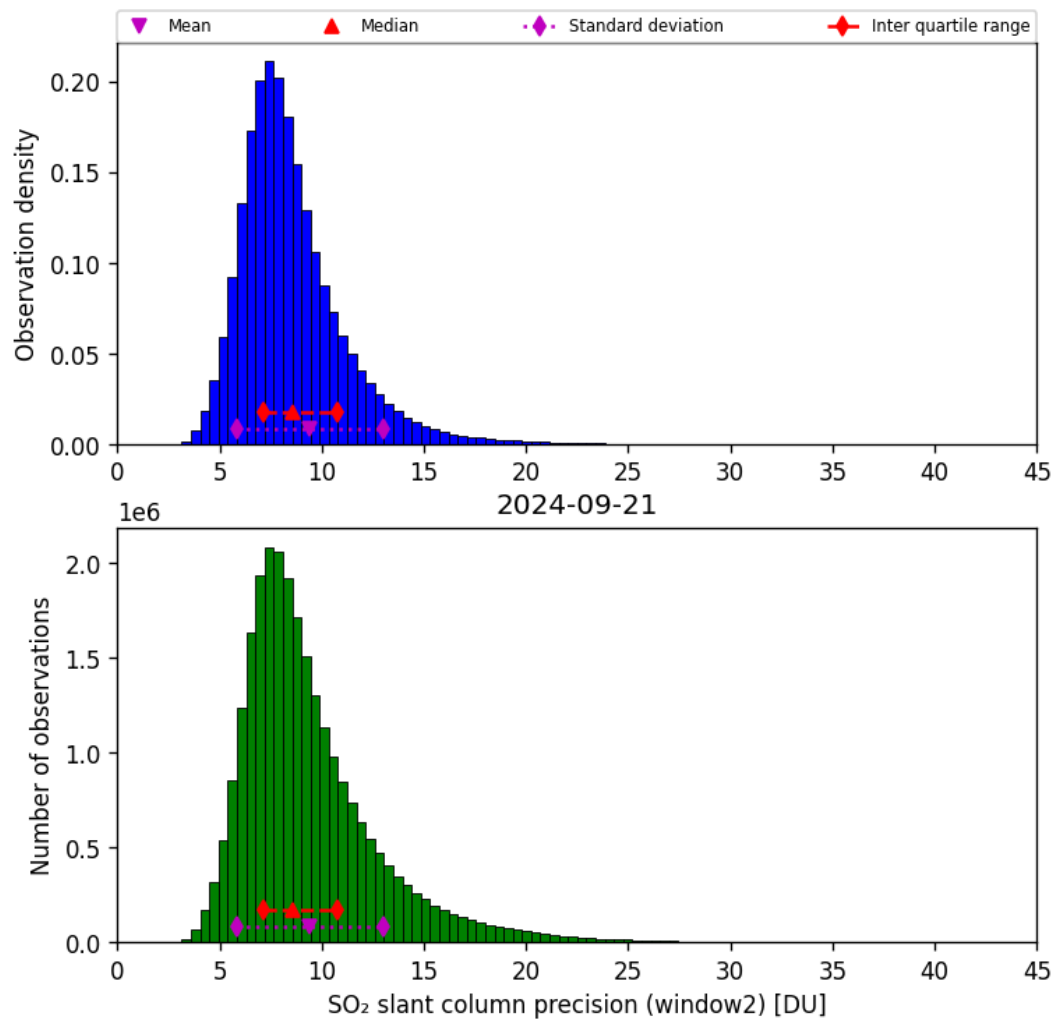
Figure 61: Histogram of “SO 2 slant column precision (window2)” for 2024-09-20 to 2024-09-22
