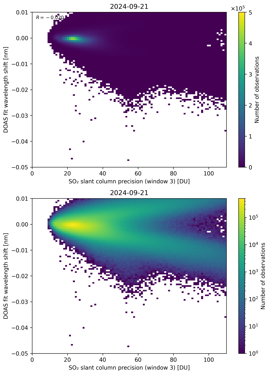
Figure 258: Scatter density plot of “SO 2 slant column precision (window 3)” against “DOAS fit wavelength shift” for 2024-09-20 to 2024-09-22.
