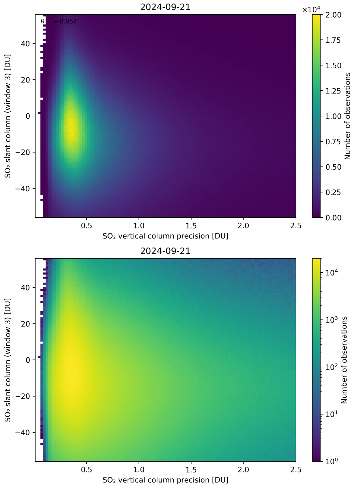
Figure 292: Scatter density plot of “SO 2 vertical column precision” against “SO 2 slant column (window 3)” for 2024-09-20 to 2024-09-22.
