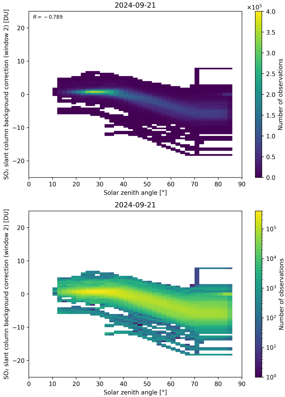
Figure 159: Scatter density plot of “Solar zenith angle” against “SO 2 slant column background correction (window 2)” for 2024-09-20 to 2024-09-22.
