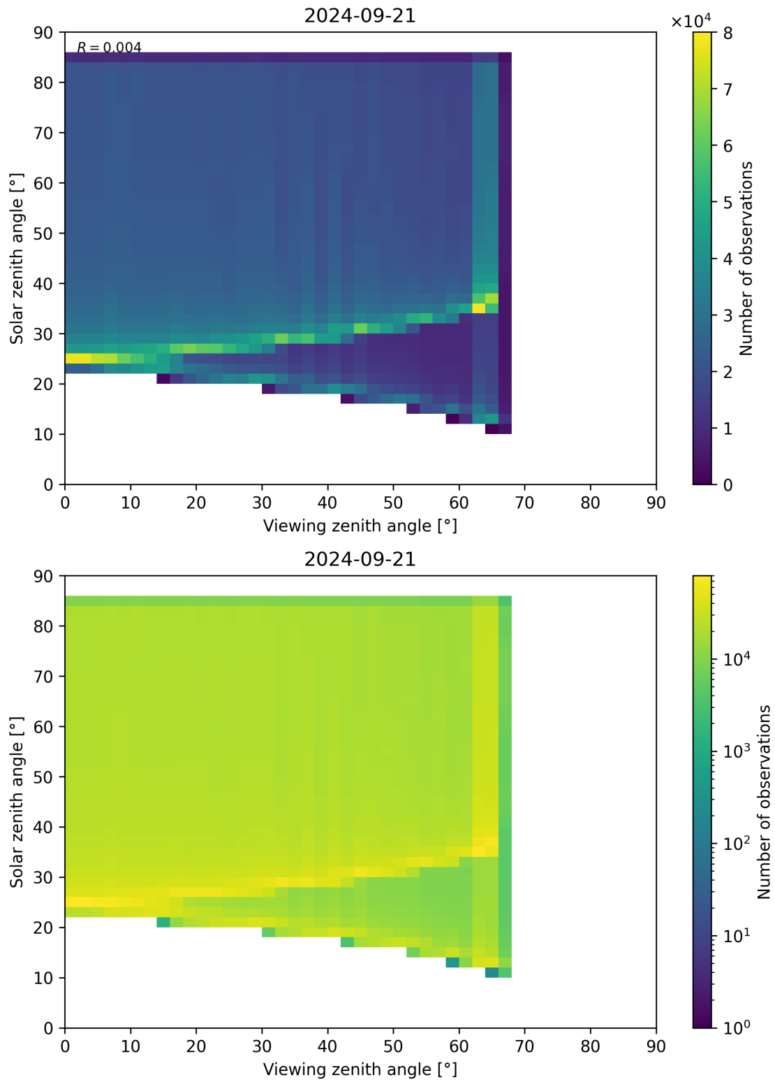
Figure 315: Scatter density plot of “Viewing zenith angle” against “Solar zenith angle” for 2024-09-20 to 2024-09-22.
