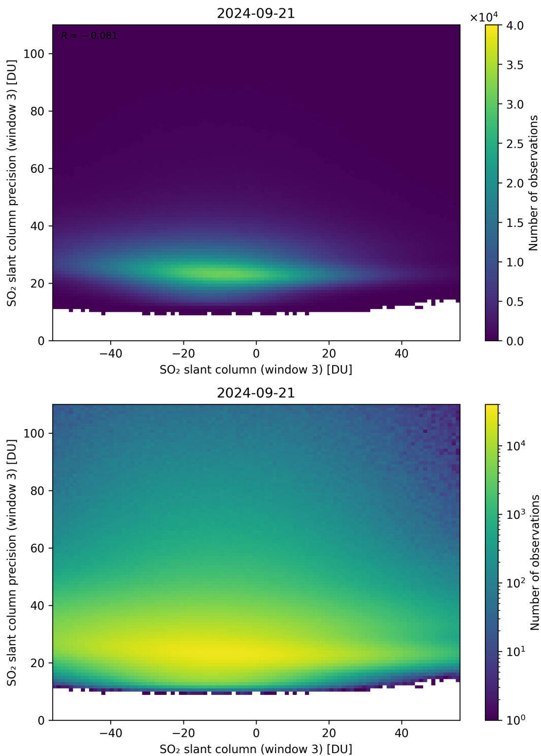
Figure 267: Scatter density plot of “SO 2 slant column (window 3)” against “SO 2 slant column precision (window 3)” for 2024-09-20 to 2024-09-22.
