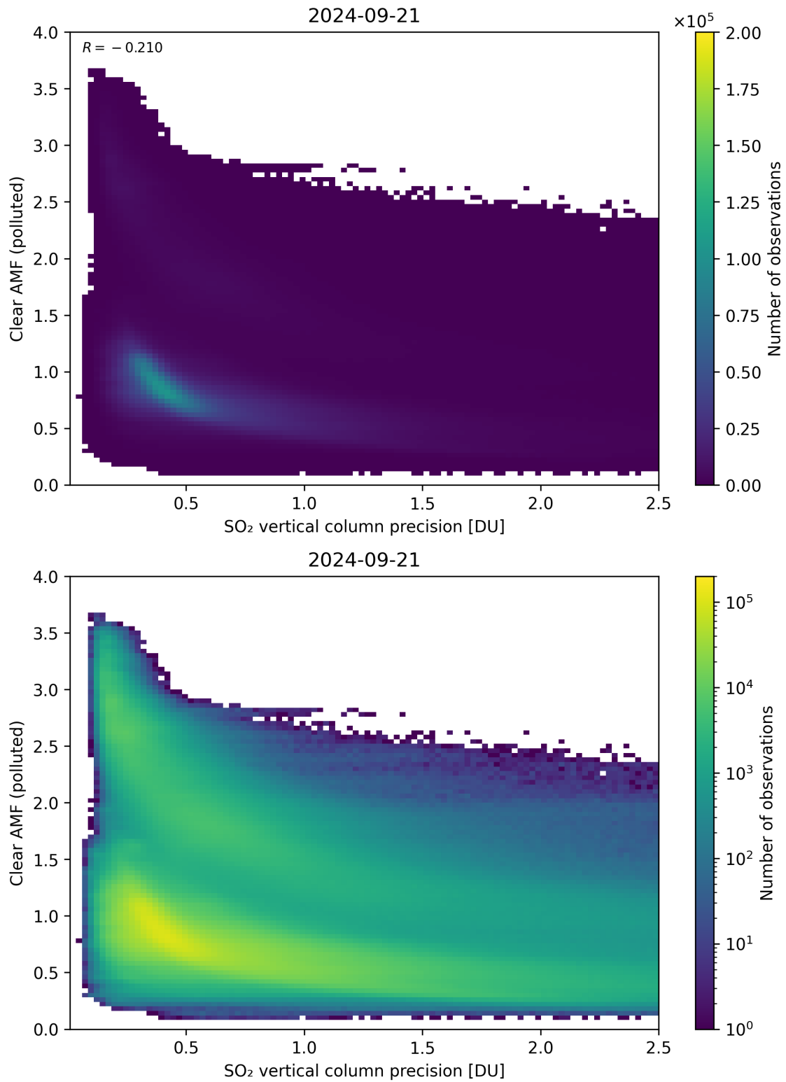
Figure 285: Scatter density plot of “SO 2 vertical column precision” against “Clear AMF (polluted)” for 2024-09-20 to 2024-09-22.
