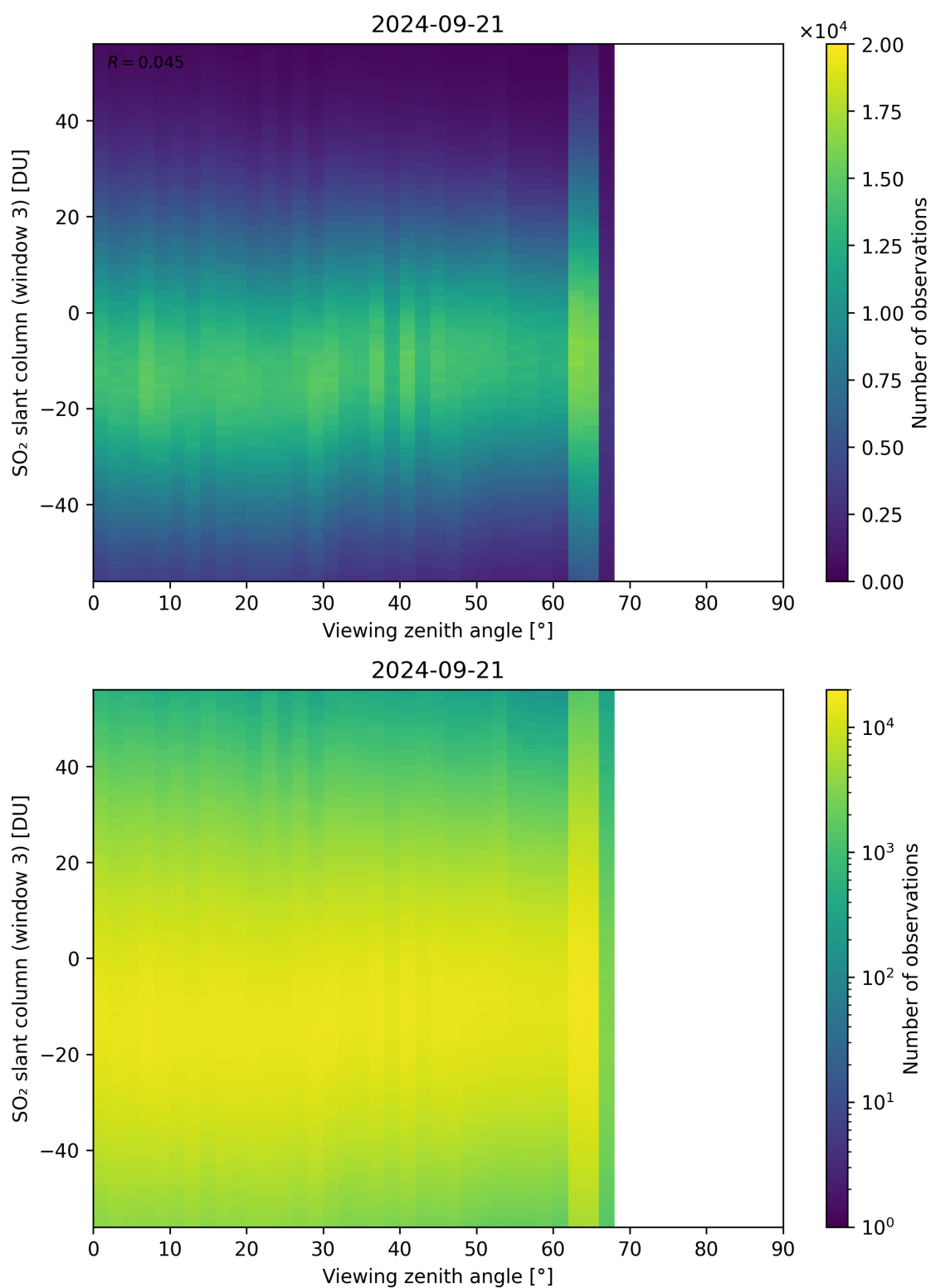
Figure 323: Scatter density plot of “Viewing zenith angle” against “SO 2 slant column (window 3)” for 2024-09-20 to 2024-09-22.
