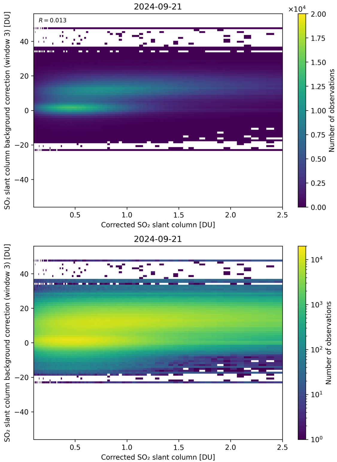
Figure 180: Scatter density plot of “Corrected SO 2 slant column” against “SO 2 slant column background correction (window 3)” for 2024-09-20 to 2024-09-22.
