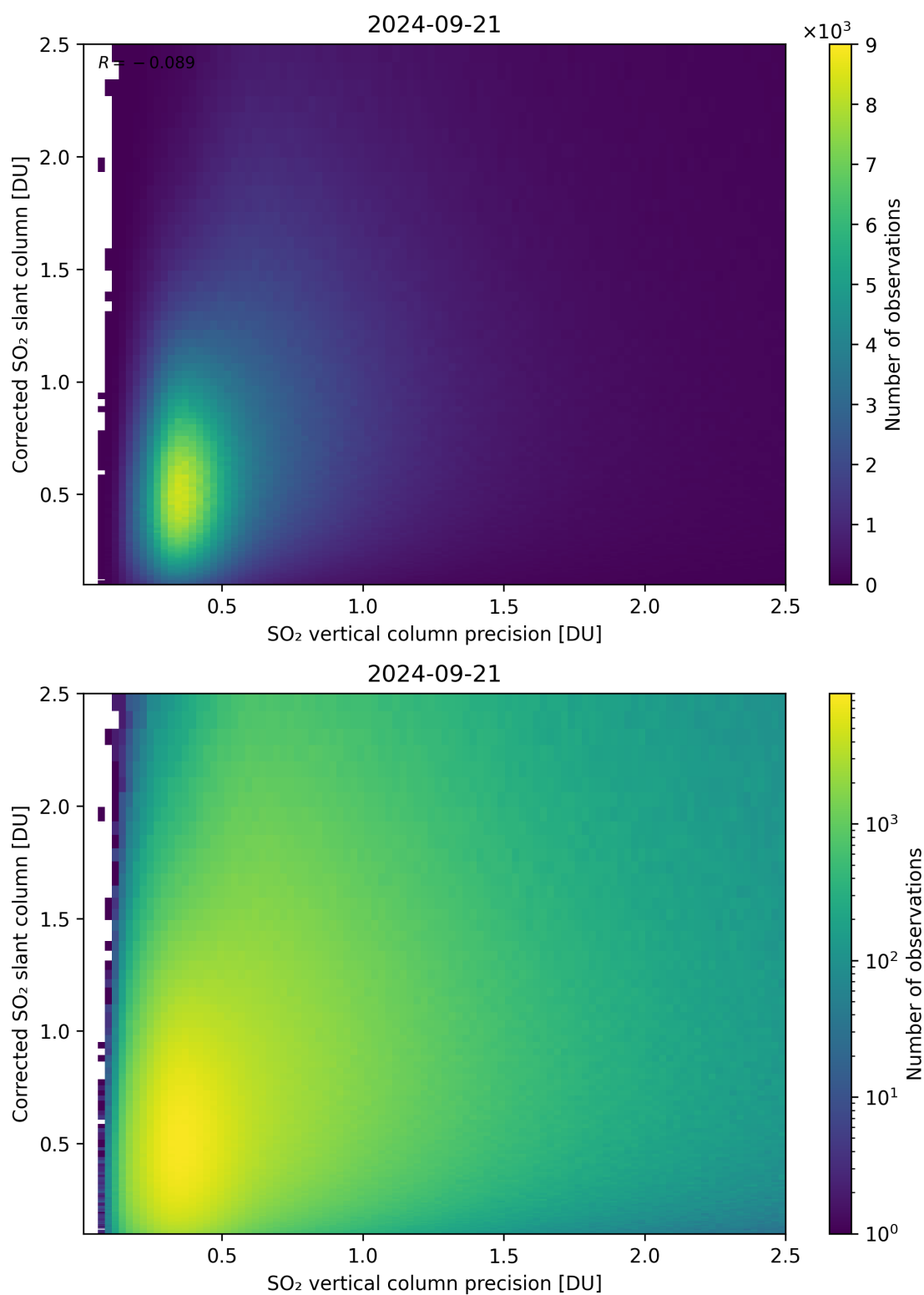
Figure 286: Scatter density plot of “SO 2 vertical column precision” against “Corrected SO 2 slant column” for 2024-09-20 to 2024-09-22.
