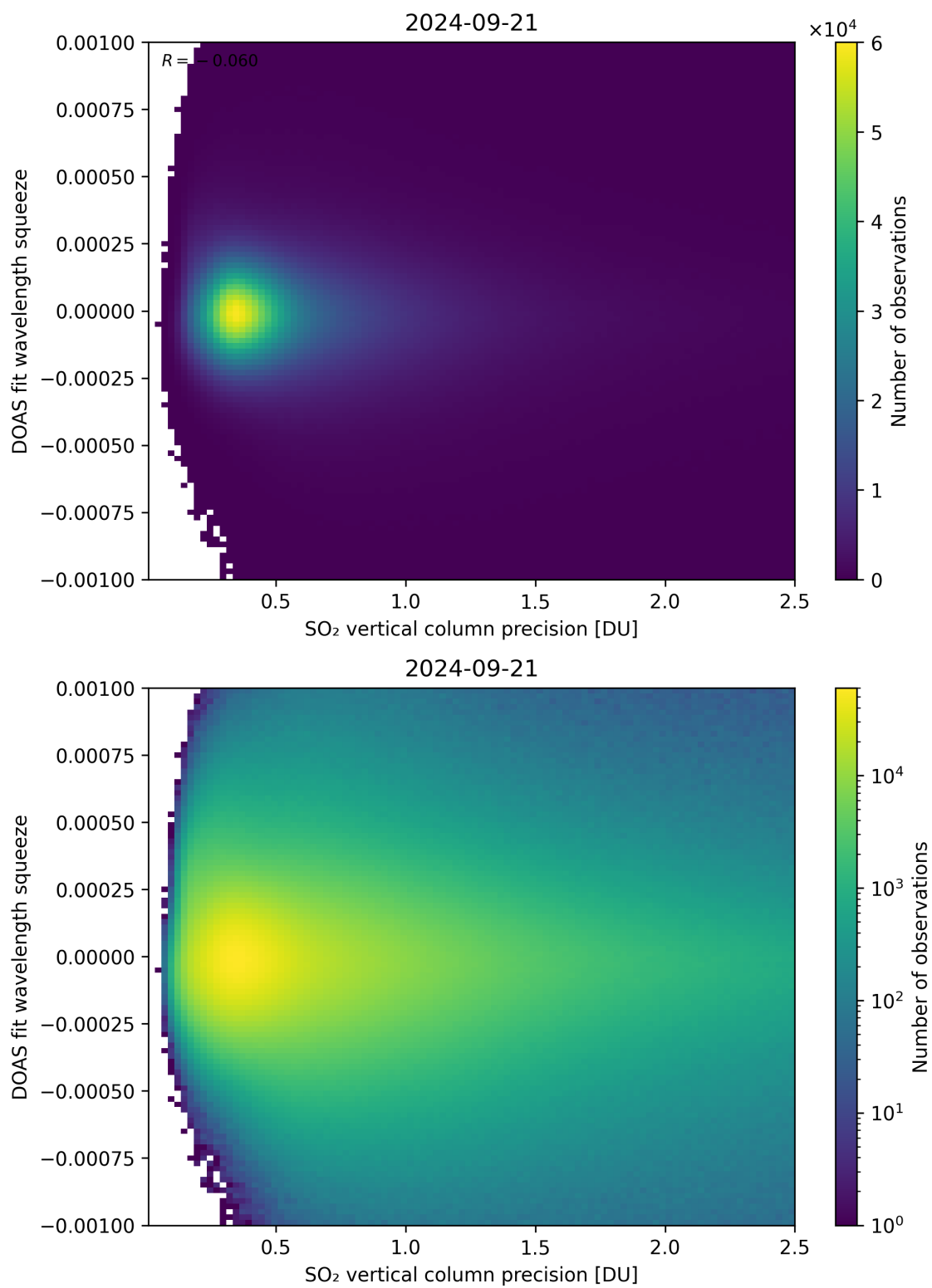
Figure 283: Scatter density plot of “SO 2 vertical column precision” against “DOAS fit wavelength squeeze” for 2024-09-20 to 2024-09-22.
