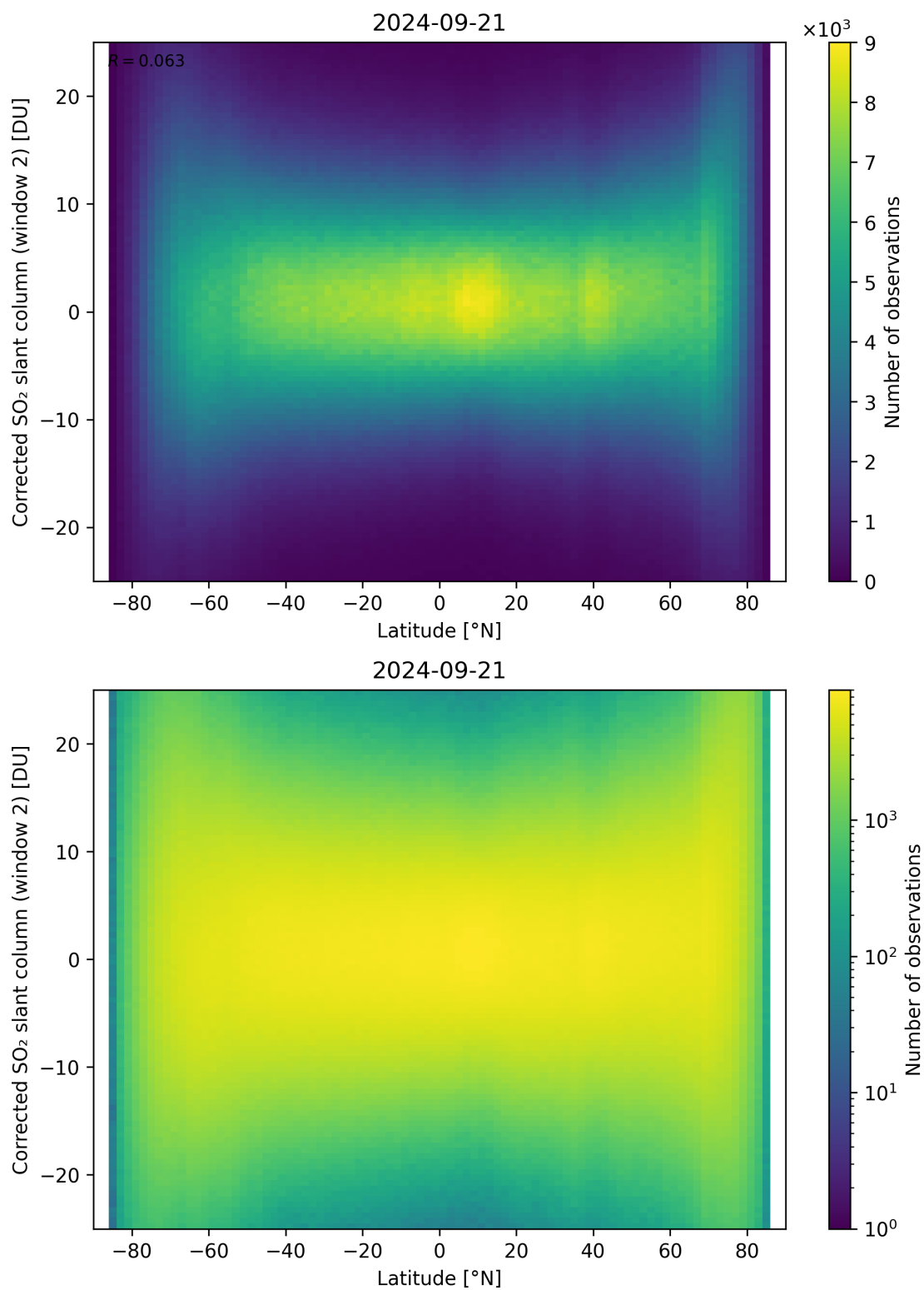
Figure 147: Scatter density plot of “Latitude” against “Corrected SO 2 slant column (window 2)” for 2024-09-20 to 2024-09-22.
