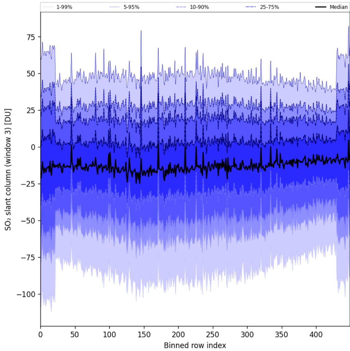
Figure 87: Along track statistics of “SO 2 slant column (window 3)” for 2024-09-20 to 2024-09-22
