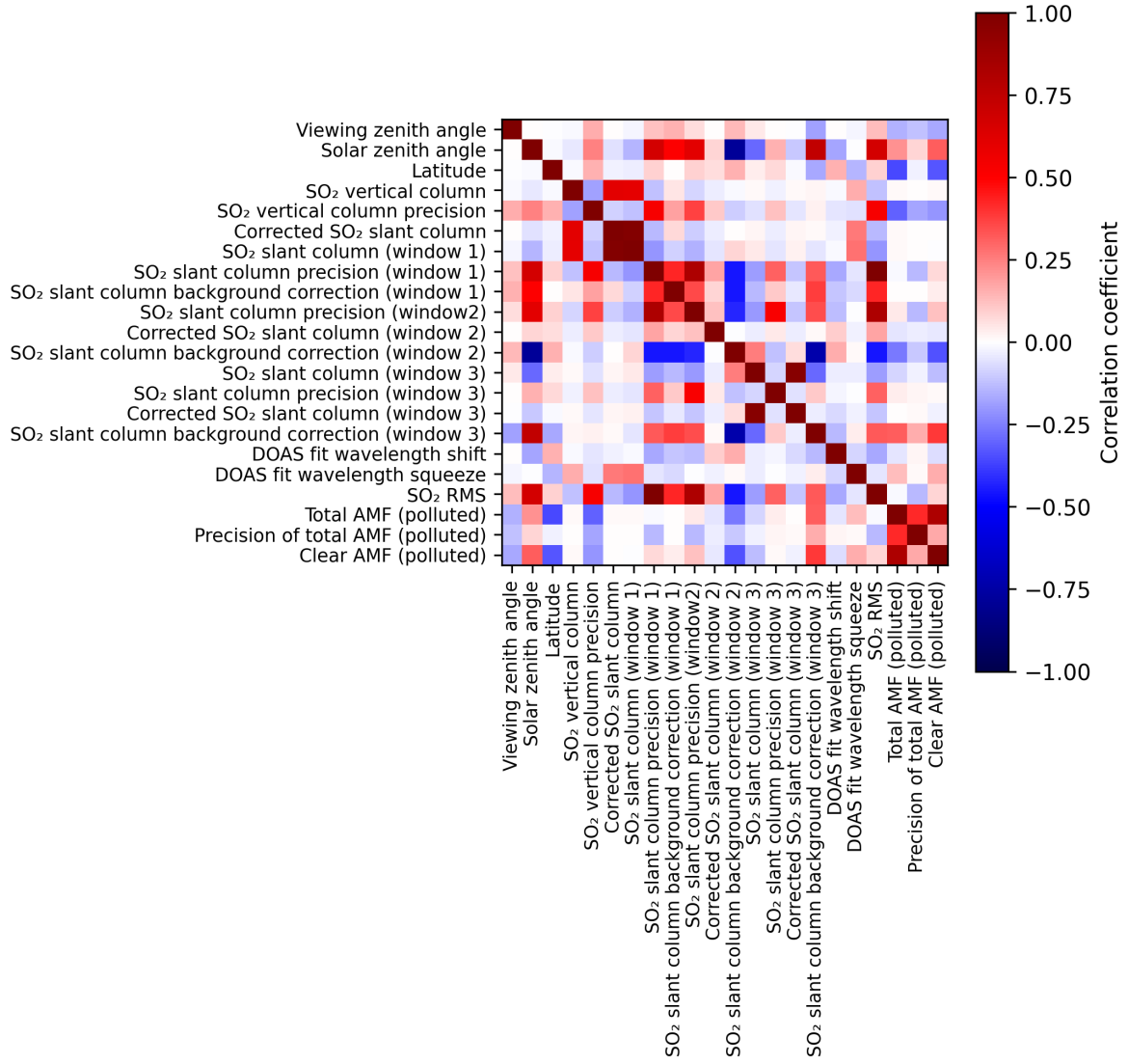
Figure 2: Map of correlation matrix for 2024-09-20 to 2024-09-22.
