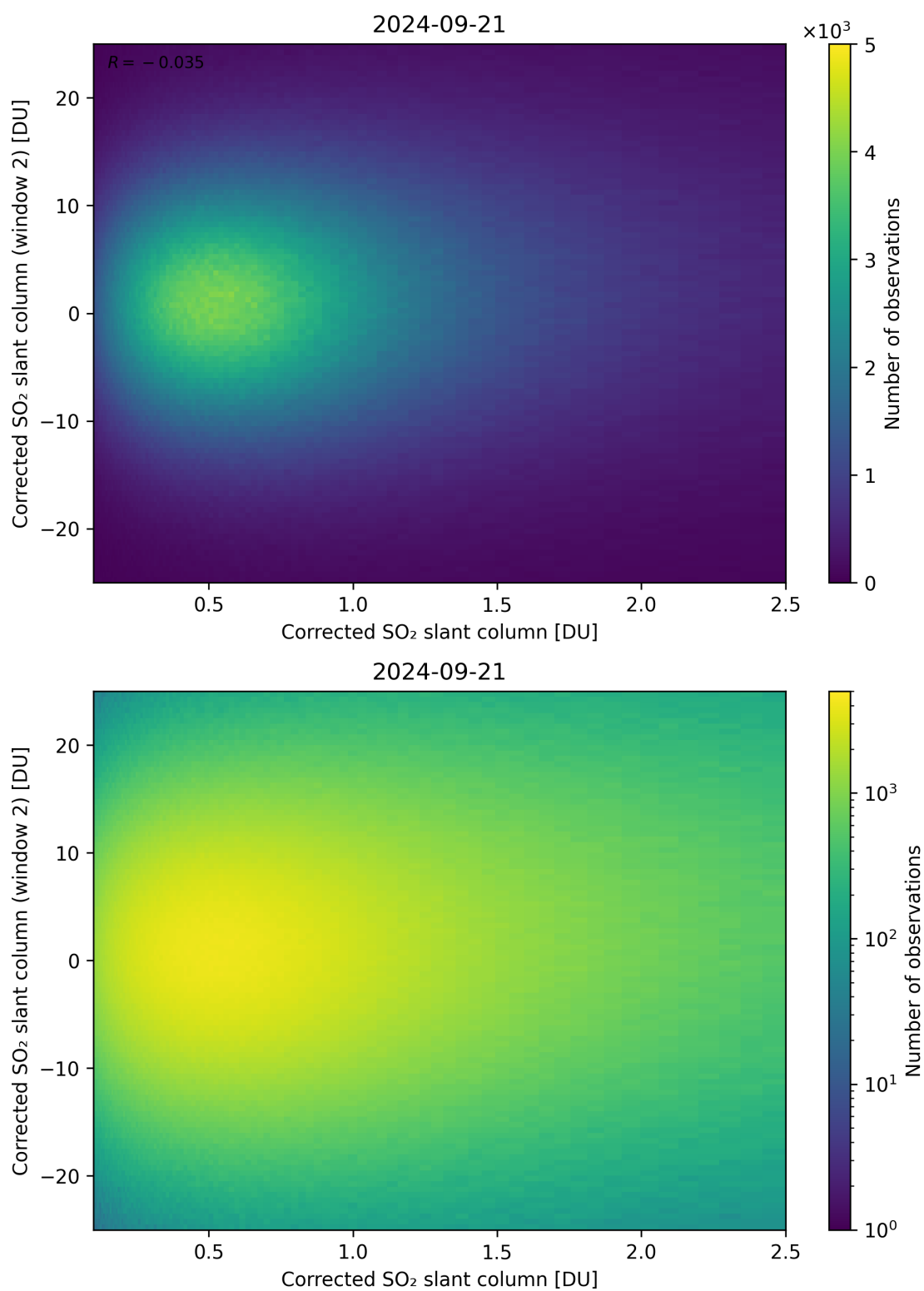
Figure 185: Scatter density plot of “Corrected SO 2 slant column” against “Corrected SO 2 slant column (window 2)” for 2024-09-20 to 2024-09-22.
