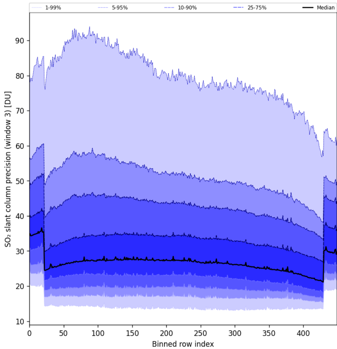
Figure 88: Along track statistics of “SO 2 slant column precision (window 3)” for 2024-09-20 to 2024-09-22
