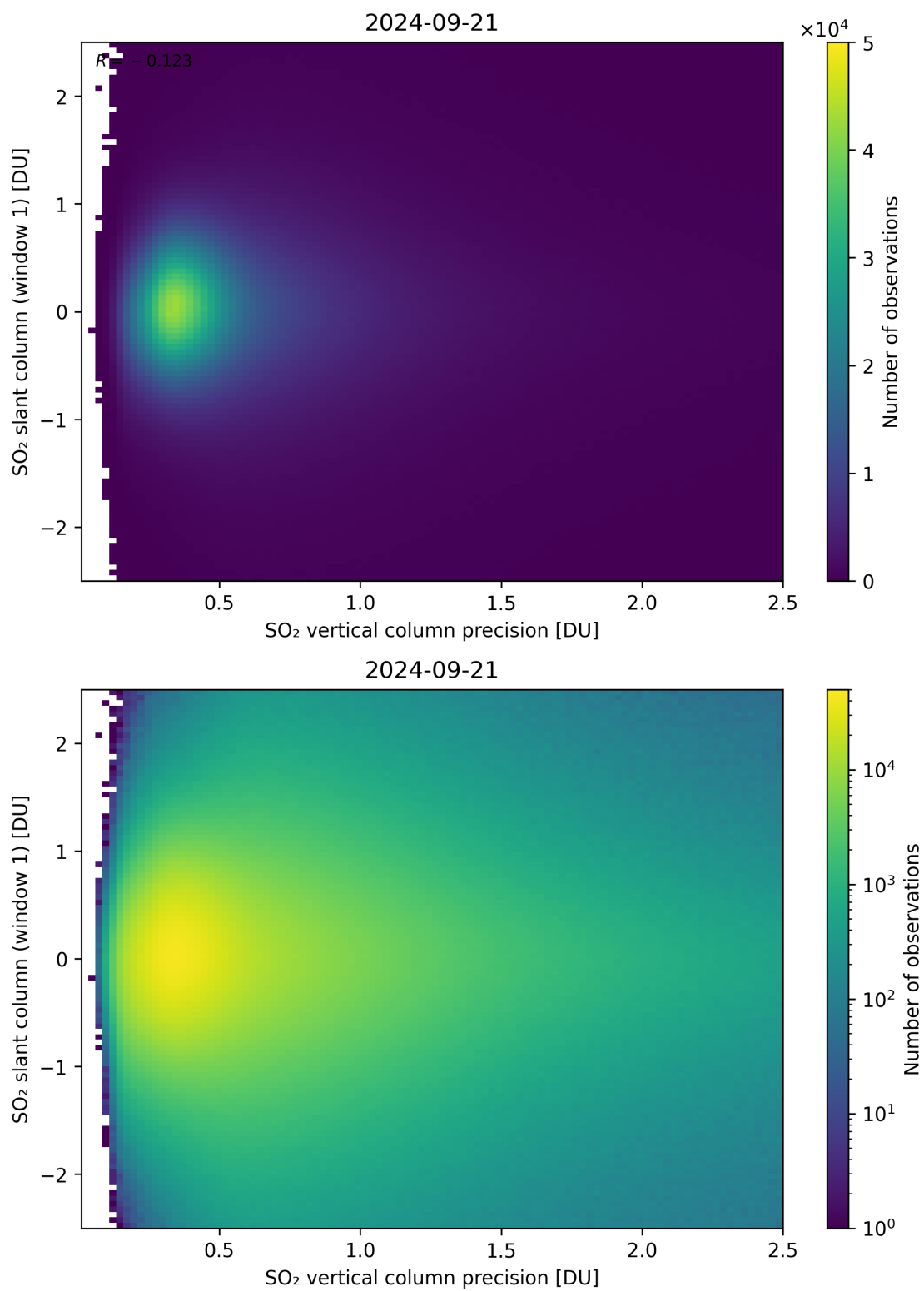
Figure 289: Scatter density plot of “SO 2 vertical column precision” against “SO 2 slant column (window 1)” for 2024-09-20 to 2024-09-22.
