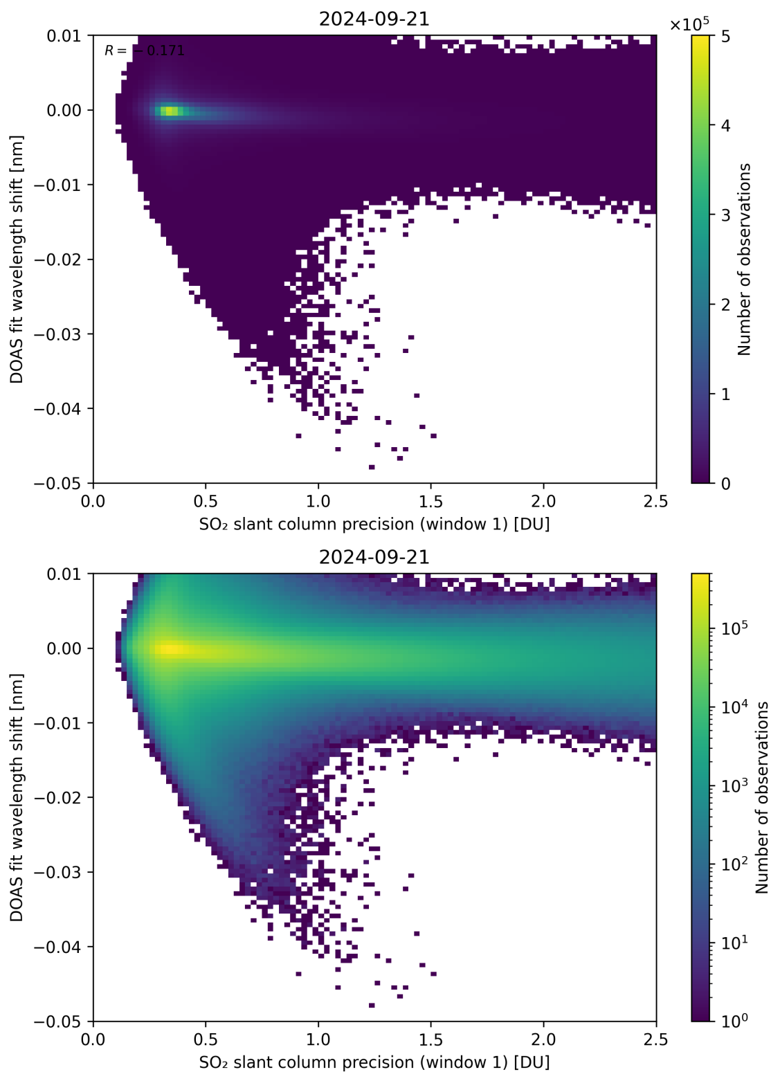
Figure 221: Scatter density plot of “SO 2 slant column precision (window 1)” against “DOAS fit wavelength shift” for 2024-09-20 to 2024-09-22.
