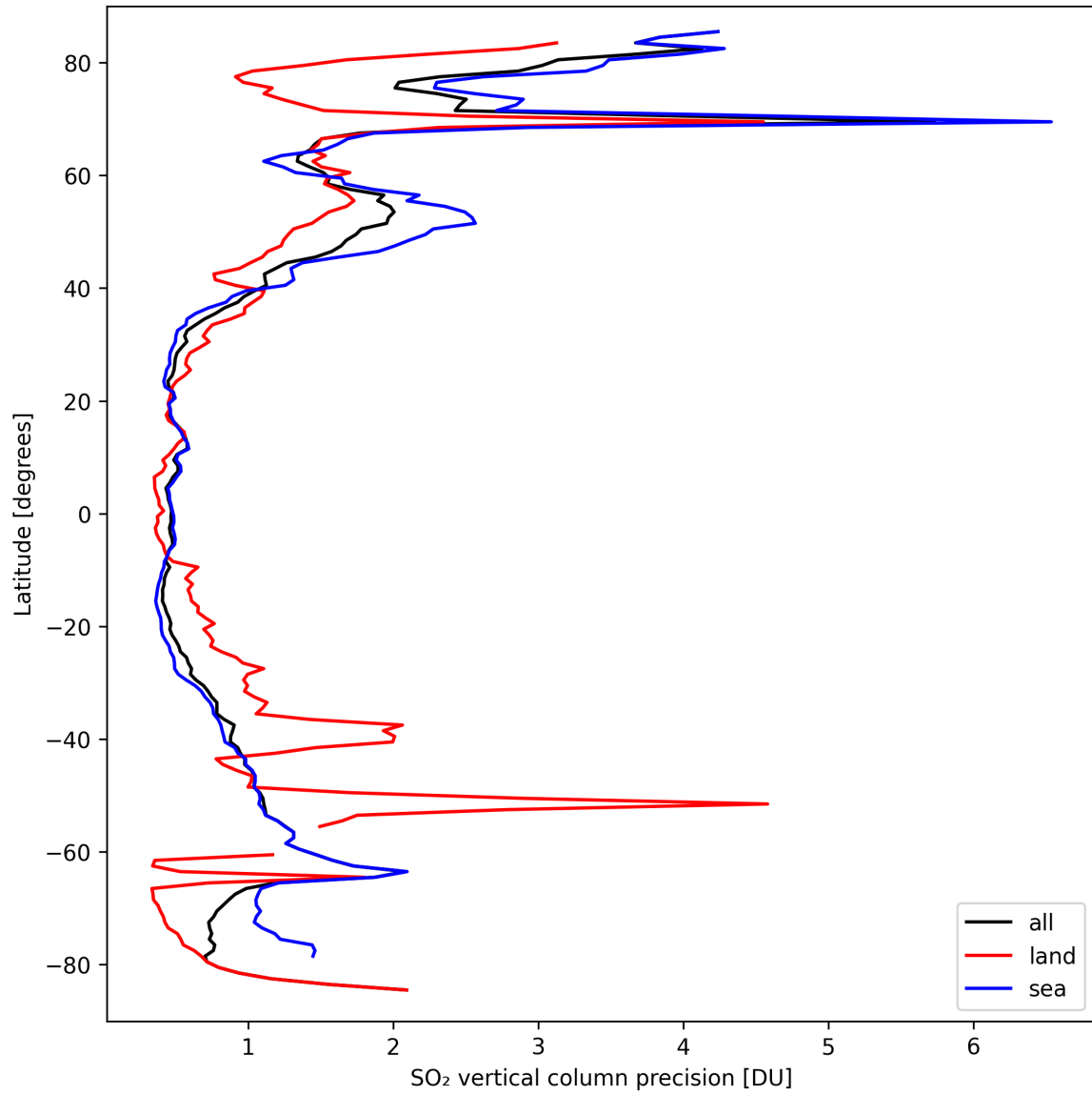
Figure 31: Zonal average of “SO 2 vertical column precision” for 2024-09-20 to 2024-09-22.
