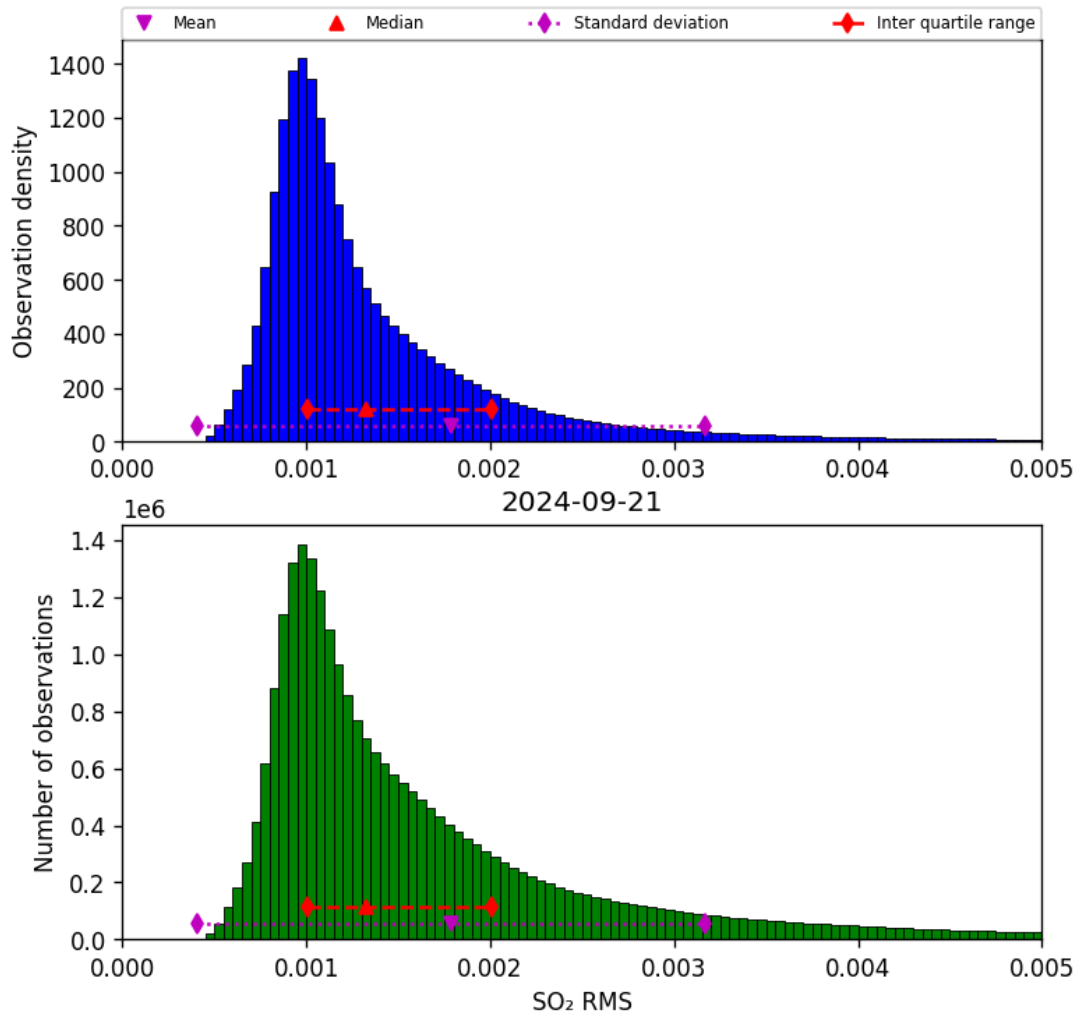
Figure 70: Histogram of “SO 2 RMS” for 2024-09-20 to 2024-09-22
