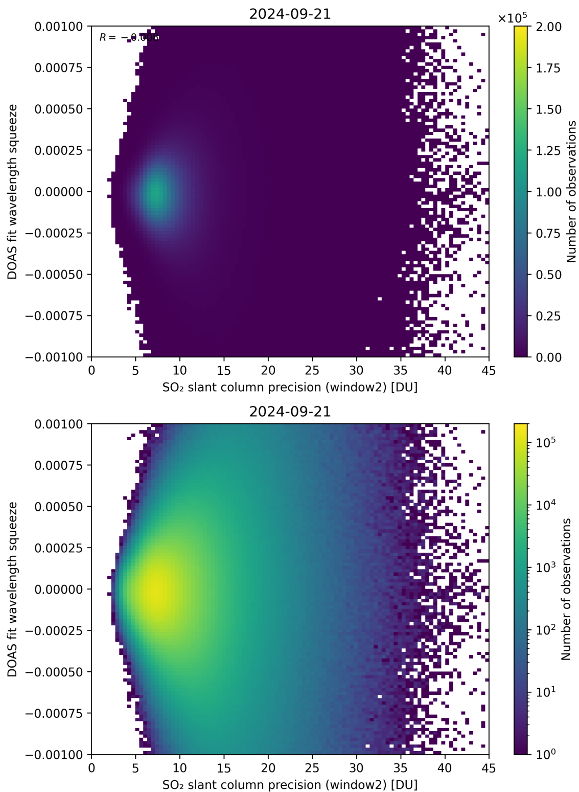
Figure 244: Scatter density plot of “SO 2 slant column precision (window2)” against “DOAS fit wavelength squeeze” for 2024-09-20 to 2024-09-22.
