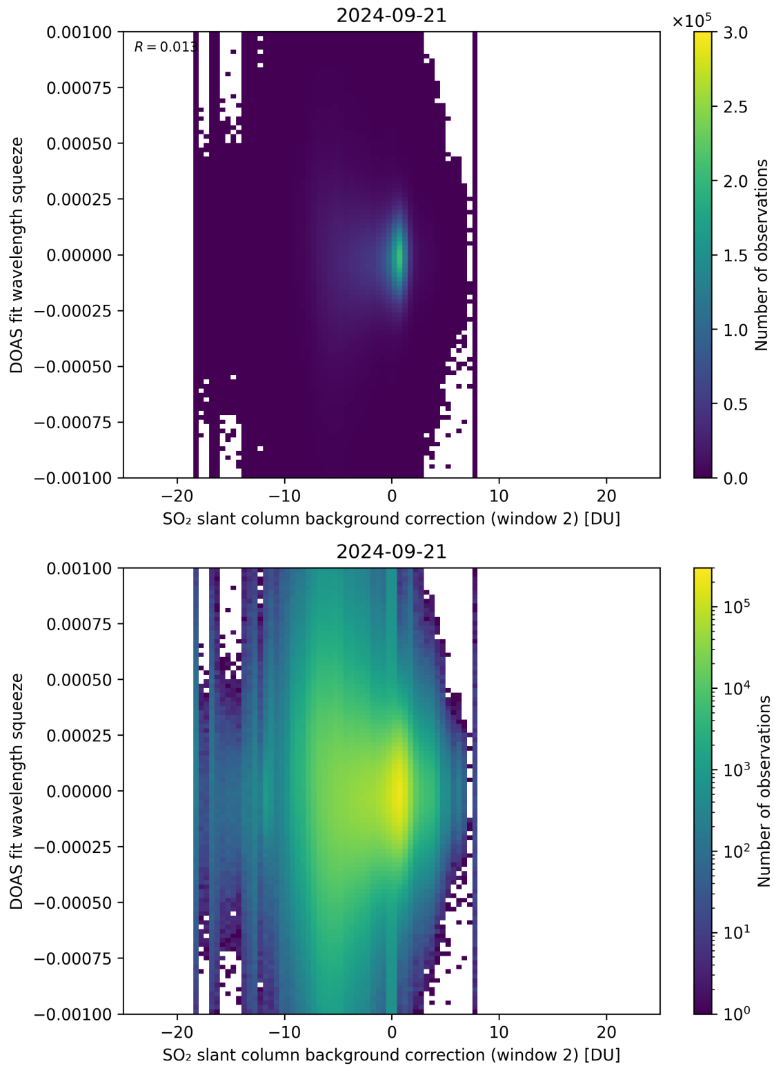
Figure 113: Scatter density plot of “SO 2 slant column background correction (window 2)” against “DOAS fit wavelength squeeze” for 2024-09-20 to 2024-09-22.
