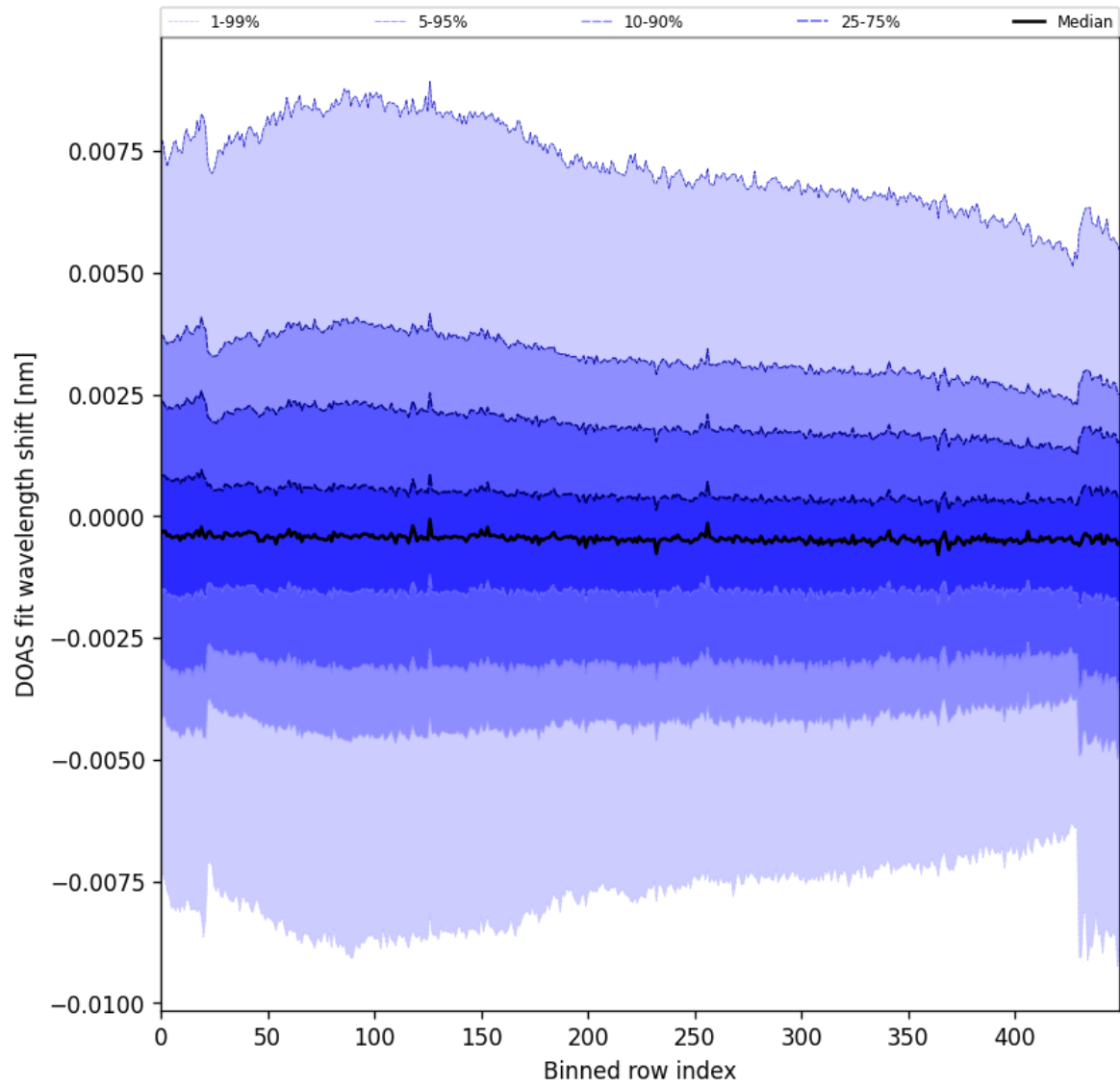
Figure 91: Along track statistics of “DOAS fit wavelength shift” for 2024-09-20 to 2024-09-22
