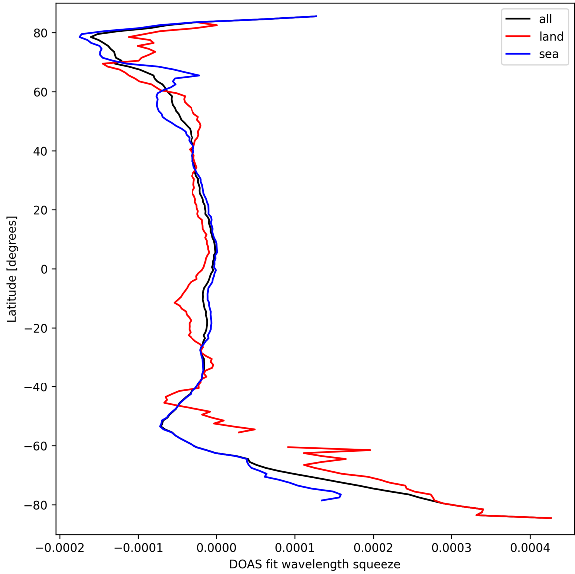
Figure 46: Zonal average of “DOAS fit wavelength squeeze” for 2024-09-20 to 2024-09-22.
