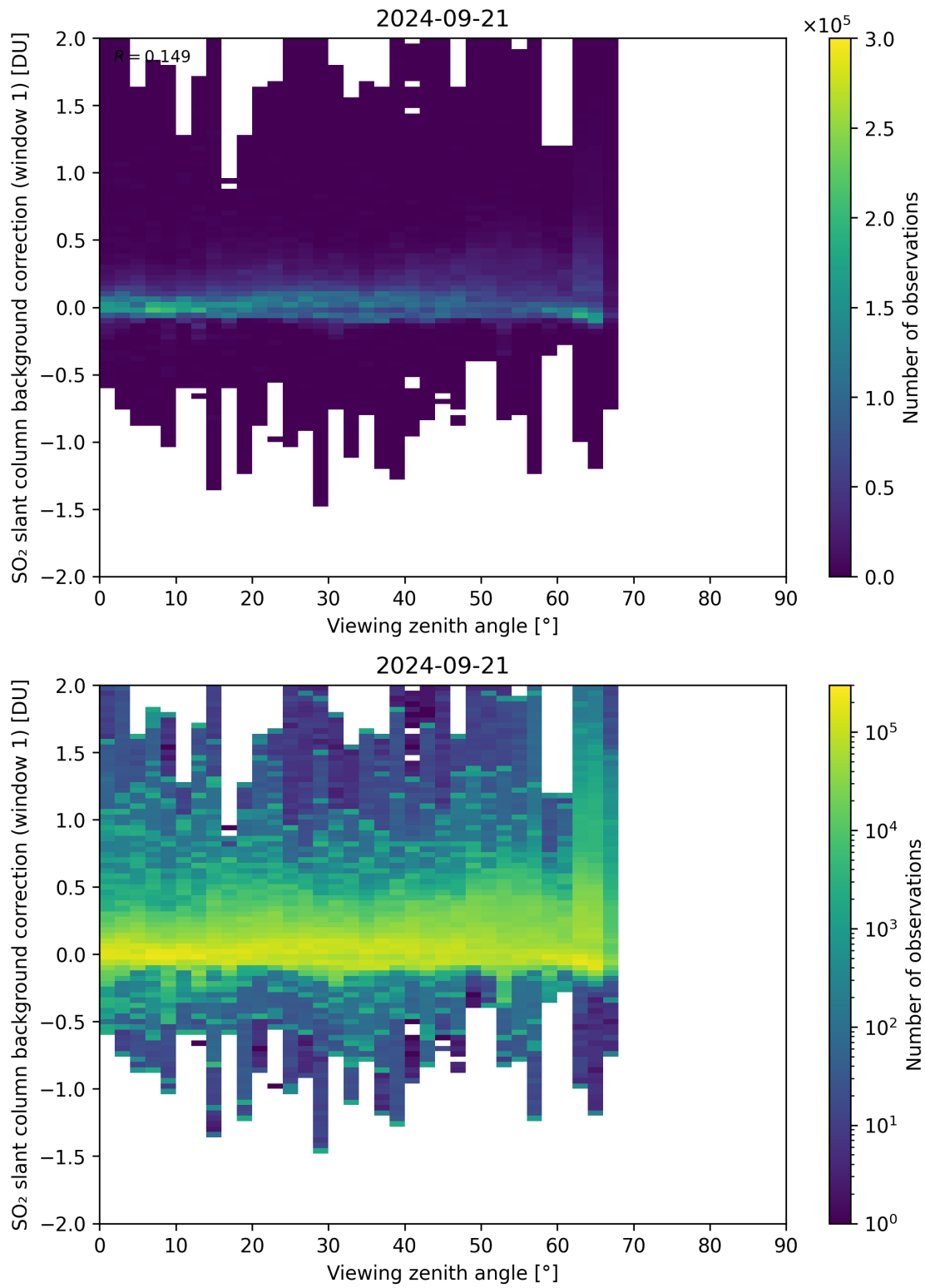
Figure 308: Scatter density plot of “Viewing zenith angle” against “SO 2 slant column background correction (window 1)” for 2024-09-20 to 2024-09-22.
