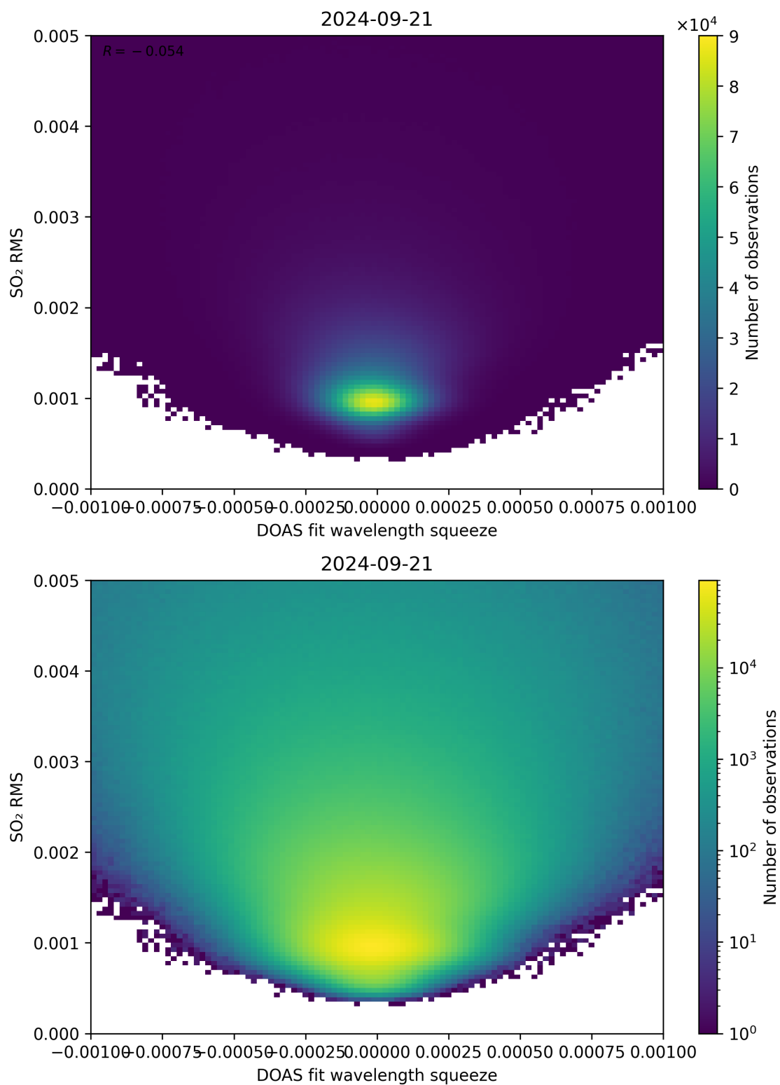
Figure 132: Scatter density plot of “DOAS fit wavelength squeeze” against “SO 2 RMS” for 2024-09-20 to 2024-09-22.
