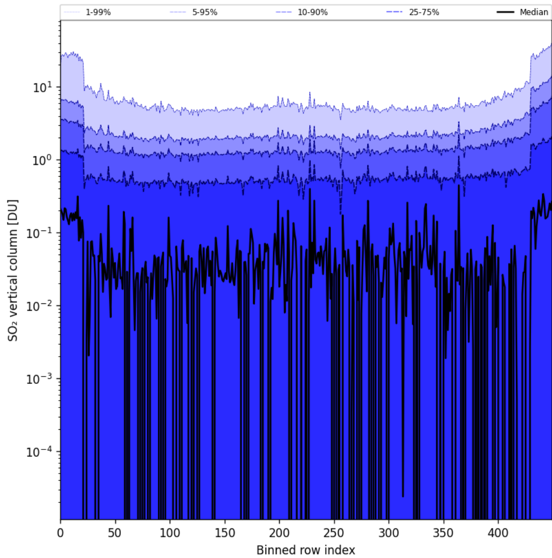
Figure 76: Along track statistics of “SO 2 vertical column” for 2024-09-20 to 2024-09-22
