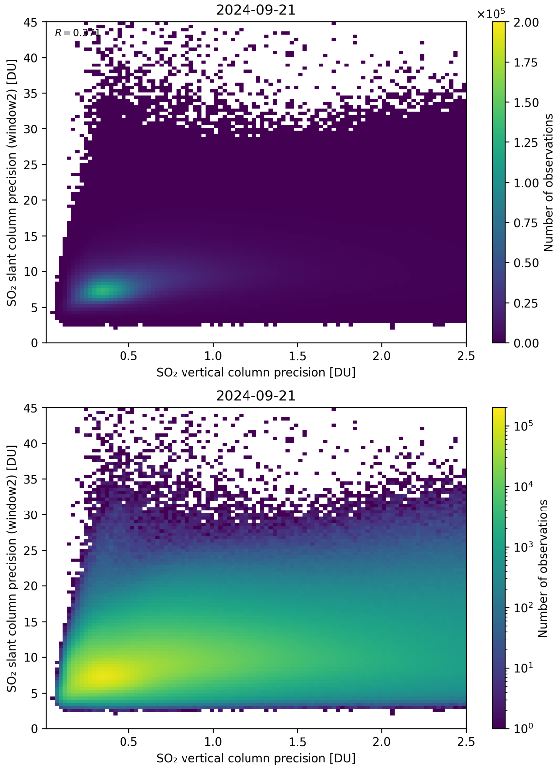
Figure 291: Scatter density plot of “SO 2 vertical column precision” against “SO 2 slant column precision (window2)” for 2024-09-20 to 2024-09-22.
