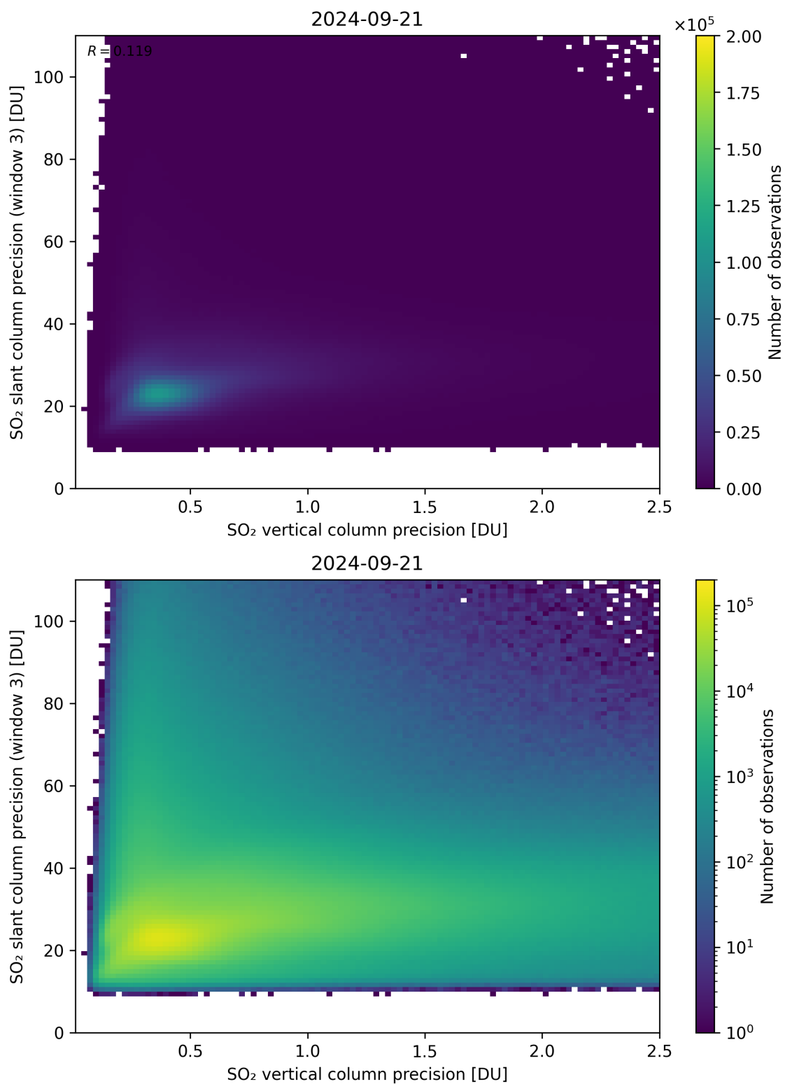
Figure 293: Scatter density plot of “SO 2 vertical column precision” against “SO 2 slant column precision (window 3)” for 2024-09-20 to 2024-09-22.
