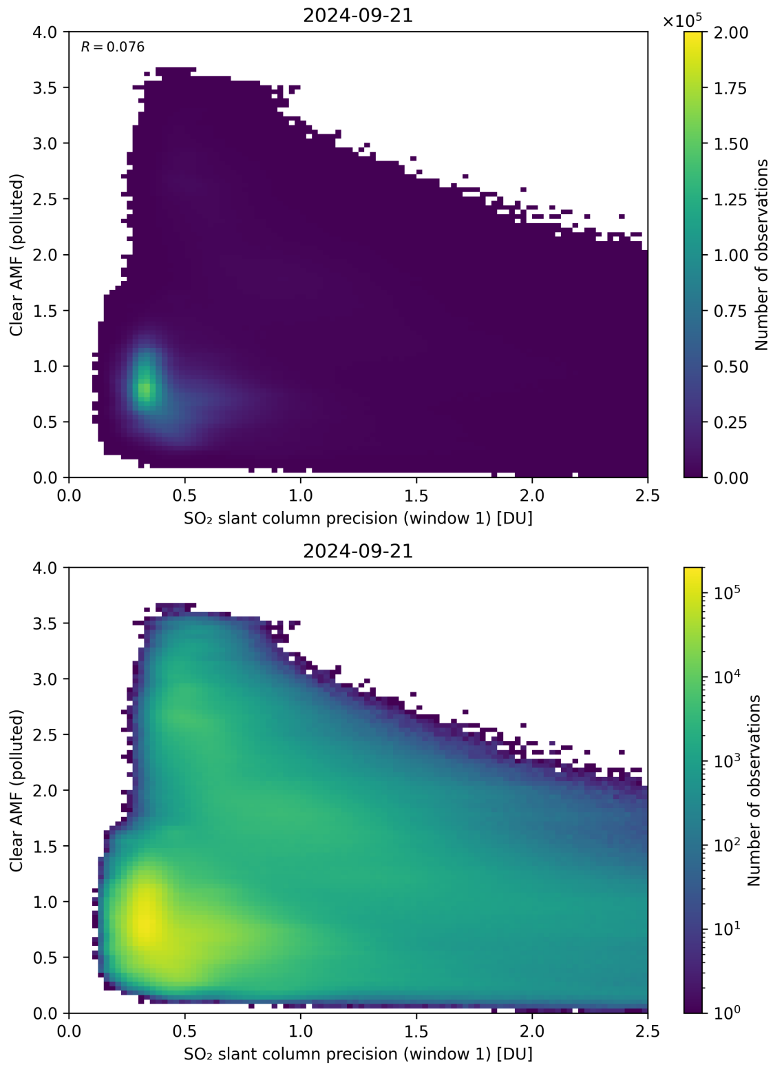
Figure 224: Scatter density plot of “SO 2 slant column precision (window 1)” against “Clear AMF (polluted)” for 2024-09-20 to 2024-09-22.
