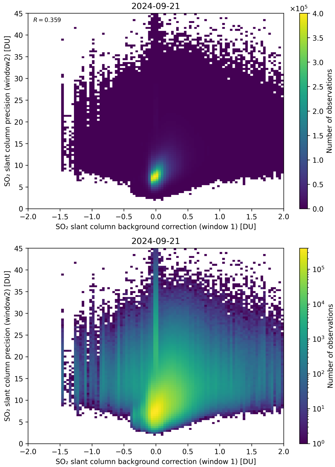
Figure 106: Scatter density plot of “SO 2 slant column background correction (window 1)” against “SO 2 slant column precision (window2)” for 2024-09-20 to 2024-09-22.
