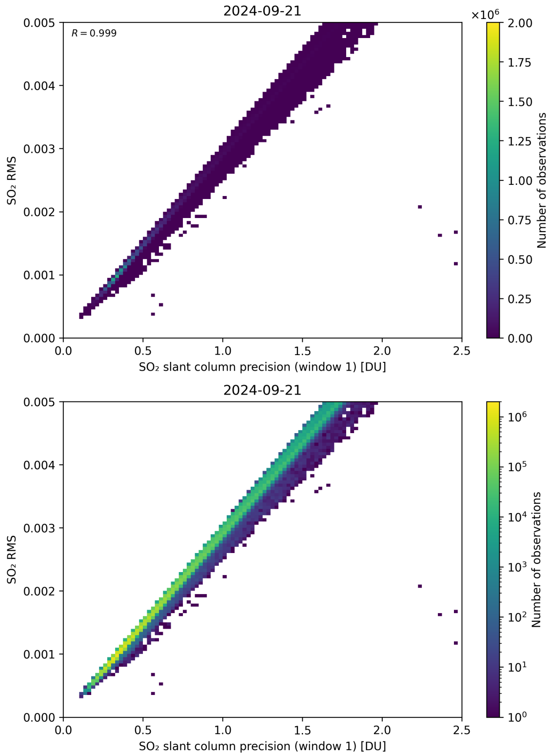
Figure 223: Scatter density plot of “SO 2 slant column precision (window 1)” against “SO 2 RMS” for 2024-09-20 to 2024-09-22.
