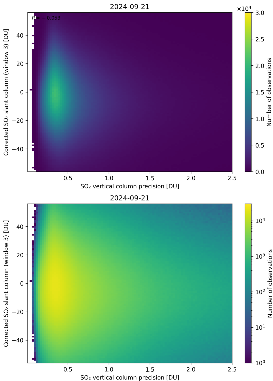
Figure 288: Scatter density plot of “SO 2 vertical column precision” against “Corrected SO 2 slant column (window 3)” for 2024-09-20 to 2024-09-22.
