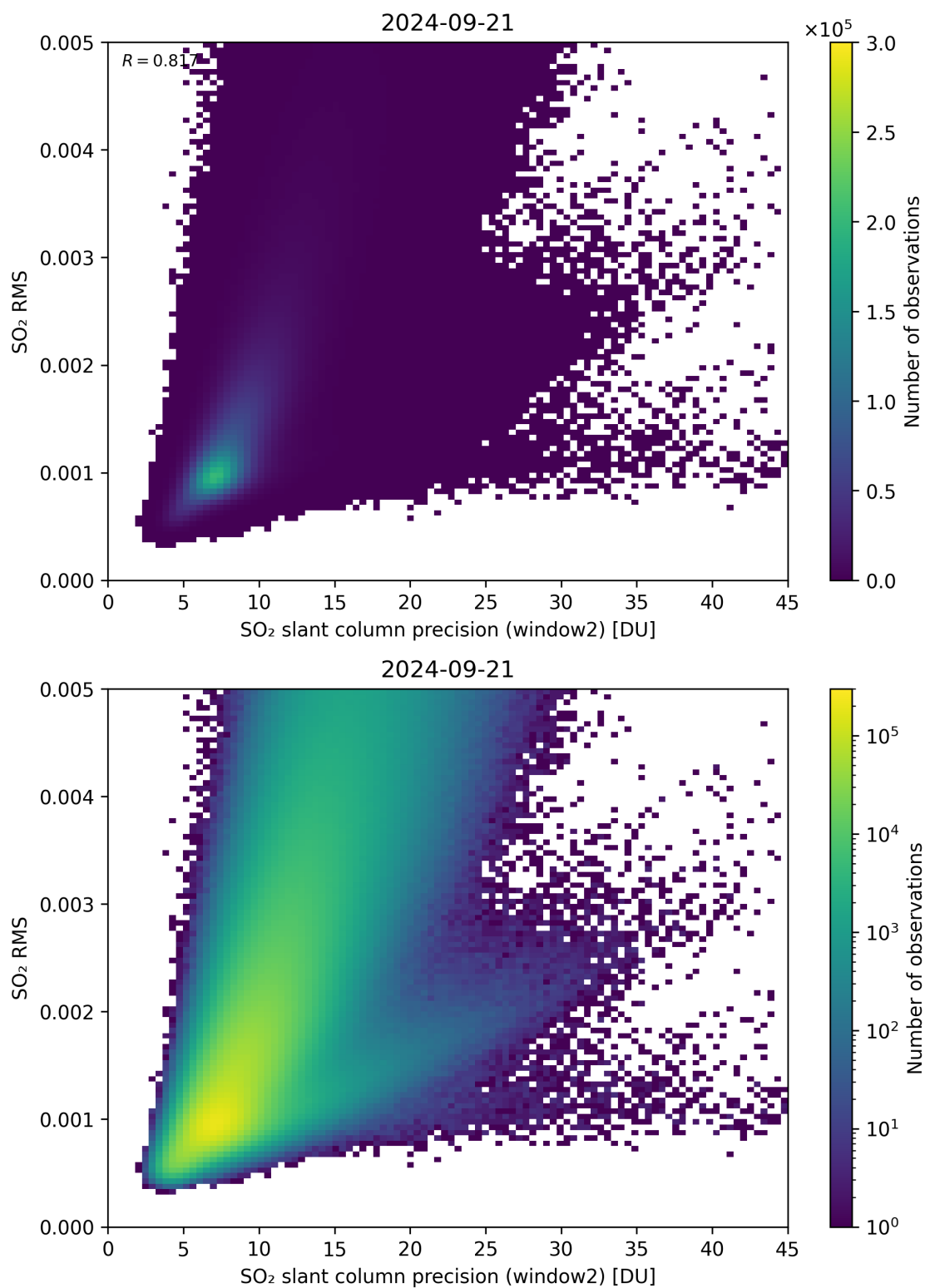
Figure 245: Scatter density plot of “SO 2 slant column precision (window2)” against “SO 2 RMS” for 2024-09-20 to 2024-09-22.
