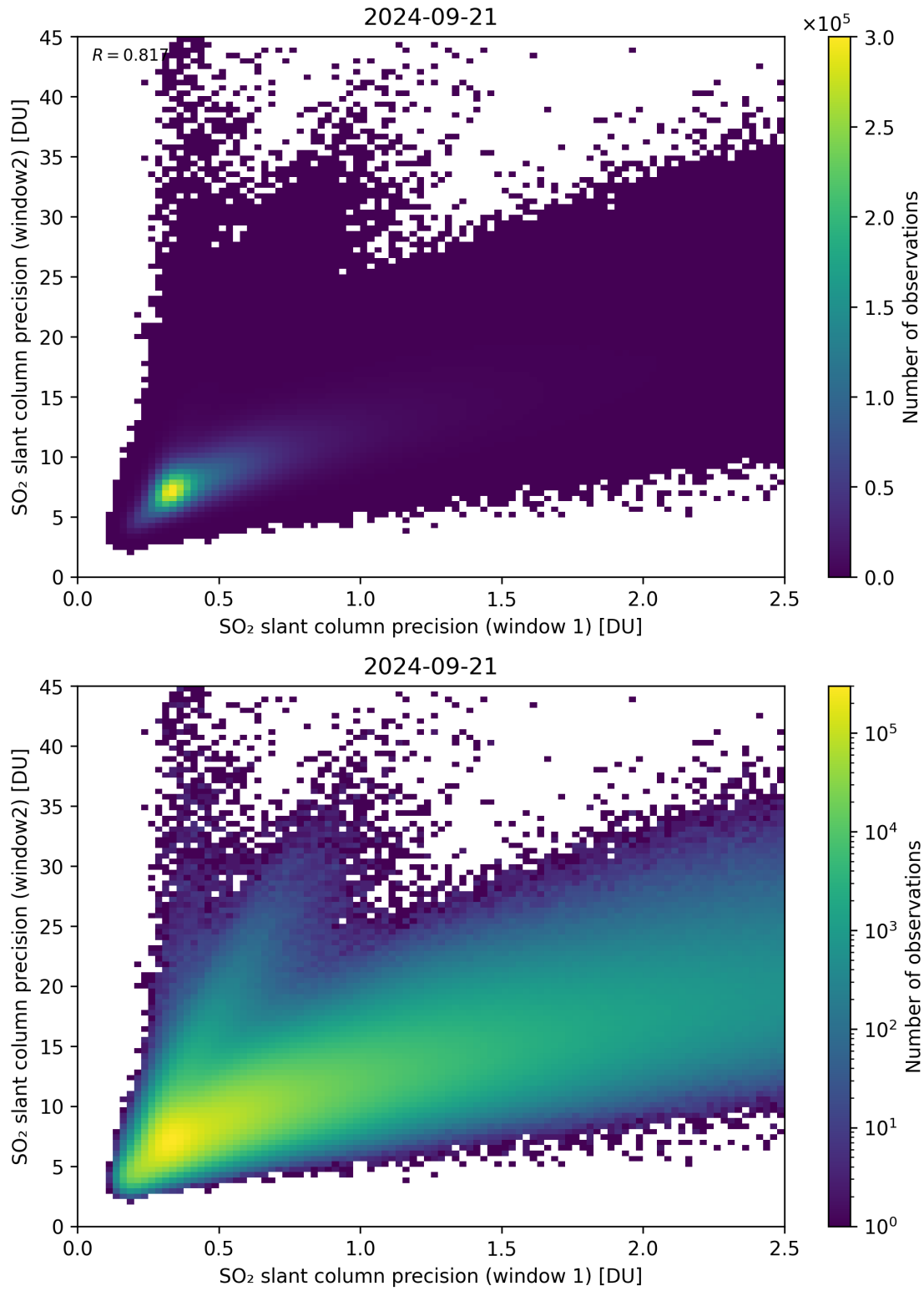
Figure 227: Scatter density plot of “SO 2 slant column precision (window 1)” against “SO 2 slant column precision (window2)” for 2024-09-20 to 2024-09-22.
