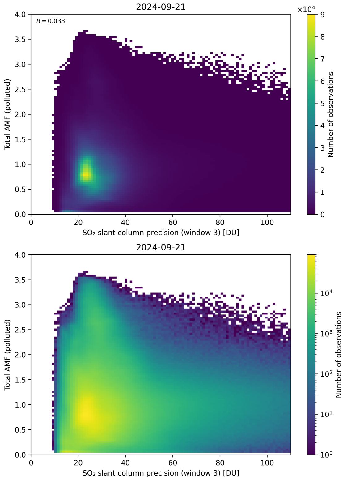
Figure 263: Scatter density plot of “SO 2 slant column precision (window 3)” against “Total AMF (polluted)” for 2024-09-20 to 2024-09-22.
