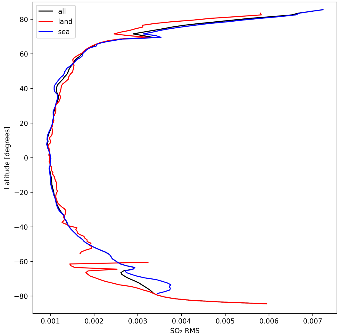
Figure 47: Zonal average of “SO 2 RMS” for 2024-09-20 to 2024-09-22.
