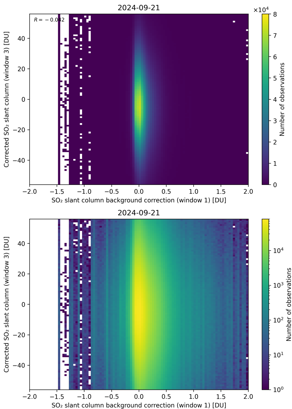
Figure 105: Scatter density plot of “SO 2 slant column background correction (window 1)” against “Corrected SO 2 slant column (window 3)” for 2024-09-20 to 2024-09-22.
