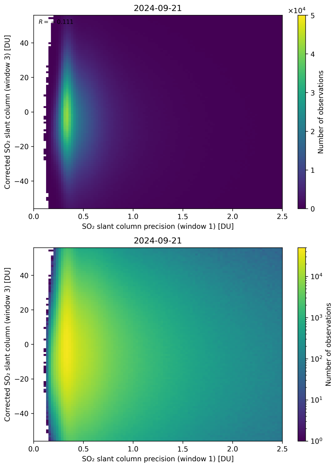
Figure 226: Scatter density plot of “SO 2 slant column precision (window 1)” against “Corrected SO 2 slant column (window 3)” for 2024-09-20 to 2024-09-22.
