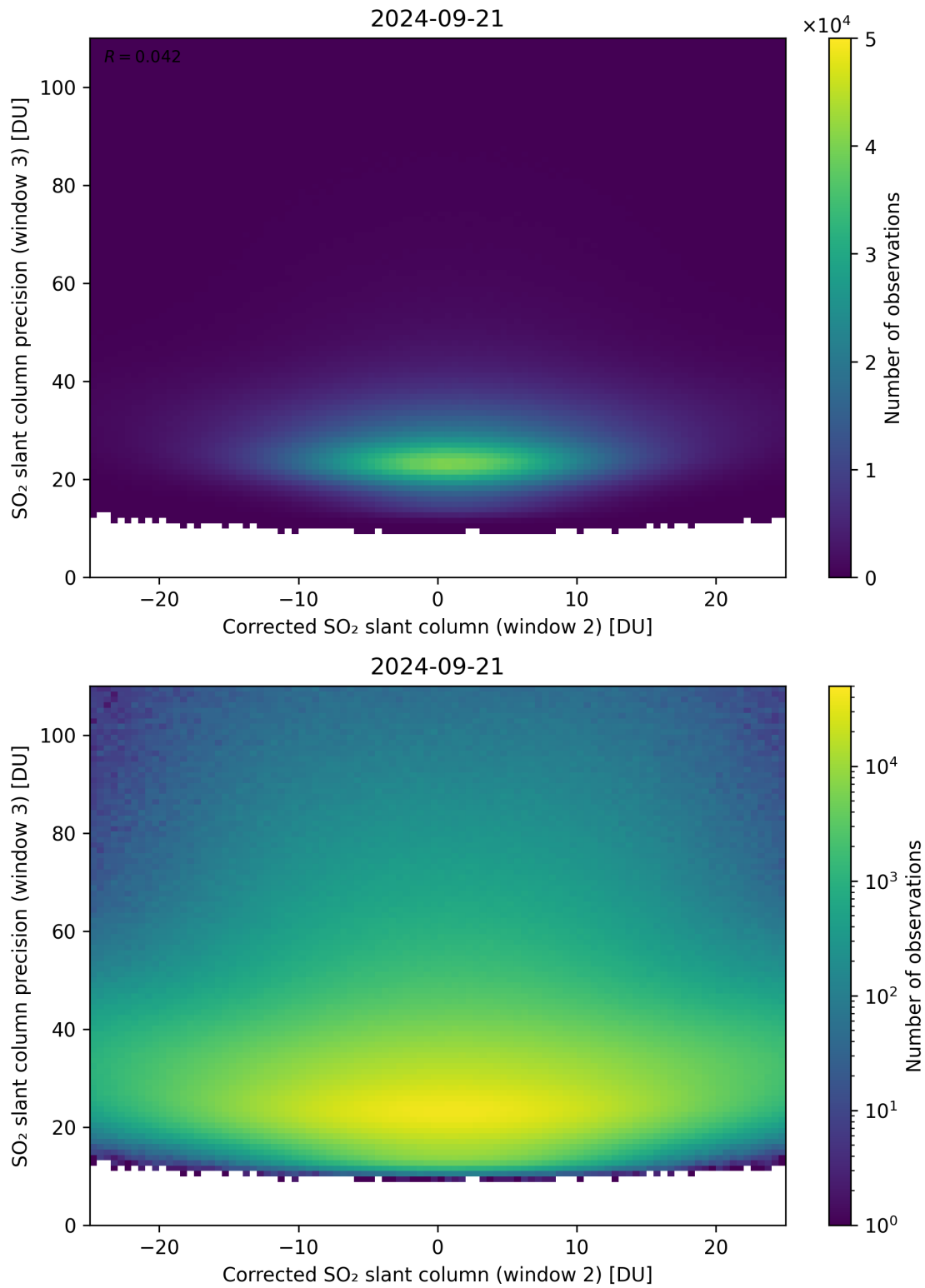
Figure 202: Scatter density plot of “Corrected SO 2 slant column (window 2)” against “SO 2 slant column precision (window 3)” for 2024-09-20 to 2024-09-22.
