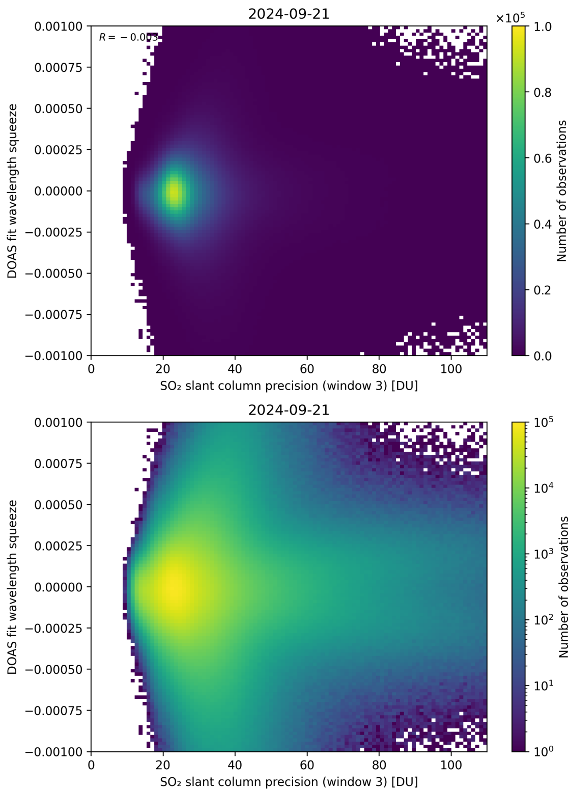
Figure 259: Scatter density plot of “SO 2 slant column precision (window 3)” against “DOAS fit wavelength squeeze” for 2024-09-20 to 2024-09-22.
