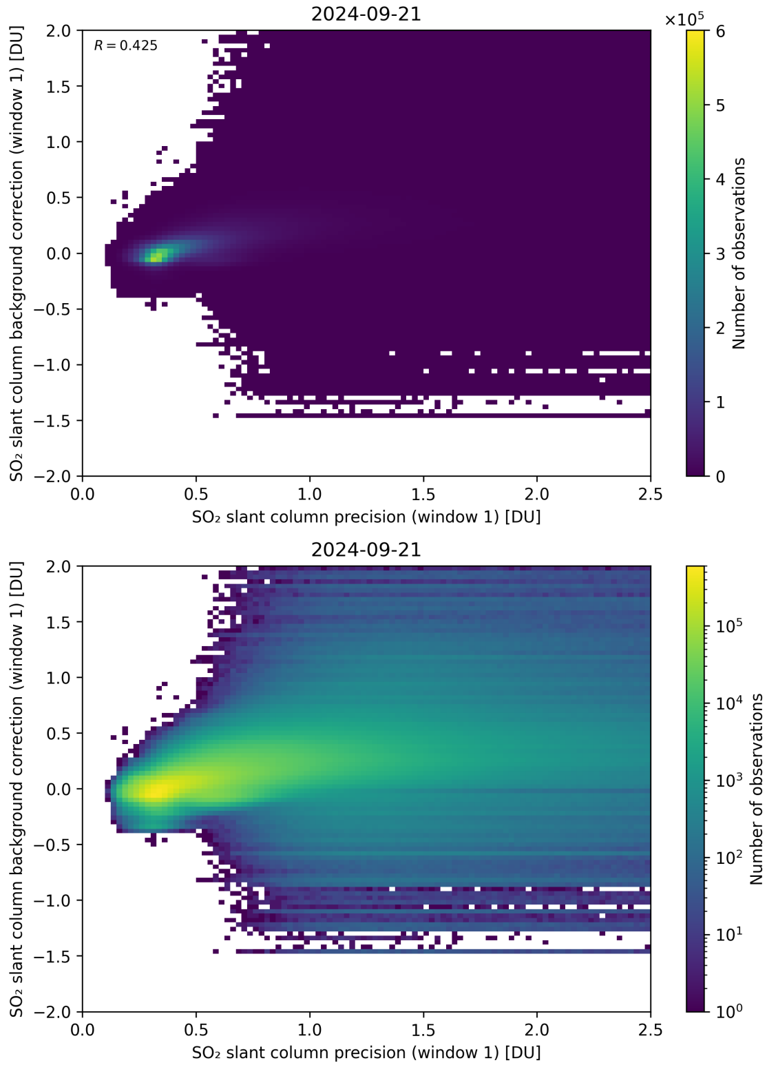
Figure 218: Scatter density plot of “SO 2 slant column precision (window 1)” against “SO 2 slant column background correction (window 1)” for 2024-09-20 to 2024-09-22.
