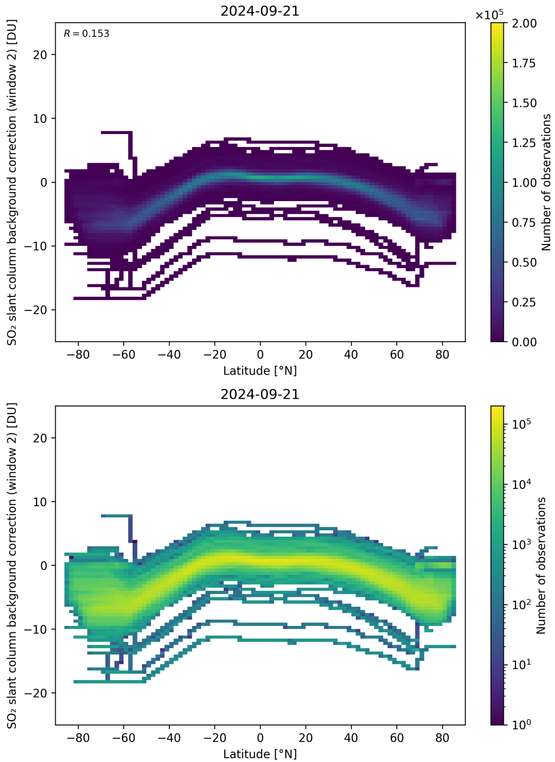
Figure 140: Scatter density plot of “Latitude” against “SO 2 slant column background correction (window 2)” for 2024-09-20 to 2024-09-22.
