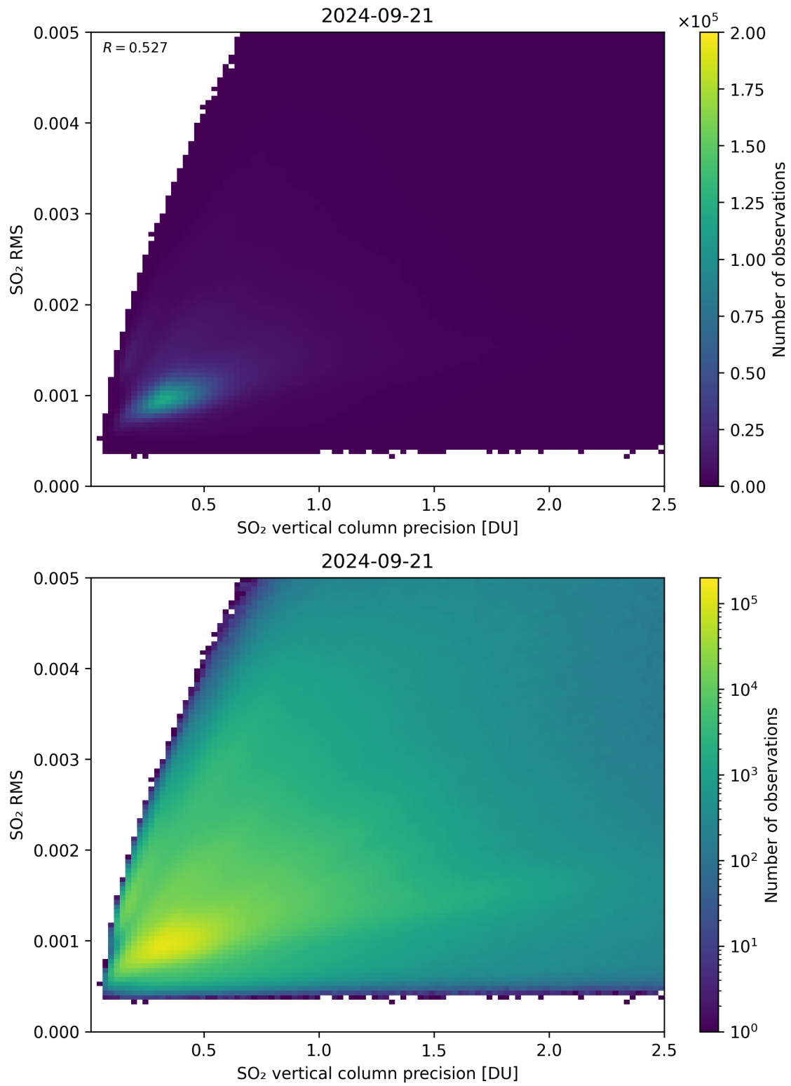
Figure 284: Scatter density plot of “SO 2 vertical column precision” against “SO 2 RMS” for 2024-09-20 to 2024-09-22.
