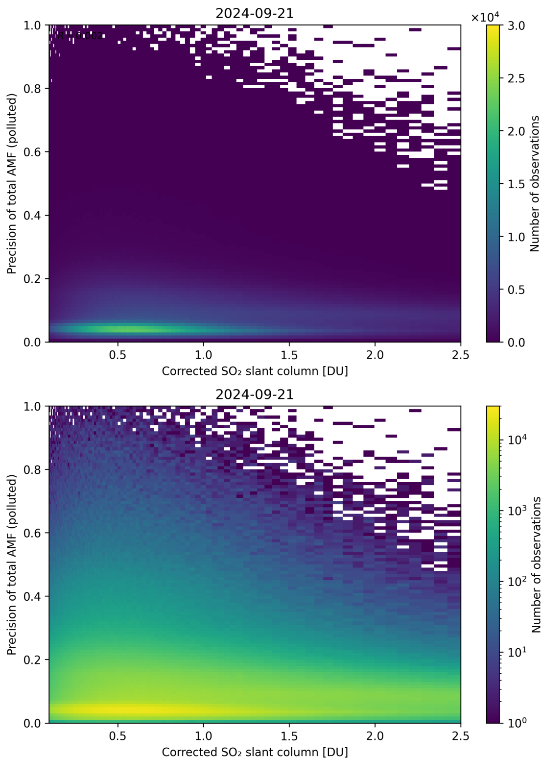
Figure 193: Scatter density plot of “Corrected SO 2 slant column” against “Precision of total AMF (polluted)” for 2024-09-20 to 2024-09-22.
