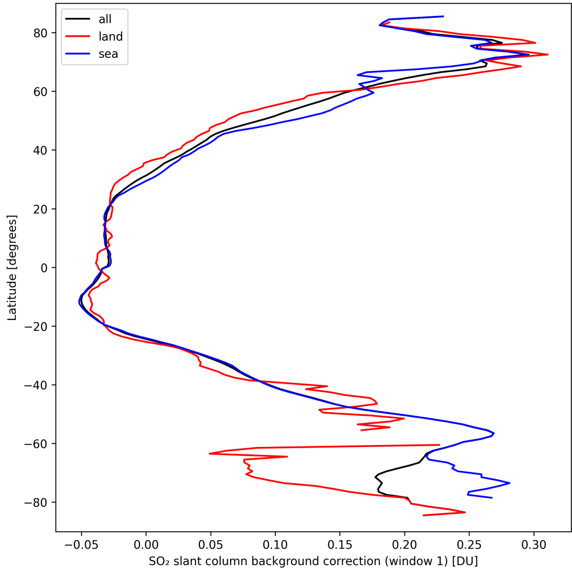
Figure 36: Zonal average of “SO 2 slant column background correction (window 1)” for 2024-09-20 to 2024-09-22.
