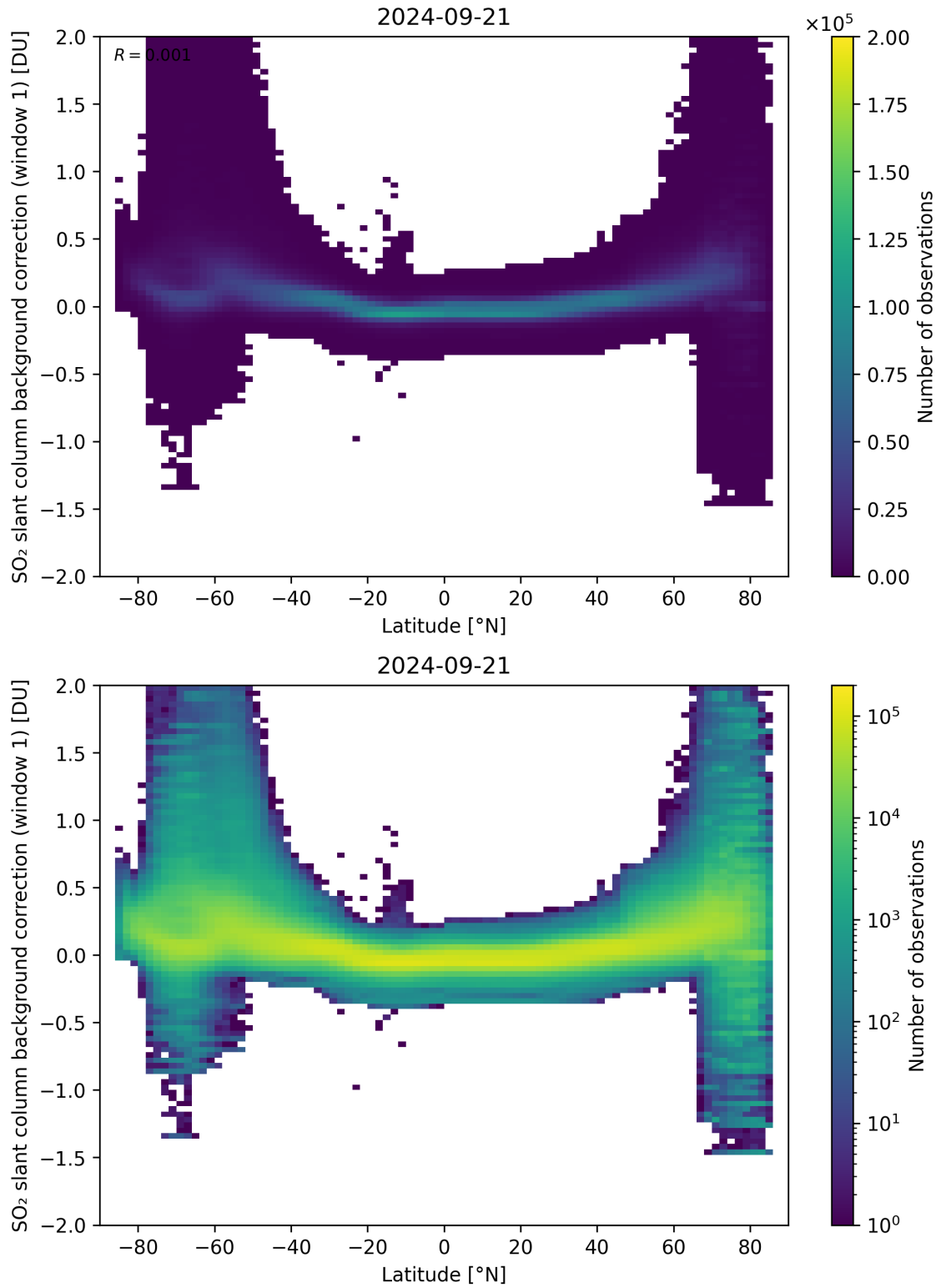
Figure 139: Scatter density plot of “Latitude” against “SO 2 slant column background correction (window 1)” for 2024-09-20 to 2024-09-22.
