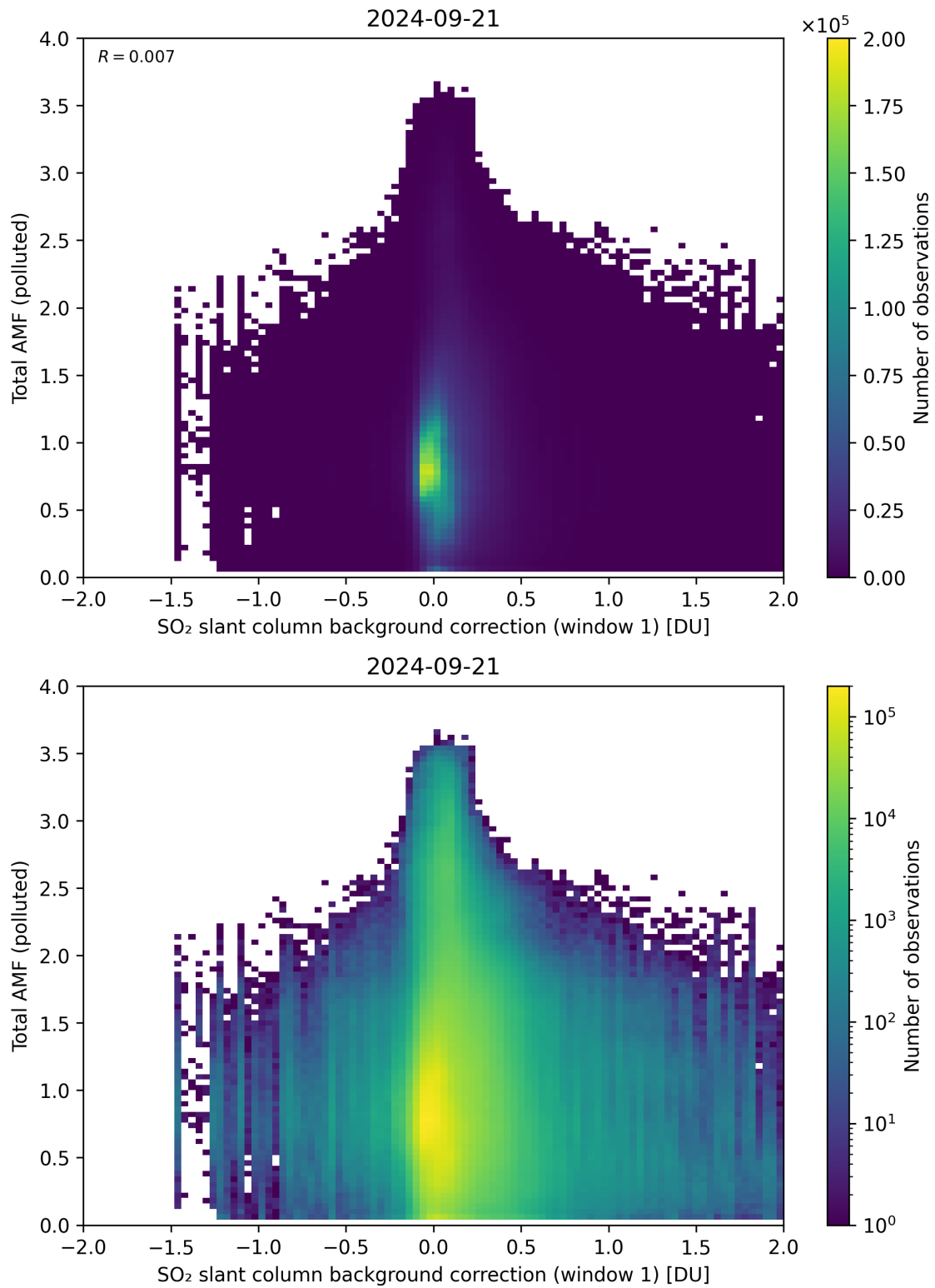
Figure 109: Scatter density plot of “SO 2 slant column background correction (window 1)” against “Total AMF (polluted)” for 2024-09-20 to 2024-09-22.
