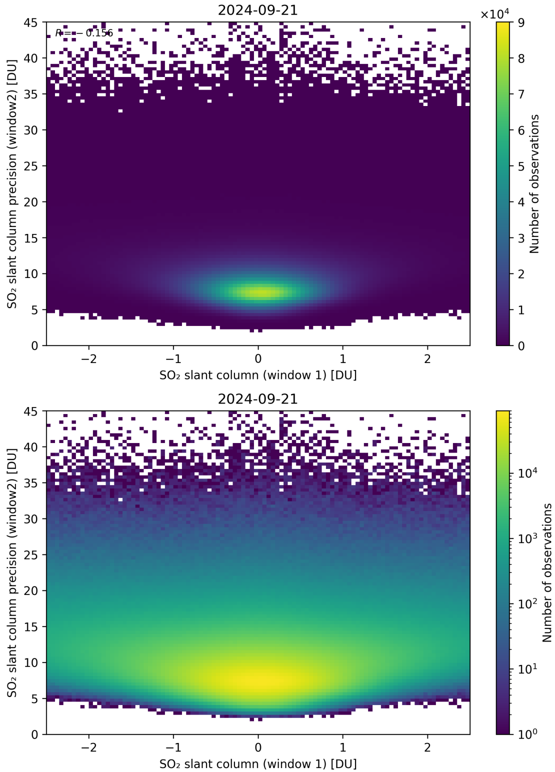
Figure 236: Scatter density plot of “SO 2 slant column (window 1)” against “SO 2 slant column precision (window2)” for 2024-09-20 to 2024-09-22.
