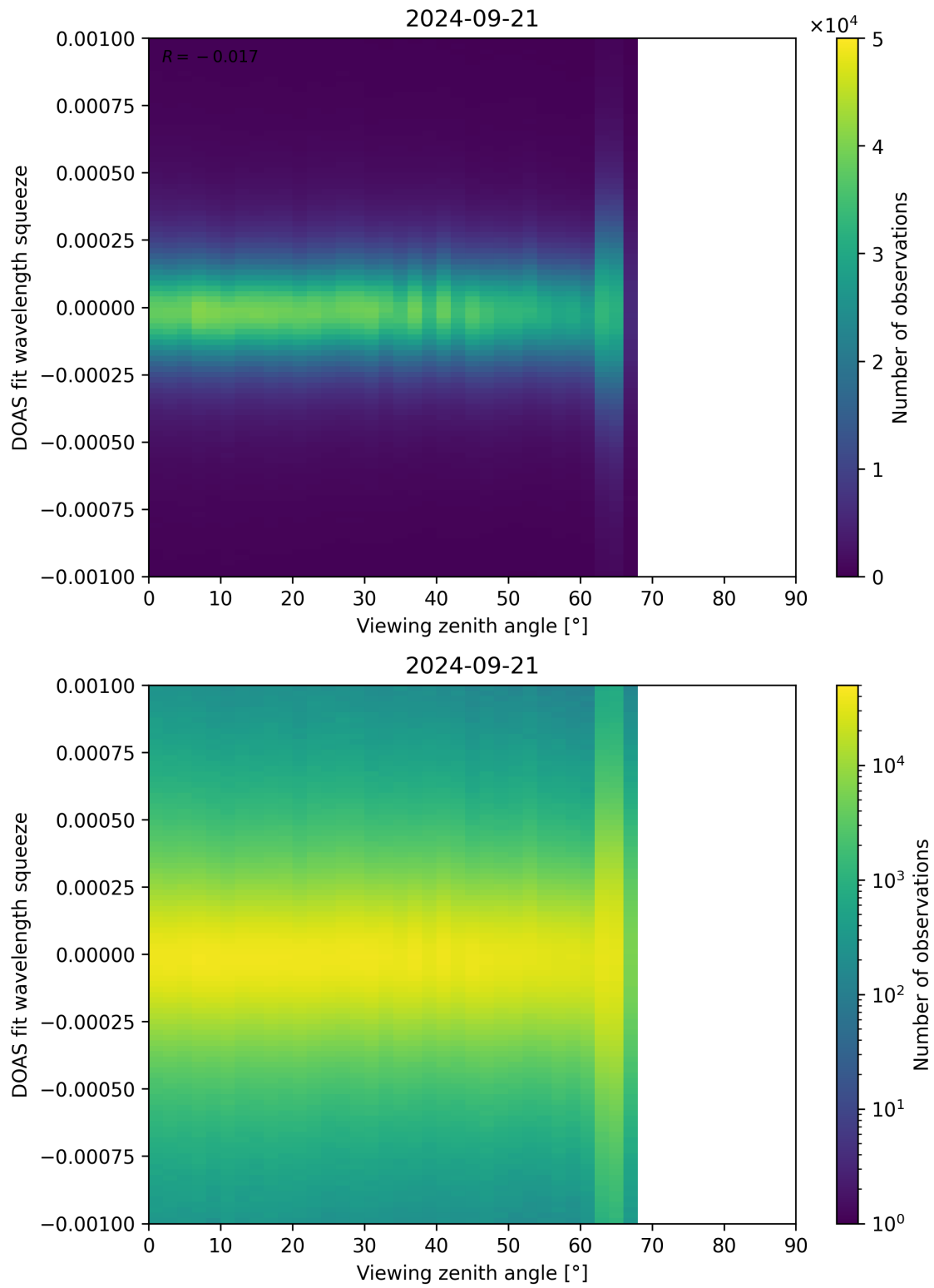
Figure 312: Scatter density plot of “Viewing zenith angle” against “DOAS fit wavelength squeeze” for 2024-09-20 to 2024-09-22.
