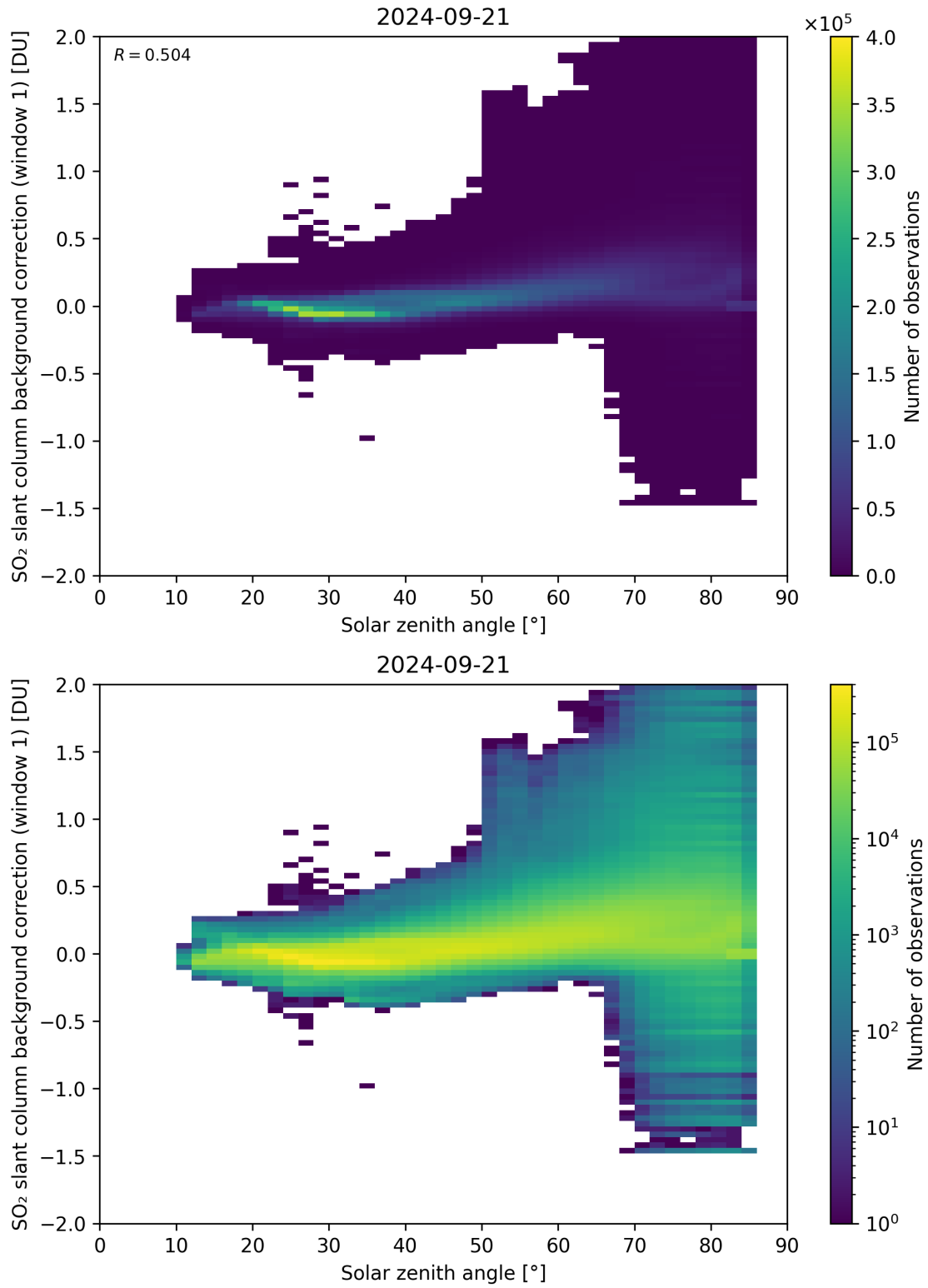
Figure 158: Scatter density plot of “Solar zenith angle” against “SO 2 slant column background correction (window 1)” for 2024-09-20 to 2024-09-22.
