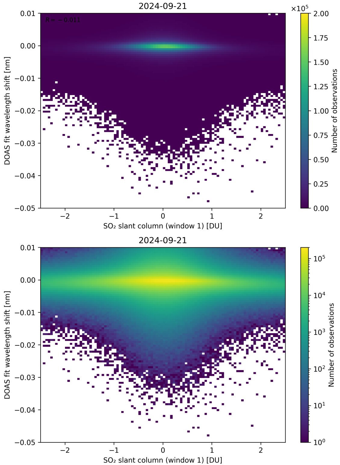
Figure 215: Scatter density plot of “SO 2 slant column (window 1)” against “DOAS fit wavelength shift” for 2024-09-20 to 2024-09-22.
