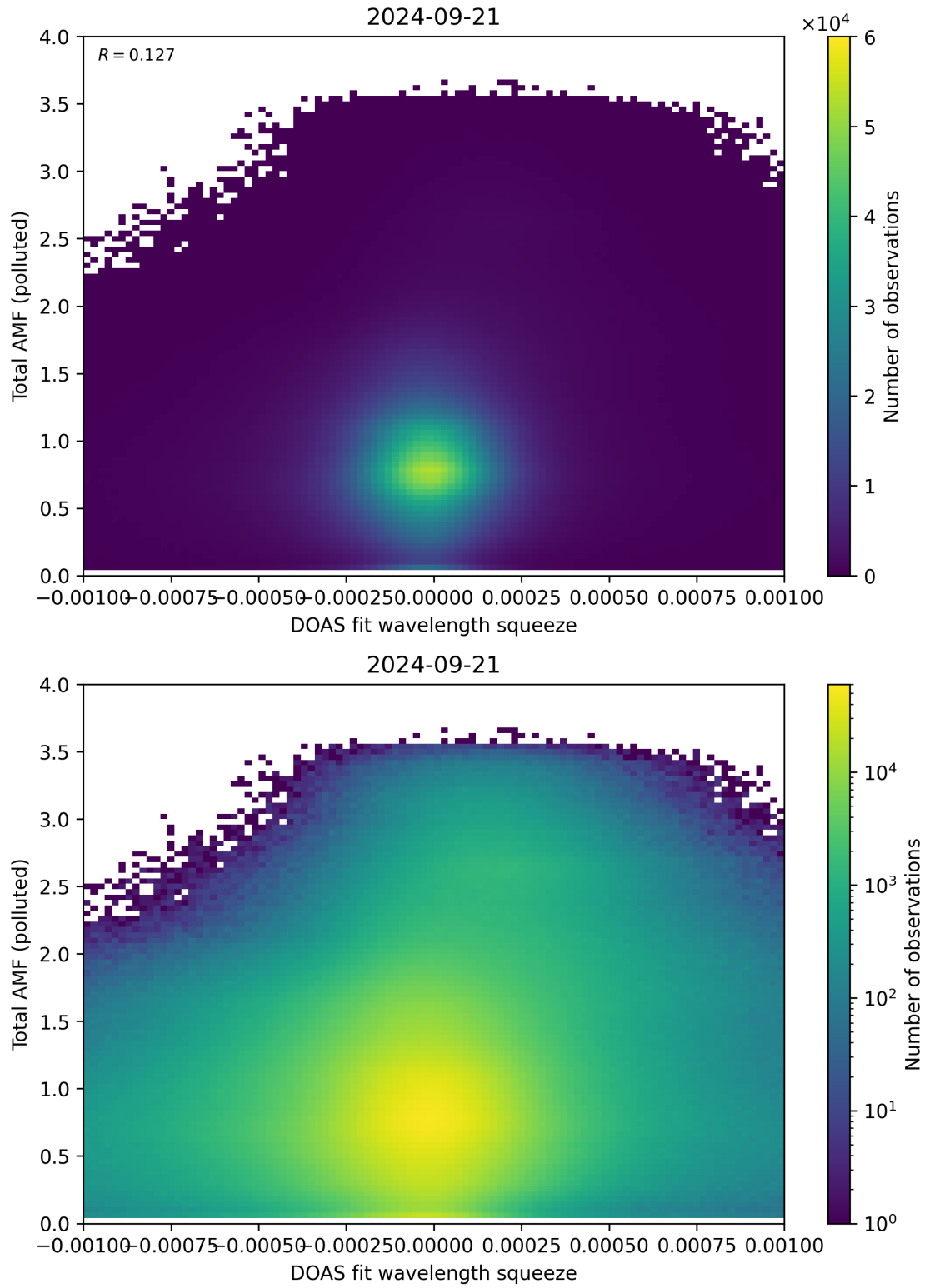
Figure 134: Scatter density plot of “DOAS fit wavelength squeeze” against “Total AMF (polluted)” for 2024-09-20 to 2024-09-22.
