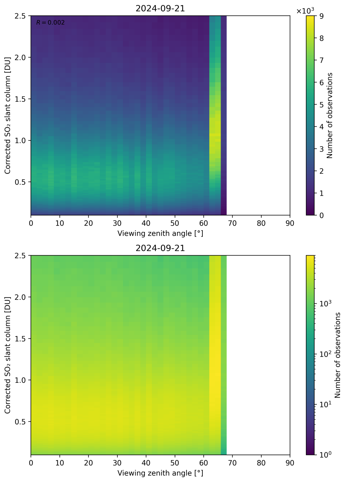
Figure 317: Scatter density plot of “Viewing zenith angle” against “Corrected SO 2 slant column” for 2024-09-20 to 2024-09-22.
