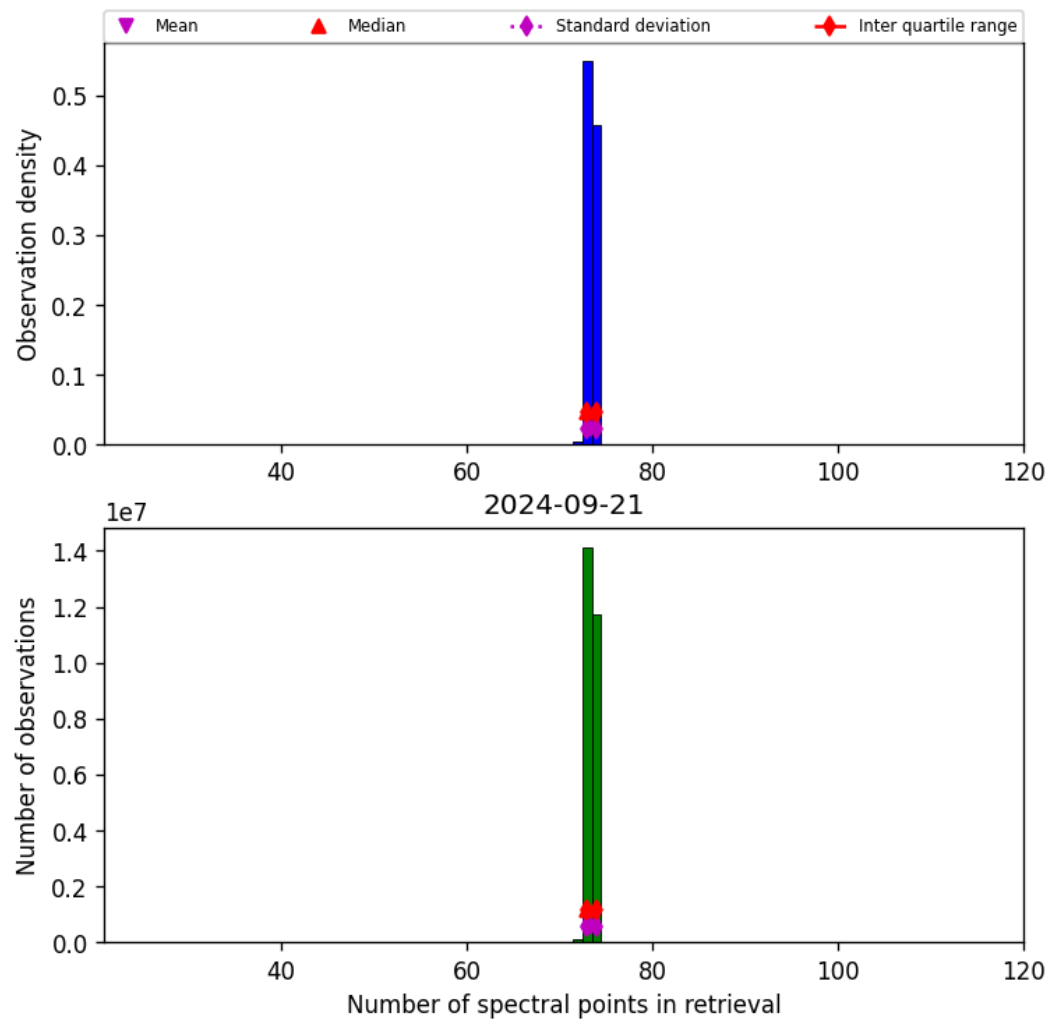
Figure 74: Histogram of “Number of spectral points in retrieval” for 2024-09-20 to 2024-09-22
