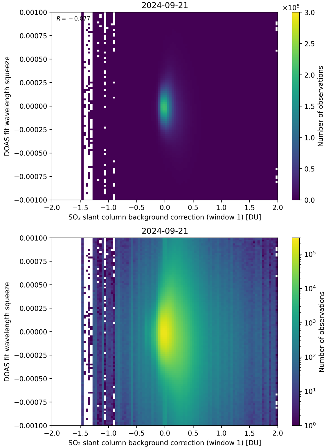
Figure 101: Scatter density plot of “SO 2 slant column background correction (window 1)” against “DOAS fit wavelength squeeze” for 2024-09-20 to 2024-09-22.
