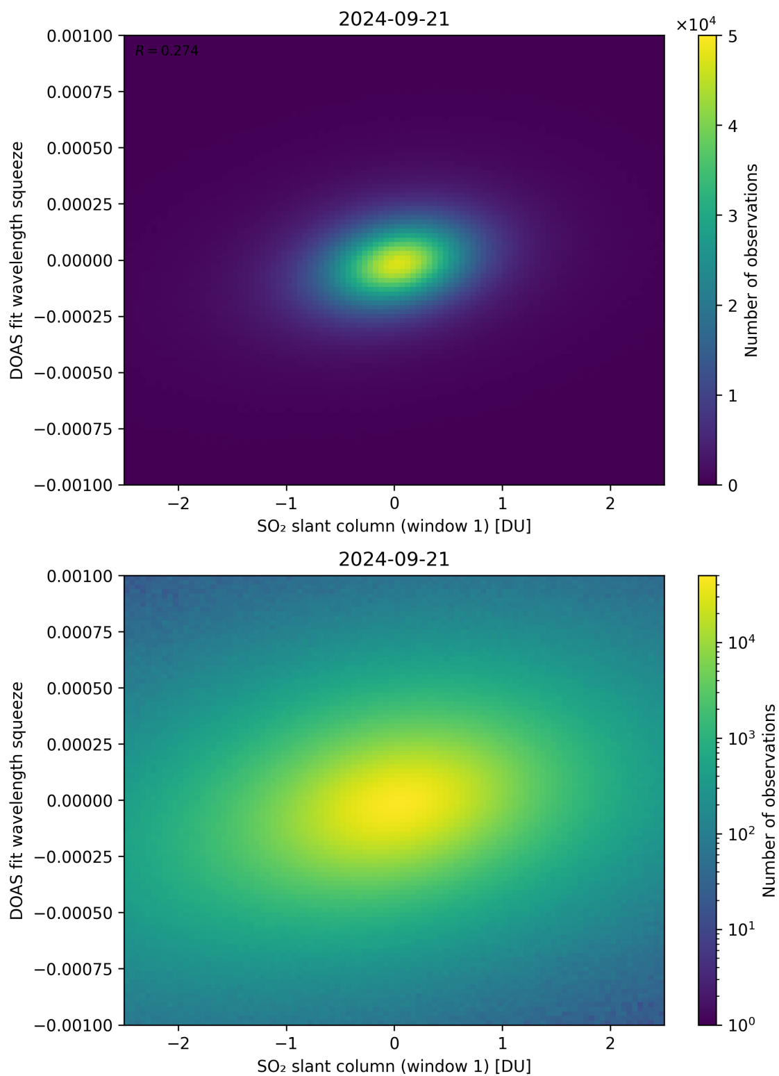
Figure 216: Scatter density plot of “SO 2 slant column (window 1)” against “DOAS fit wavelength squeeze” for 2024-09-20 to 2024-09-22.
