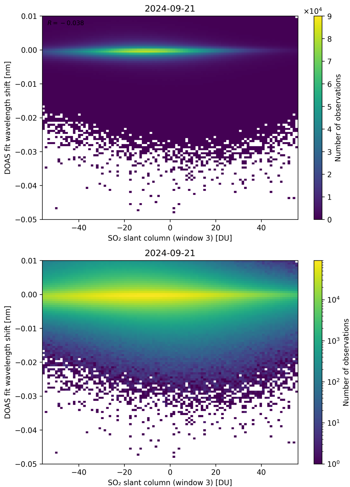
Figure 254: Scatter density plot of “SO 2 slant column (window 3)” against “DOAS fit wavelength shift” for 2024-09-20 to 2024-09-22.
