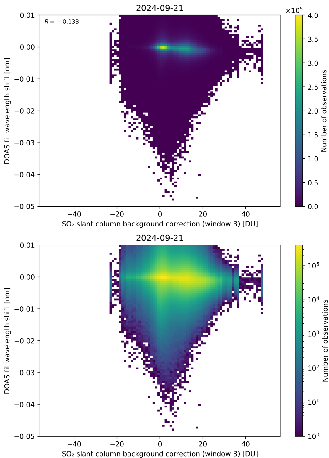
Figure 121: Scatter density plot of “SO 2 slant column background correction (window 3)” against “DOAS fit wavelength shift” for 2024-09-20 to 2024-09-22.
