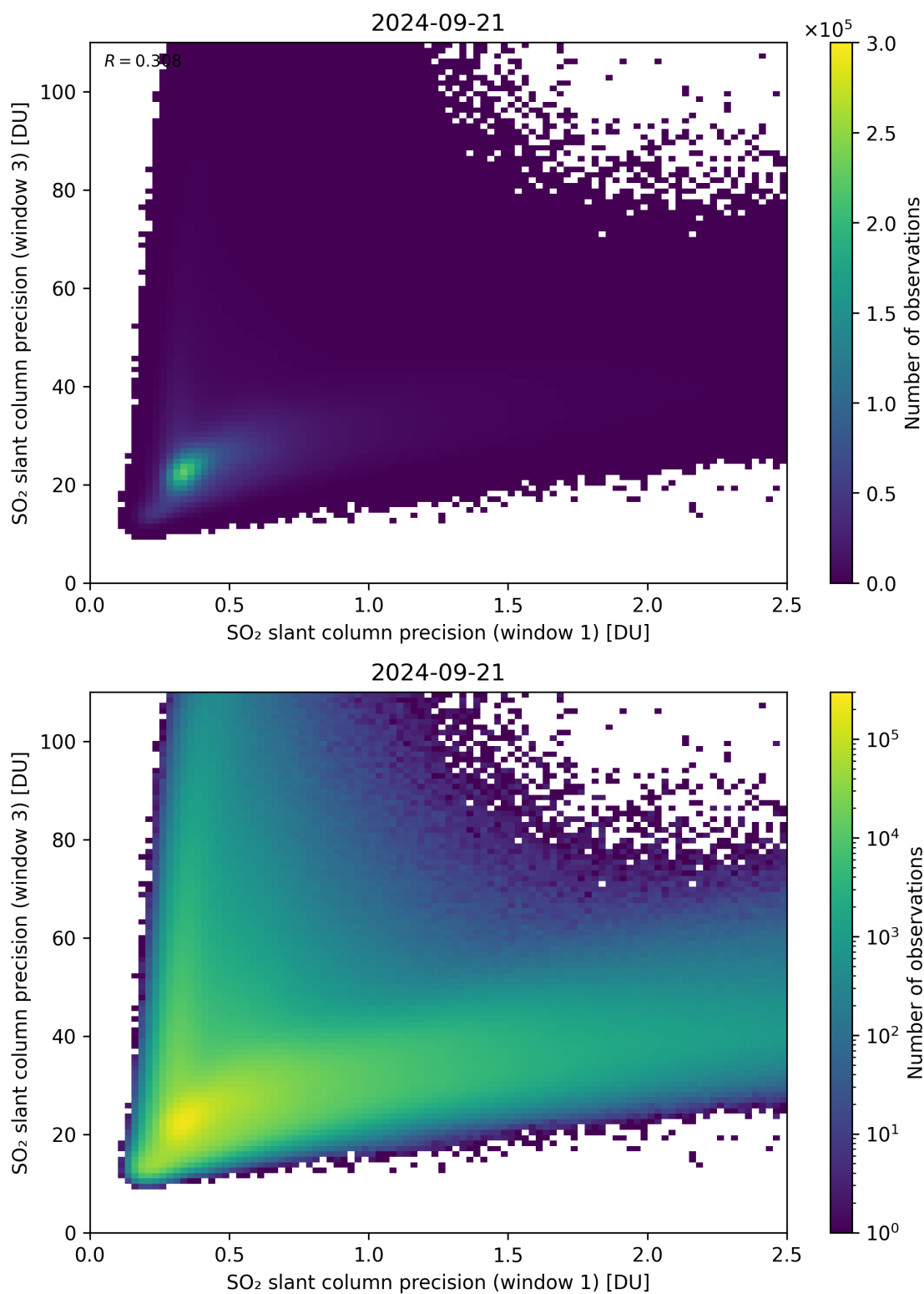
Figure 229: Scatter density plot of “SO 2 slant column precision (window 1)” against “SO 2 slant column precision (window 3)” for 2024-09-20 to 2024-09-22.
