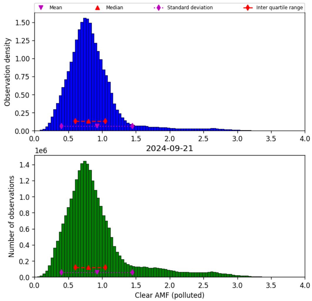
Figure 73: Histogram of “Clear AMF (polluted)” for 2024-09-20 to 2024-09-22
