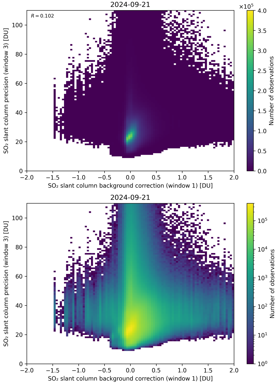
Figure 108: Scatter density plot of “SO 2 slant column background correction (window 1)” against “SO 2 slant column precision (window 3)” for 2024-09-20 to 2024-09-22.
