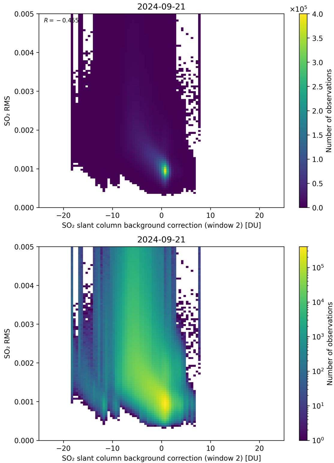
Figure 114: Scatter density plot of “SO 2 slant column background correction (window 2)” against “SO 2 RMS” for 2024-09-20 to 2024-09-22.
