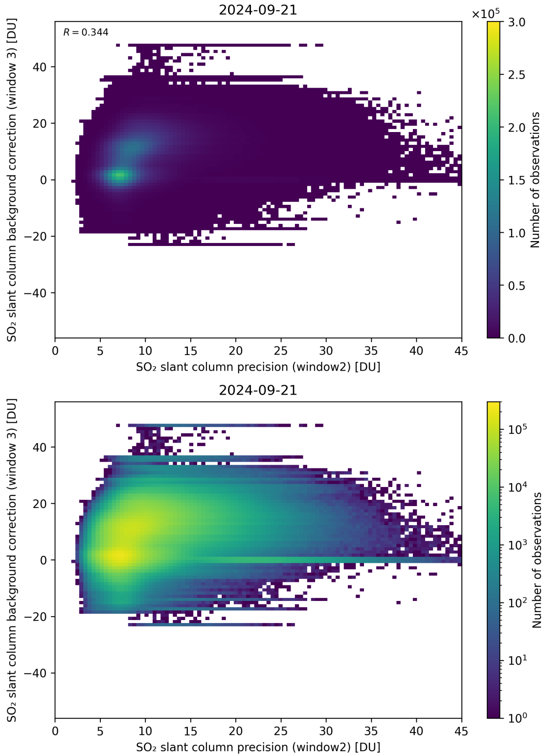
Figure 242: Scatter density plot of “SO 2 slant column precision (window2)” against “SO 2 slant column background correction (window 3)” for 2024-09-20 to 2024-09-22.
