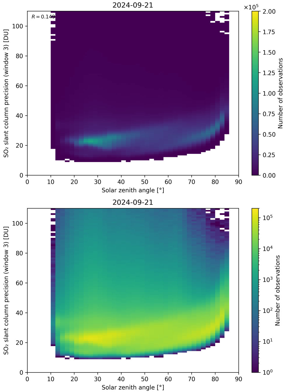
Figure 173: Scatter density plot of “Solar zenith angle” against “SO 2 slant column precision (window 3)” for 2024-09-20 to 2024-09-22.
