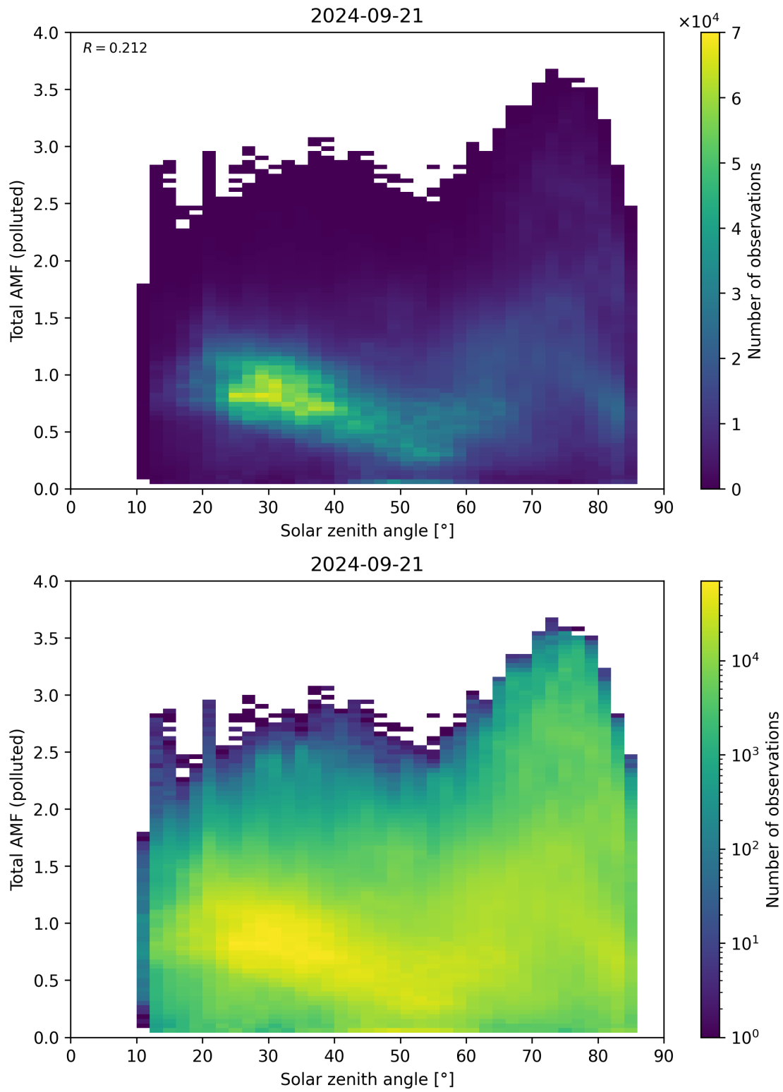
Figure 174: Scatter density plot of “Solar zenith angle” against “Total AMF (polluted)” for 2024-09-20 to 2024-09-22.
