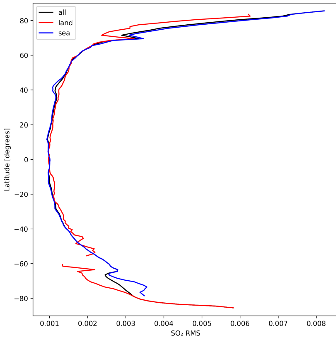
Figure 47: Zonal average of “SO 2 RMS” for 2024-09-22 to 2024-09-23.
