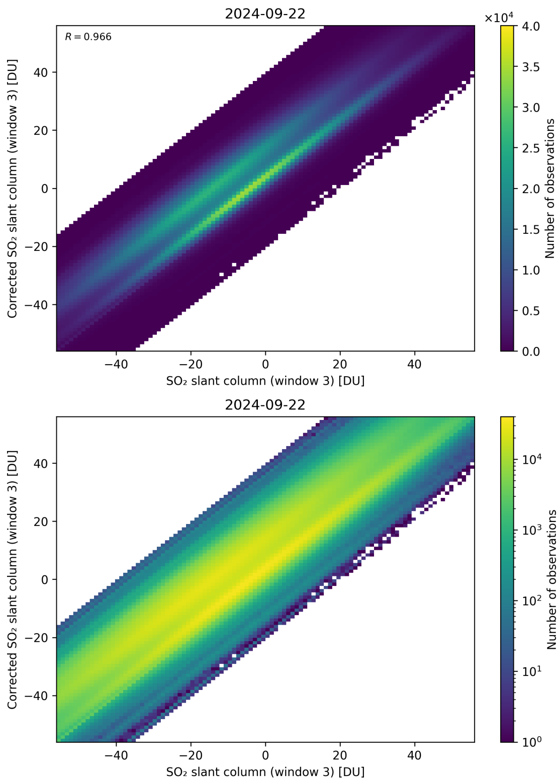
Figure 266: Scatter density plot of “SO 2 slant column (window 3)” against “Corrected SO 2 slant column (window 3)” for 2024-09-22 to 2024-09-23.
