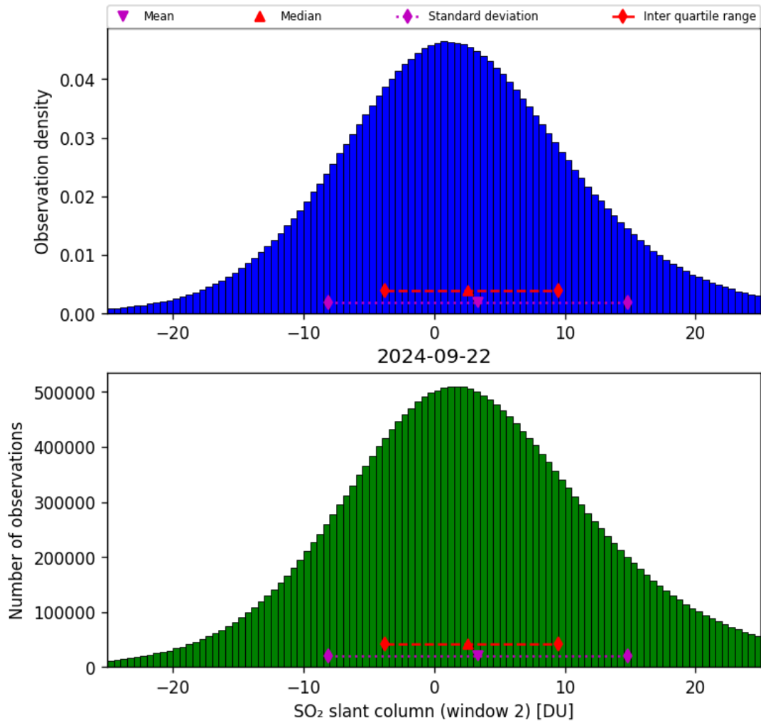
Figure 60: Histogram of “SO 2 slant column (window 2)” for 2024-09-22 to 2024-09-23
