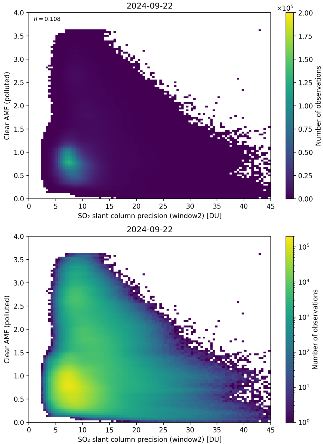
Figure 246: Scatter density plot of “SO 2 slant column precision (window2)” against “Clear AMF (polluted)” for 2024-09-22 to 2024-09-23.
