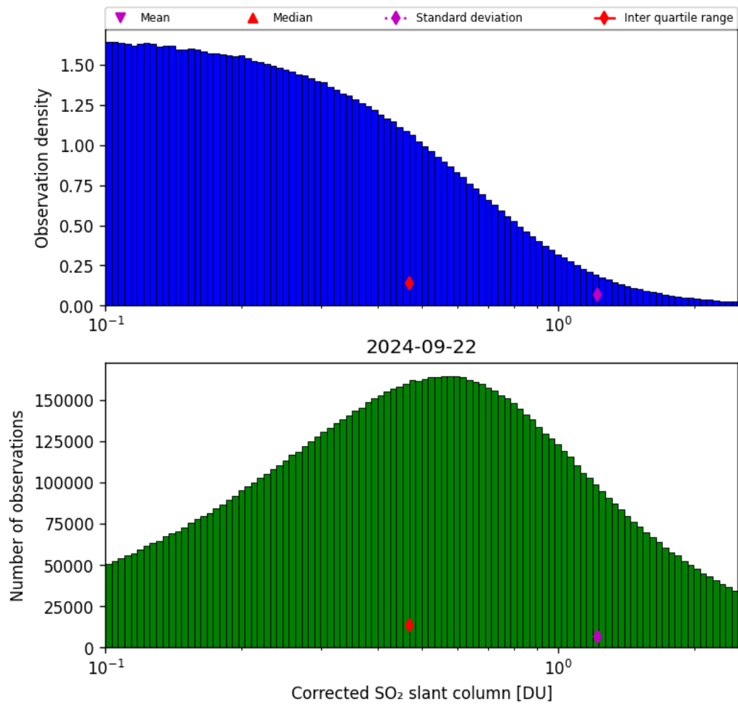
Figure 55: Histogram of “Corrected SO 2 slant column” for 2024-09-22 to 2024-09-23
