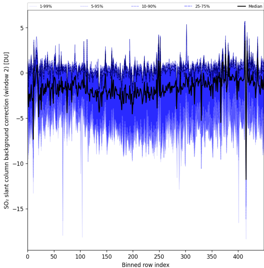
Figure 86: Along track statistics of “SO 2 slant column background correction (window 2)” for 2024-09-22 to 2024-09-23
