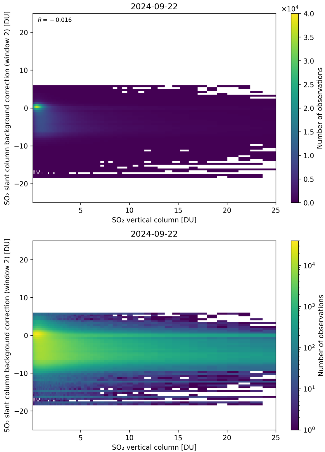
Figure 274: Scatter density plot of “SO 2 vertical column” against “SO 2 slant column background correction (window 2)” for 2024-09-22 to 2024-09-23.
