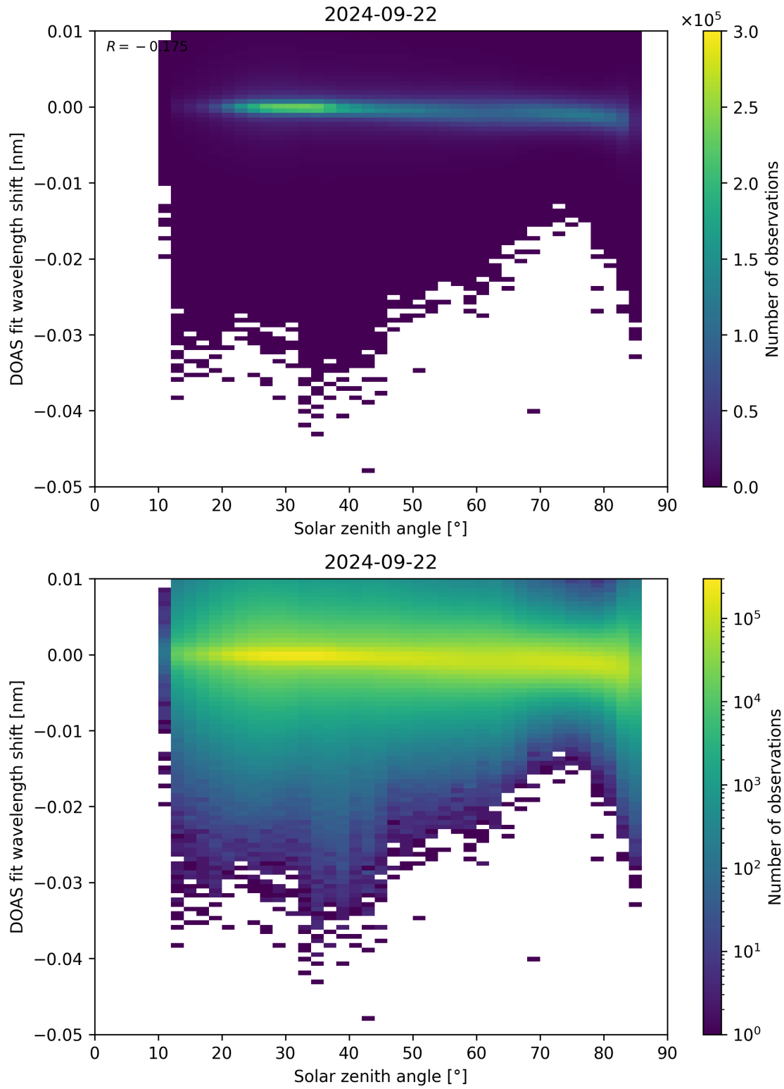
Figure 161: Scatter density plot of “Solar zenith angle” against “DOAS fit wavelength shift” for 2024-09-22 to 2024-09-23.
