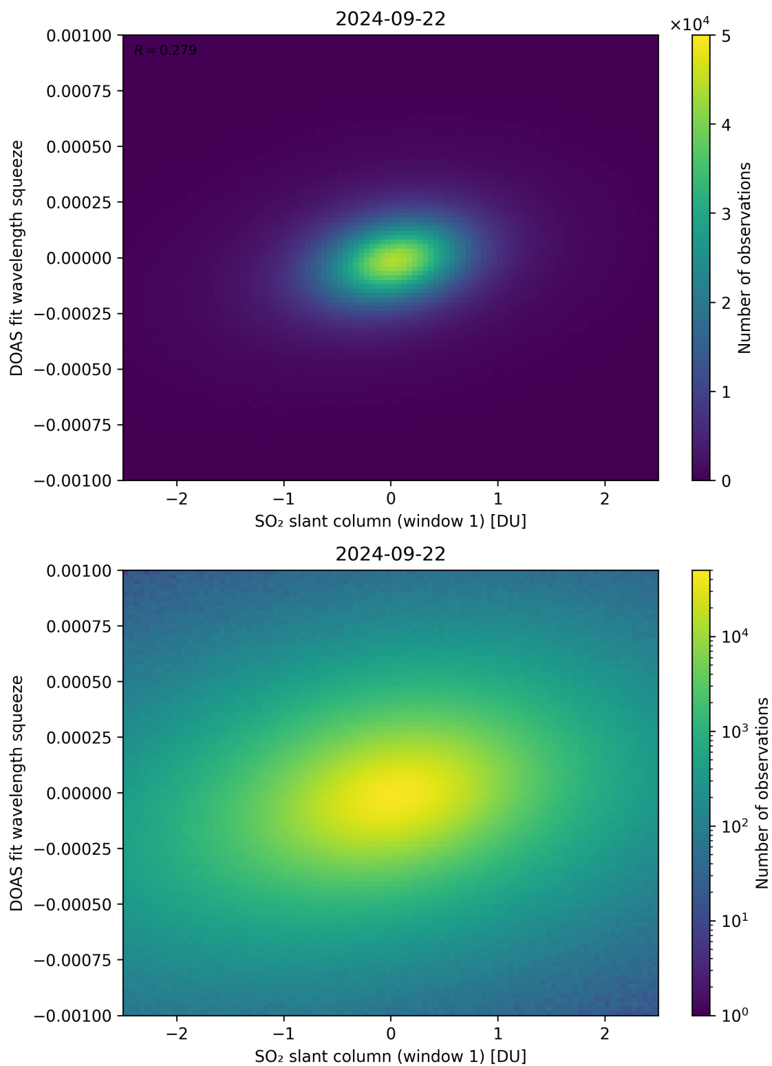
Figure 216: Scatter density plot of “SO 2 slant column (window 1)” against “DOAS fit wavelength squeeze” for 2024-09-22 to 2024-09-23.
