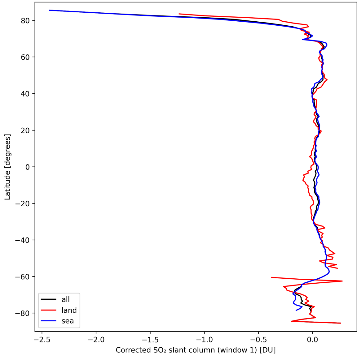
Figure 35: Zonal average of “Corrected SO 2 slant column (window 1)” for 2024-09-22 to 2024-09-23.
