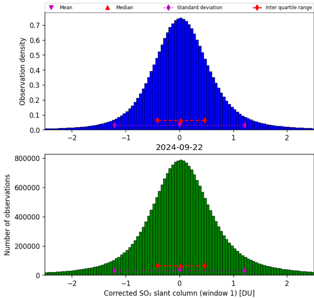
Figure 58: Histogram of “Corrected SO 2 slant column (window 1)” for 2024-09-22 to 2024-09-23
