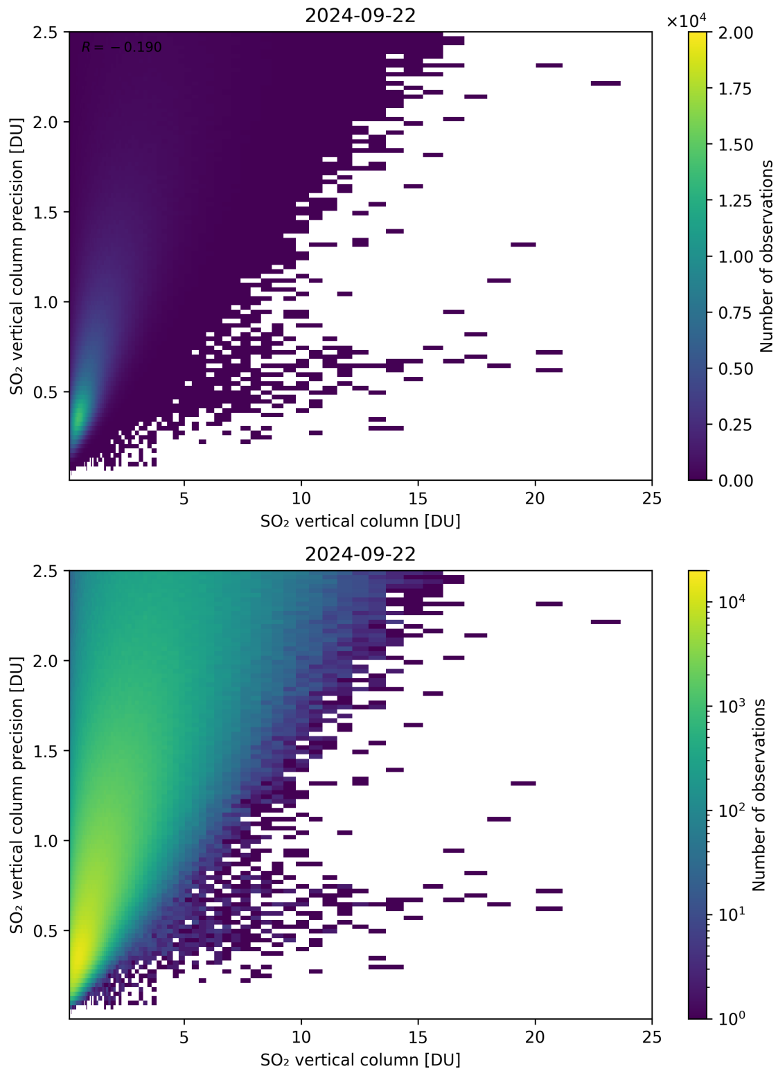
Figure 307: Scatter density plot of “SO 2 vertical column” against “SO 2 vertical column precision” for 2024-09-22 to 2024-09-23.
