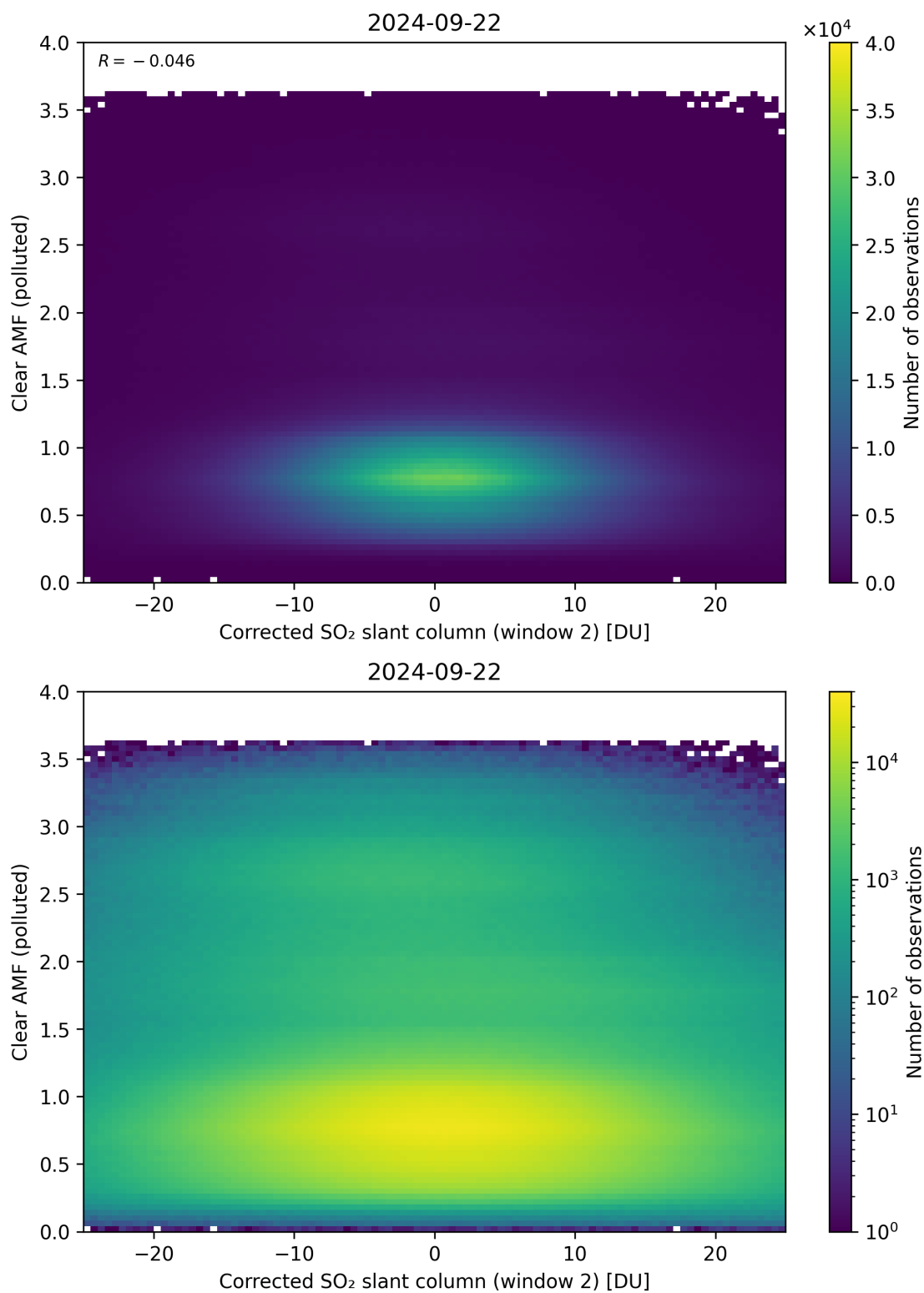
Figure 199: Scatter density plot of “Corrected SO 2 slant column (window 2)” against “Clear AMF (polluted)” for 2024-09-22 to 2024-09-23.
