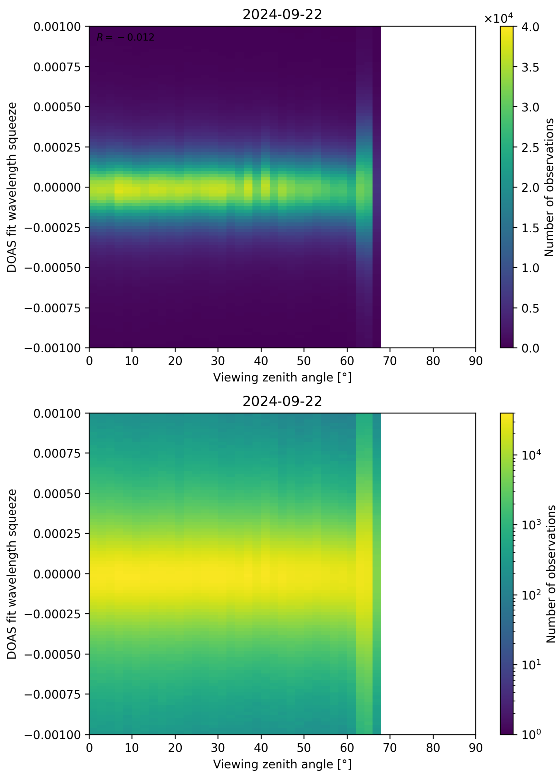
Figure 312: Scatter density plot of “Viewing zenith angle” against “DOAS fit wavelength squeeze” for 2024-09-22 to 2024-09-23.
