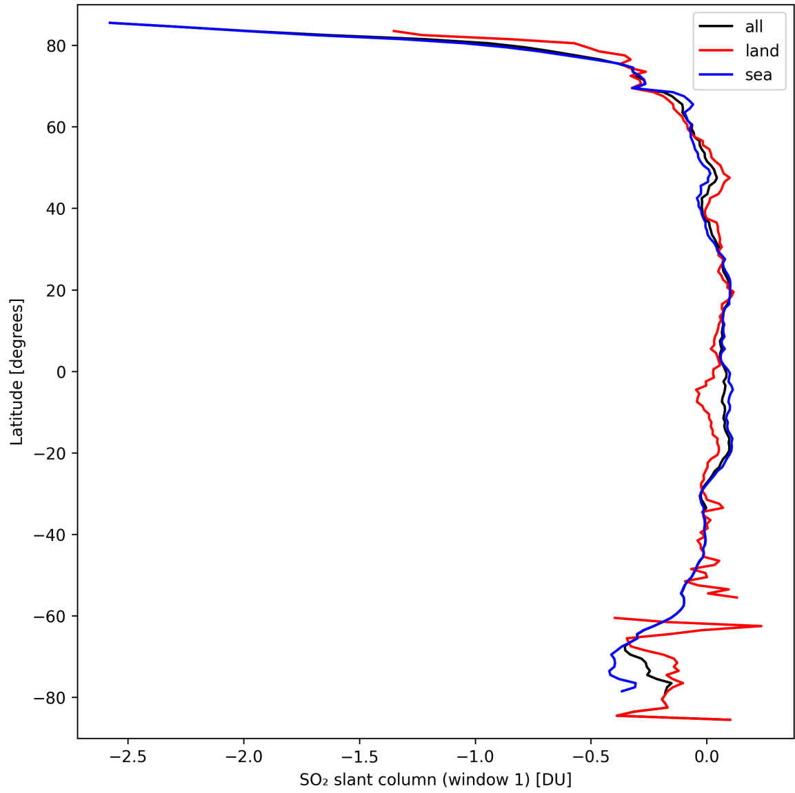
Figure 33: Zonal average of “SO 2 slant column (window 1)” for 2024-09-22 to 2024-09-23.
