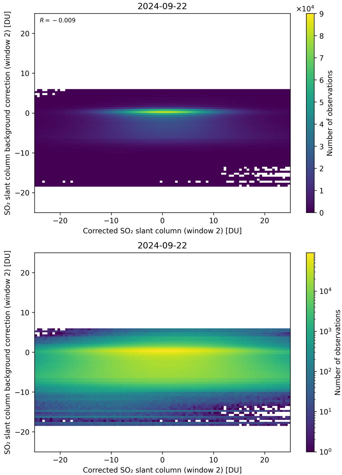
Figure 194: Scatter density plot of “Corrected SO 2 slant column (window 2)” against “SO 2 slant column background correction (window 2)” for 2024-09-22 to 2024-09-23.
