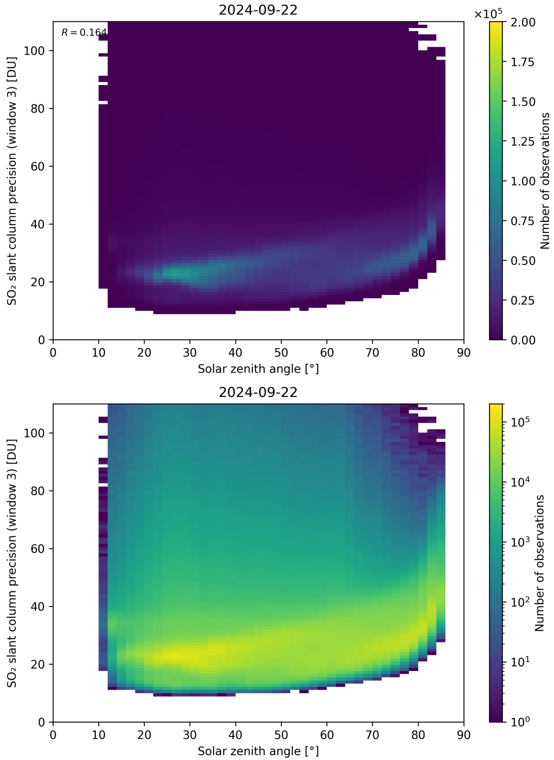
Figure 173: Scatter density plot of “Solar zenith angle” against “SO 2 slant column precision (window 3)” for 2024-09-22 to 2024-09-23.
