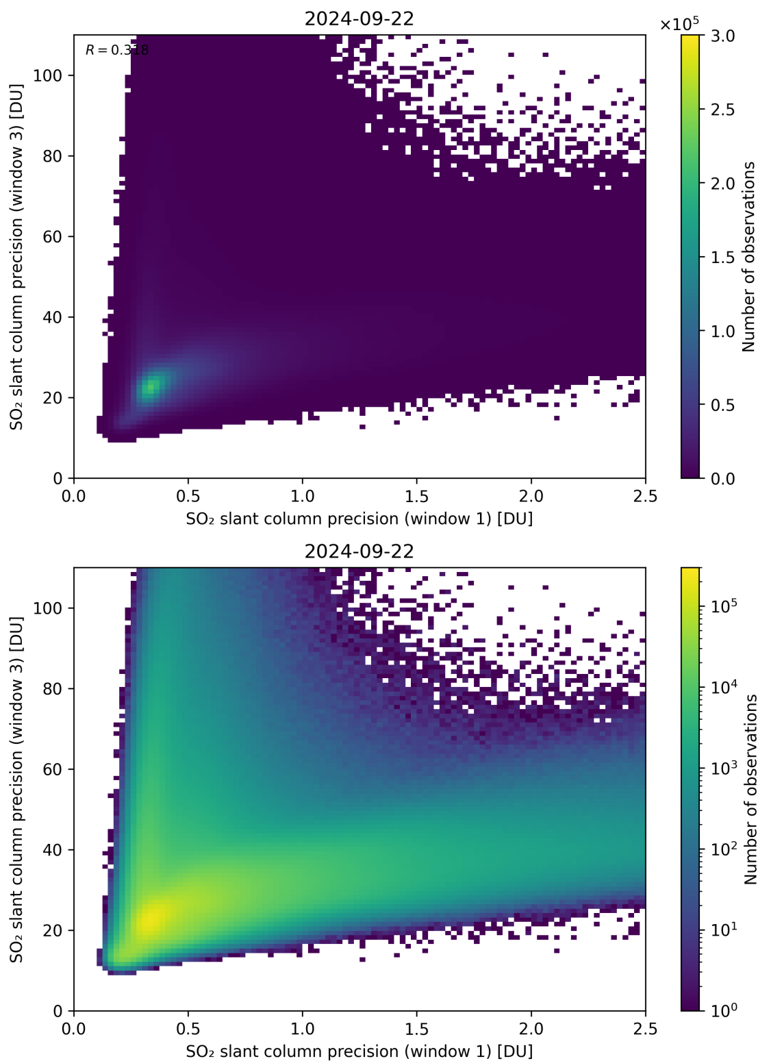
Figure 229: Scatter density plot of “SO 2 slant column precision (window 1)” against “SO 2 slant column precision (window 3)” for 2024-09-22 to 2024-09-23.
