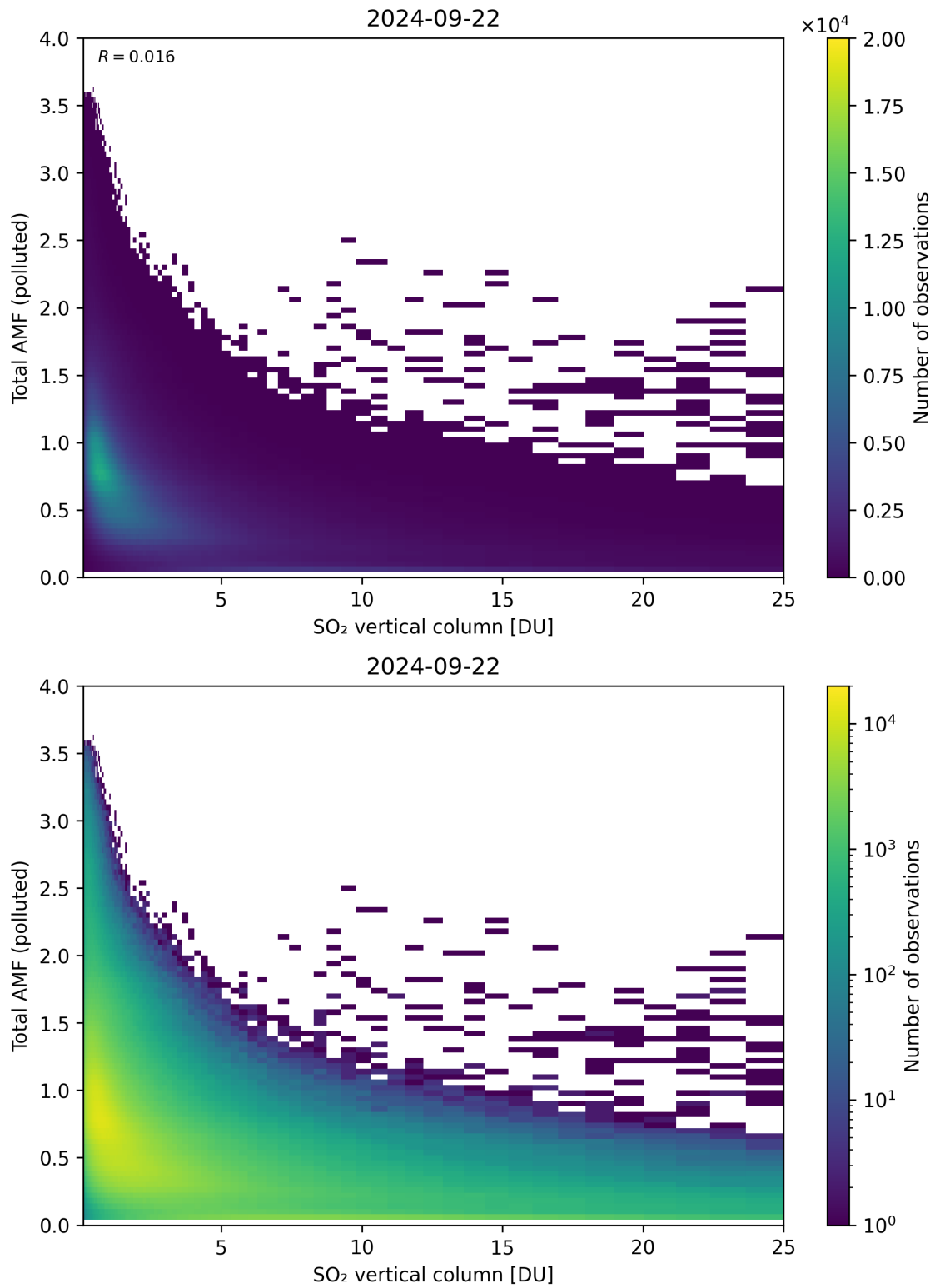
Figure 305: Scatter density plot of “SO 2 vertical column” against “Total AMF (polluted)” for 2024-09-22 to 2024-09-23.
