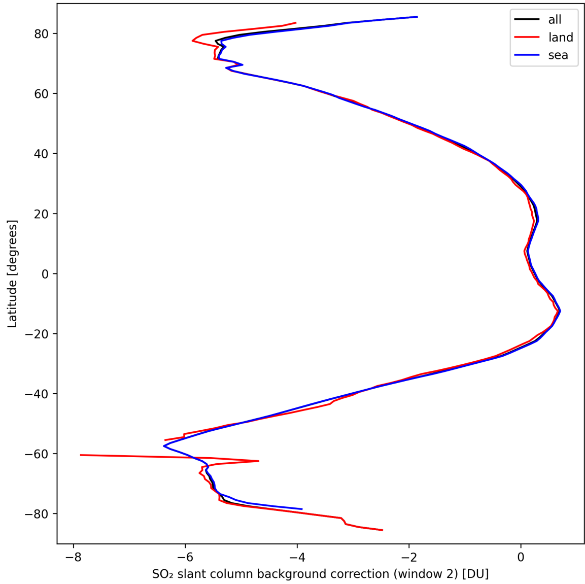
Figure 40: Zonal average of “SO 2 slant column background correction (window 2)” for 2024-09-22 to 2024-09-23.
