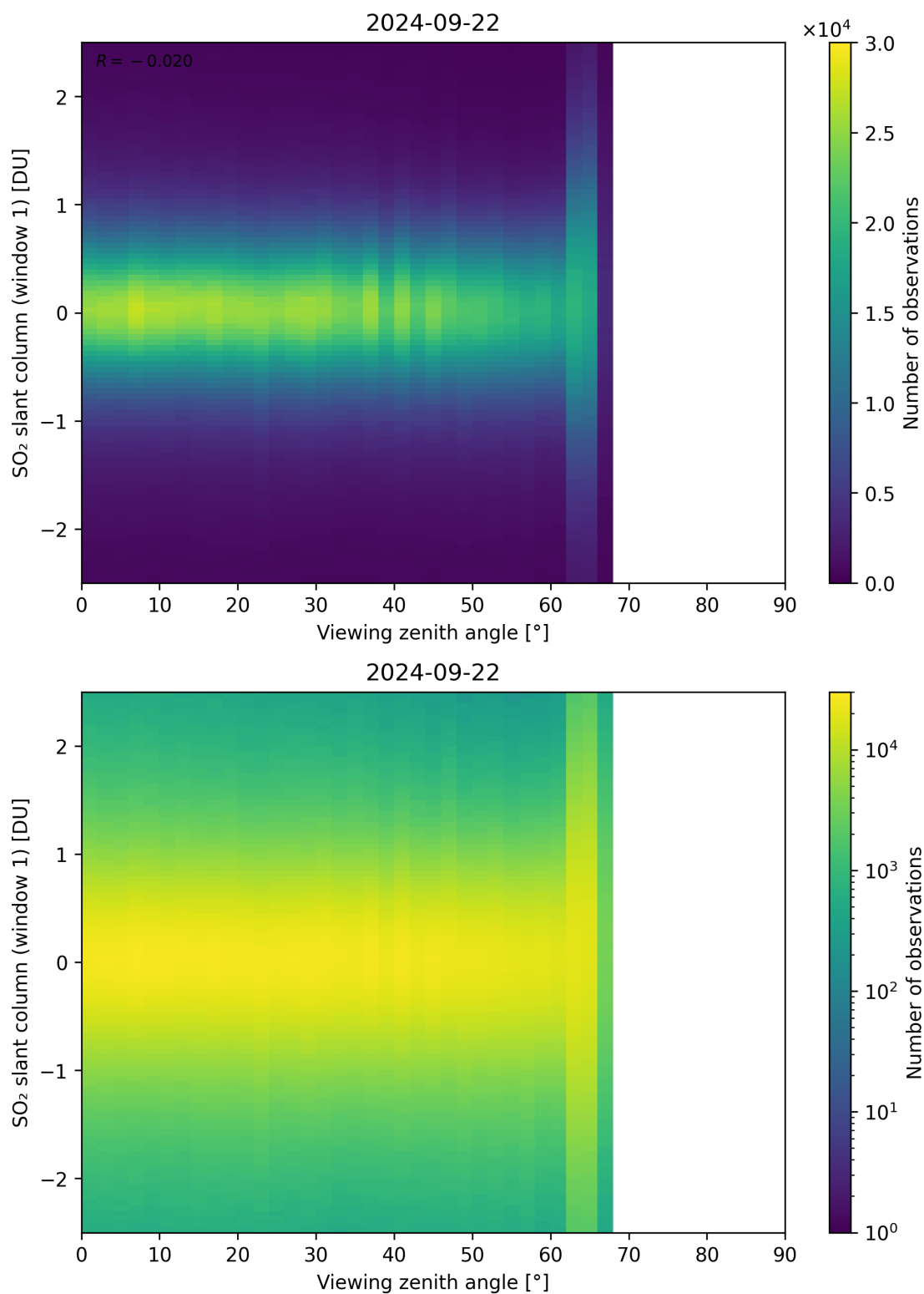
Figure 320: Scatter density plot of “Viewing zenith angle” against “SO 2 slant column (window 1)” for 2024-09-22 to 2024-09-23.
