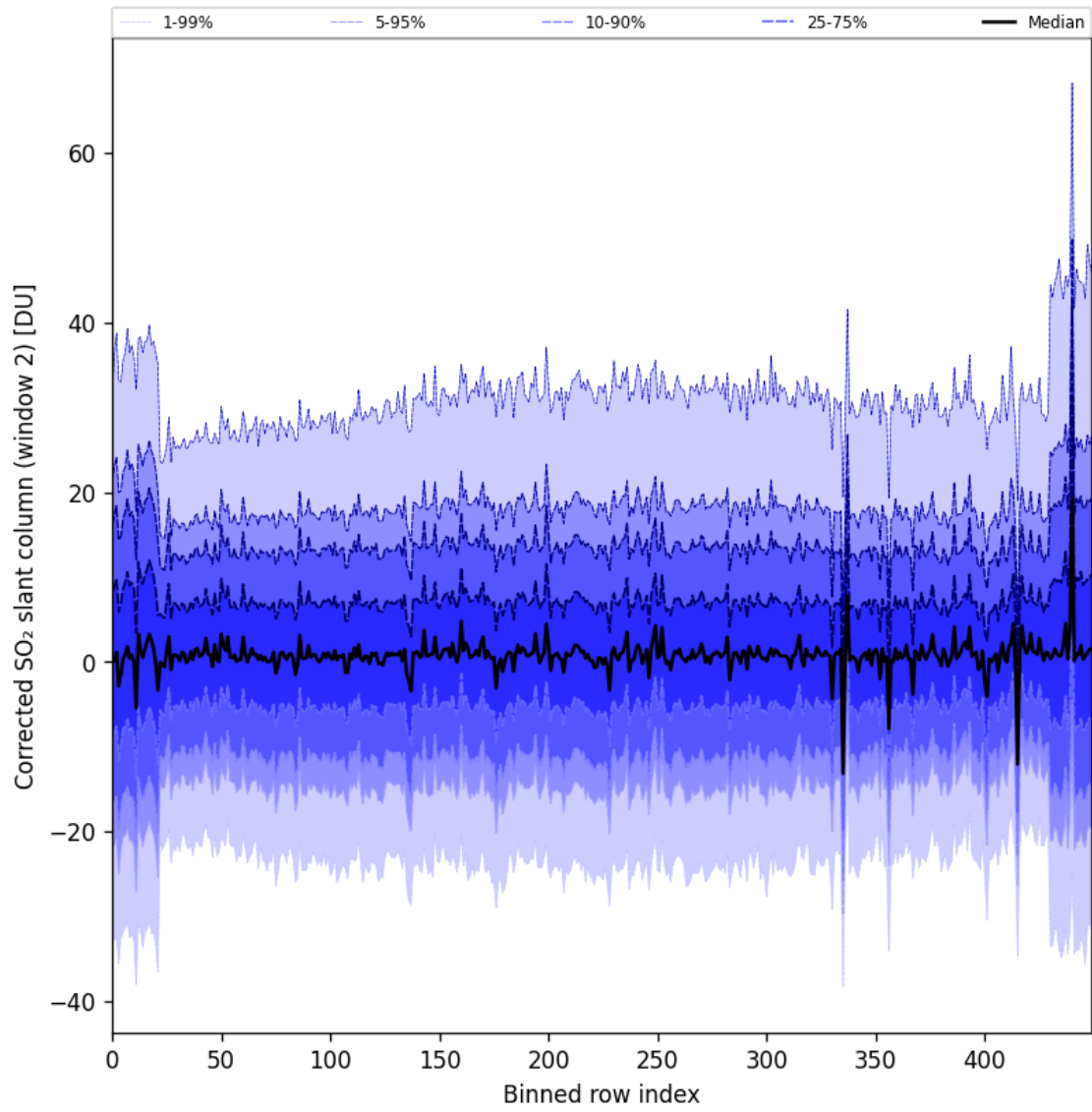
Figure 85: Along track statistics of “Corrected SO 2 slant column (window 2)” for 2024-09-22 to 2024-09-23
