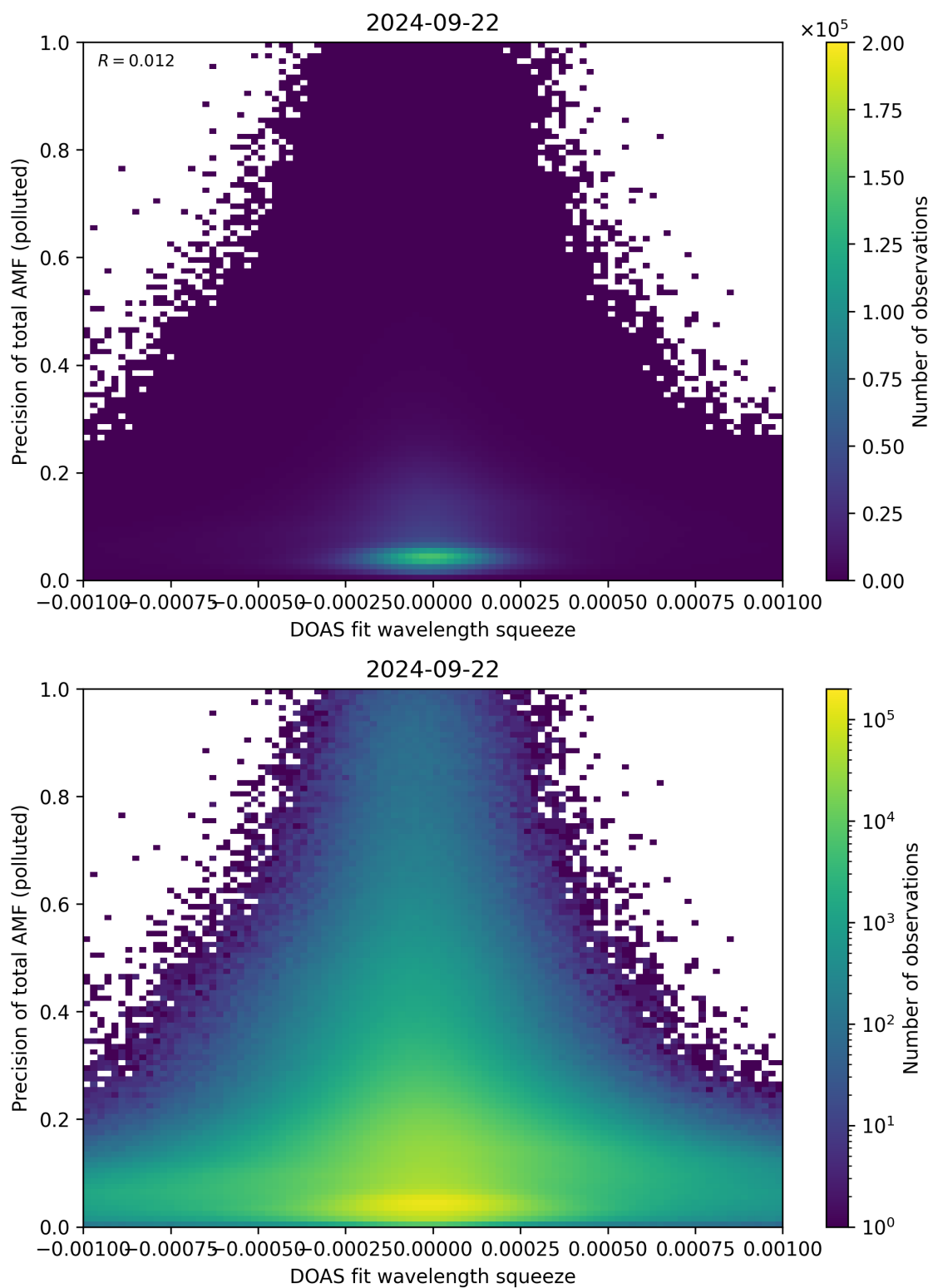
Figure 135: Scatter density plot of “DOAS fit wavelength squeeze” against “Precision of total AMF (polluted)” for 2024-09-22 to 2024-09-23.
