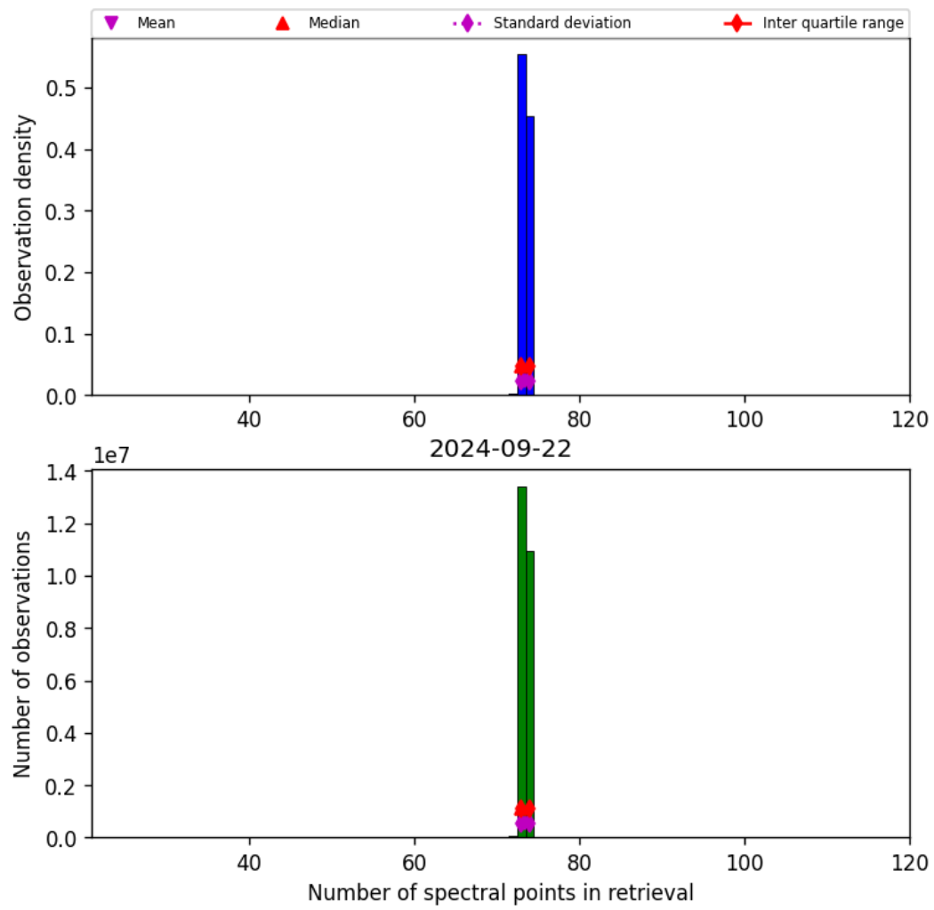
Figure 74: Histogram of “Number of spectral points in retrieval” for 2024-09-22 to 2024-09-23
