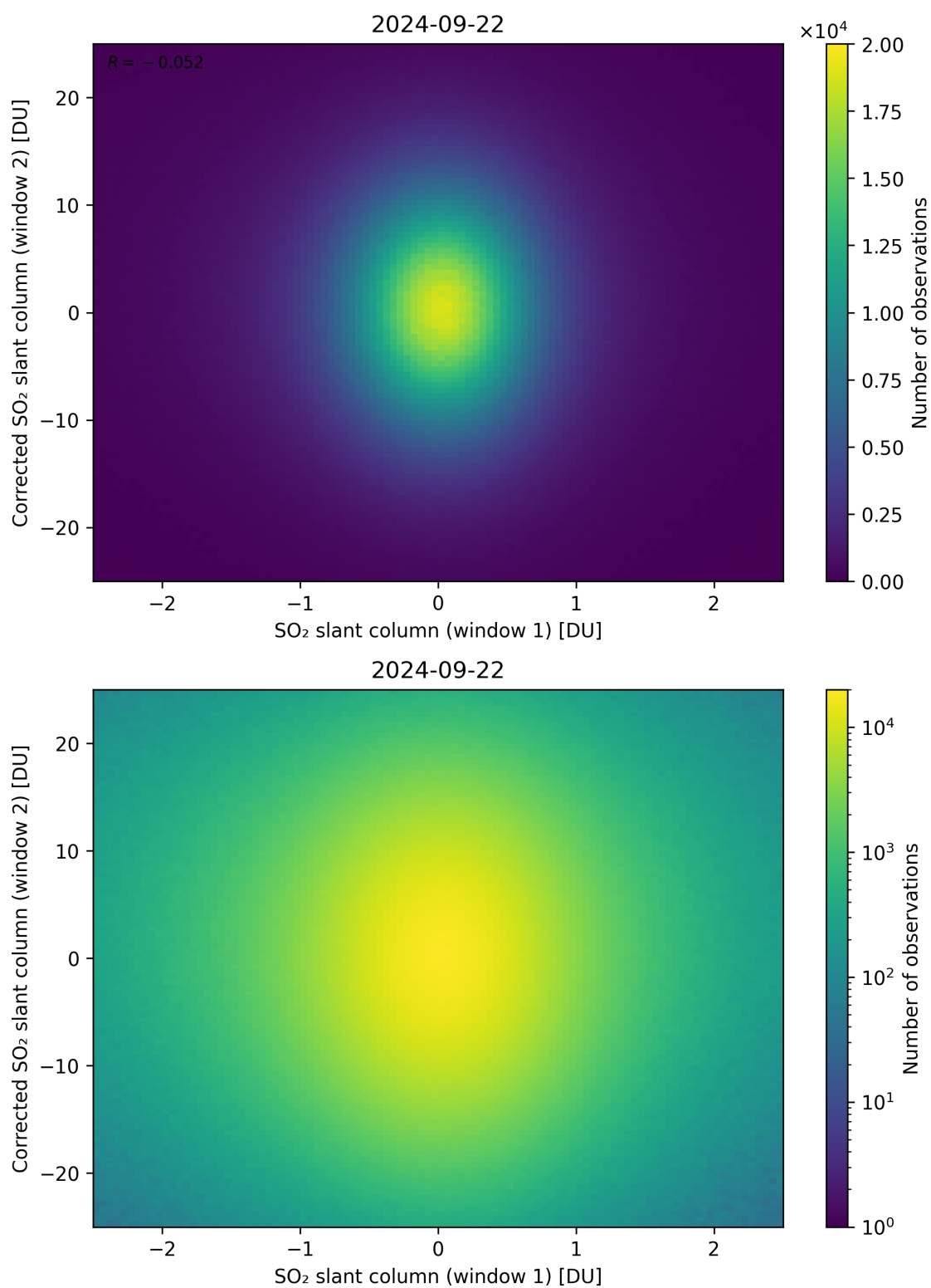
Figure 233: Scatter density plot of “SO 2 slant column (window 1)” against “Corrected SO 2 slant column (window 2)” for 2024-09-22 to 2024-09-23.
