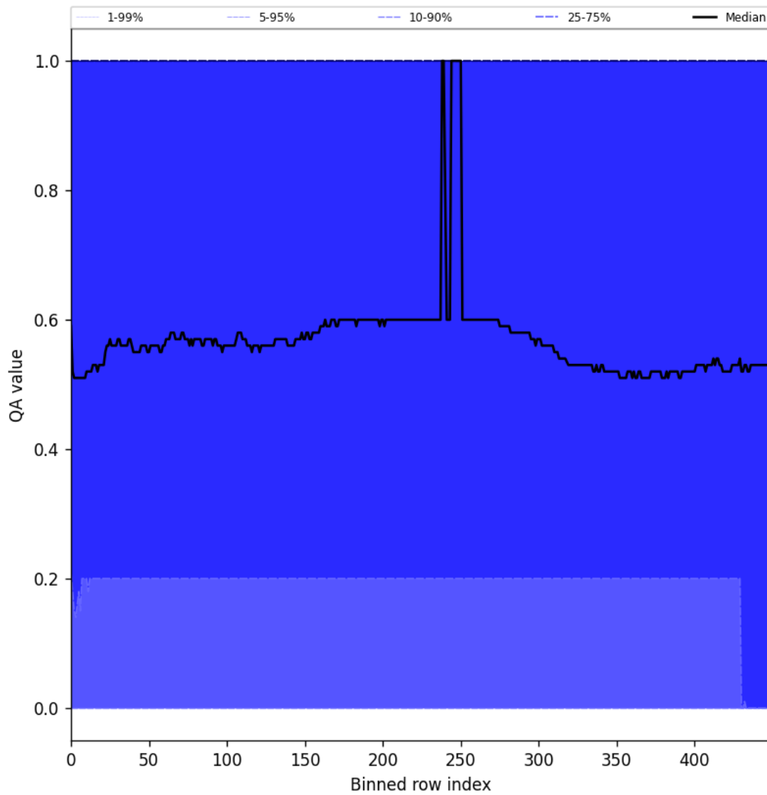
Figure 75: Along track statistics of “QA value” for 2024-09-22 to 2024-09-23
