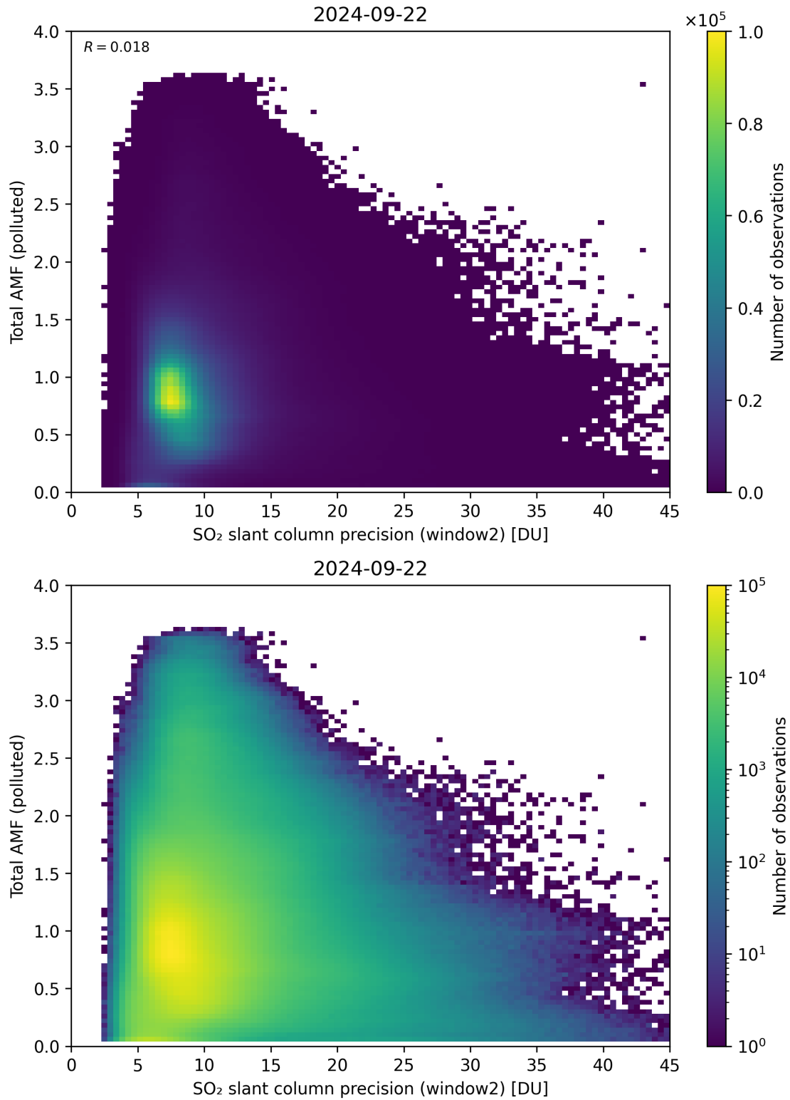
Figure 251: Scatter density plot of “SO 2 slant column precision (window2)” against “Total AMF (polluted)” for 2024-09-22 to 2024-09-23.
