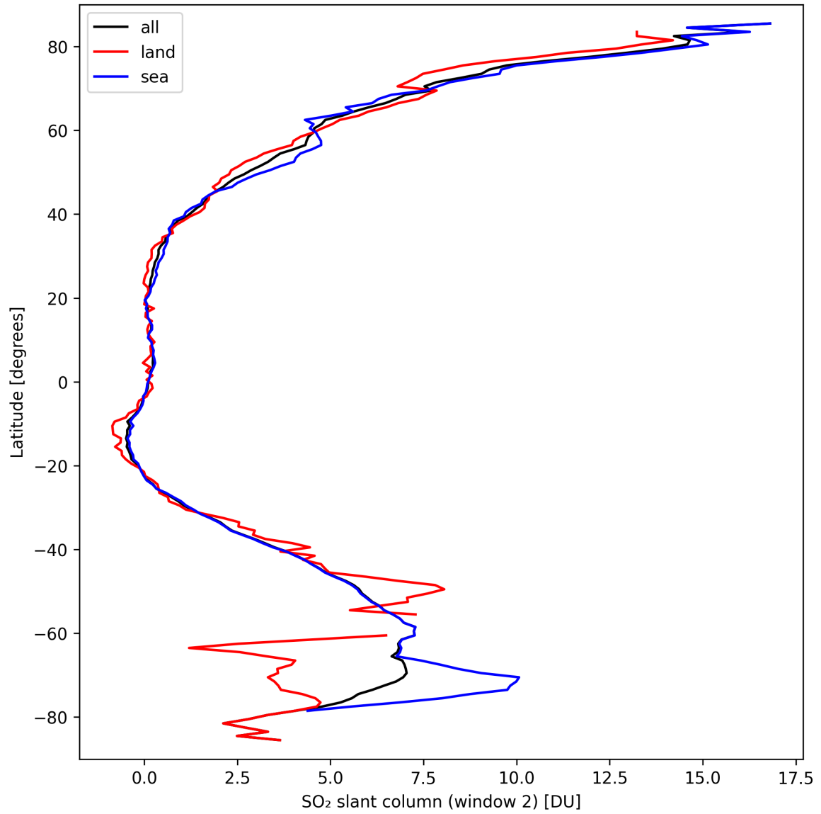
Figure 37: Zonal average of “SO 2 slant column (window 2)” for 2024-09-22 to 2024-09-23.
