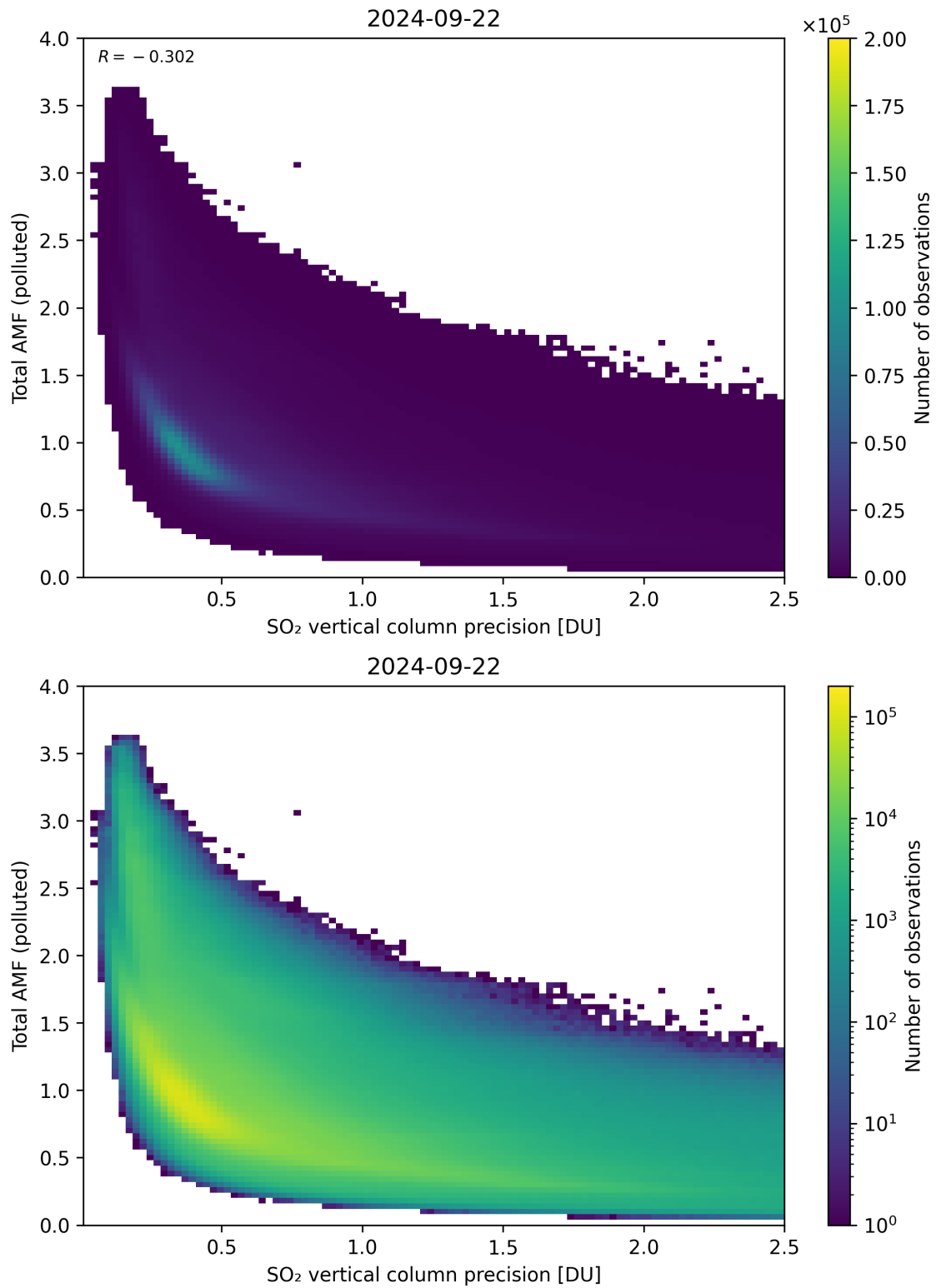
Figure 294: Scatter density plot of “SO 2 vertical column precision” against “Total AMF (polluted)” for 2024-09-22 to 2024-09-23.
