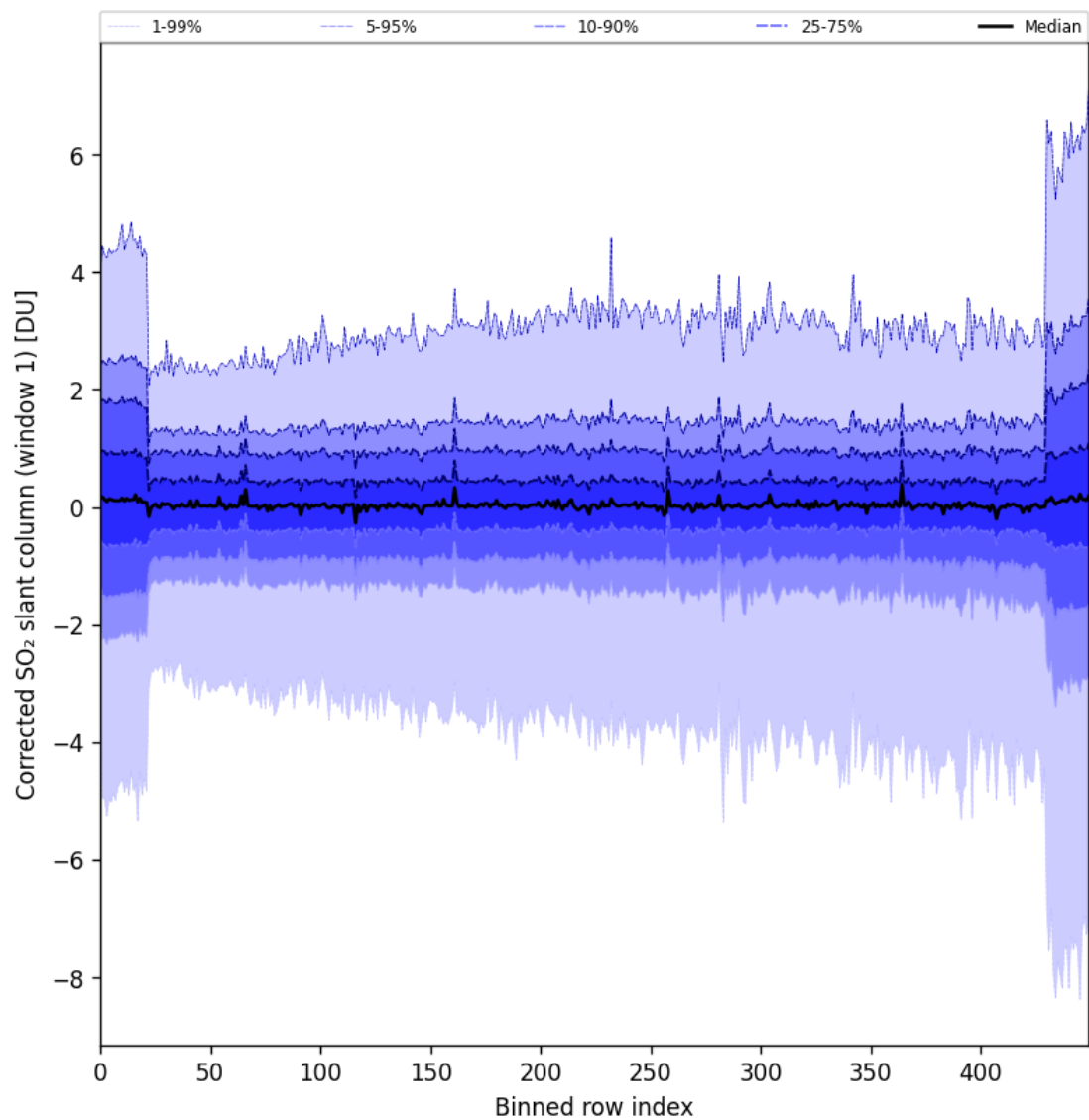
Figure 81: Along track statistics of “Corrected SO 2 slant column (window 1)” for 2024-09-22 to 2024-09-23
