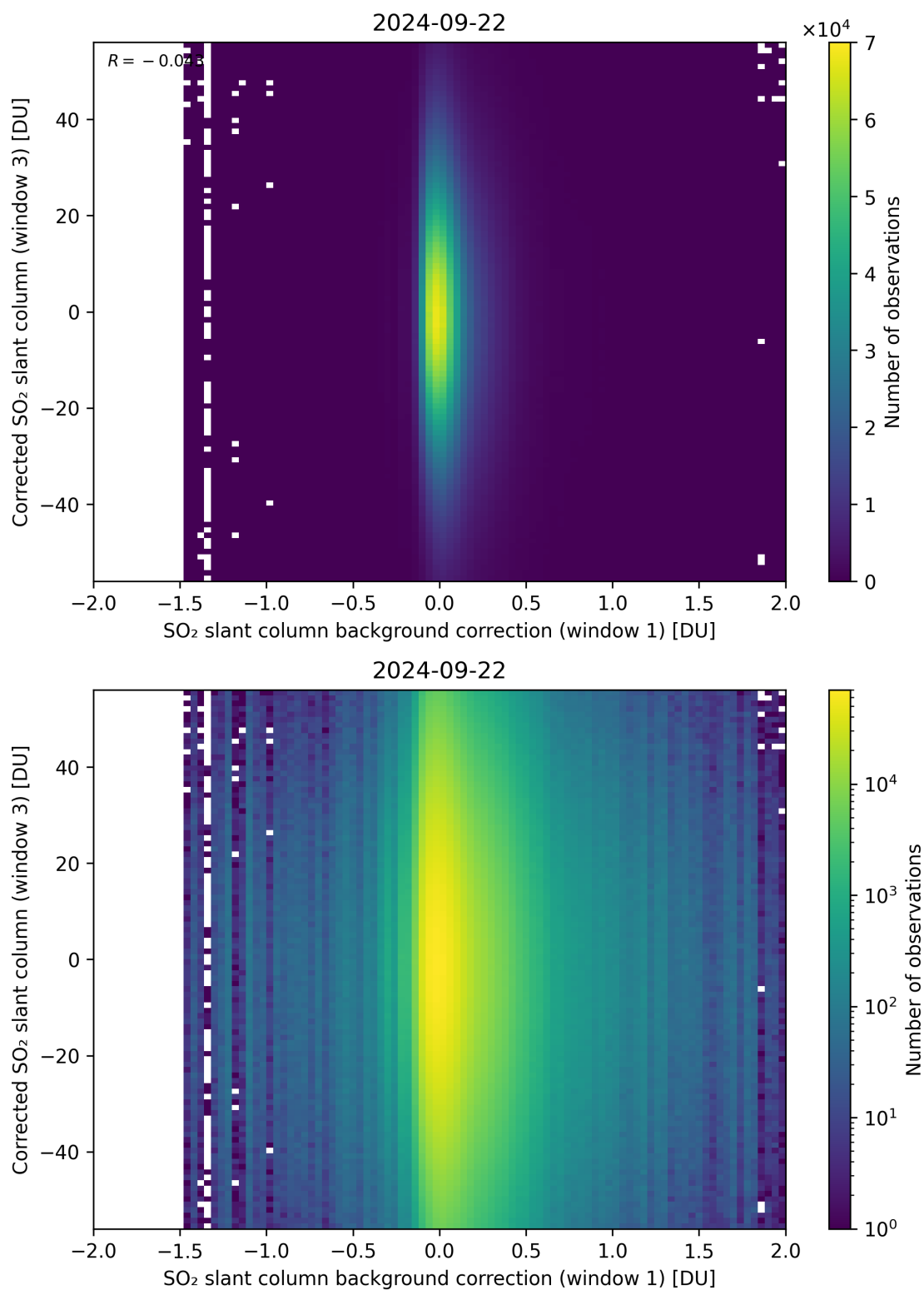
Figure 105: Scatter density plot of “SO 2 slant column background correction (window 1)” against “Corrected SO 2 slant column (window 3)” for 2024-09-22 to 2024-09-23.
