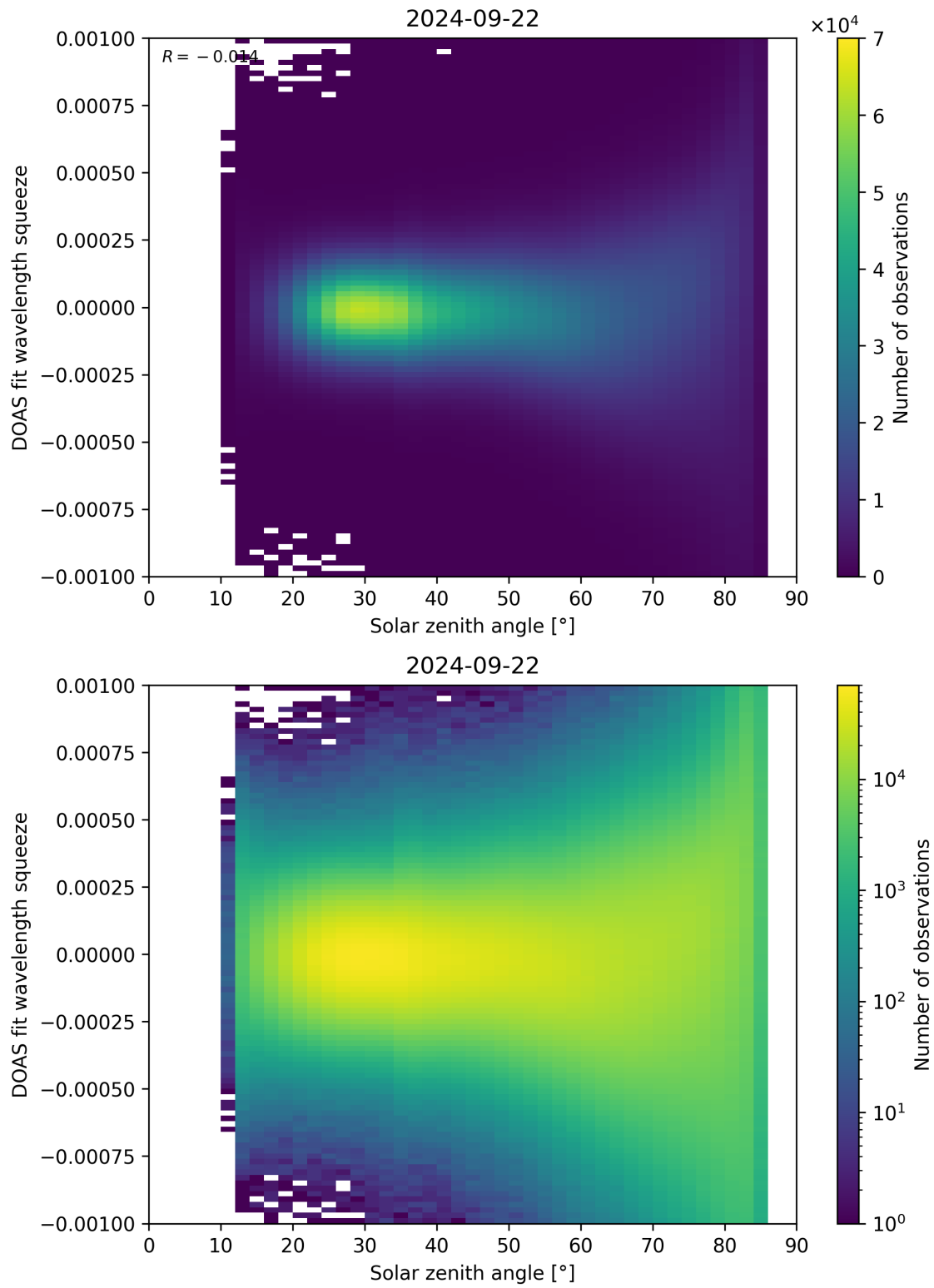
Figure 162: Scatter density plot of “Solar zenith angle” against “DOAS fit wavelength squeeze” for 2024-09-22 to 2024-09-23.
