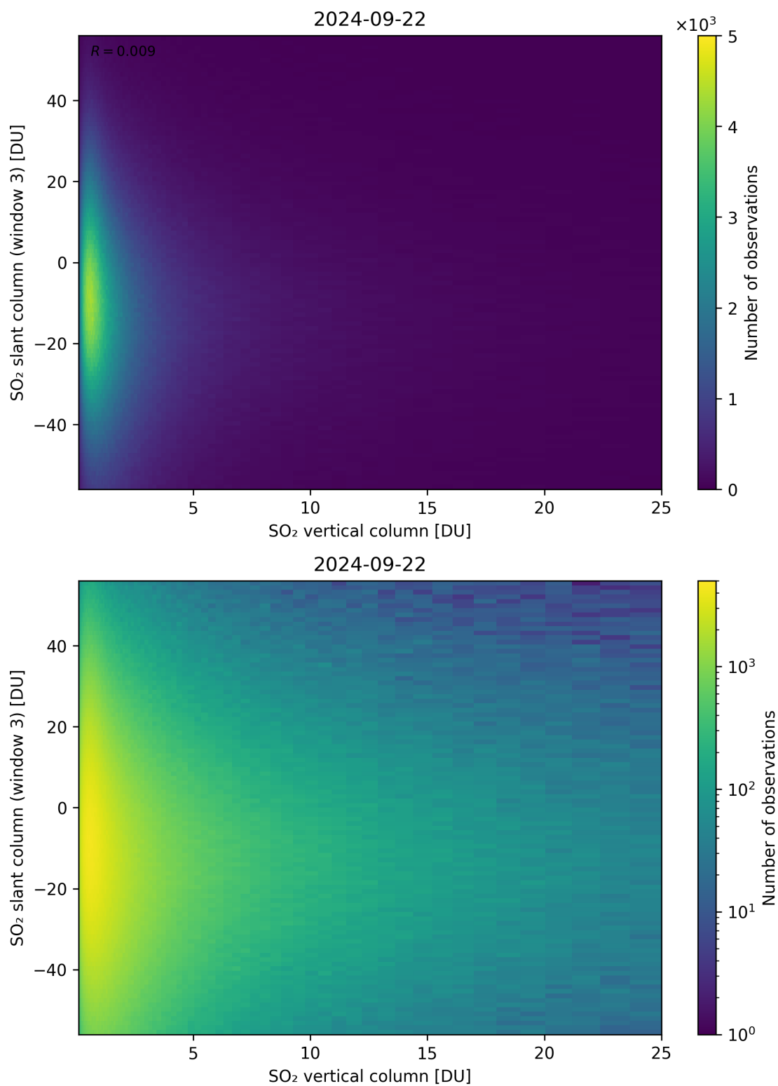
Figure 303: Scatter density plot of “SO 2 vertical column” against “SO 2 slant column (window 3)” for 2024-09-22 to 2024-09-23.
