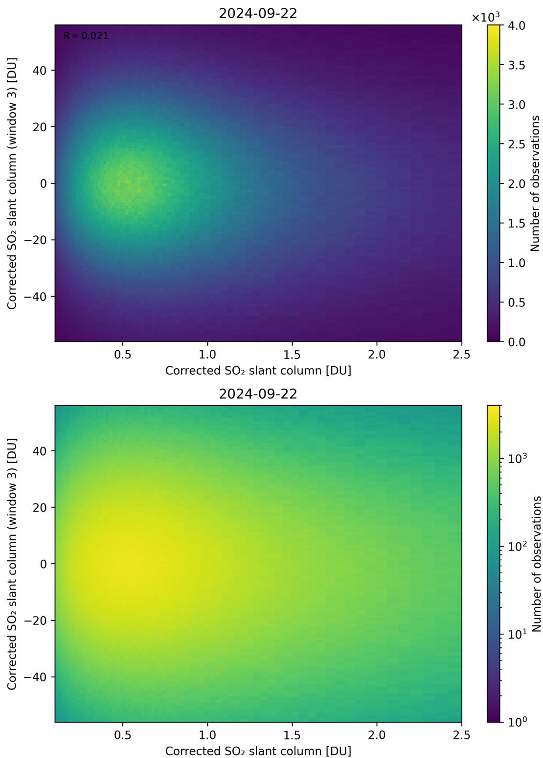
Figure 186: Scatter density plot of “Corrected SO 2 slant column” against “Corrected SO 2 slant column (window 3)” for 2024-09-22 to 2024-09-23.
