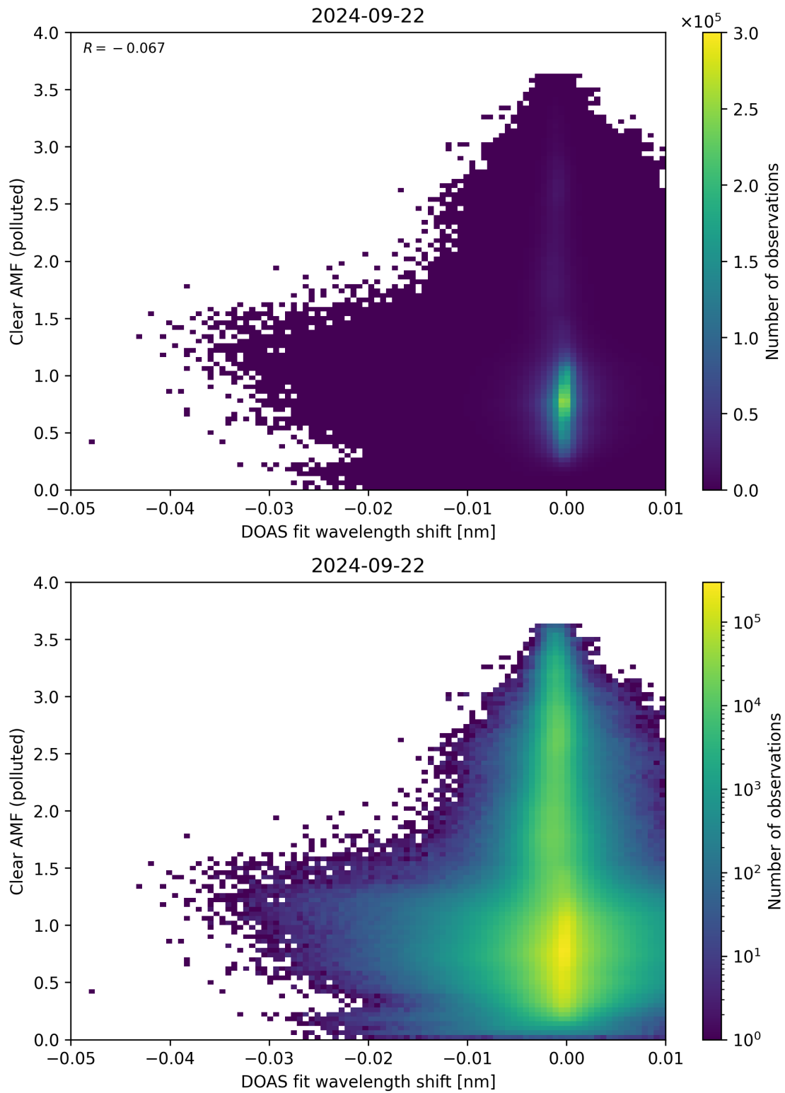
Figure 129: Scatter density plot of “DOAS fit wavelength shift” against “Clear AMF (polluted)” for 2024-09-22 to 2024-09-23.
