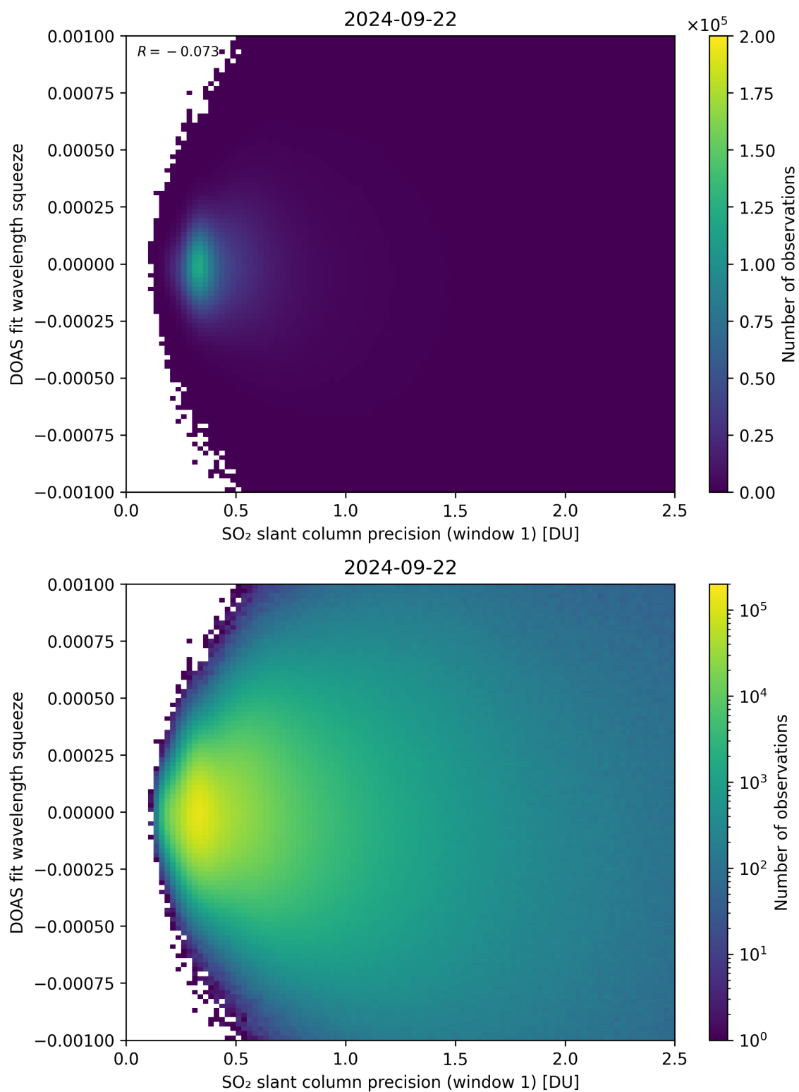
Figure 222: Scatter density plot of “SO 2 slant column precision (window 1)” against “DOAS fit wavelength squeeze” for 2024-09-22 to 2024-09-23.
