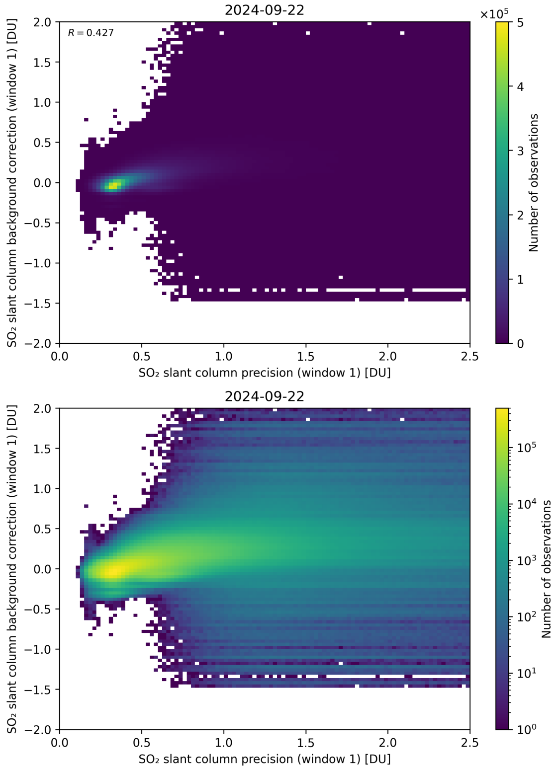
Figure 218: Scatter density plot of “SO 2 slant column precision (window 1)” against “SO 2 slant column background correction (window 1)” for 2024-09-22 to 2024-09-23.
