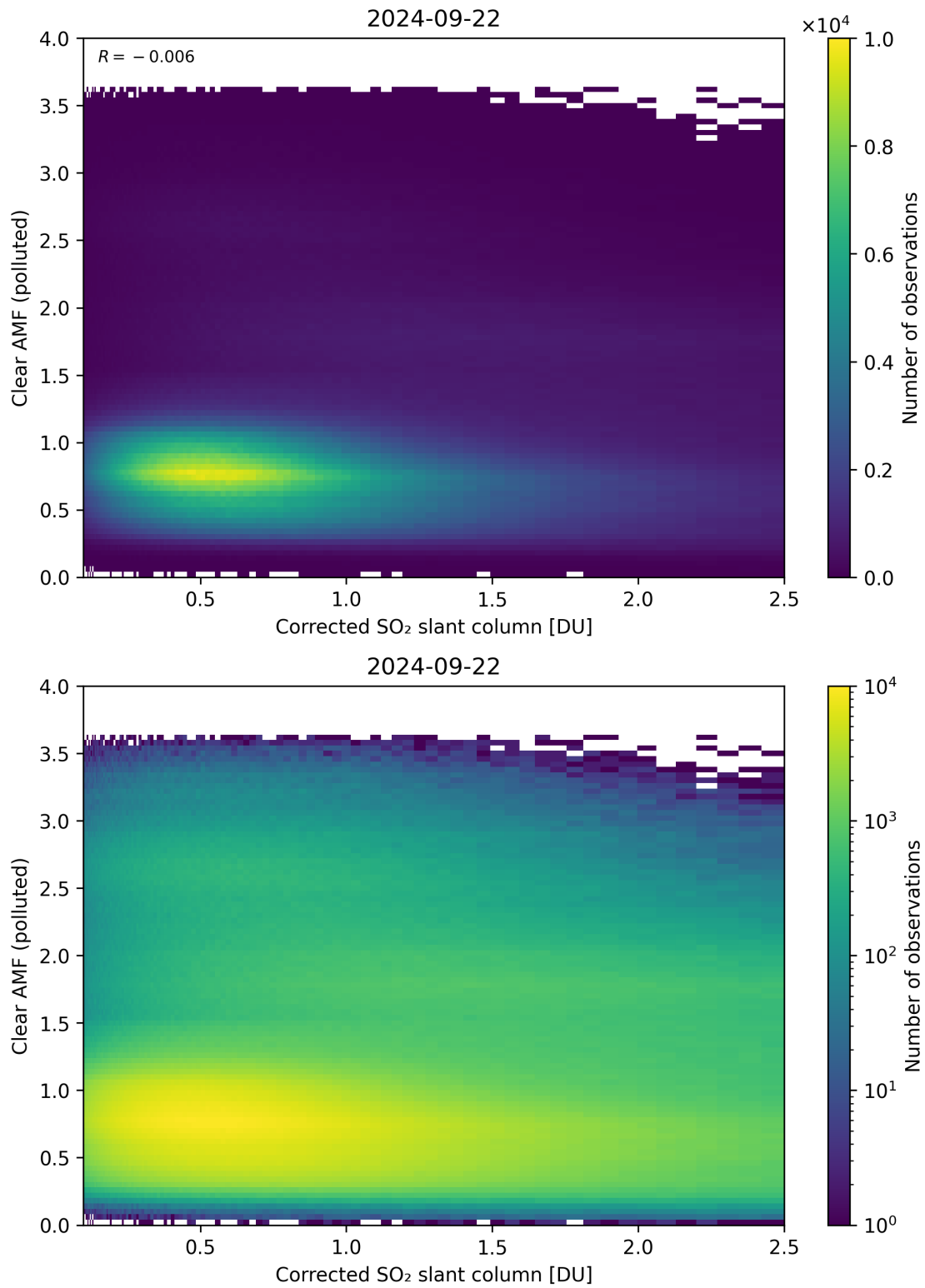
Figure 184: Scatter density plot of “Corrected SO 2 slant column” against “Clear AMF (polluted)” for 2024-09-22 to 2024-09-23.
