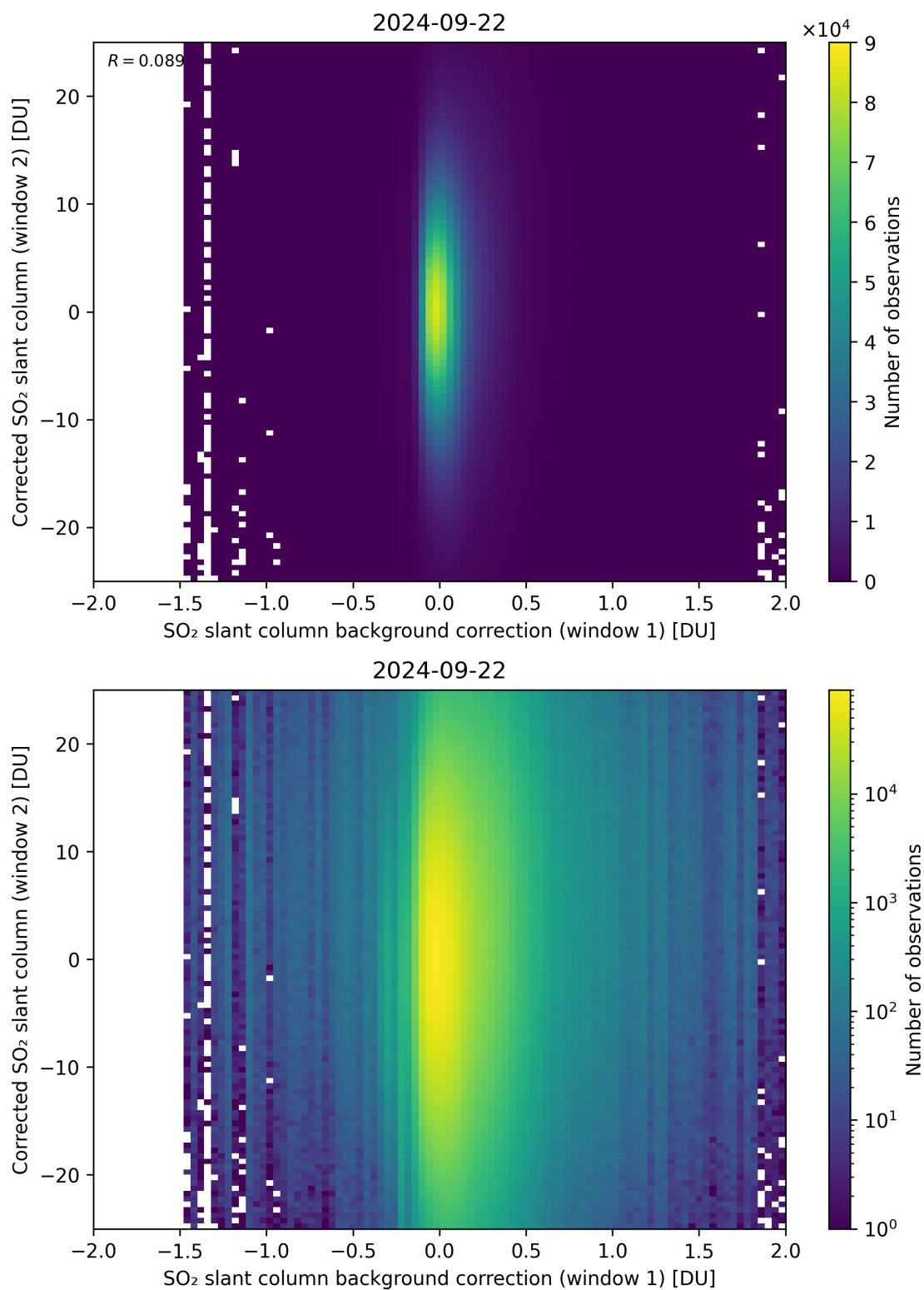
Figure 104: Scatter density plot of “SO 2 slant column background correction (window 1)” against “Corrected SO 2 slant column (window 2)” for 2024-09-22 to 2024-09-23.
