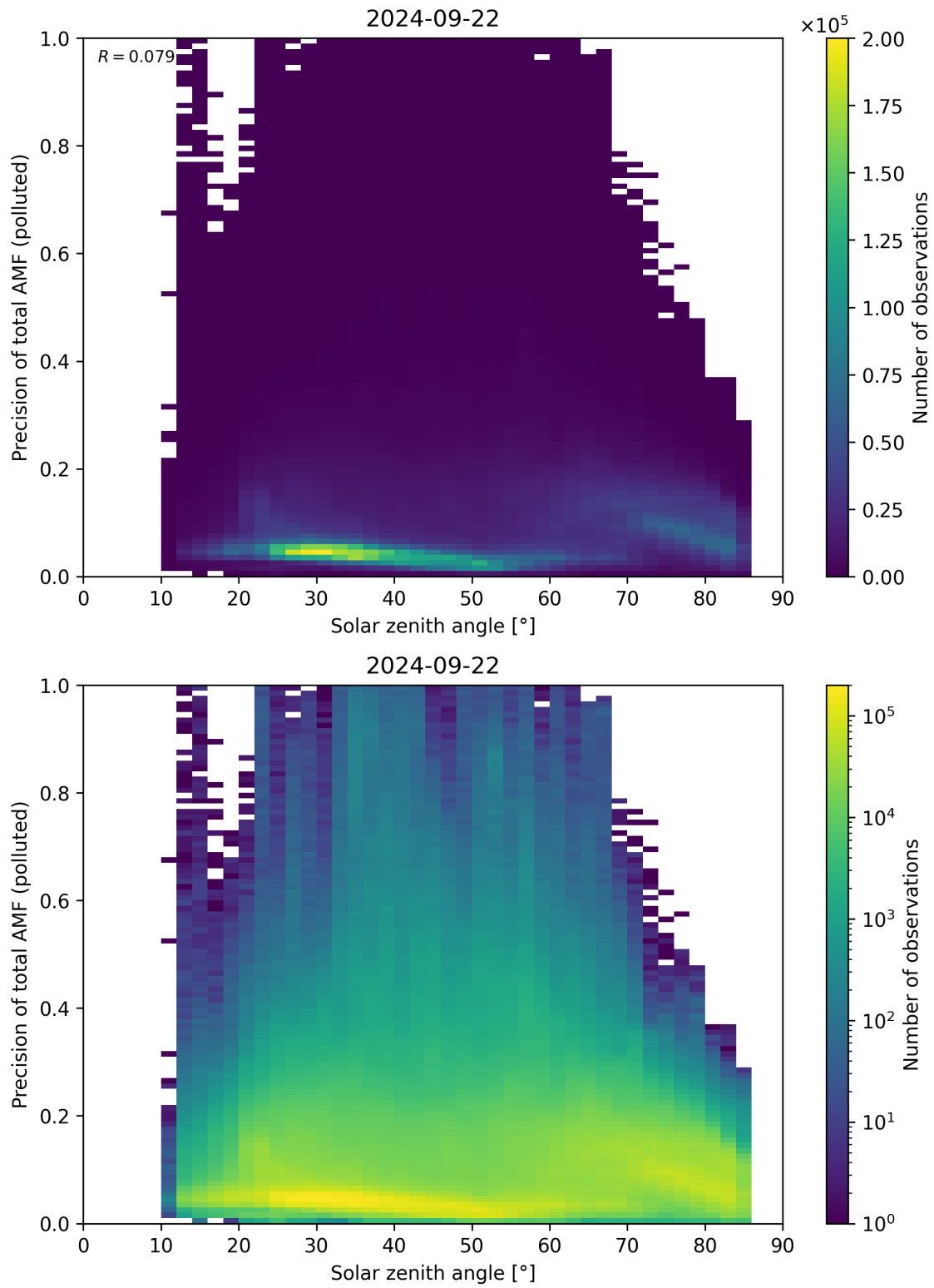
Figure 175: Scatter density plot of “Solar zenith angle” against “Precision of total AMF (polluted)” for 2024-09-22 to 2024-09-23.
