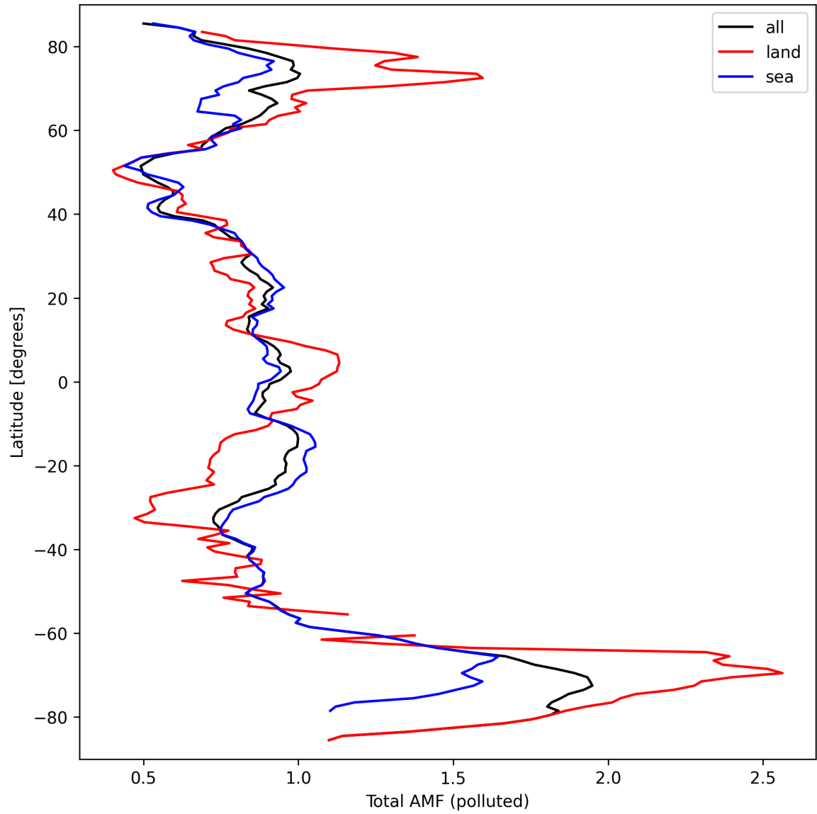
Figure 48: Zonal average of “Total AMF (polluted)” for 2024-09-22 to 2024-09-23.
