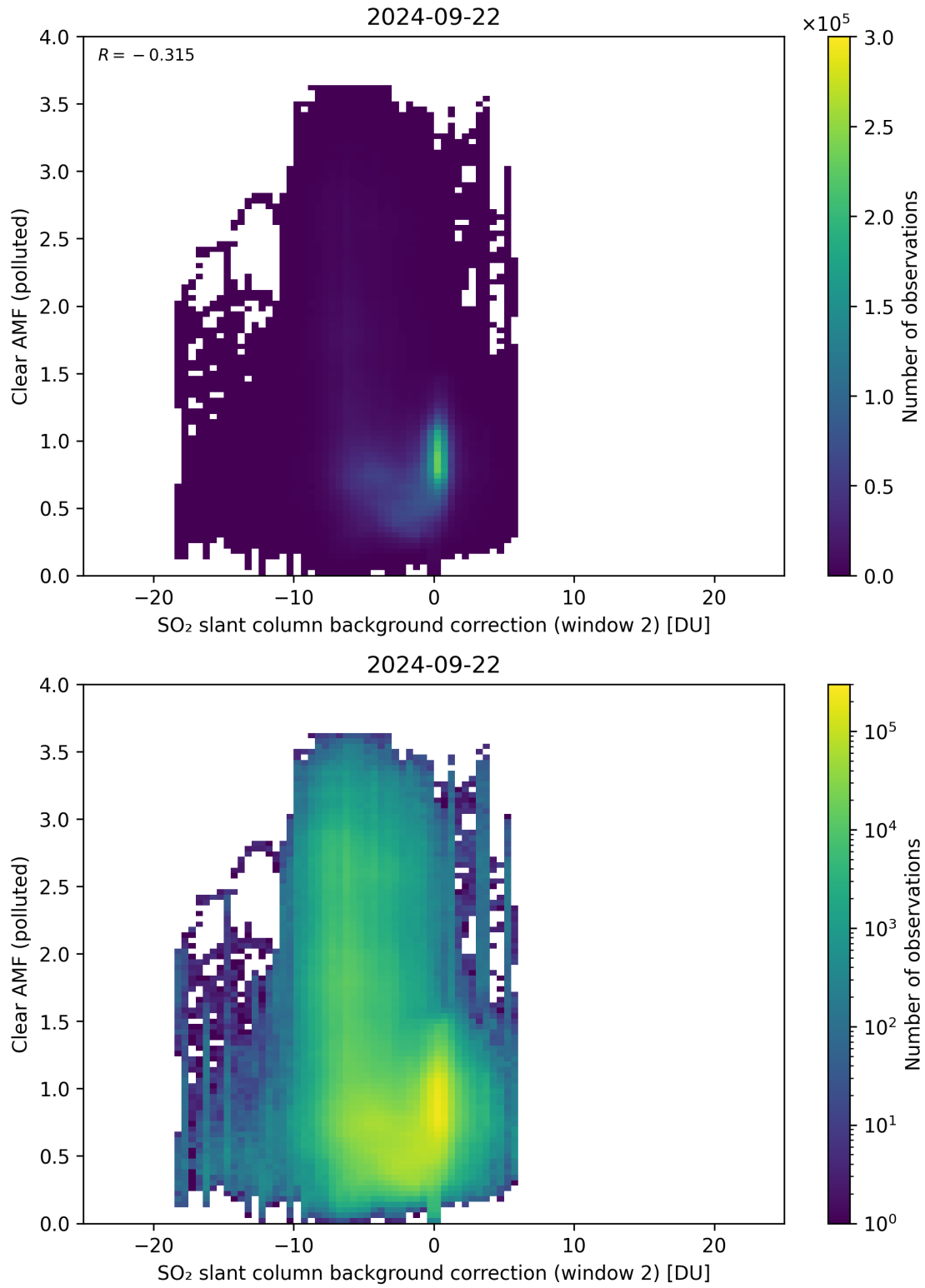
Figure 115: Scatter density plot of “SO 2 slant column background correction (window 2)” against “Clear AMF (polluted)” for 2024-09-22 to 2024-09-23.
