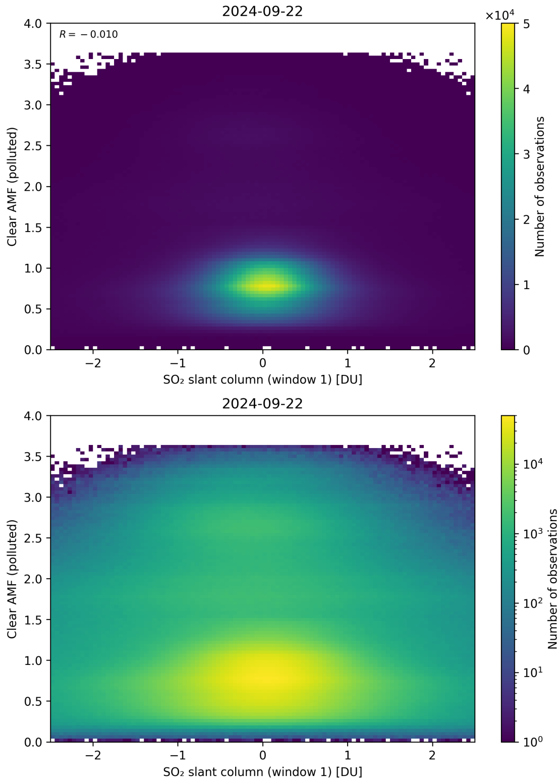
Figure 232: Scatter density plot of “SO 2 slant column (window 1)” against “Clear AMF (polluted)” for 2024-09-22 to 2024-09-23.
