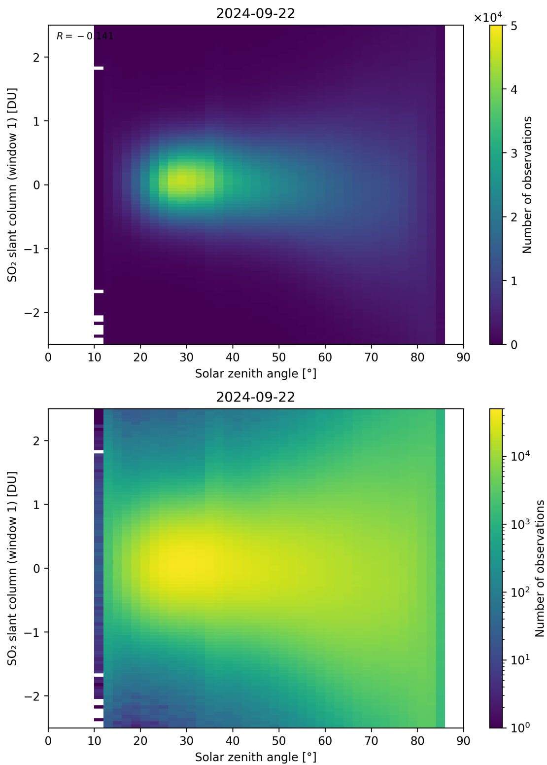
Figure 169: Scatter density plot of “Solar zenith angle” against “SO 2 slant column (window 1)” for 2024-09-22 to 2024-09-23.
