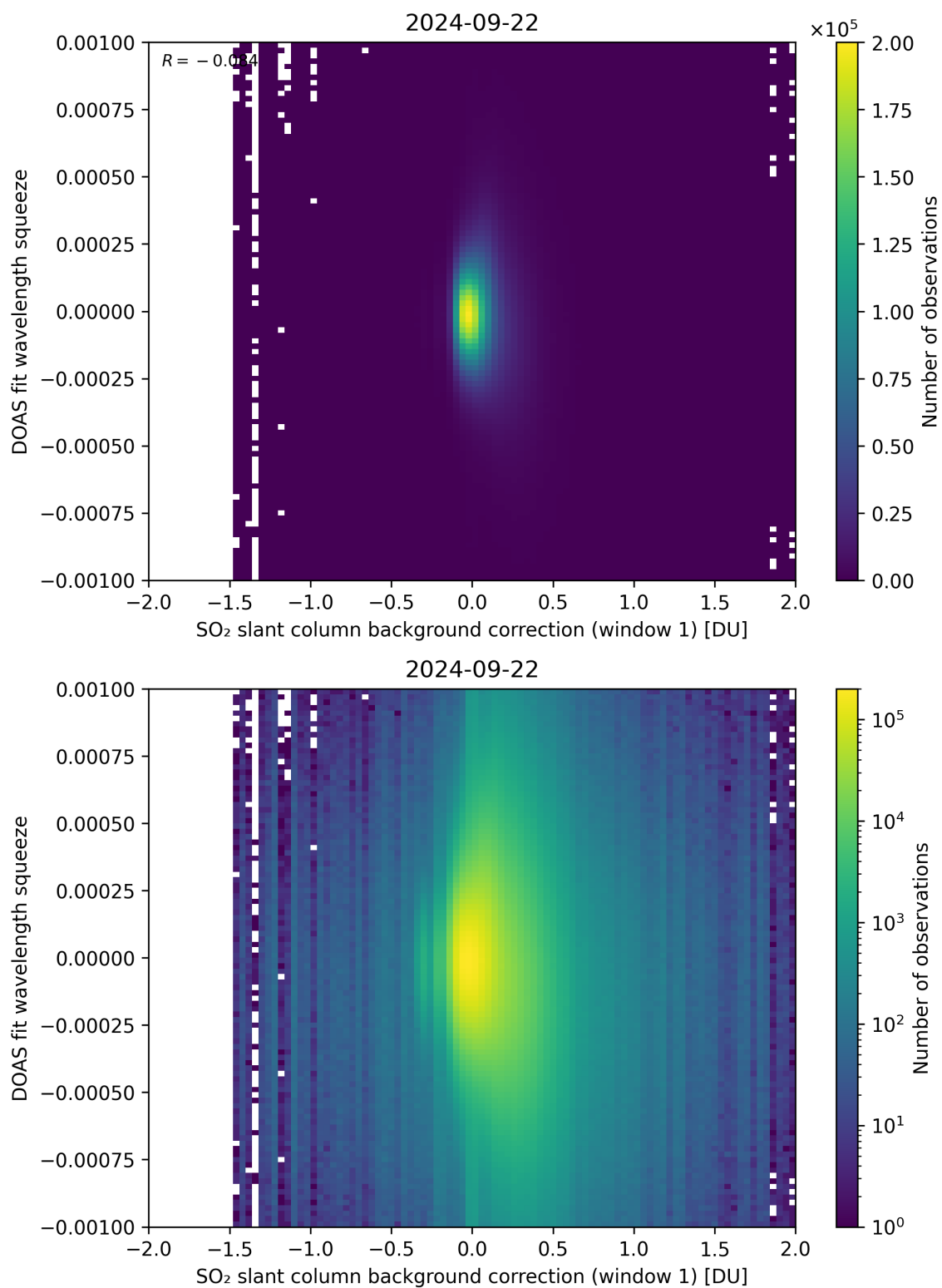
Figure 101: Scatter density plot of “SO 2 slant column background correction (window 1)” against “DOAS fit wavelength squeeze” for 2024-09-22 to 2024-09-23.
