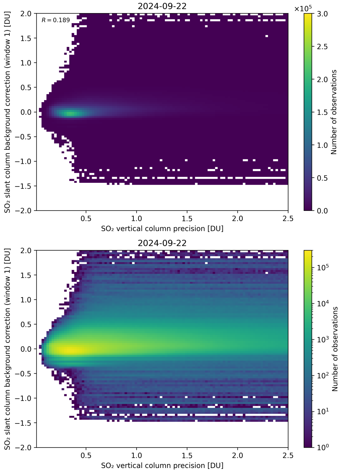
Figure 279: Scatter density plot of “SO 2 vertical column precision” against “SO 2 slant column background correction (window 1)” for 2024-09-22 to 2024-09-23.
