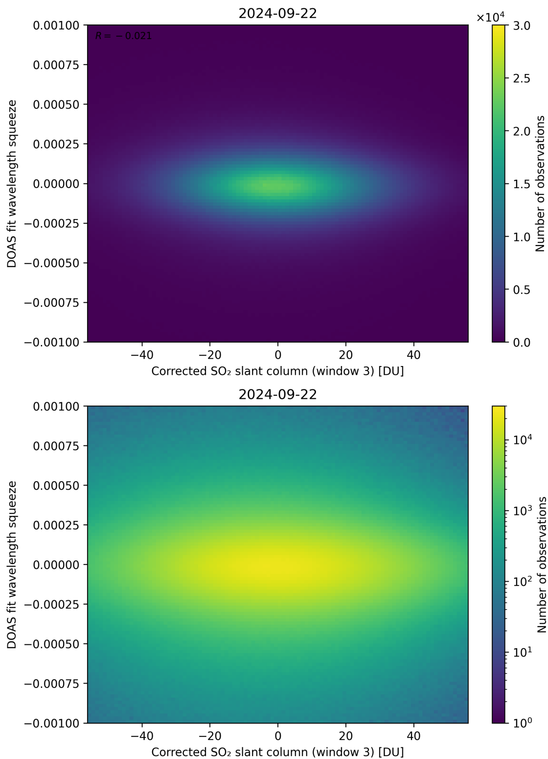
Figure 207: Scatter density plot of “Corrected SO 2 slant column (window 3)” against “DOAS fit wavelength squeeze” for 2024-09-22 to 2024-09-23.
