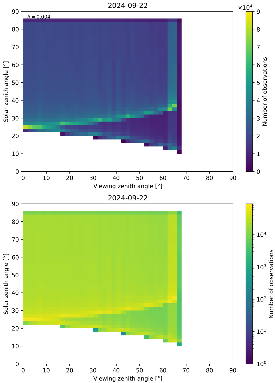
Figure 315: Scatter density plot of “Viewing zenith angle” against “Solar zenith angle” for 2024-09-22 to 2024-09-23.
