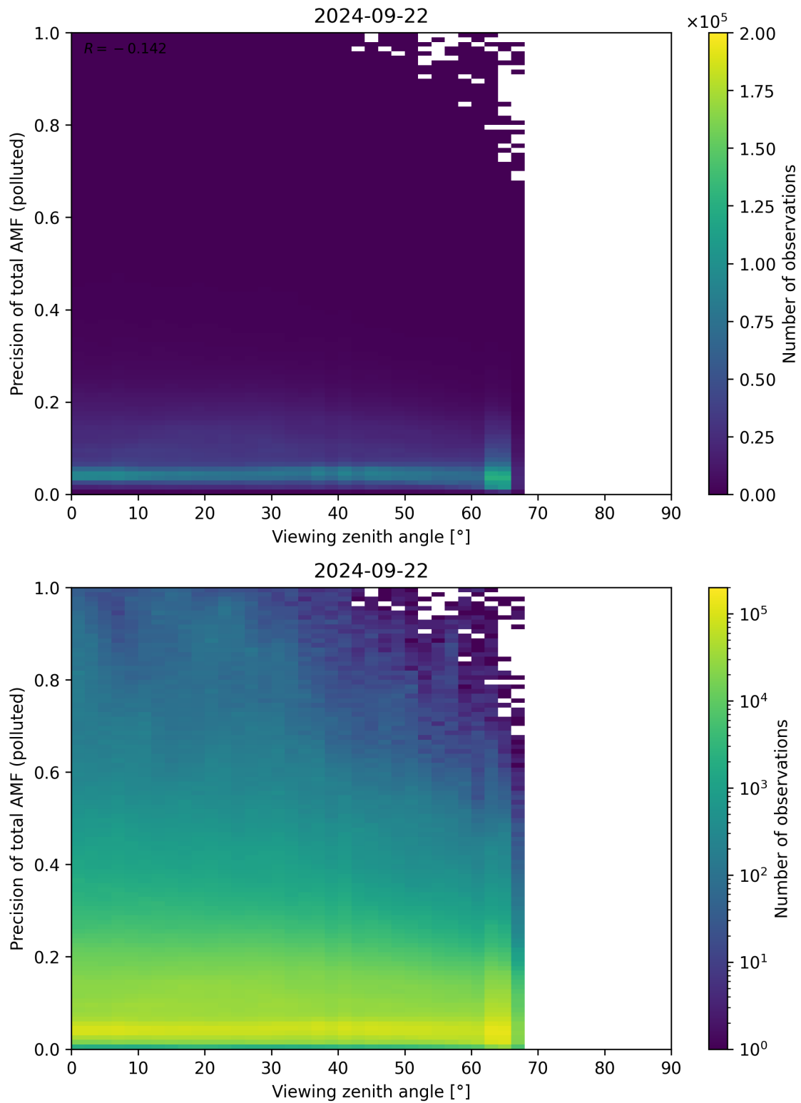
Figure 326: Scatter density plot of “Viewing zenith angle” against “Precision of total AMF (polluted)” for 2024-09-22 to 2024-09-23.
