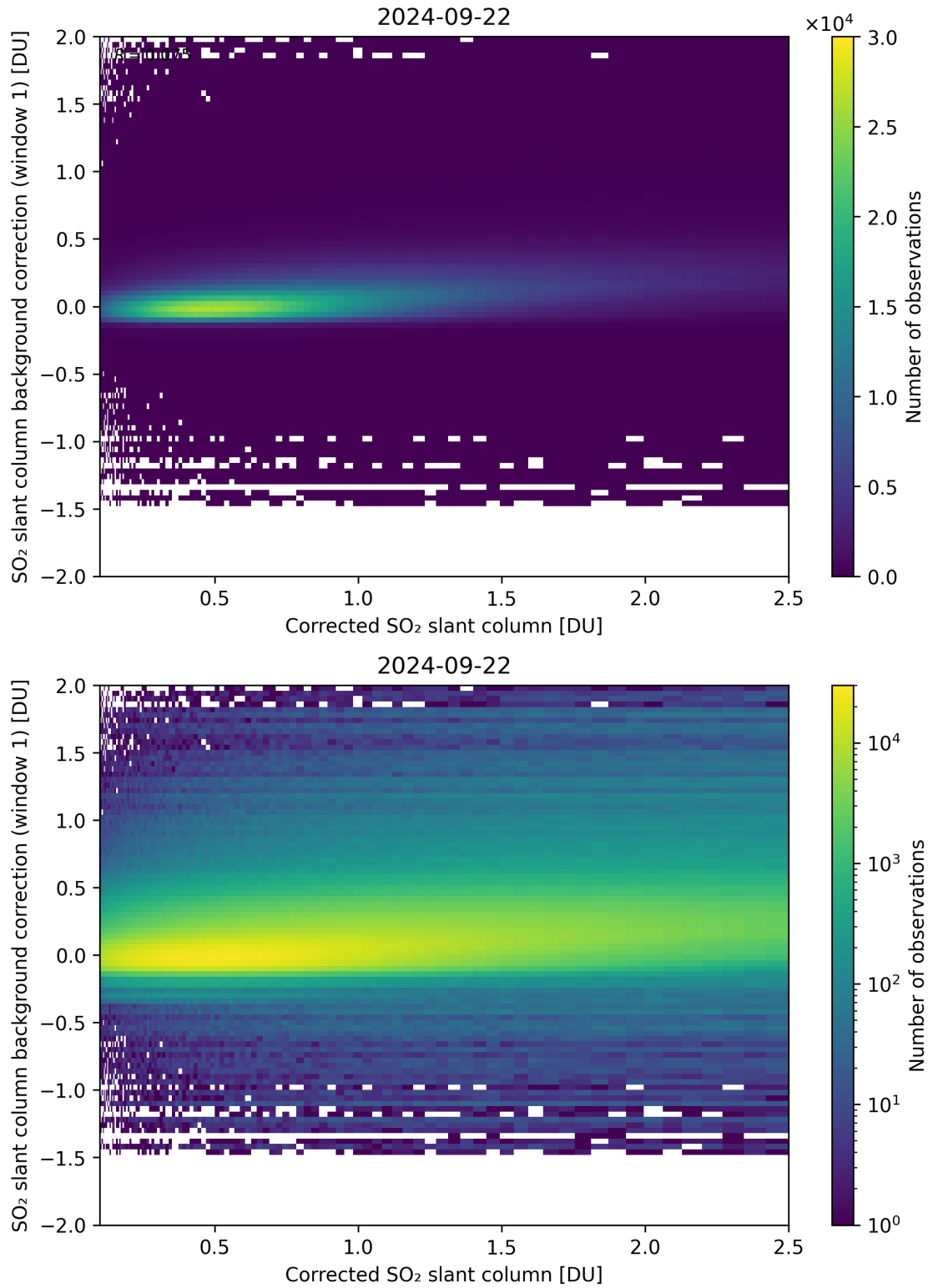
Figure 178: Scatter density plot of “Corrected SO 2 slant column” against “SO 2 slant column background correction (window 1)” for 2024-09-22 to 2024-09-23.
