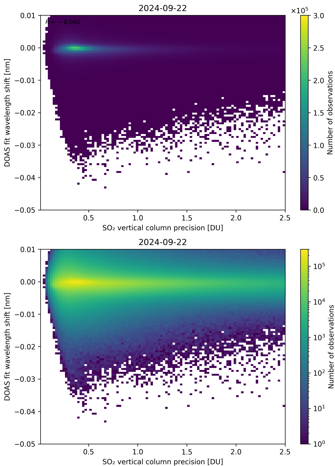
Figure 282: Scatter density plot of “SO 2 vertical column precision” against “DOAS fit wavelength shift” for 2024-09-22 to 2024-09-23.
