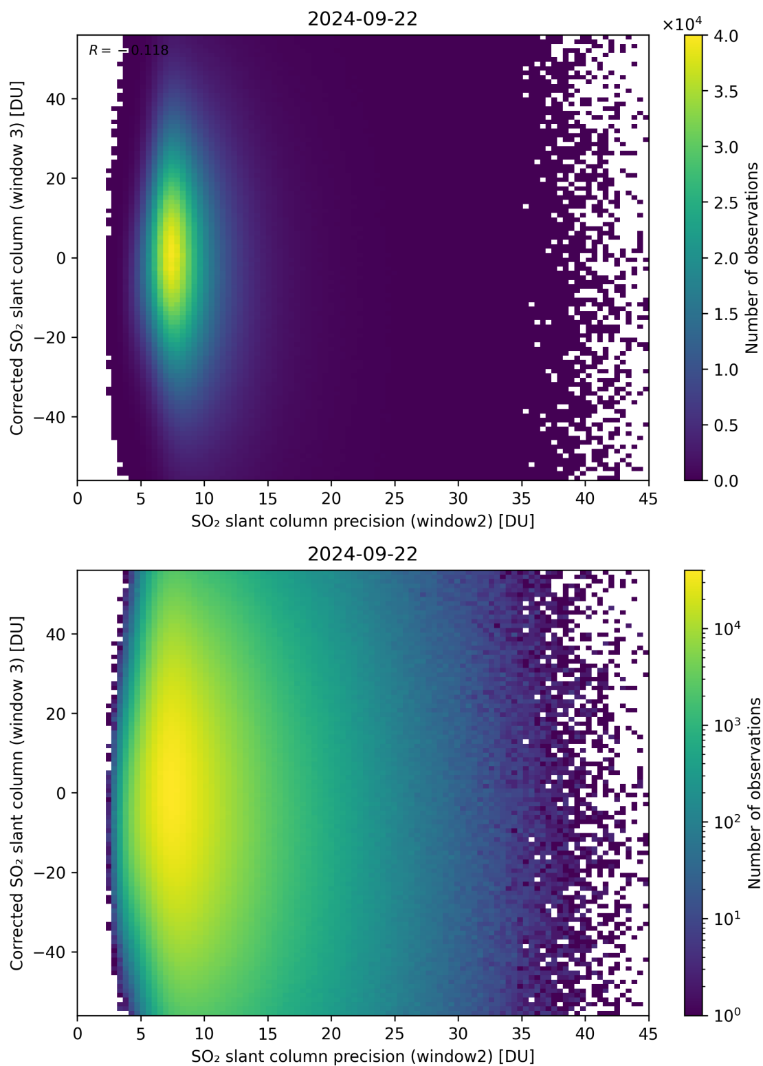
Figure 248: Scatter density plot of “SO 2 slant column precision (window2)” against “Corrected SO 2 slant column (window 3)” for 2024-09-22 to 2024-09-23.
