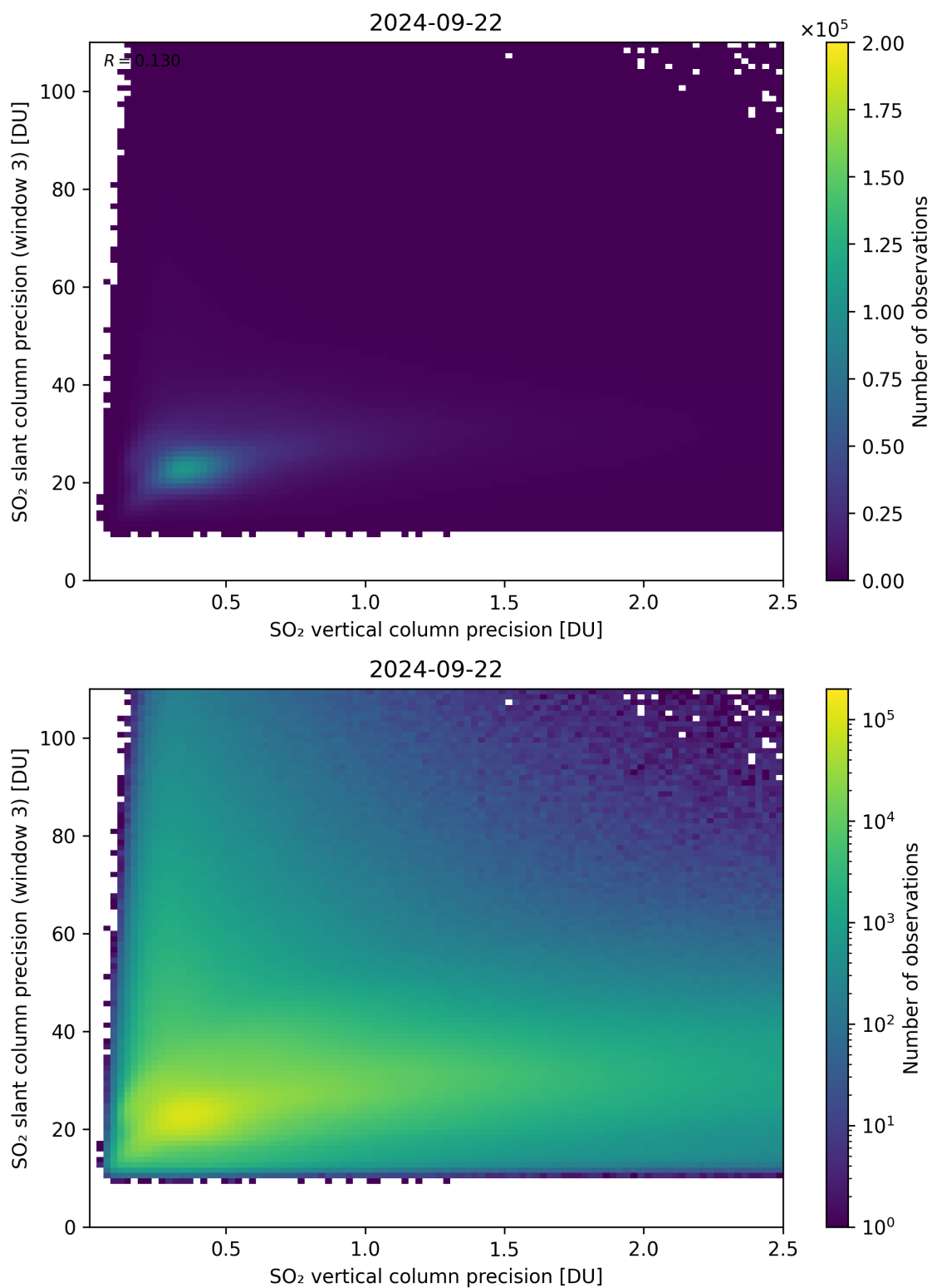
Figure 293: Scatter density plot of “SO 2 vertical column precision” against “SO 2 slant column precision (window 3)” for 2024-09-22 to 2024-09-23.
