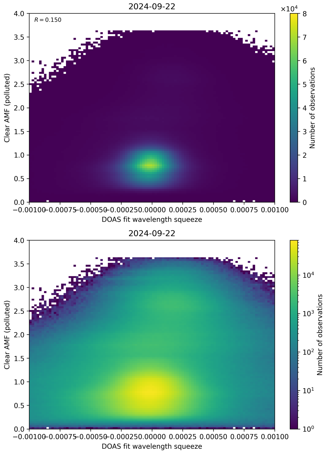
Figure 133: Scatter density plot of “DOAS fit wavelength squeeze” against “Clear AMF (polluted)” for 2024-09-22 to 2024-09-23.
