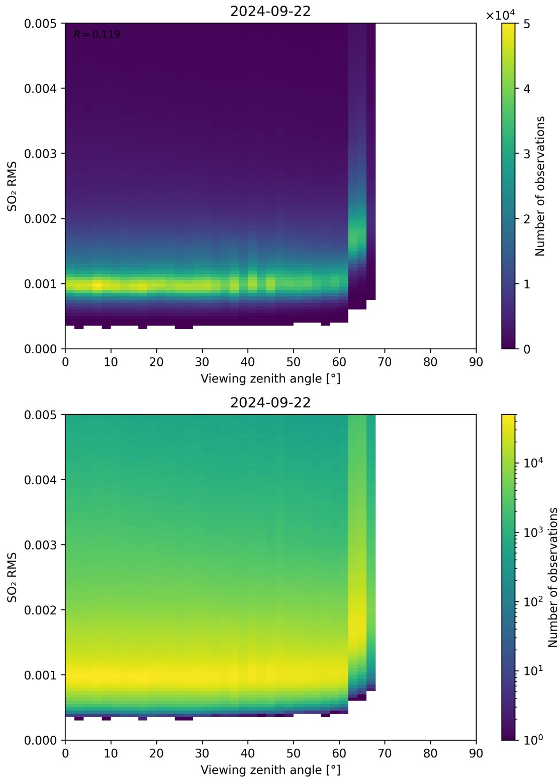
Figure 313: Scatter density plot of “Viewing zenith angle” against “SO 2 RMS” for 2024-09-22 to 2024-09-23.
