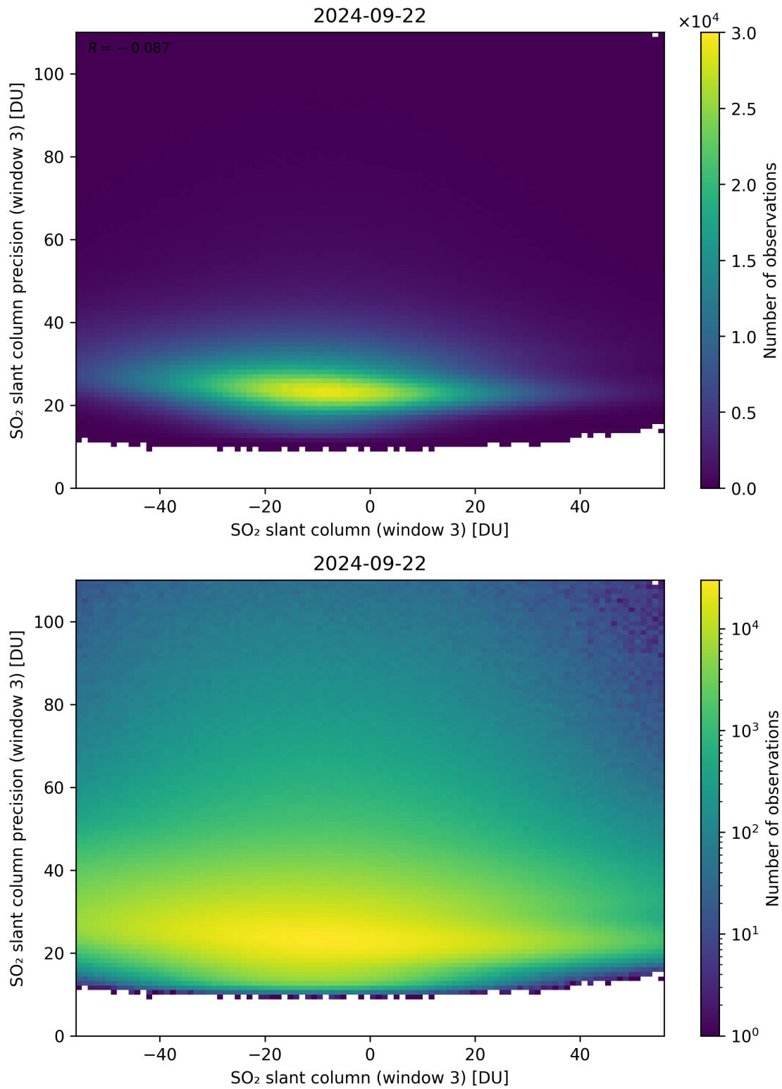
Figure 267: Scatter density plot of “SO 2 slant column (window 3)” against “SO 2 slant column precision (window 3)” for 2024-09-22 to 2024-09-23.
