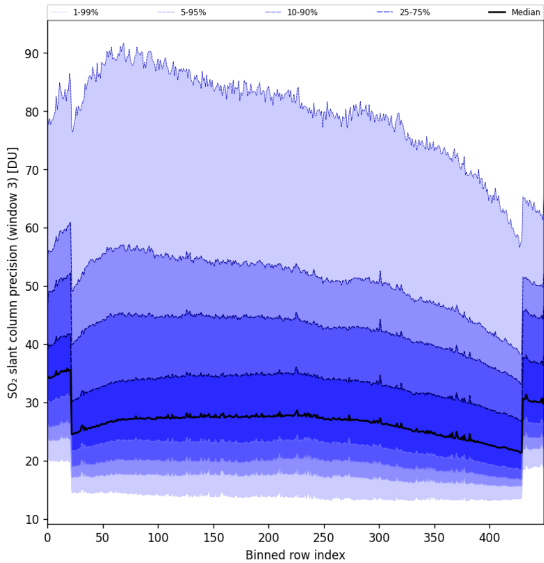
Figure 88: Along track statistics of “SO 2 slant column precision (window 3)” for 2024-09-22 to 2024-09-23
