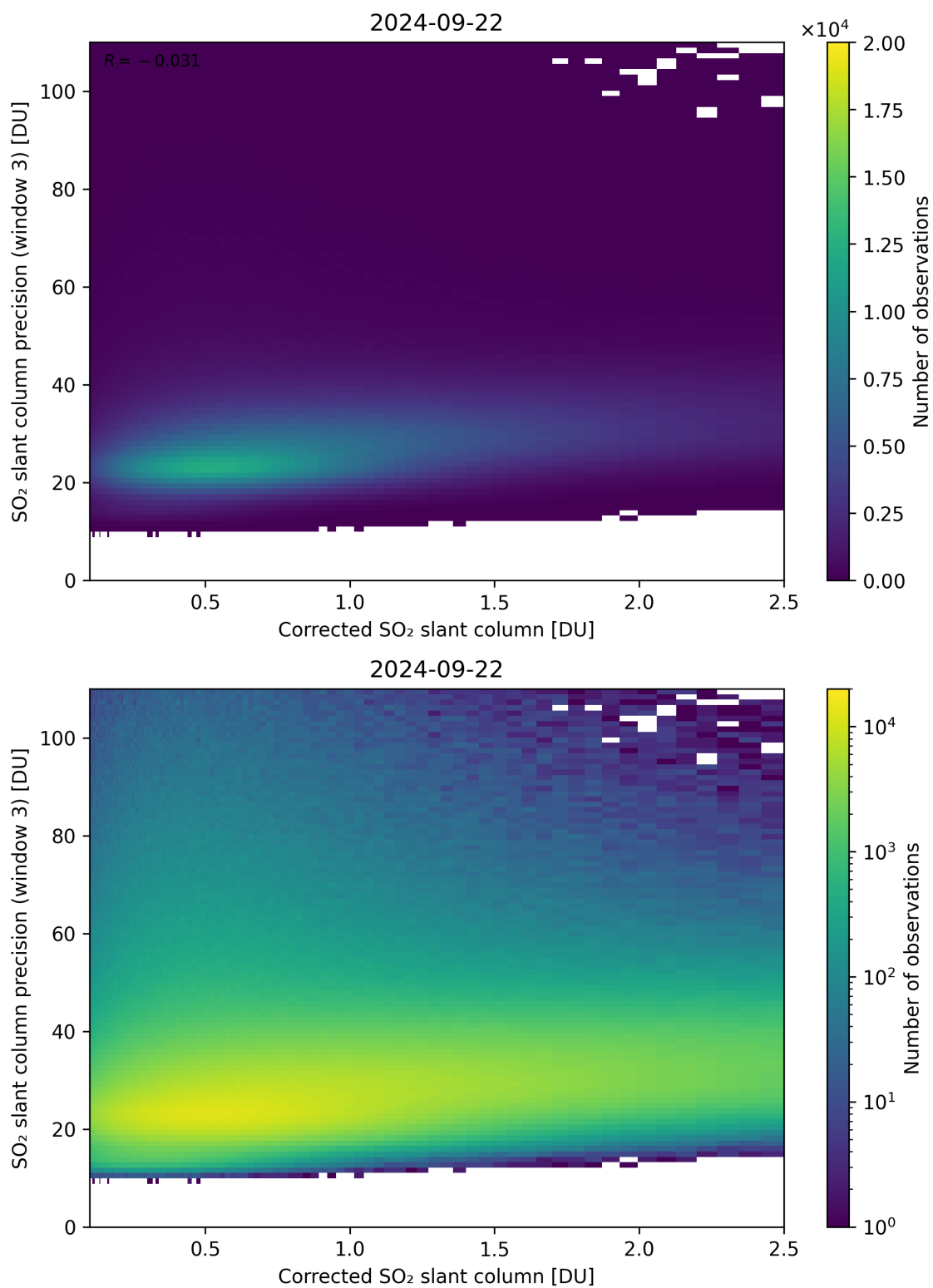
Figure 191: Scatter density plot of “Corrected SO 2 slant column” against “SO 2 slant column precision (window 3)” for 2024-09-22 to 2024-09-23.
