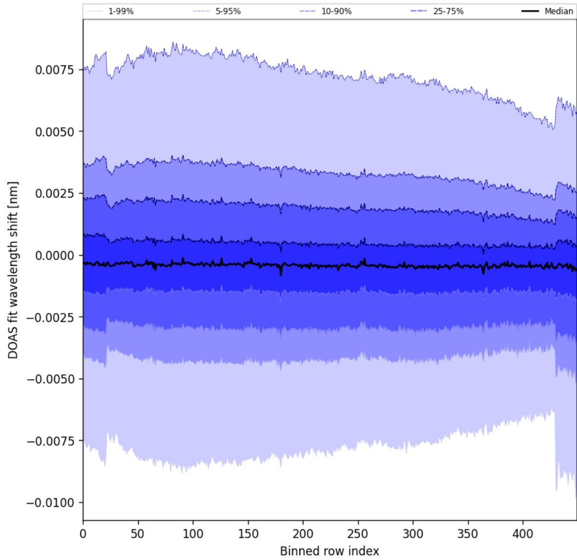
Figure 91: Along track statistics of “DOAS fit wavelength shift” for 2024-09-22 to 2024-09-23
