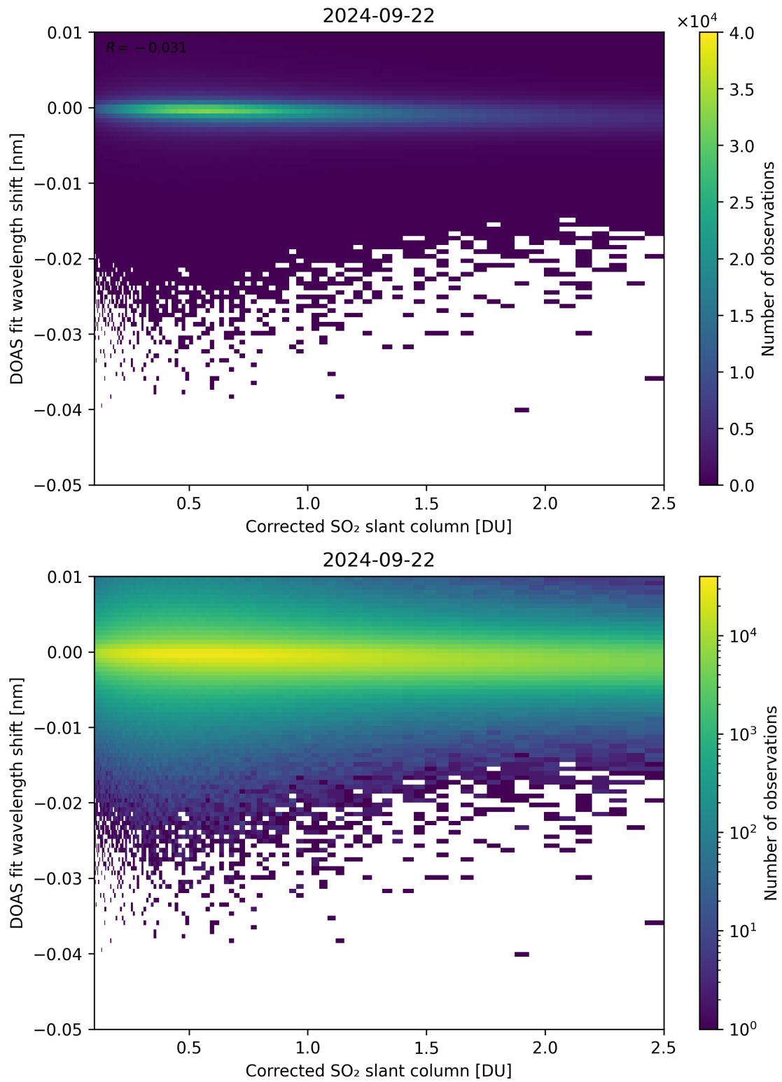
Figure 181: Scatter density plot of “Corrected SO 2 slant column” against “DOAS fit wavelength shift” for 2024-09-22 to 2024-09-23.
