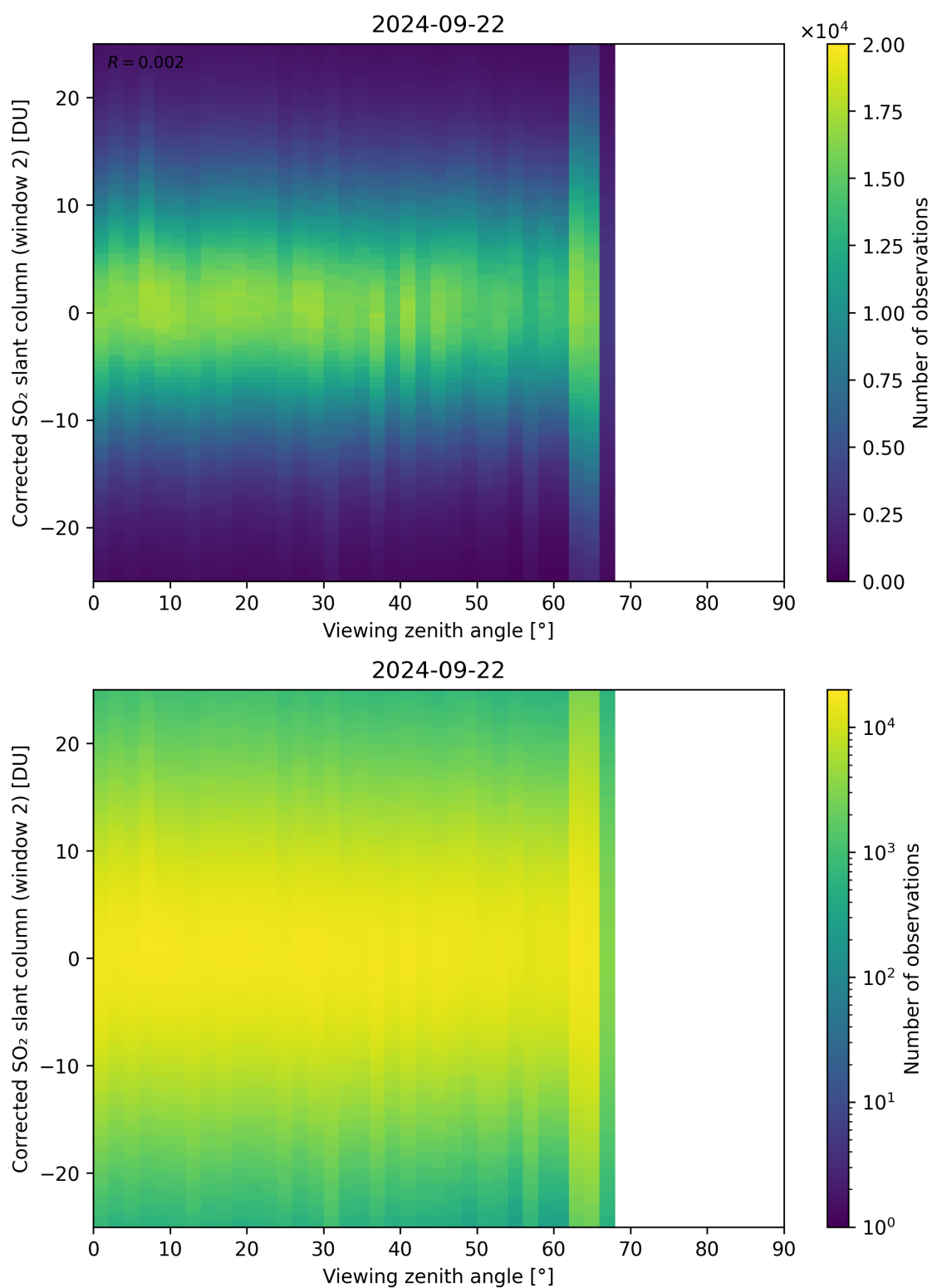
Figure 318: Scatter density plot of “Viewing zenith angle” against “Corrected SO 2 slant column (window 2)” for 2024-09-22 to 2024-09-23.
