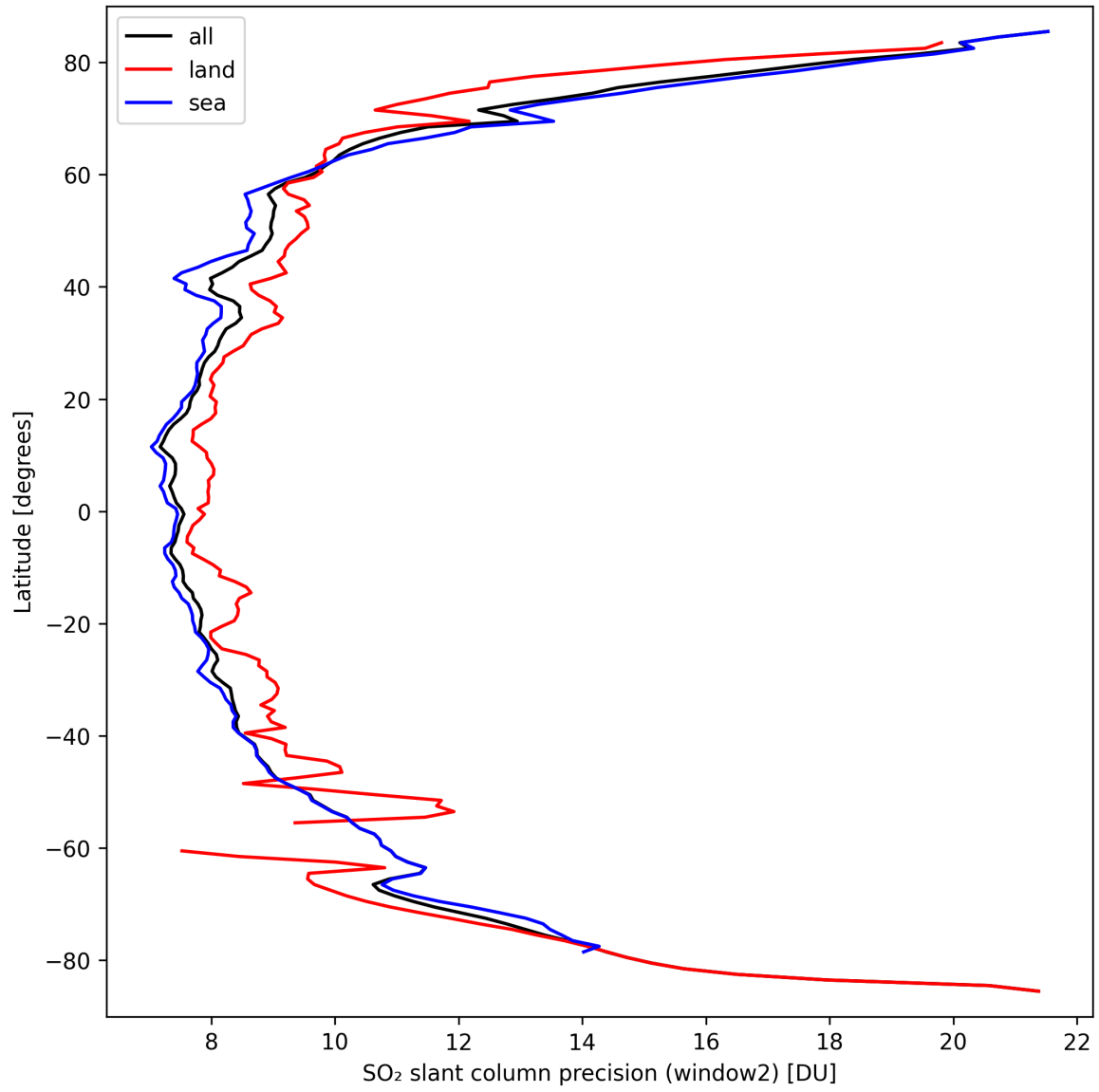
Figure 38: Zonal average of “SO 2 slant column precision (window2)” for 2024-09-22 to 2024-09-23.
