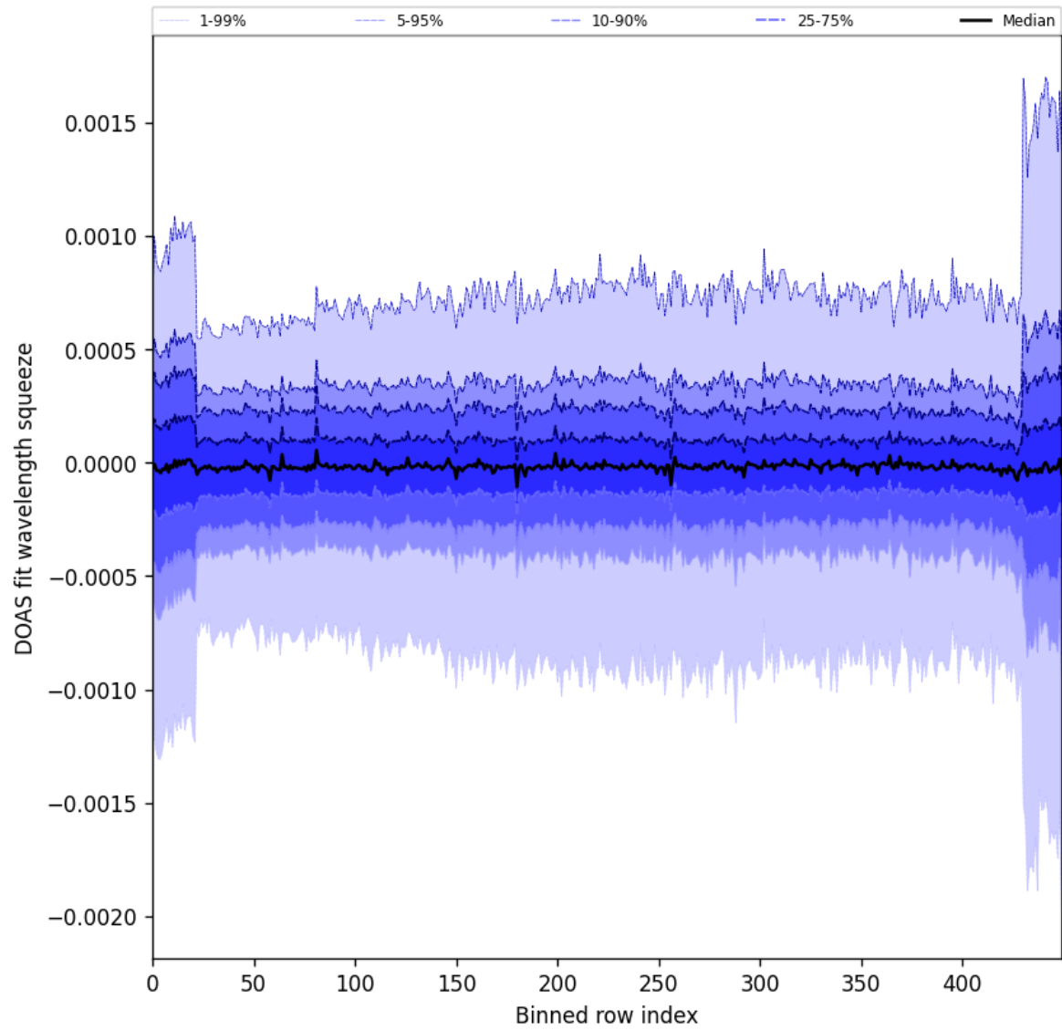
Figure 92: Along track statistics of “DOAS fit wavelength squeeze” for 2024-09-22 to 2024-09-23
