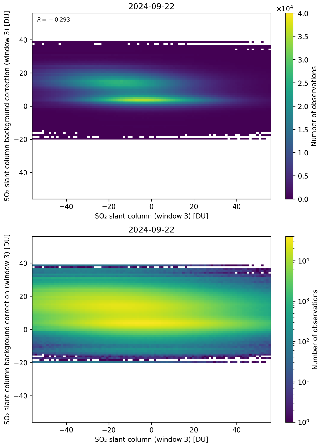
Figure 253: Scatter density plot of “SO 2 slant column (window 3)” against “SO 2 slant column background correction (window 3)” for 2024-09-22 to 2024-09-23.
