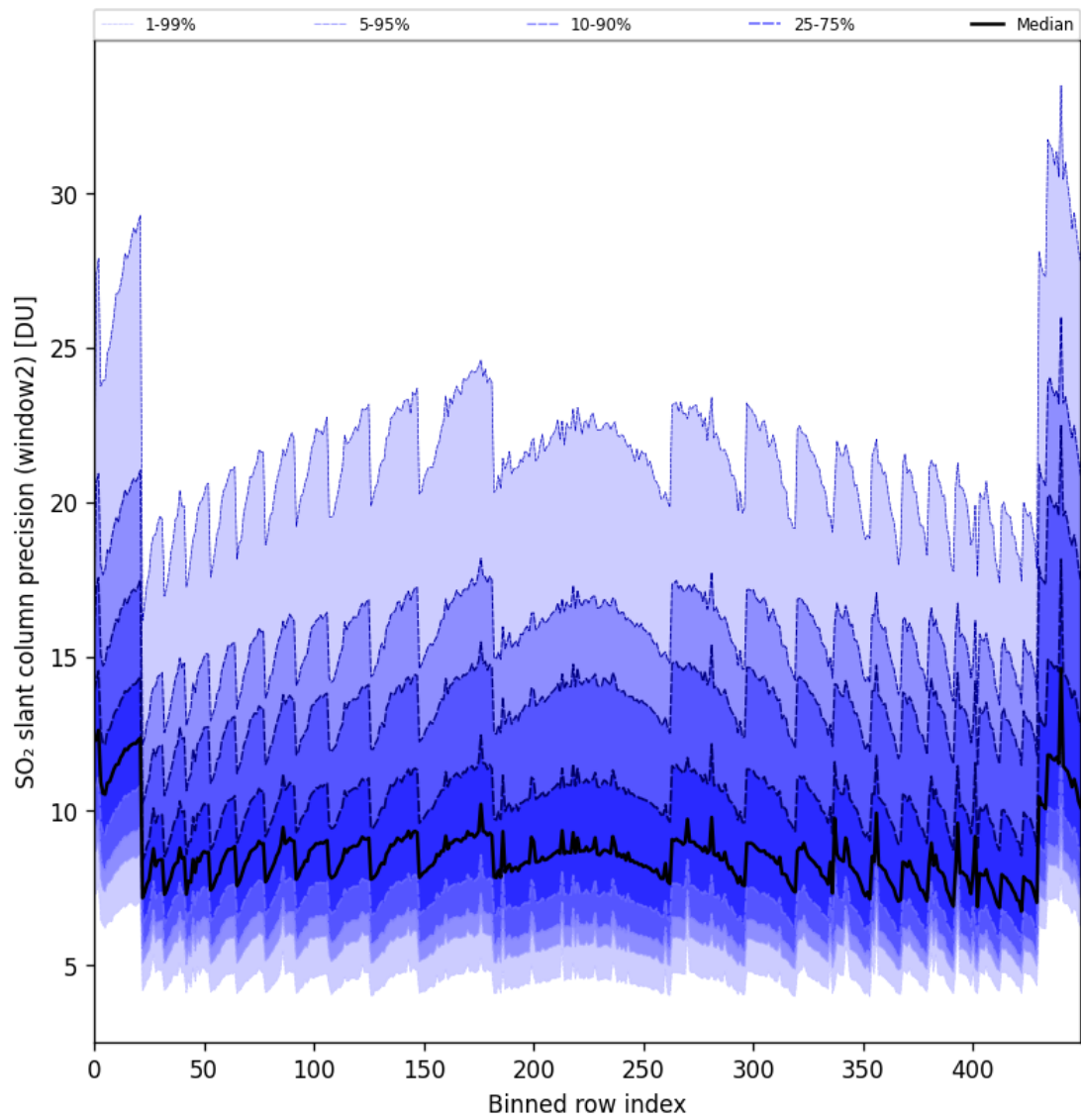
Figure 84: Along track statistics of “SO 2 slant column precision (window2)” for 2024-09-22 to 2024-09-23
