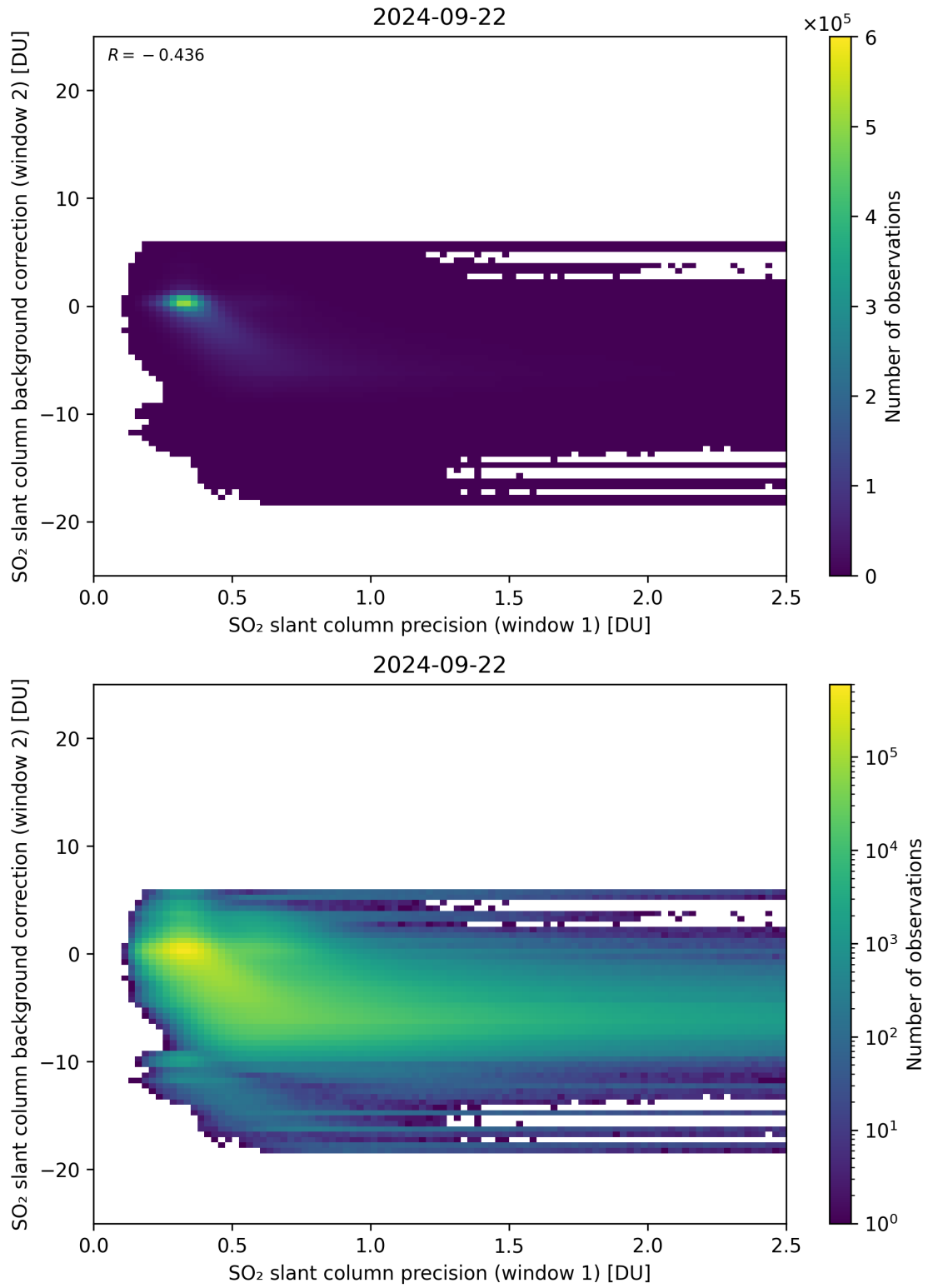
Figure 219: Scatter density plot of “SO 2 slant column precision (window 1)” against “SO 2 slant column background correction (window 2)” for 2024-09-22 to 2024-09-23.
