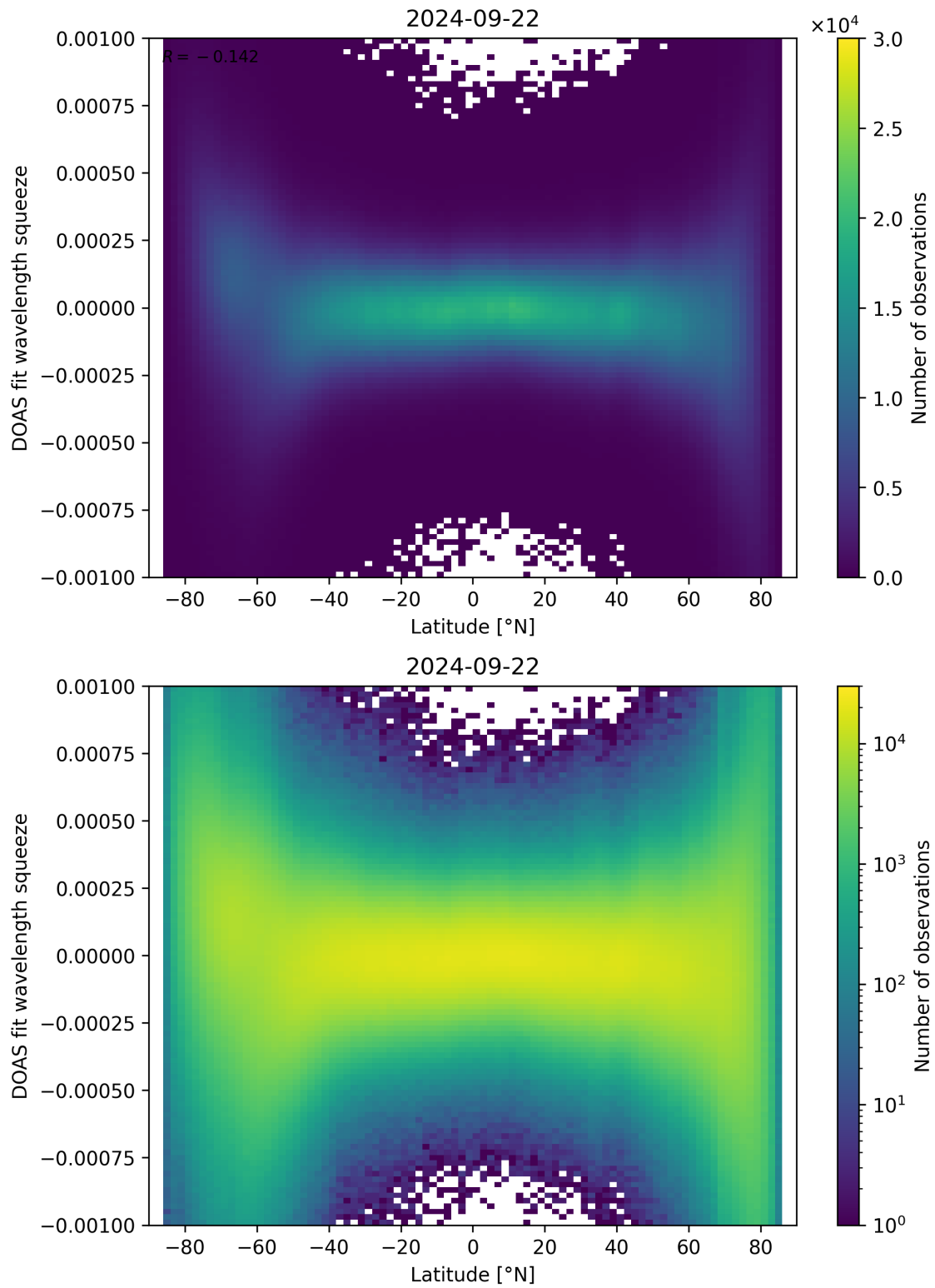
Figure 143: Scatter density plot of “Latitude” against “DOAS fit wavelength squeeze” for 2024-09-22 to 2024-09-23.
