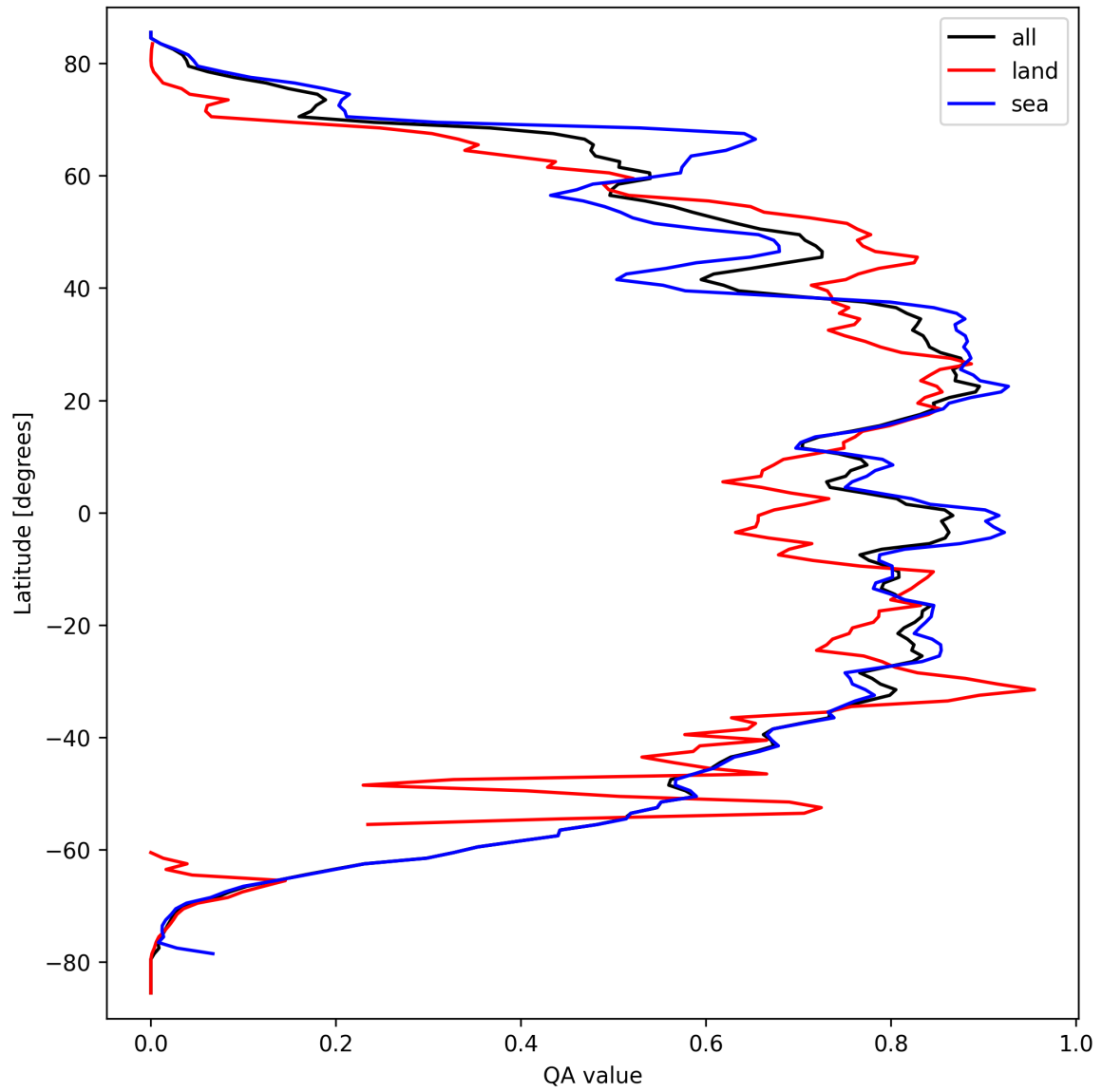
Figure 29: Zonal average of “QA value” for 2024-09-22 to 2024-09-23.
