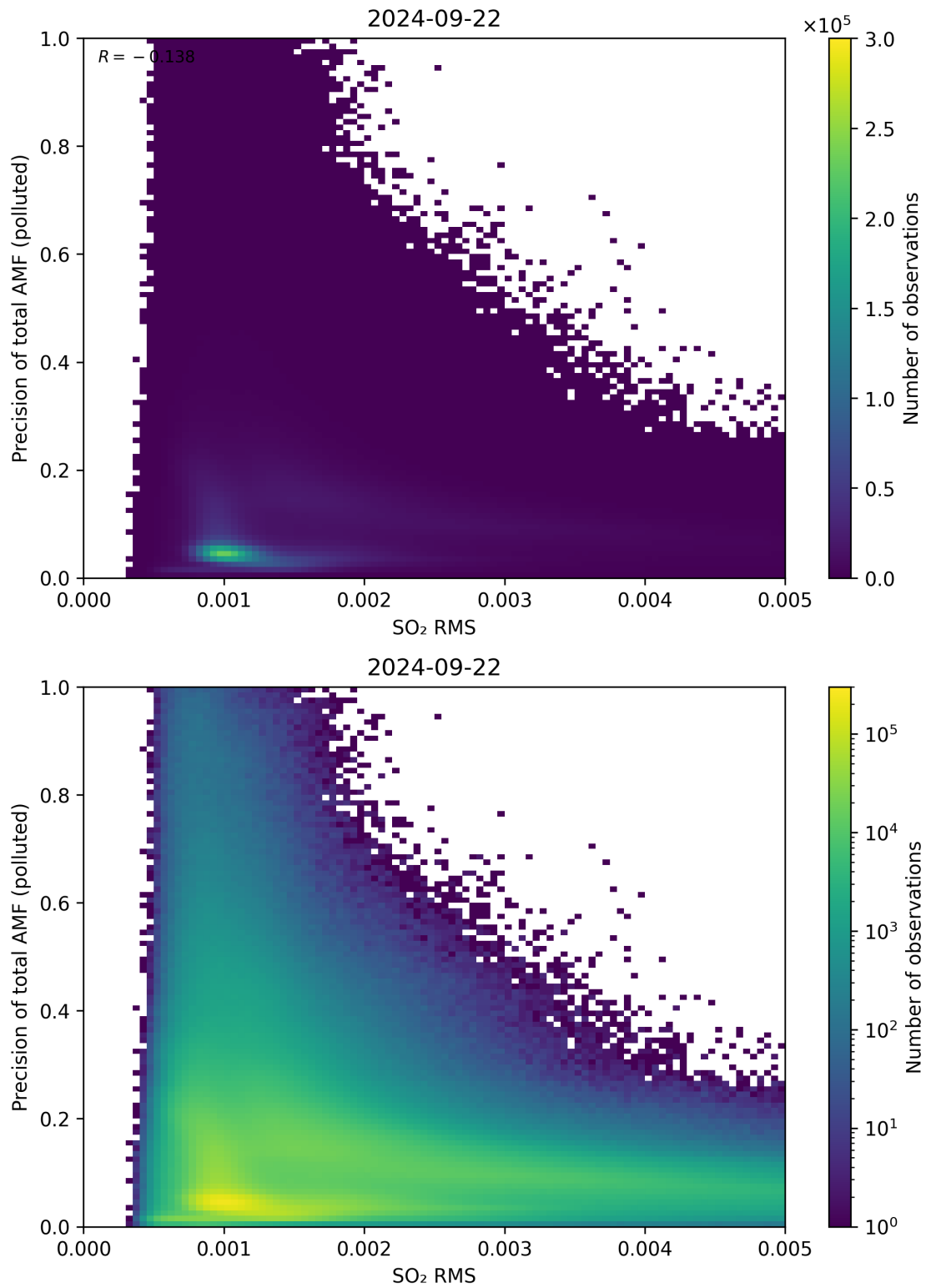
Figure 138: Scatter density plot of “SO 2 RMS” against “Precision of total AMF (polluted)” for 2024-09-22 to 2024-09-23.
