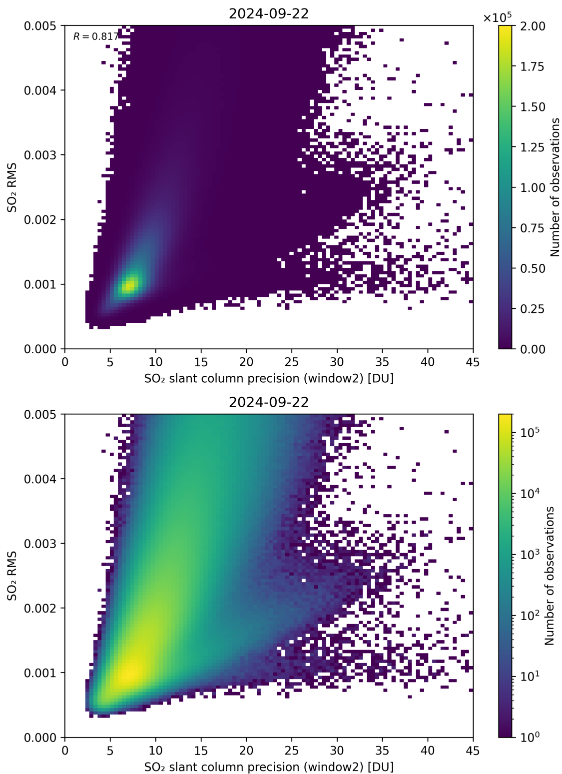
Figure 245: Scatter density plot of “SO 2 slant column precision (window2)” against “SO 2 RMS” for 2024-09-22 to 2024-09-23.
