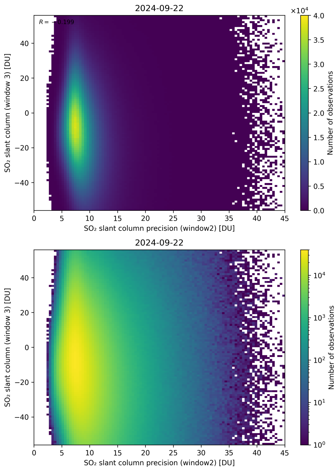
Figure 249: Scatter density plot of “SO 2 slant column precision (window2)” against “SO 2 slant column (window 3)” for 2024-09-22 to 2024-09-23.
