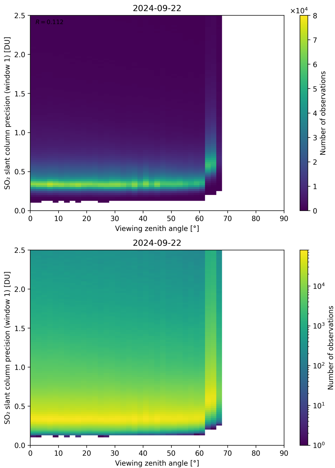
Figure 321: Scatter density plot of “Viewing zenith angle” against “SO 2 slant column precision (window 1)” for 2024-09-22 to 2024-09-23.
