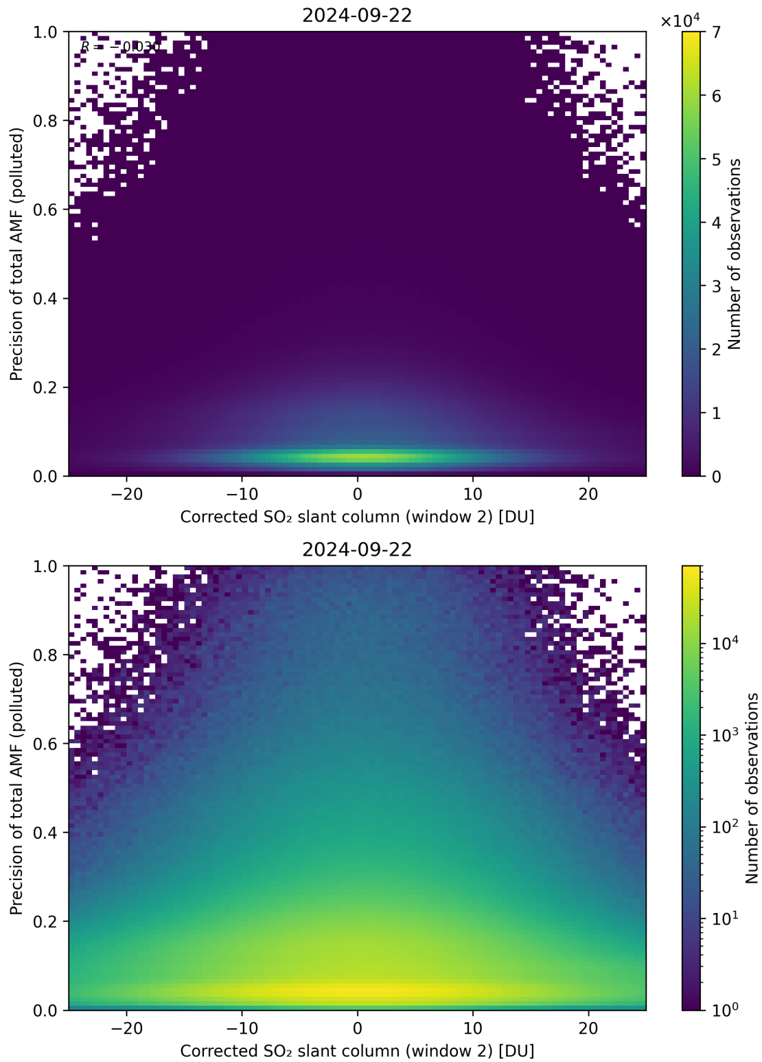
Figure 204: Scatter density plot of “Corrected SO 2 slant column (window 2)” against “Precision of total AMF (polluted)” for 2024-09-22 to 2024-09-23.
