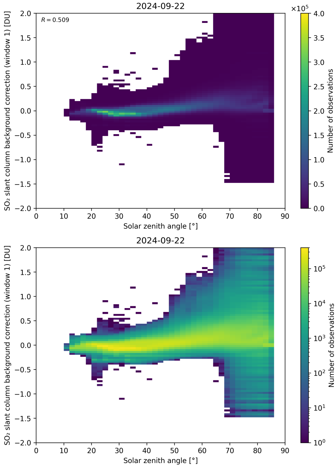
Figure 158: Scatter density plot of “Solar zenith angle” against “SO 2 slant column background correction (window 1)” for 2024-09-22 to 2024-09-23.
