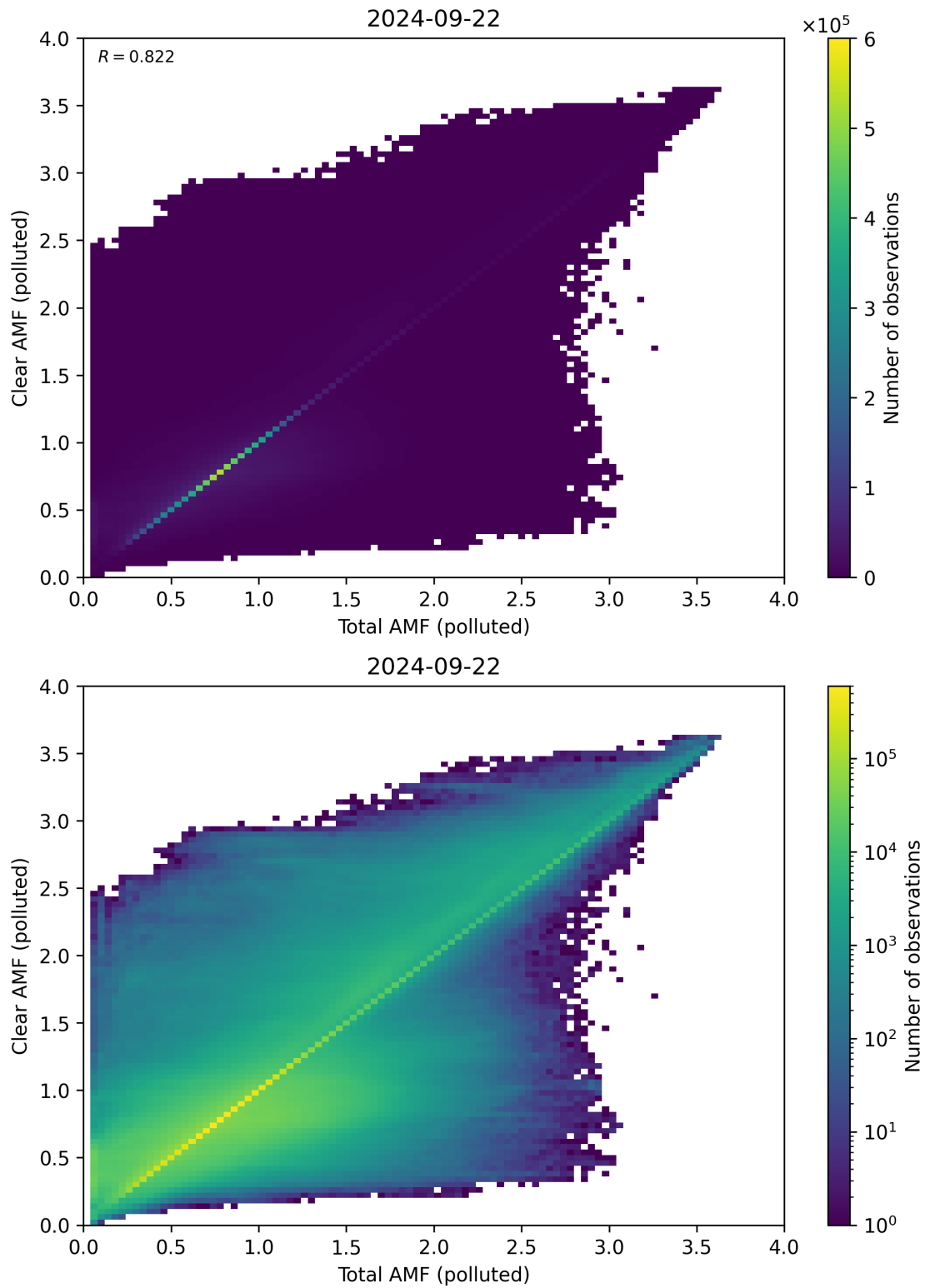
Figure 271: Scatter density plot of “Total AMF (polluted)” against “Clear AMF (polluted)” for 2024-09-22 to 2024-09-23.
