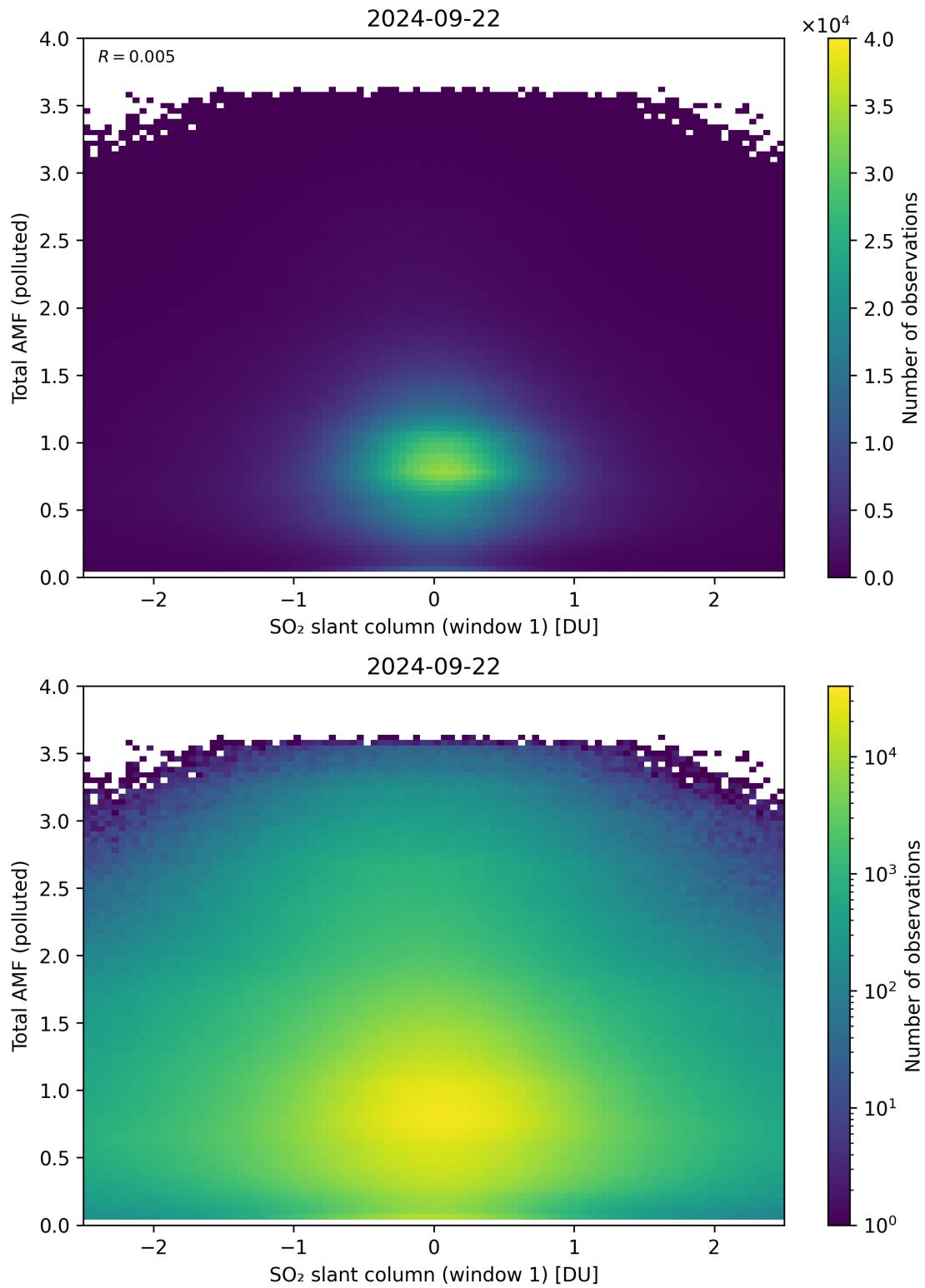
Figure 239: Scatter density plot of “SO 2 slant column (window 1)” against “Total AMF (polluted)” for 2024-09-22 to 2024-09-23.
