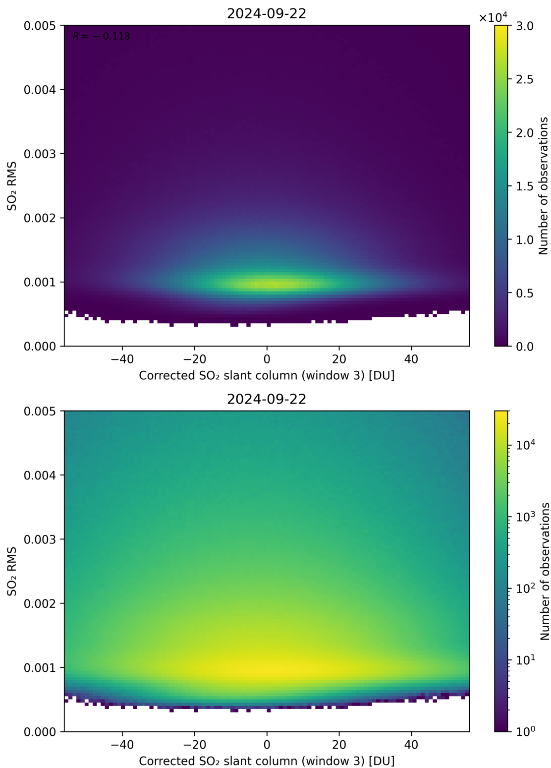
Figure 208: Scatter density plot of “Corrected SO 2 slant column (window 3)” against “SO 2 RMS” for 2024-09-22 to 2024-09-23.
