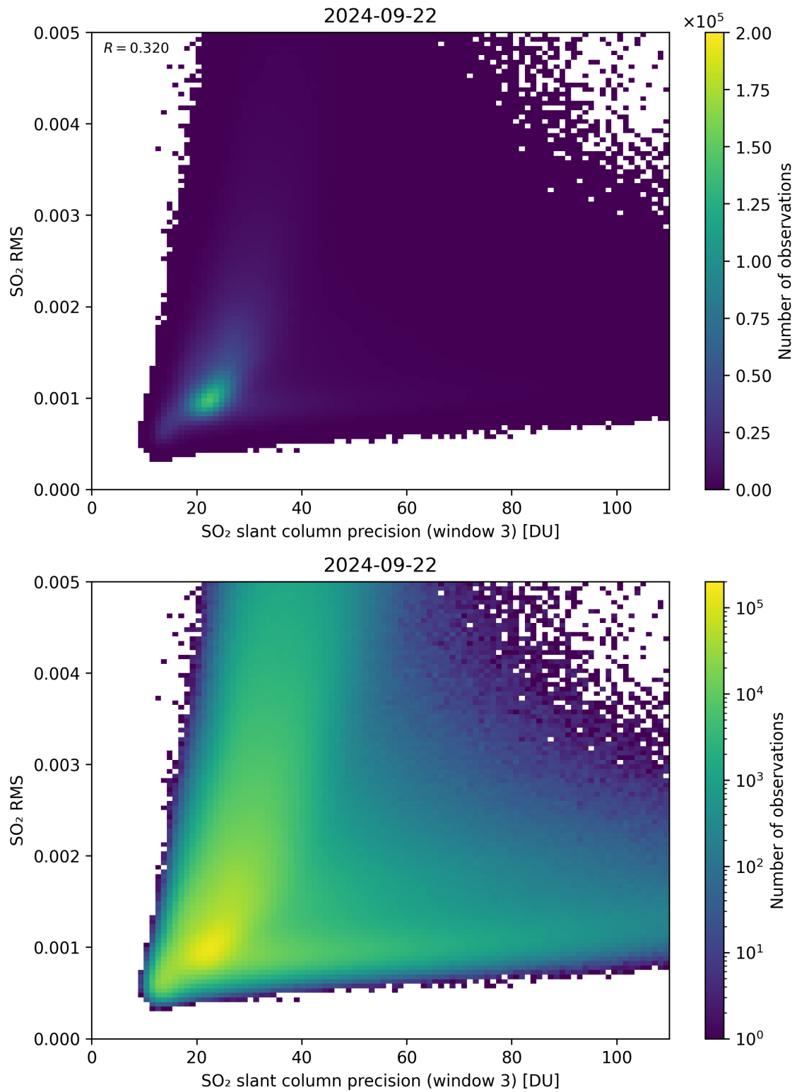
Figure 260: Scatter density plot of “SO 2 slant column precision (window 3)” against “SO 2 RMS” for 2024-09-22 to 2024-09-23.
