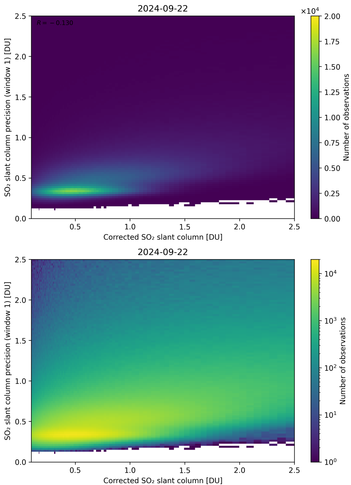
Figure 188: Scatter density plot of “Corrected SO 2 slant column” against “SO 2 slant column precision (window 1)” for 2024-09-22 to 2024-09-23.
