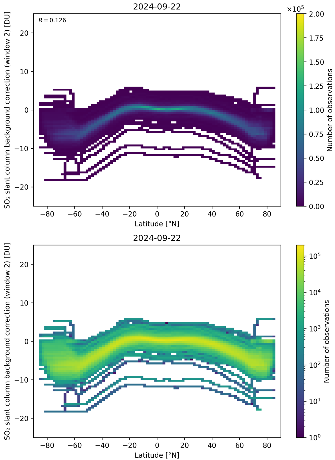
Figure 140: Scatter density plot of “Latitude” against “SO 2 slant column background correction (window 2)” for 2024-09-22 to 2024-09-23.
