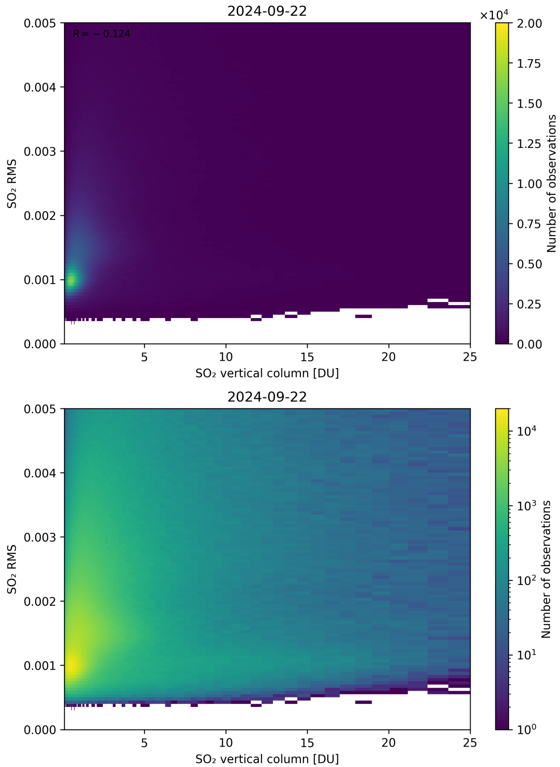
Figure 278: Scatter density plot of “SO 2 vertical column” against “SO 2 RMS” for 2024-09-22 to 2024-09-23.
