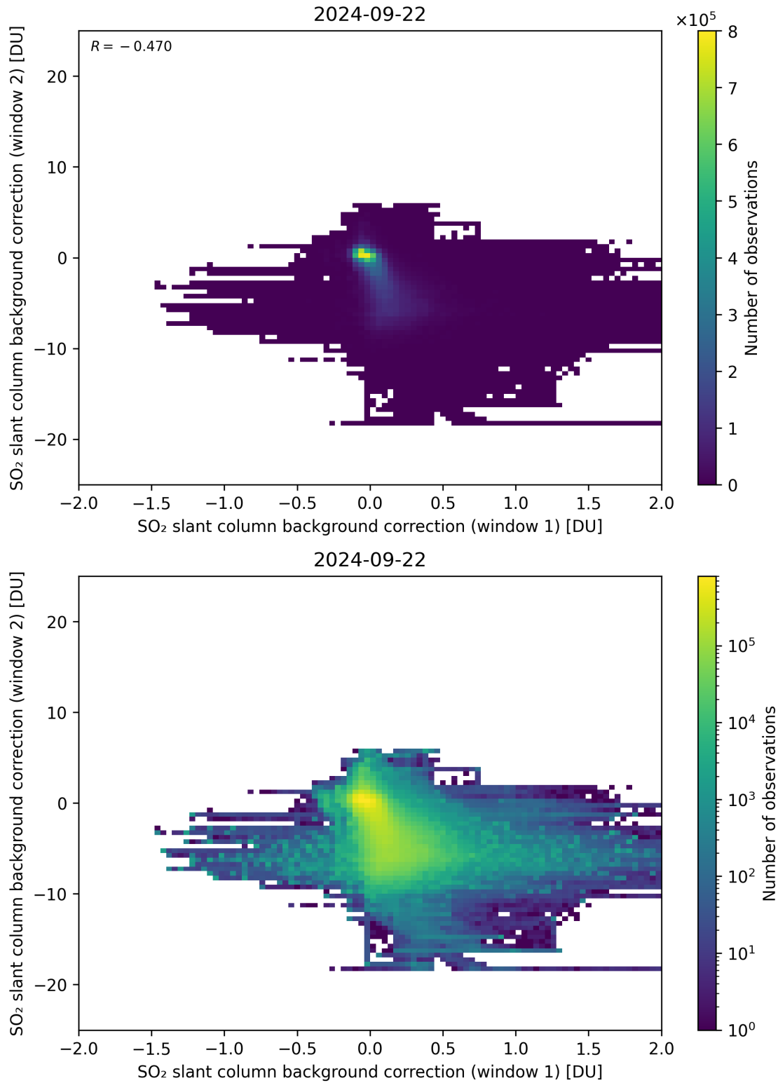
Figure 98: Scatter density plot of “SO 2 slant column background correction (window 1)” against “SO 2 slant column background correction (window 2)” for 2024-09-22 to 2024-09-23.
