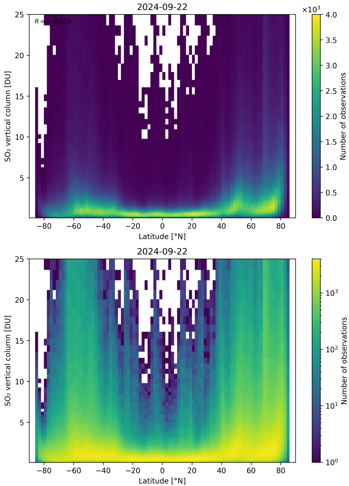
Figure 156: Scatter density plot of “Latitude” against “SO 2 vertical column” for 2024-09-22 to 2024-09-23.
