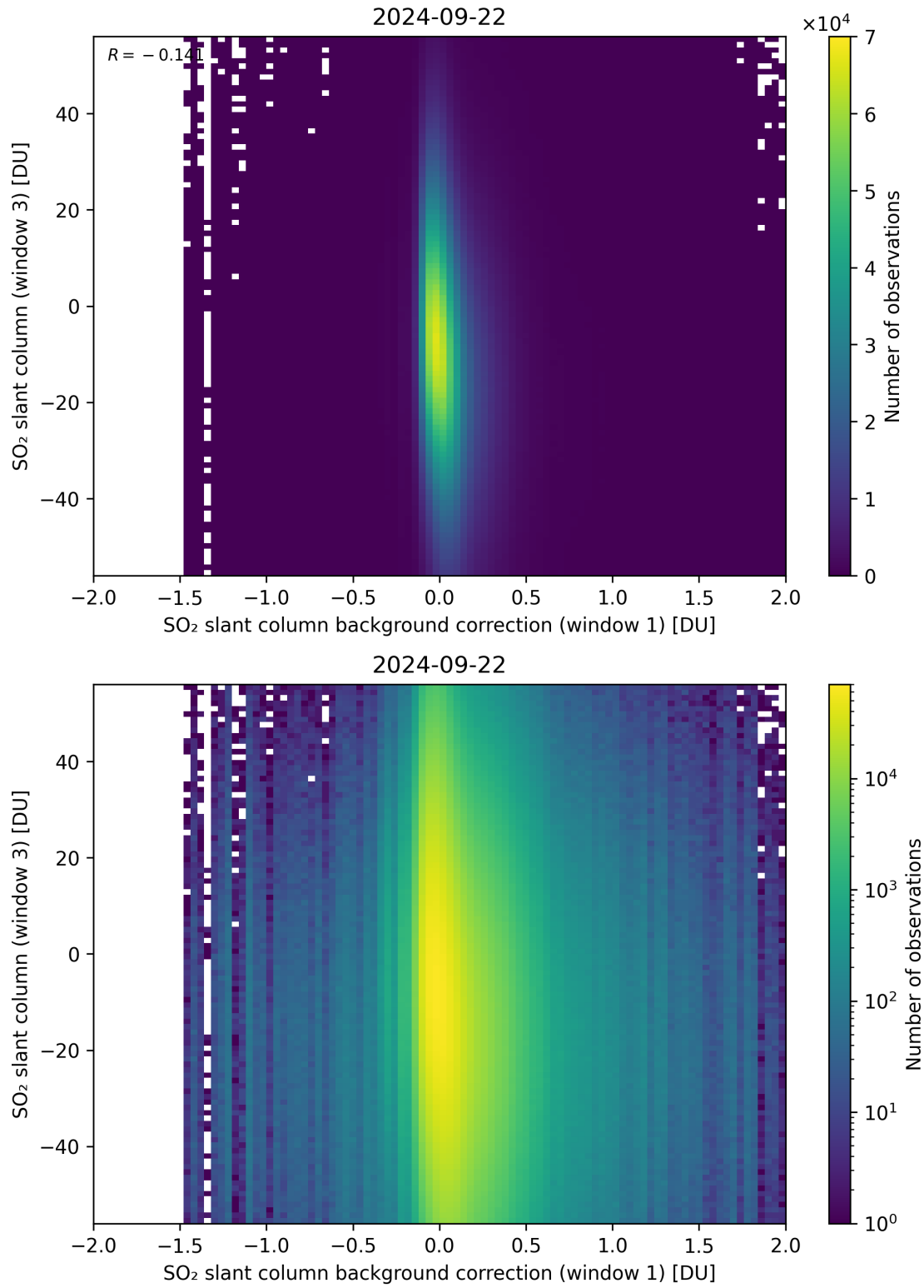
Figure 107: Scatter density plot of “SO 2 slant column background correction (window 1)” against “SO 2 slant column (window 3)” for 2024-09-22 to 2024-09-23.
