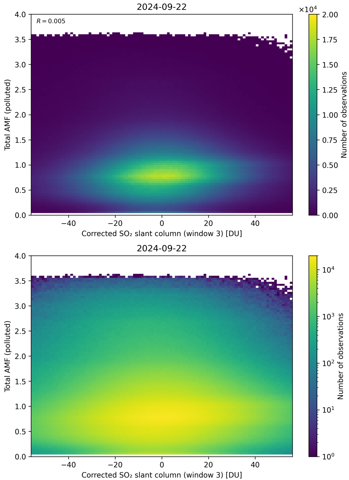
Figure 210: Scatter density plot of “Corrected SO 2 slant column (window 3)” against “Total AMF (polluted)” for 2024-09-22 to 2024-09-23.
