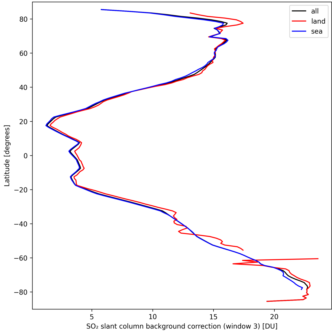
Figure 44: Zonal average of “SO 2 slant column background correction (window 3)” for 2024-09-22 to 2024-09-23.
