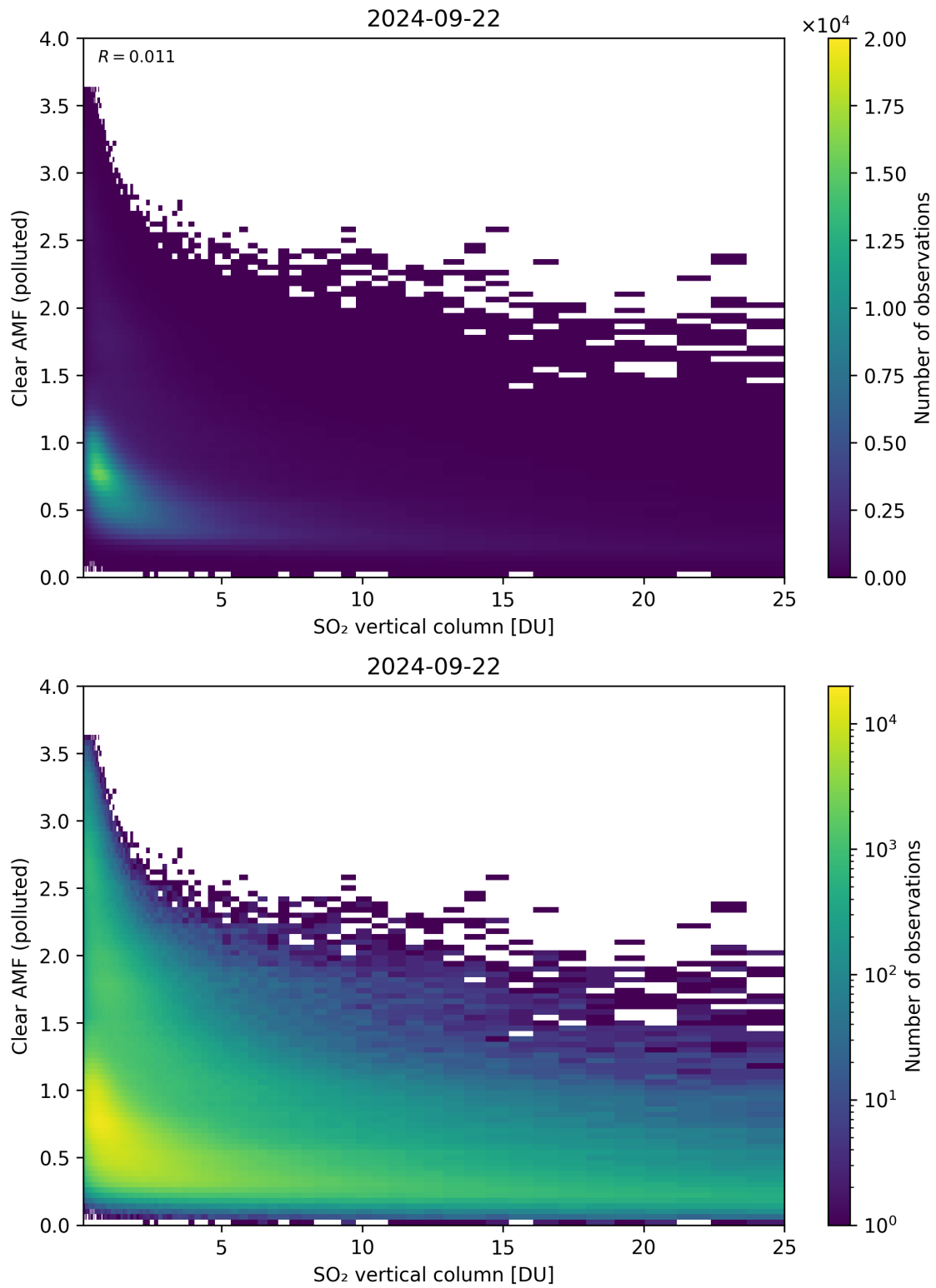
Figure 296: Scatter density plot of “SO 2 vertical column” against “Clear AMF (polluted)” for 2024-09-22 to 2024-09-23.
