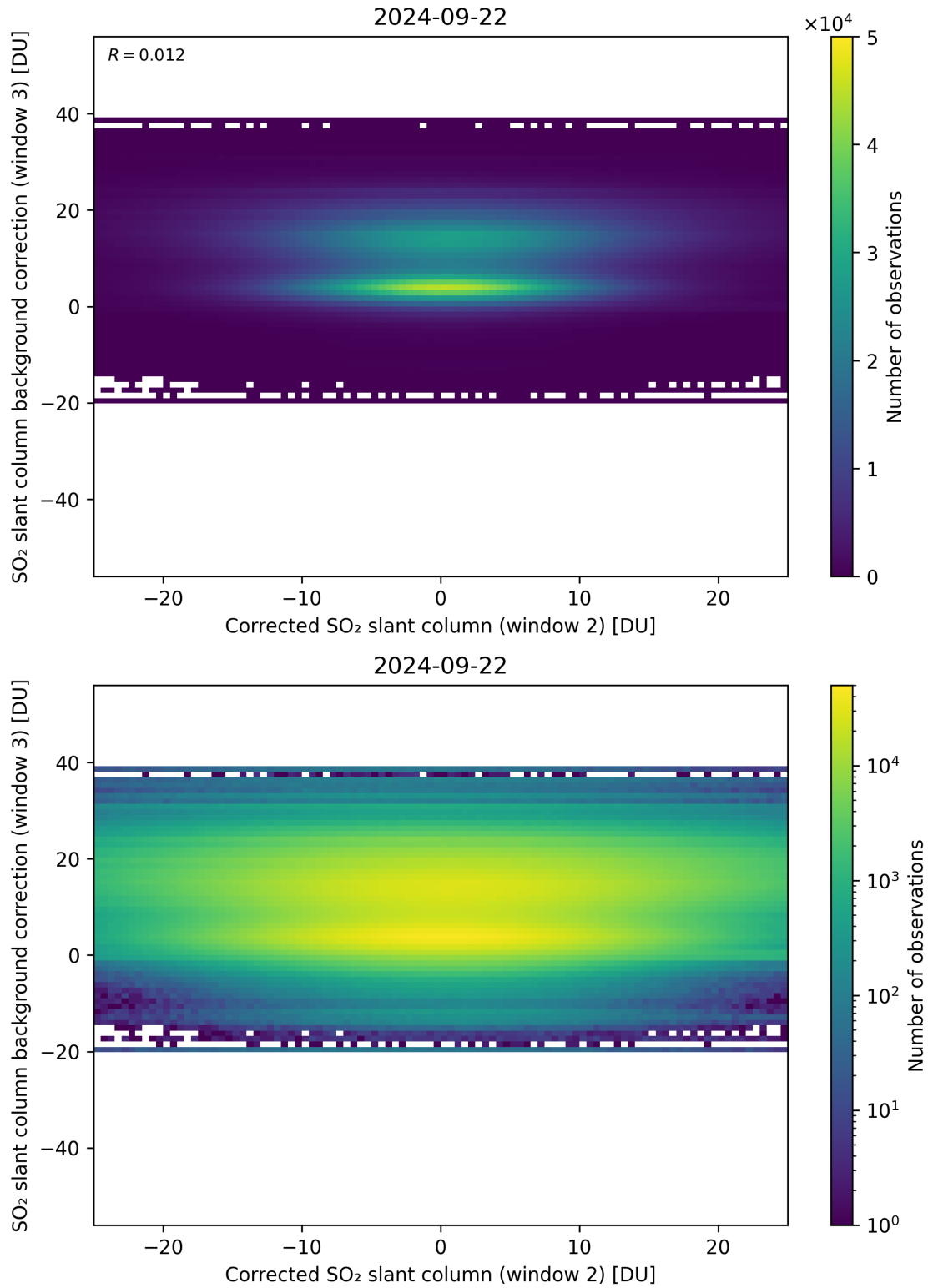
Figure 195: Scatter density plot of “Corrected SO 2 slant column (window 2)” against “SO 2 slant column background correction (window 3)” for 2024-09-22 to 2024-09-23.
