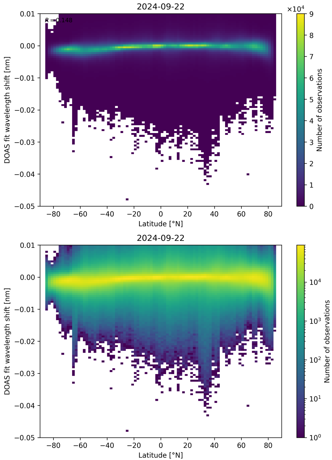
Figure 142: Scatter density plot of “Latitude” against “DOAS fit wavelength shift” for 2024-09-22 to 2024-09-23.
