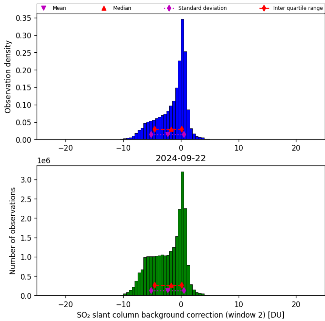
Figure 63: Histogram of “SO 2 slant column background correction (window 2)” for 2024-09-22 to 2024-09-23
