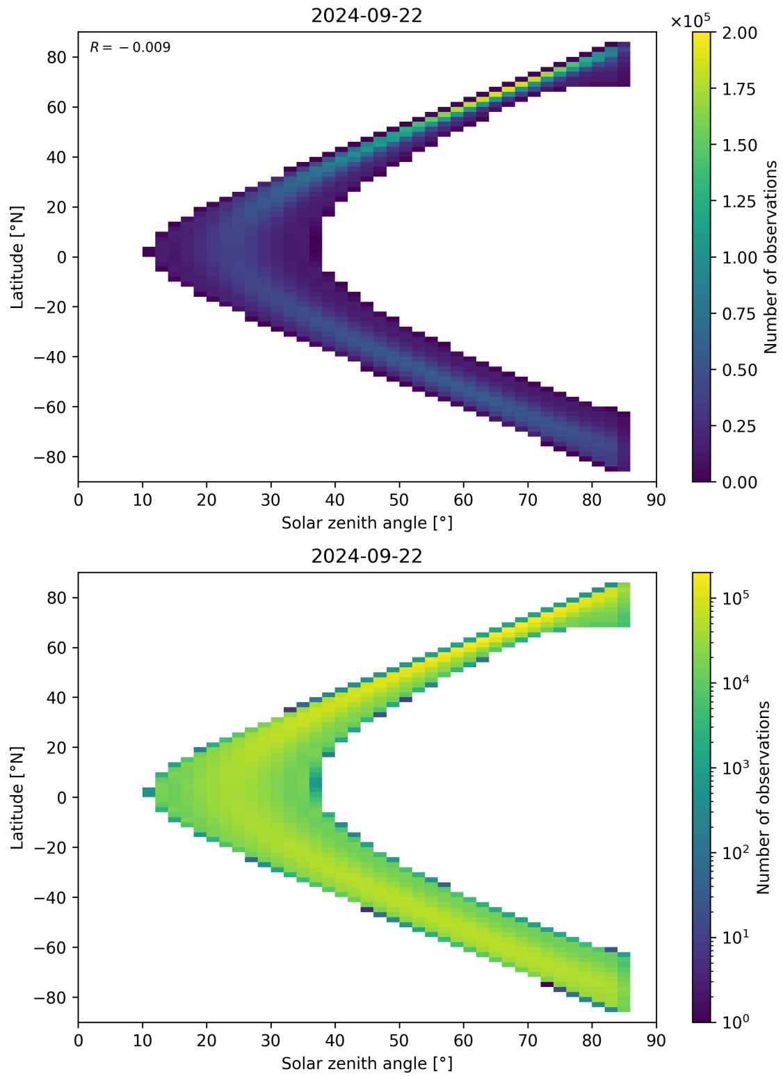
Figure 164: Scatter density plot of “Solar zenith angle” against “Latitude” for 2024-09-22 to 2024-09-23.
