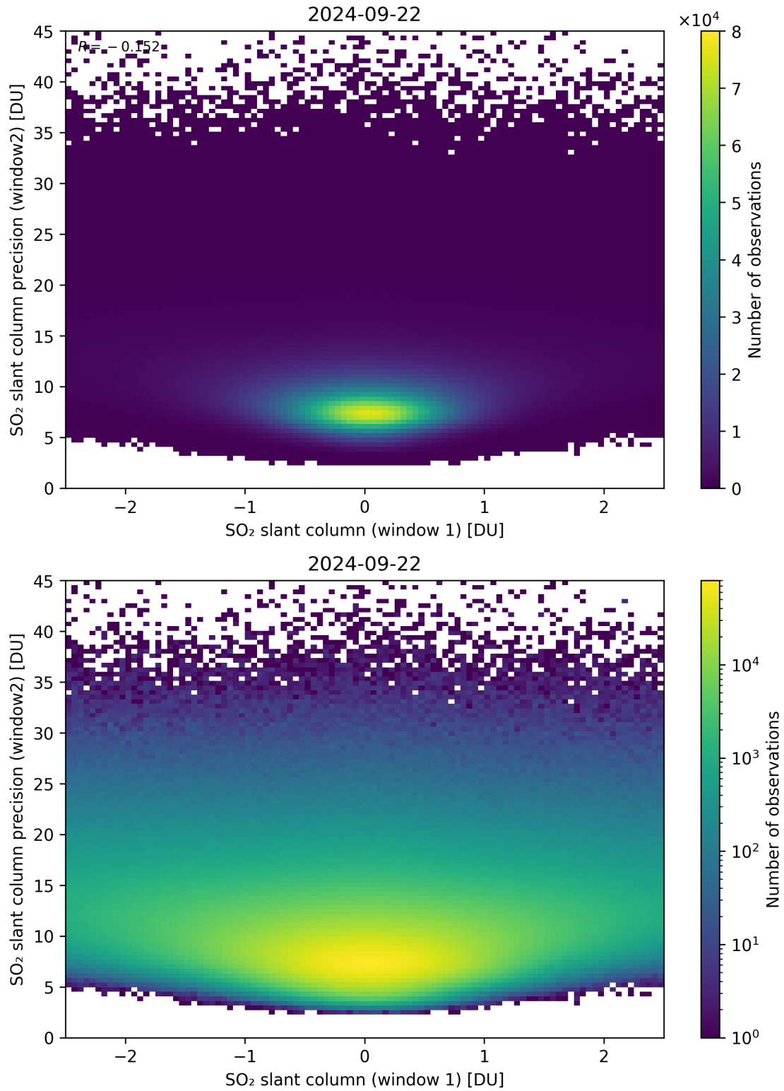
Figure 236: Scatter density plot of “SO 2 slant column (window 1)” against “SO 2 slant column precision (window2)” for 2024-09-22 to 2024-09-23.
