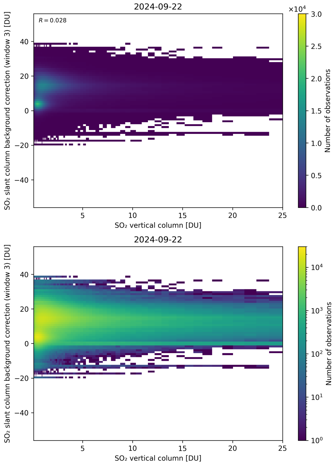
Figure 275: Scatter density plot of “SO 2 vertical column” against “SO 2 slant column background correction (window 3)” for 2024-09-22 to 2024-09-23.
