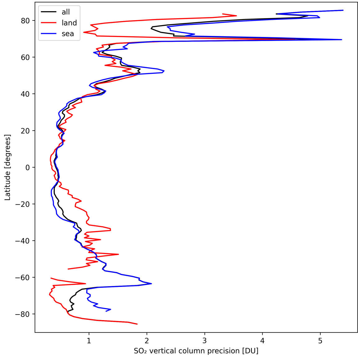
Figure 31: Zonal average of “SO 2 vertical column precision” for 2024-09-22 to 2024-09-23.
