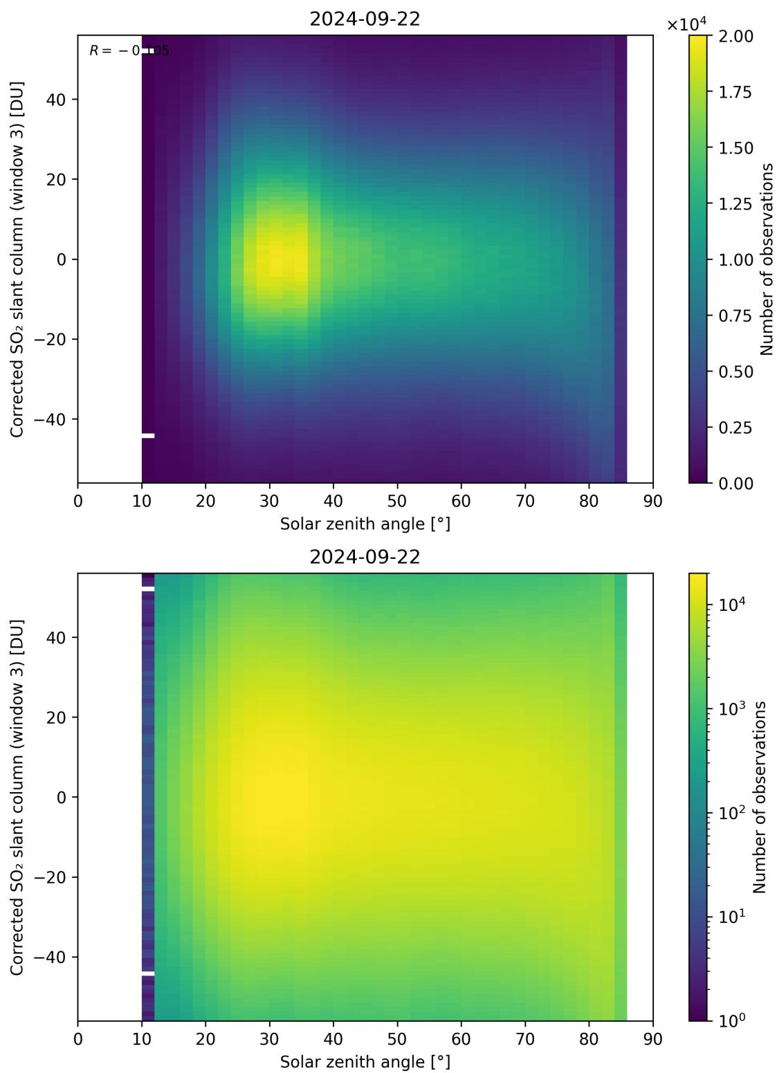
Figure 168: Scatter density plot of “Solar zenith angle” against “Corrected SO 2 slant column (window 3)” for 2024-09-22 to 2024-09-23.
