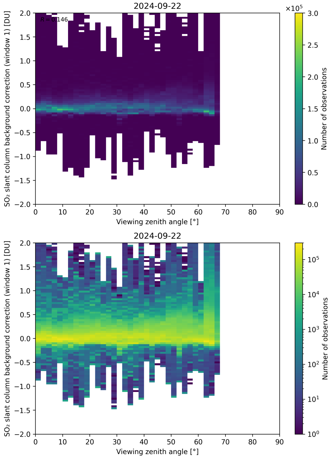
Figure 308: Scatter density plot of “Viewing zenith angle” against “SO 2 slant column background correction (window 1)” for 2024-09-22 to 2024-09-23.
