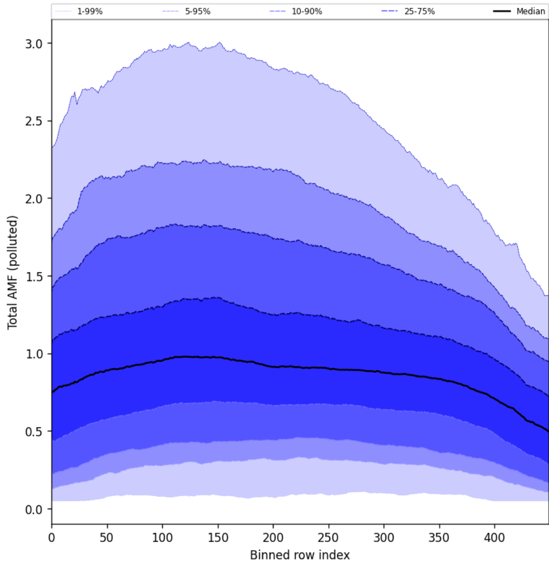
Figure 94: Along track statistics of “Total AMF (polluted)” for 2024-09-22 to 2024-09-23
