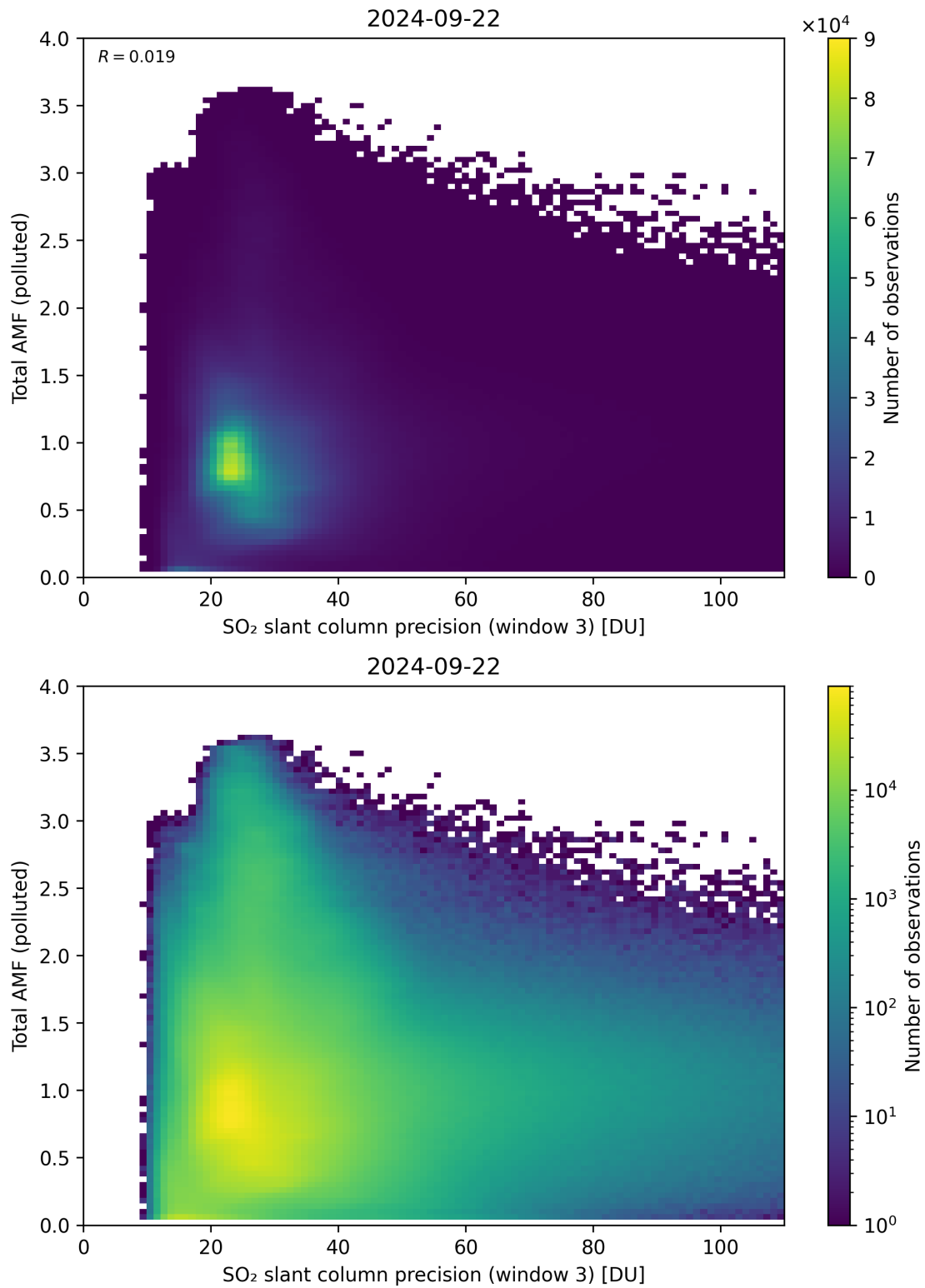
Figure 263: Scatter density plot of “SO 2 slant column precision (window 3)” against “Total AMF (polluted)” for 2024-09-22 to 2024-09-23.
