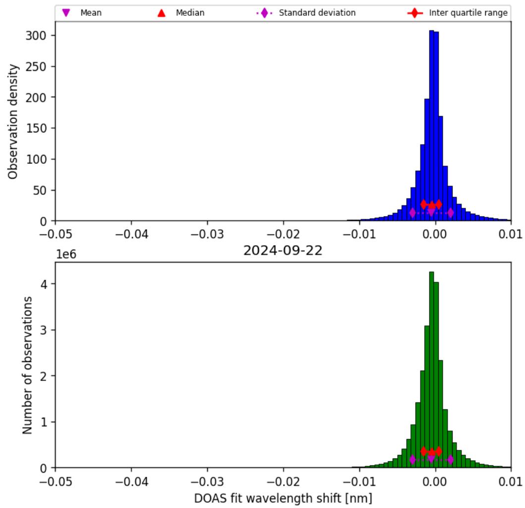
Figure 68: Histogram of “DOAS fit wavelength shift” for 2024-09-22 to 2024-09-23
