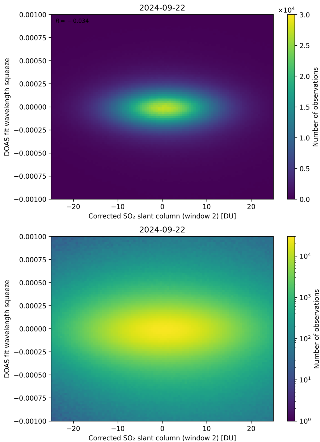
Figure 197: Scatter density plot of “Corrected SO 2 slant column (window 2)” against “DOAS fit wavelength squeeze” for 2024-09-22 to 2024-09-23.
