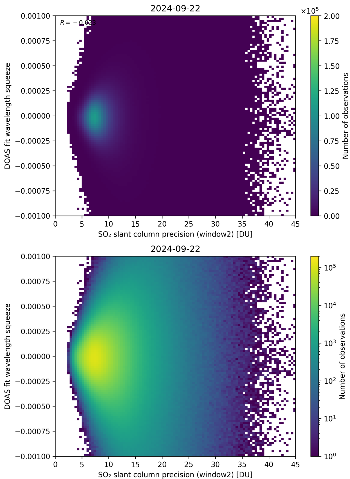
Figure 244: Scatter density plot of “SO 2 slant column precision (window2)” against “DOAS fit wavelength squeeze” for 2024-09-22 to 2024-09-23.
