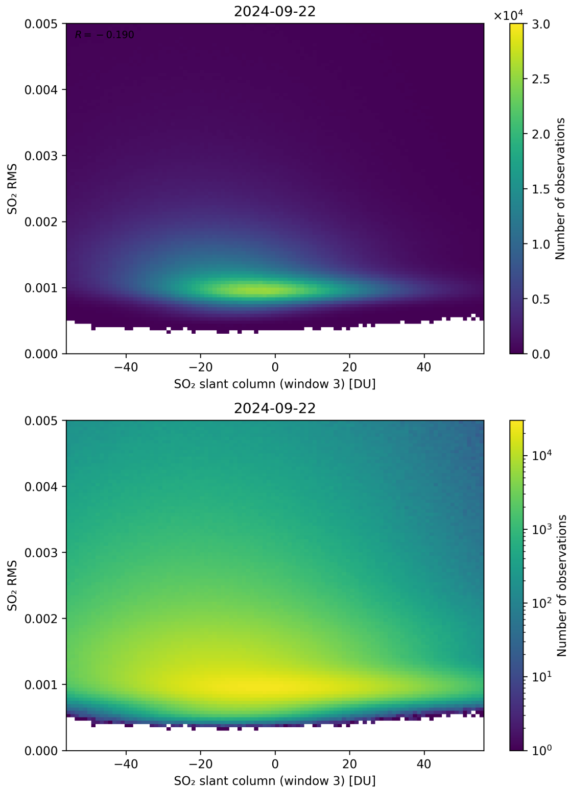
Figure 256: Scatter density plot of “SO 2 slant column (window 3)” against “SO 2 RMS” for 2024-09-22 to 2024-09-23.
