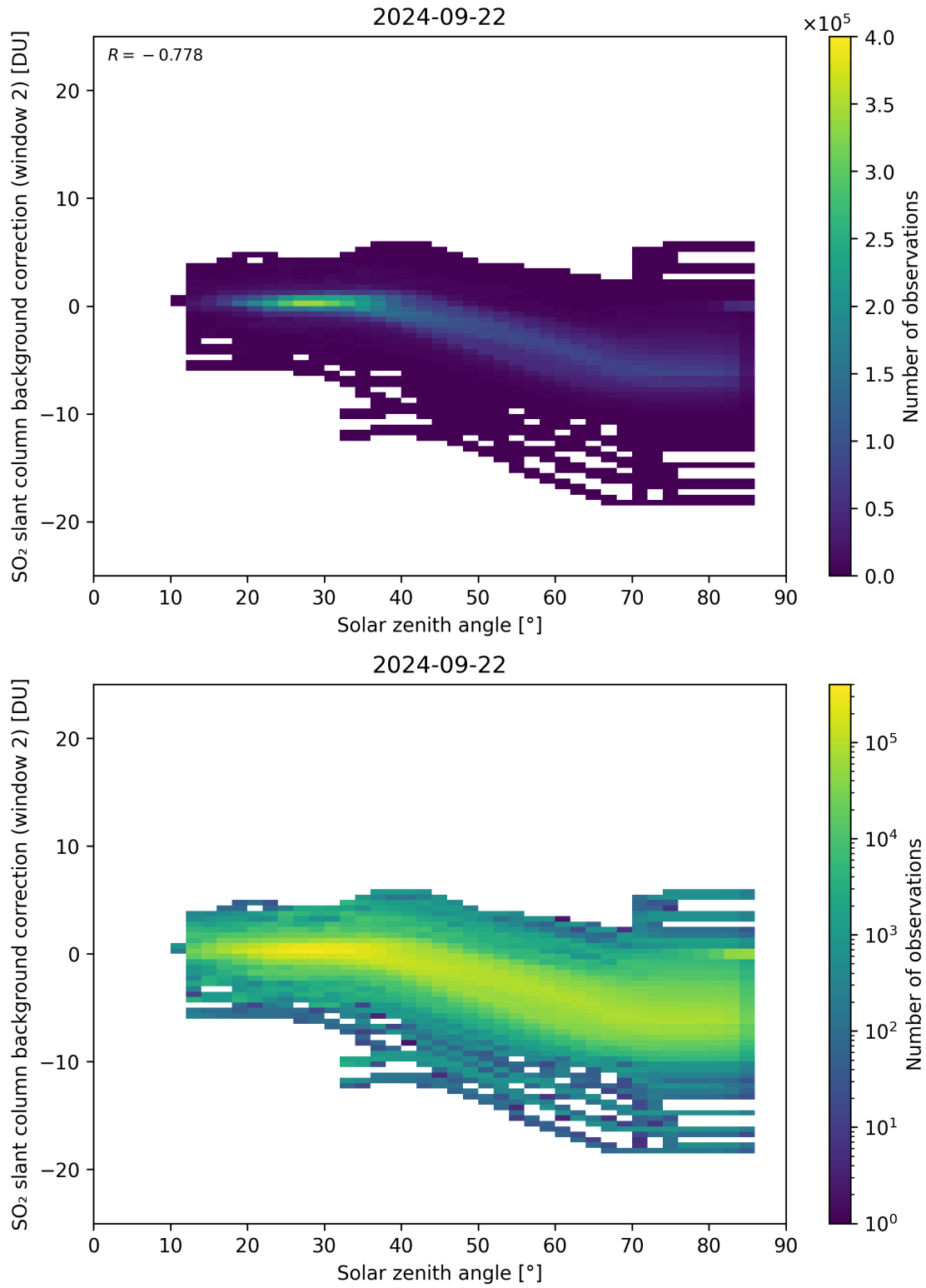
Figure 159: Scatter density plot of “Solar zenith angle” against “SO 2 slant column background correction (window 2)” for 2024-09-22 to 2024-09-23.
