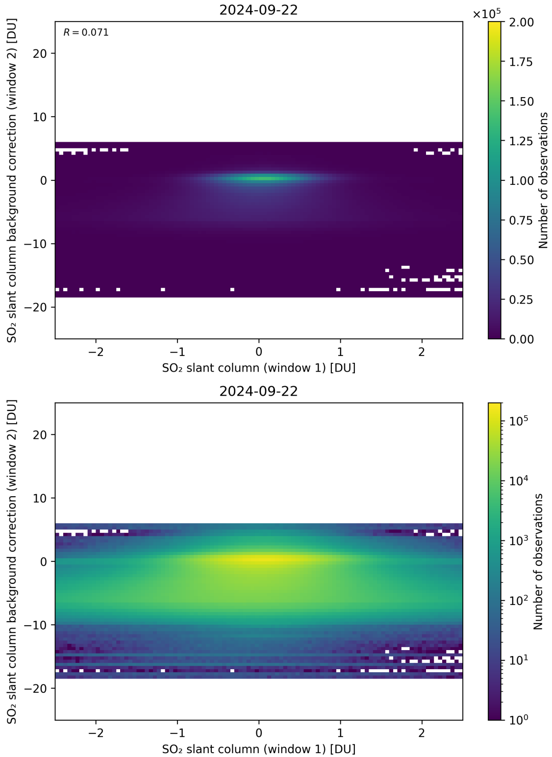
Figure 213: Scatter density plot of “SO 2 slant column (window 1)” against “SO 2 slant column background correction (window 2)” for 2024-09-22 to 2024-09-23.
