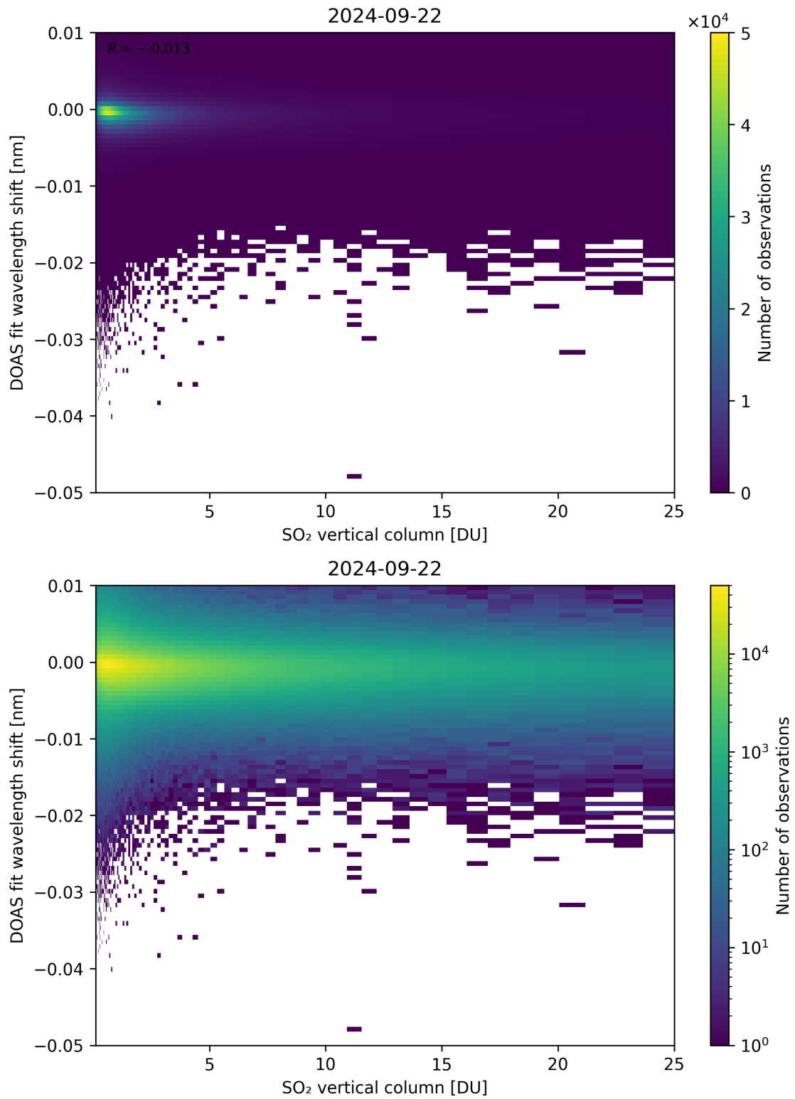
Figure 276: Scatter density plot of “SO 2 vertical column” against “DOAS fit wavelength shift” for 2024-09-22 to 2024-09-23.
