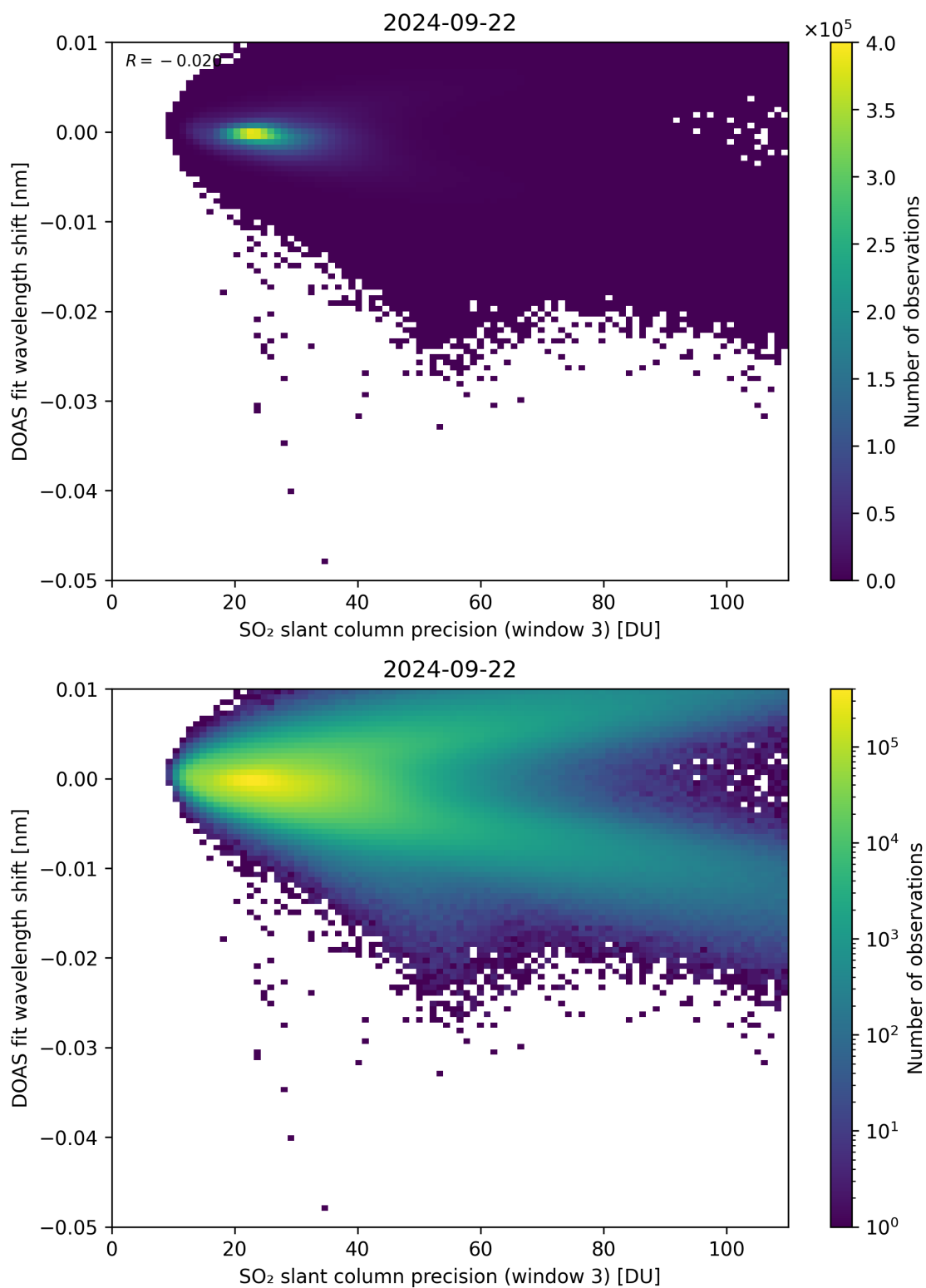
Figure 258: Scatter density plot of “SO 2 slant column precision (window 3)” against “DOAS fit wavelength shift” for 2024-09-22 to 2024-09-23.
