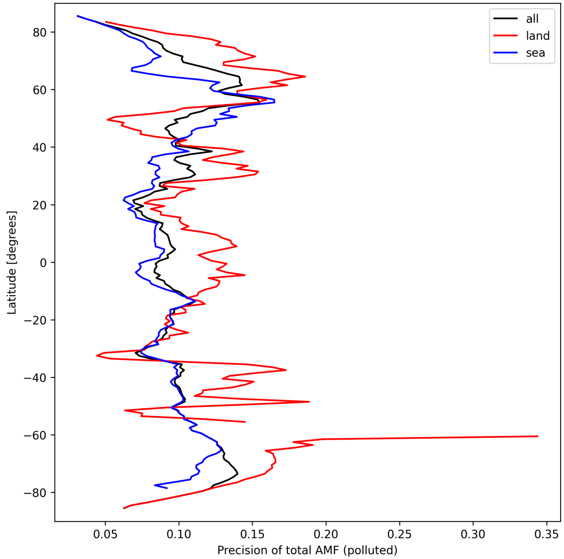
Figure 49: Zonal average of “Precision of total AMF (polluted)” for 2024-09-22 to 2024-09-23.
