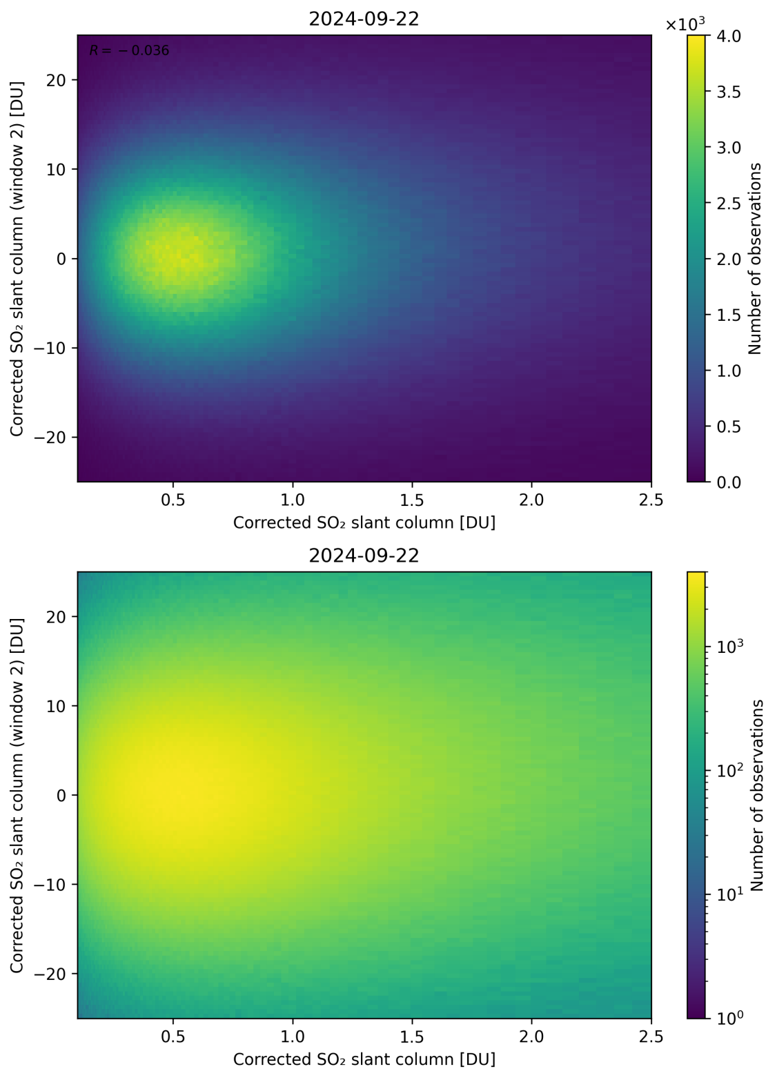
Figure 185: Scatter density plot of “Corrected SO 2 slant column” against “Corrected SO 2 slant column (window 2)” for 2024-09-22 to 2024-09-23.
