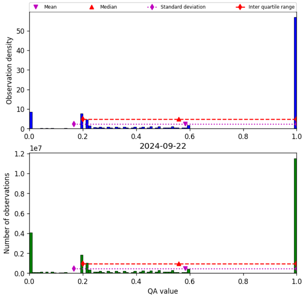
Figure 52: Histogram of “QA value” for 2024-09-22 to 2024-09-23
