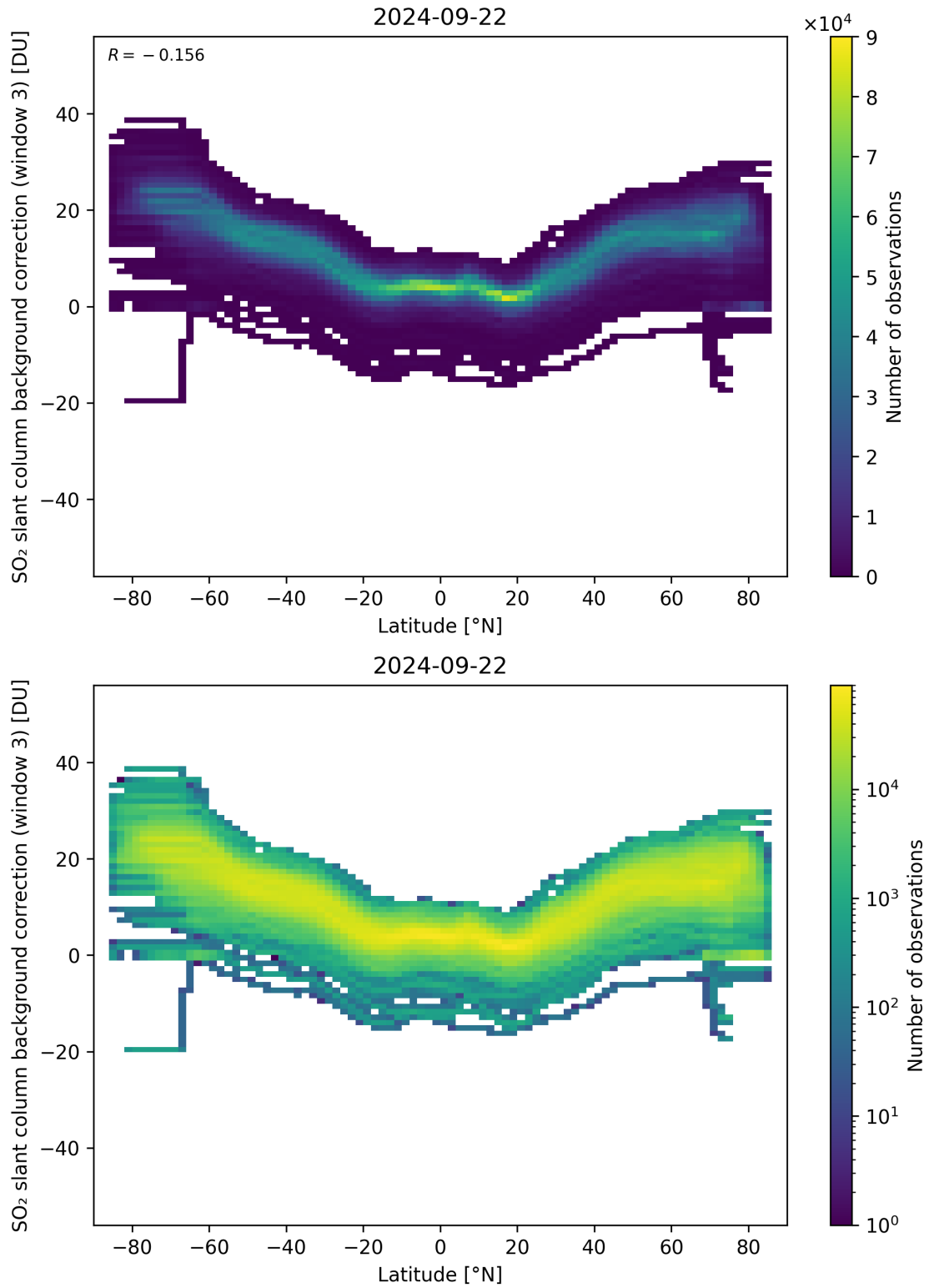
Figure 141: Scatter density plot of “Latitude” against “SO 2 slant column background correction (window 3)” for 2024-09-22 to 2024-09-23.
