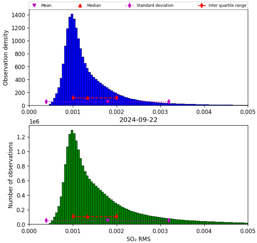
Figure 70: Histogram of “SO 2 RMS” for 2024-09-22 to 2024-09-23
