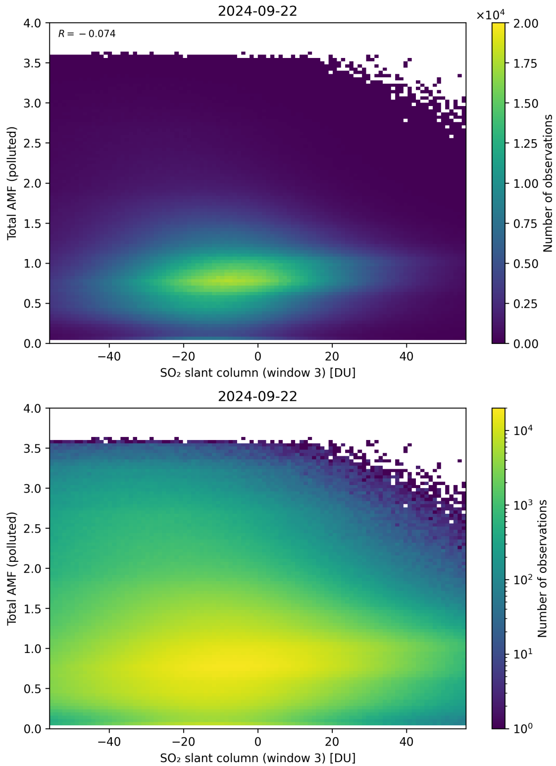
Figure 268: Scatter density plot of “SO 2 slant column (window 3)” against “Total AMF (polluted)” for 2024-09-22 to 2024-09-23.
