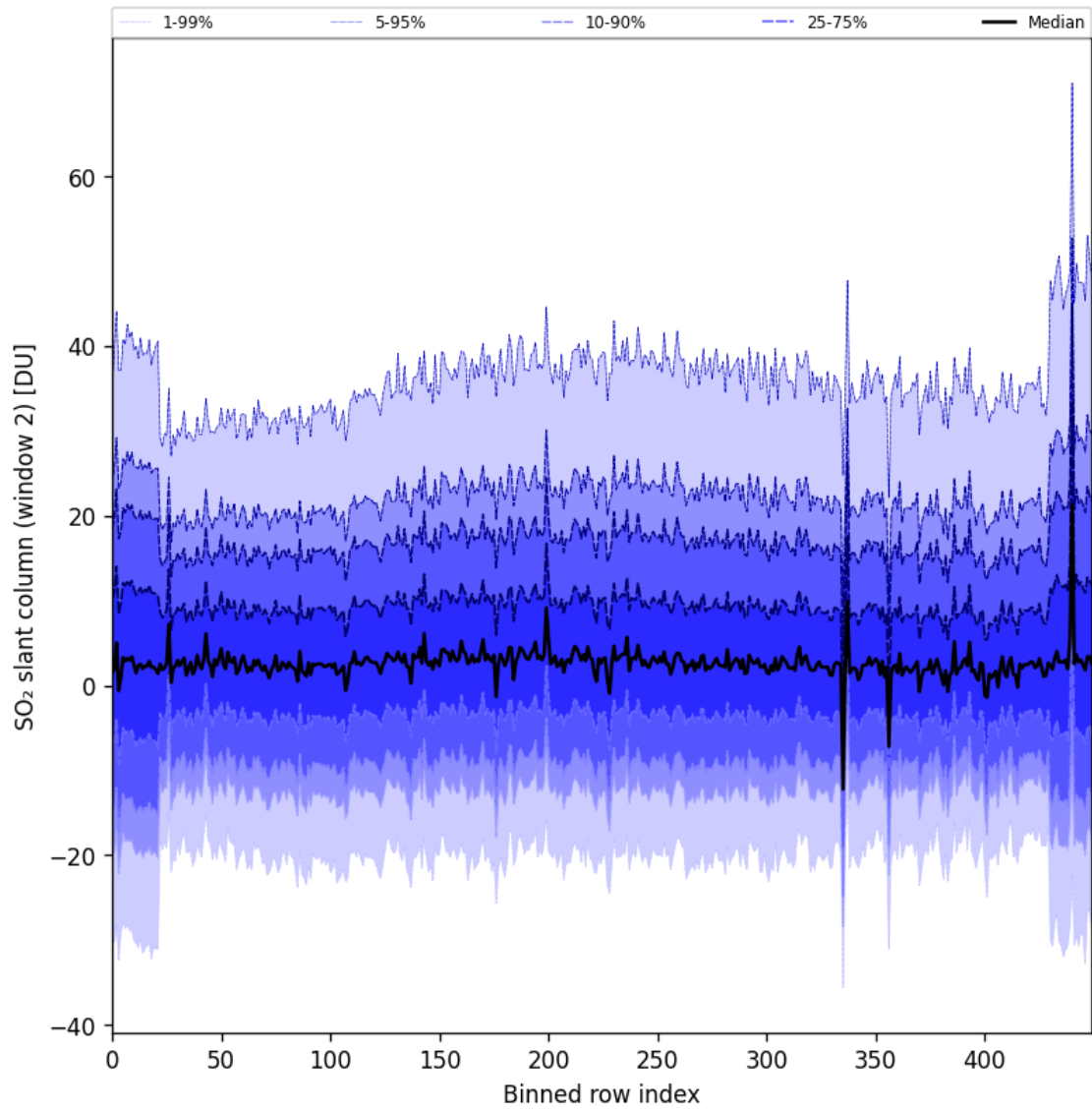
Figure 83: Along track statistics of “SO 2 slant column (window 2)” for 2024-09-22 to 2024-09-23
