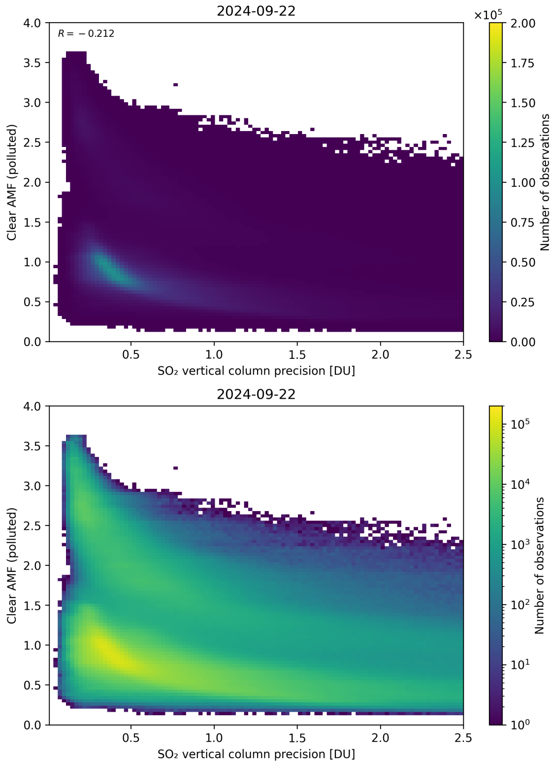
Figure 285: Scatter density plot of “SO 2 vertical column precision” against “Clear AMF (polluted)” for 2024-09-22 to 2024-09-23.
