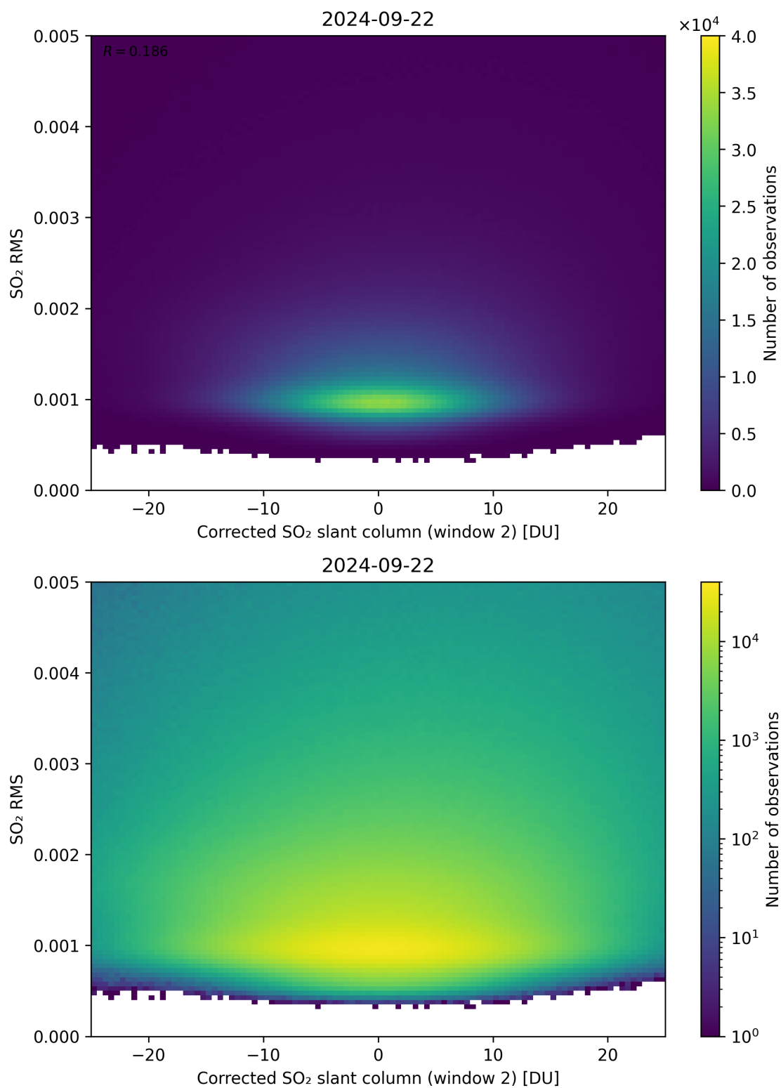
Figure 198: Scatter density plot of “Corrected SO 2 slant column (window 2)” against “SO 2 RMS” for 2024-09-22 to 2024-09-23.
