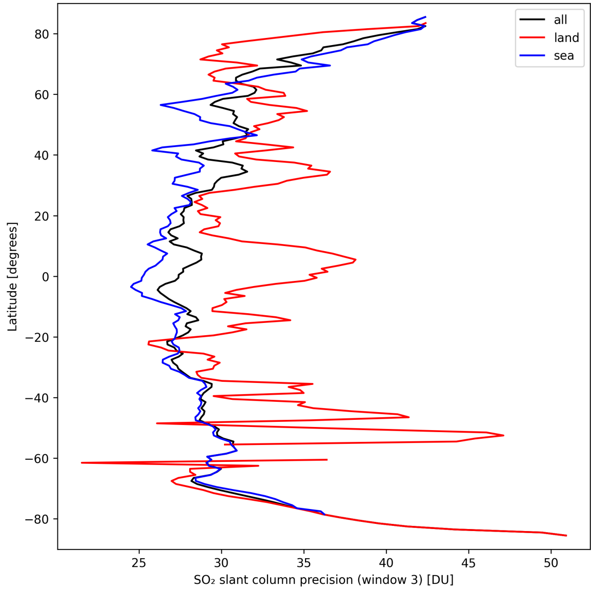
Figure 42: Zonal average of “SO 2 slant column precision (window 3)” for 2024-09-22 to 2024-09-23.
