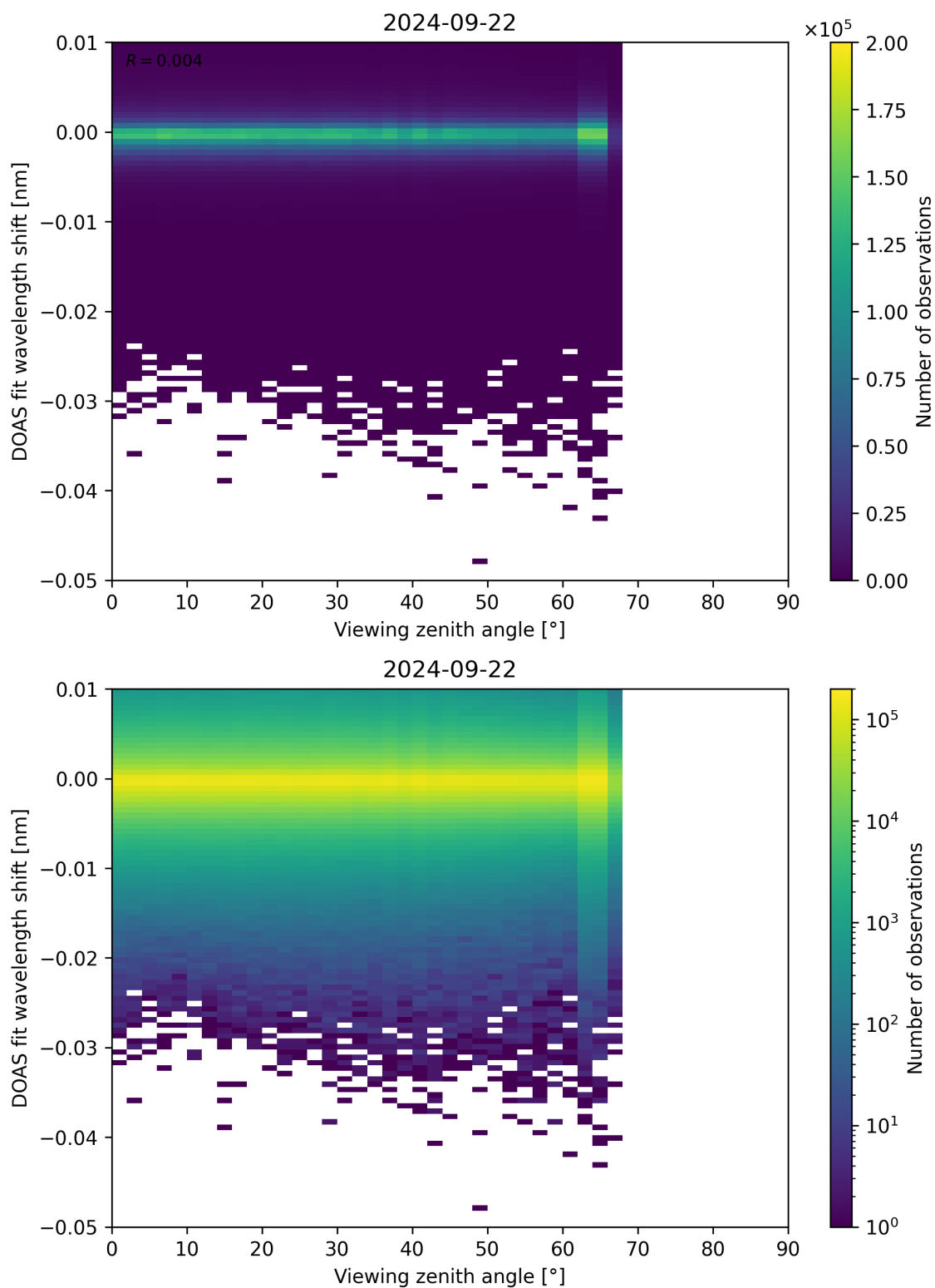
Figure 311: Scatter density plot of “Viewing zenith angle” against “DOAS fit wavelength shift” for 2024-09-22 to 2024-09-23.
