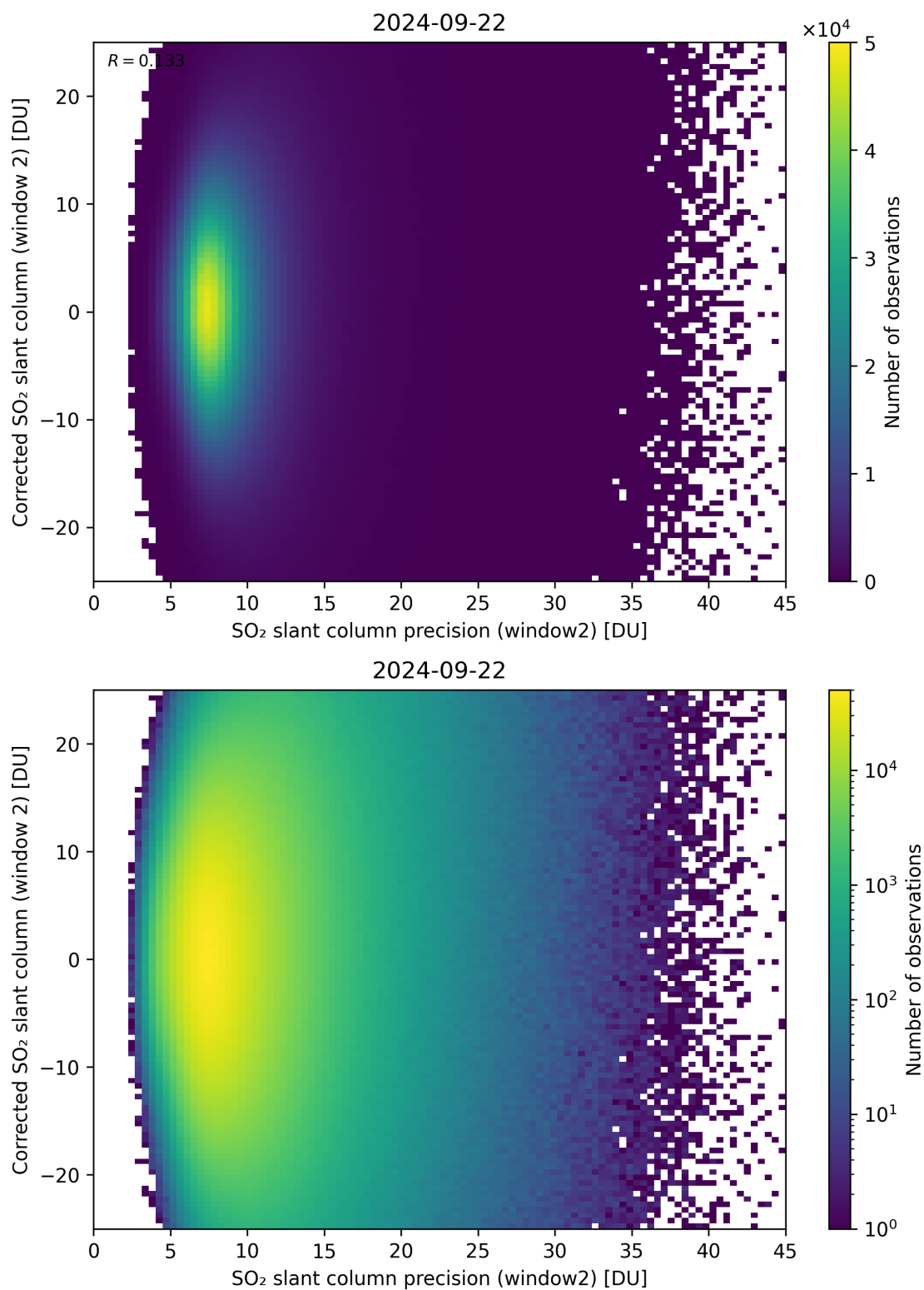
Figure 247: Scatter density plot of “SO 2 slant column precision (window2)” against “Corrected SO 2 slant column (window 2)” for 2024-09-22 to 2024-09-23.
