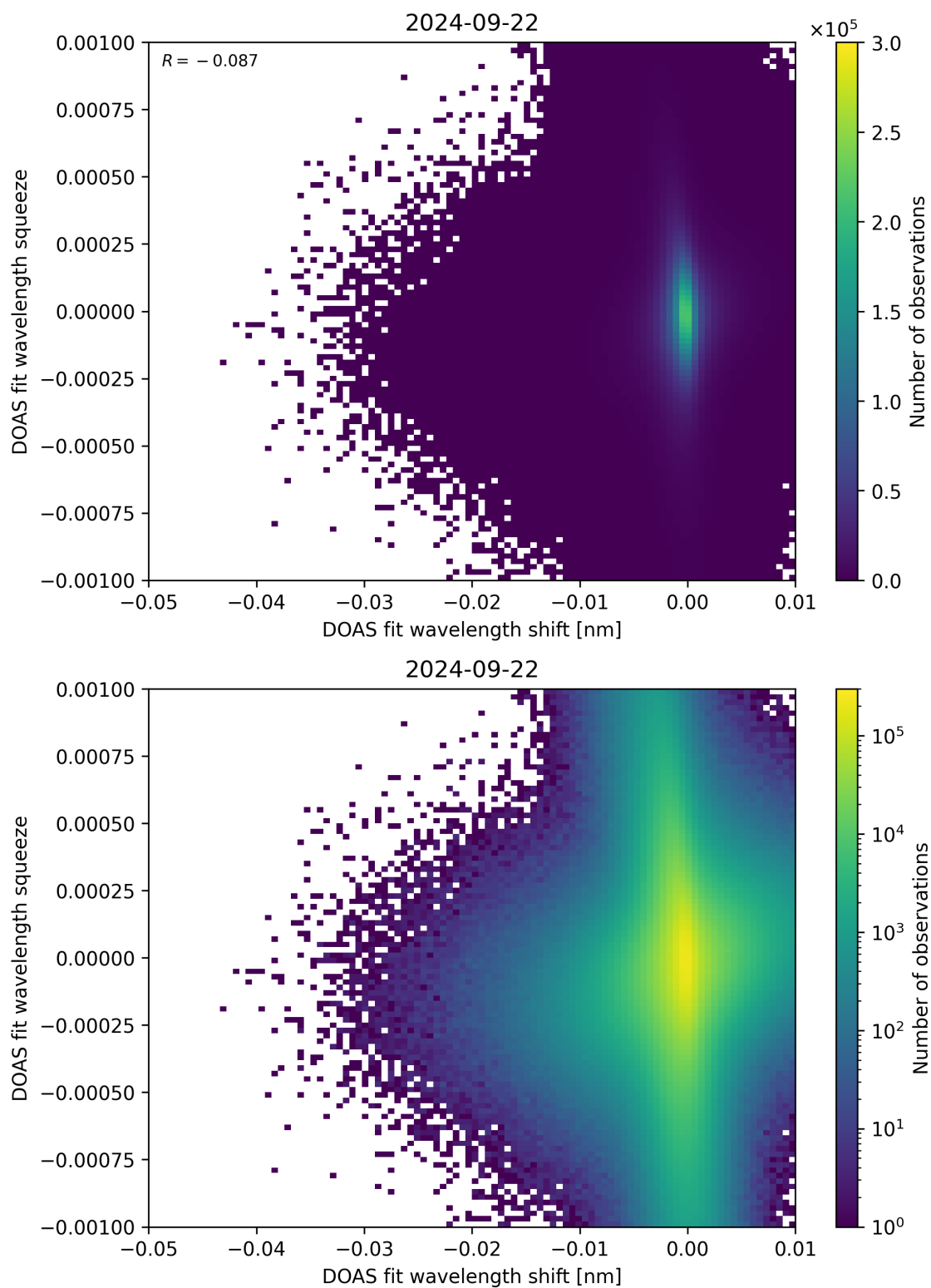
Figure 127: Scatter density plot of “DOAS fit wavelength shift” against “DOAS fit wavelength squeeze” for 2024-09-22 to 2024-09-23.
