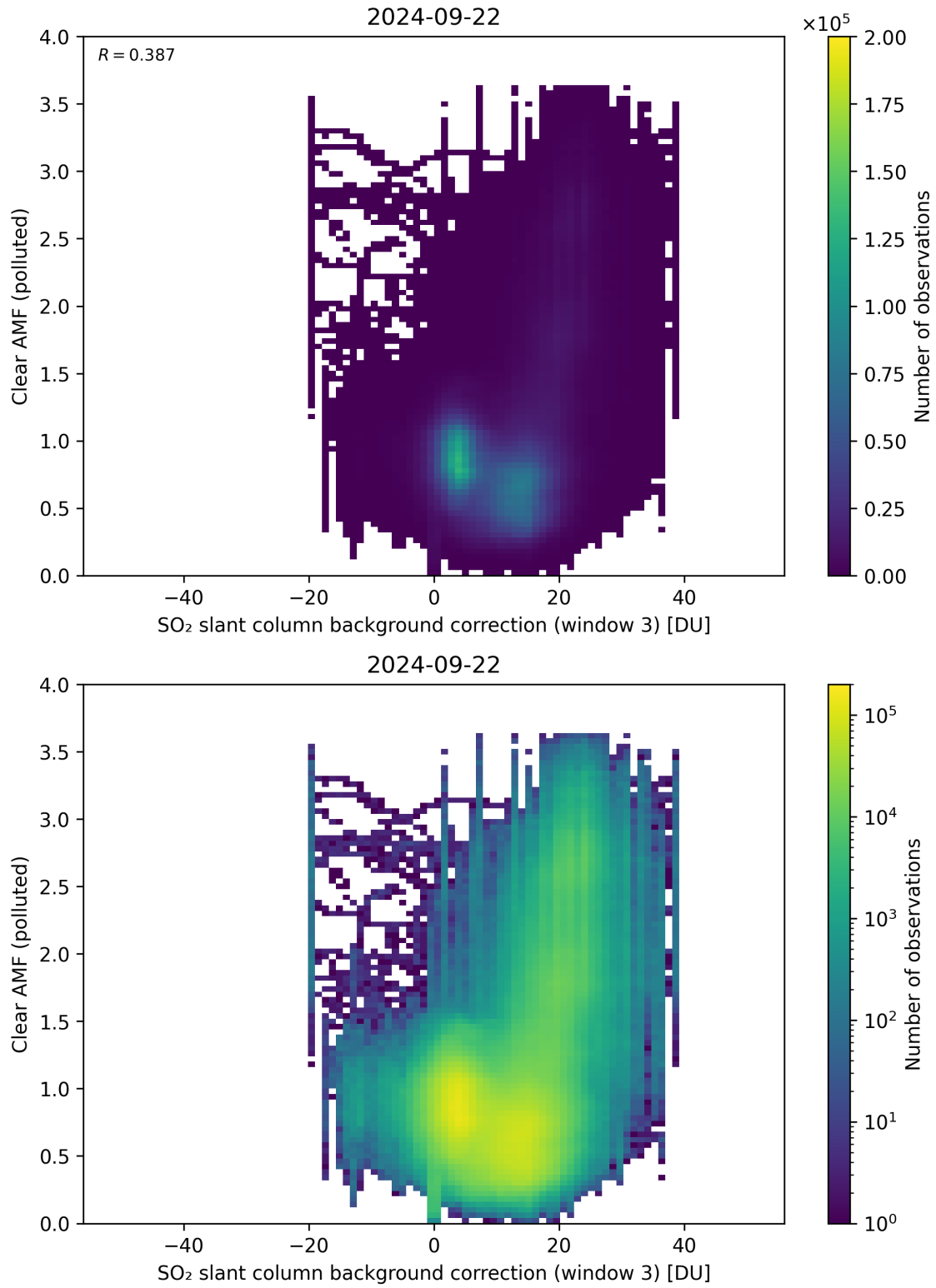
Figure 124: Scatter density plot of “SO 2 slant column background correction (window 3)” against “Clear AMF (polluted)” for 2024-09-22 to 2024-09-23.
