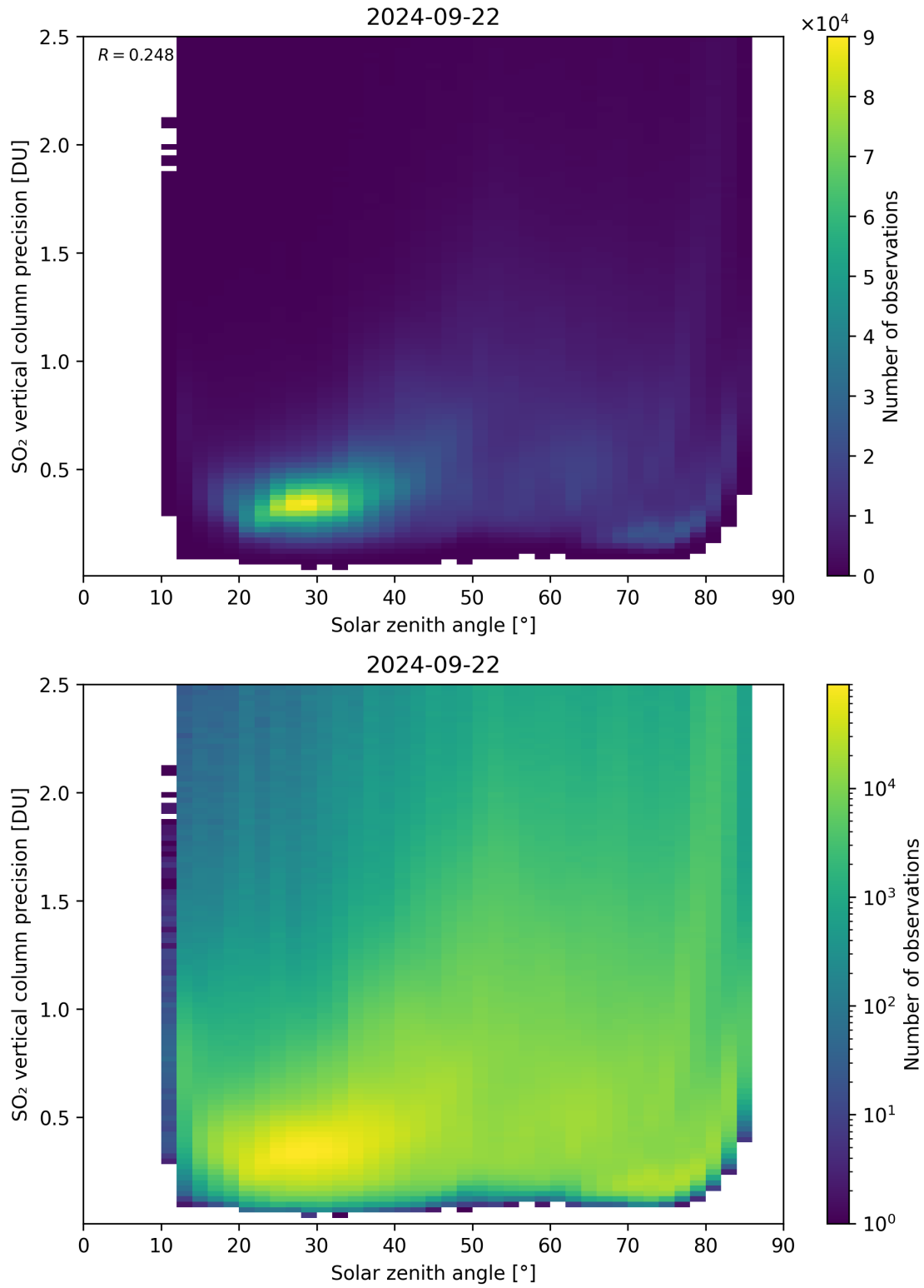
Figure 177: Scatter density plot of “Solar zenith angle” against “SO 2 vertical column precision” for 2024-09-22 to 2024-09-23.
