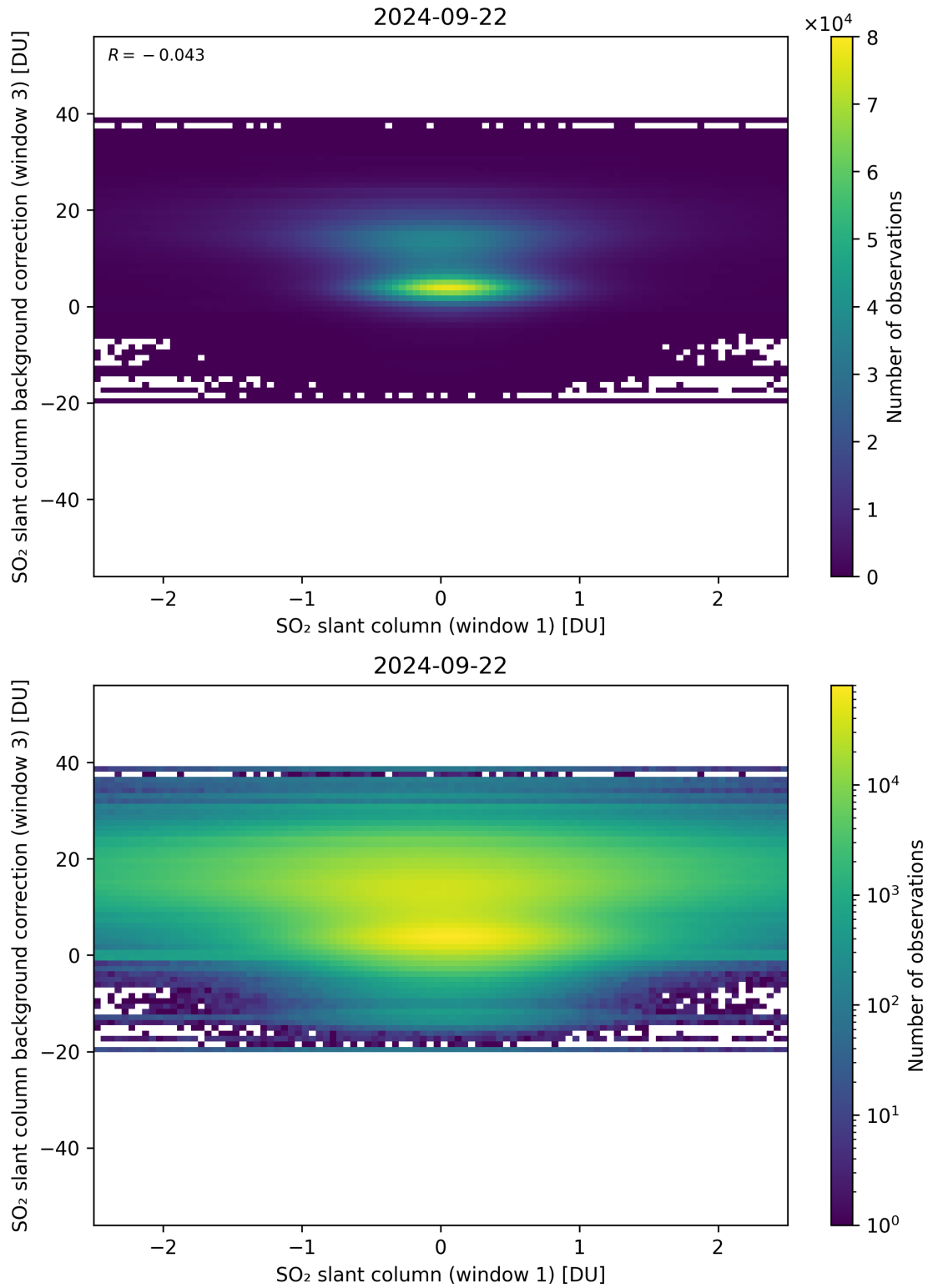
Figure 214: Scatter density plot of “SO 2 slant column (window 1)” against “SO 2 slant column background correction (window 3)” for 2024-09-22 to 2024-09-23.
