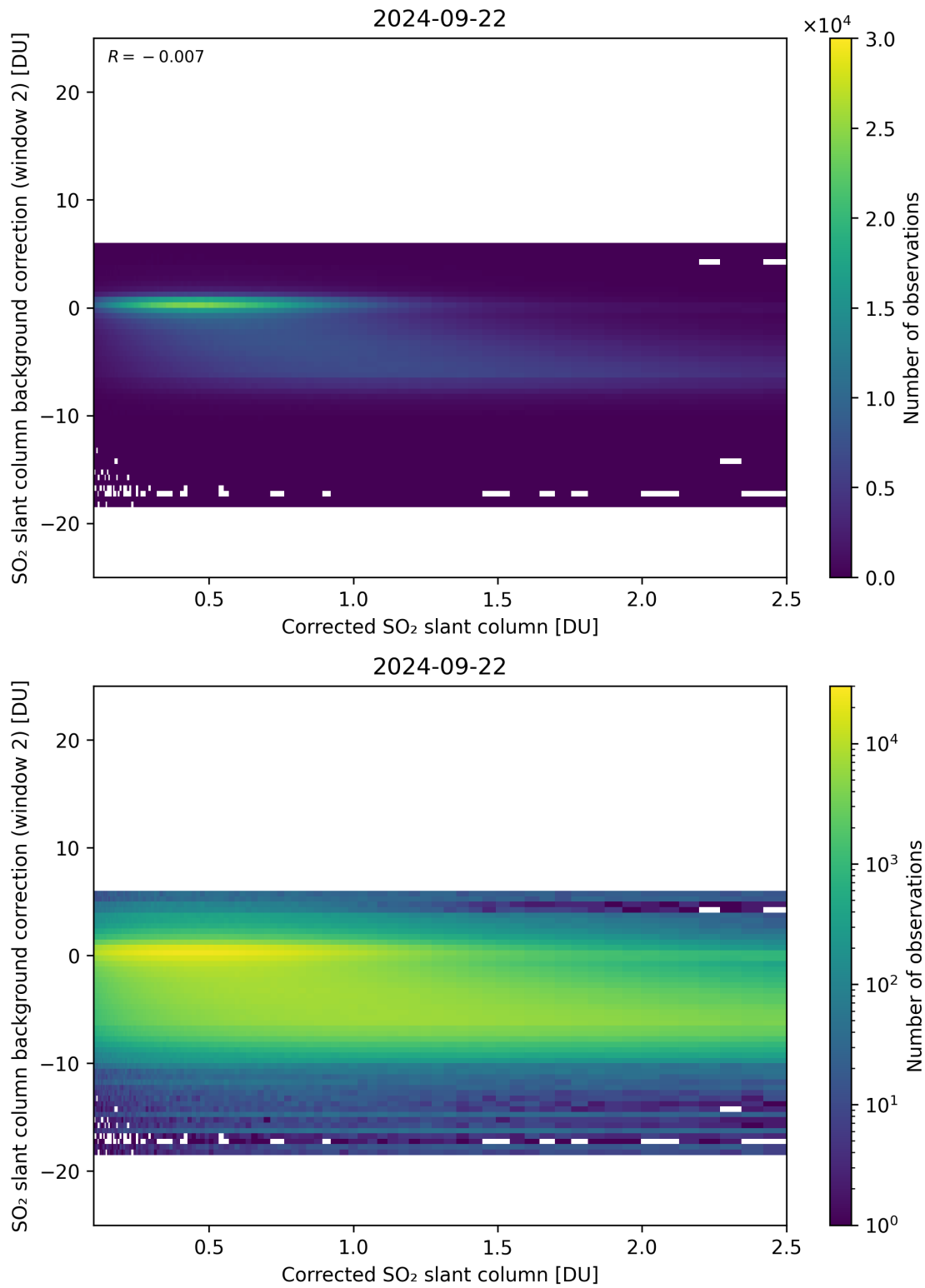
Figure 179: Scatter density plot of “Corrected SO 2 slant column” against “SO 2 slant column background correction (window 2)” for 2024-09-22 to 2024-09-23.
