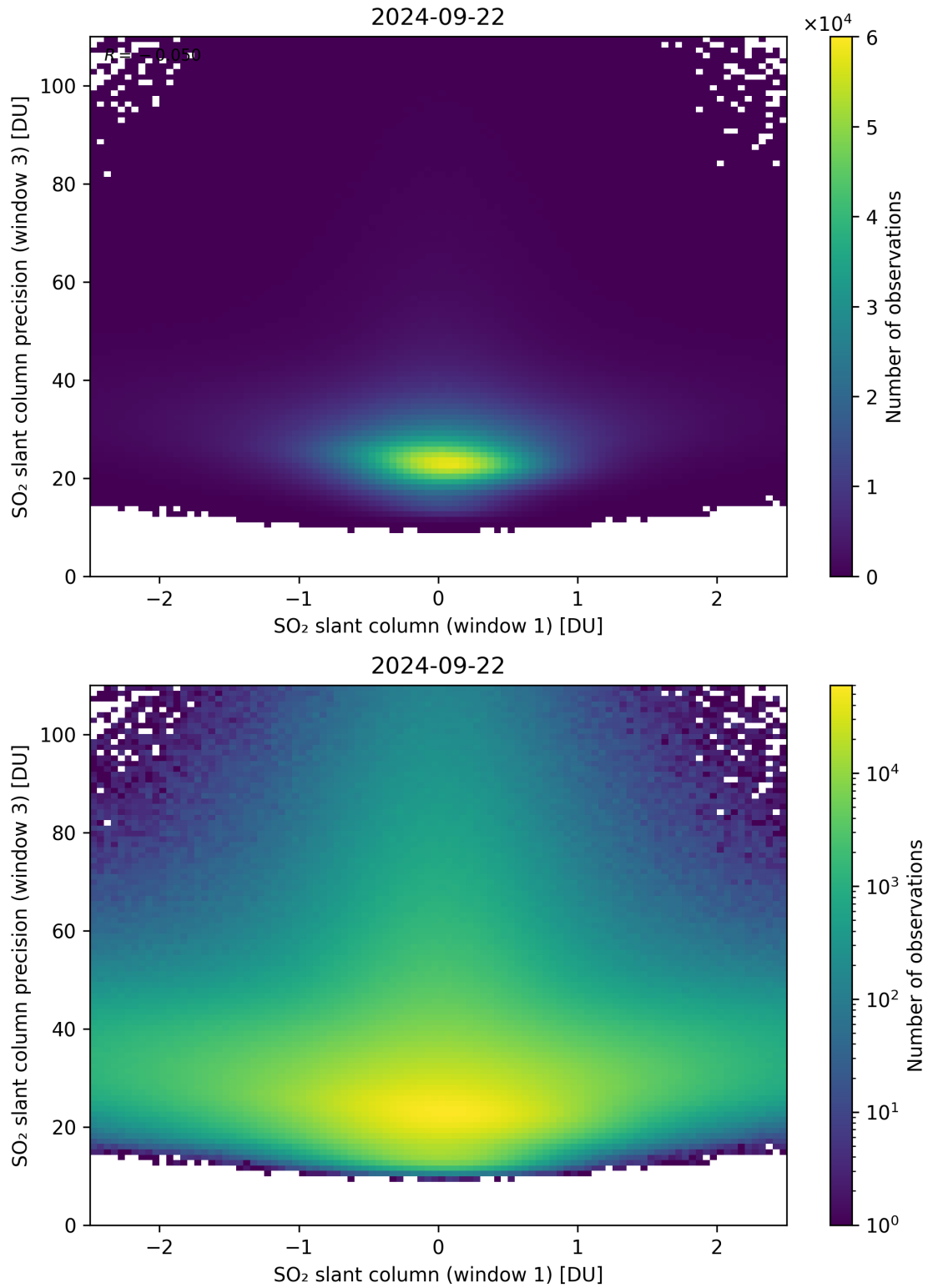
Figure 238: Scatter density plot of “SO 2 slant column (window 1)” against “SO 2 slant column precision (window 3)” for 2024-09-22 to 2024-09-23.
