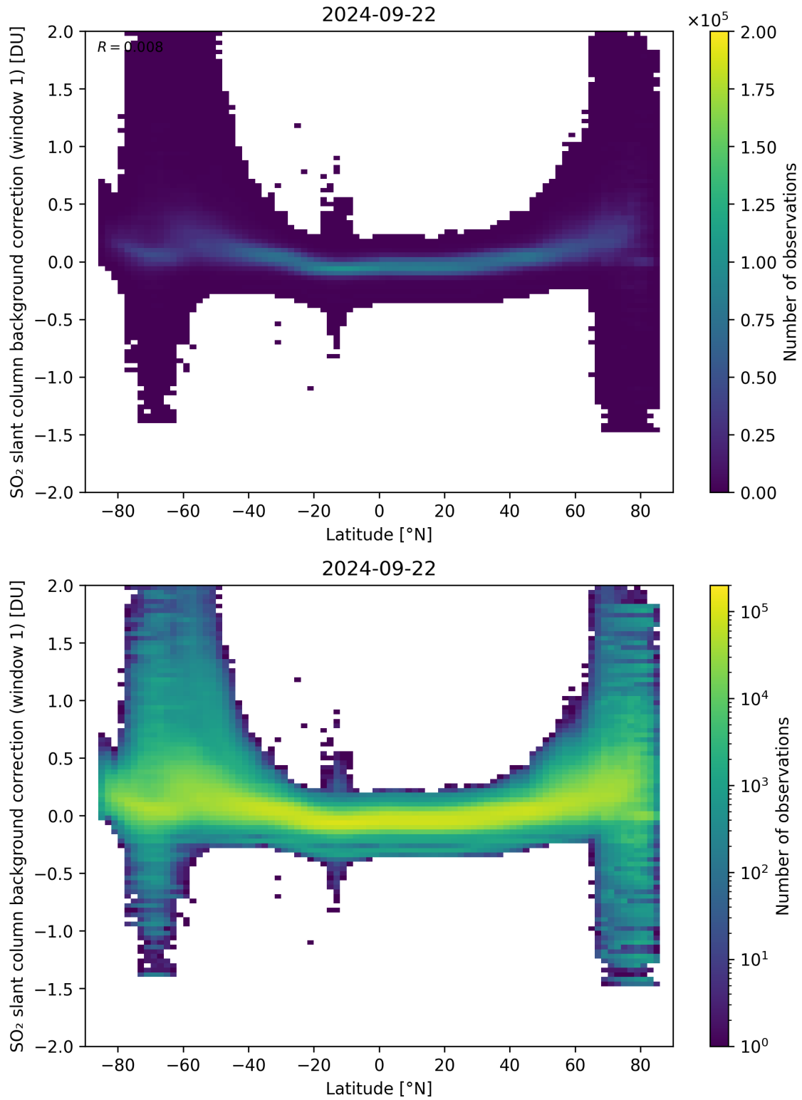
Figure 139: Scatter density plot of “Latitude” against “SO 2 slant column background correction (window 1)” for 2024-09-22 to 2024-09-23.
