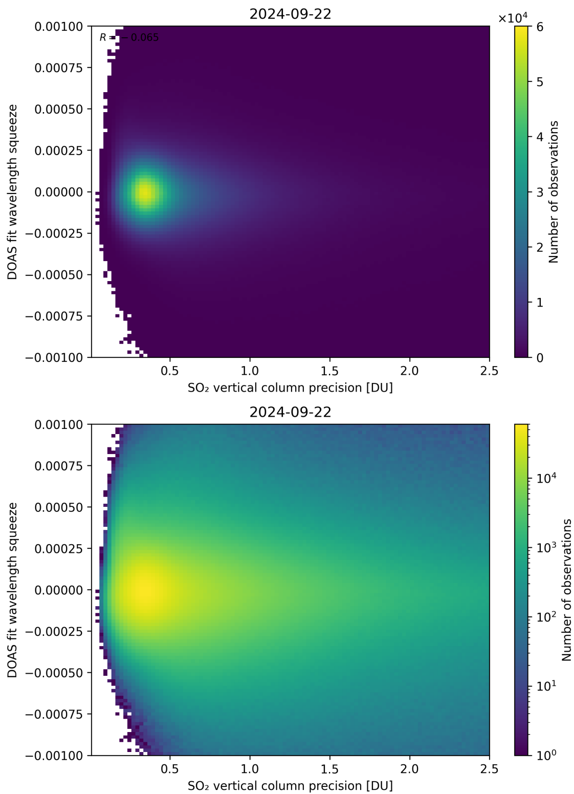
Figure 283: Scatter density plot of “SO 2 vertical column precision” against “DOAS fit wavelength squeeze” for 2024-09-22 to 2024-09-23.
