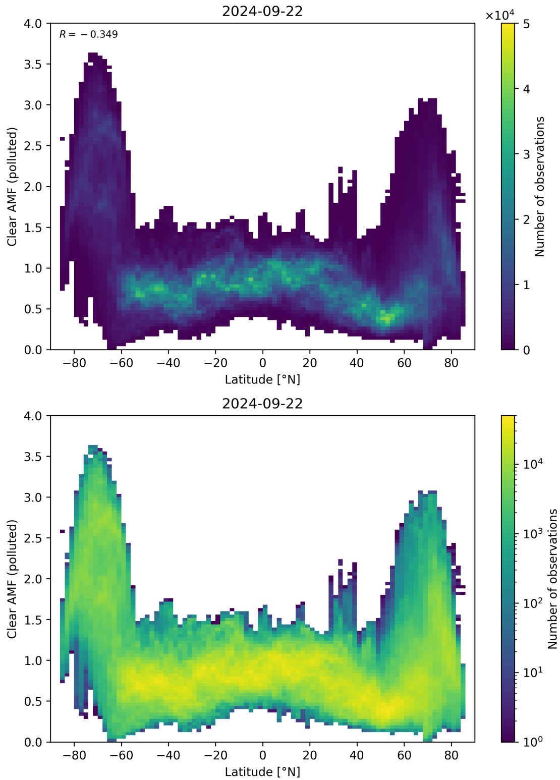
Figure 145: Scatter density plot of “Latitude” against “Clear AMF (polluted)” for 2024-09-22 to 2024-09-23.
