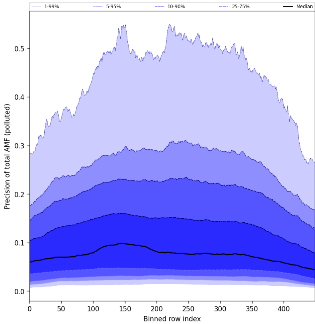
Figure 95: Along track statistics of “Precision of total AMF (polluted)” for 2024-09-22 to 2024-09-23
