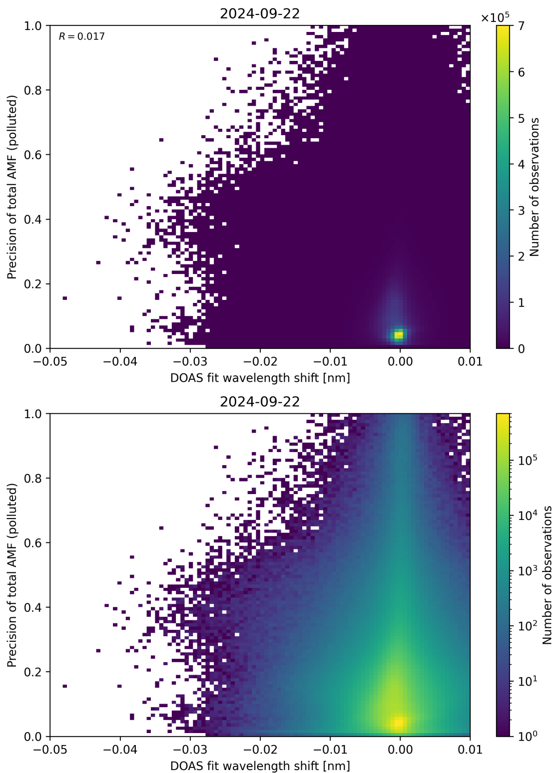
Figure 131: Scatter density plot of “DOAS fit wavelength shift” against “Precision of total AMF (polluted)” for 2024-09-22 to 2024-09-23.
