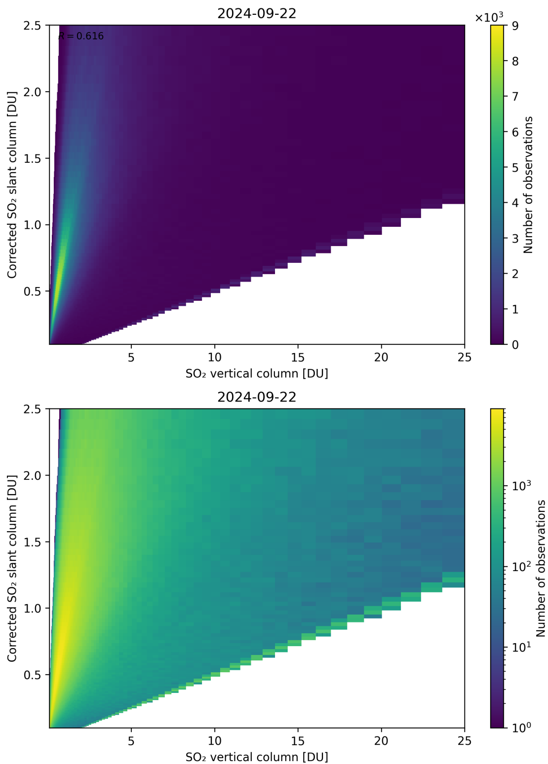
Figure 297: Scatter density plot of “SO 2 vertical column” against “Corrected SO 2 slant column” for 2024-09-22 to 2024-09-23.
