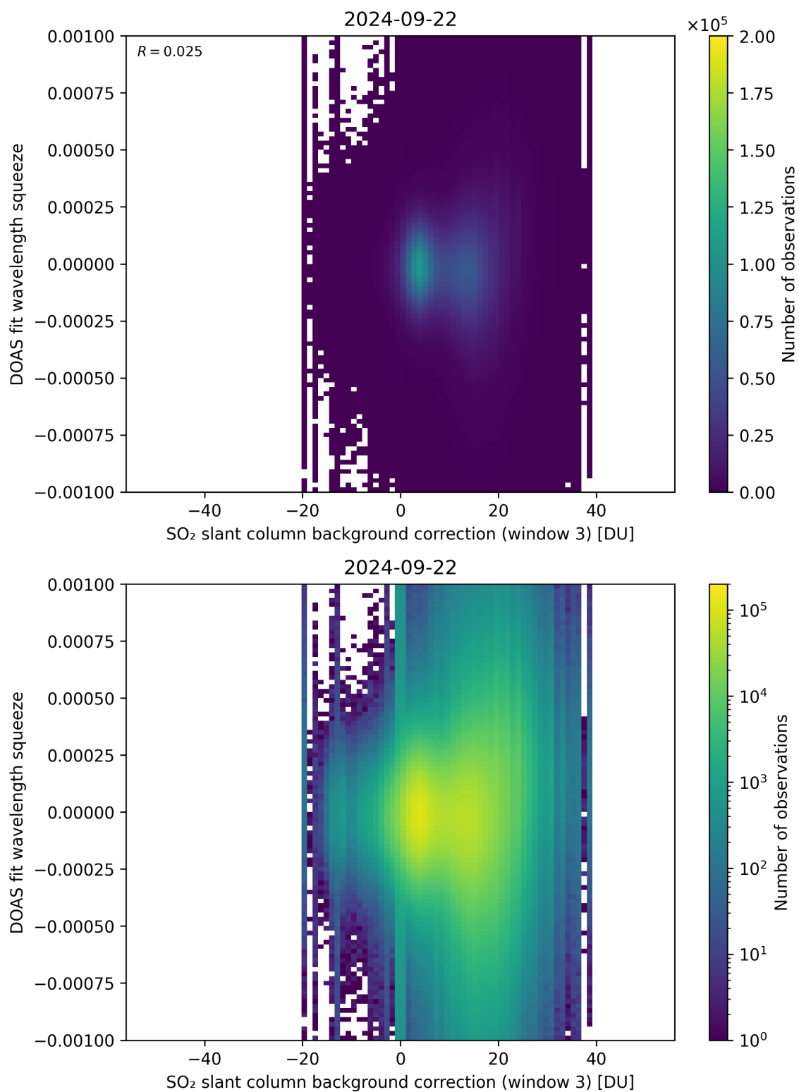
Figure 122: Scatter density plot of “SO 2 slant column background correction (window 3)” against “DOAS fit wavelength squeeze” for 2024-09-22 to 2024-09-23.
