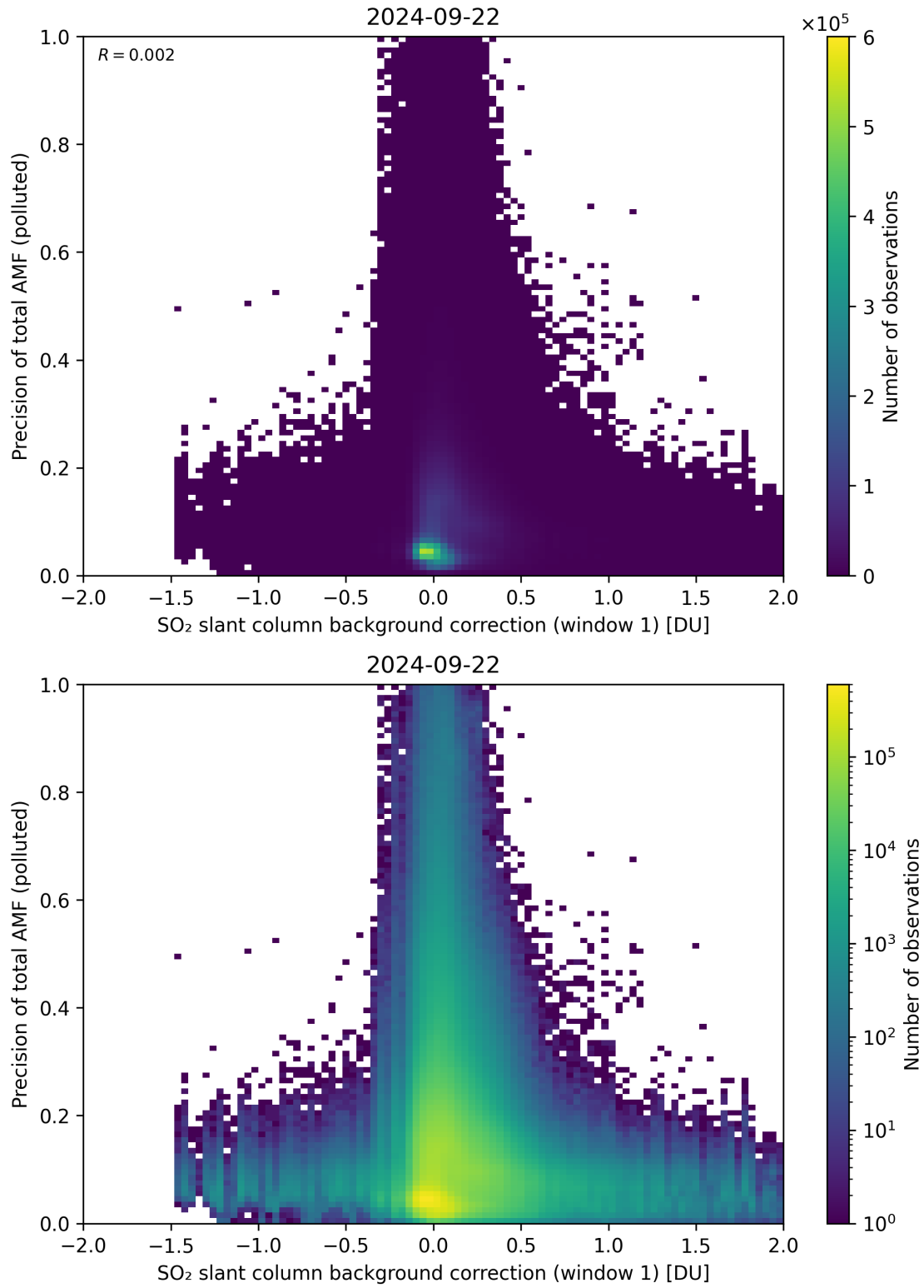
Figure 110: Scatter density plot of “SO 2 slant column background correction (window 1)” against “Precision of total AMF (polluted)” for 2024-09-22 to 2024-09-23.
