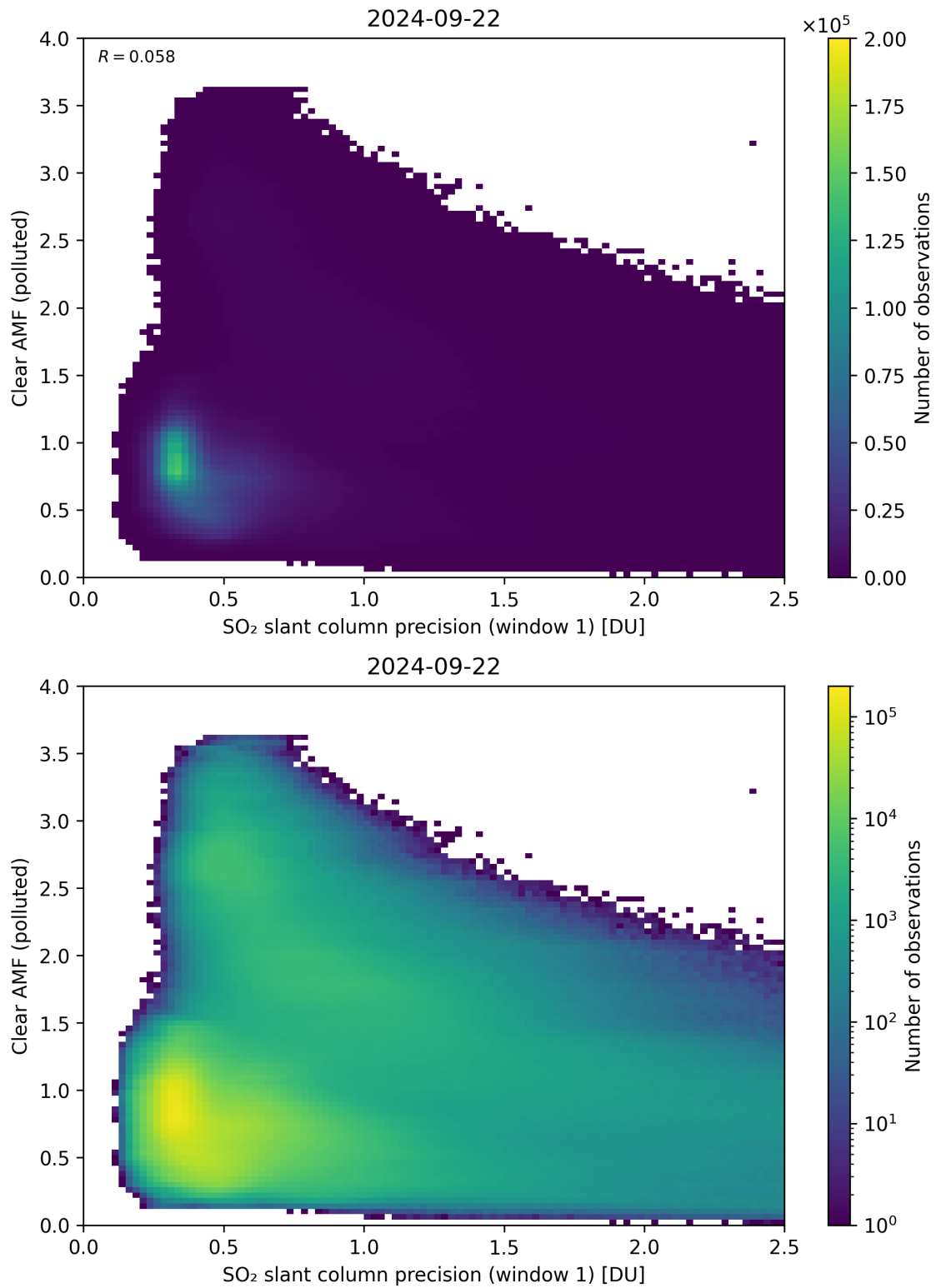
Figure 224: Scatter density plot of “SO 2 slant column precision (window 1)” against “Clear AMF (polluted)” for 2024-09-22 to 2024-09-23.
