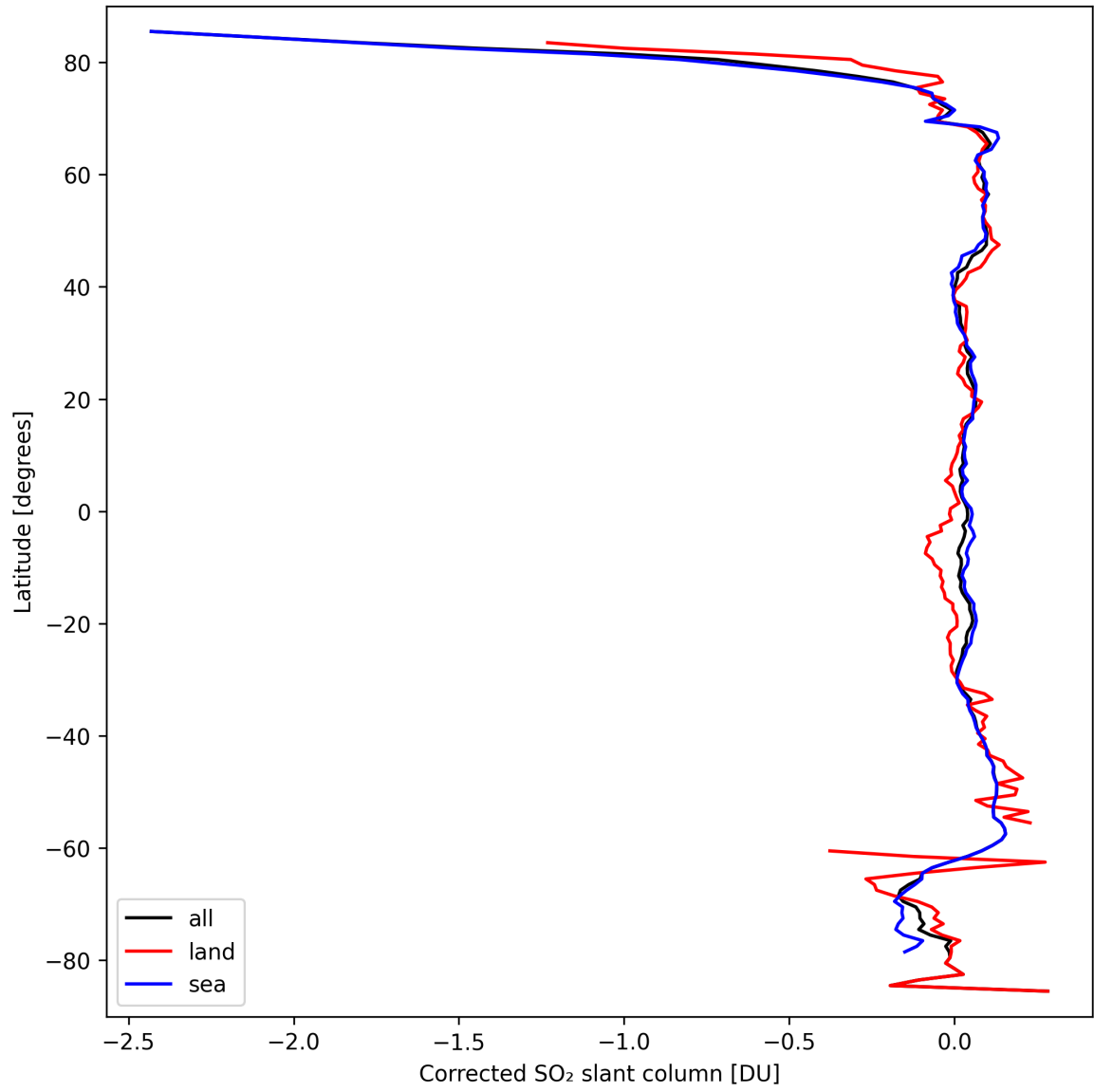
Figure 32: Zonal average of “Corrected SO 2 slant column” for 2024-09-22 to 2024-09-23.
