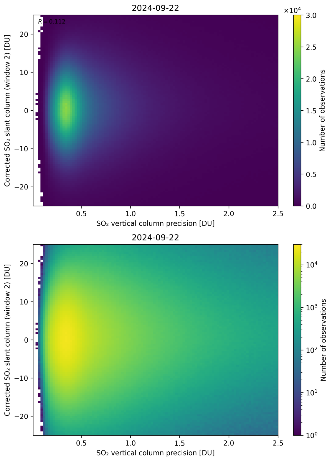
Figure 287: Scatter density plot of “SO 2 vertical column precision” against “Corrected SO 2 slant column (window 2)” for 2024-09-22 to 2024-09-23.
