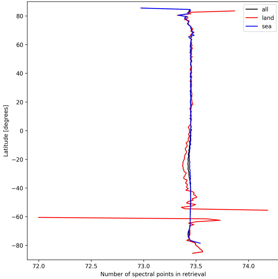
Figure 51: Zonal average of “Number of spectral points in retrieval” for 2024-09-22 to 2024-09-23.
