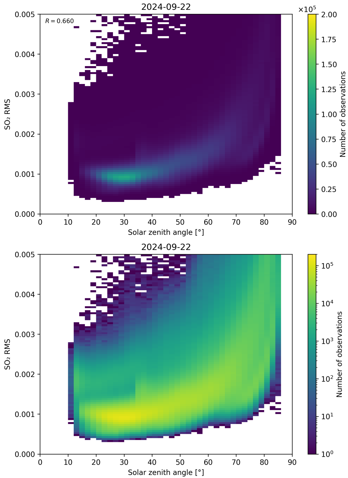
Figure 163: Scatter density plot of “Solar zenith angle” against “SO 2 RMS” for 2024-09-22 to 2024-09-23.
