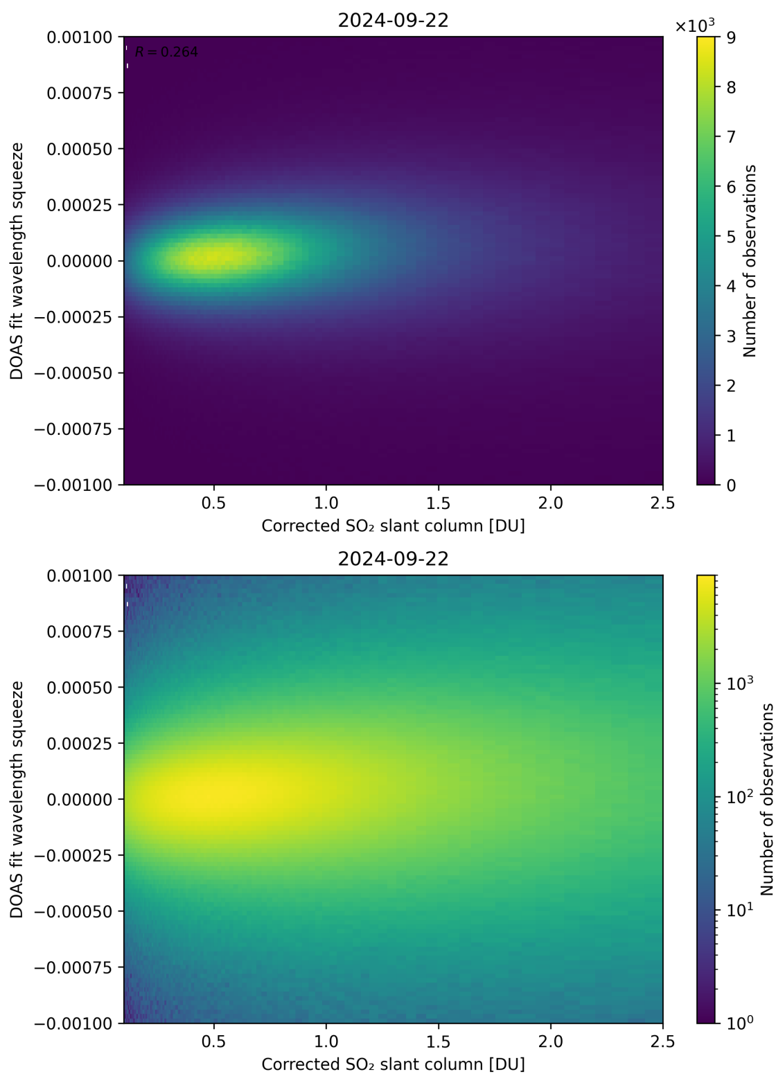
Figure 182: Scatter density plot of “Corrected SO 2 slant column” against “DOAS fit wavelength squeeze” for 2024-09-22 to 2024-09-23.
