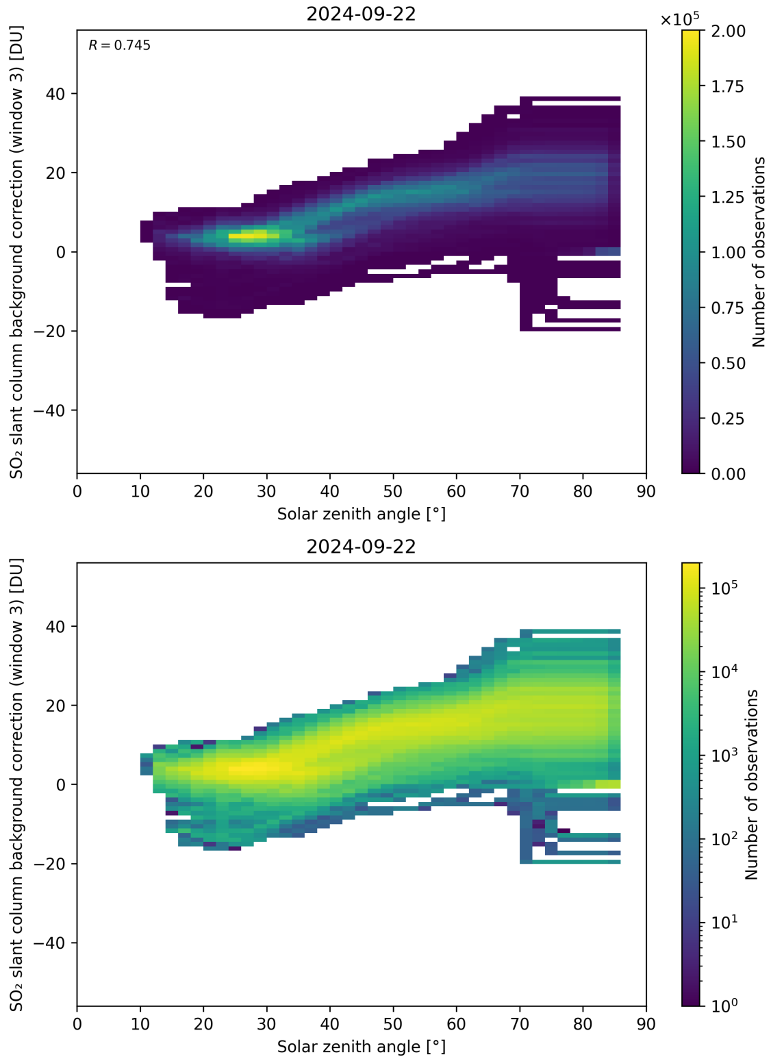
Figure 160: Scatter density plot of “Solar zenith angle” against “SO 2 slant column background correction (window 3)” for 2024-09-22 to 2024-09-23.
