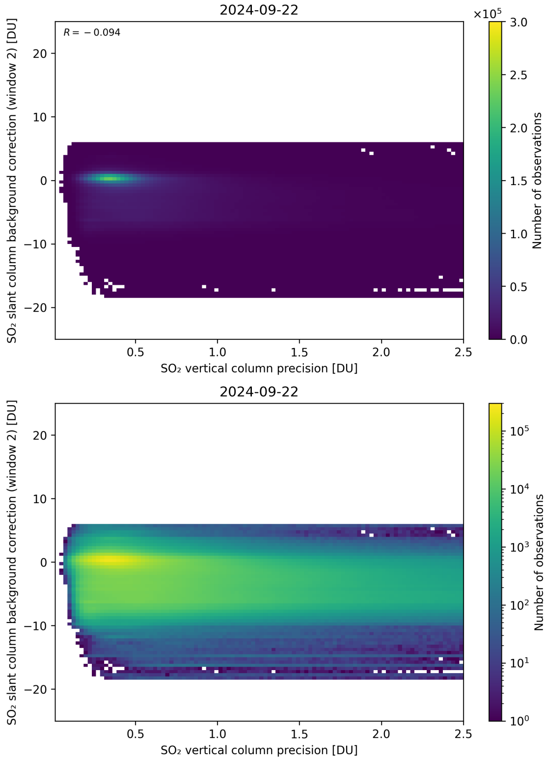
Figure 280: Scatter density plot of “SO 2 vertical column precision” against “SO 2 slant column background correction (window 2)” for 2024-09-22 to 2024-09-23.
