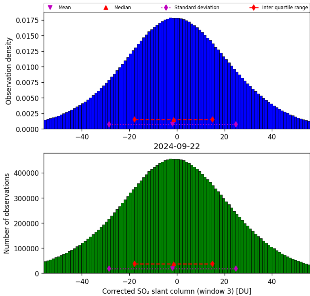
Figure 66: Histogram of “Corrected SO 2 slant column (window 3)” for 2024-09-22 to 2024-09-23
