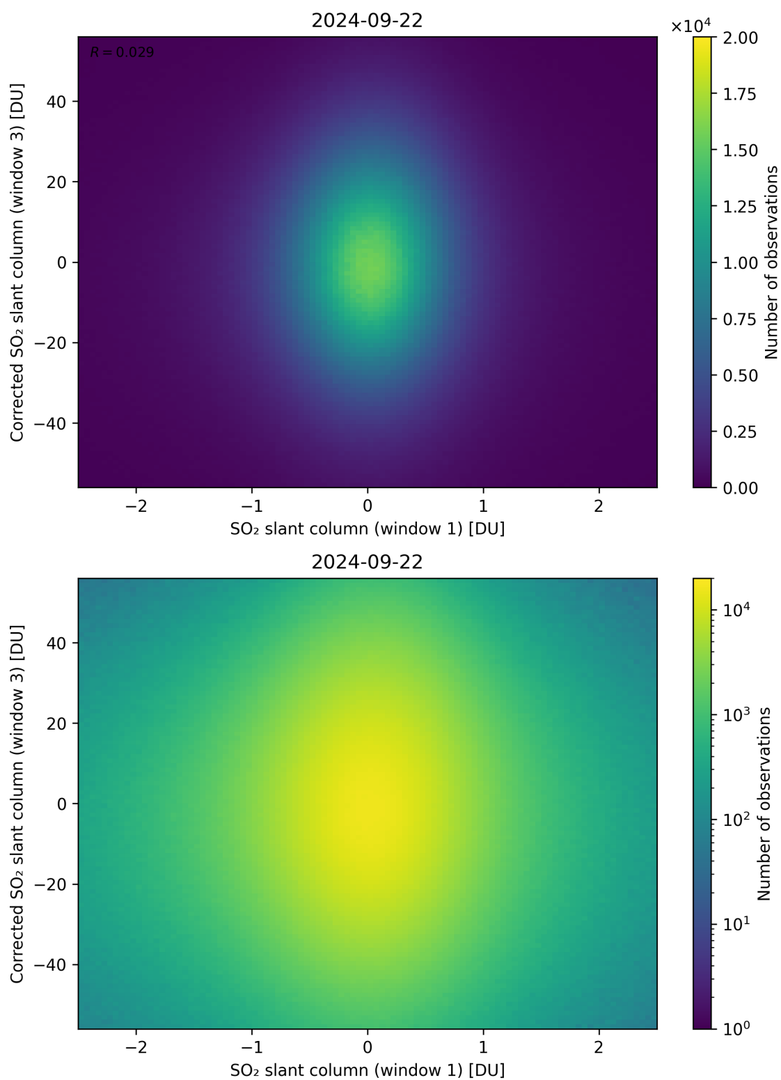
Figure 234: Scatter density plot of “SO 2 slant column (window 1)” against “Corrected SO 2 slant column (window 3)” for 2024-09-22 to 2024-09-23.
