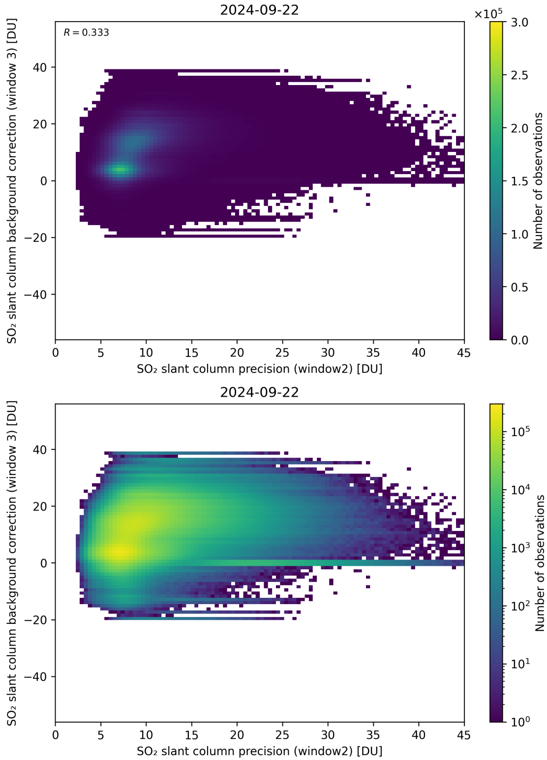
Figure 242: Scatter density plot of “SO 2 slant column precision (window2)” against “SO 2 slant column background correction (window 3)” for 2024-09-22 to 2024-09-23.
