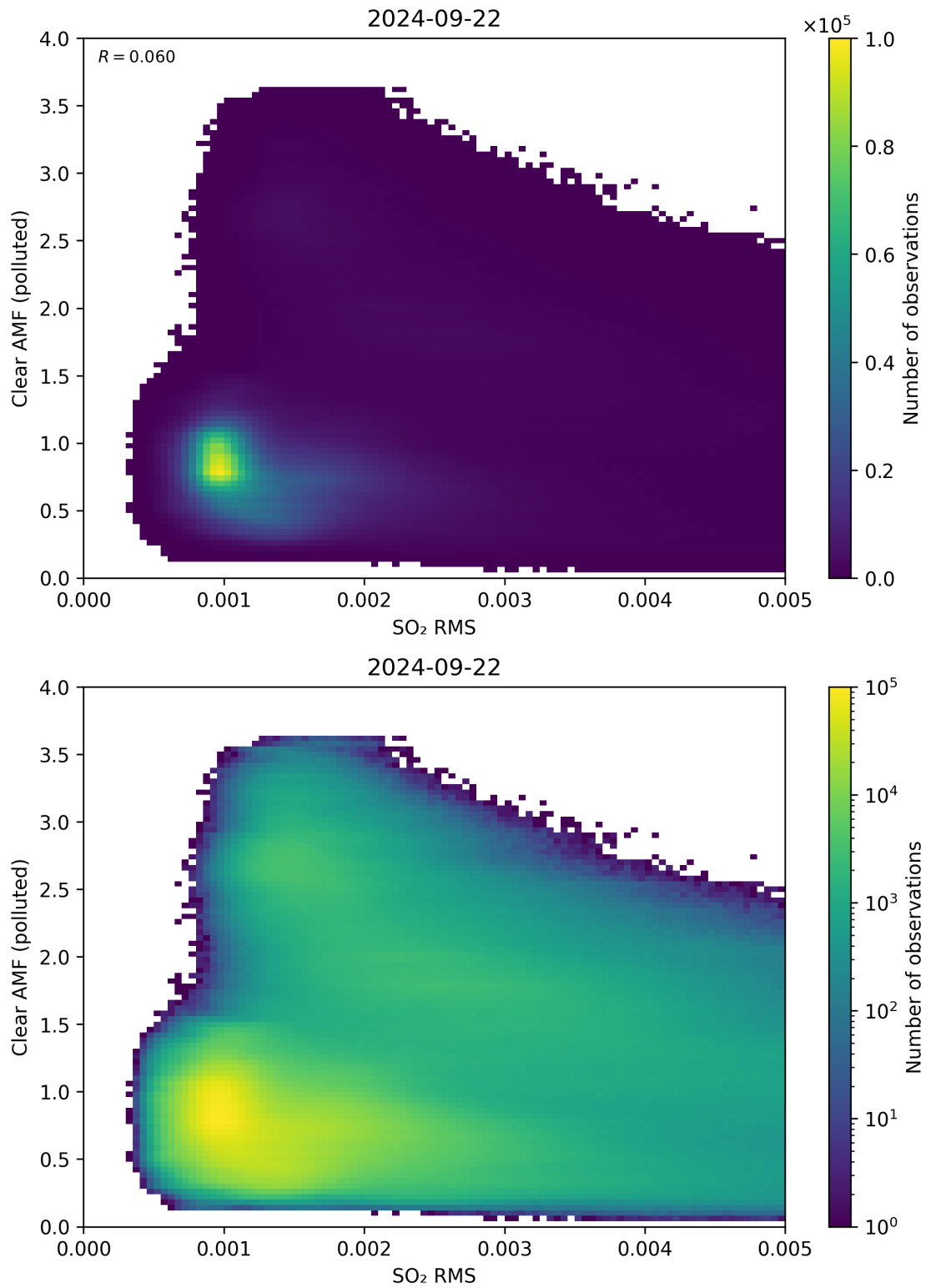
Figure 136: Scatter density plot of “SO 2 RMS” against “Clear AMF (polluted)” for 2024-09-22 to 2024-09-23.
