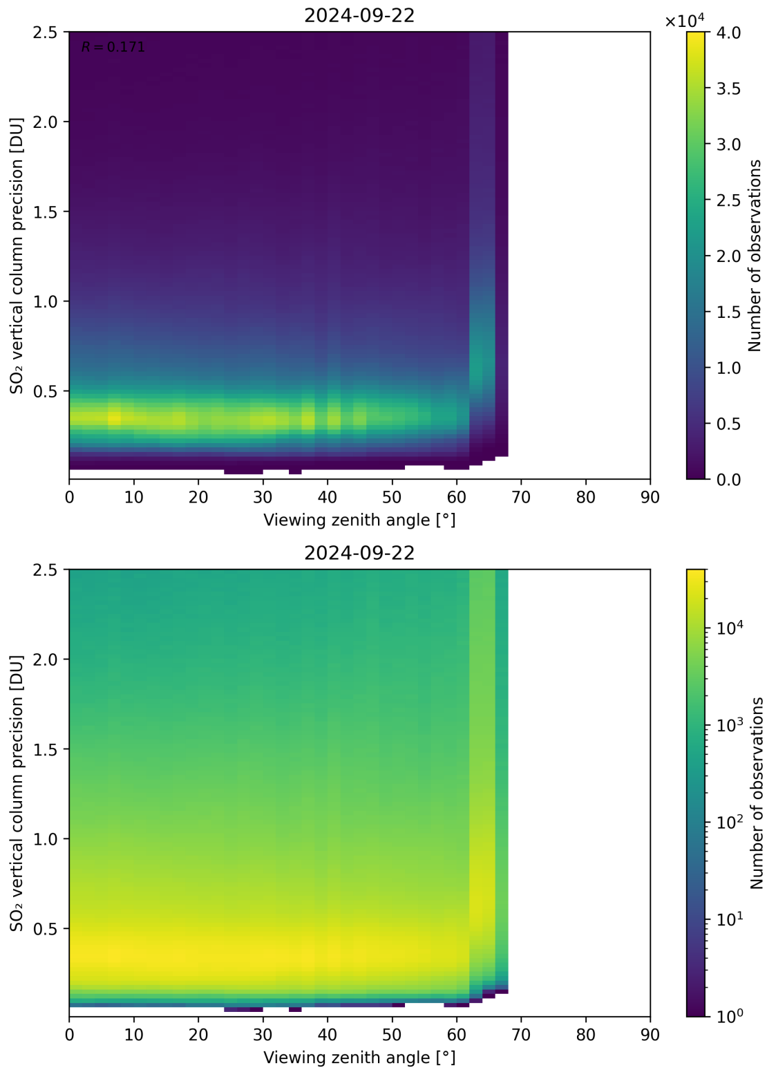
Figure 328: Scatter density plot of “Viewing zenith angle” against “SO 2 vertical column precision” for 2024-09-22 to 2024-09-23.
