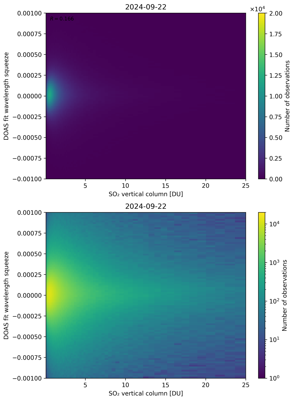
Figure 277: Scatter density plot of “SO 2 vertical column” against “DOAS fit wavelength squeeze” for 2024-09-22 to 2024-09-23.
