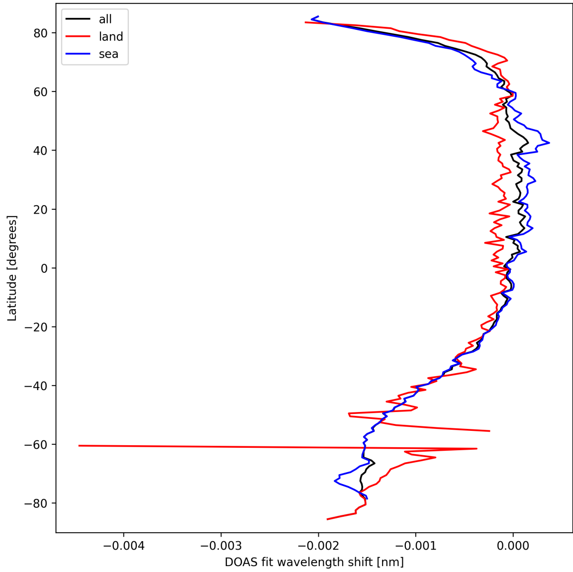
Figure 45: Zonal average of “DOAS fit wavelength shift” for 2024-09-22 to 2024-09-23.
