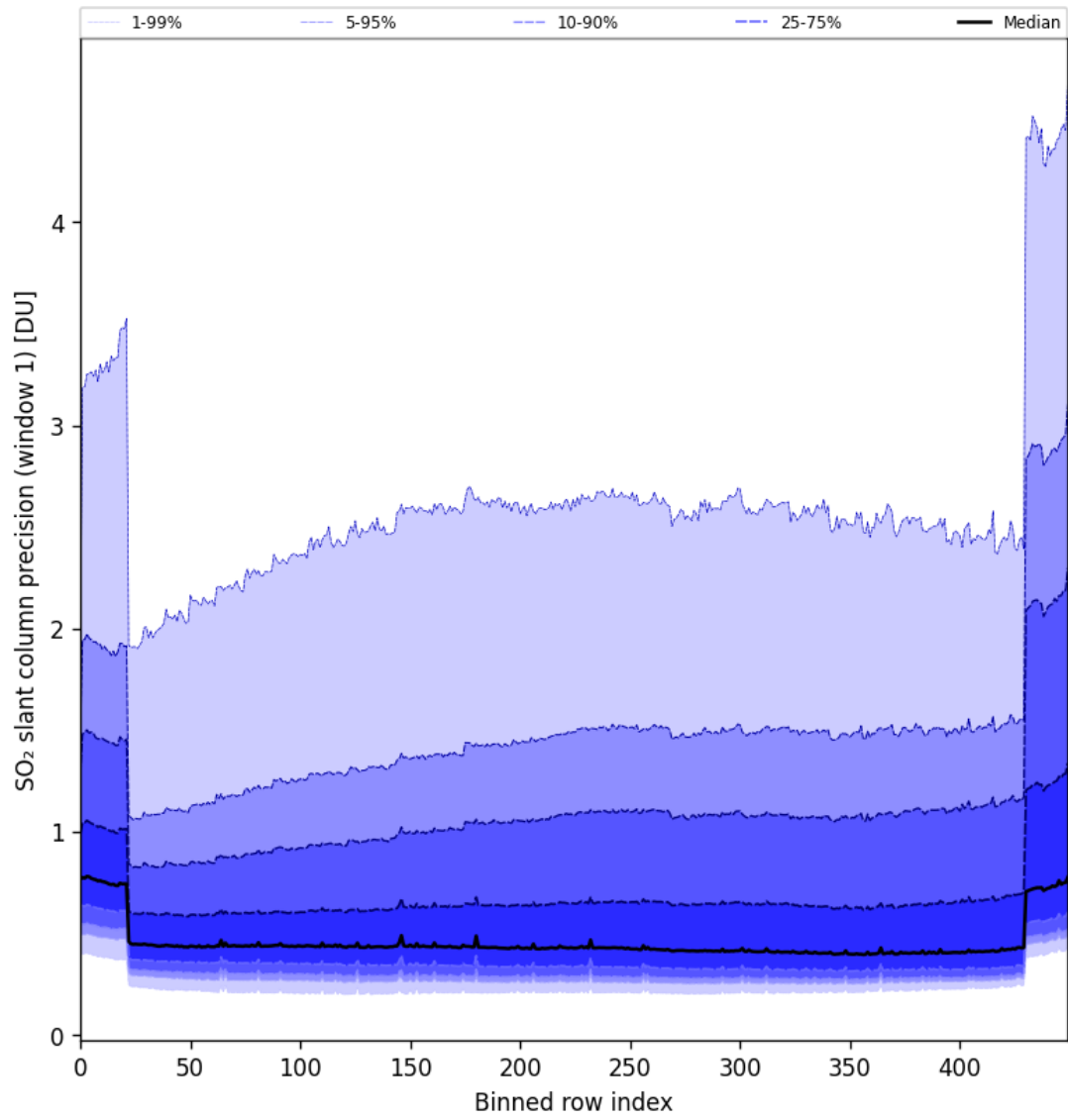
Figure 80: Along track statistics of “SO 2 slant column precision (window 1)” for 2024-09-22 to 2024-09-23
