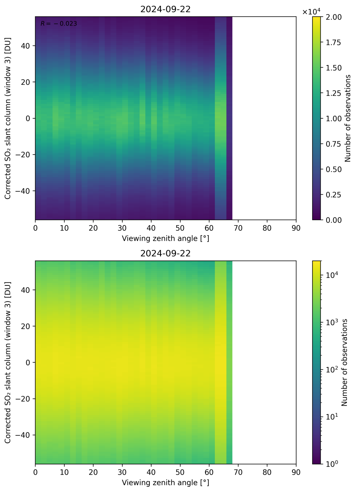
Figure 319: Scatter density plot of “Viewing zenith angle” against “Corrected SO 2 slant column (window 3)” for 2024-09-22 to 2024-09-23.
