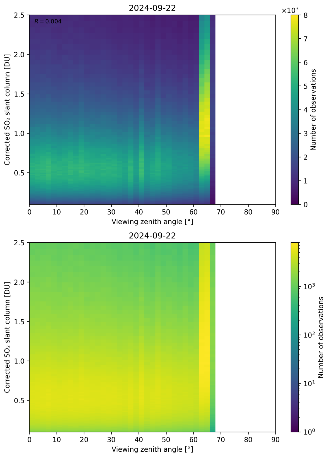
Figure 317: Scatter density plot of “Viewing zenith angle” against “Corrected SO 2 slant column” for 2024-09-22 to 2024-09-23.
