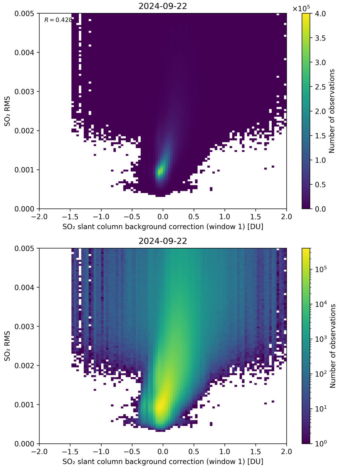
Figure 102: Scatter density plot of “SO 2 slant column background correction (window 1)” against “SO 2 RMS” for 2024-09-22 to 2024-09-23.
