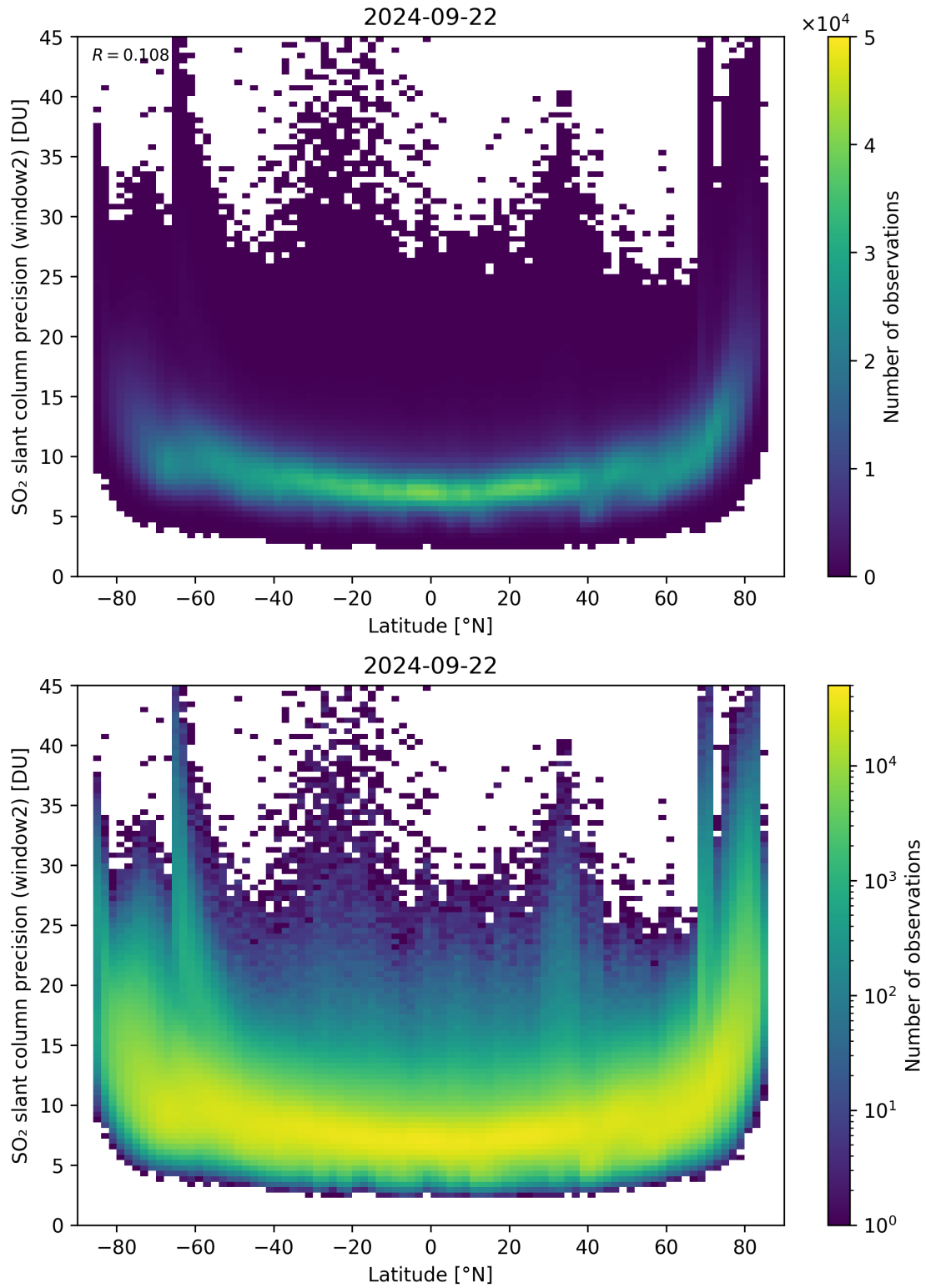
Figure 151: Scatter density plot of “Latitude” against “SO 2 slant column precision (window2)” for 2024-09-22 to 2024-09-23.
