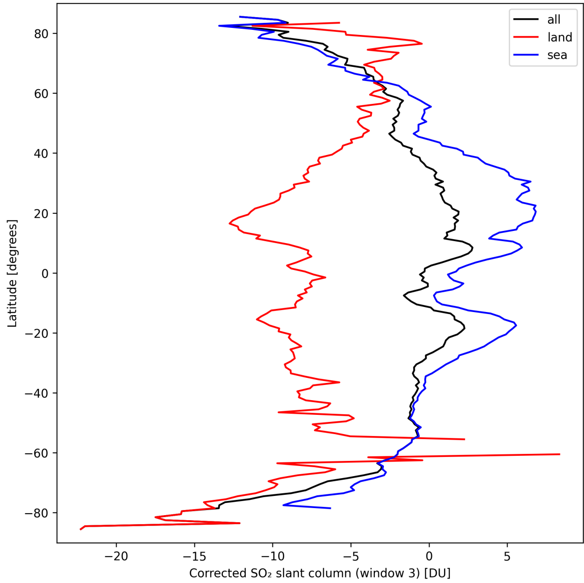
Figure 43: Zonal average of “Corrected SO 2 slant column (window 3)” for 2024-09-22 to 2024-09-23.
