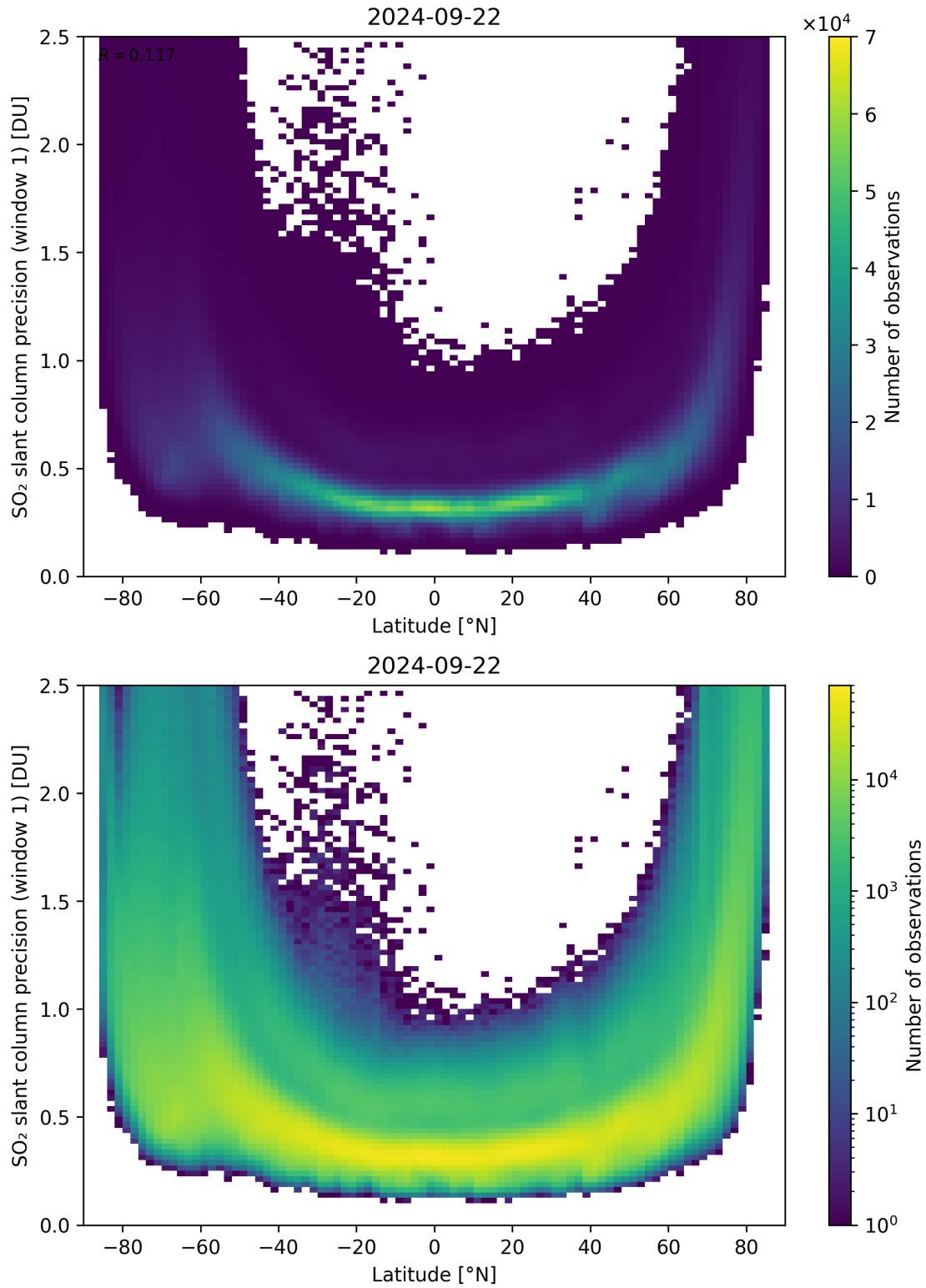
Figure 150: Scatter density plot of “Latitude” against “SO 2 slant column precision (window 1)” for 2024-09-22 to 2024-09-23.
