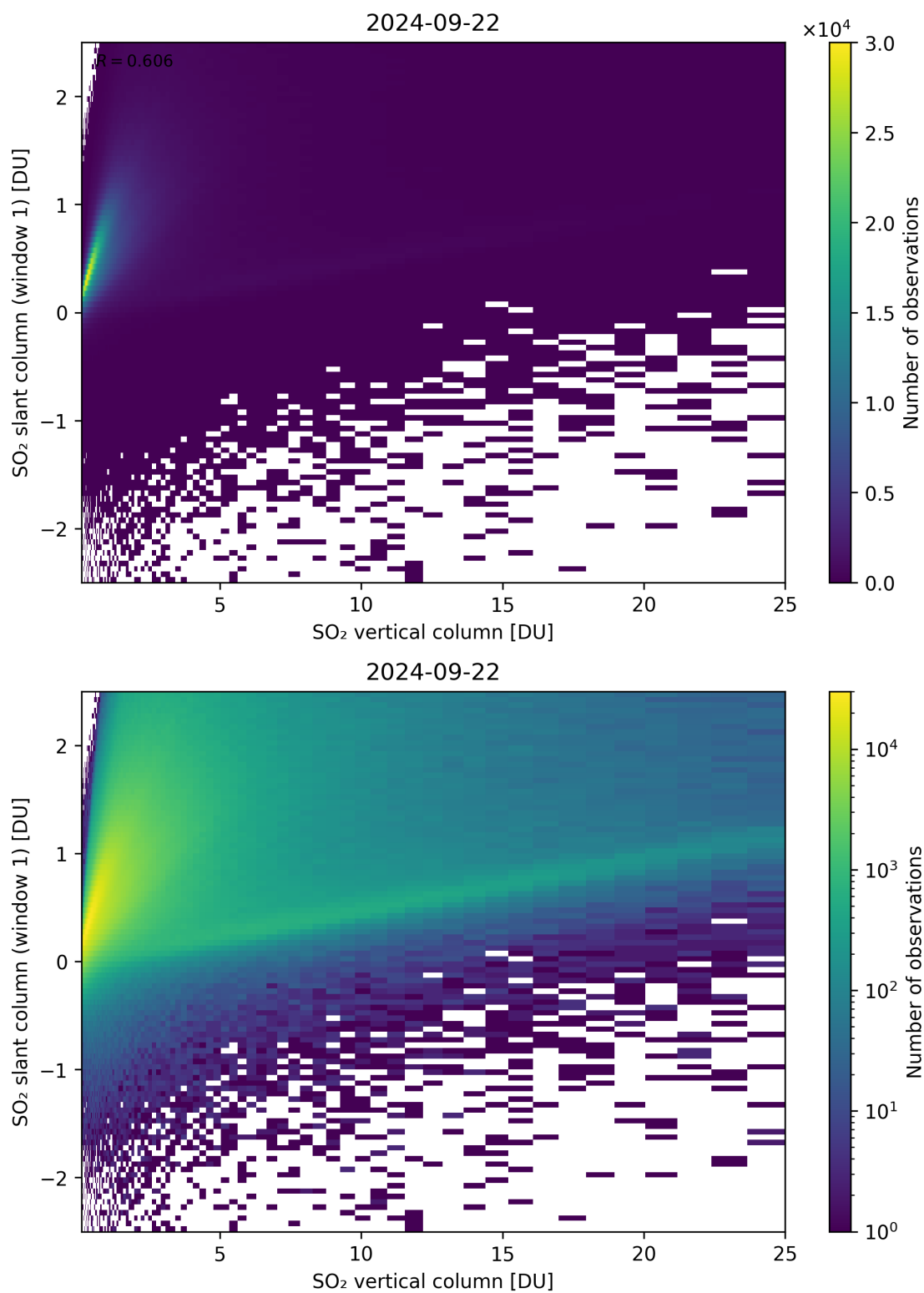
Figure 300: Scatter density plot of “SO 2 vertical column” against “SO 2 slant column (window 1)” for 2024-09-22 to 2024-09-23.
