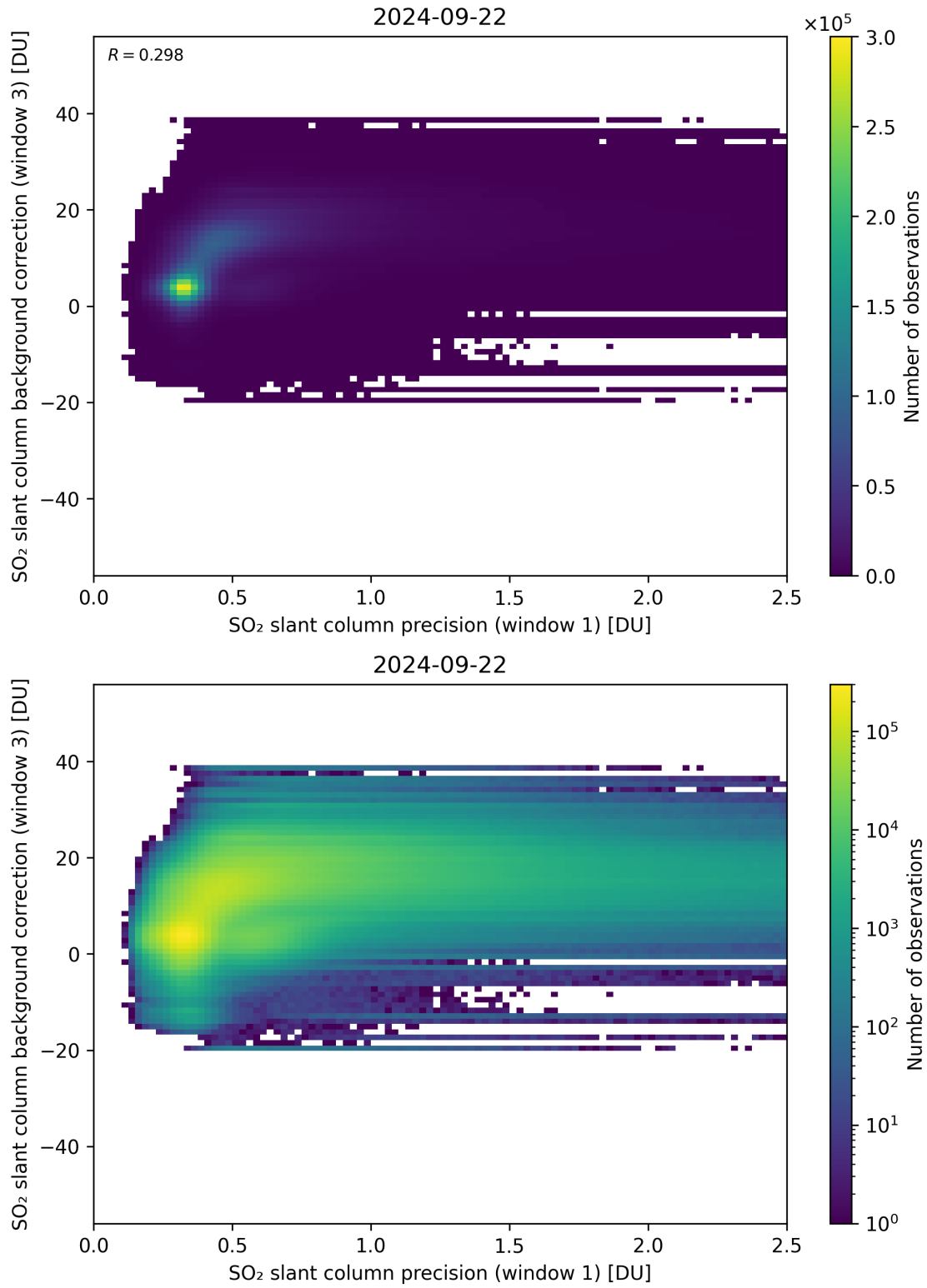
Figure 220: Scatter density plot of “SO 2 slant column precision (window 1)” against “SO 2 slant column background correction (window 3)” for 2024-09-22 to 2024-09-23.
