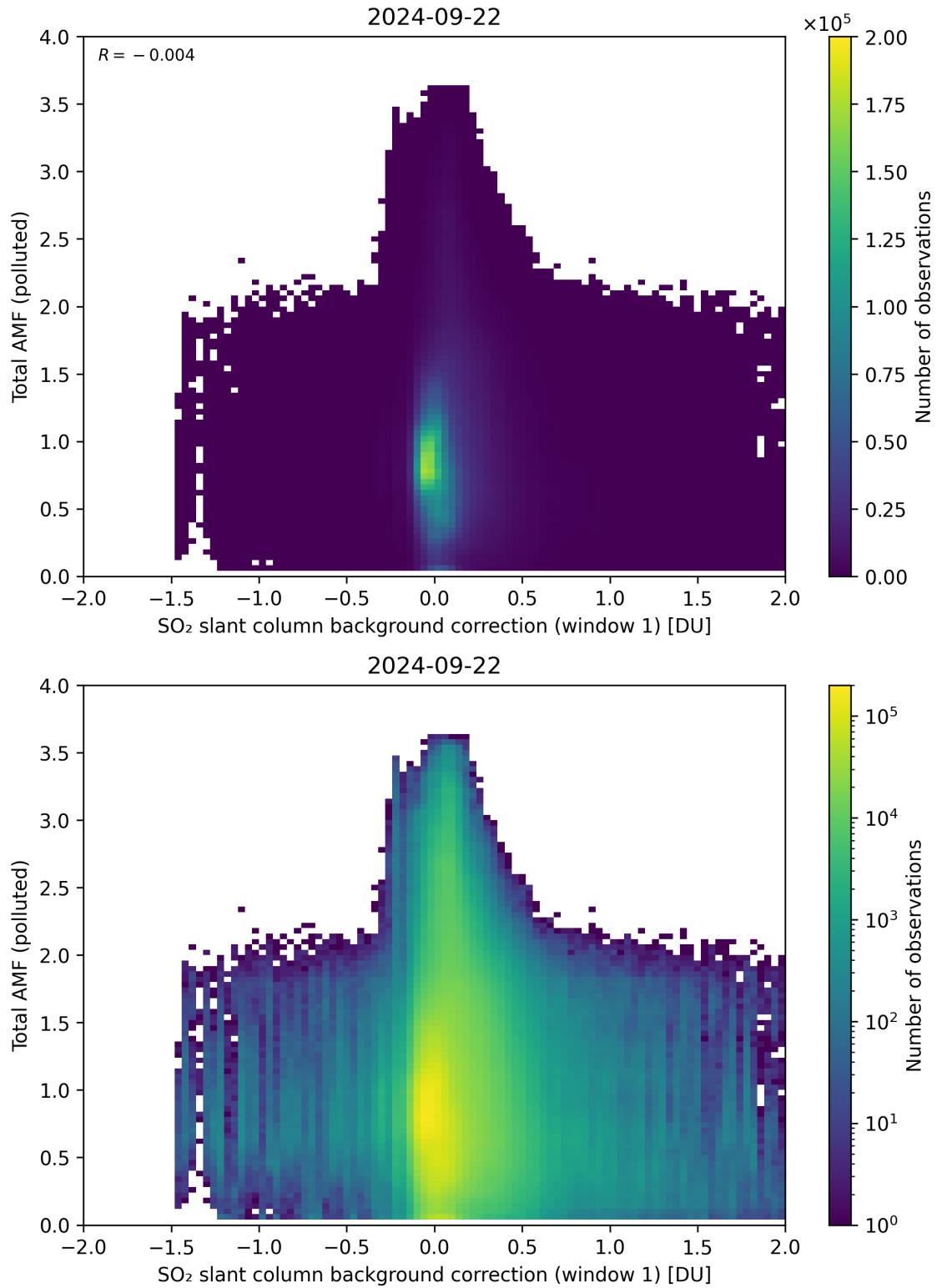
Figure 109: Scatter density plot of “SO 2 slant column background correction (window 1)” against “Total AMF (polluted)” for 2024-09-22 to 2024-09-23.
