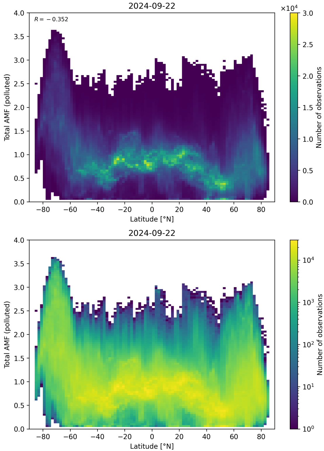
Figure 154: Scatter density plot of “Latitude” against “Total AMF (polluted)” for 2024-09-22 to 2024-09-23.
