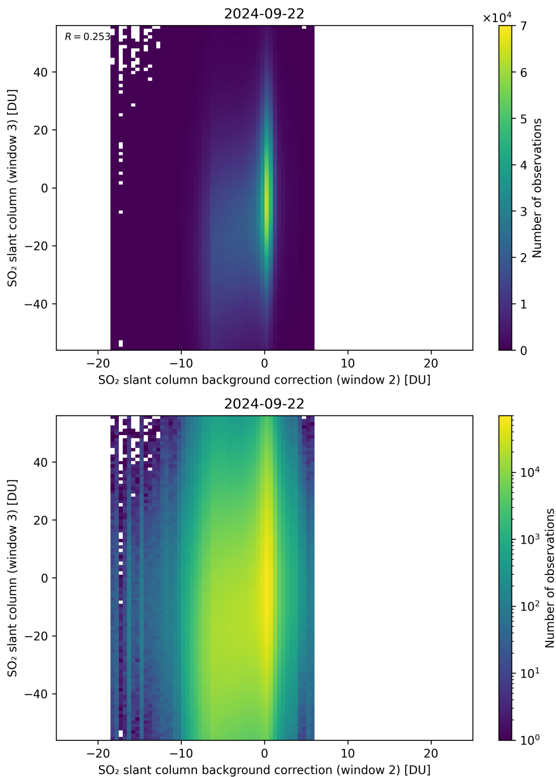
Figure 117: Scatter density plot of “SO 2 slant column background correction (window 2)” against “SO 2 slant column (window 3)” for 2024-09-22 to 2024-09-23.
