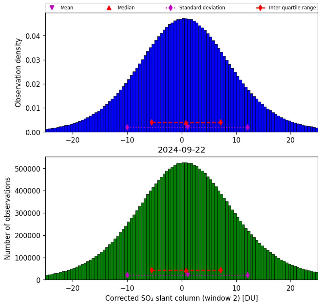
Figure 62: Histogram of “Corrected SO 2 slant column (window 2)” for 2024-09-22 to 2024-09-23
