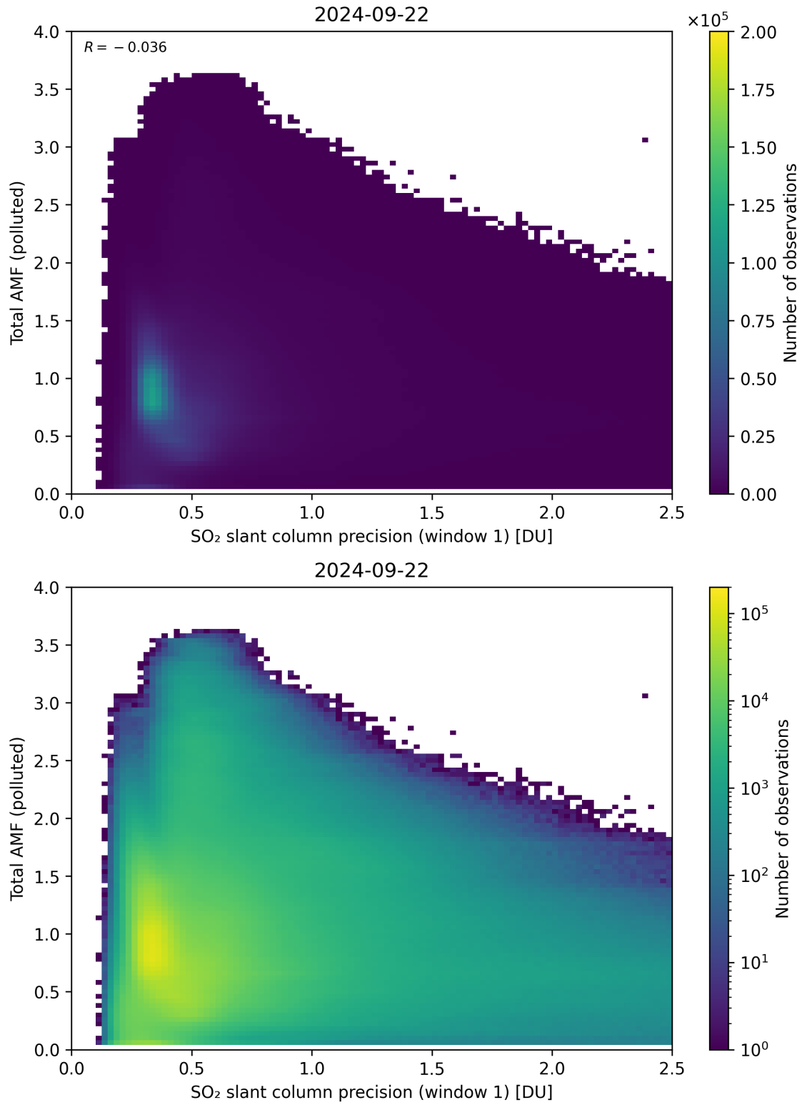
Figure 230: Scatter density plot of “SO 2 slant column precision (window 1)” against “Total AMF (polluted)” for 2024-09-22 to 2024-09-23.
