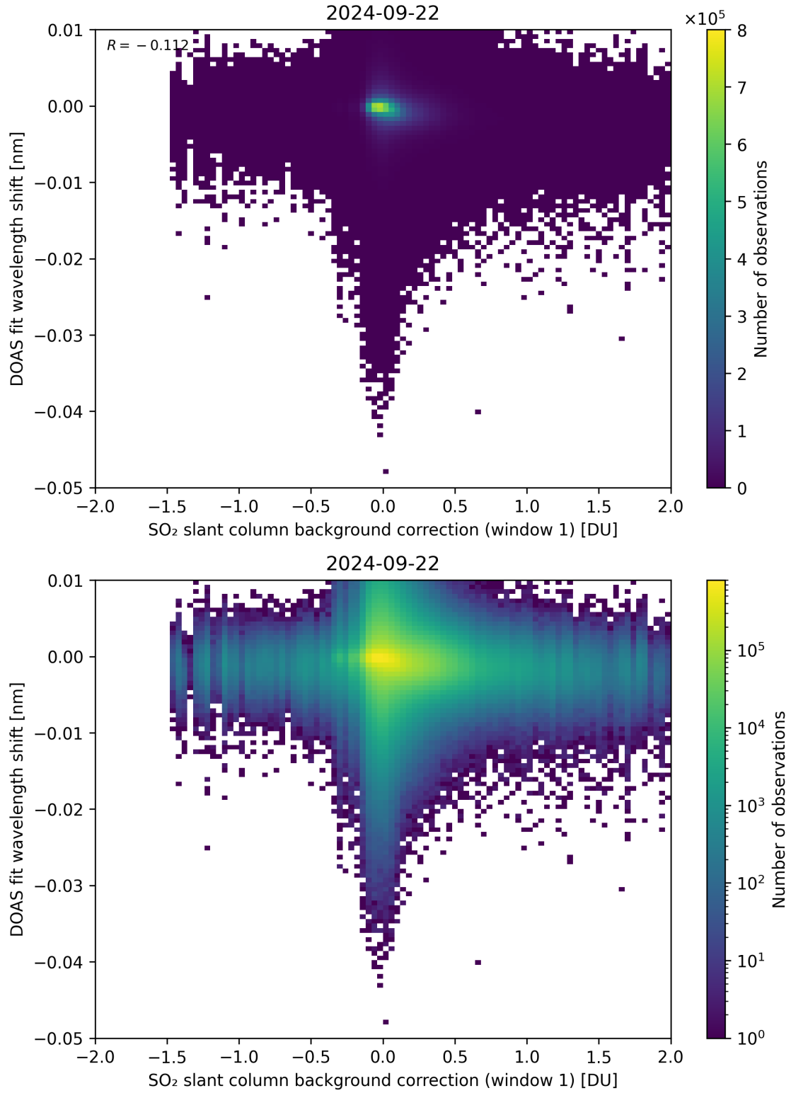
Figure 100: Scatter density plot of “SO 2 slant column background correction (window 1)” against “DOAS fit wavelength shift” for 2024-09-22 to 2024-09-23.
