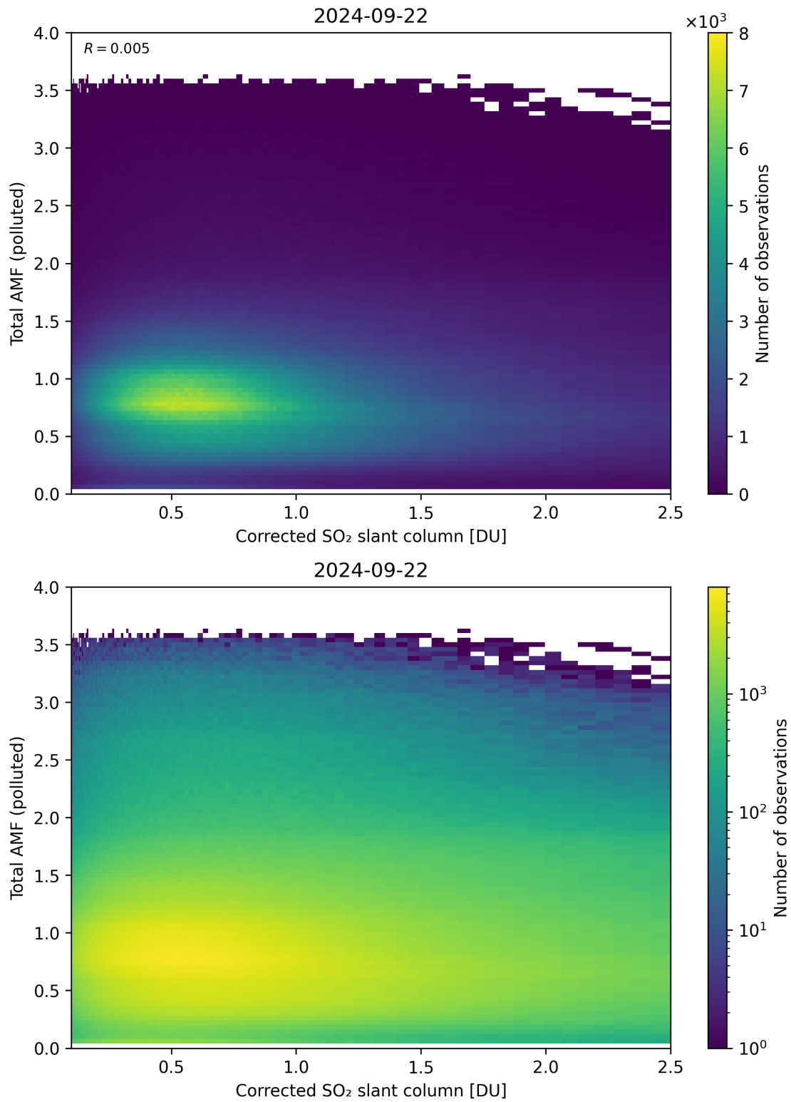
Figure 192: Scatter density plot of “Corrected SO 2 slant column” against “Total AMF (polluted)” for 2024-09-22 to 2024-09-23.
