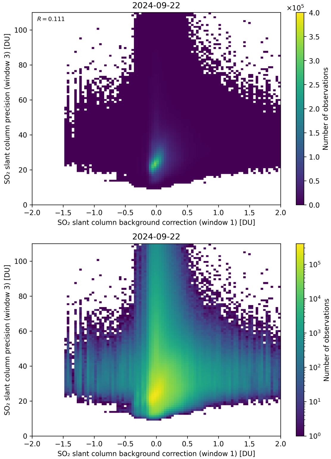
Figure 108: Scatter density plot of “SO 2 slant column background correction (window 1)” against “SO 2 slant column precision (window 3)” for 2024-09-22 to 2024-09-23.
