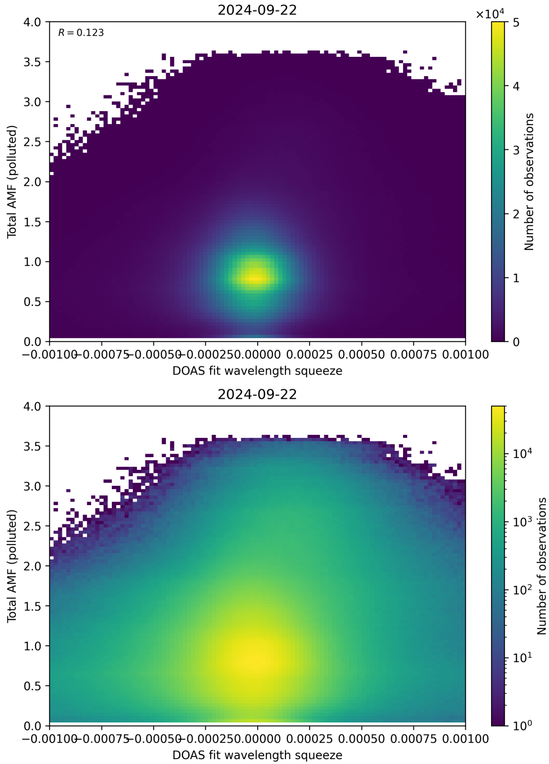
Figure 134: Scatter density plot of “DOAS fit wavelength squeeze” against “Total AMF (polluted)” for 2024-09-22 to 2024-09-23.
