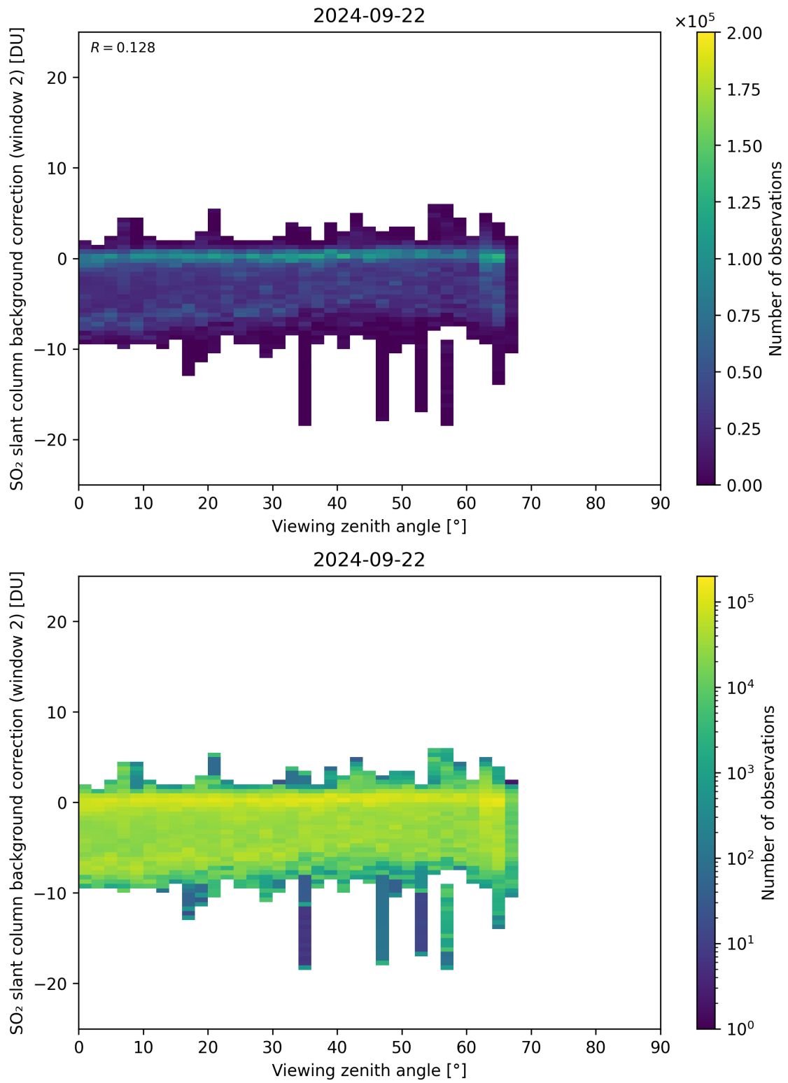
Figure 309: Scatter density plot of “Viewing zenith angle” against “SO 2 slant column background correction (window 2)” for 2024-09-22 to 2024-09-23.
