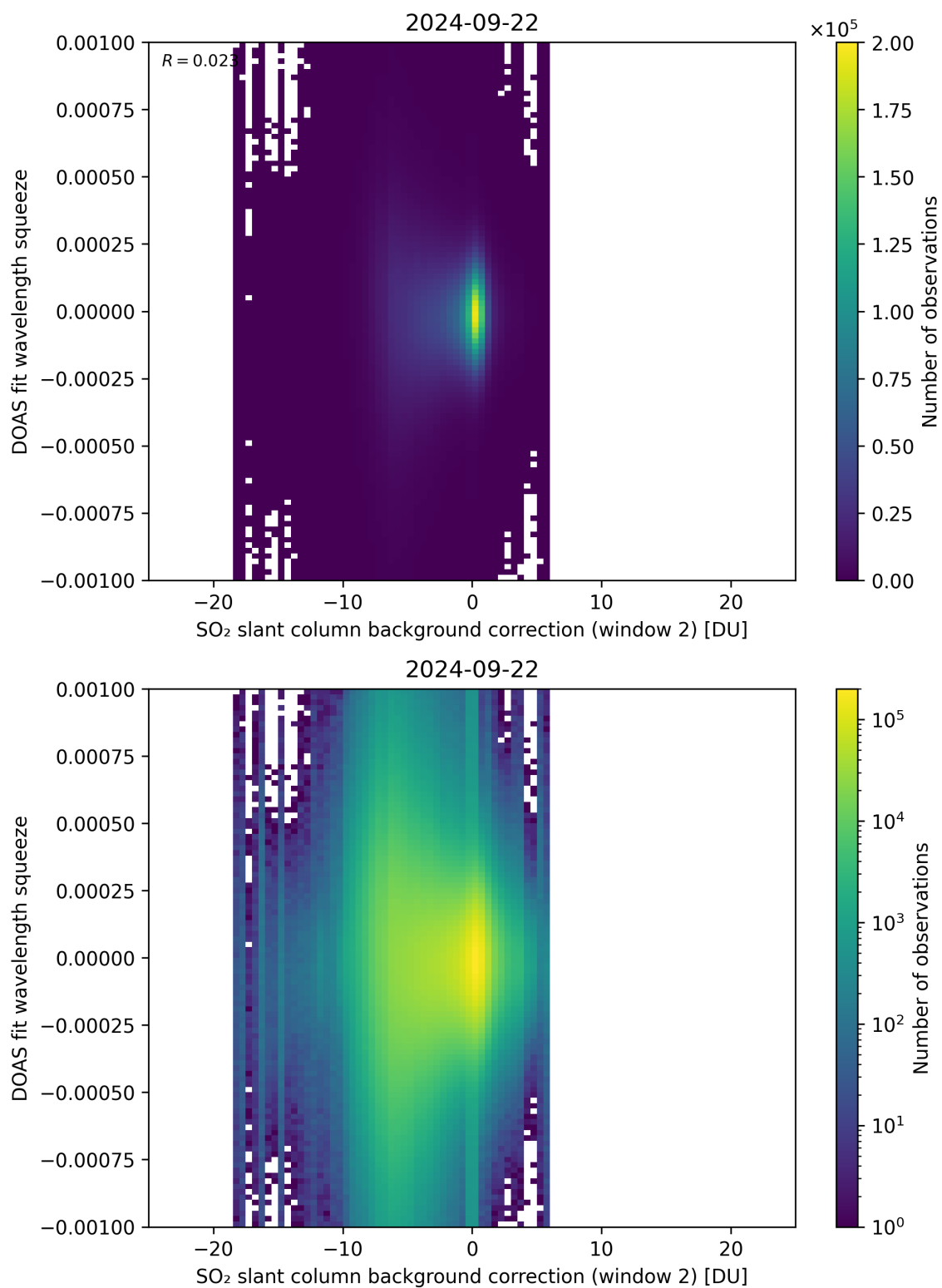
Figure 113: Scatter density plot of “SO 2 slant column background correction (window 2)” against “DOAS fit wavelength squeeze” for 2024-09-22 to 2024-09-23.
