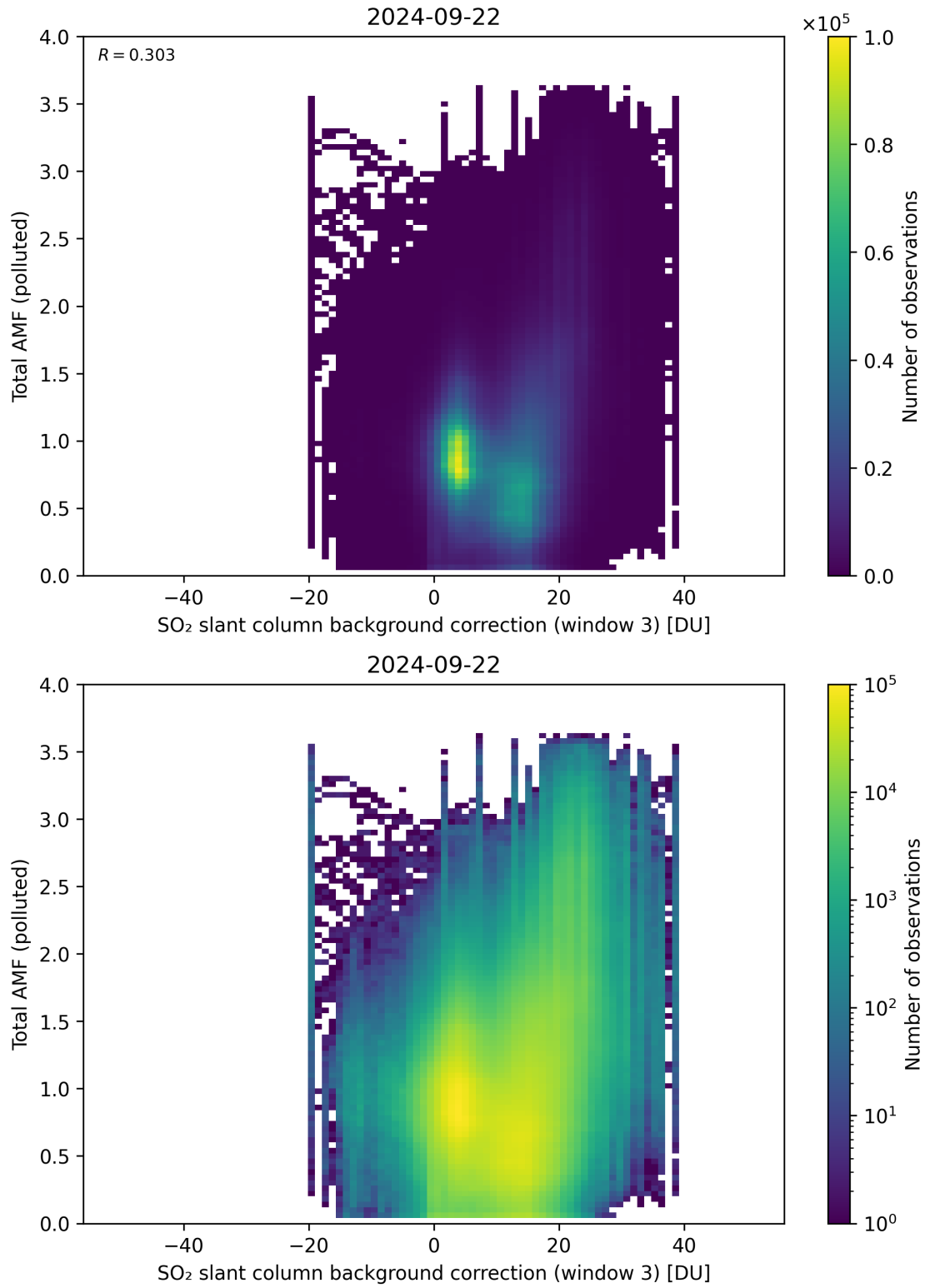
Figure 125: Scatter density plot of “SO 2 slant column background correction (window 3)” against “Total AMF (polluted)” for 2024-09-22 to 2024-09-23.
