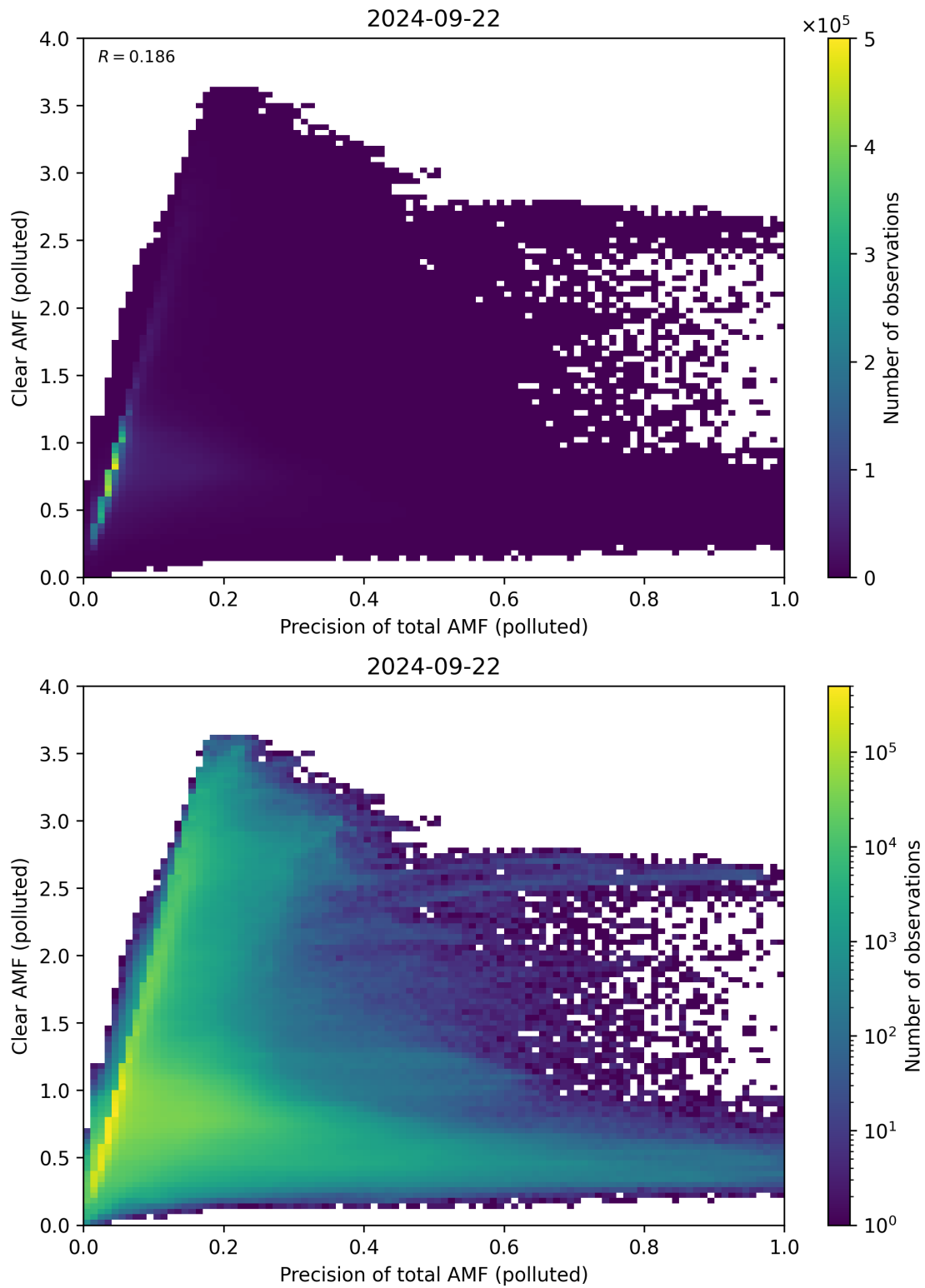
Figure 270: Scatter density plot of “Precision of total AMF (polluted)” against “Clear AMF (polluted)” for 2024-09-22 to 2024-09-23.
