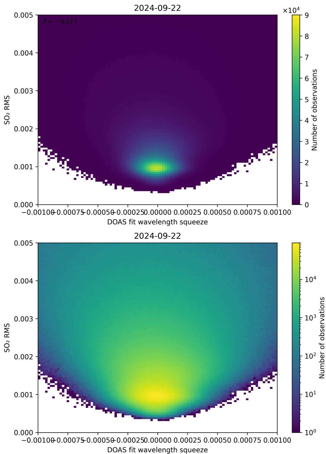
Figure 132: Scatter density plot of “DOAS fit wavelength squeeze” against “SO 2 RMS” for 2024-09-22 to 2024-09-23.
