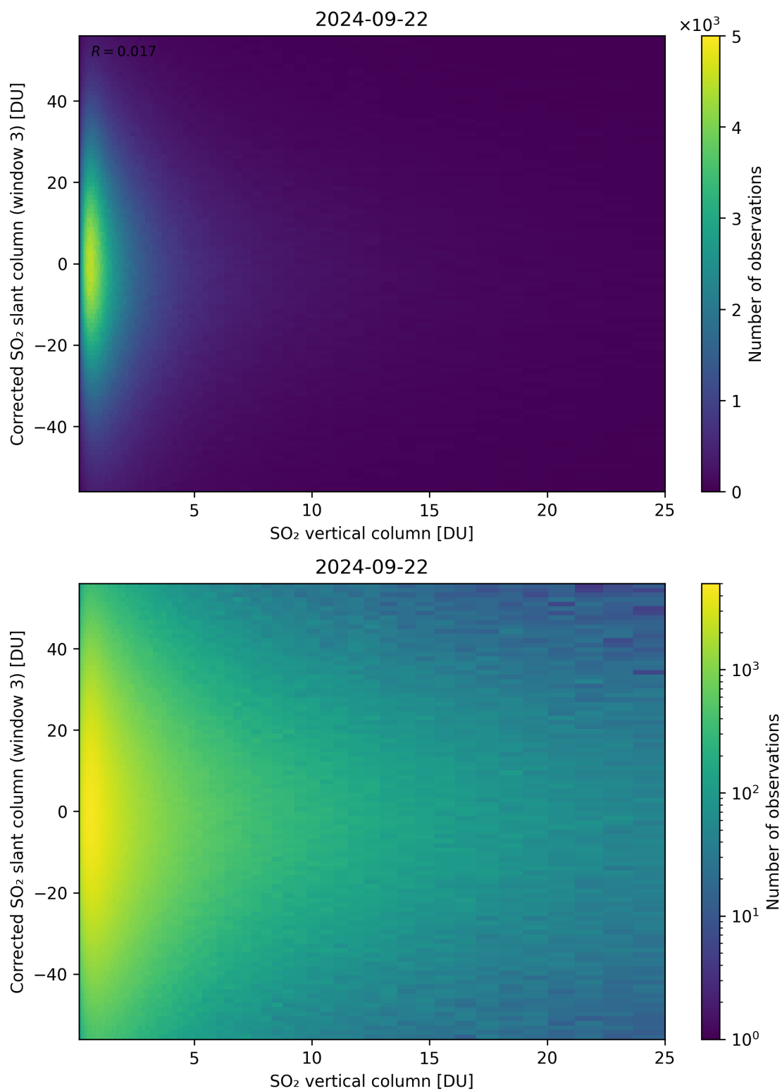
Figure 299: Scatter density plot of “SO 2 vertical column” against “Corrected SO 2 slant column (window 3)” for 2024-09-22 to 2024-09-23.
