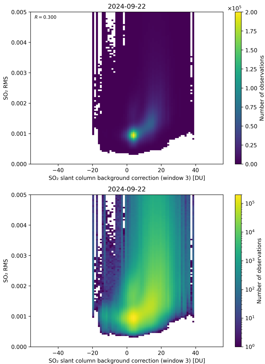
Figure 123: Scatter density plot of “SO 2 slant column background correction (window 3)” against “SO 2 RMS” for 2024-09-22 to 2024-09-23.
