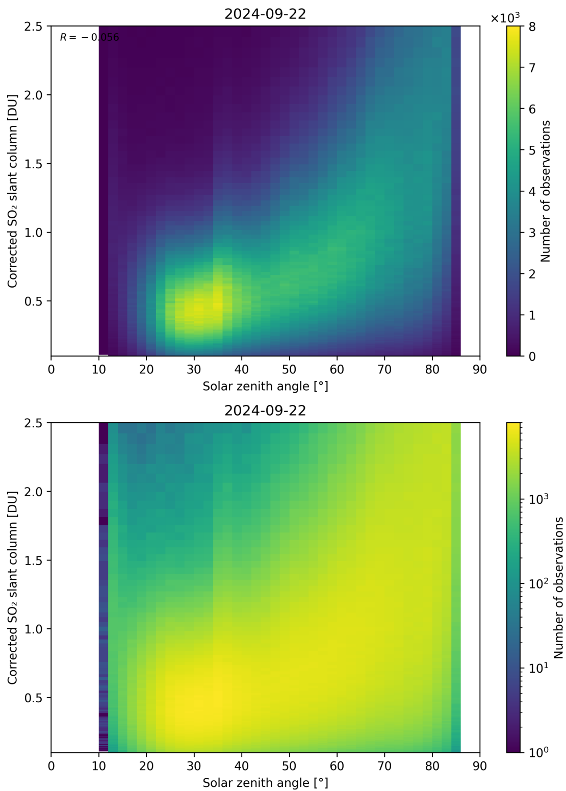
Figure 166: Scatter density plot of “Solar zenith angle” against “Corrected SO 2 slant column” for 2024-09-22 to 2024-09-23.
