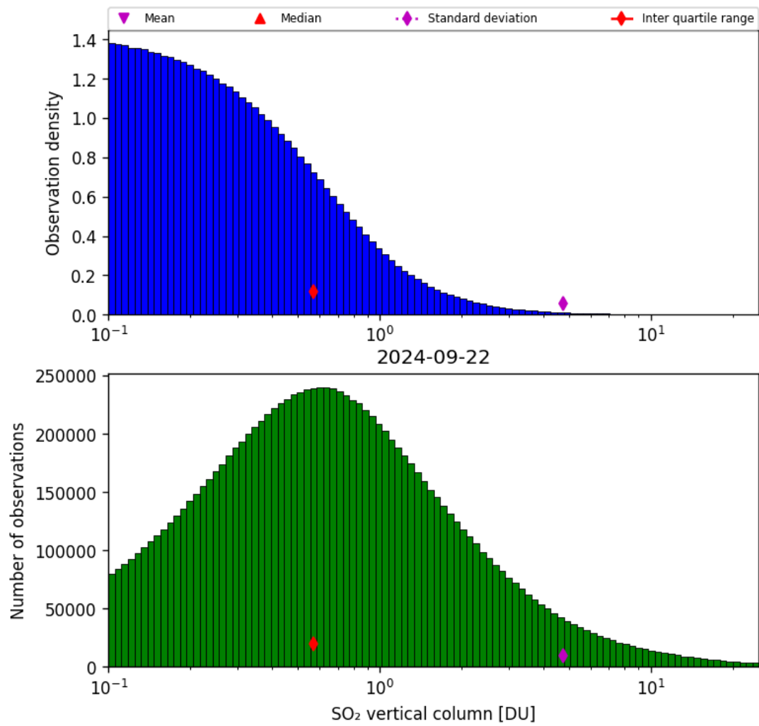
Figure 53: Histogram of “SO 2 vertical column” for 2024-09-22 to 2024-09-23
