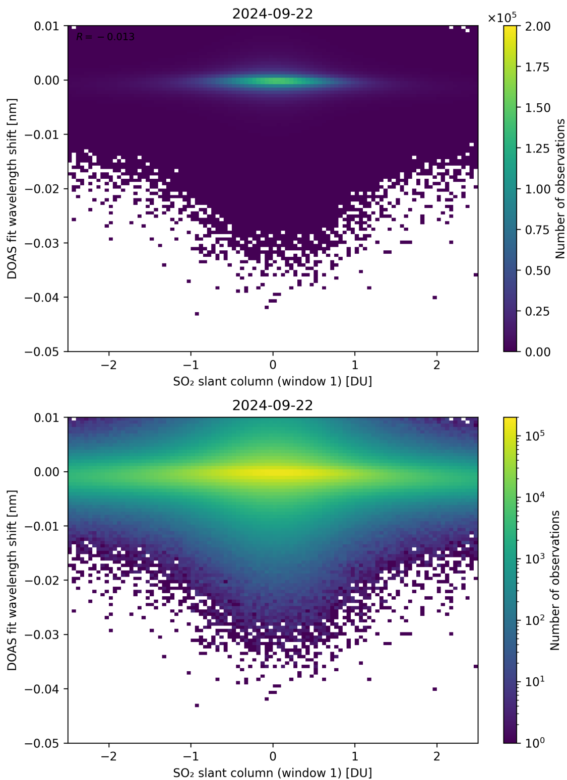
Figure 215: Scatter density plot of “SO 2 slant column (window 1)” against “DOAS fit wavelength shift” for 2024-09-22 to 2024-09-23.
