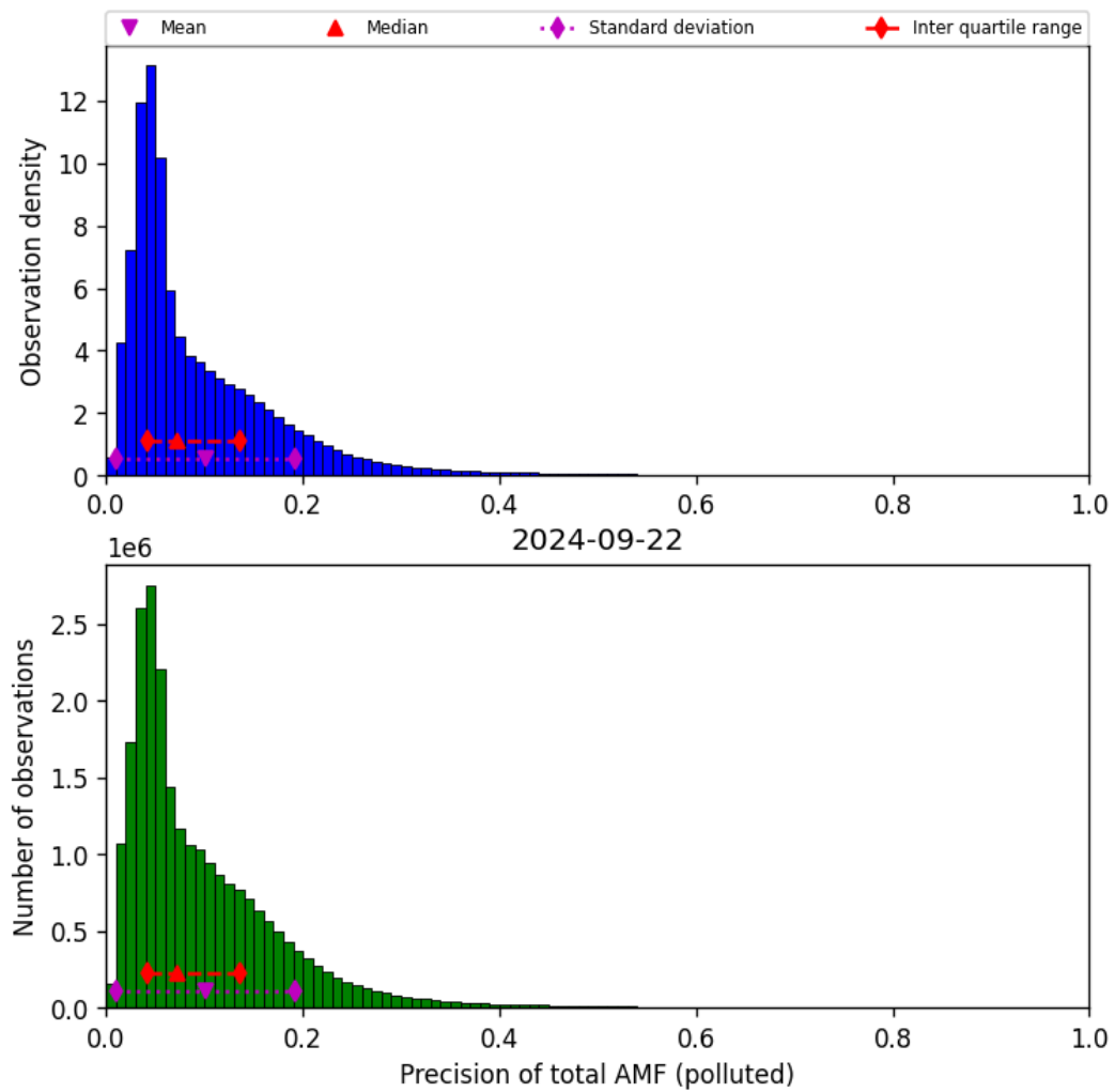
Figure 72: Histogram of “Precision of total AMF (polluted)” for 2024-09-22 to 2024-09-23
