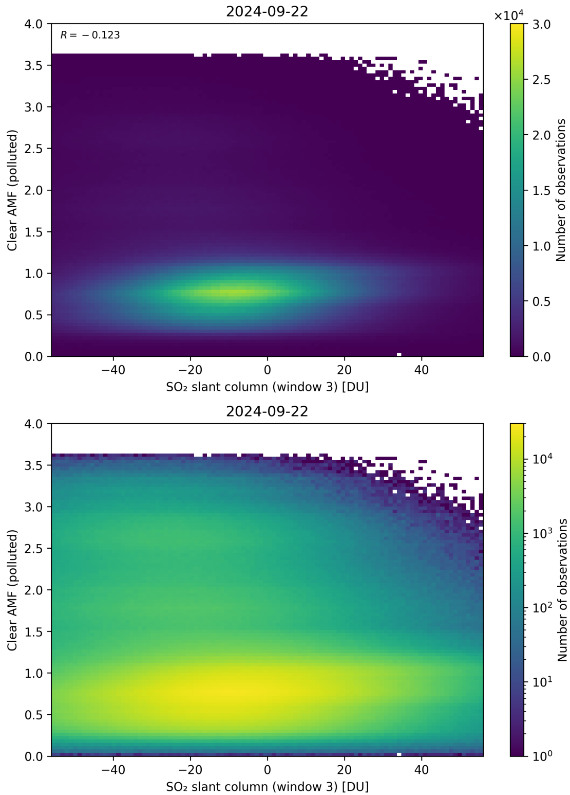
Figure 265: Scatter density plot of “SO 2 slant column (window 3)” against “Clear AMF (polluted)” for 2024-09-22 to 2024-09-23.
