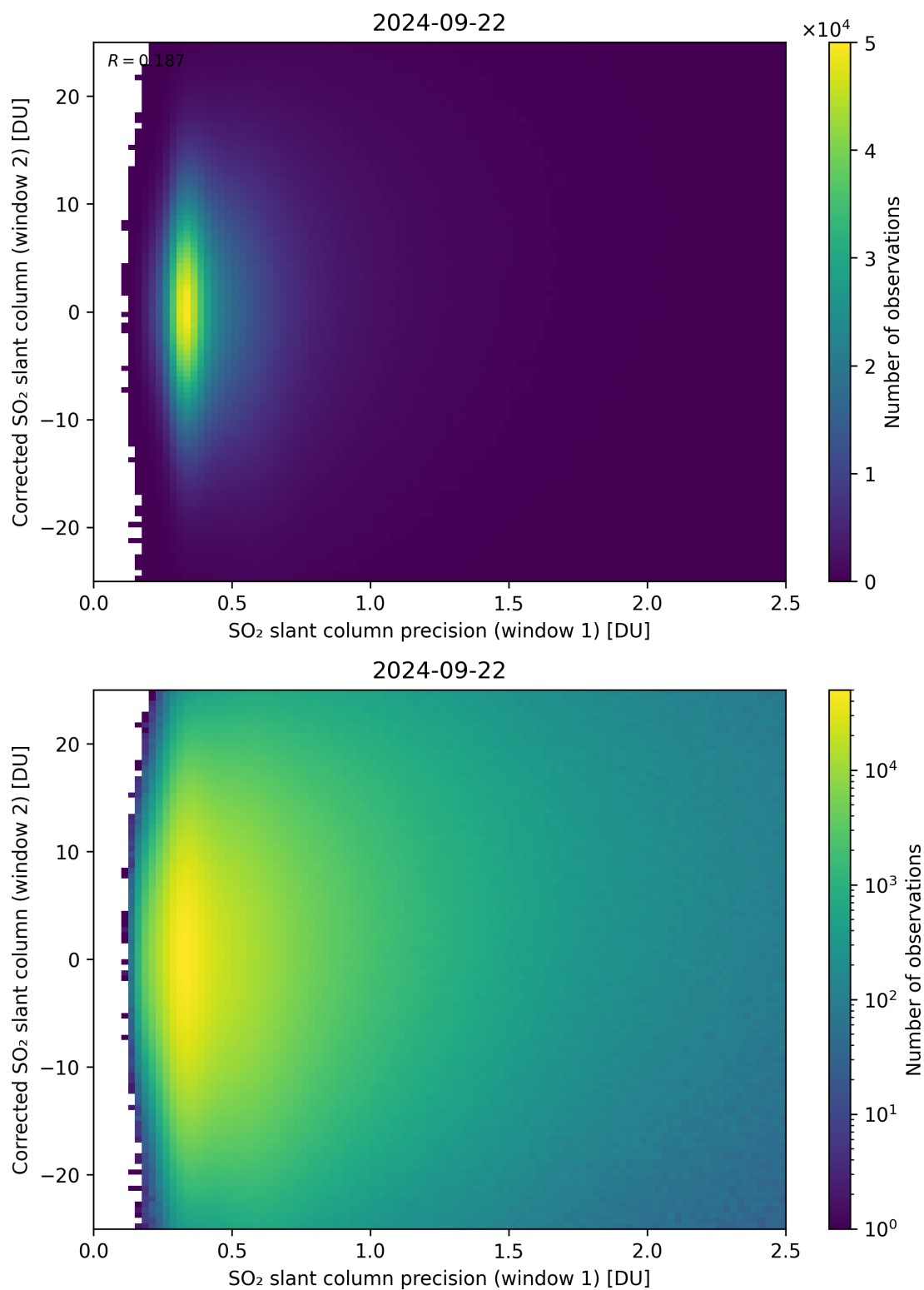
Figure 225: Scatter density plot of “SO 2 slant column precision (window 1)” against “Corrected SO 2 slant column (window 2)” for 2024-09-22 to 2024-09-23.
