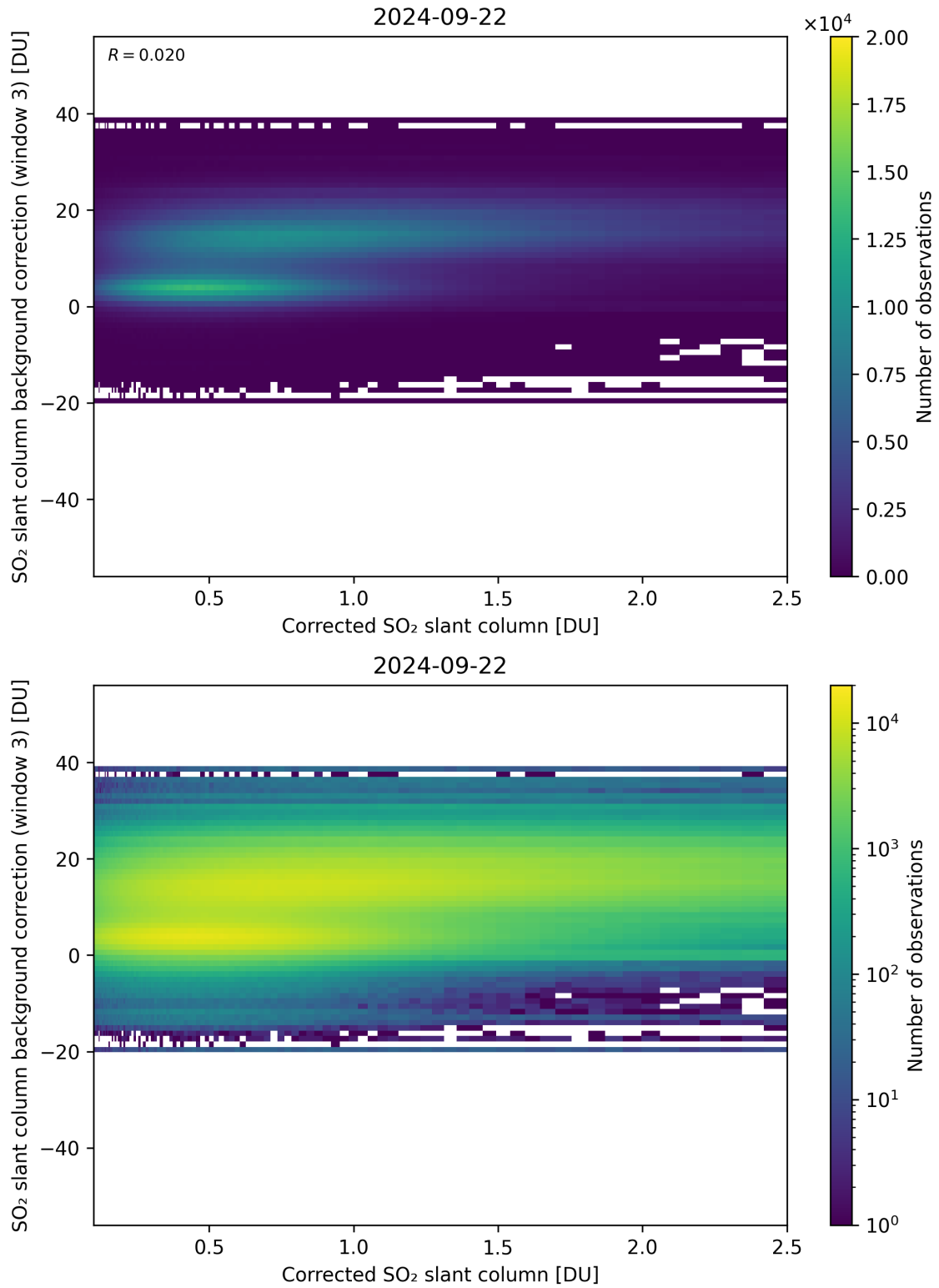
Figure 180: Scatter density plot of “Corrected SO 2 slant column” against “SO 2 slant column background correction (window 3)” for 2024-09-22 to 2024-09-23.
