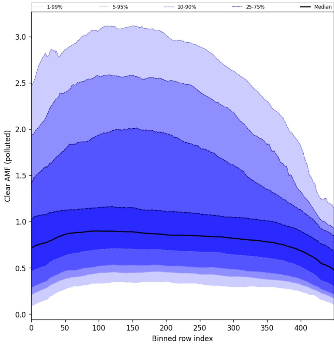
Figure 96: Along track statistics of “Clear AMF (polluted)” for 2024-09-22 to 2024-09-23
