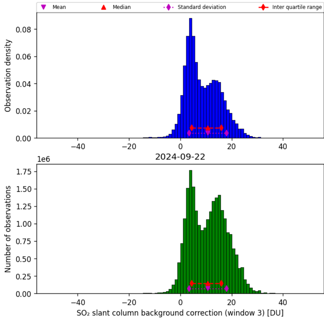
Figure 67: Histogram of “SO 2 slant column background correction (window 3)” for 2024-09-22 to 2024-09-23
