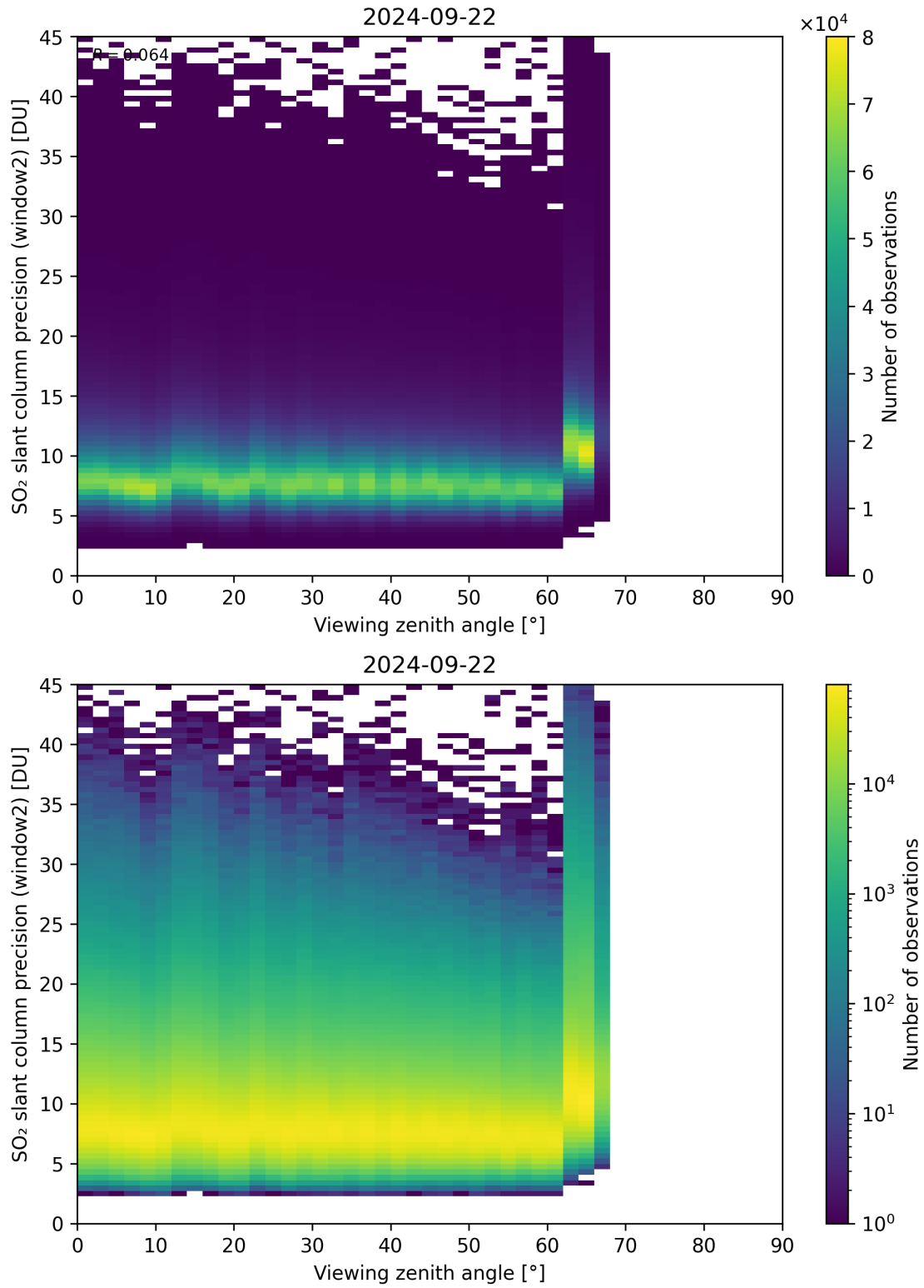
Figure 322: Scatter density plot of “Viewing zenith angle” against “SO 2 slant column precision (window2)” for 2024-09-22 to 2024-09-23.
