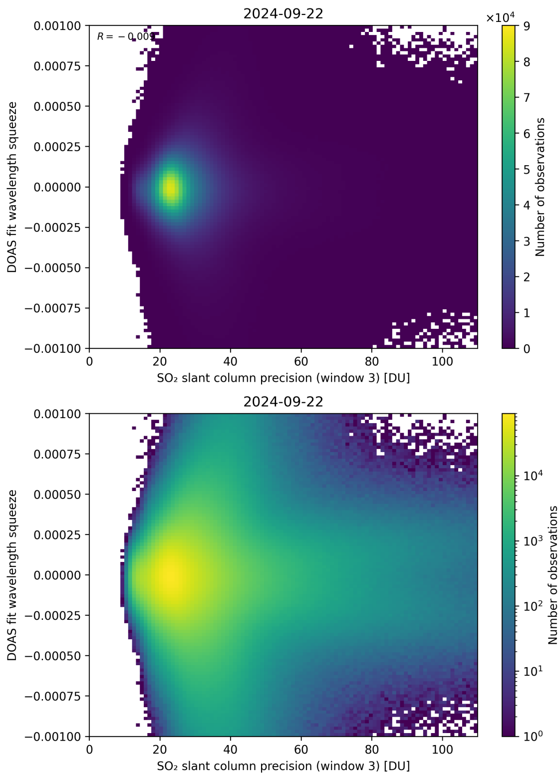
Figure 259: Scatter density plot of “SO 2 slant column precision (window 3)” against “DOAS fit wavelength squeeze” for 2024-09-22 to 2024-09-23.
