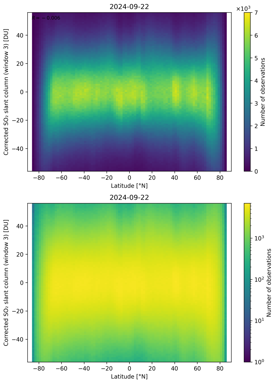
Figure 148: Scatter density plot of “Latitude” against “Corrected SO 2 slant column (window 3)” for 2024-09-22 to 2024-09-23.
