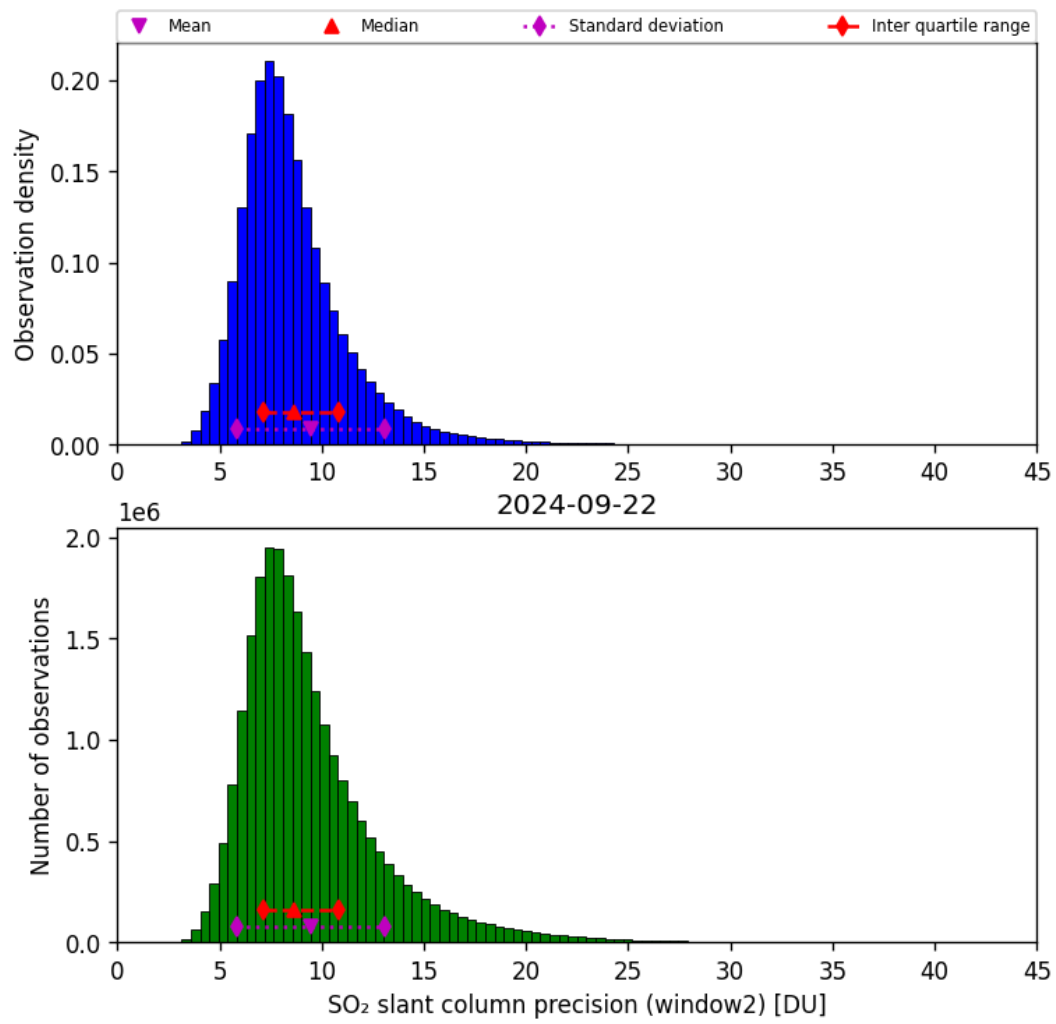
Figure 61: Histogram of “SO 2 slant column precision (window2)” for 2024-09-22 to 2024-09-23
