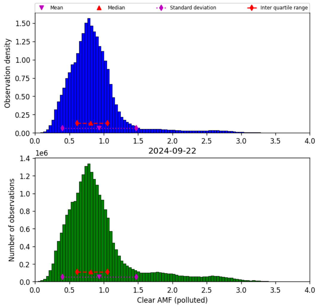
Figure 73: Histogram of “Clear AMF (polluted)” for 2024-09-22 to 2024-09-23
