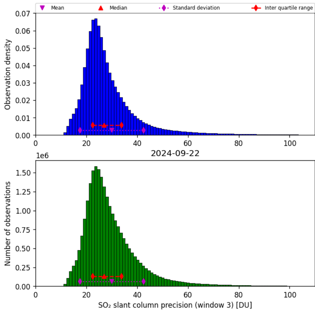
Figure 65: Histogram of “SO 2 slant column precision (window 3)” for 2024-09-22 to 2024-09-23
