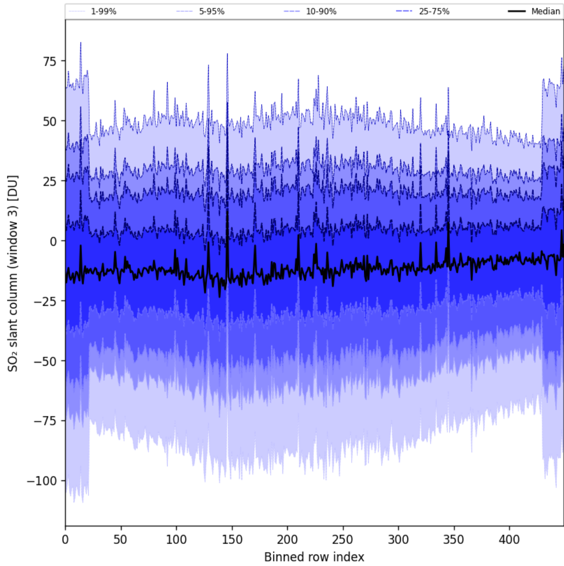
Figure 87: Along track statistics of “SO 2 slant column (window 3)” for 2024-09-22 to 2024-09-23
