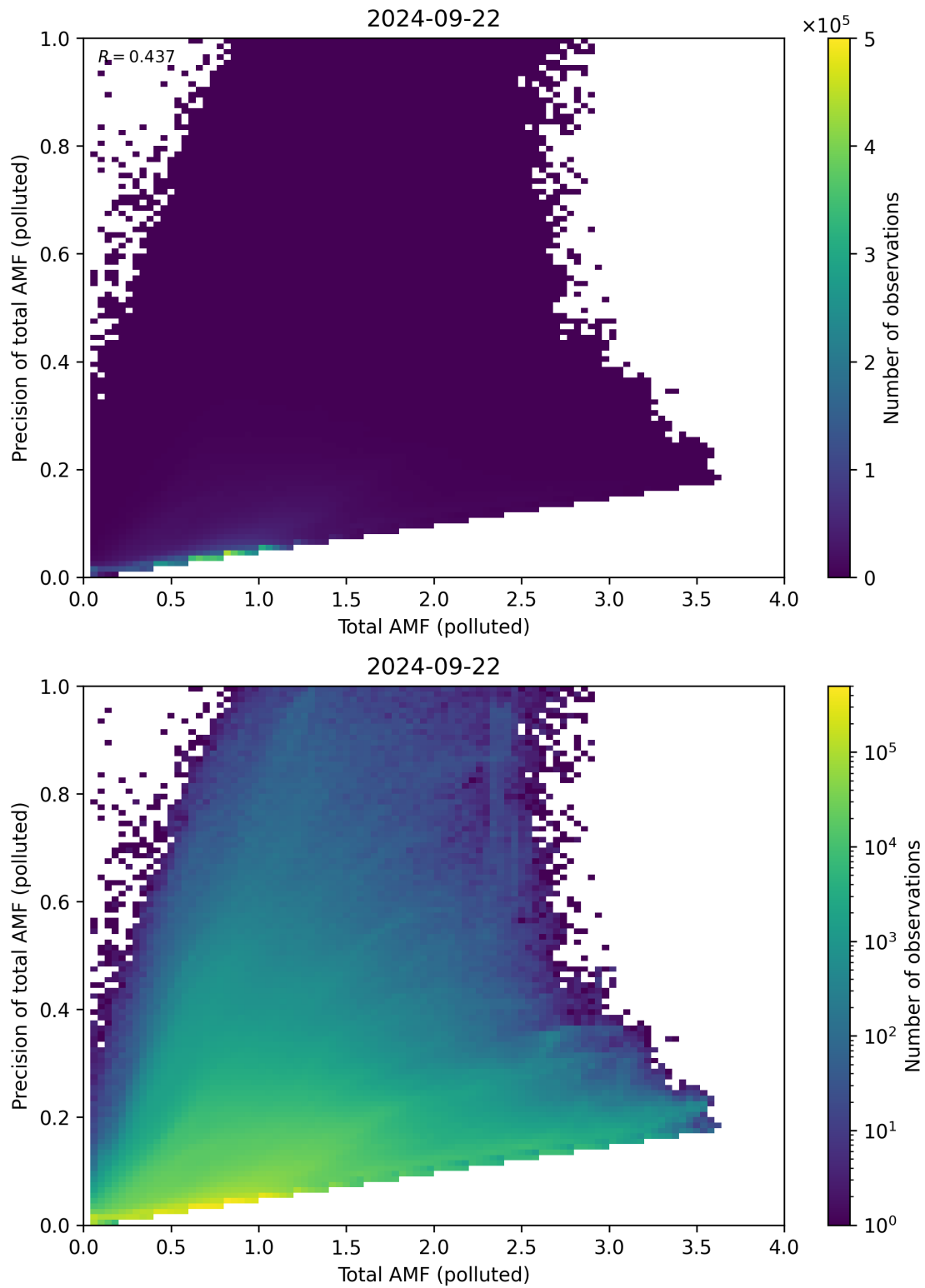
Figure 272: Scatter density plot of “Total AMF (polluted)” against “Precision of total AMF (polluted)” for 2024-09-22 to 2024-09-23.
