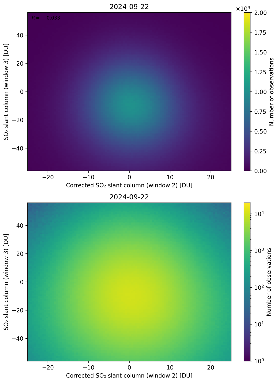
Figure 201: Scatter density plot of “Corrected SO 2 slant column (window 2)” against “SO 2 slant column (window 3)” for 2024-09-22 to 2024-09-23.
