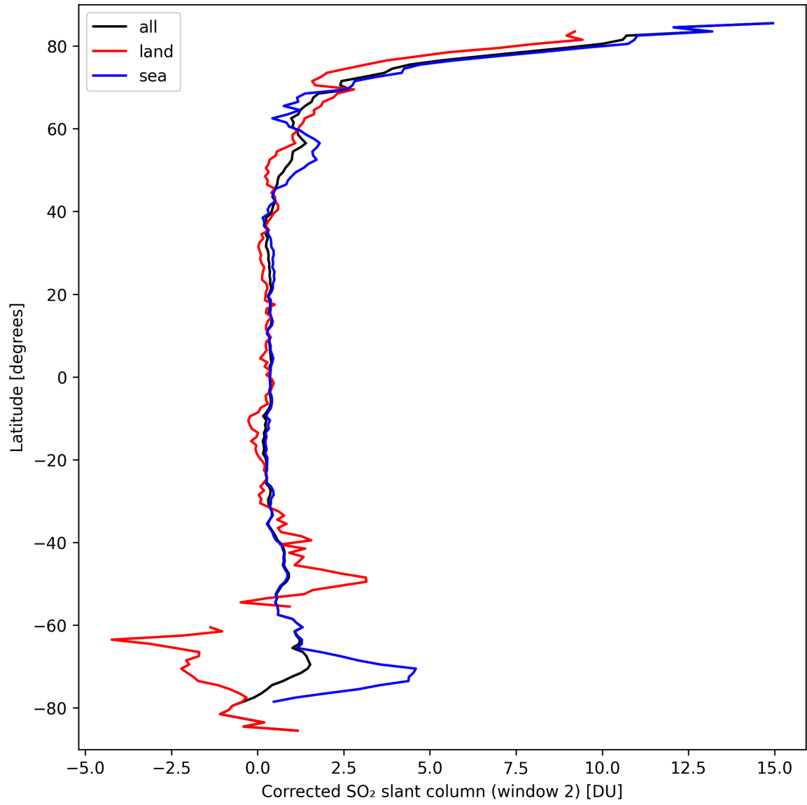
Figure 39: Zonal average of “Corrected SO 2 slant column (window 2)” for 2024-09-22 to 2024-09-23.
