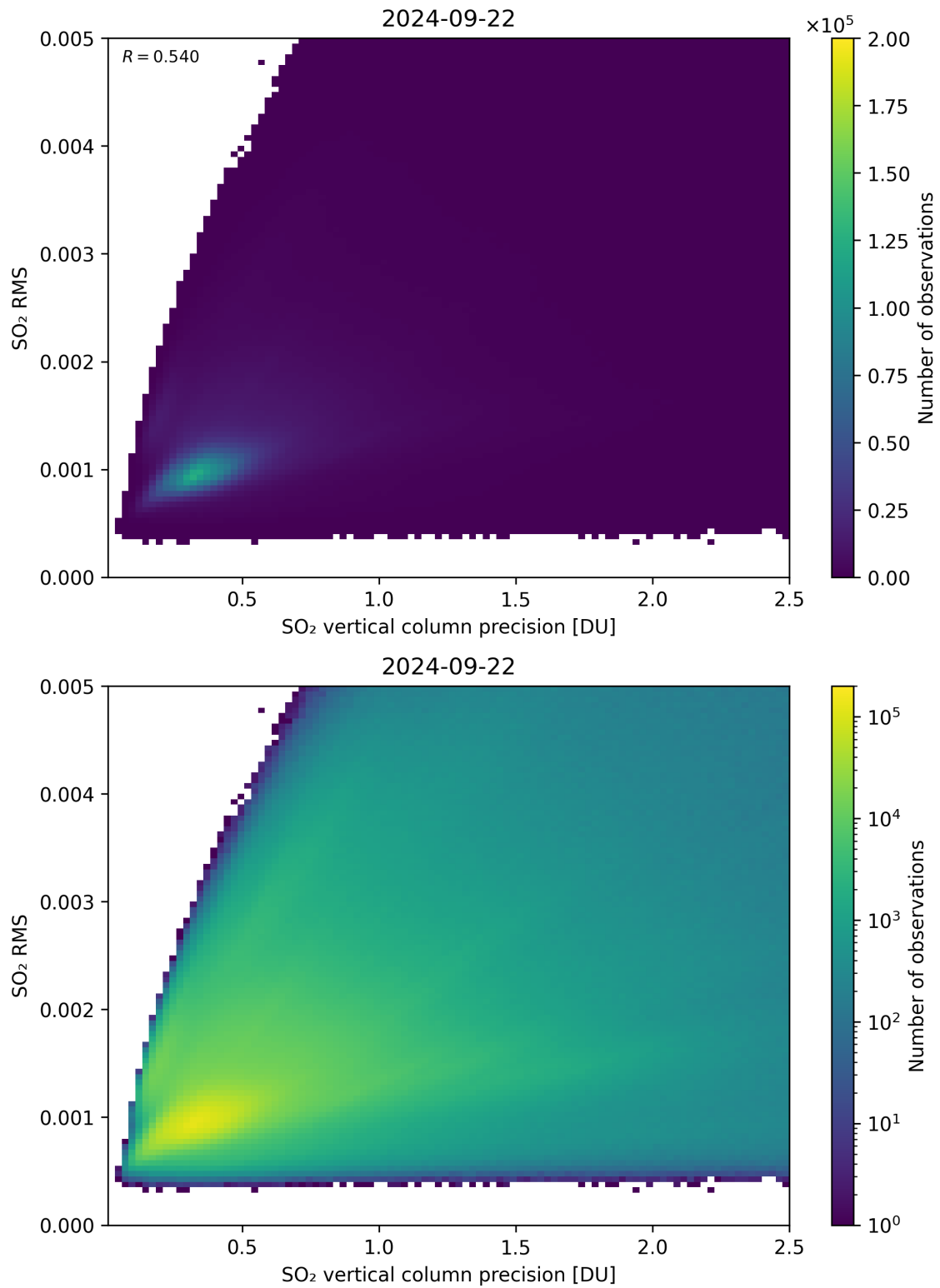
Figure 284: Scatter density plot of “SO 2 vertical column precision” against “SO 2 RMS” for 2024-09-22 to 2024-09-23.
