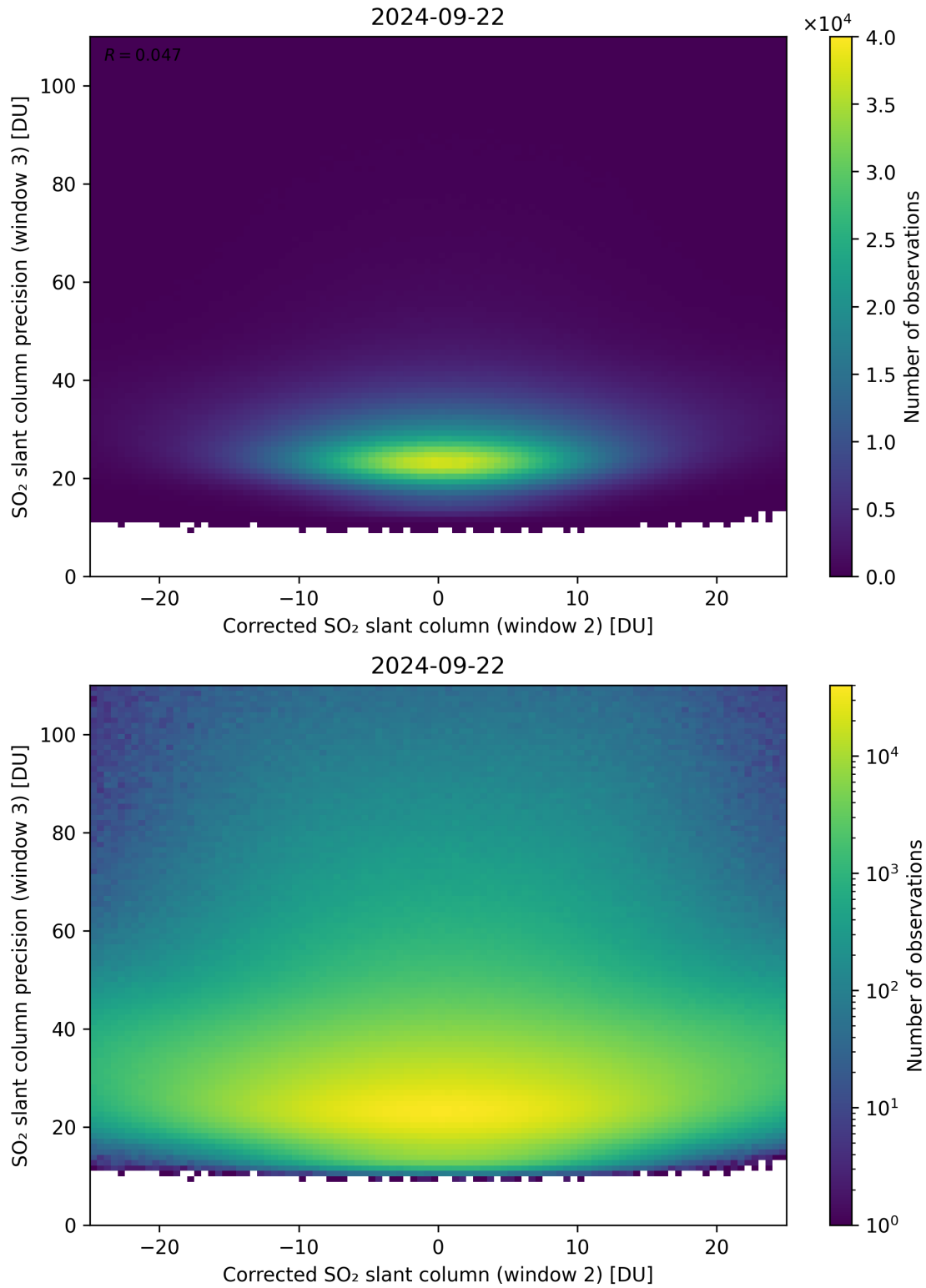
Figure 202: Scatter density plot of “Corrected SO 2 slant column (window 2)” against “SO 2 slant column precision (window 3)” for 2024-09-22 to 2024-09-23.
