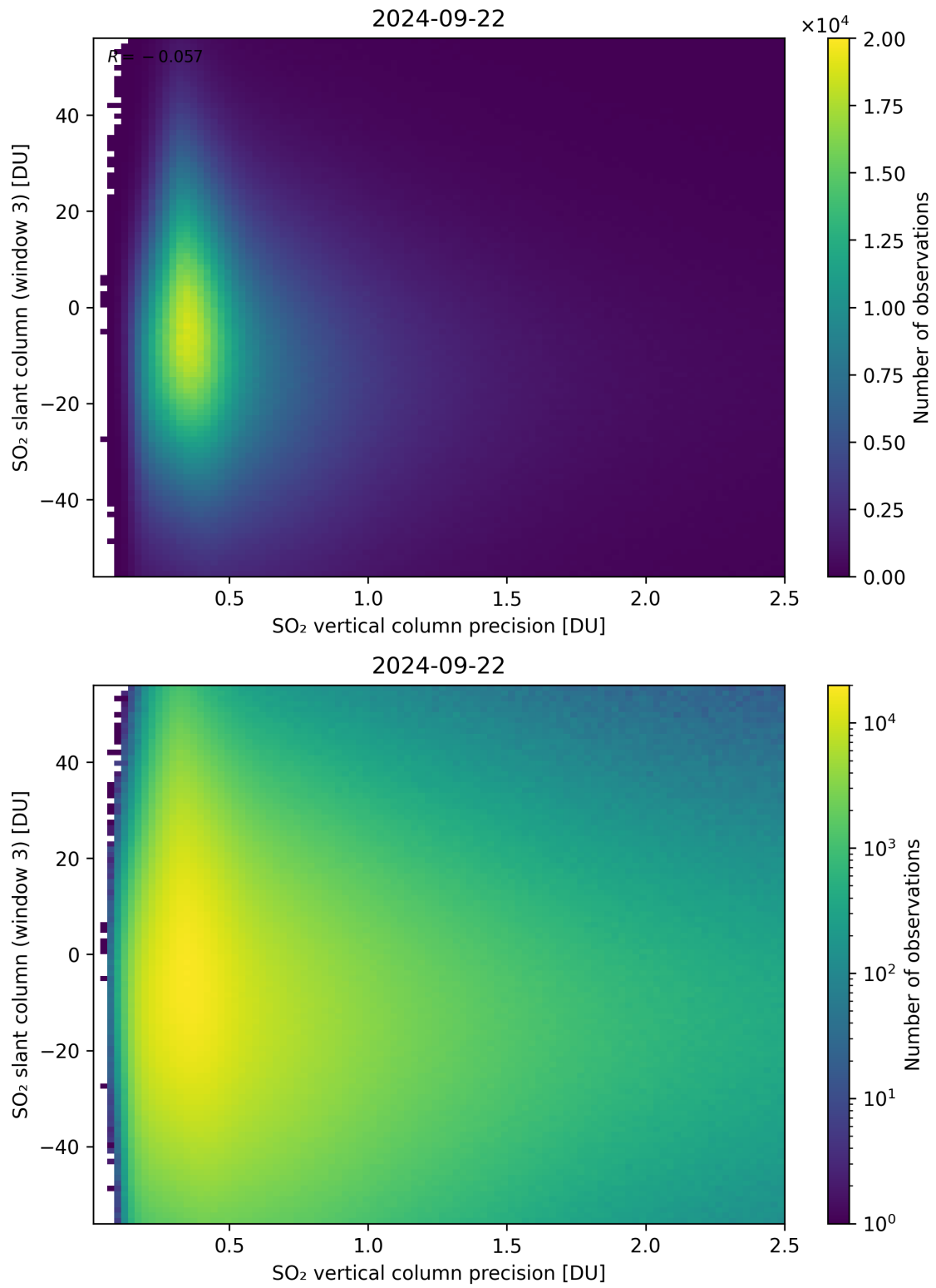
Figure 292: Scatter density plot of “SO 2 vertical column precision” against “SO 2 slant column (window 3)” for 2024-09-22 to 2024-09-23.
