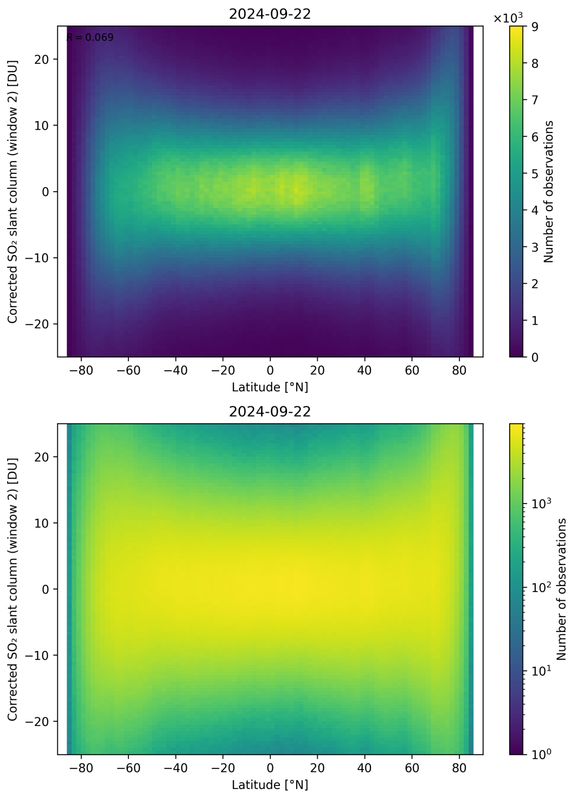
Figure 147: Scatter density plot of “Latitude” against “Corrected SO 2 slant column (window 2)” for 2024-09-22 to 2024-09-23.
