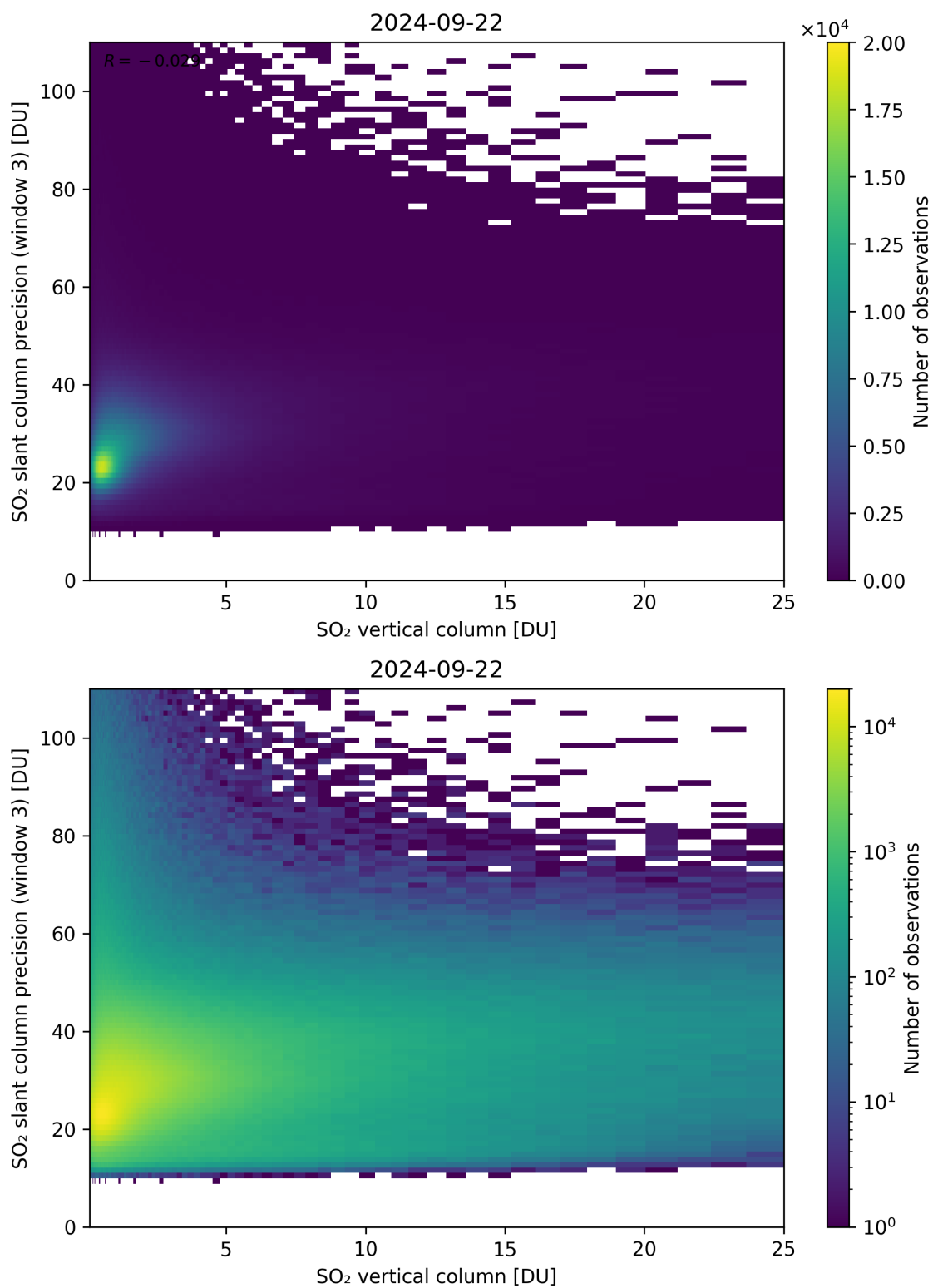
Figure 304: Scatter density plot of “SO 2 vertical column” against “SO 2 slant column precision (window 3)” for 2024-09-22 to 2024-09-23.
