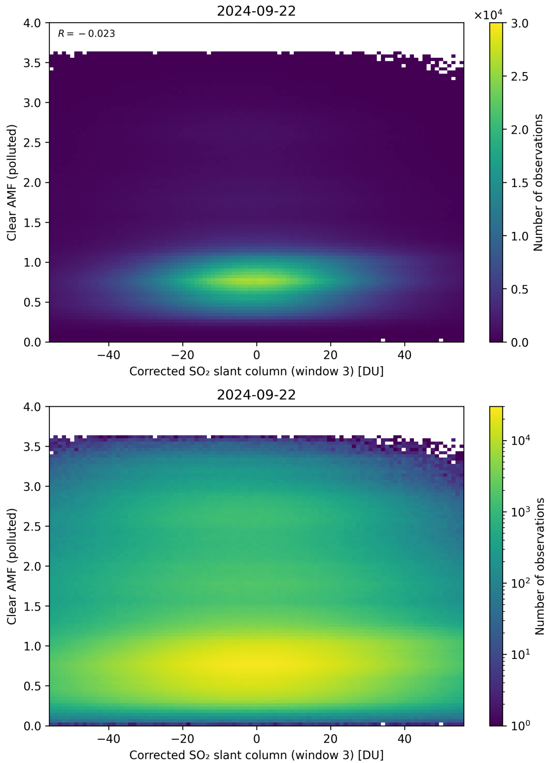
Figure 209: Scatter density plot of “Corrected SO 2 slant column (window 3)” against “Clear AMF (polluted)” for 2024-09-22 to 2024-09-23.
