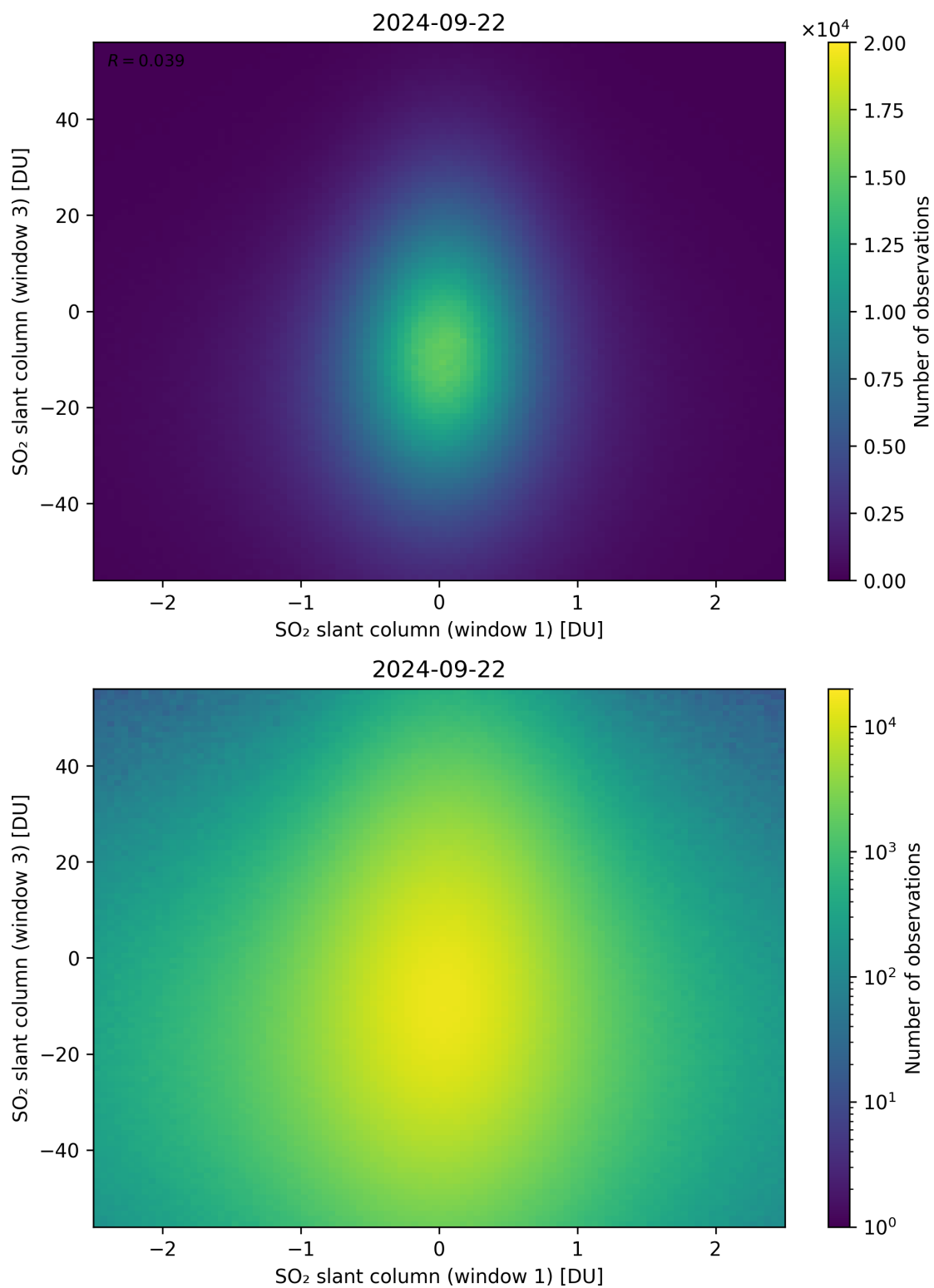
Figure 237: Scatter density plot of “SO 2 slant column (window 1)” against “SO 2 slant column (window 3)” for 2024-09-22 to 2024-09-23.
