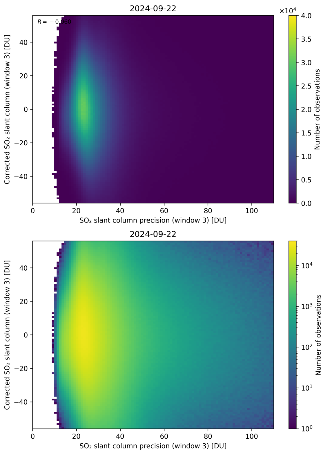
Figure 262: Scatter density plot of “SO 2 slant column precision (window 3)” against “Corrected SO 2 slant column (window 3)” for 2024-09-22 to 2024-09-23.
