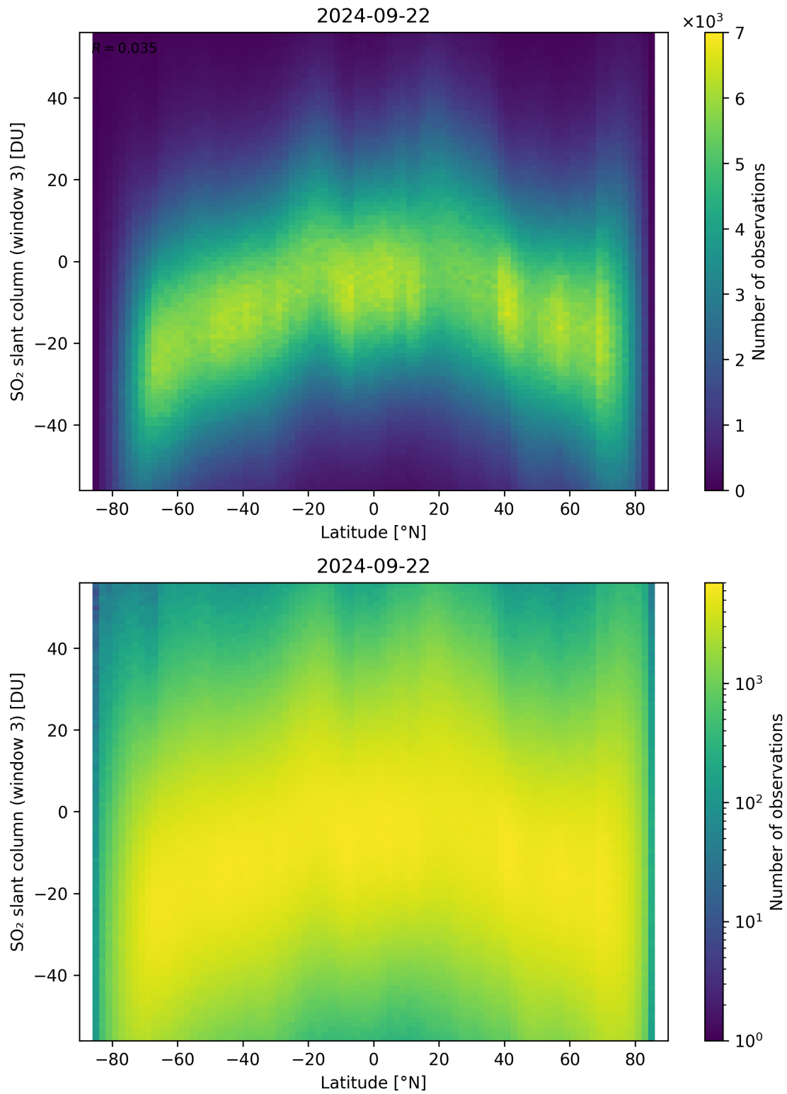
Figure 152: Scatter density plot of “Latitude” against “SO 2 slant column (window 3)” for 2024-09-22 to 2024-09-23.
