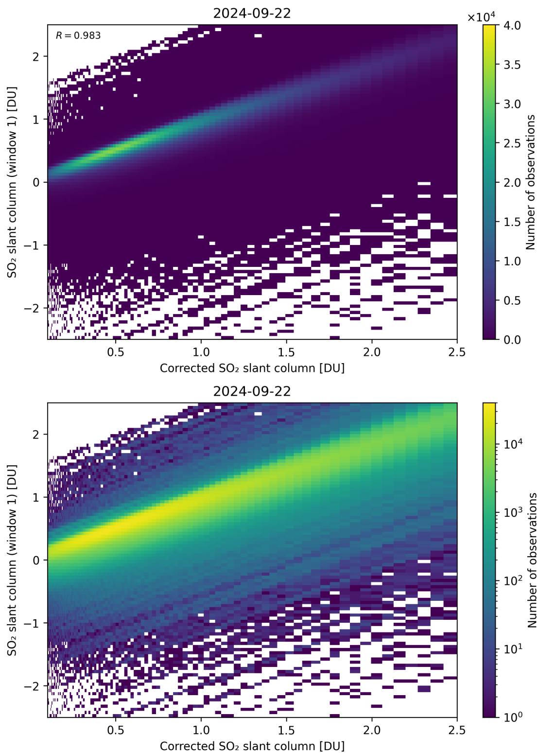
Figure 187: Scatter density plot of “Corrected SO 2 slant column” against “SO 2 slant column (window 1)” for 2024-09-22 to 2024-09-23.
