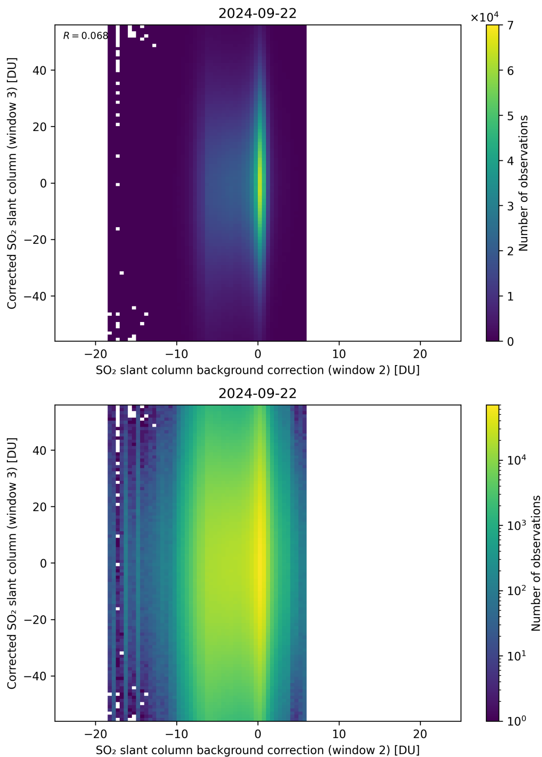
Figure 116: Scatter density plot of “SO 2 slant column background correction (window 2)” against “Corrected SO 2 slant column (window 3)” for 2024-09-22 to 2024-09-23.
