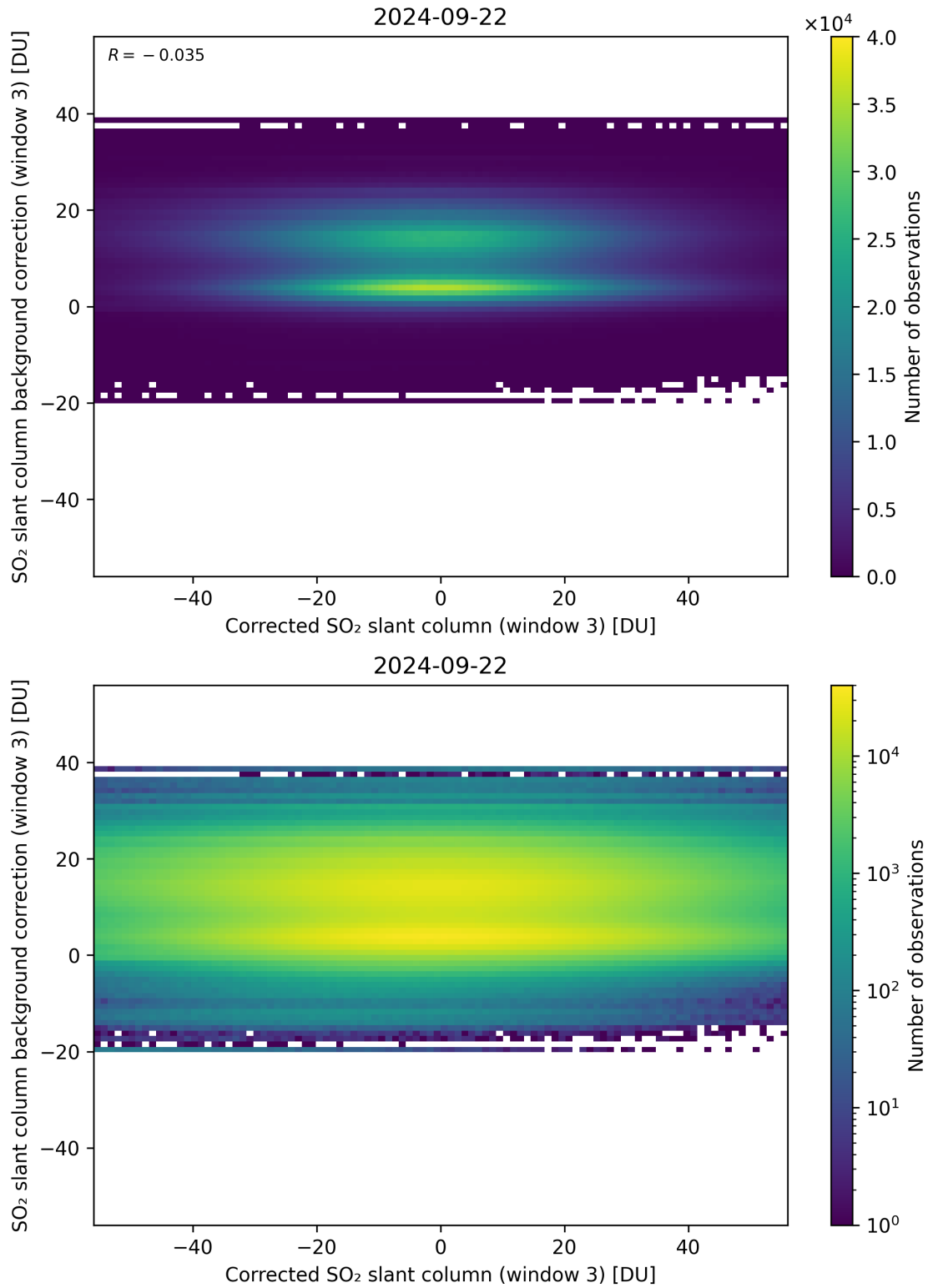
Figure 205: Scatter density plot of “Corrected SO 2 slant column (window 3)” against “SO 2 slant column background correction (window 3)” for 2024-09-22 to 2024-09-23.
