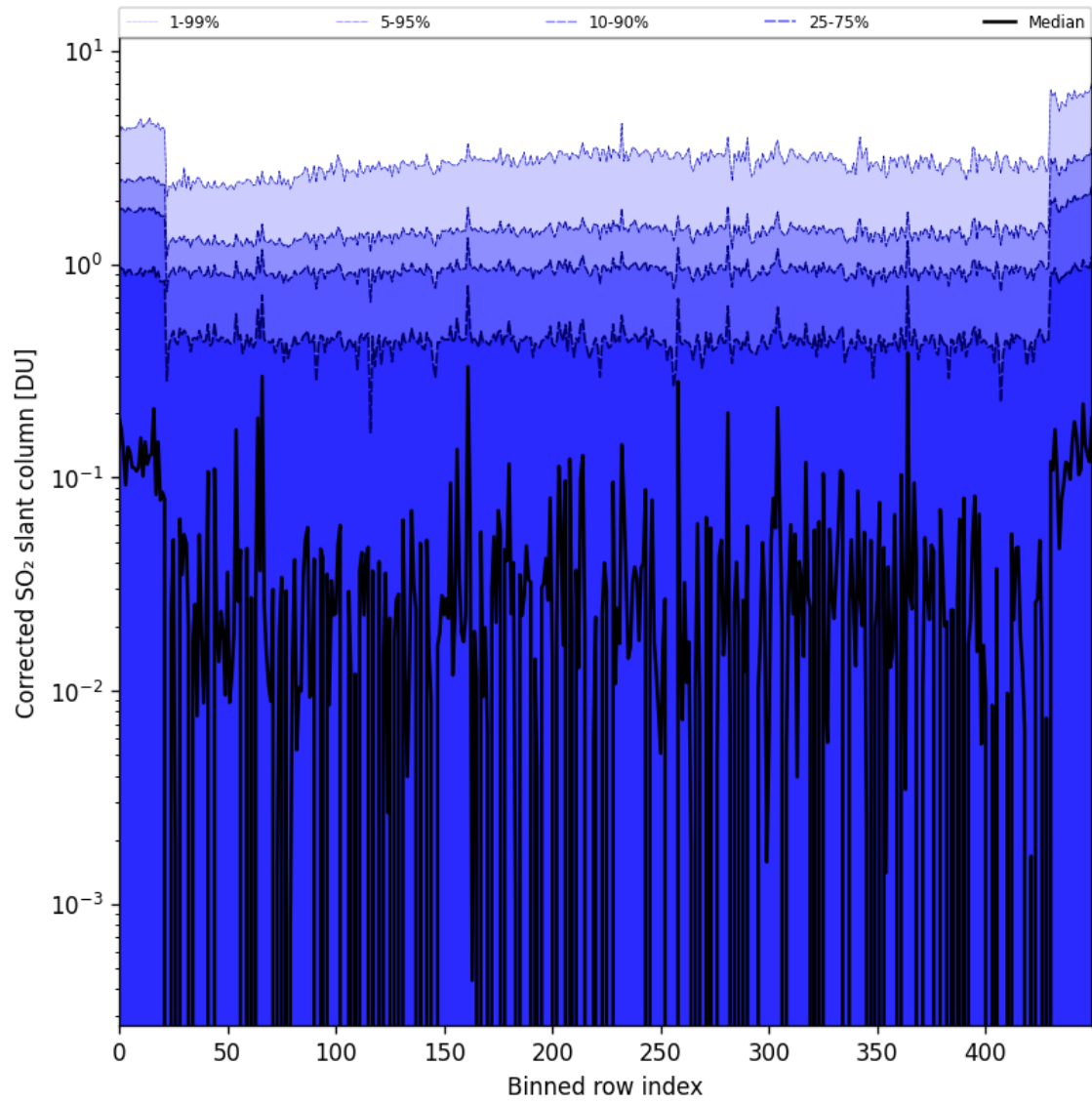
Figure 78: Along track statistics of “Corrected SO 2 slant column” for 2024-09-22 to 2024-09-23
