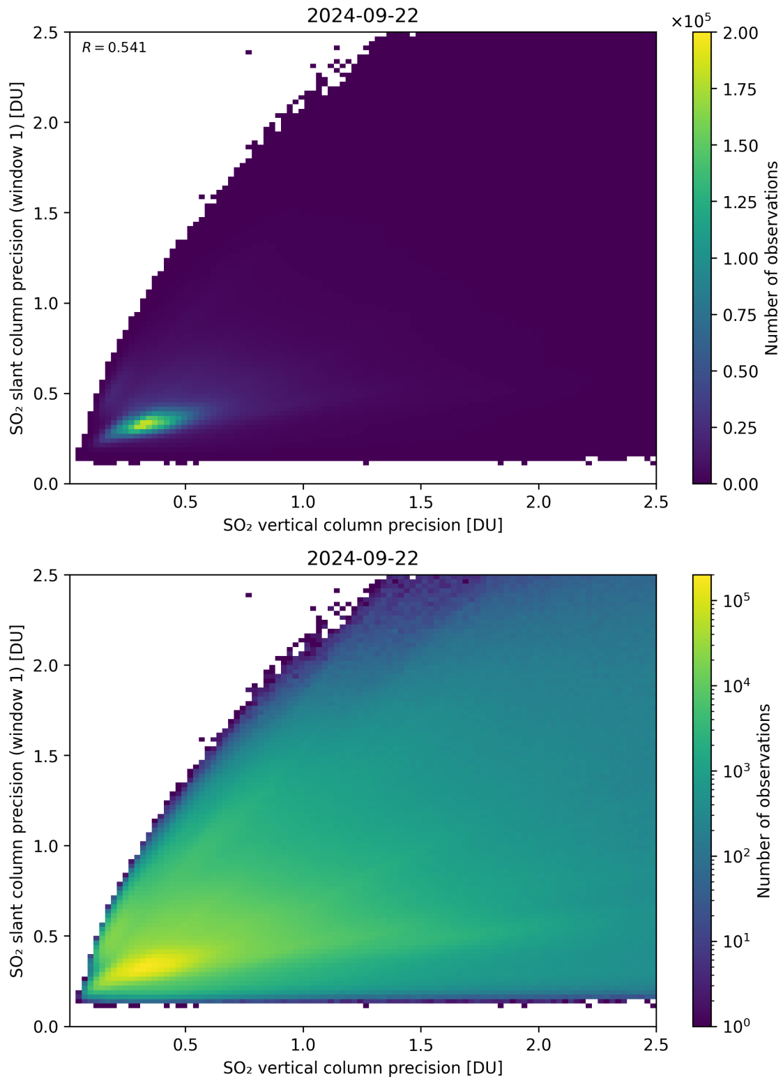
Figure 290: Scatter density plot of “SO 2 vertical column precision” against “SO 2 slant column precision (window 1)” for 2024-09-22 to 2024-09-23.
