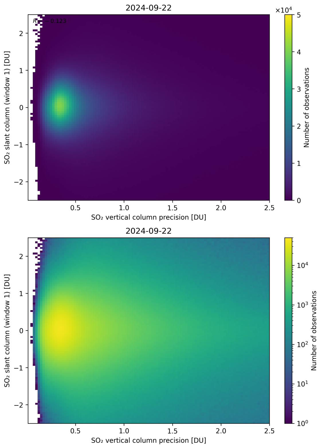
Figure 289: Scatter density plot of “SO 2 vertical column precision” against “SO 2 slant column (window 1)” for 2024-09-22 to 2024-09-23.
