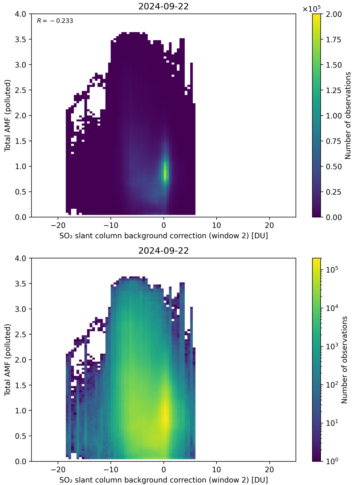
Figure 119: Scatter density plot of “SO 2 slant column background correction (window 2)” against “Total AMF (polluted)” for 2024-09-22 to 2024-09-23.
