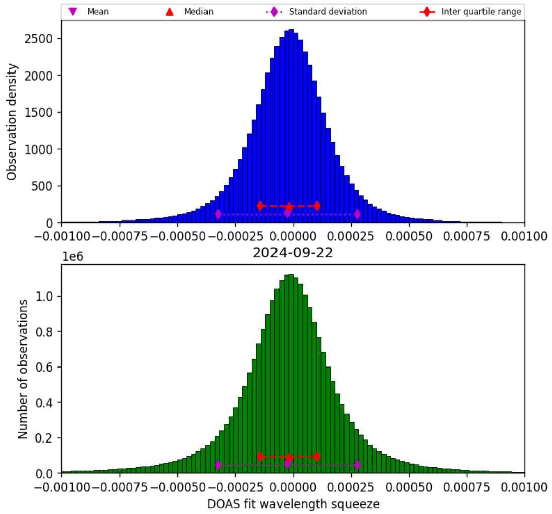
Figure 69: Histogram of “DOAS fit wavelength squeeze” for 2024-09-22 to 2024-09-23
