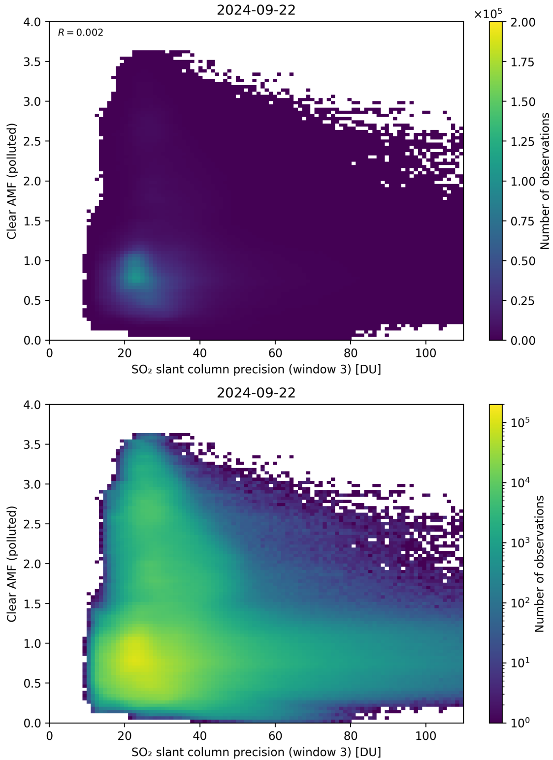
Figure 261: Scatter density plot of “SO 2 slant column precision (window 3)” against “Clear AMF (polluted)” for 2024-09-22 to 2024-09-23.
