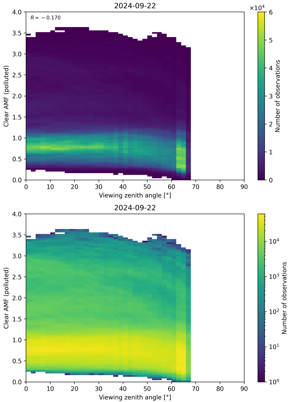
Figure 316: Scatter density plot of “Viewing zenith angle” against “Clear AMF (polluted)” for 2024-09-22 to 2024-09-23.
