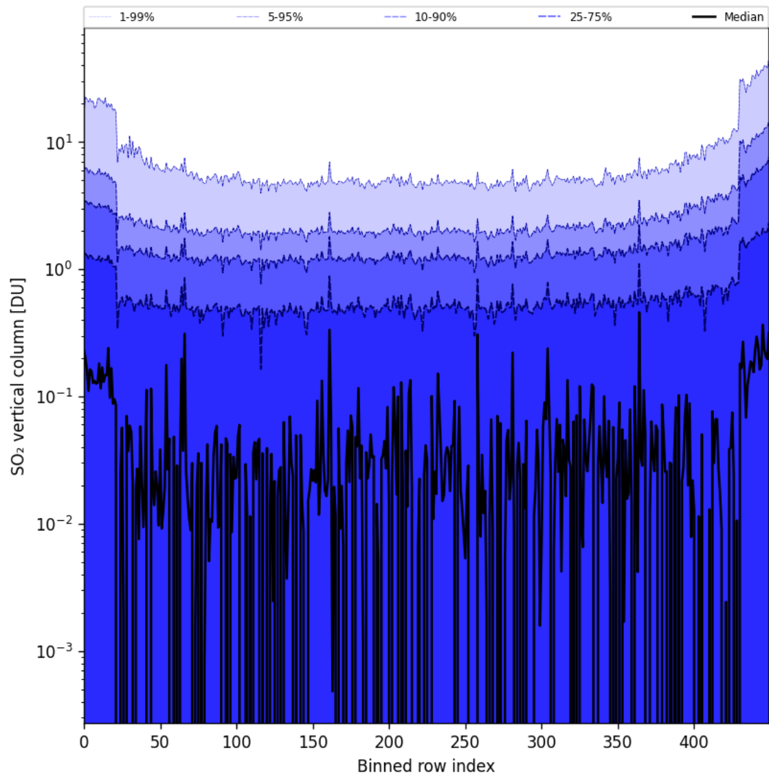
Figure 76: Along track statistics of “SO 2 vertical column” for 2024-09-22 to 2024-09-23
