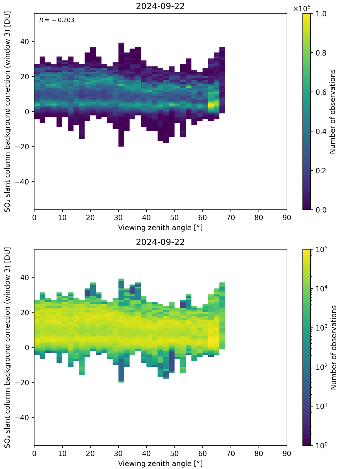
Figure 310: Scatter density plot of “Viewing zenith angle” against “SO 2 slant column background correction (window 3)” for 2024-09-22 to 2024-09-23.
