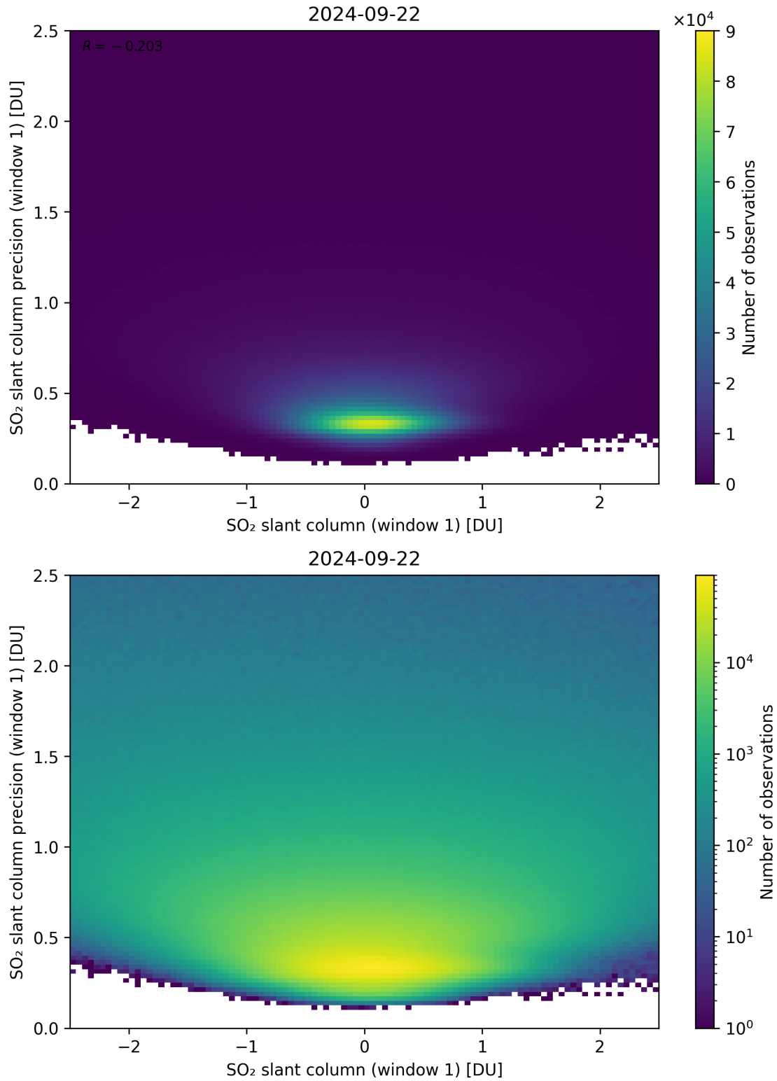
Figure 235: Scatter density plot of “SO 2 slant column (window 1)” against “SO 2 slant column precision (window 1)” for 2024-09-22 to 2024-09-23.
