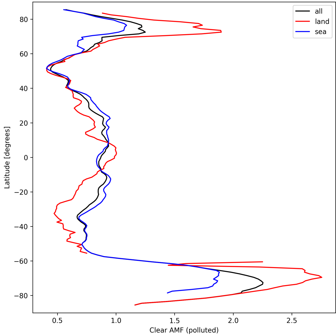
Figure 50: Zonal average of “Clear AMF (polluted)” for 2024-09-22 to 2024-09-23.
