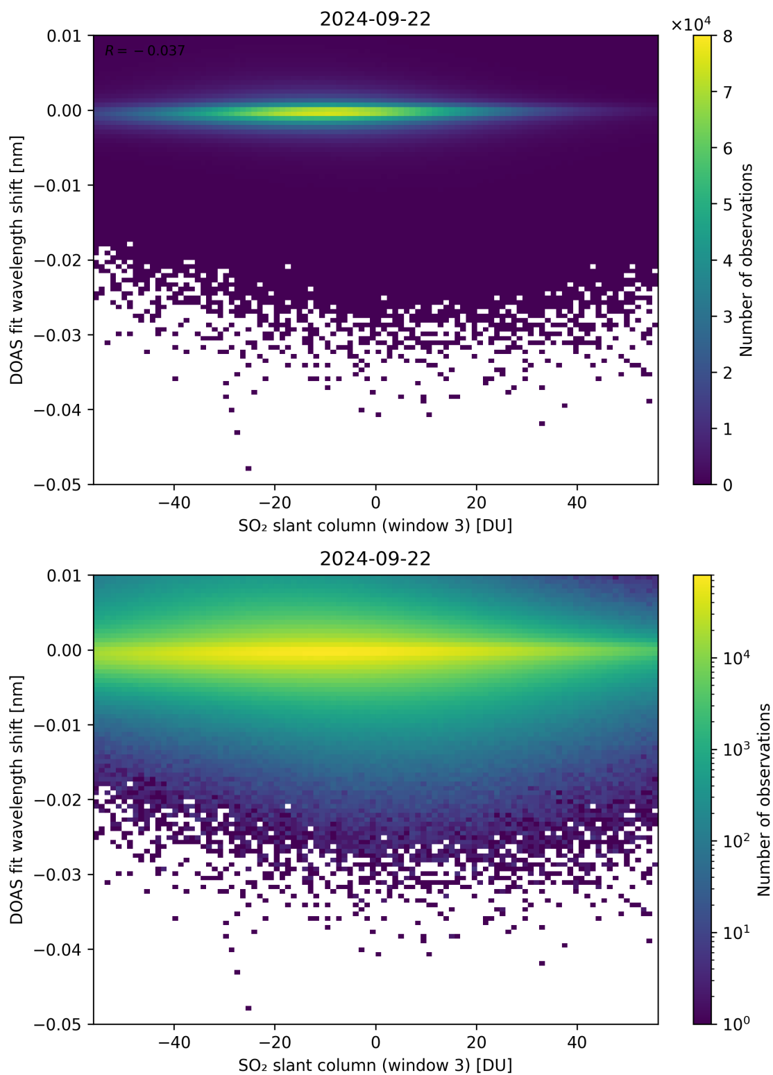
Figure 254: Scatter density plot of “SO 2 slant column (window 3)” against “DOAS fit wavelength shift” for 2024-09-22 to 2024-09-23.
