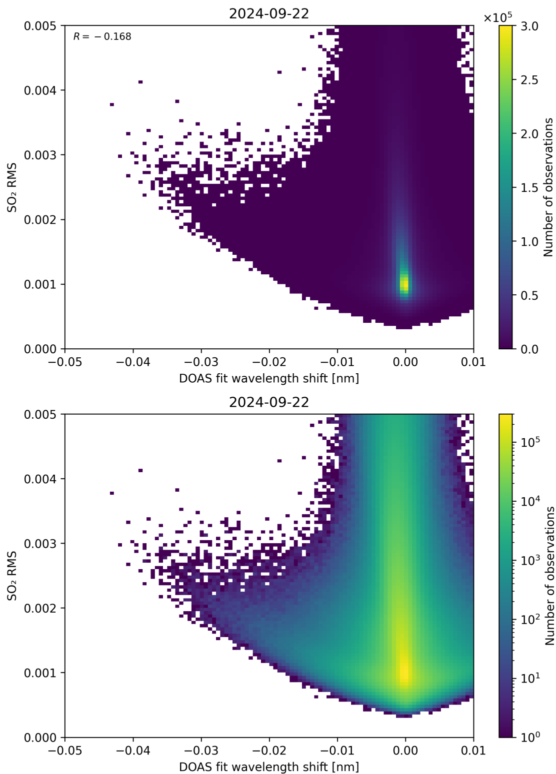
Figure 128: Scatter density plot of “DOAS fit wavelength shift” against “SO 2 RMS” for 2024-09-22 to 2024-09-23.
