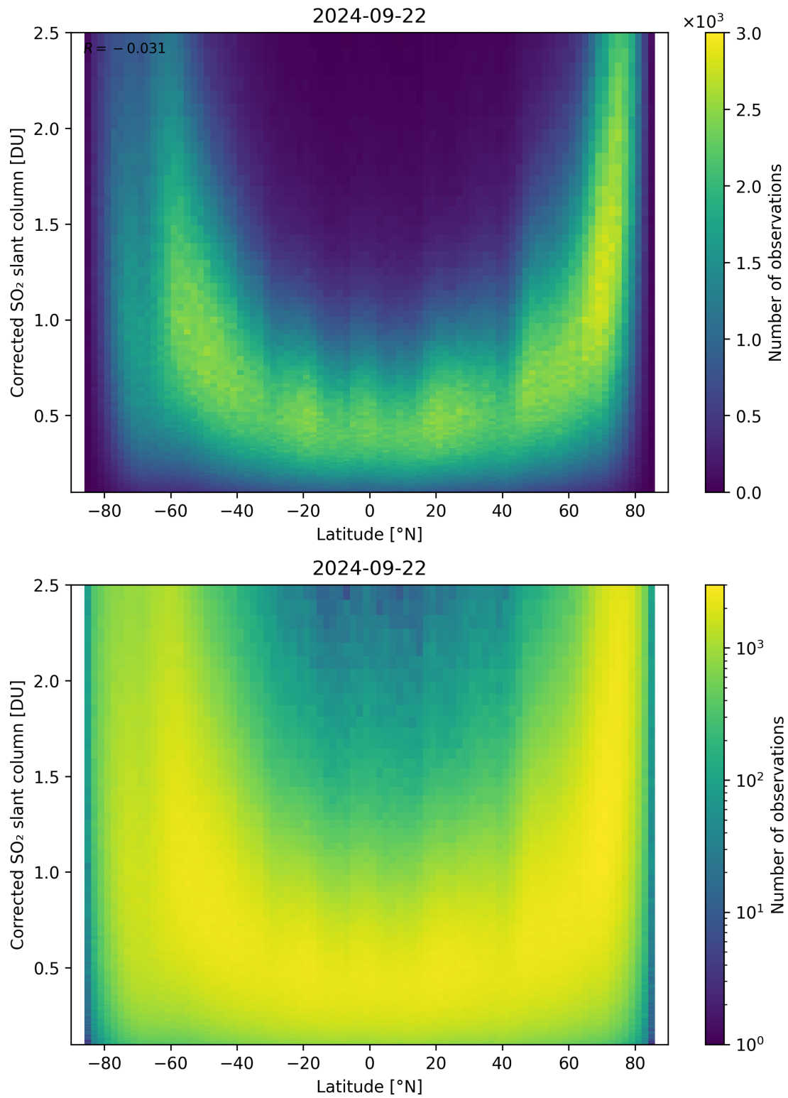
Figure 146: Scatter density plot of “Latitude” against “Corrected SO 2 slant column” for 2024-09-22 to 2024-09-23.
