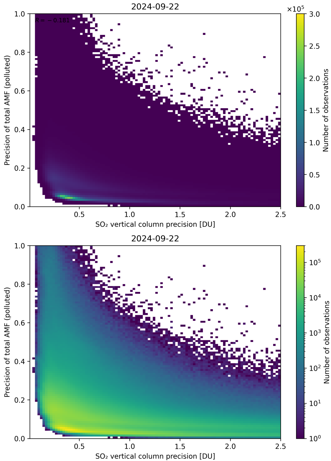
Figure 295: Scatter density plot of “SO 2 vertical column precision” against “Precision of total AMF (polluted)” for 2024-09-22 to 2024-09-23.
