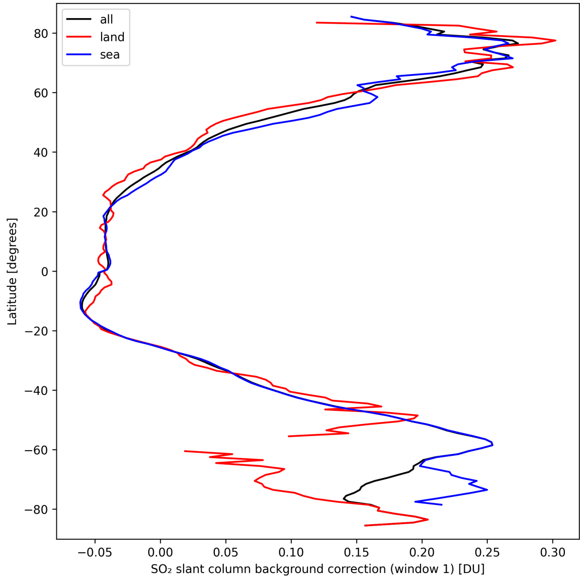
Figure 36: Zonal average of “SO 2 slant column background correction (window 1)” for 2024-09-22 to 2024-09-23.
