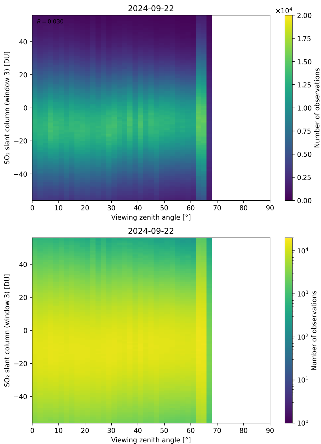
Figure 323: Scatter density plot of “Viewing zenith angle” against “SO 2 slant column (window 3)” for 2024-09-22 to 2024-09-23.
