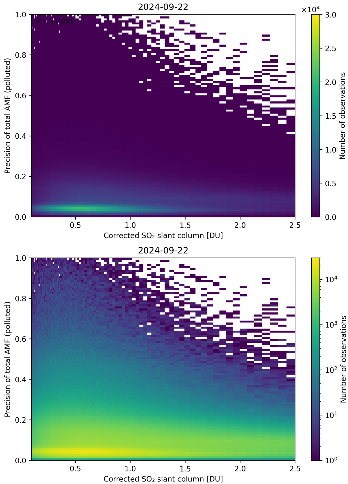
Figure 193: Scatter density plot of “Corrected SO 2 slant column” against “Precision of total AMF (polluted)” for 2024-09-22 to 2024-09-23.
