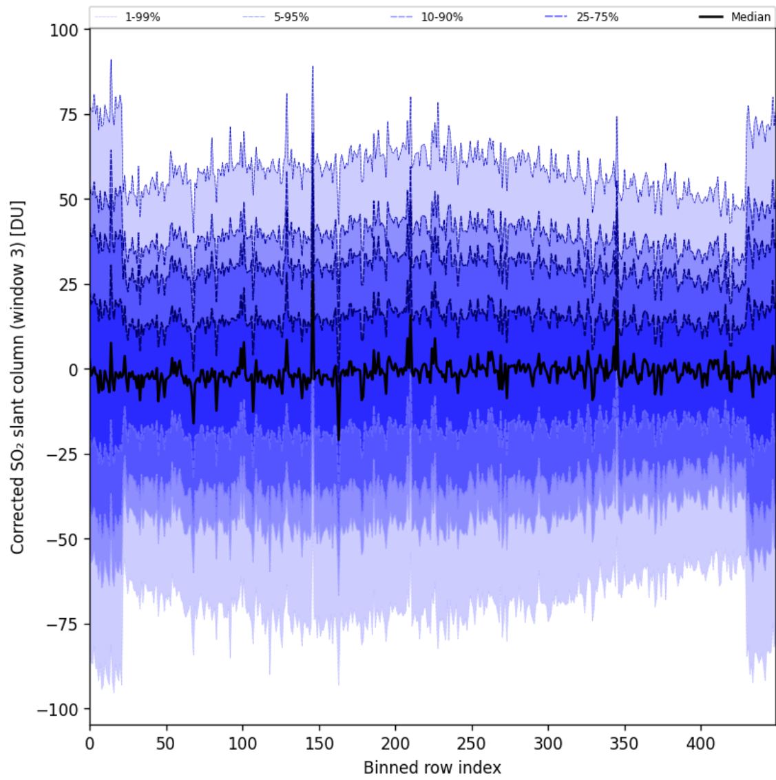
Figure 89: Along track statistics of “Corrected SO 2 slant column (window 3)” for 2024-09-22 to 2024-09-23
