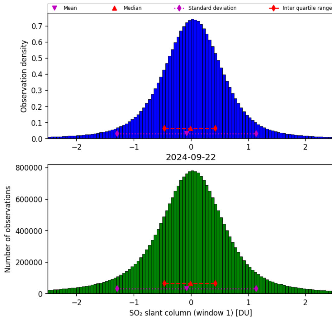
Figure 56: Histogram of “SO 2 slant column (window 1)” for 2024-09-22 to 2024-09-23
