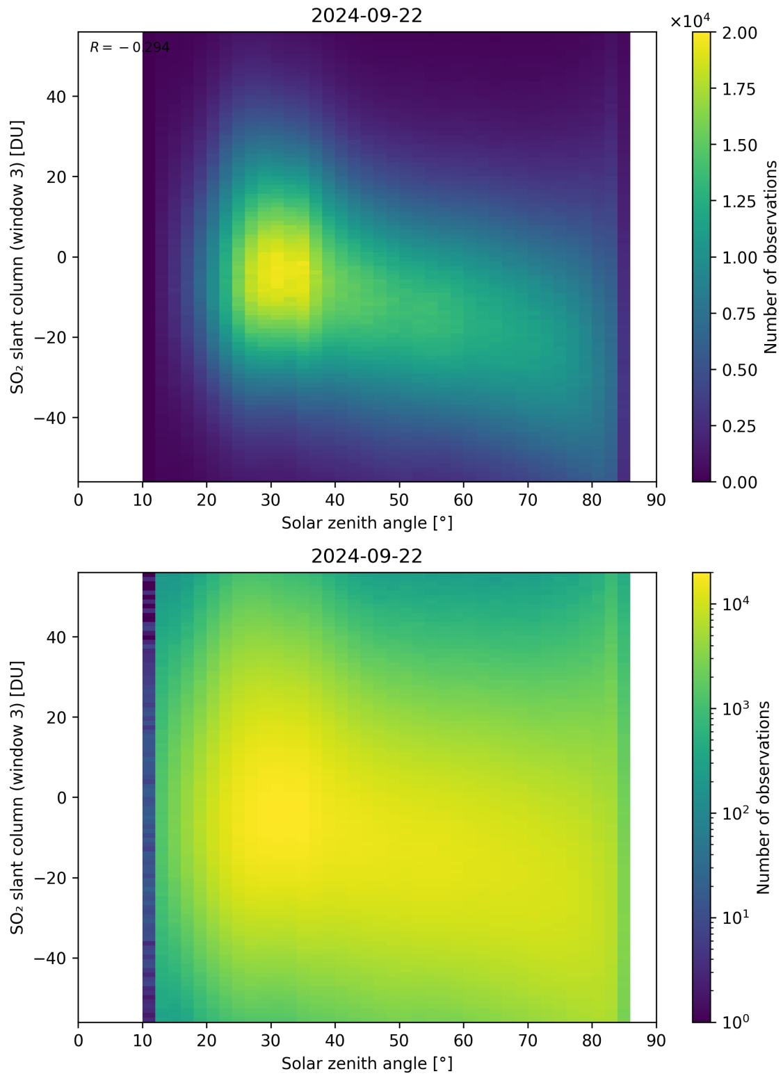
Figure 172: Scatter density plot of “Solar zenith angle” against “SO 2 slant column (window 3)” for 2024-09-22 to 2024-09-23.
