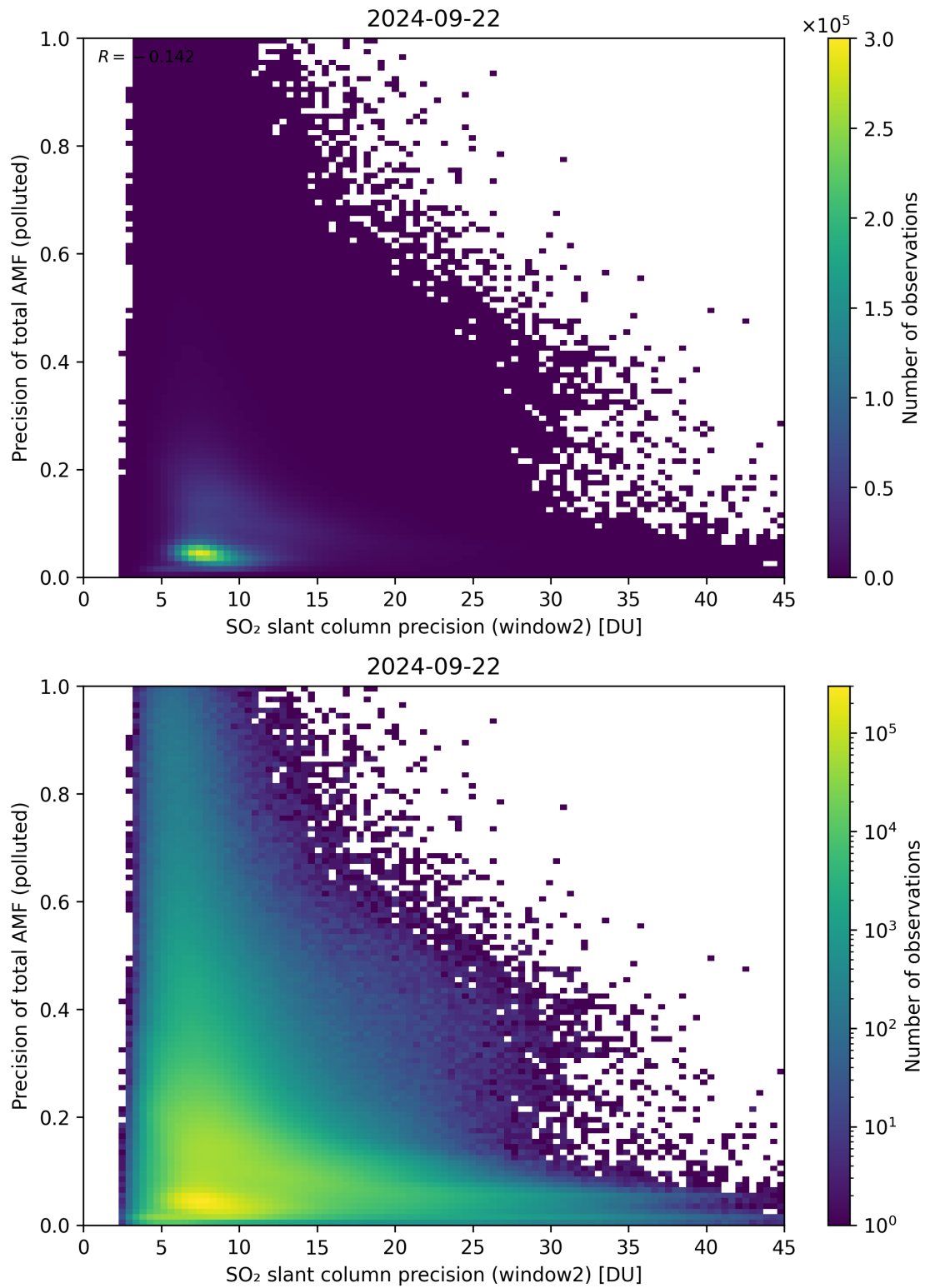
Figure 252: Scatter density plot of “SO 2 slant column precision (window2)” against “Precision of total AMF (polluted)” for 2024-09-22 to 2024-09-23.
