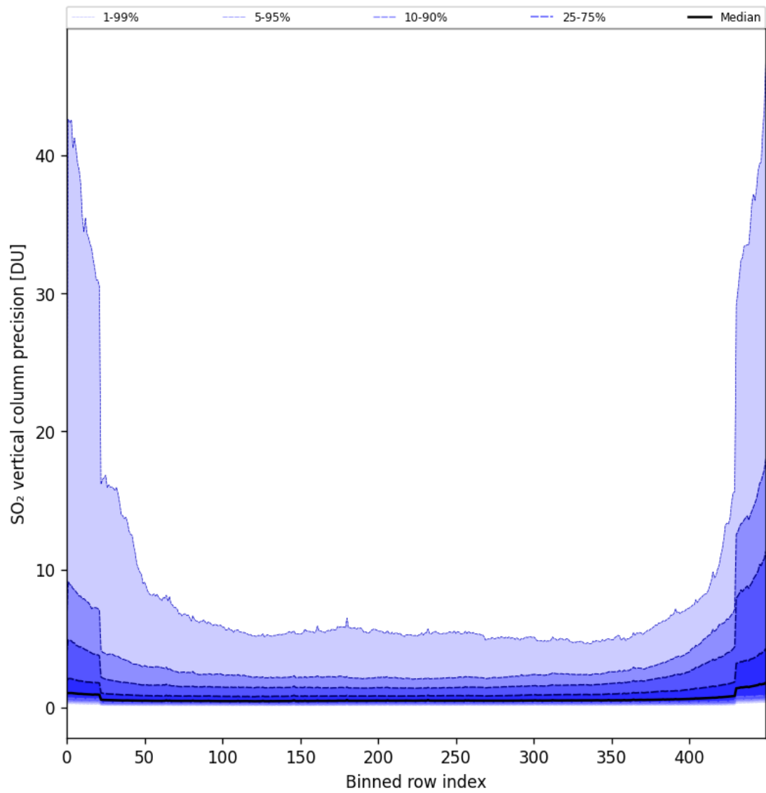
Figure 77: Along track statistics of “SO 2 vertical column precision” for 2024-09-22 to 2024-09-23
