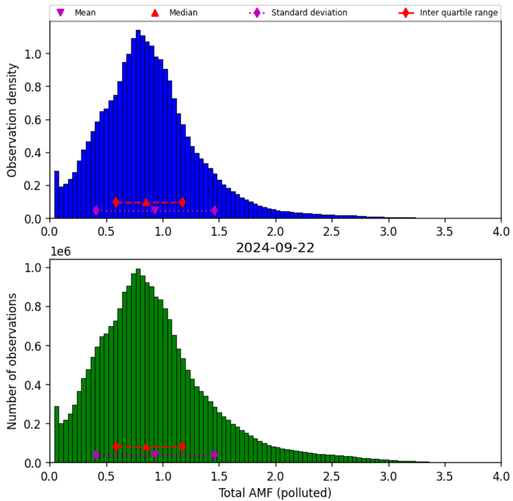
Figure 71: Histogram of “Total AMF (polluted)” for 2024-09-22 to 2024-09-23
