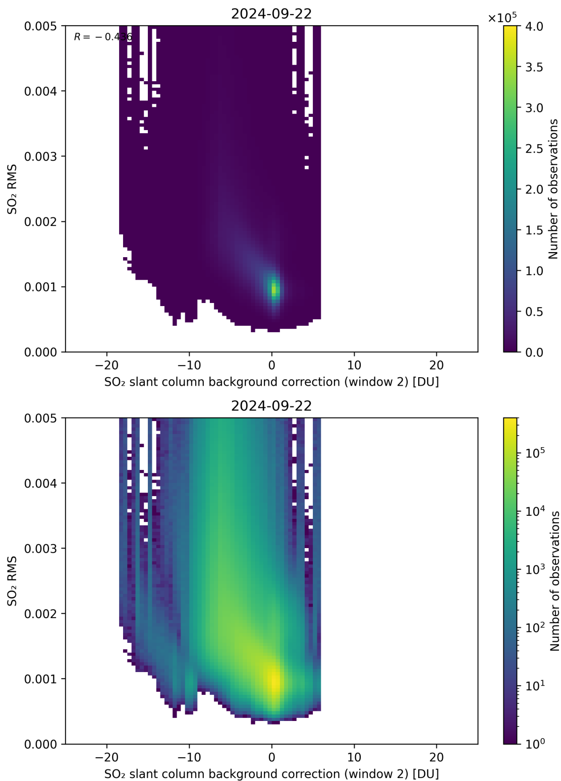
Figure 114: Scatter density plot of “SO 2 slant column background correction (window 2)” against “SO 2 RMS” for 2024-09-22 to 2024-09-23.
