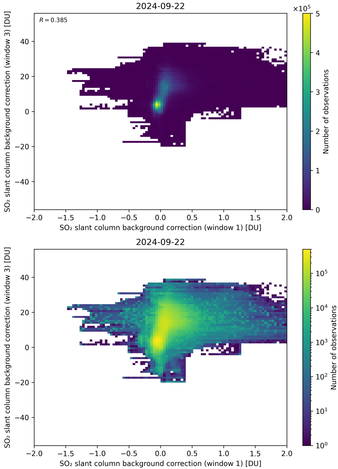
Figure 99: Scatter density plot of “SO 2 slant column background correction (window 1)” against “SO 2 slant column background correction (window 3)” for 2024-09-22 to 2024-09-23.
