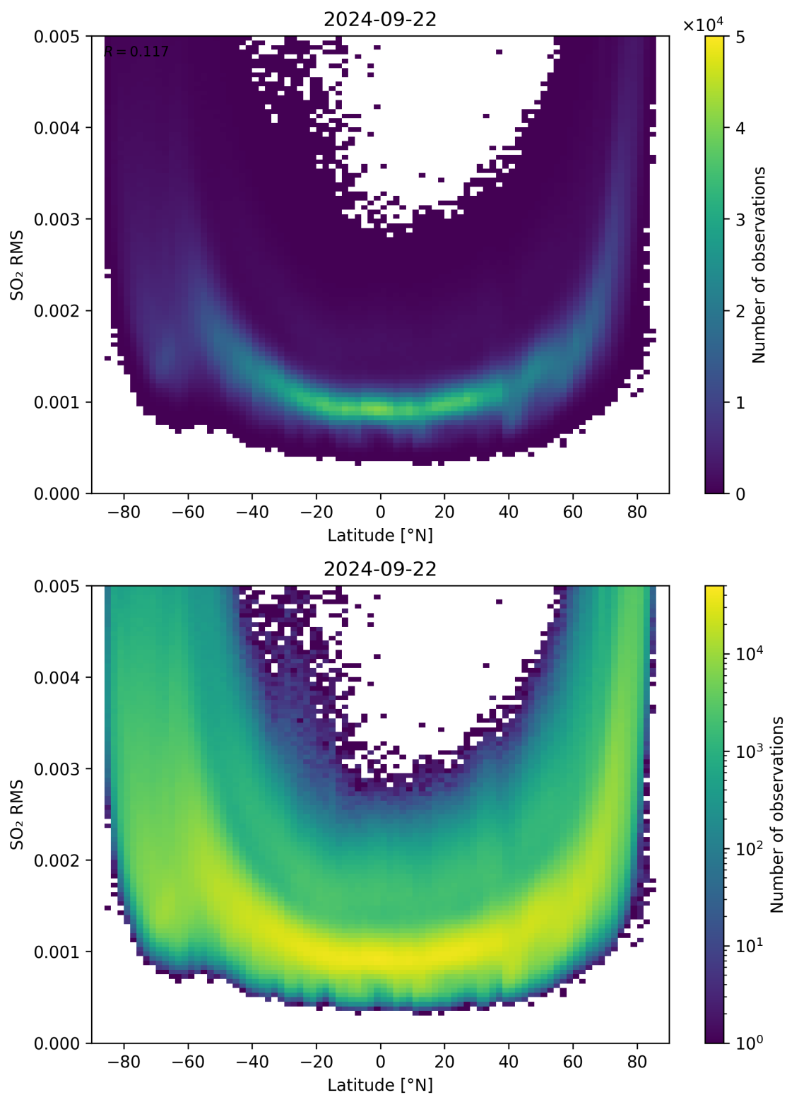
Figure 144: Scatter density plot of “Latitude” against “SO 2 RMS” for 2024-09-22 to 2024-09-23.
