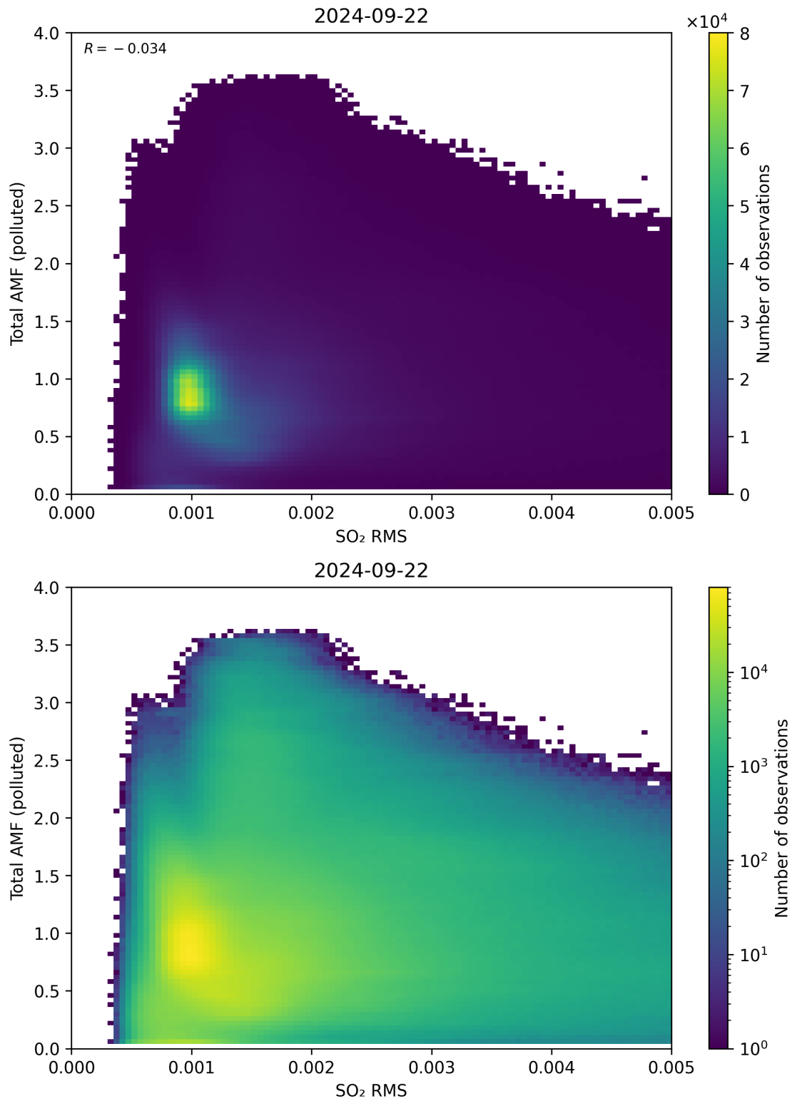
Figure 137: Scatter density plot of “SO 2 RMS” against “Total AMF (polluted)” for 2024-09-22 to 2024-09-23.
