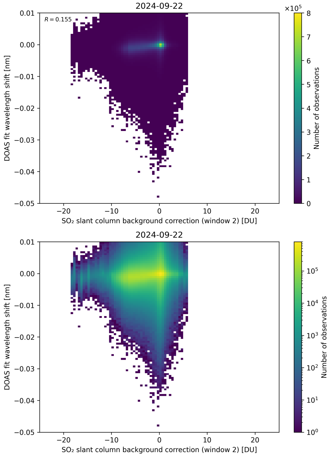
Figure 112: Scatter density plot of “SO 2 slant column background correction (window 2)” against “DOAS fit wavelength shift” for 2024-09-22 to 2024-09-23.
