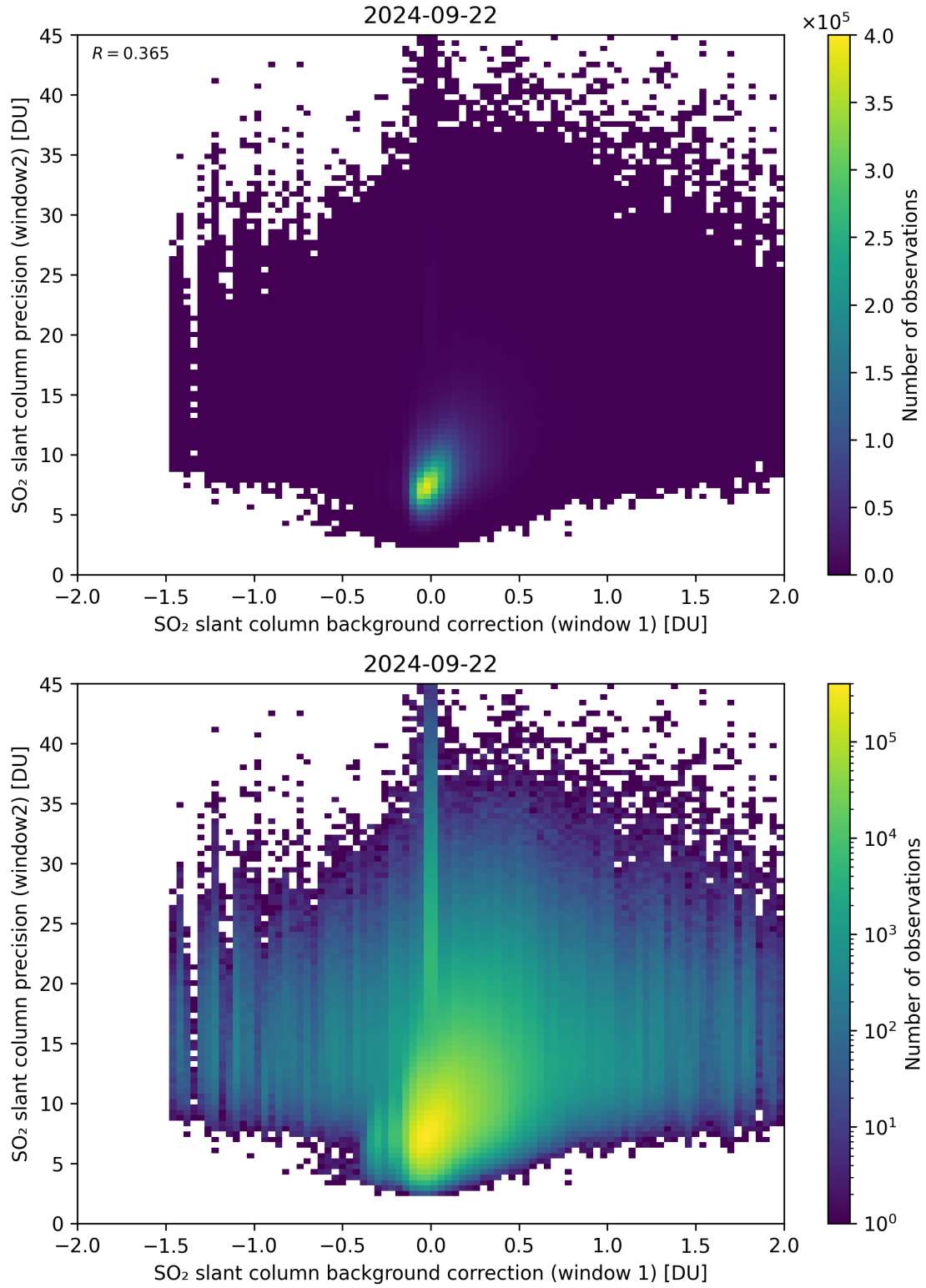
Figure 106: Scatter density plot of “SO 2 slant column background correction (window 1)” against “SO 2 slant column precision (window2)” for 2024-09-22 to 2024-09-23.
