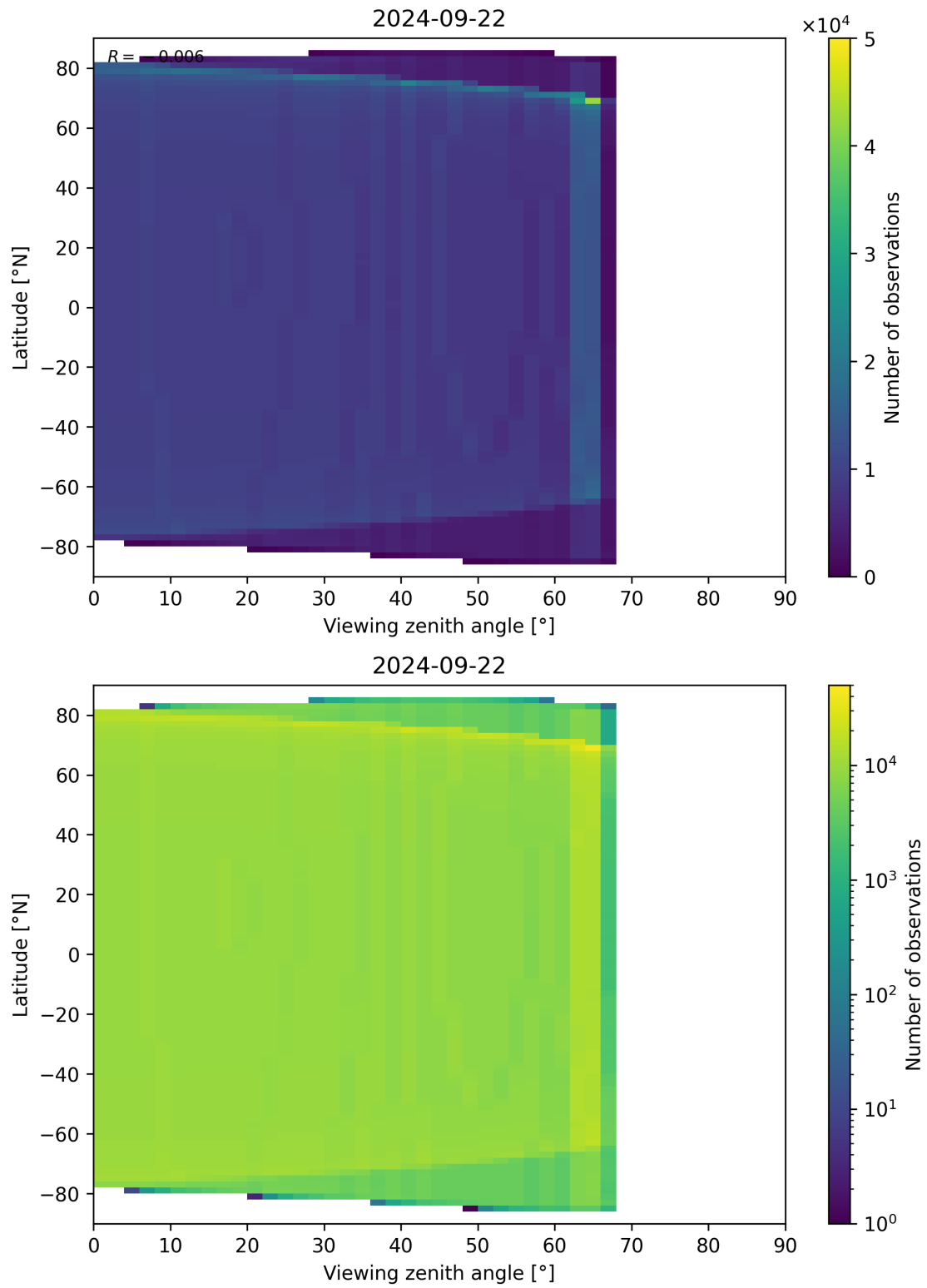
Figure 314: Scatter density plot of “Viewing zenith angle” against “Latitude” for 2024-09-22 to 2024-09-23.
