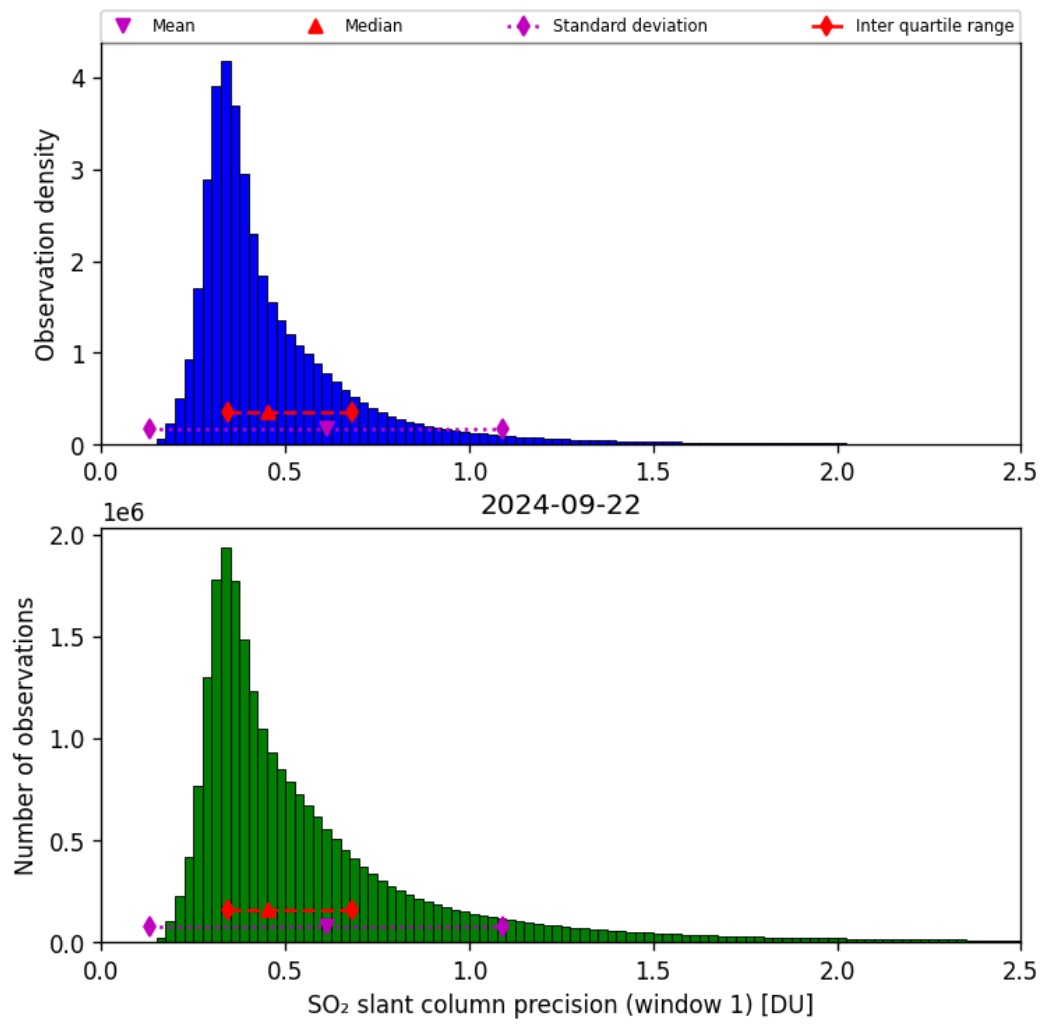
Figure 57: Histogram of “SO 2 slant column precision (window 1)” for 2024-09-22 to 2024-09-23
