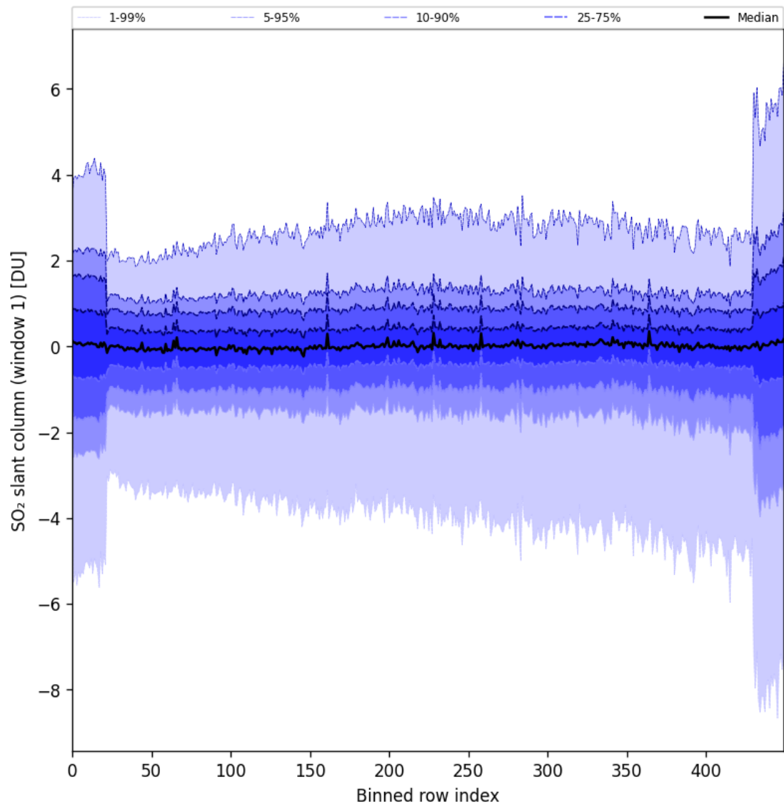
Figure 79: Along track statistics of “SO 2 slant column (window 1)” for 2024-09-22 to 2024-09-23
