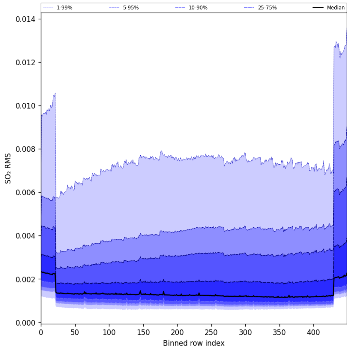
Figure 93: Along track statistics of “SO 2 RMS” for 2024-09-22 to 2024-09-23
