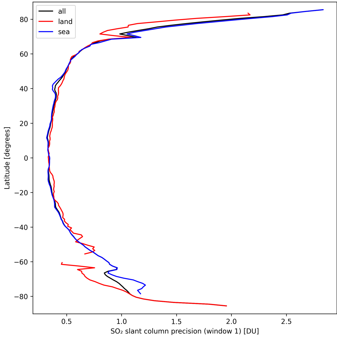
Figure 34: Zonal average of “SO 2 slant column precision (window 1)” for 2024-09-22 to 2024-09-23.
