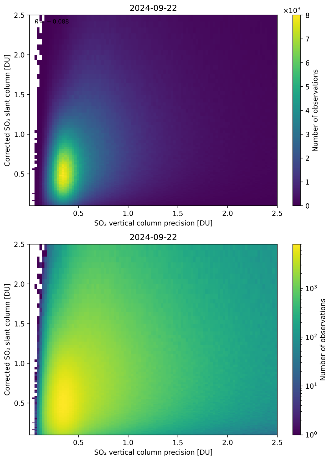
Figure 286: Scatter density plot of “SO 2 vertical column precision” against “Corrected SO 2 slant column” for 2024-09-22 to 2024-09-23.
