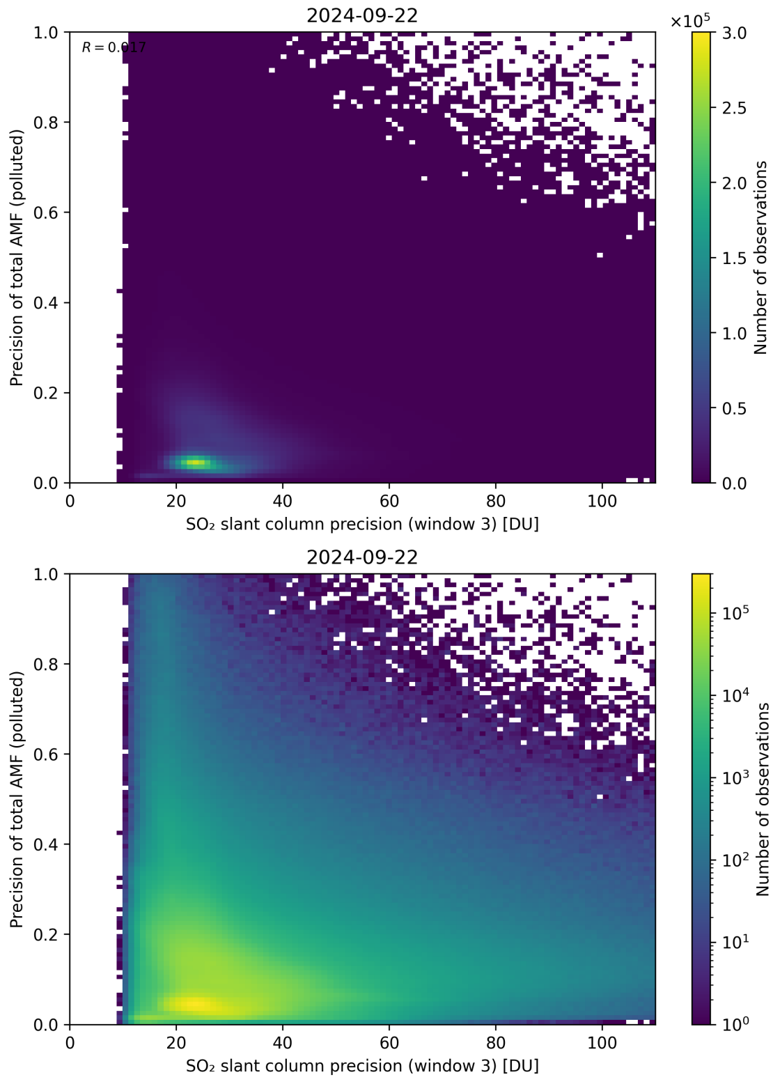
Figure 264: Scatter density plot of “SO 2 slant column precision (window 3)” against “Precision of total AMF (polluted)” for 2024-09-22 to 2024-09-23.
