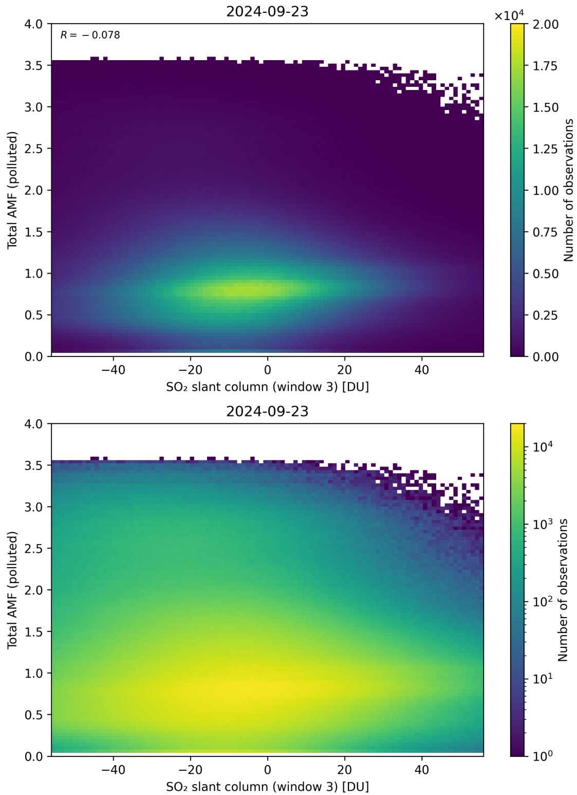
Figure 268: Scatter density plot of “SO 2 slant column (window 3)” against “Total AMF (polluted)” for 2024-09-22 to 2024-09-24.
