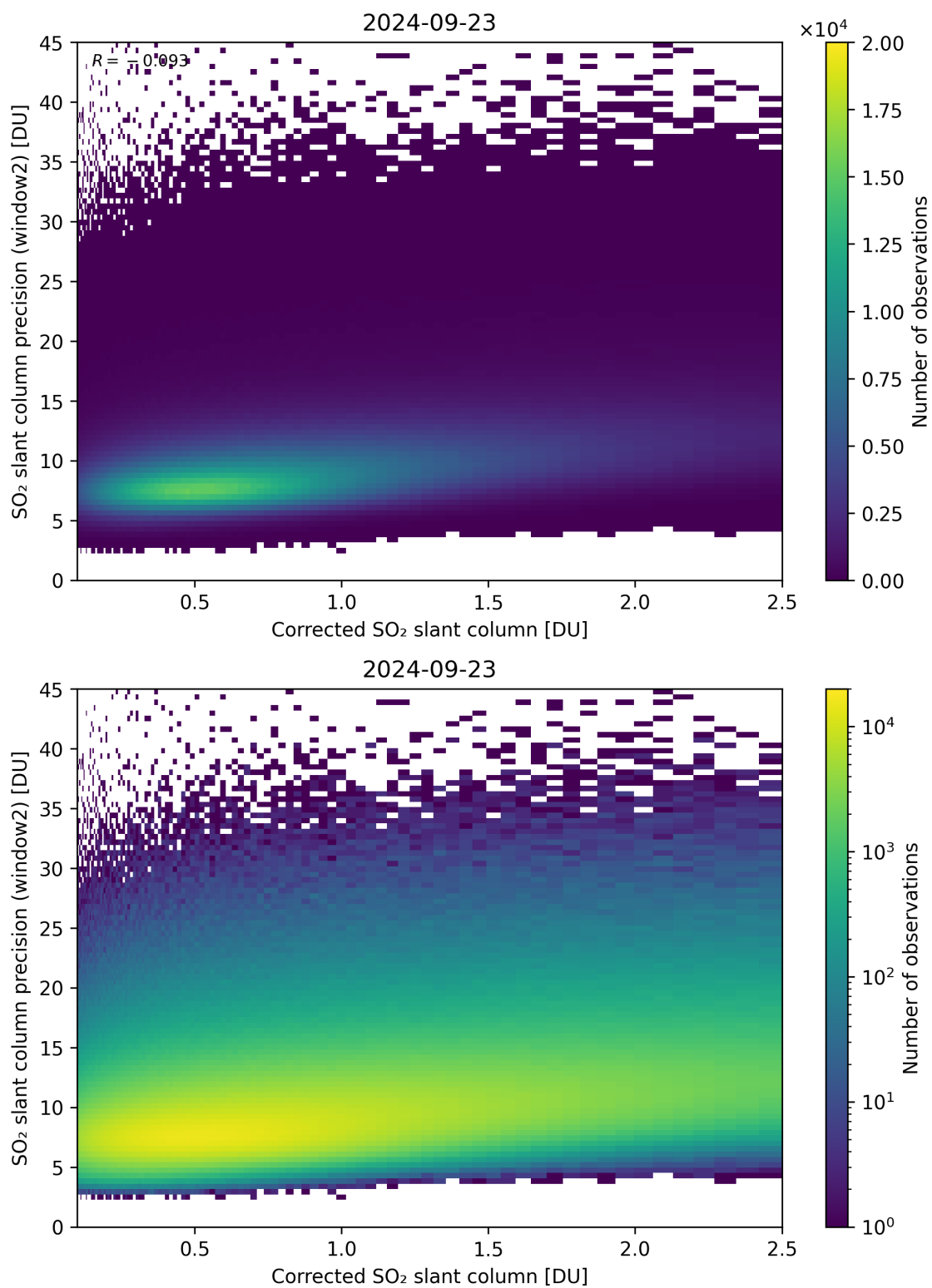
Figure 189: Scatter density plot of “Corrected SO 2 slant column” against “SO 2 slant column precision (window2)” for 2024-09-22 to 2024-09-24.
