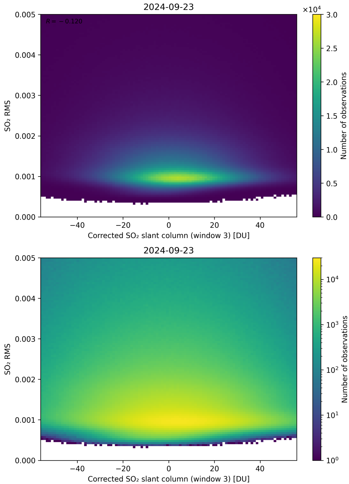
Figure 208: Scatter density plot of “Corrected SO 2 slant column (window 3)” against “SO 2 RMS” for 2024-09-22 to 2024-09-24.
