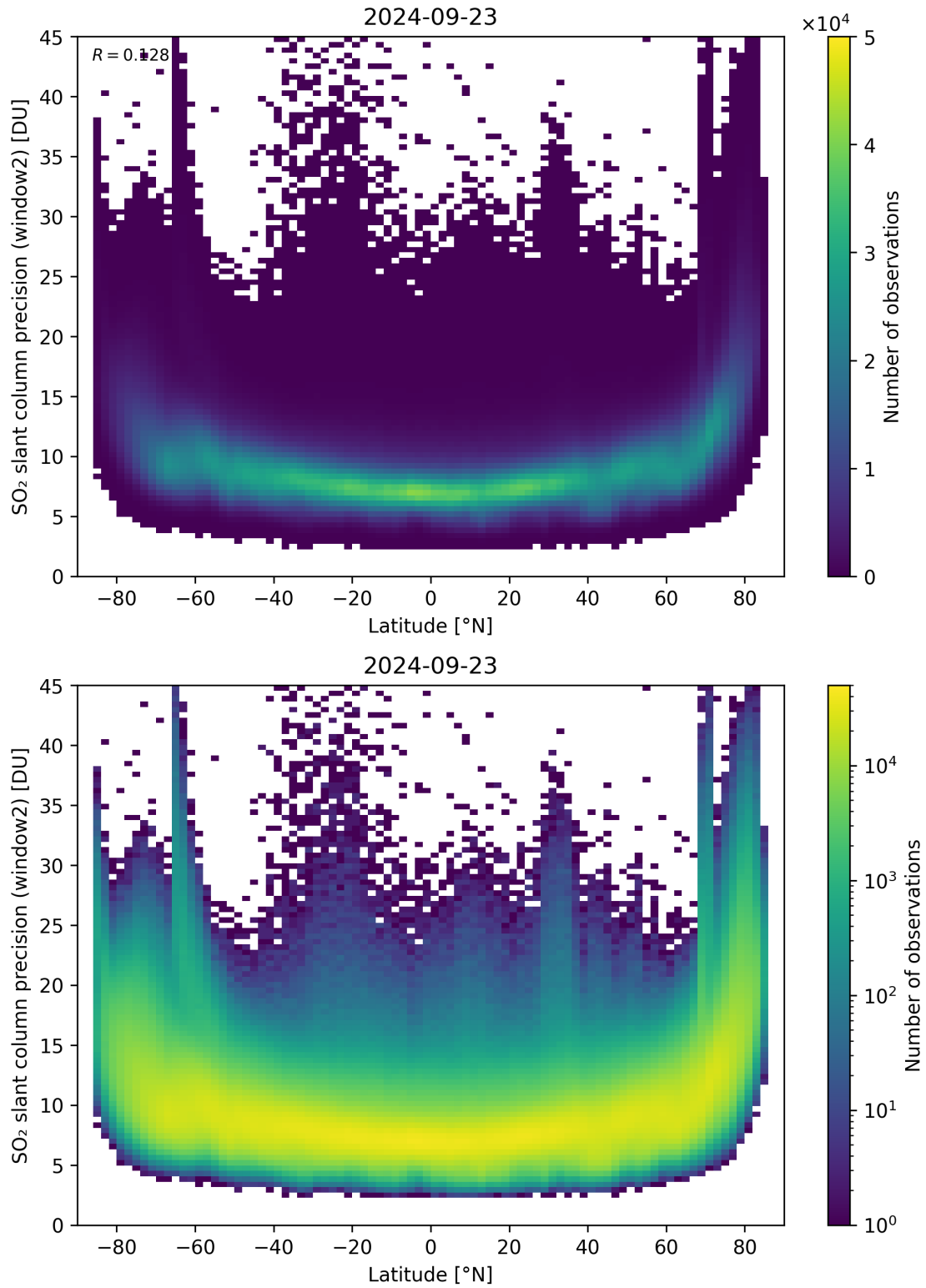
Figure 151: Scatter density plot of “Latitude” against “SO 2 slant column precision (window2)” for 2024-09-22 to 2024-09-24.
