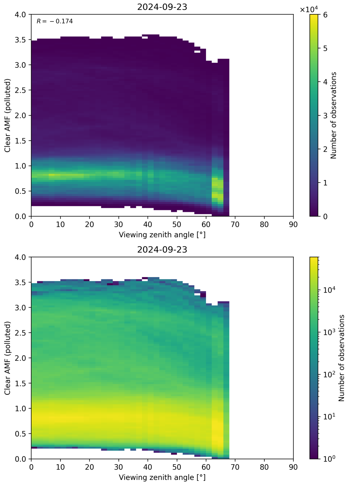
Figure 316: Scatter density plot of “Viewing zenith angle” against “Clear AMF (polluted)” for 2024-09-22 to 2024-09-24.
