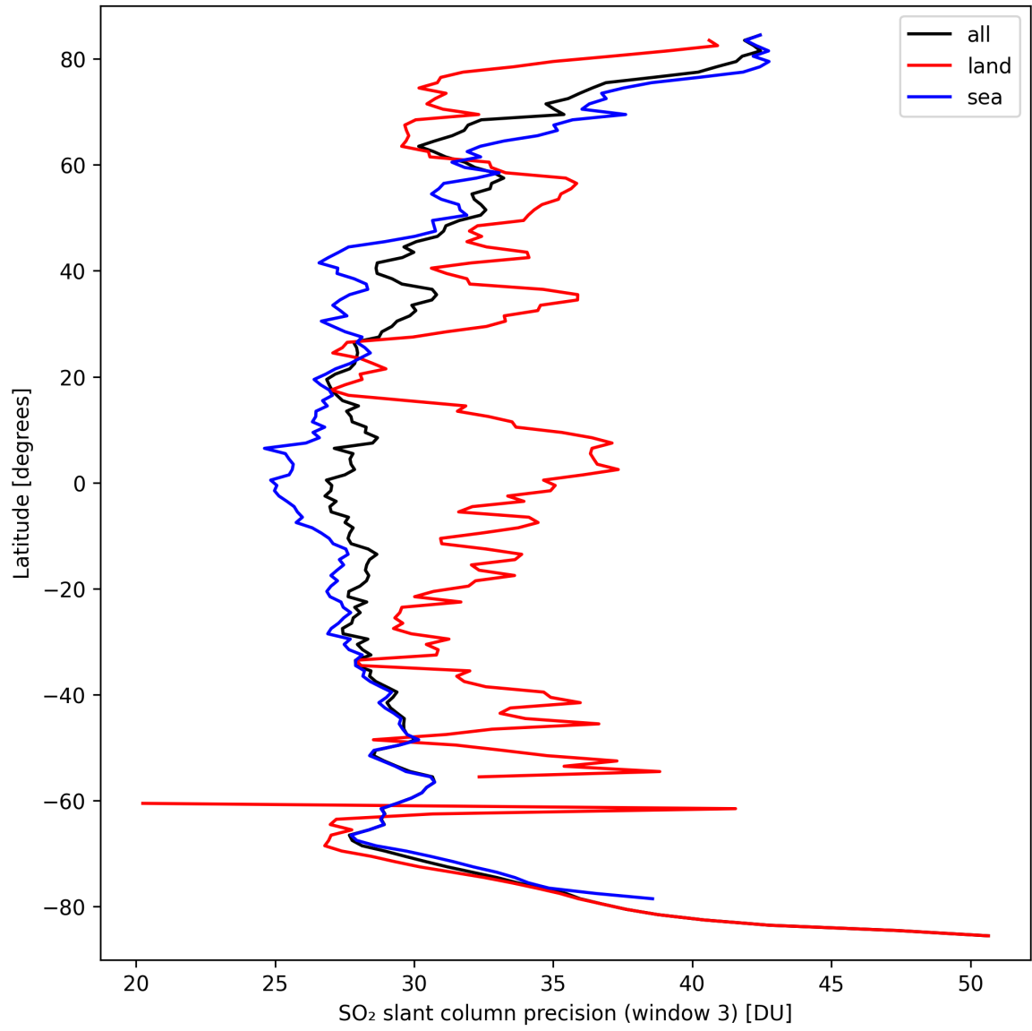
Figure 42: Zonal average of “SO 2 slant column precision (window 3)” for 2024-09-22 to 2024-09-24.
