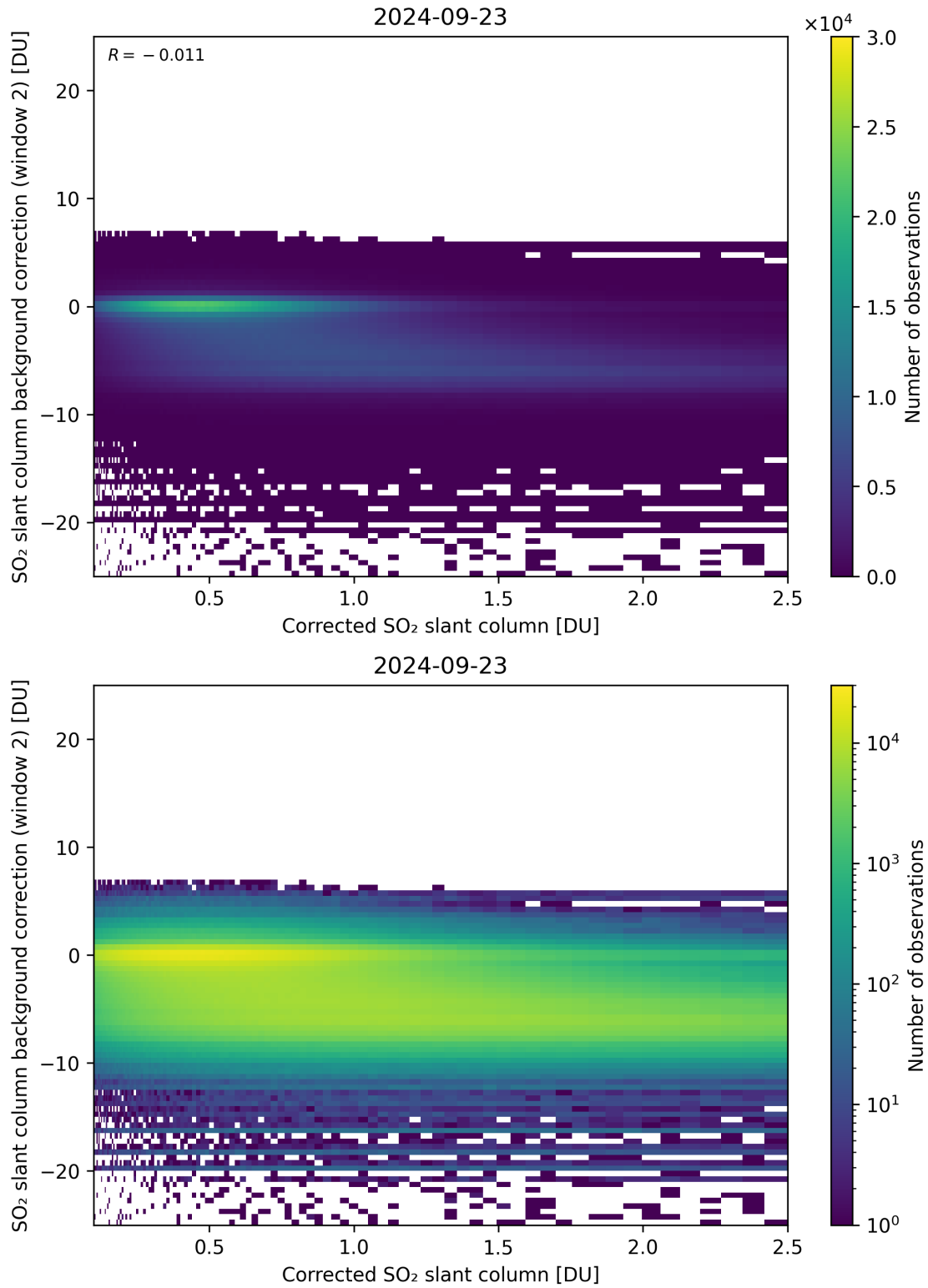
Figure 179: Scatter density plot of “Corrected SO 2 slant column” against “SO 2 slant column background correction (window 2)” for 2024-09-22 to 2024-09-24.
