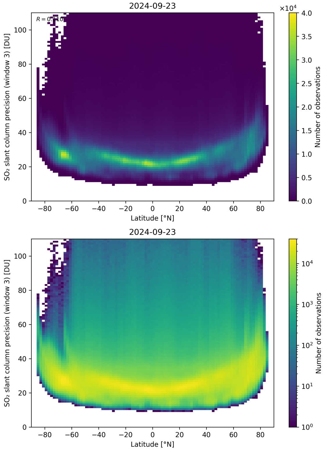
Figure 153: Scatter density plot of “Latitude” against “SO 2 slant column precision (window 3)” for 2024-09-22 to 2024-09-24.
