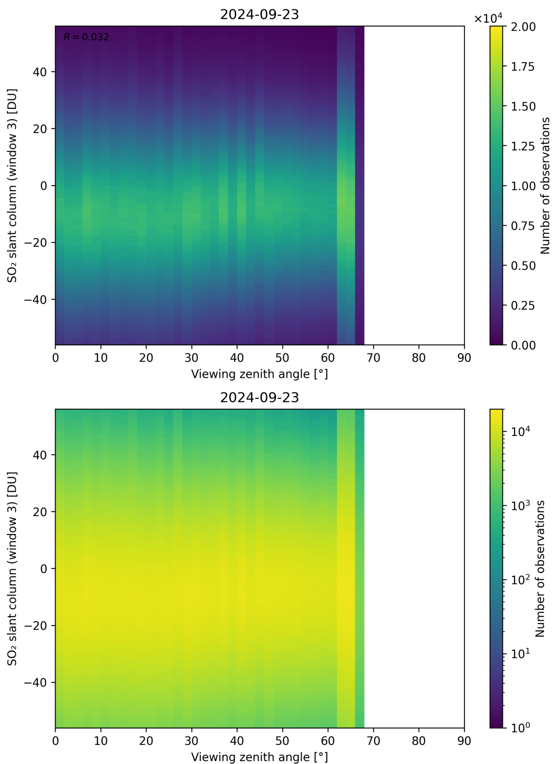
Figure 323: Scatter density plot of “Viewing zenith angle” against “SO 2 slant column (window 3)” for 2024-09-22 to 2024-09-24.
