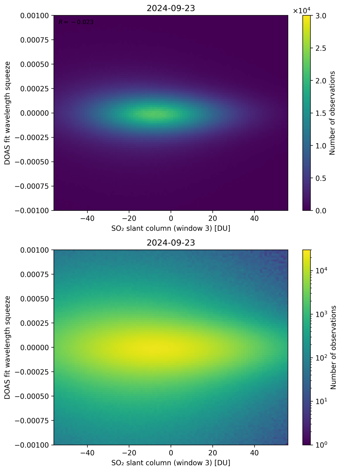
Figure 255: Scatter density plot of “SO 2 slant column (window 3)” against “DOAS fit wavelength squeeze” for 2024-09-22 to 2024-09-24.
