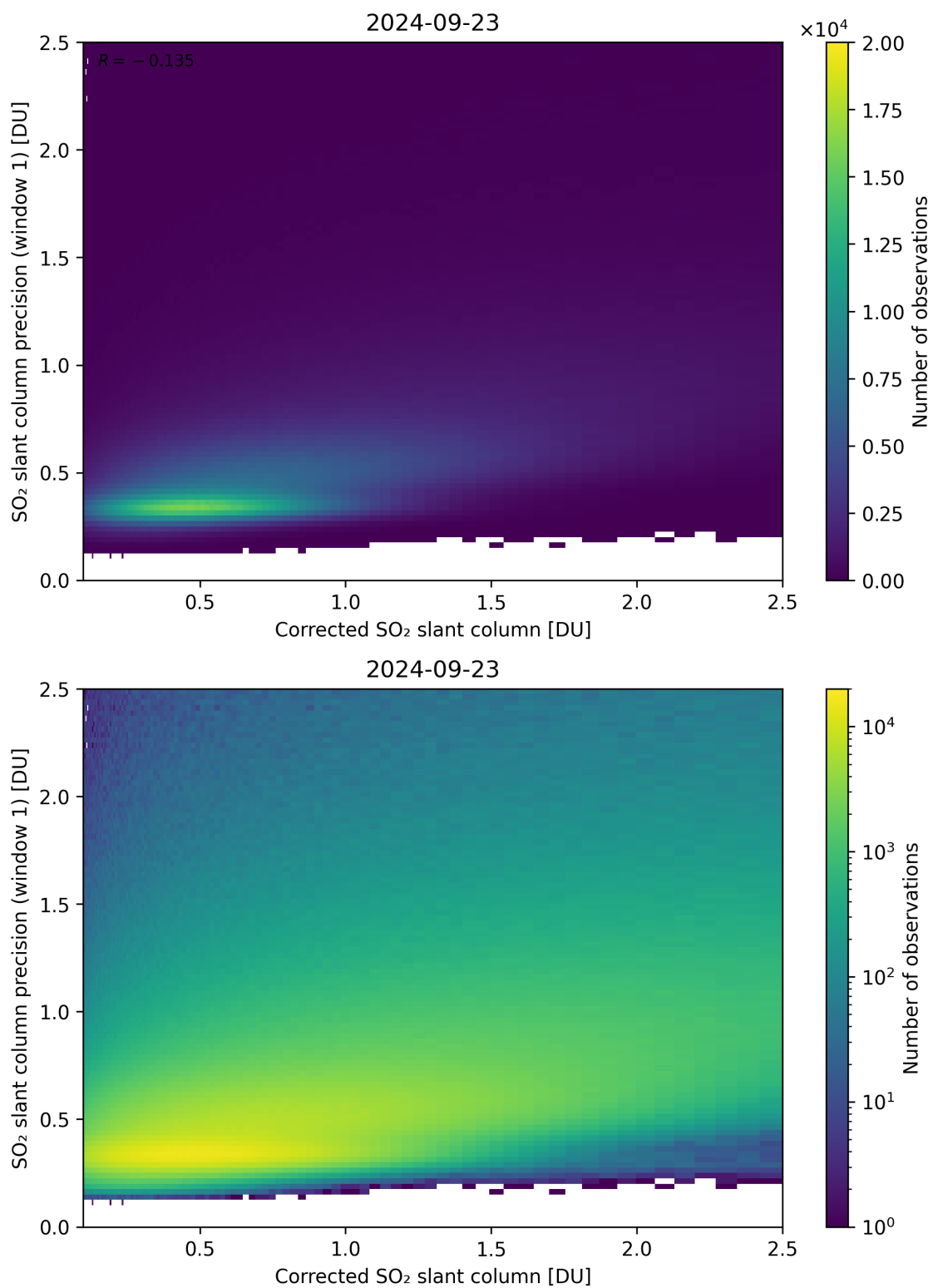
Figure 188: Scatter density plot of “Corrected SO 2 slant column” against “SO 2 slant column precision (window 1)” for 2024-09-22 to 2024-09-24.
