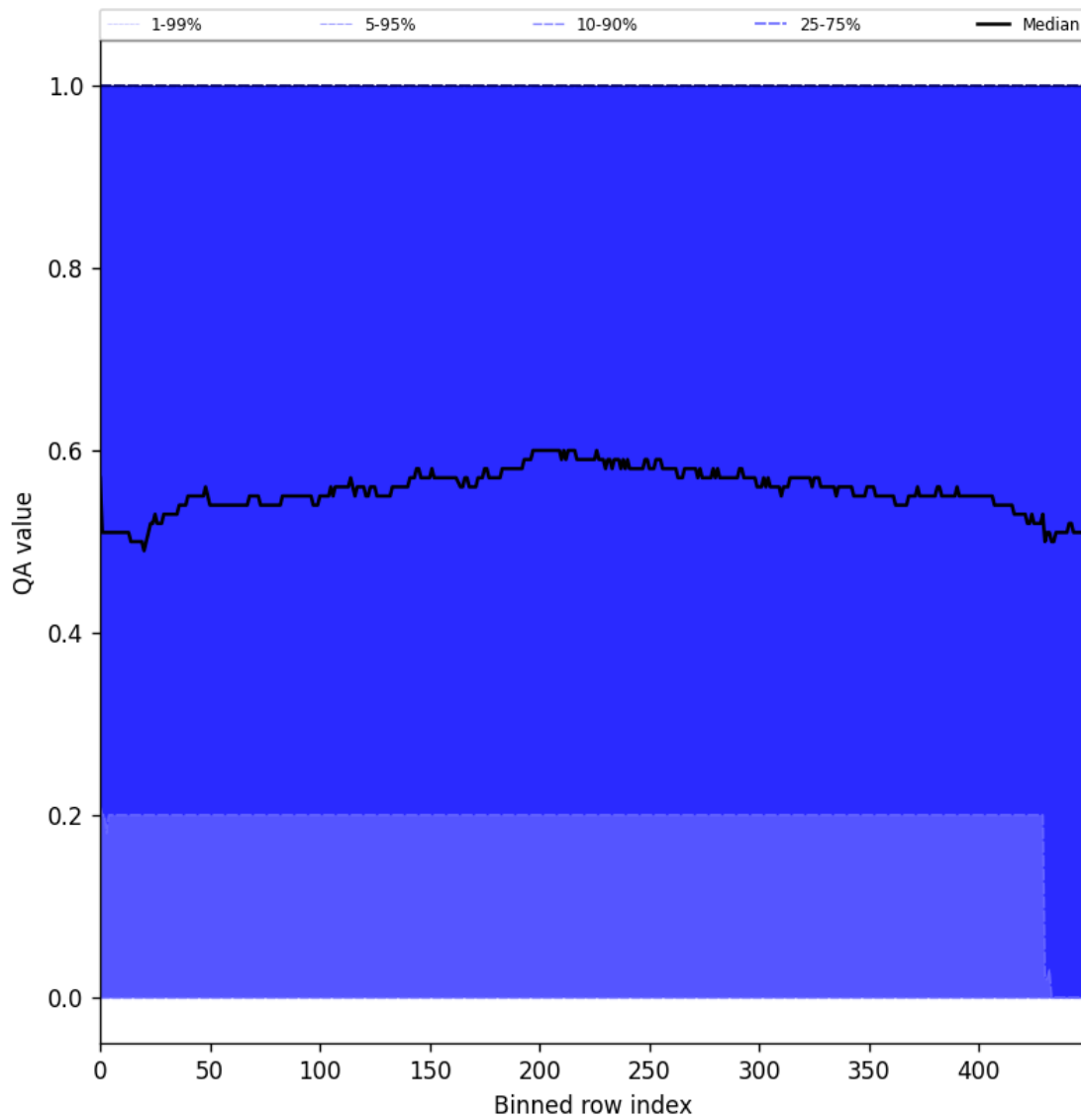
Figure 75: Along track statistics of “QA value” for 2024-09-22 to 2024-09-24
