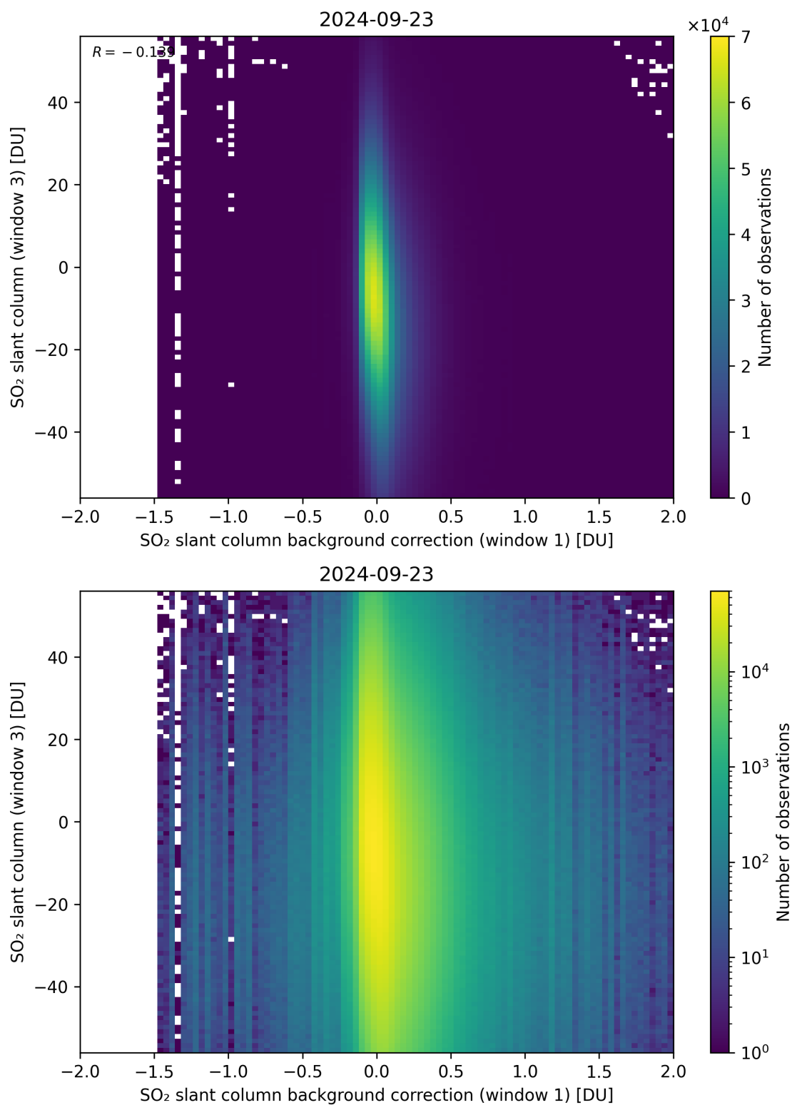
Figure 107: Scatter density plot of “SO 2 slant column background correction (window 1)” against “SO 2 slant column (window 3)” for 2024-09-22 to 2024-09-24.
