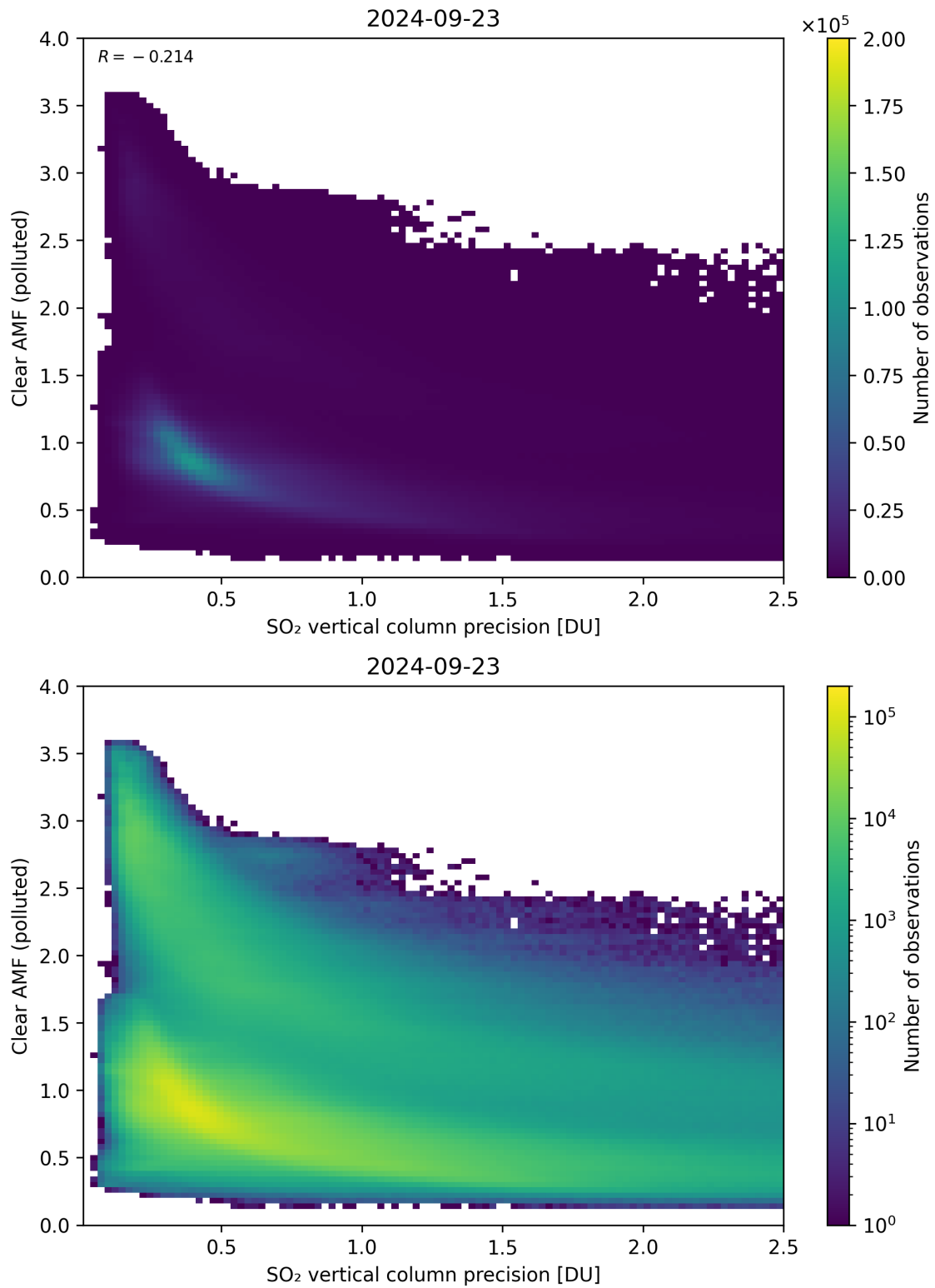
Figure 285: Scatter density plot of “SO 2 vertical column precision” against “Clear AMF (polluted)” for 2024-09-22 to 2024-09-24.
