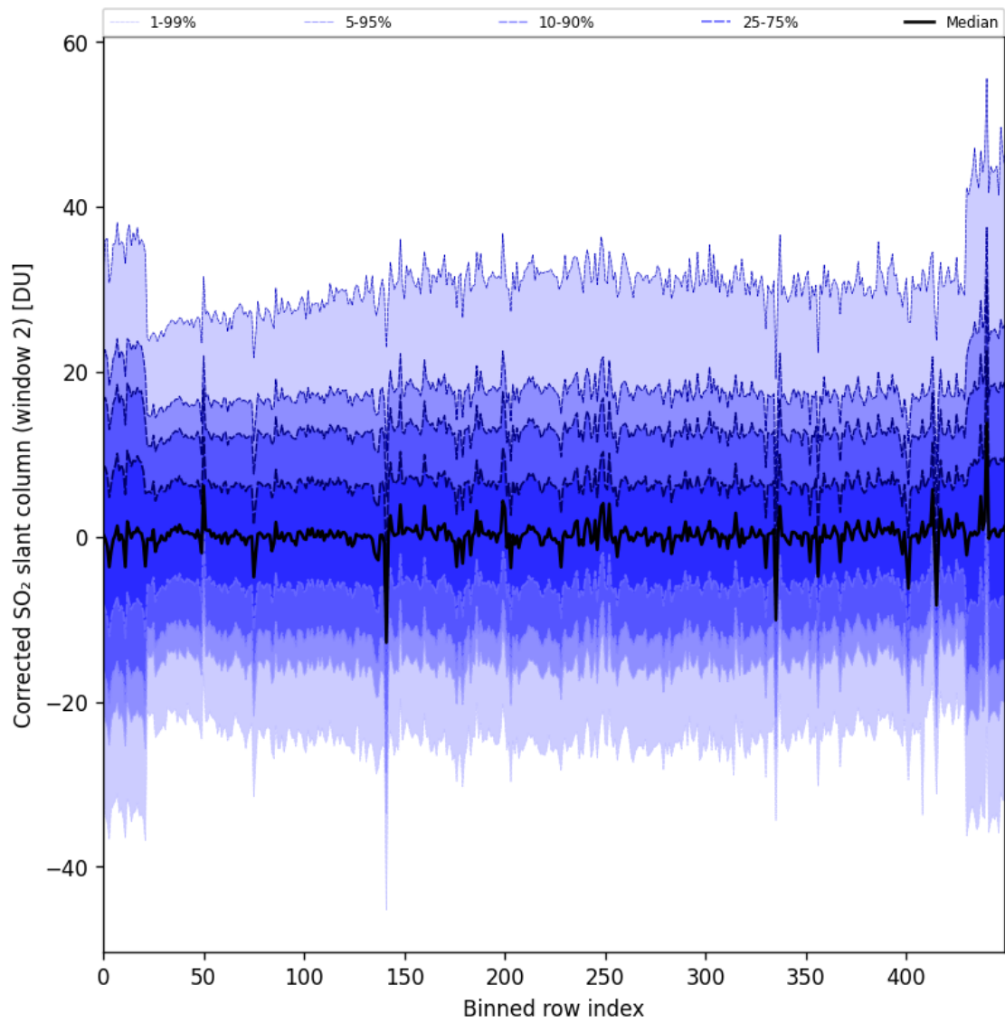
Figure 85: Along track statistics of “Corrected SO 2 slant column (window 2)” for 2024-09-22 to 2024-09-24
