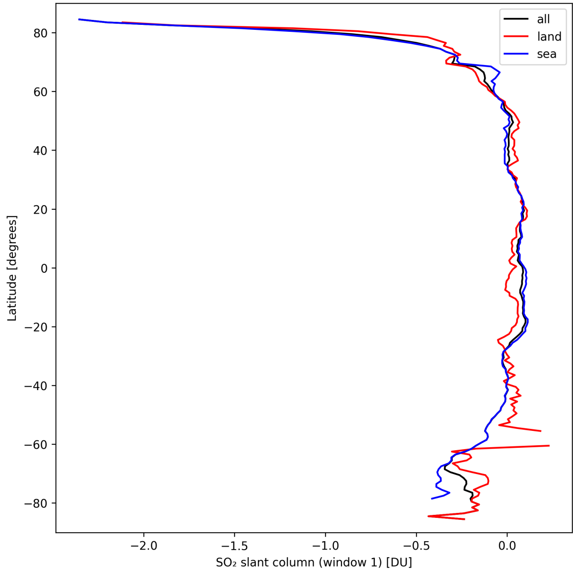
Figure 33: Zonal average of “SO 2 slant column (window 1)” for 2024-09-22 to 2024-09-24.
