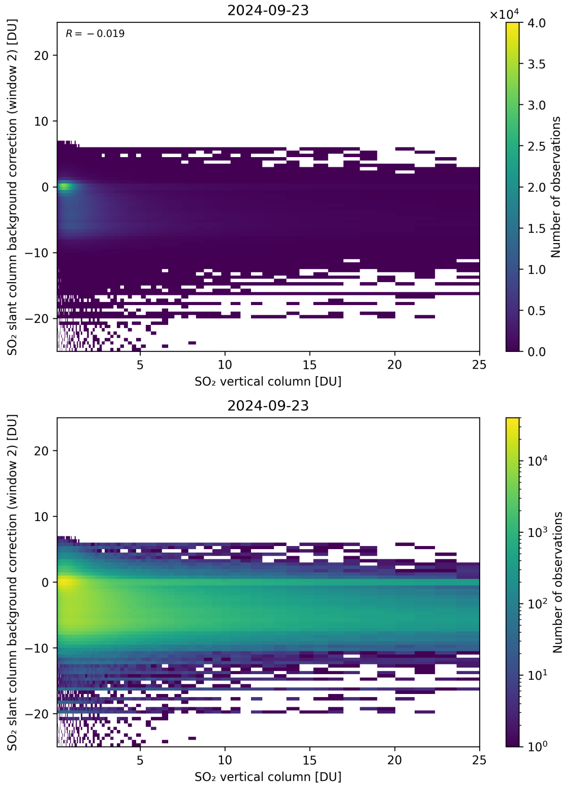
Figure 274: Scatter density plot of “SO 2 vertical column” against “SO 2 slant column background correction (window 2)” for 2024-09-22 to 2024-09-24.
