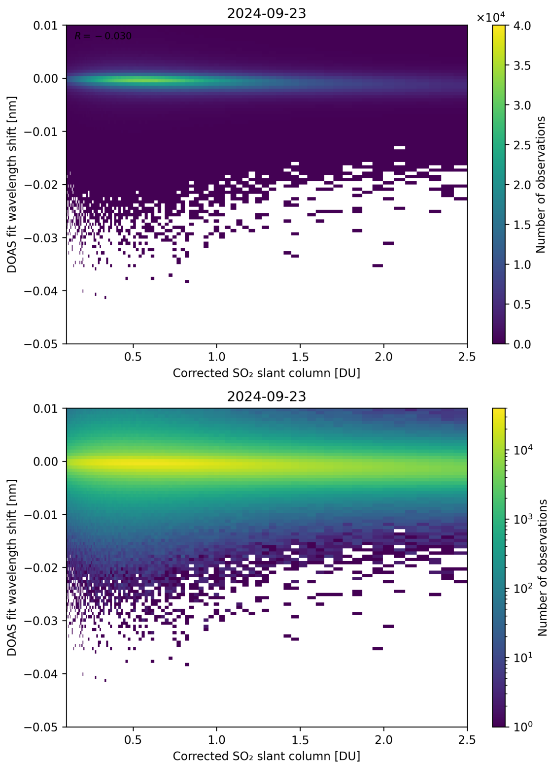
Figure 181: Scatter density plot of “Corrected SO 2 slant column” against “DOAS fit wavelength shift” for 2024-09-22 to 2024-09-24.
