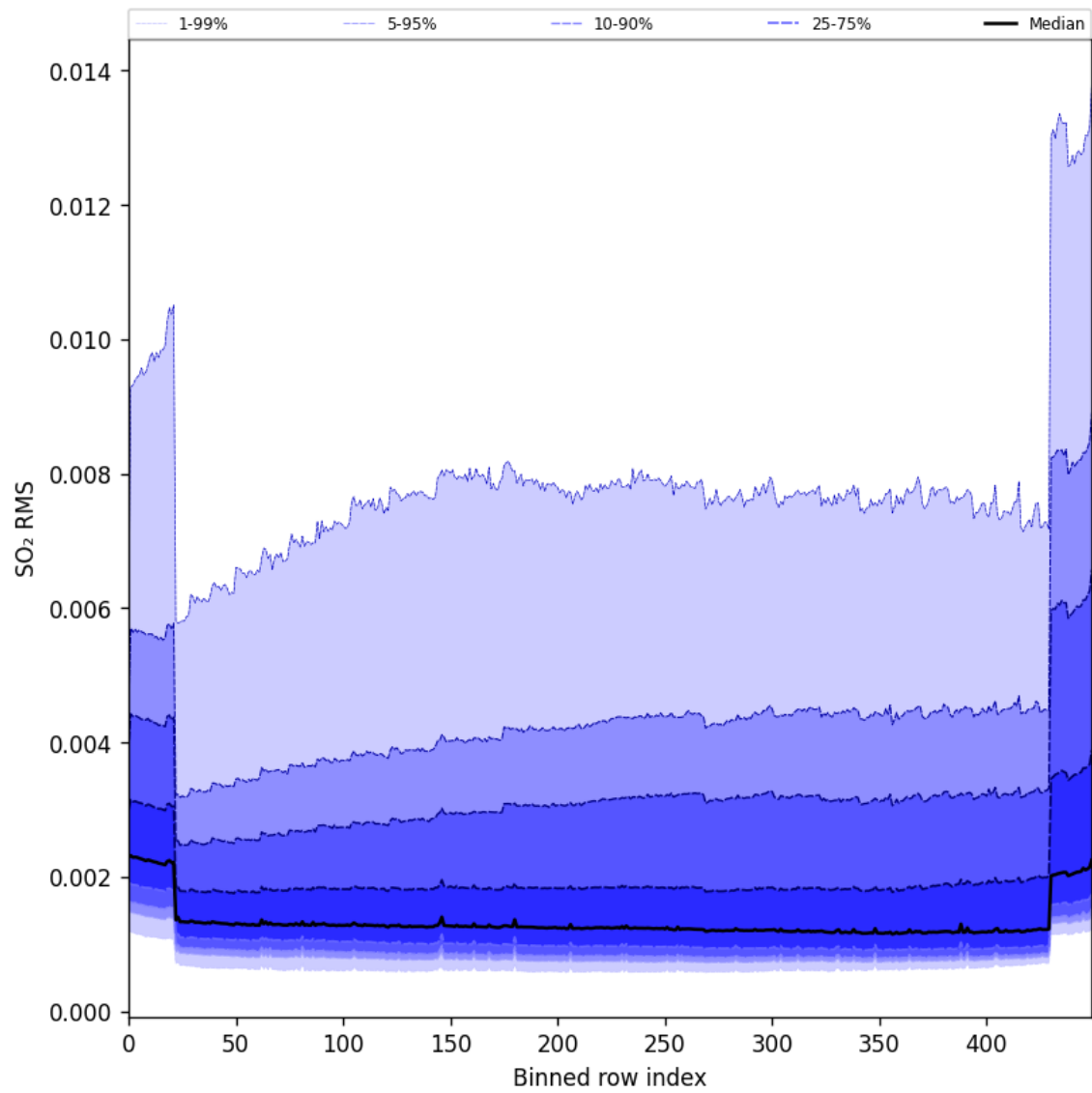
Figure 93: Along track statistics of “SO 2 RMS” for 2024-09-22 to 2024-09-24
