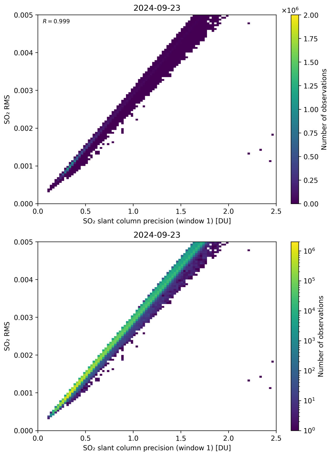
Figure 223: Scatter density plot of “SO 2 slant column precision (window 1)” against “SO 2 RMS” for 2024-09-22 to 2024-09-24.
