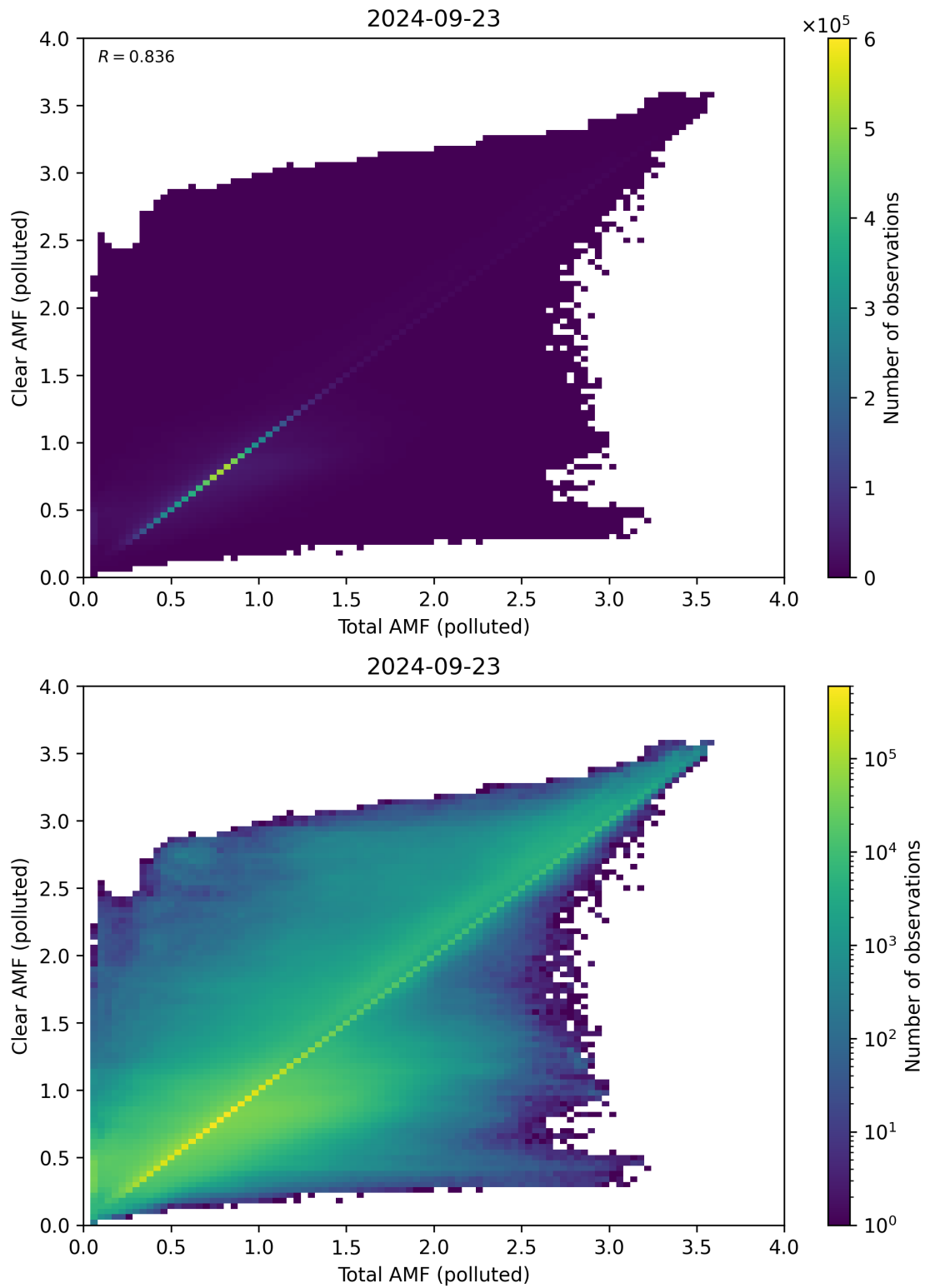
Figure 271: Scatter density plot of “Total AMF (polluted)” against “Clear AMF (polluted)” for 2024-09-22 to 2024-09-24.
