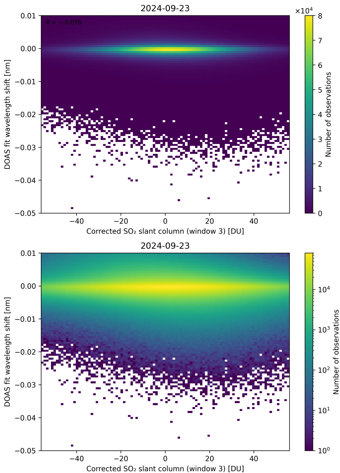
Figure 206: Scatter density plot of “Corrected SO 2 slant column (window 3)” against “DOAS fit wavelength shift” for 2024-09-22 to 2024-09-24.
