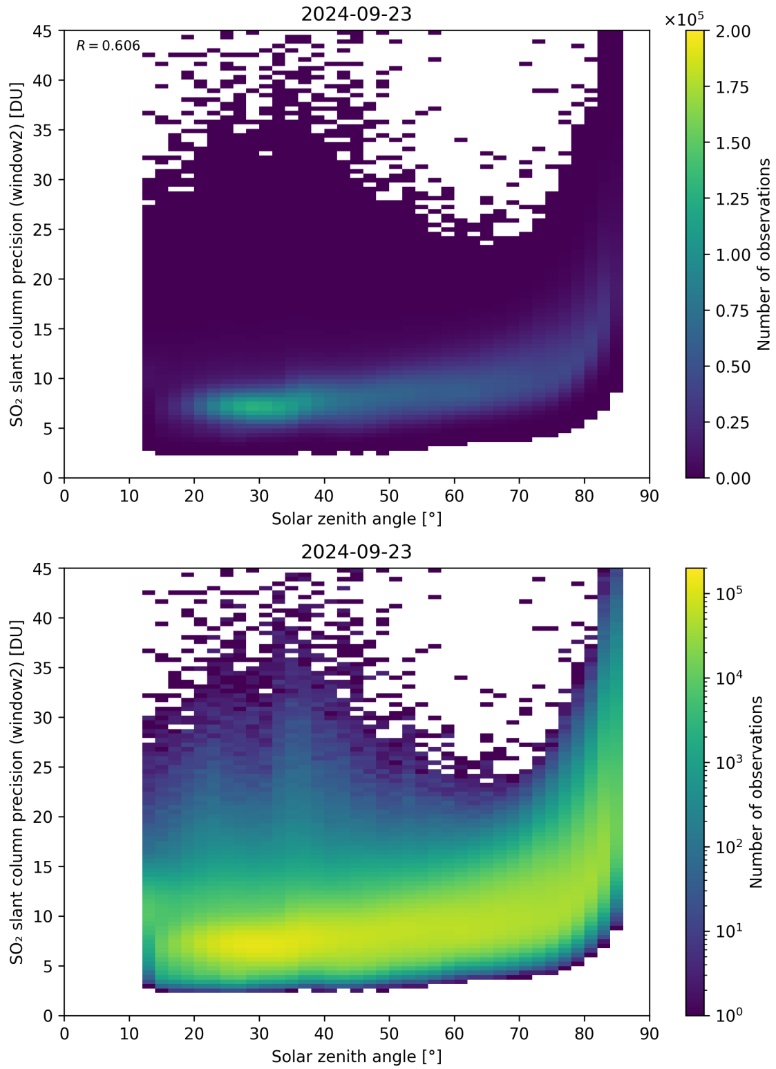
Figure 171: Scatter density plot of “Solar zenith angle” against “SO 2 slant column precision (window2)” for 2024-09-22 to 2024-09-24.
