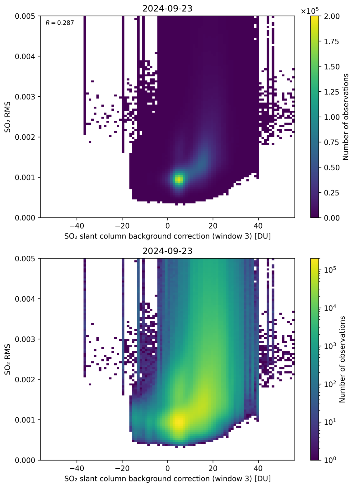
Figure 123: Scatter density plot of “SO 2 slant column background correction (window 3)” against “SO 2 RMS” for 2024-09-22 to 2024-09-24.
