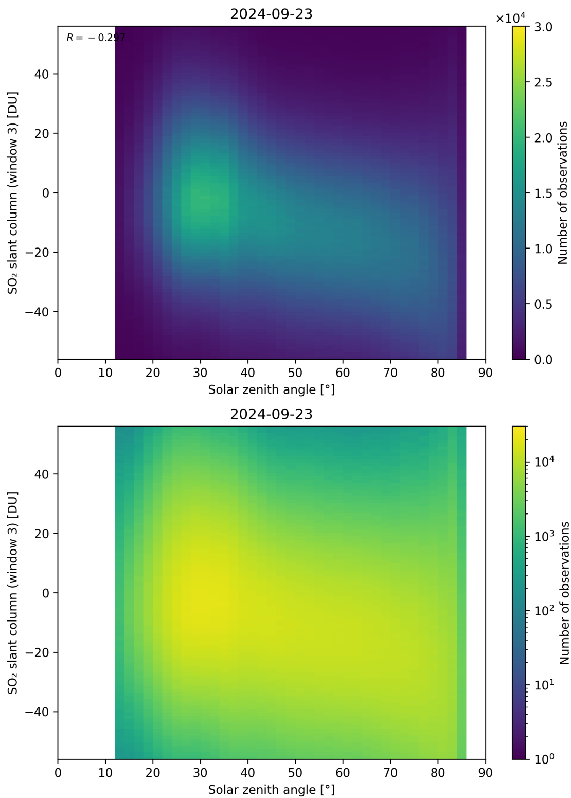
Figure 172: Scatter density plot of “Solar zenith angle” against “SO 2 slant column (window 3)” for 2024-09-22 to 2024-09-24.
