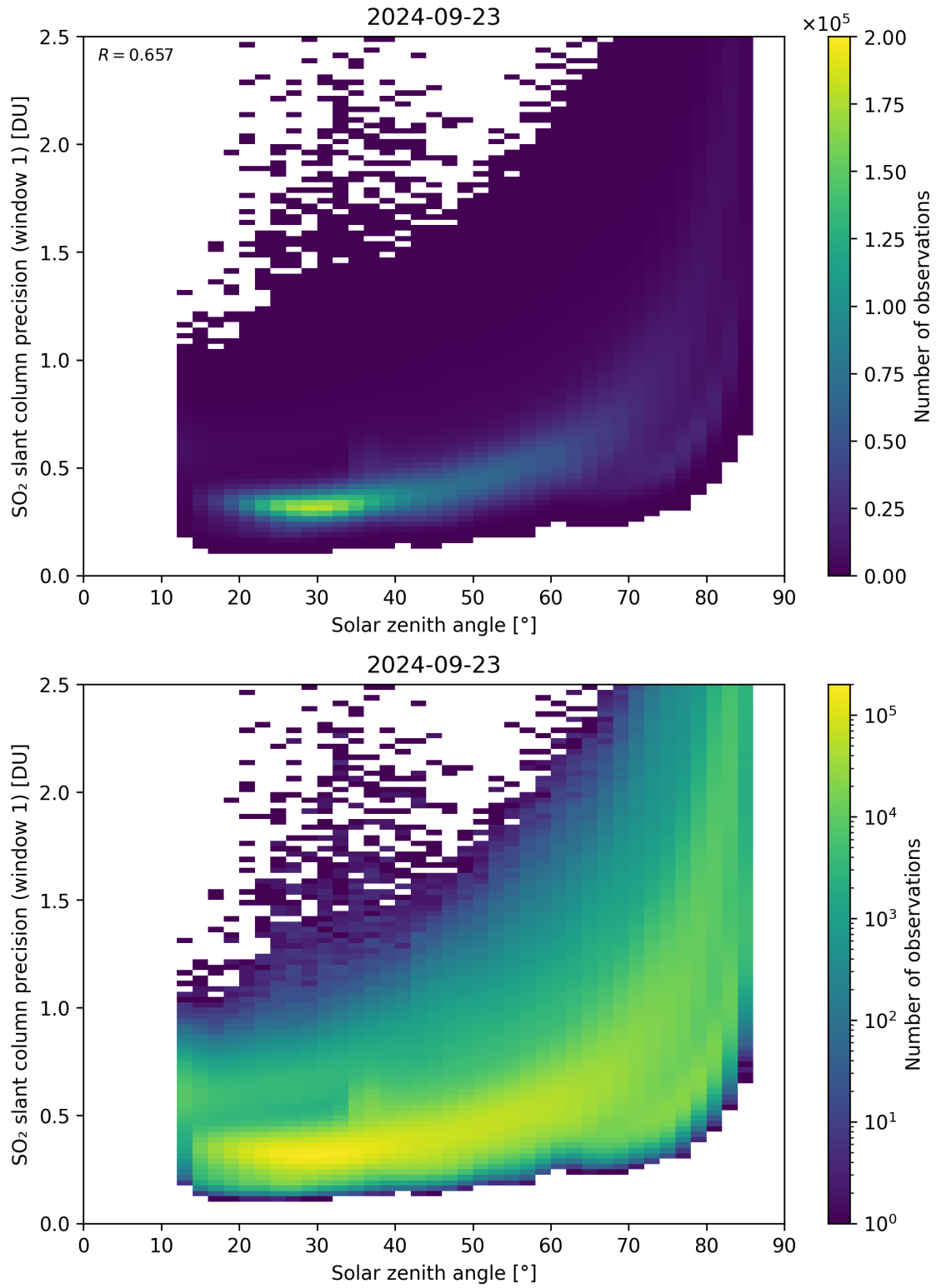
Figure 170: Scatter density plot of “Solar zenith angle” against “SO 2 slant column precision (window 1)” for 2024-09-22 to 2024-09-24.
