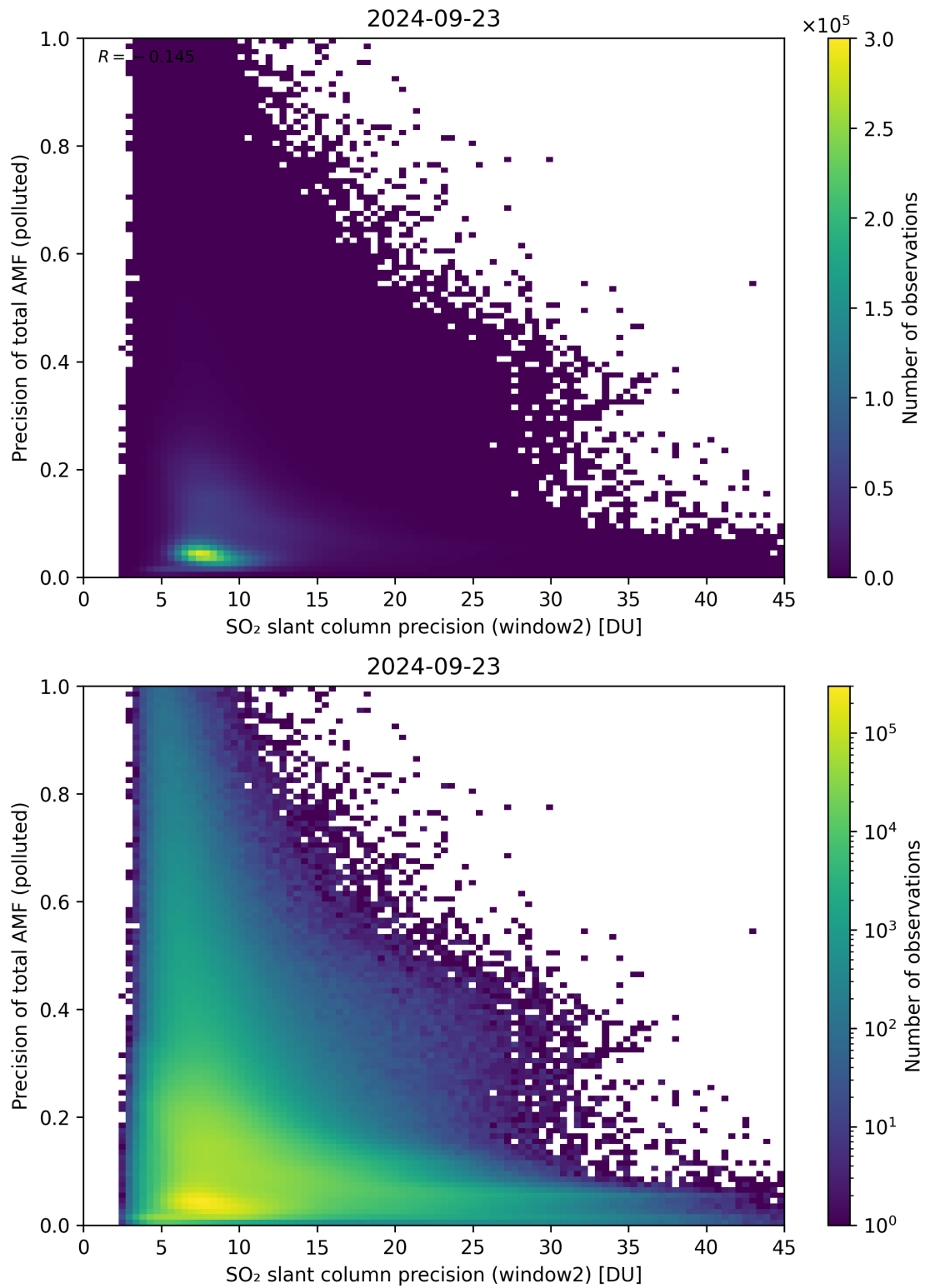
Figure 252: Scatter density plot of “SO 2 slant column precision (window2)” against “Precision of total AMF (polluted)” for 2024-09-22 to 2024-09-24.
