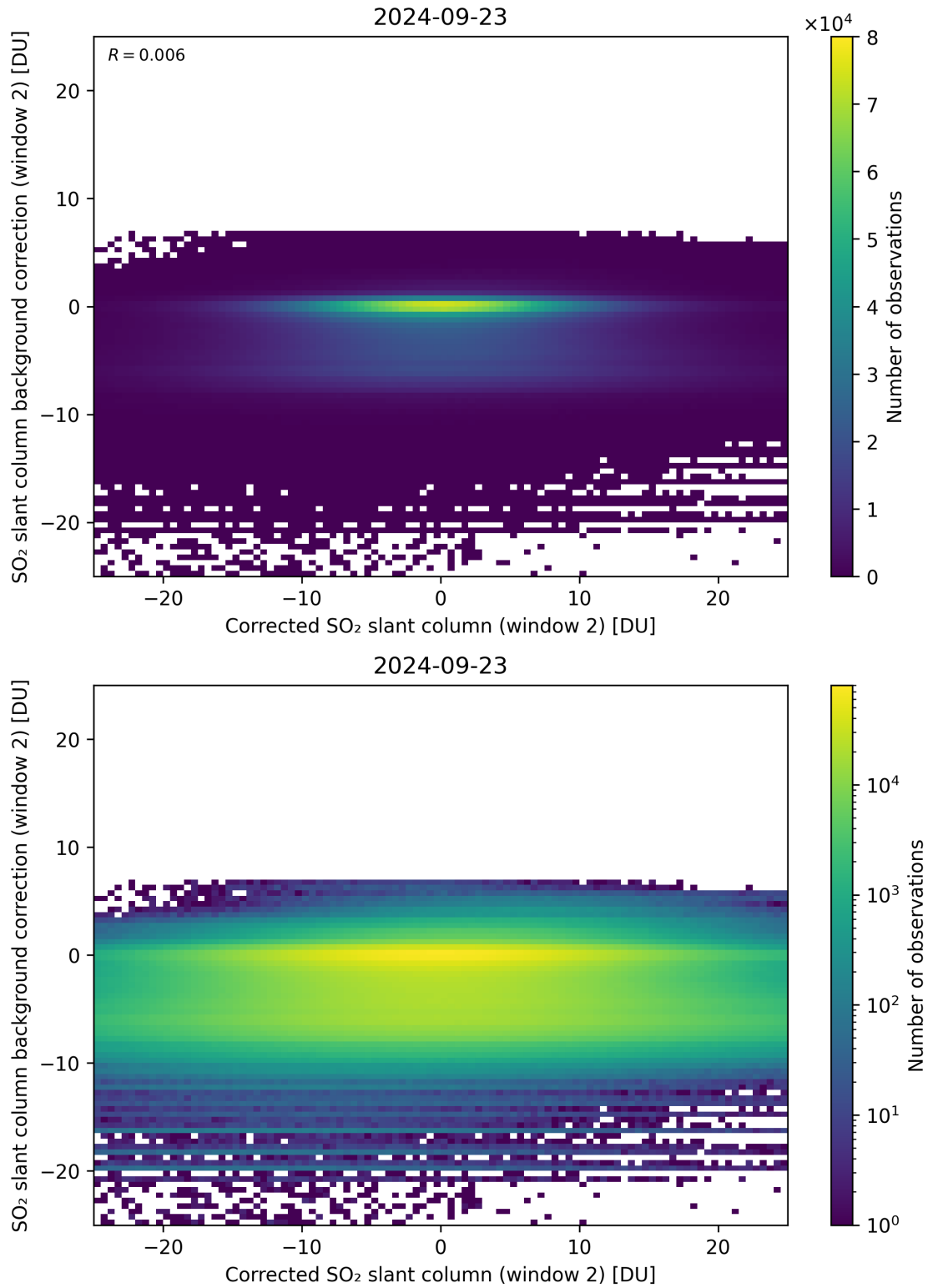
Figure 194: Scatter density plot of “Corrected SO 2 slant column (window 2)” against “SO 2 slant column background correction (window 2)” for 2024-09-22 to 2024-09-24.
