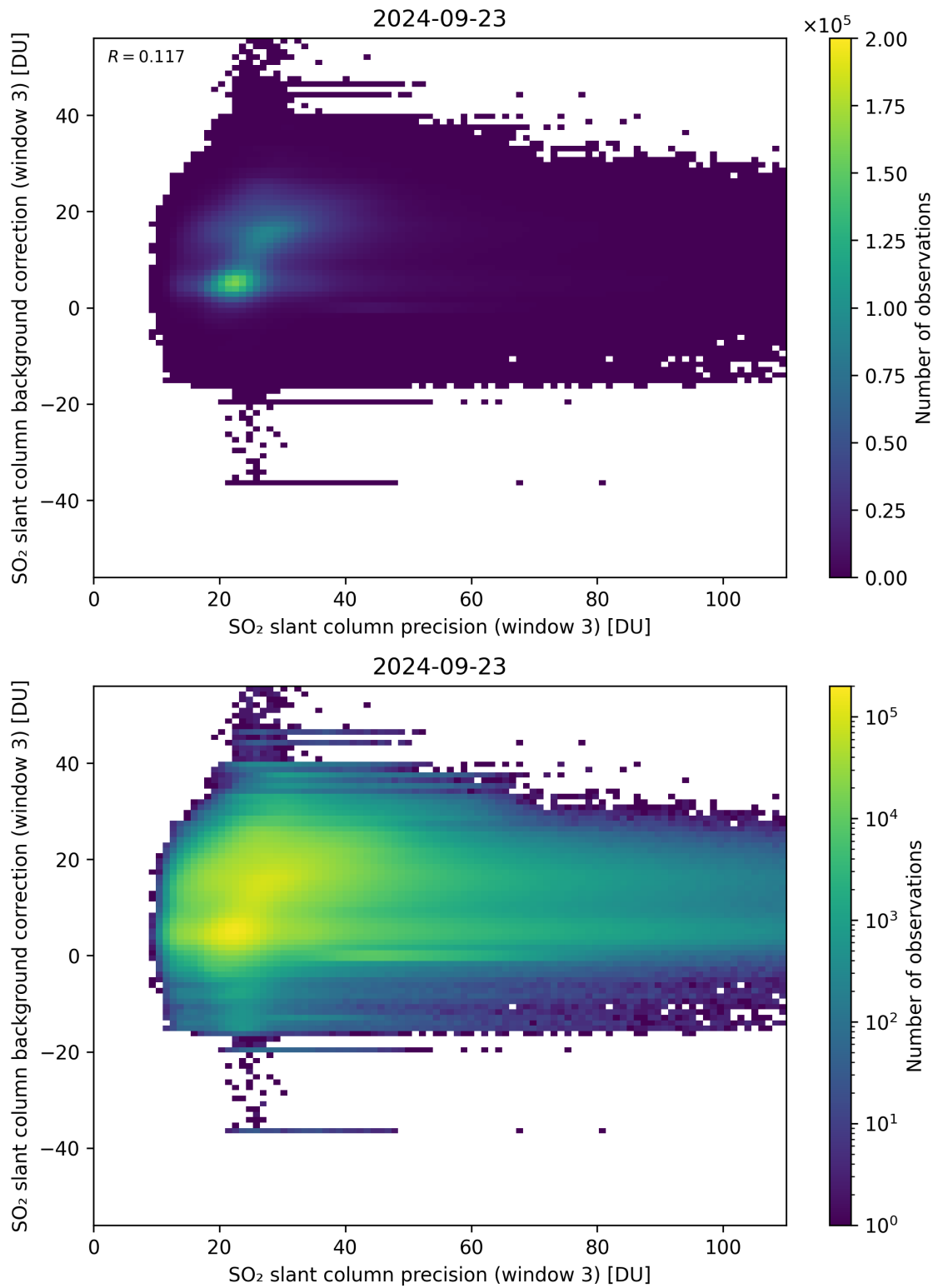
Figure 257: Scatter density plot of “SO 2 slant column precision (window 3)” against “SO 2 slant column background correction (window 3)” for 2024-09-22 to 2024-09-24.
