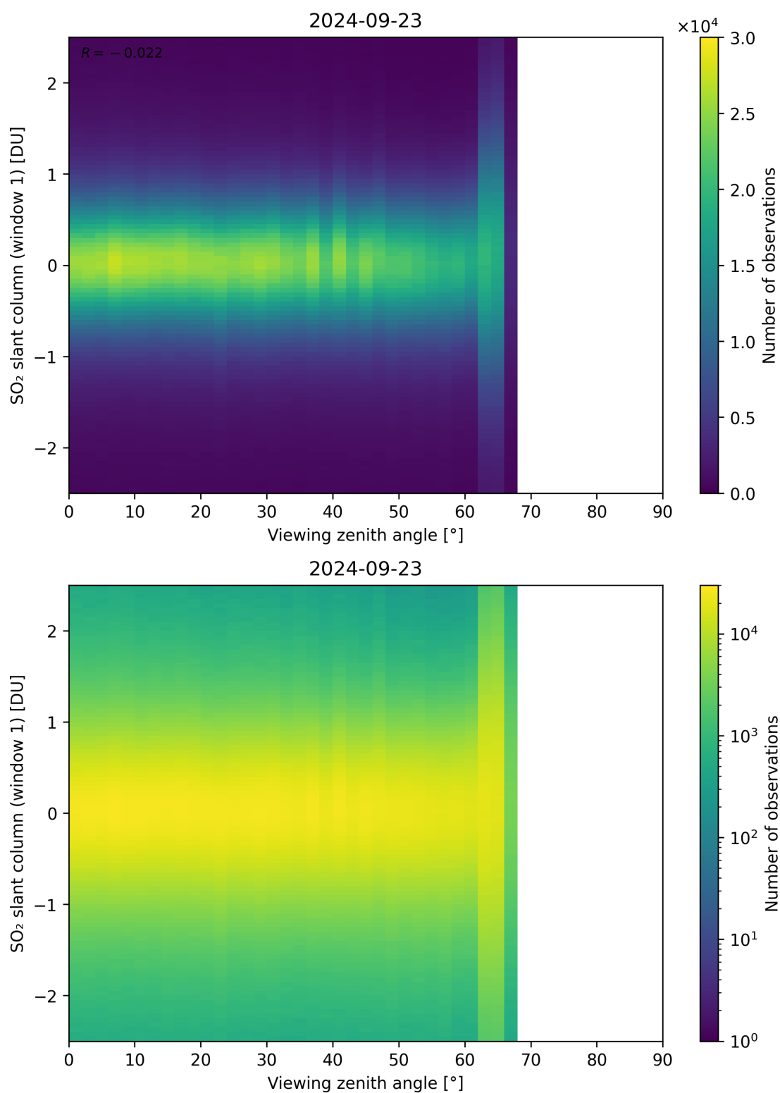
Figure 320: Scatter density plot of “Viewing zenith angle” against “SO 2 slant column (window 1)” for 2024-09-22 to 2024-09-24.
