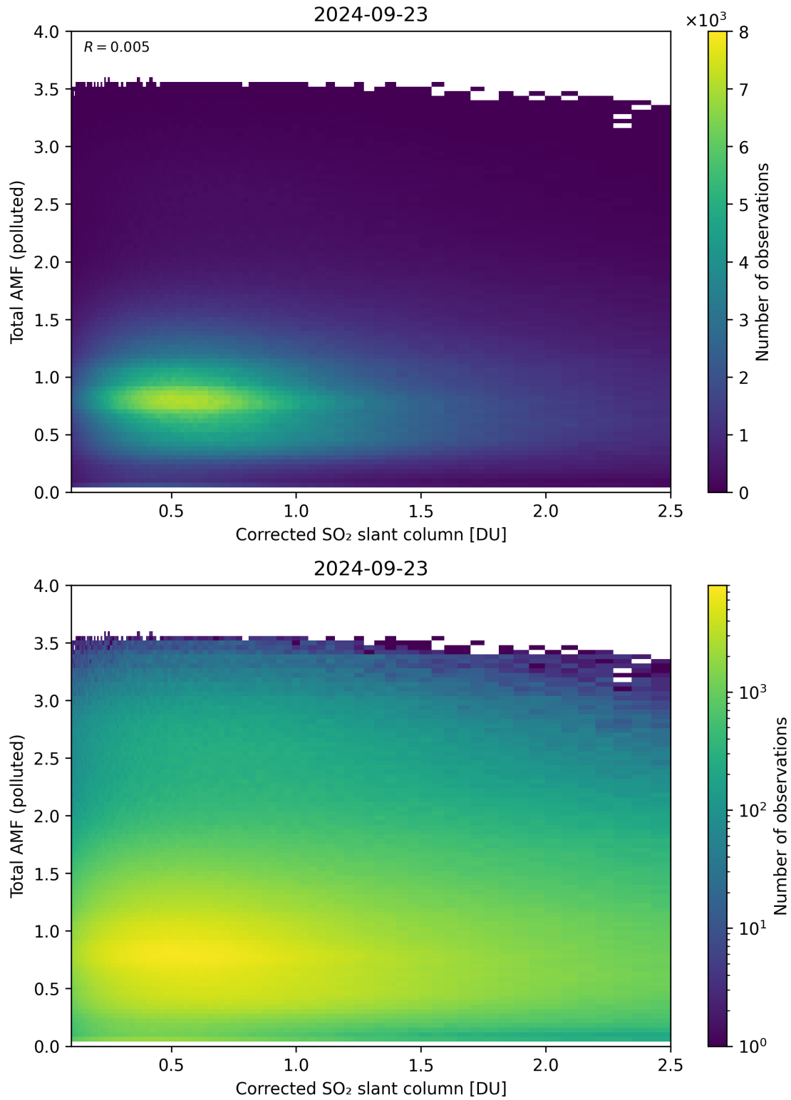
Figure 192: Scatter density plot of “Corrected SO 2 slant column” against “Total AMF (polluted)” for 2024-09-22 to 2024-09-24.
