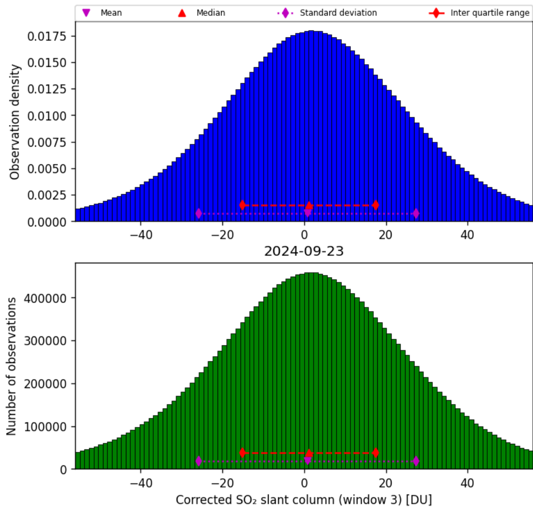
Figure 66: Histogram of “Corrected SO 2 slant column (window 3)” for 2024-09-22 to 2024-09-24
