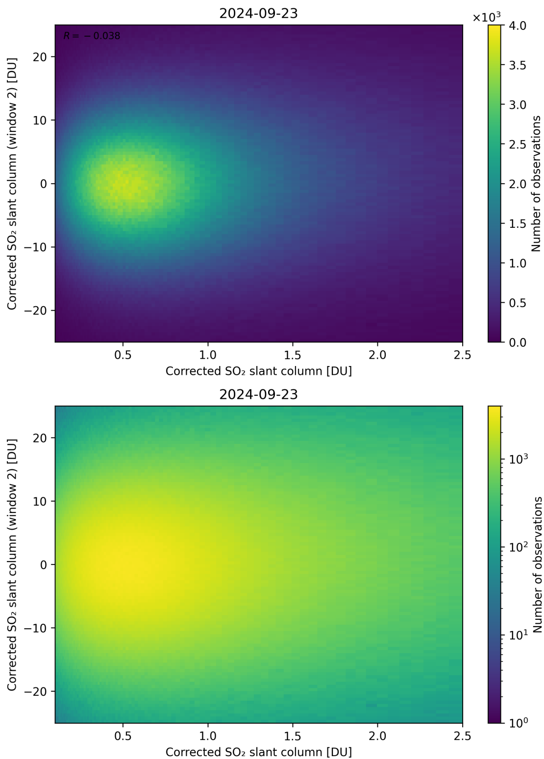
Figure 185: Scatter density plot of “Corrected SO 2 slant column” against “Corrected SO 2 slant column (window 2)” for 2024-09-22 to 2024-09-24.
