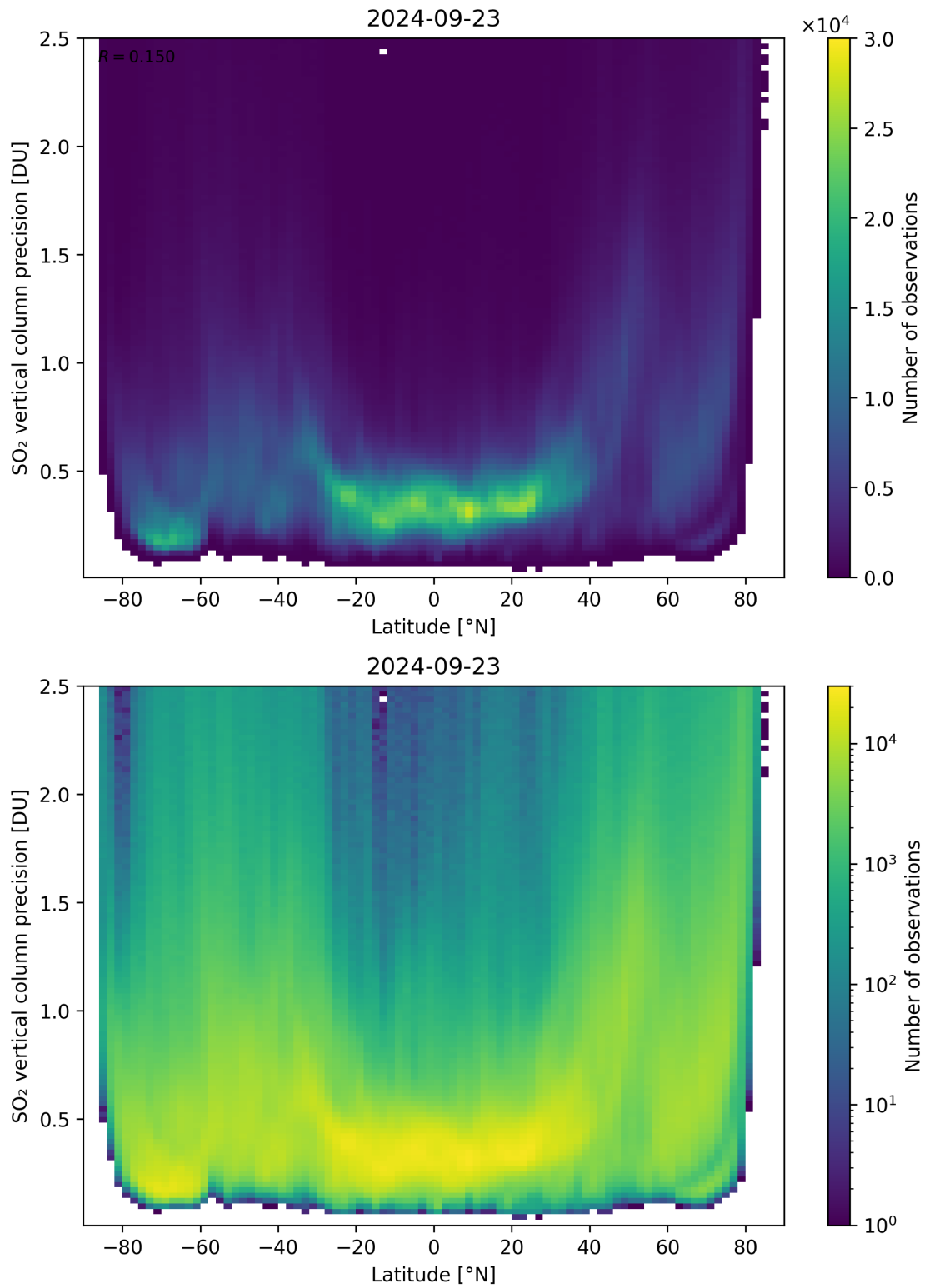
Figure 157: Scatter density plot of “Latitude” against “SO 2 vertical column precision” for 2024-09-22 to 2024-09-24.
