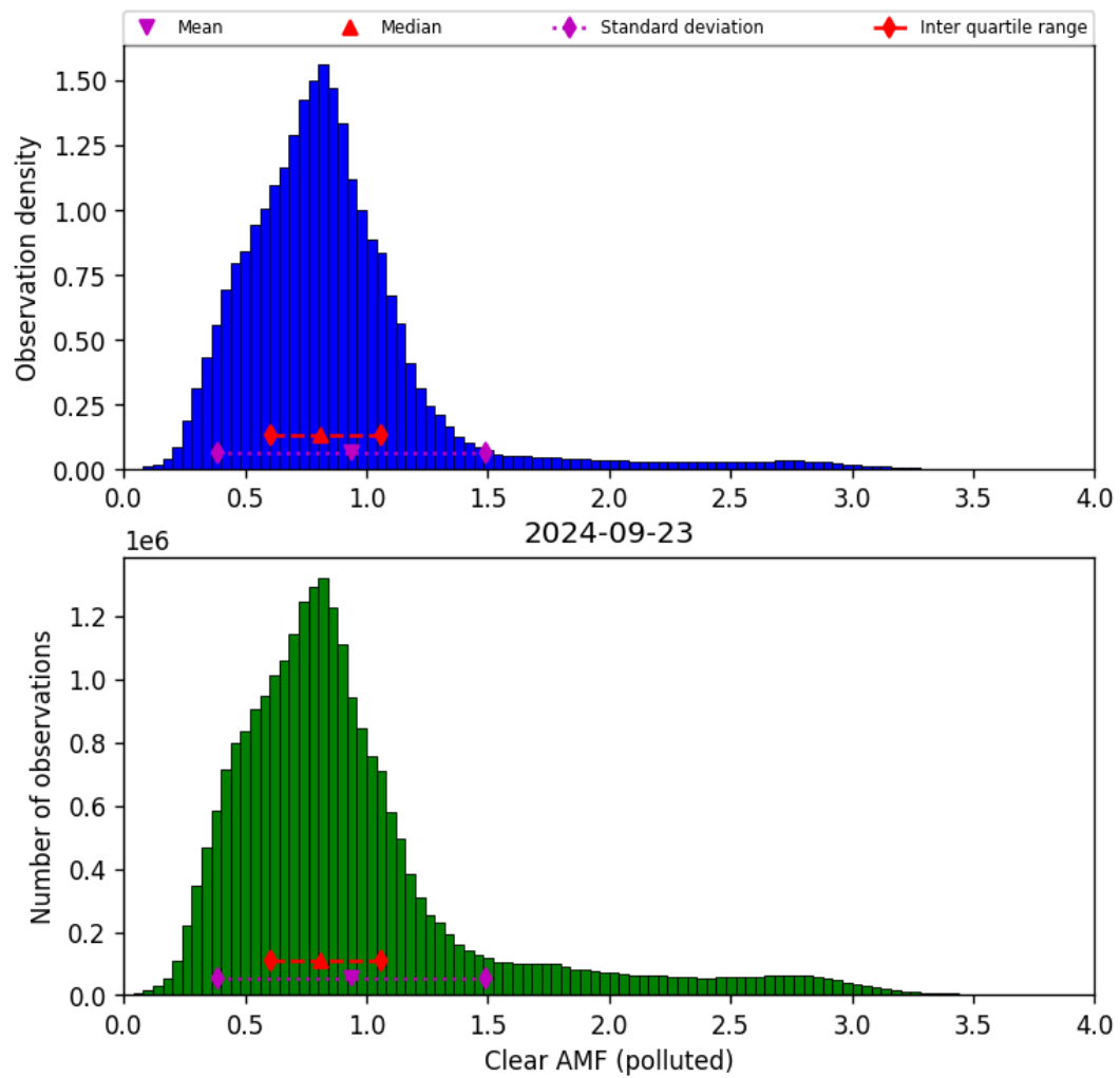
Figure 73: Histogram of “Clear AMF (polluted)” for 2024-09-22 to 2024-09-24
