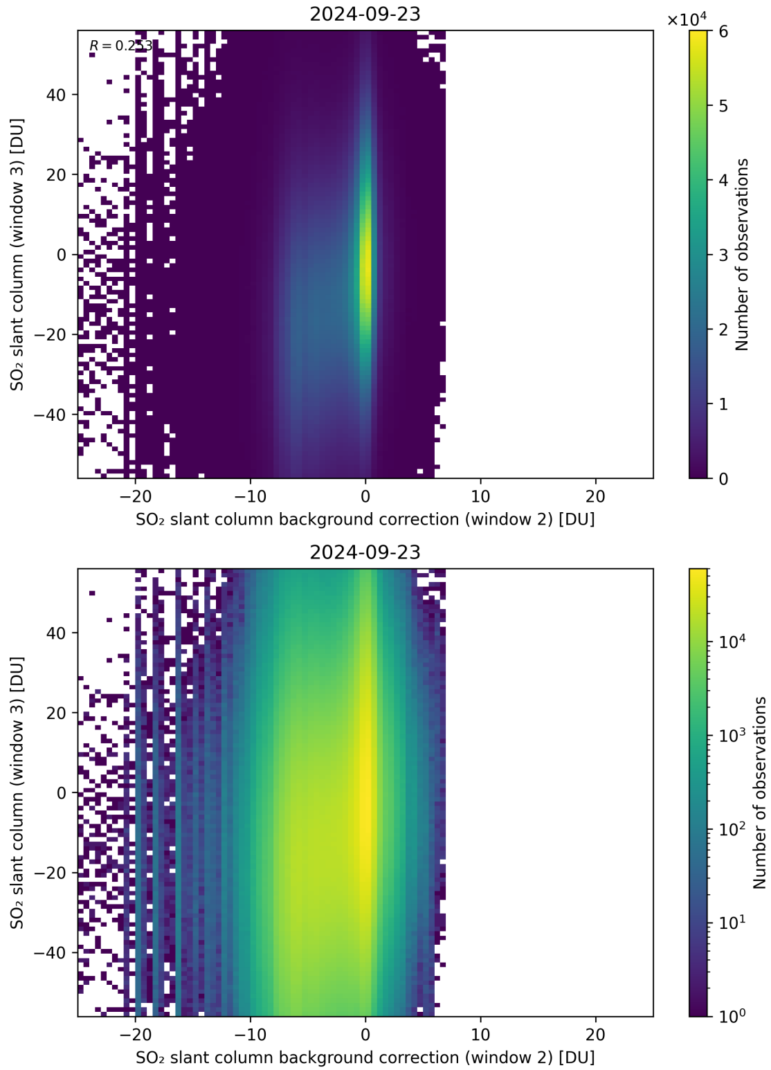
Figure 117: Scatter density plot of “SO 2 slant column background correction (window 2)” against “SO 2 slant column (window 3)” for 2024-09-22 to 2024-09-24.
