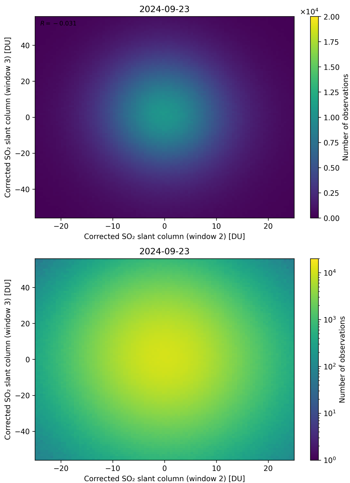
Figure 200: Scatter density plot of “Corrected SO 2 slant column (window 2)” against “Corrected SO 2 slant column (window 3)” for 2024-09-22 to 2024-09-24.
