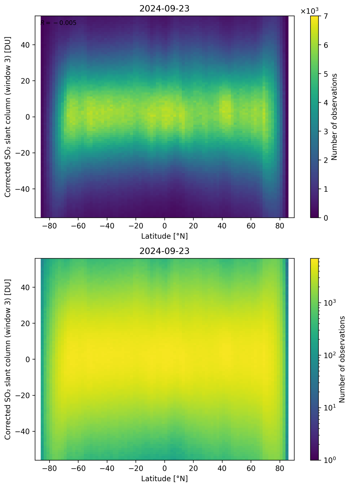
Figure 148: Scatter density plot of “Latitude” against “Corrected SO 2 slant column (window 3)” for 2024-09-22 to 2024-09-24.
