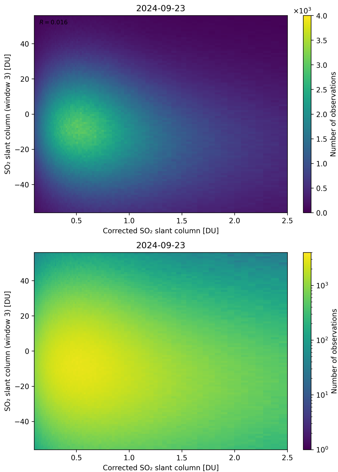
Figure 190: Scatter density plot of “Corrected SO 2 slant column” against “SO 2 slant column (window 3)” for 2024-09-22 to 2024-09-24.
