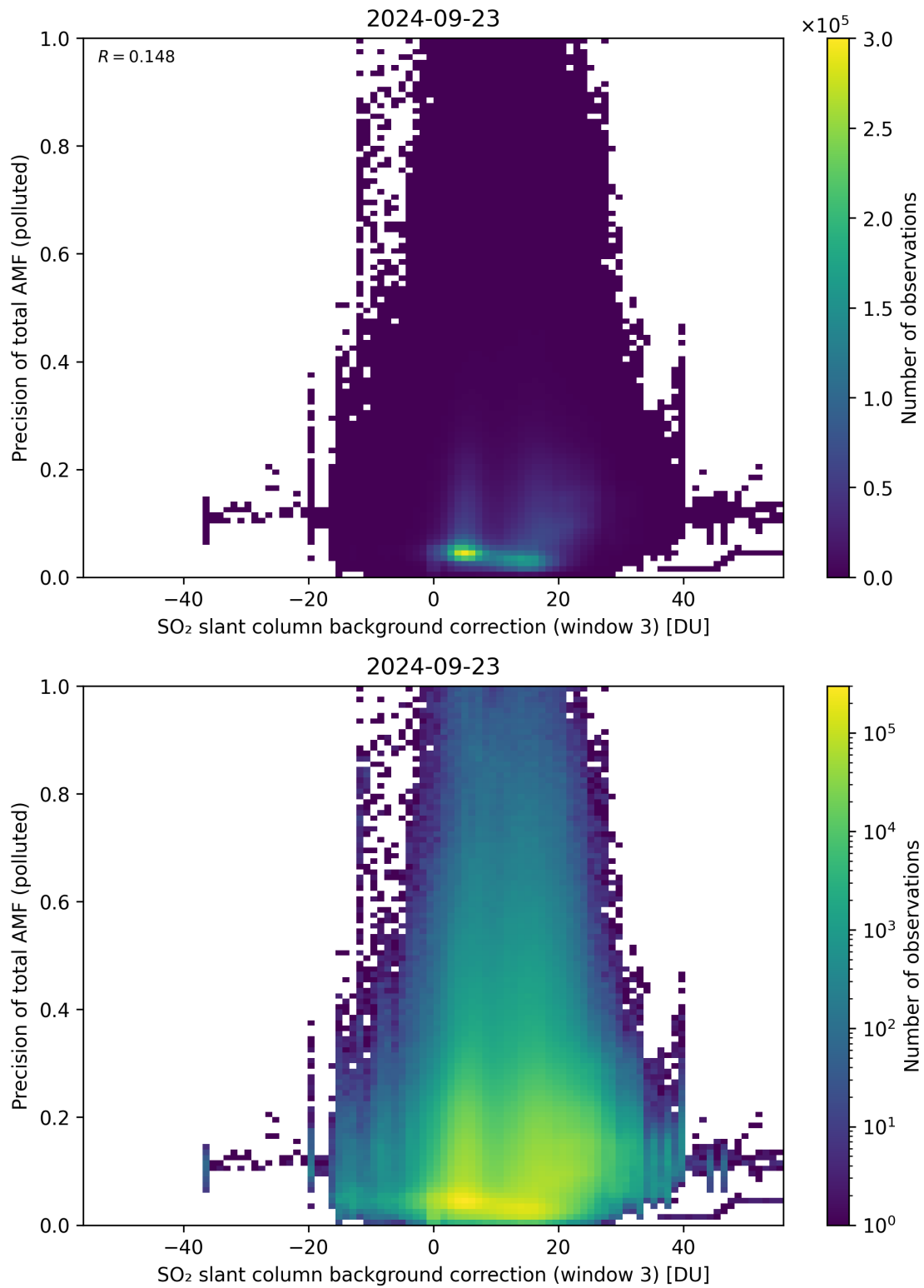
Figure 126: Scatter density plot of “SO 2 slant column background correction (window 3)” against “Precision of total AMF (polluted)” for 2024-09-22 to 2024-09-24.
