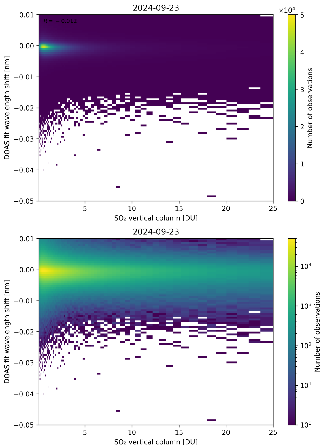
Figure 276: Scatter density plot of “SO 2 vertical column” against “DOAS fit wavelength shift” for 2024-09-22 to 2024-09-24.
