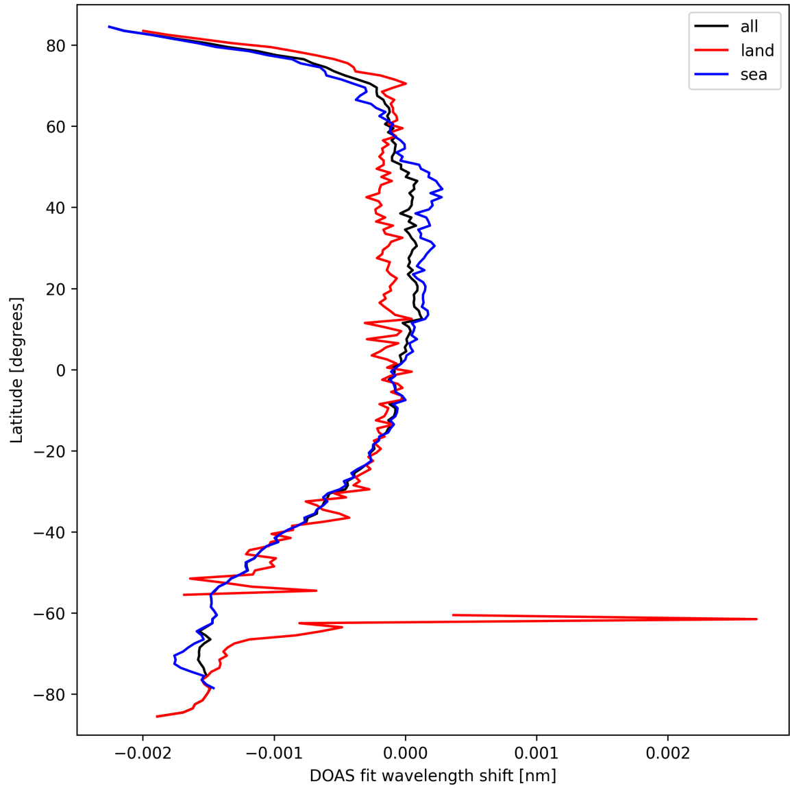
Figure 45: Zonal average of “DOAS fit wavelength shift” for 2024-09-22 to 2024-09-24.
