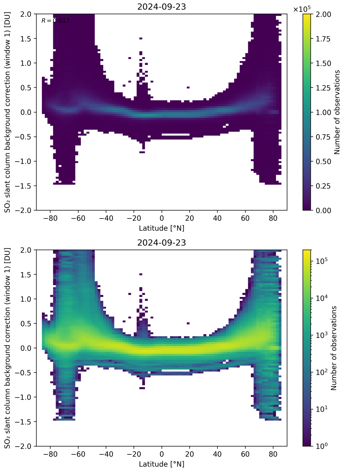
Figure 139: Scatter density plot of “Latitude” against “SO 2 slant column background correction (window 1)” for 2024-09-22 to 2024-09-24.
