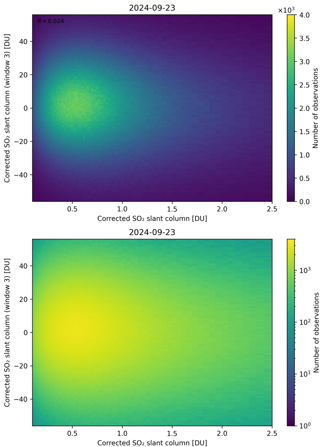
Figure 186: Scatter density plot of “Corrected SO 2 slant column” against “Corrected SO 2 slant column (window 3)” for 2024-09-22 to 2024-09-24.
