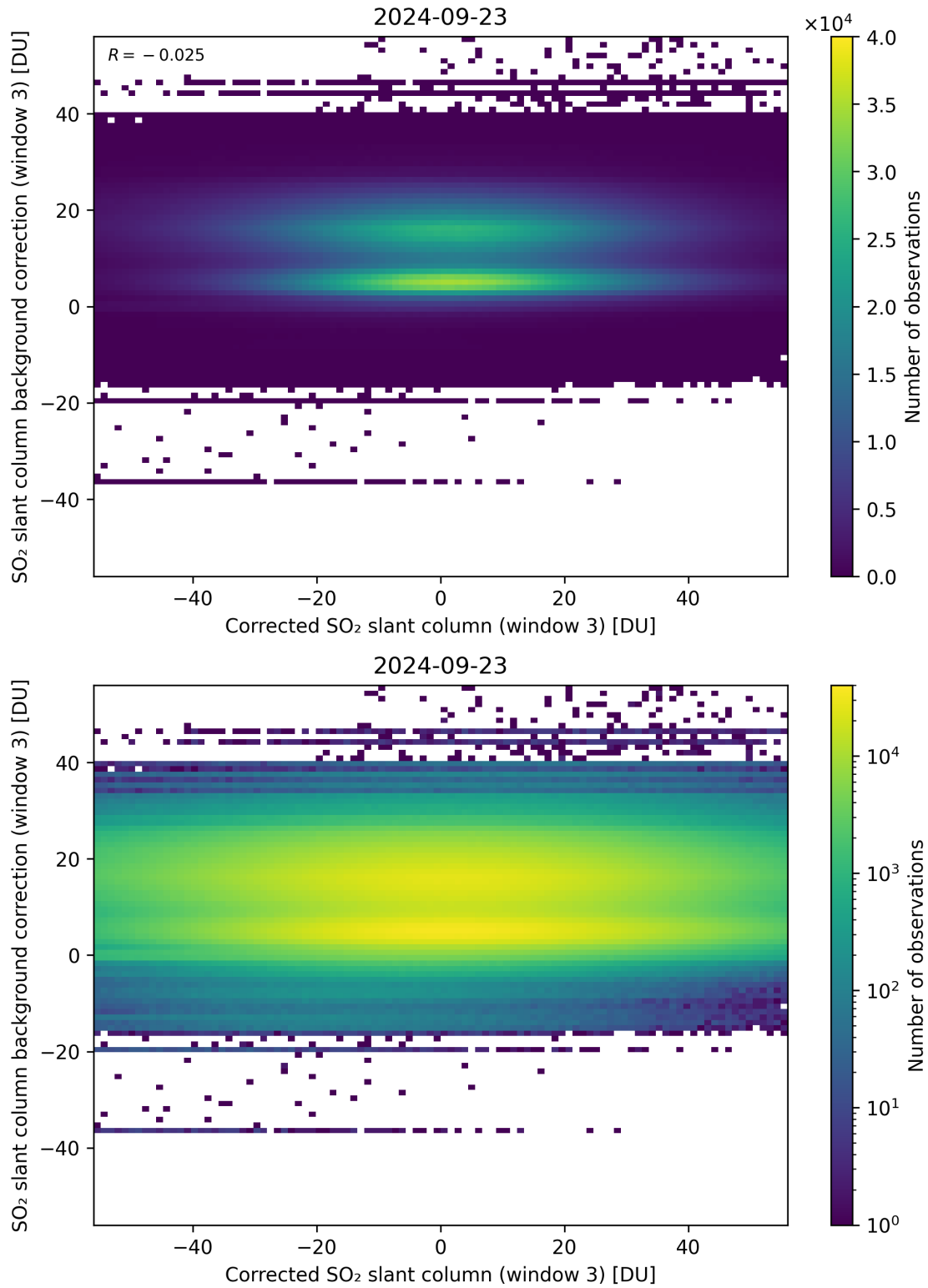
Figure 205: Scatter density plot of “Corrected SO 2 slant column (window 3)” against “SO 2 slant column background correction (window 3)” for 2024-09-22 to 2024-09-24.
