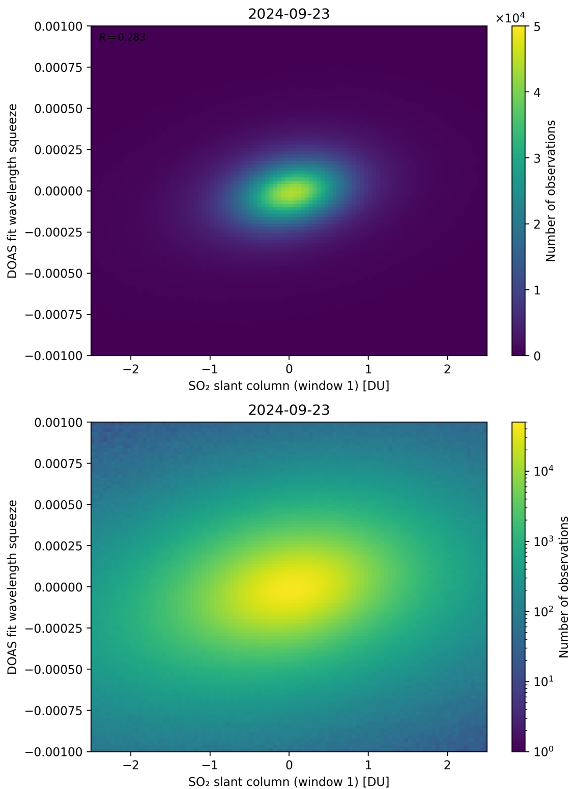
Figure 216: Scatter density plot of “SO 2 slant column (window 1)” against “DOAS fit wavelength squeeze” for 2024-09-22 to 2024-09-24.
