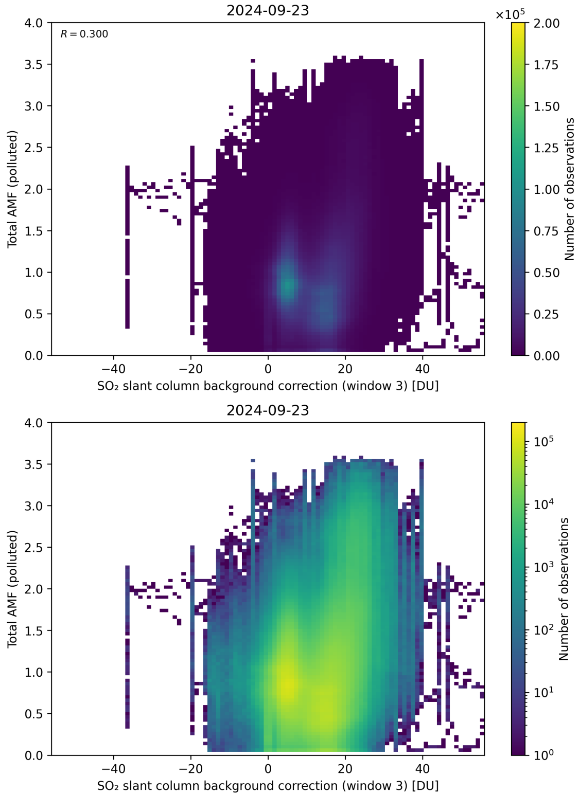
Figure 125: Scatter density plot of “SO 2 slant column background correction (window 3)” against “Total AMF (polluted)” for 2024-09-22 to 2024-09-24.
