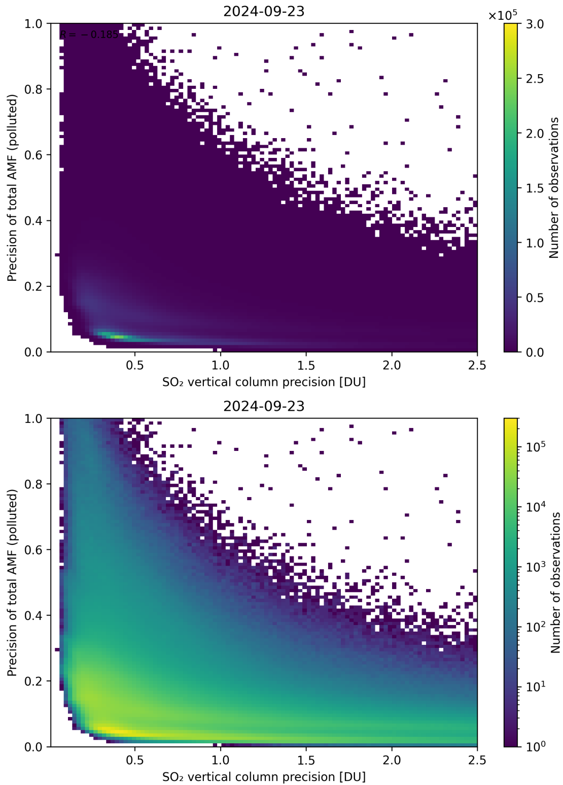
Figure 295: Scatter density plot of “SO 2 vertical column precision” against “Precision of total AMF (polluted)” for 2024-09-22 to 2024-09-24.
