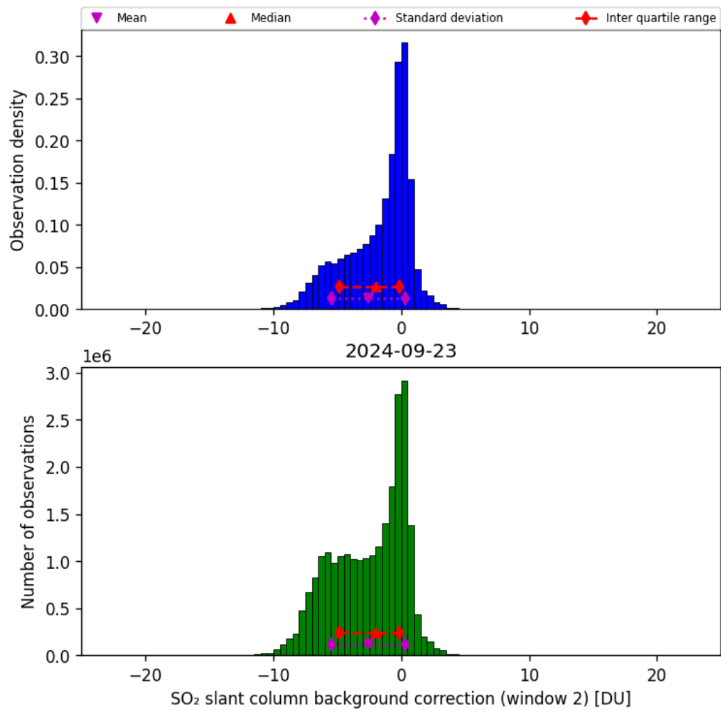
Figure 63: Histogram of “SO 2 slant column background correction (window 2)” for 2024-09-22 to 2024-09-24
