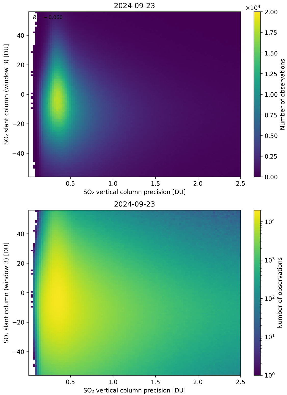
Figure 292: Scatter density plot of “SO 2 vertical column precision” against “SO 2 slant column (window 3)” for 2024-09-22 to 2024-09-24.
