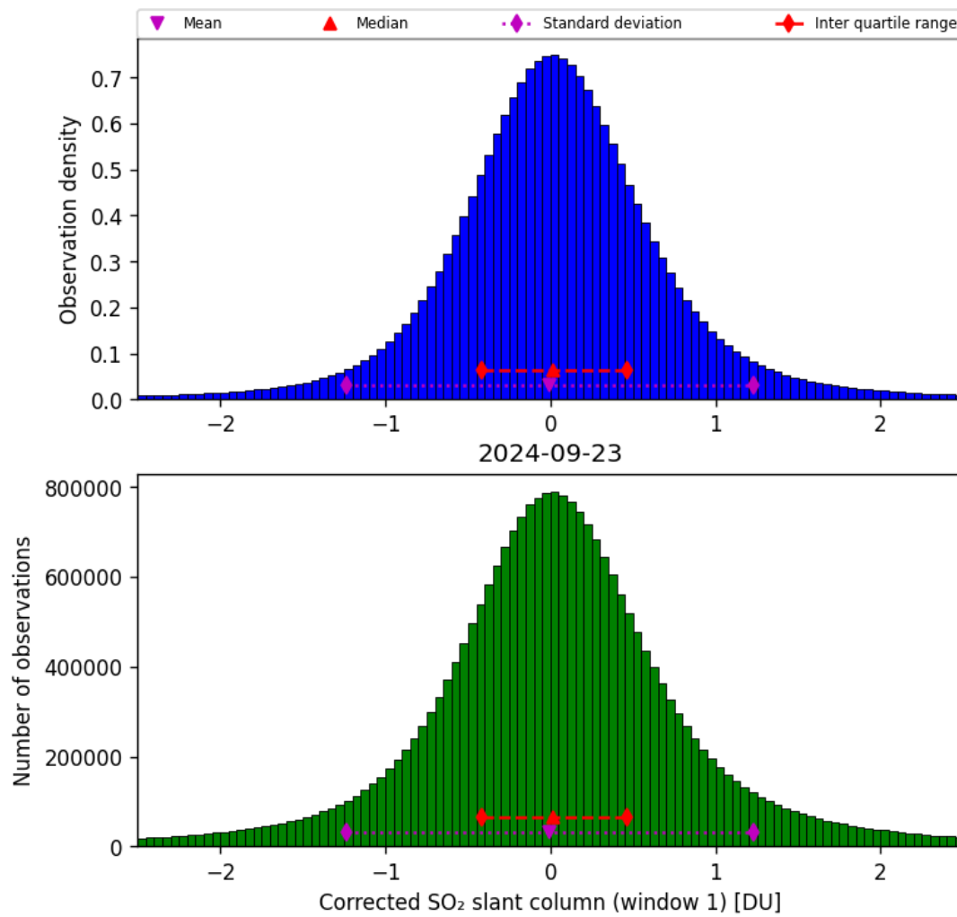
Figure 58: Histogram of “Corrected SO 2 slant column (window 1)” for 2024-09-22 to 2024-09-24
