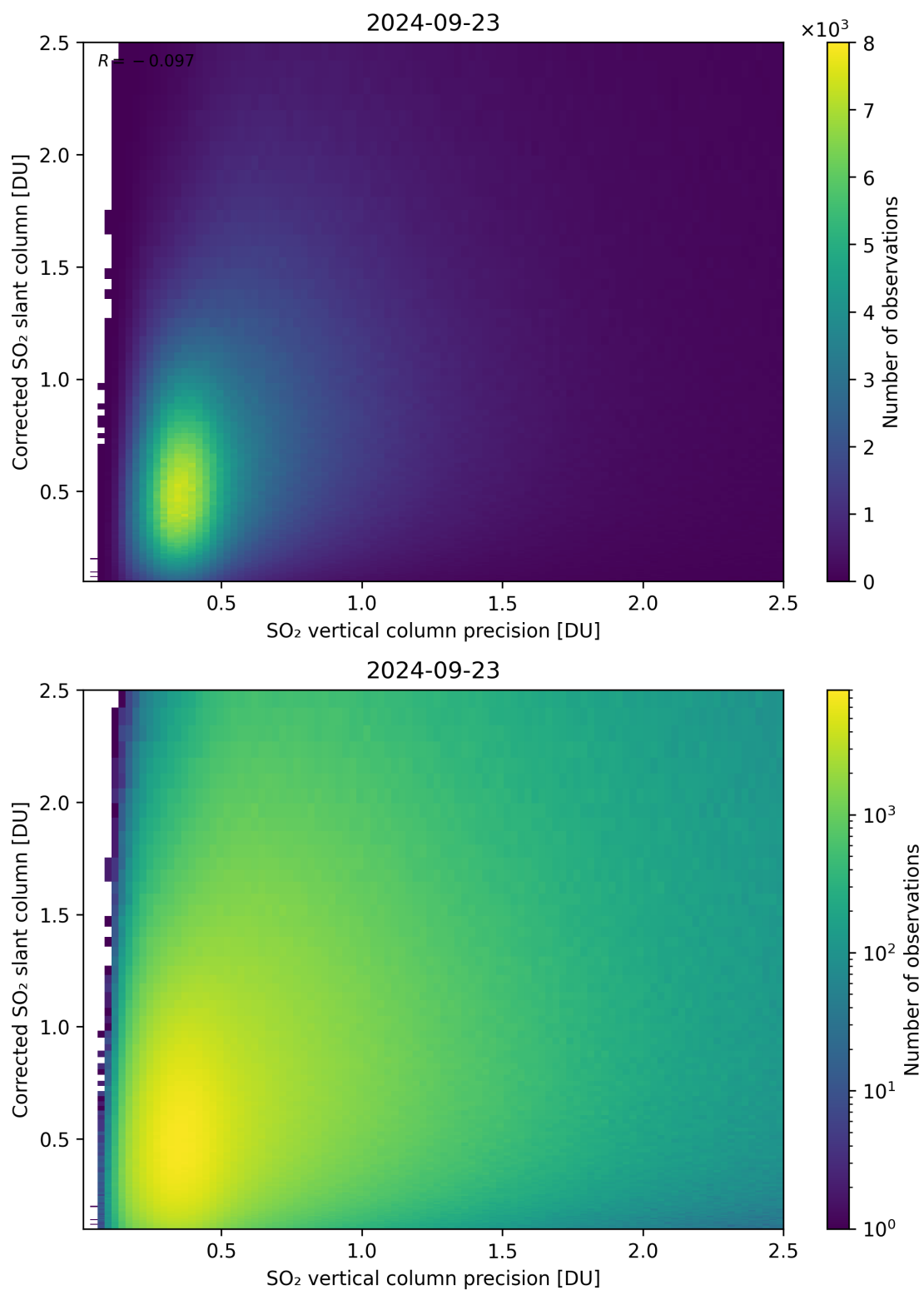
Figure 286: Scatter density plot of “SO 2 vertical column precision” against “Corrected SO 2 slant column” for 2024-09-22 to 2024-09-24.
