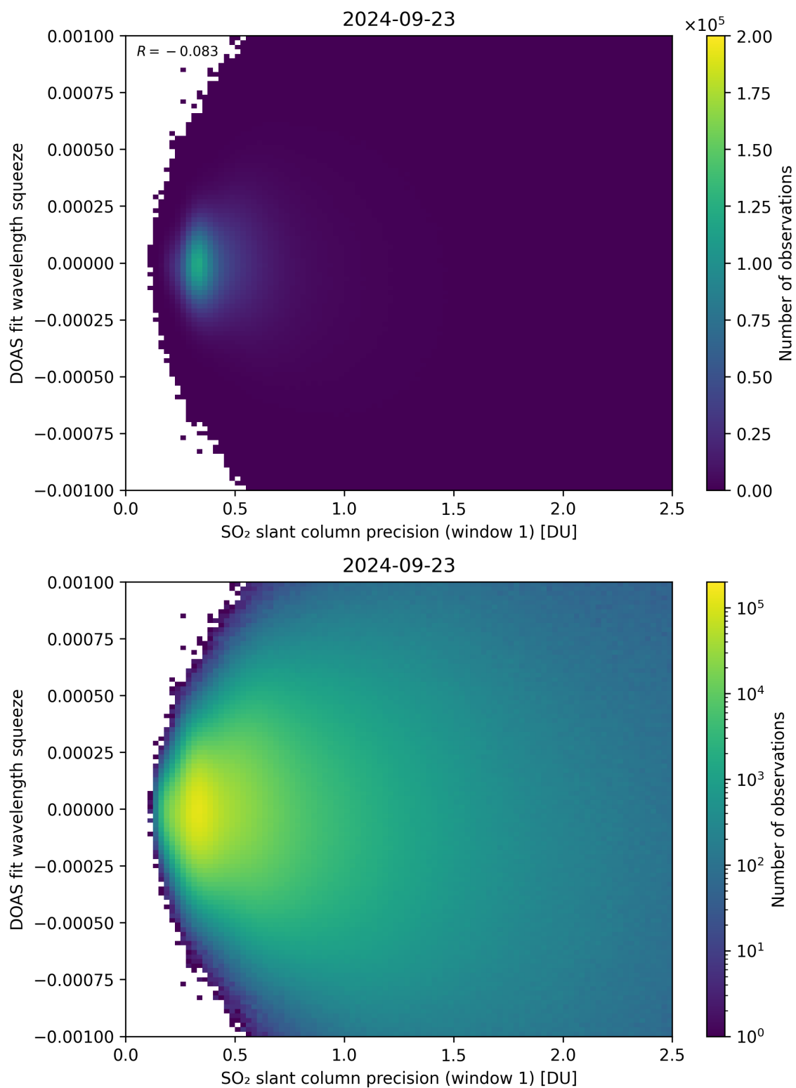
Figure 222: Scatter density plot of “SO 2 slant column precision (window 1)” against “DOAS fit wavelength squeeze” for 2024-09-22 to 2024-09-24.
