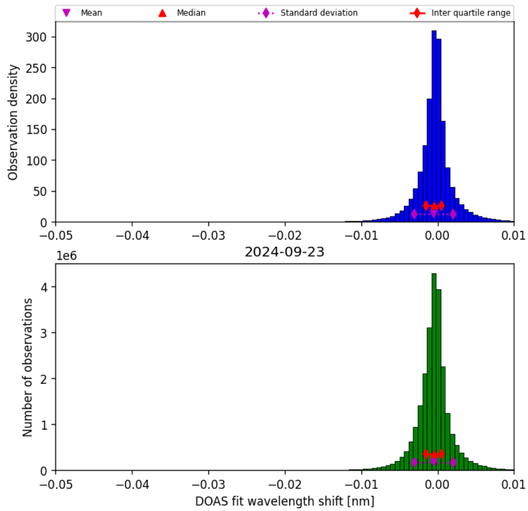
Figure 68: Histogram of “DOAS fit wavelength shift” for 2024-09-22 to 2024-09-24
