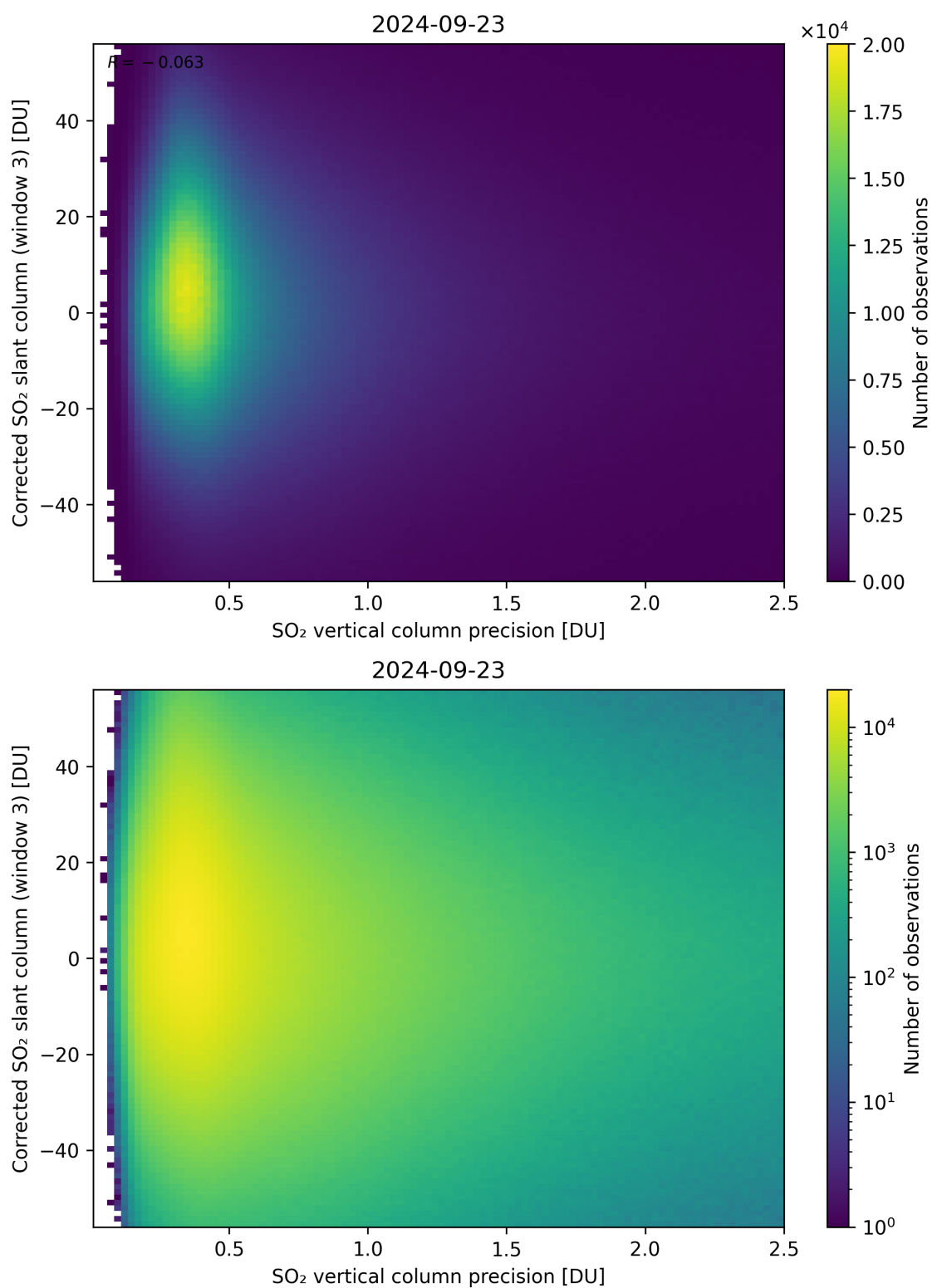
Figure 288: Scatter density plot of “SO 2 vertical column precision” against “Corrected SO 2 slant column (window 3)” for 2024-09-22 to 2024-09-24.
