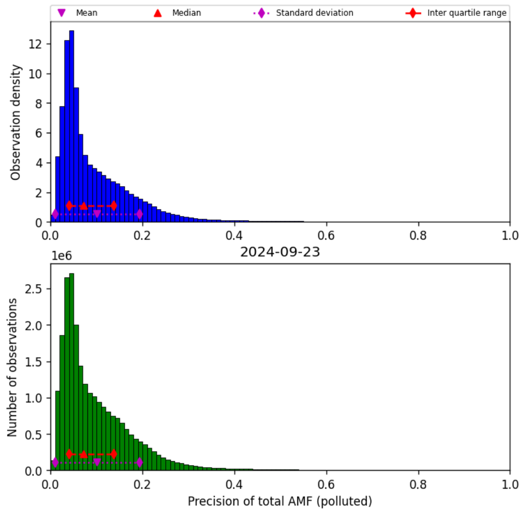
Figure 72: Histogram of “Precision of total AMF (polluted)” for 2024-09-22 to 2024-09-24
