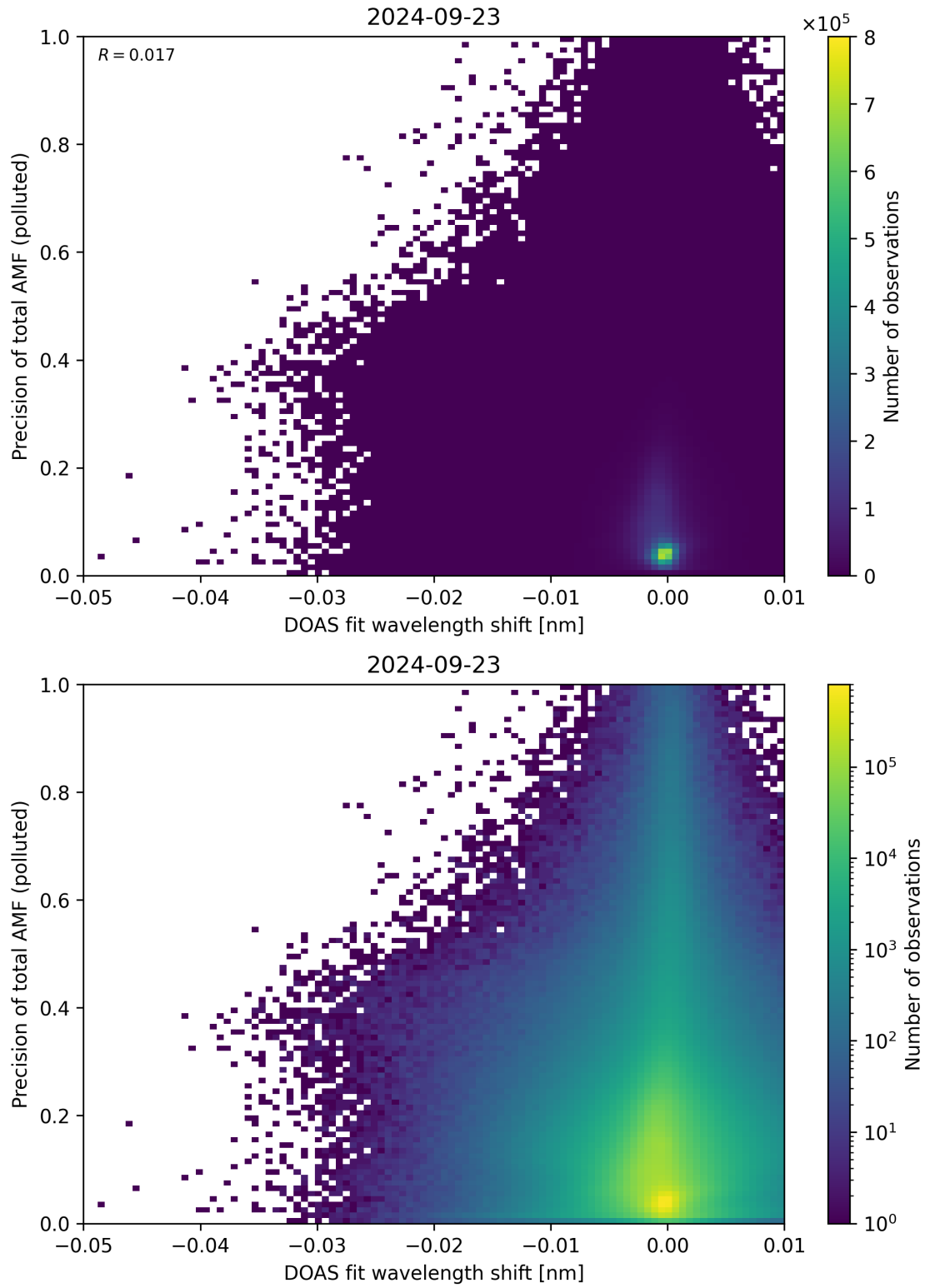
Figure 131: Scatter density plot of “DOAS fit wavelength shift” against “Precision of total AMF (polluted)” for 2024-09-22 to 2024-09-24.
