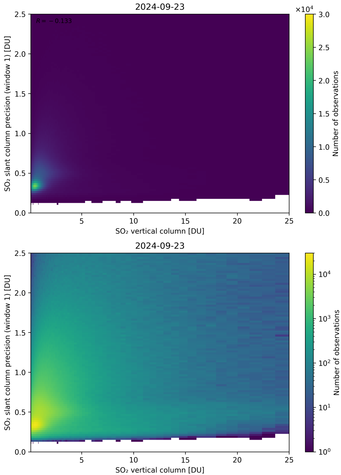
Figure 301: Scatter density plot of “SO 2 vertical column” against “SO 2 slant column precision (window 1)” for 2024-09-22 to 2024-09-24.
