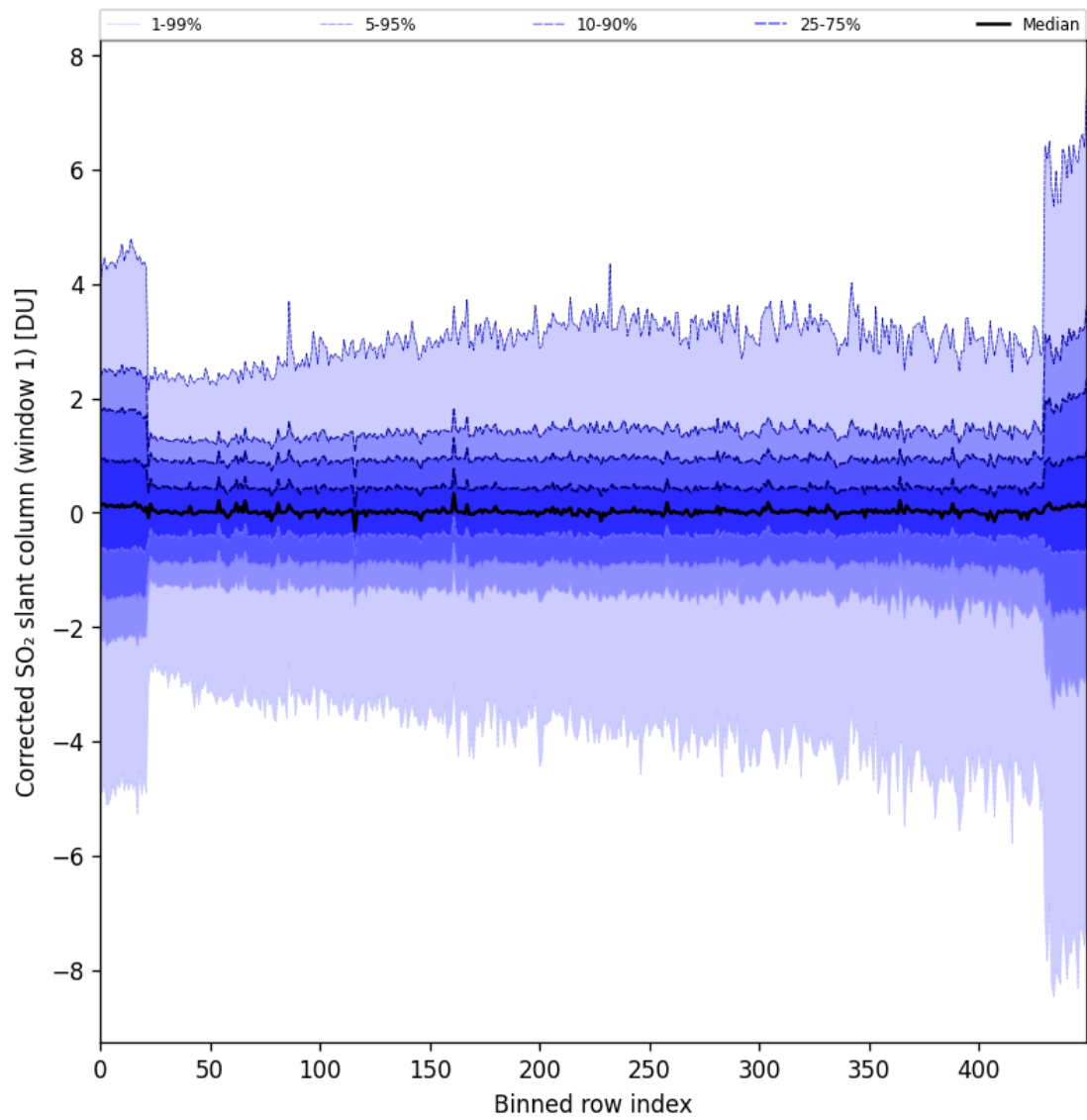
Figure 81: Along track statistics of "Corrected SO 2 slant column (window 1)" for 2024-09-22 to 2024-09-24
