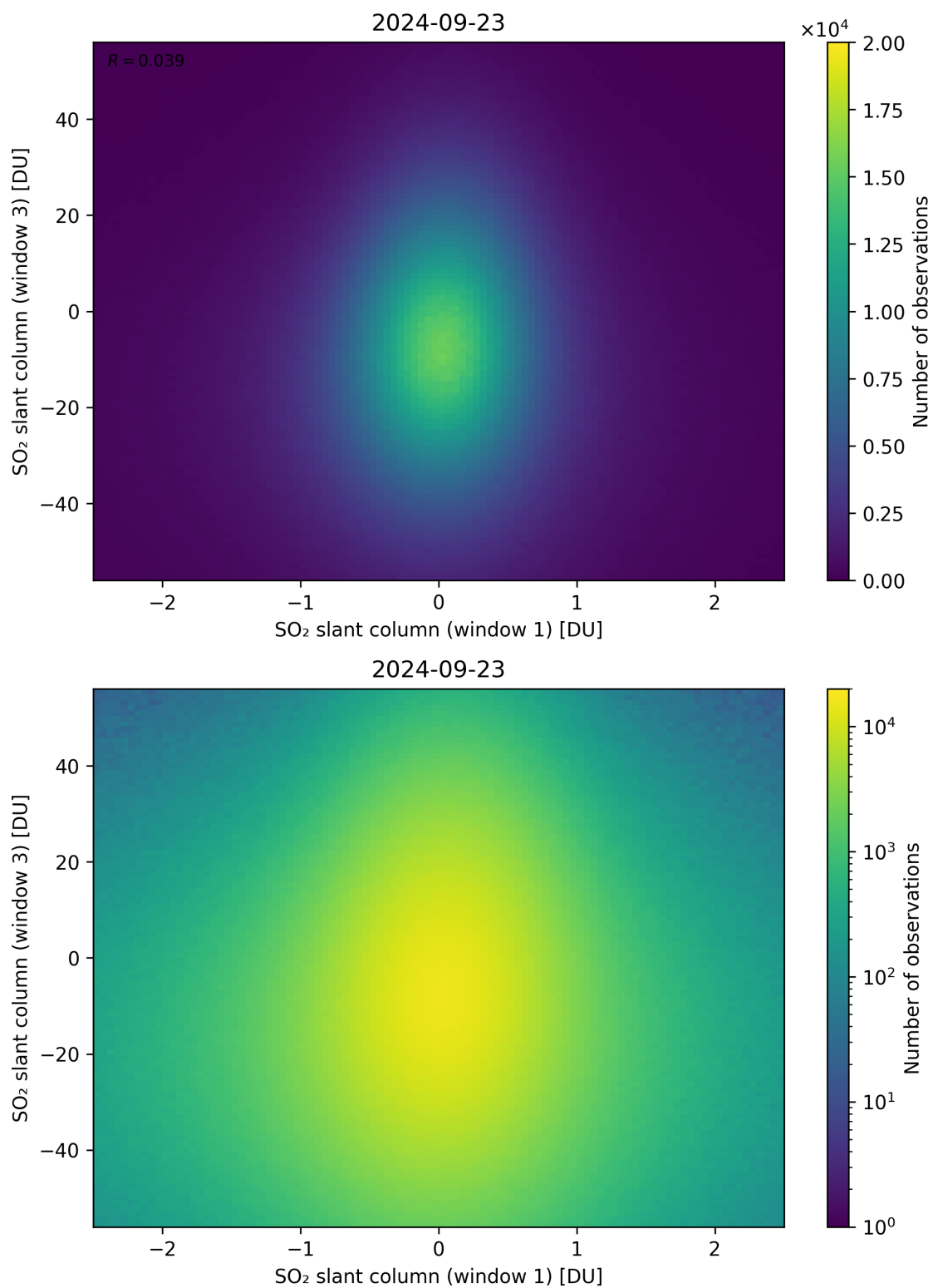
Figure 237: Scatter density plot of “SO 2 slant column (window 1)” against “SO 2 slant column (window 3)” for 2024-09-22 to 2024-09-24.
