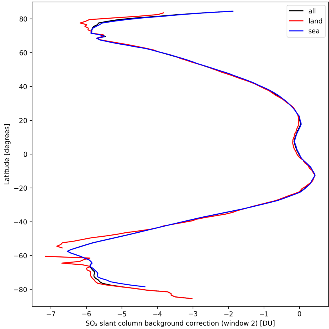
Figure 40: Zonal average of “SO 2 slant column background correction (window 2)” for 2024-09-22 to 2024-09-24.
