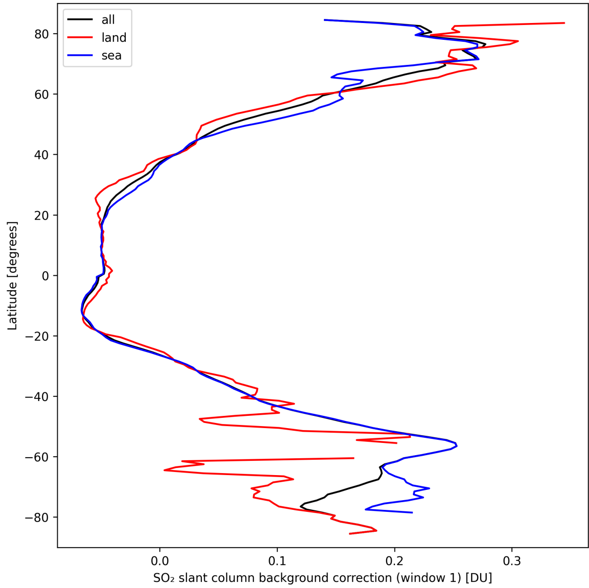
Figure 36: Zonal average of “SO 2 slant column background correction (window 1)” for 2024-09-22 to 2024-09-24.
