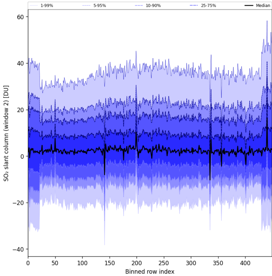
Figure 83: Along track statistics of “SO 2 slant column (window 2)” for 2024-09-22 to 2024-09-24
