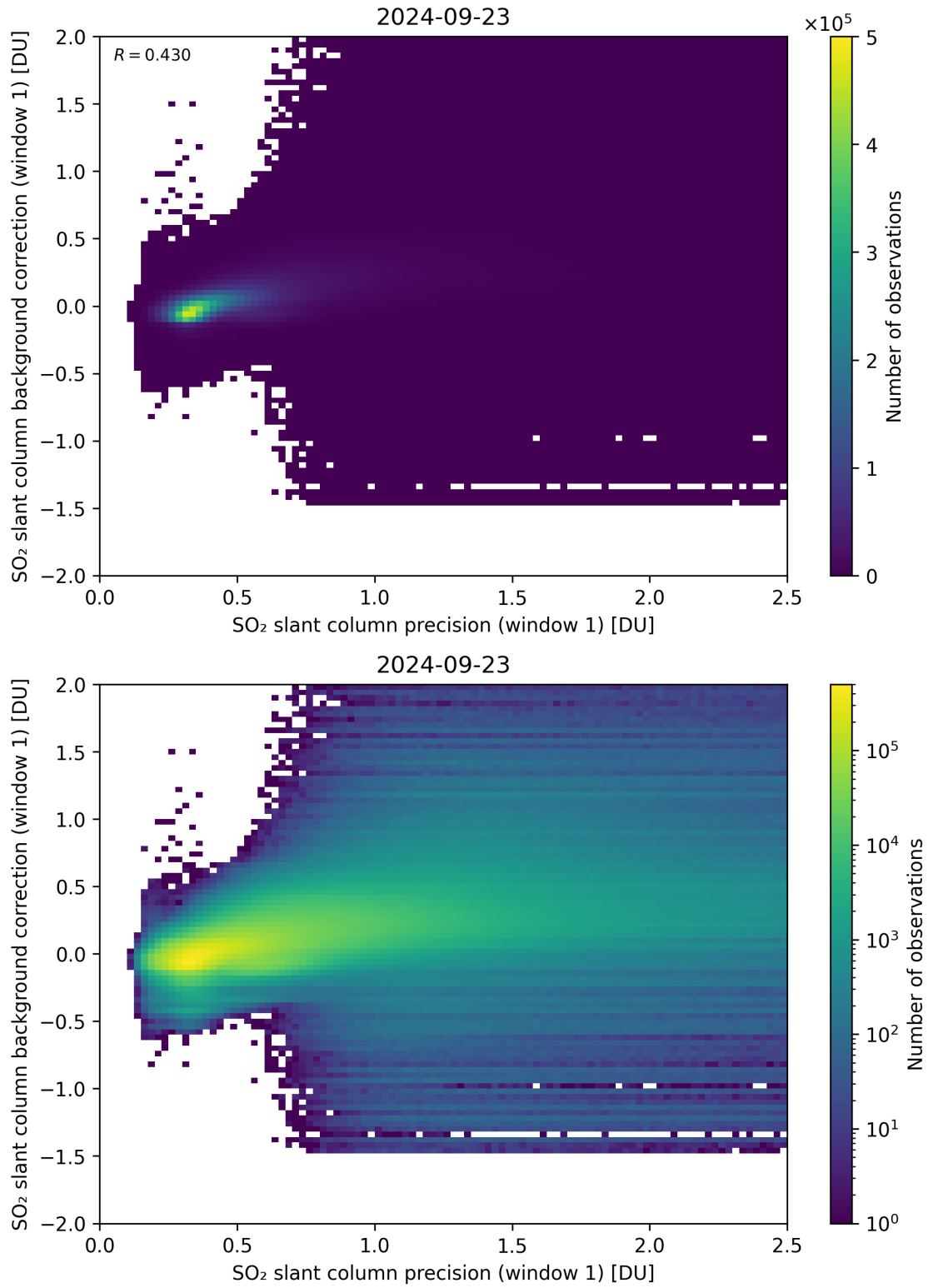
Figure 218: Scatter density plot of “SO 2 slant column precision (window 1)” against “SO 2 slant column background correction (window 1)” for 2024-09-22 to 2024-09-24.
