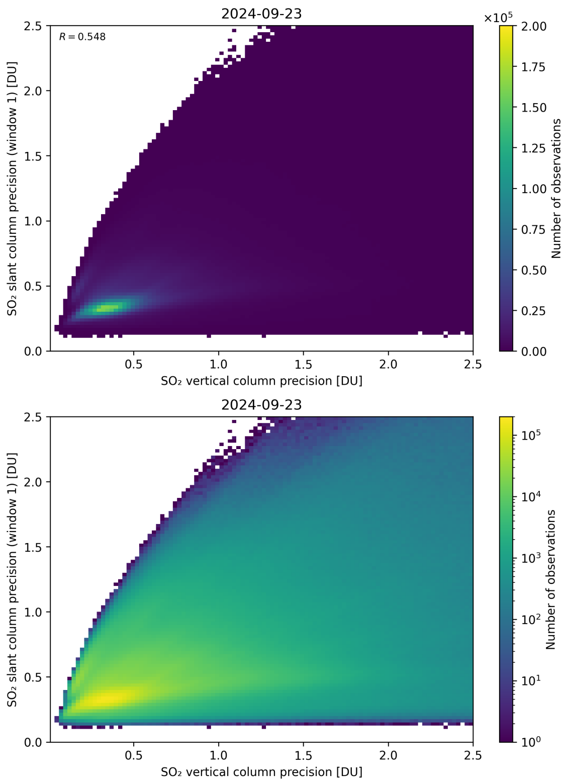
Figure 290: Scatter density plot of “SO 2 vertical column precision” against “SO 2 slant column precision (window 1)” for 2024-09-22 to 2024-09-24.
