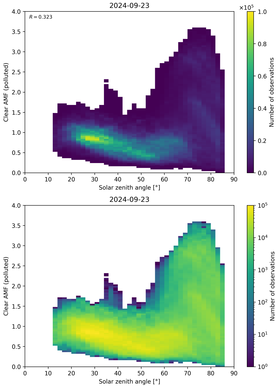
Figure 165: Scatter density plot of “Solar zenith angle” against “Clear AMF (polluted)” for 2024-09-22 to 2024-09-24.
