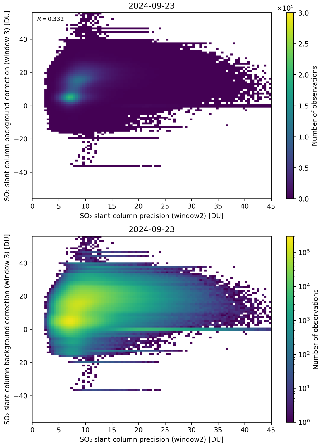
Figure 242: Scatter density plot of “SO 2 slant column precision (window2)” against “SO 2 slant column background correction (window 3)” for 2024-09-22 to 2024-09-24.
