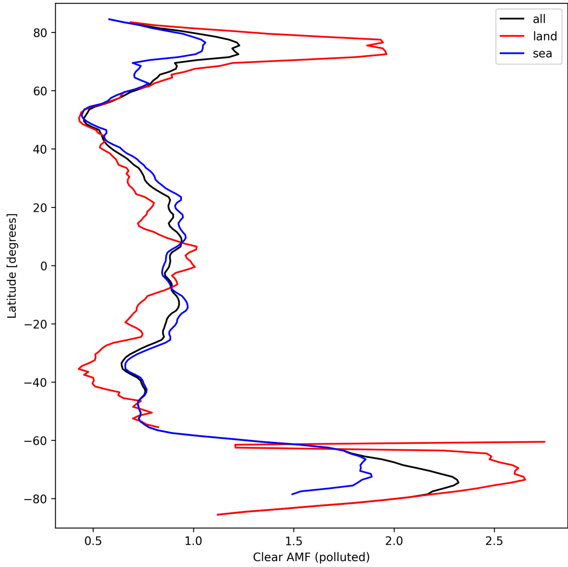
Figure 50: Zonal average of “Clear AMF (polluted)” for 2024-09-22 to 2024-09-24.
