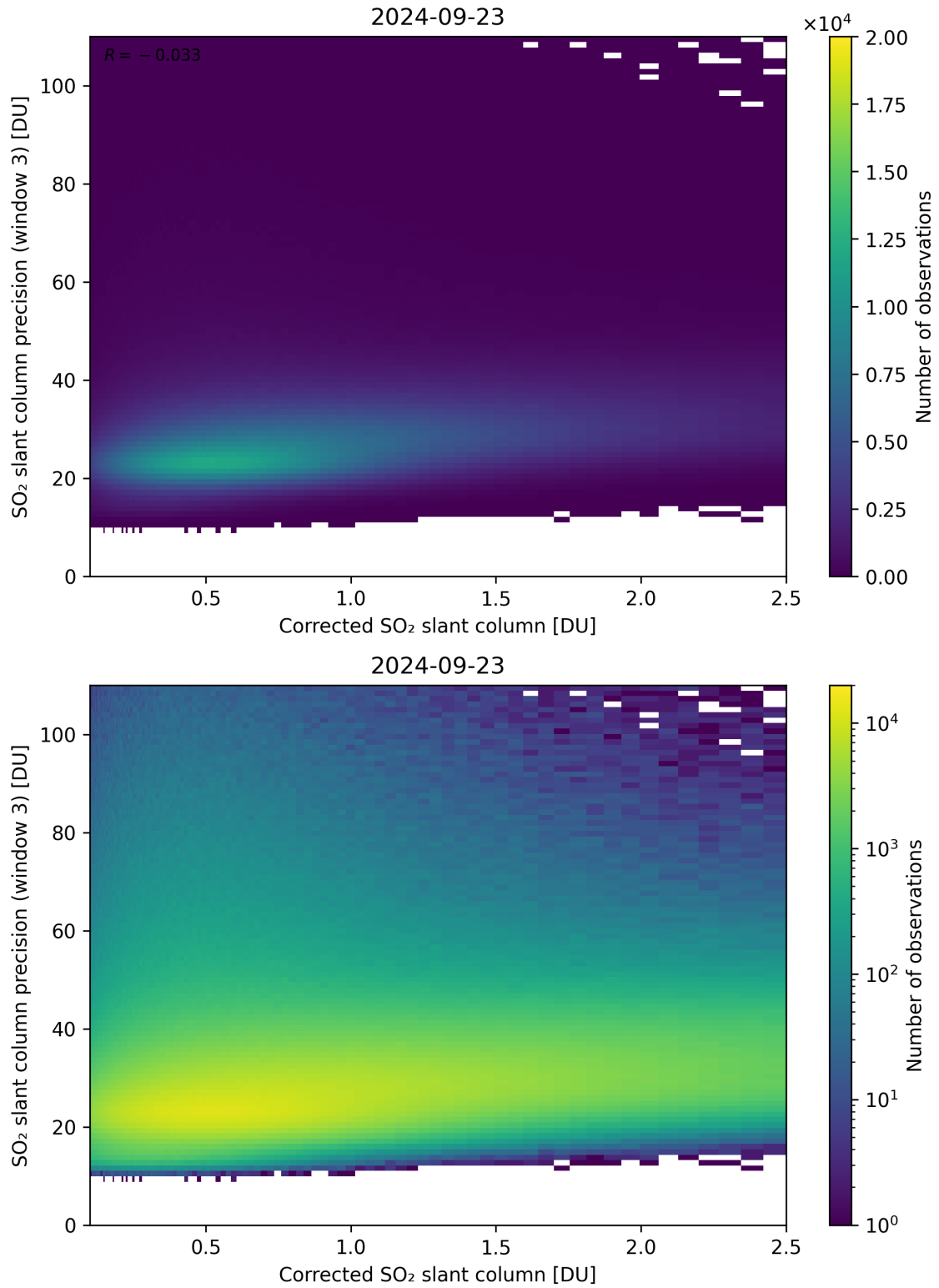
Figure 191: Scatter density plot of “Corrected SO 2 slant column” against “SO 2 slant column precision (window 3)” for 2024-09-22 to 2024-09-24.
