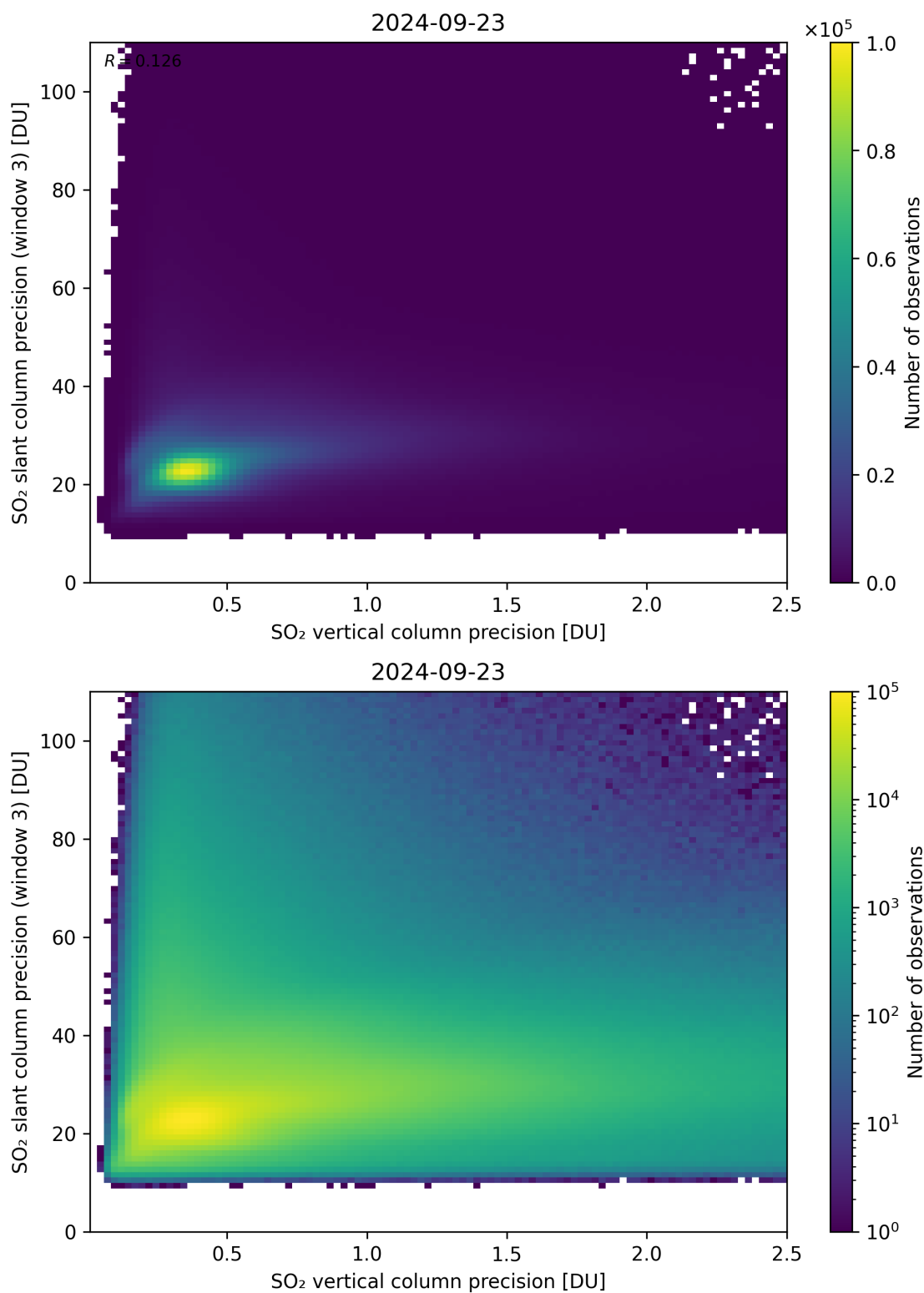
Figure 293: Scatter density plot of “SO 2 vertical column precision” against “SO 2 slant column precision (window 3)” for 2024-09-22 to 2024-09-24.
