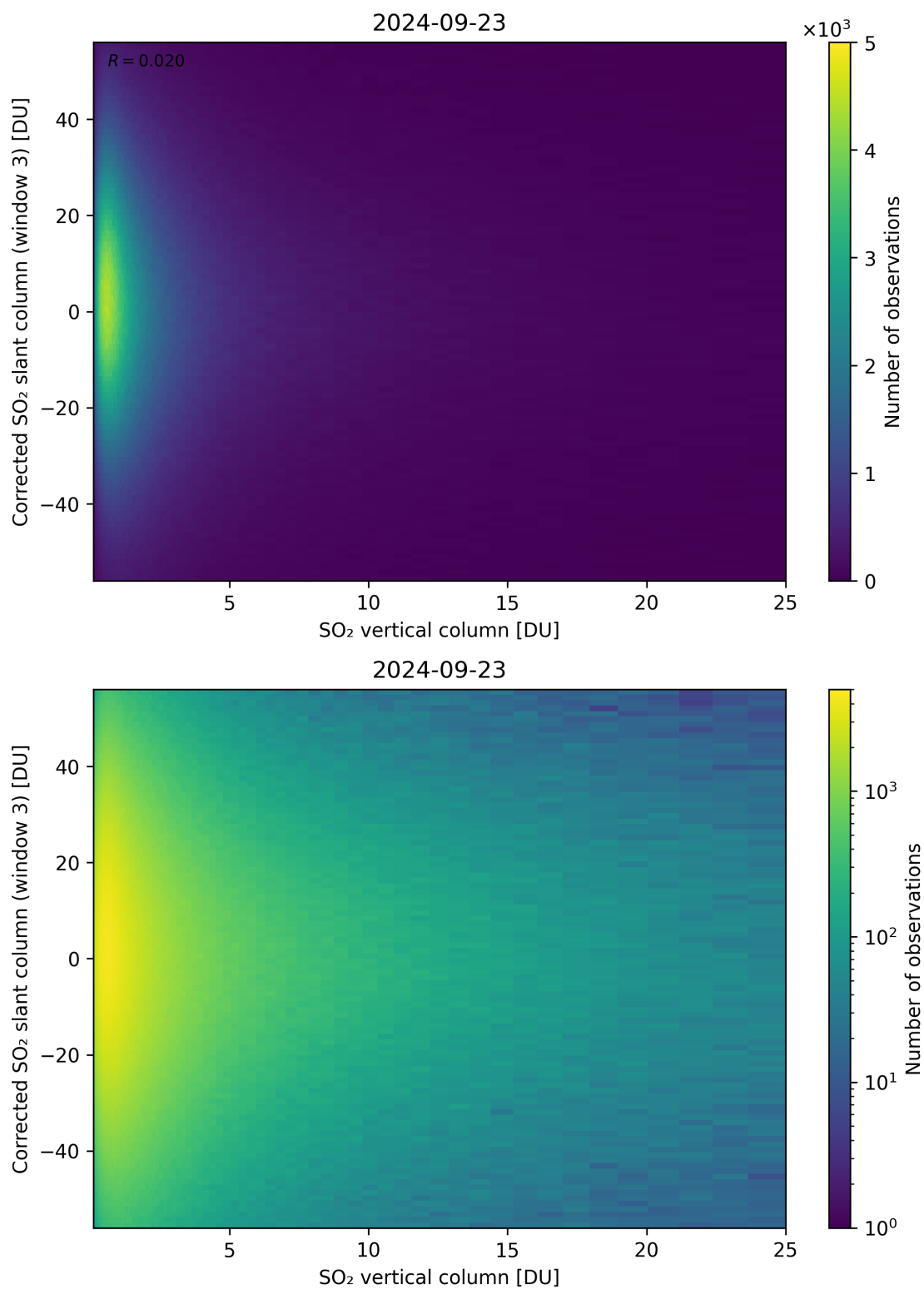
Figure 299: Scatter density plot of “SO 2 vertical column” against “Corrected SO 2 slant column (window 3)” for 2024-09-22 to 2024-09-24.
