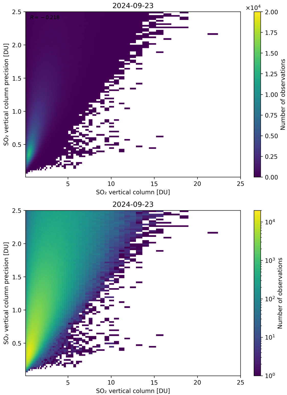
Figure 307: Scatter density plot of “SO 2 vertical column” against “SO 2 vertical column precision” for 2024-09-22 to 2024-09-24.
