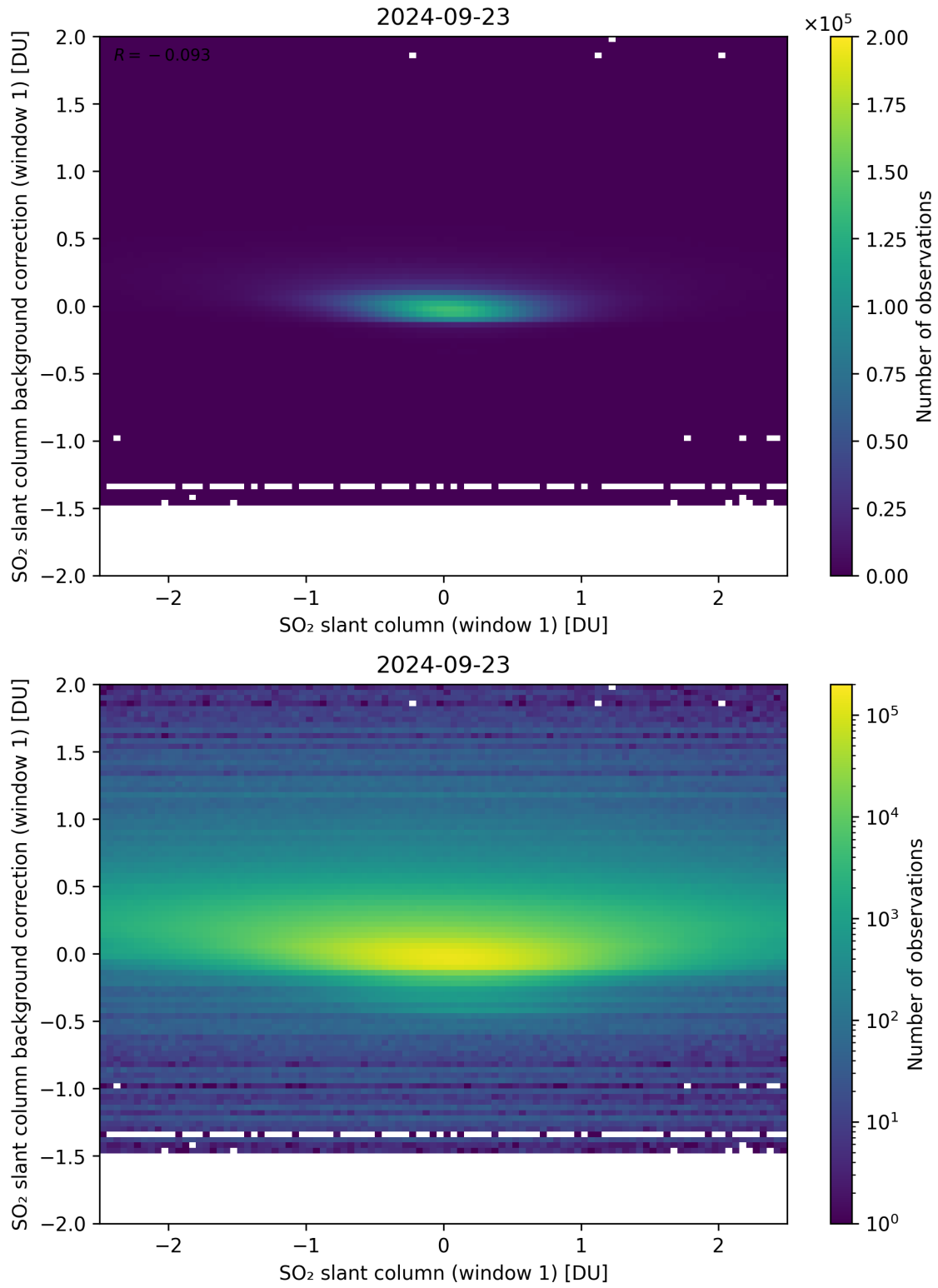
Figure 212: Scatter density plot of “SO 2 slant column (window 1)” against “SO 2 slant column background correction (window 1)” for 2024-09-22 to 2024-09-24.
