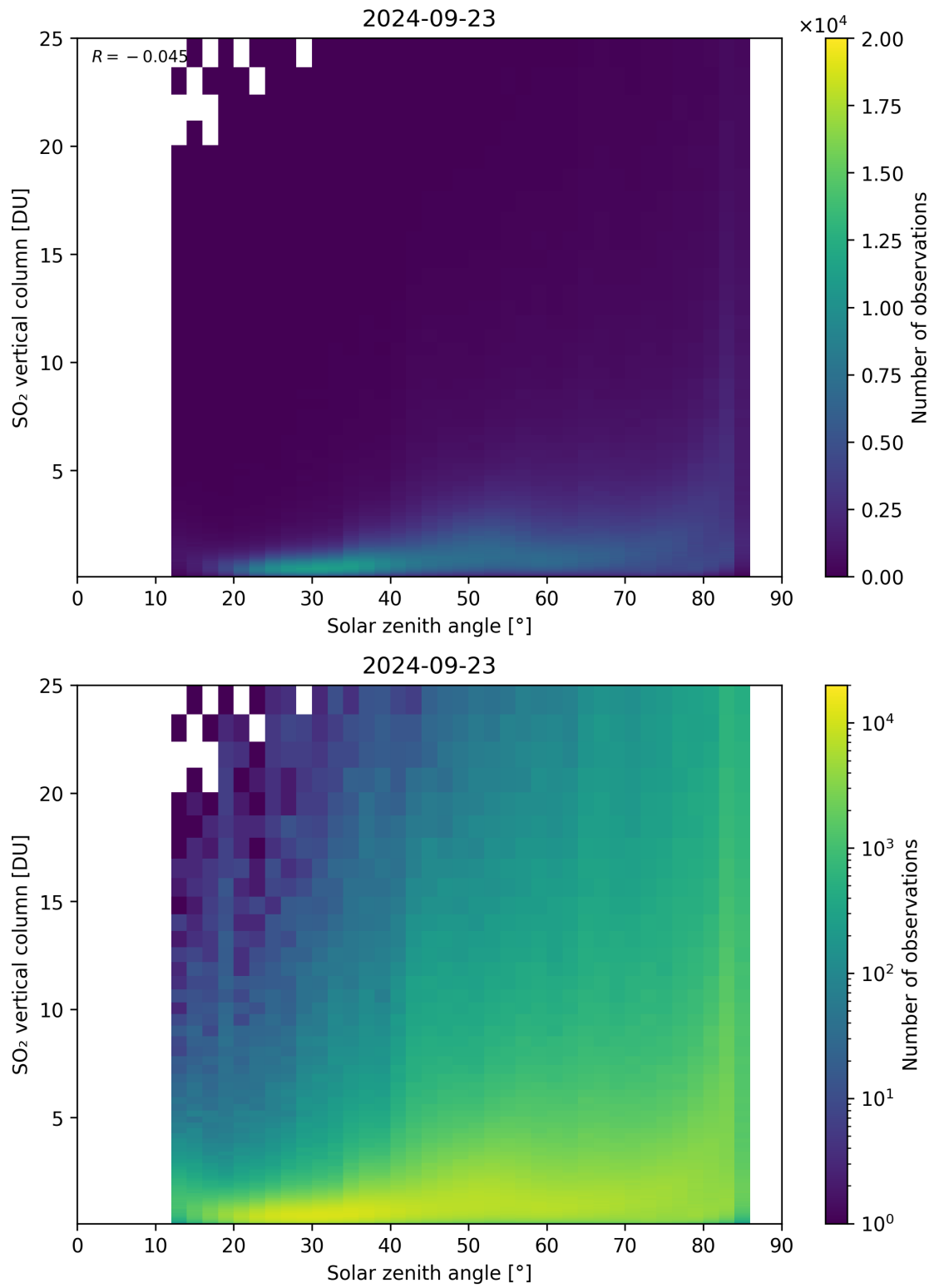
Figure 176: Scatter density plot of “Solar zenith angle” against “SO 2 vertical column” for 2024-09-22 to 2024-09-24.
