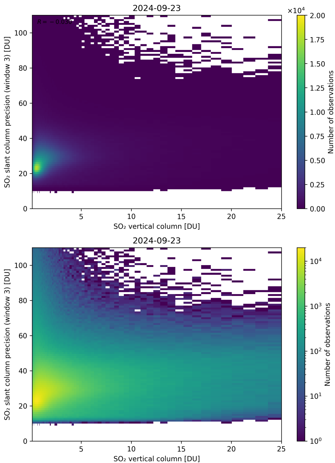
Figure 304: Scatter density plot of “SO 2 vertical column” against “SO 2 slant column precision (window 3)” for 2024-09-22 to 2024-09-24.
