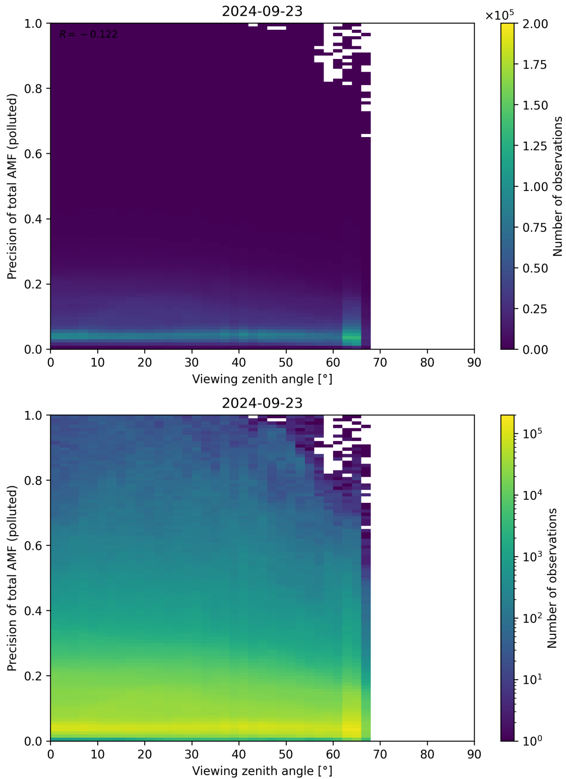
Figure 326: Scatter density plot of “Viewing zenith angle” against “Precision of total AMF (polluted)” for 2024-09-22 to 2024-09-24.
