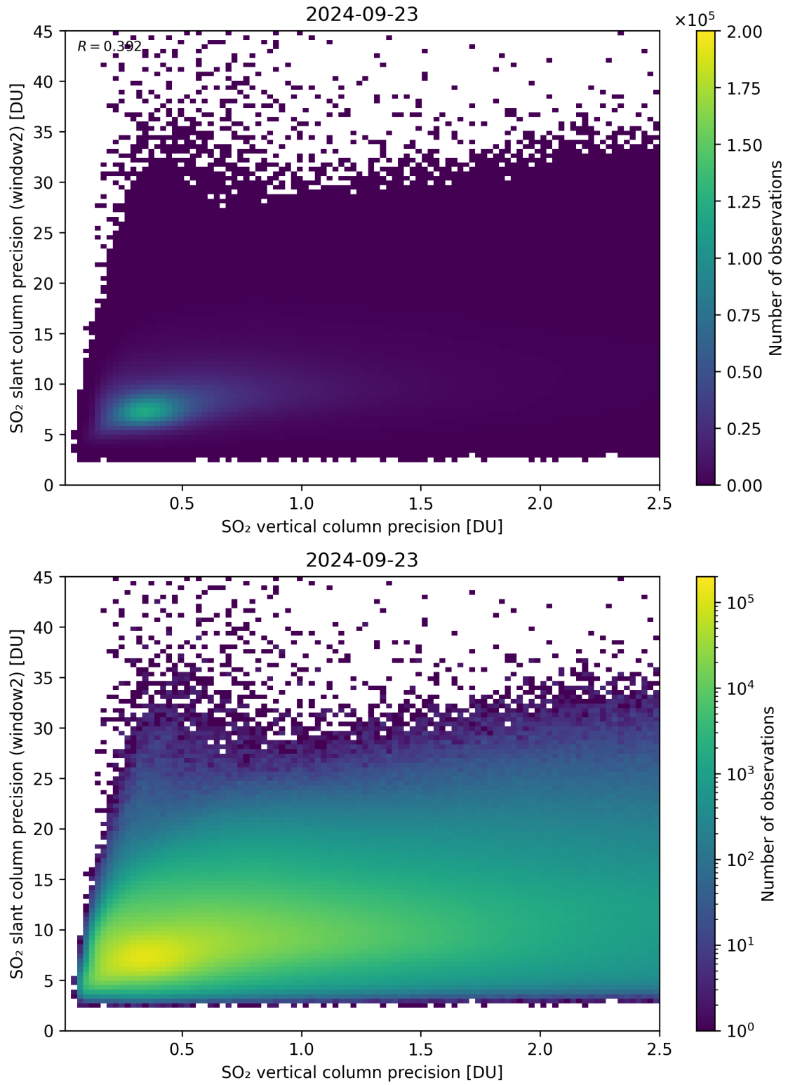
Figure 291: Scatter density plot of “SO 2 vertical column precision” against “SO 2 slant column precision (window2)” for 2024-09-22 to 2024-09-24.
