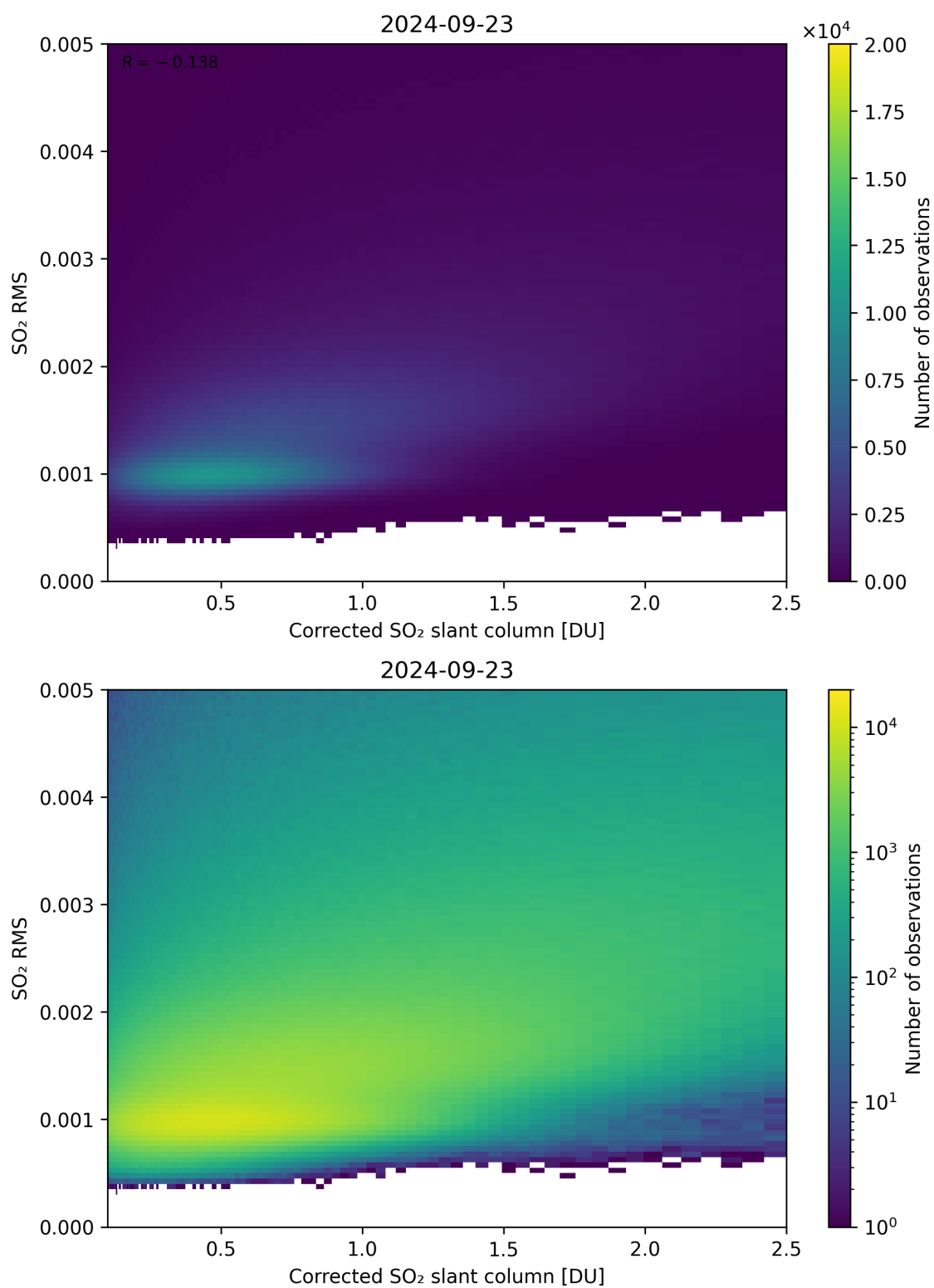
Figure 183: Scatter density plot of “Corrected SO 2 slant column” against “SO 2 RMS” for 2024-09-22 to 2024-09-24.
