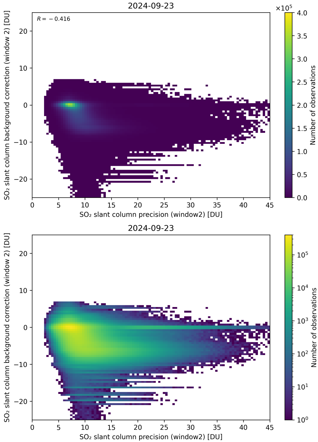
Figure 241: Scatter density plot of “SO 2 slant column precision (window2)” against “SO 2 slant column background correction (window 2)” for 2024-09-22 to 2024-09-24.
