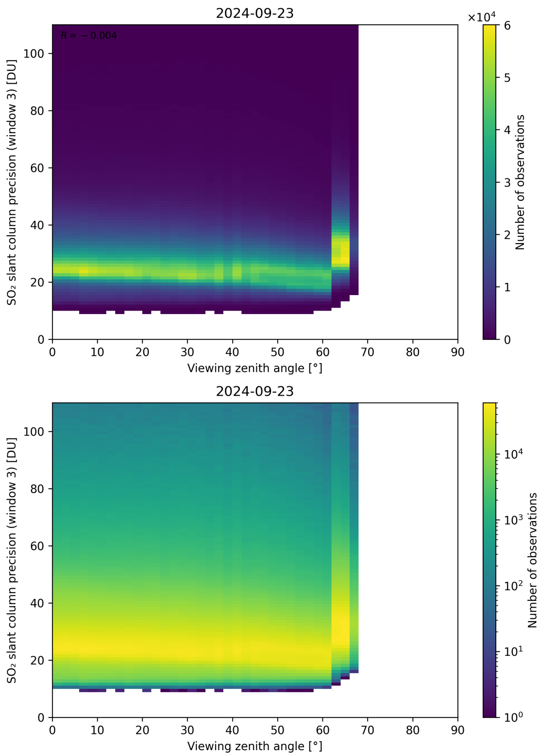
Figure 324: Scatter density plot of “Viewing zenith angle” against “SO 2 slant column precision (window 3)” for 2024-09-22 to 2024-09-24.
