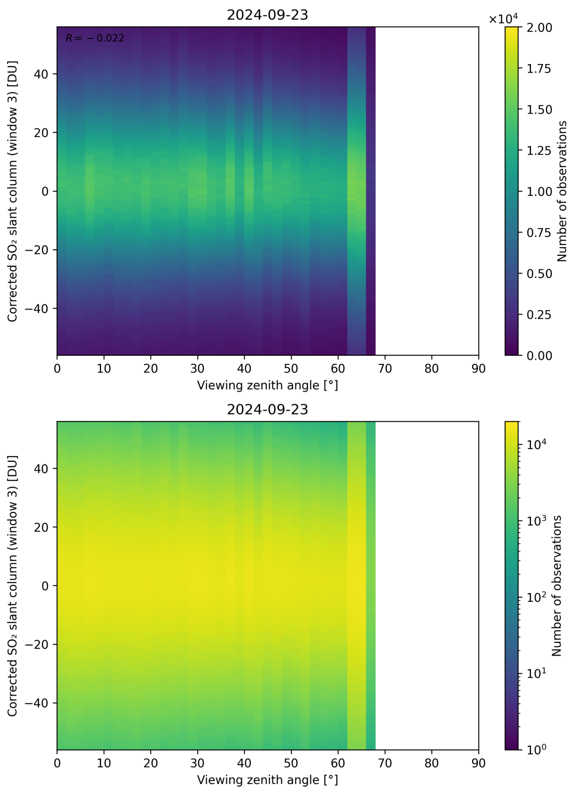
Figure 319: Scatter density plot of “Viewing zenith angle” against “Corrected SO 2 slant column (window 3)” for 2024-09-22 to 2024-09-24.
