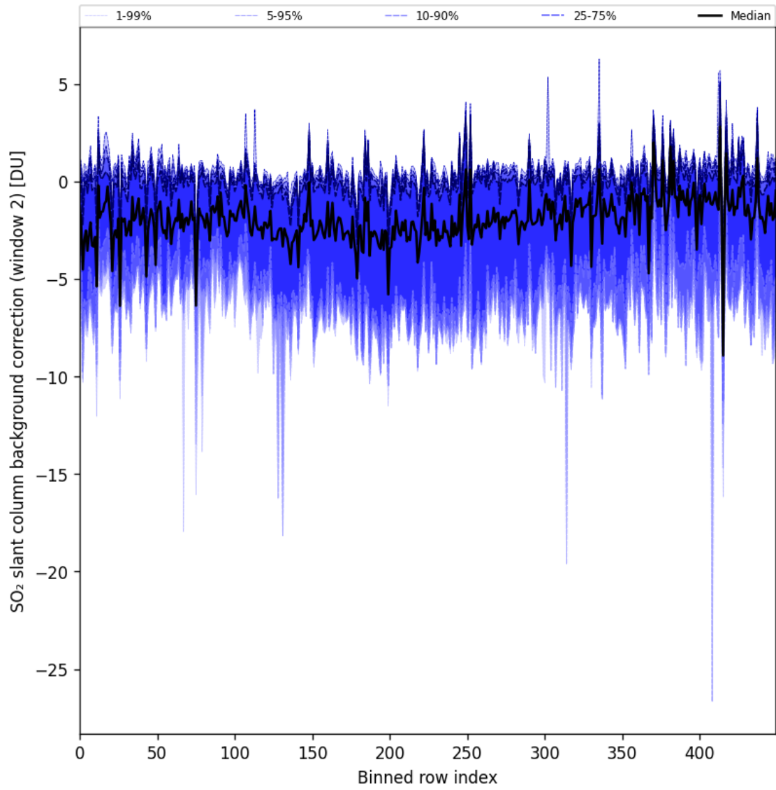
Figure 86: Along track statistics of “SO 2 slant column background correction (window 2)” for 2024-09-22 to 2024-09-24
