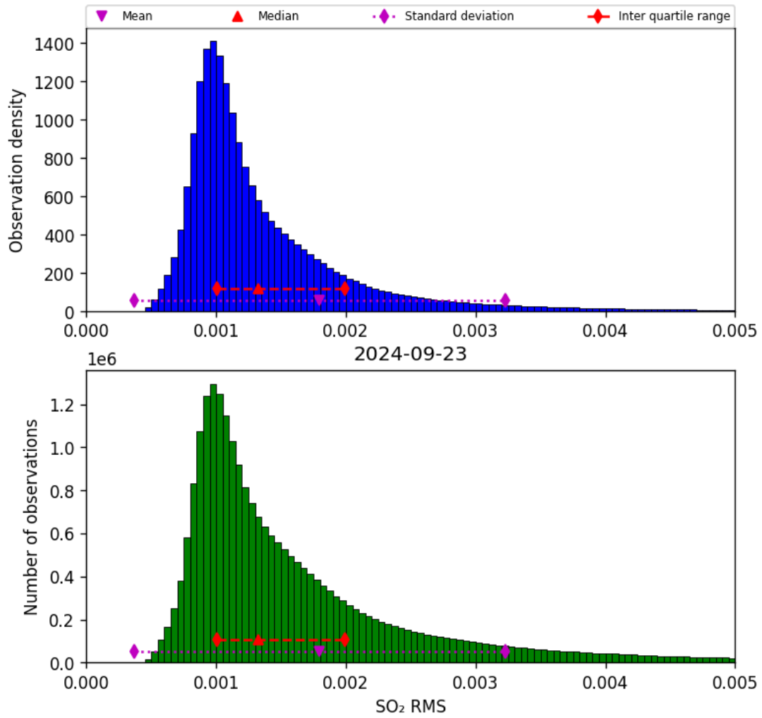
Figure 70: Histogram of “SO 2 RMS” for 2024-09-22 to 2024-09-24
