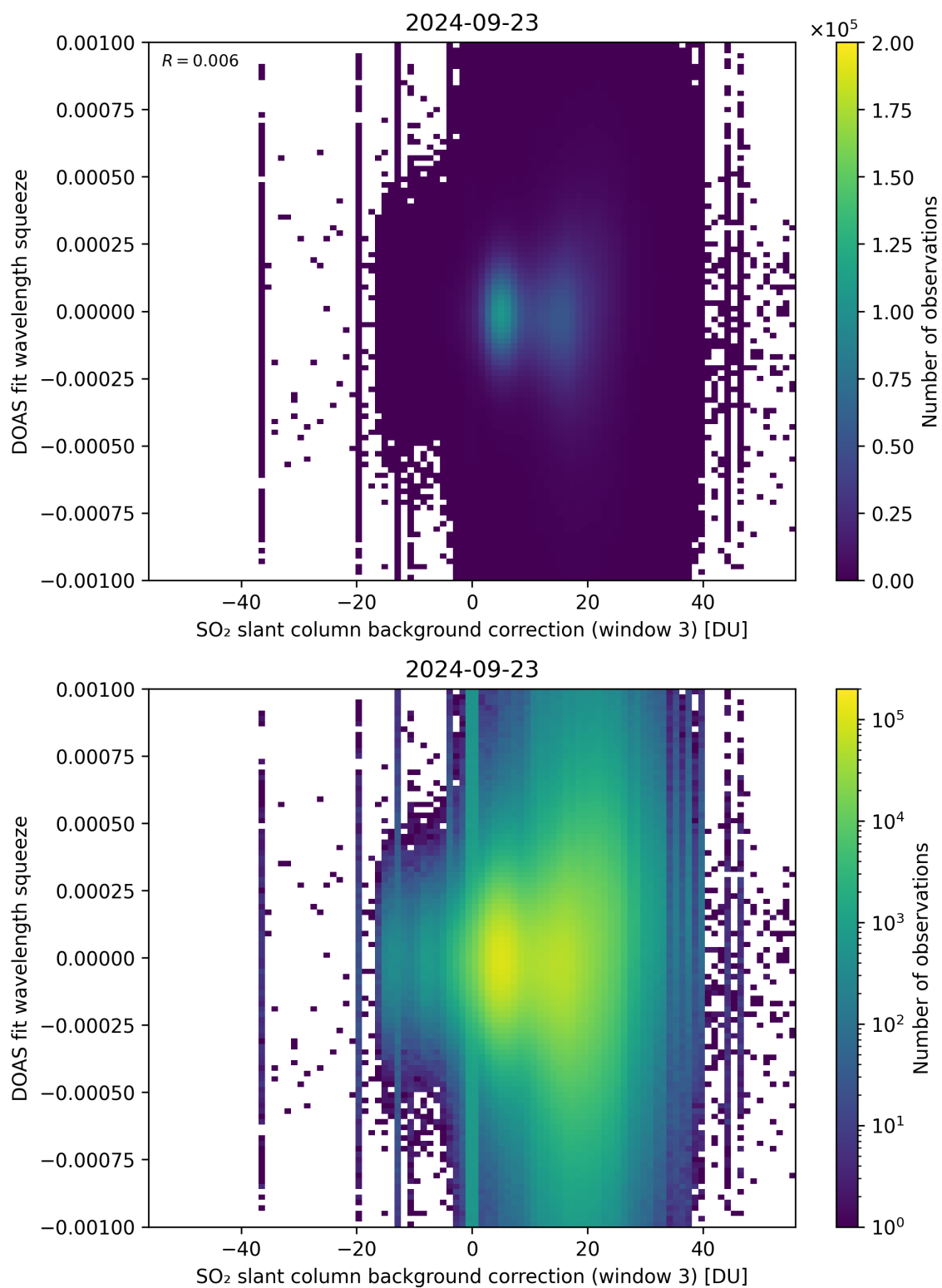
Figure 122: Scatter density plot of “SO 2 slant column background correction (window 3)” against “DOAS fit wavelength squeeze” for 2024-09-22 to 2024-09-24.
