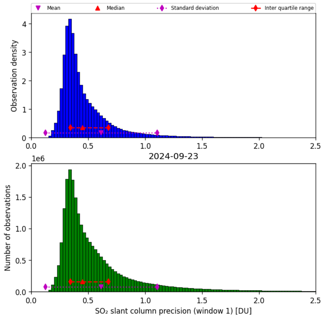
Figure 57: Histogram of “SO 2 slant column precision (window 1)” for 2024-09-22 to 2024-09-24
