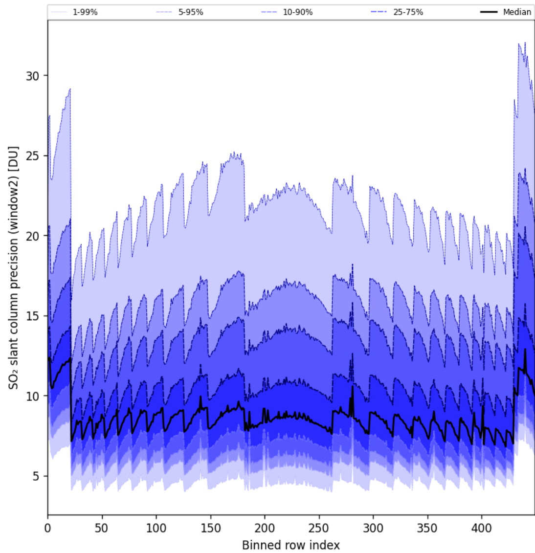
Figure 84: Along track statistics of “SO 2 slant column precision (window2)” for 2024-09-22 to 2024-09-24
