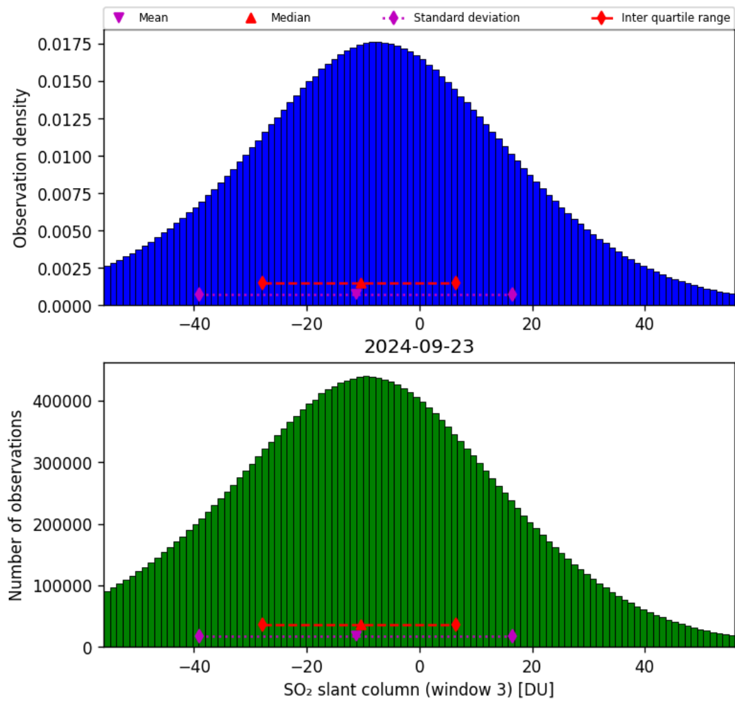
Figure 64: Histogram of “SO 2 slant column (window 3)” for 2024-09-22 to 2024-09-24
