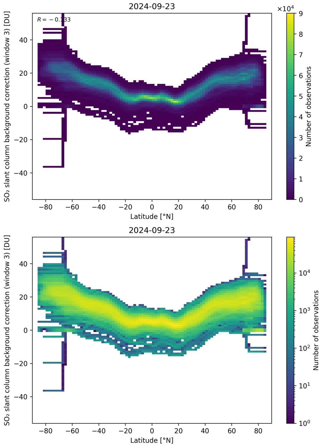
Figure 141: Scatter density plot of “Latitude” against “SO 2 slant column background correction (window 3)” for 2024-09-22 to 2024-09-24.
