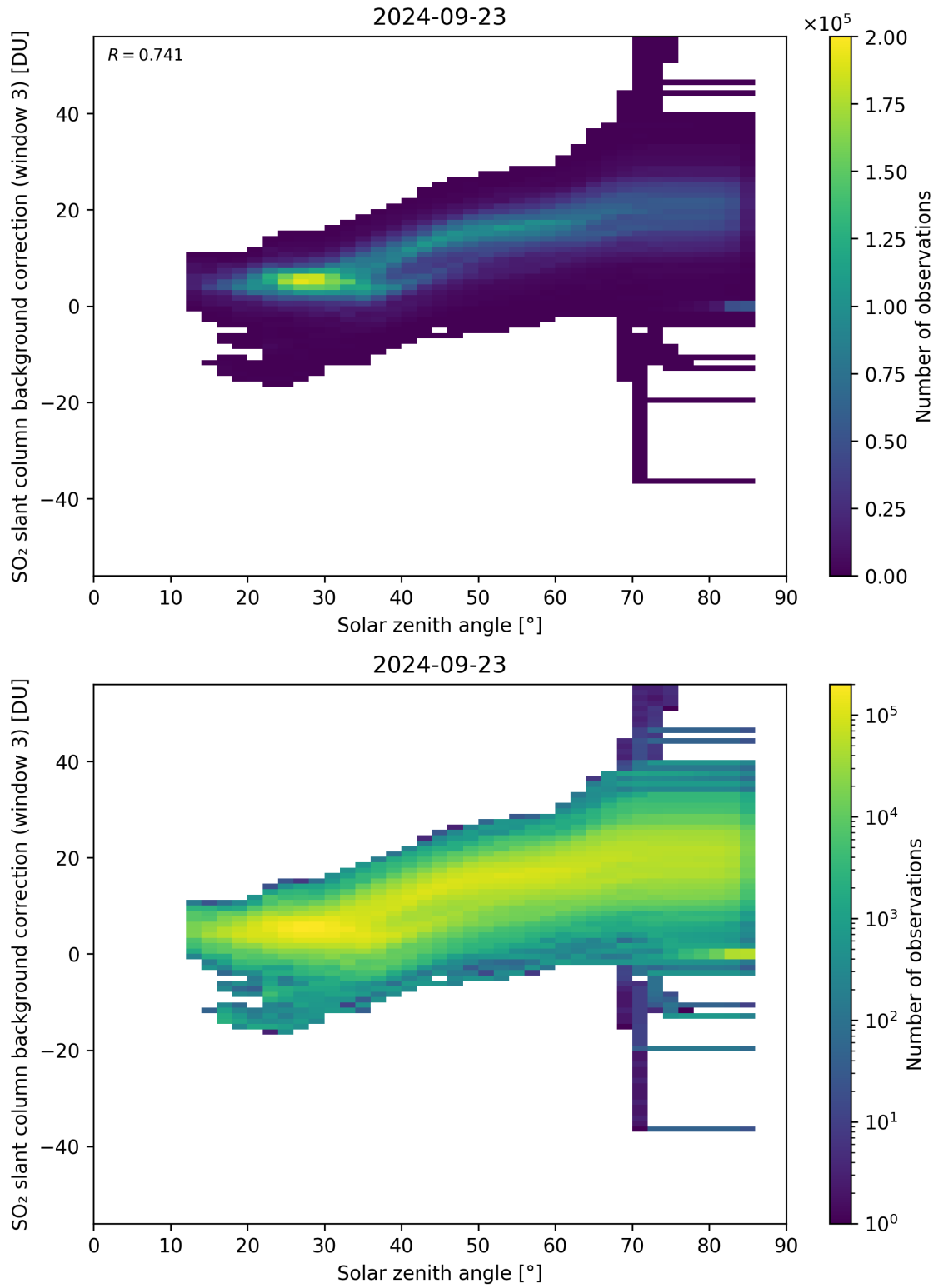
Figure 160: Scatter density plot of “Solar zenith angle” against “SO 2 slant column background correction (window 3)” for 2024-09-22 to 2024-09-24.
