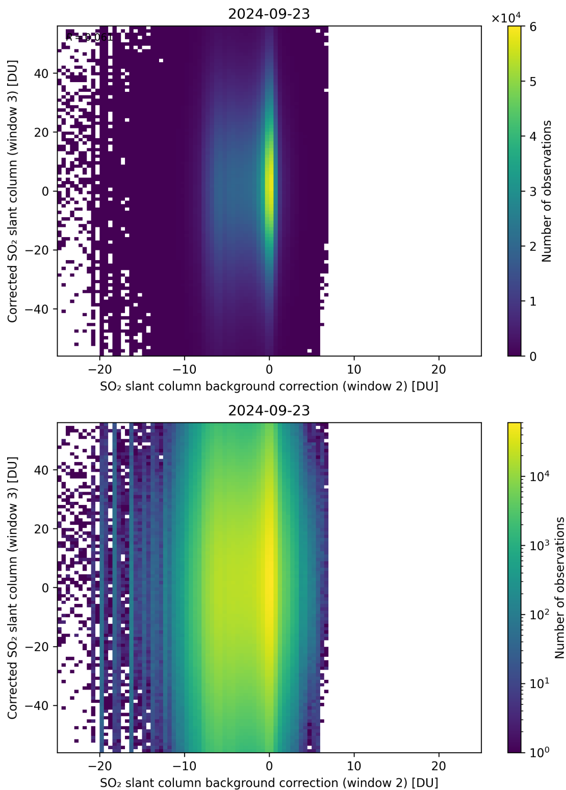
Figure 116: Scatter density plot of “SO 2 slant column background correction (window 2)” against “Corrected SO 2 slant column (window 3)” for 2024-09-22 to 2024-09-24.
