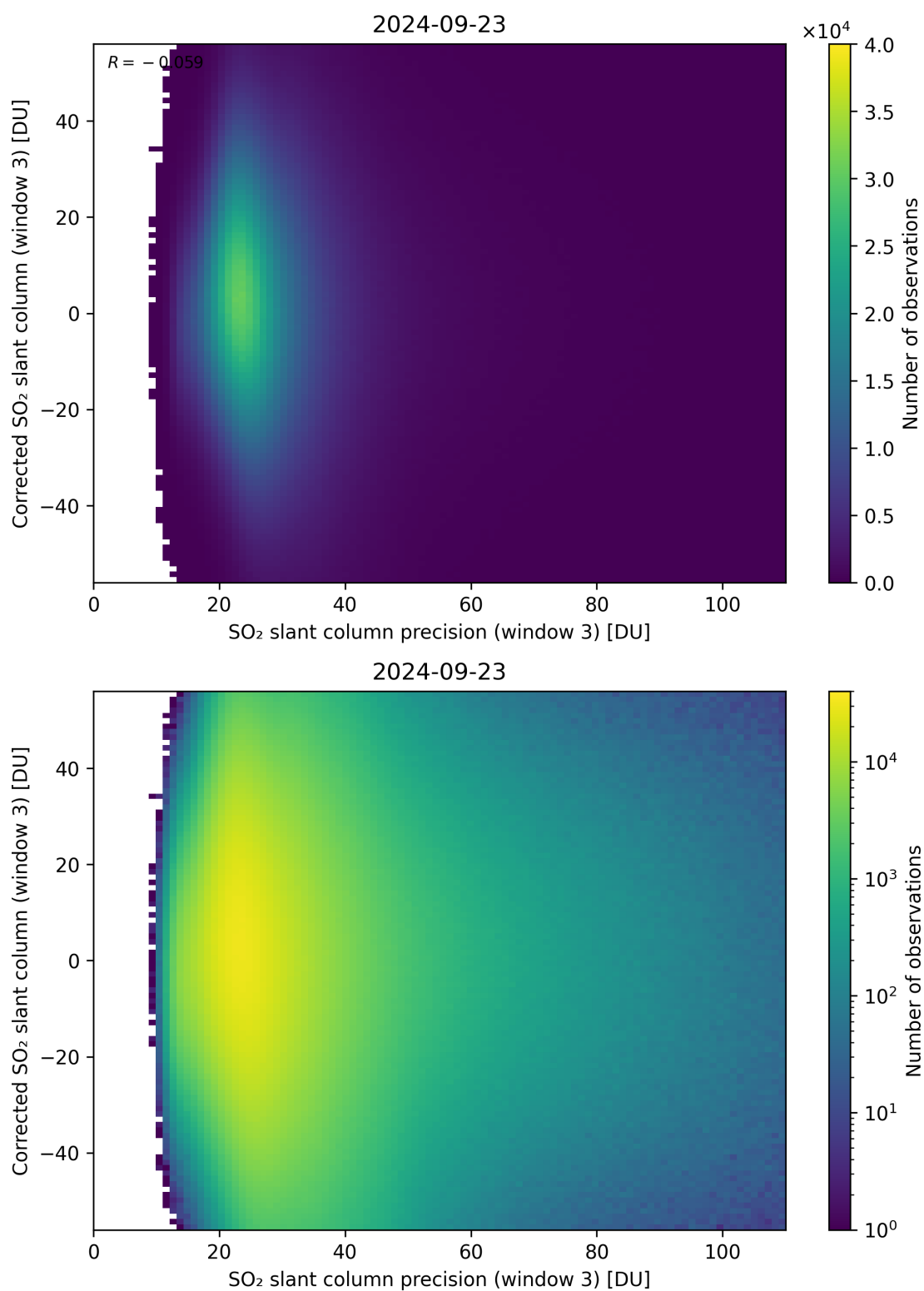
Figure 262: Scatter density plot of “SO 2 slant column precision (window 3)” against “Corrected SO 2 slant column (window 3)” for 2024-09-22 to 2024-09-24.
