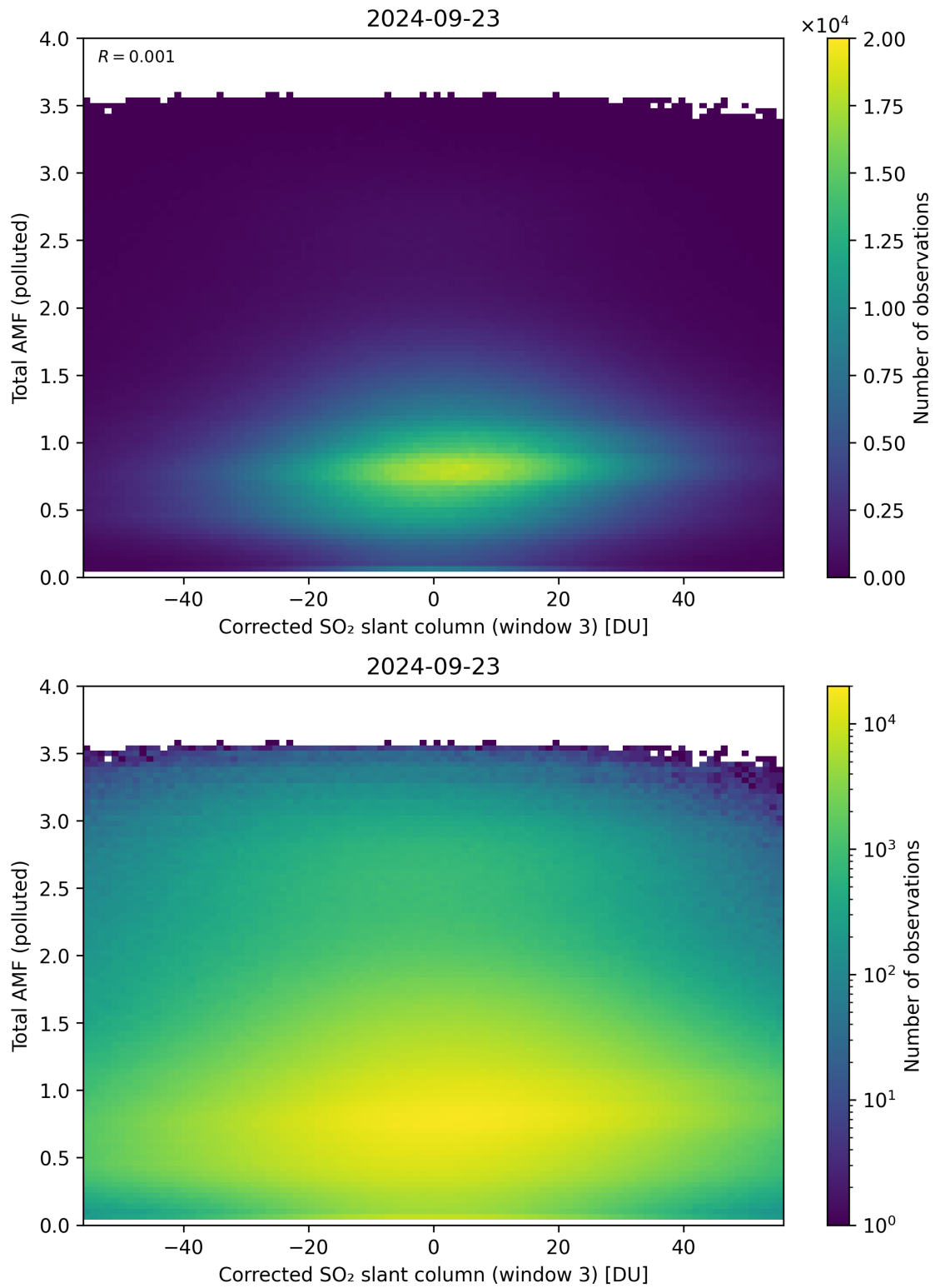
Figure 210: Scatter density plot of “Corrected SO 2 slant column (window 3)” against “Total AMF (polluted)” for 2024-09-22 to 2024-09-24.
