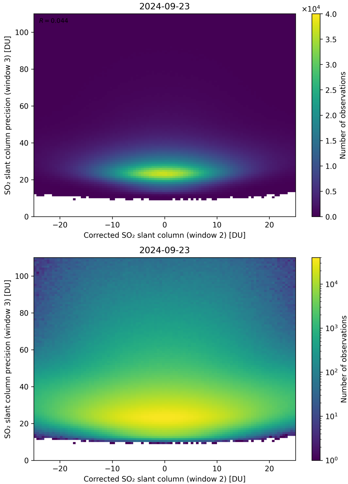
Figure 202: Scatter density plot of “Corrected SO 2 slant column (window 2)” against “SO 2 slant column precision (window 3)” for 2024-09-22 to 2024-09-24.
