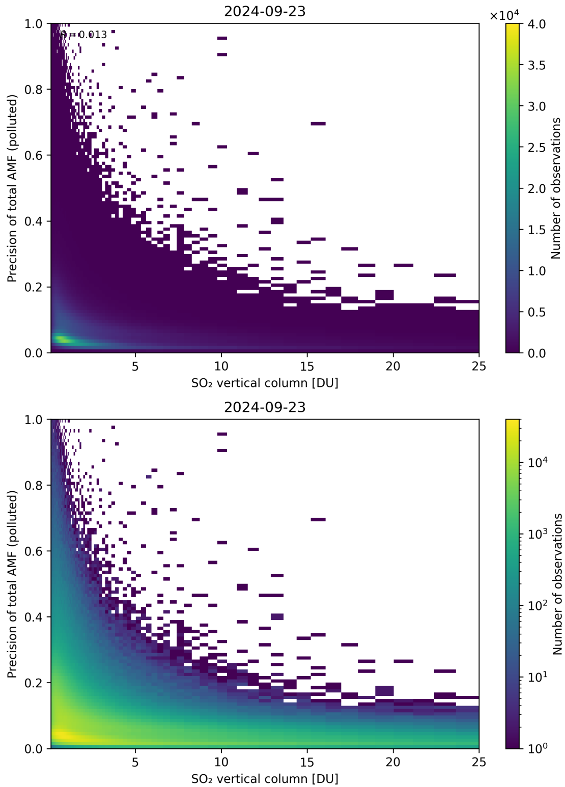
Figure 306: Scatter density plot of “SO 2 vertical column” against “Precision of total AMF (polluted)” for 2024-09-22 to 2024-09-24.
