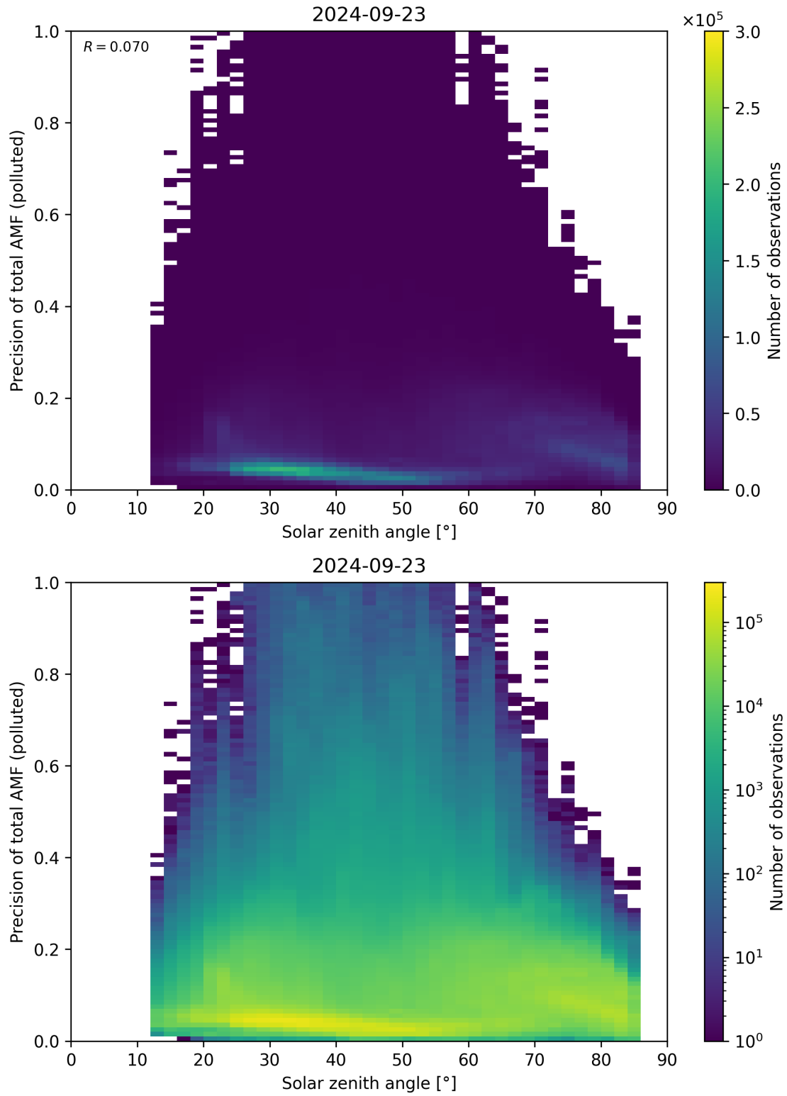
Figure 175: Scatter density plot of “Solar zenith angle” against “Precision of total AMF (polluted)” for 2024-09-22 to 2024-09-24.
