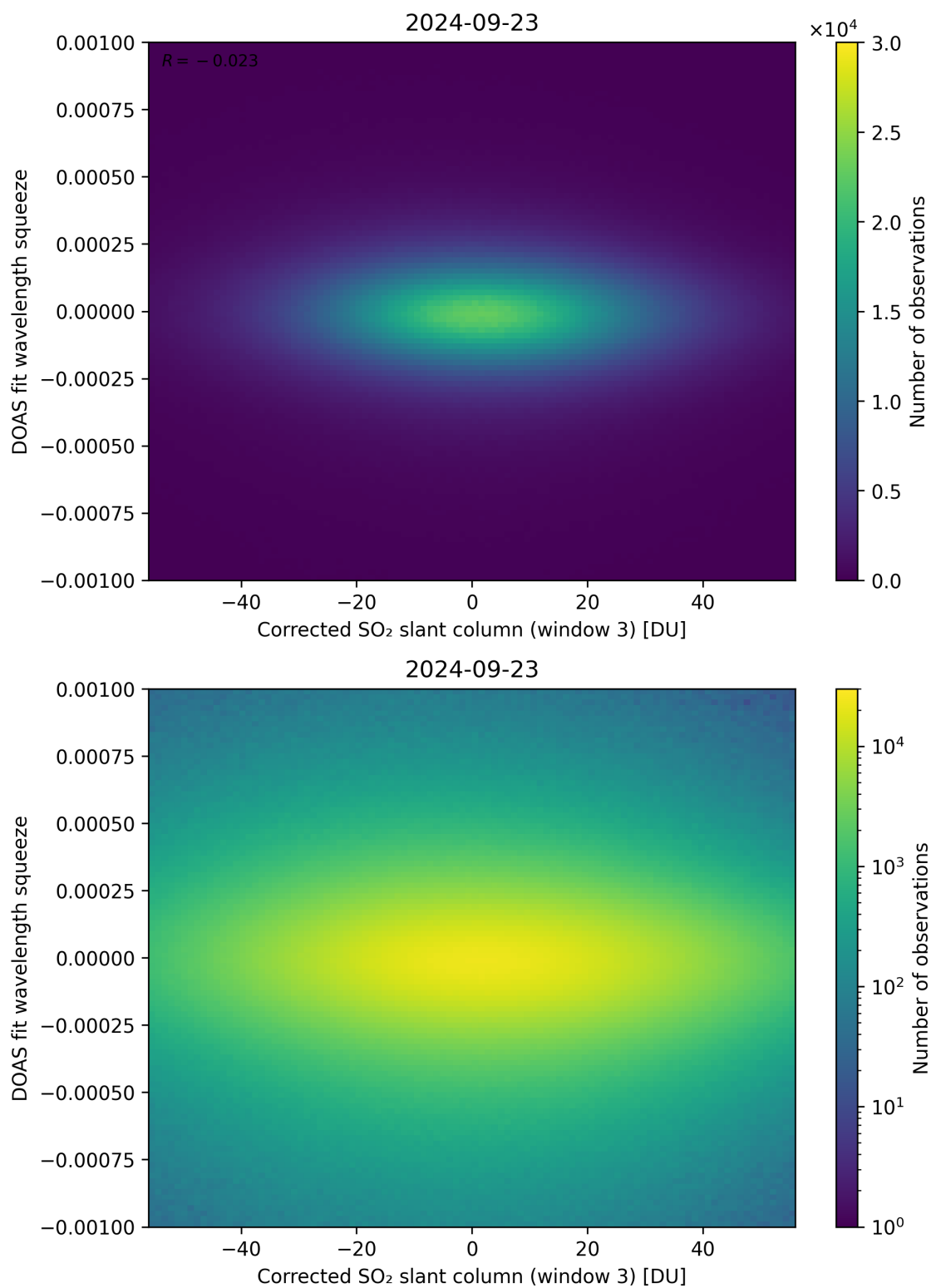
Figure 207: Scatter density plot of “Corrected SO 2 slant column (window 3)” against “DOAS fit wavelength squeeze” for 2024-09-22 to 2024-09-24.
