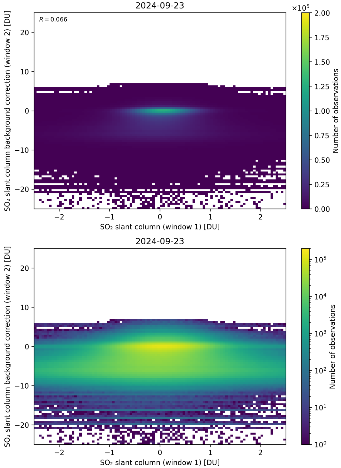
Figure 213: Scatter density plot of “SO 2 slant column (window 1)” against “SO 2 slant column background correction (window 2)” for 2024-09-22 to 2024-09-24.
