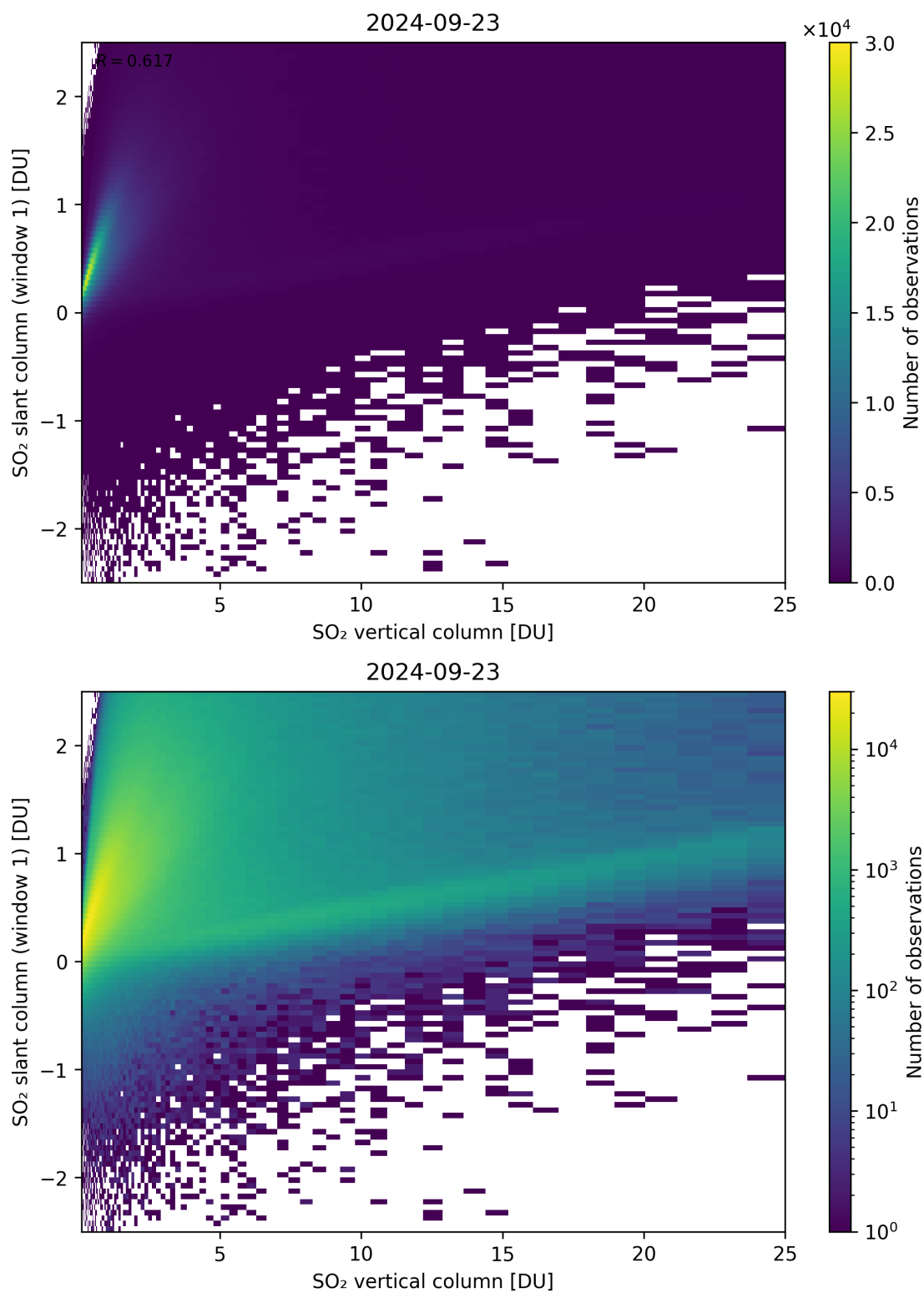
Figure 300: Scatter density plot of “SO 2 vertical column” against “SO 2 slant column (window 1)” for 2024-09-22 to 2024-09-24.
