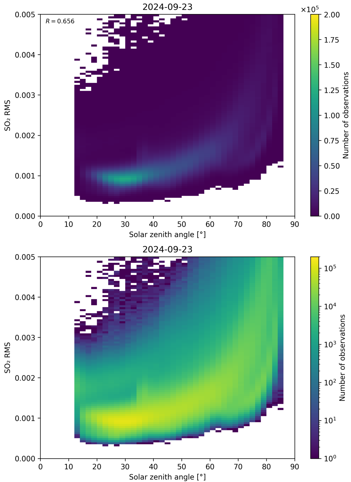
Figure 163: Scatter density plot of “Solar zenith angle” against “SO 2 RMS” for 2024-09-22 to 2024-09-24.
