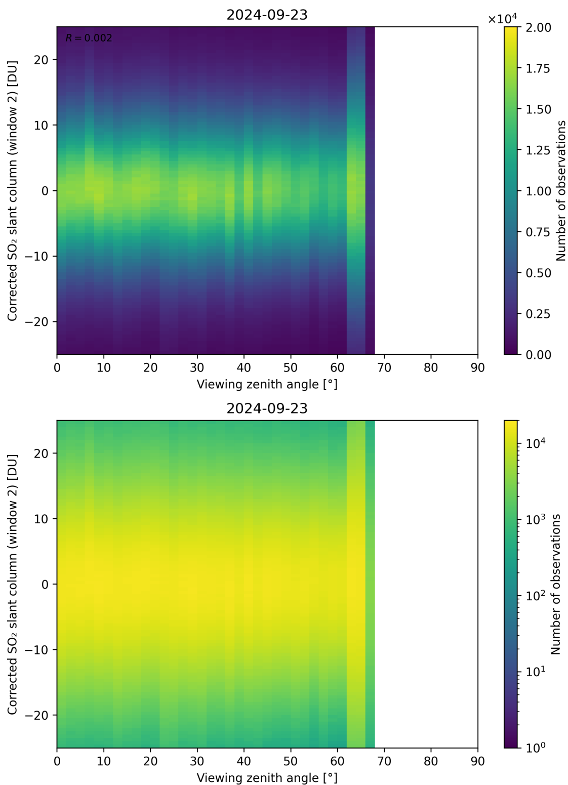
Figure 318: Scatter density plot of “Viewing zenith angle” against “Corrected SO 2 slant column (window 2)” for 2024-09-22 to 2024-09-24.
