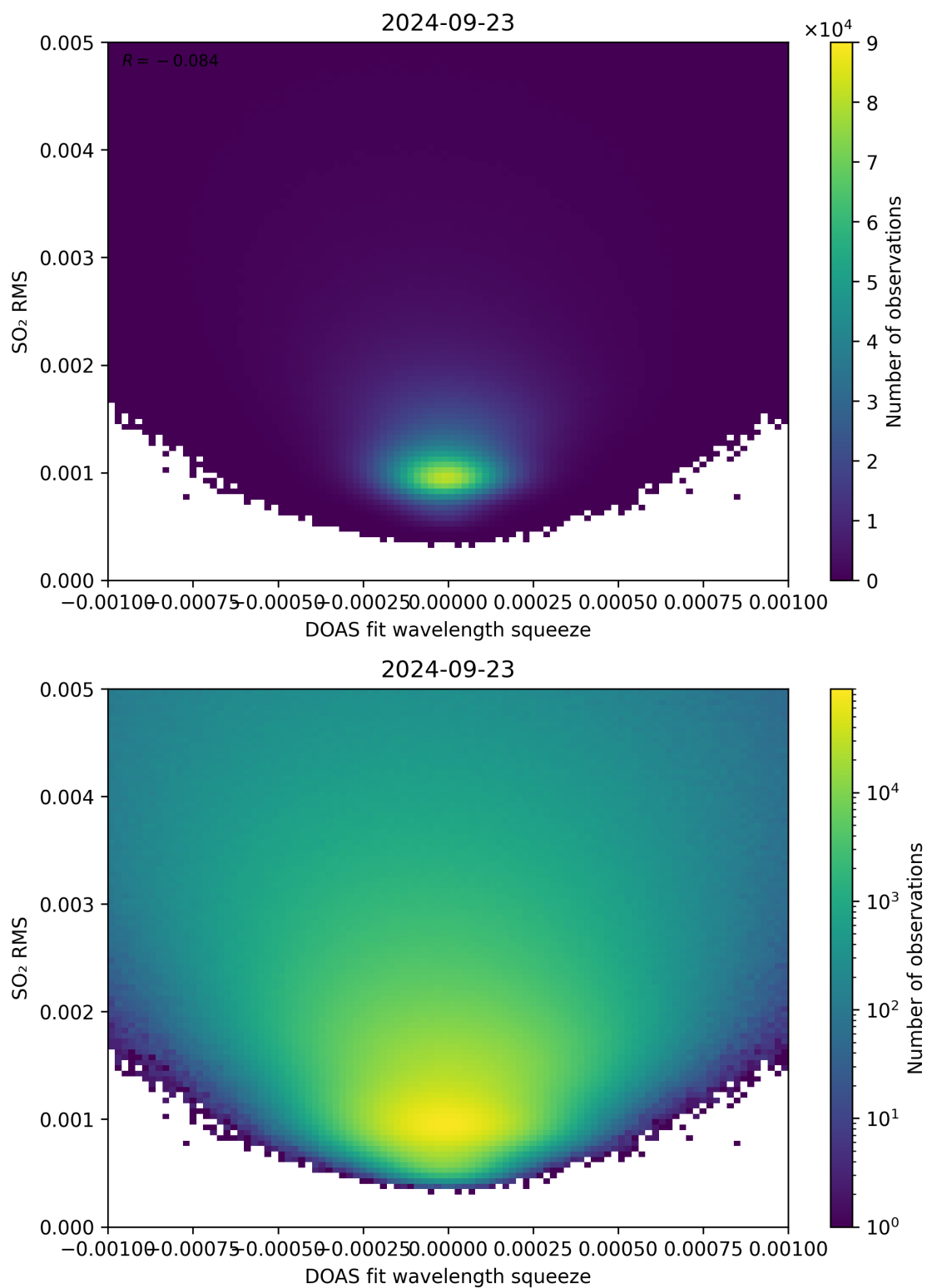
Figure 132: Scatter density plot of “DOAS fit wavelength squeeze” against “SO 2 RMS” for 2024-09-22 to 2024-09-24.
