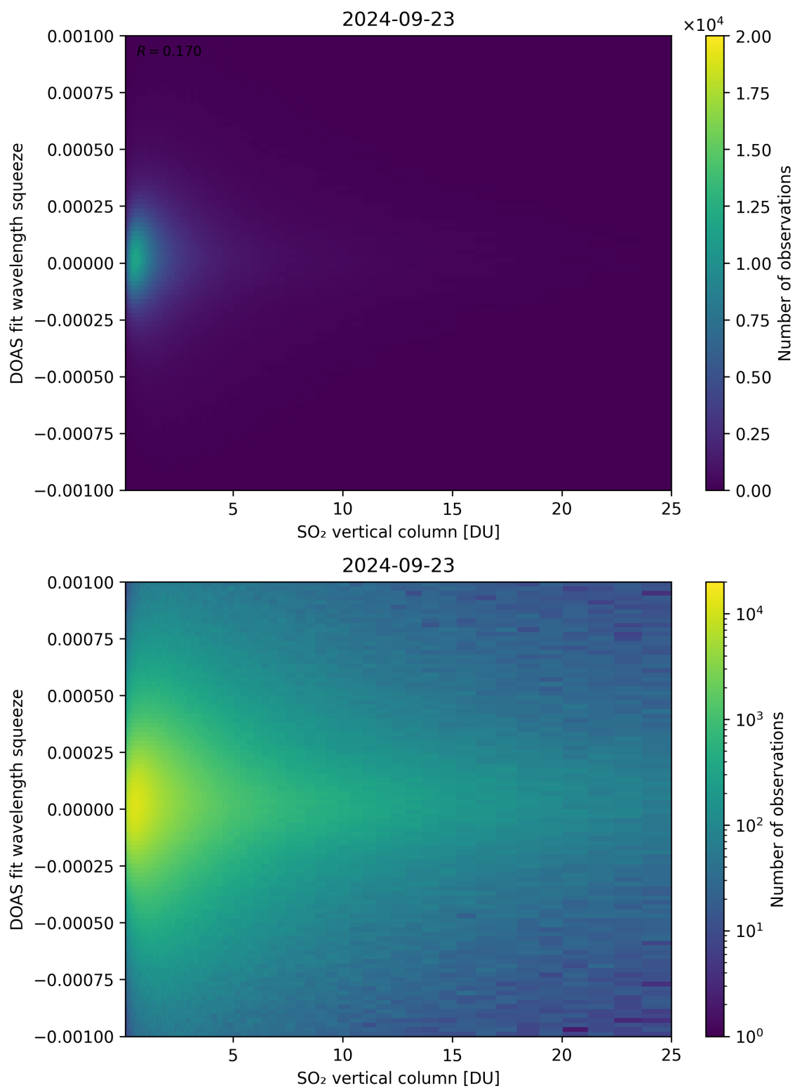
Figure 277: Scatter density plot of “SO 2 vertical column” against “DOAS fit wavelength squeeze” for 2024-09-22 to 2024-09-24.
