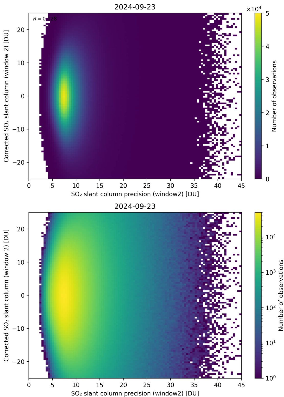
Figure 247: Scatter density plot of “SO 2 slant column precision (window2)” against “Corrected SO 2 slant column (window 2)” for 2024-09-22 to 2024-09-24.
