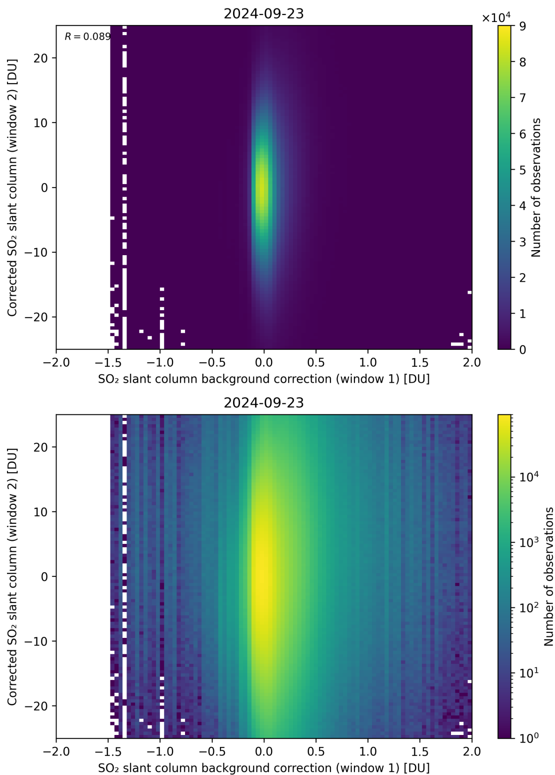
Figure 104: Scatter density plot of “SO 2 slant column background correction (window 1)” against “Corrected SO 2 slant column (window 2)” for 2024-09-22 to 2024-09-24.
