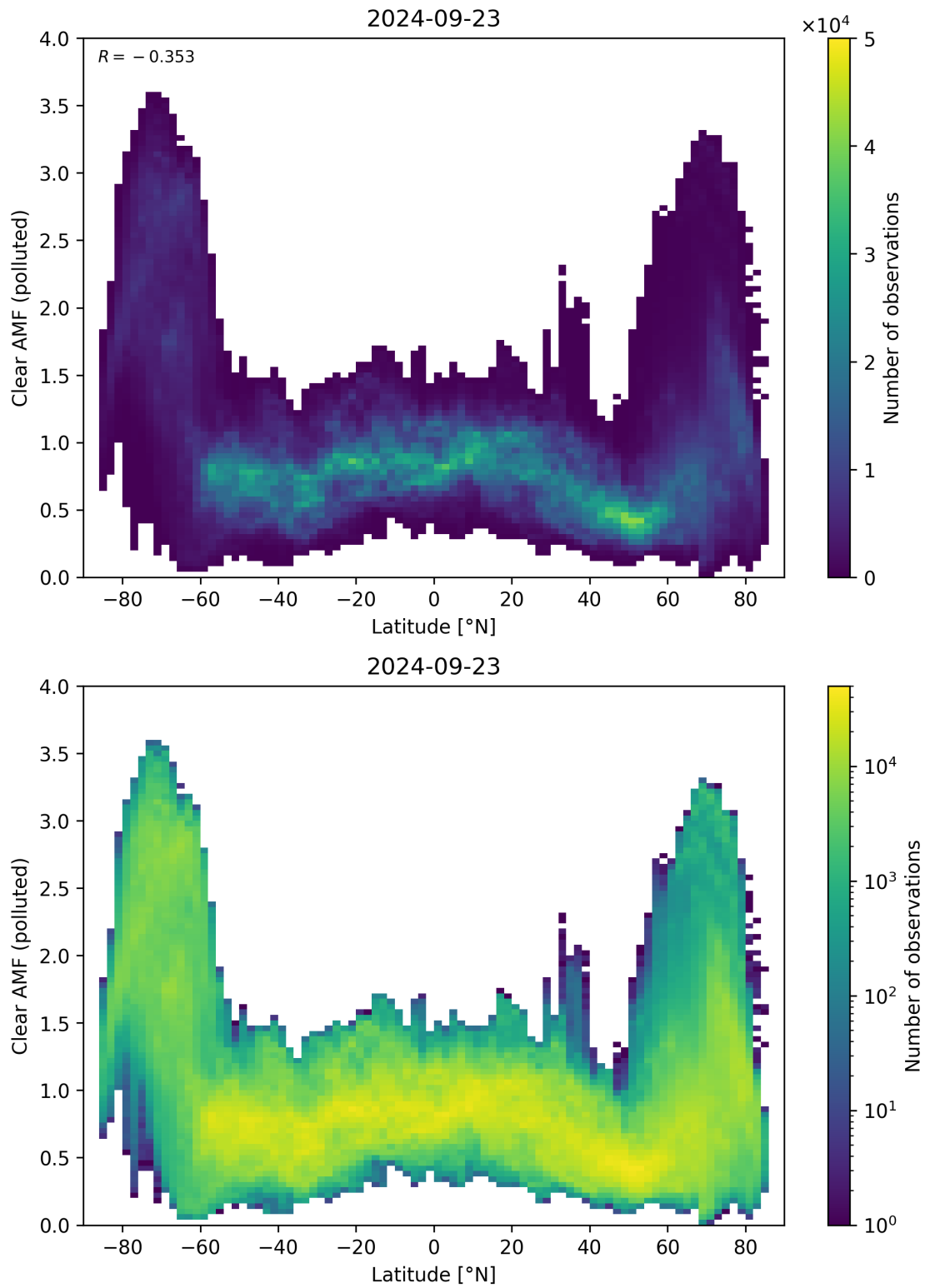
Figure 145: Scatter density plot of “Latitude” against “Clear AMF (polluted)” for 2024-09-22 to 2024-09-24.
