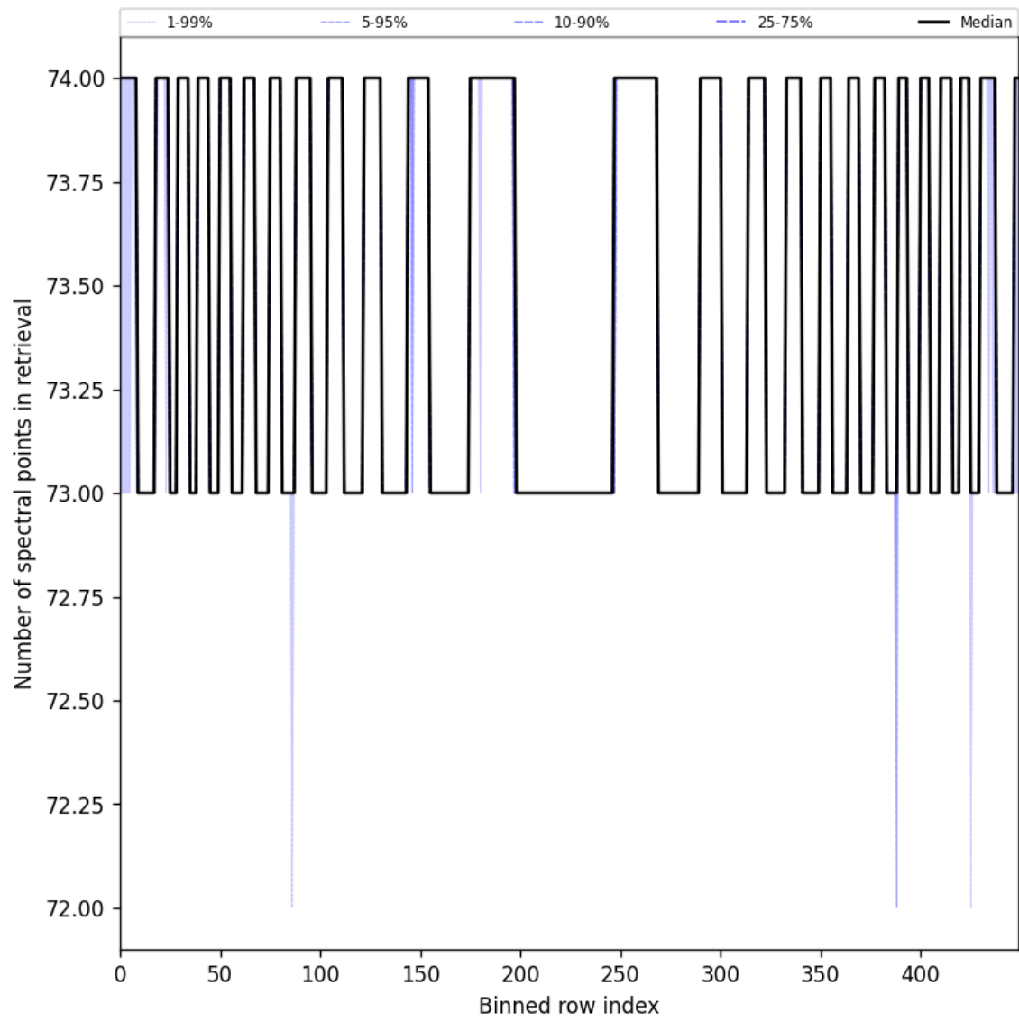
Figure 97: Along track statistics of “Number of spectral points in retrieval” for 2024-09-22 to 2024-09-24
