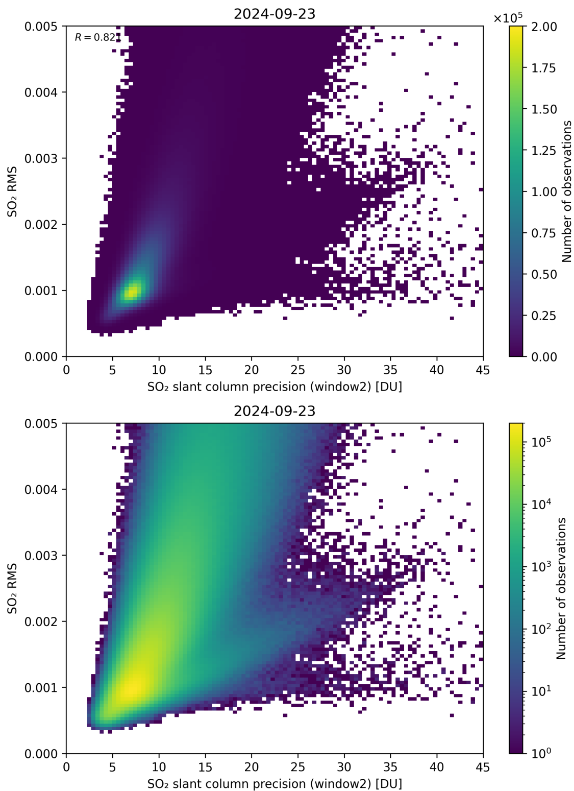
Figure 245: Scatter density plot of “SO 2 slant column precision (window2)” against “SO 2 RMS” for 2024-09-22 to 2024-09-24.
