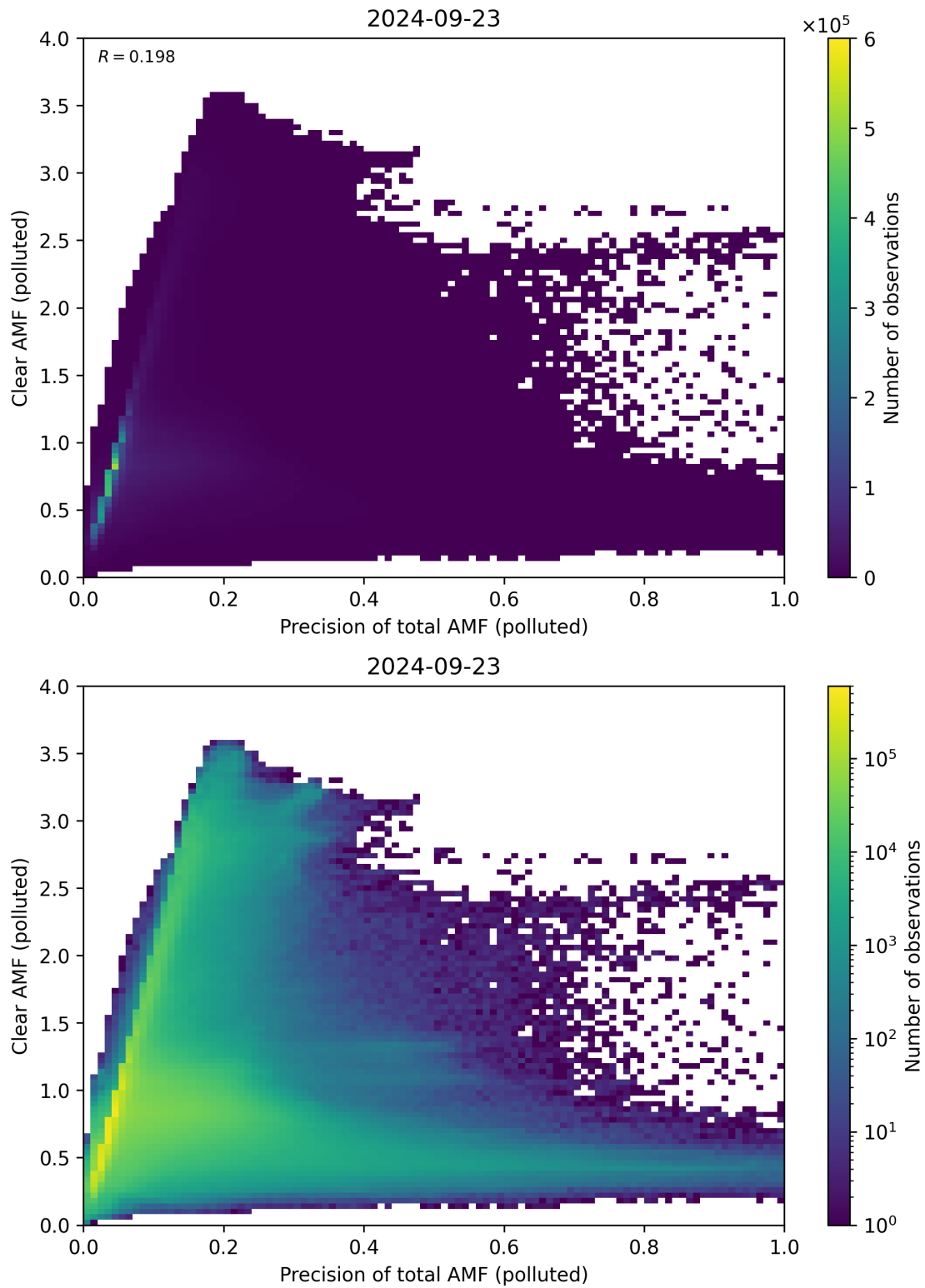
Figure 270: Scatter density plot of “Precision of total AMF (polluted)” against “Clear AMF (polluted)” for 2024-09-22 to 2024-09-24.
