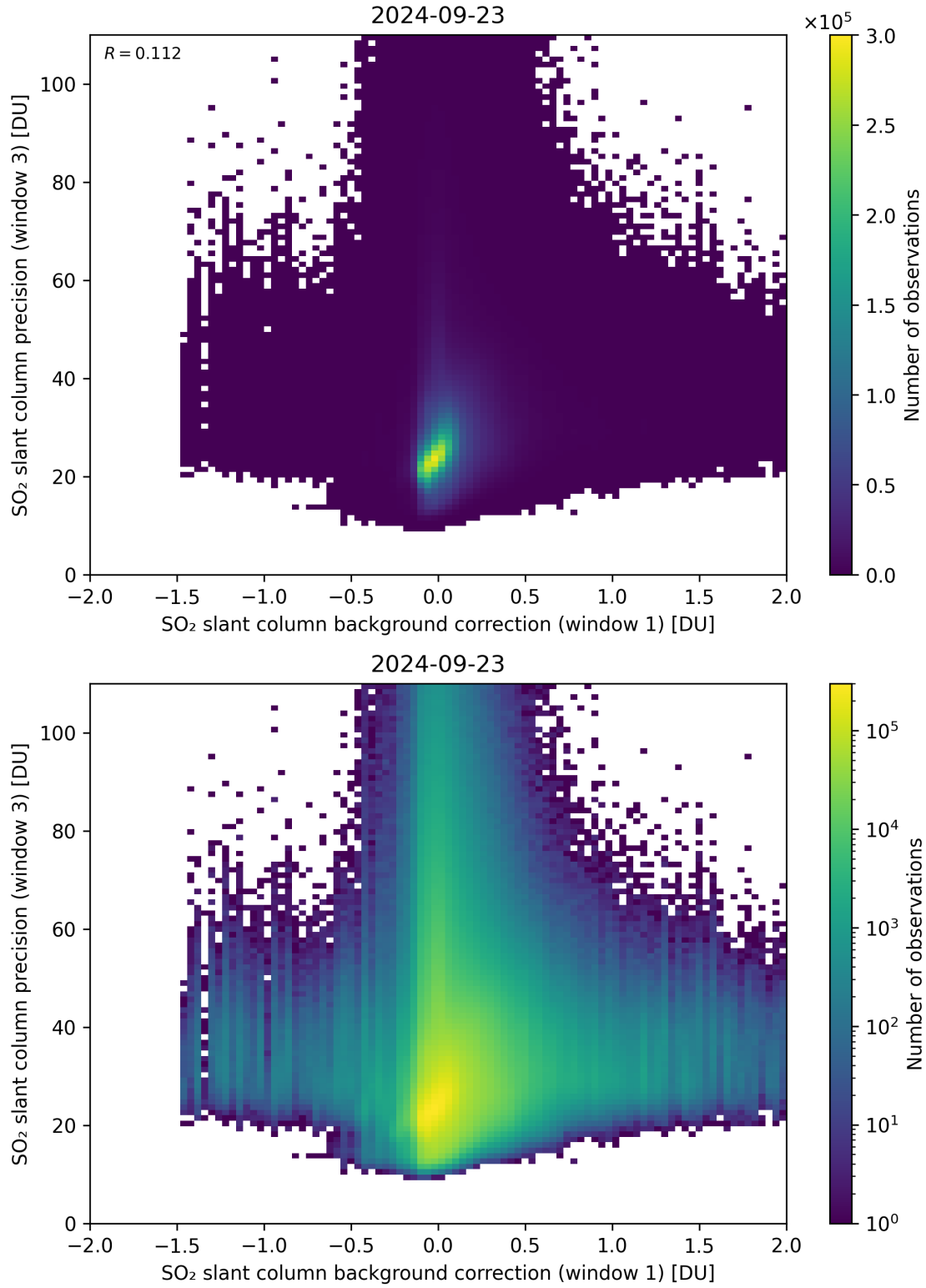
Figure 108: Scatter density plot of “SO 2 slant column background correction (window 1)” against “SO 2 slant column precision (window 3)” for 2024-09-22 to 2024-09-24.
