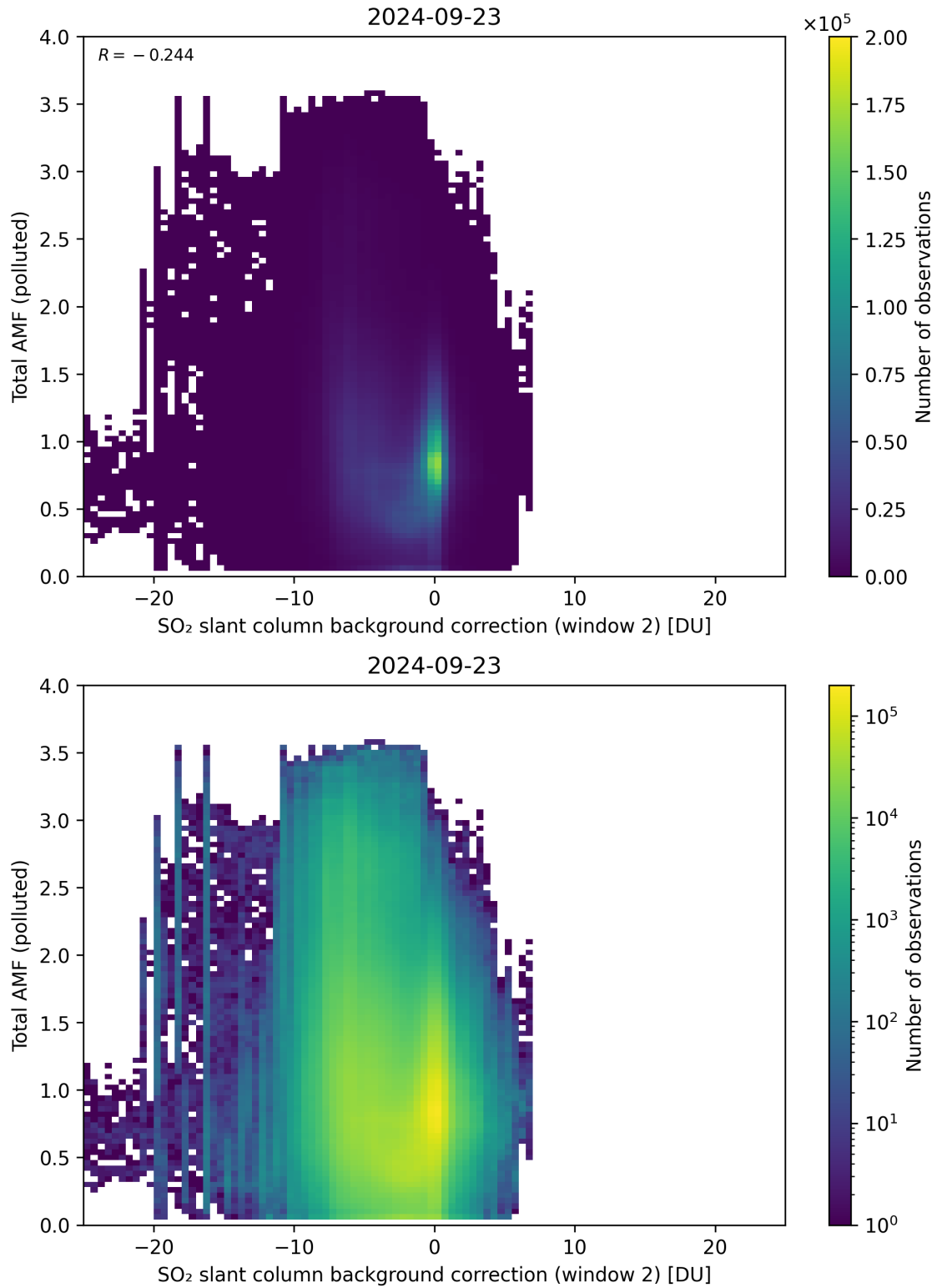
Figure 119: Scatter density plot of “SO 2 slant column background correction (window 2)” against “Total AMF (polluted)” for 2024-09-22 to 2024-09-24.
