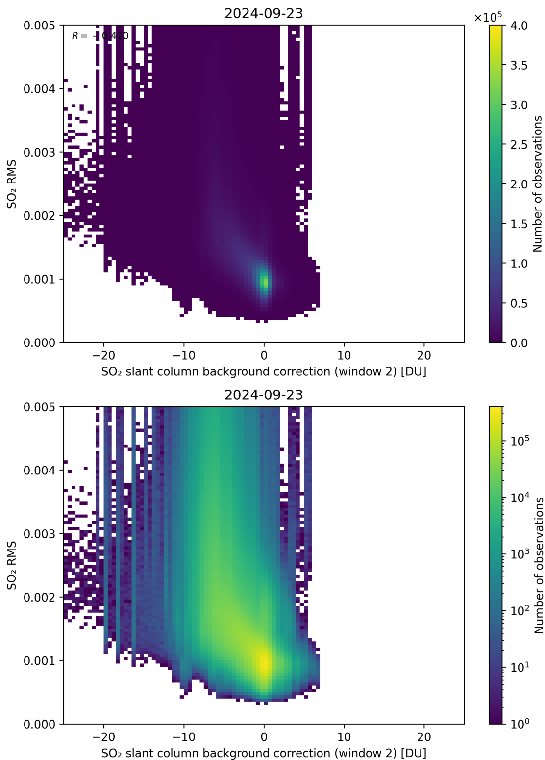
Figure 114: Scatter density plot of “SO 2 slant column background correction (window 2)” against “SO 2 RMS” for 2024-09-22 to 2024-09-24.
