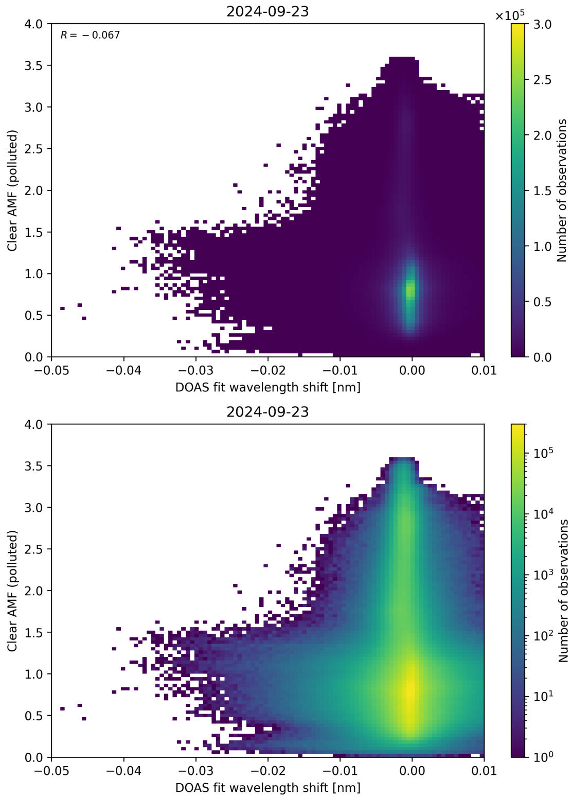
Figure 129: Scatter density plot of “DOAS fit wavelength shift” against “Clear AMF (polluted)” for 2024-09-22 to 2024-09-24.
