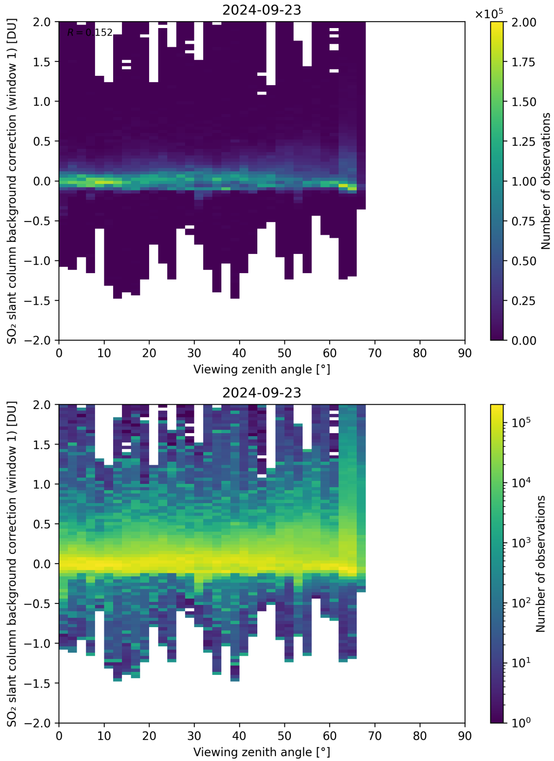
Figure 308: Scatter density plot of “Viewing zenith angle” against “SO 2 slant column background correction (window 1)” for 2024-09-22 to 2024-09-24.
