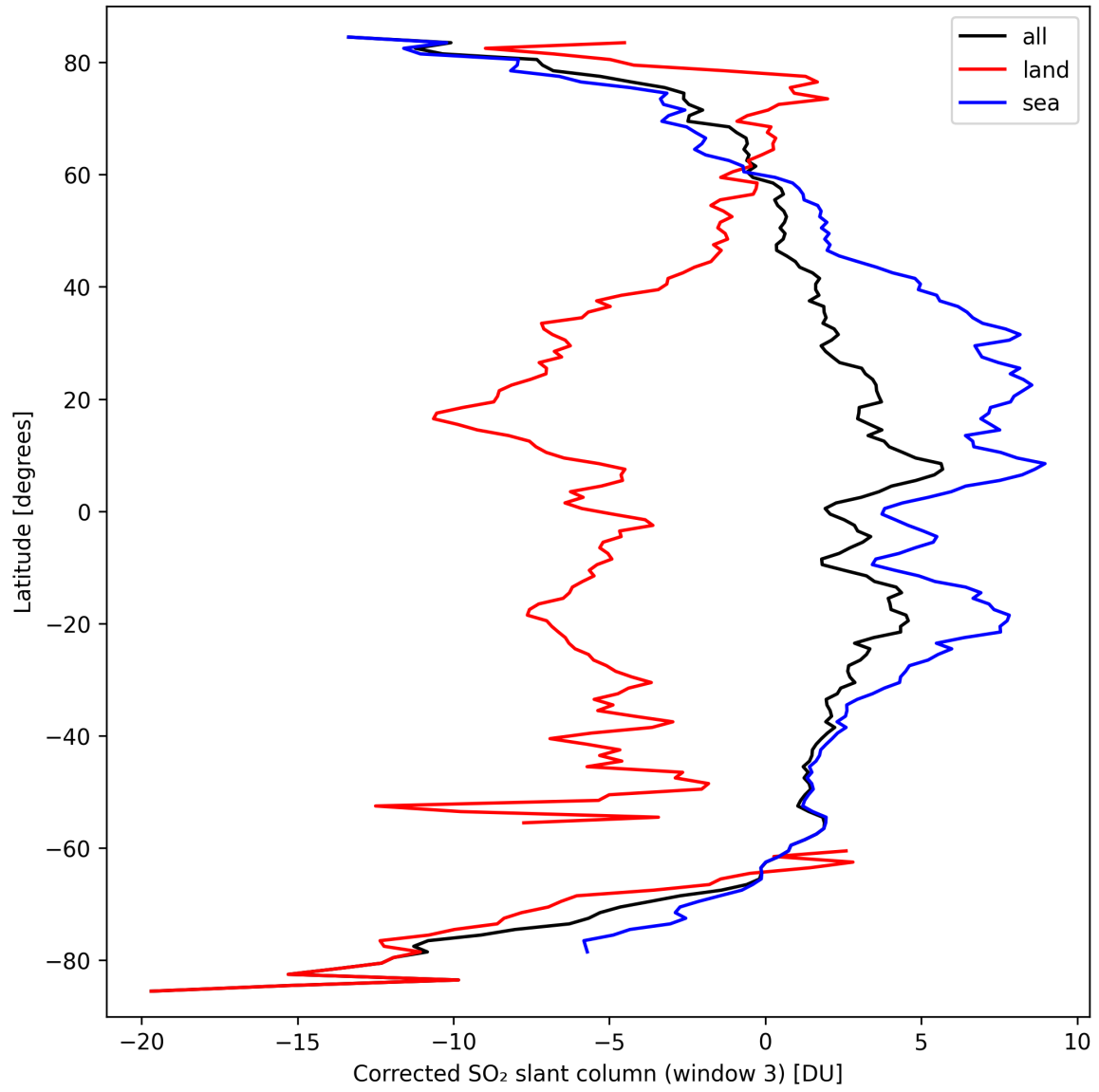
Figure 43: Zonal average of “Corrected SO 2 slant column (window 3)” for 2024-09-22 to 2024-09-24.
