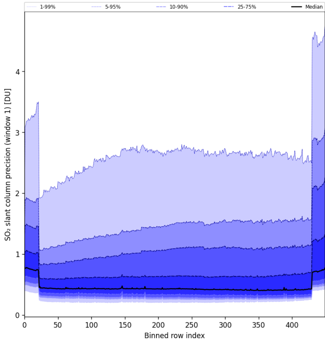
Figure 80: Along track statistics of “SO 2 slant column precision (window 1)” for 2024-09-22 to 2024-09-24
