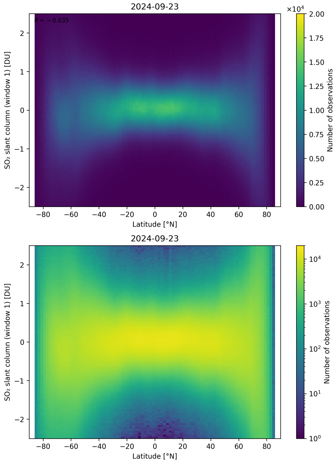
Figure 149: Scatter density plot of “Latitude” against “SO 2 slant column (window 1)” for 2024-09-22 to 2024-09-24.
