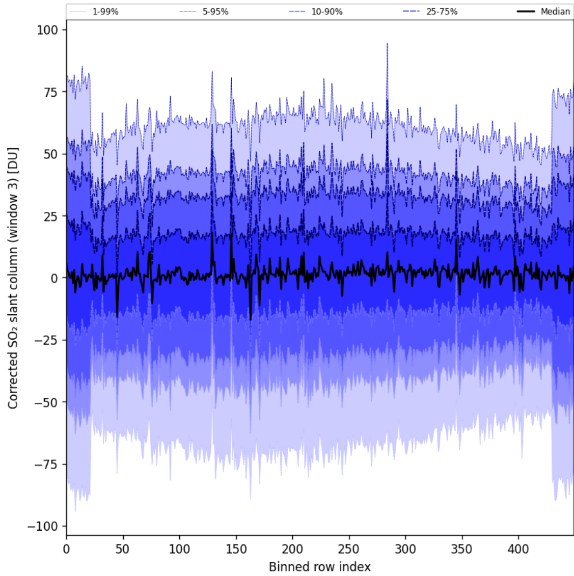
Figure 89: Along track statistics of “Corrected SO 2 slant column (window 3)” for 2024-09-22 to 2024-09-24
