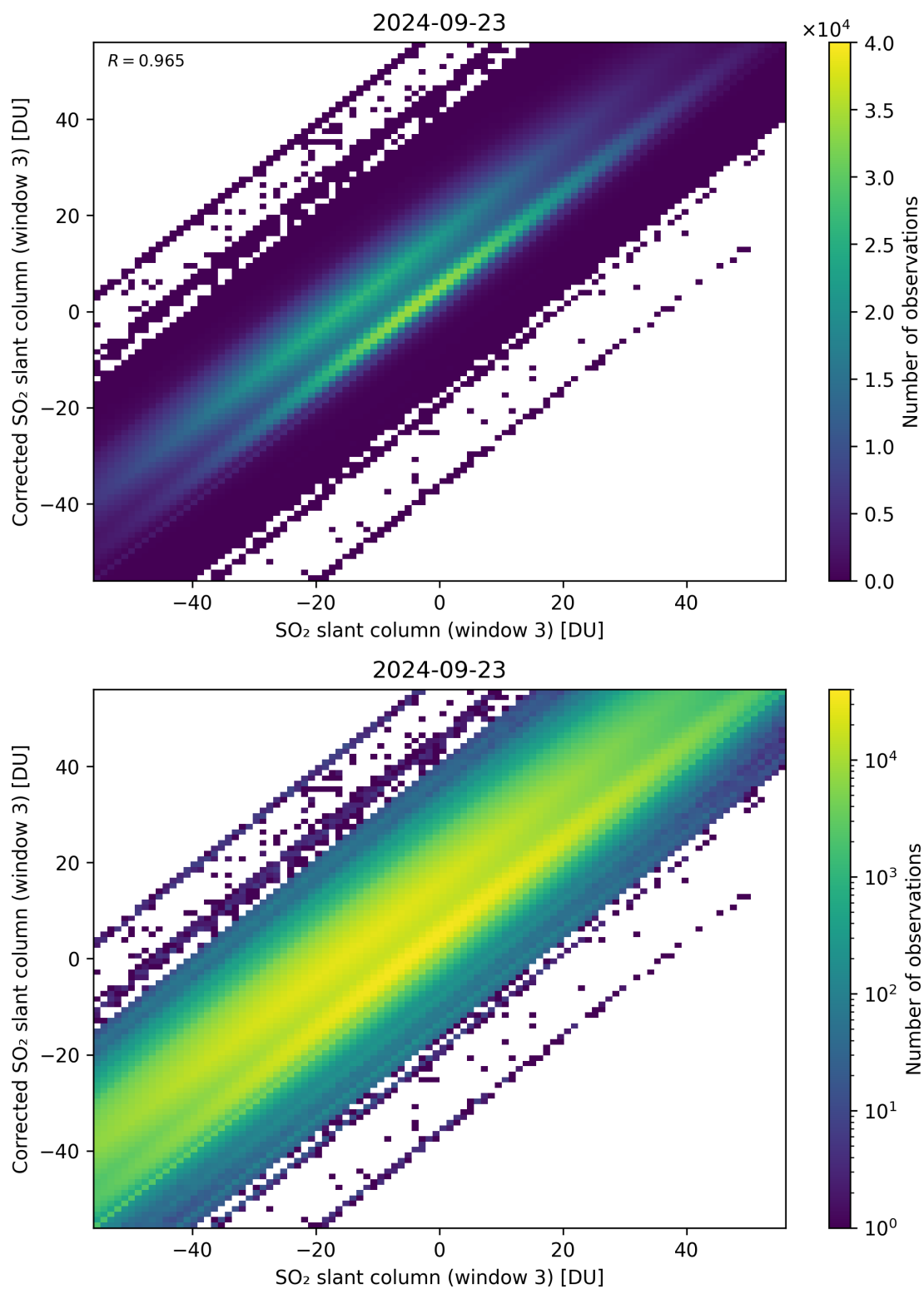
Figure 266: Scatter density plot of “SO 2 slant column (window 3)” against “Corrected SO 2 slant column (window 3)” for 2024-09-22 to 2024-09-24.
