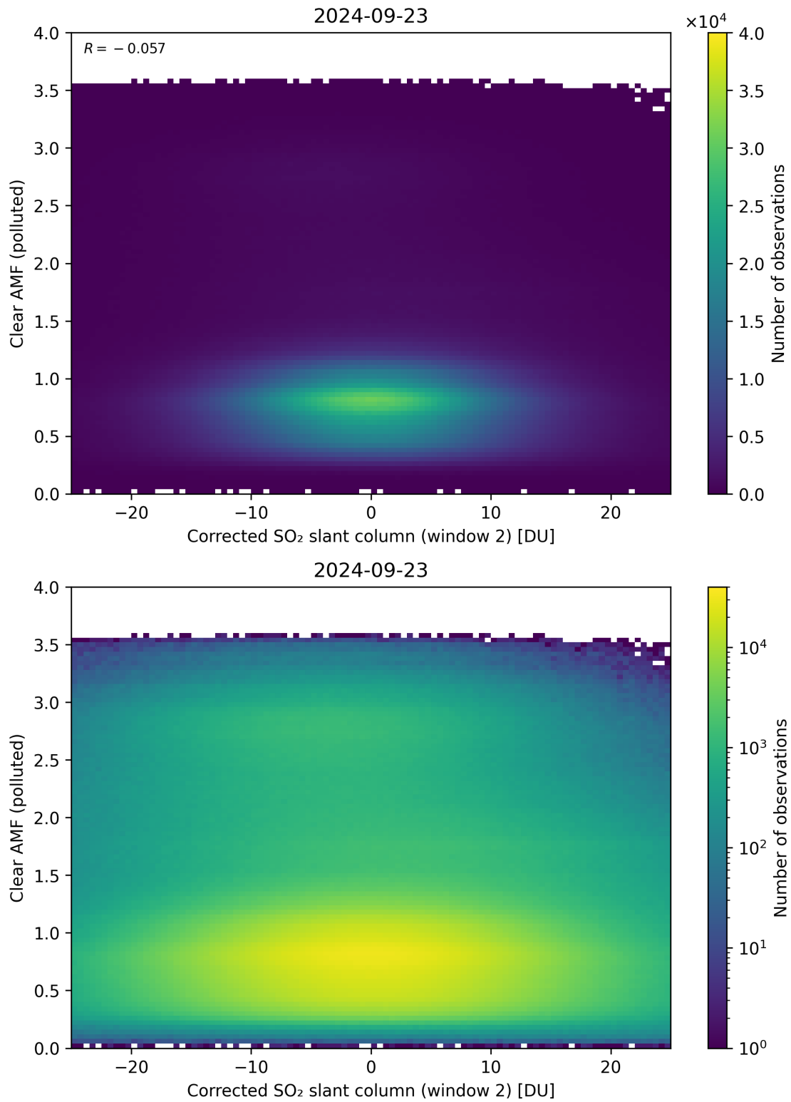
Figure 199: Scatter density plot of “Corrected SO 2 slant column (window 2)” against “Clear AMF (polluted)” for 2024-09-22 to 2024-09-24.
