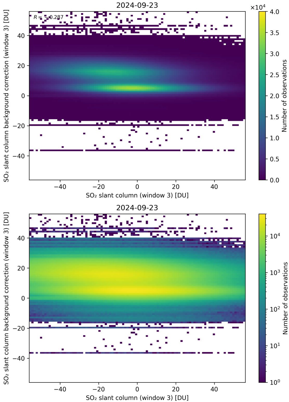
Figure 253: Scatter density plot of “SO 2 slant column (window 3)” against “SO 2 slant column background correction (window 3)” for 2024-09-22 to 2024-09-24.
