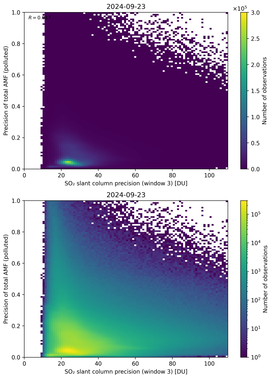
Figure 264: Scatter density plot of “SO 2 slant column precision (window 3)” against “Precision of total AMF (polluted)” for 2024-09-22 to 2024-09-24.
