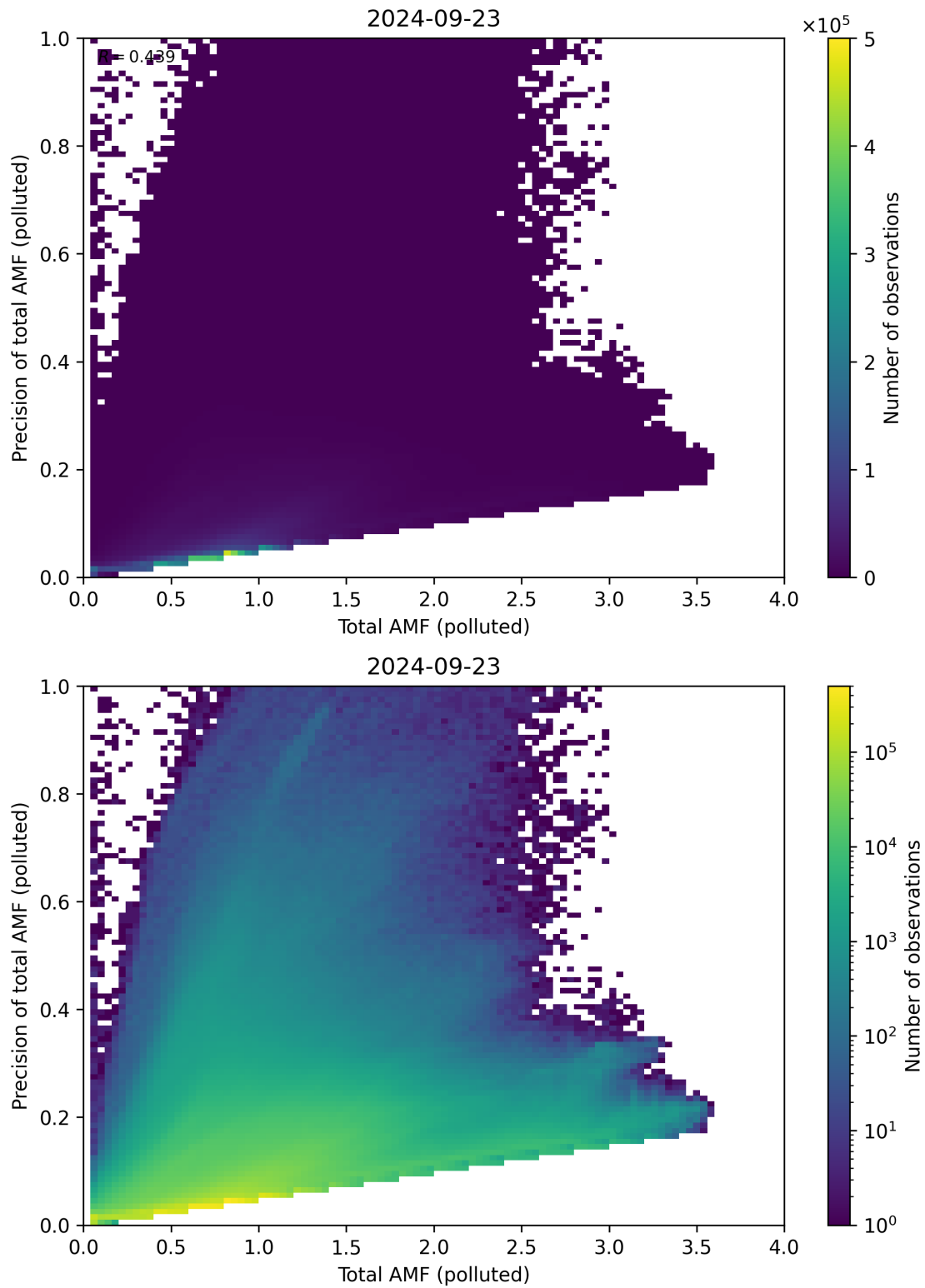
Figure 272: Scatter density plot of “Total AMF (polluted)” against “Precision of total AMF (polluted)” for 2024-09-22 to 2024-09-24.
