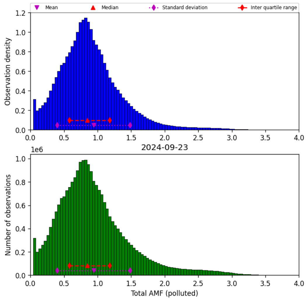
Figure 71: Histogram of “Total AMF (polluted)” for 2024-09-22 to 2024-09-24
