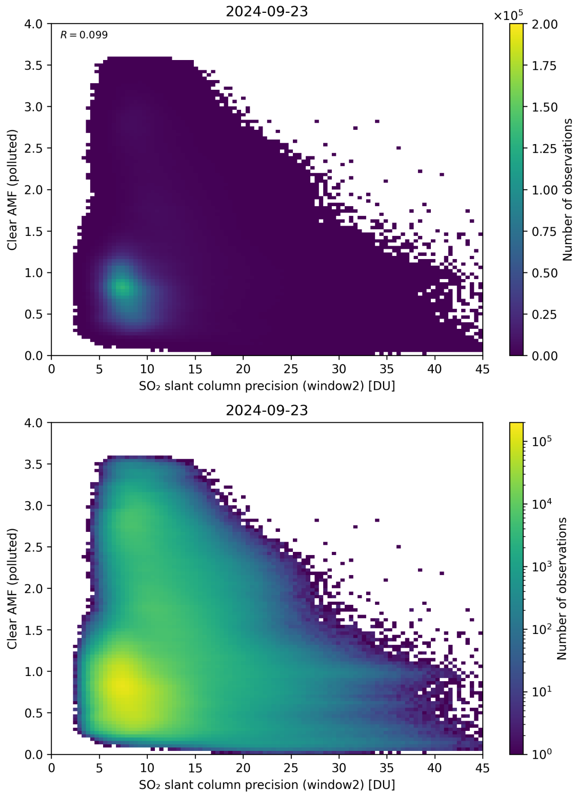
Figure 246: Scatter density plot of “SO 2 slant column precision (window2)” against “Clear AMF (polluted)” for 2024-09-22 to 2024-09-24.
