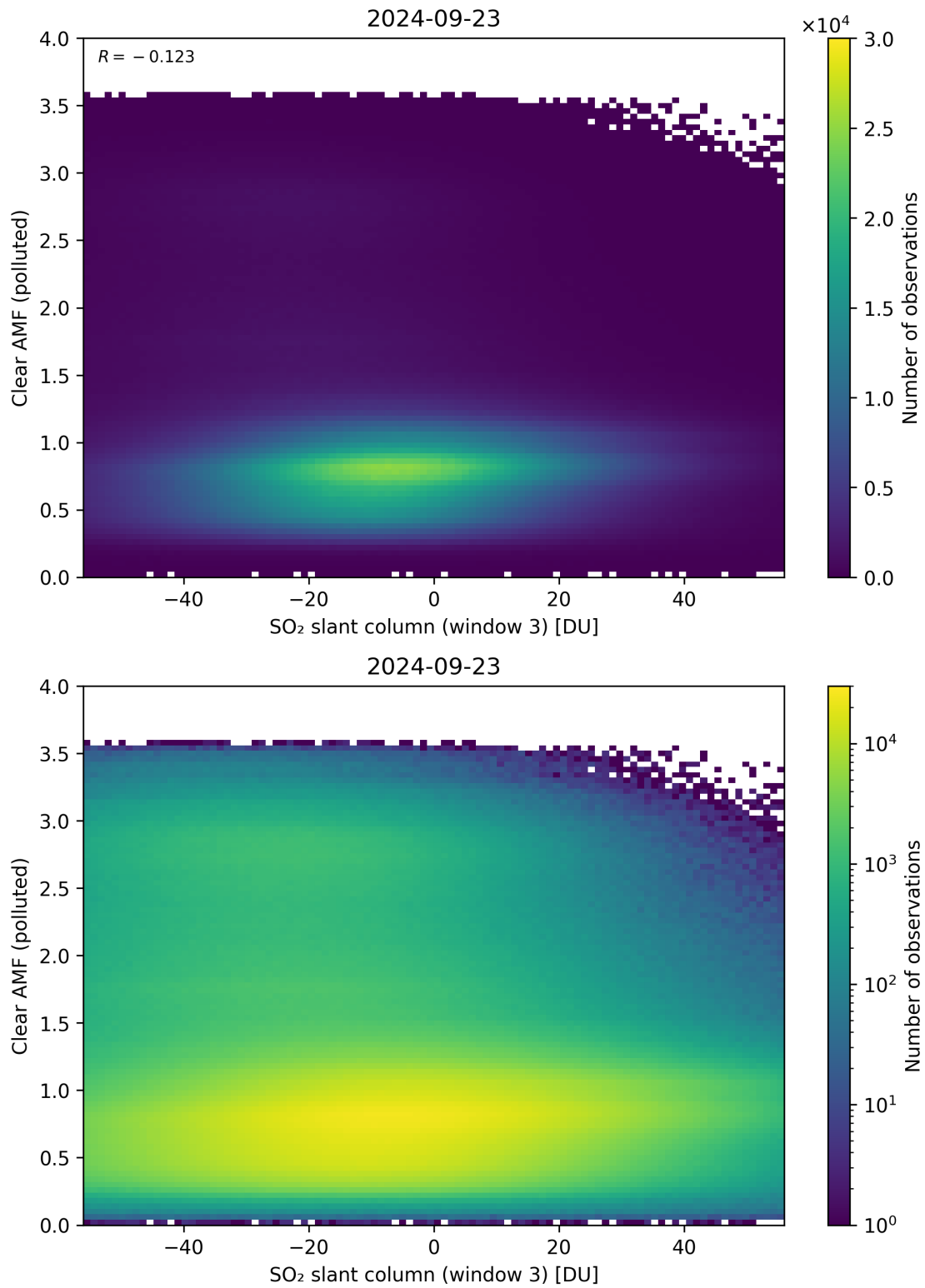
Figure 265: Scatter density plot of “SO 2 slant column (window 3)” against “Clear AMF (polluted)” for 2024-09-22 to 2024-09-24.
