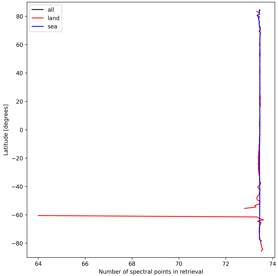
Figure 51: Zonal average of “Number of spectral points in retrieval” for 2024-09-22 to 2024-09-24.
