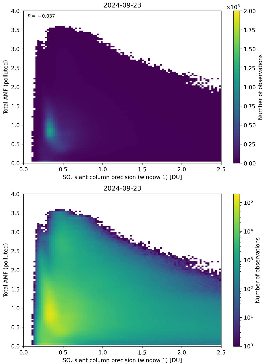
Figure 230: Scatter density plot of “SO 2 slant column precision (window 1)” against “Total AMF (polluted)” for 2024-09-22 to 2024-09-24.
