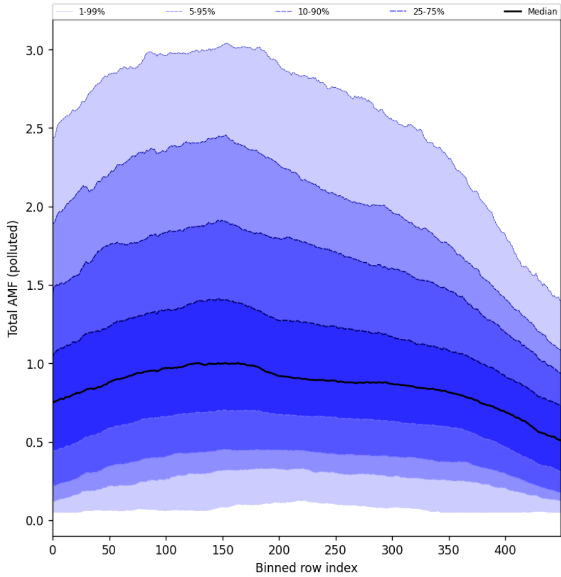
Figure 94: Along track statistics of “Total AMF (polluted)” for 2024-09-22 to 2024-09-24
