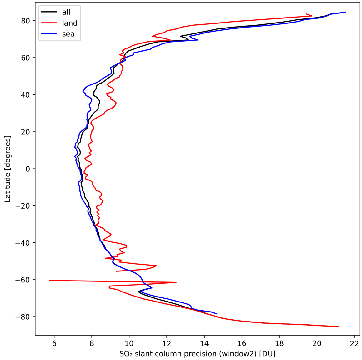
Figure 38: Zonal average of “SO 2 slant column precision (window2)” for 2024-09-22 to 2024-09-24.
