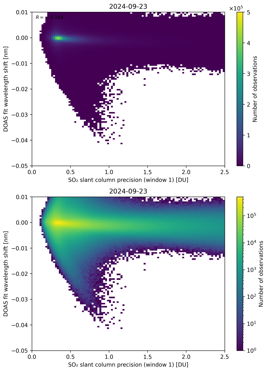
Figure 221: Scatter density plot of “SO 2 slant column precision (window 1)” against “DOAS fit wavelength shift” for 2024-09-22 to 2024-09-24.
