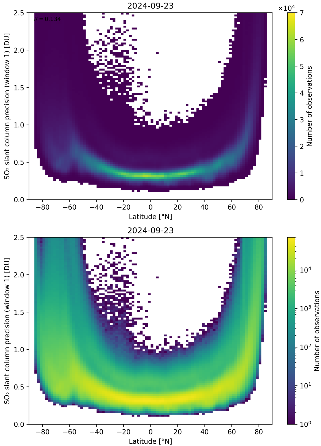
Figure 150: Scatter density plot of “Latitude” against “SO 2 slant column precision (window 1)” for 2024-09-22 to 2024-09-24.
