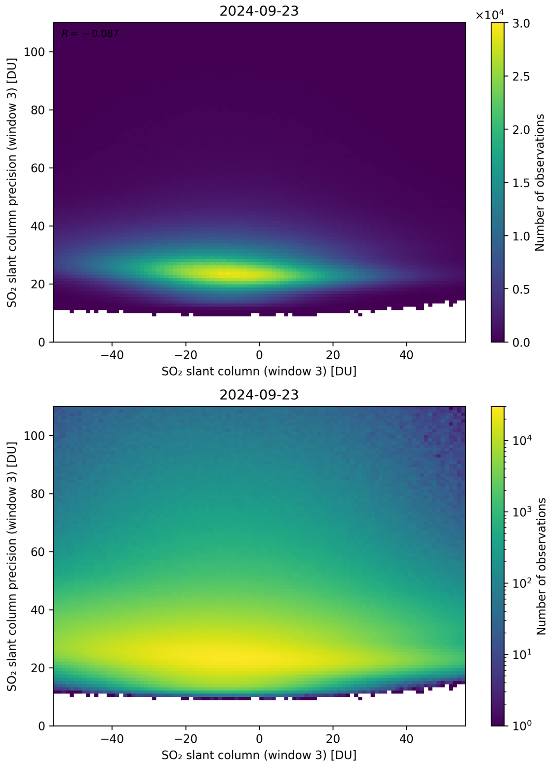
Figure 267: Scatter density plot of “SO 2 slant column (window 3)” against “SO 2 slant column precision (window 3)” for 2024-09-22 to 2024-09-24.
