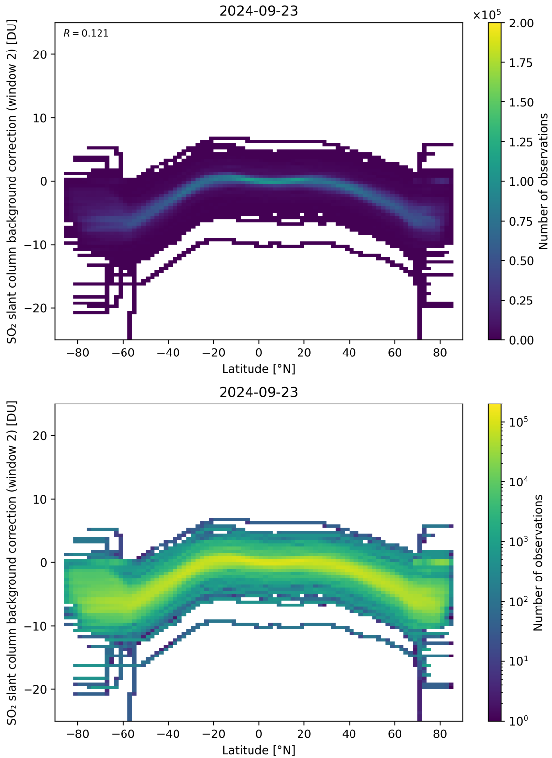
Figure 140: Scatter density plot of “Latitude” against “SO 2 slant column background correction (window 2)” for 2024-09-22 to 2024-09-24.
