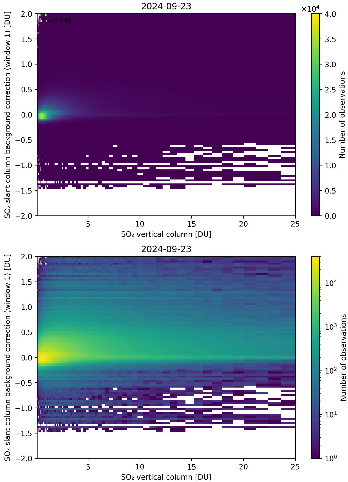
Figure 273: Scatter density plot of “SO 2 vertical column” against “SO 2 slant column background correction (window 1)” for 2024-09-22 to 2024-09-24.
