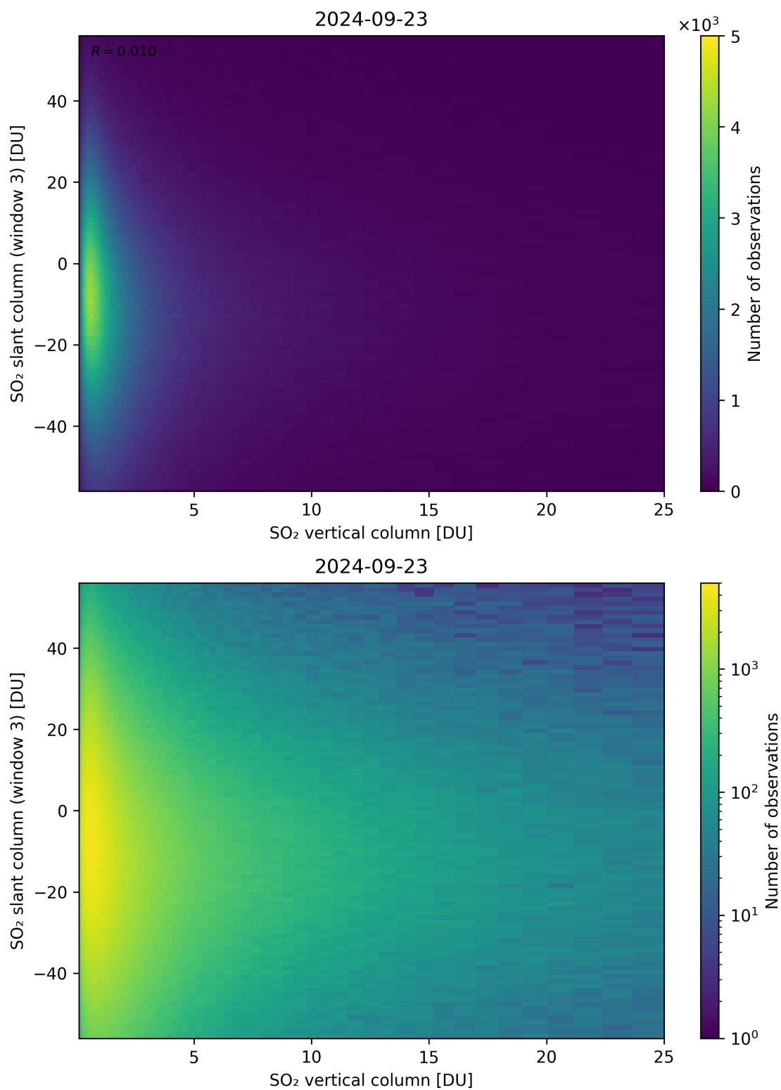
Figure 303: Scatter density plot of “SO 2 vertical column” against “SO 2 slant column (window 3)” for 2024-09-22 to 2024-09-24.
