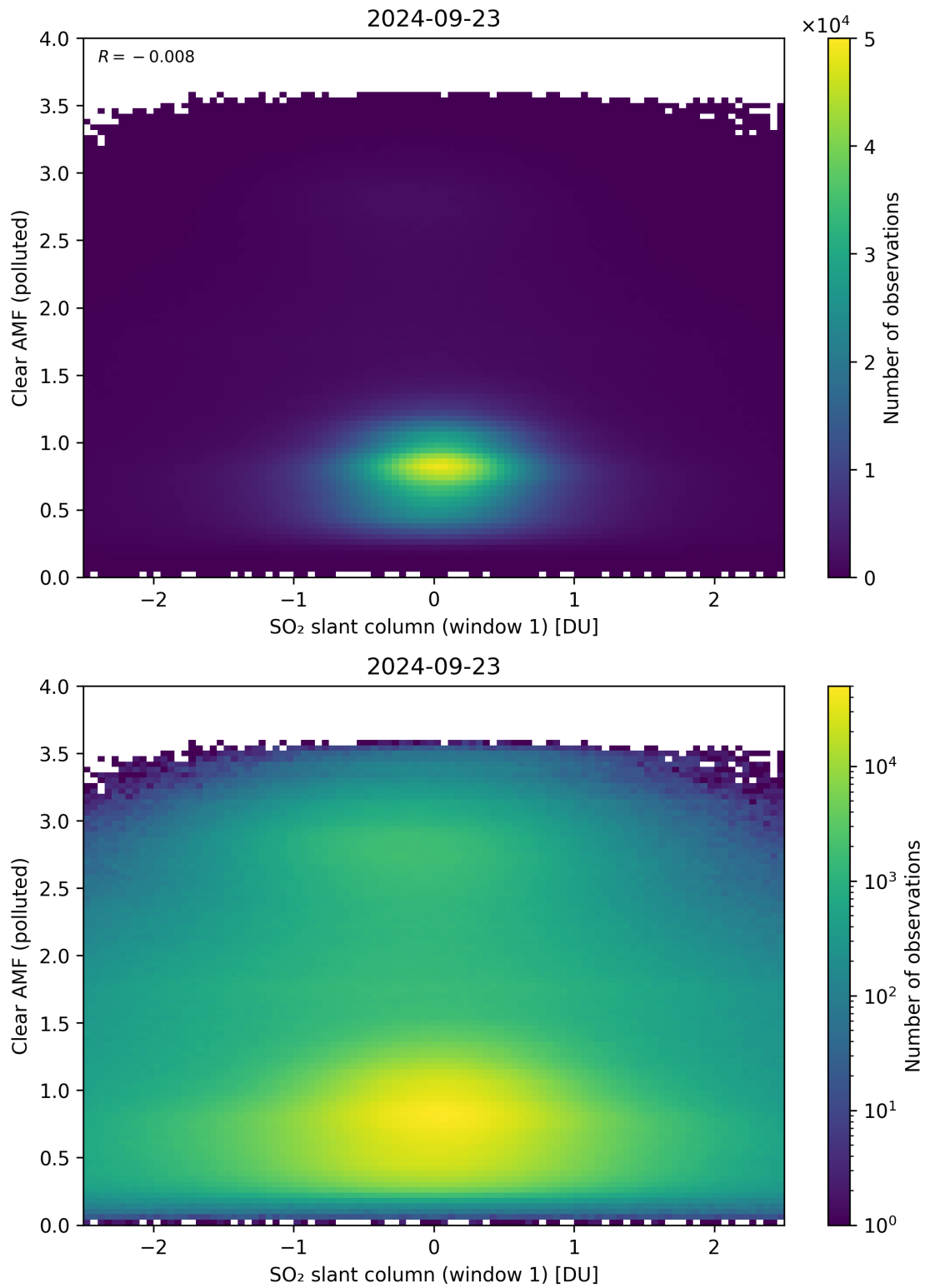
Figure 232: Scatter density plot of “SO 2 slant column (window 1)” against “Clear AMF (polluted)” for 2024-09-22 to 2024-09-24.
