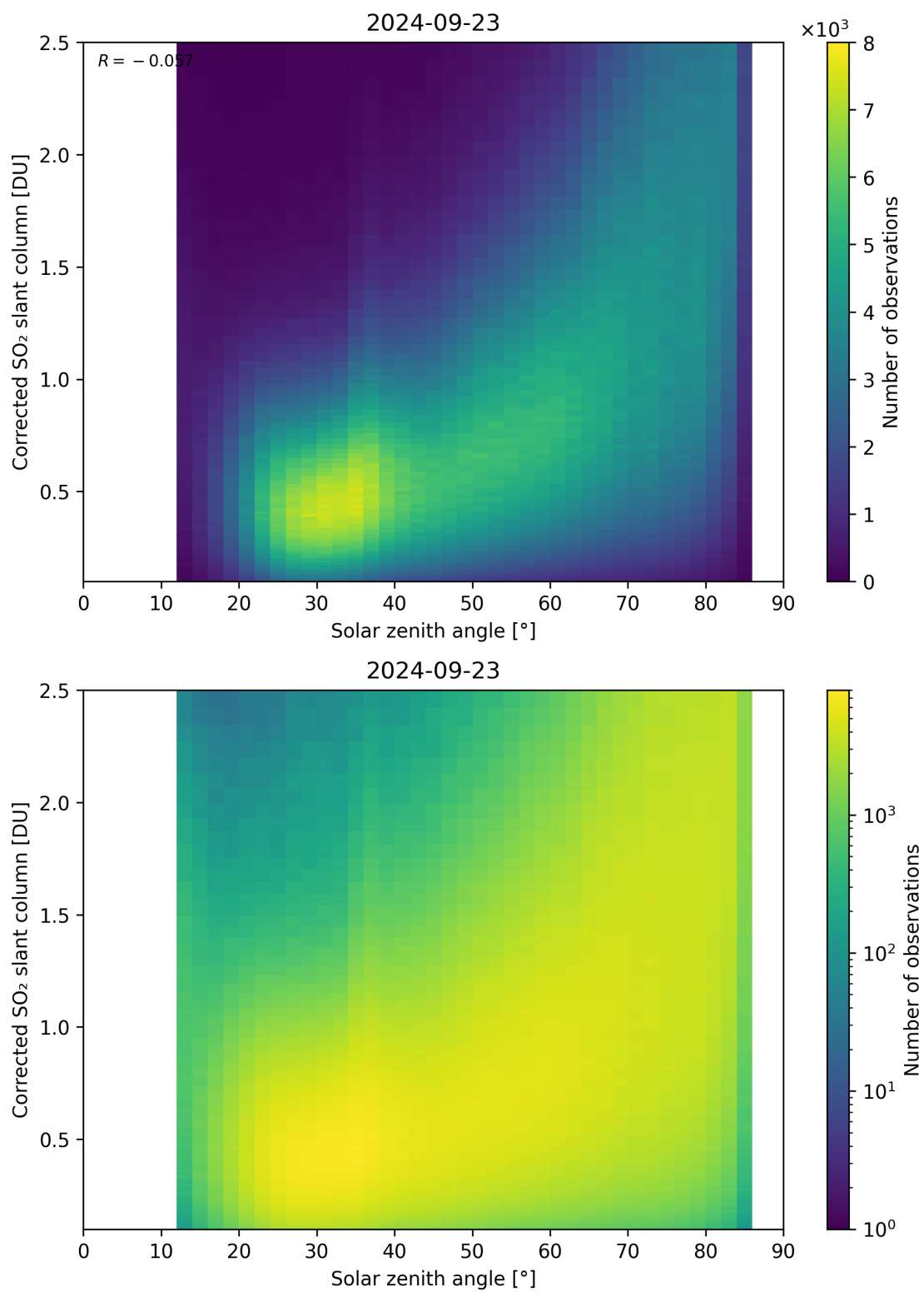
Figure 166: Scatter density plot of “Solar zenith angle” against “Corrected SO 2 slant column” for 2024-09-22 to 2024-09-24.
