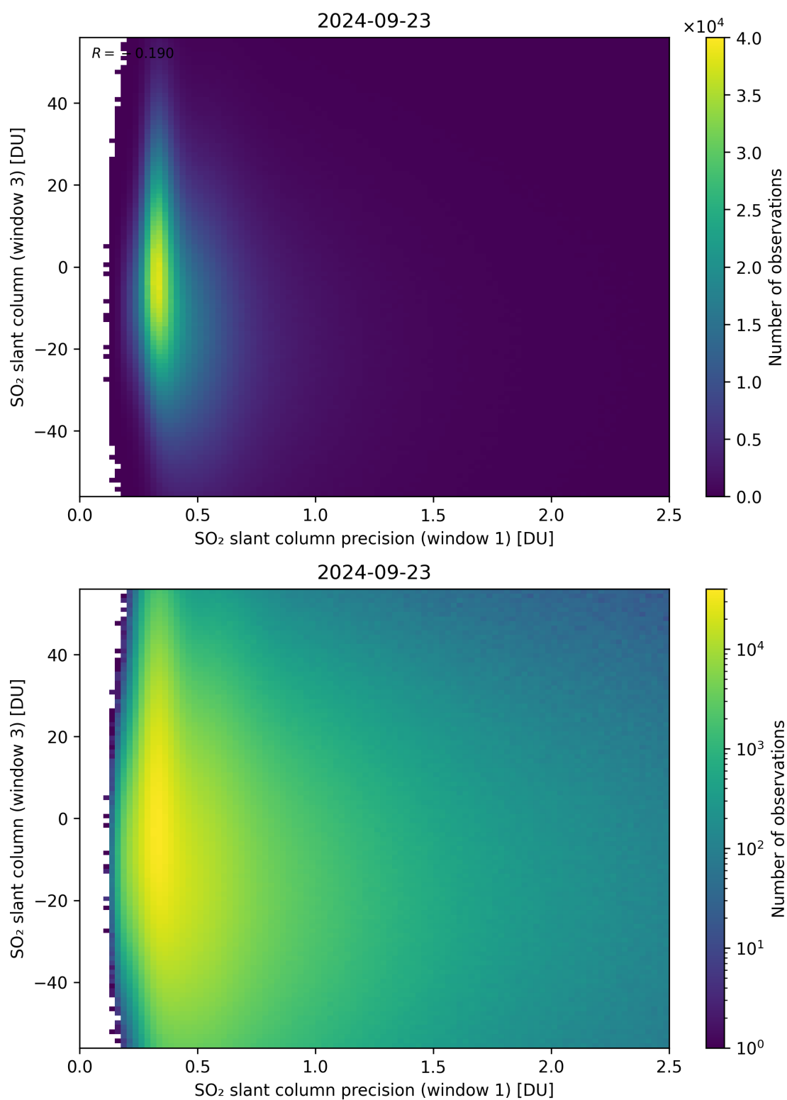
Figure 228: Scatter density plot of “SO 2 slant column precision (window 1)” against “SO 2 slant column (window 3)” for 2024-09-22 to 2024-09-24.
