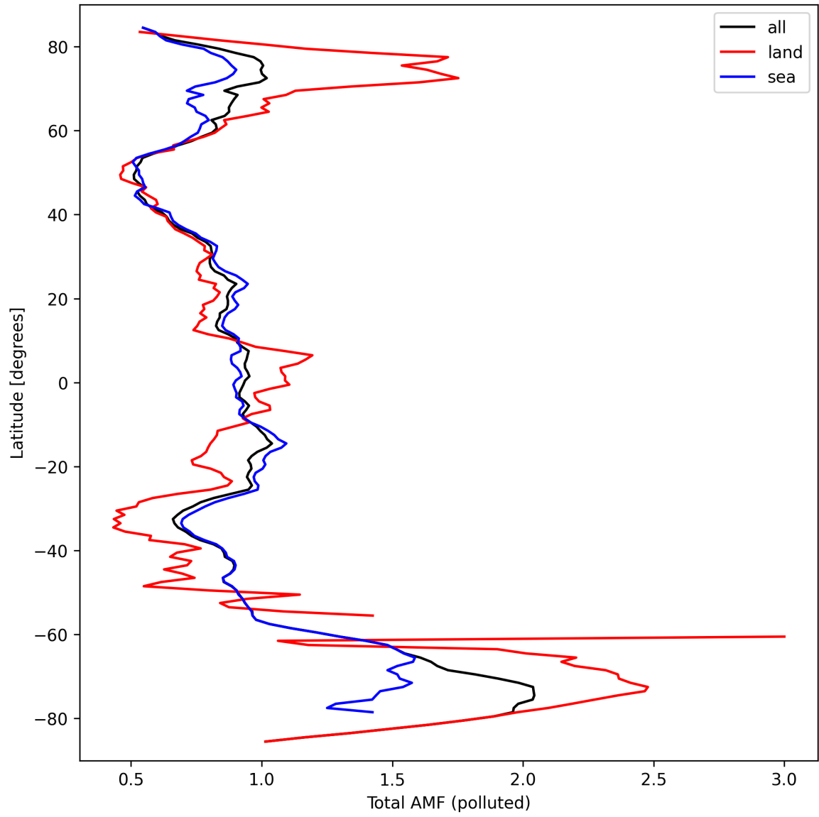
Figure 48: Zonal average of “Total AMF (polluted)” for 2024-09-22 to 2024-09-24.
