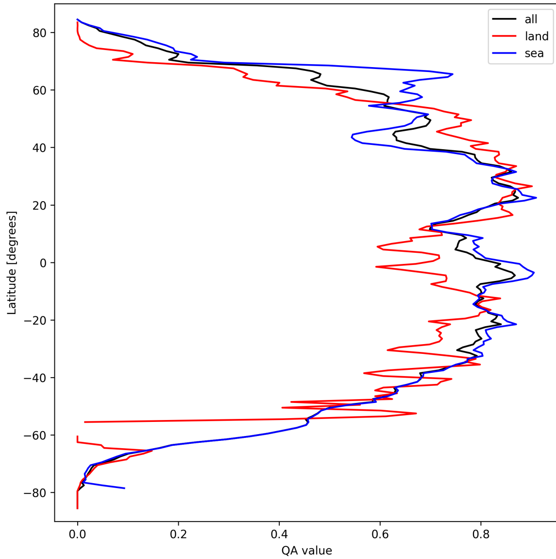
Figure 29: Zonal average of “QA value” for 2024-09-22 to 2024-09-24.
