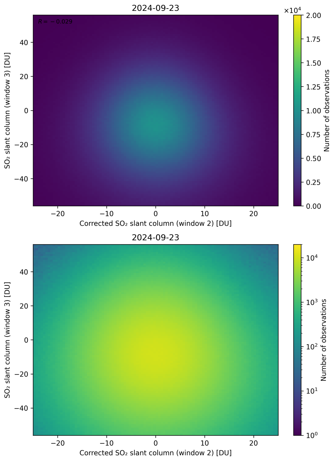
Figure 201: Scatter density plot of “Corrected SO 2 slant column (window 2)” against “SO 2 slant column (window 3)” for 2024-09-22 to 2024-09-24.
