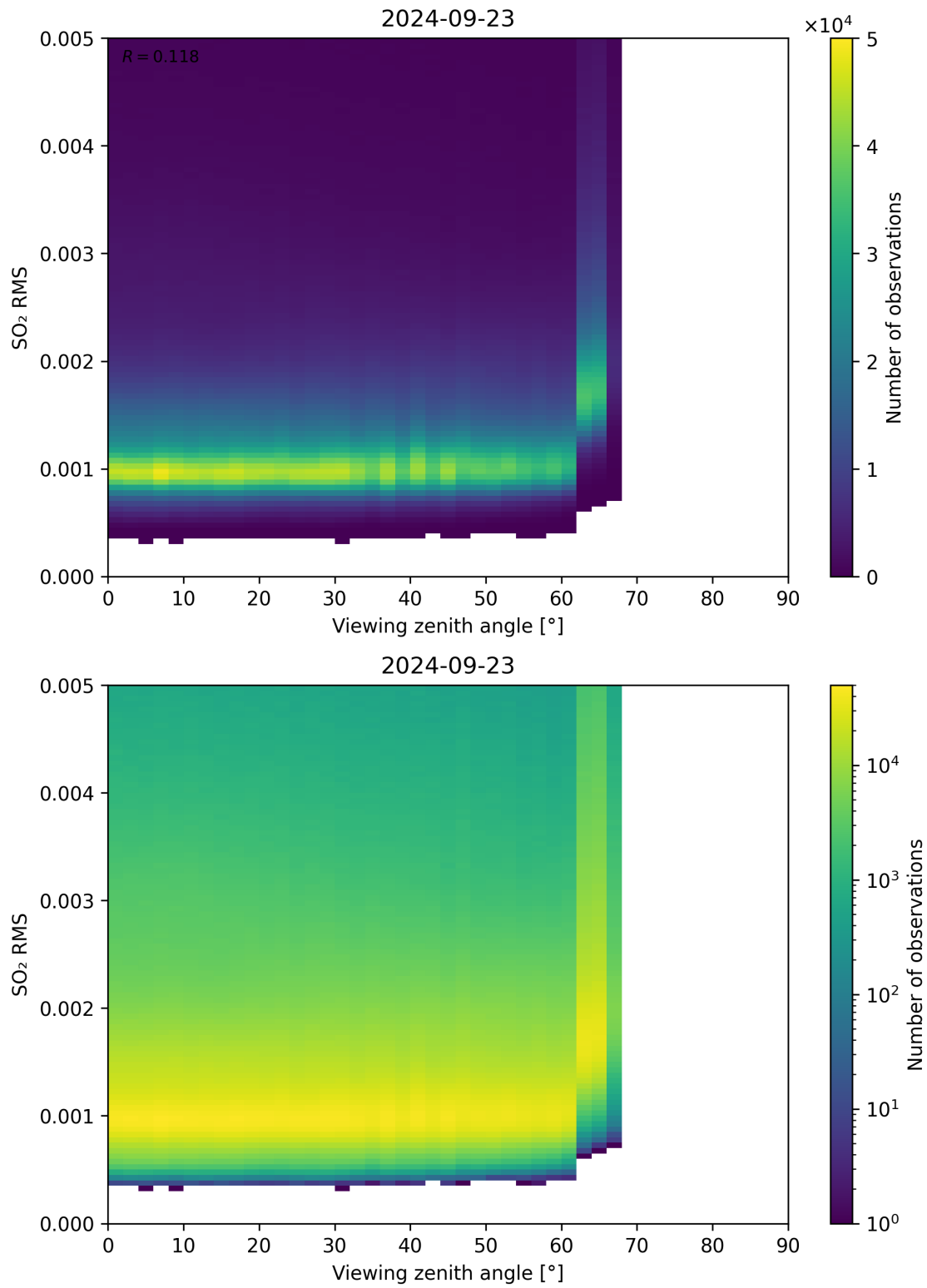
Figure 313: Scatter density plot of “Viewing zenith angle” against “SO 2 RMS” for 2024-09-22 to 2024-09-24.
