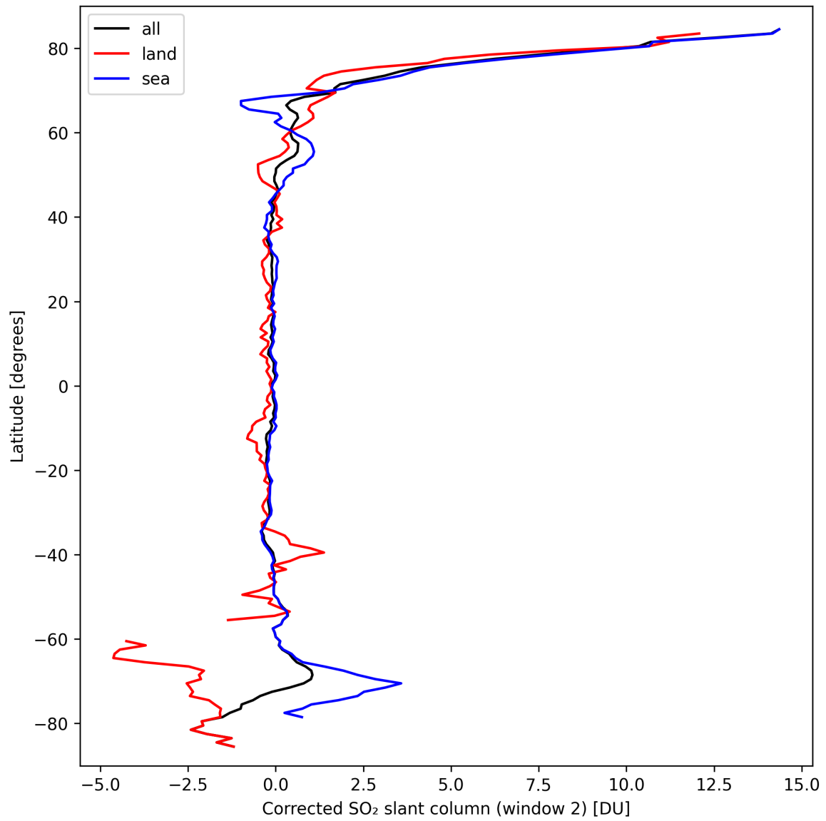
Figure 39: Zonal average of “Corrected SO 2 slant column (window 2)” for 2024-09-22 to 2024-09-24.
