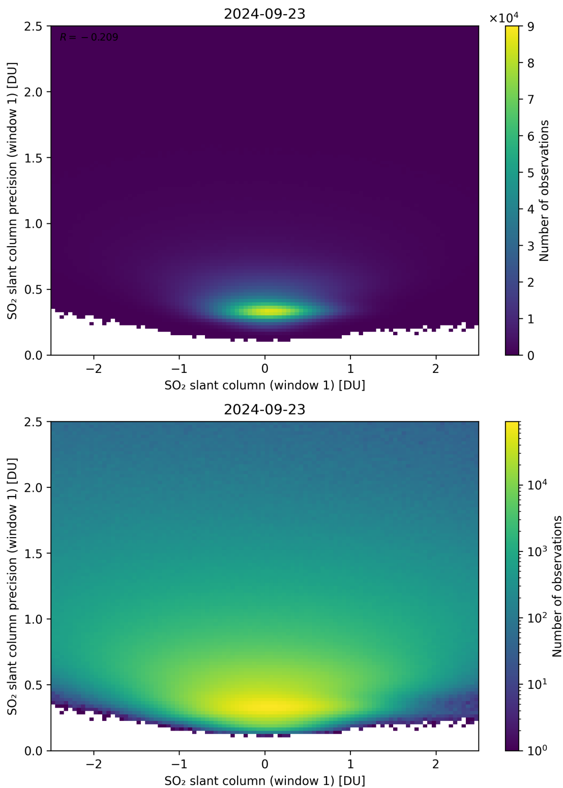
Figure 235: Scatter density plot of “SO 2 slant column (window 1)” against “SO 2 slant column precision (window 1)” for 2024-09-22 to 2024-09-24.
