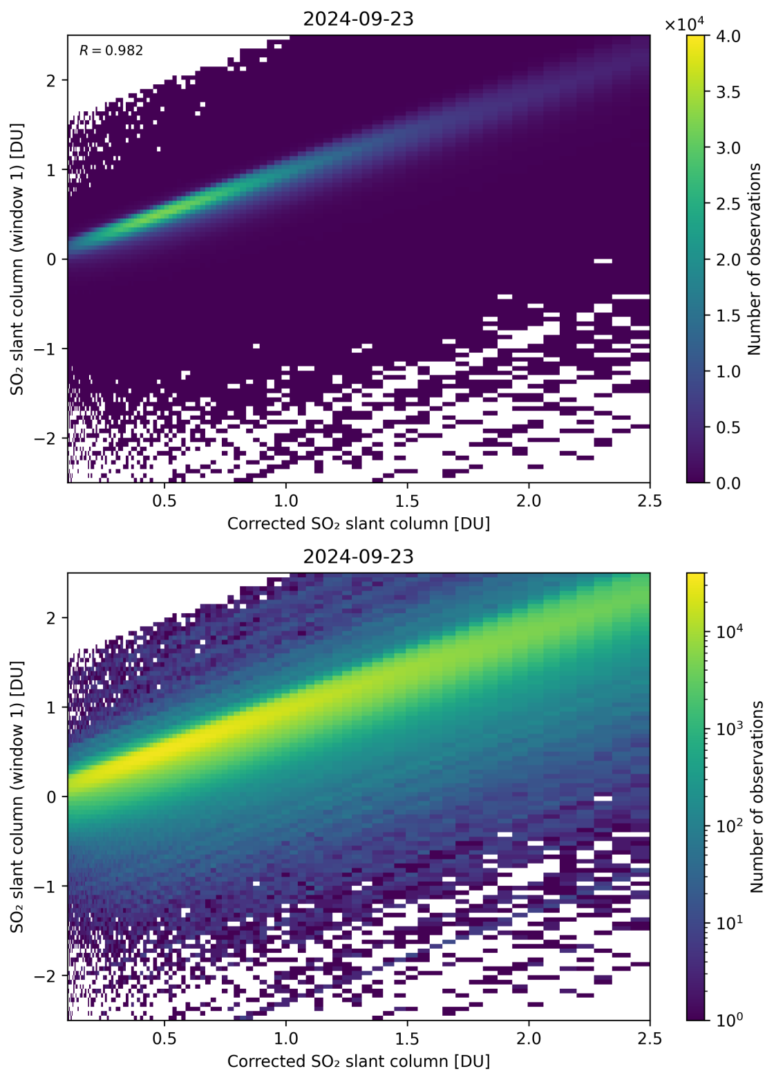
Figure 187: Scatter density plot of “Corrected SO 2 slant column” against “SO 2 slant column (window 1)” for 2024-09-22 to 2024-09-24.
