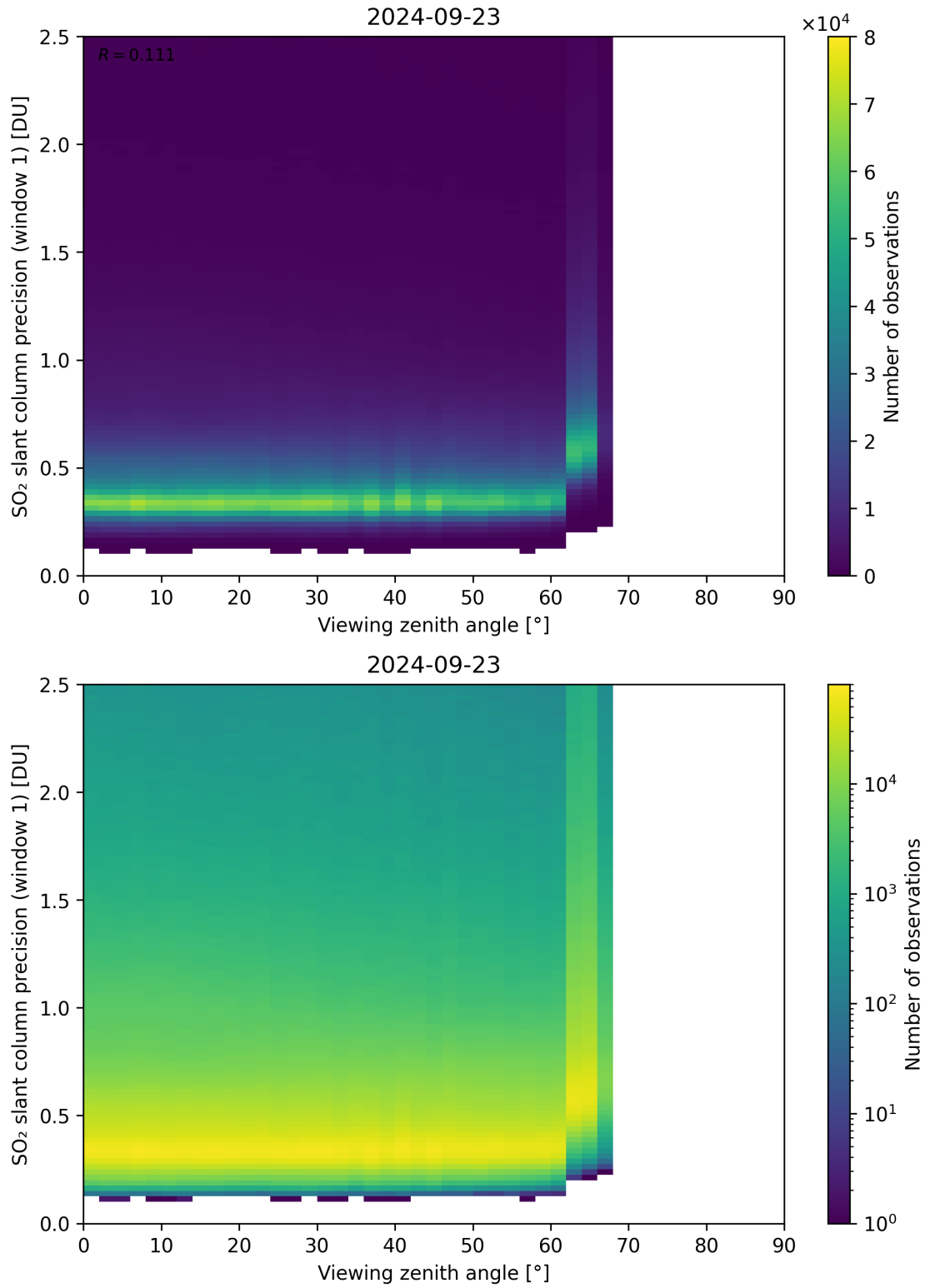
Figure 321: Scatter density plot of “Viewing zenith angle” against “SO 2 slant column precision (window 1)” for 2024-09-22 to 2024-09-24.
