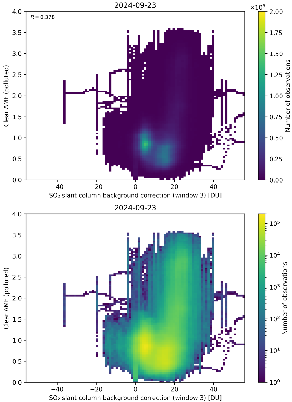
Figure 124: Scatter density plot of “SO 2 slant column background correction (window 3)” against “Clear AMF (polluted)” for 2024-09-22 to 2024-09-24.
