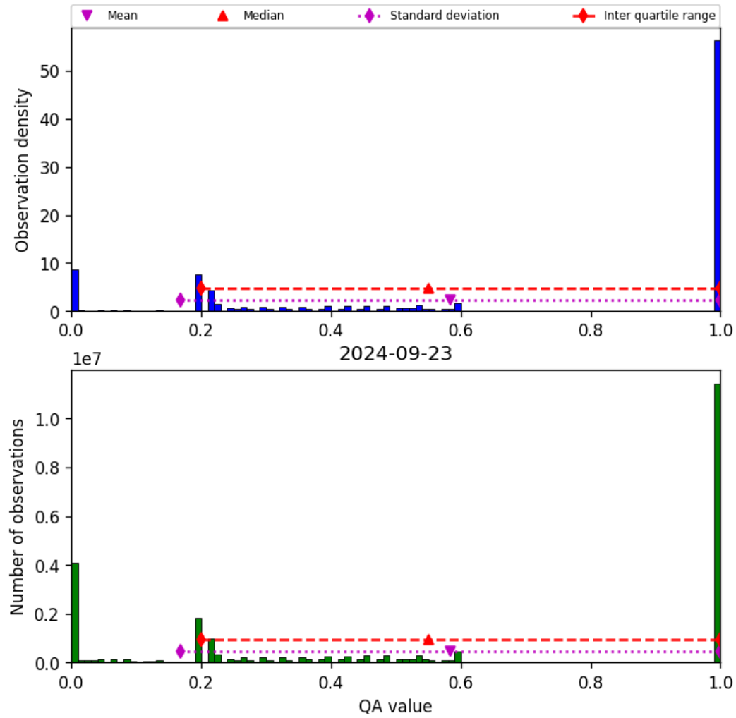
Figure 52: Histogram of “QA value” for 2024-09-22 to 2024-09-24
