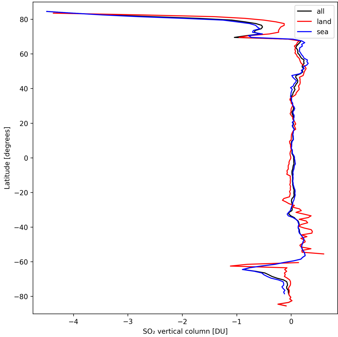
Figure 30: Zonal average of “SO 2 vertical column” for 2024-09-22 to 2024-09-24.
