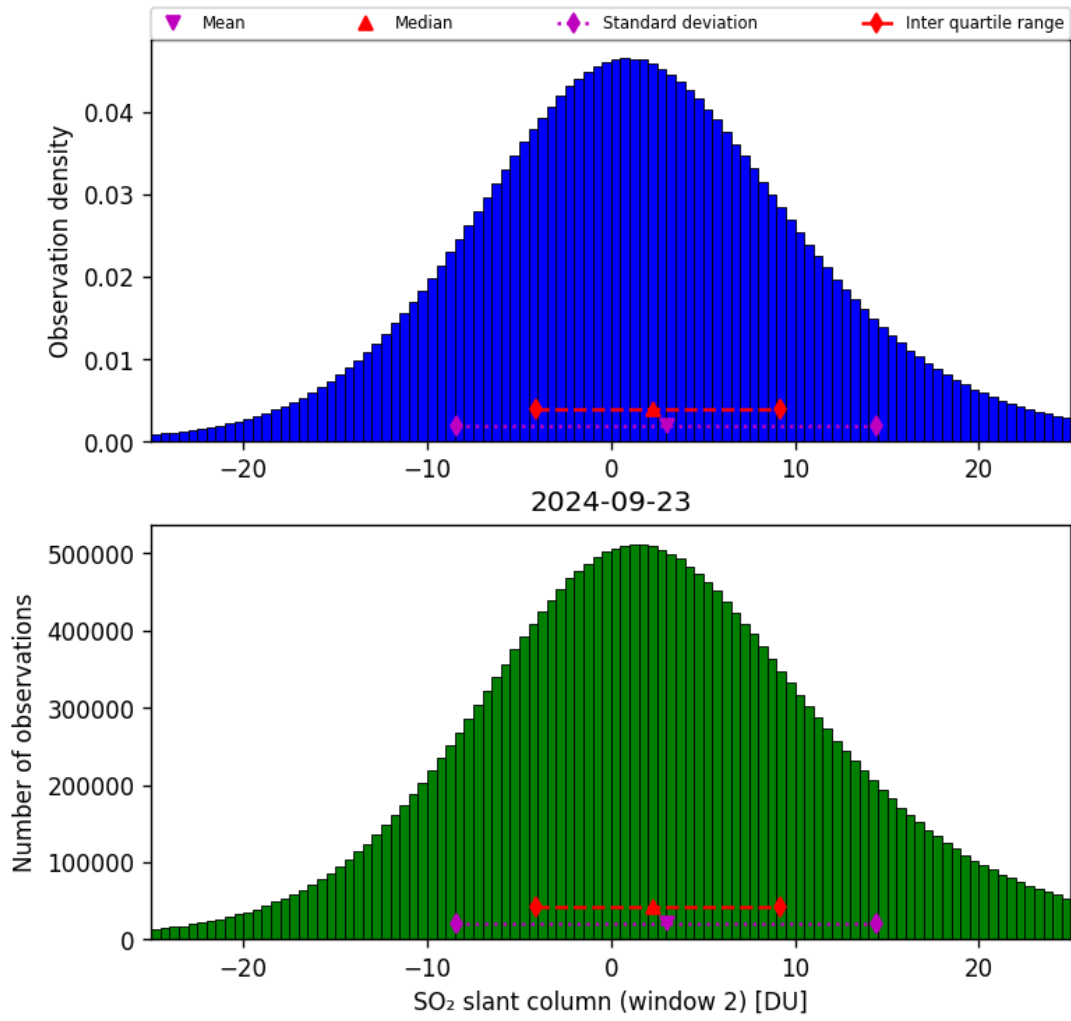
Figure 60: Histogram of “SO 2 slant column (window 2)” for 2024-09-22 to 2024-09-24
