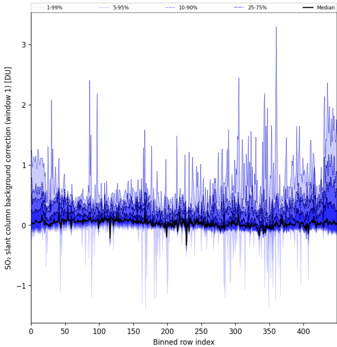
Figure 82: Along track statistics of “SO 2 slant column background correction (window 1)” for 2024-09-22 to 2024-09-24
