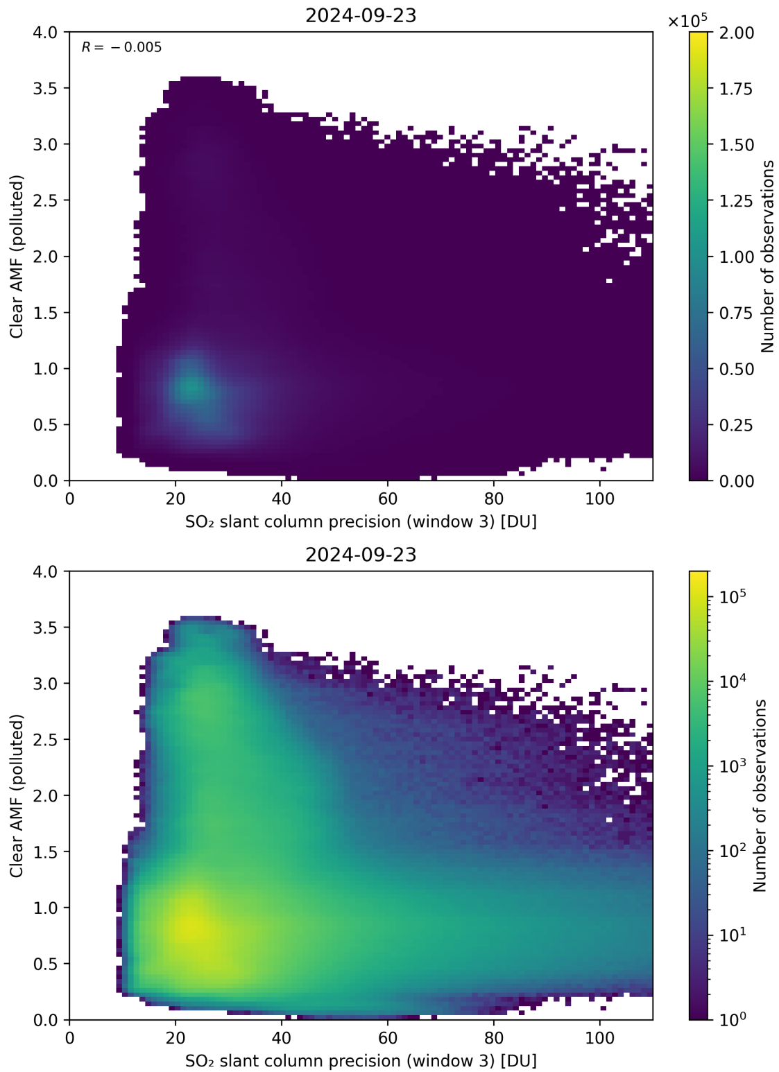
Figure 261: Scatter density plot of “SO 2 slant column precision (window 3)” against “Clear AMF (polluted)” for 2024-09-22 to 2024-09-24.
