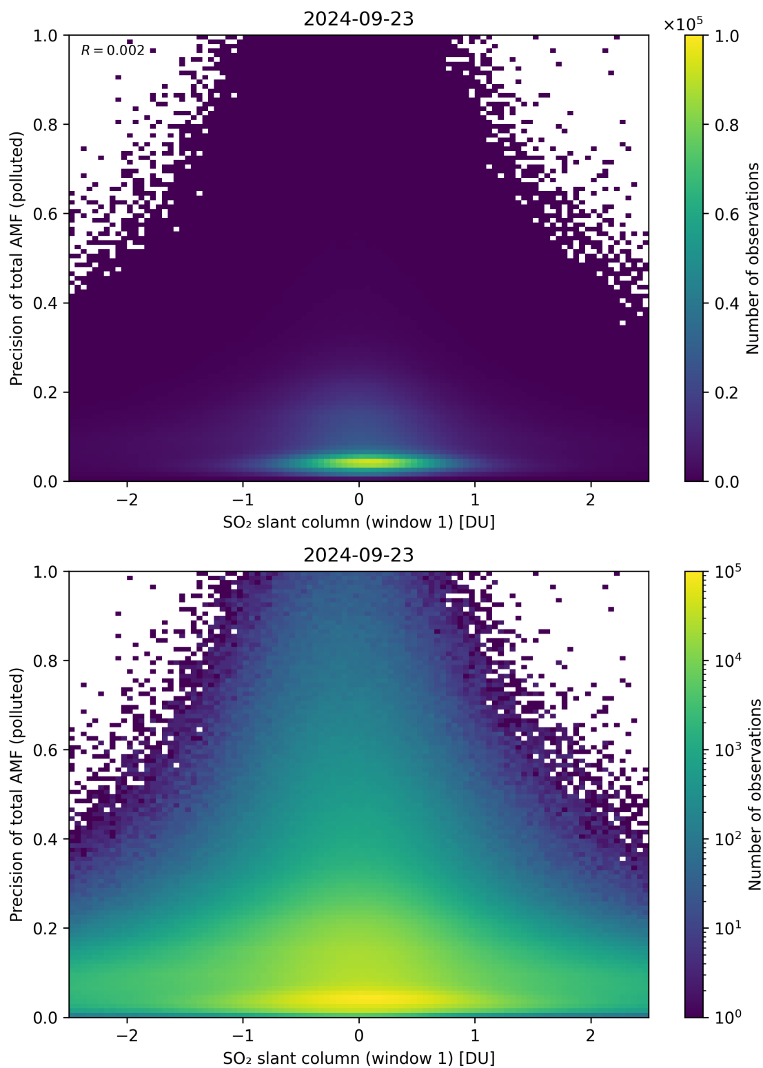
Figure 240: Scatter density plot of “SO 2 slant column (window 1)” against “Precision of total AMF (polluted)” for 2024-09-22 to 2024-09-24.
