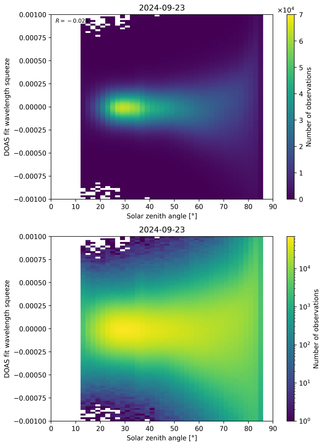
Figure 162: Scatter density plot of “Solar zenith angle” against “DOAS fit wavelength squeeze” for 2024-09-22 to 2024-09-24.
