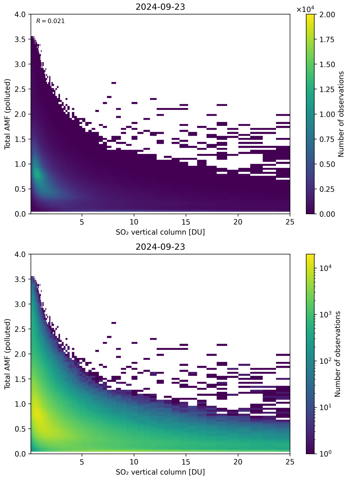
Figure 305: Scatter density plot of “SO 2 vertical column” against “Total AMF (polluted)” for 2024-09-22 to 2024-09-24.
