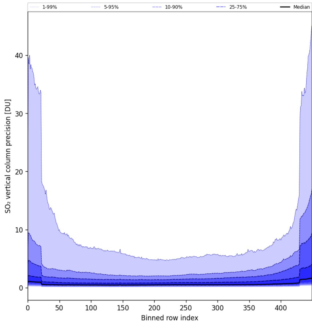
Figure 77: Along track statistics of “SO 2 vertical column precision” for 2024-09-22 to 2024-09-24
