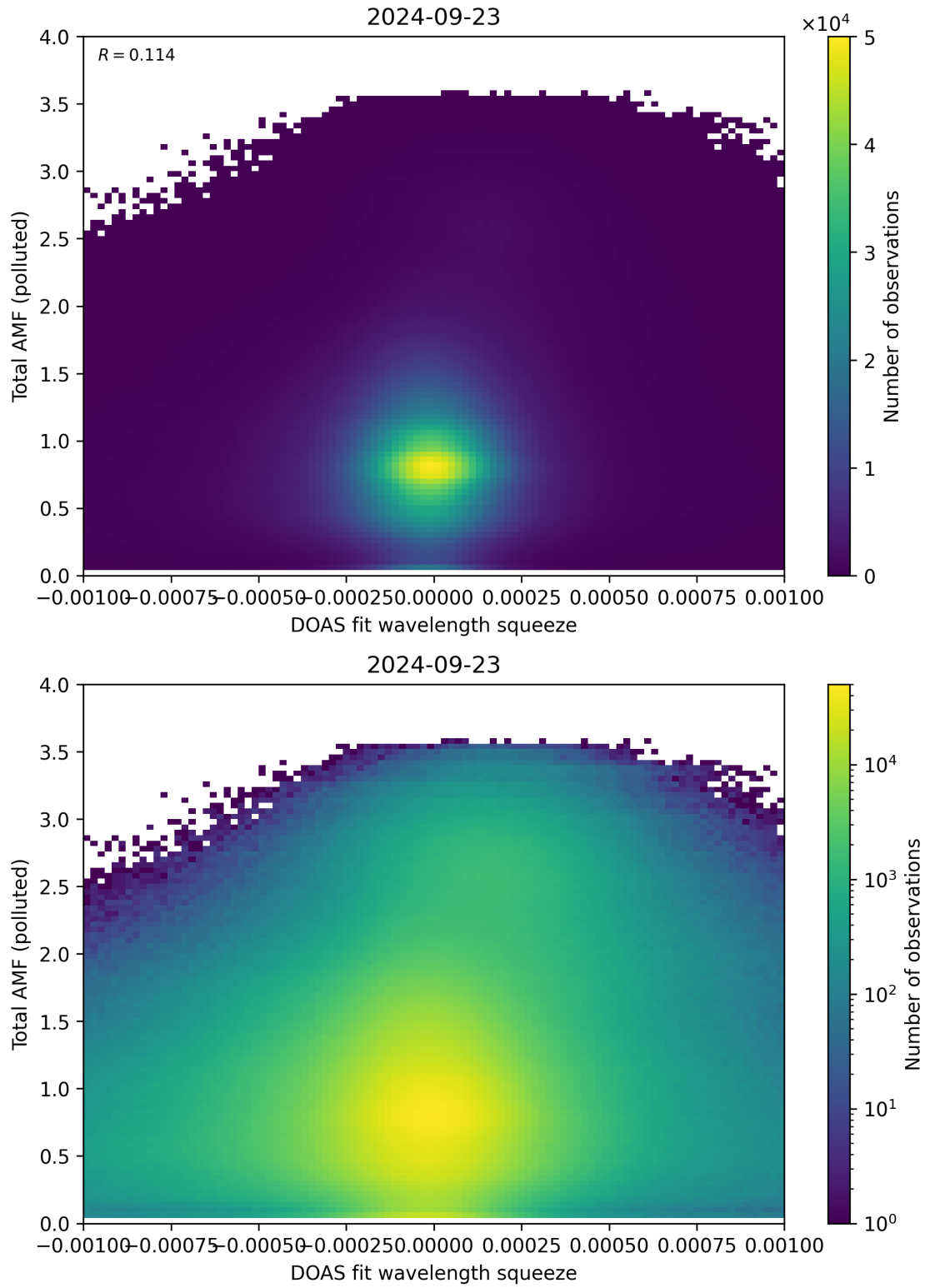
Figure 134: Scatter density plot of “DOAS fit wavelength squeeze” against “Total AMF (polluted)” for 2024-09-22 to 2024-09-24.
