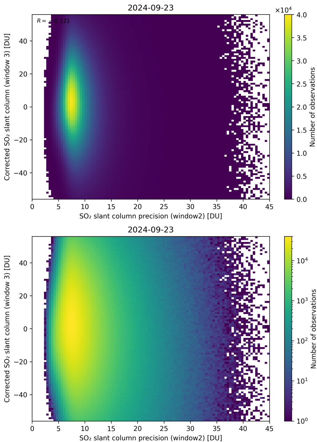
Figure 248: Scatter density plot of “SO 2 slant column precision (window2)” against “Corrected SO 2 slant column (window 3)” for 2024-09-22 to 2024-09-24.
