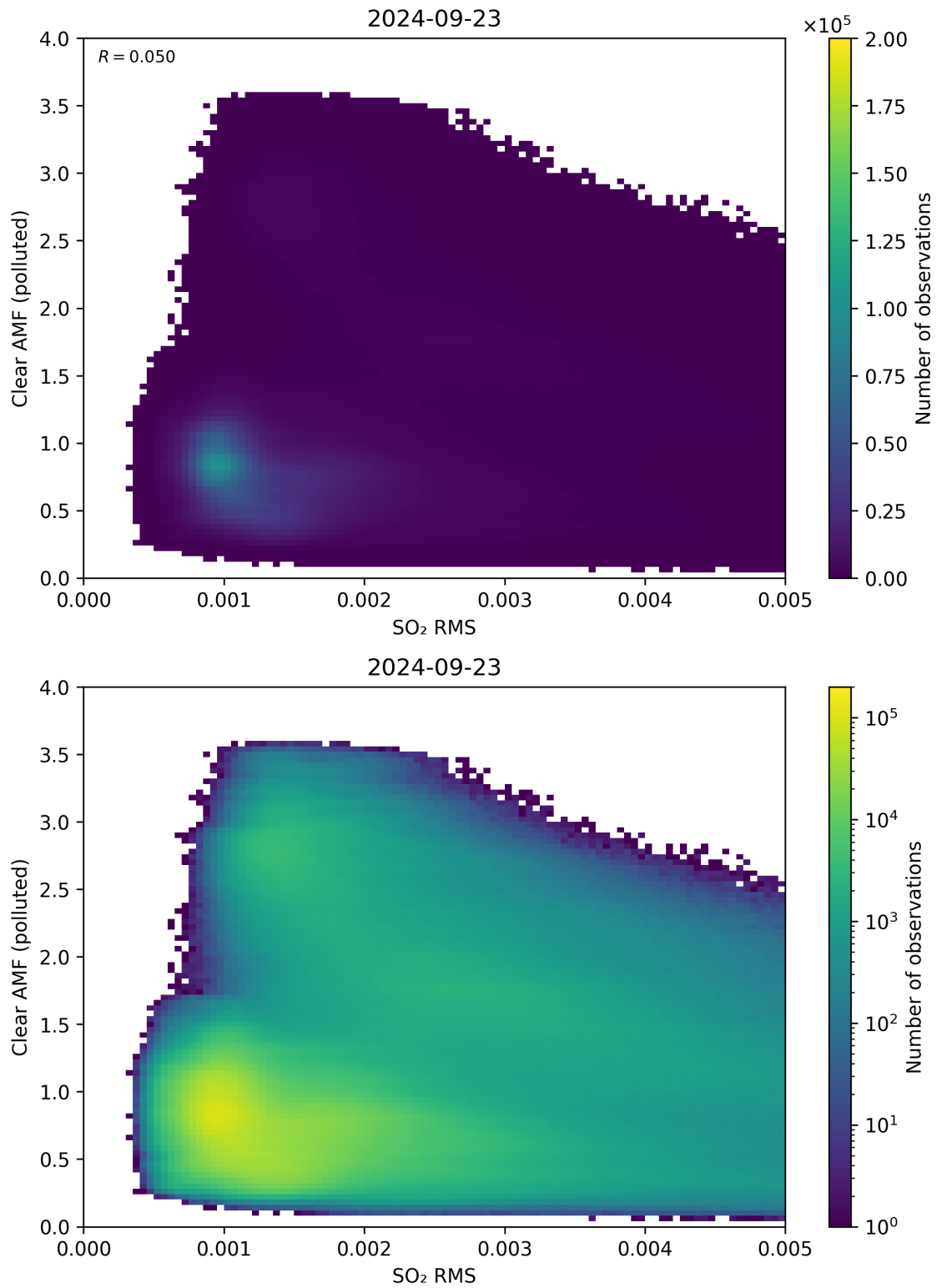
Figure 136: Scatter density plot of “SO 2 RMS” against “Clear AMF (polluted)” for 2024-09-22 to 2024-09-24.
