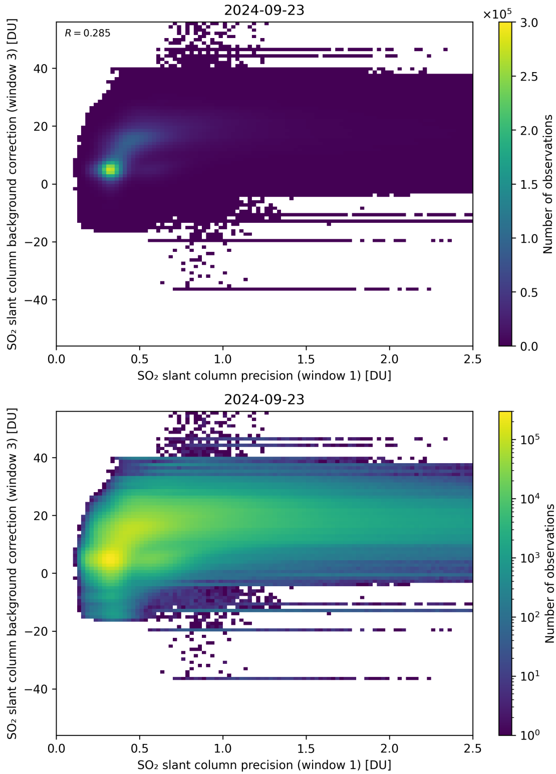
Figure 220: Scatter density plot of “SO 2 slant column precision (window 1)” against “SO 2 slant column background correction (window 3)” for 2024-09-22 to 2024-09-24.
