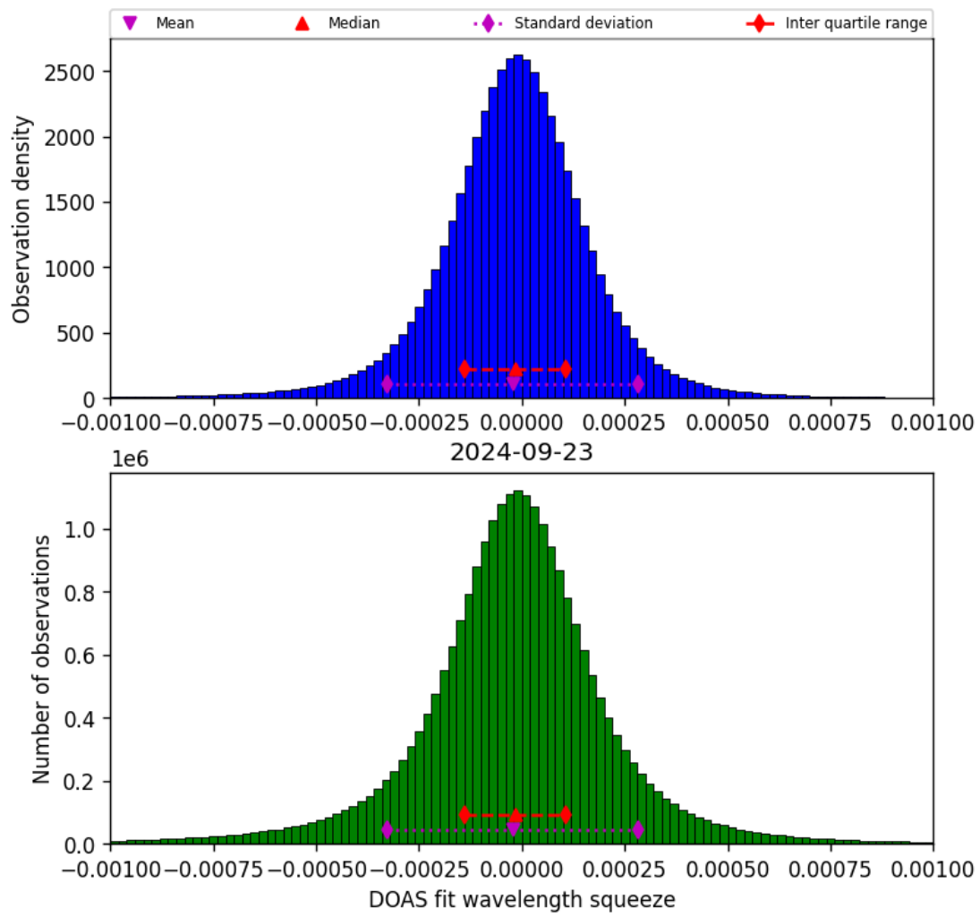
Figure 69: Histogram of “DOAS fit wavelength squeeze” for 2024-09-22 to 2024-09-24
