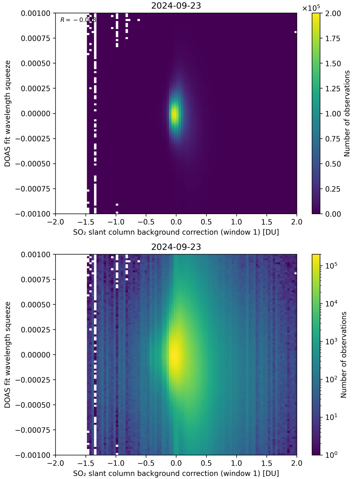
Figure 101: Scatter density plot of “SO 2 slant column background correction (window 1)” against “DOAS fit wavelength squeeze” for 2024-09-22 to 2024-09-24.
