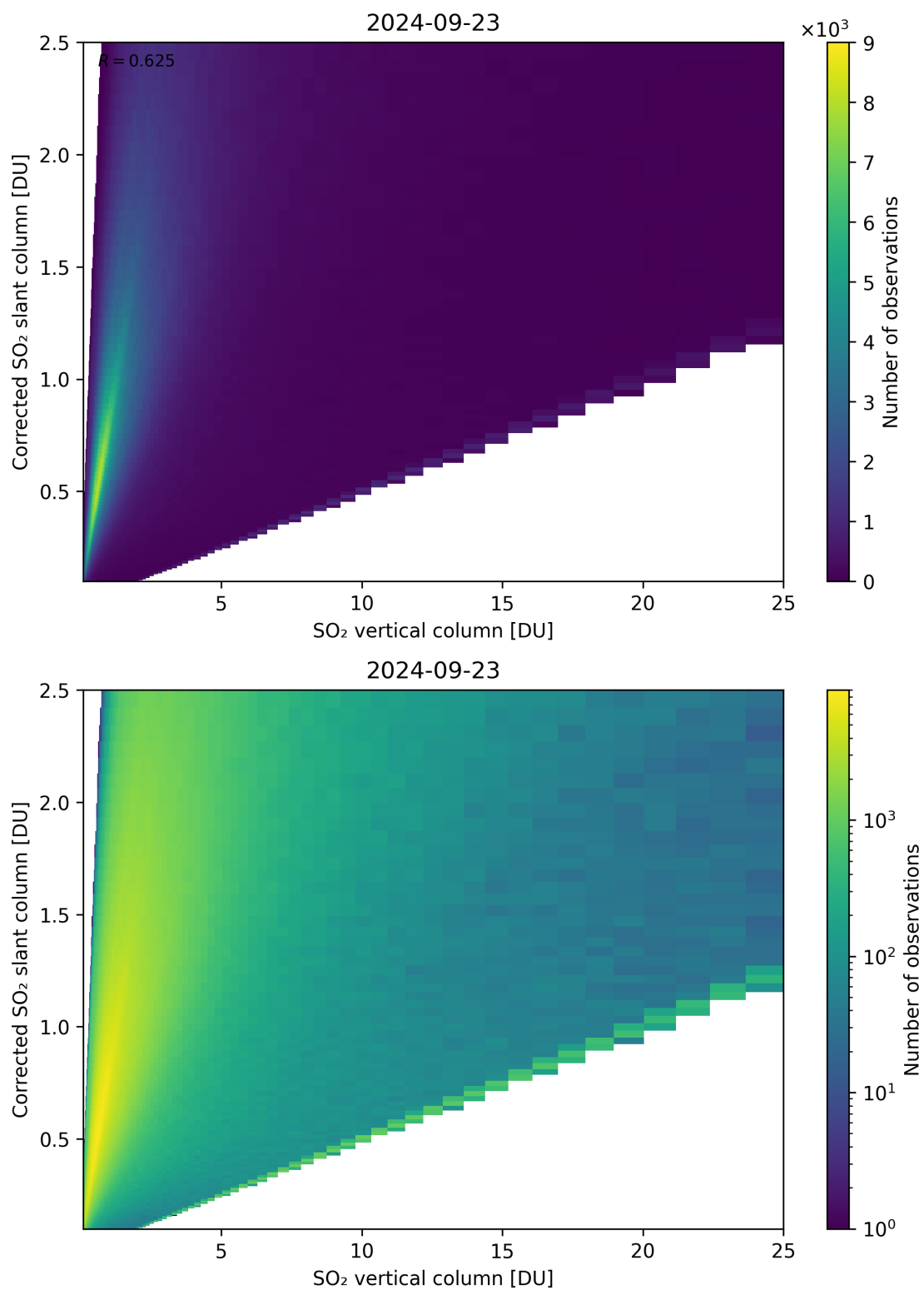
Figure 297: Scatter density plot of “SO 2 vertical column” against “Corrected SO 2 slant column” for 2024-09-22 to 2024-09-24.
