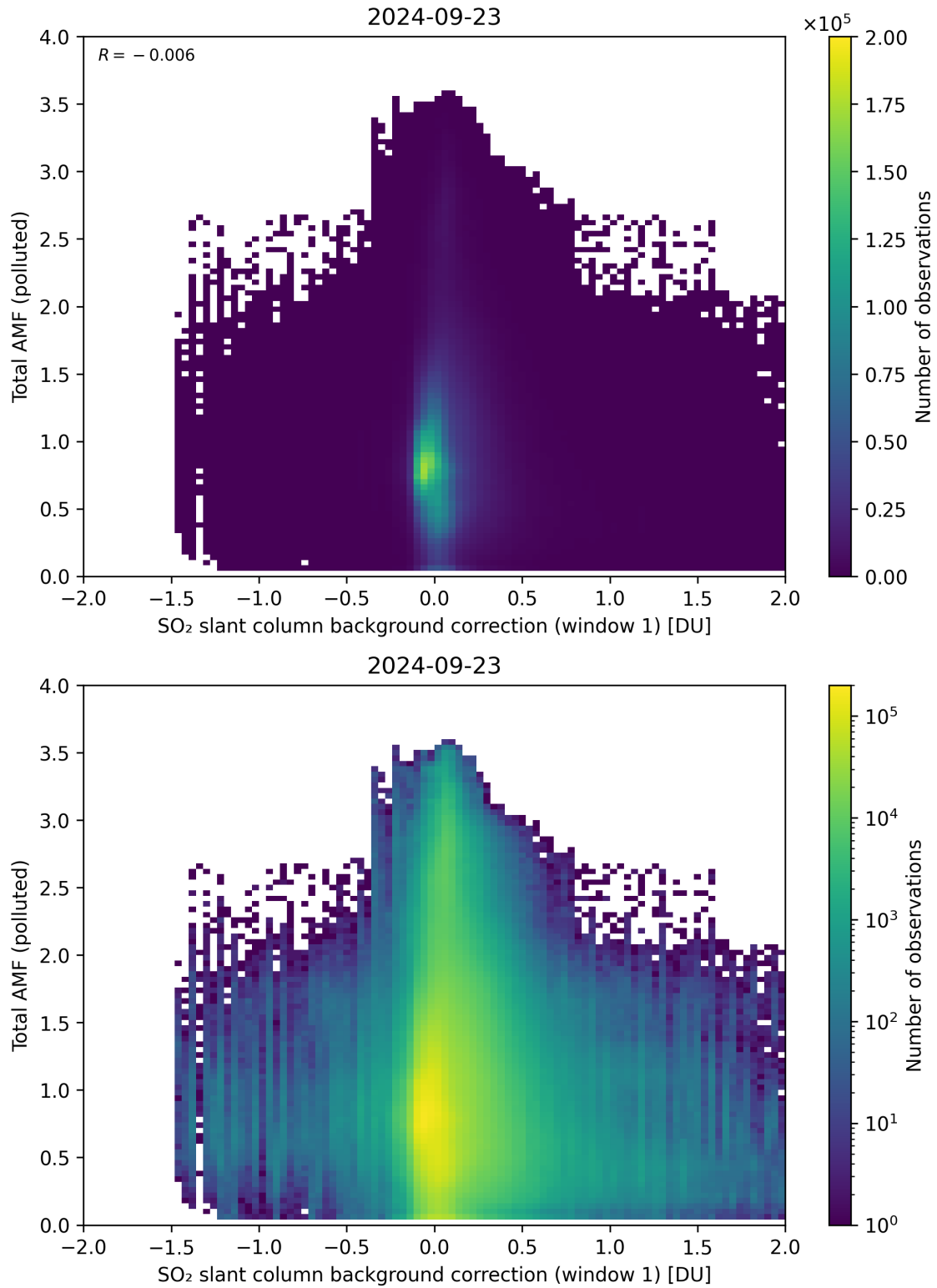
Figure 109: Scatter density plot of “SO 2 slant column background correction (window 1)” against “Total AMF (polluted)” for 2024-09-22 to 2024-09-24.
