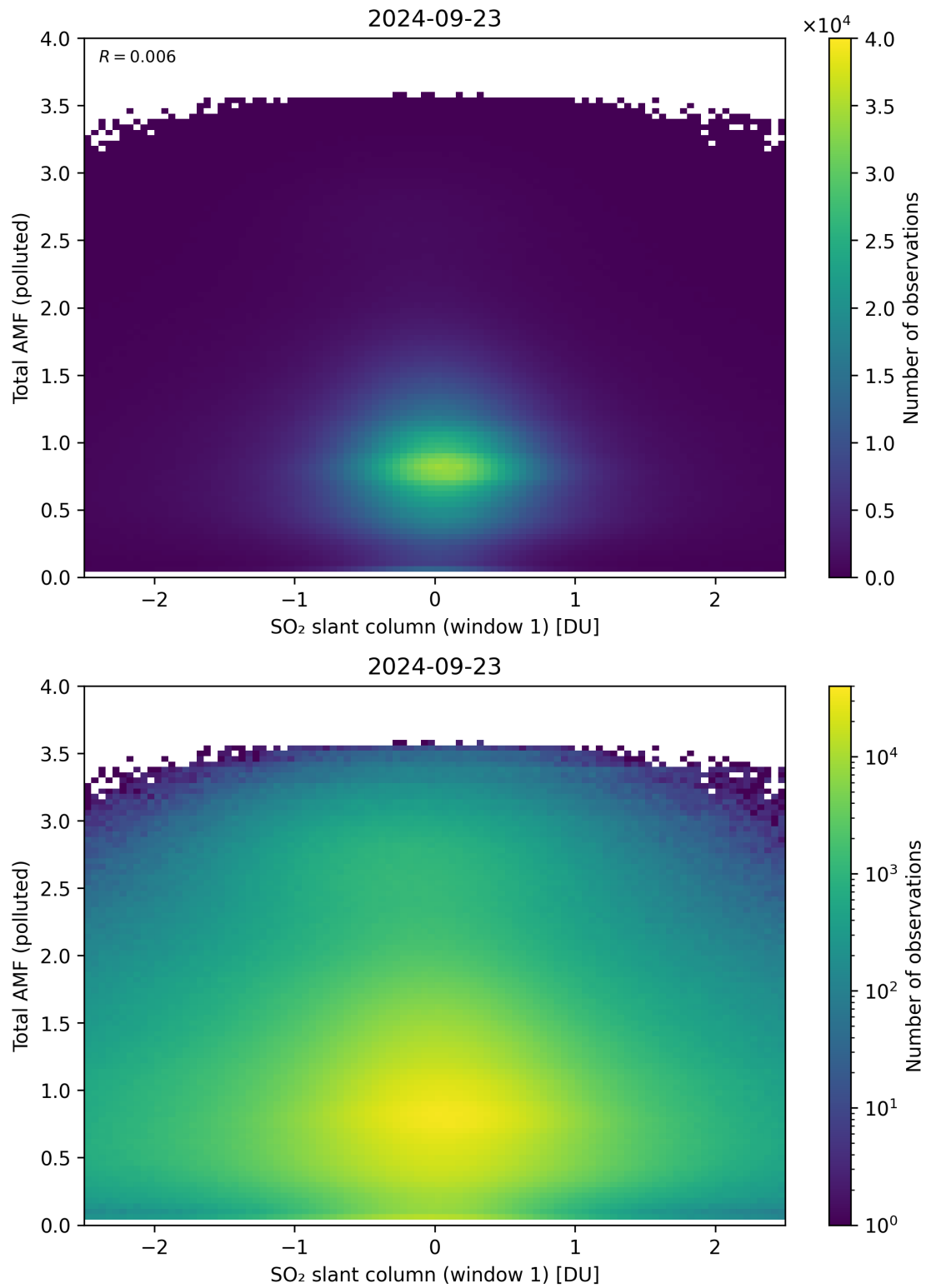
Figure 239: Scatter density plot of “SO 2 slant column (window 1)” against “Total AMF (polluted)” for 2024-09-22 to 2024-09-24.
