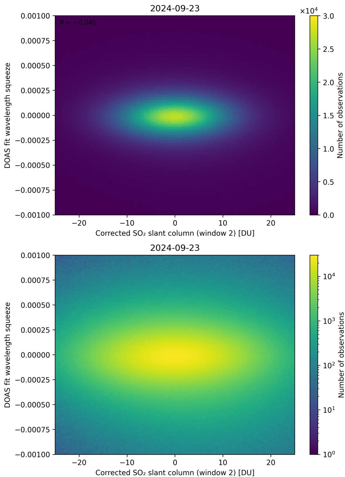
Figure 197: Scatter density plot of “Corrected SO 2 slant column (window 2)” against “DOAS fit wavelength squeeze” for 2024-09-22 to 2024-09-24.
