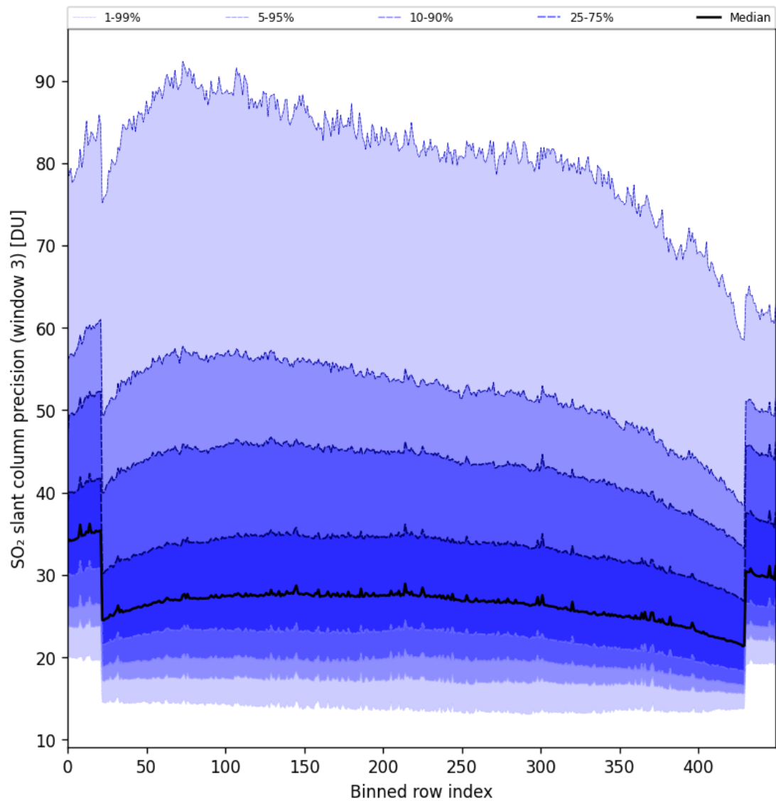
Figure 88: Along track statistics of “SO 2 slant column precision (window 3)” for 2024-09-22 to 2024-09-24
