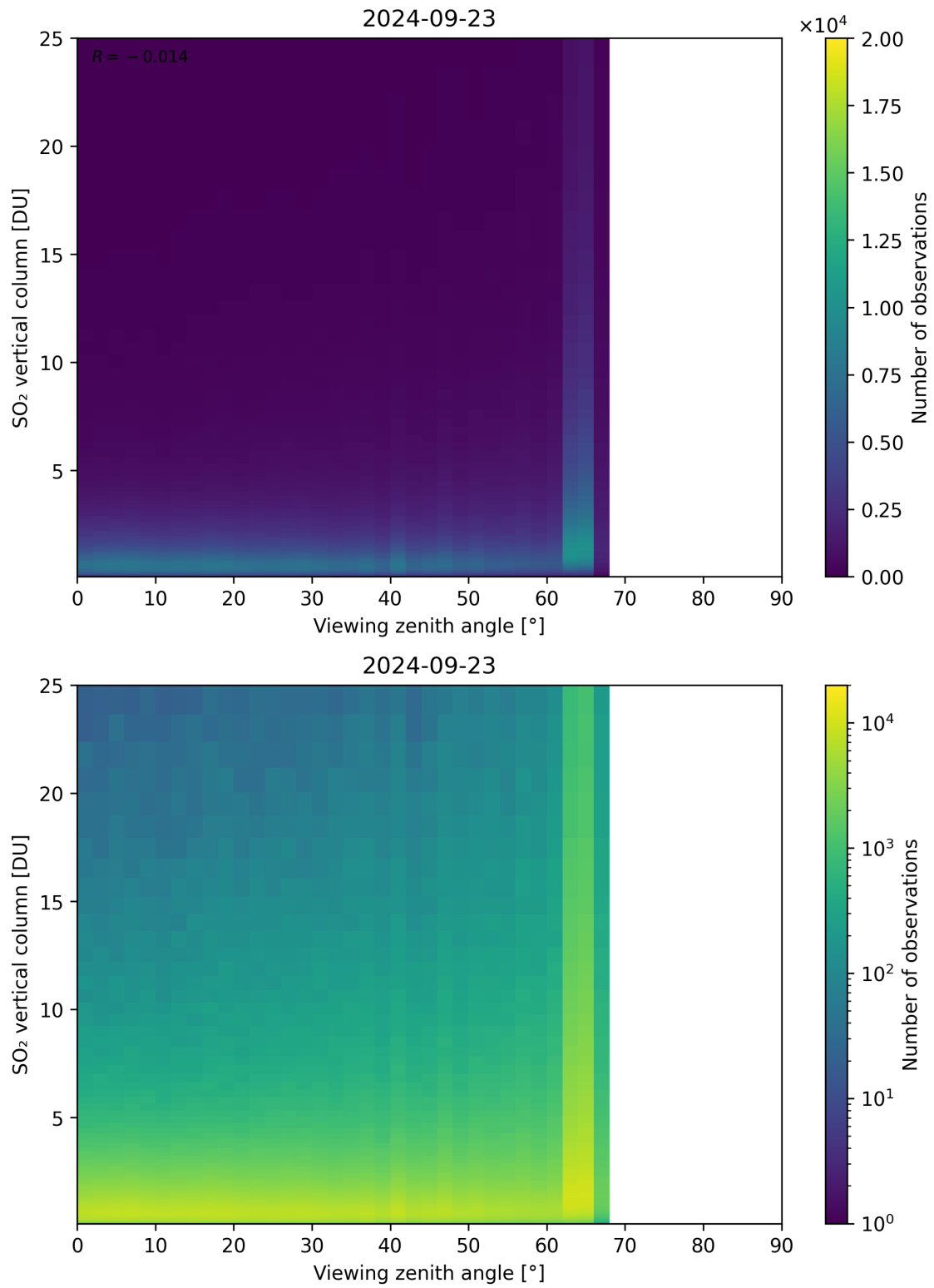
Figure 327: Scatter density plot of “Viewing zenith angle” against “SO 2 vertical column” for 2024-09-22 to 2024-09-24.
