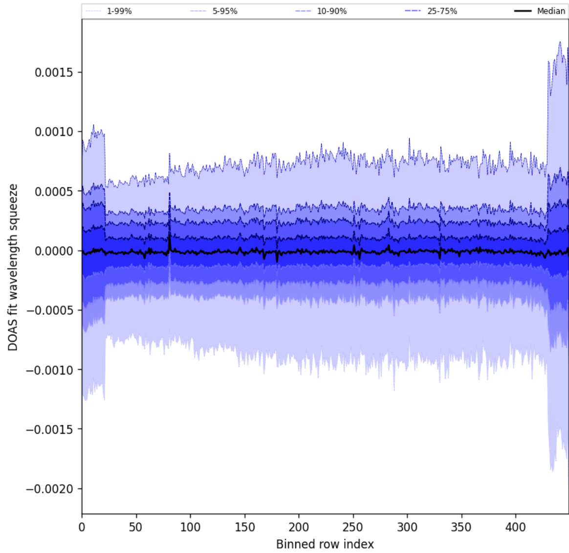
Figure 92: Along track statistics of “DOAS fit wavelength squeeze” for 2024-09-22 to 2024-09-24
