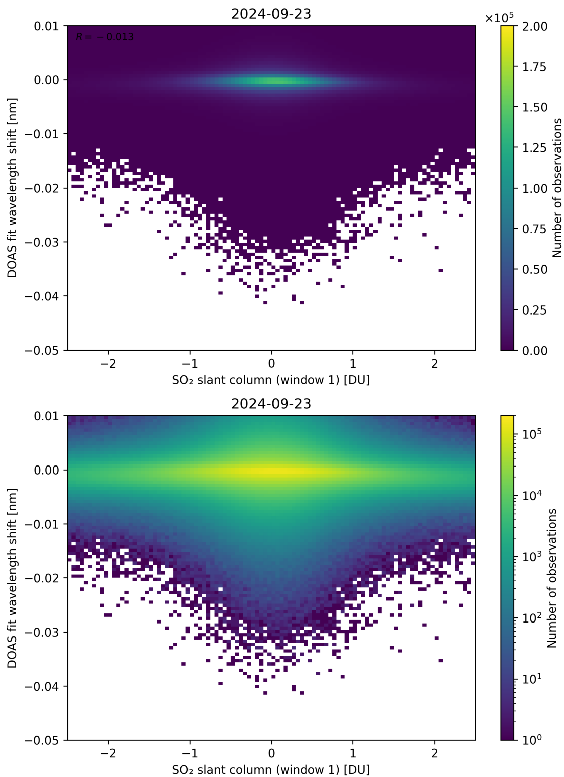
Figure 215: Scatter density plot of “SO 2 slant column (window 1)” against “DOAS fit wavelength shift” for 2024-09-22 to 2024-09-24.
