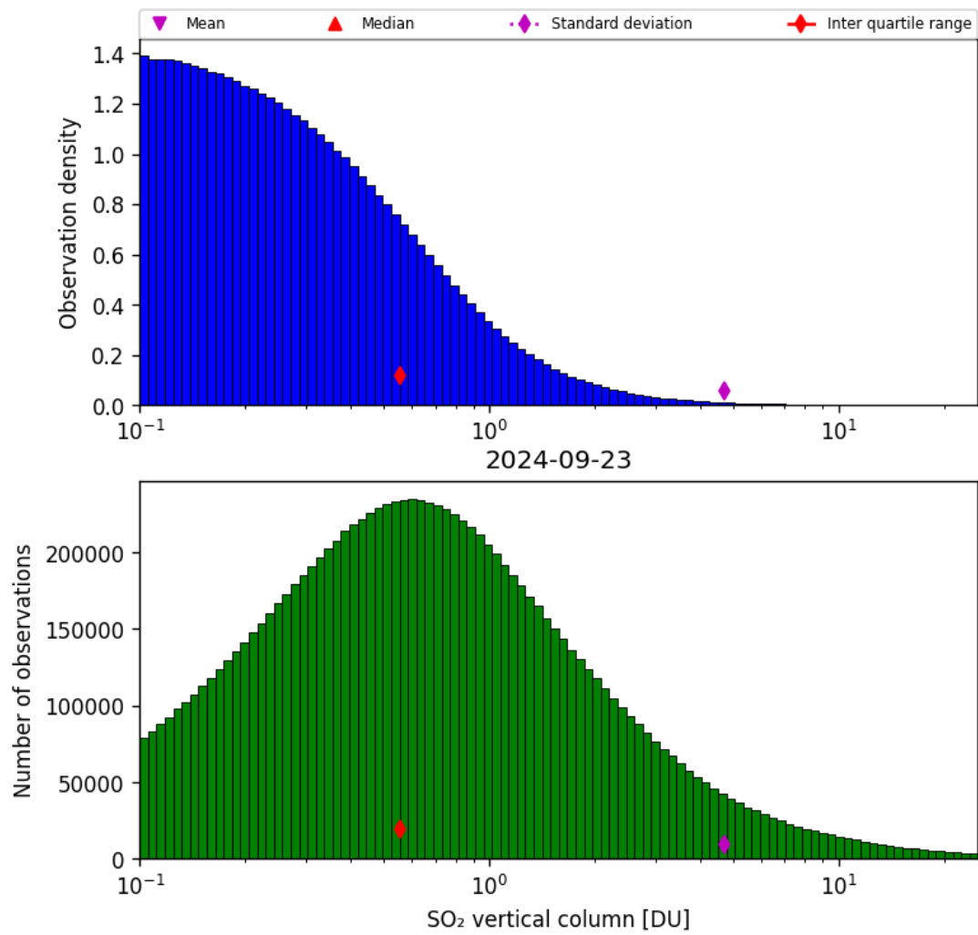
Figure 53: Histogram of “SO 2 vertical column” for 2024-09-22 to 2024-09-24
