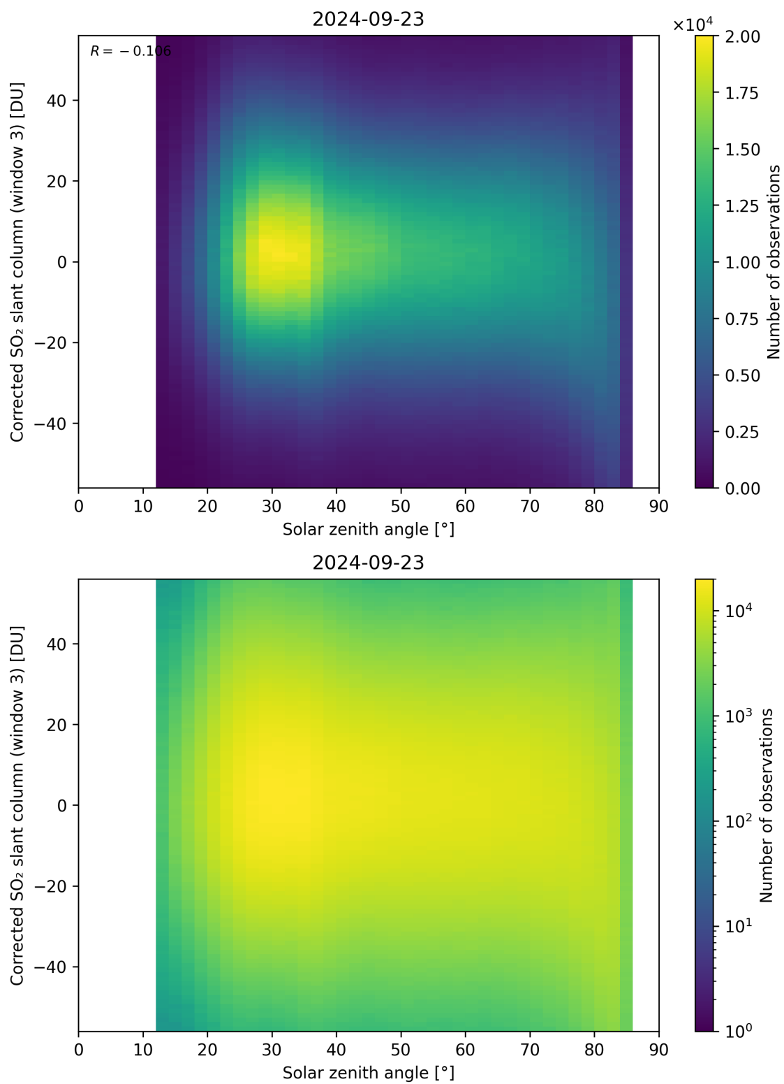
Figure 168: Scatter density plot of “Solar zenith angle” against “Corrected SO 2 slant column (window 3)” for 2024-09-22 to 2024-09-24.
