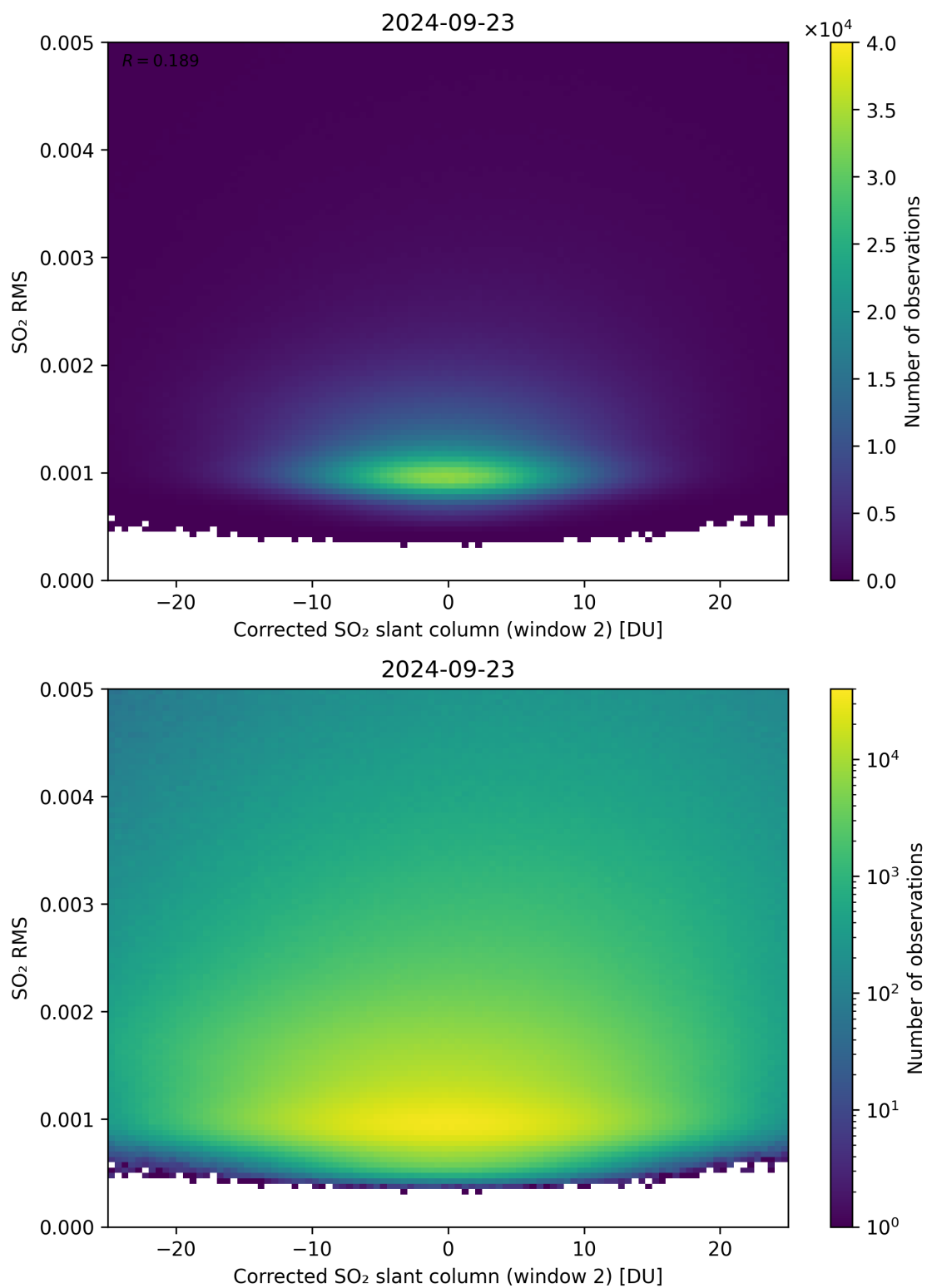
Figure 198: Scatter density plot of “Corrected SO 2 slant column (window 2)” against “SO 2 RMS” for 2024-09-22 to 2024-09-24.
