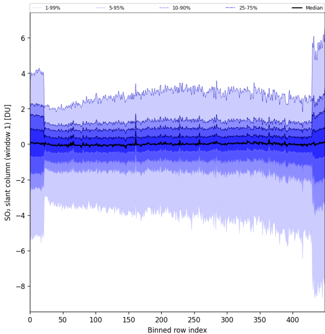
Figure 79: Along track statistics of “SO 2 slant column (window 1)” for 2024-09-22 to 2024-09-24
