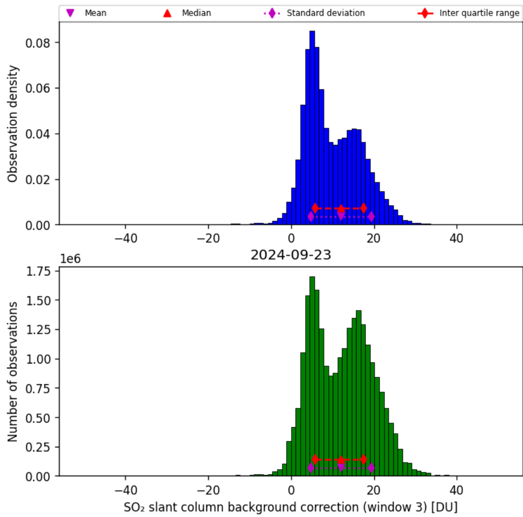
Figure 67: Histogram of “SO 2 slant column background correction (window 3)” for 2024-09-22 to 2024-09-24
