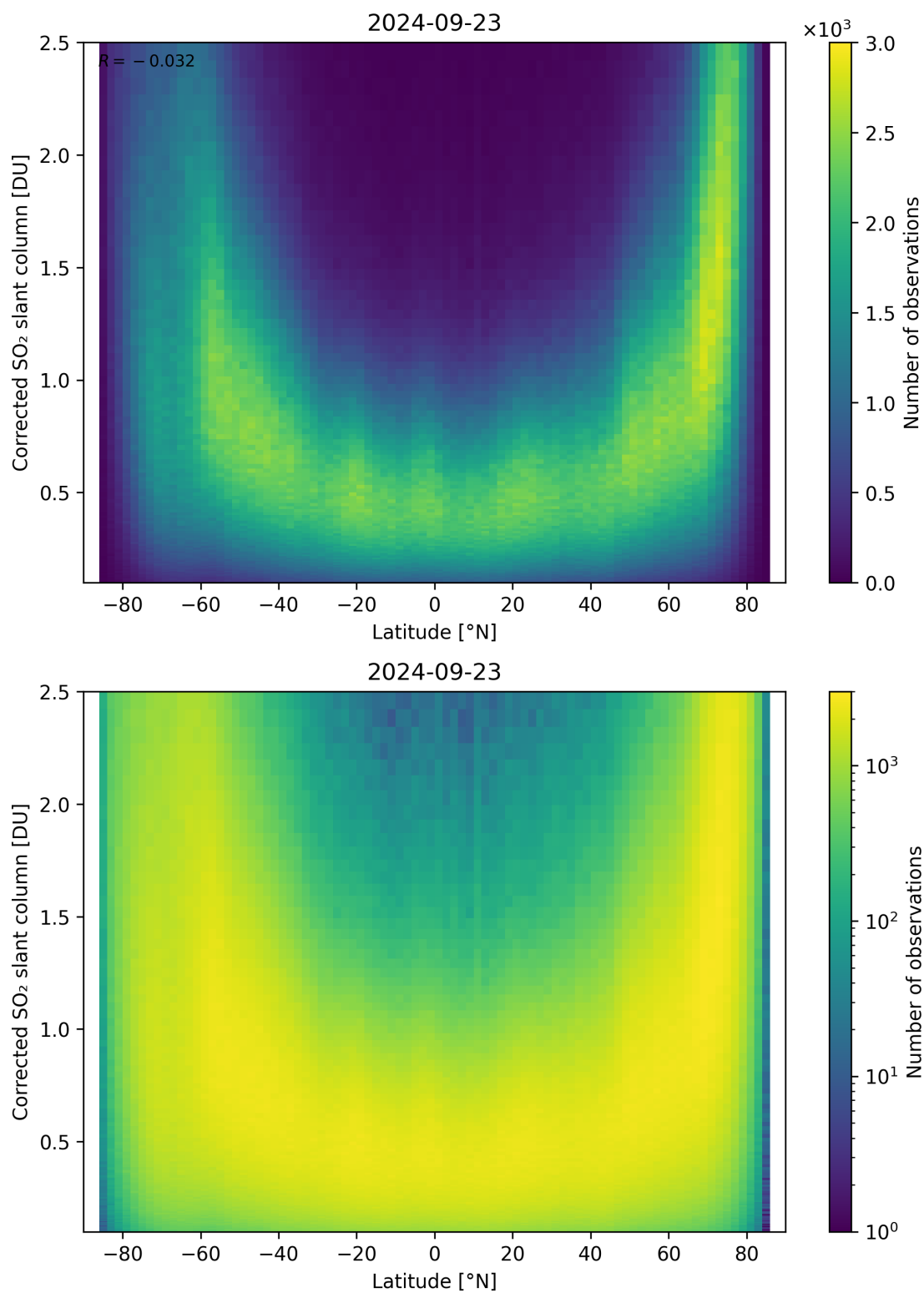
Figure 146: Scatter density plot of “Latitude” against “Corrected SO 2 slant column” for 2024-09-22 to 2024-09-24.
