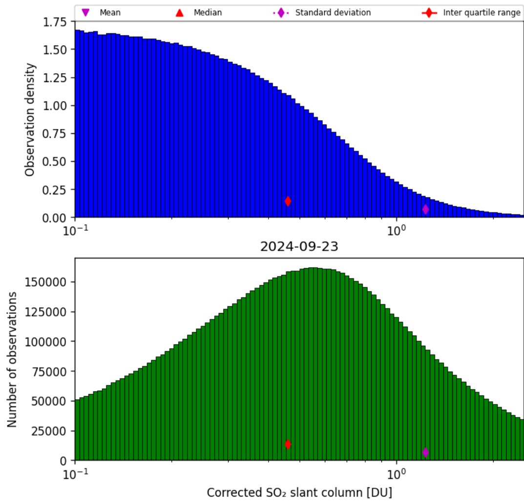
Figure 55: Histogram of “Corrected SO 2 slant column” for 2024-09-22 to 2024-09-24
