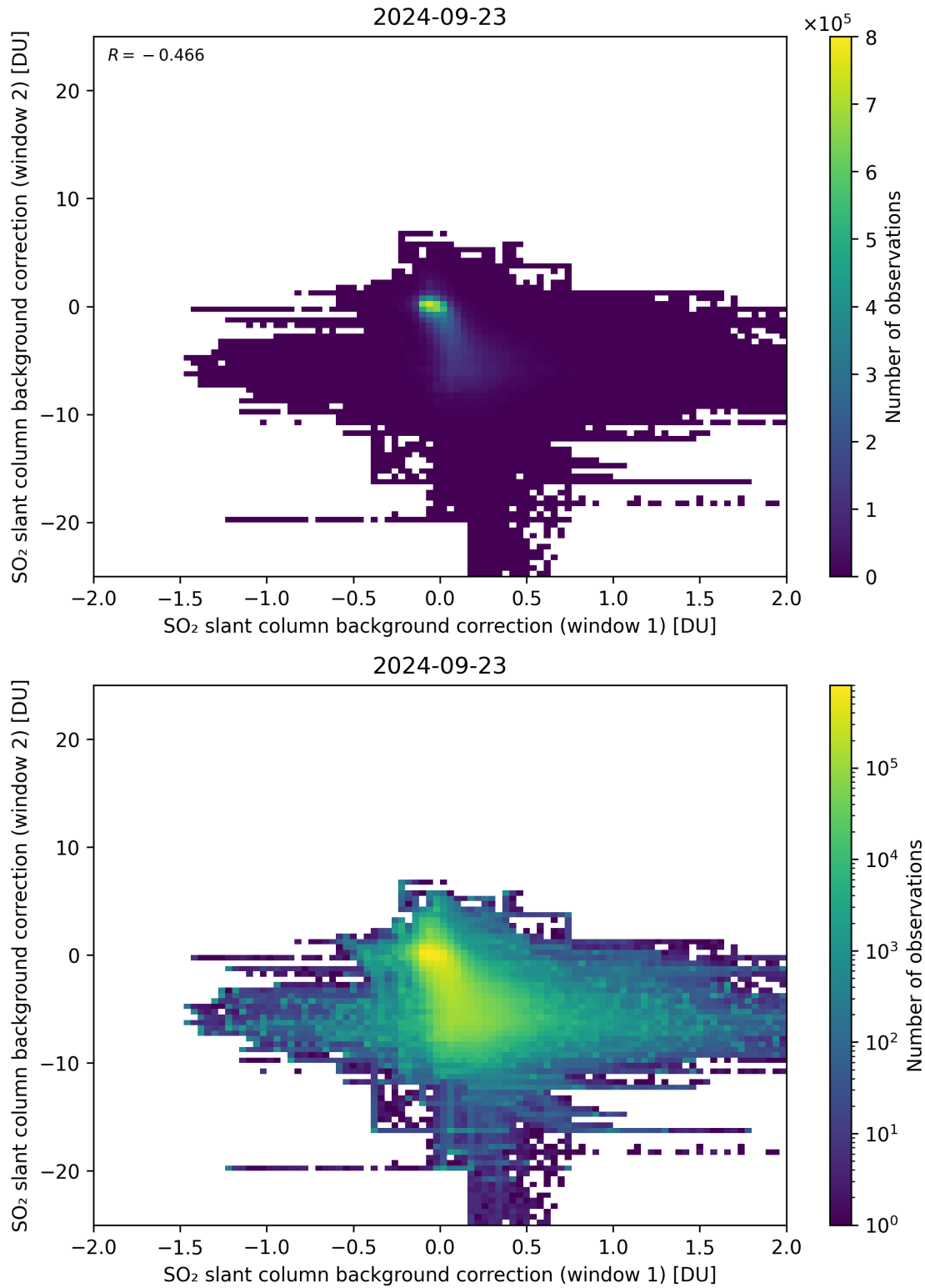
Figure 98: Scatter density plot of “SO 2 slant column background correction (window 1)” against “SO 2 slant column background correction (window 2)” for 2024-09-22 to 2024-09-24.
