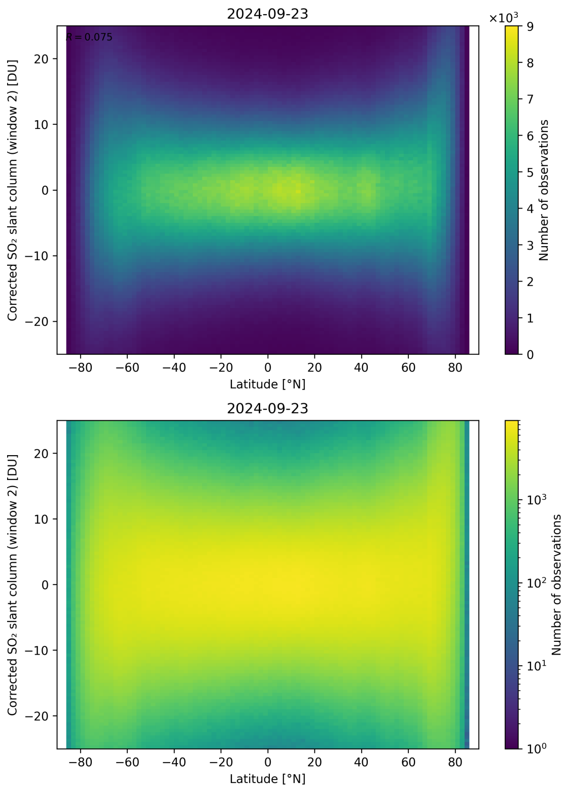
Figure 147: Scatter density plot of “Latitude” against “Corrected SO 2 slant column (window 2)” for 2024-09-22 to 2024-09-24.
