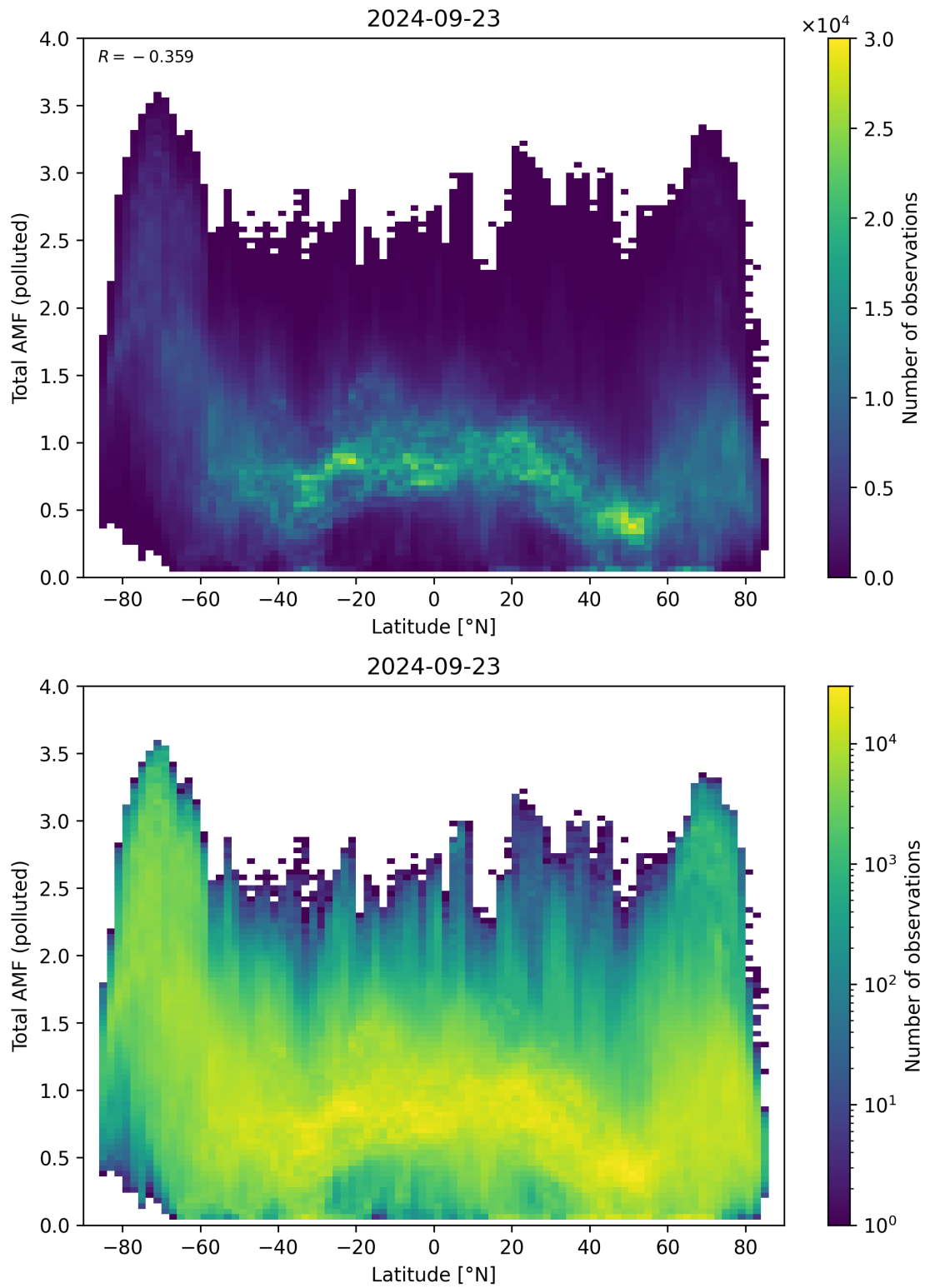
Figure 154: Scatter density plot of “Latitude” against “Total AMF (polluted)” for 2024-09-22 to 2024-09-24.
