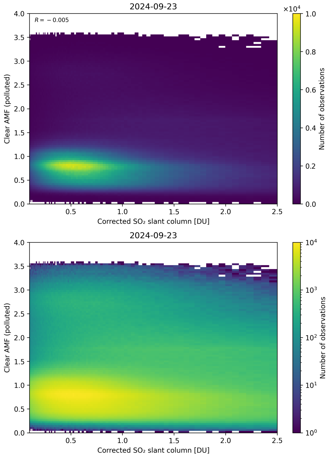
Figure 184: Scatter density plot of “Corrected SO 2 slant column” against “Clear AMF (polluted)” for 2024-09-22 to 2024-09-24.
