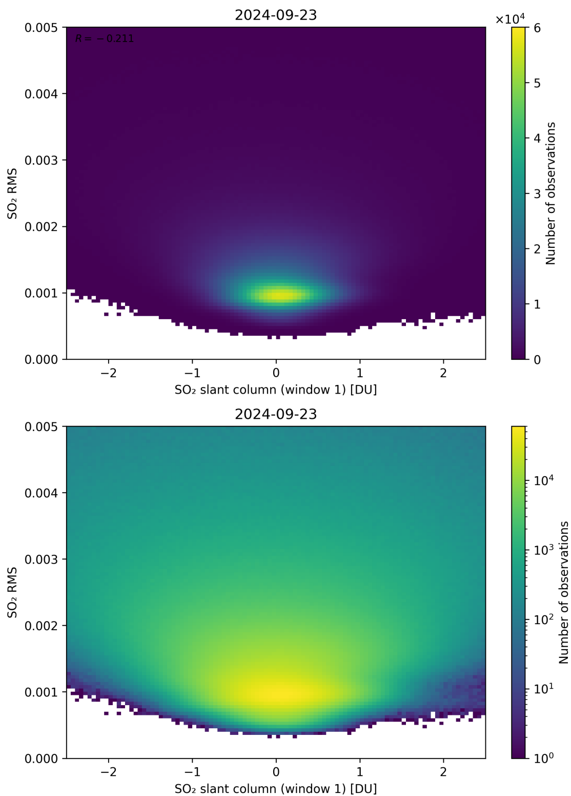
Figure 217: Scatter density plot of “SO 2 slant column (window 1)” against “SO 2 RMS” for 2024-09-22 to 2024-09-24.
