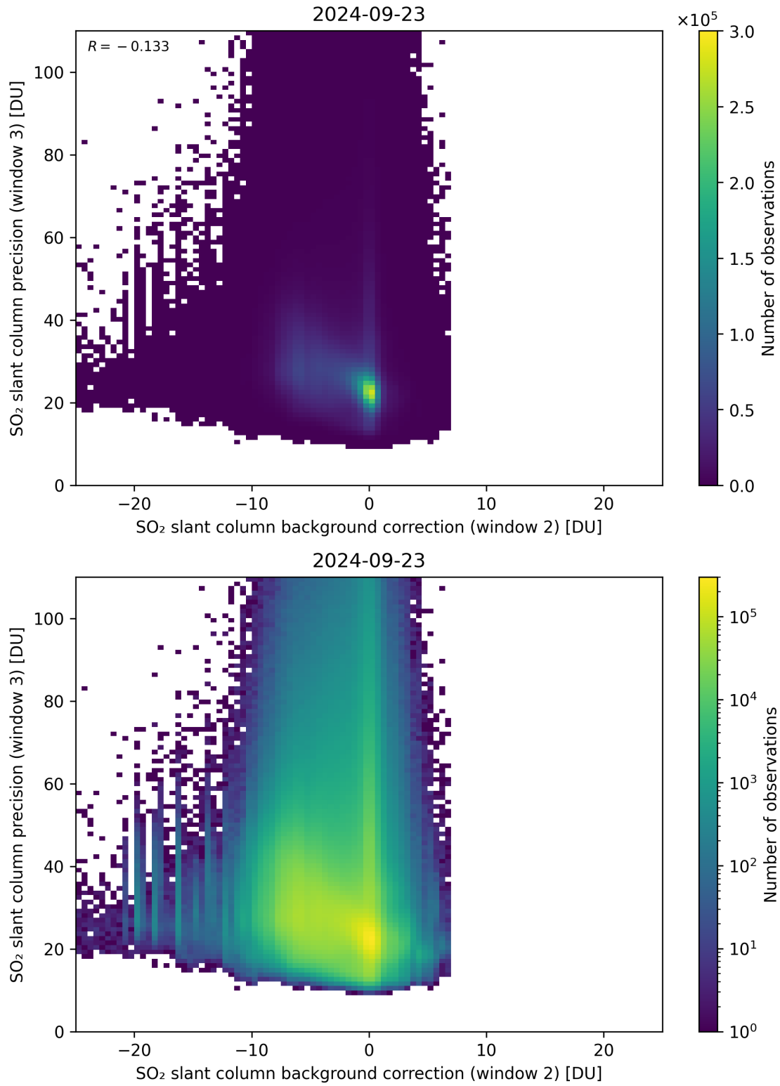
Figure 118: Scatter density plot of “SO 2 slant column background correction (window 2)” against “SO 2 slant column precision (window 3)” for 2024-09-22 to 2024-09-24.
