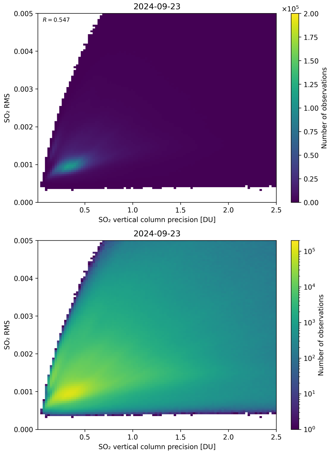
Figure 284: Scatter density plot of “SO 2 vertical column precision” against “SO 2 RMS” for 2024-09-22 to 2024-09-24.
