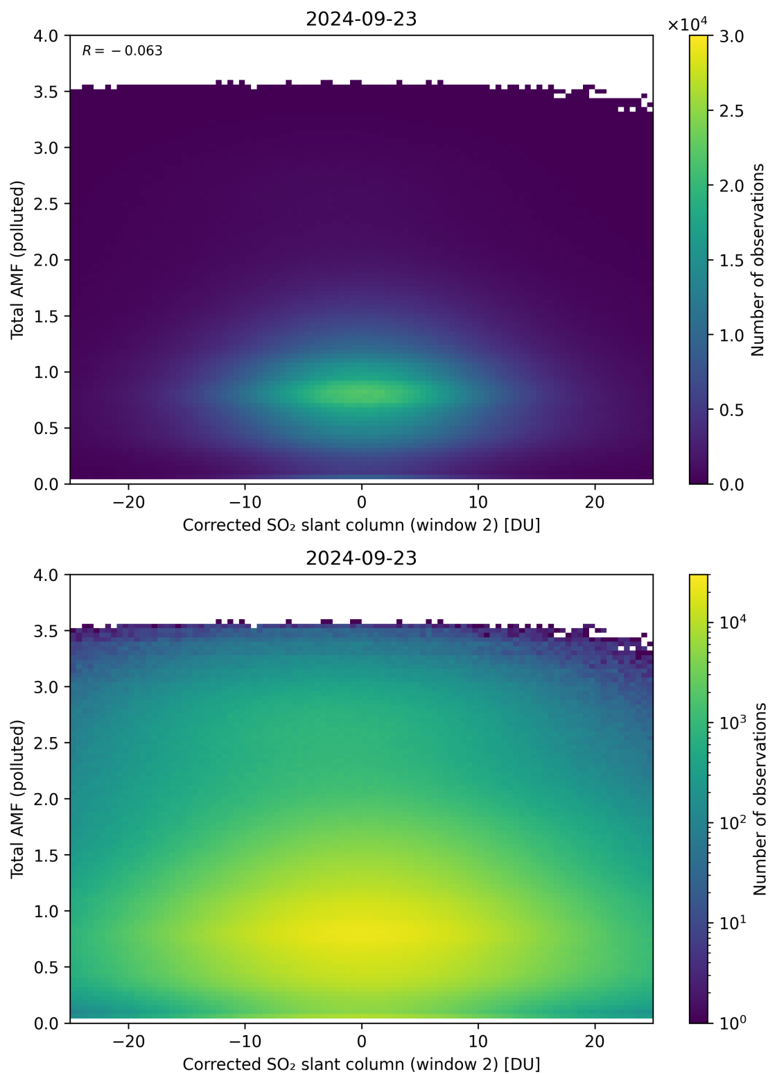
Figure 203: Scatter density plot of “Corrected SO 2 slant column (window 2)” against “Total AMF (polluted)” for 2024-09-22 to 2024-09-24.
