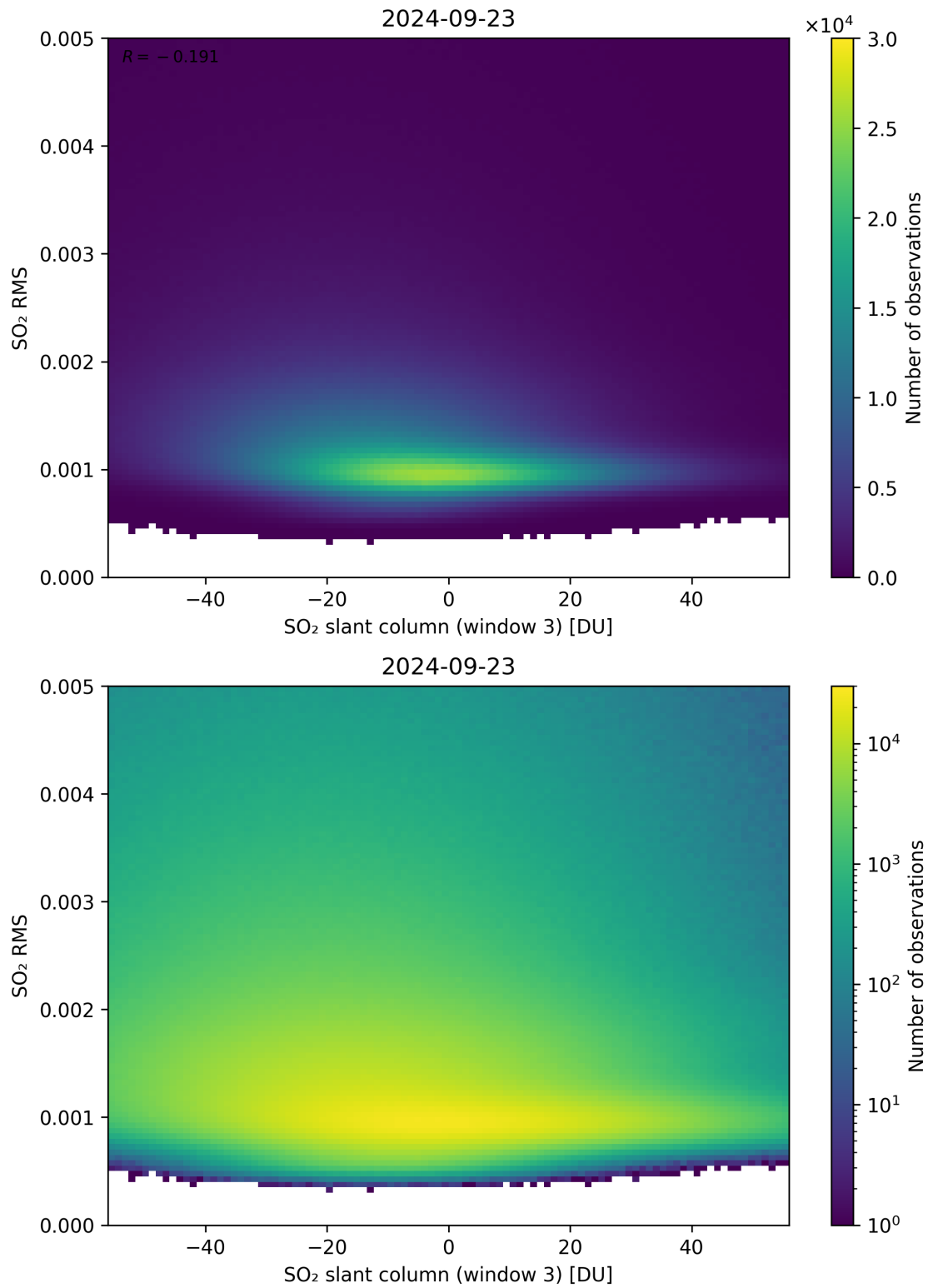
Figure 256: Scatter density plot of “SO 2 slant column (window 3)” against “SO 2 RMS” for 2024-09-22 to 2024-09-24.
