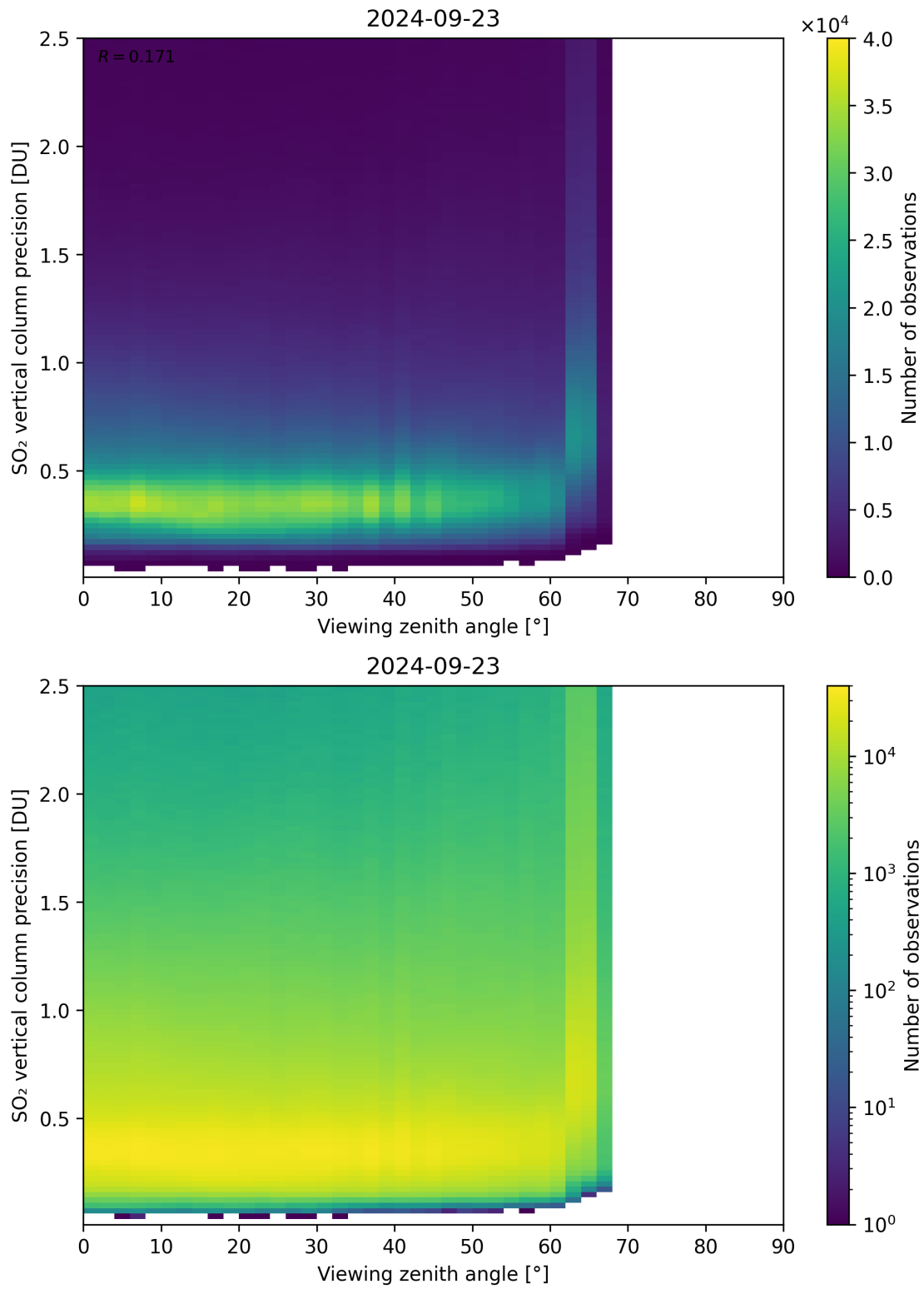
Figure 328: Scatter density plot of “Viewing zenith angle” against “SO 2 vertical column precision” for 2024-09-22 to 2024-09-24.
