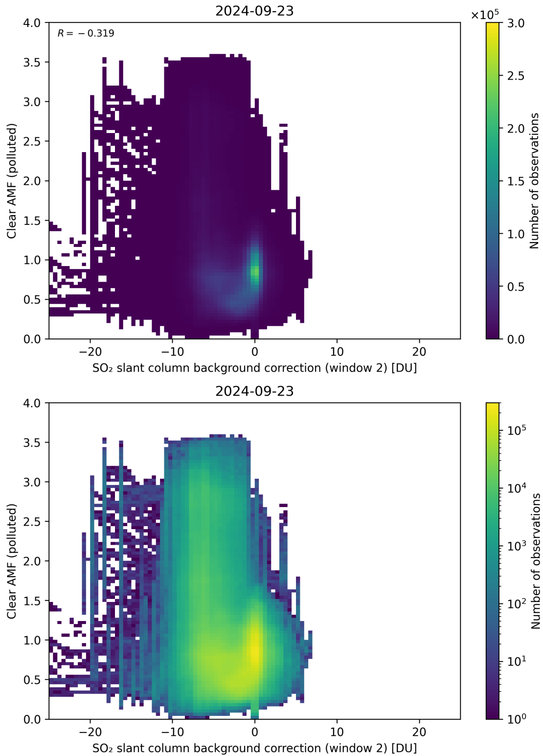
Figure 115: Scatter density plot of “SO 2 slant column background correction (window 2)” against “Clear AMF (polluted)” for 2024-09-22 to 2024-09-24.
