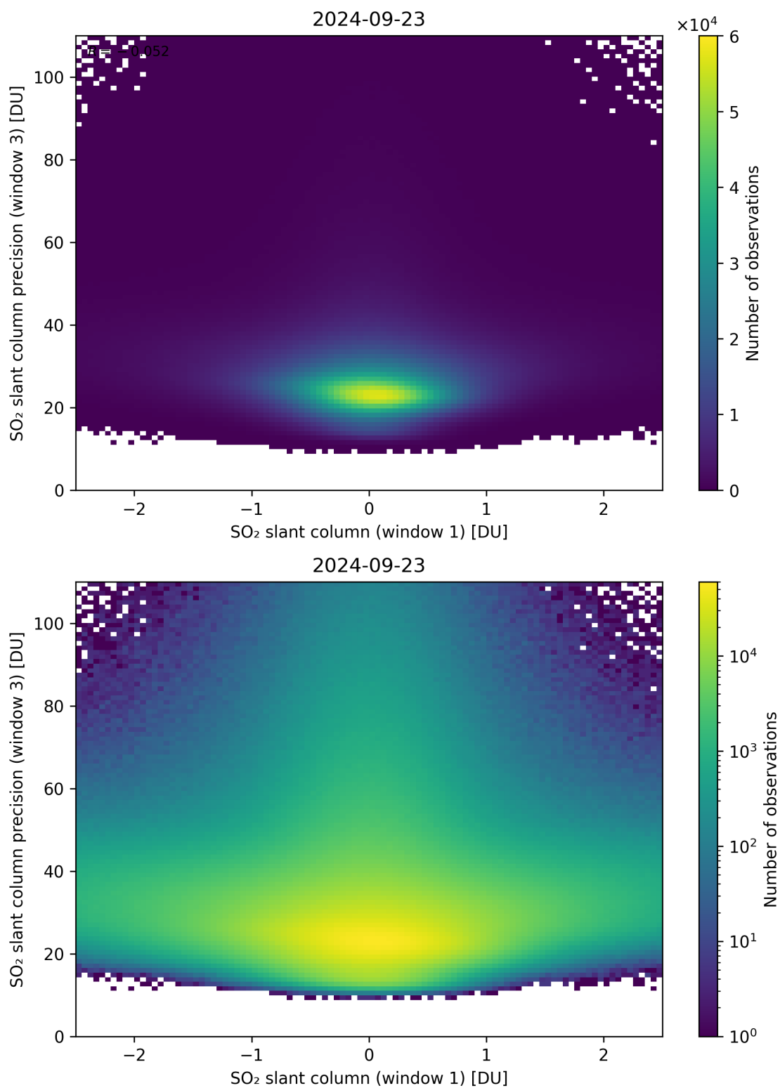
Figure 238: Scatter density plot of “SO 2 slant column (window 1)” against “SO 2 slant column precision (window 3)” for 2024-09-22 to 2024-09-24.
