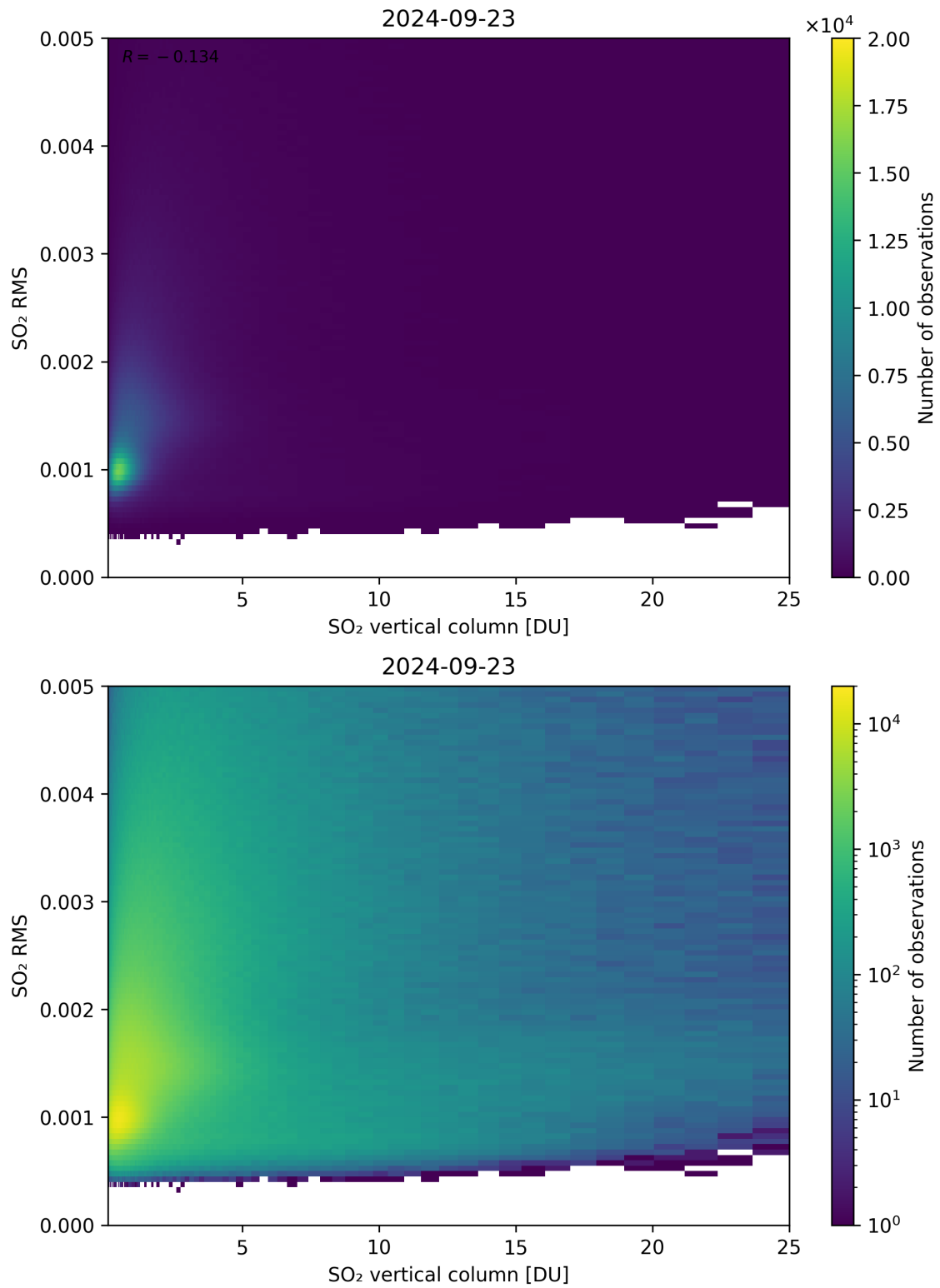
Figure 278: Scatter density plot of “SO 2 vertical column” against “SO 2 RMS” for 2024-09-22 to 2024-09-24.
