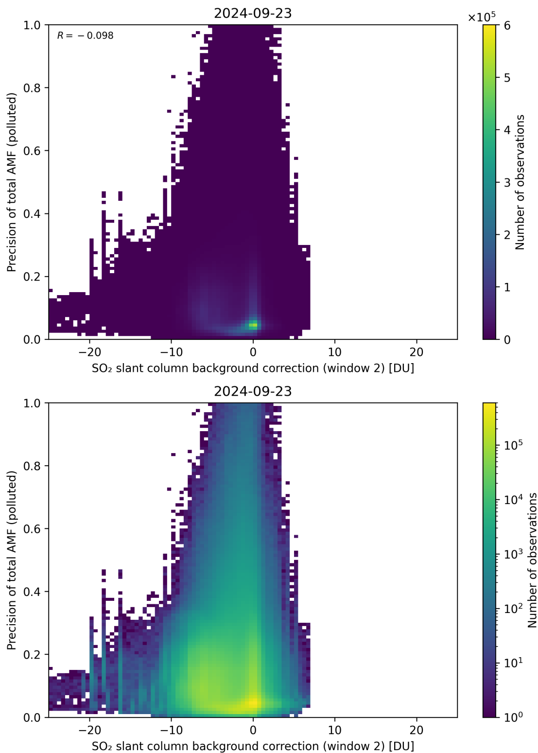
Figure 120: Scatter density plot of “SO 2 slant column background correction (window 2)” against “Precision of total AMF (polluted)” for 2024-09-22 to 2024-09-24.
