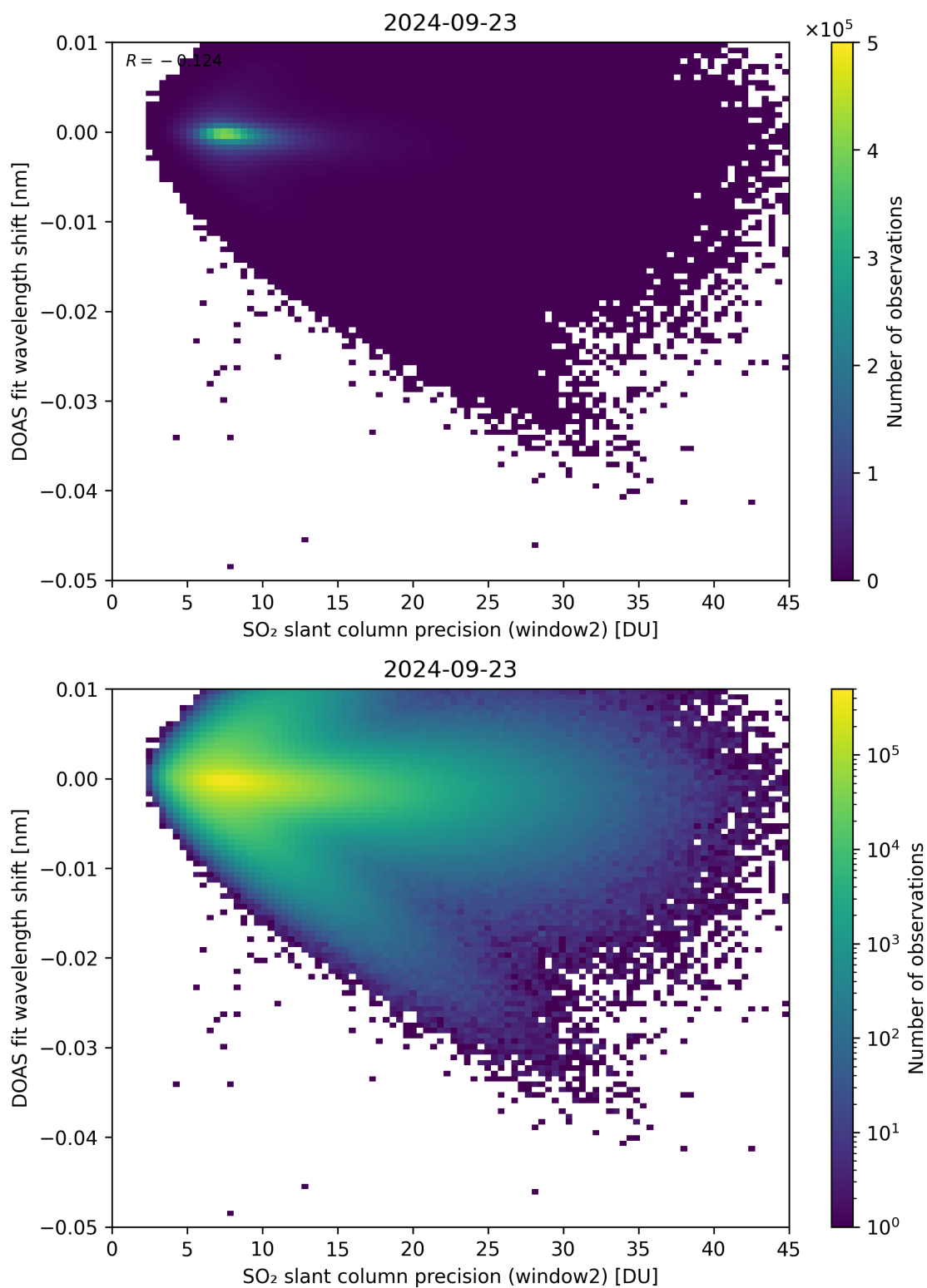
Figure 243: Scatter density plot of “SO 2 slant column precision (window2)” against “DOAS fit wavelength shift” for 2024-09-22 to 2024-09-24.
