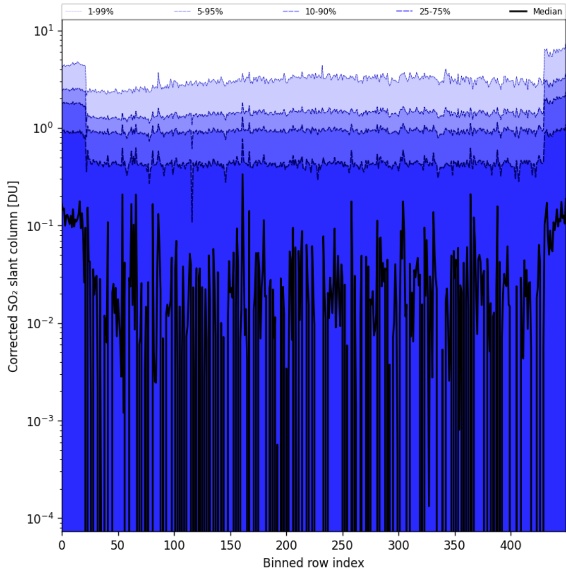
Figure 78: Along track statistics of “Corrected SO 2 slant column” for 2024-09-22 to 2024-09-24
