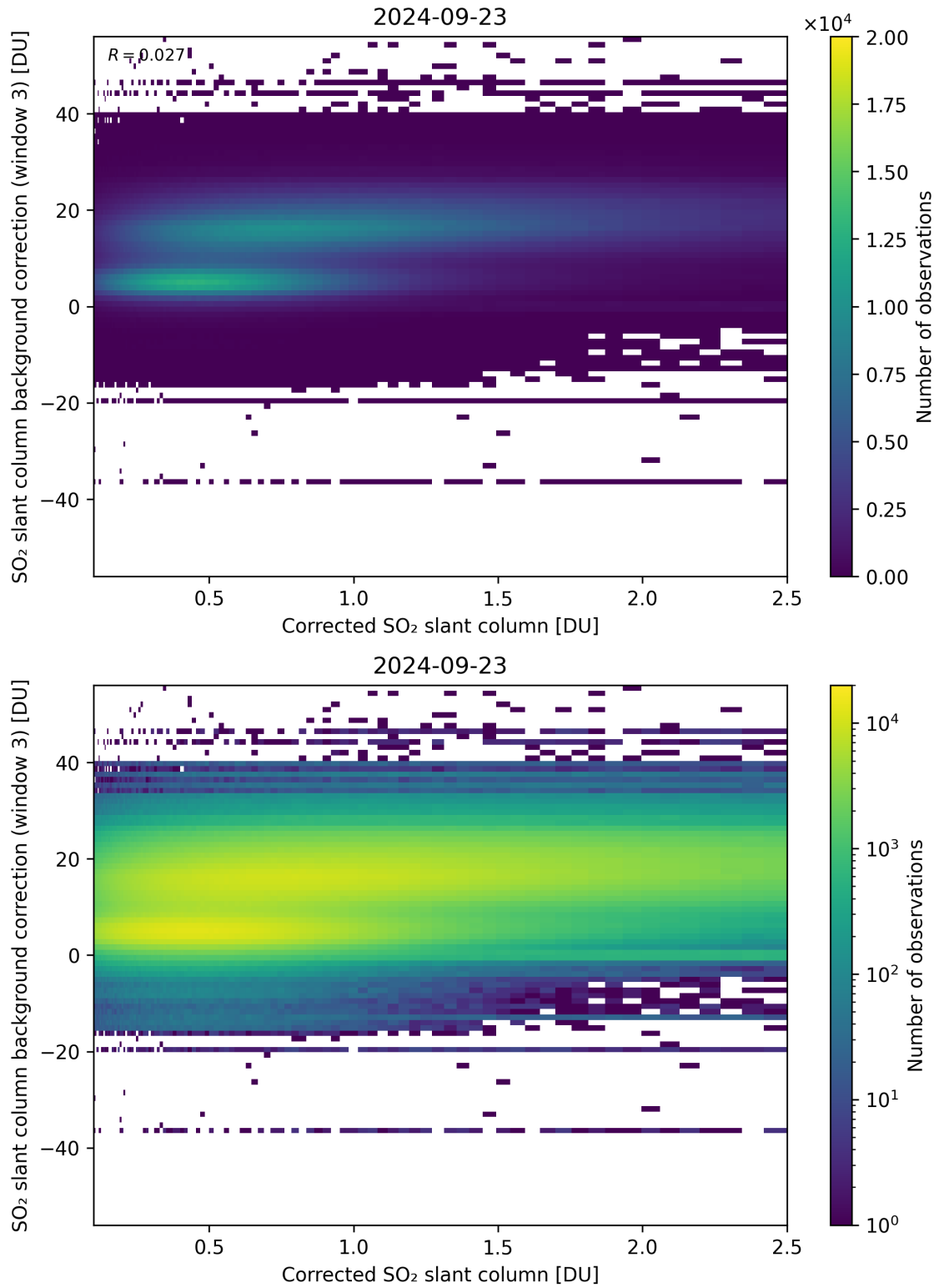
Figure 180: Scatter density plot of “Corrected SO 2 slant column” against “SO 2 slant column background correction (window 3)” for 2024-09-22 to 2024-09-24.
