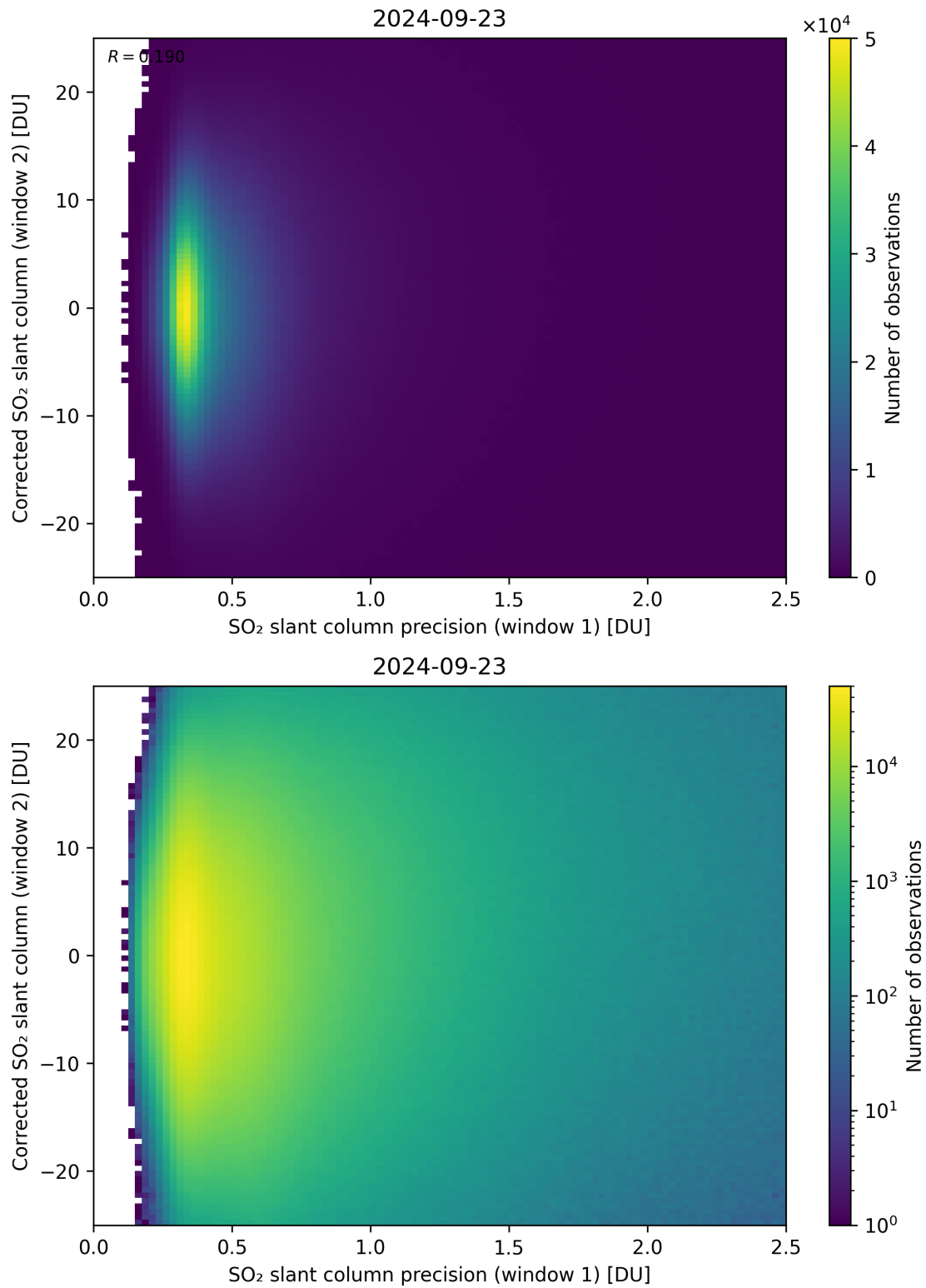
Figure 225: Scatter density plot of “SO 2 slant column precision (window 1)” against “Corrected SO 2 slant column (window 2)” for 2024-09-22 to 2024-09-24.
