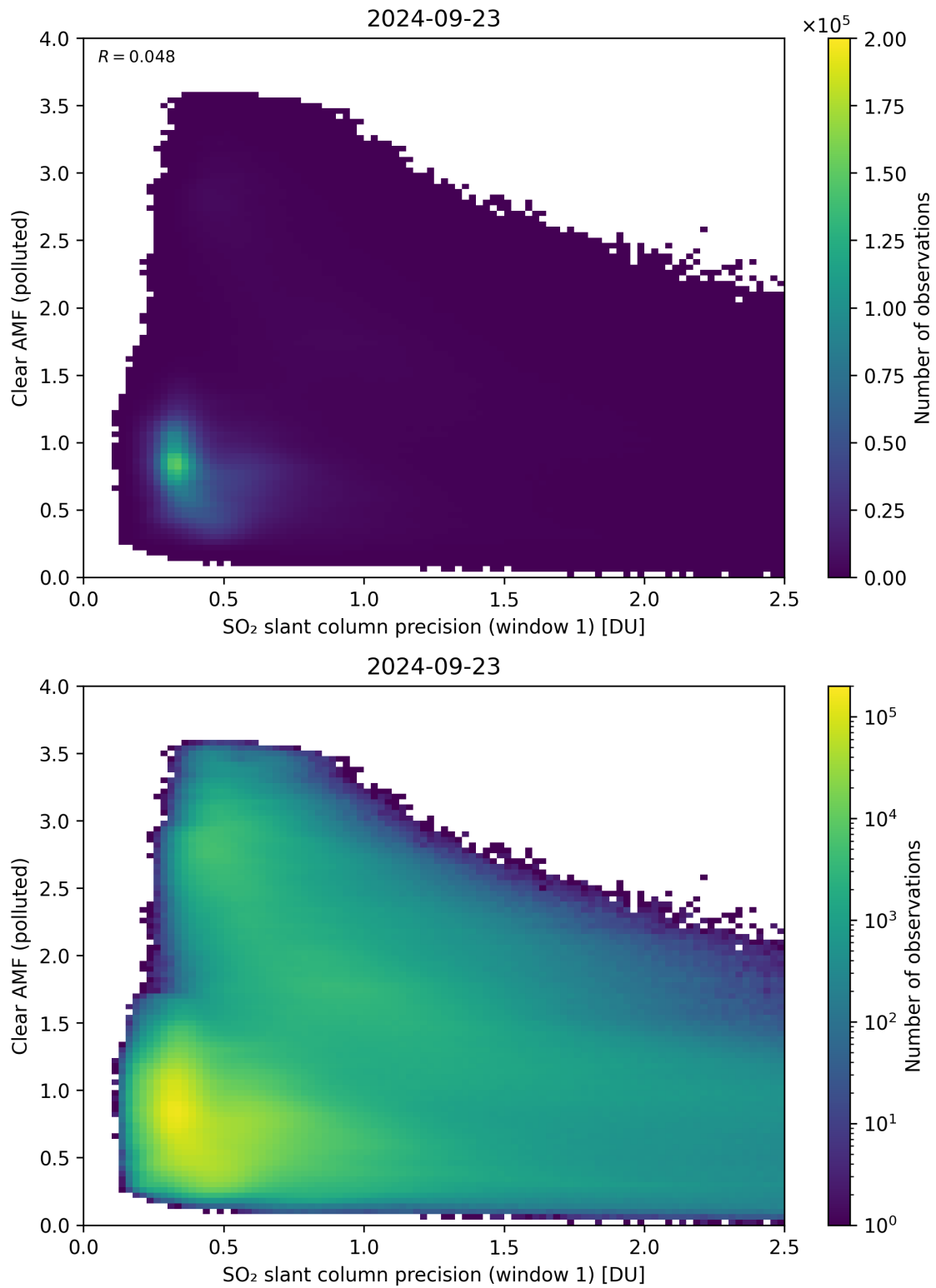
Figure 224: Scatter density plot of “SO 2 slant column precision (window 1)” against “Clear AMF (polluted)” for 2024-09-22 to 2024-09-24.
