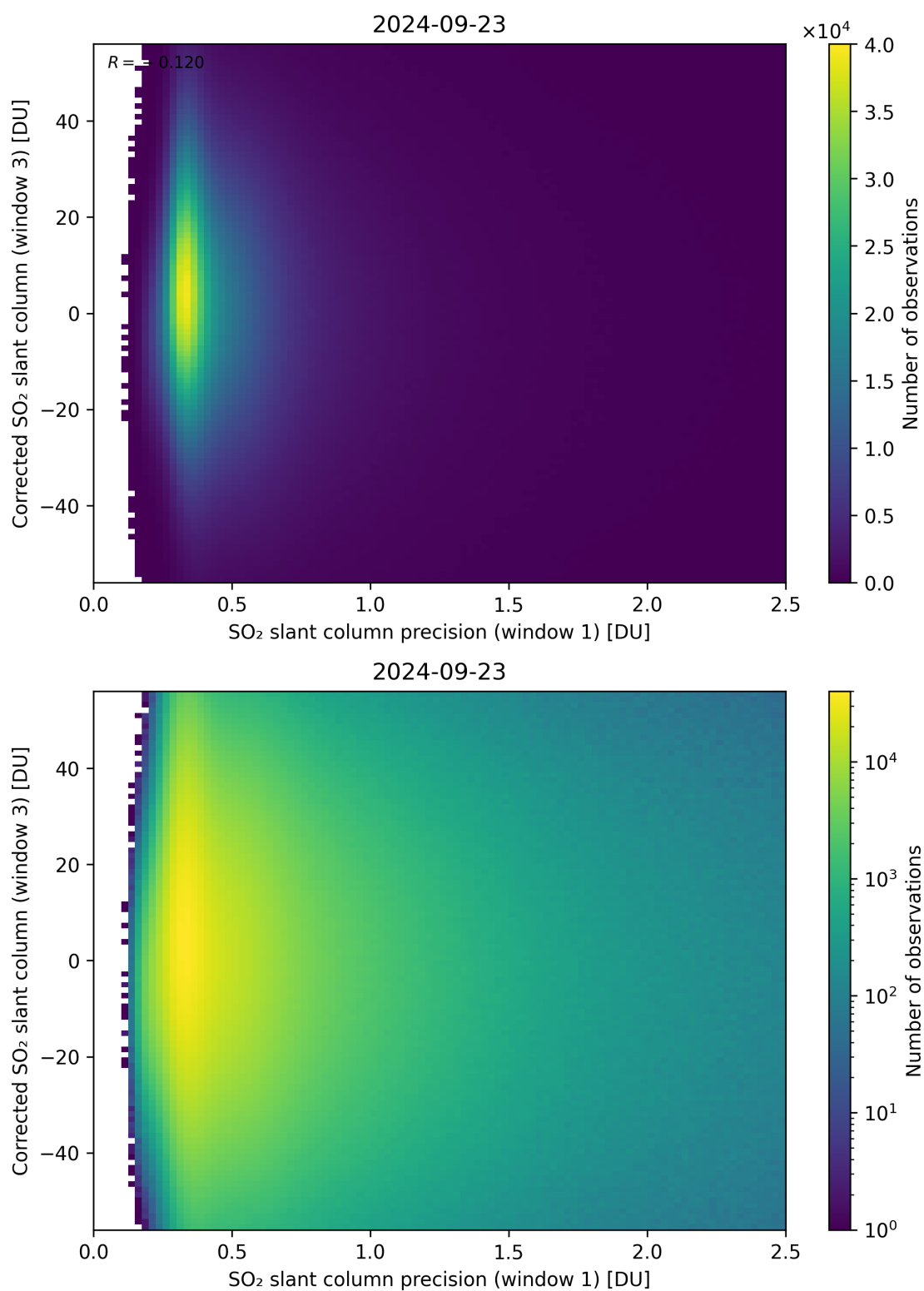
Figure 226: Scatter density plot of “SO 2 slant column precision (window 1)” against “Corrected SO 2 slant column (window 3)” for 2024-09-22 to 2024-09-24.
