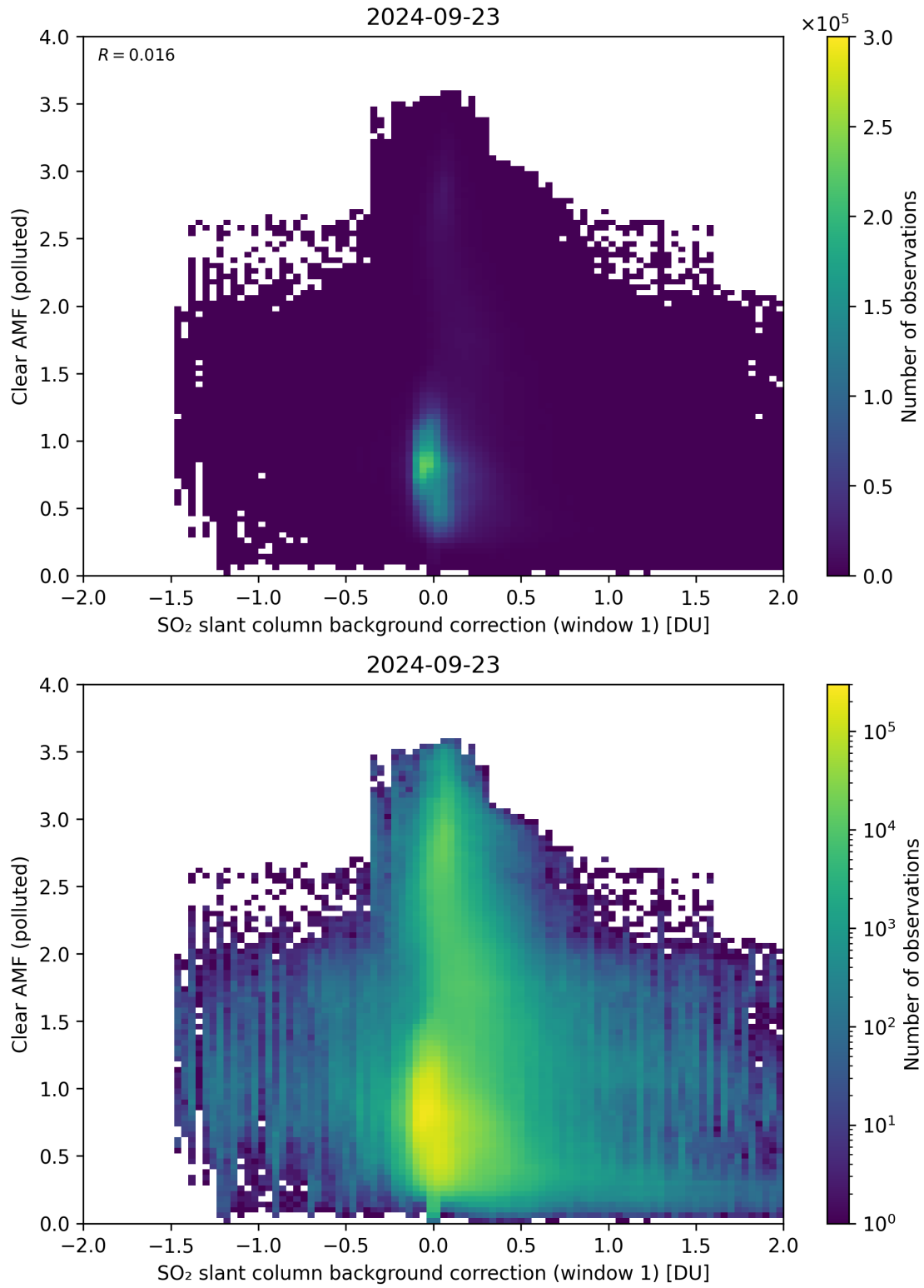
Figure 103: Scatter density plot of “SO 2 slant column background correction (window 1)” against “Clear AMF (polluted)” for 2024-09-22 to 2024-09-24.
