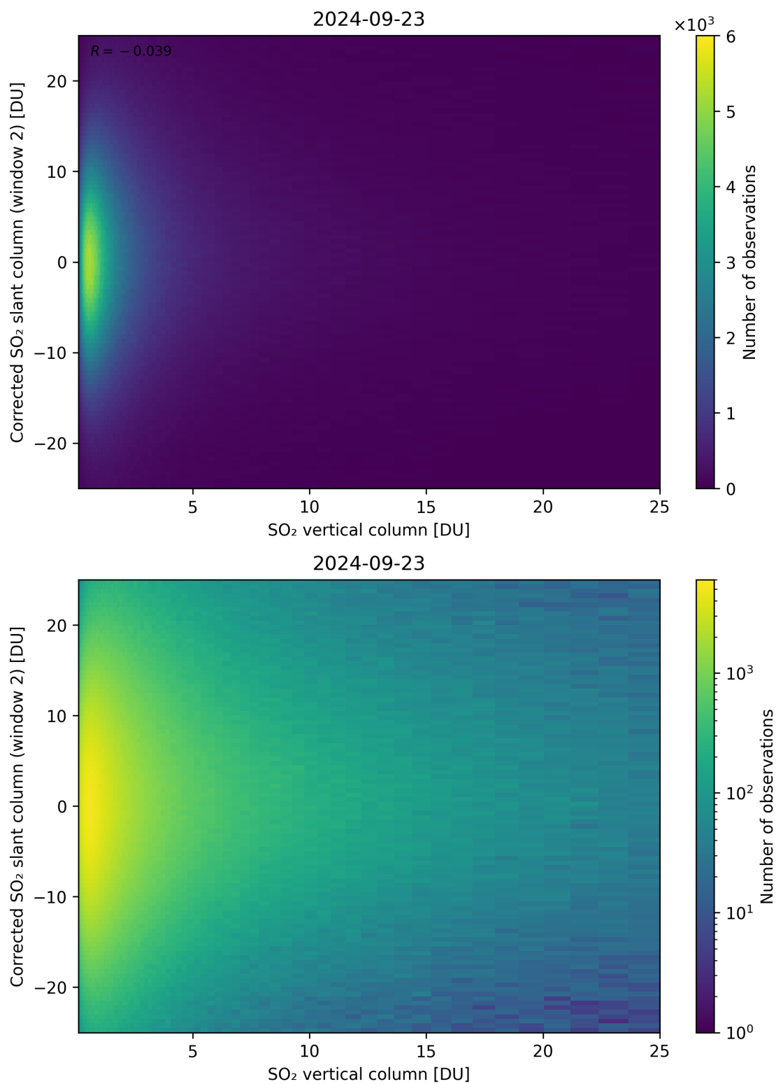
Figure 298: Scatter density plot of “SO 2 vertical column” against “Corrected SO 2 slant column (window 2)” for 2024-09-22 to 2024-09-24.
