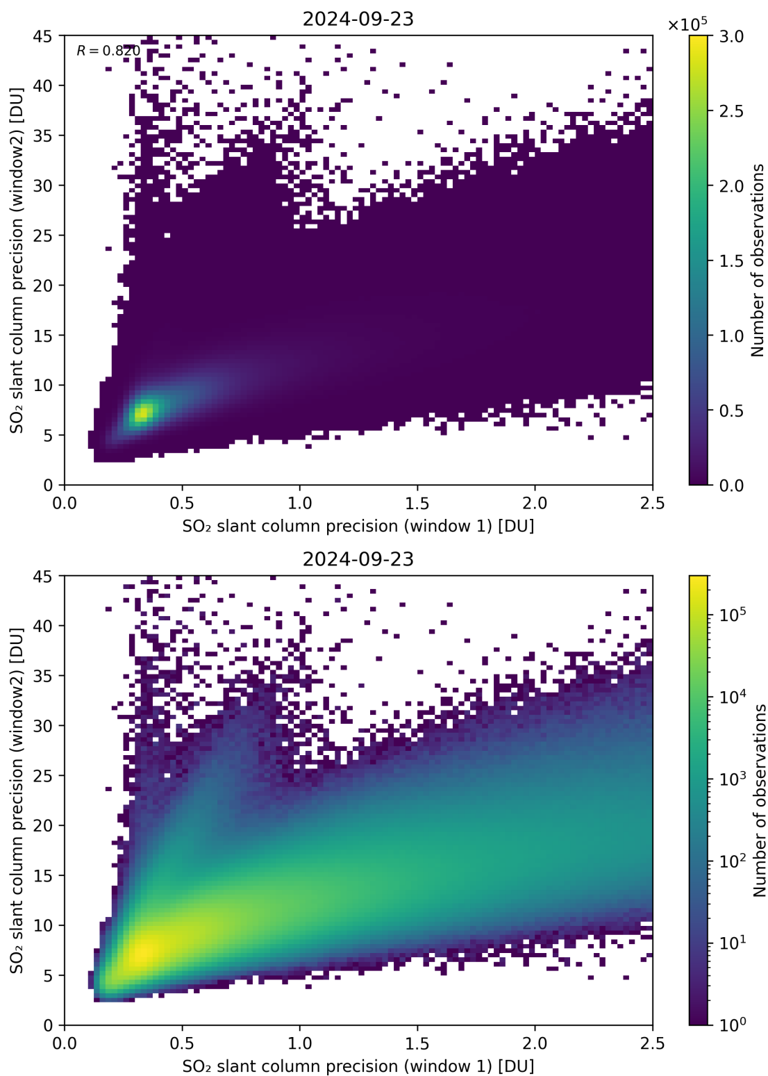
Figure 227: Scatter density plot of “SO 2 slant column precision (window 1)” against “SO 2 slant column precision (window 2)” for 2024-09-22 to 2024-09-24.
