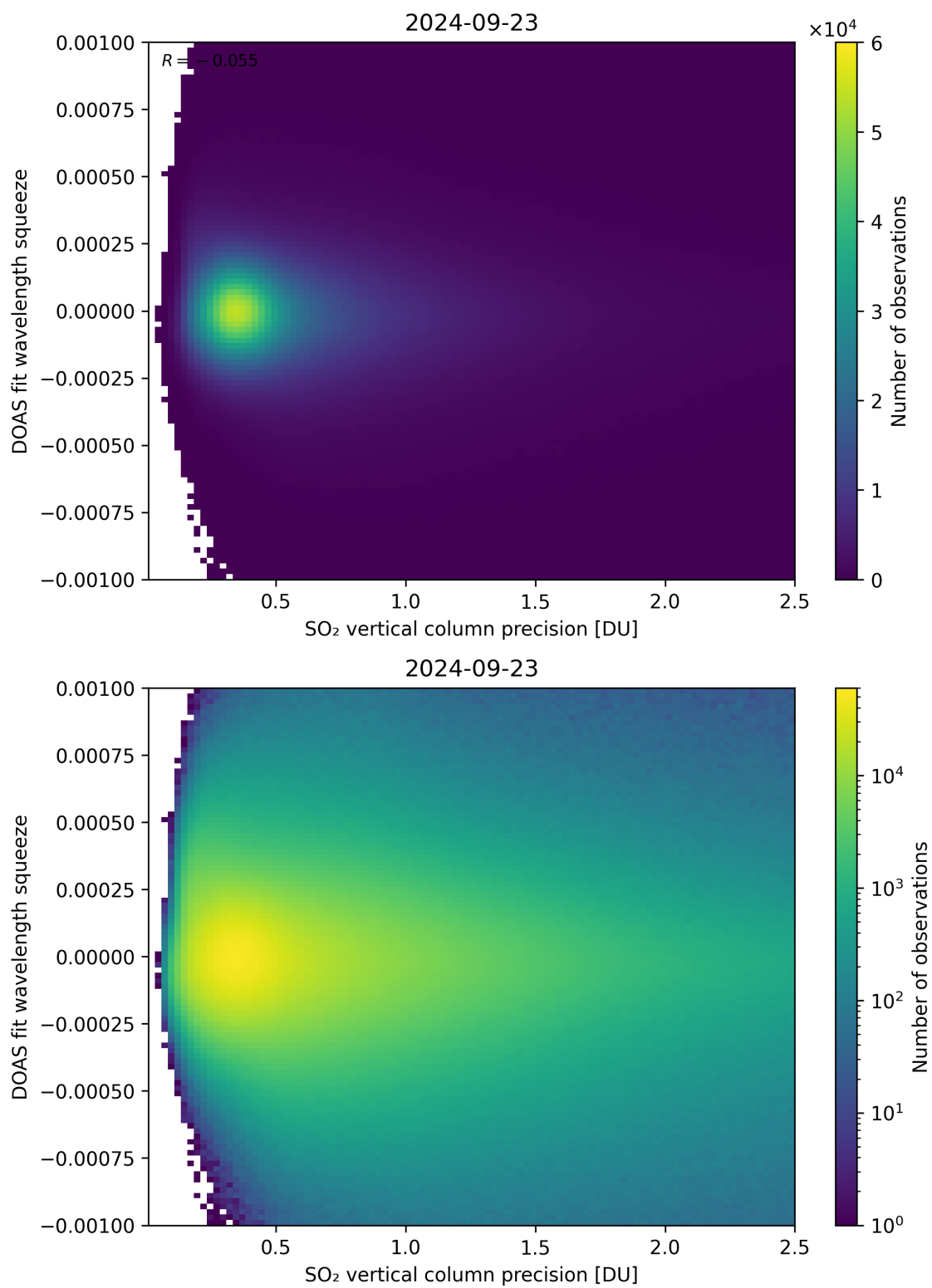
Figure 283: Scatter density plot of “SO 2 vertical column precision” against “DOAS fit wavelength squeeze” for 2024-09-22 to 2024-09-24.
