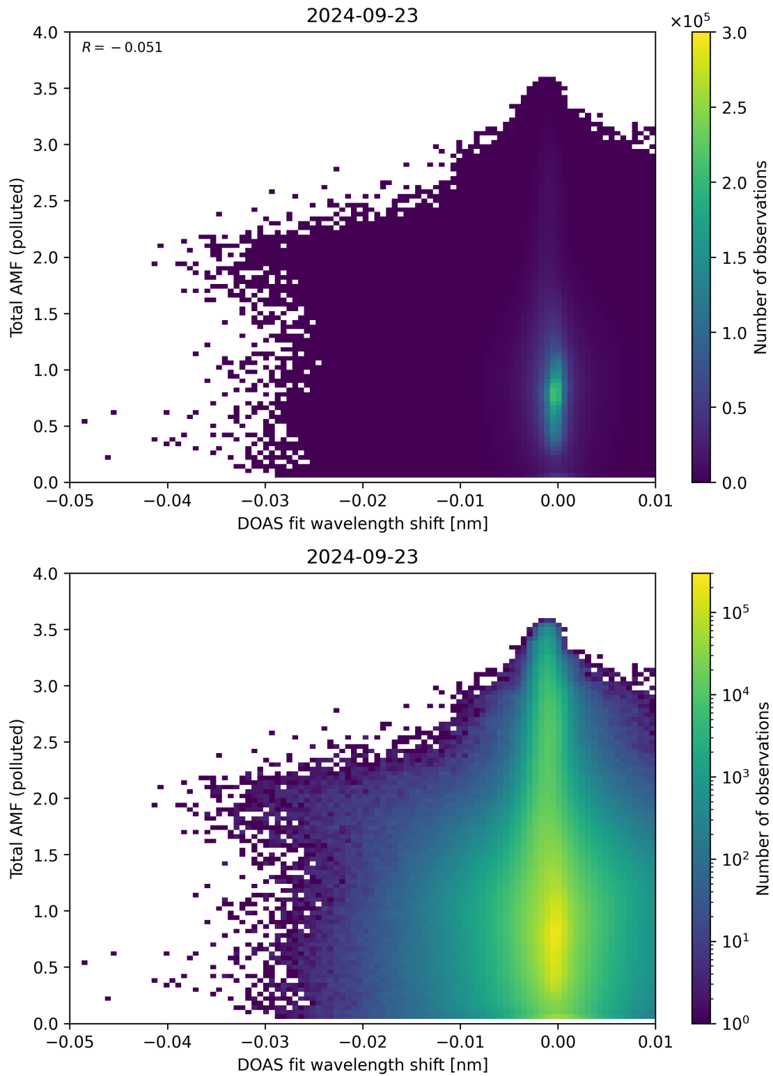
Figure 130: Scatter density plot of “DOAS fit wavelength shift” against “Total AMF (polluted)” for 2024-09-22 to 2024-09-24.
