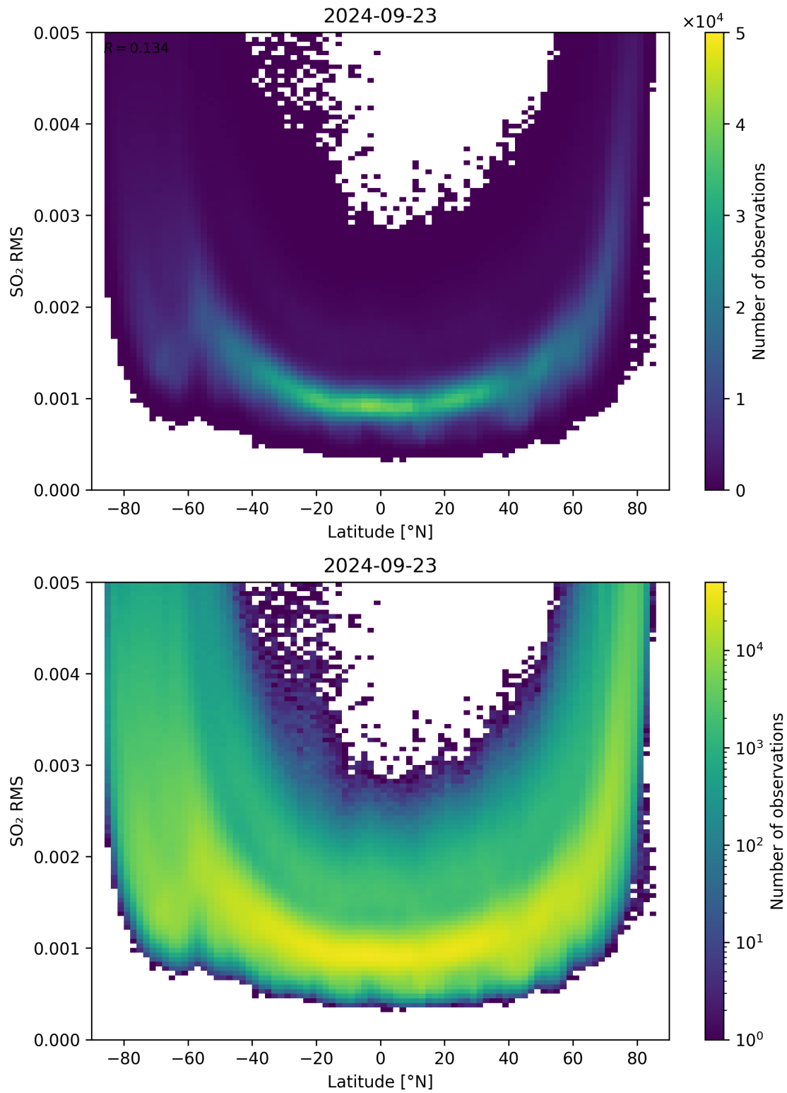
Figure 144: Scatter density plot of “Latitude” against “SO 2 RMS” for 2024-09-22 to 2024-09-24.
