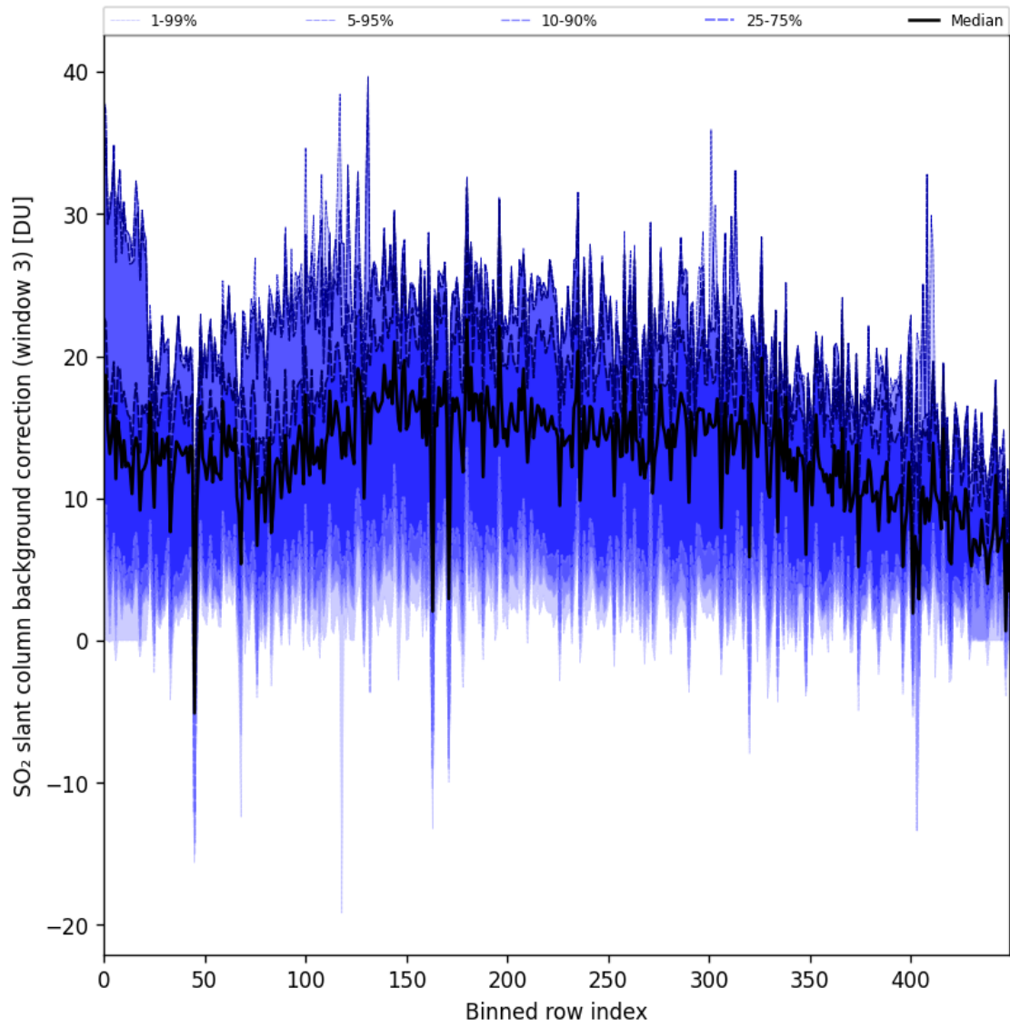
Figure 90: Along track statistics of “SO 2 slant column background correction (window 3)” for 2024-09-22 to 2024-09-24
