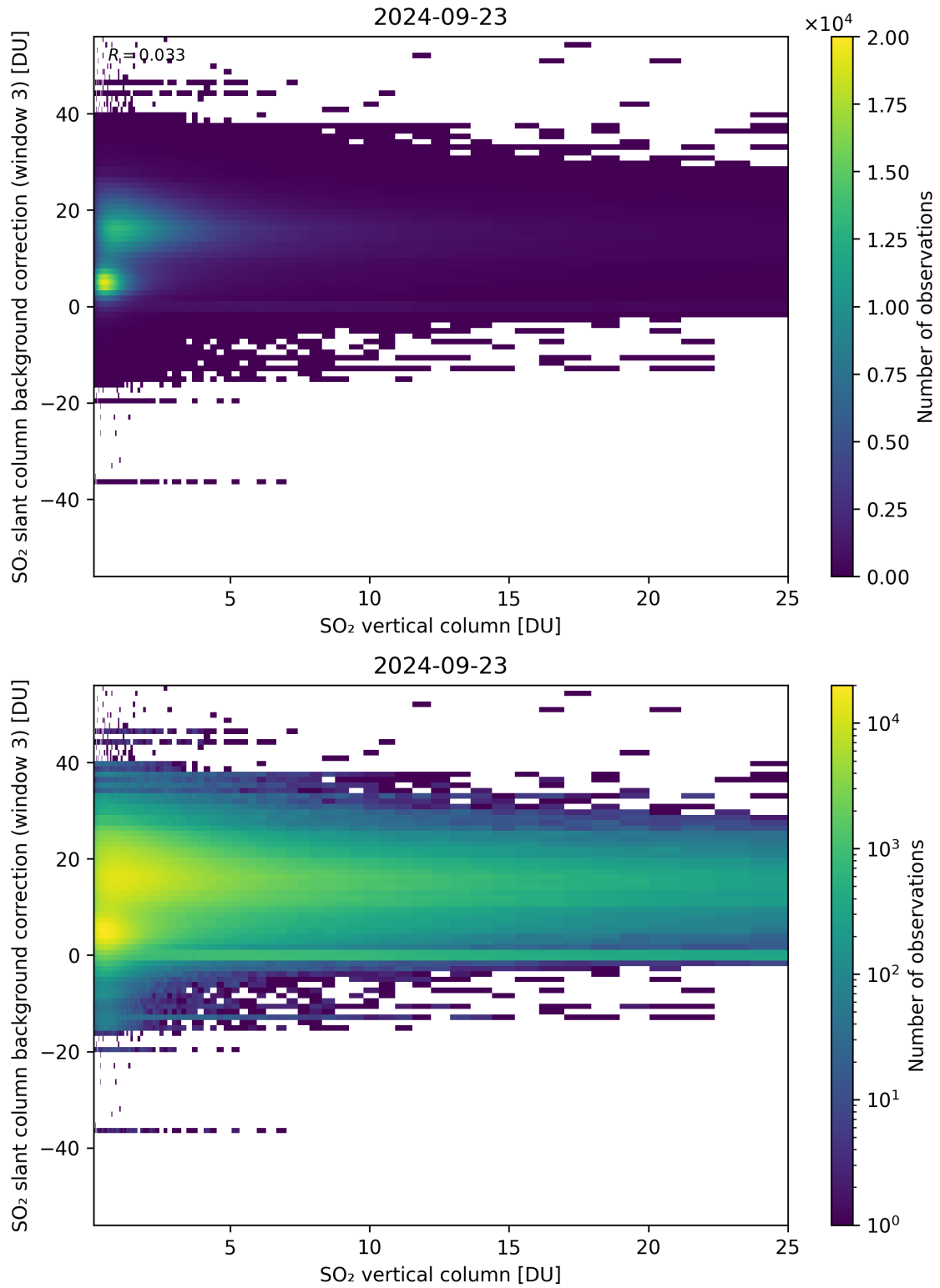
Figure 275: Scatter density plot of “SO 2 vertical column” against “SO 2 slant column background correction (window 3)” for 2024-09-22 to 2024-09-24.
