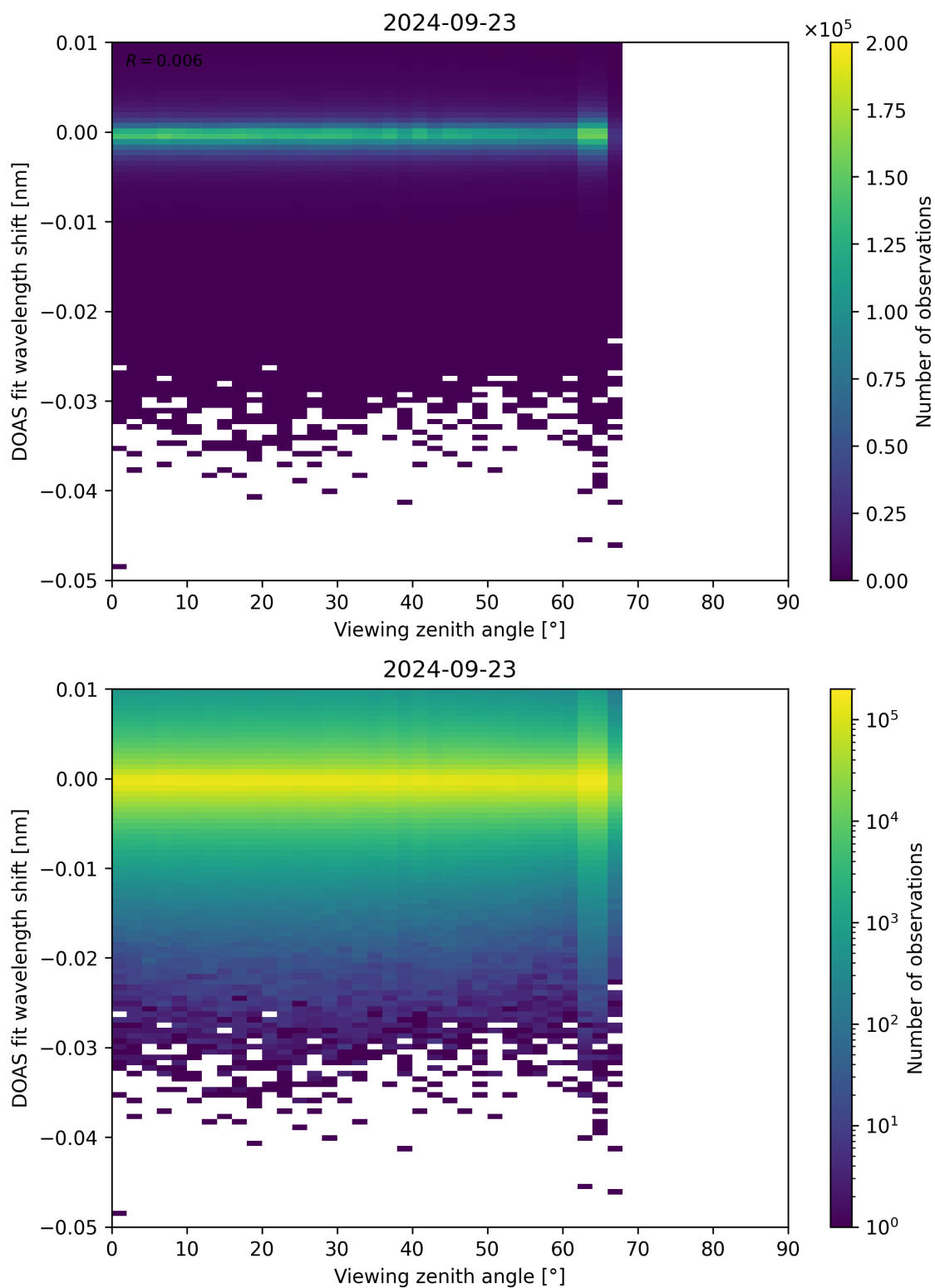
Figure 311: Scatter density plot of “Viewing zenith angle” against “DOAS fit wavelength shift” for 2024-09-22 to 2024-09-24.
