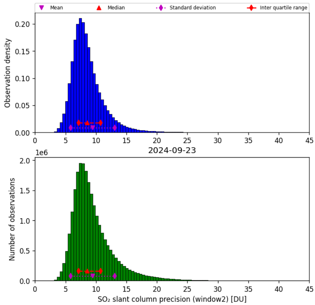
Figure 61: Histogram of “SO 2 slant column precision (window2)” for 2024-09-22 to 2024-09-24
