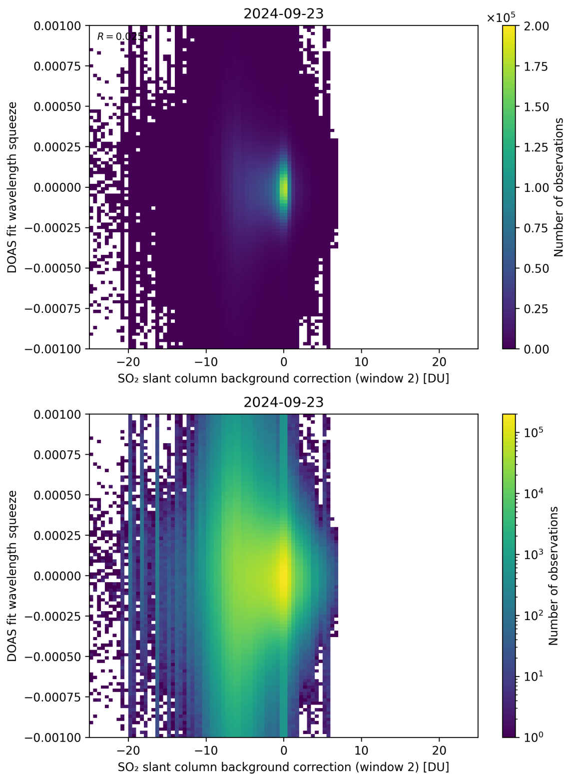
Figure 113: Scatter density plot of “SO 2 slant column background correction (window 2)” against “DOAS fit wavelength squeeze” for 2024-09-22 to 2024-09-24.
