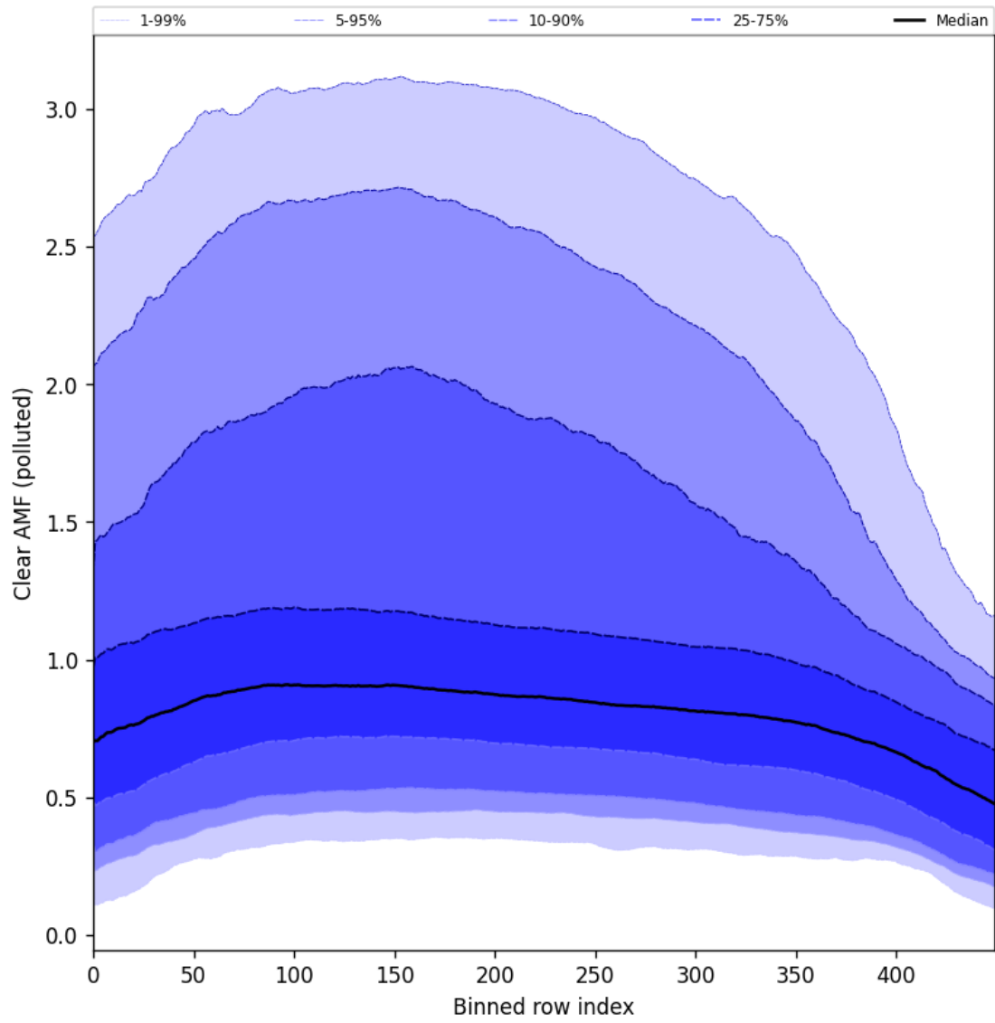
Figure 96: Along track statistics of “Clear AMF (polluted)” for 2024-09-22 to 2024-09-24
