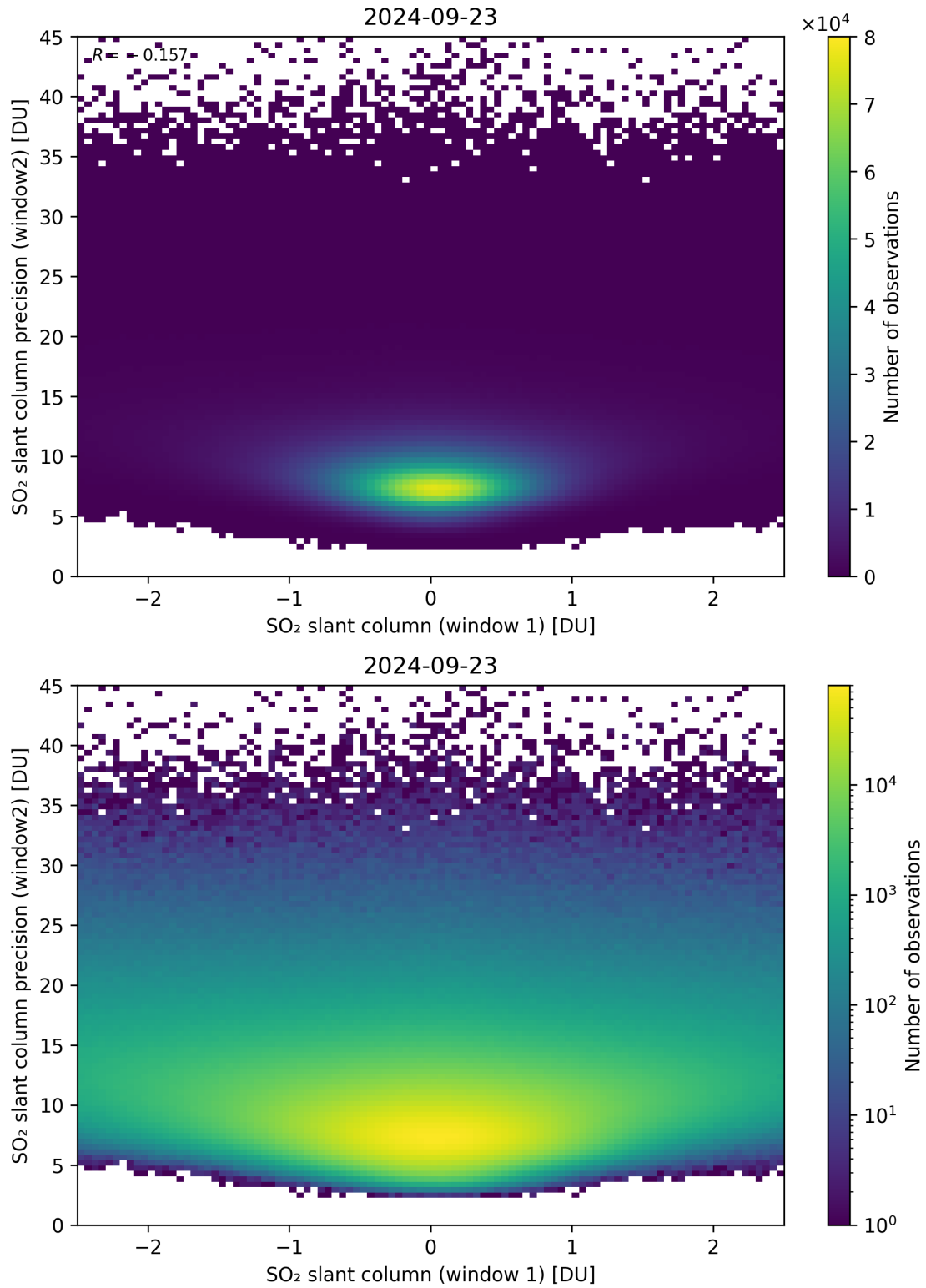
Figure 236: Scatter density plot of “SO 2 slant column (window 1)” against “SO 2 slant column precision (window2)” for 2024-09-22 to 2024-09-24.
