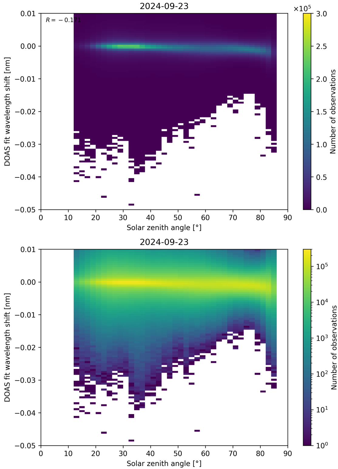
Figure 161: Scatter density plot of “Solar zenith angle” against “DOAS fit wavelength shift” for 2024-09-22 to 2024-09-24.
