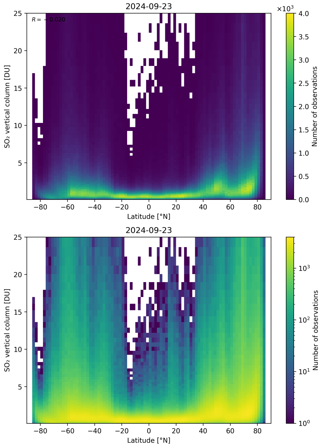
Figure 156: Scatter density plot of “Latitude” against “SO 2 vertical column” for 2024-09-22 to 2024-09-24.
