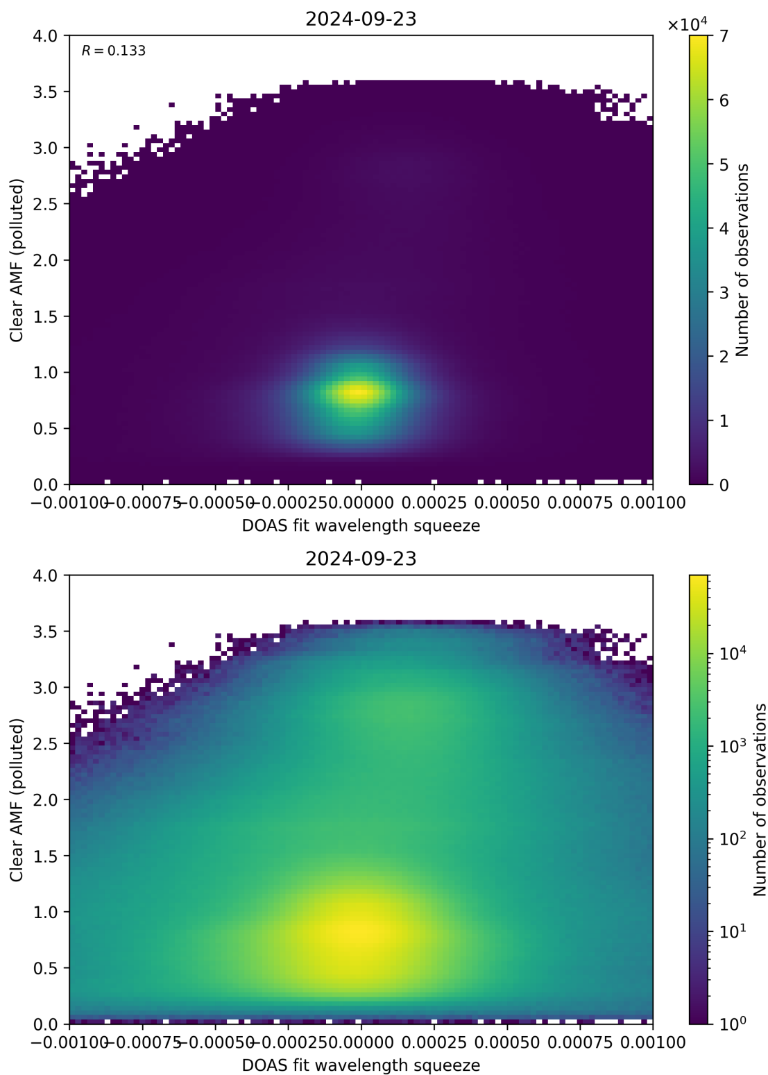
Figure 133: Scatter density plot of “DOAS fit wavelength squeeze” against “Clear AMF (polluted)” for 2024-09-22 to 2024-09-24.
