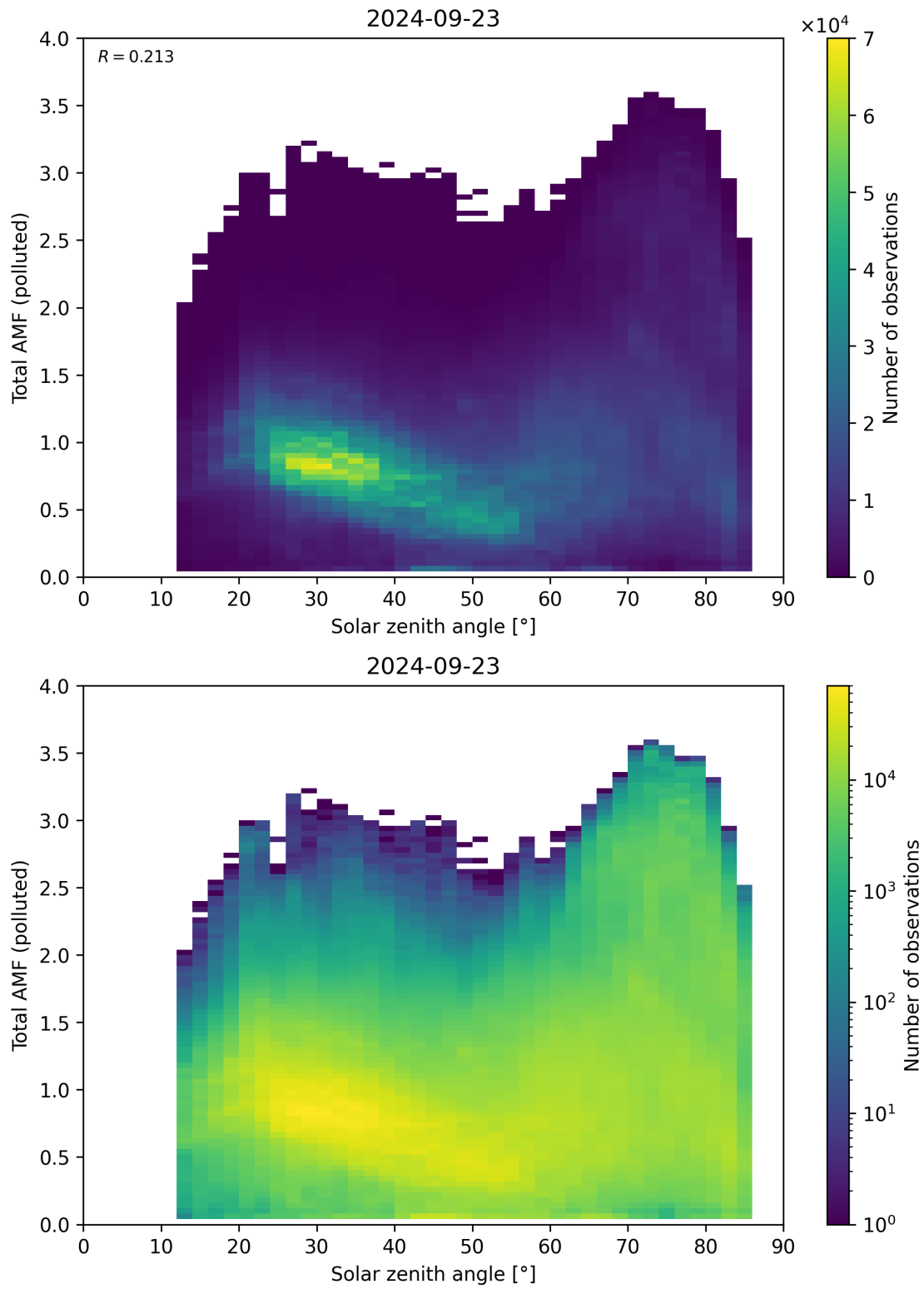
Figure 174: Scatter density plot of “Solar zenith angle” against “Total AMF (polluted)” for 2024-09-22 to 2024-09-24.
