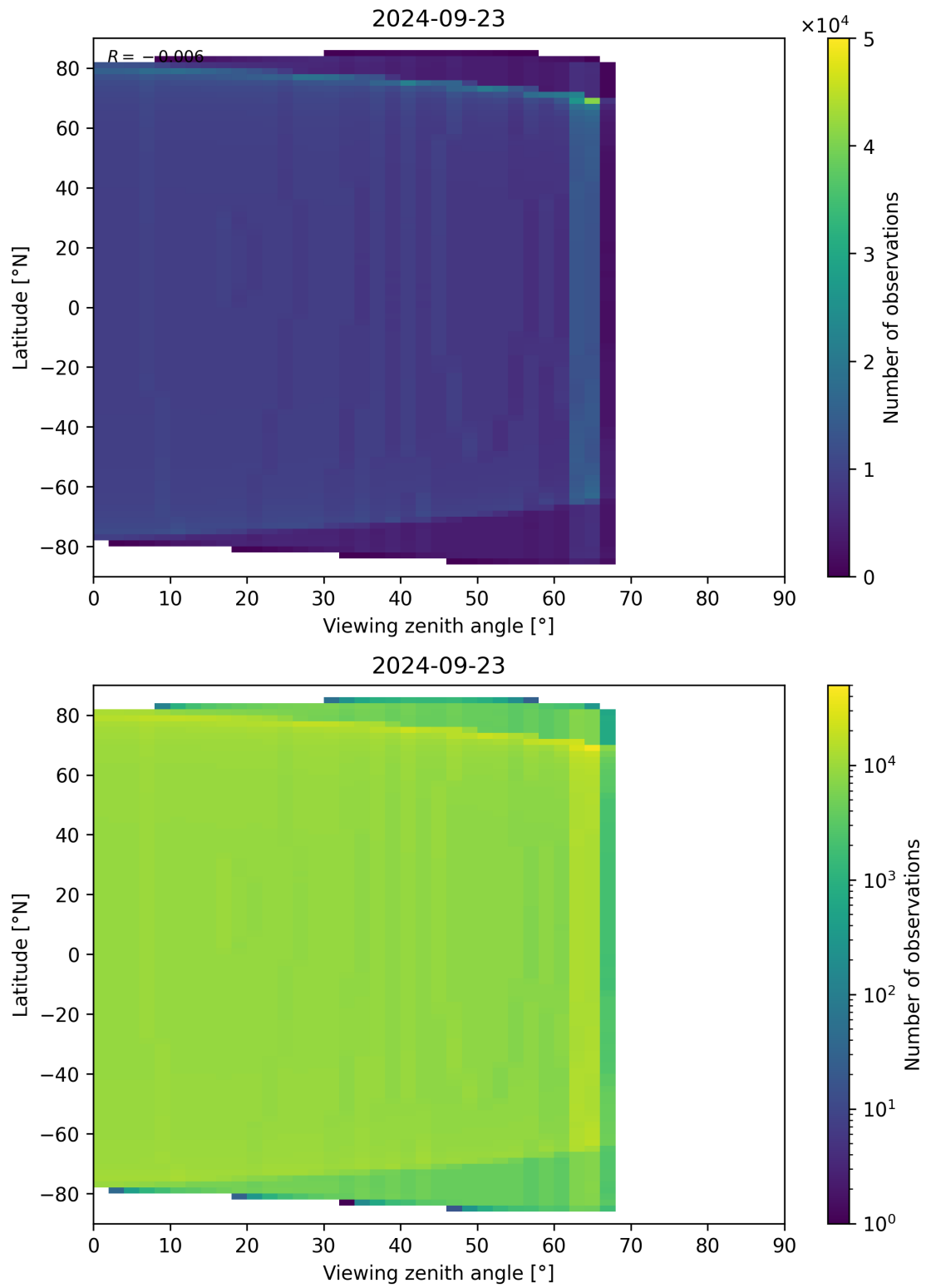
Figure 314: Scatter density plot of “Viewing zenith angle” against “Latitude” for 2024-09-22 to 2024-09-24.
