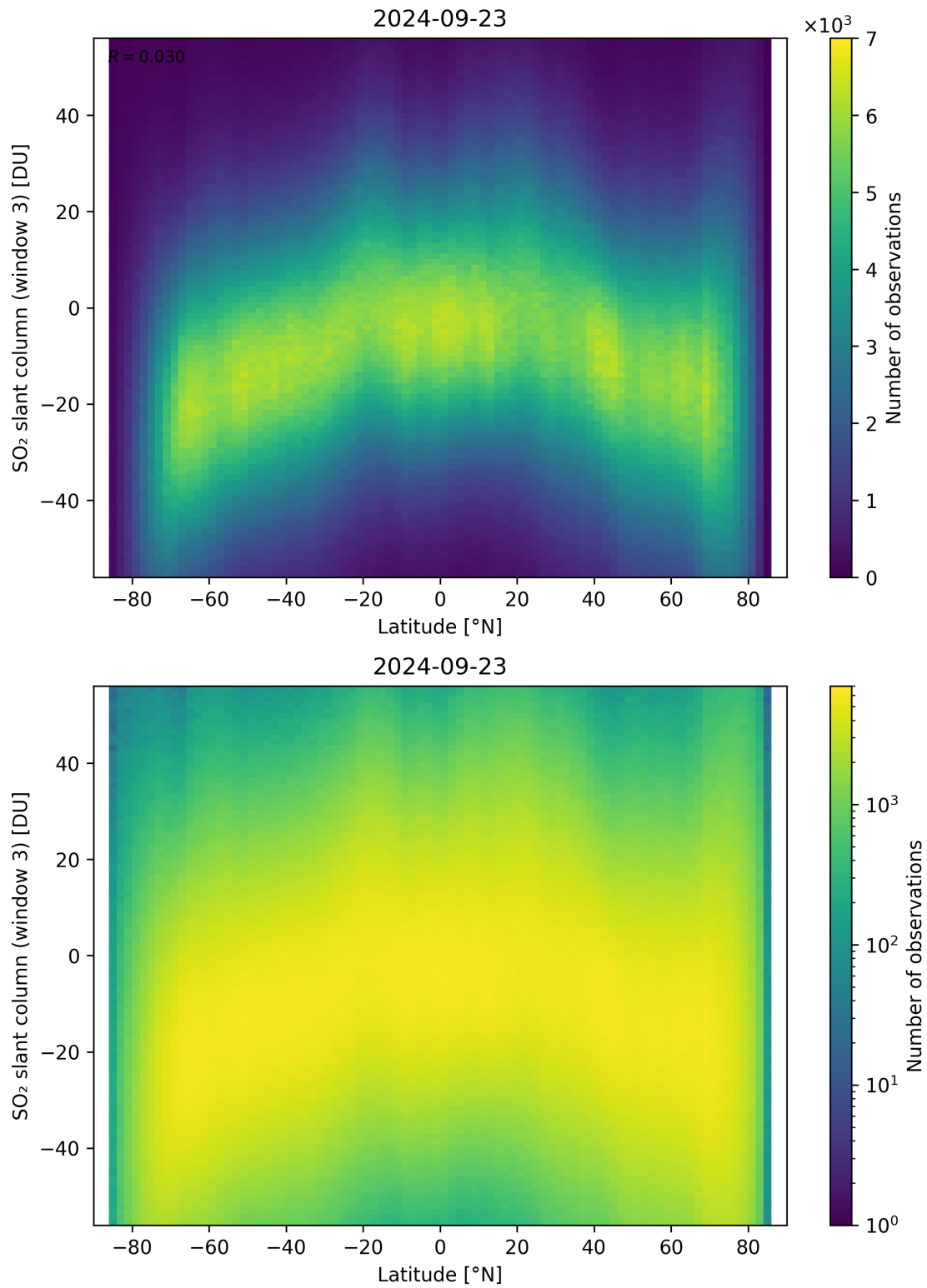
Figure 152: Scatter density plot of “Latitude” against “SO 2 slant column (window 3)” for 2024-09-22 to 2024-09-24.
