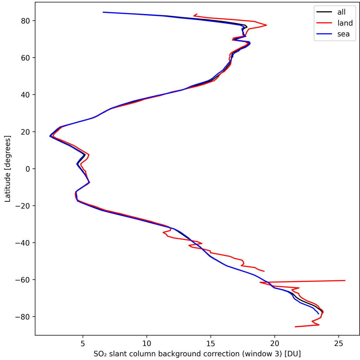
Figure 44: Zonal average of “SO 2 slant column background correction (window 3)” for 2024-09-22 to 2024-09-24.
