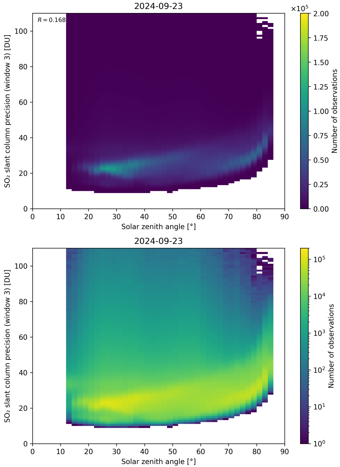
Figure 173: Scatter density plot of “Solar zenith angle” against “SO 2 slant column precision (window 3)” for 2024-09-22 to 2024-09-24.
