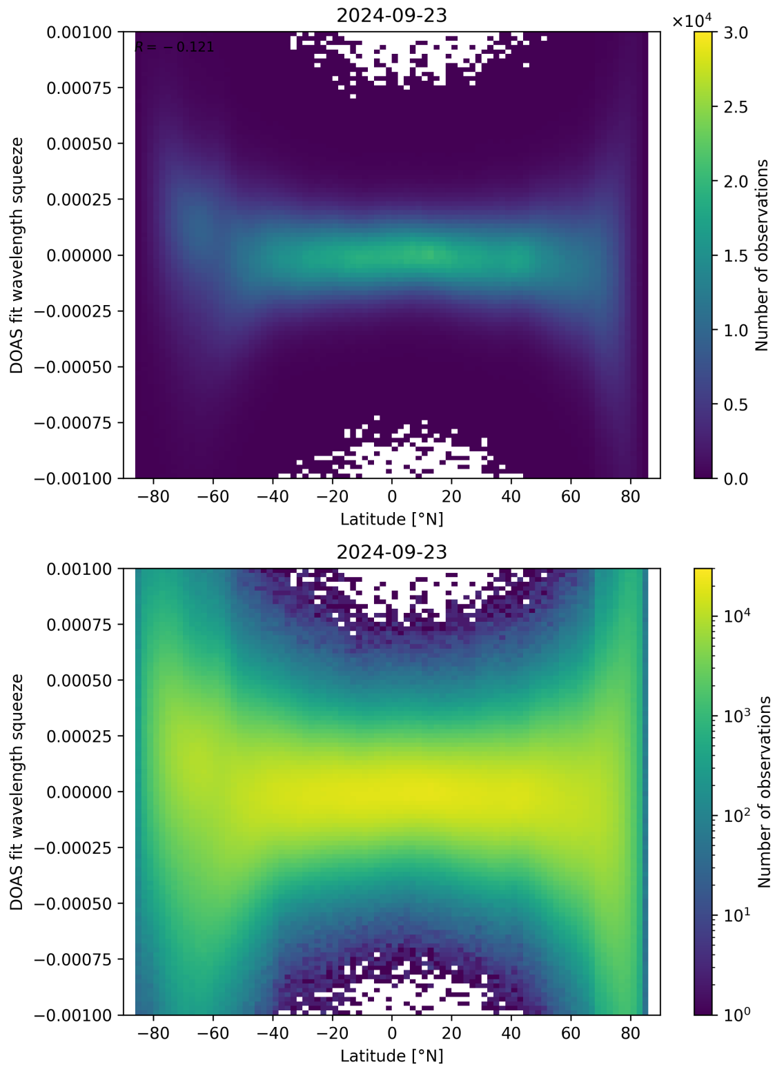
Figure 143: Scatter density plot of “Latitude” against “DOAS fit wavelength squeeze” for 2024-09-22 to 2024-09-24.
