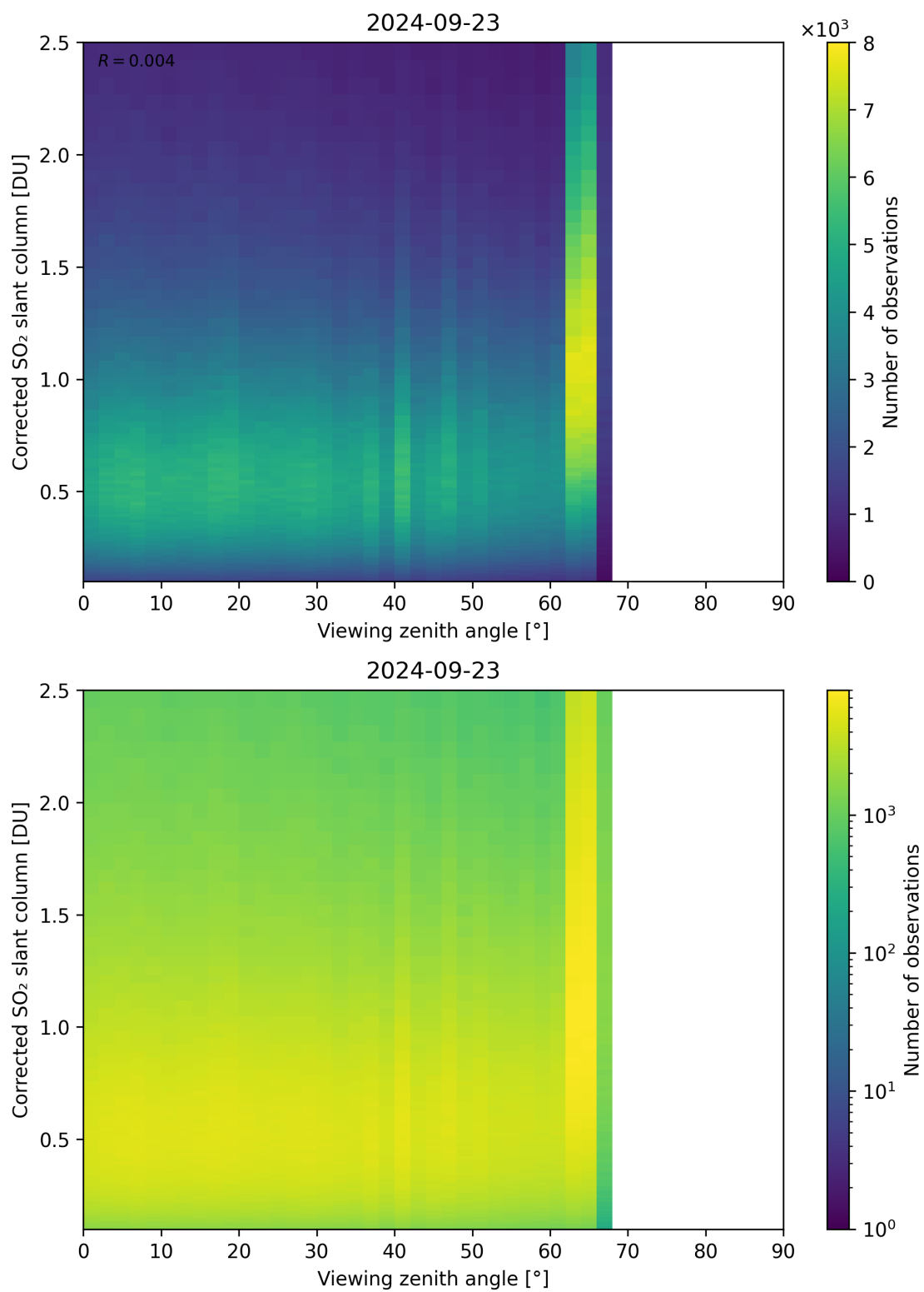
Figure 317: Scatter density plot of “Viewing zenith angle” against “Corrected SO 2 slant column” for 2024-09-22 to 2024-09-24.
