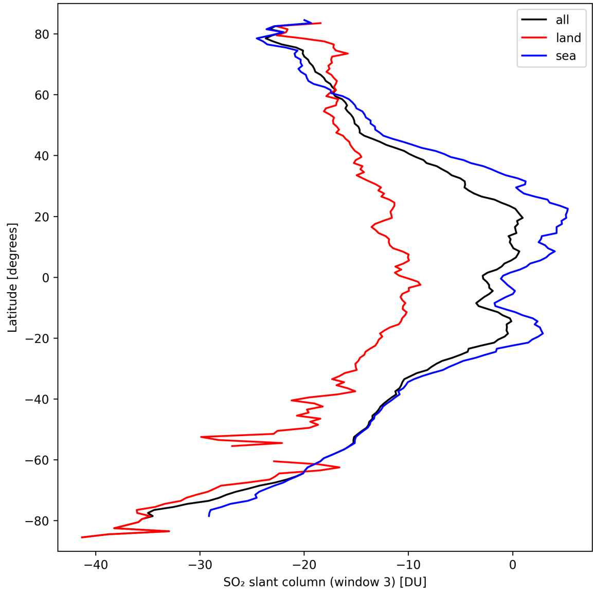
Figure 41: Zonal average of “SO 2 slant column (window 3)” for 2024-09-22 to 2024-09-24.
