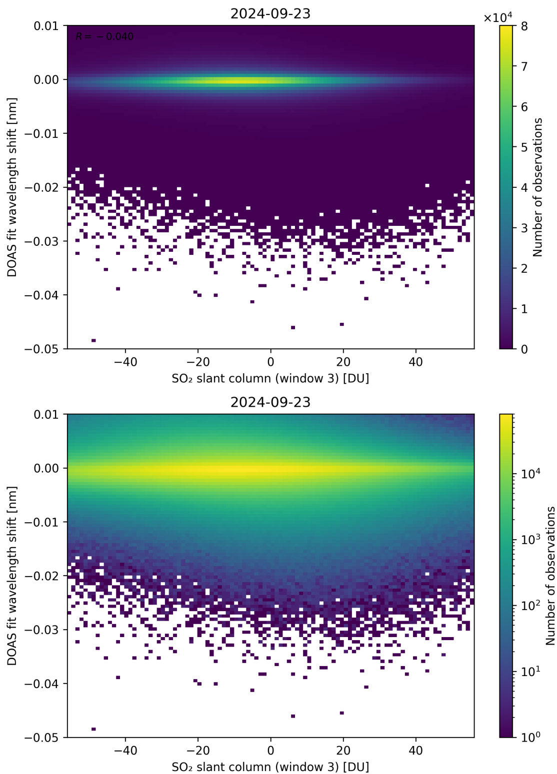
Figure 254: Scatter density plot of “SO 2 slant column (window 3)” against “DOAS fit wavelength shift” for 2024-09-22 to 2024-09-24.
