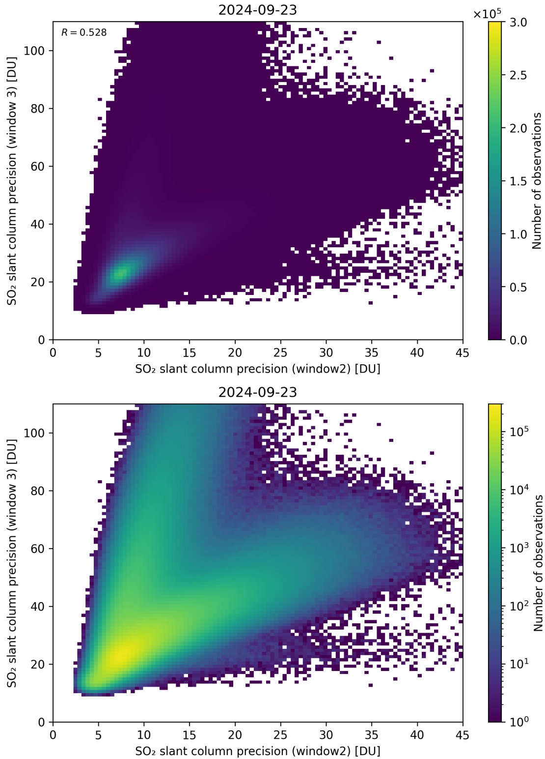
Figure 250: Scatter density plot of “SO 2 slant column precision (window2)” against “SO 2 slant column precision (window 3)” for 2024-09-22 to 2024-09-24.
