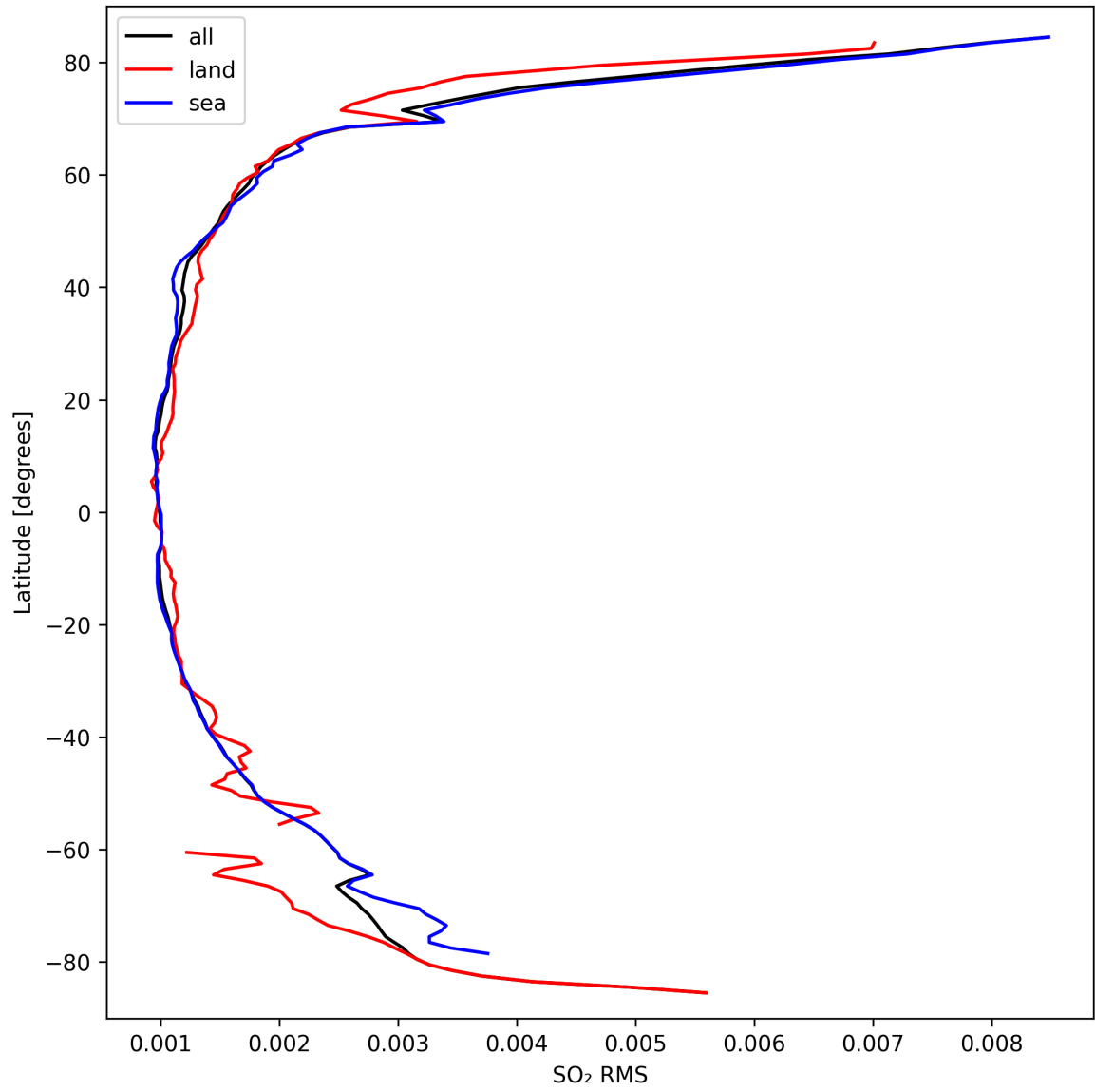
Figure 47: Zonal average of “SO 2 RMS” for 2024-09-22 to 2024-09-24.
