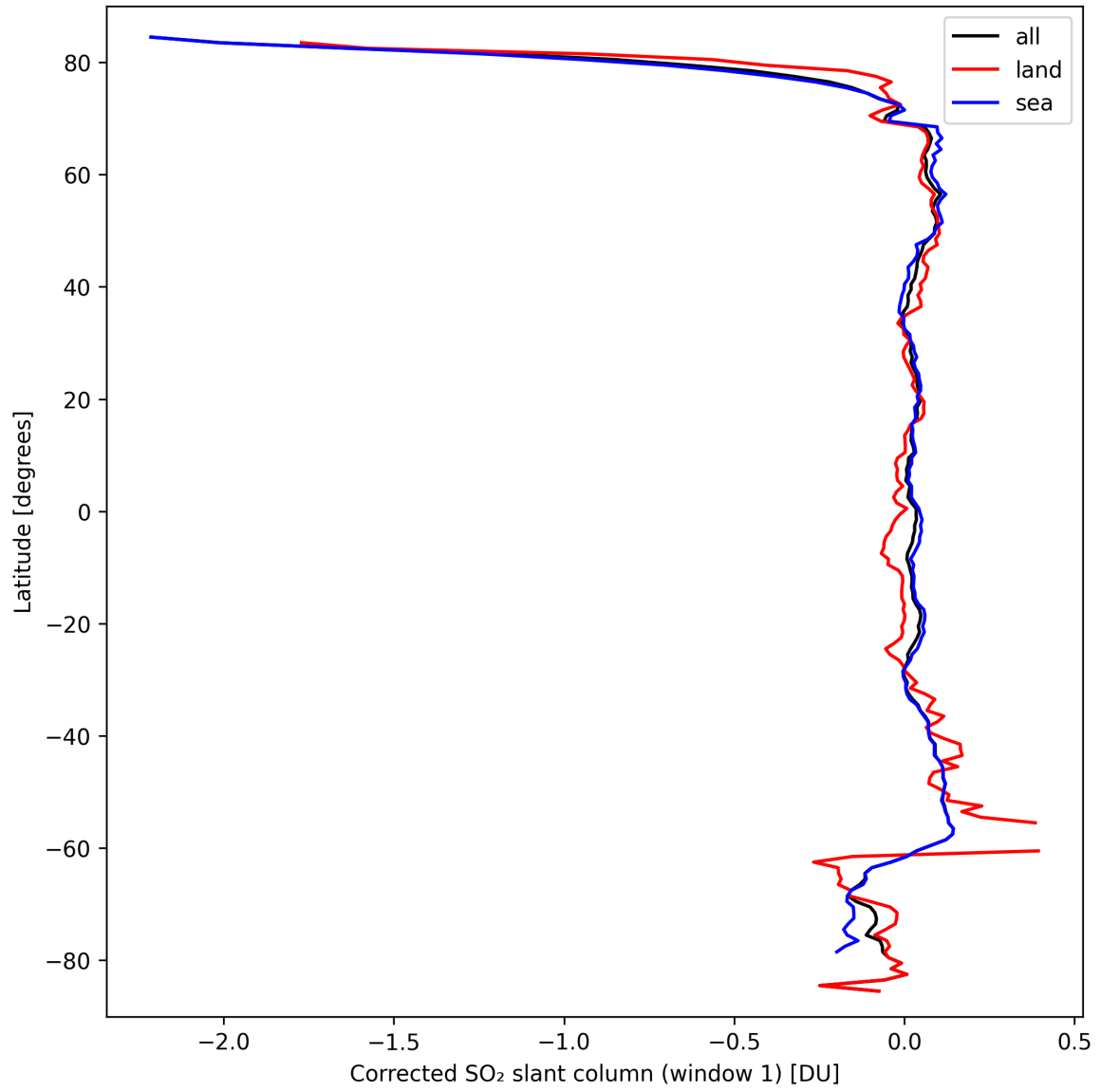
Figure 35: Zonal average of “Corrected SO 2 slant column (window 1)” for 2024-09-22 to 2024-09-24.
