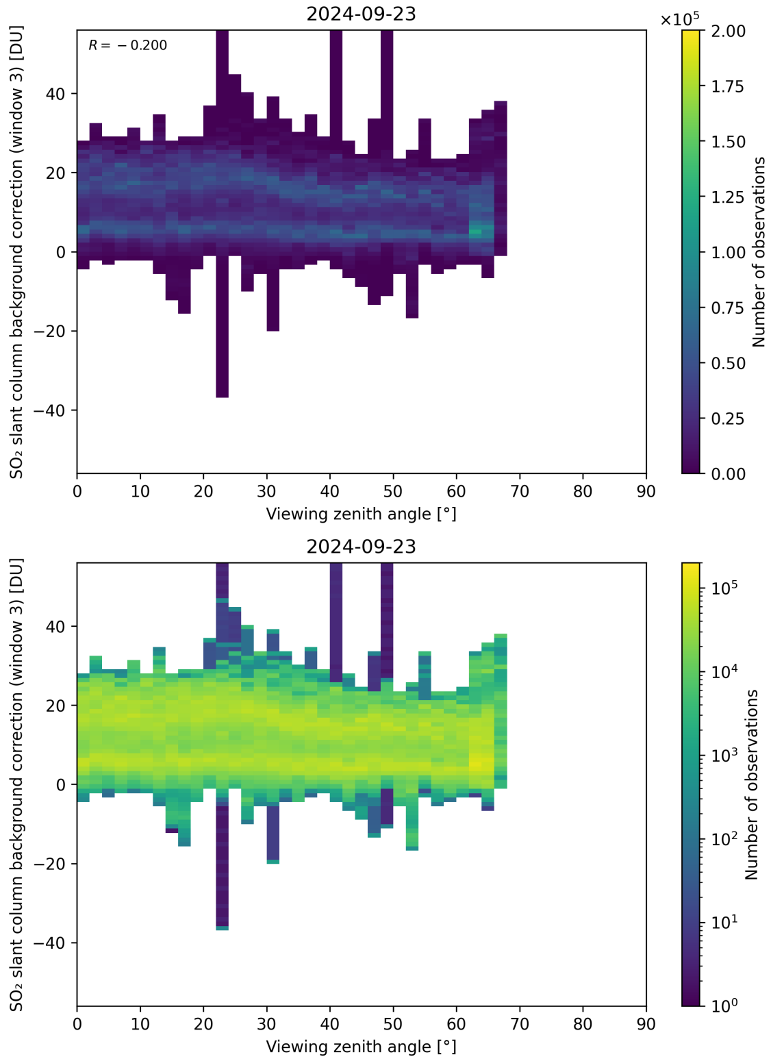
Figure 310: Scatter density plot of “Viewing zenith angle” against “SO 2 slant column background correction (window 3)” for 2024-09-22 to 2024-09-24.
