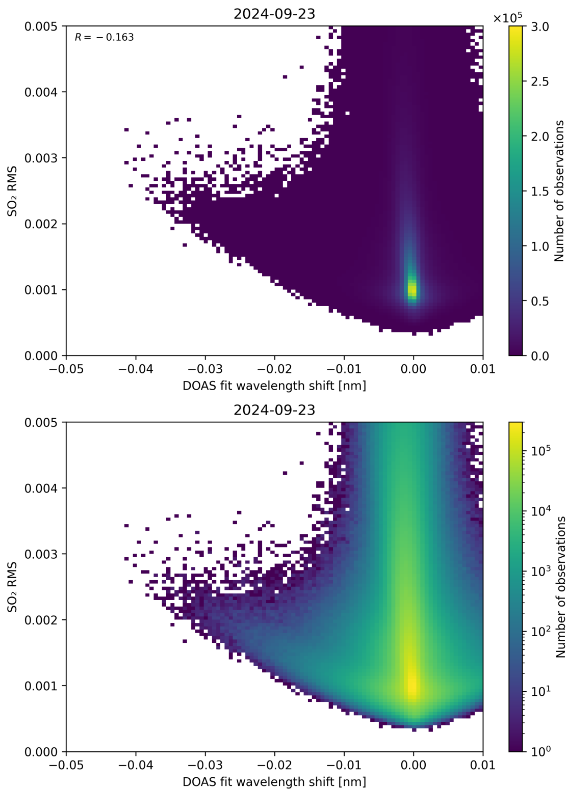
Figure 128: Scatter density plot of “DOAS fit wavelength shift” against “SO 2 RMS” for 2024-09-22 to 2024-09-24.
