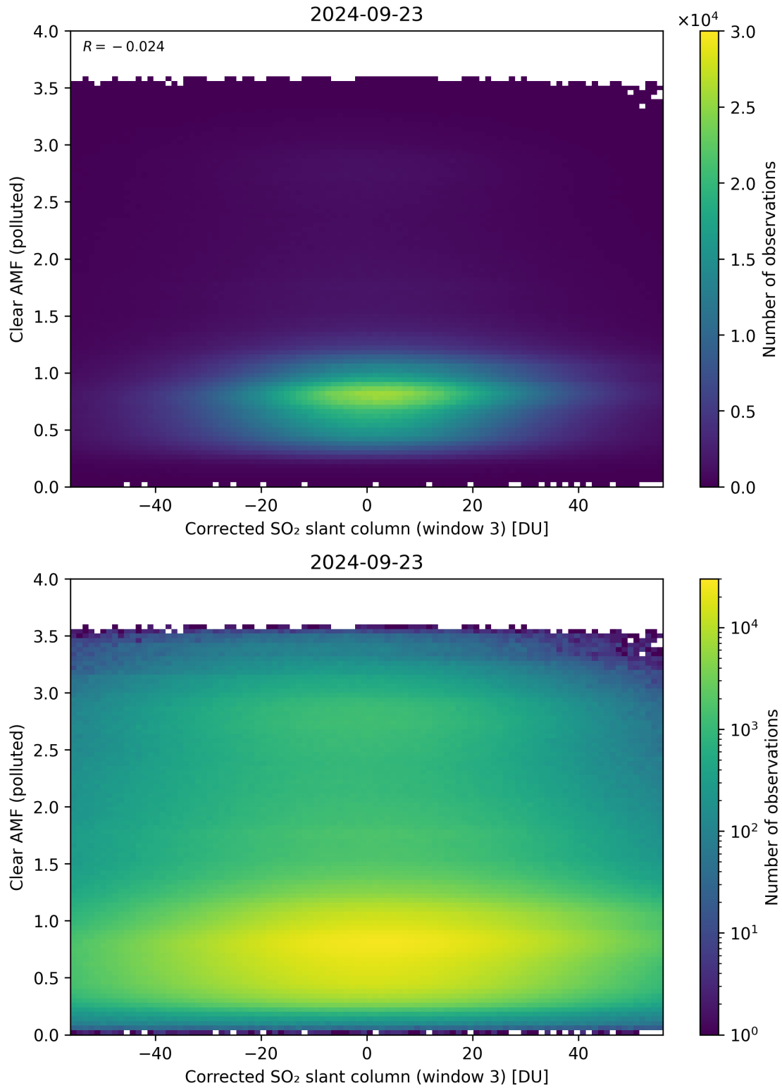
Figure 209: Scatter density plot of “Corrected SO 2 slant column (window 3)” against “Clear AMF (polluted)” for 2024-09-22 to 2024-09-24.
