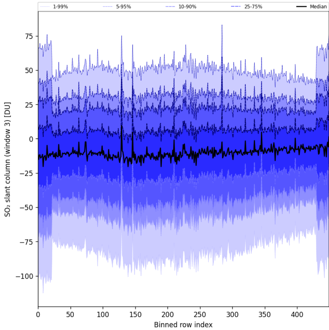
Figure 87: Along track statistics of “SO 2 slant column (window 3)” for 2024-09-22 to 2024-09-24
