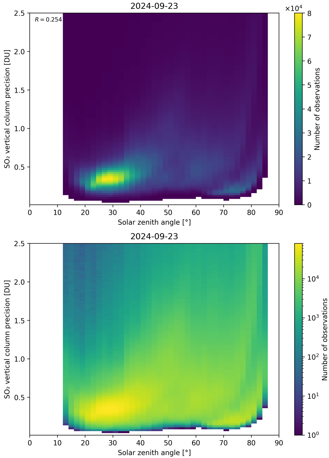
Figure 177: Scatter density plot of “Solar zenith angle” against “SO 2 vertical column precision” for 2024-09-22 to 2024-09-24.
