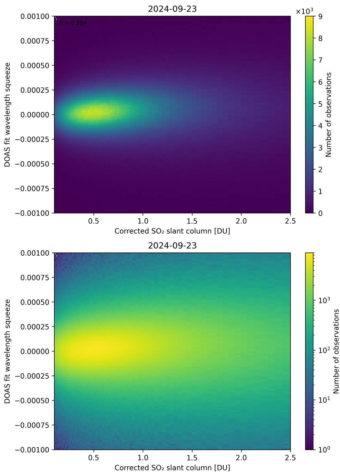
Figure 182: Scatter density plot of “Corrected SO 2 slant column” against “DOAS fit wavelength squeeze” for 2024-09-22 to 2024-09-24.
