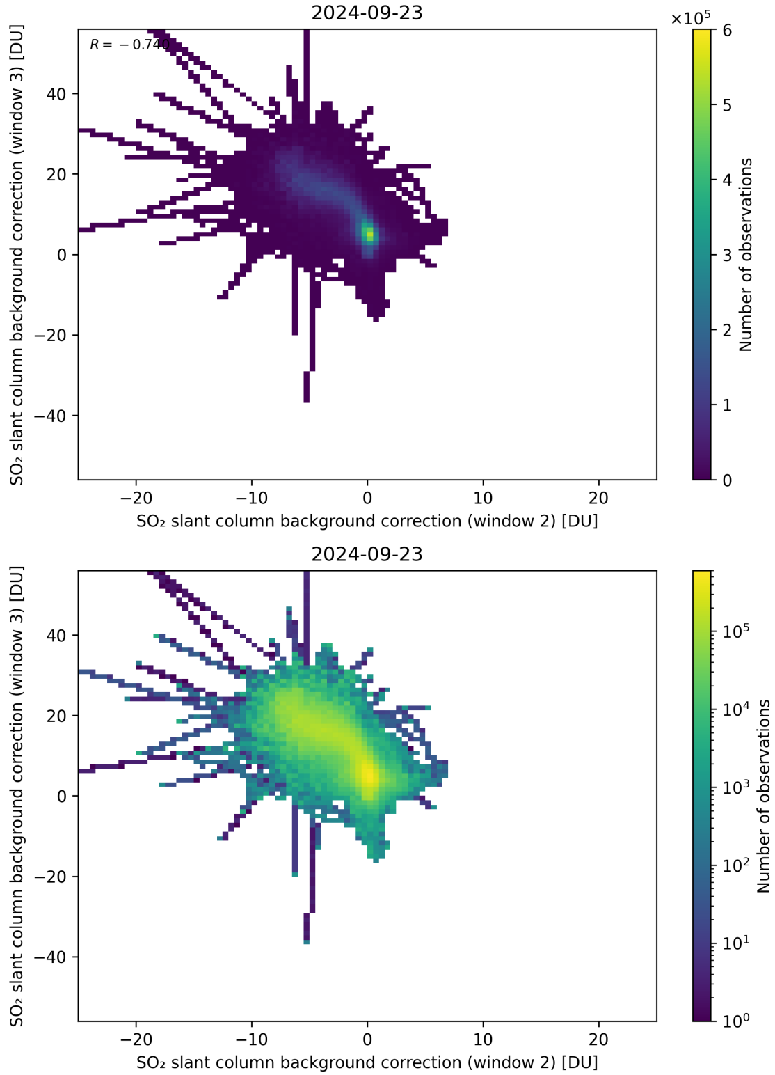
Figure 111: Scatter density plot of “SO 2 slant column background correction (window 2)” against “SO 2 slant column background correction (window 3)” for 2024-09-22 to 2024-09-24.
