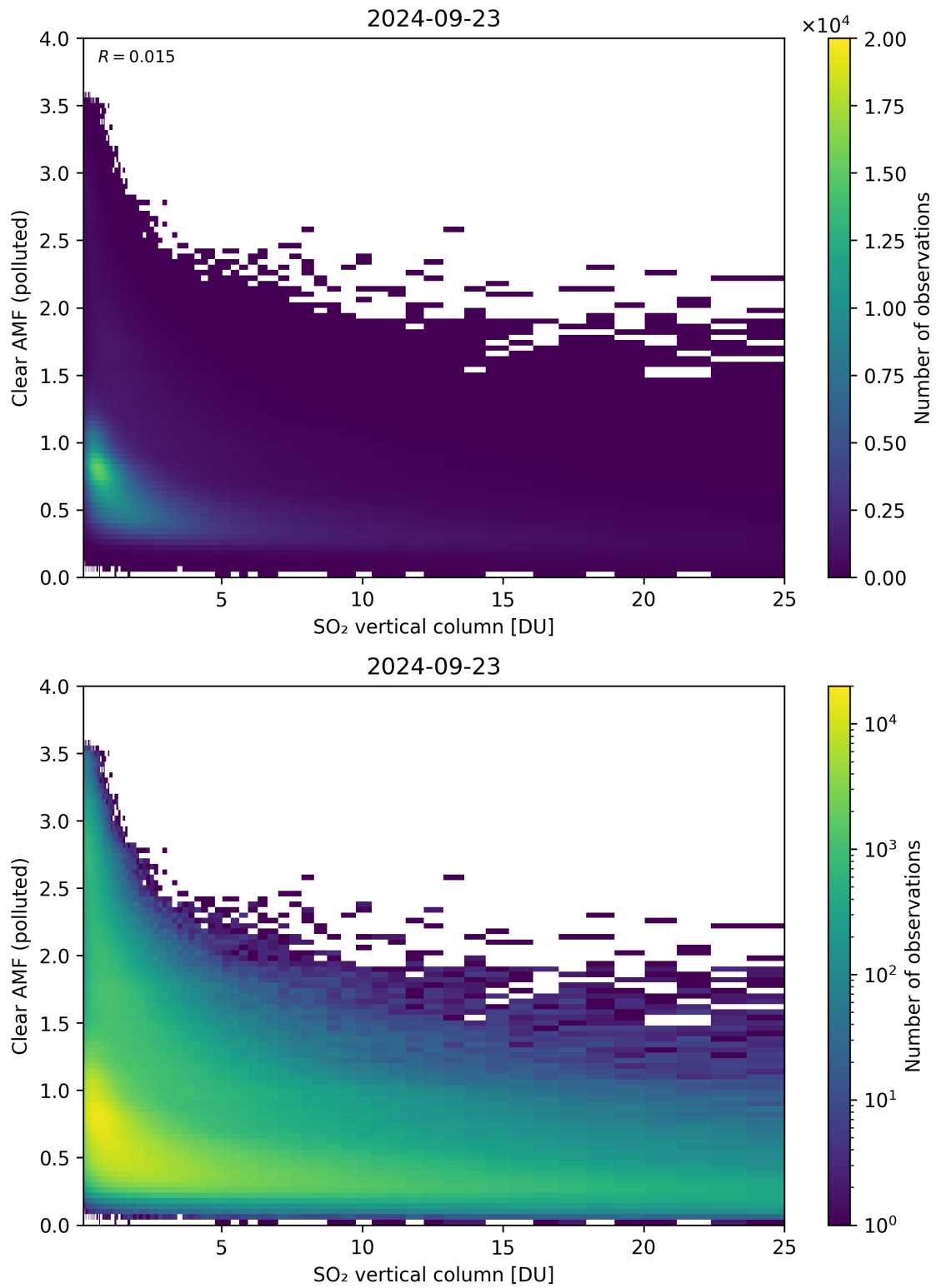
Figure 296: Scatter density plot of “SO 2 vertical column” against “Clear AMF (polluted)” for 2024-09-22 to 2024-09-24.
