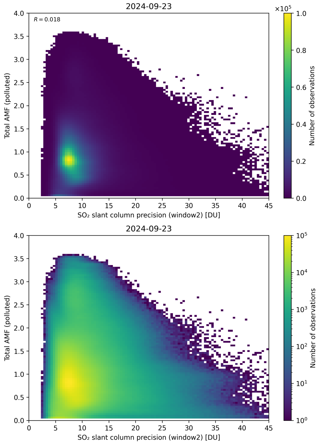
Figure 251: Scatter density plot of “SO 2 slant column precision (window2)” against “Total AMF (polluted)” for 2024-09-22 to 2024-09-24.
