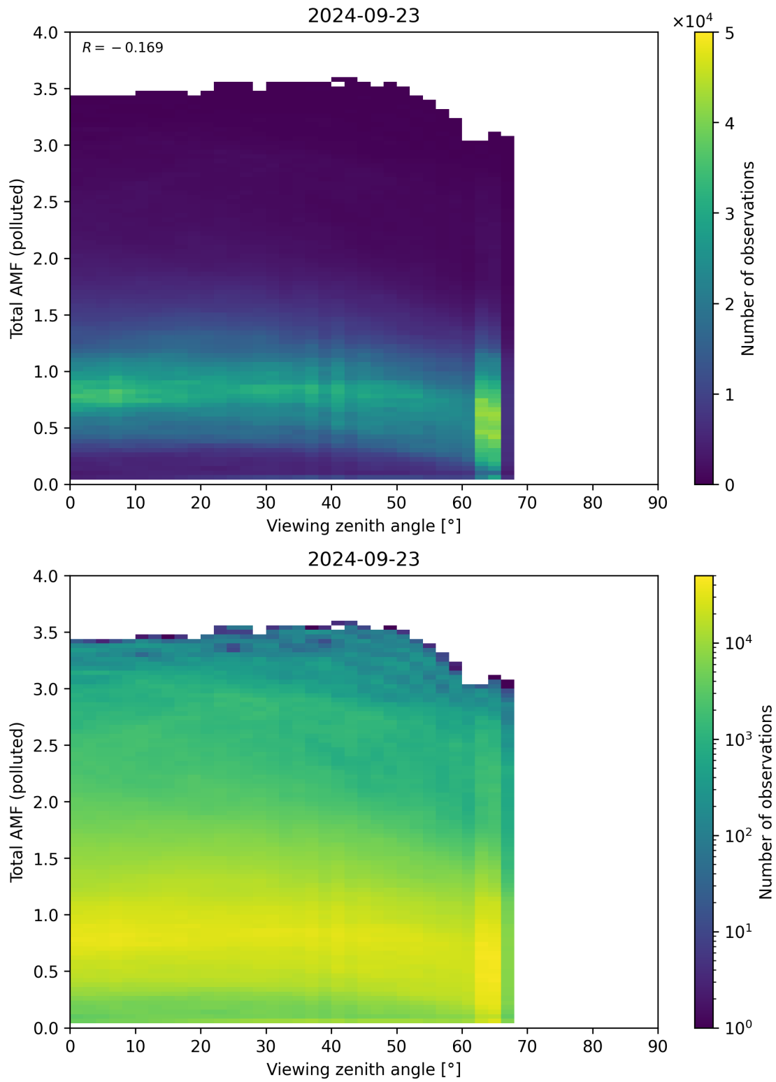
Figure 325: Scatter density plot of “Viewing zenith angle” against “Total AMF (polluted)” for 2024-09-22 to 2024-09-24.
