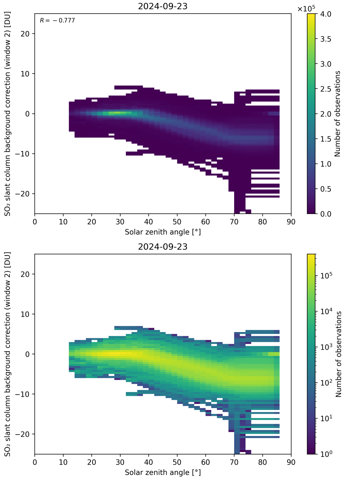
Figure 159: Scatter density plot of “Solar zenith angle” against “SO 2 slant column background correction (window 2)” for 2024-09-22 to 2024-09-24.
