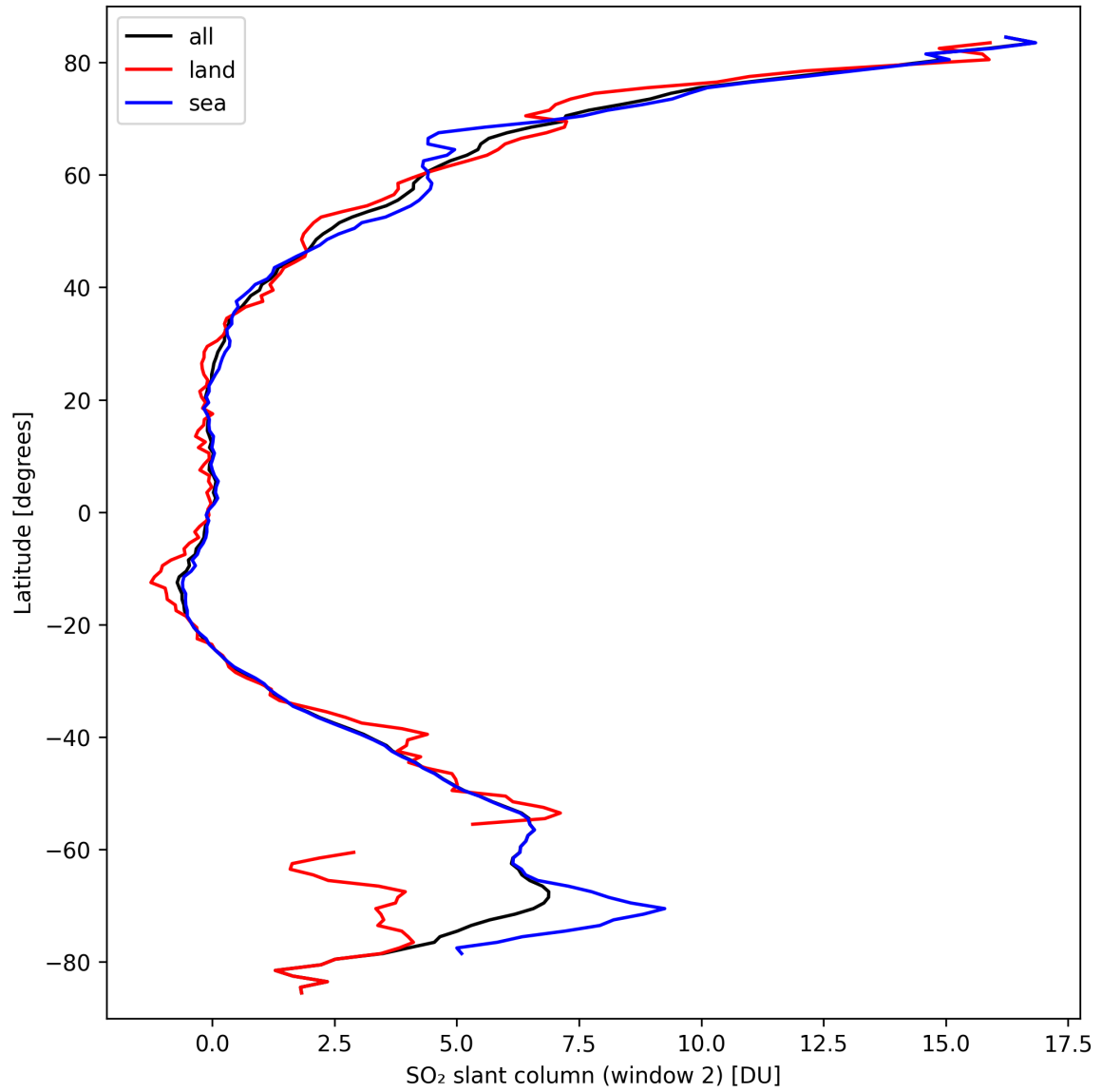
Figure 37: Zonal average of “SO 2 slant column (window 2)” for 2024-09-22 to 2024-09-24.
