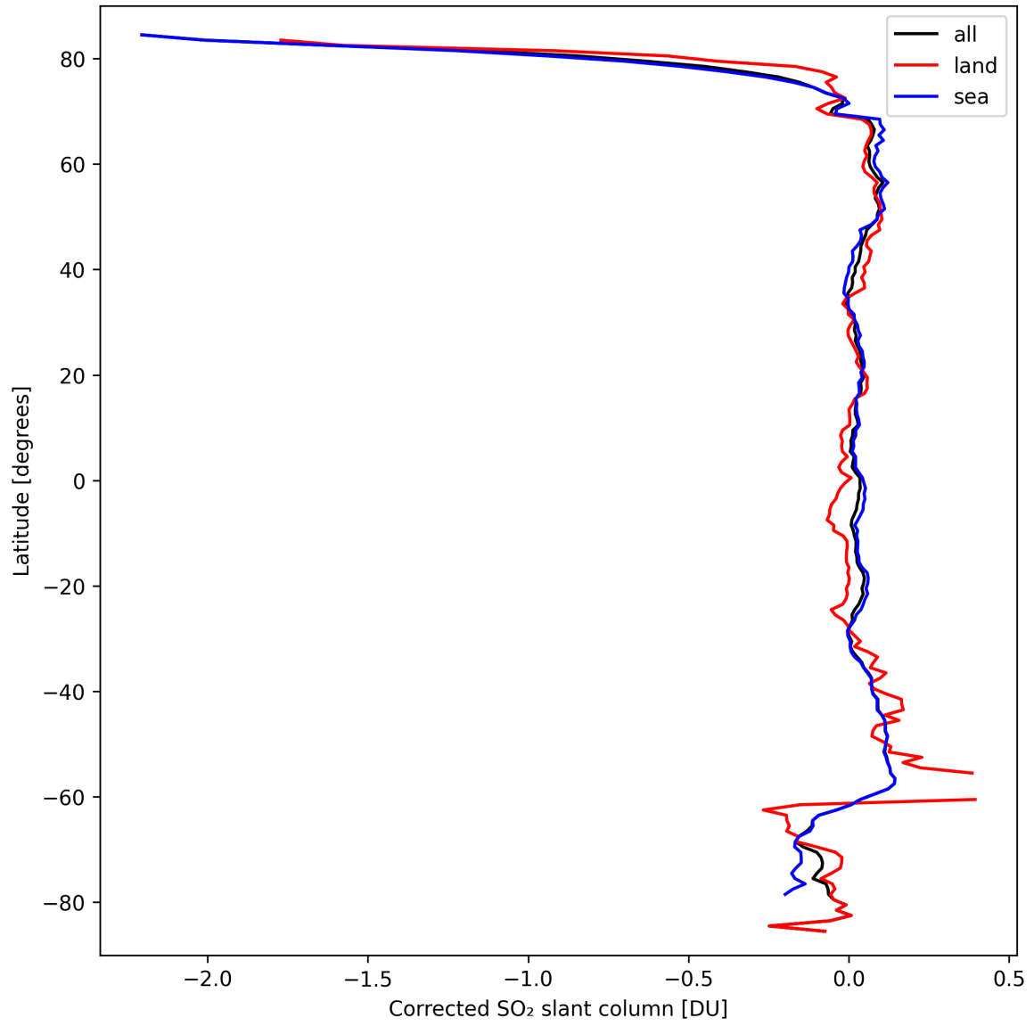
Figure 32: Zonal average of “Corrected SO 2 slant column” for 2024-09-22 to 2024-09-24.
