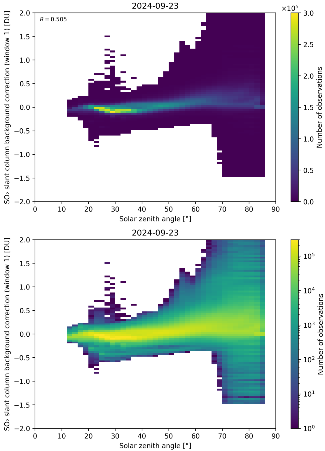
Figure 158: Scatter density plot of “Solar zenith angle” against “SO 2 slant column background correction (window 1)” for 2024-09-22 to 2024-09-24.
