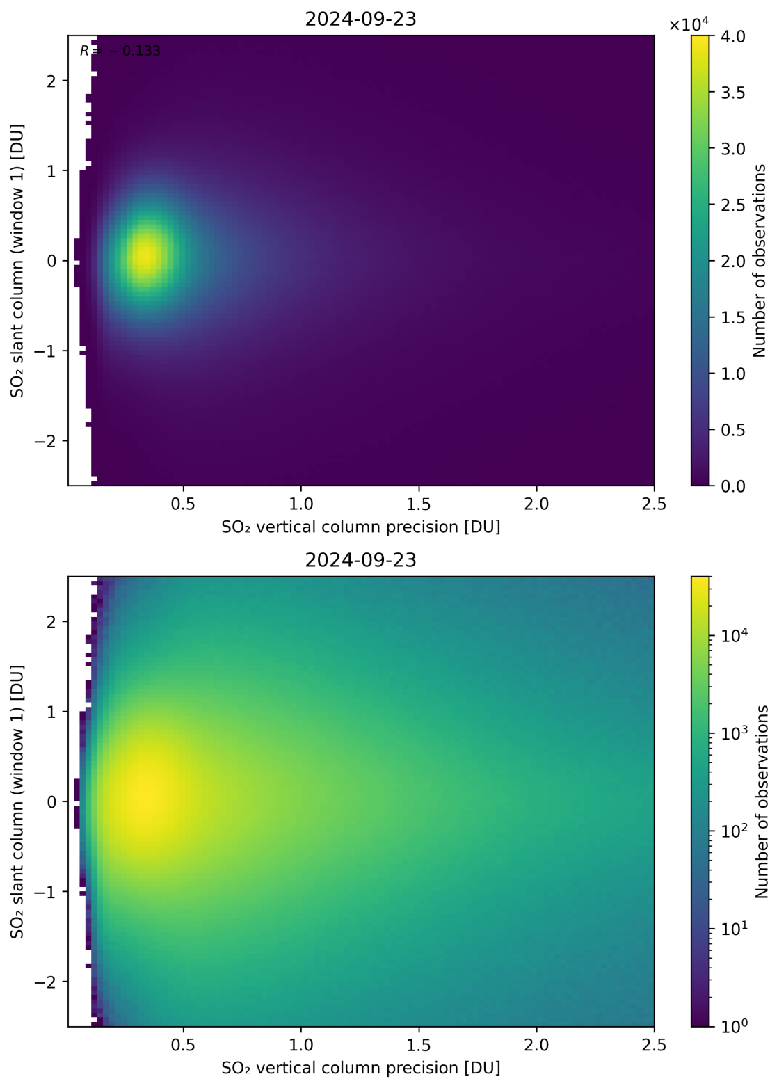
Figure 289: Scatter density plot of “SO 2 vertical column precision” against “SO 2 slant column (window 1)” for 2024-09-22 to 2024-09-24.
