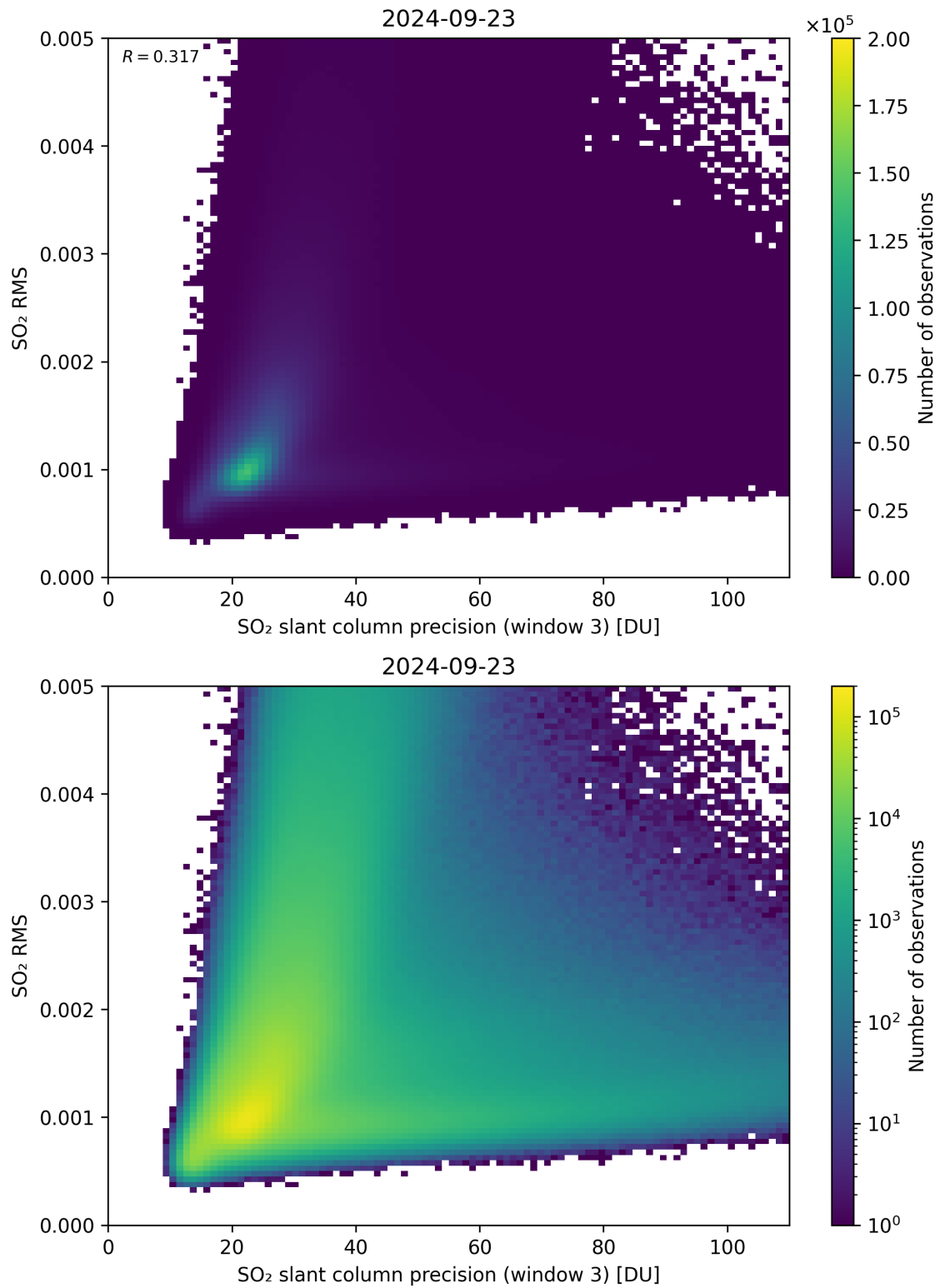
Figure 260: Scatter density plot of “SO 2 slant column precision (window 3)” against “SO 2 RMS” for 2024-09-22 to 2024-09-24.
