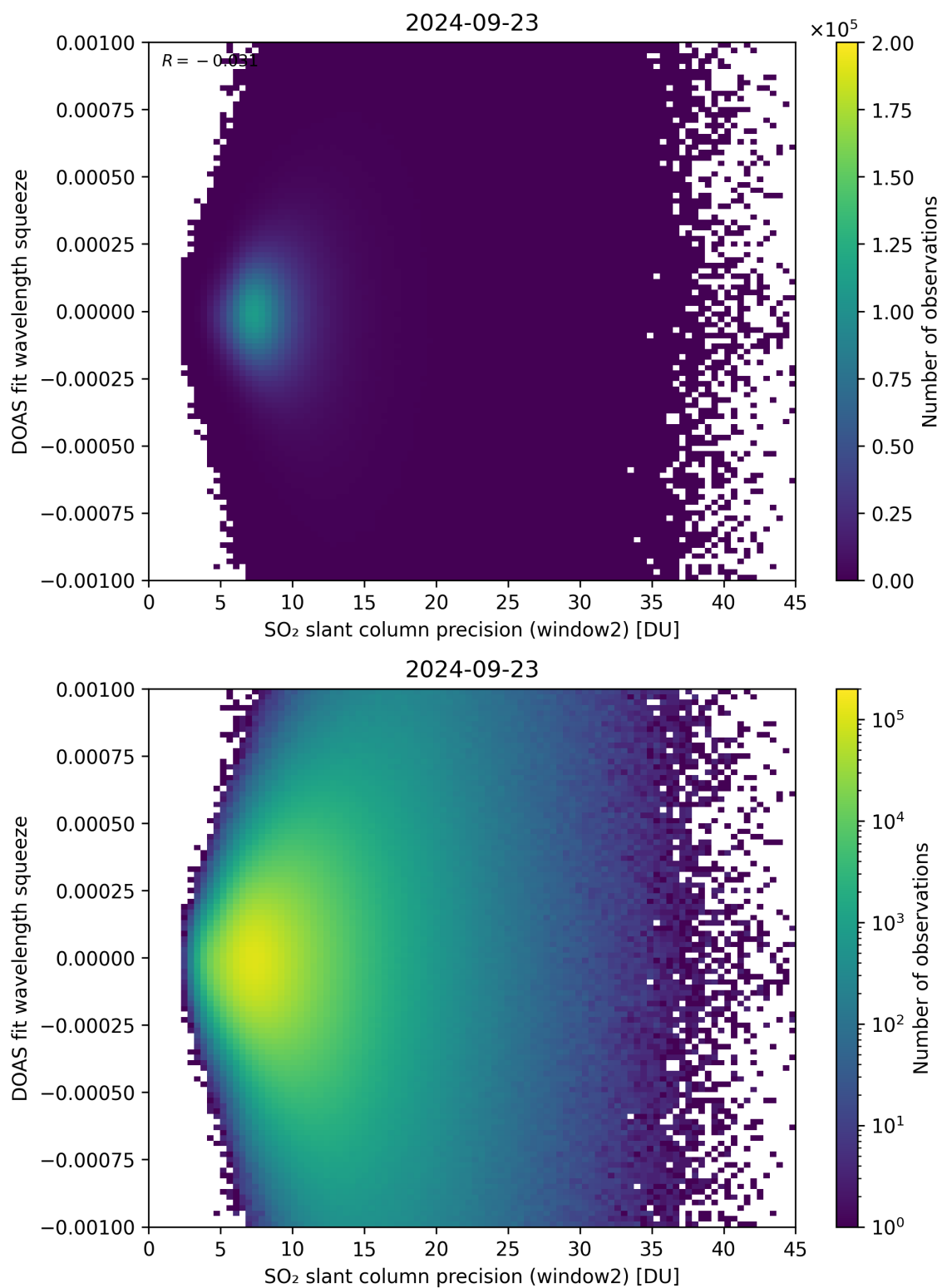
Figure 244: Scatter density plot of “SO 2 slant column precision (window2)” against “DOAS fit wavelength squeeze” for 2024-09-22 to 2024-09-24.
