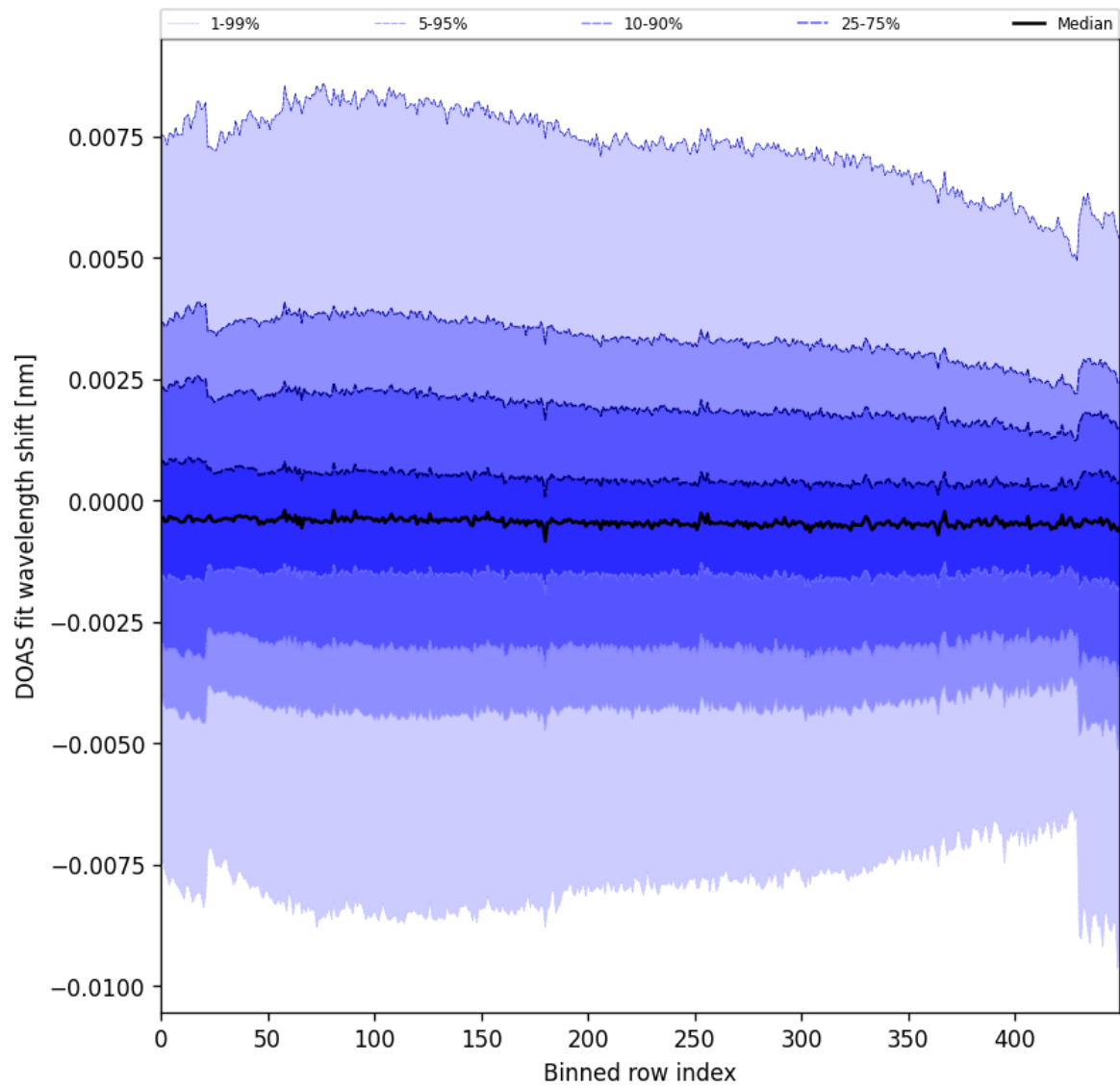
Figure 91: Along track statistics of “DOAS fit wavelength shift” for 2024-09-22 to 2024-09-24
