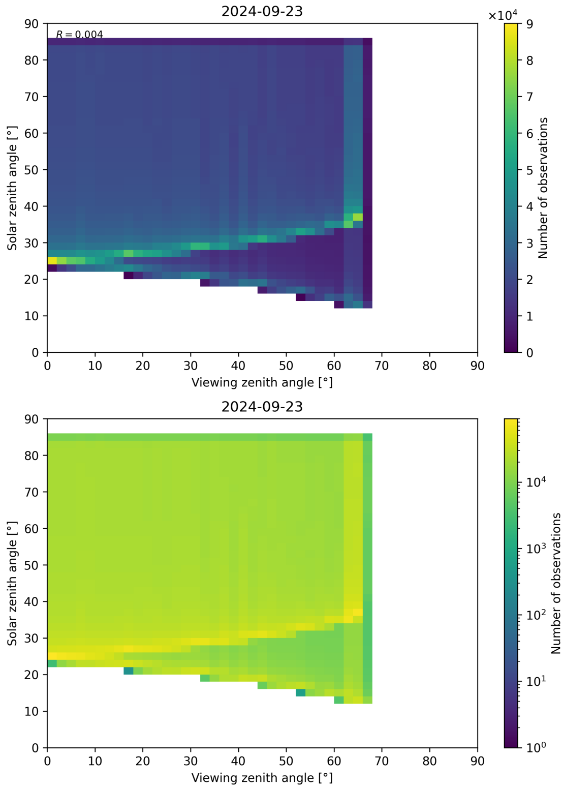
Figure 315: Scatter density plot of “Viewing zenith angle” against “Solar zenith angle” for 2024-09-22 to 2024-09-24.
