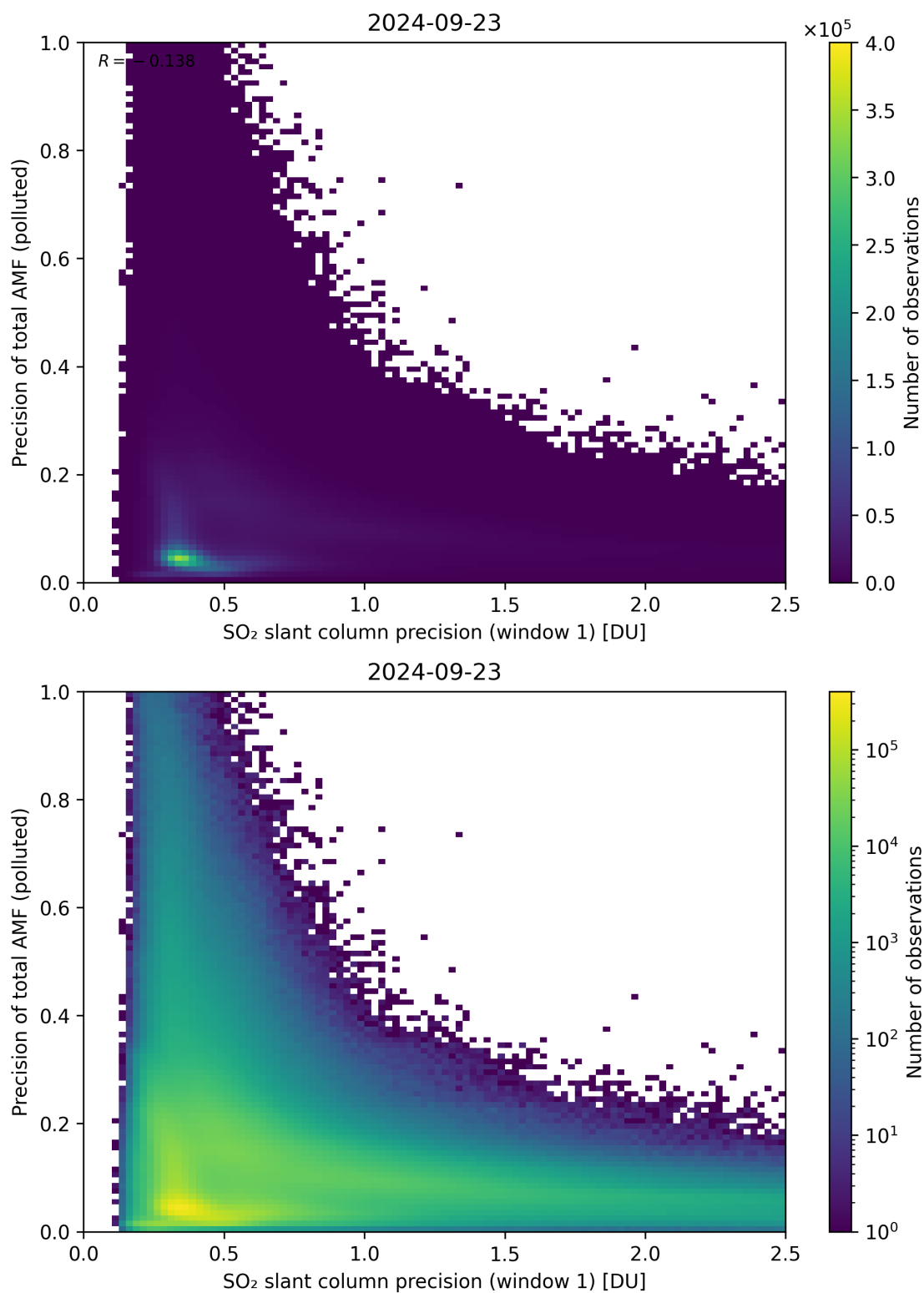
Figure 231: Scatter density plot of “SO 2 slant column precision (window 1)” against “Precision of total AMF (polluted)” for 2024-09-22 to 2024-09-24.
