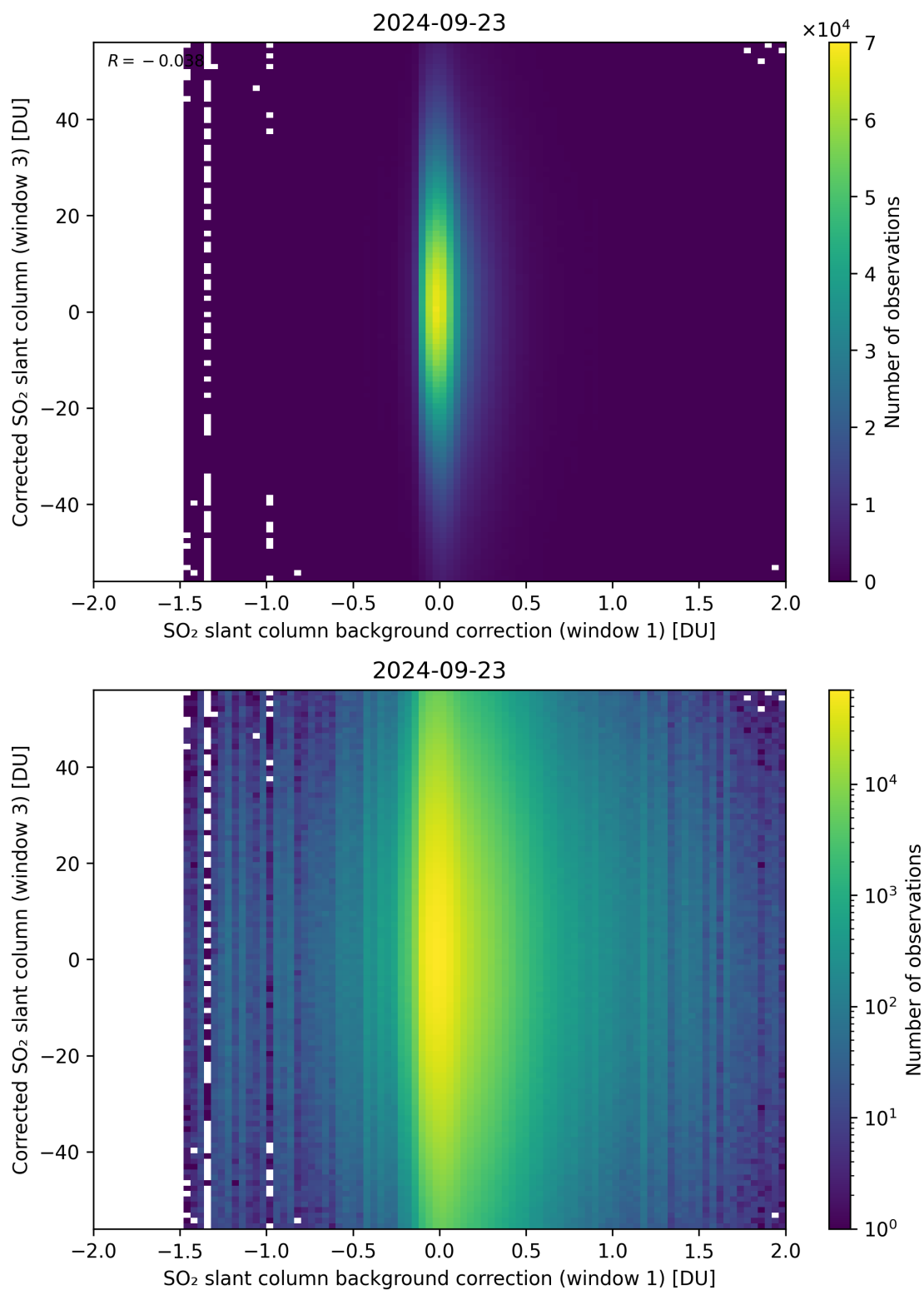
Figure 105: Scatter density plot of “SO 2 slant column background correction (window 1)” against “Corrected SO 2 slant column (window 3)” for 2024-09-22 to 2024-09-24.
