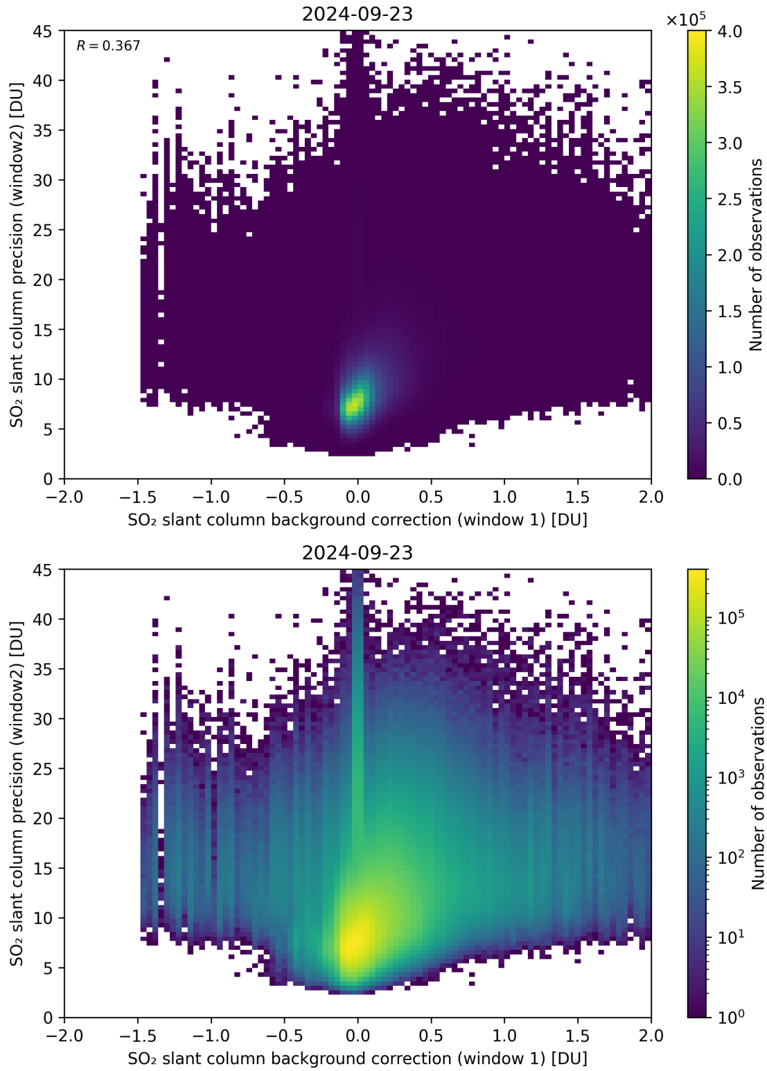
Figure 106: Scatter density plot of “SO 2 slant column background correction (window 1)” against “SO 2 slant column precision (window2)” for 2024-09-22 to 2024-09-24.
