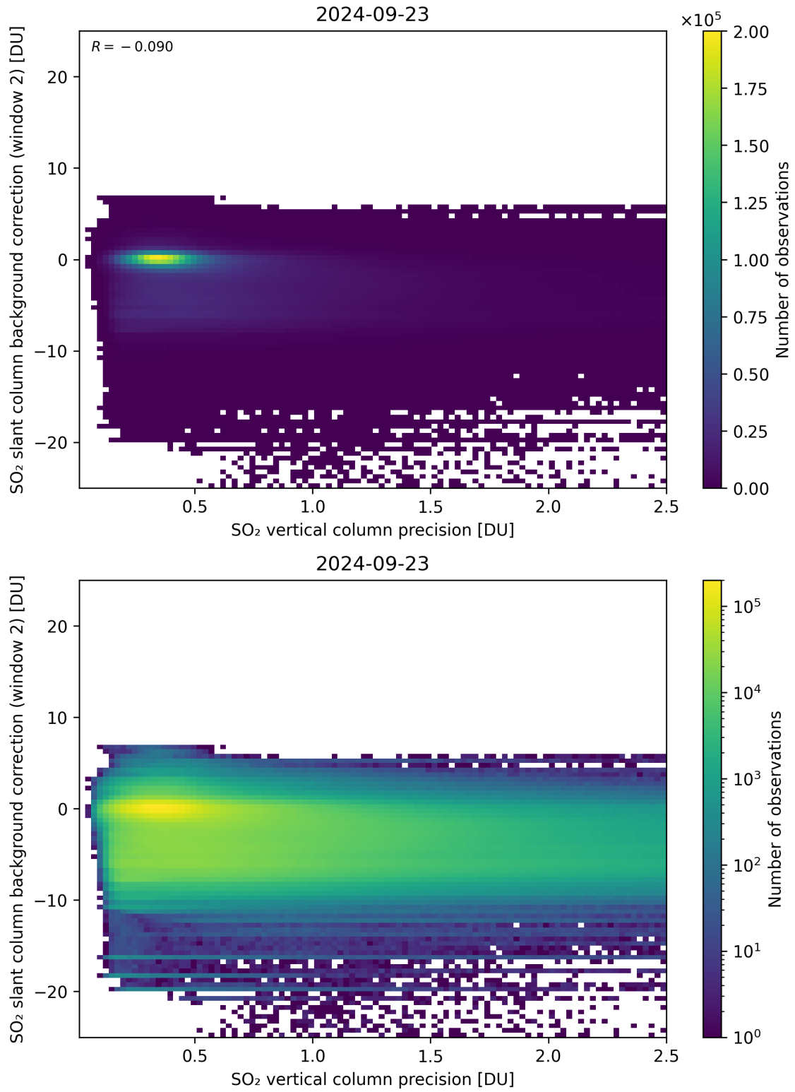
Figure 280: Scatter density plot of “SO 2 vertical column precision” against “SO 2 slant column background correction (window 2)” for 2024-09-22 to 2024-09-24.
