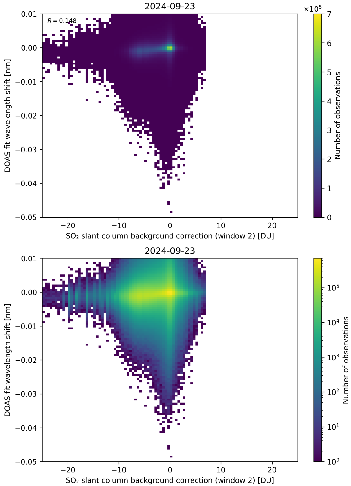
Figure 112: Scatter density plot of “SO 2 slant column background correction (window 2)” against “DOAS fit wavelength shift” for 2024-09-22 to 2024-09-24.
