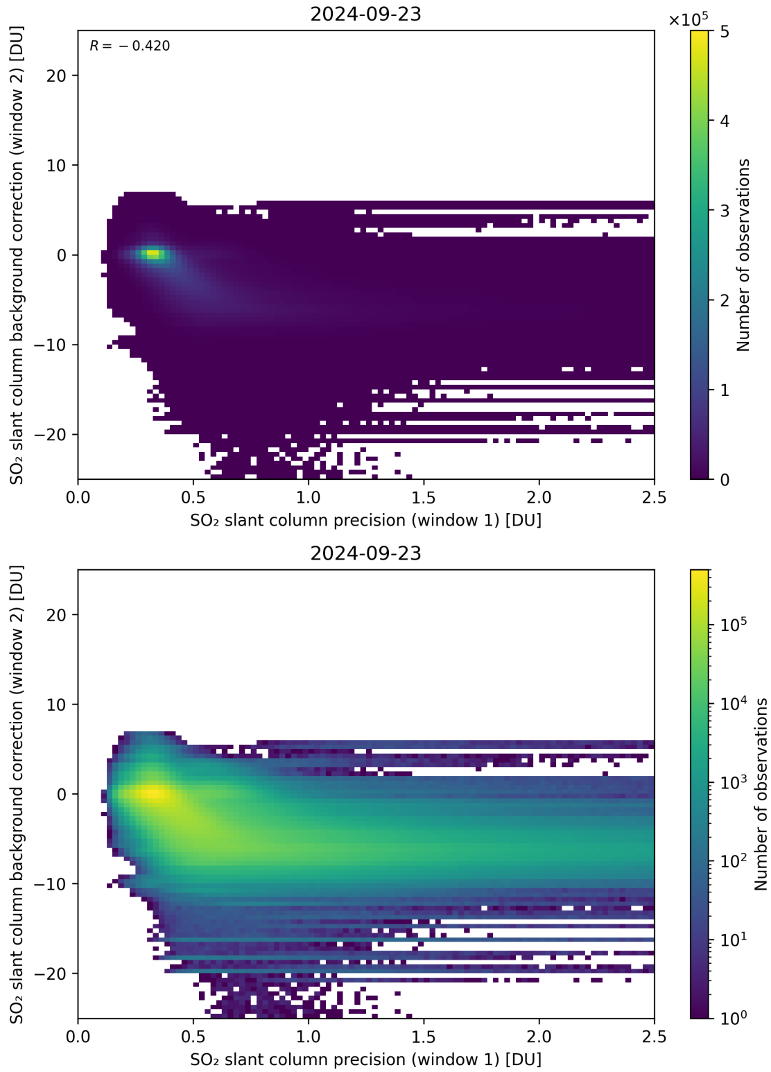
Figure 219: Scatter density plot of “SO 2 slant column precision (window 1)” against “SO 2 slant column background correction (window 2)” for 2024-09-22 to 2024-09-24.
