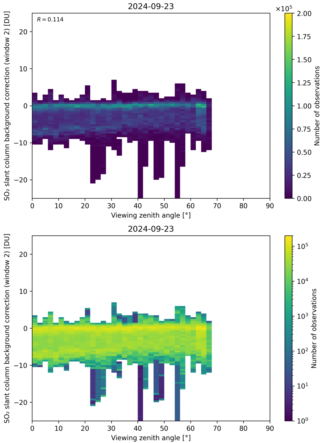
Figure 309: Scatter density plot of “Viewing zenith angle” against “SO 2 slant column background correction (window 2)” for 2024-09-22 to 2024-09-24.
