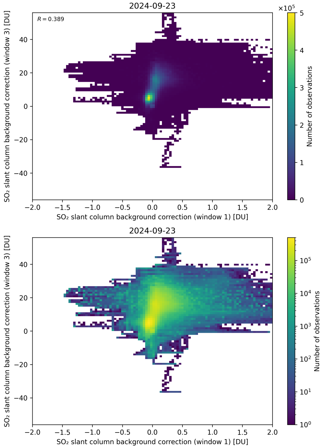
Figure 99: Scatter density plot of “SO 2 slant column background correction (window 1)” against “SO 2 slant column background correction (window 3)” for 2024-09-22 to 2024-09-24.
