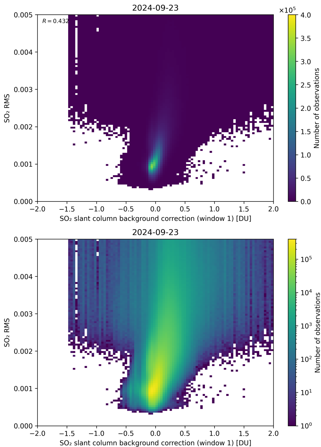
Figure 102: Scatter density plot of “SO 2 slant column background correction (window 1)” against “SO 2 RMS” for 2024-09-22 to 2024-09-24.
