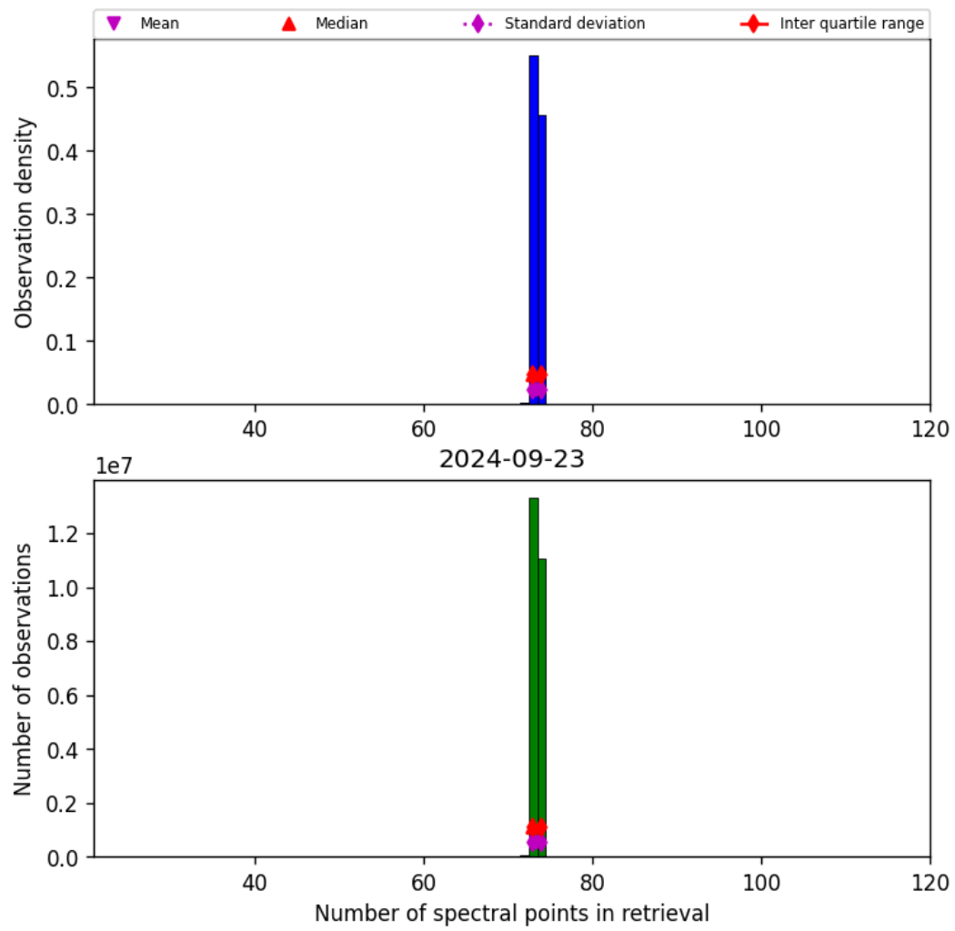
Figure 74: Histogram of “Number of spectral points in retrieval” for 2024-09-22 to 2024-09-24
