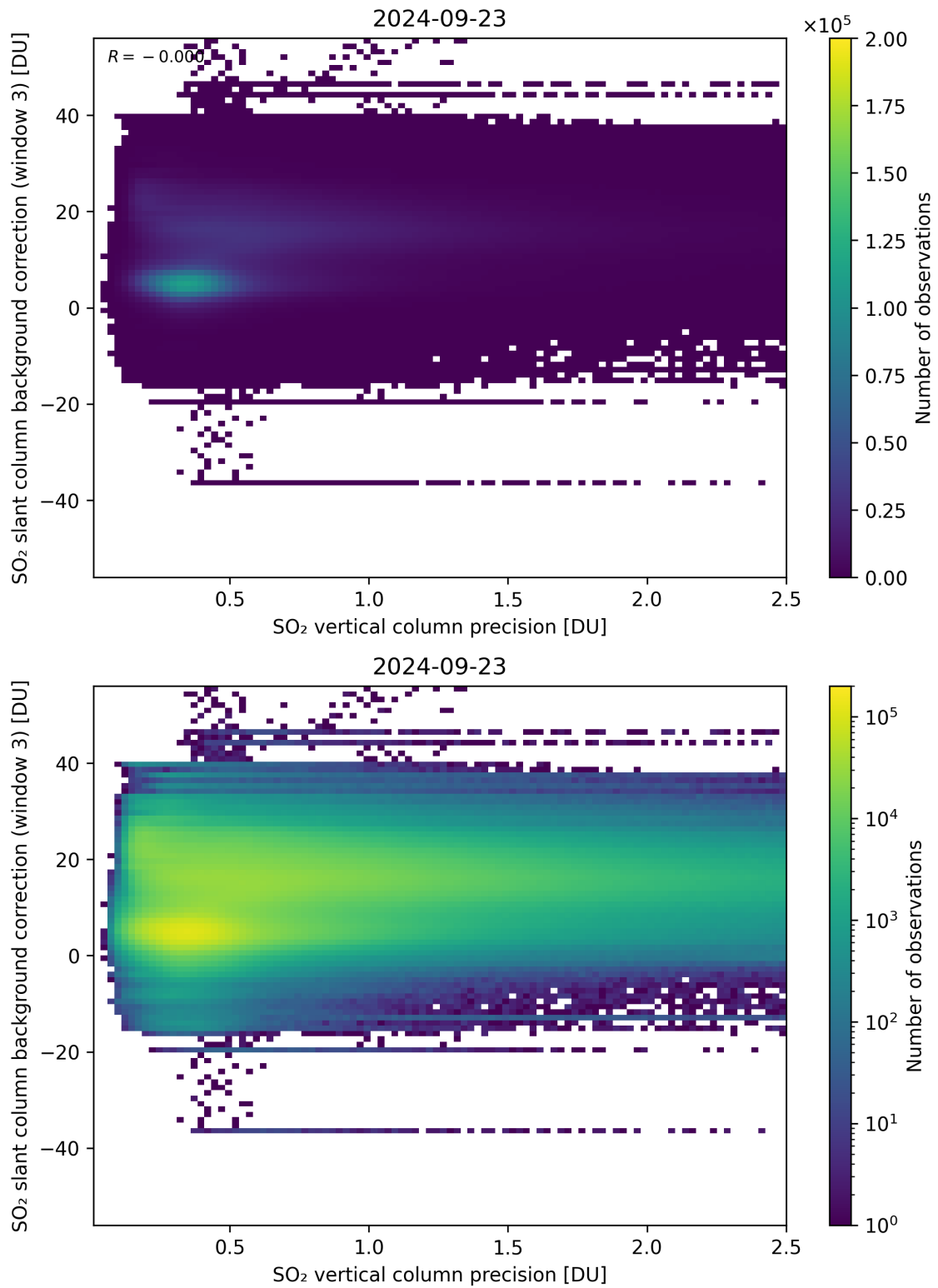
Figure 281: Scatter density plot of “SO 2 vertical column precision” against “SO 2 slant column background correction (window 3)” for 2024-09-22 to 2024-09-24.
