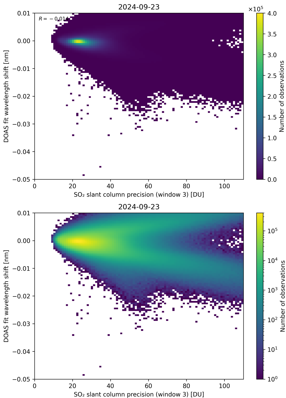
Figure 258: Scatter density plot of “SO 2 slant column precision (window 3)” against “DOAS fit wavelength shift” for 2024-09-22 to 2024-09-24.
