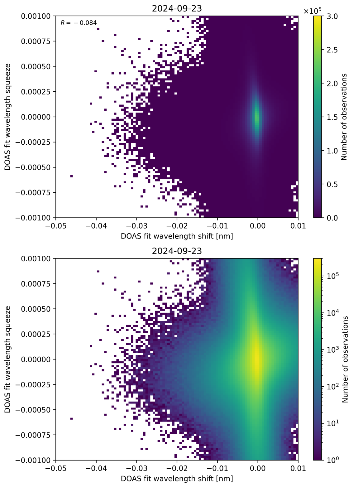
Figure 127: Scatter density plot of “DOAS fit wavelength shift” against “DOAS fit wavelength squeeze” for 2024-09-22 to 2024-09-24.
