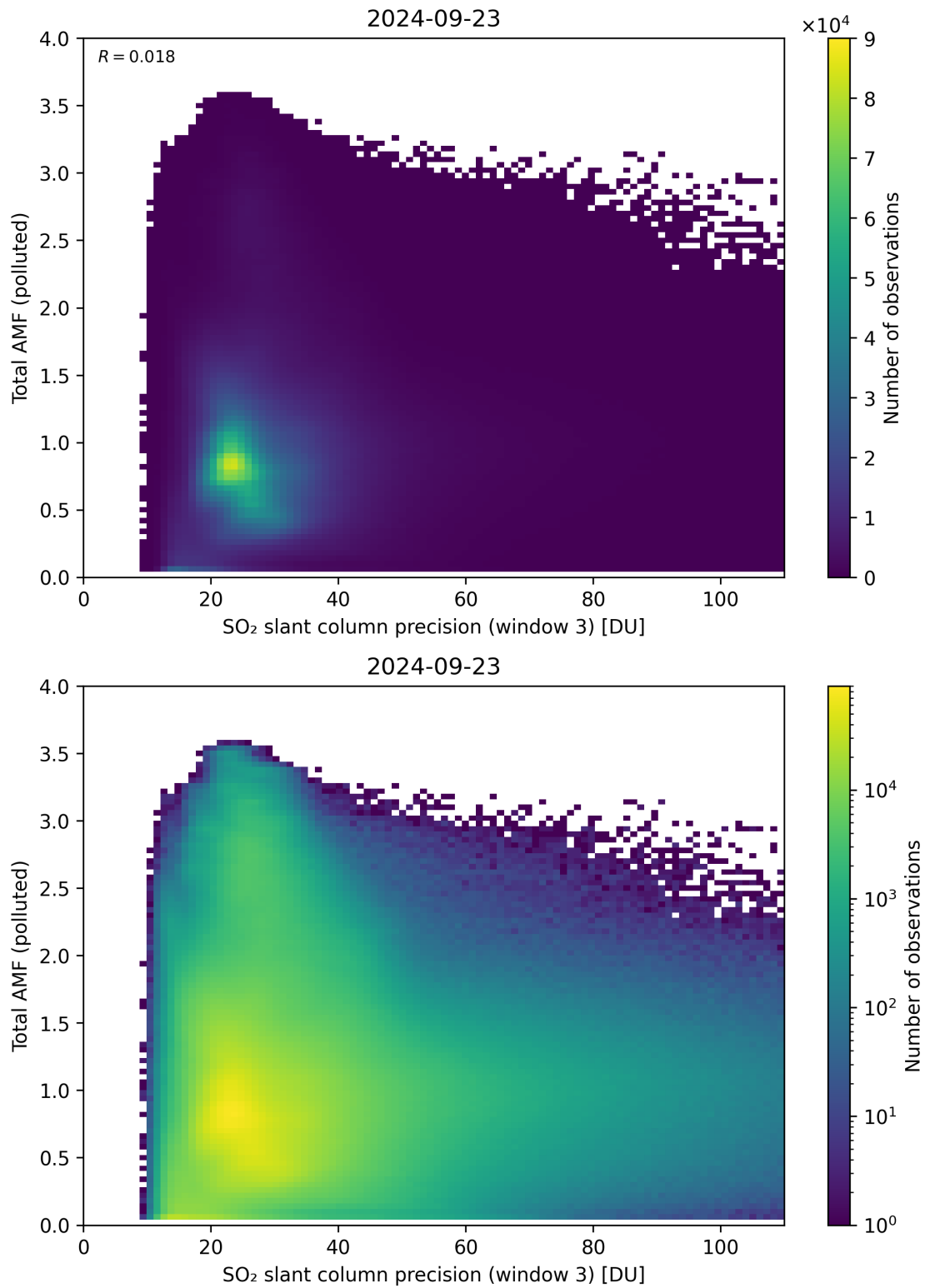
Figure 263: Scatter density plot of “SO 2 slant column precision (window 3)” against “Total AMF (polluted)” for 2024-09-22 to 2024-09-24.
