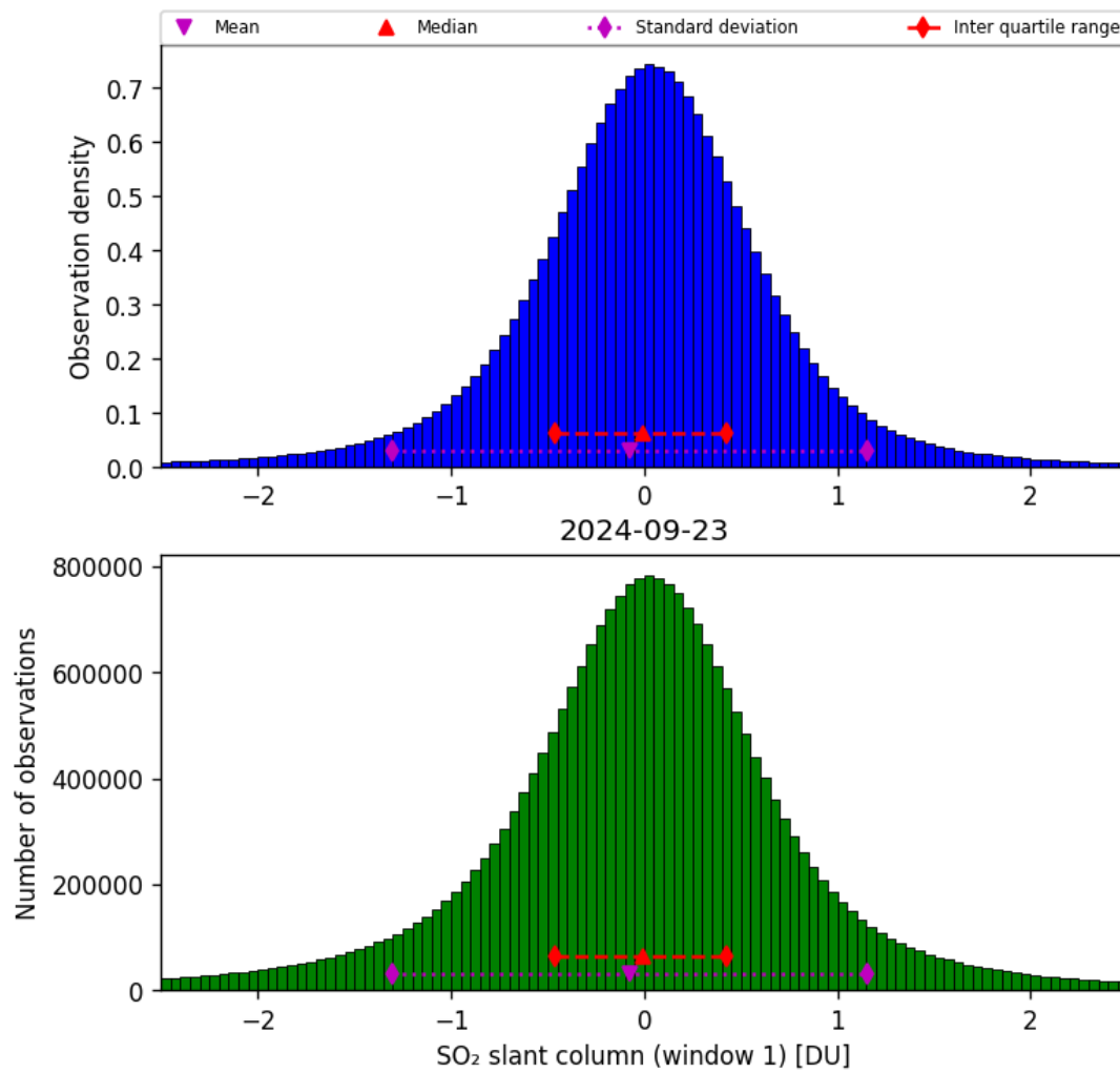
Figure 56: Histogram of “SO 2 slant column (window 1)” for 2024-09-22 to 2024-09-24
