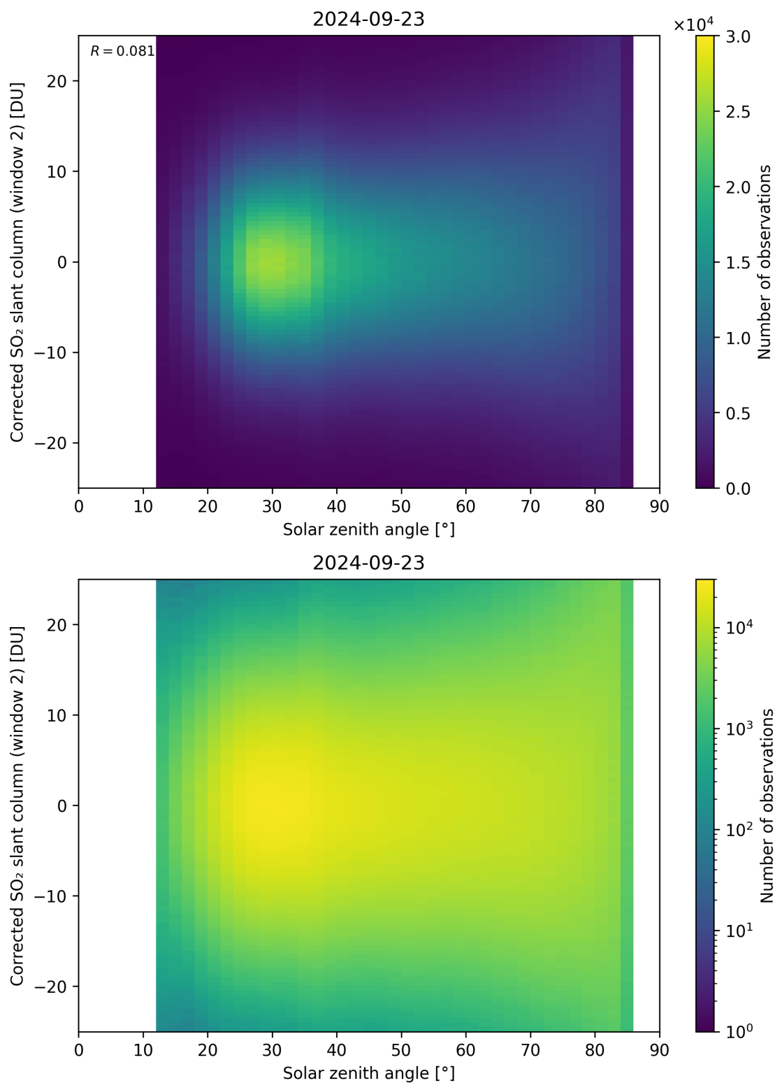
Figure 167: Scatter density plot of “Solar zenith angle” against “Corrected SO 2 slant column (window 2)” for 2024-09-22 to 2024-09-24.
