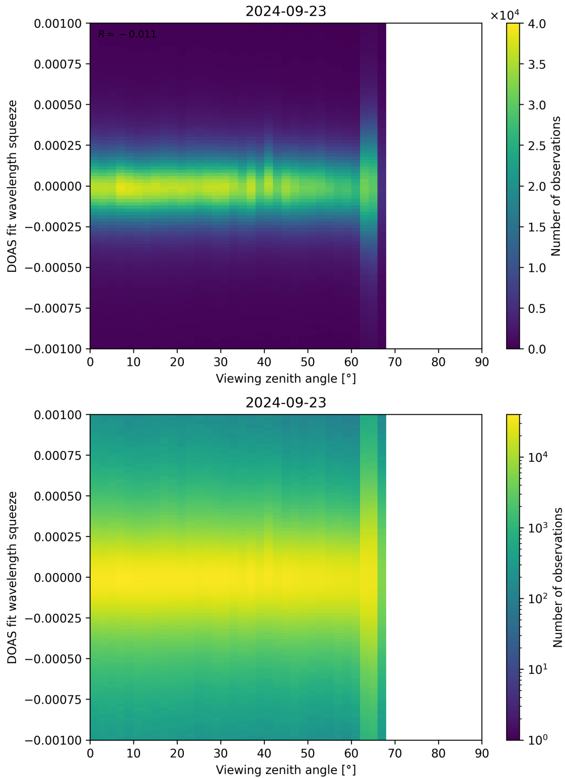
Figure 312: Scatter density plot of “Viewing zenith angle” against “DOAS fit wavelength squeeze” for 2024-09-22 to 2024-09-24.
