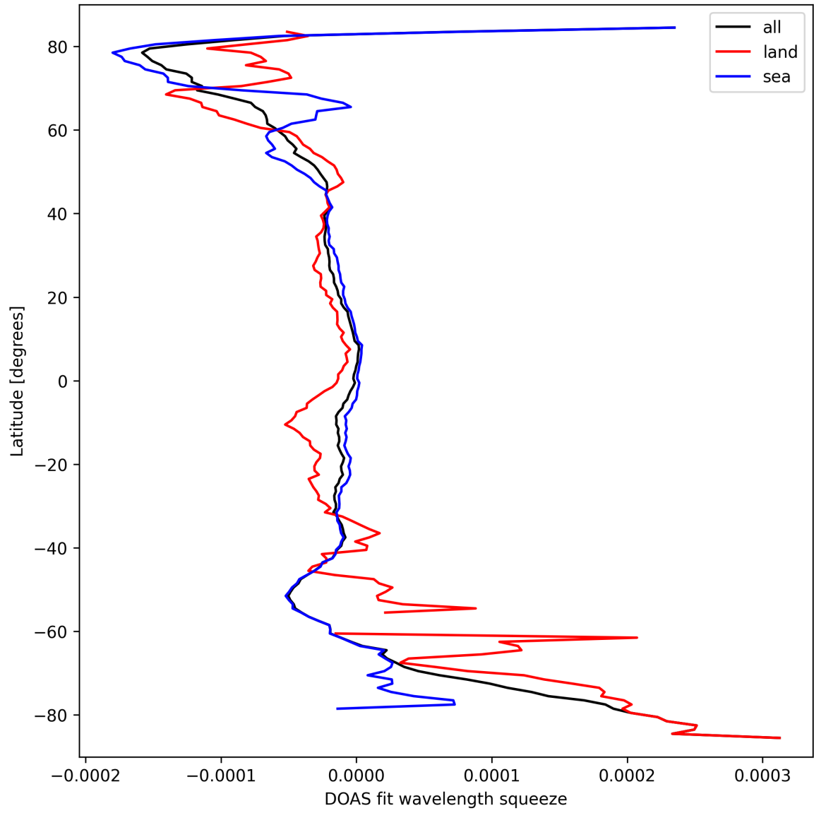
Figure 46: Zonal average of “DOAS fit wavelength squeeze” for 2024-09-22 to 2024-09-24.
