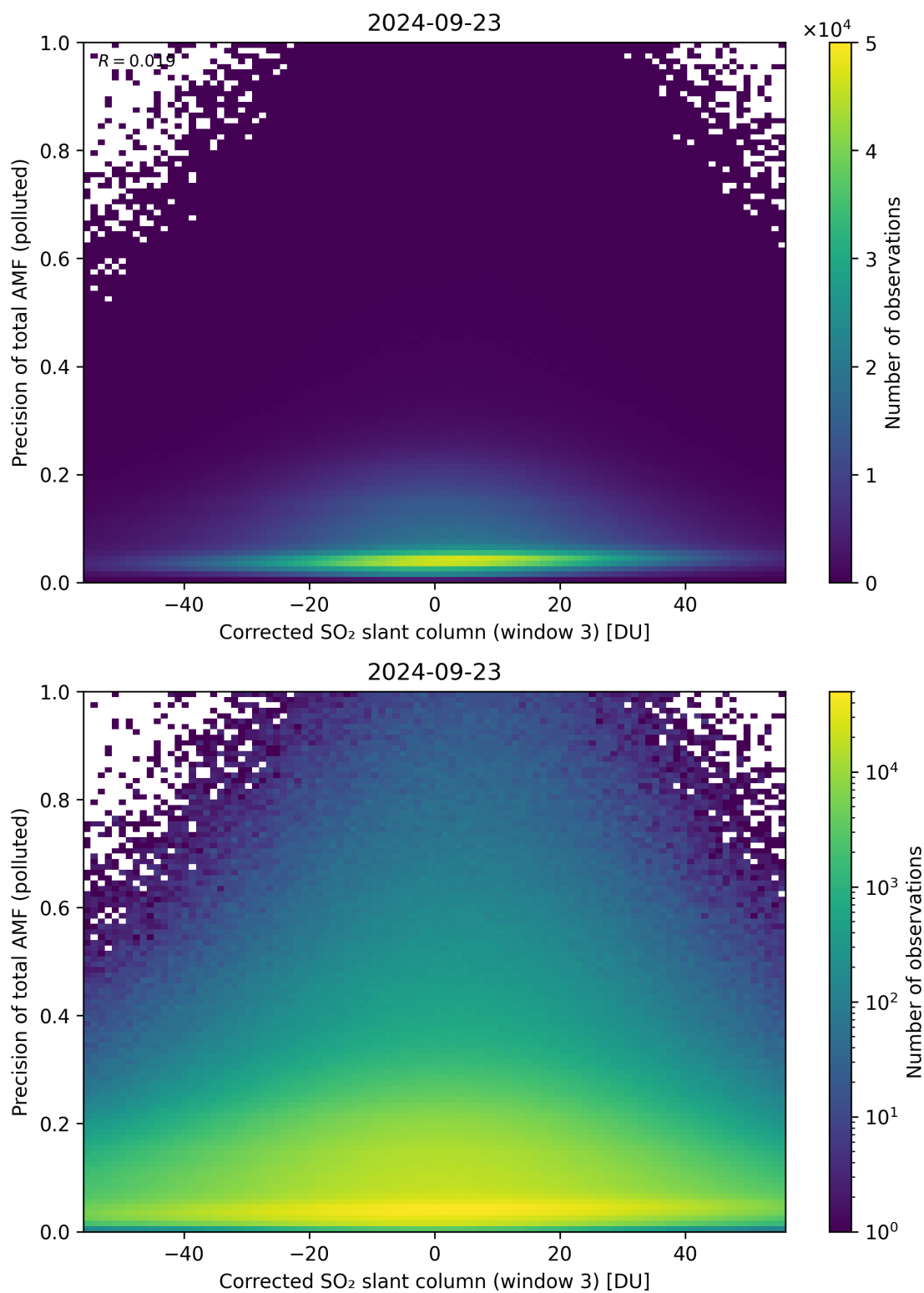
Figure 211: Scatter density plot of “Corrected SO 2 slant column (window 3)” against “Precision of total AMF (polluted)” for 2024-09-22 to 2024-09-24.
