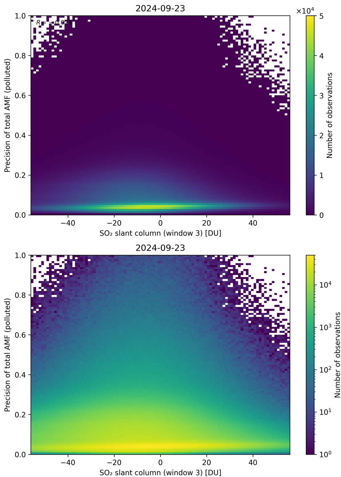
Figure 269: Scatter density plot of “SO 2 slant column (window 3)” against “Precision of total AMF (polluted)” for 2024-09-22 to 2024-09-24.
