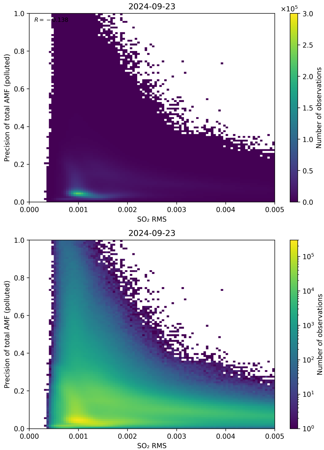
Figure 138: Scatter density plot of “SO 2 RMS” against “Precision of total AMF (polluted)” for 2024-09-22 to 2024-09-24.
