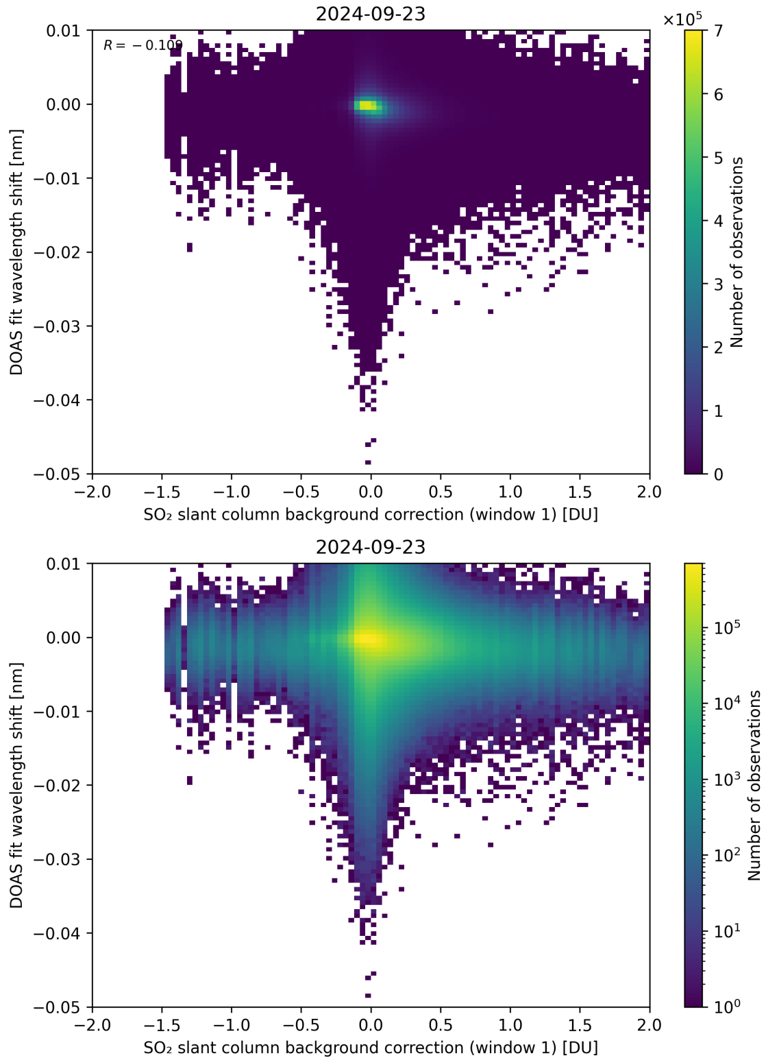
Figure 100: Scatter density plot of “SO 2 slant column background correction (window 1)” against “DOAS fit wavelength shift” for 2024-09-22 to 2024-09-24.
