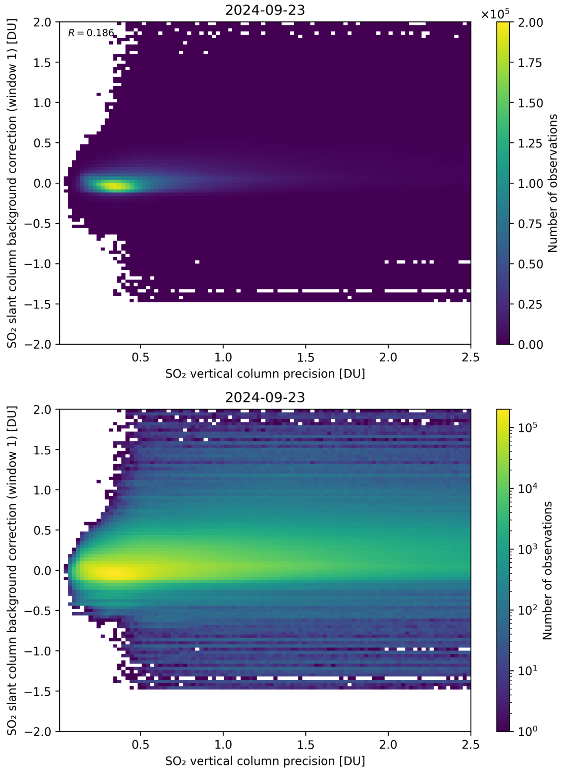
Figure 279: Scatter density plot of “SO 2 vertical column precision” against “SO 2 slant column background correction (window 1)” for 2024-09-22 to 2024-09-24.
