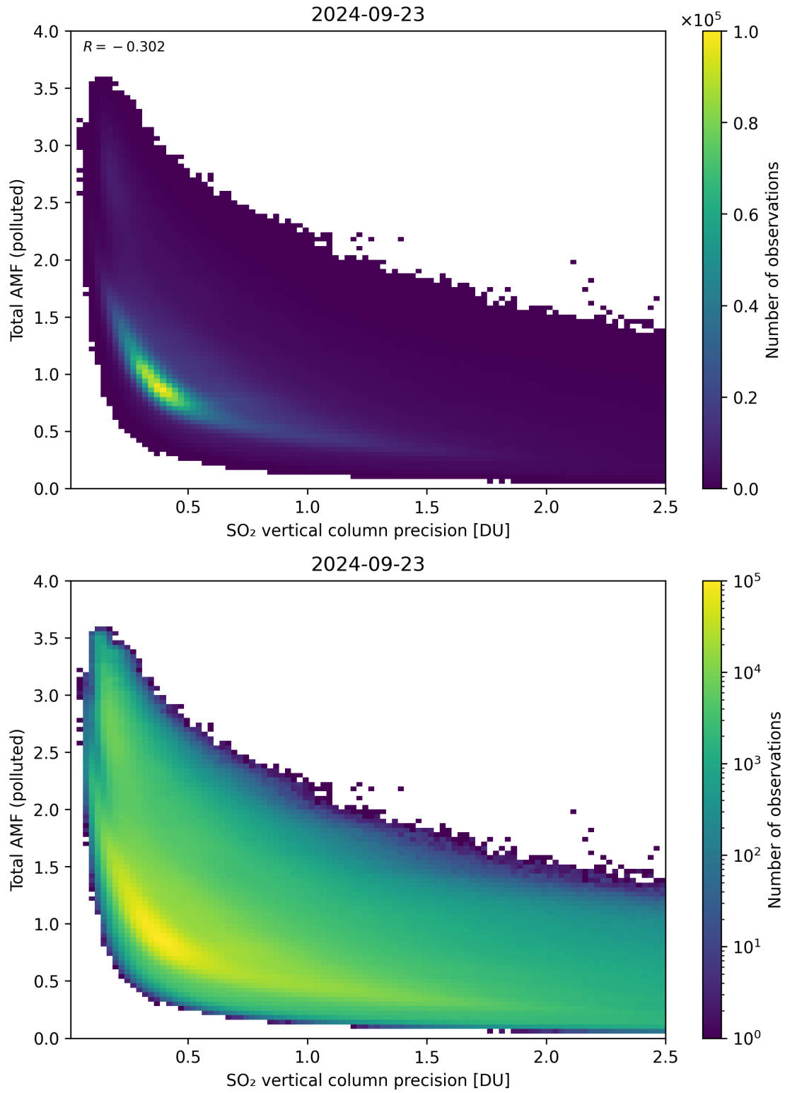
Figure 294: Scatter density plot of “SO 2 vertical column precision” against “Total AMF (polluted)” for 2024-09-22 to 2024-09-24.
