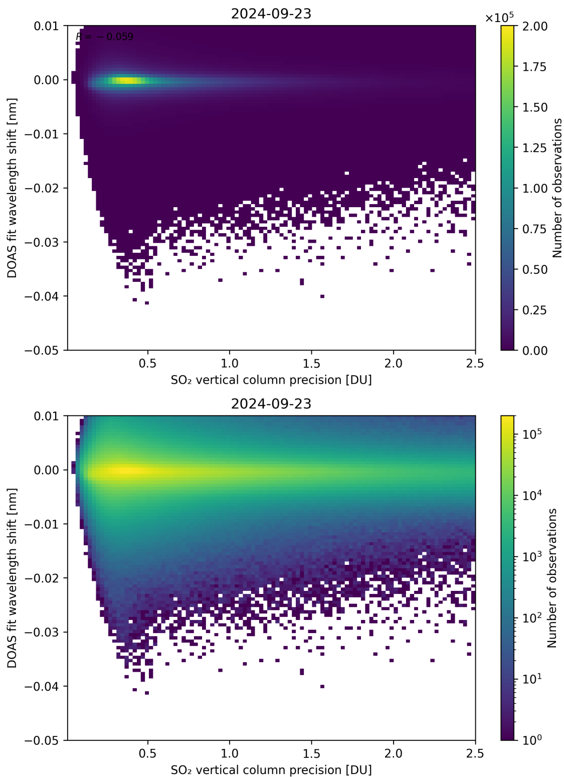
Figure 282: Scatter density plot of “SO 2 vertical column precision” against “DOAS fit wavelength shift” for 2024-09-22 to 2024-09-24.
