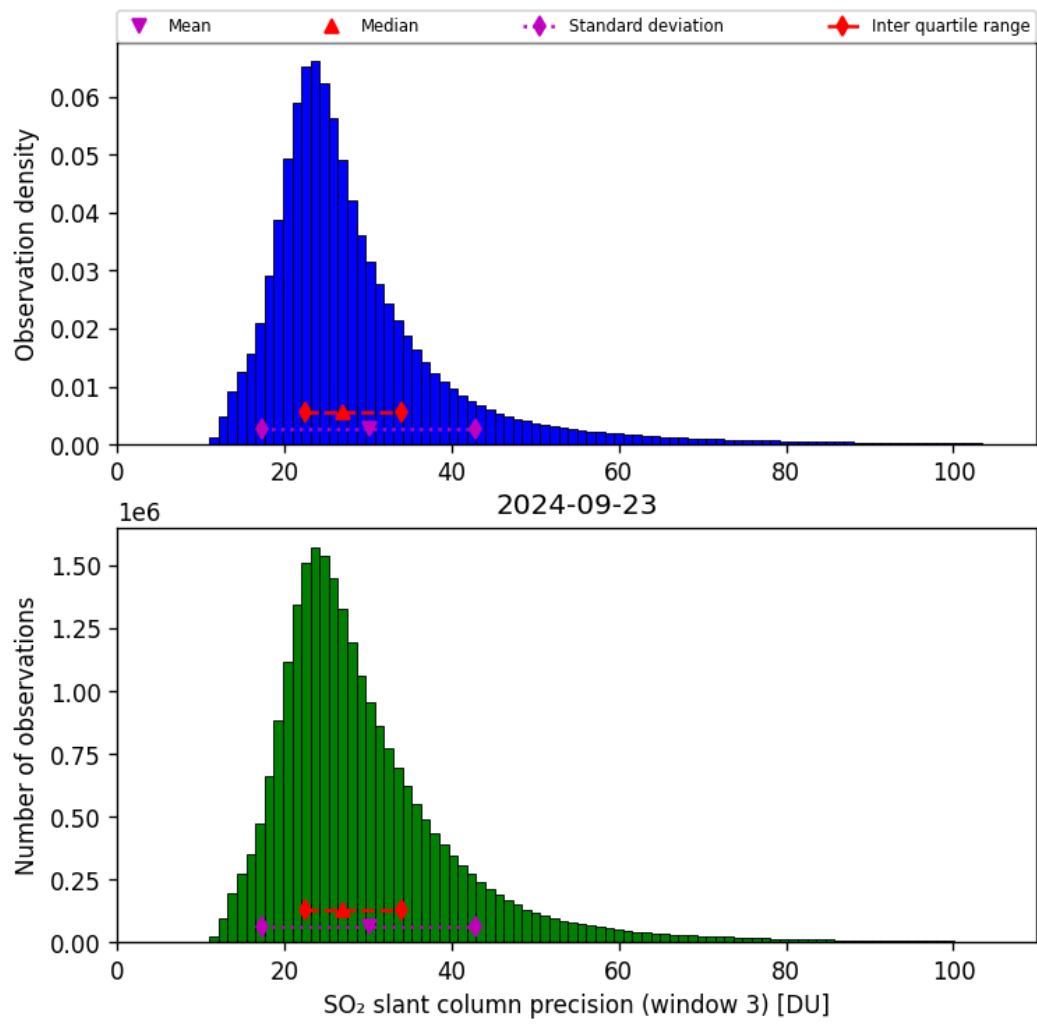
Figure 65: Histogram of “SO 2 slant column precision (window 3)” for 2024-09-22 to 2024-09-24
