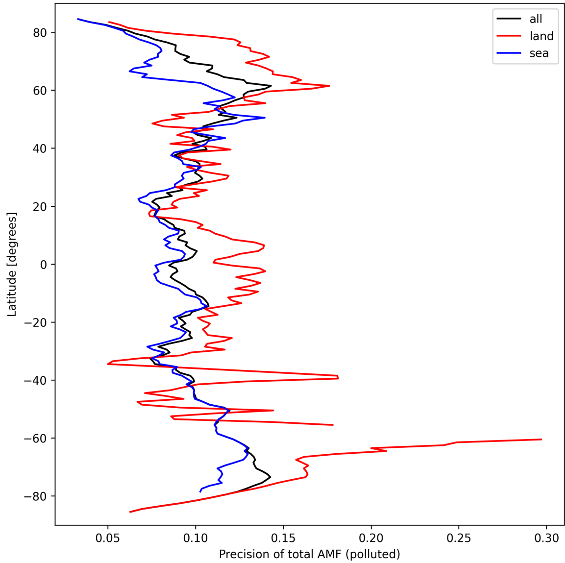
Figure 49: Zonal average of “Precision of total AMF (polluted)” for 2024-09-22 to 2024-09-24.
