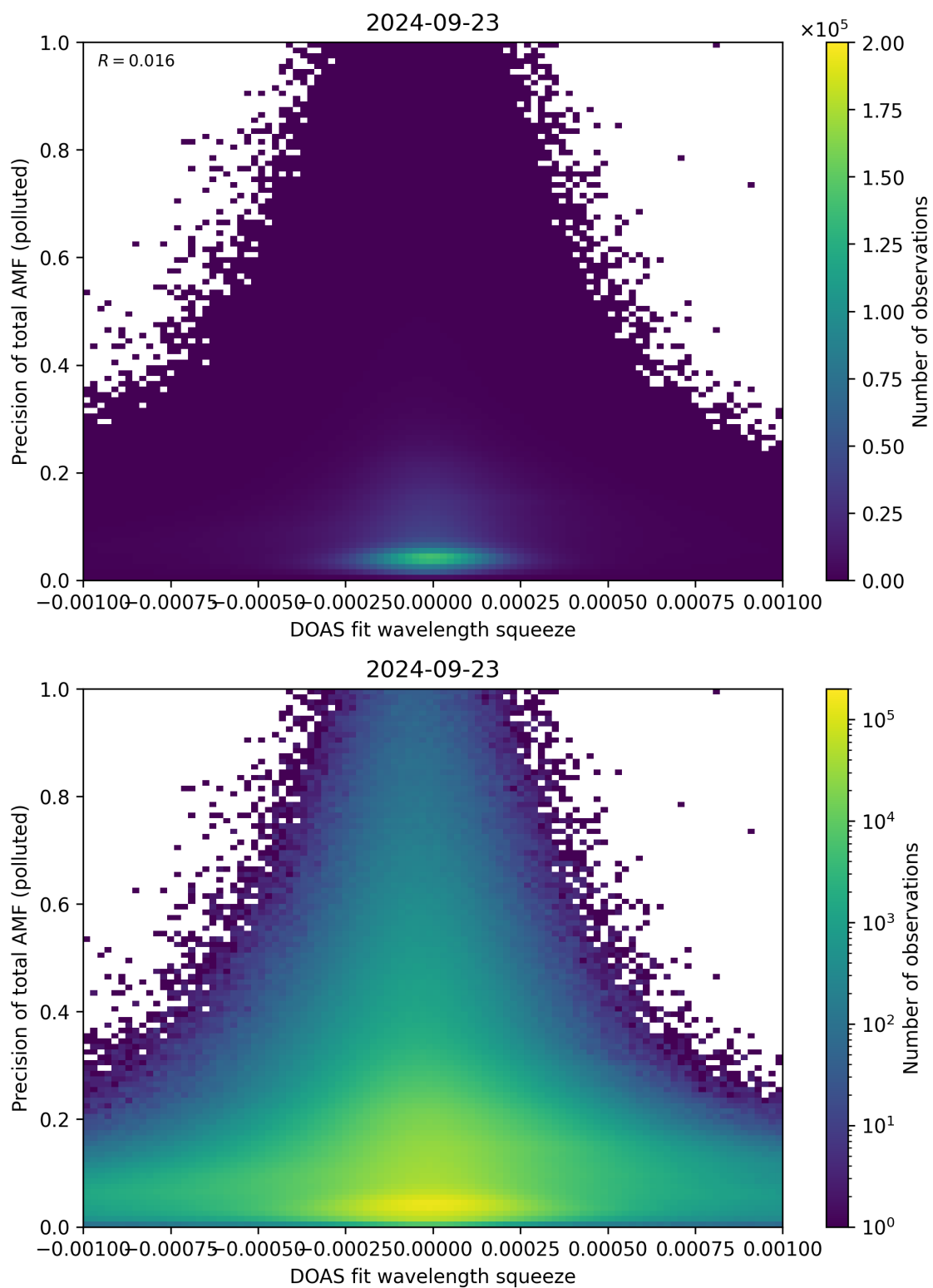
Figure 135: Scatter density plot of “DOAS fit wavelength squeeze” against “Precision of total AMF (polluted)” for 2024-09-22 to 2024-09-24.
