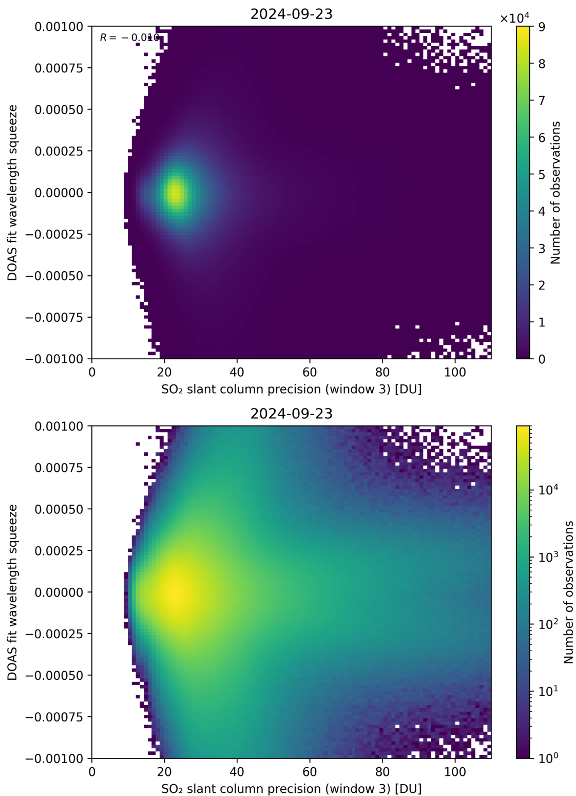
Figure 259: Scatter density plot of “SO 2 slant column precision (window 3)” against “DOAS fit wavelength squeeze” for 2024-09-22 to 2024-09-24.
