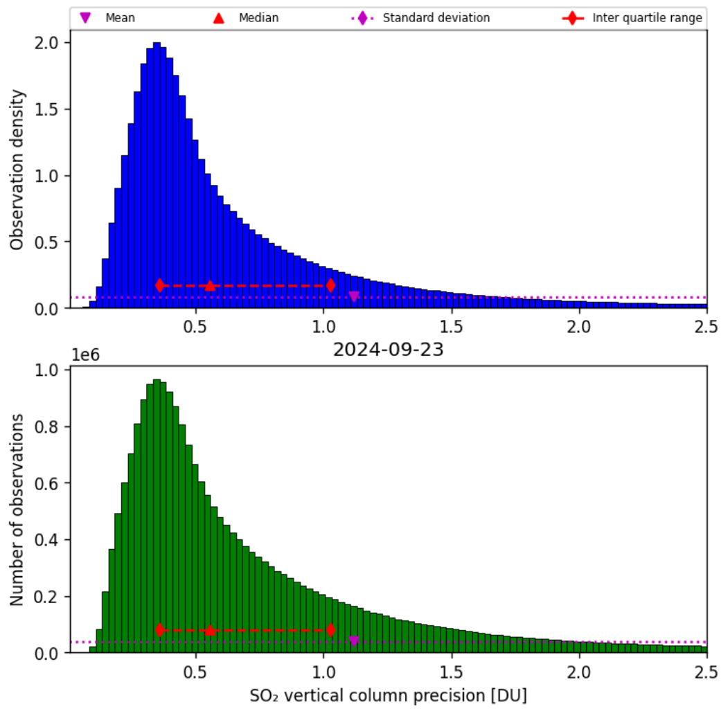
Figure 54: Histogram of “SO 2 vertical column precision” for 2024-09-22 to 2024-09-24
