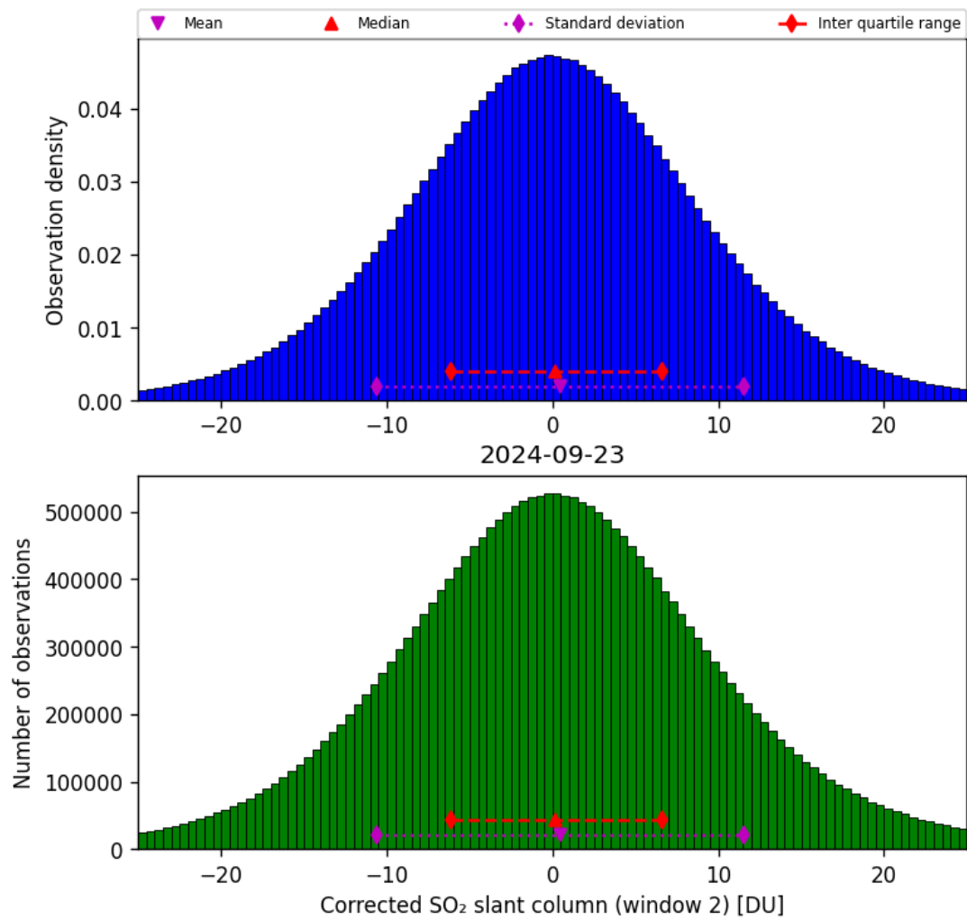
Figure 62: Histogram of “Corrected SO 2 slant column (window 2)” for 2024-09-22 to 2024-09-24
