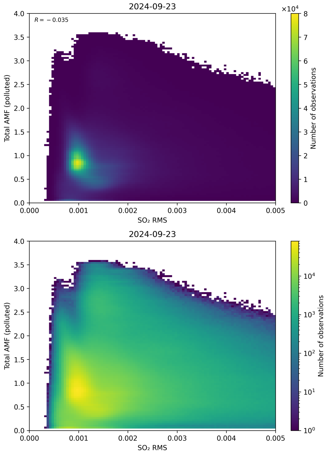
Figure 137: Scatter density plot of “SO 2 RMS” against “Total AMF (polluted)” for 2024-09-22 to 2024-09-24.
