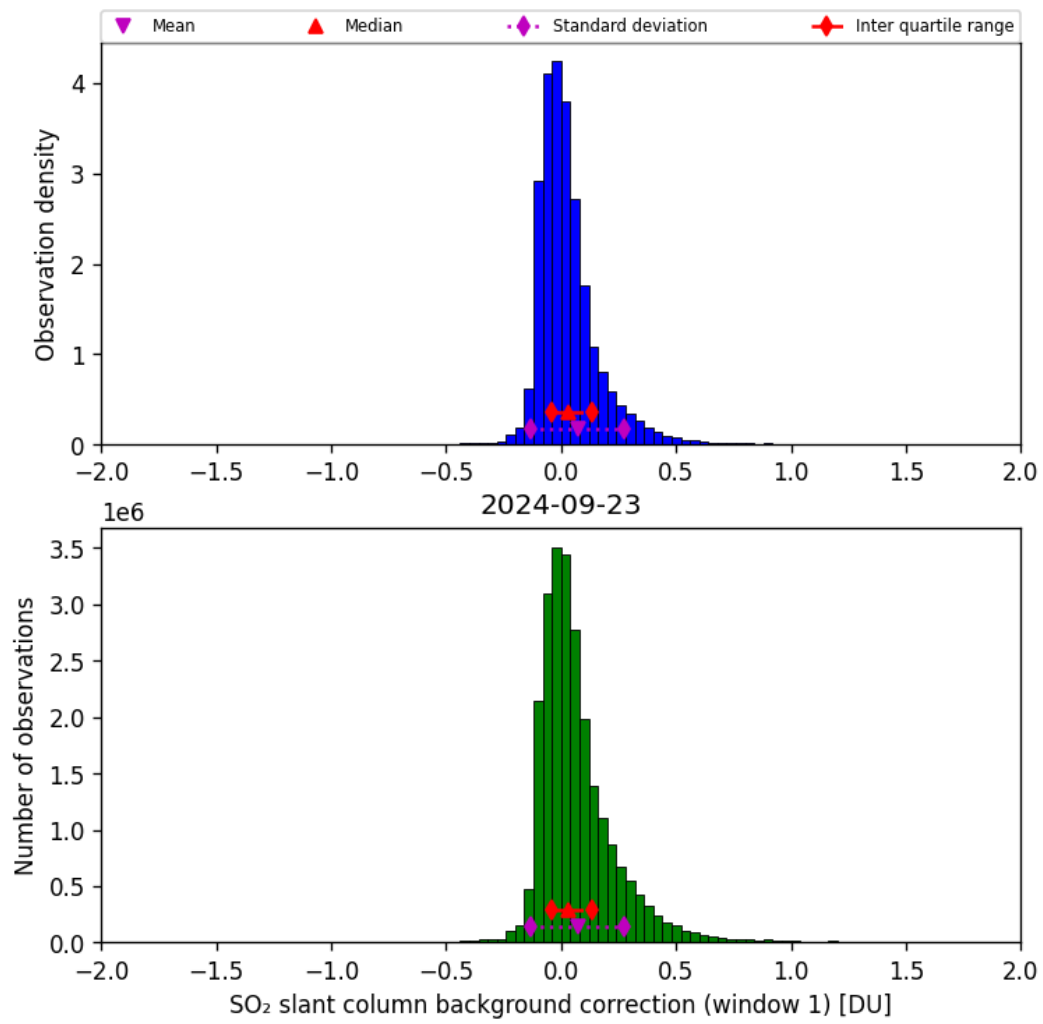
Figure 59: Histogram of “SO 2 slant column background correction (window 1)” for 2024-09-22 to 2024-09-24
