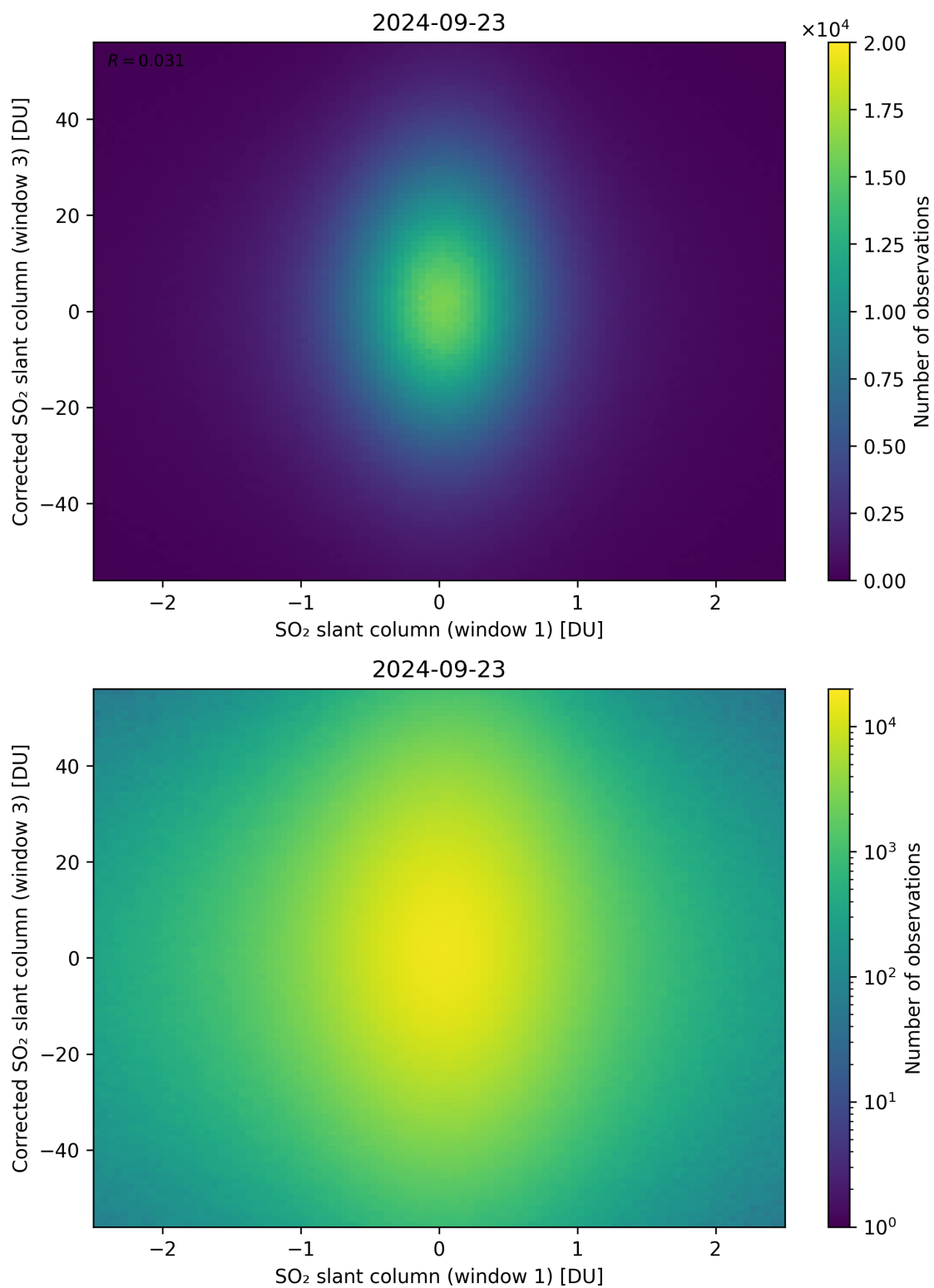
Figure 234: Scatter density plot of “SO 2 slant column (window 1)” against “Corrected SO 2 slant column (window 3)” for 2024-09-22 to 2024-09-24.
