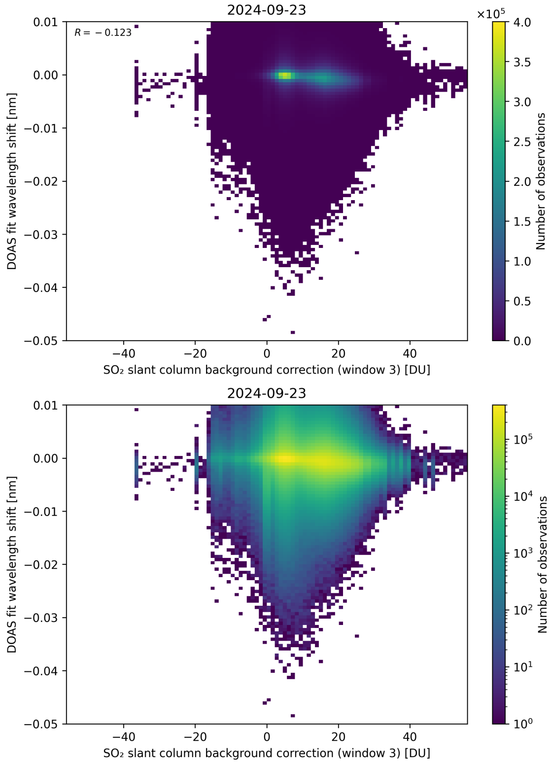
Figure 121: Scatter density plot of “SO 2 slant column background correction (window 3)” against “DOAS fit wavelength shift” for 2024-09-22 to 2024-09-24.
