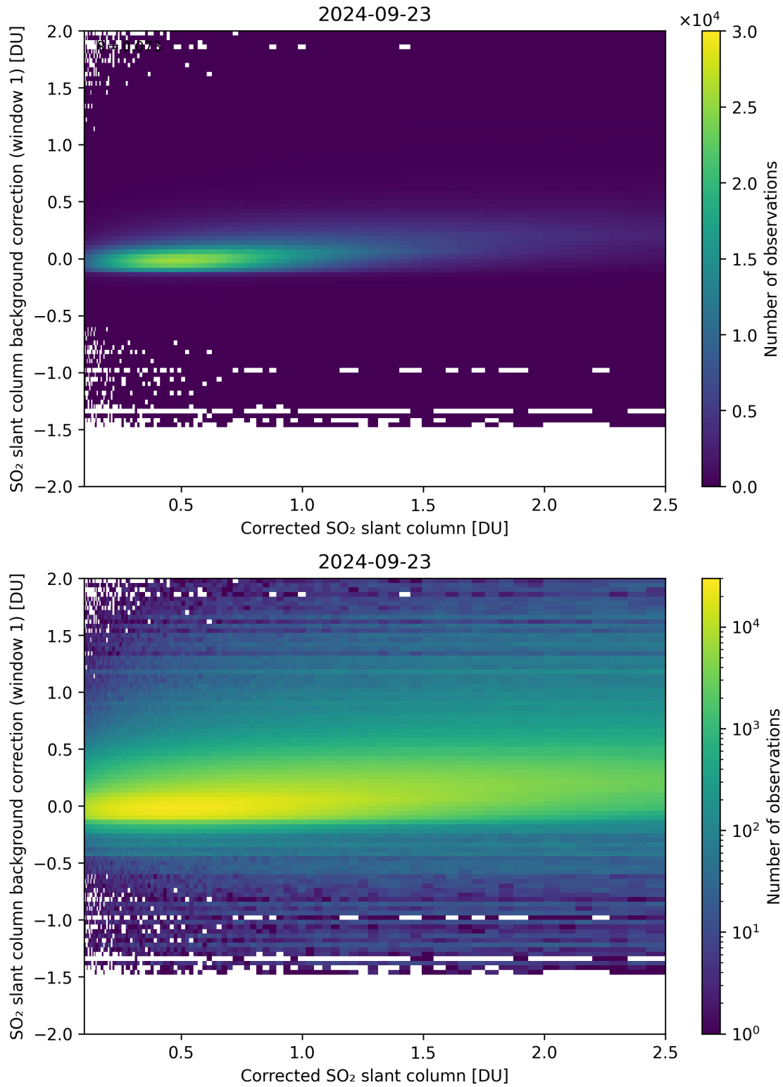
Figure 178: Scatter density plot of “Corrected SO 2 slant column” against “SO 2 slant column background correction (window 1)” for 2024-09-22 to 2024-09-24.
