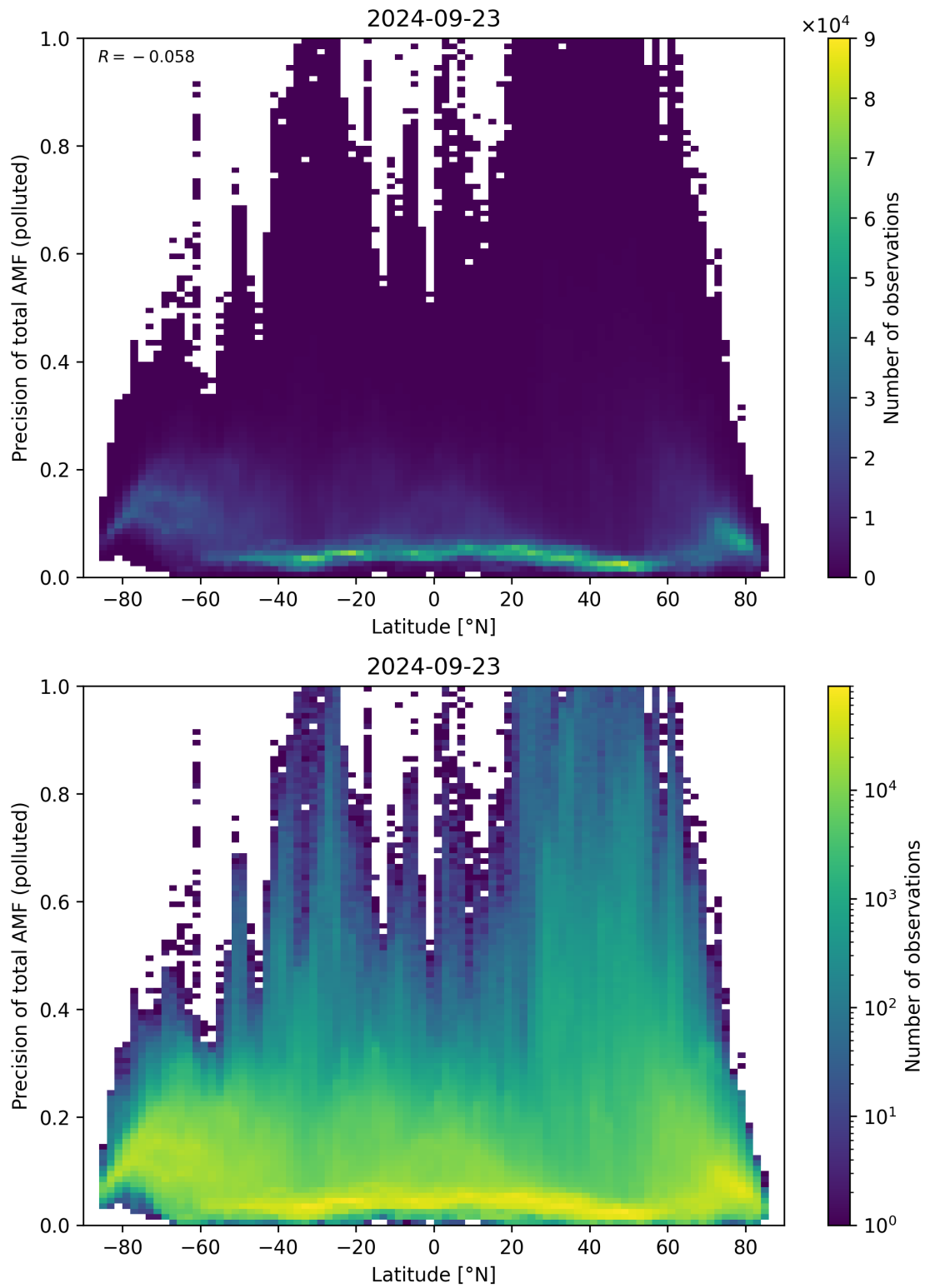
Figure 155: Scatter density plot of “Latitude” against “Precision of total AMF (polluted)” for 2024-09-22 to 2024-09-24.
