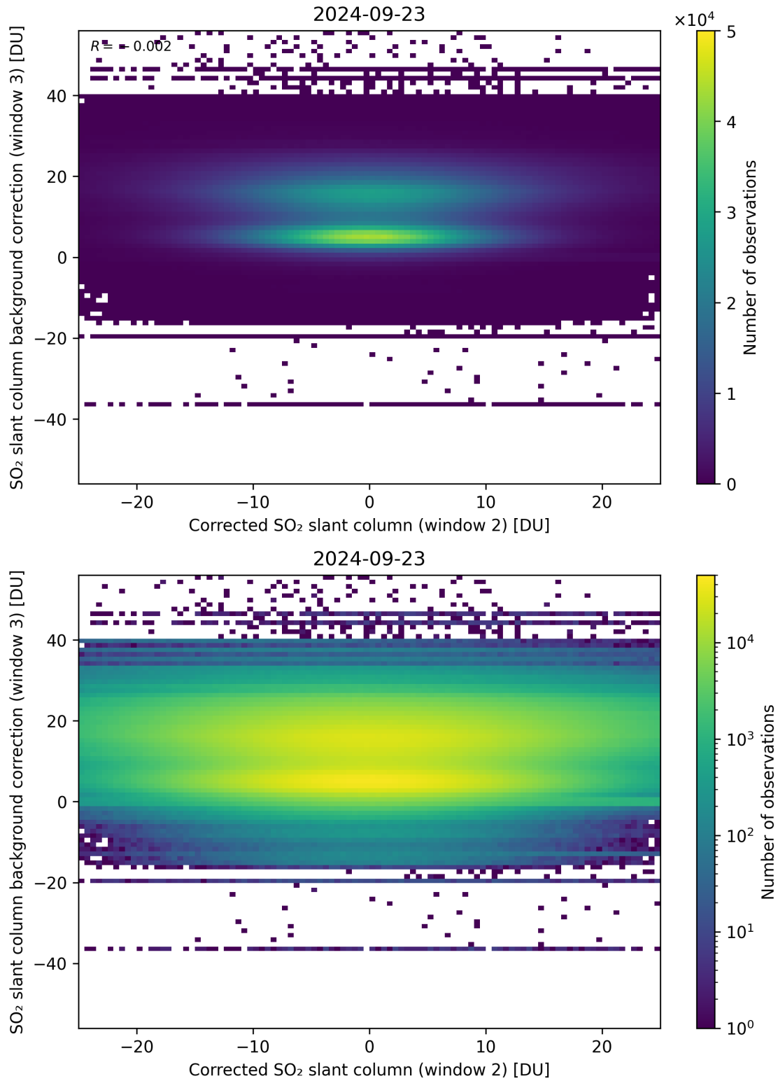
Figure 195: Scatter density plot of “Corrected SO 2 slant column (window 2)” against “SO 2 slant column background correction (window 3)” for 2024-09-22 to 2024-09-24.
