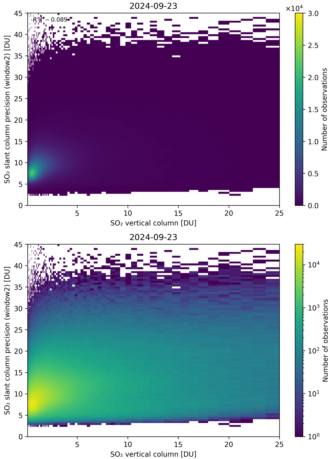
Figure 302: Scatter density plot of “SO 2 vertical column” against “SO 2 slant column precision (window2)” for 2024-09-22 to 2024-09-24.
