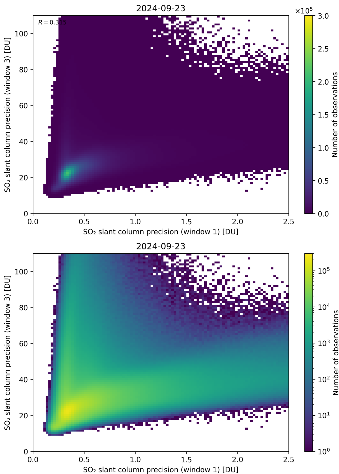
Figure 229: Scatter density plot of “SO 2 slant column precision (window 1)” against “SO 2 slant column precision (window 3)” for 2024-09-22 to 2024-09-24.
