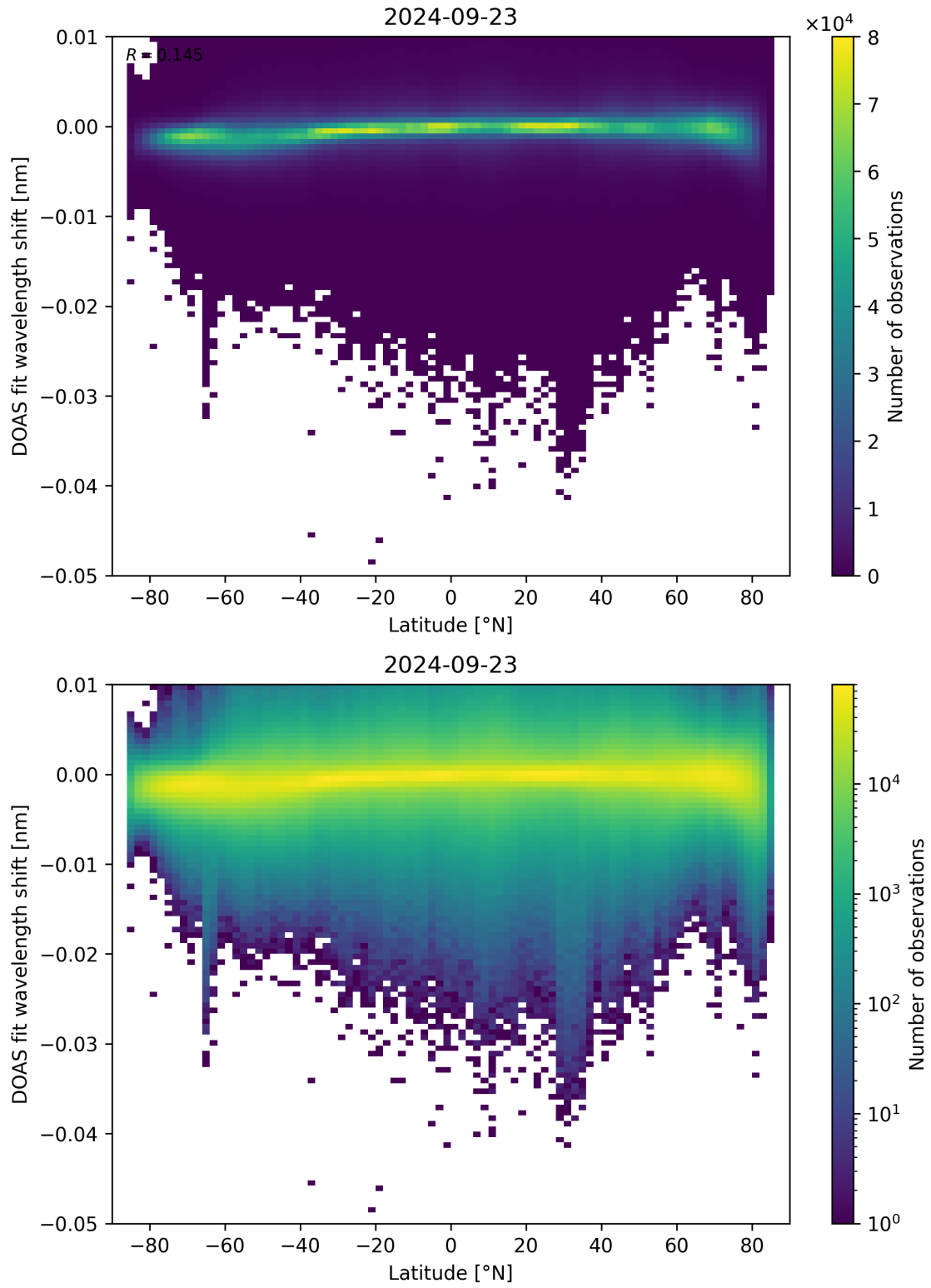
Figure 142: Scatter density plot of “Latitude” against “DOAS fit wavelength shift” for 2024-09-22 to 2024-09-24.
