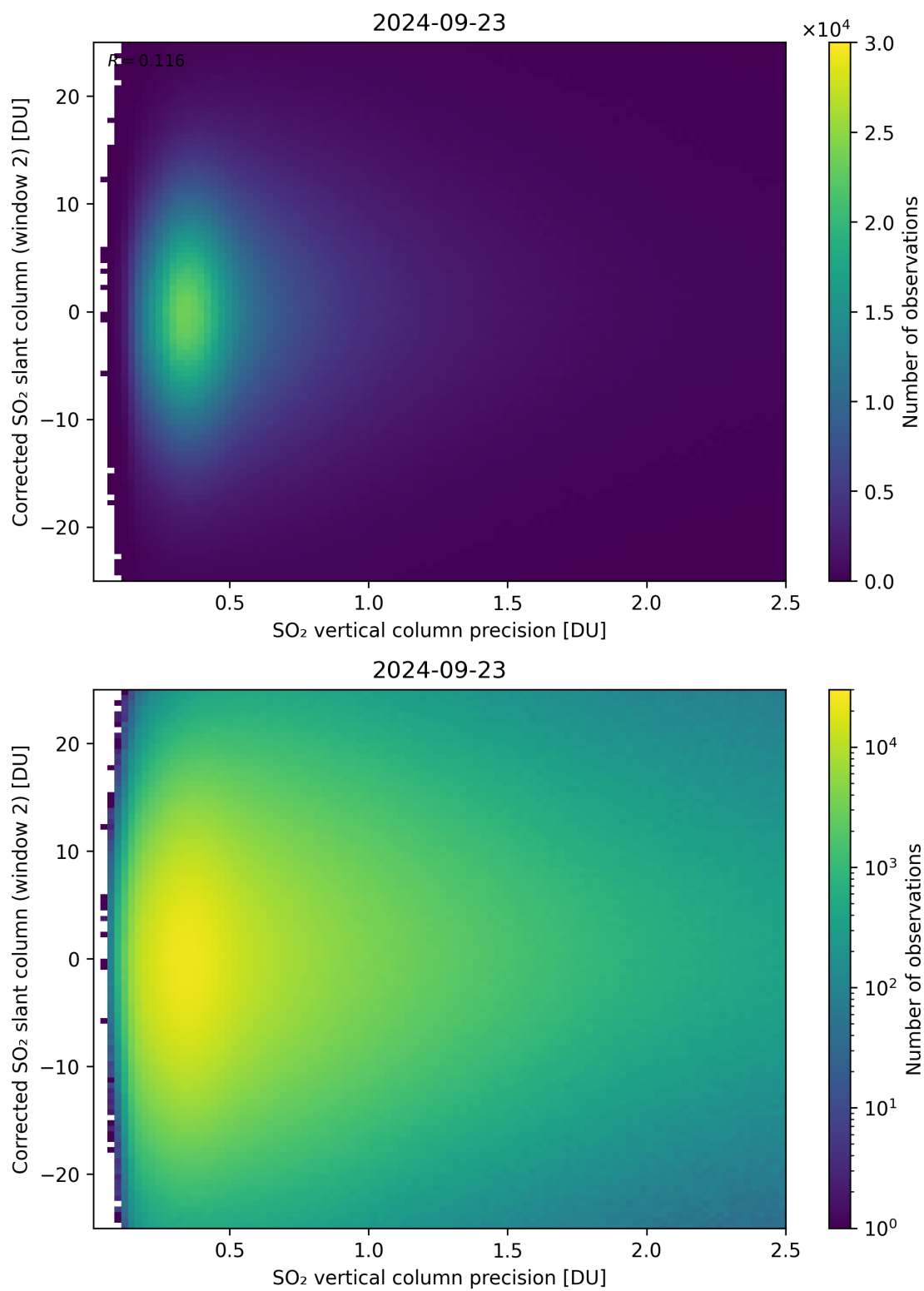
Figure 287: Scatter density plot of “SO 2 vertical column precision” against “Corrected SO 2 slant column (window 2)” for 2024-09-22 to 2024-09-24.
