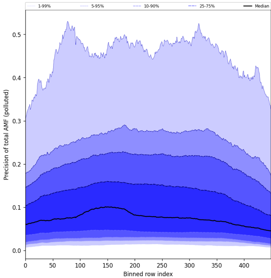
Figure 95: Along track statistics of “Precision of total AMF (polluted)” for 2024-09-22 to 2024-09-24
