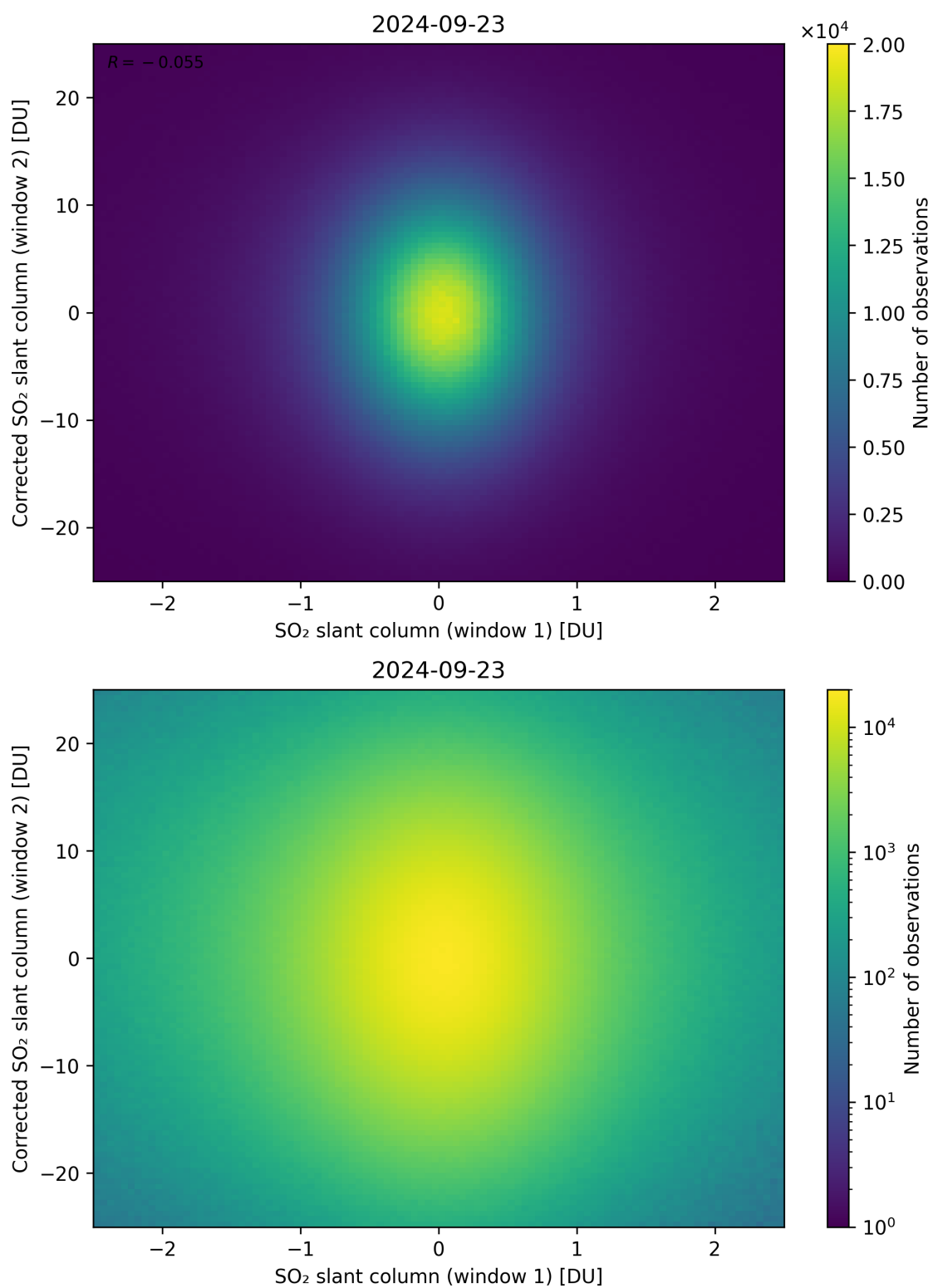
Figure 233: Scatter density plot of “SO 2 slant column (window 1)” against “Corrected SO 2 slant column (window 2)” for 2024-09-22 to 2024-09-24.
