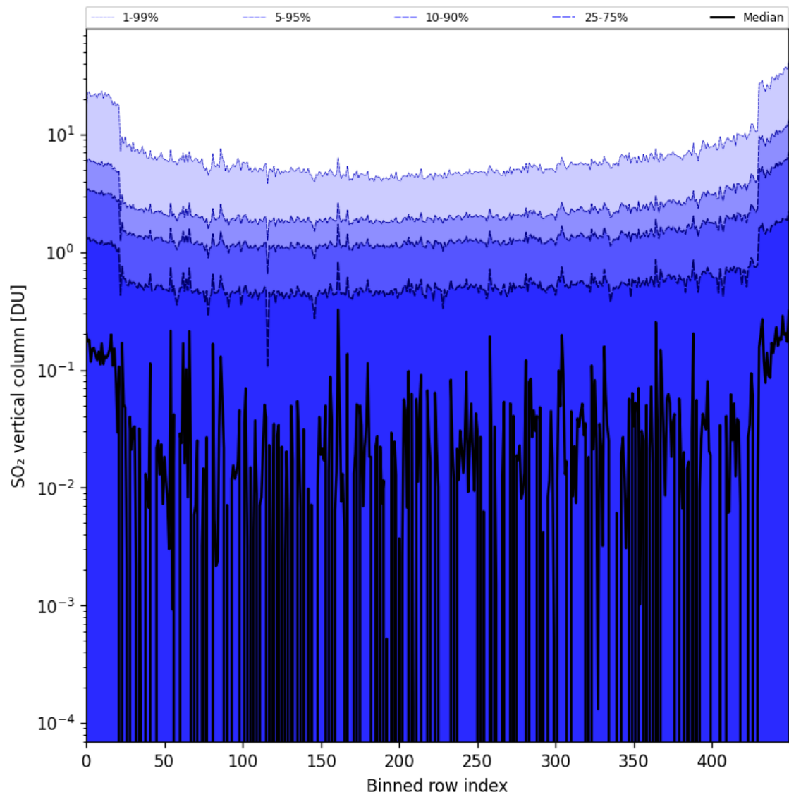
Figure 76: Along track statistics of “SO 2 vertical column” for 2024-09-22 to 2024-09-24
