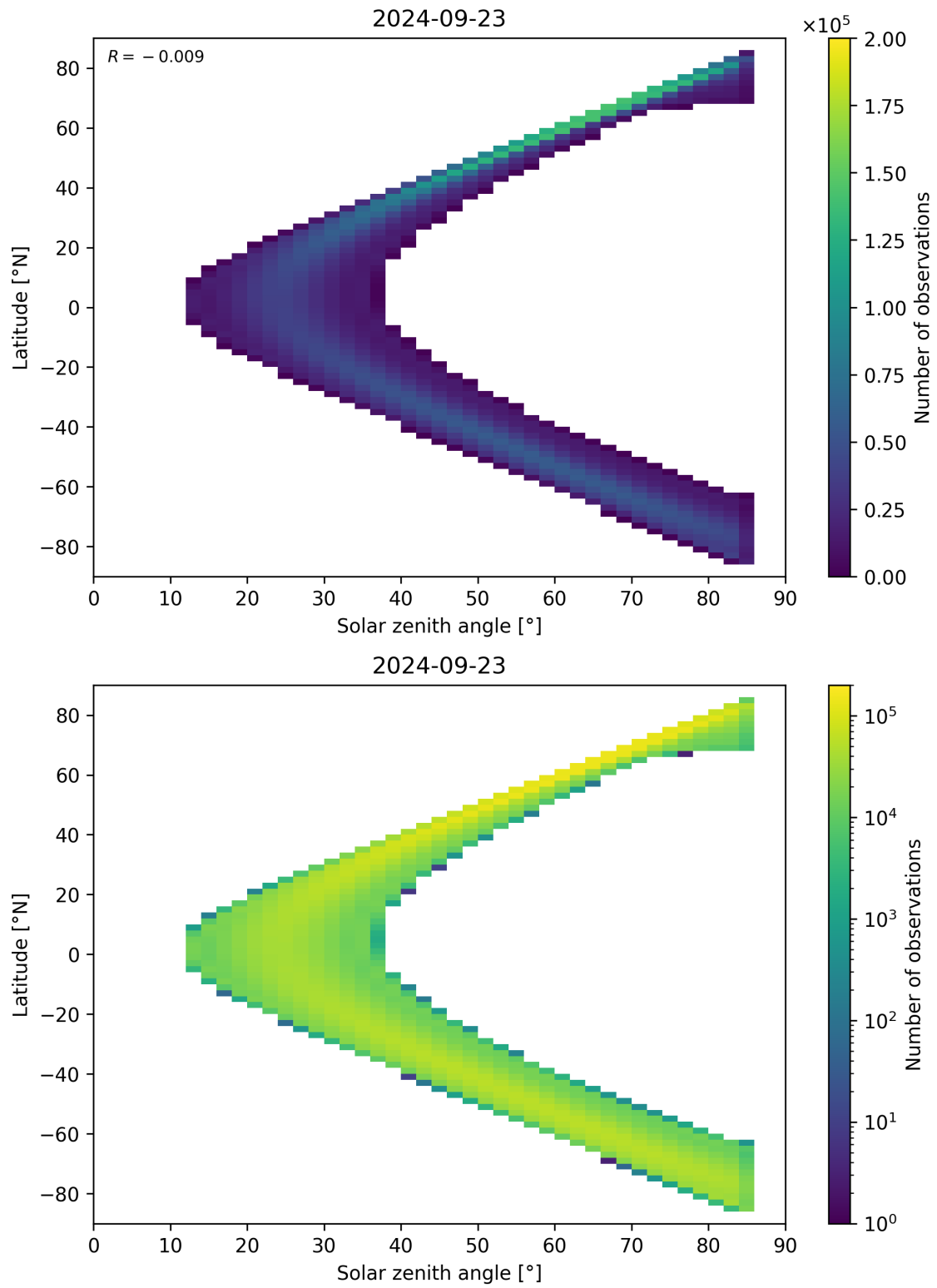
Figure 164: Scatter density plot of “Solar zenith angle” against “Latitude” for 2024-09-22 to 2024-09-24.
