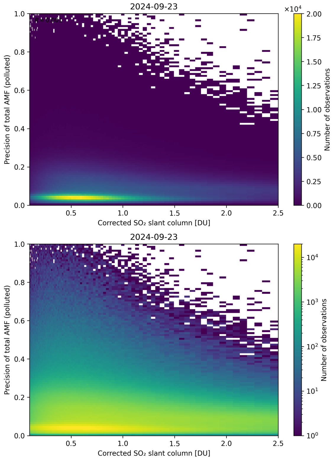
Figure 193: Scatter density plot of “Corrected SO 2 slant column” against “Precision of total AMF (polluted)” for 2024-09-22 to 2024-09-24.
