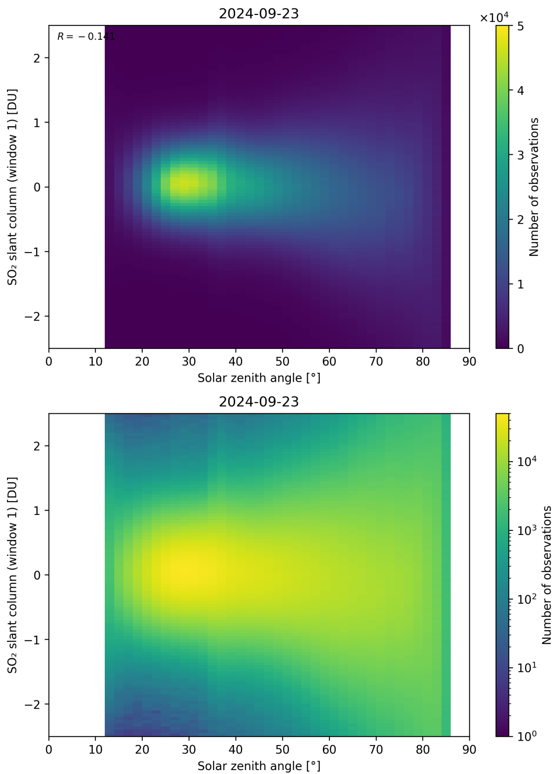
Figure 169: Scatter density plot of “Solar zenith angle” against “SO 2 slant column (window 1)” for 2024-09-22 to 2024-09-24.
