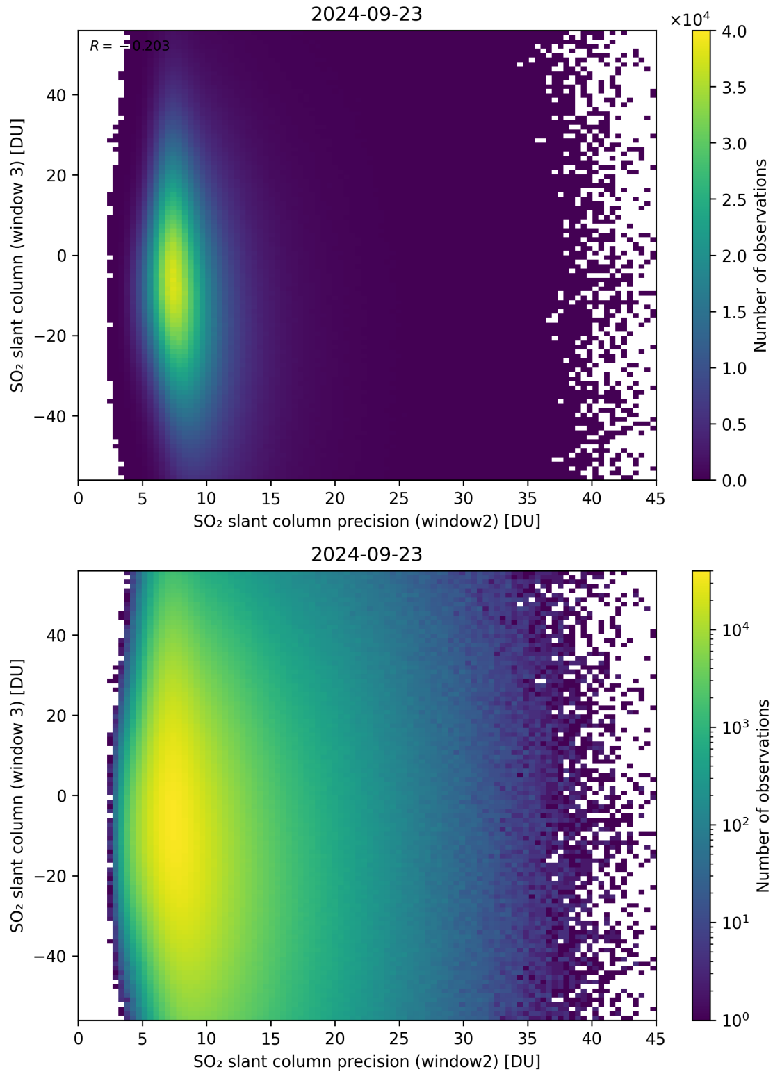
Figure 249: Scatter density plot of “SO 2 slant column precision (window2)” against “SO 2 slant column (window 3)” for 2024-09-22 to 2024-09-24.
