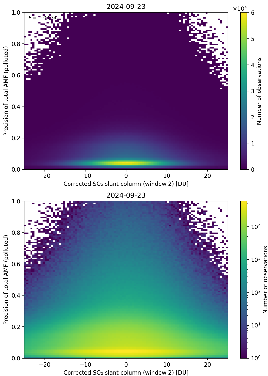
Figure 204: Scatter density plot of “Corrected SO 2 slant column (window 2)” against “Precision of total AMF (polluted)” for 2024-09-22 to 2024-09-24.
