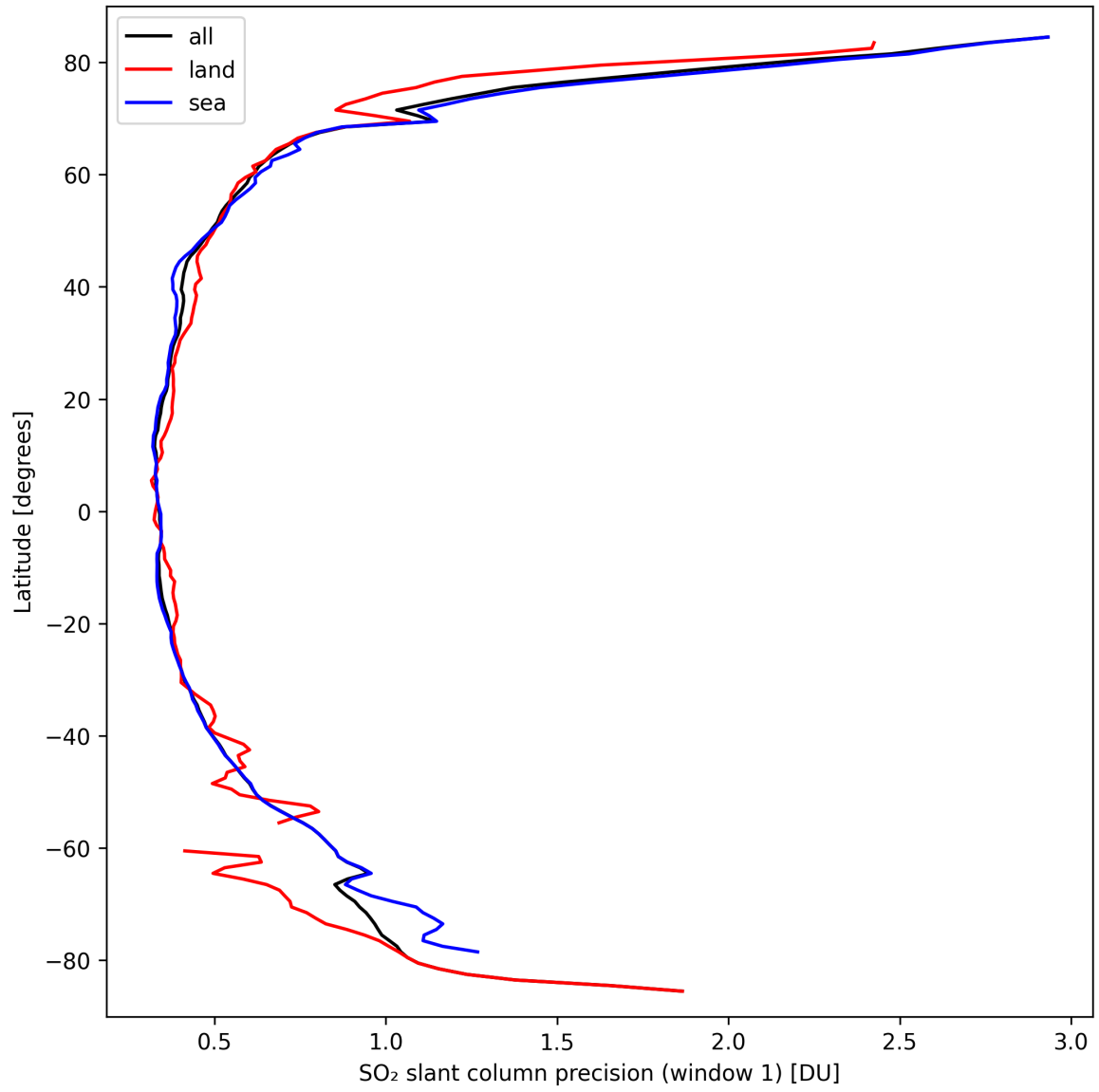
Figure 34: Zonal average of “SO 2 slant column precision (window 1)” for 2024-09-22 to 2024-09-24.
