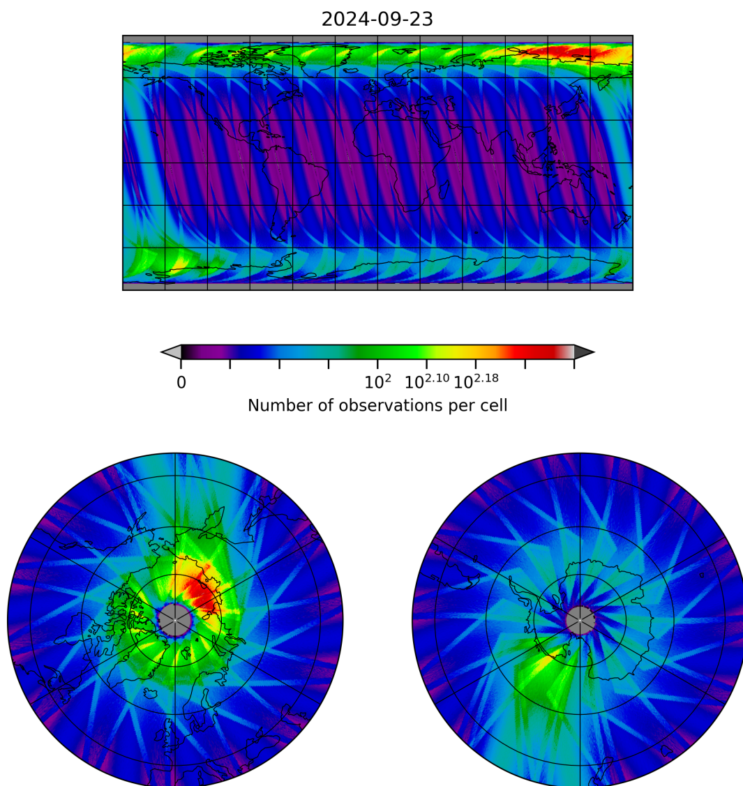
Figure 28: Map of the number of observations for 2024-09-22 to 2024-09-24
