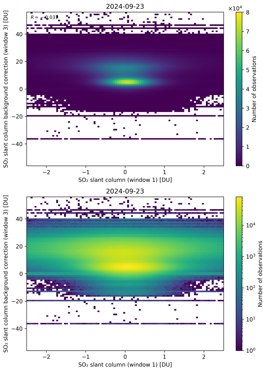
Figure 214: Scatter density plot of “SO 2 slant column (window 1)” against “SO 2 slant column background correction (window 3)” for 2024-09-22 to 2024-09-24.
