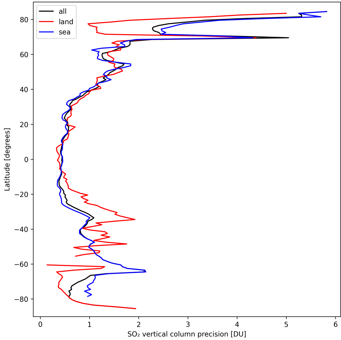
Figure 31: Zonal average of “SO 2 vertical column precision” for 2024-09-22 to 2024-09-24.
