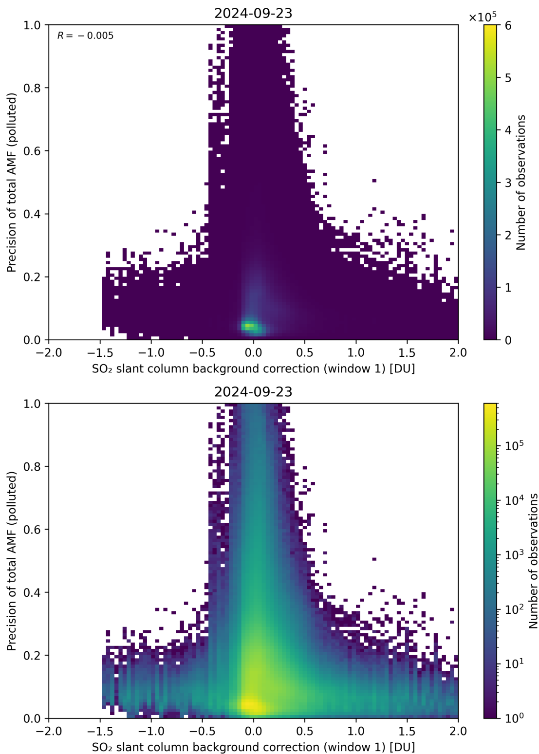
Figure 110: Scatter density plot of “SO 2 slant column background correction (window 1)” against “Precision of total AMF (polluted)” for 2024-09-22 to 2024-09-24.
