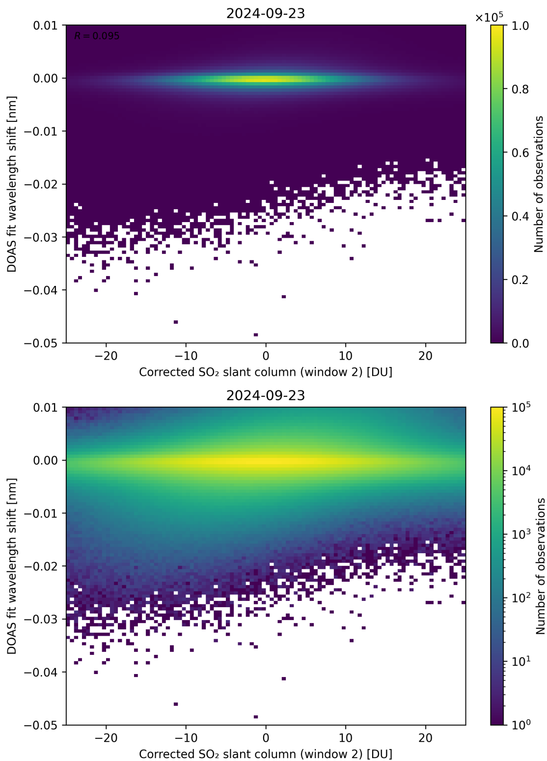
Figure 196: Scatter density plot of “Corrected SO 2 slant column (window 2)” against “DOAS fit wavelength shift” for 2024-09-22 to 2024-09-24.
