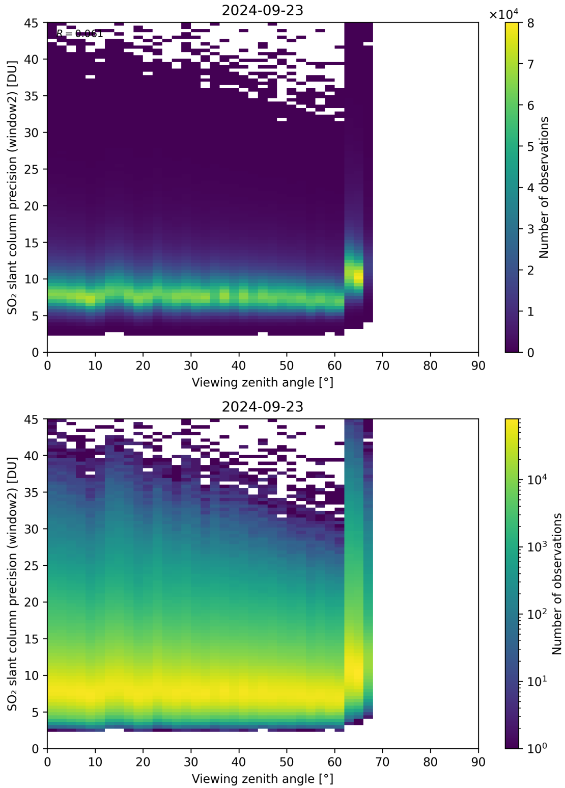
Figure 322: Scatter density plot of “Viewing zenith angle” against “SO 2 slant column precision (window2)” for 2024-09-22 to 2024-09-24.
