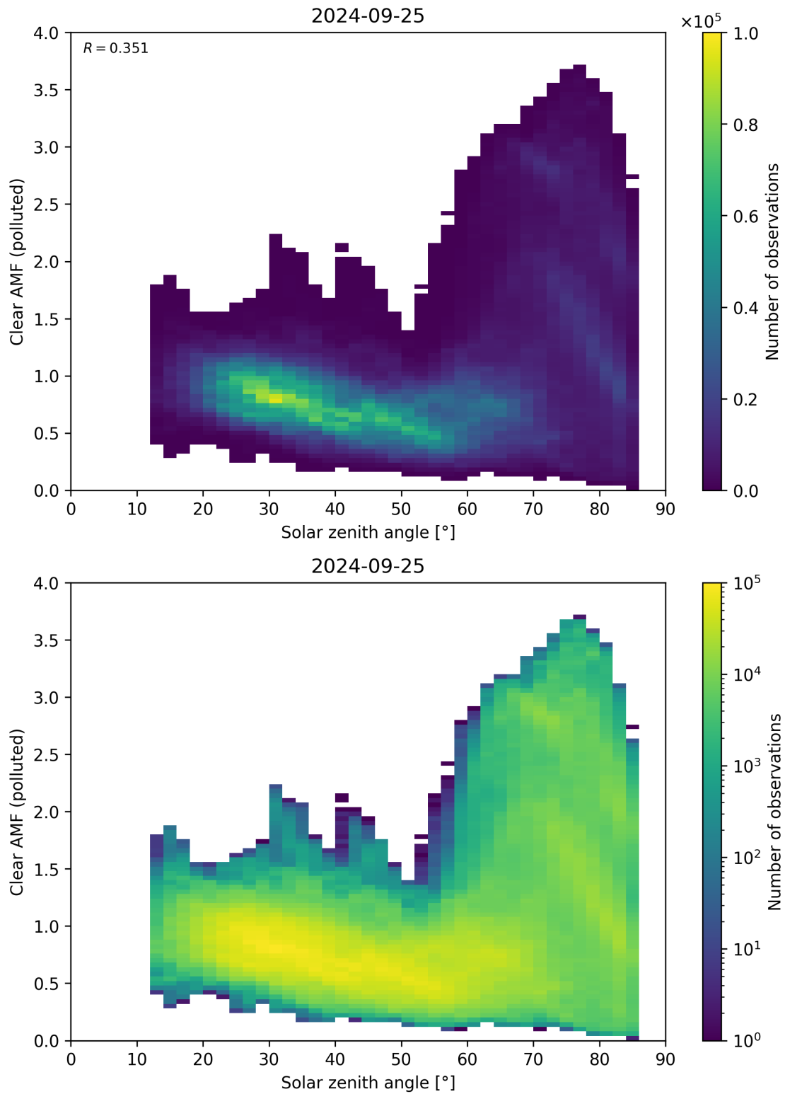
Figure 165: Scatter density plot of “Solar zenith angle” against “Clear AMF (polluted)” for 2024-09-24 to 2024-09-26.
