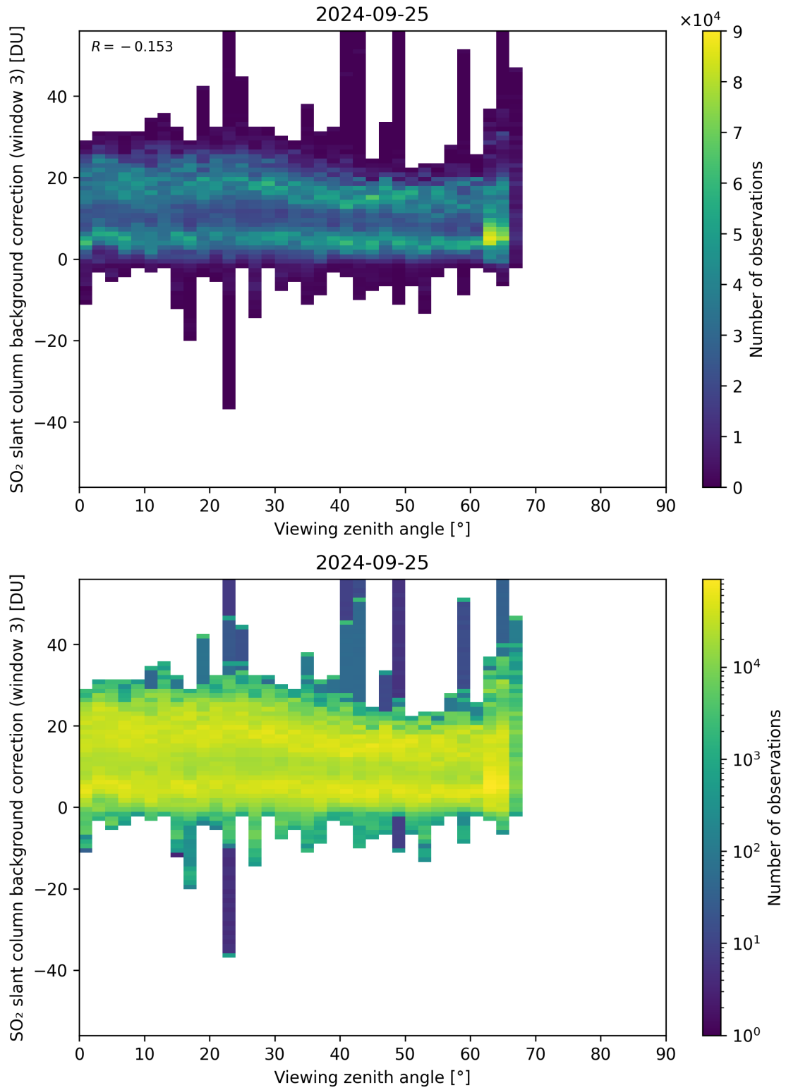
Figure 310: Scatter density plot of “Viewing zenith angle” against “SO 2 slant column background correction (window 3)” for 2024-09-24 to 2024-09-26.
