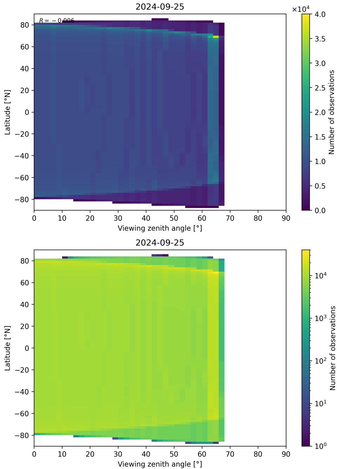
Figure 314: Scatter density plot of “Viewing zenith angle” against “Latitude” for 2024-09-24 to 2024-09-26.
