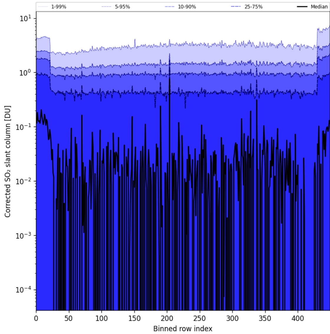
Figure 78: Along track statistics of “Corrected SO 2 slant column” for 2024-09-24 to 2024-09-26
