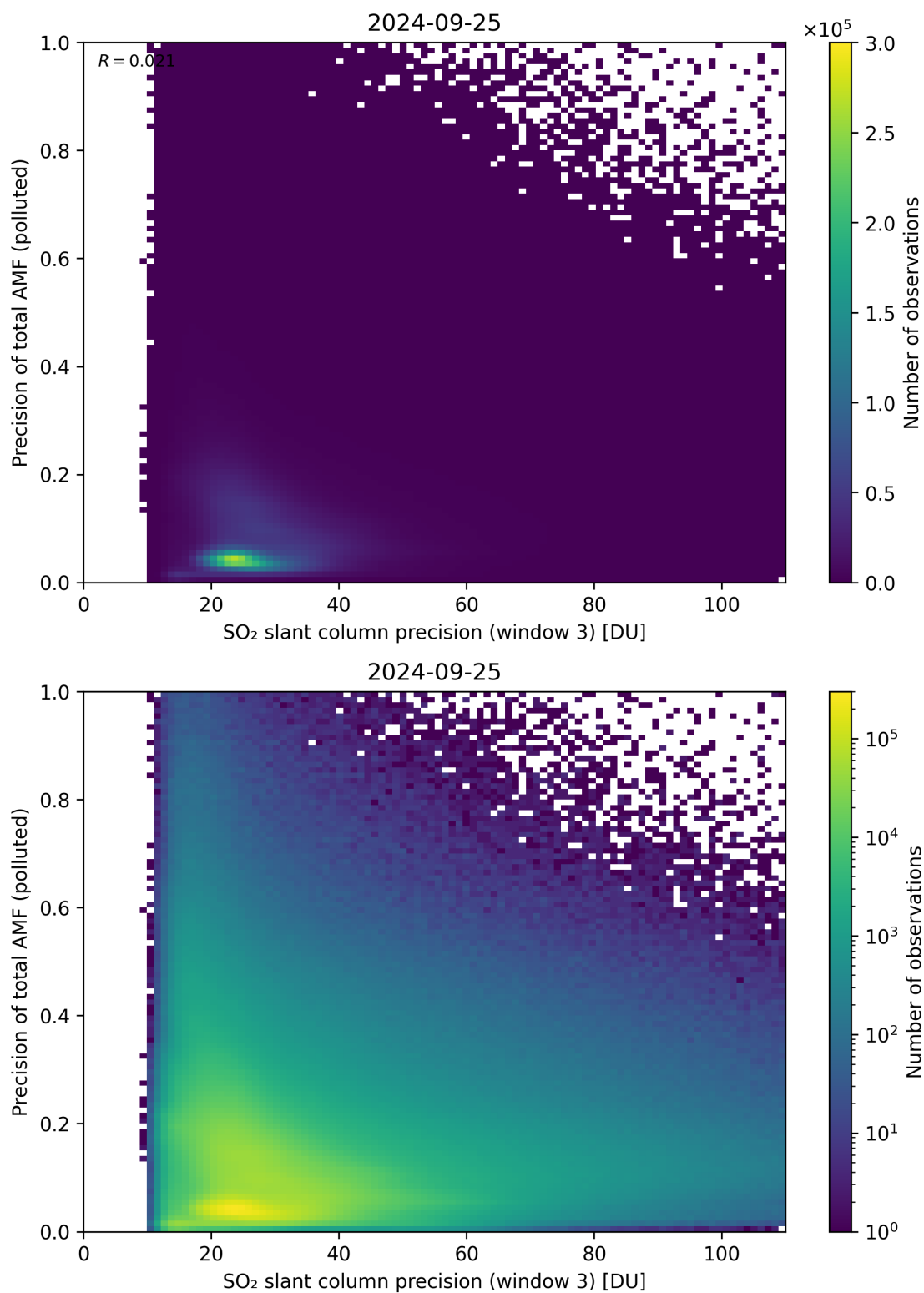
Figure 264: Scatter density plot of “SO 2 slant column precision (window 3)” against “Precision of total AMF (polluted)” for 2024-09-24 to 2024-09-26.
