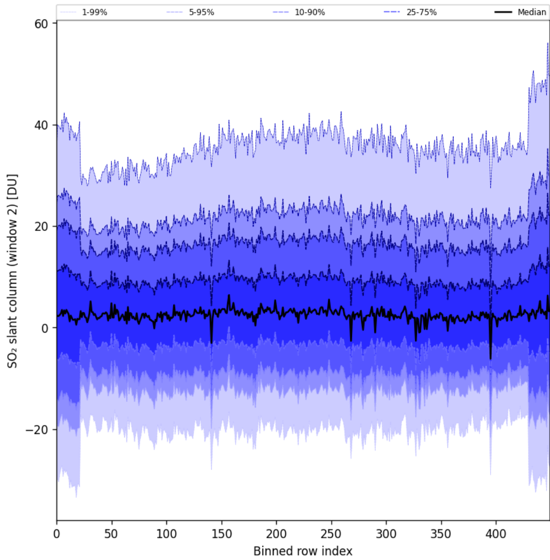
Figure 83: Along track statistics of “SO 2 slant column (window 2)” for 2024-09-24 to 2024-09-26
