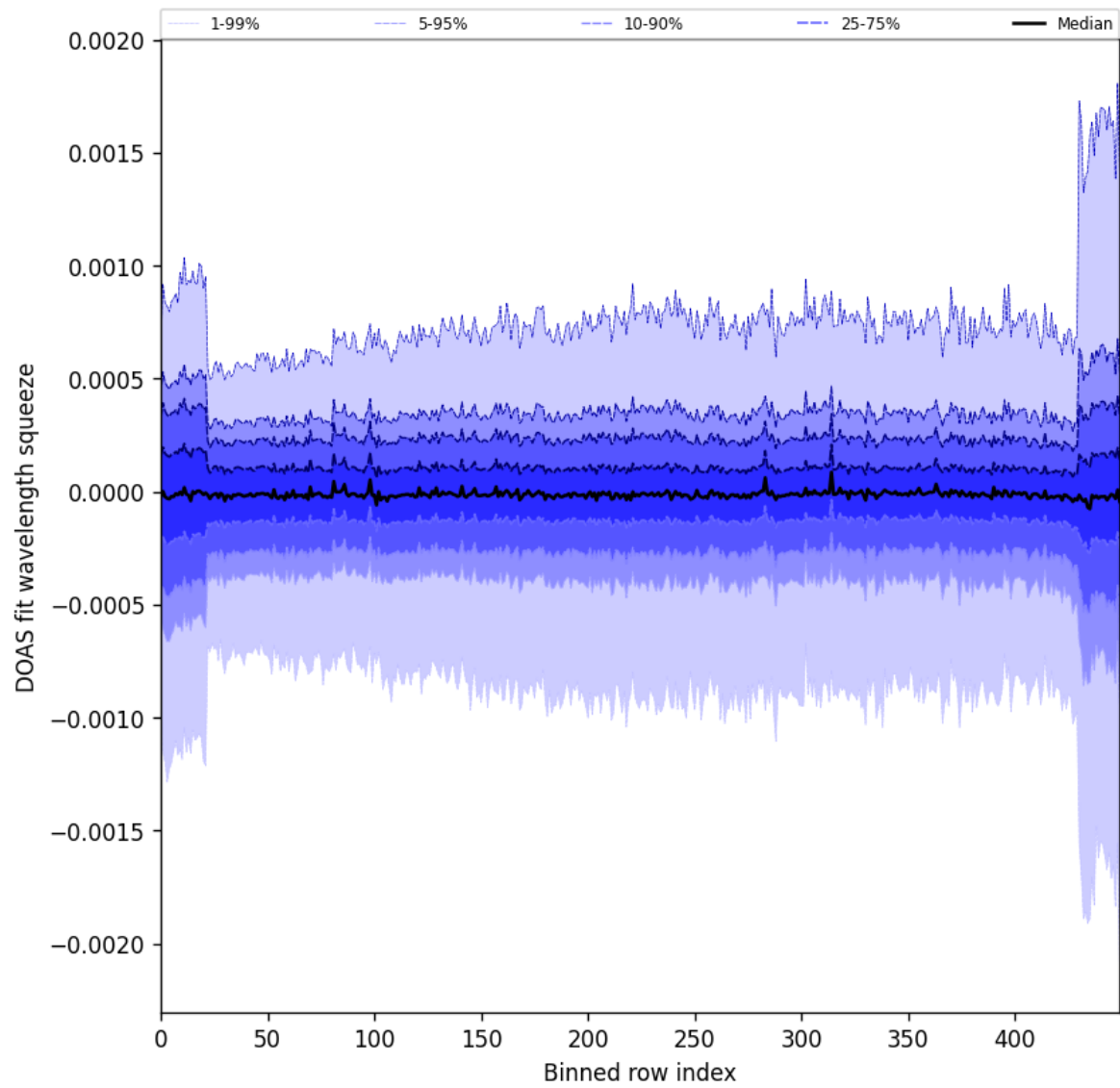
Figure 92: Along track statistics of “DOAS fit wavelength squeeze” for 2024-09-24 to 2024-09-26
