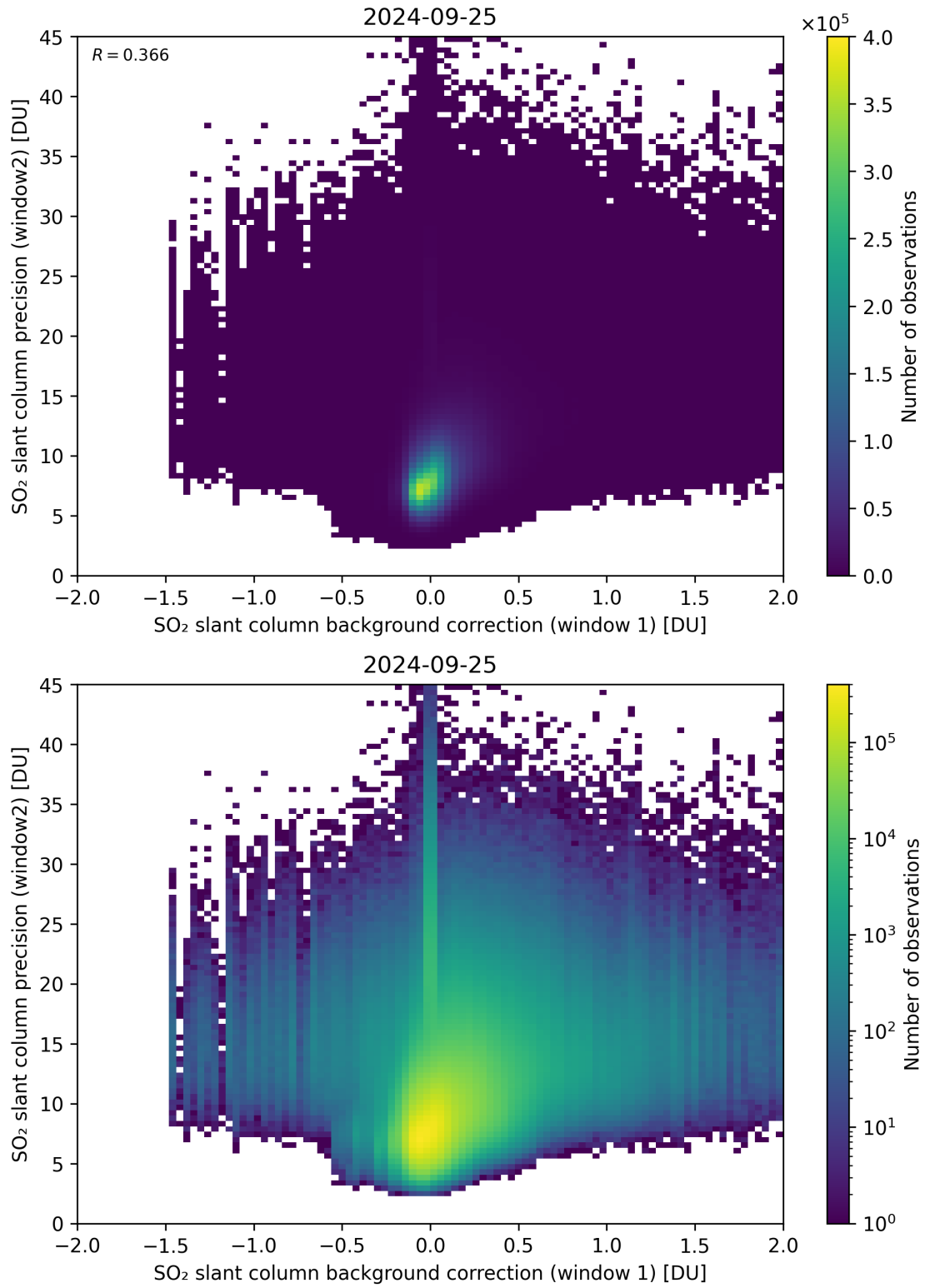
Figure 106: Scatter density plot of “SO 2 slant column background correction (window 1)” against “SO 2 slant column precision (window2)” for 2024-09-24 to 2024-09-26.
