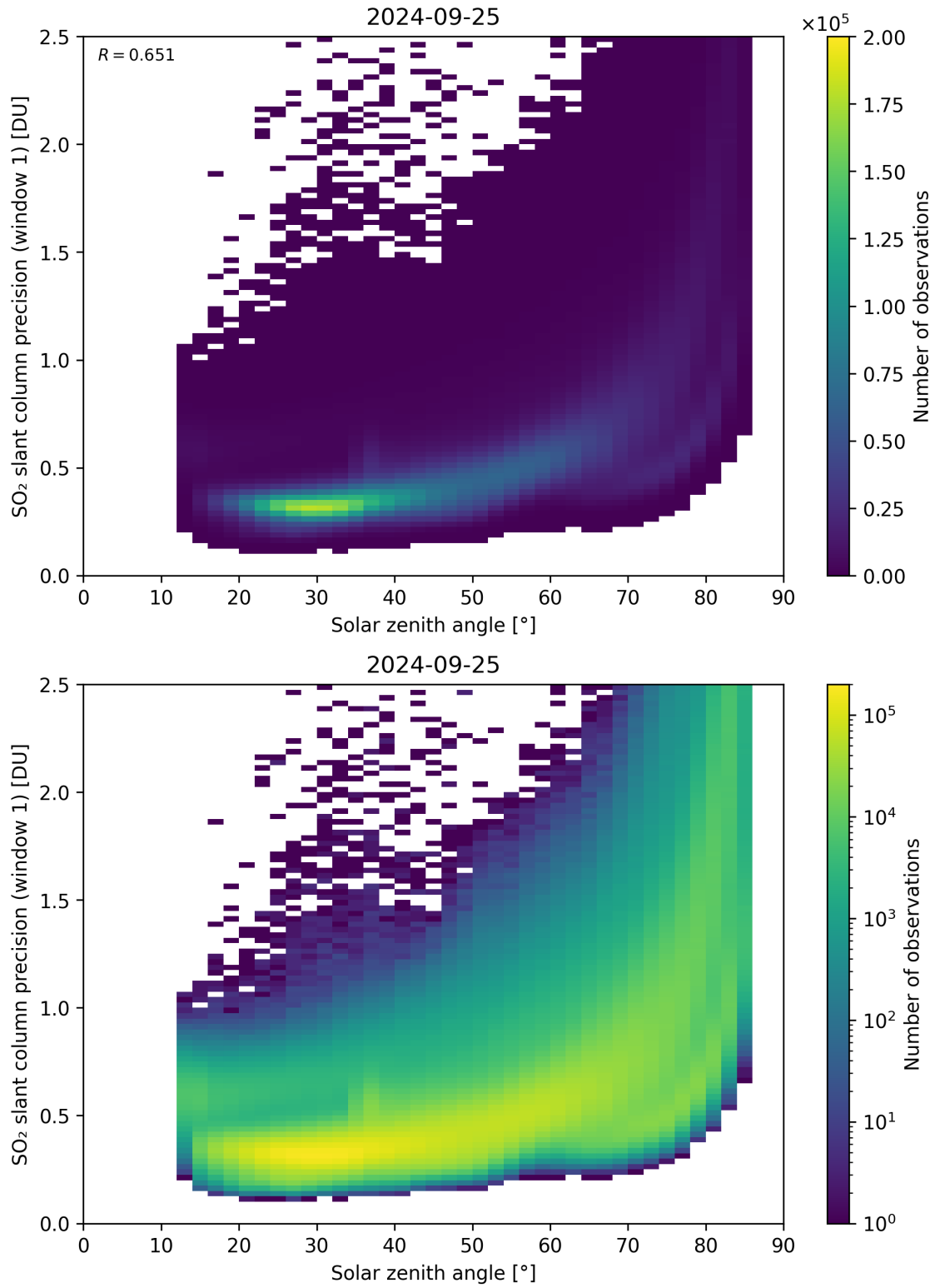
Figure 170: Scatter density plot of “Solar zenith angle” against “SO 2 slant column precision (window 1)” for 2024-09-24 to 2024-09-26.
