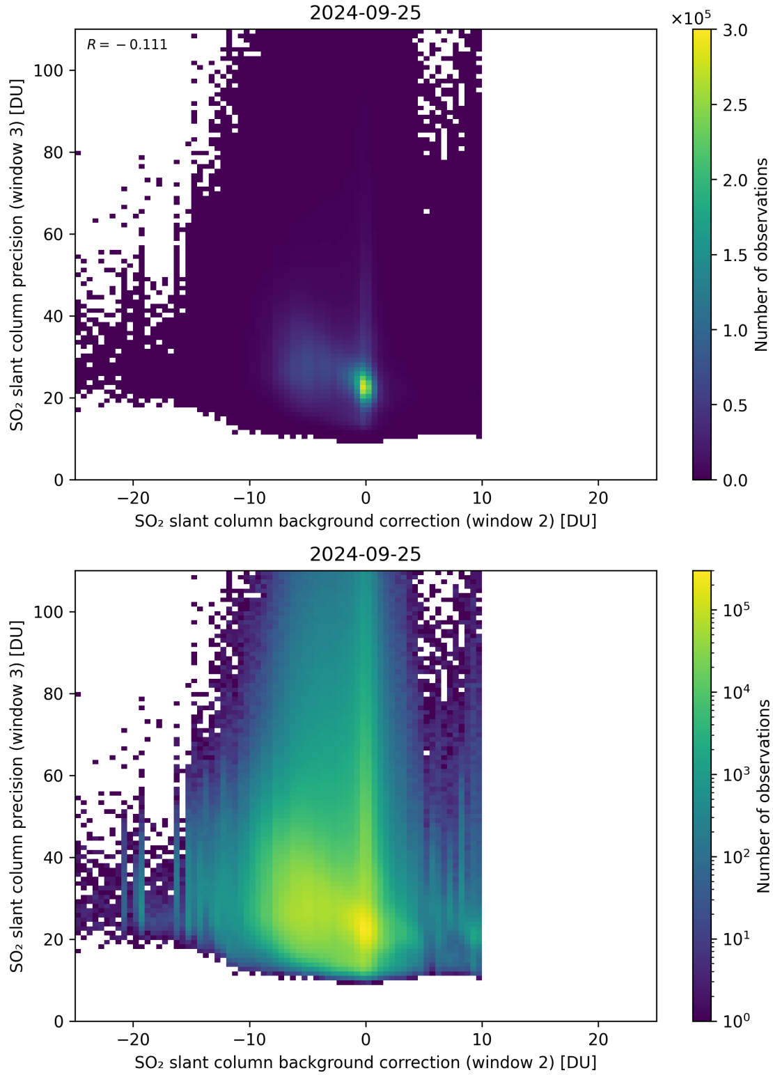
Figure 118: Scatter density plot of “SO 2 slant column background correction (window 2)” against “SO 2 slant column precision (window 3)” for 2024-09-24 to 2024-09-26.
