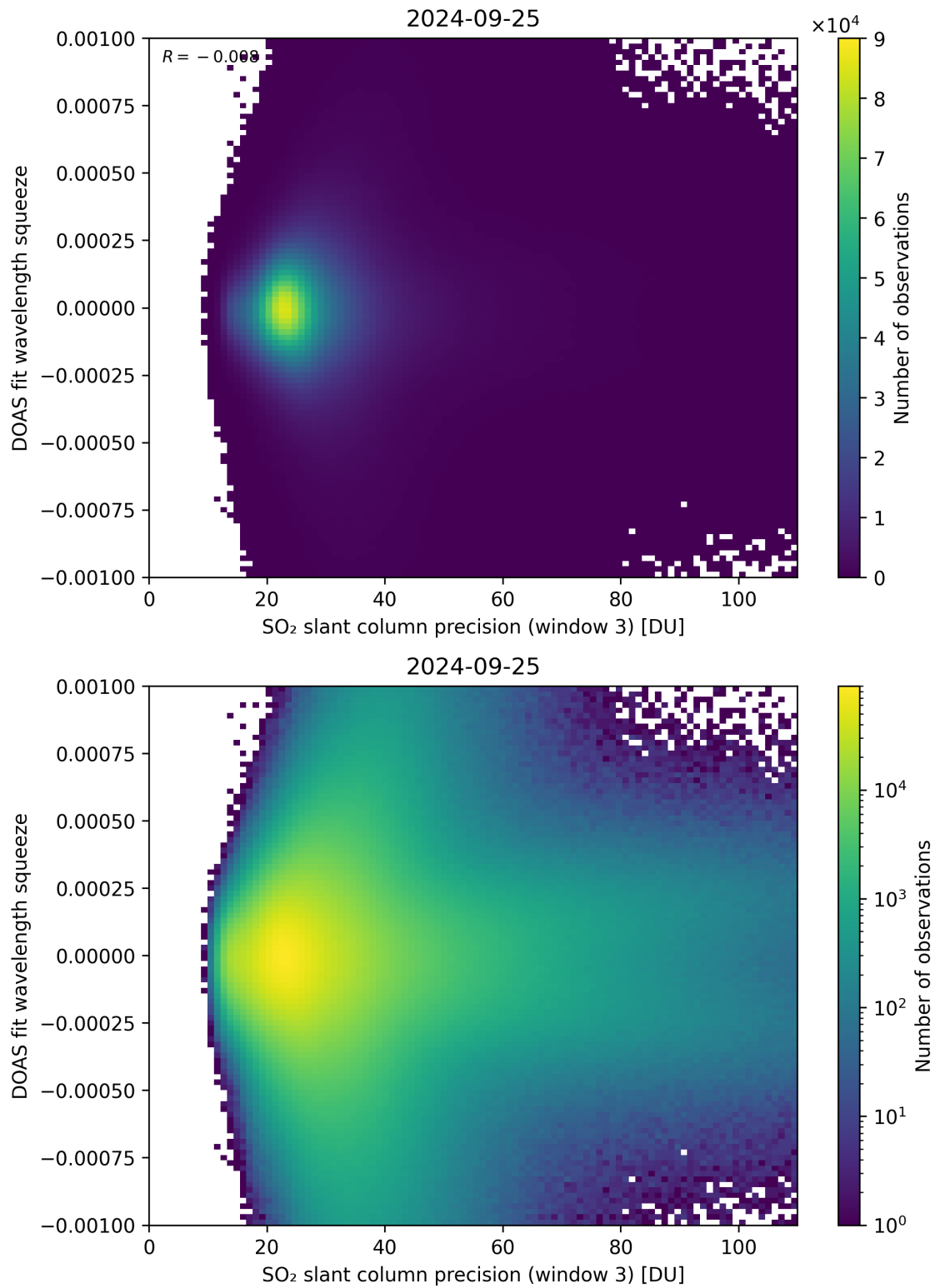
Figure 259: Scatter density plot of “SO 2 slant column precision (window 3)” against “DOAS fit wavelength squeeze” for 2024-09-24 to 2024-09-26.
