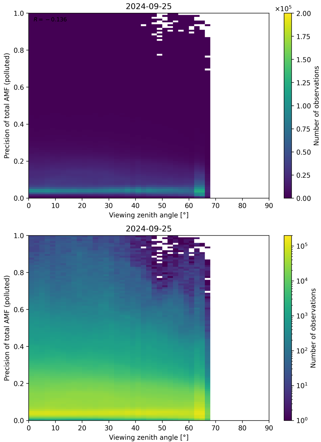
Figure 326: Scatter density plot of “Viewing zenith angle” against “Precision of total AMF (polluted)” for 2024-09-24 to 2024-09-26.
