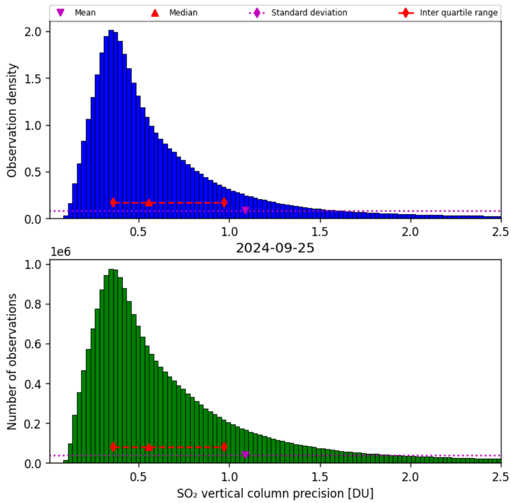
Figure 54: Histogram of “SO 2 vertical column precision” for 2024-09-24 to 2024-09-26
