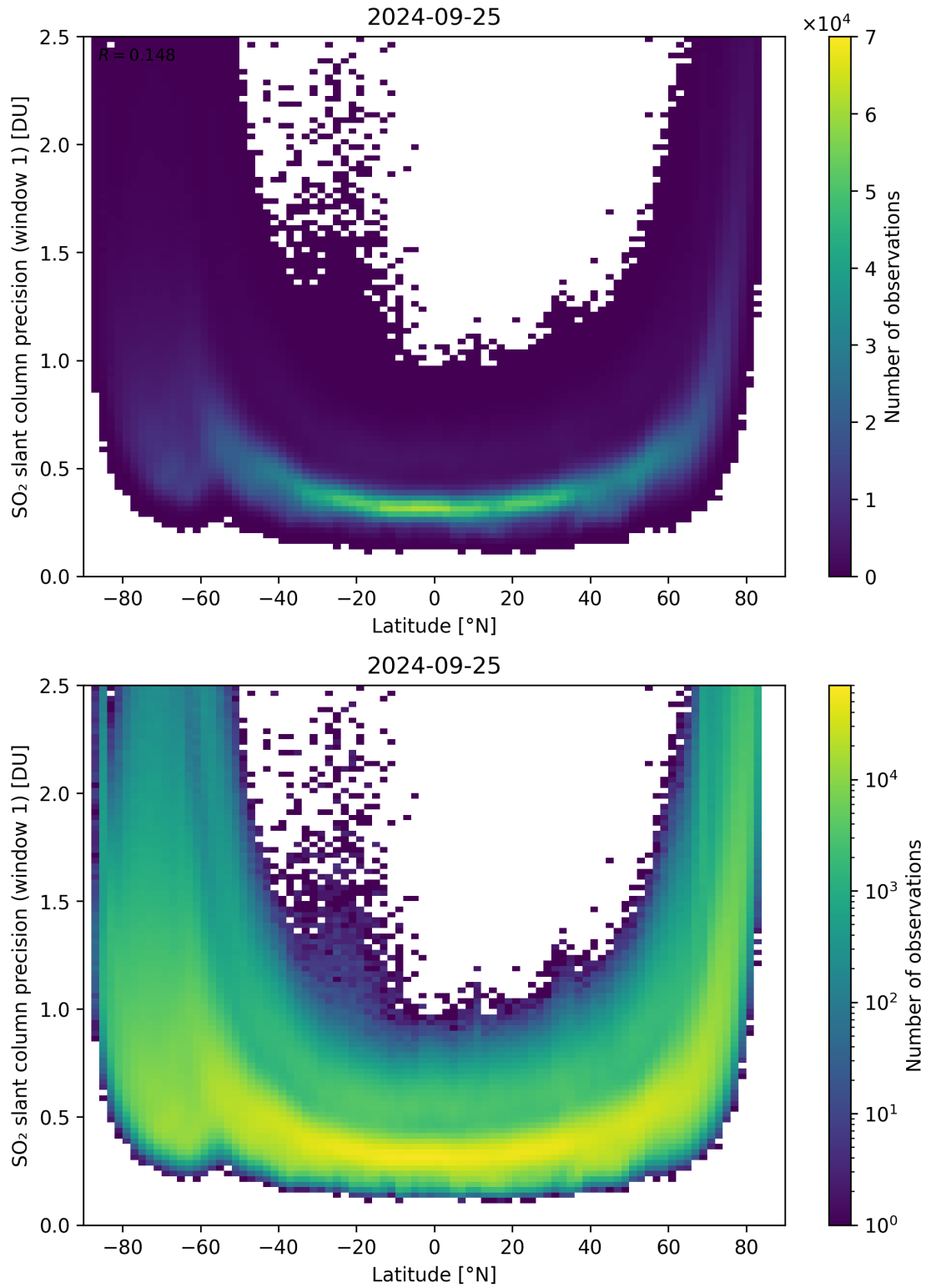
Figure 150: Scatter density plot of “Latitude” against “SO 2 slant column precision (window 1)” for 2024-09-24 to 2024-09-26.
