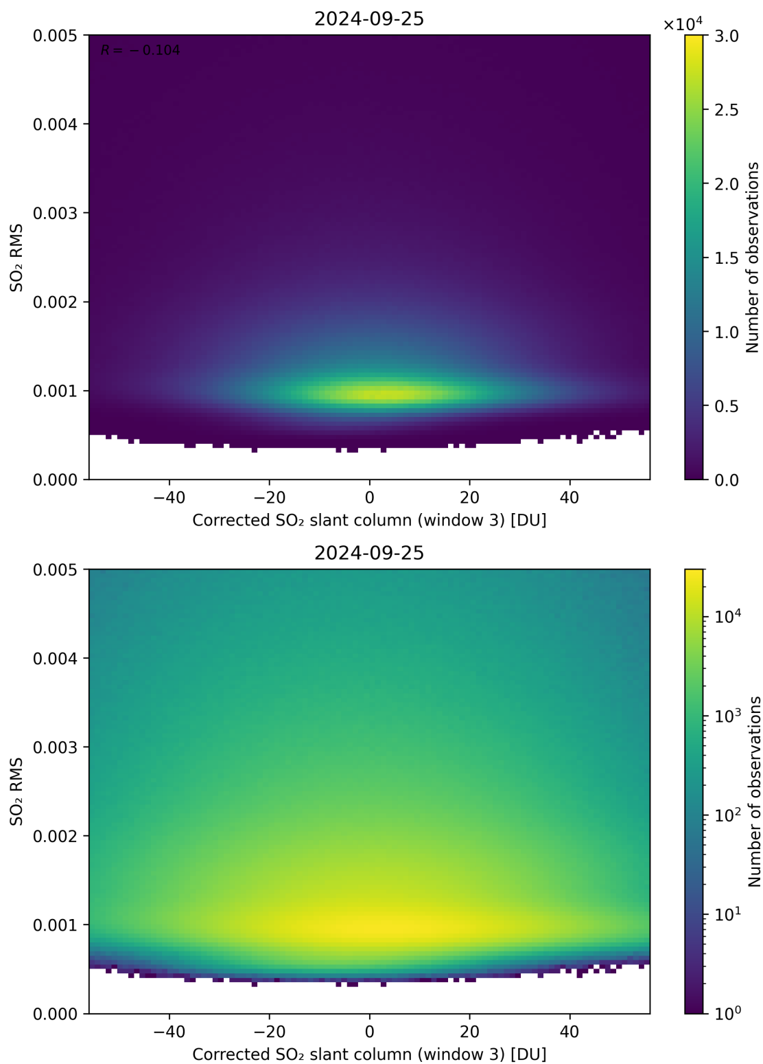
Figure 208: Scatter density plot of “Corrected SO 2 slant column (window 3)” against “SO 2 RMS” for 2024-09-24 to 2024-09-26.
