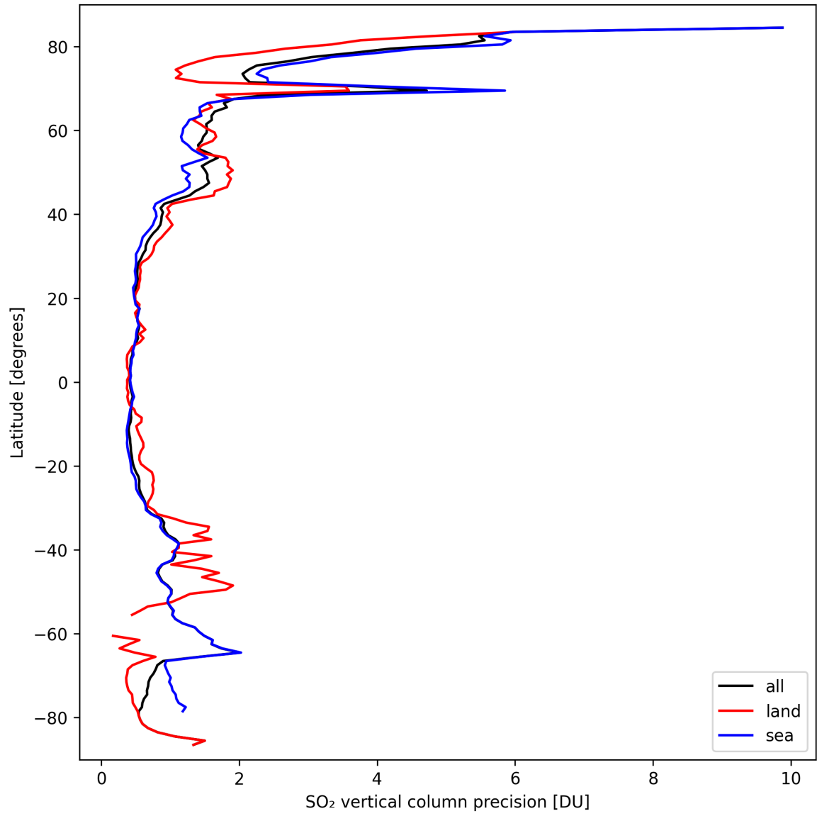
Figure 31: Zonal average of “SO 2 vertical column precision” for 2024-09-24 to 2024-09-26.
