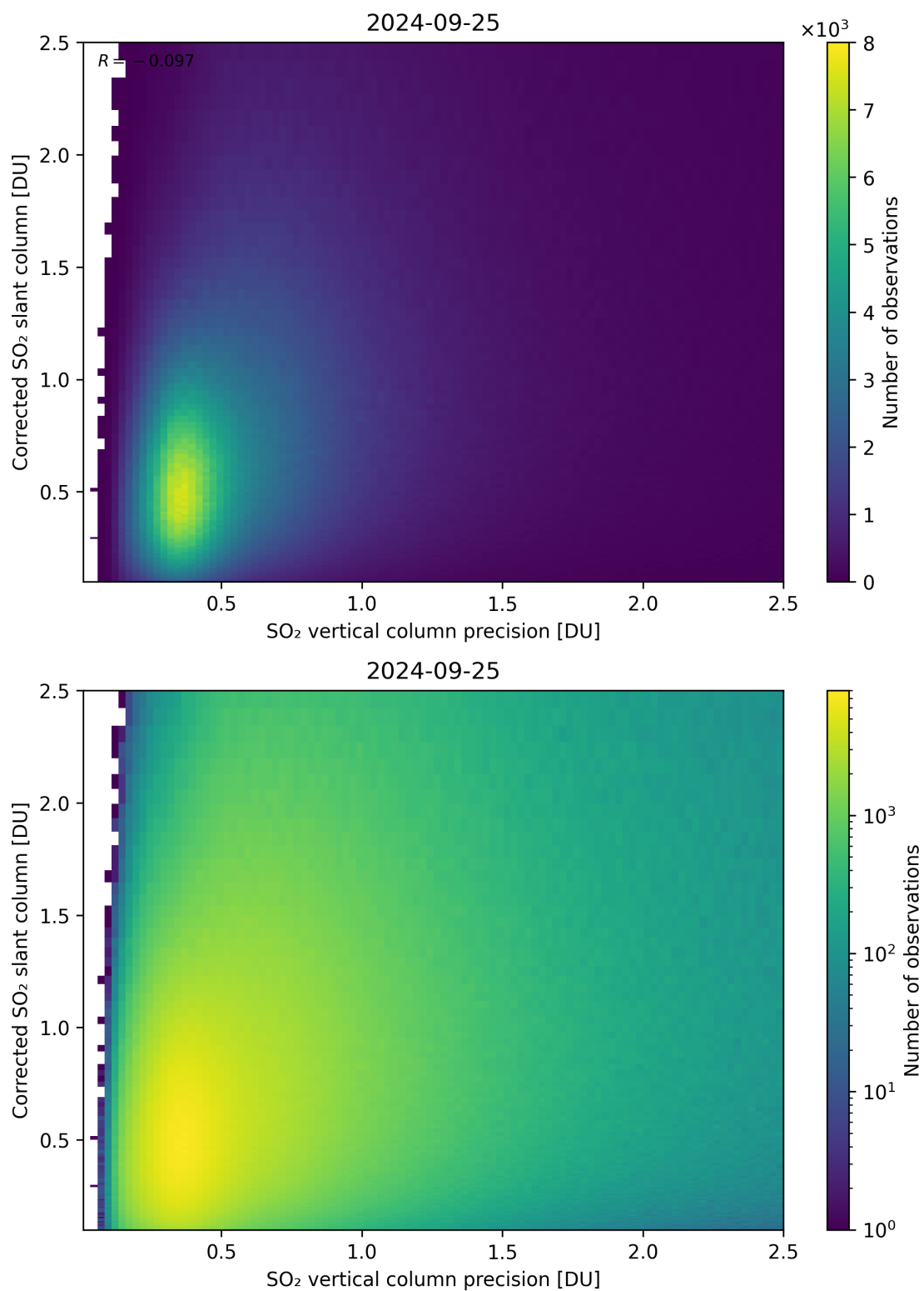
Figure 286: Scatter density plot of “SO 2 vertical column precision” against “Corrected SO 2 slant column” for 2024-09-24 to 2024-09-26.
