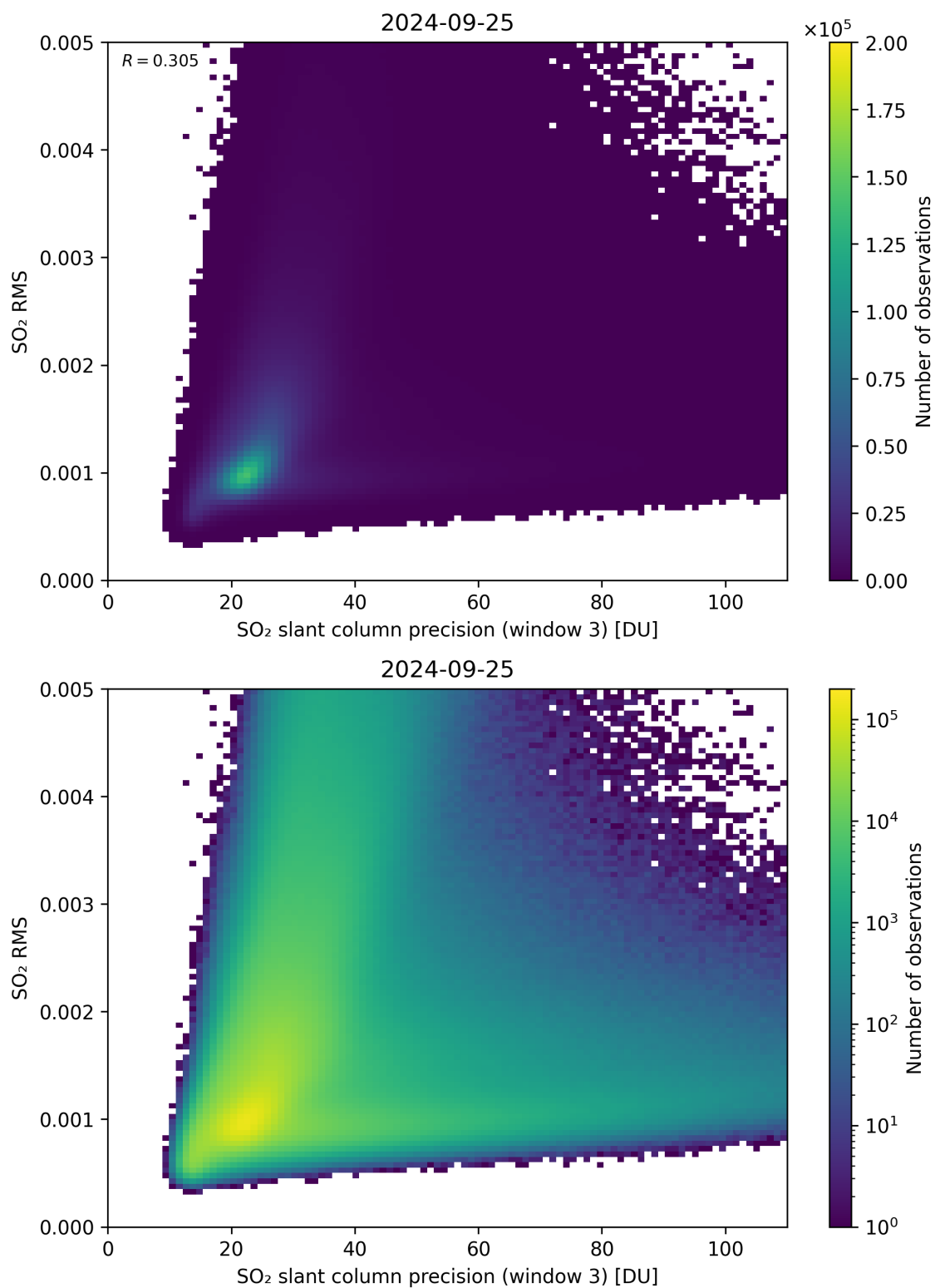
Figure 260: Scatter density plot of “SO 2 slant column precision (window 3)” against “SO 2 RMS” for 2024-09-24 to 2024-09-26.
