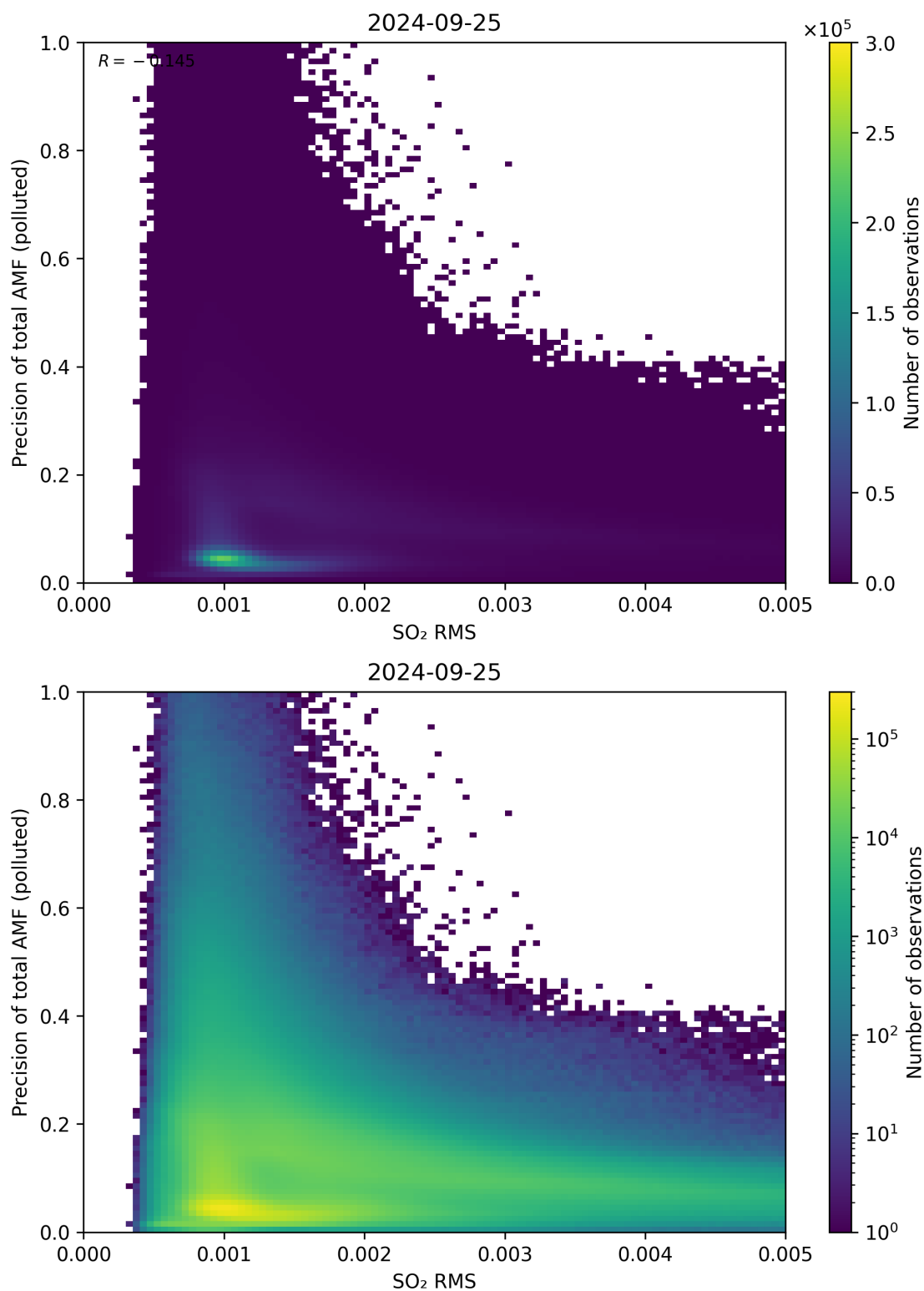
Figure 138: Scatter density plot of “SO 2 RMS” against “Precision of total AMF (polluted)” for 2024-09-24 to 2024-09-26.
