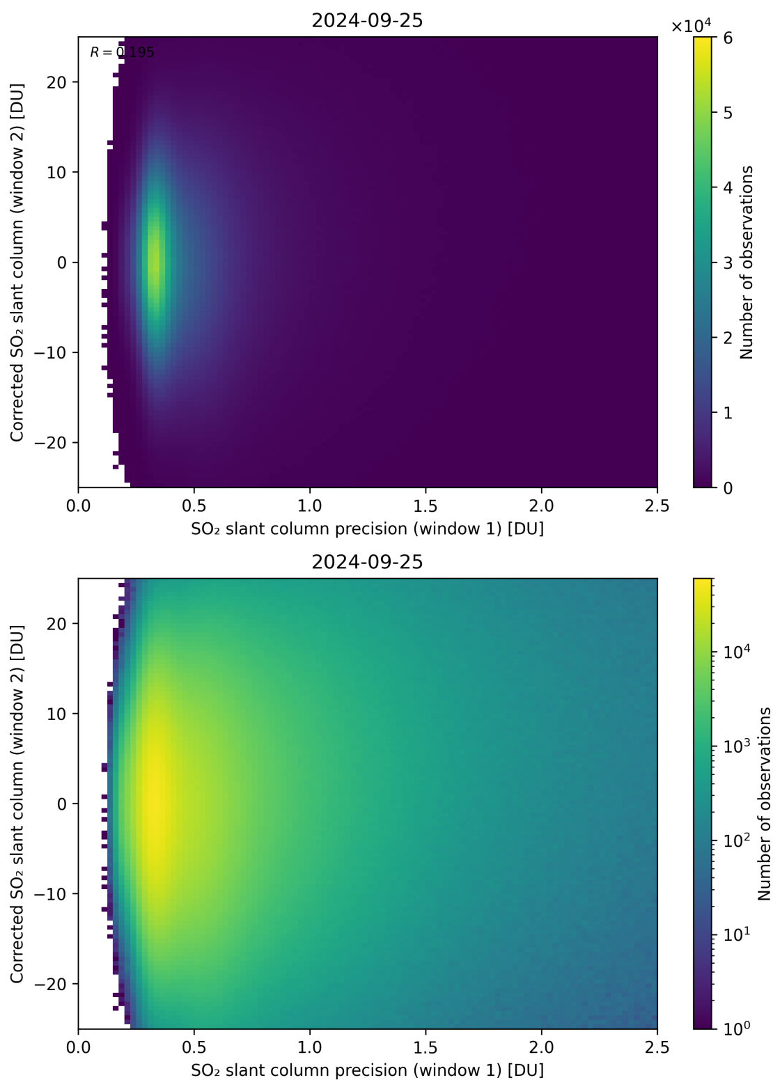
Figure 225: Scatter density plot of “SO 2 slant column precision (window 1)” against “Corrected SO 2 slant column (window 2)” for 2024-09-24 to 2024-09-26.
