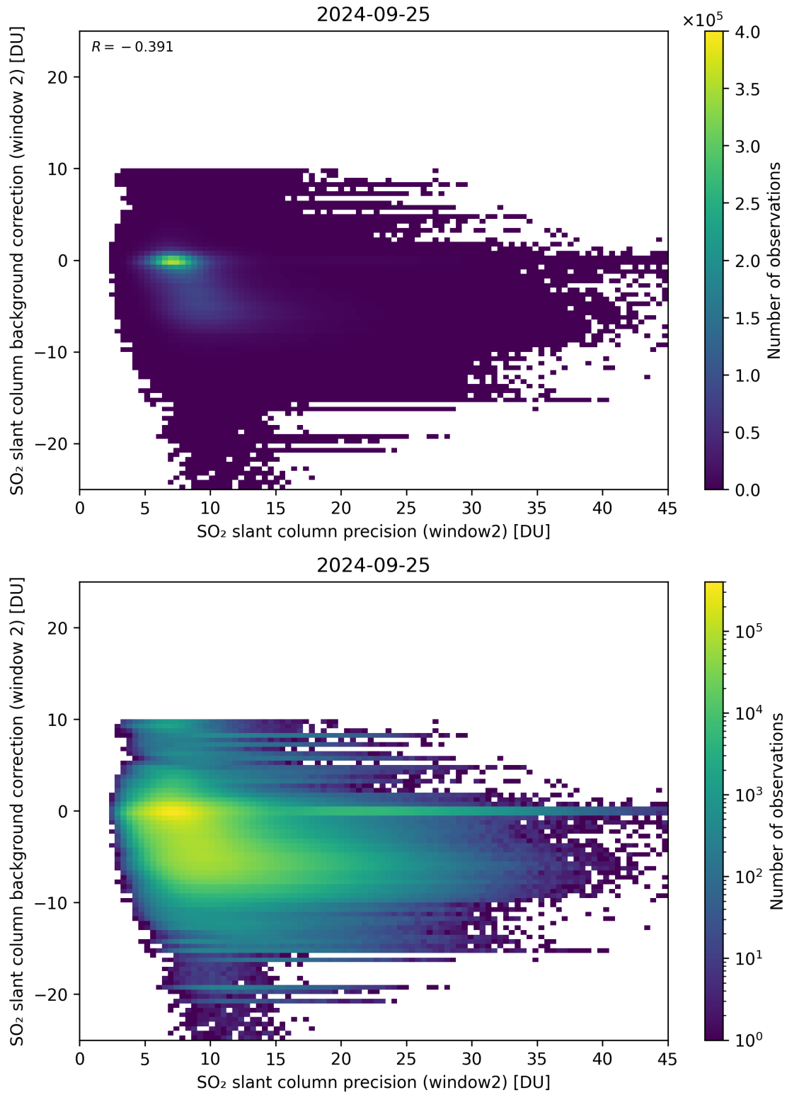
Figure 241: Scatter density plot of “SO 2 slant column precision (window2)” against “SO 2 slant column background correction (window 2)” for 2024-09-24 to 2024-09-26.
