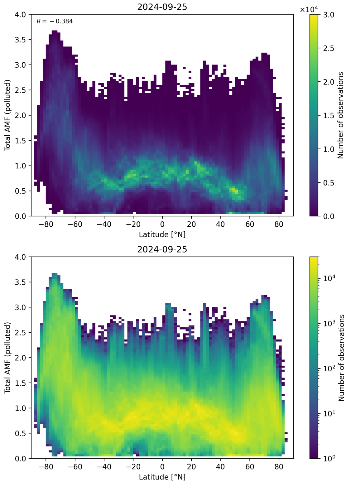
Figure 154: Scatter density plot of “Latitude” against “Total AMF (polluted)” for 2024-09-24 to 2024-09-26.
