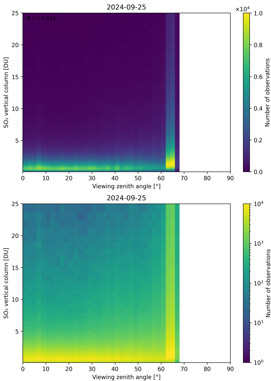
Figure 327: Scatter density plot of “Viewing zenith angle” against “SO 2 vertical column” for 2024-09-24 to 2024-09-26.
