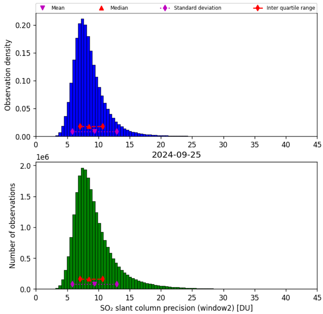
Figure 61: Histogram of “SO 2 slant column precision (window2)” for 2024-09-24 to 2024-09-26
