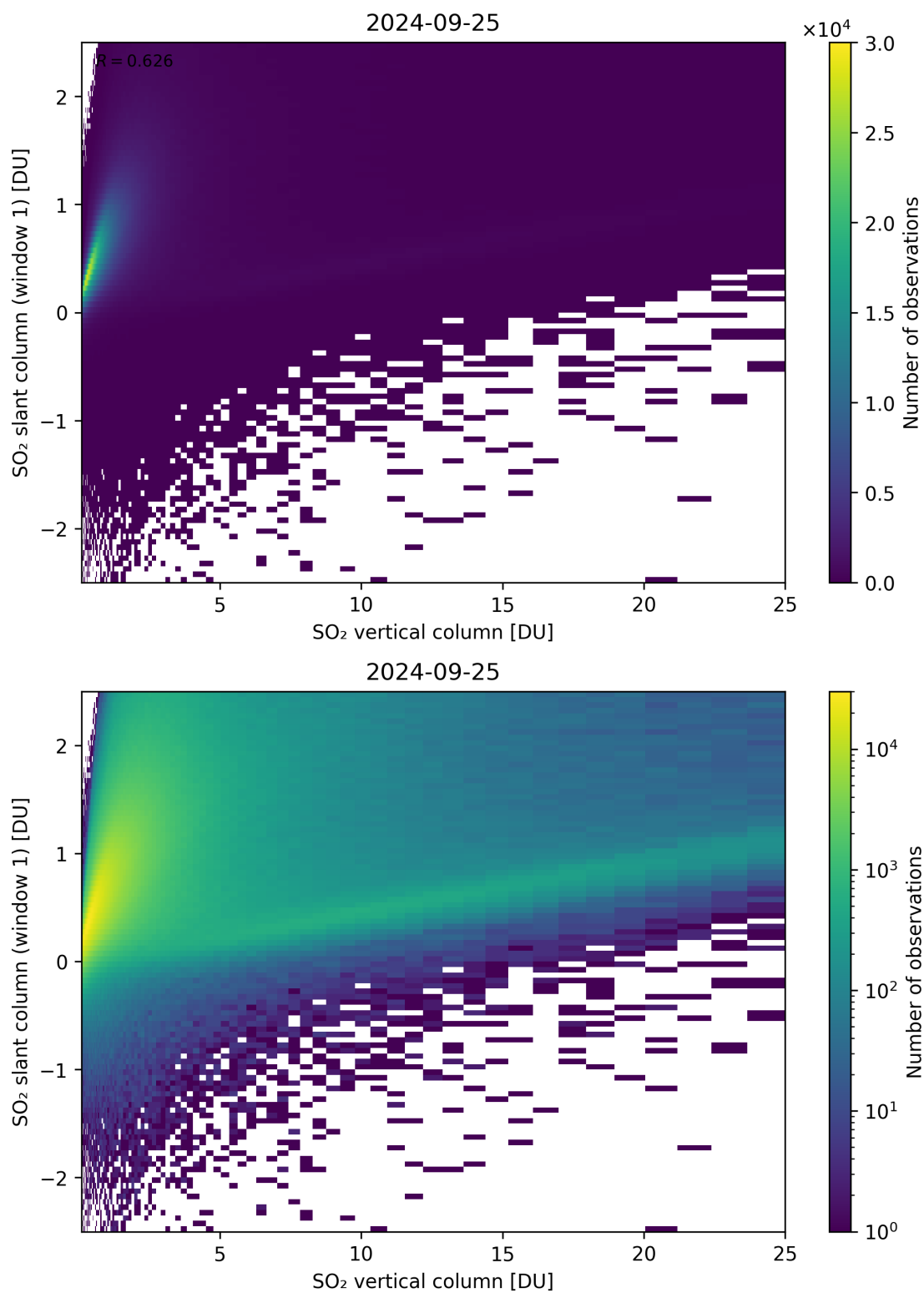
Figure 300: Scatter density plot of “SO 2 vertical column” against “SO 2 slant column (window 1)” for 2024-09-24 to 2024-09-26.
