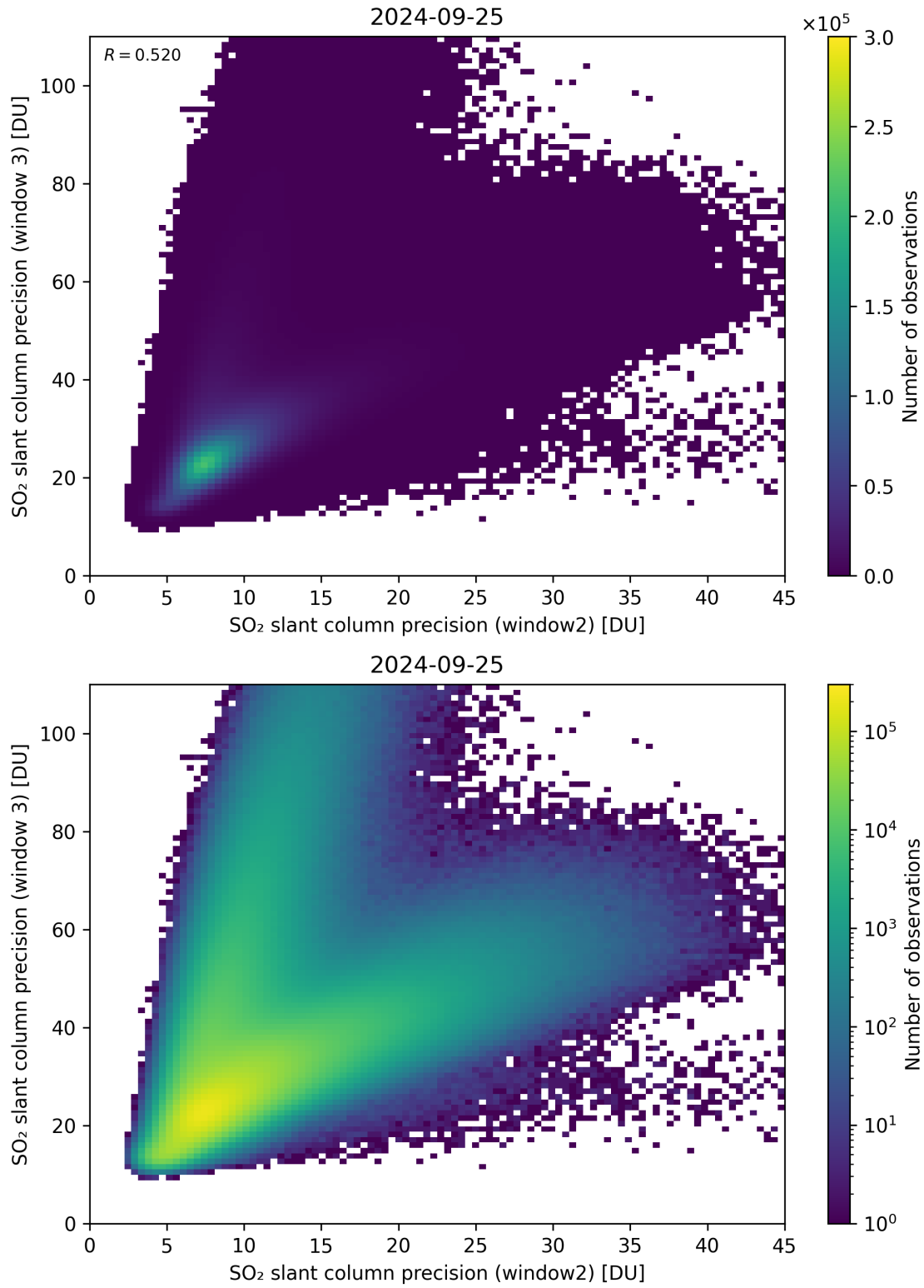
Figure 250: Scatter density plot of “SO 2 slant column precision (window2)” against “SO 2 slant column precision (window 3)” for 2024-09-24 to 2024-09-26.
