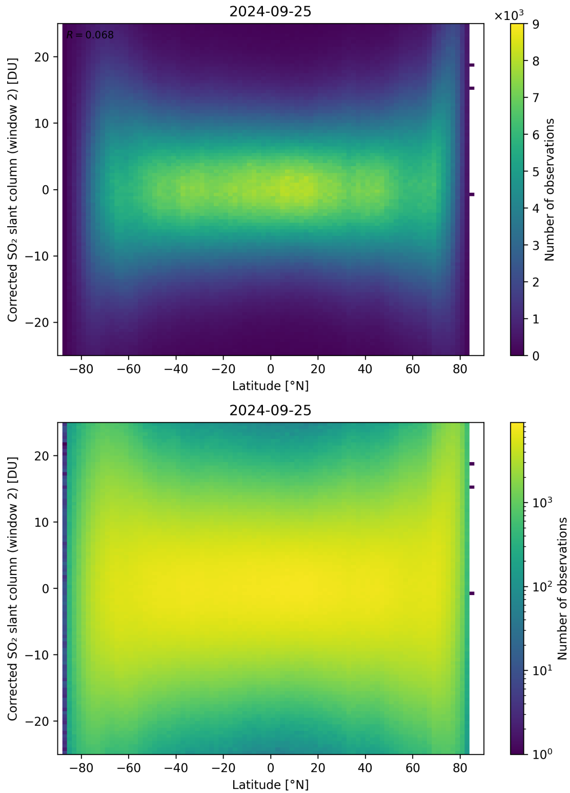
Figure 147: Scatter density plot of “Latitude” against “Corrected SO 2 slant column (window 2)” for 2024-09-24 to 2024-09-26.
