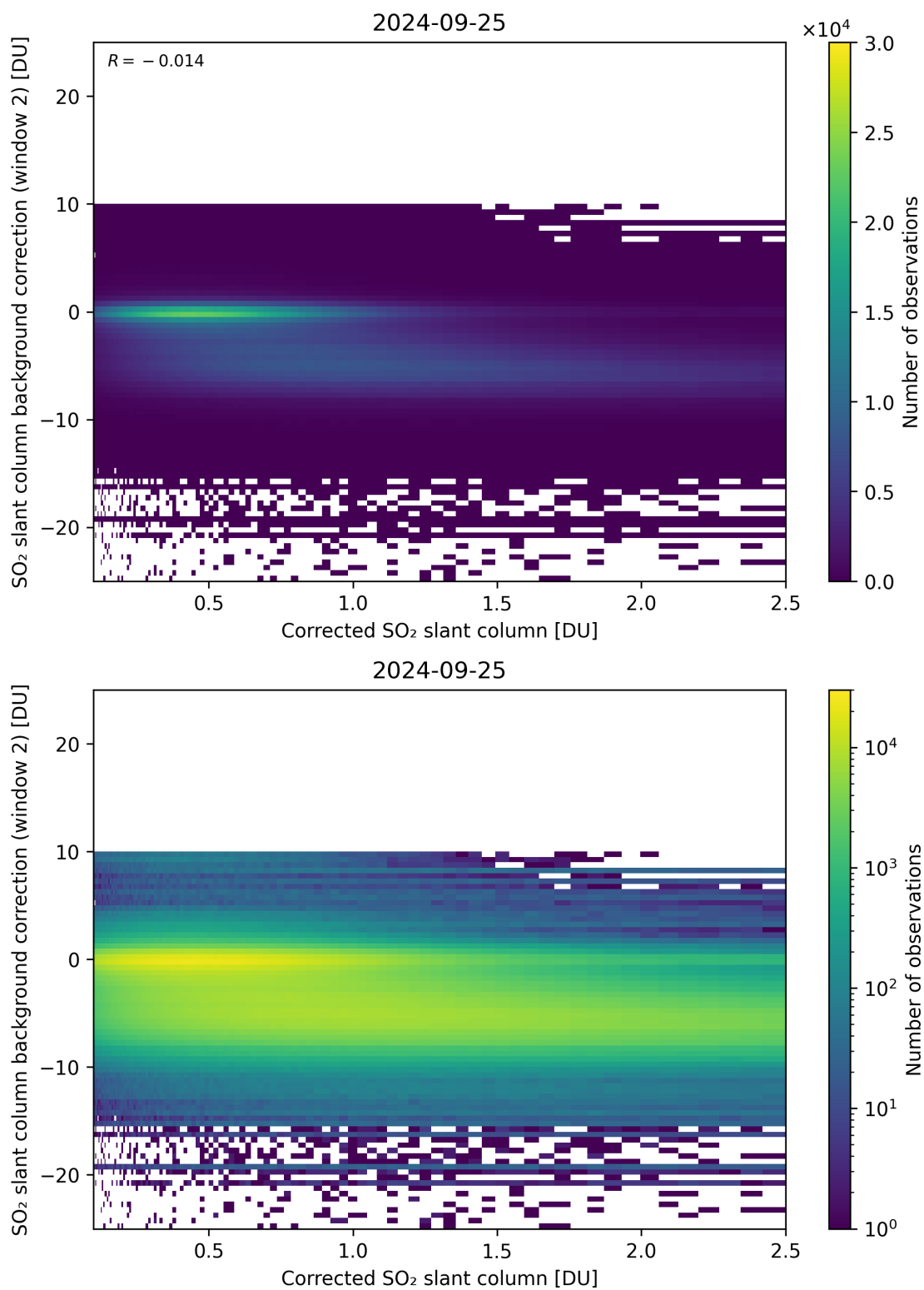
Figure 179: Scatter density plot of “Corrected SO 2 slant column” against “SO 2 slant column background correction (window 2)” for 2024-09-24 to 2024-09-26.
