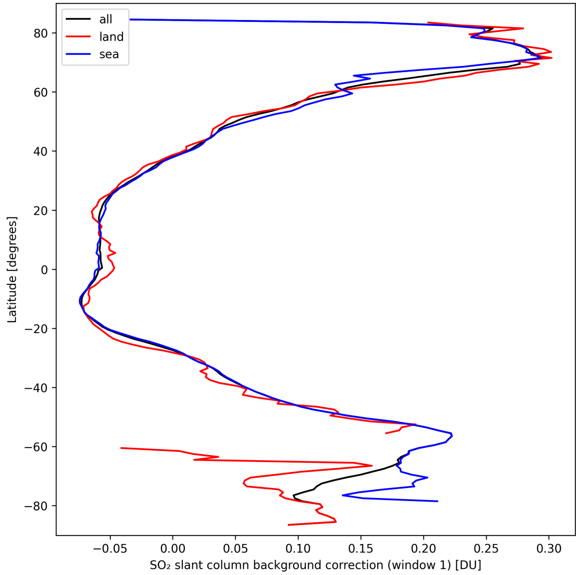
Figure 36: Zonal average of "SO 2 slant column background correction (window 1)" for 2024-09-24 to 2024-09-26.
