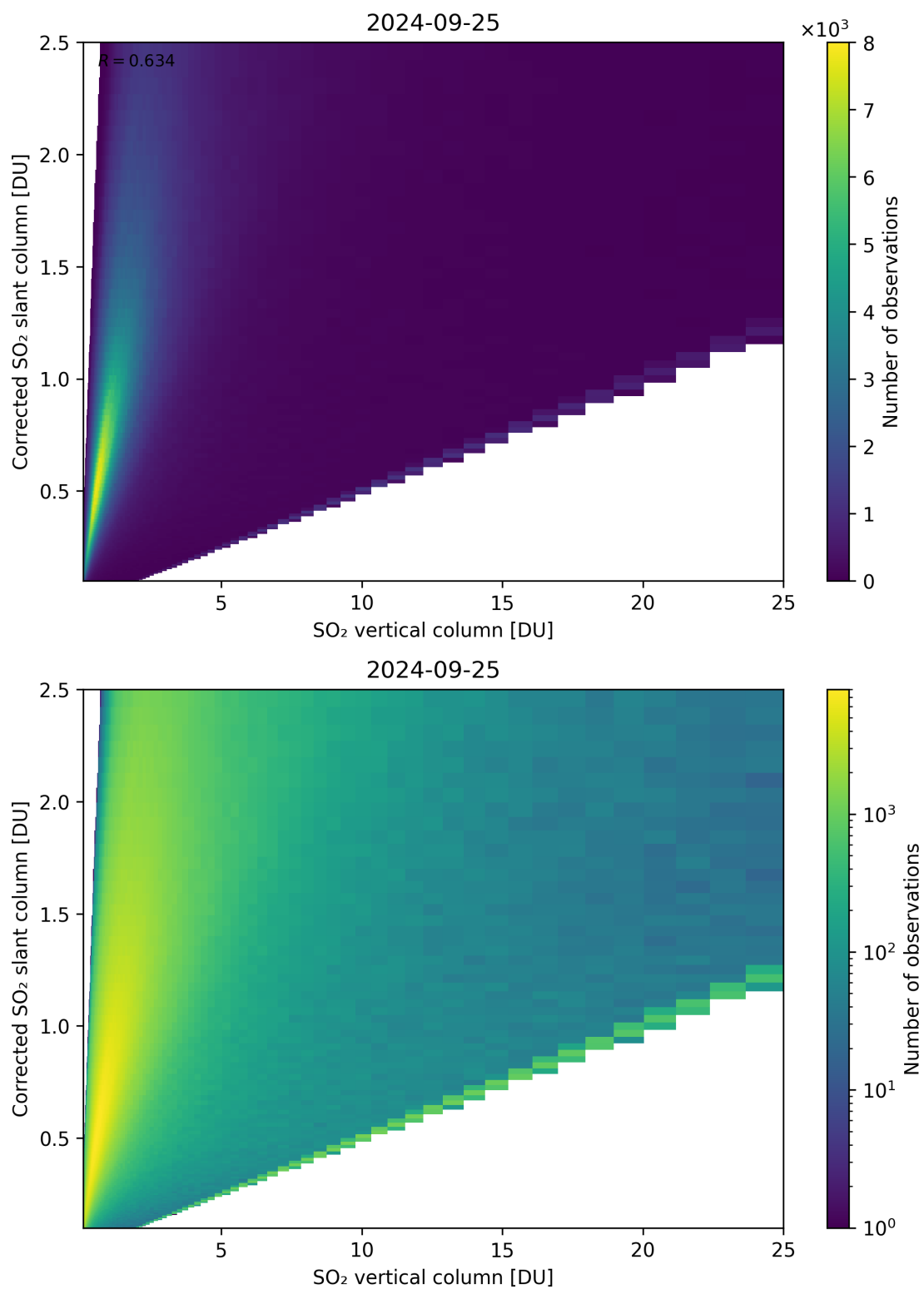
Figure 297: Scatter density plot of “SO 2 vertical column” against “Corrected SO 2 slant column” for 2024-09-24 to 2024-09-26.
