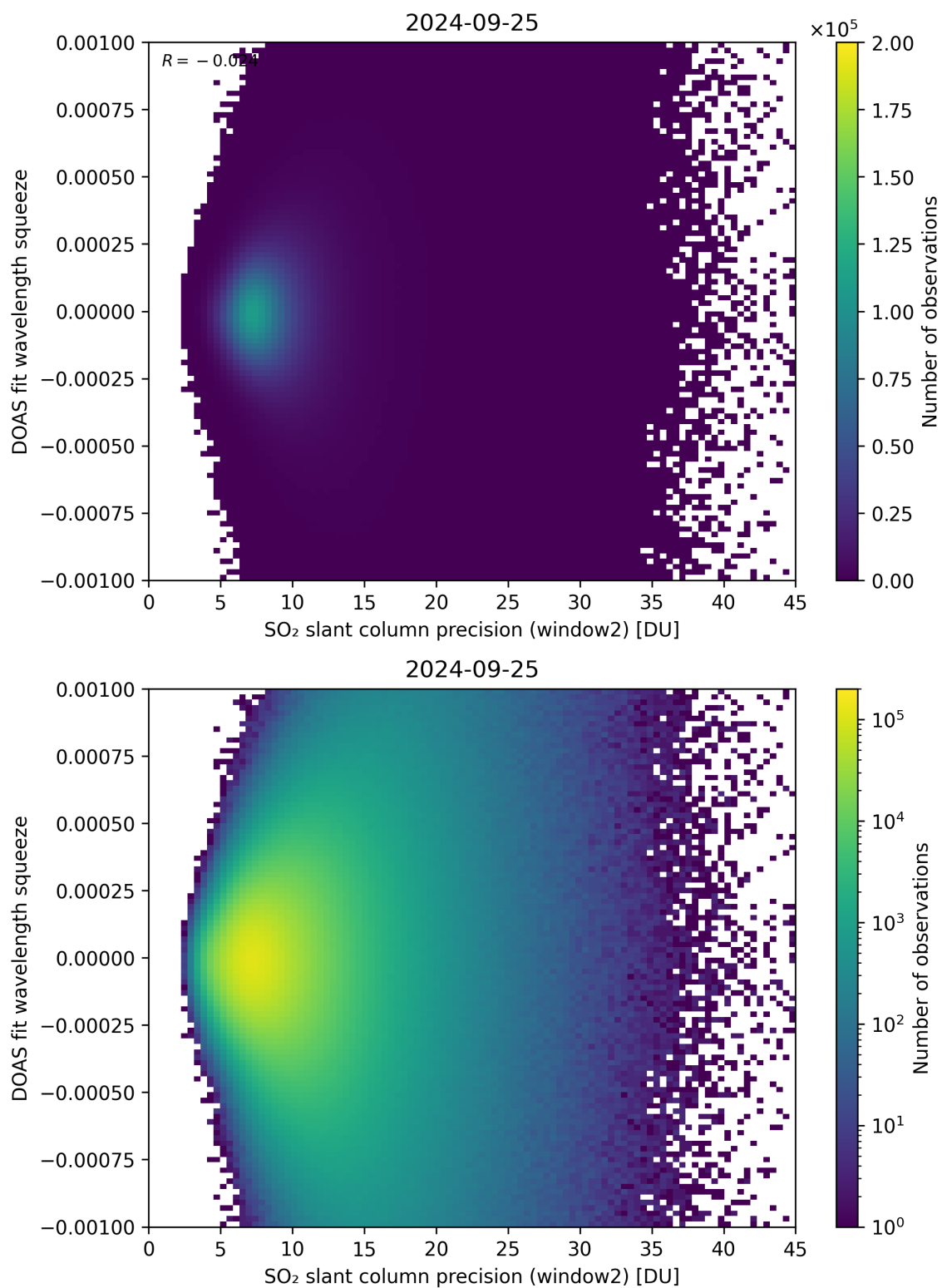
Figure 244: Scatter density plot of “SO 2 slant column precision (window2)” against “DOAS fit wavelength squeeze” for 2024-09-24 to 2024-09-26.
