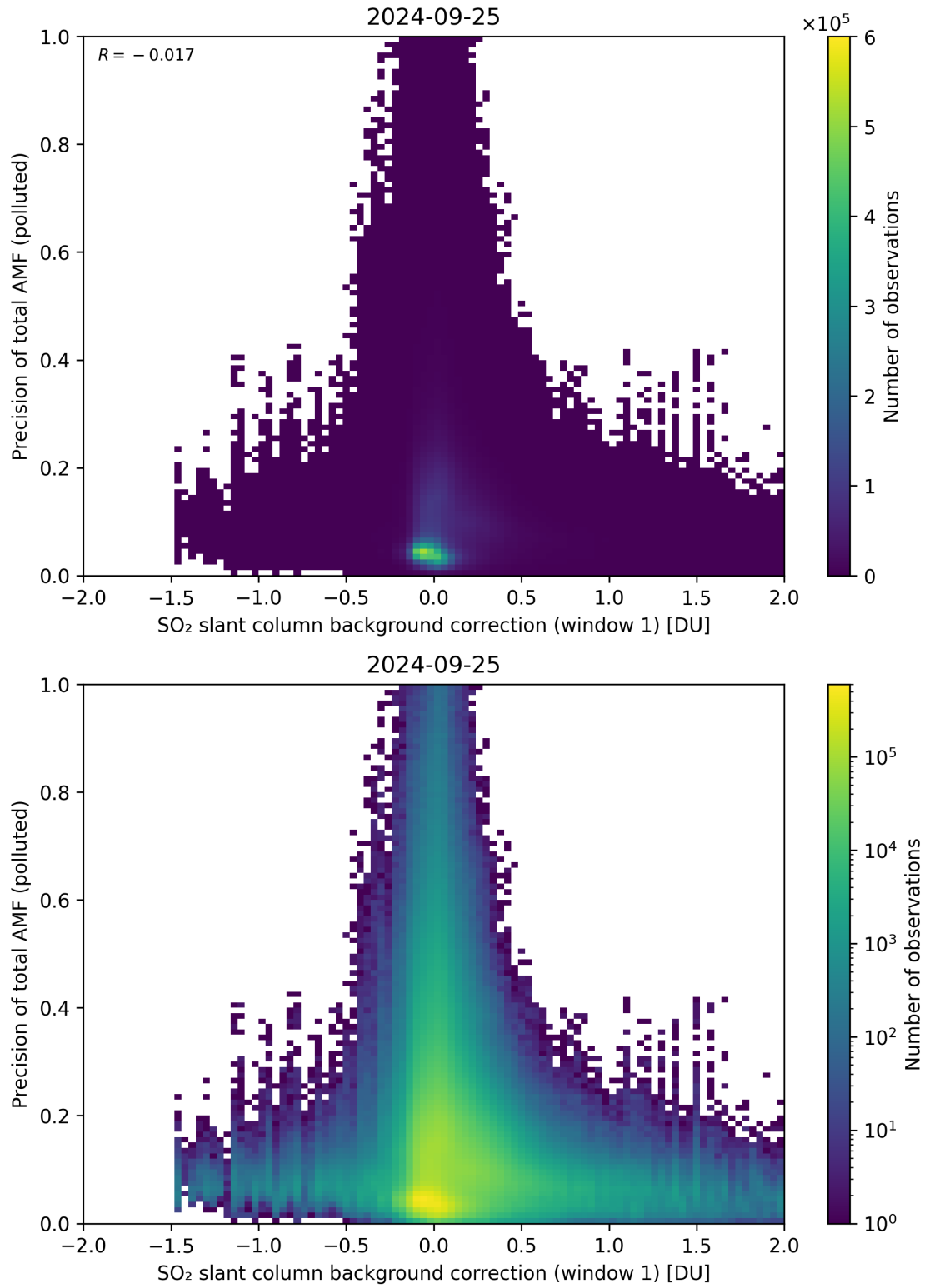
Figure 110: Scatter density plot of “SO 2 slant column background correction (window 1)” against “Precision of total AMF (polluted)” for 2024-09-24 to 2024-09-26.
