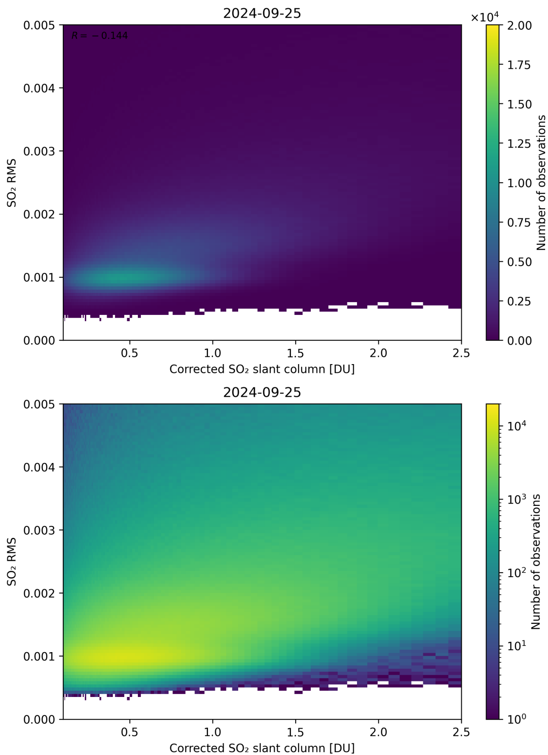
Figure 183: Scatter density plot of “Corrected SO 2 slant column” against “SO 2 RMS” for 2024-09-24 to 2024-09-26.
