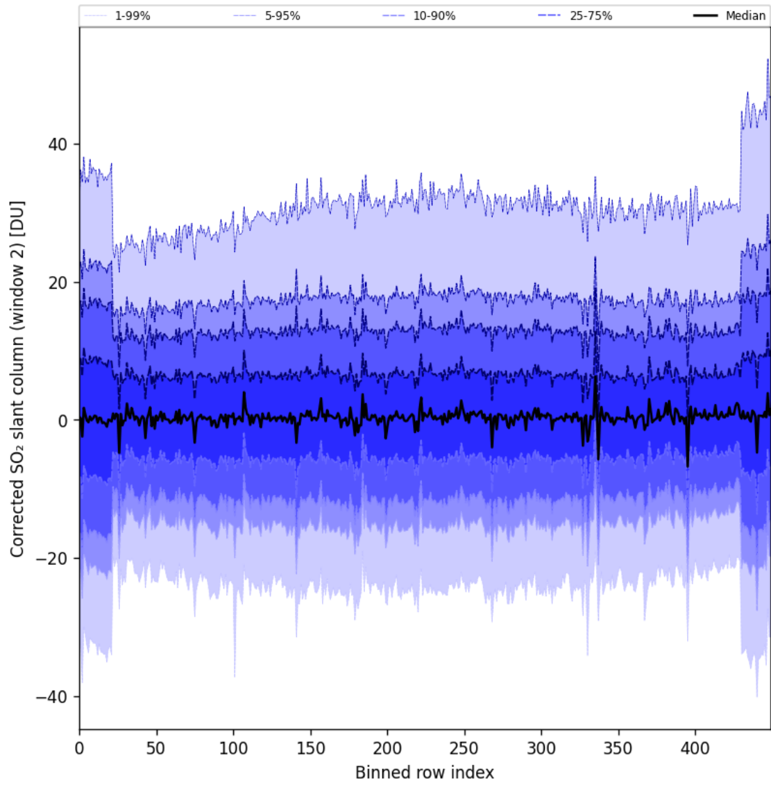
Figure 85: Along track statistics of "Corrected SO 2 slant column (window 2)" for 2024-09-24 to 2024-09-26
