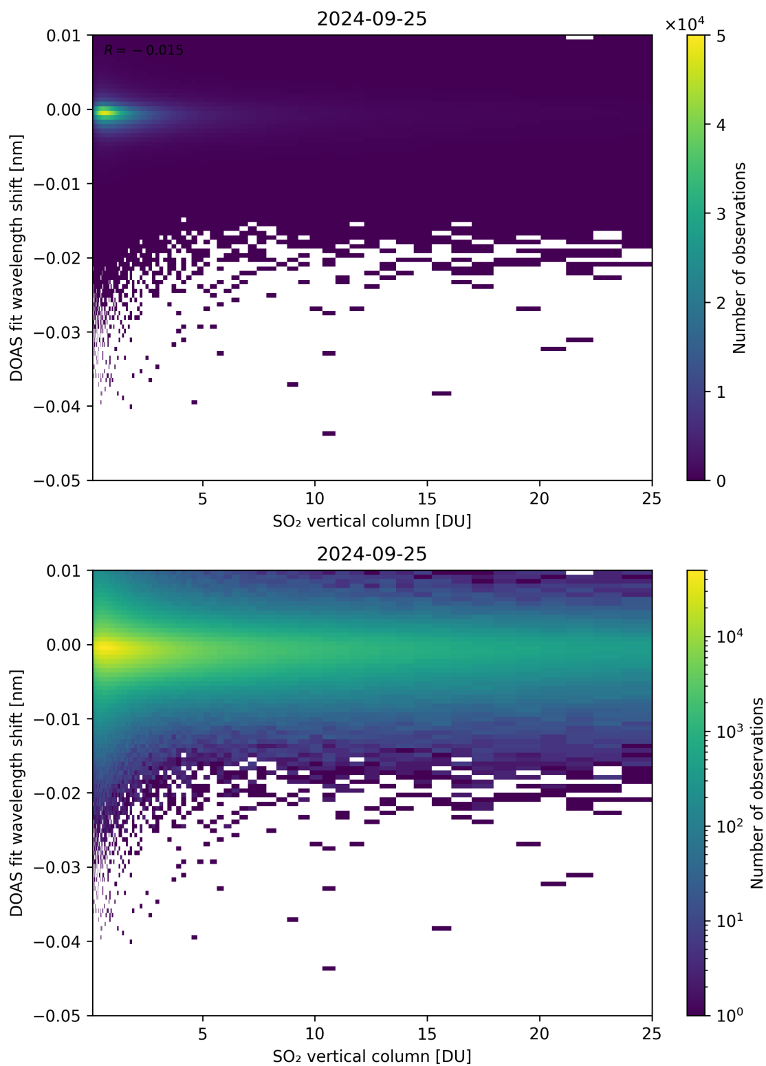
Figure 276: Scatter density plot of “SO 2 vertical column” against “DOAS fit wavelength shift” for 2024-09-24 to 2024-09-26.
