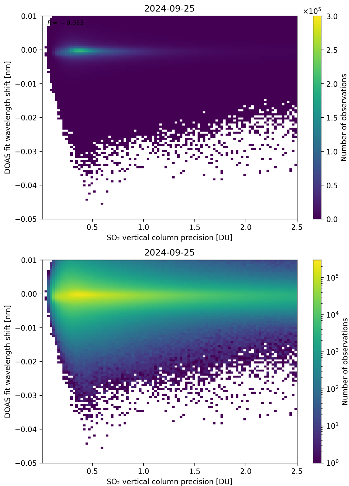
Figure 282: Scatter density plot of “SO 2 vertical column precision” against “DOAS fit wavelength shift” for 2024-09-24 to 2024-09-26.
