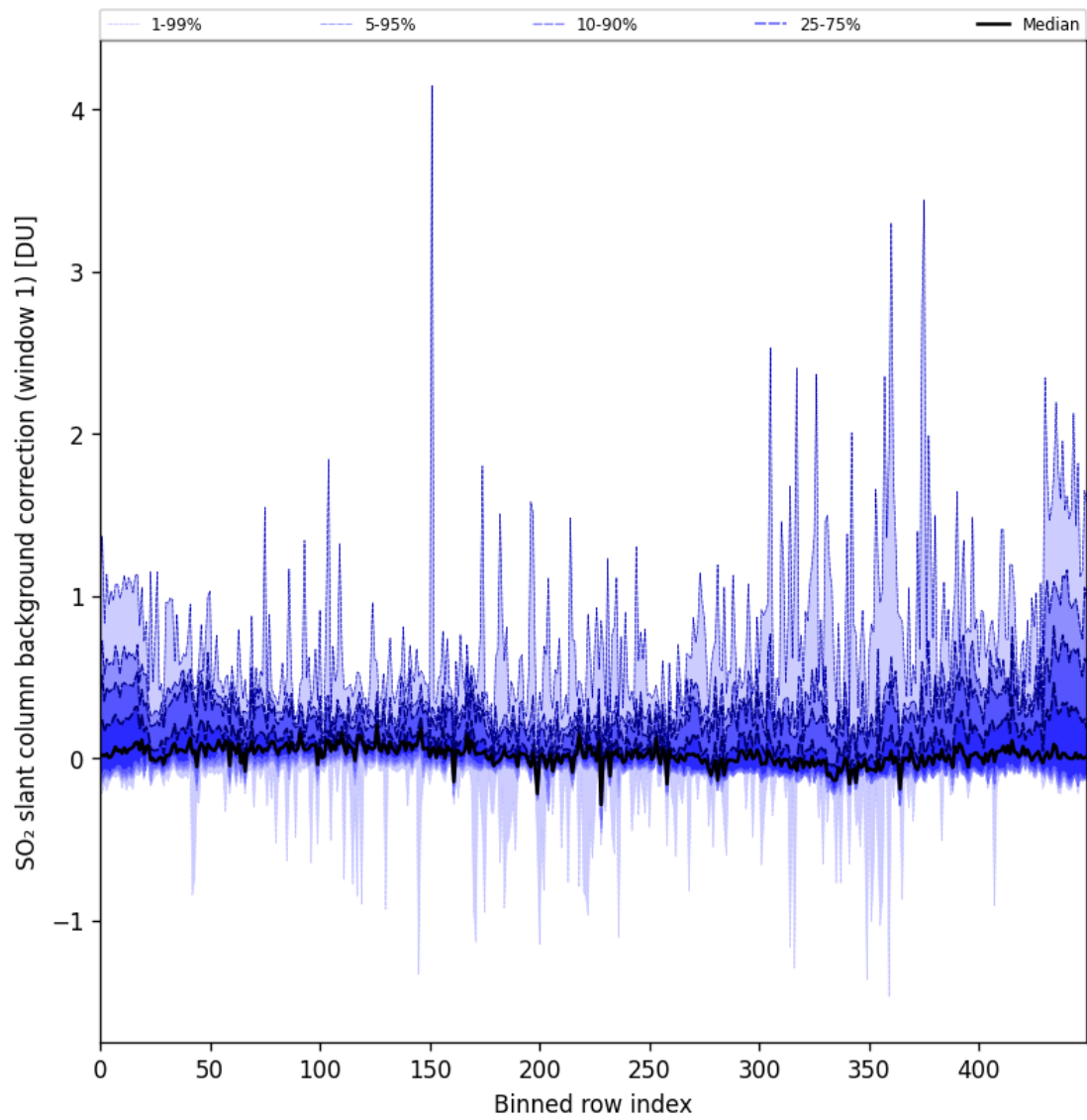
Figure 82: Along track statistics of “SO 2 slant column background correction (window 1)” for 2024-09-24 to 2024-09-26
