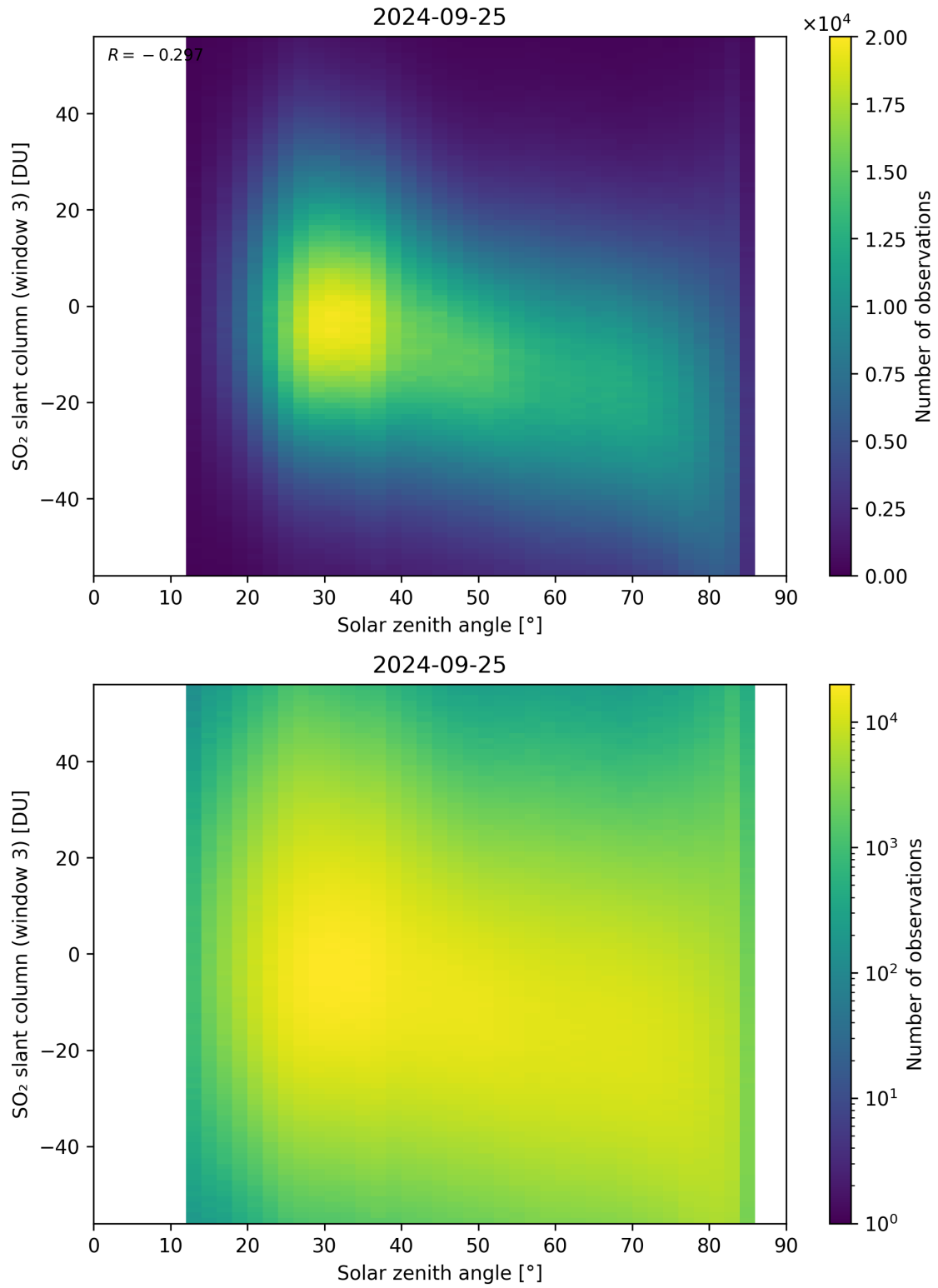
Figure 172: Scatter density plot of “Solar zenith angle” against “SO 2 slant column (window 3)” for 2024-09-24 to 2024-09-26.
