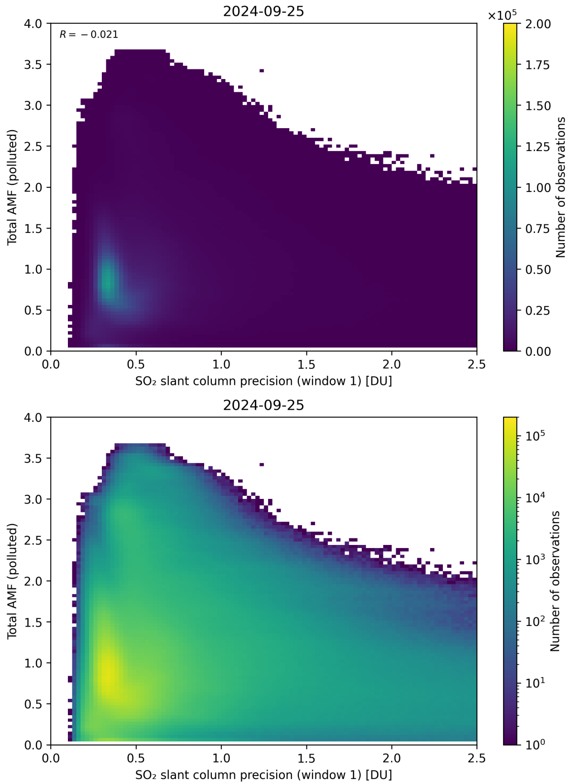
Figure 230: Scatter density plot of “SO 2 slant column precision (window 1)” against “Total AMF (polluted)” for 2024-09-24 to 2024-09-26.
