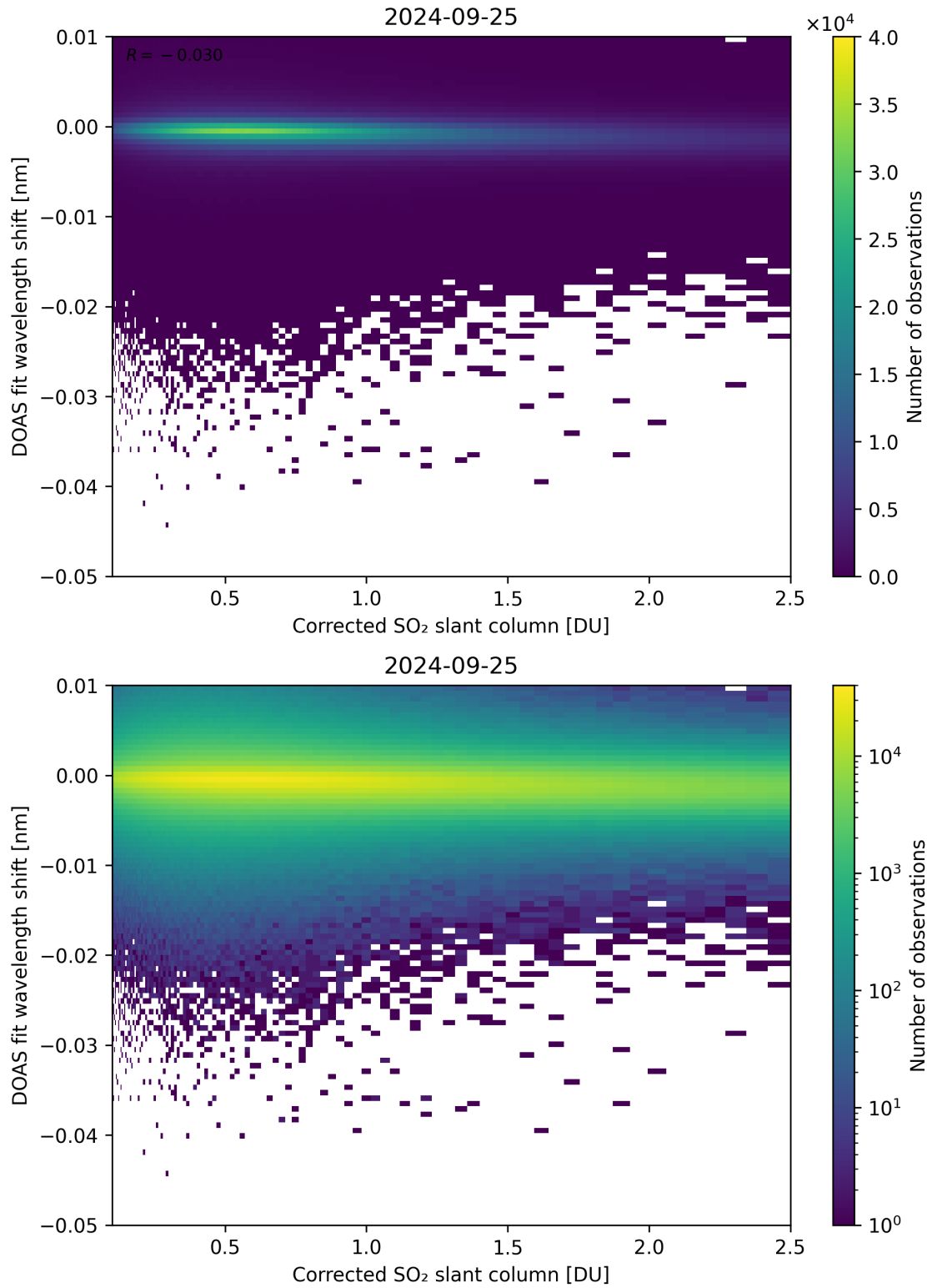
Figure 181: Scatter density plot of “Corrected SO 2 slant column” against “DOAS fit wavelength shift” for 2024-09-24 to 2024-09-26.
