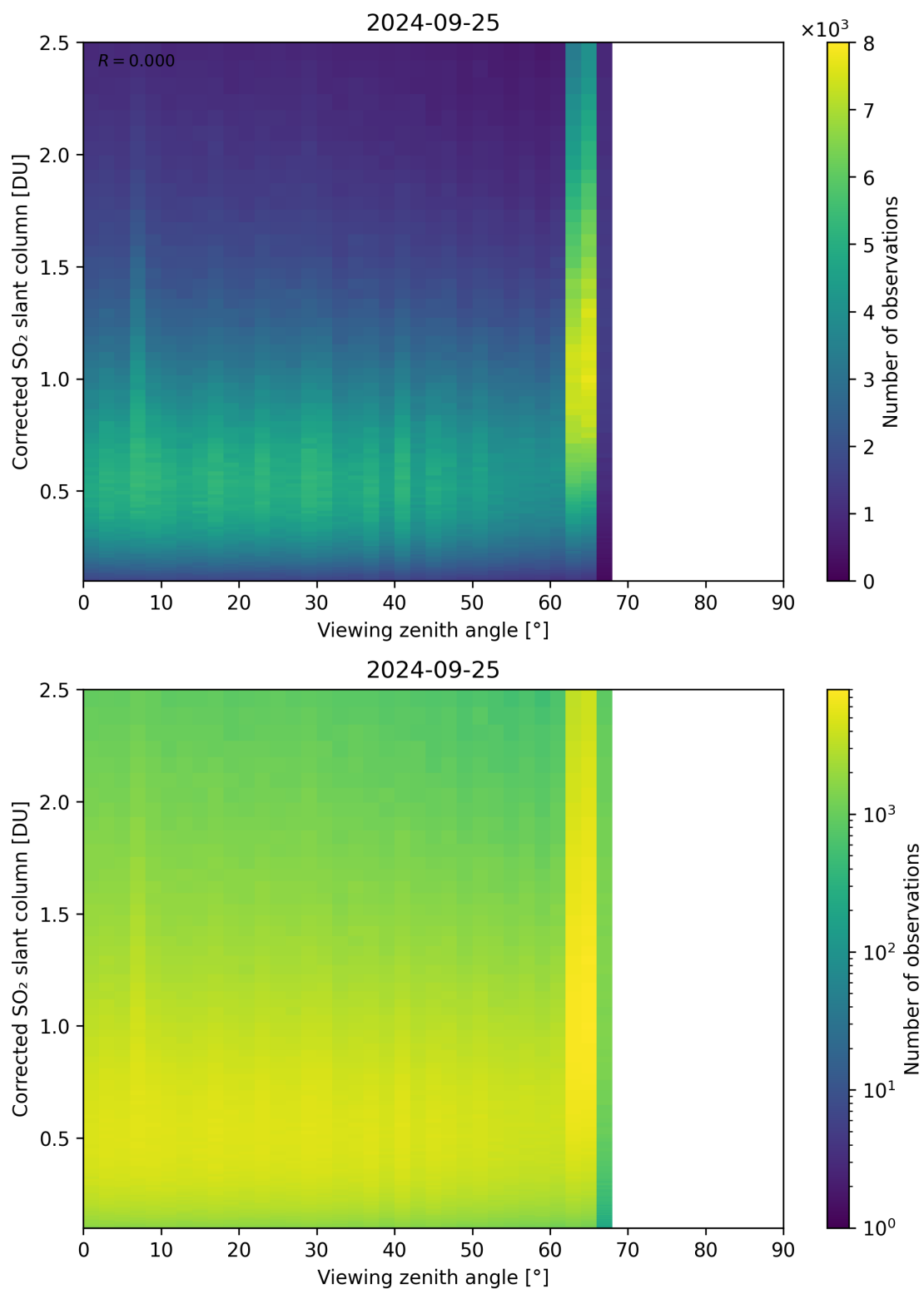
Figure 317: Scatter density plot of “Viewing zenith angle” against “Corrected SO 2 slant column” for 2024-09-24 to 2024-09-26.
