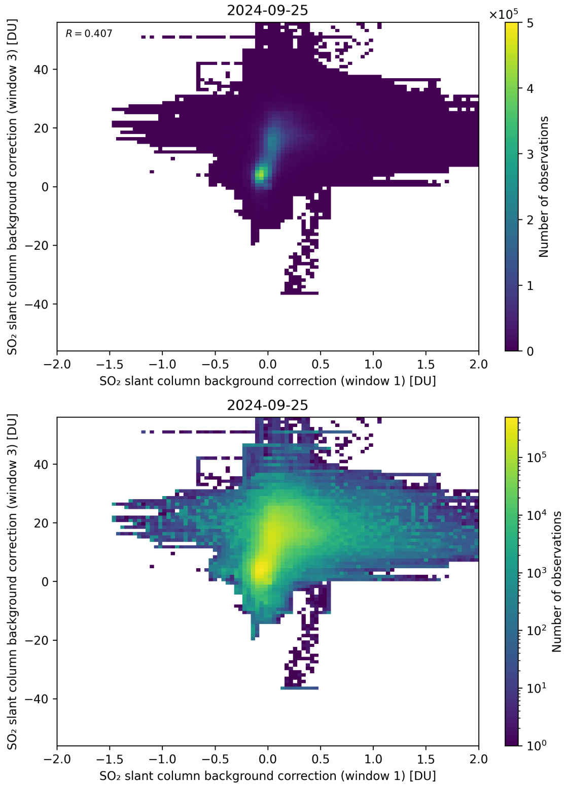
Figure 99: Scatter density plot of “SO 2 slant column background correction (window 1)” against “SO 2 slant column background correction (window 3)” for 2024-09-24 to 2024-09-26.
