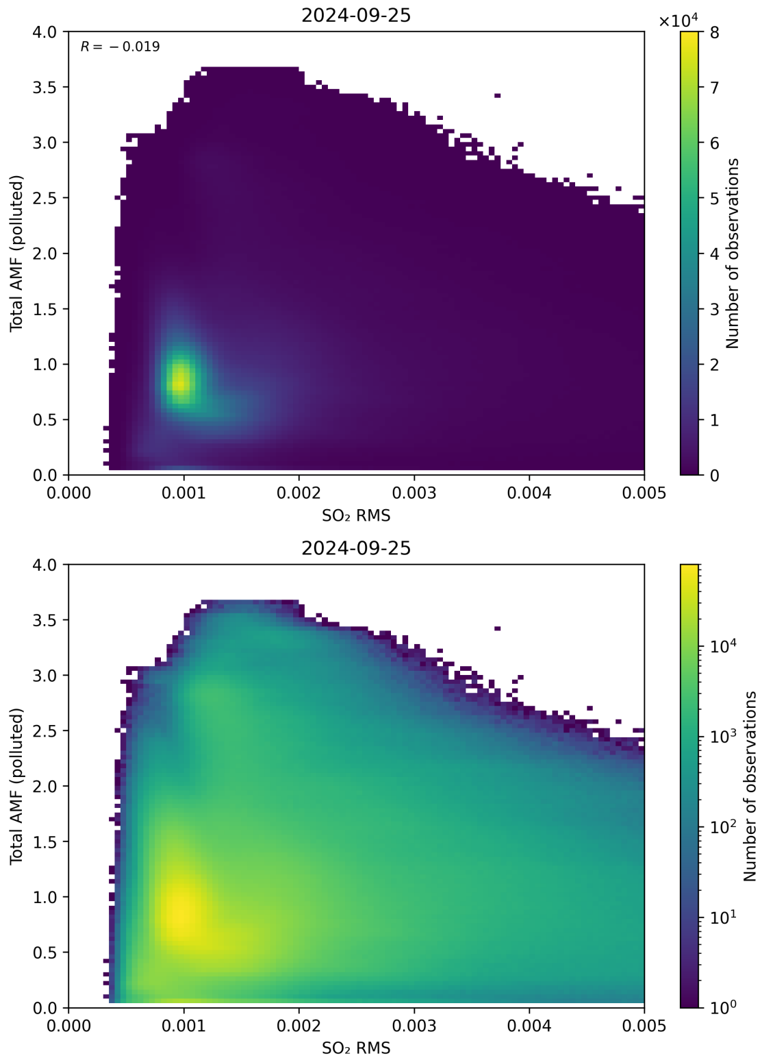
Figure 137: Scatter density plot of “SO 2 RMS” against “Total AMF (polluted)” for 2024-09-24 to 2024-09-26.
