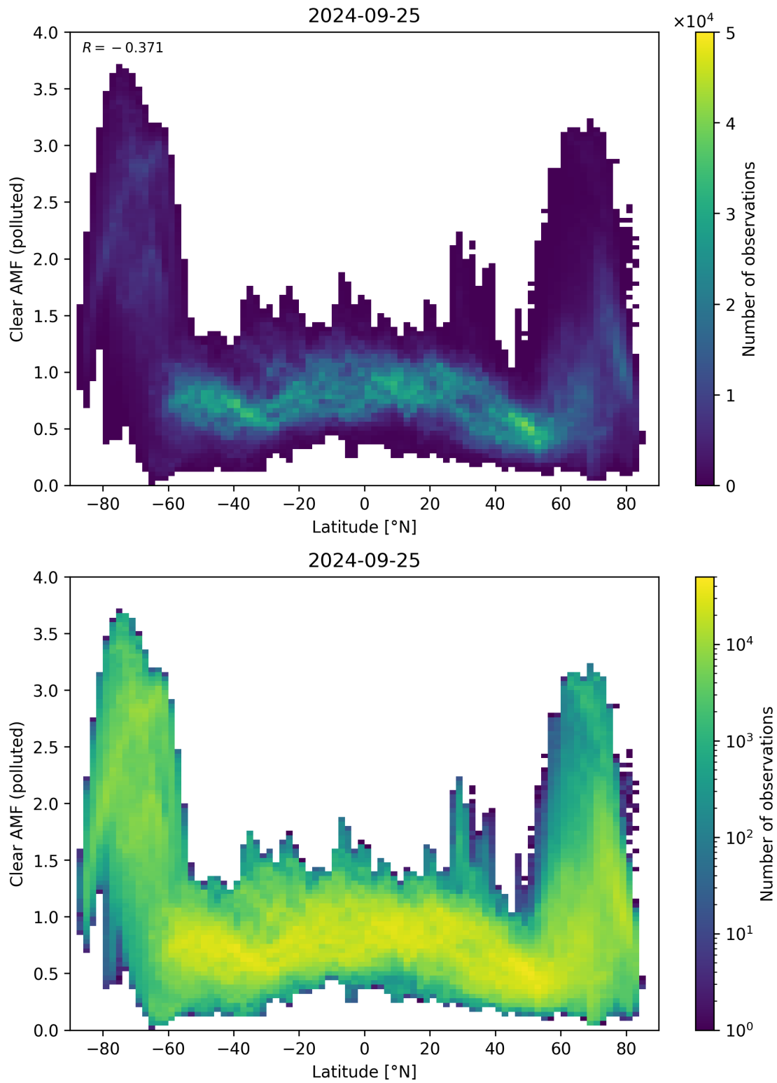
Figure 145: Scatter density plot of “Latitude” against “Clear AMF (polluted)” for 2024-09-24 to 2024-09-26.
