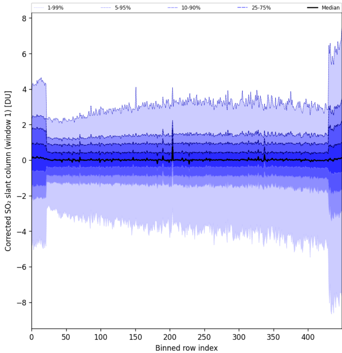
Figure 81: Along track statistics of “Corrected SO 2 slant column (window 1)” for 2024-09-24 to 2024-09-26
