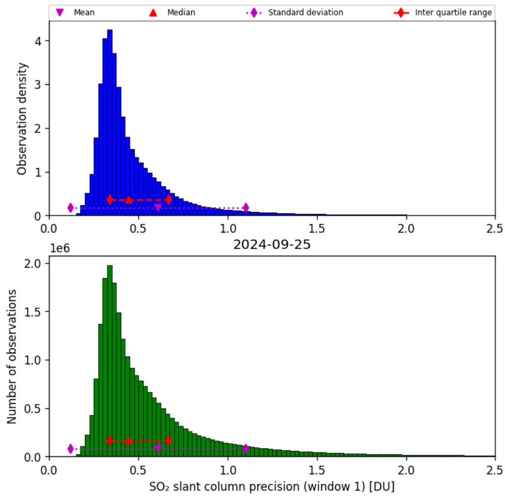
Figure 57: Histogram of “SO 2 slant column precision (window 1)” for 2024-09-24 to 2024-09-26
