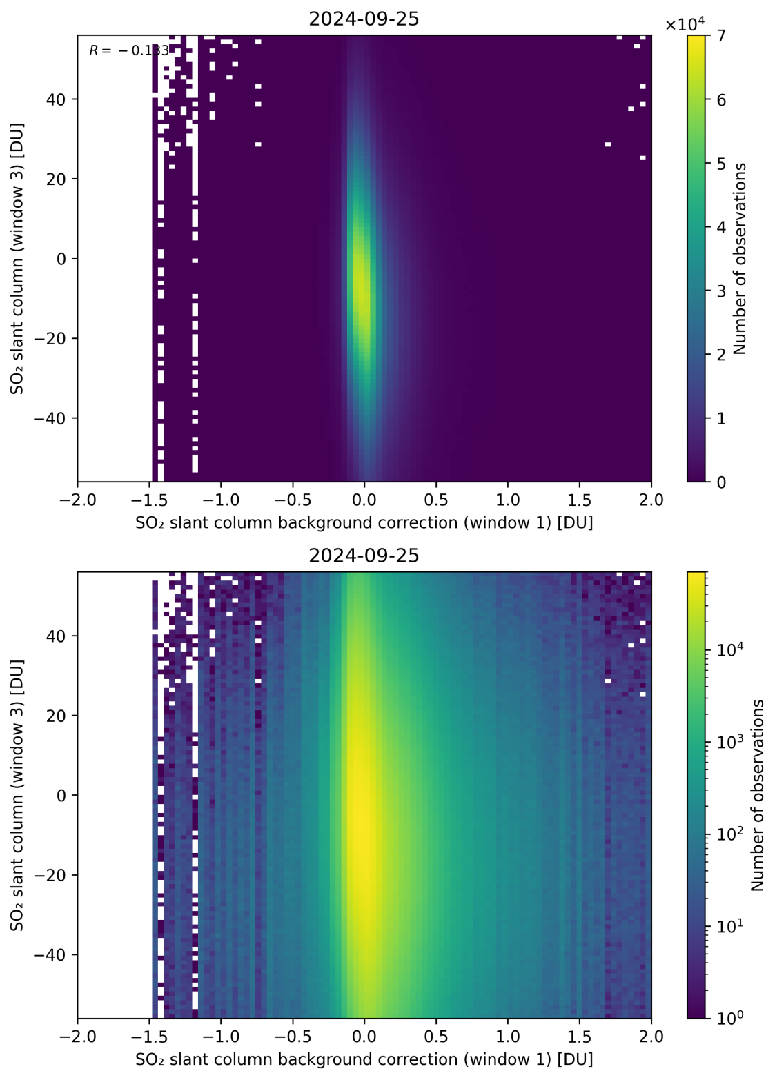
Figure 107: Scatter density plot of “SO 2 slant column background correction (window 1)” against “SO 2 slant column (window 3)” for 2024-09-24 to 2024-09-26.
