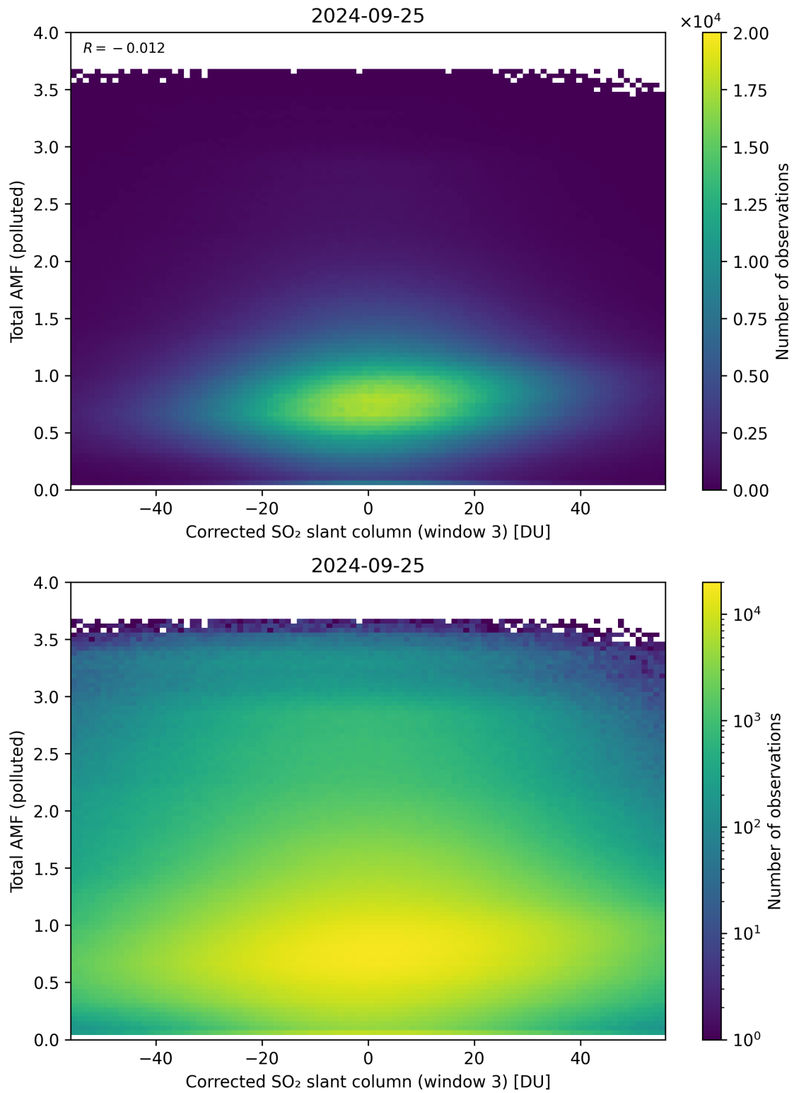
Figure 210: Scatter density plot of “Corrected SO 2 slant column (window 3)” against “Total AMF (polluted)” for 2024-09-24 to 2024-09-26.
