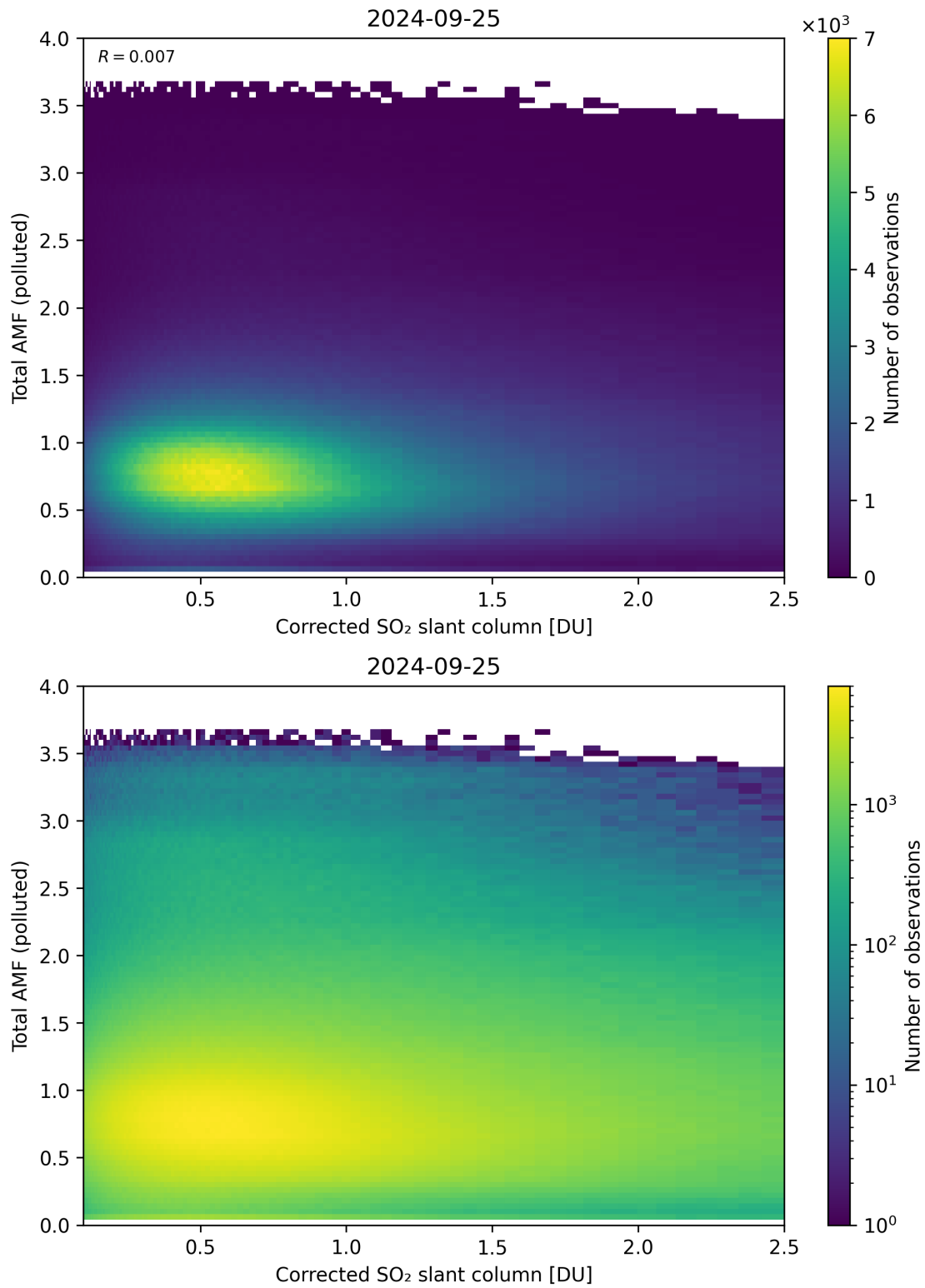
Figure 192: Scatter density plot of “Corrected SO 2 slant column” against “Total AMF (polluted)” for 2024-09-24 to 2024-09-26.
