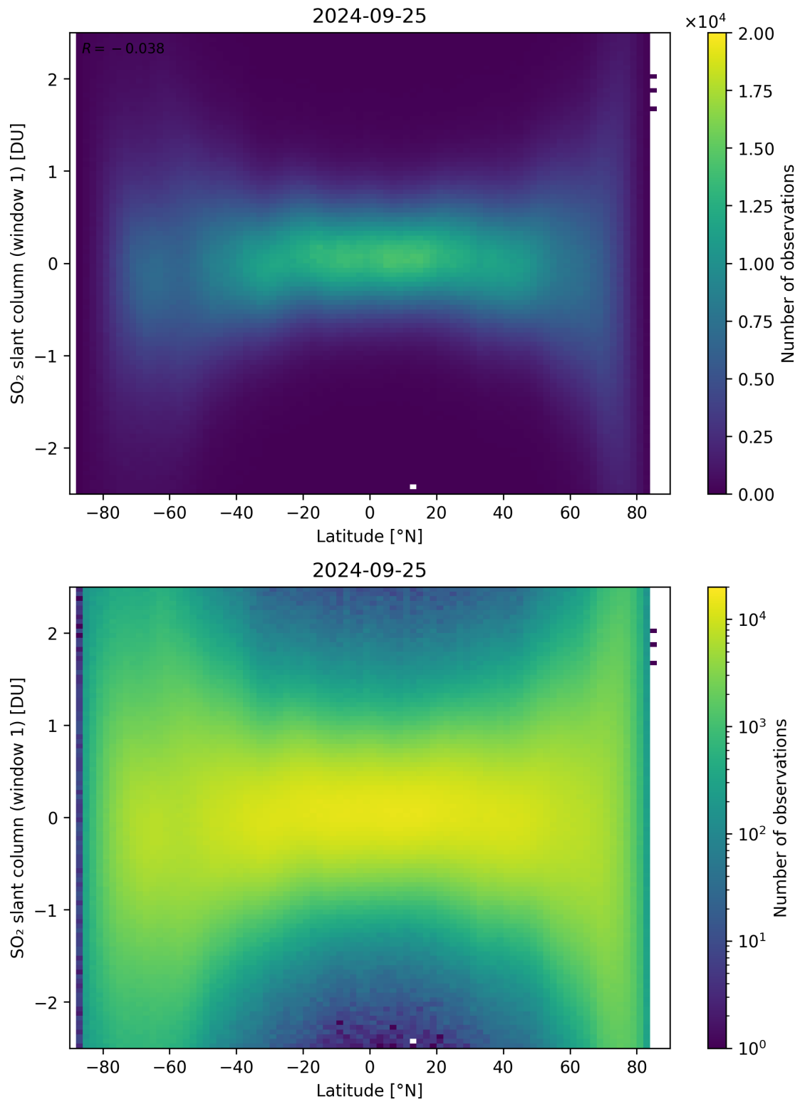
Figure 149: Scatter density plot of “Latitude” against “SO 2 slant column (window 1)” for 2024-09-24 to 2024-09-26.
