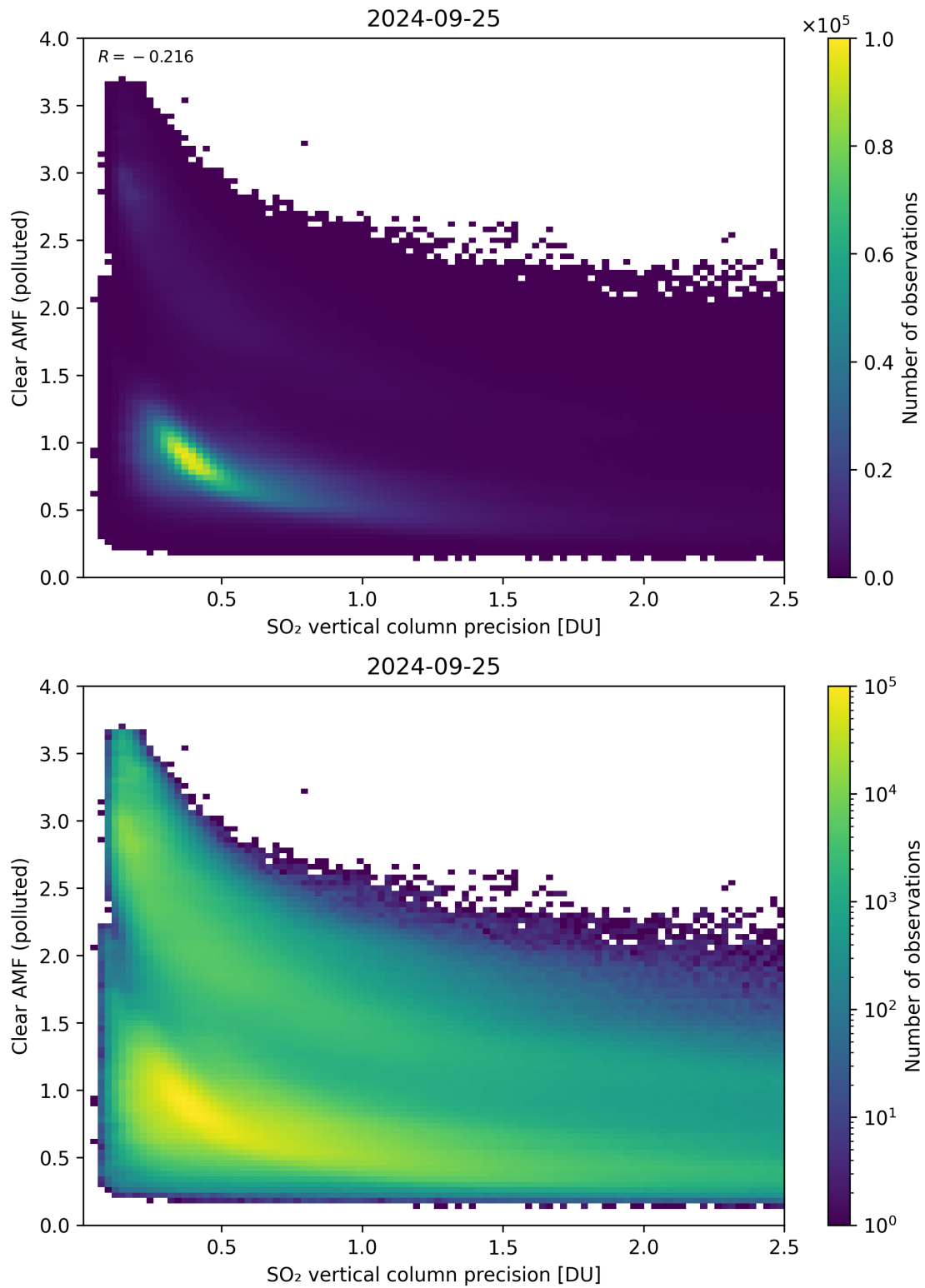
Figure 285: Scatter density plot of “SO 2 vertical column precision” against “Clear AMF (polluted)” for 2024-09-24 to 2024-09-26.
