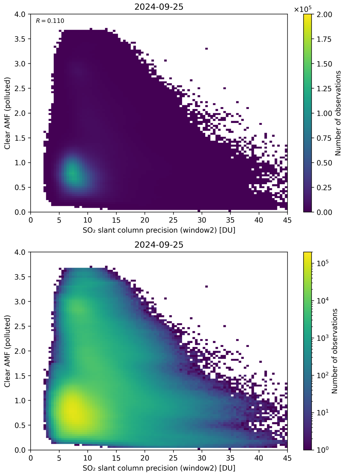
Figure 246: Scatter density plot of “SO 2 slant column precision (window2)” against “Clear AMF (polluted)” for 2024-09-24 to 2024-09-26.
