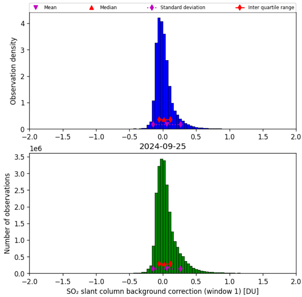
Figure 59: Histogram of “SO 2 slant column background correction (window 1)” for 2024-09-24 to 2024-09-26
