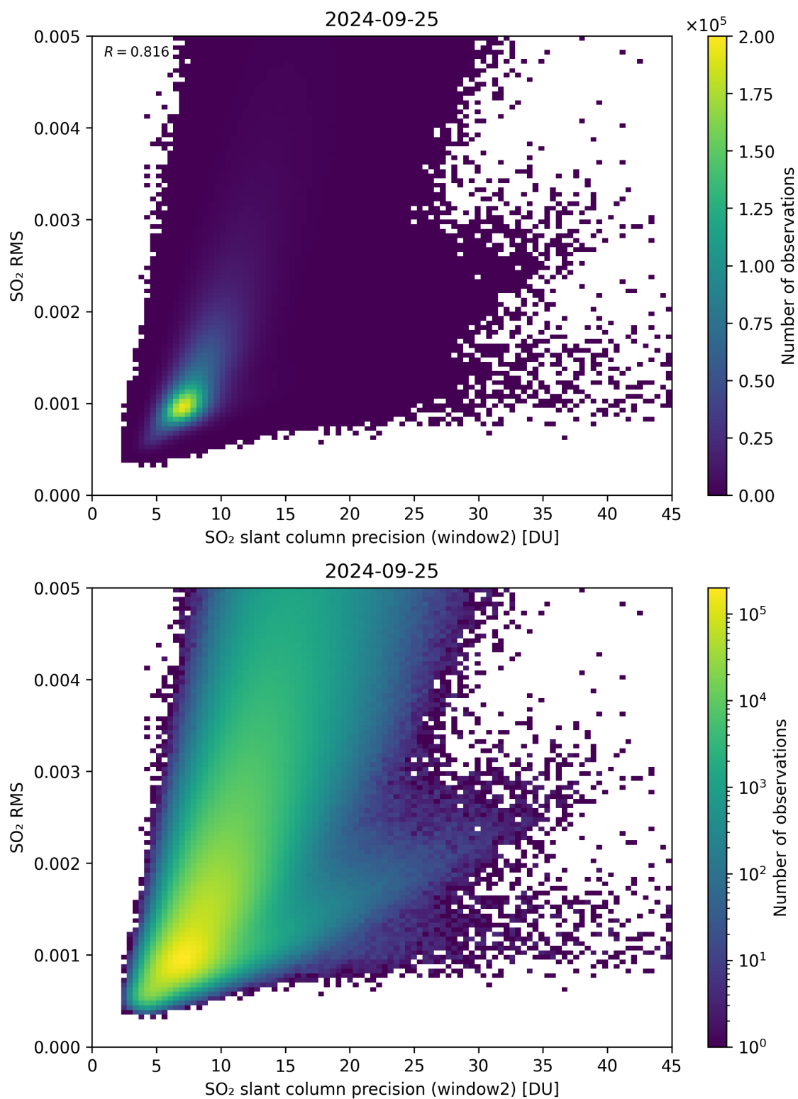
Figure 245: Scatter density plot of “SO 2 slant column precision (window2)” against “SO 2 RMS” for 2024-09-24 to 2024-09-26.
