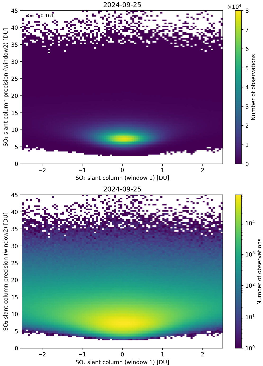
Figure 236: Scatter density plot of “SO 2 slant column (window 1)” against “SO 2 slant column precision (window2)” for 2024-09-24 to 2024-09-26.
