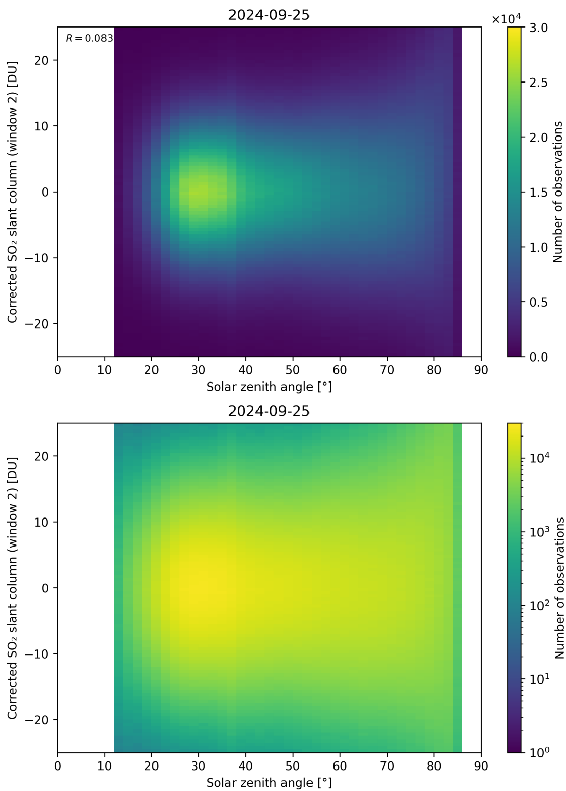
Figure 167: Scatter density plot of “Solar zenith angle” against “Corrected SO 2 slant column (window 2)” for 2024-09-24 to 2024-09-26.
