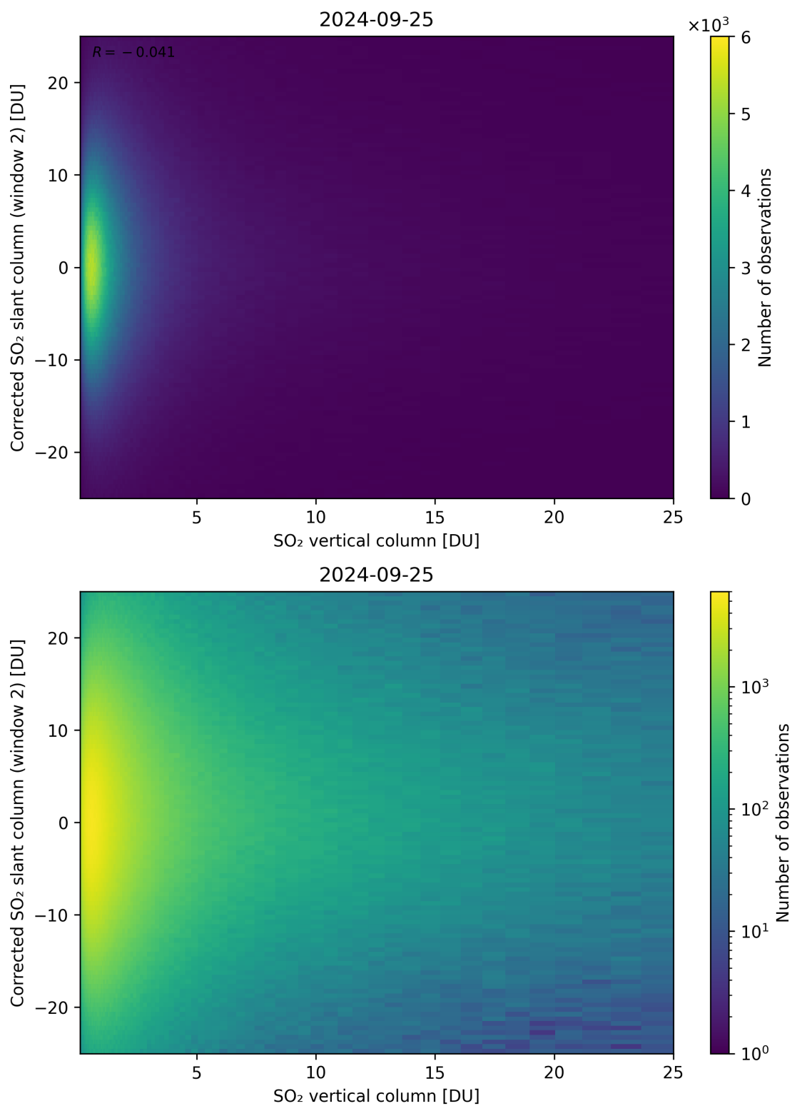
Figure 298: Scatter density plot of “SO 2 vertical column” against “Corrected SO 2 slant column (window 2)” for 2024-09-24 to 2024-09-26.
