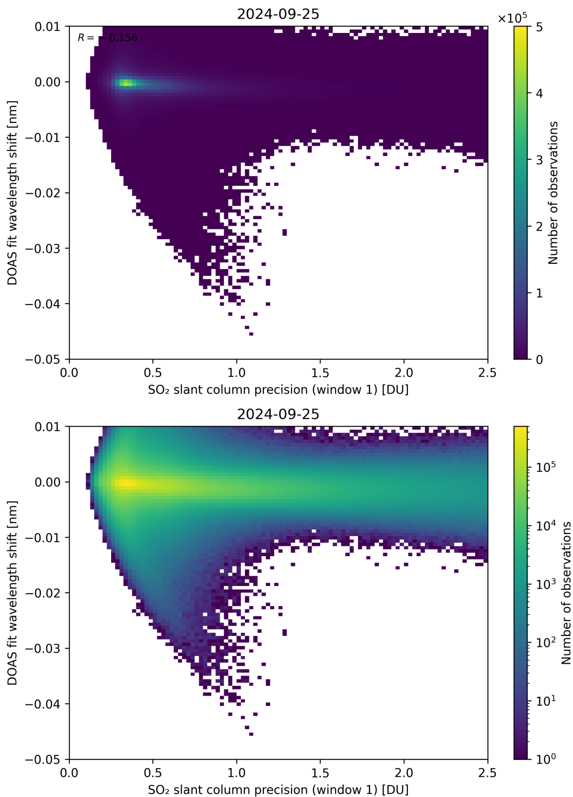
Figure 221: Scatter density plot of “SO 2 slant column precision (window 1)” against “DOAS fit wavelength shift” for 2024-09-24 to 2024-09-26.
