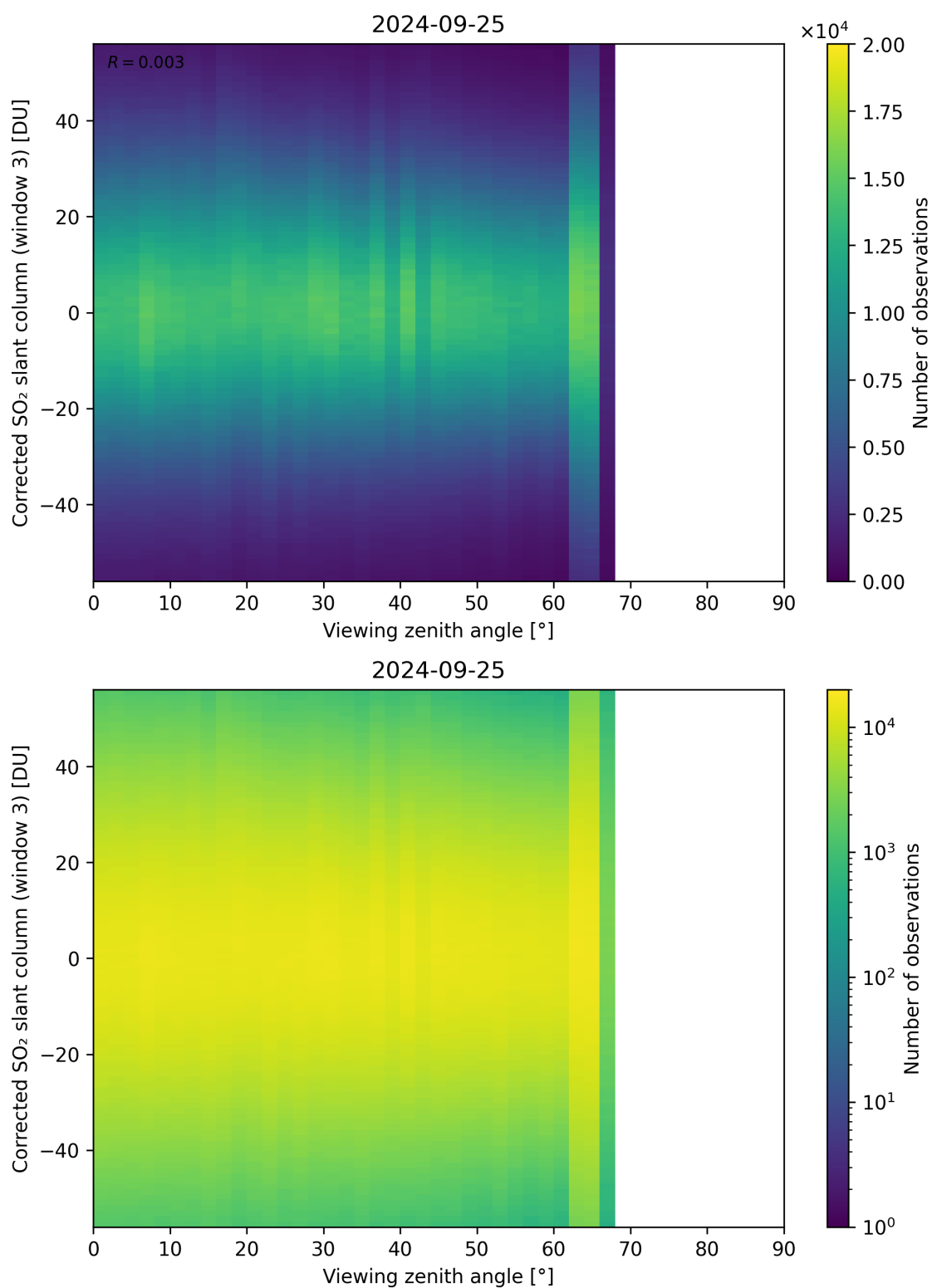
Figure 319: Scatter density plot of “Viewing zenith angle” against “Corrected SO 2 slant column (window 3)” for 2024-09-24 to 2024-09-26.
