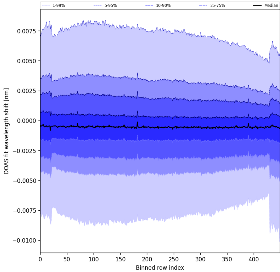
Figure 91: Along track statistics of “DOAS fit wavelength shift” for 2024-09-24 to 2024-09-26
