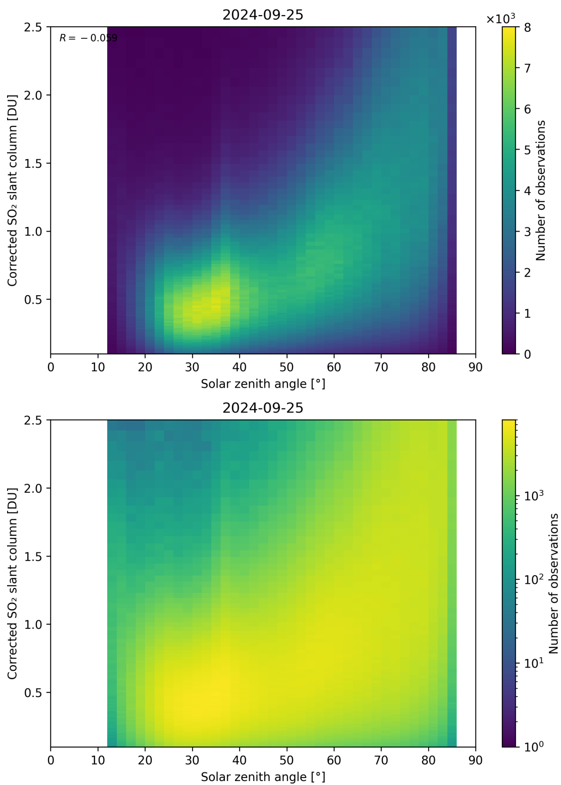
Figure 166: Scatter density plot of “Solar zenith angle” against “Corrected SO 2 slant column” for 2024-09-24 to 2024-09-26.
