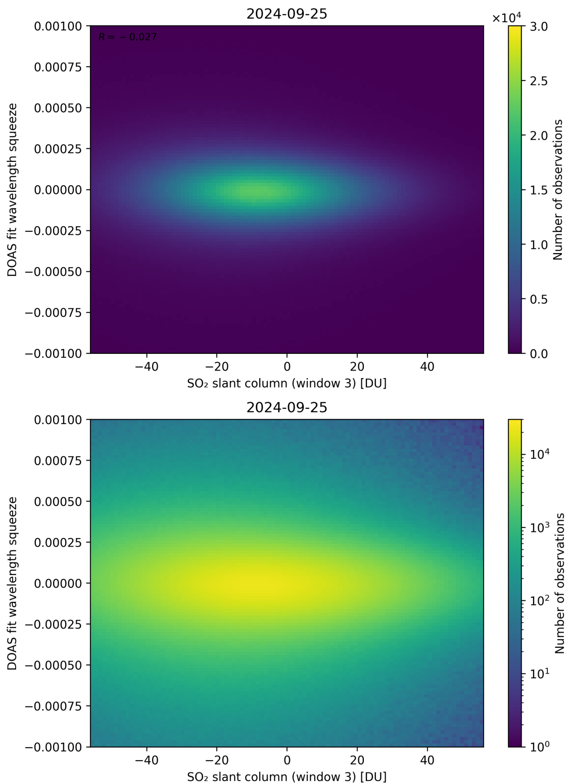
Figure 255: Scatter density plot of “SO 2 slant column (window 3)” against “DOAS fit wavelength squeeze” for 2024-09-24 to 2024-09-26.
