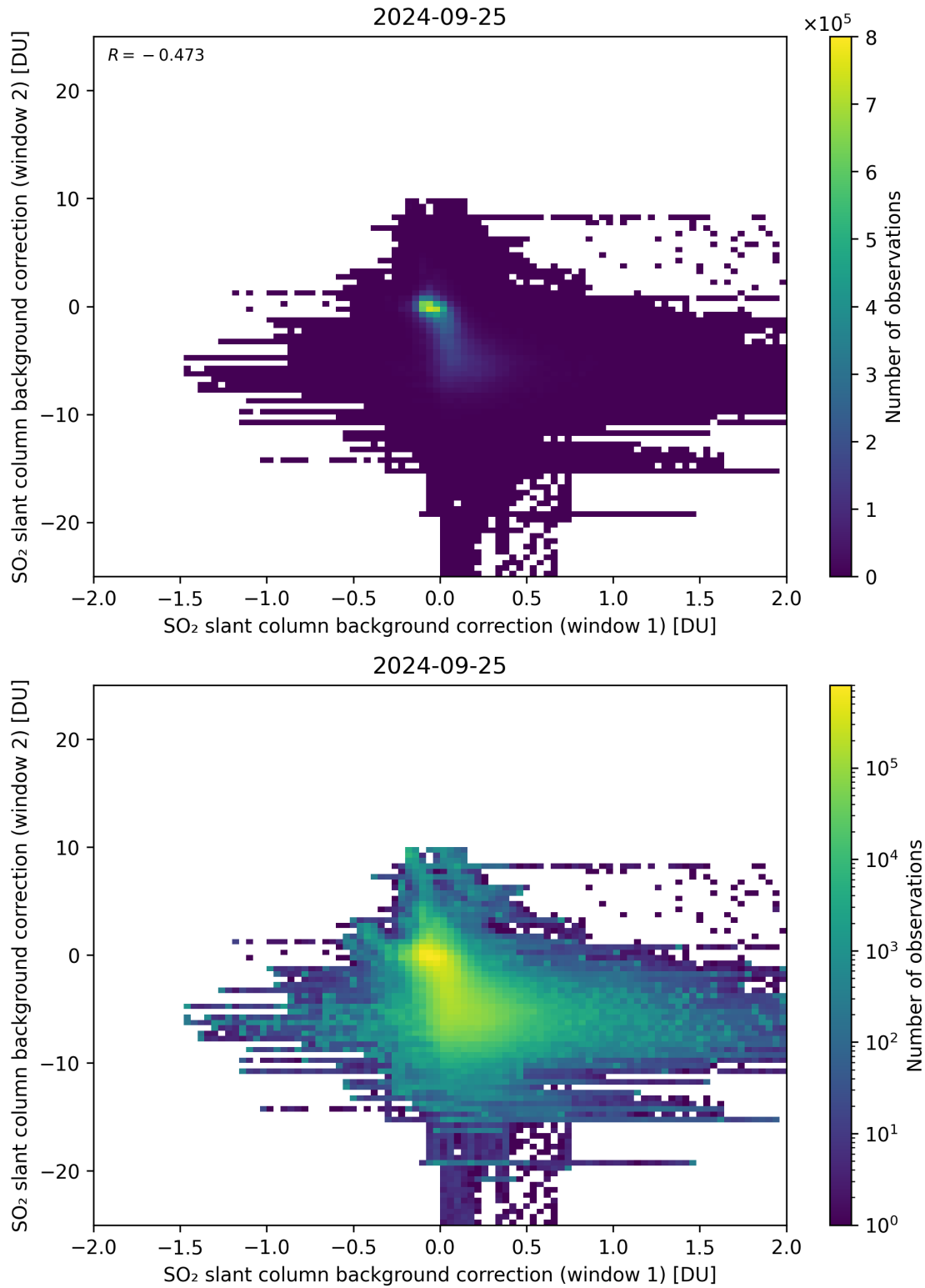
Figure 98: Scatter density plot of “SO 2 slant column background correction (window 1)” against “SO 2 slant column background correction (window 2)” for 2024-09-24 to 2024-09-26.
