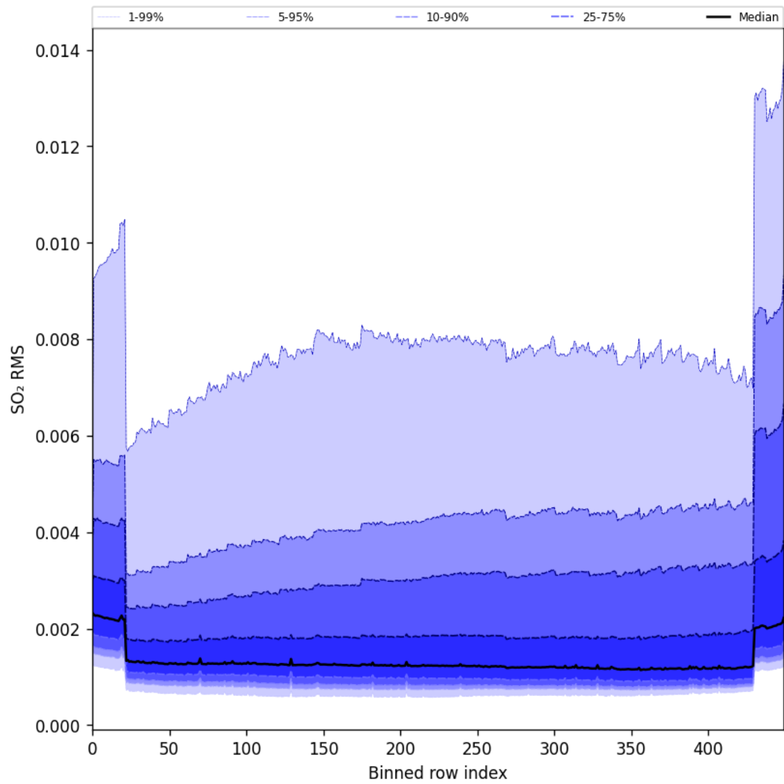
Figure 93: Along track statistics of “SO 2 RMS” for 2024-09-24 to 2024-09-26
