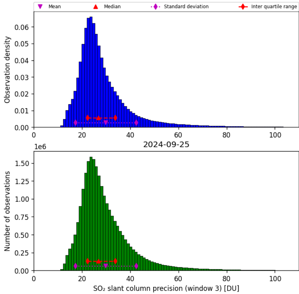
Figure 65: Histogram of “SO 2 slant column precision (window 3)” for 2024-09-24 to 2024-09-26
