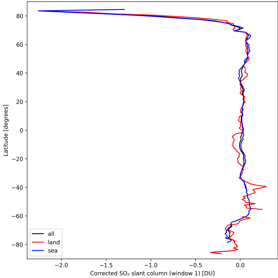
Figure 35: Zonal average of “Corrected SO 2 slant column (window 1)” for 2024-09-24 to 2024-09-26.
