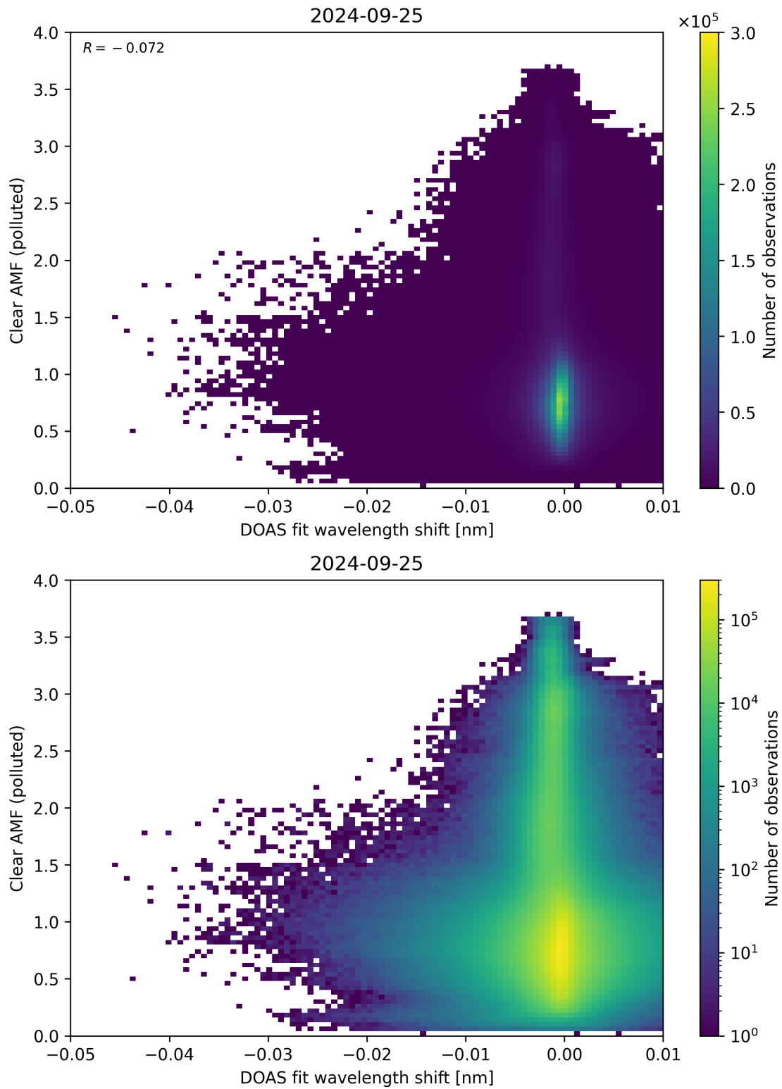
Figure 129: Scatter density plot of “DOAS fit wavelength shift” against “Clear AMF (polluted)” for 2024-09-24 to 2024-09-26.
