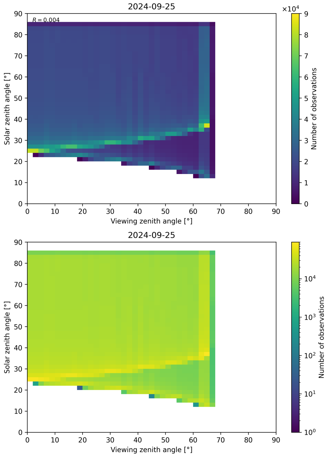
Figure 315: Scatter density plot of “Viewing zenith angle” against “Solar zenith angle” for 2024-09-24 to 2024-09-26.
