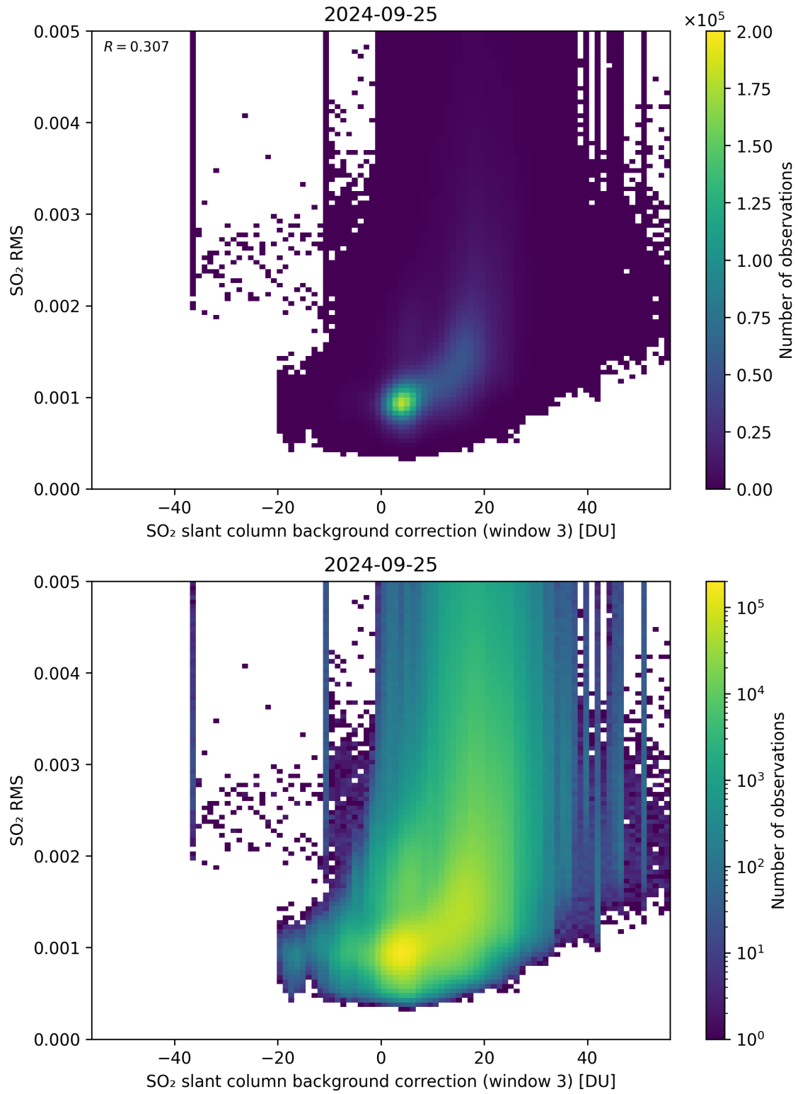
Figure 123: Scatter density plot of “SO 2 slant column background correction (window 3)” against “SO 2 RMS” for 2024-09-24 to 2024-09-26.
