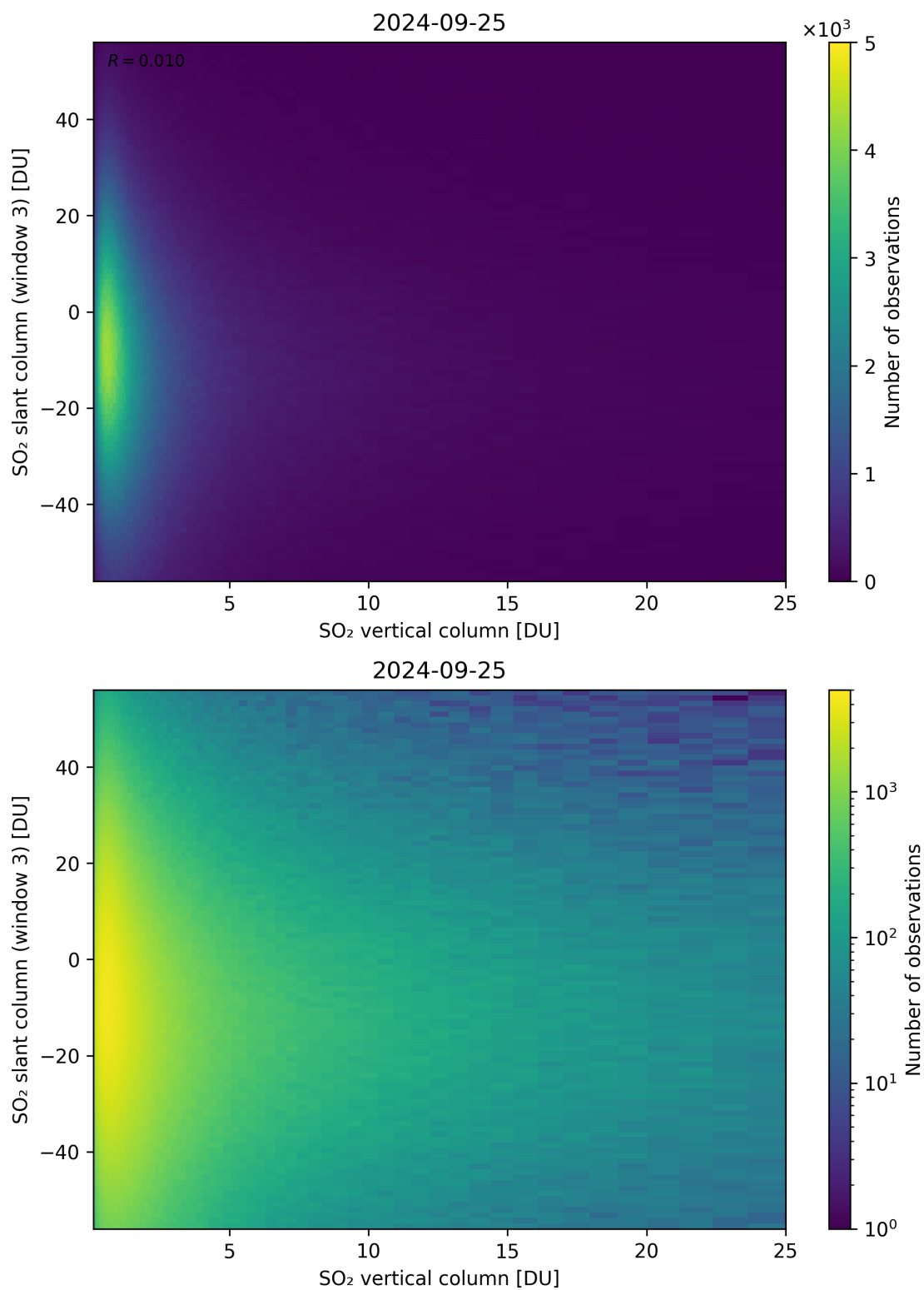
Figure 303: Scatter density plot of “SO 2 vertical column” against “SO 2 slant column (window 3)” for 2024-09-24 to 2024-09-26.
