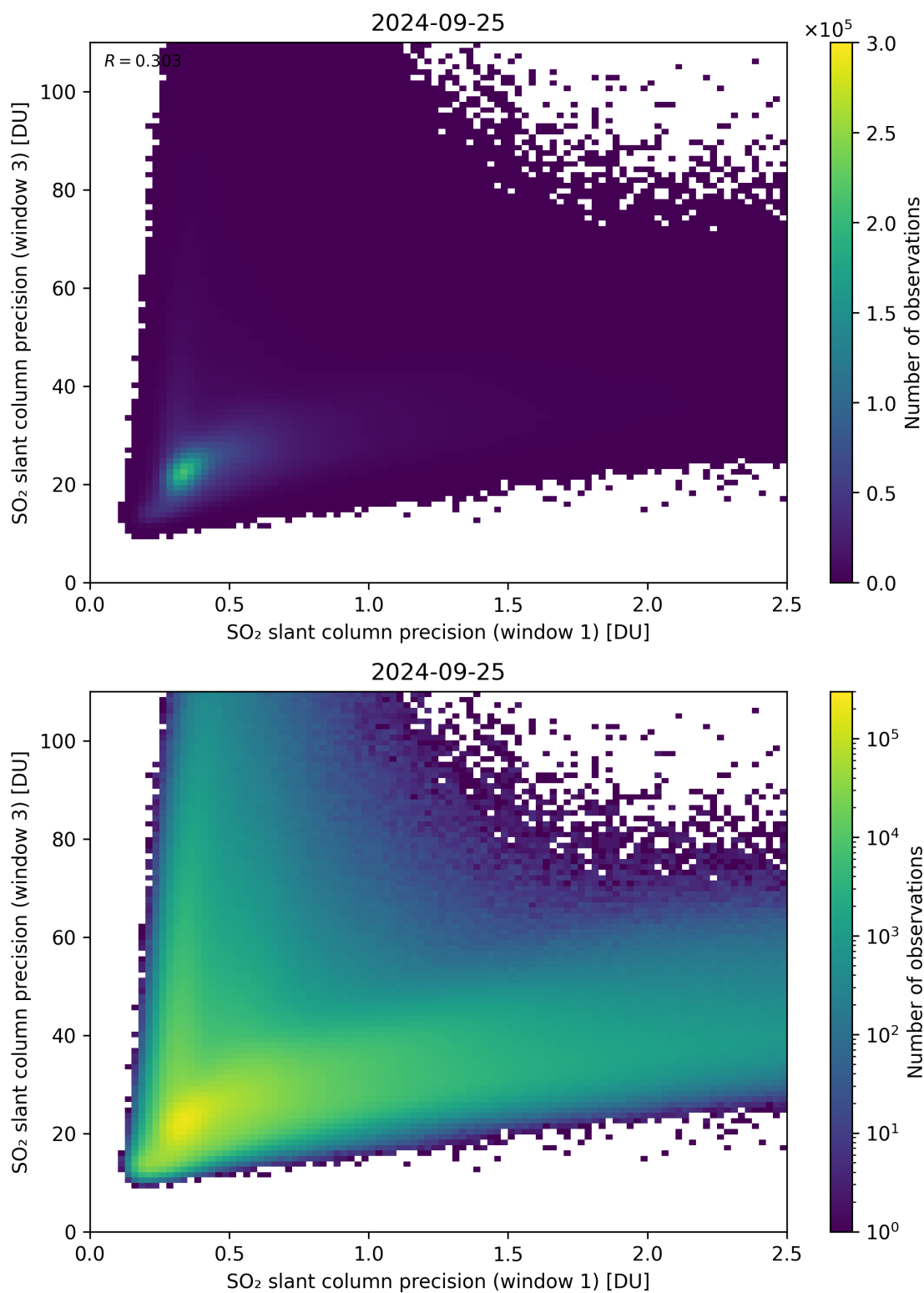
Figure 229: Scatter density plot of “SO 2 slant column precision (window 1)” against “SO 2 slant column precision (window 3)” for 2024-09-24 to 2024-09-26.
