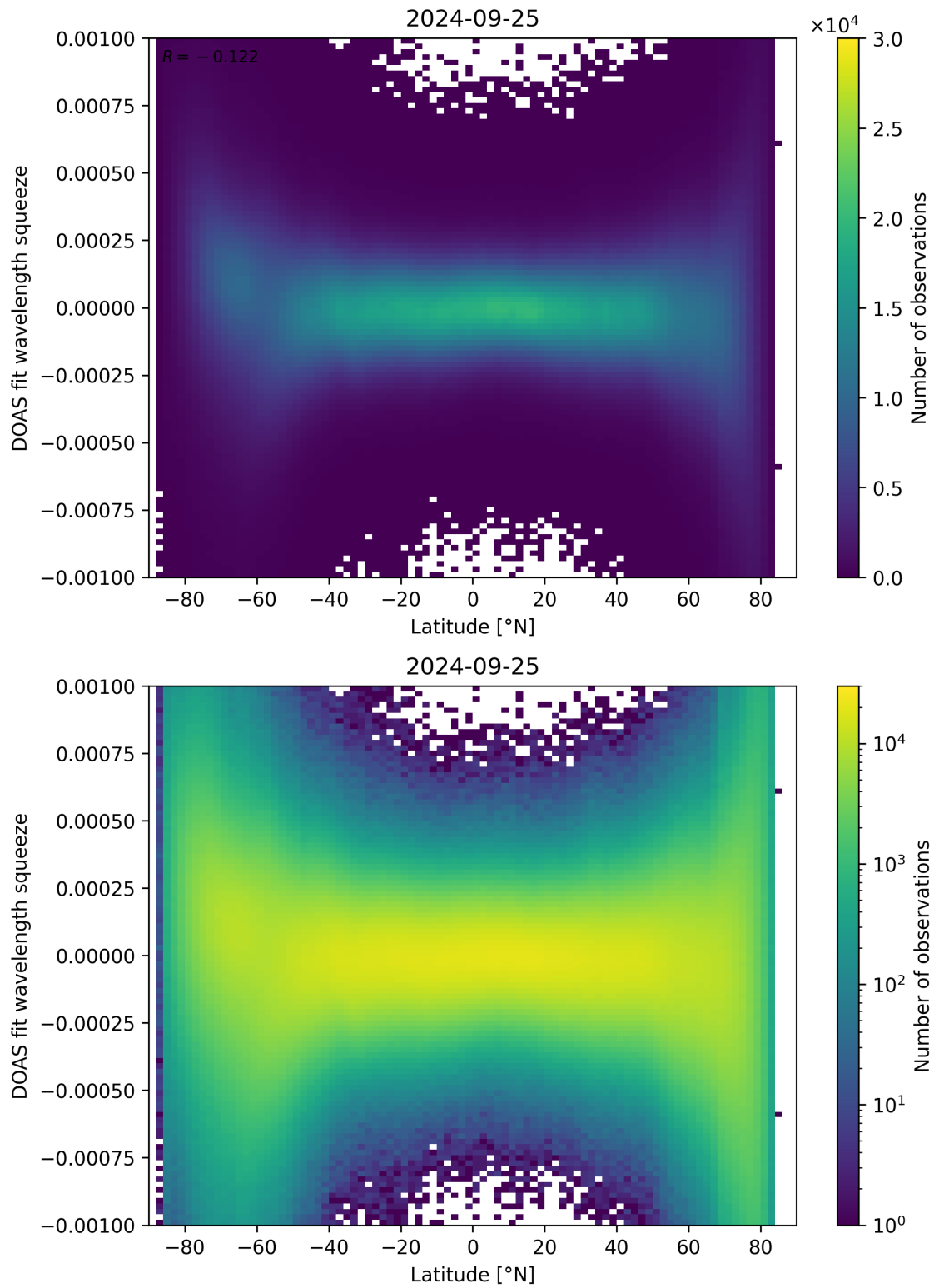
Figure 143: Scatter density plot of “Latitude” against “DOAS fit wavelength squeeze” for 2024-09-24 to 2024-09-26.
