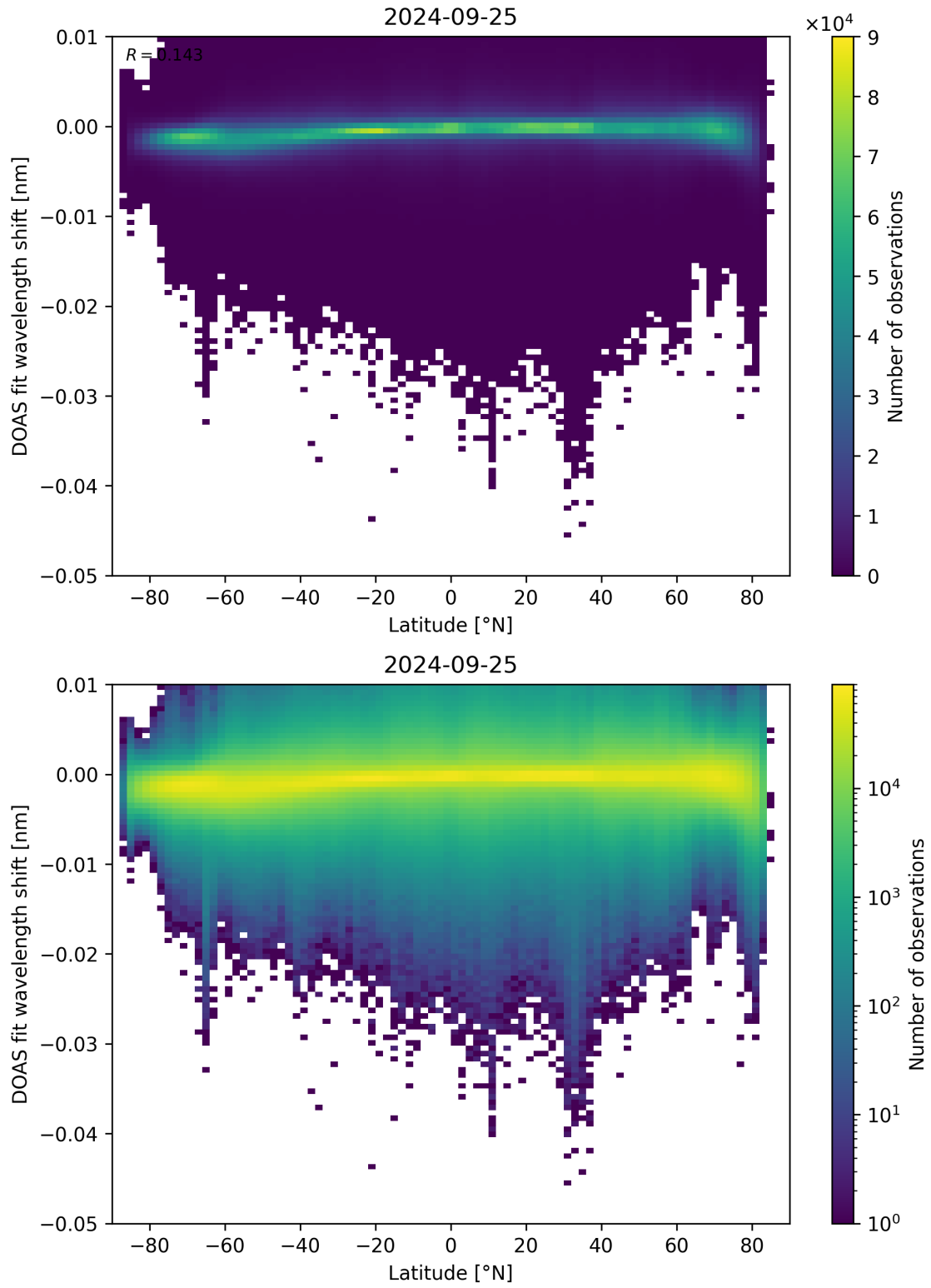
Figure 142: Scatter density plot of “Latitude” against “DOAS fit wavelength shift” for 2024-09-24 to 2024-09-26.
