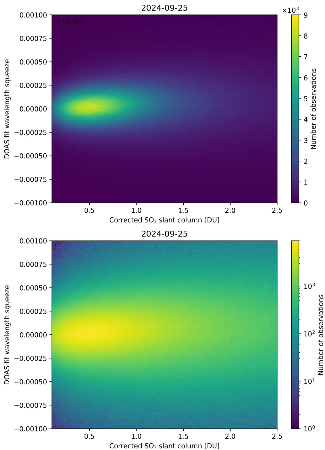
Figure 182: Scatter density plot of “Corrected SO 2 slant column” against “DOAS fit wavelength squeeze” for 2024-09-24 to 2024-09-26.
