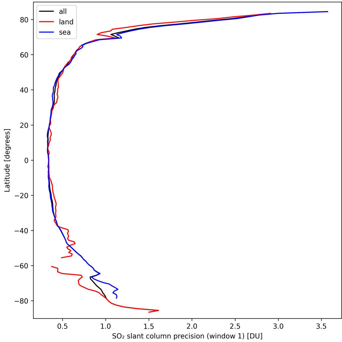
Figure 34: Zonal average of “SO 2 slant column precision (window 1)” for 2024-09-24 to 2024-09-26.
