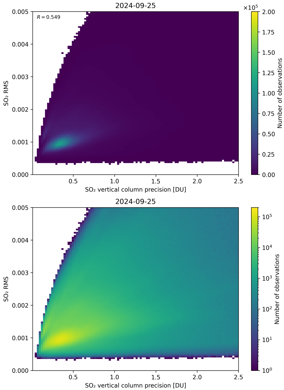
Figure 284: Scatter density plot of “SO 2 vertical column precision” against “SO 2 RMS” for 2024-09-24 to 2024-09-26.
