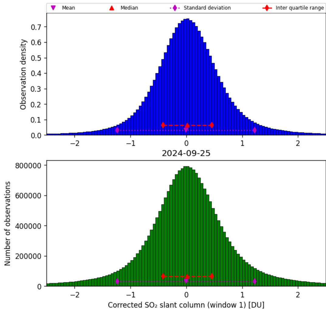
Figure 58: Histogram of “Corrected SO 2 slant column (window 1)” for 2024-09-24 to 2024-09-26
