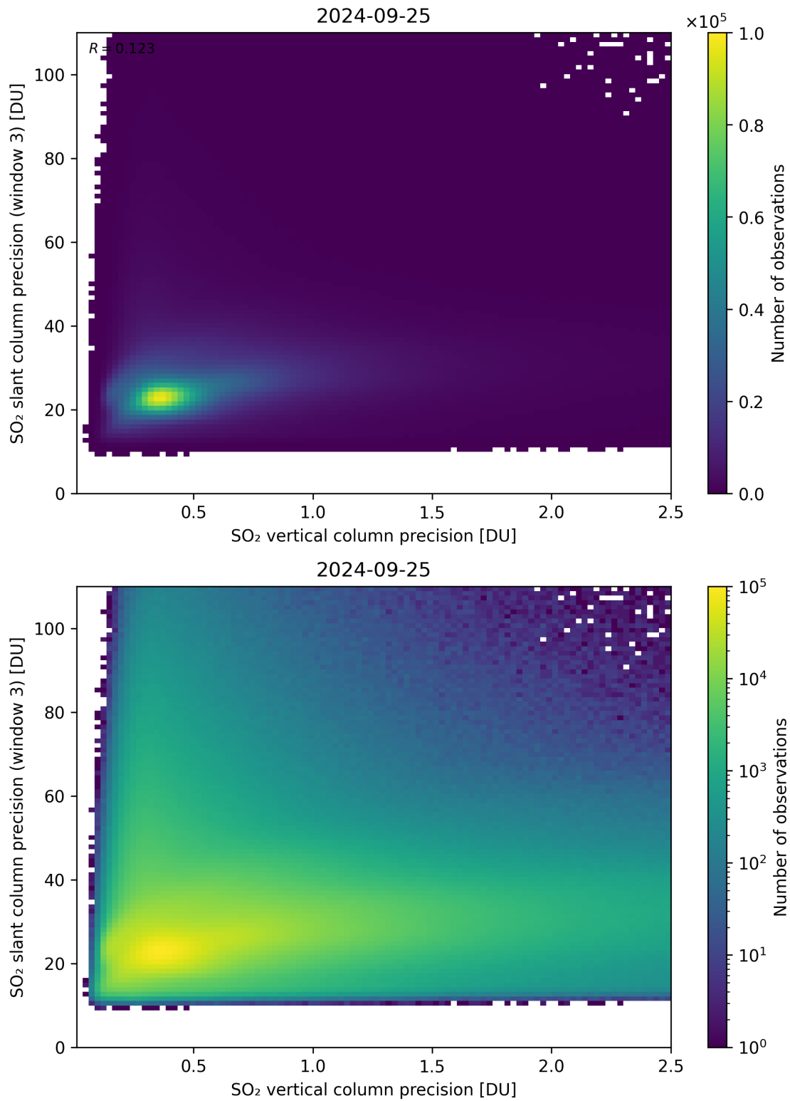
Figure 293: Scatter density plot of “SO 2 vertical column precision” against “SO 2 slant column precision (window 3)” for 2024-09-24 to 2024-09-26.
