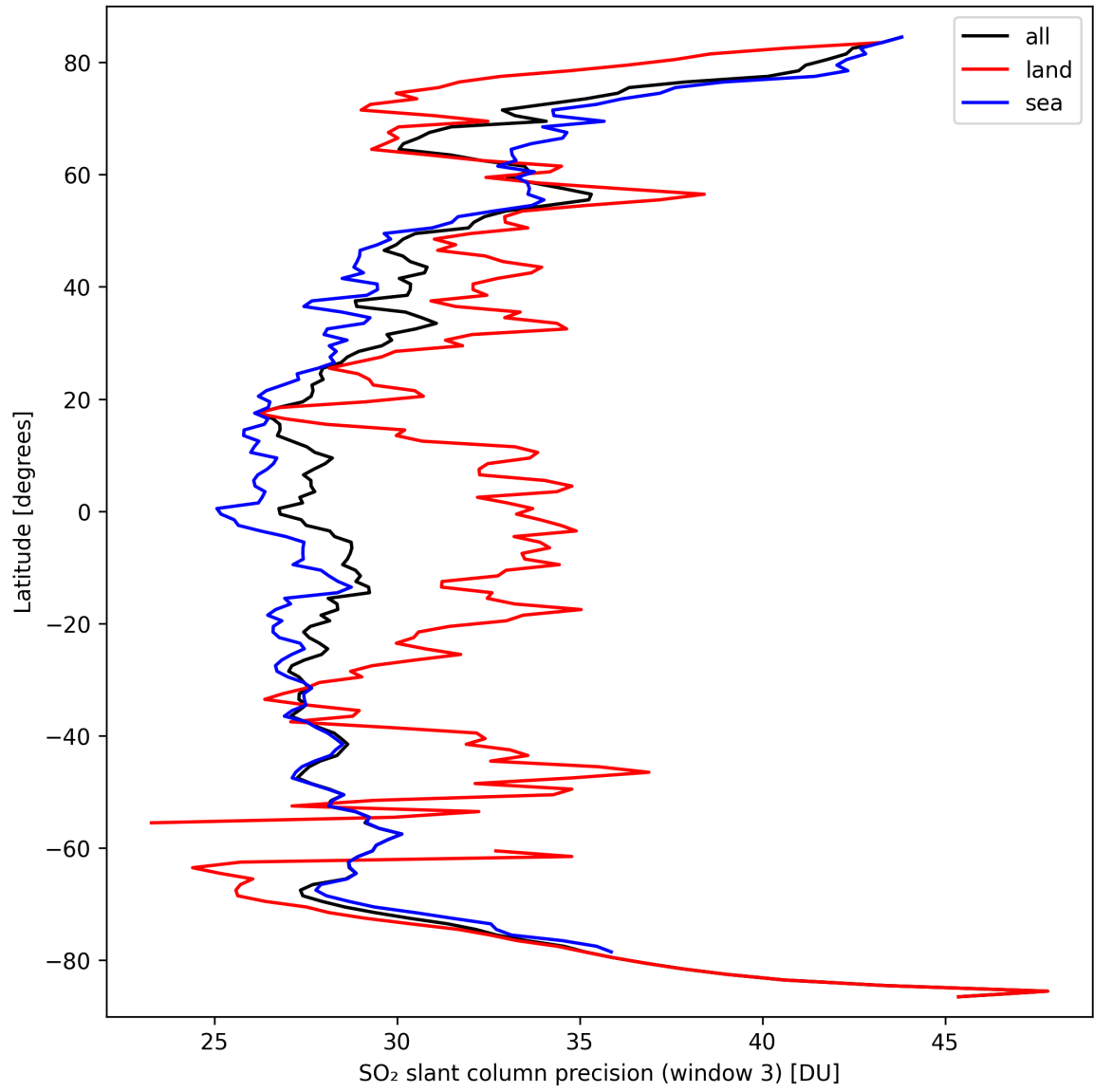
Figure 42: Zonal average of “SO 2 slant column precision (window 3)” for 2024-09-24 to 2024-09-26.
