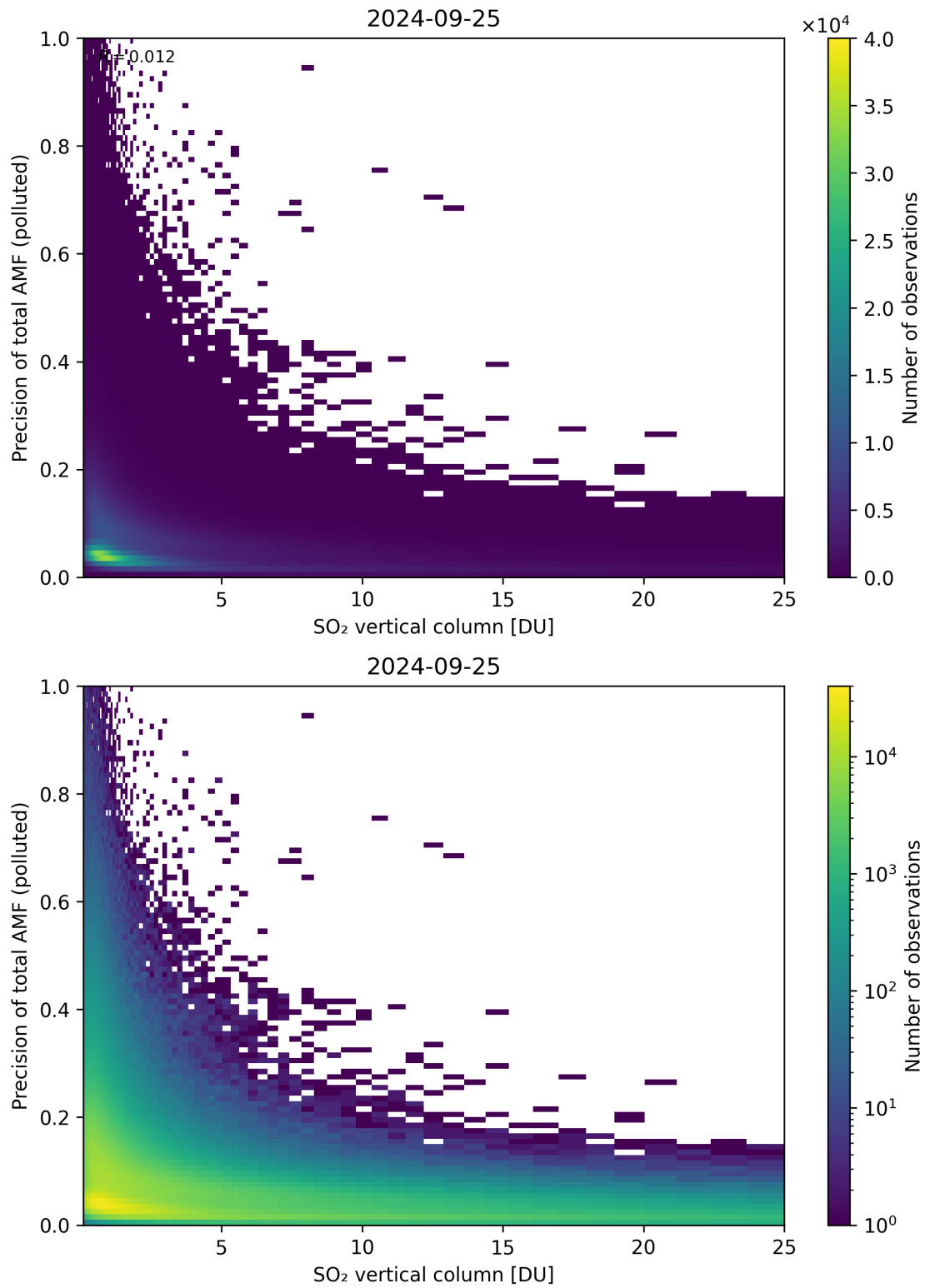
Figure 306: Scatter density plot of “SO 2 vertical column” against “Precision of total AMF (polluted)” for 2024-09-24 to 2024-09-26.
