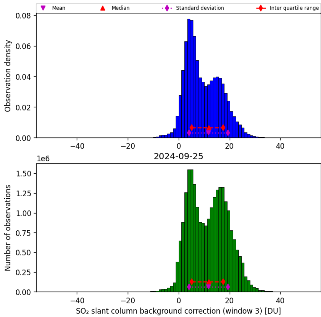
Figure 67: Histogram of “SO 2 slant column background correction (window 3)” for 2024-09-24 to 2024-09-26
