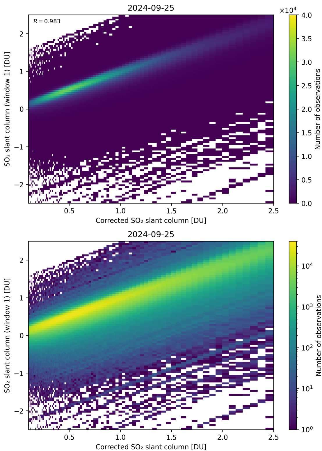
Figure 187: Scatter density plot of “Corrected SO 2 slant column” against “SO 2 slant column (window 1)” for 2024-09-24 to 2024-09-26.
