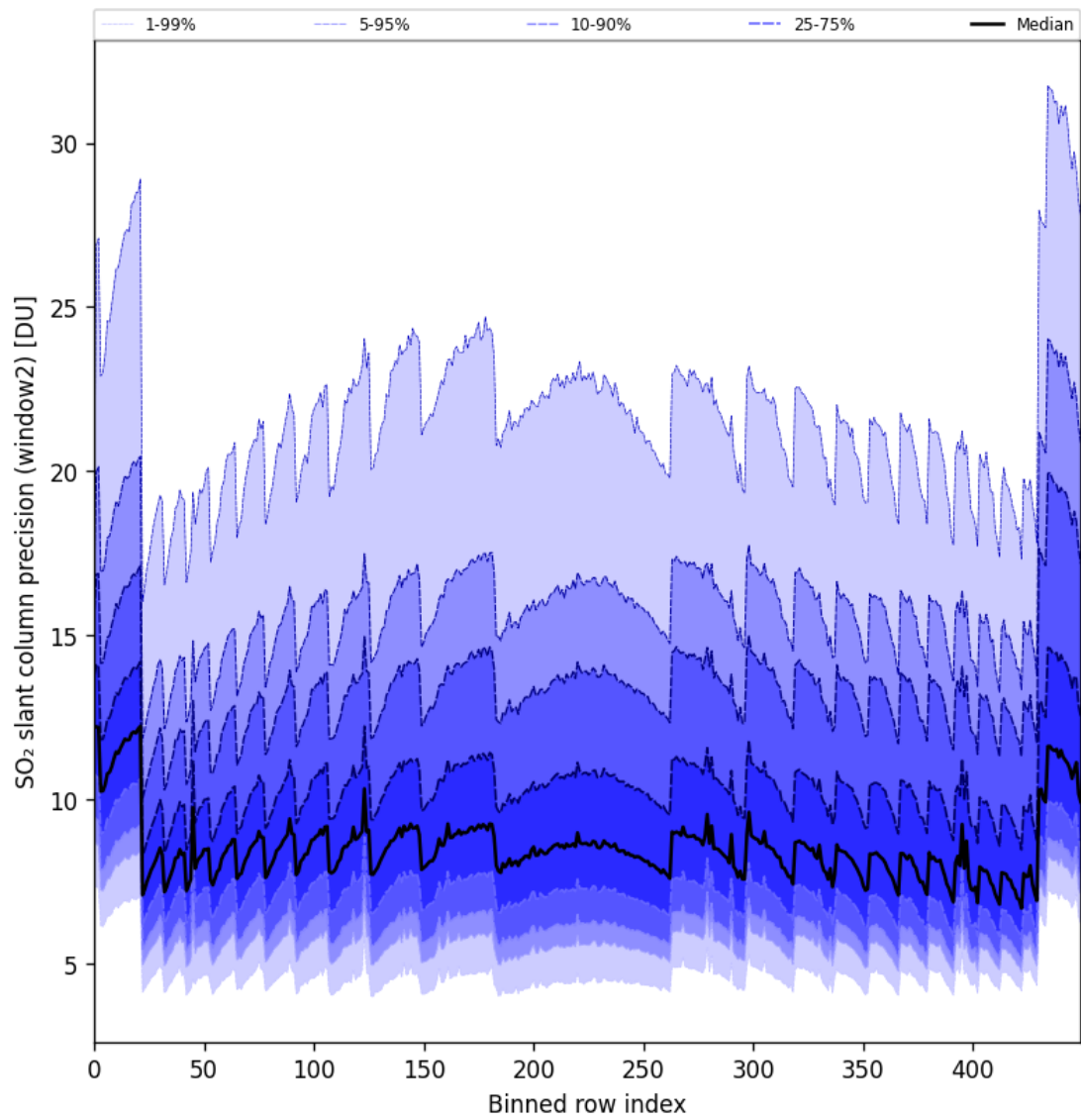
Figure 84: Along track statistics of “SO 2 slant column precision (window2)” for 2024-09-24 to 2024-09-26
