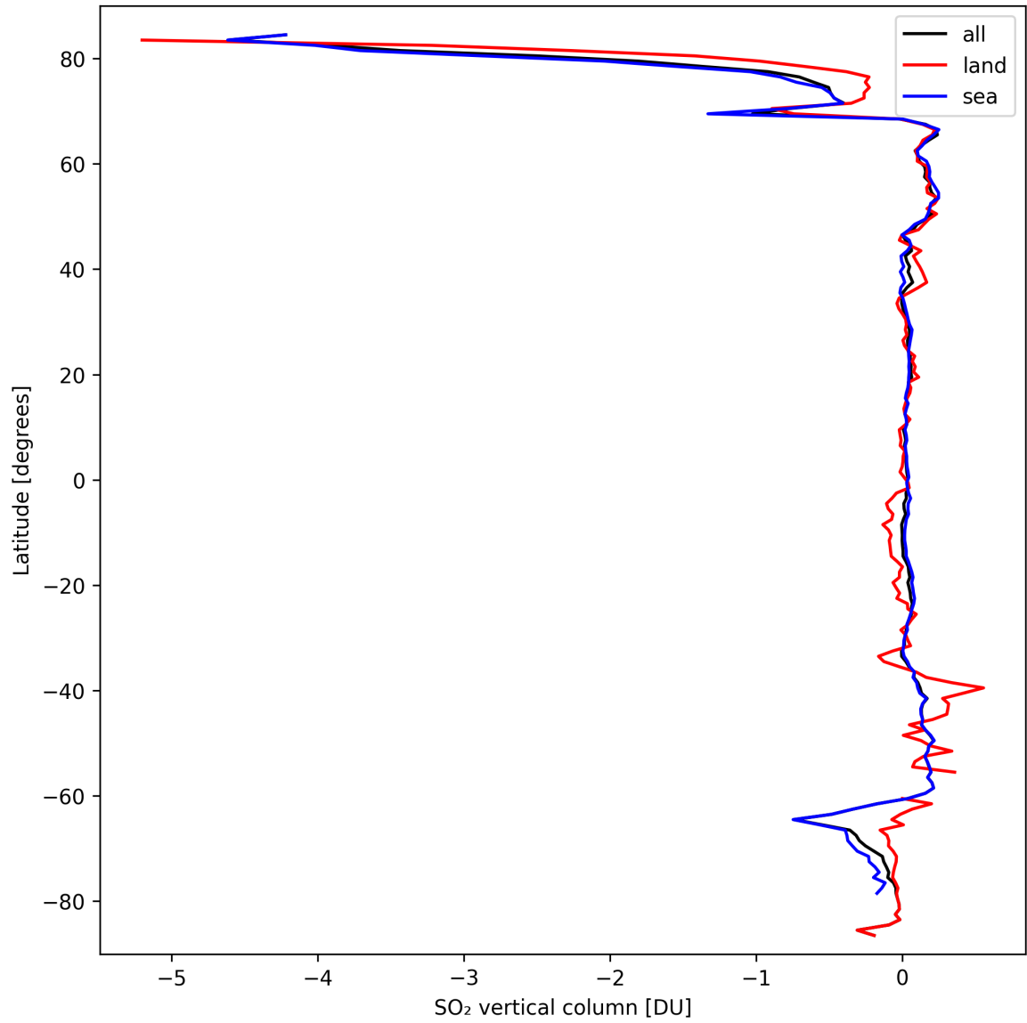
Figure 30: Zonal average of “SO 2 vertical column” for 2024-09-24 to 2024-09-26.
