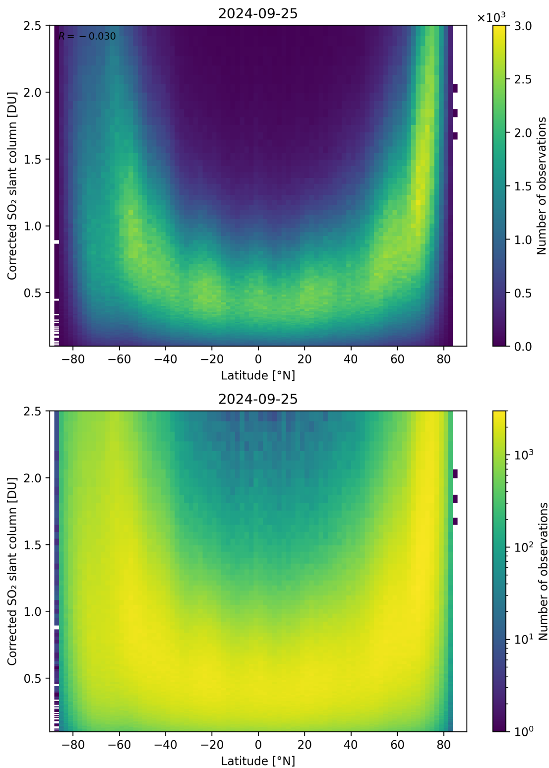
Figure 146: Scatter density plot of “Latitude” against “Corrected SO 2 slant column” for 2024-09-24 to 2024-09-26.
