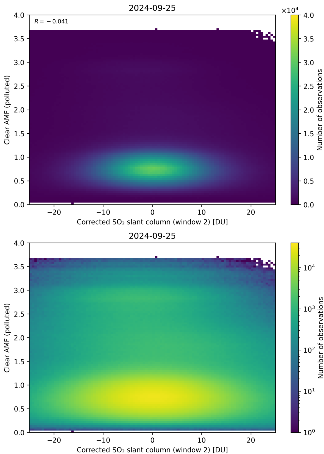
Figure 199: Scatter density plot of “Corrected SO 2 slant column (window 2)” against “Clear AMF (polluted)” for 2024-09-24 to 2024-09-26.
