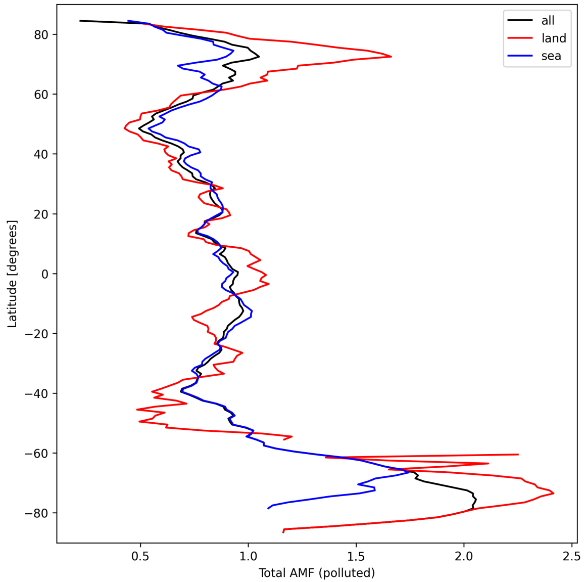
Figure 48: Zonal average of “Total AMF (polluted)” for 2024-09-24 to 2024-09-26.
