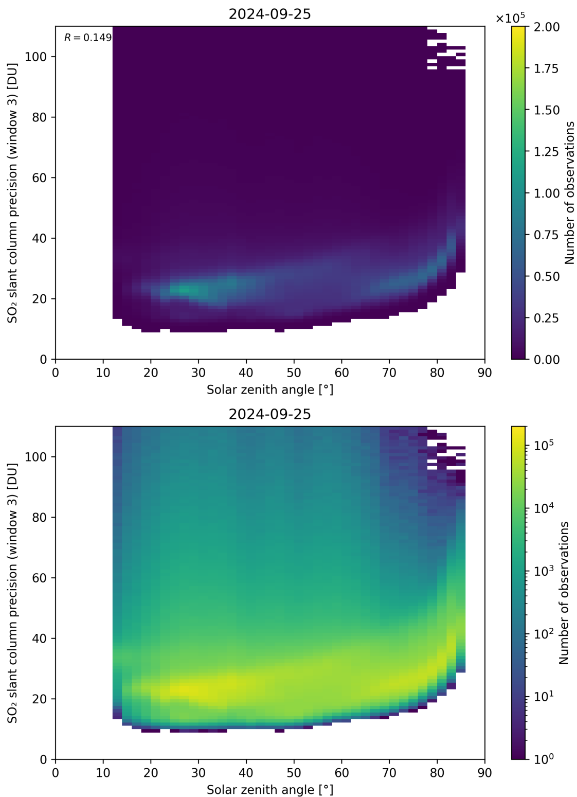
Figure 173: Scatter density plot of “Solar zenith angle” against “SO 2 slant column precision (window 3)” for 2024-09-24 to 2024-09-26.
