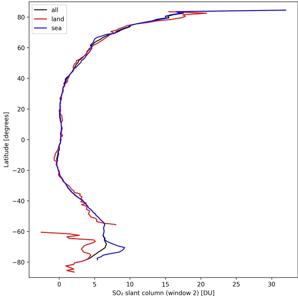
Figure 37: Zonal average of “SO 2 slant column (window 2)” for 2024-09-24 to 2024-09-26.
