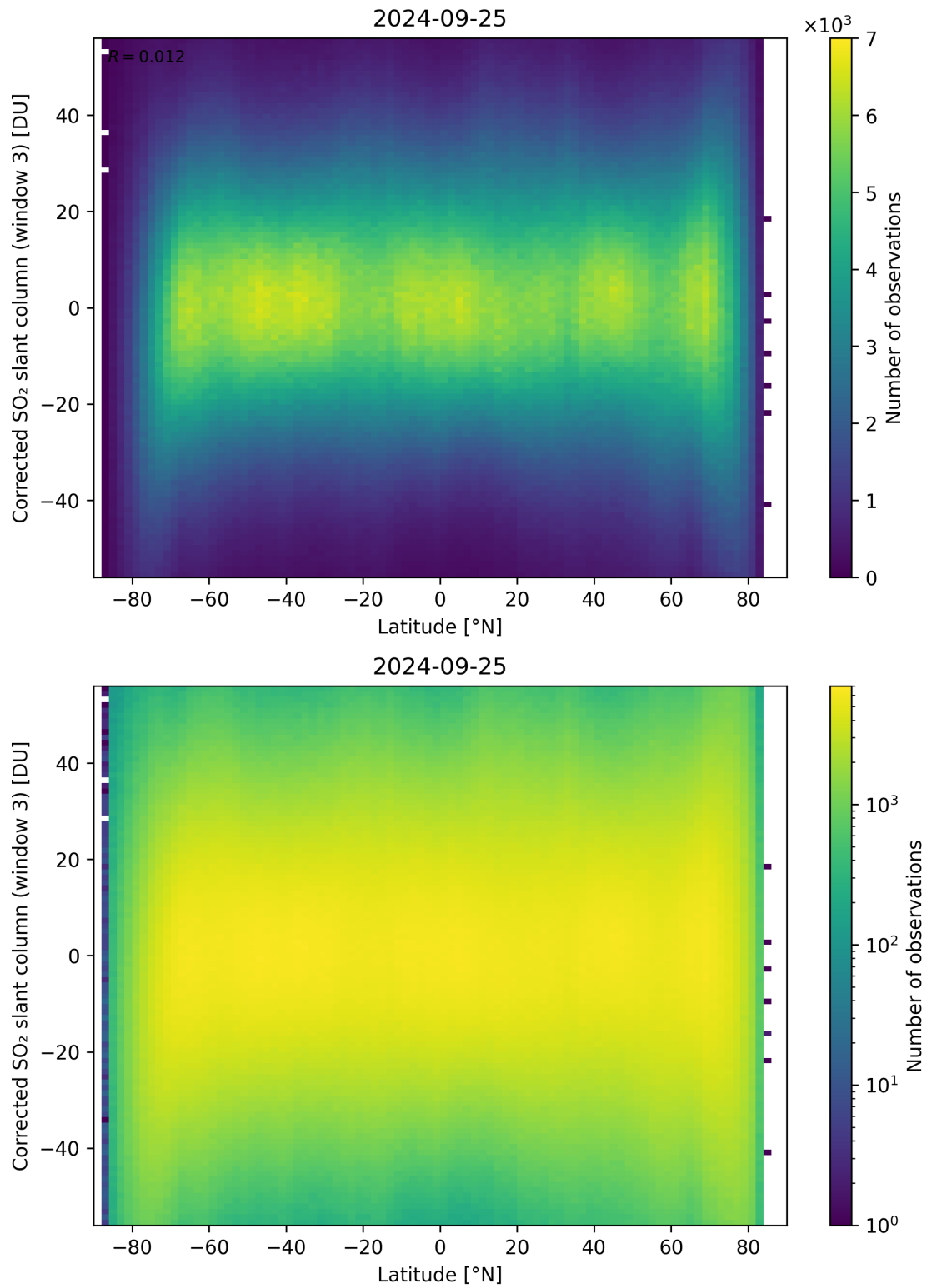
Figure 148: Scatter density plot of “Latitude” against “Corrected SO 2 slant column (window 3)” for 2024-09-24 to 2024-09-26.
