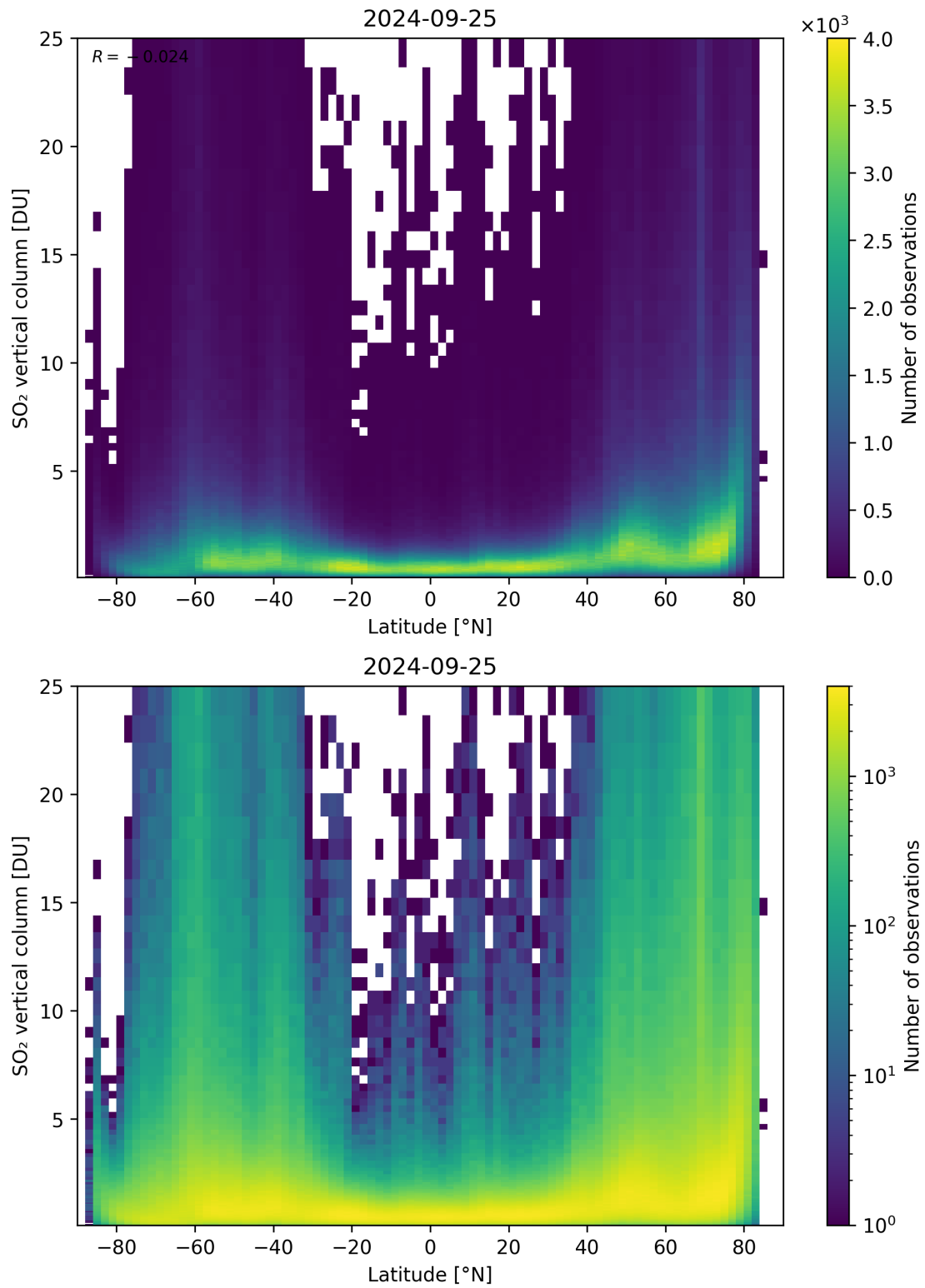
Figure 156: Scatter density plot of “Latitude” against “SO 2 vertical column” for 2024-09-24 to 2024-09-26.
