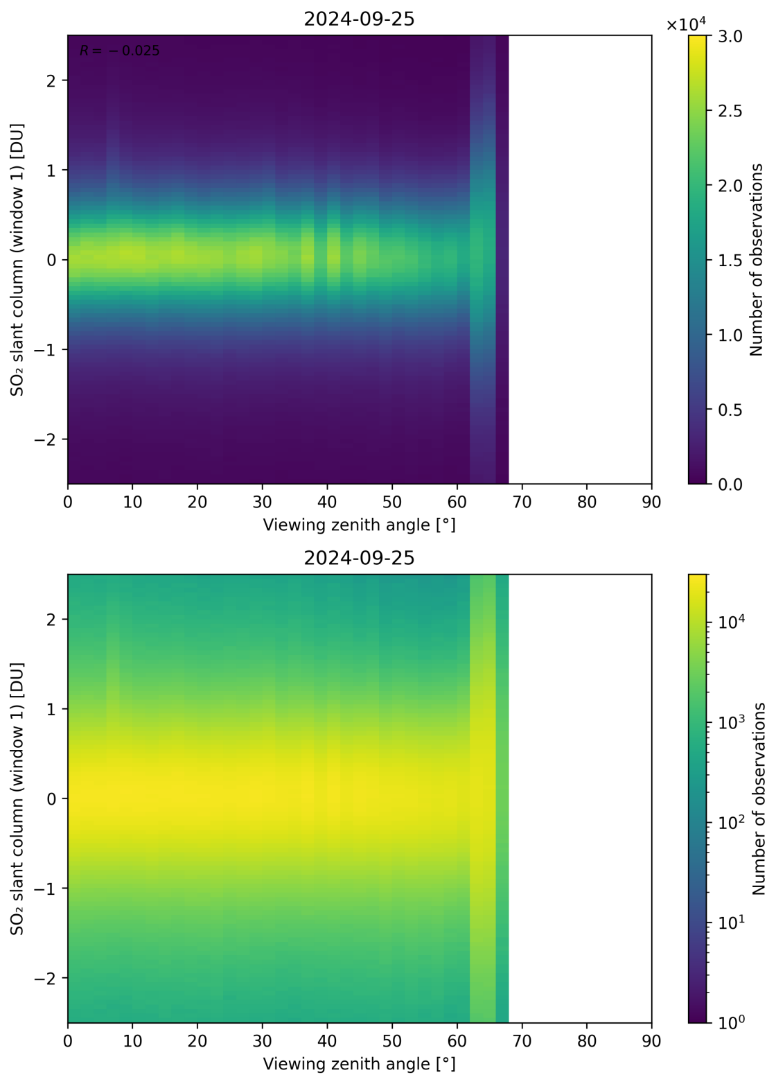
Figure 320: Scatter density plot of “Viewing zenith angle” against “SO 2 slant column (window 1)” for 2024-09-24 to 2024-09-26.
