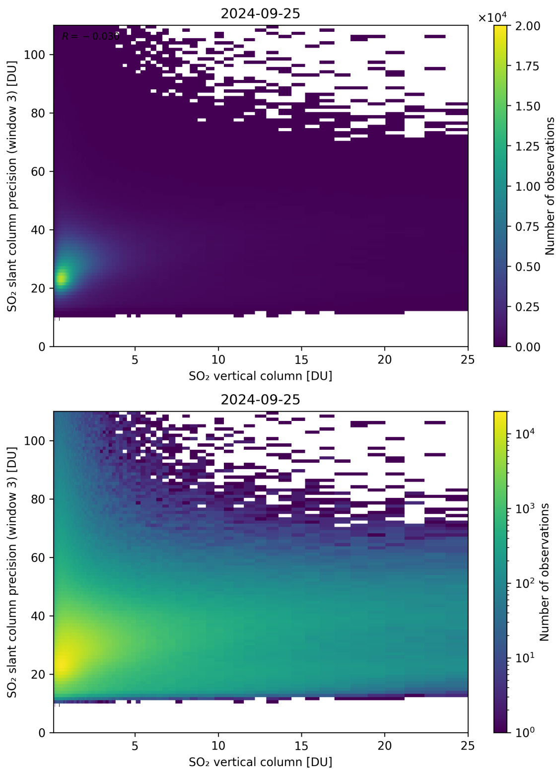
Figure 304: Scatter density plot of “SO 2 vertical column” against “SO 2 slant column precision (window 3)” for 2024-09-24 to 2024-09-26.
