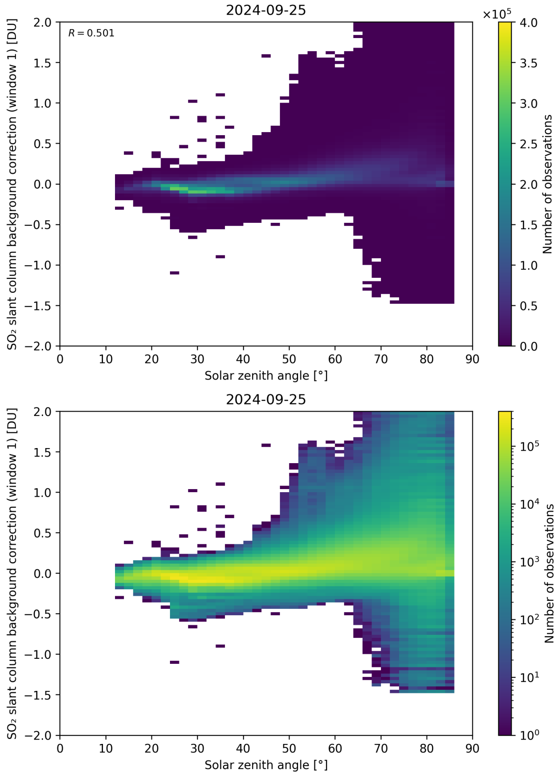
Figure 158: Scatter density plot of “Solar zenith angle” against “SO 2 slant column background correction (window 1)” for 2024-09-24 to 2024-09-26.
