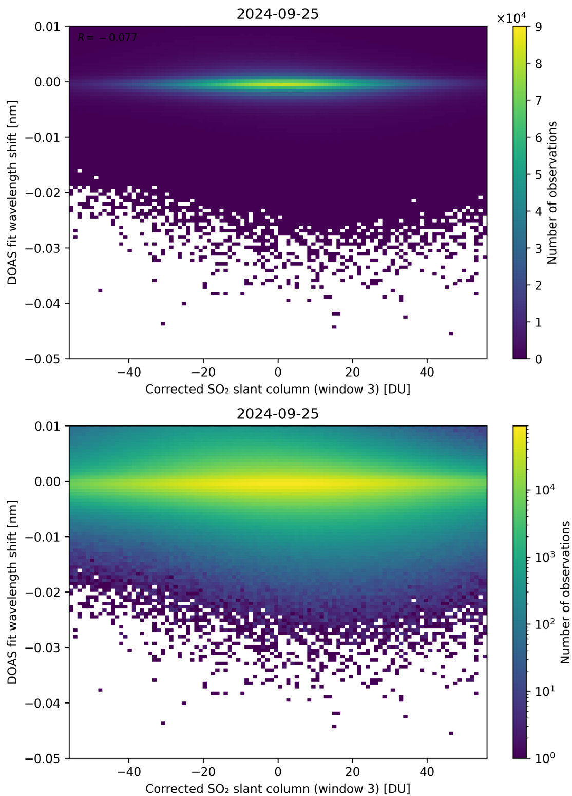
Figure 206: Scatter density plot of “Corrected SO 2 slant column (window 3)” against “DOAS fit wavelength shift” for 2024-09-24 to 2024-09-26.
