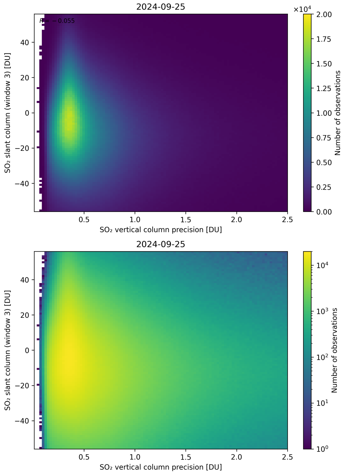
Figure 292: Scatter density plot of “SO 2 vertical column precision” against “SO 2 slant column (window 3)” for 2024-09-24 to 2024-09-26.
