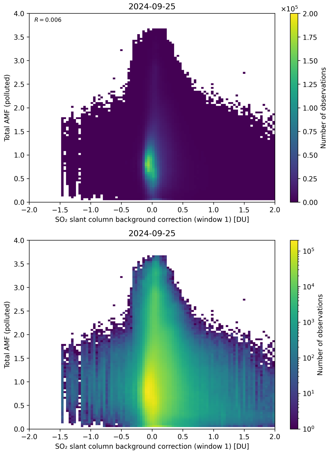
Figure 109: Scatter density plot of “SO 2 slant column background correction (window 1)” against “Total AMF (polluted)” for 2024-09-24 to 2024-09-26.
