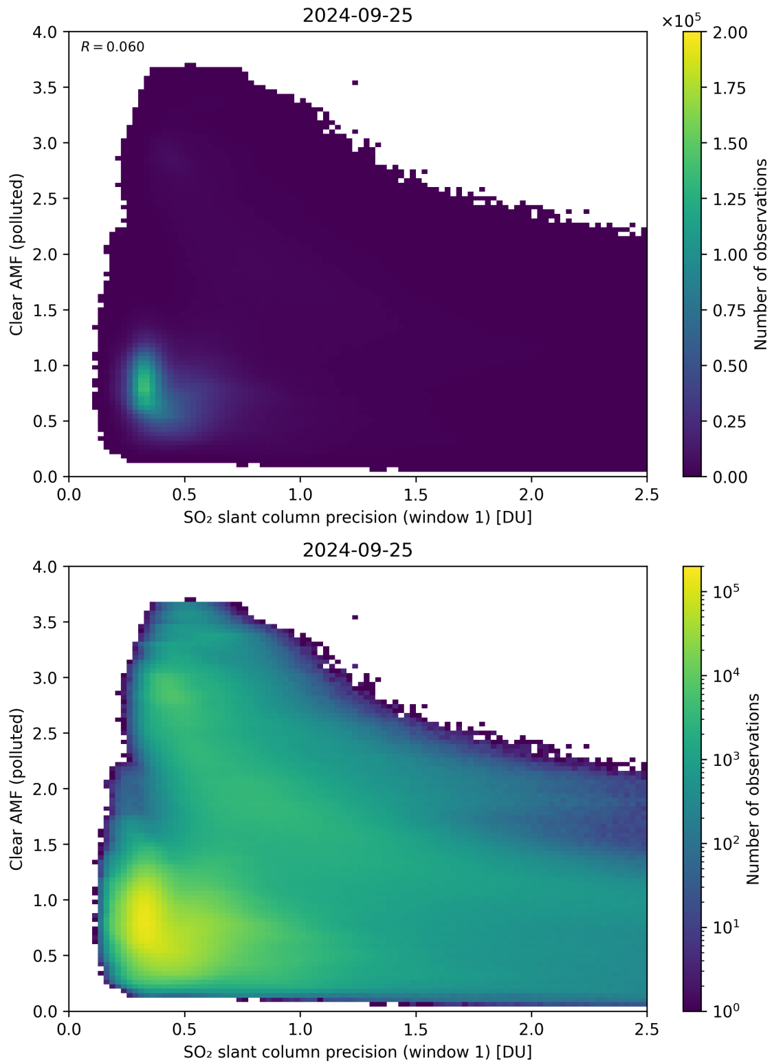
Figure 224: Scatter density plot of “SO 2 slant column precision (window 1)” against “Clear AMF (polluted)” for 2024-09-24 to 2024-09-26.
