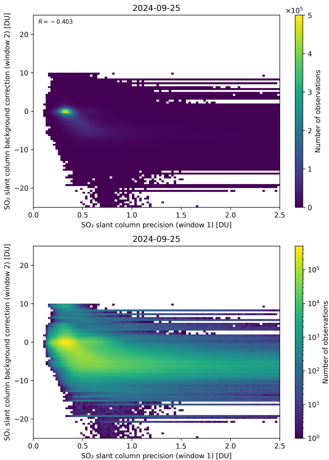
Figure 219: Scatter density plot of “SO 2 slant column precision (window 1)” against “SO 2 slant column background correction (window 2)” for 2024-09-24 to 2024-09-26.
