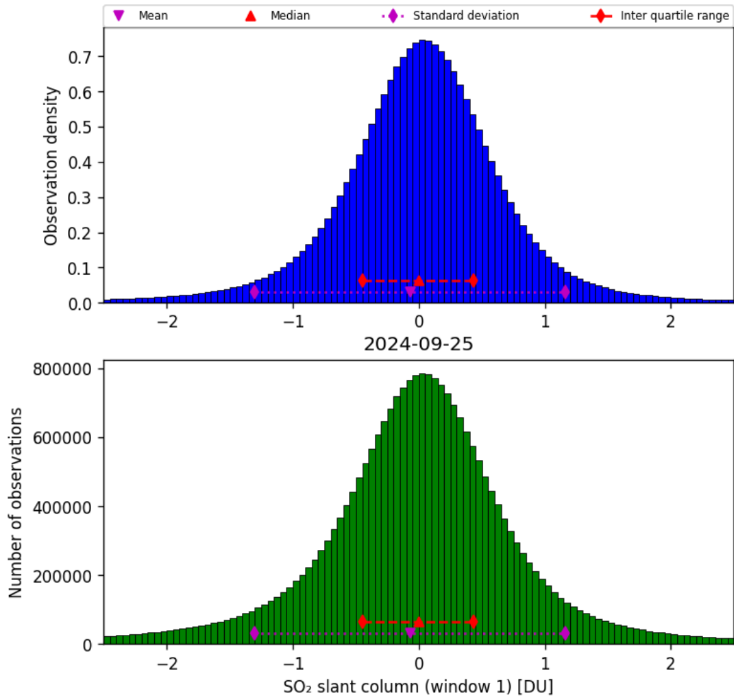
Figure 56: Histogram of “SO 2 slant column (window 1)” for 2024-09-24 to 2024-09-26
