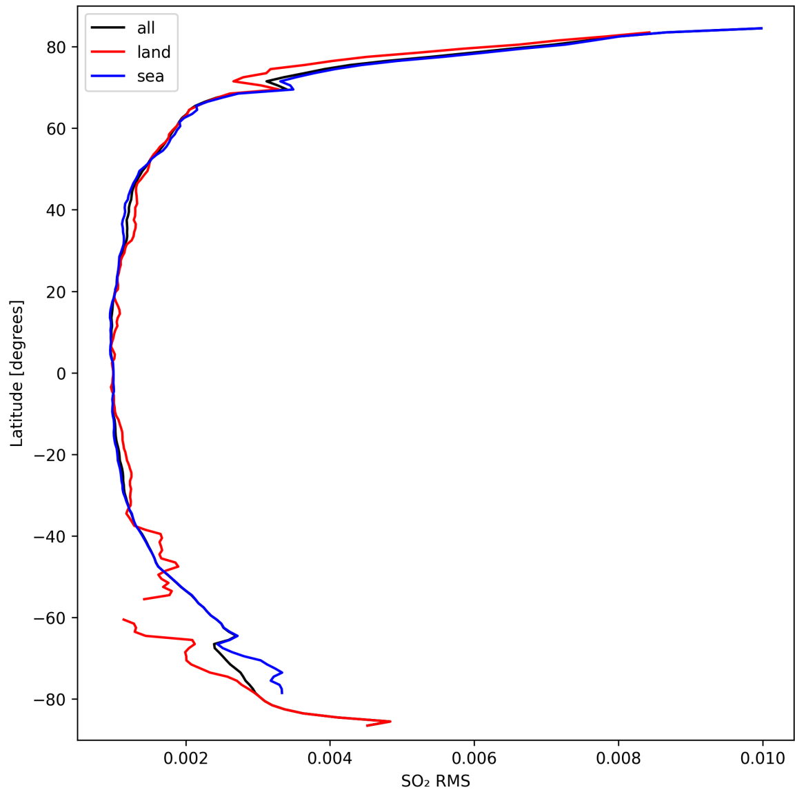
Figure 47: Zonal average of “SO 2 RMS” for 2024-09-24 to 2024-09-26.
