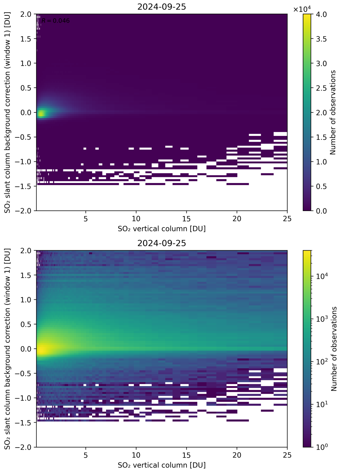
Figure 273: Scatter density plot of “SO 2 vertical column” against “SO 2 slant column background correction (window 1)” for 2024-09-24 to 2024-09-26.
