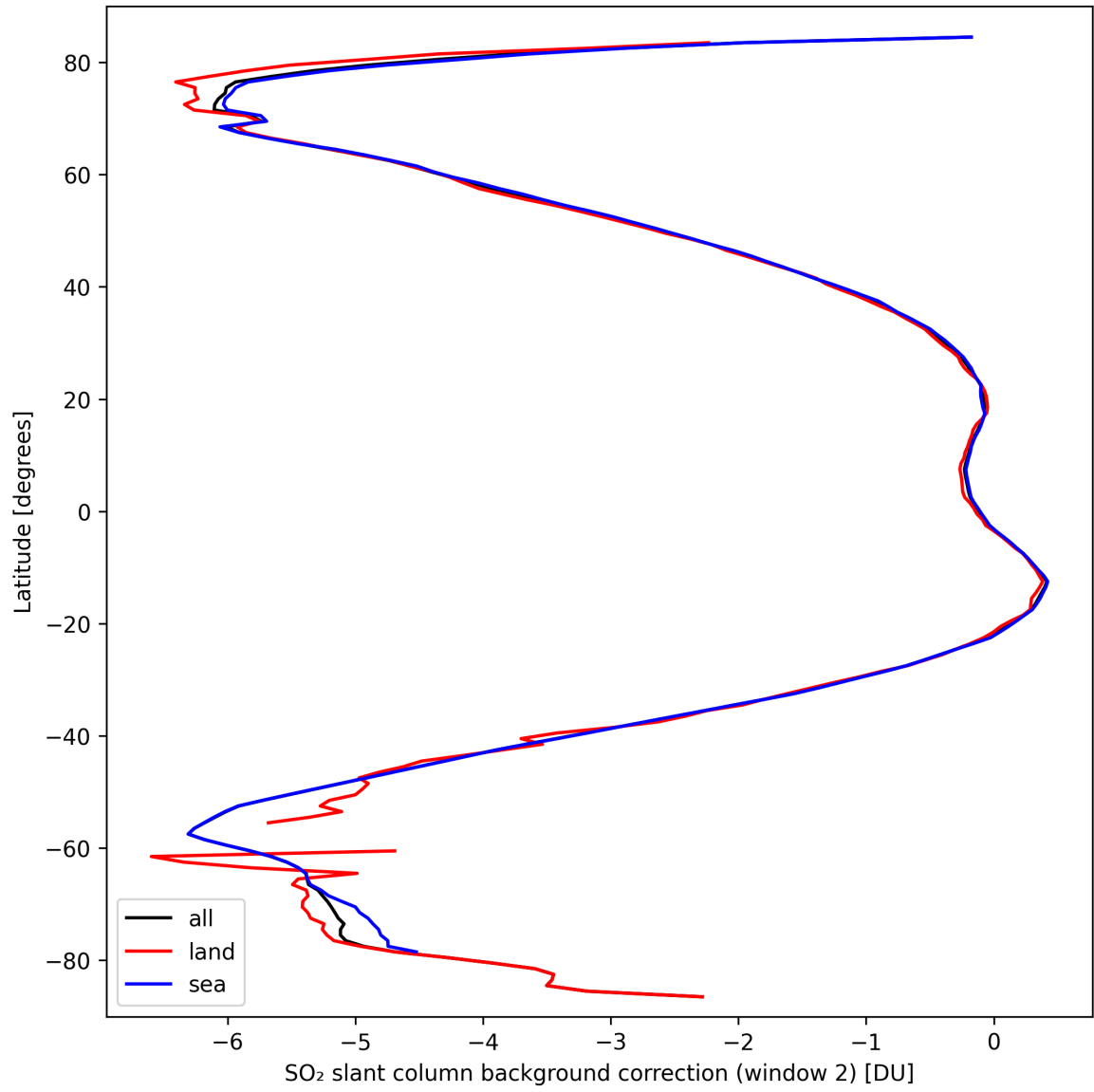
Figure 40: Zonal average of “SO 2 slant column background correction (window 2)” for 2024-09-24 to 2024-09-26.
