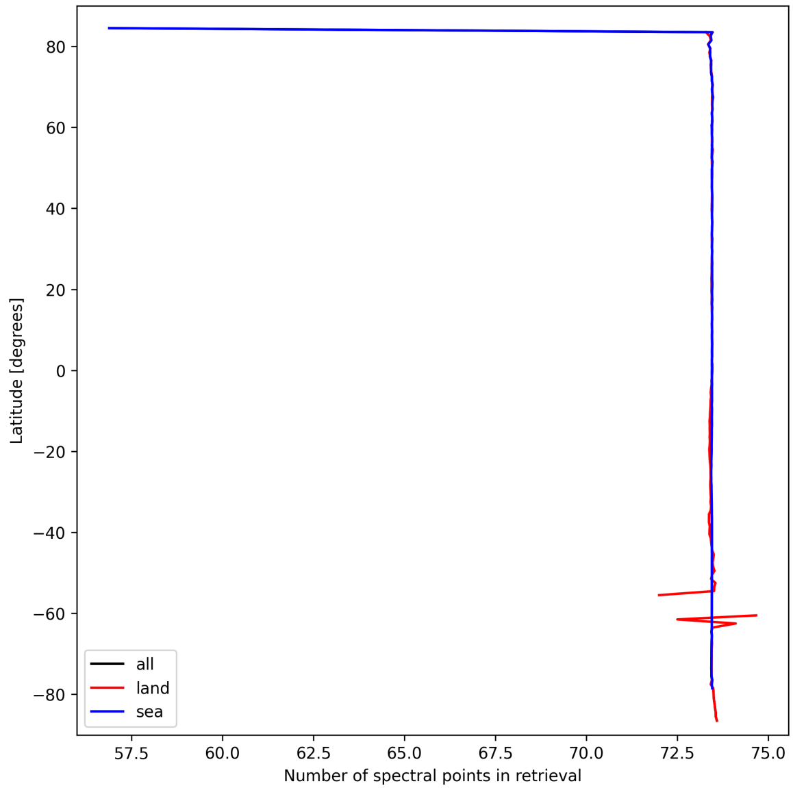
Figure 51: Zonal average of “Number of spectral points in retrieval” for 2024-09-24 to 2024-09-26.
