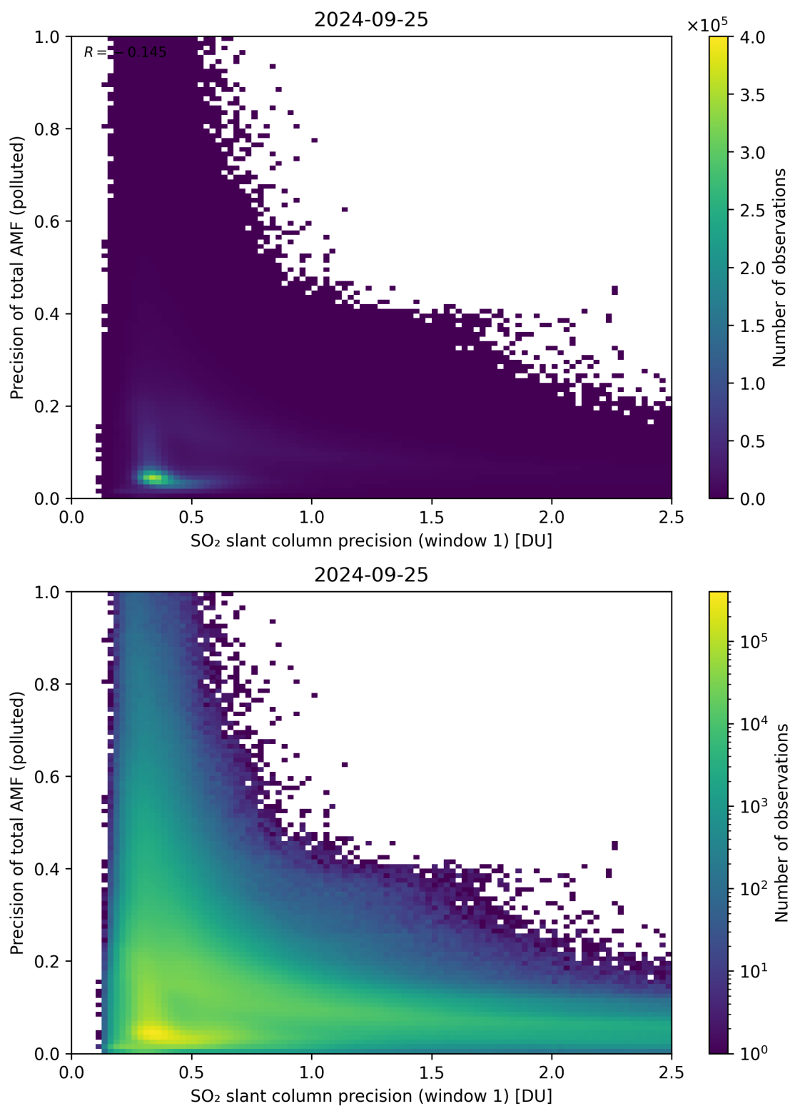
Figure 231: Scatter density plot of “SO 2 slant column precision (window 1)” against “Precision of total AMF (polluted)” for 2024-09-24 to 2024-09-26.
