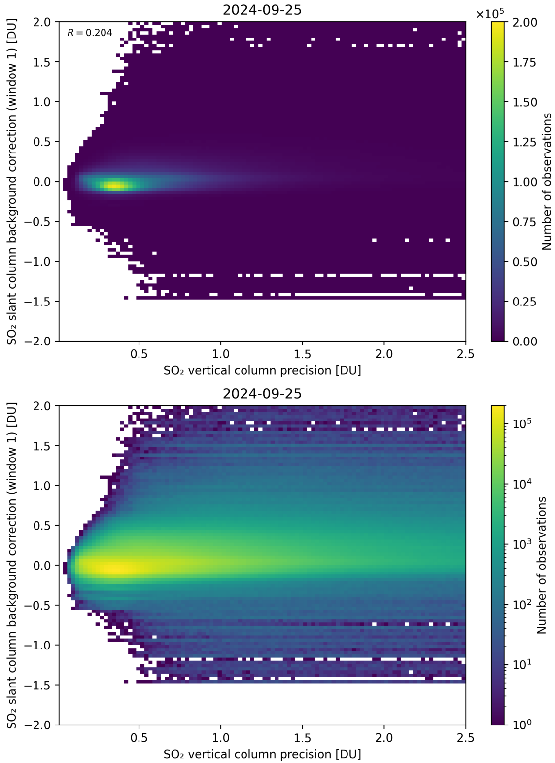
Figure 279: Scatter density plot of “SO 2 vertical column precision” against “SO 2 slant column background correction (window 1)” for 2024-09-24 to 2024-09-26.
