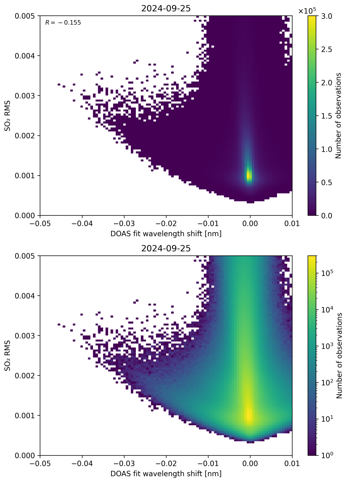
Figure 128: Scatter density plot of “DOAS fit wavelength shift” against “SO 2 RMS” for 2024-09-24 to 2024-09-26.
