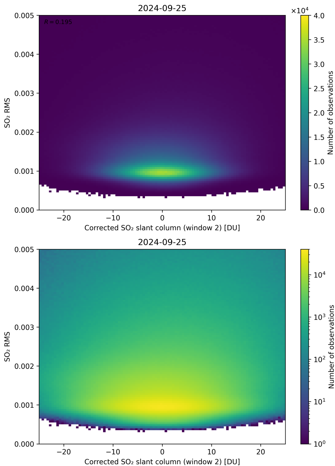
Figure 198: Scatter density plot of “Corrected SO 2 slant column (window 2)” against “SO 2 RMS” for 2024-09-24 to 2024-09-26.
