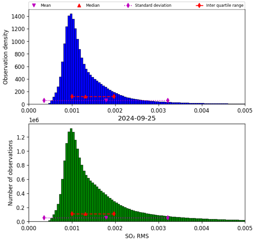
Figure 70: Histogram of “SO 2 RMS” for 2024-09-24 to 2024-09-26
