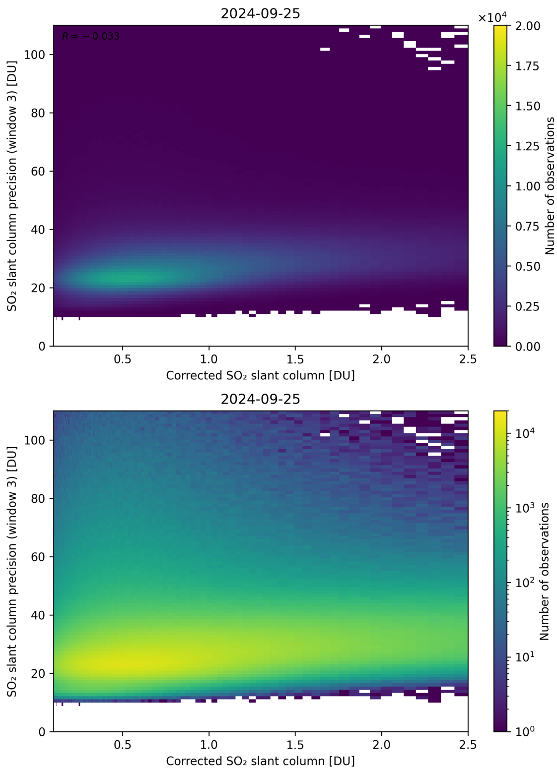
Figure 191: Scatter density plot of “Corrected SO 2 slant column” against “SO 2 slant column precision (window 3)” for 2024-09-24 to 2024-09-26.
