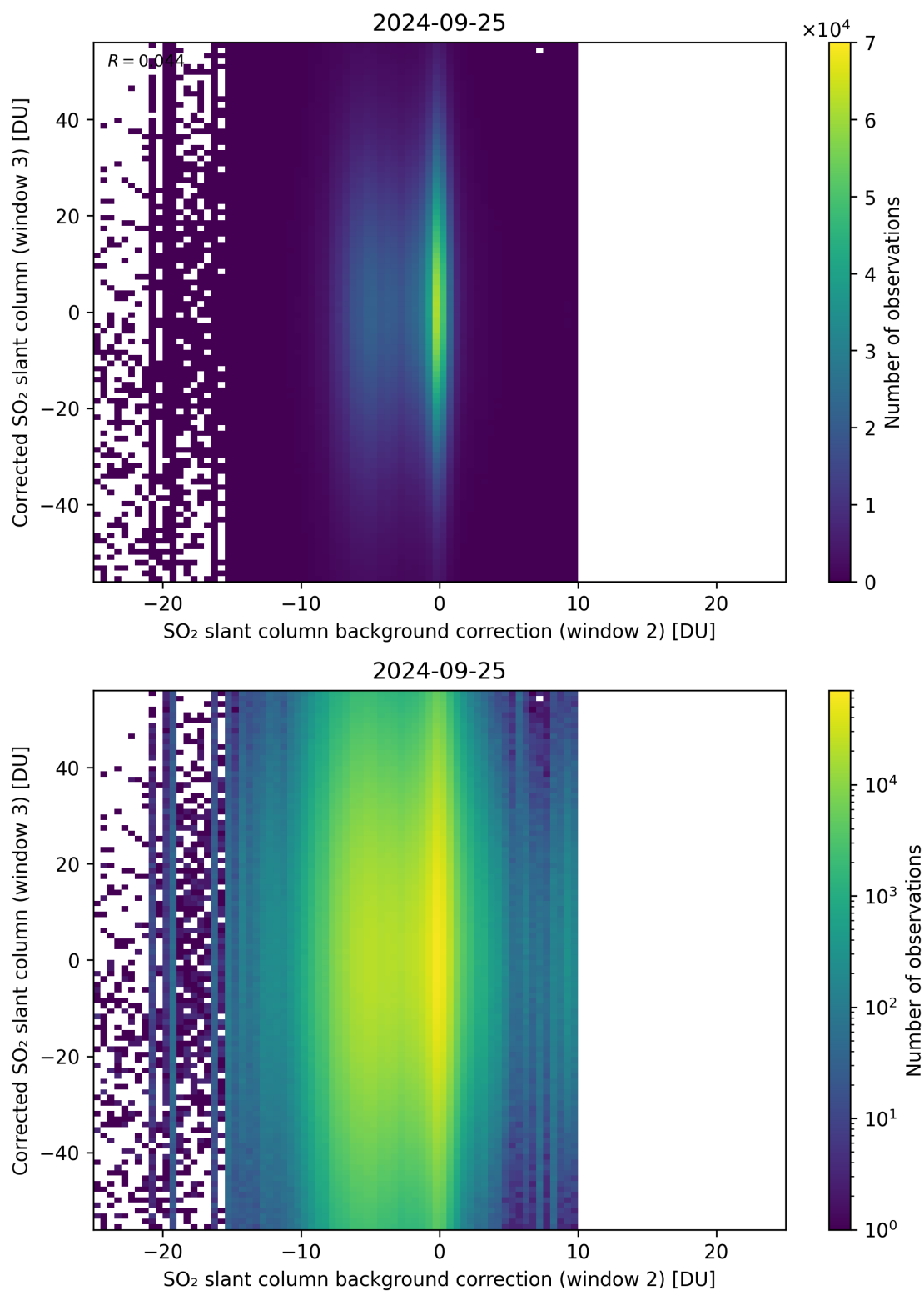
Figure 116: Scatter density plot of “SO 2 slant column background correction (window 2)” against “Corrected SO 2 slant column (window 3)” for 2024-09-24 to 2024-09-26.
