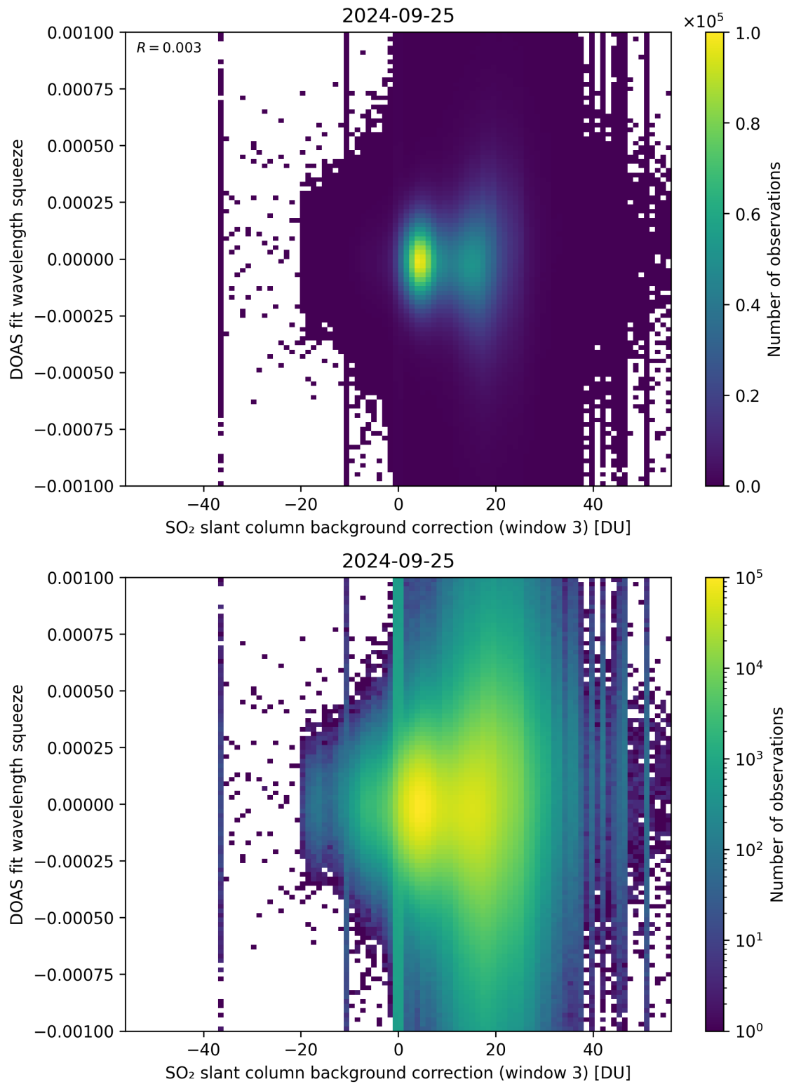
Figure 122: Scatter density plot of “SO 2 slant column background correction (window 3)” against “DOAS fit wavelength squeeze” for 2024-09-24 to 2024-09-26.
