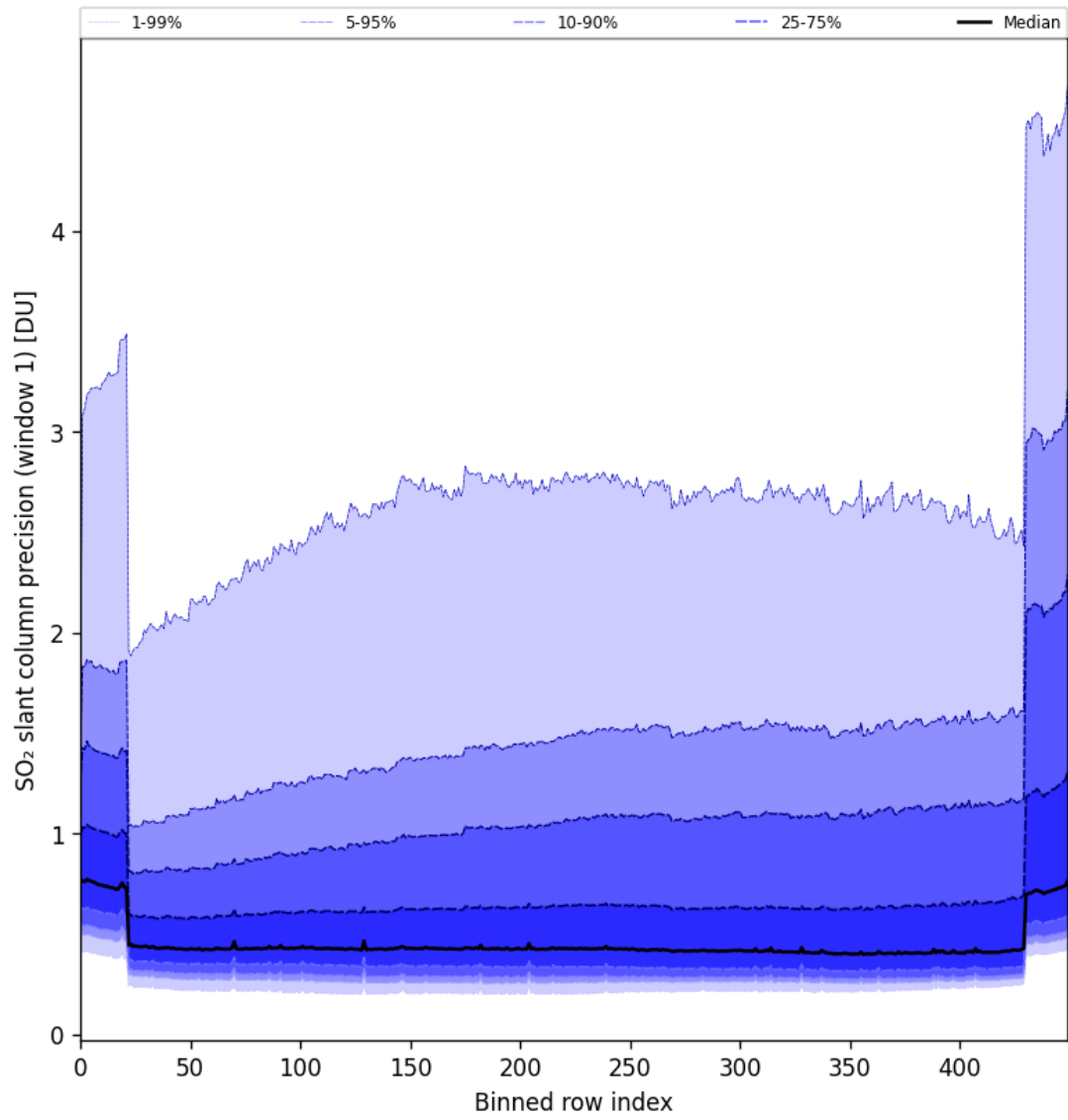
Figure 80: Along track statistics of “SO 2 slant column precision (window 1)” for 2024-09-24 to 2024-09-26
