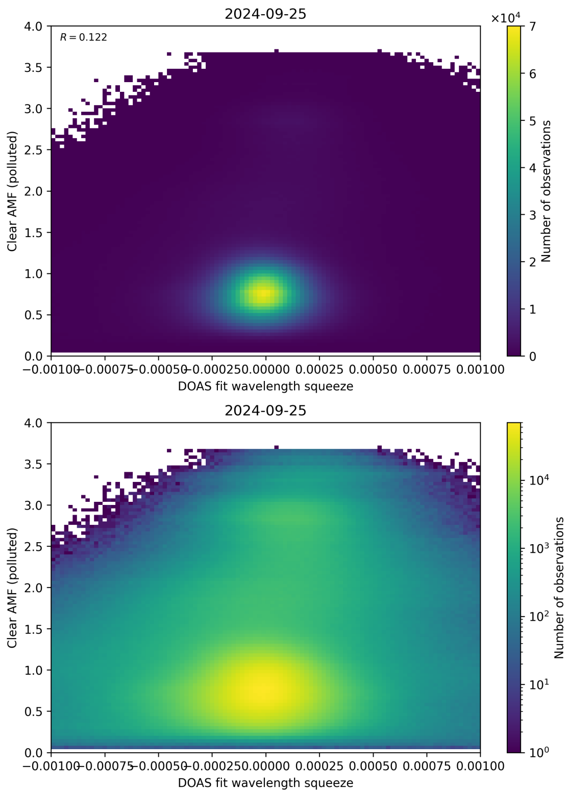
Figure 133: Scatter density plot of “DOAS fit wavelength squeeze” against “Clear AMF (polluted)” for 2024-09-24 to 2024-09-26.
