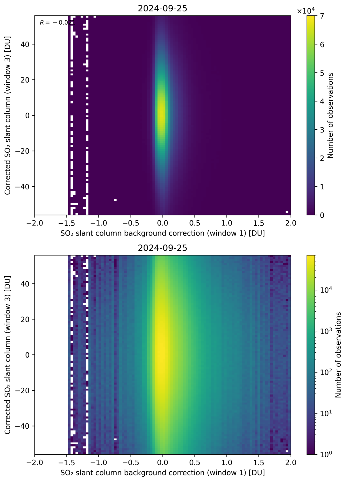
Figure 105: Scatter density plot of “SO 2 slant column background correction (window 1)” against “Corrected SO 2 slant column (window 3)” for 2024-09-24 to 2024-09-26.
