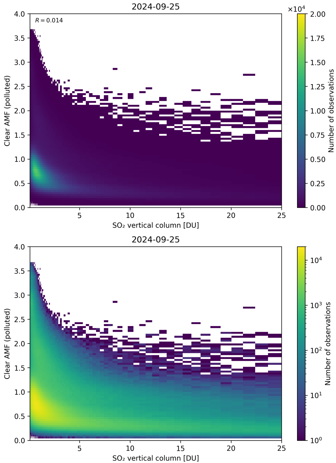
Figure 296: Scatter density plot of “SO 2 vertical column” against “Clear AMF (polluted)” for 2024-09-24 to 2024-09-26.
