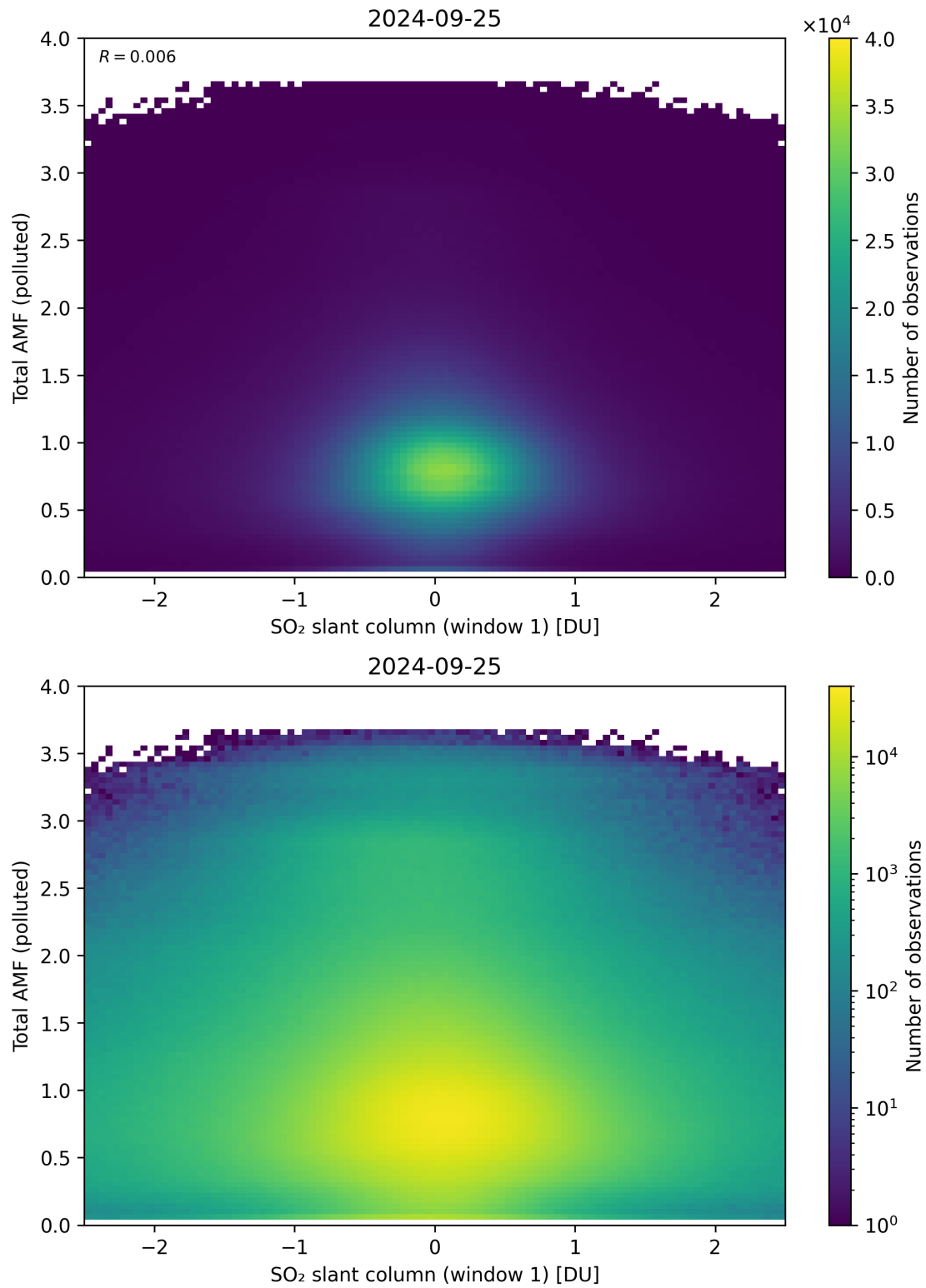
Figure 239: Scatter density plot of “SO 2 slant column (window 1)” against “Total AMF (polluted)” for 2024-09-24 to 2024-09-26.
