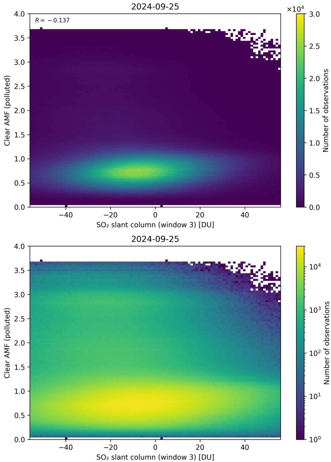
Figure 265: Scatter density plot of “SO 2 slant column (window 3)” against “Clear AMF (polluted)” for 2024-09-24 to 2024-09-26.
