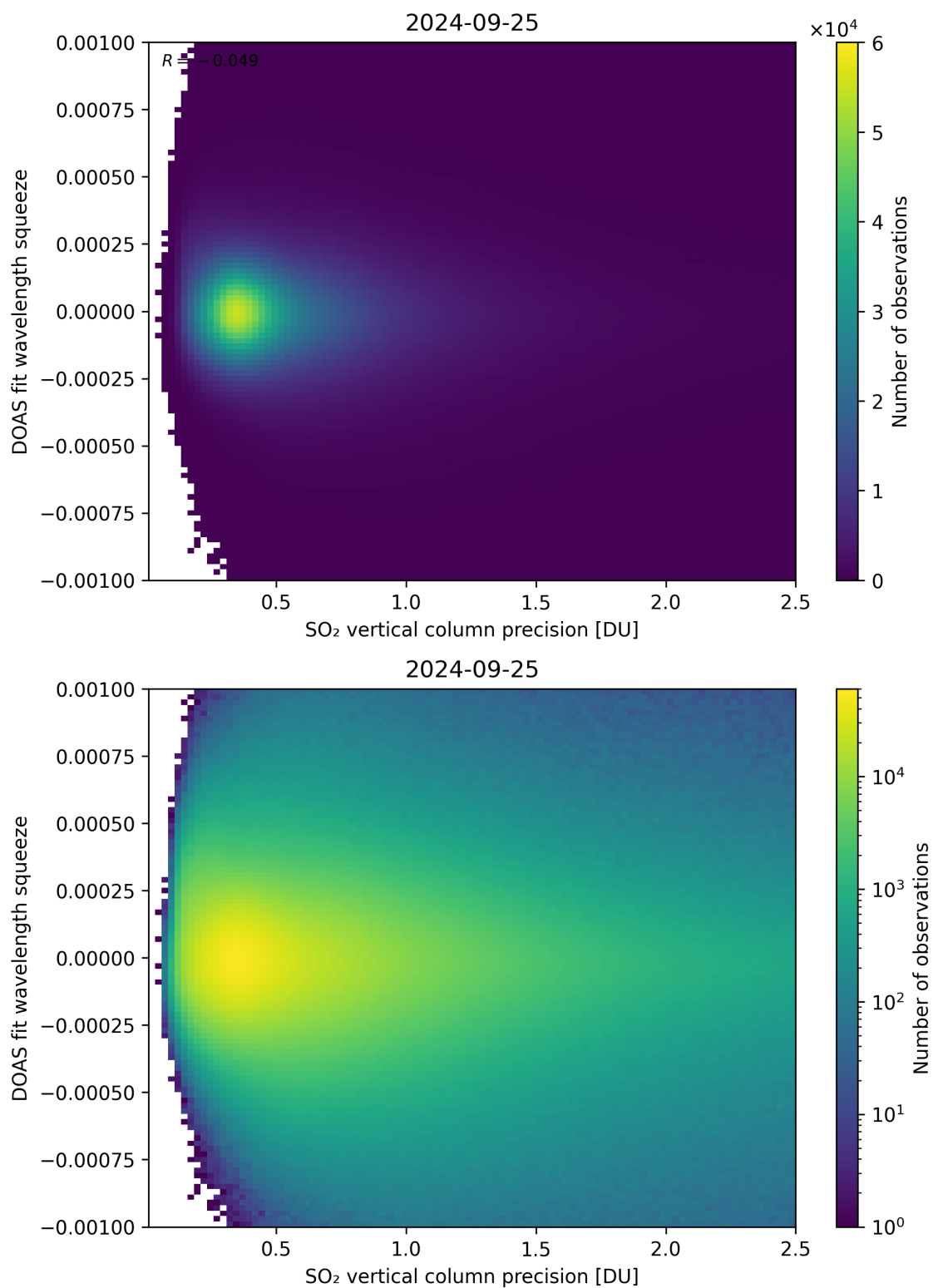
Figure 283: Scatter density plot of “SO 2 vertical column precision” against “DOAS fit wavelength squeeze” for 2024-09-24 to 2024-09-26.
