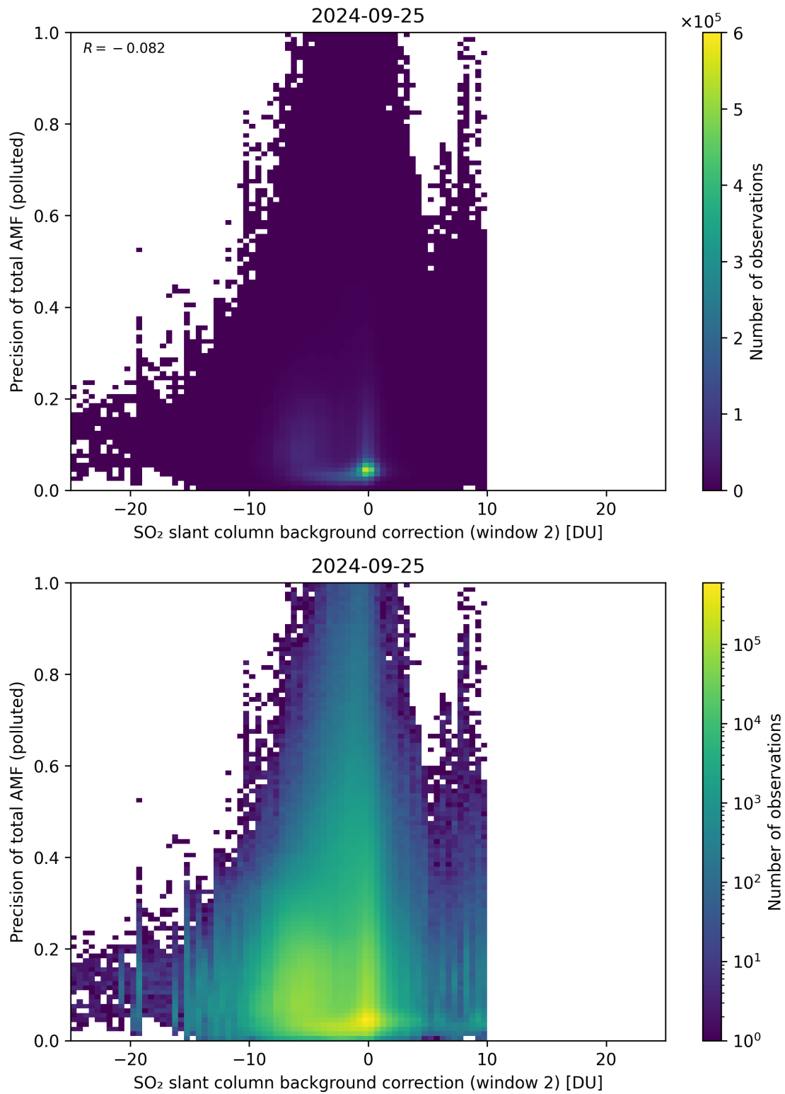
Figure 120: Scatter density plot of “SO 2 slant column background correction (window 2)” against “Precision of total AMF (polluted)” for 2024-09-24 to 2024-09-26.
