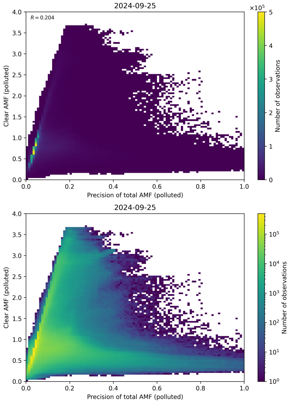
Figure 270: Scatter density plot of “Precision of total AMF (polluted)” against “Clear AMF (polluted)” for 2024-09-24 to 2024-09-26.
