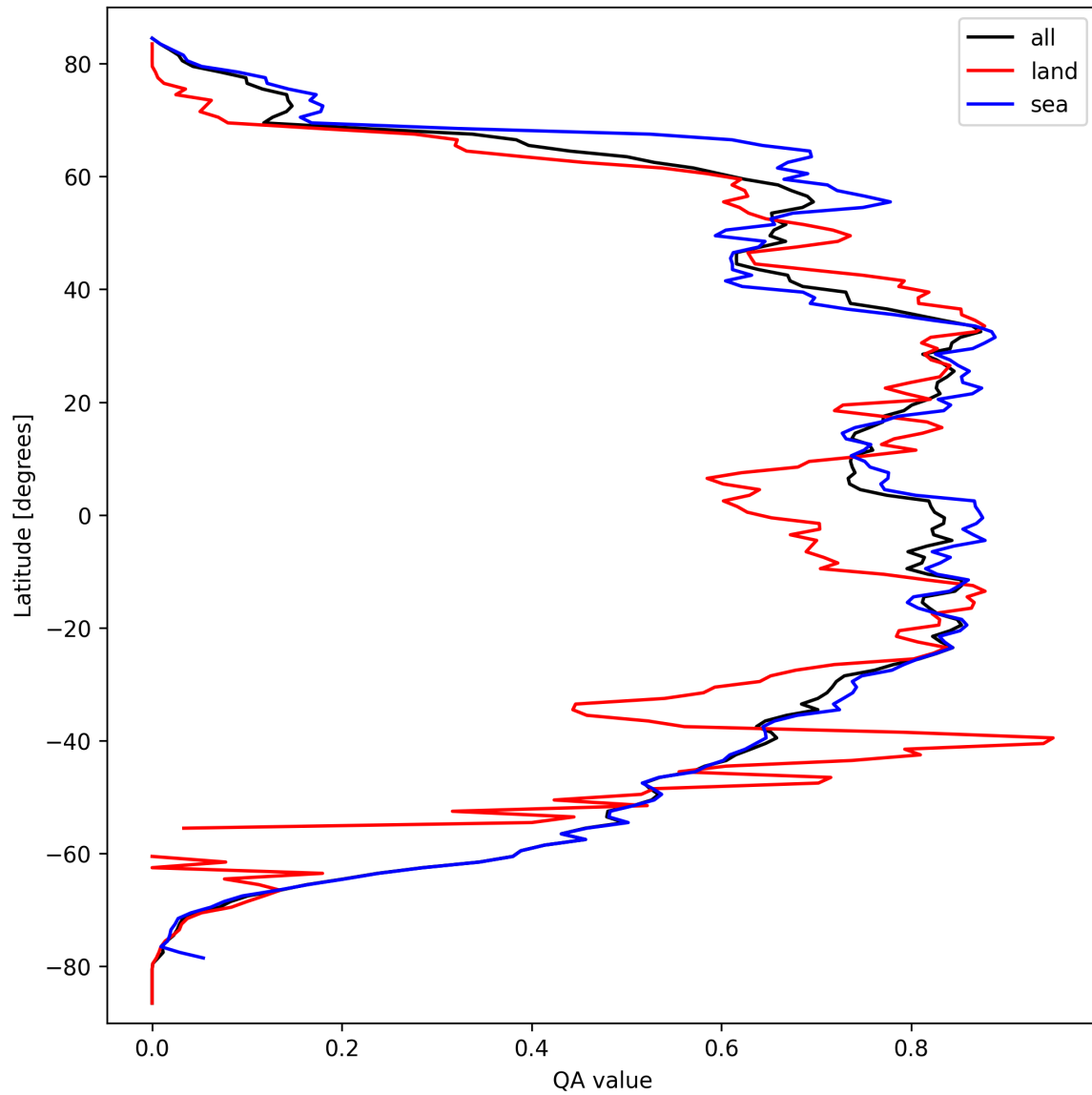
Figure 29: Zonal average of “QA value” for 2024-09-24 to 2024-09-26.
