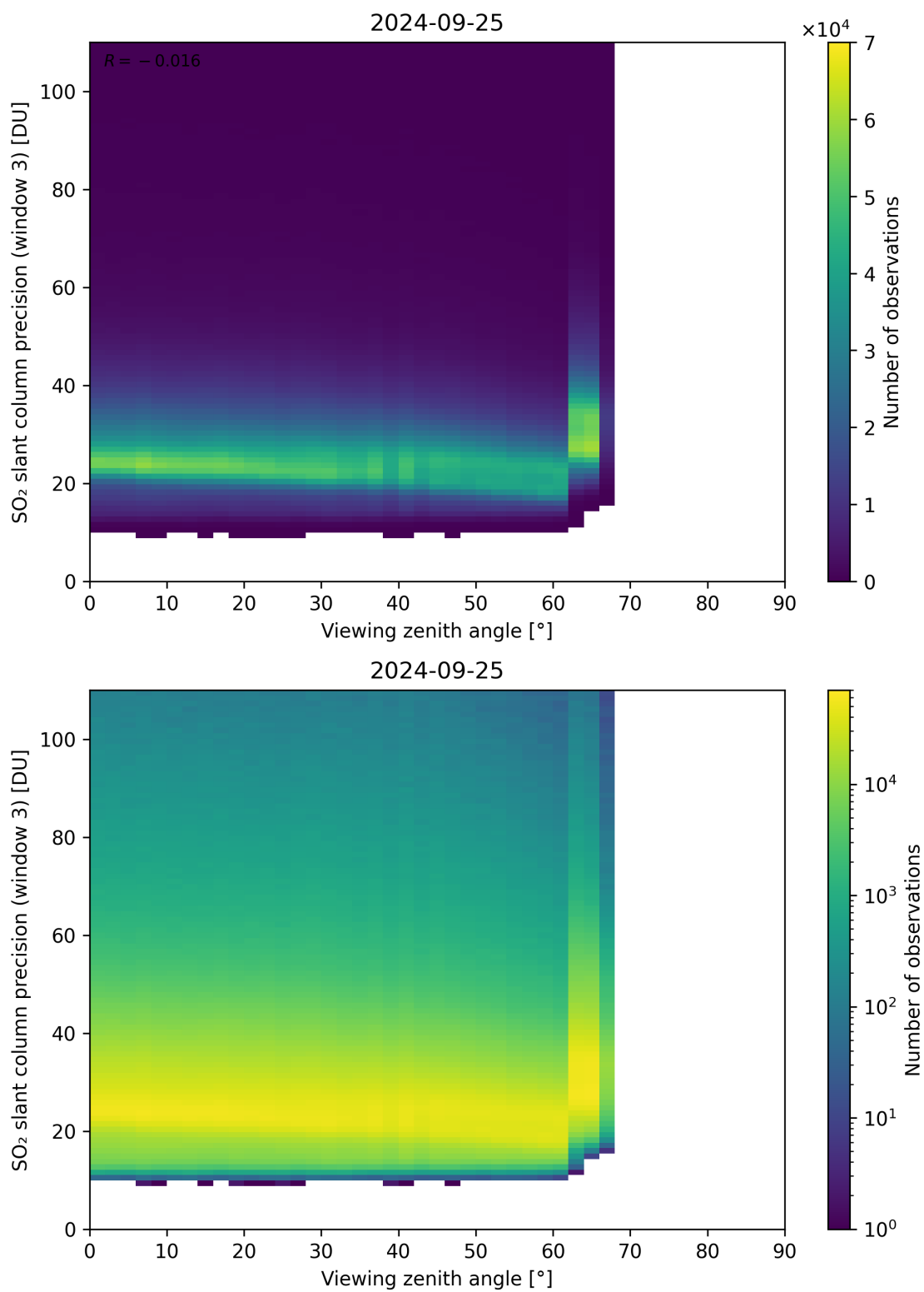
Figure 324: Scatter density plot of “Viewing zenith angle” against “SO 2 slant column precision (window 3)” for 2024-09-24 to 2024-09-26.
