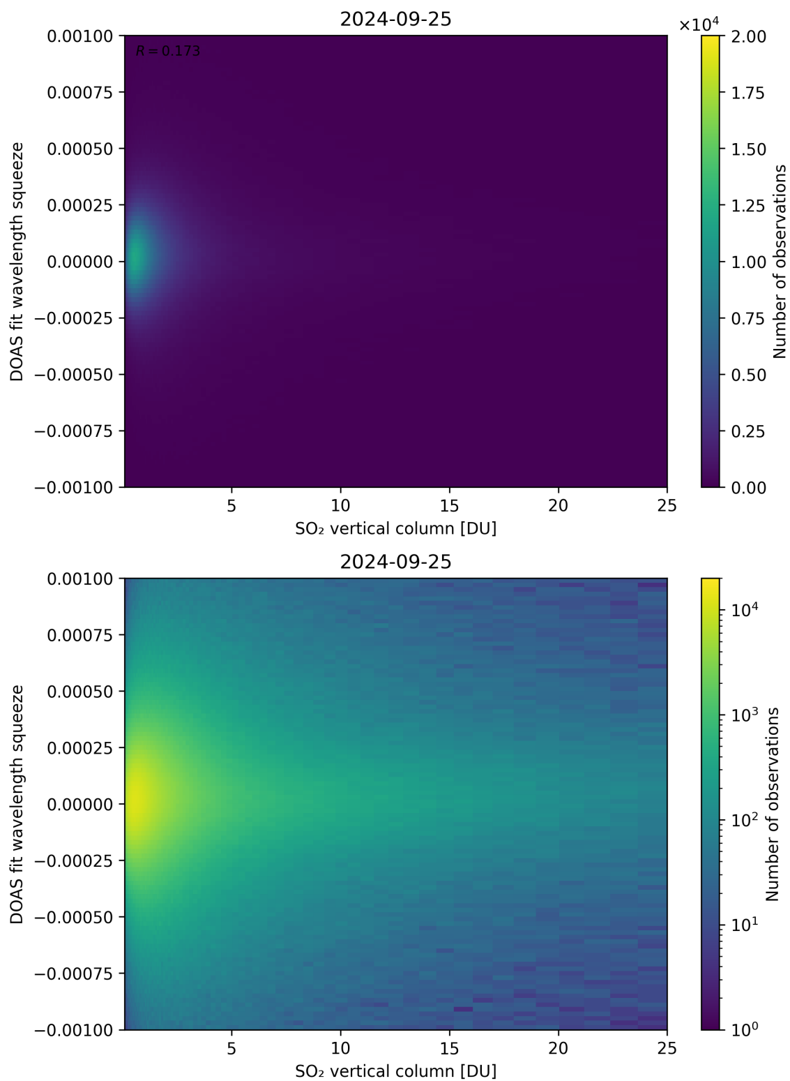
Figure 277: Scatter density plot of “SO 2 vertical column” against “DOAS fit wavelength squeeze” for 2024-09-24 to 2024-09-26.
