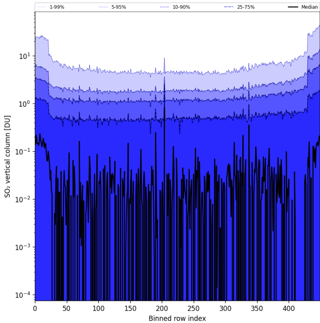
Figure 76: Along track statistics of “SO 2 vertical column” for 2024-09-24 to 2024-09-26
