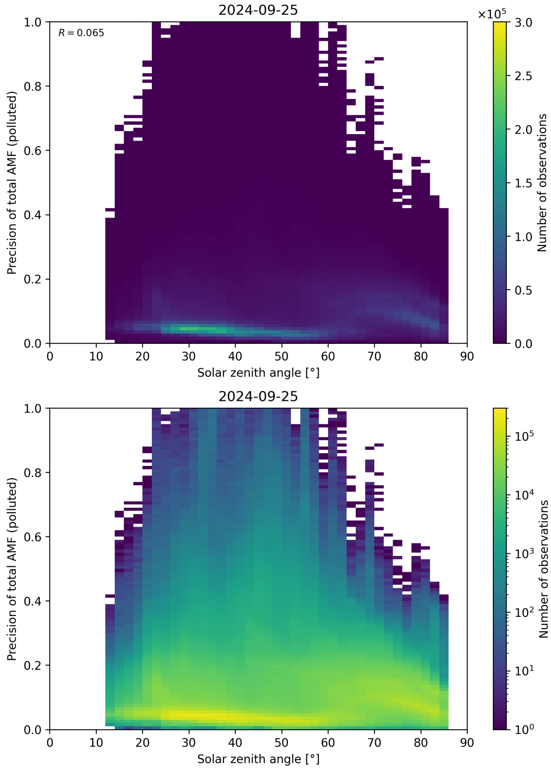
Figure 175: Scatter density plot of “Solar zenith angle” against “Precision of total AMF (polluted)” for 2024-09-24 to 2024-09-26.
