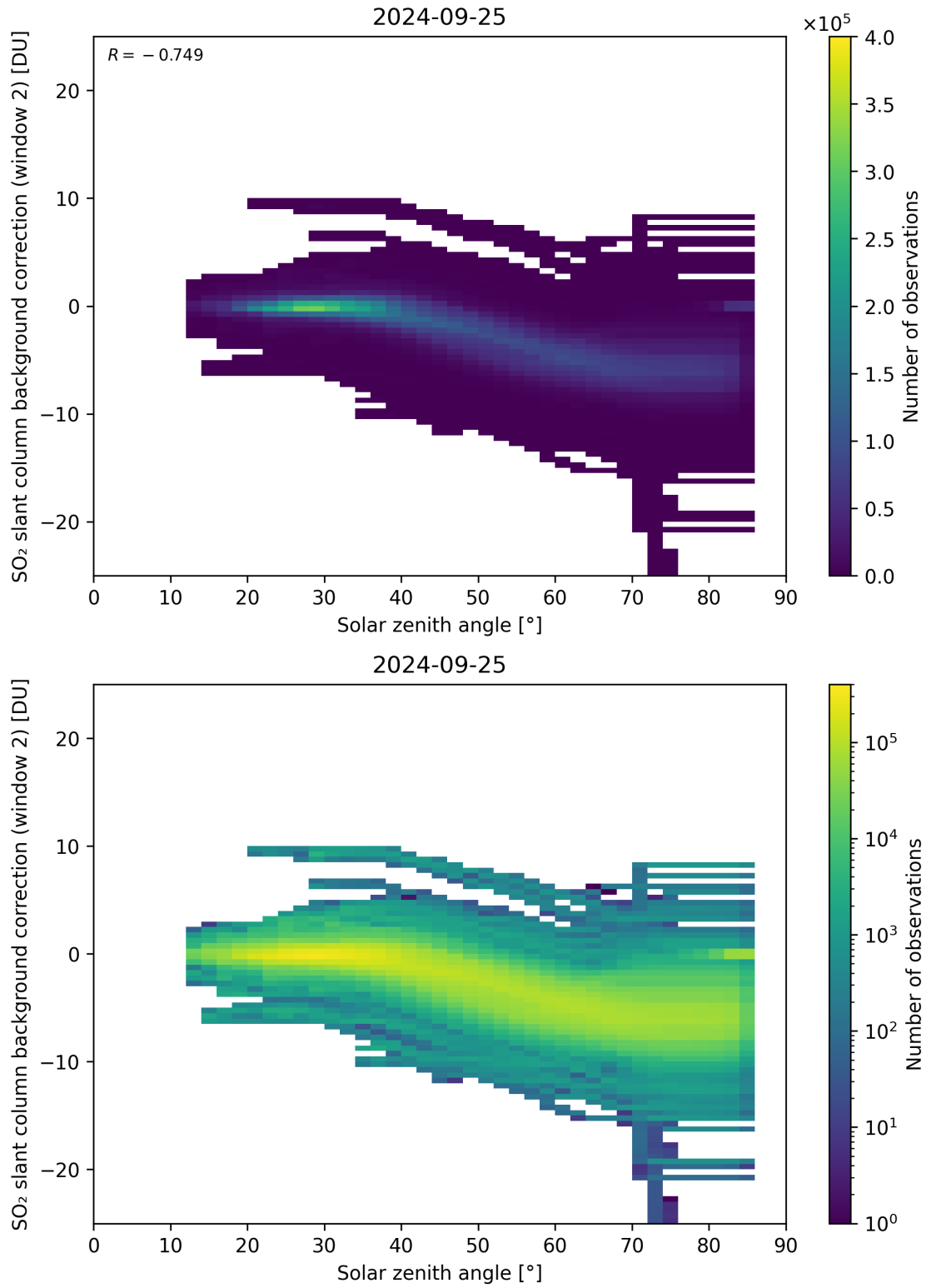
Figure 159: Scatter density plot of “Solar zenith angle” against “SO 2 slant column background correction (window 2)” for 2024-09-24 to 2024-09-26.
