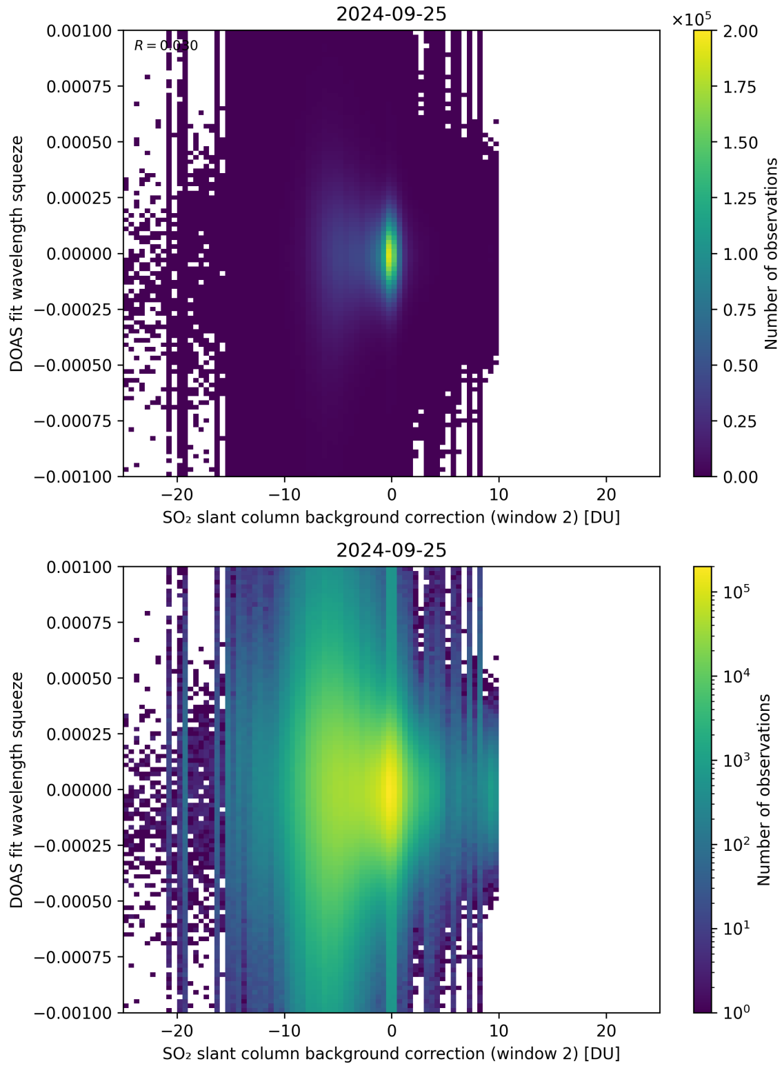
Figure 113: Scatter density plot of “SO 2 slant column background correction (window 2)” against “DOAS fit wavelength squeeze” for 2024-09-24 to 2024-09-26.
