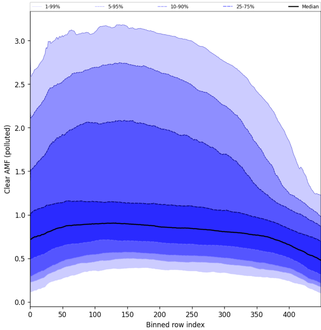
Figure 96: Along track statistics of “Clear AMF (polluted)” for 2024-09-24 to 2024-09-26
