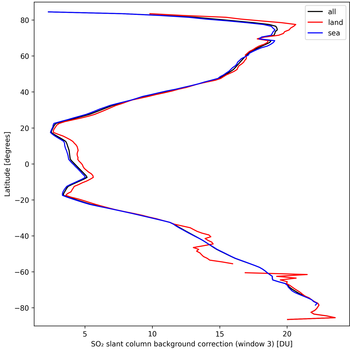
Figure 44: Zonal average of “SO 2 slant column background correction (window 3)” for 2024-09-24 to 2024-09-26.
