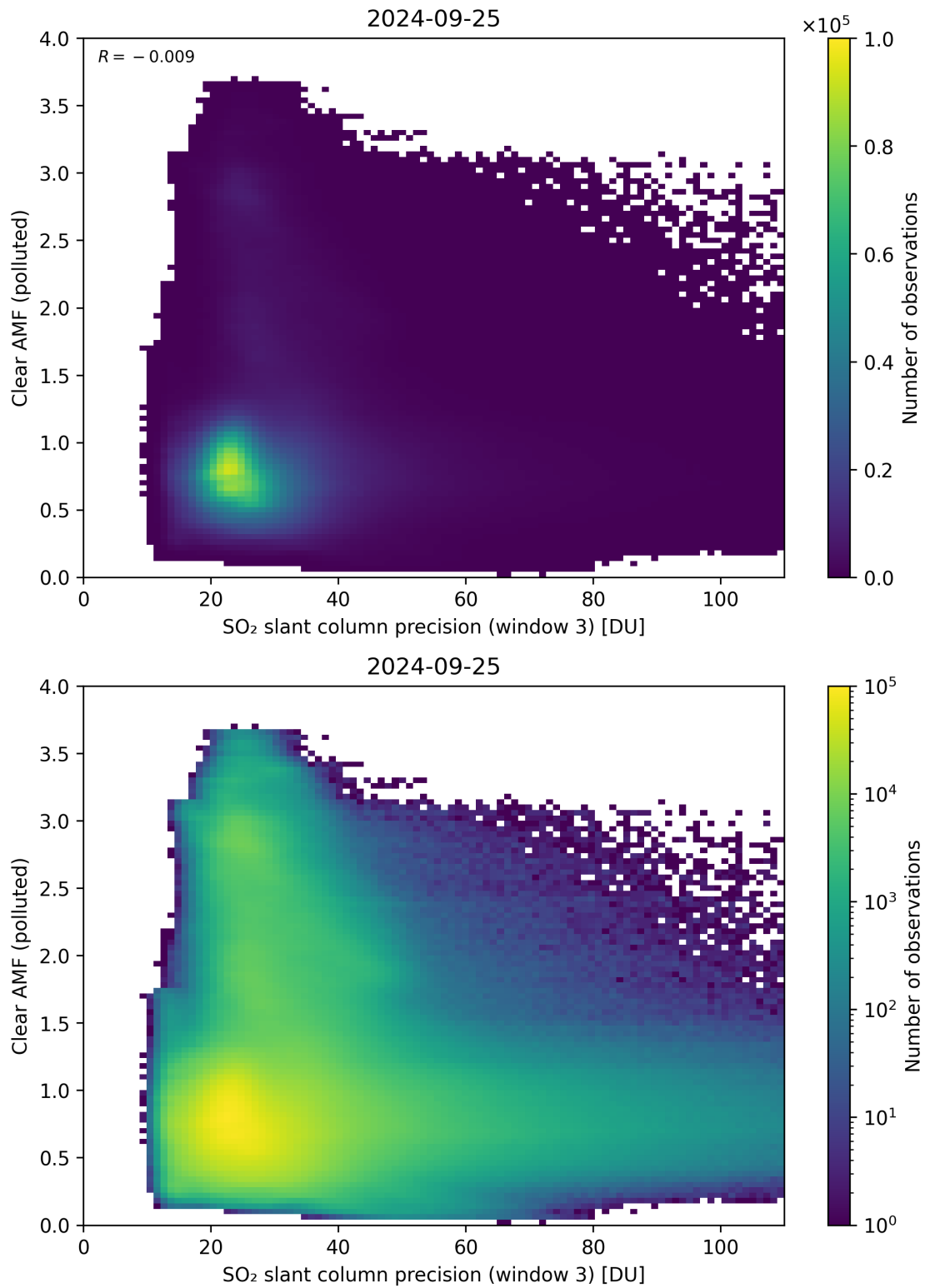
Figure 261: Scatter density plot of “SO 2 slant column precision (window 3)” against “Clear AMF (polluted)” for 2024-09-24 to 2024-09-26.
