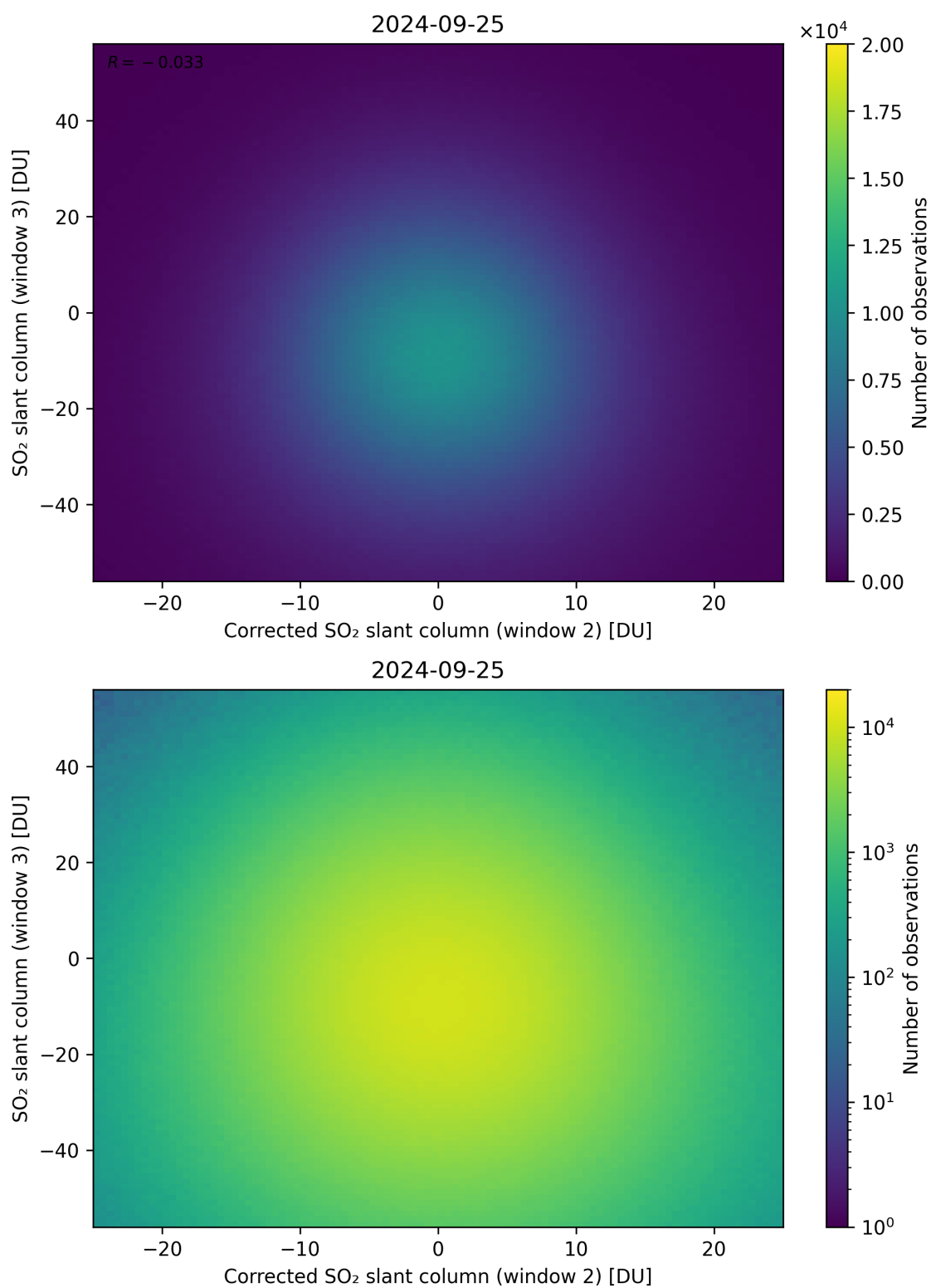
Figure 201: Scatter density plot of “Corrected SO 2 slant column (window 2)” against “SO 2 slant column (window 3)” for 2024-09-24 to 2024-09-26.
