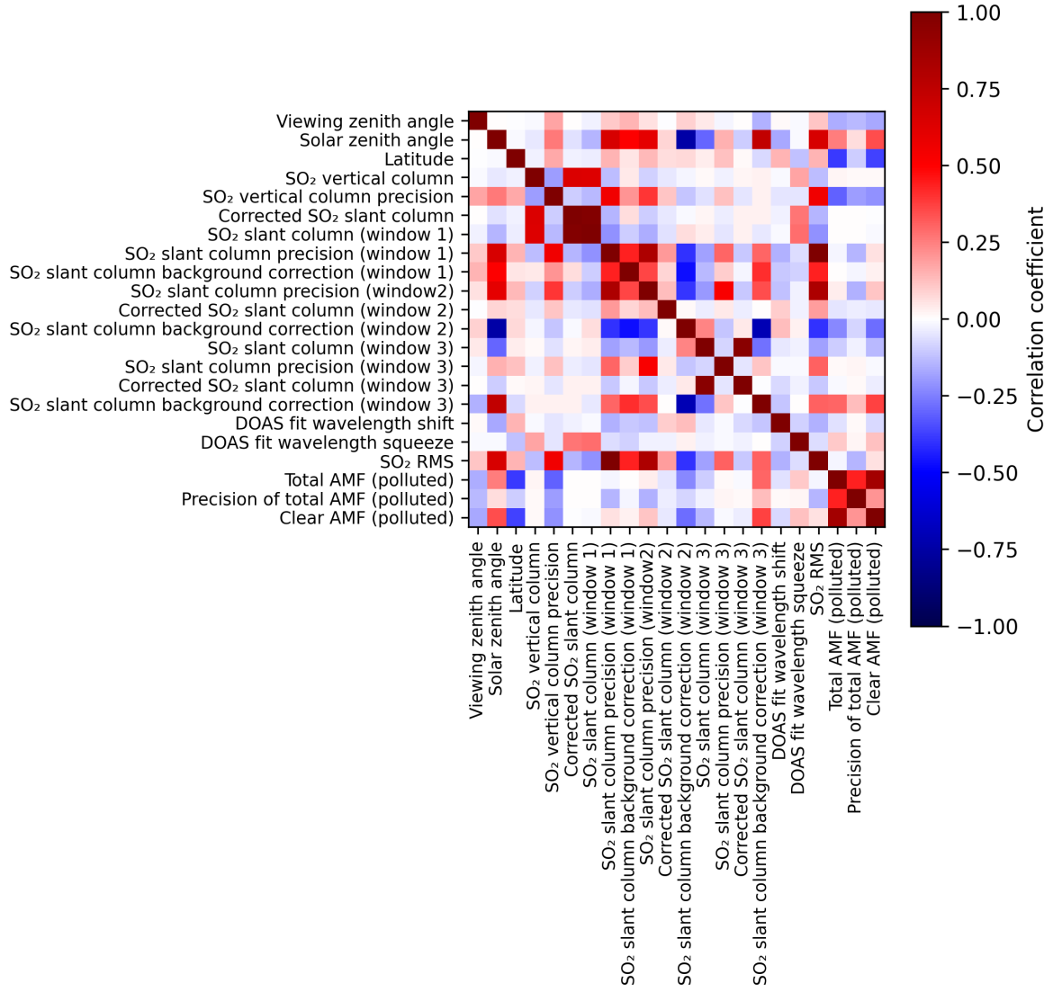
Figure 2: Map of correlation matrix for 2024-09-24 to 2024-09-26.
