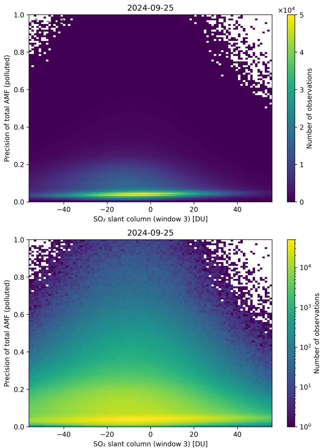
Figure 269: Scatter density plot of “SO 2 slant column (window 3)” against “Precision of total AMF (polluted)” for 2024-09-24 to 2024-09-26.
