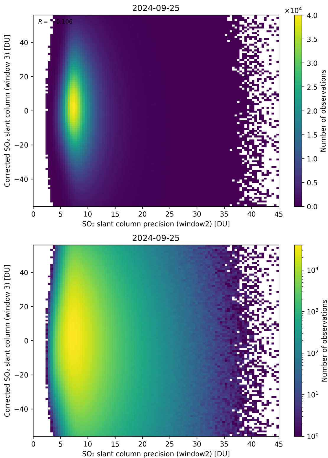
Figure 248: Scatter density plot of “SO 2 slant column precision (window2)” against “Corrected SO 2 slant column (window 3)” for 2024-09-24 to 2024-09-26.
