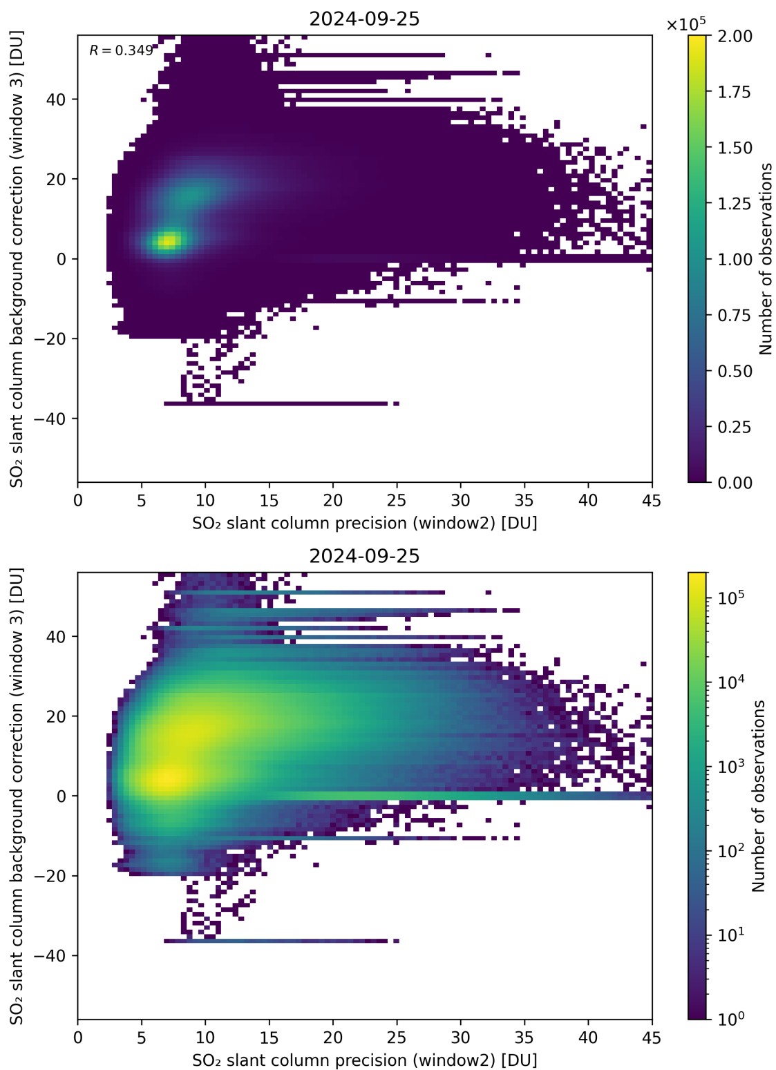
Figure 242: Scatter density plot of “SO 2 slant column precision (window2)” against “SO 2 slant column background correction (window 3)” for 2024-09-24 to 2024-09-26.
