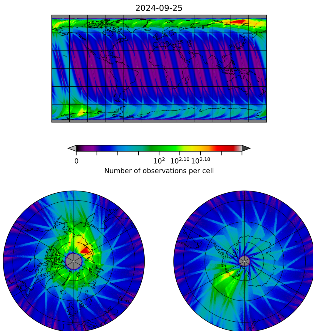
Figure 28: Map of the number of observations for 2024-09-24 to 2024-09-26
