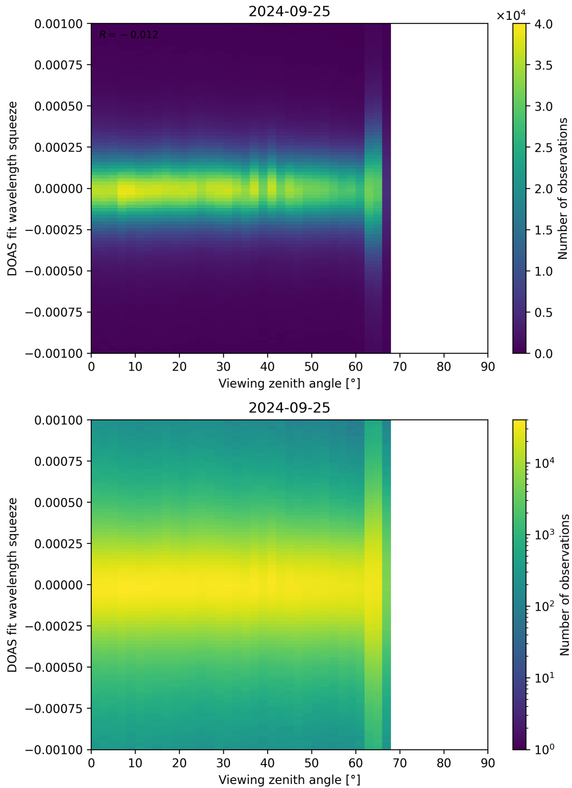
Figure 312: Scatter density plot of “Viewing zenith angle” against “DOAS fit wavelength squeeze” for 2024-09-24 to 2024-09-26.
