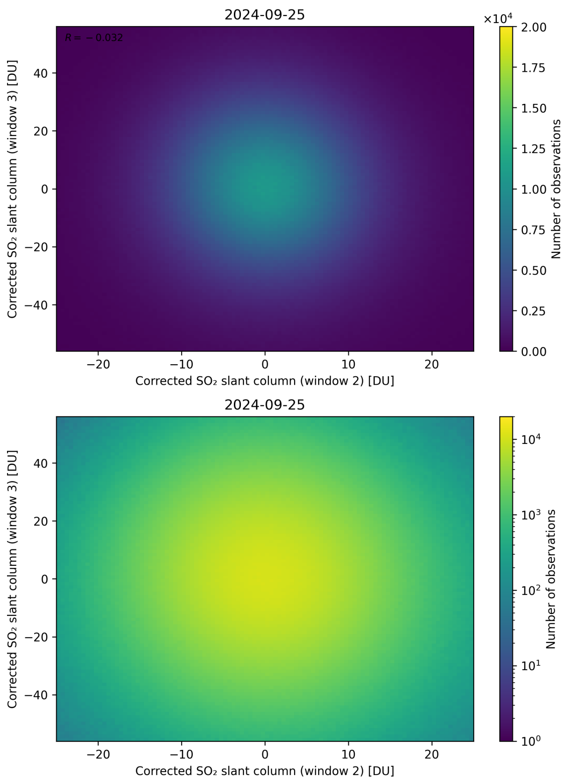
Figure 200: Scatter density plot of “Corrected SO 2 slant column (window 2)” against “Corrected SO 2 slant column (window 3)” for 2024-09-24 to 2024-09-26.
