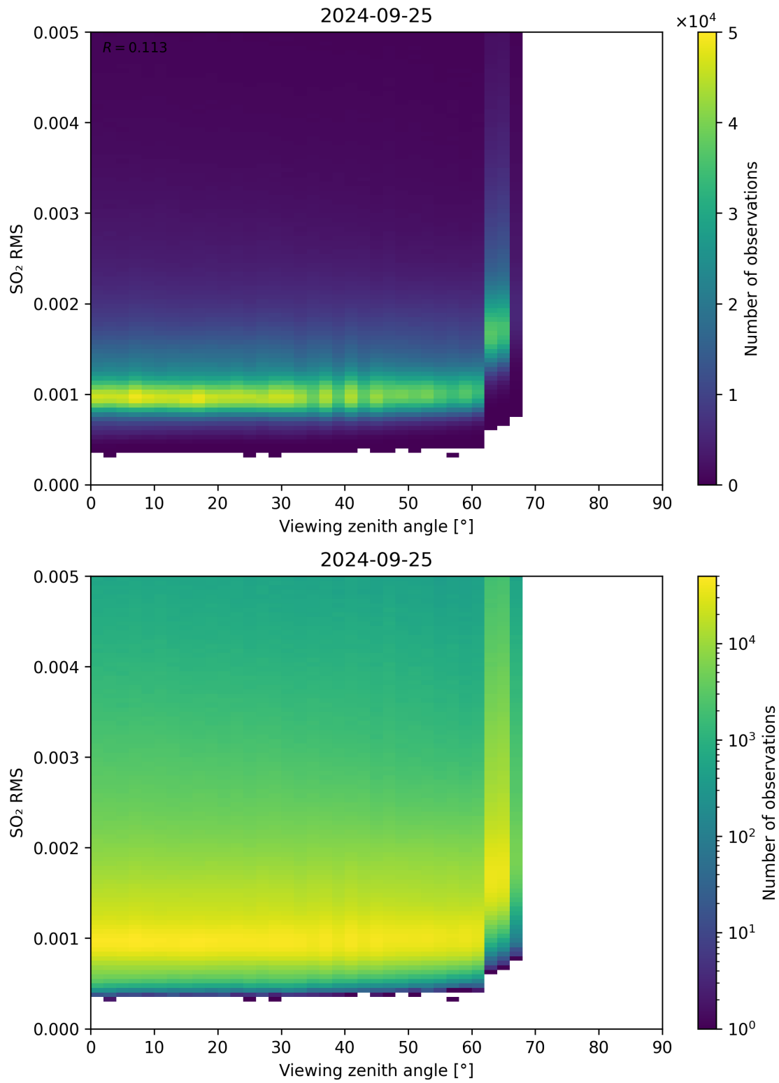
Figure 313: Scatter density plot of “Viewing zenith angle” against “SO 2 RMS” for 2024-09-24 to 2024-09-26.
