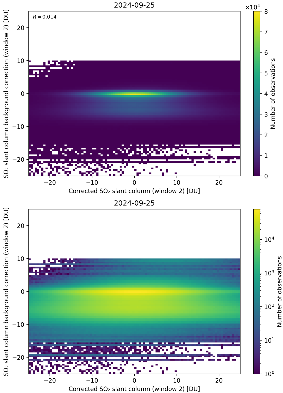
Figure 194: Scatter density plot of “Corrected SO 2 slant column (window 2)” against “SO 2 slant column background correction (window 2)” for 2024-09-24 to 2024-09-26.
