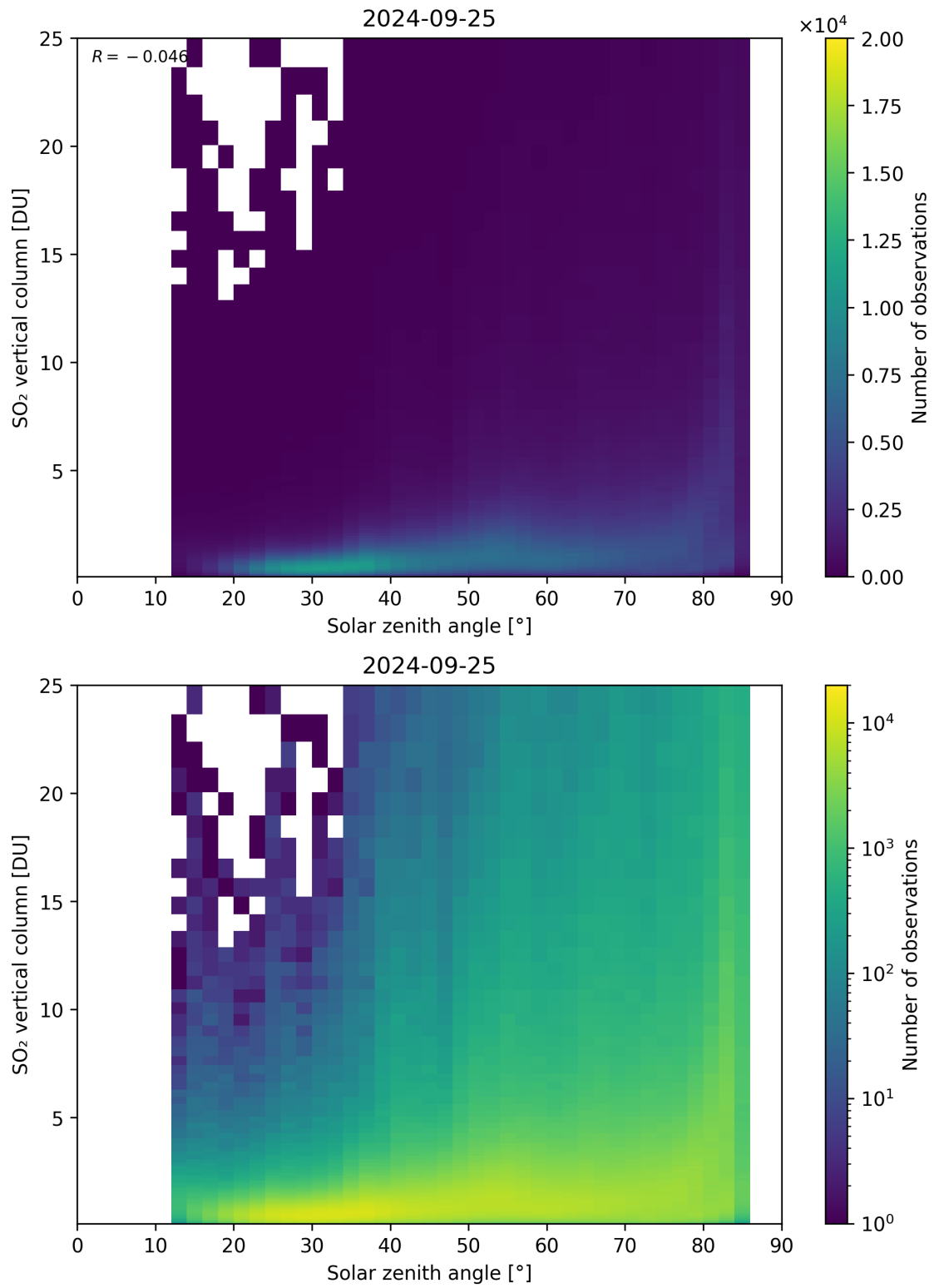
Figure 176: Scatter density plot of “Solar zenith angle” against “SO 2 vertical column” for 2024-09-24 to 2024-09-26.
