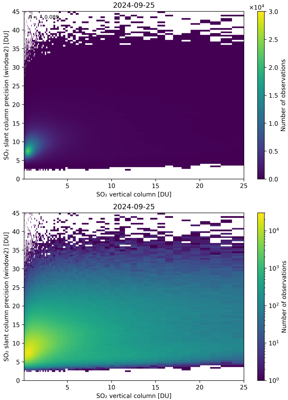
Figure 302: Scatter density plot of “SO 2 vertical column” against “SO 2 slant column precision (window2)” for 2024-09-24 to 2024-09-26.
