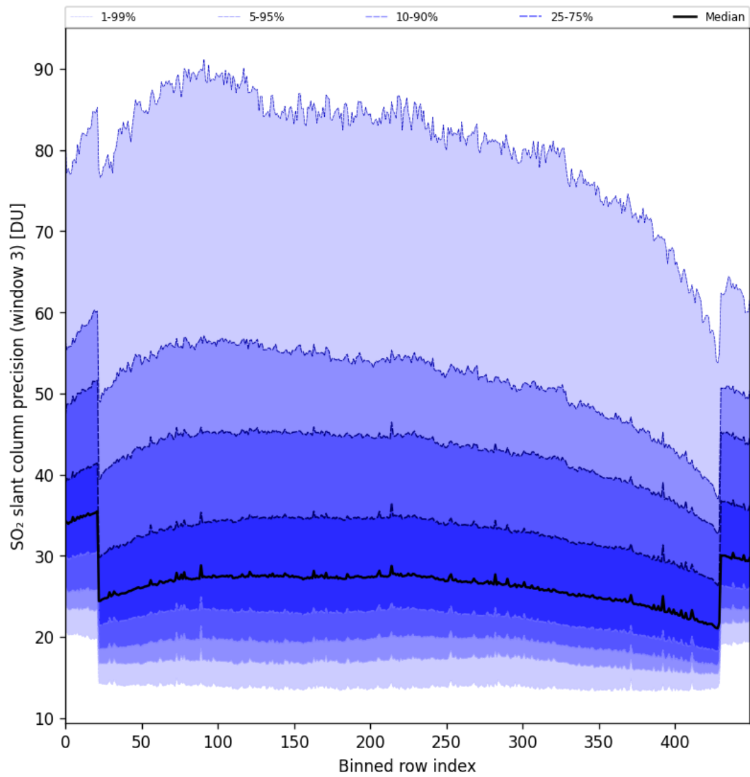
Figure 88: Along track statistics of “SO 2 slant column precision (window 3)” for 2024-09-24 to 2024-09-26
