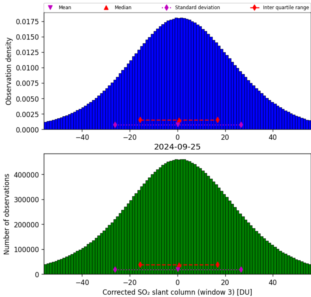
Figure 66: Histogram of “Corrected SO 2 slant column (window 3)” for 2024-09-24 to 2024-09-26
