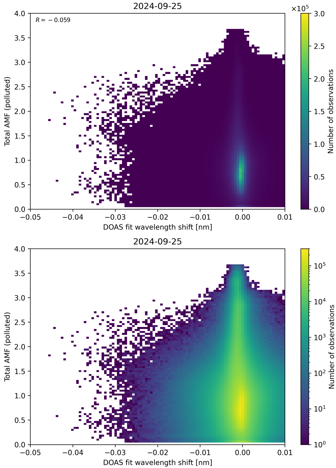
Figure 130: Scatter density plot of “DOAS fit wavelength shift” against “Total AMF (polluted)” for 2024-09-24 to 2024-09-26.
