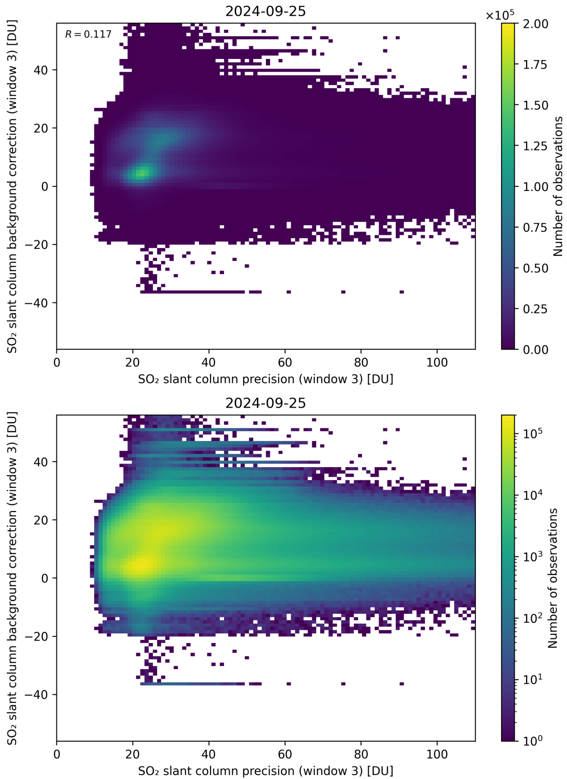
Figure 257: Scatter density plot of “SO 2 slant column precision (window 3)” against “SO 2 slant column background correction (window 3)” for 2024-09-24 to 2024-09-26.
