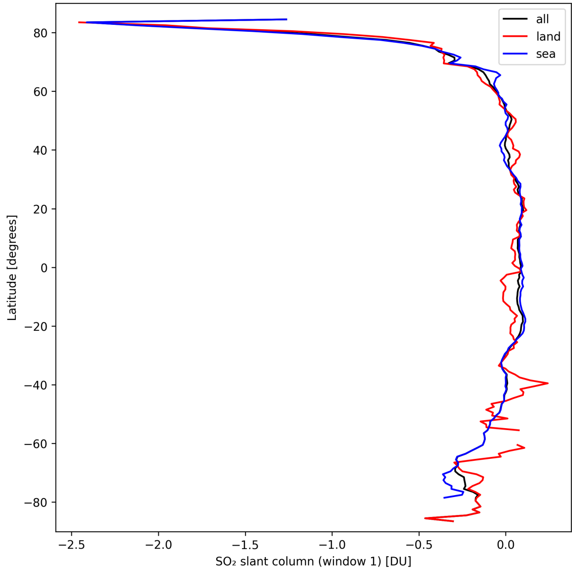
Figure 33: Zonal average of “SO 2 slant column (window 1)” for 2024-09-24 to 2024-09-26.
