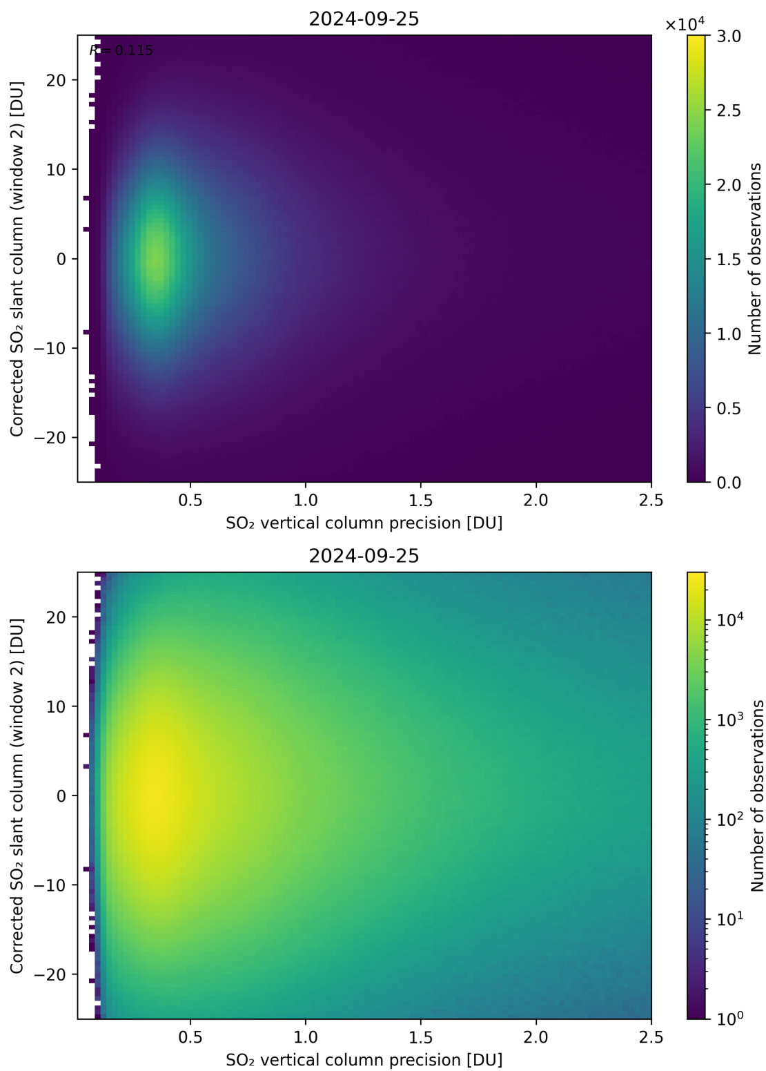
Figure 287: Scatter density plot of “SO 2 vertical column precision” against “Corrected SO 2 slant column (window 2)” for 2024-09-24 to 2024-09-26.
