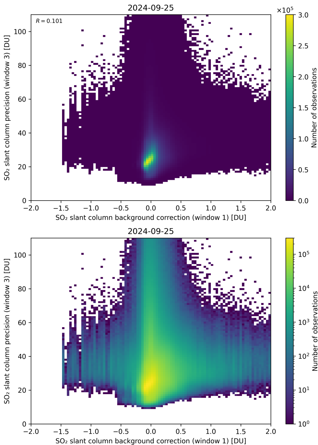
Figure 108: Scatter density plot of “SO 2 slant column background correction (window 1)” against “SO 2 slant column precision (window 3)” for 2024-09-24 to 2024-09-26.
