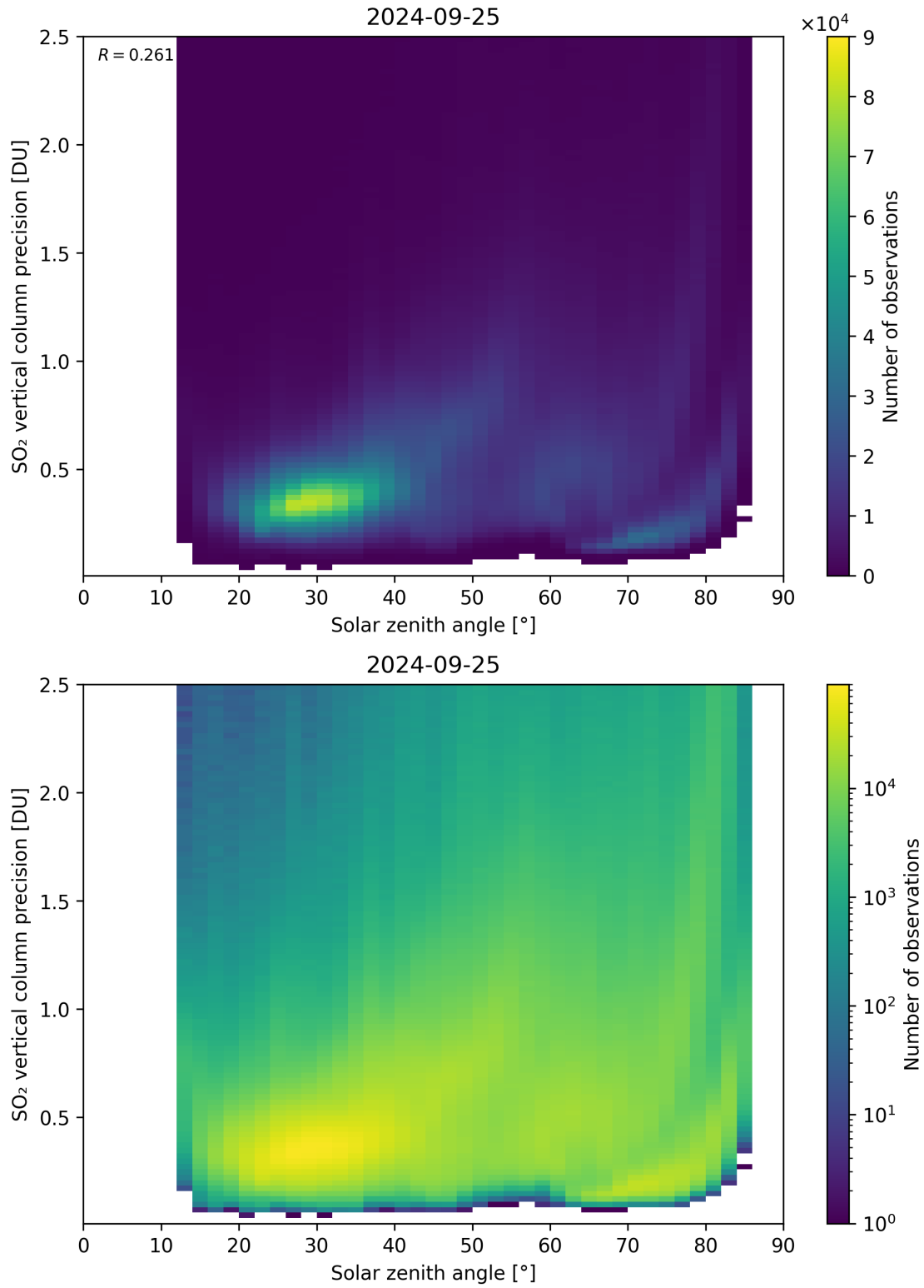
Figure 177: Scatter density plot of “Solar zenith angle” against “SO 2 vertical column precision” for 2024-09-24 to 2024-09-26.
