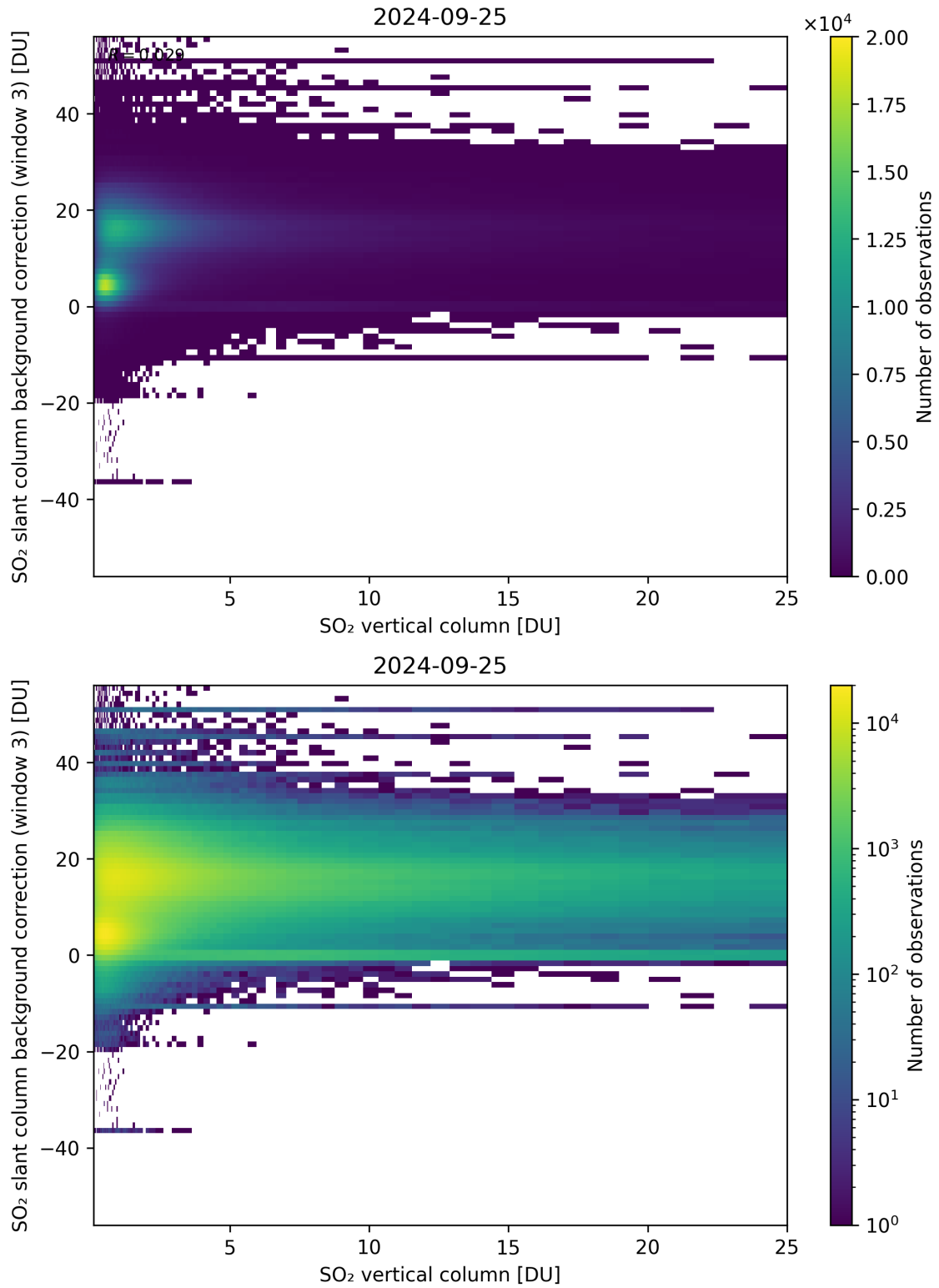
Figure 275: Scatter density plot of “SO 2 vertical column” against “SO 2 slant column background correction (window 3)” for 2024-09-24 to 2024-09-26.
