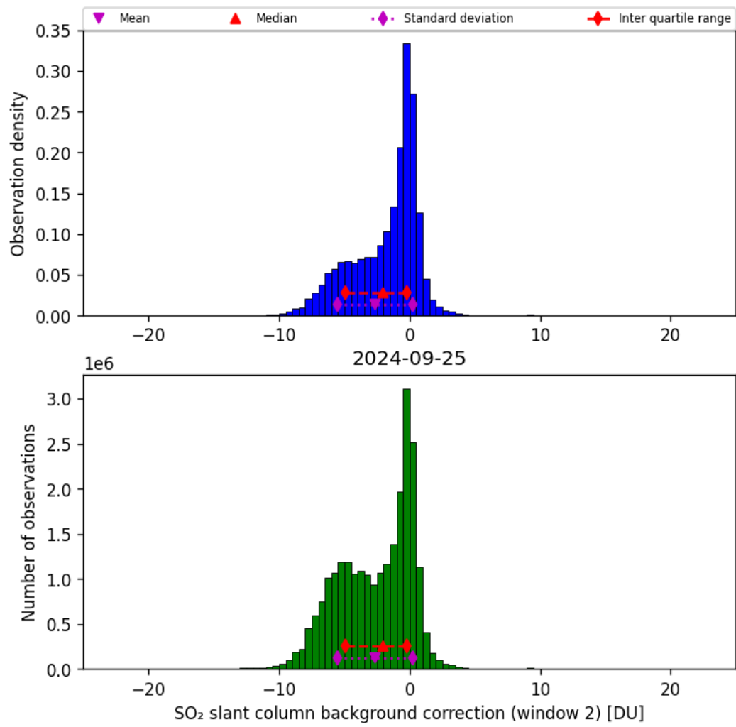
Figure 63: Histogram of “SO 2 slant column background correction (window 2)” for 2024-09-24 to 2024-09-26
