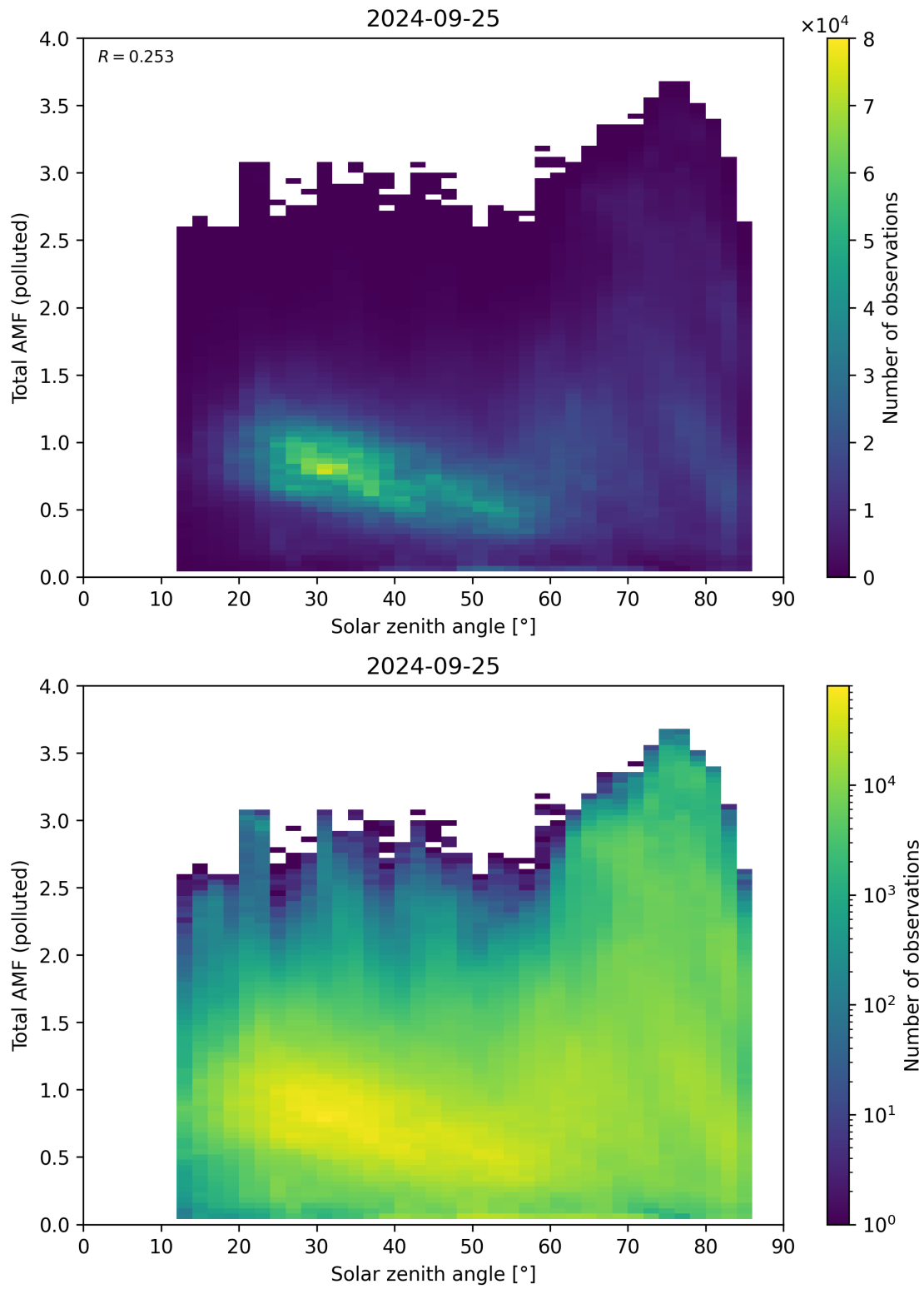
Figure 174: Scatter density plot of “Solar zenith angle” against “Total AMF (polluted)” for 2024-09-24 to 2024-09-26.
