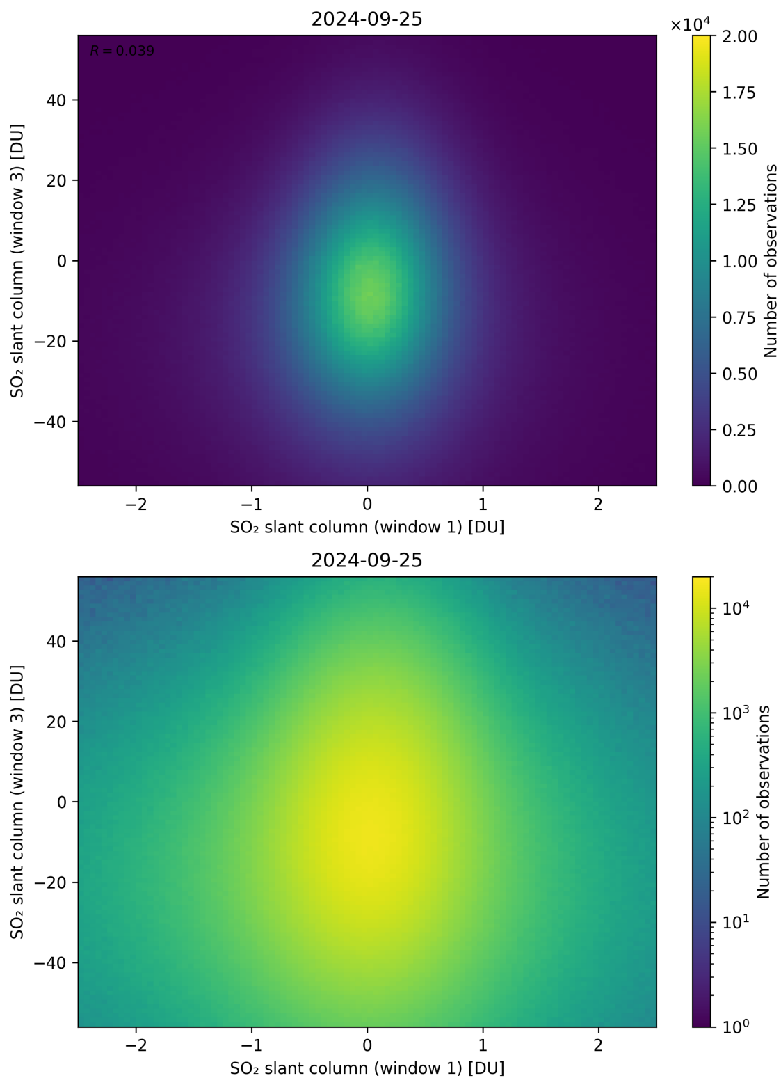
Figure 237: Scatter density plot of “SO 2 slant column (window 1)” against “SO 2 slant column (window 3)” for 2024-09-24 to 2024-09-26.
