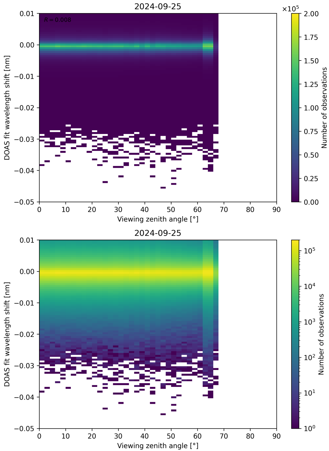
Figure 311: Scatter density plot of “Viewing zenith angle” against “DOAS fit wavelength shift” for 2024-09-24 to 2024-09-26.
