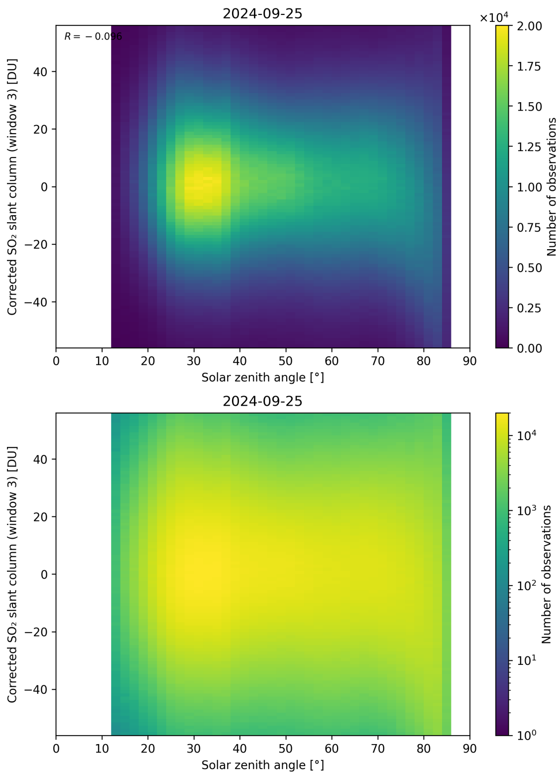
Figure 168: Scatter density plot of “Solar zenith angle” against “Corrected SO 2 slant column (window 3)” for 2024-09-24 to 2024-09-26.
