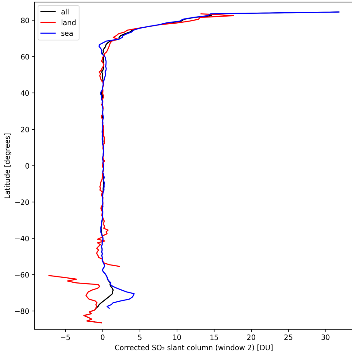
Figure 39: Zonal average of “Corrected SO 2 slant column (window 2)” for 2024-09-24 to 2024-09-26.
