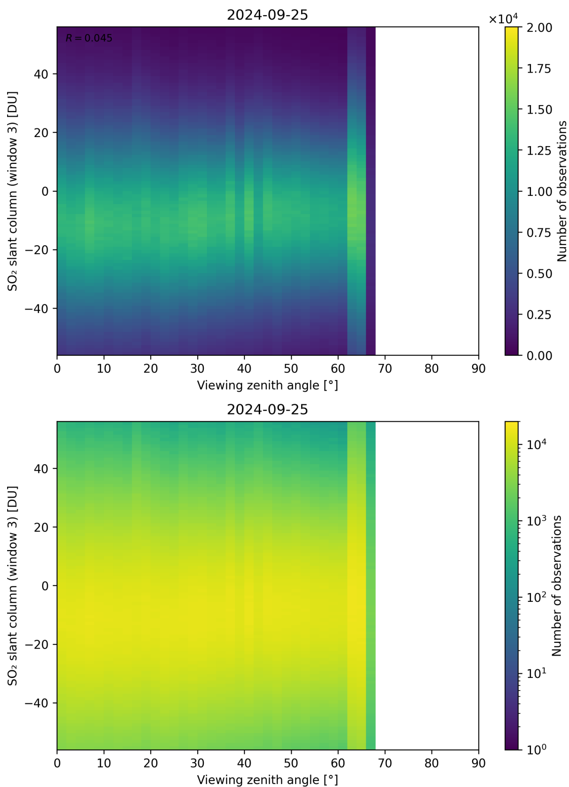
Figure 323: Scatter density plot of “Viewing zenith angle” against “SO 2 slant column (window 3)” for 2024-09-24 to 2024-09-26.
