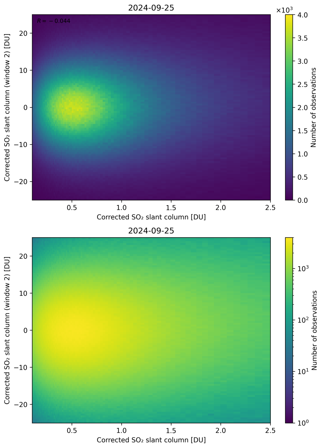
Figure 185: Scatter density plot of “Corrected SO 2 slant column” against “Corrected SO 2 slant column (window 2)” for 2024-09-24 to 2024-09-26.
