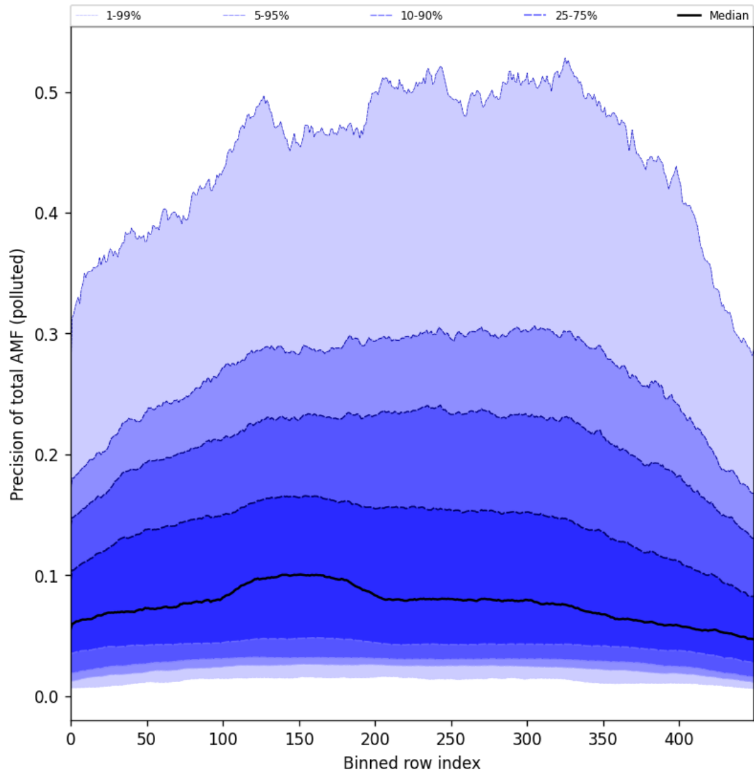
Figure 95: Along track statistics of “Precision of total AMF (polluted)” for 2024-09-24 to 2024-09-26
