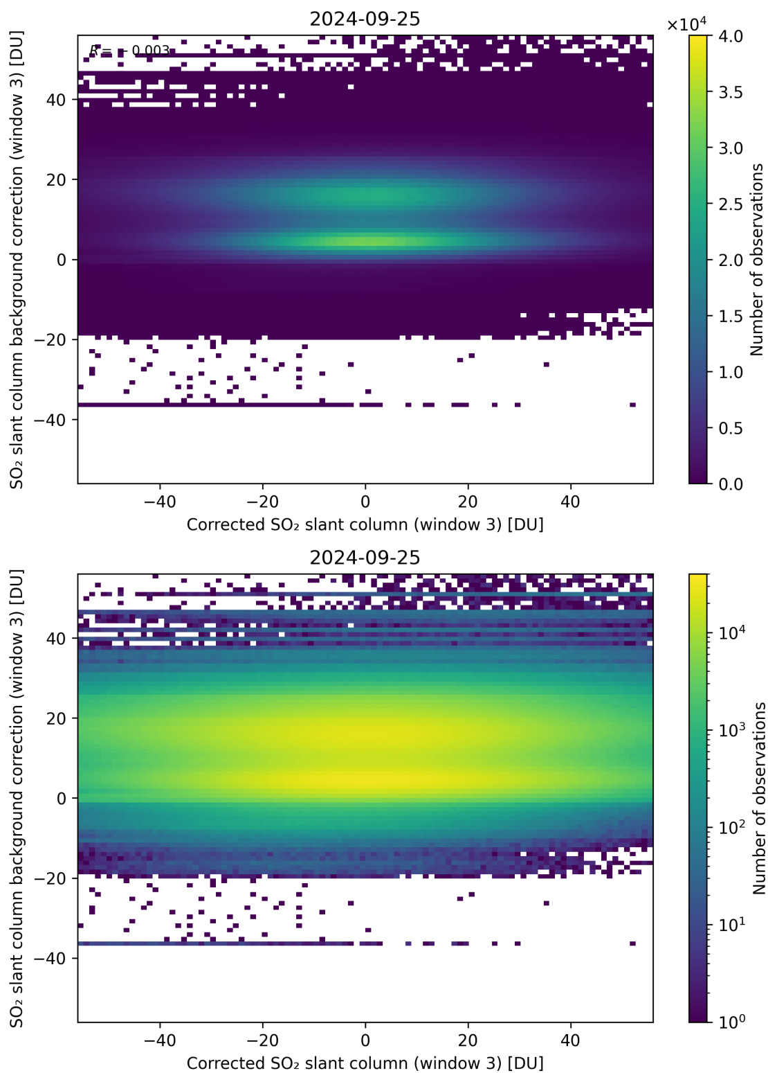
Figure 205: Scatter density plot of “Corrected SO 2 slant column (window 3)” against “SO 2 slant column background correction (window 3)” for 2024-09-24 to 2024-09-26.
