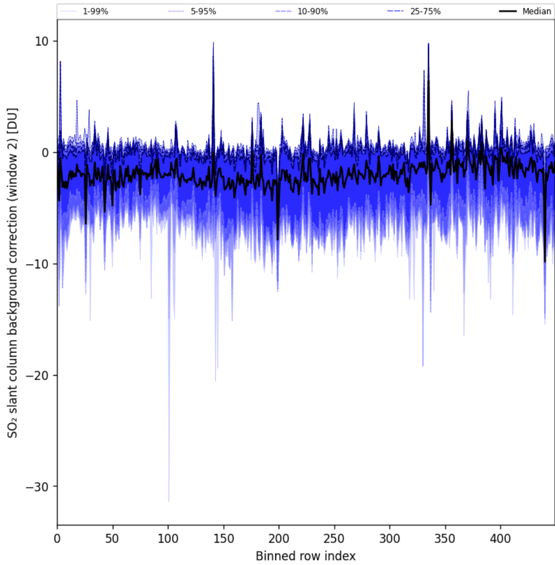
Figure 86: Along track statistics of “SO 2 slant column background correction (window 2)” for 2024-09-24 to 2024-09-26
