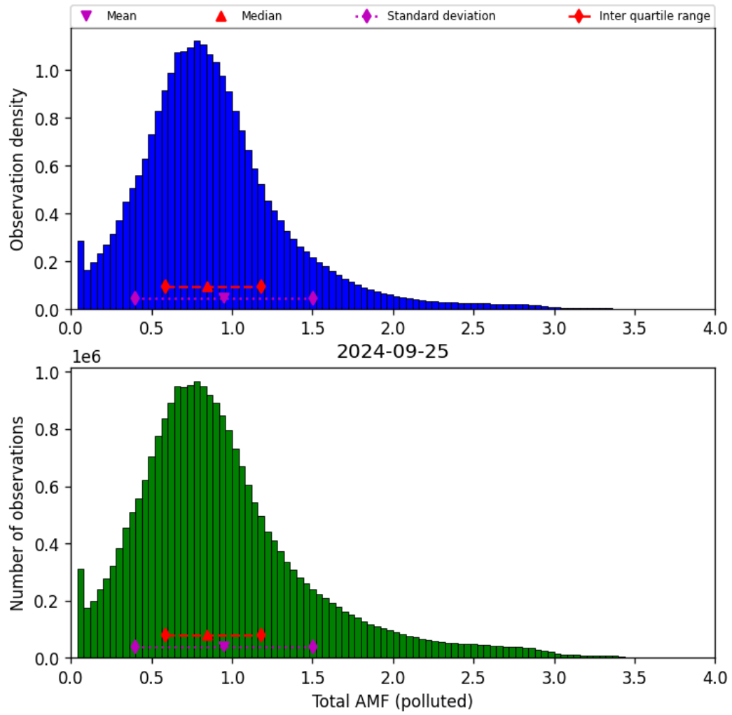
Figure 71: Histogram of “Total AMF (polluted)” for 2024-09-24 to 2024-09-26
