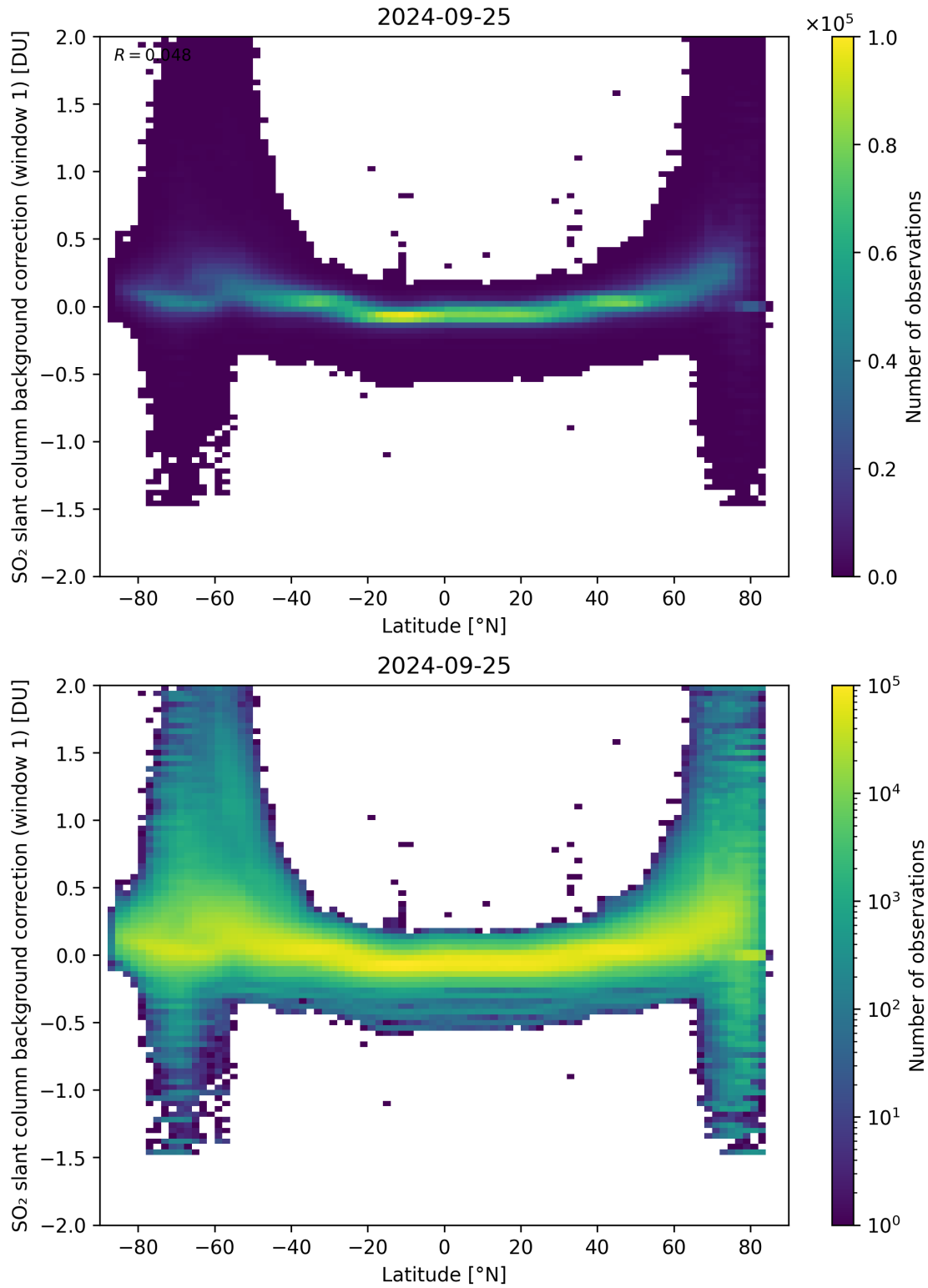
Figure 139: Scatter density plot of “Latitude” against “SO 2 slant column background correction (window 1)” for 2024-09-24 to 2024-09-26.
