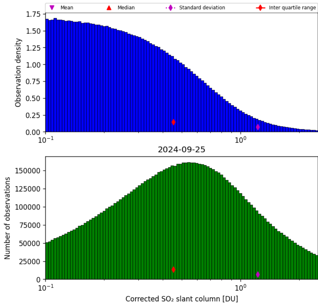
Figure 55: Histogram of “Corrected SO 2 slant column” for 2024-09-24 to 2024-09-26
