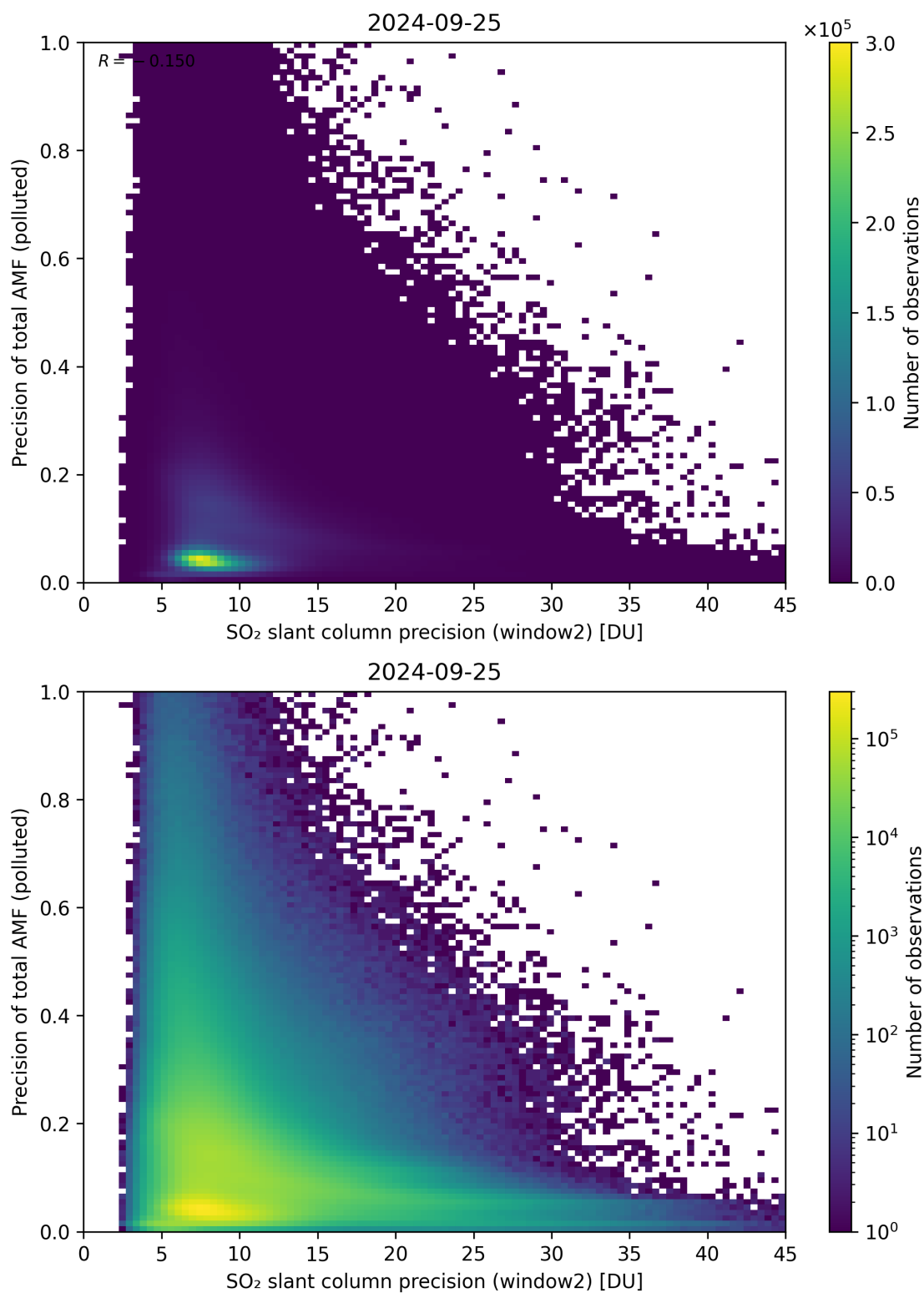
Figure 252: Scatter density plot of “SO 2 slant column precision (window2)” against “Precision of total AMF (polluted)” for 2024-09-24 to 2024-09-26.
