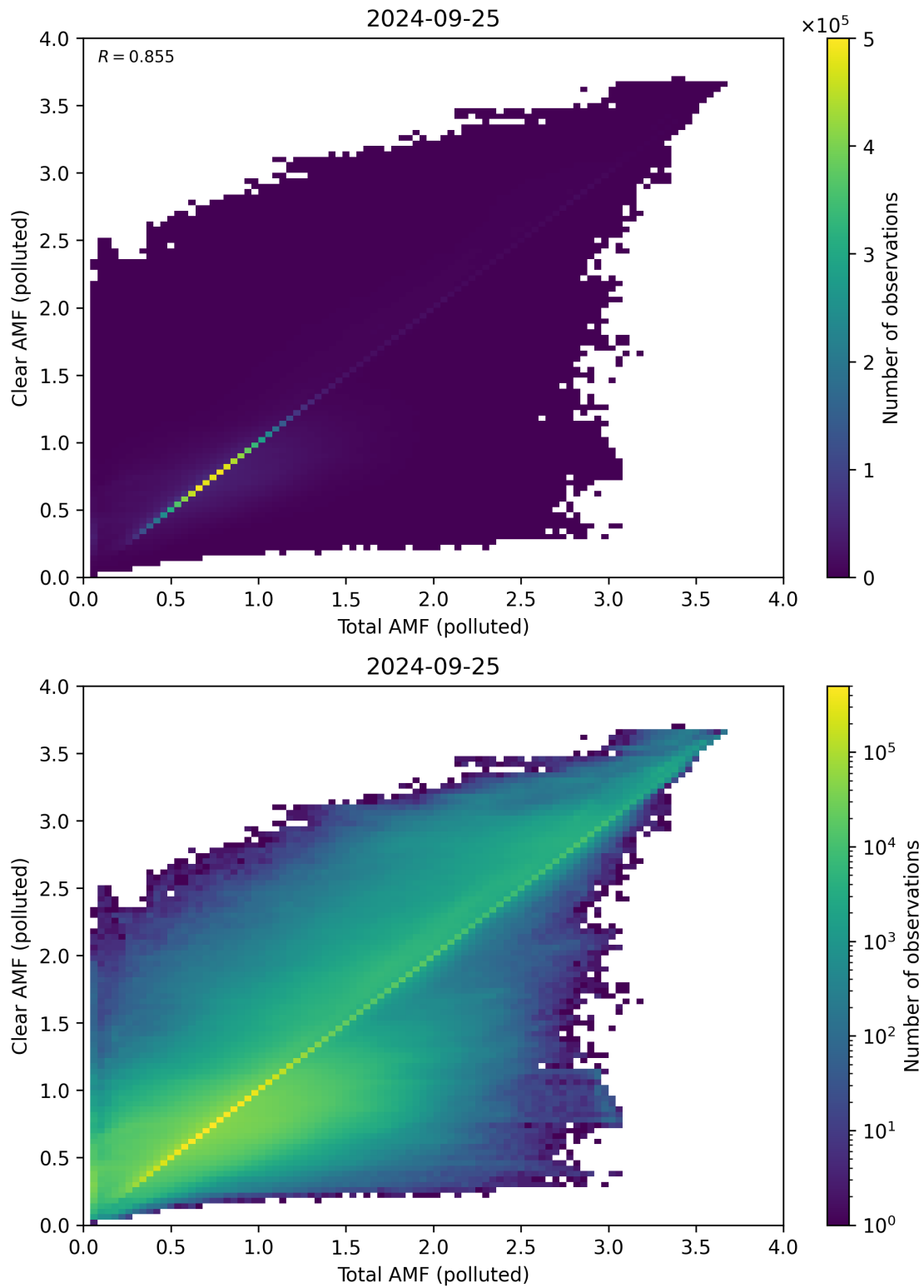
Figure 271: Scatter density plot of “Total AMF (polluted)” against “Clear AMF (polluted)” for 2024-09-24 to 2024-09-26.
