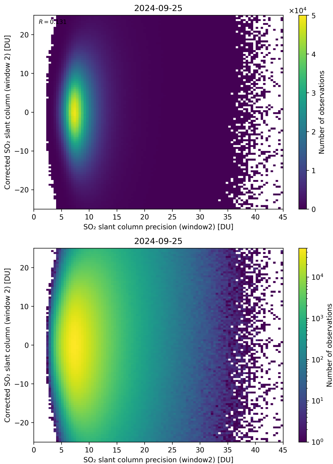
Figure 247: Scatter density plot of “SO 2 slant column precision (window2)” against “Corrected SO 2 slant column (window 2)” for 2024-09-24 to 2024-09-26.
