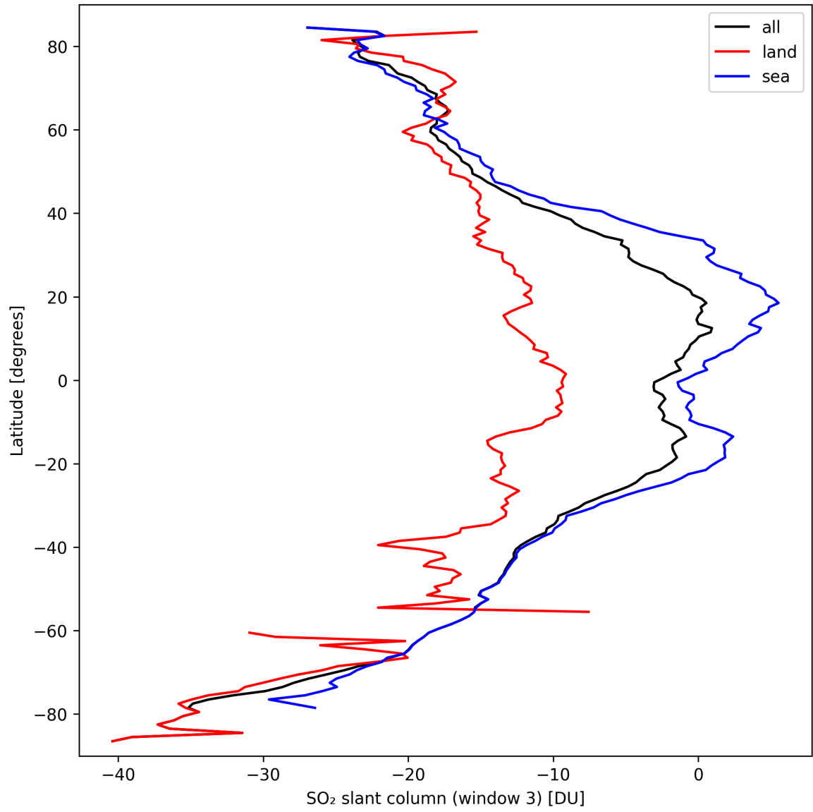
Figure 41: Zonal average of “SO 2 slant column (window 3)” for 2024-09-24 to 2024-09-26.
