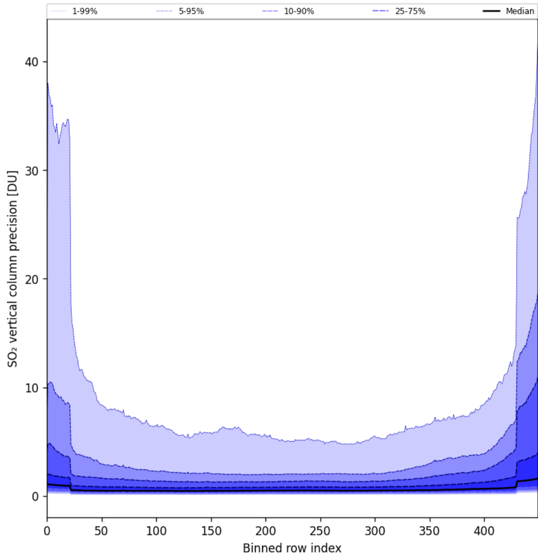
Figure 77: Along track statistics of “SO 2 vertical column precision” for 2024-09-24 to 2024-09-26
