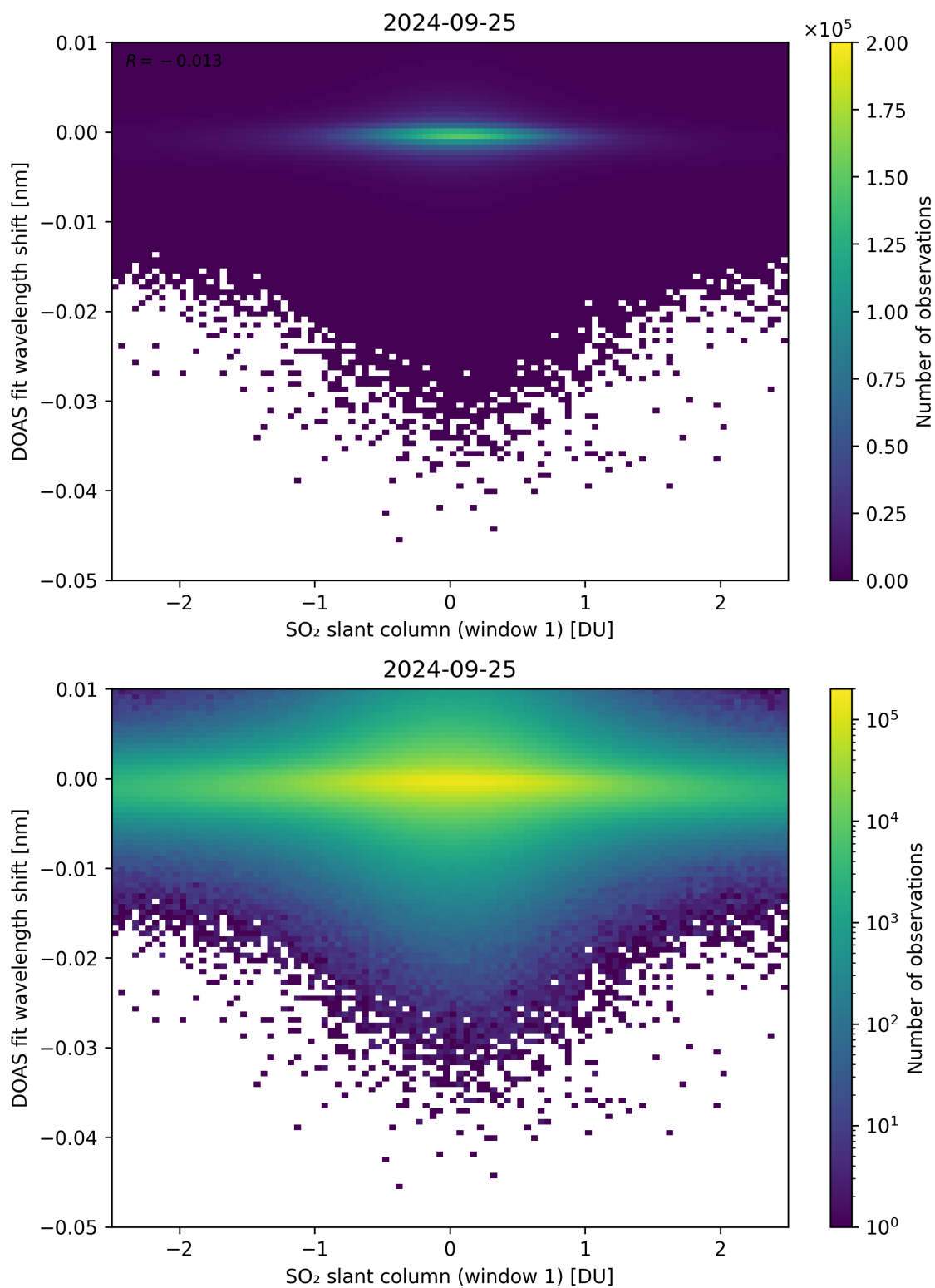
Figure 215: Scatter density plot of “SO 2 slant column (window 1)” against “DOAS fit wavelength shift” for 2024-09-24 to 2024-09-26.
