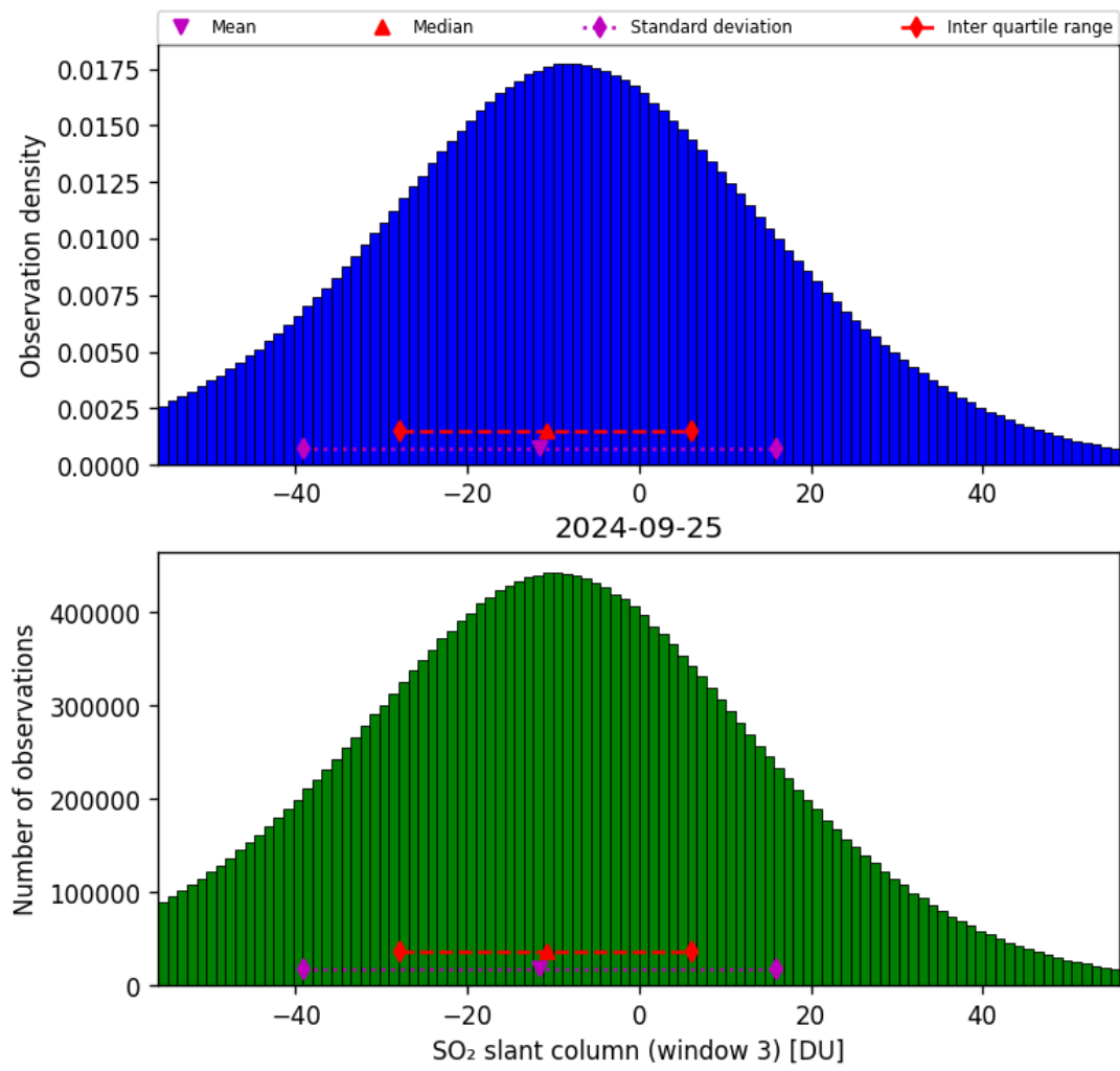
Figure 64: Histogram of “SO 2 slant column (window 3)” for 2024-09-24 to 2024-09-26
