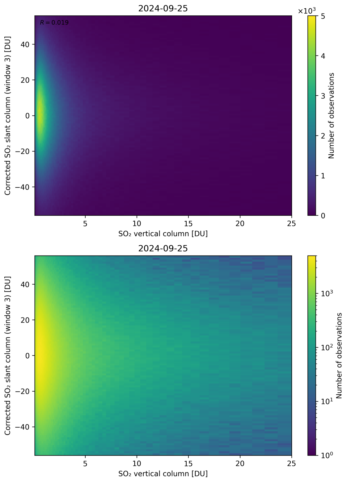
Figure 299: Scatter density plot of “SO 2 vertical column” against “Corrected SO 2 slant column (window 3)” for 2024-09-24 to 2024-09-26.
