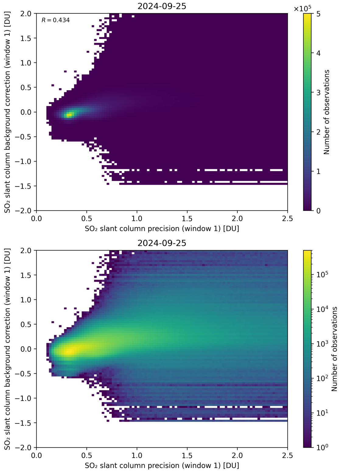
Figure 218: Scatter density plot of “SO 2 slant column precision (window 1)” against “SO 2 slant column background correction (window 1)” for 2024-09-24 to 2024-09-26.
