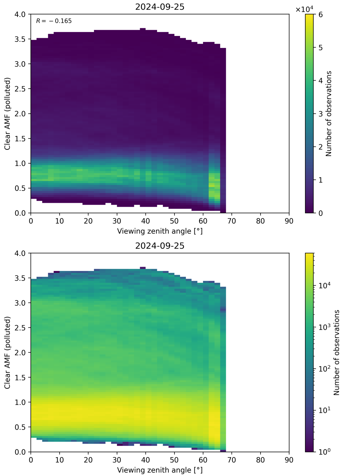
Figure 316: Scatter density plot of “Viewing zenith angle” against “Clear AMF (polluted)” for 2024-09-24 to 2024-09-26.
