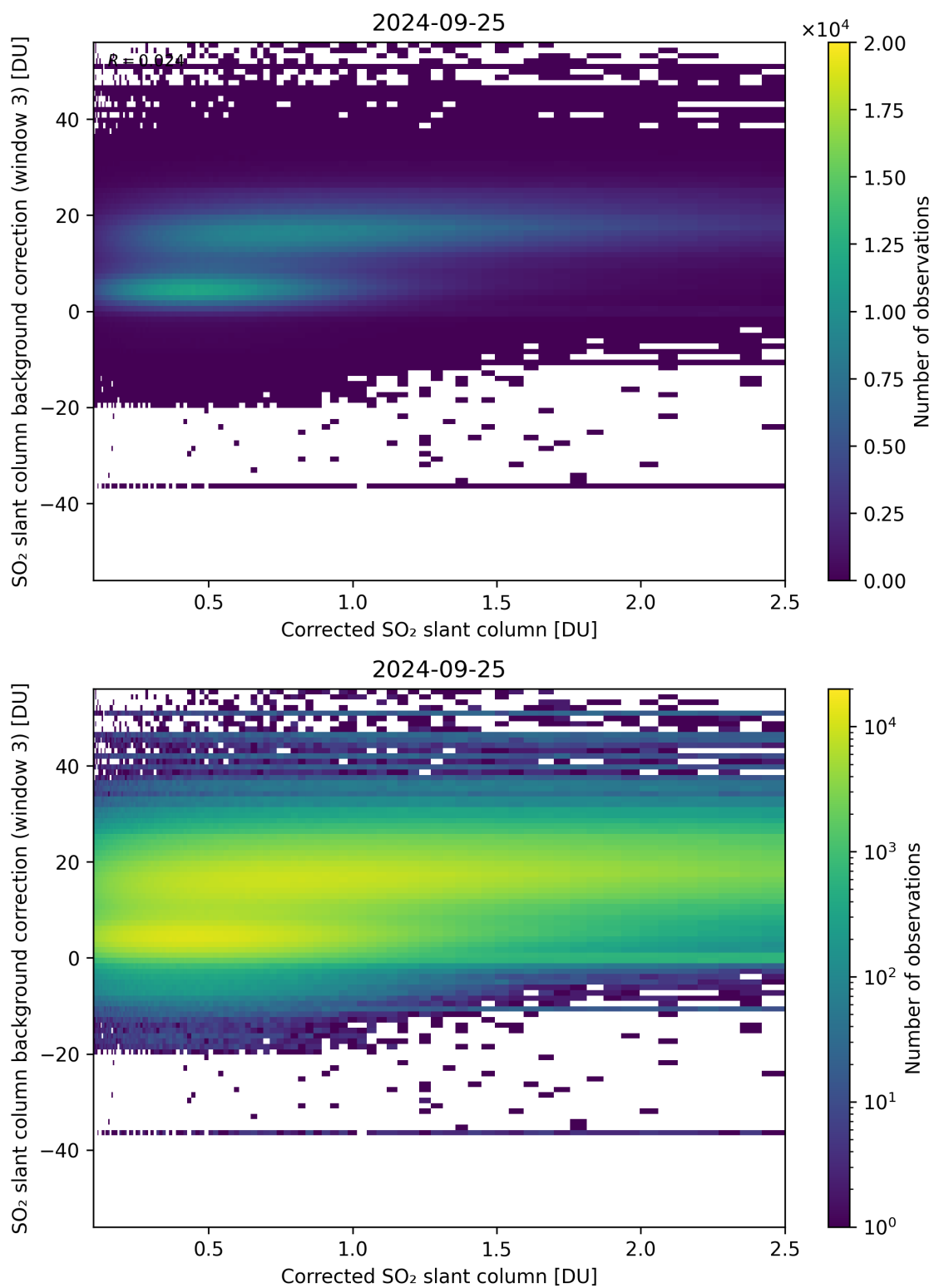
Figure 180: Scatter density plot of “Corrected SO 2 slant column” against “SO 2 slant column background correction (window 3)” for 2024-09-24 to 2024-09-26.
