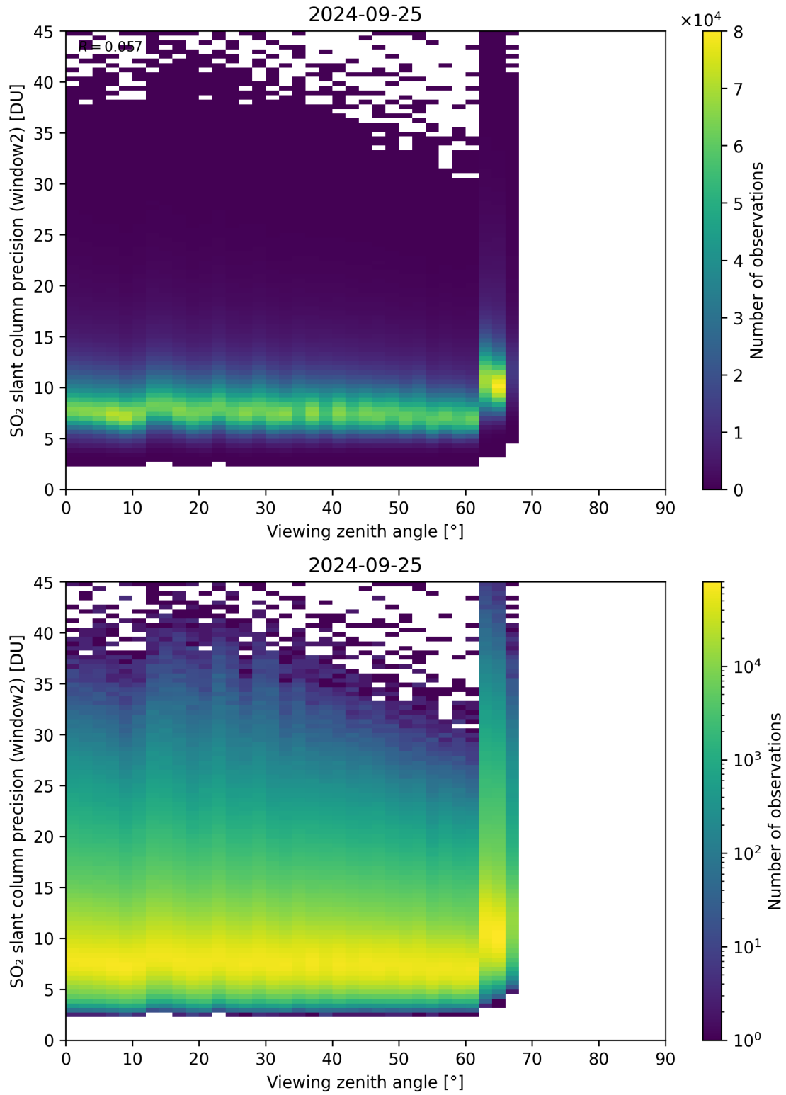
Figure 322: Scatter density plot of “Viewing zenith angle” against “SO 2 slant column precision (window2)” for 2024-09-24 to 2024-09-26.
