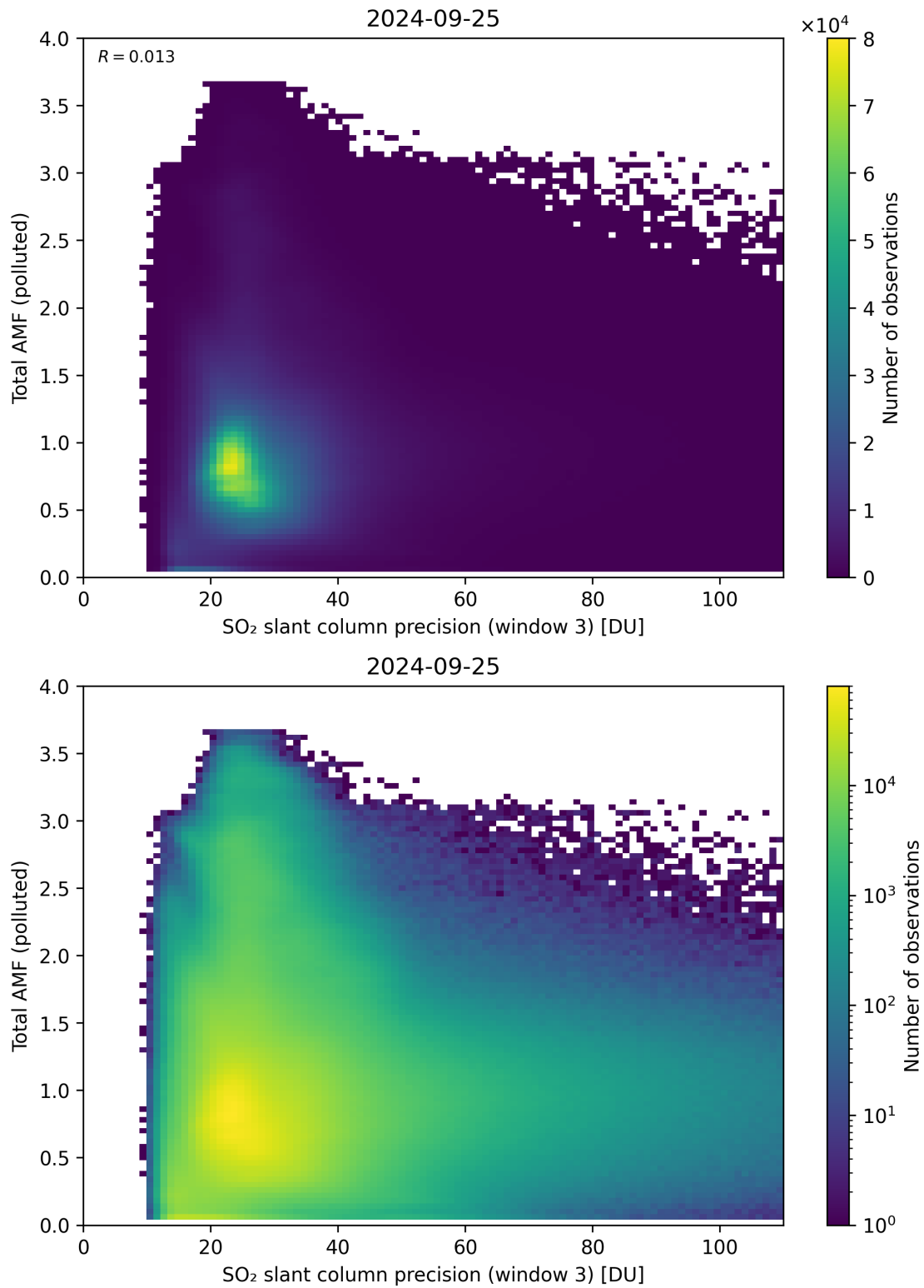
Figure 263: Scatter density plot of “SO 2 slant column precision (window 3)” against “Total AMF (polluted)” for 2024-09-24 to 2024-09-26.
