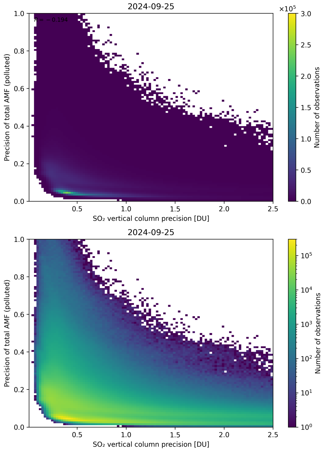
Figure 295: Scatter density plot of “SO 2 vertical column precision” against “Precision of total AMF (polluted)” for 2024-09-24 to 2024-09-26.
