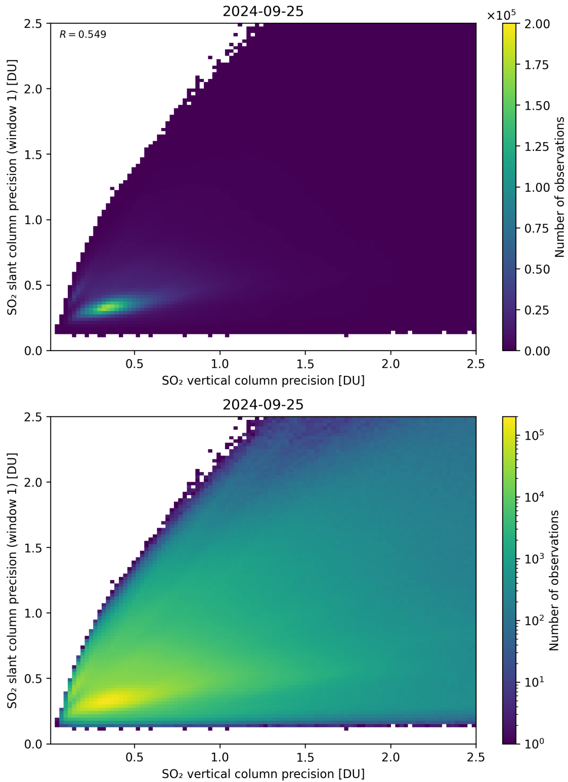
Figure 290: Scatter density plot of “SO 2 vertical column precision” against “SO 2 slant column precision (window 1)” for 2024-09-24 to 2024-09-26.
