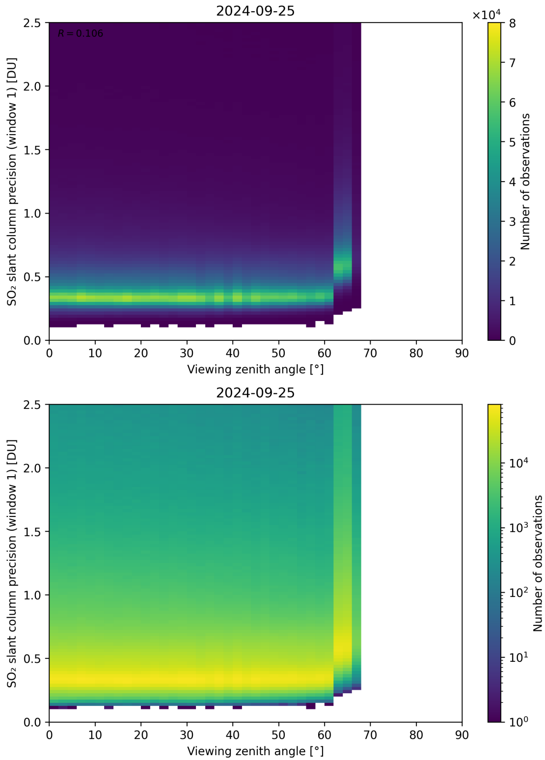
Figure 321: Scatter density plot of “Viewing zenith angle” against “SO 2 slant column precision (window 1)” for 2024-09-24 to 2024-09-26.
