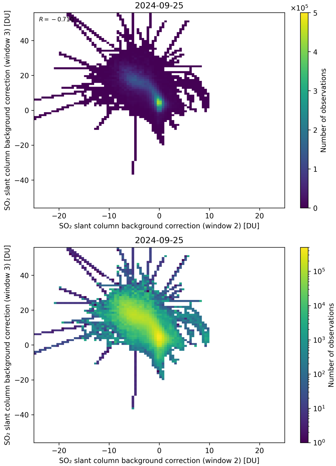
Figure 111: Scatter density plot of “SO 2 slant column background correction (window 2)” against “SO 2 slant column background correction (window 3)” for 2024-09-24 to 2024-09-26.
