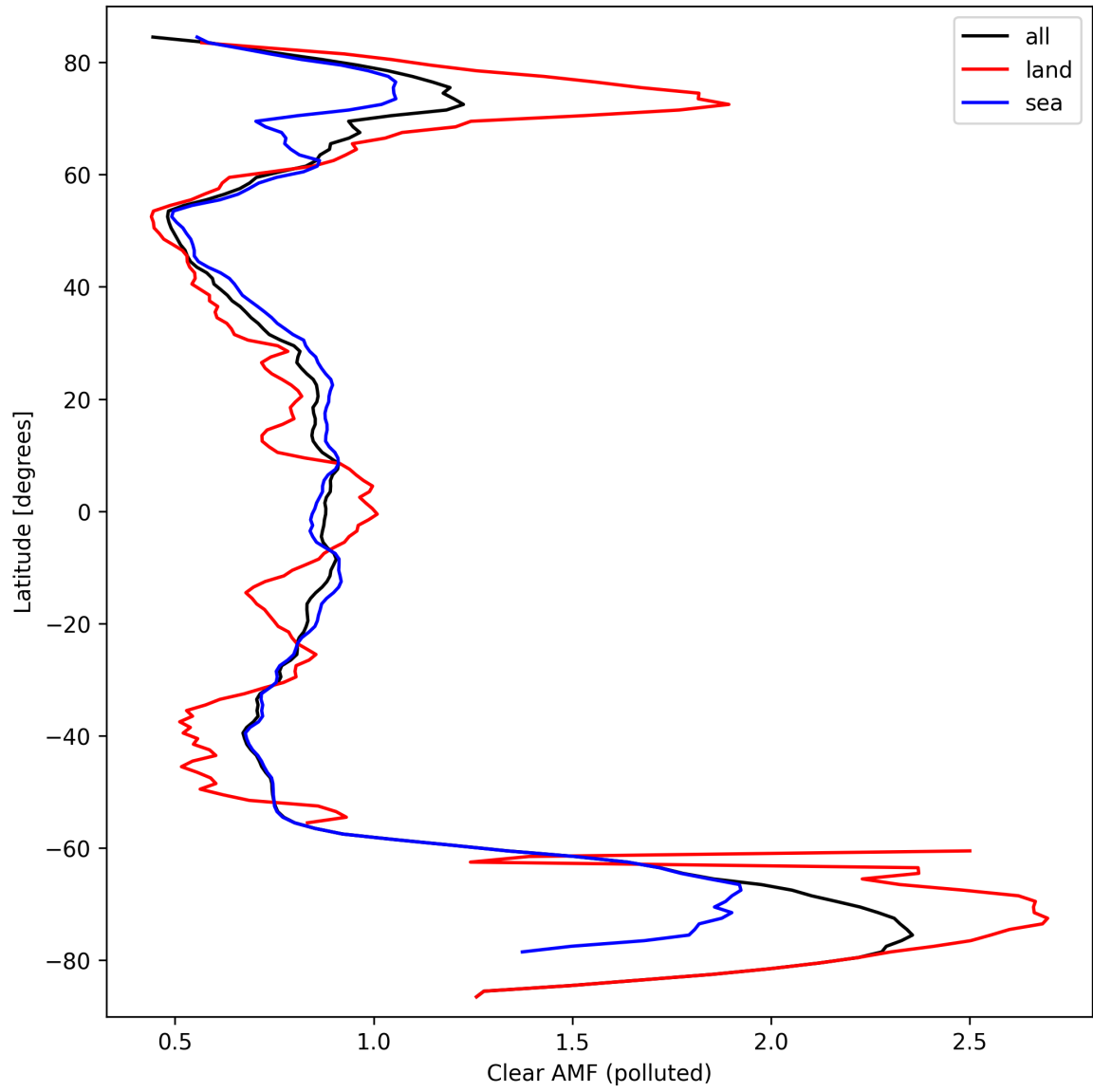
Figure 50: Zonal average of “Clear AMF (polluted)” for 2024-09-24 to 2024-09-26.
