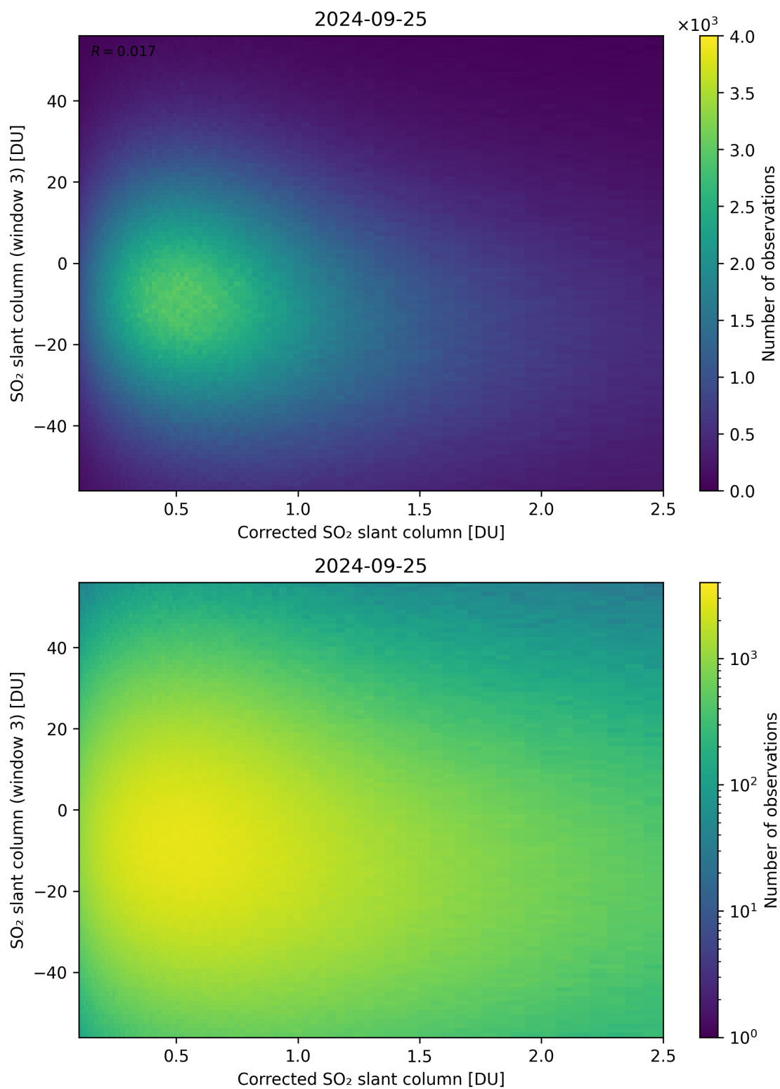
Figure 190: Scatter density plot of “Corrected SO 2 slant column” against “SO 2 slant column (window 3)” for 2024-09-24 to 2024-09-26.
