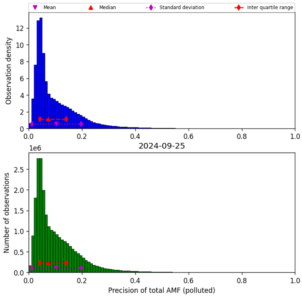
Figure 72: Histogram of “Precision of total AMF (polluted)” for 2024-09-24 to 2024-09-26
