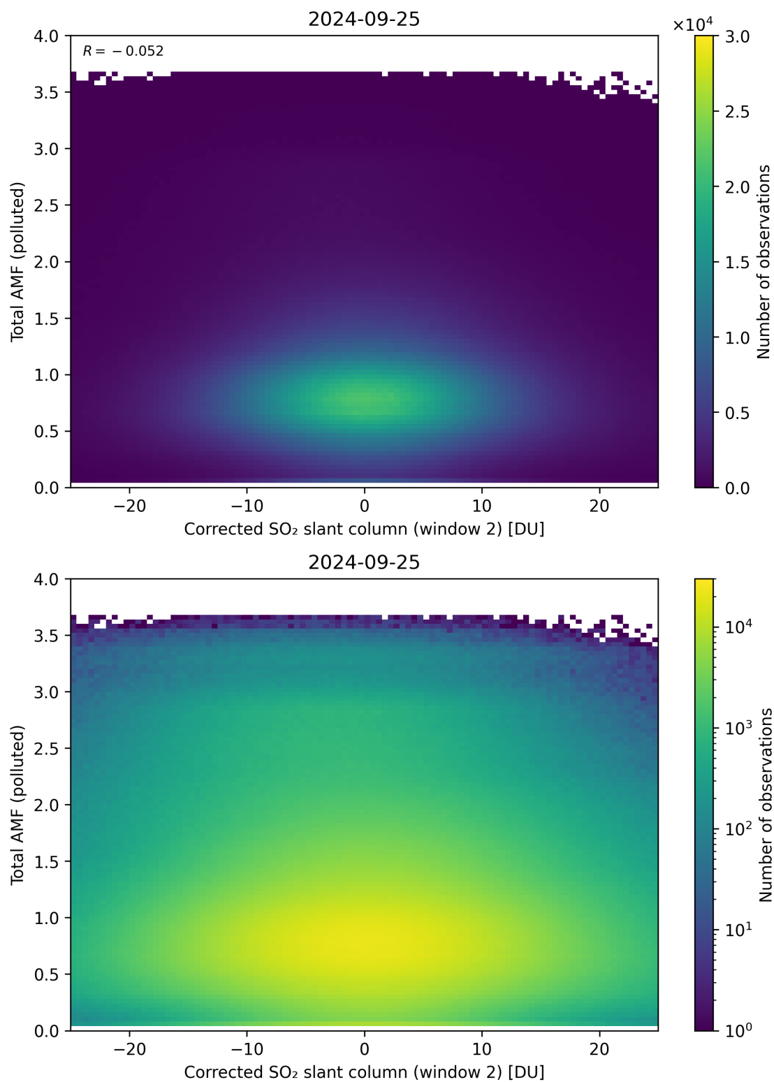
Figure 203: Scatter density plot of “Corrected SO 2 slant column (window 2)” against “Total AMF (polluted)” for 2024-09-24 to 2024-09-26.
