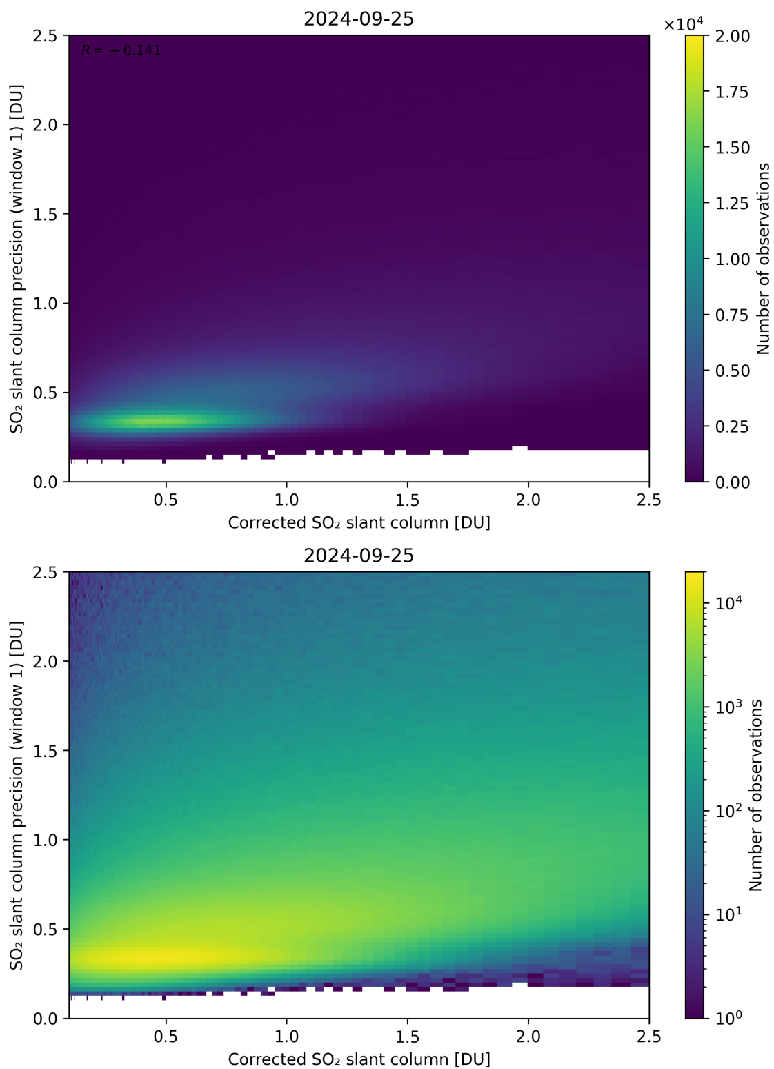
Figure 188: Scatter density plot of “Corrected SO 2 slant column” against “SO 2 slant column precision (window 1)” for 2024-09-24 to 2024-09-26.
