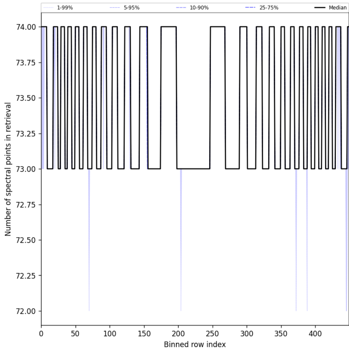
Figure 97: Along track statistics of “Number of spectral points in retrieval” for 2024-09-24 to 2024-09-26
