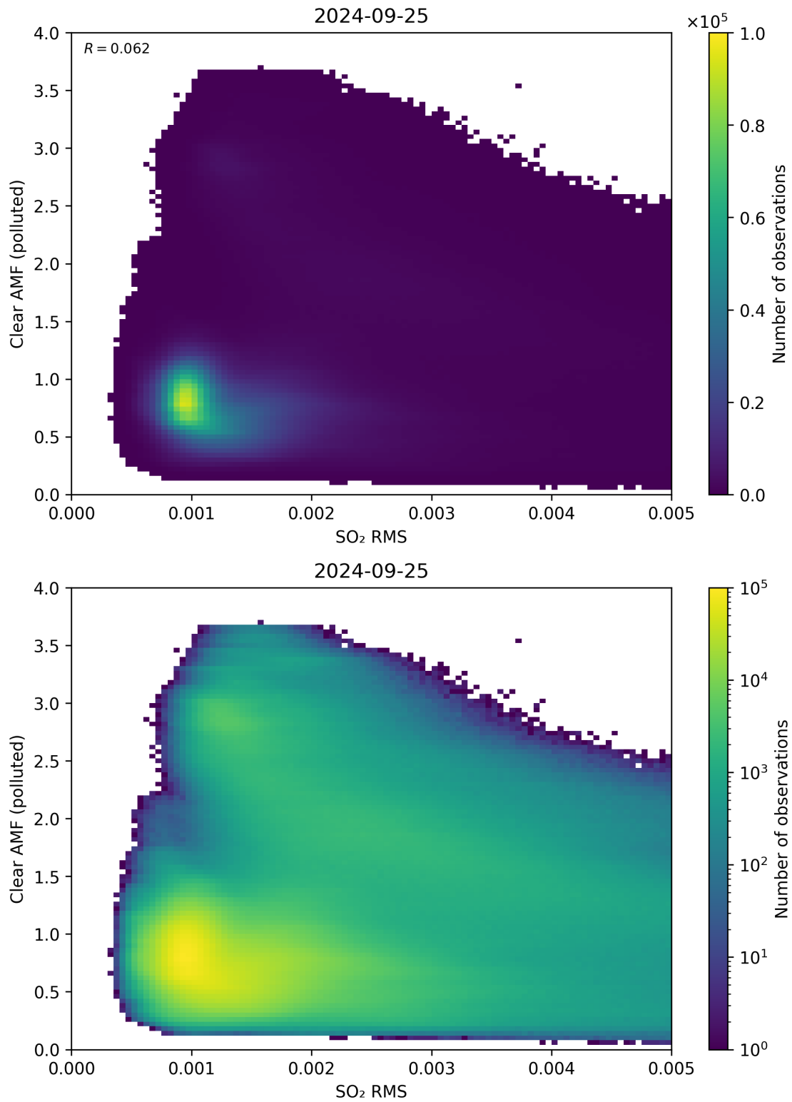
Figure 136: Scatter density plot of “SO 2 RMS” against “Clear AMF (polluted)” for 2024-09-24 to 2024-09-26.
