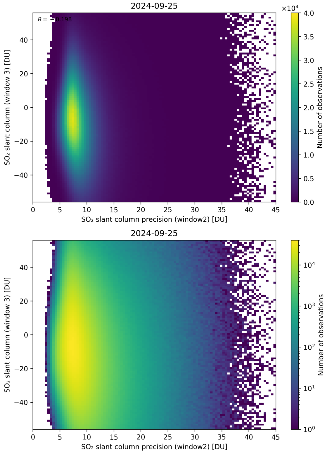
Figure 249: Scatter density plot of “SO 2 slant column precision (window2)” against “SO 2 slant column (window 3)” for 2024-09-24 to 2024-09-26.
