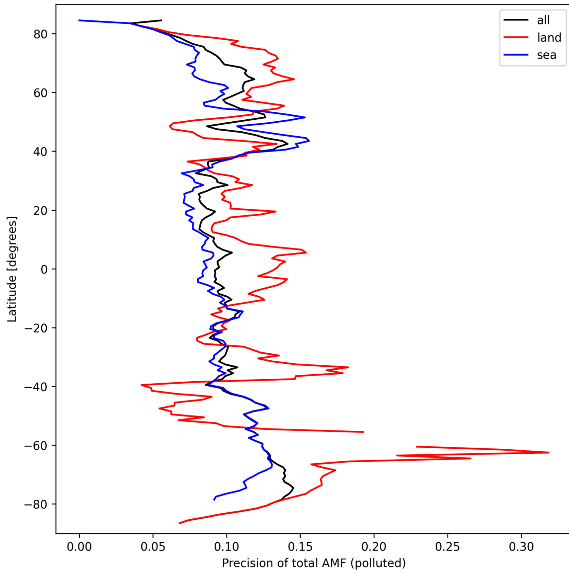
Figure 49: Zonal average of “Precision of total AMF (polluted)” for 2024-09-24 to 2024-09-26.
