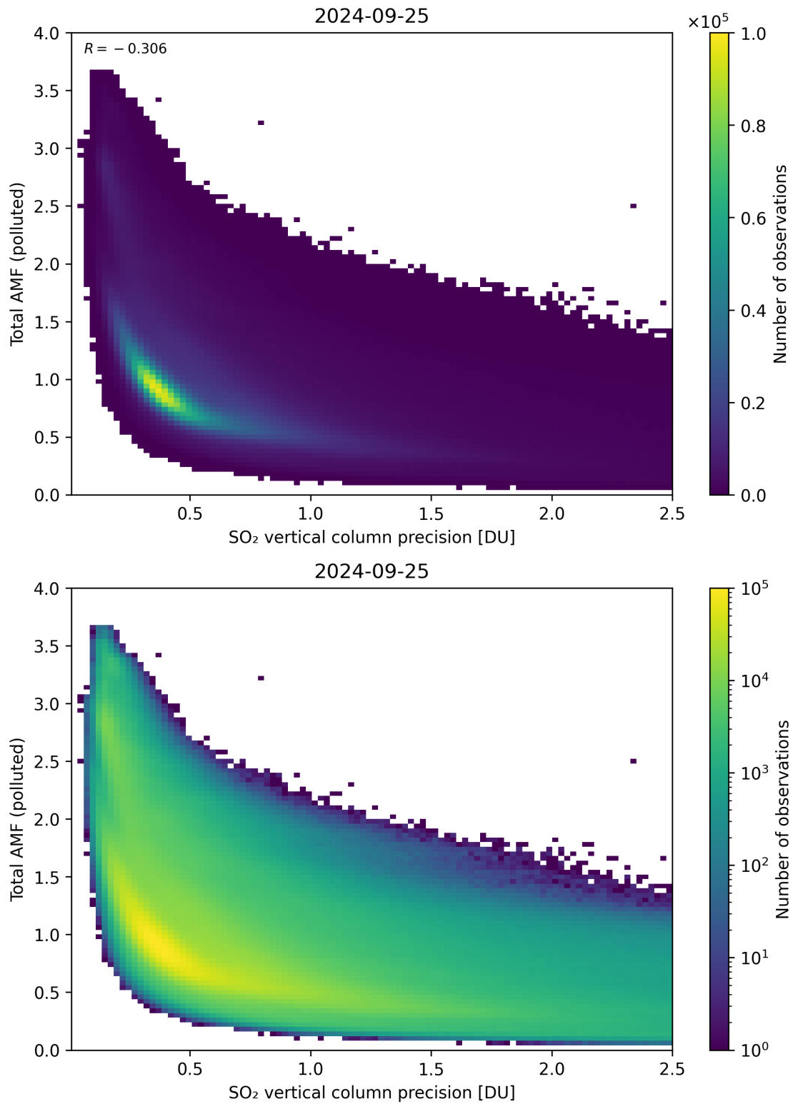
Figure 294: Scatter density plot of “SO 2 vertical column precision” against “Total AMF (polluted)” for 2024-09-24 to 2024-09-26.
