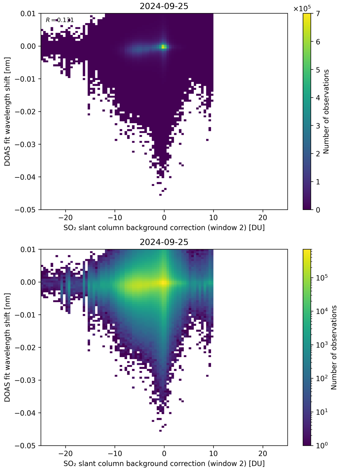
Figure 112: Scatter density plot of “SO 2 slant column background correction (window 2)” against “DOAS fit wavelength shift” for 2024-09-24 to 2024-09-26.
