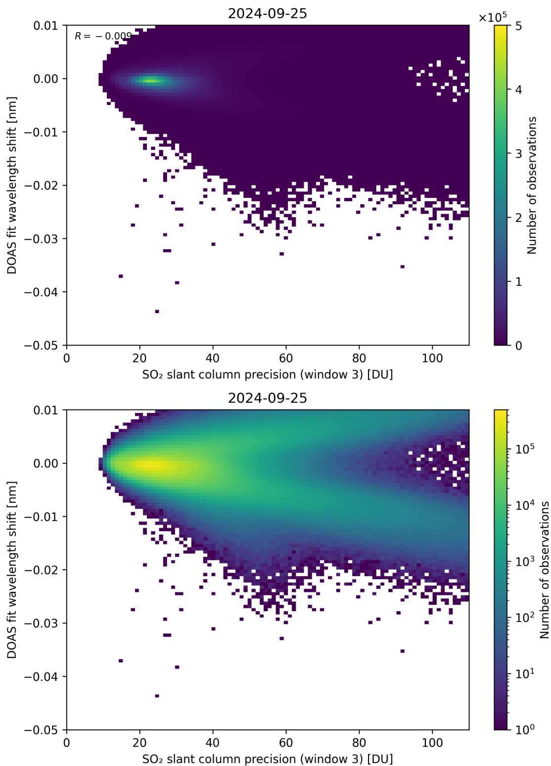
Figure 258: Scatter density plot of “SO 2 slant column precision (window 3)” against “DOAS fit wavelength shift” for 2024-09-24 to 2024-09-26.
