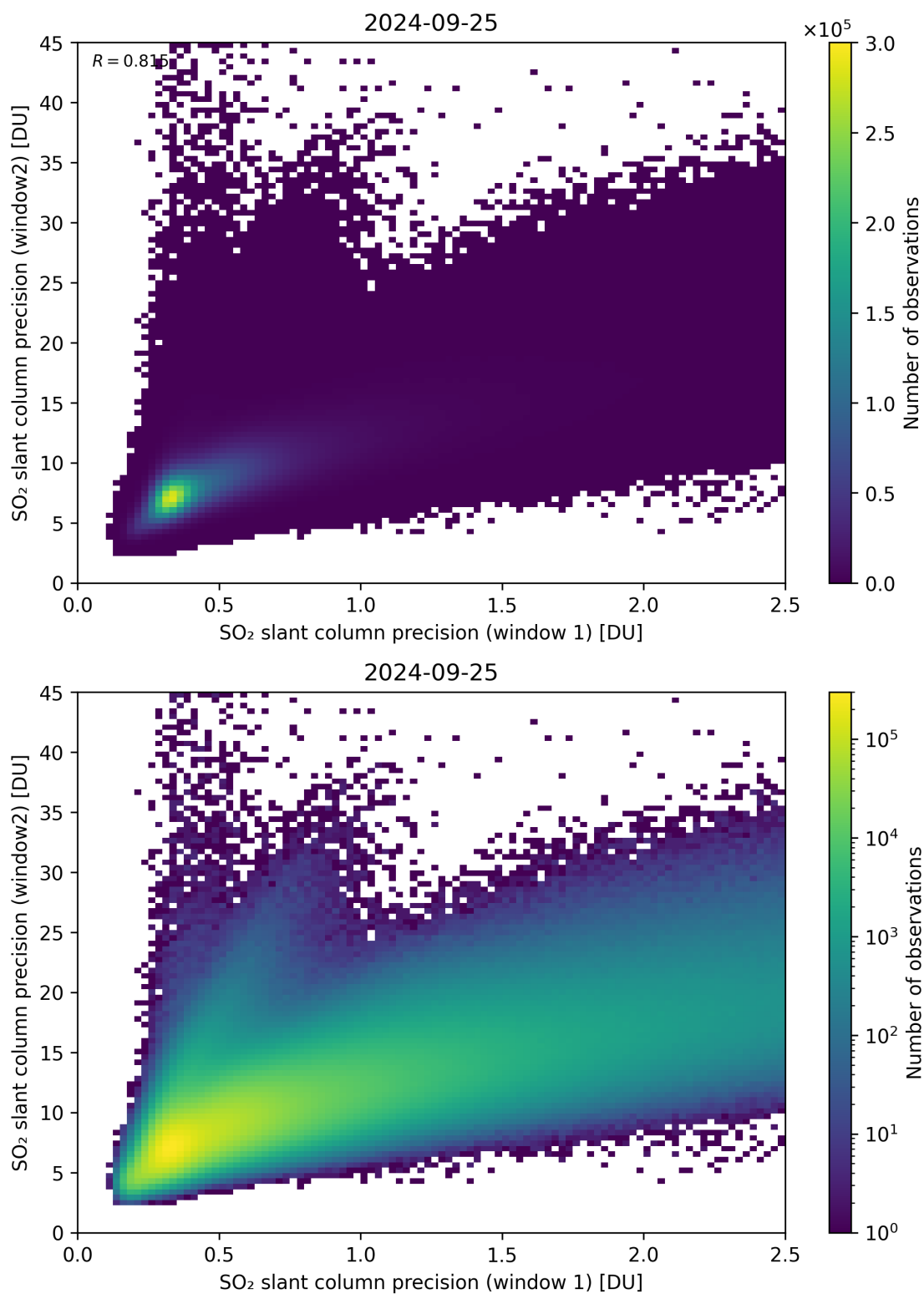
Figure 227: Scatter density plot of “SO 2 slant column precision (window 1)” against “SO 2 slant column precision (window2)” for 2024-09-24 to 2024-09-26.
