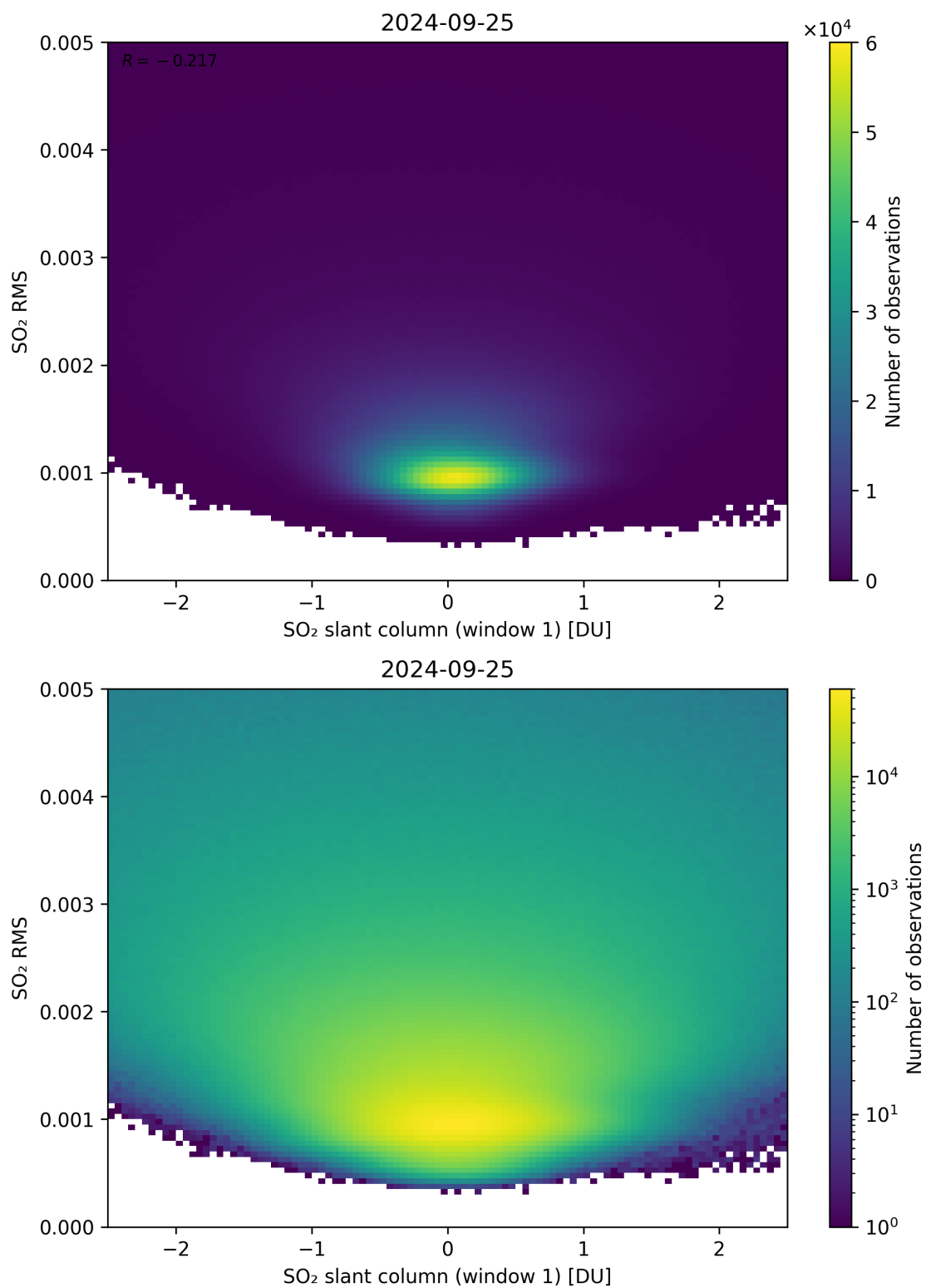
Figure 217: Scatter density plot of “SO 2 slant column (window 1)” against “SO 2 RMS” for 2024-09-24 to 2024-09-26.
