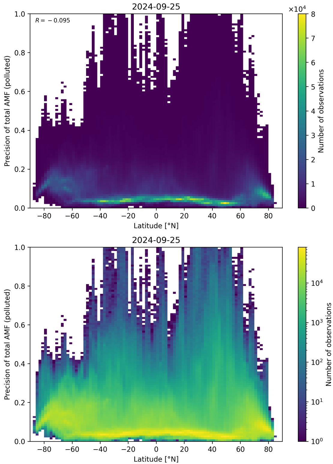
Figure 155: Scatter density plot of “Latitude” against “Precision of total AMF (polluted)” for 2024-09-24 to 2024-09-26.
