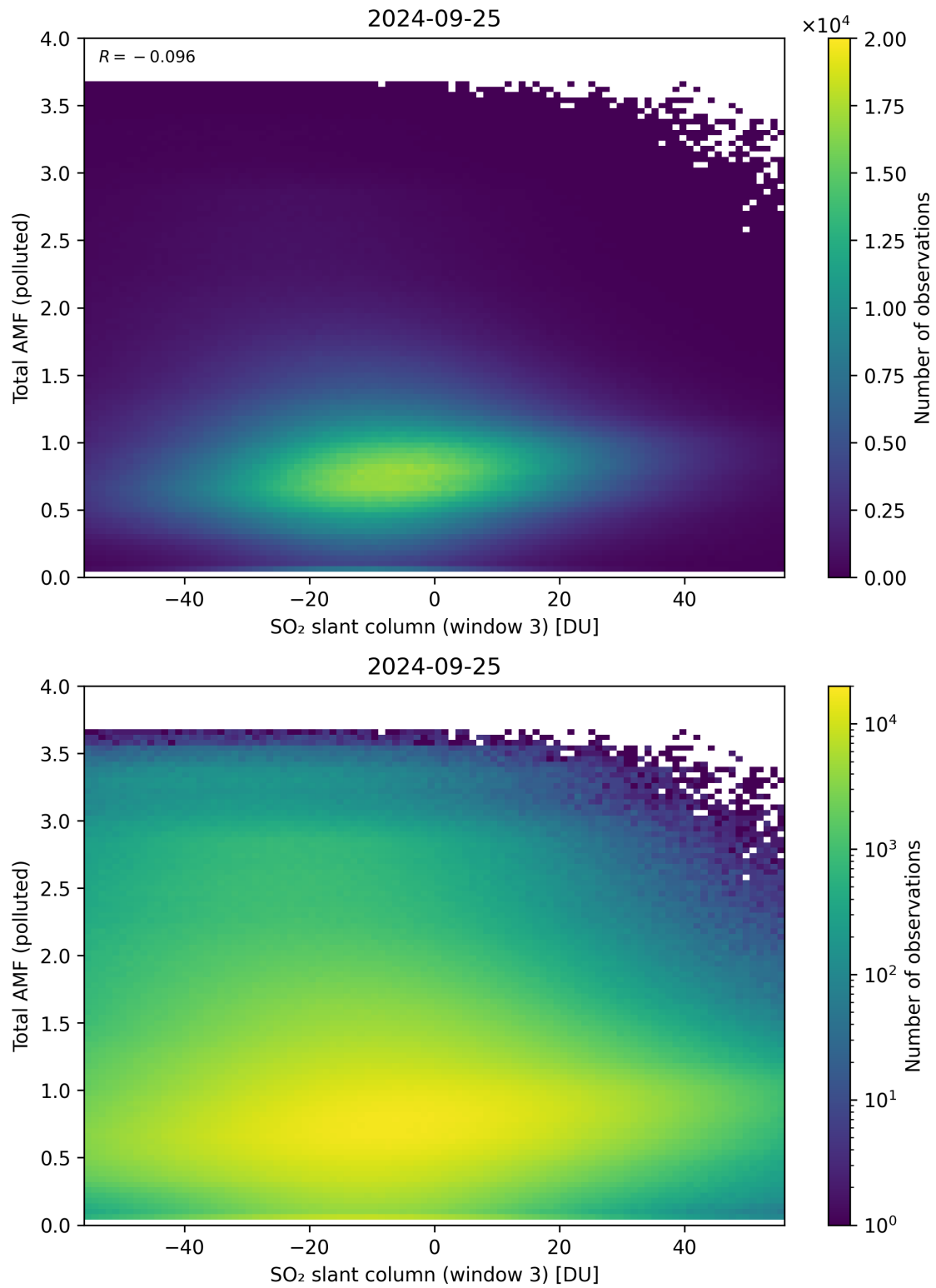
Figure 268: Scatter density plot of “SO 2 slant column (window 3)” against “Total AMF (polluted)” for 2024-09-24 to 2024-09-26.
