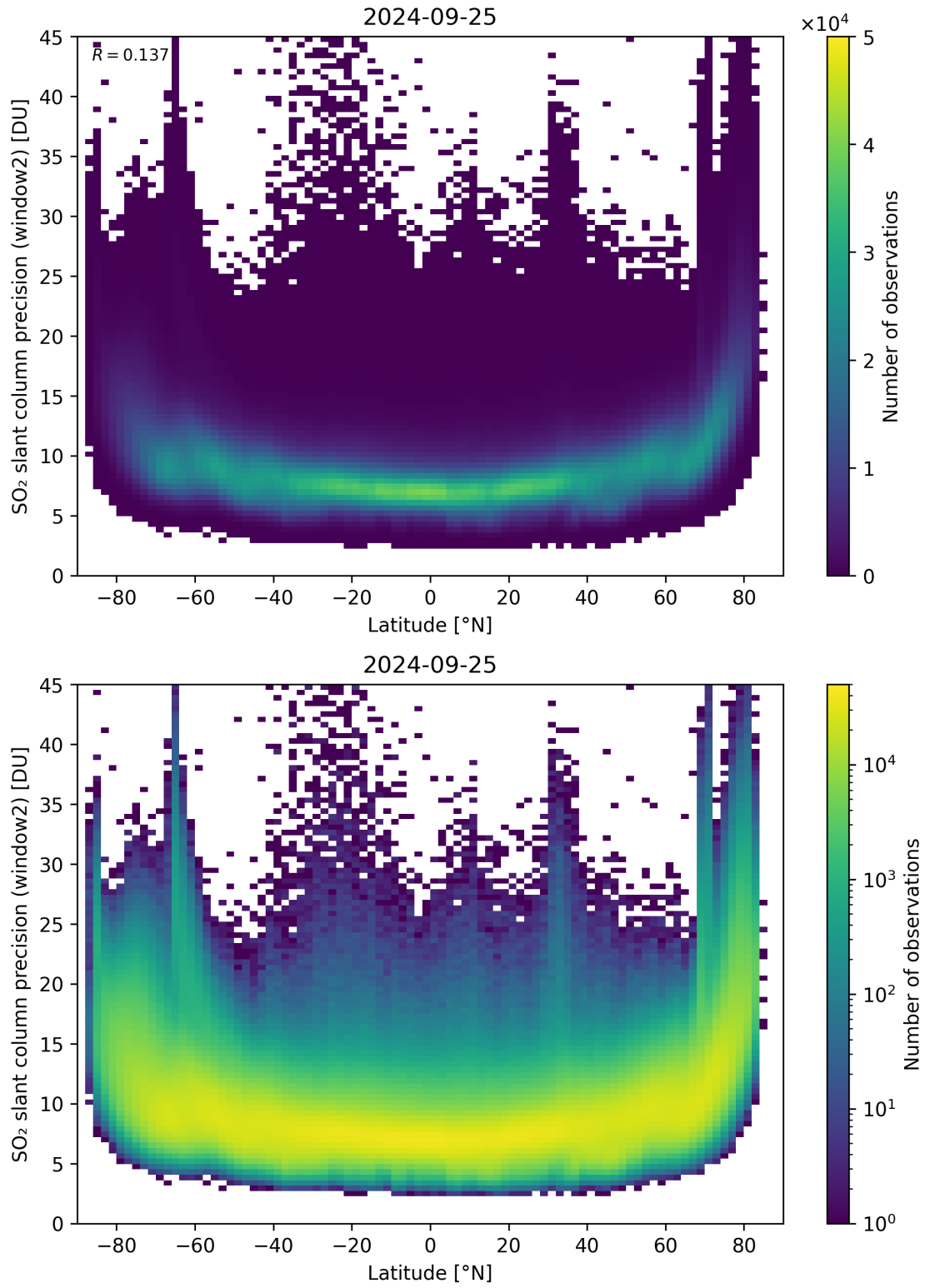
Figure 151: Scatter density plot of “Latitude” against “SO 2 slant column precision (window2)” for 2024-09-24 to 2024-09-26.
