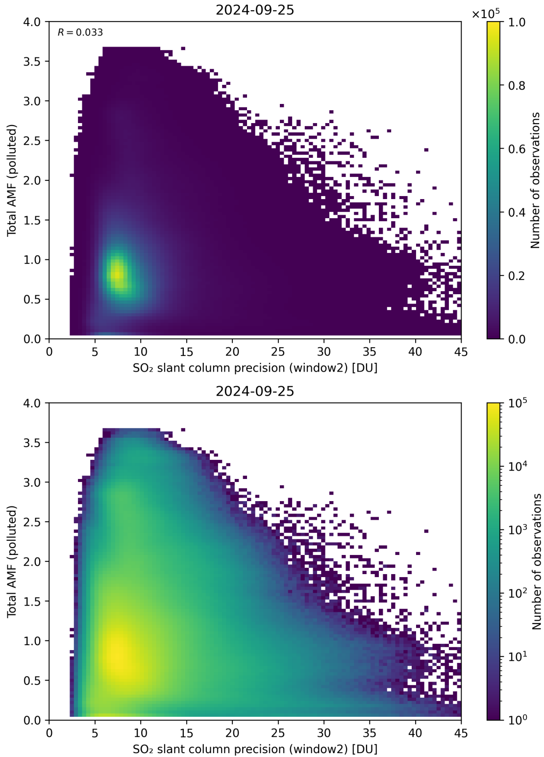
Figure 251: Scatter density plot of “SO 2 slant column precision (window2)” against “Total AMF (polluted)” for 2024-09-24 to 2024-09-26.
