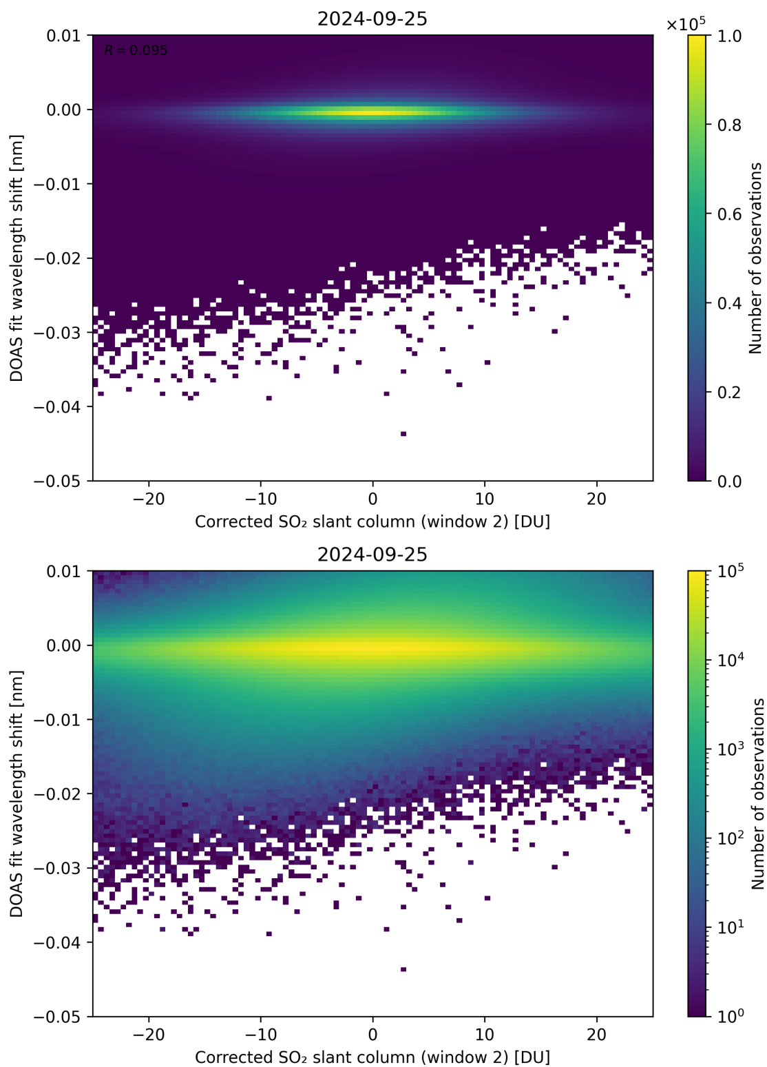
Figure 196: Scatter density plot of “Corrected SO 2 slant column (window 2)” against “DOAS fit wavelength shift” for 2024-09-24 to 2024-09-26.
