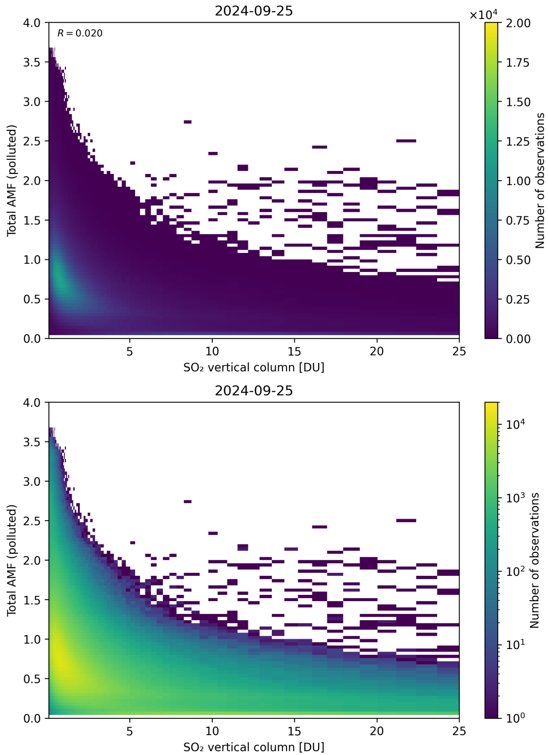
Figure 305: Scatter density plot of “SO 2 vertical column” against “Total AMF (polluted)” for 2024-09-24 to 2024-09-26.
