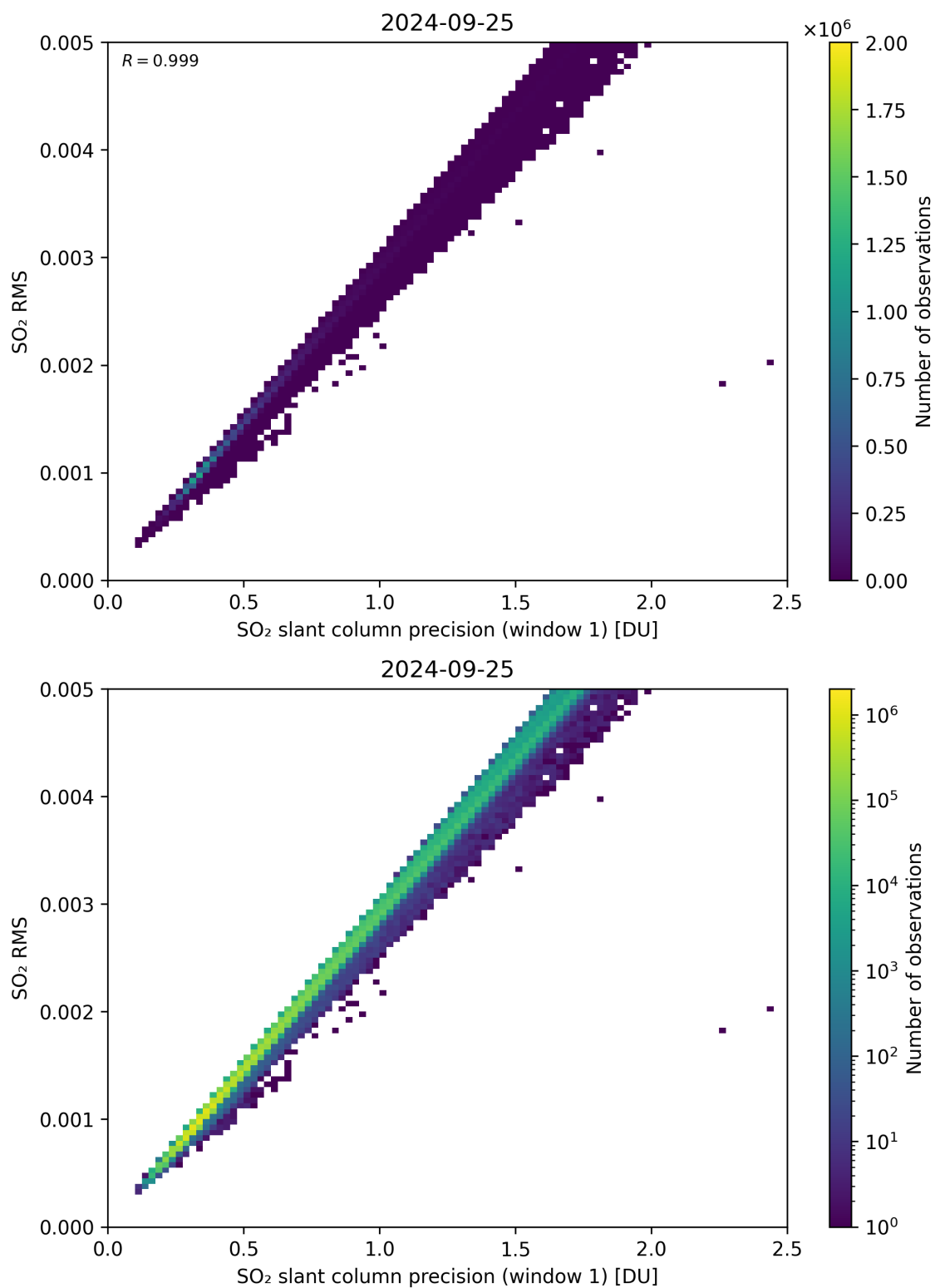
Figure 223: Scatter density plot of “SO 2 slant column precision (window 1)” against “SO 2 RMS” for 2024-09-24 to 2024-09-26.
