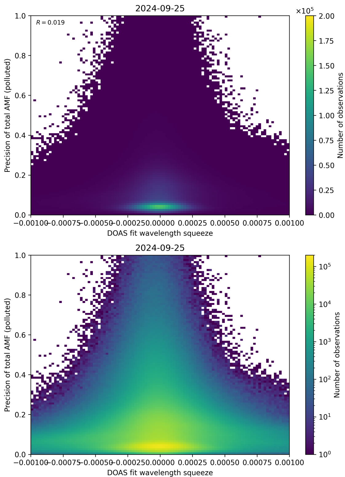
Figure 135: Scatter density plot of “DOAS fit wavelength squeeze” against “Precision of total AMF (polluted)” for 2024-09-24 to 2024-09-26.
