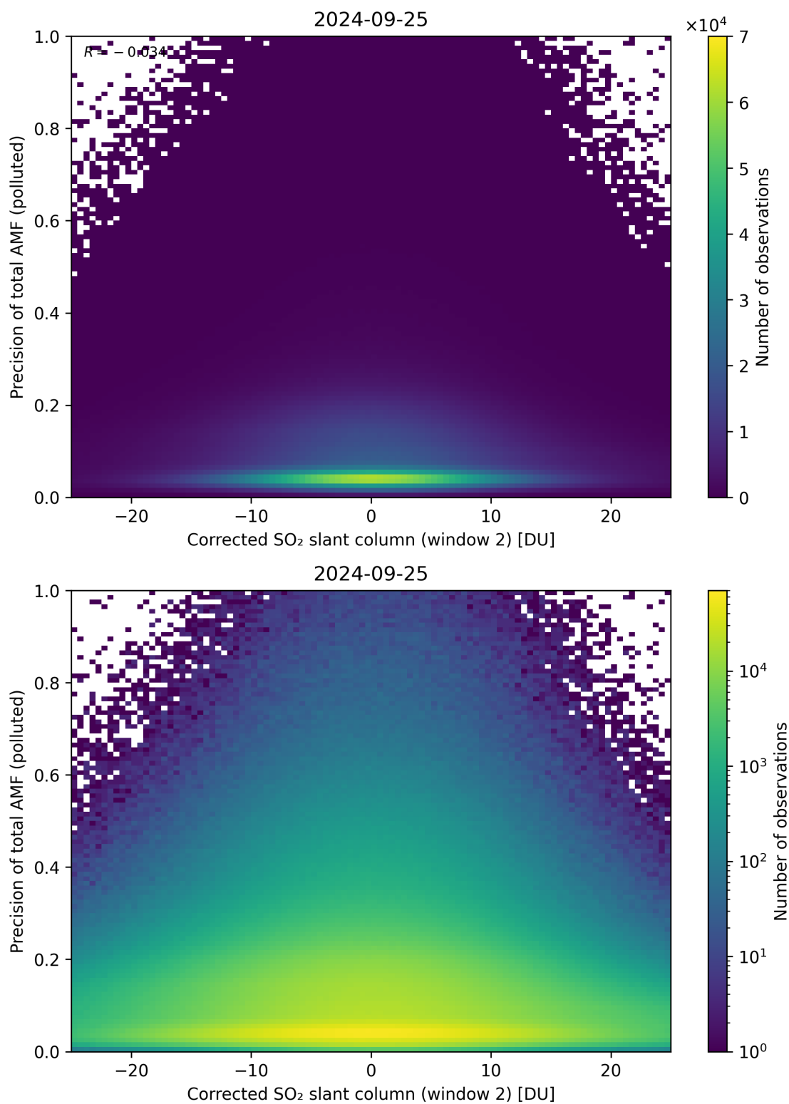
Figure 204: Scatter density plot of “Corrected SO 2 slant column (window 2)” against “Precision of total AMF (polluted)” for 2024-09-24 to 2024-09-26.
