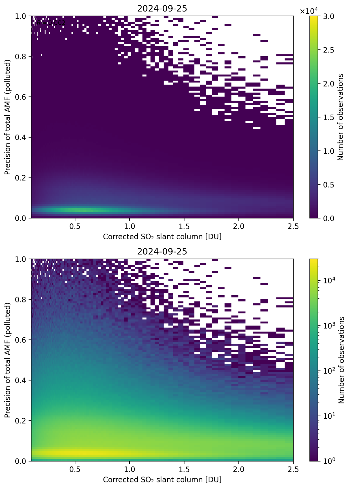
Figure 193: Scatter density plot of “Corrected SO 2 slant column” against “Precision of total AMF (polluted)” for 2024-09-24 to 2024-09-26.
