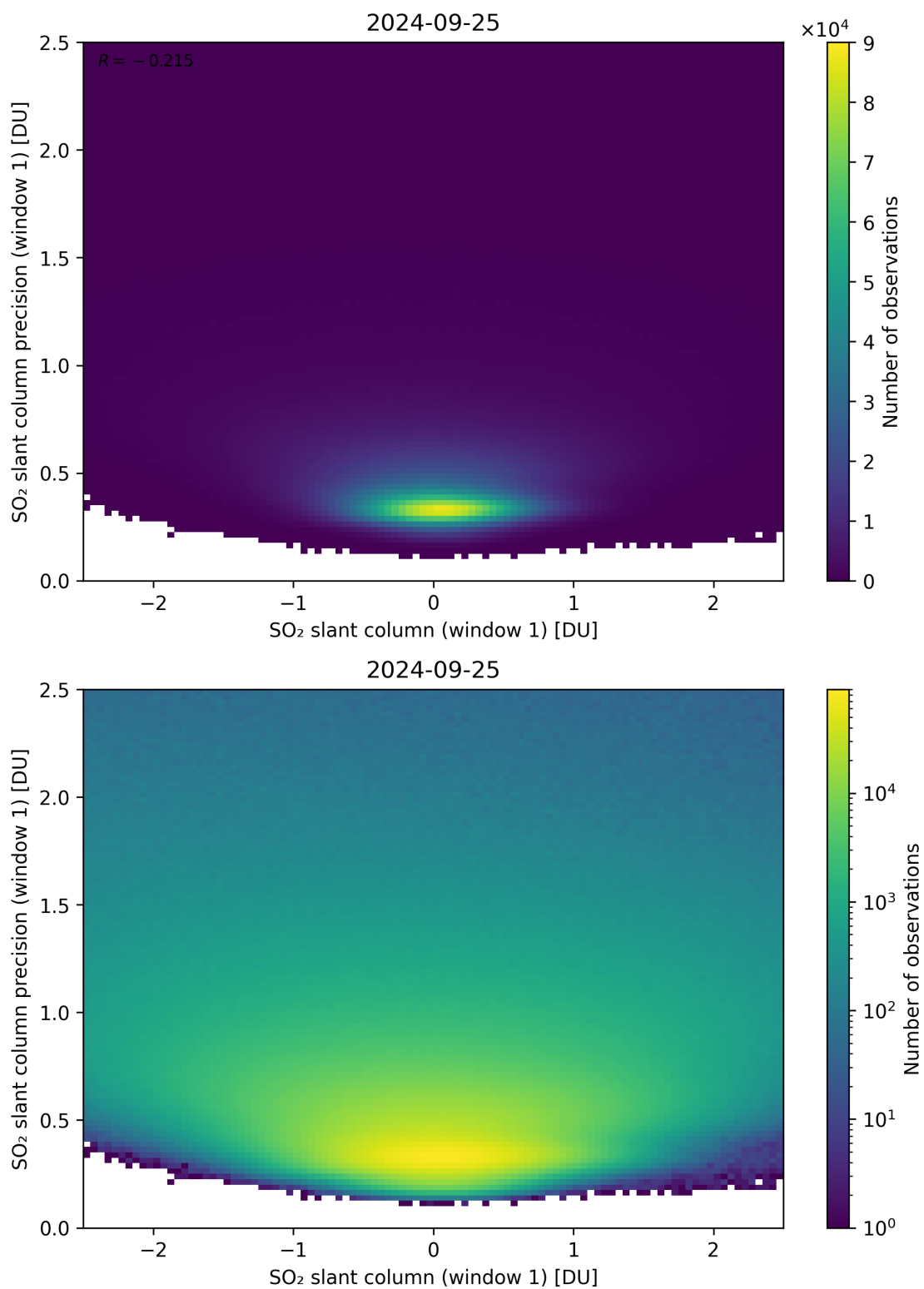
Figure 235: Scatter density plot of “SO 2 slant column (window 1)” against “SO 2 slant column precision (window 1)” for 2024-09-24 to 2024-09-26.
