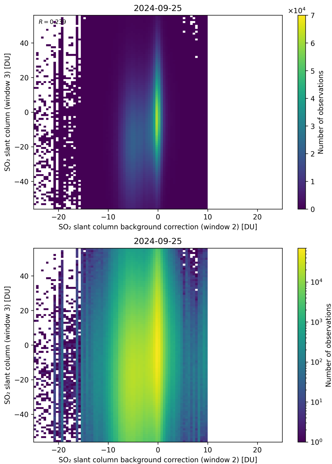
Figure 117: Scatter density plot of “SO 2 slant column background correction (window 2)” against “SO 2 slant column (window 3)” for 2024-09-24 to 2024-09-26.
