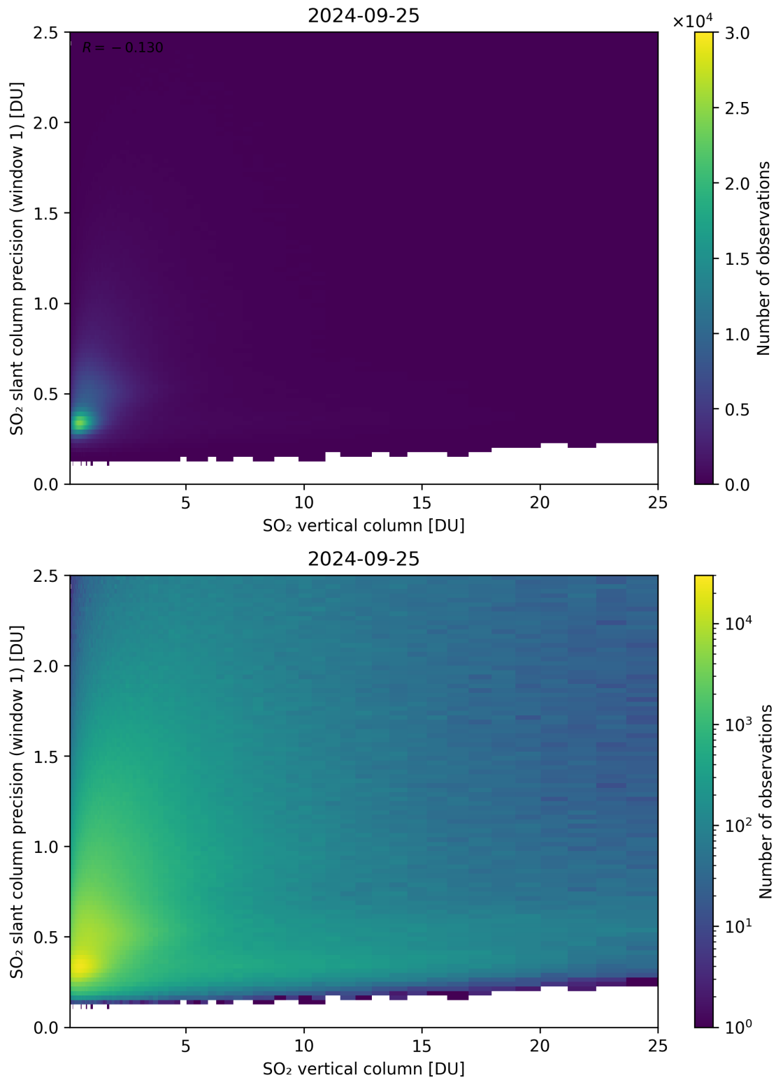
Figure 301: Scatter density plot of “SO 2 vertical column” against “SO 2 slant column precision (window 1)” for 2024-09-24 to 2024-09-26.
