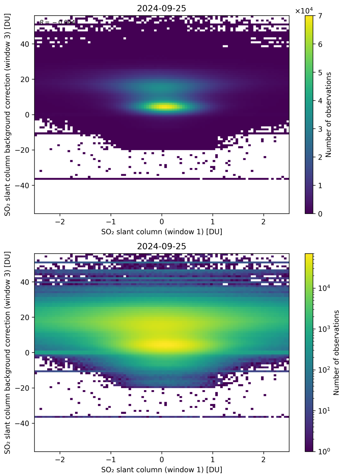
Figure 214: Scatter density plot of “SO 2 slant column (window 1)” against “SO 2 slant column background correction (window 3)” for 2024-09-24 to 2024-09-26.
