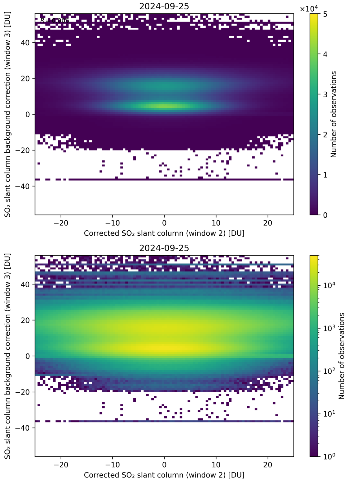
Figure 195: Scatter density plot of “Corrected SO 2 slant column (window 2)” against “SO 2 slant column background correction (window 3)” for 2024-09-24 to 2024-09-26.
