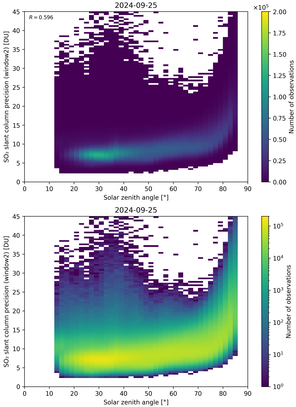
Figure 171: Scatter density plot of “Solar zenith angle” against “SO 2 slant column precision (window2)” for 2024-09-24 to 2024-09-26.
