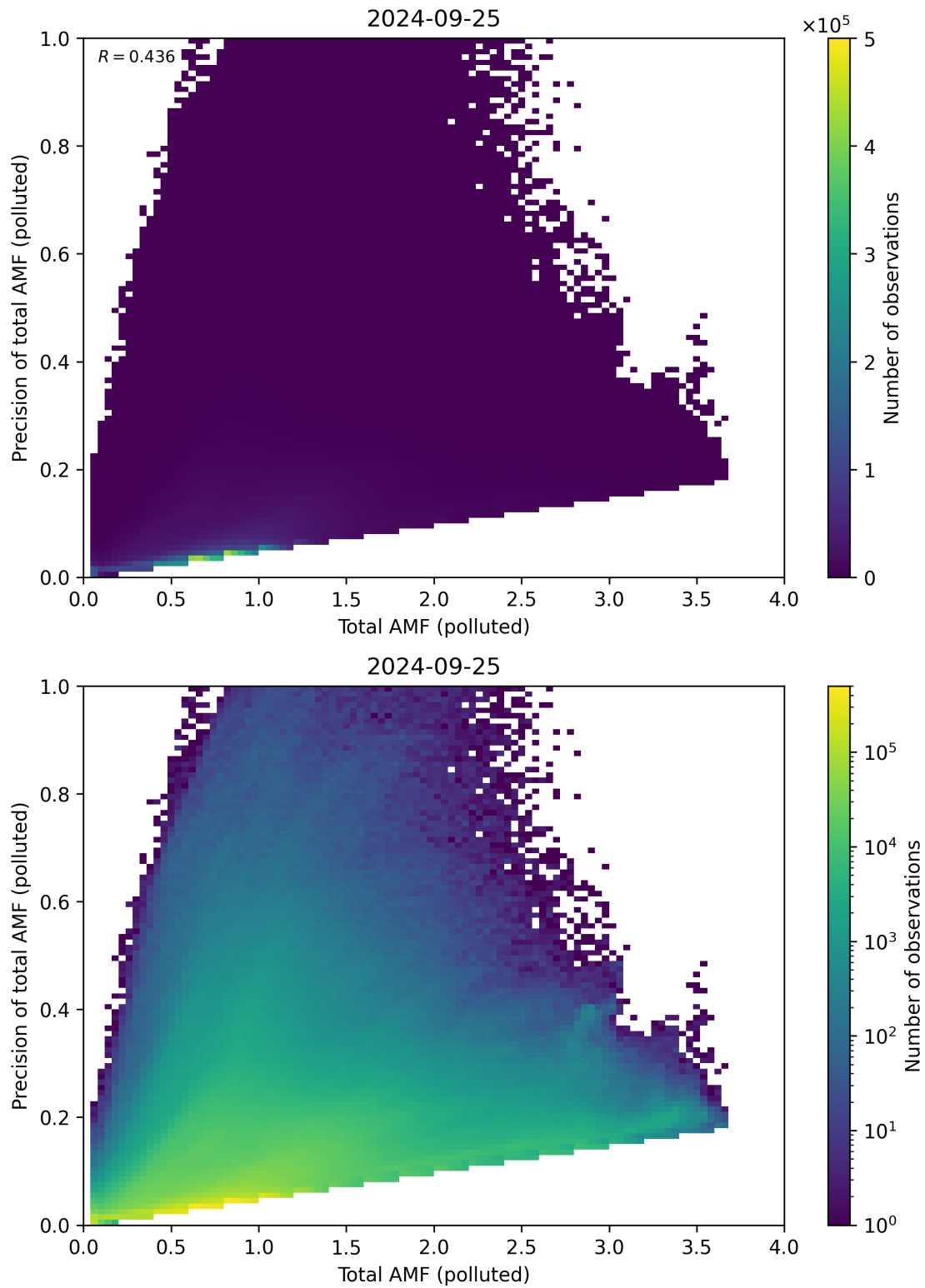
Figure 272: Scatter density plot of “Total AMF (polluted)” against “Precision of total AMF (polluted)” for 2024-09-24 to 2024-09-26.
