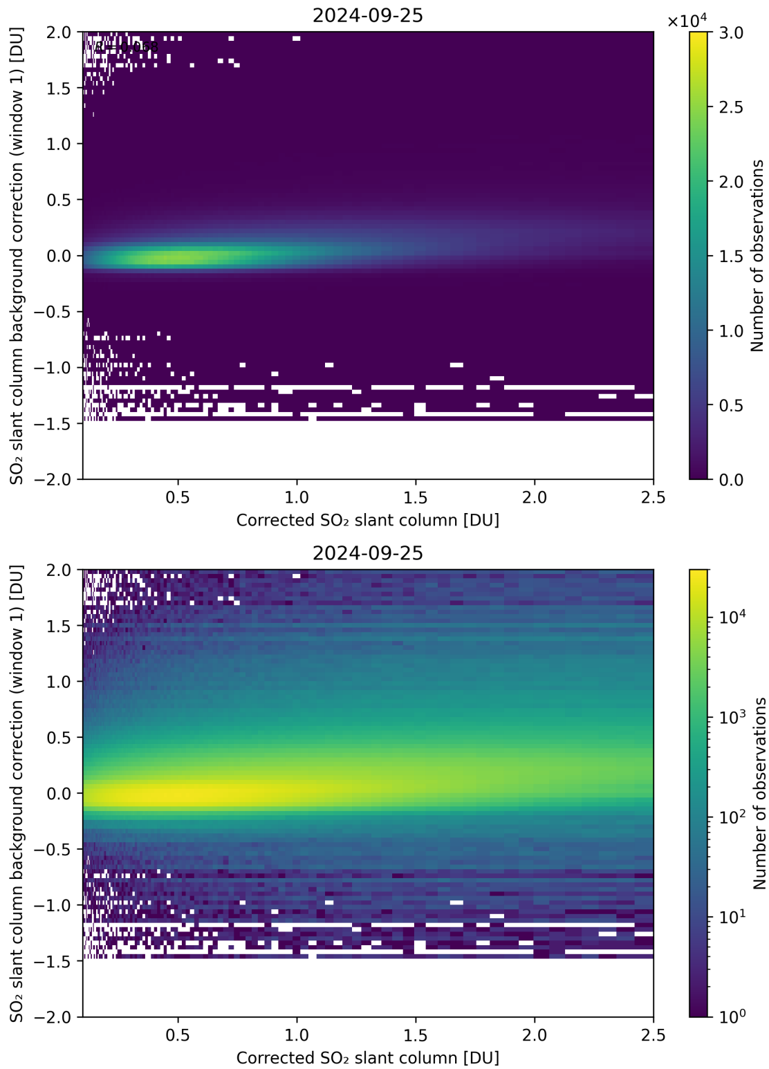
Figure 178: Scatter density plot of “Corrected SO 2 slant column” against “SO 2 slant column background correction (window 1)” for 2024-09-24 to 2024-09-26.
