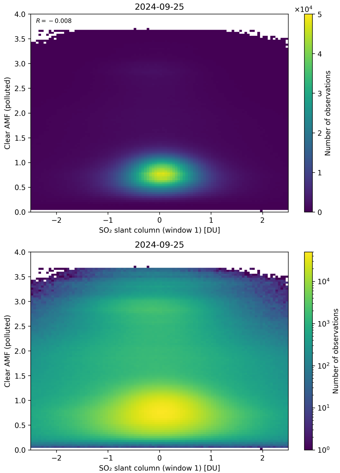
Figure 232: Scatter density plot of “SO 2 slant column (window 1)” against “Clear AMF (polluted)” for 2024-09-24 to 2024-09-26.
