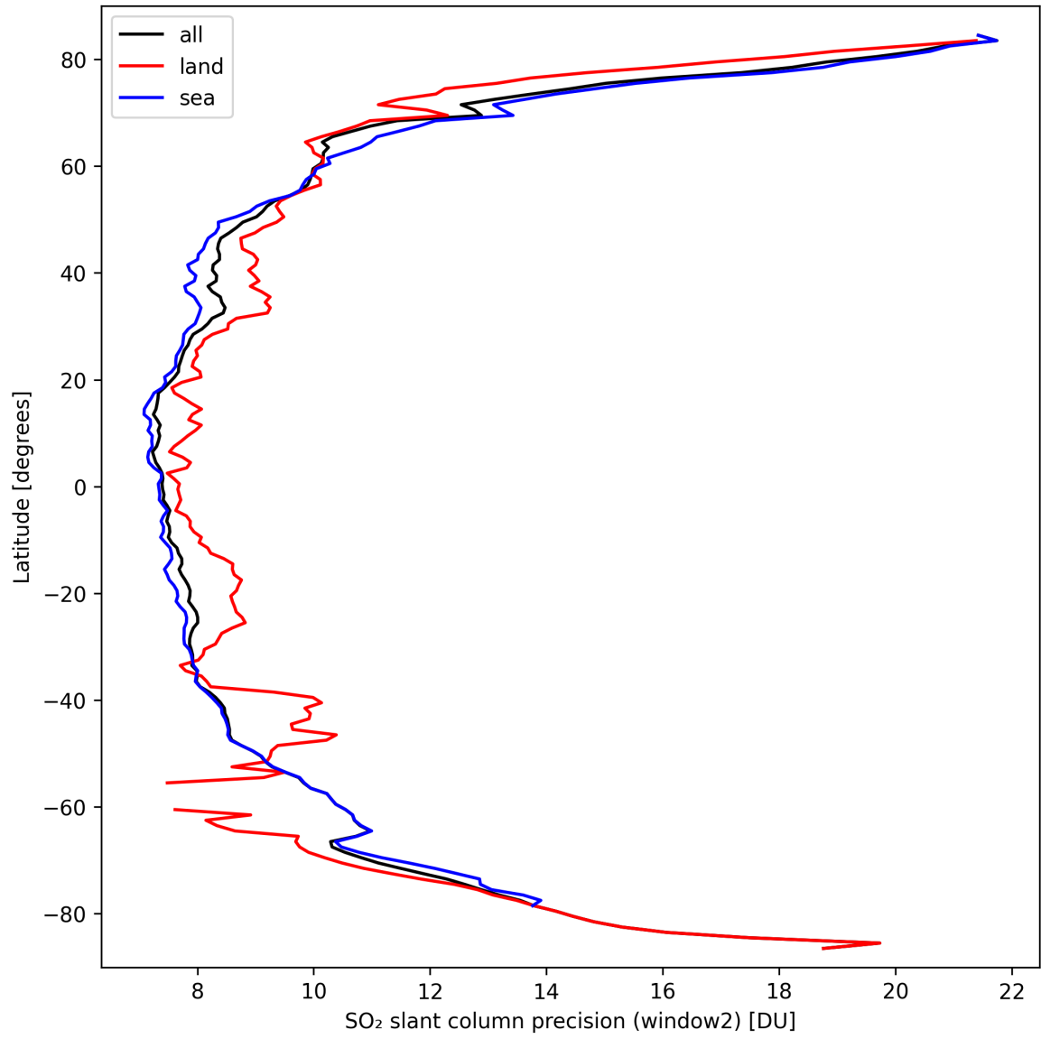
Figure 38: Zonal average of “SO 2 slant column precision (window2)” for 2024-09-24 to 2024-09-26.
