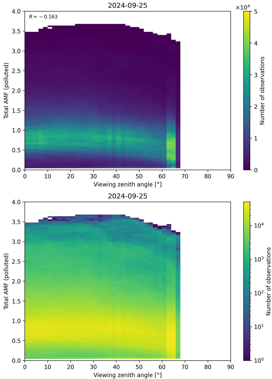
Figure 325: Scatter density plot of “Viewing zenith angle” against “Total AMF (polluted)” for 2024-09-24 to 2024-09-26.
