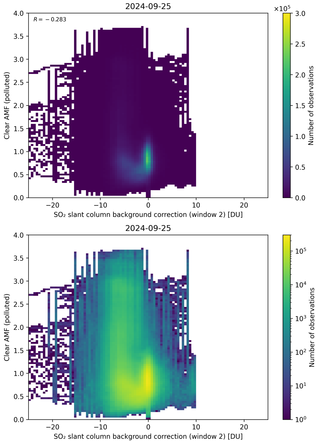
Figure 115: Scatter density plot of “SO 2 slant column background correction (window 2)” against “Clear AMF (polluted)” for 2024-09-24 to 2024-09-26.
