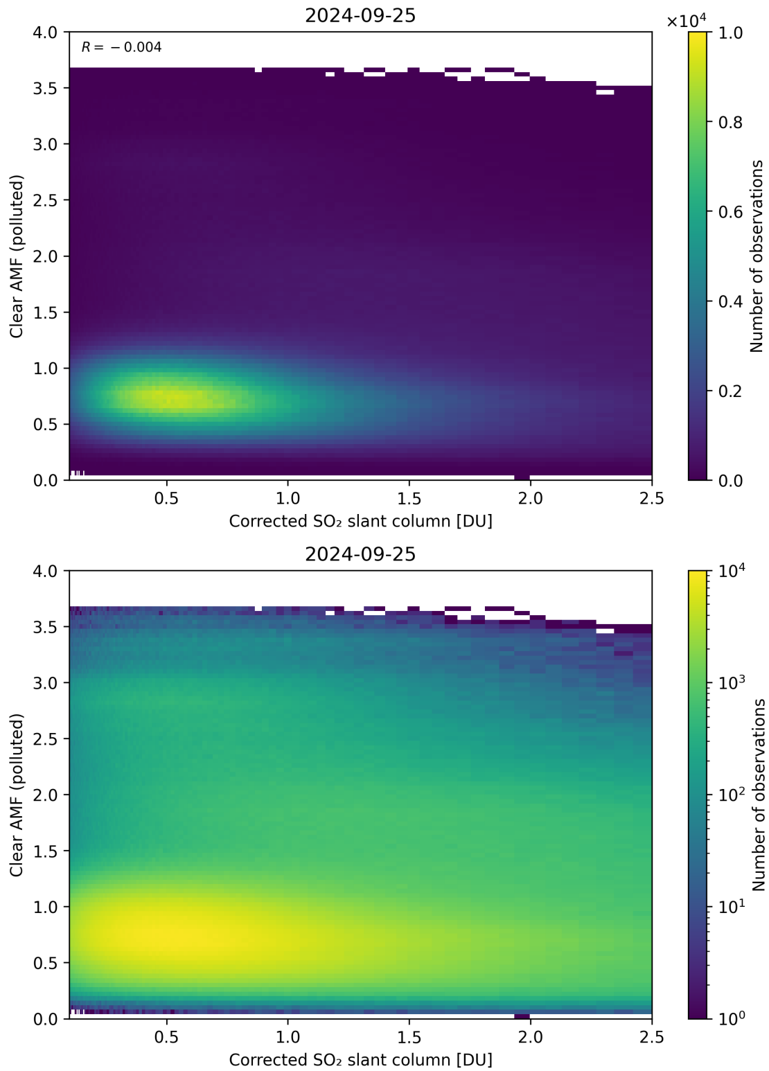
Figure 184: Scatter density plot of “Corrected SO 2 slant column” against “Clear AMF (polluted)” for 2024-09-24 to 2024-09-26.
