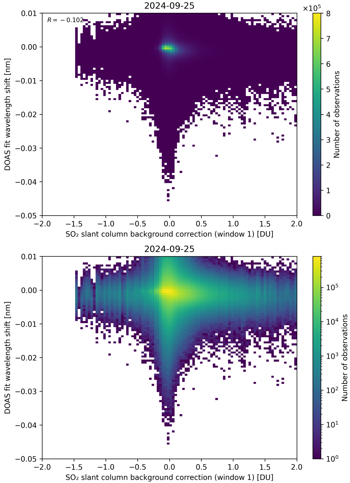
Figure 100: Scatter density plot of “SO 2 slant column background correction (window 1)” against “DOAS fit wavelength shift” for 2024-09-24 to 2024-09-26.
