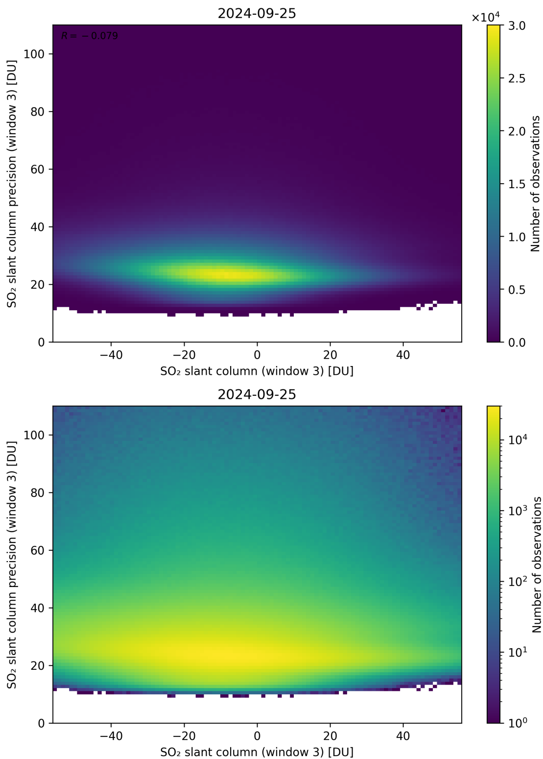
Figure 267: Scatter density plot of “SO 2 slant column (window 3)” against “SO 2 slant column precision (window 3)” for 2024-09-24 to 2024-09-26.
