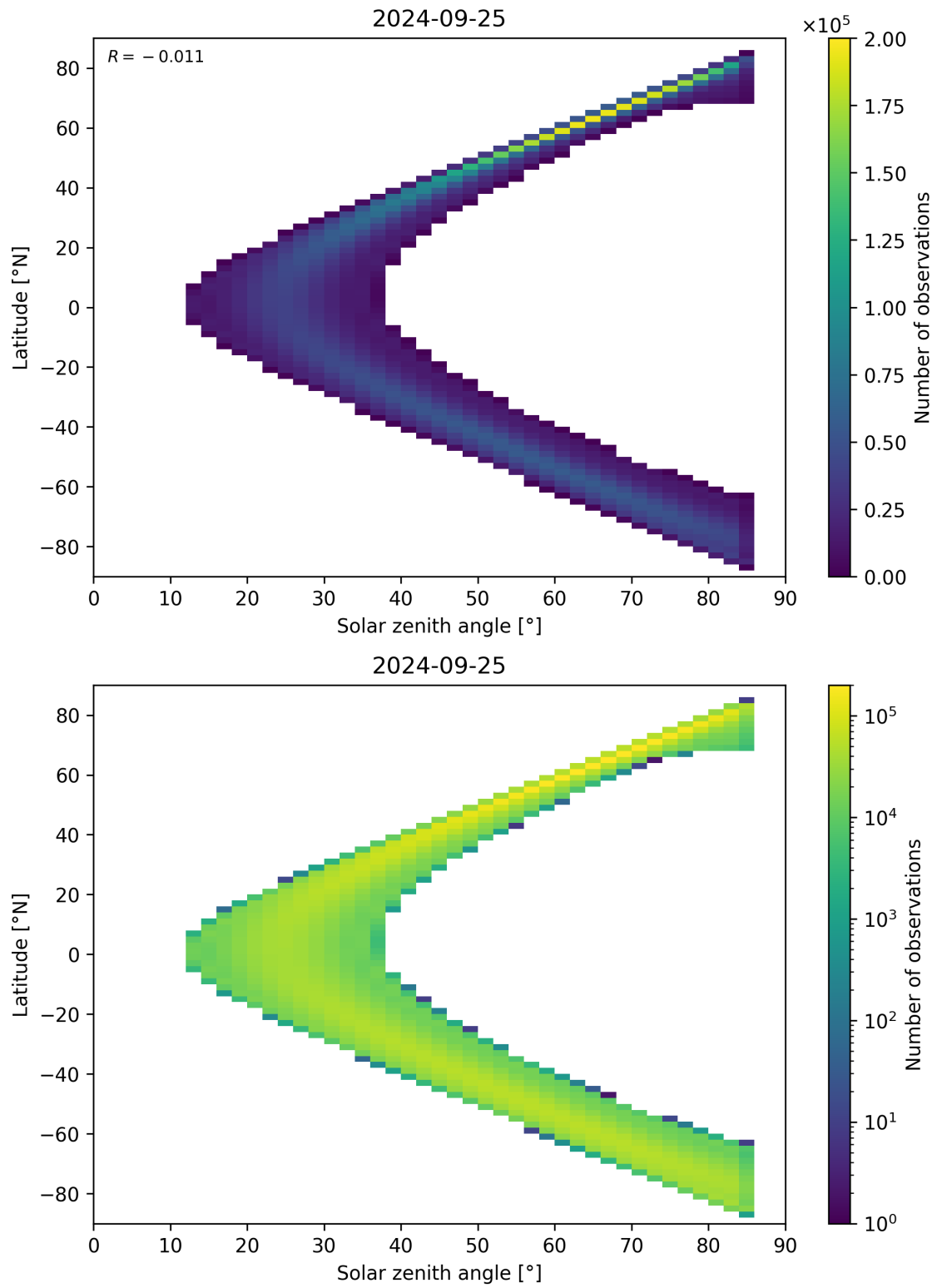
Figure 164: Scatter density plot of “Solar zenith angle” against “Latitude” for 2024-09-24 to 2024-09-26.
