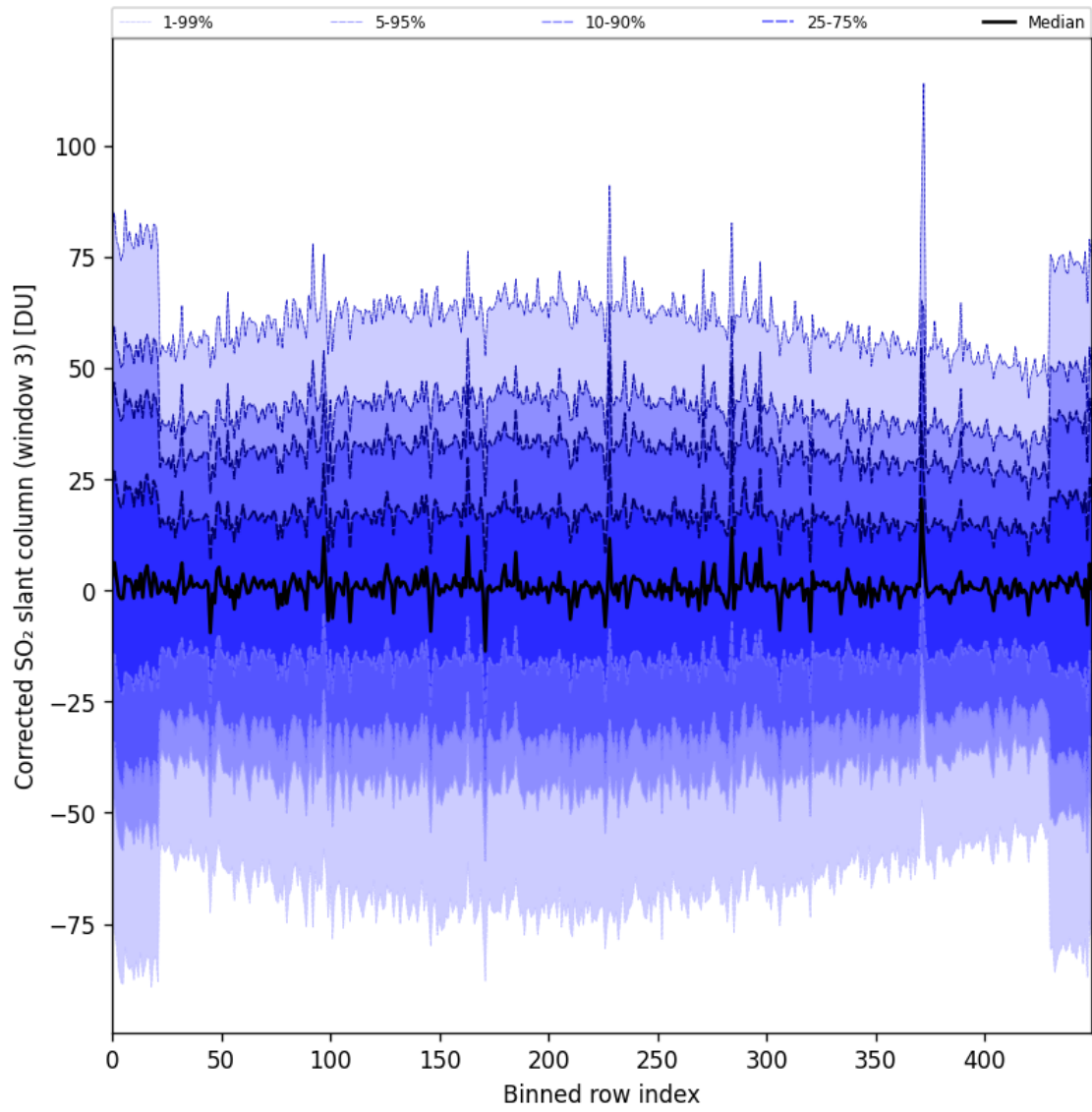
Figure 89: Along track statistics of “Corrected SO 2 slant column (window 3)” for 2024-09-24 to 2024-09-26
