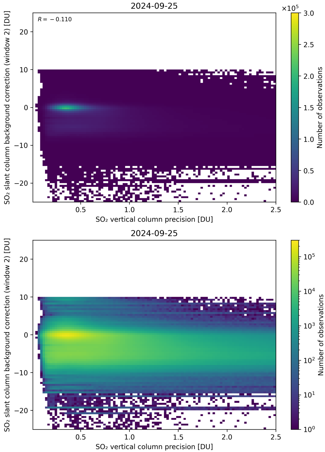
Figure 280: Scatter density plot of “SO 2 vertical column precision” against “SO 2 slant column background correction (window 2)” for 2024-09-24 to 2024-09-26.
