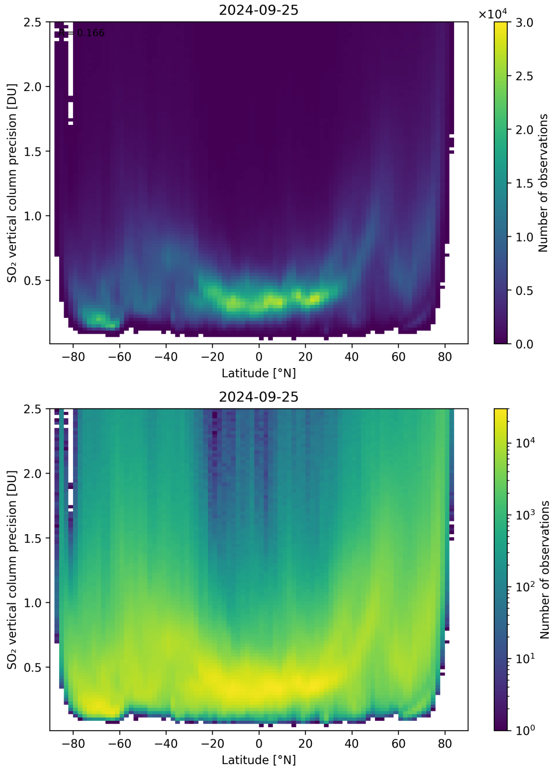
Figure 157: Scatter density plot of “Latitude” against “SO 2 vertical column precision” for 2024-09-24 to 2024-09-26.
