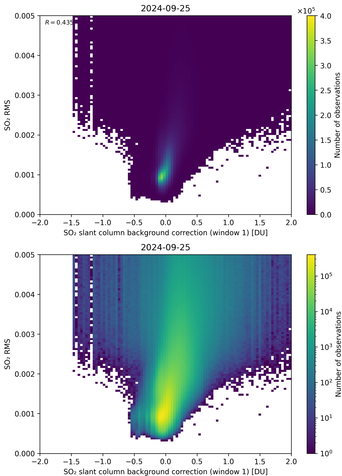
Figure 102: Scatter density plot of “SO 2 slant column background correction (window 1)” against “SO 2 RMS” for 2024-09-24 to 2024-09-26.
