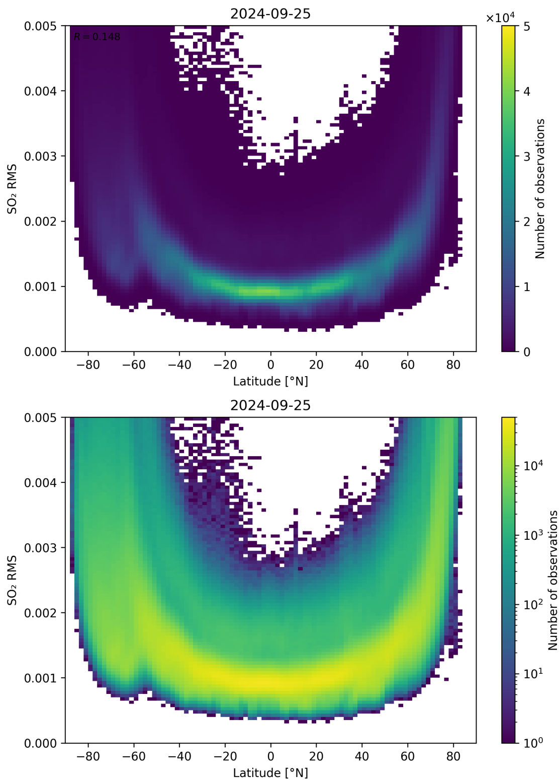
Figure 144: Scatter density plot of “Latitude” against “SO 2 RMS” for 2024-09-24 to 2024-09-26.
