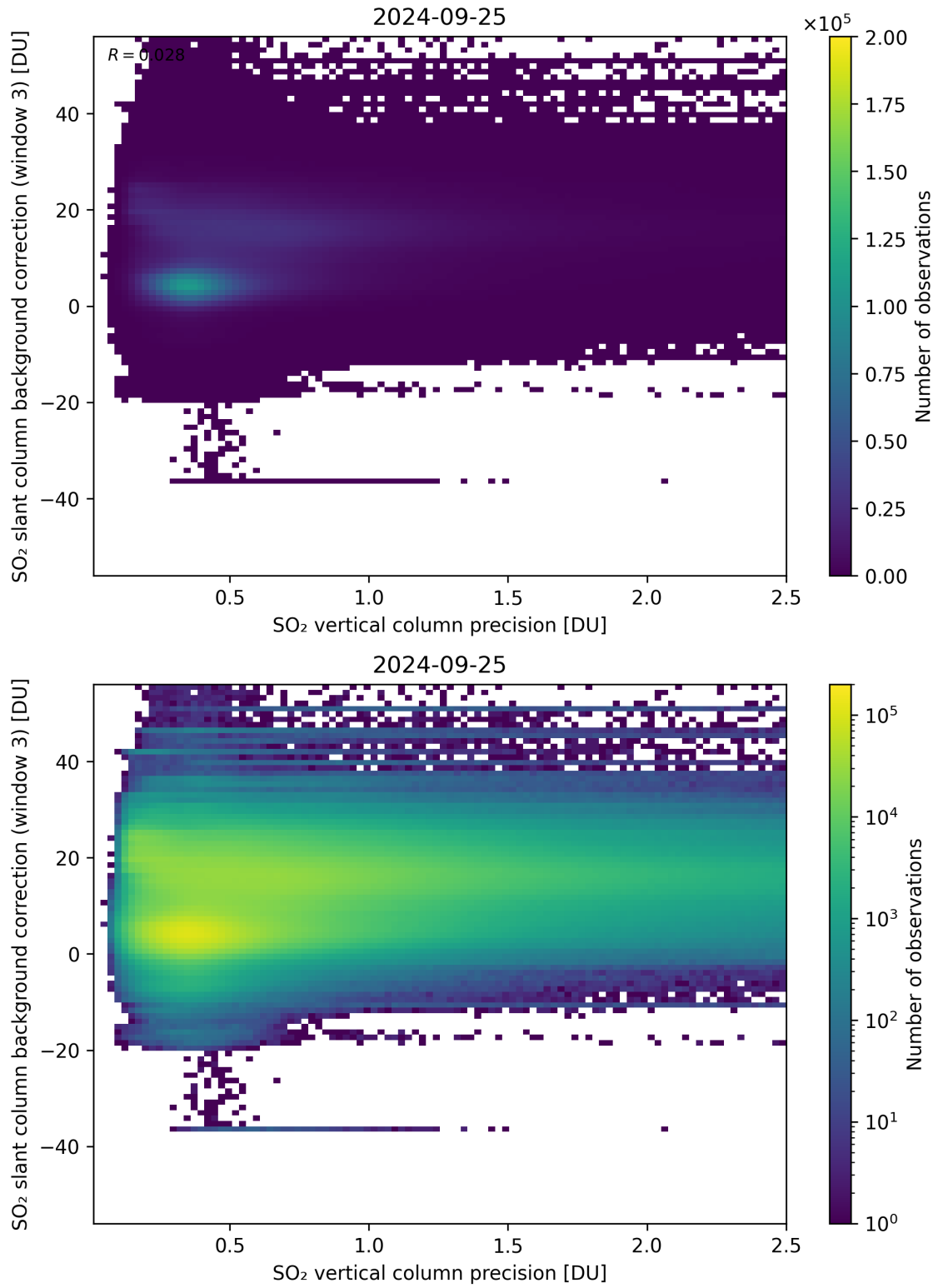
Figure 281: Scatter density plot of “SO 2 vertical column precision” against “SO 2 slant column background correction (window 3)” for 2024-09-24 to 2024-09-26.
