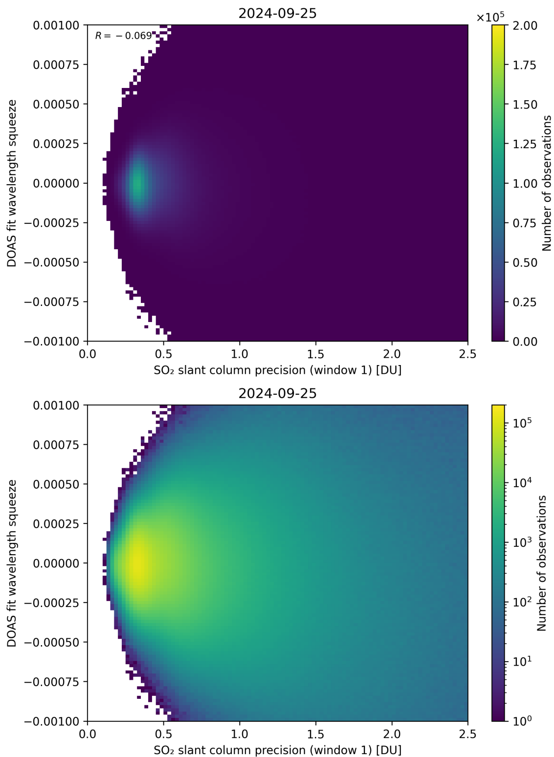
Figure 222: Scatter density plot of “SO 2 slant column precision (window 1)” against “DOAS fit wavelength squeeze” for 2024-09-24 to 2024-09-26.
