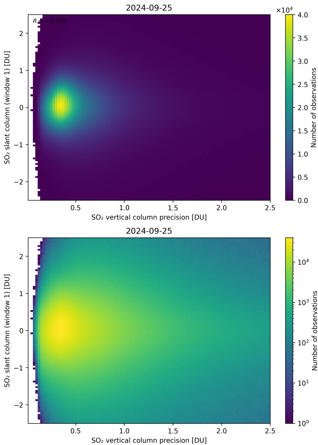
Figure 289: Scatter density plot of “SO 2 vertical column precision” against “SO 2 slant column (window 1)” for 2024-09-24 to 2024-09-26.
