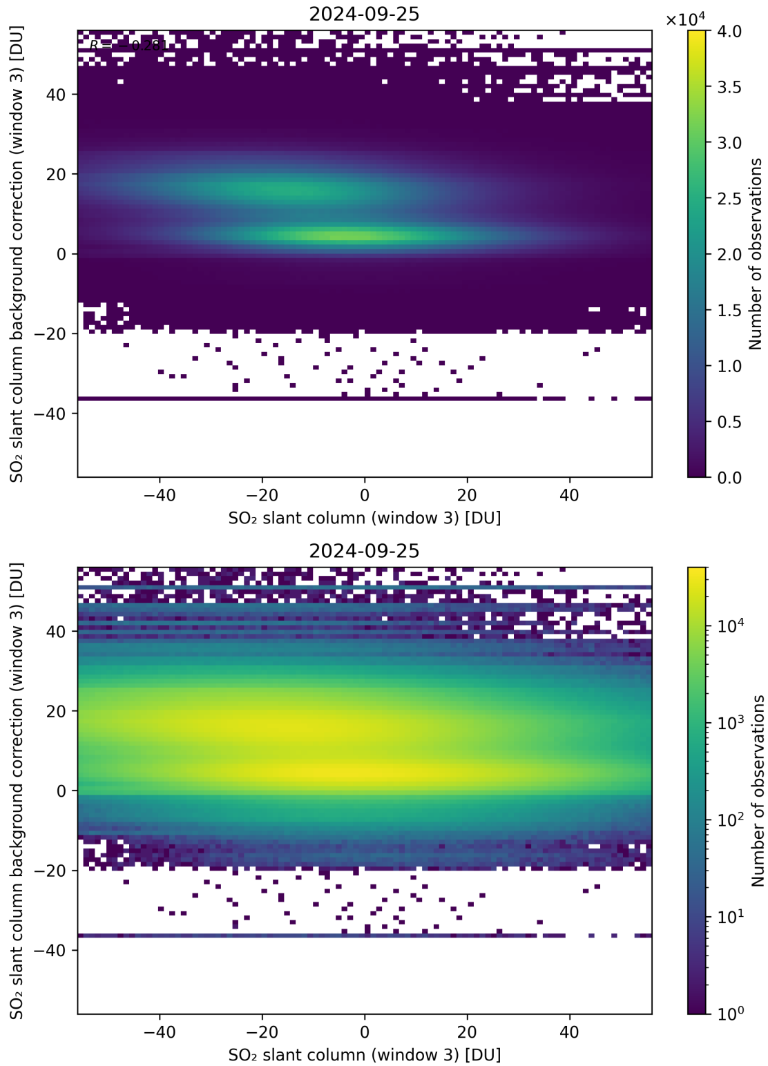
Figure 253: Scatter density plot of “SO 2 slant column (window 3)” against “SO 2 slant column background correction (window 3)” for 2024-09-24 to 2024-09-26.
