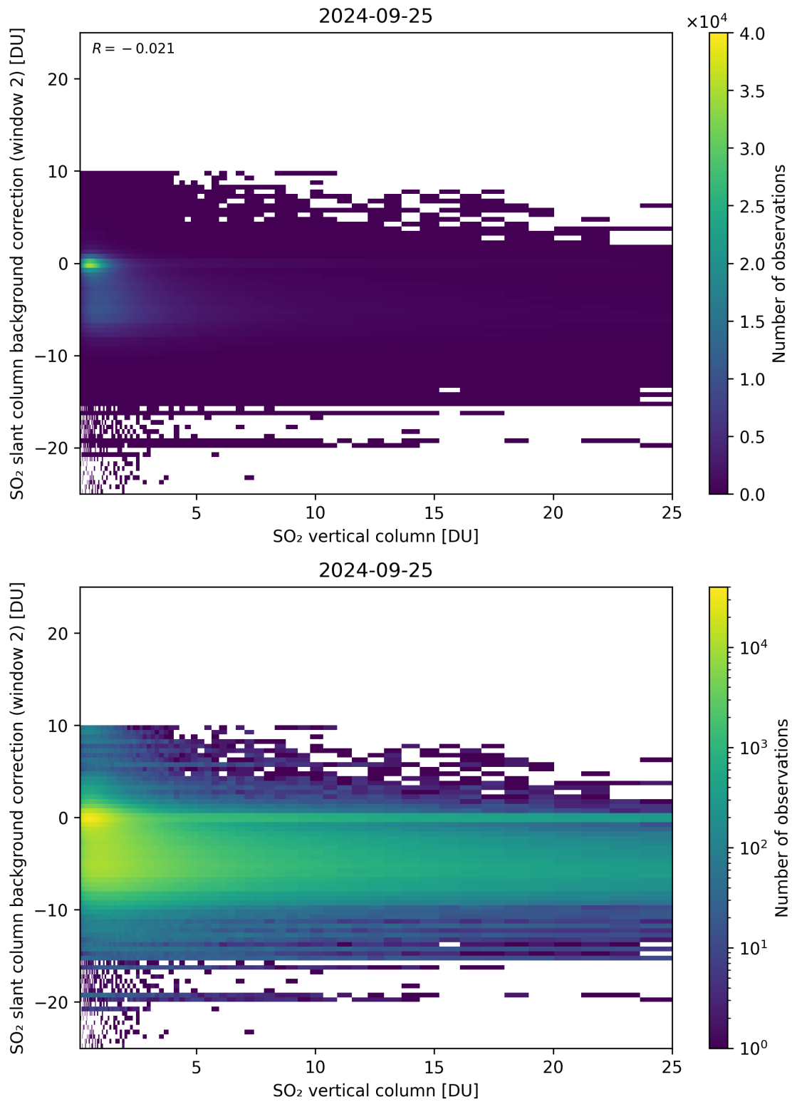
Figure 274: Scatter density plot of “SO 2 vertical column” against “SO 2 slant column background correction (window 2)” for 2024-09-24 to 2024-09-26.
