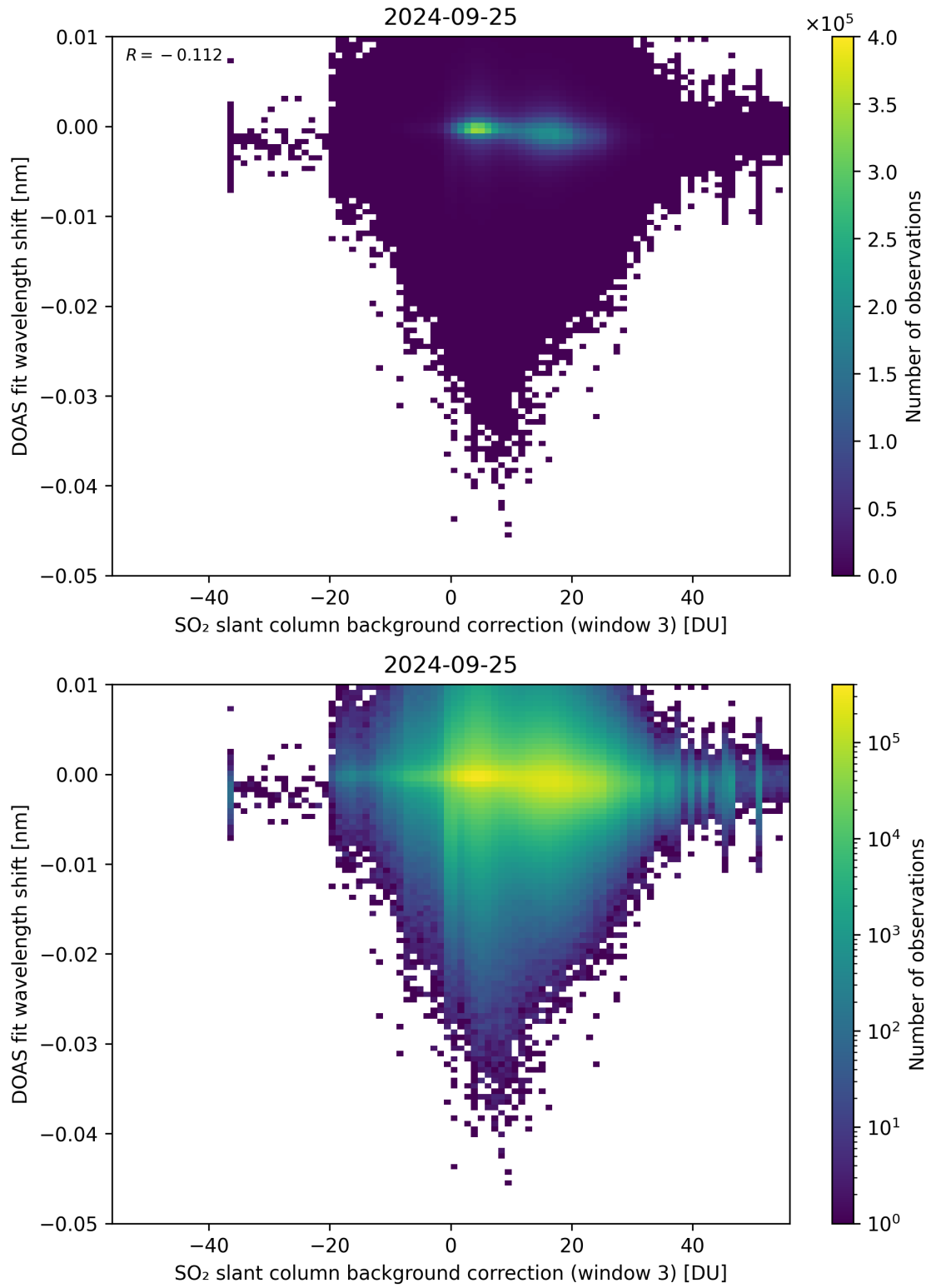
Figure 121: Scatter density plot of “SO 2 slant column background correction (window 3)” against “DOAS fit wavelength shift” for 2024-09-24 to 2024-09-26.
