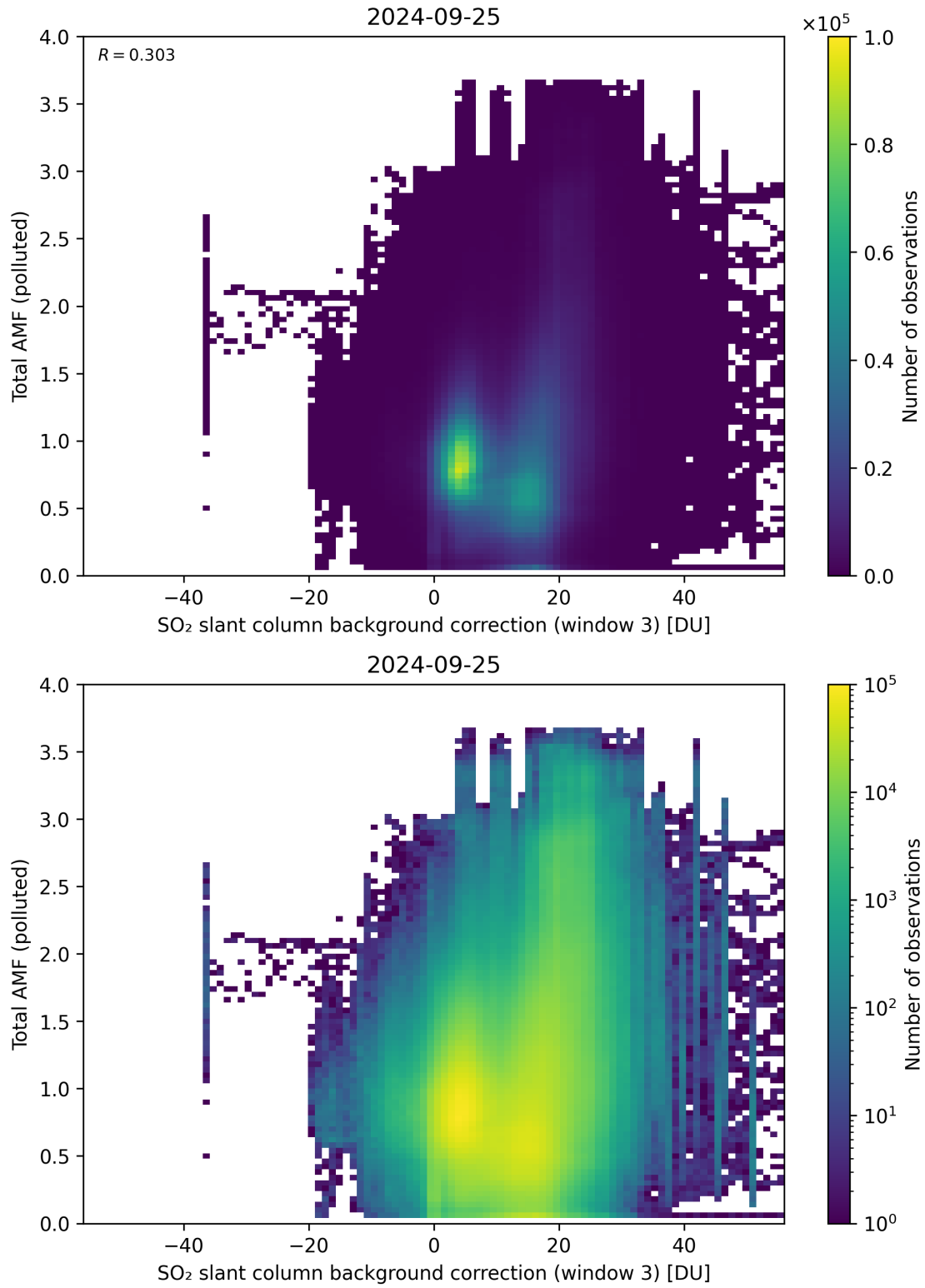
Figure 125: Scatter density plot of “SO 2 slant column background correction (window 3)” against “Total AMF (polluted)” for 2024-09-24 to 2024-09-26.
