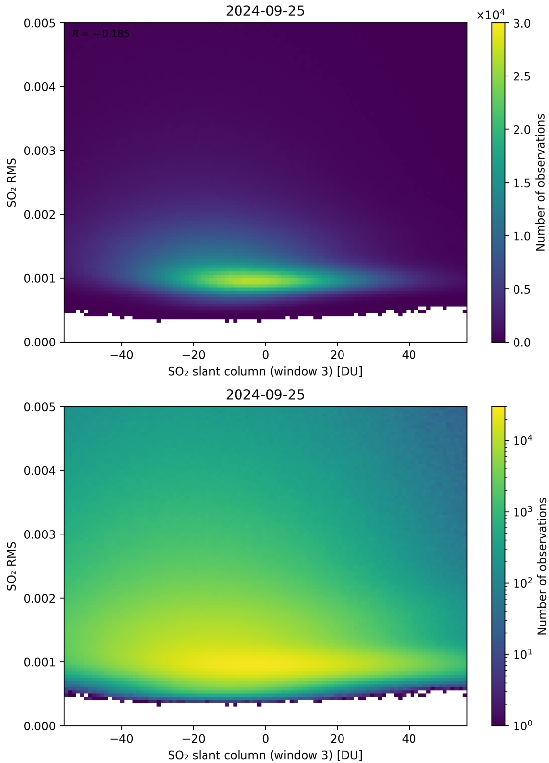
Figure 256: Scatter density plot of “SO 2 slant column (window 3)” against “SO 2 RMS” for 2024-09-24 to 2024-09-26.
