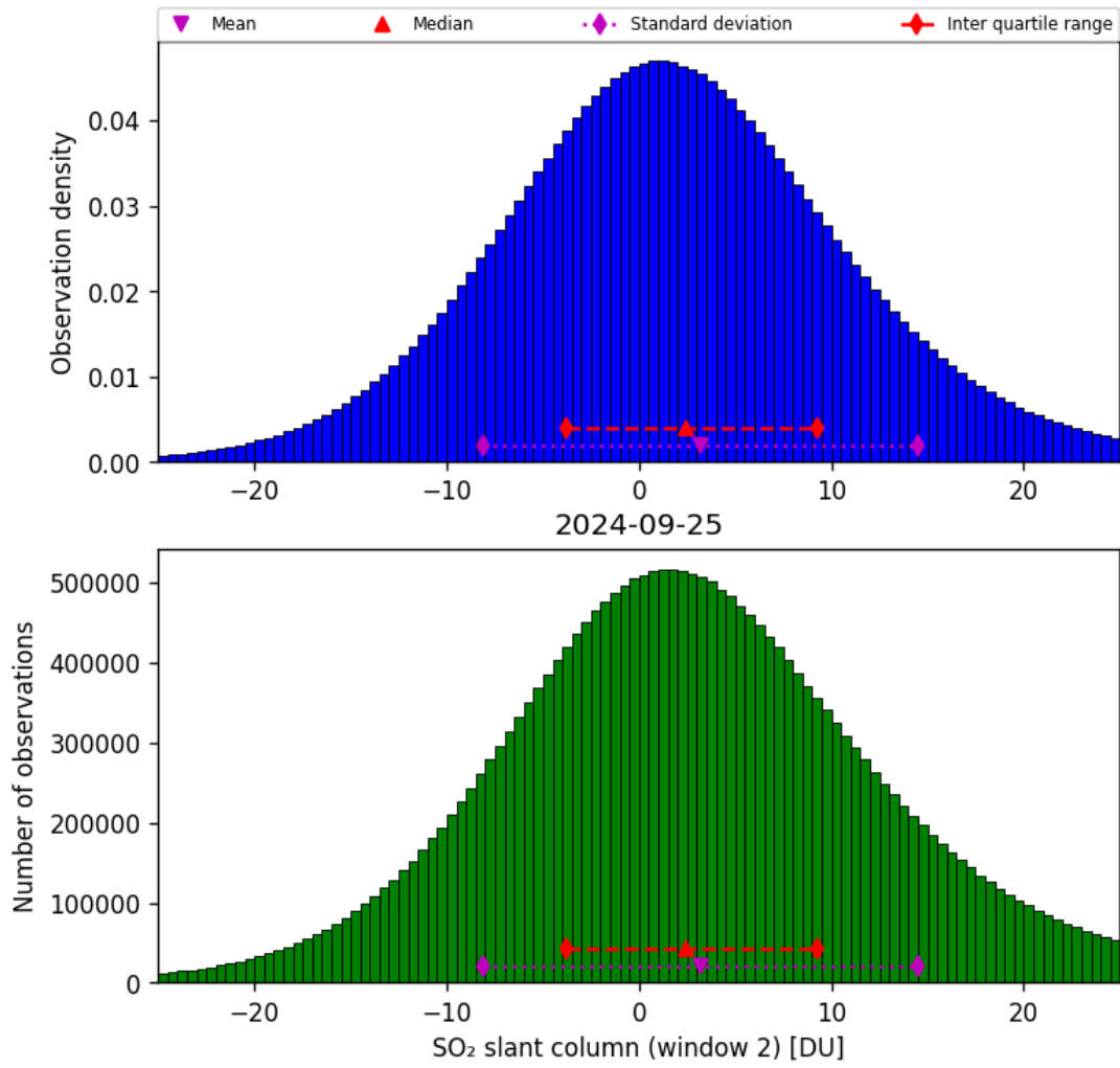
Figure 60: Histogram of “SO 2 slant column (window 2)” for 2024-09-24 to 2024-09-26
