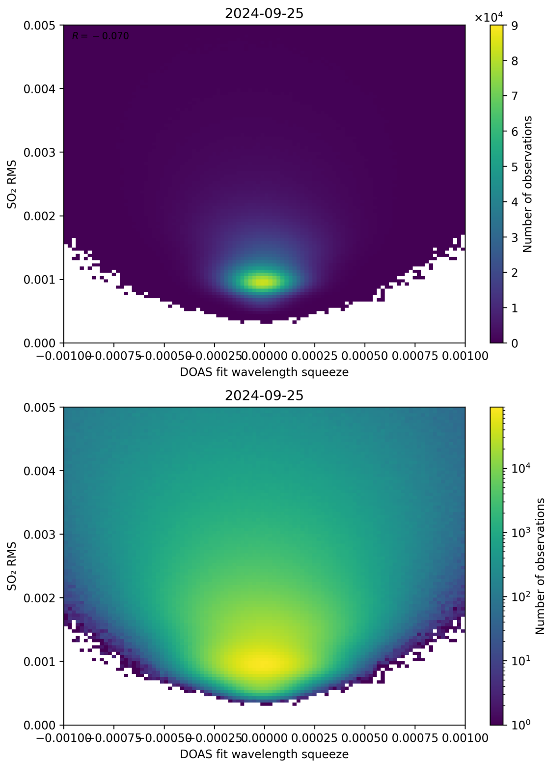
Figure 132: Scatter density plot of “DOAS fit wavelength squeeze” against “SO 2 RMS” for 2024-09-24 to 2024-09-26.
