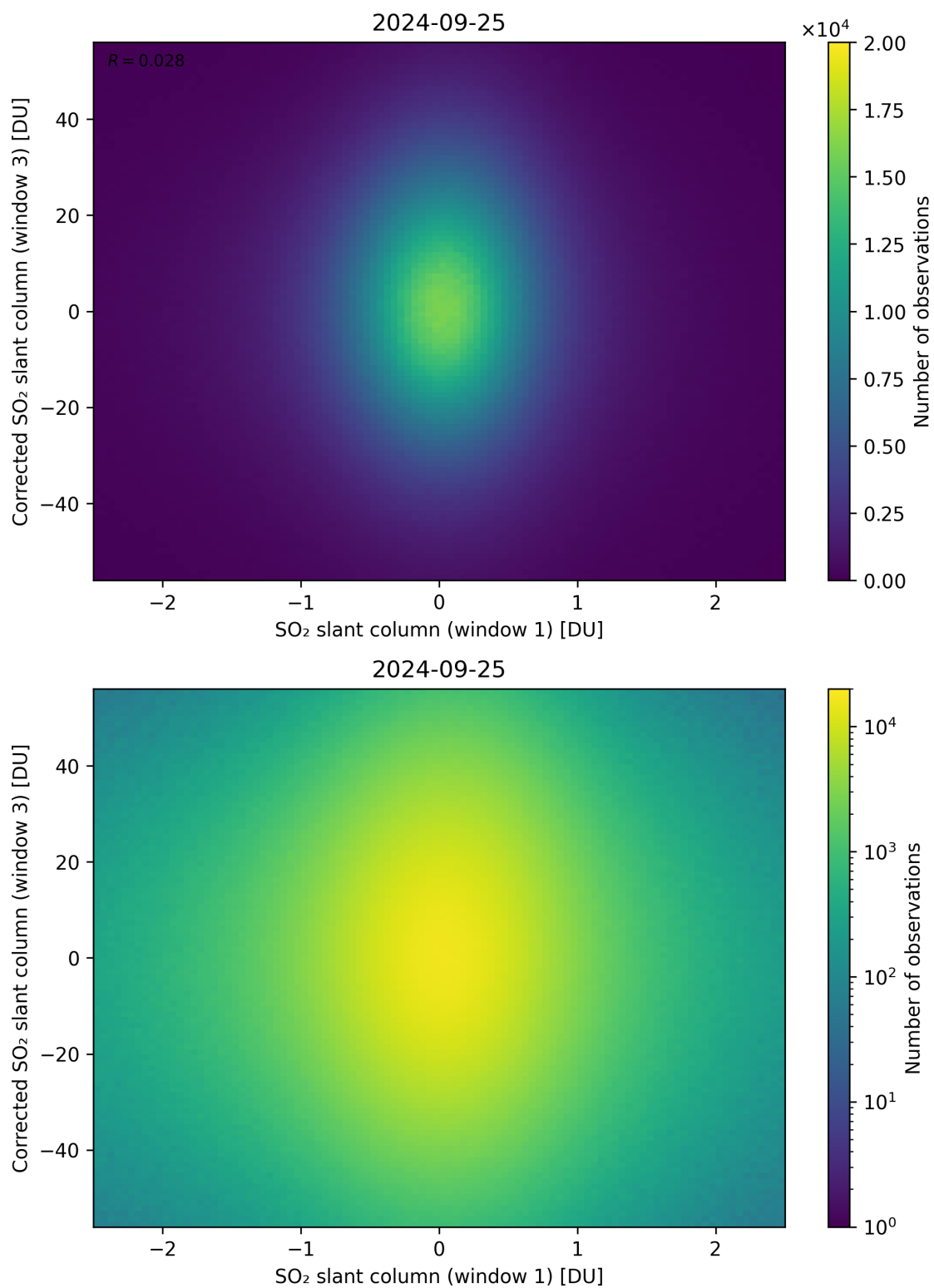
Figure 234: Scatter density plot of “SO 2 slant column (window 1)” against “Corrected SO 2 slant column (window 3)” for 2024-09-24 to 2024-09-26.
