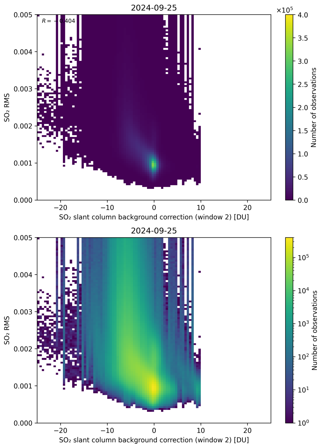
Figure 114: Scatter density plot of “SO 2 slant column background correction (window 2)” against “SO 2 RMS” for 2024-09-24 to 2024-09-26.
