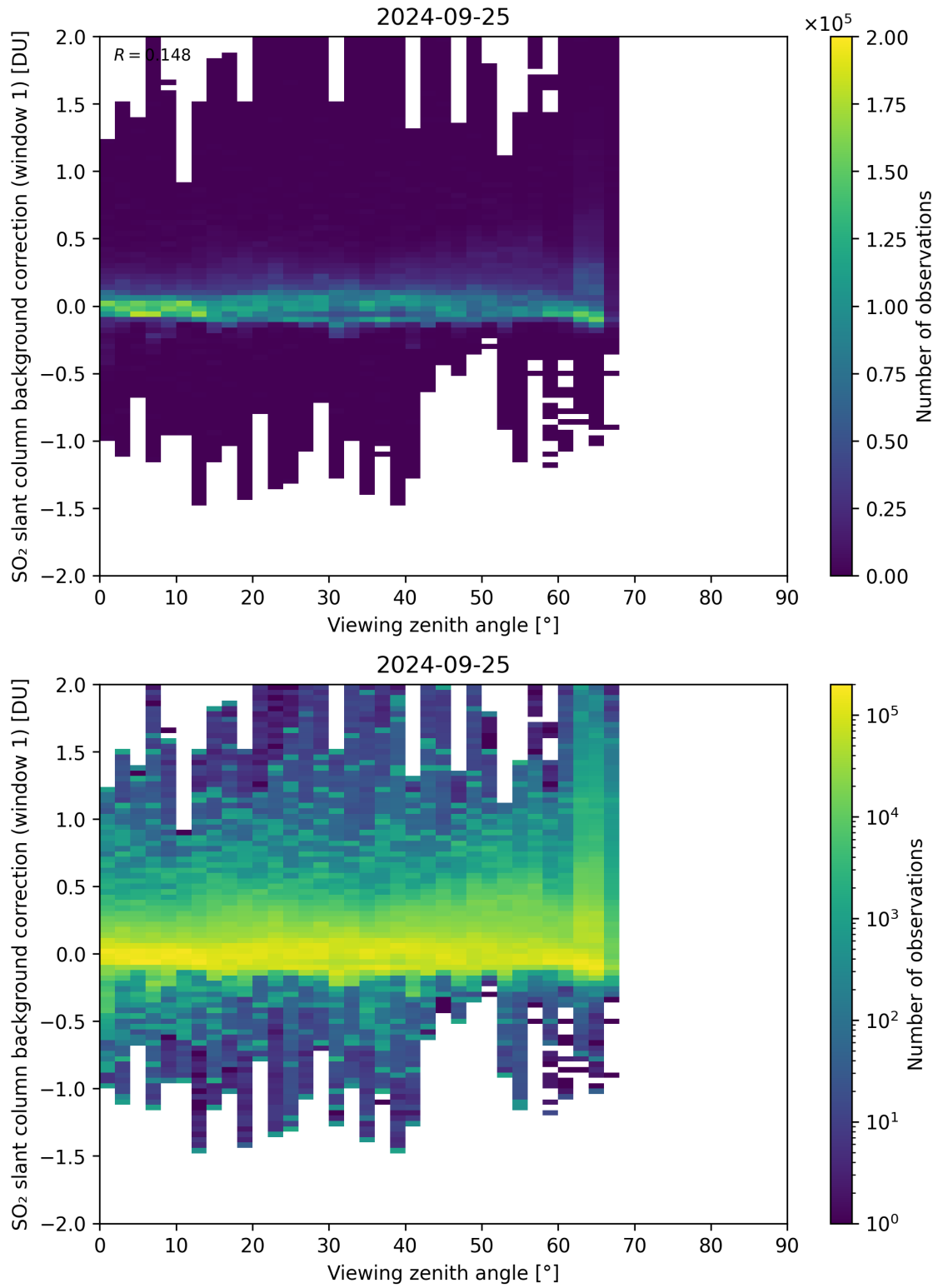
Figure 308: Scatter density plot of “Viewing zenith angle” against “SO 2 slant column background correction (window 1)” for 2024-09-24 to 2024-09-26.
