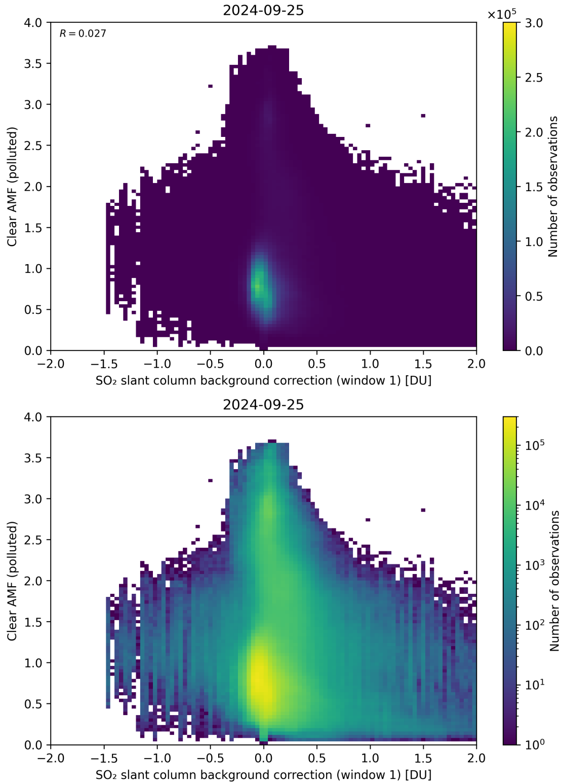
Figure 103: Scatter density plot of “SO 2 slant column background correction (window 1)” against “Clear AMF (polluted)” for 2024-09-24 to 2024-09-26.
