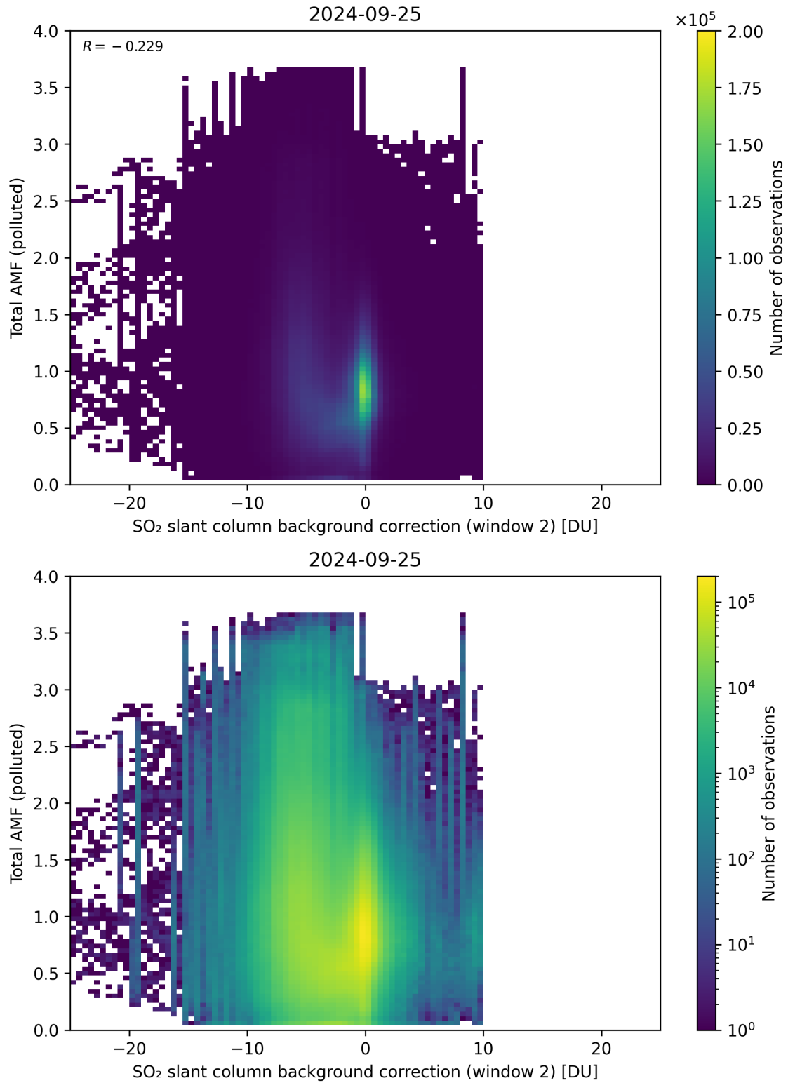
Figure 119: Scatter density plot of “SO 2 slant column background correction (window 2)” against “Total AMF (polluted)” for 2024-09-24 to 2024-09-26.
