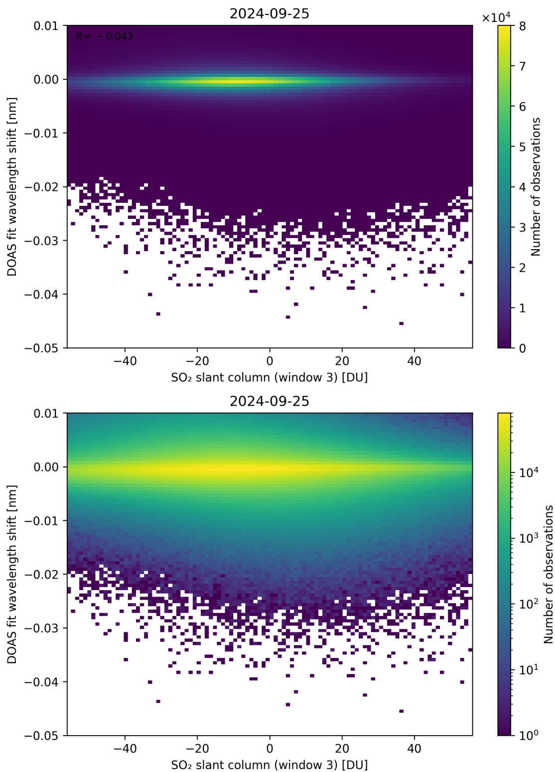
Figure 254: Scatter density plot of “SO 2 slant column (window 3)” against “DOAS fit wavelength shift” for 2024-09-24 to 2024-09-26.
