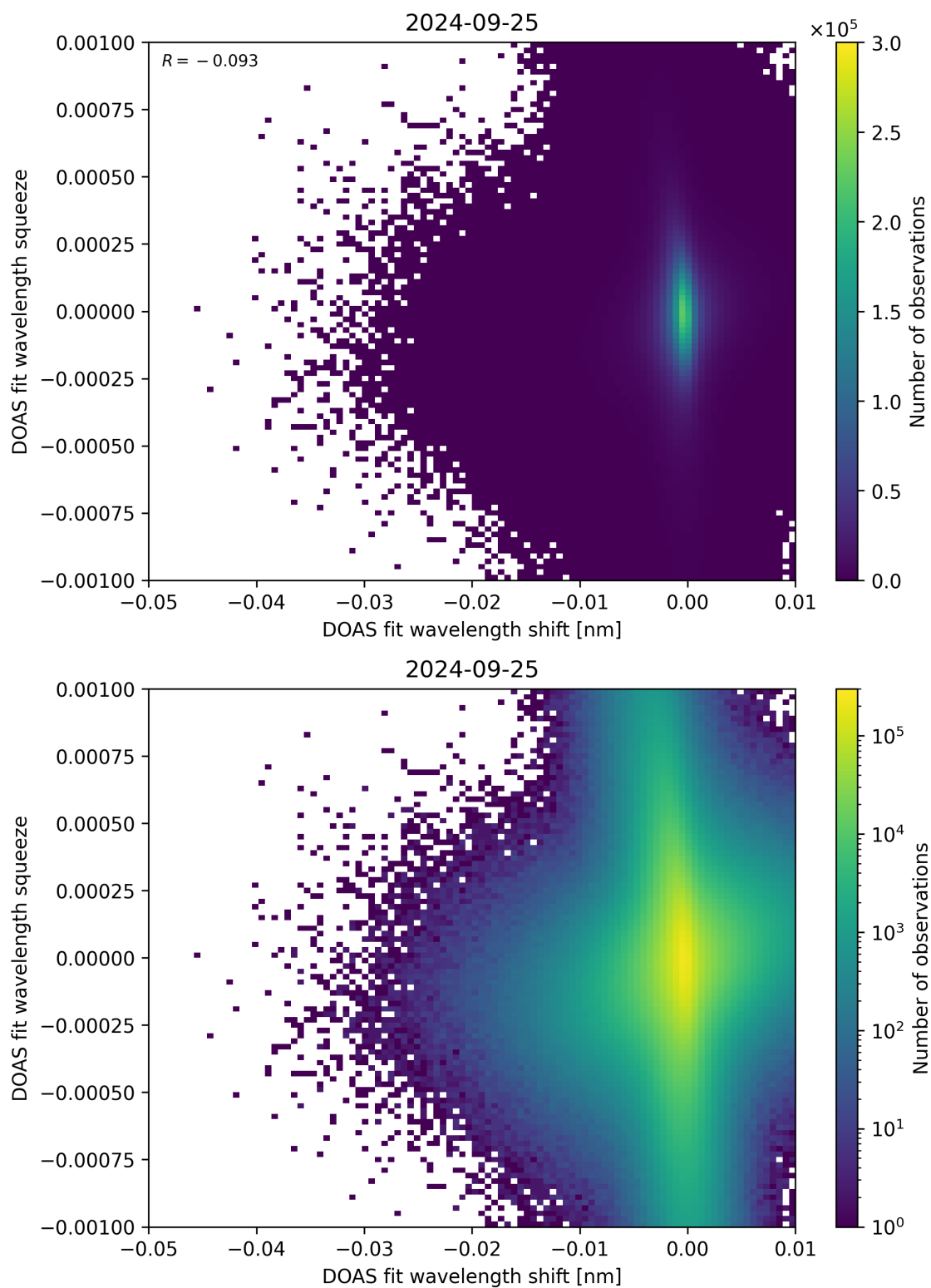
Figure 127: Scatter density plot of “DOAS fit wavelength shift” against “DOAS fit wavelength squeeze” for 2024-09-24 to 2024-09-26.
