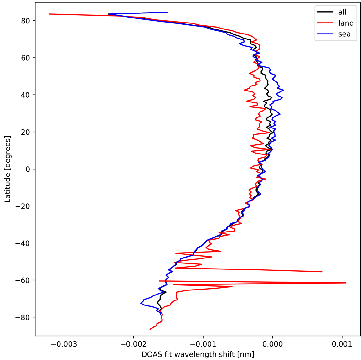
Figure 45: Zonal average of “DOAS fit wavelength shift” for 2024-09-24 to 2024-09-26.
