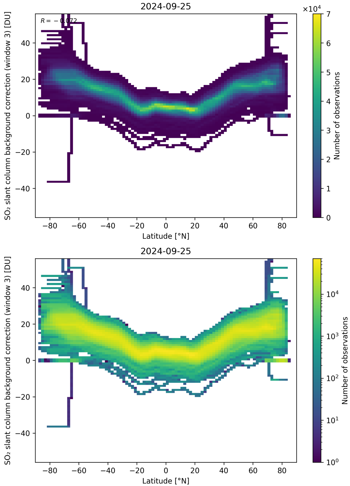
Figure 141: Scatter density plot of “Latitude” against “SO 2 slant column background correction (window 3)” for 2024-09-24 to 2024-09-26.
