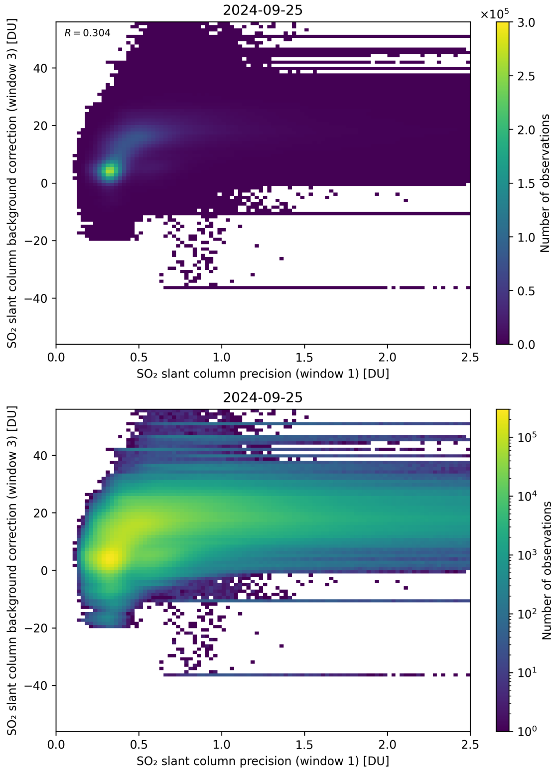
Figure 220: Scatter density plot of “SO 2 slant column precision (window 1)” against “SO 2 slant column background correction (window 3)” for 2024-09-24 to 2024-09-26.
