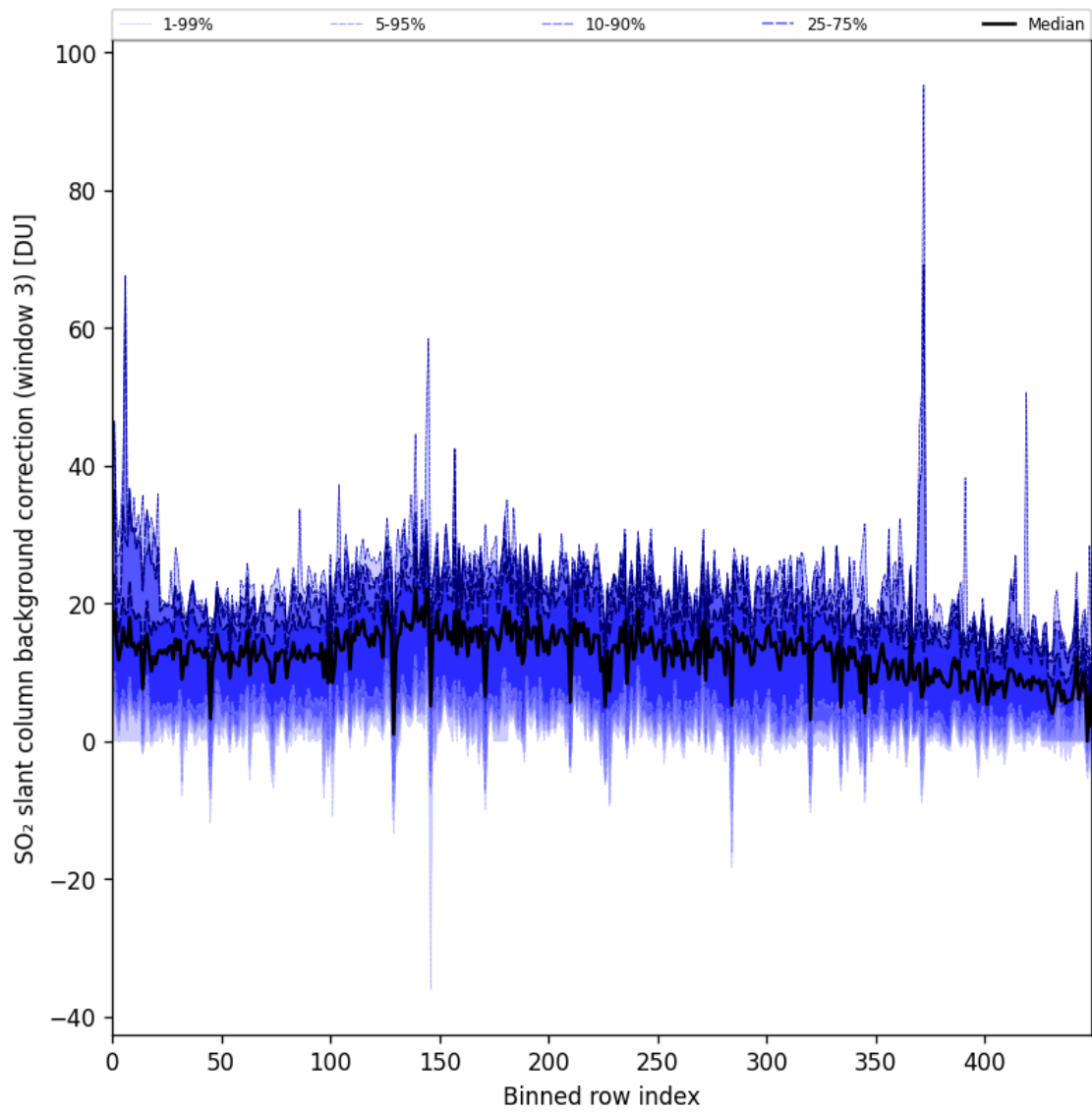
Figure 90: Along track statistics of “SO 2 slant column background correction (window 3)” for 2024-09-24 to 2024-09-26
