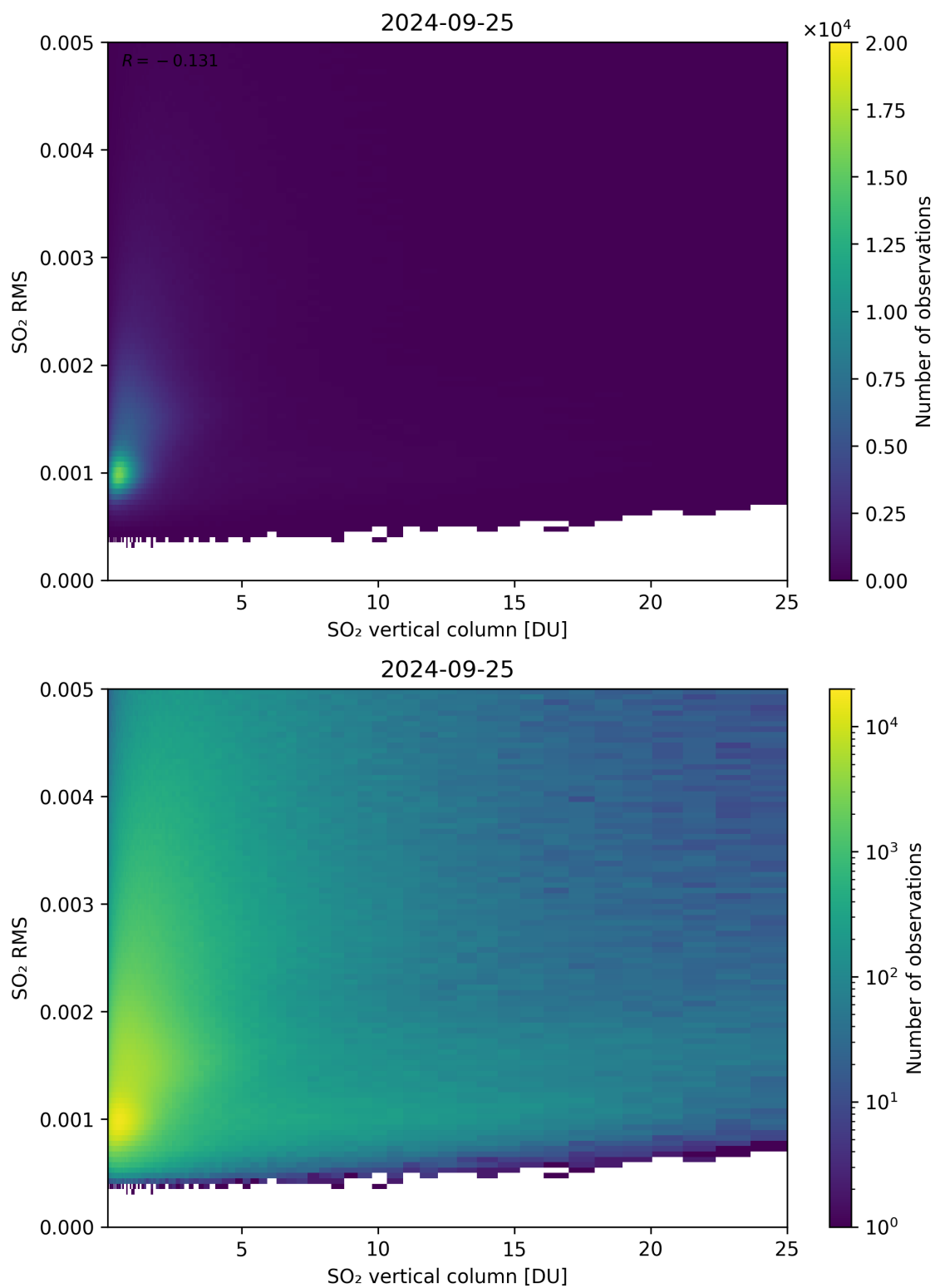
Figure 278: Scatter density plot of “SO 2 vertical column” against “SO 2 RMS” for 2024-09-24 to 2024-09-26.
