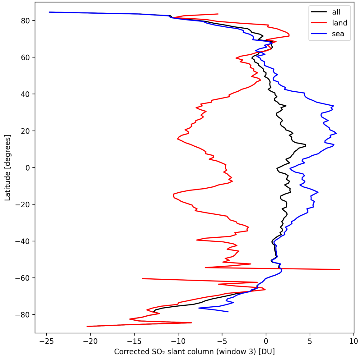
Figure 43: Zonal average of “Corrected SO 2 slant column (window 3)” for 2024-09-24 to 2024-09-26.
