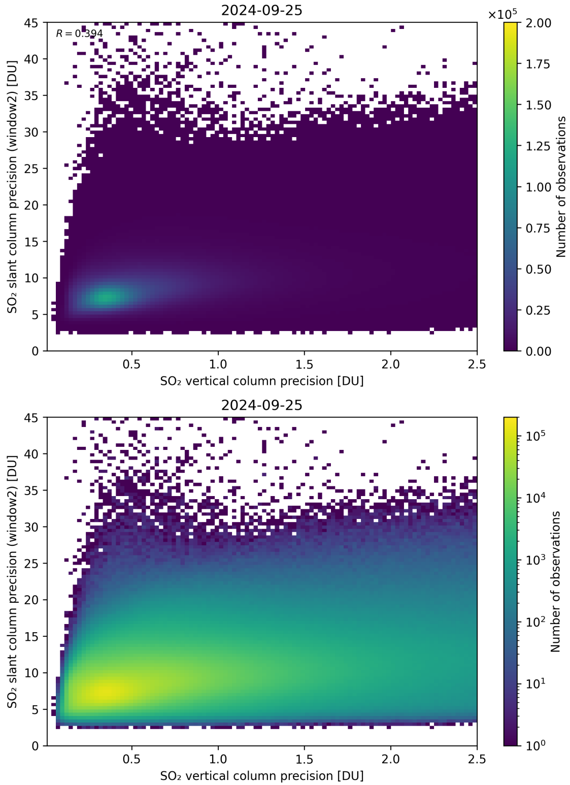
Figure 291: Scatter density plot of “SO 2 vertical column precision” against “SO 2 slant column precision (window2)” for 2024-09-24 to 2024-09-26.
