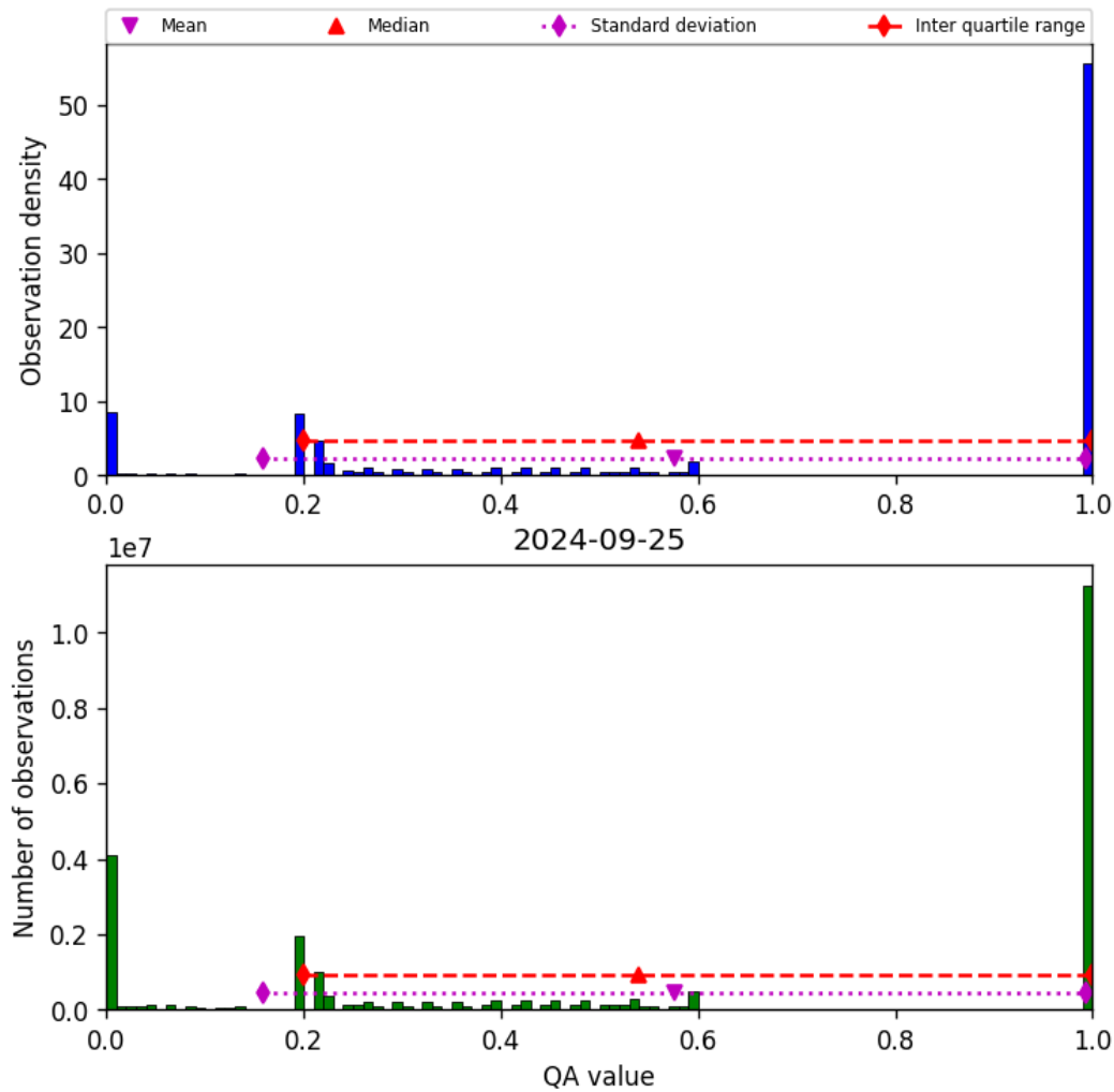
Figure 52: Histogram of “QA value” for 2024-09-24 to 2024-09-26
