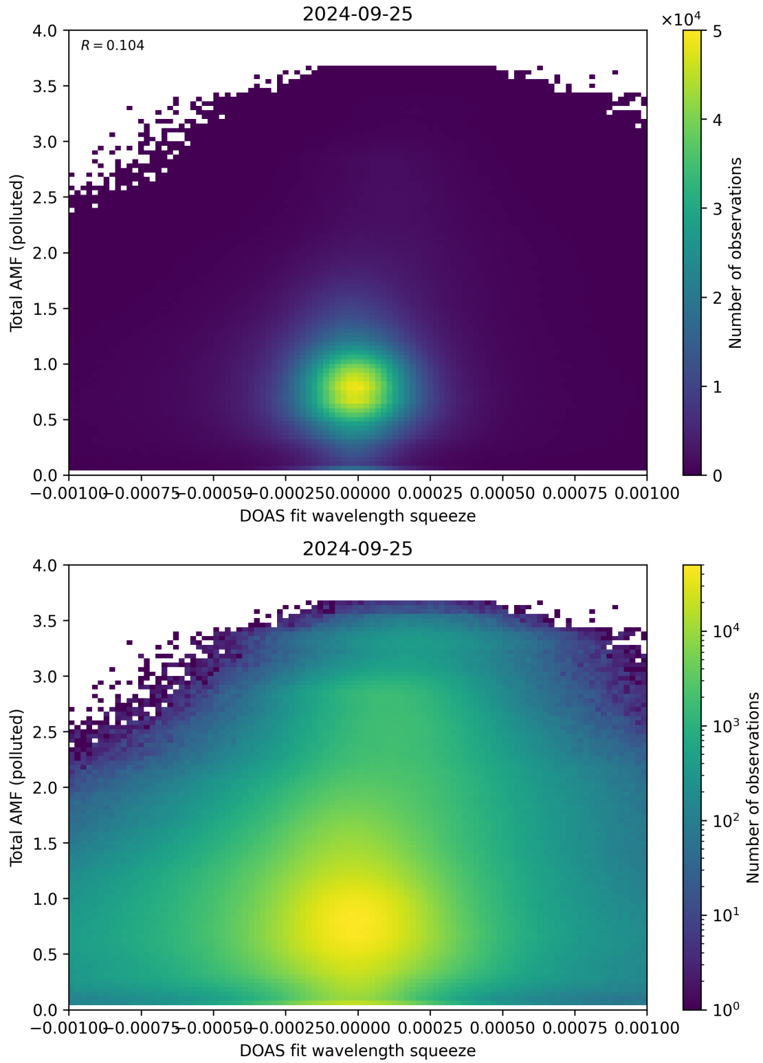
Figure 134: Scatter density plot of “DOAS fit wavelength squeeze” against “Total AMF (polluted)” for 2024-09-24 to 2024-09-26.
