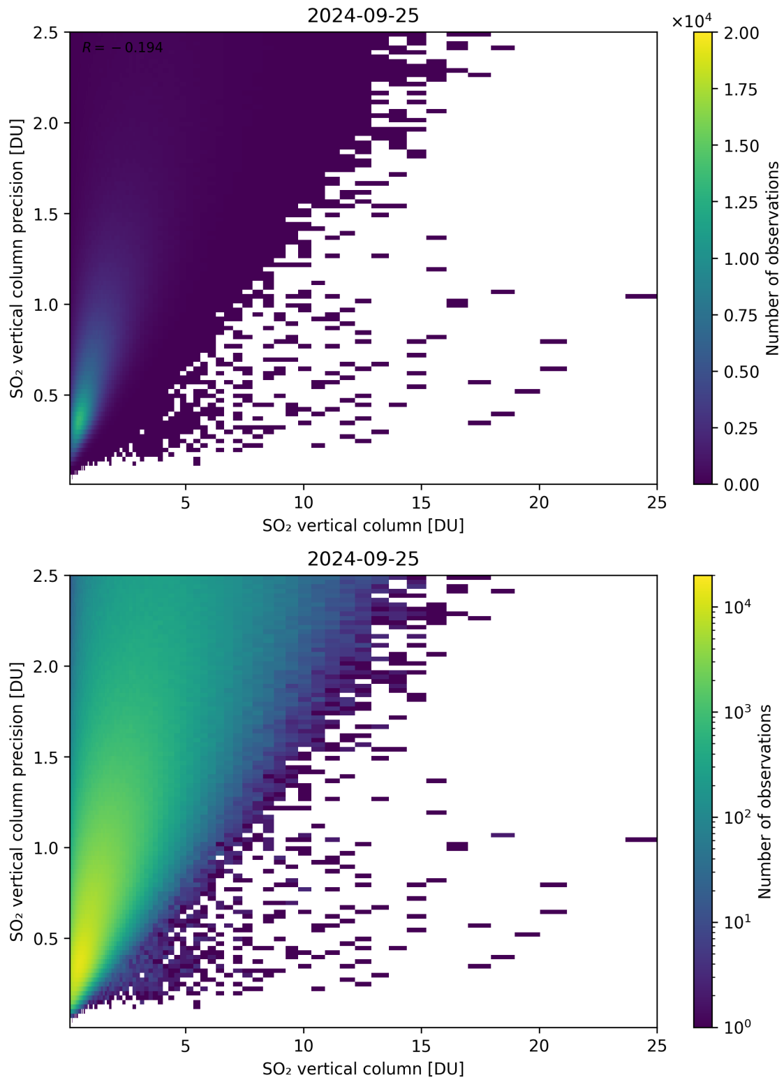
Figure 307: Scatter density plot of “SO 2 vertical column” against “SO 2 vertical column precision” for 2024-09-24 to 2024-09-26.
