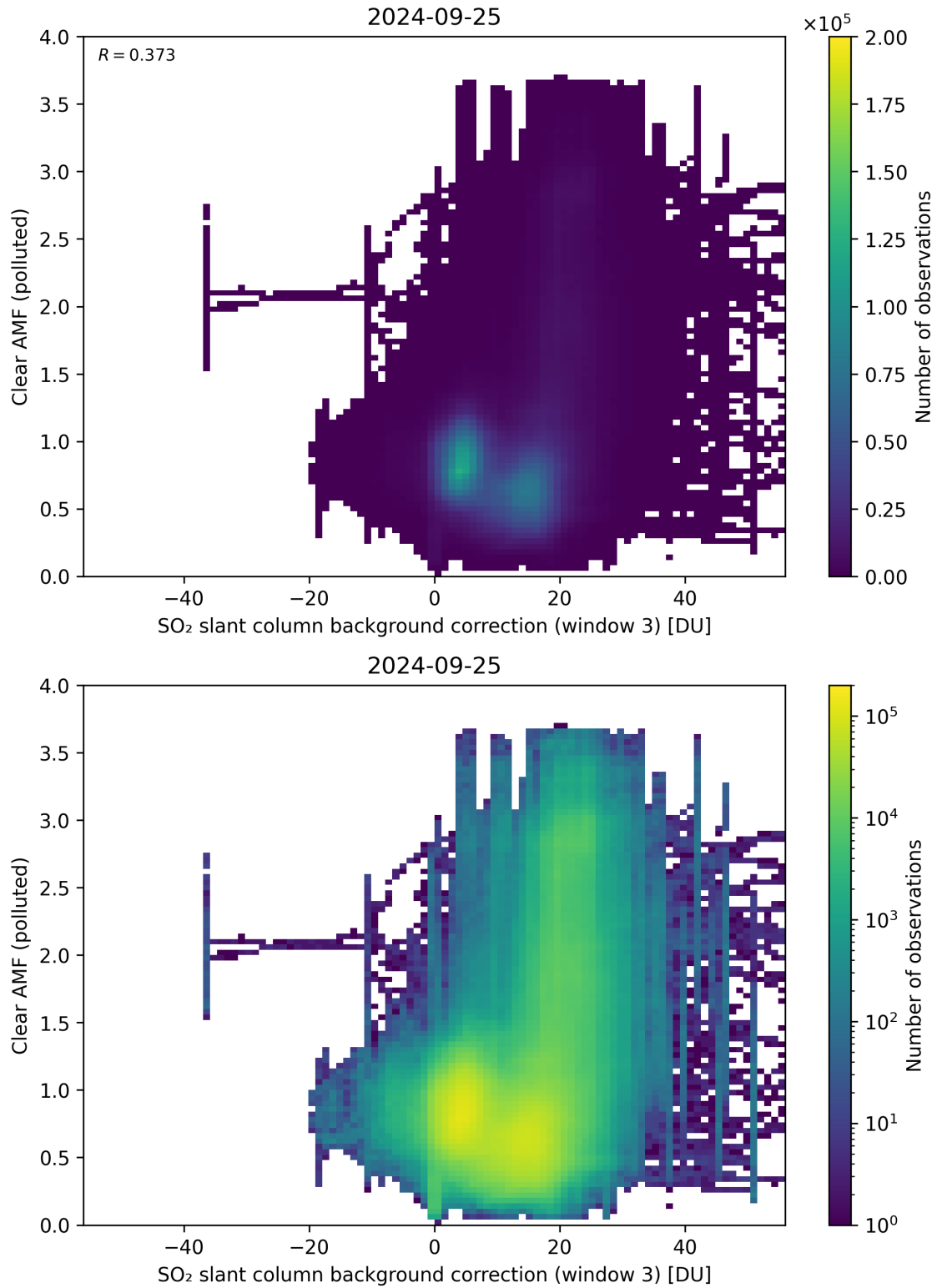
Figure 124: Scatter density plot of “SO 2 slant column background correction (window 3)” against “Clear AMF (polluted)” for 2024-09-24 to 2024-09-26.
