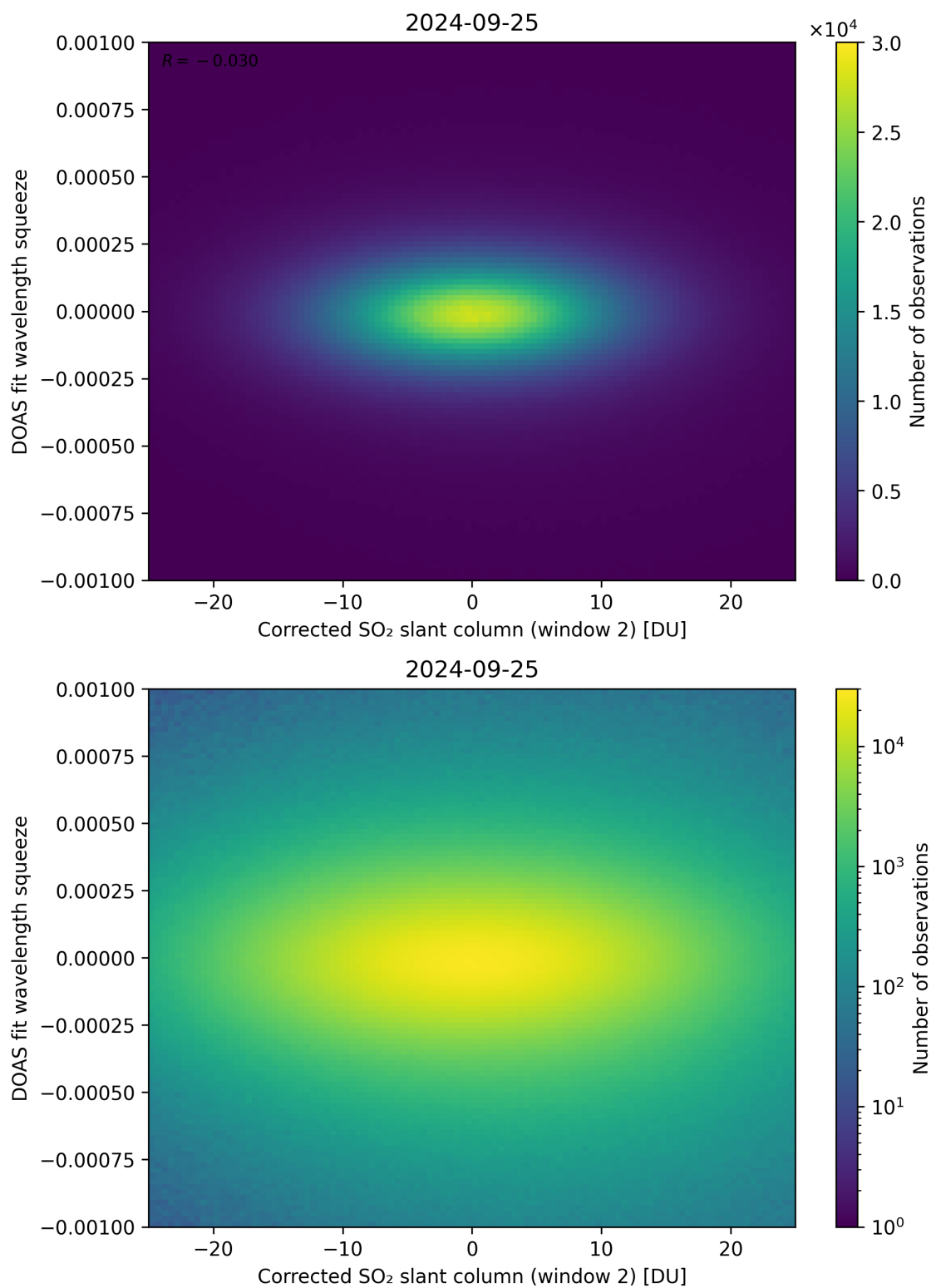
Figure 197: Scatter density plot of “Corrected SO 2 slant column (window 2)” against “DOAS fit wavelength squeeze” for 2024-09-24 to 2024-09-26.
