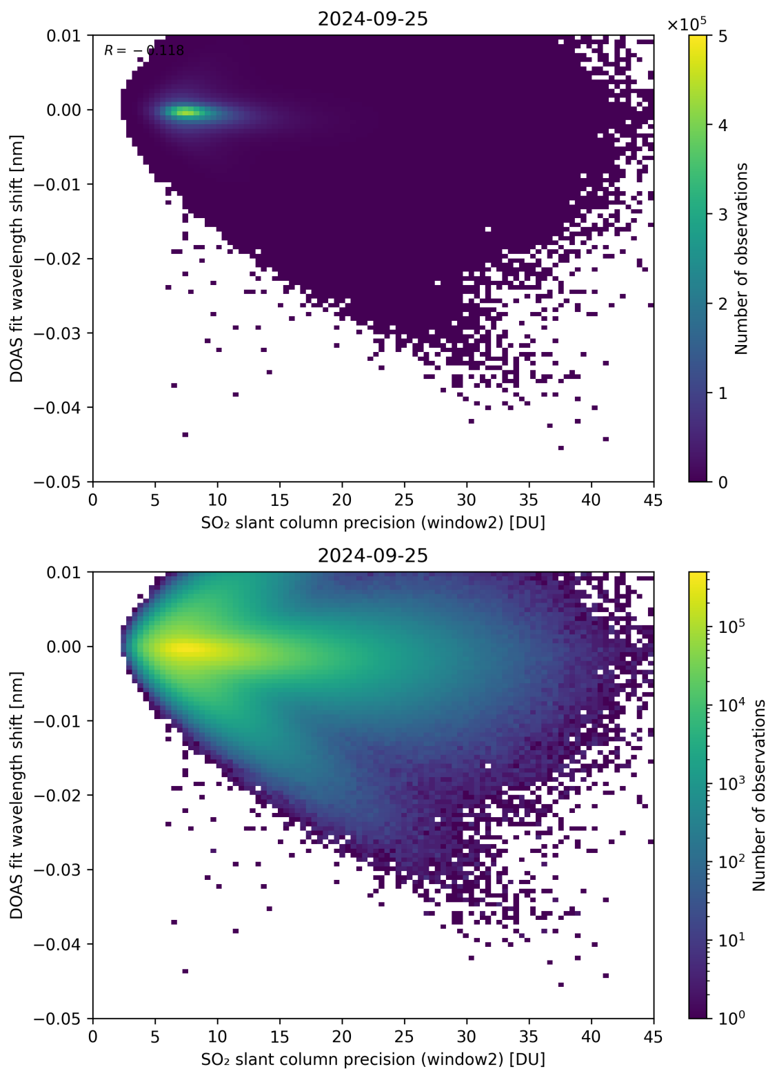
Figure 243: Scatter density plot of “SO 2 slant column precision (window2)” against “DOAS fit wavelength shift” for 2024-09-24 to 2024-09-26.
