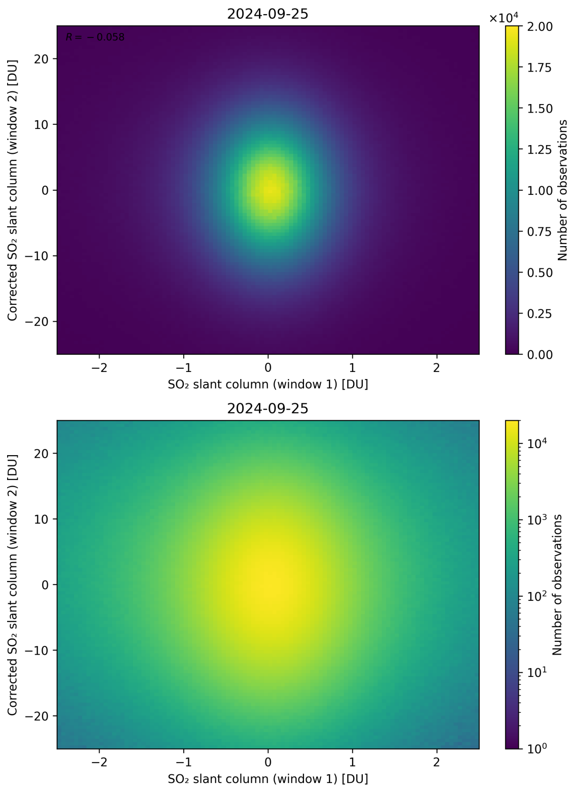
Figure 233: Scatter density plot of “SO 2 slant column (window 1)” against “Corrected SO 2 slant column (window 2)” for 2024-09-24 to 2024-09-26.
