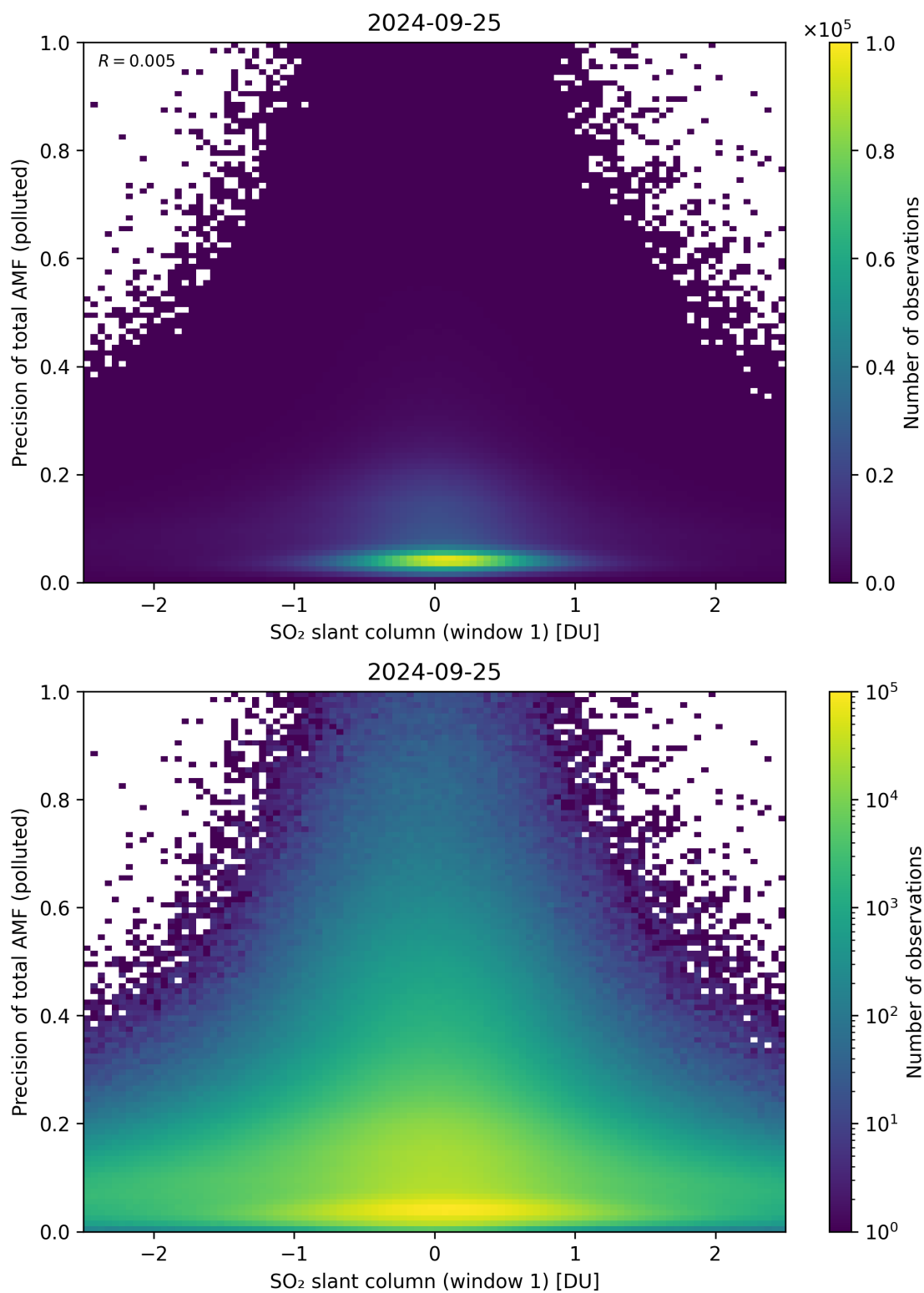
Figure 240: Scatter density plot of “SO 2 slant column (window 1)” against “Precision of total AMF (polluted)” for 2024-09-24 to 2024-09-26.
