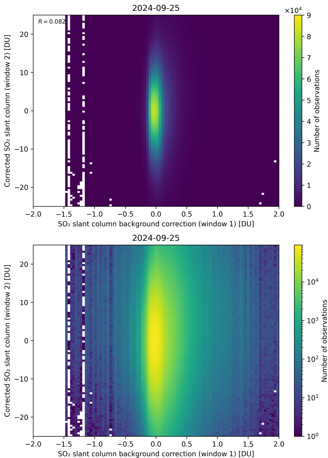
Figure 104: Scatter density plot of “SO 2 slant column background correction (window 1)” against “Corrected SO 2 slant column (window 2)” for 2024-09-24 to 2024-09-26.
