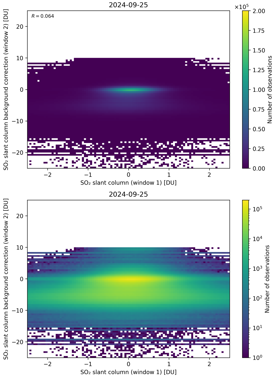
Figure 213: Scatter density plot of “SO 2 slant column (window 1)” against “SO 2 slant column background correction (window 2)” for 2024-09-24 to 2024-09-26.
