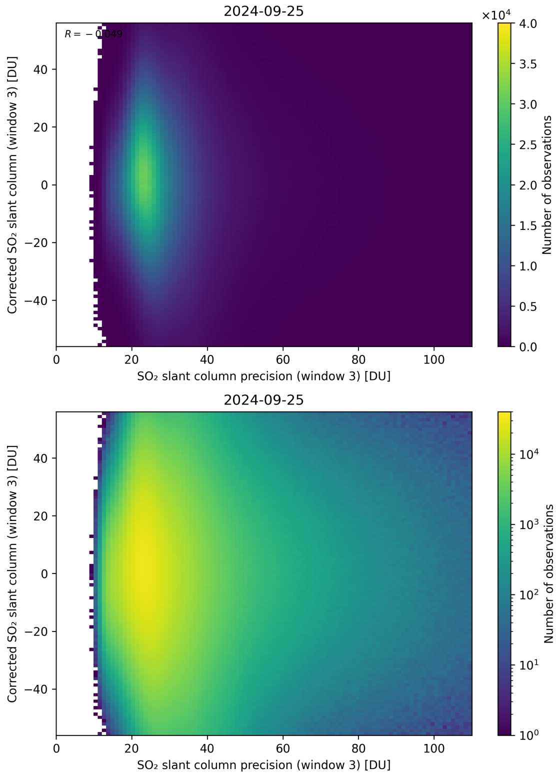
Figure 262: Scatter density plot of “SO 2 slant column precision (window 3)” against “Corrected SO 2 slant column (window 3)” for 2024-09-24 to 2024-09-26.
