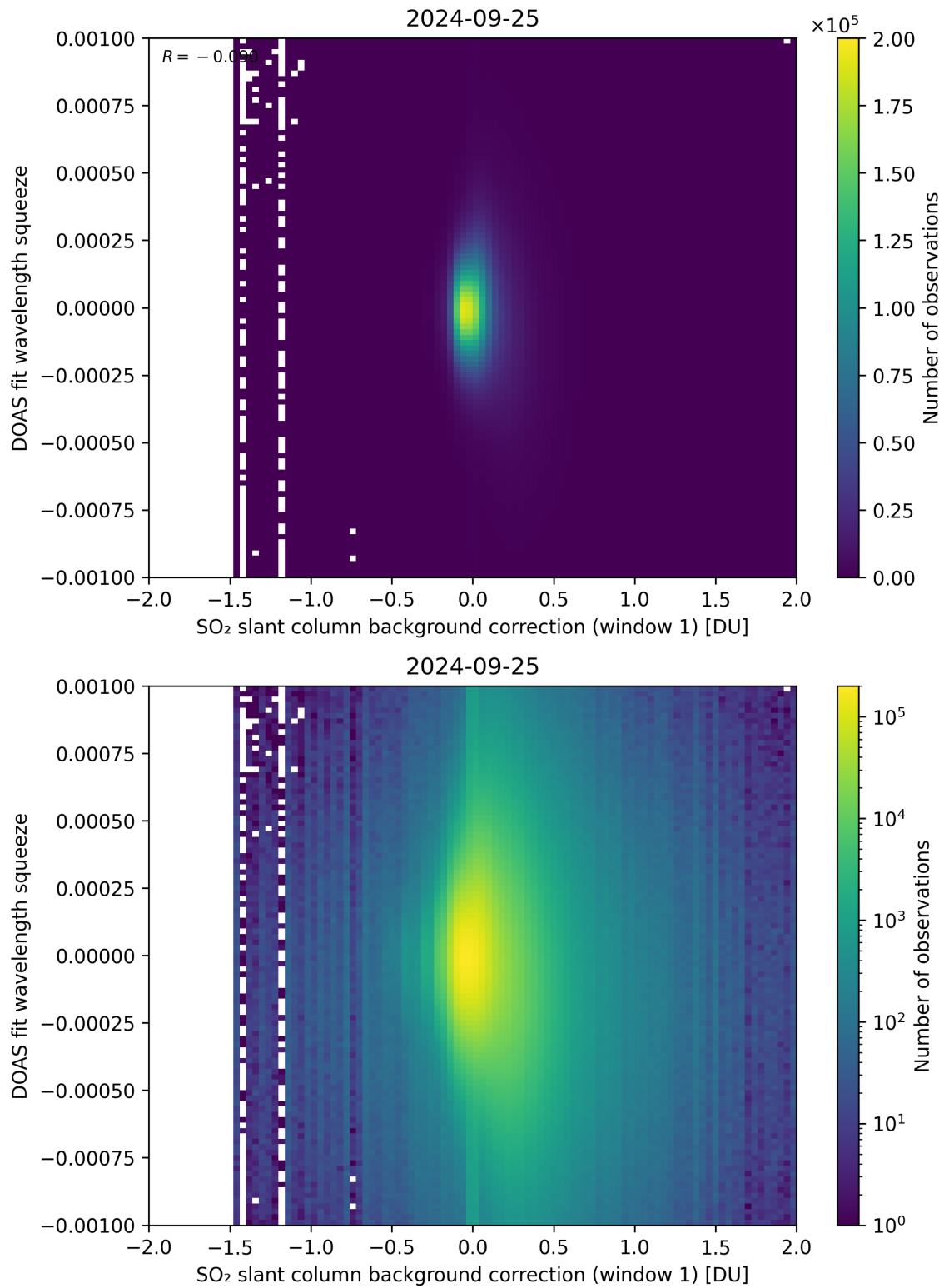
Figure 101: Scatter density plot of “SO 2 slant column background correction (window 1)” against “DOAS fit wavelength squeeze” for 2024-09-24 to 2024-09-26.
