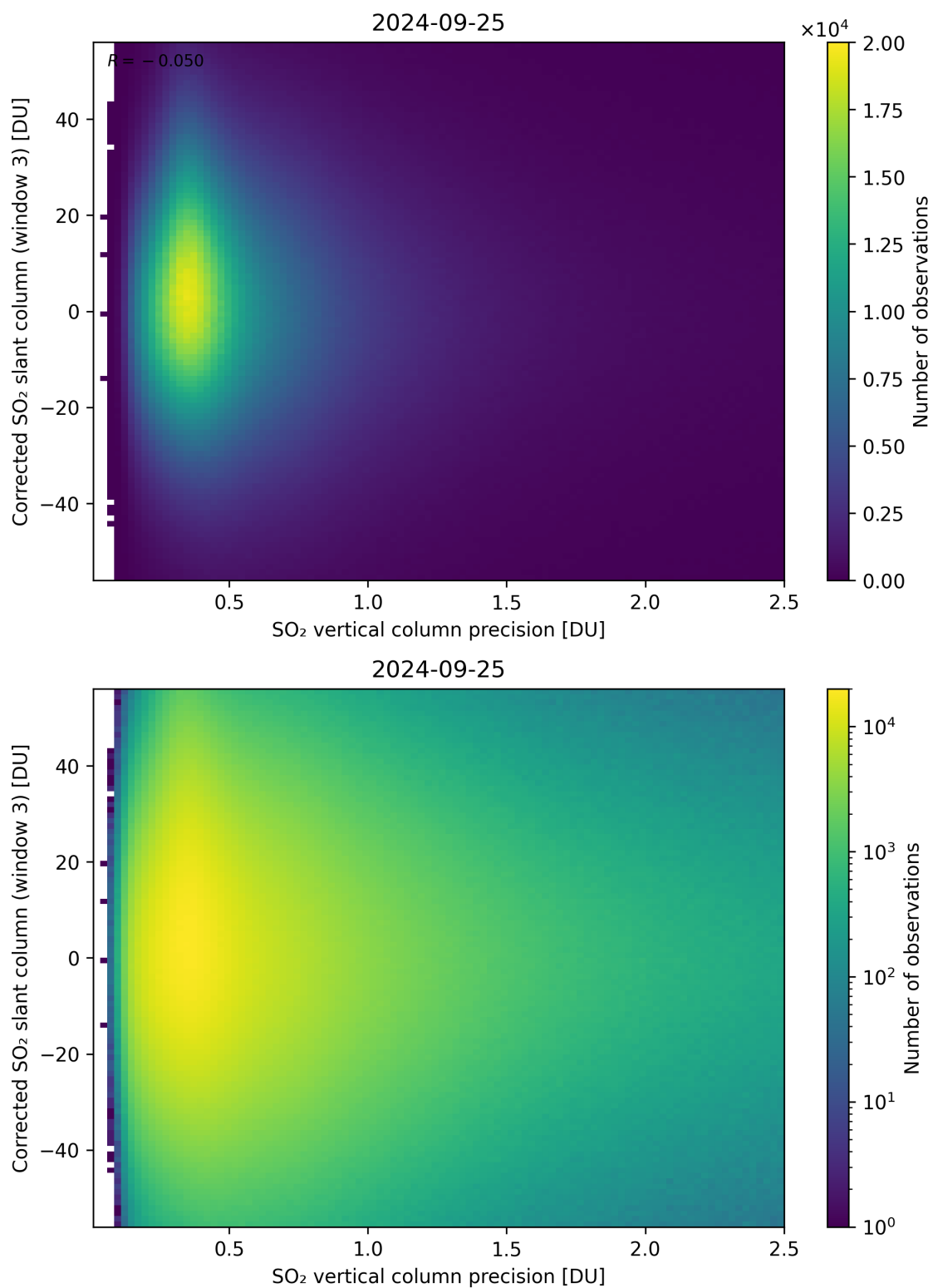
Figure 288: Scatter density plot of “SO 2 vertical column precision” against “Corrected SO 2 slant column (window 3)” for 2024-09-24 to 2024-09-26.
