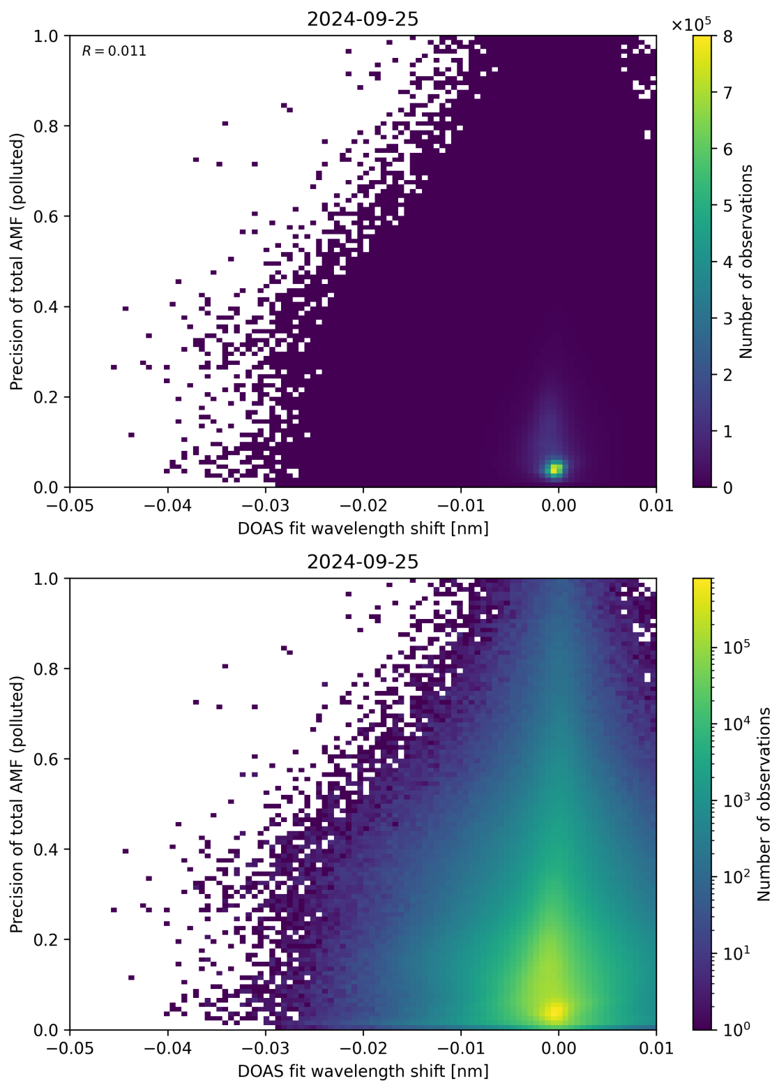
Figure 131: Scatter density plot of “DOAS fit wavelength shift” against “Precision of total AMF (polluted)” for 2024-09-24 to 2024-09-26.
