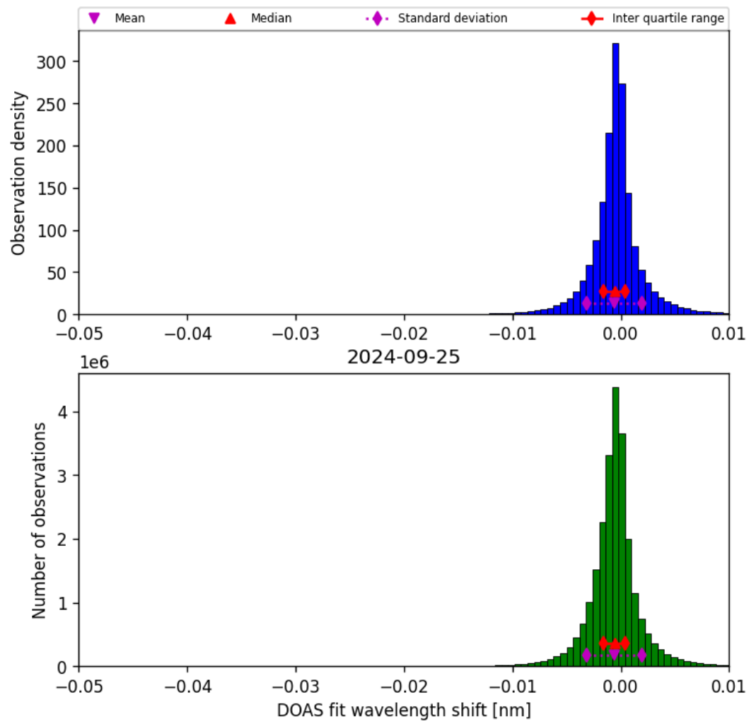
Figure 68: Histogram of “DOAS fit wavelength shift” for 2024-09-24 to 2024-09-26
