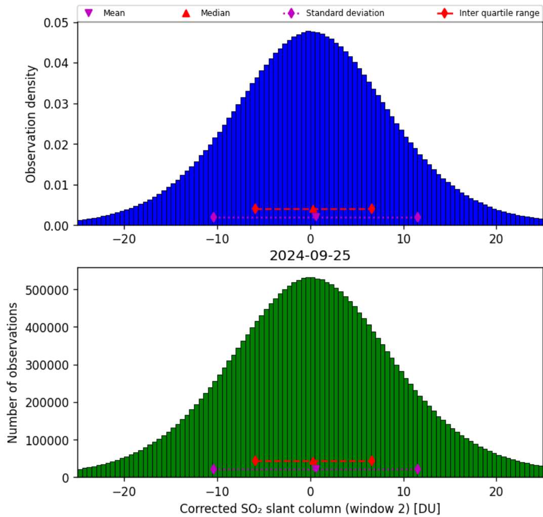
Figure 62: Histogram of “Corrected SO 2 slant column (window 2)” for 2024-09-24 to 2024-09-26
