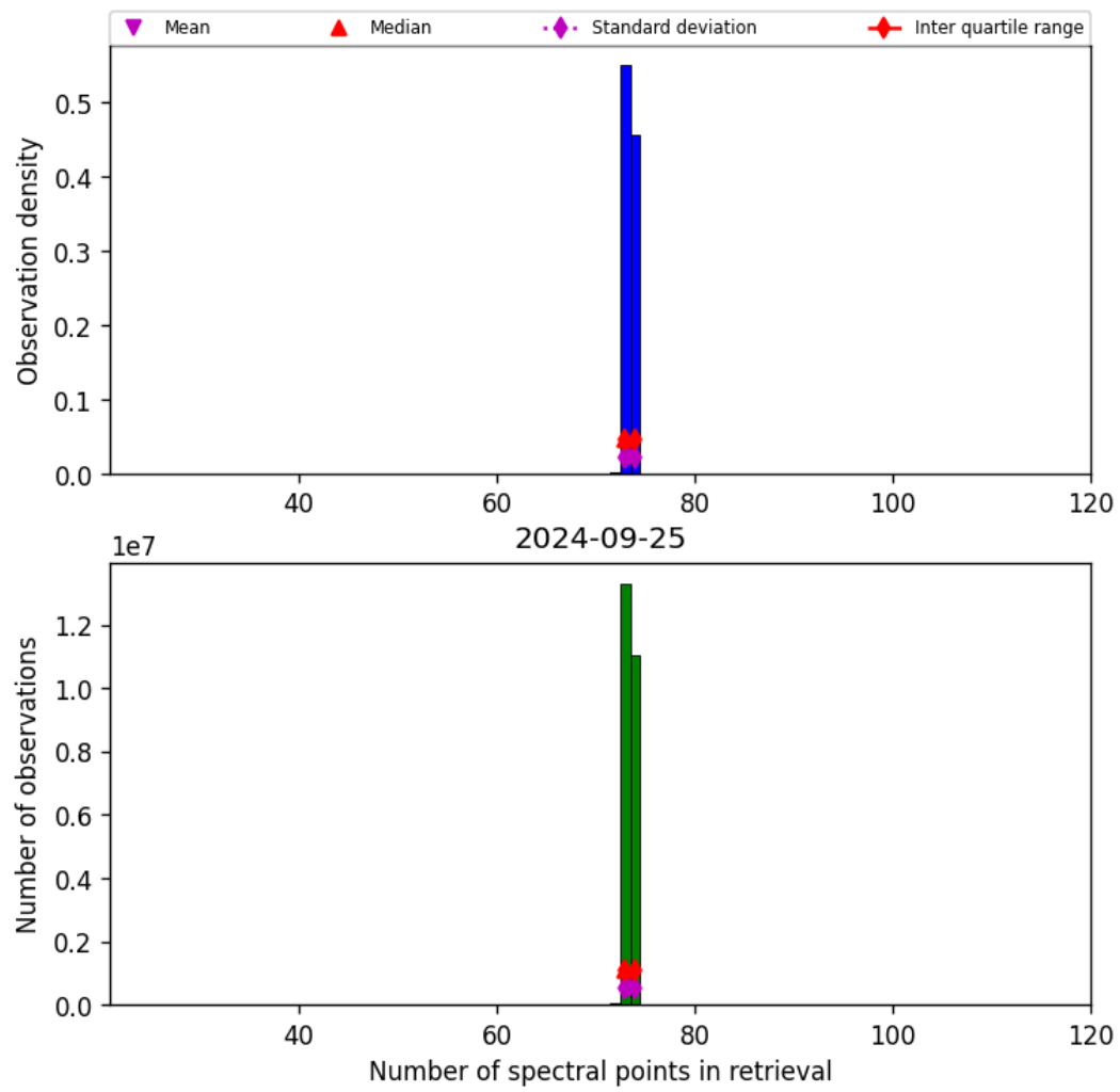
Figure 74: Histogram of “Number of spectral points in retrieval” for 2024-09-24 to 2024-09-26
