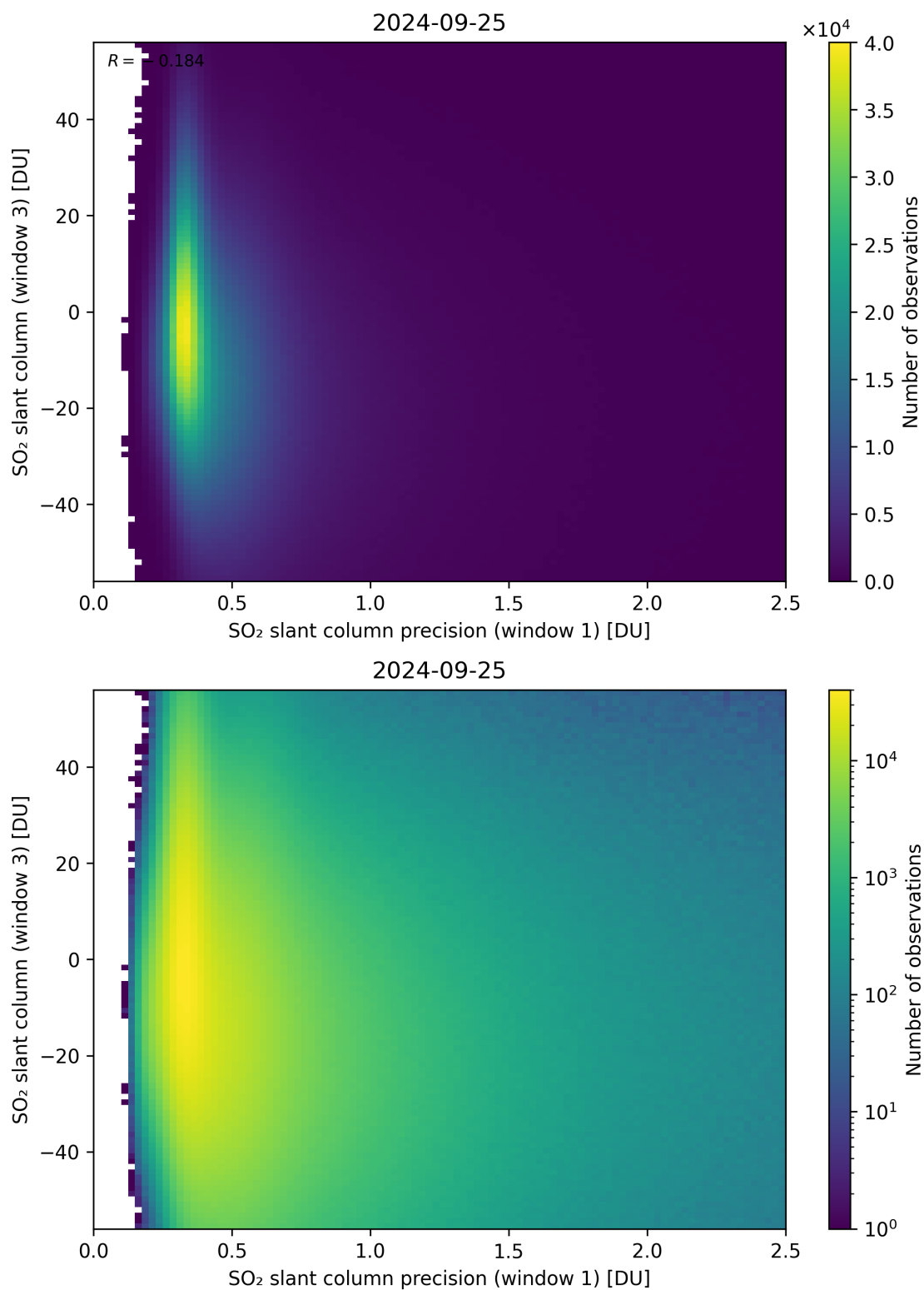
Figure 228: Scatter density plot of “SO 2 slant column precision (window 1)” against “SO 2 slant column (window 3)” for 2024-09-24 to 2024-09-26.
