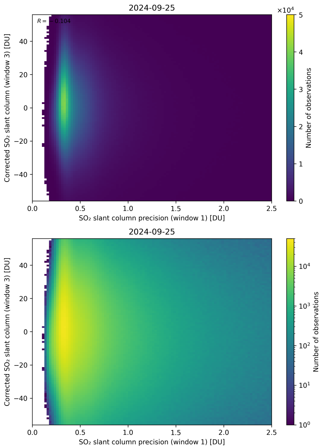
Figure 226: Scatter density plot of “SO 2 slant column precision (window 1)” against “Corrected SO 2 slant column (window 3)” for 2024-09-24 to 2024-09-26.
