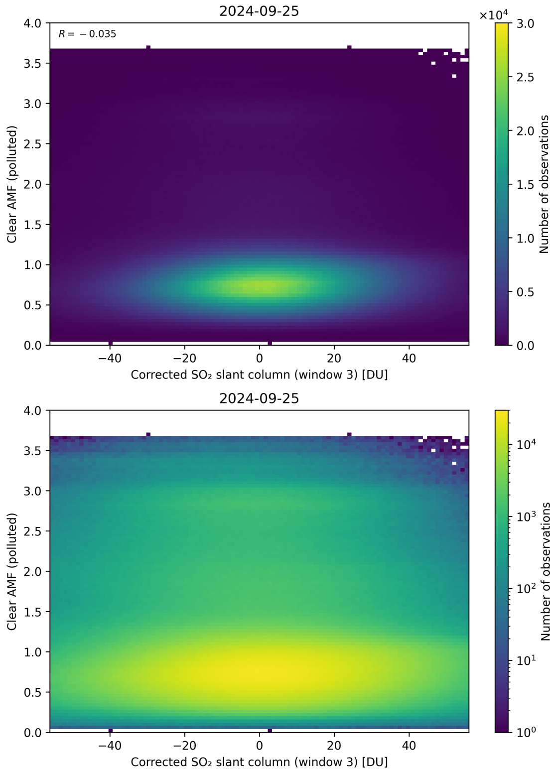
Figure 209: Scatter density plot of “Corrected SO 2 slant column (window 3)” against “Clear AMF (polluted)” for 2024-09-24 to 2024-09-26.
