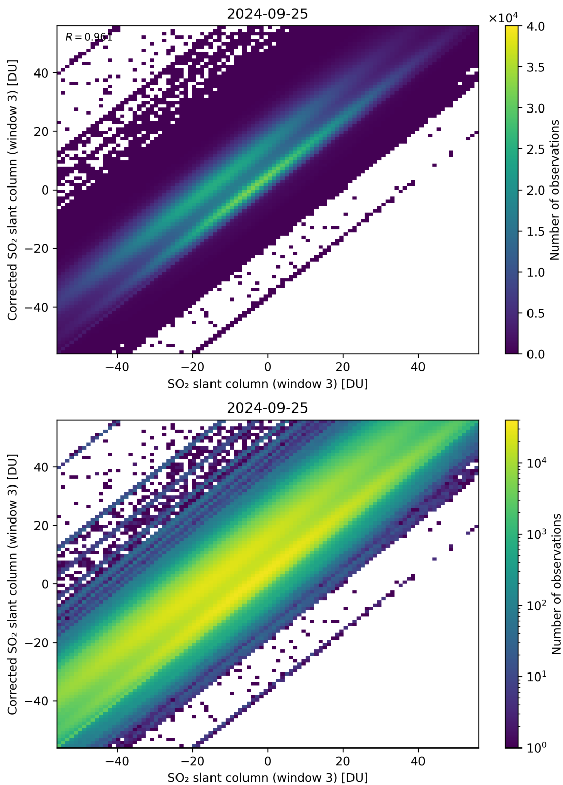
Figure 266: Scatter density plot of “SO 2 slant column (window 3)” against “Corrected SO 2 slant column (window 3)” for 2024-09-24 to 2024-09-26.
