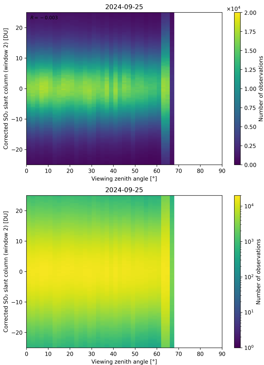
Figure 318: Scatter density plot of “Viewing zenith angle” against “Corrected SO 2 slant column (window 2)” for 2024-09-24 to 2024-09-26.
