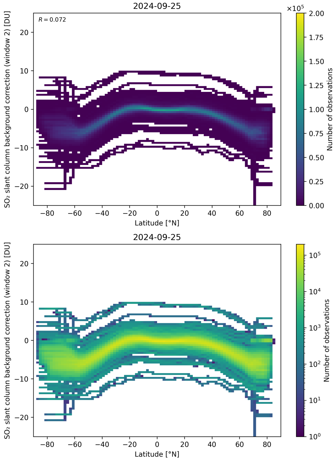
Figure 140: Scatter density plot of “Latitude” against “SO 2 slant column background correction (window 2)” for 2024-09-24 to 2024-09-26.
