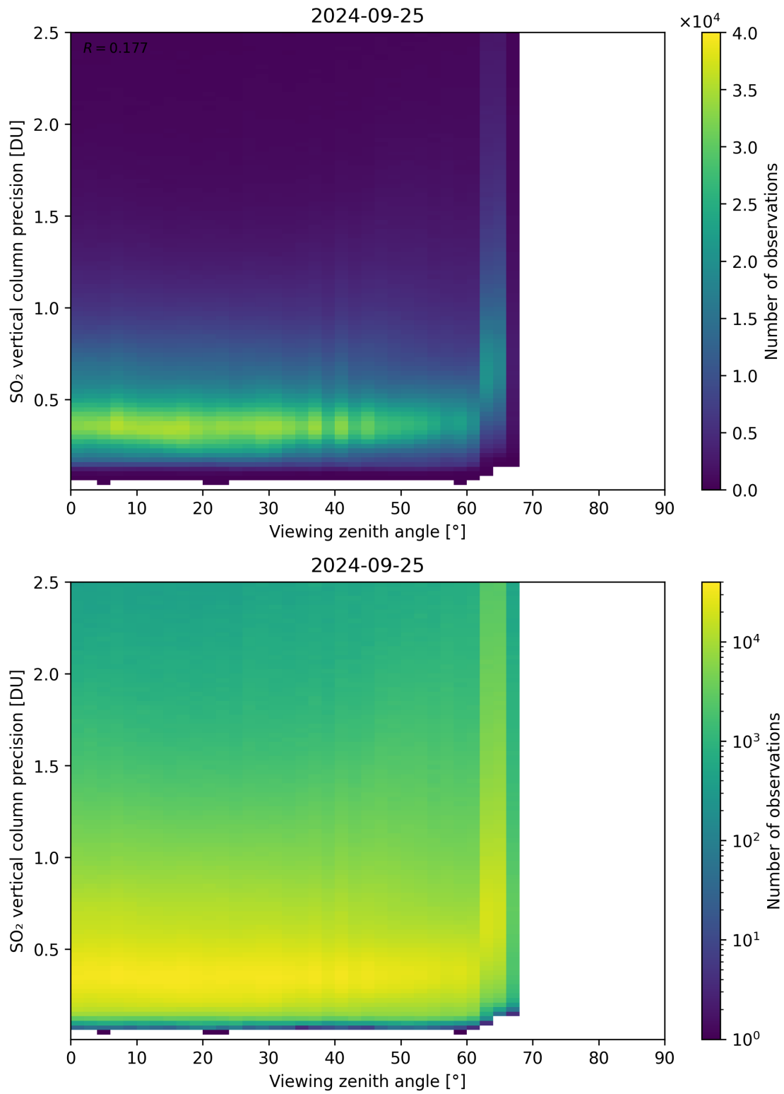
Figure 328: Scatter density plot of “Viewing zenith angle” against “SO 2 vertical column precision” for 2024-09-24 to 2024-09-26.
