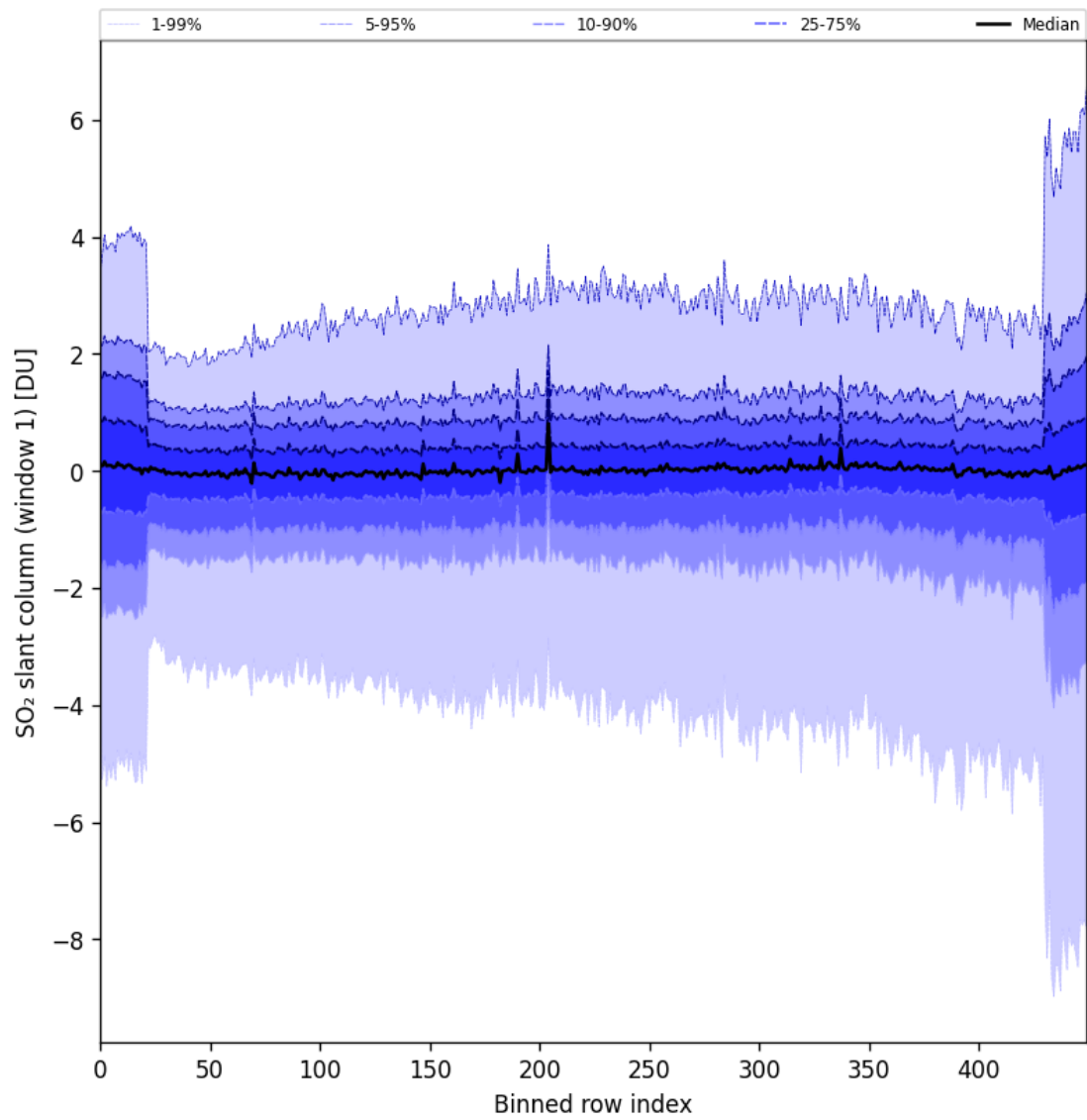
Figure 79: Along track statistics of “SO 2 slant column (window 1)” for 2024-09-24 to 2024-09-26
