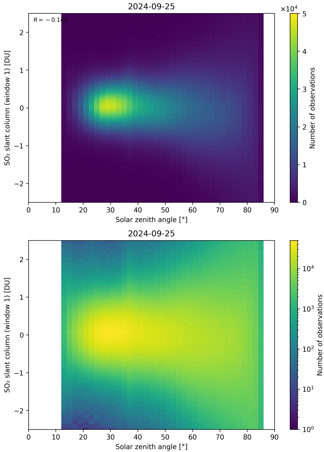
Figure 169: Scatter density plot of “Solar zenith angle” against “SO 2 slant column (window 1)” for 2024-09-24 to 2024-09-26.
