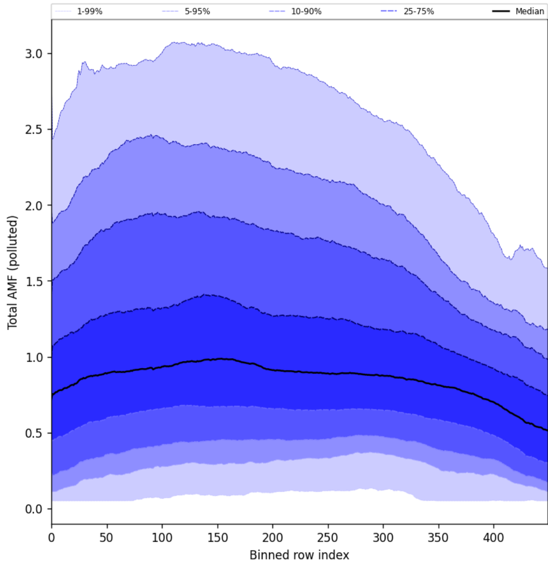
Figure 94: Along track statistics of “Total AMF (polluted)” for 2024-09-24 to 2024-09-26
