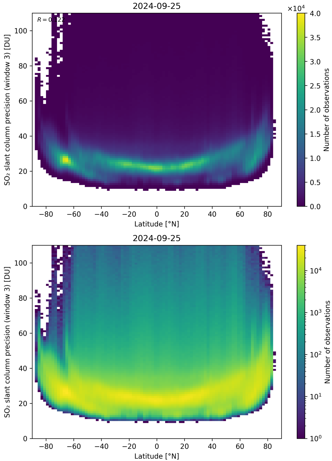
Figure 153: Scatter density plot of “Latitude” against “SO 2 slant column precision (window 3)” for 2024-09-24 to 2024-09-26.
