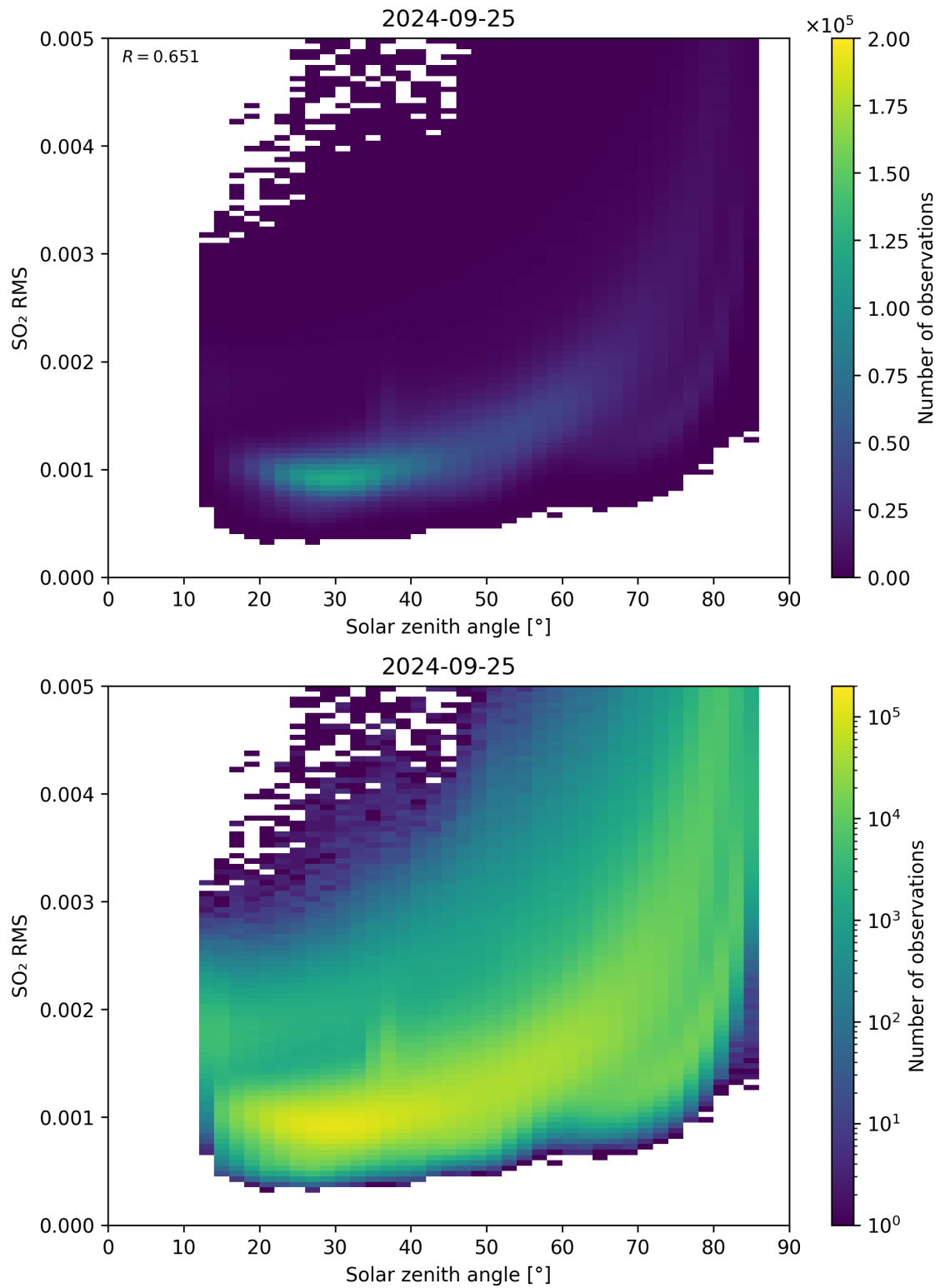
Figure 163: Scatter density plot of “Solar zenith angle” against “SO 2 RMS” for 2024-09-24 to 2024-09-26.
