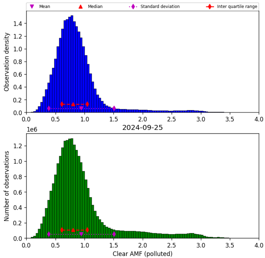
Figure 73: Histogram of “Clear AMF (polluted)” for 2024-09-24 to 2024-09-26
