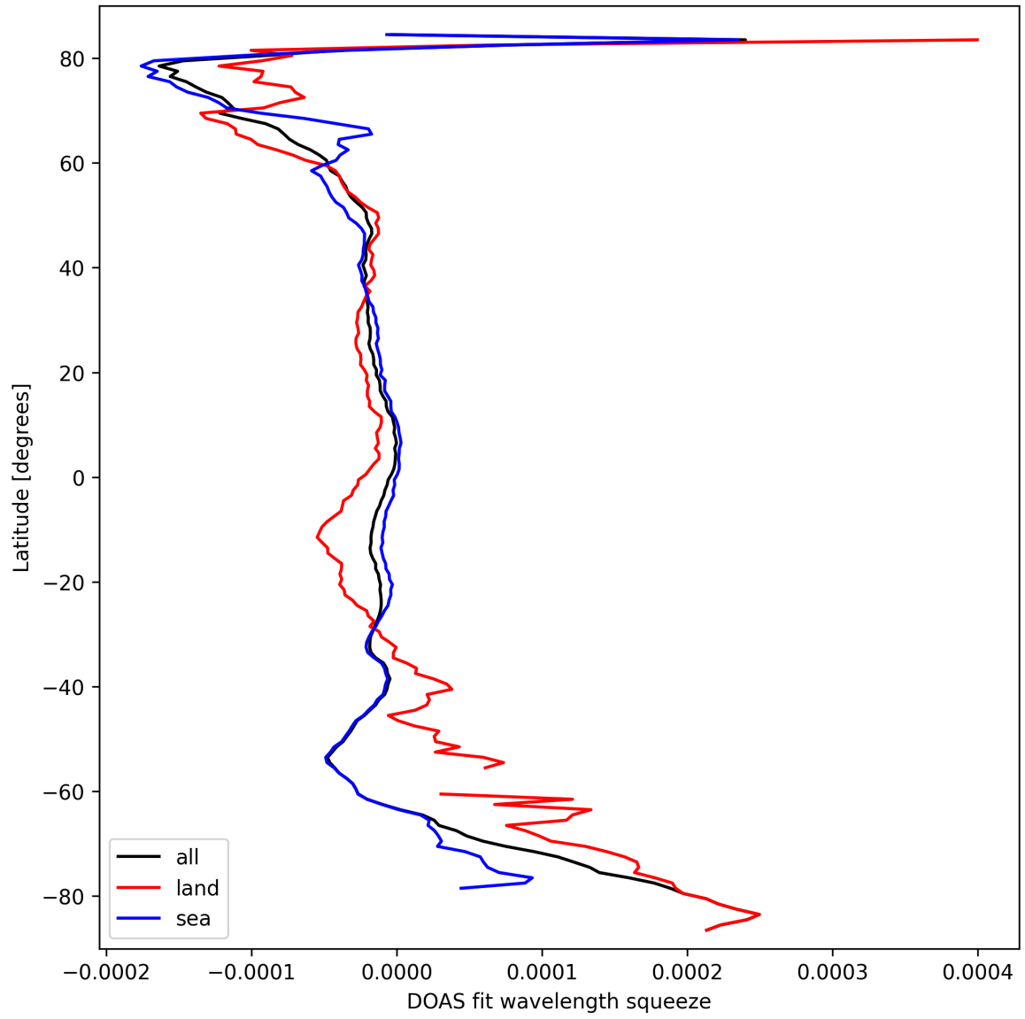
Figure 46: Zonal average of “DOAS fit wavelength squeeze” for 2024-09-24 to 2024-09-26.
