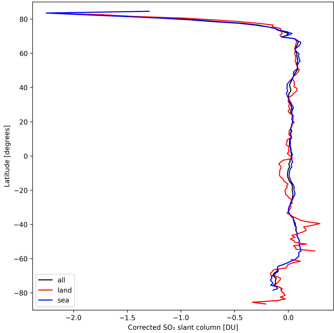
Figure 32: Zonal average of “Corrected SO 2 slant column” for 2024-09-24 to 2024-09-26.
