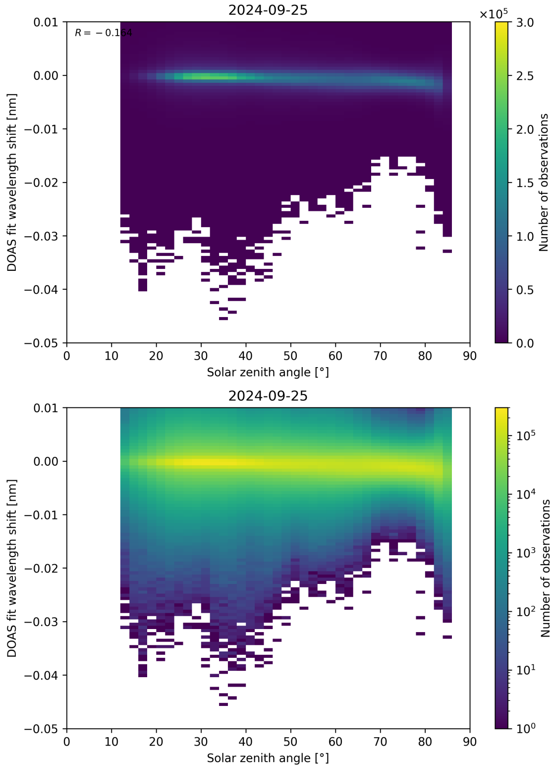
Figure 161: Scatter density plot of “Solar zenith angle” against “DOAS fit wavelength shift” for 2024-09-24 to 2024-09-26.
