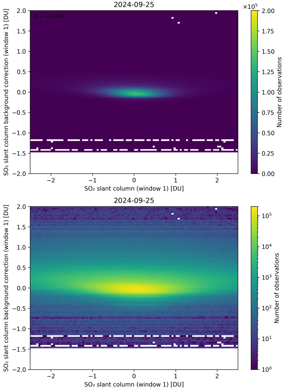
Figure 212: Scatter density plot of “SO 2 slant column (window 1)” against “SO 2 slant column background correction (window 1)” for 2024-09-24 to 2024-09-26.
