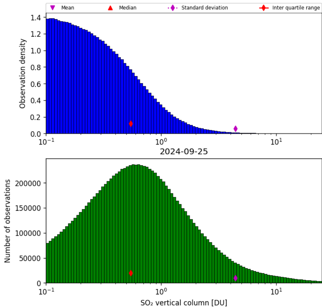
Figure 53: Histogram of “SO 2 vertical column” for 2024-09-24 to 2024-09-26
