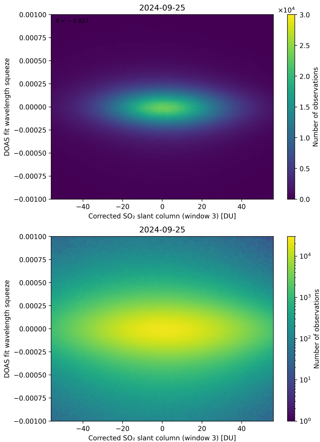
Figure 207: Scatter density plot of “Corrected SO 2 slant column (window 3)” against “DOAS fit wavelength squeeze” for 2024-09-24 to 2024-09-26.
