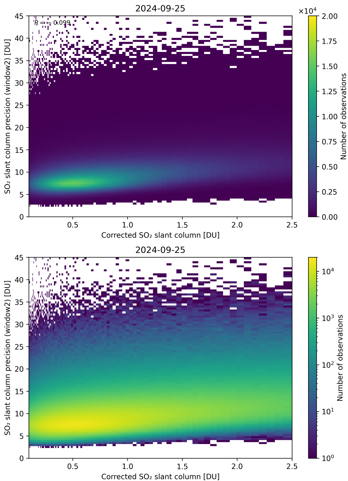
Figure 189: Scatter density plot of “Corrected SO 2 slant column” against “SO 2 slant column precision (window2)” for 2024-09-24 to 2024-09-26.
