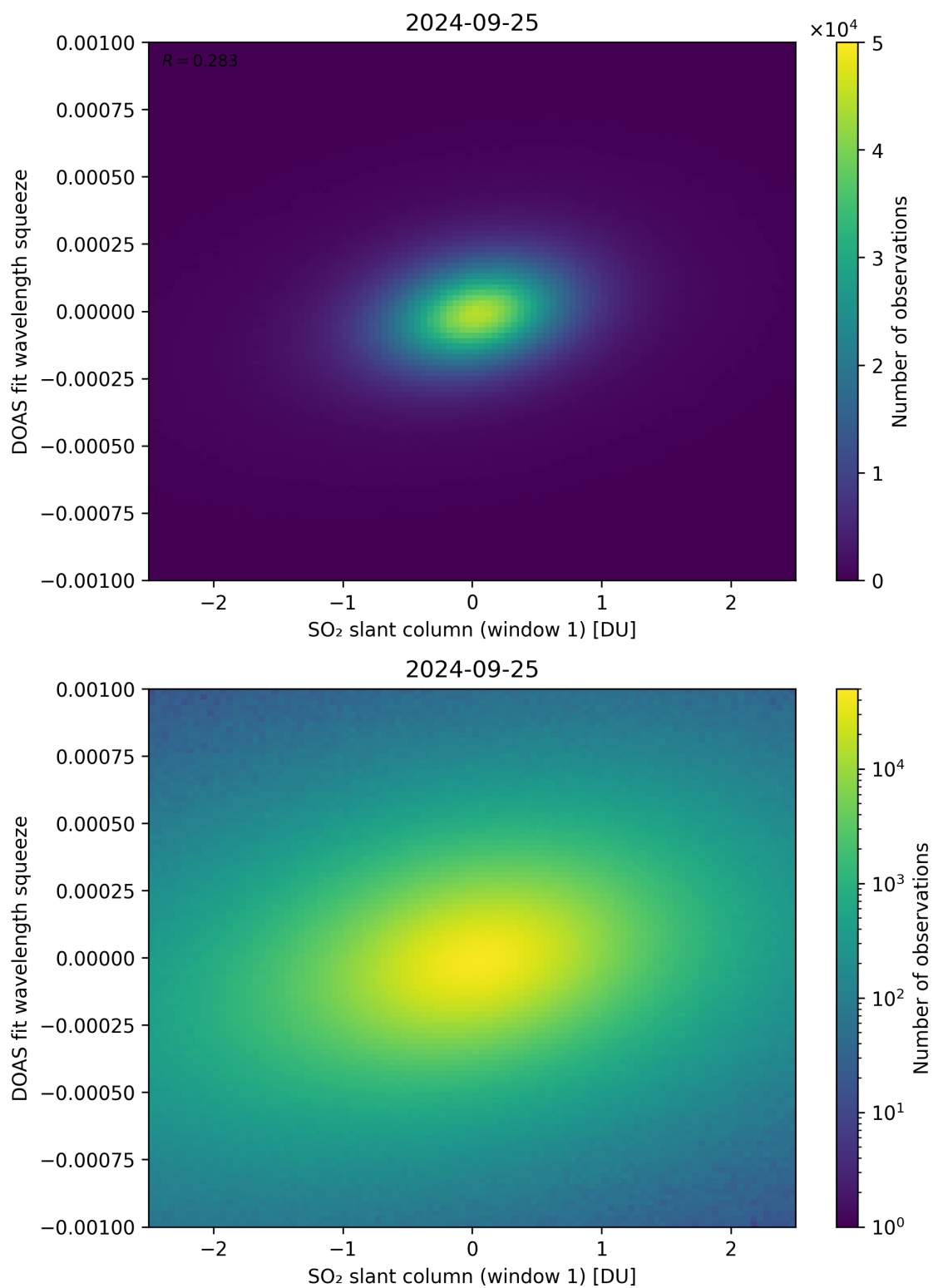
Figure 216: Scatter density plot of “SO 2 slant column (window 1)” against “DOAS fit wavelength squeeze” for 2024-09-24 to 2024-09-26.
