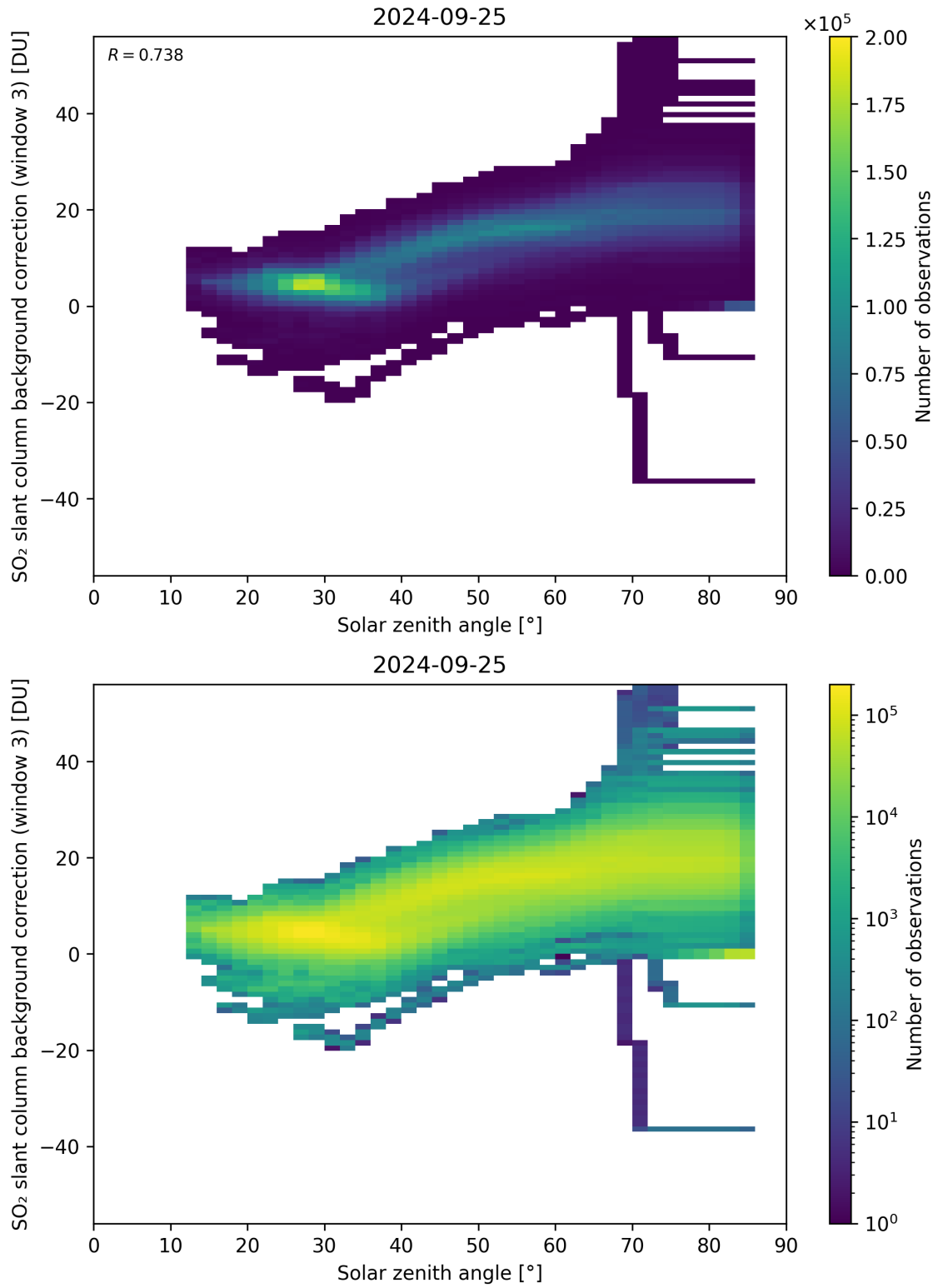
Figure 160: Scatter density plot of “Solar zenith angle” against “SO 2 slant column background correction (window 3)” for 2024-09-24 to 2024-09-26.
