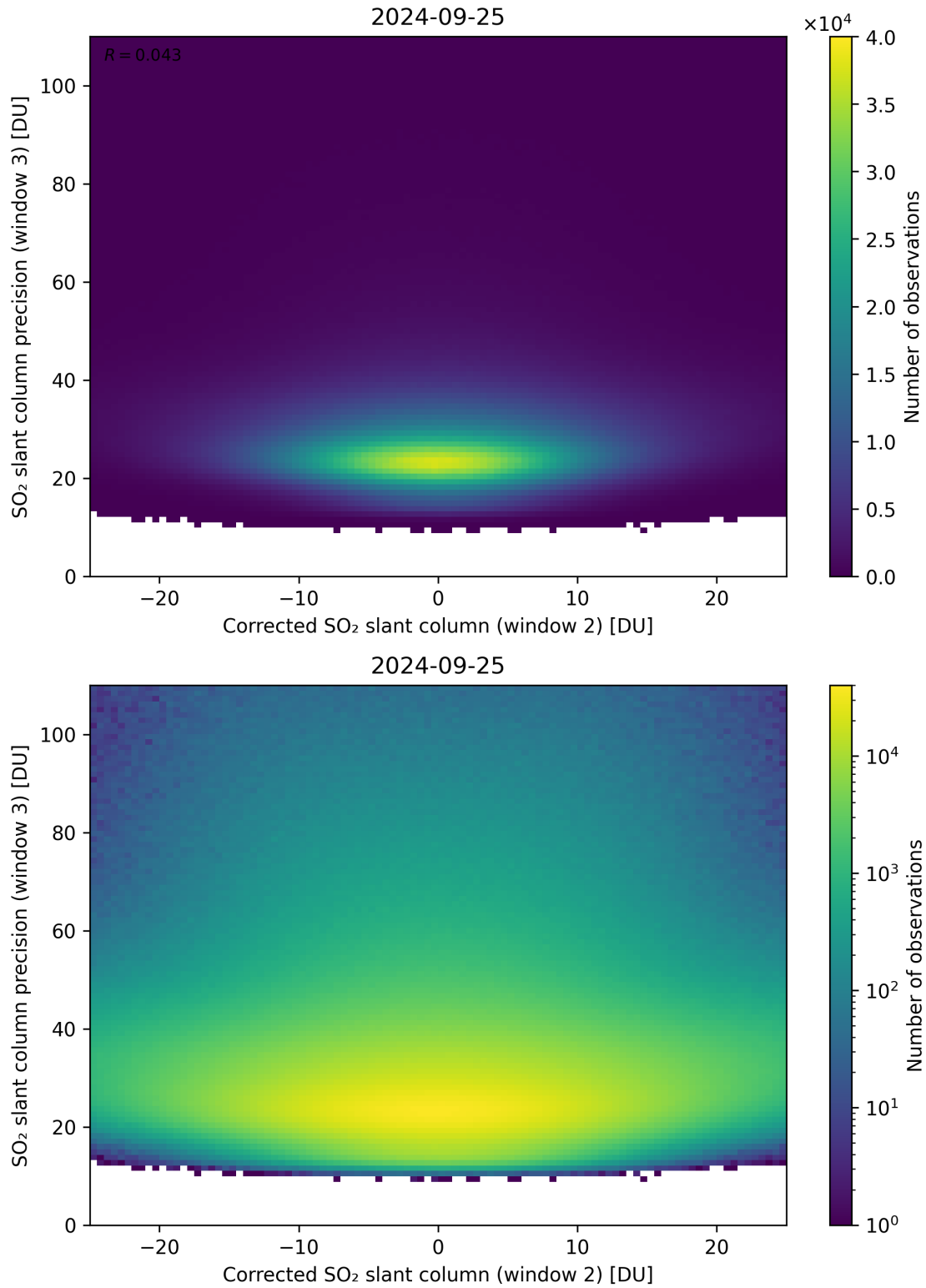
Figure 202: Scatter density plot of “Corrected SO 2 slant column (window 2)” against “SO 2 slant column precision (window 3)” for 2024-09-24 to 2024-09-26.
