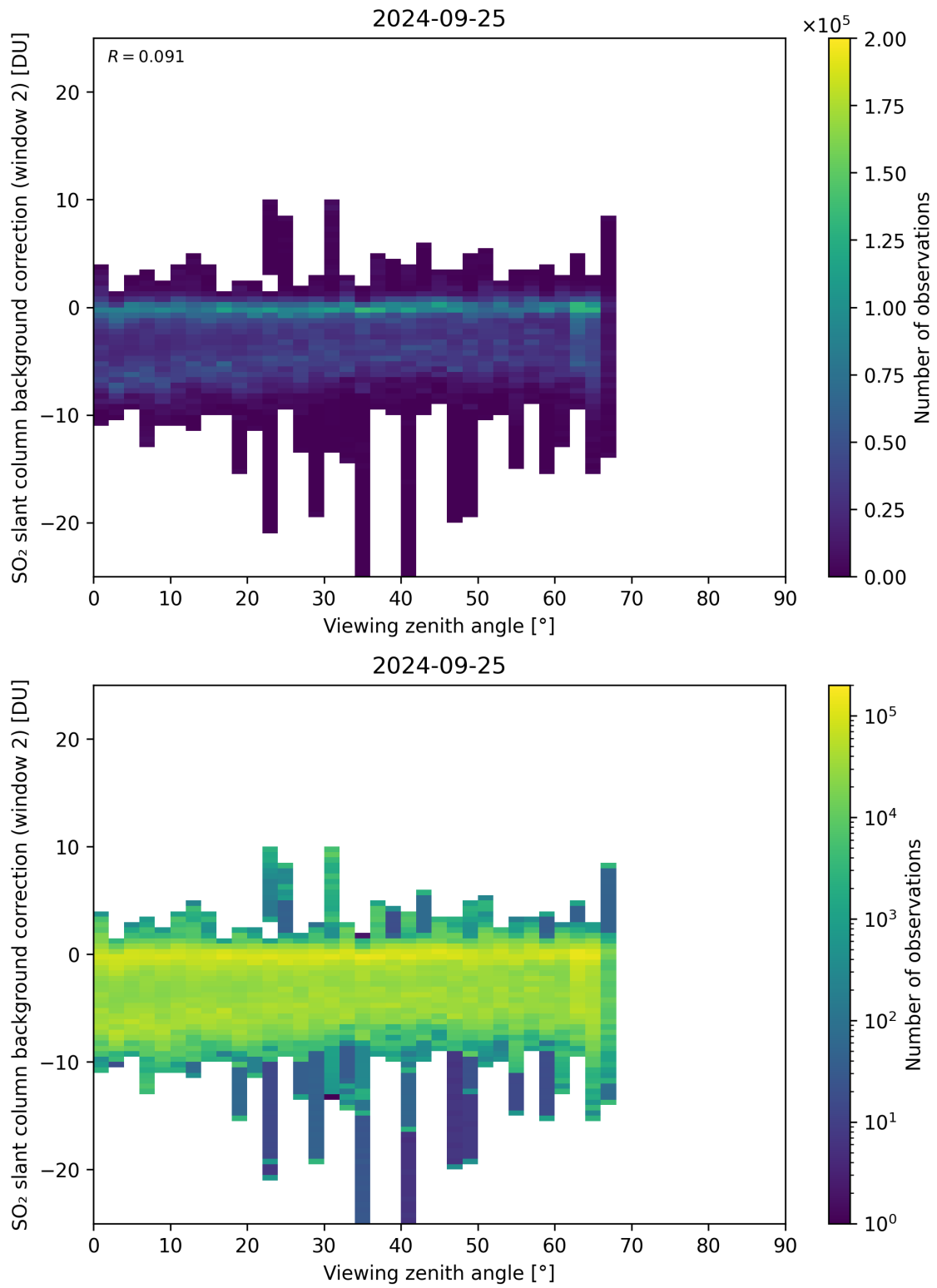
Figure 309: Scatter density plot of “Viewing zenith angle” against “SO 2 slant column background correction (window 2)” for 2024-09-24 to 2024-09-26.
