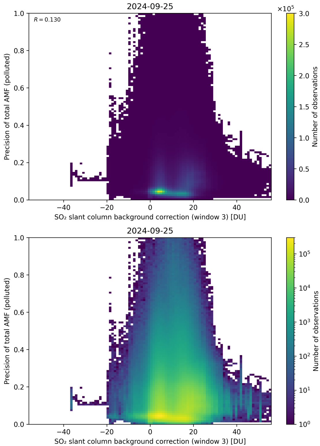
Figure 126: Scatter density plot of “SO 2 slant column background correction (window 3)” against “Precision of total AMF (polluted)” for 2024-09-24 to 2024-09-26.
