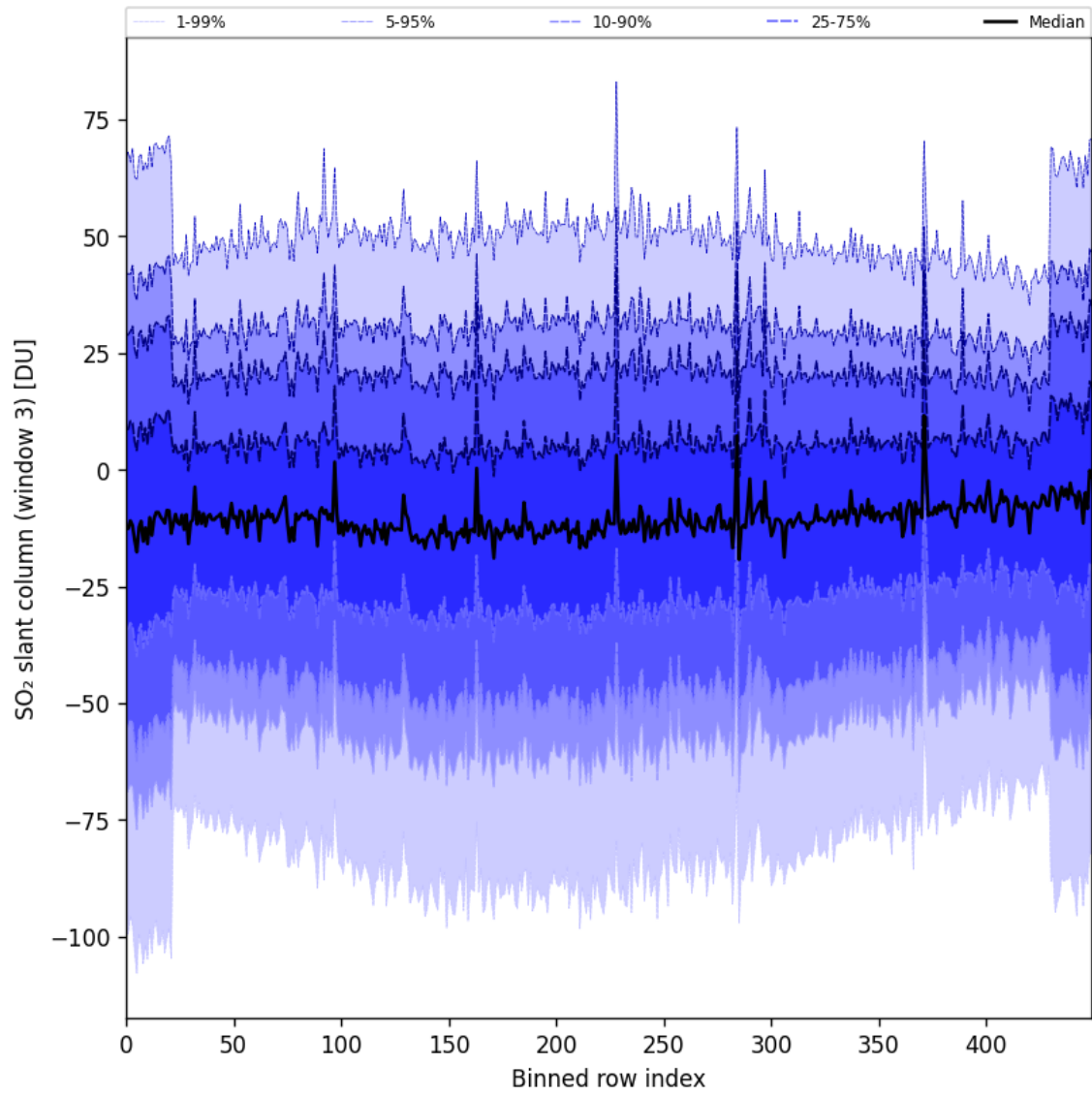
Figure 87: Along track statistics of “SO 2 slant column (window 3)” for 2024-09-24 to 2024-09-26
