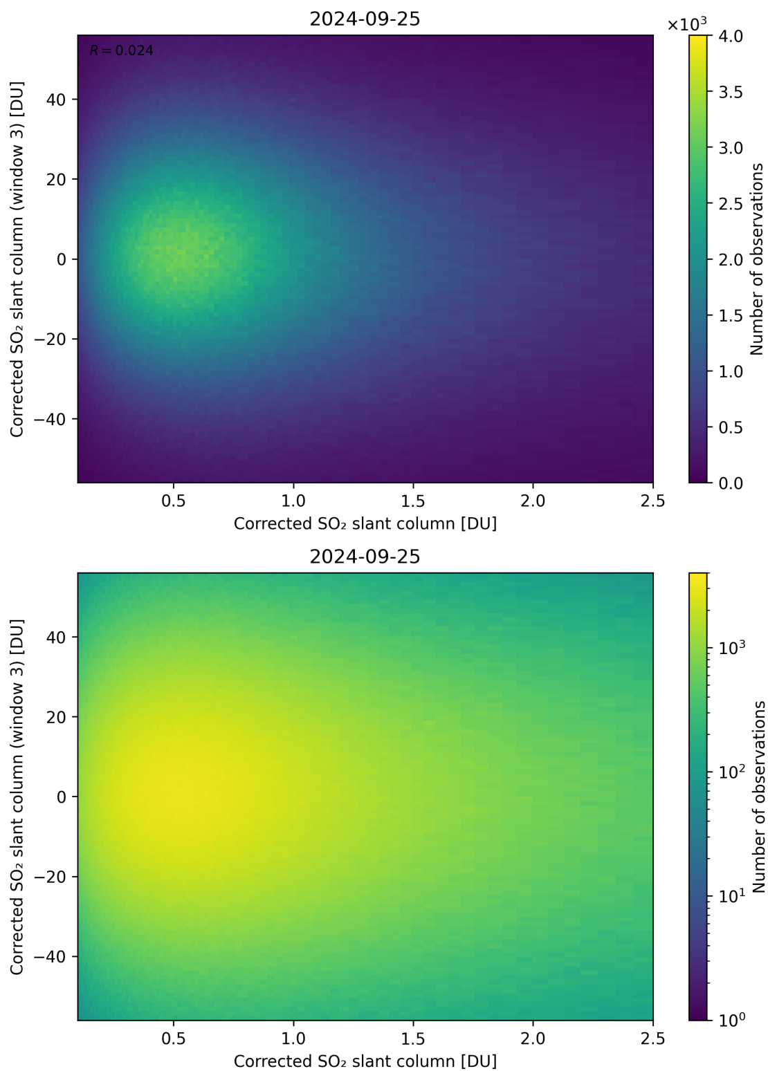
Figure 186: Scatter density plot of “Corrected SO 2 slant column” against “Corrected SO 2 slant column (window 3)” for 2024-09-24 to 2024-09-26.
