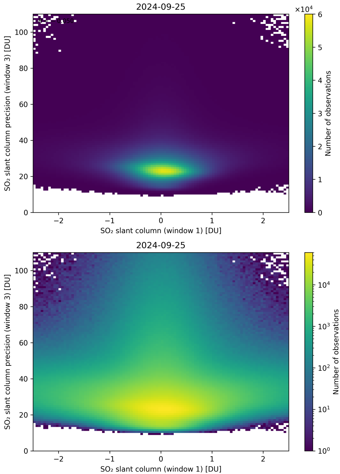
Figure 238: Scatter density plot of “SO 2 slant column (window 1)” against “SO 2 slant column precision (window 3)” for 2024-09-24 to 2024-09-26.
