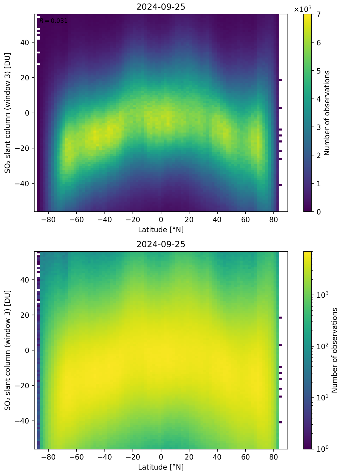
Figure 152: Scatter density plot of “Latitude” against “SO 2 slant column (window 3)” for 2024-09-24 to 2024-09-26.
