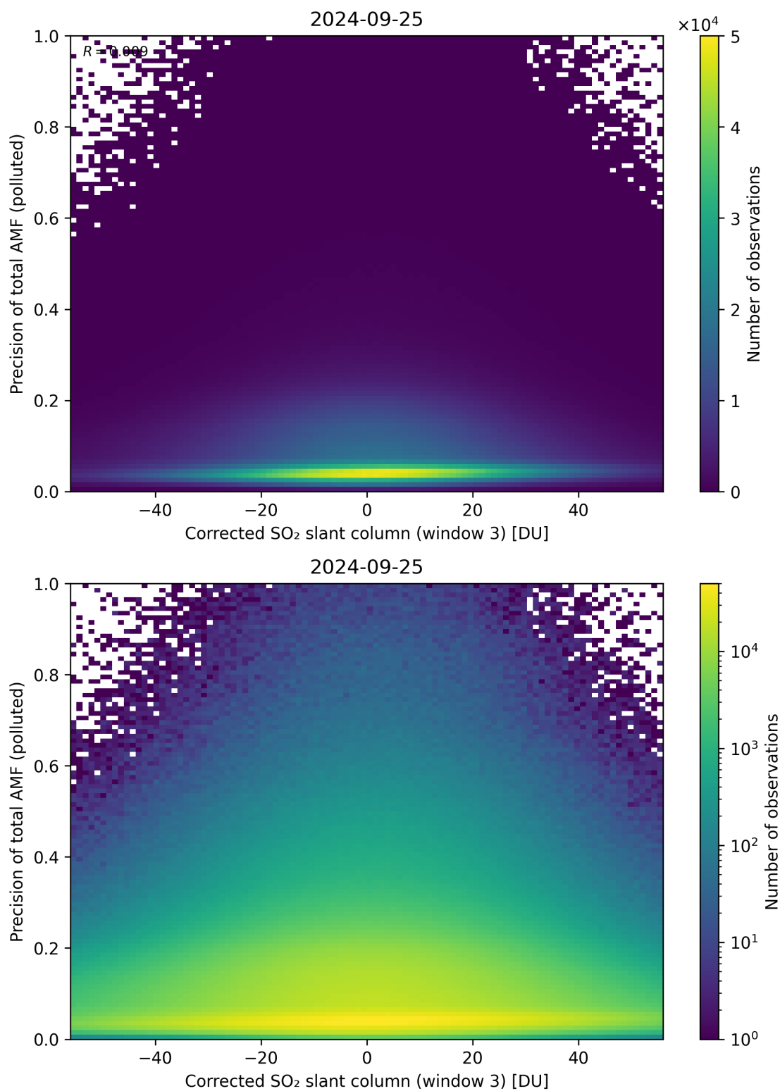
Figure 211: Scatter density plot of “Corrected SO 2 slant column (window 3)” against “Precision of total AMF (polluted)” for 2024-09-24 to 2024-09-26.
