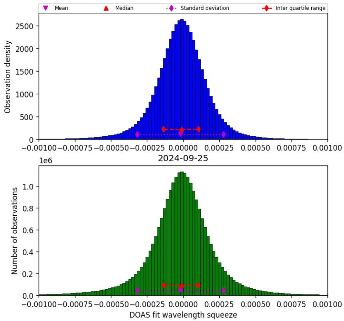
Figure 69: Histogram of “DOAS fit wavelength squeeze” for 2024-09-24 to 2024-09-26
