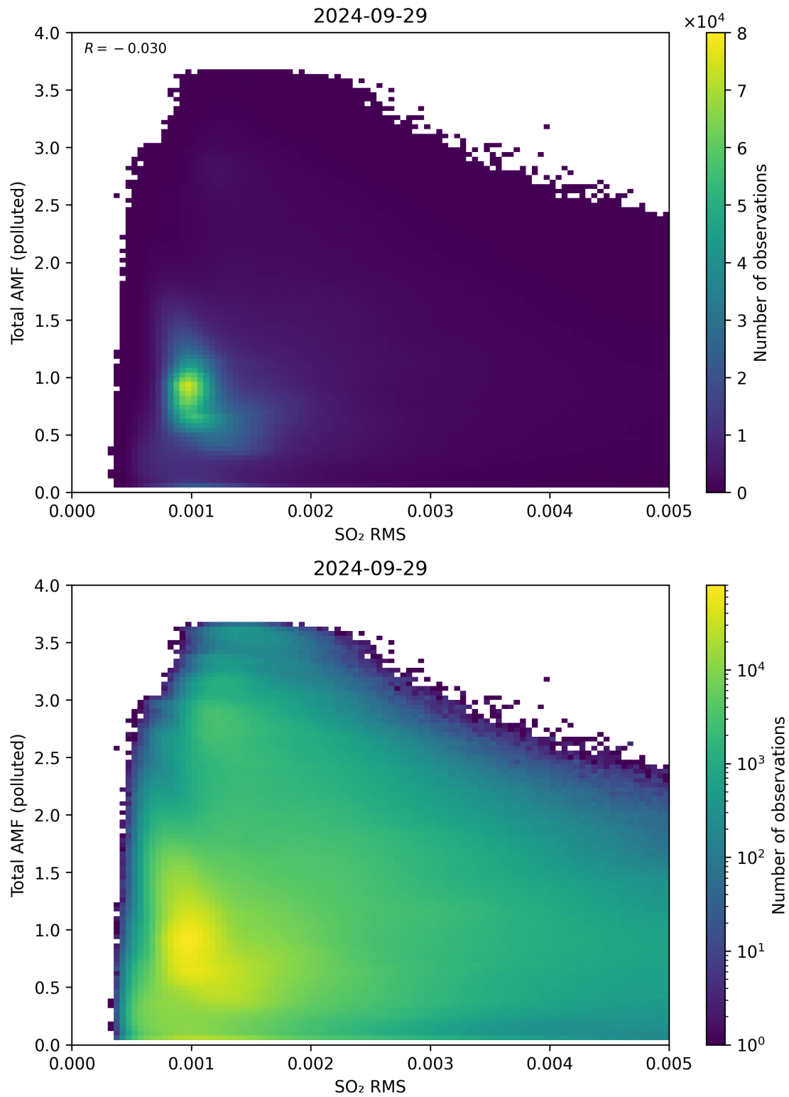
Figure 137: Scatter density plot of “SO 2 RMS” against “Total AMF (polluted)” for 2024-09-28 to 2024-09-30.
