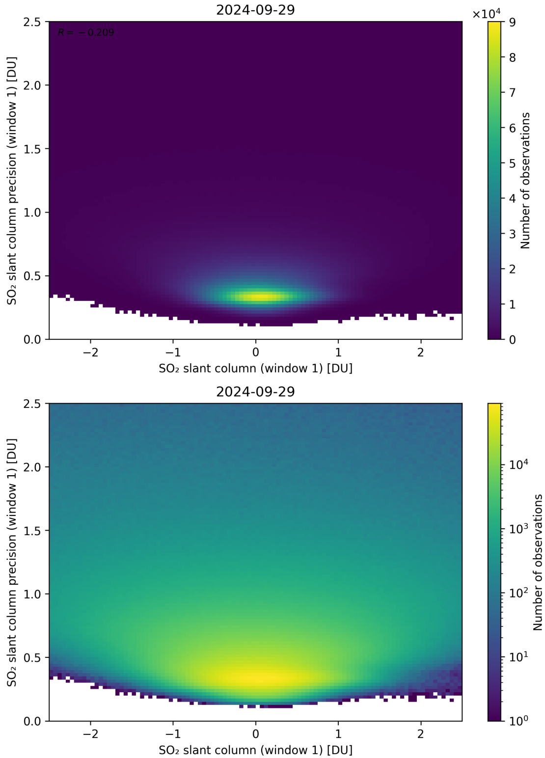
Figure 235: Scatter density plot of “SO 2 slant column (window 1)” against “SO 2 slant column precision (window 1)” for 2024-09-28 to 2024-09-30.
