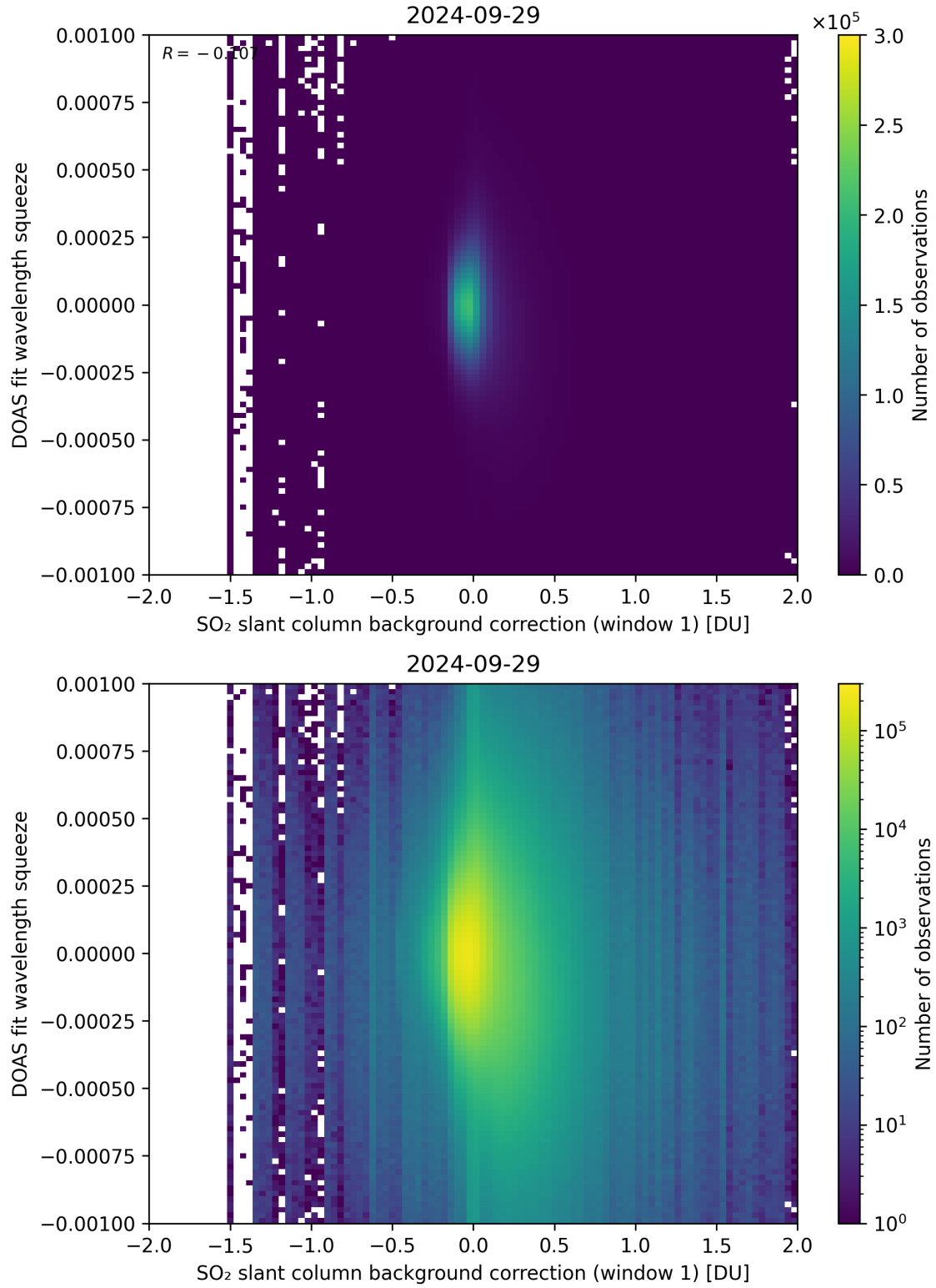
Figure 101: Scatter density plot of “SO 2 slant column background correction (window 1)” against “DOAS fit wavelength squeeze” for 2024-09-28 to 2024-09-30.
