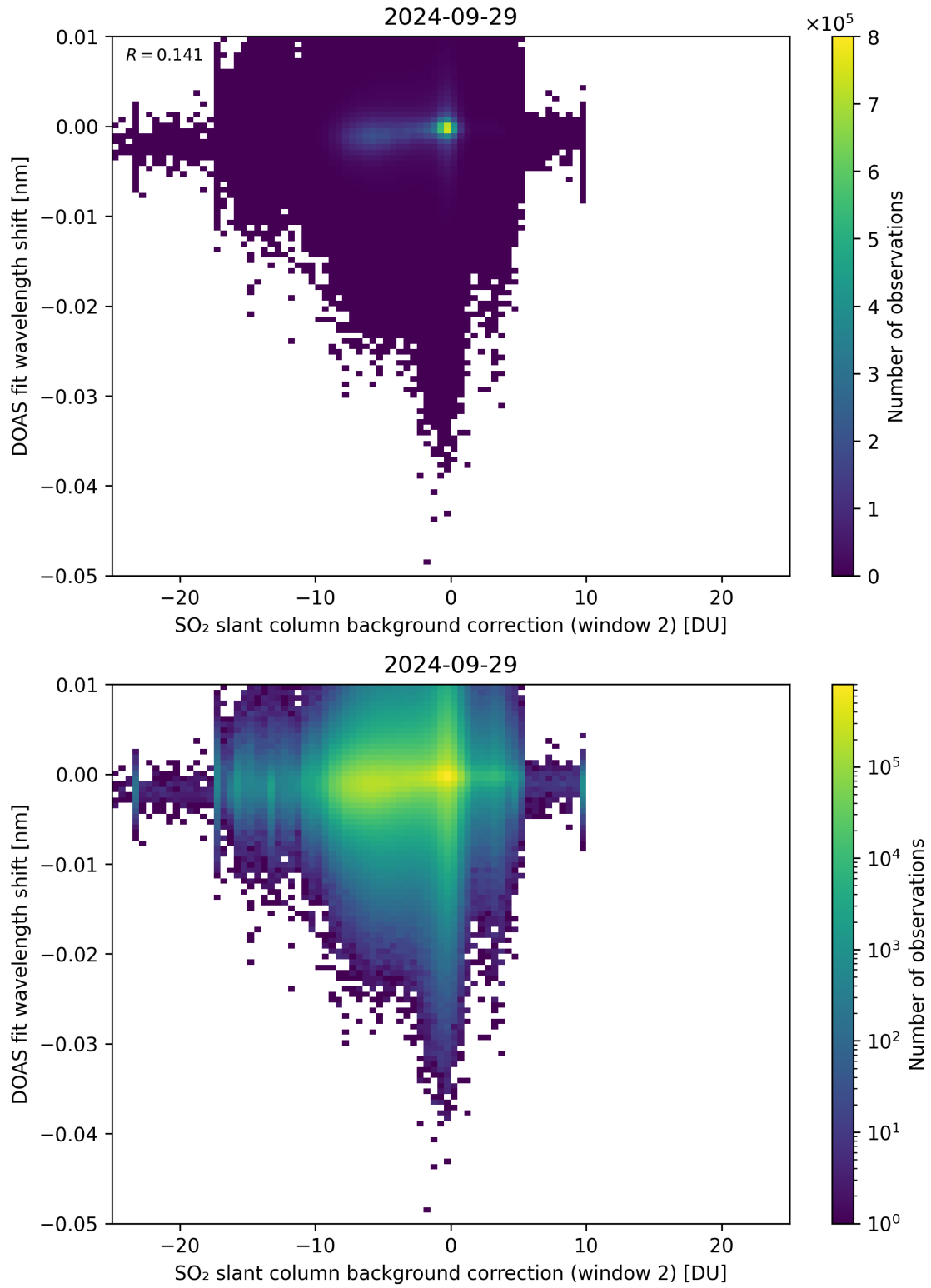
Figure 112: Scatter density plot of “SO 2 slant column background correction (window 2)” against “DOAS fit wavelength shift” for 2024-09-28 to 2024-09-30.
