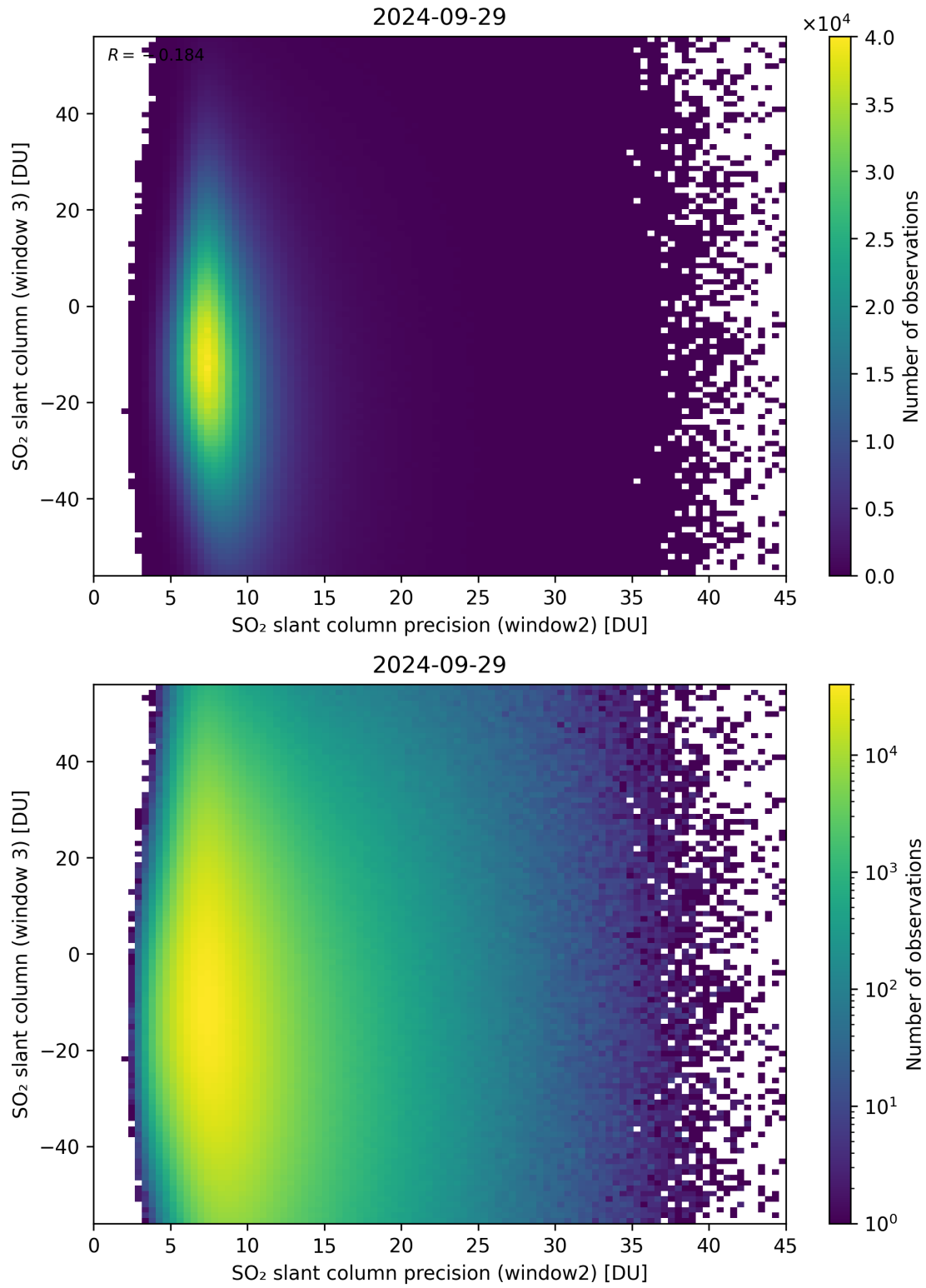
Figure 249: Scatter density plot of “SO 2 slant column precision (window2)” against “SO 2 slant column (window 3)” for 2024-09-28 to 2024-09-30.
