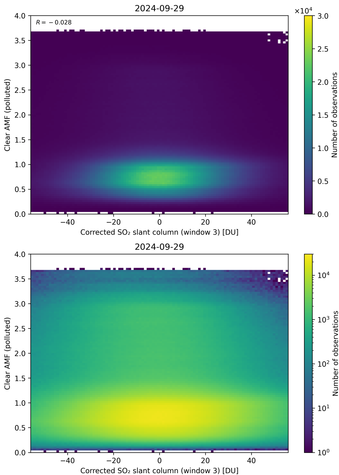
Figure 209: Scatter density plot of “Corrected SO 2 slant column (window 3)” against “Clear AMF (polluted)” for 2024-09-28 to 2024-09-30.
