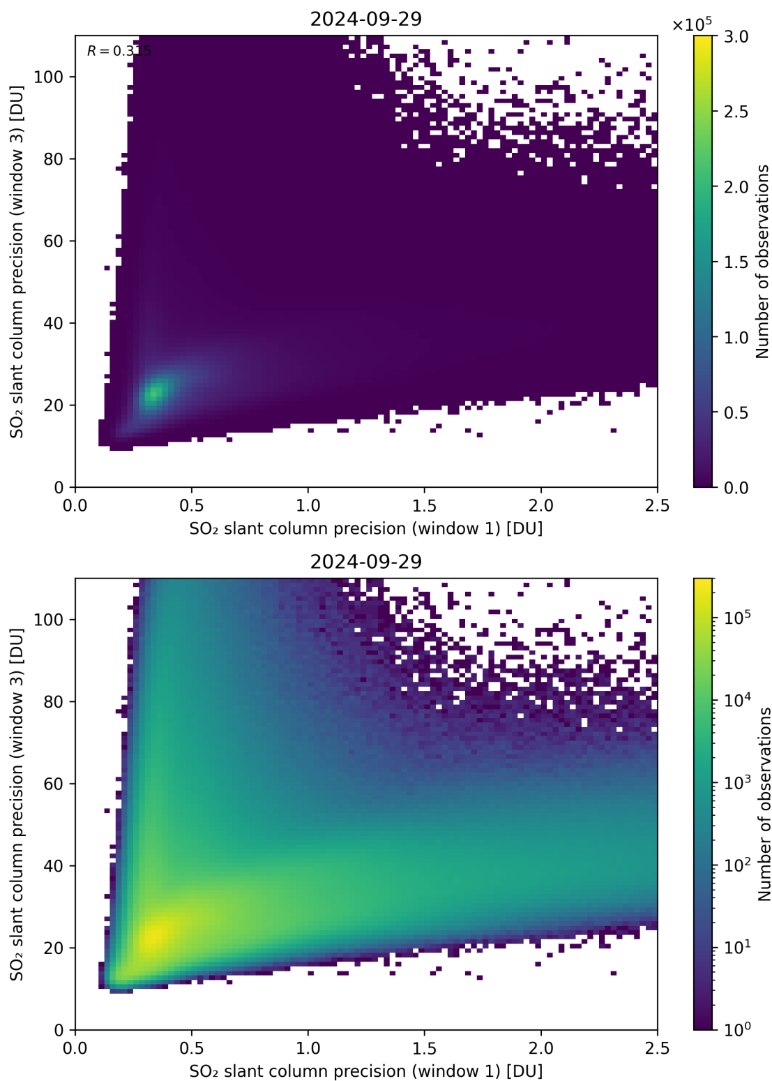
Figure 229: Scatter density plot of “SO 2 slant column precision (window 1)” against “SO 2 slant column precision (window 3)” for 2024-09-28 to 2024-09-30.
