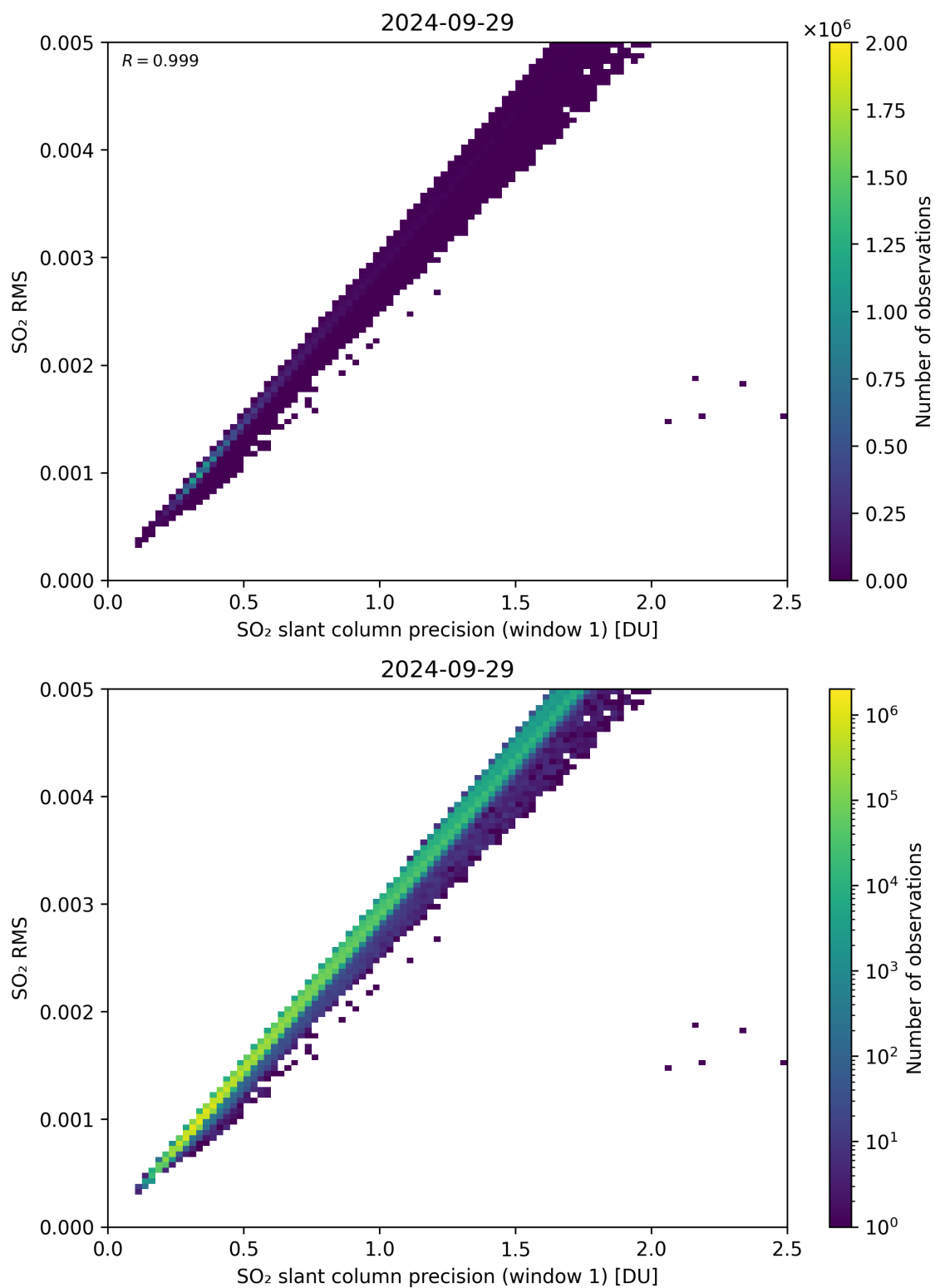
Figure 223: Scatter density plot of “SO 2 slant column precision (window 1)” against “SO 2 RMS” for 2024-09-28 to 2024-09-30.
