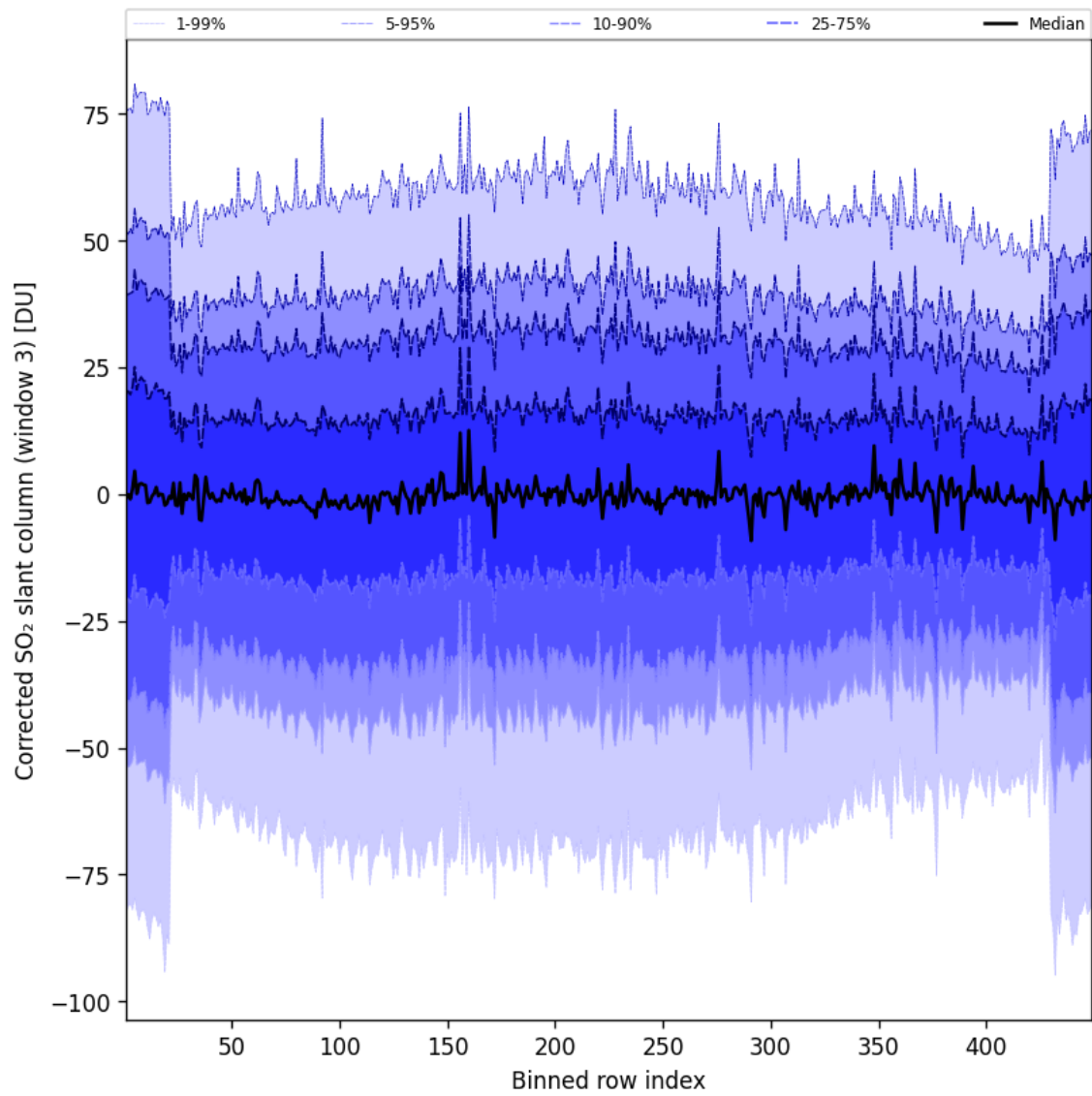
Figure 89: Along track statistics of “Corrected SO 2 slant column (window 3)” for 2024-09-28 to 2024-09-30
