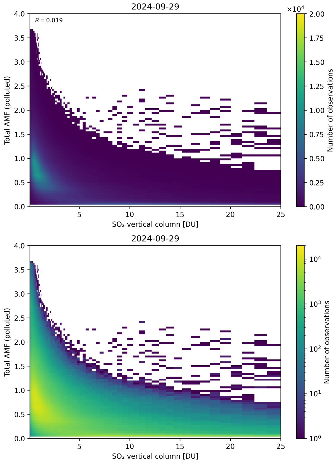
Figure 305: Scatter density plot of “SO 2 vertical column” against “Total AMF (polluted)” for 2024-09-28 to 2024-09-30.
