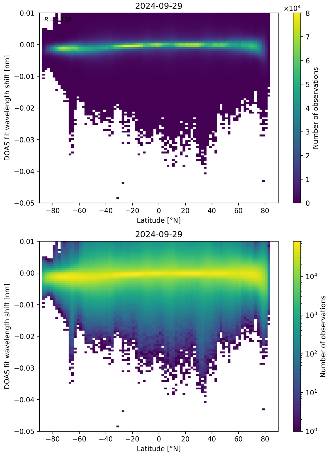
Figure 142: Scatter density plot of “Latitude” against “DOAS fit wavelength shift” for 2024-09-28 to 2024-09-30.
