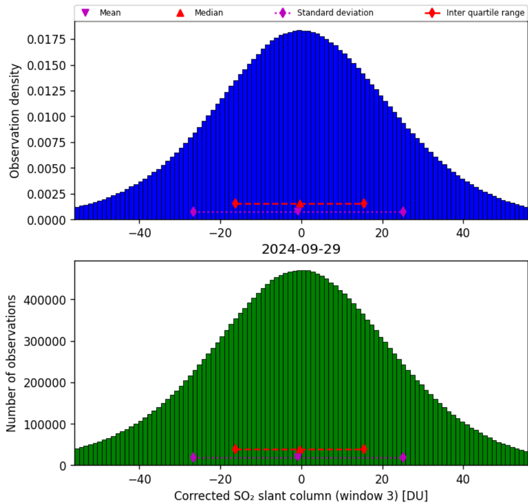
Figure 66: Histogram of “Corrected SO 2 slant column (window 3)” for 2024-09-28 to 2024-09-30
