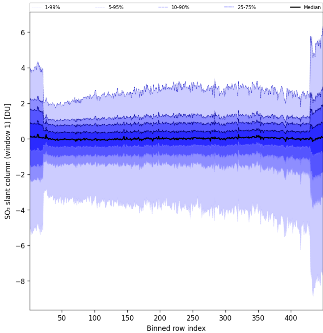
Figure 79: Along track statistics of “SO 2 slant column (window 1)” for 2024-09-28 to 2024-09-30
