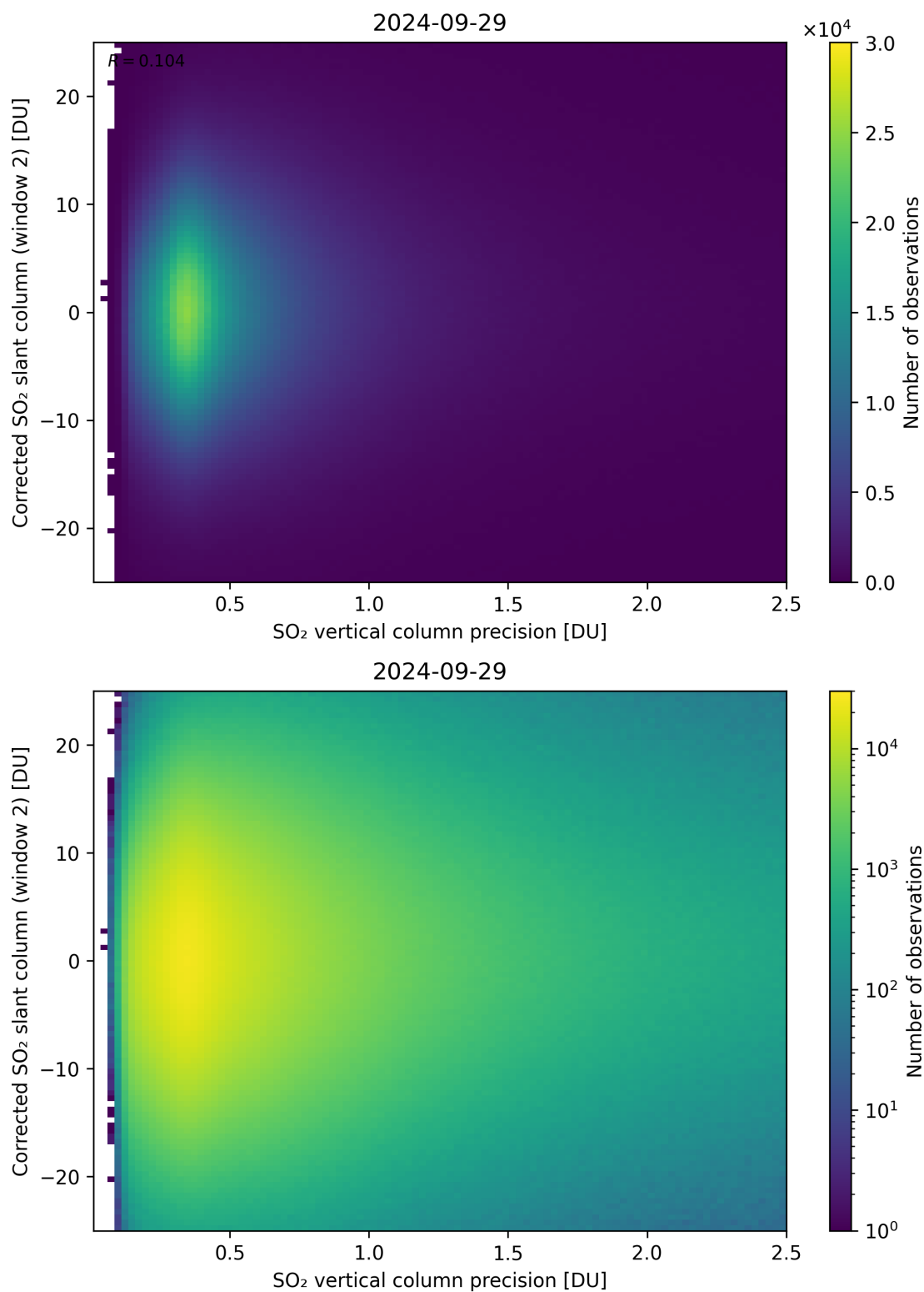
Figure 287: Scatter density plot of “SO 2 vertical column precision” against “Corrected SO 2 slant column (window 2)” for 2024-09-28 to 2024-09-30.
