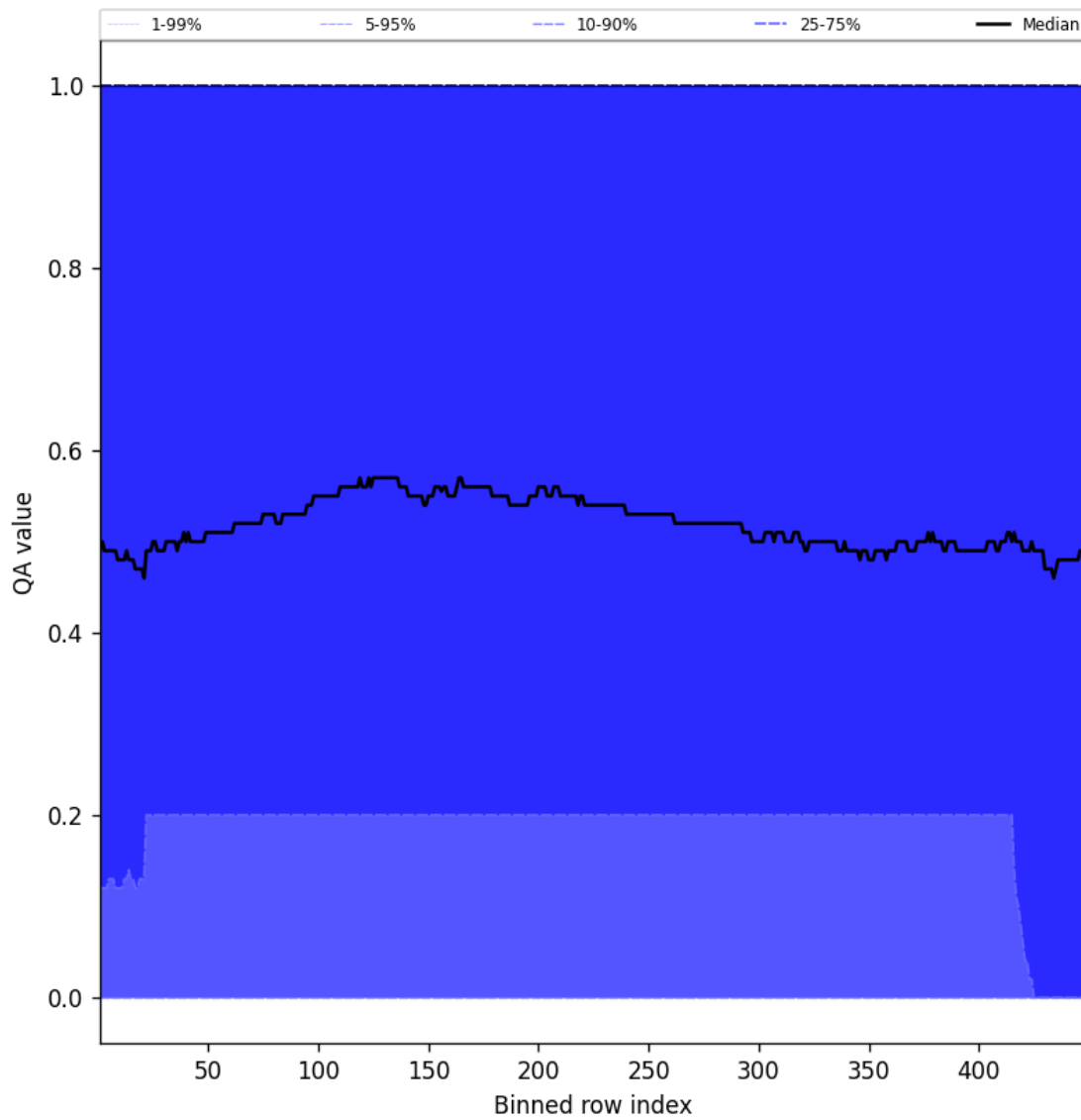
Figure 75: Along track statistics of “QA value” for 2024-09-28 to 2024-09-30
