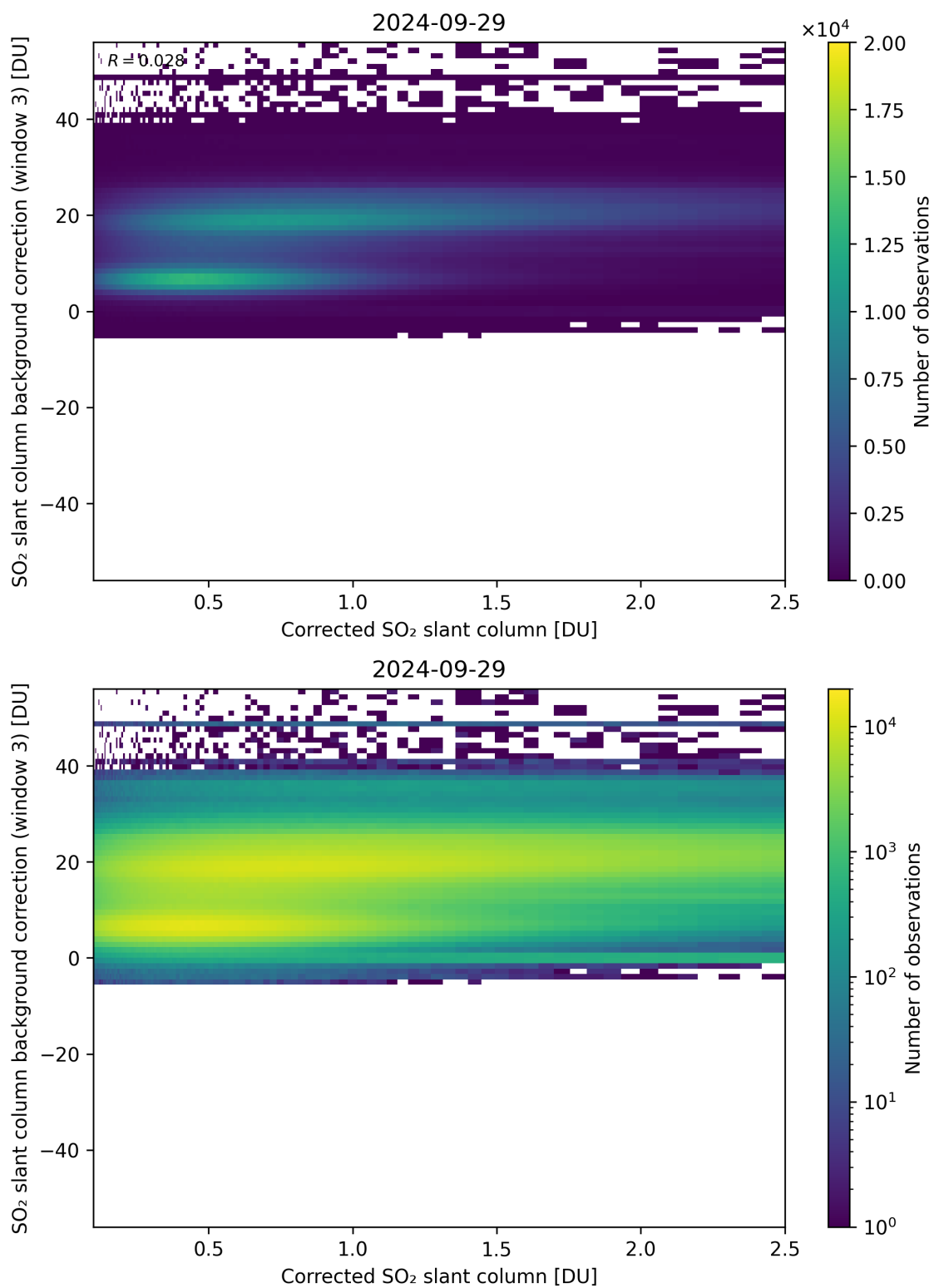
Figure 180: Scatter density plot of “Corrected SO 2 slant column” against “SO 2 slant column background correction (window 3)” for 2024-09-28 to 2024-09-30.
