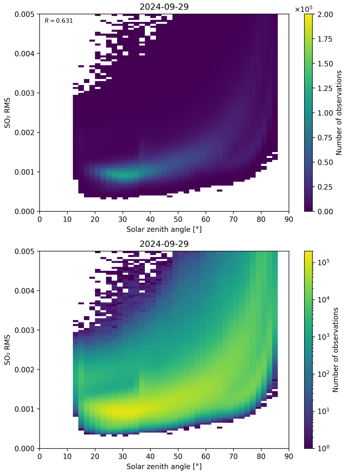
Figure 163: Scatter density plot of “Solar zenith angle” against “SO 2 RMS” for 2024-09-28 to 2024-09-30.
