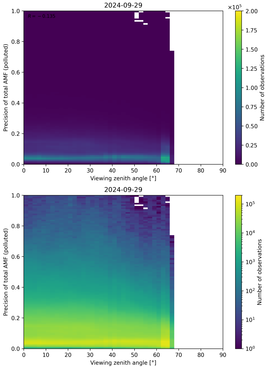
Figure 326: Scatter density plot of “Viewing zenith angle” against “Precision of total AMF (polluted)” for 2024-09-28 to 2024-09-30.
