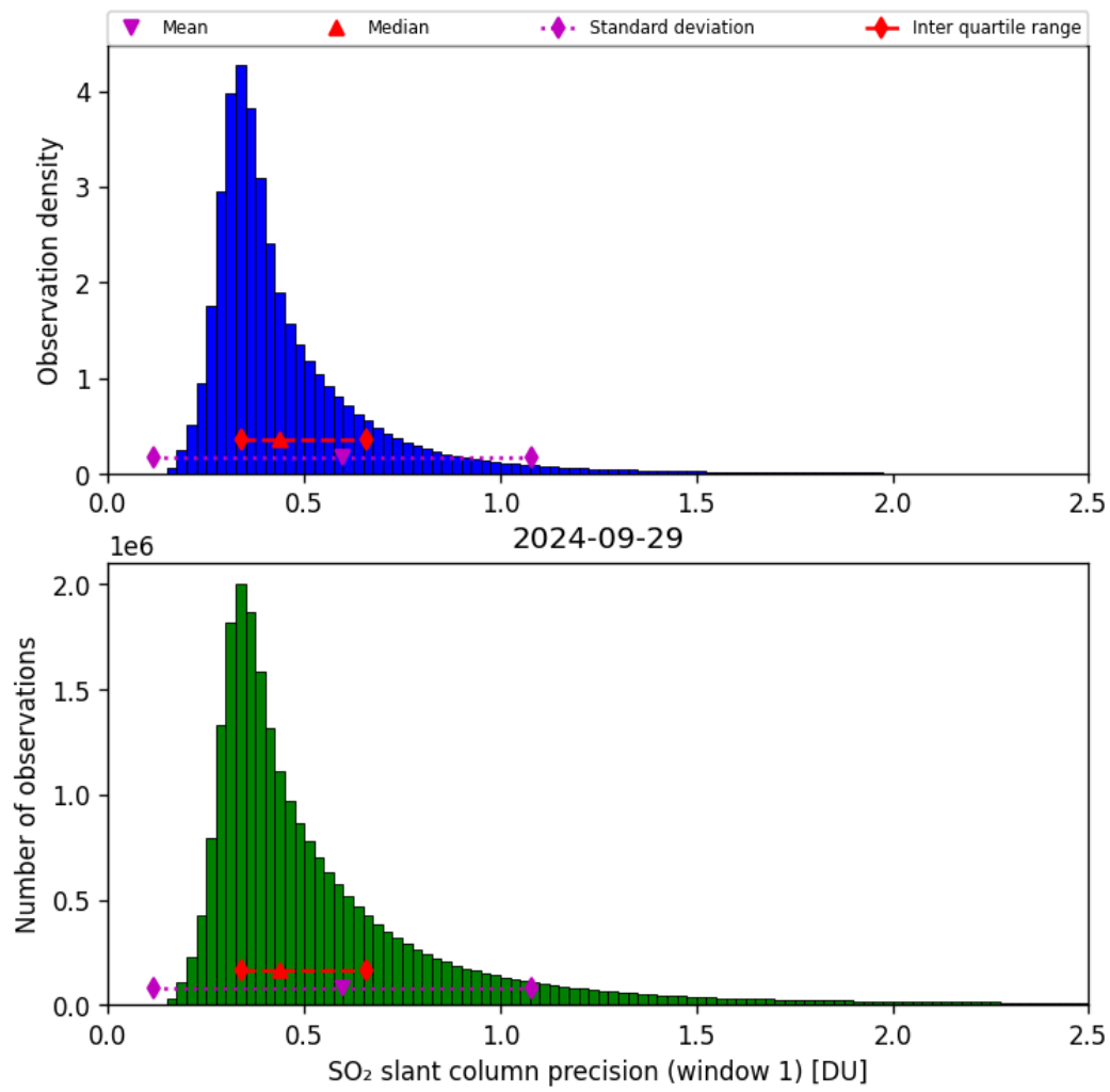
Figure 57: Histogram of “SO 2 slant column precision (window 1)” for 2024-09-28 to 2024-09-30
