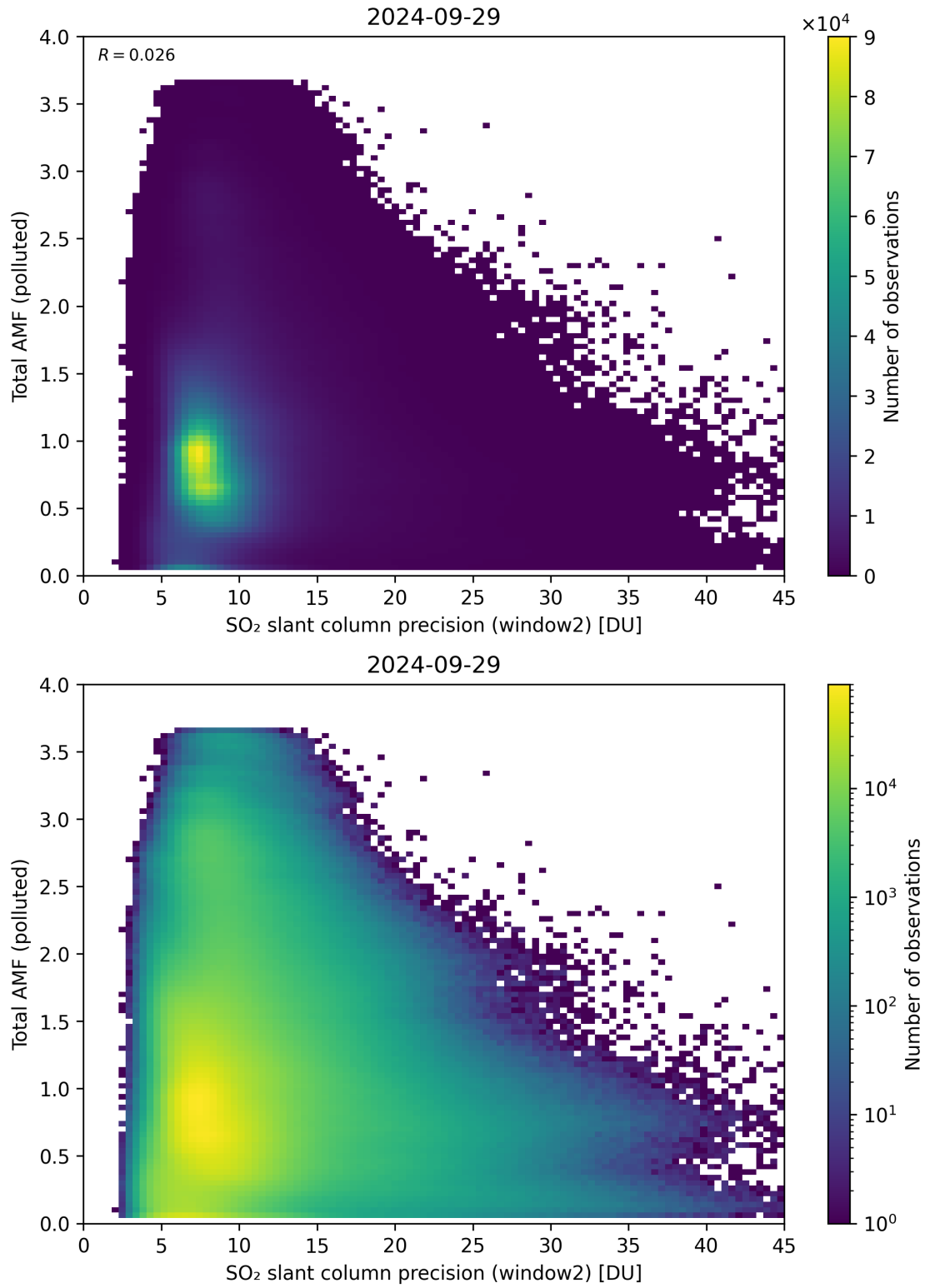
Figure 251: Scatter density plot of “SO 2 slant column precision (window2)” against “Total AMF (polluted)” for 2024-09-28 to 2024-09-30.
