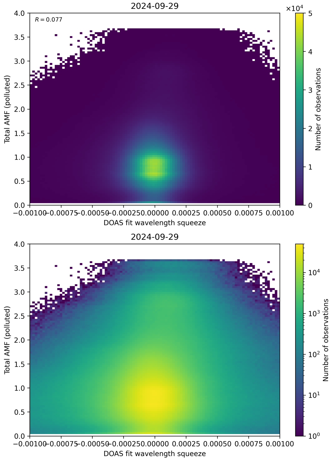
Figure 134: Scatter density plot of “DOAS fit wavelength squeeze” against “Total AMF (polluted)” for 2024-09-28 to 2024-09-30.
