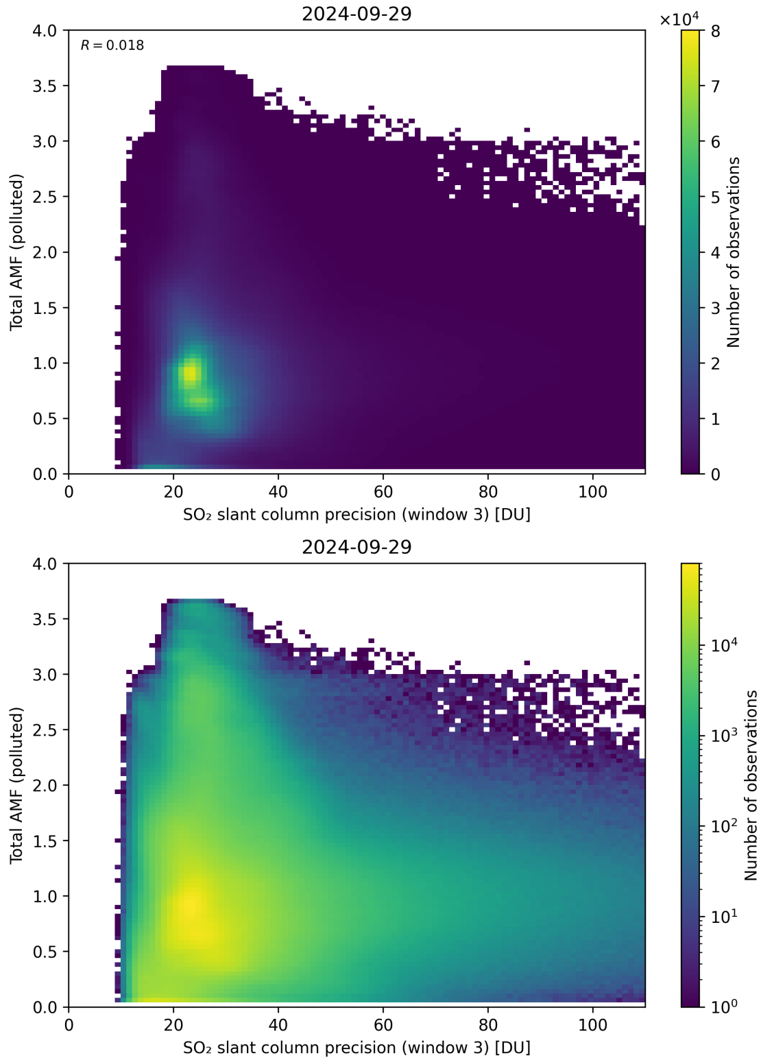
Figure 263: Scatter density plot of “SO 2 slant column precision (window 3)” against “Total AMF (polluted)” for 2024-09-28 to 2024-09-30.
