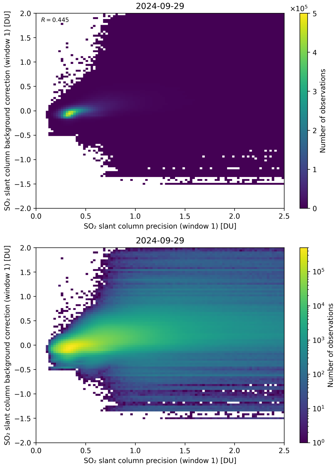
Figure 218: Scatter density plot of “SO 2 slant column precision (window 1)” against “SO 2 slant column background correction (window 1)” for 2024-09-28 to 2024-09-30.
