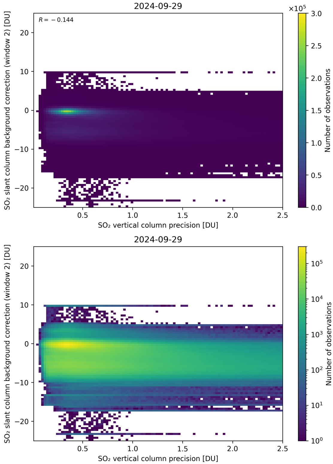
Figure 280: Scatter density plot of “SO 2 vertical column precision” against “SO 2 slant column background correction (window 2)” for 2024-09-28 to 2024-09-30.
