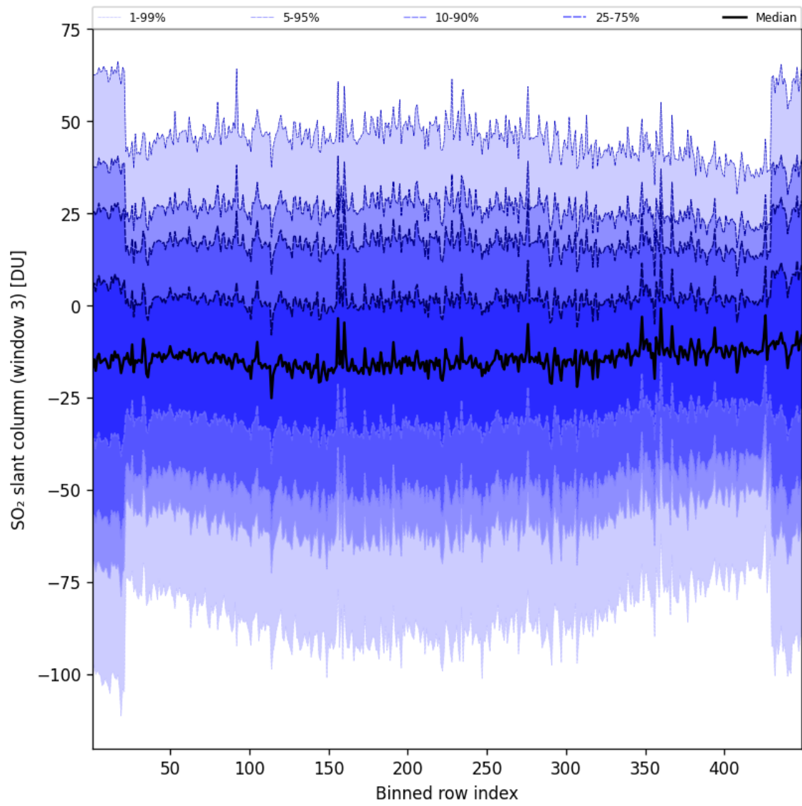
Figure 87: Along track statistics of “SO 2 slant column (window 3)” for 2024-09-28 to 2024-09-30
