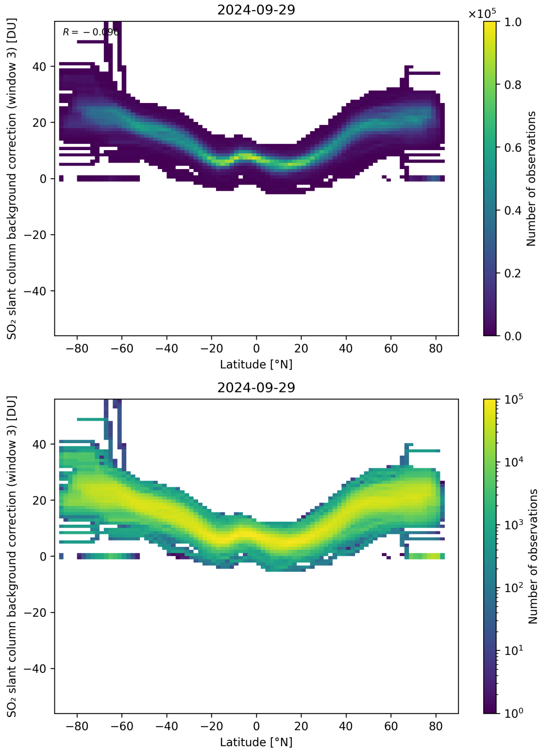
Figure 141: Scatter density plot of “Latitude” against “SO 2 slant column background correction (window 3)” for 2024-09-28 to 2024-09-30.
