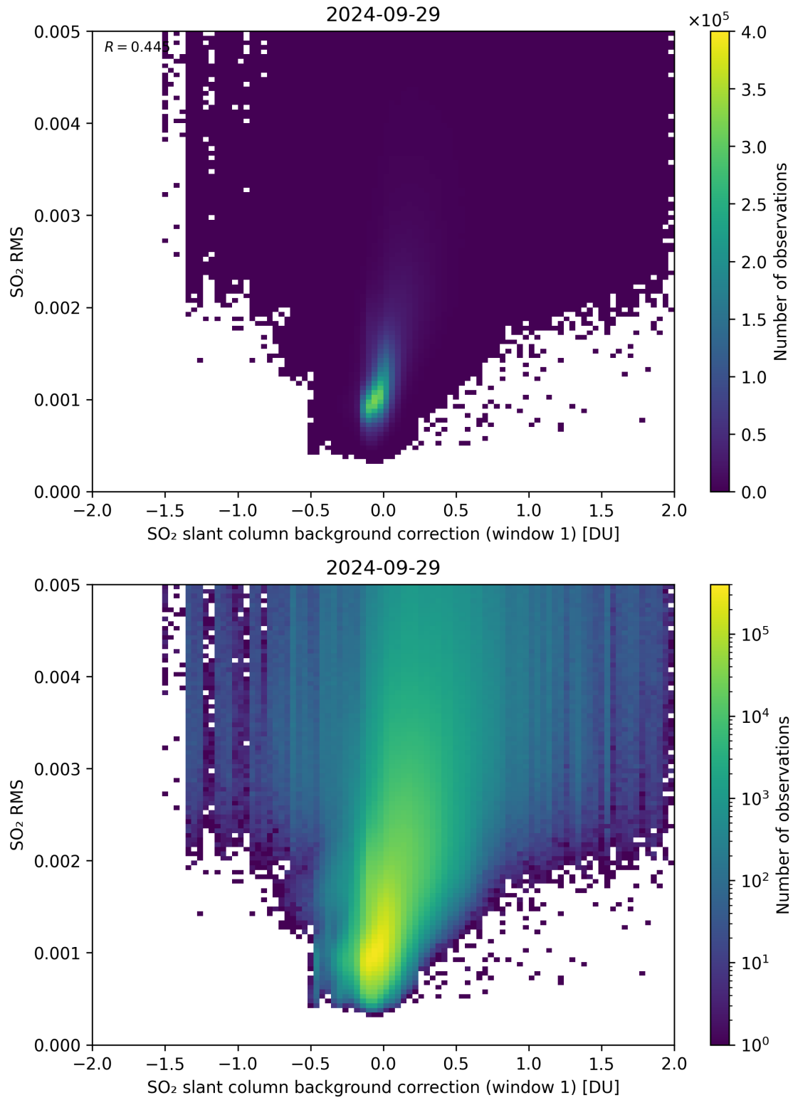
Figure 102: Scatter density plot of “SO 2 slant column background correction (window 1)” against “SO 2 RMS” for 2024-09-28 to 2024-09-30.
