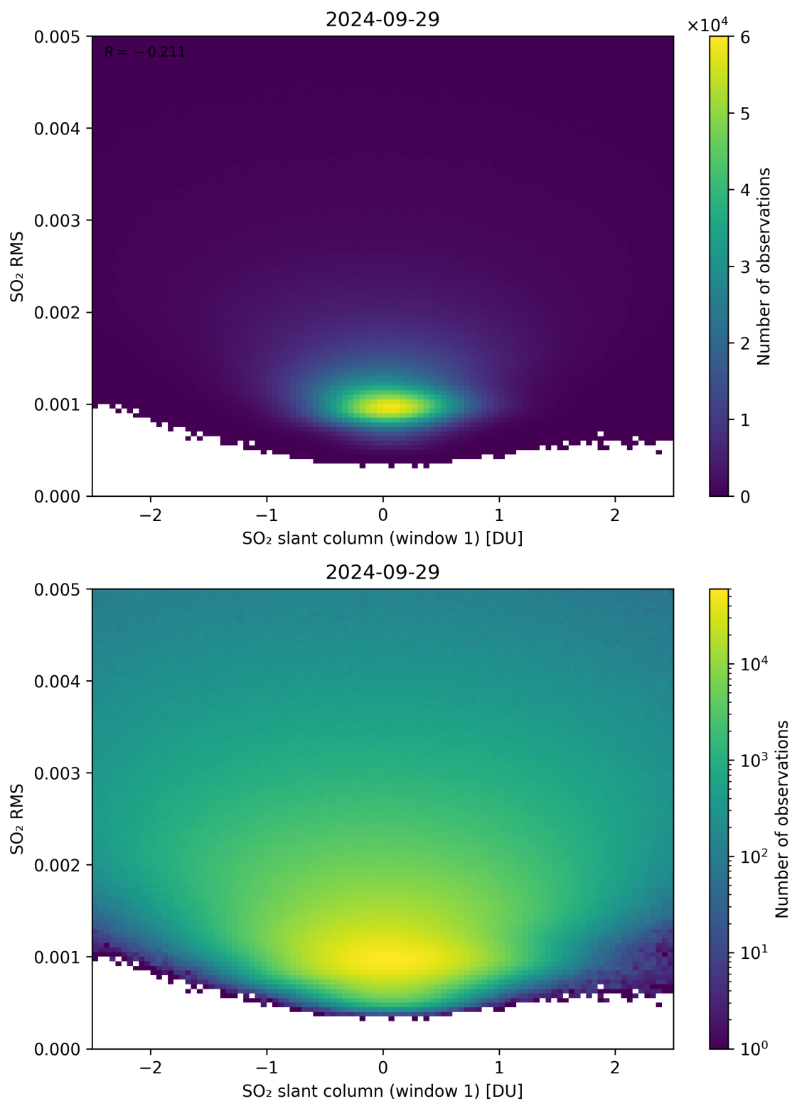
Figure 217: Scatter density plot of “SO 2 slant column (window 1)” against “SO 2 RMS” for 2024-09-28 to 2024-09-30.
