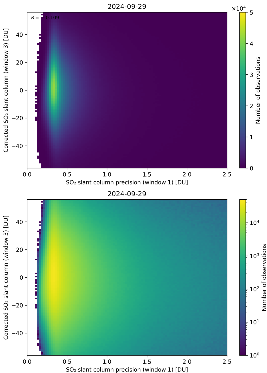
Figure 226: Scatter density plot of “SO 2 slant column precision (window 1)” against “Corrected SO 2 slant column (window 3)” for 2024-09-28 to 2024-09-30.
