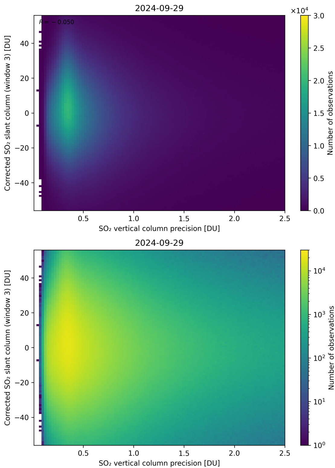
Figure 288: Scatter density plot of “SO 2 vertical column precision” against “Corrected SO 2 slant column (window 3)” for 2024-09-28 to 2024-09-30.
