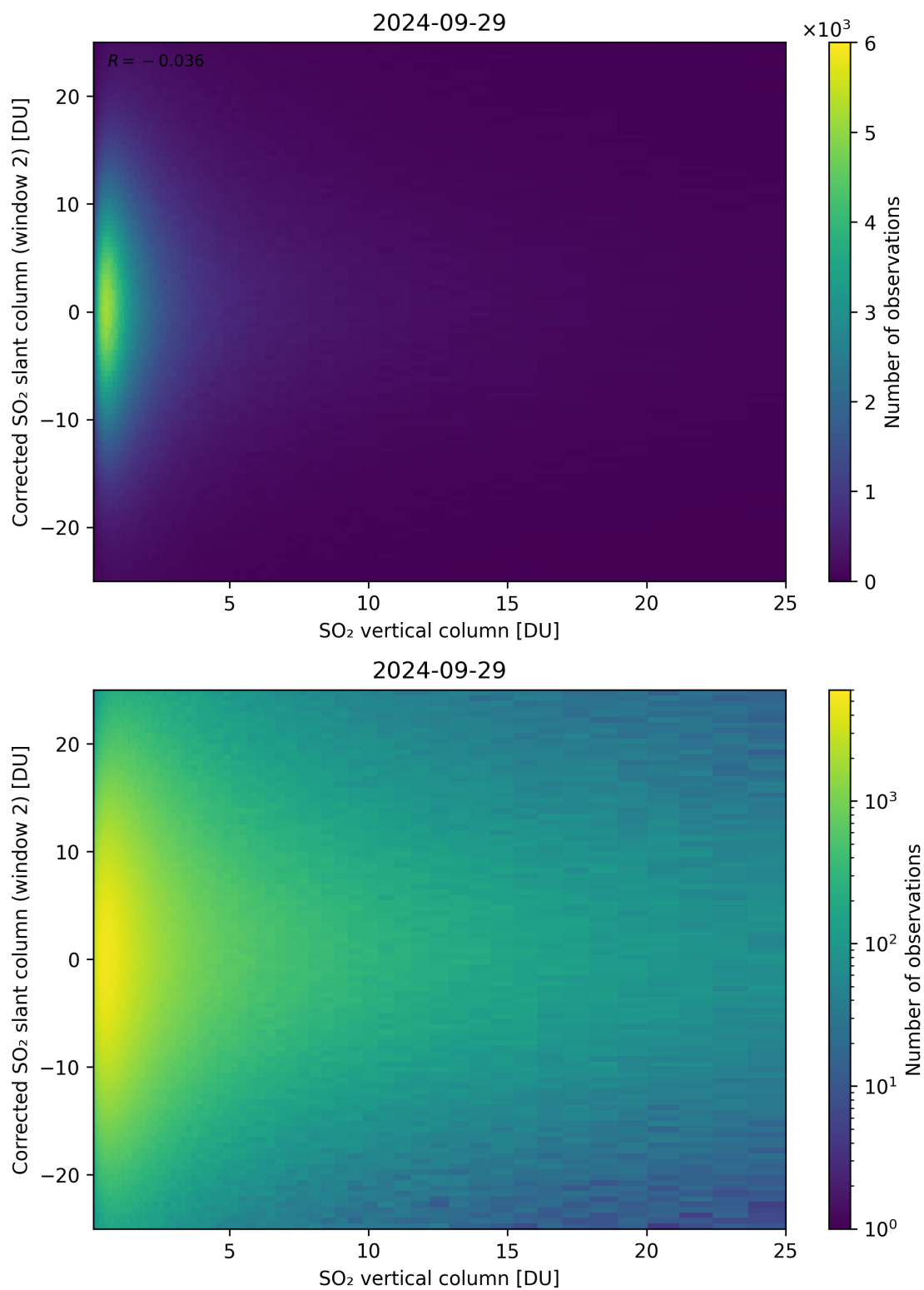
Figure 298: Scatter density plot of “SO 2 vertical column” against “Corrected SO 2 slant column (window 2)” for 2024-09-28 to 2024-09-30.
