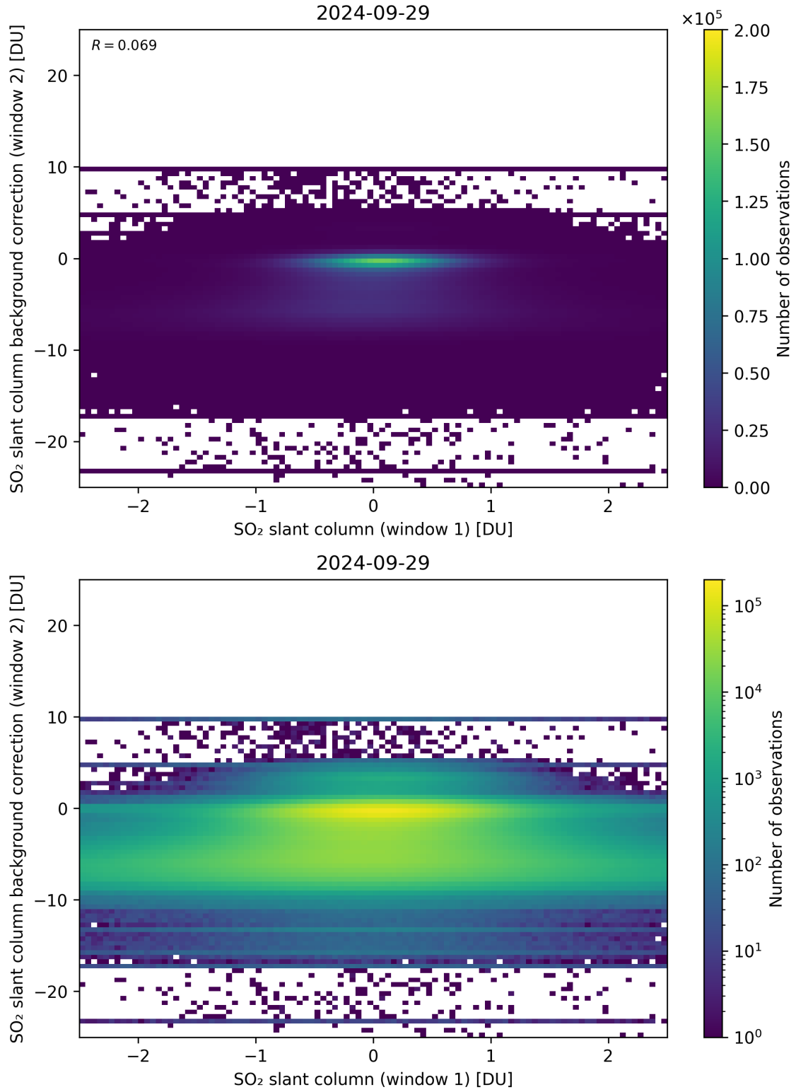
Figure 213: Scatter density plot of “SO 2 slant column (window 1)” against “SO 2 slant column background correction (window 2)” for 2024-09-28 to 2024-09-30.
