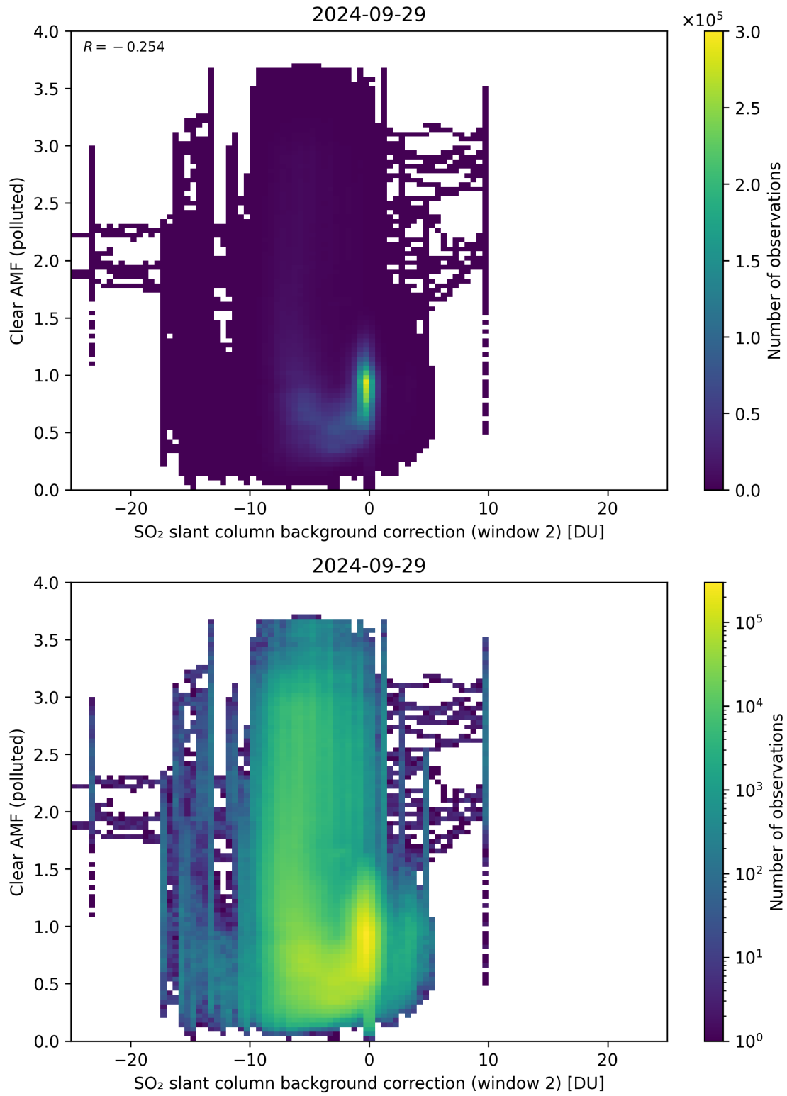
Figure 115: Scatter density plot of “SO 2 slant column background correction (window 2)” against “Clear AMF (polluted)” for 2024-09-28 to 2024-09-30.
