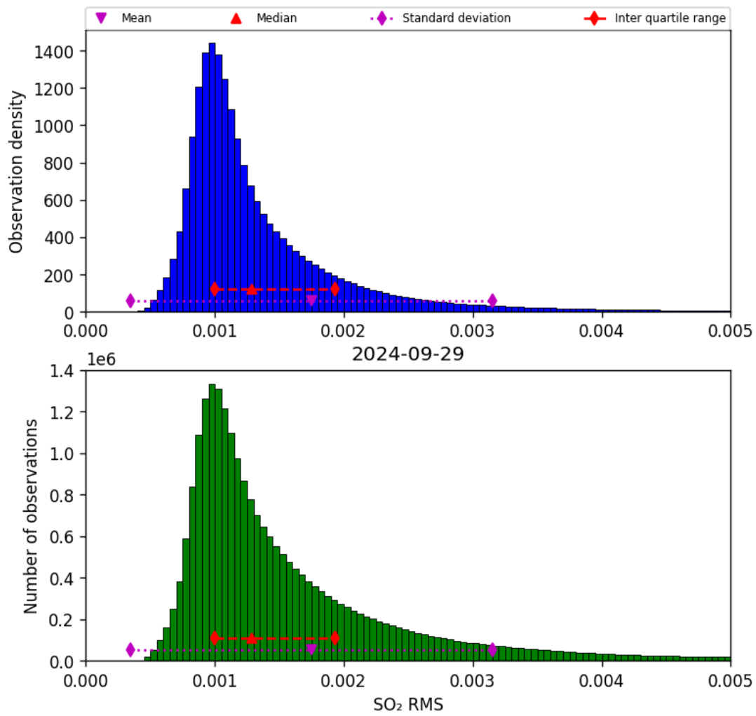
Figure 70: Histogram of “SO 2 RMS” for 2024-09-28 to 2024-09-30
