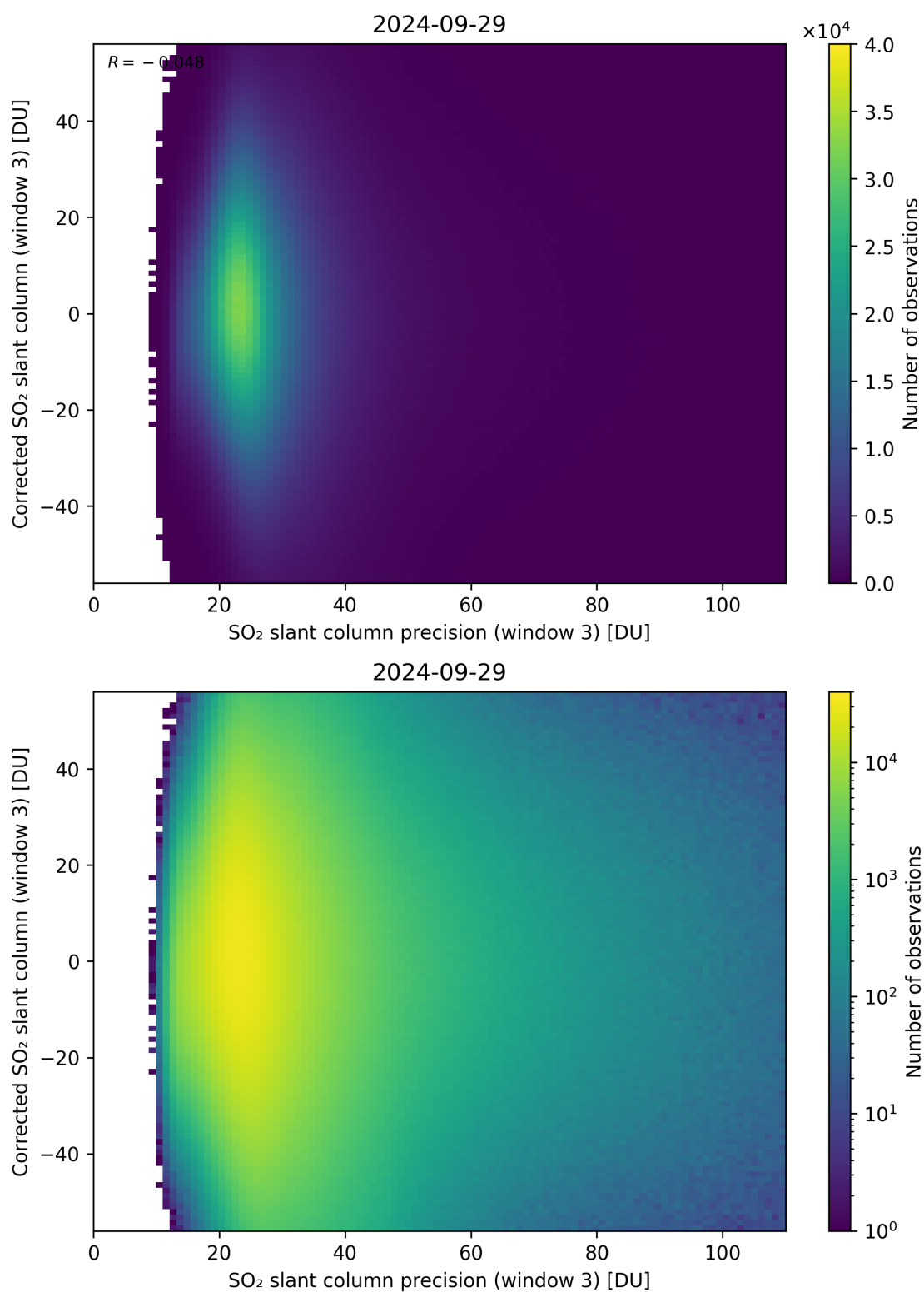
Figure 262: Scatter density plot of “SO 2 slant column precision (window 3)” against “Corrected SO 2 slant column (window 3)” for 2024-09-28 to 2024-09-30.
