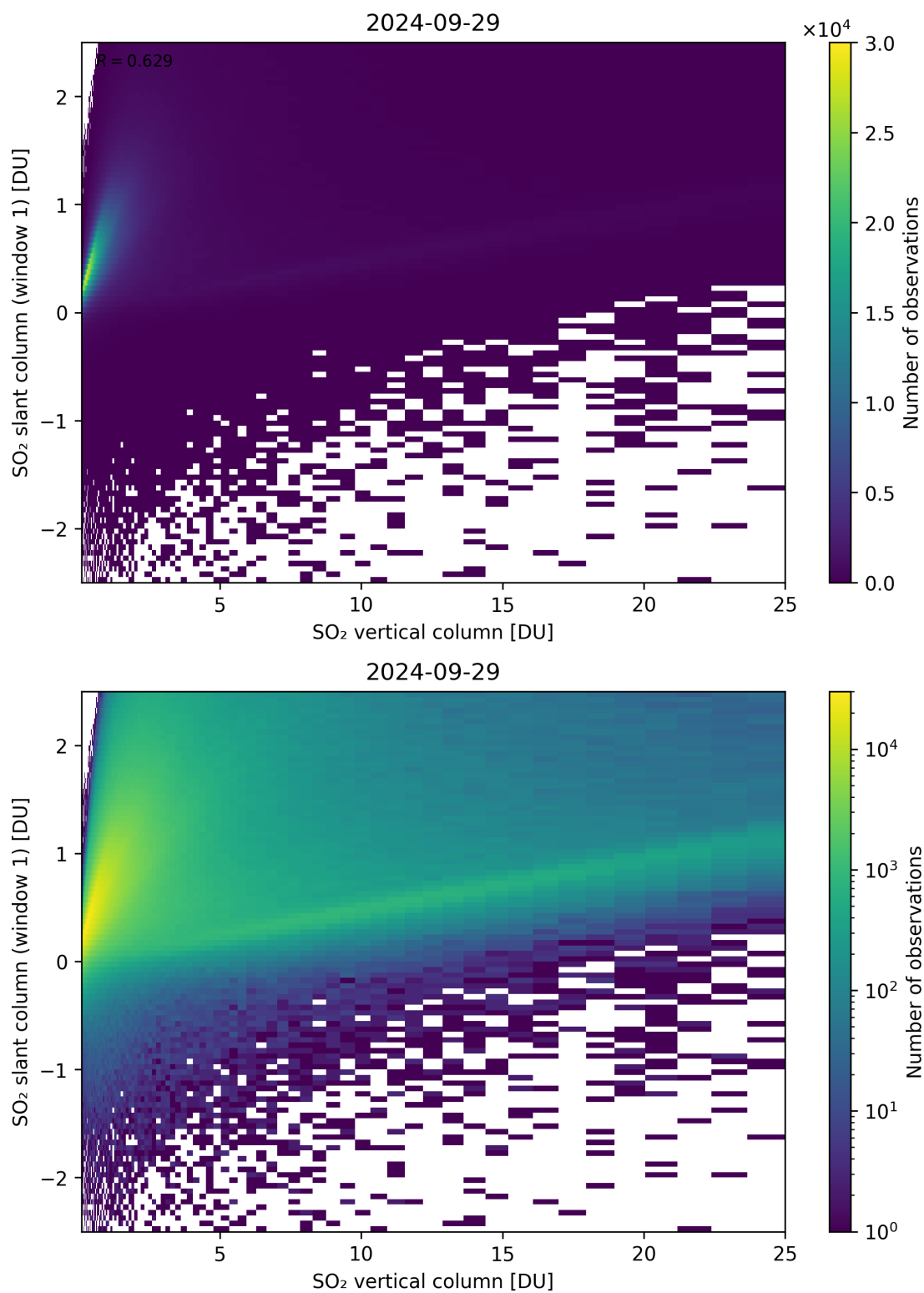
Figure 300: Scatter density plot of “SO 2 vertical column” against “SO 2 slant column (window 1)” for 2024-09-28 to 2024-09-30.
