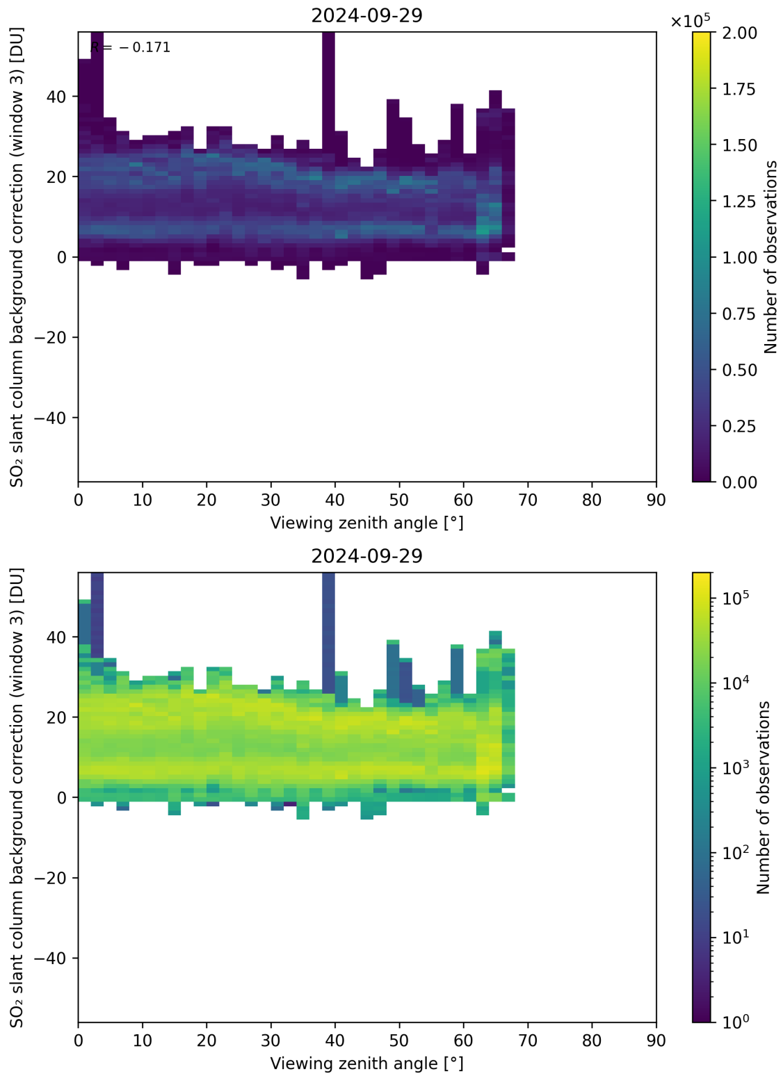
Figure 310: Scatter density plot of “Viewing zenith angle” against “SO 2 slant column background correction (window 3)” for 2024-09-28 to 2024-09-30.
