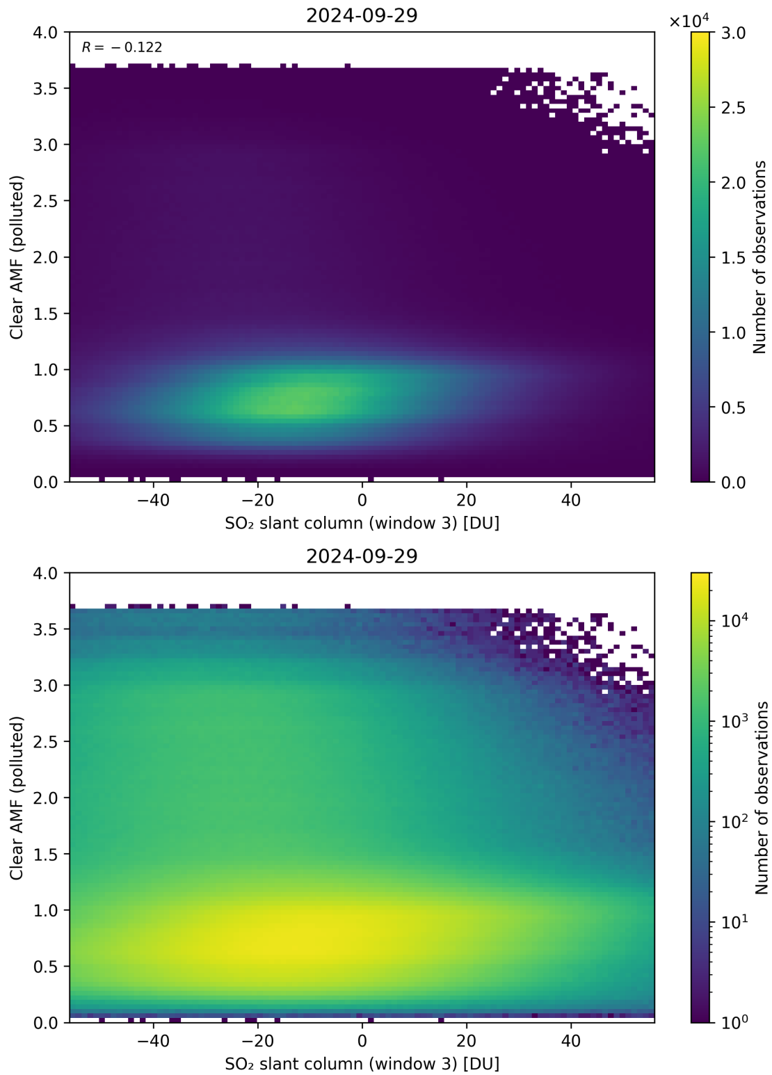
Figure 265: Scatter density plot of “SO 2 slant column (window 3)” against “Clear AMF (polluted)” for 2024-09-28 to 2024-09-30.
