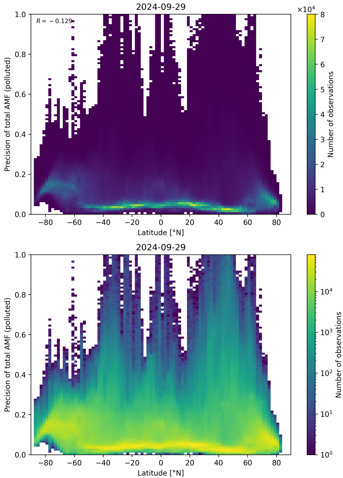
Figure 155: Scatter density plot of “Latitude” against “Precision of total AMF (polluted)” for 2024-09-28 to 2024-09-30.
