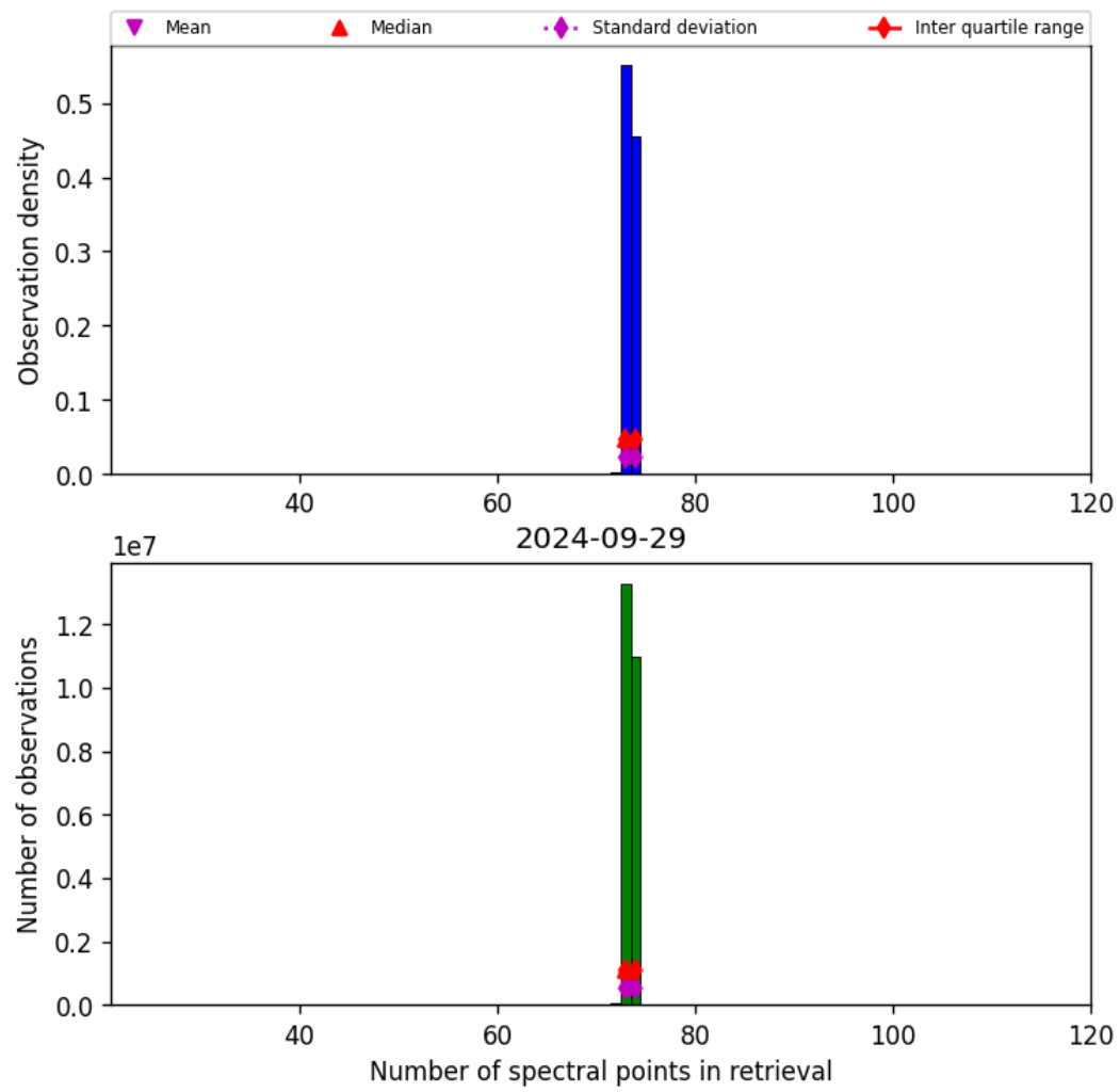
Figure 74: Histogram of “Number of spectral points in retrieval” for 2024-09-28 to 2024-09-30
