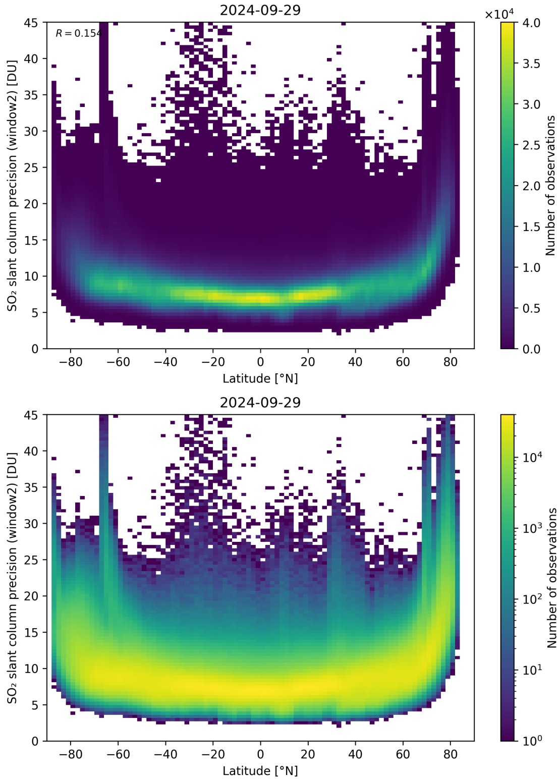
Figure 151: Scatter density plot of “Latitude” against “SO 2 slant column precision (window2)” for 2024-09-28 to 2024-09-30.
