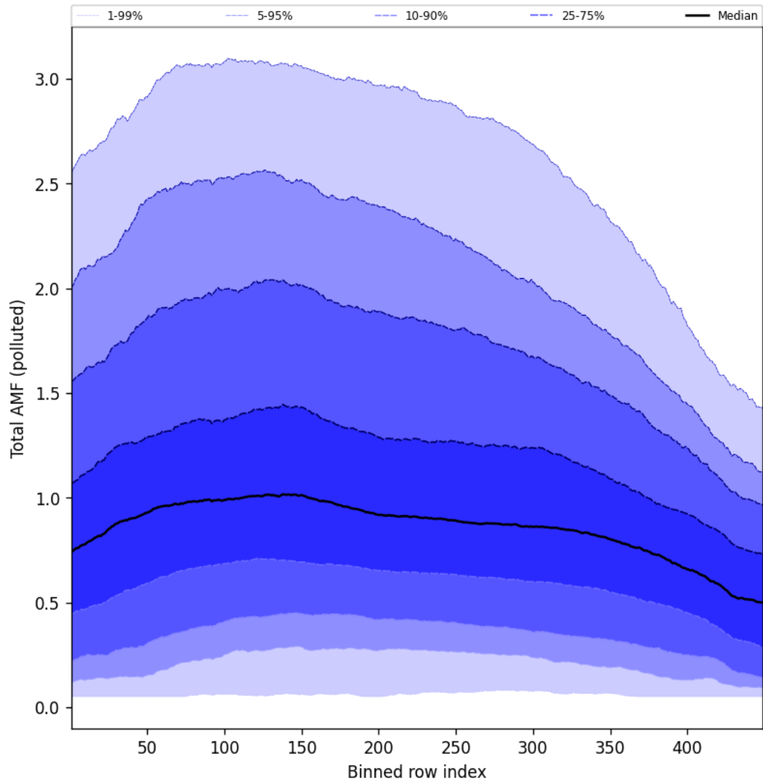
Figure 94: Along track statistics of “Total AMF (polluted)” for 2024-09-28 to 2024-09-30
