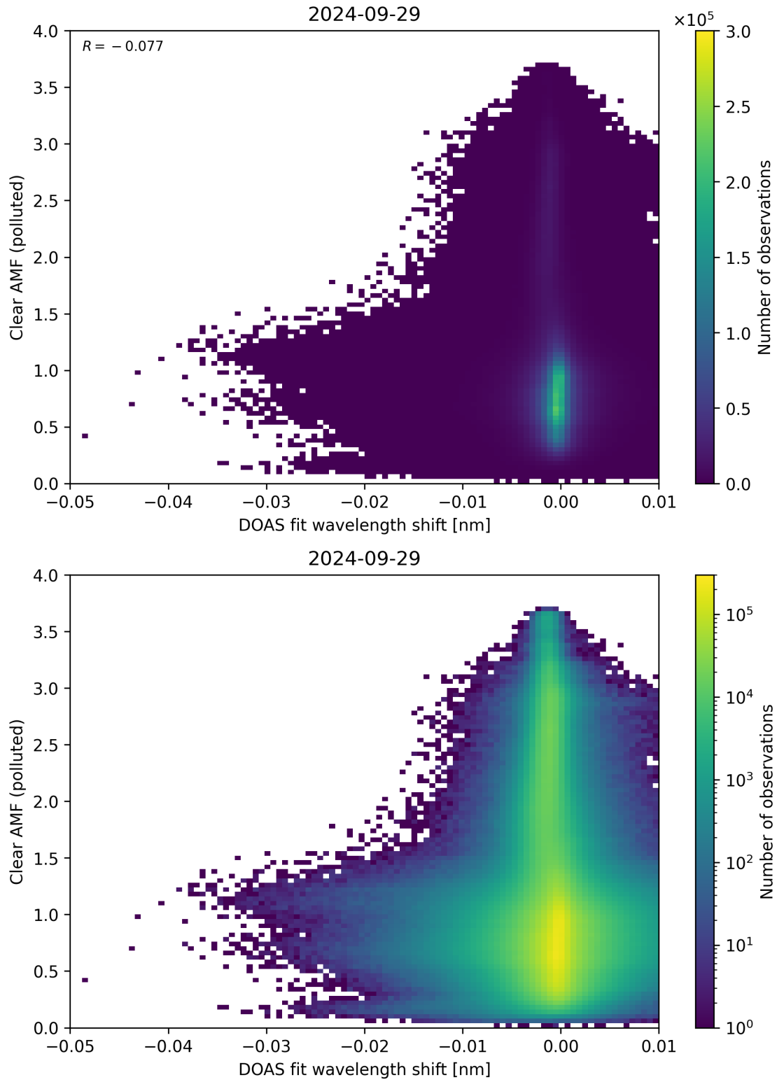
Figure 129: Scatter density plot of “DOAS fit wavelength shift” against “Clear AMF (polluted)” for 2024-09-28 to 2024-09-30.
