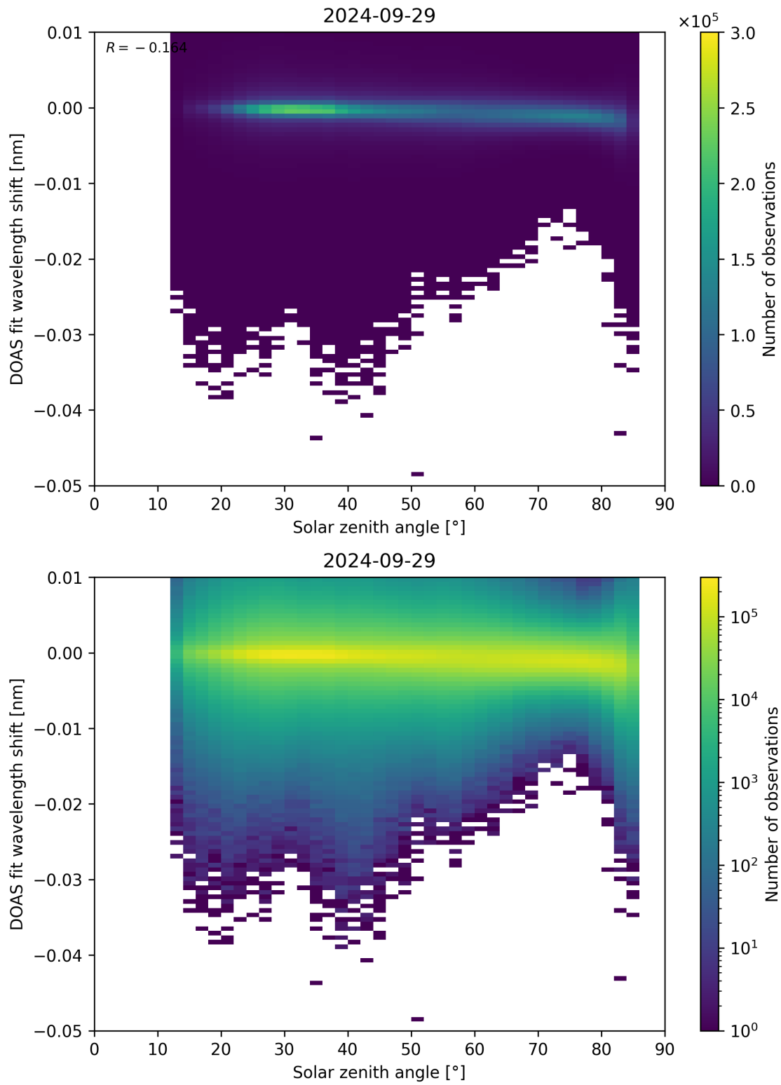
Figure 161: Scatter density plot of “Solar zenith angle” against “DOAS fit wavelength shift” for 2024-09-28 to 2024-09-30.
