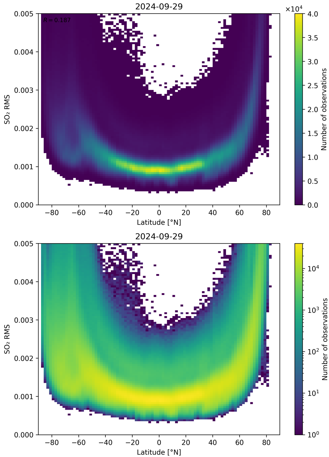
Figure 144: Scatter density plot of “Latitude” against “SO 2 RMS” for 2024-09-28 to 2024-09-30.
