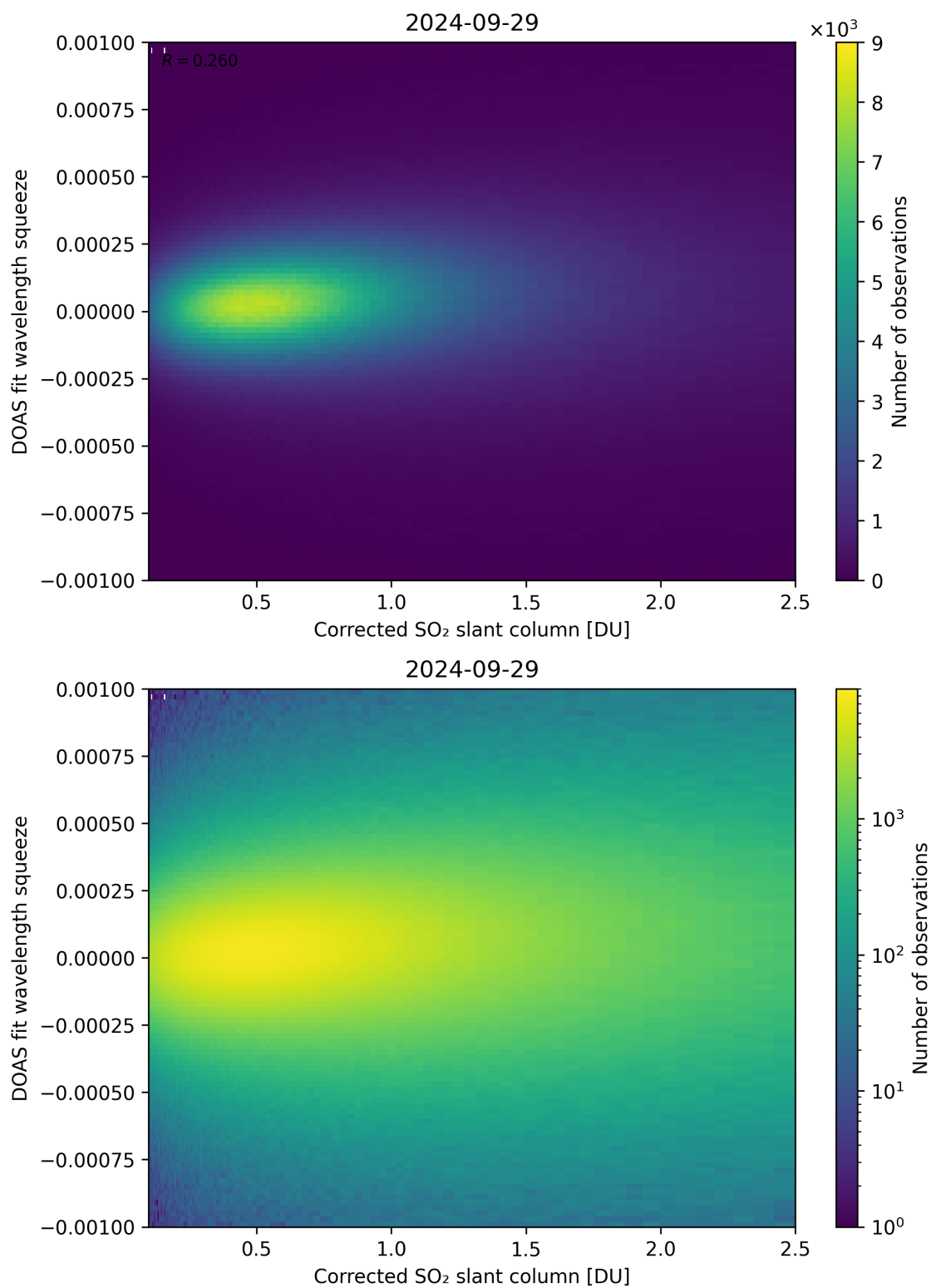
Figure 182: Scatter density plot of “Corrected SO 2 slant column” against “DOAS fit wavelength squeeze” for 2024-09-28 to 2024-09-30.
