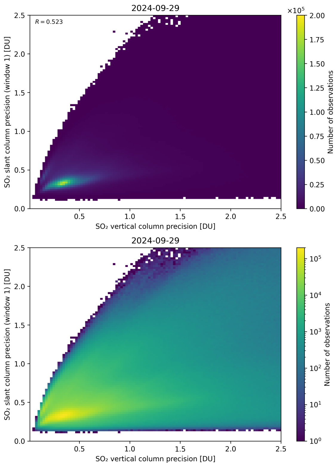
Figure 290: Scatter density plot of “SO 2 vertical column precision” against “SO 2 slant column precision (window 1)” for 2024-09-28 to 2024-09-30.
