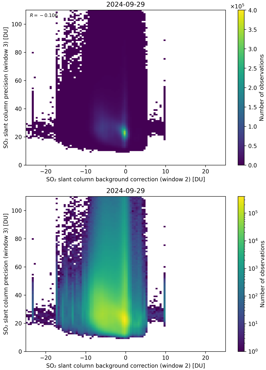
Figure 118: Scatter density plot of “SO 2 slant column background correction (window 2)” against “SO 2 slant column precision (window 3)” for 2024-09-28 to 2024-09-30.
