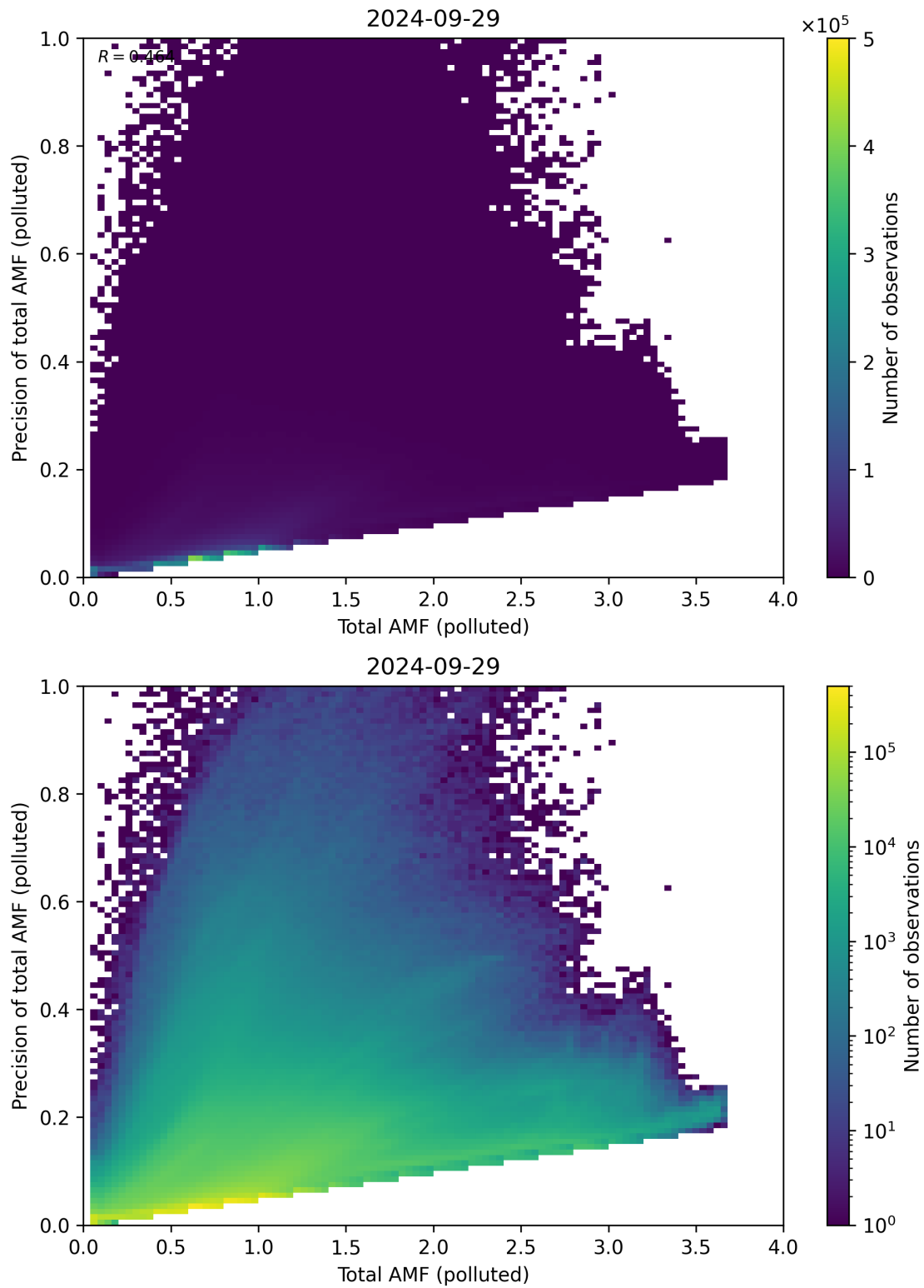
Figure 272: Scatter density plot of “Total AMF (polluted)” against “Precision of total AMF (polluted)” for 2024-09-28 to 2024-09-30.
