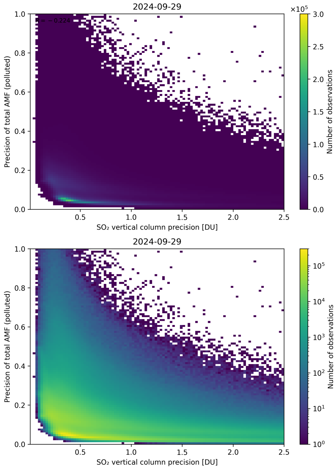
Figure 295: Scatter density plot of “SO 2 vertical column precision” against “Precision of total AMF (polluted)” for 2024-09-28 to 2024-09-30.
