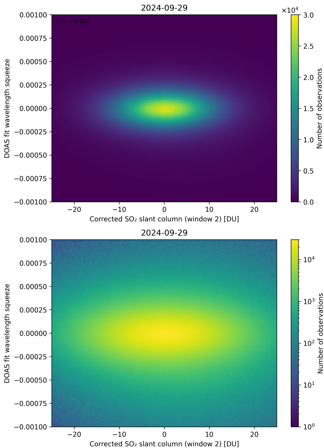
Figure 197: Scatter density plot of “Corrected SO 2 slant column (window 2)” against “DOAS fit wavelength squeeze” for 2024-09-28 to 2024-09-30.
