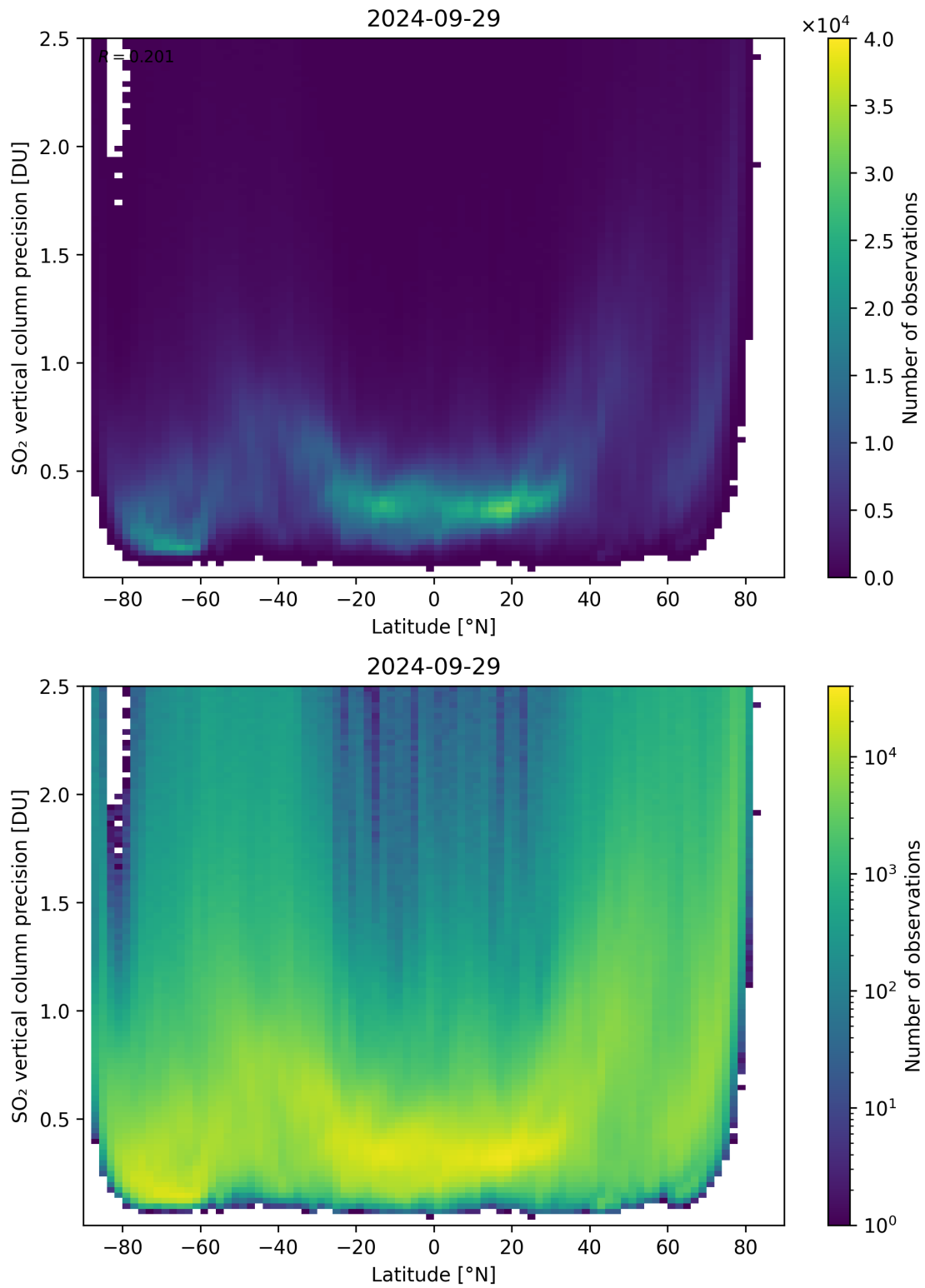
Figure 157: Scatter density plot of “Latitude” against “SO 2 vertical column precision” for 2024-09-28 to 2024-09-30.
