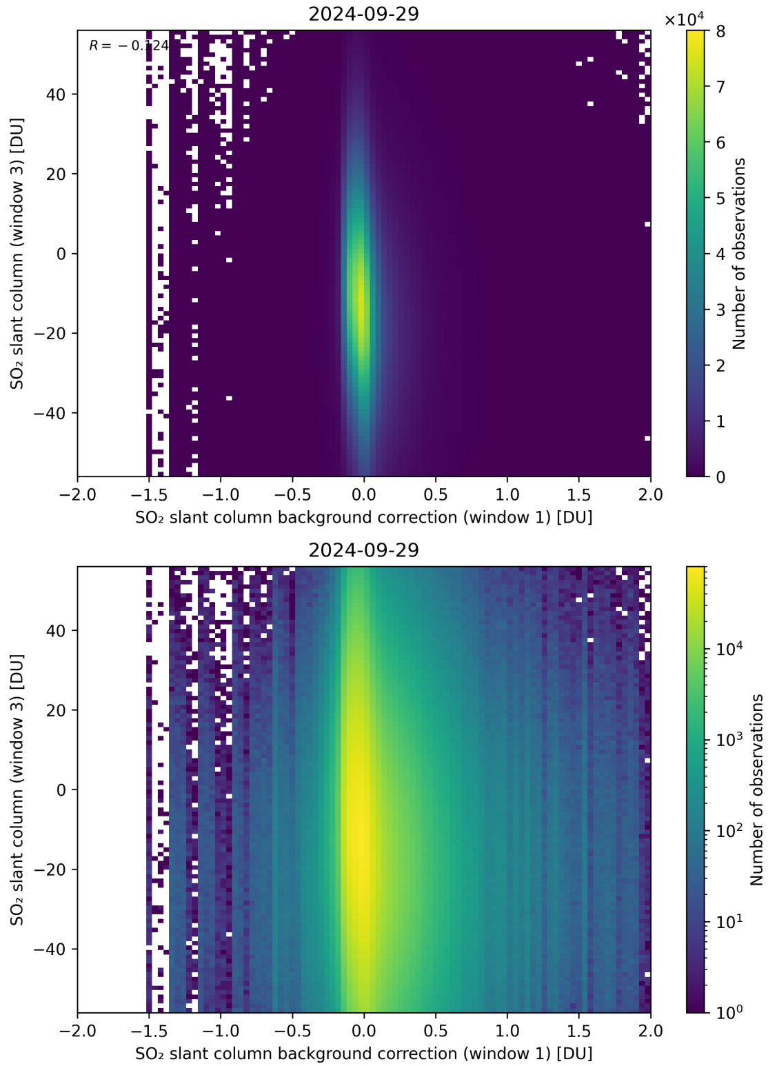
Figure 107: Scatter density plot of “SO 2 slant column background correction (window 1)” against “SO 2 slant column (window 3)” for 2024-09-28 to 2024-09-30.
