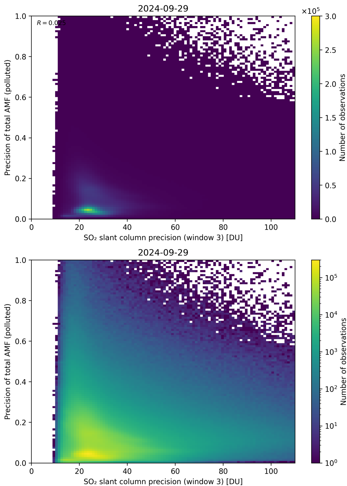
Figure 264: Scatter density plot of “SO 2 slant column precision (window 3)” against “Precision of total AMF (polluted)” for 2024-09-28 to 2024-09-30.
