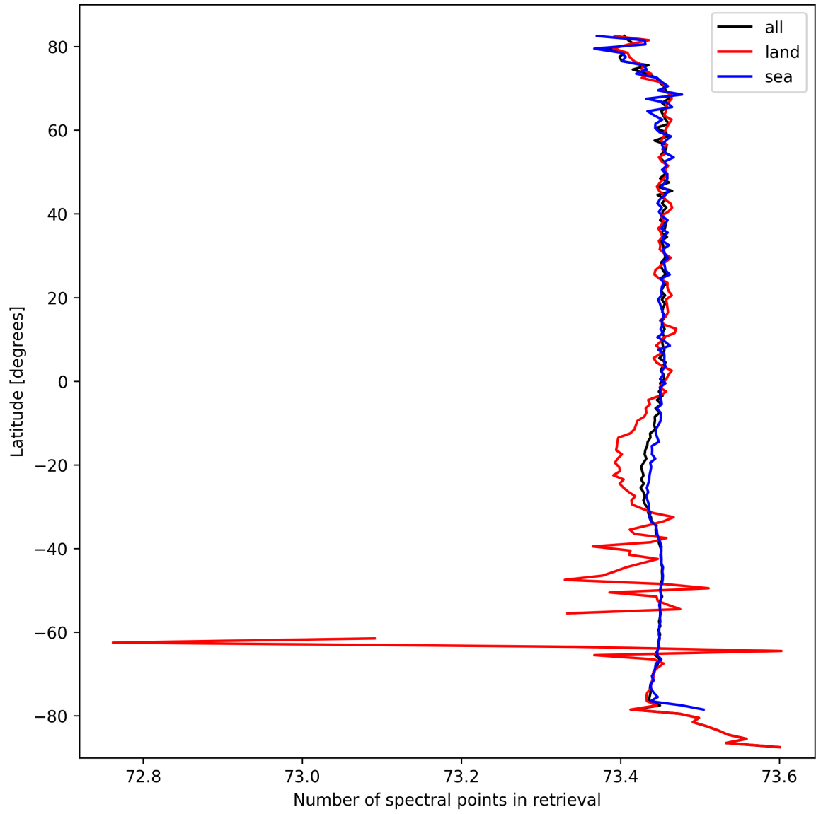
Figure 51: Zonal average of “Number of spectral points in retrieval” for 2024-09-28 to 2024-09-30.
