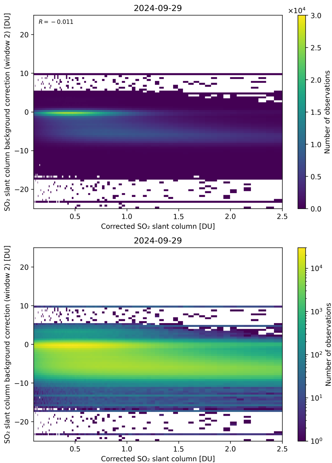
Figure 179: Scatter density plot of “Corrected SO 2 slant column” against “SO 2 slant column background correction (window 2)” for 2024-09-28 to 2024-09-30.
