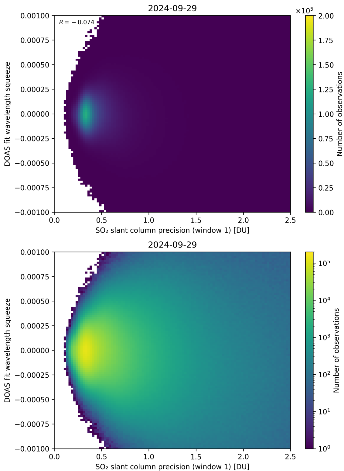
Figure 222: Scatter density plot of “SO 2 slant column precision (window 1)” against “DOAS fit wavelength squeeze” for 2024-09-28 to 2024-09-30.
