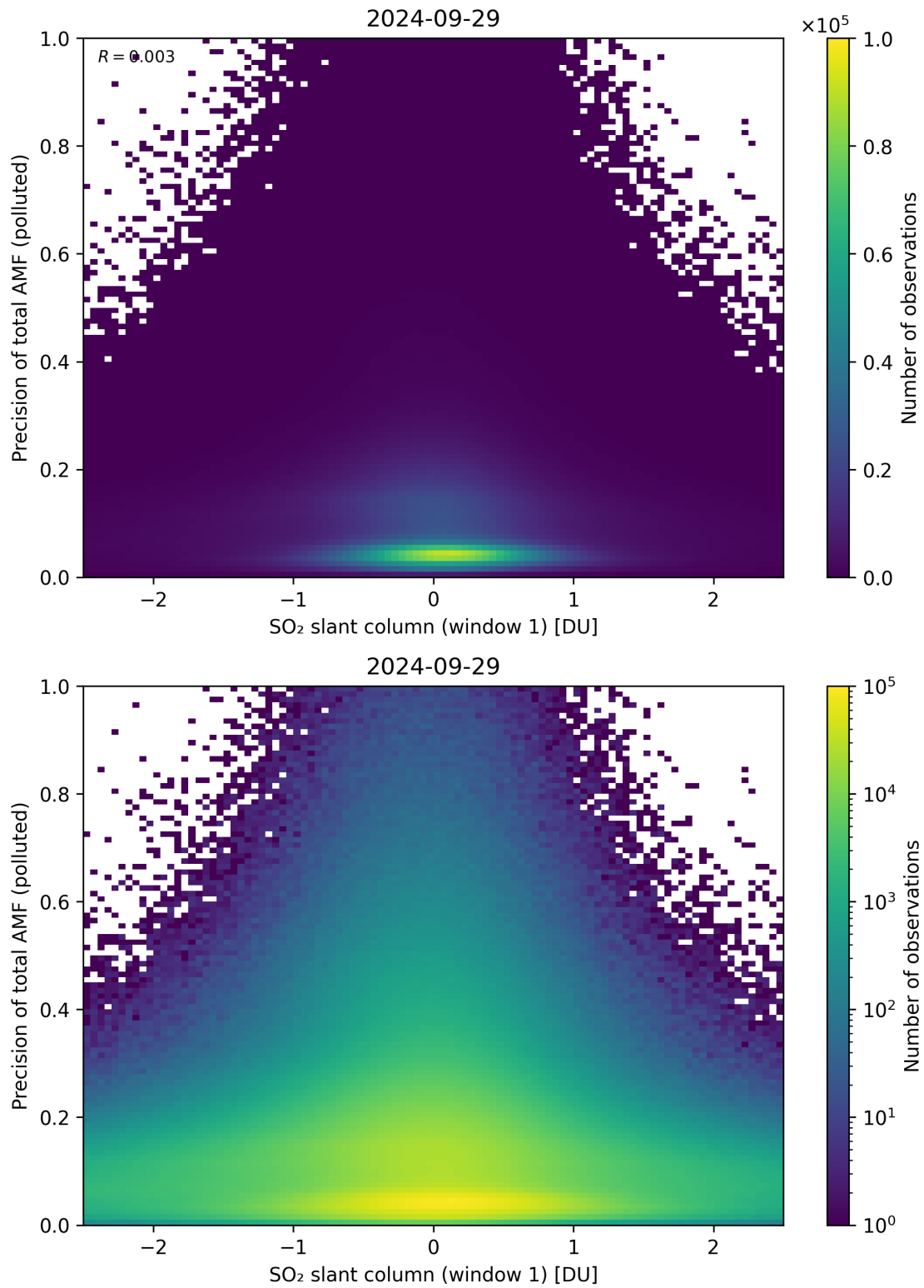
Figure 240: Scatter density plot of “SO 2 slant column (window 1)” against “Precision of total AMF (polluted)” for 2024-09-28 to 2024-09-30.
