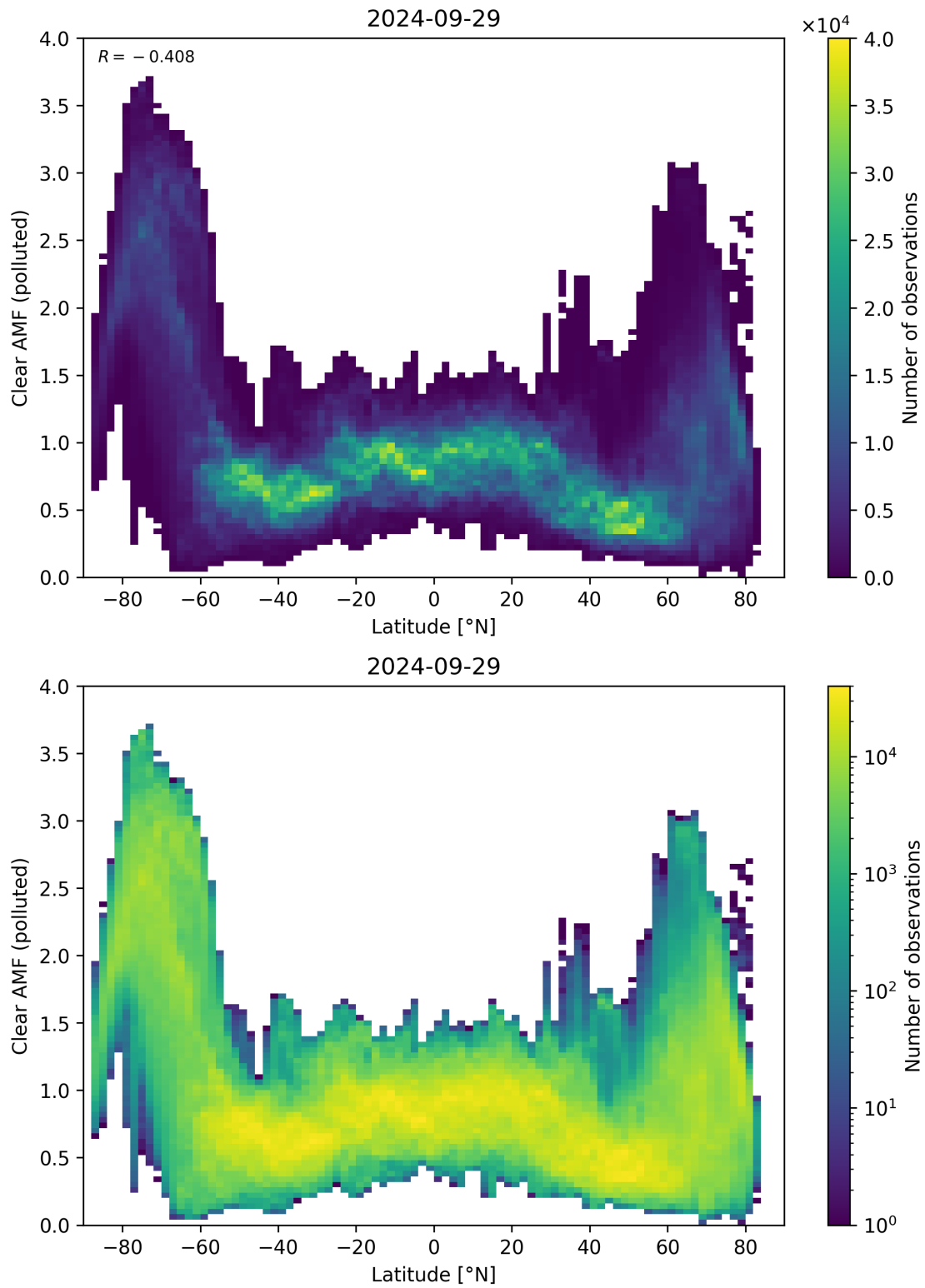
Figure 145: Scatter density plot of “Latitude” against “Clear AMF (polluted)” for 2024-09-28 to 2024-09-30.
