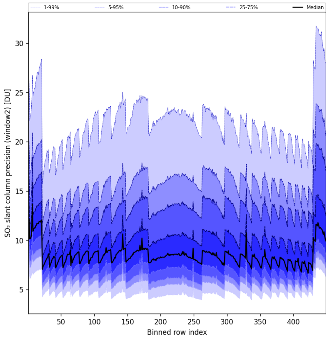
Figure 84: Along track statistics of “SO 2 slant column precision (window2)” for 2024-09-28 to 2024-09-30
