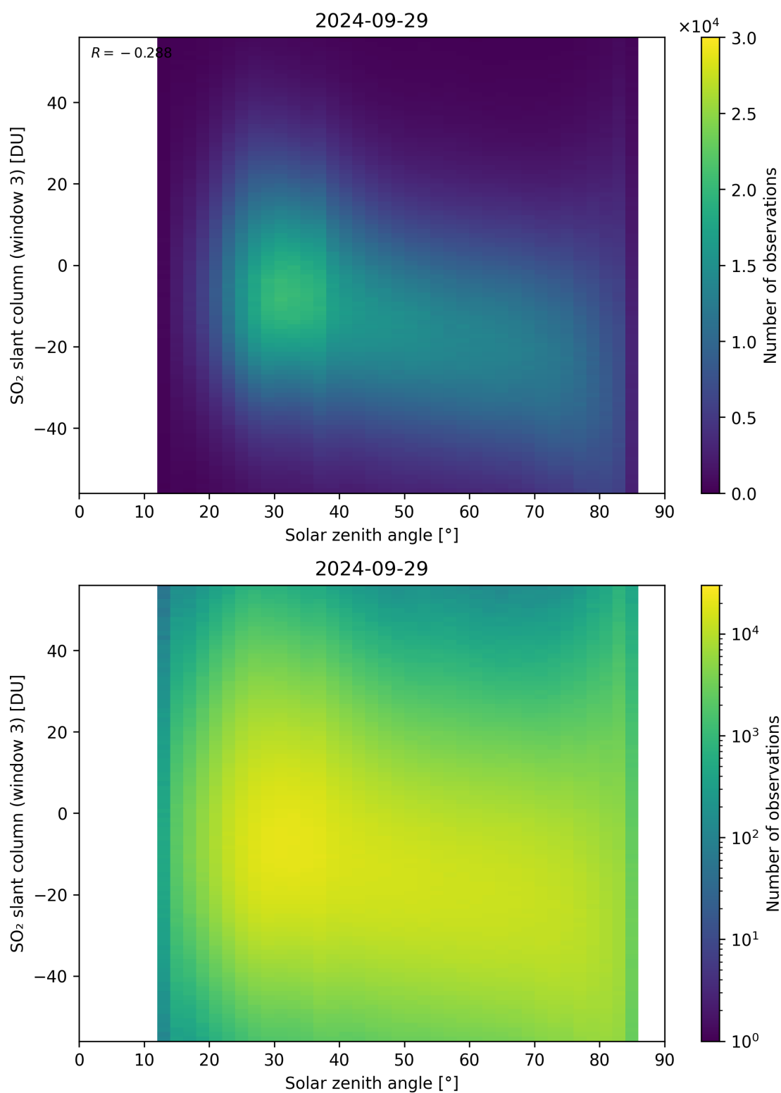
Figure 172: Scatter density plot of “Solar zenith angle” against “SO 2 slant column (window 3)” for 2024-09-28 to 2024-09-30.
