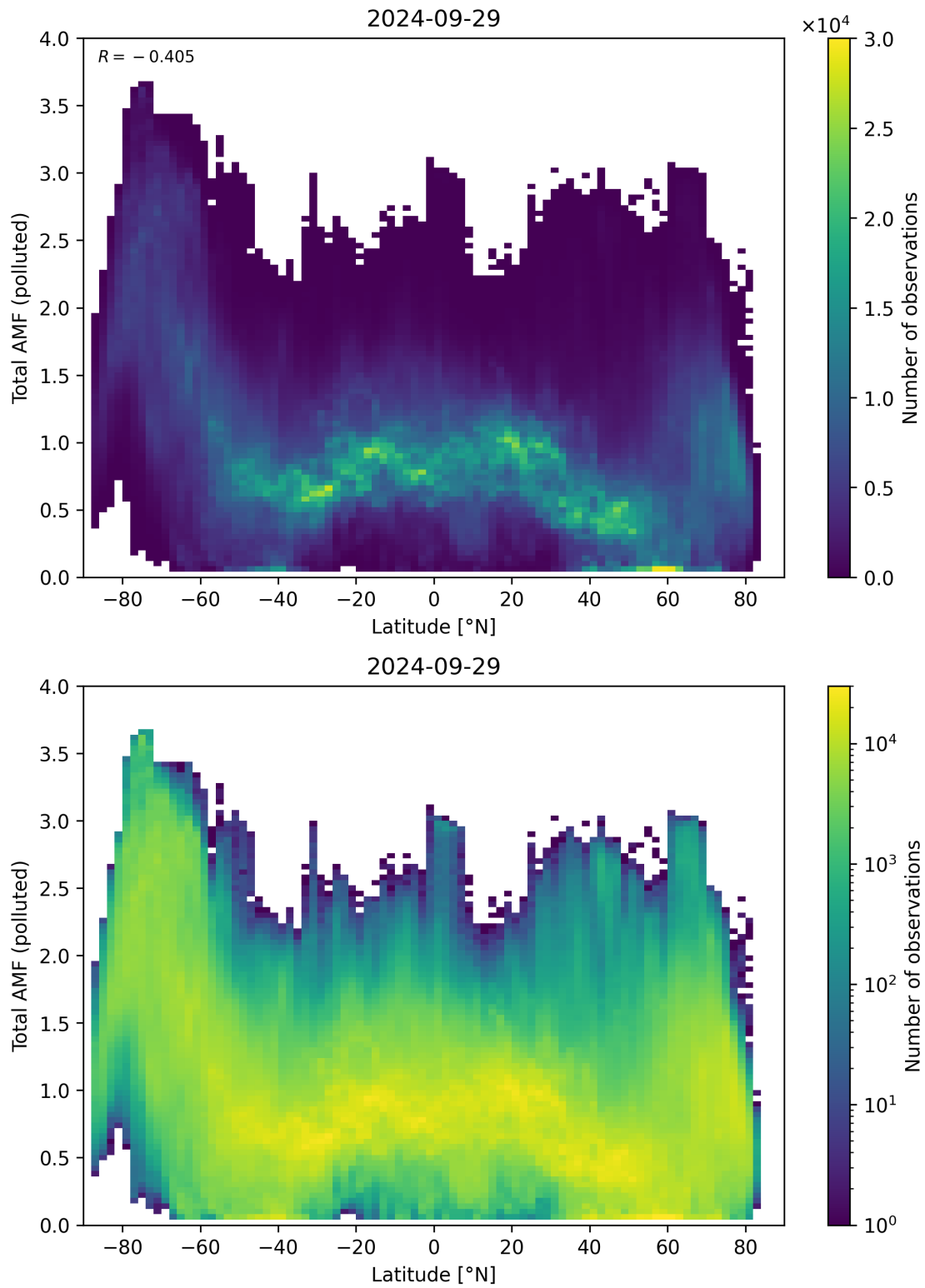
Figure 154: Scatter density plot of “Latitude” against “Total AMF (polluted)” for 2024-09-28 to 2024-09-30.
