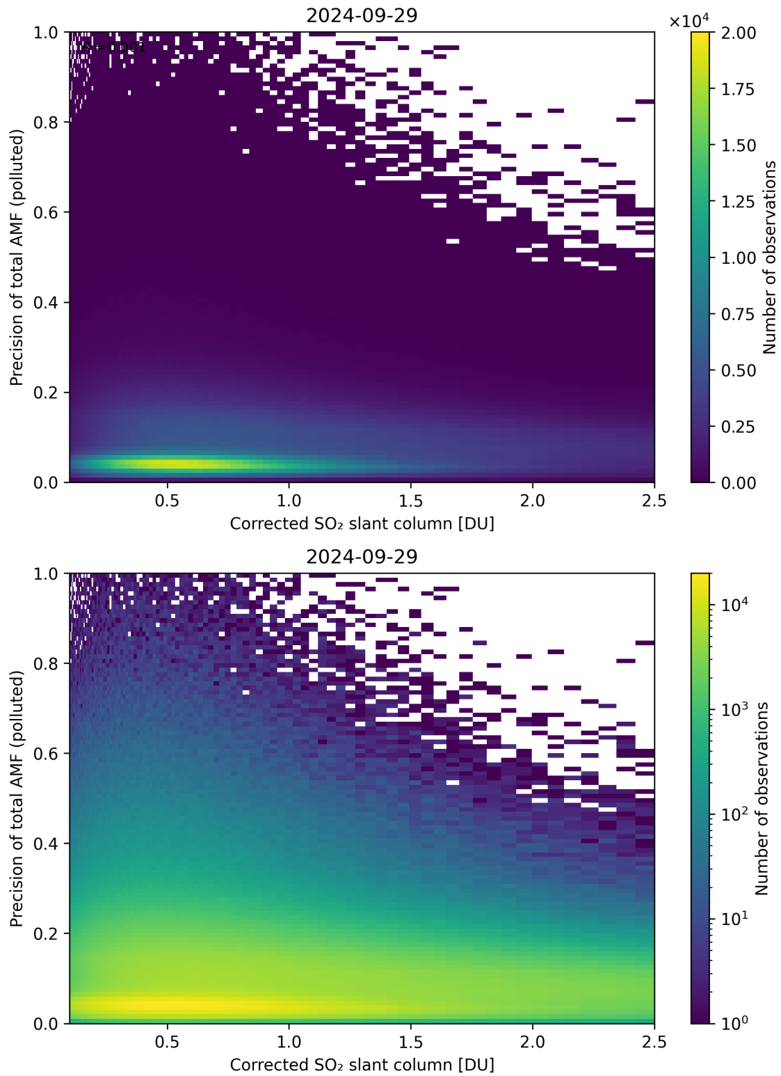
Figure 193: Scatter density plot of “Corrected SO 2 slant column” against “Precision of total AMF (polluted)” for 2024-09-28 to 2024-09-30.
