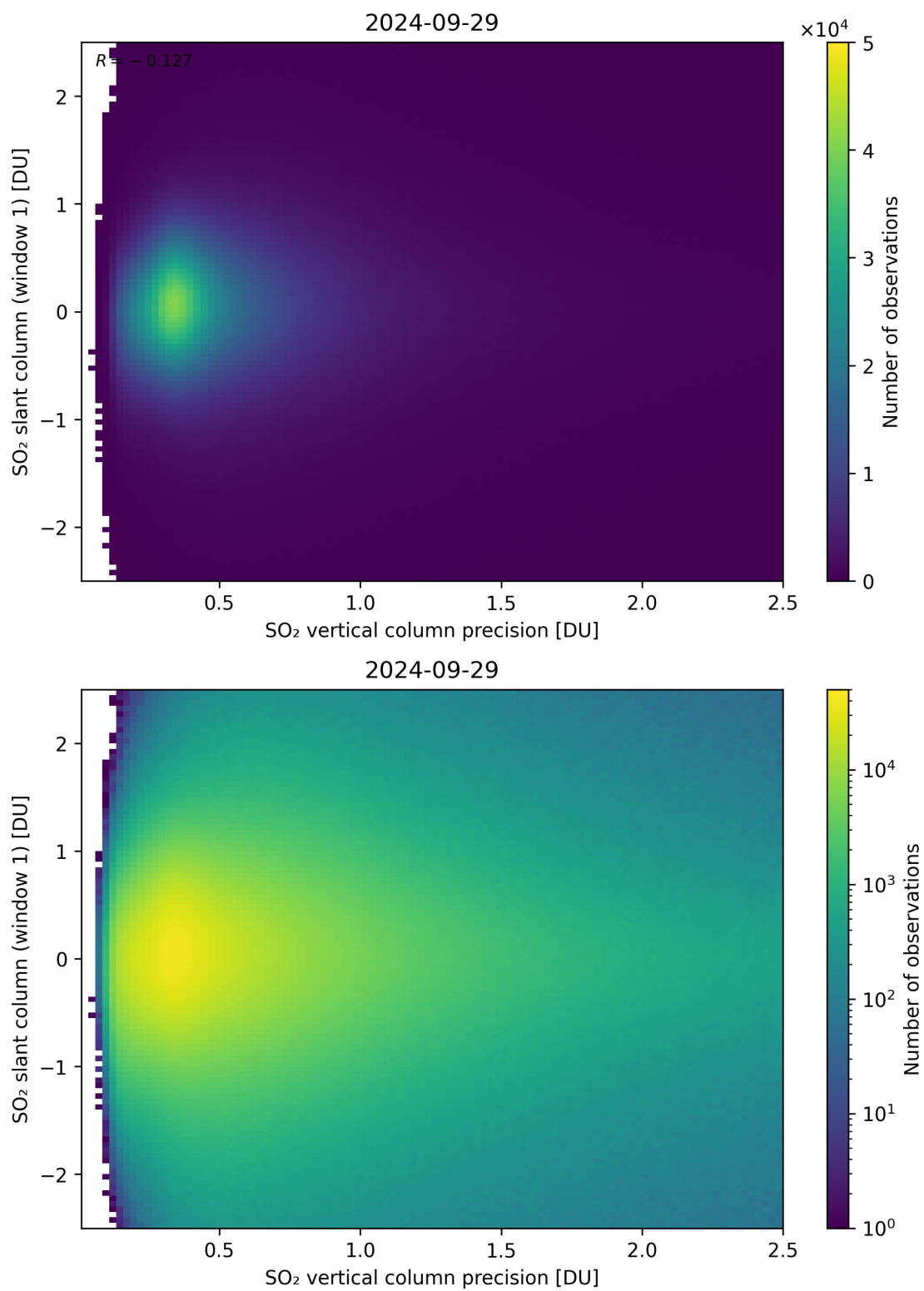
Figure 289: Scatter density plot of “SO 2 vertical column precision” against “SO 2 slant column (window 1)” for 2024-09-28 to 2024-09-30.
