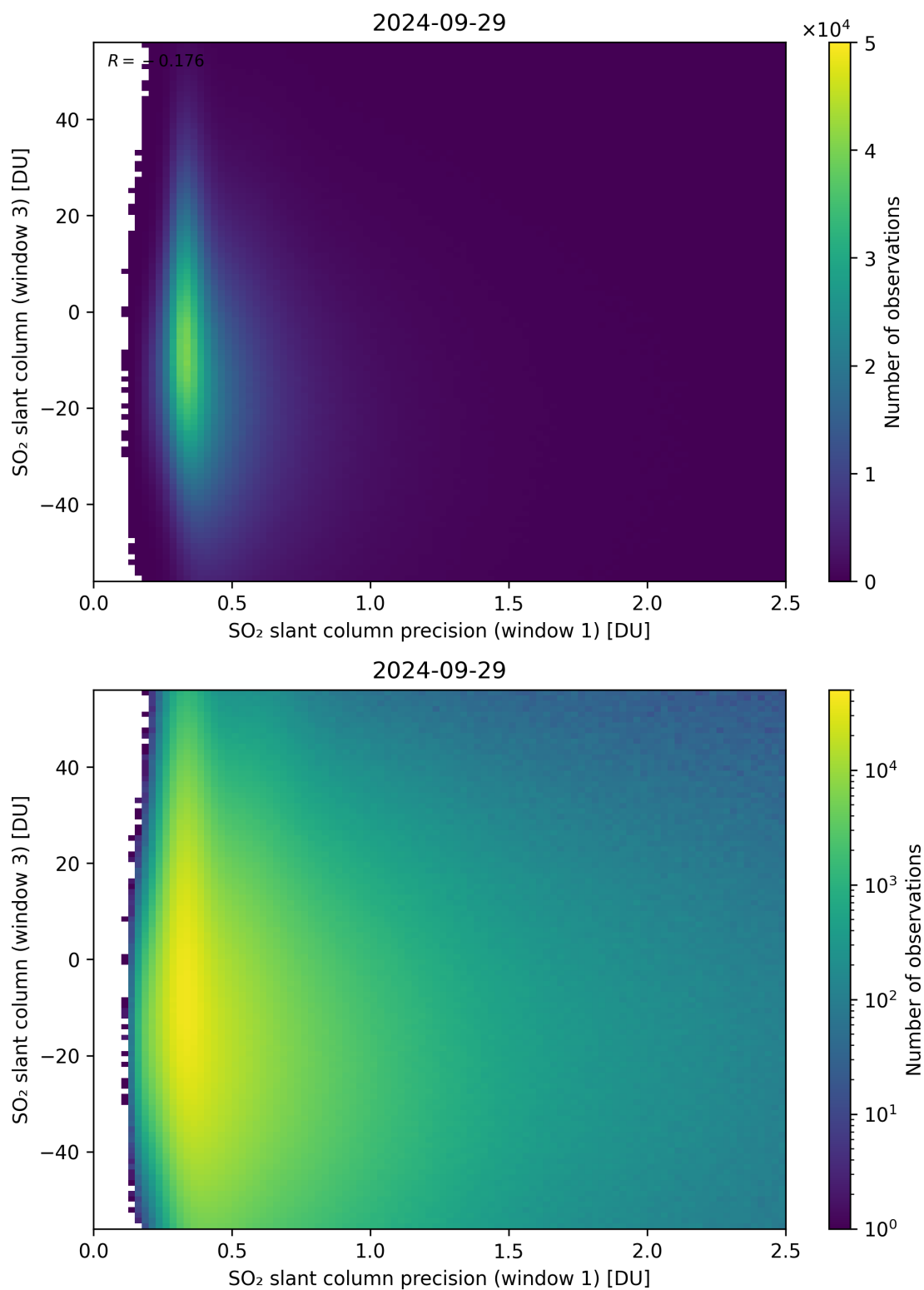
Figure 228: Scatter density plot of “SO 2 slant column precision (window 1)” against “SO 2 slant column (window 3)” for 2024-09-28 to 2024-09-30.
