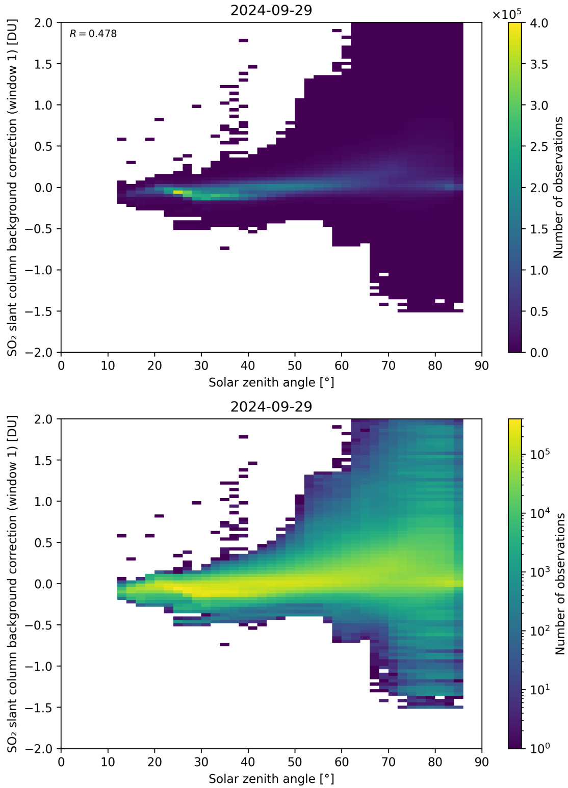
Figure 158: Scatter density plot of “Solar zenith angle” against “SO 2 slant column background correction (window 1)” for 2024-09-28 to 2024-09-30.
