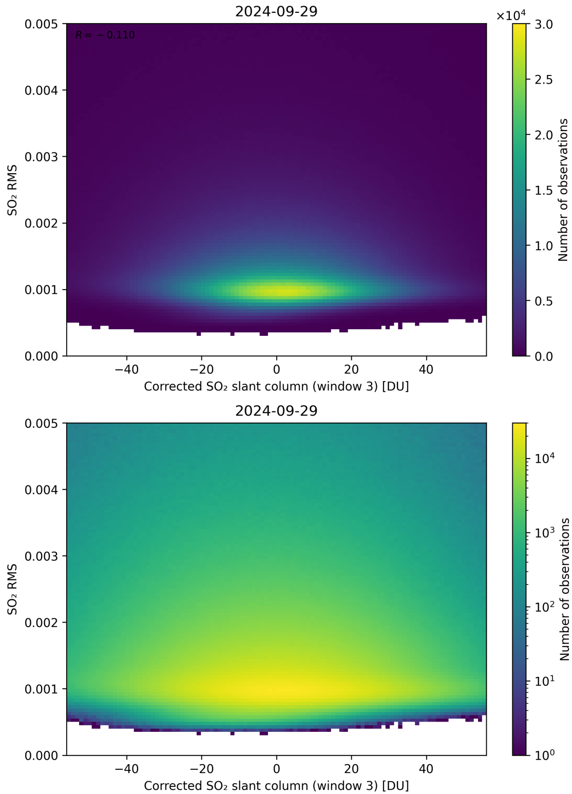
Figure 208: Scatter density plot of “Corrected SO 2 slant column (window 3)” against “SO 2 RMS” for 2024-09-28 to 2024-09-30.
