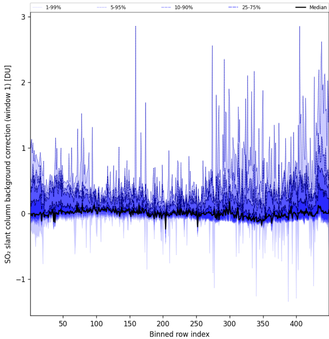
Figure 82: Along track statistics of “SO 2 slant column background correction (window 1)” for 2024-09-28 to 2024-09-30
