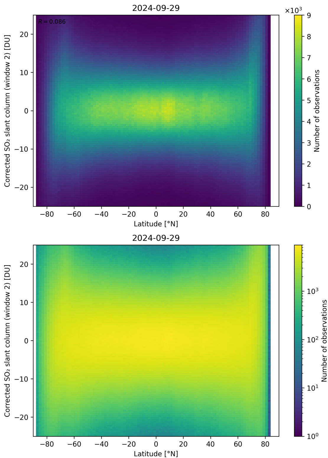
Figure 147: Scatter density plot of “Latitude” against “Corrected SO 2 slant column (window 2)” for 2024-09-28 to 2024-09-30.
