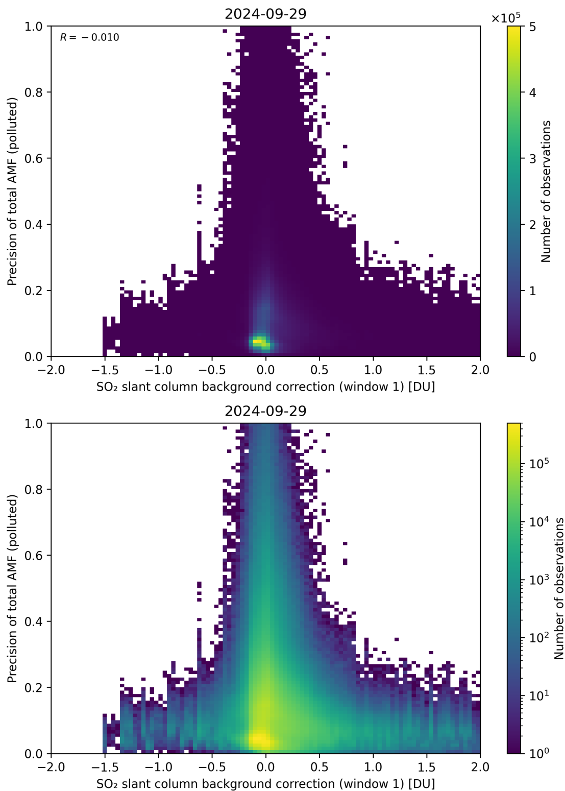
Figure 110: Scatter density plot of “SO 2 slant column background correction (window 1)” against “Precision of total AMF (polluted)” for 2024-09-28 to 2024-09-30.
