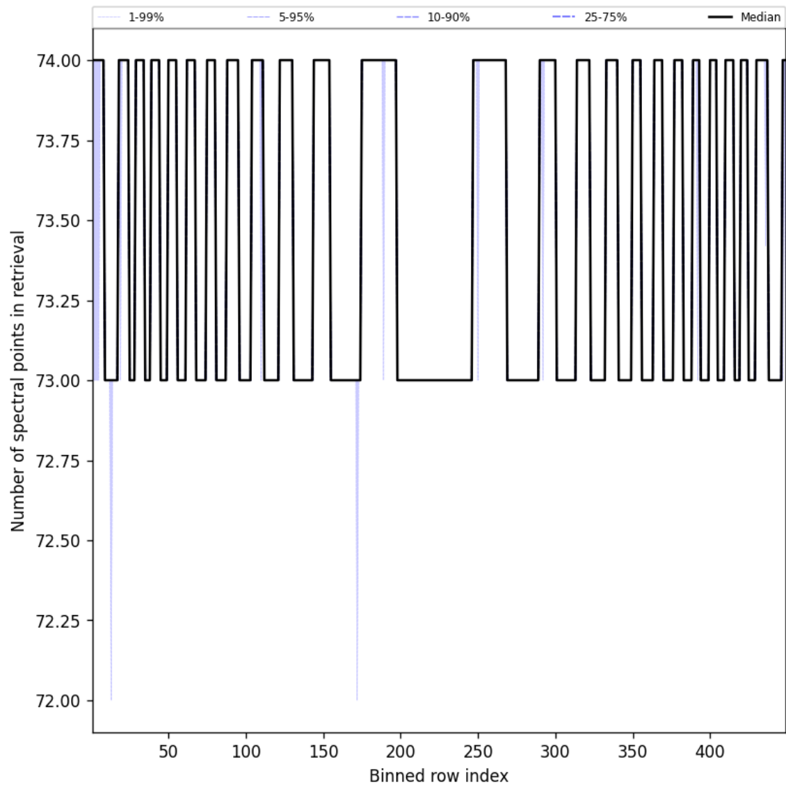
Figure 97: Along track statistics of “Number of spectral points in retrieval” for 2024-09-28 to 2024-09-30
