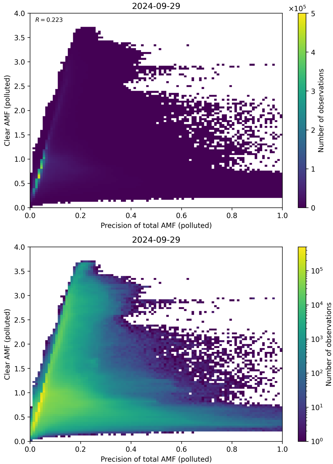
Figure 270: Scatter density plot of “Precision of total AMF (polluted)” against “Clear AMF (polluted)” for 2024-09-28 to 2024-09-30.
