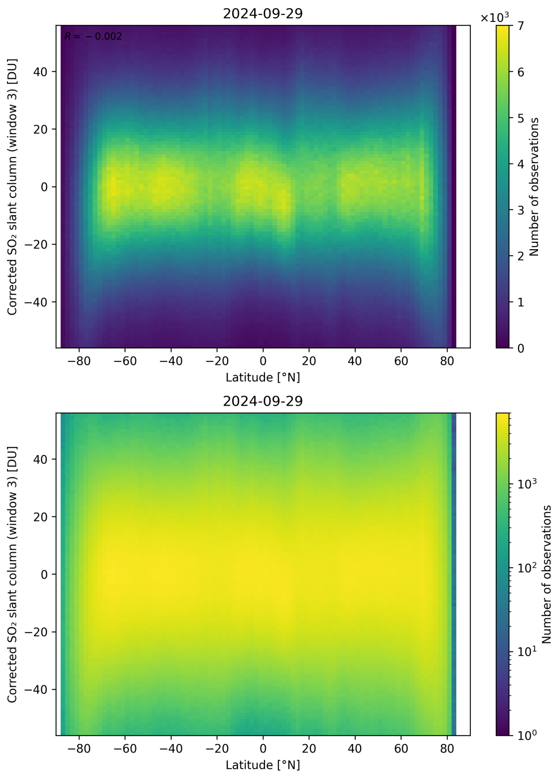
Figure 148: Scatter density plot of “Latitude” against “Corrected SO 2 slant column (window 3)” for 2024-09-28 to 2024-09-30.
