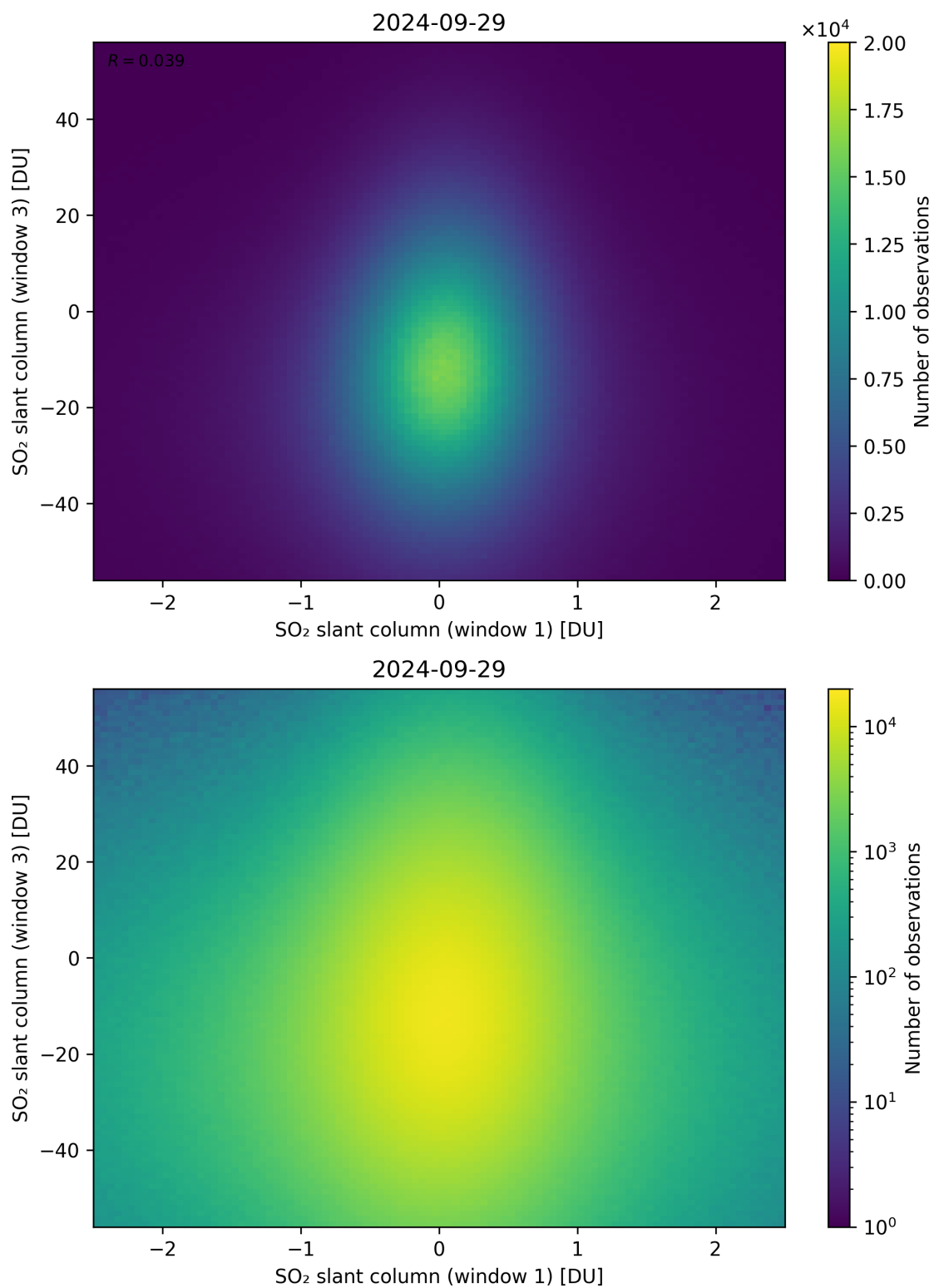
Figure 237: Scatter density plot of “SO 2 slant column (window 1)” against “SO 2 slant column (window 3)” for 2024-09-28 to 2024-09-30.
