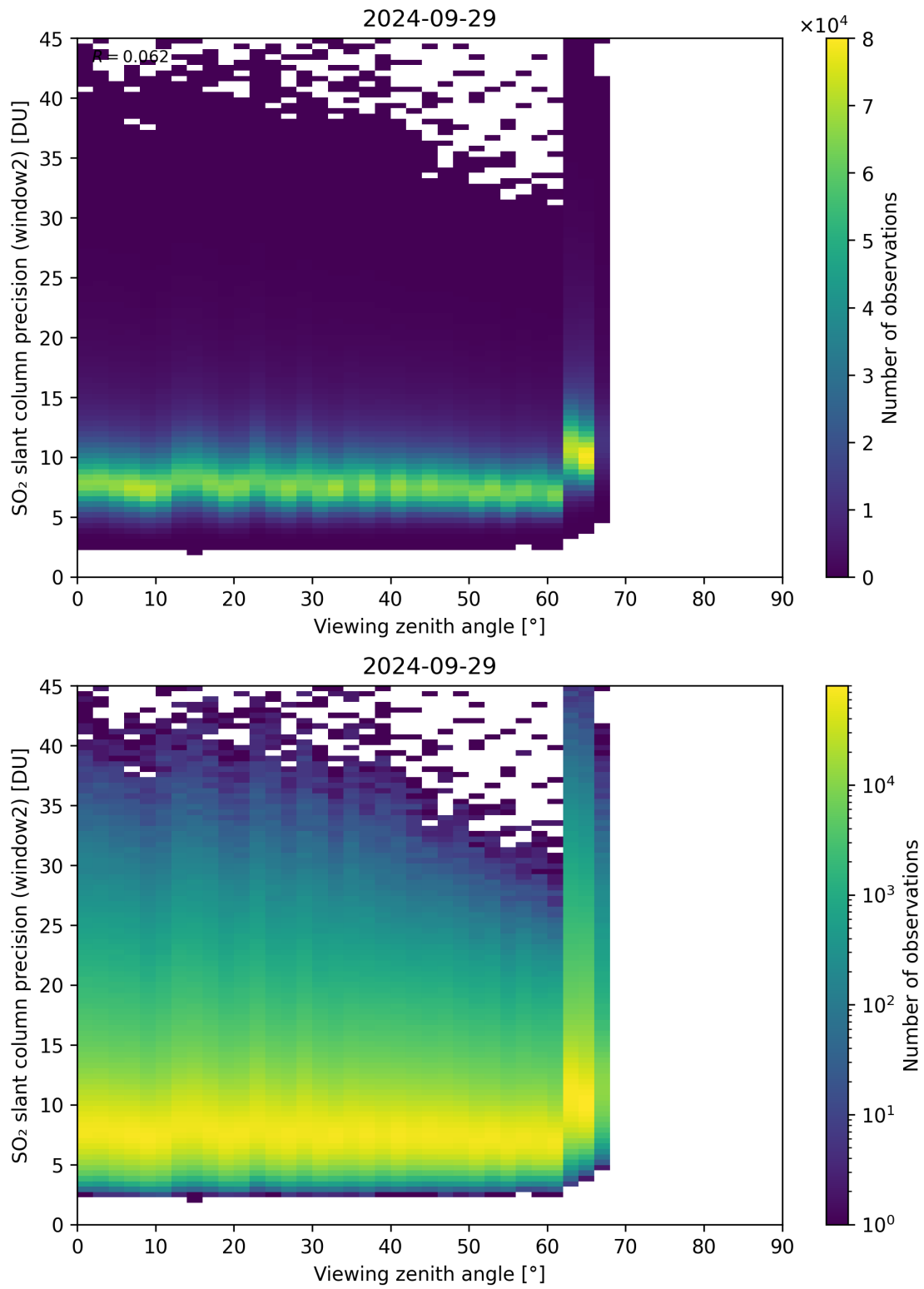
Figure 322: Scatter density plot of “Viewing zenith angle” against “SO 2 slant column precision (window2)” for 2024-09-28 to 2024-09-30.
