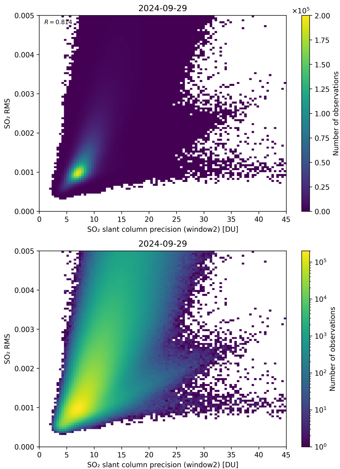
Figure 245: Scatter density plot of “SO 2 slant column precision (window2)” against “SO 2 RMS” for 2024-09-28 to 2024-09-30.
