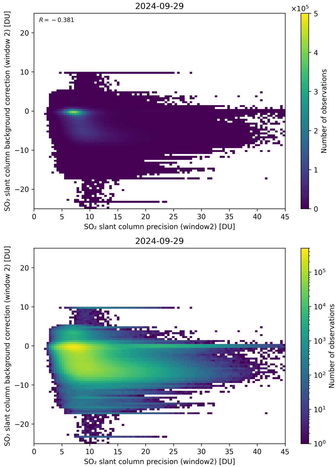
Figure 241: Scatter density plot of “SO 2 slant column precision (window2)” against “SO 2 slant column background correction (window 2)” for 2024-09-28 to 2024-09-30.
