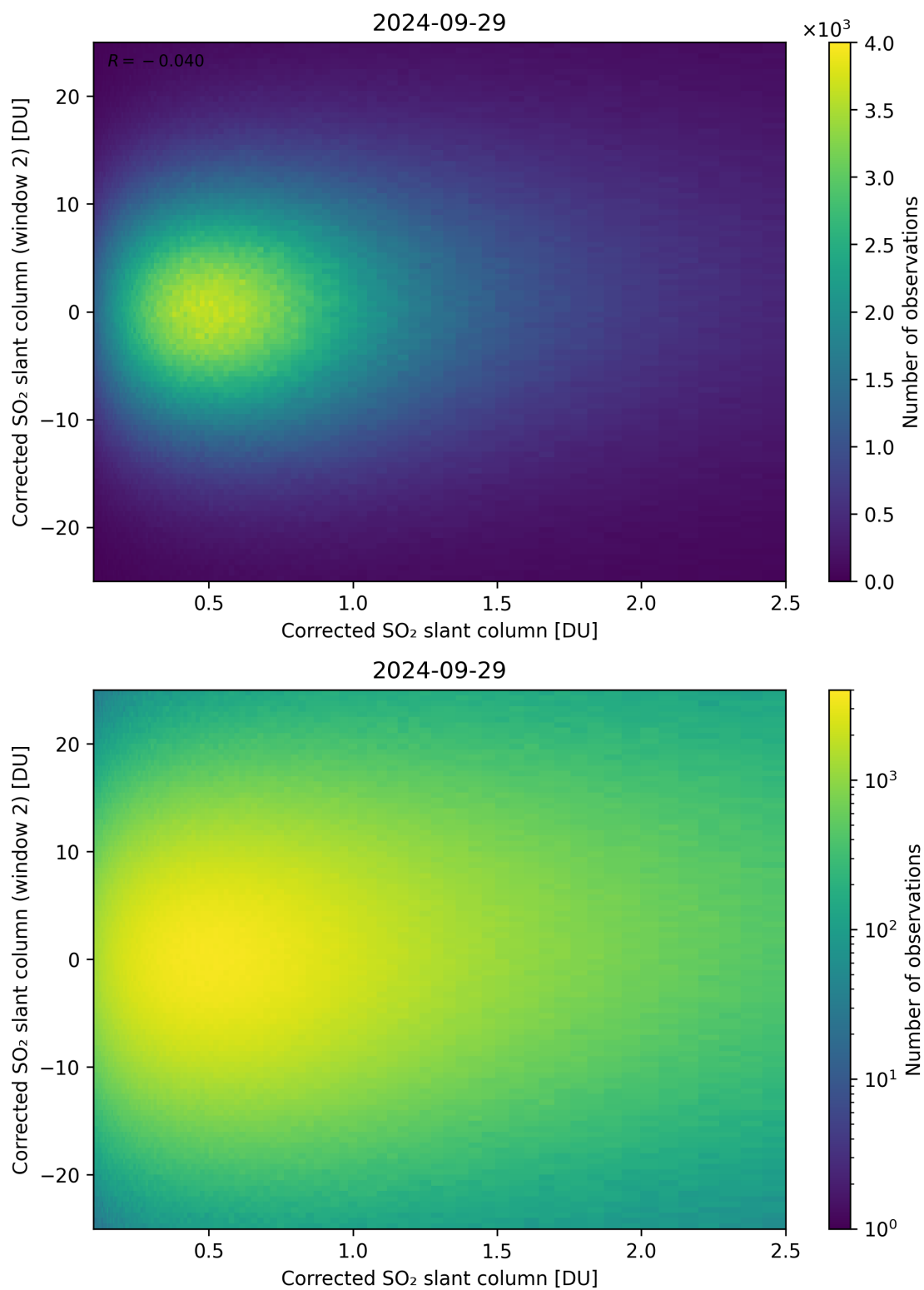
Figure 185: Scatter density plot of “Corrected SO 2 slant column” against “Corrected SO 2 slant column (window 2)” for 2024-09-28 to 2024-09-30.
