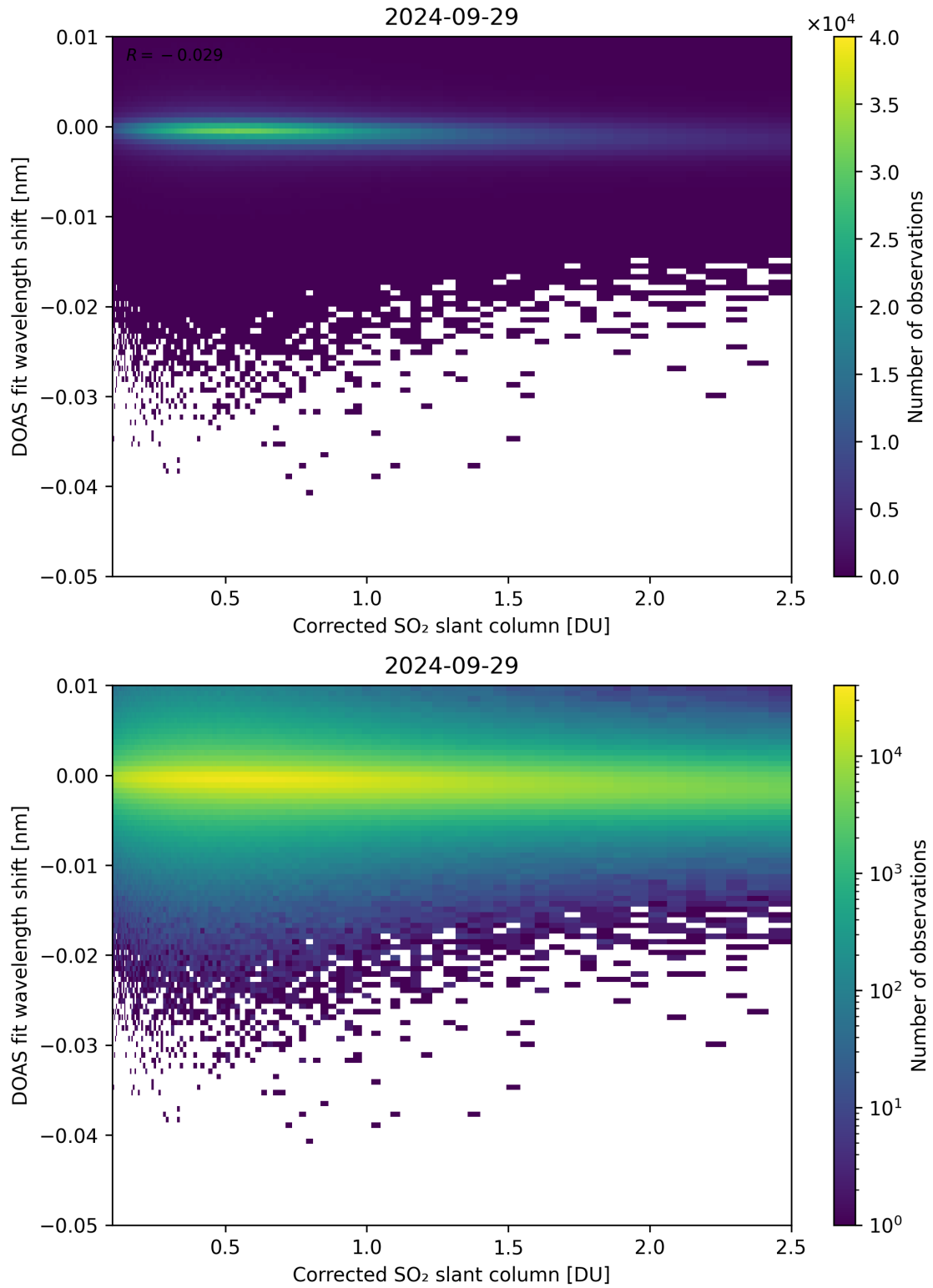
Figure 181: Scatter density plot of “Corrected SO 2 slant column” against “DOAS fit wavelength shift” for 2024-09-28 to 2024-09-30.
