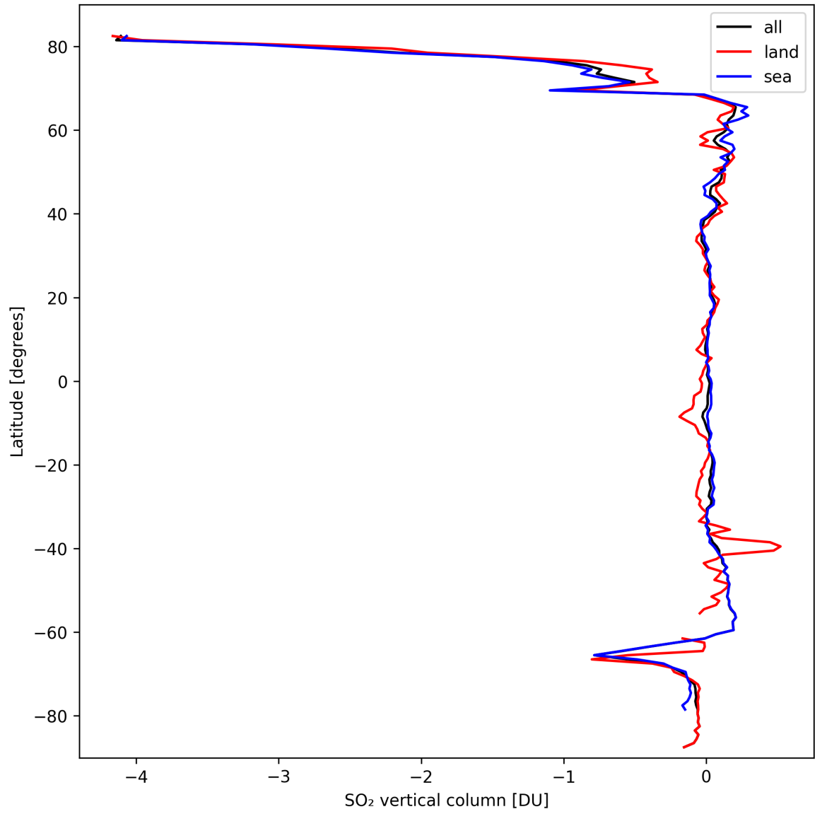
Figure 30: Zonal average of “SO 2 vertical column” for 2024-09-28 to 2024-09-30.
