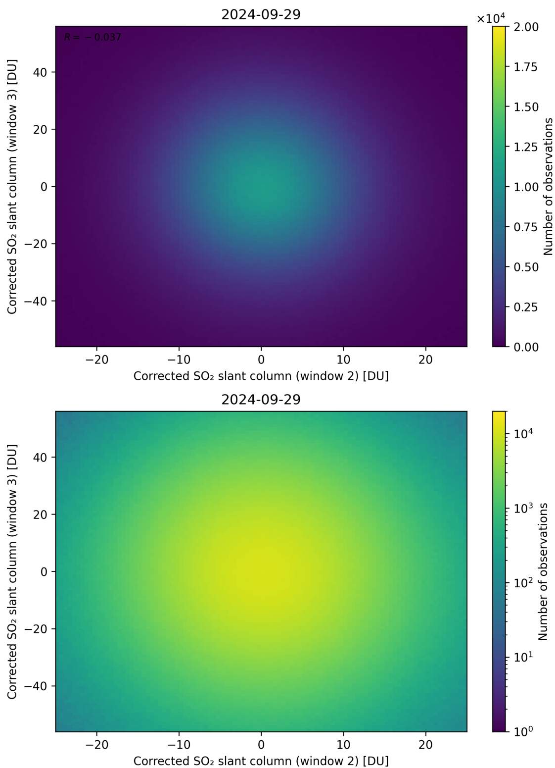
Figure 200: Scatter density plot of “Corrected SO 2 slant column (window 2)” against “Corrected SO 2 slant column (window 3)” for 2024-09-28 to 2024-09-30.
