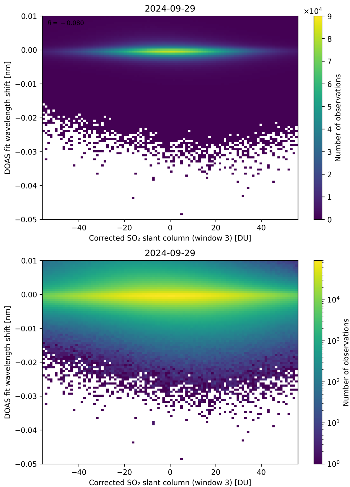
Figure 206: Scatter density plot of “Corrected SO 2 slant column (window 3)” against “DOAS fit wavelength shift” for 2024-09-28 to 2024-09-30.
