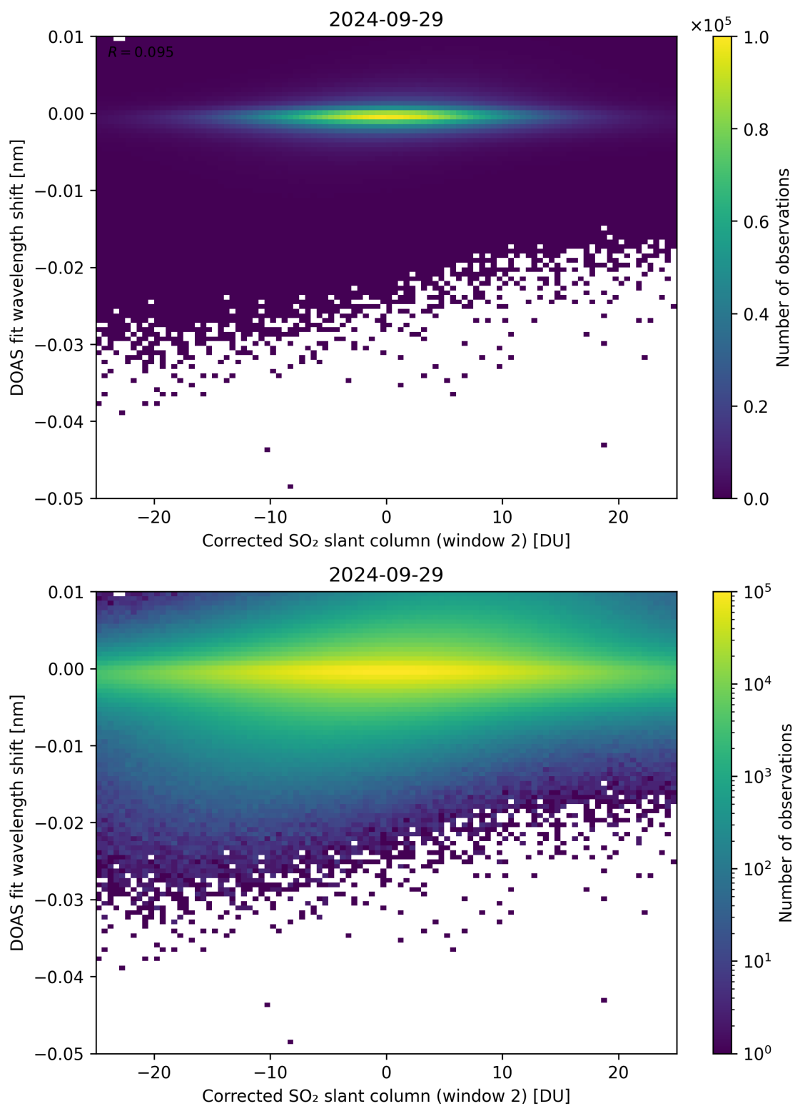
Figure 196: Scatter density plot of “Corrected SO 2 slant column (window 2)” against “DOAS fit wavelength shift” for 2024-09-28 to 2024-09-30.
