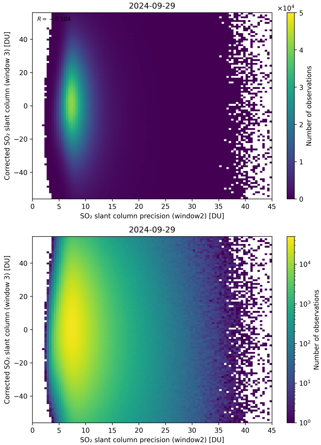
Figure 248: Scatter density plot of “SO 2 slant column precision (window2)” against “Corrected SO 2 slant column (window 3)” for 2024-09-28 to 2024-09-30.
