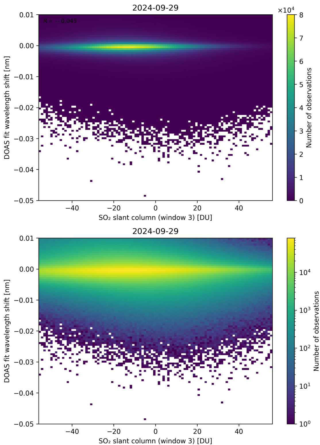
Figure 254: Scatter density plot of “SO 2 slant column (window 3)” against “DOAS fit wavelength shift” for 2024-09-28 to 2024-09-30.
