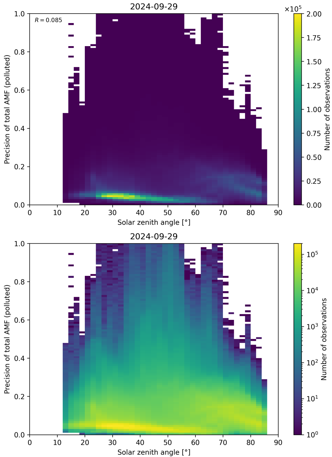
Figure 175: Scatter density plot of “Solar zenith angle” against “Precision of total AMF (polluted)” for 2024-09-28 to 2024-09-30.
