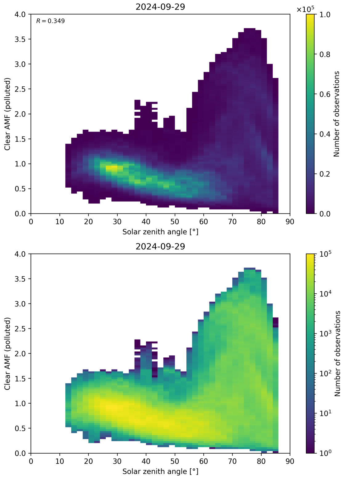
Figure 165: Scatter density plot of “Solar zenith angle” against “Clear AMF (polluted)” for 2024-09-28 to 2024-09-30.
