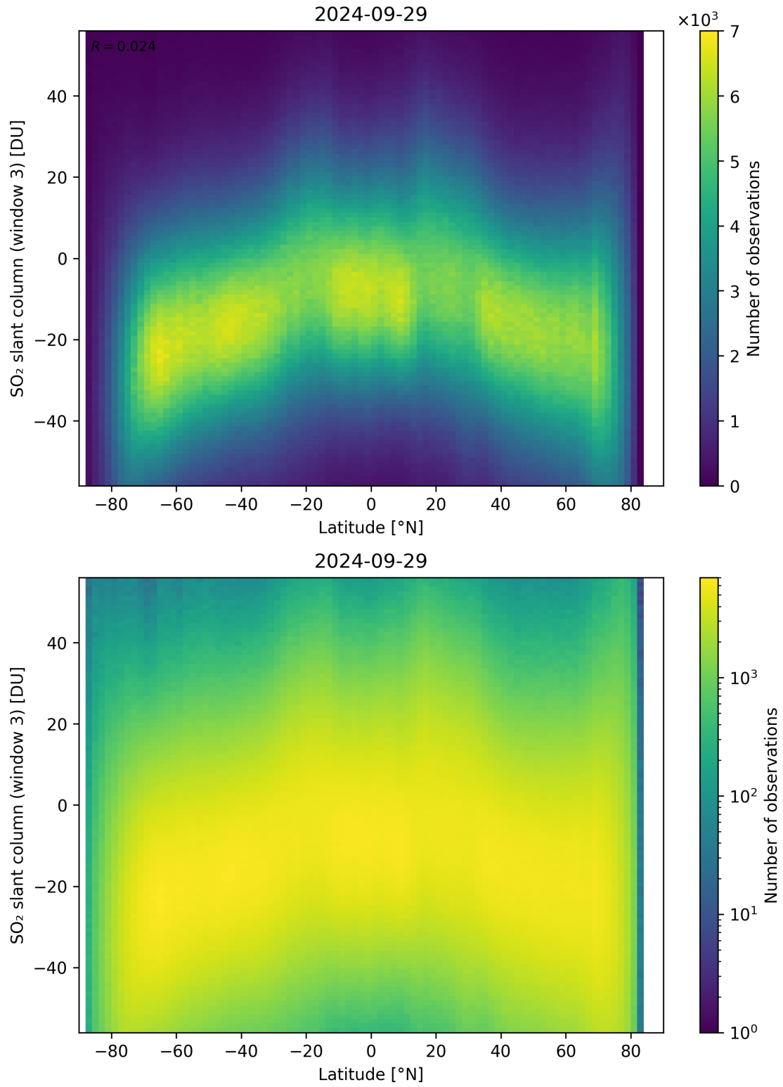
Figure 152: Scatter density plot of “Latitude” against “SO 2 slant column (window 3)” for 2024-09-28 to 2024-09-30.
