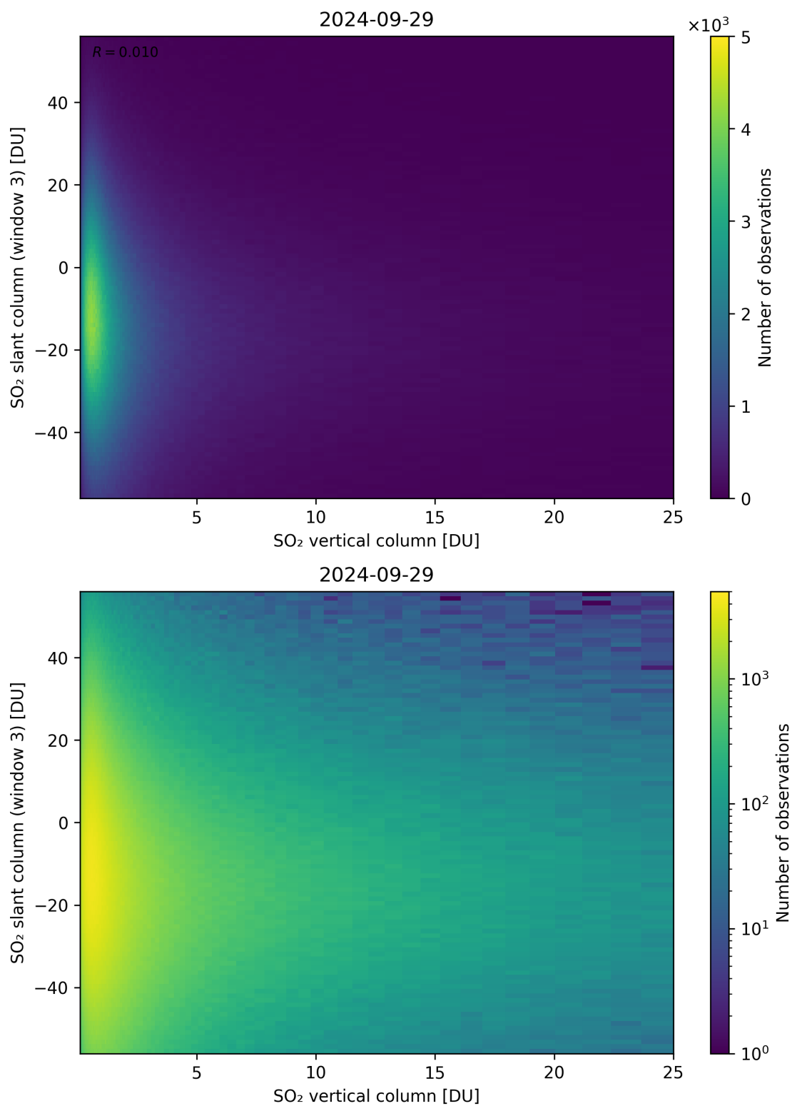
Figure 303: Scatter density plot of “SO 2 vertical column” against “SO 2 slant column (window 3)” for 2024-09-28 to 2024-09-30.
