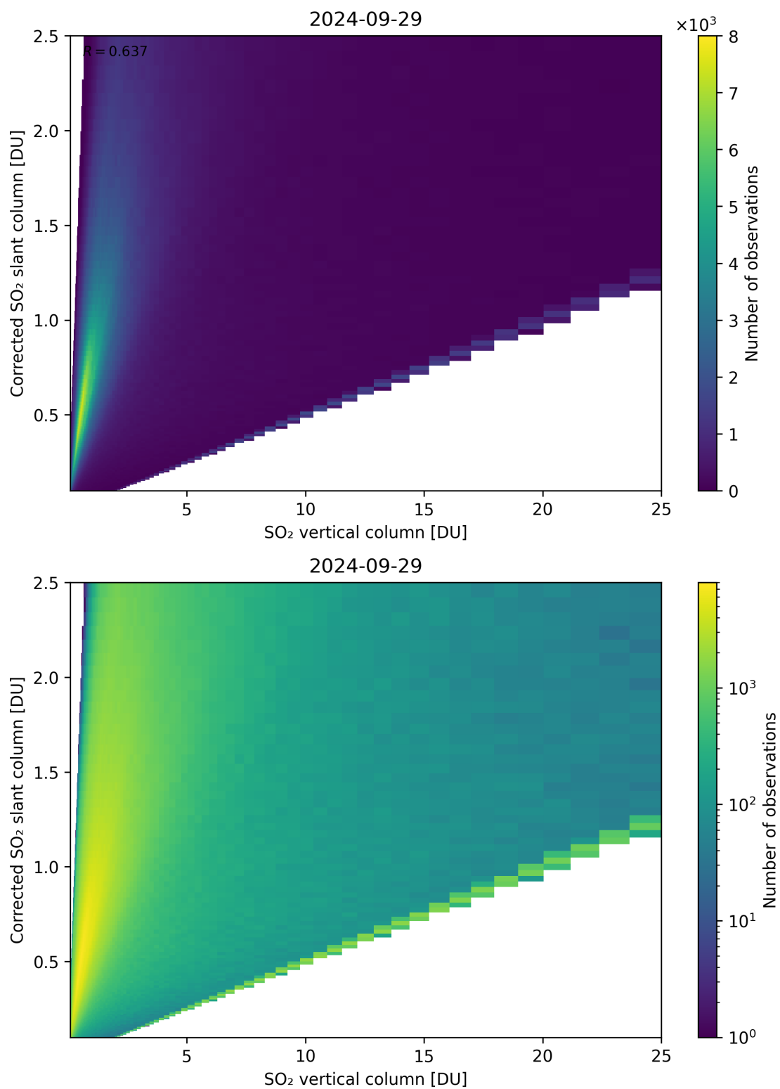
Figure 297: Scatter density plot of “SO 2 vertical column” against “Corrected SO 2 slant column” for 2024-09-28 to 2024-09-30.
