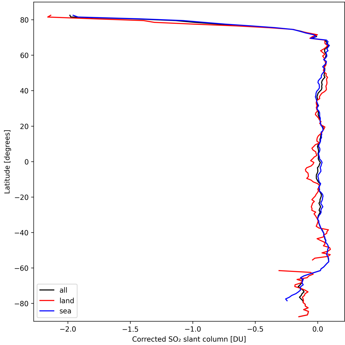
Figure 32: Zonal average of “Corrected SO 2 slant column” for 2024-09-28 to 2024-09-30.
