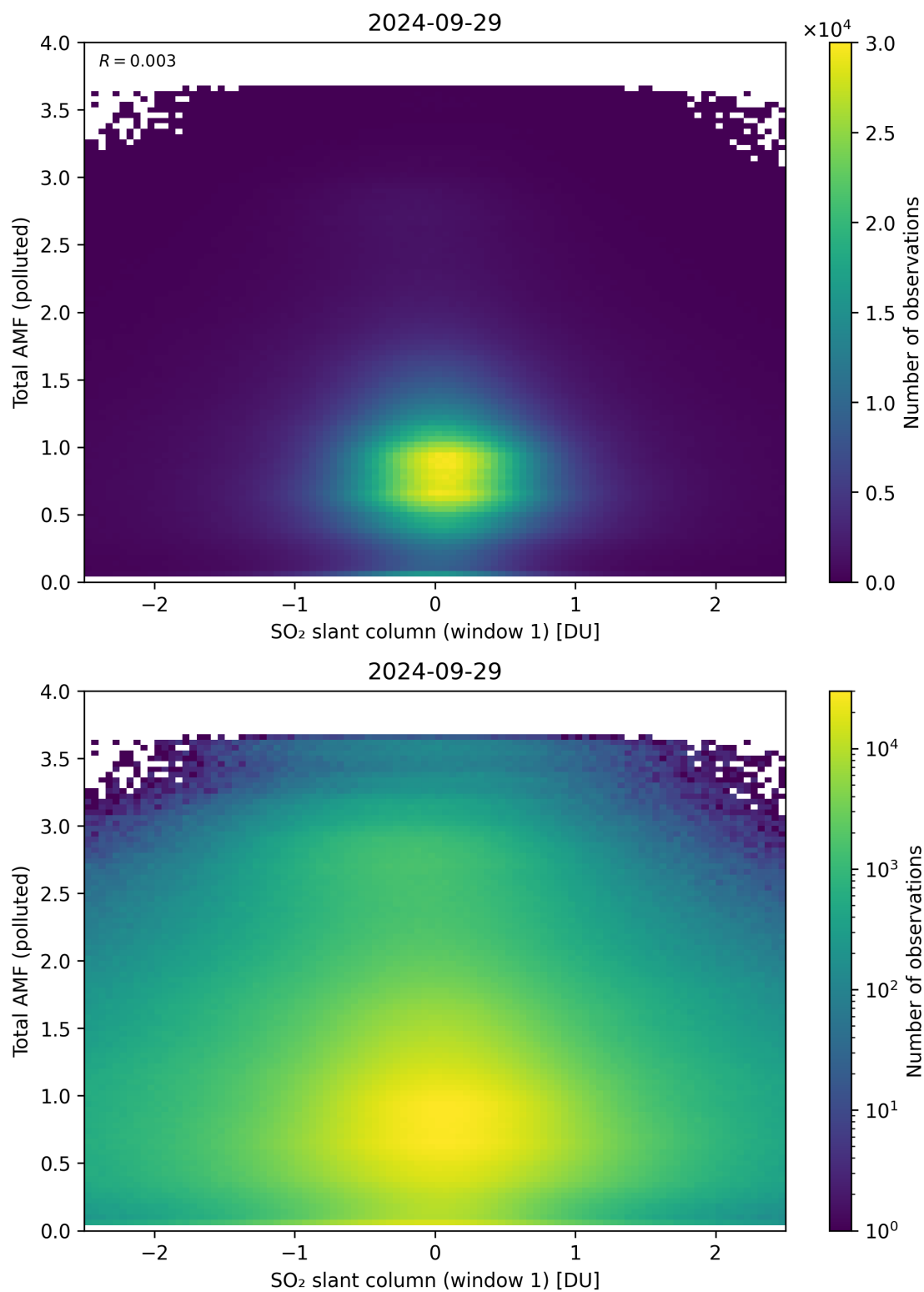
Figure 239: Scatter density plot of “SO 2 slant column (window 1)” against “Total AMF (polluted)” for 2024-09-28 to 2024-09-30.
