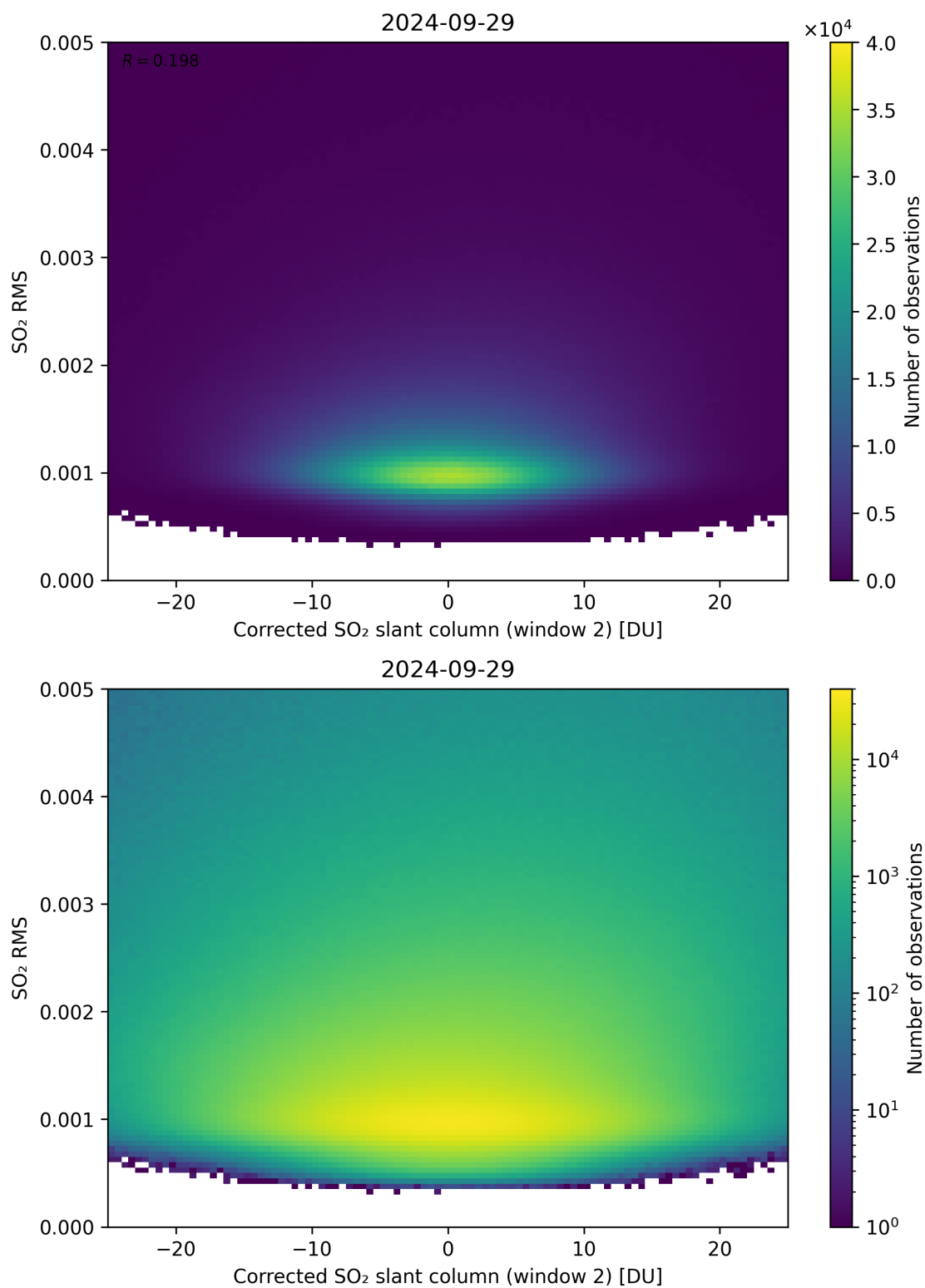
Figure 198: Scatter density plot of “Corrected SO 2 slant column (window 2)” against “SO 2 RMS” for 2024-09-28 to 2024-09-30.
