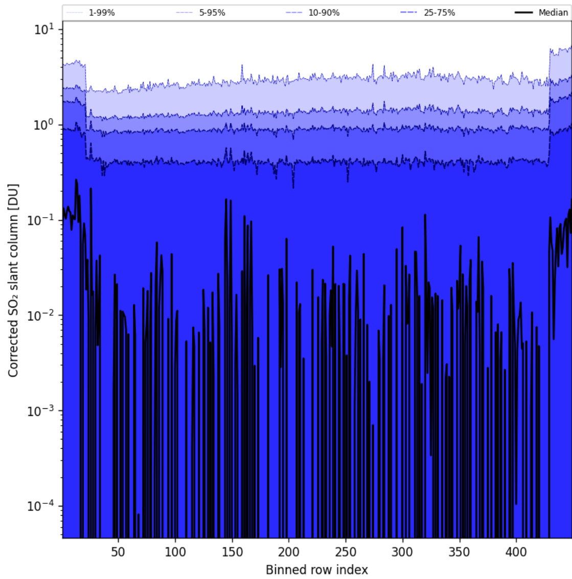
Figure 78: Along track statistics of “Corrected SO 2 slant column” for 2024-09-28 to 2024-09-30
