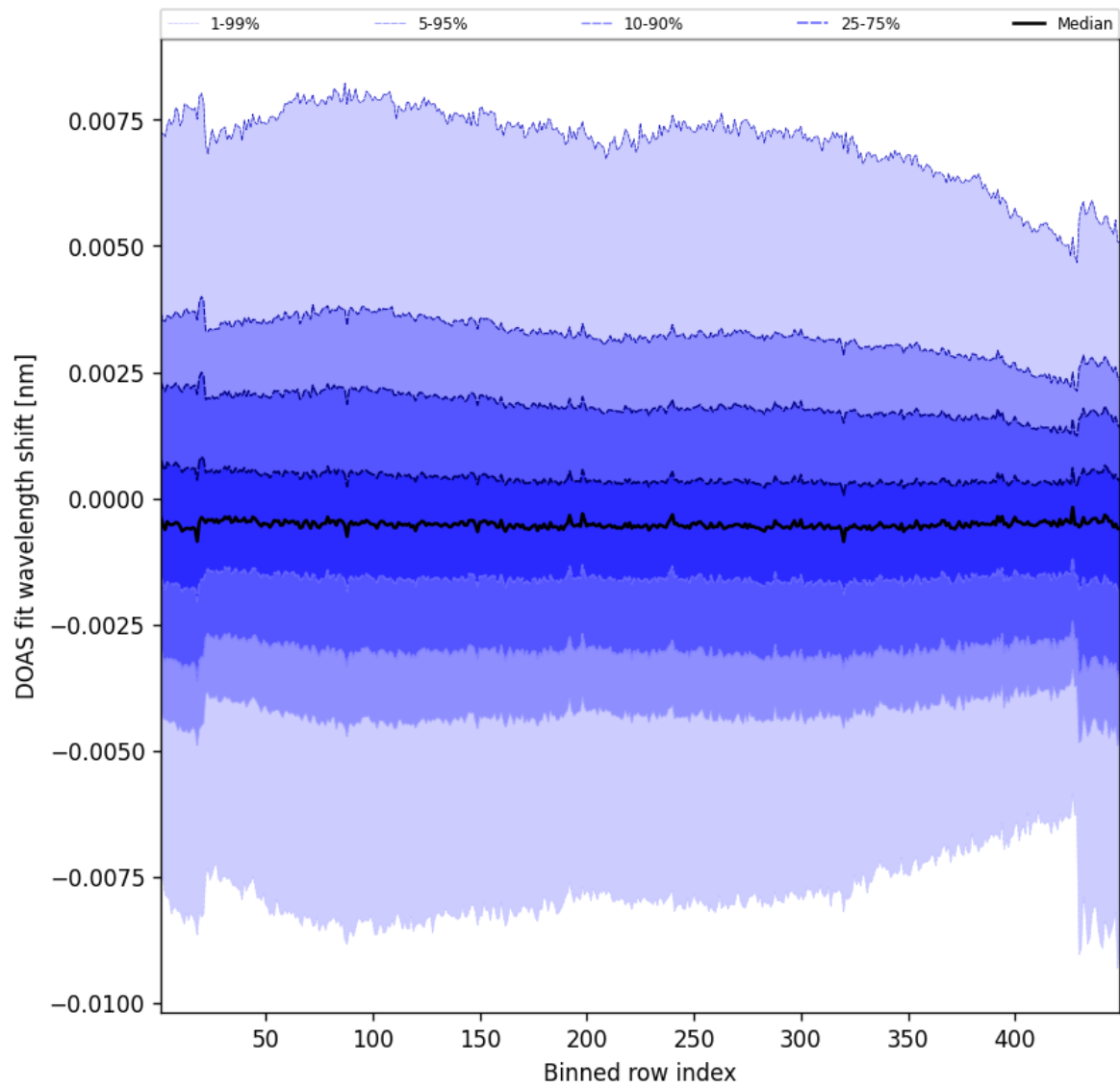
Figure 91: Along track statistics of “DOAS fit wavelength shift” for 2024-09-28 to 2024-09-30
