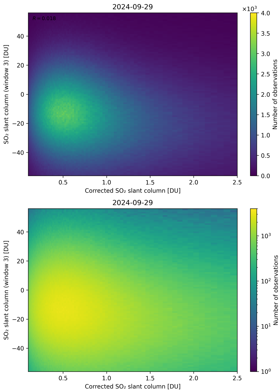
Figure 190: Scatter density plot of “Corrected SO 2 slant column” against “SO 2 slant column (window 3)” for 2024-09-28 to 2024-09-30.
