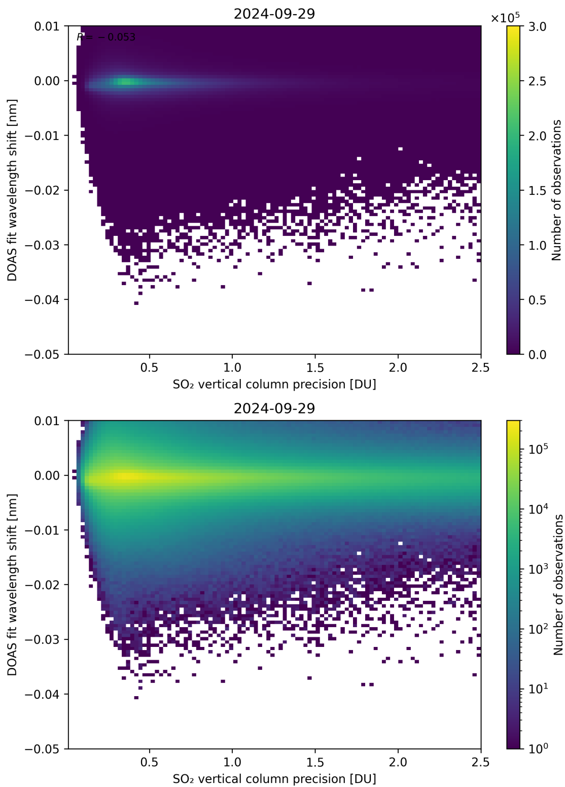
Figure 282: Scatter density plot of “SO 2 vertical column precision” against “DOAS fit wavelength shift” for 2024-09-28 to 2024-09-30.
