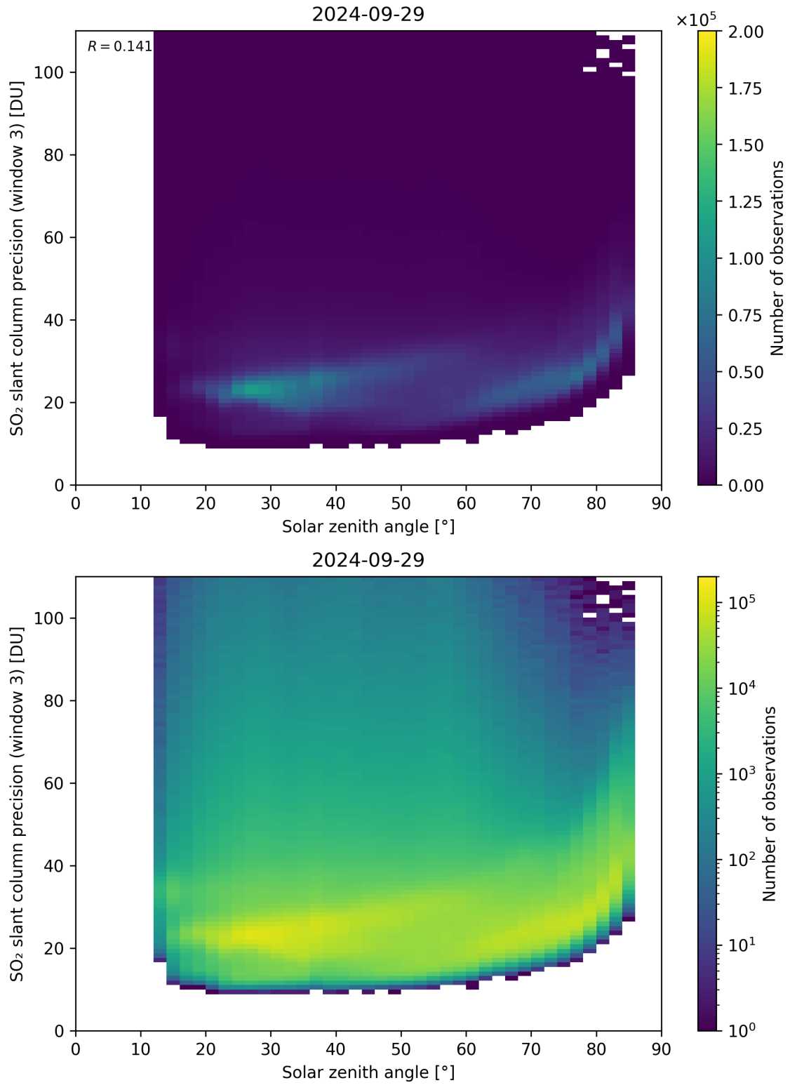
Figure 173: Scatter density plot of “Solar zenith angle” against “SO 2 slant column precision (window 3)” for 2024-09-28 to 2024-09-30.
