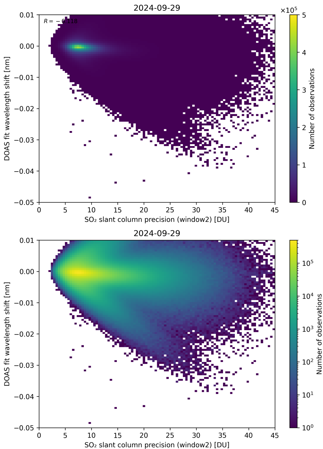
Figure 243: Scatter density plot of “SO 2 slant column precision (window2)” against “DOAS fit wavelength shift” for 2024-09-28 to 2024-09-30.
