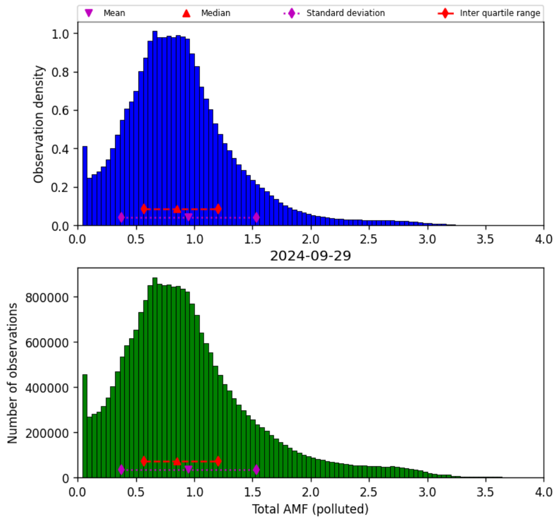
Figure 71: Histogram of “Total AMF (polluted)” for 2024-09-28 to 2024-09-30
