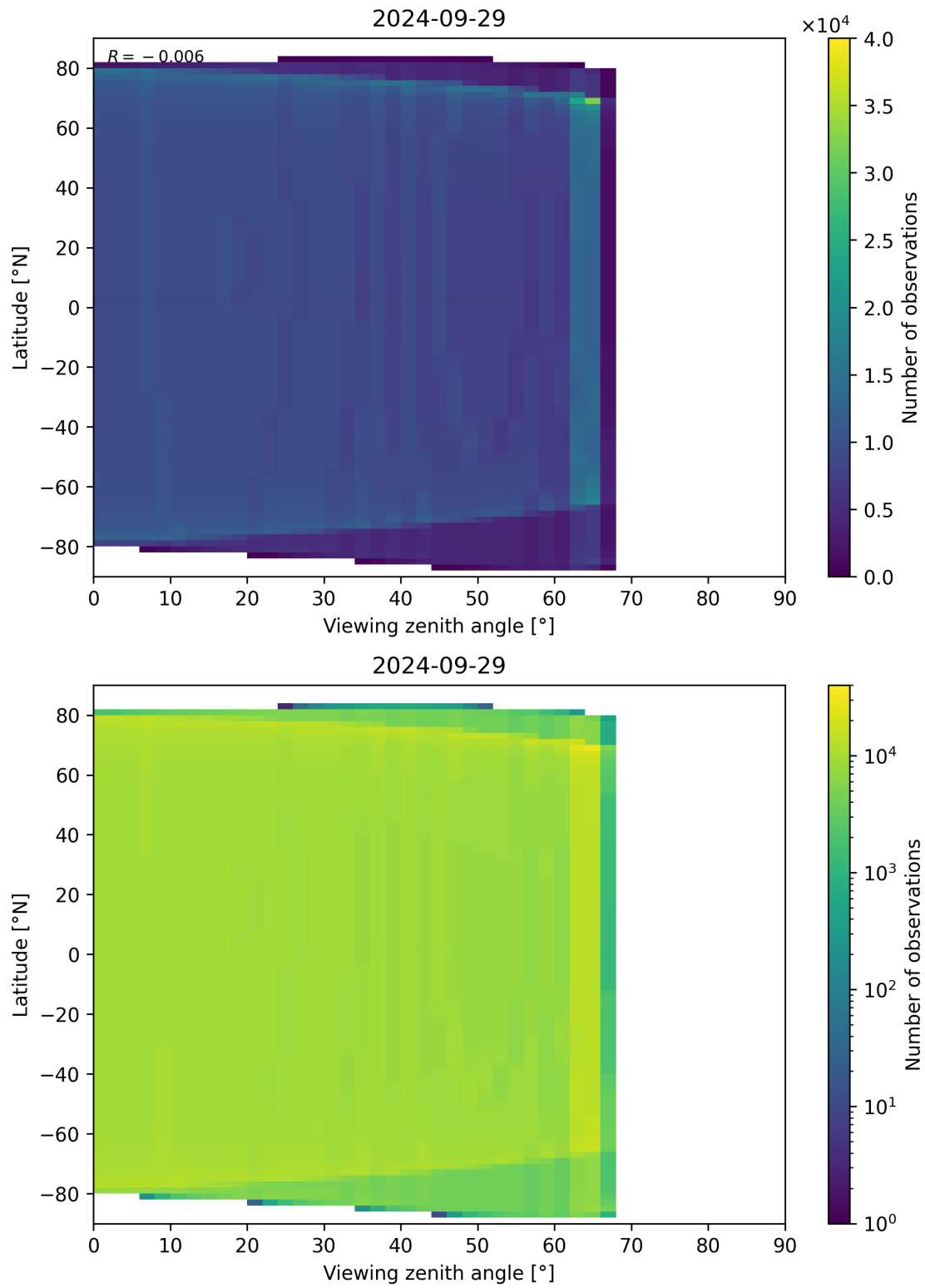
Figure 314: Scatter density plot of “Viewing zenith angle” against “Latitude” for 2024-09-28 to 2024-09-30.
