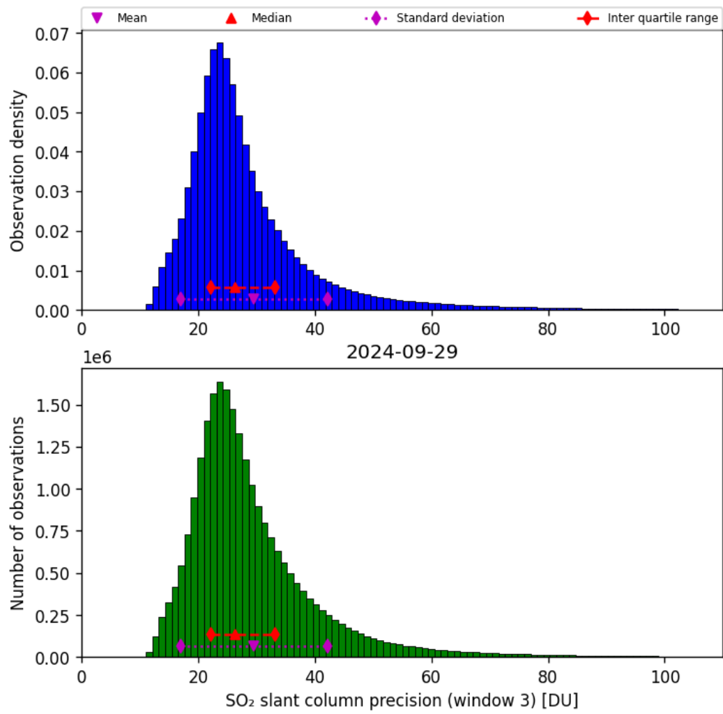
Figure 65: Histogram of “SO 2 slant column precision (window 3)” for 2024-09-28 to 2024-09-30
