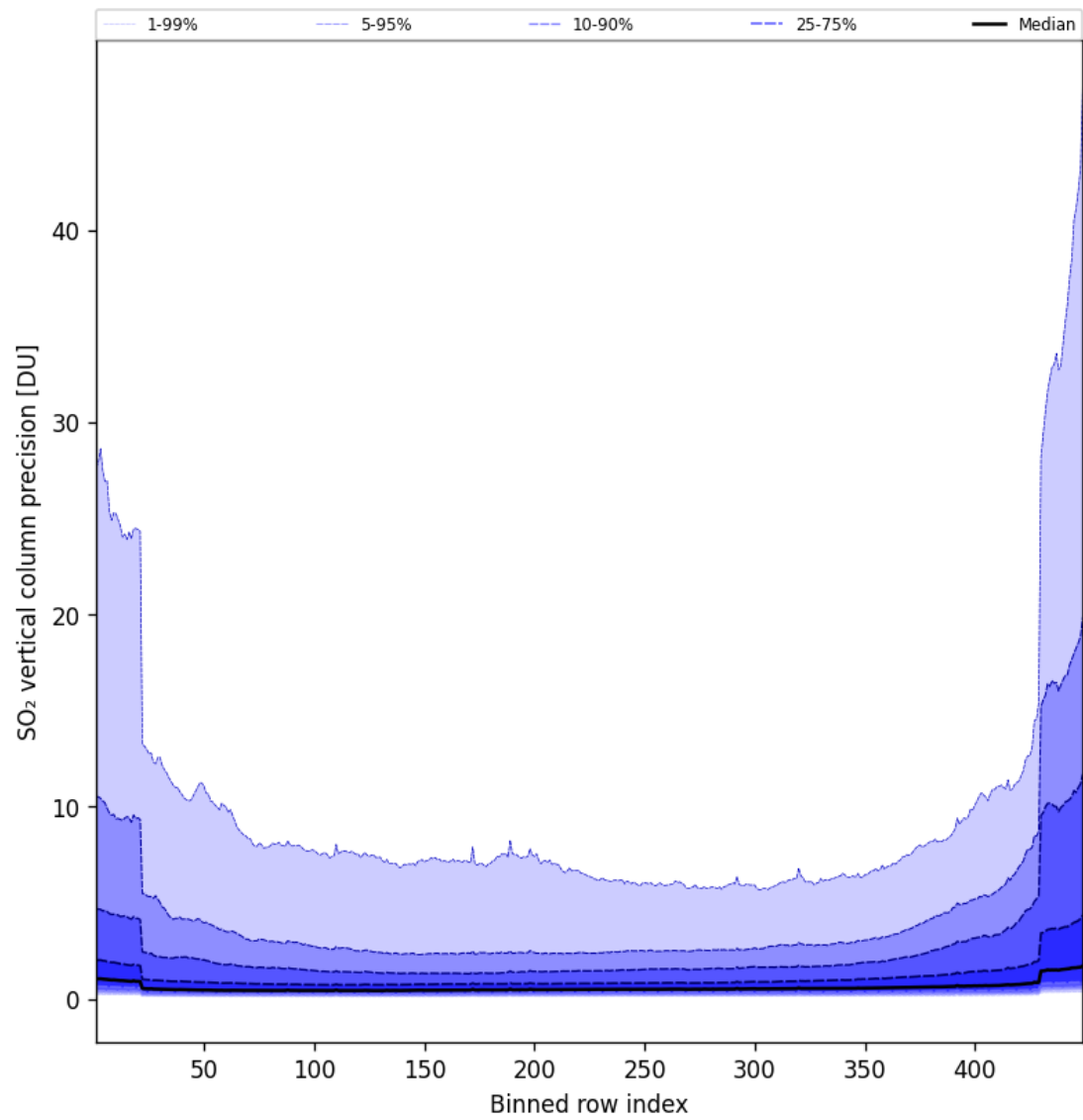
Figure 77: Along track statistics of “SO 2 vertical column precision” for 2024-09-28 to 2024-09-30
