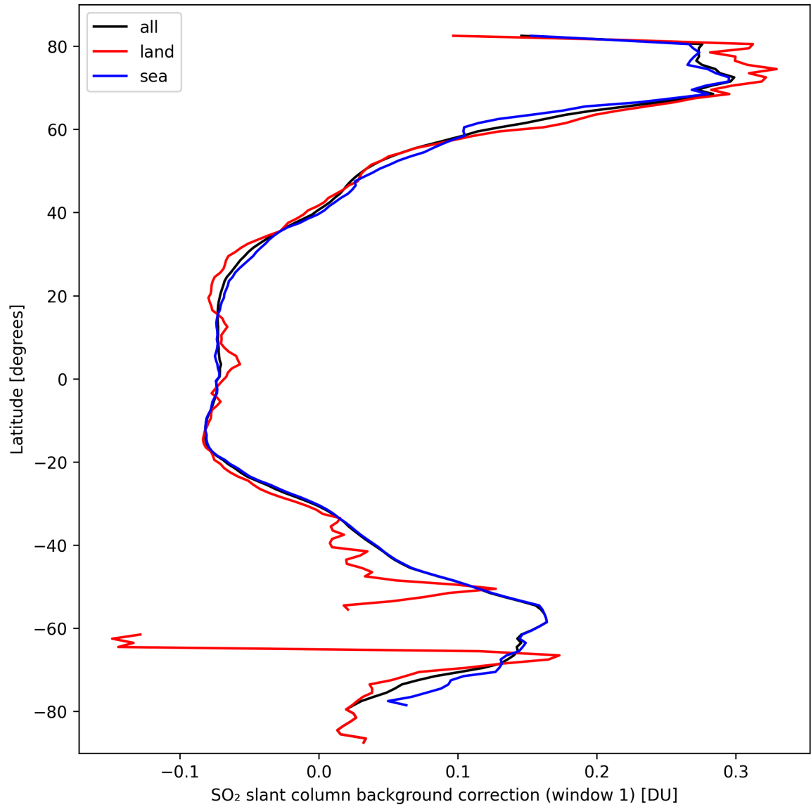
Figure 36: Zonal average of “SO 2 slant column background correction (window 1)” for 2024-09-28 to 2024-09-30.
