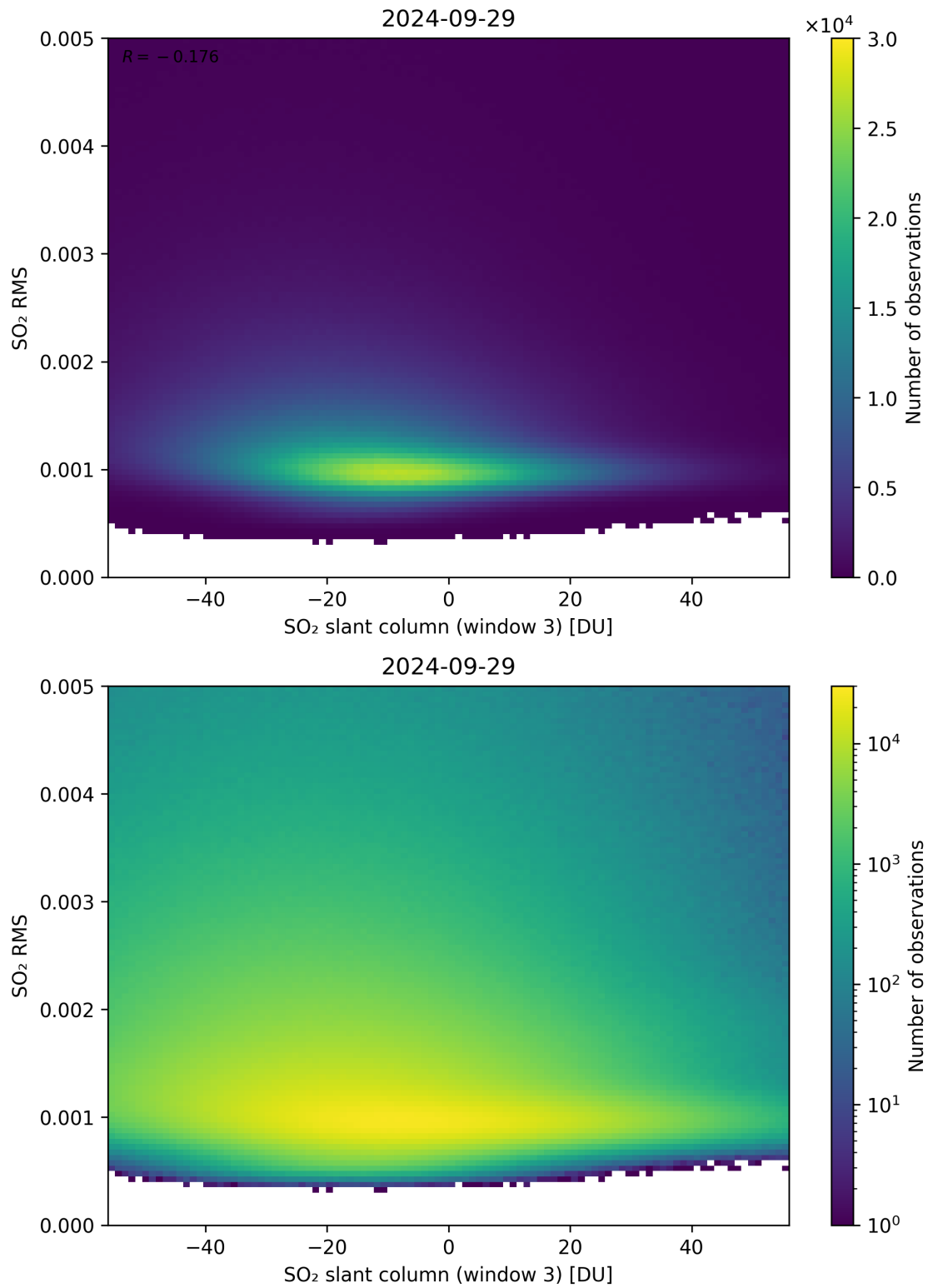
Figure 256: Scatter density plot of “SO 2 slant column (window 3)” against “SO 2 RMS” for 2024-09-28 to 2024-09-30.
