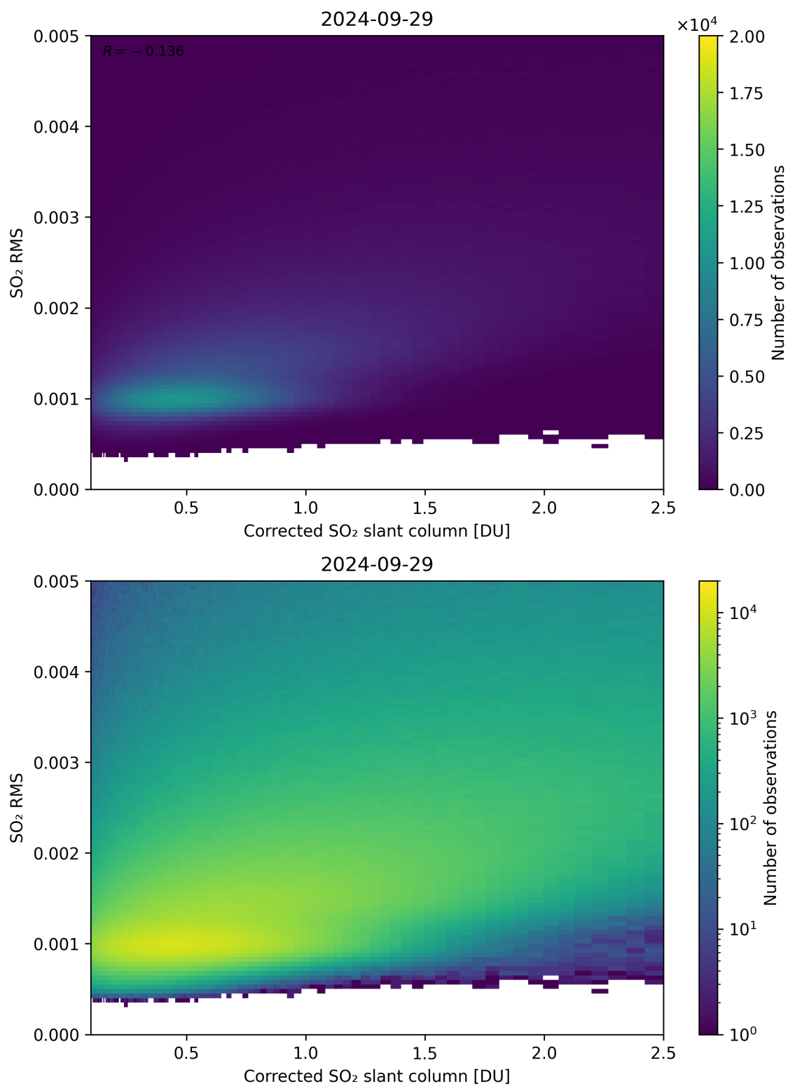
Figure 183: Scatter density plot of “Corrected SO 2 slant column” against “SO 2 RMS” for 2024-09-28 to 2024-09-30.
