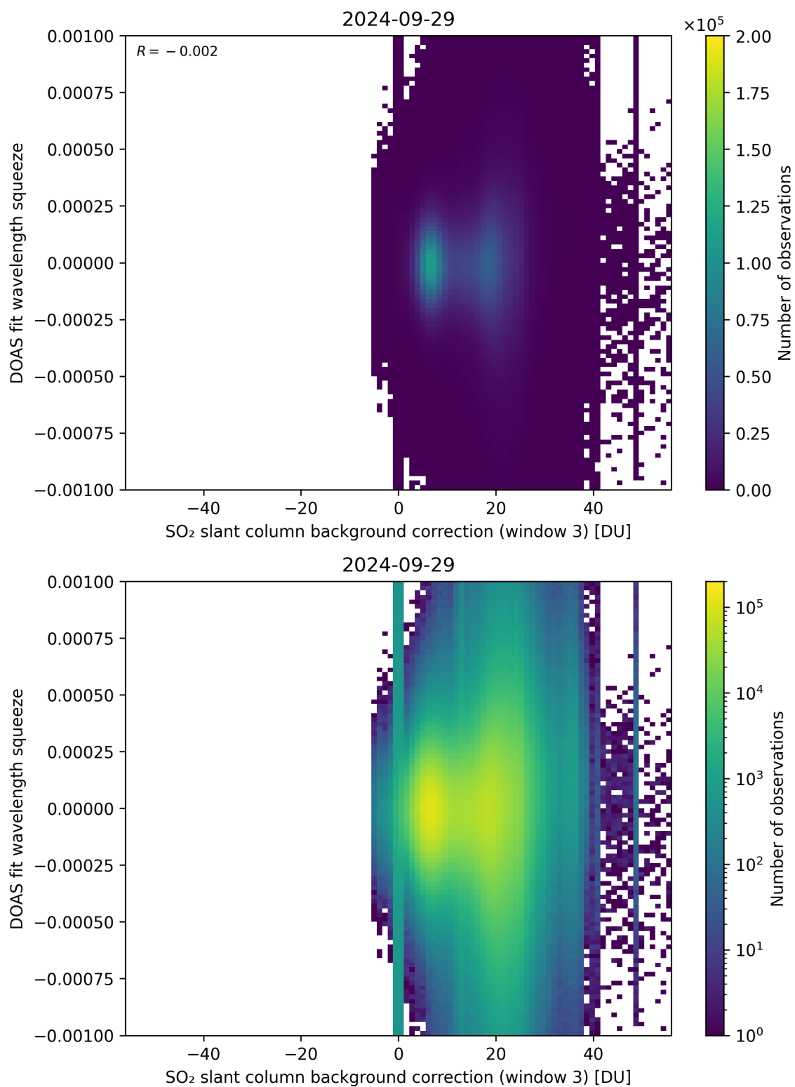
Figure 122: Scatter density plot of “SO 2 slant column background correction (window 3)” against “DOAS fit wavelength squeeze” for 2024-09-28 to 2024-09-30.
