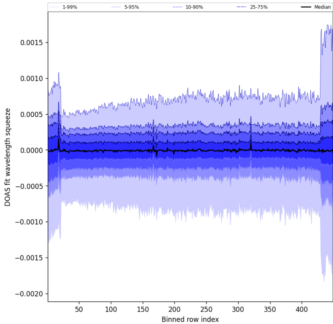
Figure 92: Along track statistics of “DOAS fit wavelength squeeze” for 2024-09-28 to 2024-09-30
