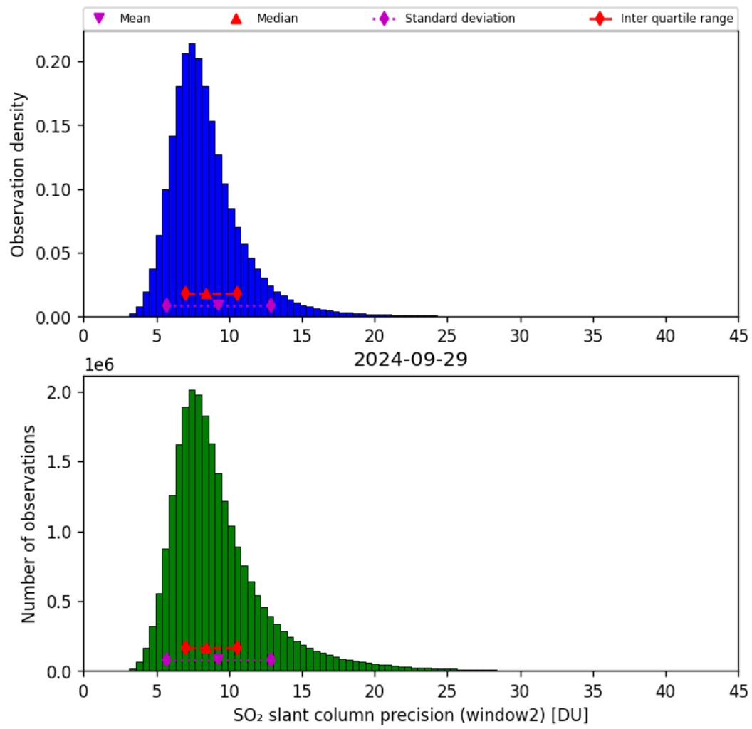
Figure 61: Histogram of “SO 2 slant column precision (window2)” for 2024-09-28 to 2024-09-30
