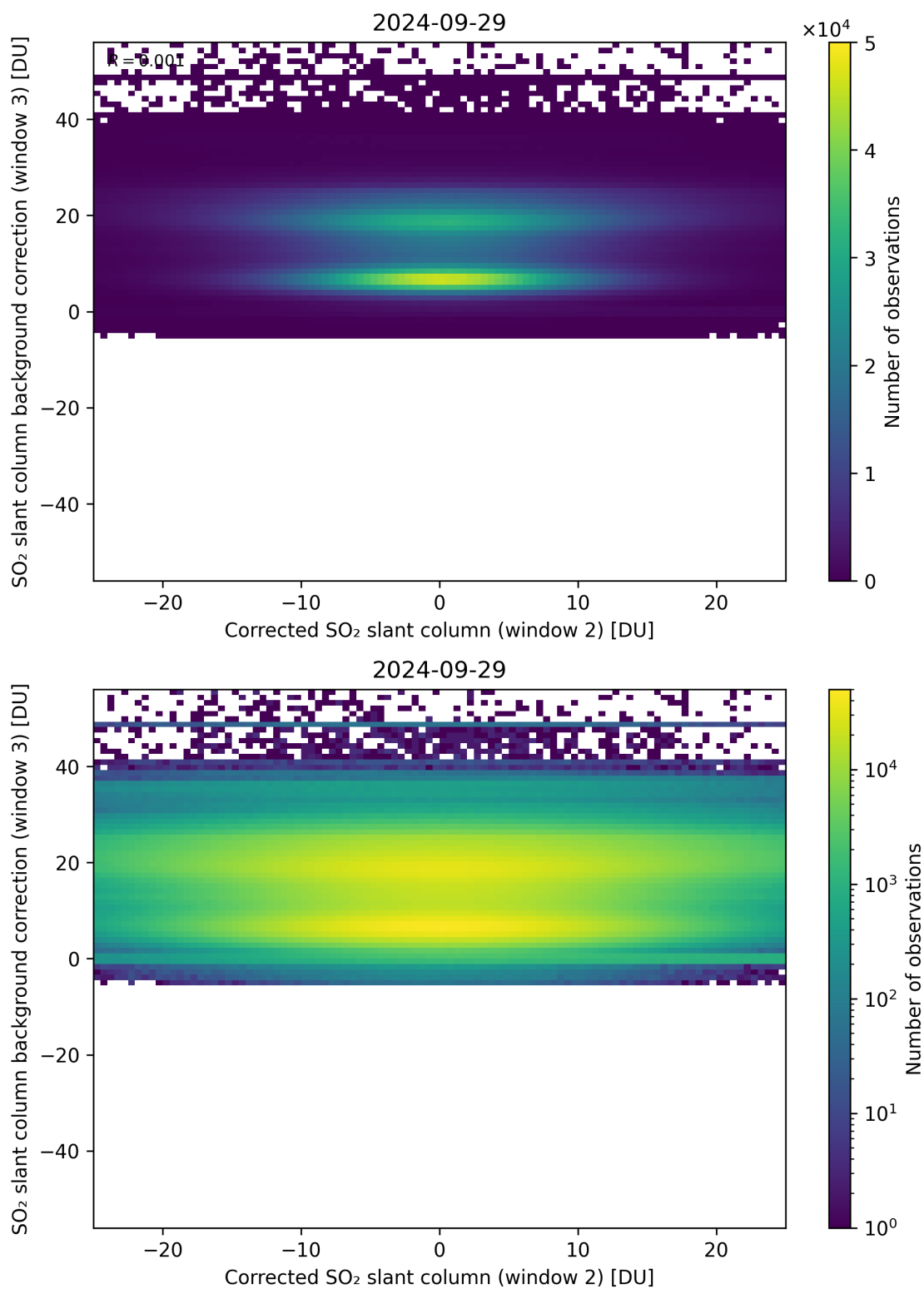
Figure 195: Scatter density plot of “Corrected SO 2 slant column (window 2)” against “SO 2 slant column background correction (window 3)” for 2024-09-28 to 2024-09-30.
