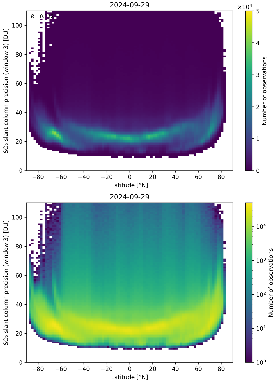
Figure 153: Scatter density plot of “Latitude” against “SO 2 slant column precision (window 3)” for 2024-09-28 to 2024-09-30.
