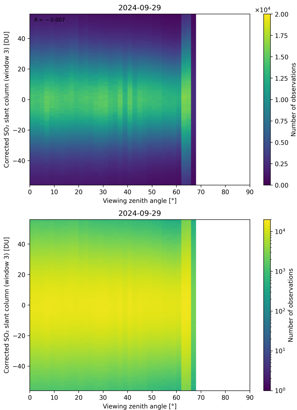
Figure 319: Scatter density plot of “Viewing zenith angle” against “Corrected SO 2 slant column (window 3)” for 2024-09-28 to 2024-09-30.
