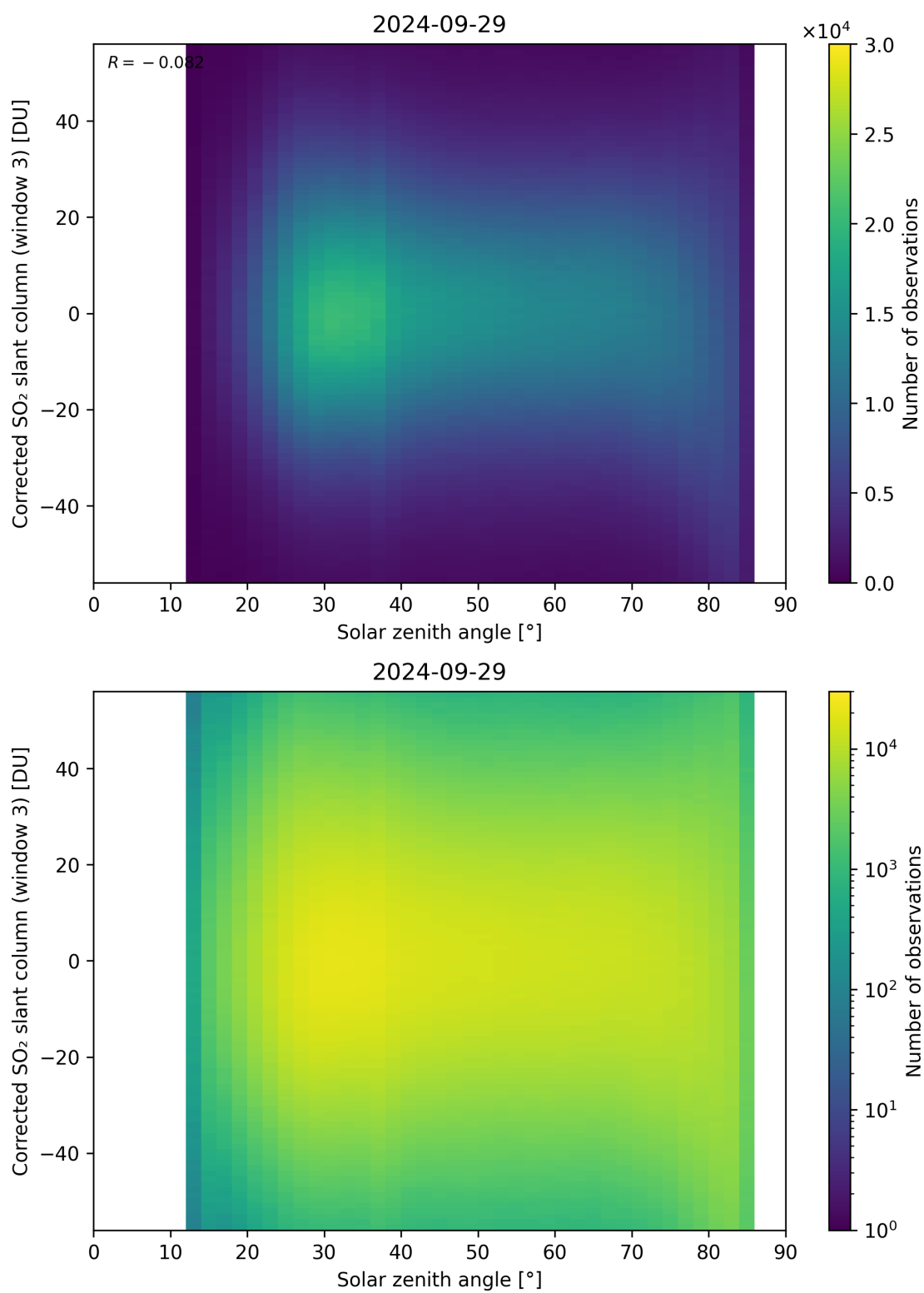
Figure 168: Scatter density plot of “Solar zenith angle” against “Corrected SO 2 slant column (window 3)” for 2024-09-28 to 2024-09-30.
