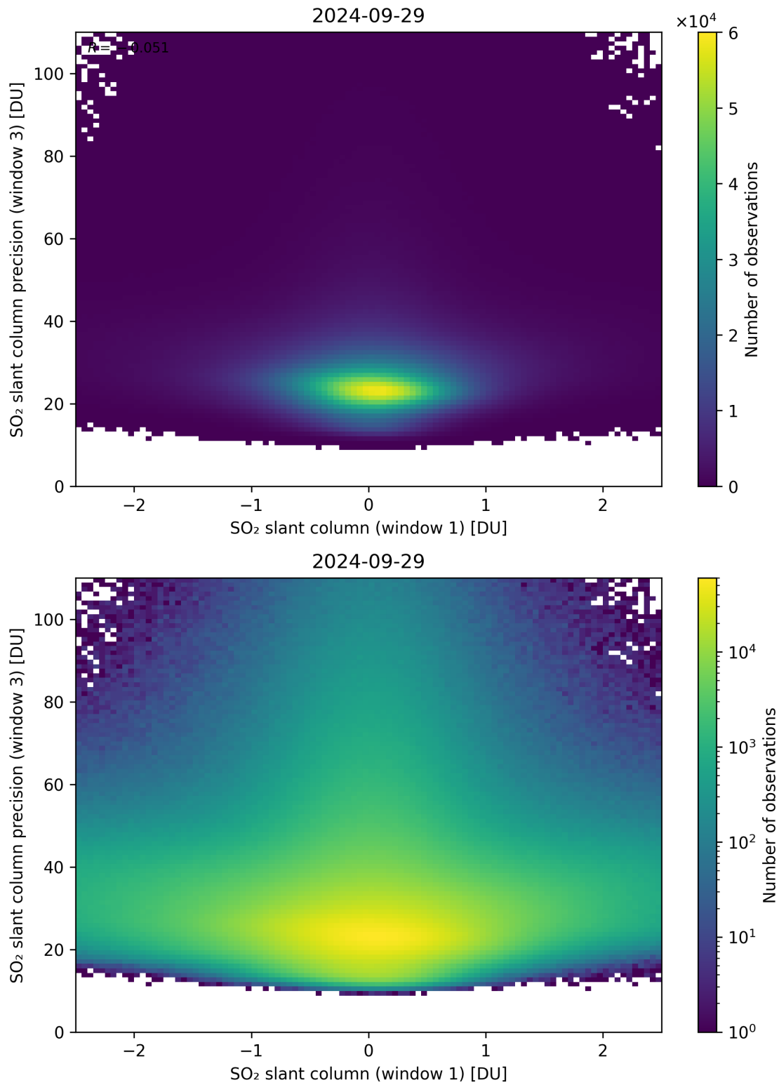
Figure 238: Scatter density plot of “SO 2 slant column (window 1)” against “SO 2 slant column precision (window 3)” for 2024-09-28 to 2024-09-30.
