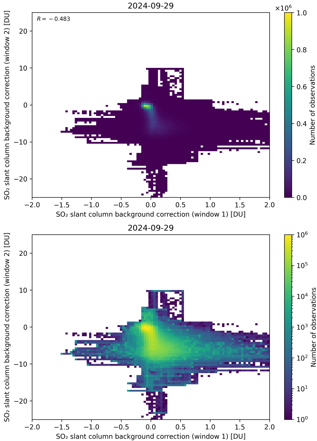
Figure 98: Scatter density plot of “SO 2 slant column background correction (window 1)” against “SO 2 slant column background correction (window 2)” for 2024-09-28 to 2024-09-30.
