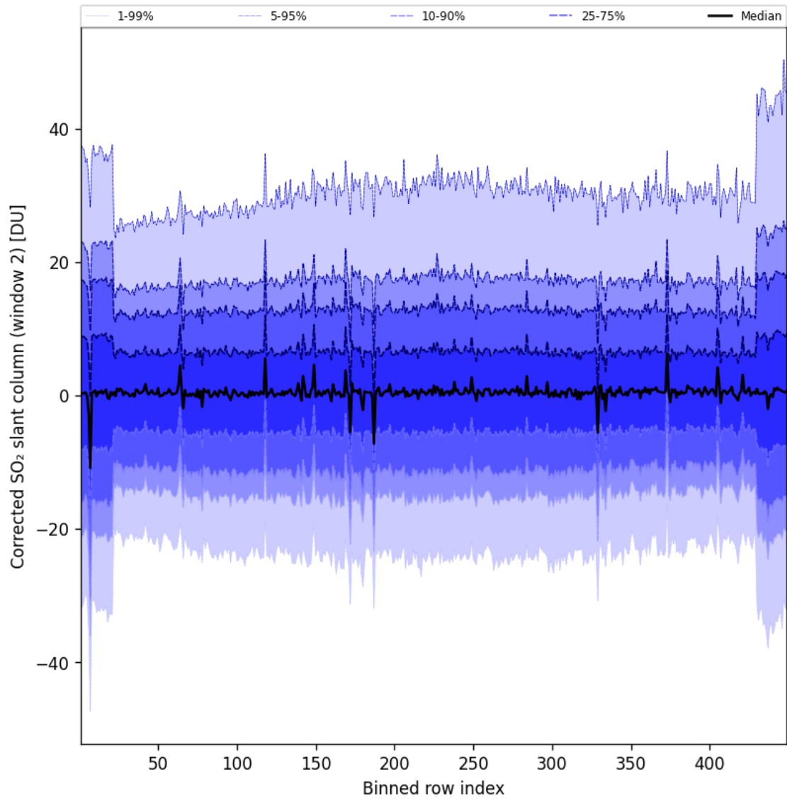
Figure 85: Along track statistics of “Corrected SO 2 slant column (window 2)” for 2024-09-28 to 2024-09-30
