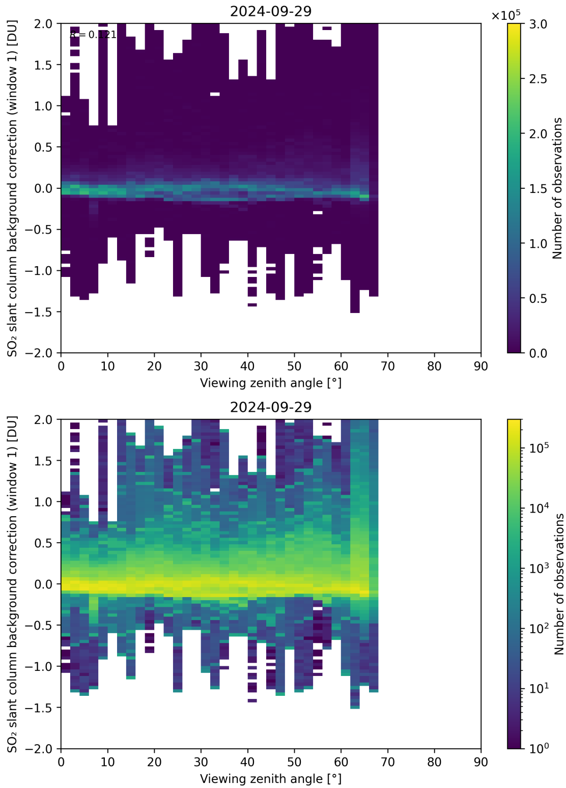
Figure 308: Scatter density plot of “Viewing zenith angle” against “SO 2 slant column background correction (window 1)” for 2024-09-28 to 2024-09-30.
