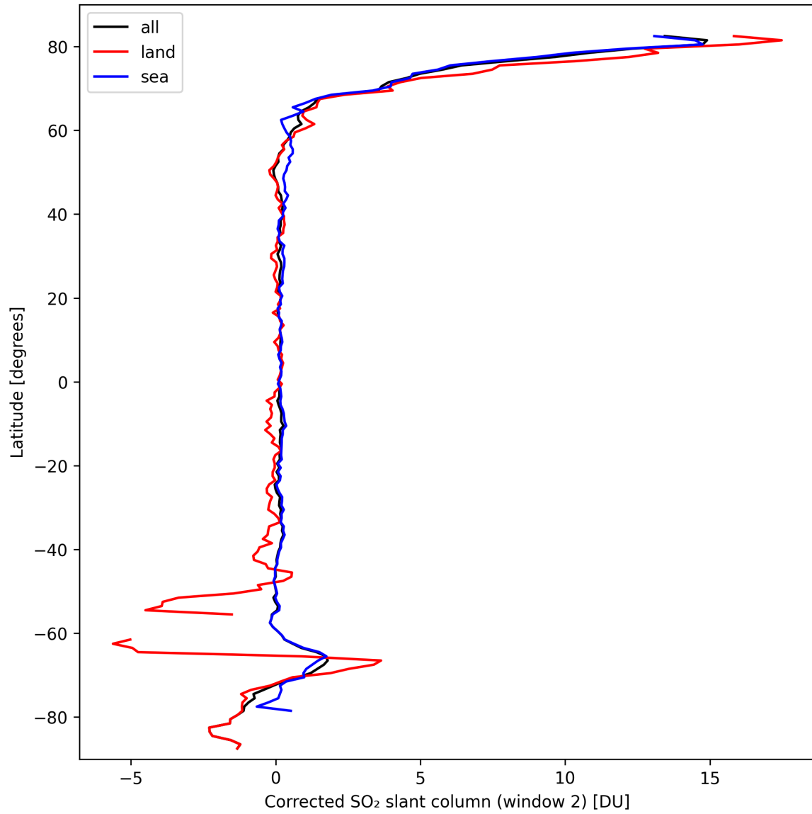
Figure 39: Zonal average of “Corrected SO 2 slant column (window 2)” for 2024-09-28 to 2024-09-30.
