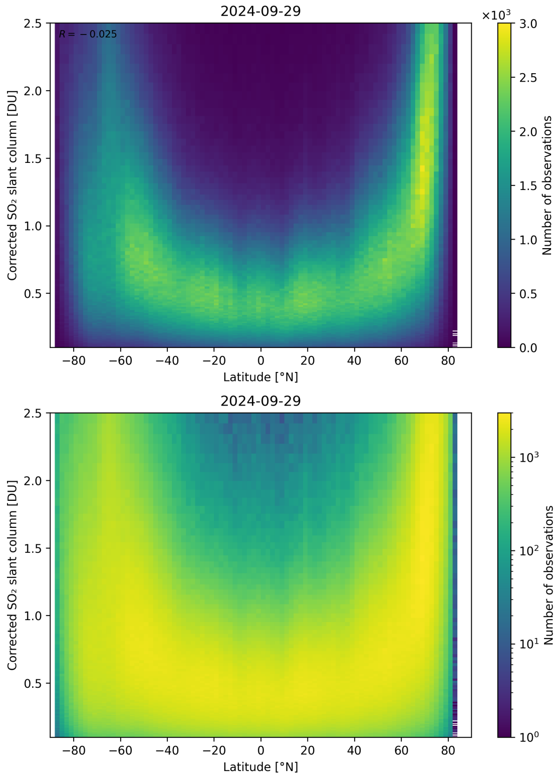
Figure 146: Scatter density plot of “Latitude” against “Corrected SO 2 slant column” for 2024-09-28 to 2024-09-30.
