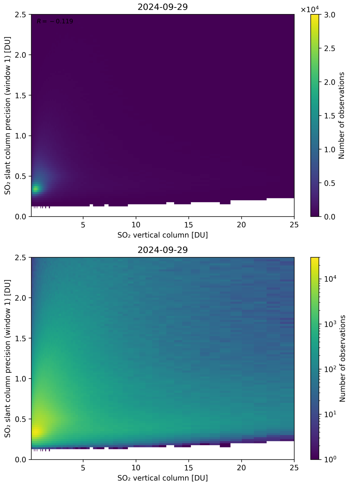
Figure 301: Scatter density plot of “SO 2 vertical column” against “SO 2 slant column precision (window 1)” for 2024-09-28 to 2024-09-30.
