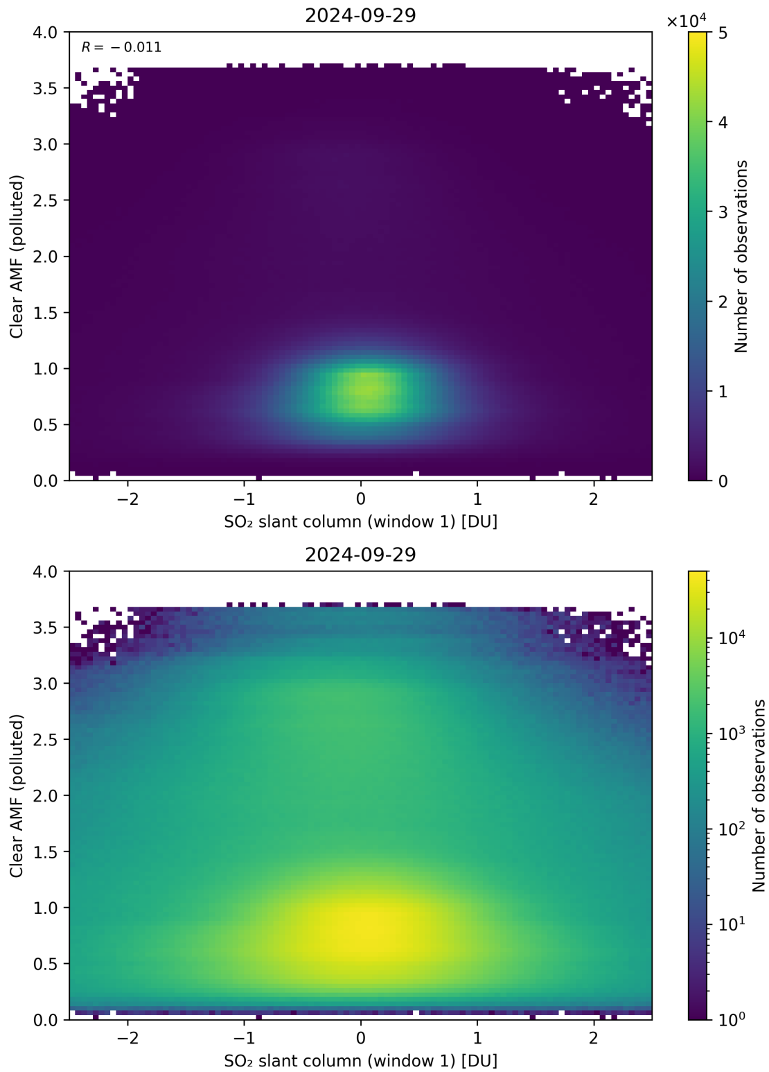
Figure 232: Scatter density plot of “SO 2 slant column (window 1)” against “Clear AMF (polluted)” for 2024-09-28 to 2024-09-30.
