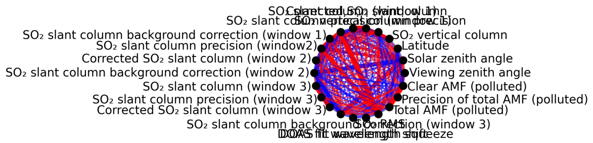
Figure 1: Map of correlation graph for 2024-09-28 to 2024-09-30.
