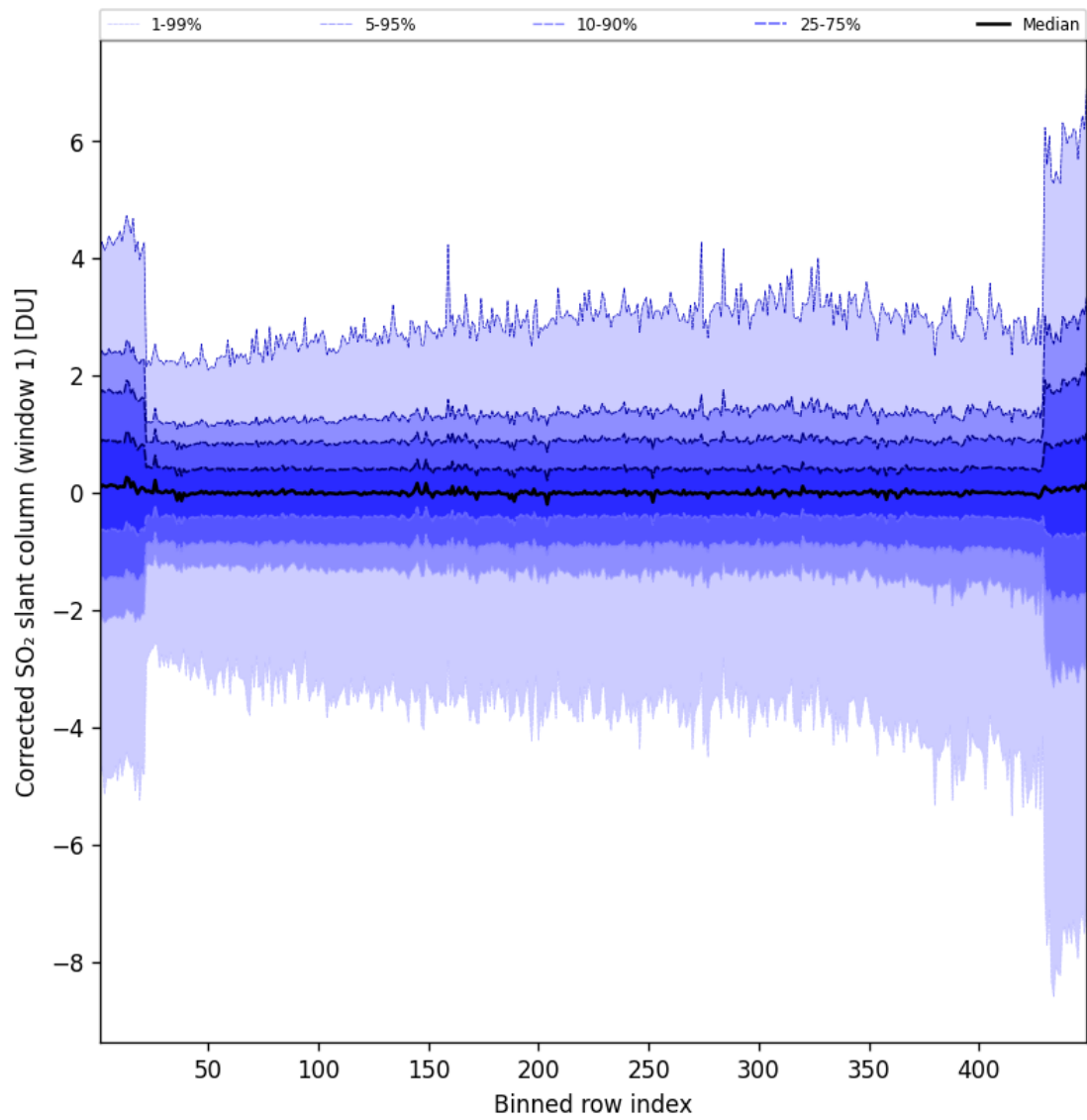
Figure 81: Along track statistics of “Corrected SO 2 slant column (window 1)” for 2024-09-28 to 2024-09-30
