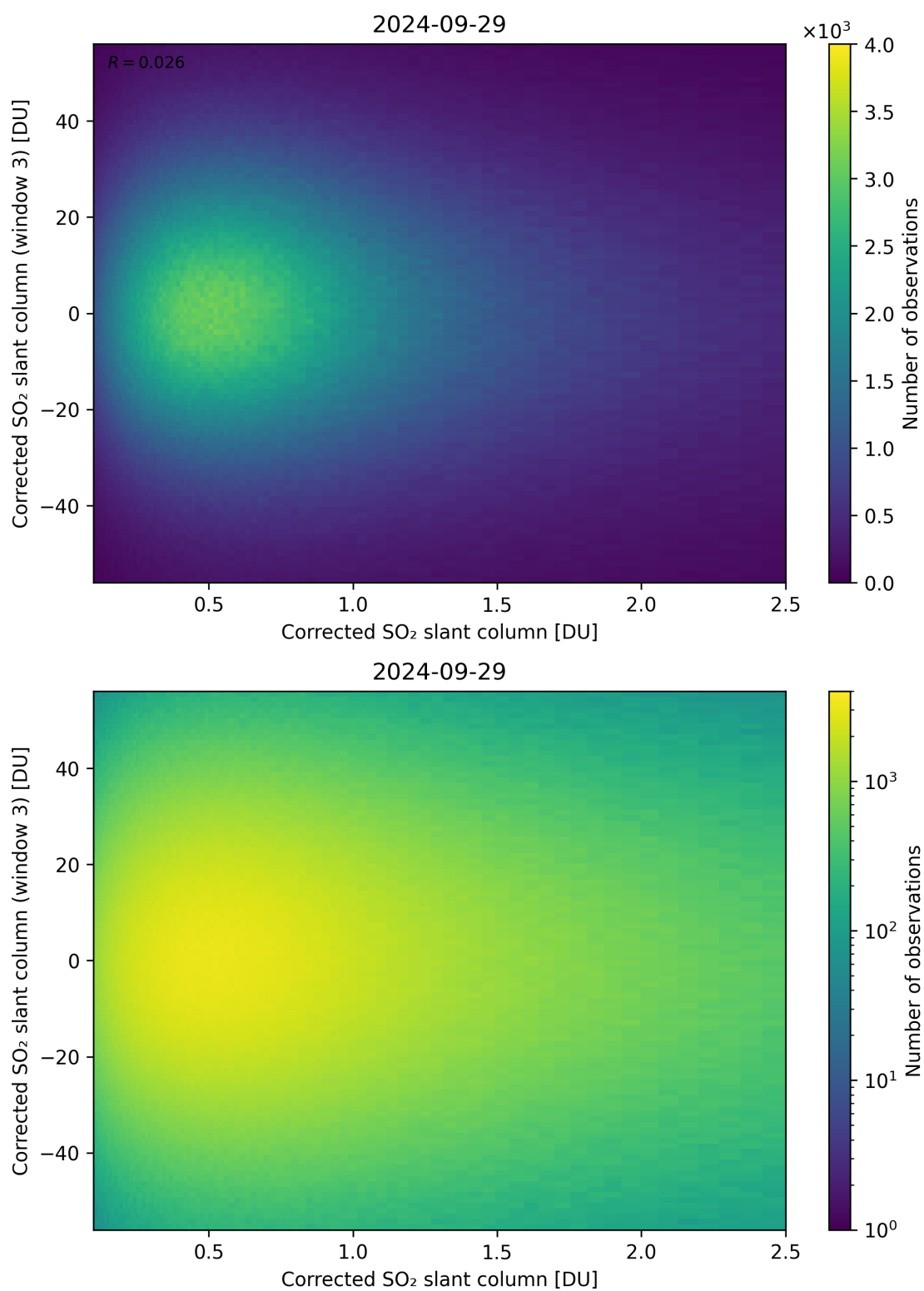
Figure 186: Scatter density plot of “Corrected SO 2 slant column” against “Corrected SO 2 slant column (window 3)” for 2024-09-28 to 2024-09-30.
