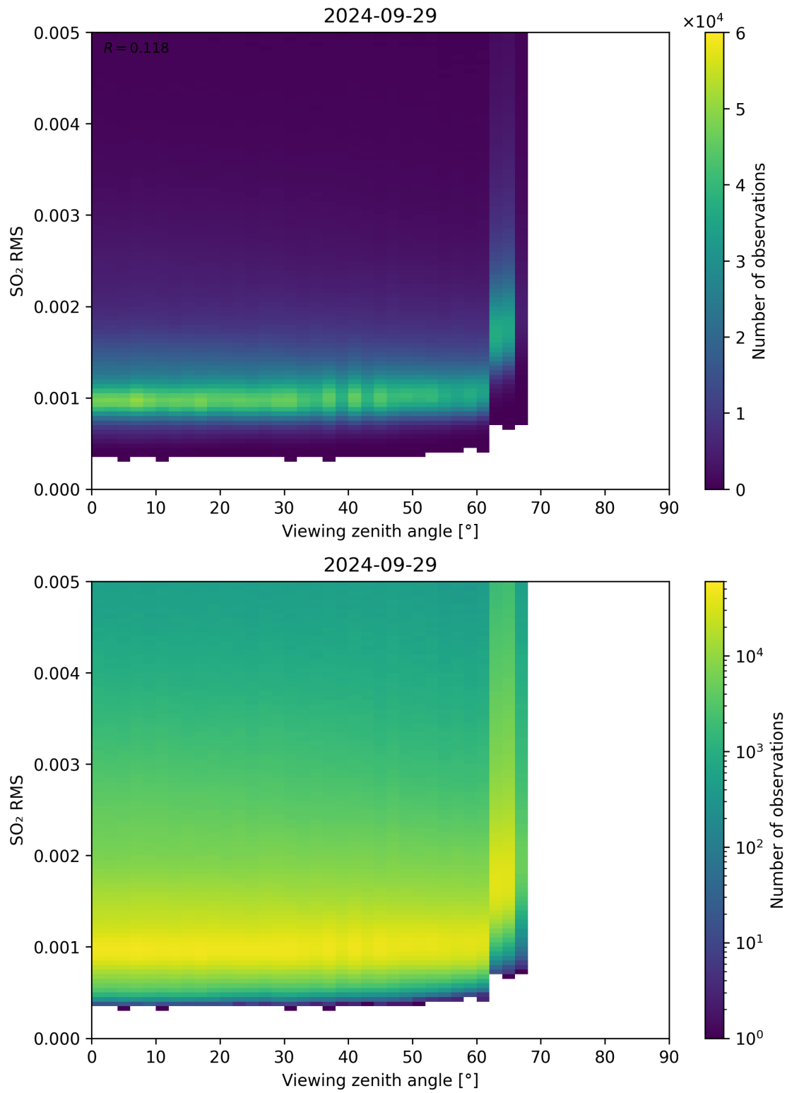
Figure 313: Scatter density plot of “Viewing zenith angle” against “SO 2 RMS” for 2024-09-28 to 2024-09-30.
