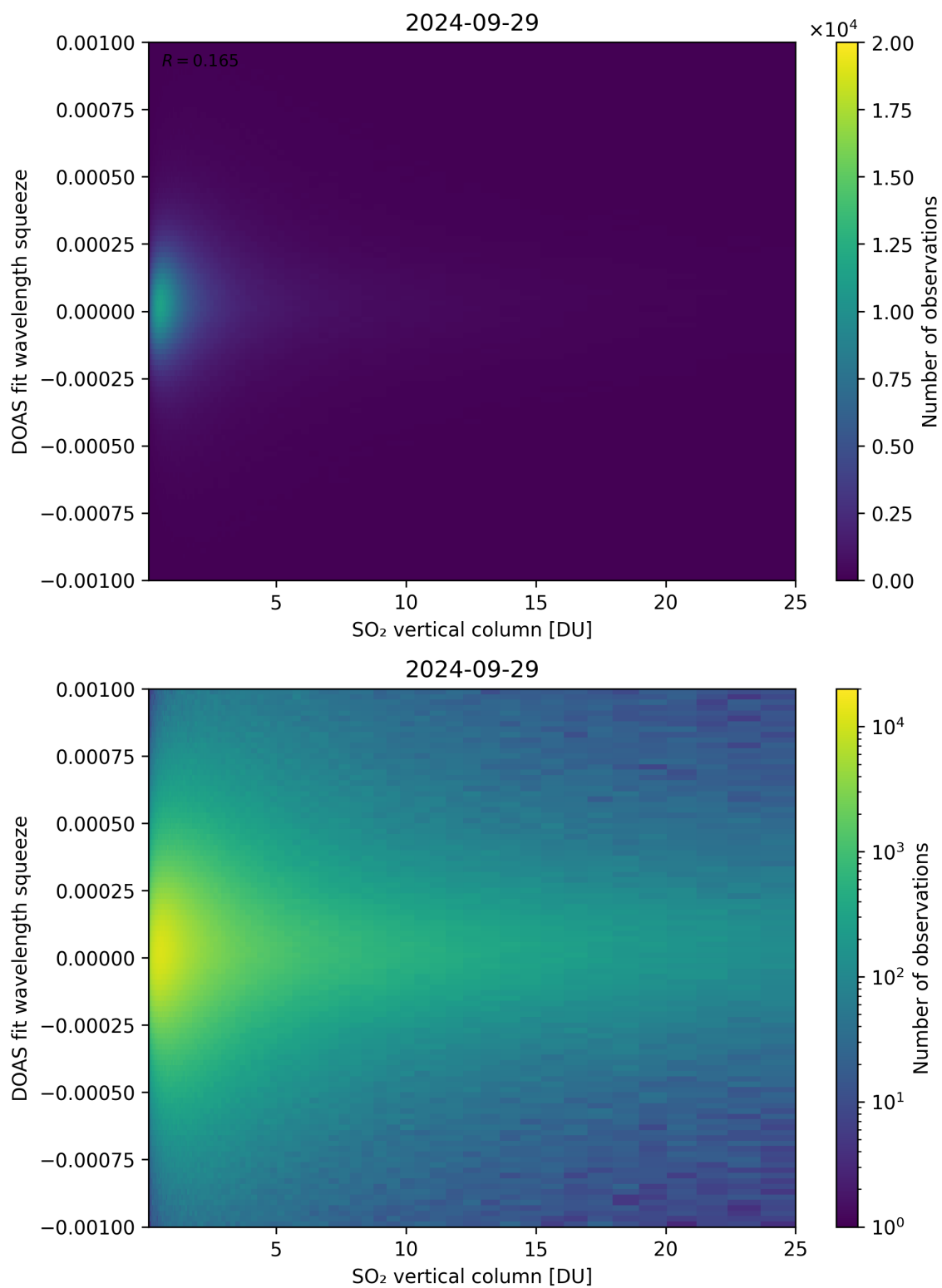
Figure 277: Scatter density plot of “SO 2 vertical column” against “DOAS fit wavelength squeeze” for 2024-09-28 to 2024-09-30.
