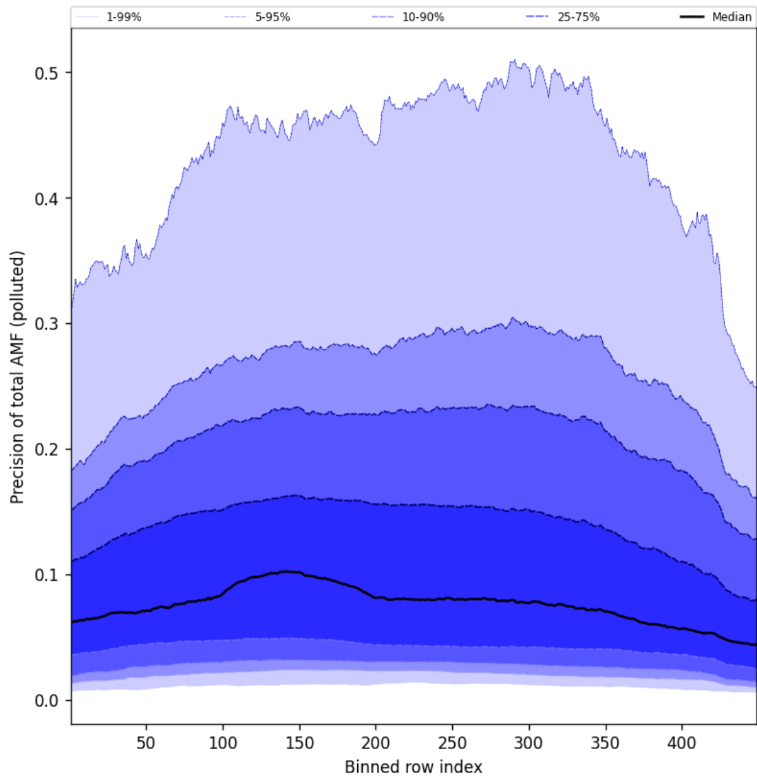
Figure 95: Along track statistics of “Precision of total AMF (polluted)” for 2024-09-28 to 2024-09-30
