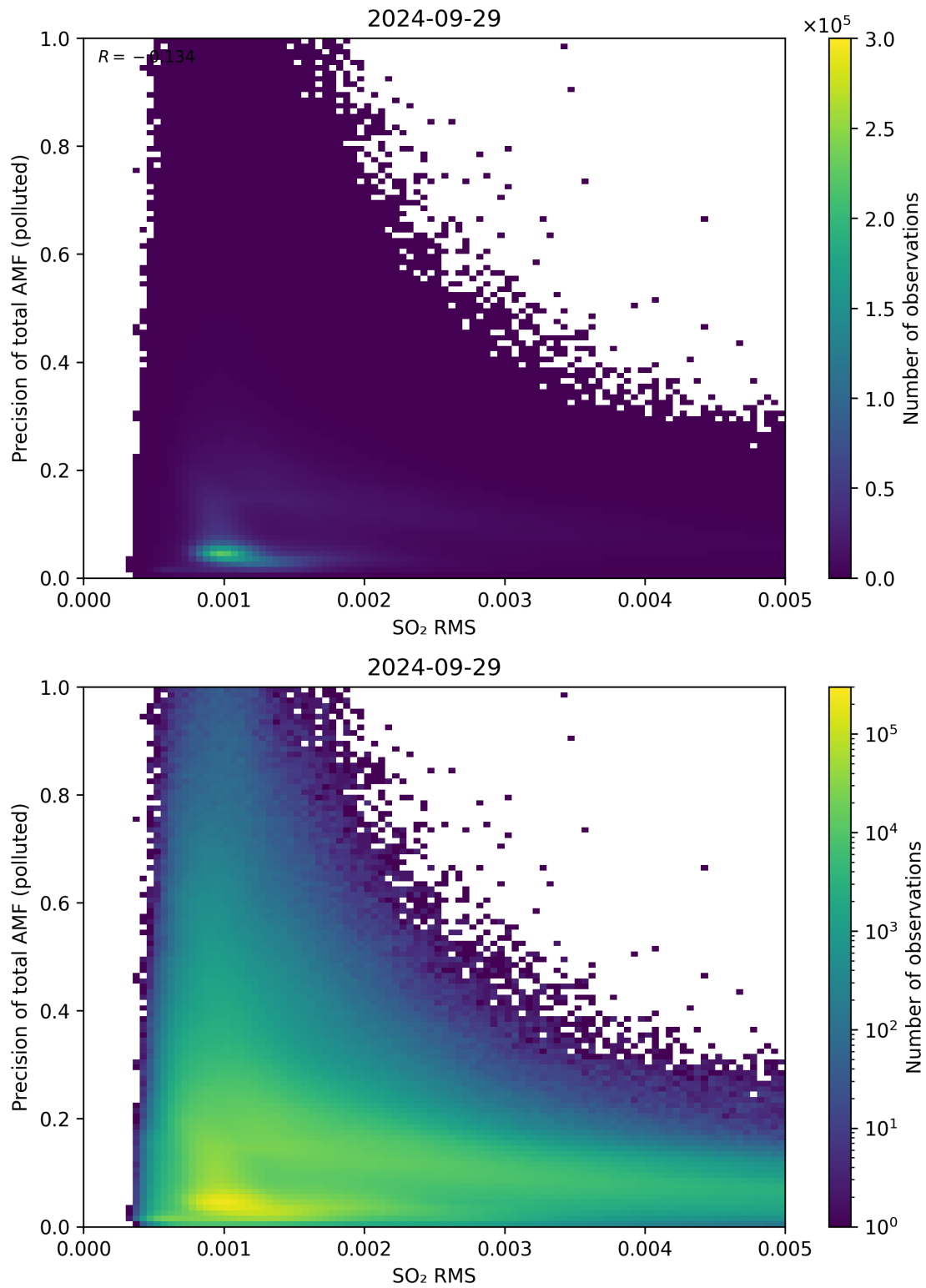
Figure 138: Scatter density plot of “SO 2 RMS” against “Precision of total AMF (polluted)” for 2024-09-28 to 2024-09-30.
