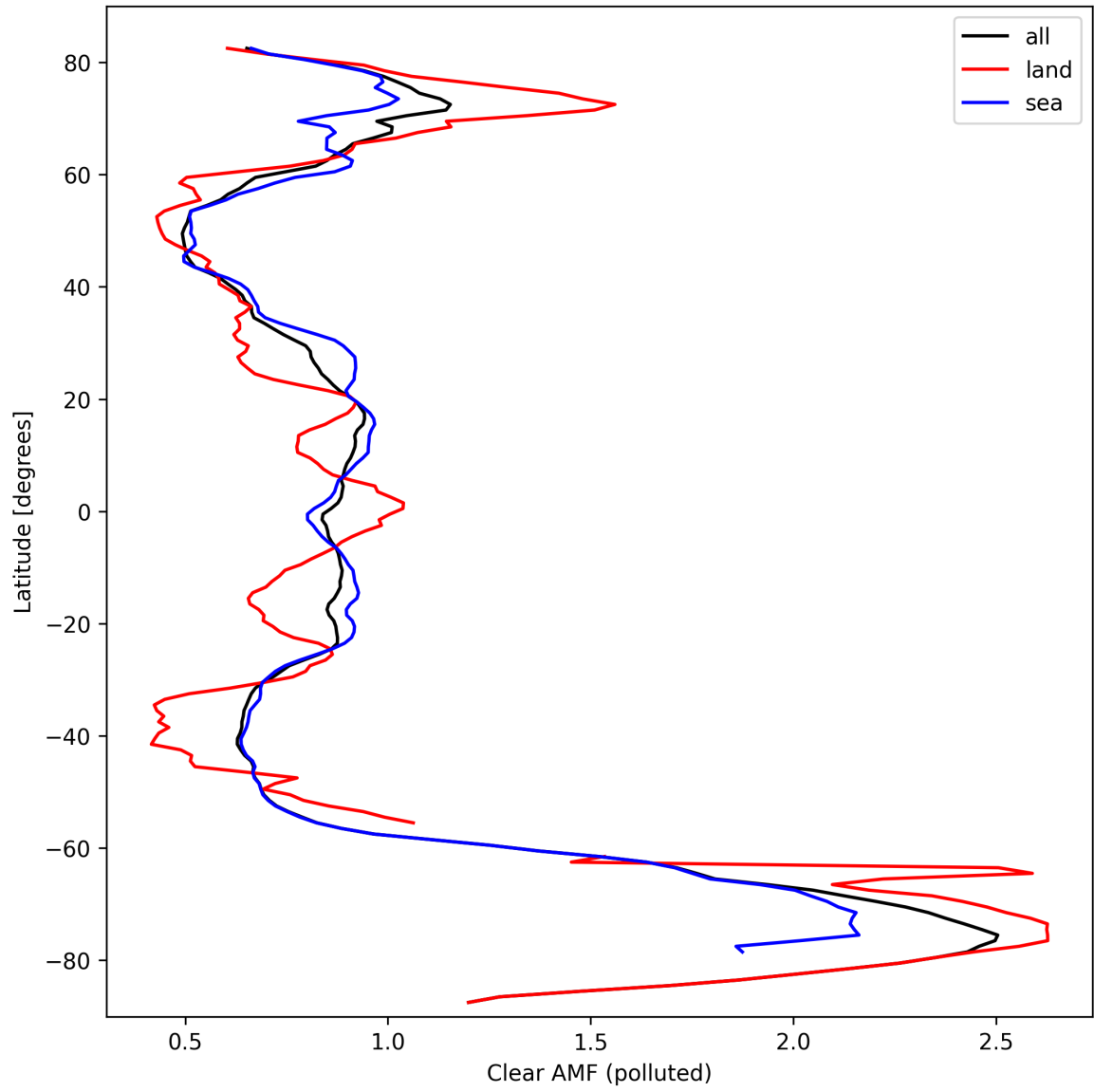
Figure 50: Zonal average of “Clear AMF (polluted)” for 2024-09-28 to 2024-09-30.
