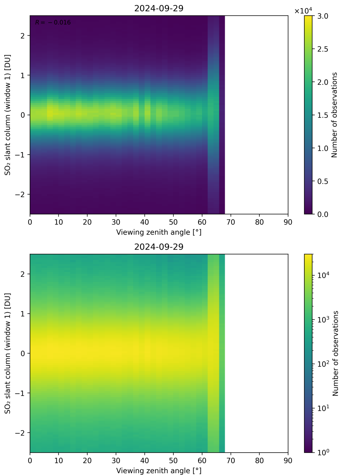
Figure 320: Scatter density plot of “Viewing zenith angle” against “SO 2 slant column (window 1)” for 2024-09-28 to 2024-09-30.
