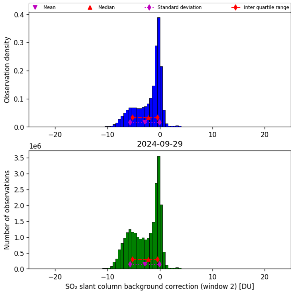
Figure 63: Histogram of “SO 2 slant column background correction (window 2)” for 2024-09-28 to 2024-09-30
