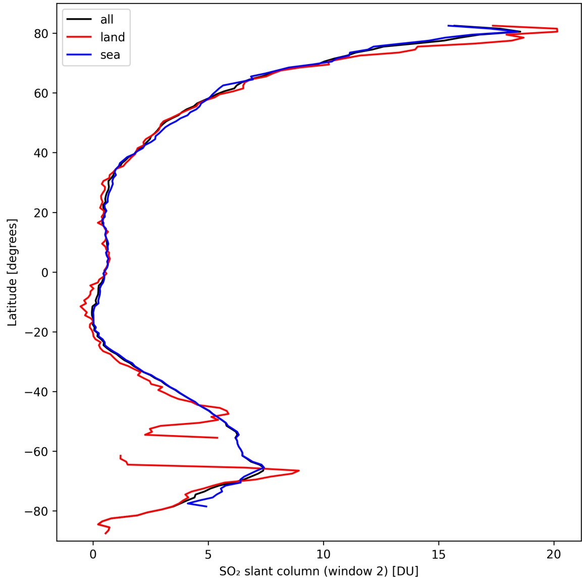
Figure 37: Zonal average of “SO 2 slant column (window 2)” for 2024-09-28 to 2024-09-30.
