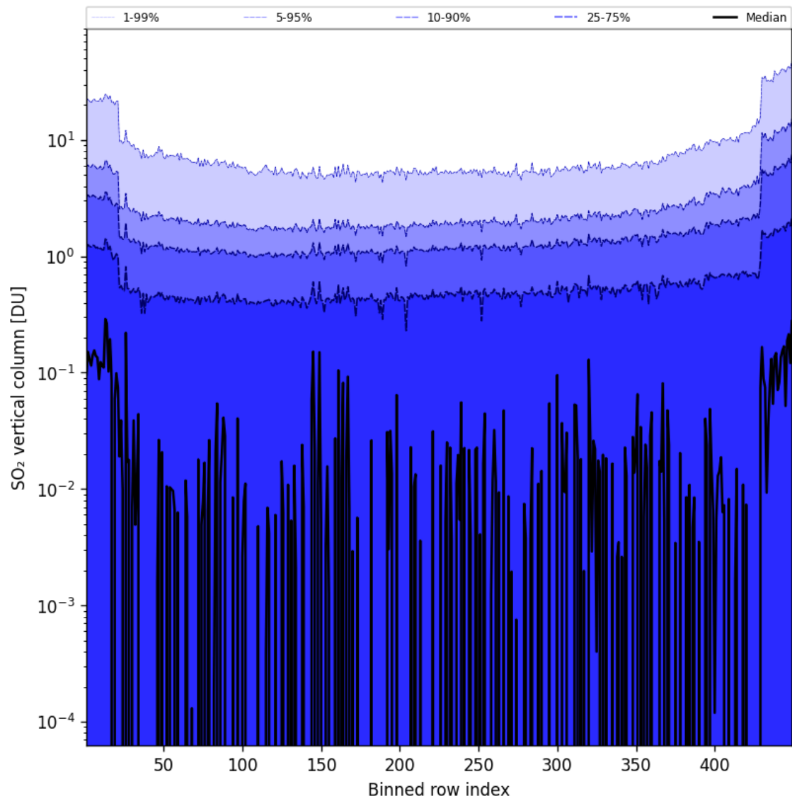
Figure 76: Along track statistics of “SO 2 vertical column” for 2024-09-28 to 2024-09-30
