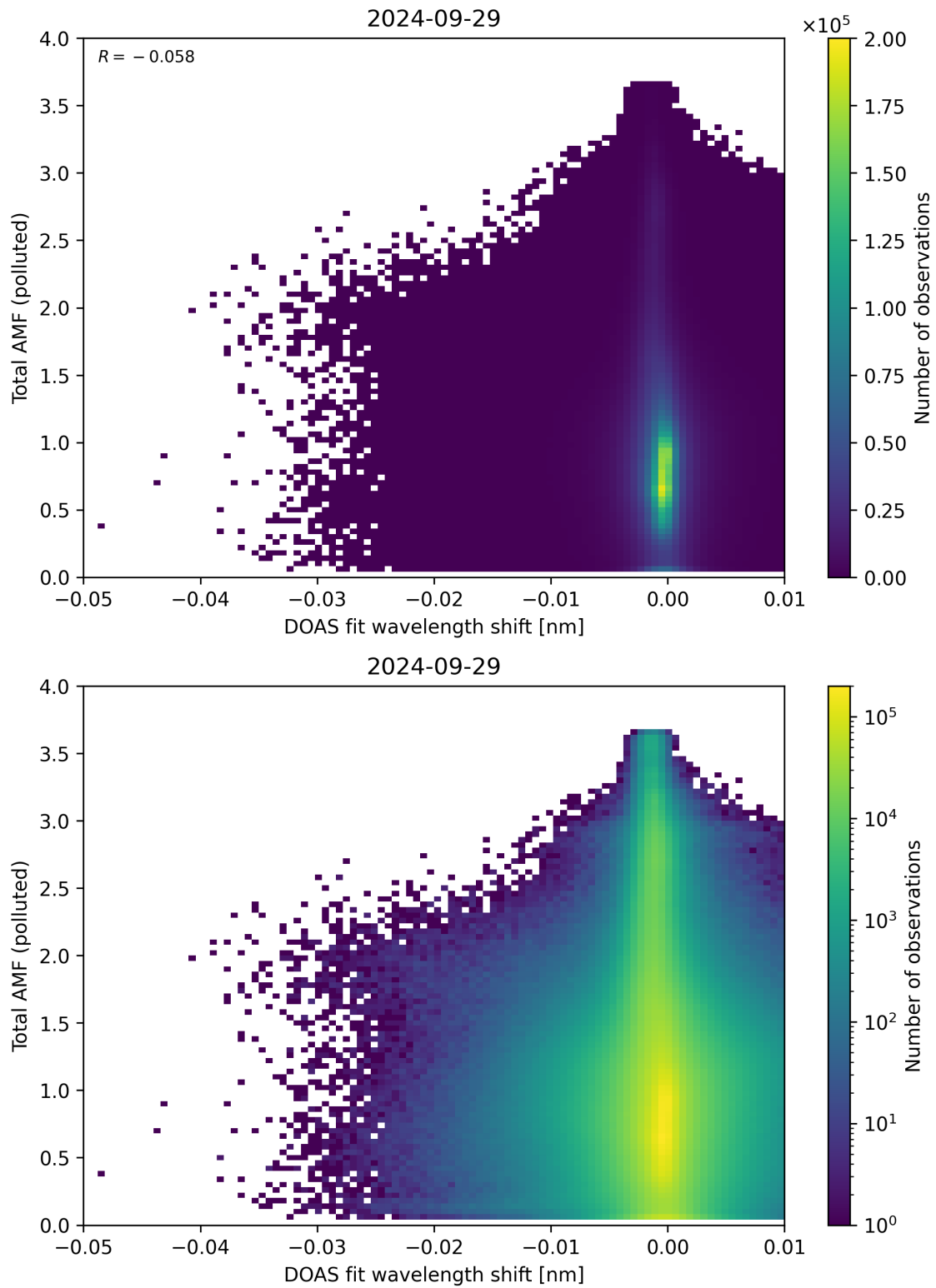
Figure 130: Scatter density plot of “DOAS fit wavelength shift” against “Total AMF (polluted)” for 2024-09-28 to 2024-09-30.
