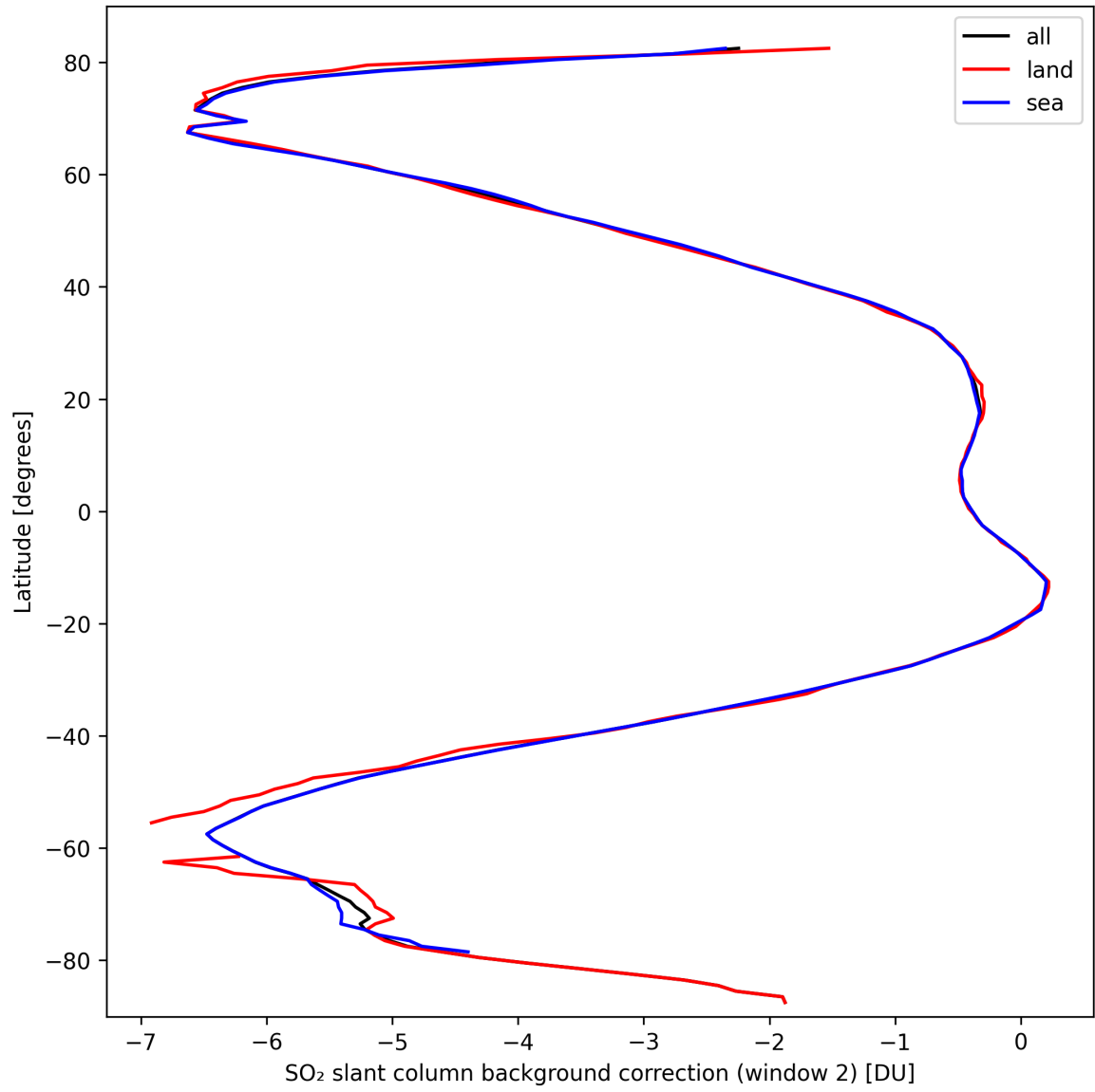
Figure 40: Zonal average of "SO 2 slant column background correction (window 2)" for 2024-09-28 to 2024-09-30.
