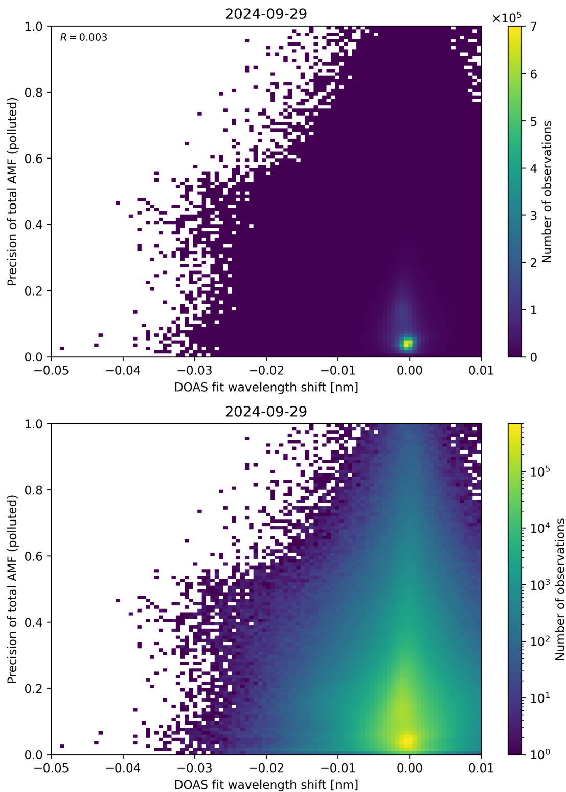
Figure 131: Scatter density plot of “DOAS fit wavelength shift” against “Precision of total AMF (polluted)” for 2024-09-28 to 2024-09-30.
