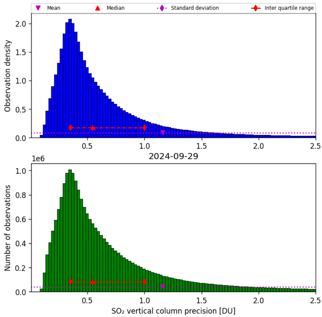
Figure 54: Histogram of “SO 2 vertical column precision” for 2024-09-28 to 2024-09-30
