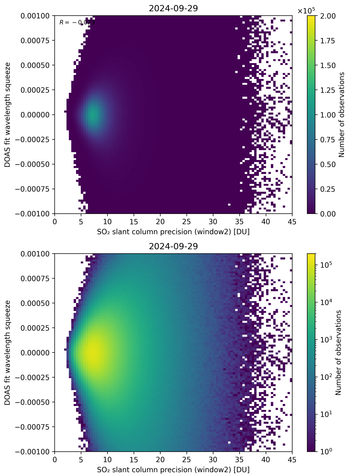
Figure 244: Scatter density plot of “SO 2 slant column precision (window2)” against “DOAS fit wavelength squeeze” for 2024-09-28 to 2024-09-30.
