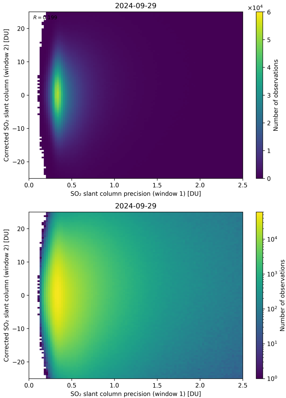
Figure 225: Scatter density plot of “SO 2 slant column precision (window 1)” against “Corrected SO 2 slant column (window 2)” for 2024-09-28 to 2024-09-30.
