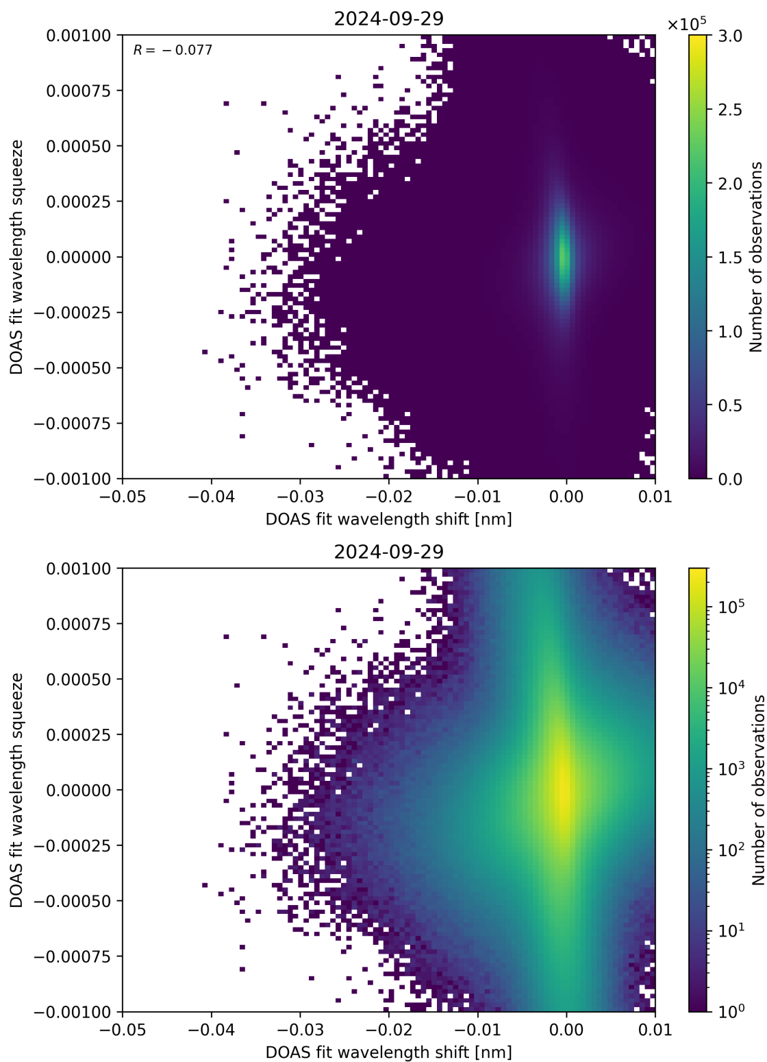
Figure 127: Scatter density plot of “DOAS fit wavelength shift” against “DOAS fit wavelength squeeze” for 2024-09-28 to 2024-09-30.
