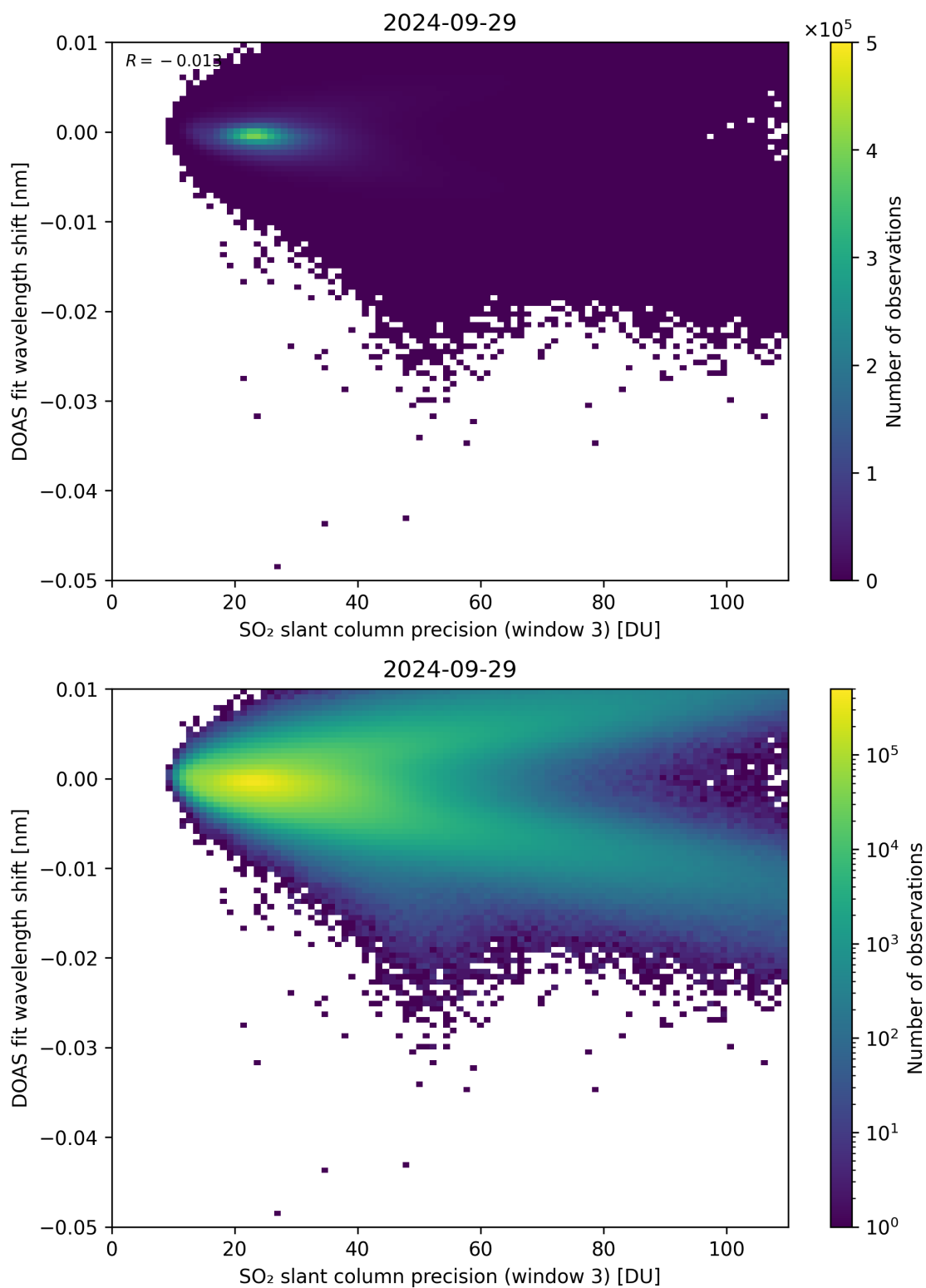
Figure 258: Scatter density plot of “SO 2 slant column precision (window 3)” against “DOAS fit wavelength shift” for 2024-09-28 to 2024-09-30.
