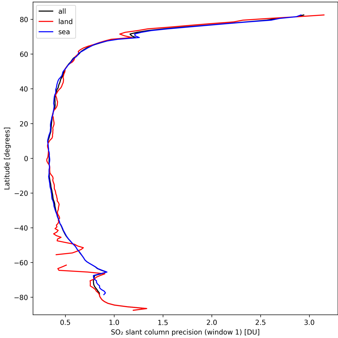
Figure 34: Zonal average of “SO 2 slant column precision (window 1)” for 2024-09-28 to 2024-09-30.
