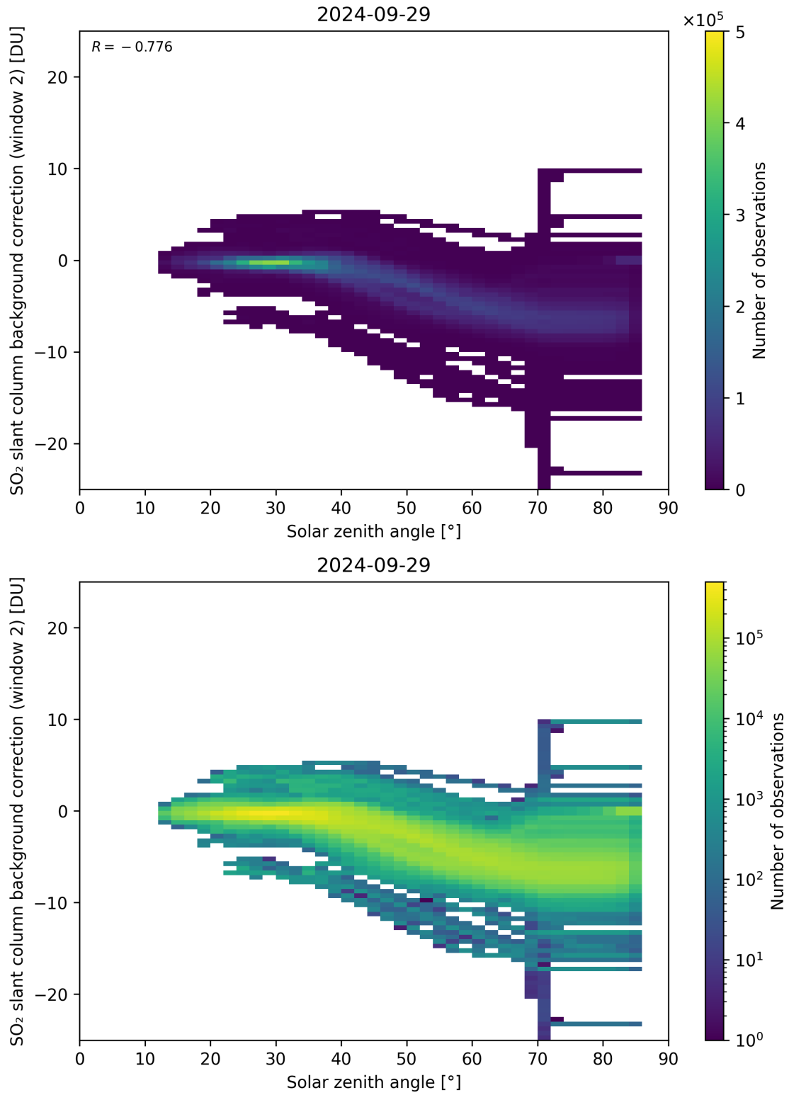
Figure 159: Scatter density plot of “Solar zenith angle” against “SO 2 slant column background correction (window 2)” for 2024-09-28 to 2024-09-30.
