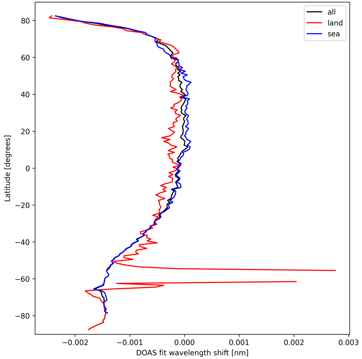
Figure 45: Zonal average of “DOAS fit wavelength shift” for 2024-09-28 to 2024-09-30.
