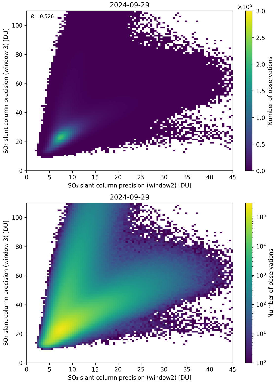
Figure 250: Scatter density plot of “SO 2 slant column precision (window2)” against “SO 2 slant column precision (window 3)” for 2024-09-28 to 2024-09-30.
