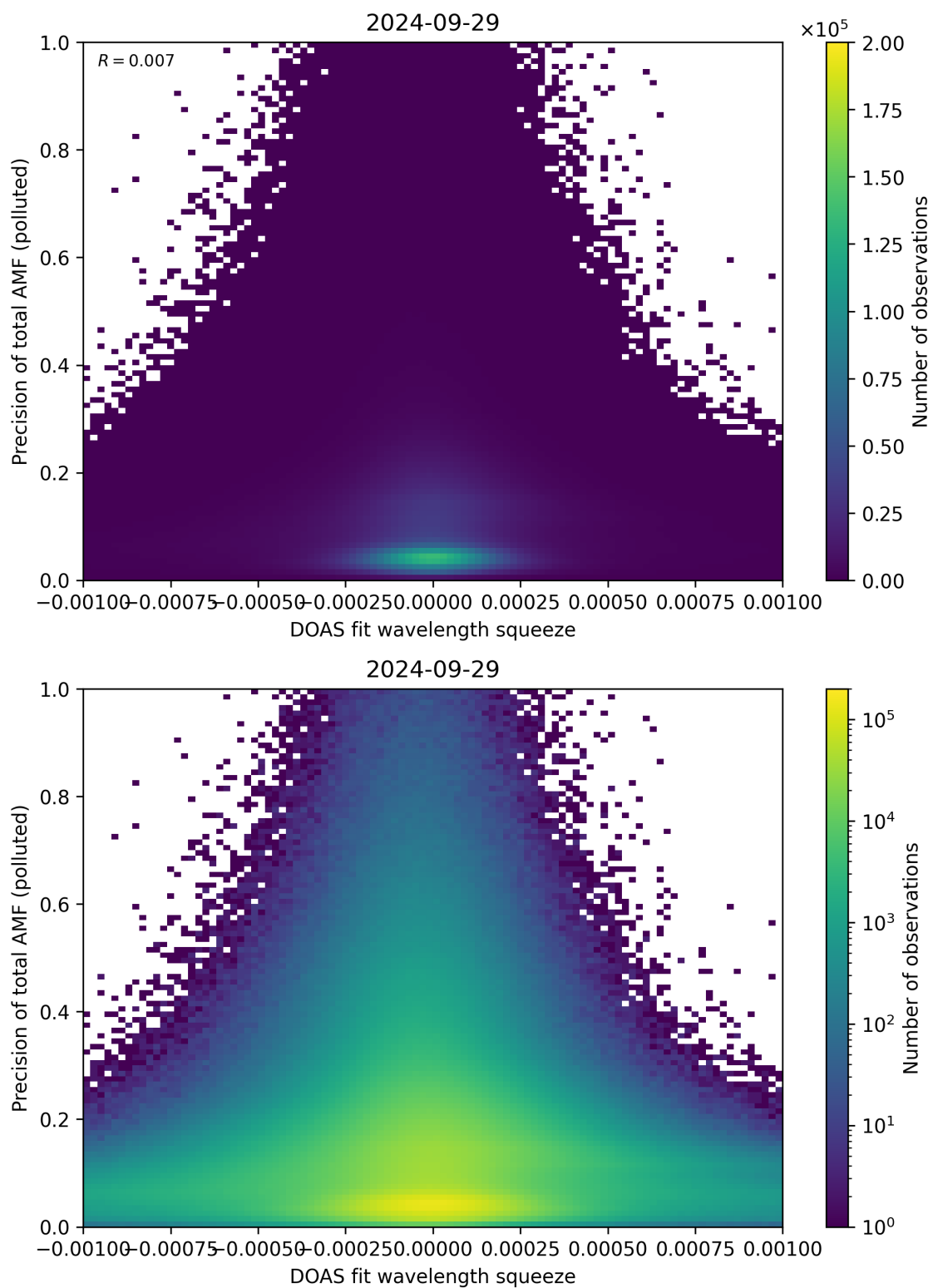
Figure 135: Scatter density plot of “DOAS fit wavelength squeeze” against “Precision of total AMF (polluted)” for 2024-09-28 to 2024-09-30.
