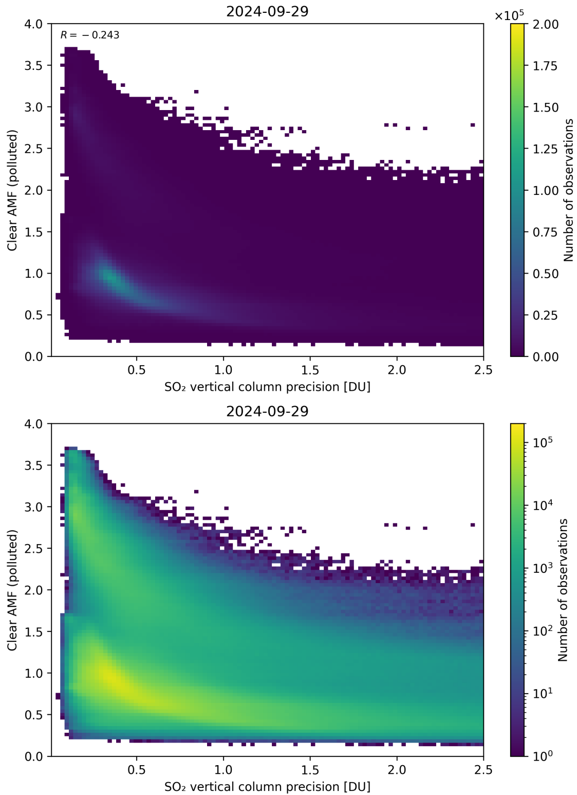
Figure 285: Scatter density plot of “SO 2 vertical column precision” against “Clear AMF (polluted)” for 2024-09-28 to 2024-09-30.
