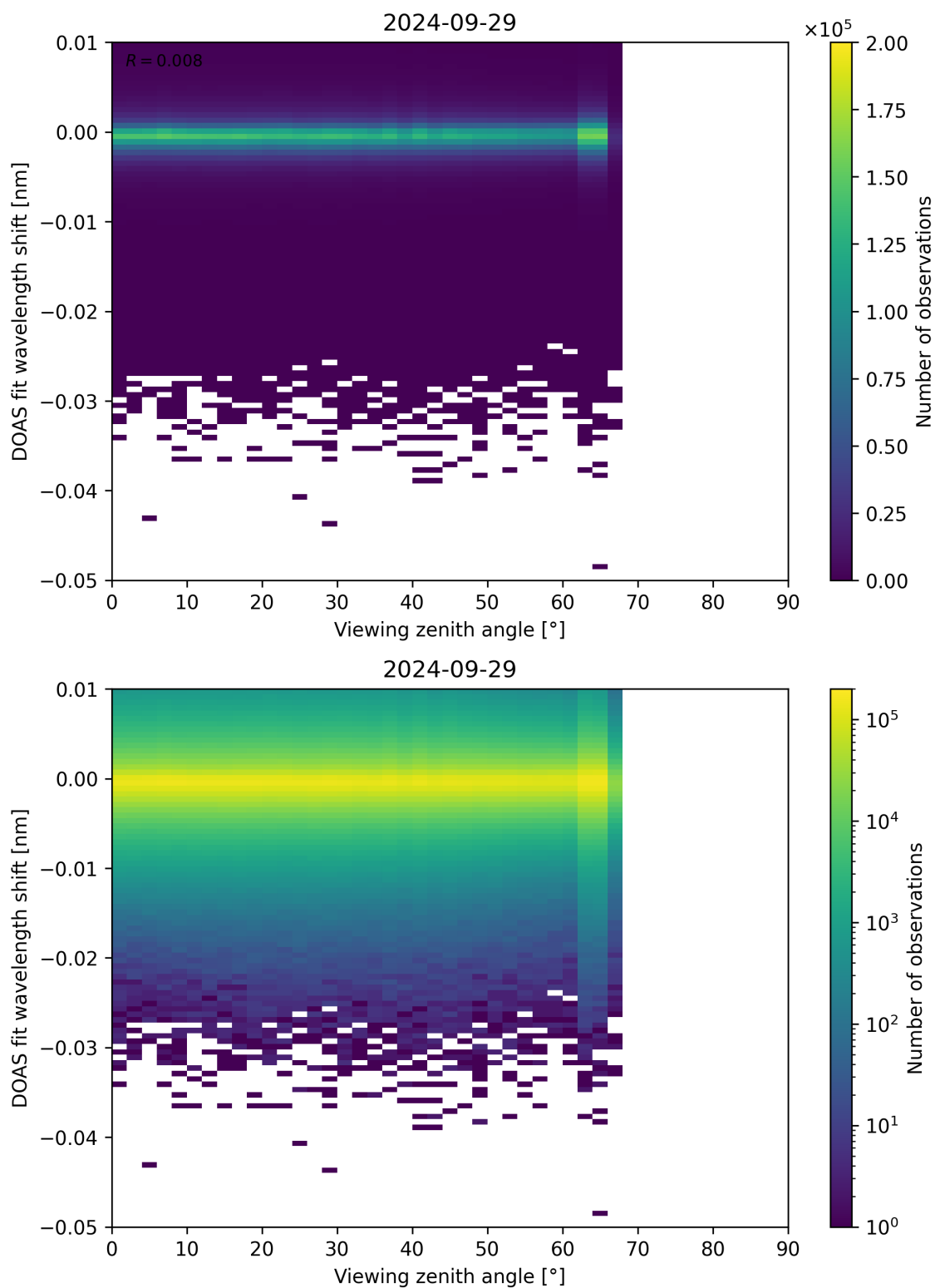
Figure 311: Scatter density plot of “Viewing zenith angle” against “DOAS fit wavelength shift” for 2024-09-28 to 2024-09-30.
