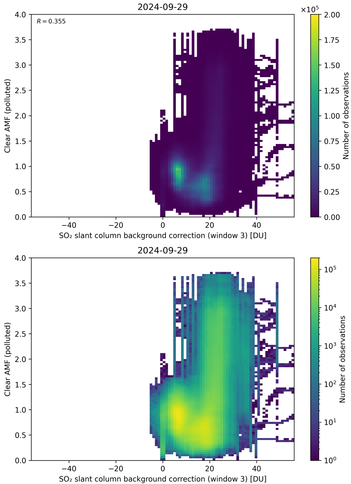
Figure 124: Scatter density plot of “SO 2 slant column background correction (window 3)” against “Clear AMF (polluted)” for 2024-09-28 to 2024-09-30.
