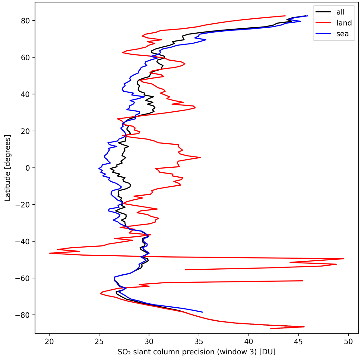
Figure 42: Zonal average of “SO 2 slant column precision (window 3)” for 2024-09-28 to 2024-09-30.
