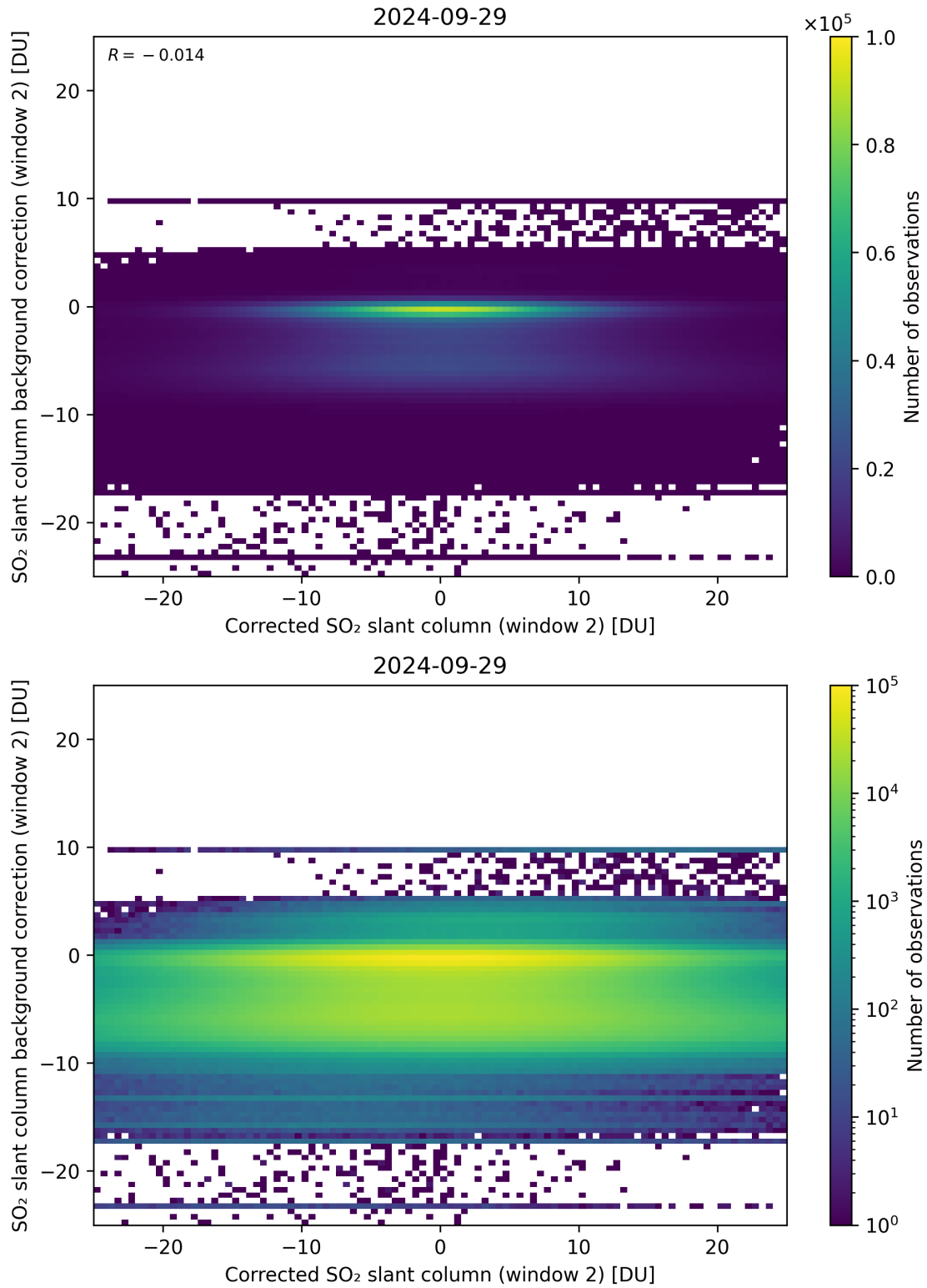
Figure 194: Scatter density plot of “Corrected SO 2 slant column (window 2)” against “SO 2 slant column background correction (window 2)” for 2024-09-28 to 2024-09-30.
