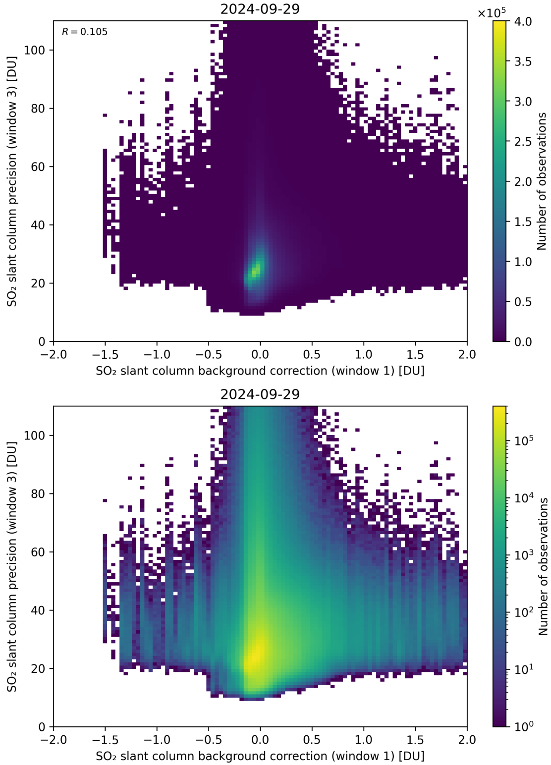
Figure 108: Scatter density plot of “SO 2 slant column background correction (window 1)” against “SO 2 slant column precision (window 3)” for 2024-09-28 to 2024-09-30.
