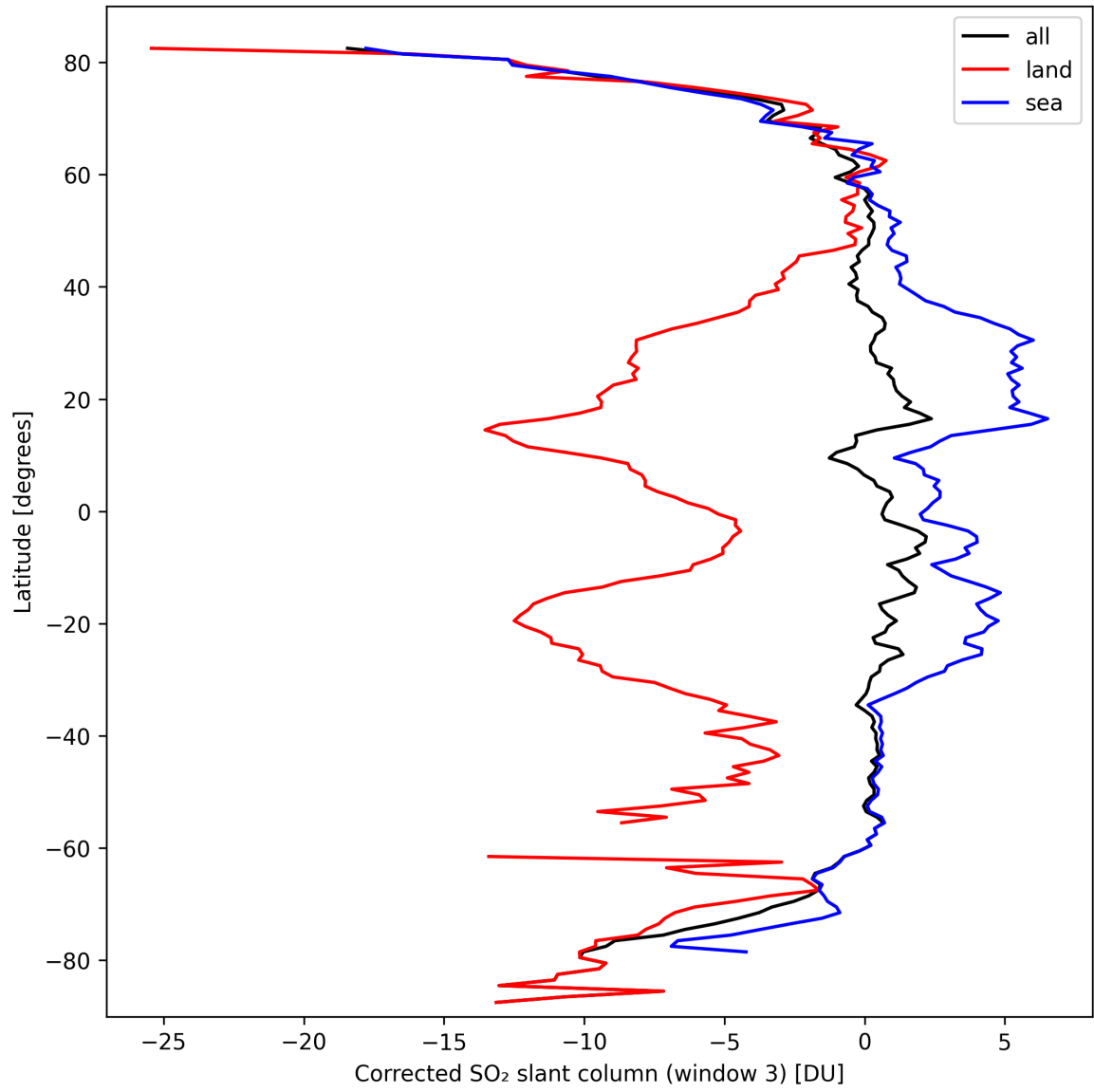
Figure 43: Zonal average of “Corrected SO 2 slant column (window 3)” for 2024-09-28 to 2024-09-30.
