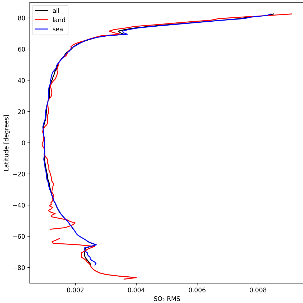
Figure 47: Zonal average of “SO 2 RMS” for 2024-09-28 to 2024-09-30.
