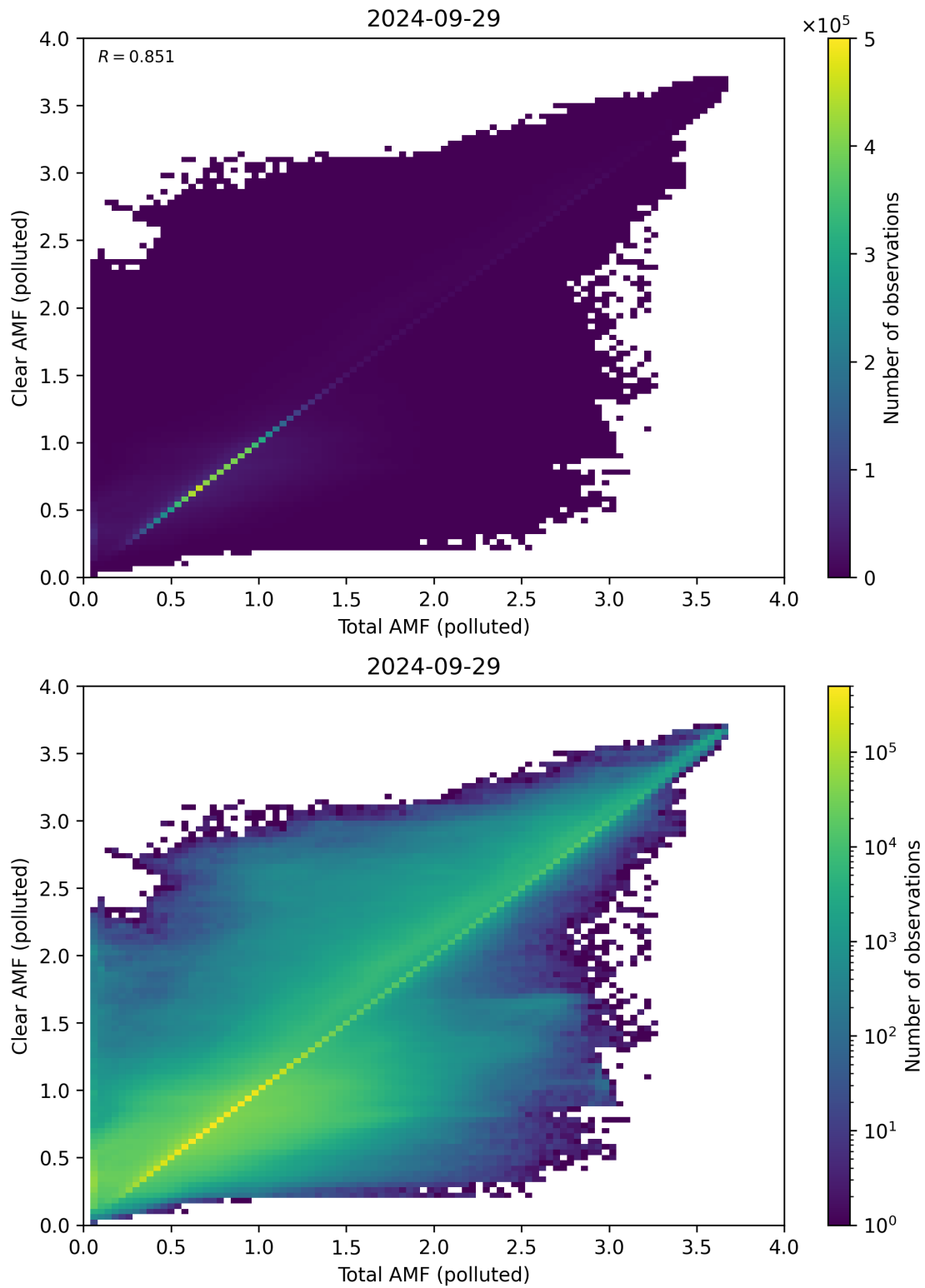
Figure 271: Scatter density plot of “Total AMF (polluted)” against “Clear AMF (polluted)” for 2024-09-28 to 2024-09-30.
