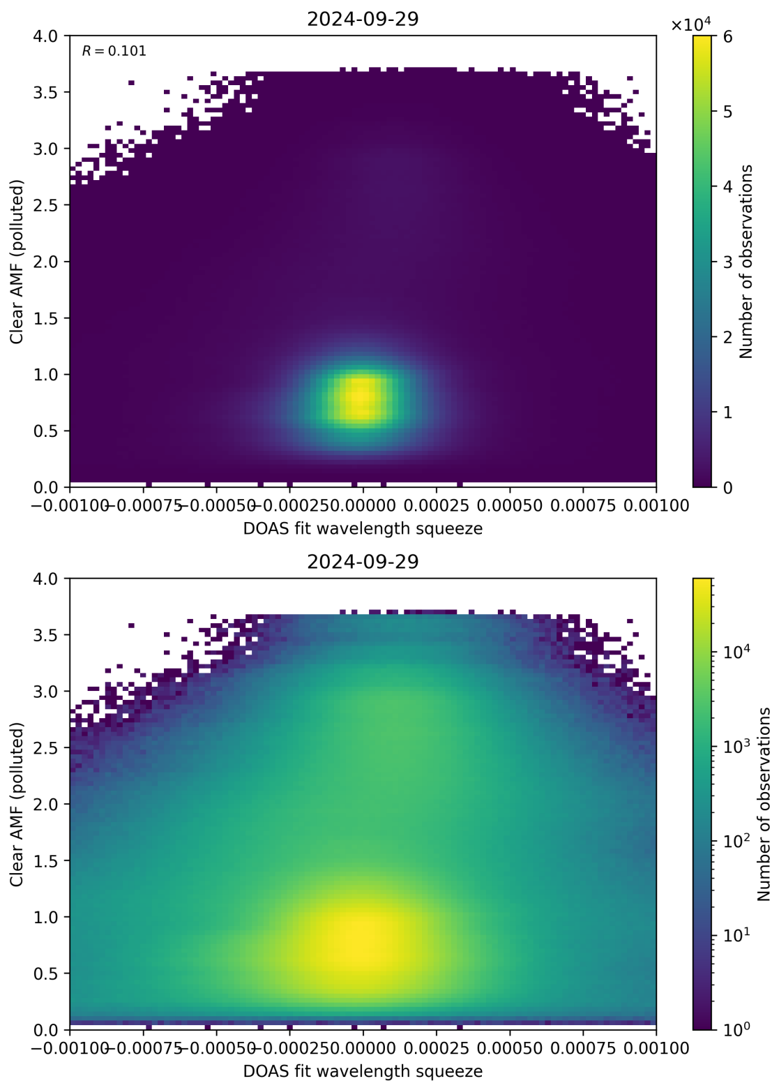
Figure 133: Scatter density plot of “DOAS fit wavelength squeeze” against “Clear AMF (polluted)” for 2024-09-28 to 2024-09-30.
