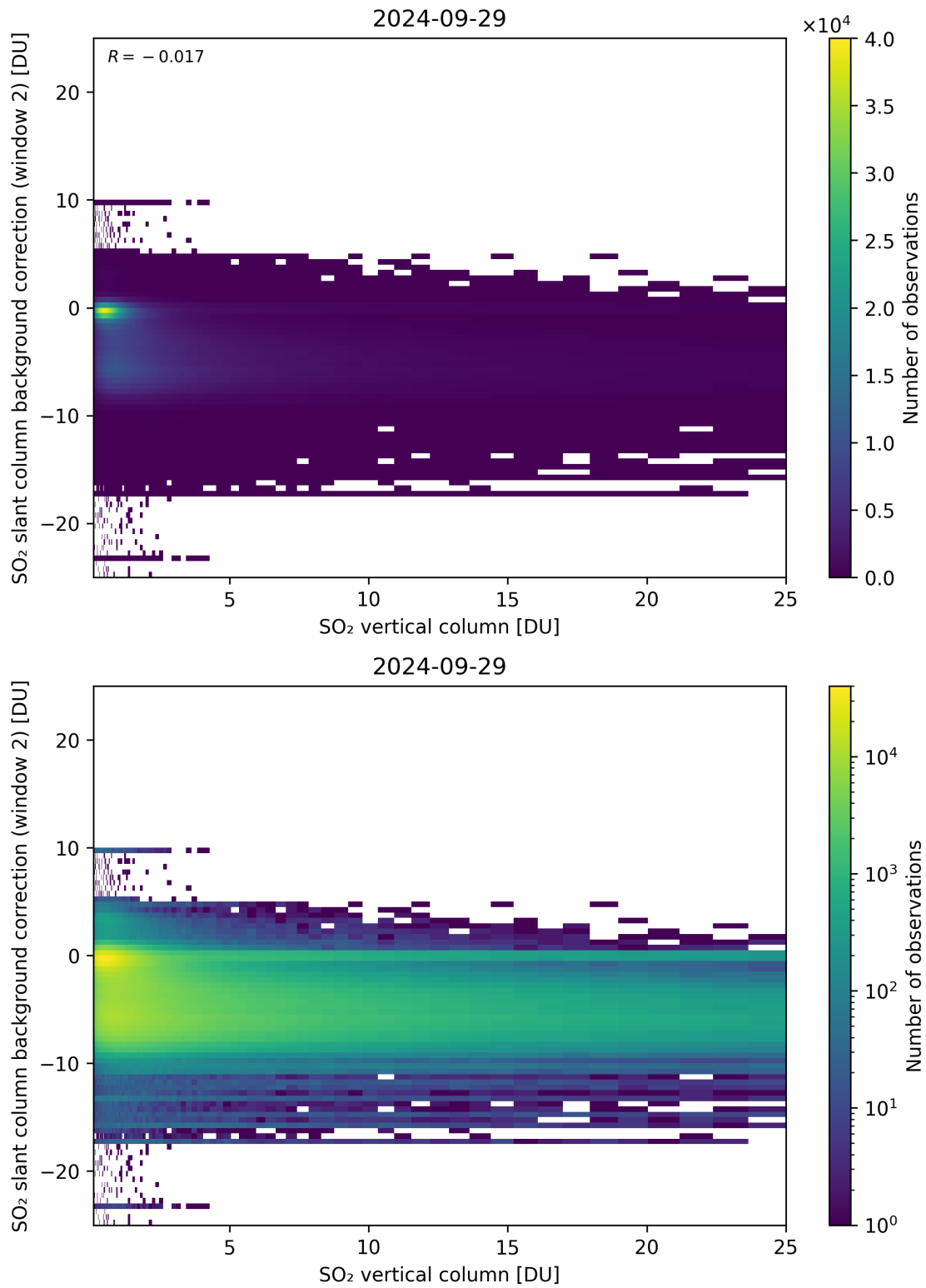
Figure 274: Scatter density plot of “SO 2 vertical column” against “SO 2 slant column background correction (window 2)” for 2024-09-28 to 2024-09-30.
