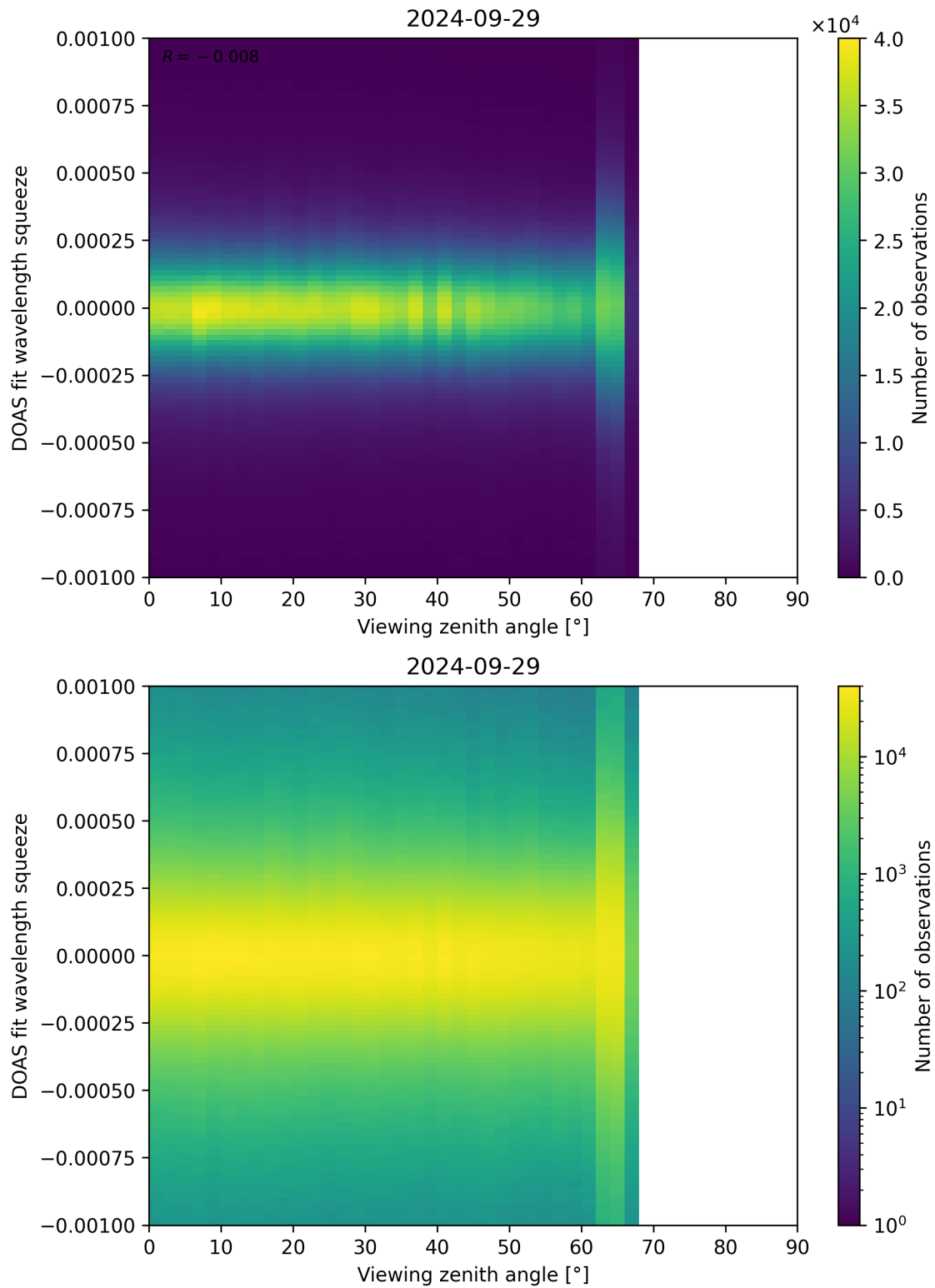
Figure 312: Scatter density plot of “Viewing zenith angle” against “DOAS fit wavelength squeeze” for 2024-09-28 to 2024-09-30.
