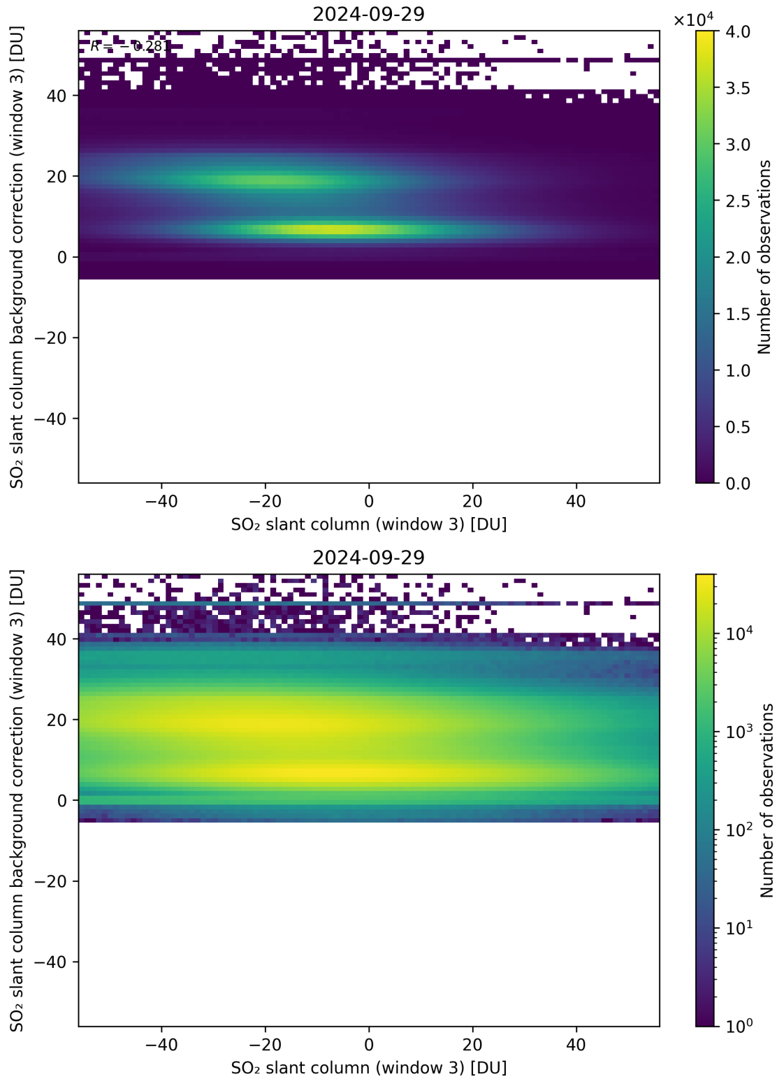
Figure 253: Scatter density plot of “SO 2 slant column (window 3)” against “SO 2 slant column background correction (window 3)” for 2024-09-28 to 2024-09-30.
