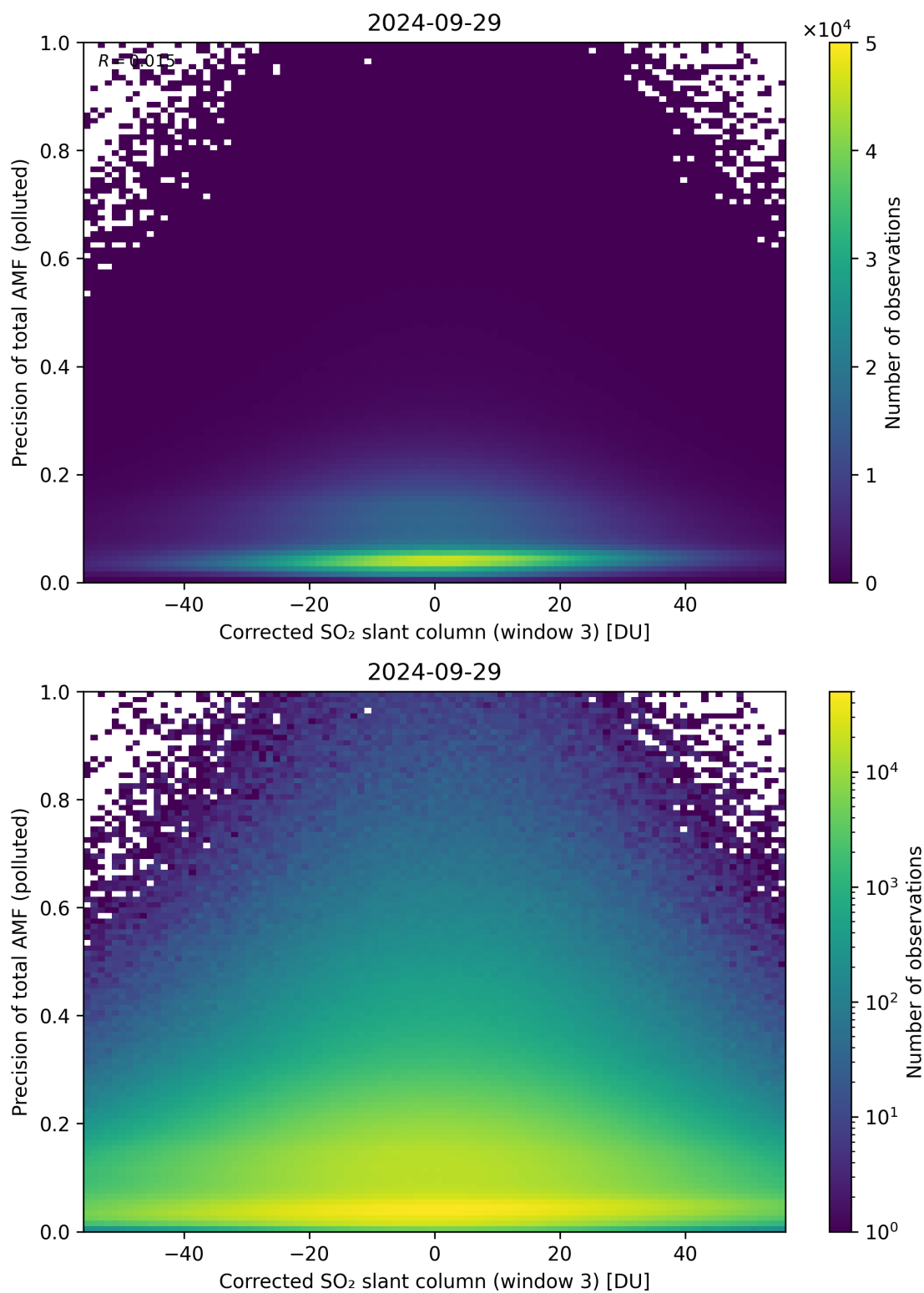
Figure 211: Scatter density plot of “Corrected SO 2 slant column (window 3)” against “Precision of total AMF (polluted)” for 2024-09-28 to 2024-09-30.
