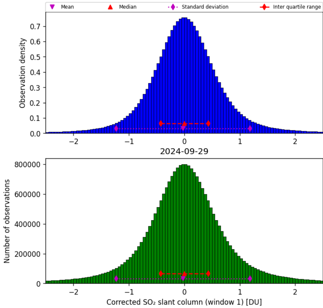
Figure 58: Histogram of “Corrected SO 2 slant column (window 1)” for 2024-09-28 to 2024-09-30
