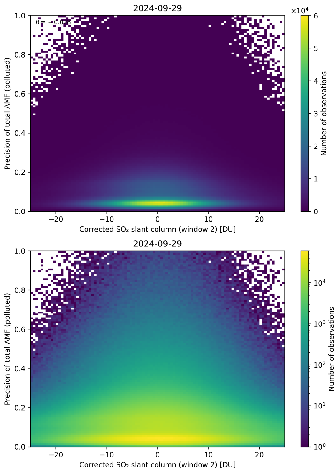
Figure 204: Scatter density plot of “Corrected SO 2 slant column (window 2)” against “Precision of total AMF (polluted)” for 2024-09-28 to 2024-09-30.
