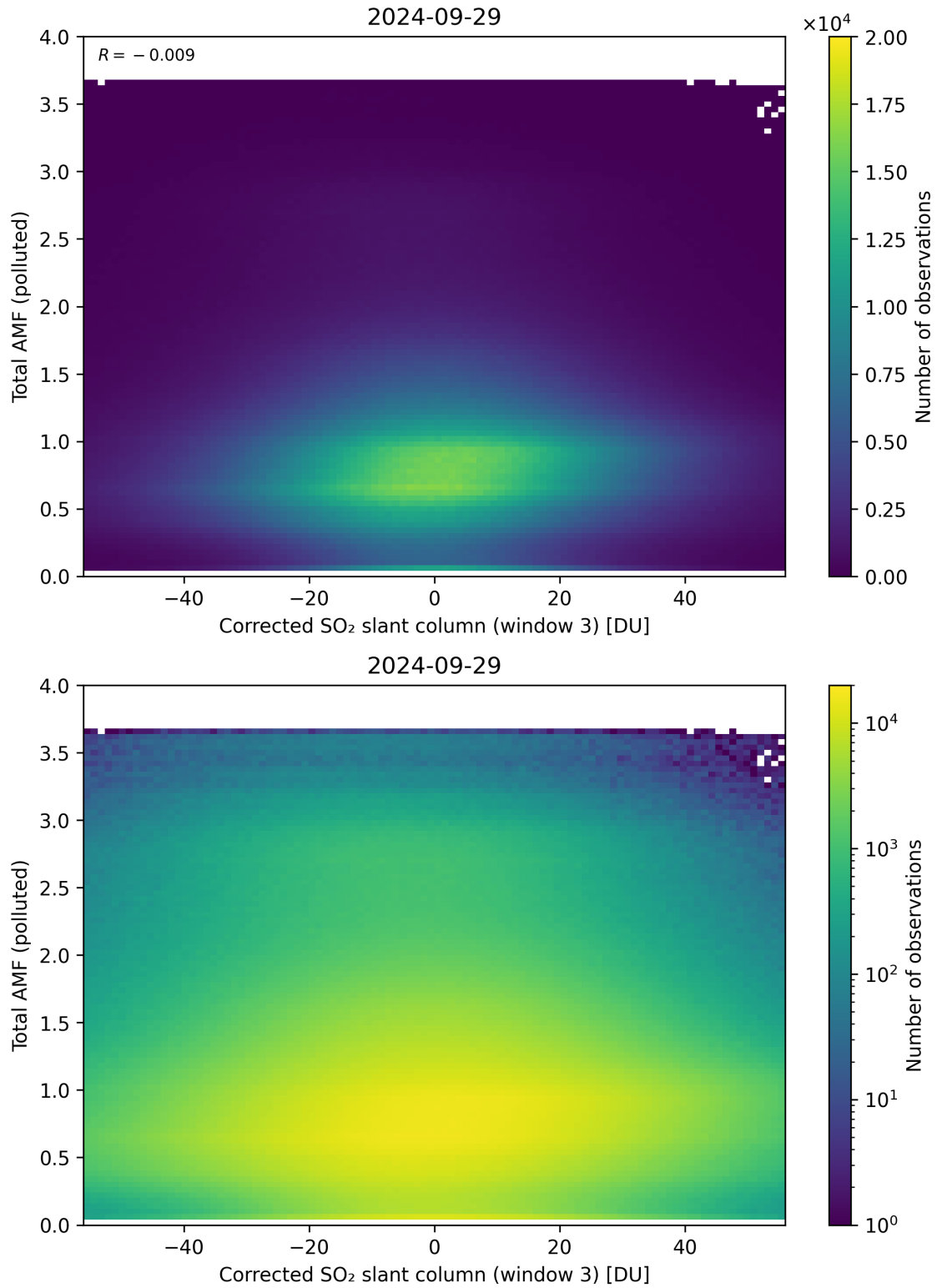
Figure 210: Scatter density plot of “Corrected SO 2 slant column (window 3)” against “Total AMF (polluted)” for 2024-09-28 to 2024-09-30.
