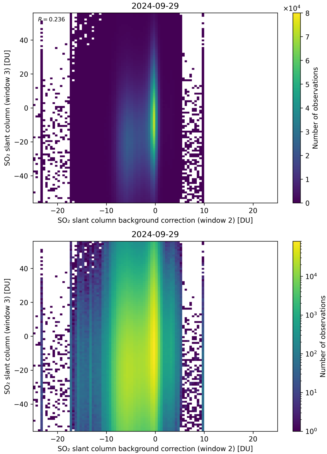
Figure 117: Scatter density plot of “SO 2 slant column background correction (window 2)” against “SO 2 slant column (window 3)” for 2024-09-28 to 2024-09-30.
