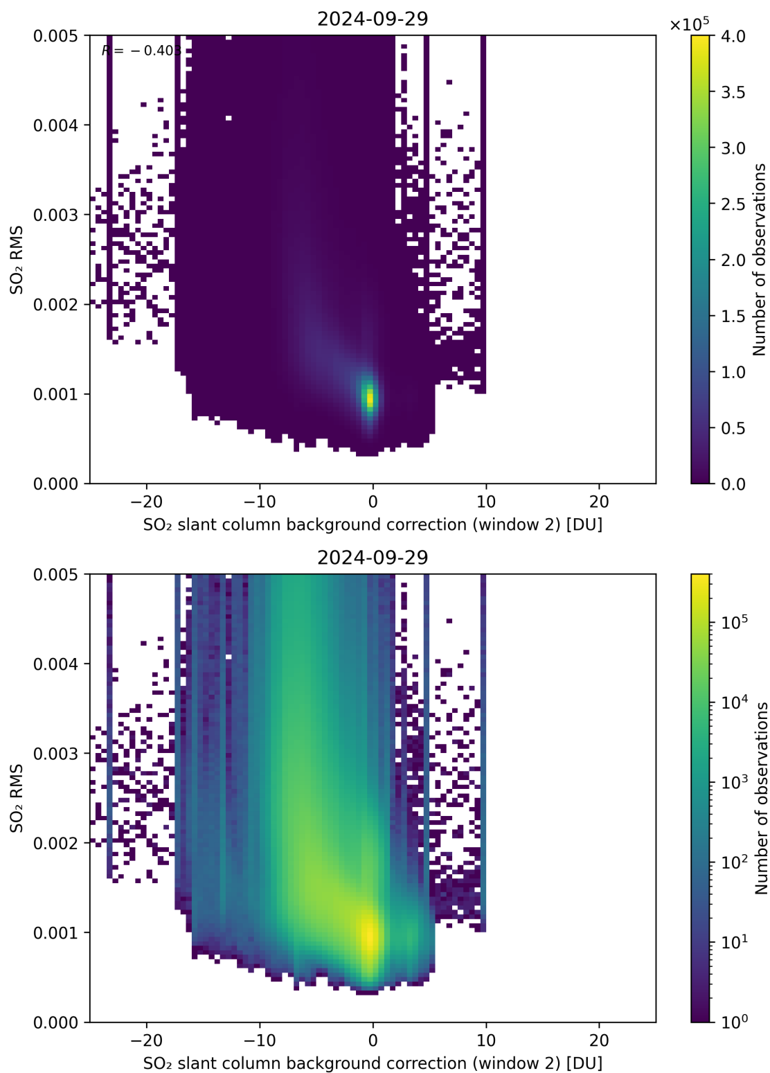
Figure 114: Scatter density plot of “SO 2 slant column background correction (window 2)” against “SO 2 RMS” for 2024-09-28 to 2024-09-30.
