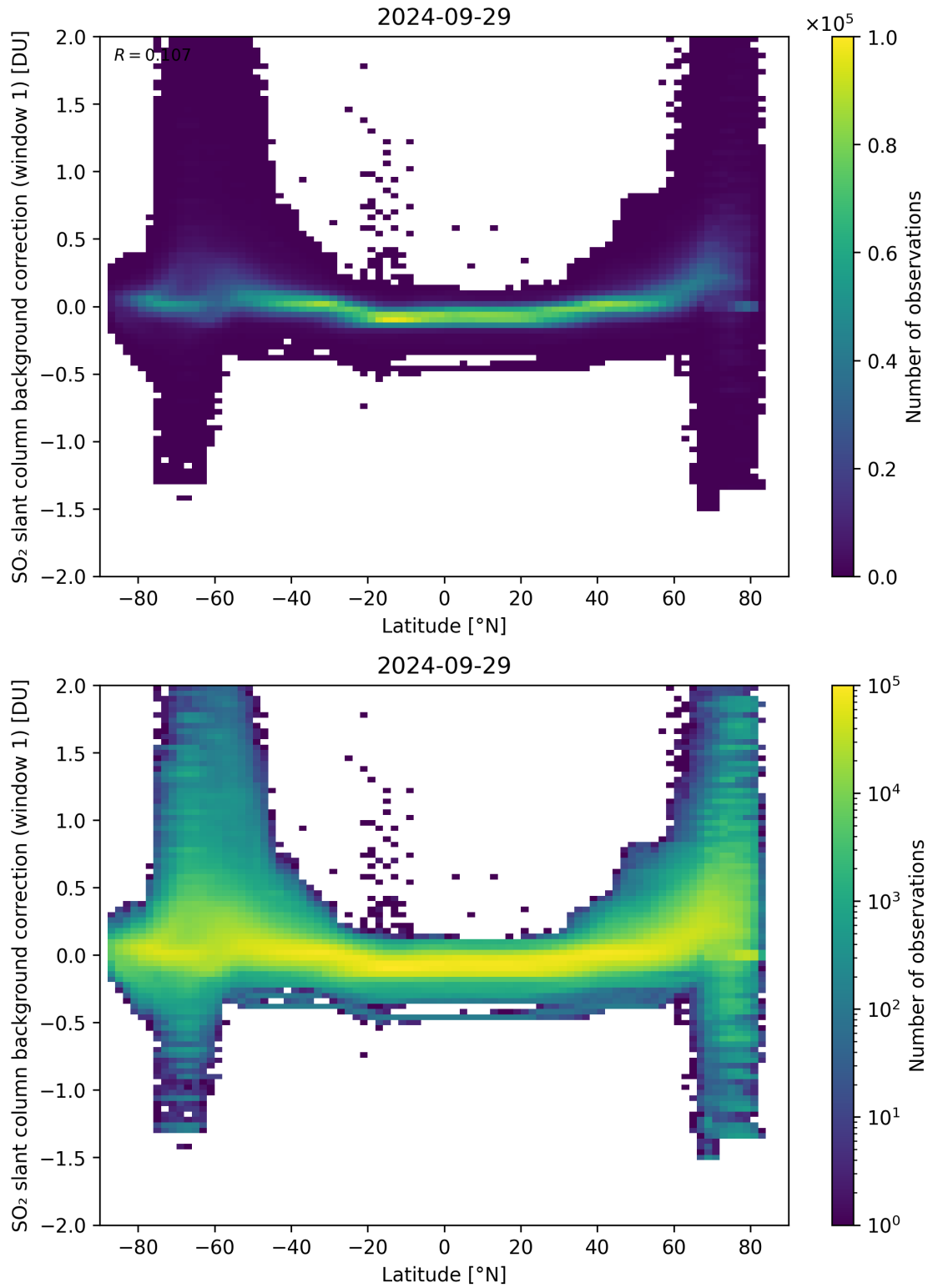
Figure 139: Scatter density plot of “Latitude” against “SO 2 slant column background correction (window 1)” for 2024-09-28 to 2024-09-30.
