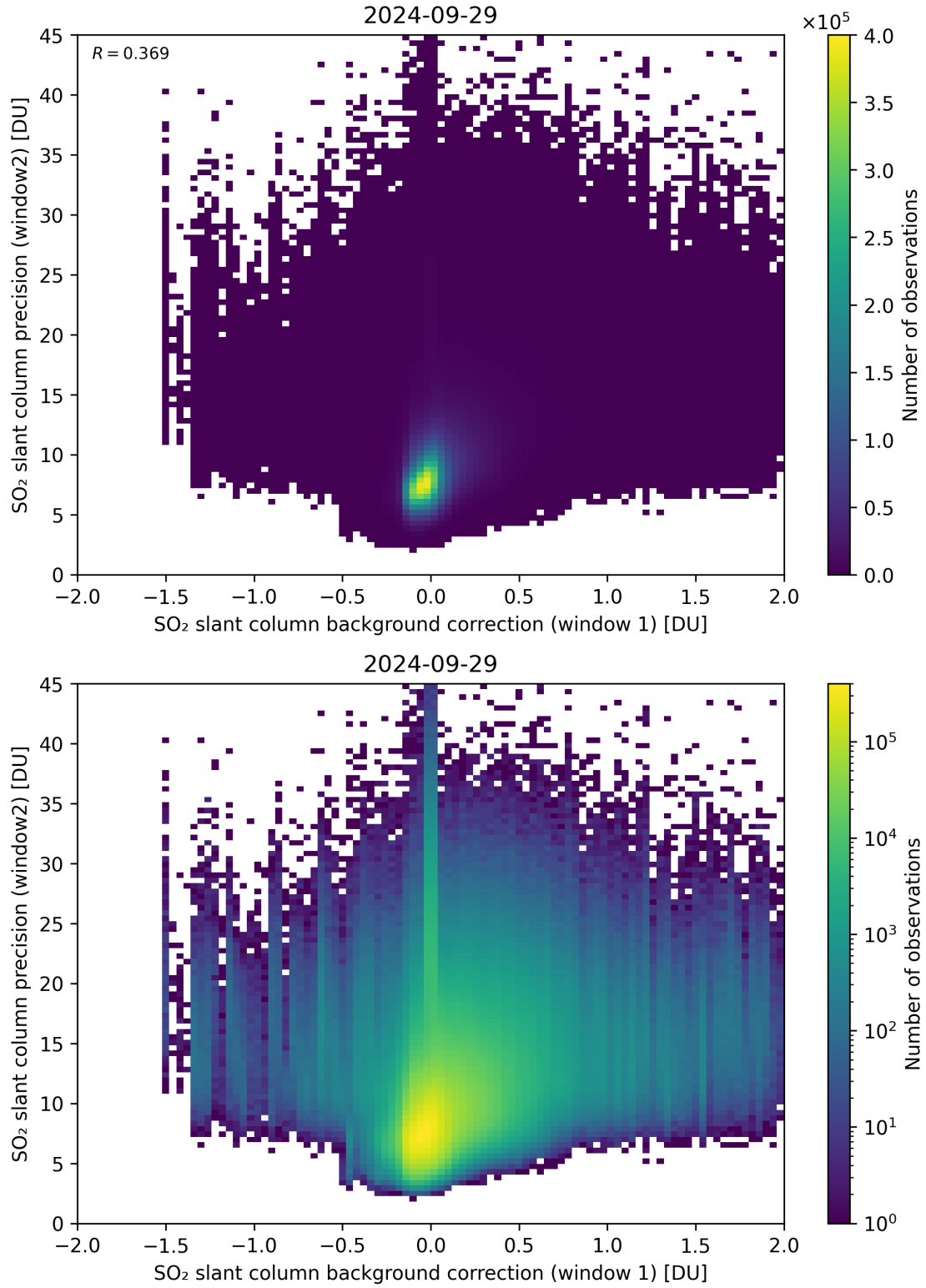
Figure 106: Scatter density plot of “SO 2 slant column background correction (window 1)” against “SO 2 slant column precision (window2)” for 2024-09-28 to 2024-09-30.
