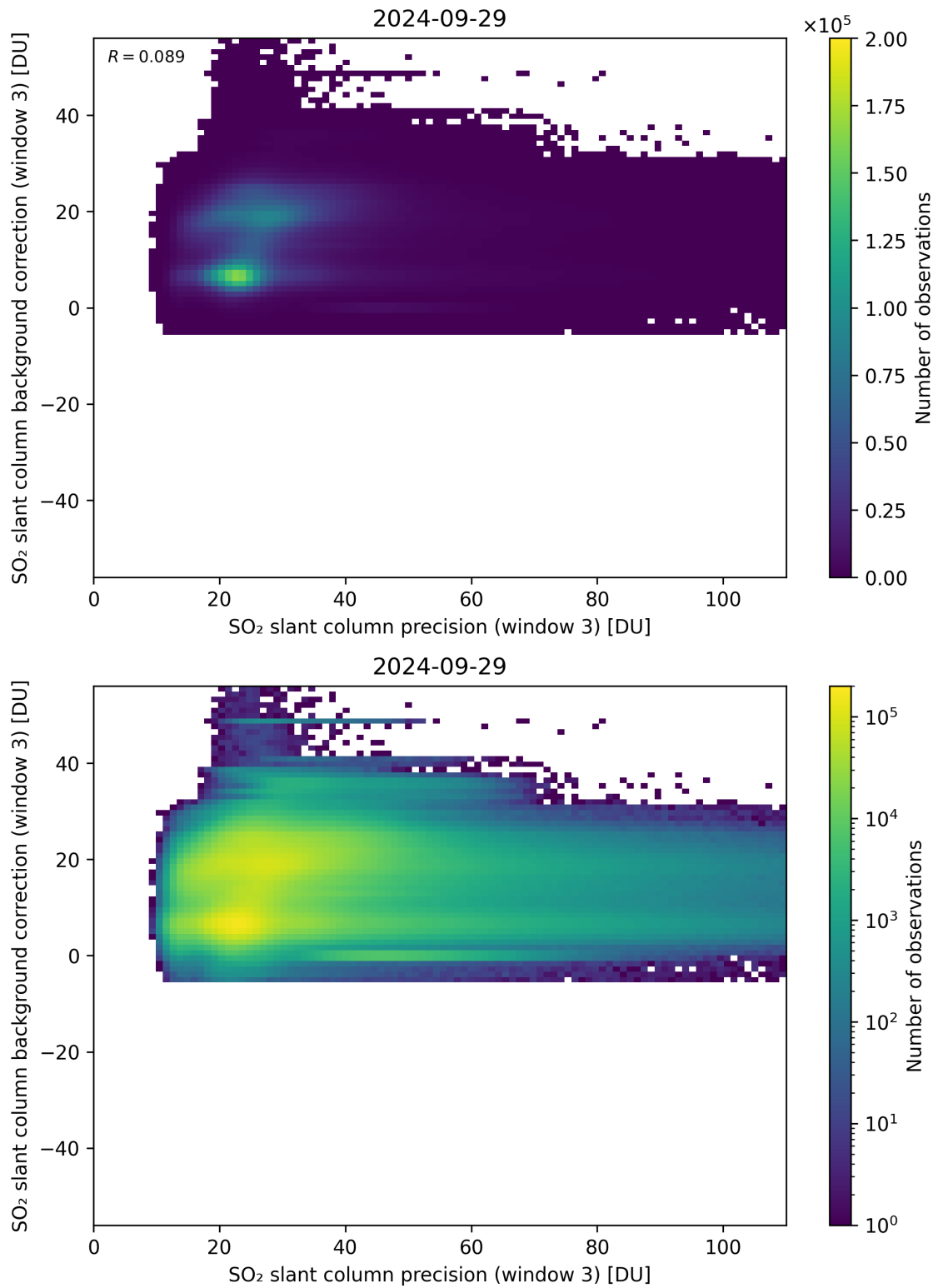
Figure 257: Scatter density plot of “SO 2 slant column precision (window 3)” against “SO 2 slant column background correction (window 3)” for 2024-09-28 to 2024-09-30.
