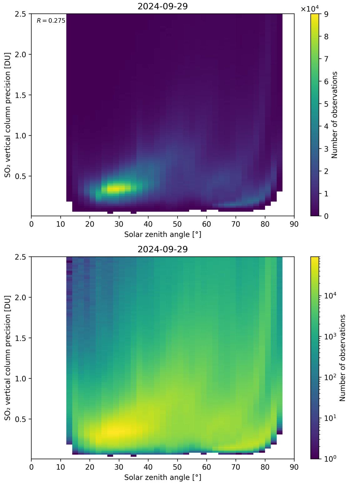
Figure 177: Scatter density plot of “Solar zenith angle” against “SO 2 vertical column precision” for 2024-09-28 to 2024-09-30.
