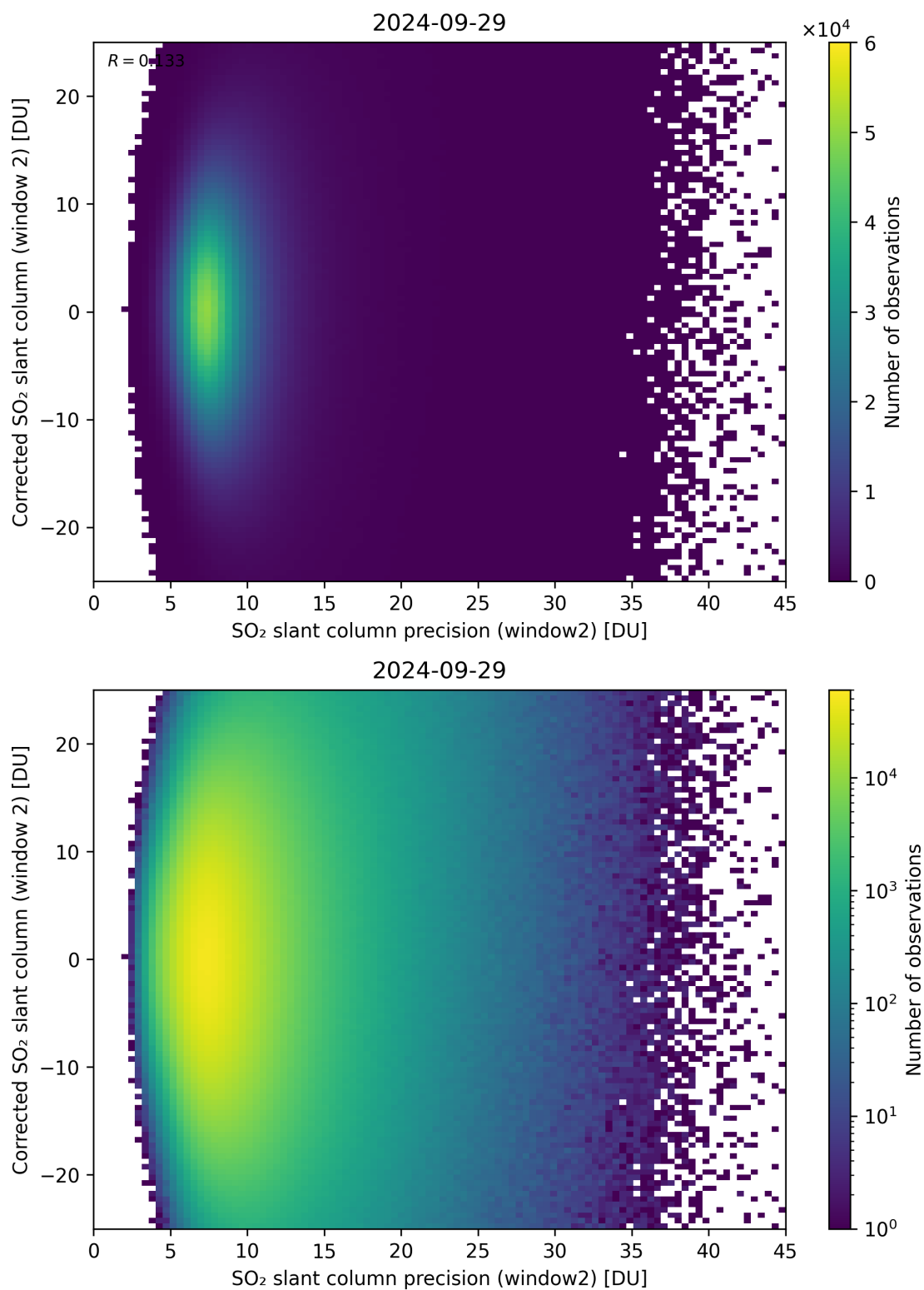
Figure 247: Scatter density plot of “SO 2 slant column precision (window2)” against “Corrected SO 2 slant column (window 2)” for 2024-09-28 to 2024-09-30.
