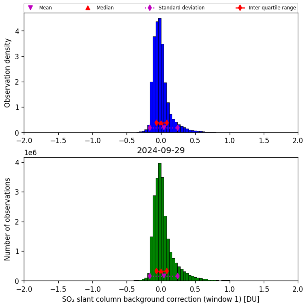
Figure 59: Histogram of “SO 2 slant column background correction (window 1)” for 2024-09-28 to 2024-09-30
