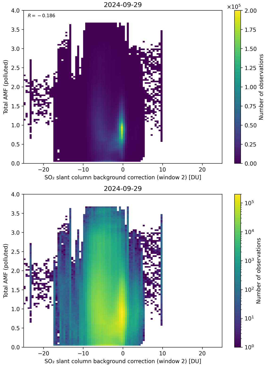
Figure 119: Scatter density plot of “SO 2 slant column background correction (window 2)” against “Total AMF (polluted)” for 2024-09-28 to 2024-09-30.
