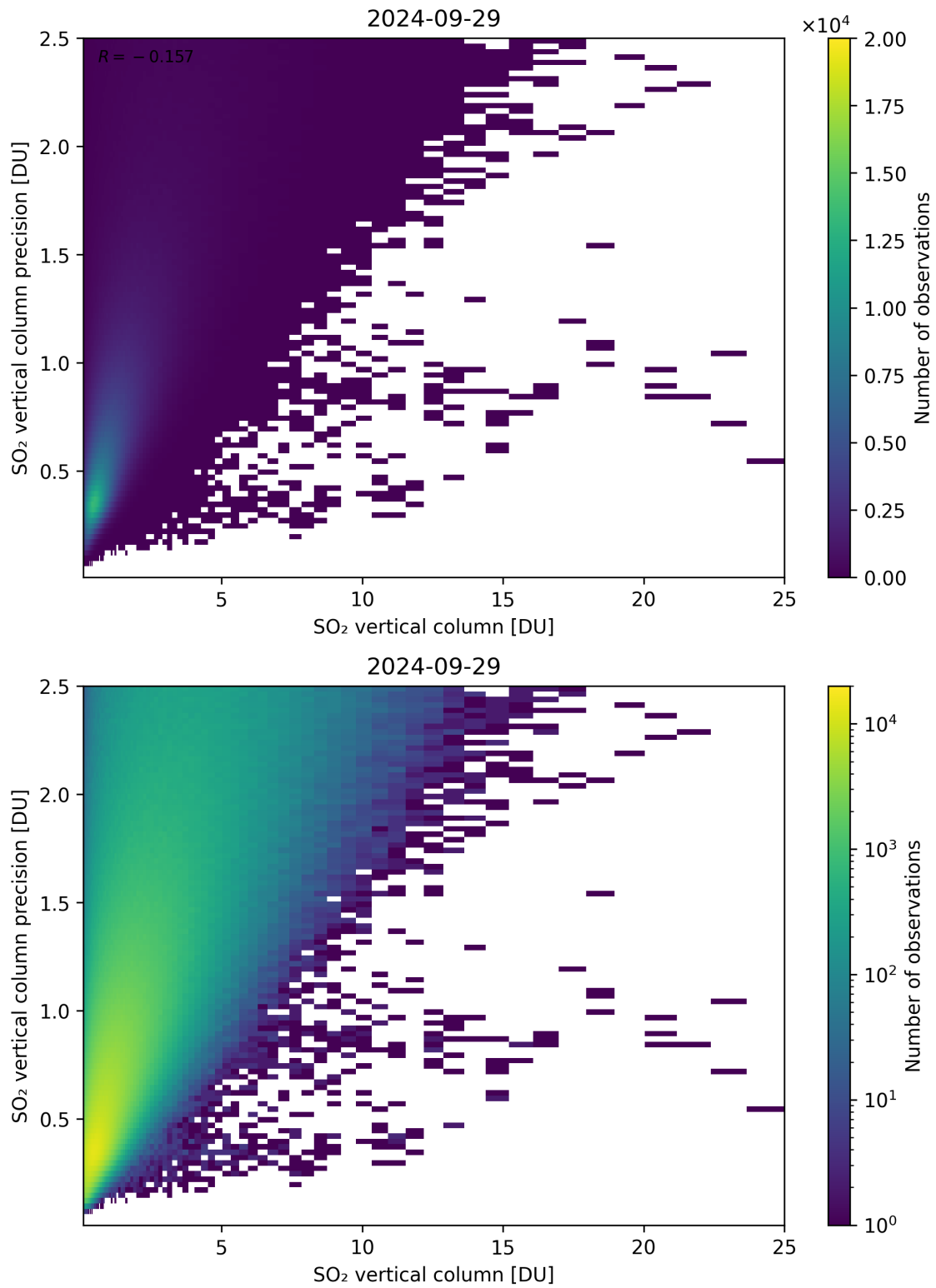
Figure 307: Scatter density plot of “SO 2 vertical column” against “SO 2 vertical column precision” for 2024-09-28 to 2024-09-30.
