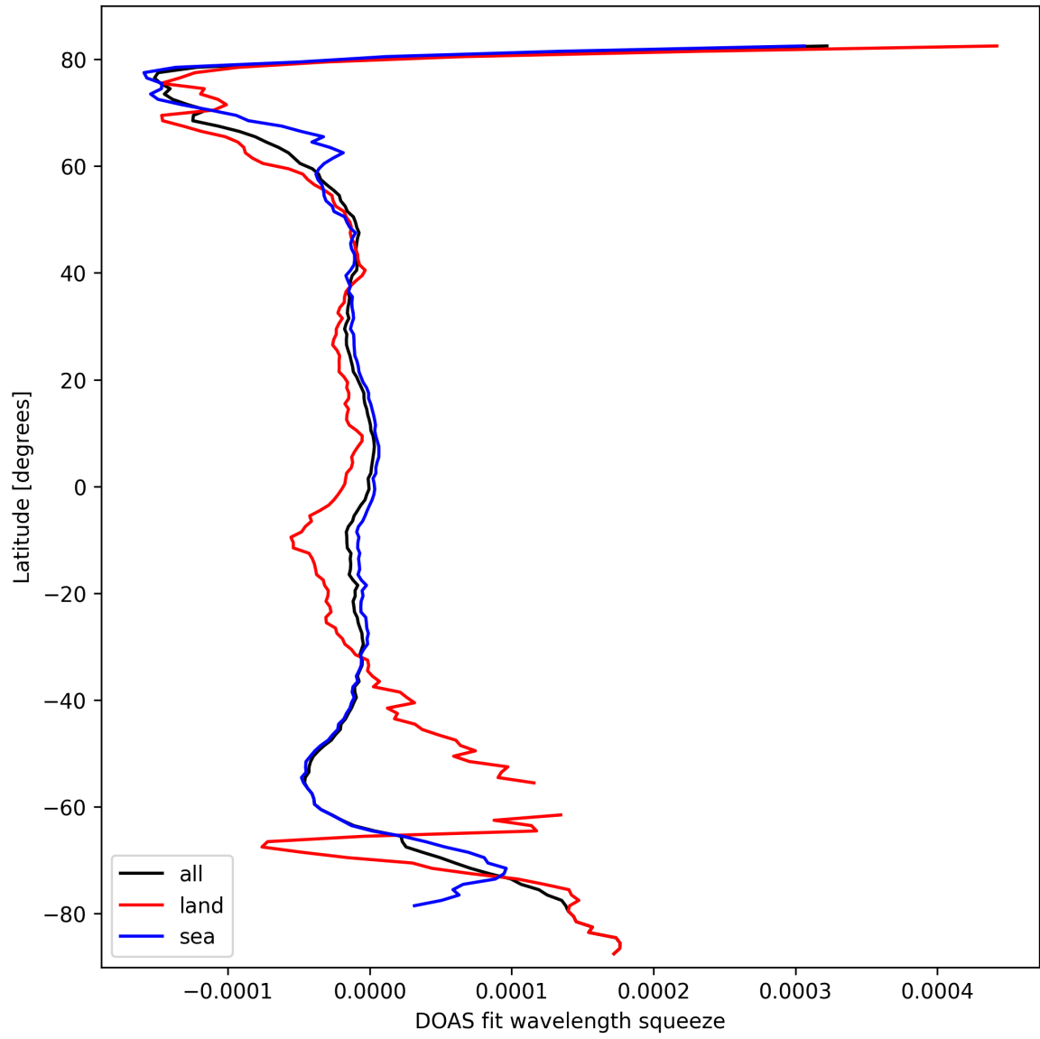
Figure 46: Zonal average of “DOAS fit wavelength squeeze” for 2024-09-28 to 2024-09-30.
