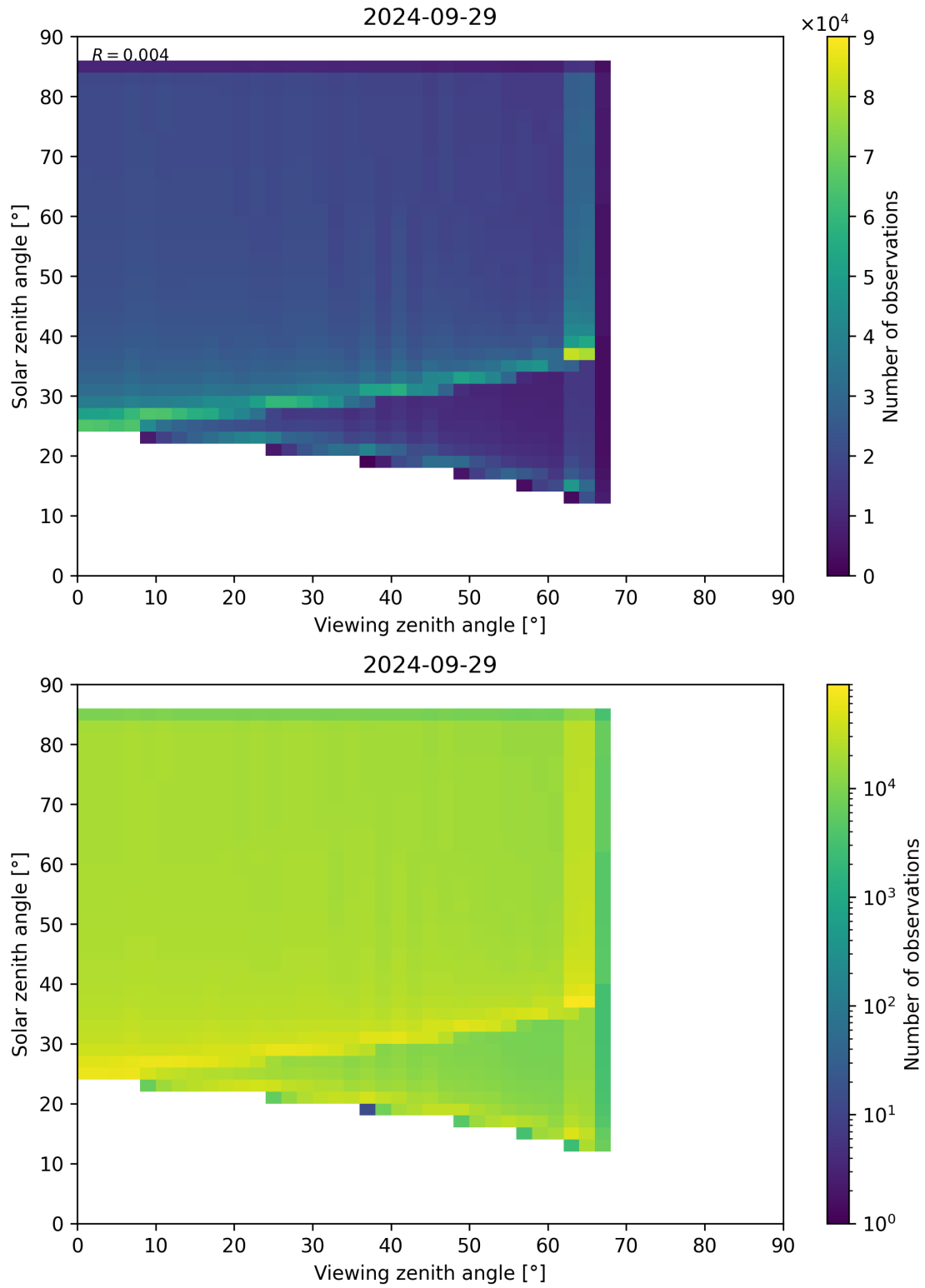
Figure 315: Scatter density plot of “Viewing zenith angle” against “Solar zenith angle” for 2024-09-28 to 2024-09-30.
