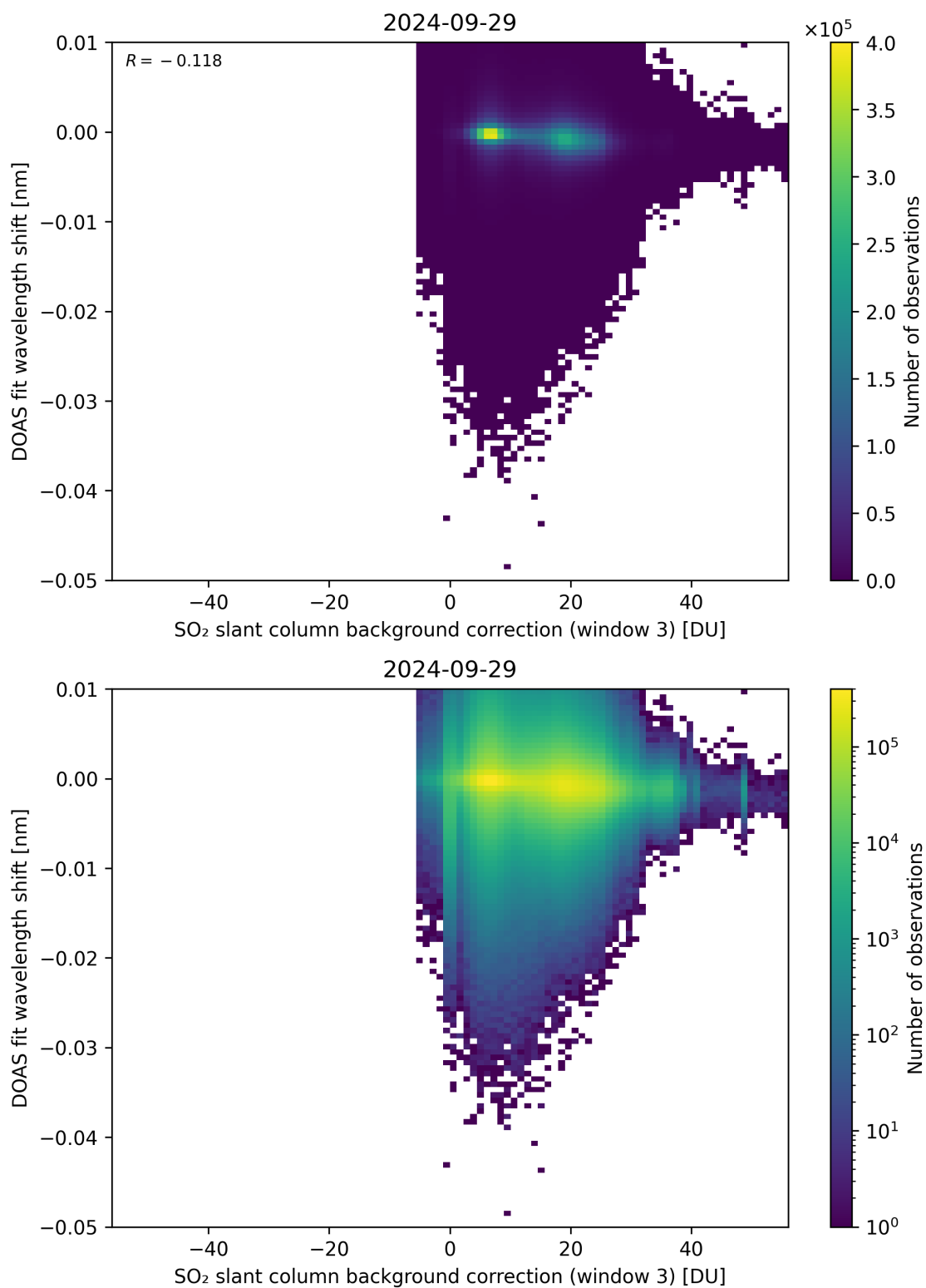
Figure 121: Scatter density plot of “SO 2 slant column background correction (window 3)” against “DOAS fit wavelength shift” for 2024-09-28 to 2024-09-30.
