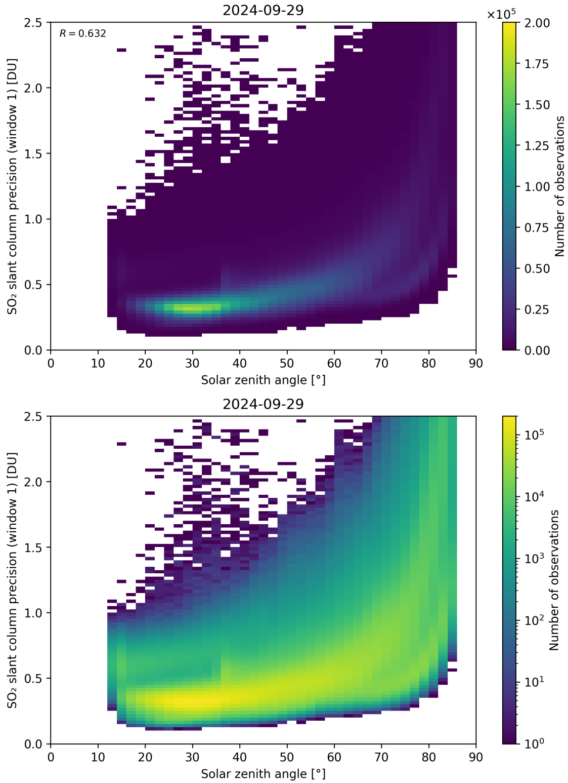
Figure 170: Scatter density plot of “Solar zenith angle” against “SO 2 slant column precision (window 1)” for 2024-09-28 to 2024-09-30.
