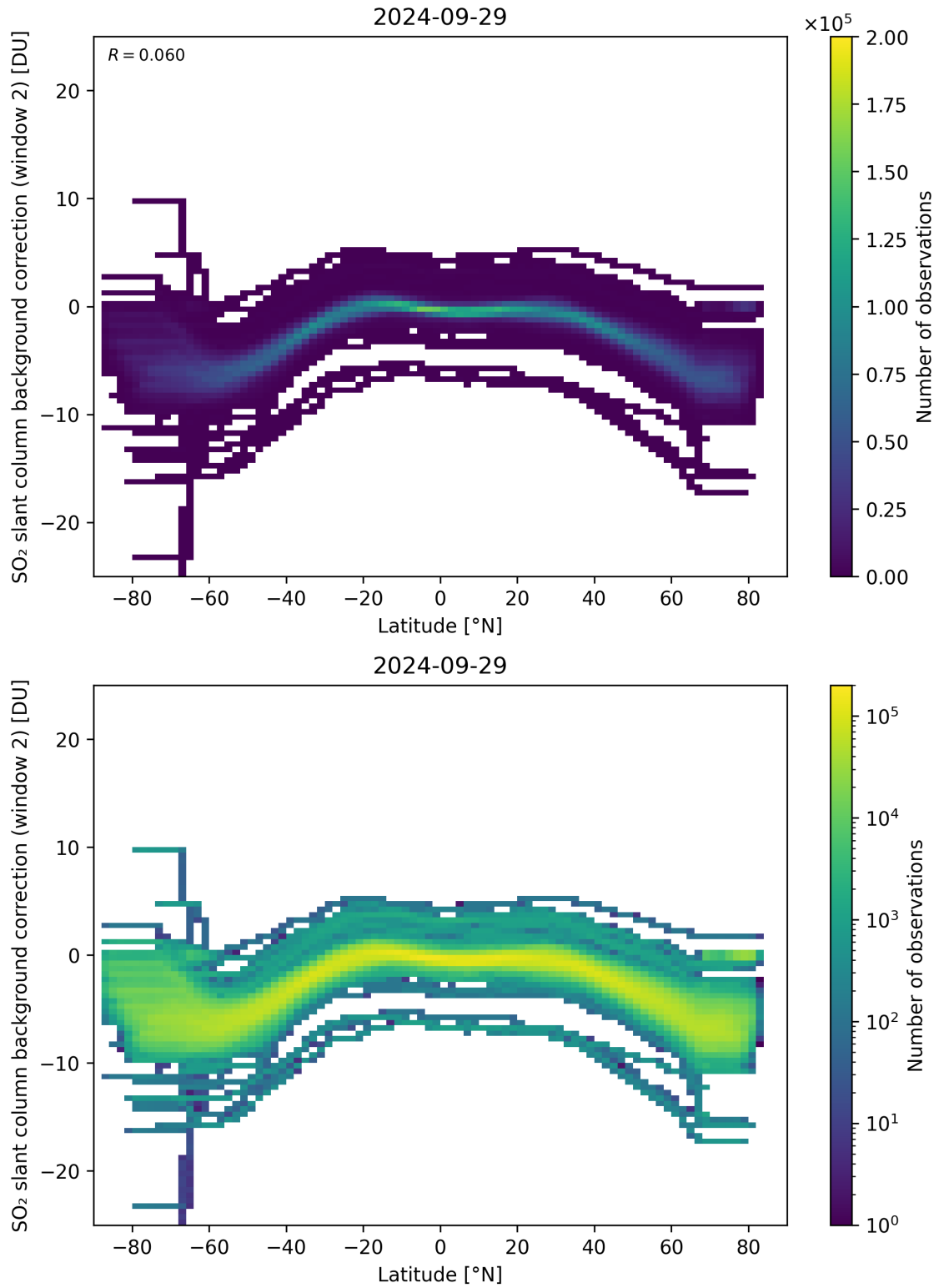
Figure 140: Scatter density plot of “Latitude” against “SO 2 slant column background correction (window 2)” for 2024-09-28 to 2024-09-30.
