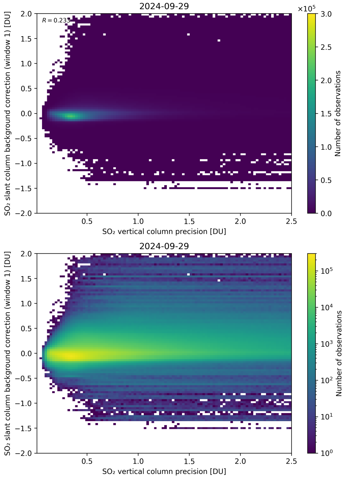
Figure 279: Scatter density plot of “SO 2 vertical column precision” against “SO 2 slant column background correction (window 1)” for 2024-09-28 to 2024-09-30.
