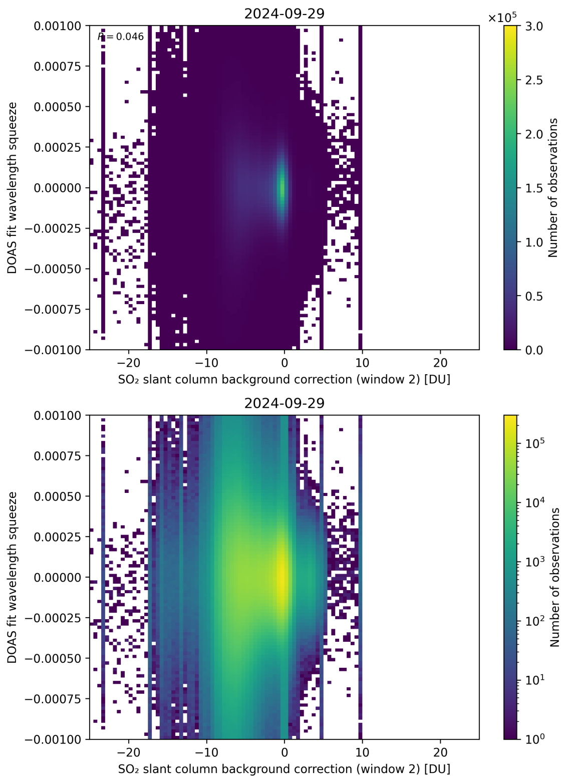
Figure 113: Scatter density plot of “SO 2 slant column background correction (window 2)” against “DOAS fit wavelength squeeze” for 2024-09-28 to 2024-09-30.
