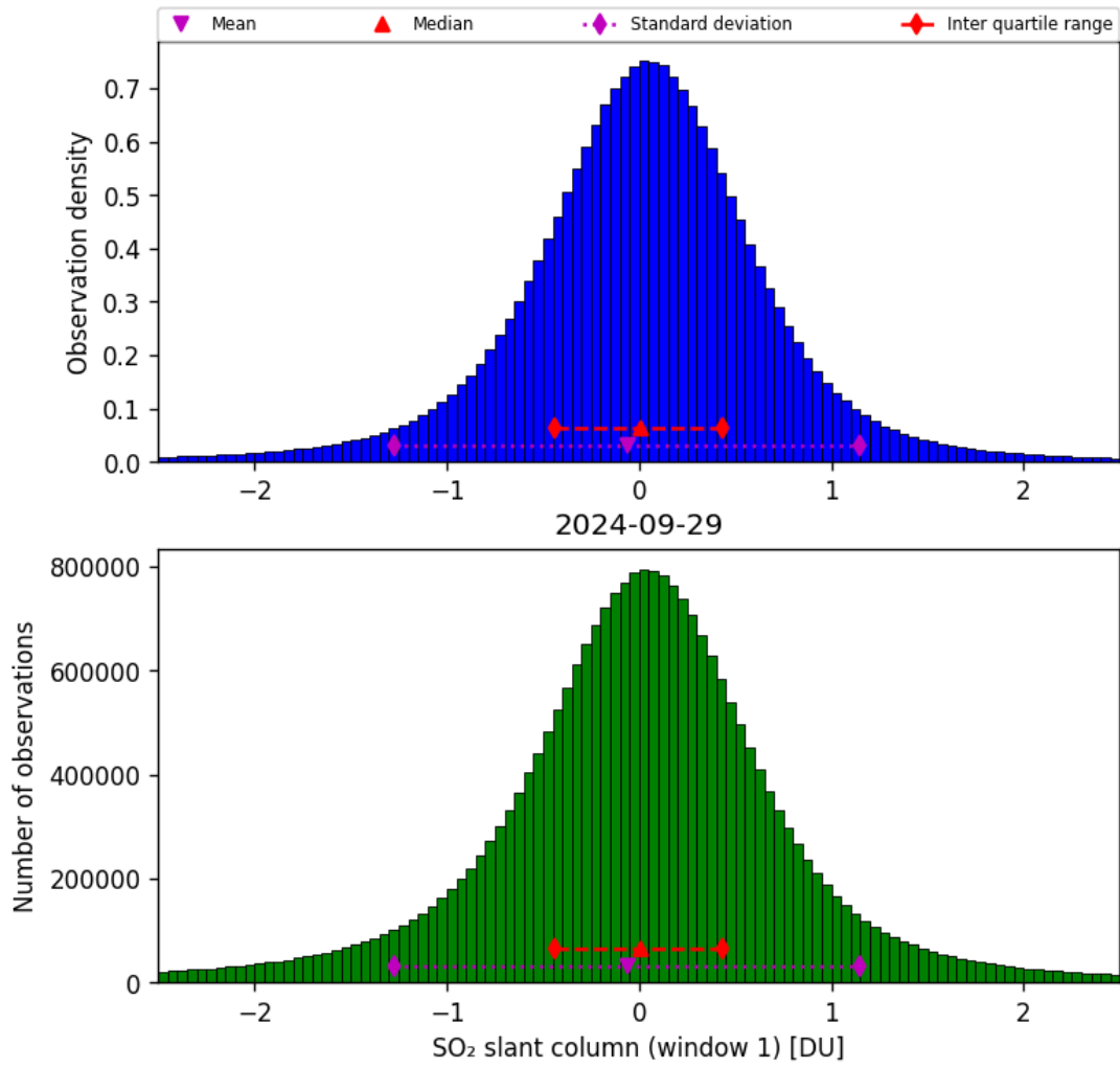
Figure 56: Histogram of “SO 2 slant column (window 1)” for 2024-09-28 to 2024-09-30
