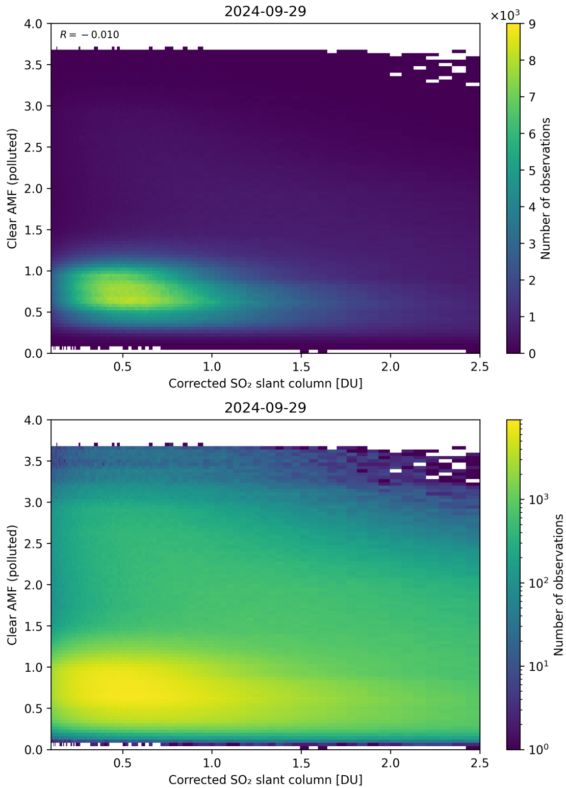
Figure 184: Scatter density plot of “Corrected SO 2 slant column” against “Clear AMF (polluted)” for 2024-09-28 to 2024-09-30.
