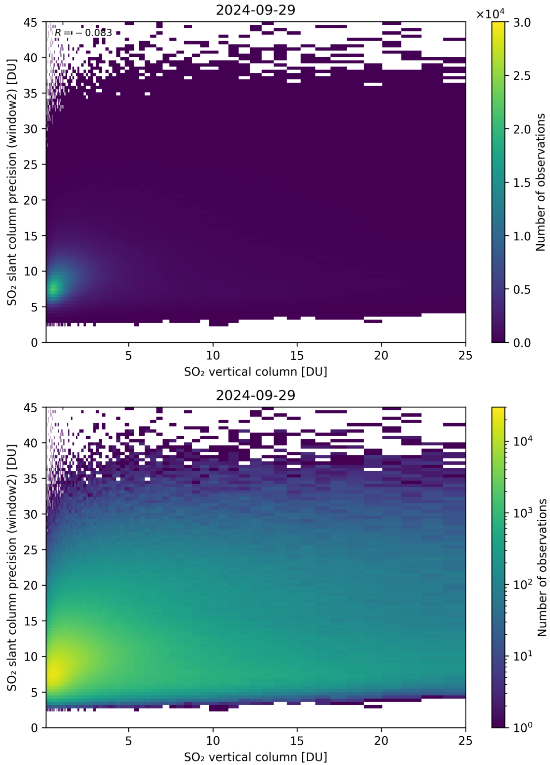
Figure 302: Scatter density plot of “SO 2 vertical column” against “SO 2 slant column precision (window2)” for 2024-09-28 to 2024-09-30.
