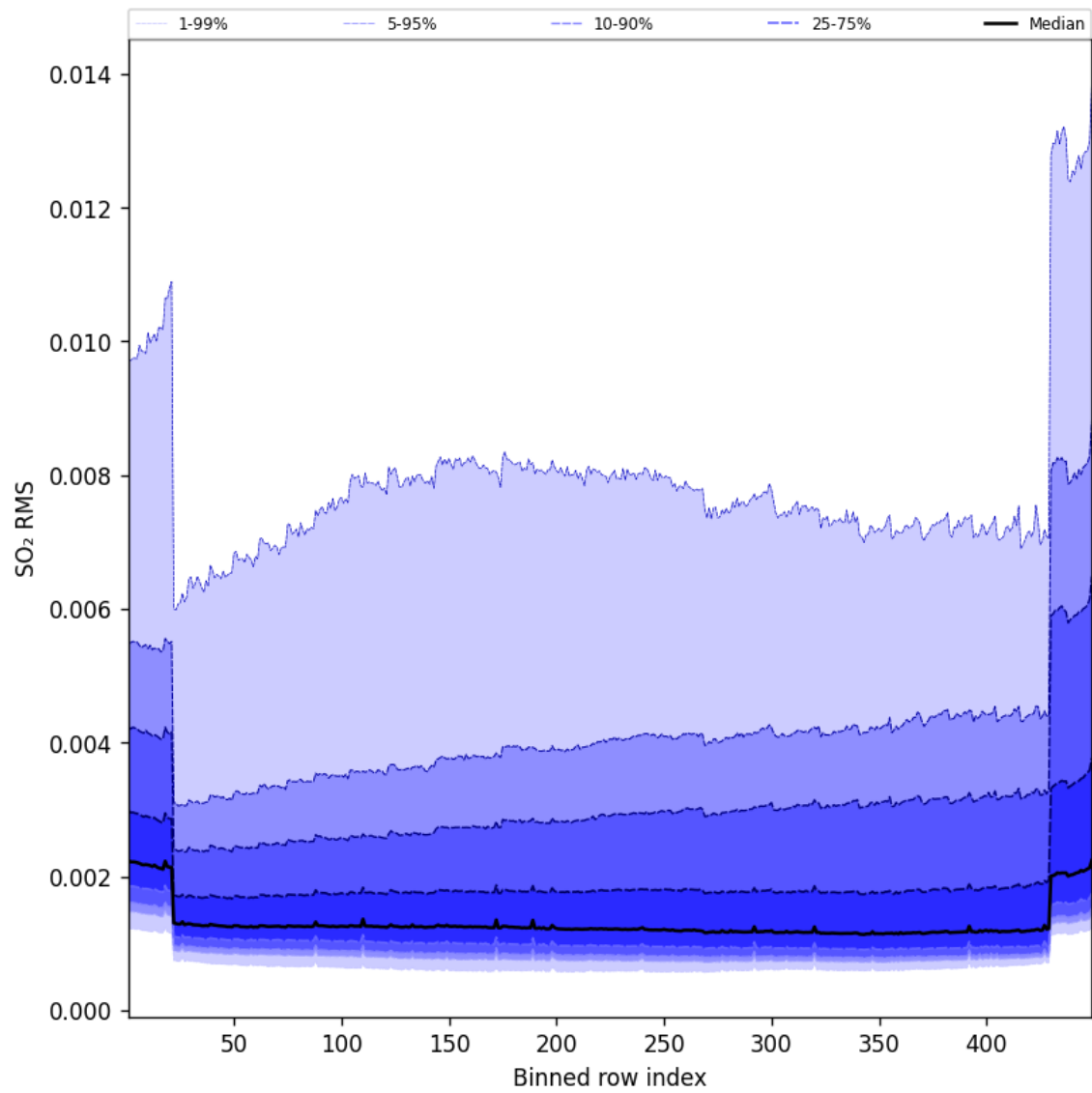
Figure 93: Along track statistics of “SO 2 RMS” for 2024-09-28 to 2024-09-30
