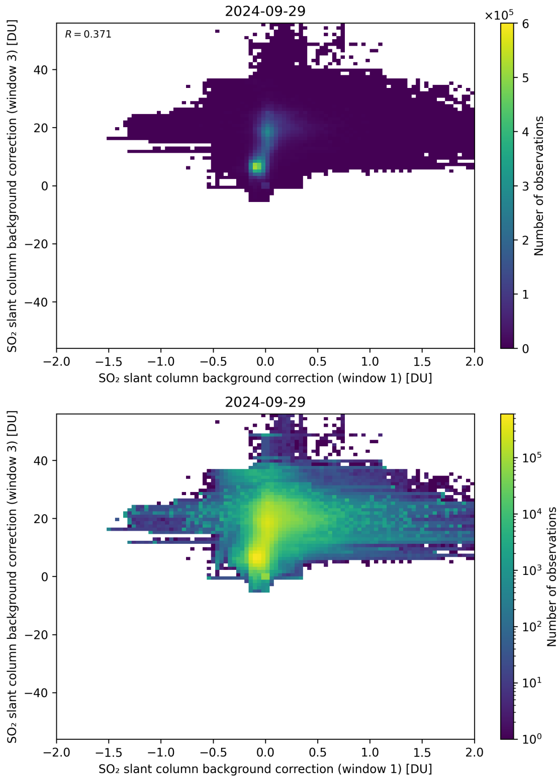
Figure 99: Scatter density plot of “SO 2 slant column background correction (window 1)” against “SO 2 slant column background correction (window 3)” for 2024-09-28 to 2024-09-30.
