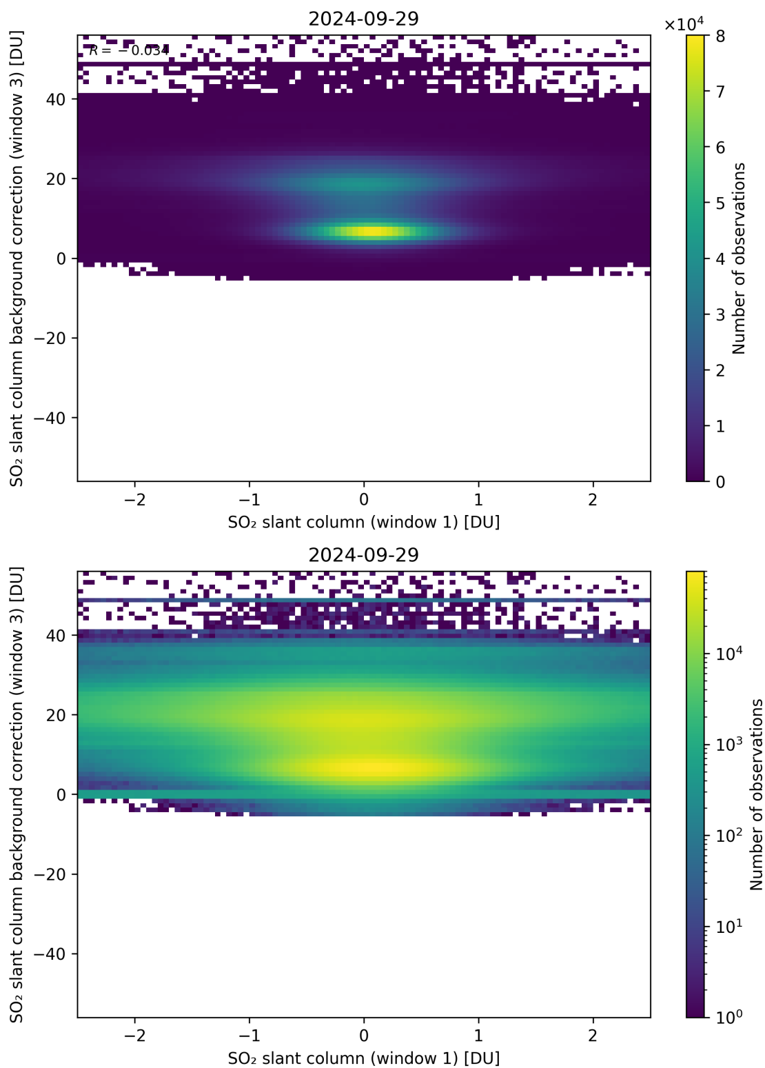
Figure 214: Scatter density plot of “SO 2 slant column (window 1)” against “SO 2 slant column background correction (window 3)” for 2024-09-28 to 2024-09-30.
