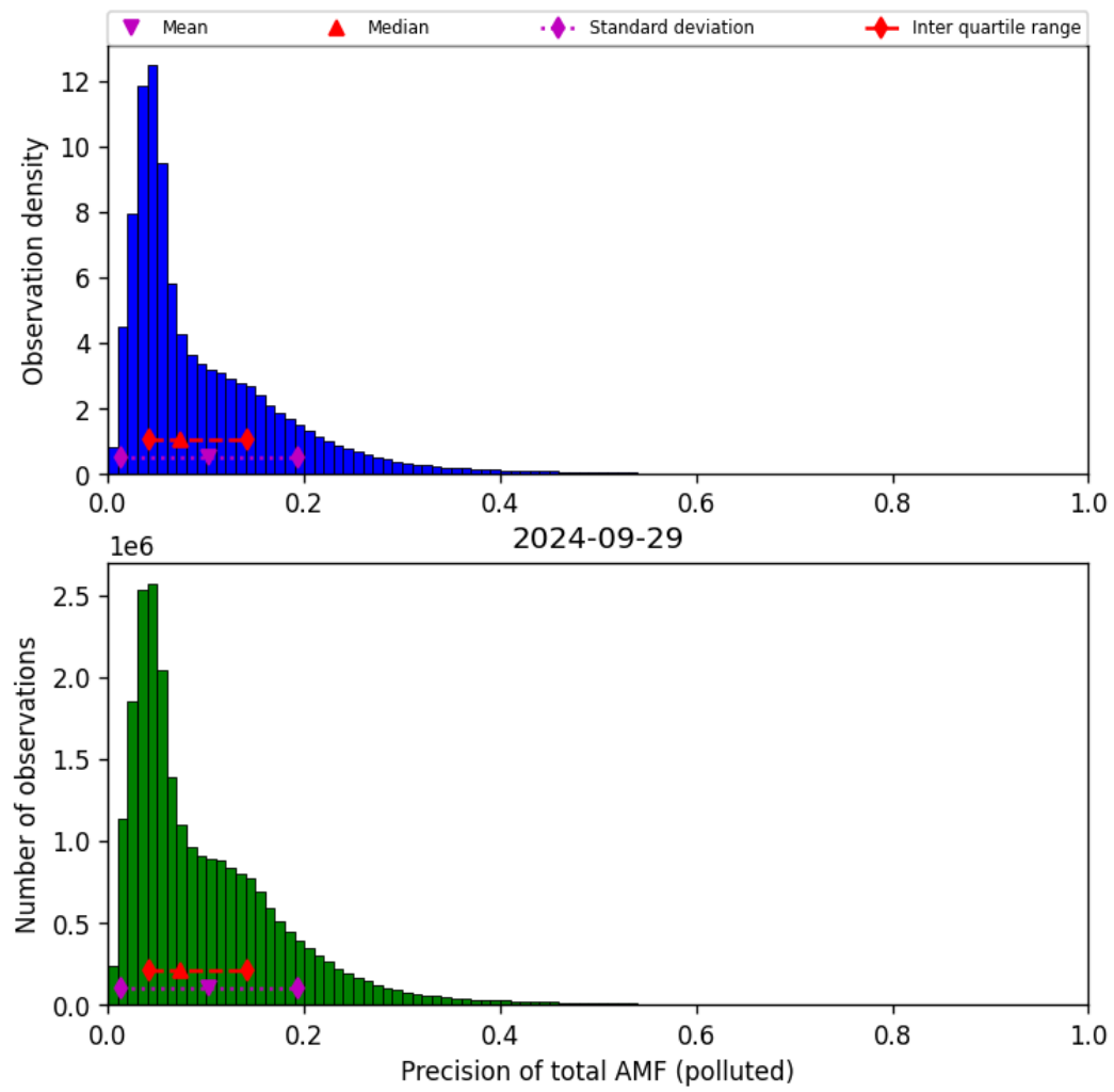
Figure 72: Histogram of “Precision of total AMF (polluted)” for 2024-09-28 to 2024-09-30
