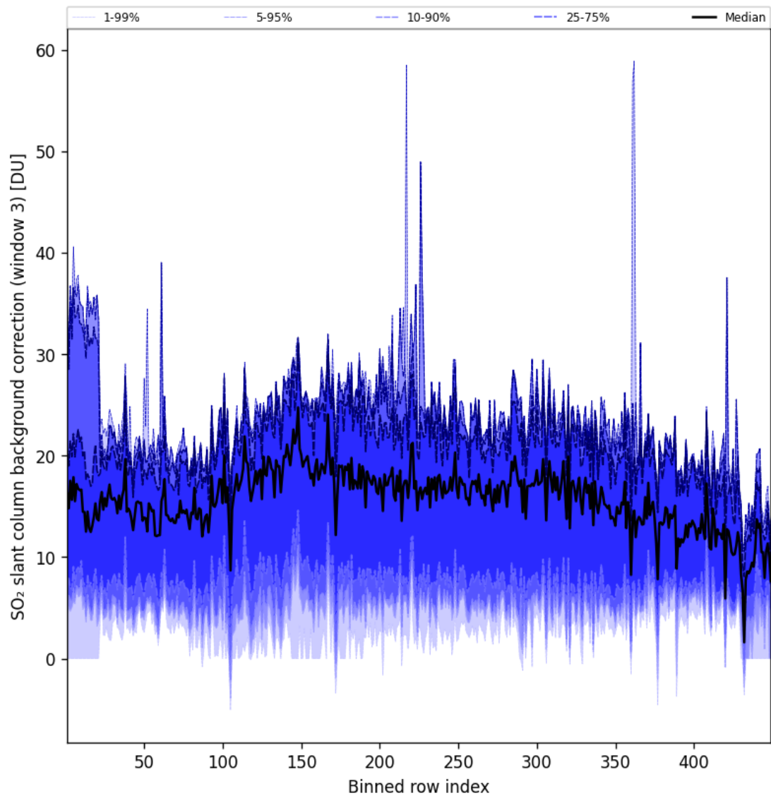
Figure 90: Along track statistics of “SO 2 slant column background correction (window 3)” for 2024-09-28 to 2024-09-30
