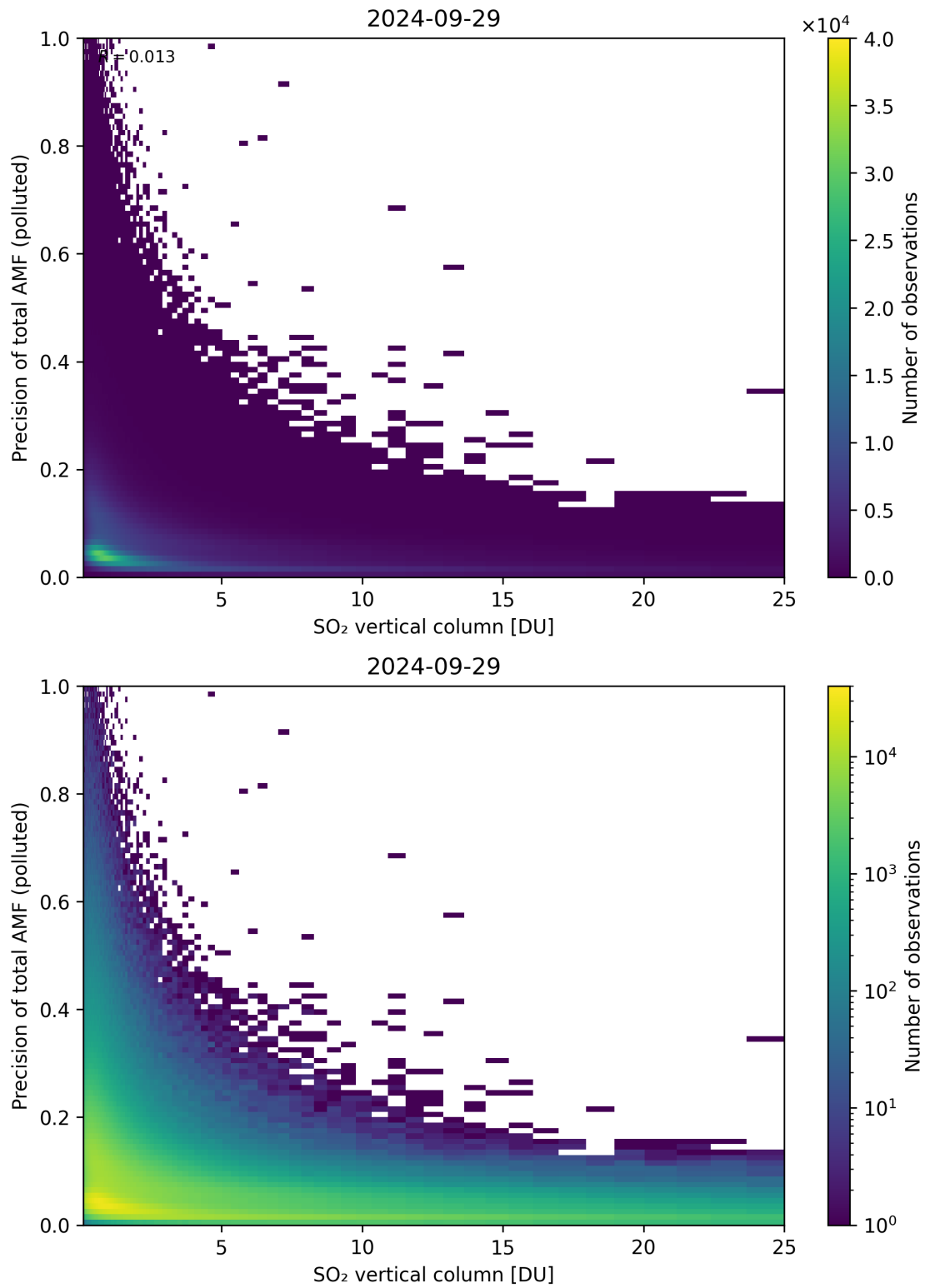
Figure 306: Scatter density plot of “SO 2 vertical column” against “Precision of total AMF (polluted)” for 2024-09-28 to 2024-09-30.
