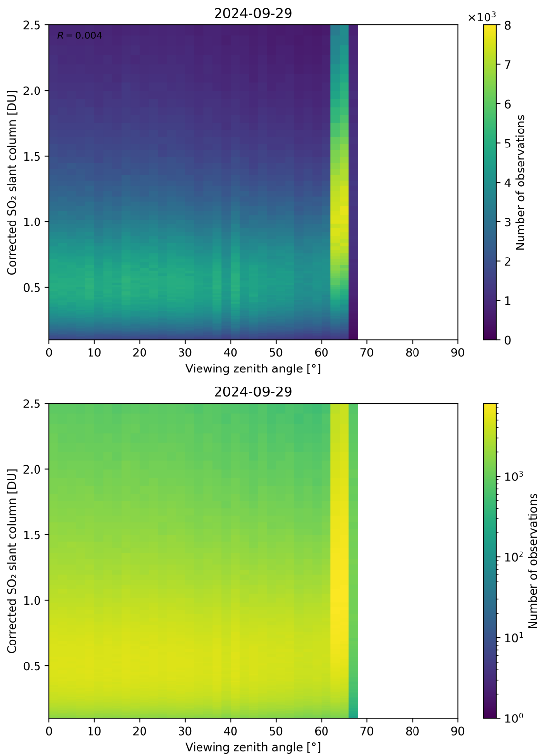
Figure 317: Scatter density plot of “Viewing zenith angle” against “Corrected SO 2 slant column” for 2024-09-28 to 2024-09-30.
