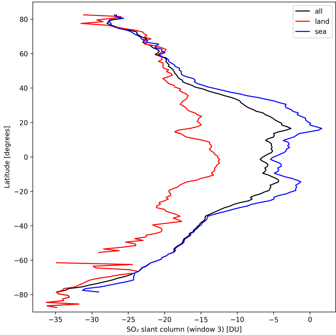
Figure 41: Zonal average of “SO 2 slant column (window 3)” for 2024-09-28 to 2024-09-30.
