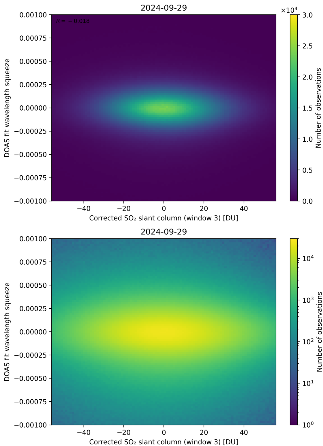
Figure 207: Scatter density plot of “Corrected SO 2 slant column (window 3)” against “DOAS fit wavelength squeeze” for 2024-09-28 to 2024-09-30.
