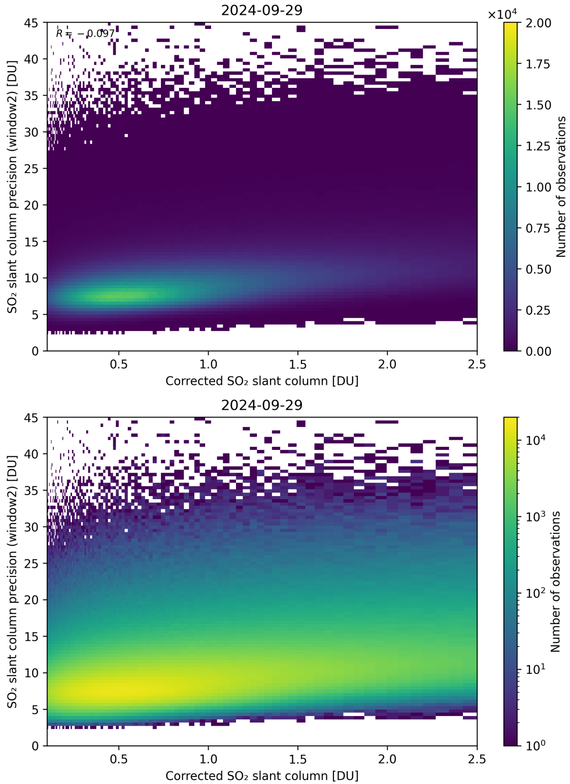
Figure 189: Scatter density plot of “Corrected SO 2 slant column” against “SO 2 slant column precision (window2)” for 2024-09-28 to 2024-09-30.
