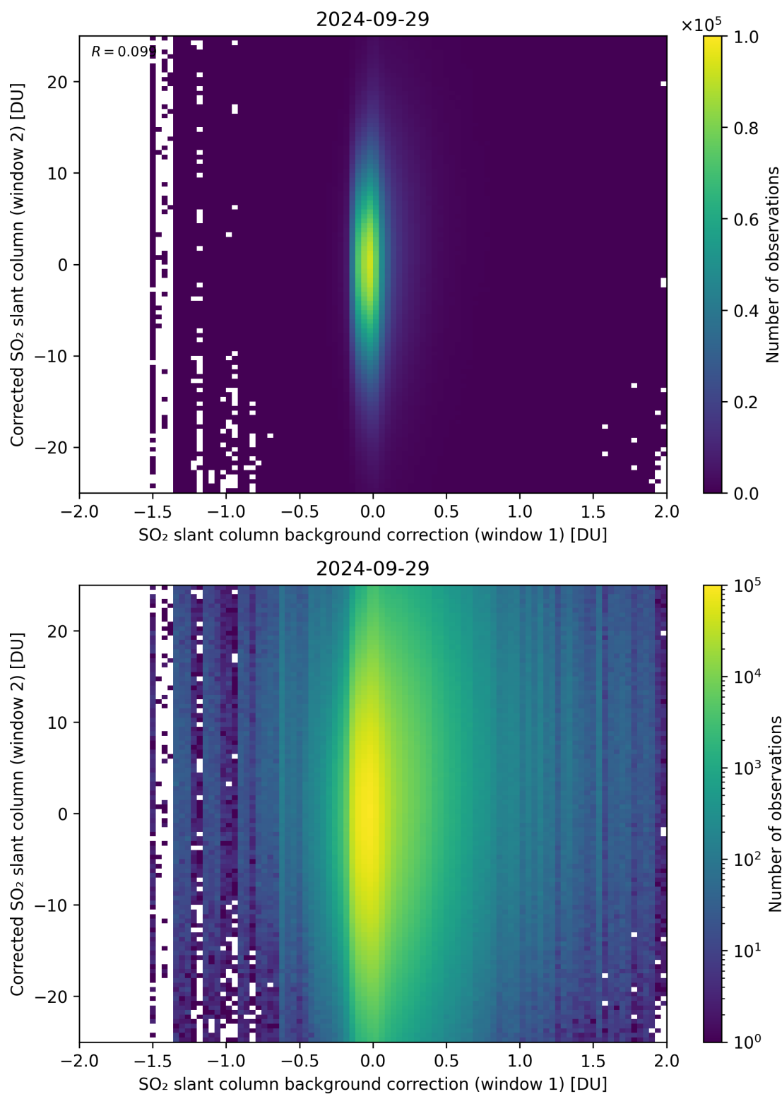
Figure 104: Scatter density plot of “SO 2 slant column background correction (window 1)” against “Corrected SO 2 slant column (window 2)” for 2024-09-28 to 2024-09-30.
