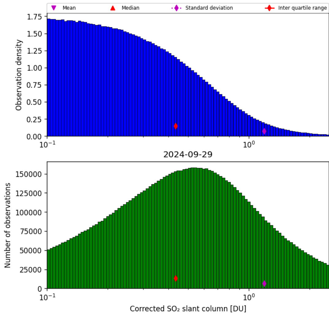
Figure 55: Histogram of “Corrected SO 2 slant column” for 2024-09-28 to 2024-09-30
