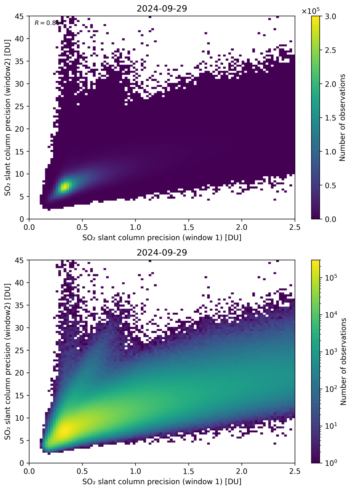
Figure 227: Scatter density plot of “SO 2 slant column precision (window 1)” against “SO 2 slant column precision (window2)” for 2024-09-28 to 2024-09-30.
