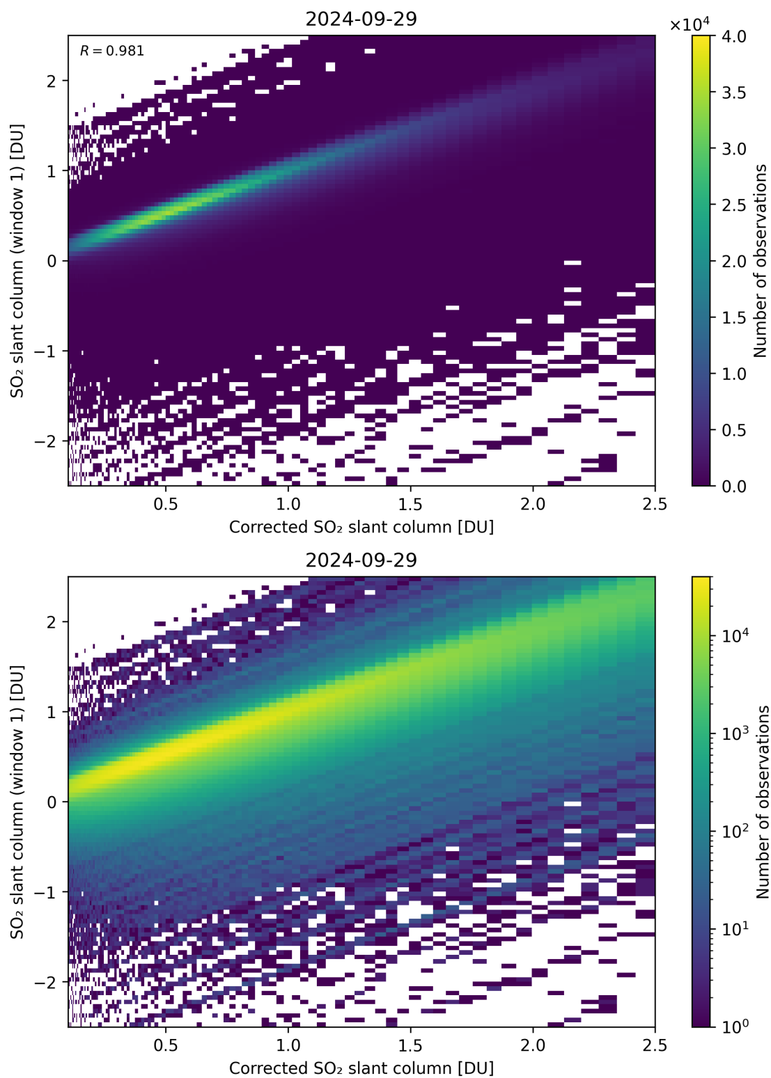
Figure 187: Scatter density plot of “Corrected SO 2 slant column” against “SO 2 slant column (window 1)” for 2024-09-28 to 2024-09-30.
