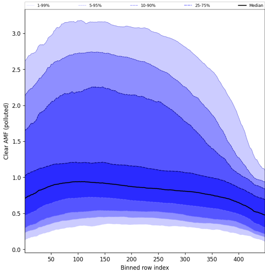
Figure 96: Along track statistics of “Clear AMF (polluted)” for 2024-09-28 to 2024-09-30
