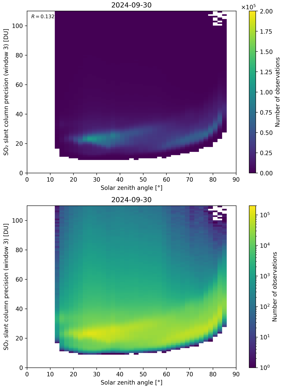
Figure 173: Scatter density plot of “Solar zenith angle” against “SO 2 slant column precision (window 3)” for 2024-09-29 to 2024-10-01.
