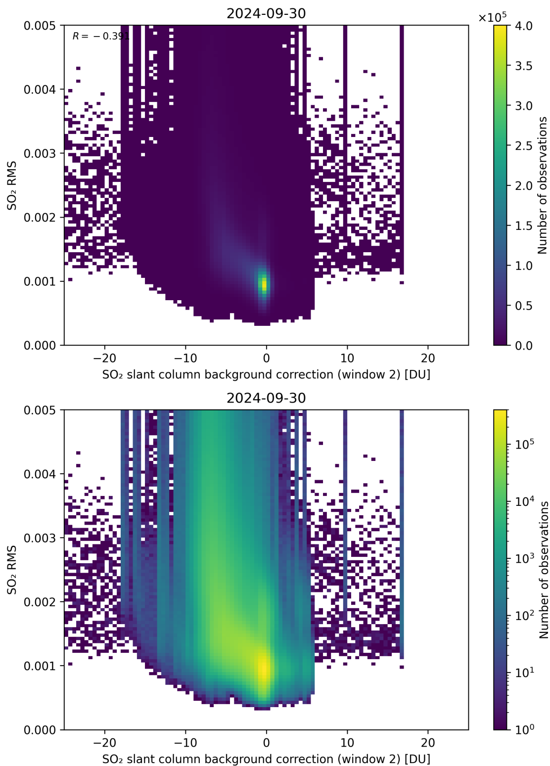
Figure 114: Scatter density plot of “SO 2 slant column background correction (window 2)” against “SO 2 RMS” for 2024-09-29 to 2024-10-01.
