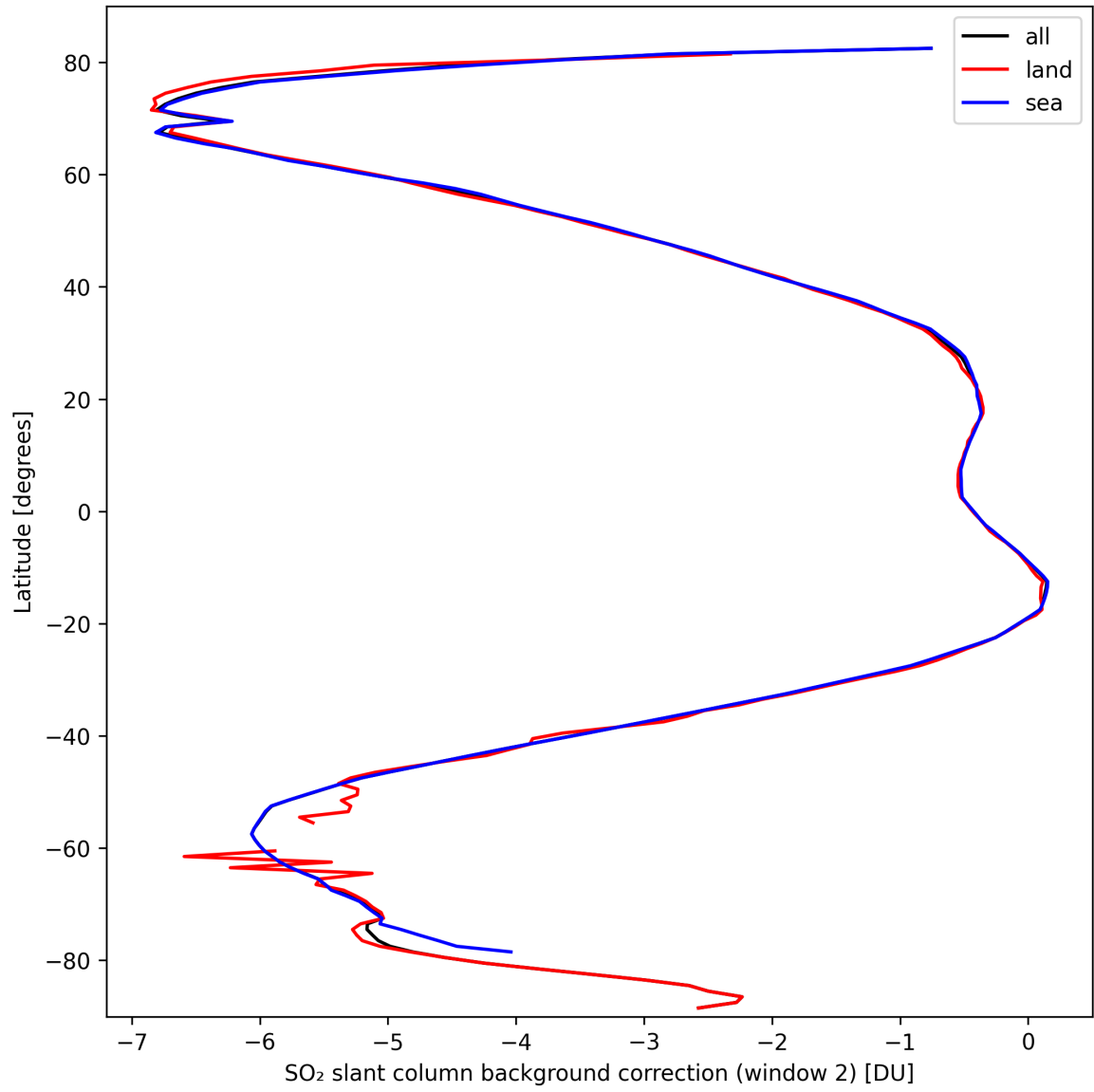
Figure 40: Zonal average of “SO 2 slant column background correction (window 2)” for 2024-09-29 to 2024-10-01.
