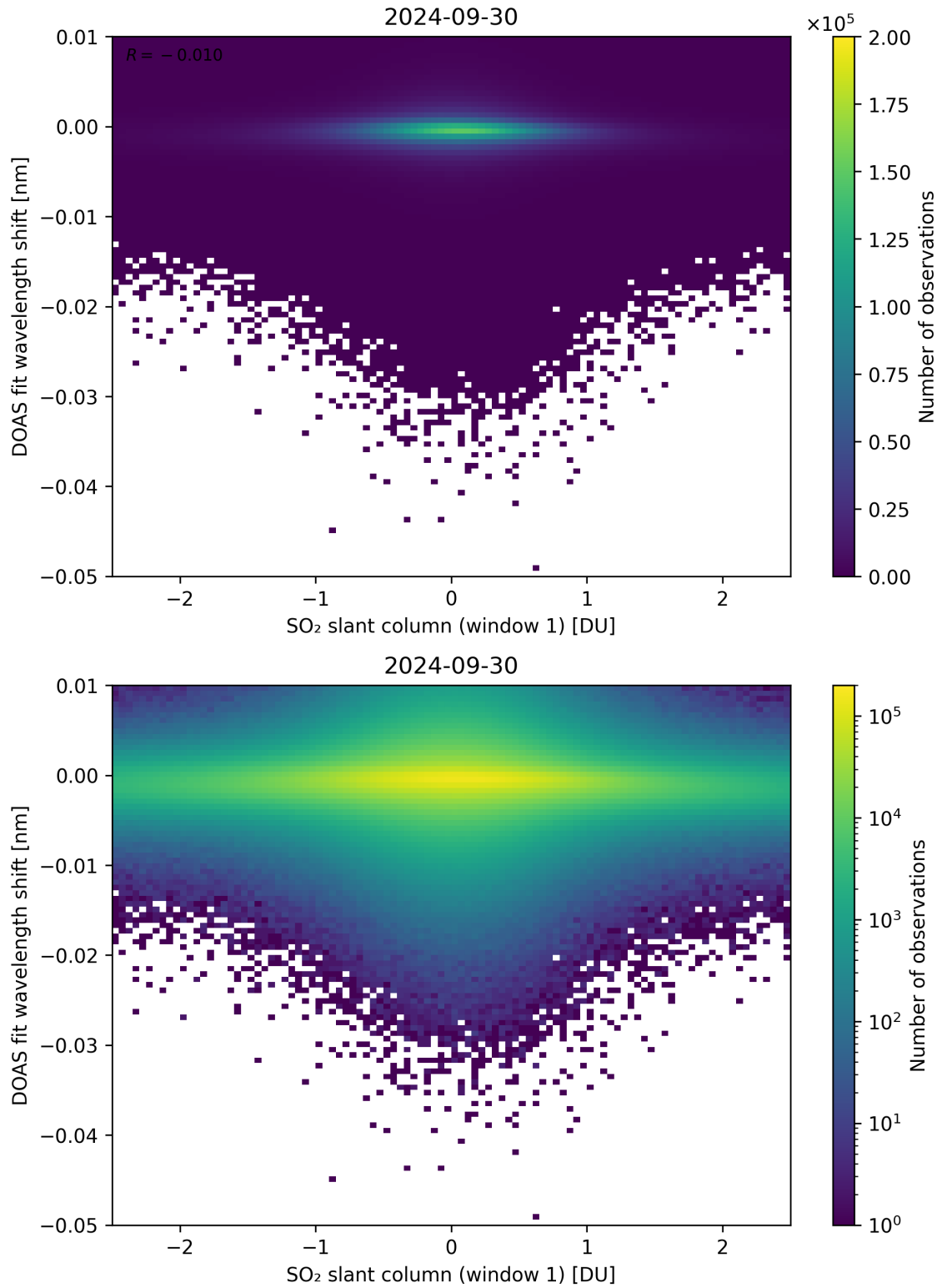
Figure 215: Scatter density plot of “SO 2 slant column (window 1)” against “DOAS fit wavelength shift” for 2024-09-29 to 2024-10-01.
