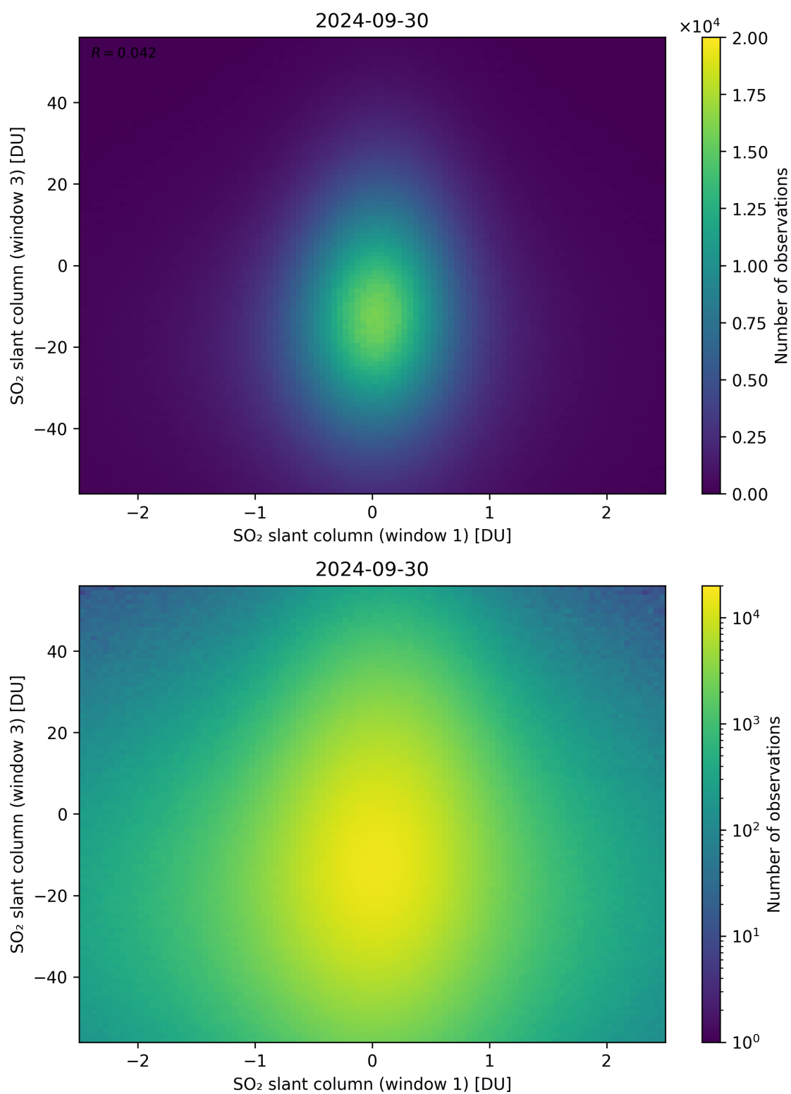
Figure 237: Scatter density plot of “SO 2 slant column (window 1)” against “SO 2 slant column (window 3)” for 2024-09-29 to 2024-10-01.
