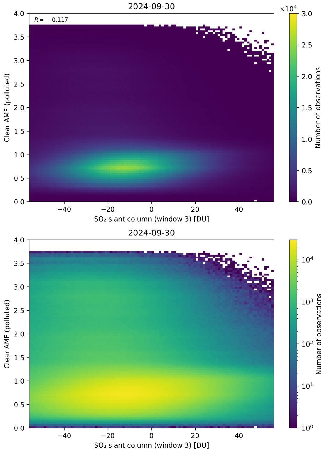
Figure 265: Scatter density plot of “SO 2 slant column (window 3)” against “Clear AMF (polluted)” for 2024-09-29 to 2024-10-01.
