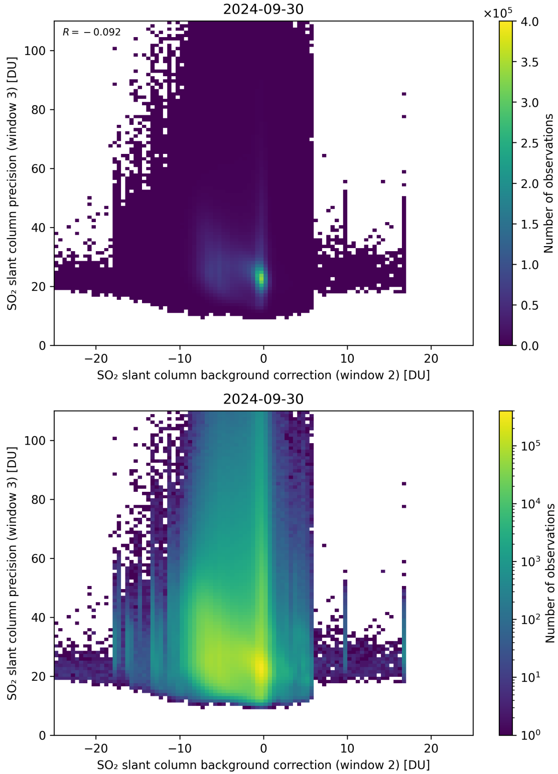
Figure 118: Scatter density plot of “SO 2 slant column background correction (window 2)” against “SO 2 slant column precision (window 3)” for 2024-09-29 to 2024-10-01.
