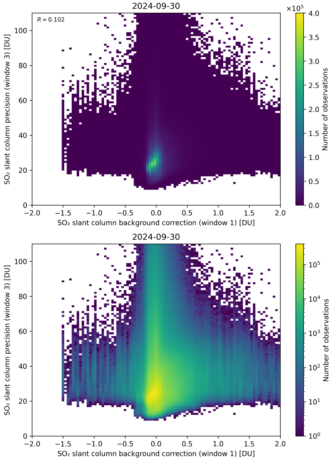
Figure 108: Scatter density plot of “SO 2 slant column background correction (window 1)” against “SO 2 slant column precision (window 3)” for 2024-09-29 to 2024-10-01.
