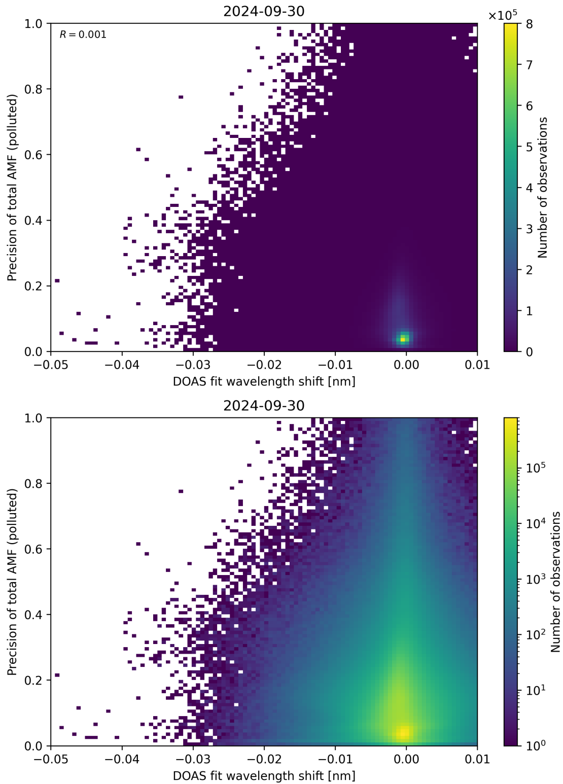
Figure 131: Scatter density plot of “DOAS fit wavelength shift” against “Precision of total AMF (polluted)” for 2024-09-29 to 2024-10-01.
