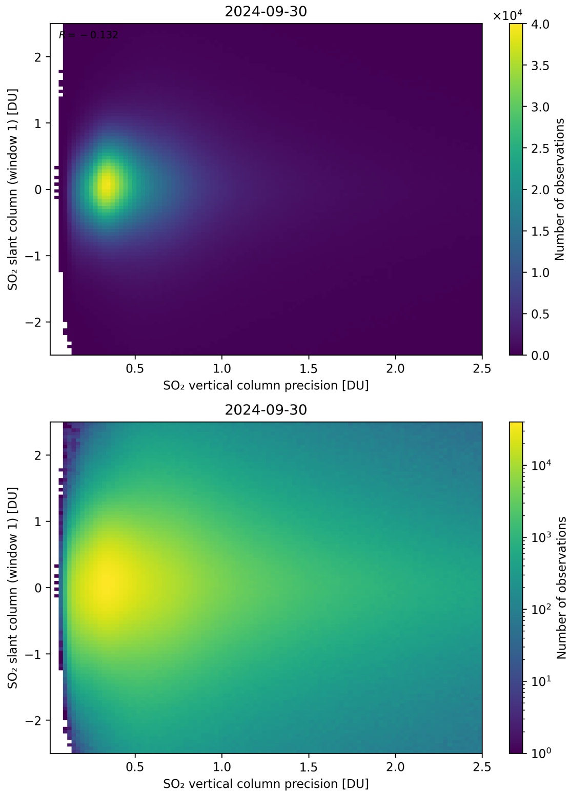
Figure 289: Scatter density plot of “SO 2 vertical column precision” against “SO 2 slant column (window 1)” for 2024-09-29 to 2024-10-01.
