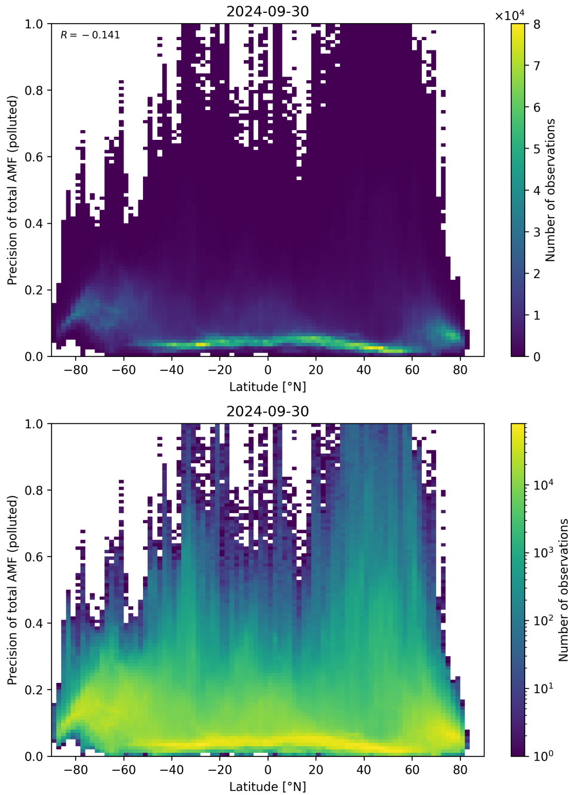
Figure 155: Scatter density plot of “Latitude” against “Precision of total AMF (polluted)” for 2024-09-29 to 2024-10-01.
