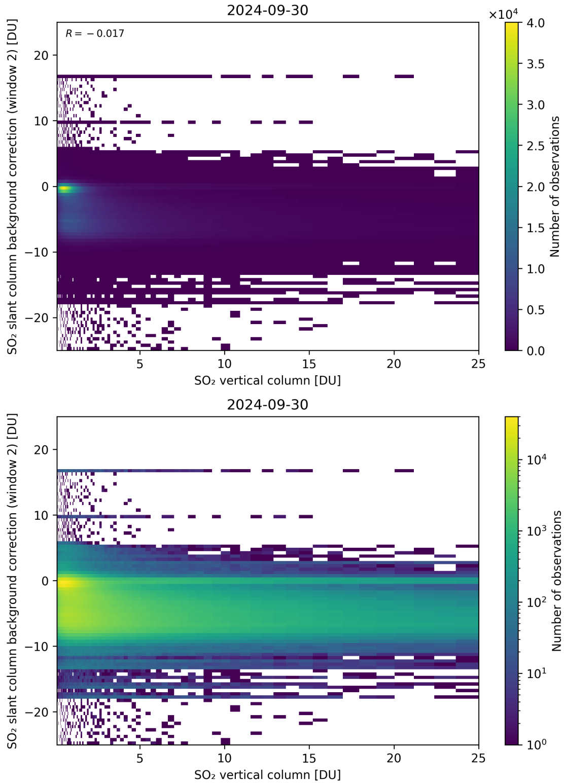
Figure 274: Scatter density plot of “SO 2 vertical column” against “SO 2 slant column background correction (window 2)” for 2024-09-29 to 2024-10-01.
