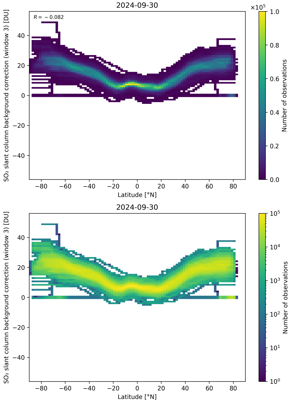
Figure 141: Scatter density plot of “Latitude” against “SO 2 slant column background correction (window 3)” for 2024-09-29 to 2024-10-01.
