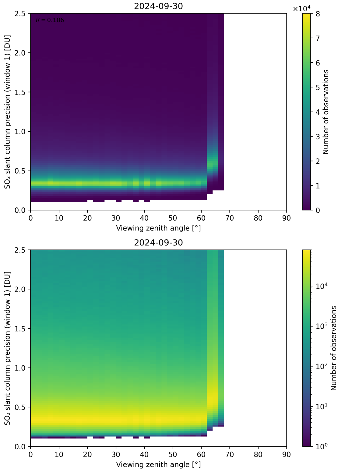
Figure 321: Scatter density plot of “Viewing zenith angle” against “SO 2 slant column precision (window 1)” for 2024-09-29 to 2024-10-01.
