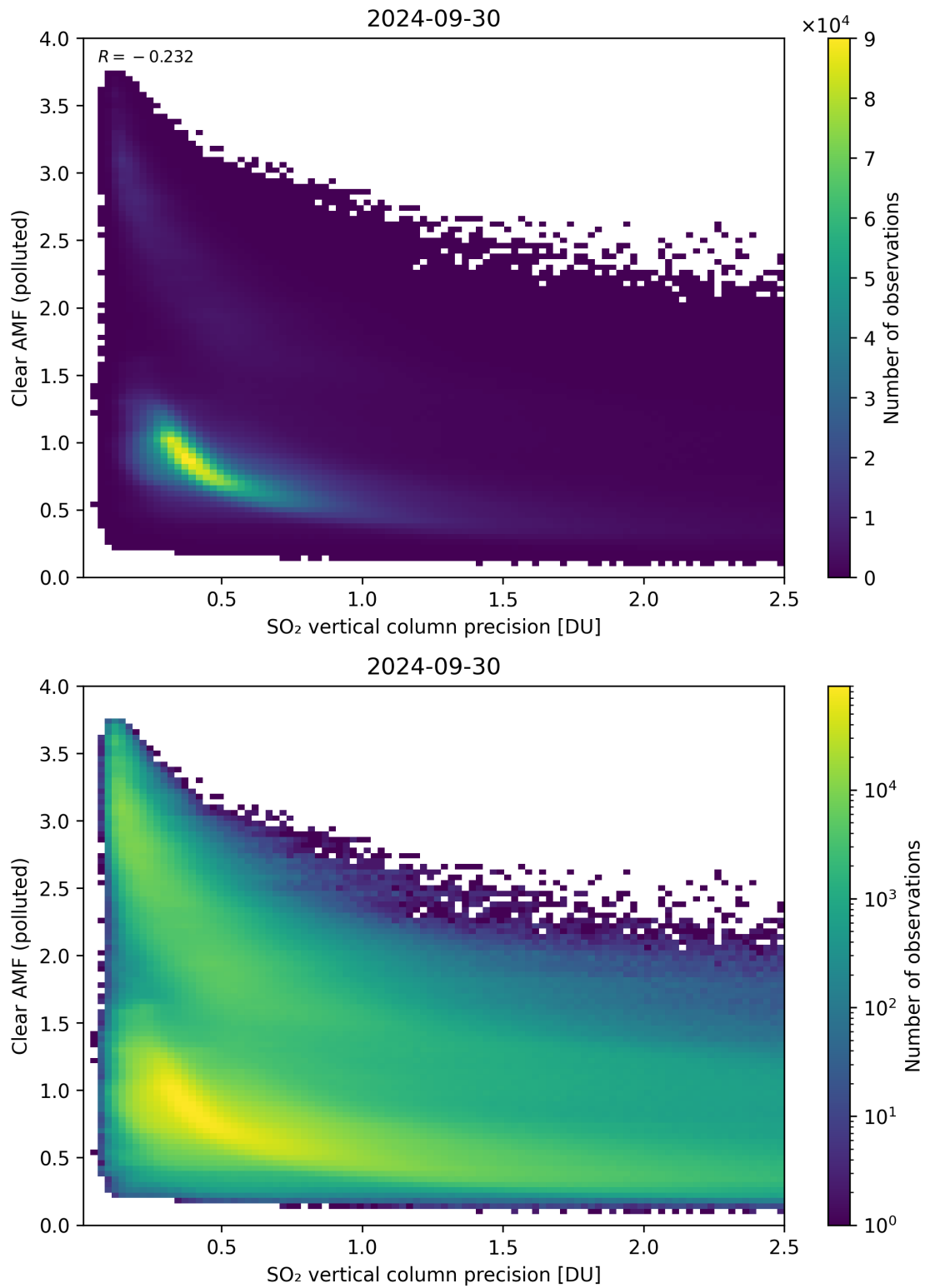
Figure 285: Scatter density plot of “SO 2 vertical column precision” against “Clear AMF (polluted)” for 2024-09-29 to 2024-10-01.
