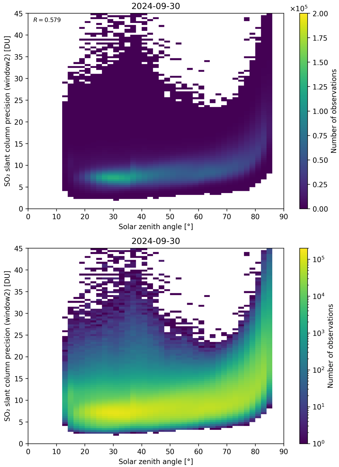
Figure 171: Scatter density plot of “Solar zenith angle” against “SO 2 slant column precision (window2)” for 2024-09-29 to 2024-10-01.
