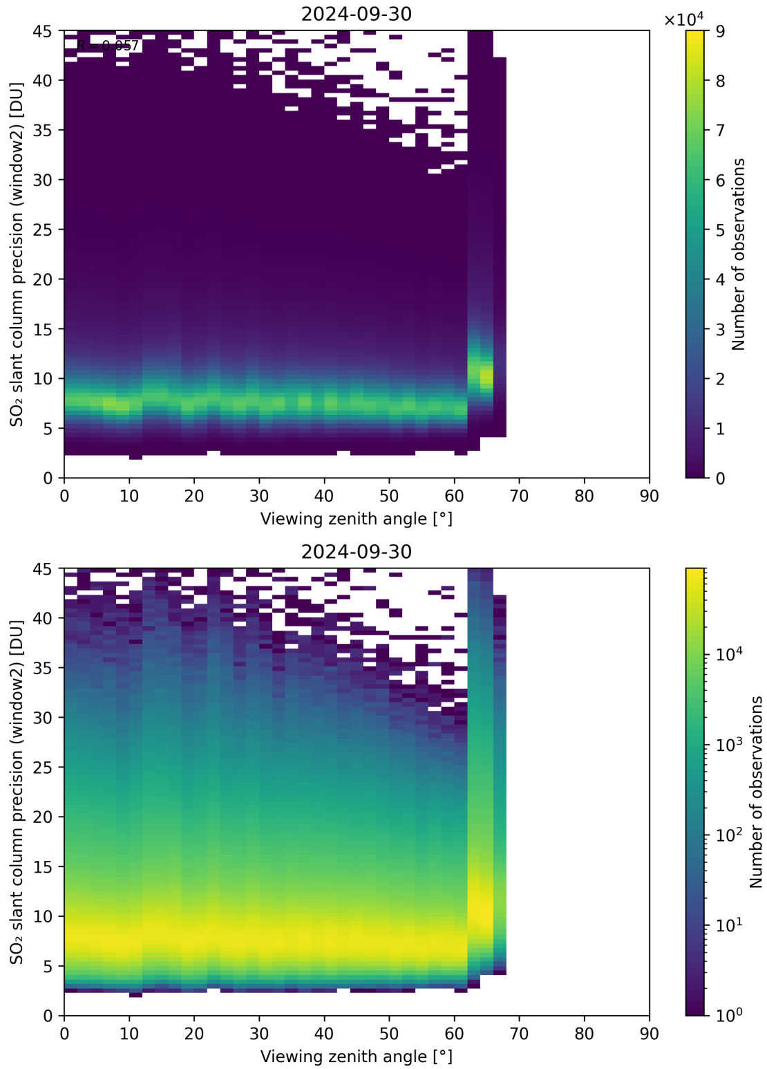
Figure 322: Scatter density plot of “Viewing zenith angle” against “SO 2 slant column precision (window2)” for 2024-09-29 to 2024-10-01.
