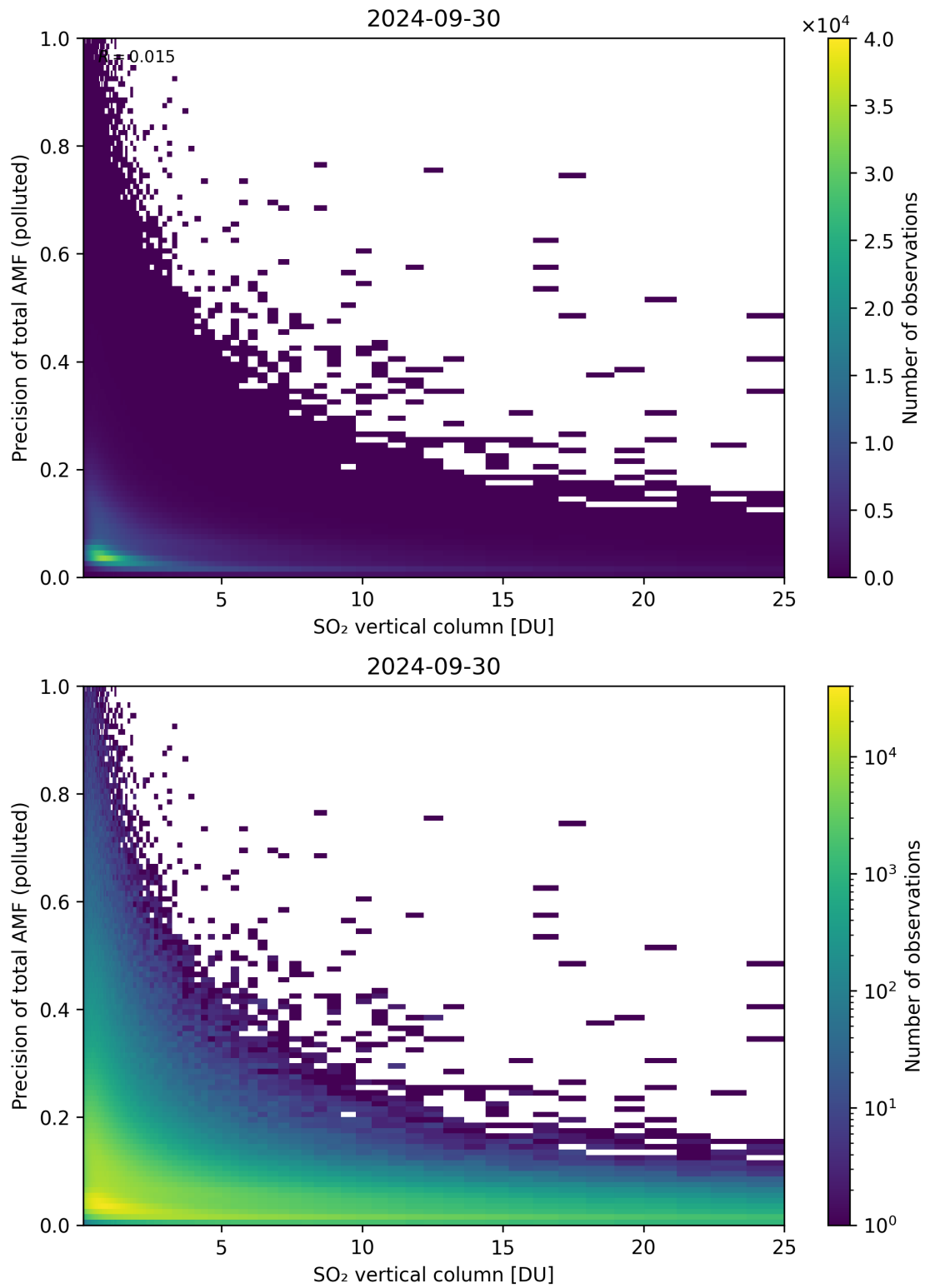
Figure 306: Scatter density plot of “SO 2 vertical column” against “Precision of total AMF (polluted)” for 2024-09-29 to 2024-10-01.
