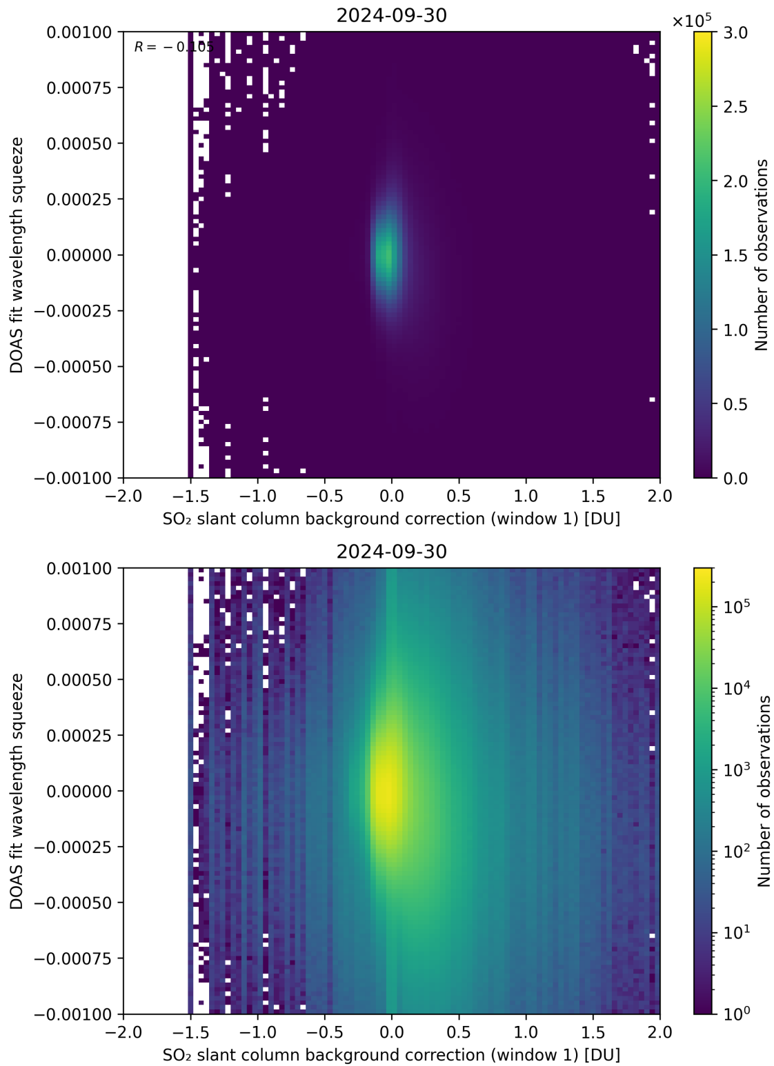
Figure 101: Scatter density plot of “SO 2 slant column background correction (window 1)” against “DOAS fit wavelength squeeze” for 2024-09-29 to 2024-10-01.
