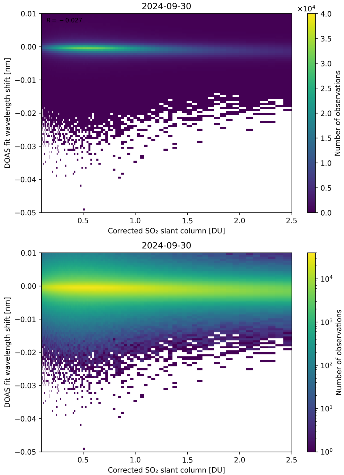
Figure 181: Scatter density plot of “Corrected SO 2 slant column” against “DOAS fit wavelength shift” for 2024-09-29 to 2024-10-01.
