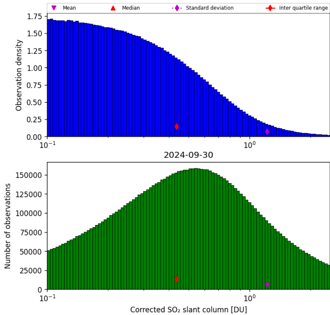
Figure 55: Histogram of “Corrected SO 2 slant column” for 2024-09-29 to 2024-10-01
