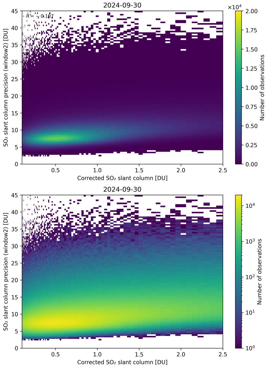
Figure 189: Scatter density plot of “Corrected SO 2 slant column” against “SO 2 slant column precision (window2)” for 2024-09-29 to 2024-10-01.
