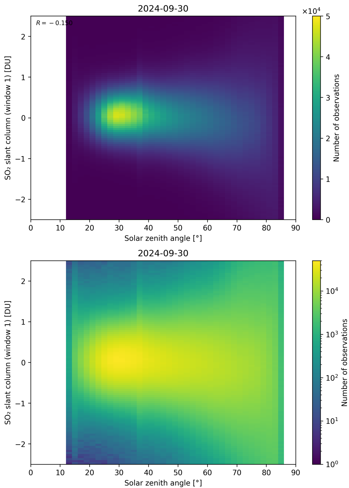
Figure 169: Scatter density plot of “Solar zenith angle” against “SO 2 slant column (window 1)” for 2024-09-29 to 2024-10-01.
