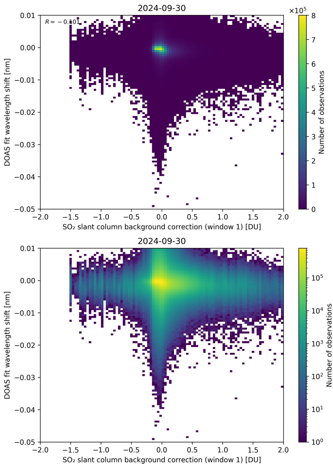
Figure 100: Scatter density plot of “SO 2 slant column background correction (window 1)” against “DOAS fit wavelength shift” for 2024-09-29 to 2024-10-01.
