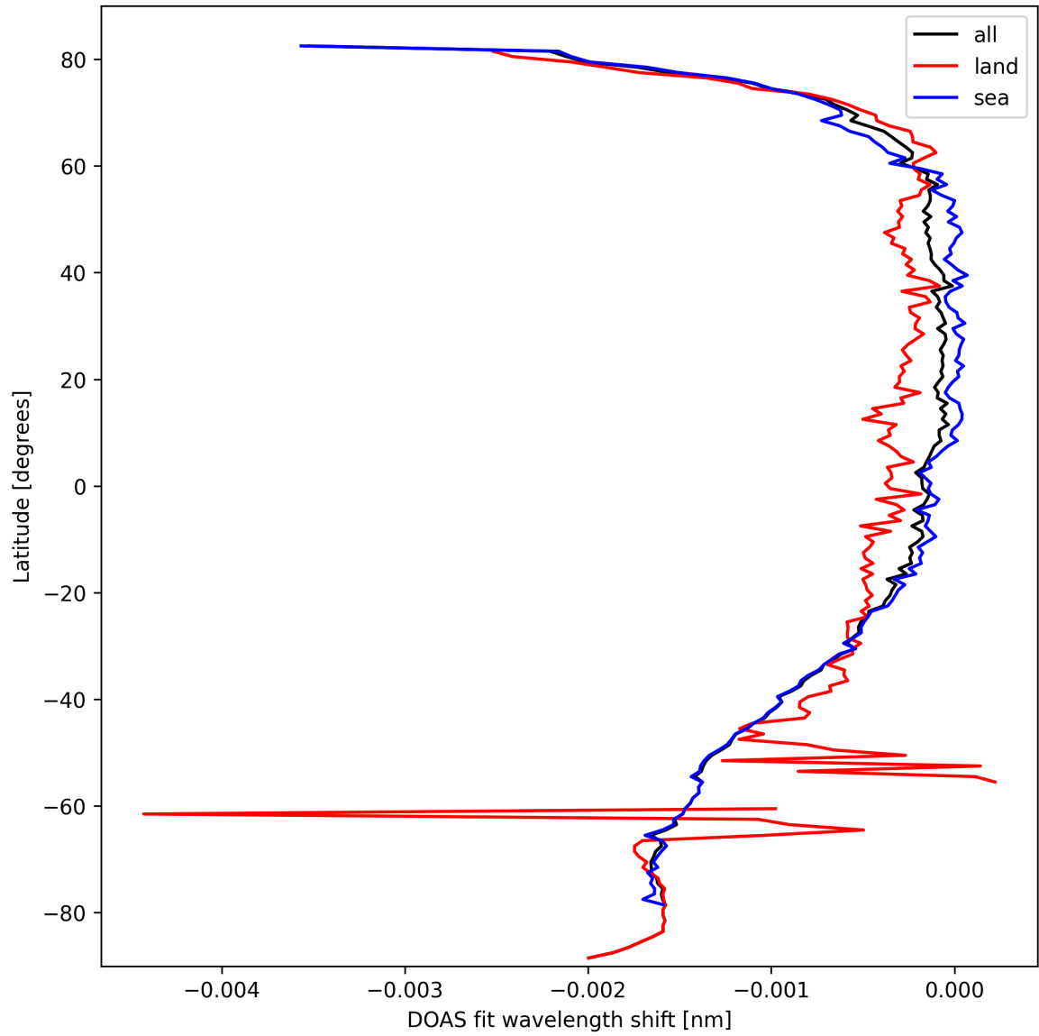
Figure 45: Zonal average of “DOAS fit wavelength shift” for 2024-09-29 to 2024-10-01.
