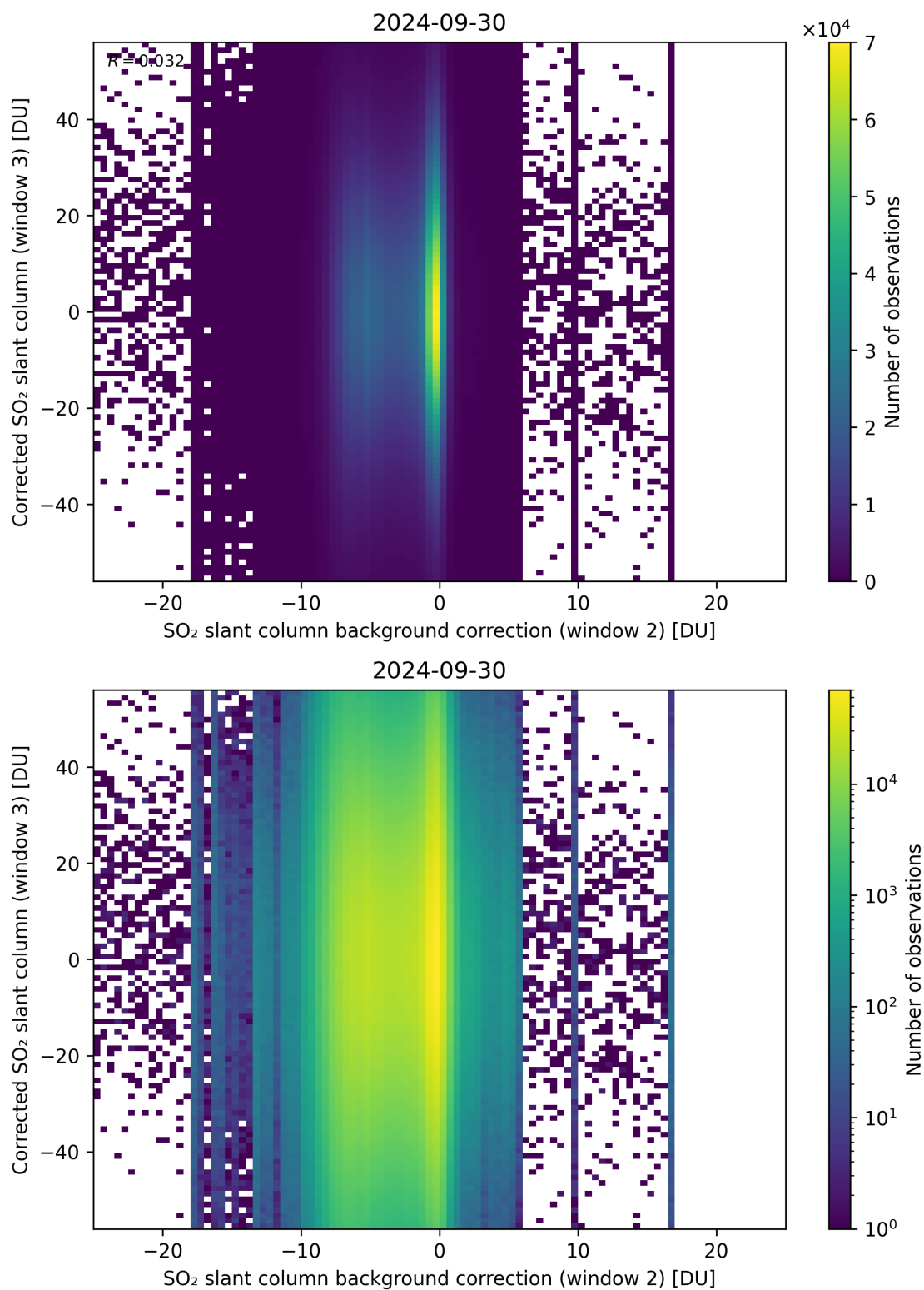
Figure 116: Scatter density plot of “SO 2 slant column background correction (window 2)” against “Corrected SO 2 slant column (window 3)” for 2024-09-29 to 2024-10-01.
