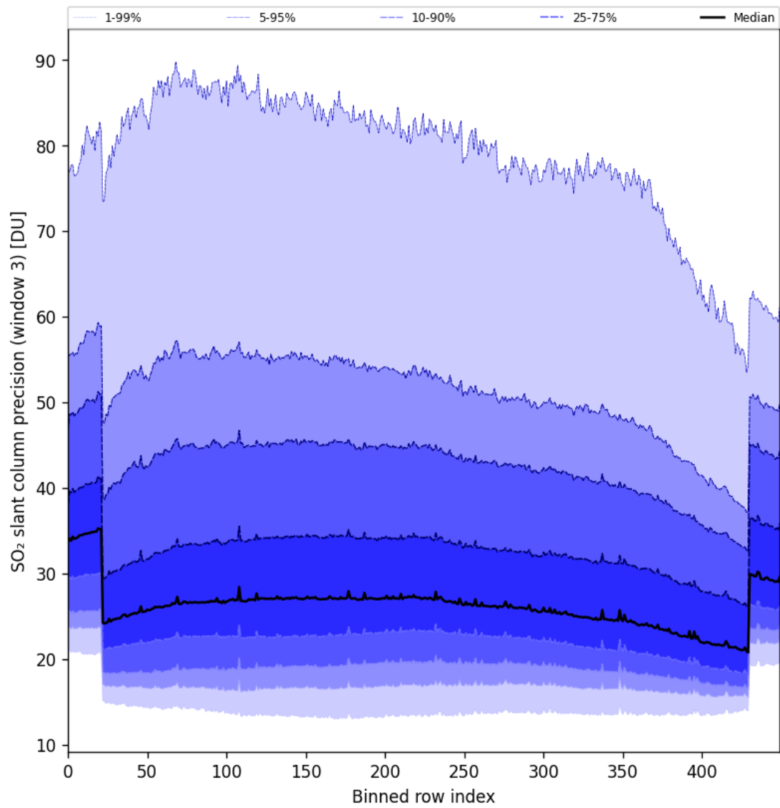
Figure 88: Along track statistics of “SO 2 slant column precision (window 3)” for 2024-09-29 to 2024-10-01
