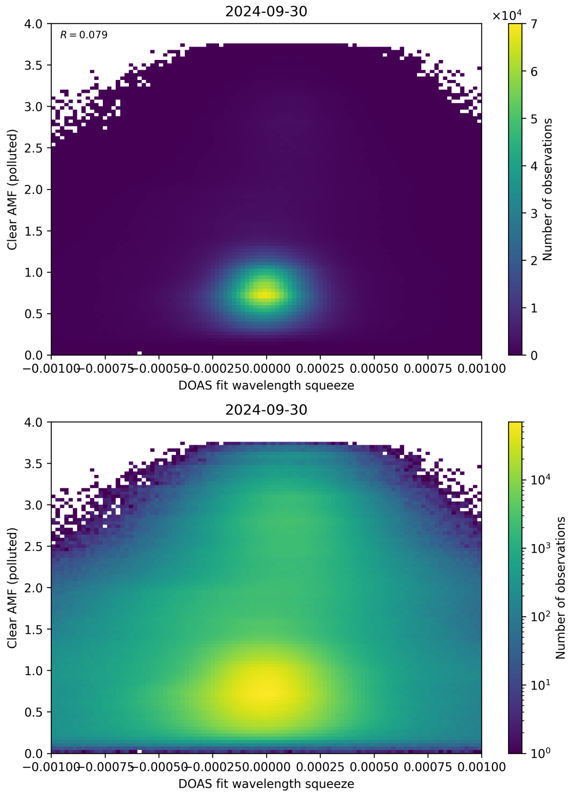
Figure 133: Scatter density plot of “DOAS fit wavelength squeeze” against “Clear AMF (polluted)” for 2024-09-29 to 2024-10-01.
