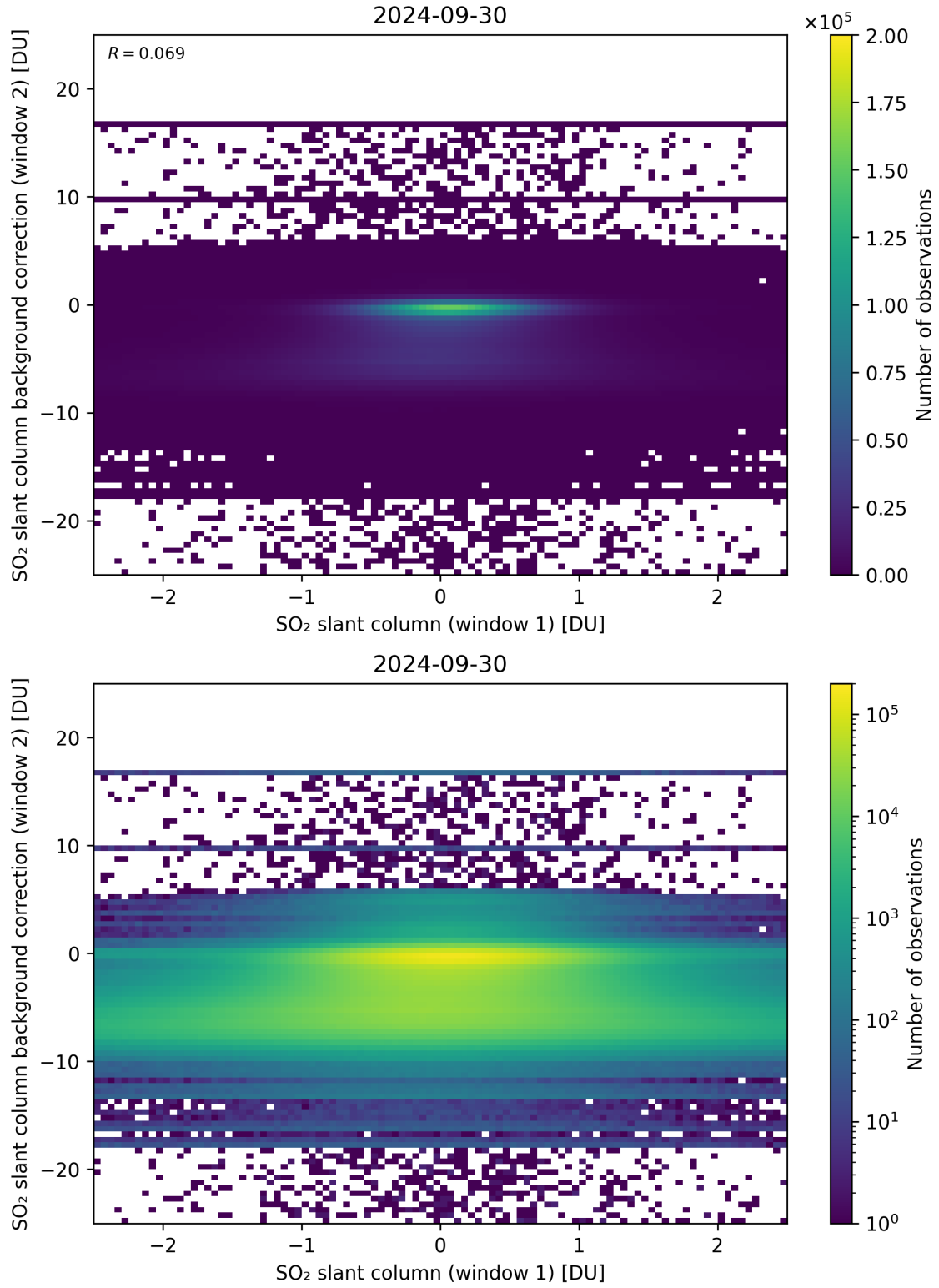
Figure 213: Scatter density plot of “SO 2 slant column (window 1)” against “SO 2 slant column background correction (window 2)” for 2024-09-29 to 2024-10-01.
