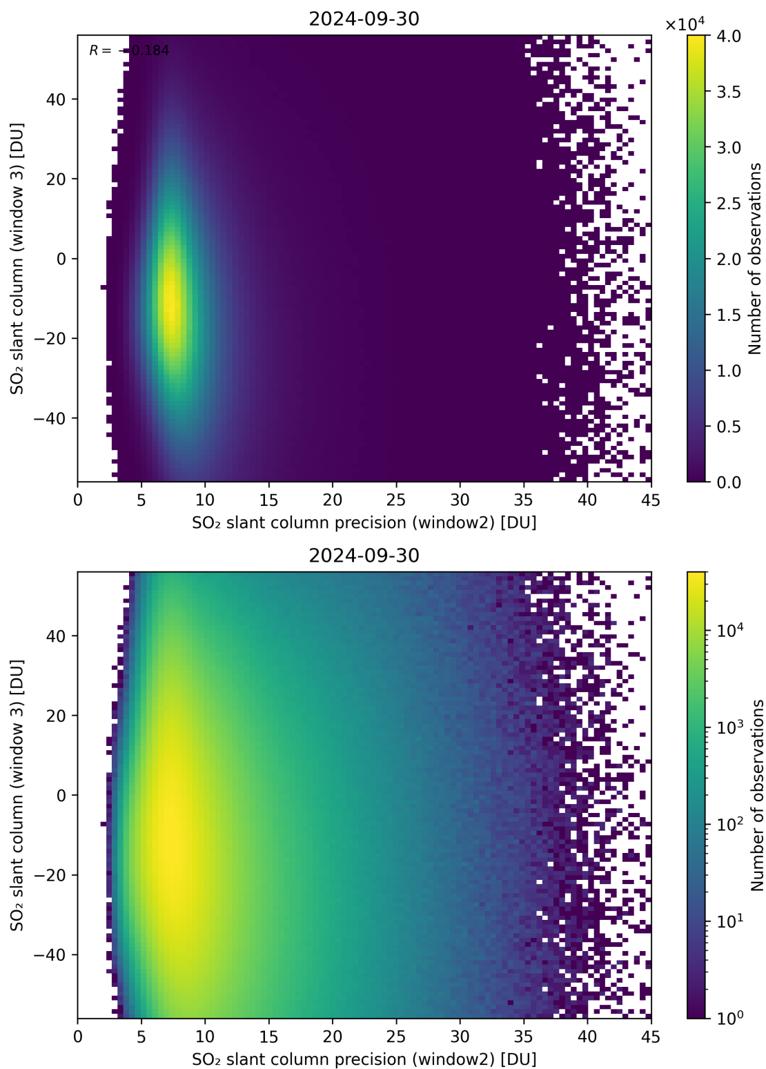
Figure 249: Scatter density plot of “SO 2 slant column precision (window2)” against “SO 2 slant column (window 3)” for 2024-09-29 to 2024-10-01.
