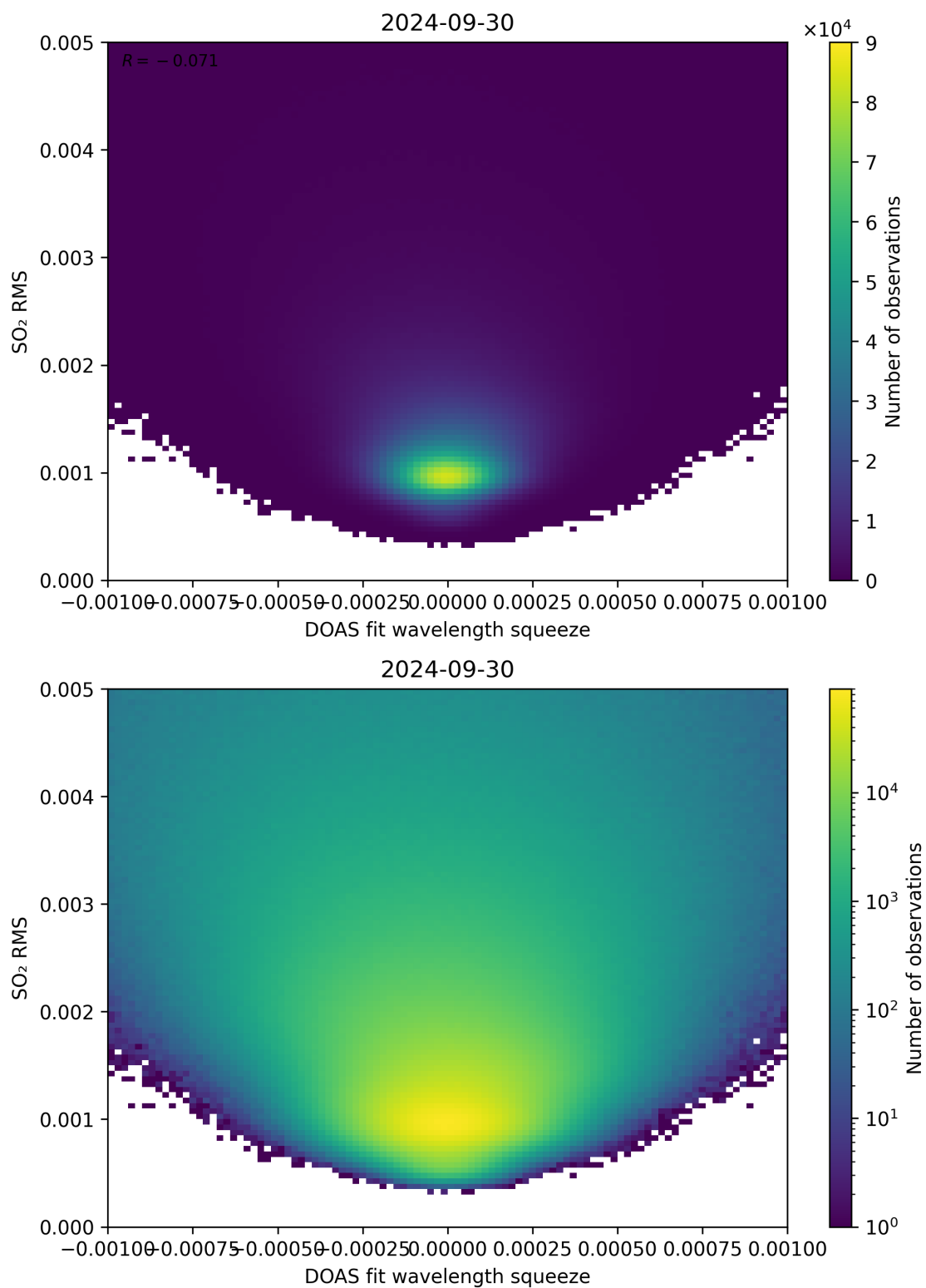
Figure 132: Scatter density plot of “DOAS fit wavelength squeeze” against “SO 2 RMS” for 2024-09-29 to 2024-10-01.
