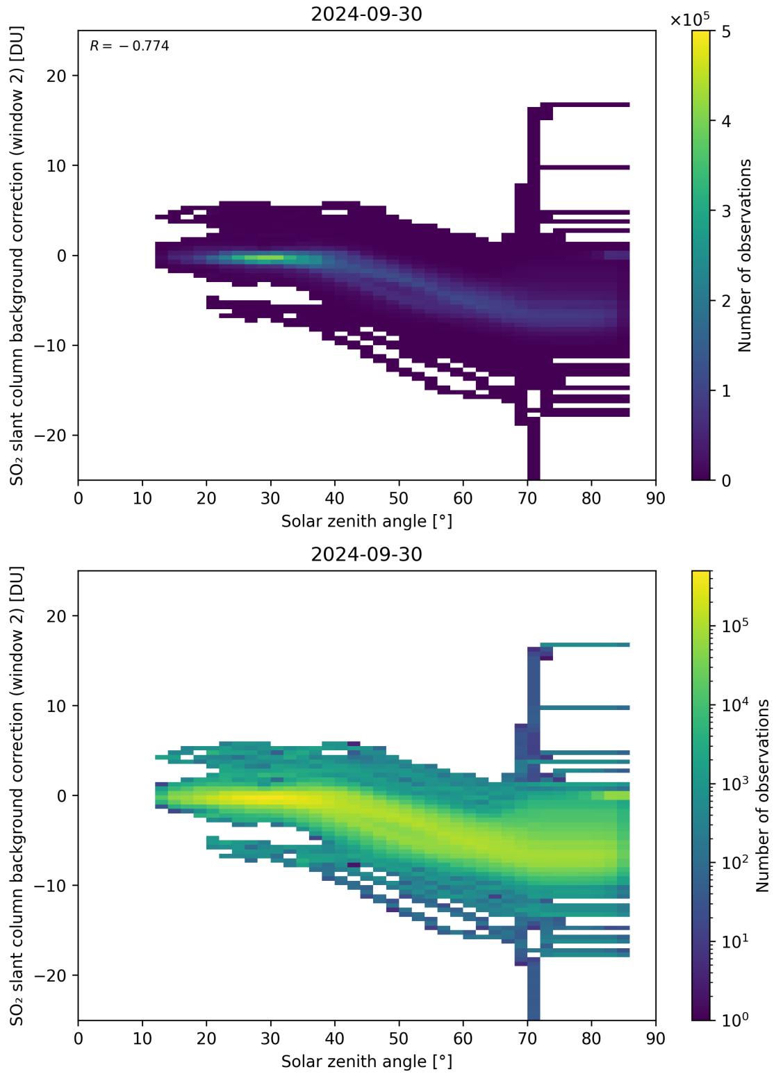
Figure 159: Scatter density plot of “Solar zenith angle” against “SO 2 slant column background correction (window 2)” for 2024-09-29 to 2024-10-01.
