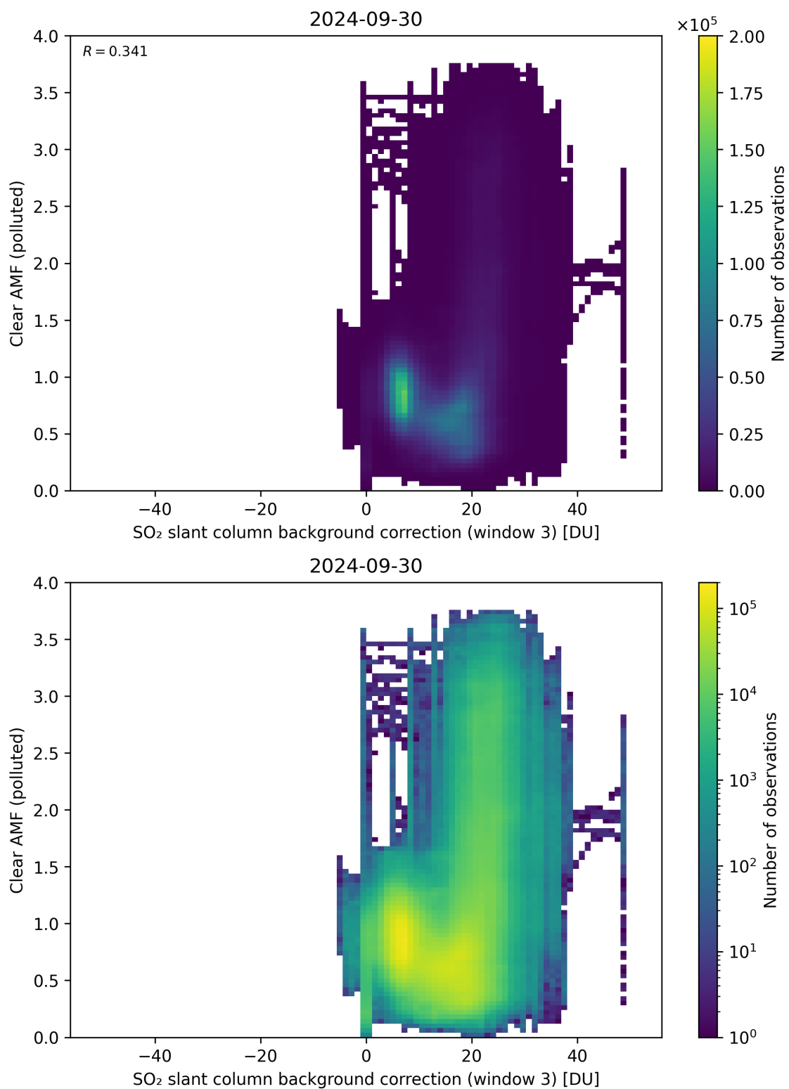
Figure 124: Scatter density plot of “SO 2 slant column background correction (window 3)” against “Clear AMF (polluted)” for 2024-09-29 to 2024-10-01.
