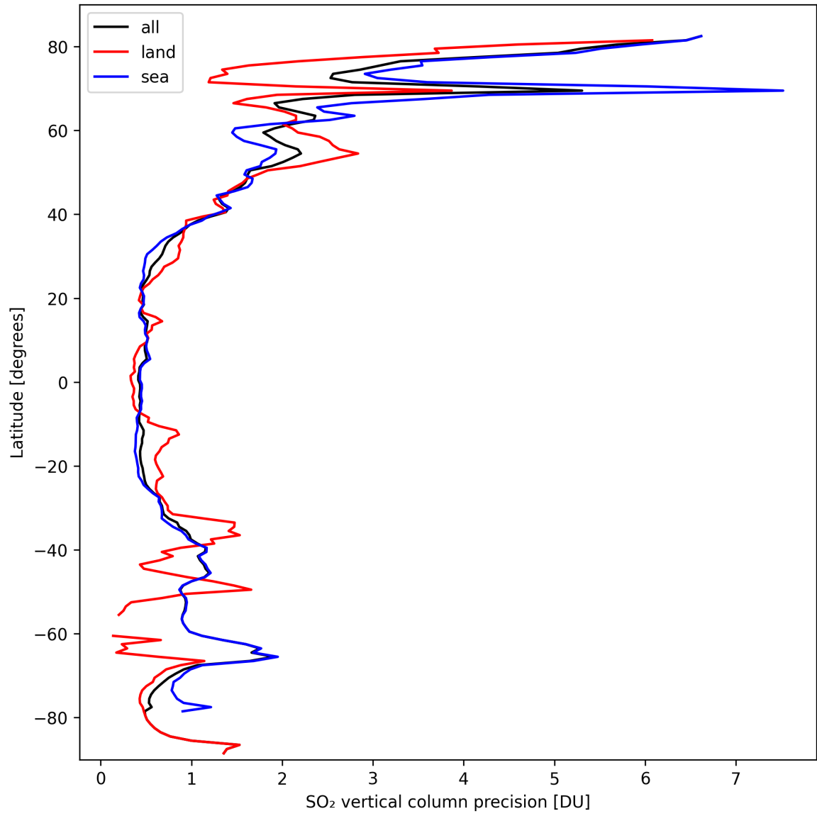
Figure 31: Zonal average of “SO 2 vertical column precision” for 2024-09-29 to 2024-10-01.
