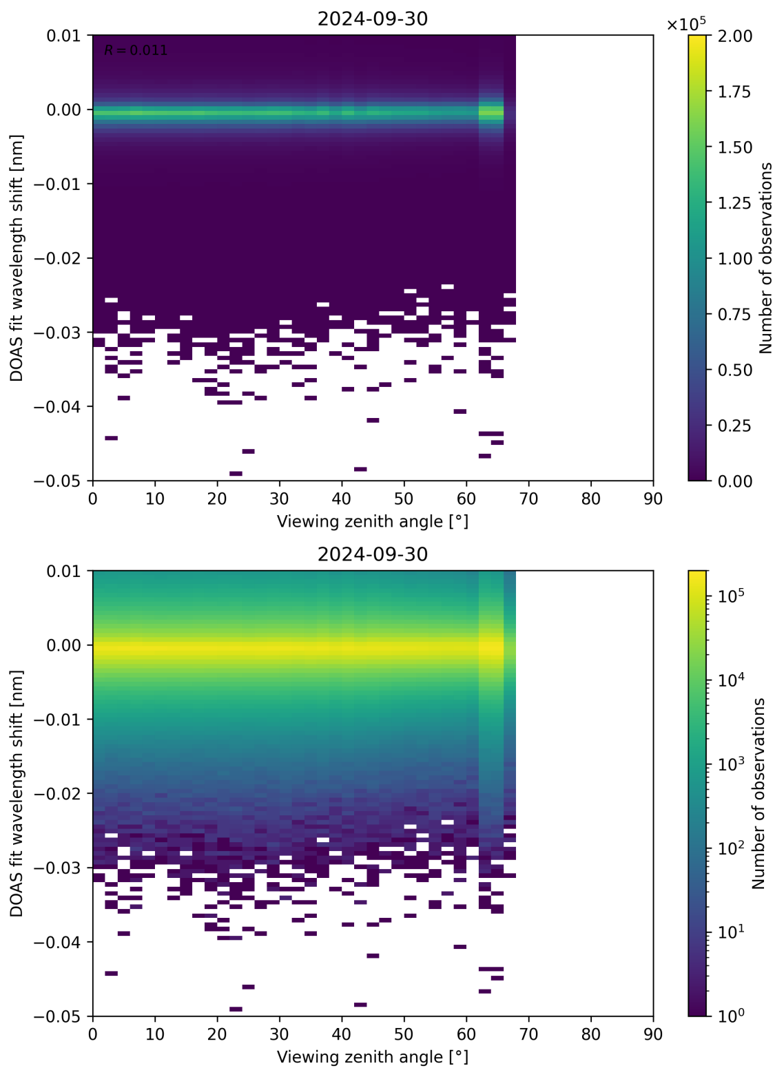
Figure 311: Scatter density plot of “Viewing zenith angle” against “DOAS fit wavelength shift” for 2024-09-29 to 2024-10-01.
