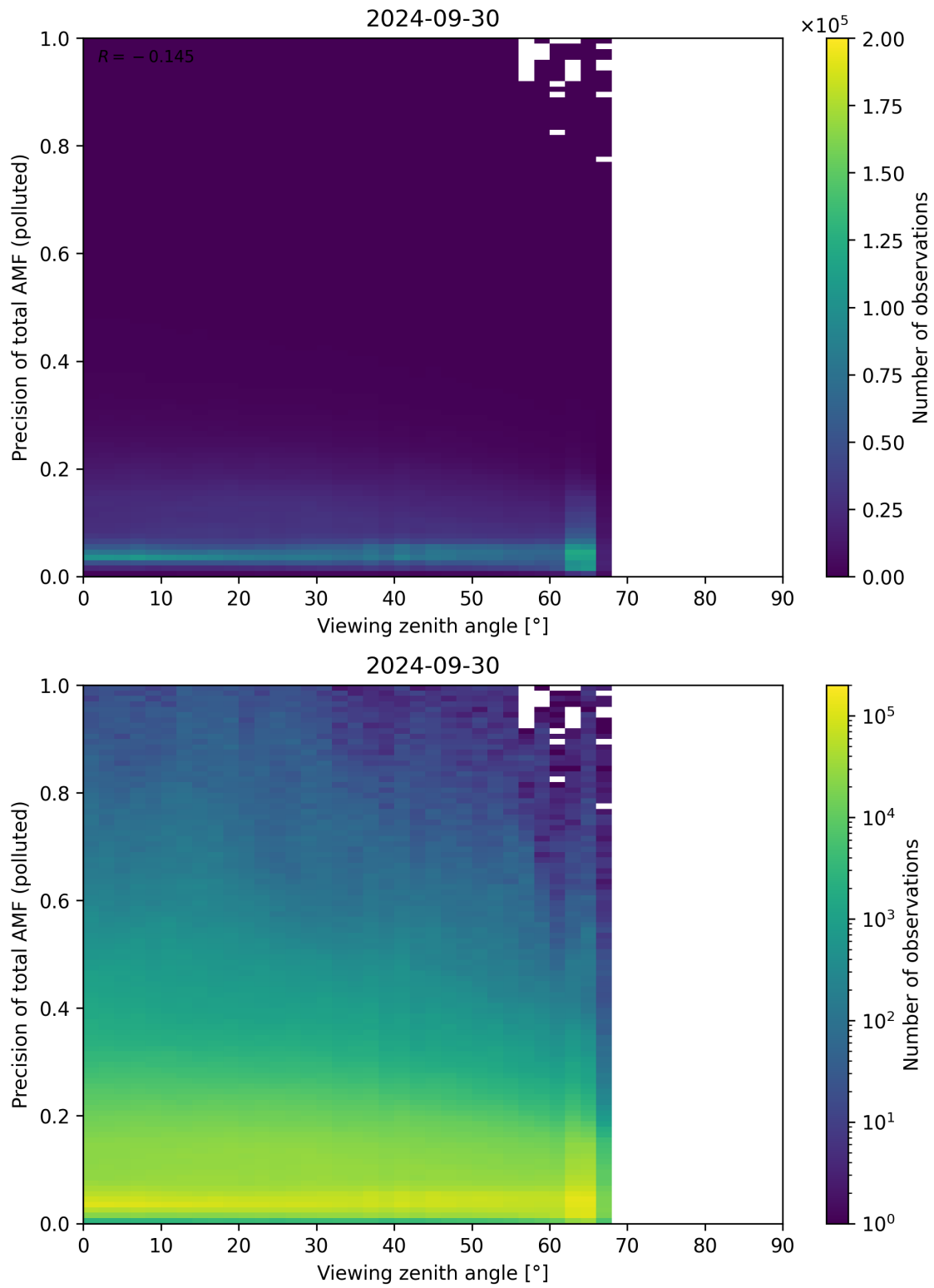
Figure 326: Scatter density plot of “Viewing zenith angle” against “Precision of total AMF (polluted)” for 2024-09-29 to 2024-10-01.
