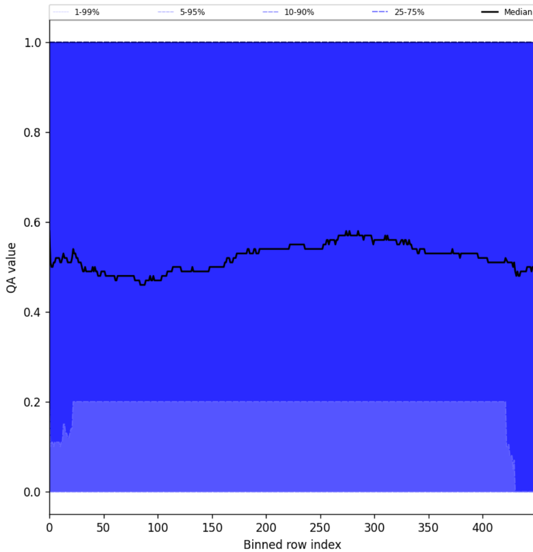
Figure 75: Along track statistics of “QA value” for 2024-09-29 to 2024-10-01
