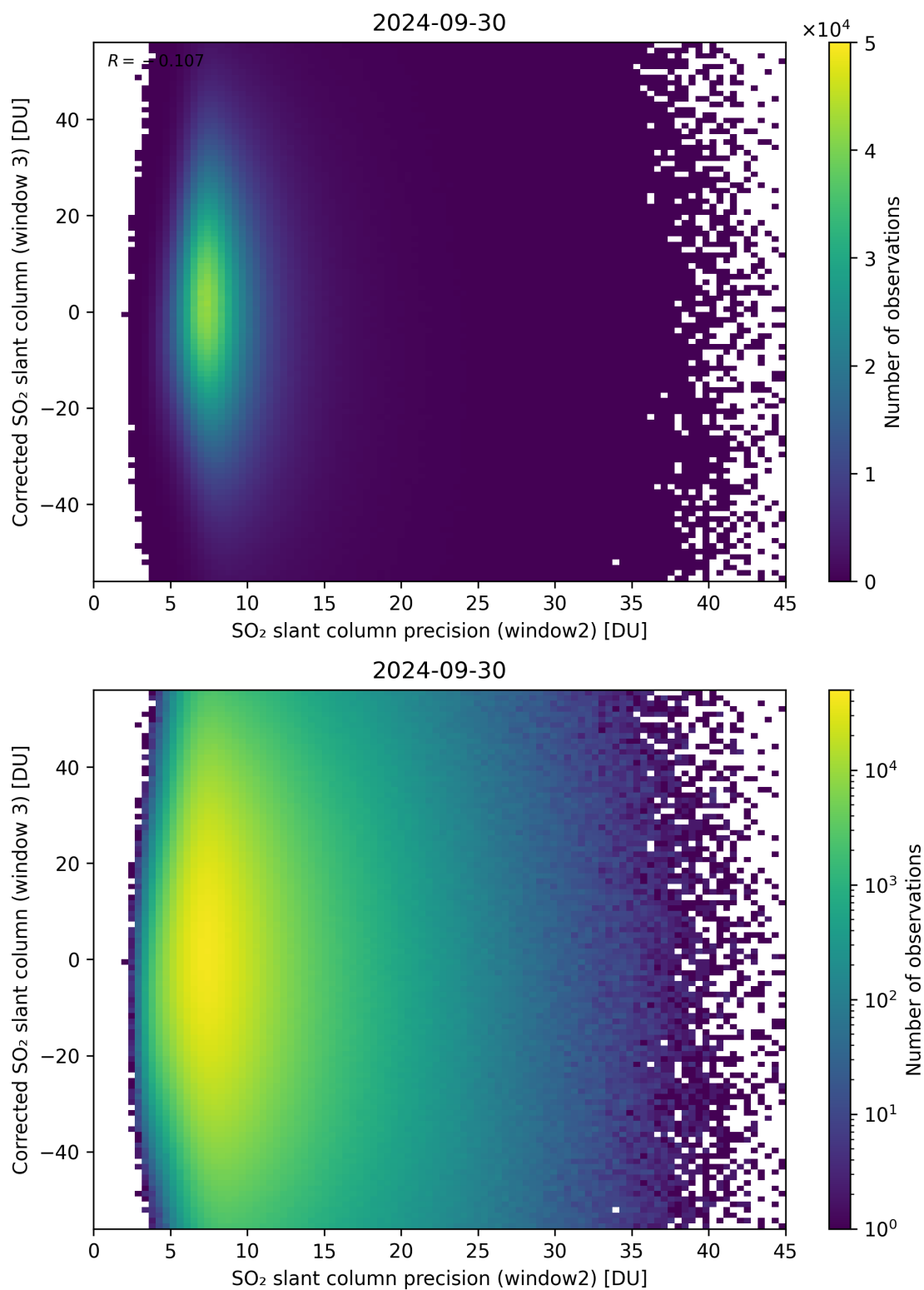
Figure 248: Scatter density plot of “SO 2 slant column precision (window2)” against “Corrected SO 2 slant column (window 3)” for 2024-09-29 to 2024-10-01.
