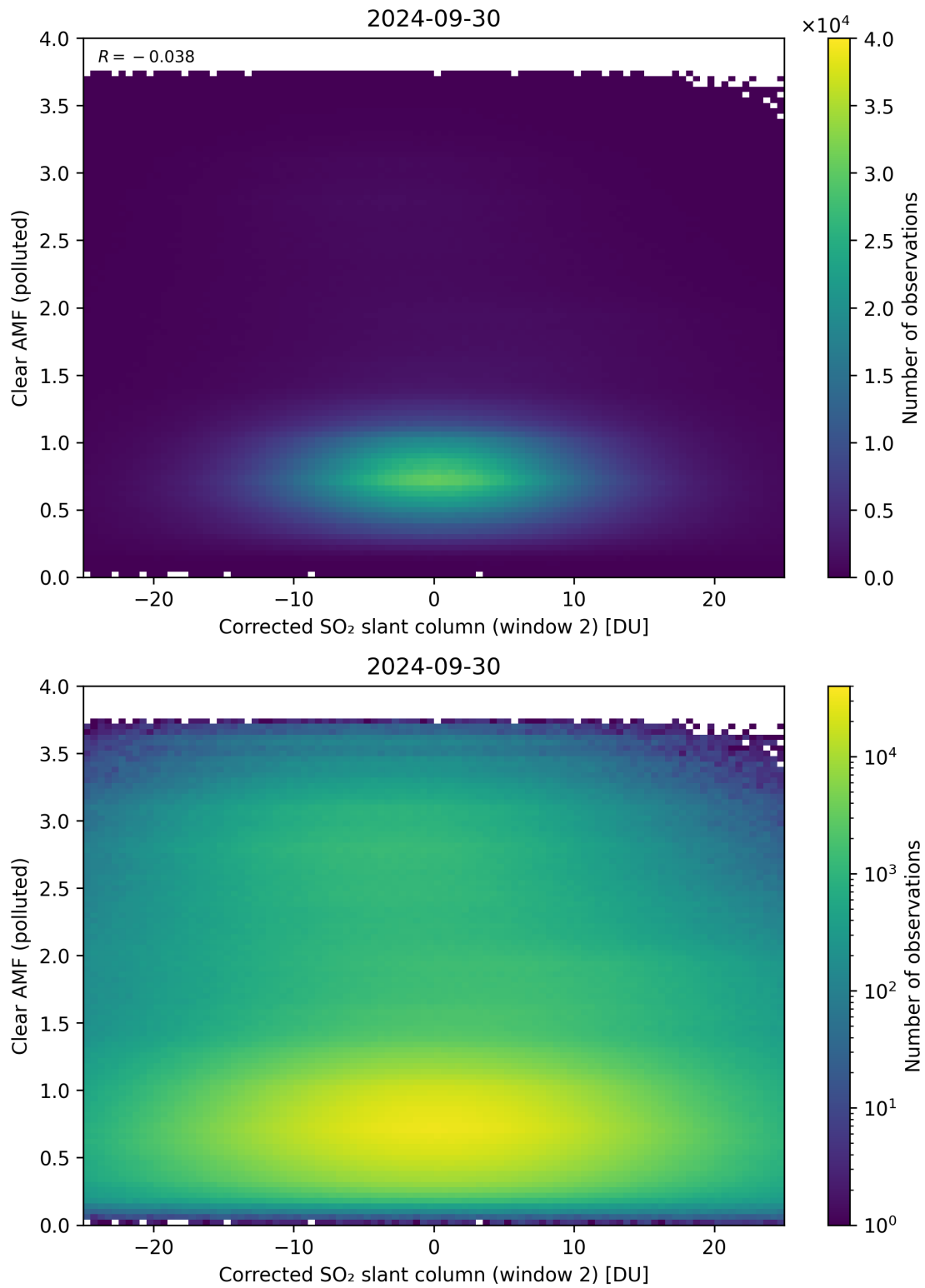
Figure 199: Scatter density plot of “Corrected SO 2 slant column (window 2)” against “Clear AMF (polluted)” for 2024-09-29 to 2024-10-01.
