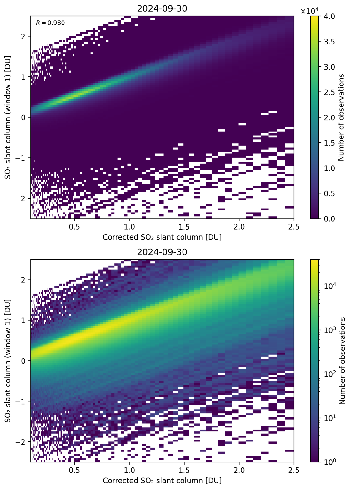
Figure 187: Scatter density plot of “Corrected SO 2 slant column” against “SO 2 slant column (window 1)” for 2024-09-29 to 2024-10-01.
