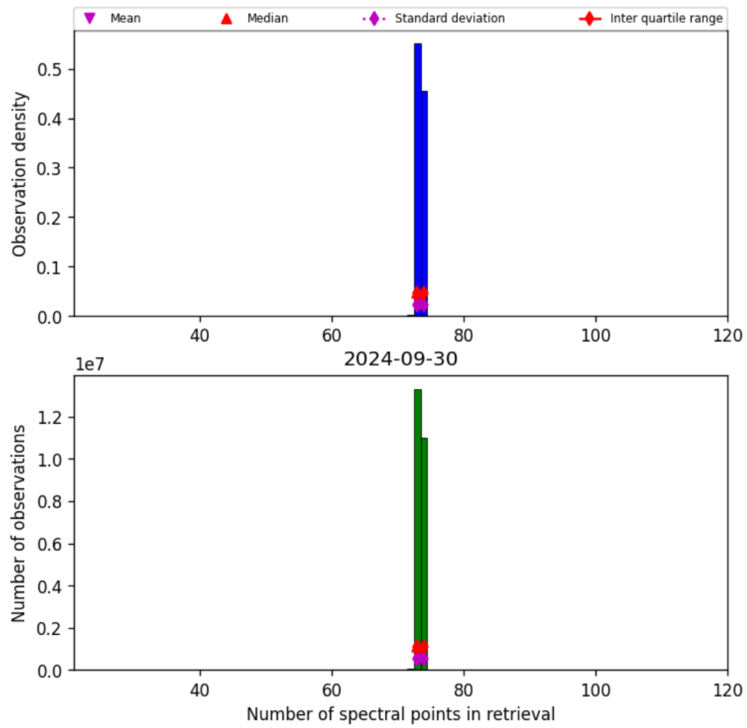
Figure 74: Histogram of “Number of spectral points in retrieval” for 2024-09-29 to 2024-10-01
