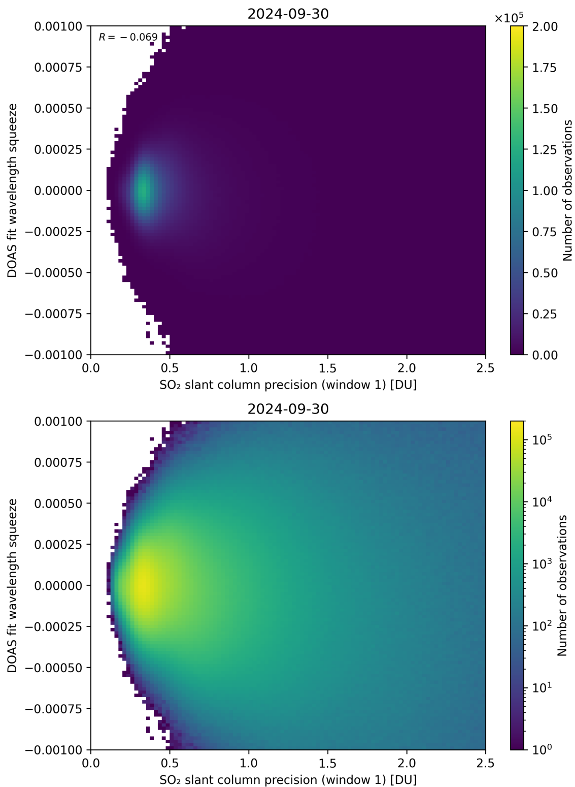
Figure 222: Scatter density plot of “SO 2 slant column precision (window 1)” against “DOAS fit wavelength squeeze” for 2024-09-29 to 2024-10-01.
