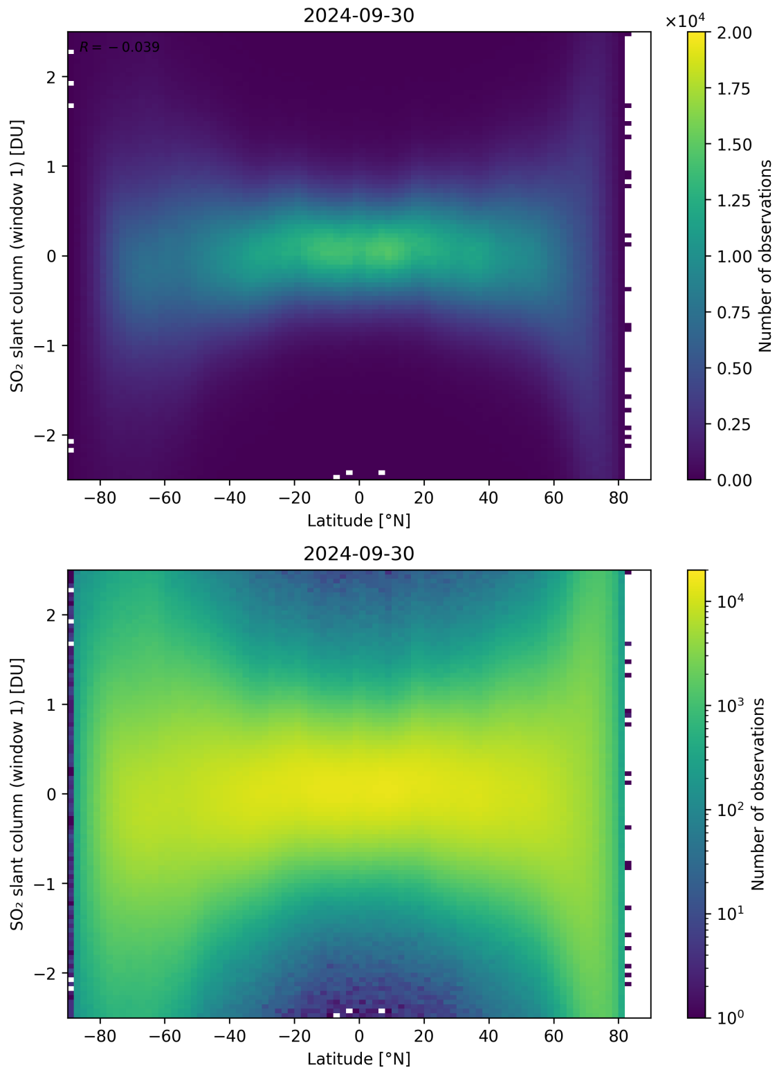
Figure 149: Scatter density plot of “Latitude” against “SO 2 slant column (window 1)” for 2024-09-29 to 2024-10-01.
