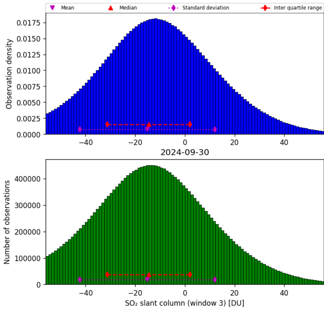
Figure 64: Histogram of “SO 2 slant column (window 3)” for 2024-09-29 to 2024-10-01
