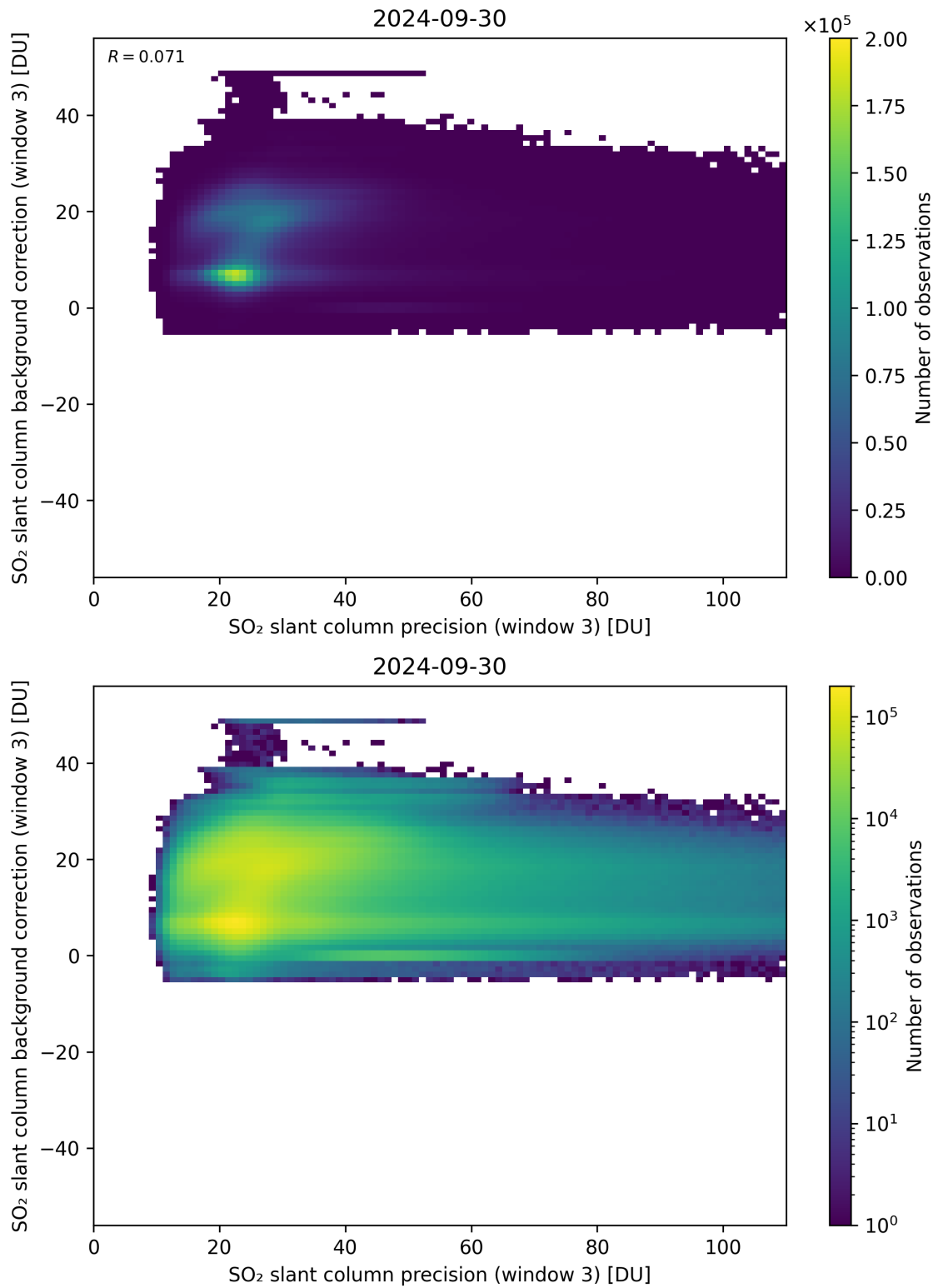
Figure 257: Scatter density plot of “SO 2 slant column precision (window 3)” against “SO 2 slant column background correction (window 3)” for 2024-09-29 to 2024-10-01.
