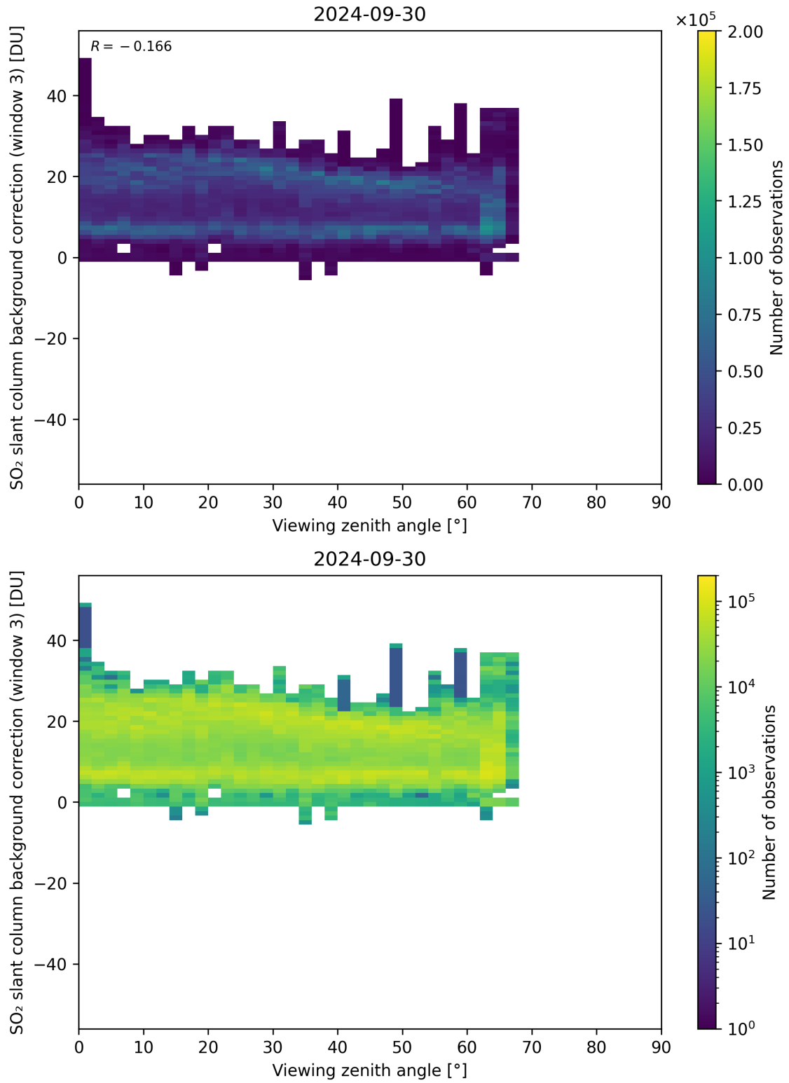
Figure 310: Scatter density plot of “Viewing zenith angle” against “SO 2 slant column background correction (window 3)” for 2024-09-29 to 2024-10-01.
