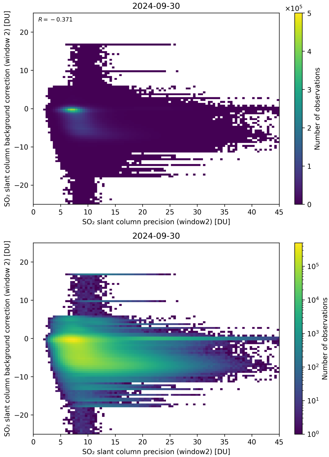
Figure 241: Scatter density plot of “SO 2 slant column precision (window2)” against “SO 2 slant column background correction (window 2)” for 2024-09-29 to 2024-10-01.
