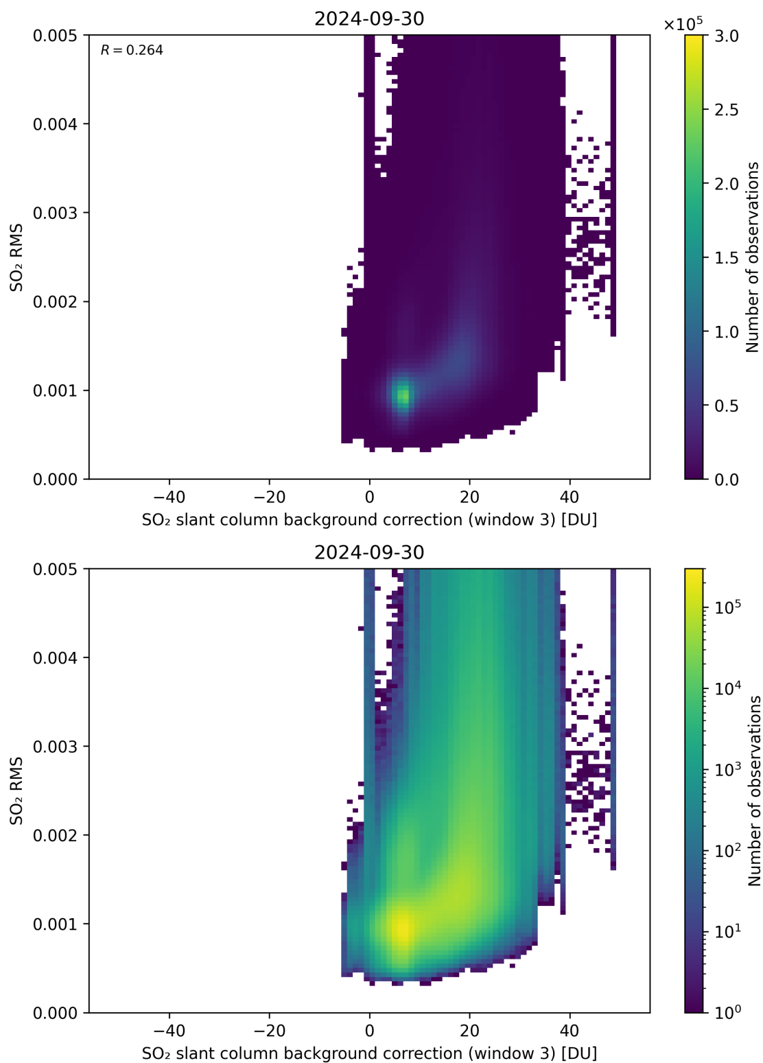
Figure 123: Scatter density plot of “SO 2 slant column background correction (window 3)” against “SO 2 RMS” for 2024-09-29 to 2024-10-01.
