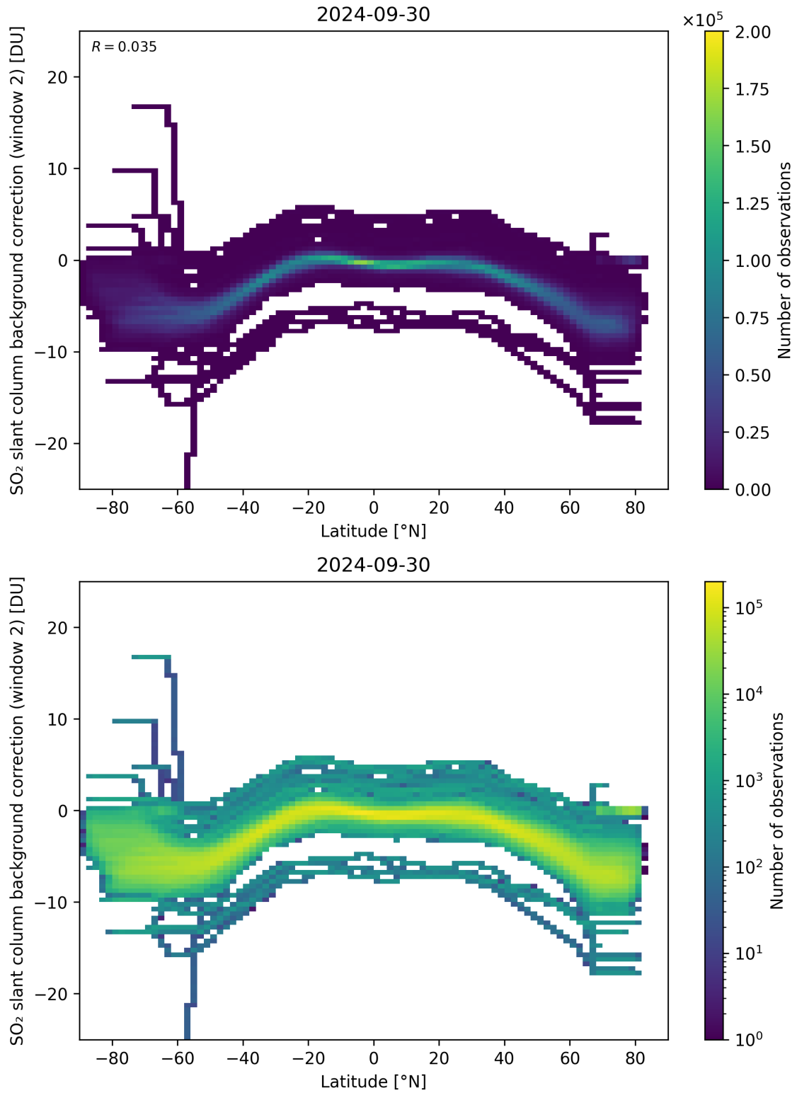
Figure 140: Scatter density plot of “Latitude” against “SO 2 slant column background correction (window 2)” for 2024-09-29 to 2024-10-01.
