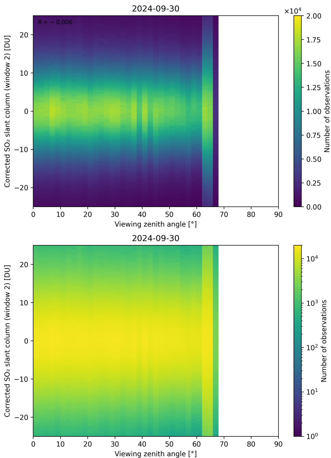
Figure 318: Scatter density plot of “Viewing zenith angle” against “Corrected SO 2 slant column (window 2)” for 2024-09-29 to 2024-10-01.
