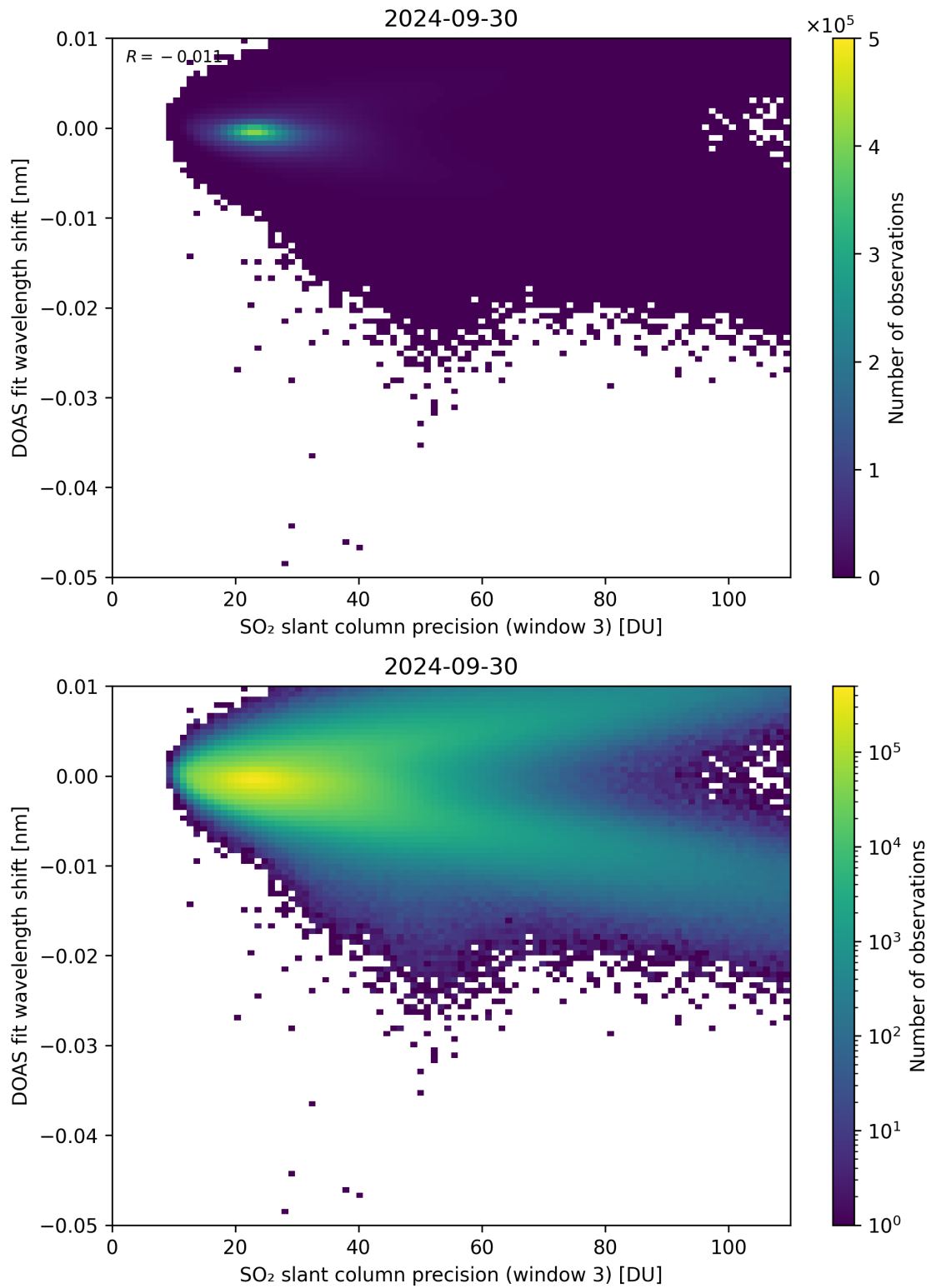
Figure 258: Scatter density plot of “SO 2 slant column precision (window 3)” against “DOAS fit wavelength shift” for 2024-09-29 to 2024-10-01.
