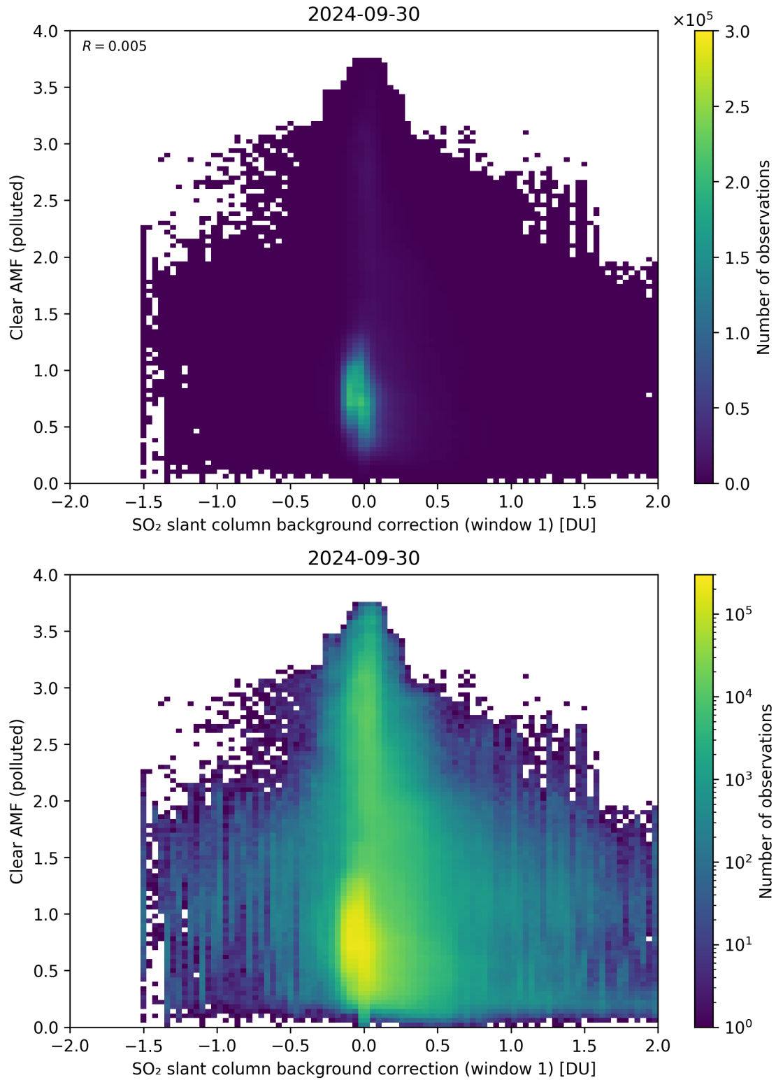
Figure 103: Scatter density plot of “SO 2 slant column background correction (window 1)” against “Clear AMF (polluted)” for 2024-09-29 to 2024-10-01.
