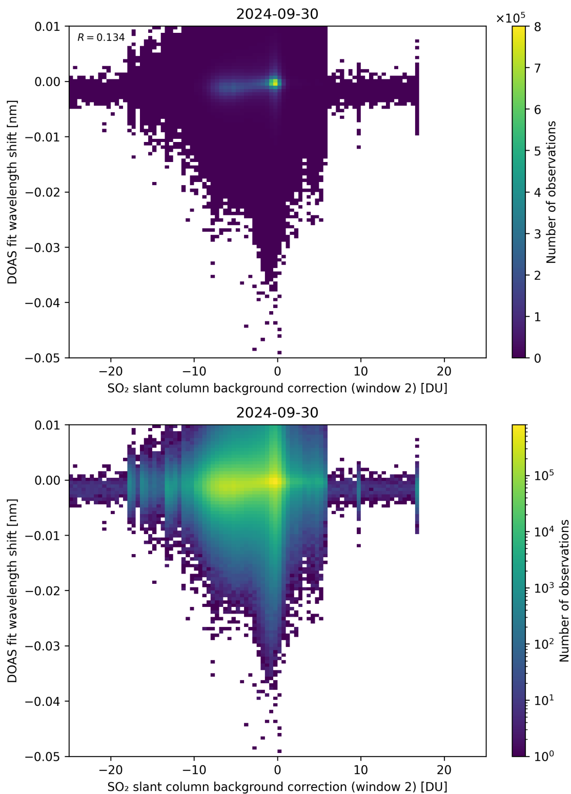
Figure 112: Scatter density plot of “SO 2 slant column background correction (window 2)” against “DOAS fit wavelength shift” for 2024-09-29 to 2024-10-01.
