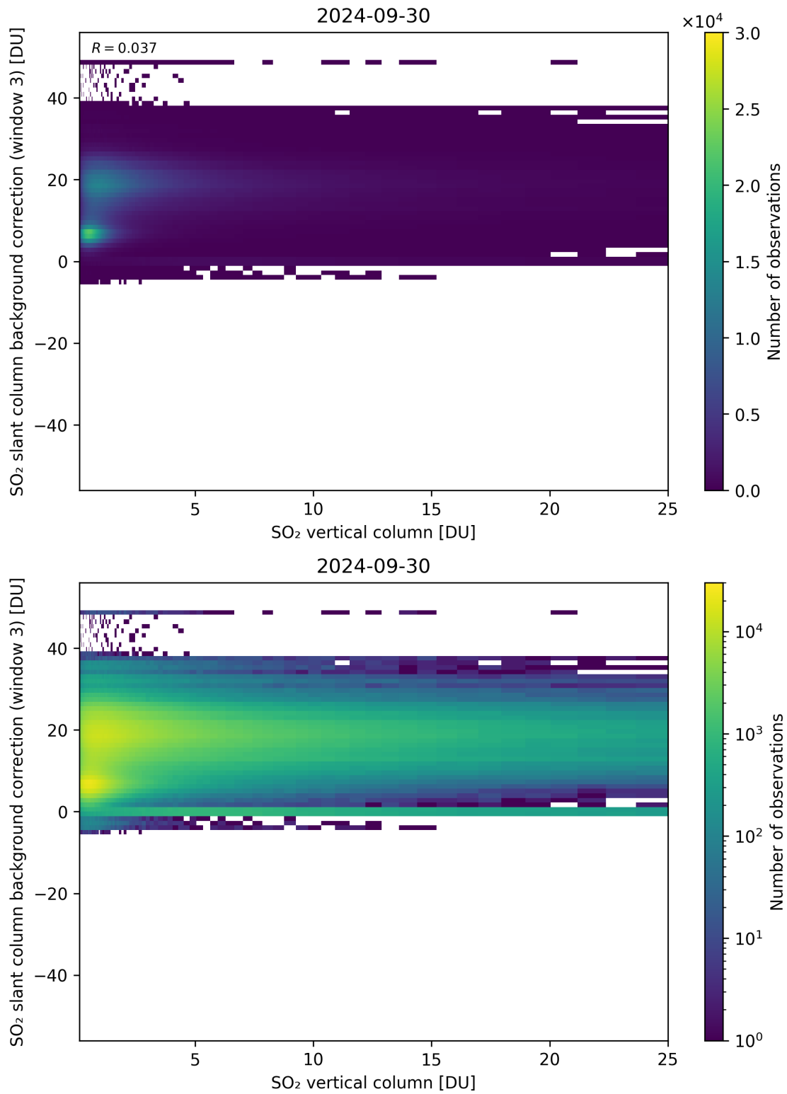
Figure 275: Scatter density plot of “SO 2 vertical column” against “SO 2 slant column background correction (window 3)” for 2024-09-29 to 2024-10-01.
