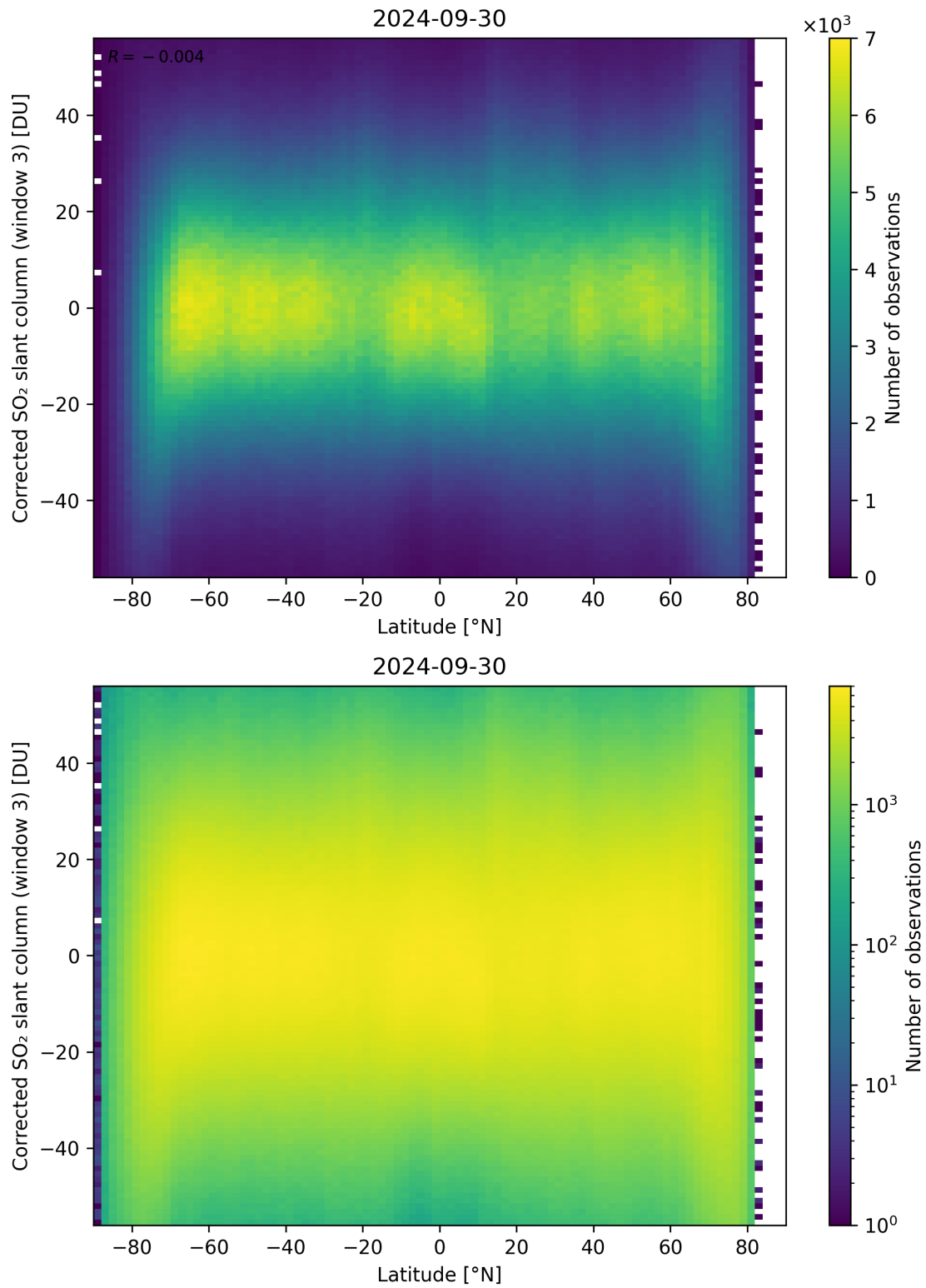
Figure 148: Scatter density plot of “Latitude” against “Corrected SO 2 slant column (window 3)” for 2024-09-29 to 2024-10-01.
