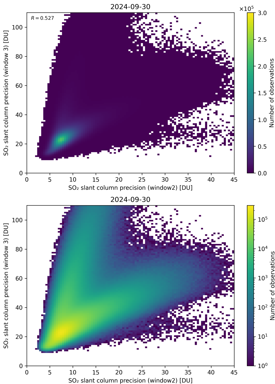
Figure 250: Scatter density plot of “SO 2 slant column precision (window2)” against “SO 2 slant column precision (window 3)” for 2024-09-29 to 2024-10-01.
