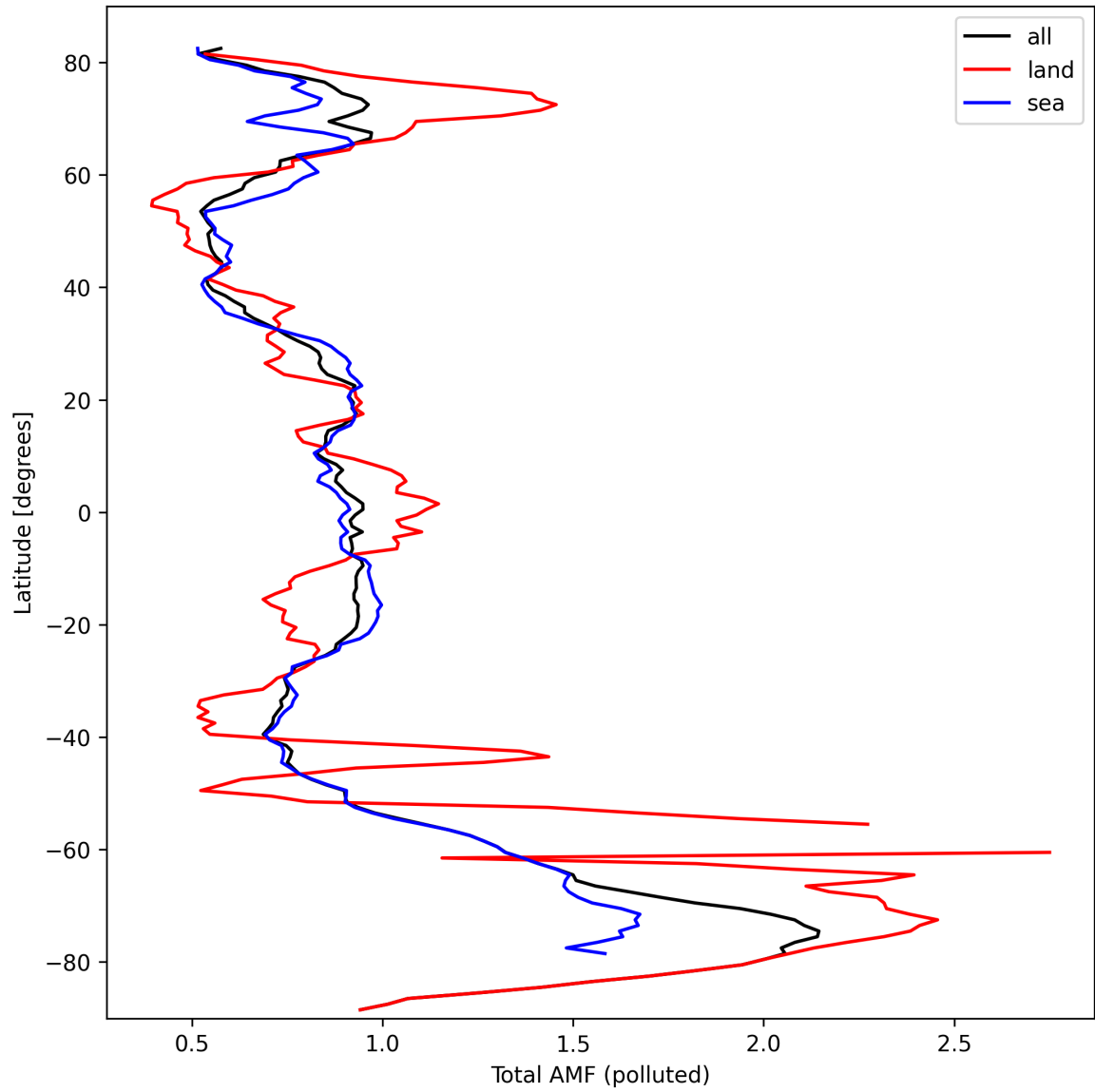
Figure 48: Zonal average of “Total AMF (polluted)” for 2024-09-29 to 2024-10-01.
