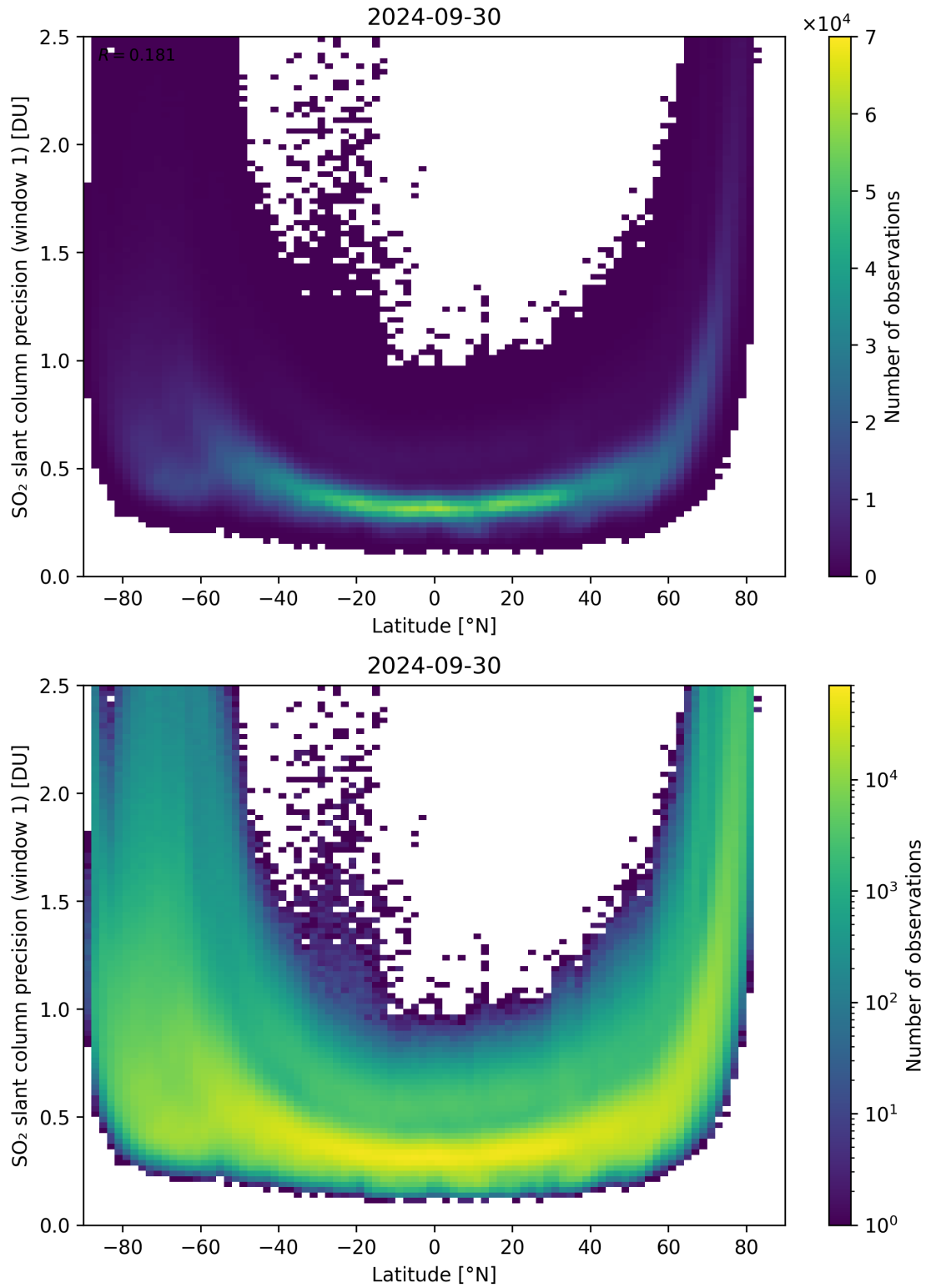
Figure 150: Scatter density plot of “Latitude” against “SO 2 slant column precision (window 1)” for 2024-09-29 to 2024-10-01.
