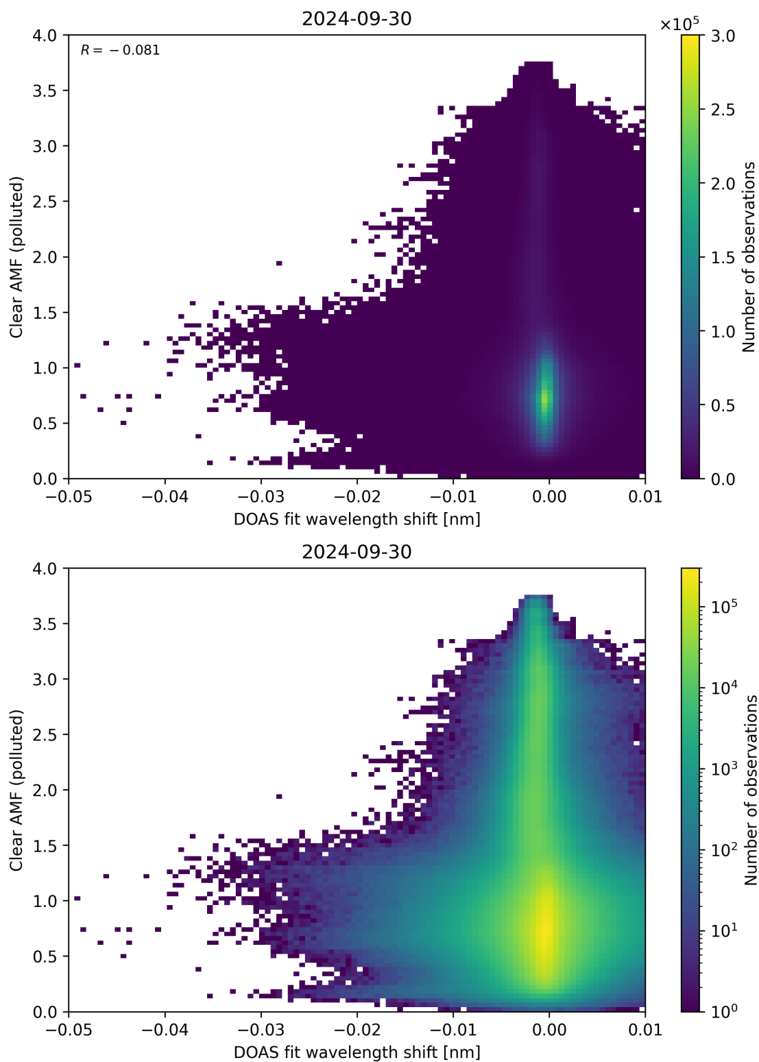
Figure 129: Scatter density plot of “DOAS fit wavelength shift” against “Clear AMF (polluted)” for 2024-09-29 to 2024-10-01.
