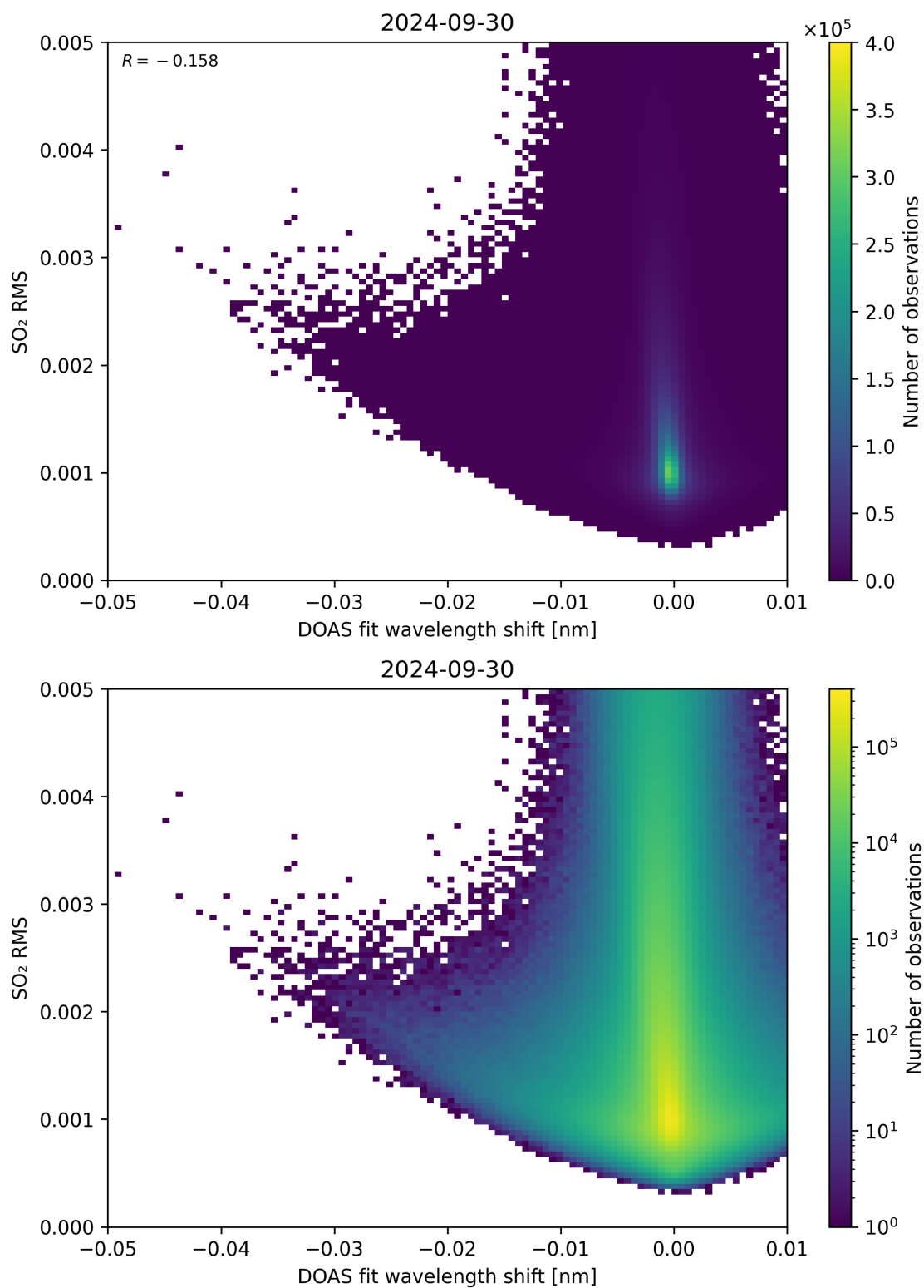
Figure 128: Scatter density plot of “DOAS fit wavelength shift” against “SO 2 RMS” for 2024-09-29 to 2024-10-01.
