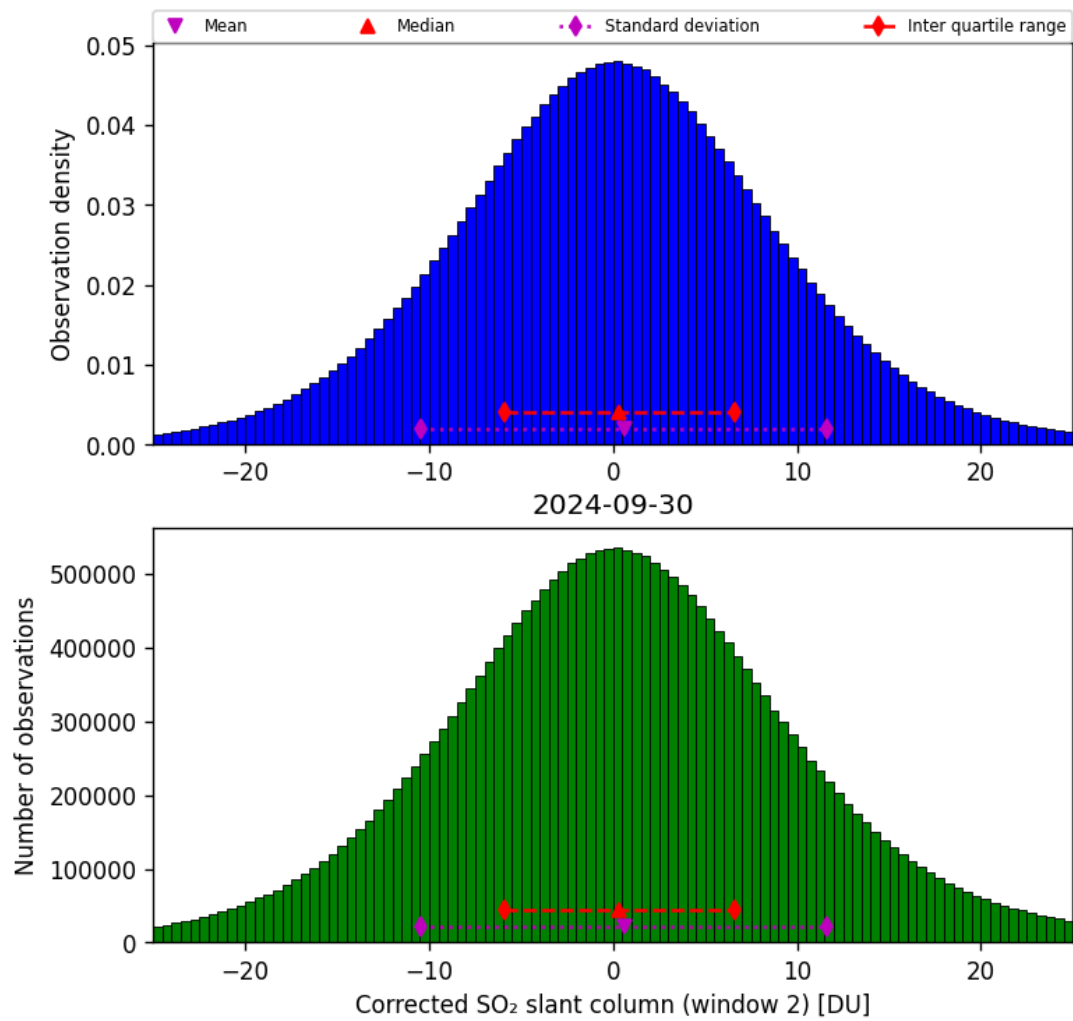
Figure 62: Histogram of “Corrected SO 2 slant column (window 2)” for 2024-09-29 to 2024-10-01
