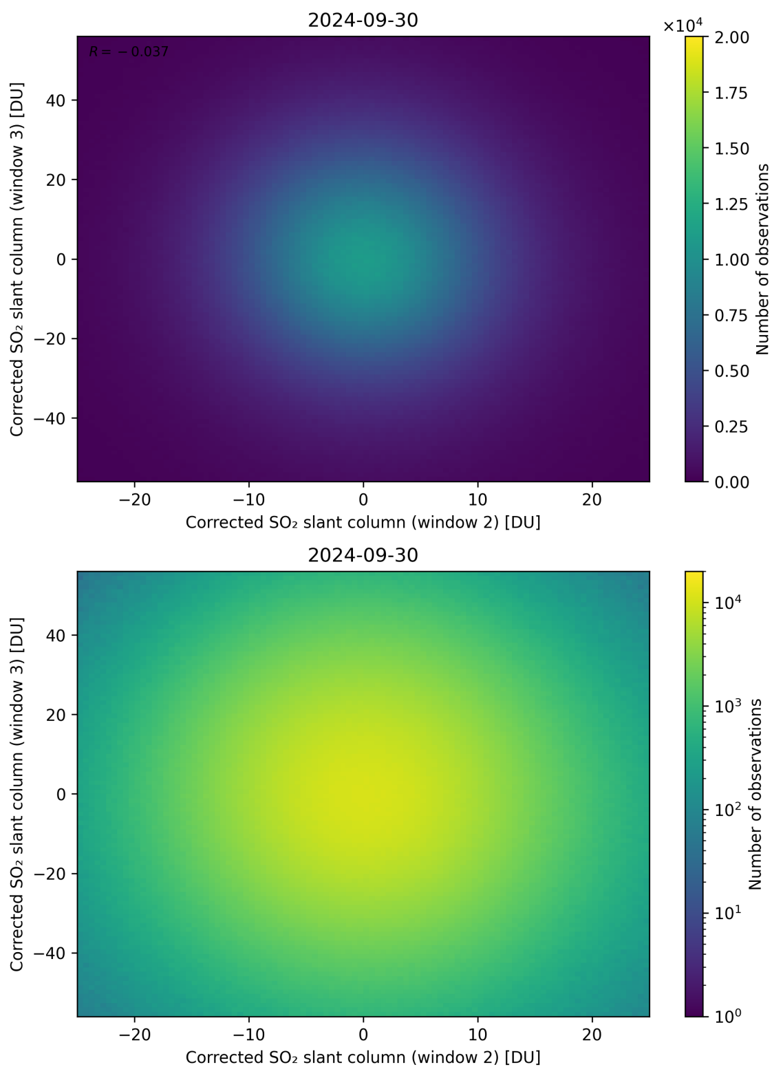
Figure 200: Scatter density plot of “Corrected SO 2 slant column (window 2)” against “Corrected SO 2 slant column (window 3)” for 2024-09-29 to 2024-10-01.
