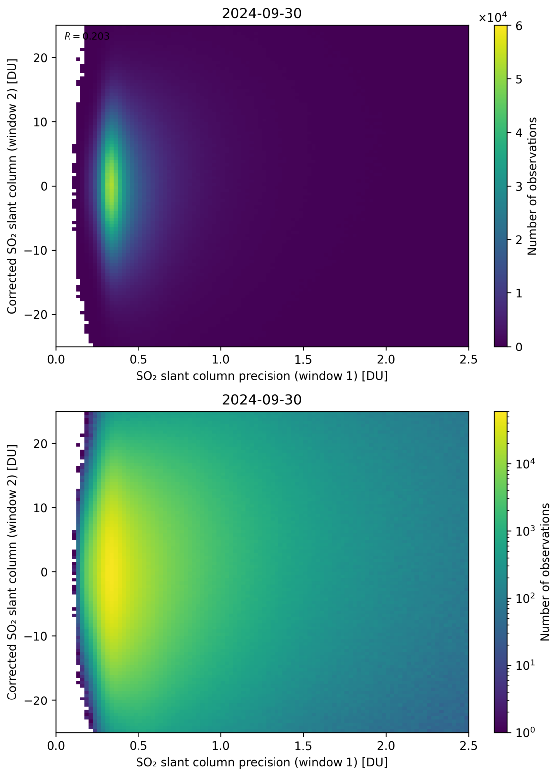
Figure 225: Scatter density plot of “SO 2 slant column precision (window 1)” against “Corrected SO 2 slant column (window 2)” for 2024-09-29 to 2024-10-01.
