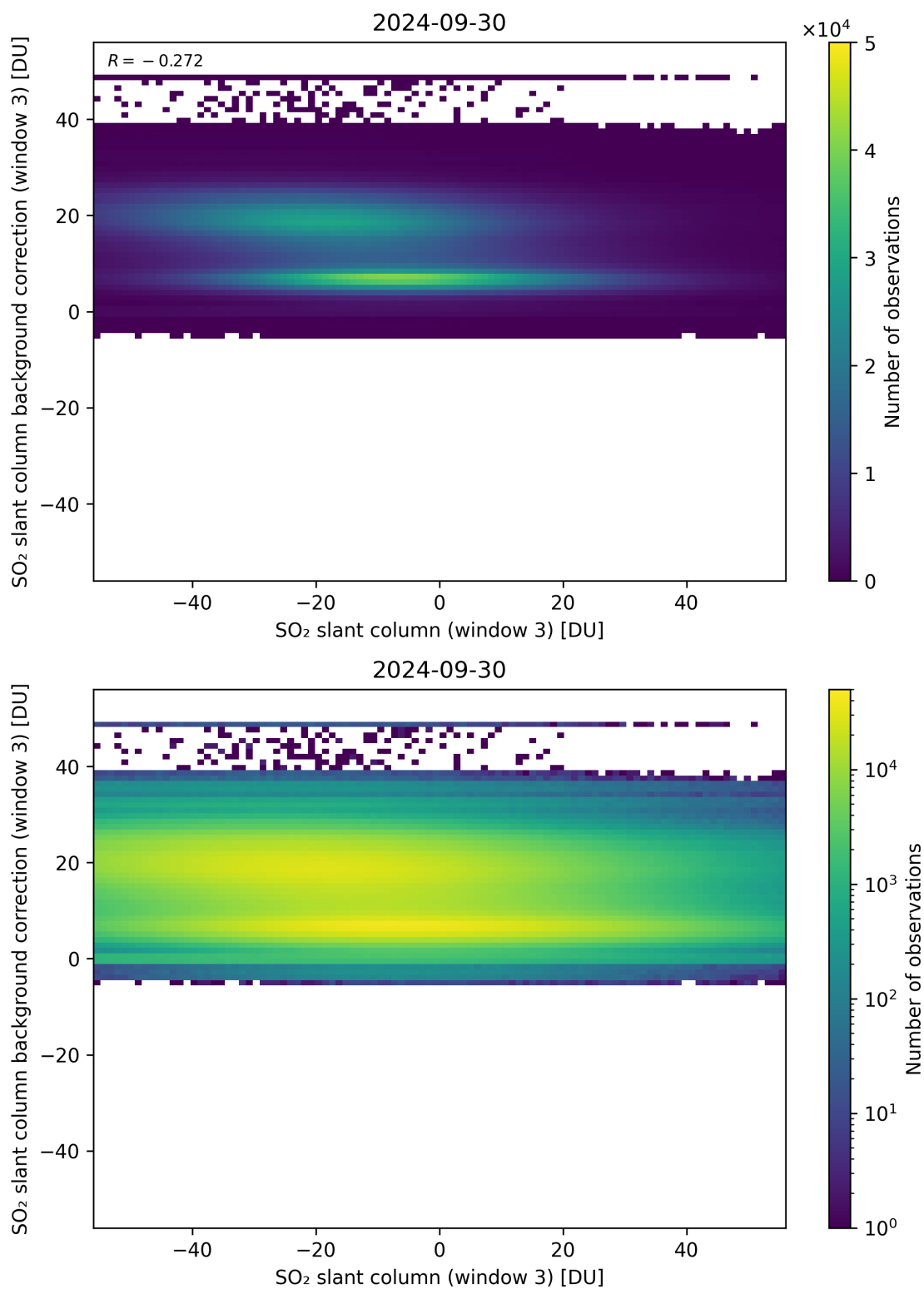
Figure 253: Scatter density plot of “SO 2 slant column (window 3)” against “SO 2 slant column background correction (window 3)” for 2024-09-29 to 2024-10-01.
