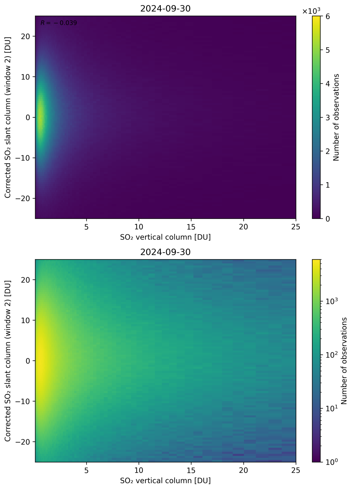
Figure 298: Scatter density plot of “SO 2 vertical column” against “Corrected SO 2 slant column (window 2)” for 2024-09-29 to 2024-10-01.
