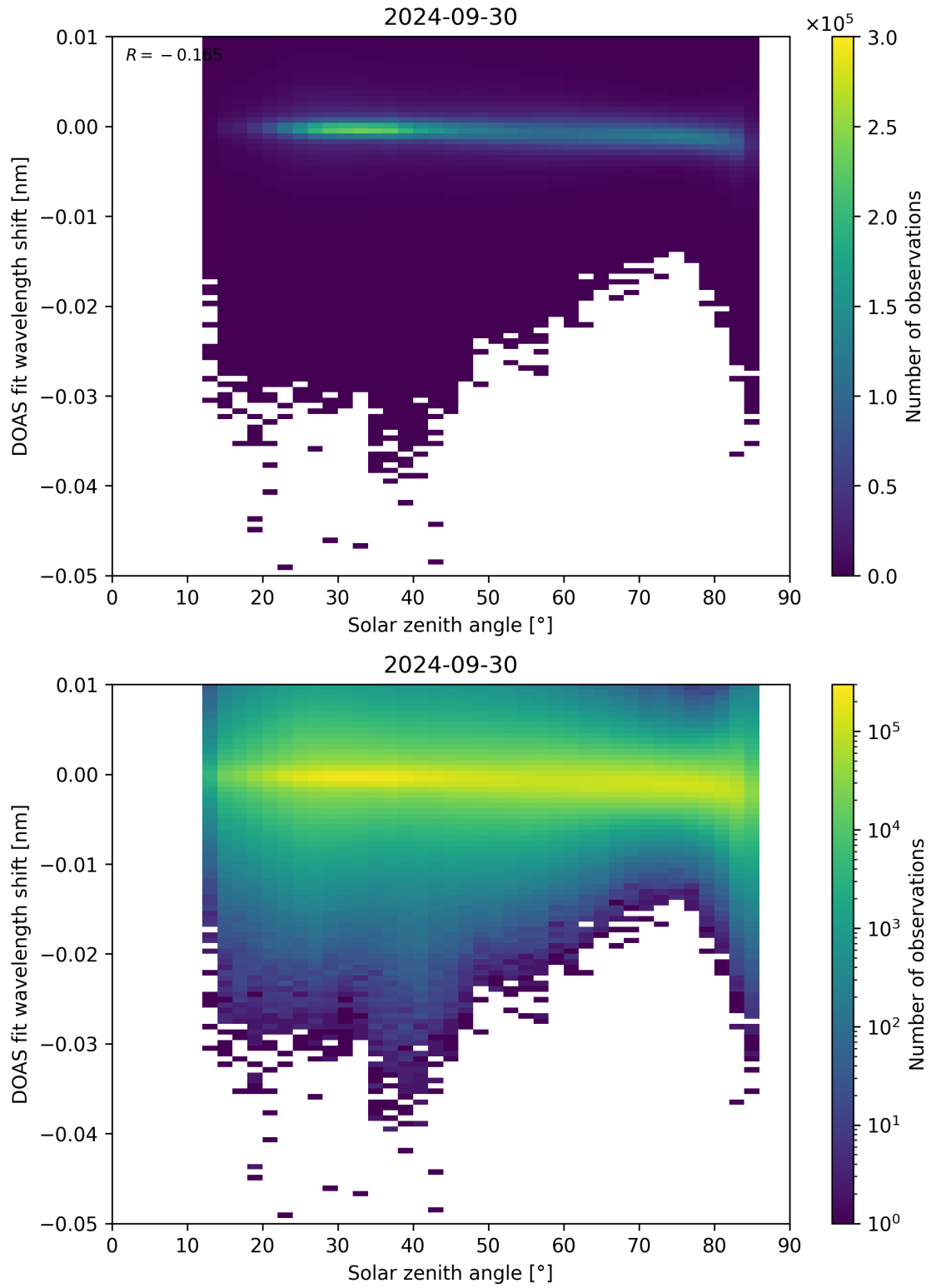
Figure 161: Scatter density plot of “Solar zenith angle” against “DOAS fit wavelength shift” for 2024-09-29 to 2024-10-01.
