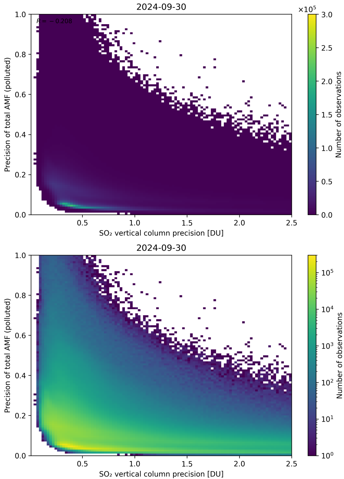
Figure 295: Scatter density plot of “SO 2 vertical column precision” against “Precision of total AMF (polluted)” for 2024-09-29 to 2024-10-01.
