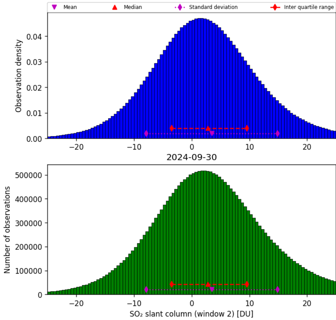
Figure 60: Histogram of “SO 2 slant column (window 2)” for 2024-09-29 to 2024-10-01
