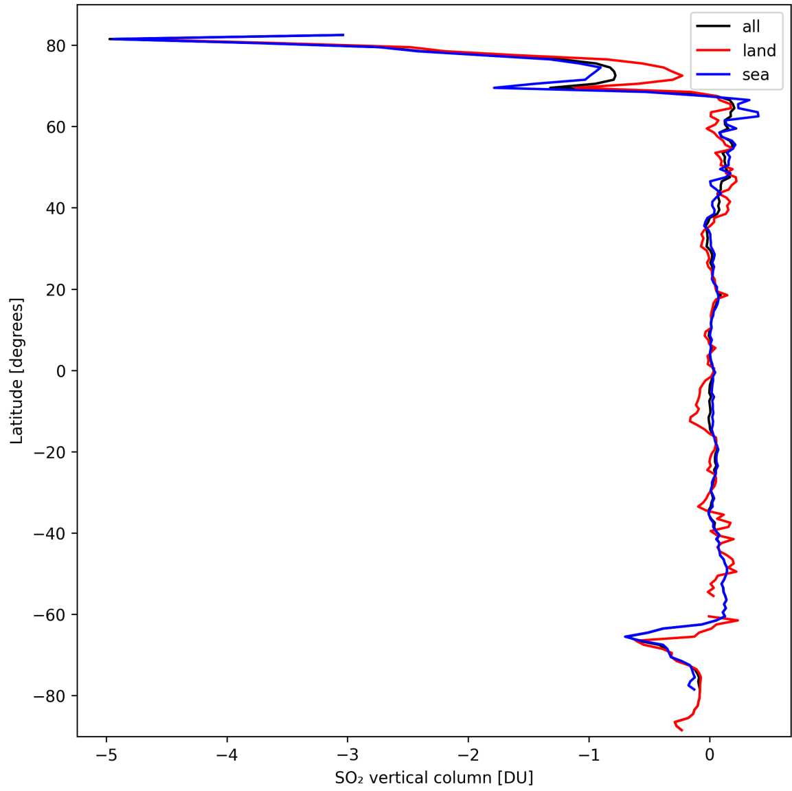
Figure 30: Zonal average of “SO 2 vertical column” for 2024-09-29 to 2024-10-01.
