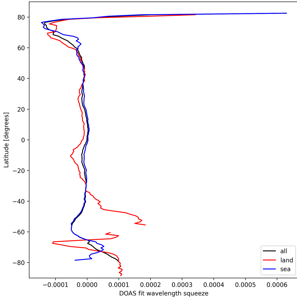
Figure 46: Zonal average of “DOAS fit wavelength squeeze” for 2024-09-29 to 2024-10-01.
