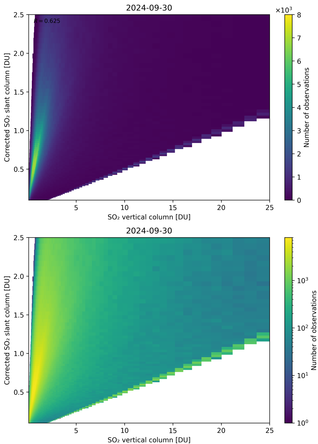
Figure 297: Scatter density plot of “SO 2 vertical column” against “Corrected SO 2 slant column” for 2024-09-29 to 2024-10-01.
