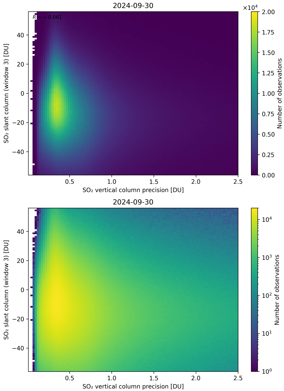
Figure 292: Scatter density plot of “SO 2 vertical column precision” against “SO 2 slant column (window 3)” for 2024-09-29 to 2024-10-01.
