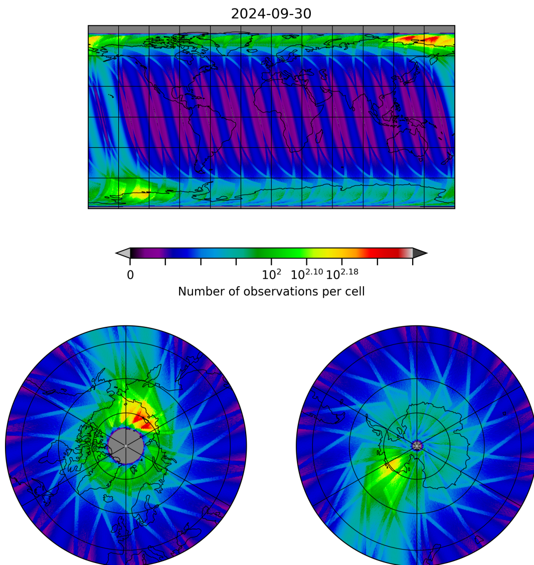
Figure 28: Map of the number of observations for 2024-09-29 to 2024-10-01
