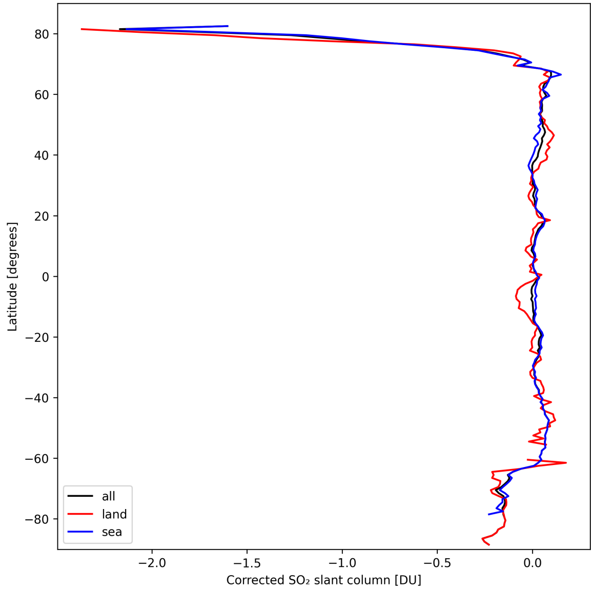
Figure 32: Zonal average of “Corrected SO 2 slant column” for 2024-09-29 to 2024-10-01.
