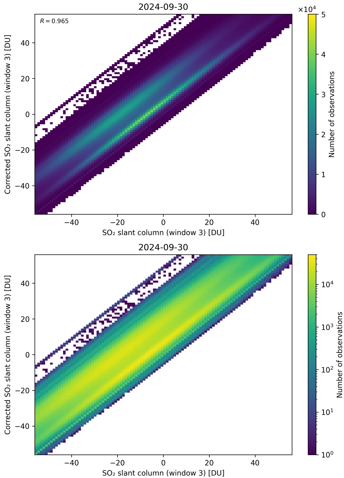
Figure 266: Scatter density plot of “SO 2 slant column (window 3)” against “Corrected SO 2 slant column (window 3)” for 2024-09-29 to 2024-10-01.
