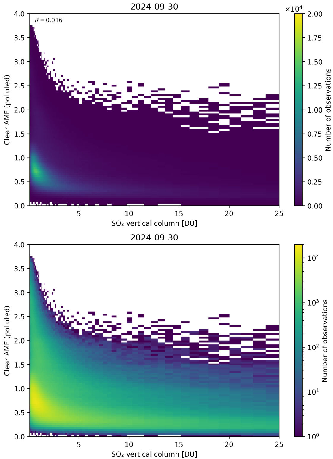
Figure 296: Scatter density plot of “SO 2 vertical column” against “Clear AMF (polluted)” for 2024-09-29 to 2024-10-01.
