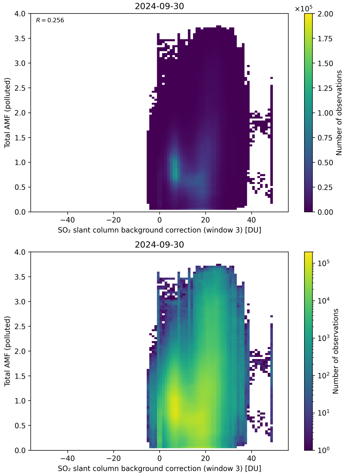
Figure 125: Scatter density plot of “SO 2 slant column background correction (window 3)” against “Total AMF (polluted)” for 2024-09-29 to 2024-10-01.
