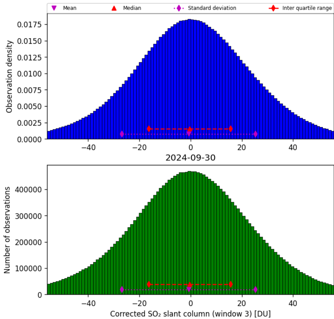
Figure 66: Histogram of “Corrected SO 2 slant column (window 3)” for 2024-09-29 to 2024-10-01
