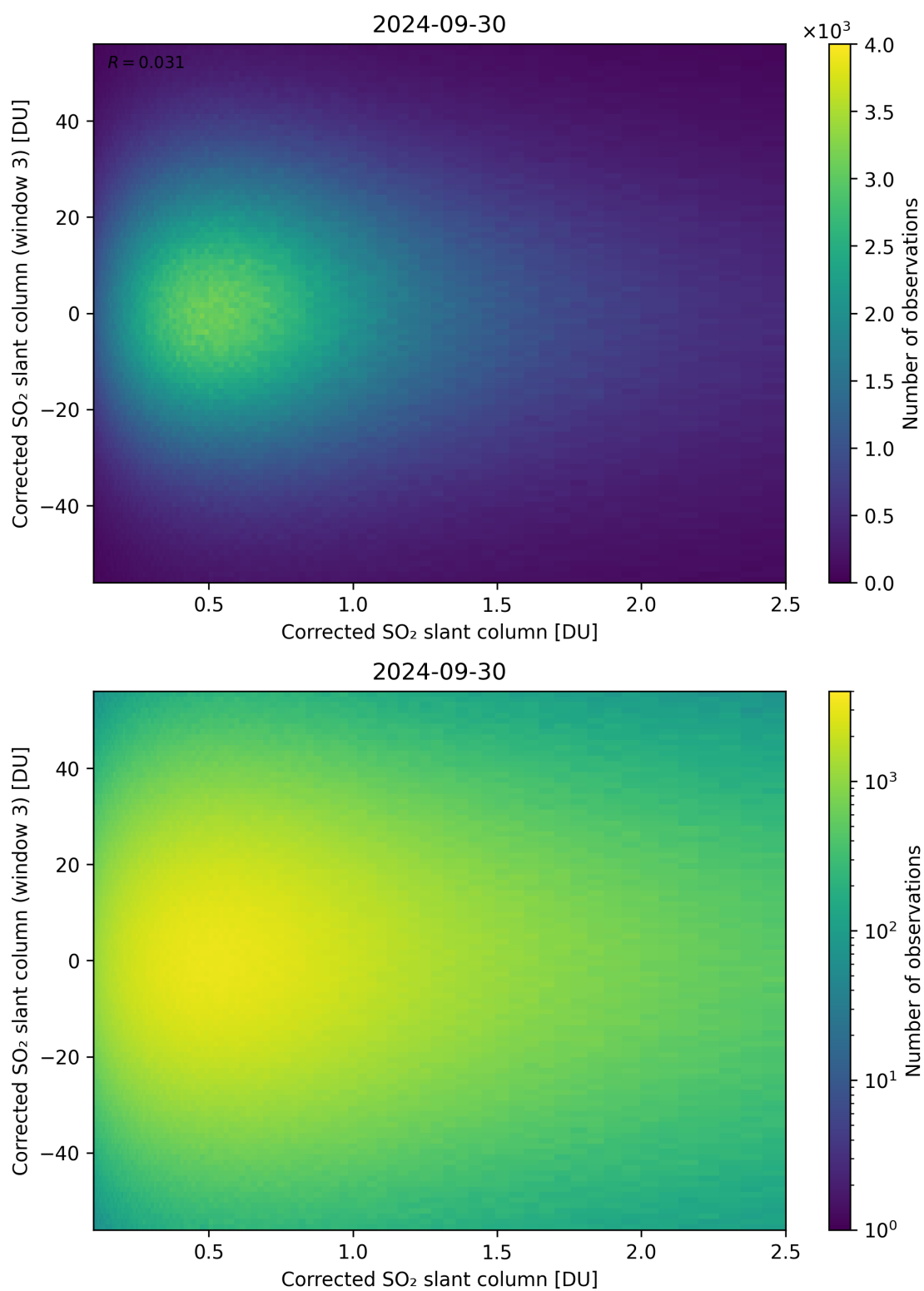
Figure 186: Scatter density plot of “Corrected SO 2 slant column” against “Corrected SO 2 slant column (window 3)” for 2024-09-29 to 2024-10-01.
