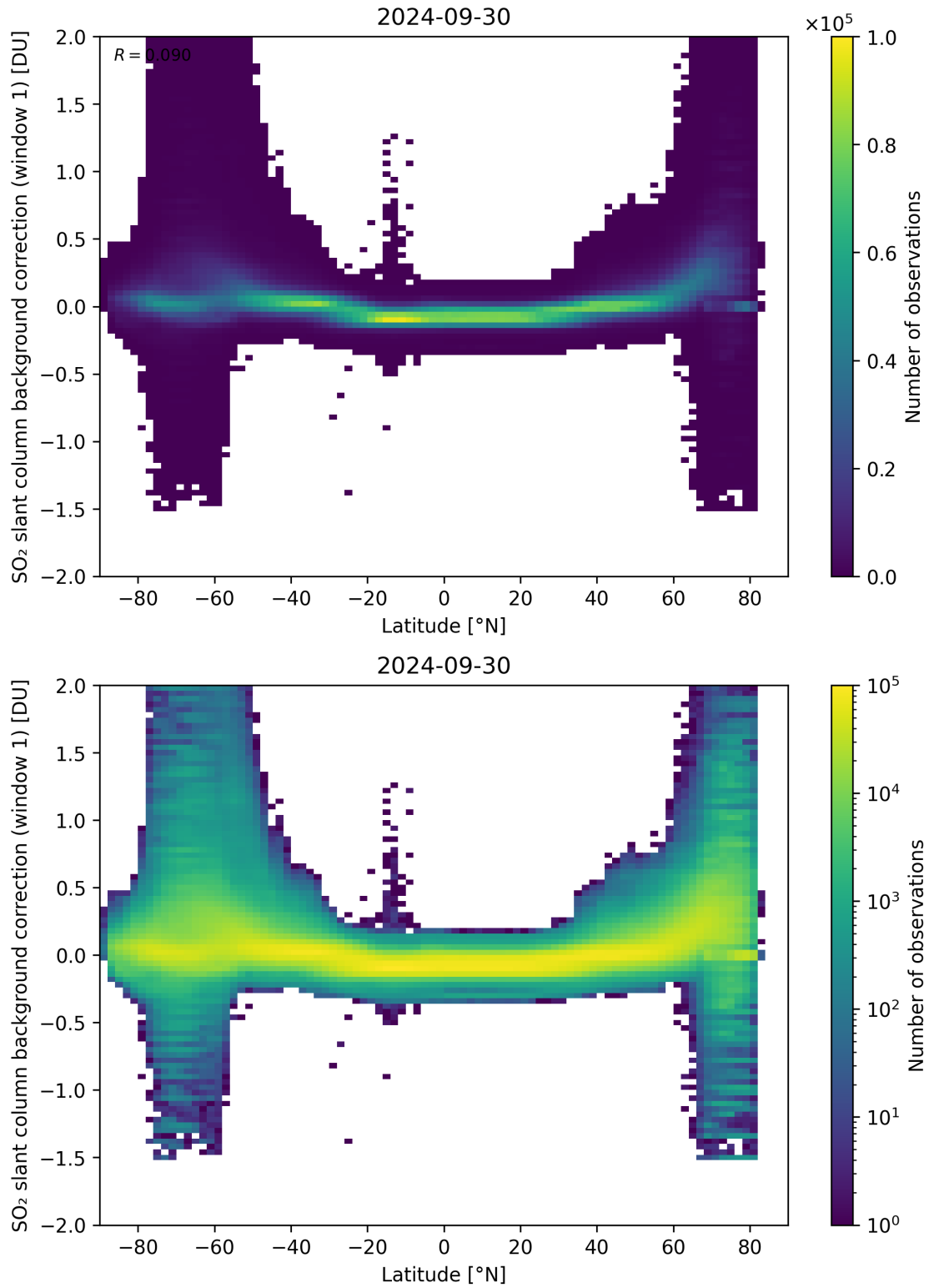
Figure 139: Scatter density plot of “Latitude” against “SO 2 slant column background correction (window 1)” for 2024-09-29 to 2024-10-01.
