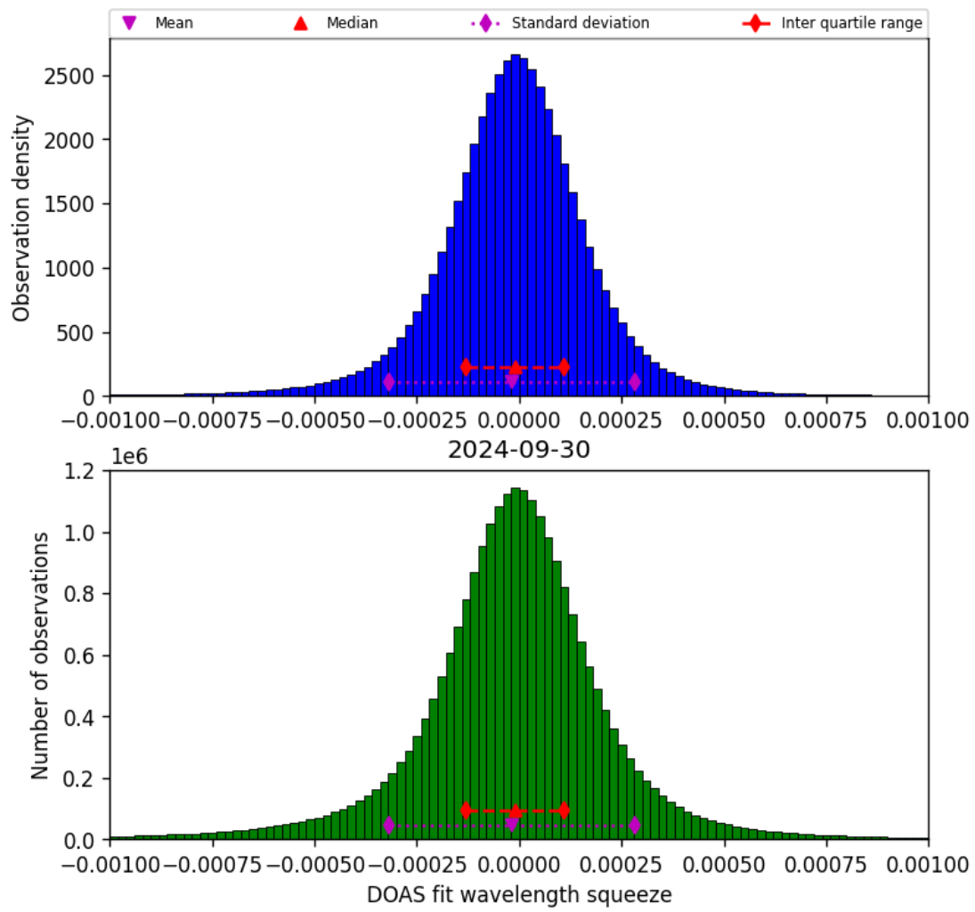
Figure 69: Histogram of “DOAS fit wavelength squeeze” for 2024-09-29 to 2024-10-01
