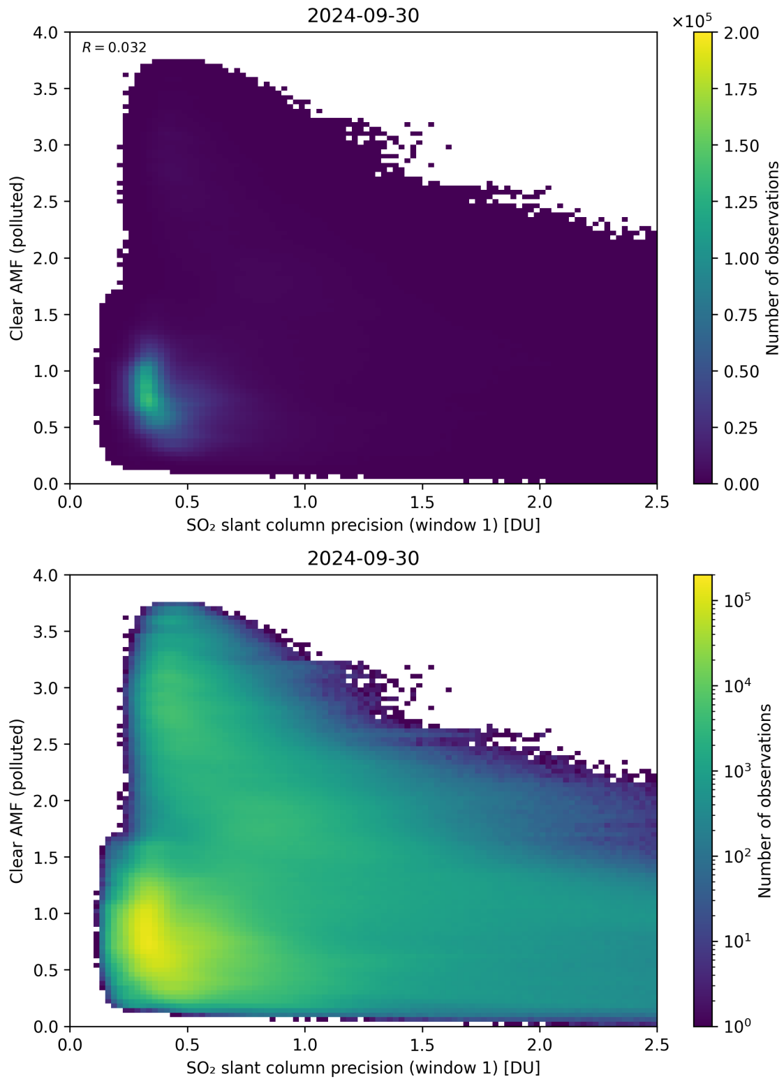
Figure 224: Scatter density plot of “SO 2 slant column precision (window 1)” against “Clear AMF (polluted)” for 2024-09-29 to 2024-10-01.
