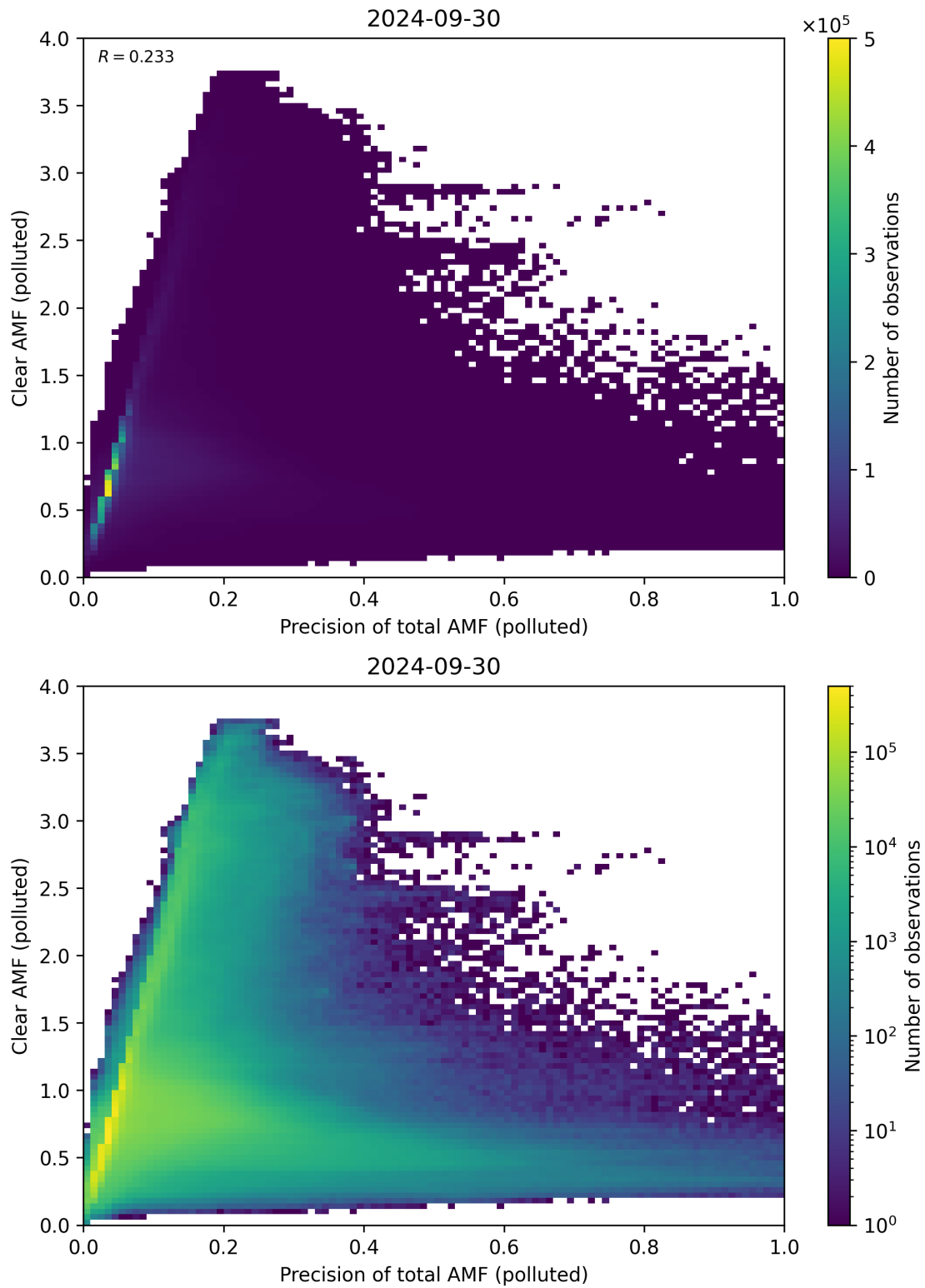
Figure 270: Scatter density plot of “Precision of total AMF (polluted)” against “Clear AMF (polluted)” for 2024-09-29 to 2024-10-01.
