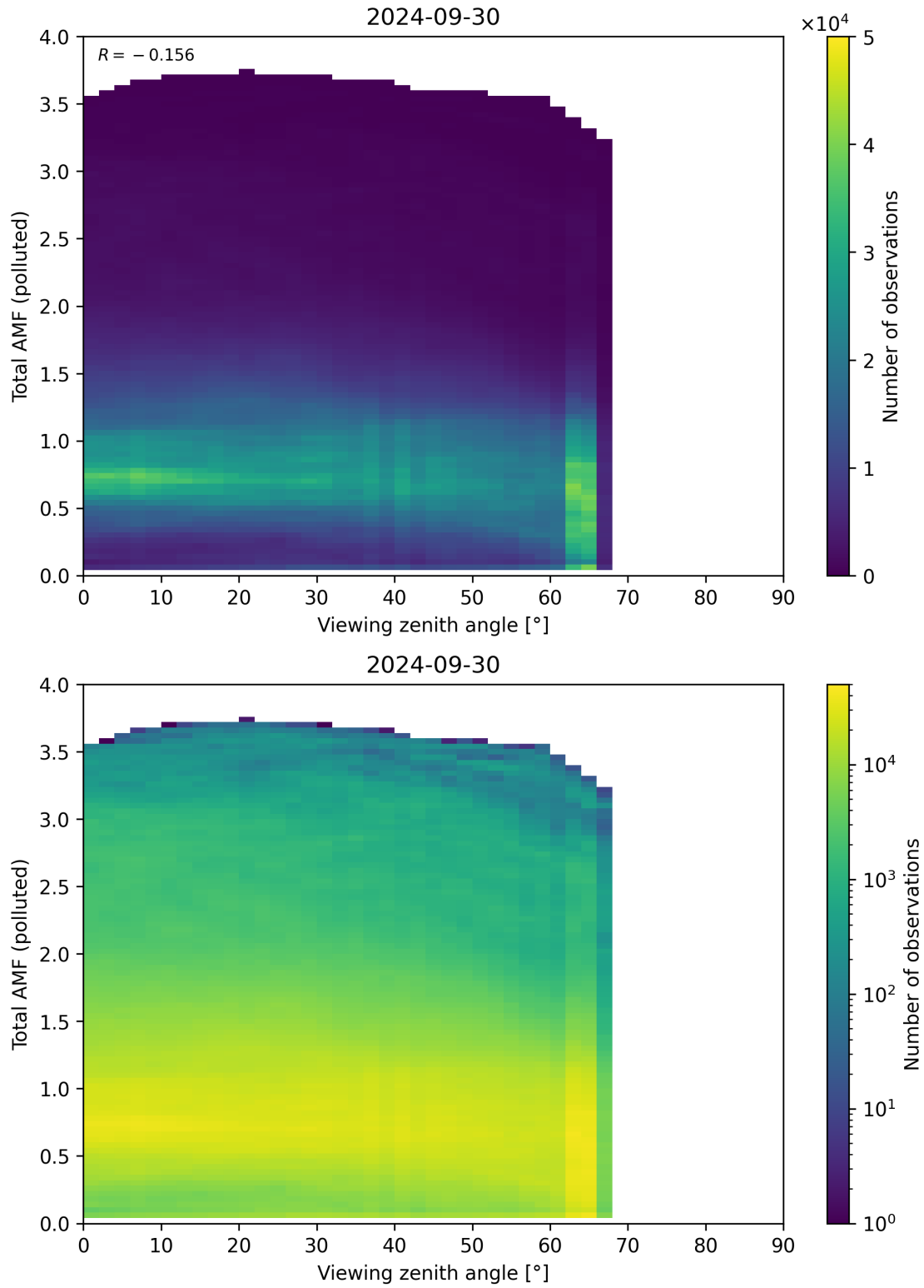
Figure 325: Scatter density plot of “Viewing zenith angle” against “Total AMF (polluted)” for 2024-09-29 to 2024-10-01.
