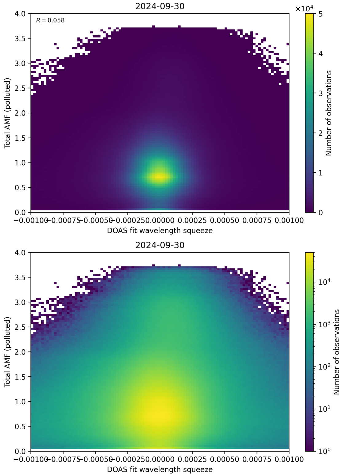
Figure 134: Scatter density plot of “DOAS fit wavelength squeeze” against “Total AMF (polluted)” for 2024-09-29 to 2024-10-01.
