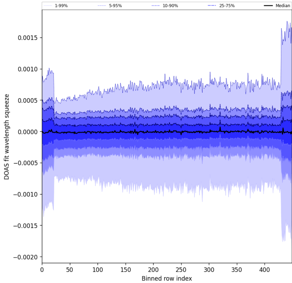
Figure 92: Along track statistics of “DOAS fit wavelength squeeze” for 2024-09-29 to 2024-10-01
