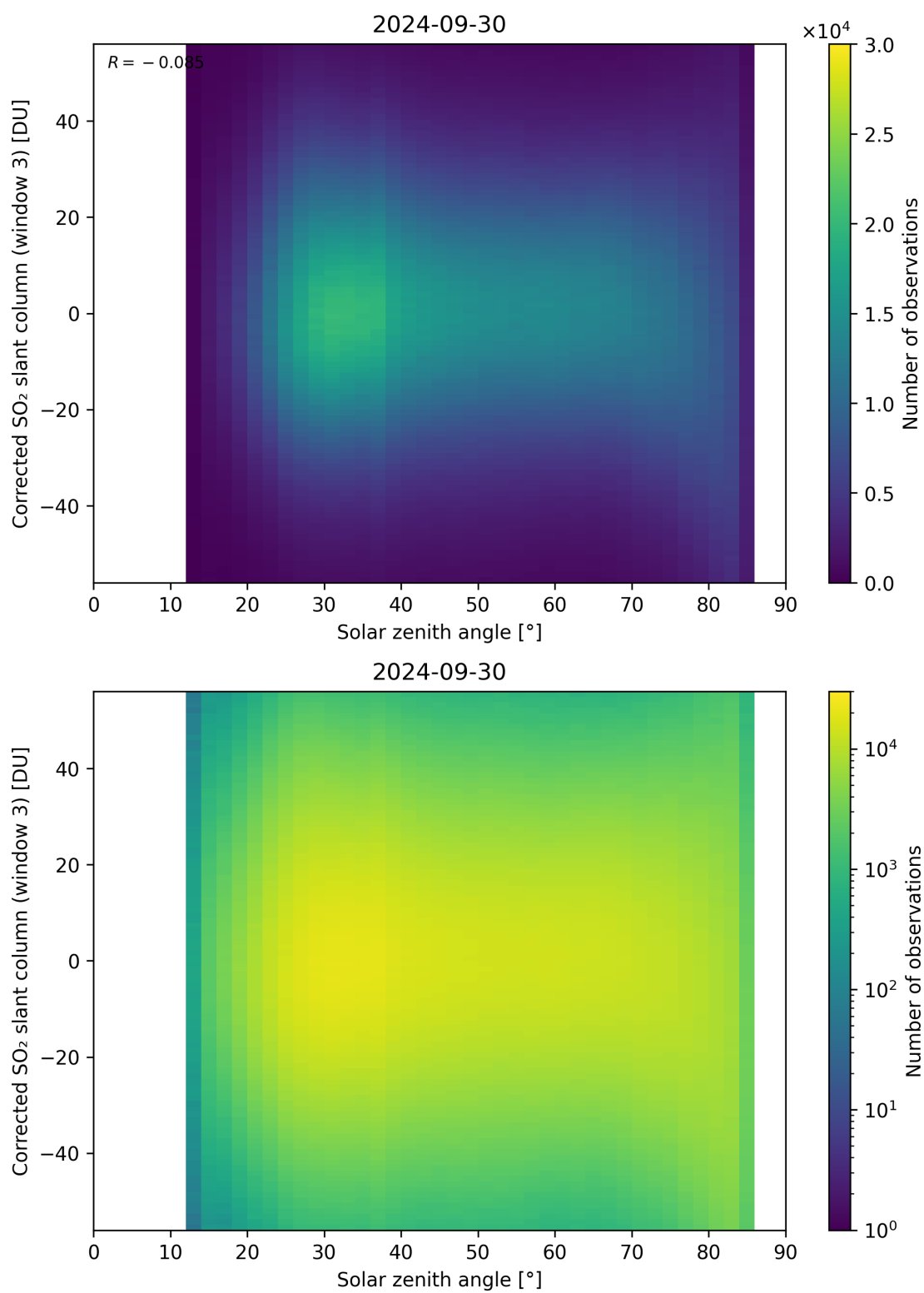
Figure 168: Scatter density plot of “Solar zenith angle” against “Corrected SO 2 slant column (window 3)” for 2024-09-29 to 2024-10-01.
