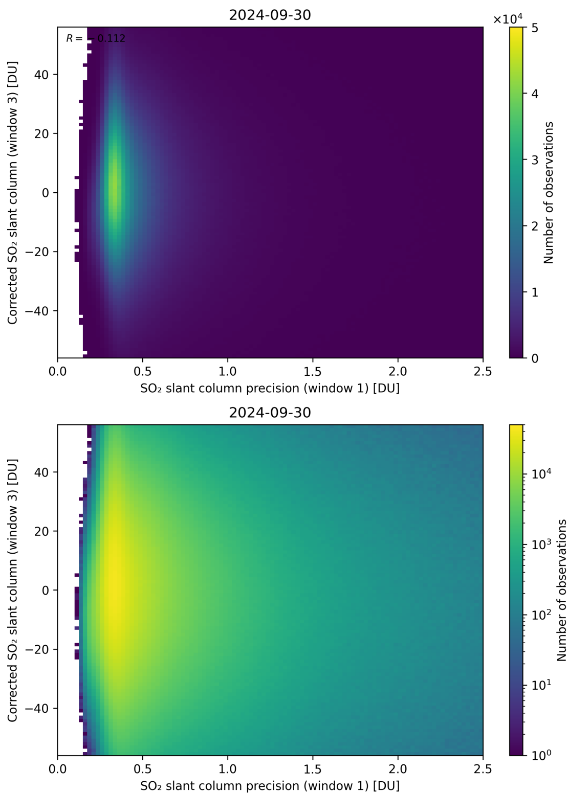
Figure 226: Scatter density plot of “SO 2 slant column precision (window 1)” against “Corrected SO 2 slant column (window 3)” for 2024-09-29 to 2024-10-01.
