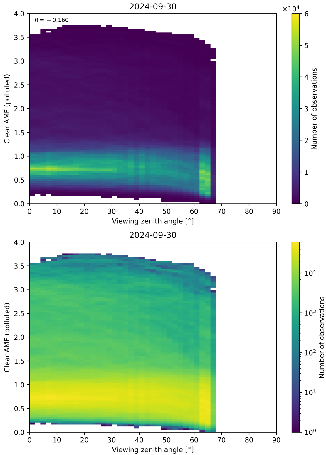
Figure 316: Scatter density plot of “Viewing zenith angle” against “Clear AMF (polluted)” for 2024-09-29 to 2024-10-01.
