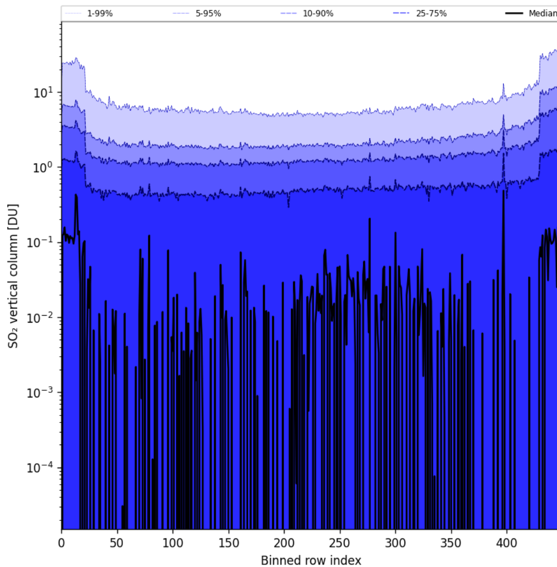
Figure 76: Along track statistics of “SO 2 vertical column” for 2024-09-29 to 2024-10-01
