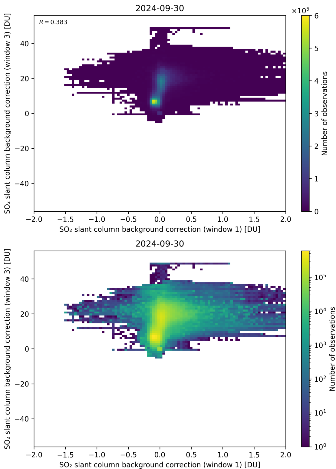
Figure 99: Scatter density plot of “SO 2 slant column background correction (window 1)” against “SO 2 slant column background correction (window 3)” for 2024-09-29 to 2024-10-01.
