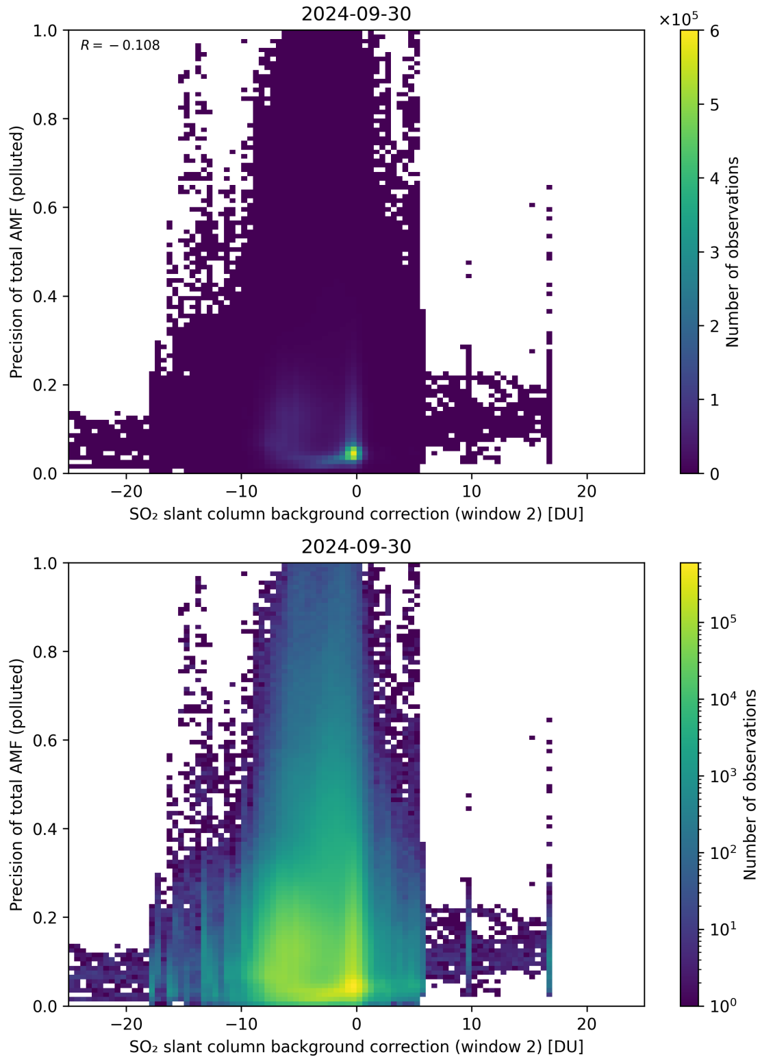
Figure 120: Scatter density plot of “SO 2 slant column background correction (window 2)” against “Precision of total AMF (polluted)” for 2024-09-29 to 2024-10-01.
