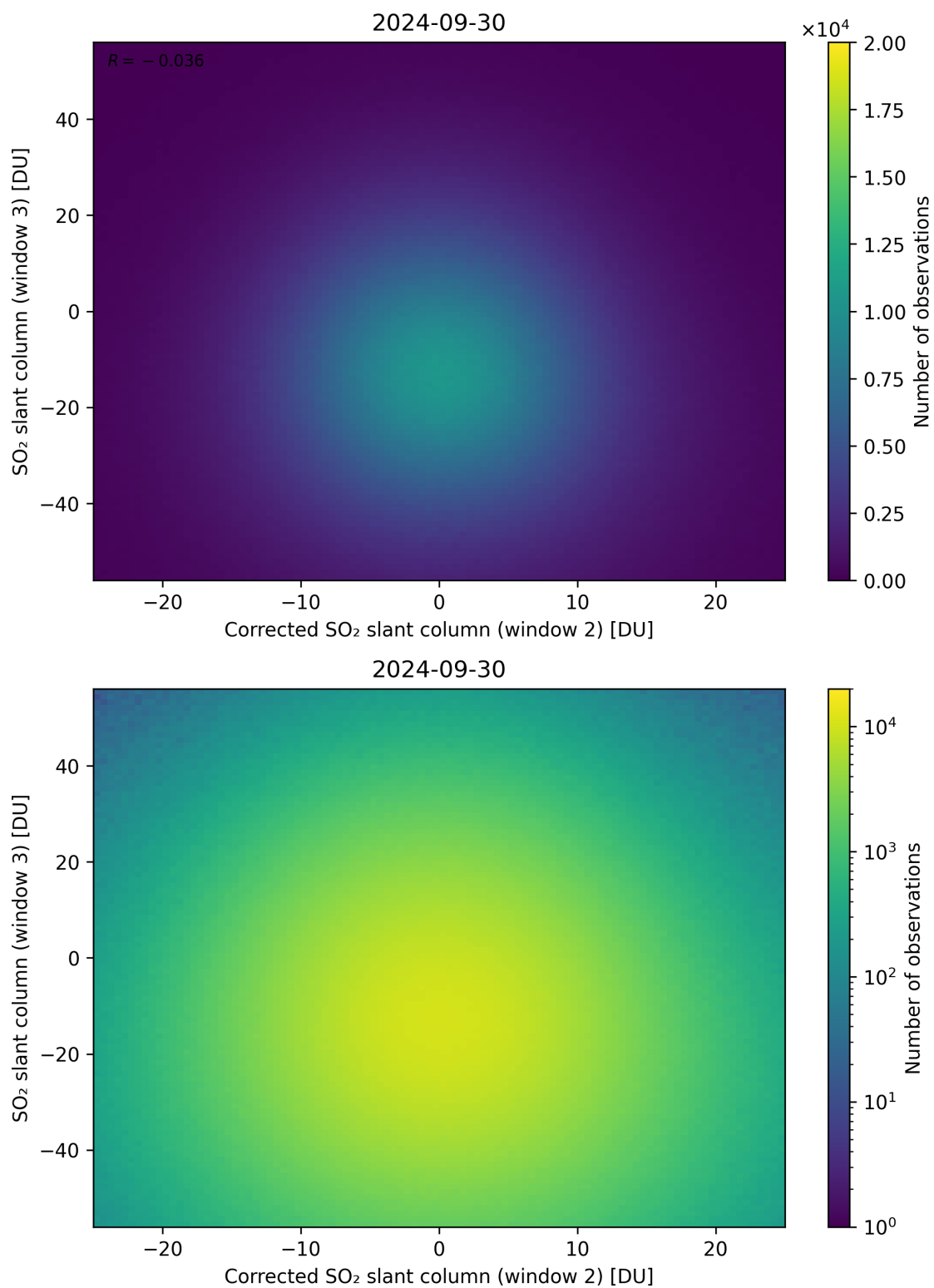
Figure 201: Scatter density plot of “Corrected SO 2 slant column (window 2)” against “SO 2 slant column (window 3)” for 2024-09-29 to 2024-10-01.
