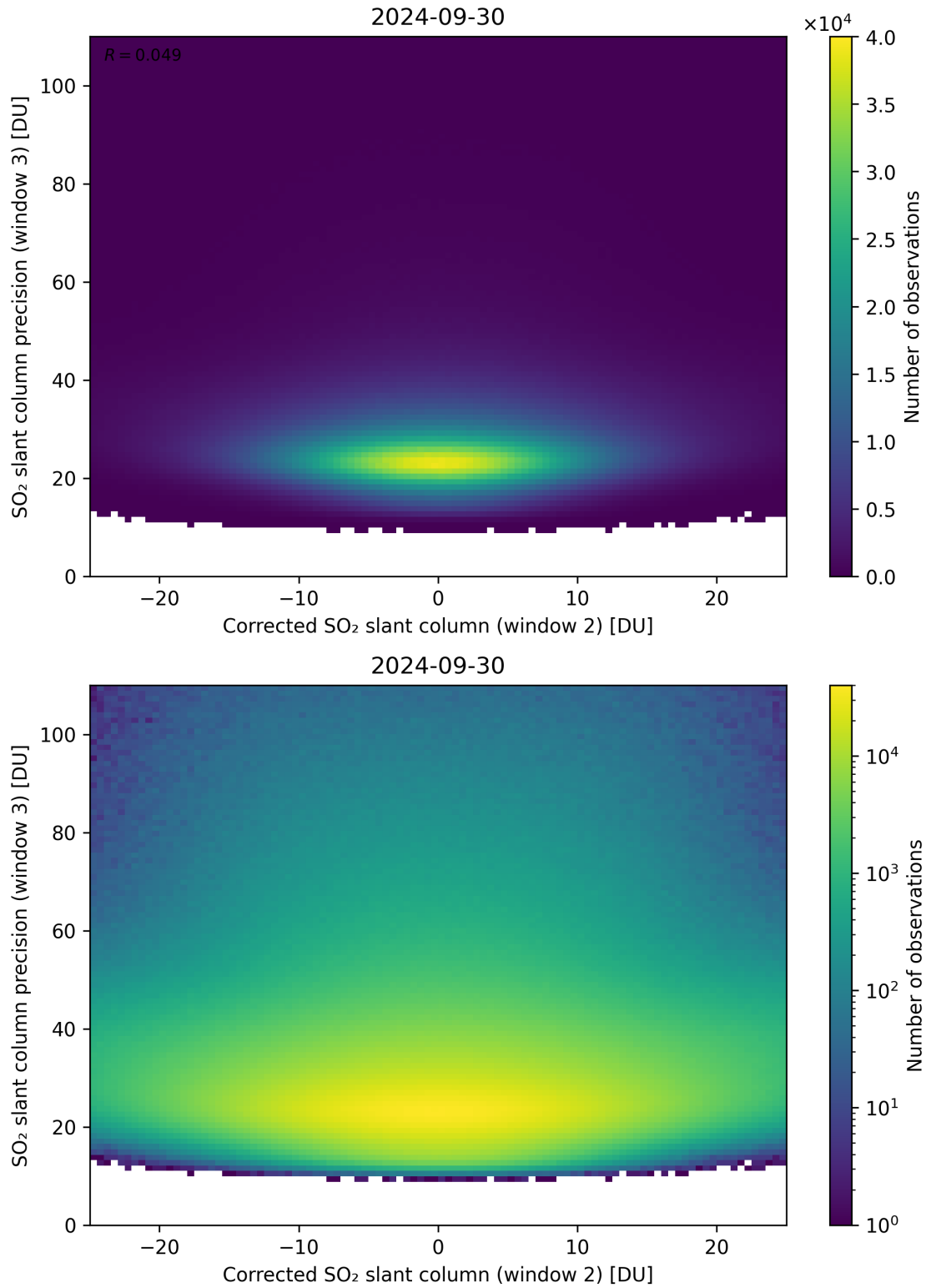
Figure 202: Scatter density plot of “Corrected SO 2 slant column (window 2)” against “SO 2 slant column precision (window 3)” for 2024-09-29 to 2024-10-01.
