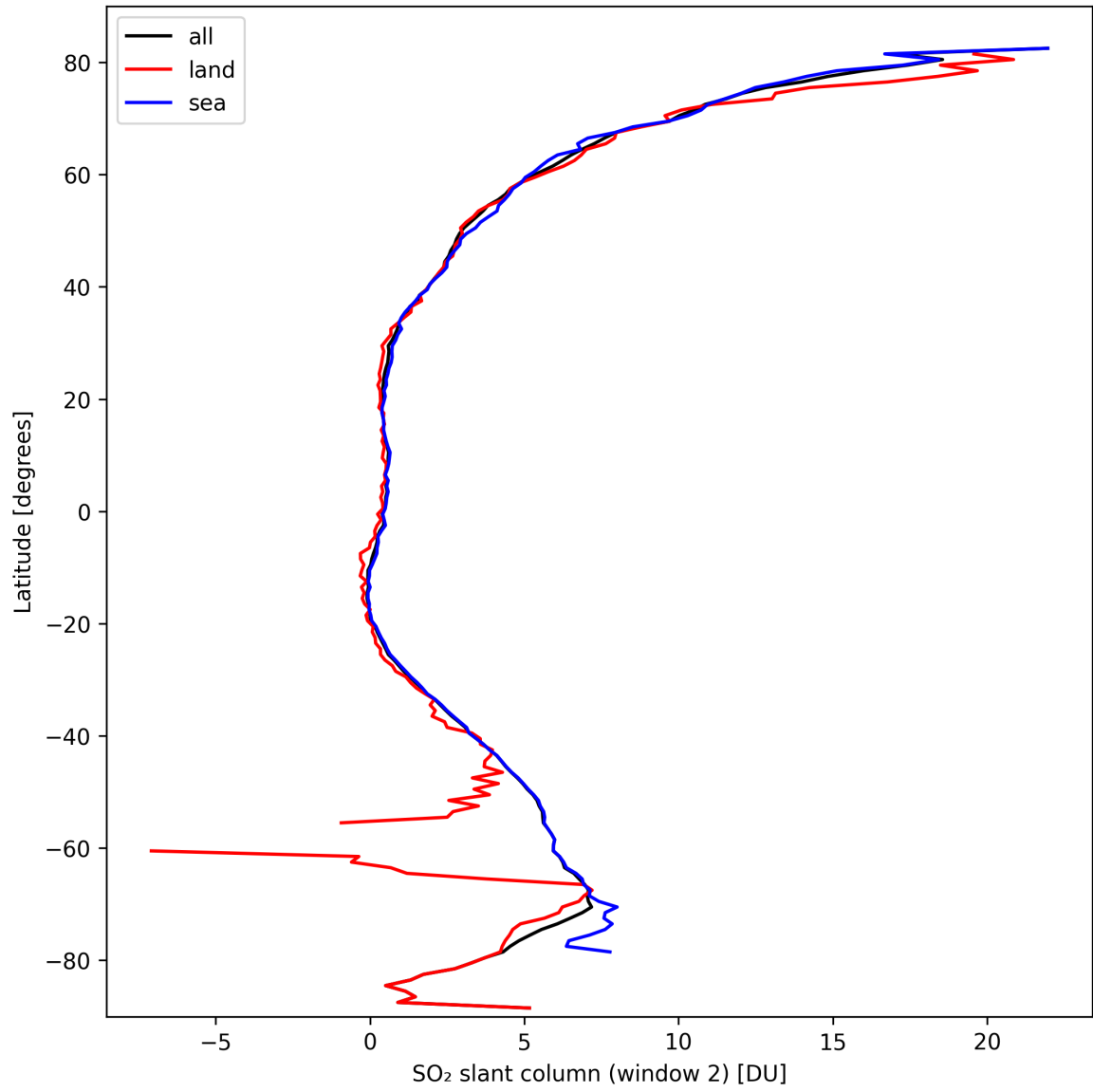
Figure 37: Zonal average of “SO 2 slant column (window 2)” for 2024-09-29 to 2024-10-01.
