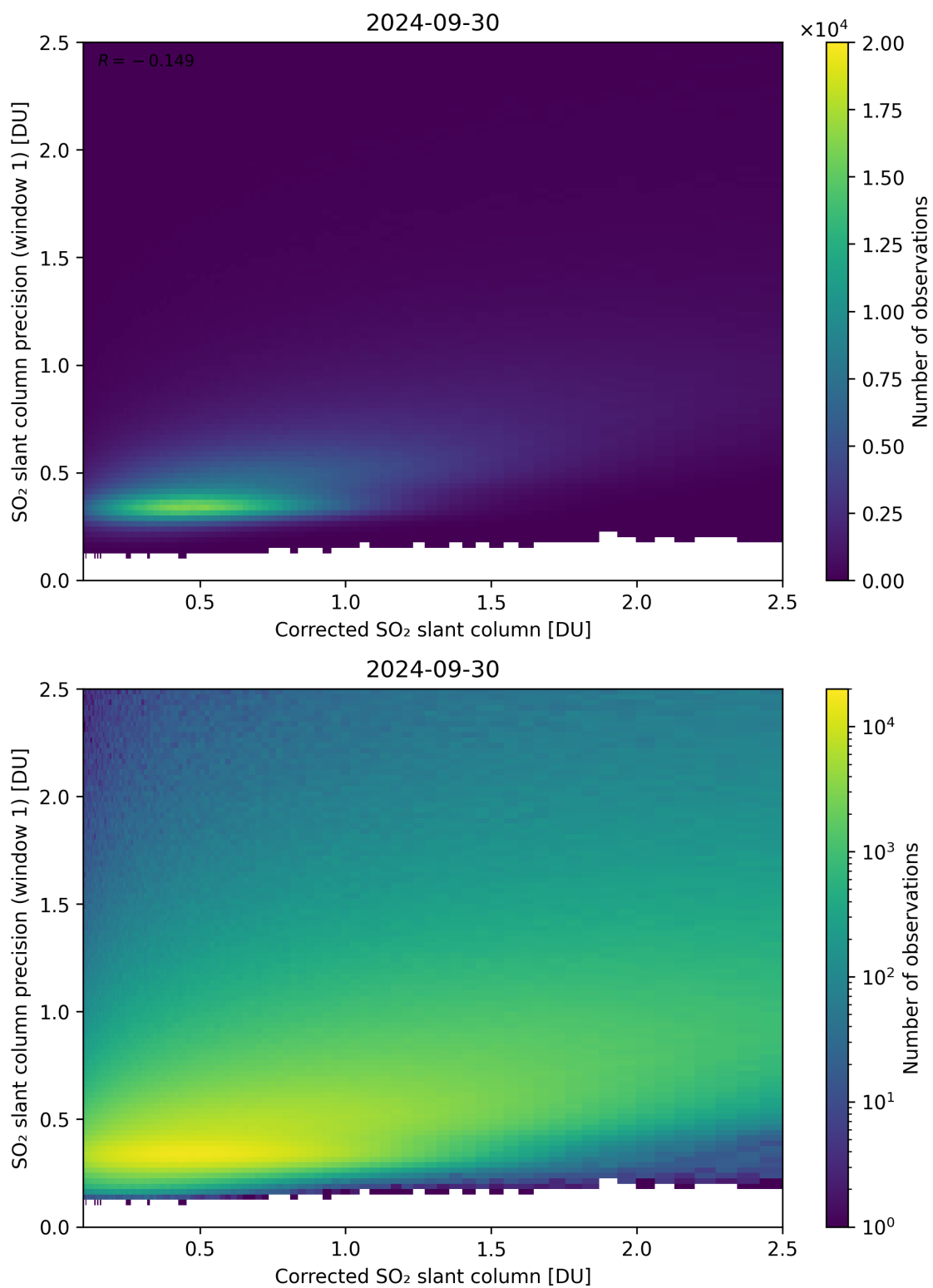
Figure 188: Scatter density plot of “Corrected SO 2 slant column” against “SO 2 slant column precision (window 1)” for 2024-09-29 to 2024-10-01.
