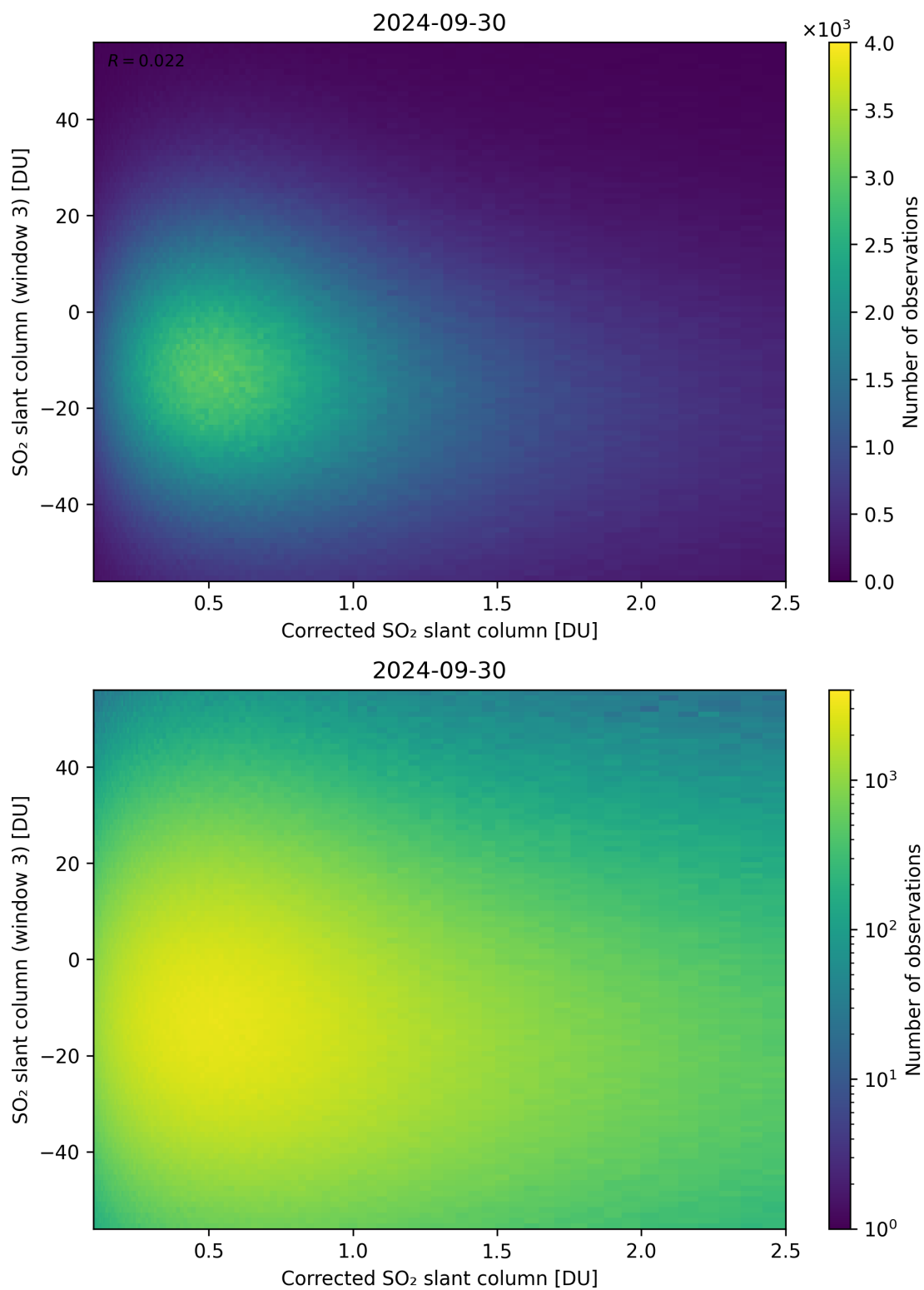
Figure 190: Scatter density plot of “Corrected SO 2 slant column” against “SO 2 slant column (window 3)” for 2024-09-29 to 2024-10-01.
