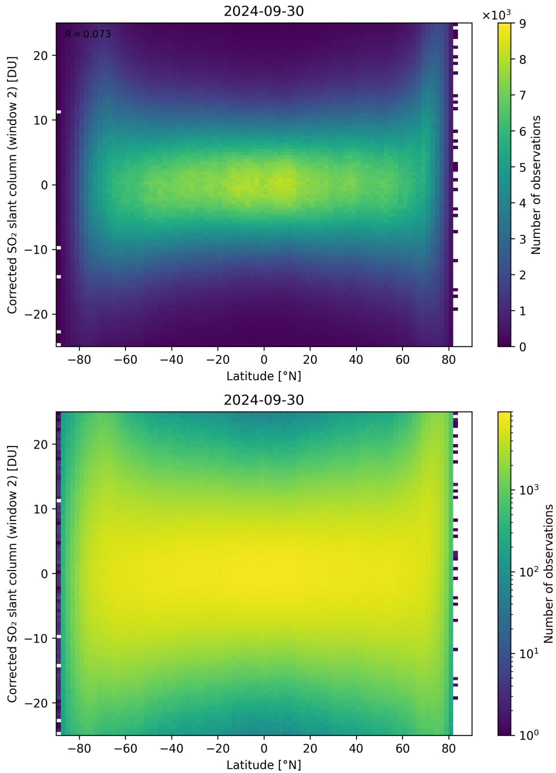
Figure 147: Scatter density plot of “Latitude” against “Corrected SO 2 slant column (window 2)” for 2024-09-29 to 2024-10-01.
