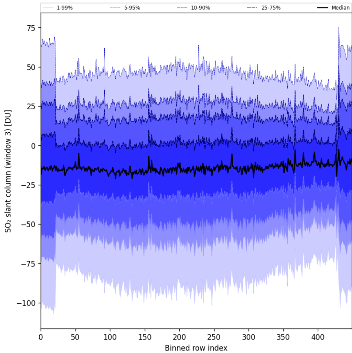
Figure 87: Along track statistics of “SO 2 slant column (window 3)” for 2024-09-29 to 2024-10-01
