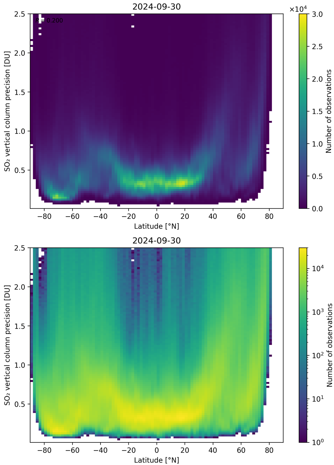
Figure 157: Scatter density plot of “Latitude” against “SO 2 vertical column precision” for 2024-09-29 to 2024-10-01.
