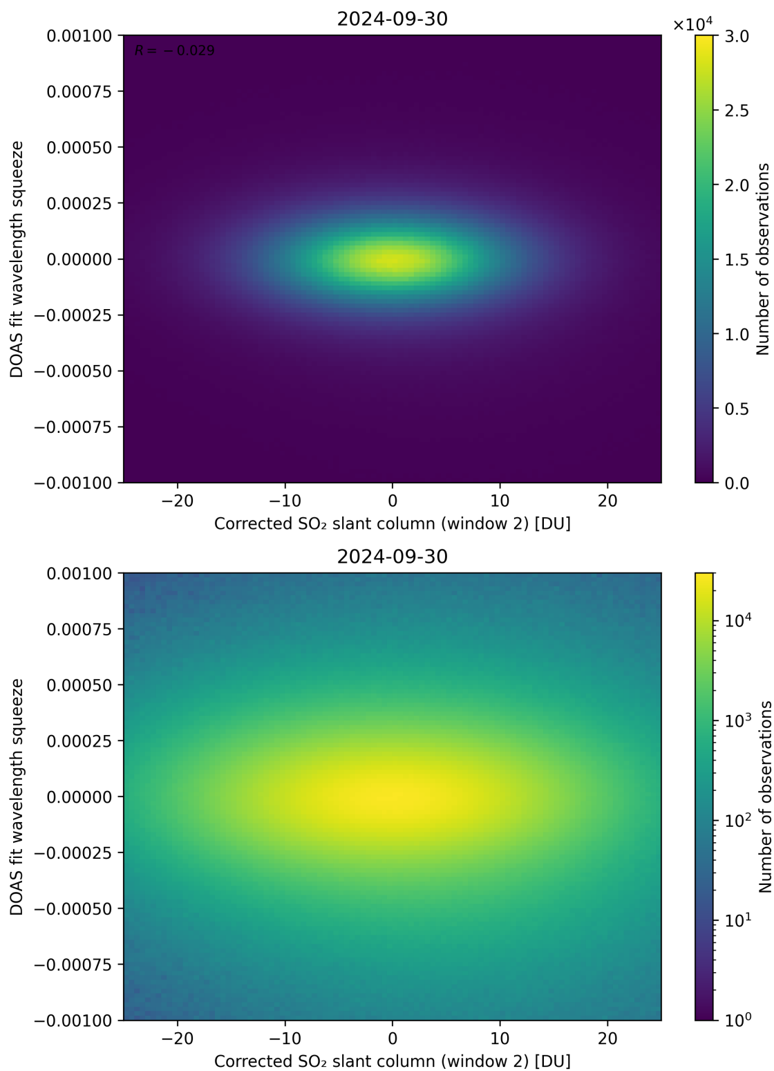
Figure 197: Scatter density plot of “Corrected SO 2 slant column (window 2)” against “DOAS fit wavelength squeeze” for 2024-09-29 to 2024-10-01.
