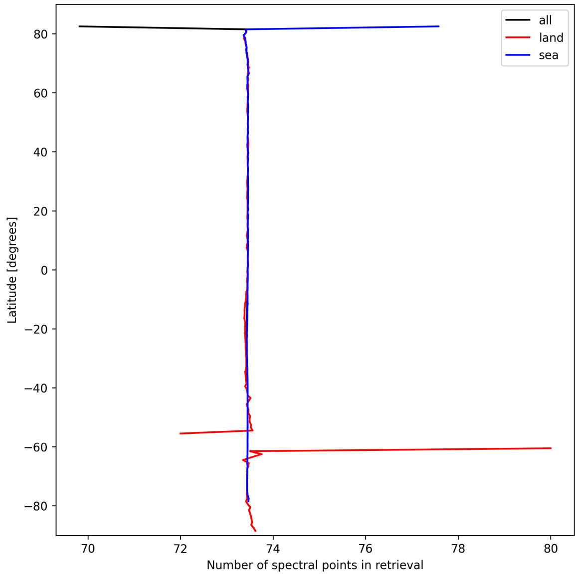
Figure 51: Zonal average of “Number of spectral points in retrieval” for 2024-09-29 to 2024-10-01.
