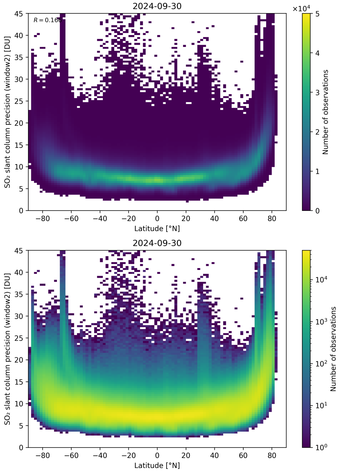
Figure 151: Scatter density plot of “Latitude” against “SO 2 slant column precision (window2)” for 2024-09-29 to 2024-10-01.
