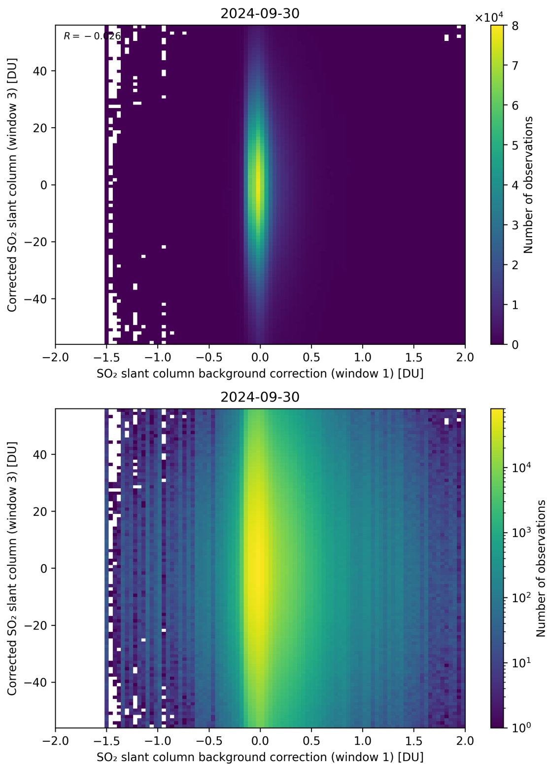
Figure 105: Scatter density plot of “SO 2 slant column background correction (window 1)” against “Corrected SO 2 slant column (window 3)” for 2024-09-29 to 2024-10-01.
