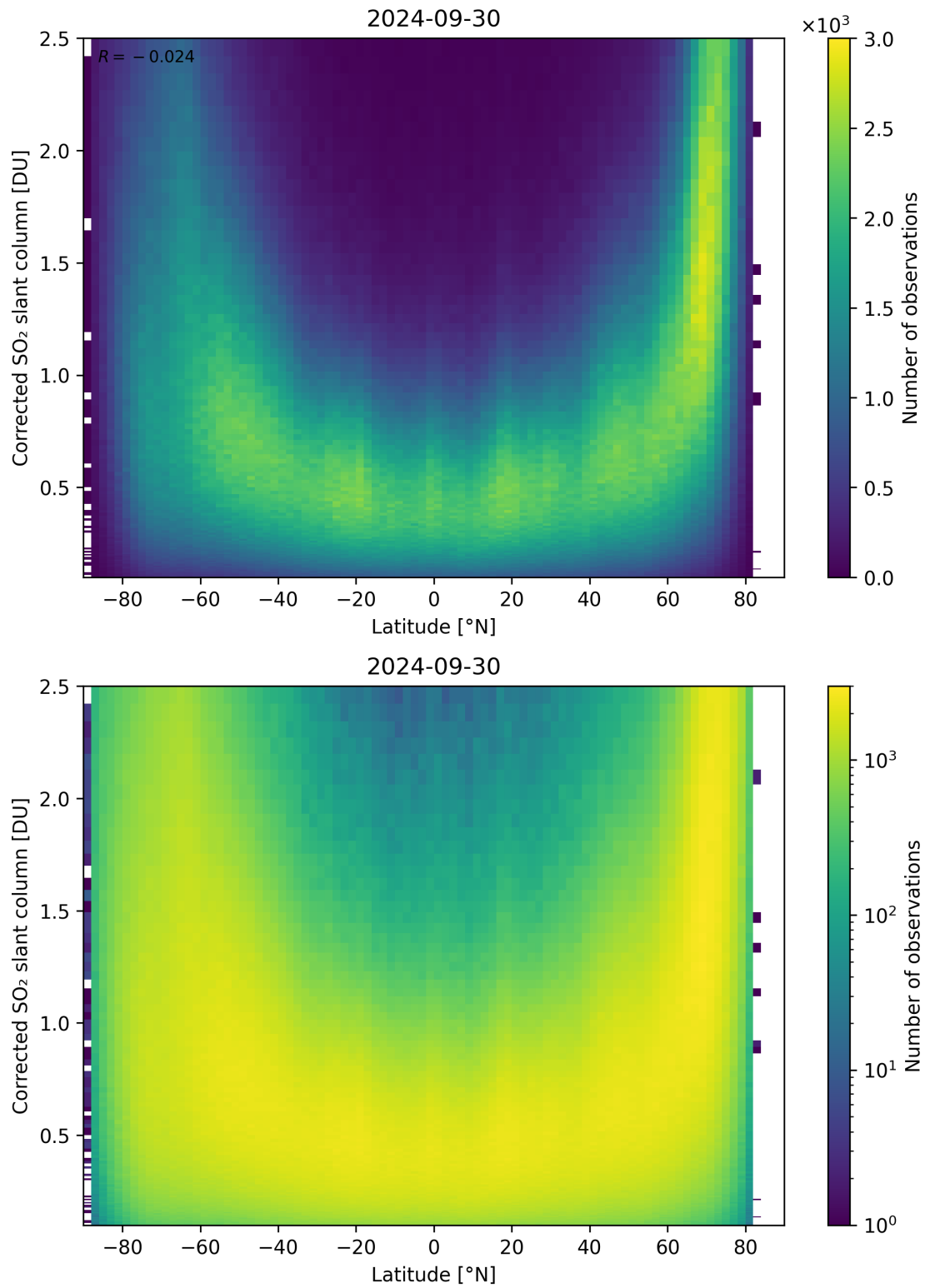
Figure 146: Scatter density plot of “Latitude” against “Corrected SO 2 slant column” for 2024-09-29 to 2024-10-01.
