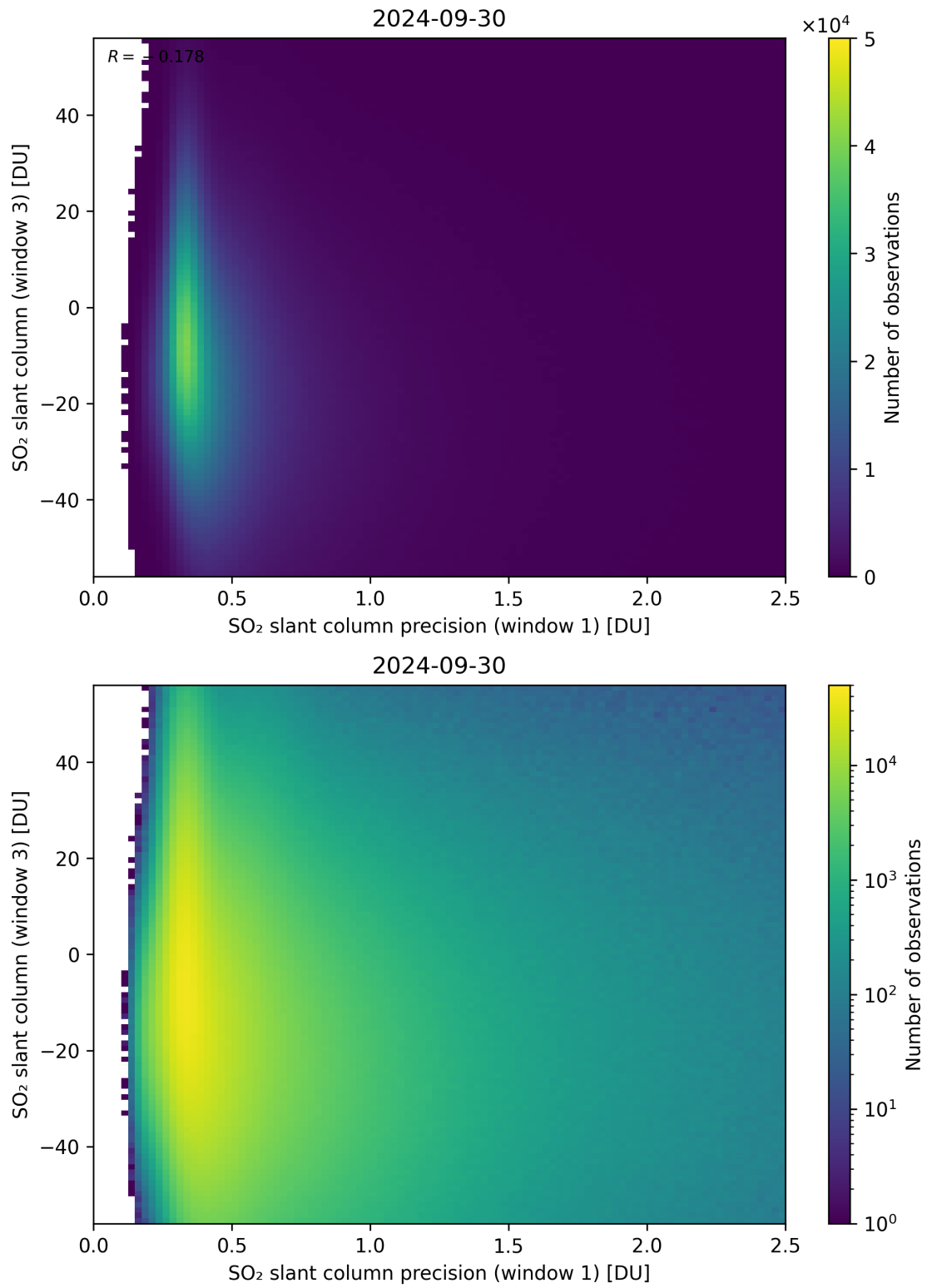
Figure 228: Scatter density plot of “SO 2 slant column precision (window 1)” against “SO 2 slant column (window 3)” for 2024-09-29 to 2024-10-01.
