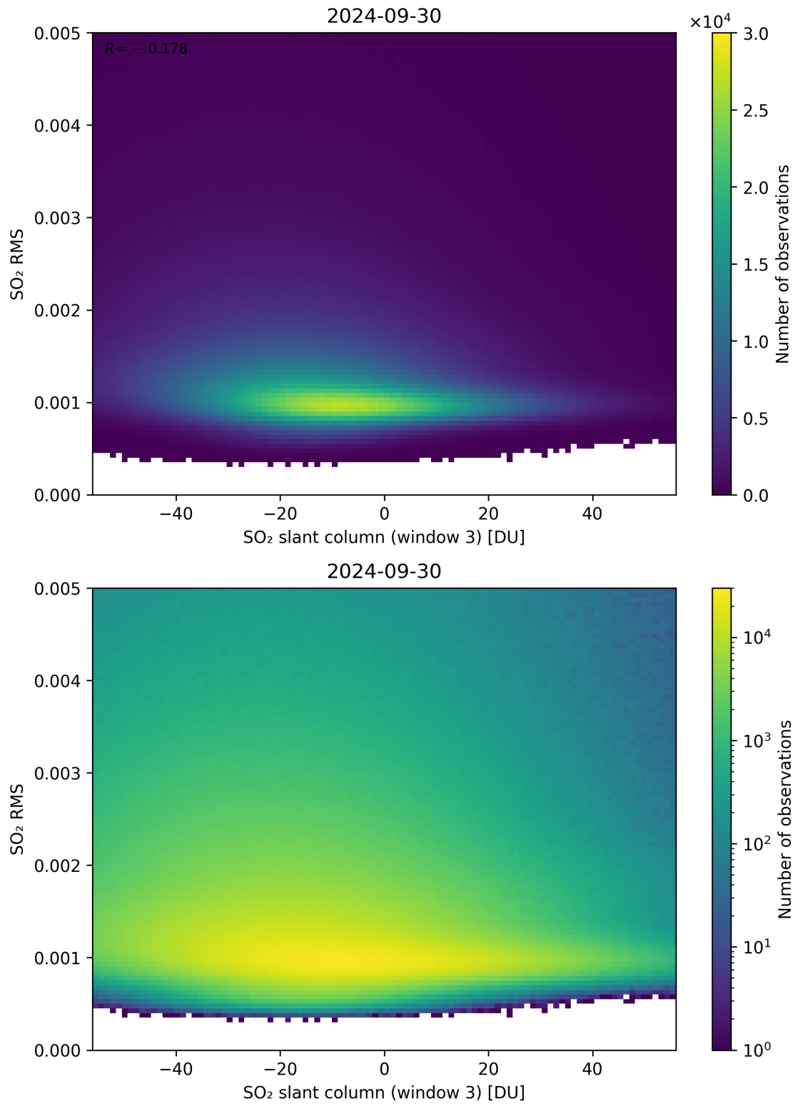
Figure 256: Scatter density plot of “SO 2 slant column (window 3)” against “SO 2 RMS” for 2024-09-29 to 2024-10-01.
