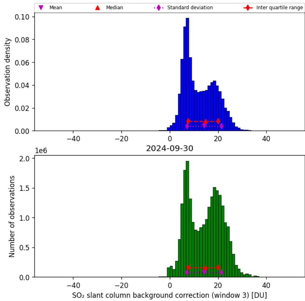
Figure 67: Histogram of “SO 2 slant column background correction (window 3)” for 2024-09-29 to 2024-10-01
