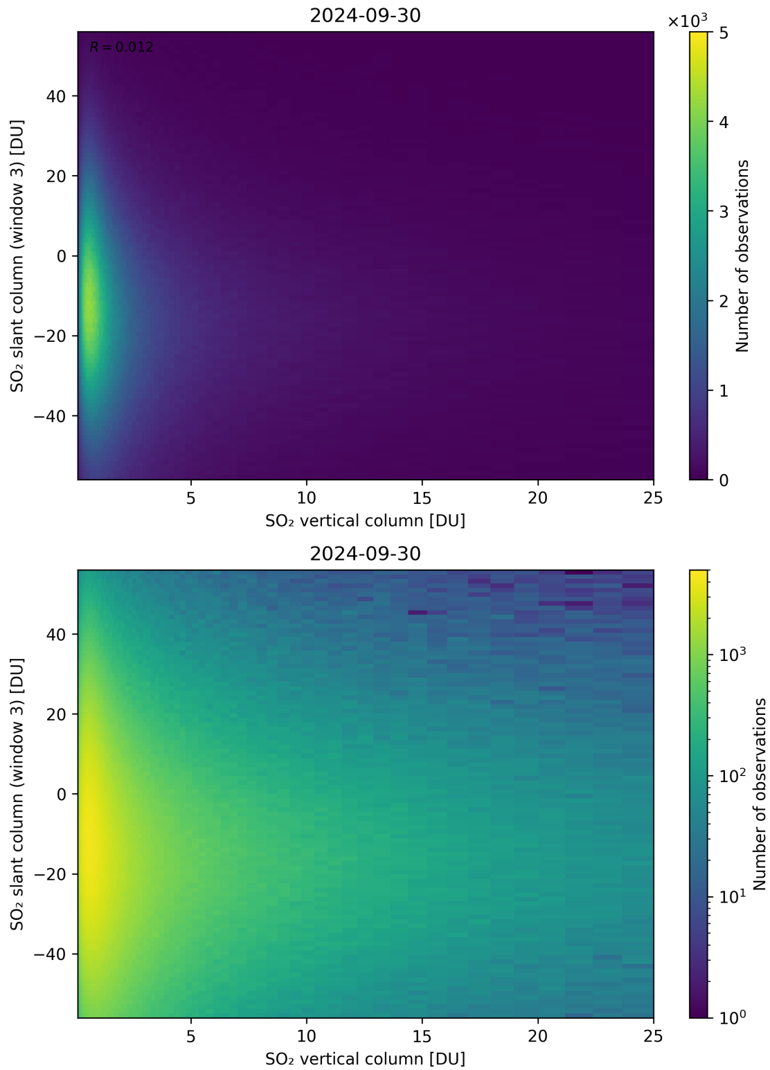
Figure 303: Scatter density plot of “SO 2 vertical column” against “SO 2 slant column (window 3)” for 2024-09-29 to 2024-10-01.
