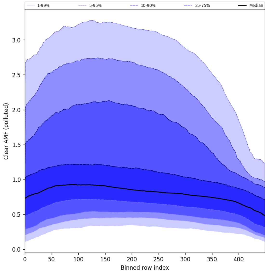
Figure 96: Along track statistics of “Clear AMF (polluted)” for 2024-09-29 to 2024-10-01
