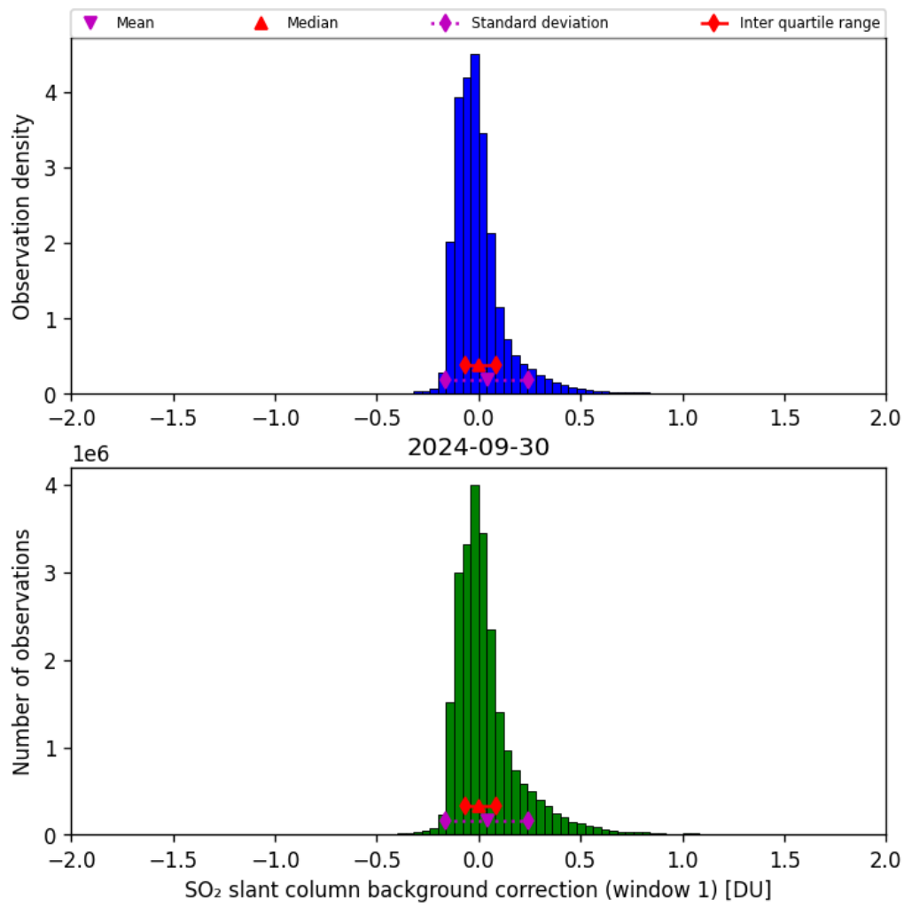
Figure 59: Histogram of “SO 2 slant column background correction (window 1)” for 2024-09-29 to 2024-10-01
