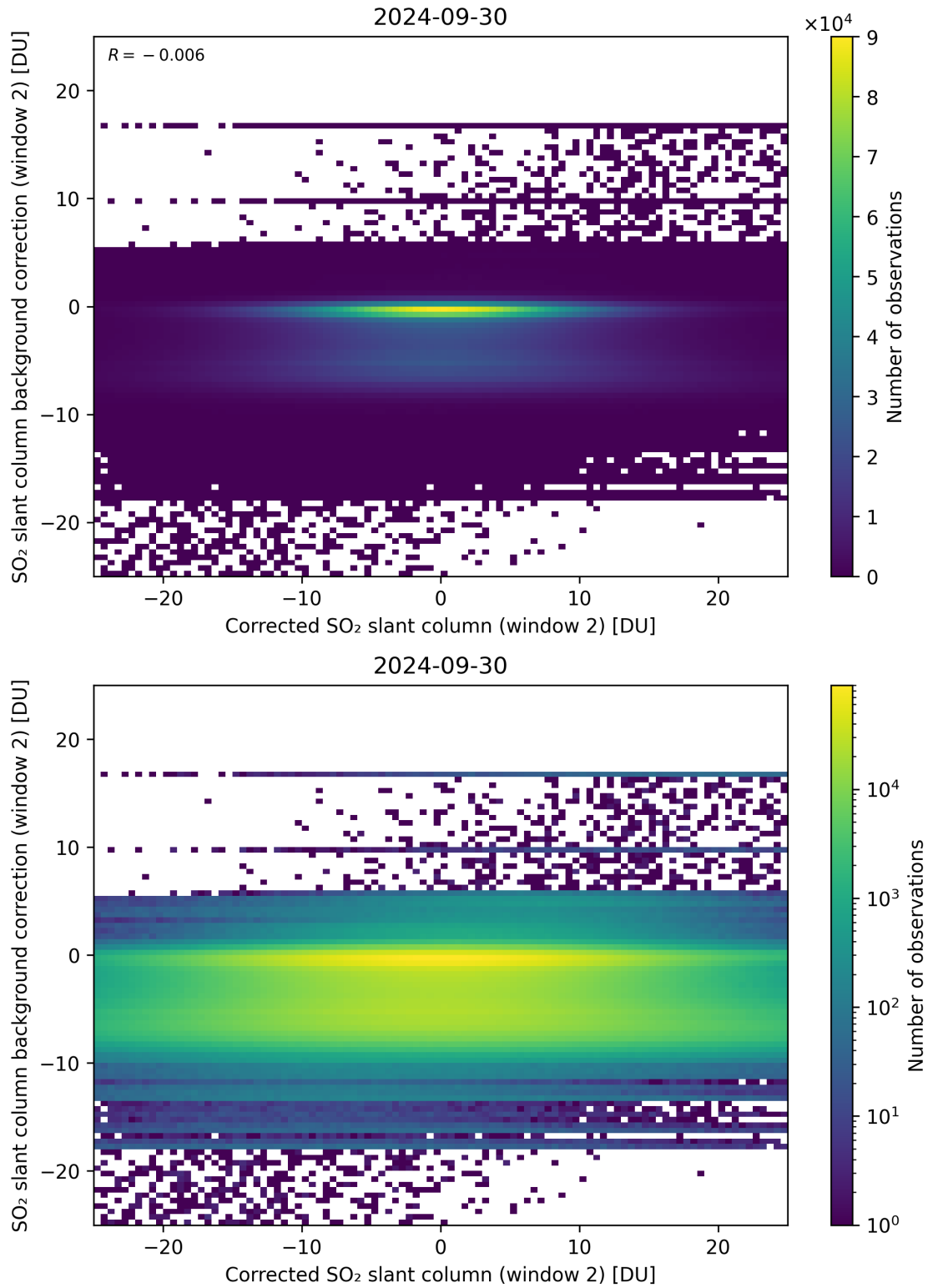
Figure 194: Scatter density plot of “Corrected SO 2 slant column (window 2)” against “SO 2 slant column background correction (window 2)” for 2024-09-29 to 2024-10-01.
