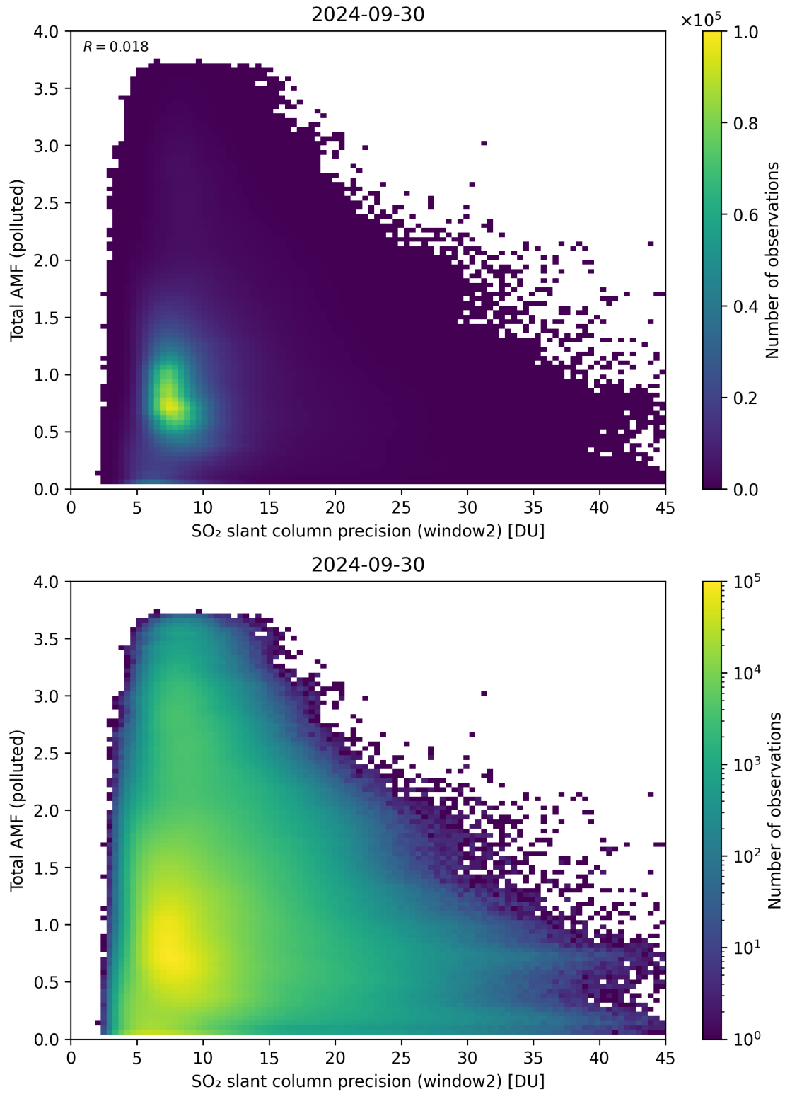
Figure 251: Scatter density plot of “SO 2 slant column precision (window2)” against “Total AMF (polluted)” for 2024-09-29 to 2024-10-01.
