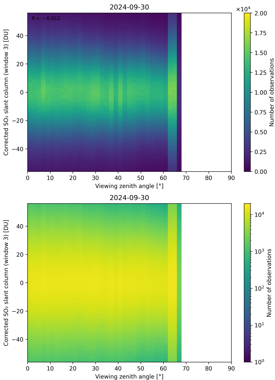
Figure 319: Scatter density plot of “Viewing zenith angle” against “Corrected SO 2 slant column (window 3)” for 2024-09-29 to 2024-10-01.
