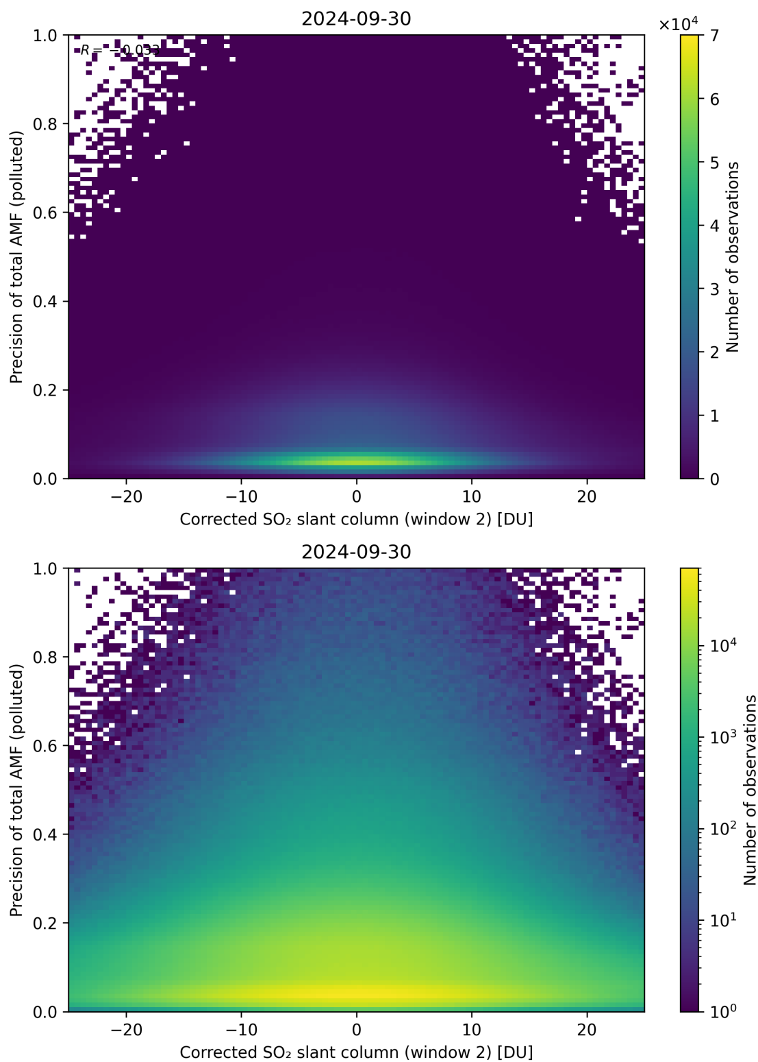
Figure 204: Scatter density plot of “Corrected SO 2 slant column (window 2)” against “Precision of total AMF (polluted)” for 2024-09-29 to 2024-10-01.
