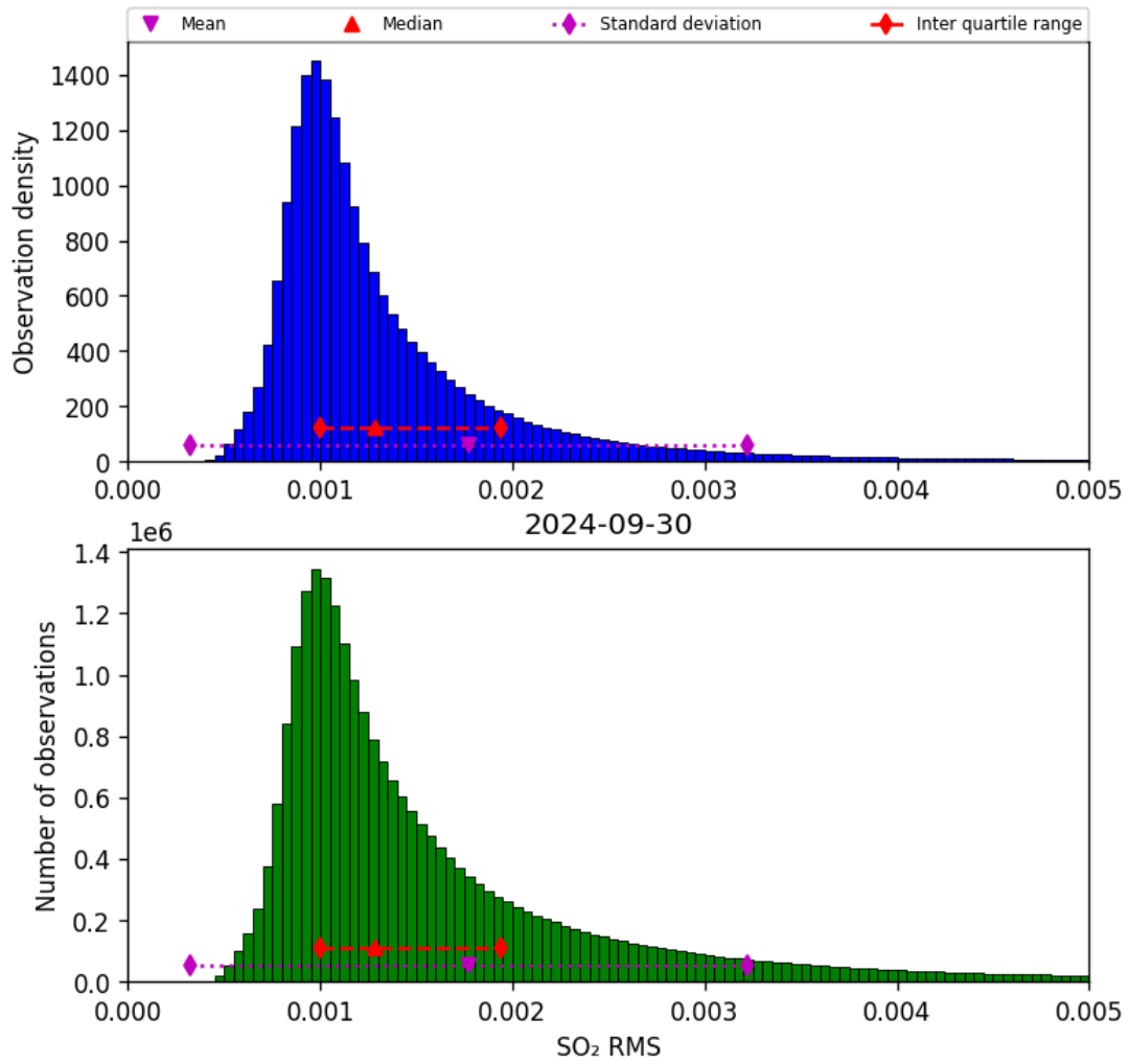
Figure 70: Histogram of “SO 2 RMS” for 2024-09-29 to 2024-10-01
