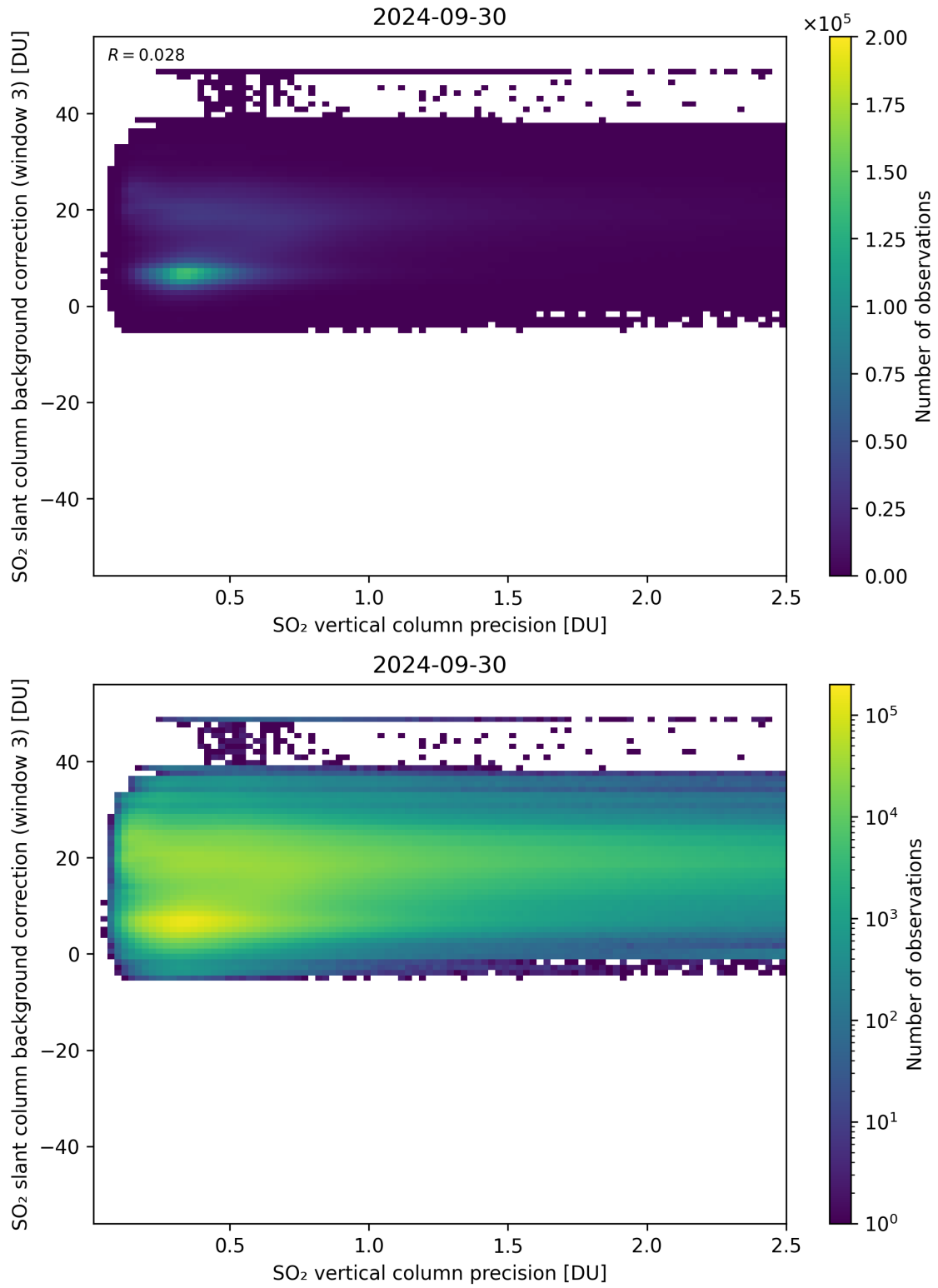
Figure 281: Scatter density plot of “SO 2 vertical column precision” against “SO 2 slant column background correction (window 3)” for 2024-09-29 to 2024-10-01.
