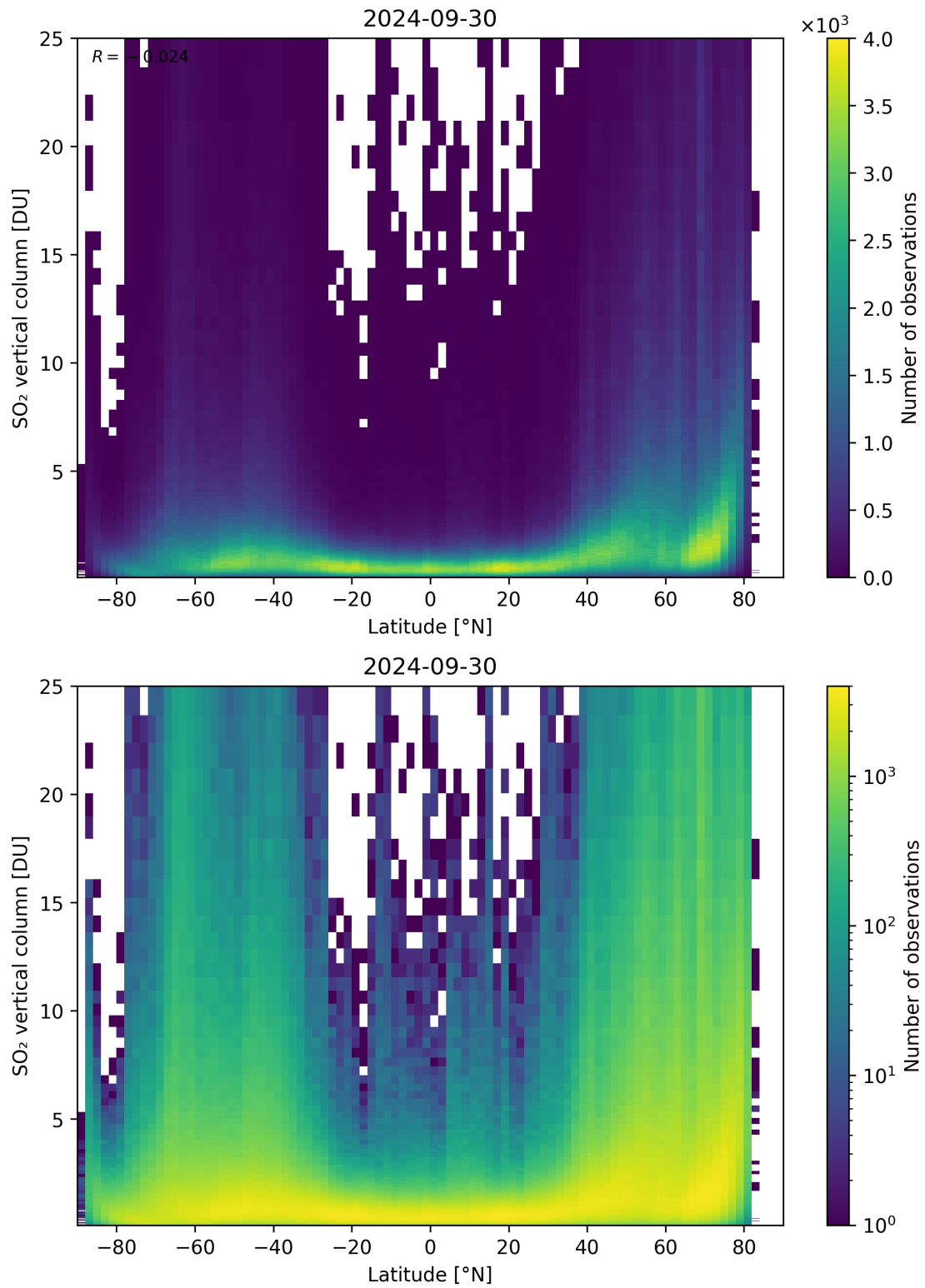
Figure 156: Scatter density plot of “Latitude” against “SO 2 vertical column” for 2024-09-29 to 2024-10-01.
