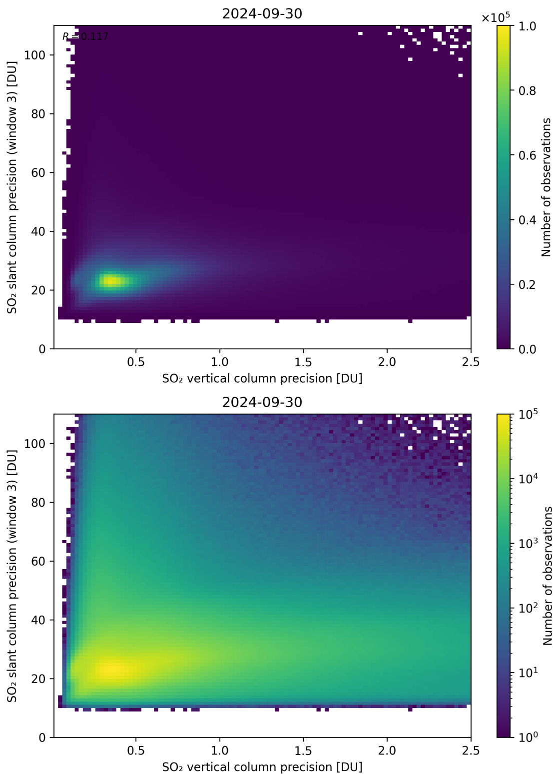
Figure 293: Scatter density plot of “SO 2 vertical column precision” against “SO 2 slant column precision (window 3)” for 2024-09-29 to 2024-10-01.
