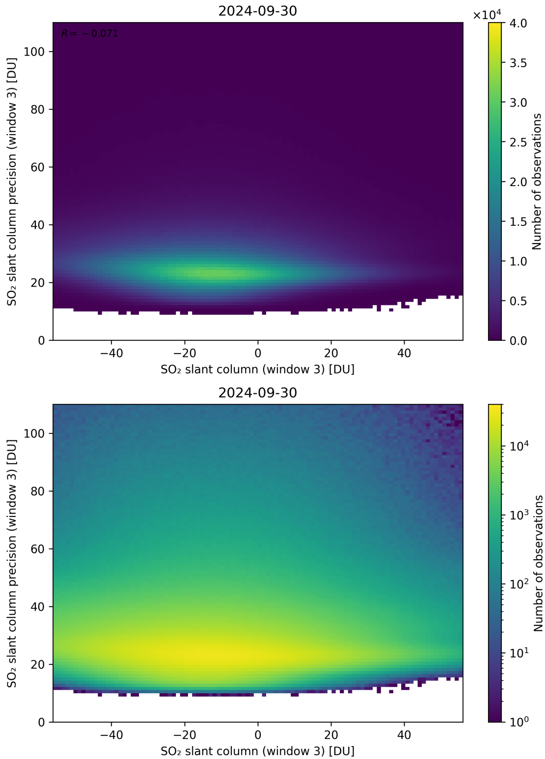
Figure 267: Scatter density plot of “SO 2 slant column (window 3)” against “SO 2 slant column precision (window 3)” for 2024-09-29 to 2024-10-01.
