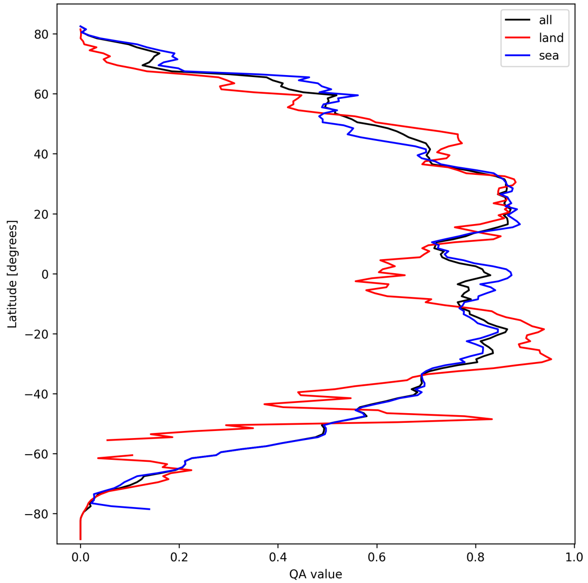
Figure 29: Zonal average of “QA value” for 2024-09-29 to 2024-10-01.
