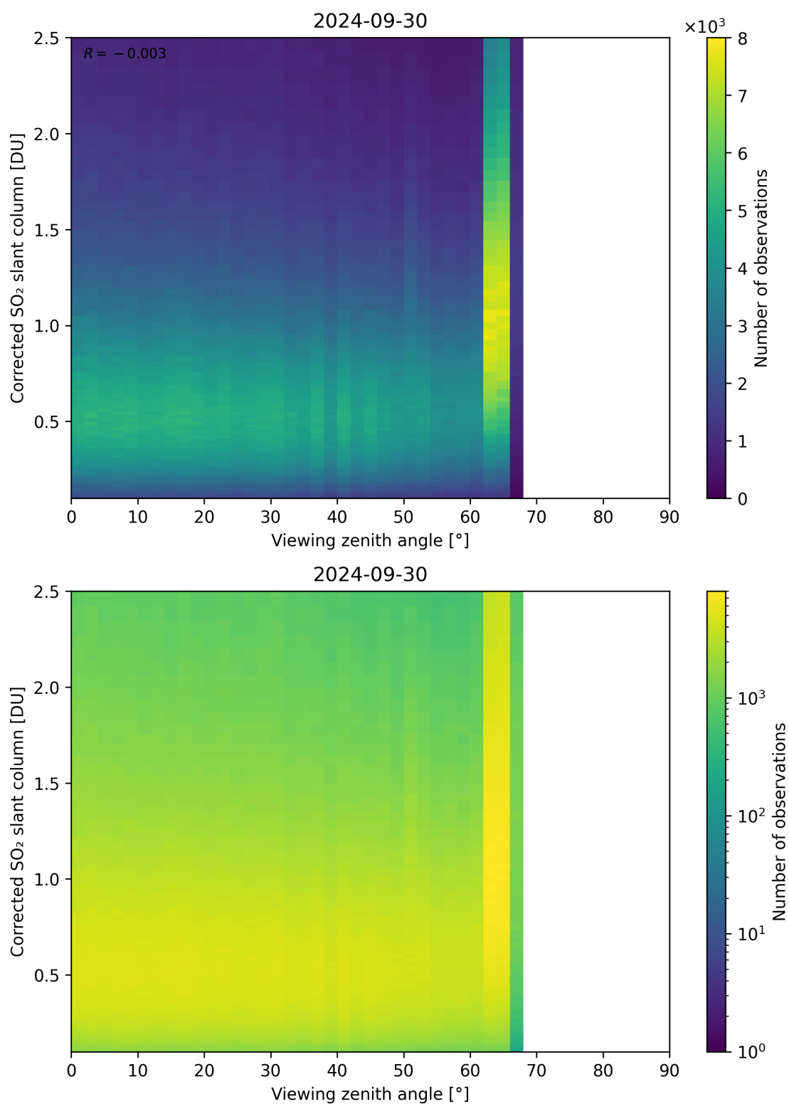
Figure 317: Scatter density plot of “Viewing zenith angle” against “Corrected SO 2 slant column” for 2024-09-29 to 2024-10-01.
