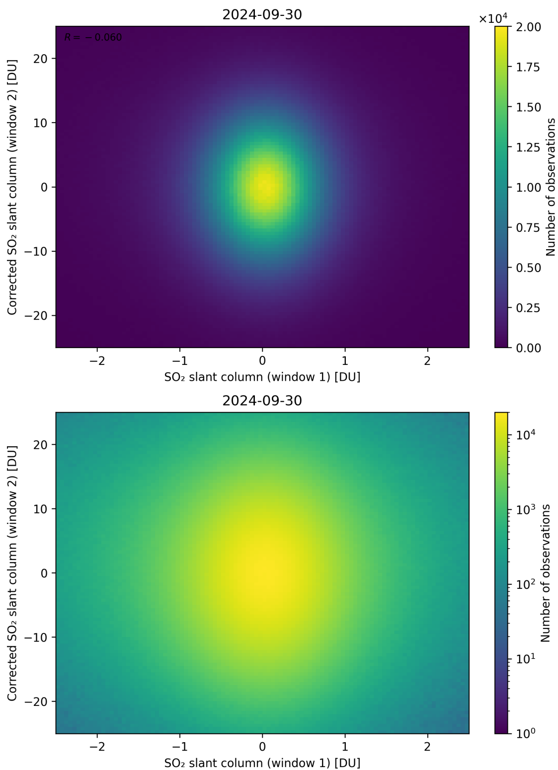
Figure 233: Scatter density plot of “SO 2 slant column (window 1)” against “Corrected SO 2 slant column (window 2)” for 2024-09-29 to 2024-10-01.
