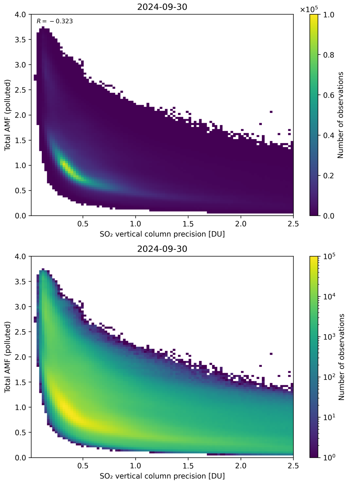
Figure 294: Scatter density plot of “SO 2 vertical column precision” against “Total AMF (polluted)” for 2024-09-29 to 2024-10-01.
