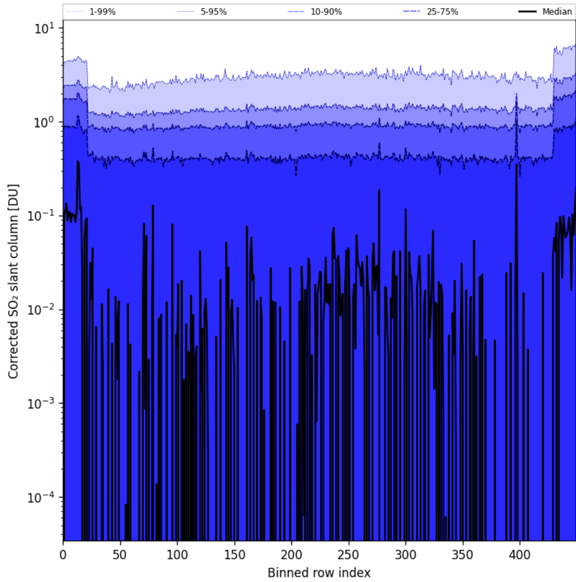
Figure 78: Along track statistics of “Corrected SO 2 slant column” for 2024-09-29 to 2024-10-01
