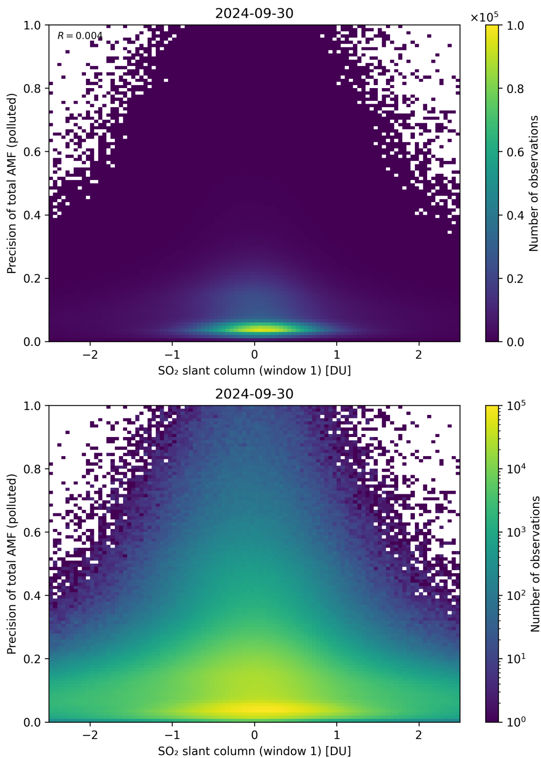
Figure 240: Scatter density plot of “SO 2 slant column (window 1)” against “Precision of total AMF (polluted)” for 2024-09-29 to 2024-10-01.
