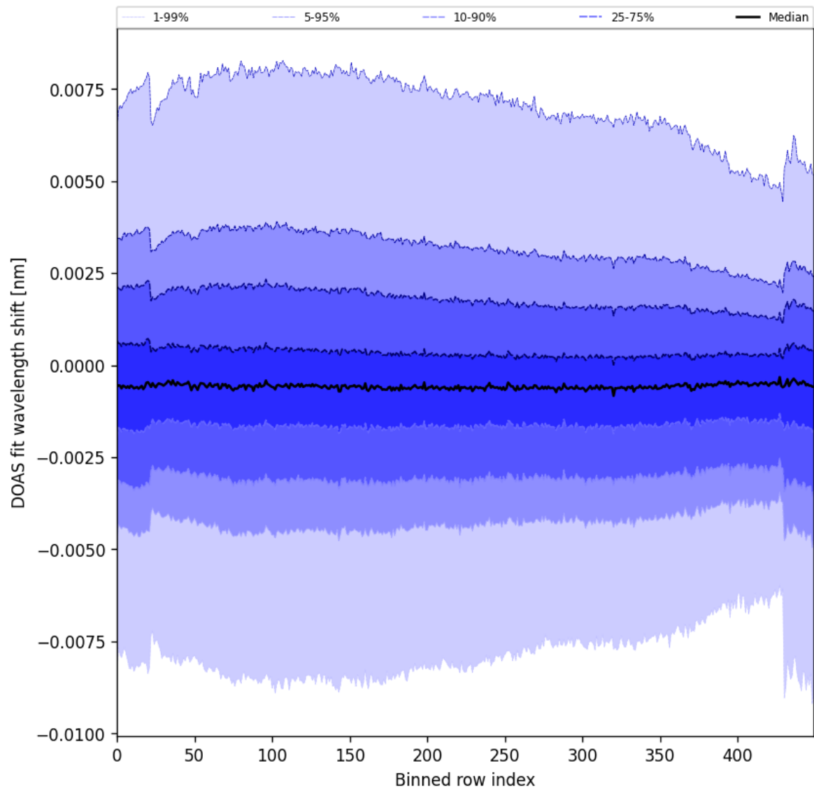
Figure 91: Along track statistics of “DOAS fit wavelength shift” for 2024-09-29 to 2024-10-01
