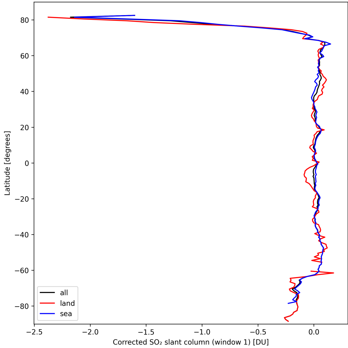
Figure 35: Zonal average of “Corrected SO 2 slant column (window 1)” for 2024-09-29 to 2024-10-01.
