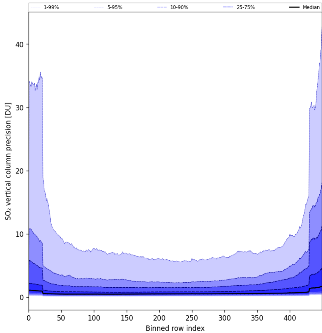
Figure 77: Along track statistics of “SO 2 vertical column precision” for 2024-09-29 to 2024-10-01
