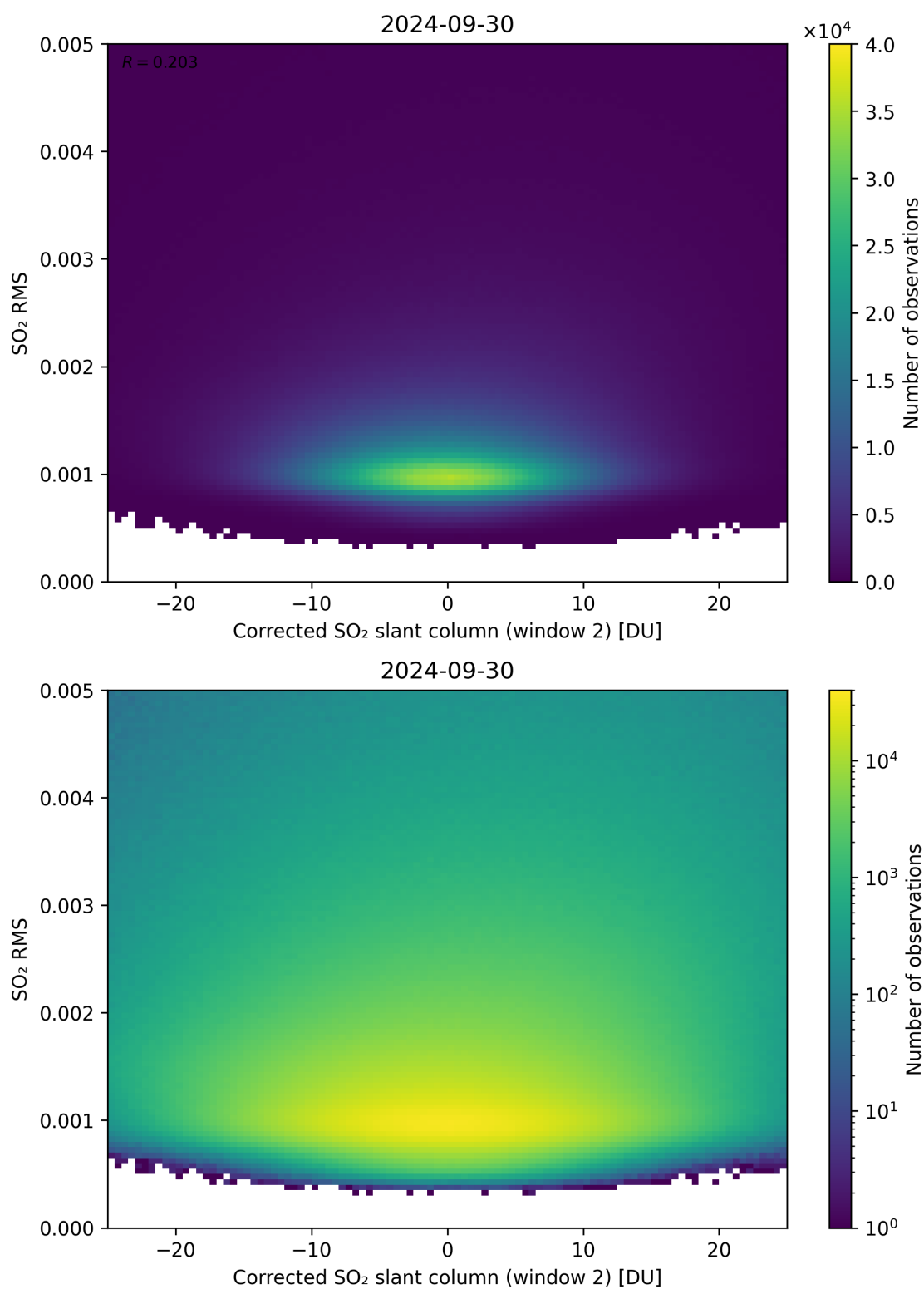
Figure 198: Scatter density plot of “Corrected SO 2 slant column (window 2)” against “SO 2 RMS” for 2024-09-29 to 2024-10-01.
