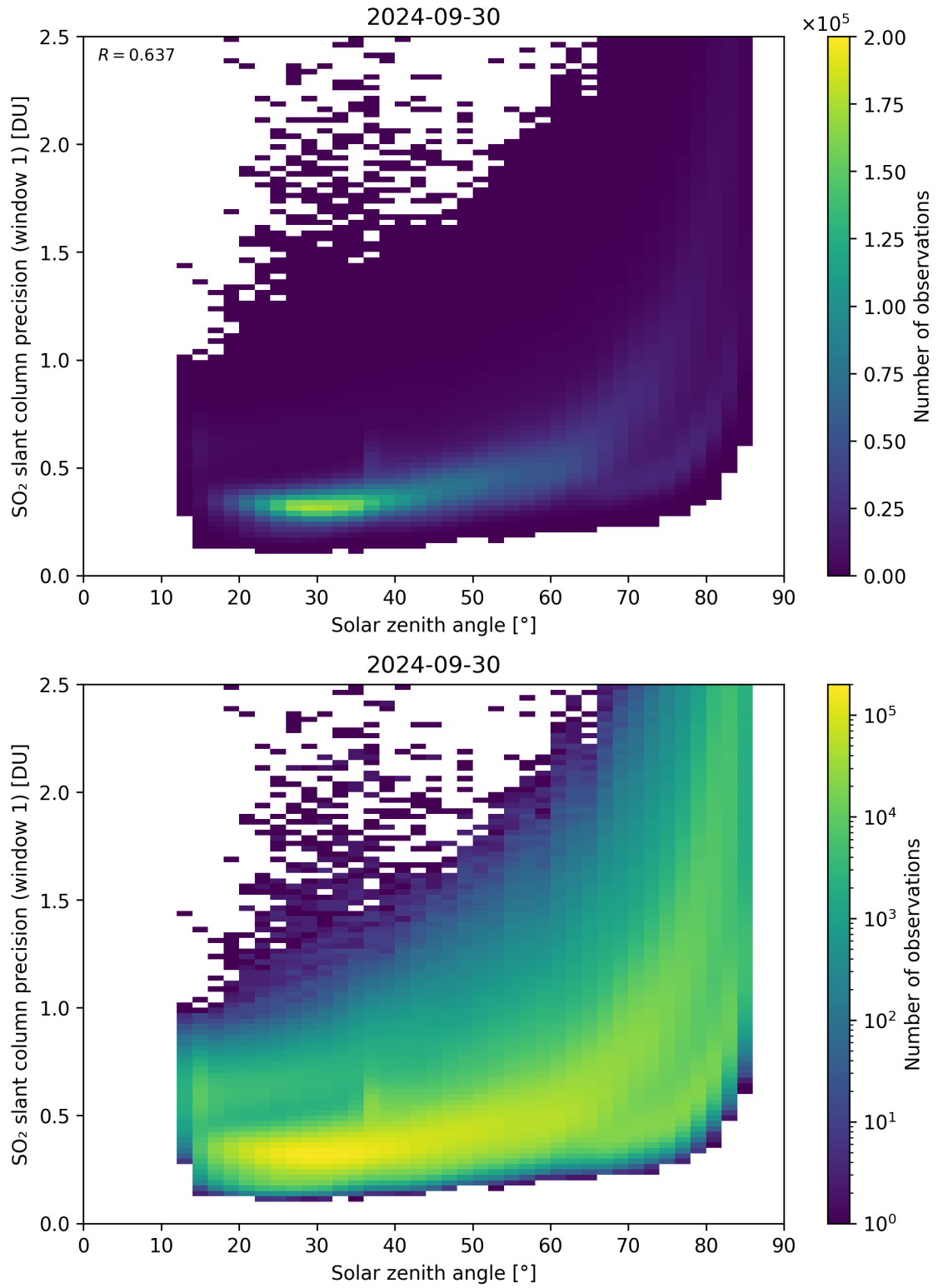
Figure 170: Scatter density plot of “Solar zenith angle” against “SO 2 slant column precision (window 1)” for 2024-09-29 to 2024-10-01.
