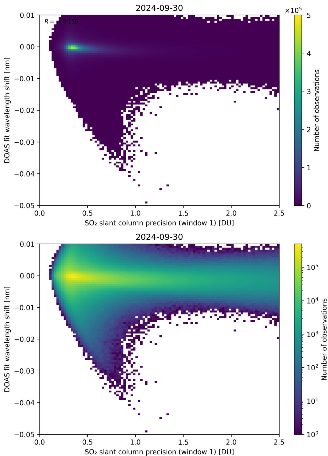
Figure 221: Scatter density plot of “SO 2 slant column precision (window 1)” against “DOAS fit wavelength shift” for 2024-09-29 to 2024-10-01.
