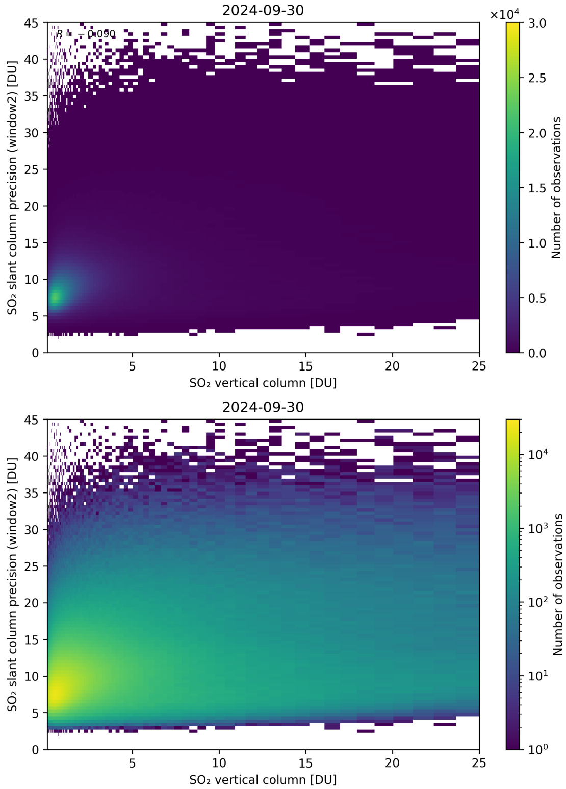
Figure 302: Scatter density plot of “SO 2 vertical column” against “SO 2 slant column precision (window2)” for 2024-09-29 to 2024-10-01.
