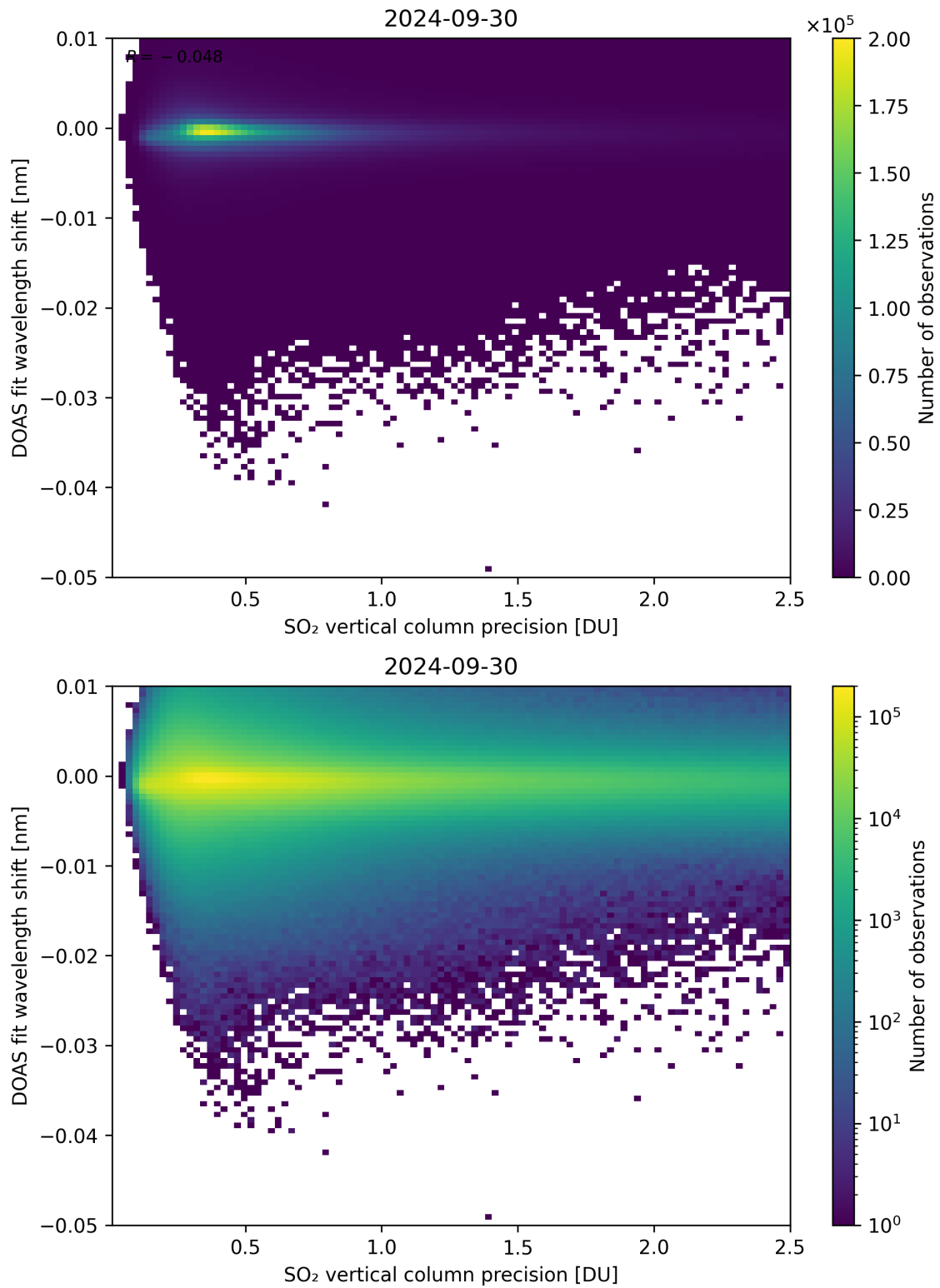
Figure 282: Scatter density plot of “SO 2 vertical column precision” against “DOAS fit wavelength shift” for 2024-09-29 to 2024-10-01.
