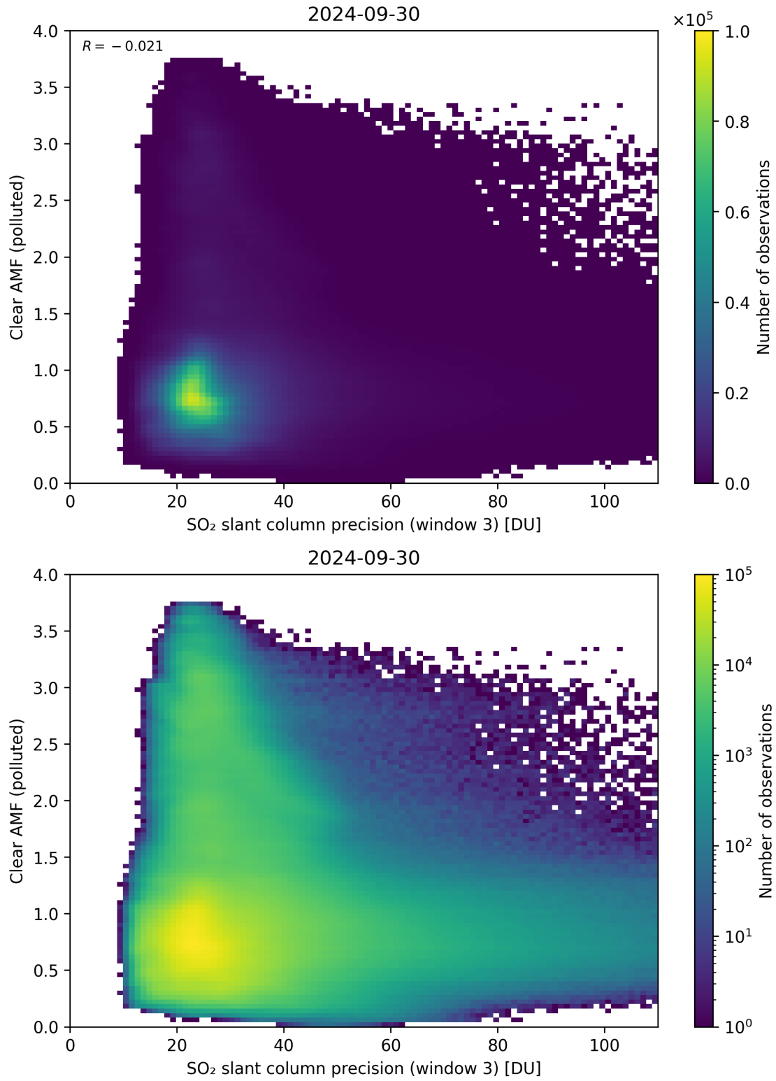
Figure 261: Scatter density plot of “SO 2 slant column precision (window 3)” against “Clear AMF (polluted)” for 2024-09-29 to 2024-10-01.
