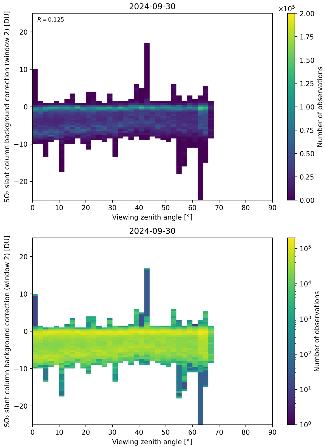
Figure 309: Scatter density plot of “Viewing zenith angle” against “SO 2 slant column background correction (window 2)” for 2024-09-29 to 2024-10-01.
