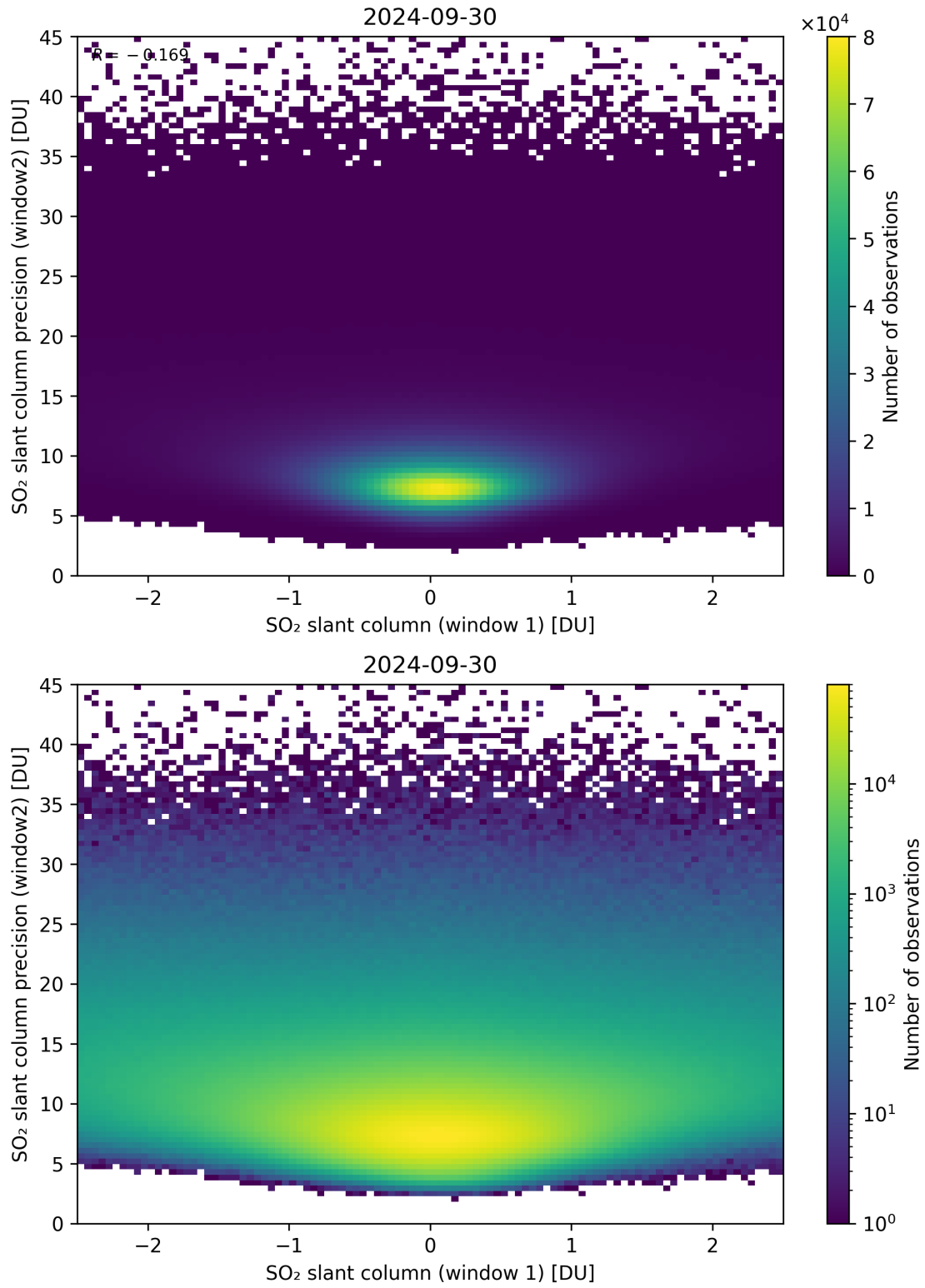
Figure 236: Scatter density plot of “SO 2 slant column (window 1)” against “SO 2 slant column precision (window2)” for 2024-09-29 to 2024-10-01.
