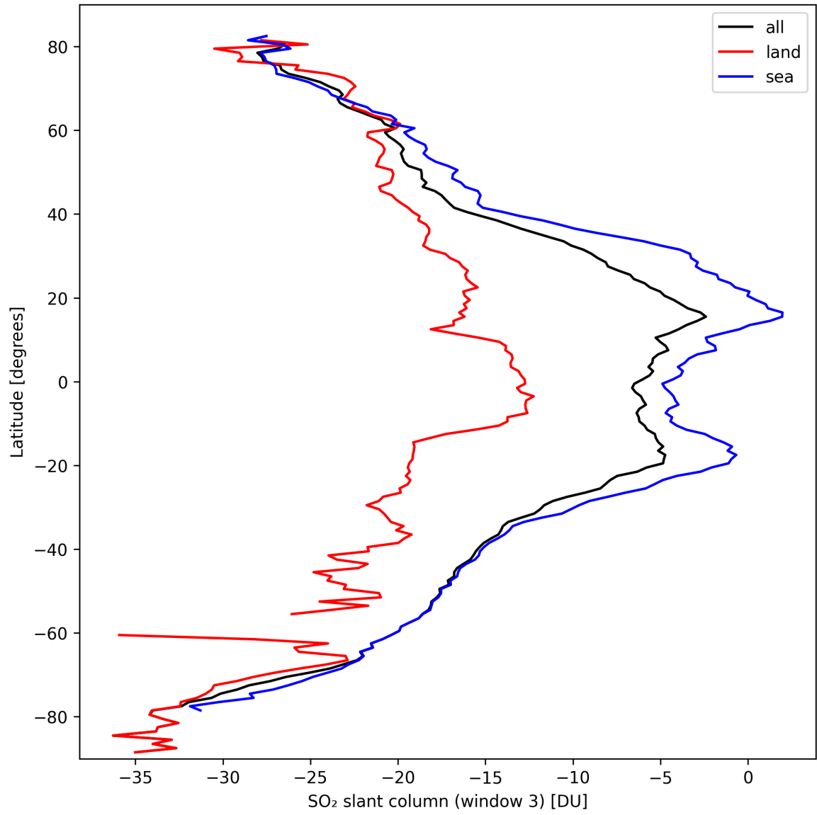
Figure 41: Zonal average of “SO 2 slant column (window 3)” for 2024-09-29 to 2024-10-01.
