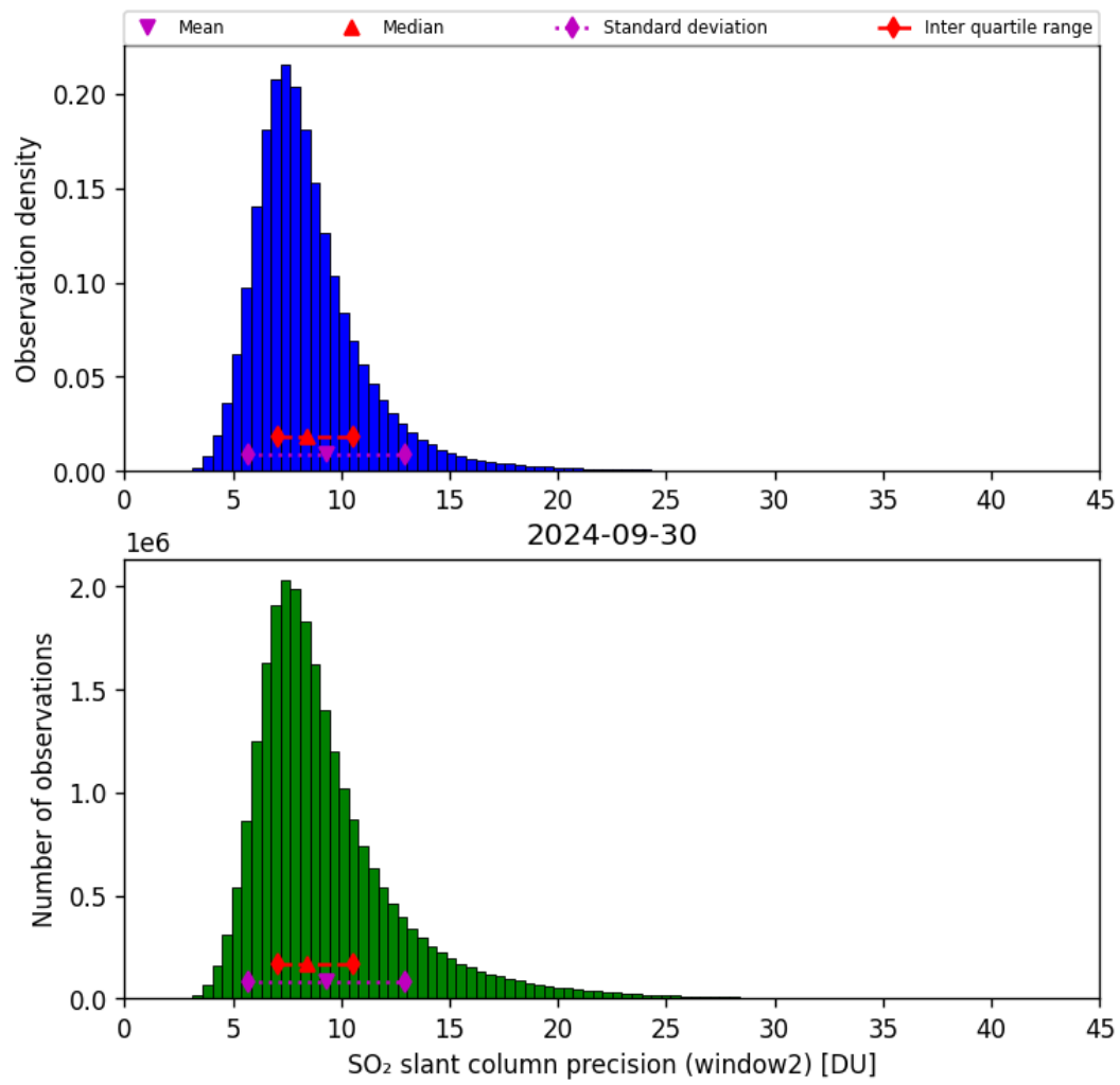
Figure 61: Histogram of “SO 2 slant column precision (window2)” for 2024-09-29 to 2024-10-01
