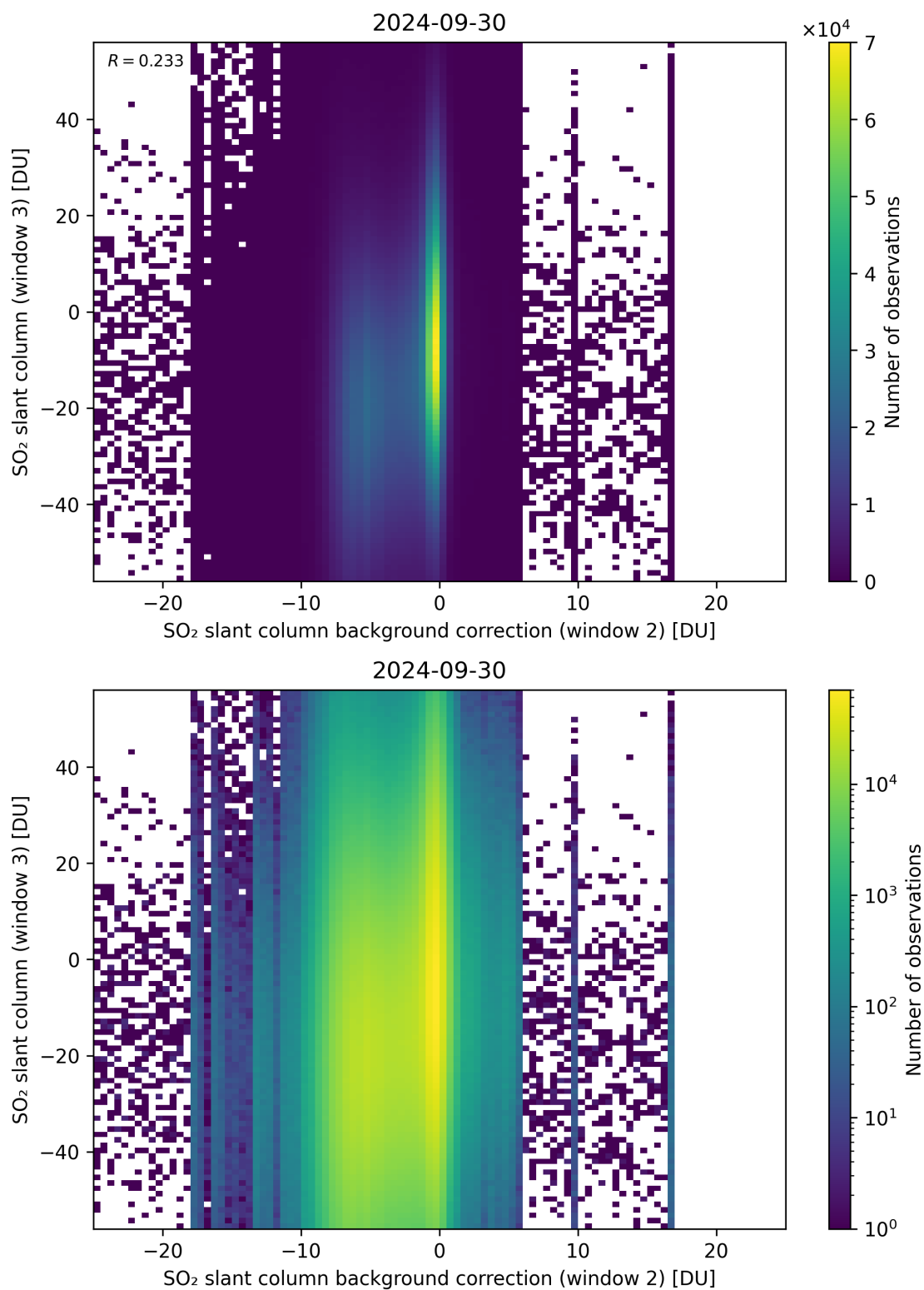
Figure 117: Scatter density plot of “SO 2 slant column background correction (window 2)” against “SO 2 slant column (window 3)” for 2024-09-29 to 2024-10-01.
