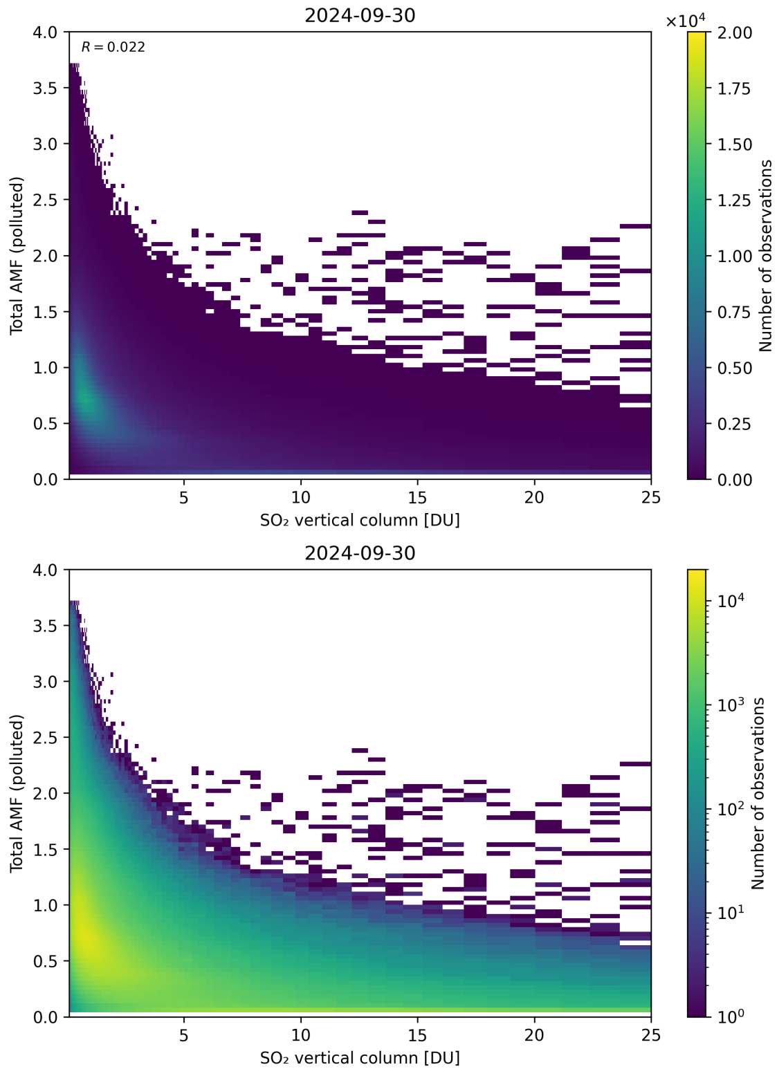
Figure 305: Scatter density plot of “SO 2 vertical column” against “Total AMF (polluted)” for 2024-09-29 to 2024-10-01.
