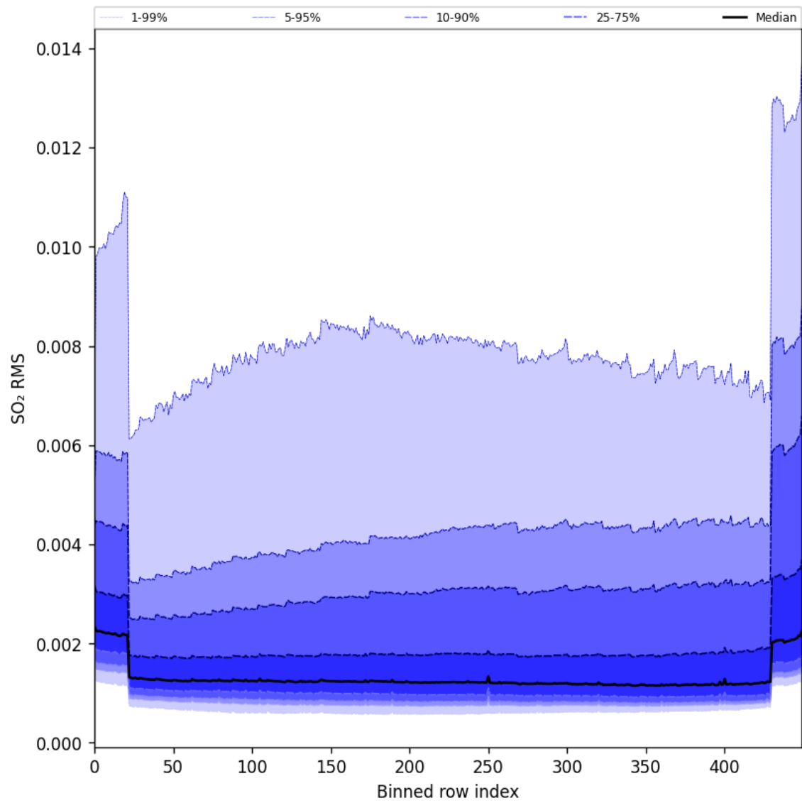
Figure 93: Along track statistics of “SO 2 RMS” for 2024-09-29 to 2024-10-01
