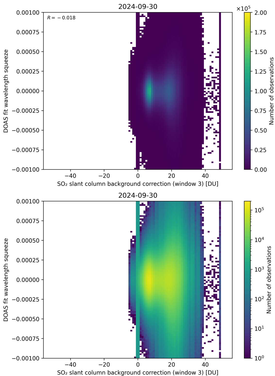
Figure 122: Scatter density plot of “SO 2 slant column background correction (window 3)” against “DOAS fit wavelength squeeze” for 2024-09-29 to 2024-10-01.
