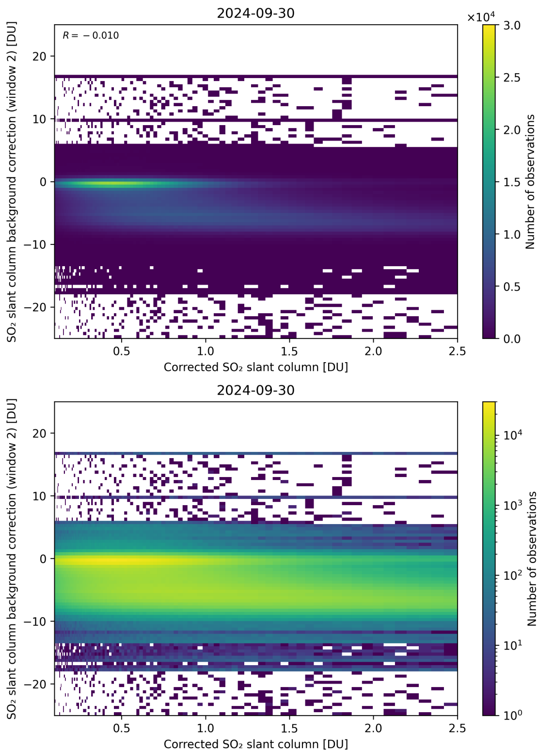
Figure 179: Scatter density plot of “Corrected SO 2 slant column” against “SO 2 slant column background correction (window 2)” for 2024-09-29 to 2024-10-01.
