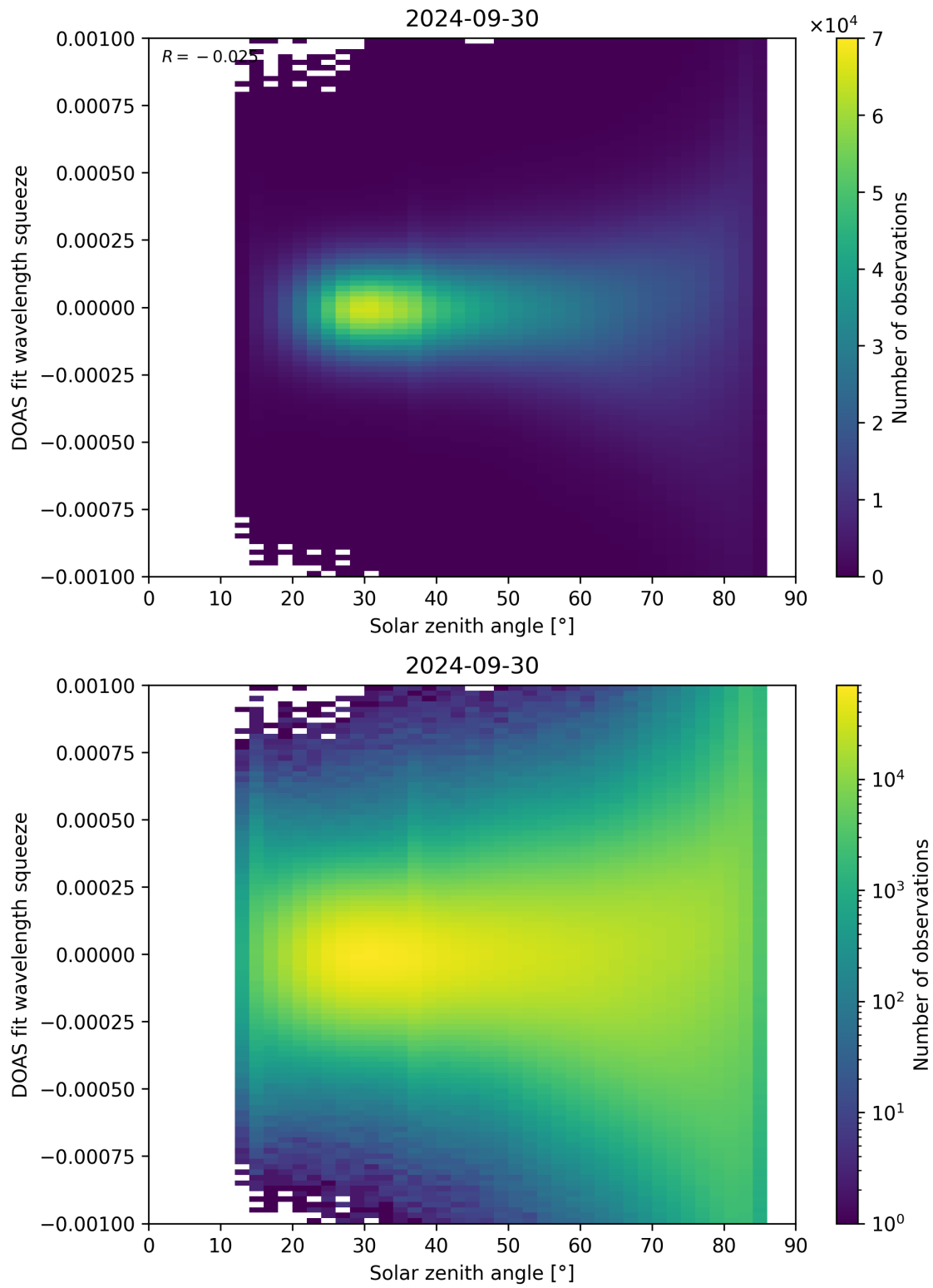
Figure 162: Scatter density plot of “Solar zenith angle” against “DOAS fit wavelength squeeze” for 2024-09-29 to 2024-10-01.
