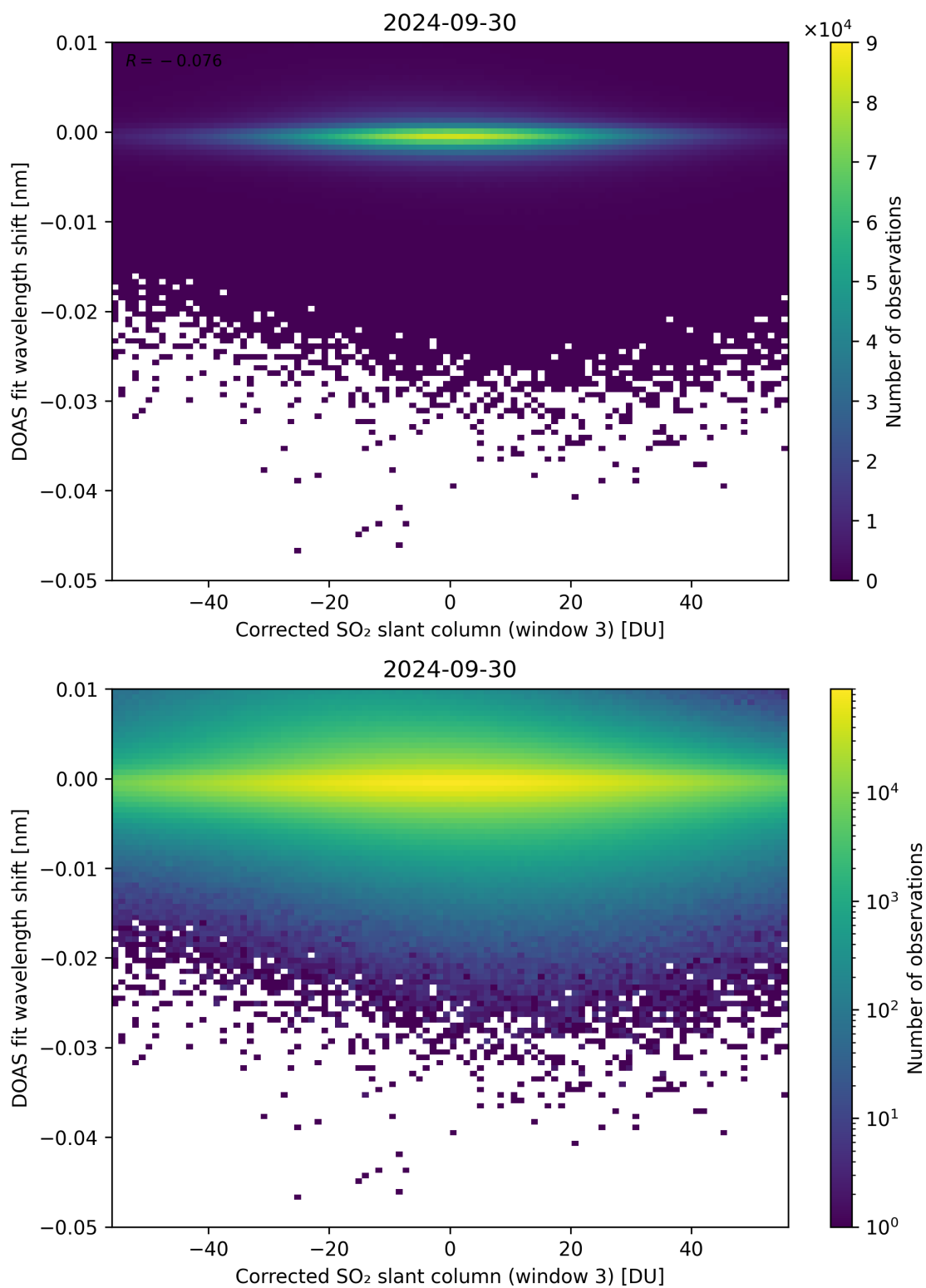
Figure 206: Scatter density plot of “Corrected SO 2 slant column (window 3)” against “DOAS fit wavelength shift” for 2024-09-29 to 2024-10-01.
