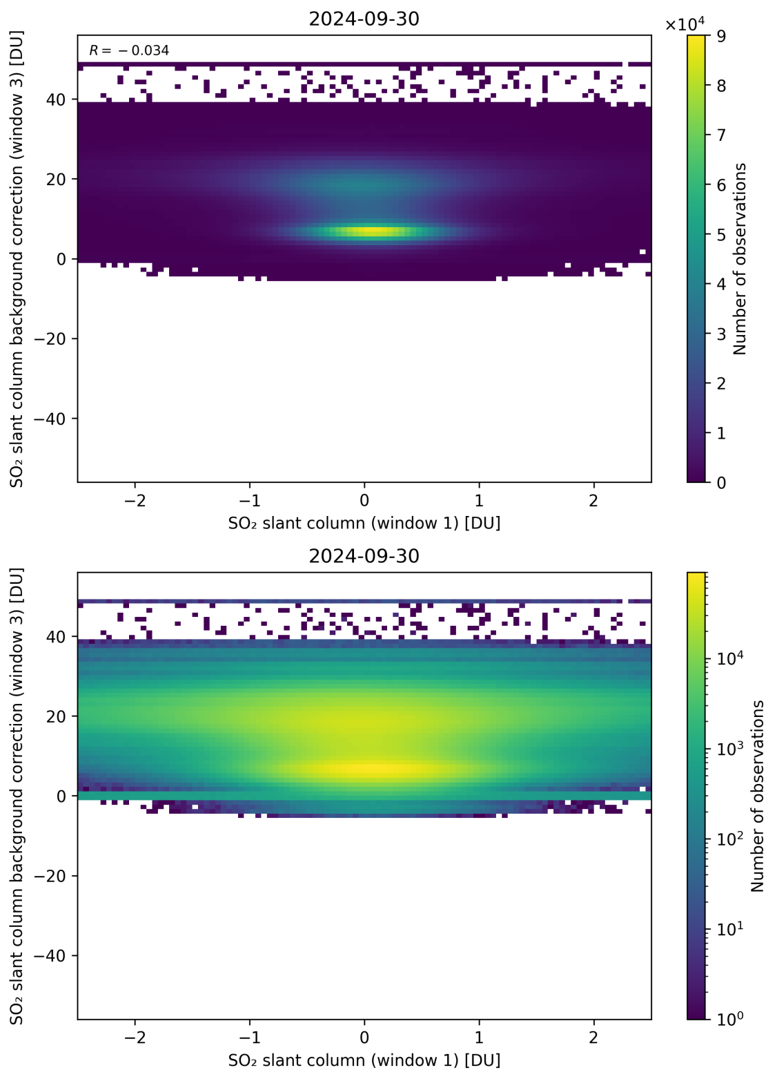
Figure 214: Scatter density plot of “SO 2 slant column (window 1)” against “SO 2 slant column background correction (window 3)” for 2024-09-29 to 2024-10-01.
