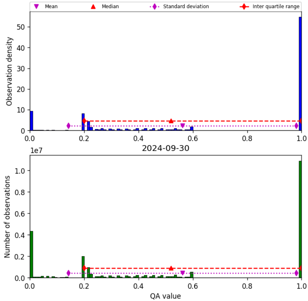
Figure 52: Histogram of “QA value” for 2024-09-29 to 2024-10-01
