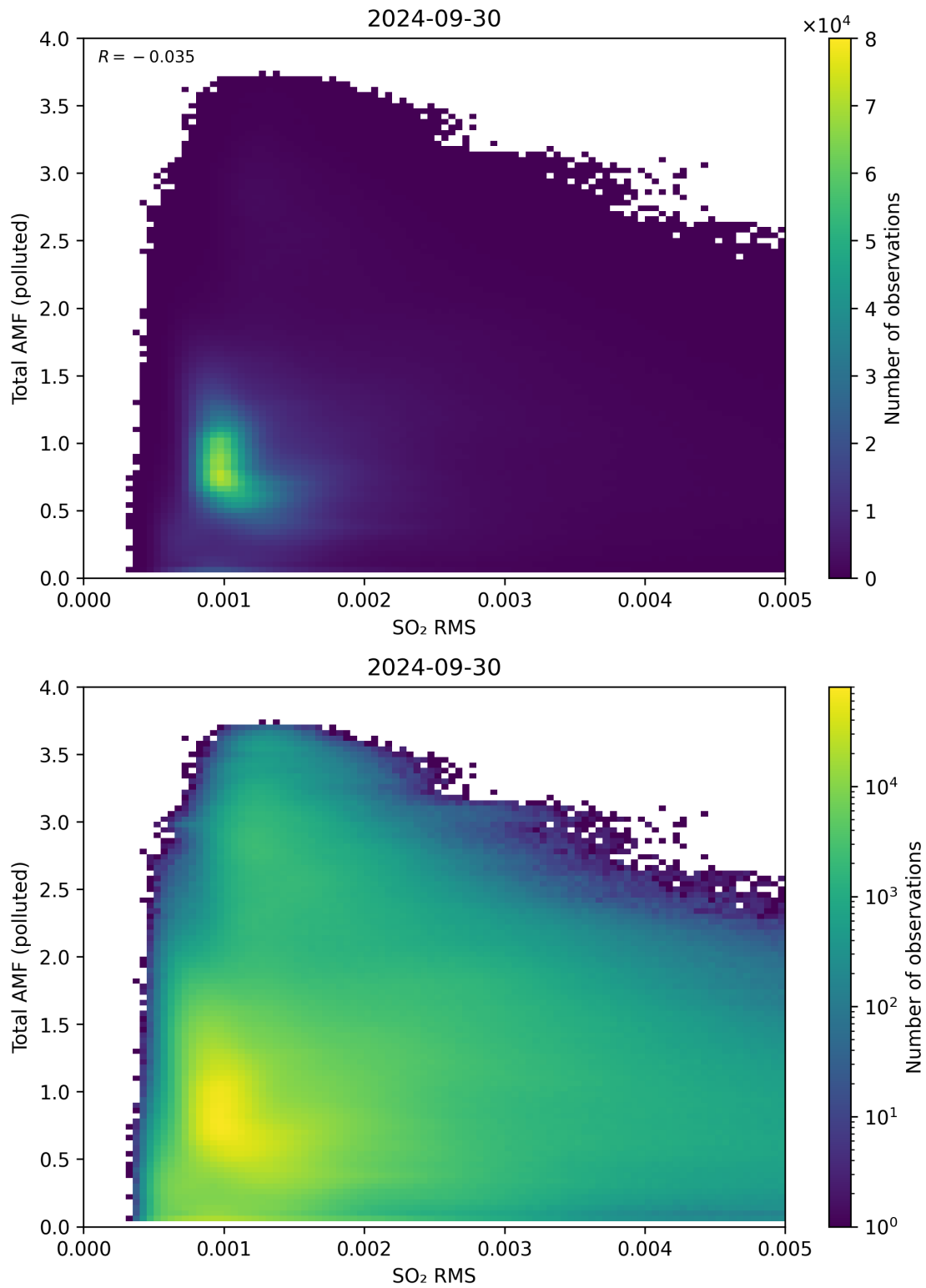
Figure 137: Scatter density plot of “SO 2 RMS” against “Total AMF (polluted)” for 2024-09-29 to 2024-10-01.
