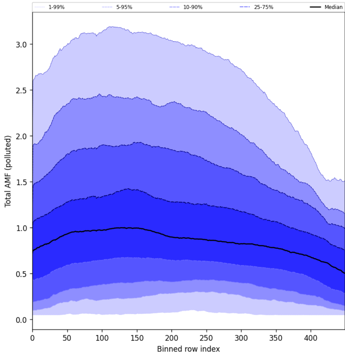
Figure 94: Along track statistics of “Total AMF (polluted)” for 2024-09-29 to 2024-10-01
