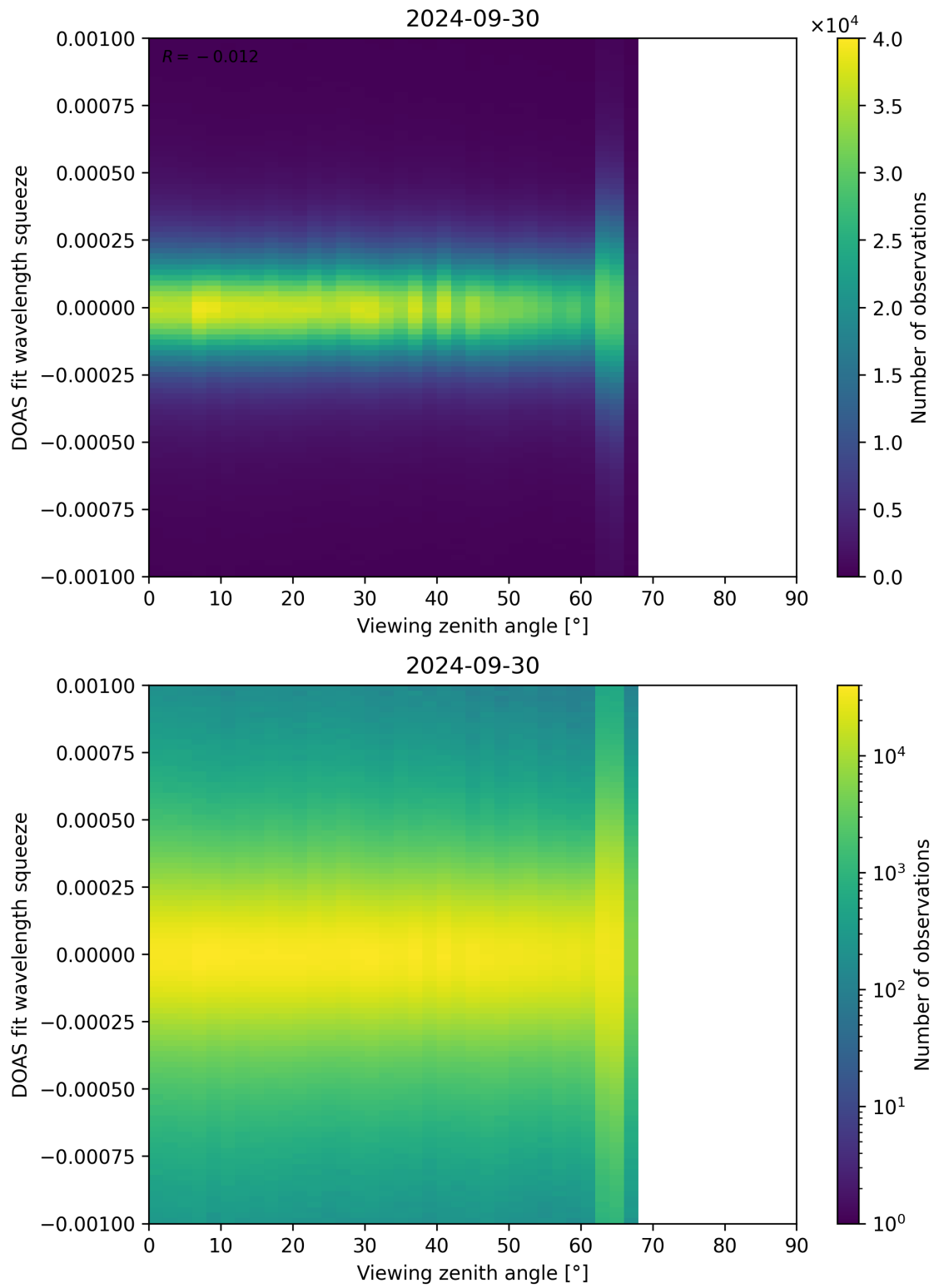
Figure 312: Scatter density plot of “Viewing zenith angle” against “DOAS fit wavelength squeeze” for 2024-09-29 to 2024-10-01.
