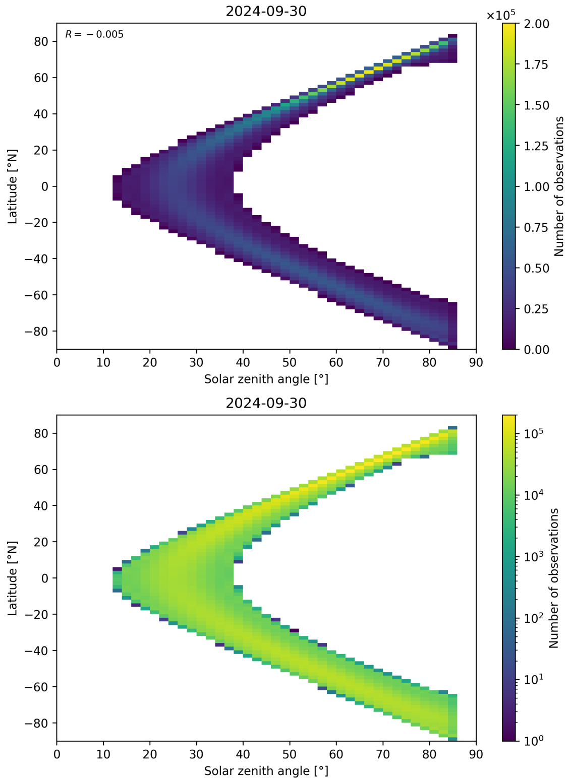
Figure 164: Scatter density plot of “Solar zenith angle” against “Latitude” for 2024-09-29 to 2024-10-01.
