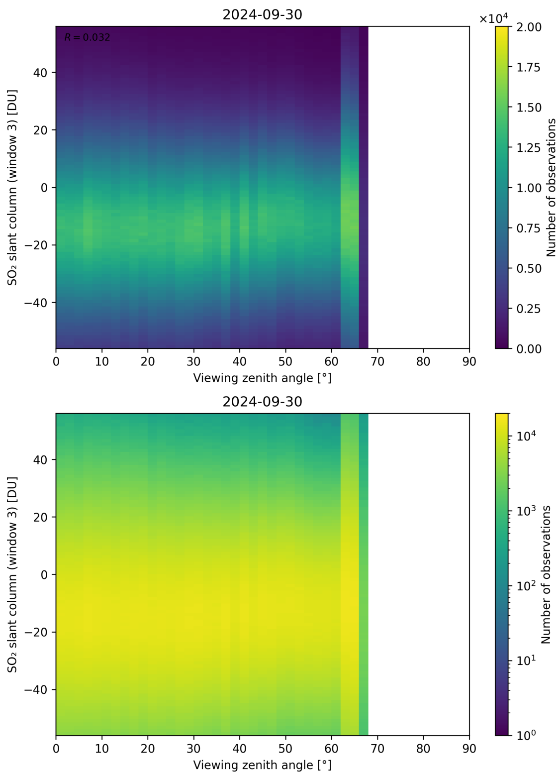
Figure 323: Scatter density plot of “Viewing zenith angle” against “SO 2 slant column (window 3)” for 2024-09-29 to 2024-10-01.
