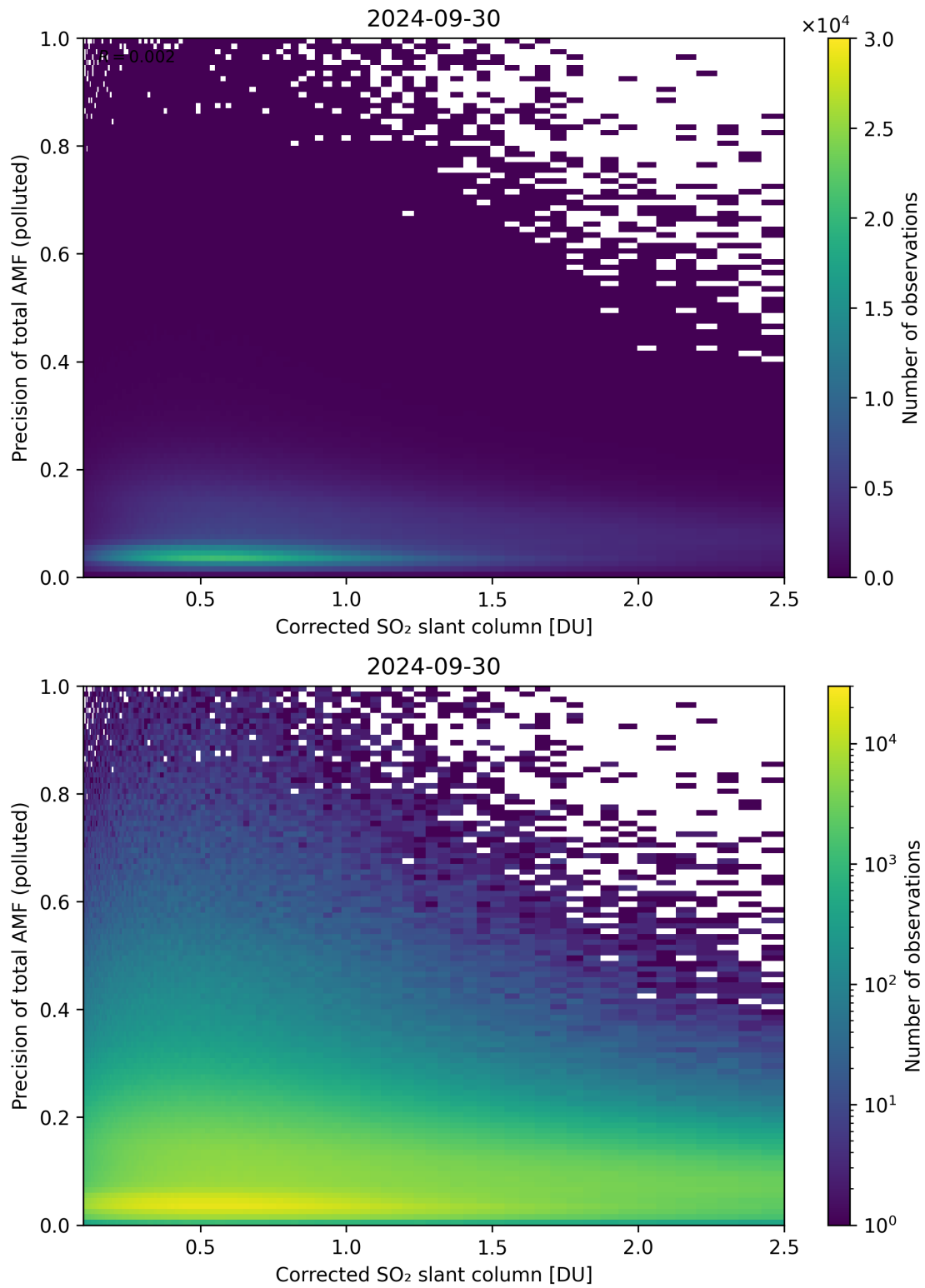
Figure 193: Scatter density plot of “Corrected SO 2 slant column” against “Precision of total AMF (polluted)” for 2024-09-29 to 2024-10-01.
