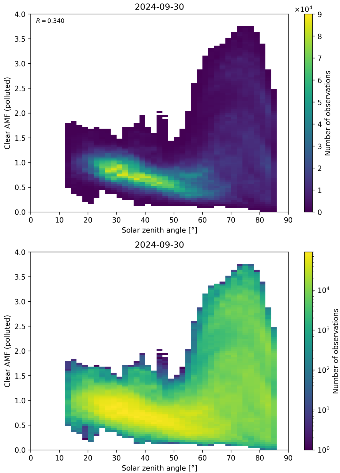
Figure 165: Scatter density plot of “Solar zenith angle” against “Clear AMF (polluted)” for 2024-09-29 to 2024-10-01.
