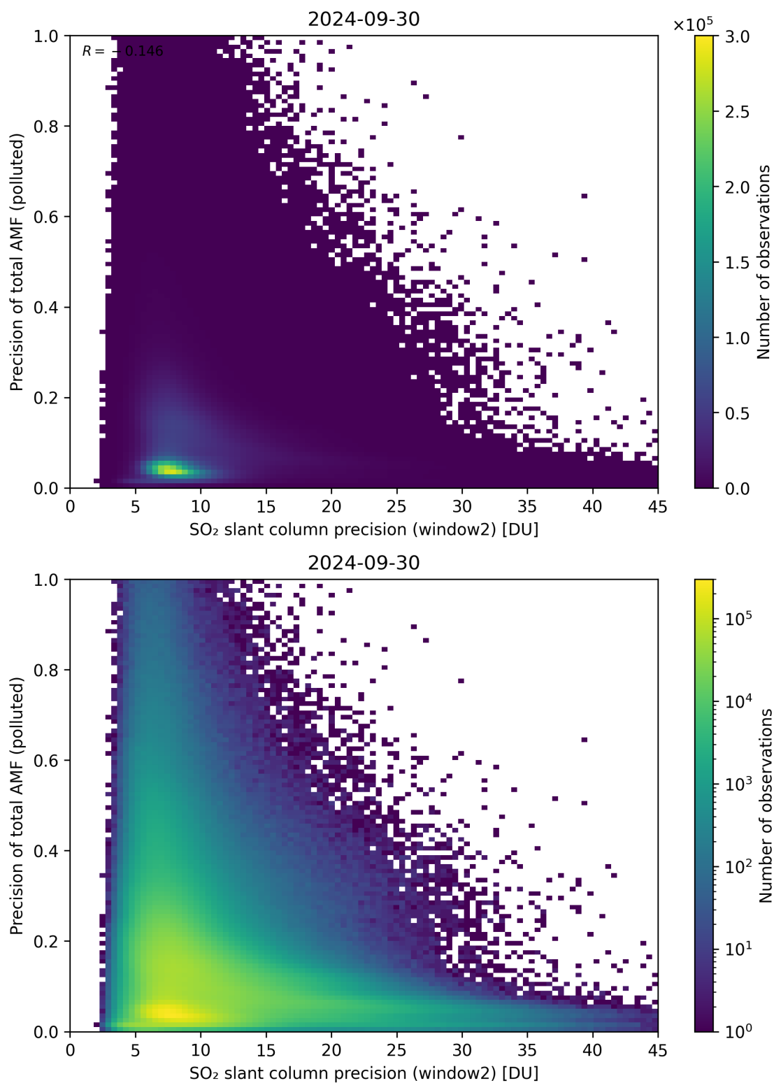
Figure 252: Scatter density plot of “SO 2 slant column precision (window2)” against “Precision of total AMF (polluted)” for 2024-09-29 to 2024-10-01.
