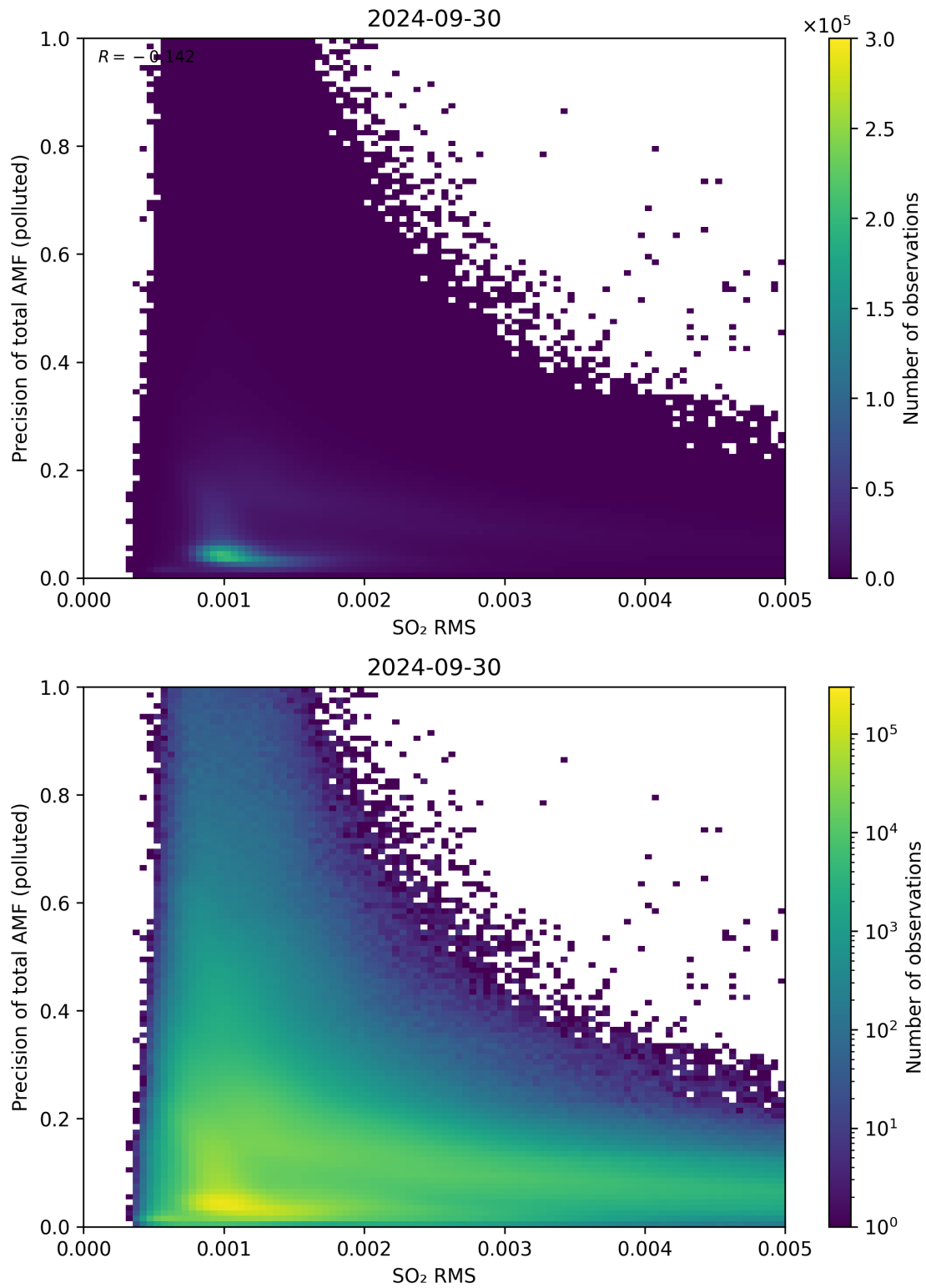
Figure 138: Scatter density plot of “SO 2 RMS” against “Precision of total AMF (polluted)” for 2024-09-29 to 2024-10-01.
