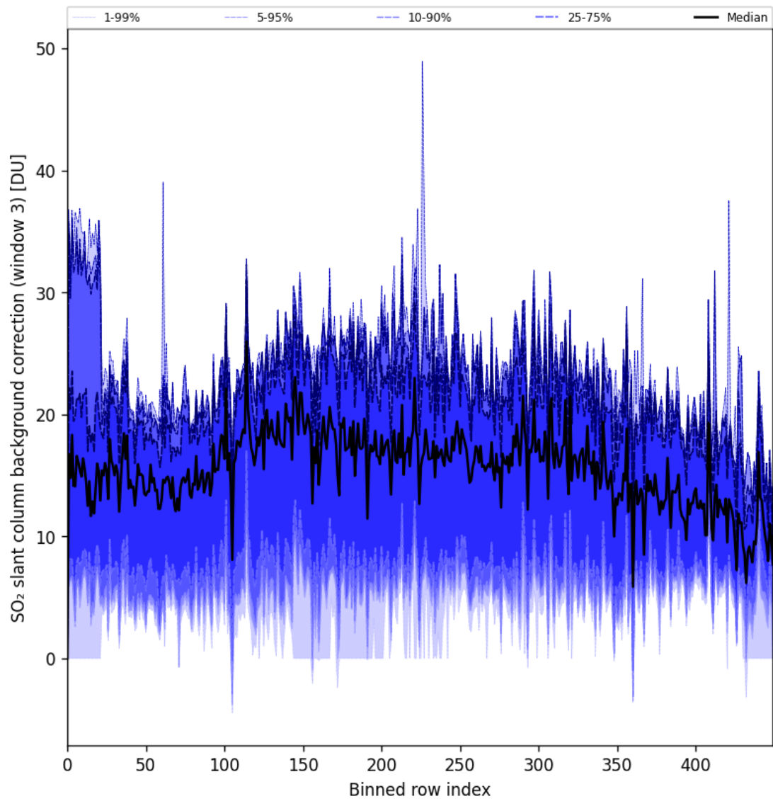
Figure 90: Along track statistics of “SO 2 slant column background correction (window 3)” for 2024-09-29 to 2024-10-01
