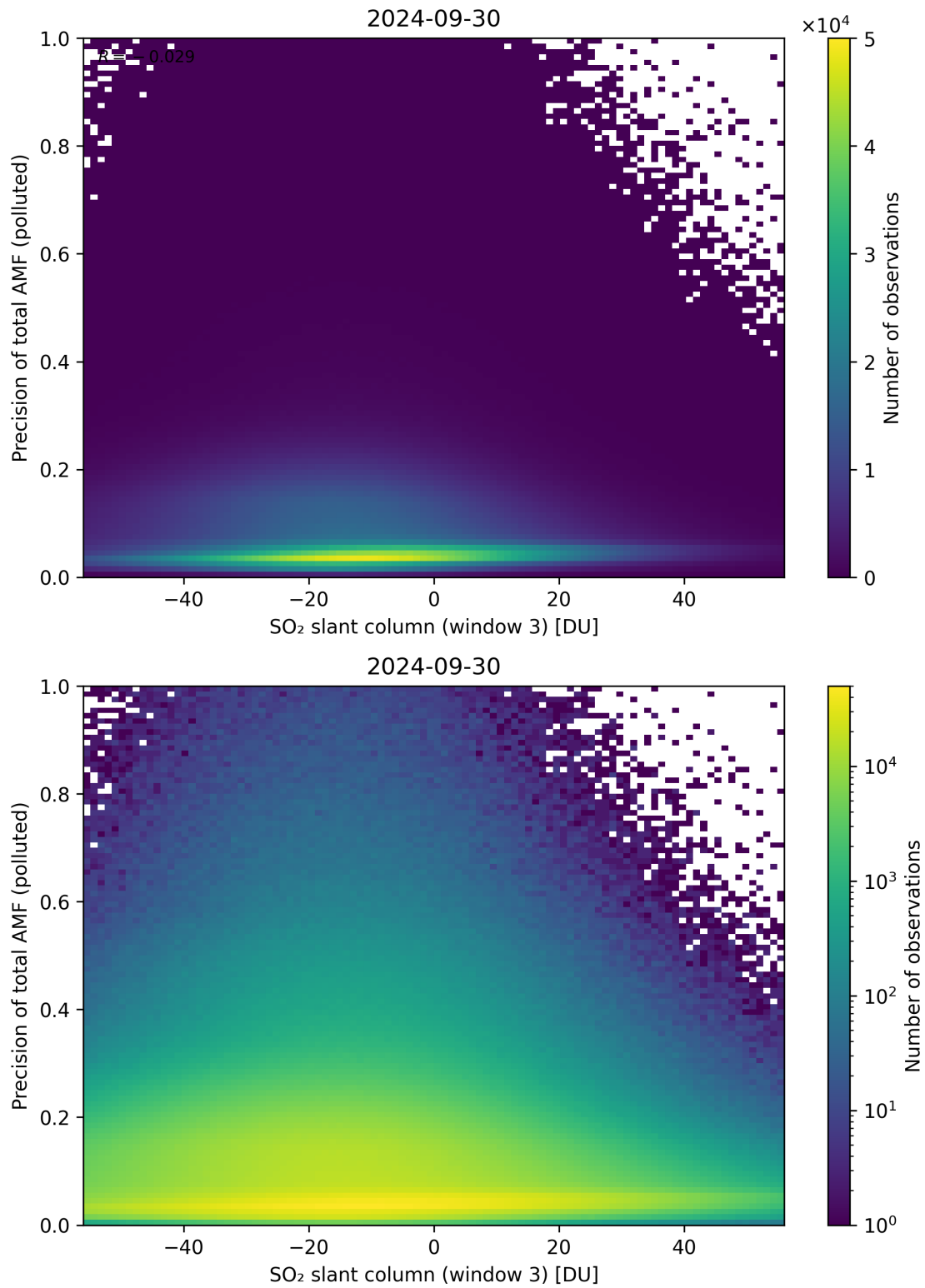
Figure 269: Scatter density plot of “SO 2 slant column (window 3)” against “Precision of total AMF (polluted)” for 2024-09-29 to 2024-10-01.
