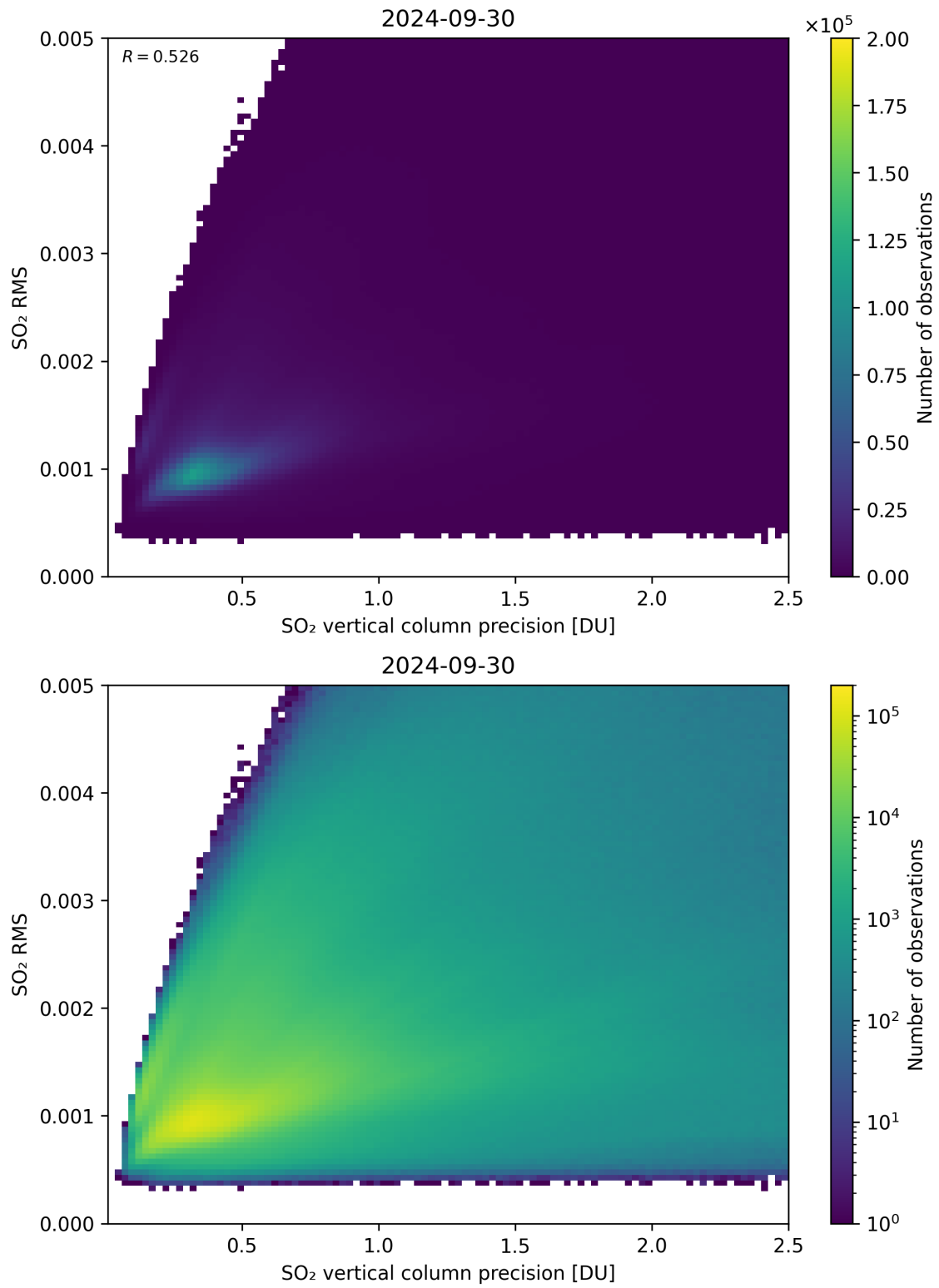
Figure 284: Scatter density plot of “SO 2 vertical column precision” against “SO 2 RMS” for 2024-09-29 to 2024-10-01.
