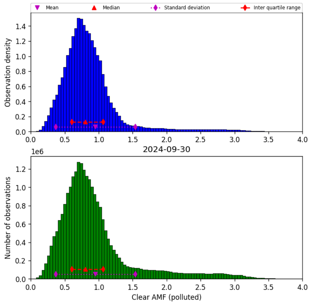
Figure 73: Histogram of “Clear AMF (polluted)” for 2024-09-29 to 2024-10-01
