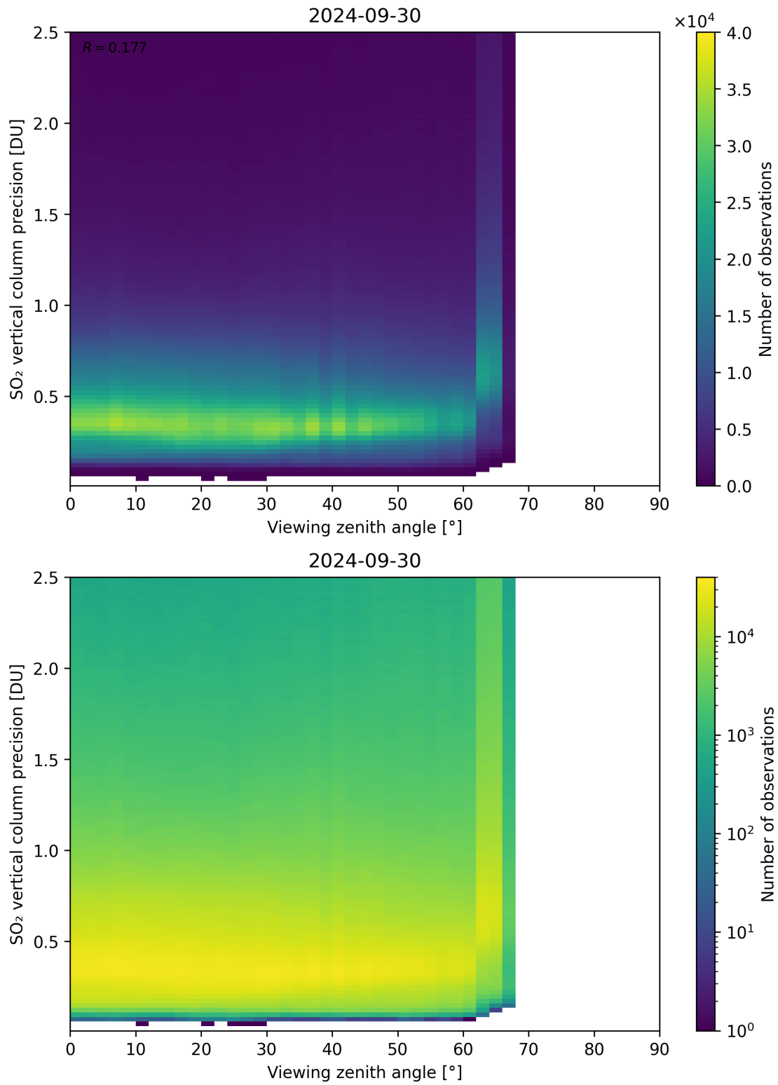
Figure 328: Scatter density plot of “Viewing zenith angle” against “SO 2 vertical column precision” for 2024-09-29 to 2024-10-01.
