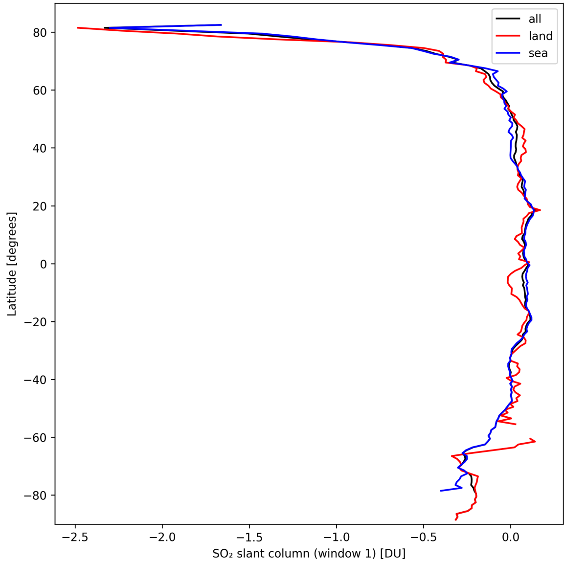
Figure 33: Zonal average of “SO 2 slant column (window 1)” for 2024-09-29 to 2024-10-01.
