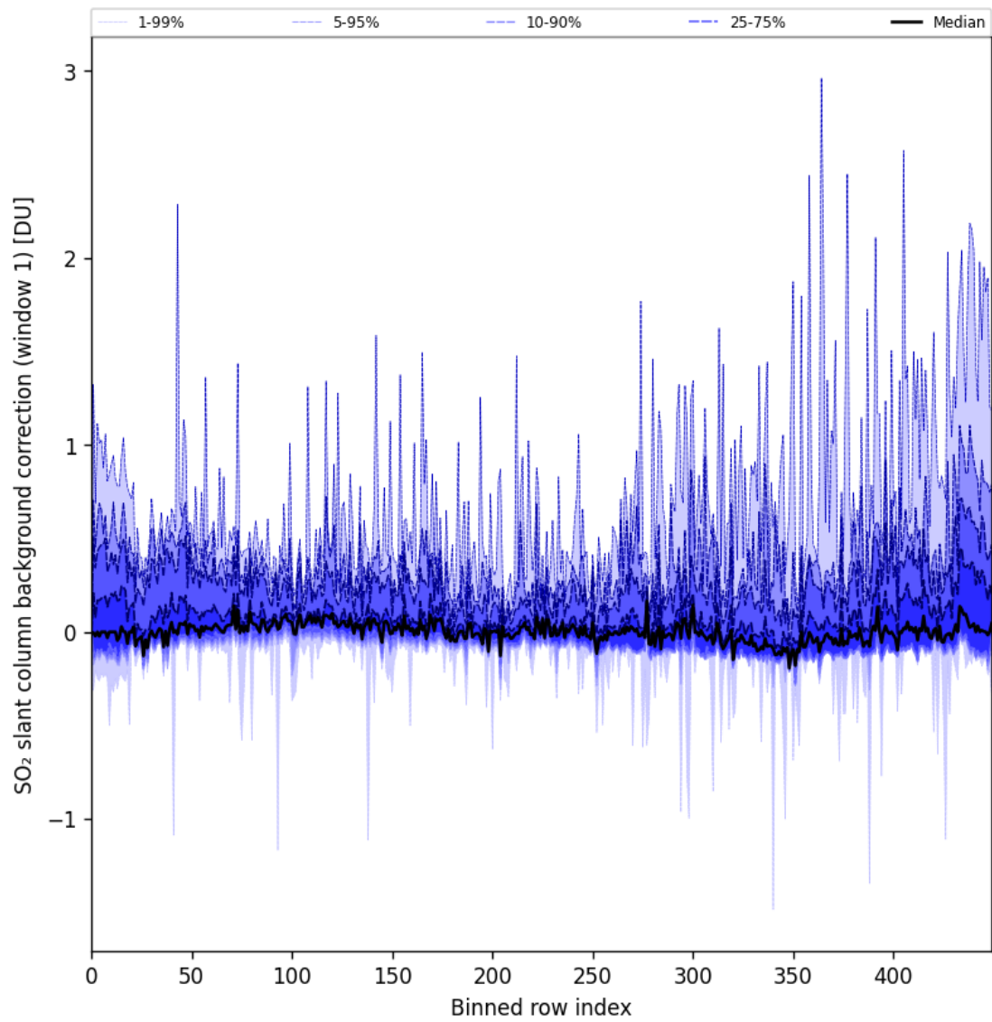
Figure 82: Along track statistics of “SO 2 slant column background correction (window 1)” for 2024-09-29 to 2024-10-01
