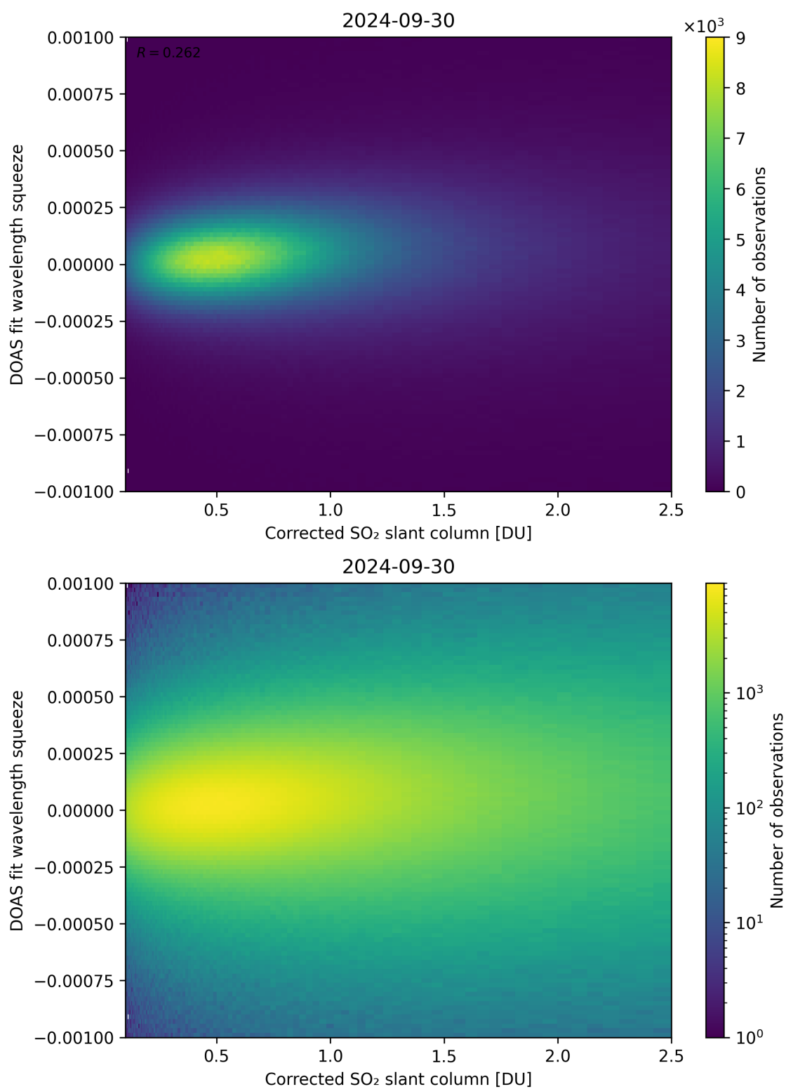
Figure 182: Scatter density plot of “Corrected SO 2 slant column” against “DOAS fit wavelength squeeze” for 2024-09-29 to 2024-10-01.
