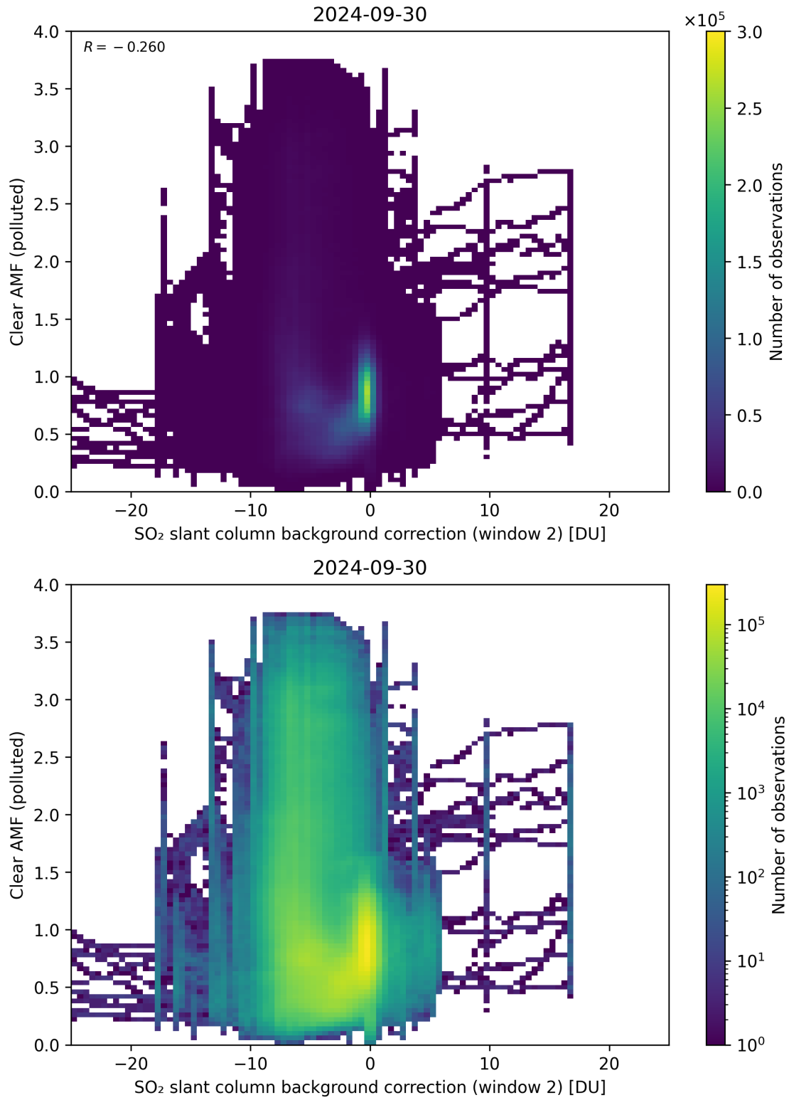
Figure 115: Scatter density plot of “SO 2 slant column background correction (window 2)” against “Clear AMF (polluted)” for 2024-09-29 to 2024-10-01.
