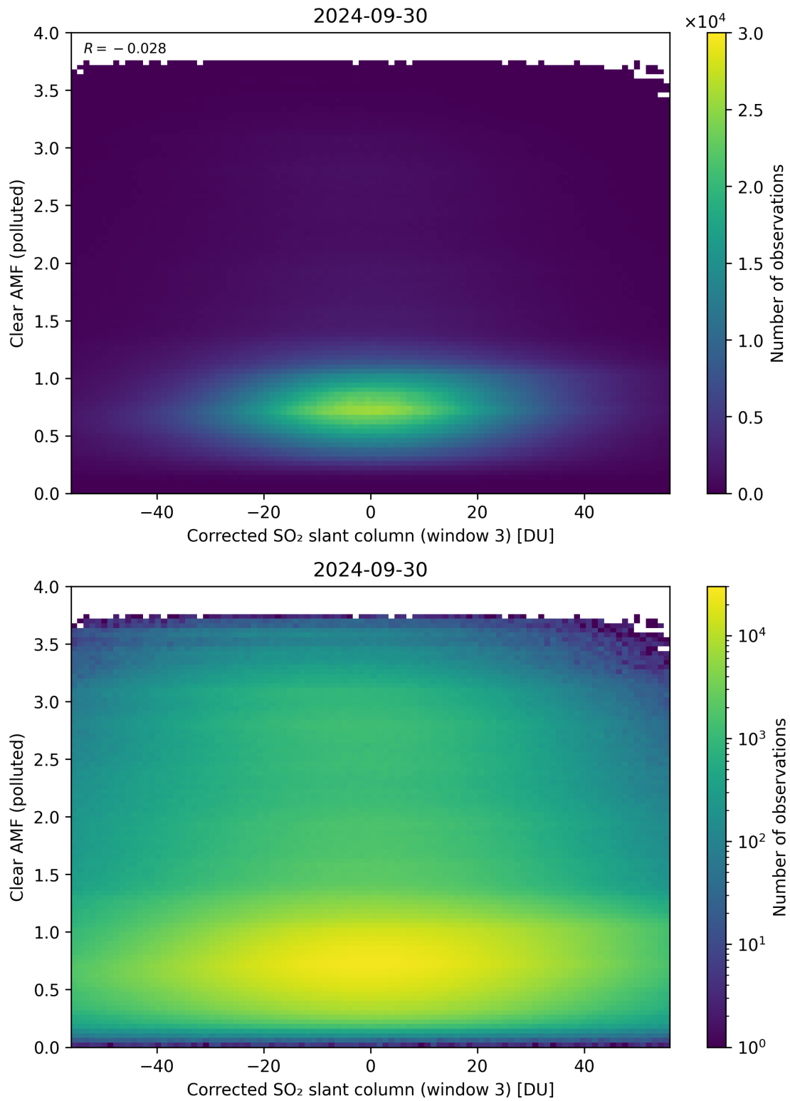
Figure 209: Scatter density plot of “Corrected SO 2 slant column (window 3)” against “Clear AMF (polluted)” for 2024-09-29 to 2024-10-01.
