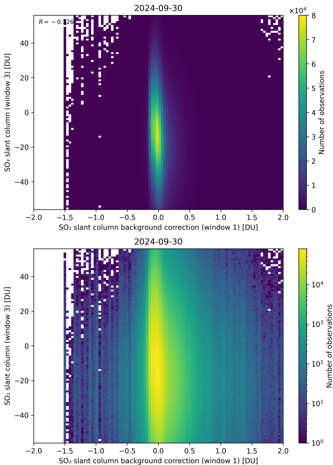
Figure 107: Scatter density plot of “SO 2 slant column background correction (window 1)” against “SO 2 slant column (window 3)” for 2024-09-29 to 2024-10-01.
