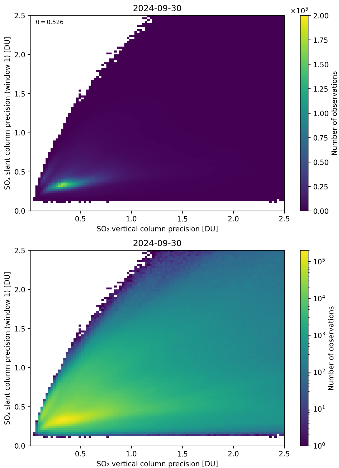
Figure 290: Scatter density plot of “SO 2 vertical column precision” against “SO 2 slant column precision (window 1)” for 2024-09-29 to 2024-10-01.
