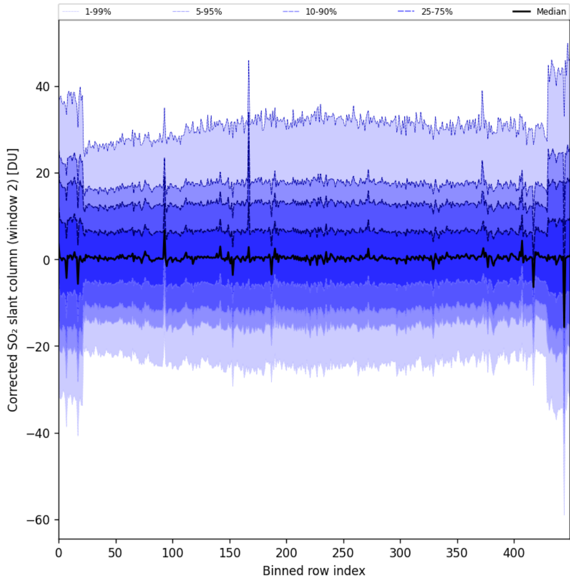
Figure 85: Along track statistics of “Corrected SO 2 slant column (window 2)” for 2024-09-29 to 2024-10-01
