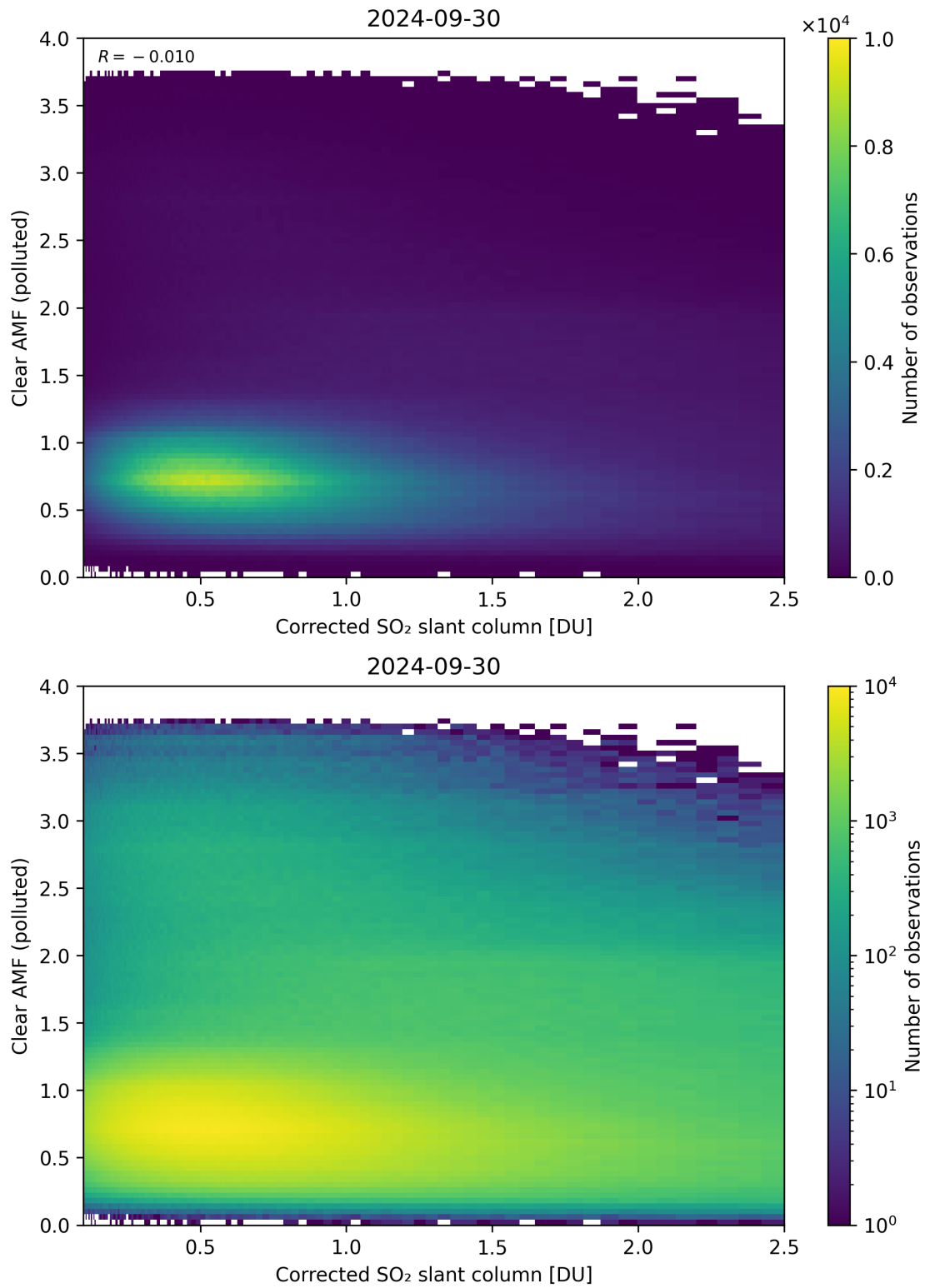
Figure 184: Scatter density plot of “Corrected SO 2 slant column” against “Clear AMF (polluted)” for 2024-09-29 to 2024-10-01.
