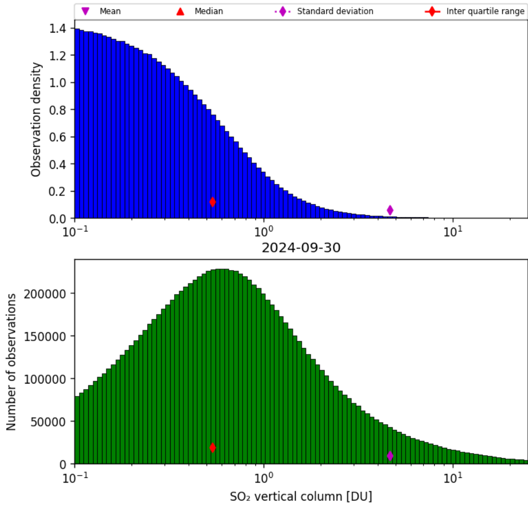
Figure 53: Histogram of “SO 2 vertical column” for 2024-09-29 to 2024-10-01
