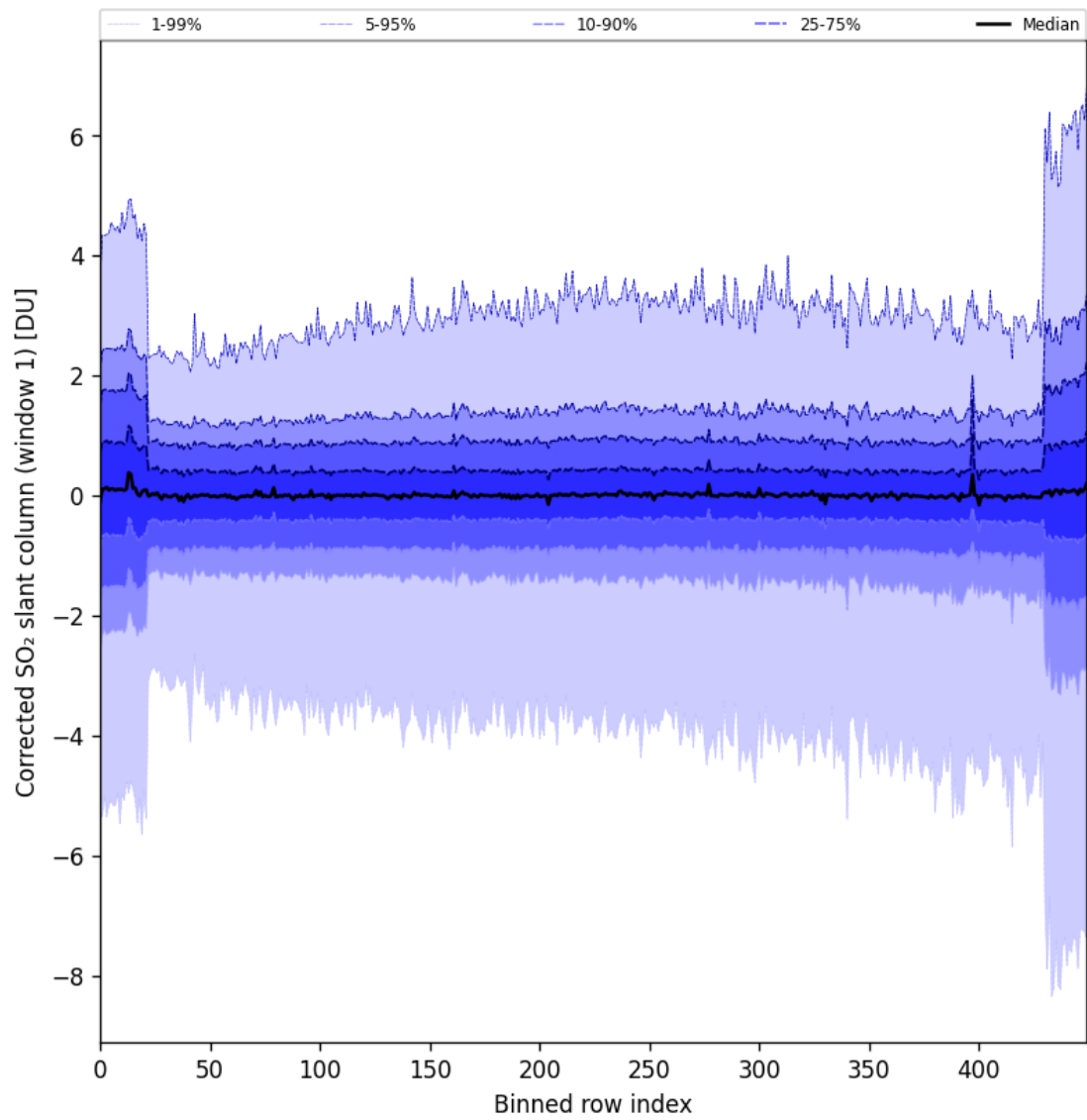
Figure 81: Along track statistics of “Corrected SO 2 slant column (window 1)” for 2024-09-29 to 2024-10-01
