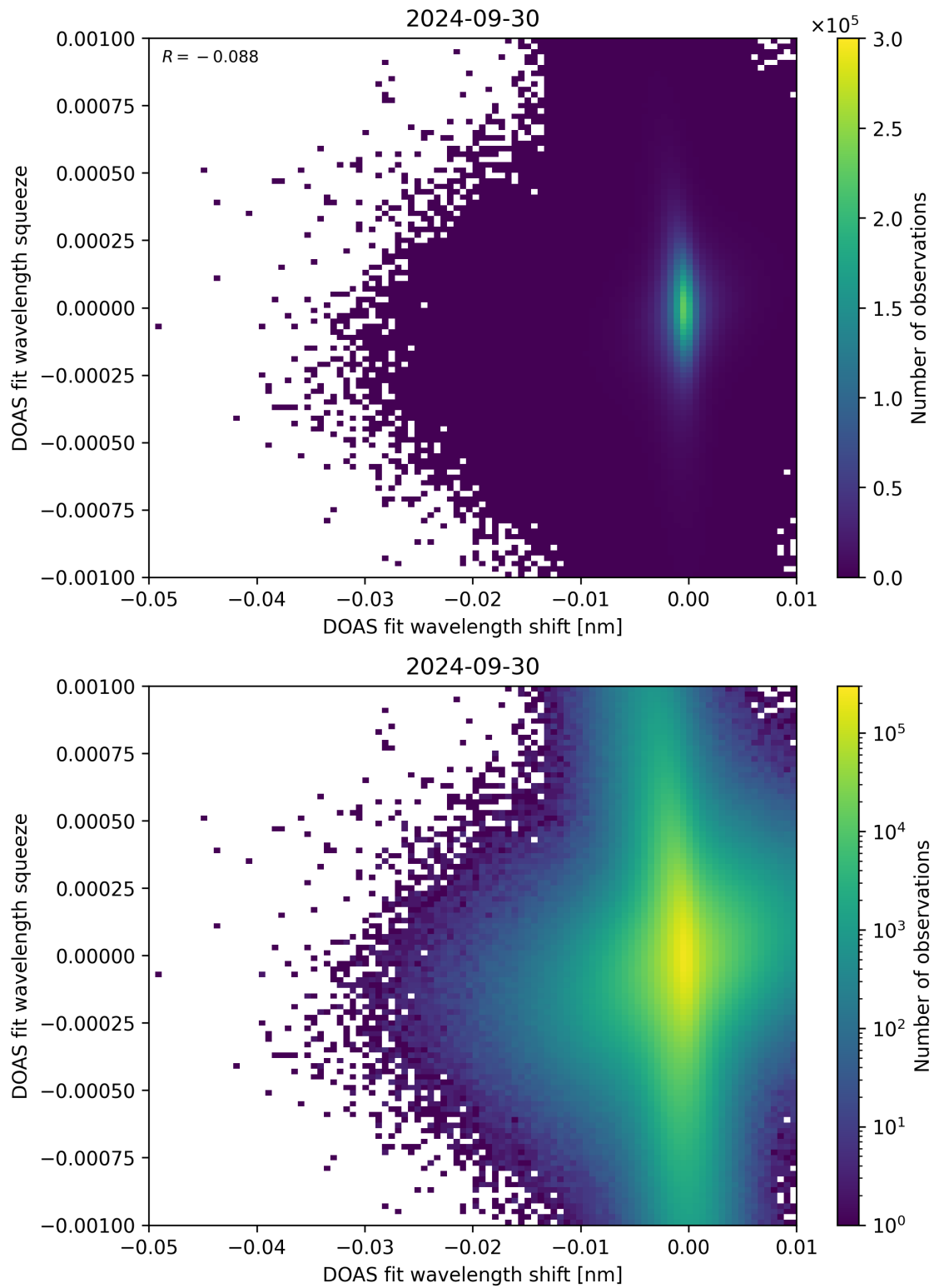
Figure 127: Scatter density plot of “DOAS fit wavelength shift” against “DOAS fit wavelength squeeze” for 2024-09-29 to 2024-10-01.
