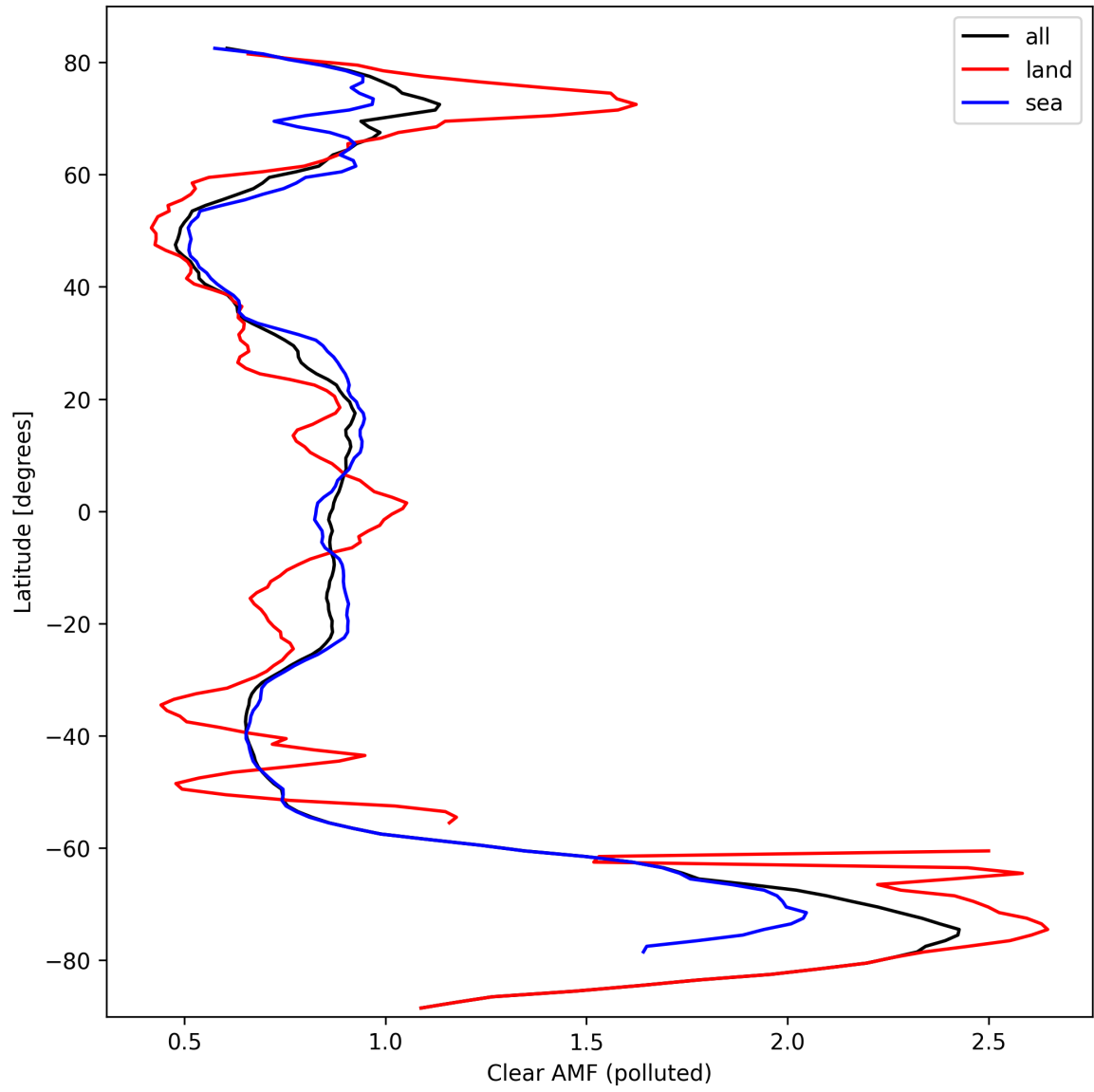
Figure 50: Zonal average of “Clear AMF (polluted)” for 2024-09-29 to 2024-10-01.
