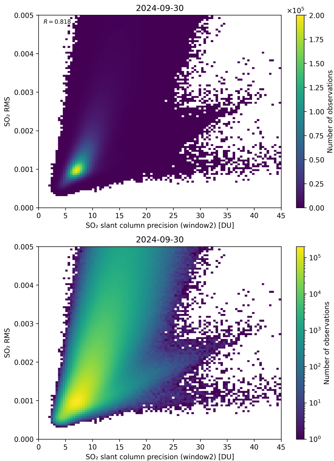
Figure 245: Scatter density plot of “SO 2 slant column precision (window2)” against “SO 2 RMS” for 2024-09-29 to 2024-10-01.
