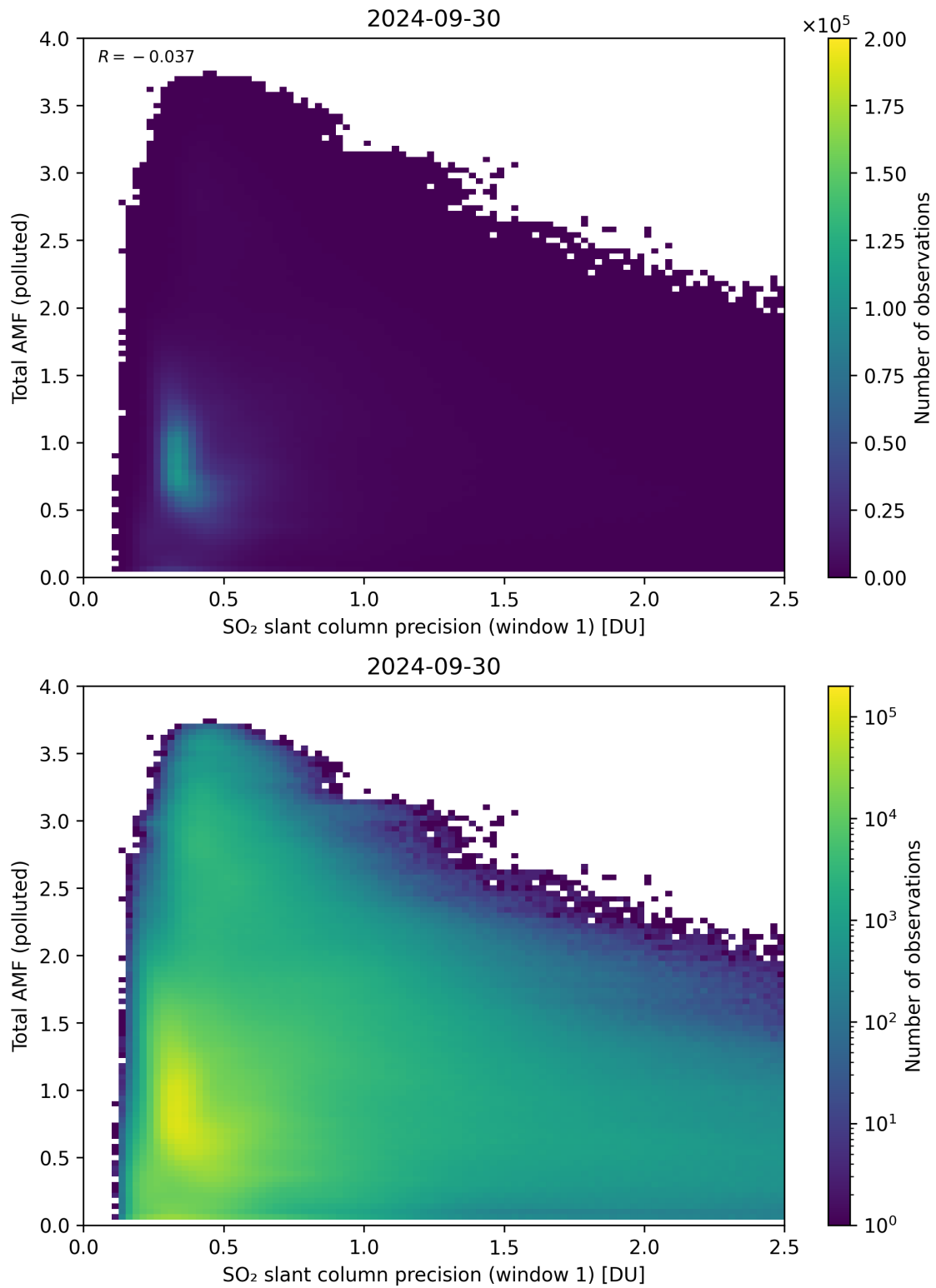
Figure 230: Scatter density plot of “SO 2 slant column precision (window 1)” against “Total AMF (polluted)” for 2024-09-29 to 2024-10-01.
