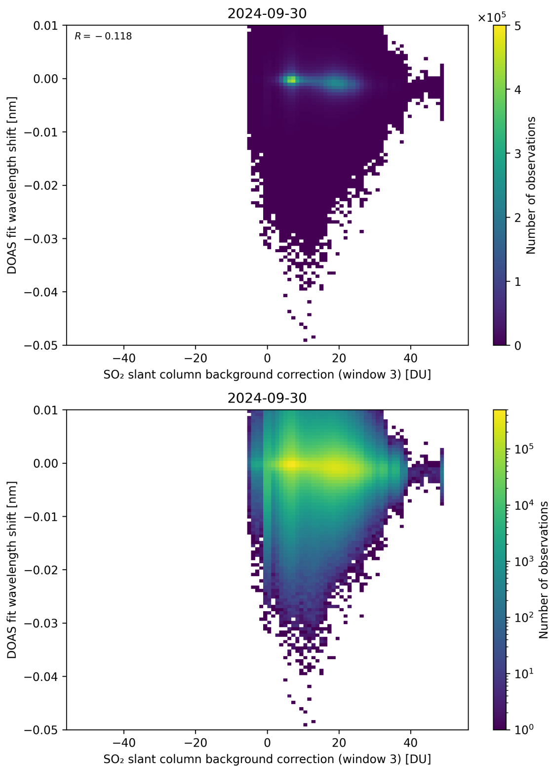
Figure 121: Scatter density plot of “SO 2 slant column background correction (window 3)” against “DOAS fit wavelength shift” for 2024-09-29 to 2024-10-01.
