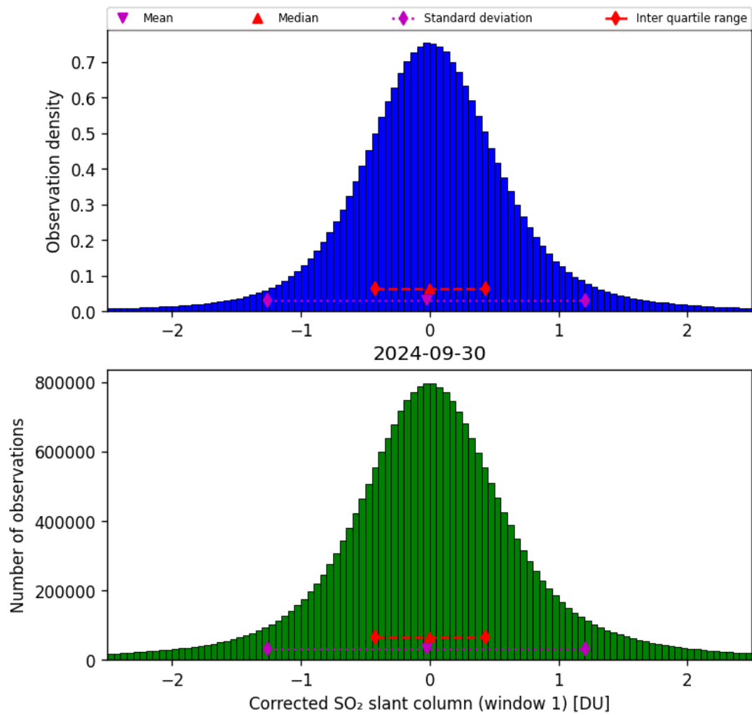
Figure 58: Histogram of “Corrected SO 2 slant column (window 1)” for 2024-09-29 to 2024-10-01
