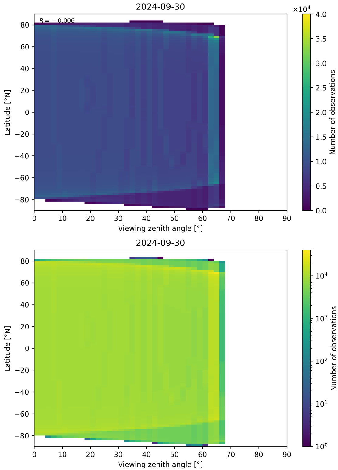
Figure 314: Scatter density plot of “Viewing zenith angle” against “Latitude” for 2024-09-29 to 2024-10-01.
