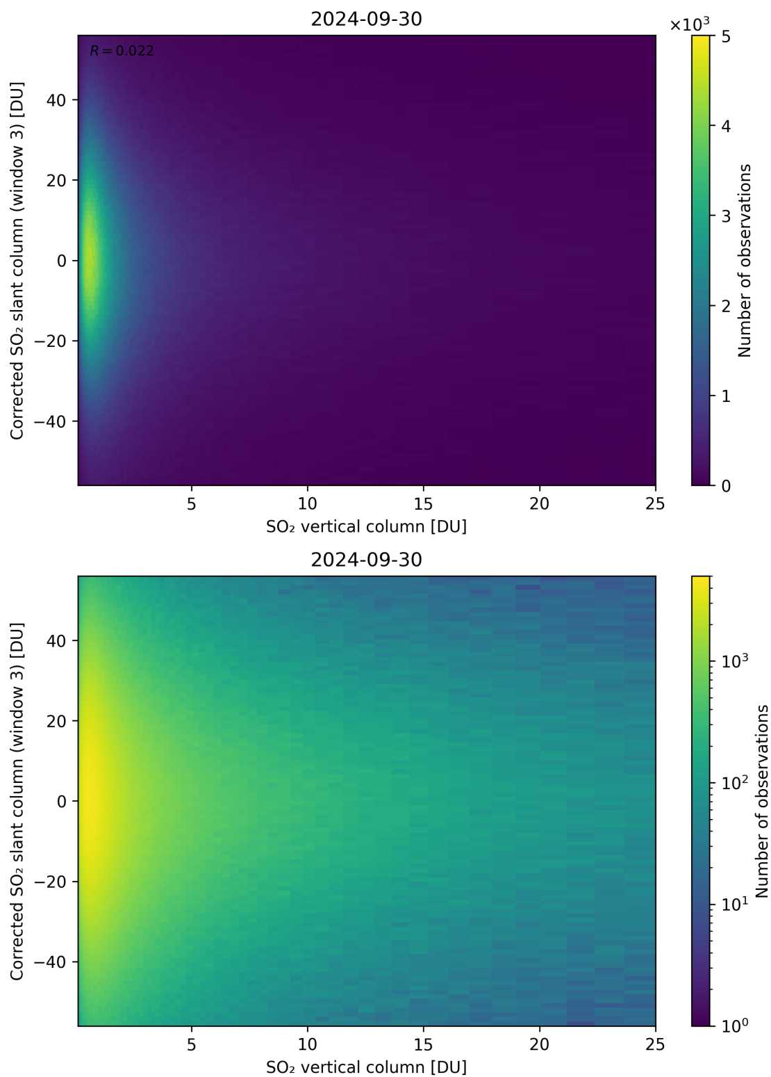
Figure 299: Scatter density plot of “SO 2 vertical column” against “Corrected SO 2 slant column (window 3)” for 2024-09-29 to 2024-10-01.
