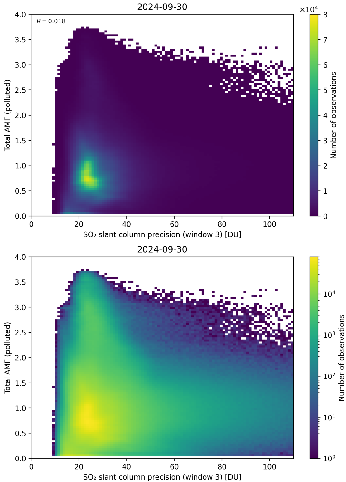
Figure 263: Scatter density plot of “SO 2 slant column precision (window 3)” against “Total AMF (polluted)” for 2024-09-29 to 2024-10-01.
