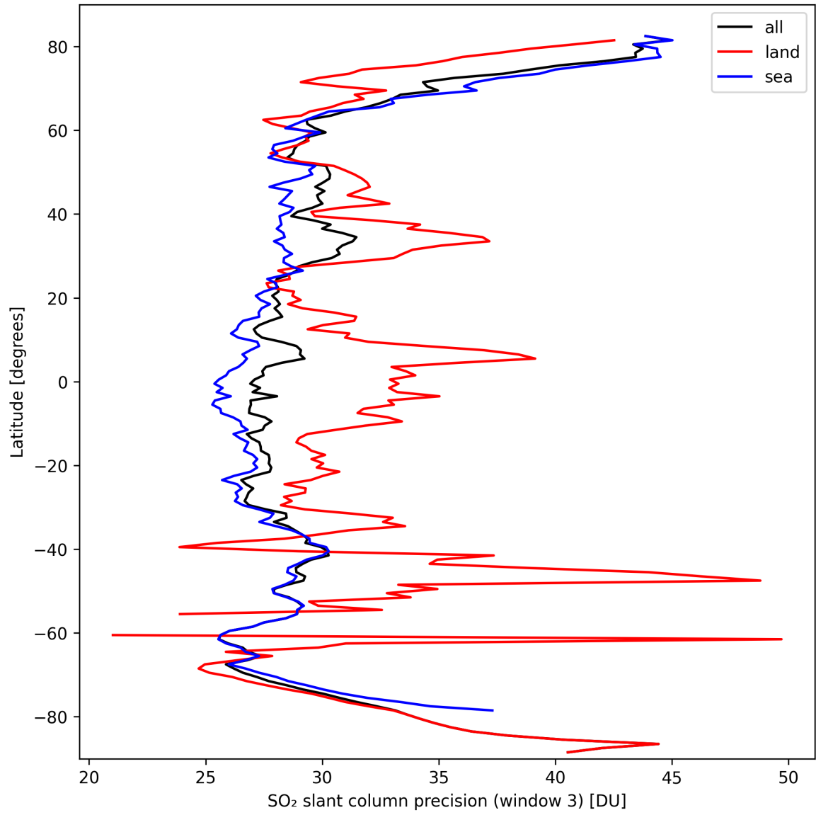
Figure 42: Zonal average of “SO 2 slant column precision (window 3)” for 2024-09-29 to 2024-10-01.
