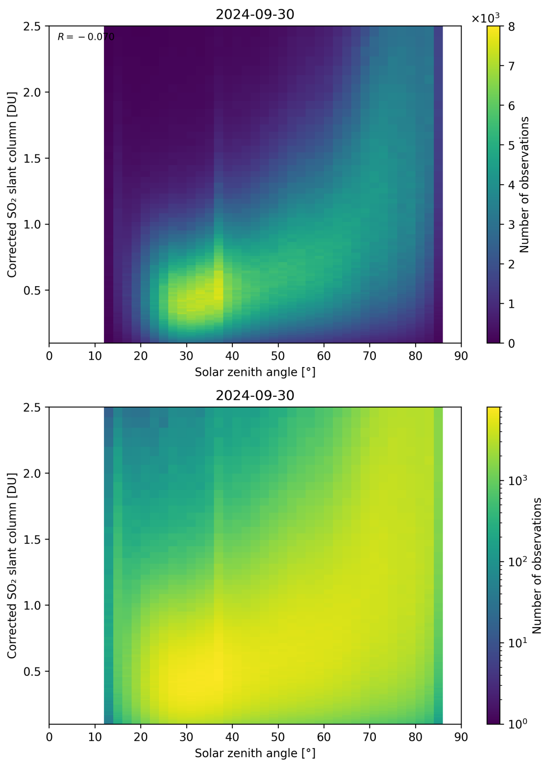
Figure 166: Scatter density plot of “Solar zenith angle” against “Corrected SO 2 slant column” for 2024-09-29 to 2024-10-01.
