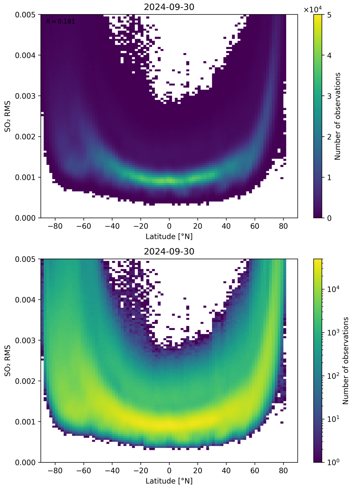
Figure 144: Scatter density plot of “Latitude” against “SO 2 RMS” for 2024-09-29 to 2024-10-01.
