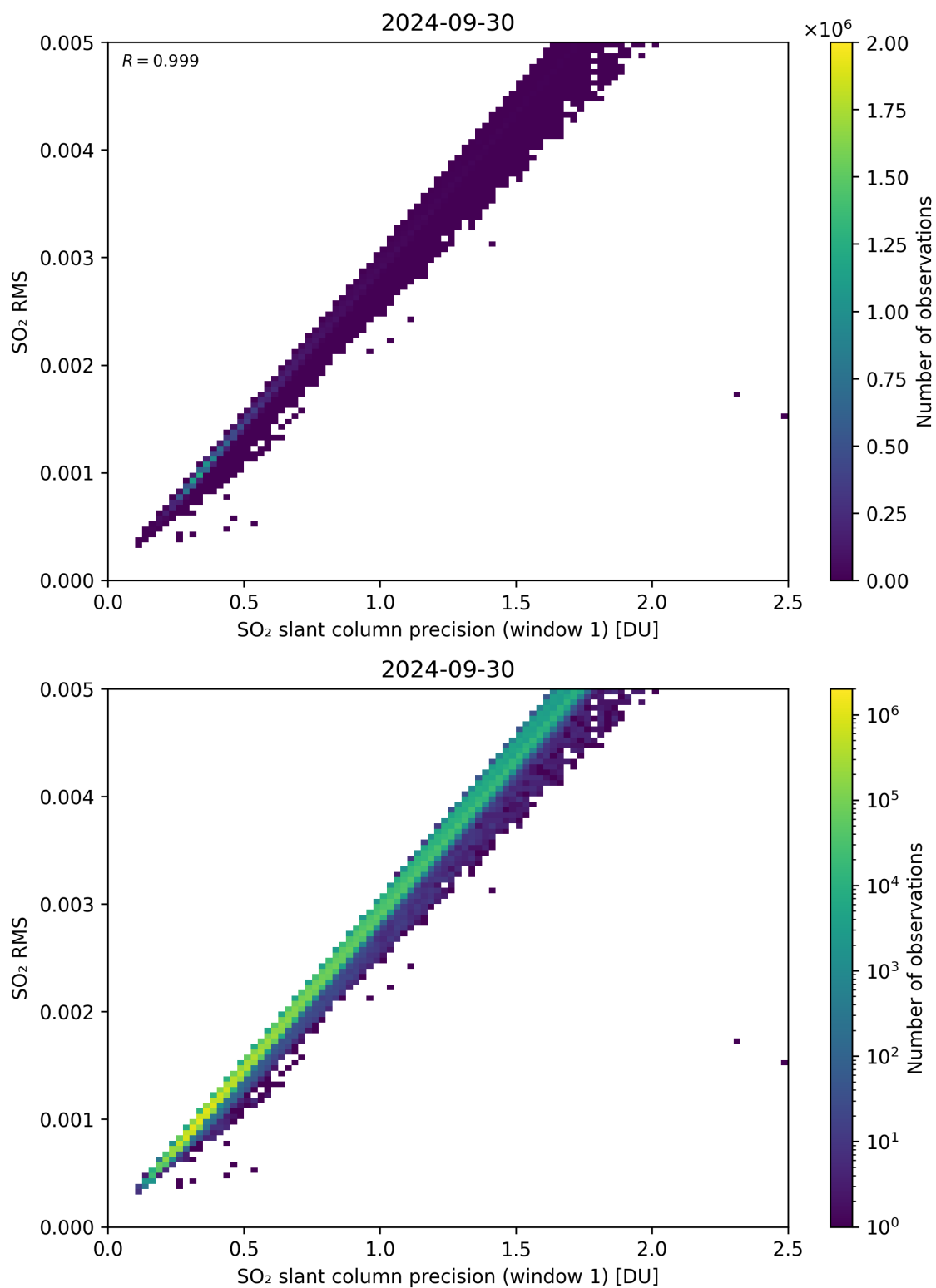
Figure 223: Scatter density plot of “SO 2 slant column precision (window 1)” against “SO 2 RMS” for 2024-09-29 to 2024-10-01.
