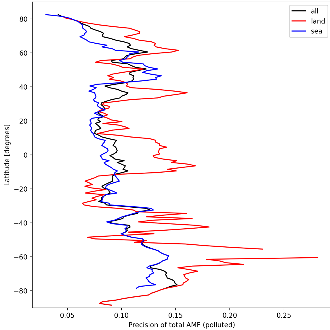
Figure 49: Zonal average of “Precision of total AMF (polluted)” for 2024-09-29 to 2024-10-01.
