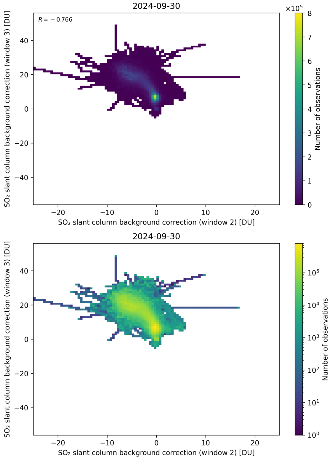
Figure 111: Scatter density plot of “SO 2 slant column background correction (window 2)” against “SO 2 slant column background correction (window 3)” for 2024-09-29 to 2024-10-01.
