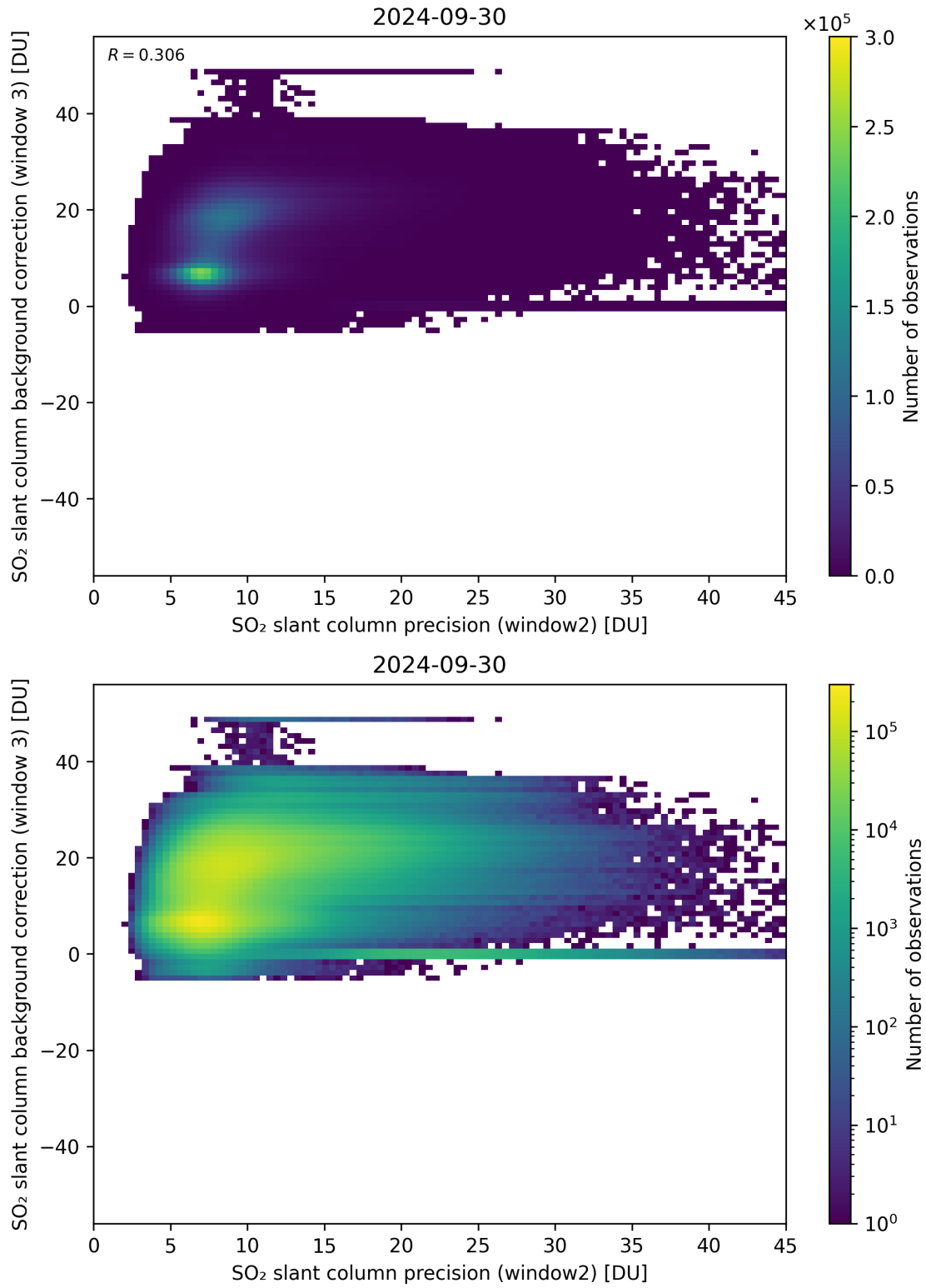
Figure 242: Scatter density plot of “SO 2 slant column precision (window2)” against “SO 2 slant column background correction (window 3)” for 2024-09-29 to 2024-10-01.
