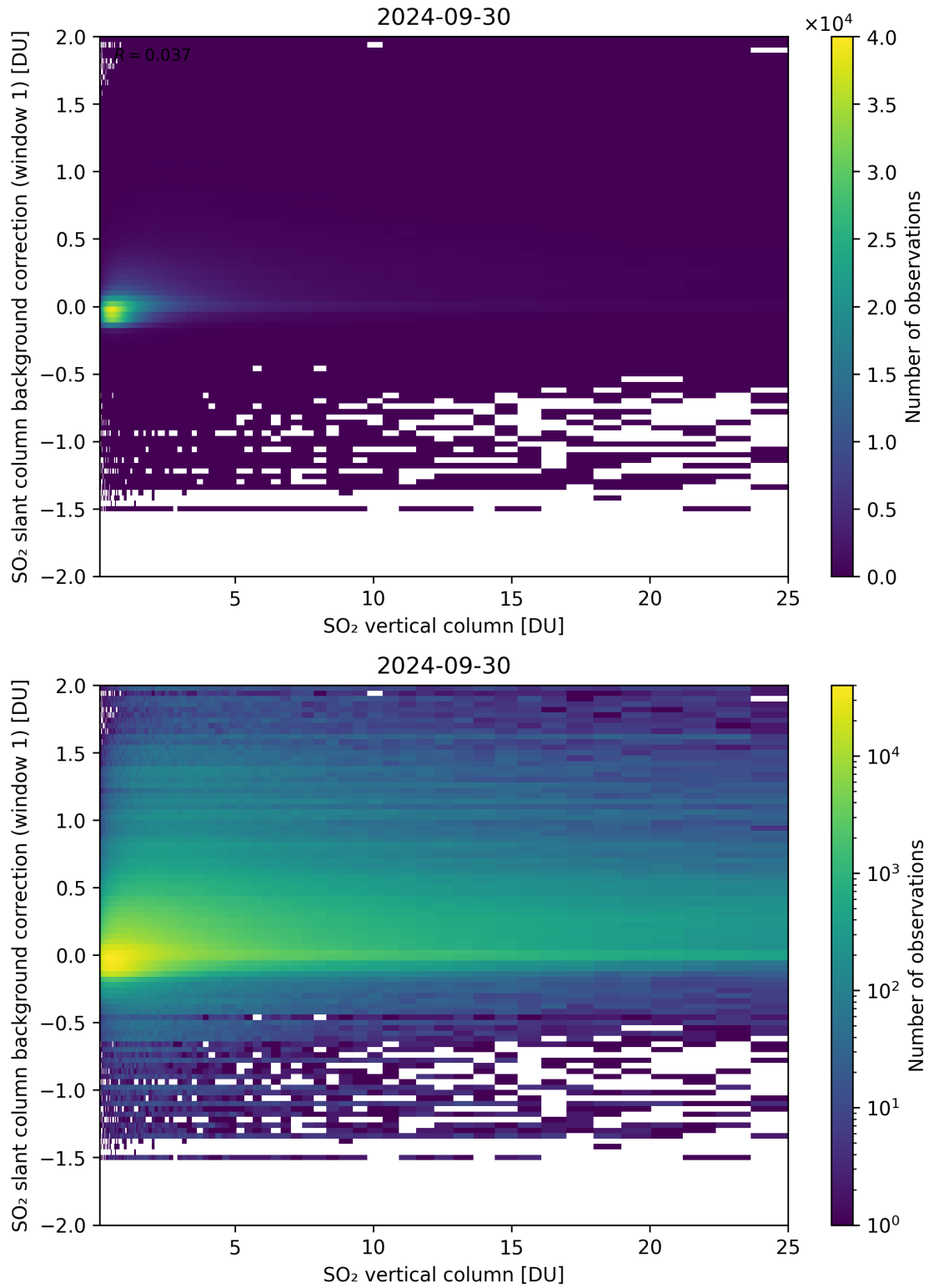
Figure 273: Scatter density plot of “SO 2 vertical column” against “SO 2 slant column background correction (window 1)” for 2024-09-29 to 2024-10-01.
