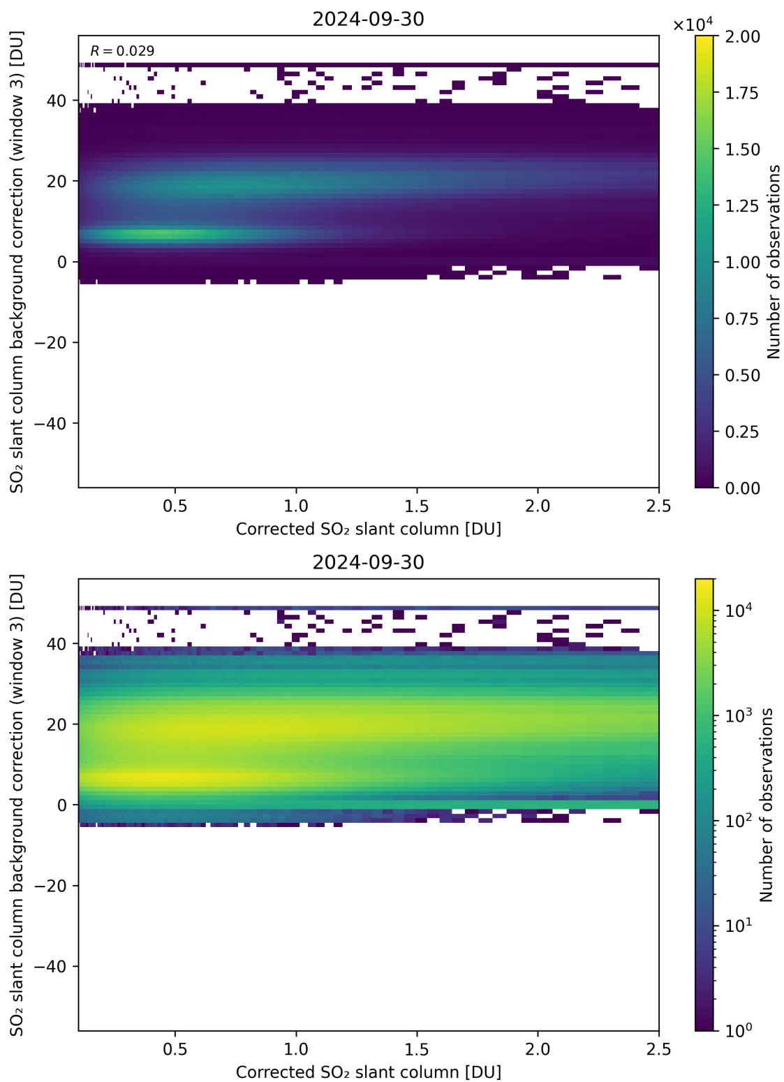
Figure 180: Scatter density plot of “Corrected SO 2 slant column” against “SO 2 slant column background correction (window 3)” for 2024-09-29 to 2024-10-01.
