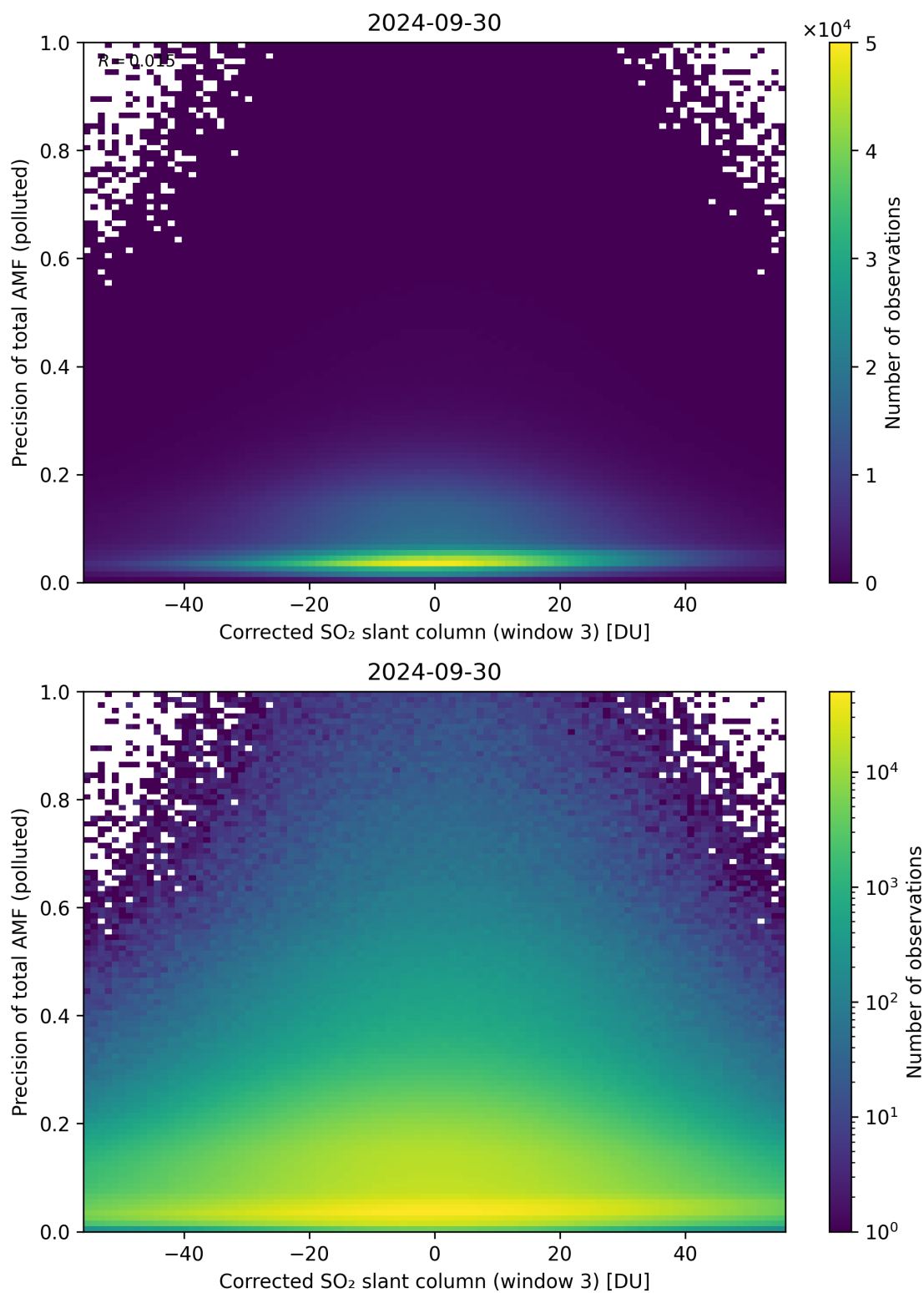
Figure 211: Scatter density plot of “Corrected SO 2 slant column (window 3)” against “Precision of total AMF (polluted)” for 2024-09-29 to 2024-10-01.
