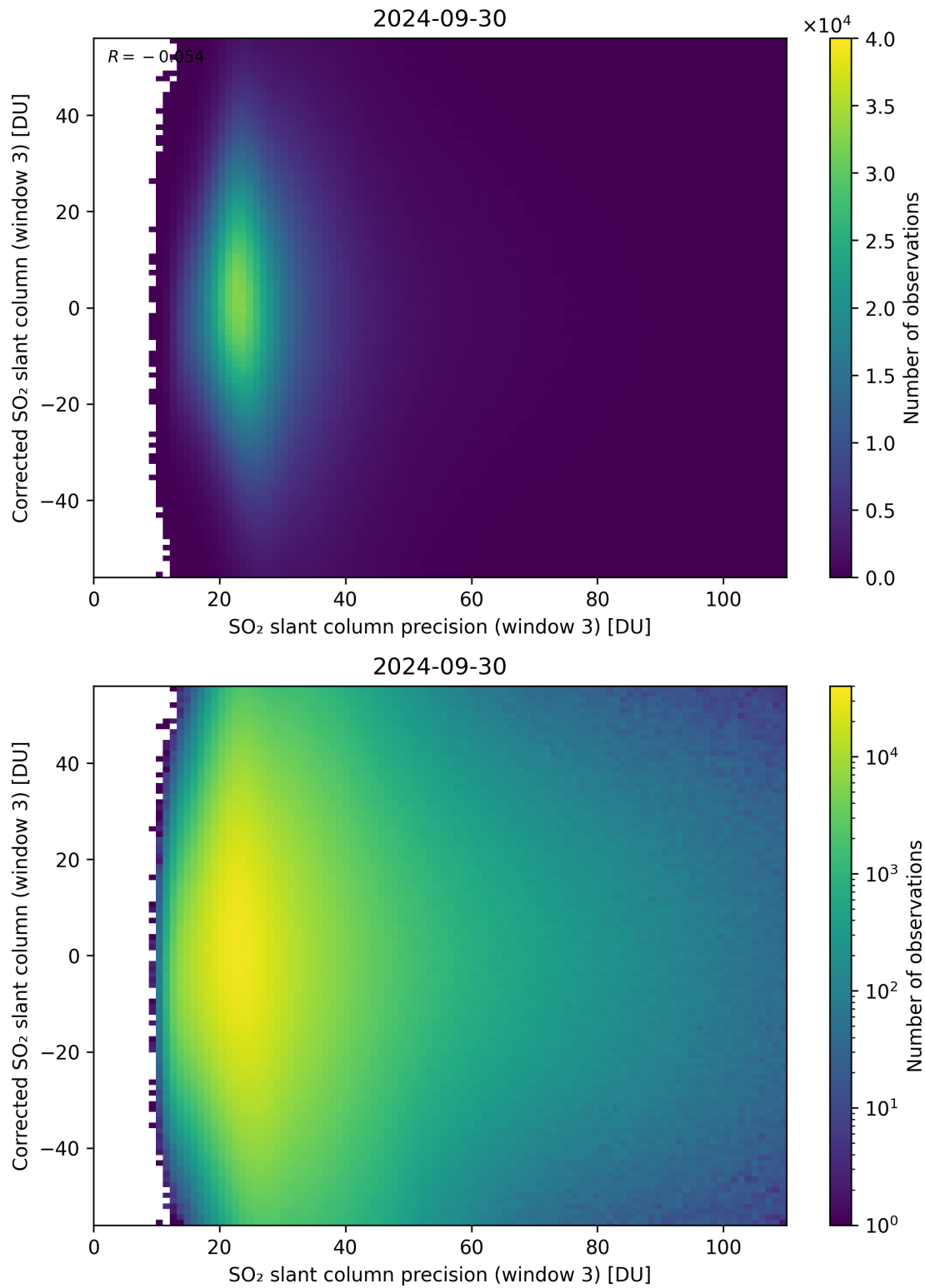
Figure 262: Scatter density plot of “SO 2 slant column precision (window 3)” against “Corrected SO 2 slant column (window 3)” for 2024-09-29 to 2024-10-01.
