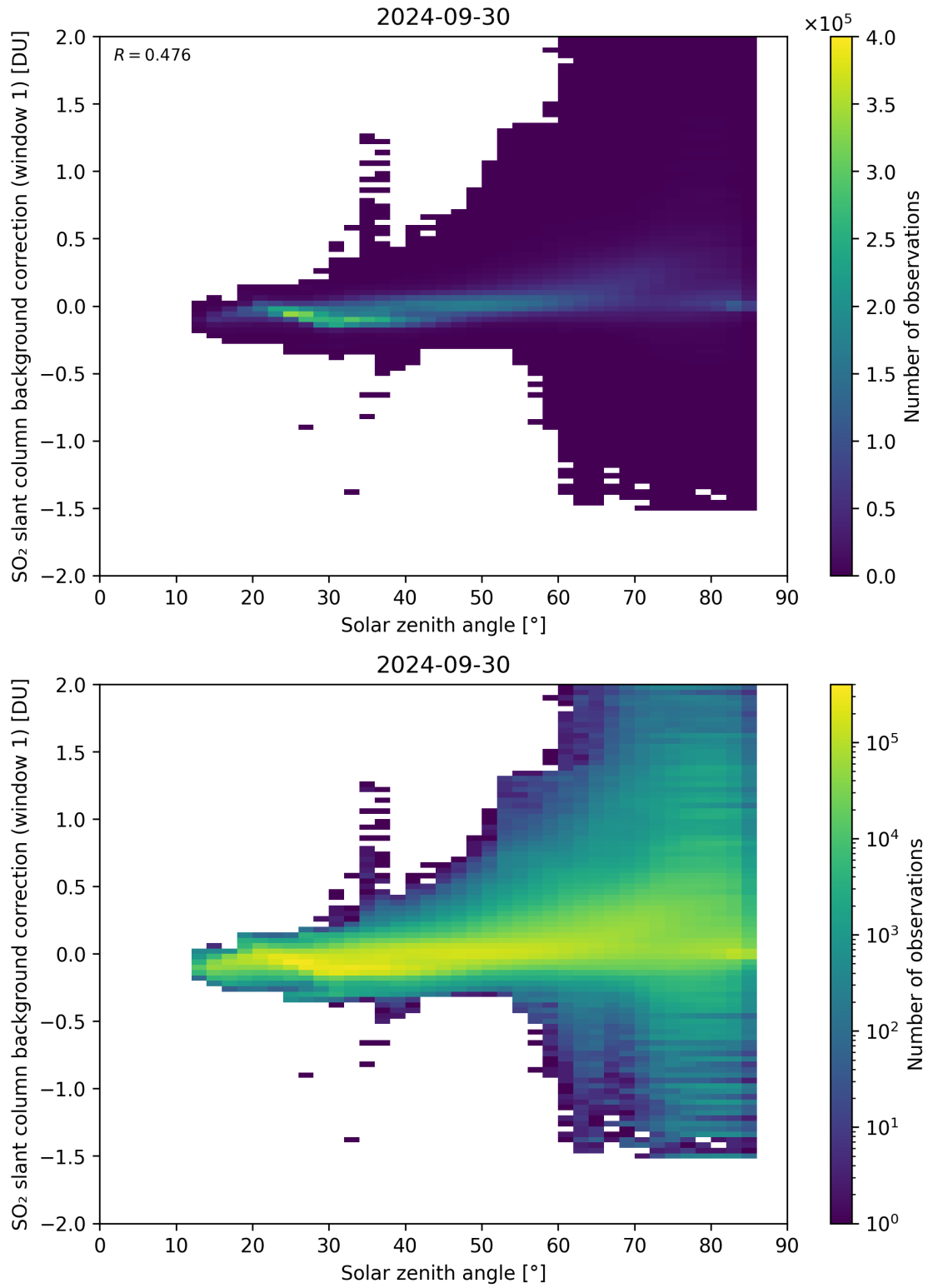
Figure 158: Scatter density plot of “Solar zenith angle” against “SO 2 slant column background correction (window 1)” for 2024-09-29 to 2024-10-01.
