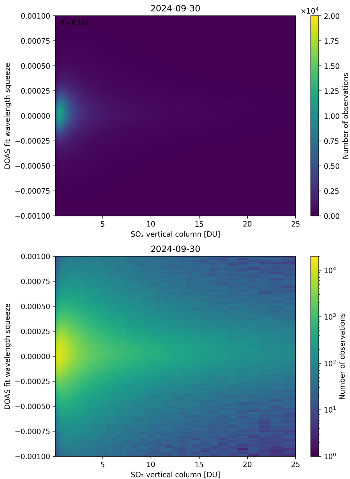
Figure 277: Scatter density plot of “SO 2 vertical column” against “DOAS fit wavelength squeeze” for 2024-09-29 to 2024-10-01.
