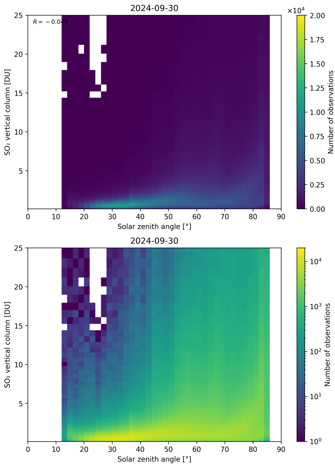
Figure 176: Scatter density plot of “Solar zenith angle” against “SO 2 vertical column” for 2024-09-29 to 2024-10-01.
