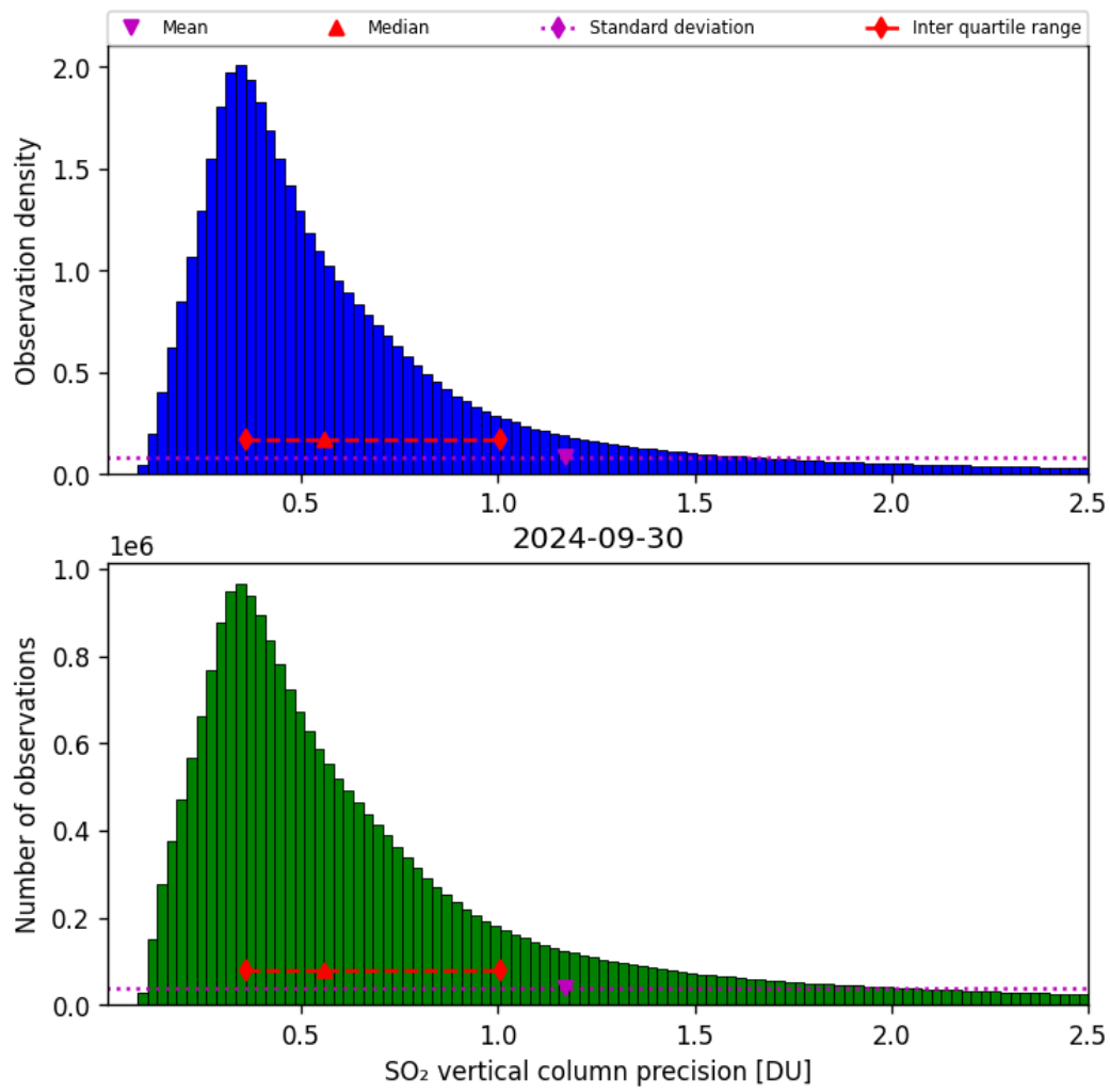
Figure 54: Histogram of “SO 2 vertical column precision” for 2024-09-29 to 2024-10-01
