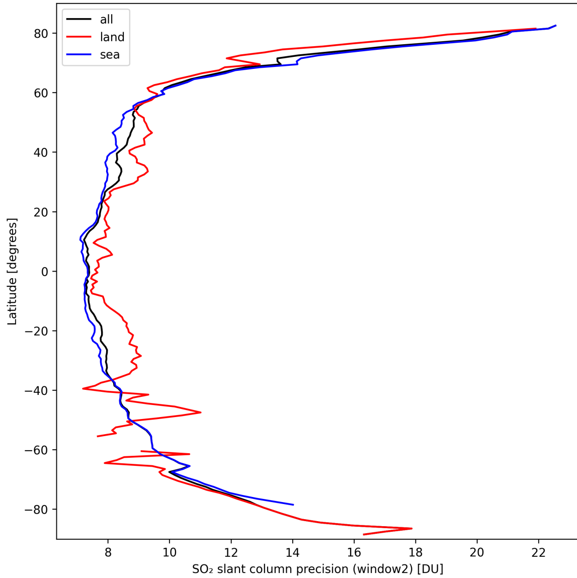
Figure 38: Zonal average of “SO 2 slant column precision (window2)” for 2024-09-29 to 2024-10-01.
