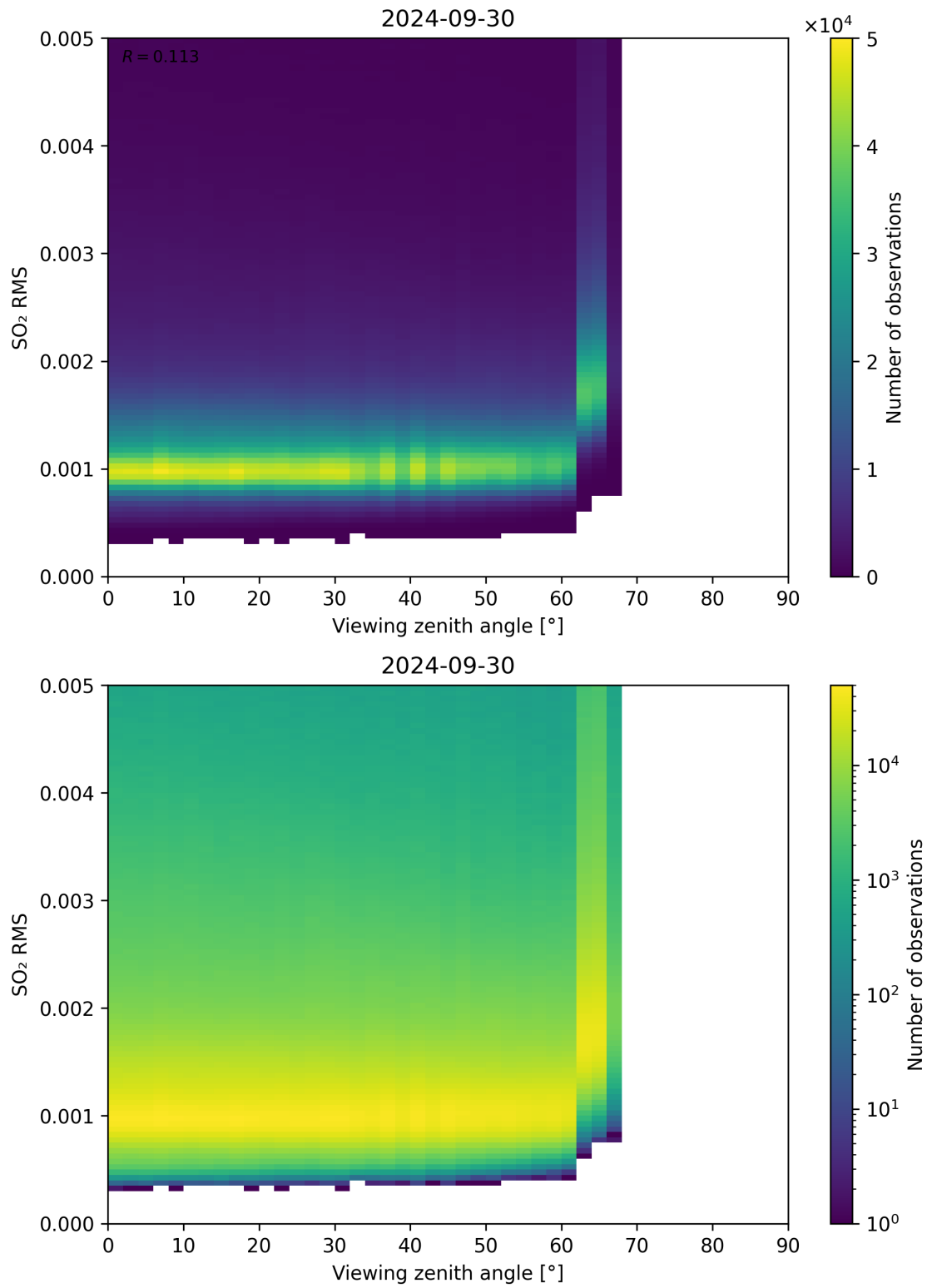
Figure 313: Scatter density plot of “Viewing zenith angle” against “SO 2 RMS” for 2024-09-29 to 2024-10-01.
