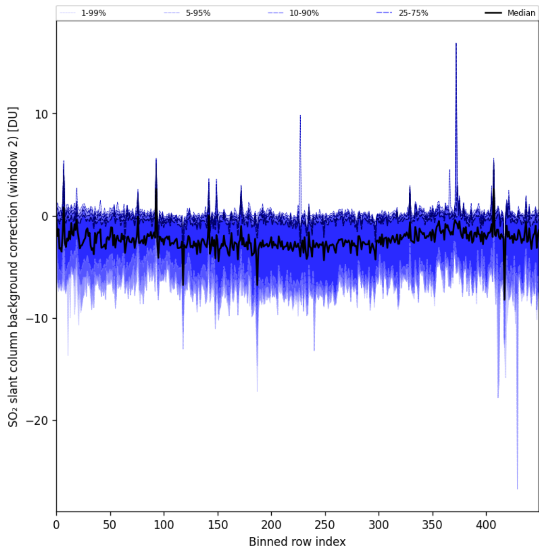
Figure 86: Along track statistics of “SO 2 slant column background correction (window 2)” for 2024-09-29 to 2024-10-01
