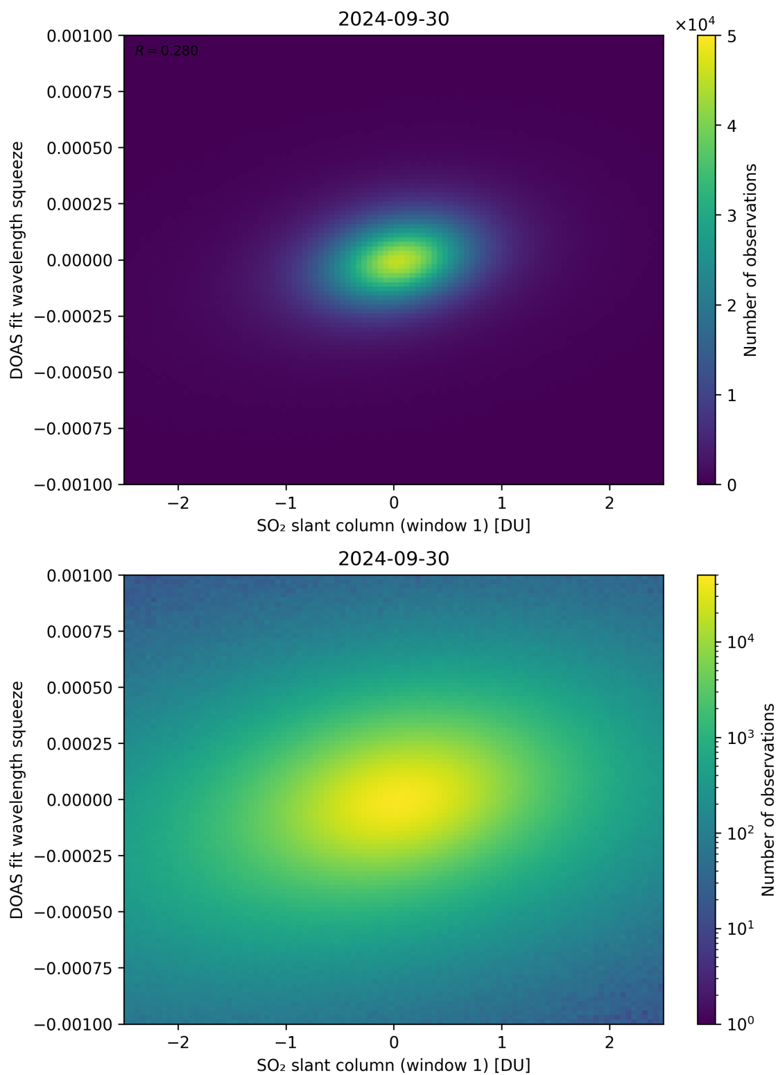
Figure 216: Scatter density plot of “SO 2 slant column (window 1)” against “DOAS fit wavelength squeeze” for 2024-09-29 to 2024-10-01.
