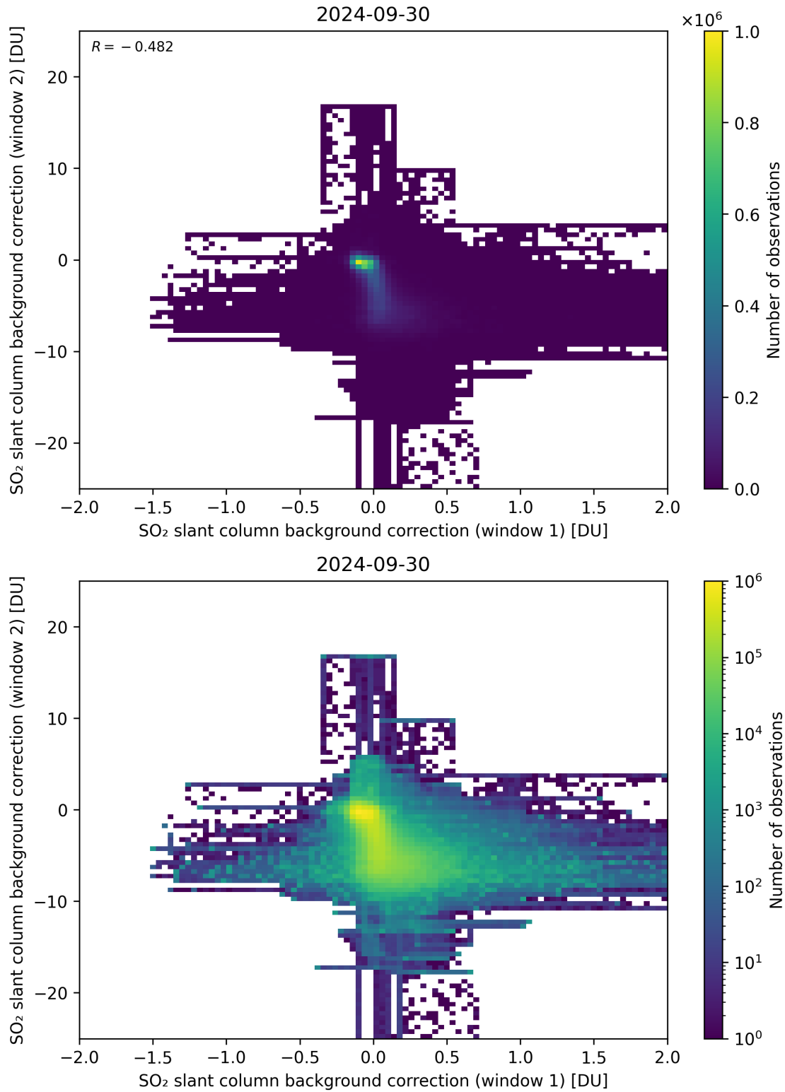
Figure 98: Scatter density plot of “SO 2 slant column background correction (window 1)” against “SO 2 slant column background correction (window 2)” for 2024-09-29 to 2024-10-01.
