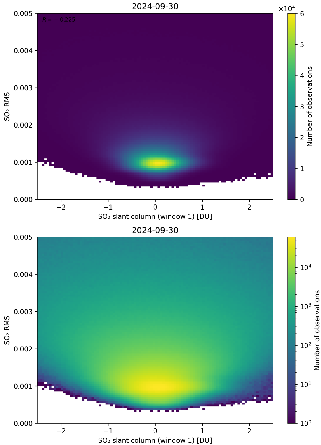
Figure 217: Scatter density plot of “SO 2 slant column (window 1)” against “SO 2 RMS” for 2024-09-29 to 2024-10-01.
