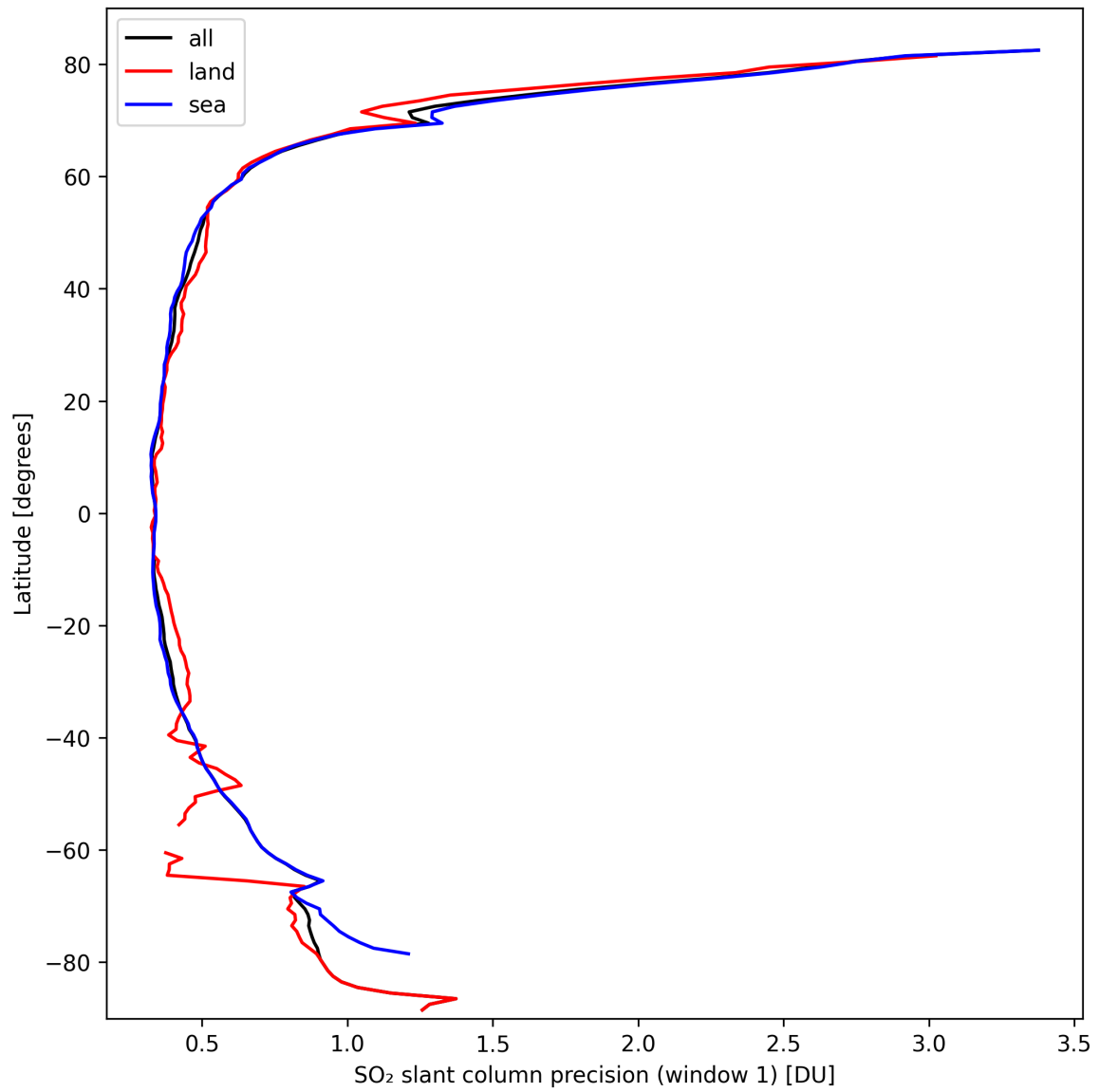
Figure 34: Zonal average of “SO 2 slant column precision (window 1)” for 2024-09-29 to 2024-10-01.
