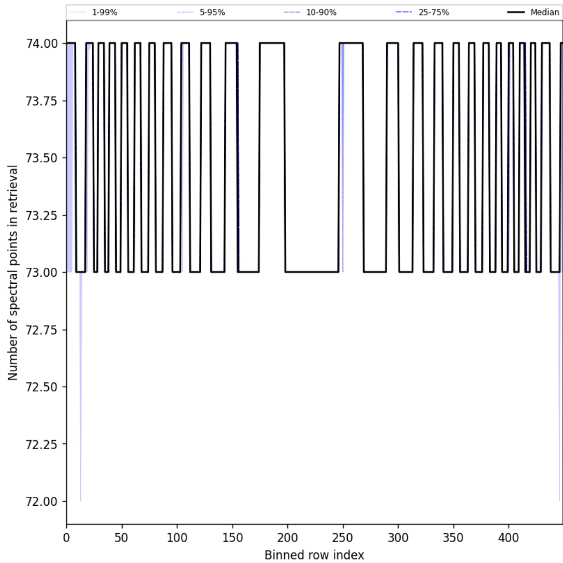
Figure 97: Along track statistics of “Number of spectral points in retrieval” for 2024-09-29 to 2024-10-01
