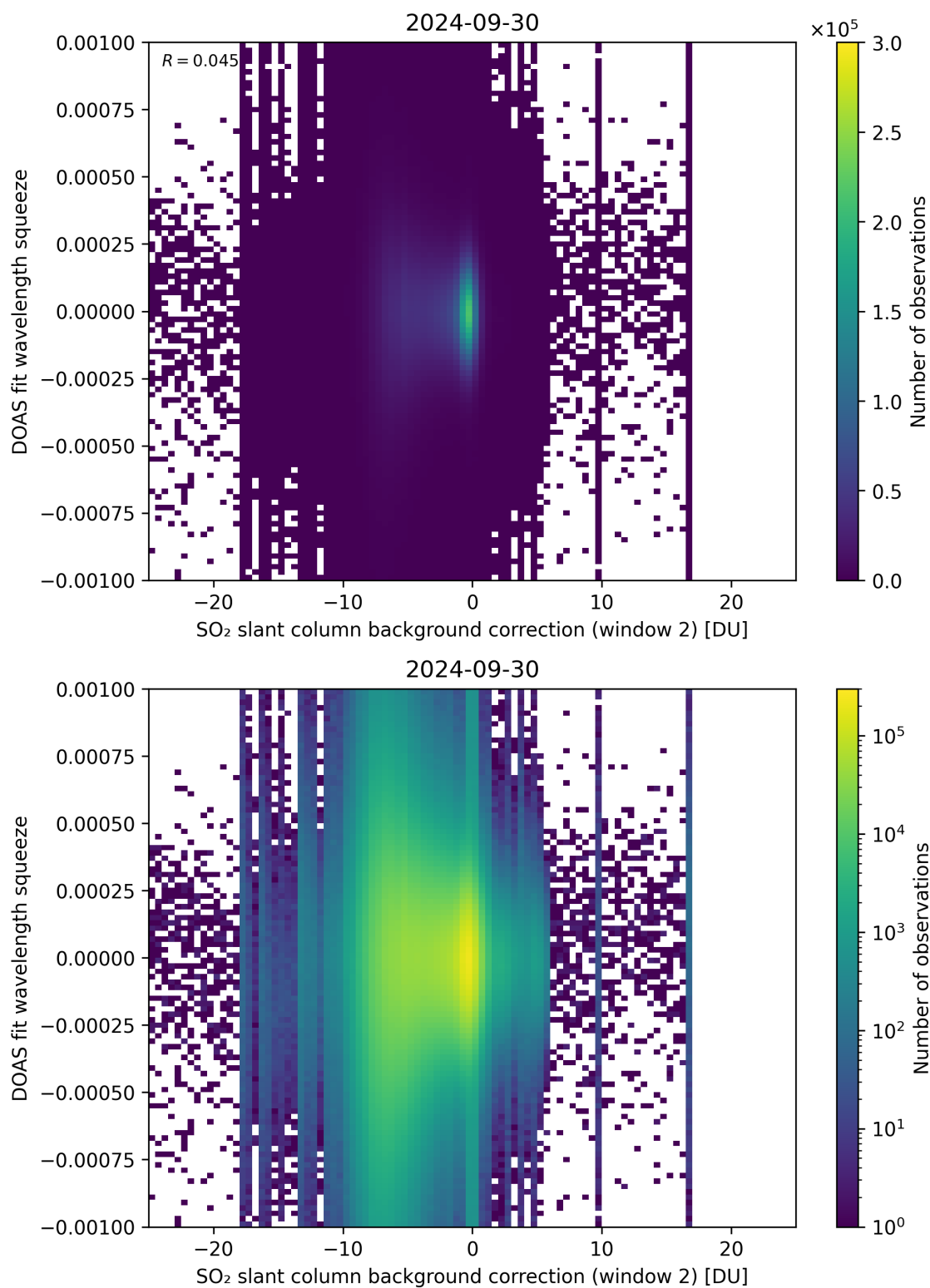
Figure 113: Scatter density plot of “SO 2 slant column background correction (window 2)” against “DOAS fit wavelength squeeze” for 2024-09-29 to 2024-10-01.
