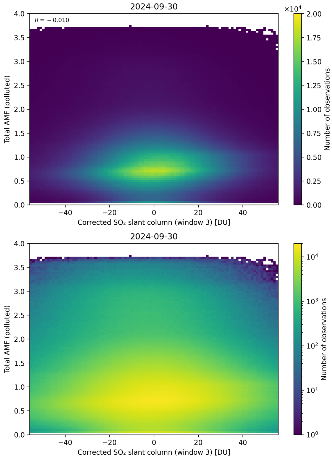
Figure 210: Scatter density plot of “Corrected SO 2 slant column (window 3)” against “Total AMF (polluted)” for 2024-09-29 to 2024-10-01.
