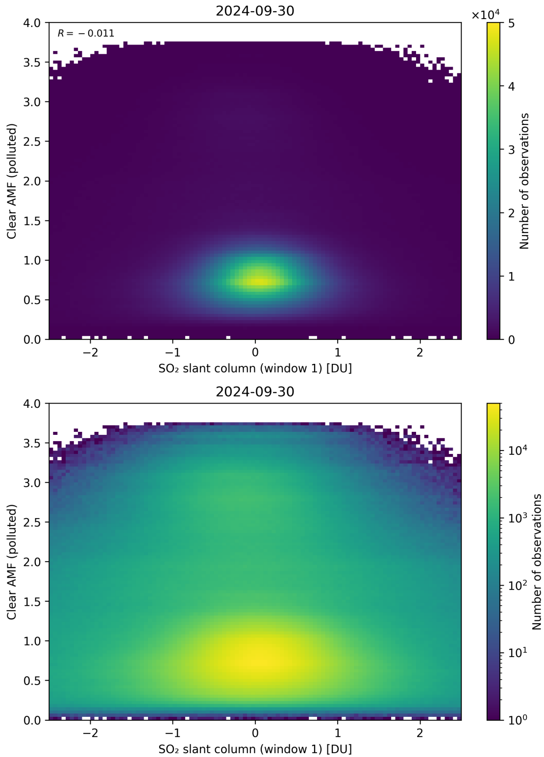
Figure 232: Scatter density plot of “SO 2 slant column (window 1)” against “Clear AMF (polluted)” for 2024-09-29 to 2024-10-01.
