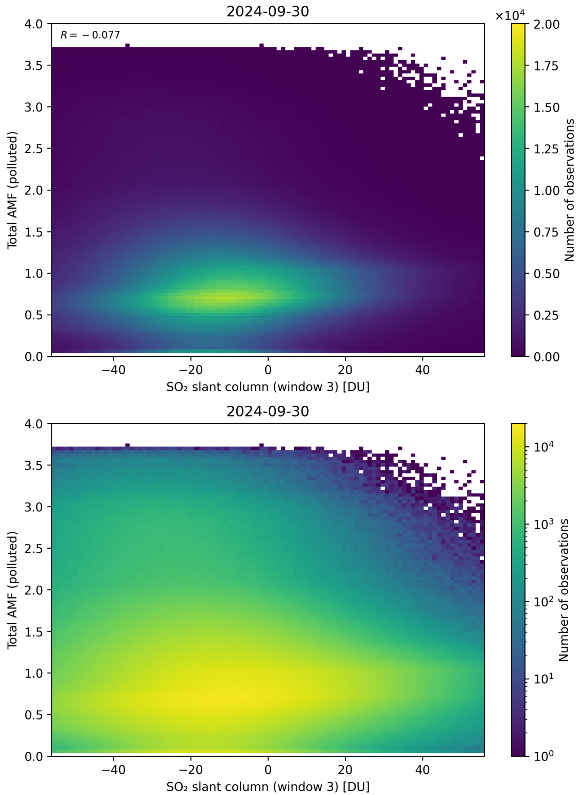
Figure 268: Scatter density plot of “SO 2 slant column (window 3)” against “Total AMF (polluted)” for 2024-09-29 to 2024-10-01.
