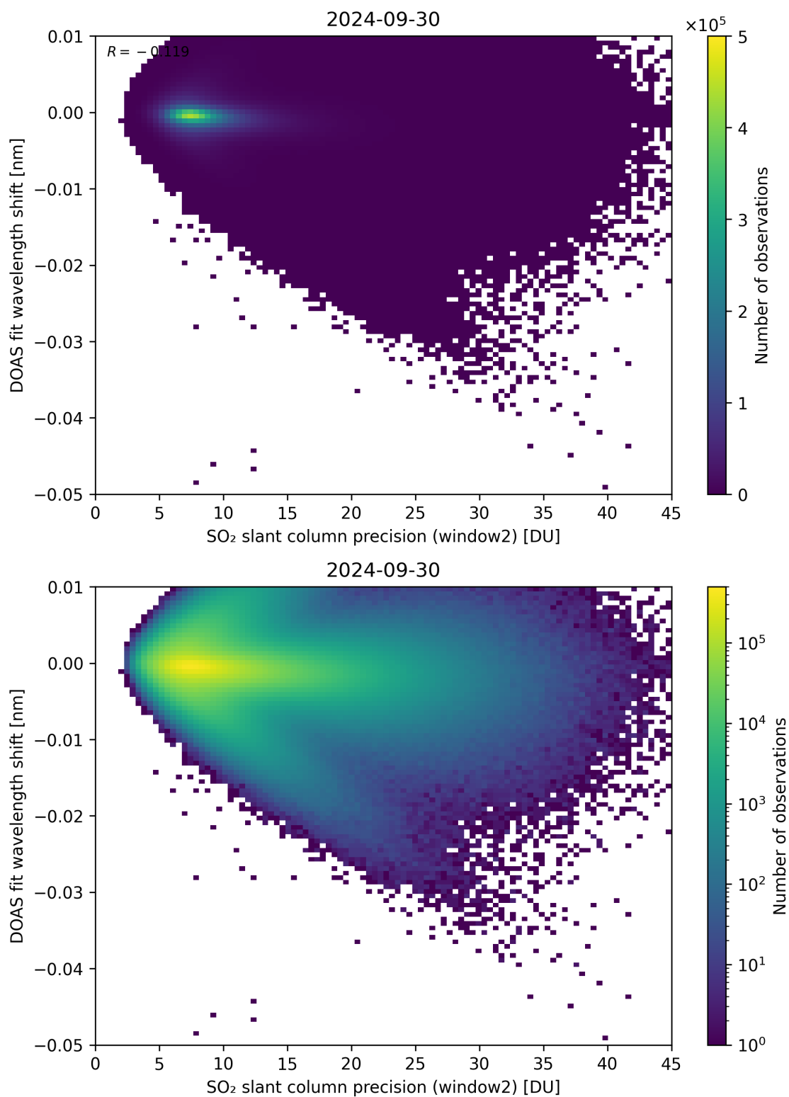
Figure 243: Scatter density plot of “SO 2 slant column precision (window2)” against “DOAS fit wavelength shift” for 2024-09-29 to 2024-10-01.
