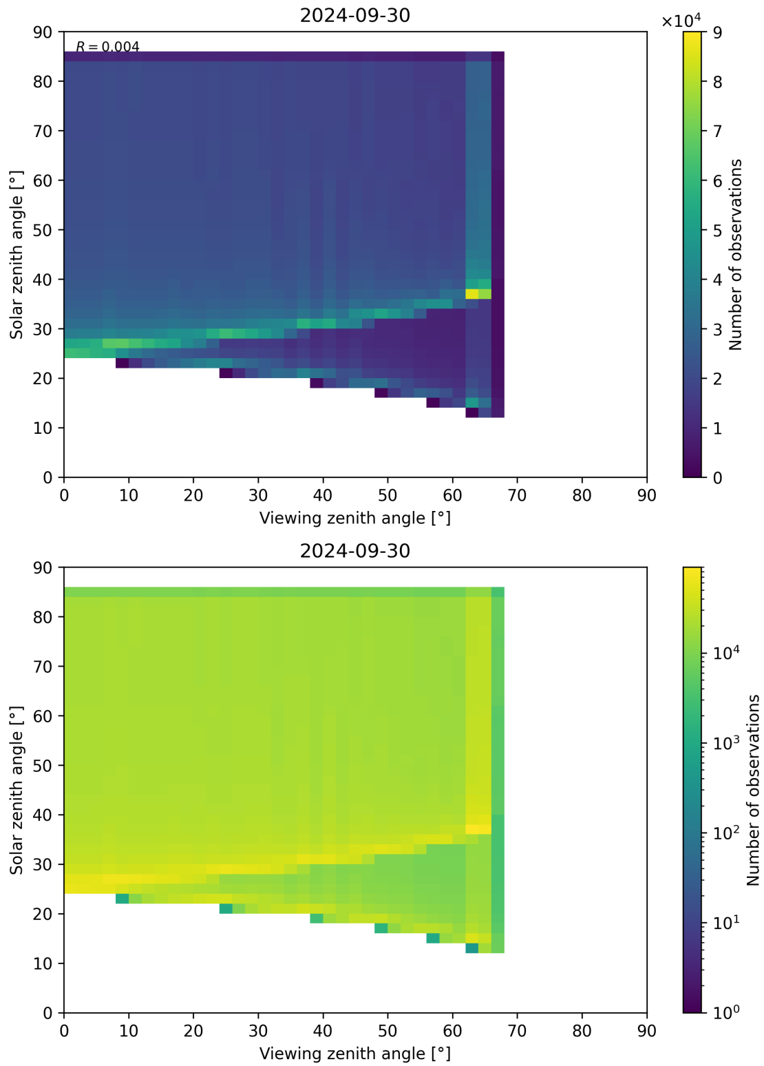
Figure 315: Scatter density plot of “Viewing zenith angle” against “Solar zenith angle” for 2024-09-29 to 2024-10-01.
