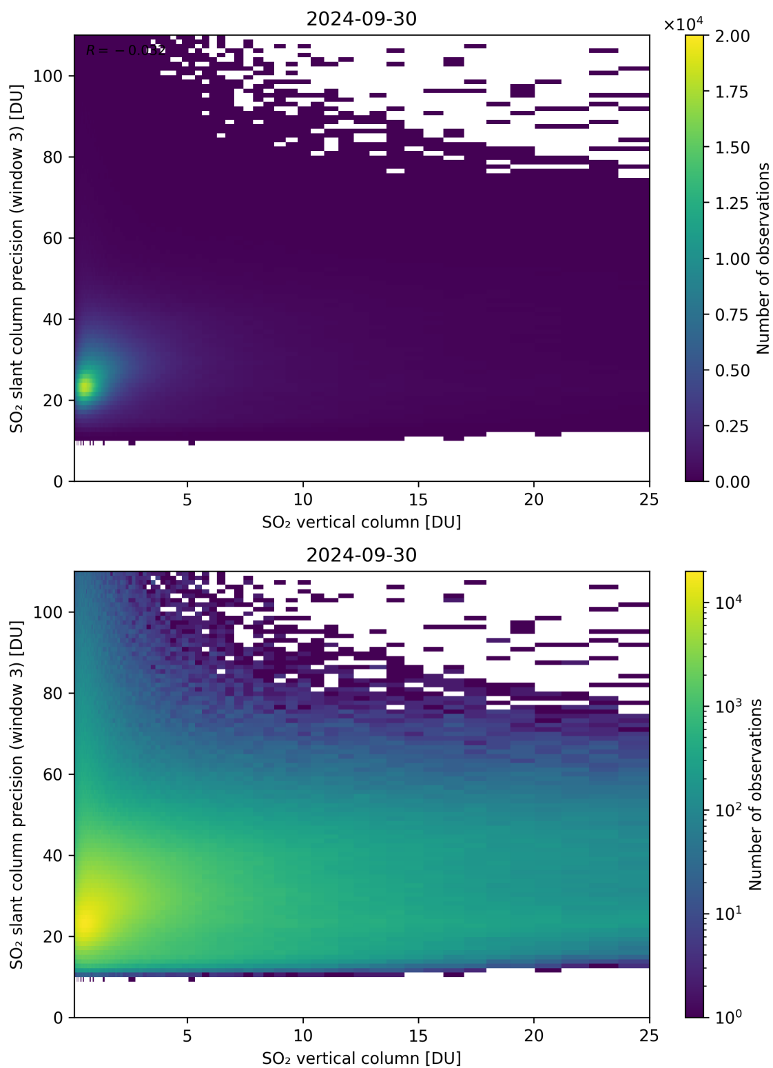
Figure 304: Scatter density plot of “SO 2 vertical column” against “SO 2 slant column precision (window 3)” for 2024-09-29 to 2024-10-01.
