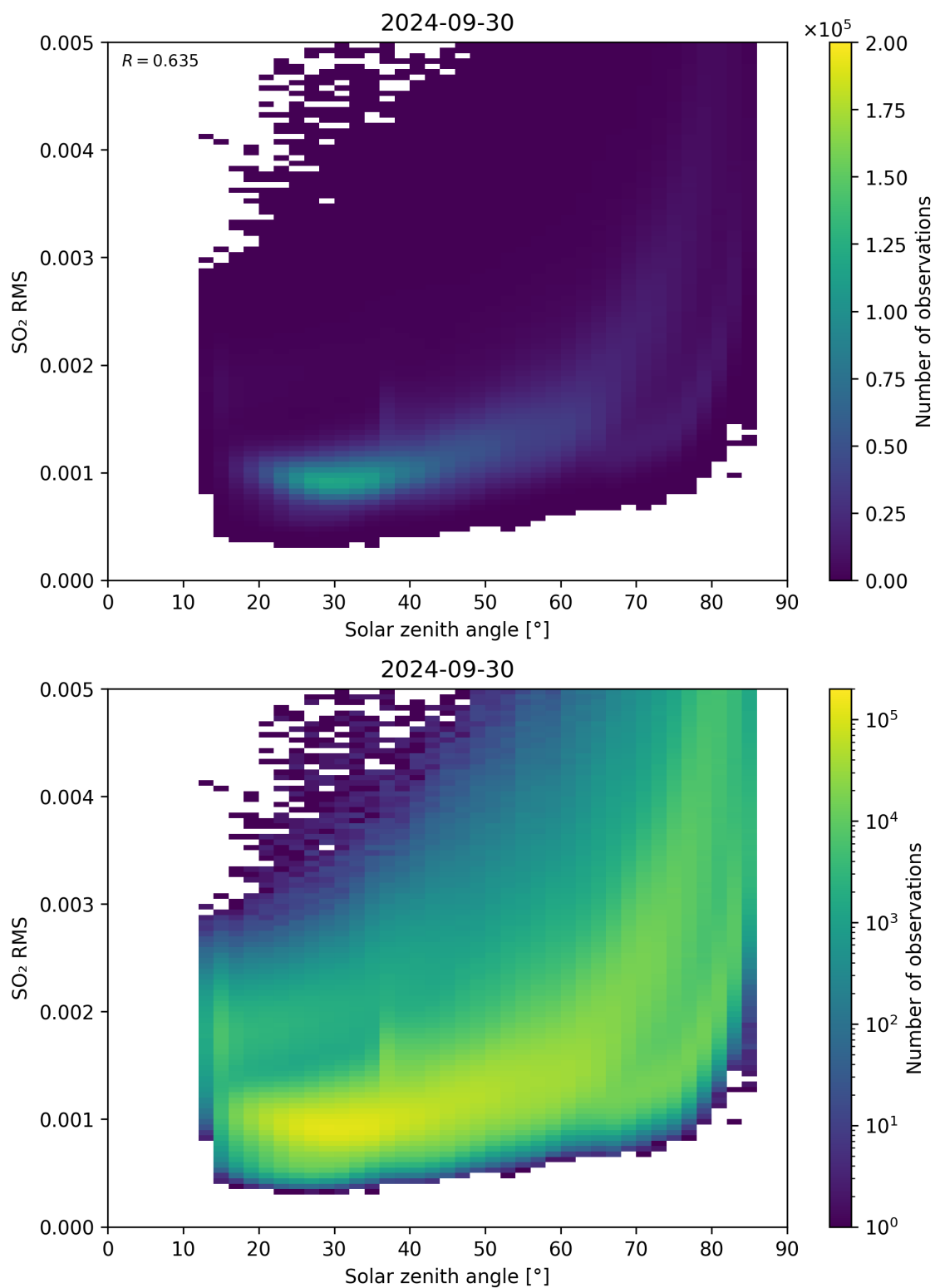
Figure 163: Scatter density plot of “Solar zenith angle” against “SO 2 RMS” for 2024-09-29 to 2024-10-01.
