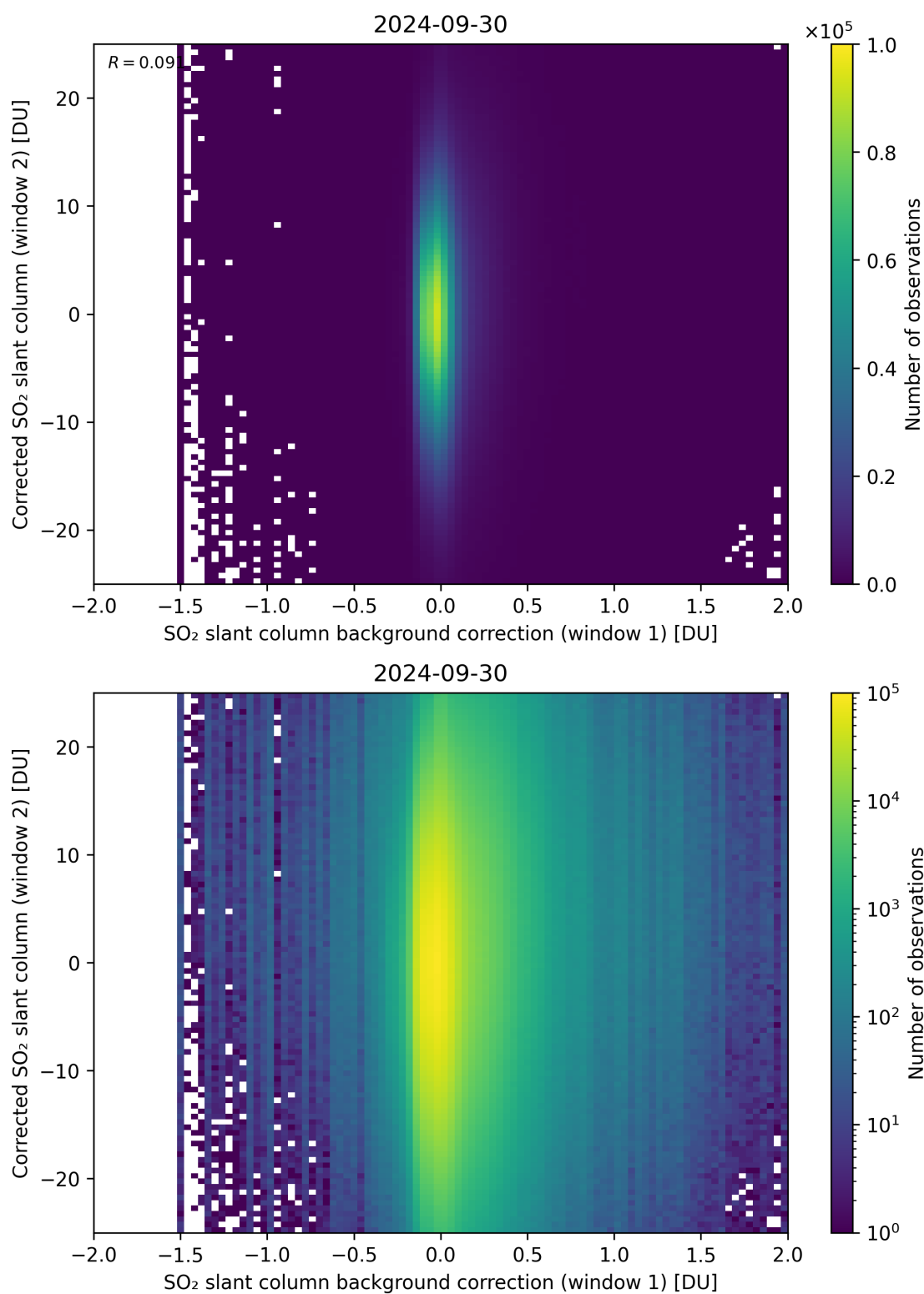
Figure 104: Scatter density plot of “SO 2 slant column background correction (window 1)” against “Corrected SO 2 slant column (window 2)” for 2024-09-29 to 2024-10-01.
