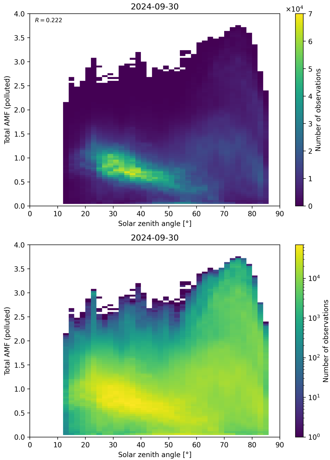
Figure 174: Scatter density plot of “Solar zenith angle” against “Total AMF (polluted)” for 2024-09-29 to 2024-10-01.
