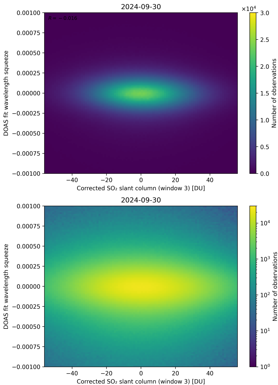
Figure 207: Scatter density plot of “Corrected SO 2 slant column (window 3)” against “DOAS fit wavelength squeeze” for 2024-09-29 to 2024-10-01.
