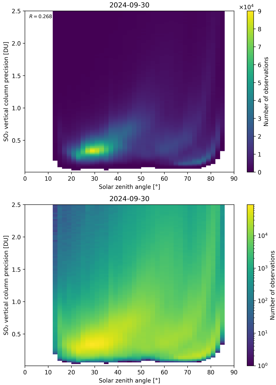
Figure 177: Scatter density plot of “Solar zenith angle” against “SO 2 vertical column precision” for 2024-09-29 to 2024-10-01.
