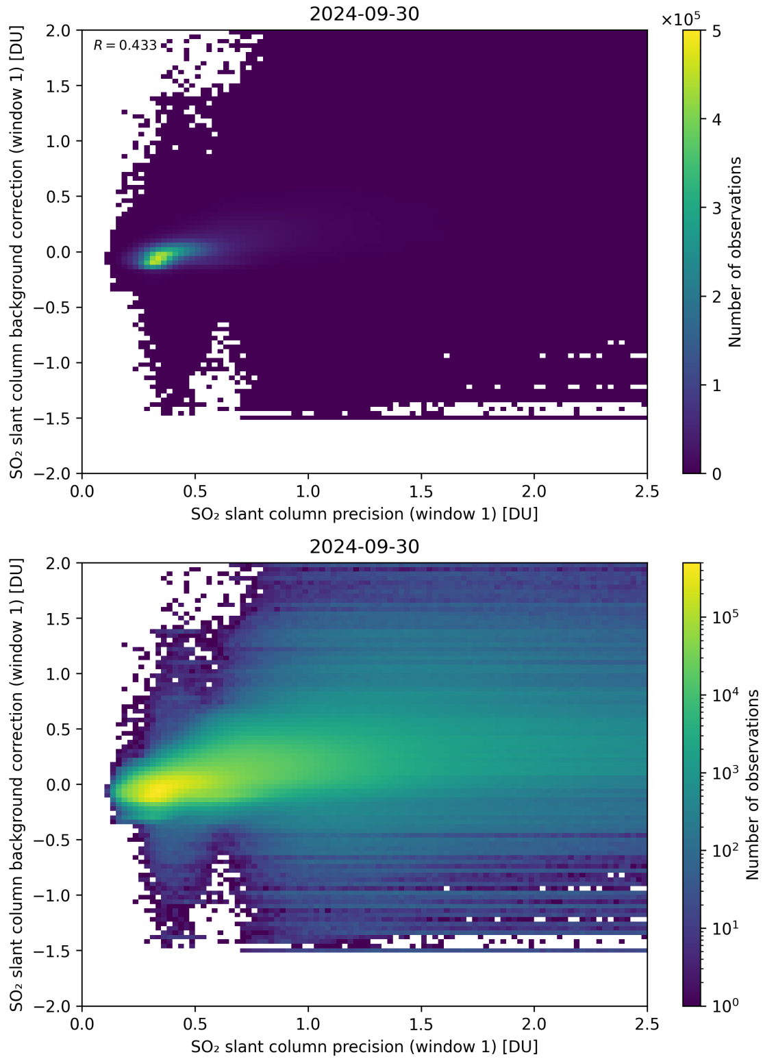
Figure 218: Scatter density plot of “SO 2 slant column precision (window 1)” against “SO 2 slant column background correction (window 1)” for 2024-09-29 to 2024-10-01.
