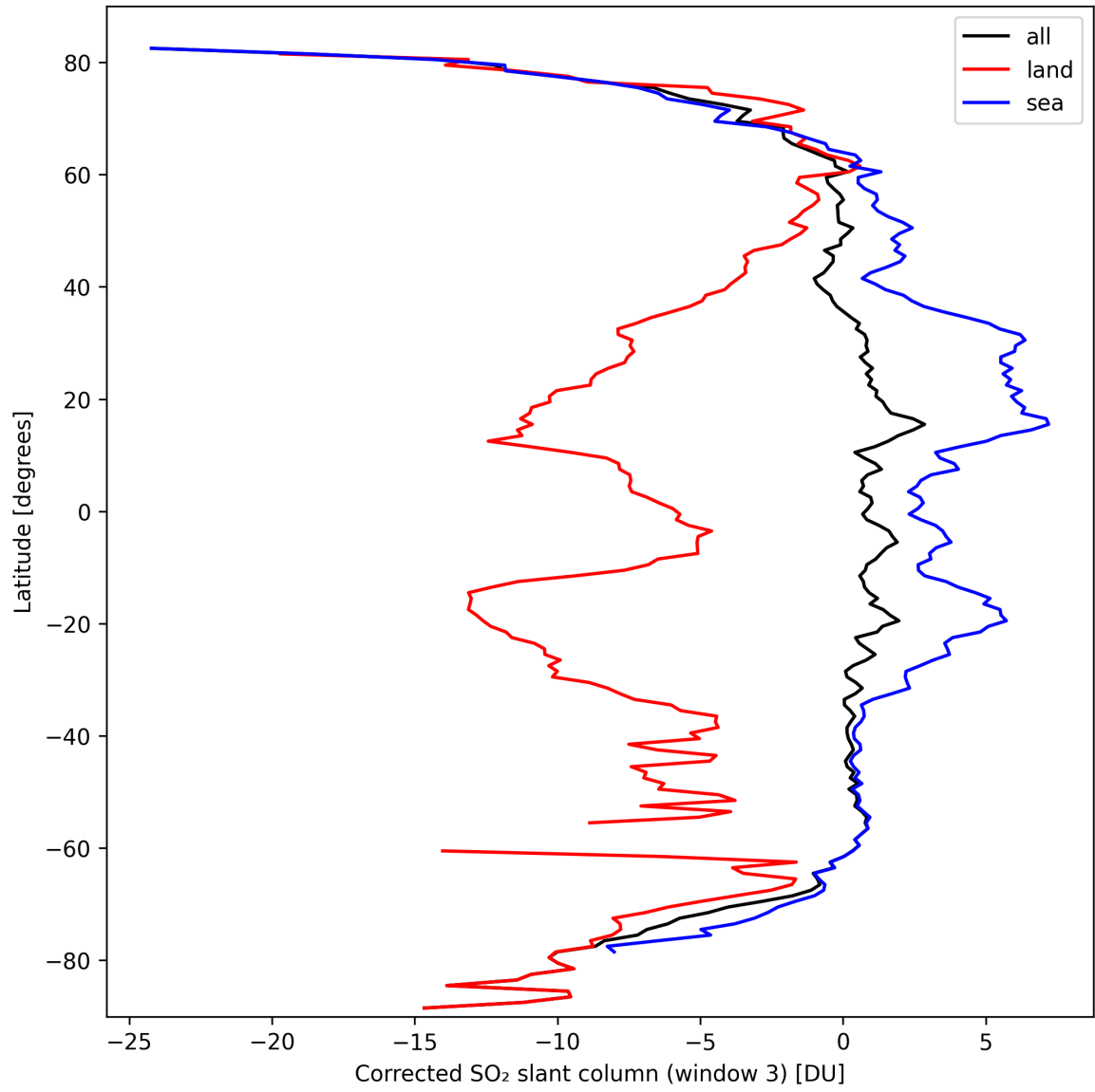
Figure 43: Zonal average of “Corrected SO 2 slant column (window 3)” for 2024-09-29 to 2024-10-01.
