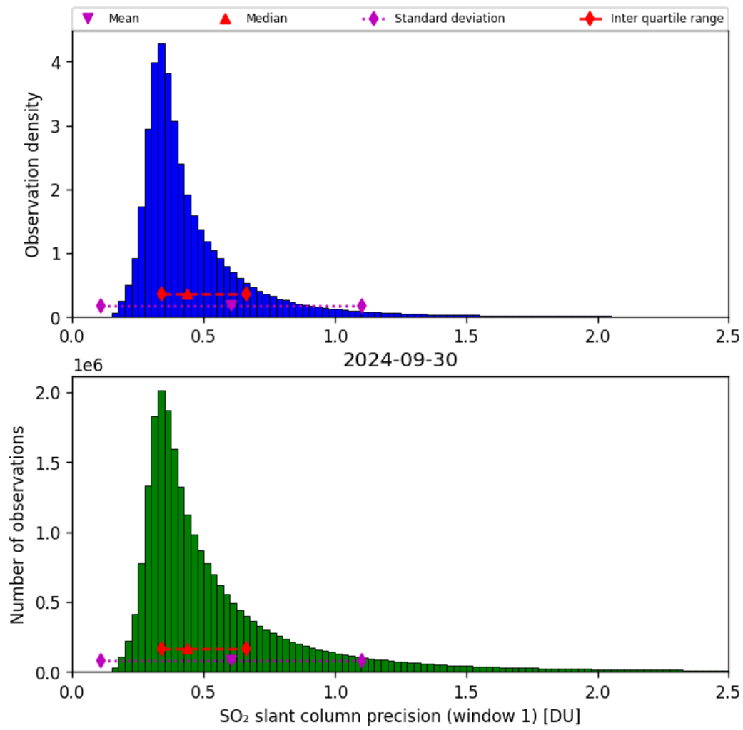
Figure 57: Histogram of “SO 2 slant column precision (window 1)” for 2024-09-29 to 2024-10-01
