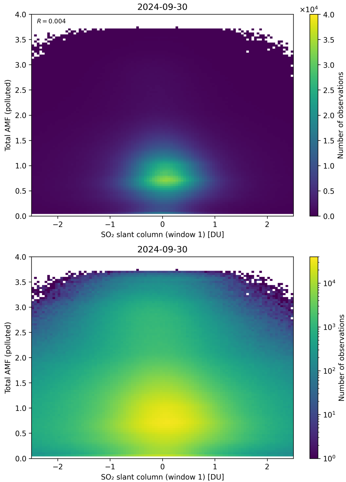
Figure 239: Scatter density plot of “SO 2 slant column (window 1)” against “Total AMF (polluted)” for 2024-09-29 to 2024-10-01.
