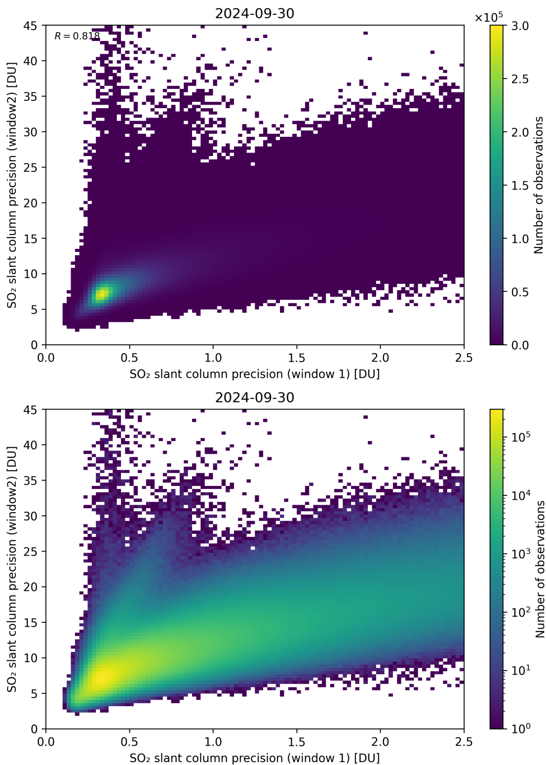
Figure 227: Scatter density plot of “SO 2 slant column precision (window 1)” against “SO 2 slant column precision (window2)” for 2024-09-29 to 2024-10-01.
