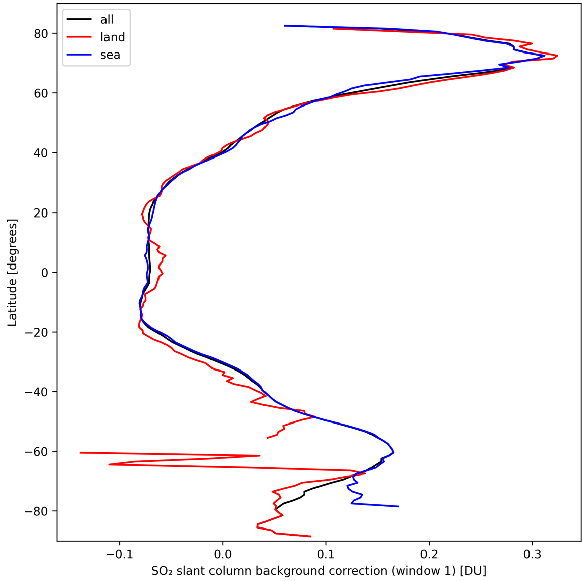
Figure 36: Zonal average of "SO 2 slant column background correction (window 1)" for 2024-09-29 to 2024-10-01.
