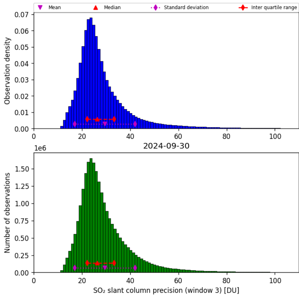
Figure 65: Histogram of “SO 2 slant column precision (window 3)” for 2024-09-29 to 2024-10-01
