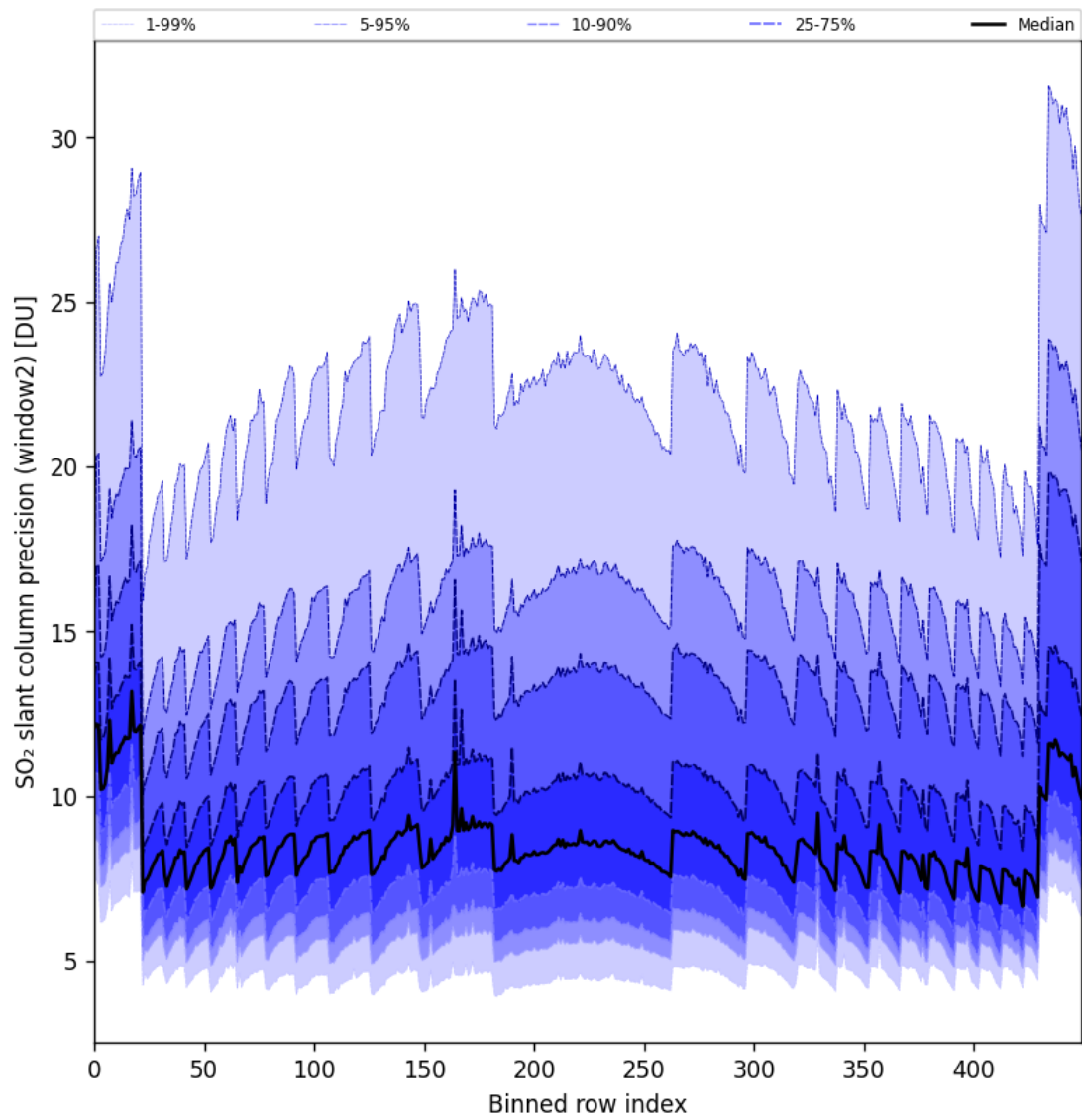
Figure 84: Along track statistics of “SO 2 slant column precision (window2)” for 2024-09-29 to 2024-10-01
