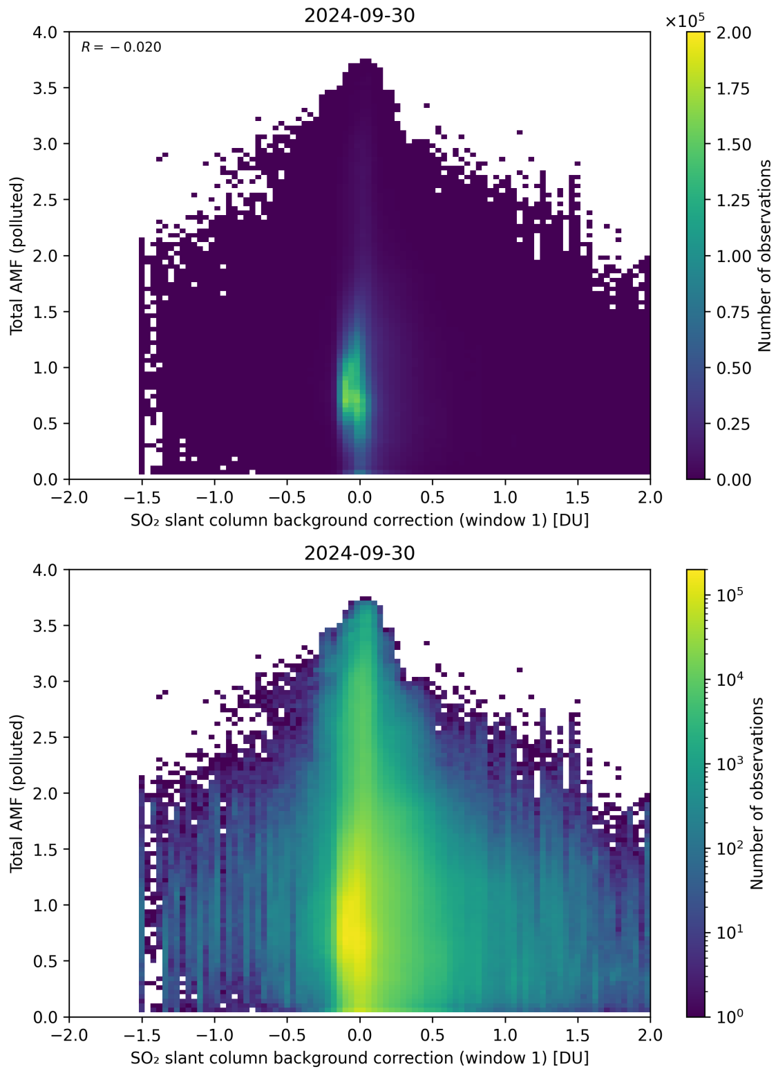
Figure 109: Scatter density plot of “SO 2 slant column background correction (window 1)” against “Total AMF (polluted)” for 2024-09-29 to 2024-10-01.
