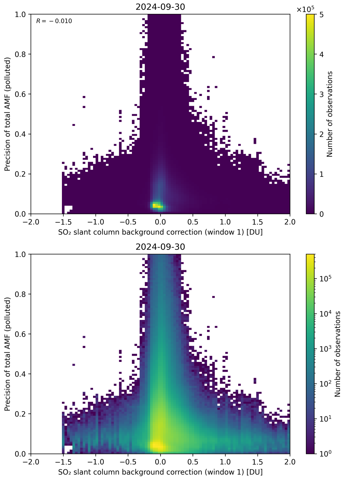
Figure 110: Scatter density plot of “SO 2 slant column background correction (window 1)” against “Precision of total AMF (polluted)” for 2024-09-29 to 2024-10-01.
