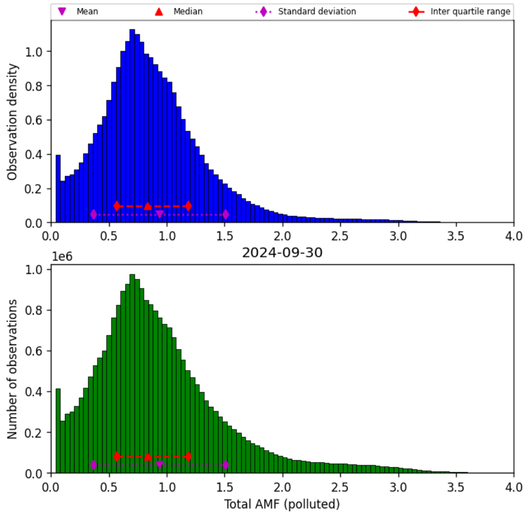
Figure 71: Histogram of “Total AMF (polluted)” for 2024-09-29 to 2024-10-01
