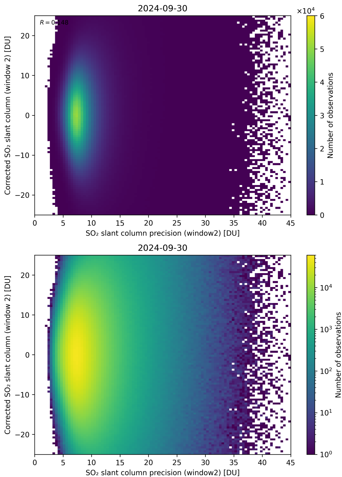
Figure 247: Scatter density plot of “SO 2 slant column precision (window2)” against “Corrected SO 2 slant column (window 2)” for 2024-09-29 to 2024-10-01.
