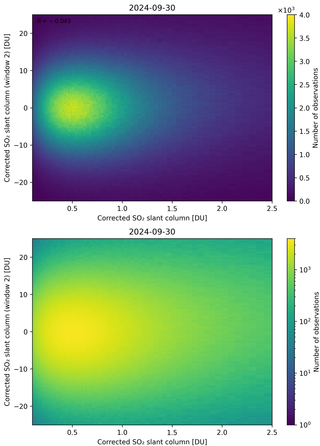
Figure 185: Scatter density plot of “Corrected SO 2 slant column” against “Corrected SO 2 slant column (window 2)” for 2024-09-29 to 2024-10-01.
