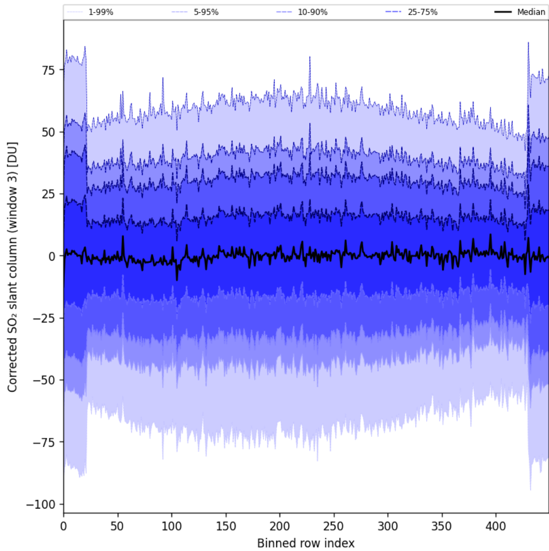
Figure 89: Along track statistics of “Corrected SO 2 slant column (window 3)” for 2024-09-29 to 2024-10-01
