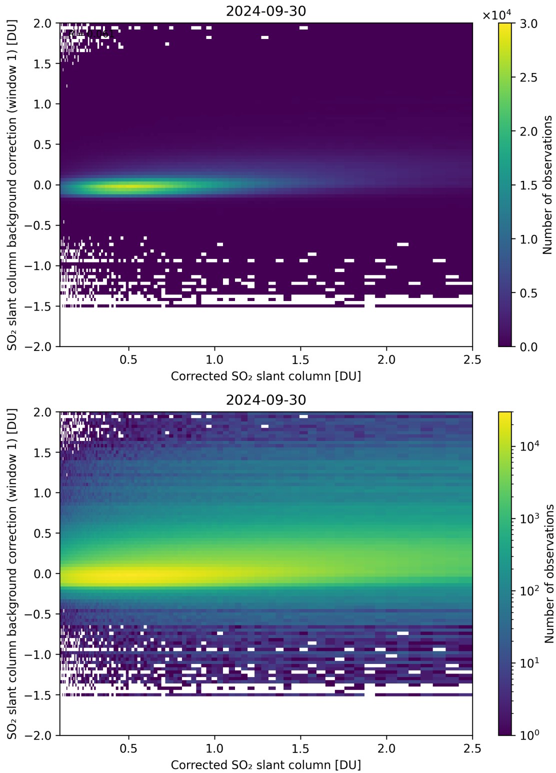
Figure 178: Scatter density plot of “Corrected SO 2 slant column” against “SO 2 slant column background correction (window 1)” for 2024-09-29 to 2024-10-01.
