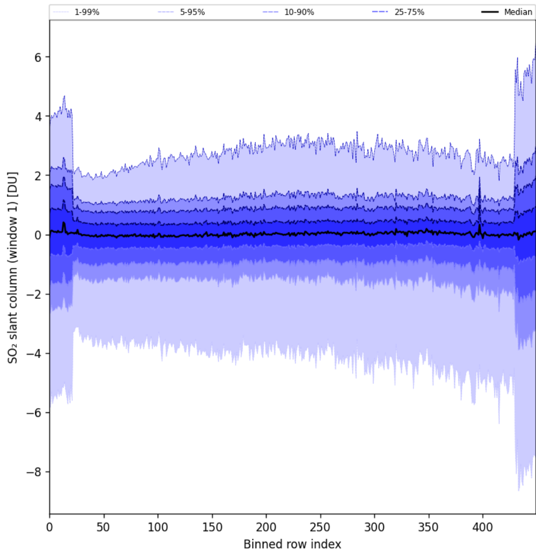
Figure 79: Along track statistics of “SO 2 slant column (window 1)” for 2024-09-29 to 2024-10-01
