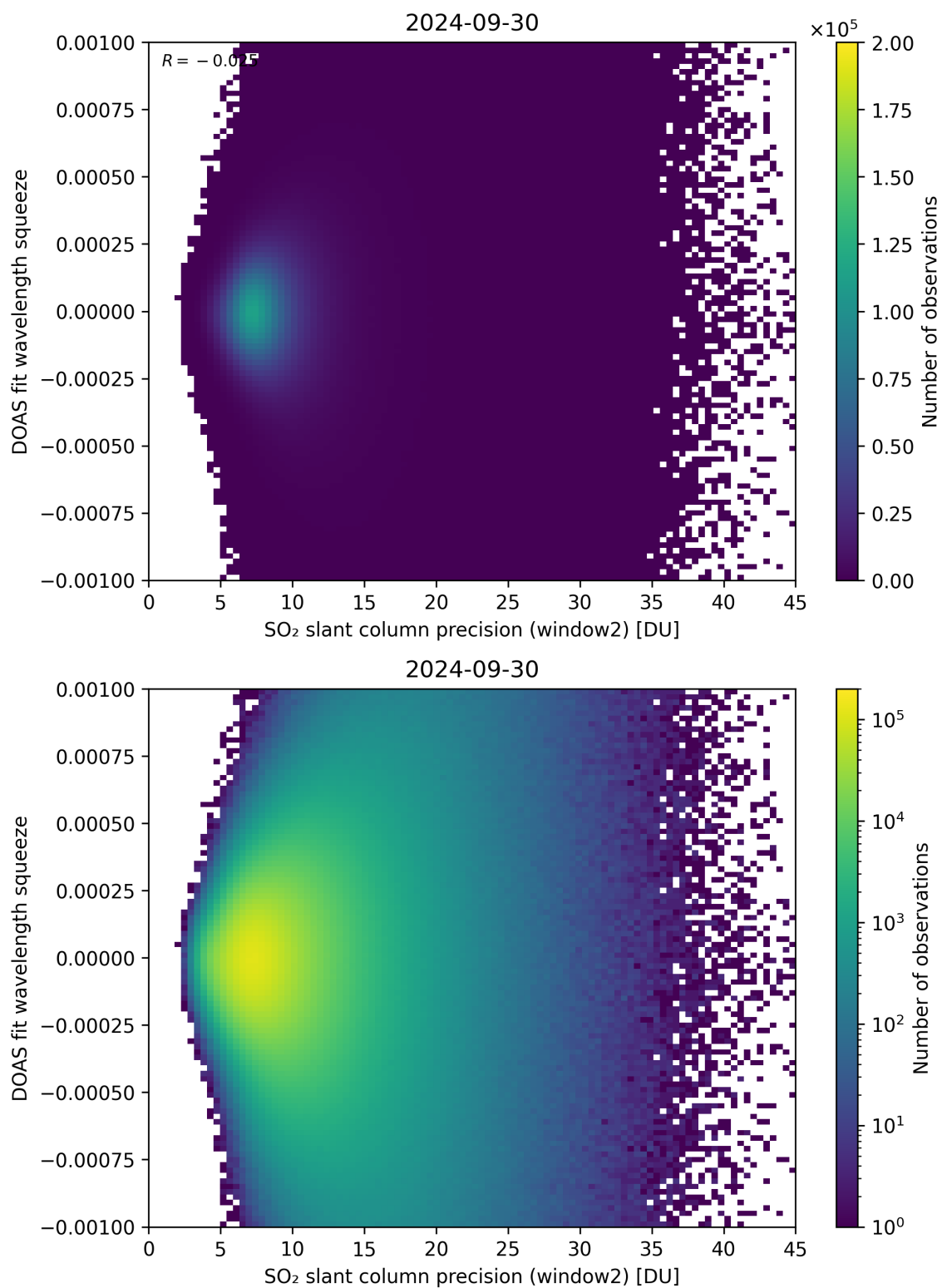
Figure 244: Scatter density plot of “SO 2 slant column precision (window2)” against “DOAS fit wavelength squeeze” for 2024-09-29 to 2024-10-01.
