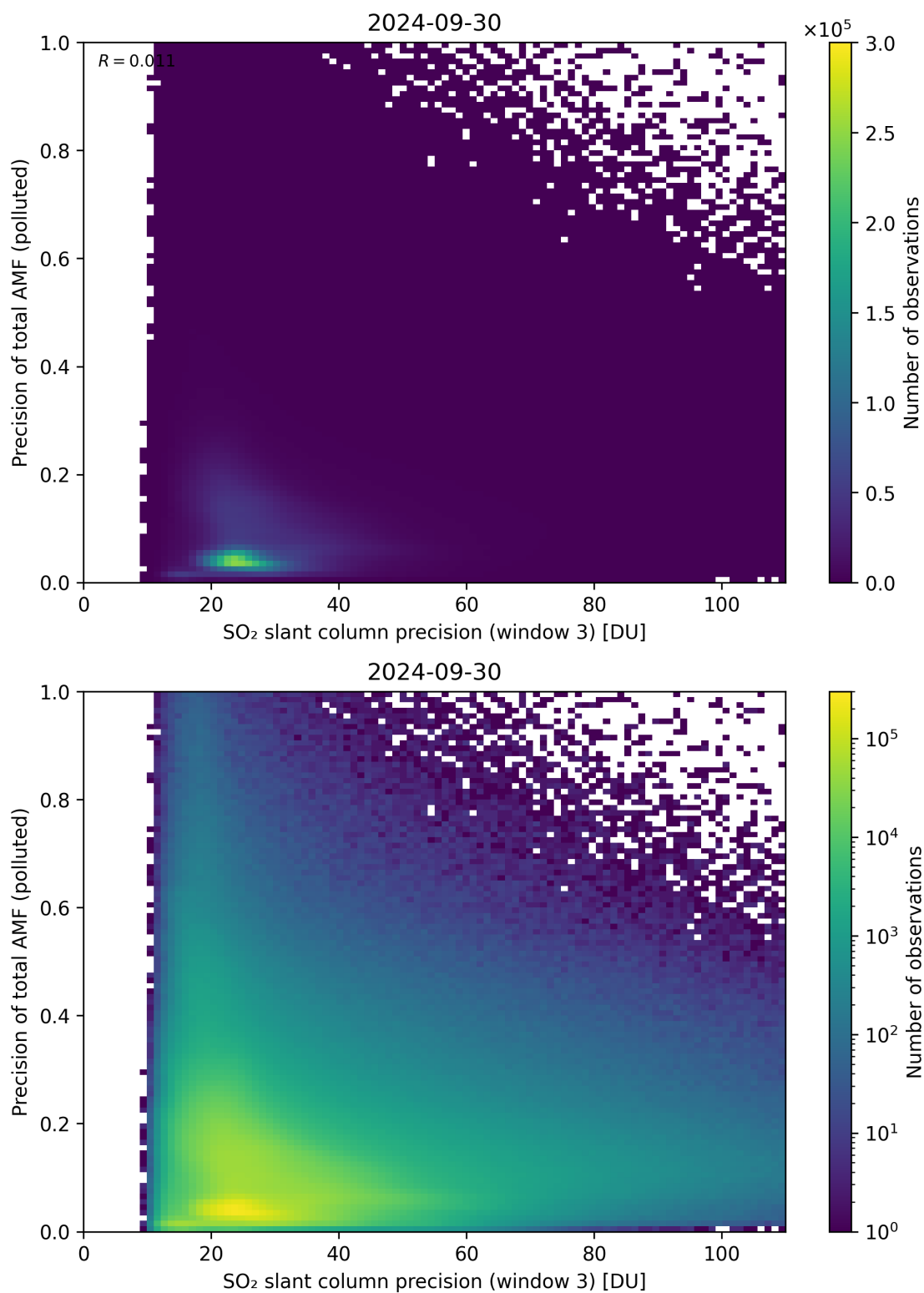
Figure 264: Scatter density plot of “SO 2 slant column precision (window 3)” against “Precision of total AMF (polluted)” for 2024-09-29 to 2024-10-01.
