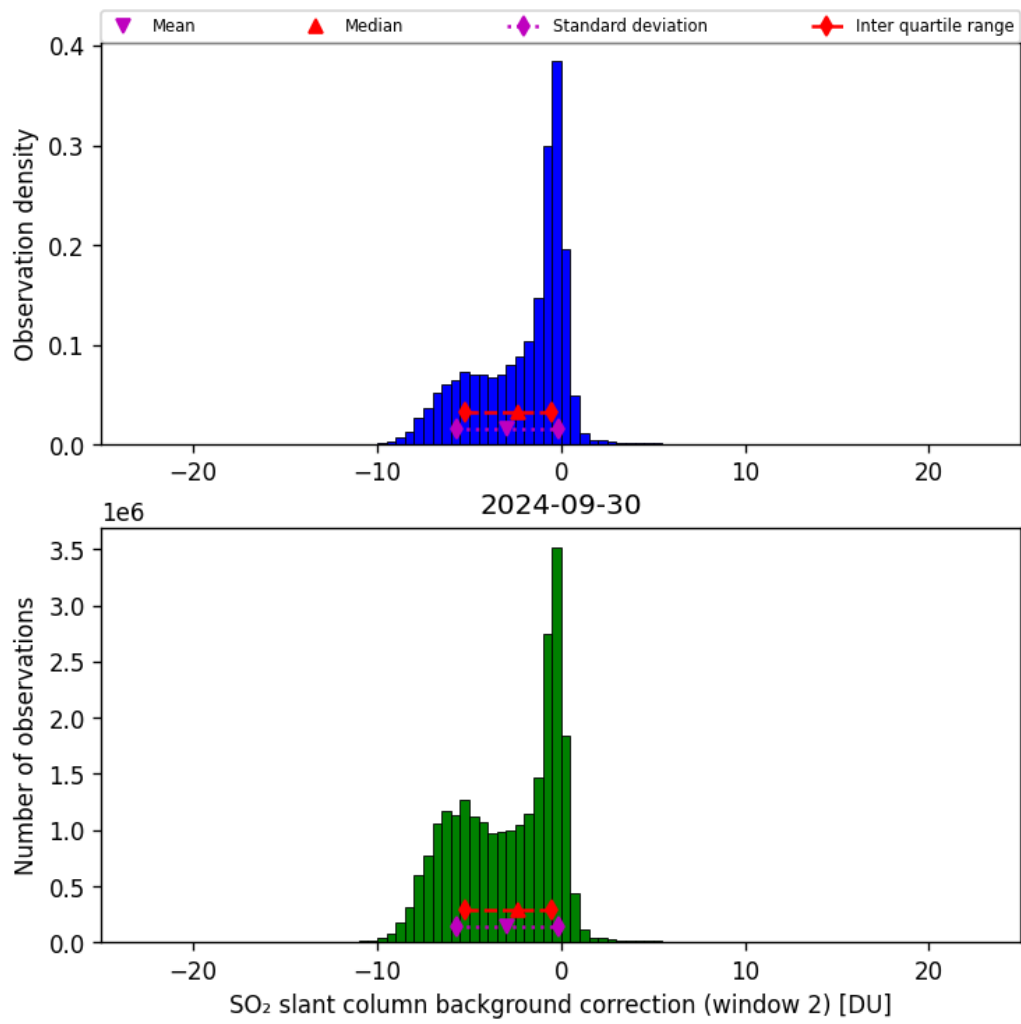
Figure 63: Histogram of “SO 2 slant column background correction (window 2)” for 2024-09-29 to 2024-10-01
