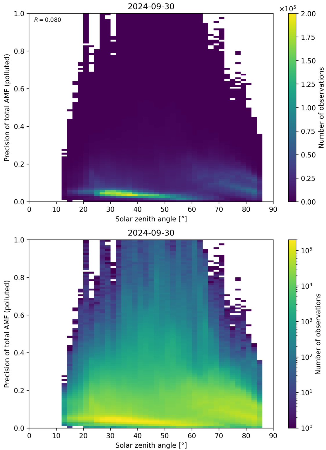
Figure 175: Scatter density plot of “Solar zenith angle” against “Precision of total AMF (polluted)” for 2024-09-29 to 2024-10-01.
