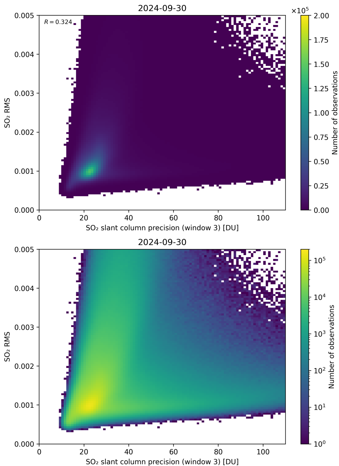
Figure 260: Scatter density plot of “SO 2 slant column precision (window 3)” against “SO 2 RMS” for 2024-09-29 to 2024-10-01.
