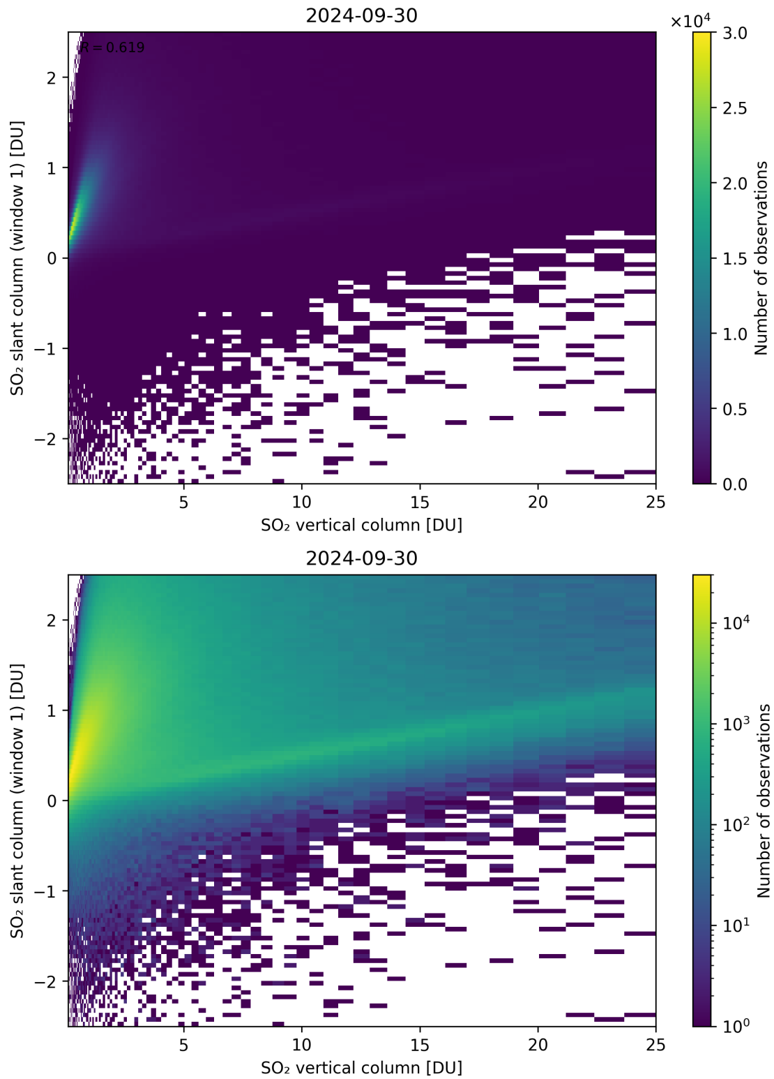
Figure 300: Scatter density plot of “SO 2 vertical column” against “SO 2 slant column (window 1)” for 2024-09-29 to 2024-10-01.
