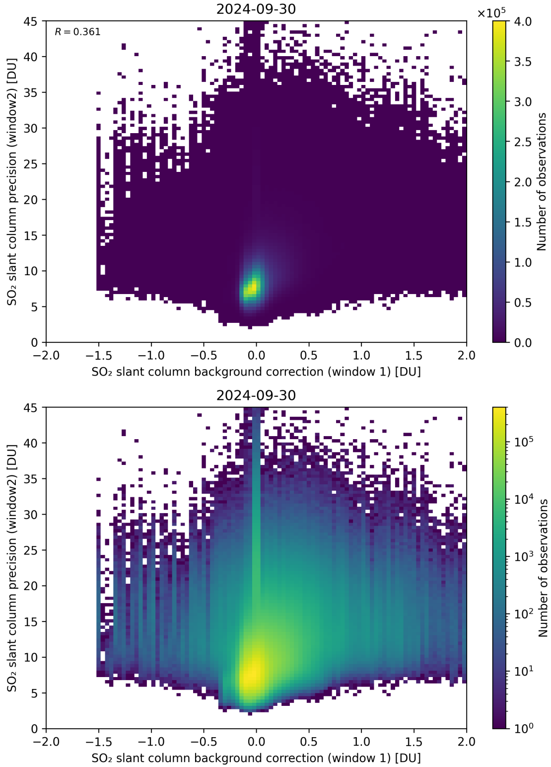
Figure 106: Scatter density plot of “SO 2 slant column background correction (window 1)” against “SO 2 slant column precision (window2)” for 2024-09-29 to 2024-10-01.
