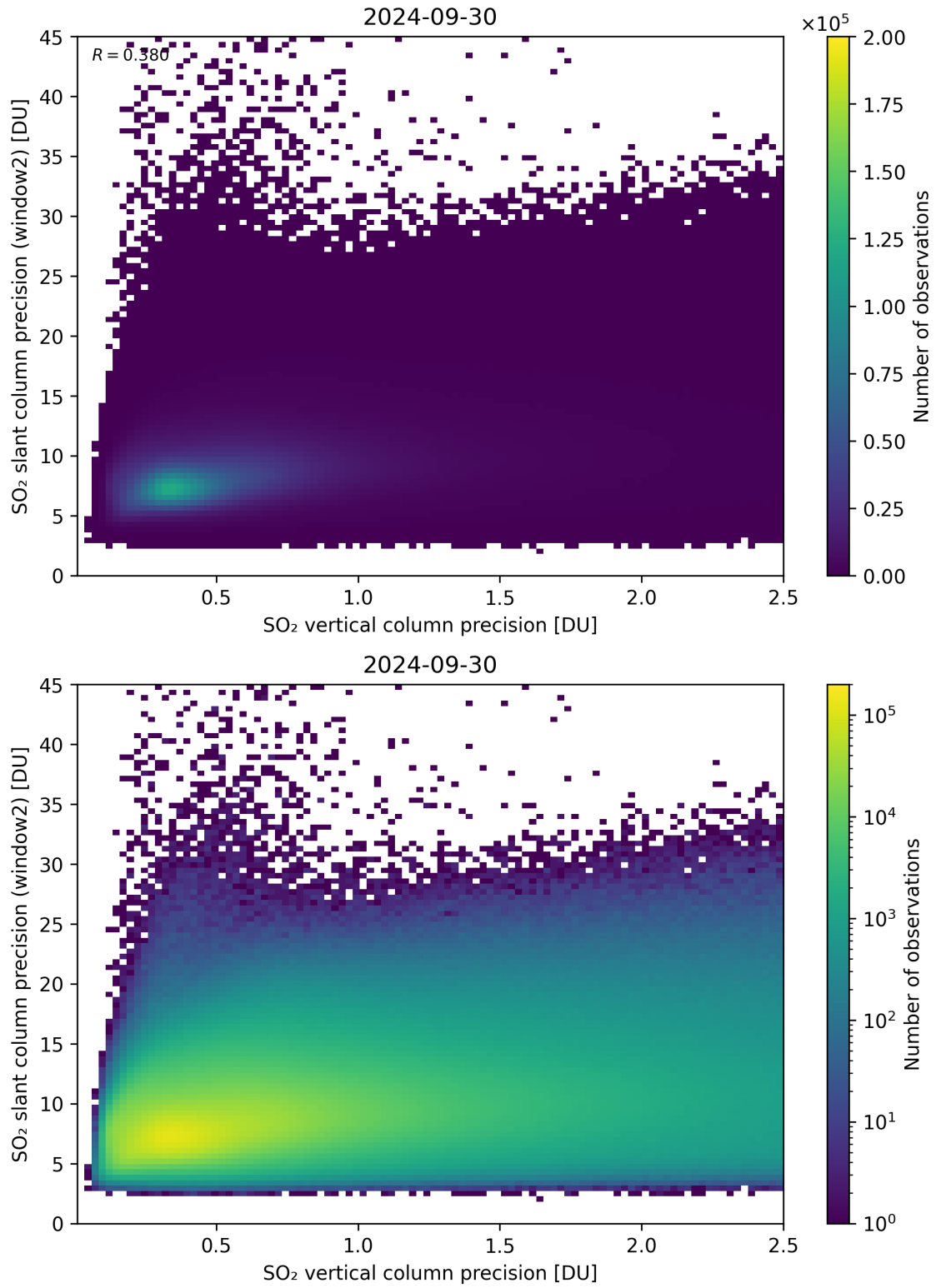
Figure 291: Scatter density plot of “SO 2 vertical column precision” against “SO 2 slant column precision (window2)” for 2024-09-29 to 2024-10-01.
