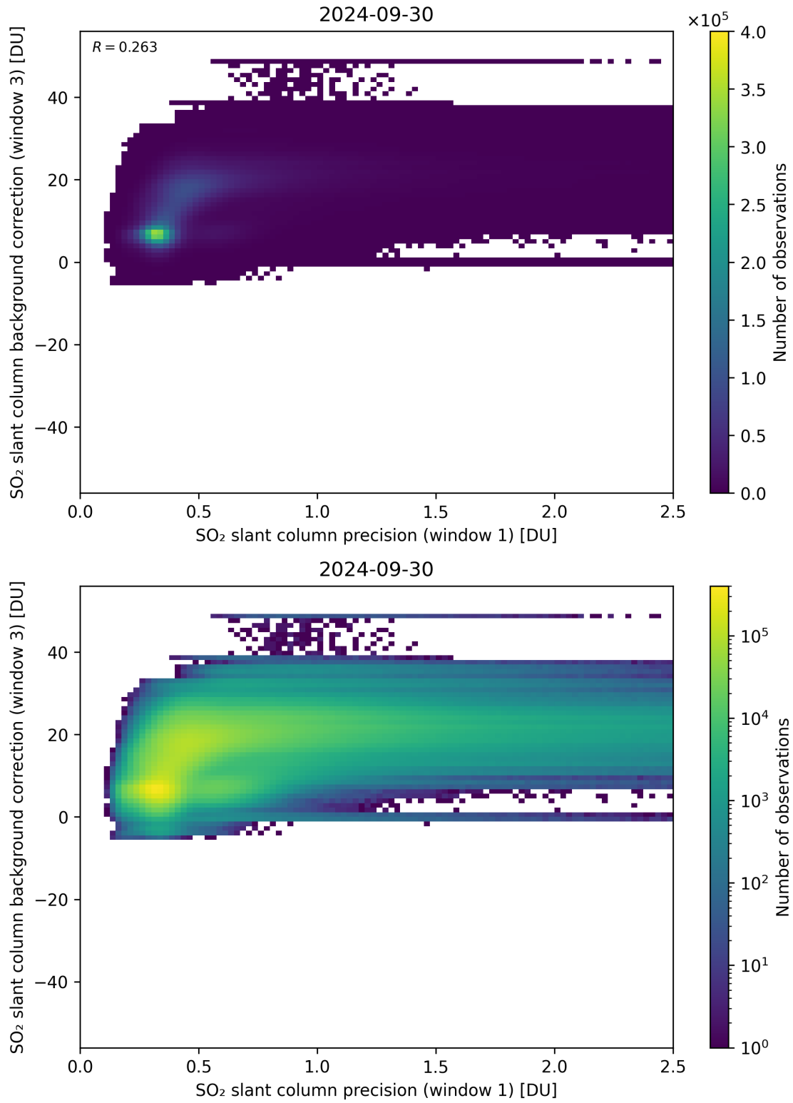
Figure 220: Scatter density plot of “SO 2 slant column precision (window 1)” against “SO 2 slant column background correction (window 3)” for 2024-09-29 to 2024-10-01.
