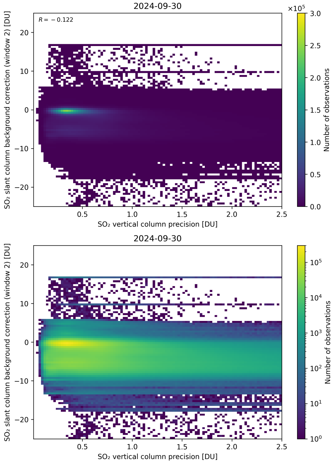
Figure 280: Scatter density plot of “SO 2 vertical column precision” against “SO 2 slant column background correction (window 2)” for 2024-09-29 to 2024-10-01.
