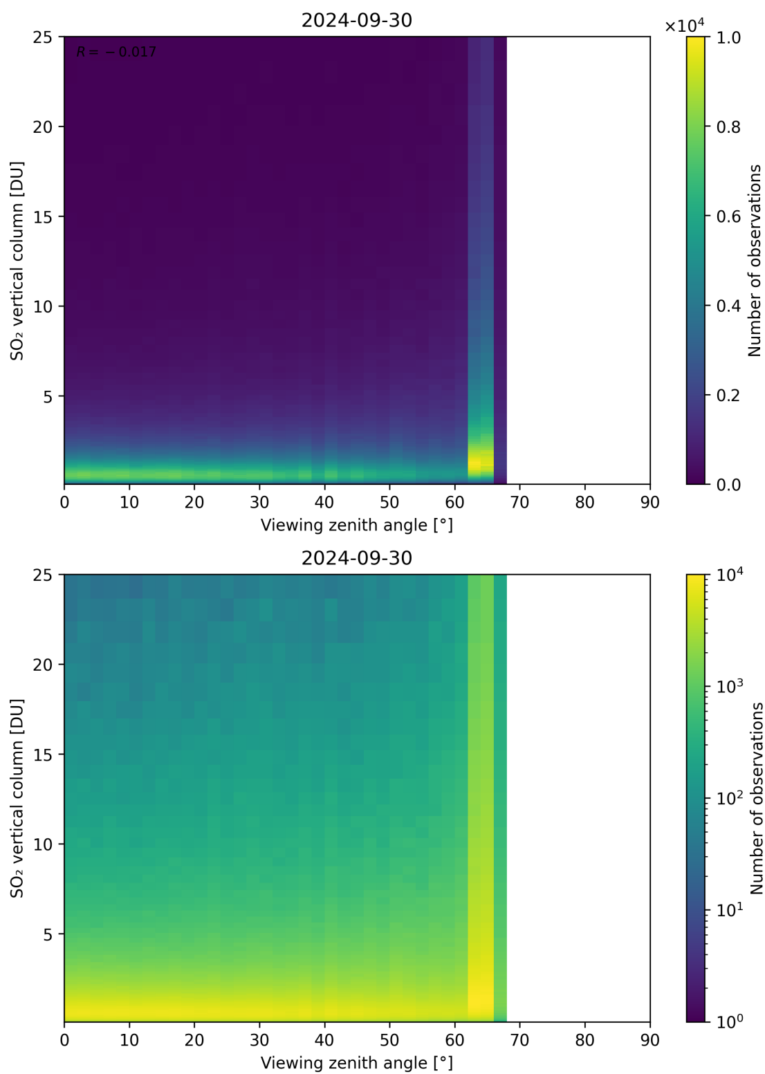
Figure 327: Scatter density plot of “Viewing zenith angle” against “SO 2 vertical column” for 2024-09-29 to 2024-10-01.
