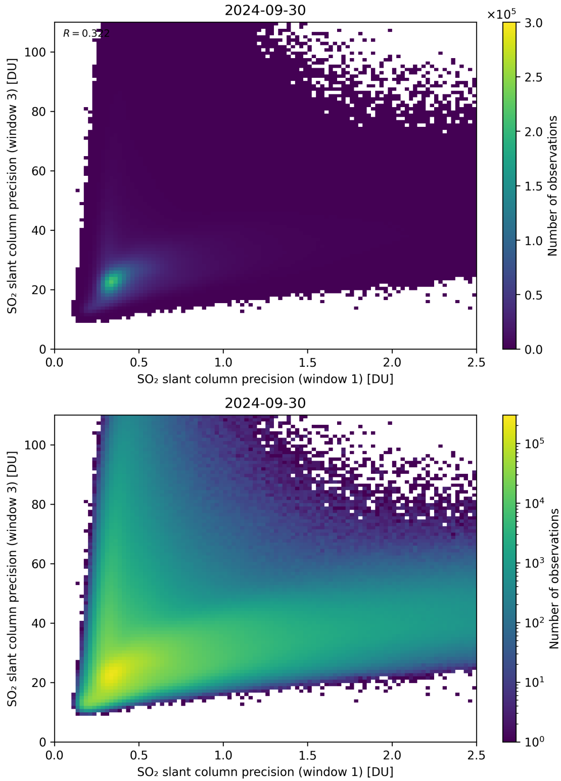
Figure 229: Scatter density plot of “SO 2 slant column precision (window 1)” against “SO 2 slant column precision (window 3)” for 2024-09-29 to 2024-10-01.
