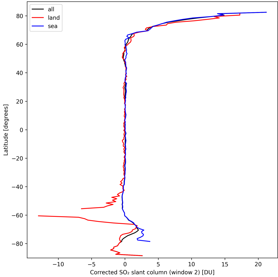
Figure 39: Zonal average of “Corrected SO 2 slant column (window 2)” for 2024-09-29 to 2024-10-01.
