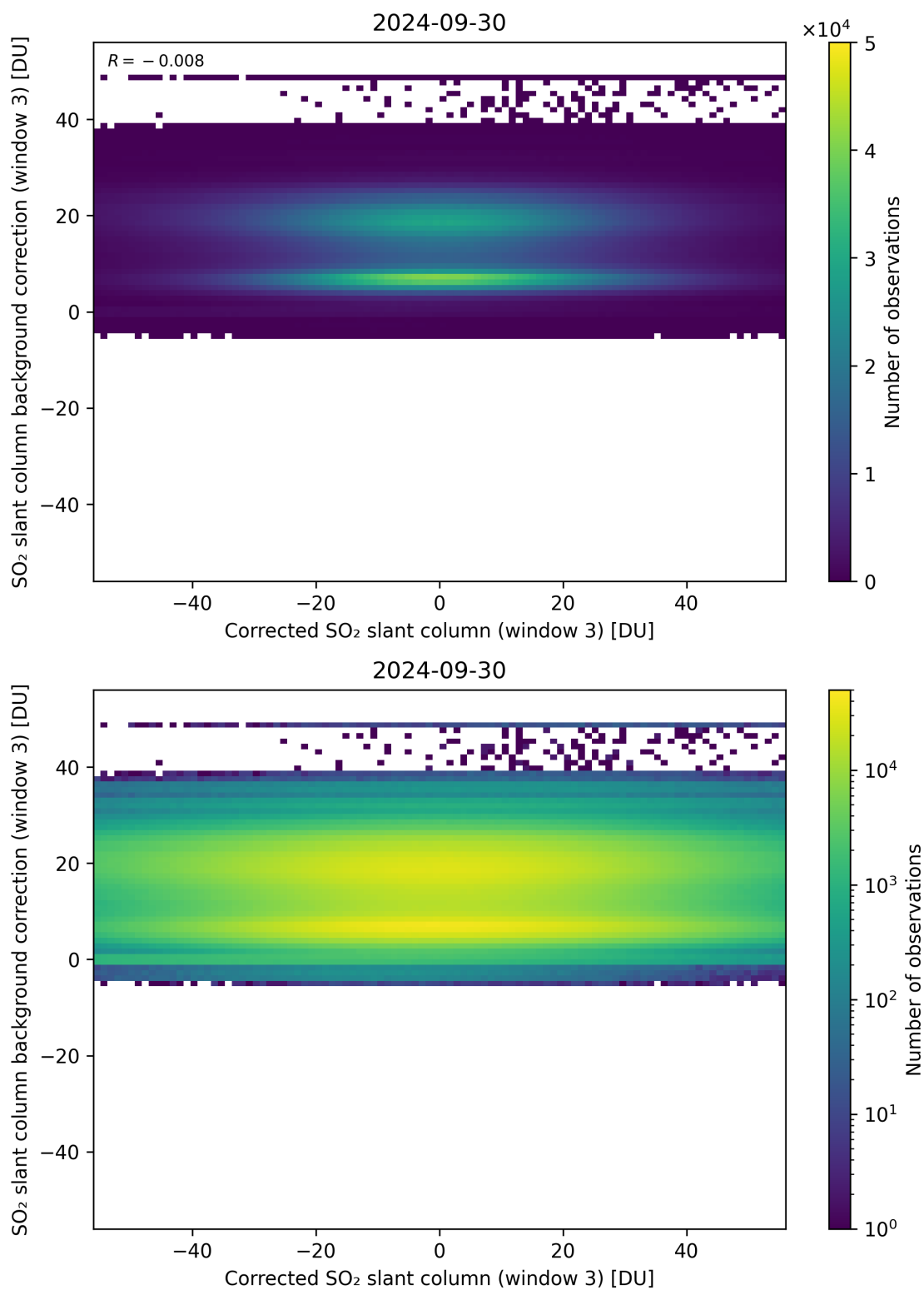
Figure 205: Scatter density plot of “Corrected SO 2 slant column (window 3)” against “SO 2 slant column background correction (window 3)” for 2024-09-29 to 2024-10-01.
