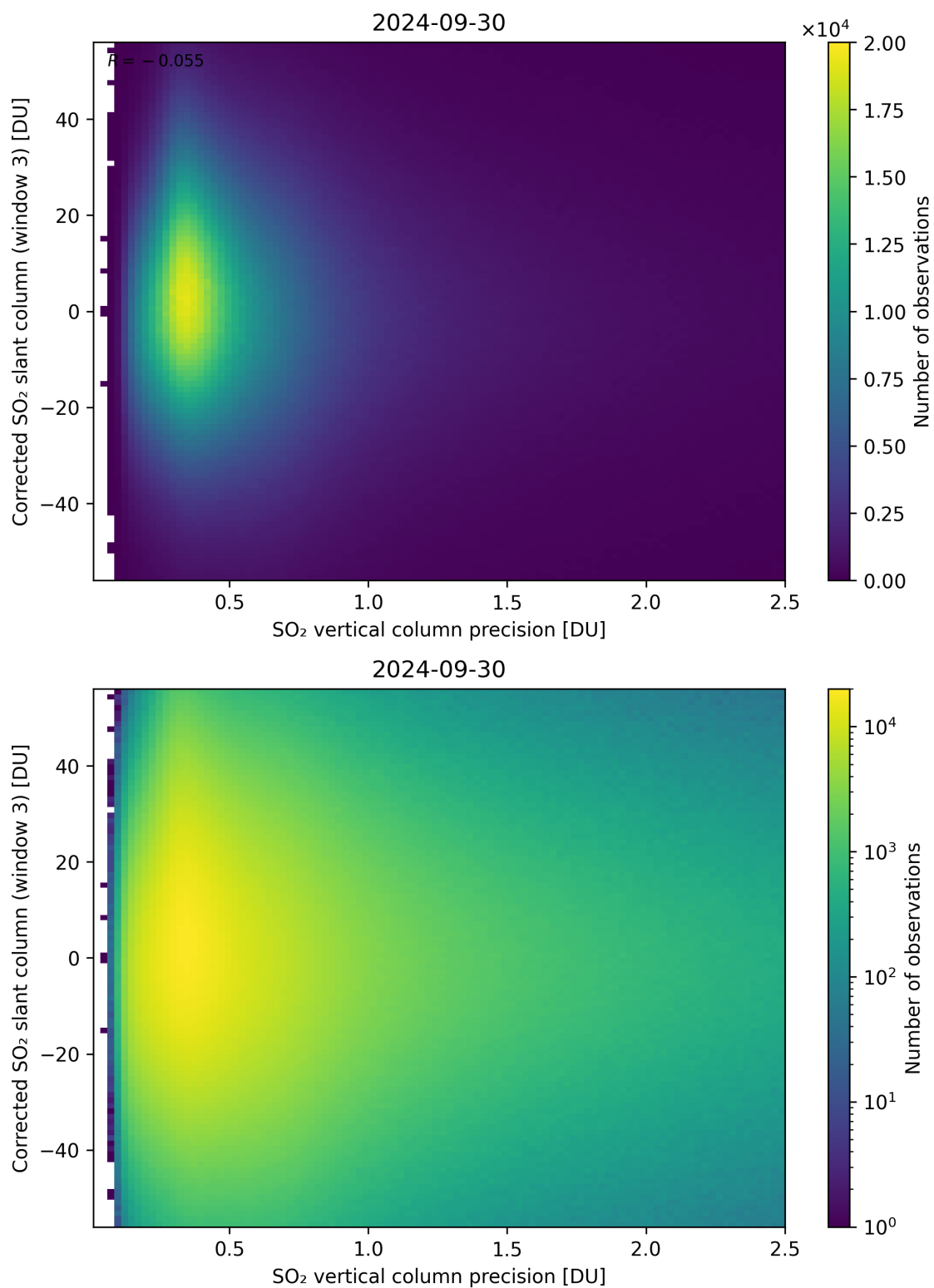
Figure 288: Scatter density plot of “SO 2 vertical column precision” against “Corrected SO 2 slant column (window 3)” for 2024-09-29 to 2024-10-01.
