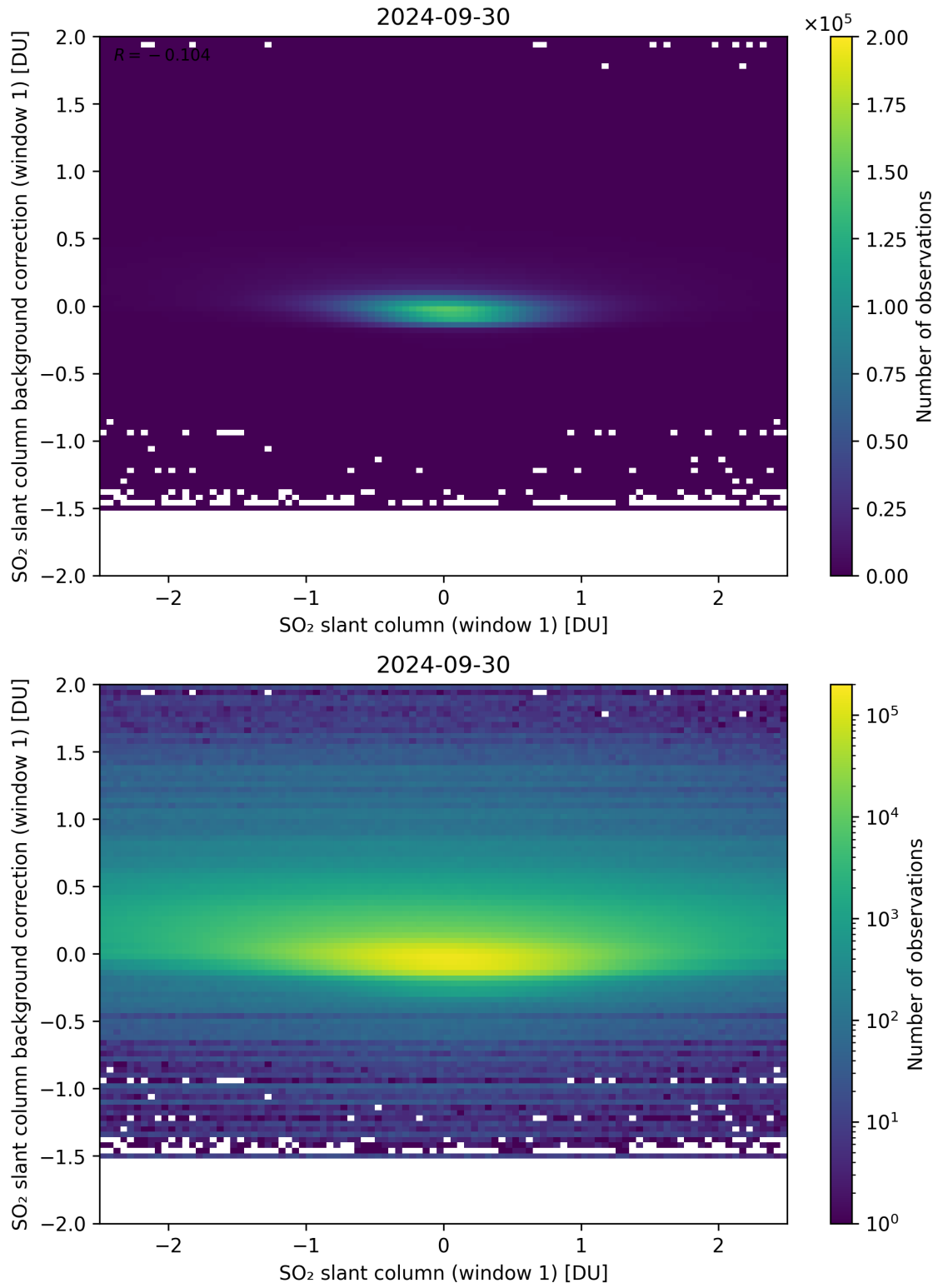
Figure 212: Scatter density plot of “SO 2 slant column (window 1)” against “SO 2 slant column background correction (window 1)” for 2024-09-29 to 2024-10-01.
