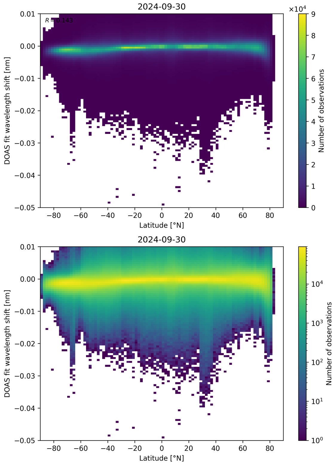
Figure 142: Scatter density plot of “Latitude” against “DOAS fit wavelength shift” for 2024-09-29 to 2024-10-01.
