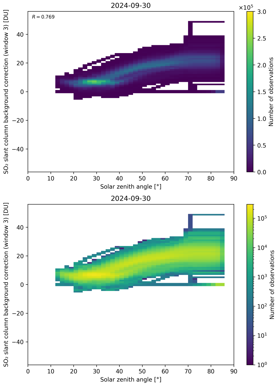
Figure 160: Scatter density plot of “Solar zenith angle” against “SO 2 slant column background correction (window 3)” for 2024-09-29 to 2024-10-01.
