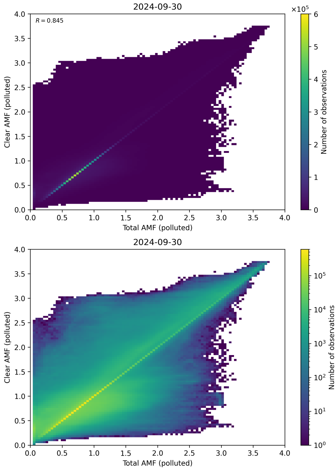
Figure 271: Scatter density plot of “Total AMF (polluted)” against “Clear AMF (polluted)” for 2024-09-29 to 2024-10-01.
