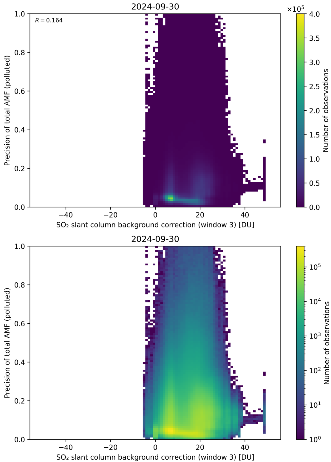
Figure 126: Scatter density plot of “SO 2 slant column background correction (window 3)” against “Precision of total AMF (polluted)” for 2024-09-29 to 2024-10-01.
