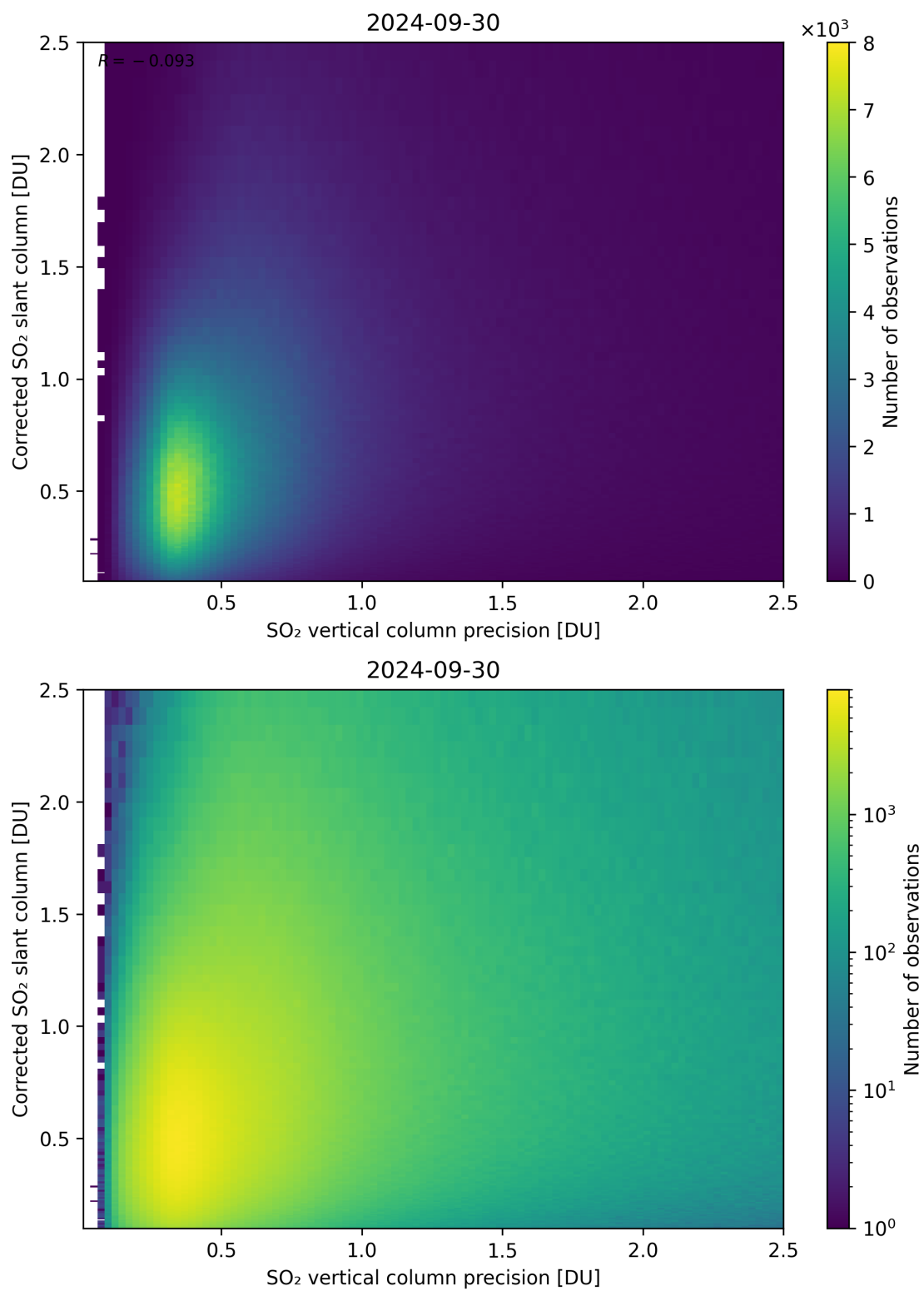
Figure 286: Scatter density plot of “SO 2 vertical column precision” against “Corrected SO 2 slant column” for 2024-09-29 to 2024-10-01.
