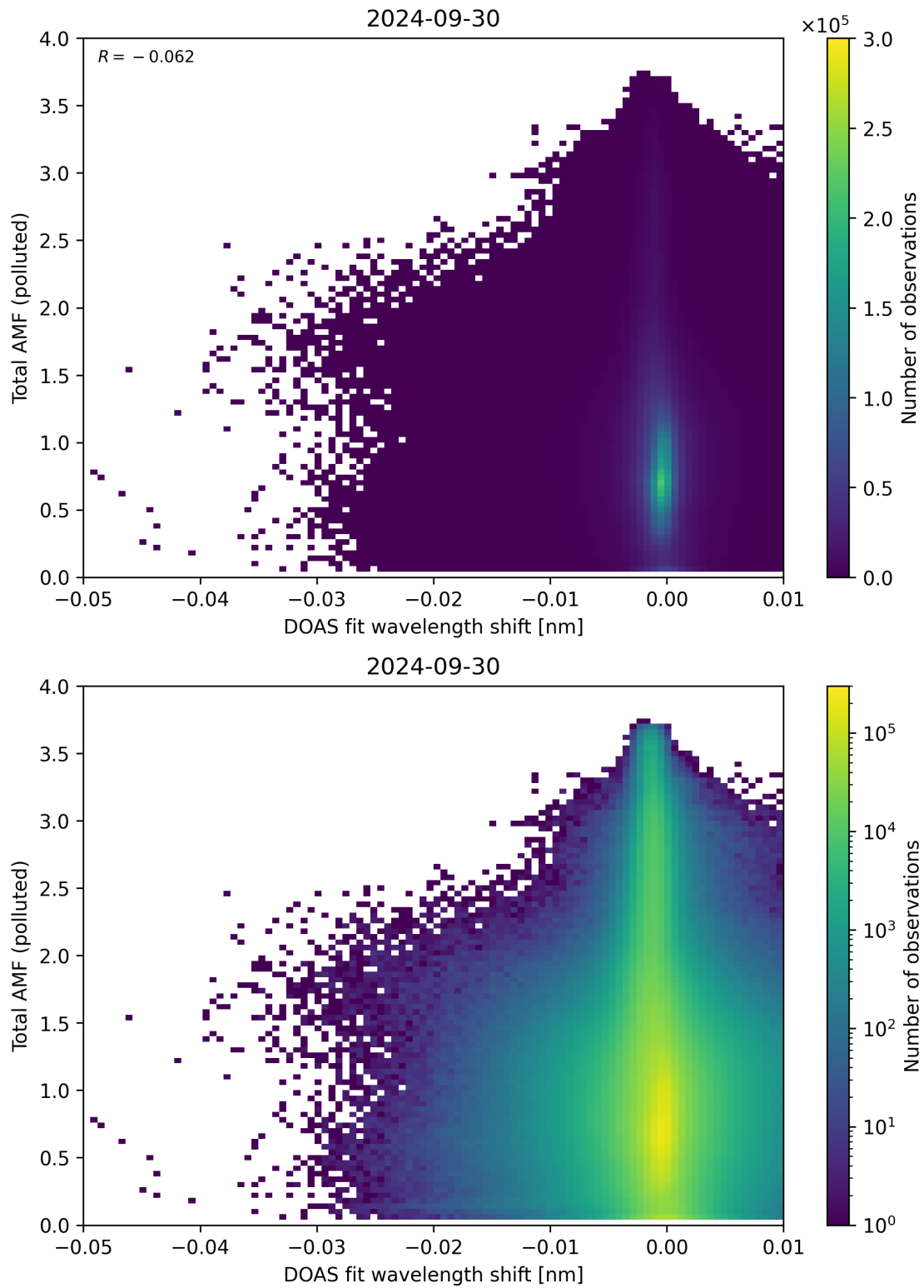
Figure 130: Scatter density plot of “DOAS fit wavelength shift” against “Total AMF (polluted)” for 2024-09-29 to 2024-10-01.
