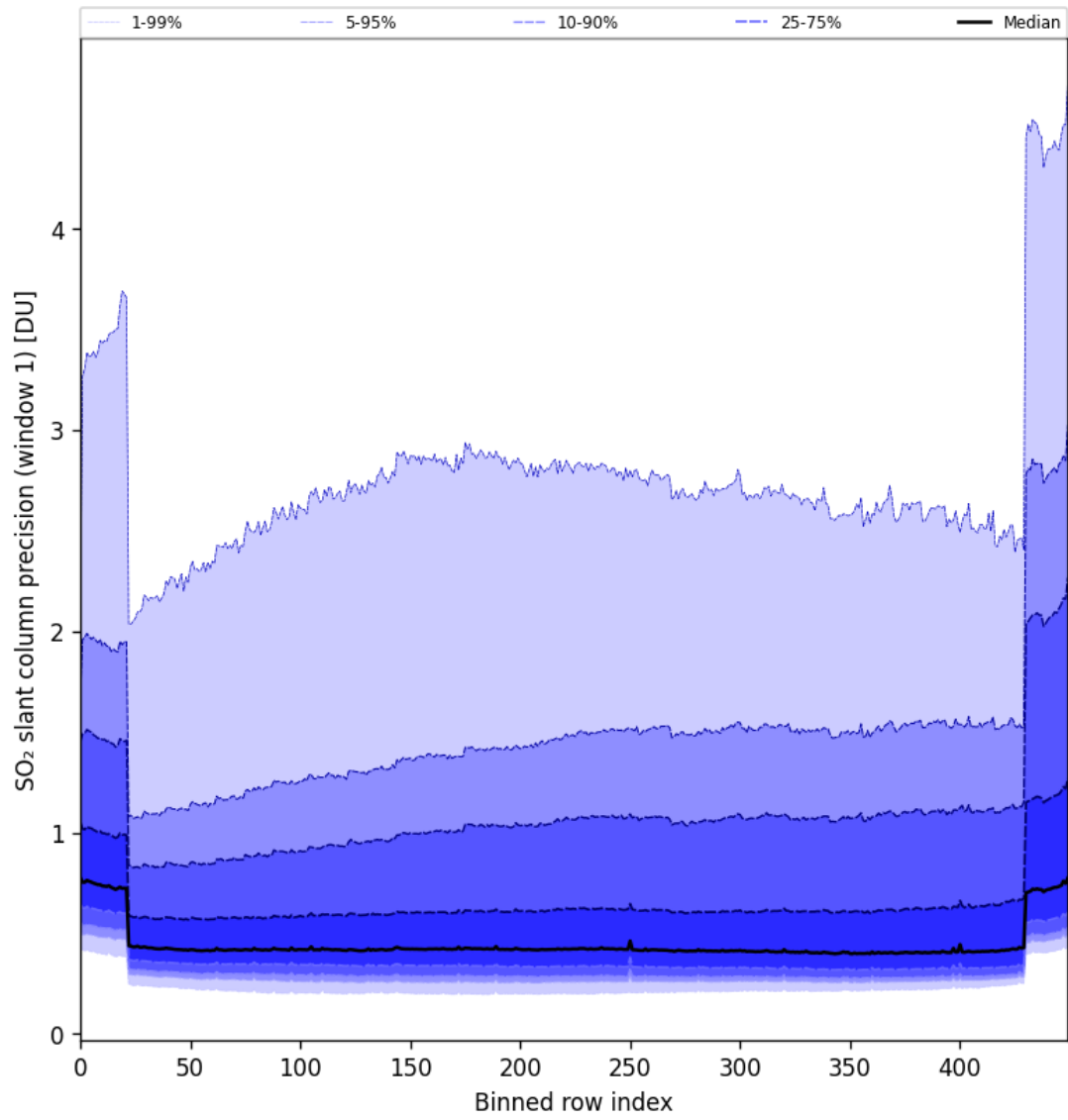
Figure 80: Along track statistics of “SO 2 slant column precision (window 1)” for 2024-09-29 to 2024-10-01
