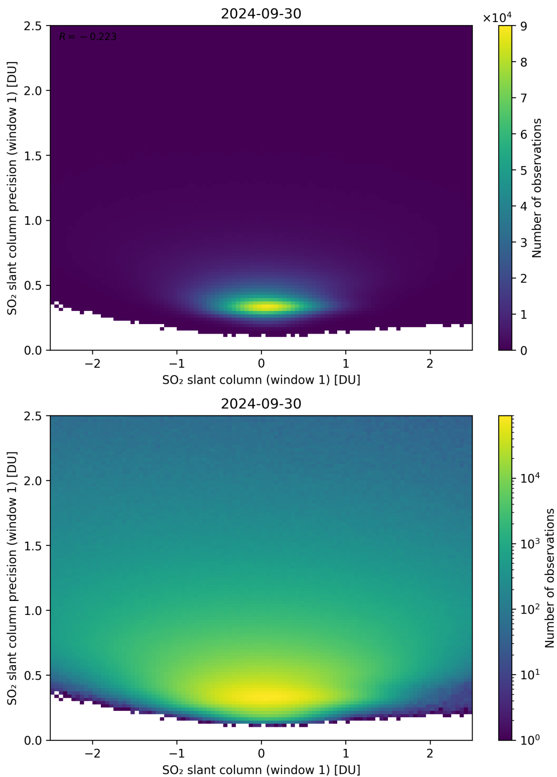
Figure 235: Scatter density plot of “SO 2 slant column (window 1)” against “SO 2 slant column precision (window 1)” for 2024-09-29 to 2024-10-01.
