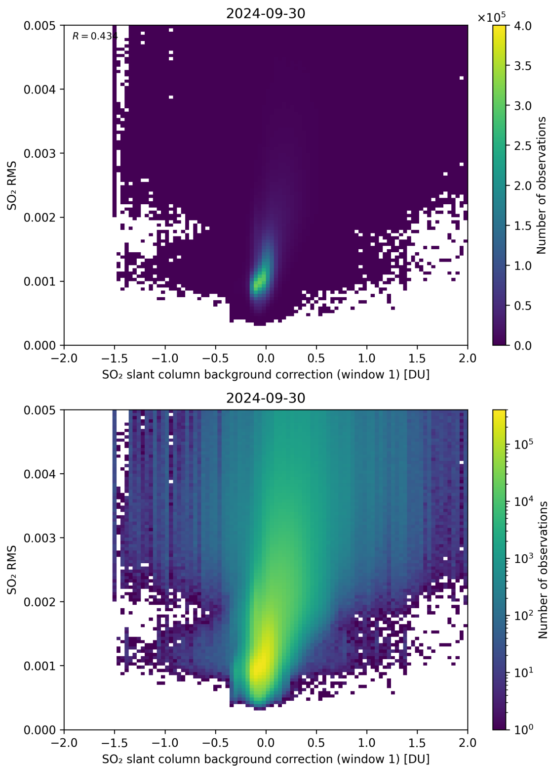
Figure 102: Scatter density plot of “SO 2 slant column background correction (window 1)” against “SO 2 RMS” for 2024-09-29 to 2024-10-01.
