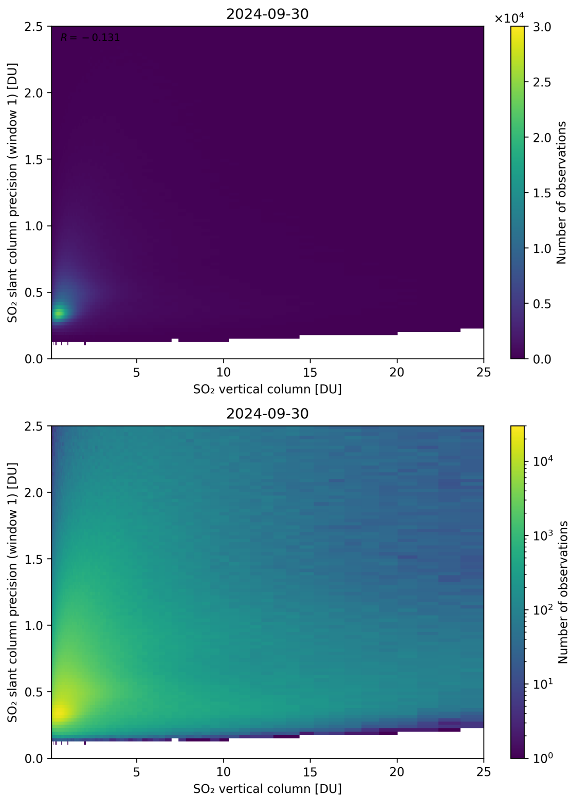
Figure 301: Scatter density plot of “SO 2 vertical column” against “SO 2 slant column precision (window 1)” for 2024-09-29 to 2024-10-01.
