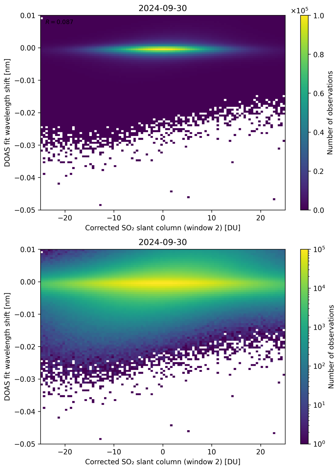
Figure 196: Scatter density plot of “Corrected SO 2 slant column (window 2)” against “DOAS fit wavelength shift” for 2024-09-29 to 2024-10-01.
