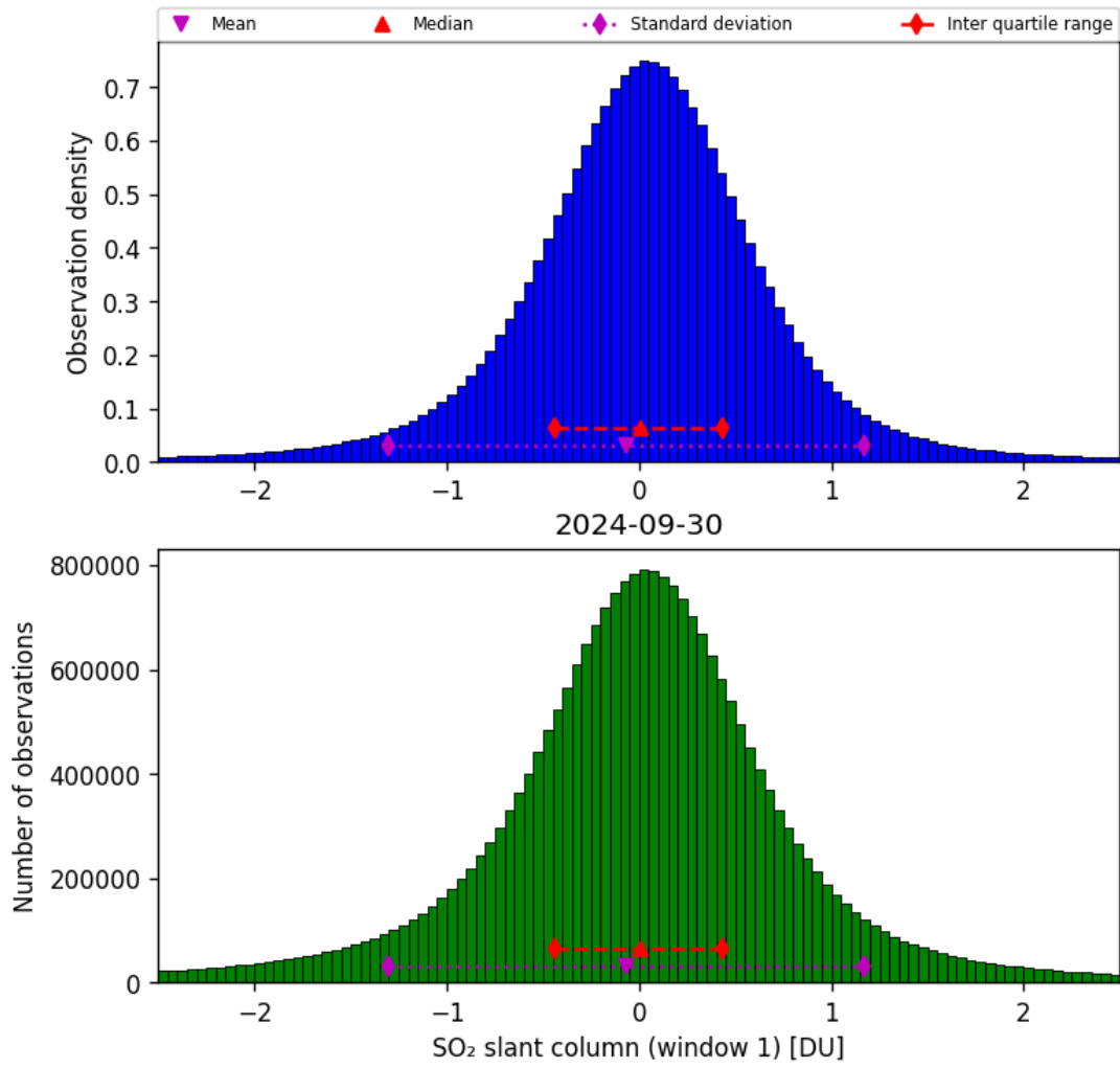
Figure 56: Histogram of “SO 2 slant column (window 1)” for 2024-09-29 to 2024-10-01
