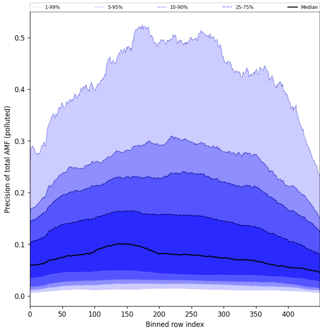
Figure 95: Along track statistics of “Precision of total AMF (polluted)” for 2024-09-29 to 2024-10-01
