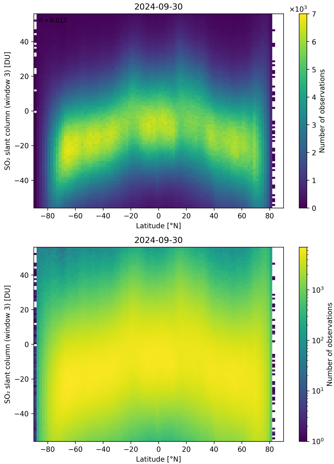
Figure 152: Scatter density plot of “Latitude” against “SO 2 slant column (window 3)” for 2024-09-29 to 2024-10-01.
