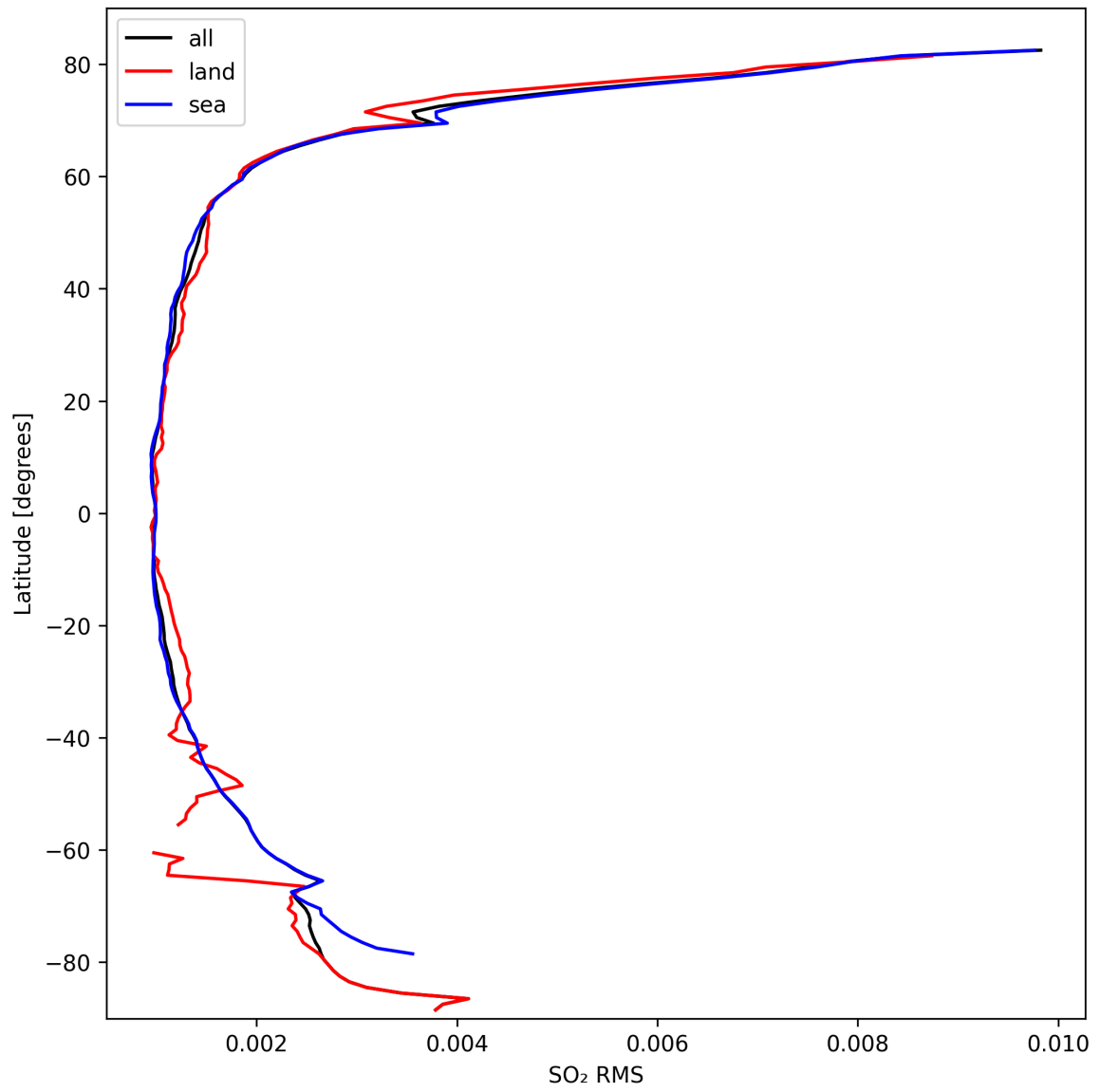
Figure 47: Zonal average of “SO 2 RMS” for 2024-09-29 to 2024-10-01.
