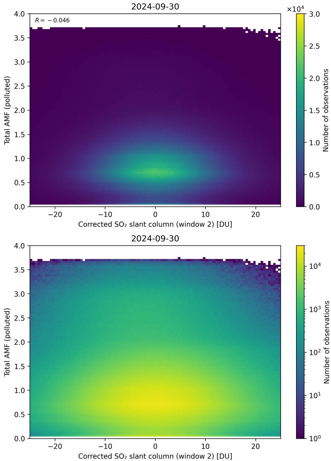
Figure 203: Scatter density plot of “Corrected SO 2 slant column (window 2)” against “Total AMF (polluted)” for 2024-09-29 to 2024-10-01.
