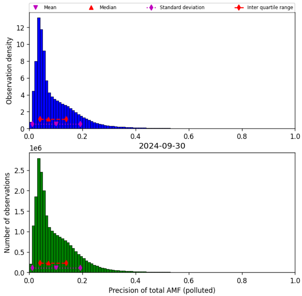
Figure 72: Histogram of “Precision of total AMF (polluted)” for 2024-09-29 to 2024-10-01
