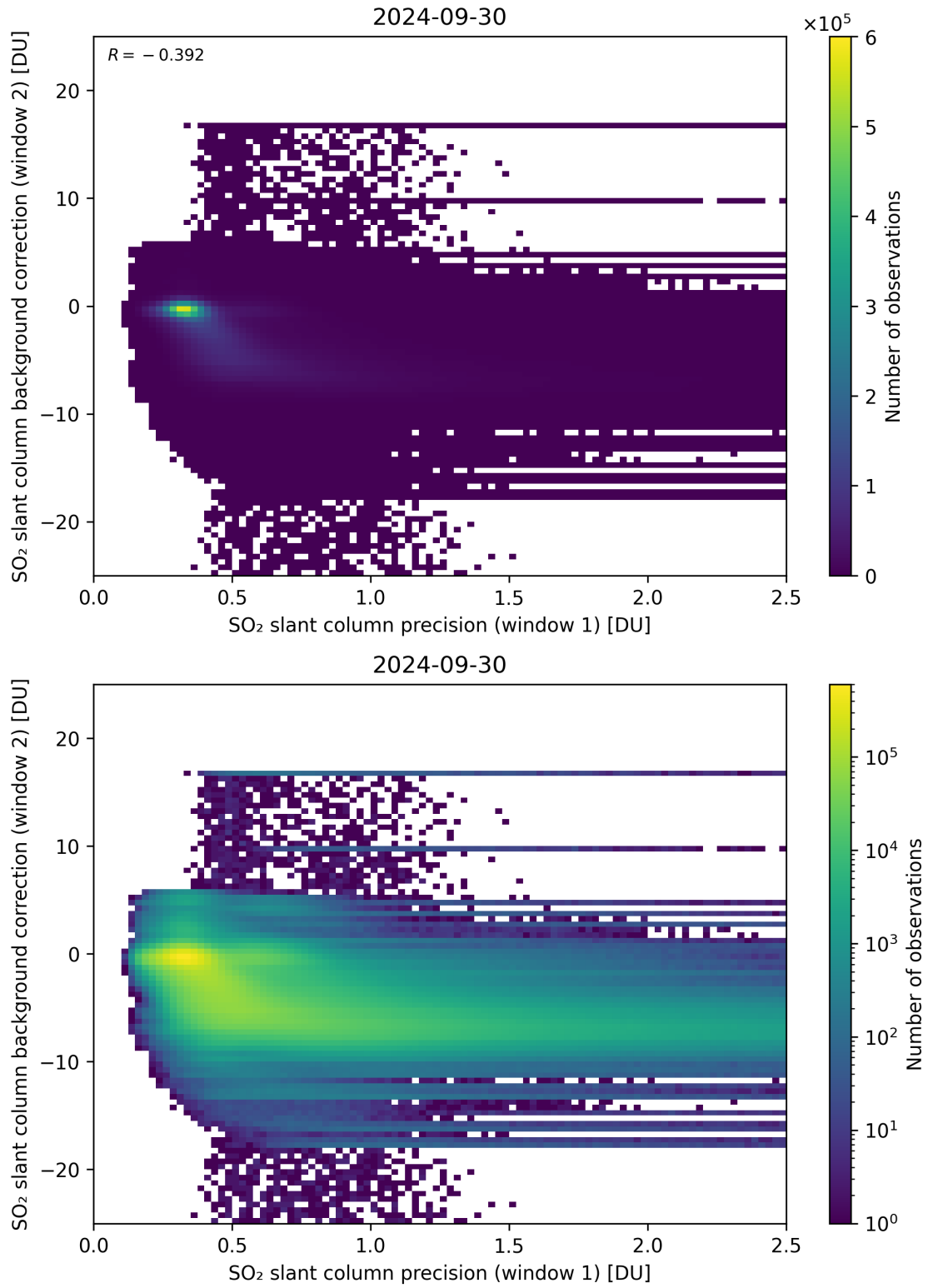
Figure 219: Scatter density plot of “SO 2 slant column precision (window 1)” against “SO 2 slant column background correction (window 2)” for 2024-09-29 to 2024-10-01.
