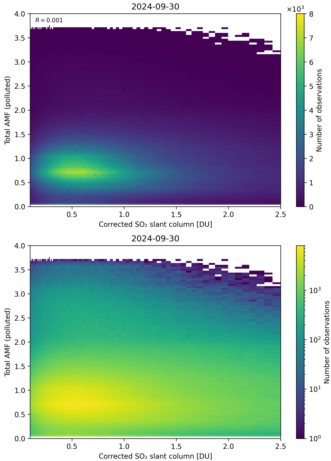
Figure 192: Scatter density plot of “Corrected SO 2 slant column” against “Total AMF (polluted)” for 2024-09-29 to 2024-10-01.
