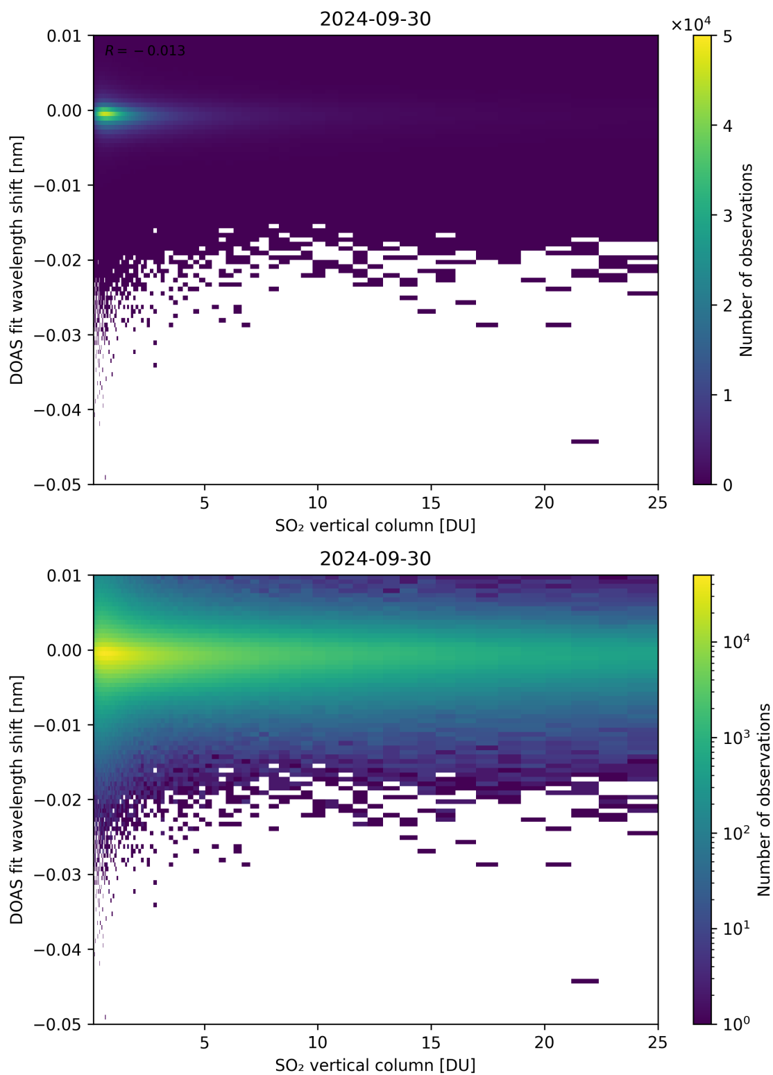
Figure 276: Scatter density plot of “SO 2 vertical column” against “DOAS fit wavelength shift” for 2024-09-29 to 2024-10-01.
