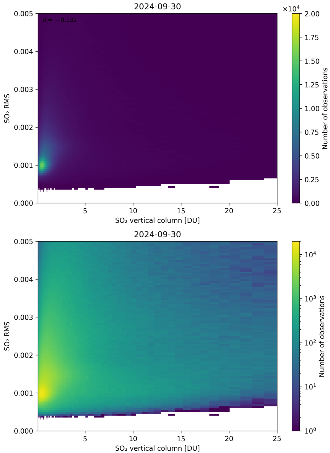
Figure 278: Scatter density plot of “SO 2 vertical column” against “SO 2 RMS” for 2024-09-29 to 2024-10-01.
