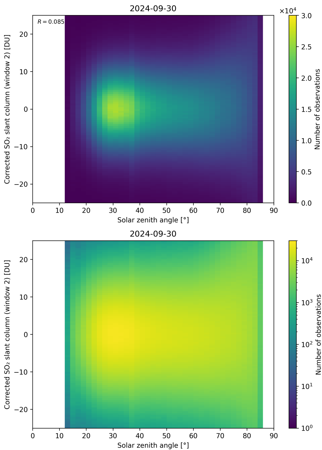
Figure 167: Scatter density plot of “Solar zenith angle” against “Corrected SO 2 slant column (window 2)” for 2024-09-29 to 2024-10-01.
