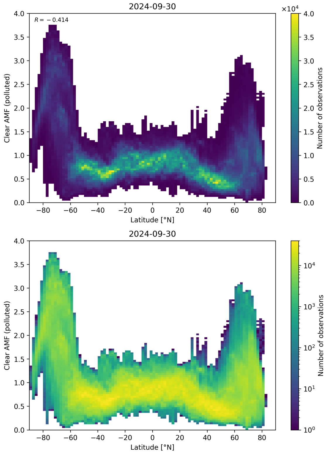
Figure 145: Scatter density plot of “Latitude” against “Clear AMF (polluted)” for 2024-09-29 to 2024-10-01.
