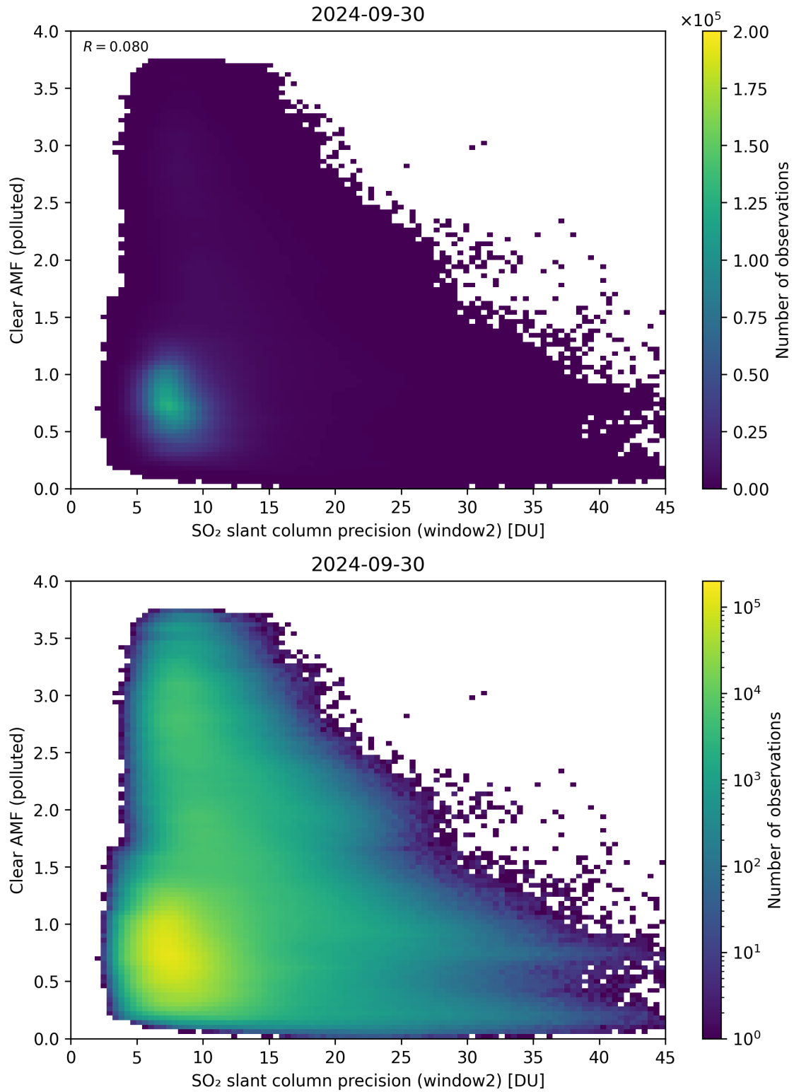
Figure 246: Scatter density plot of “SO 2 slant column precision (window2)” against “Clear AMF (polluted)” for 2024-09-29 to 2024-10-01.
