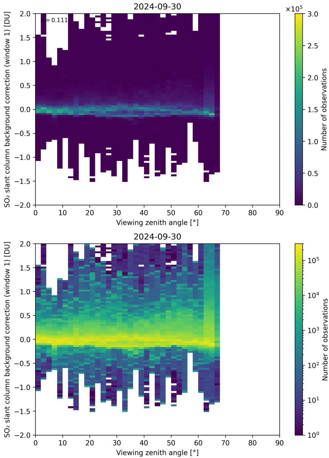
Figure 308: Scatter density plot of “Viewing zenith angle” against “SO 2 slant column background correction (window 1)” for 2024-09-29 to 2024-10-01.
