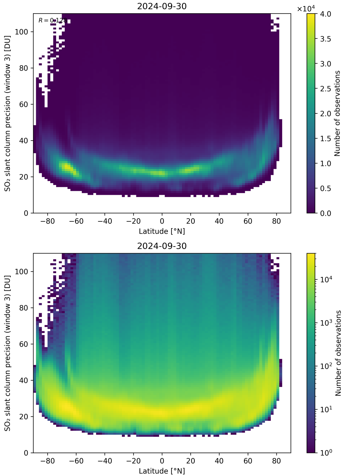
Figure 153: Scatter density plot of “Latitude” against “SO 2 slant column precision (window 3)” for 2024-09-29 to 2024-10-01.
