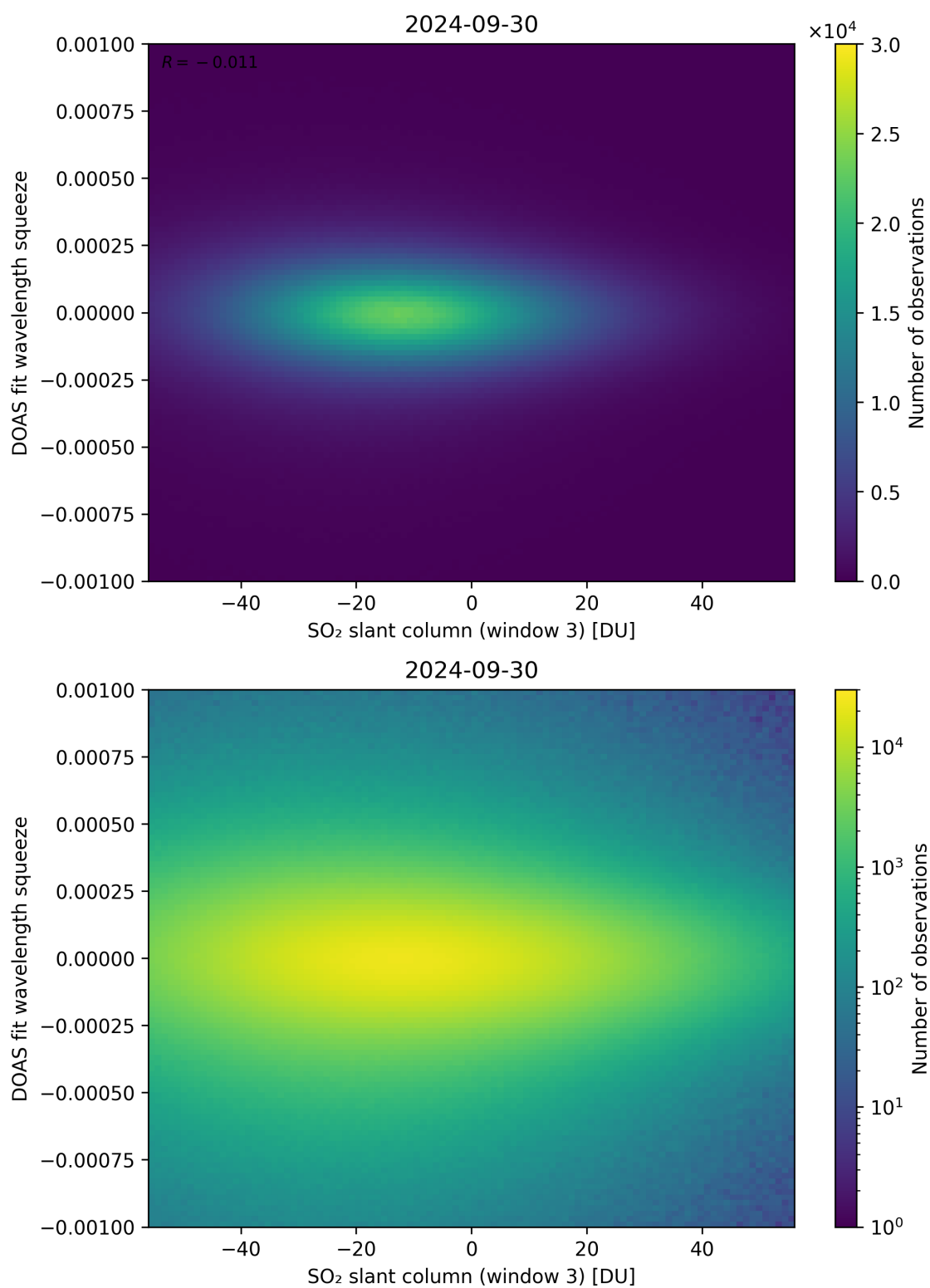
Figure 255: Scatter density plot of “SO 2 slant column (window 3)” against “DOAS fit wavelength squeeze” for 2024-09-29 to 2024-10-01.
