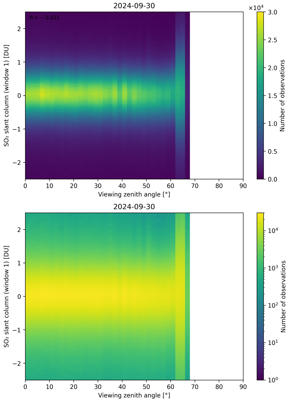
Figure 320: Scatter density plot of “Viewing zenith angle” against “SO 2 slant column (window 1)” for 2024-09-29 to 2024-10-01.
