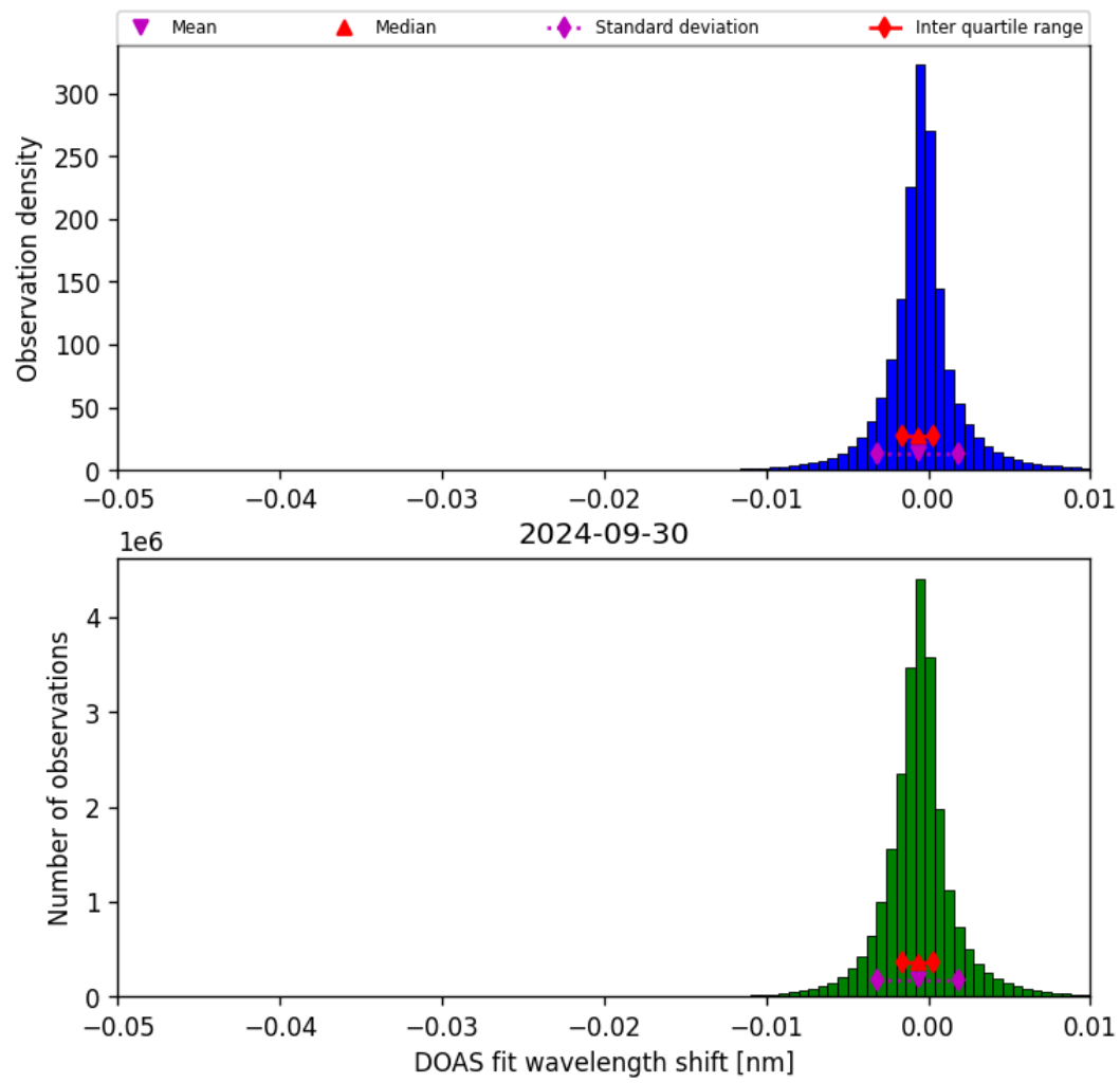
Figure 68: Histogram of “DOAS fit wavelength shift” for 2024-09-29 to 2024-10-01
