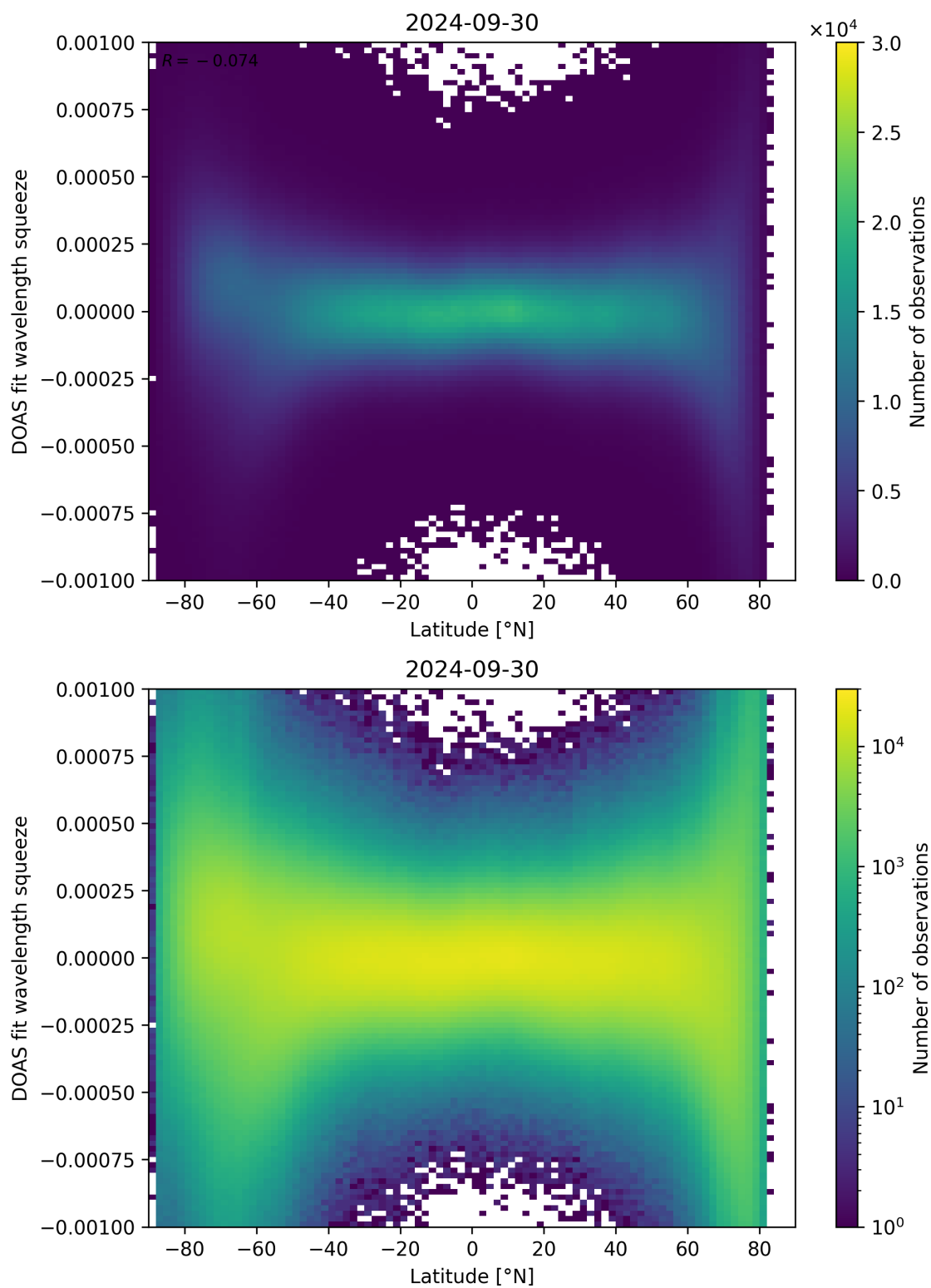
Figure 143: Scatter density plot of “Latitude” against “DOAS fit wavelength squeeze” for 2024-09-29 to 2024-10-01.
