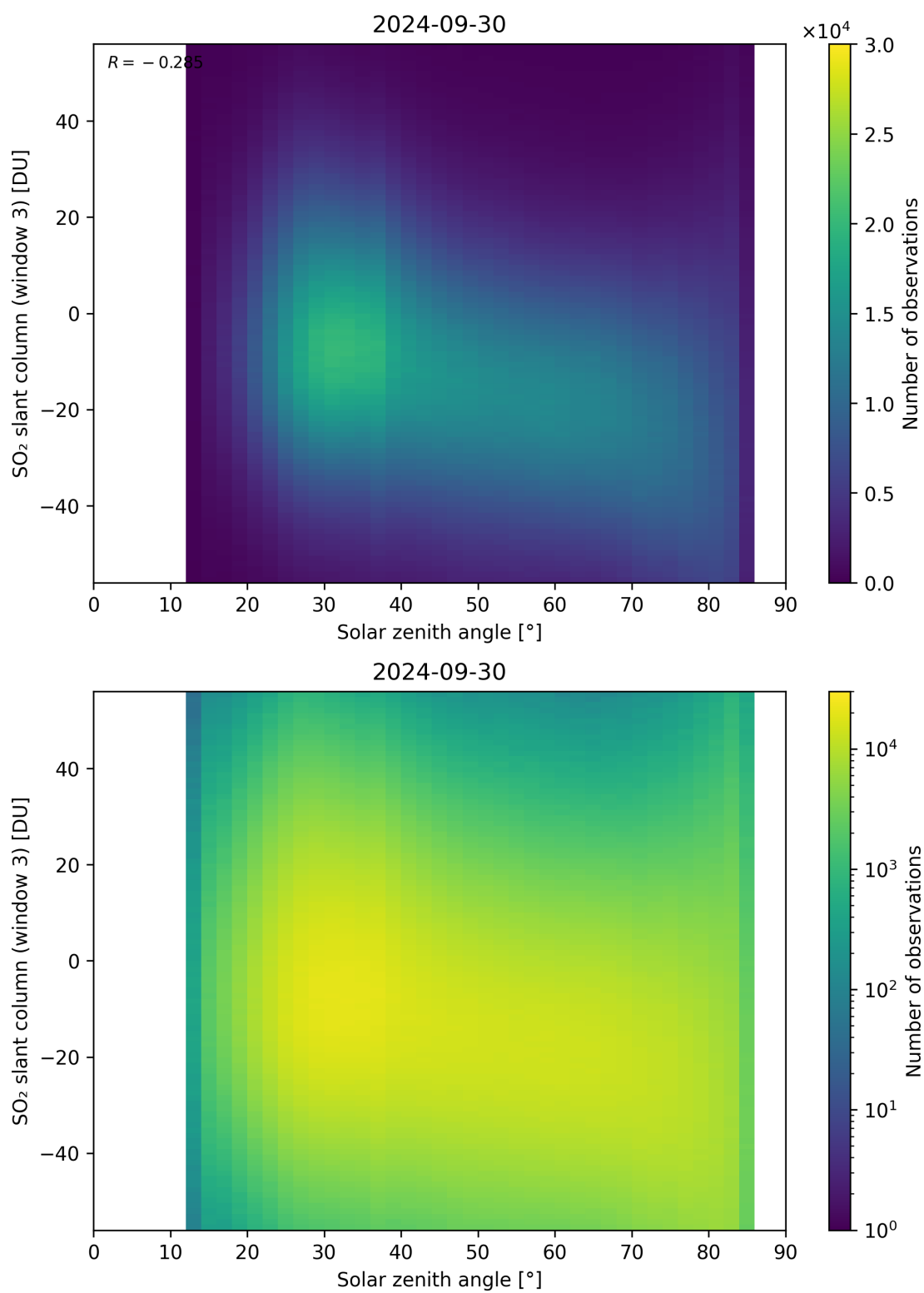
Figure 172: Scatter density plot of “Solar zenith angle” against “SO 2 slant column (window 3)” for 2024-09-29 to 2024-10-01.
