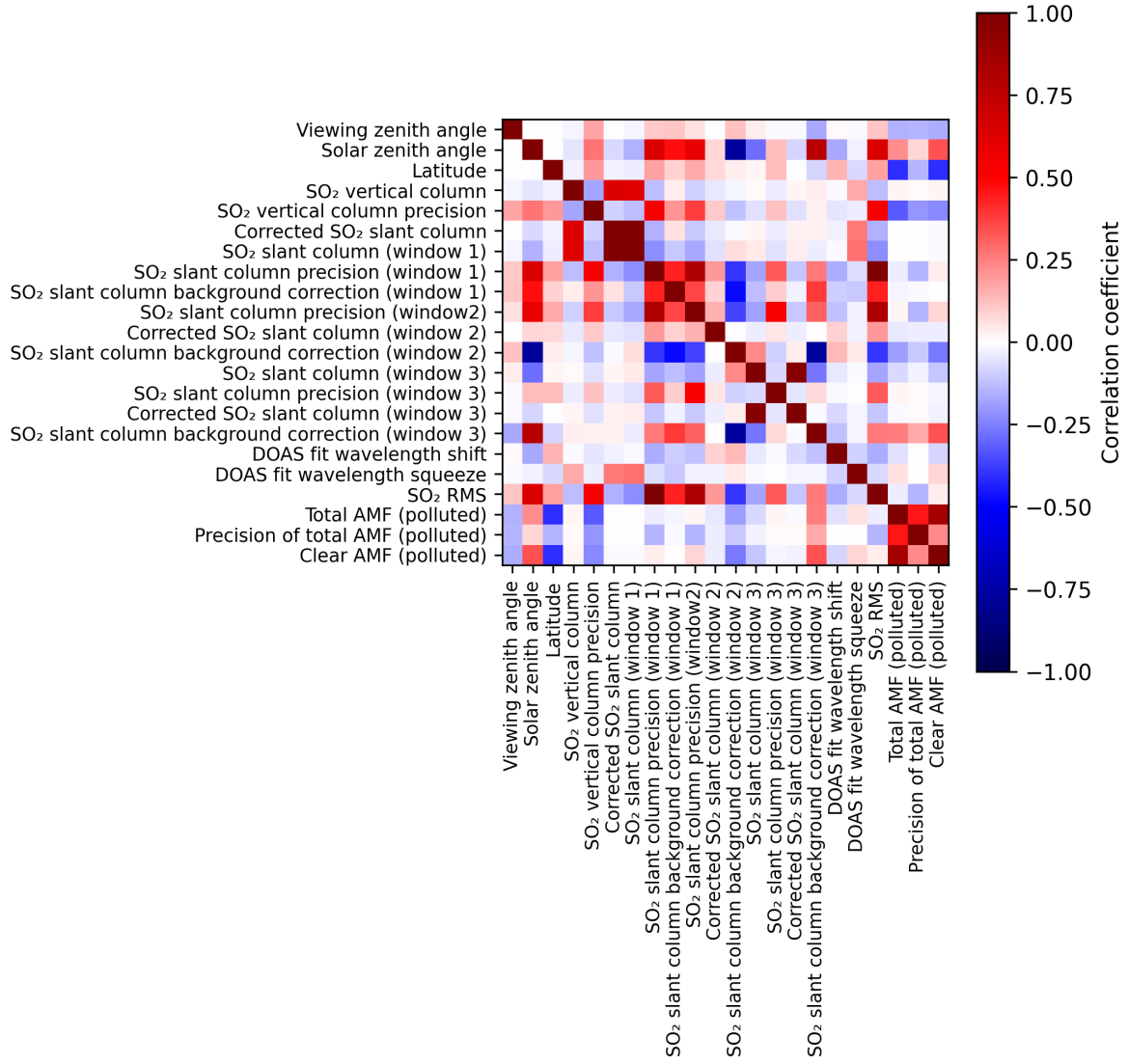
Figure 2: Map of correlation matrix for 2024-09-29 to 2024-10-01.
