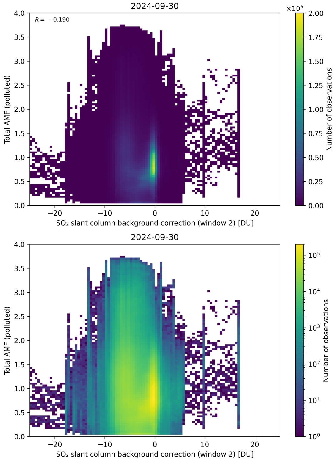
Figure 119: Scatter density plot of “SO 2 slant column background correction (window 2)” against “Total AMF (polluted)” for 2024-09-29 to 2024-10-01.
