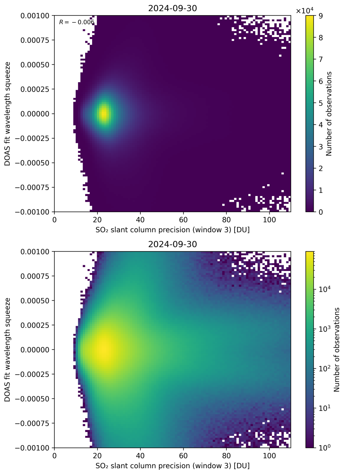
Figure 259: Scatter density plot of “SO 2 slant column precision (window 3)” against “DOAS fit wavelength squeeze” for 2024-09-29 to 2024-10-01.
