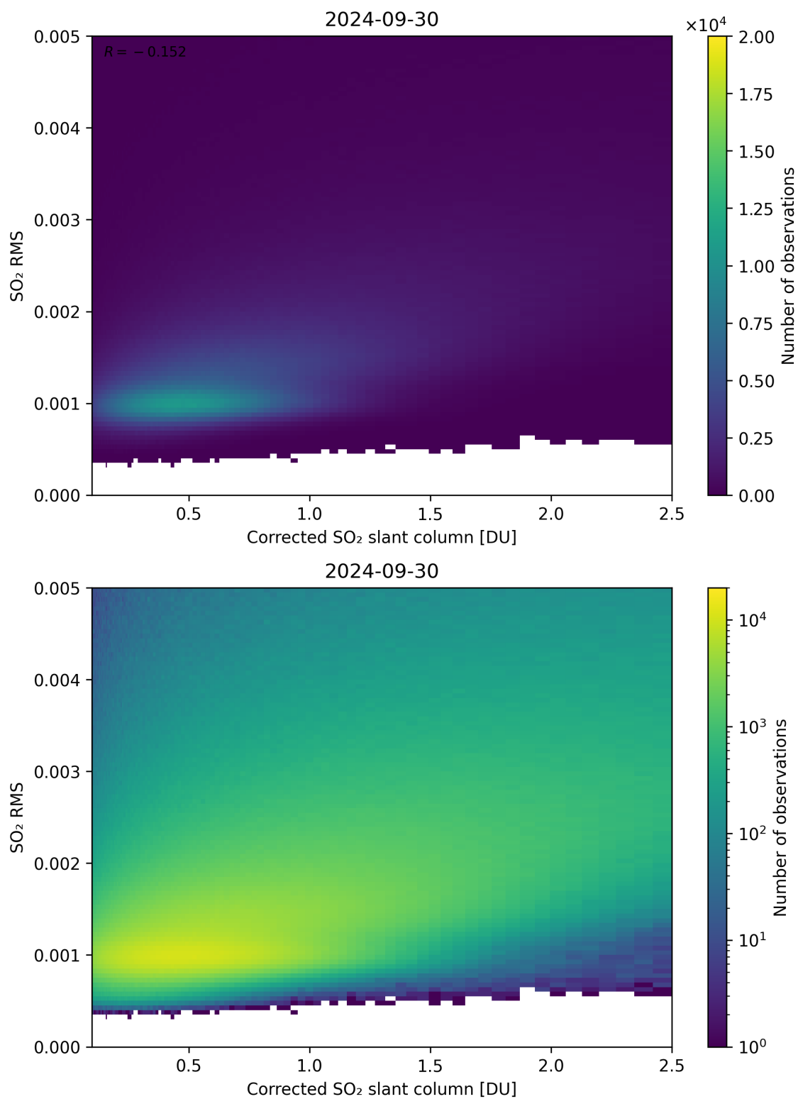
Figure 183: Scatter density plot of “Corrected SO 2 slant column” against “SO 2 RMS” for 2024-09-29 to 2024-10-01.
