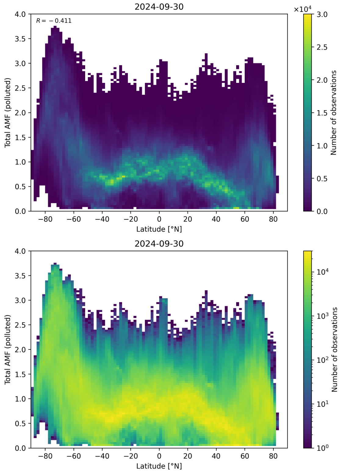
Figure 154: Scatter density plot of “Latitude” against “Total AMF (polluted)” for 2024-09-29 to 2024-10-01.
