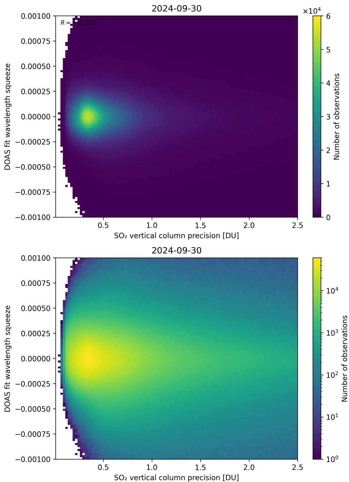
Figure 283: Scatter density plot of “SO 2 vertical column precision” against “DOAS fit wavelength squeeze” for 2024-09-29 to 2024-10-01.
