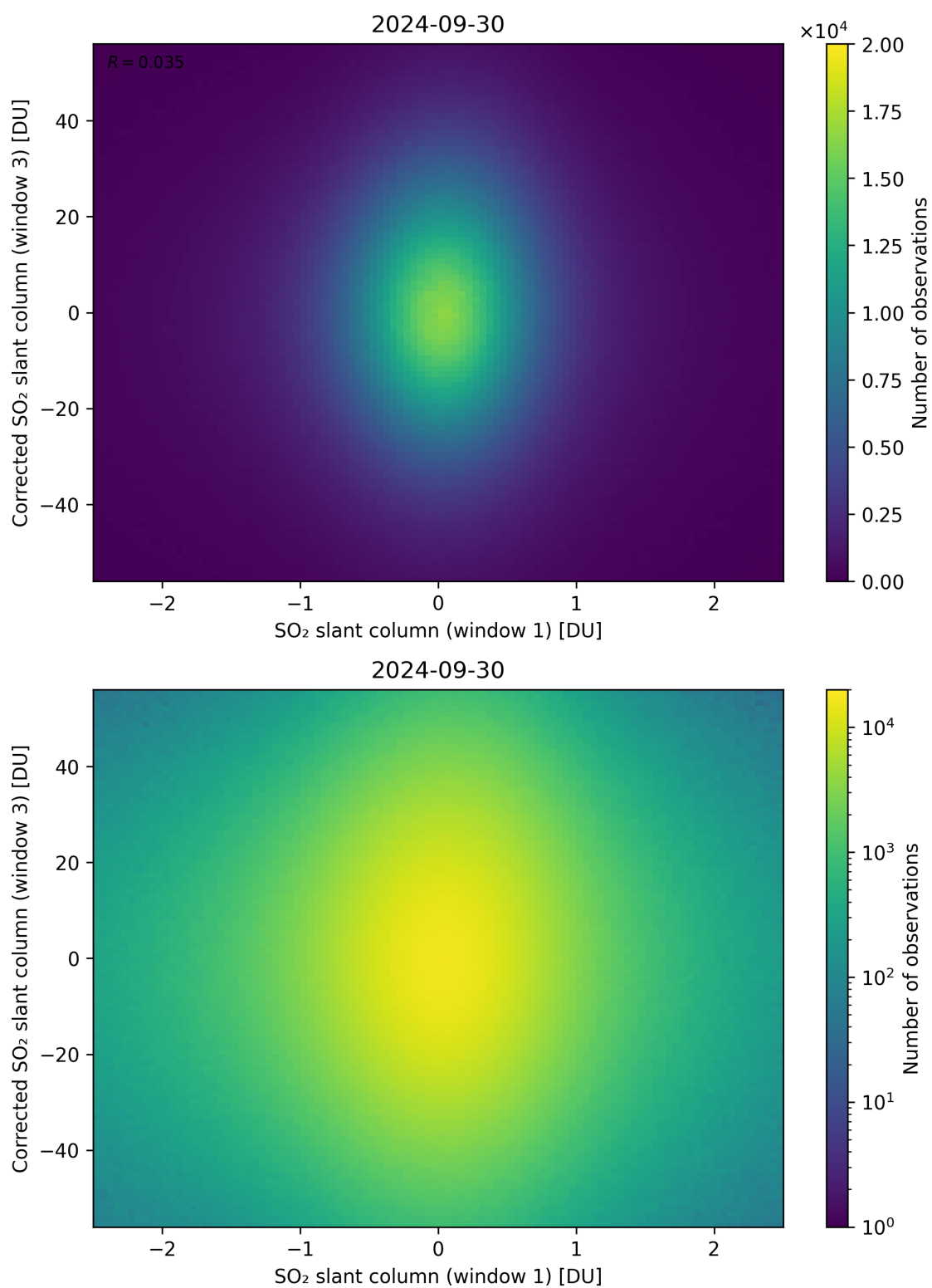
Figure 234: Scatter density plot of “SO 2 slant column (window 1)” against “Corrected SO 2 slant column (window 3)” for 2024-09-29 to 2024-10-01.
