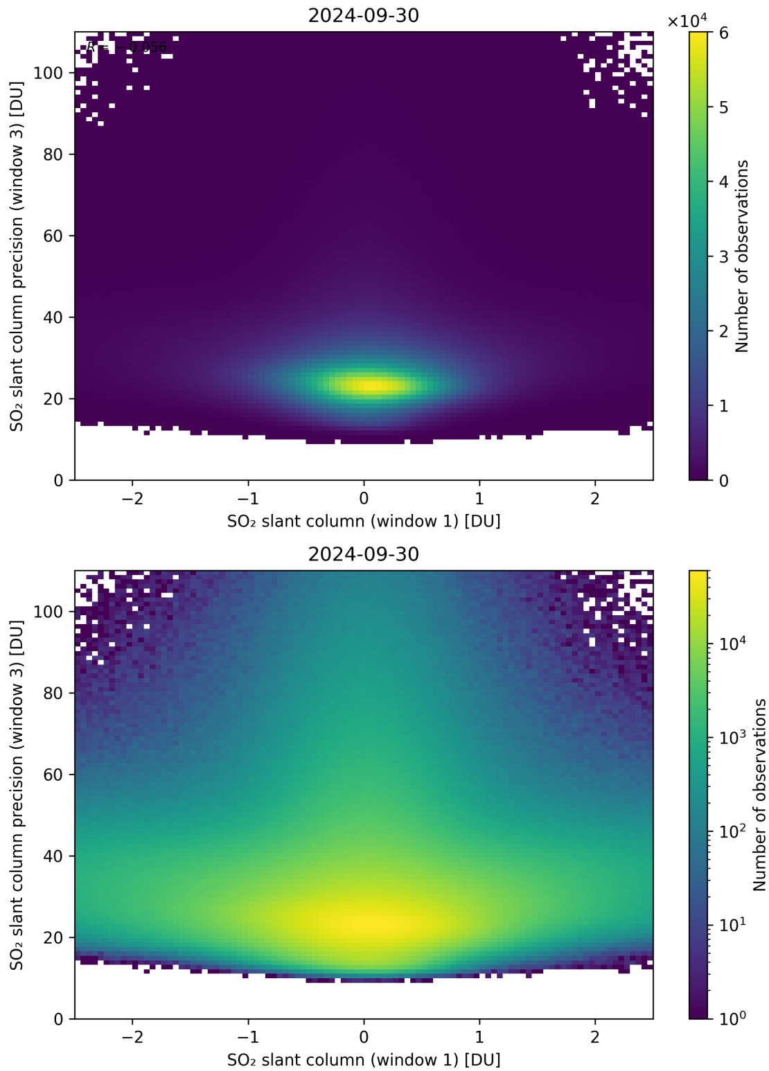
Figure 238: Scatter density plot of “SO 2 slant column (window 1)” against “SO 2 slant column precision (window 3)” for 2024-09-29 to 2024-10-01.
