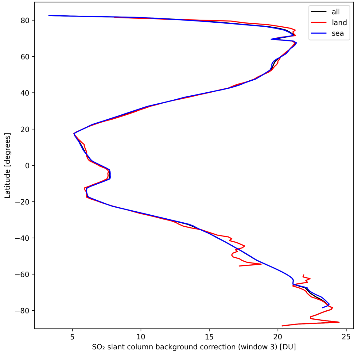
Figure 44: Zonal average of “SO 2 slant column background correction (window 3)” for 2024-09-29 to 2024-10-01.
