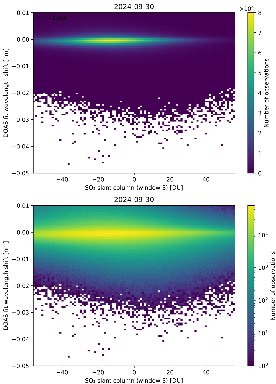
Figure 254: Scatter density plot of “SO 2 slant column (window 3)” against “DOAS fit wavelength shift” for 2024-09-29 to 2024-10-01.
