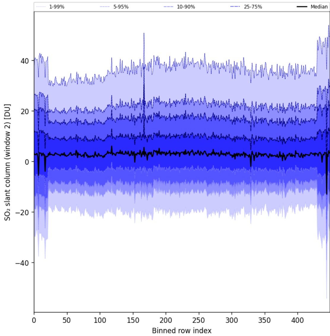
Figure 83: Along track statistics of “SO 2 slant column (window 2)” for 2024-09-29 to 2024-10-01
