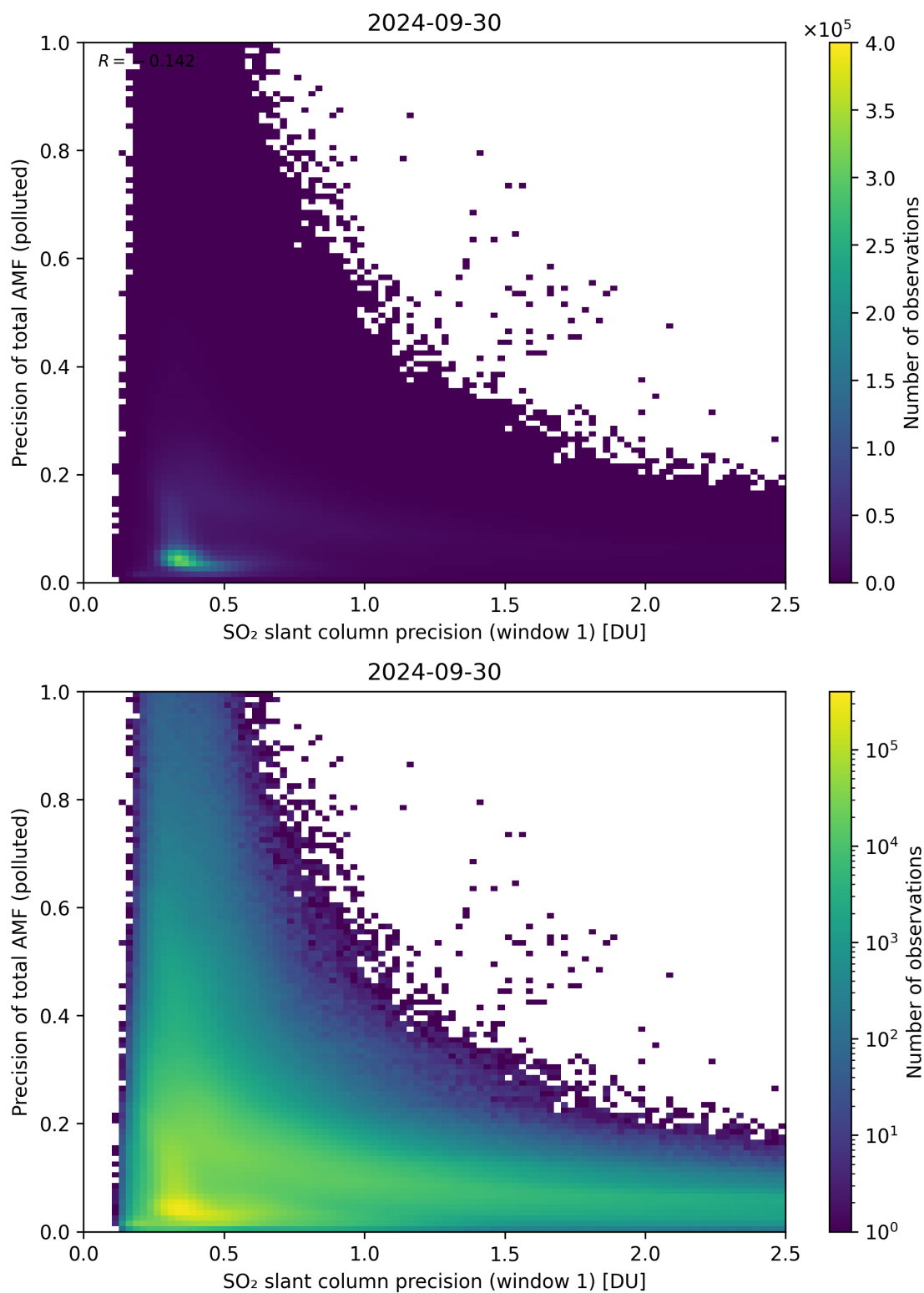
Figure 231: Scatter density plot of “SO 2 slant column precision (window 1)” against “Precision of total AMF (polluted)” for 2024-09-29 to 2024-10-01.
