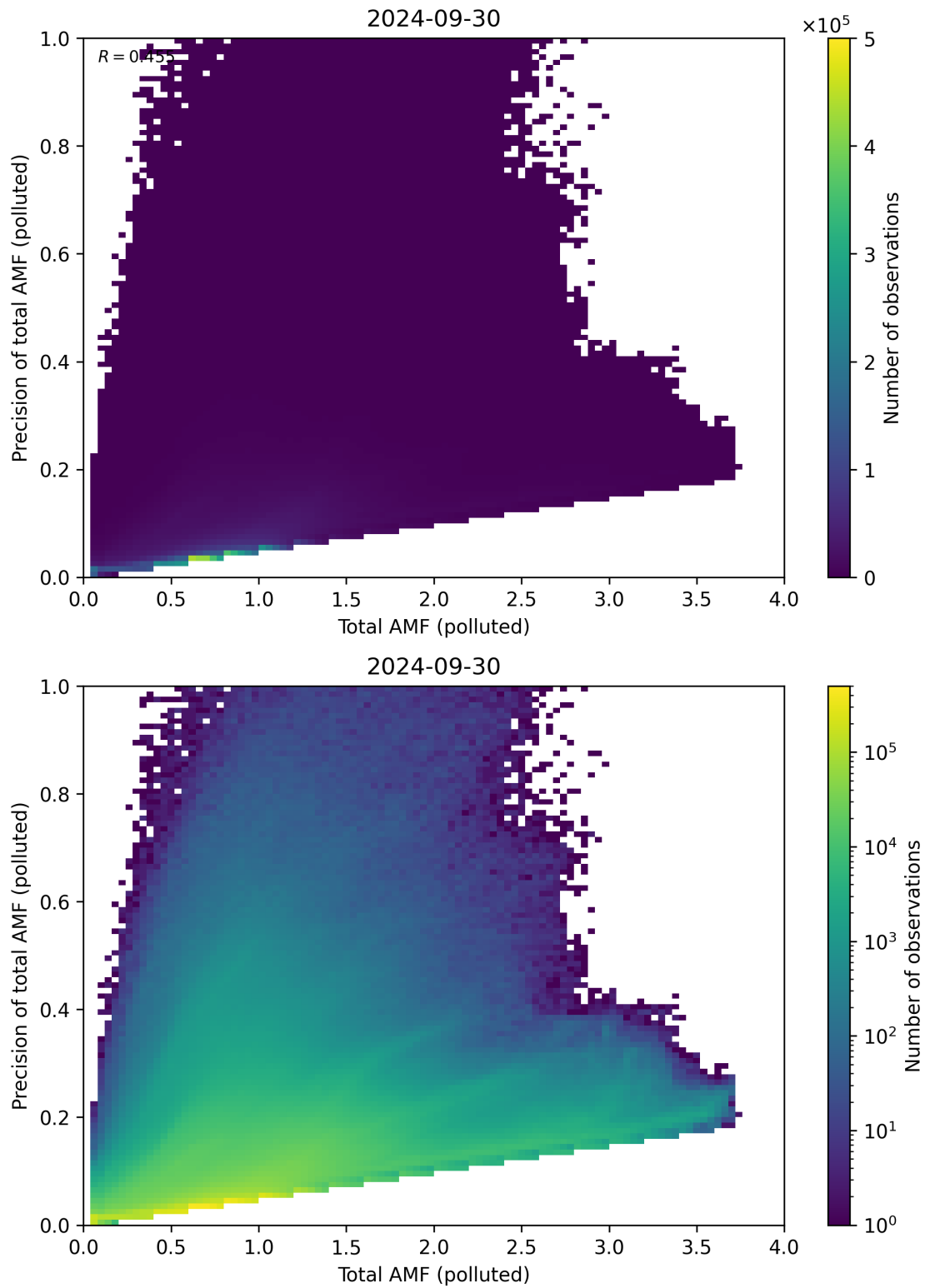
Figure 272: Scatter density plot of “Total AMF (polluted)” against “Precision of total AMF (polluted)” for 2024-09-29 to 2024-10-01.
