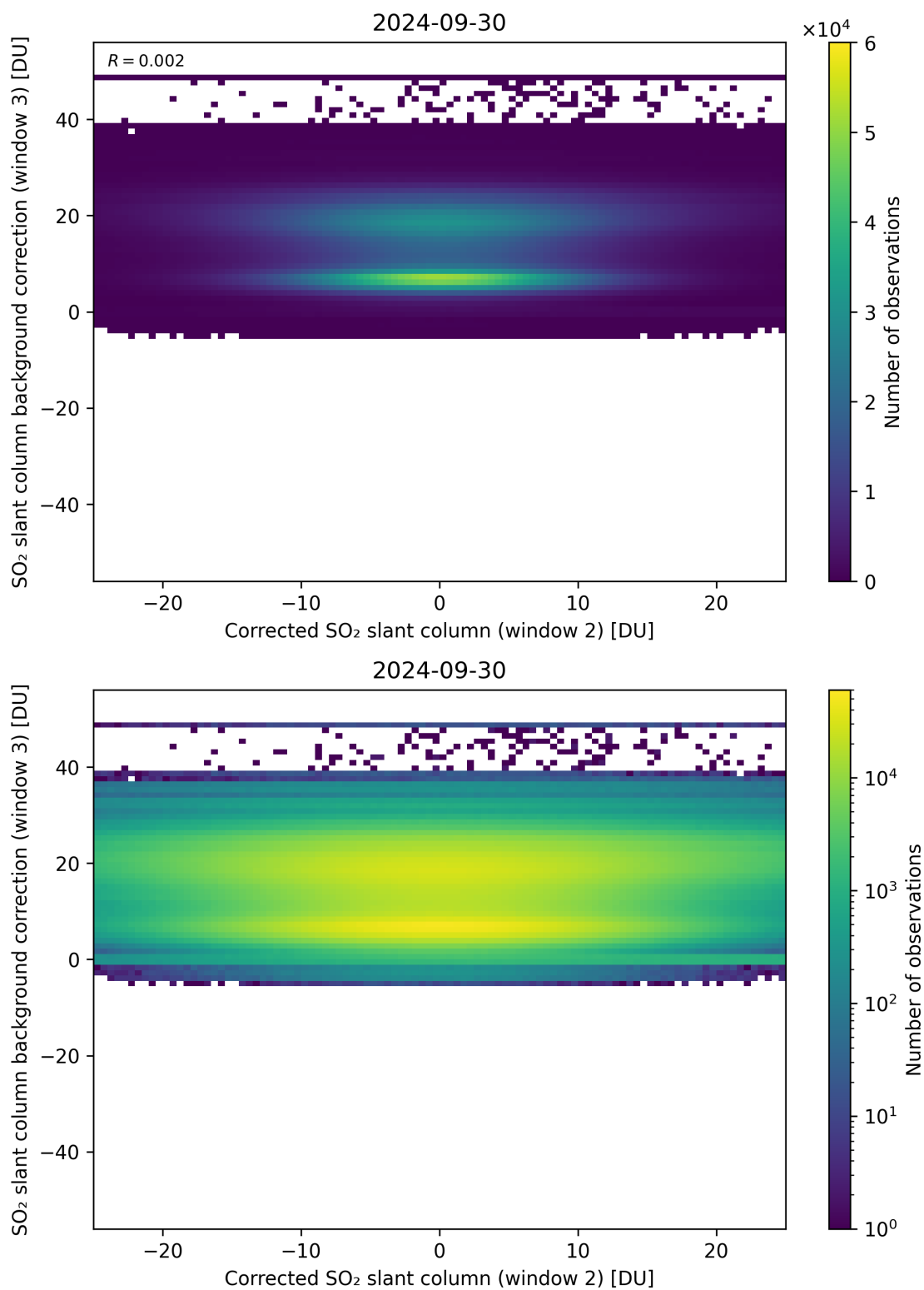
Figure 195: Scatter density plot of “Corrected SO 2 slant column (window 2)” against “SO 2 slant column background correction (window 3)” for 2024-09-29 to 2024-10-01.
