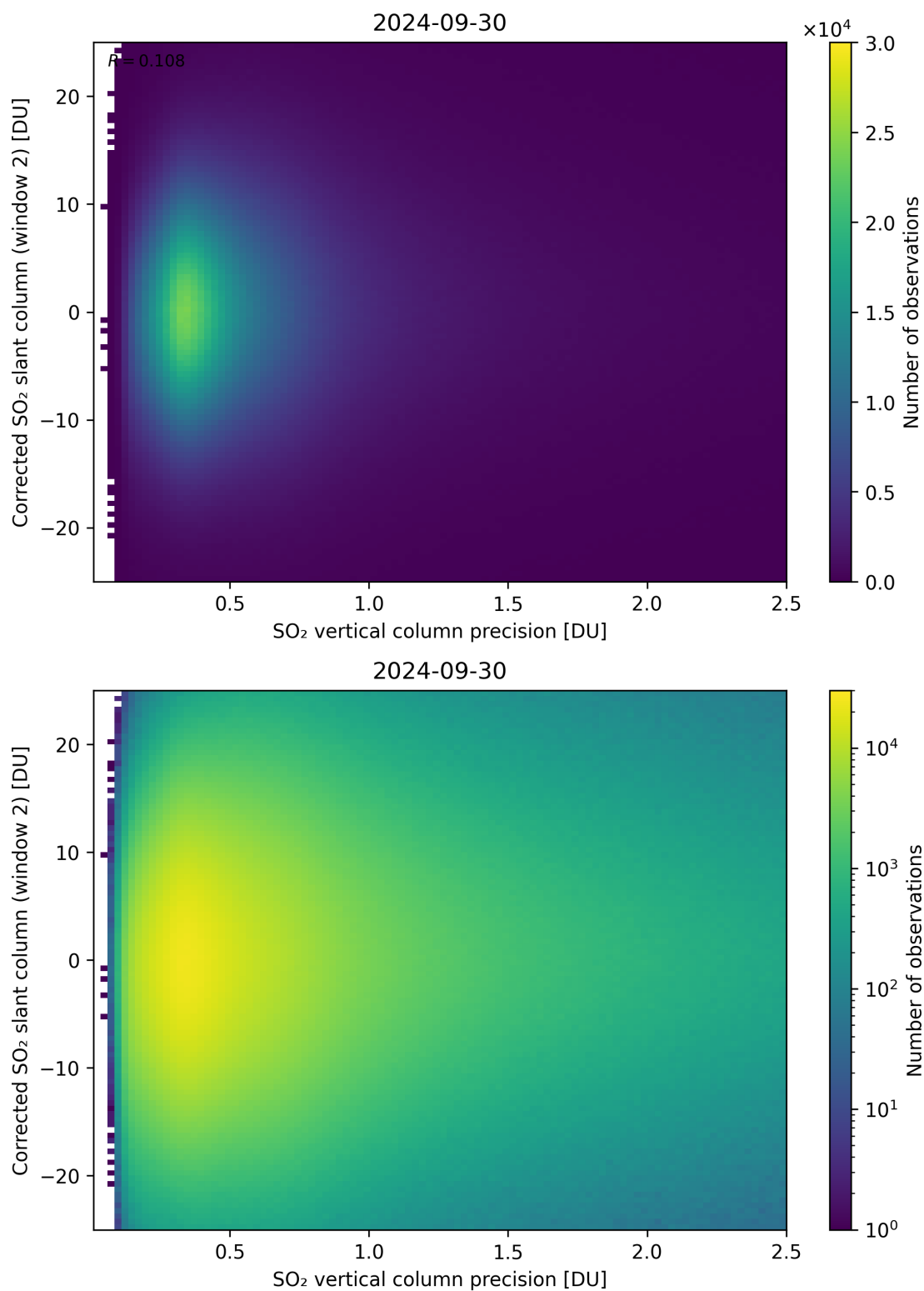
Figure 287: Scatter density plot of “SO 2 vertical column precision” against “Corrected SO 2 slant column (window 2)” for 2024-09-29 to 2024-10-01.
