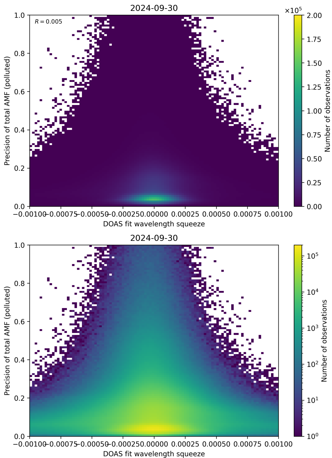
Figure 135: Scatter density plot of “DOAS fit wavelength squeeze” against “Precision of total AMF (polluted)” for 2024-09-29 to 2024-10-01.
