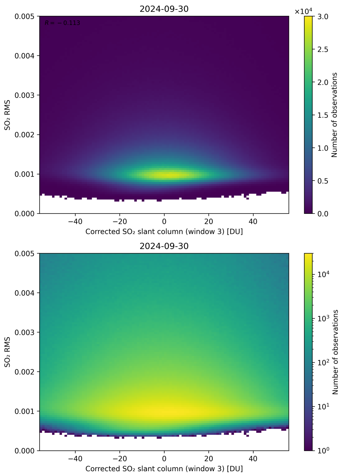
Figure 208: Scatter density plot of “Corrected SO 2 slant column (window 3)” against “SO 2 RMS” for 2024-09-29 to 2024-10-01.
