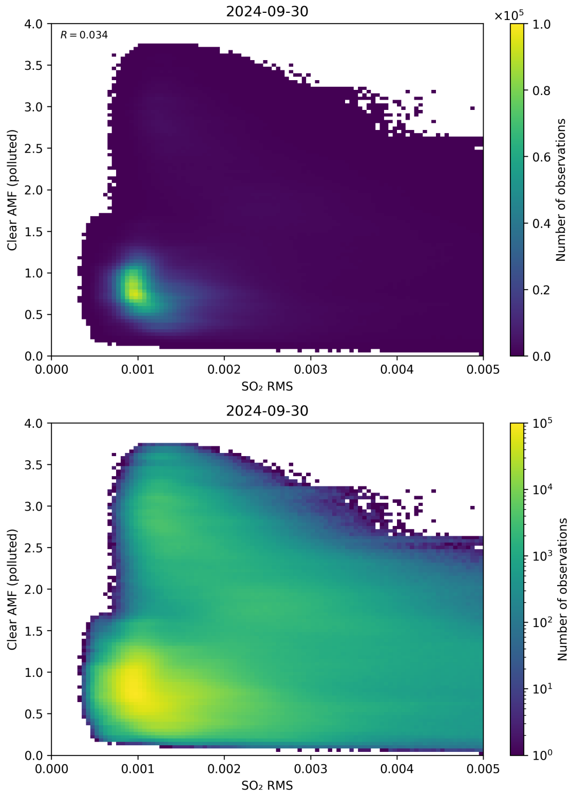
Figure 136: Scatter density plot of “SO 2 RMS” against “Clear AMF (polluted)” for 2024-09-29 to 2024-10-01.
