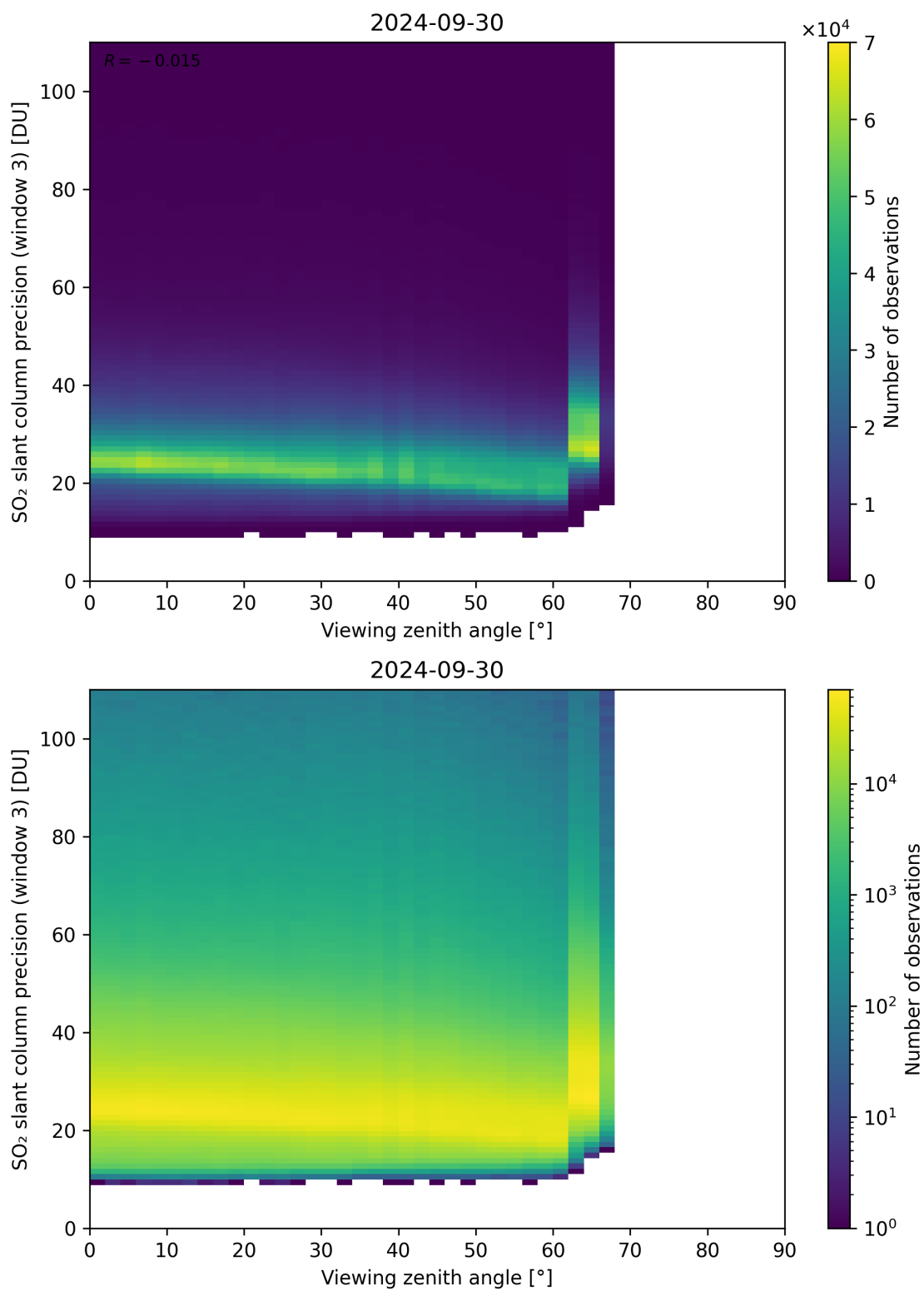
Figure 324: Scatter density plot of “Viewing zenith angle” against “SO 2 slant column precision (window 3)” for 2024-09-29 to 2024-10-01.
