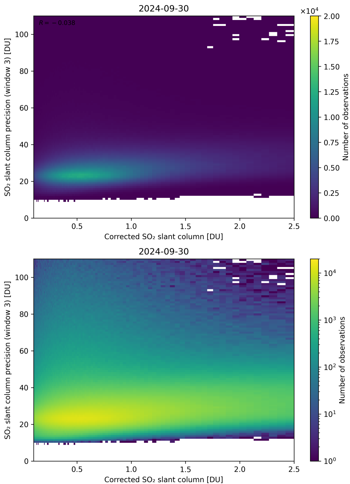
Figure 191: Scatter density plot of “Corrected SO 2 slant column” against “SO 2 slant column precision (window 3)” for 2024-09-29 to 2024-10-01.
