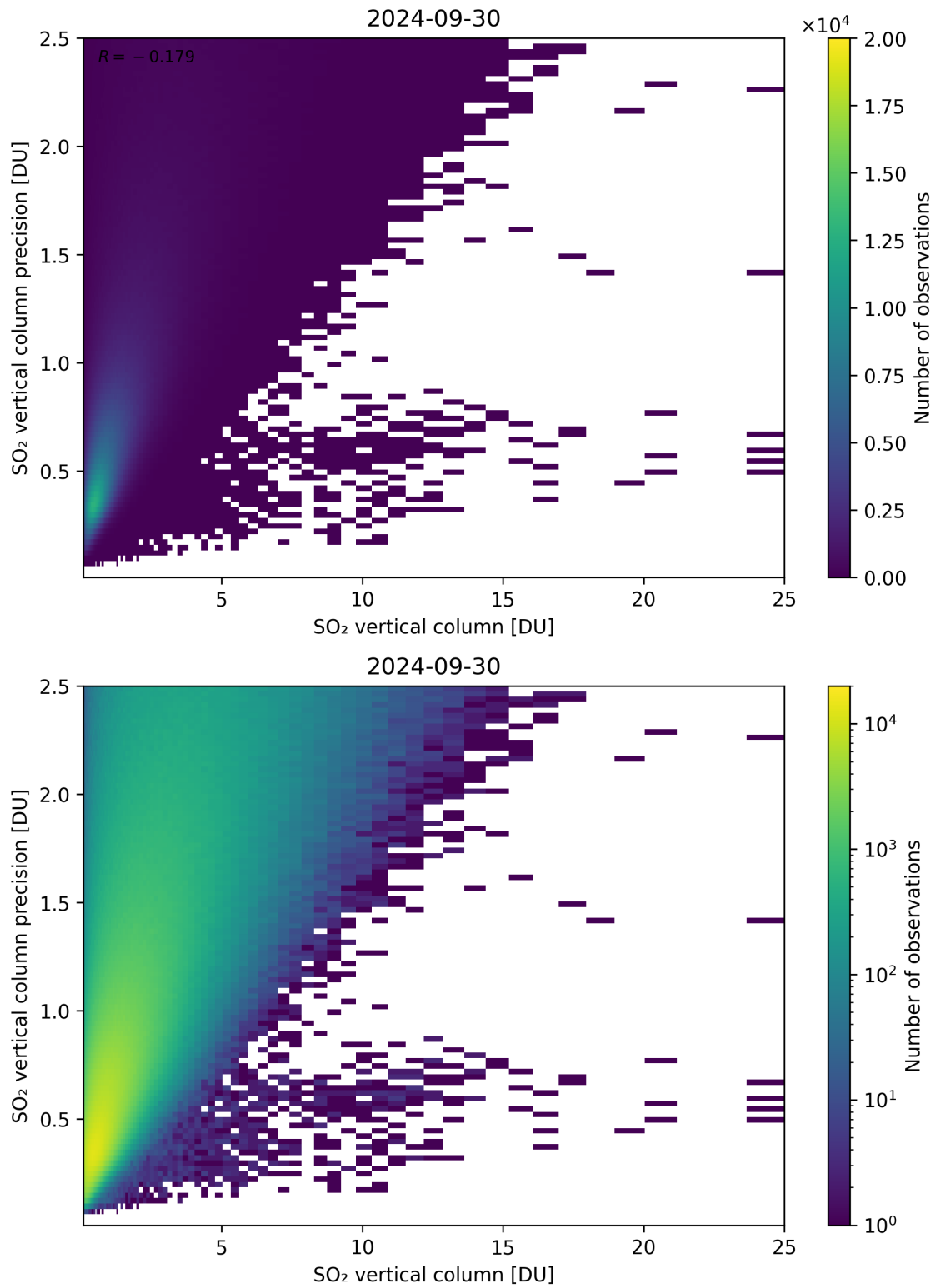
Figure 307: Scatter density plot of “SO 2 vertical column” against “SO 2 vertical column precision” for 2024-09-29 to 2024-10-01.
