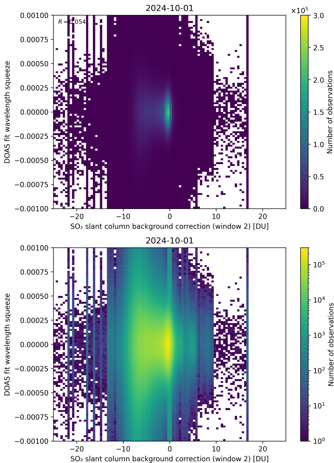
Figure 113: Scatter density plot of “SO 2 slant column background correction (window 2)” against “DOAS fit wavelength squeeze” for 2024-09-30 to 2024-10-02.
