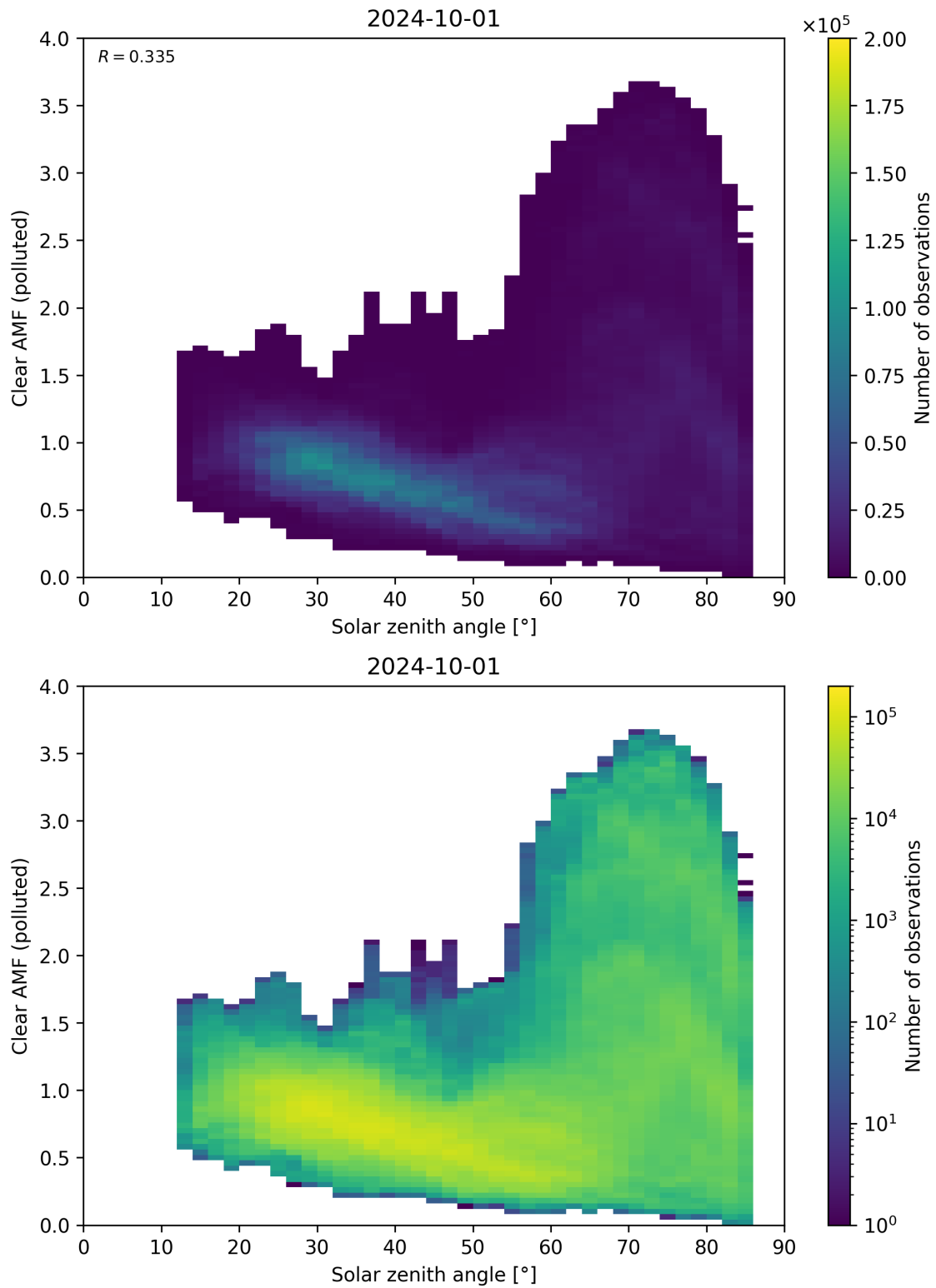
Figure 165: Scatter density plot of “Solar zenith angle” against “Clear AMF (polluted)” for 2024-09-30 to 2024-10-02.
