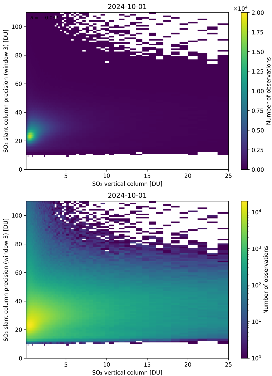
Figure 304: Scatter density plot of “SO 2 vertical column” against “SO 2 slant column precision (window 3)” for 2024-09-30 to 2024-10-02.
