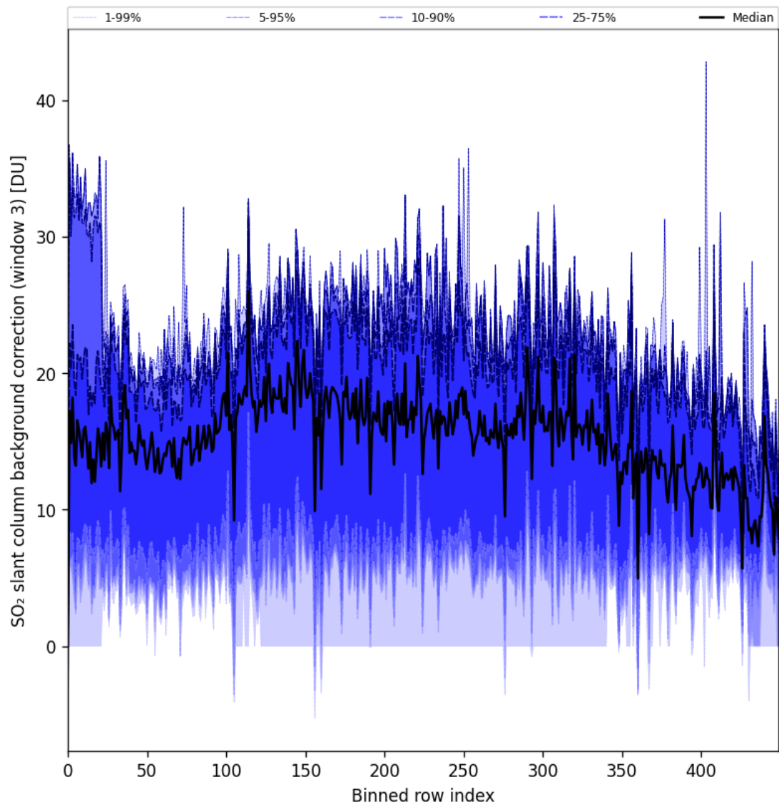
Figure 90: Along track statistics of “SO 2 slant column background correction (window 3)” for 2024-09-30 to 2024-10-02
