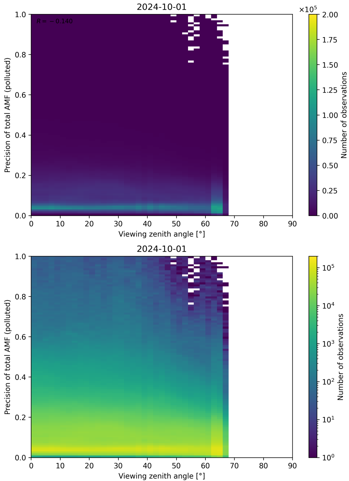
Figure 326: Scatter density plot of “Viewing zenith angle” against “Precision of total AMF (polluted)” for 2024-09-30 to 2024-10-02.
