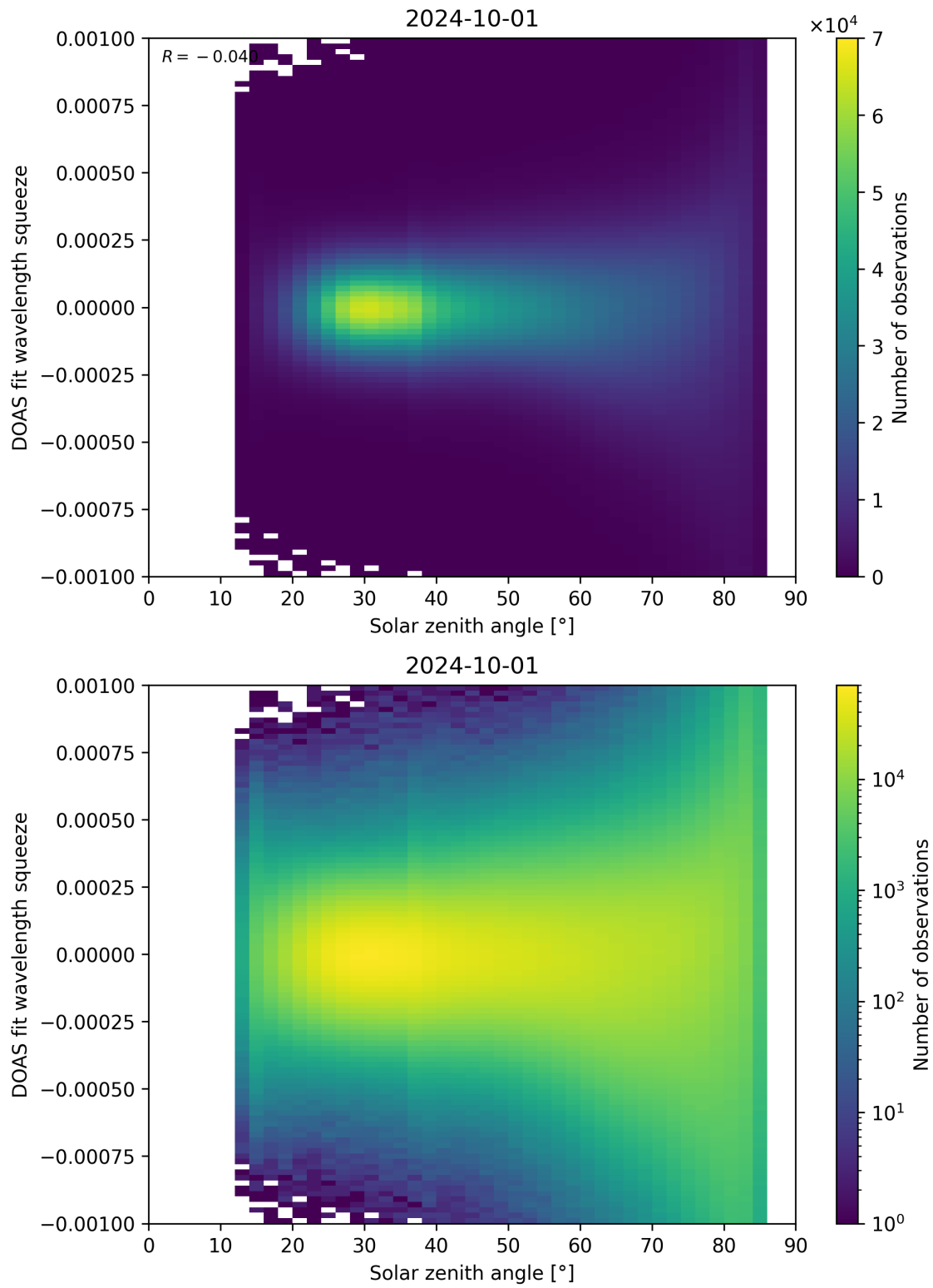
Figure 162: Scatter density plot of “Solar zenith angle” against “DOAS fit wavelength squeeze” for 2024-09-30 to 2024-10-02.
