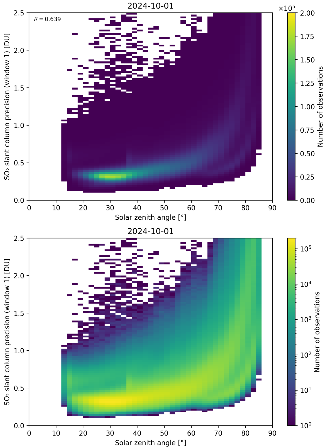
Figure 170: Scatter density plot of “Solar zenith angle” against “SO 2 slant column precision (window 1)” for 2024-09-30 to 2024-10-02.
