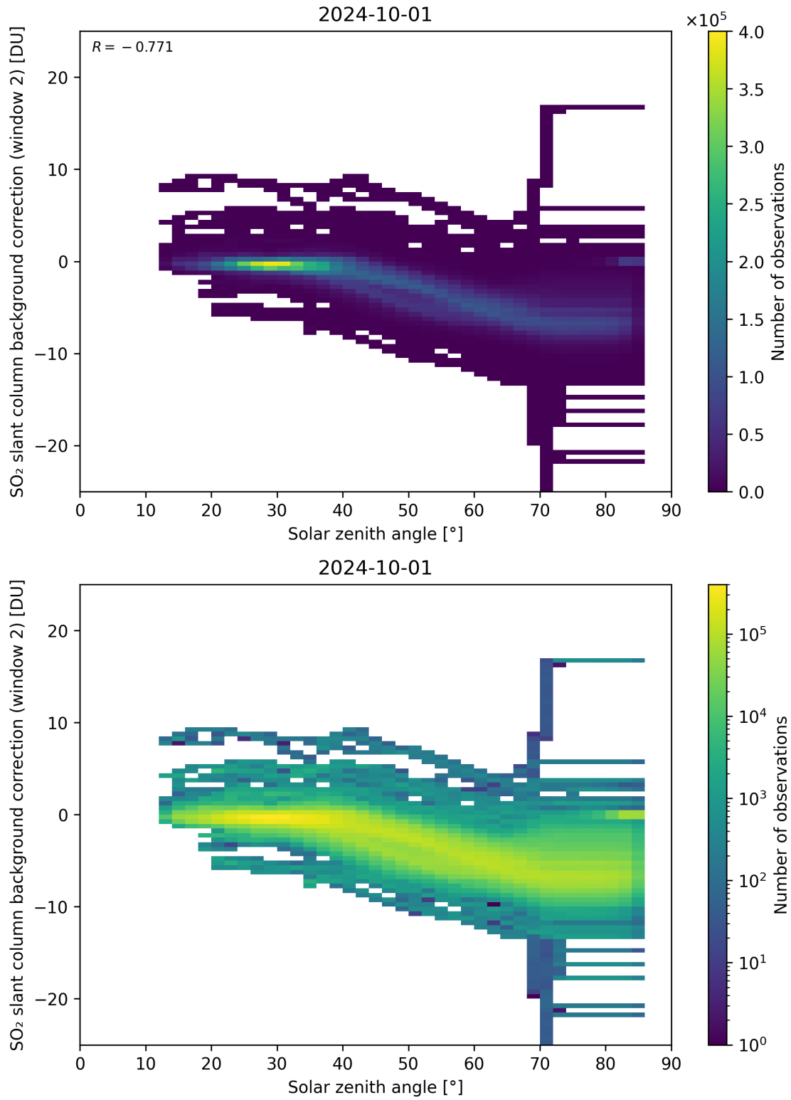
Figure 159: Scatter density plot of “Solar zenith angle” against “SO 2 slant column background correction (window 2)” for 2024-09-30 to 2024-10-02.
