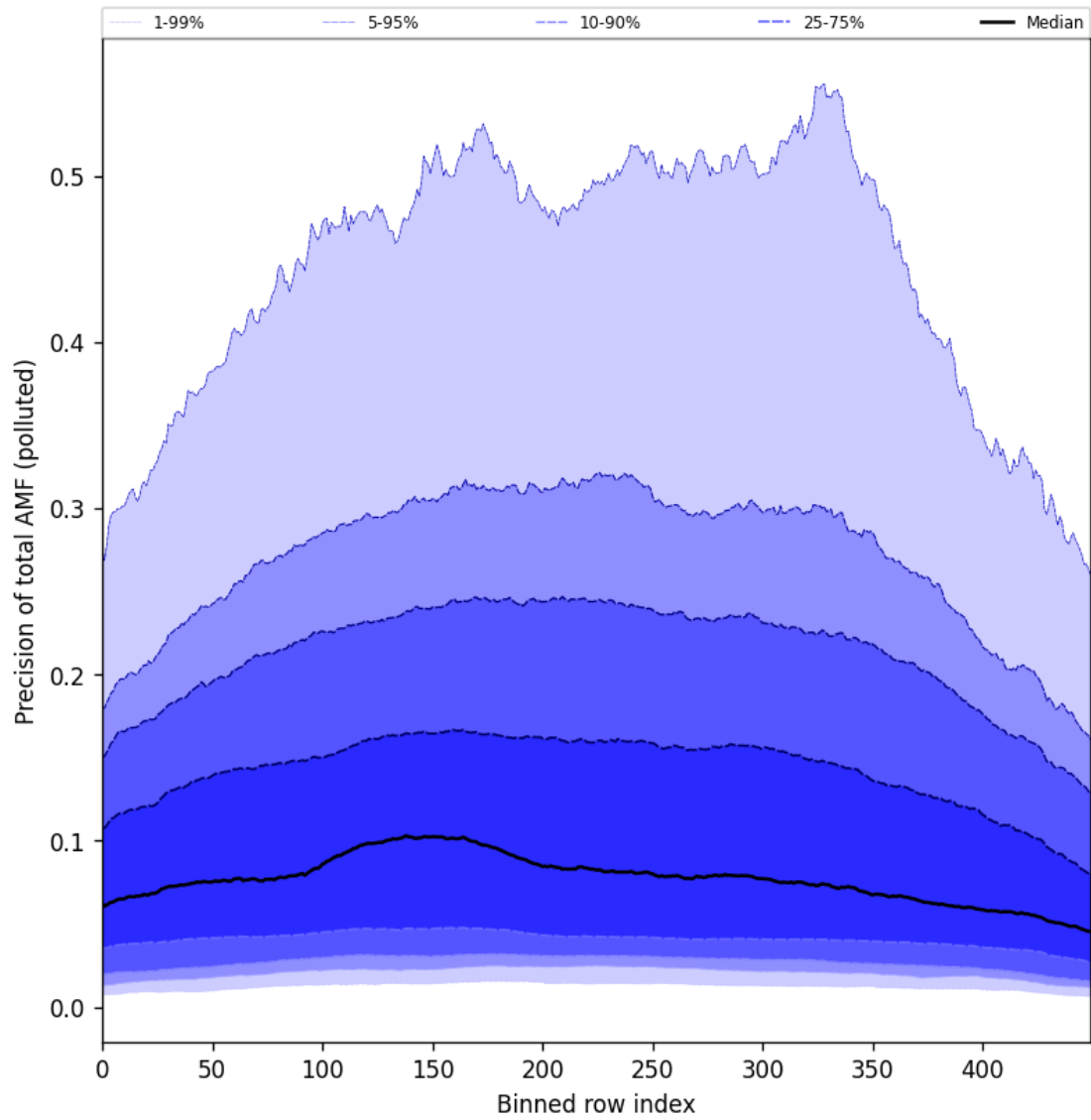
Figure 95: Along track statistics of “Precision of total AMF (polluted)” for 2024-09-30 to 2024-10-02
