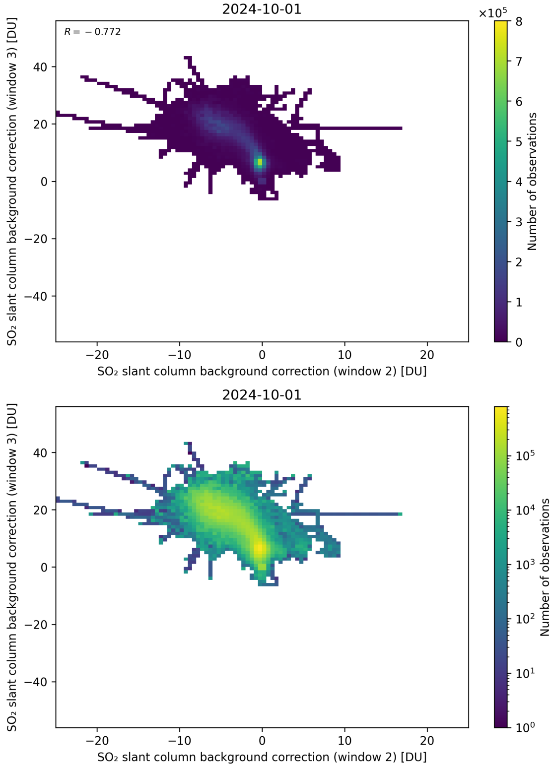
Figure 111: Scatter density plot of “SO 2 slant column background correction (window 2)” against “SO 2 slant column background correction (window 3)” for 2024-09-30 to 2024-10-02.
