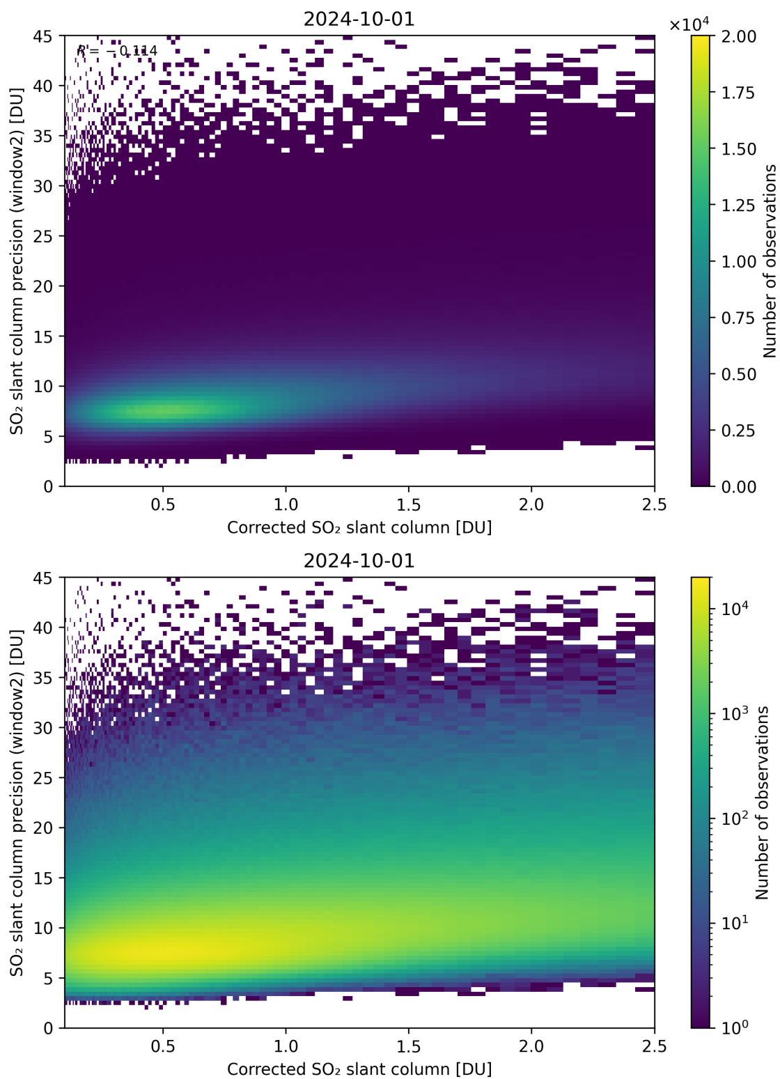
Figure 189: Scatter density plot of “Corrected SO 2 slant column” against “SO 2 slant column precision (window2)” for 2024-09-30 to 2024-10-02.
