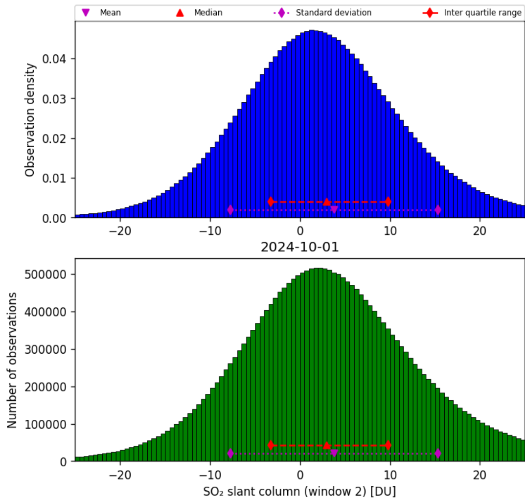
Figure 60: Histogram of “SO 2 slant column (window 2)” for 2024-09-30 to 2024-10-02
