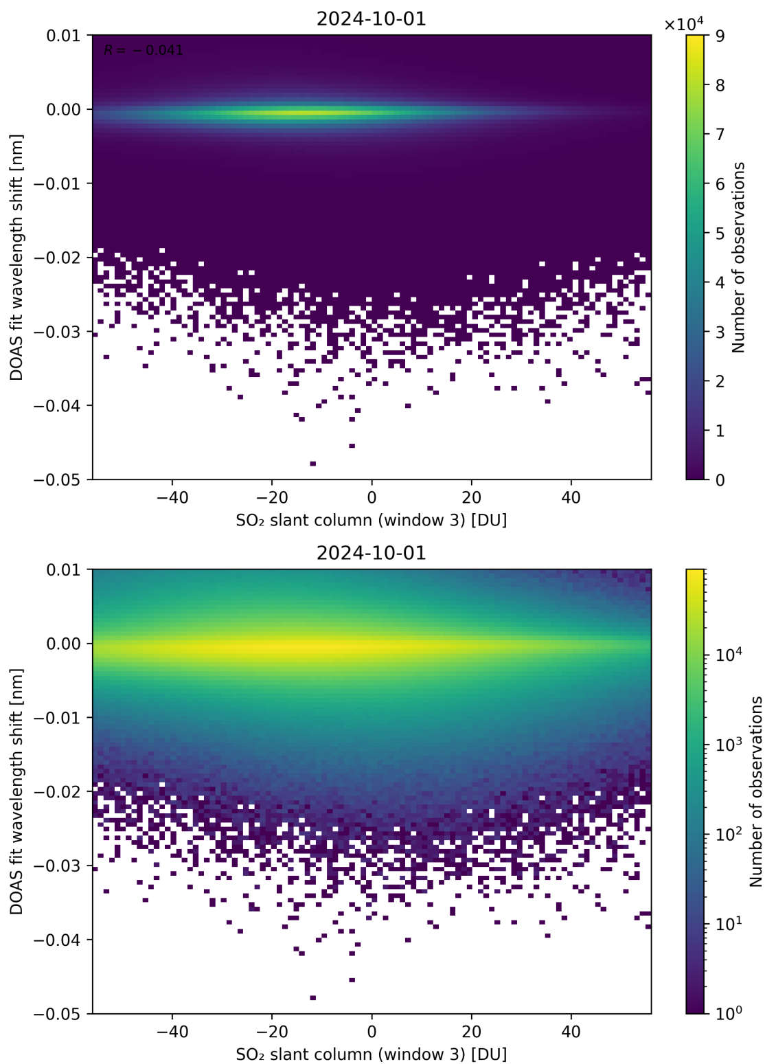
Figure 254: Scatter density plot of “SO 2 slant column (window 3)” against “DOAS fit wavelength shift” for 2024-09-30 to 2024-10-02.
