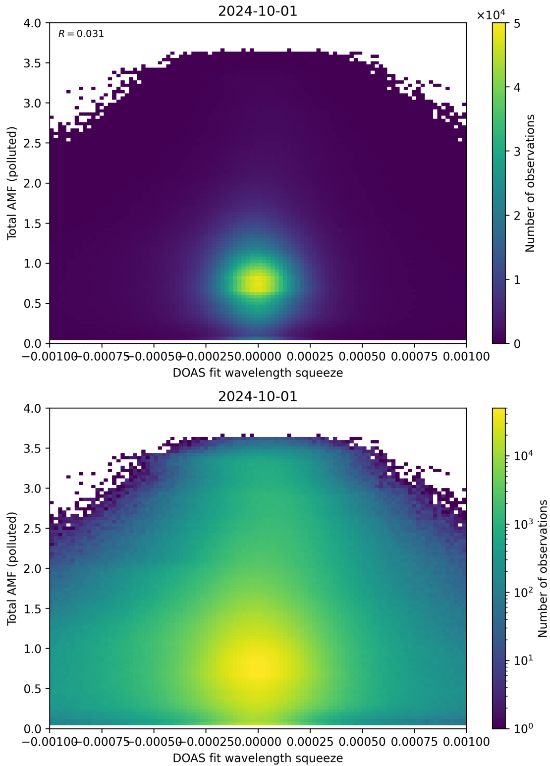
Figure 134: Scatter density plot of “DOAS fit wavelength squeeze” against “Total AMF (polluted)” for 2024-09-30 to 2024-10-02.
