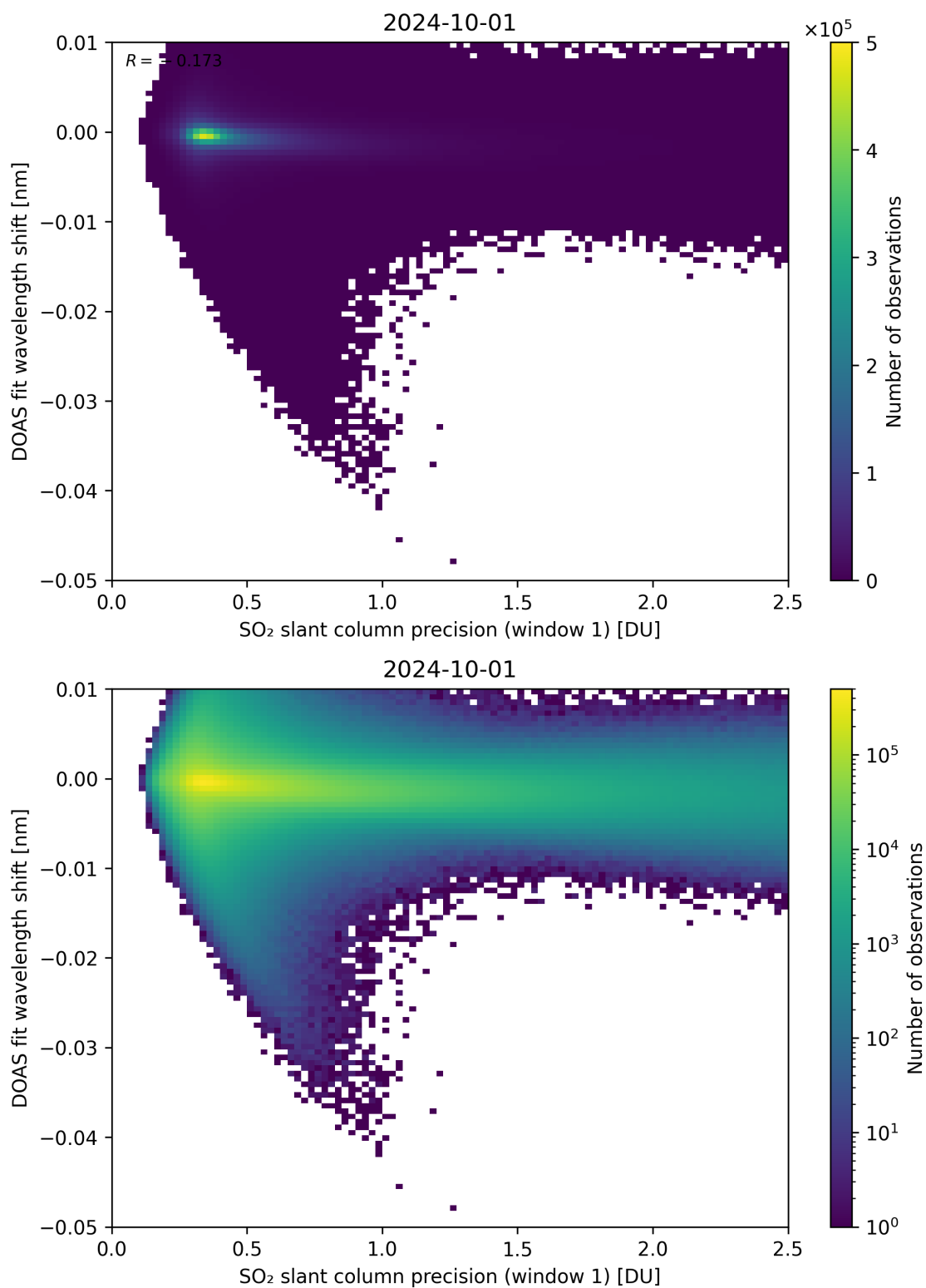
Figure 221: Scatter density plot of “SO 2 slant column precision (window 1)” against “DOAS fit wavelength shift” for 2024-09-30 to 2024-10-02.
