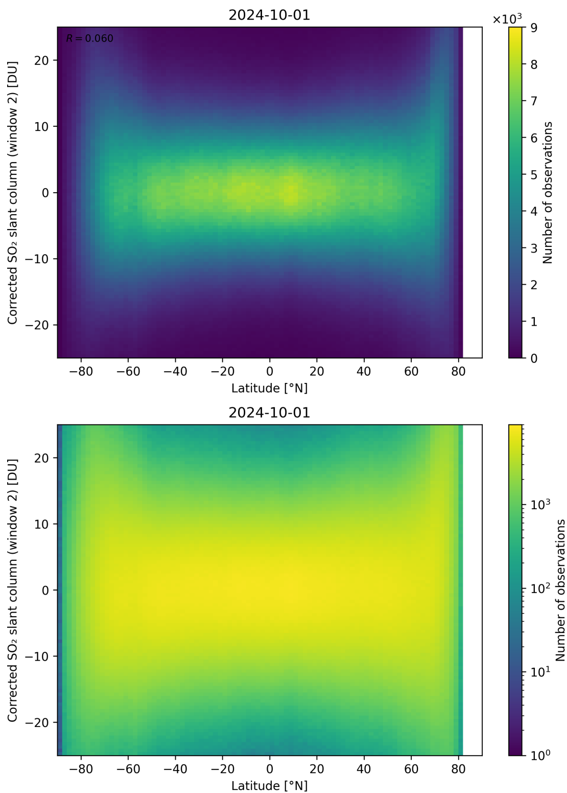
Figure 147: Scatter density plot of “Latitude” against “Corrected SO 2 slant column (window 2)” for 2024-09-30 to 2024-10-02.
