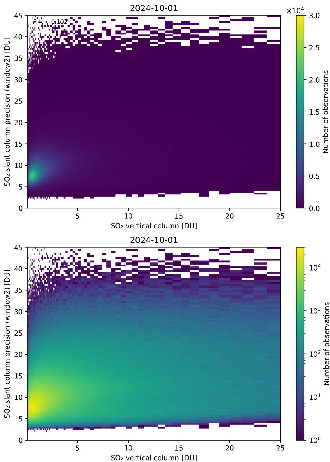
Figure 302: Scatter density plot of “SO 2 vertical column” against “SO 2 slant column precision (window2)” for 2024-09-30 to 2024-10-02.
