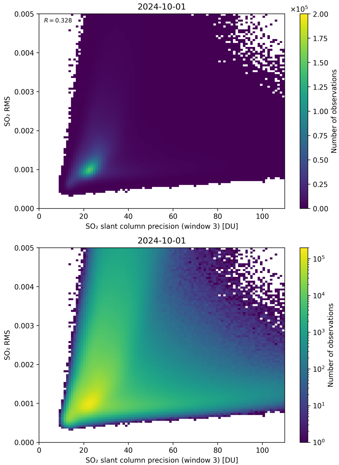
Figure 260: Scatter density plot of “SO 2 slant column precision (window 3)” against “SO 2 RMS” for 2024-09-30 to 2024-10-02.
