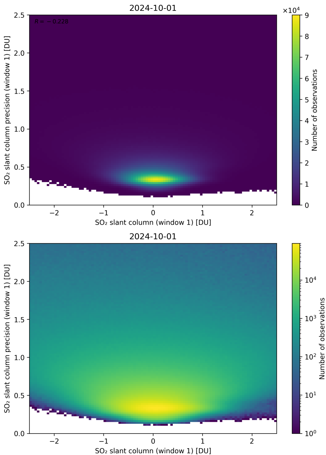
Figure 235: Scatter density plot of “SO 2 slant column (window 1)” against “SO 2 slant column precision (window 1)” for 2024-09-30 to 2024-10-02.
