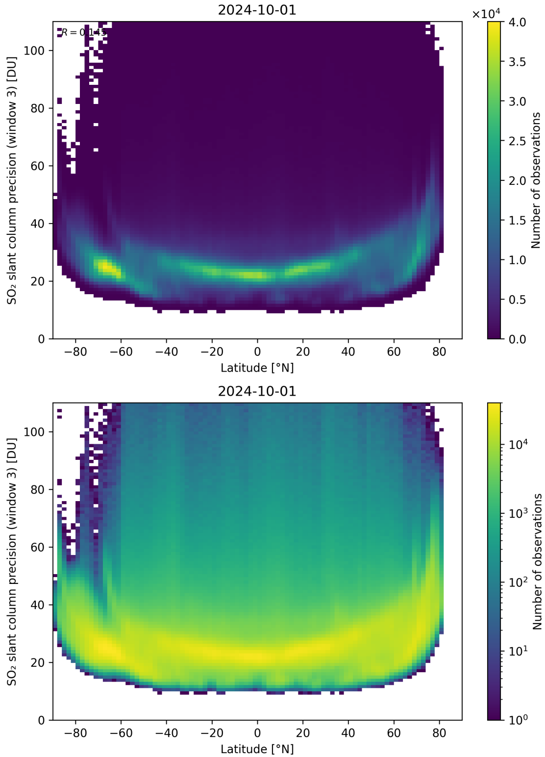
Figure 153: Scatter density plot of “Latitude” against “SO 2 slant column precision (window 3)” for 2024-09-30 to 2024-10-02.
