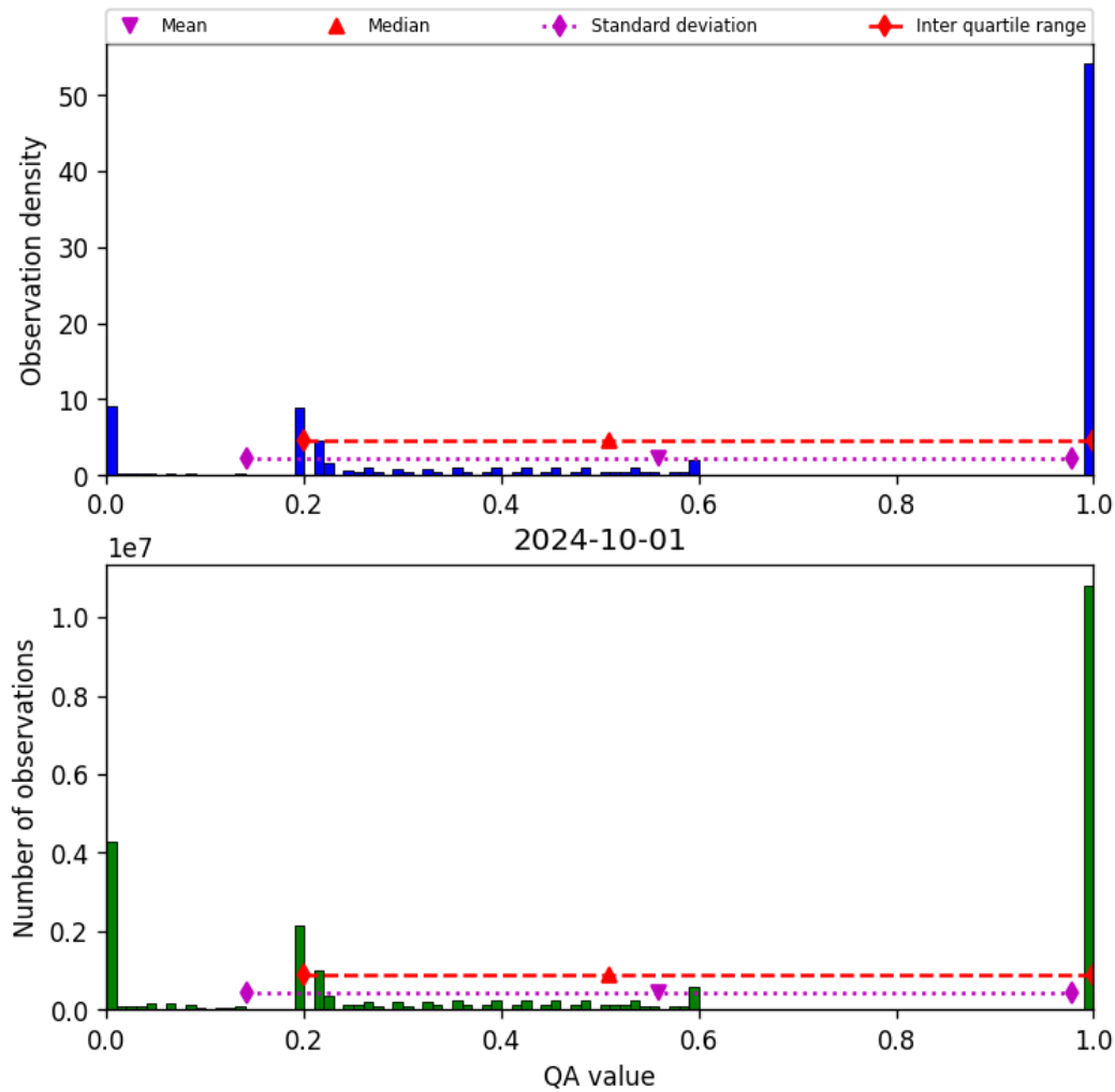
Figure 52: Histogram of “QA value” for 2024-09-30 to 2024-10-02
