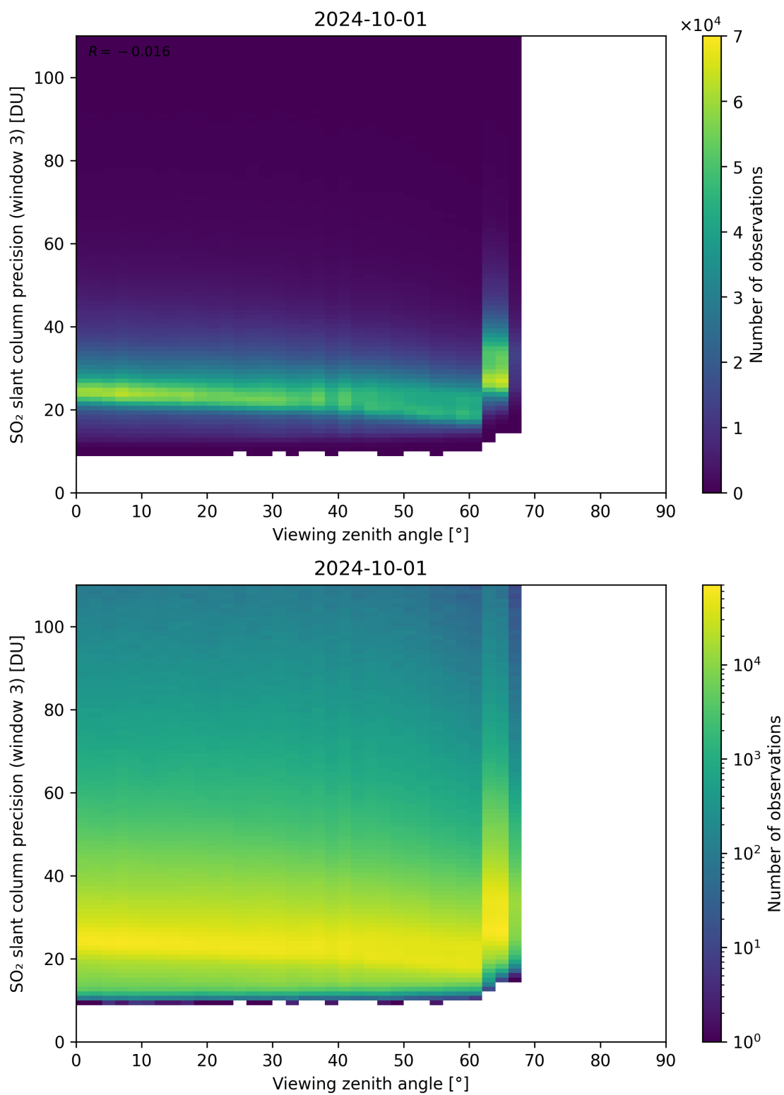
Figure 324: Scatter density plot of “Viewing zenith angle” against “SO 2 slant column precision (window 3)” for 2024-09-30 to 2024-10-02.
