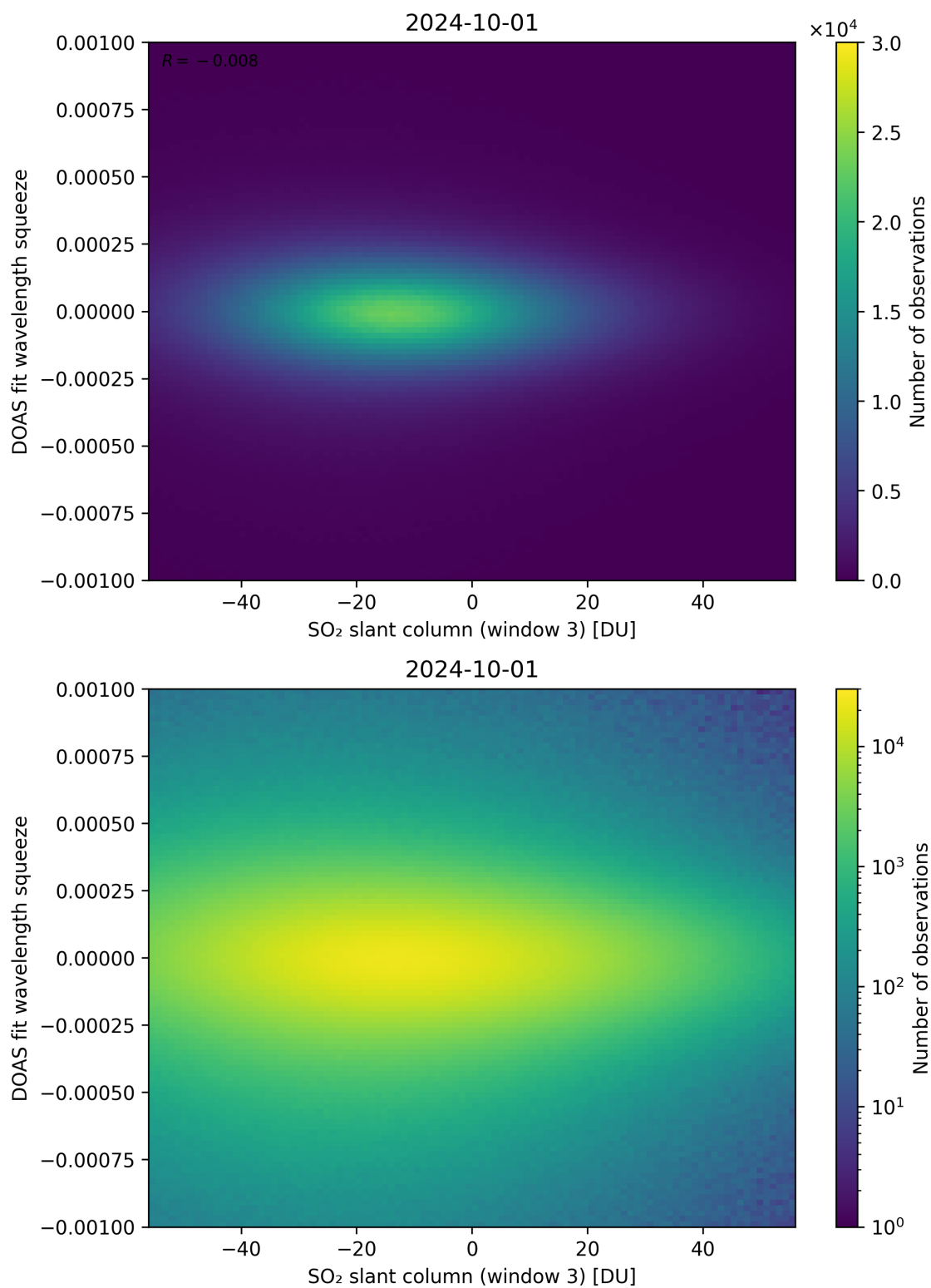
Figure 255: Scatter density plot of “SO 2 slant column (window 3)” against “DOAS fit wavelength squeeze” for 2024-09-30 to 2024-10-02.
