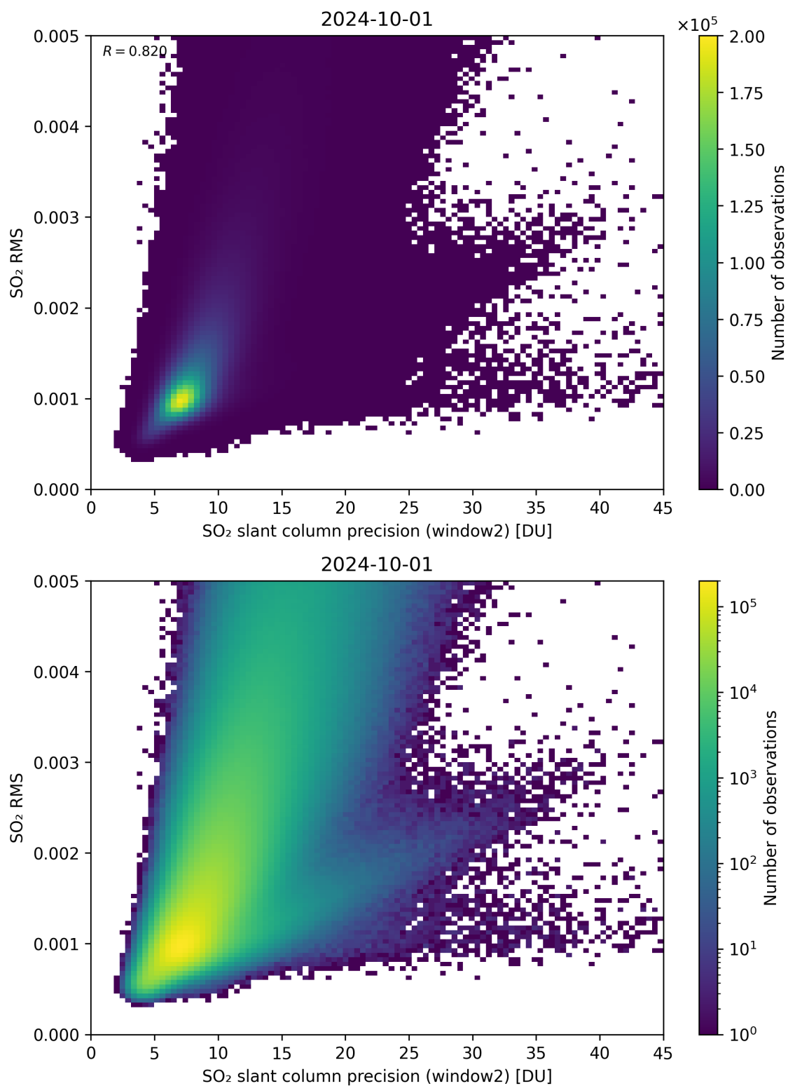
Figure 245: Scatter density plot of “SO 2 slant column precision (window2)” against “SO 2 RMS” for 2024-09-30 to 2024-10-02.
