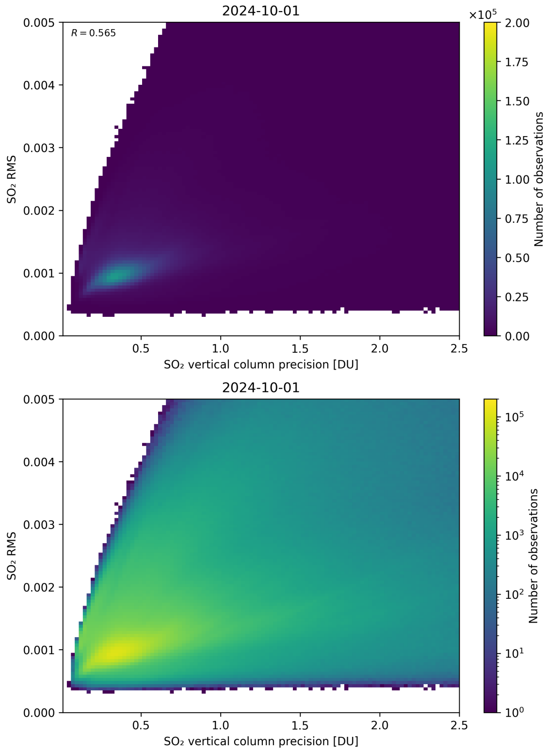
Figure 284: Scatter density plot of “SO 2 vertical column precision” against “SO 2 RMS” for 2024-09-30 to 2024-10-02.
