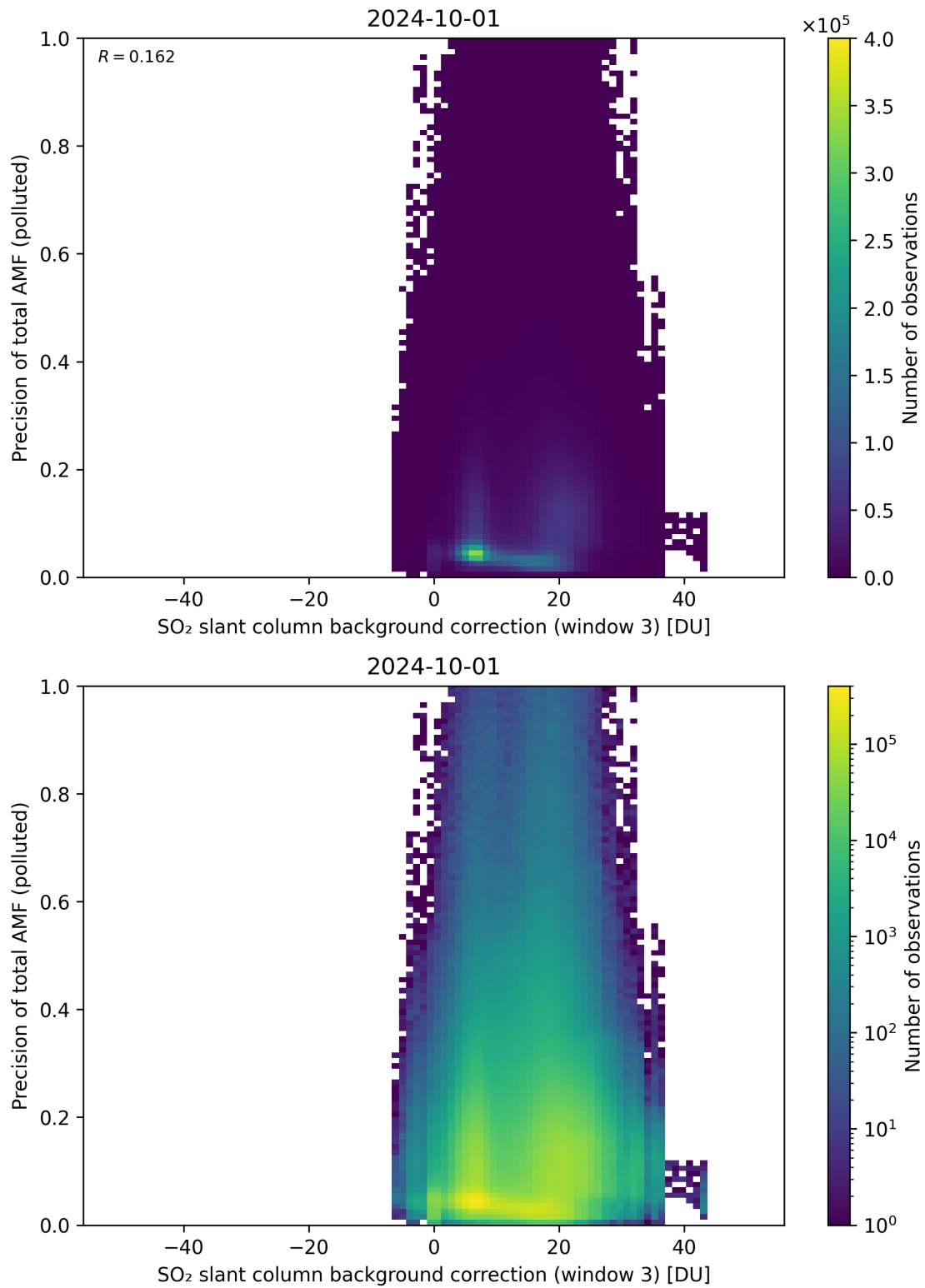
Figure 126: Scatter density plot of “SO 2 slant column background correction (window 3)” against “Precision of total AMF (polluted)” for 2024-09-30 to 2024-10-02.
