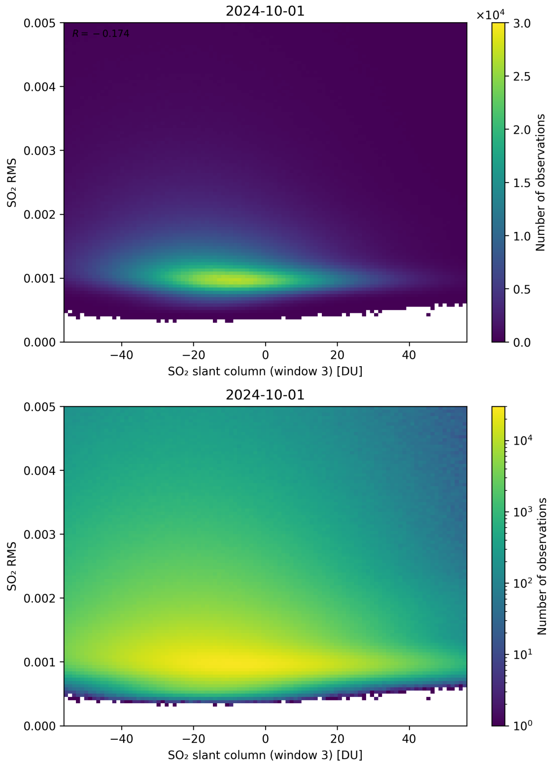
Figure 256: Scatter density plot of “SO 2 slant column (window 3)” against “SO 2 RMS” for 2024-09-30 to 2024-10-02.
