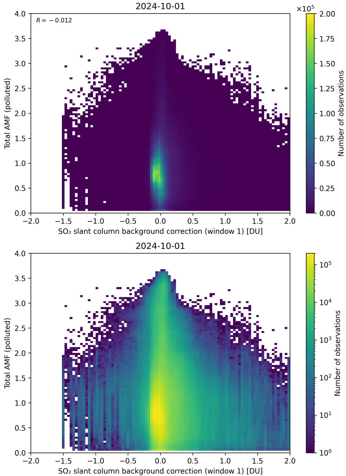
Figure 109: Scatter density plot of “SO 2 slant column background correction (window 1)” against “Total AMF (polluted)” for 2024-09-30 to 2024-10-02.
