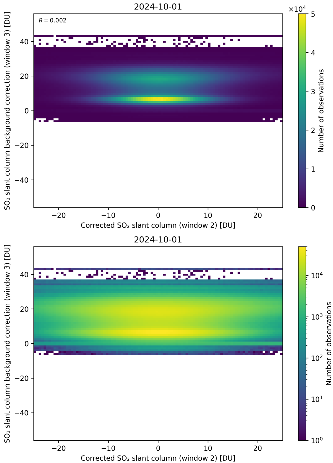
Figure 195: Scatter density plot of “Corrected SO 2 slant column (window 2)” against “SO 2 slant column background correction (window 3)” for 2024-09-30 to 2024-10-02.
