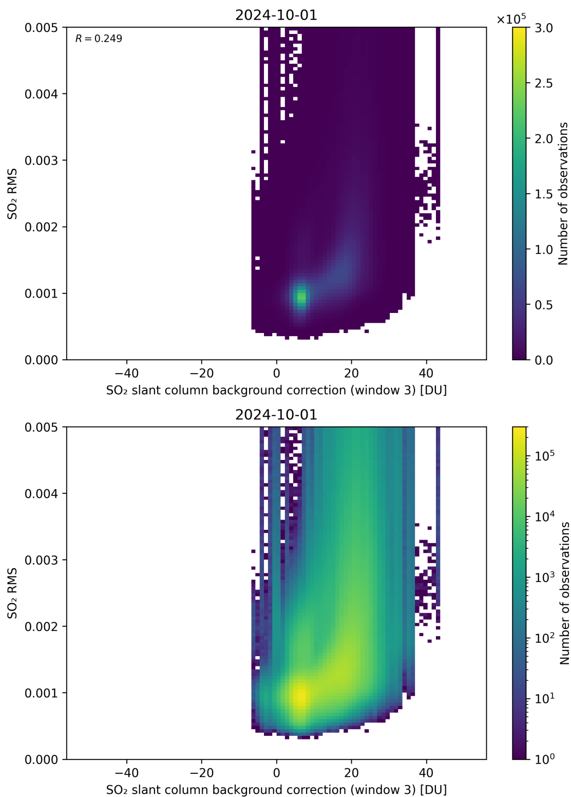
Figure 123: Scatter density plot of “SO 2 slant column background correction (window 3)” against “SO 2 RMS” for 2024-09-30 to 2024-10-02.
