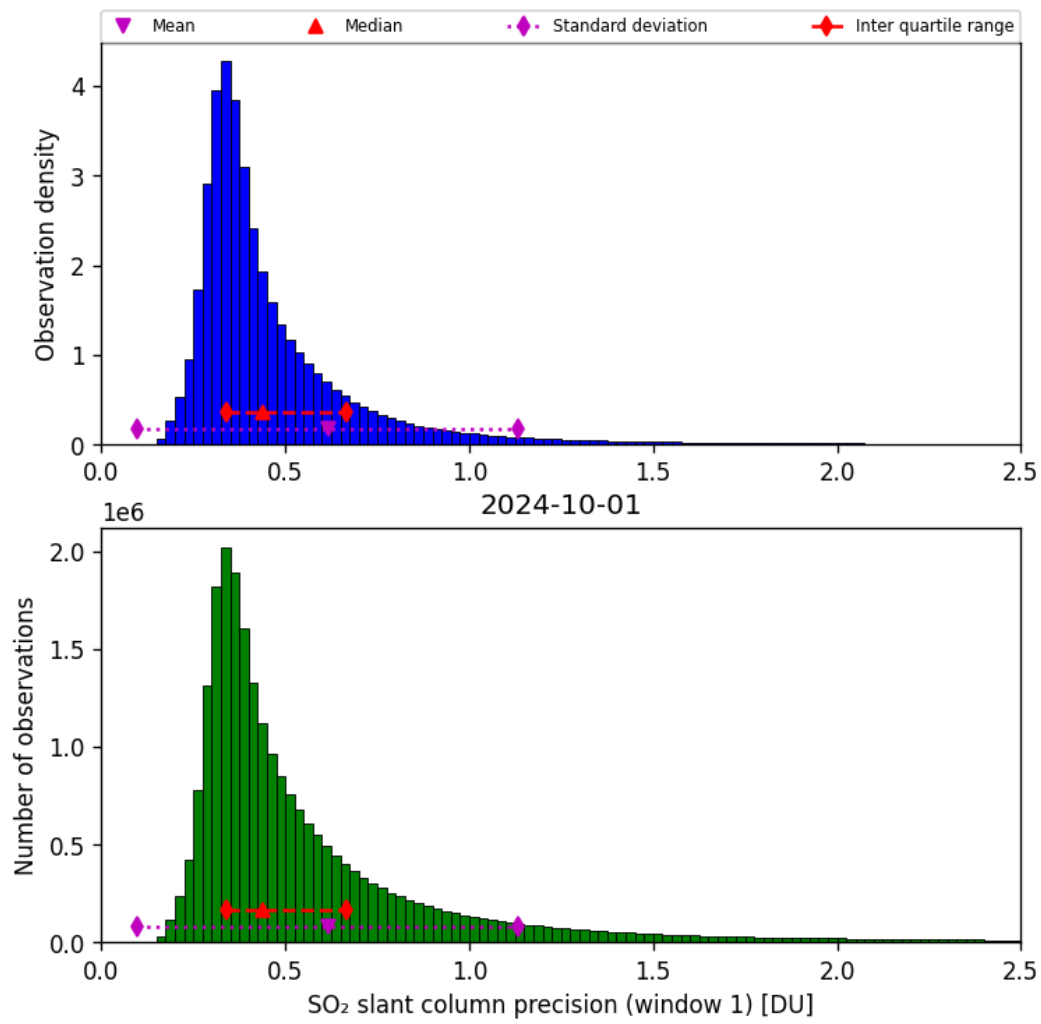
Figure 57: Histogram of “SO 2 slant column precision (window 1)” for 2024-09-30 to 2024-10-02
