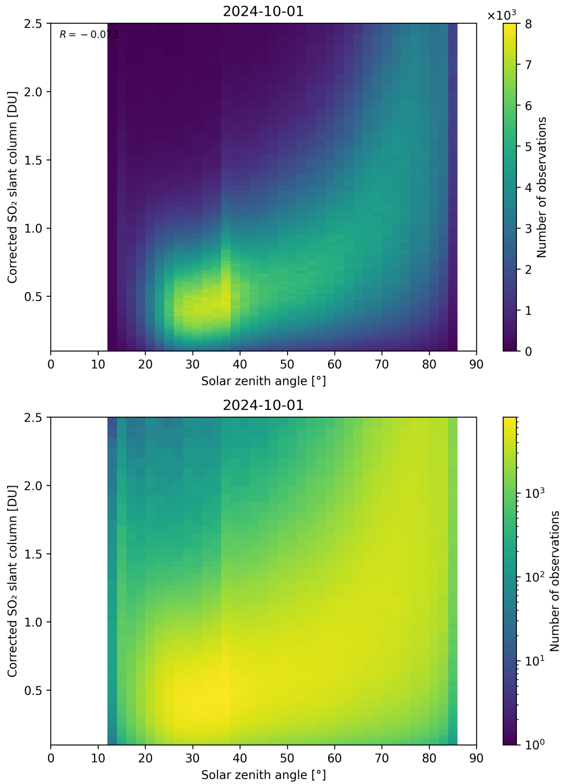
Figure 166: Scatter density plot of “Solar zenith angle” against “Corrected SO 2 slant column” for 2024-09-30 to 2024-10-02.
