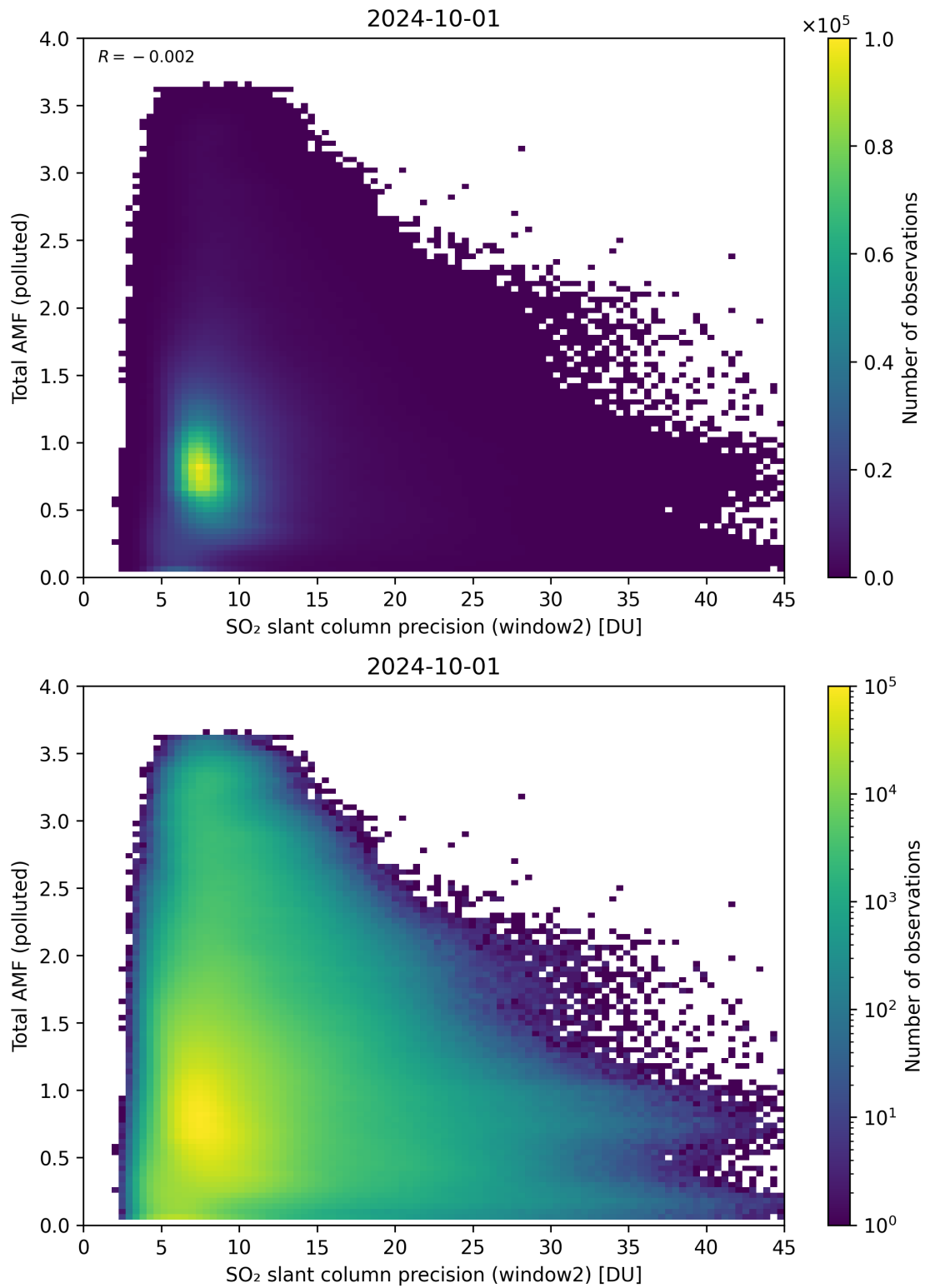
Figure 251: Scatter density plot of “SO 2 slant column precision (window2)” against “Total AMF (polluted)” for 2024-09-30 to 2024-10-02.
