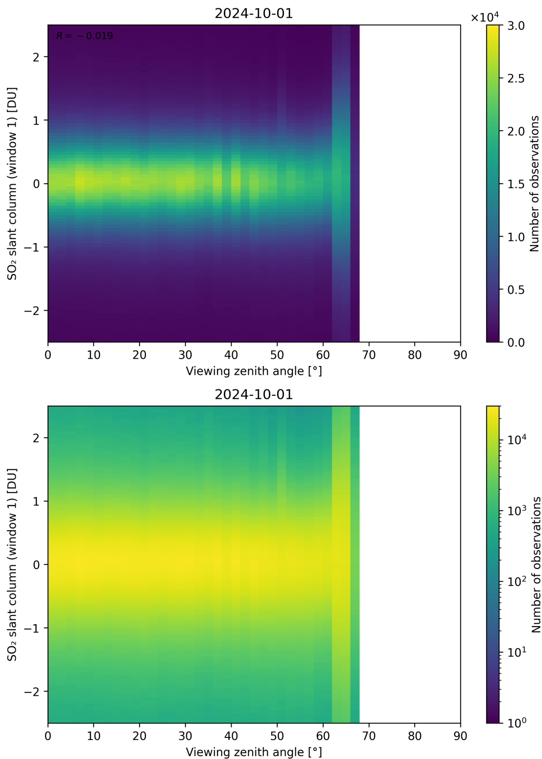
Figure 320: Scatter density plot of “Viewing zenith angle” against “SO 2 slant column (window 1)” for 2024-09-30 to 2024-10-02.
