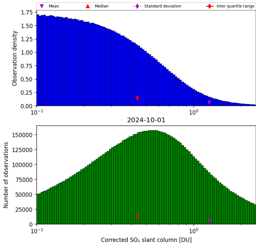
Figure 55: Histogram of “Corrected SO 2 slant column” for 2024-09-30 to 2024-10-02
