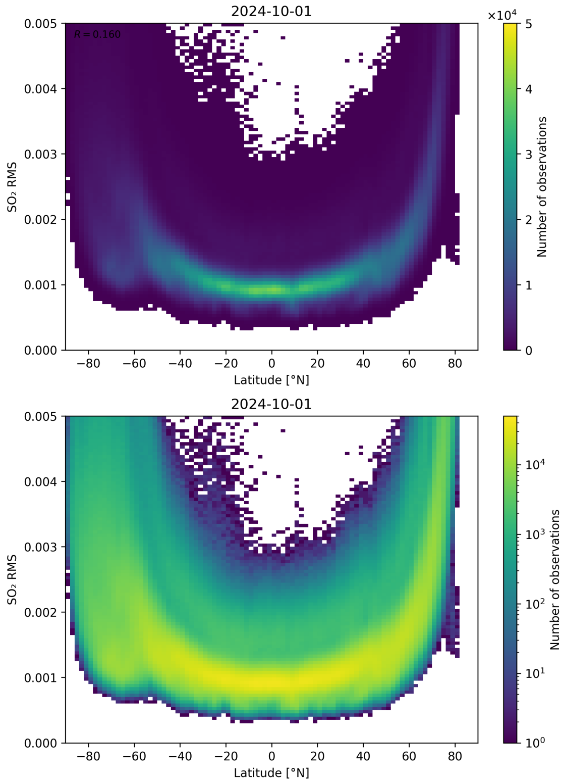
Figure 144: Scatter density plot of “Latitude” against “SO 2 RMS” for 2024-09-30 to 2024-10-02.
