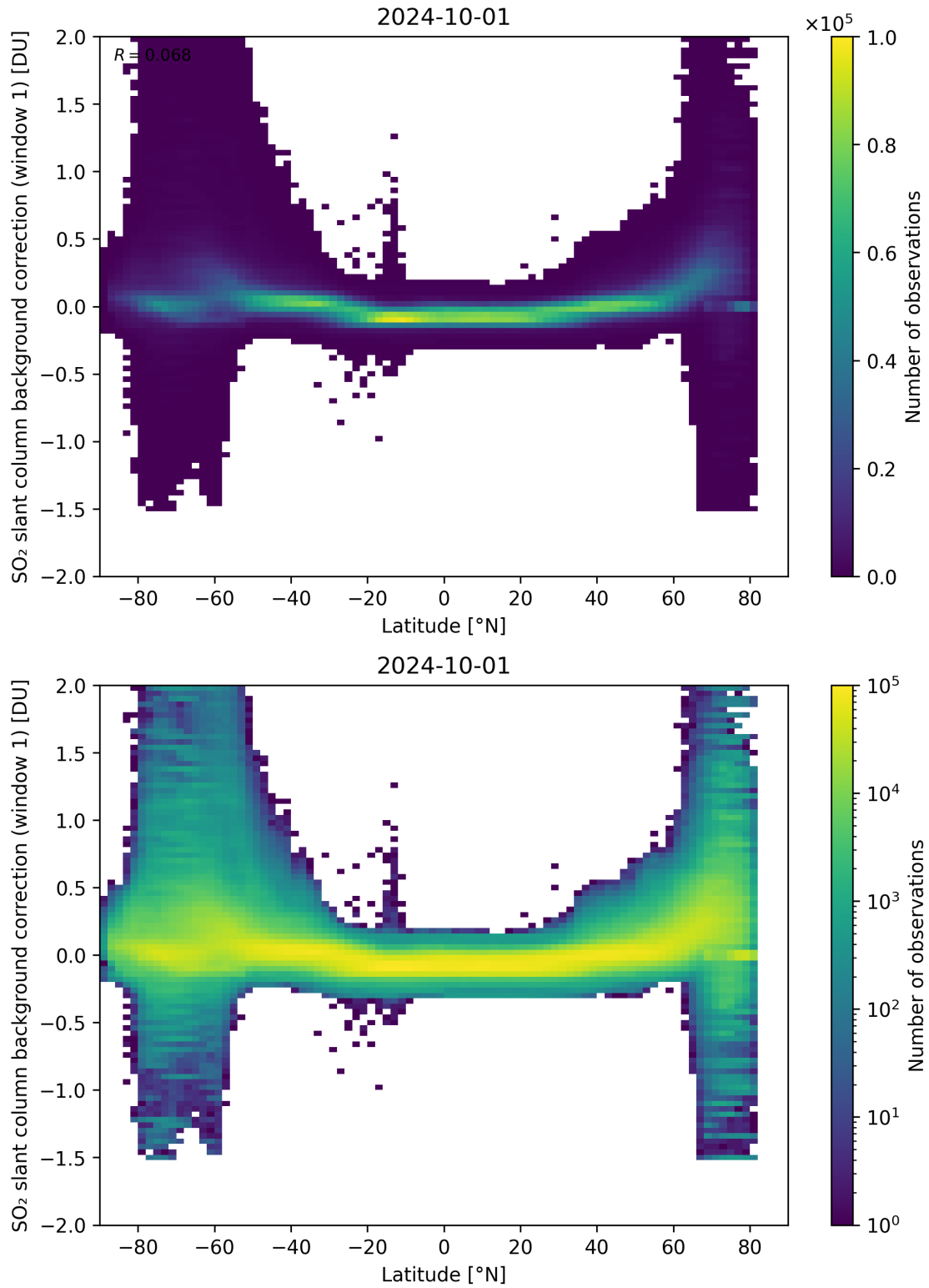
Figure 139: Scatter density plot of “Latitude” against “SO 2 slant column background correction (window 1)” for 2024-09-30 to 2024-10-02.
