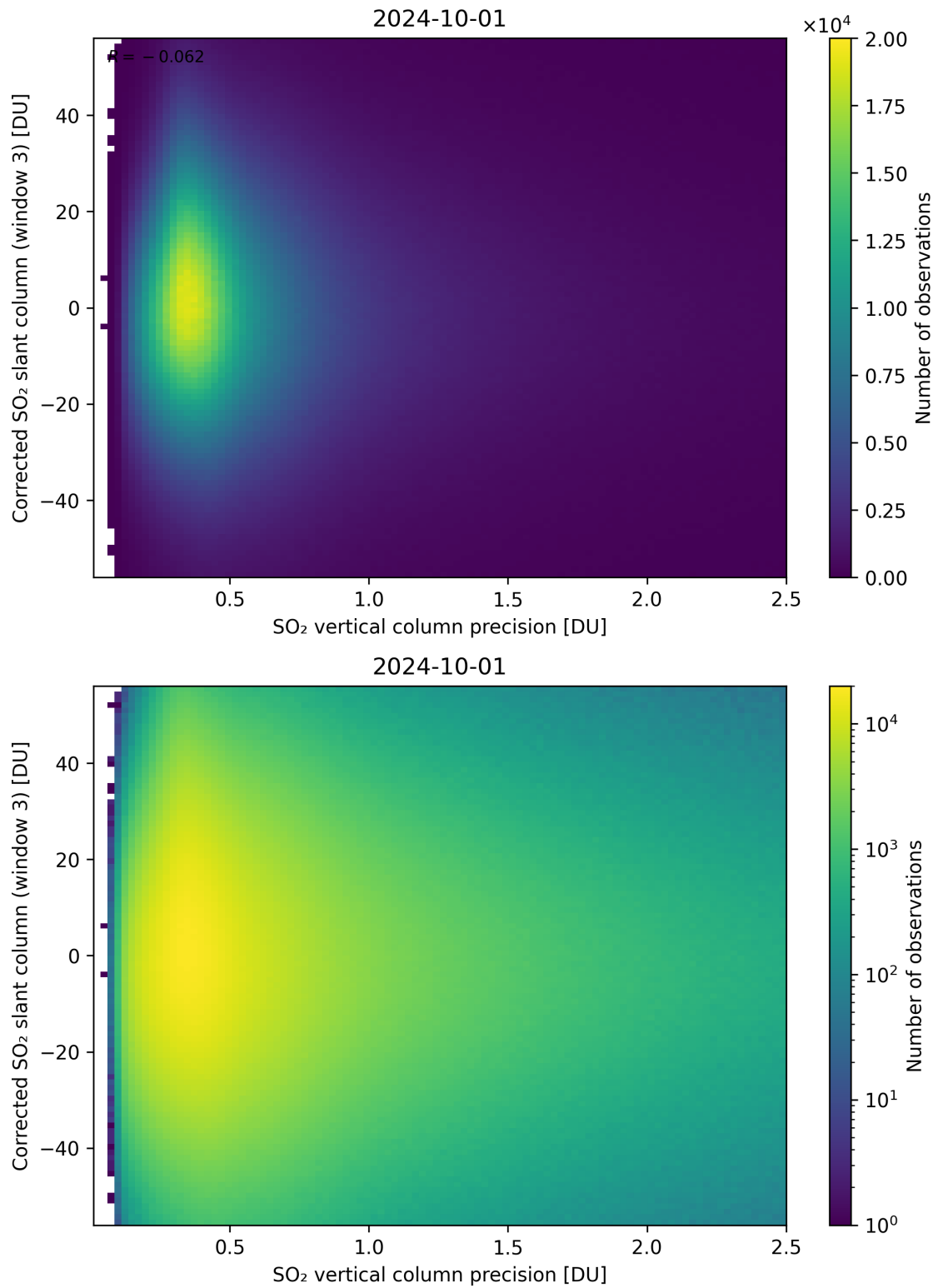
Figure 288: Scatter density plot of “SO 2 vertical column precision” against “Corrected SO 2 slant column (window 3)” for 2024-09-30 to 2024-10-02.
