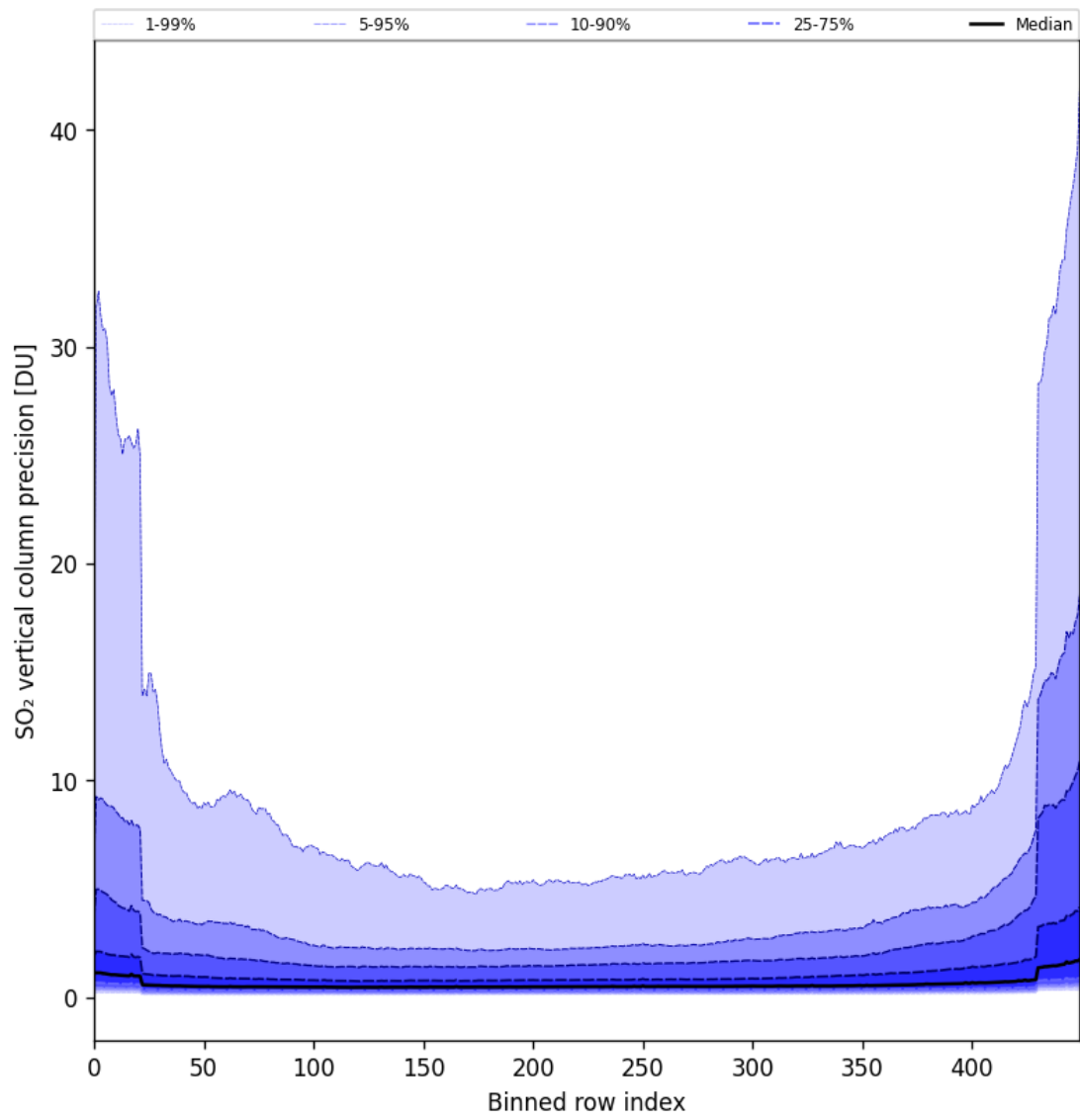
Figure 77: Along track statistics of “SO 2 vertical column precision” for 2024-09-30 to 2024-10-02
