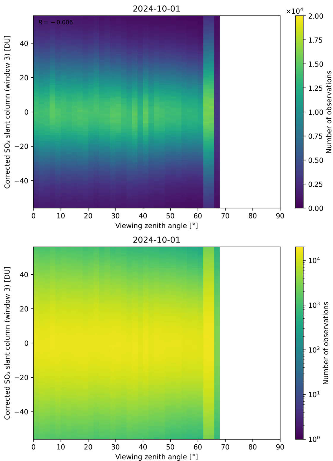
Figure 319: Scatter density plot of “Viewing zenith angle” against “Corrected SO 2 slant column (window 3)” for 2024-09-30 to 2024-10-02.
