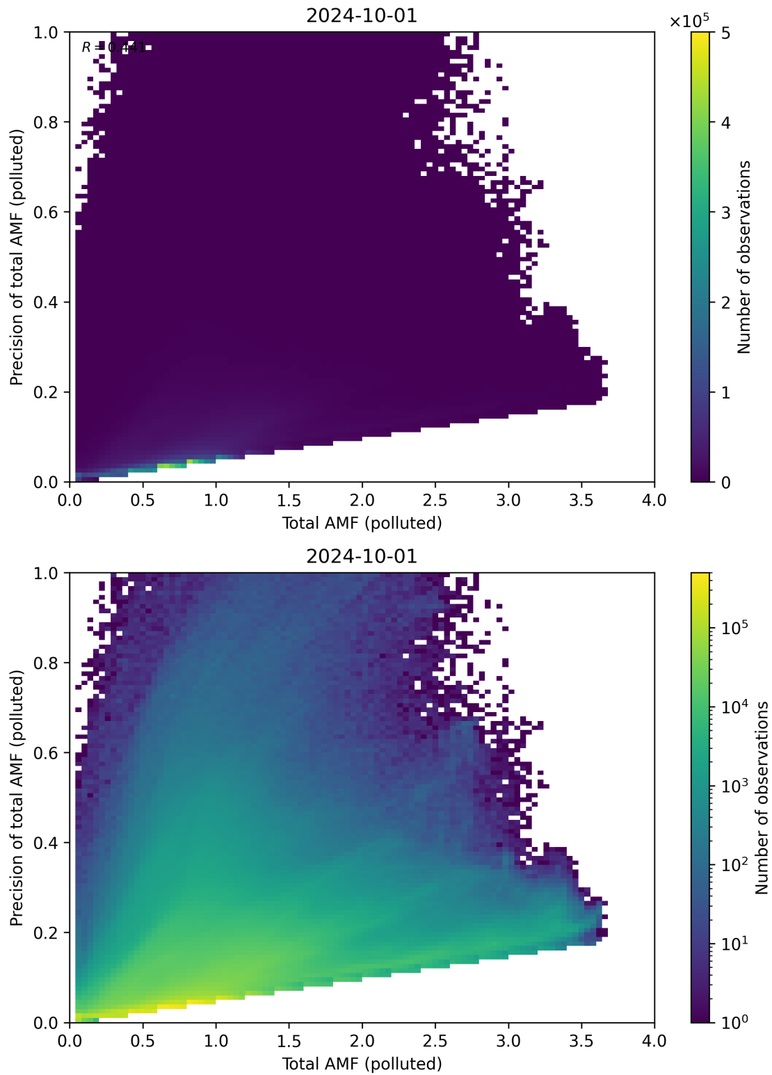
Figure 272: Scatter density plot of “Total AMF (polluted)” against “Precision of total AMF (polluted)” for 2024-09-30 to 2024-10-02.
