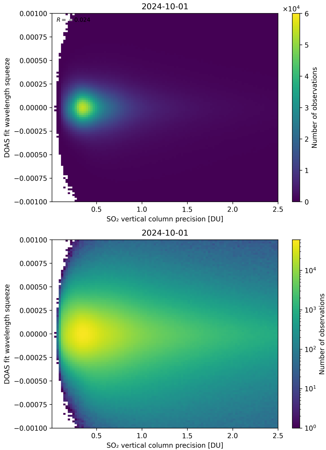
Figure 283: Scatter density plot of “SO 2 vertical column precision” against “DOAS fit wavelength squeeze” for 2024-09-30 to 2024-10-02.
