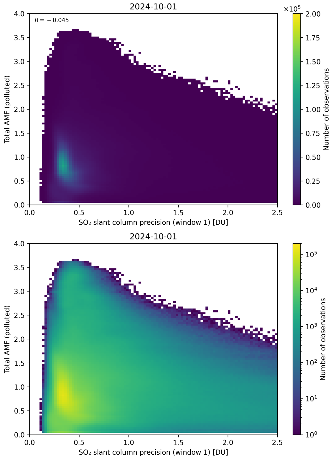
Figure 230: Scatter density plot of “SO 2 slant column precision (window 1)” against “Total AMF (polluted)” for 2024-09-30 to 2024-10-02.
