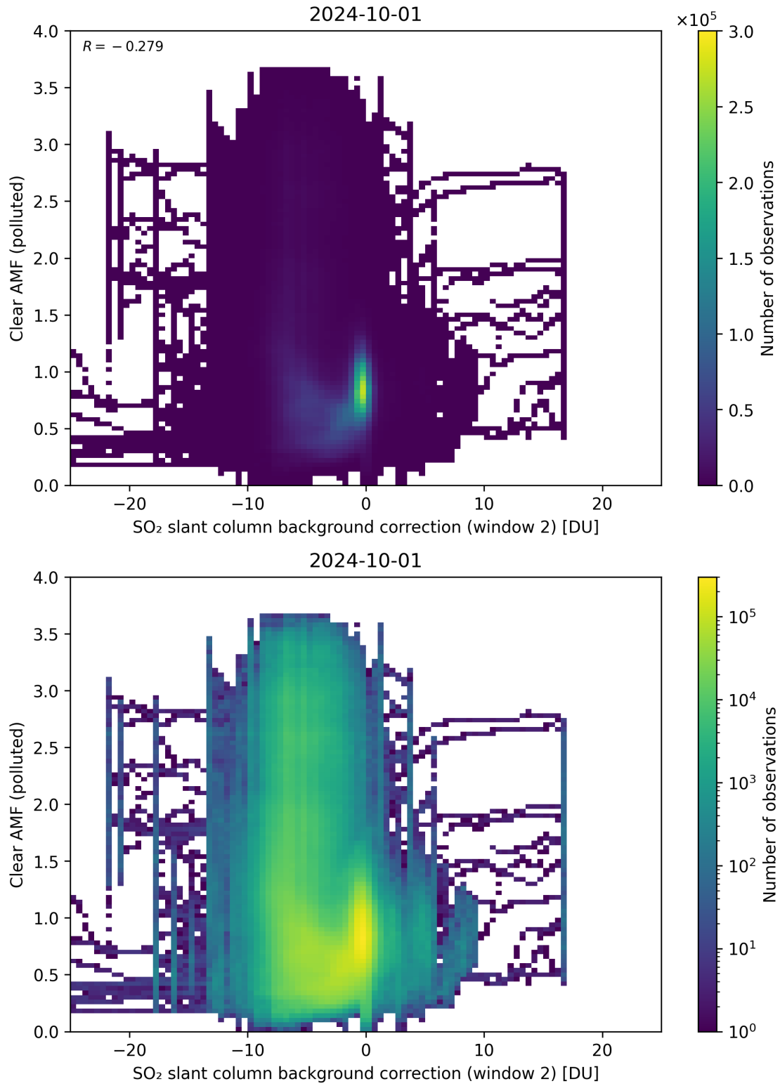
Figure 115: Scatter density plot of “SO 2 slant column background correction (window 2)” against “Clear AMF (polluted)” for 2024-09-30 to 2024-10-02.
