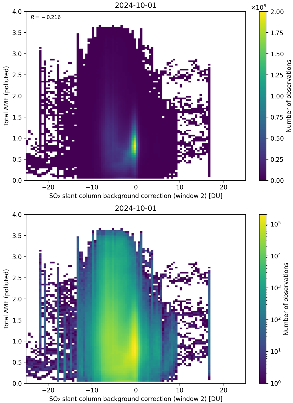
Figure 119: Scatter density plot of “SO 2 slant column background correction (window 2)” against “Total AMF (polluted)” for 2024-09-30 to 2024-10-02.
