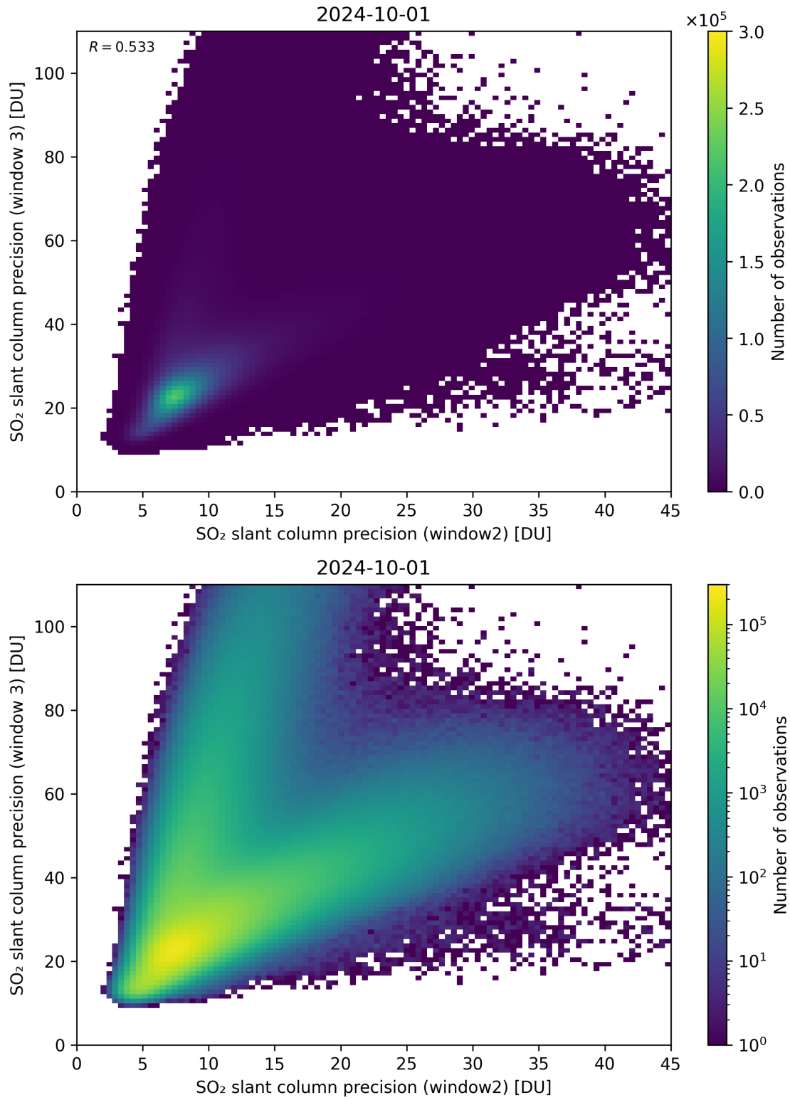
Figure 250: Scatter density plot of “SO 2 slant column precision (window2)” against “SO 2 slant column precision (window 3)” for 2024-09-30 to 2024-10-02.
