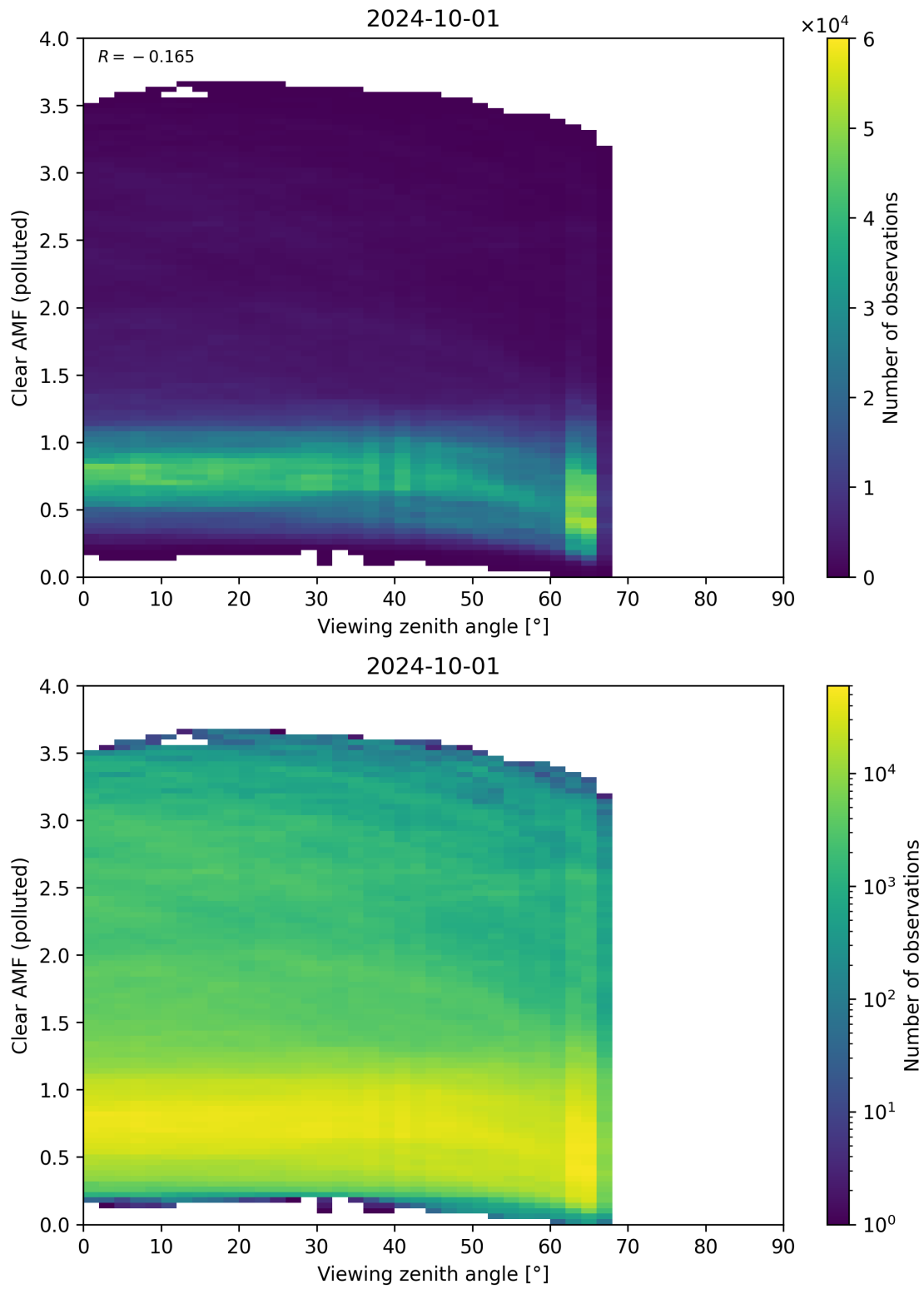
Figure 316: Scatter density plot of “Viewing zenith angle” against “Clear AMF (polluted)” for 2024-09-30 to 2024-10-02.
