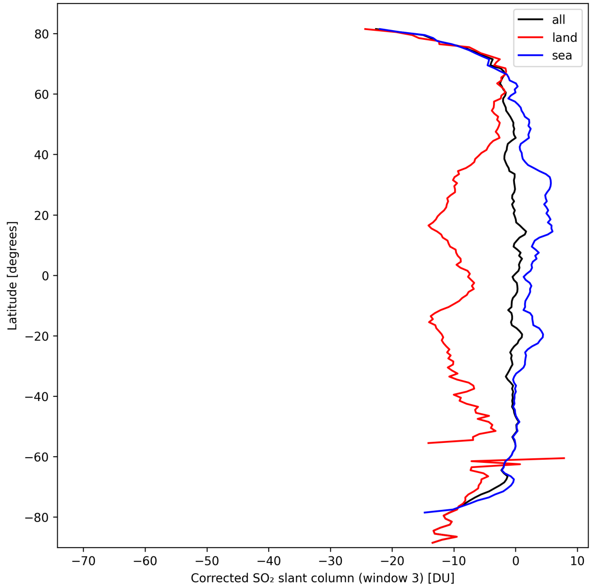
Figure 43: Zonal average of “Corrected SO 2 slant column (window 3)” for 2024-09-30 to 2024-10-02.
