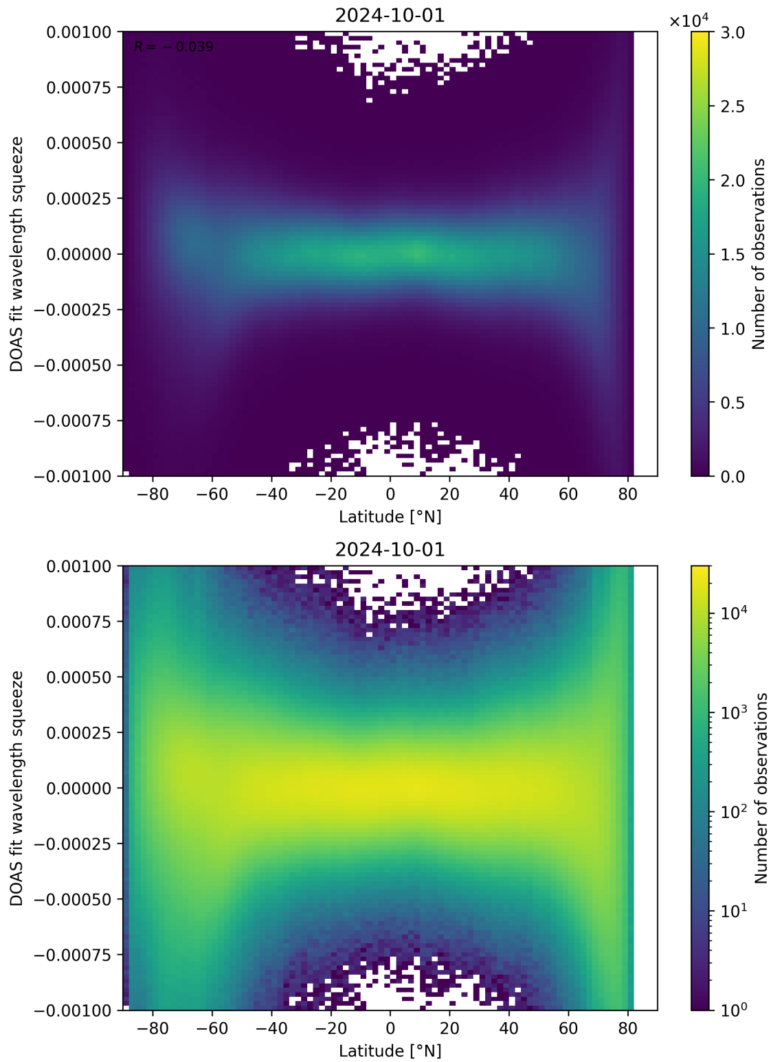
Figure 143: Scatter density plot of “Latitude” against “DOAS fit wavelength squeeze” for 2024-09-30 to 2024-10-02.
