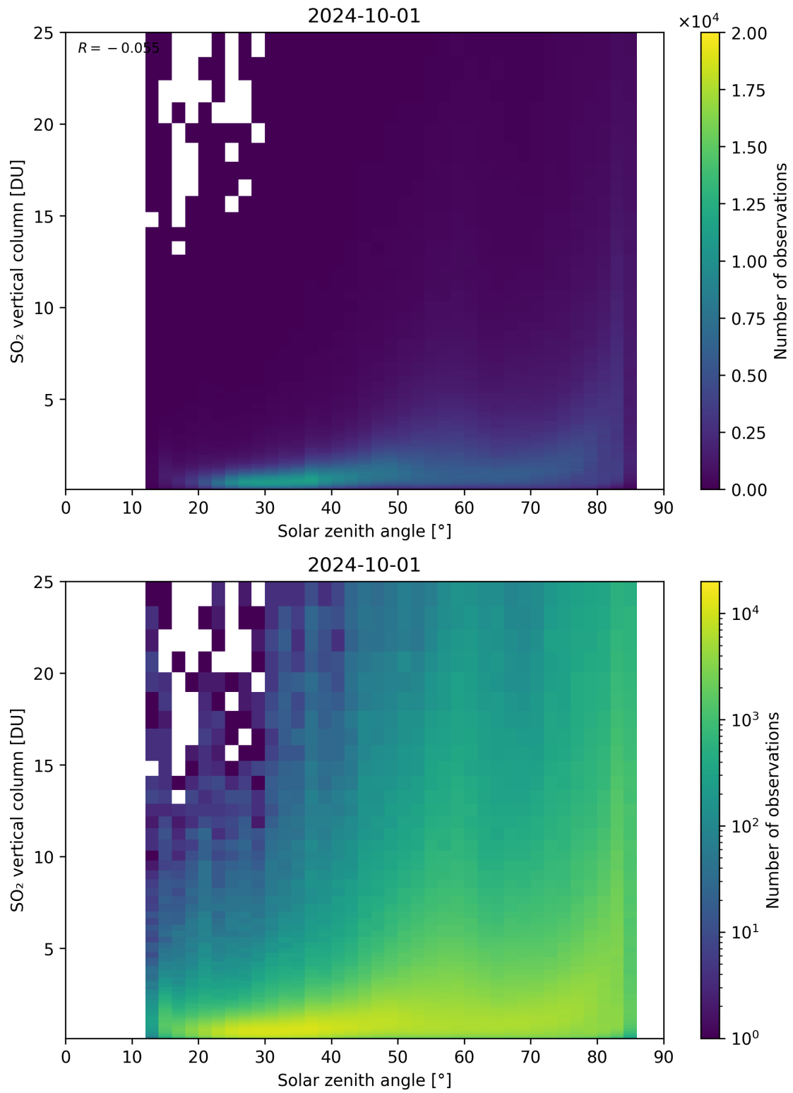
Figure 176: Scatter density plot of “Solar zenith angle” against “SO 2 vertical column” for 2024-09-30 to 2024-10-02.
