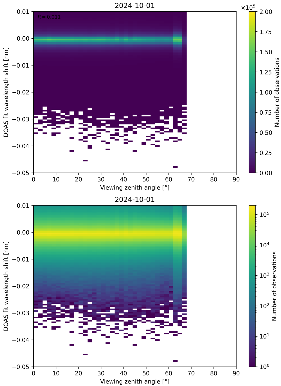
Figure 311: Scatter density plot of “Viewing zenith angle” against “DOAS fit wavelength shift” for 2024-09-30 to 2024-10-02.
