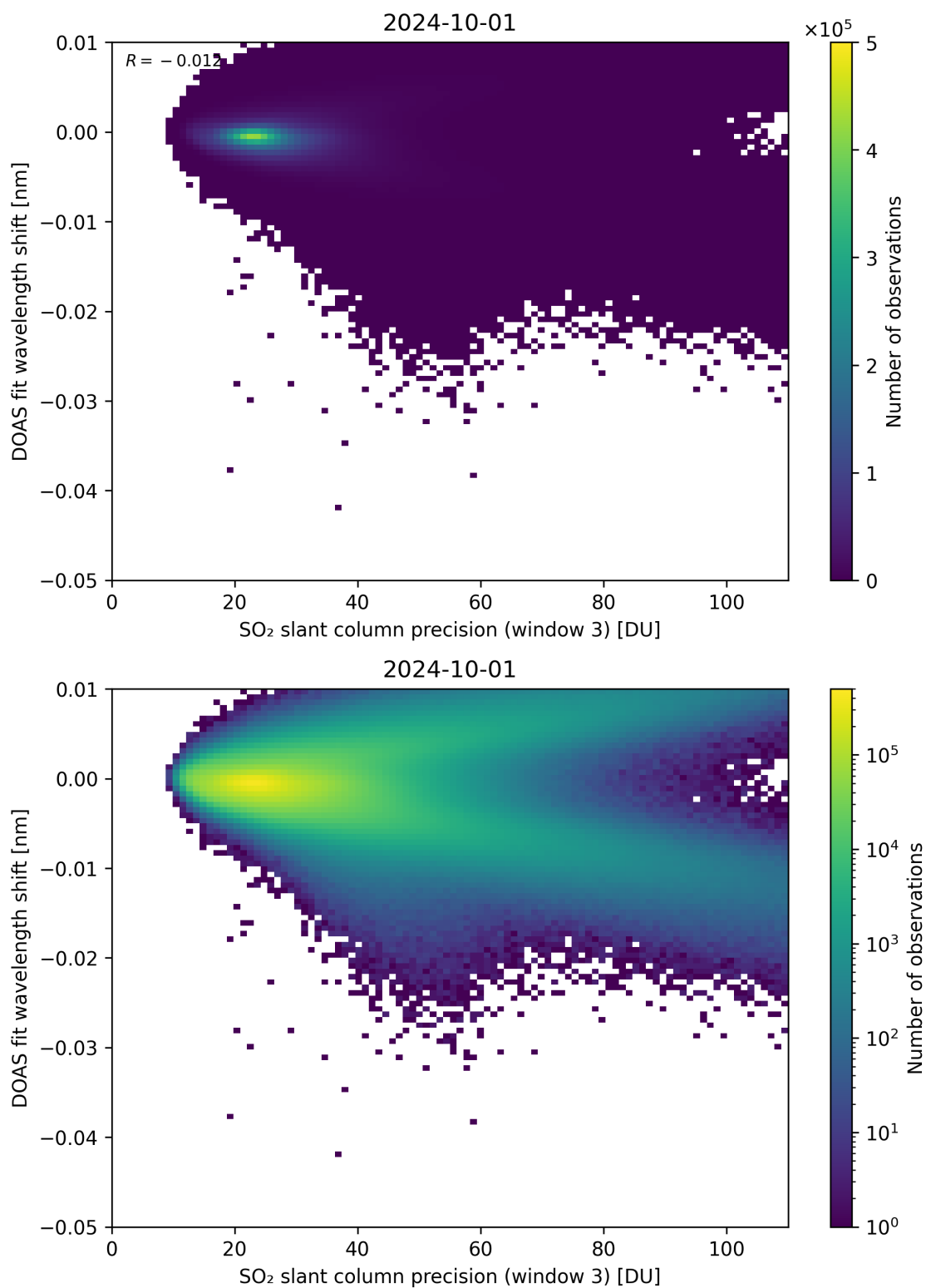
Figure 258: Scatter density plot of “SO 2 slant column precision (window 3)” against “DOAS fit wavelength shift” for 2024-09-30 to 2024-10-02.
