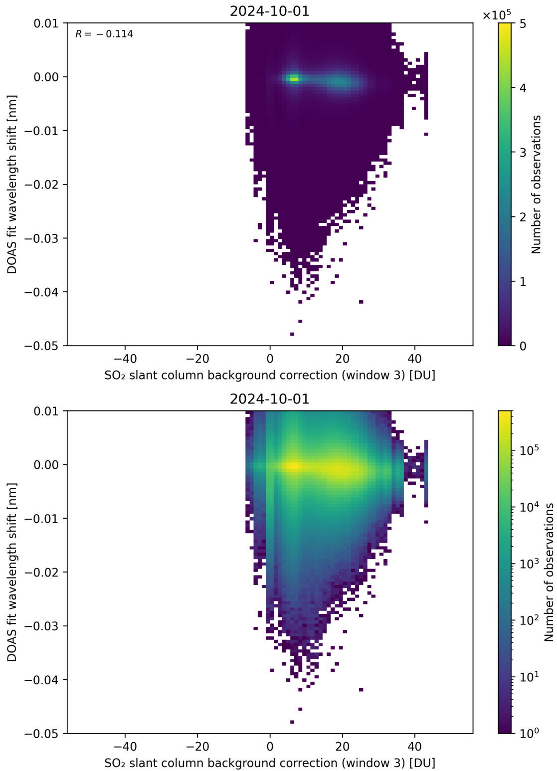
Figure 121: Scatter density plot of “SO 2 slant column background correction (window 3)” against “DOAS fit wavelength shift” for 2024-09-30 to 2024-10-02.
