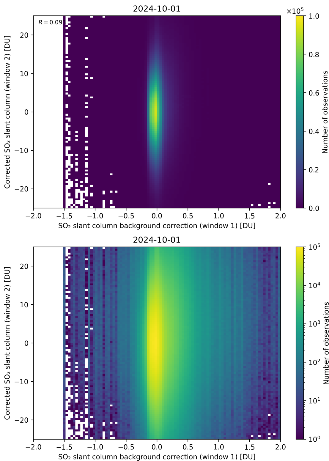
Figure 104: Scatter density plot of “SO 2 slant column background correction (window 1)” against “Corrected SO 2 slant column (window 2)” for 2024-09-30 to 2024-10-02.
