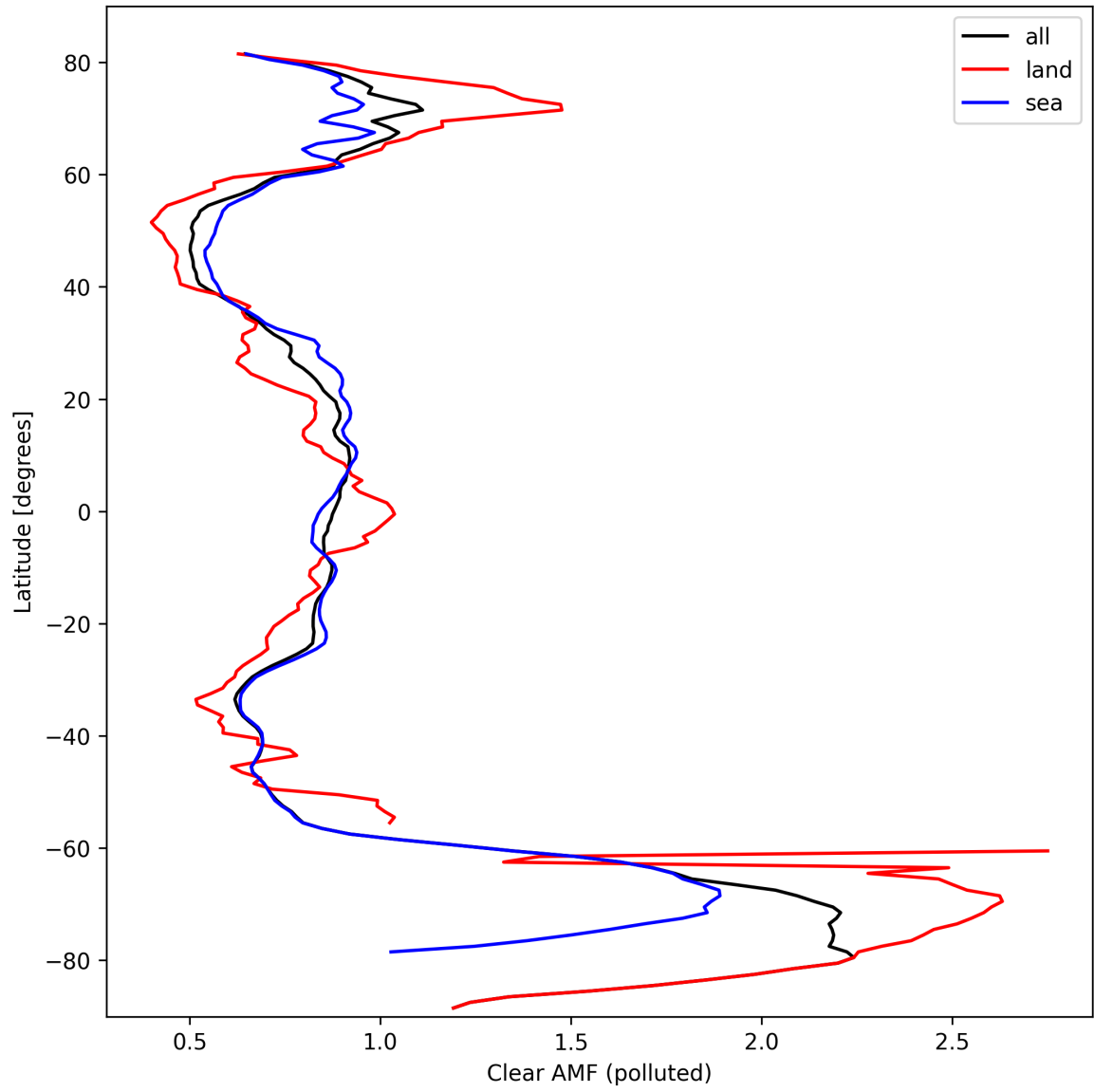
Figure 50: Zonal average of “Clear AMF (polluted)” for 2024-09-30 to 2024-10-02.
