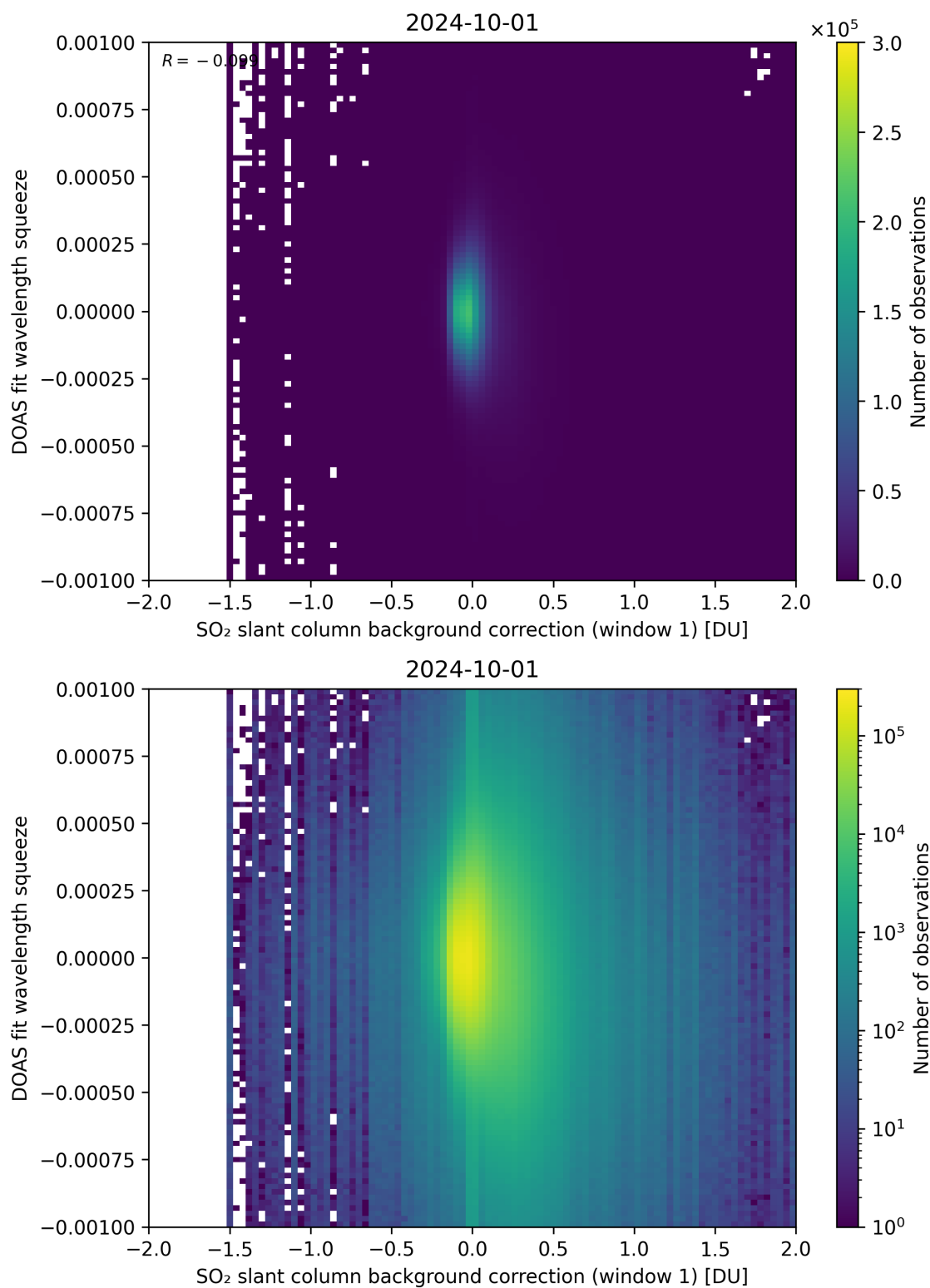
Figure 101: Scatter density plot of “SO 2 slant column background correction (window 1)” against “DOAS fit wavelength squeeze” for 2024-09-30 to 2024-10-02.
