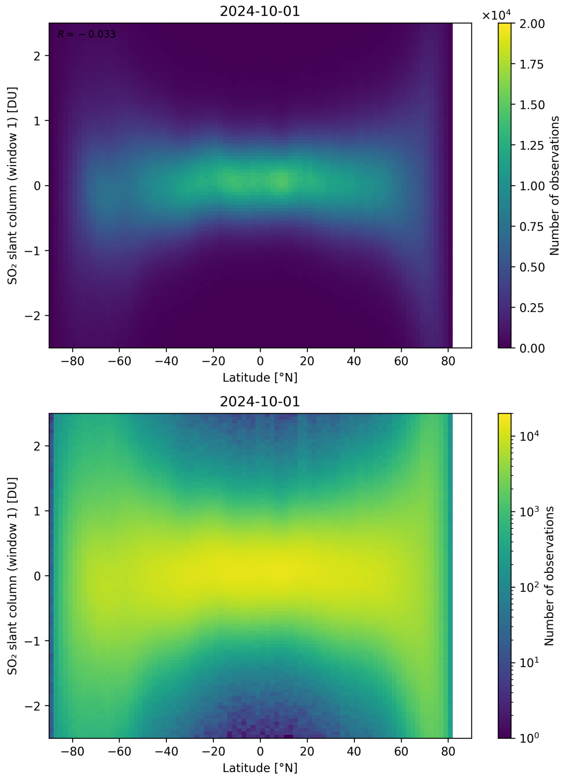
Figure 149: Scatter density plot of “Latitude” against “SO 2 slant column (window 1)” for 2024-09-30 to 2024-10-02.
