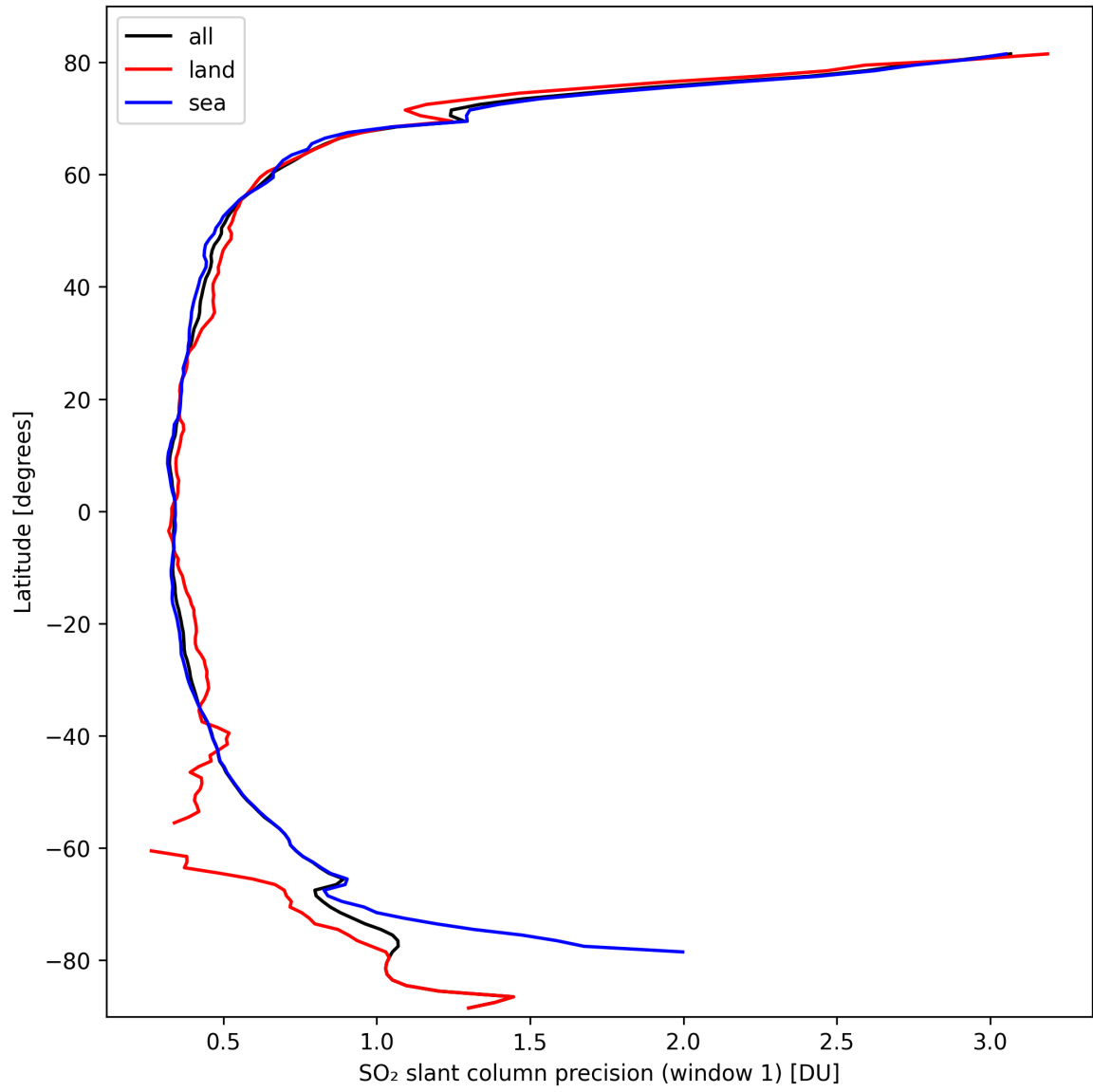
Figure 34: Zonal average of “SO 2 slant column precision (window 1)” for 2024-09-30 to 2024-10-02.
