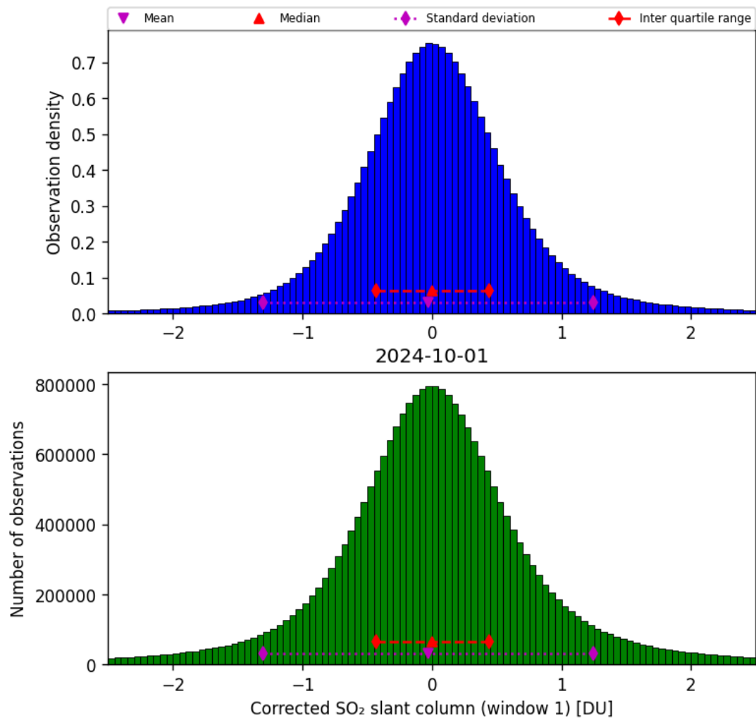
Figure 58: Histogram of “Corrected SO 2 slant column (window 1)” for 2024-09-30 to 2024-10-02
