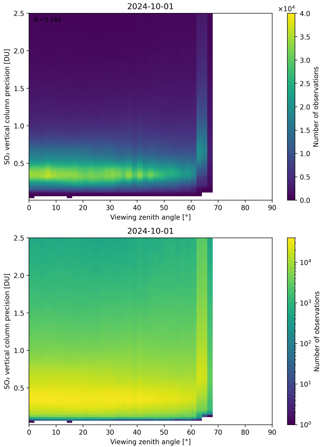
Figure 328: Scatter density plot of “Viewing zenith angle” against “SO 2 vertical column precision” for 2024-09-30 to 2024-10-02.
