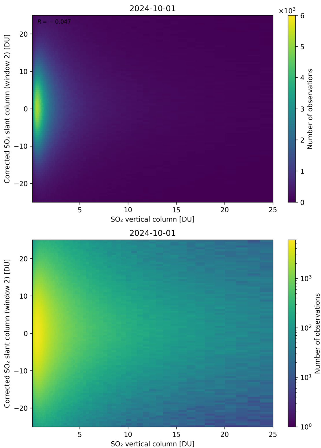
Figure 298: Scatter density plot of “SO 2 vertical column” against “Corrected SO 2 slant column (window 2)” for 2024-09-30 to 2024-10-02.
