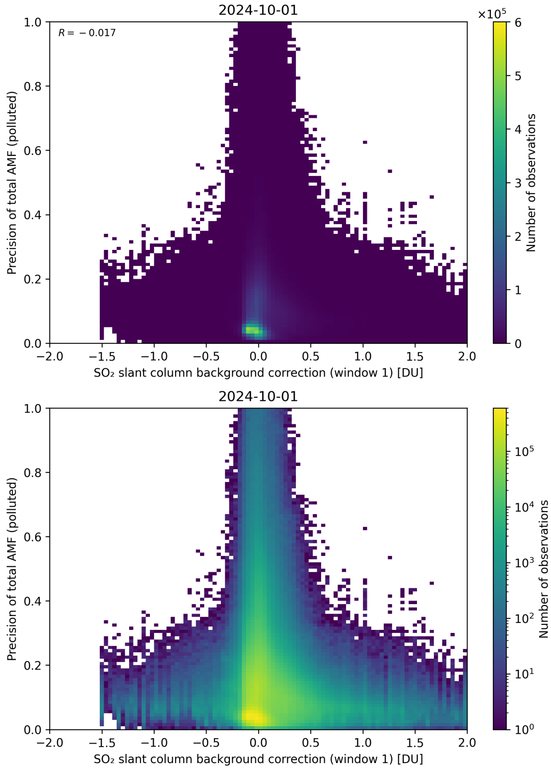
Figure 110: Scatter density plot of “SO 2 slant column background correction (window 1)” against “Precision of total AMF (polluted)” for 2024-09-30 to 2024-10-02.
