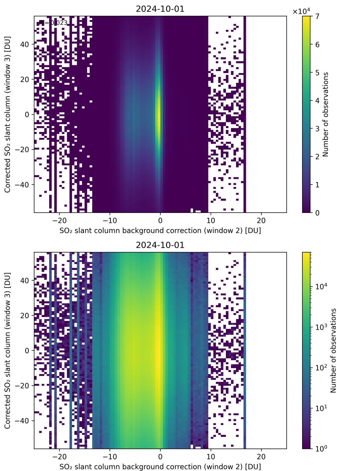
Figure 116: Scatter density plot of “SO 2 slant column background correction (window 2)” against “Corrected SO 2 slant column (window 3)” for 2024-09-30 to 2024-10-02.
