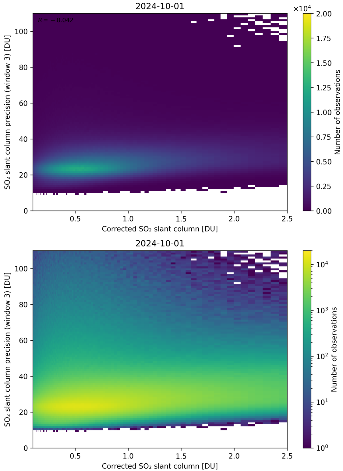
Figure 191: Scatter density plot of “Corrected SO 2 slant column” against “SO 2 slant column precision (window 3)” for 2024-09-30 to 2024-10-02.
