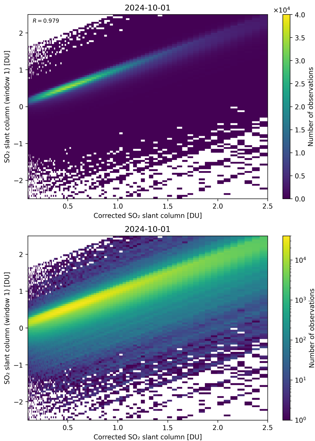
Figure 187: Scatter density plot of “Corrected SO 2 slant column” against “SO 2 slant column (window 1)” for 2024-09-30 to 2024-10-02.
