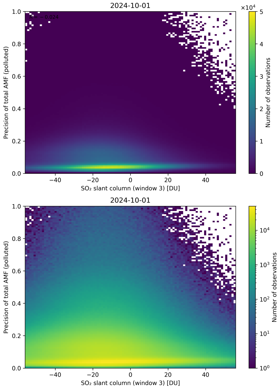
Figure 269: Scatter density plot of “SO 2 slant column (window 3)” against “Precision of total AMF (polluted)” for 2024-09-30 to 2024-10-02.
