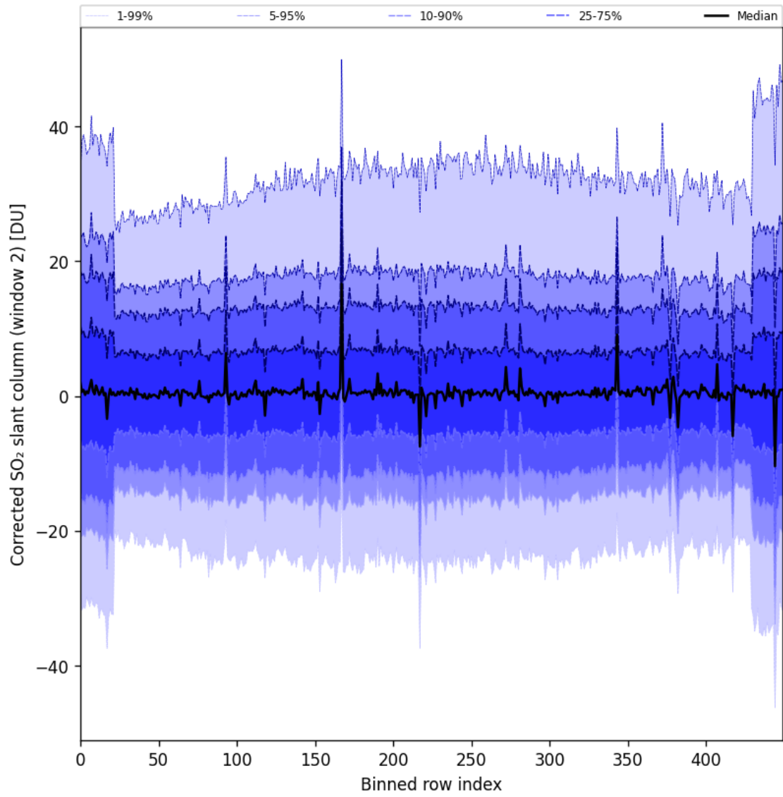
Figure 85: Along track statistics of “Corrected SO 2 slant column (window 2)” for 2024-09-30 to 2024-10-02
