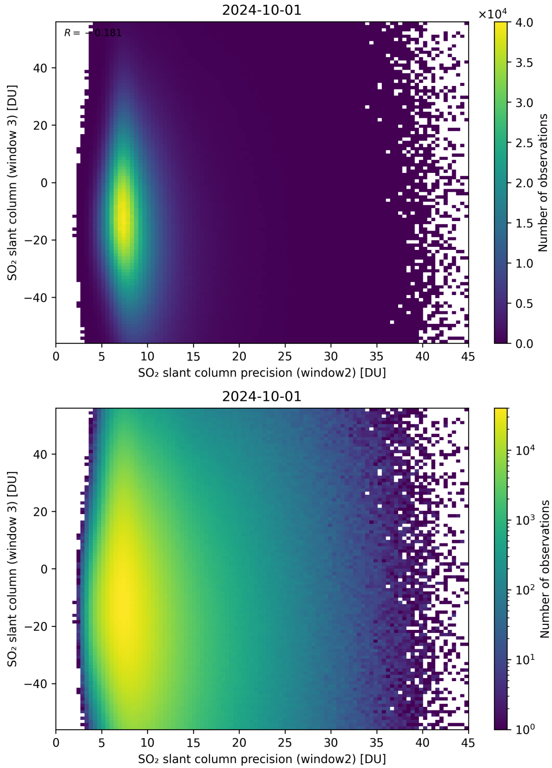
Figure 249: Scatter density plot of “SO 2 slant column precision (window2)” against “SO 2 slant column (window 3)” for 2024-09-30 to 2024-10-02.
