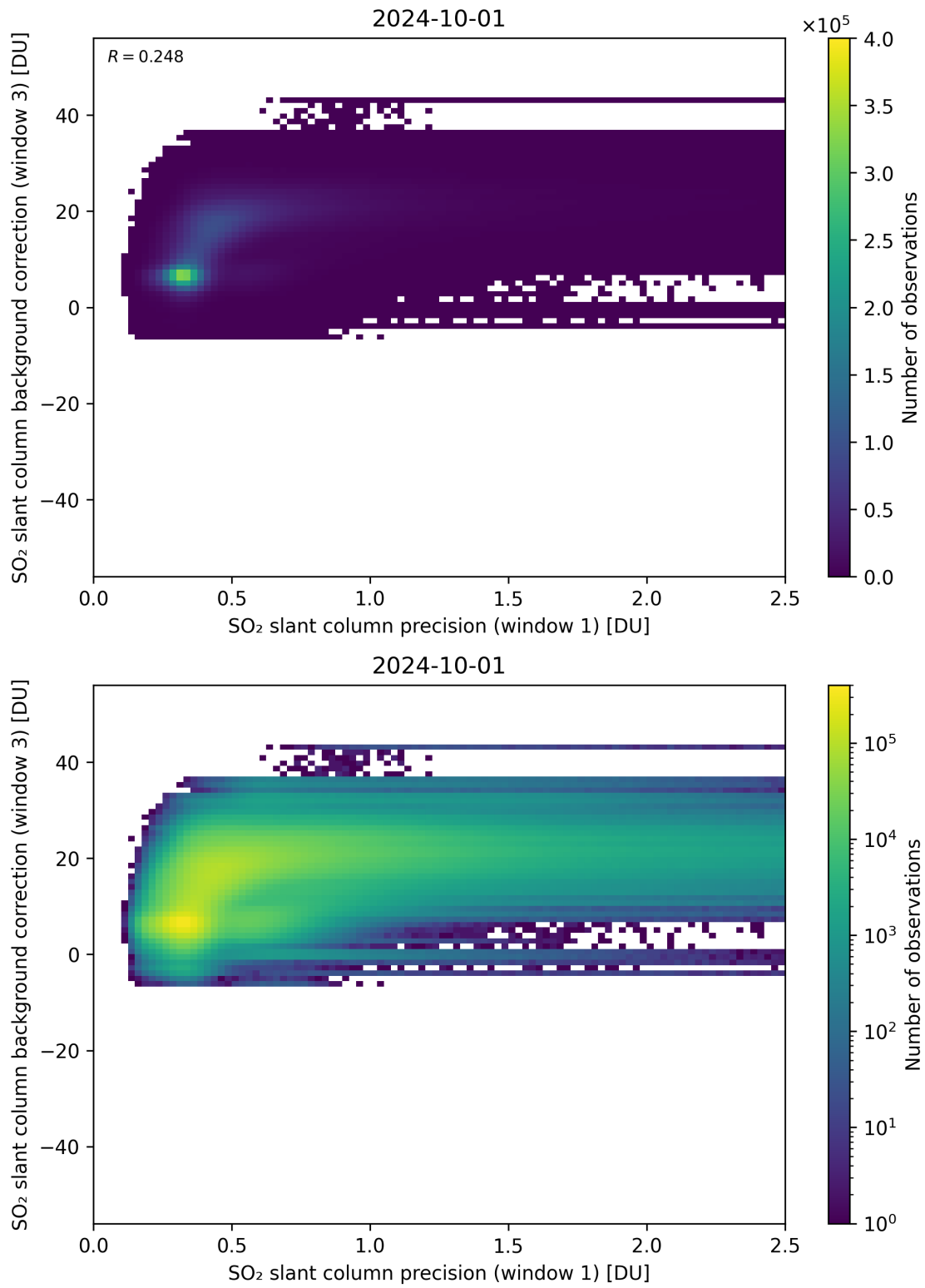
Figure 220: Scatter density plot of “SO 2 slant column precision (window 1)” against “SO 2 slant column background correction (window 3)” for 2024-09-30 to 2024-10-02.
