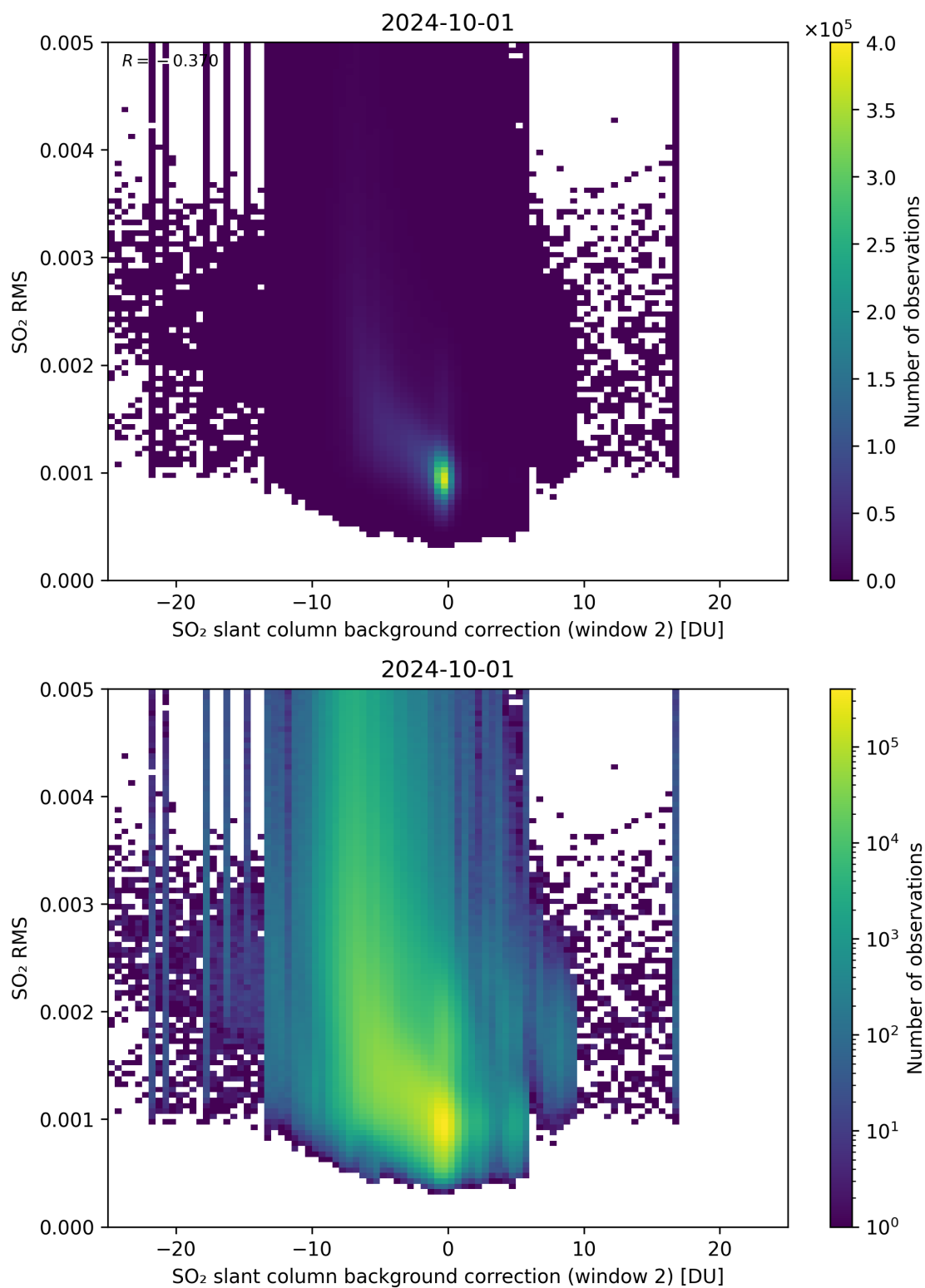
Figure 114: Scatter density plot of “SO 2 slant column background correction (window 2)” against “SO 2 RMS” for 2024-09-30 to 2024-10-02.
