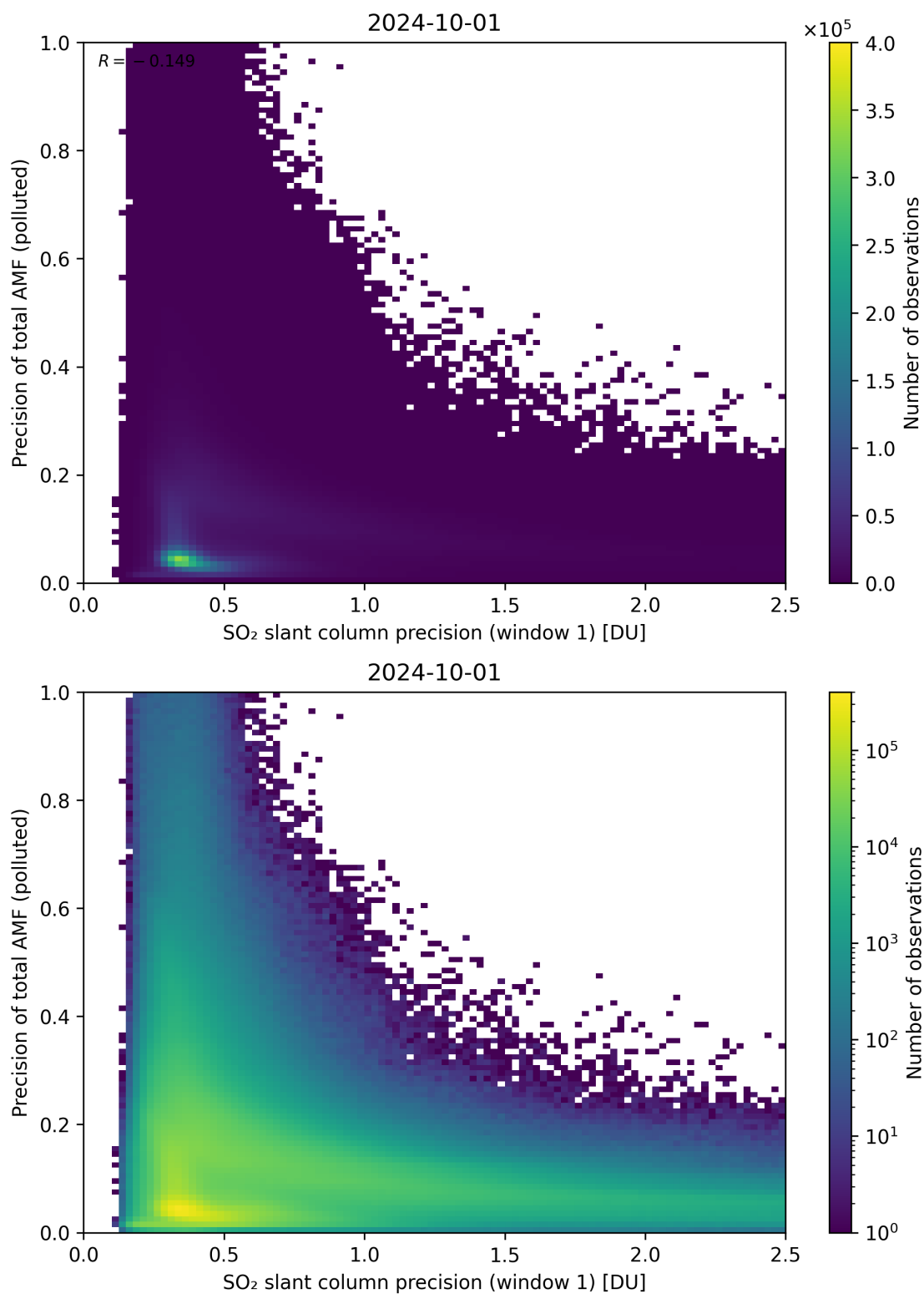
Figure 231: Scatter density plot of “SO 2 slant column precision (window 1)” against “Precision of total AMF (polluted)” for 2024-09-30 to 2024-10-02.
