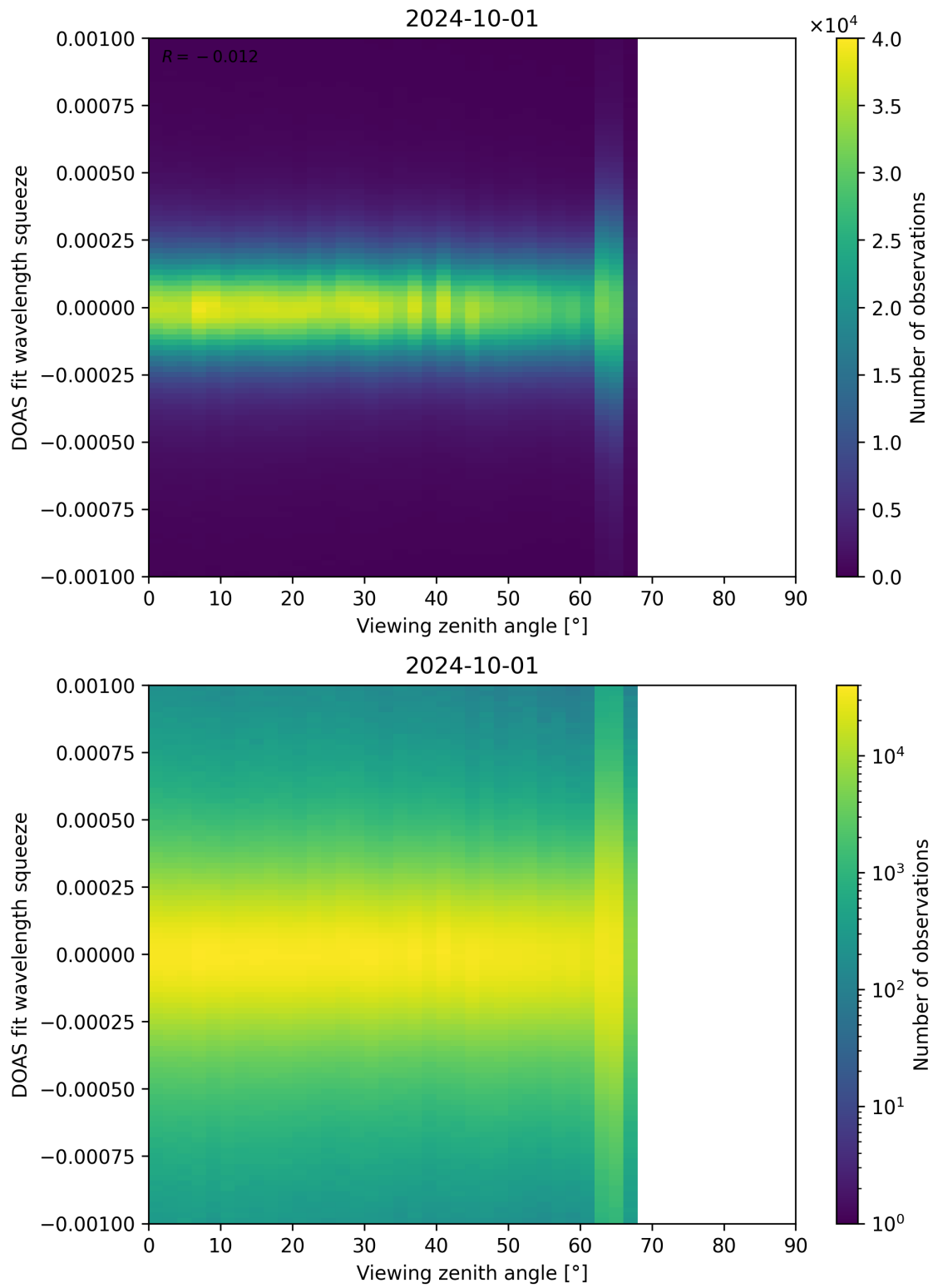
Figure 312: Scatter density plot of “Viewing zenith angle” against “DOAS fit wavelength squeeze” for 2024-09-30 to 2024-10-02.
