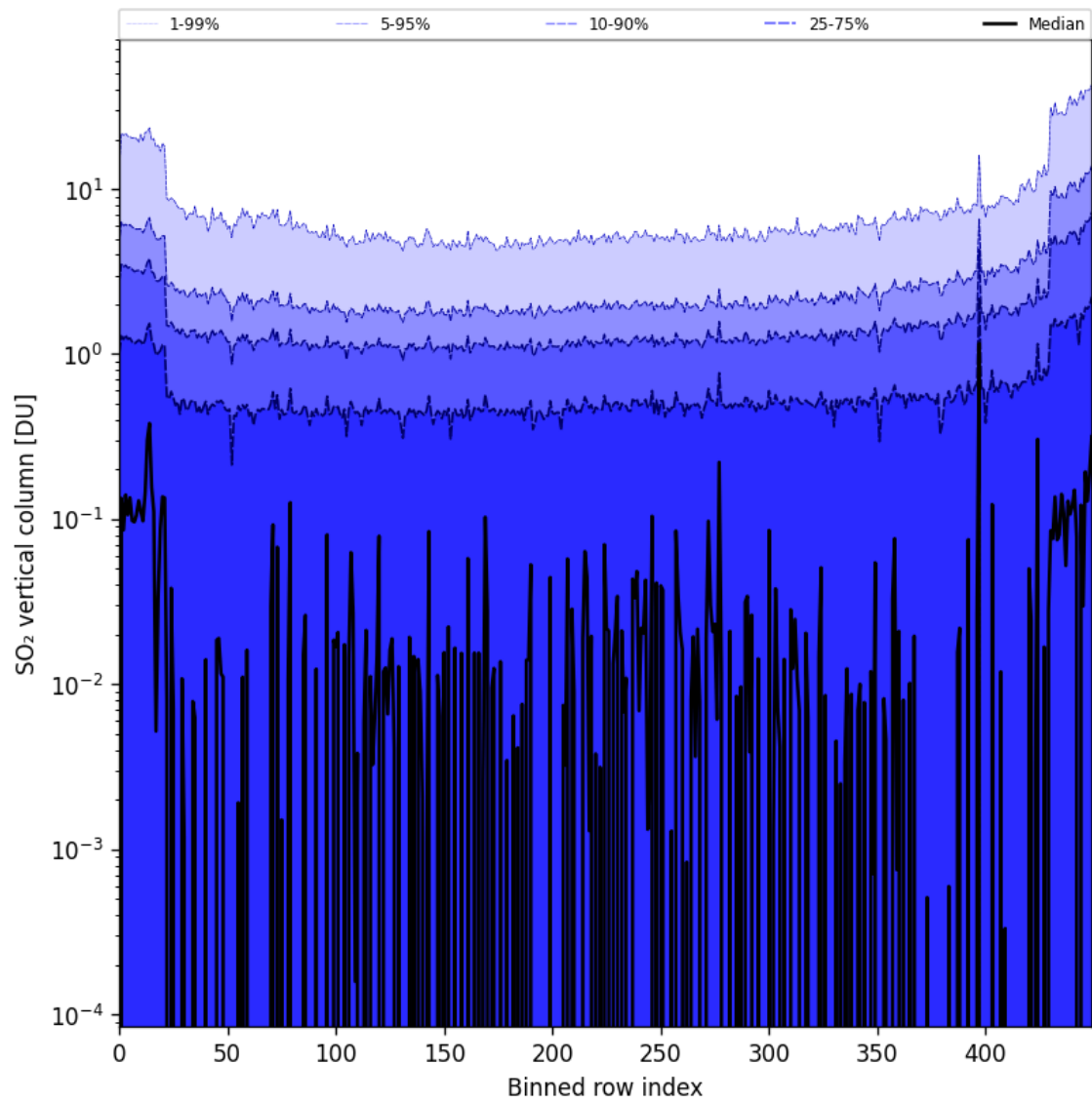
Figure 76: Along track statistics of “SO 2 vertical column” for 2024-09-30 to 2024-10-02
