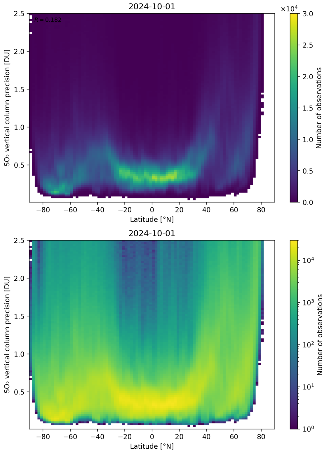
Figure 157: Scatter density plot of “Latitude” against “SO 2 vertical column precision” for 2024-09-30 to 2024-10-02.
