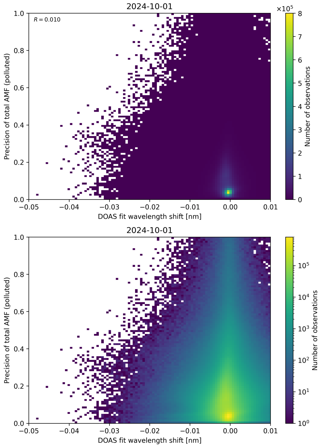
Figure 131: Scatter density plot of “DOAS fit wavelength shift” against “Precision of total AMF (polluted)” for 2024-09-30 to 2024-10-02.
