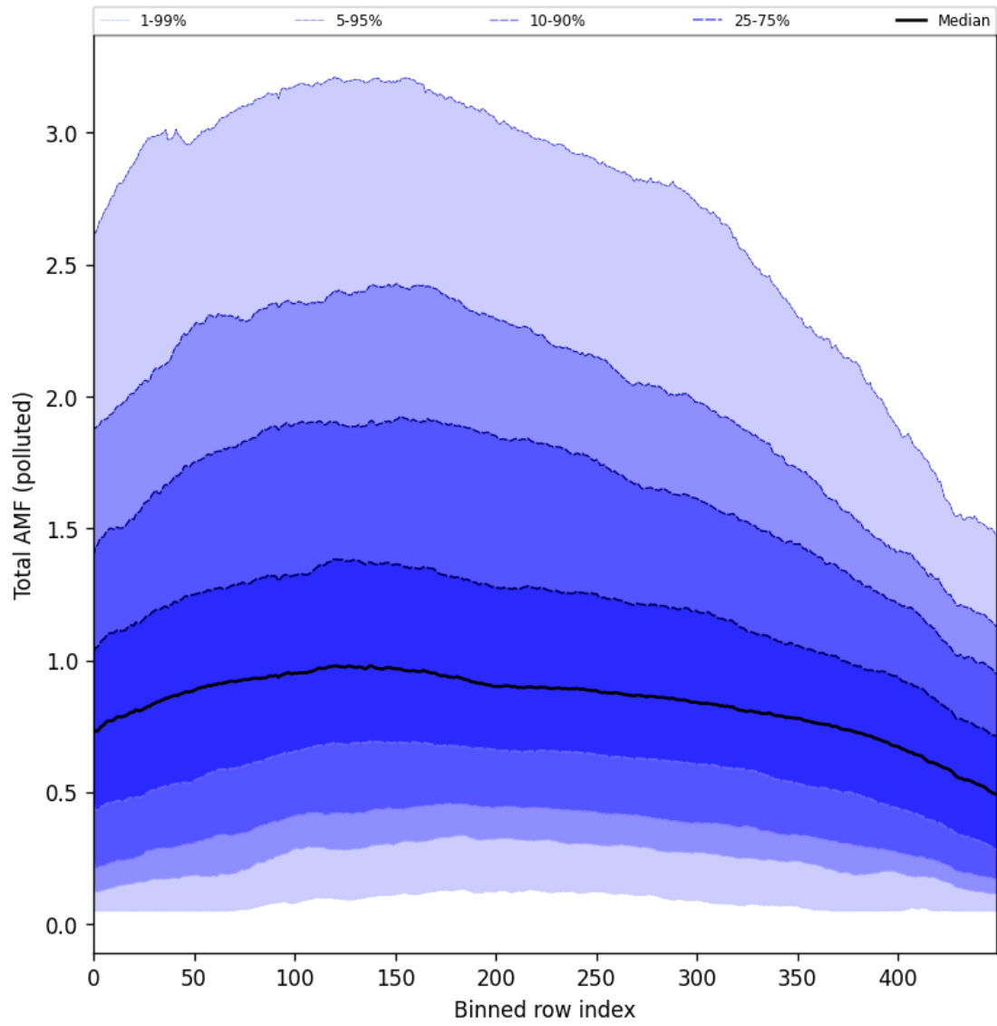
Figure 94: Along track statistics of “Total AMF (polluted)” for 2024-09-30 to 2024-10-02
