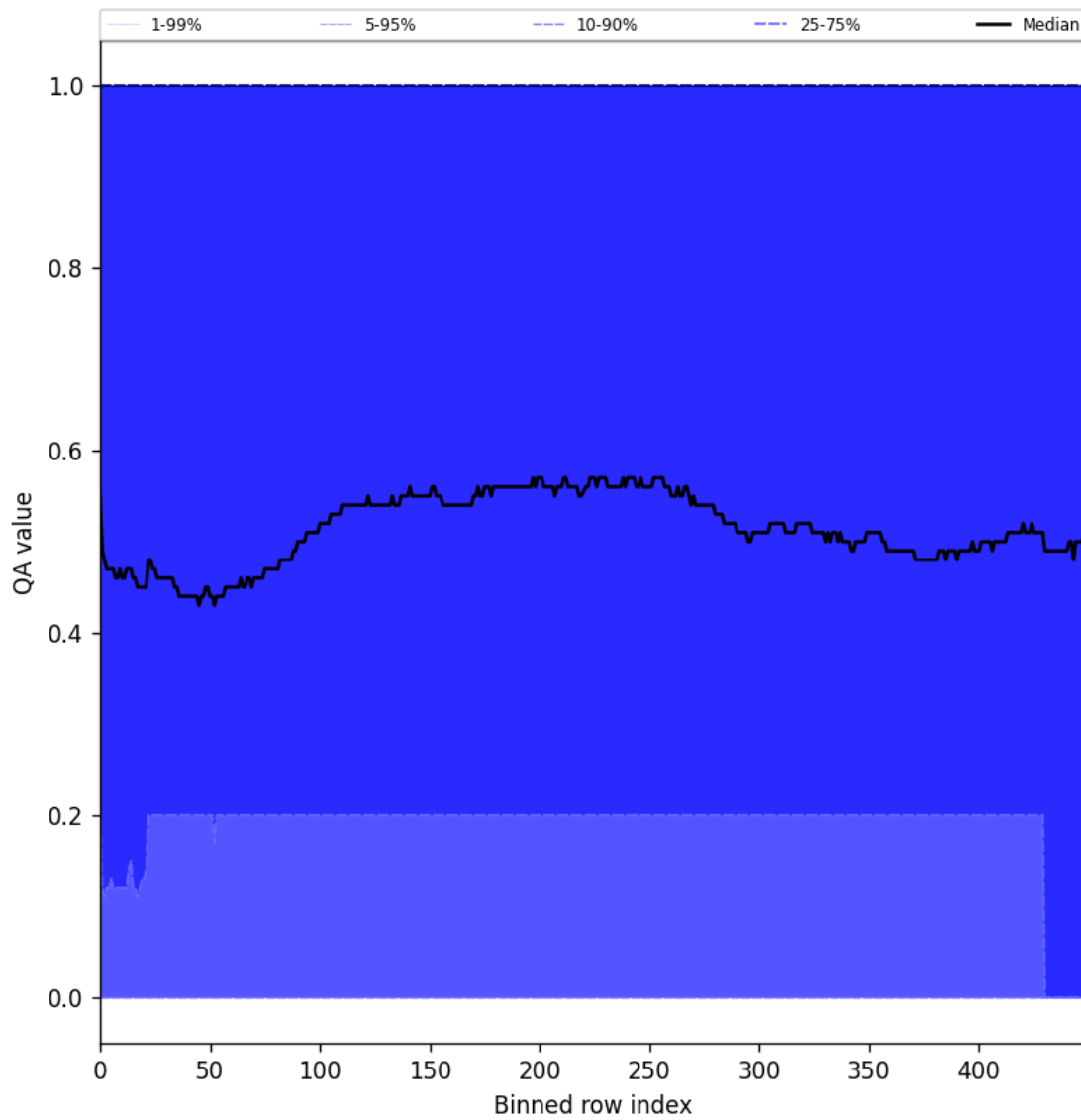
Figure 75: Along track statistics of “QA value” for 2024-09-30 to 2024-10-02
