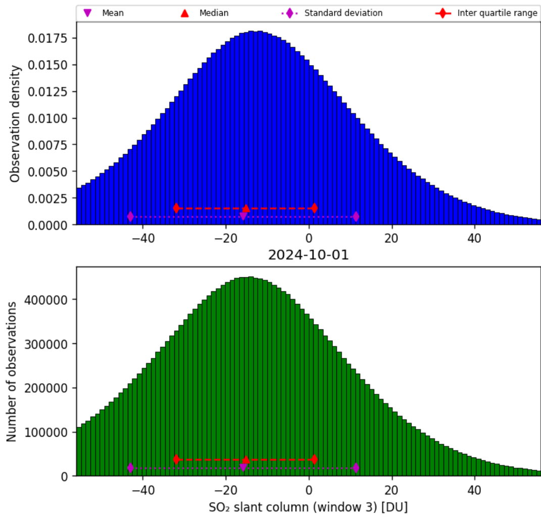
Figure 64: Histogram of “SO 2 slant column (window 3)” for 2024-09-30 to 2024-10-02
