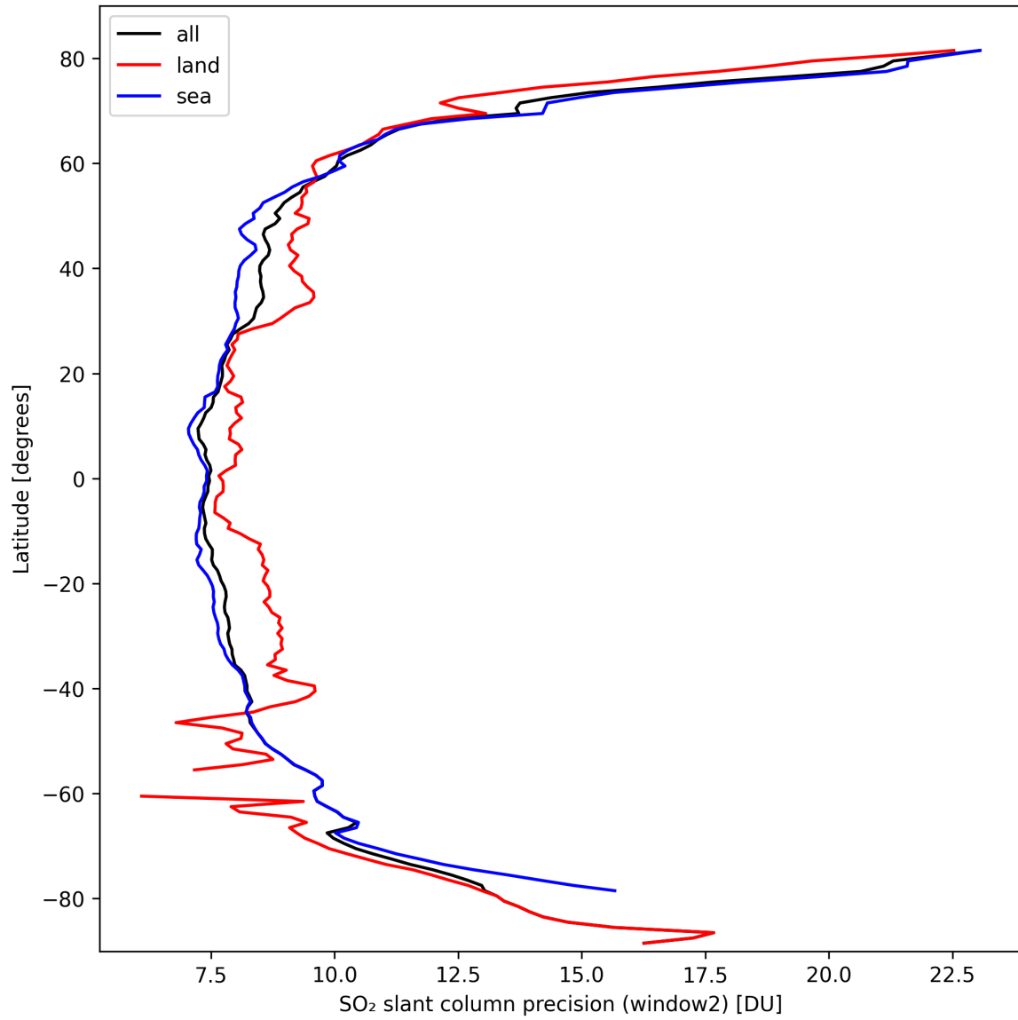
Figure 38: Zonal average of “SO 2 slant column precision (window2)” for 2024-09-30 to 2024-10-02.
