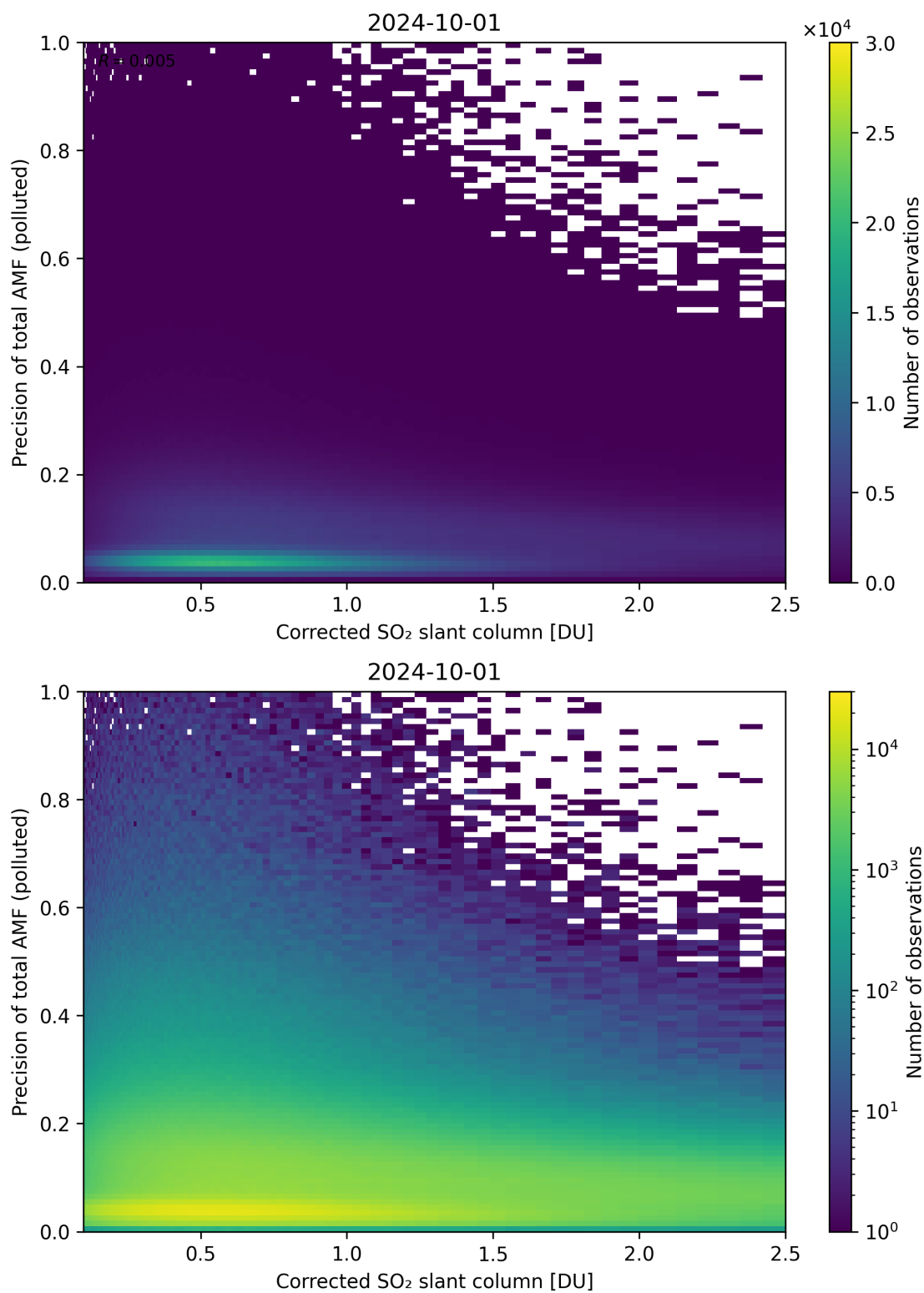
Figure 193: Scatter density plot of “Corrected SO 2 slant column” against “Precision of total AMF (polluted)” for 2024-09-30 to 2024-10-02.
