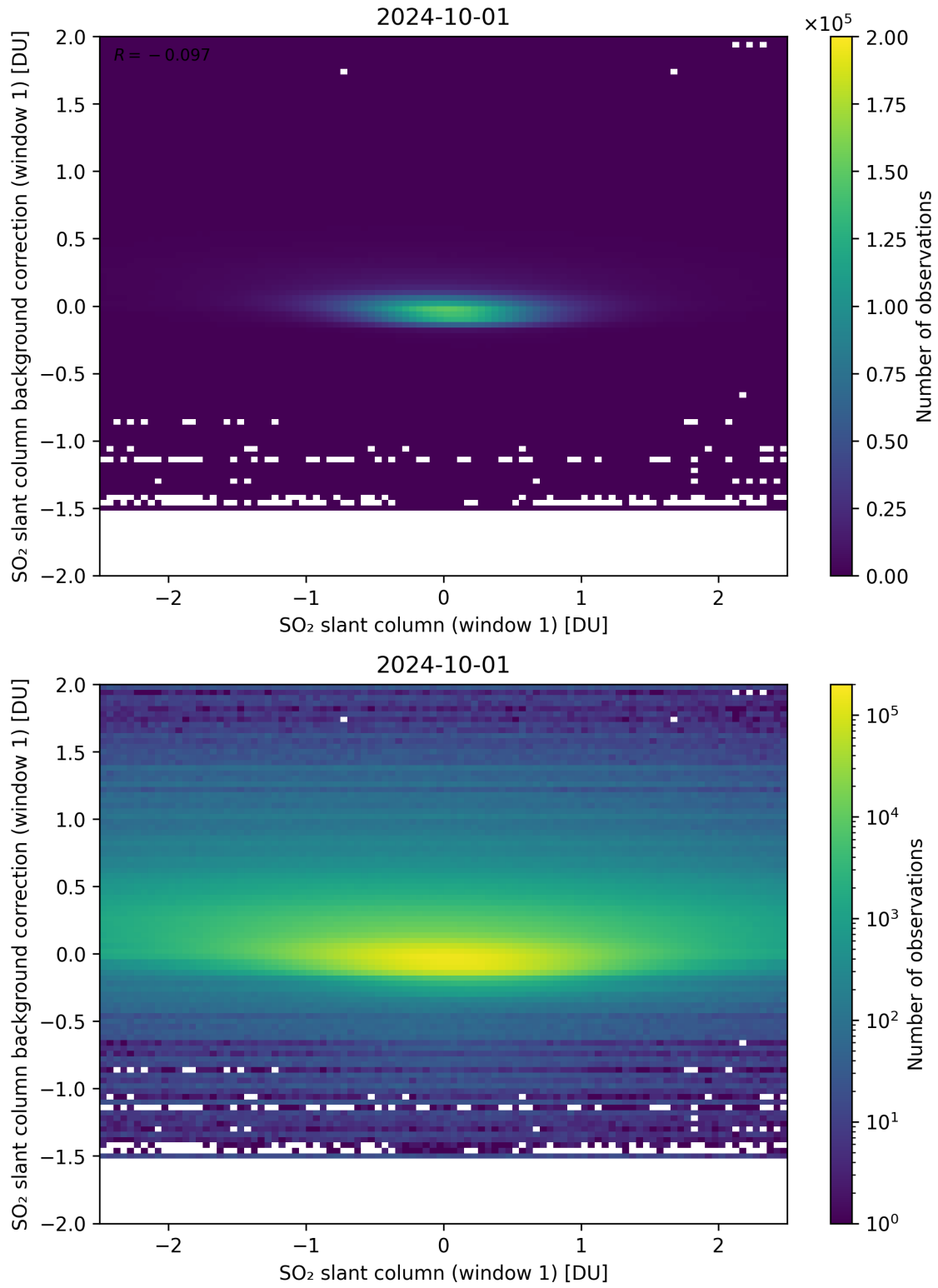
Figure 212: Scatter density plot of “SO 2 slant column (window 1)” against “SO 2 slant column background correction (window 1)” for 2024-09-30 to 2024-10-02.
