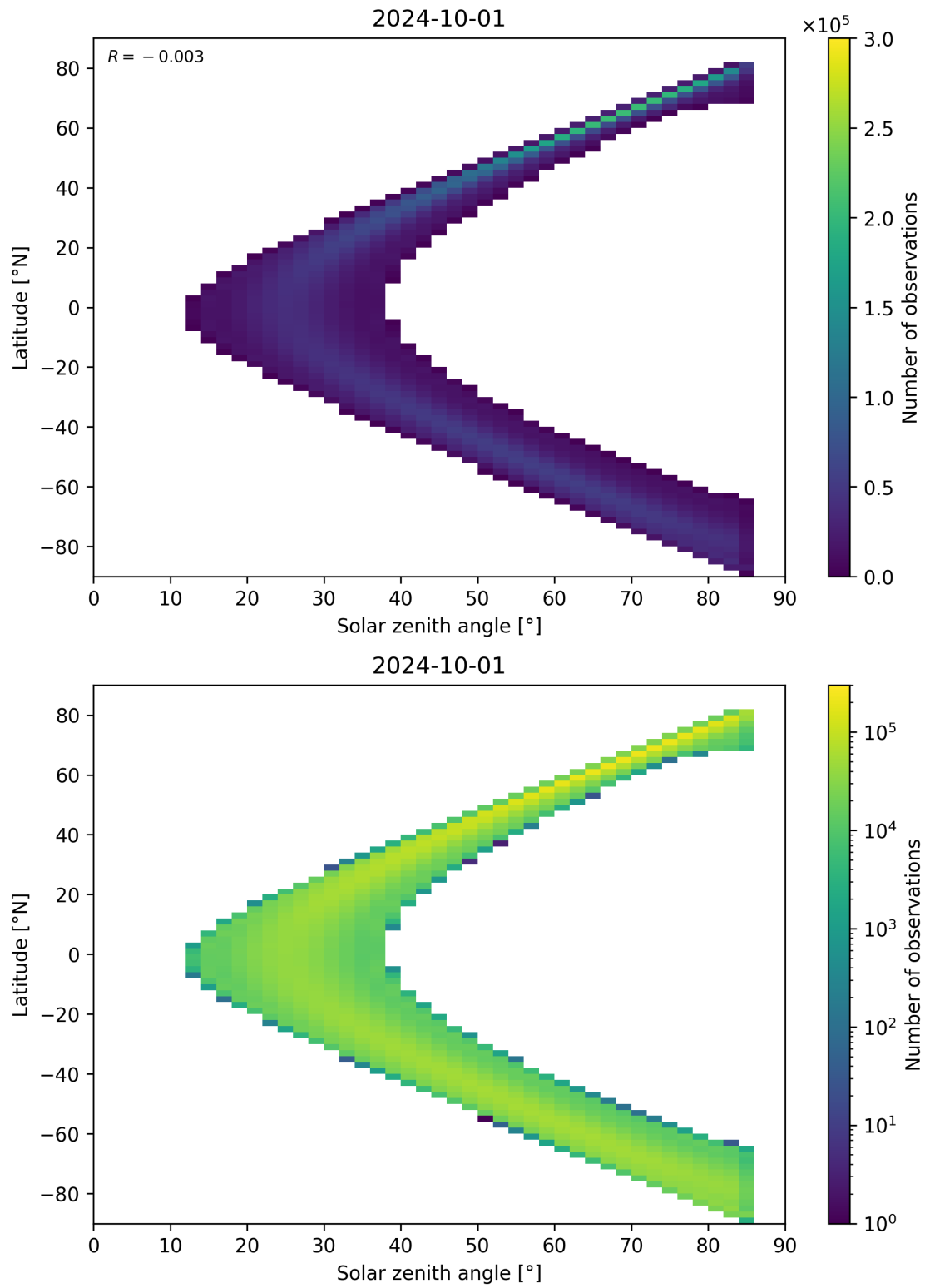
Figure 164: Scatter density plot of “Solar zenith angle” against “Latitude” for 2024-09-30 to 2024-10-02.
