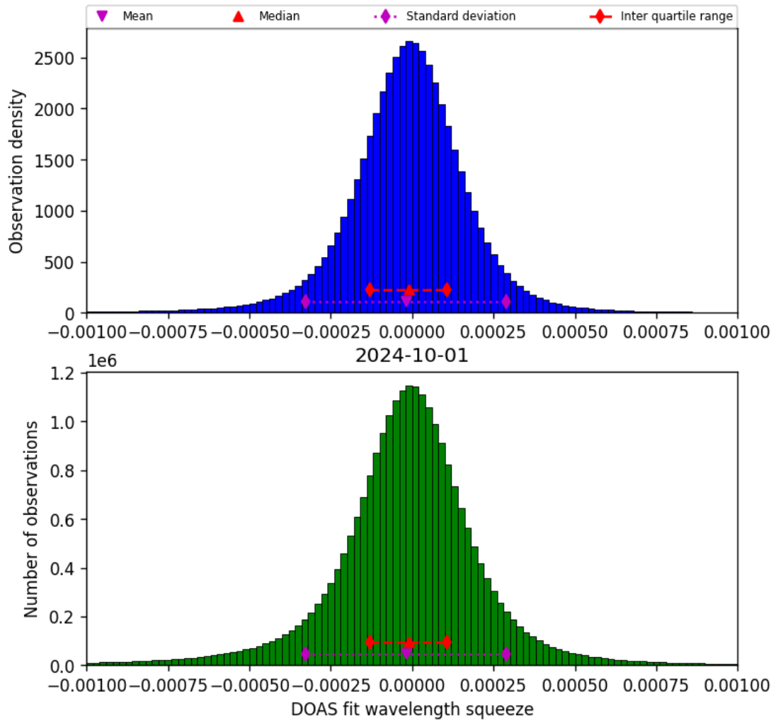
Figure 69: Histogram of “DOAS fit wavelength squeeze” for 2024-09-30 to 2024-10-02
