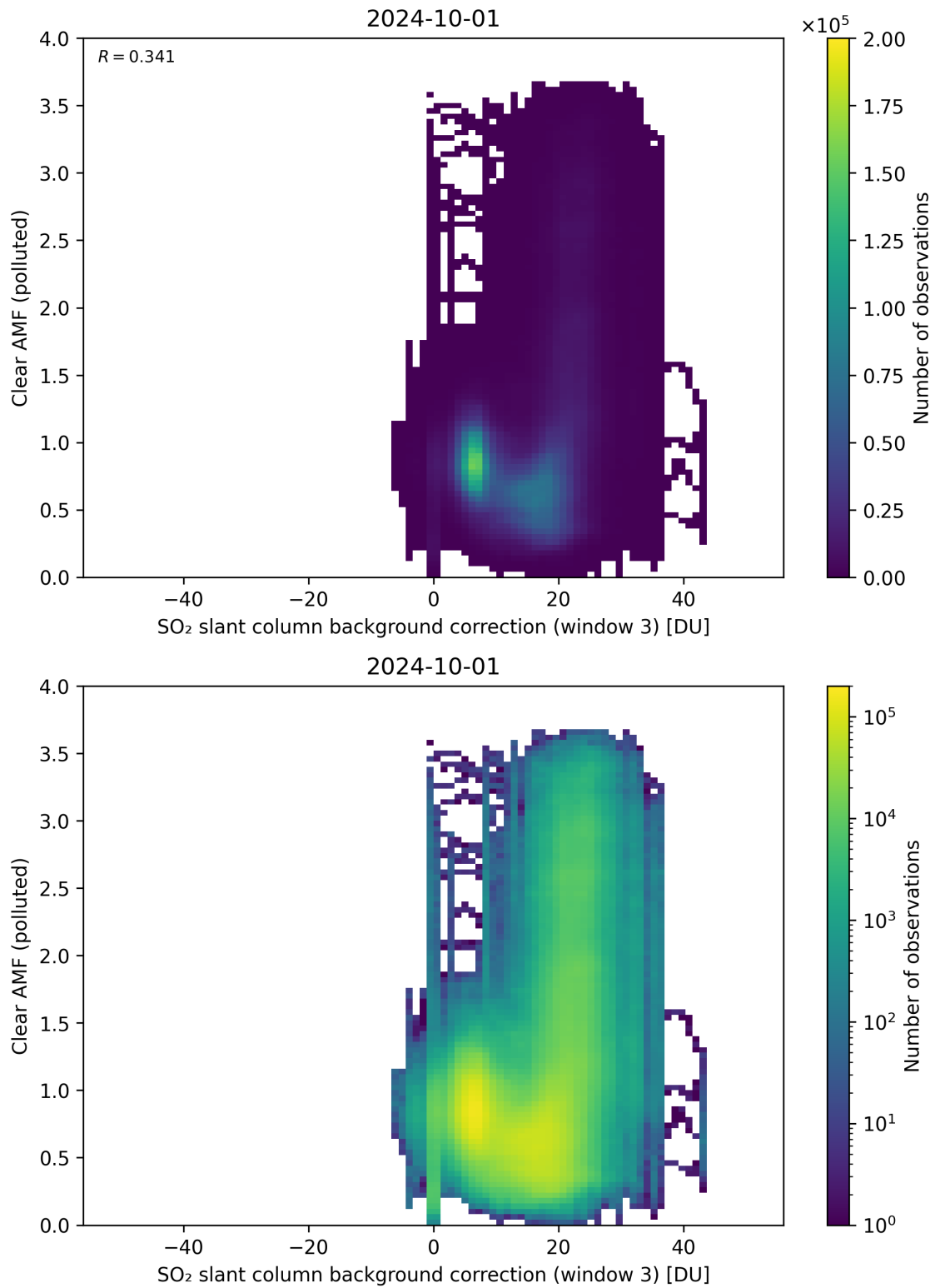
Figure 124: Scatter density plot of “SO 2 slant column background correction (window 3)” against “Clear AMF (polluted)” for 2024-09-30 to 2024-10-02.
