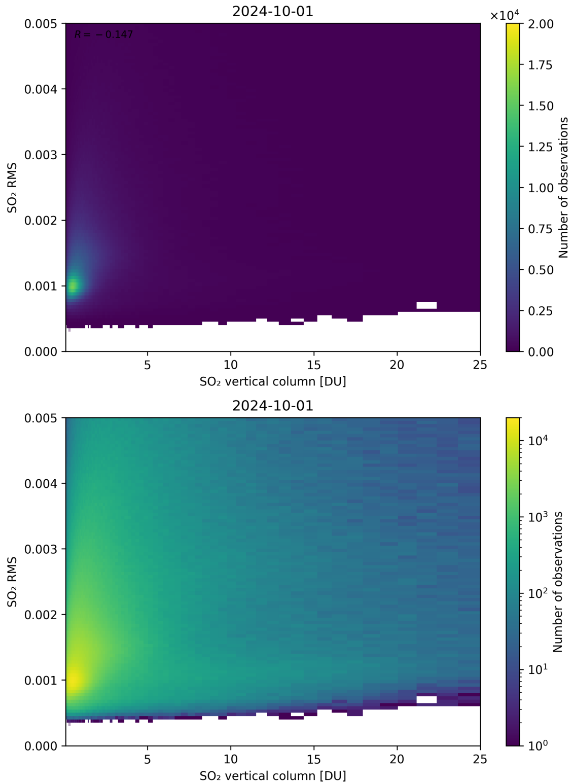
Figure 278: Scatter density plot of “SO 2 vertical column” against “SO 2 RMS” for 2024-09-30 to 2024-10-02.
