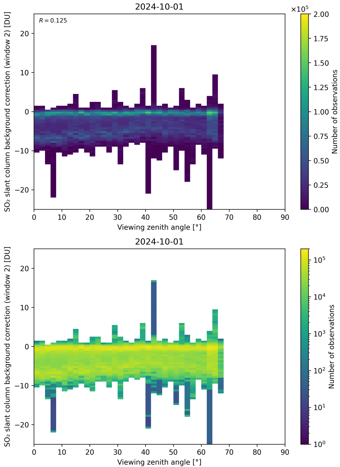
Figure 309: Scatter density plot of “Viewing zenith angle” against “SO 2 slant column background correction (window 2)” for 2024-09-30 to 2024-10-02.
