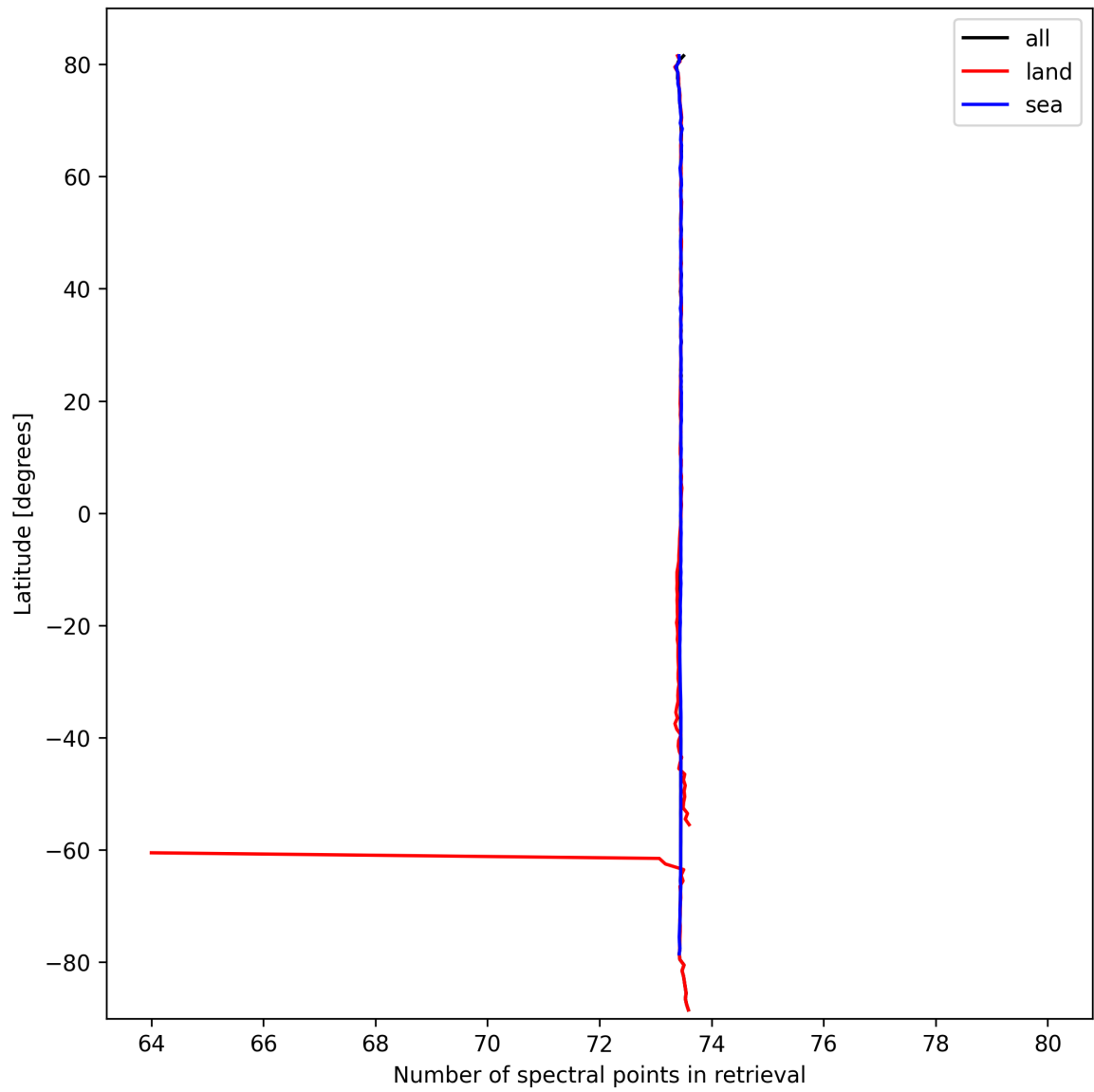
Figure 51: Zonal average of “Number of spectral points in retrieval” for 2024-09-30 to 2024-10-02.
