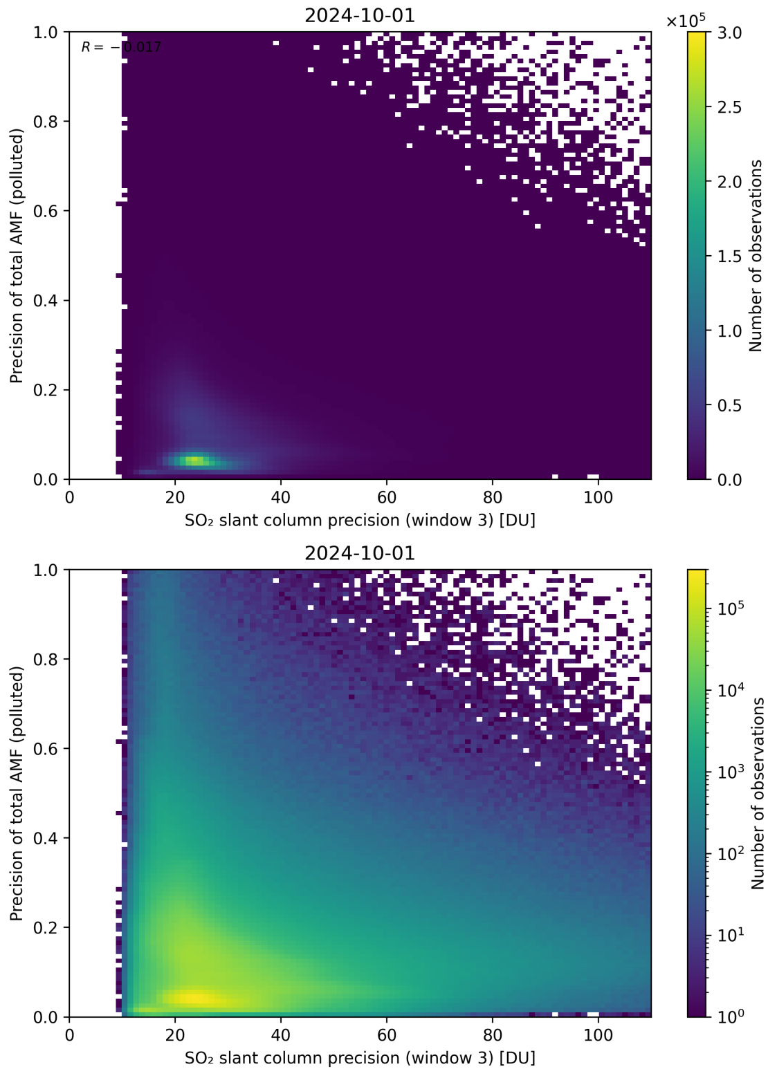
Figure 264: Scatter density plot of “SO 2 slant column precision (window 3)” against “Precision of total AMF (polluted)” for 2024-09-30 to 2024-10-02.
