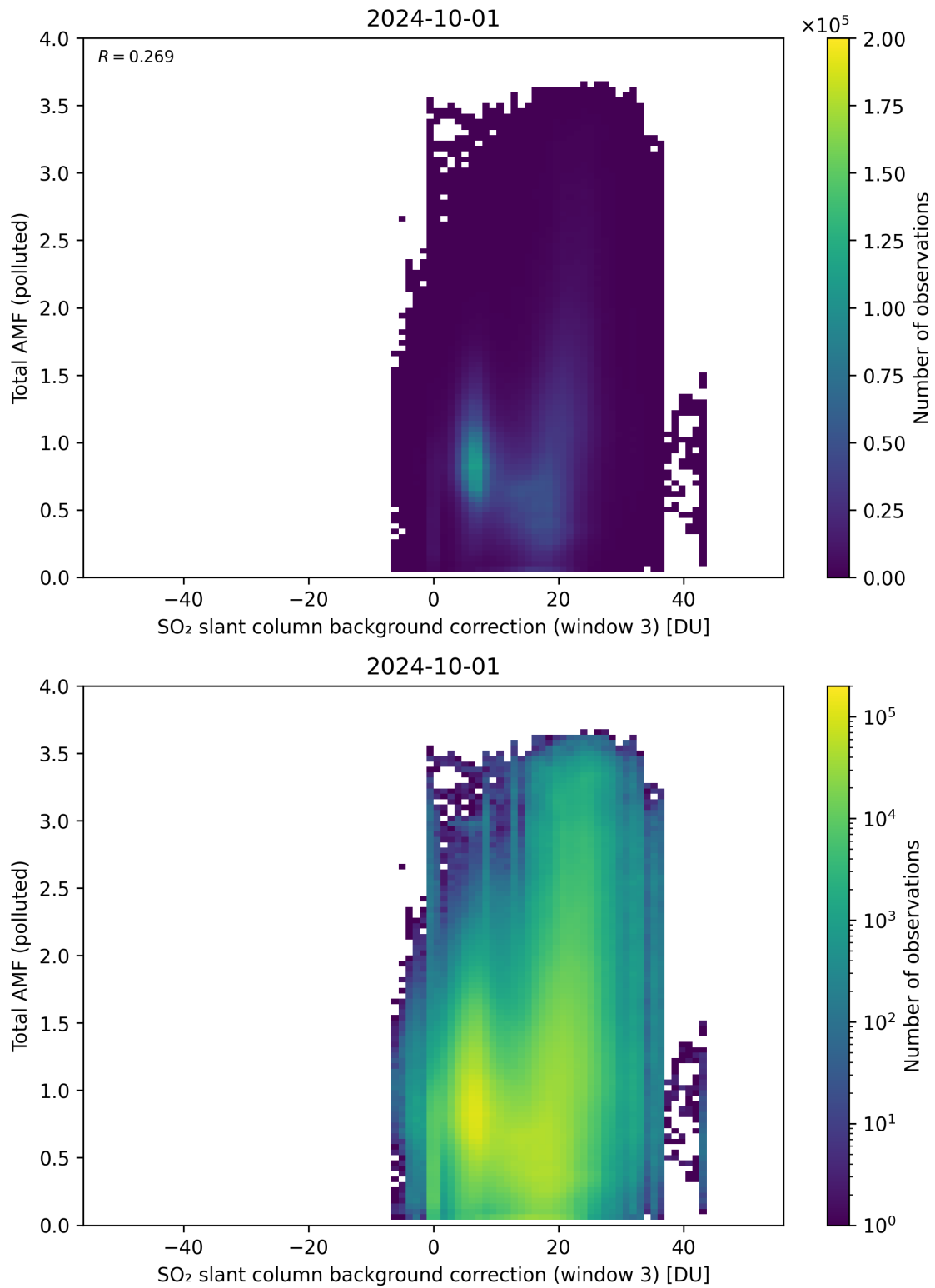
Figure 125: Scatter density plot of “SO 2 slant column background correction (window 3)” against “Total AMF (polluted)” for 2024-09-30 to 2024-10-02.
