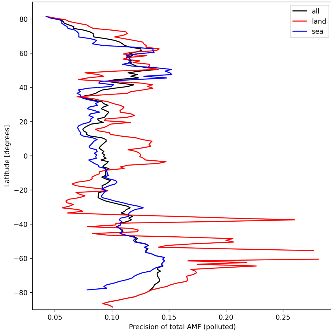
Figure 49: Zonal average of “Precision of total AMF (polluted)” for 2024-09-30 to 2024-10-02.
