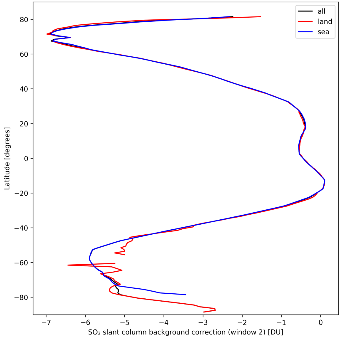
Figure 40: Zonal average of “SO 2 slant column background correction (window 2)” for 2024-09-30 to 2024-10-02.
