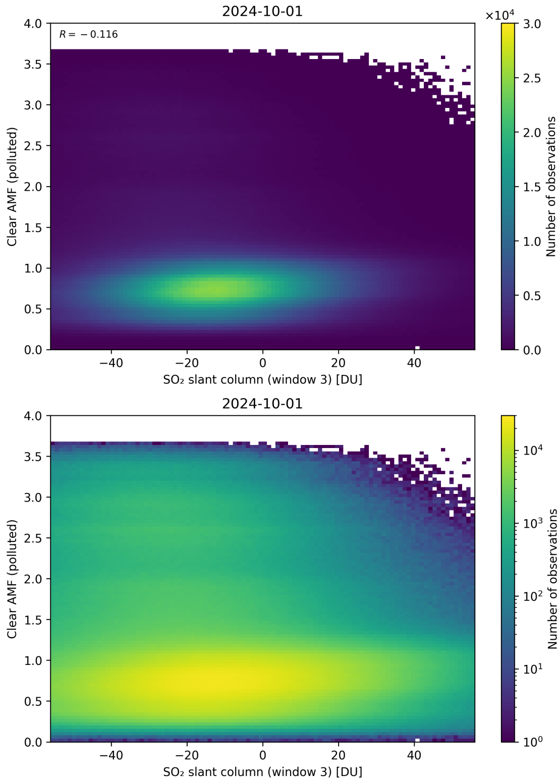
Figure 265: Scatter density plot of “SO 2 slant column (window 3)” against “Clear AMF (polluted)” for 2024-09-30 to 2024-10-02.
