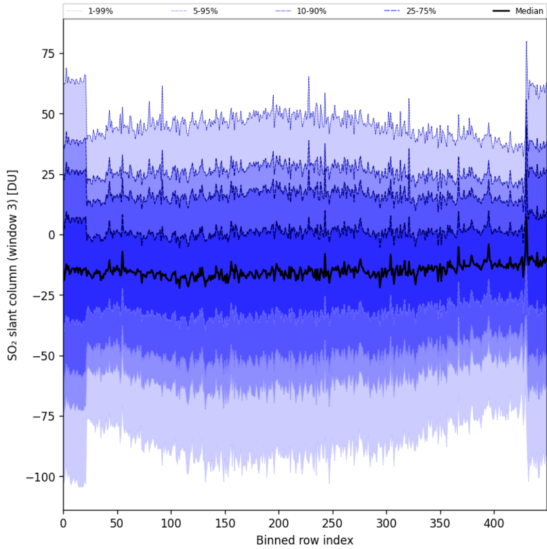
Figure 87: Along track statistics of “SO 2 slant column (window 3)” for 2024-09-30 to 2024-10-02
