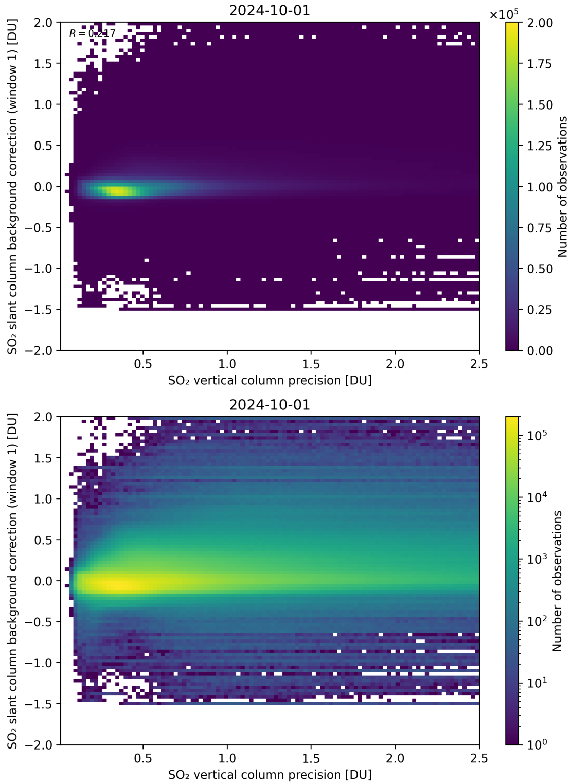
Figure 279: Scatter density plot of “SO 2 vertical column precision” against “SO 2 slant column background correction (window 1)” for 2024-09-30 to 2024-10-02.
