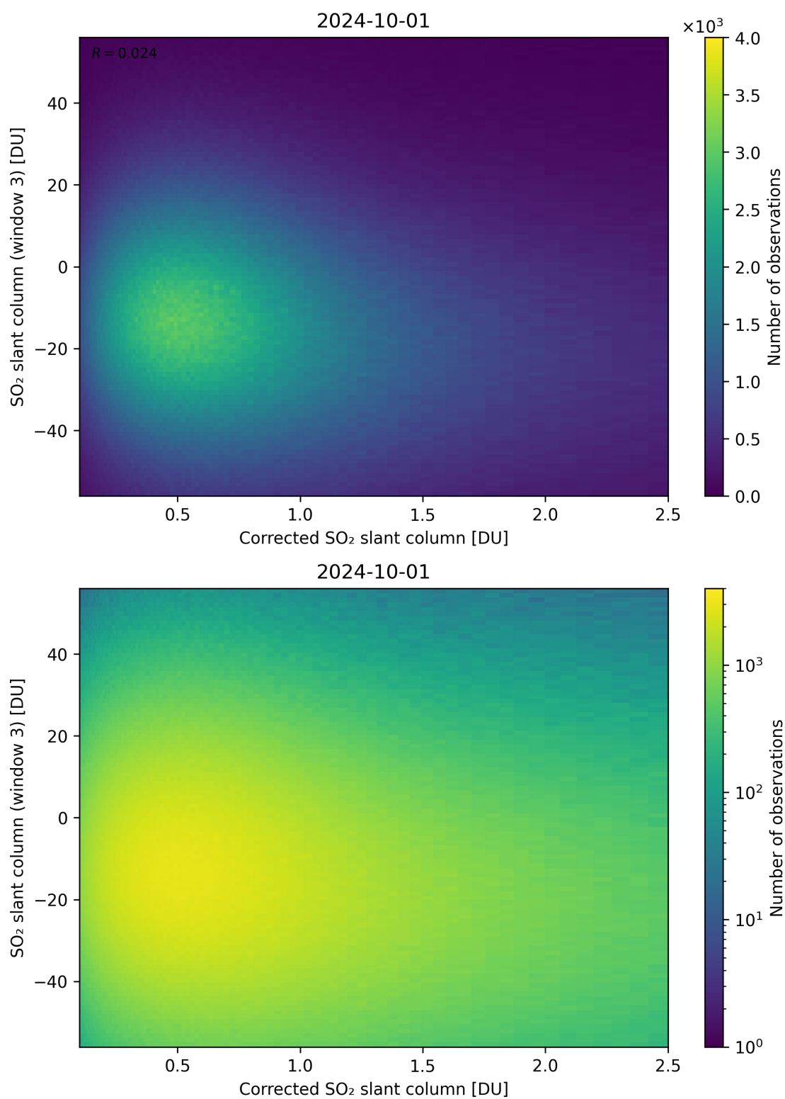
Figure 190: Scatter density plot of “Corrected SO 2 slant column” against “SO 2 slant column (window 3)” for 2024-09-30 to 2024-10-02.
