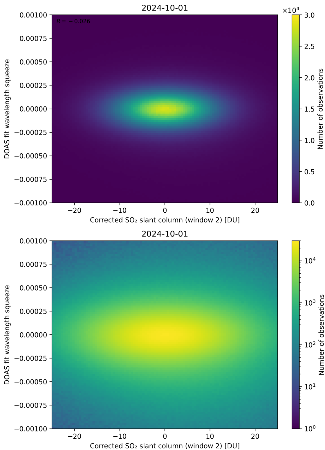
Figure 197: Scatter density plot of “Corrected SO 2 slant column (window 2)” against “DOAS fit wavelength squeeze” for 2024-09-30 to 2024-10-02.
