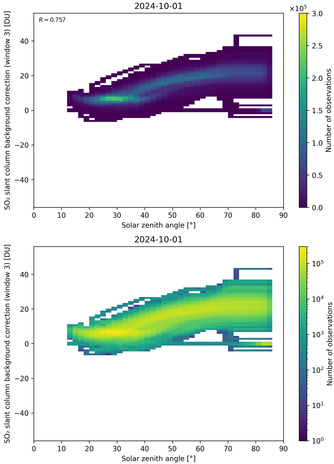
Figure 160: Scatter density plot of “Solar zenith angle” against “SO 2 slant column background correction (window 3)” for 2024-09-30 to 2024-10-02.
