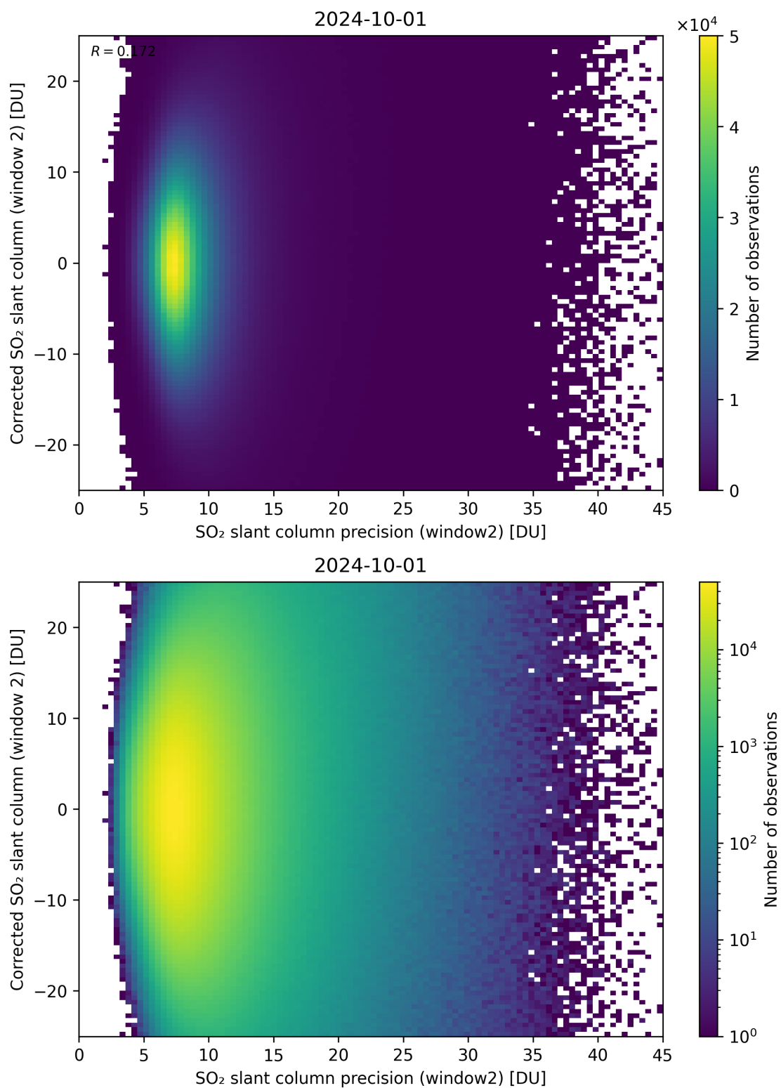
Figure 247: Scatter density plot of “SO 2 slant column precision (window2)” against “Corrected SO 2 slant column (window 2)” for 2024-09-30 to 2024-10-02.
