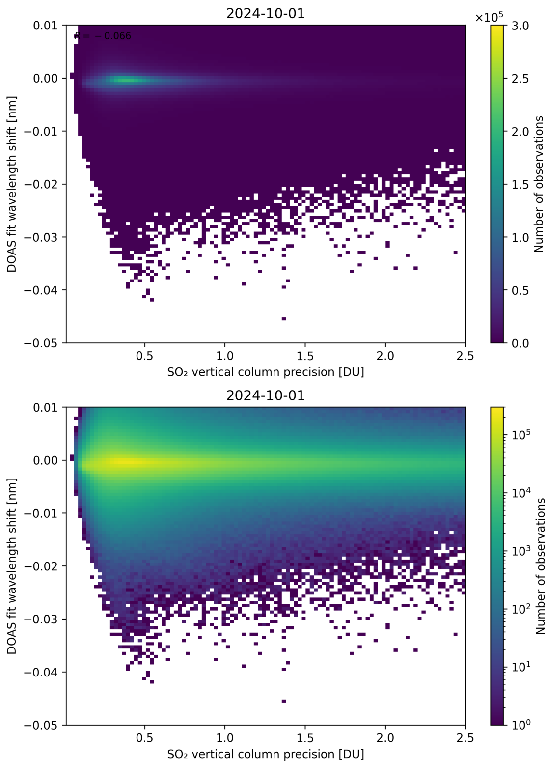
Figure 282: Scatter density plot of “SO 2 vertical column precision” against “DOAS fit wavelength shift” for 2024-09-30 to 2024-10-02.
