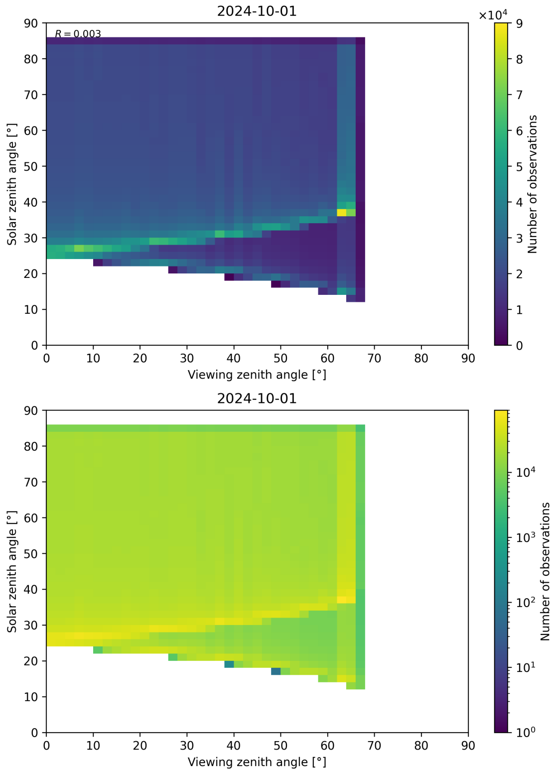
Figure 315: Scatter density plot of “Viewing zenith angle” against “Solar zenith angle” for 2024-09-30 to 2024-10-02.
