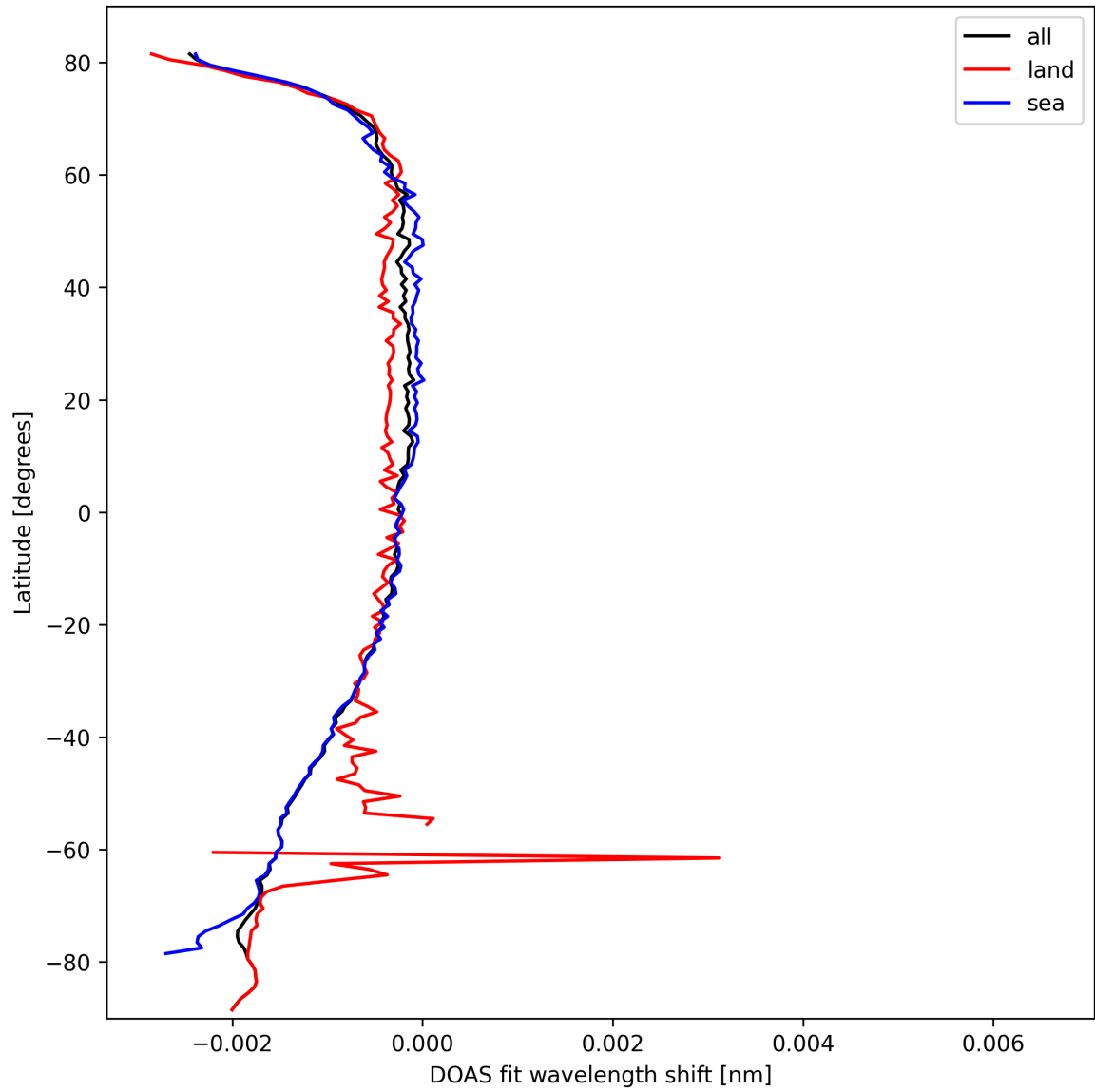
Figure 45: Zonal average of “DOAS fit wavelength shift” for 2024-09-30 to 2024-10-02.
