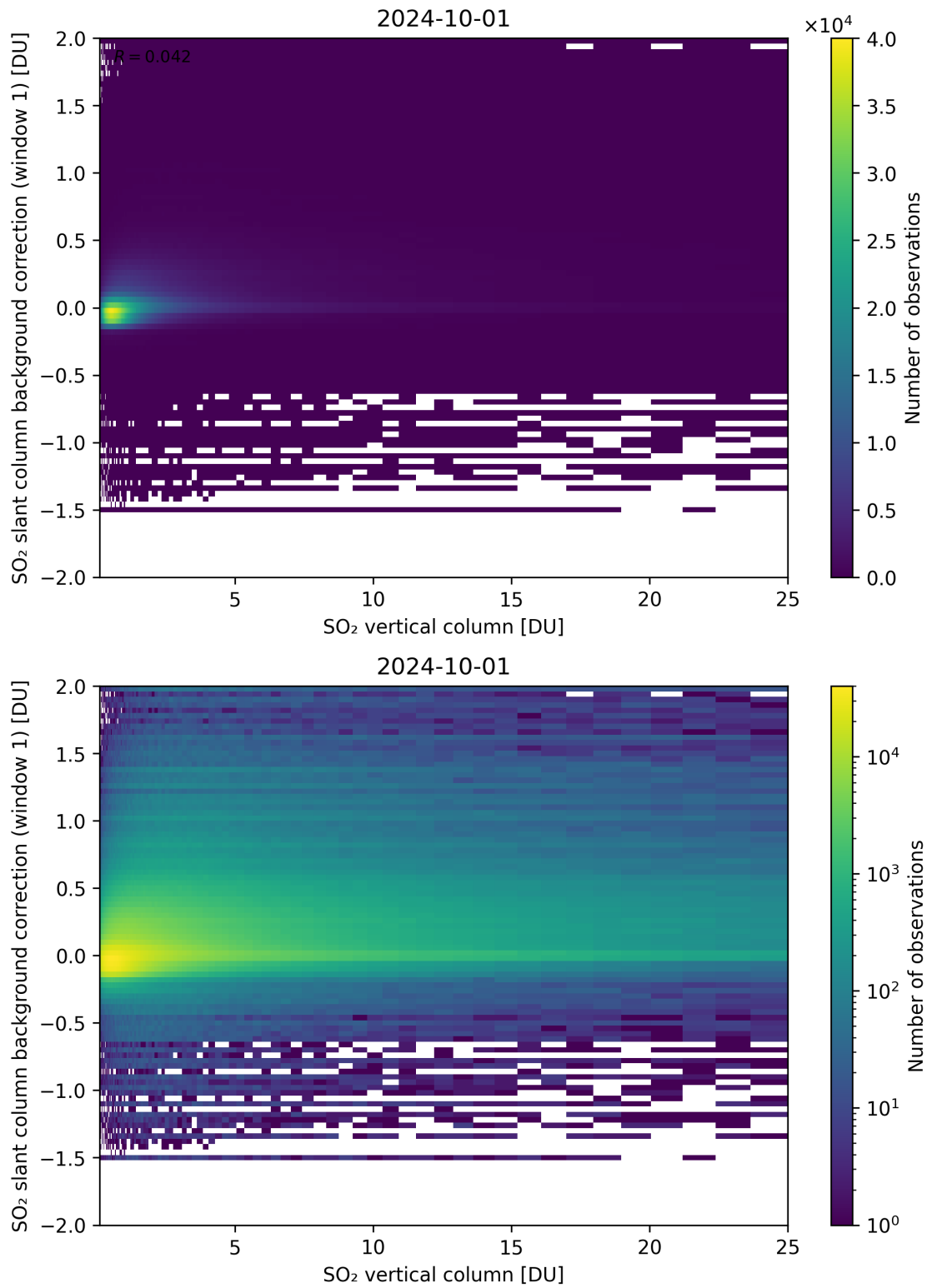
Figure 273: Scatter density plot of “SO 2 vertical column” against “SO 2 slant column background correction (window 1)” for 2024-09-30 to 2024-10-02.
