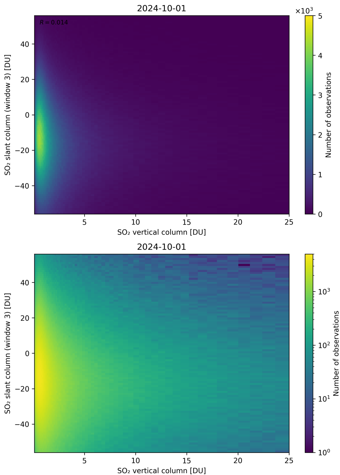
Figure 303: Scatter density plot of “SO 2 vertical column” against “SO 2 slant column (window 3)” for 2024-09-30 to 2024-10-02.
