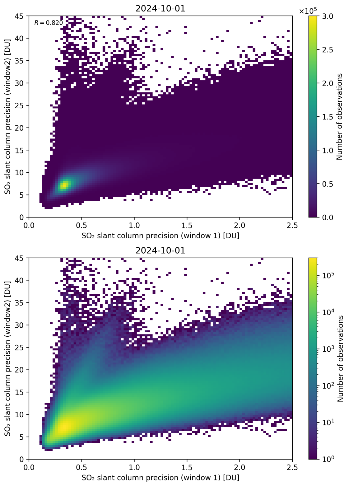
Figure 227: Scatter density plot of “SO 2 slant column precision (window 1)” against “SO 2 slant column precision (window2)” for 2024-09-30 to 2024-10-02.
