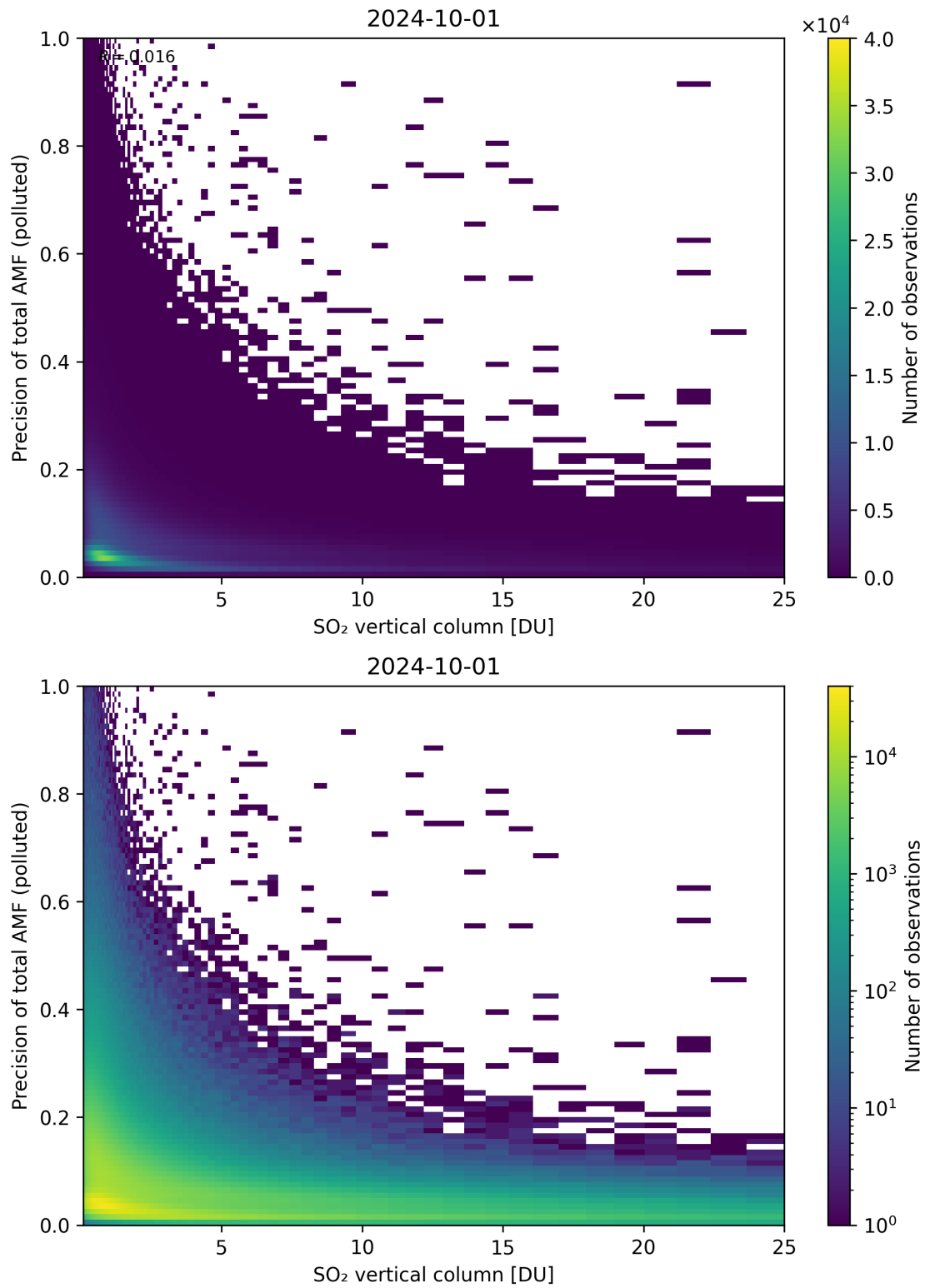
Figure 306: Scatter density plot of “SO 2 vertical column” against “Precision of total AMF (polluted)” for 2024-09-30 to 2024-10-02.
