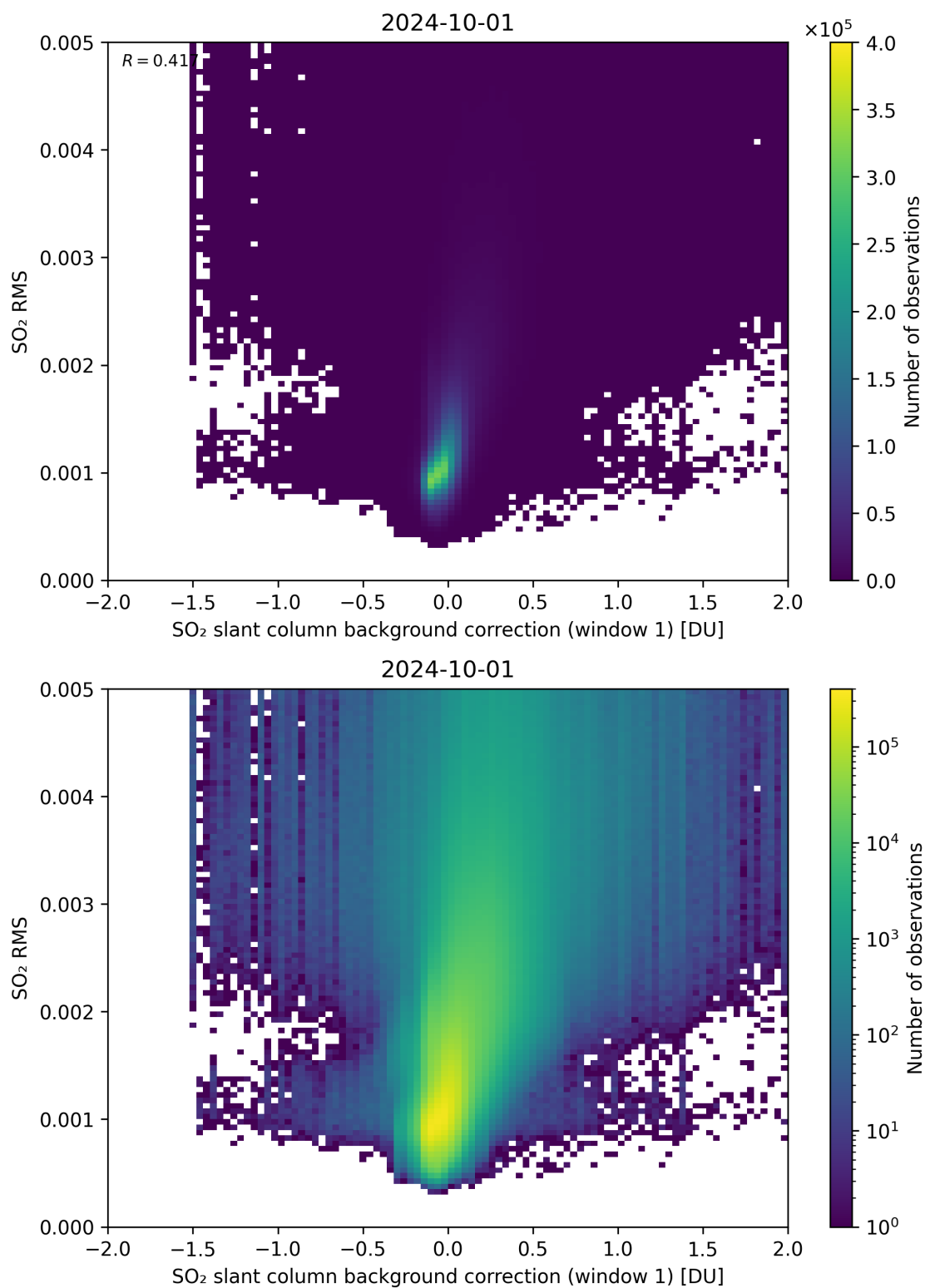
Figure 102: Scatter density plot of “SO 2 slant column background correction (window 1)” against “SO 2 RMS” for 2024-09-30 to 2024-10-02.
