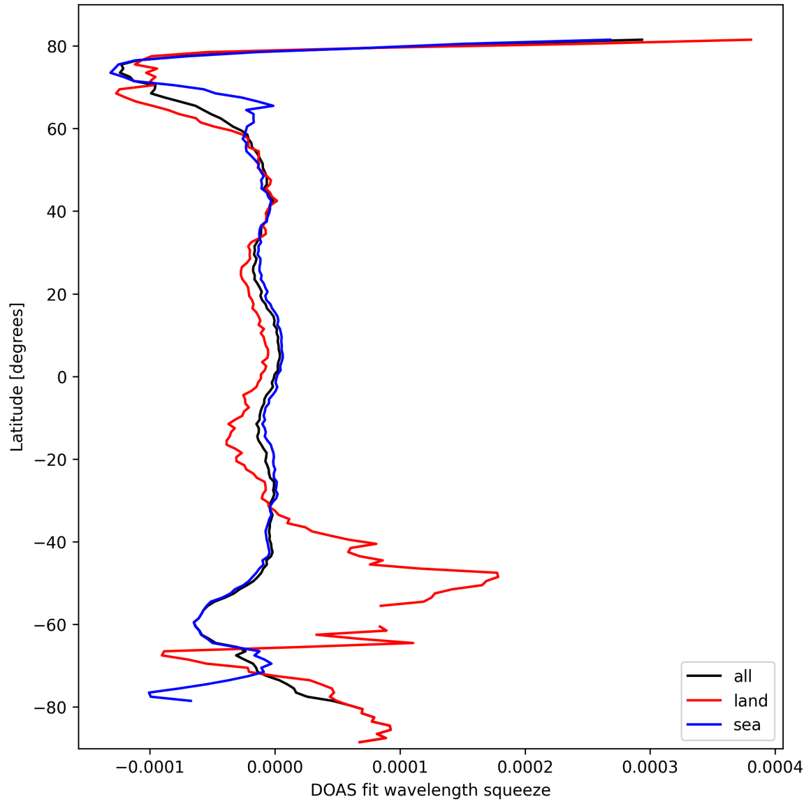
Figure 46: Zonal average of “DOAS fit wavelength squeeze” for 2024-09-30 to 2024-10-02.
