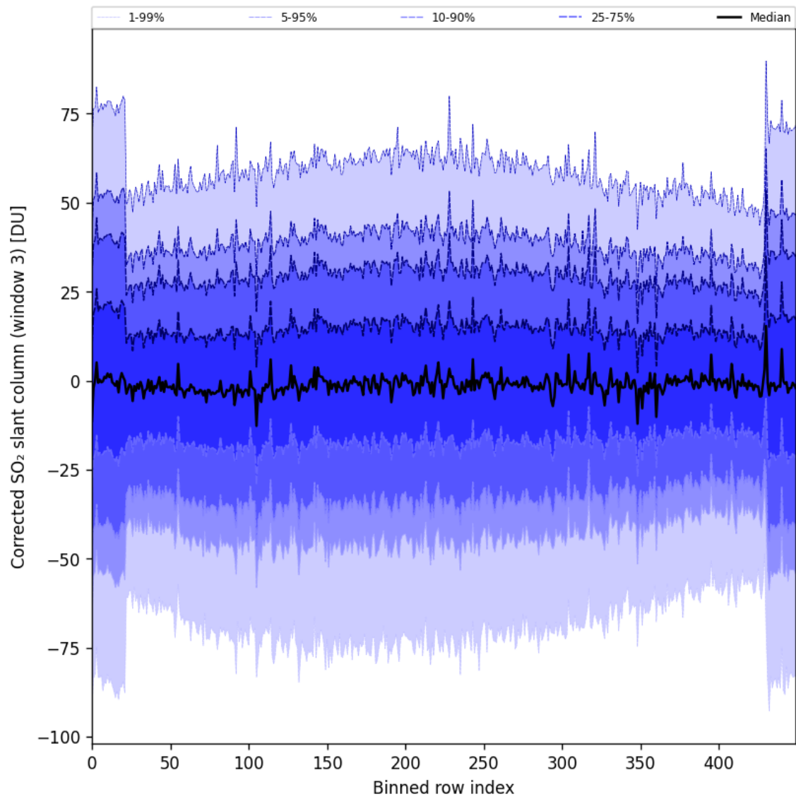
Figure 89: Along track statistics of "Corrected SO 2 slant column (window 3)" for 2024-09-30 to 2024-10-02
