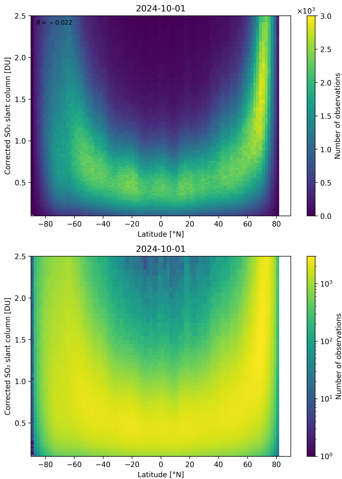
Figure 146: Scatter density plot of “Latitude” against “Corrected SO 2 slant column” for 2024-09-30 to 2024-10-02.
