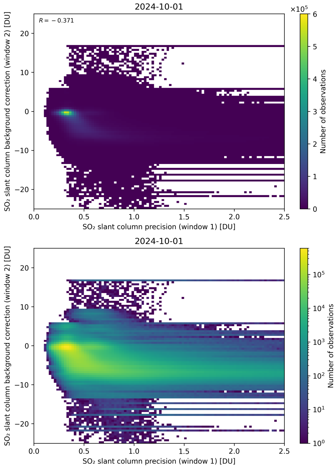
Figure 219: Scatter density plot of “SO 2 slant column precision (window 1)” against “SO 2 slant column background correction (window 2)” for 2024-09-30 to 2024-10-02.
