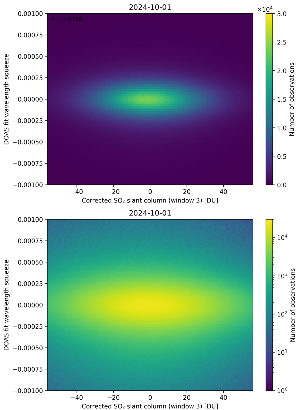
Figure 207: Scatter density plot of “Corrected SO 2 slant column (window 3)” against “DOAS fit wavelength squeeze” for 2024-09-30 to 2024-10-02.
