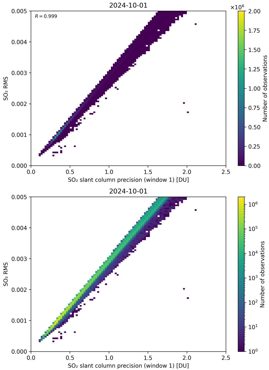
Figure 223: Scatter density plot of “SO 2 slant column precision (window 1)” against “SO 2 RMS” for 2024-09-30 to 2024-10-02.
