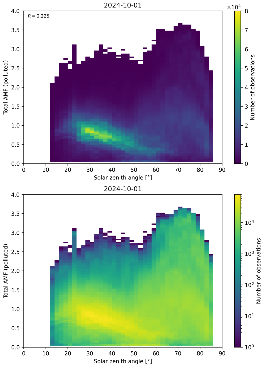
Figure 174: Scatter density plot of “Solar zenith angle” against “Total AMF (polluted)” for 2024-09-30 to 2024-10-02.
