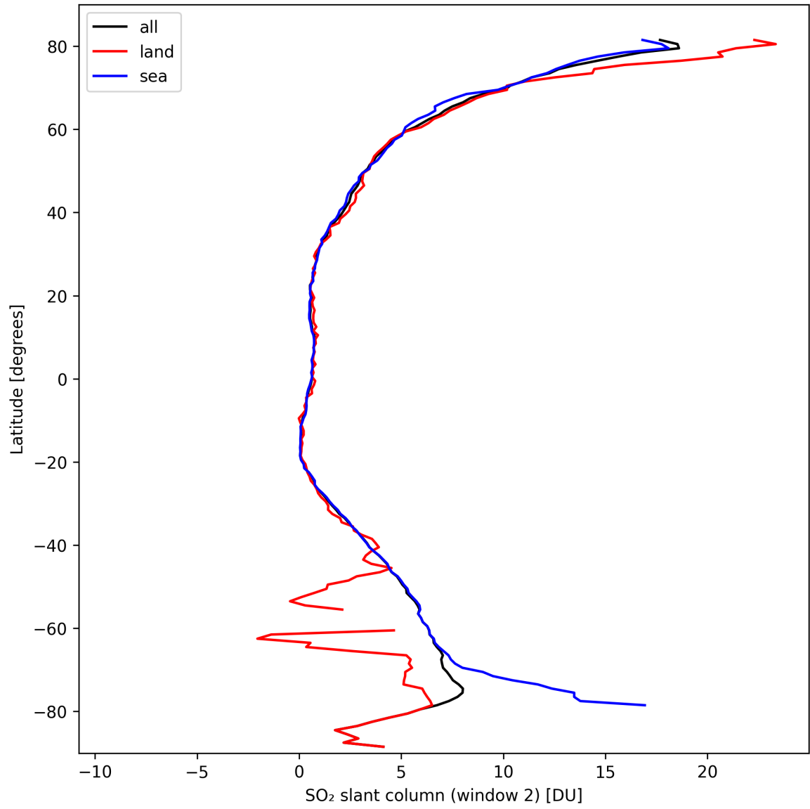
Figure 37: Zonal average of “SO 2 slant column (window 2)” for 2024-09-30 to 2024-10-02.
