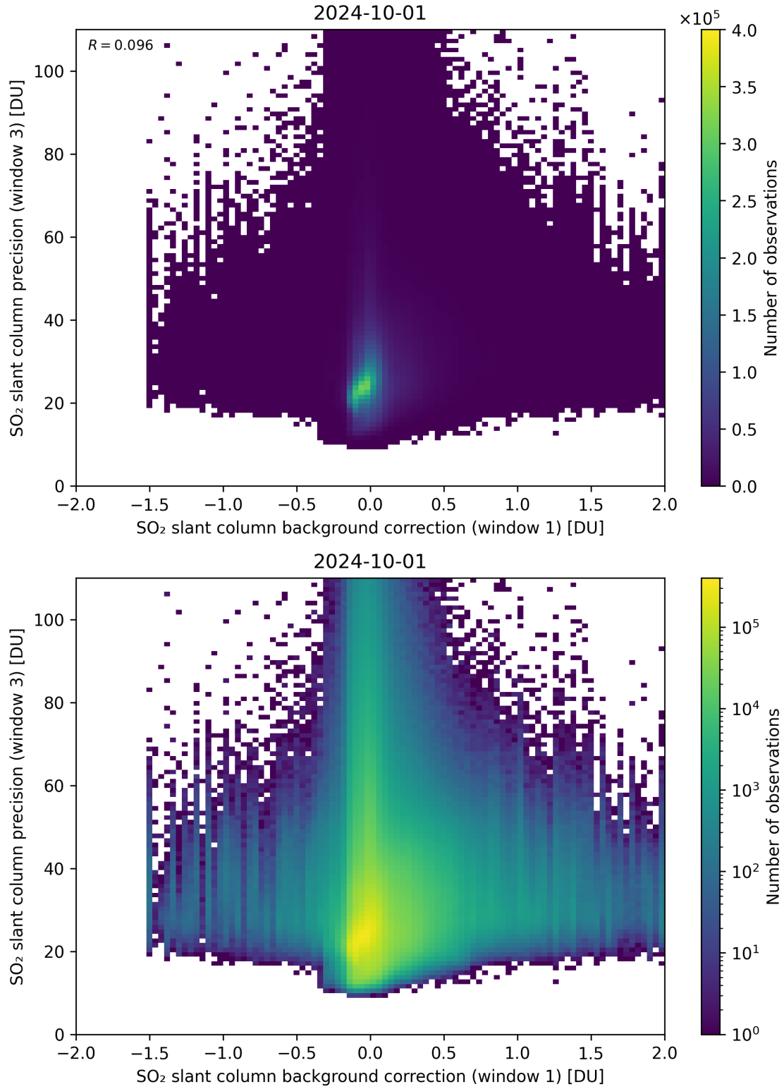
Figure 108: Scatter density plot of “SO 2 slant column background correction (window 1)” against “SO 2 slant column precision (window 3)” for 2024-09-30 to 2024-10-02.
