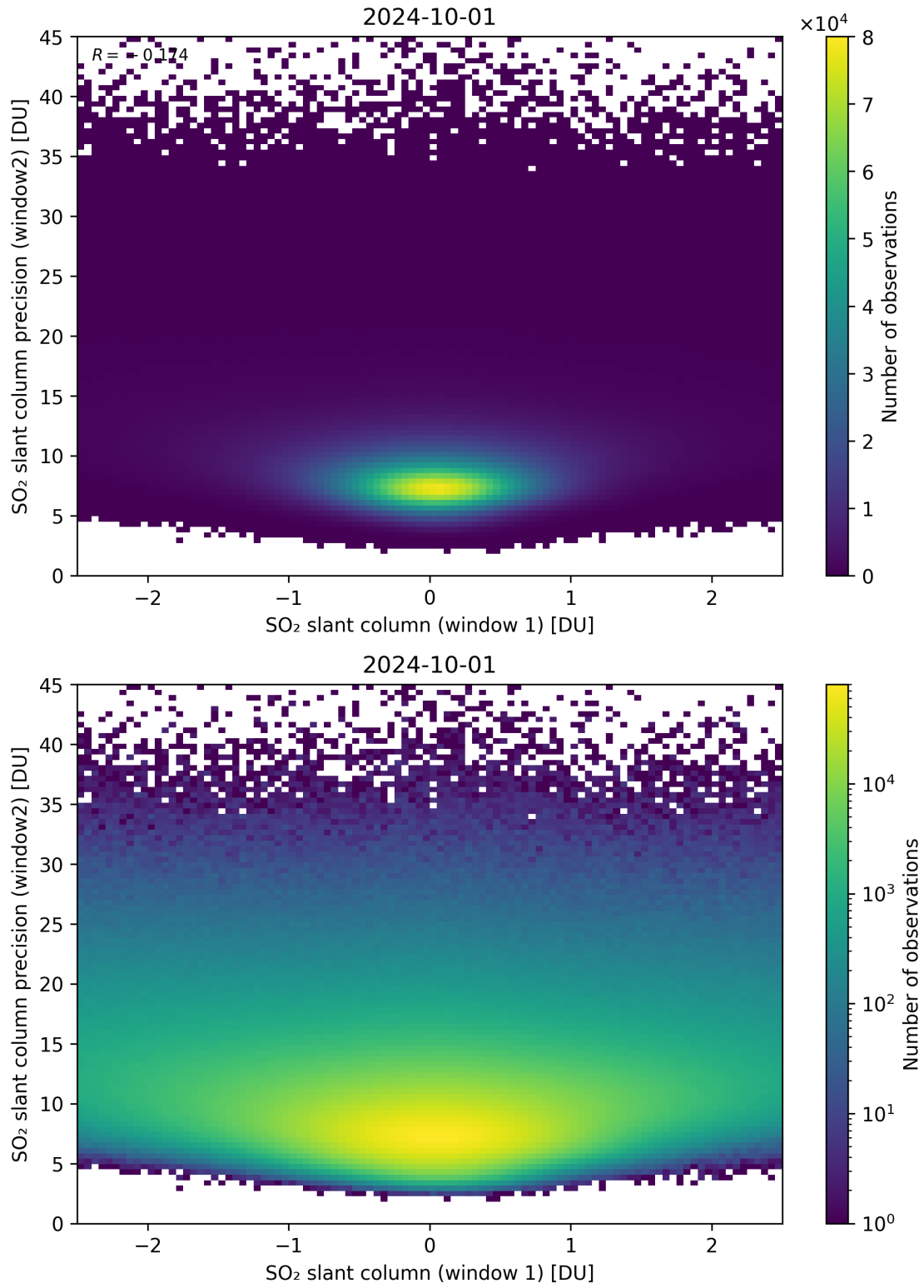
Figure 236: Scatter density plot of “SO 2 slant column (window 1)” against “SO 2 slant column precision (window2)” for 2024-09-30 to 2024-10-02.
