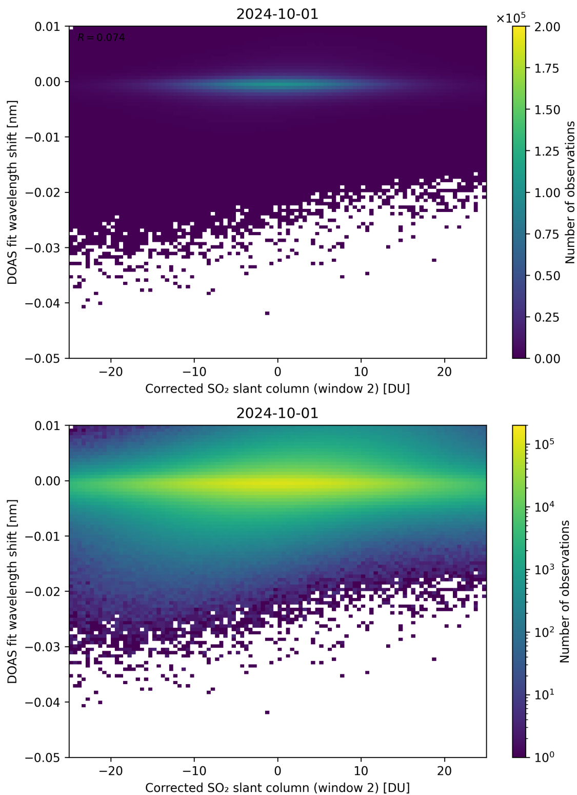
Figure 196: Scatter density plot of “Corrected SO 2 slant column (window 2)” against “DOAS fit wavelength shift” for 2024-09-30 to 2024-10-02.
