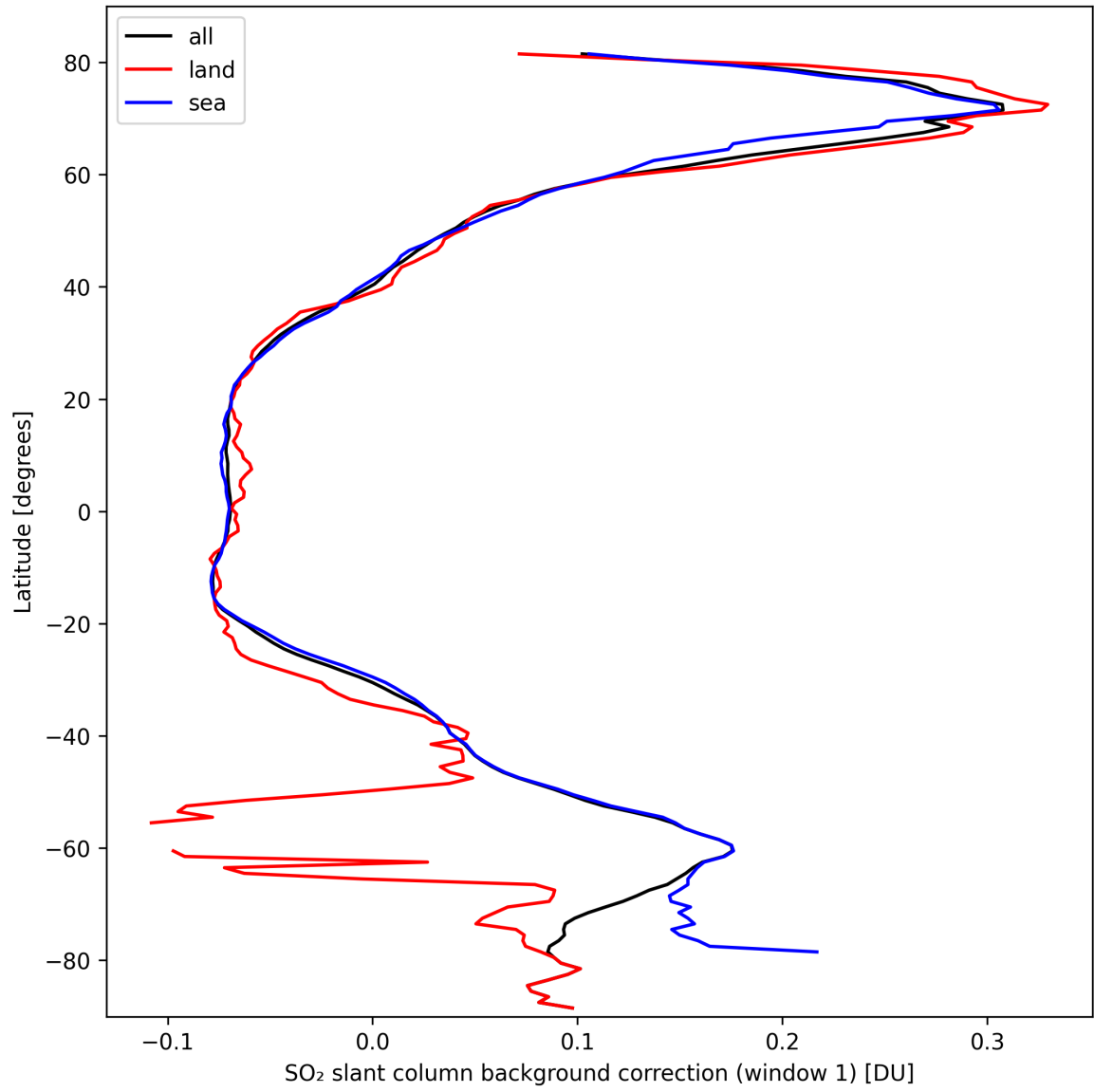
Figure 36: Zonal average of "SO 2 slant column background correction (window 1)" for 2024-09-30 to 2024-10-02.
