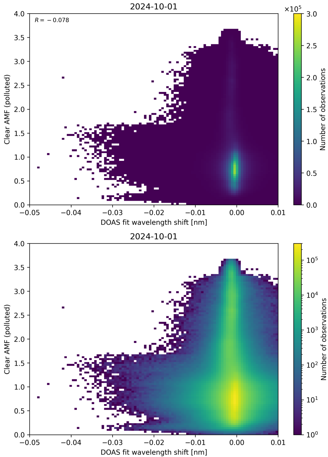
Figure 129: Scatter density plot of “DOAS fit wavelength shift” against “Clear AMF (polluted)” for 2024-09-30 to 2024-10-02.
