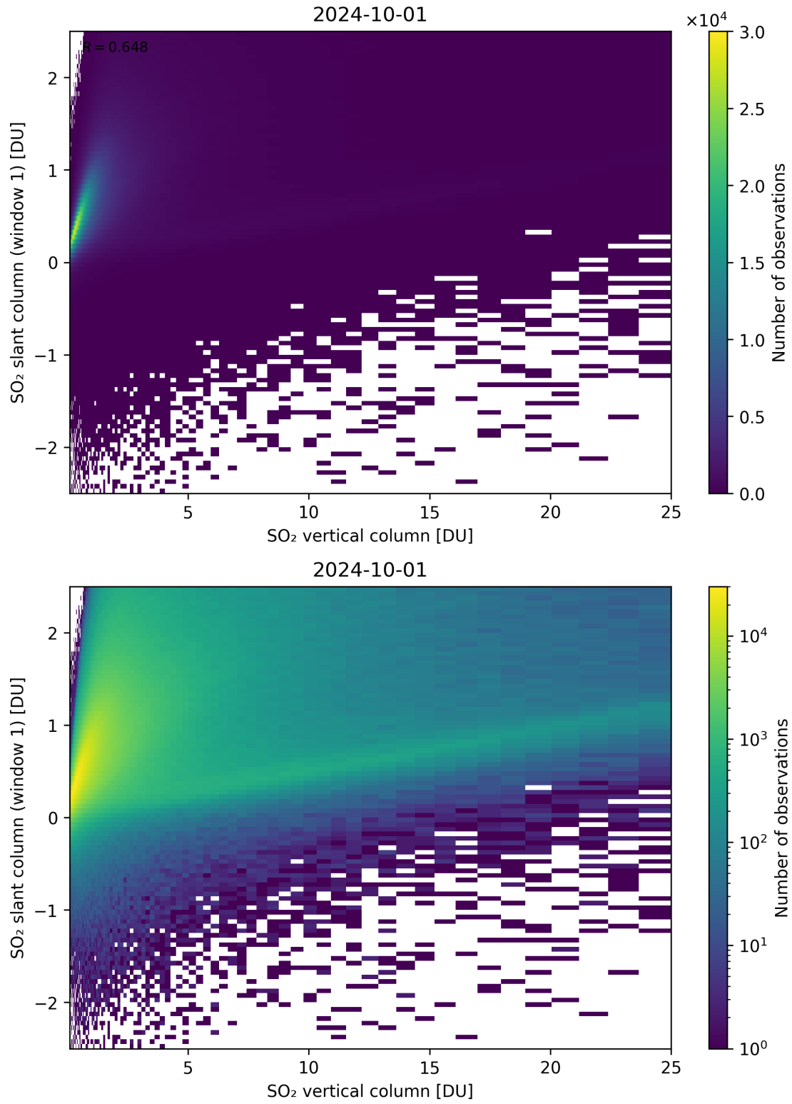
Figure 300: Scatter density plot of “SO 2 vertical column” against “SO 2 slant column (window 1)” for 2024-09-30 to 2024-10-02.
