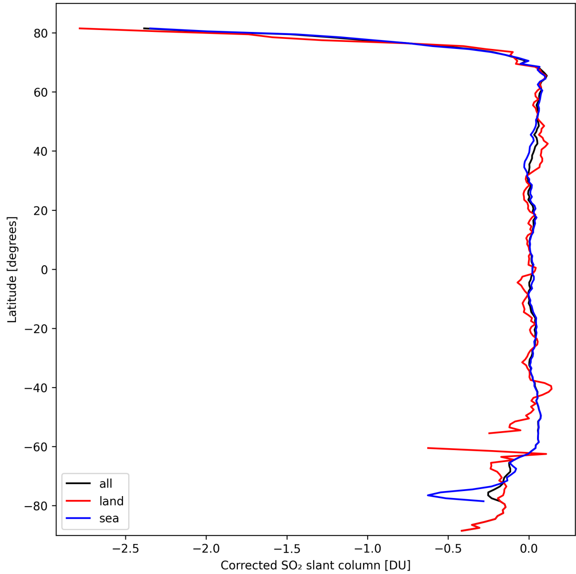
Figure 32: Zonal average of “Corrected SO 2 slant column” for 2024-09-30 to 2024-10-02.
