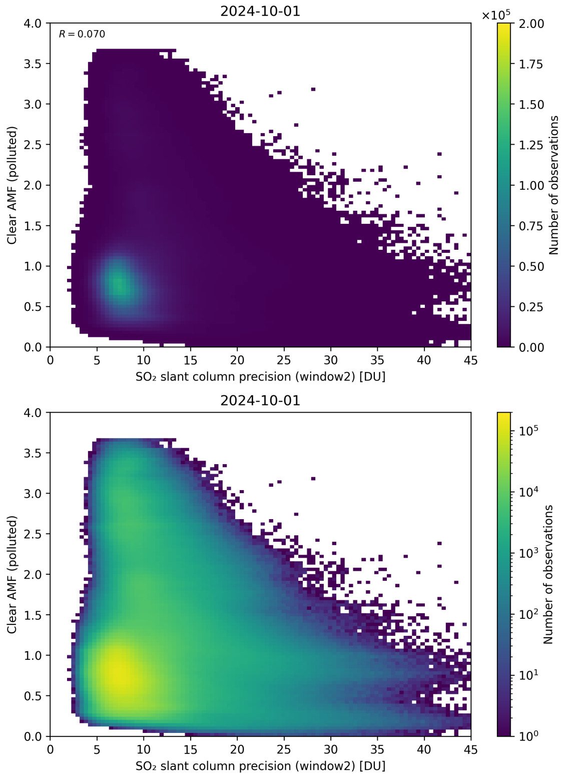
Figure 246: Scatter density plot of “SO 2 slant column precision (window2)” against “Clear AMF (polluted)” for 2024-09-30 to 2024-10-02.
