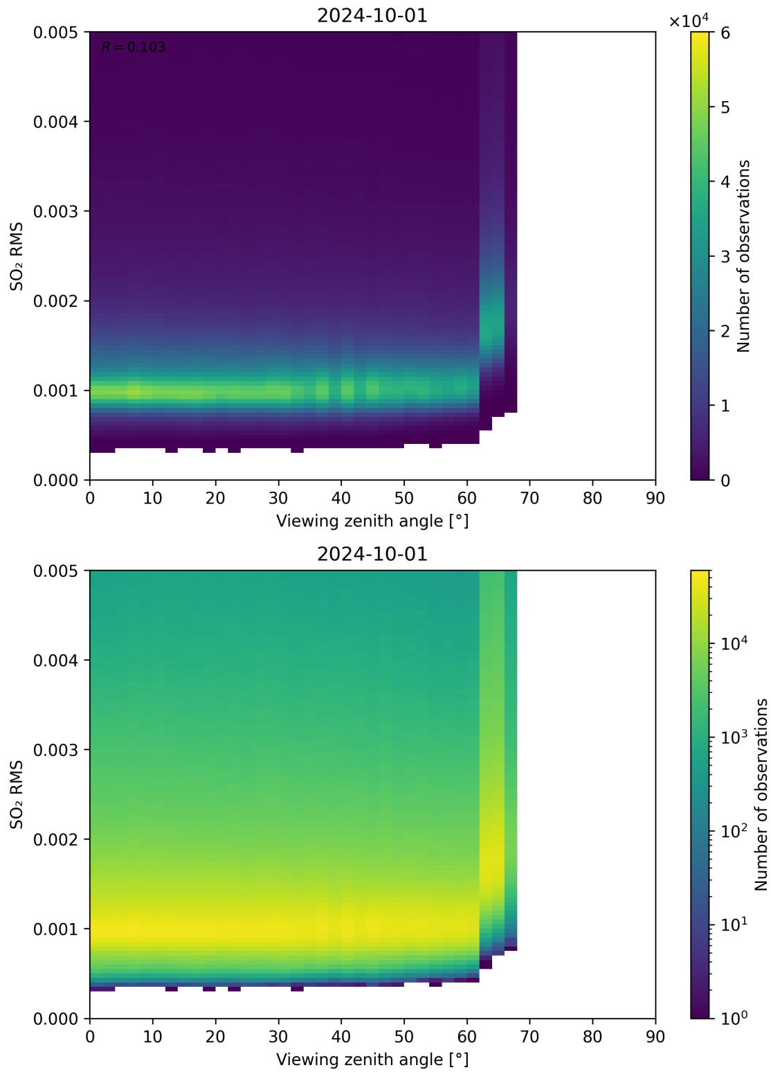
Figure 313: Scatter density plot of “Viewing zenith angle” against “SO 2 RMS” for 2024-09-30 to 2024-10-02.
