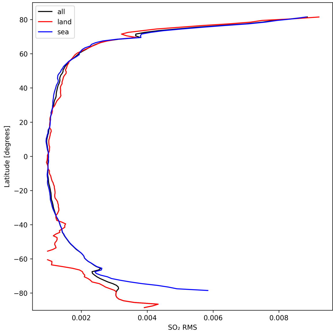
Figure 47: Zonal average of “SO 2 RMS” for 2024-09-30 to 2024-10-02.
