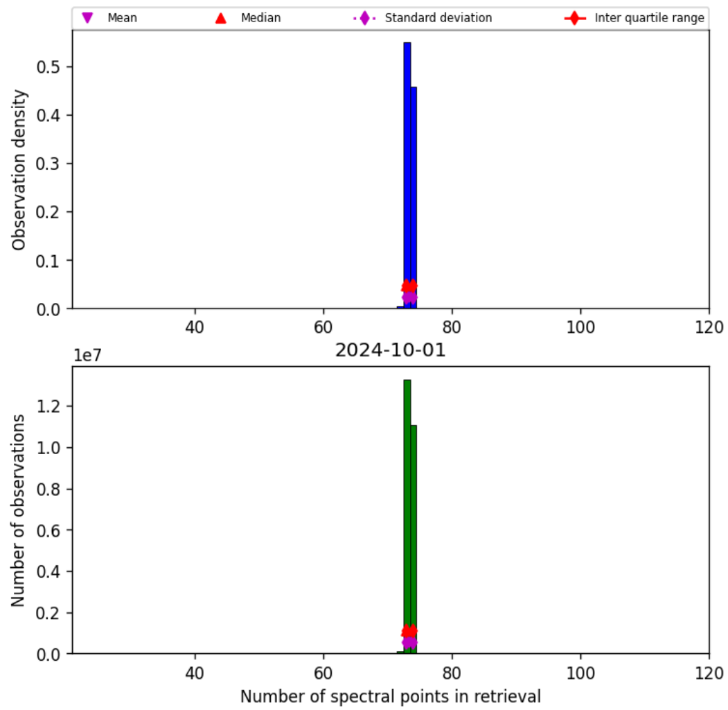
Figure 74: Histogram of “Number of spectral points in retrieval” for 2024-09-30 to 2024-10-02
