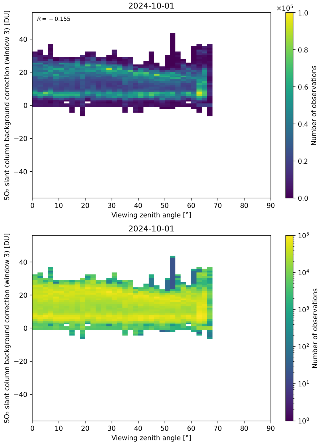
Figure 310: Scatter density plot of “Viewing zenith angle” against “SO 2 slant column background correction (window 3)” for 2024-09-30 to 2024-10-02.
