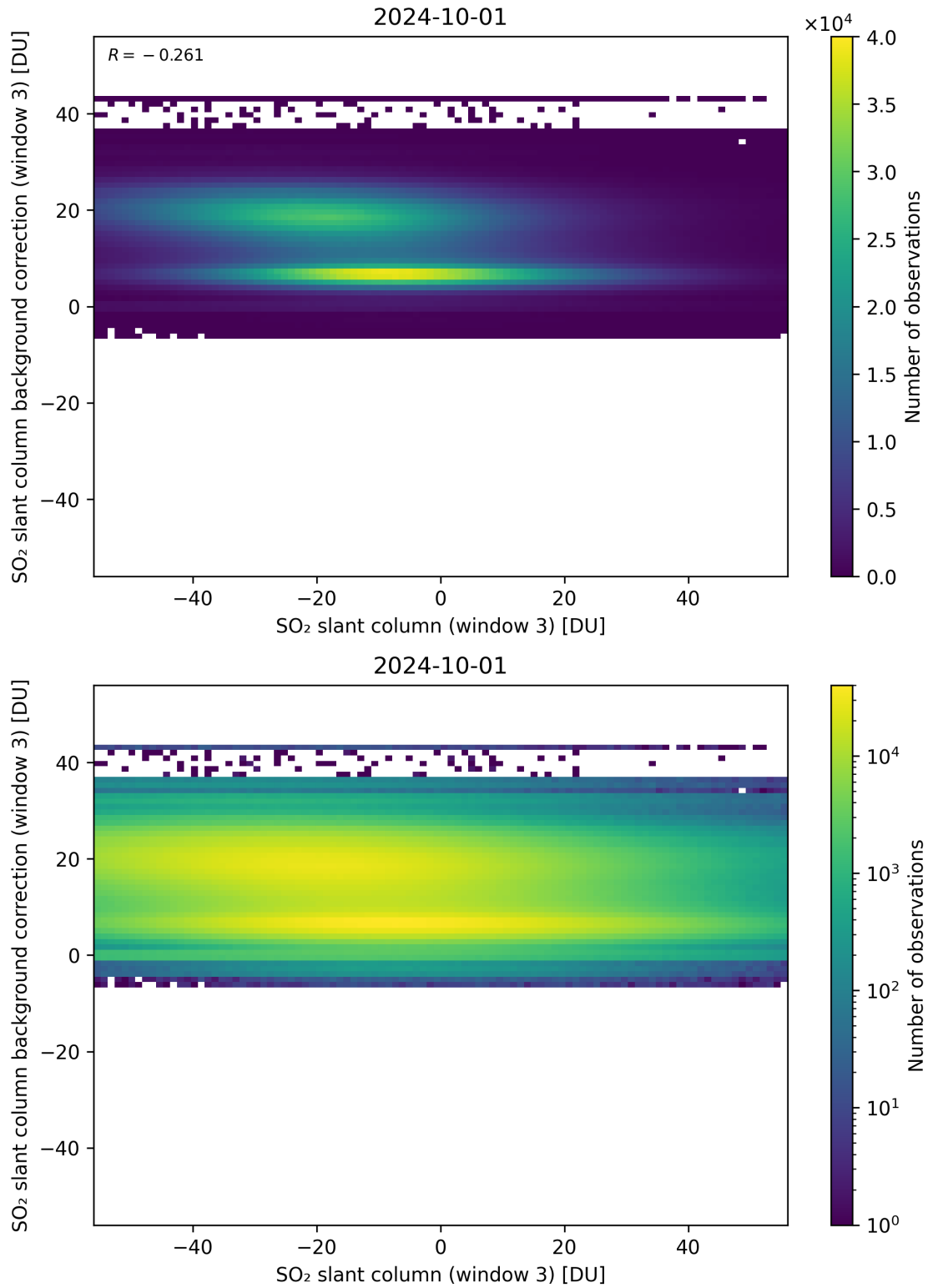
Figure 253: Scatter density plot of “SO 2 slant column (window 3)” against “SO 2 slant column background correction (window 3)” for 2024-09-30 to 2024-10-02.
