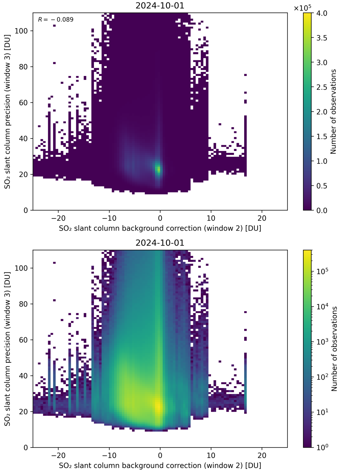
Figure 118: Scatter density plot of “SO 2 slant column background correction (window 2)” against “SO 2 slant column precision (window 3)” for 2024-09-30 to 2024-10-02.
