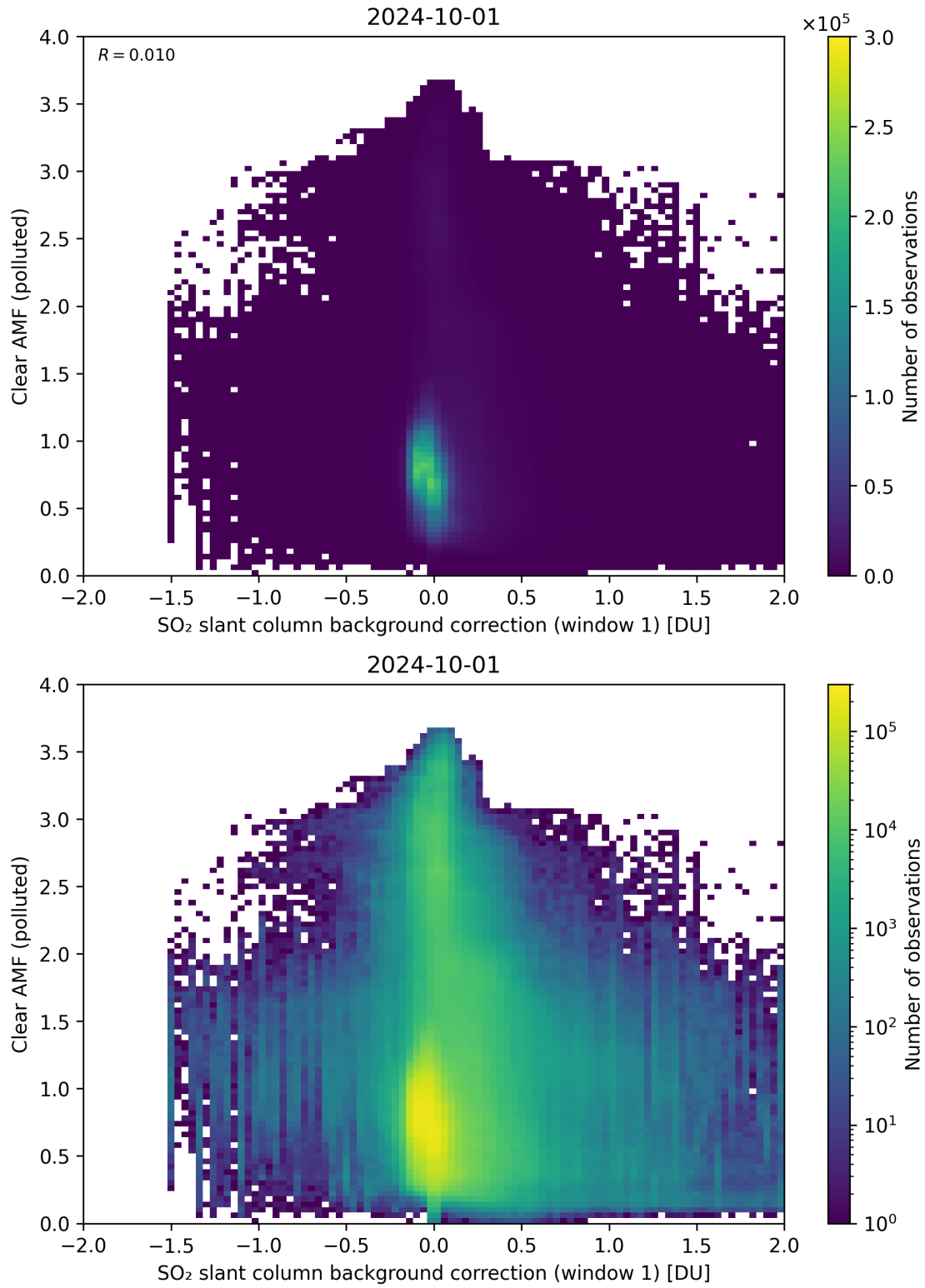
Figure 103: Scatter density plot of “SO 2 slant column background correction (window 1)” against “Clear AMF (polluted)” for 2024-09-30 to 2024-10-02.
