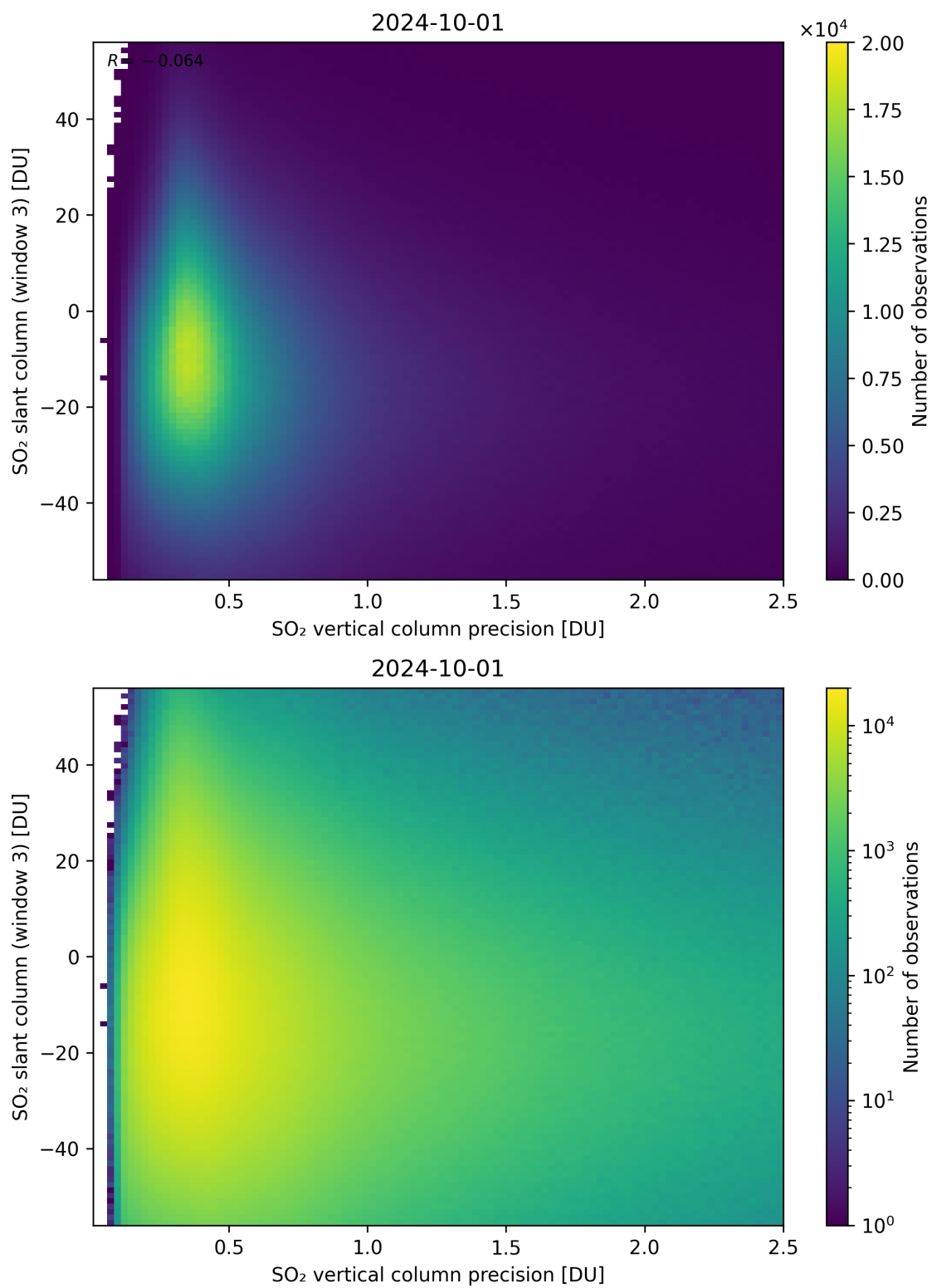
Figure 292: Scatter density plot of “SO 2 vertical column precision” against “SO 2 slant column (window 3)” for 2024-09-30 to 2024-10-02.
