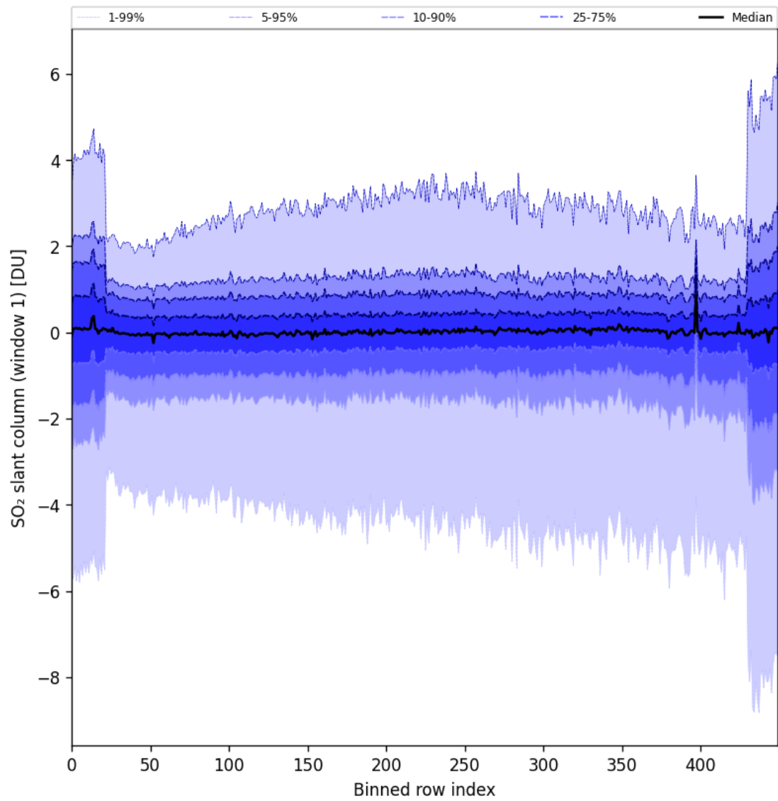
Figure 79: Along track statistics of “SO 2 slant column (window 1)” for 2024-09-30 to 2024-10-02
