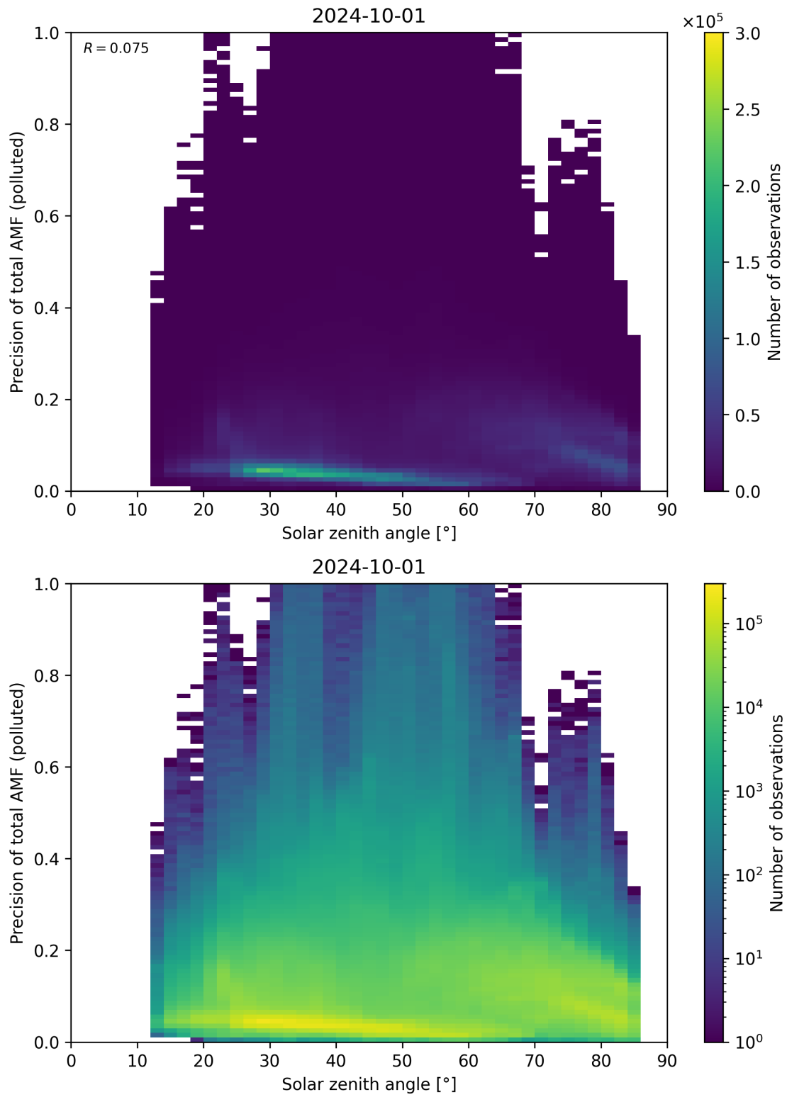
Figure 175: Scatter density plot of “Solar zenith angle” against “Precision of total AMF (polluted)” for 2024-09-30 to 2024-10-02.
