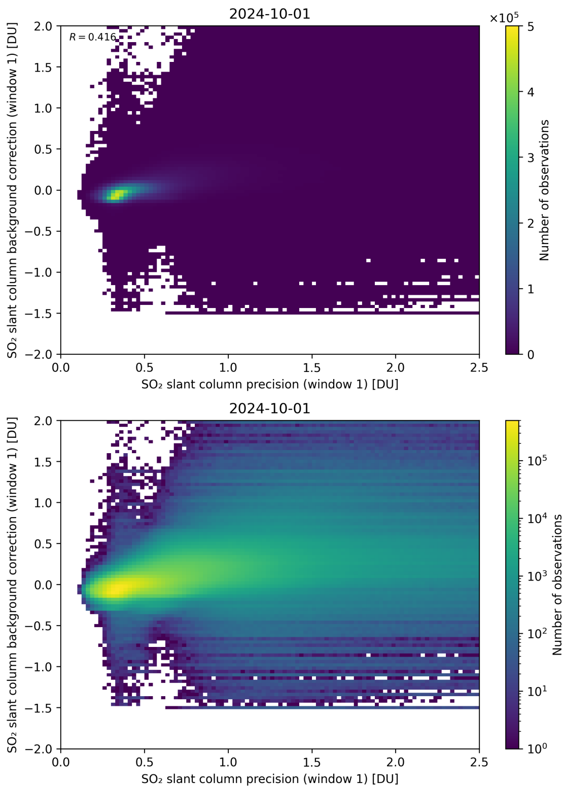
Figure 218: Scatter density plot of “SO 2 slant column precision (window 1)” against “SO 2 slant column background correction (window 1)” for 2024-09-30 to 2024-10-02.
