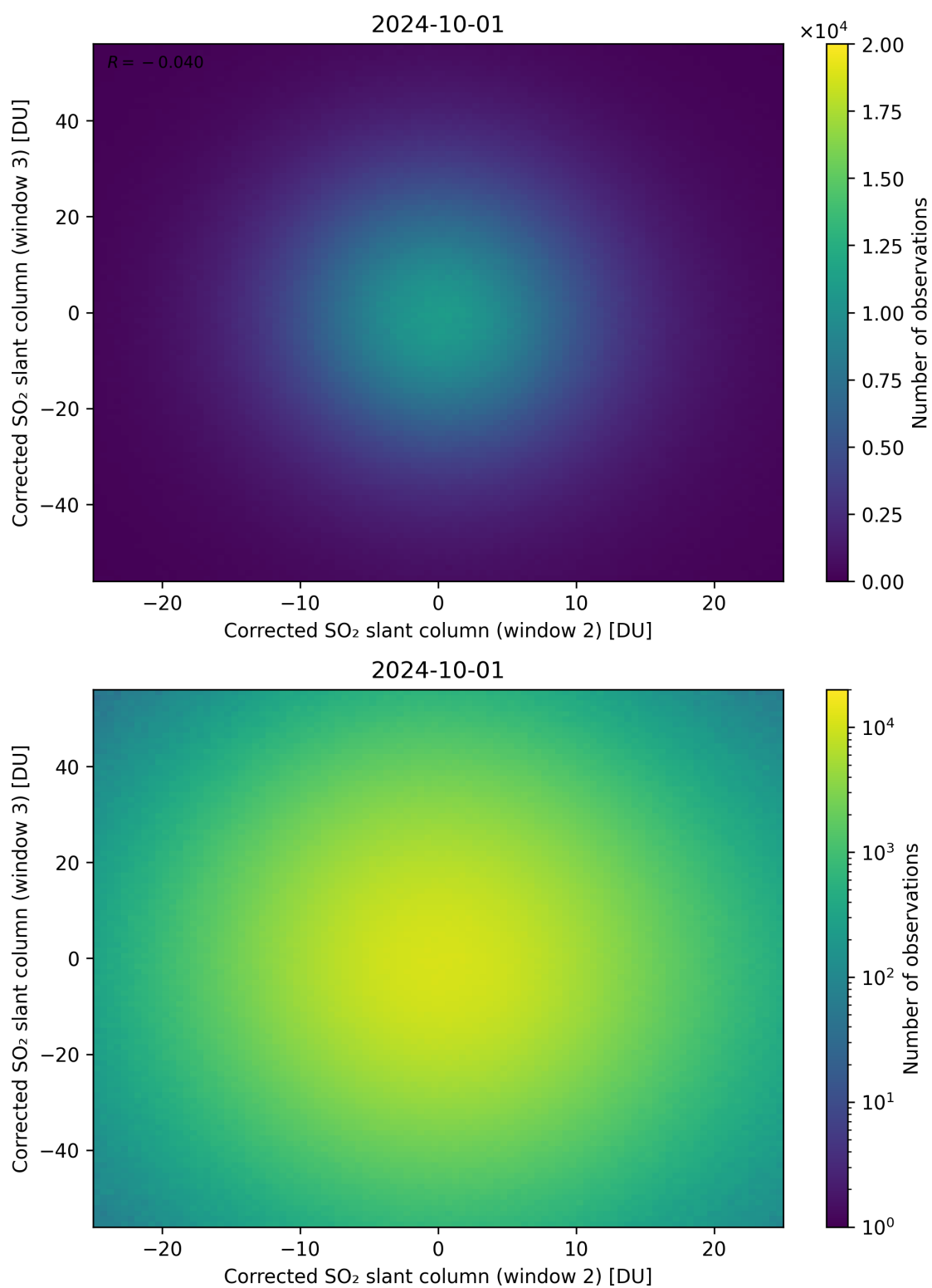
Figure 200: Scatter density plot of “Corrected SO 2 slant column (window 2)” against “Corrected SO 2 slant column (window 3)” for 2024-09-30 to 2024-10-02.
