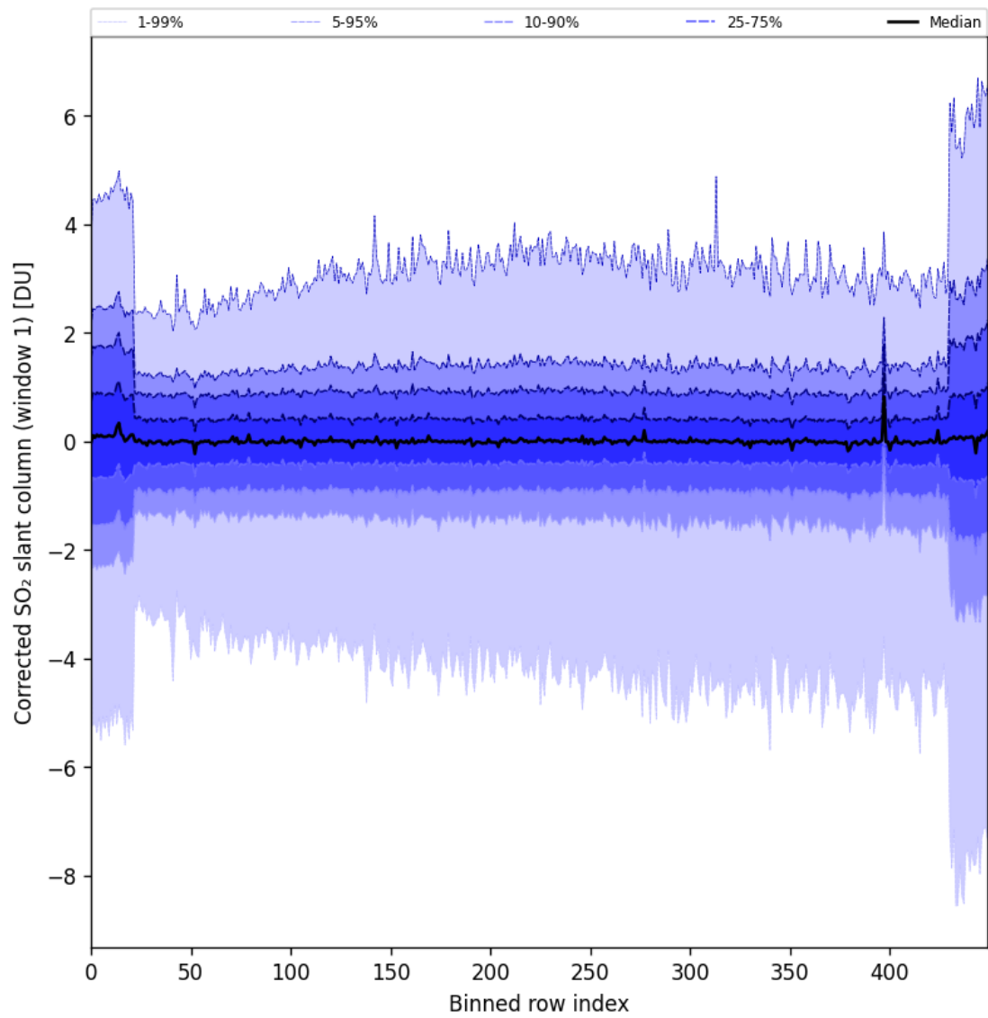
Figure 81: Along track statistics of “Corrected SO 2 slant column (window 1)” for 2024-09-30 to 2024-10-02
