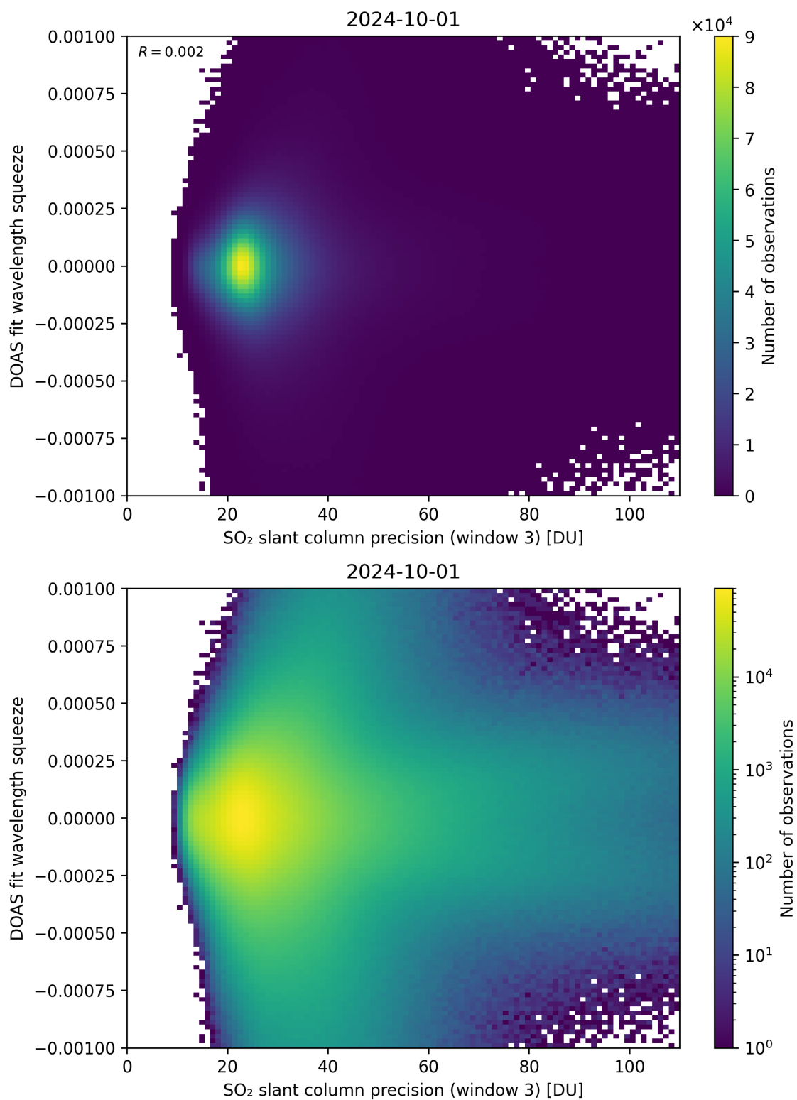
Figure 259: Scatter density plot of “SO 2 slant column precision (window 3)” against “DOAS fit wavelength squeeze” for 2024-09-30 to 2024-10-02.
