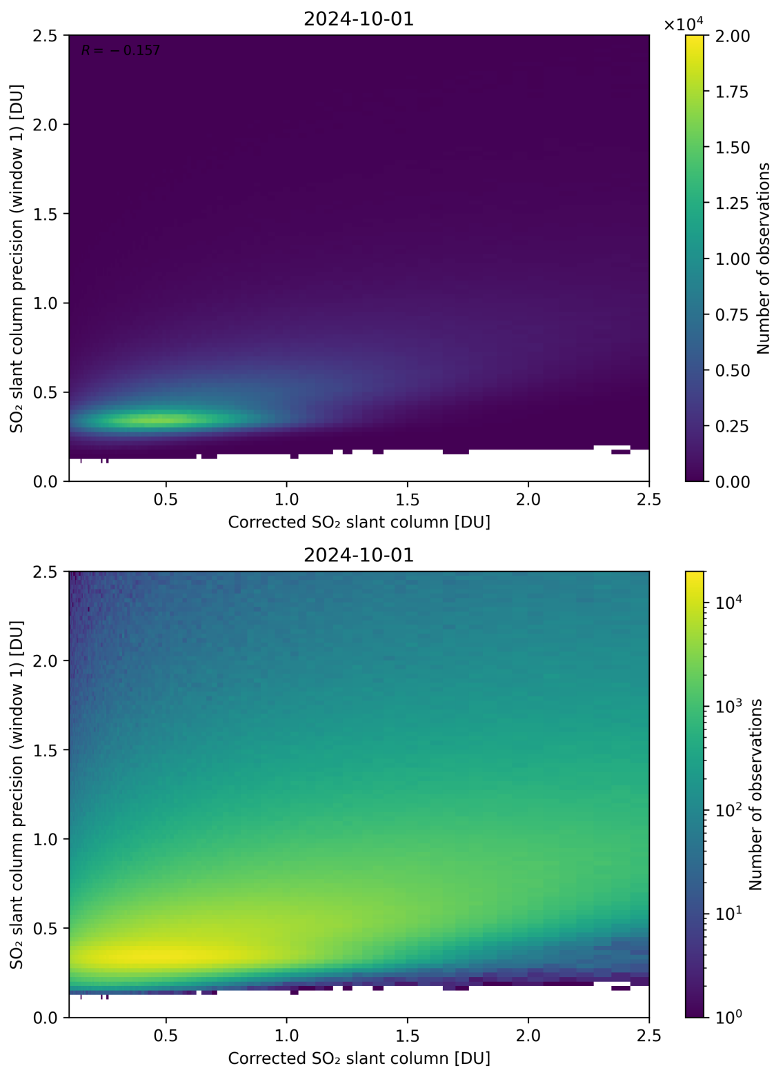
Figure 188: Scatter density plot of “Corrected SO 2 slant column” against “SO 2 slant column precision (window 1)” for 2024-09-30 to 2024-10-02.
