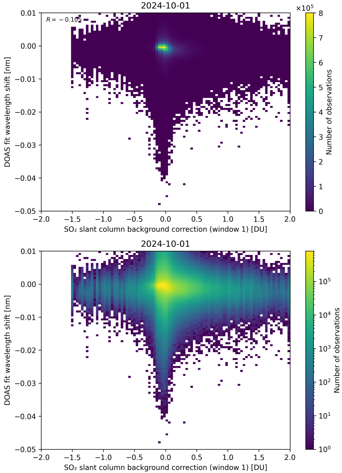
Figure 100: Scatter density plot of “SO 2 slant column background correction (window 1)” against “DOAS fit wavelength shift” for 2024-09-30 to 2024-10-02.
