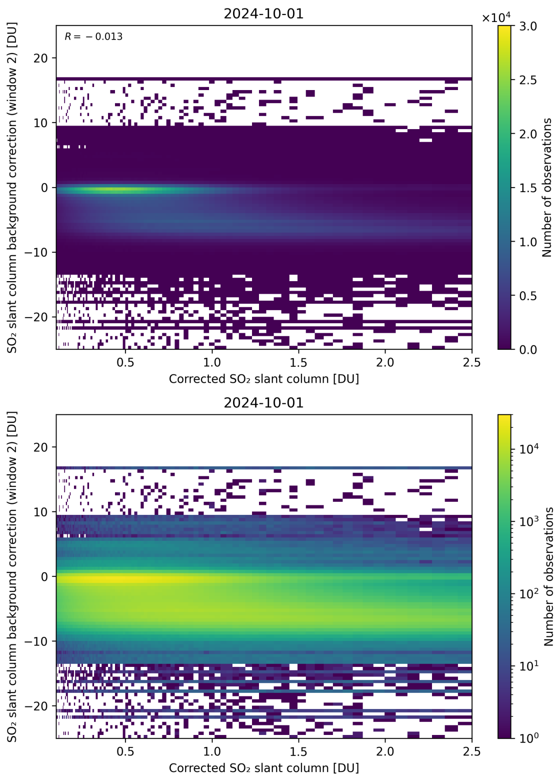
Figure 179: Scatter density plot of “Corrected SO 2 slant column” against “SO 2 slant column background correction (window 2)” for 2024-09-30 to 2024-10-02.
