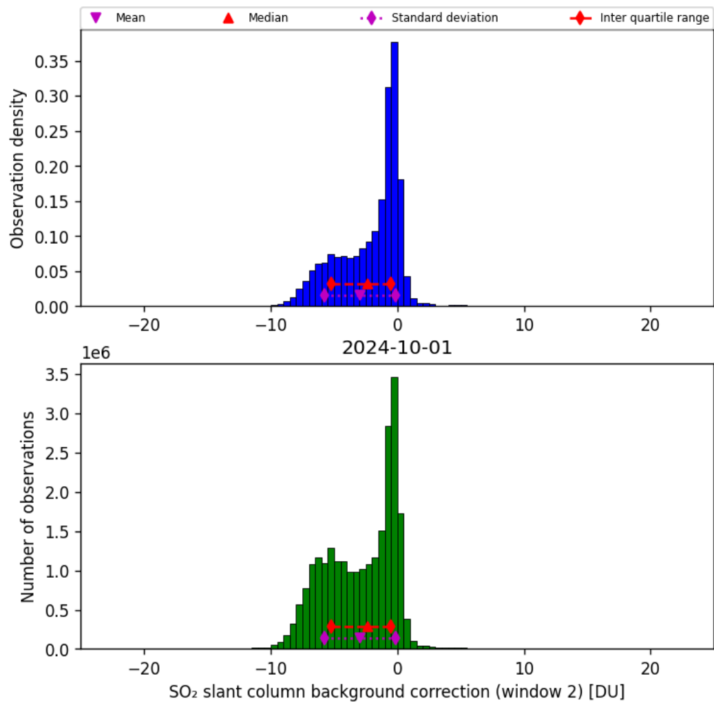
Figure 63: Histogram of “SO 2 slant column background correction (window 2)” for 2024-09-30 to 2024-10-02
