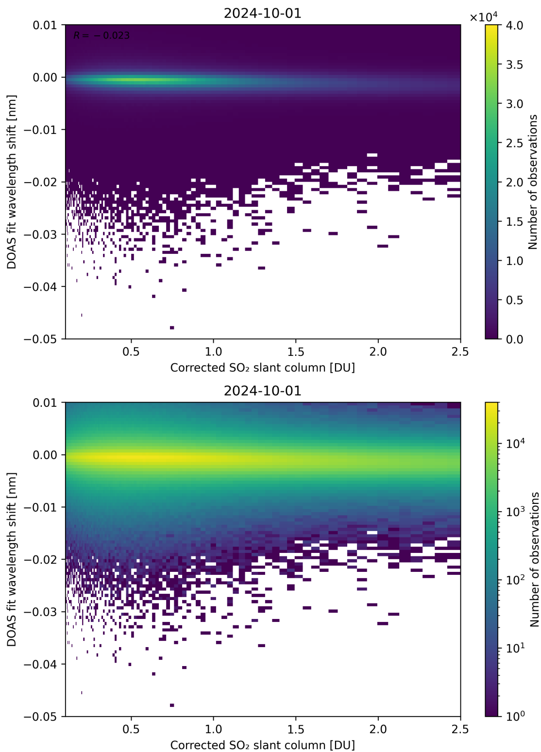
Figure 181: Scatter density plot of “Corrected SO 2 slant column” against “DOAS fit wavelength shift” for 2024-09-30 to 2024-10-02.
