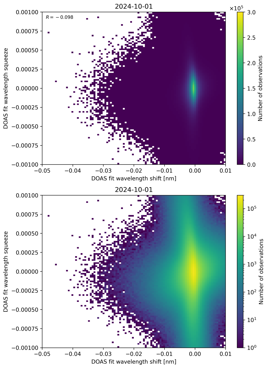
Figure 127: Scatter density plot of “DOAS fit wavelength shift” against “DOAS fit wavelength squeeze” for 2024-09-30 to 2024-10-02.
