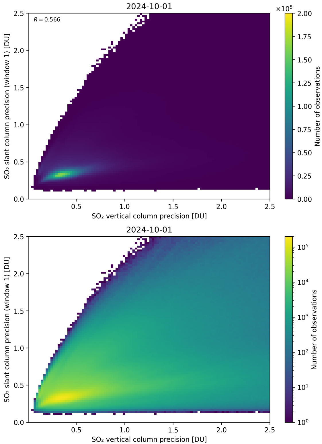
Figure 290: Scatter density plot of “SO 2 vertical column precision” against “SO 2 slant column precision (window 1)” for 2024-09-30 to 2024-10-02.
