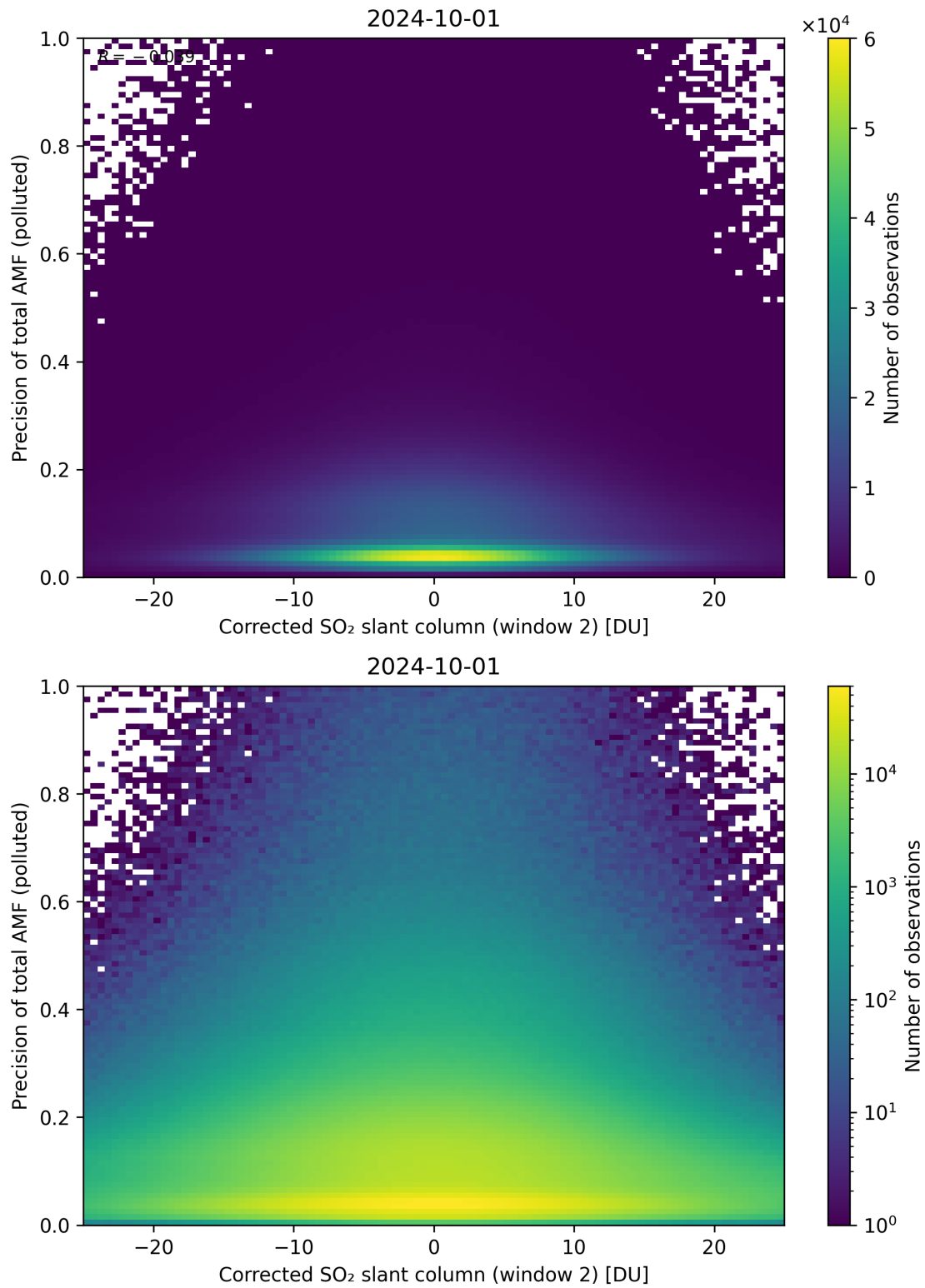
Figure 204: Scatter density plot of “Corrected SO 2 slant column (window 2)” against “Precision of total AMF (polluted)” for 2024-09-30 to 2024-10-02.
