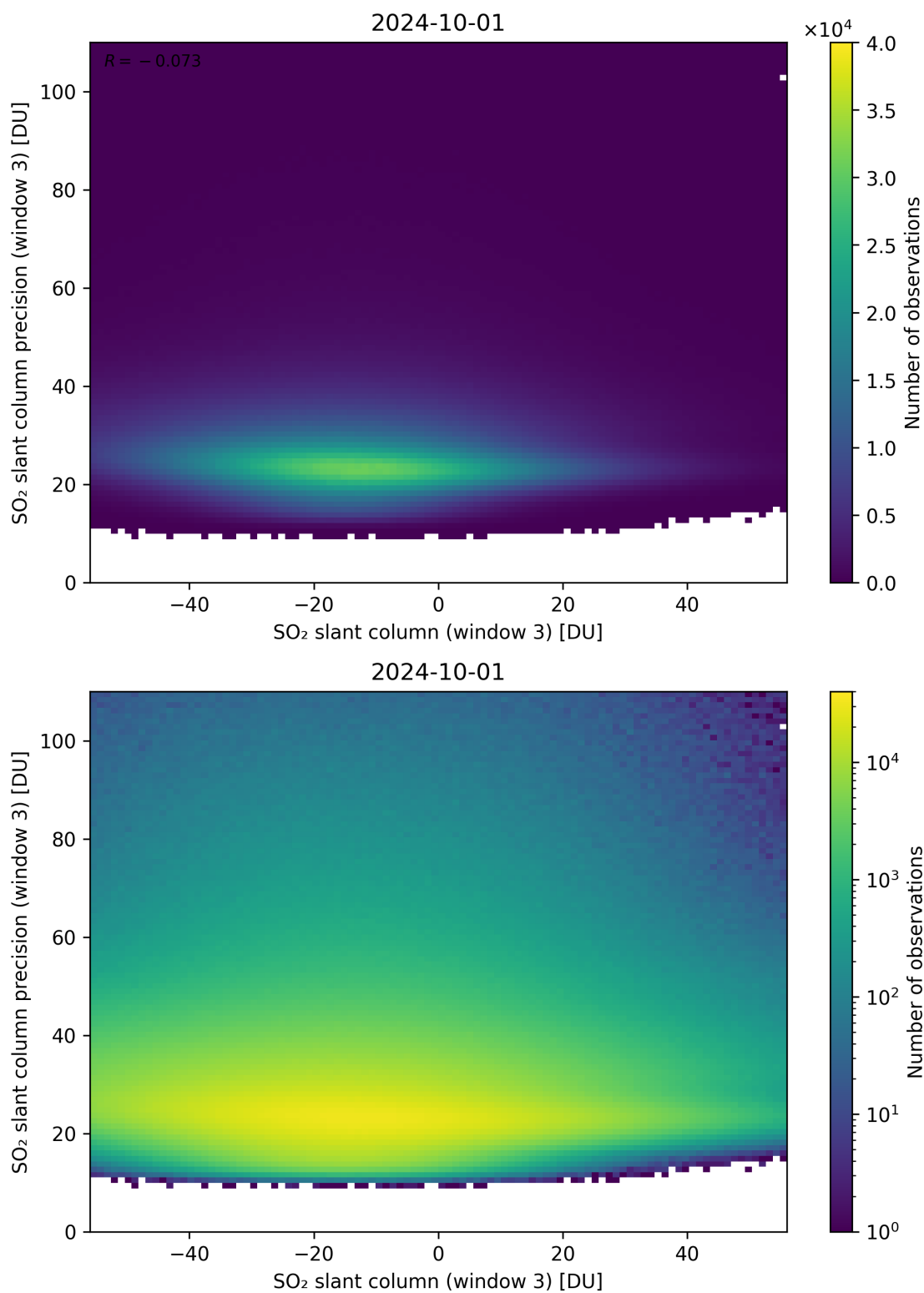
Figure 267: Scatter density plot of “SO 2 slant column (window 3)” against “SO 2 slant column precision (window 3)” for 2024-09-30 to 2024-10-02.
