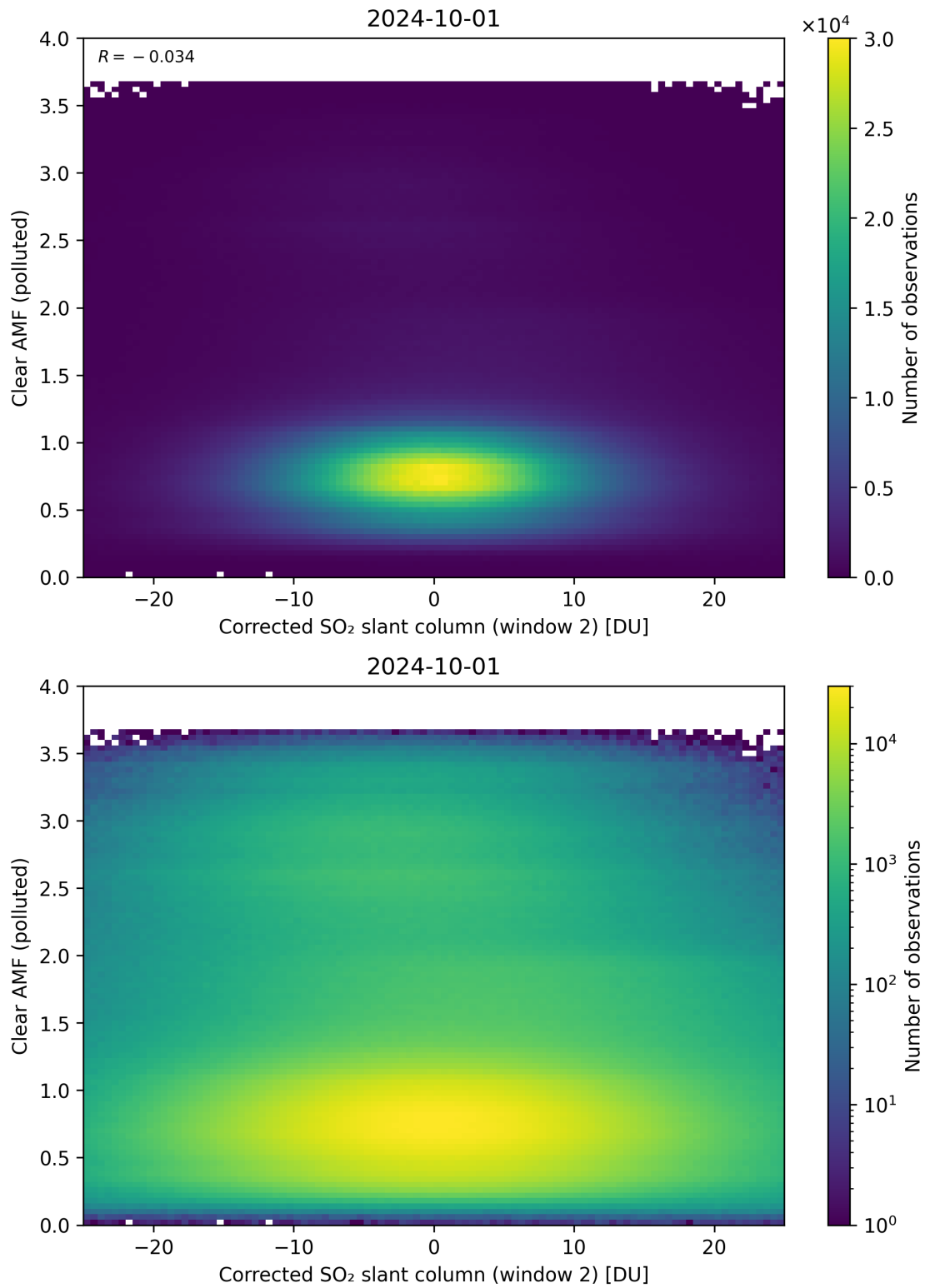
Figure 199: Scatter density plot of “Corrected SO 2 slant column (window 2)” against “Clear AMF (polluted)” for 2024-09-30 to 2024-10-02.
