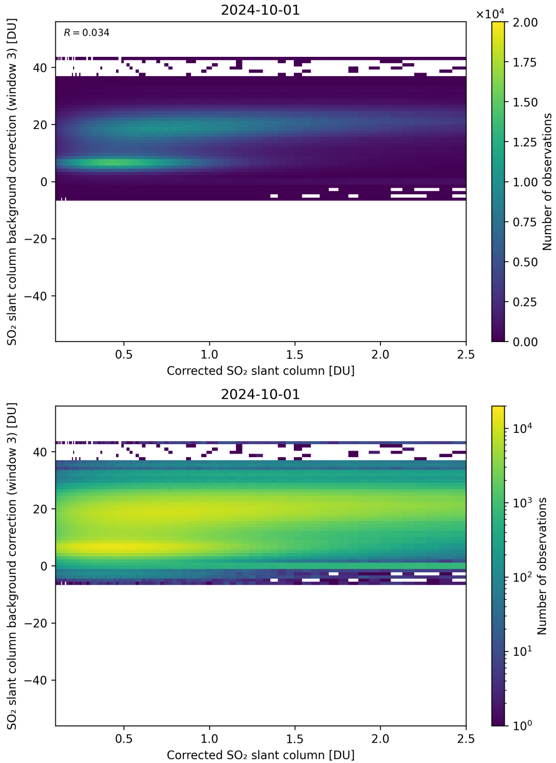
Figure 180: Scatter density plot of “Corrected SO 2 slant column” against “SO 2 slant column background correction (window 3)” for 2024-09-30 to 2024-10-02.
