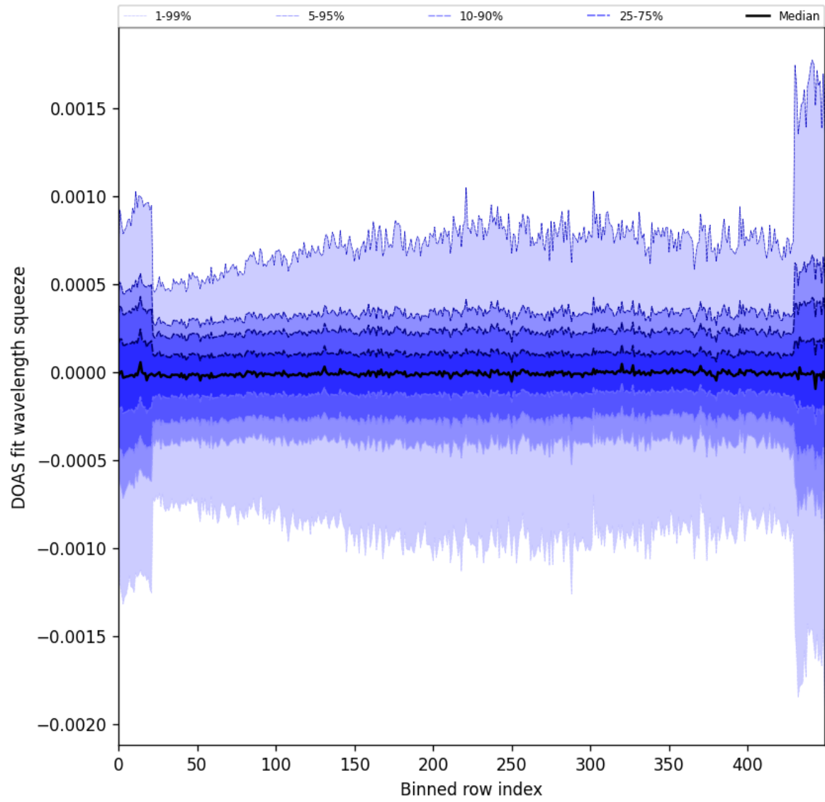
Figure 92: Along track statistics of “DOAS fit wavelength squeeze” for 2024-09-30 to 2024-10-02
