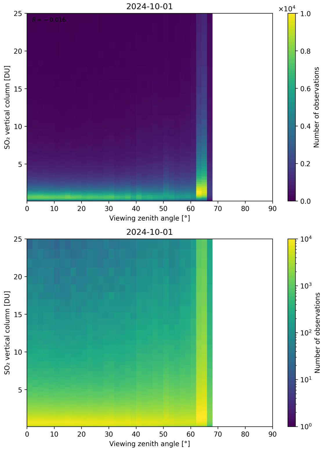
Figure 327: Scatter density plot of “Viewing zenith angle” against “SO 2 vertical column” for 2024-09-30 to 2024-10-02.
