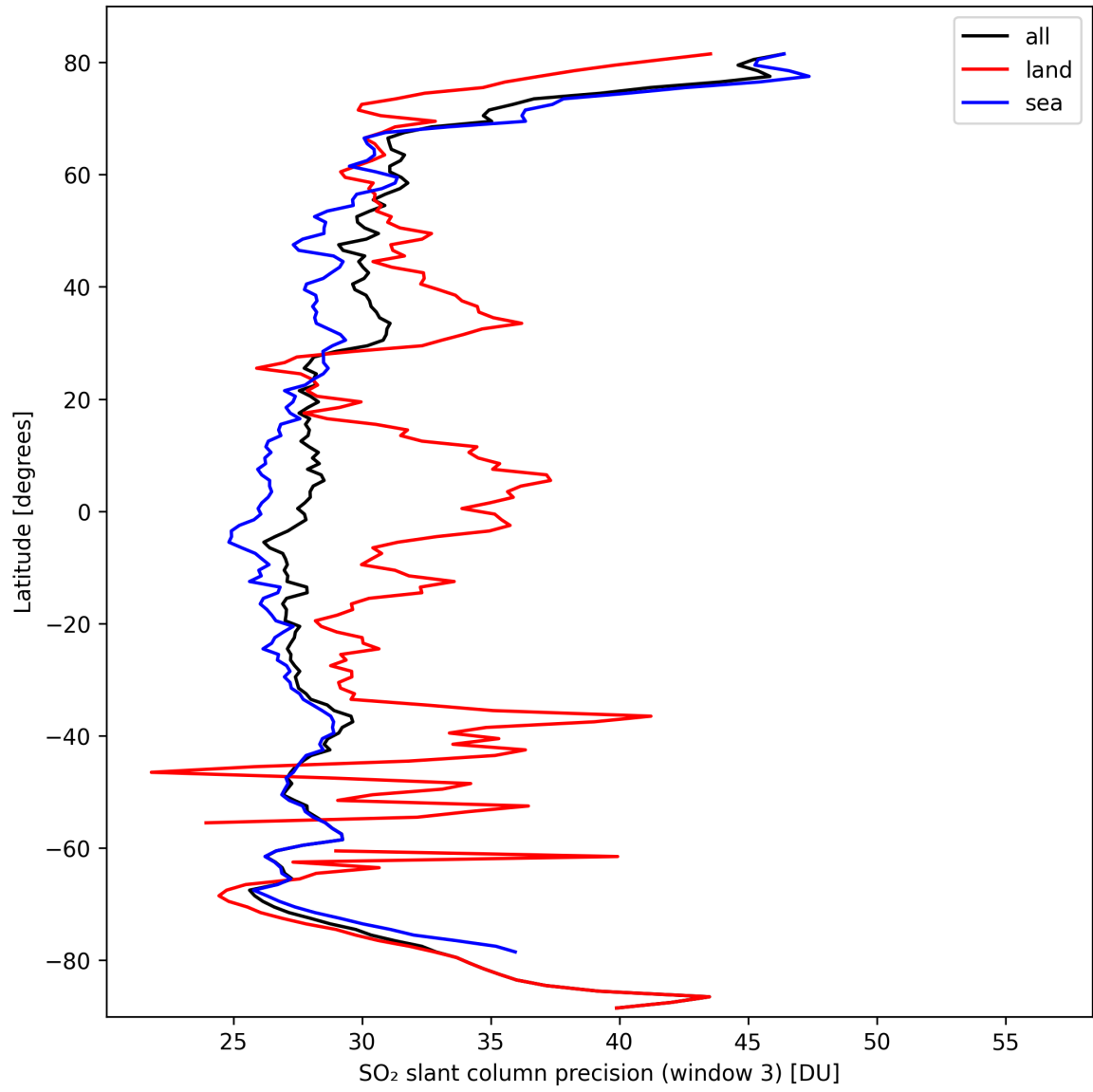
Figure 42: Zonal average of “SO 2 slant column precision (window 3)” for 2024-09-30 to 2024-10-02.
