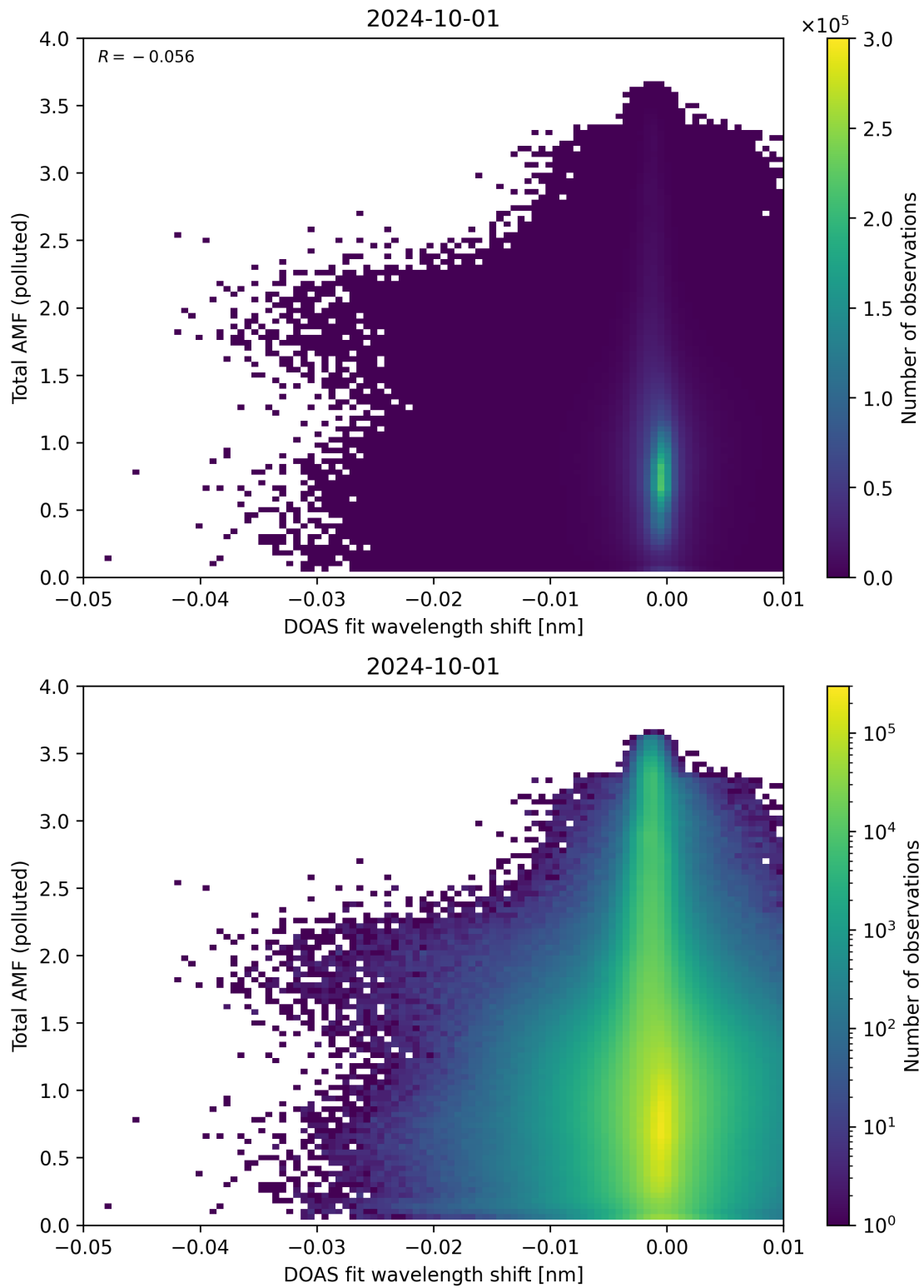
Figure 130: Scatter density plot of “DOAS fit wavelength shift” against “Total AMF (polluted)” for 2024-09-30 to 2024-10-02.
