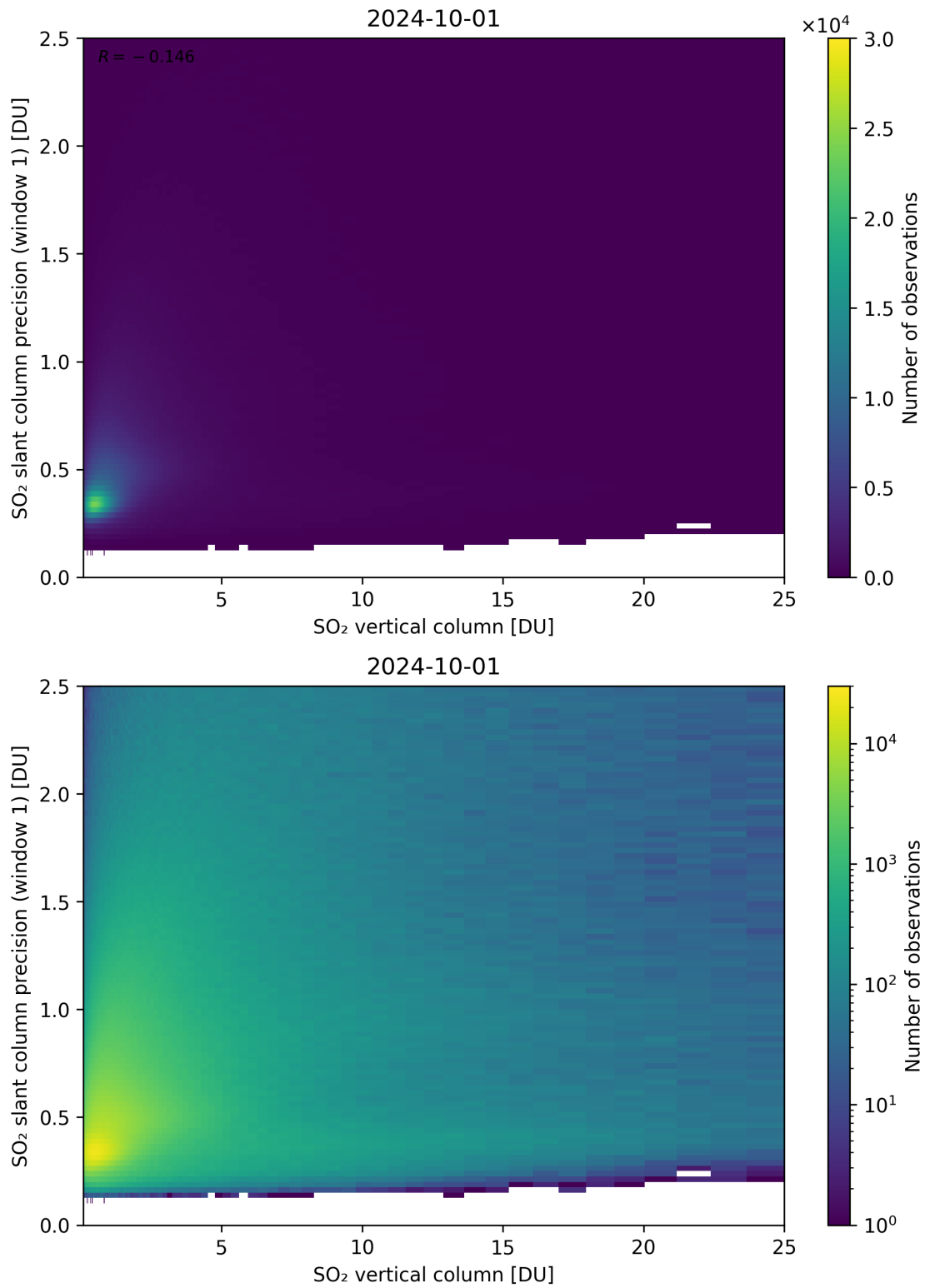
Figure 301: Scatter density plot of “SO 2 vertical column” against “SO 2 slant column precision (window 1)” for 2024-09-30 to 2024-10-02.
