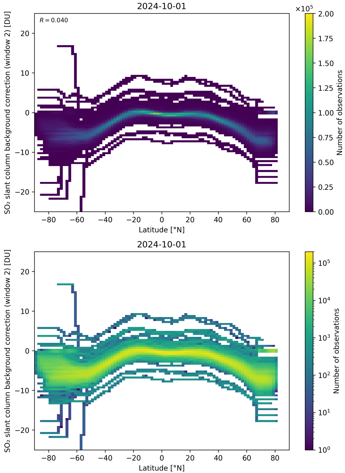
Figure 140: Scatter density plot of “Latitude” against “SO 2 slant column background correction (window 2)” for 2024-09-30 to 2024-10-02.
