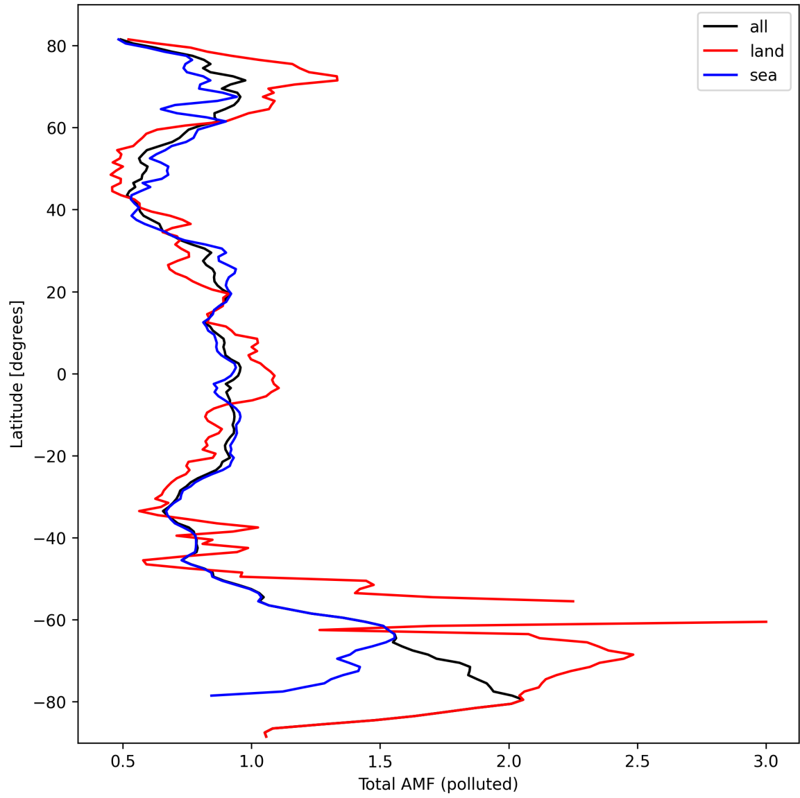
Figure 48: Zonal average of “Total AMF (polluted)” for 2024-09-30 to 2024-10-02.
