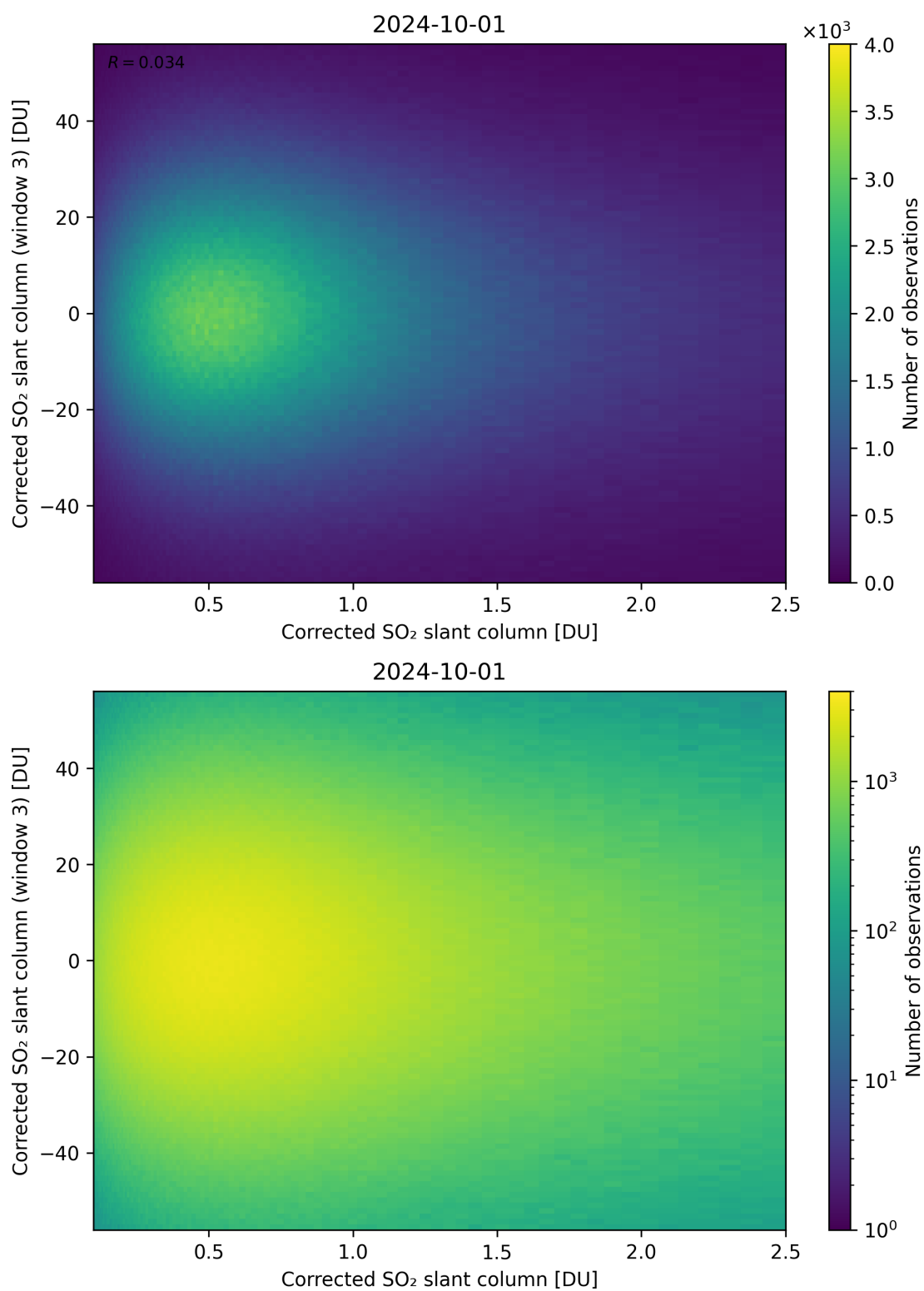
Figure 186: Scatter density plot of “Corrected SO 2 slant column” against “Corrected SO 2 slant column (window 3)” for 2024-09-30 to 2024-10-02.
