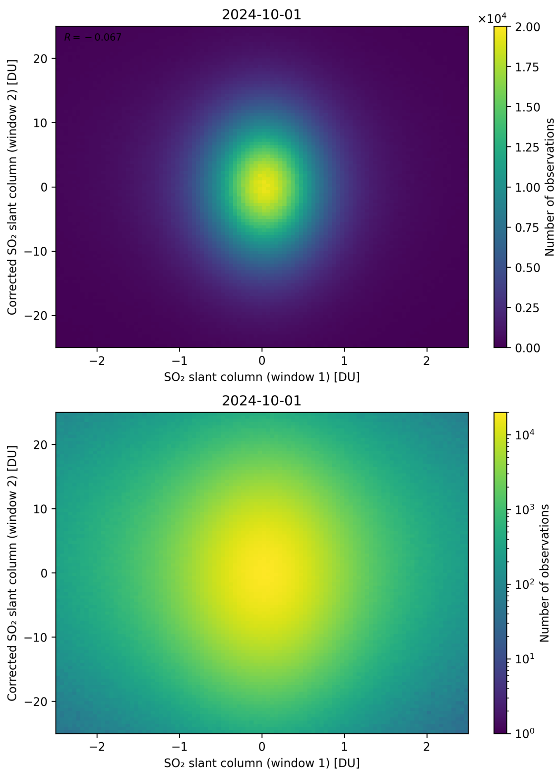
Figure 233: Scatter density plot of “SO 2 slant column (window 1)” against “Corrected SO 2 slant column (window 2)” for 2024-09-30 to 2024-10-02.
