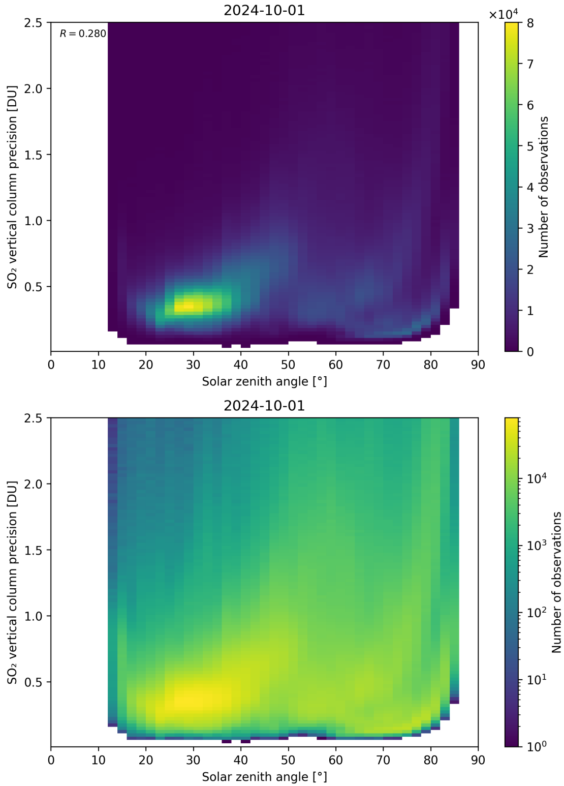
Figure 177: Scatter density plot of “Solar zenith angle” against “SO 2 vertical column precision” for 2024-09-30 to 2024-10-02.
