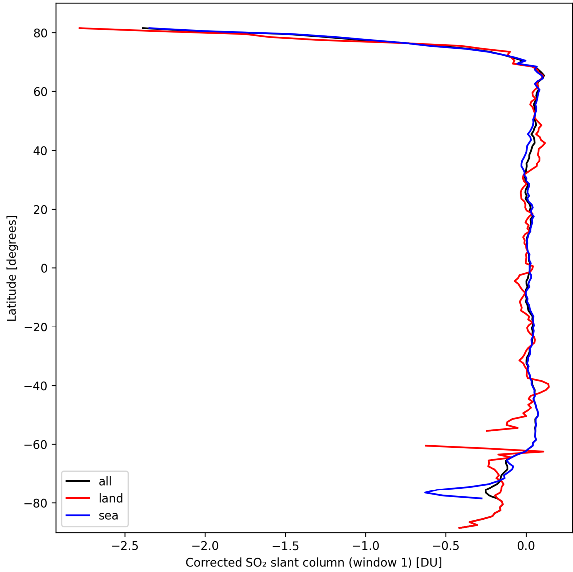
Figure 35: Zonal average of “Corrected SO 2 slant column (window 1)” for 2024-09-30 to 2024-10-02.
