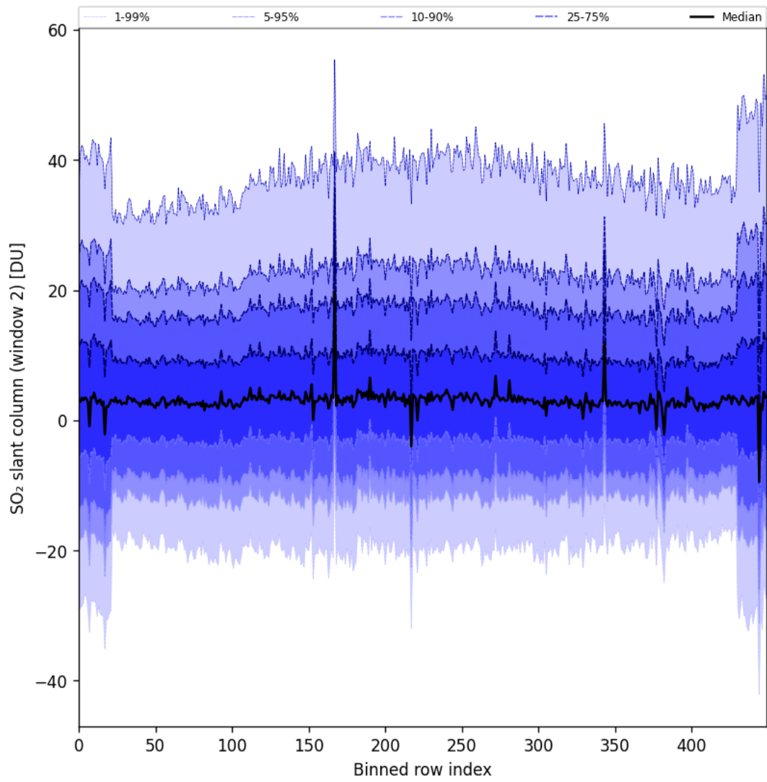
Figure 83: Along track statistics of “SO 2 slant column (window 2)” for 2024-09-30 to 2024-10-02
