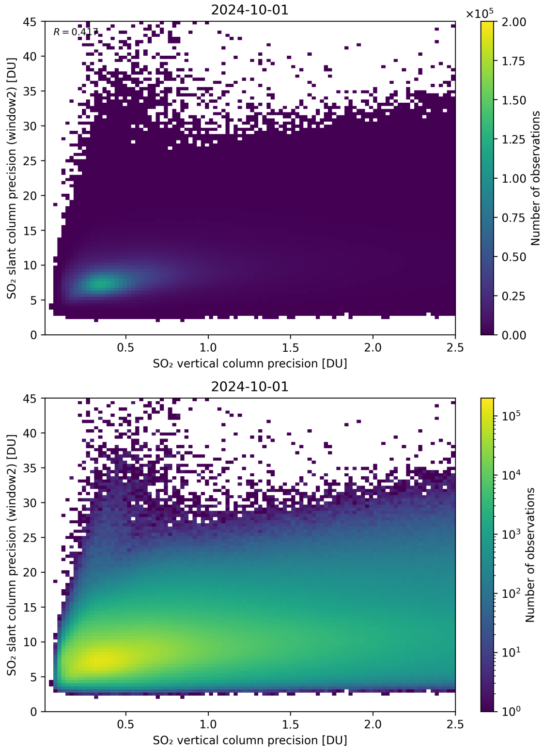
Figure 291: Scatter density plot of “SO 2 vertical column precision” against “SO 2 slant column precision (window2)” for 2024-09-30 to 2024-10-02.
