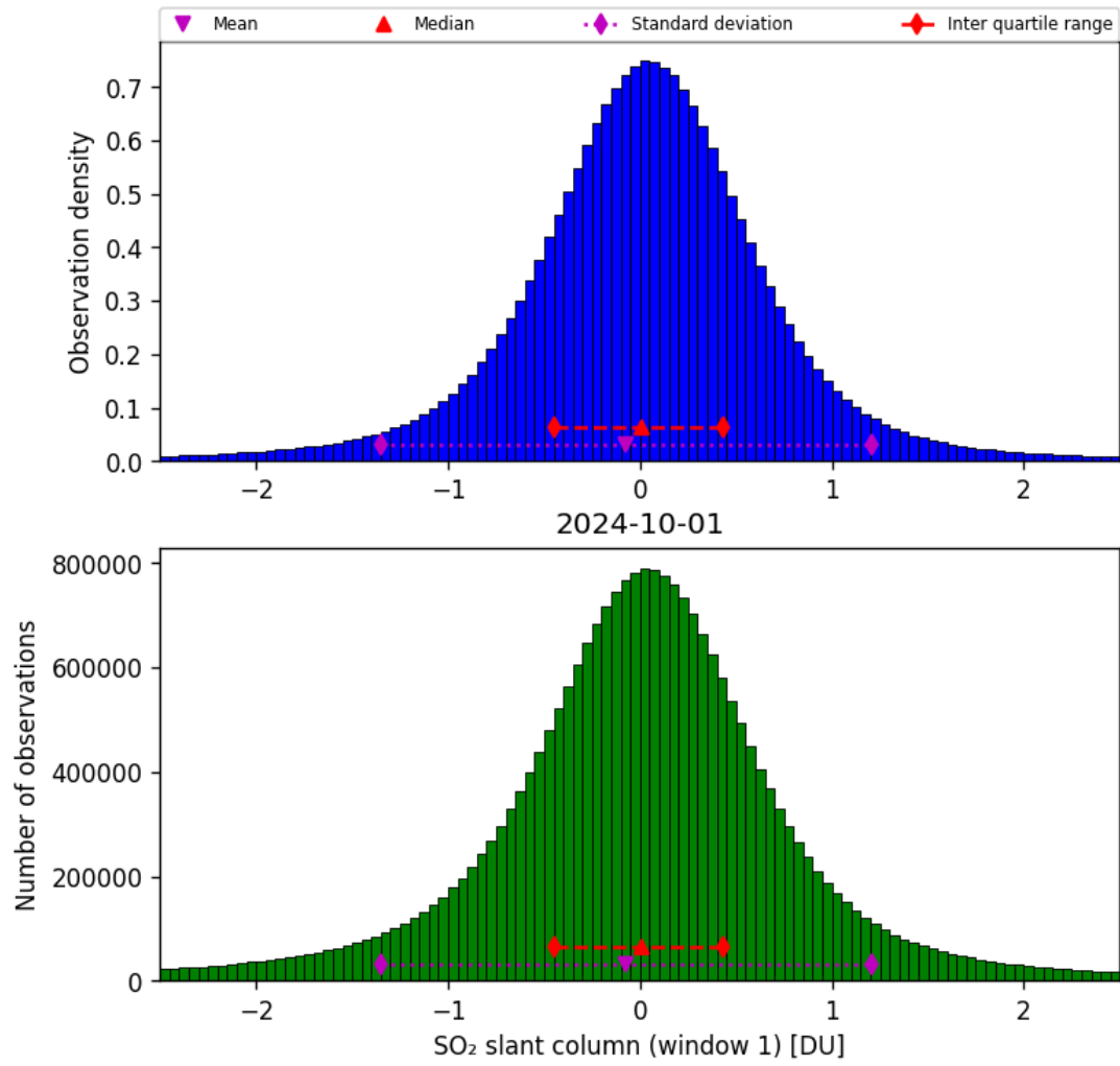
Figure 56: Histogram of “SO 2 slant column (window 1)” for 2024-09-30 to 2024-10-02
