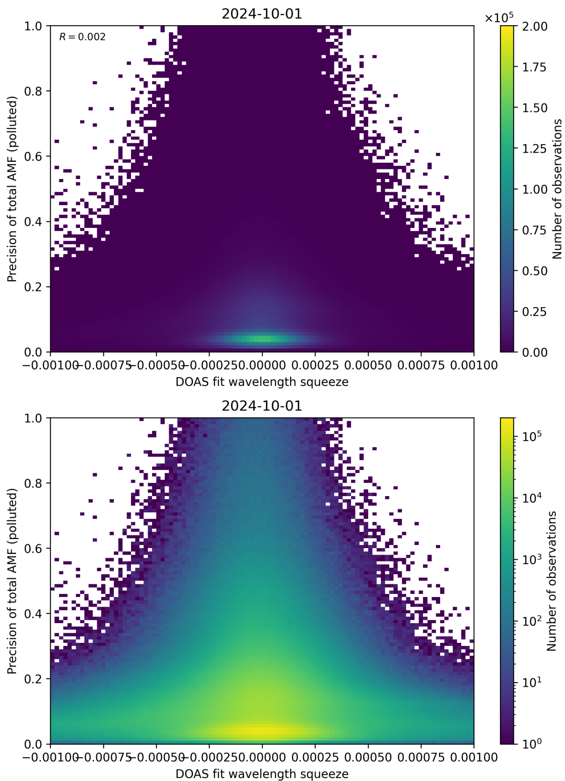
Figure 135: Scatter density plot of “DOAS fit wavelength squeeze” against “Precision of total AMF (polluted)” for 2024-09-30 to 2024-10-02.
