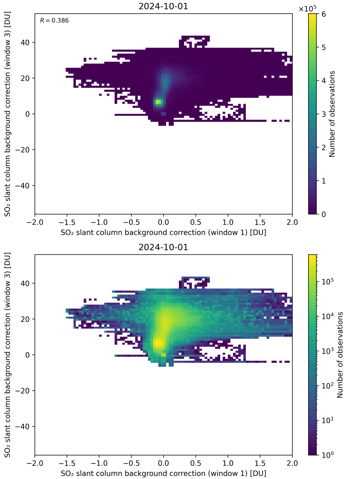
Figure 99: Scatter density plot of “SO 2 slant column background correction (window 1)” against “SO 2 slant column background correction (window 3)” for 2024-09-30 to 2024-10-02.
