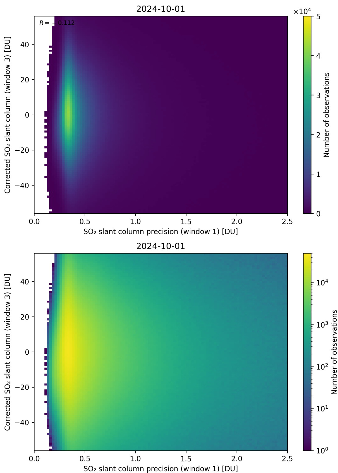
Figure 226: Scatter density plot of “SO 2 slant column precision (window 1)” against “Corrected SO 2 slant column (window 3)” for 2024-09-30 to 2024-10-02.
