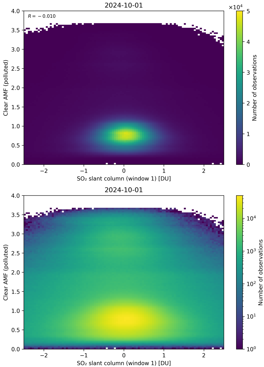
Figure 232: Scatter density plot of “SO 2 slant column (window 1)” against “Clear AMF (polluted)” for 2024-09-30 to 2024-10-02.
