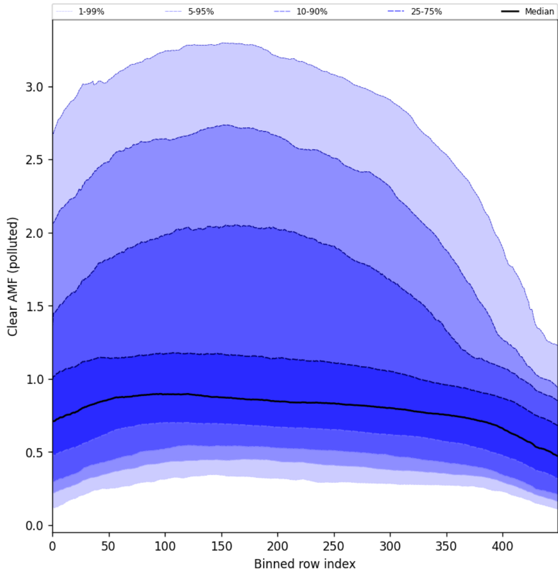
Figure 96: Along track statistics of “Clear AMF (polluted)” for 2024-09-30 to 2024-10-02
