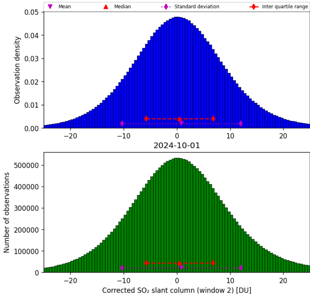
Figure 62: Histogram of “Corrected SO 2 slant column (window 2)” for 2024-09-30 to 2024-10-02
