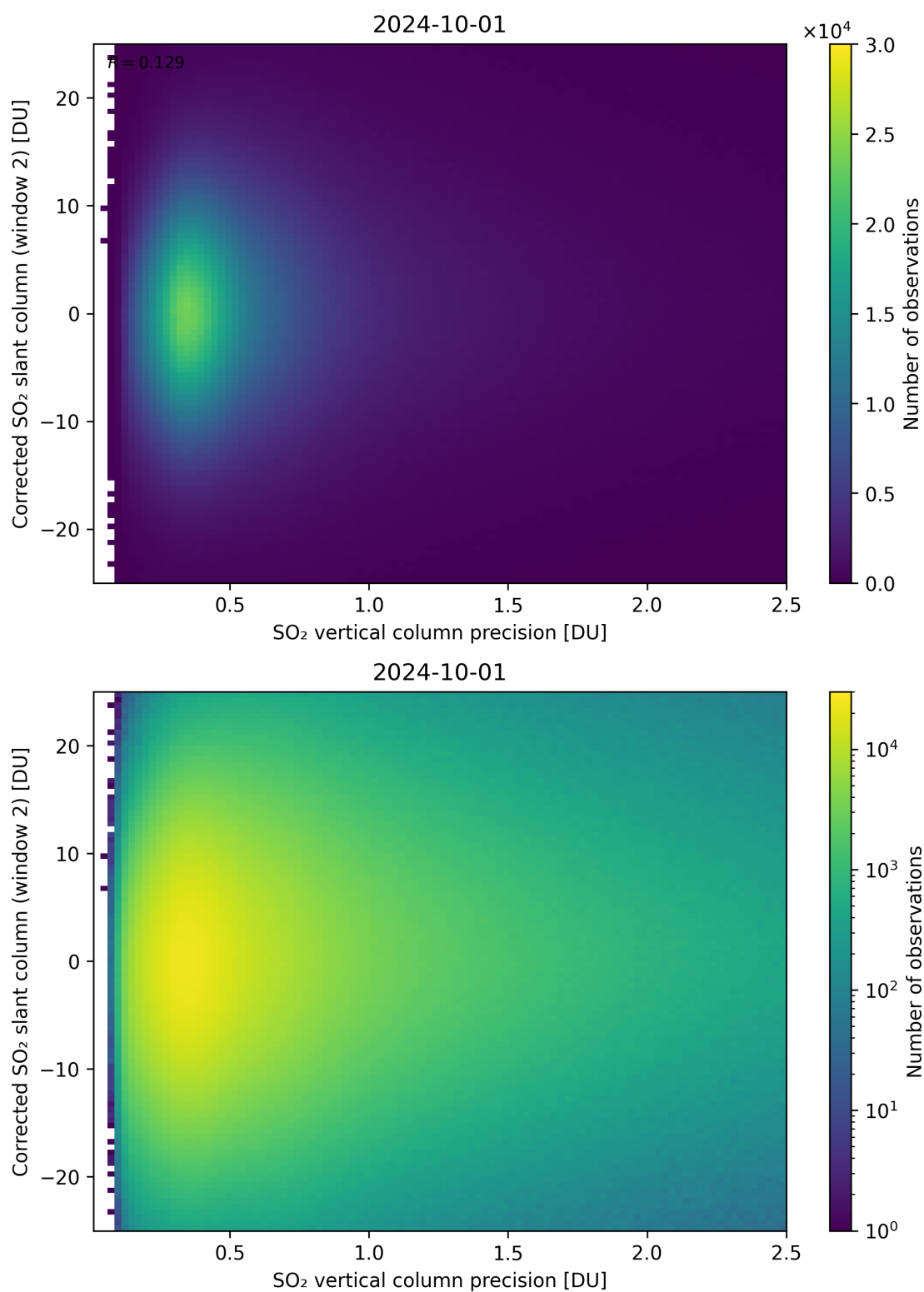
Figure 287: Scatter density plot of “SO 2 vertical column precision” against “Corrected SO 2 slant column (window 2)” for 2024-09-30 to 2024-10-02.
