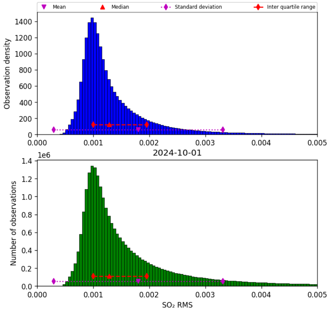
Figure 70: Histogram of “SO 2 RMS” for 2024-09-30 to 2024-10-02
