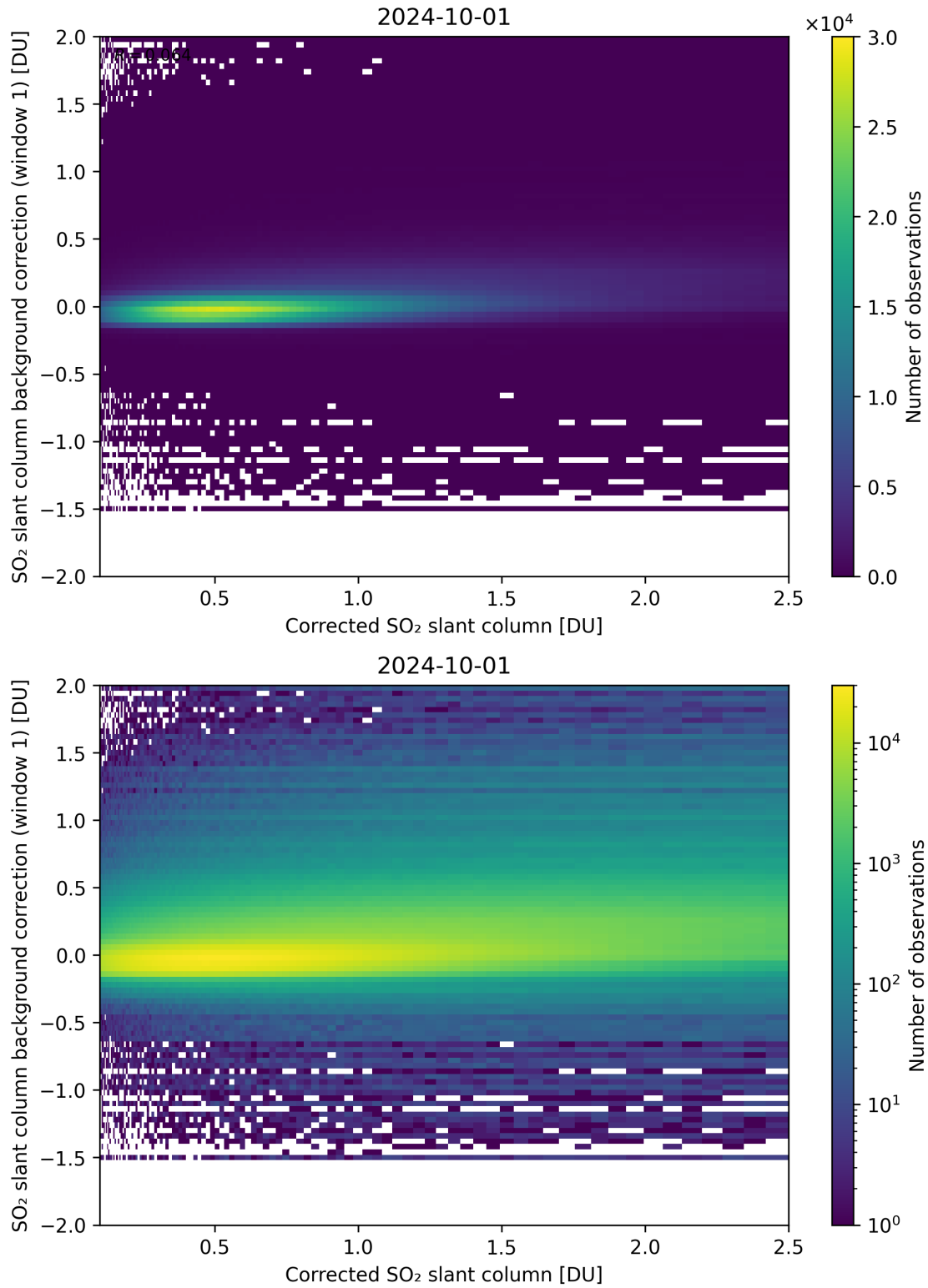
Figure 178: Scatter density plot of “Corrected SO 2 slant column” against “SO 2 slant column background correction (window 1)” for 2024-09-30 to 2024-10-02.
