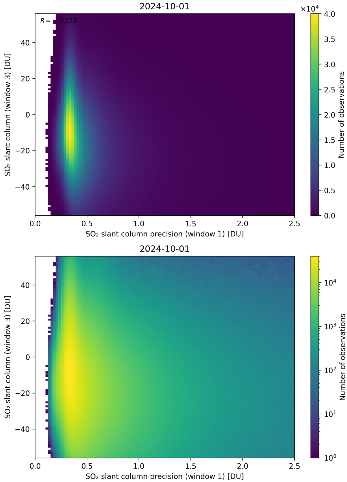
Figure 228: Scatter density plot of “SO 2 slant column precision (window 1)” against “SO 2 slant column (window 3)” for 2024-09-30 to 2024-10-02.
