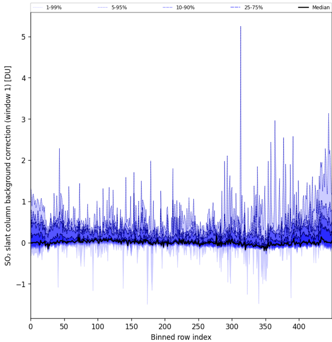
Figure 82: Along track statistics of “SO 2 slant column background correction (window 1)” for 2024-09-30 to 2024-10-02
