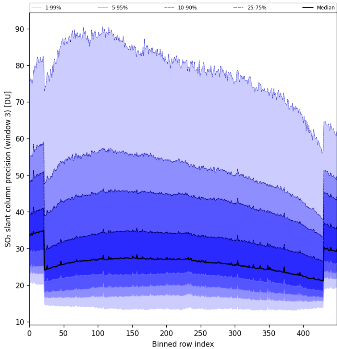
Figure 88: Along track statistics of “SO 2 slant column precision (window 3)” for 2024-09-30 to 2024-10-02
