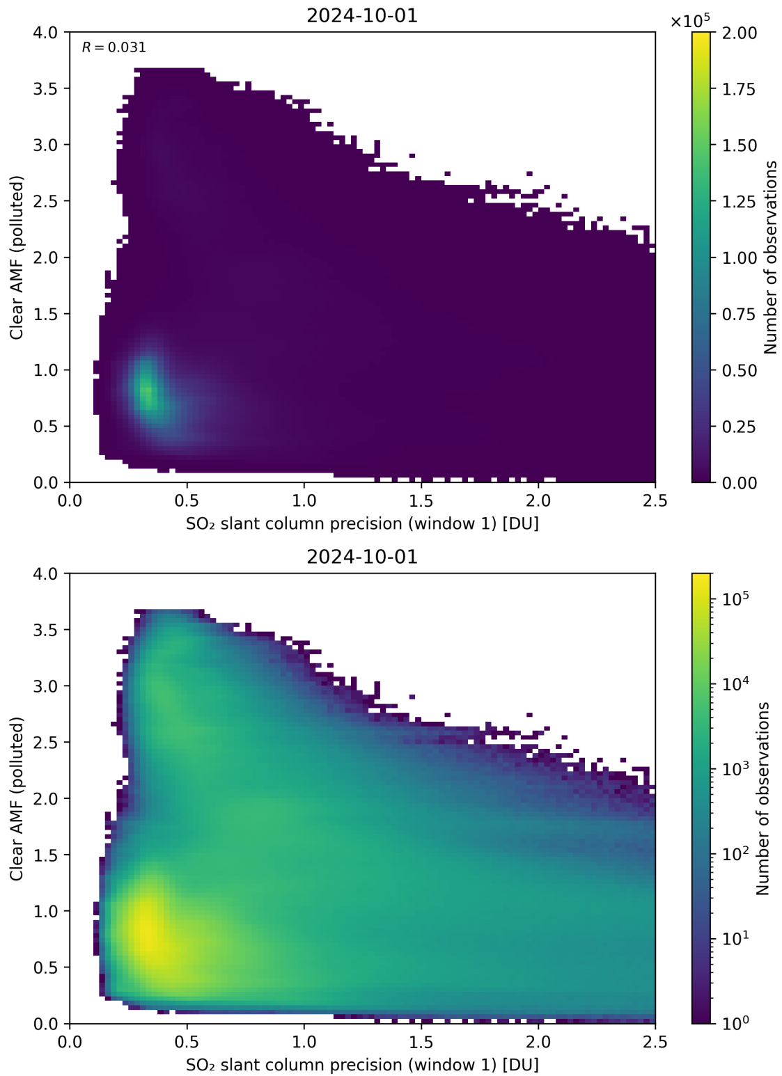
Figure 224: Scatter density plot of “SO 2 slant column precision (window 1)” against “Clear AMF (polluted)” for 2024-09-30 to 2024-10-02.
