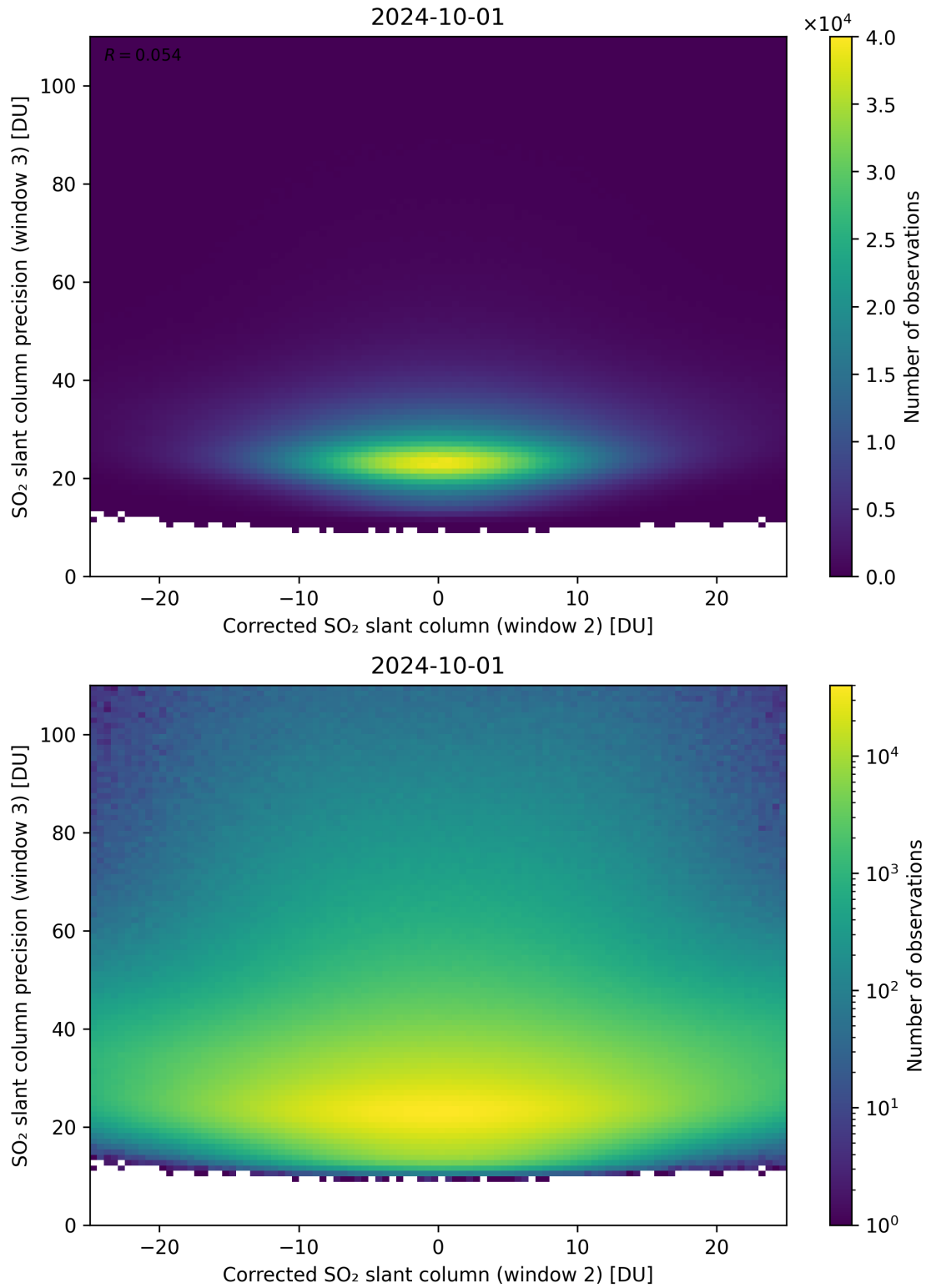
Figure 202: Scatter density plot of “Corrected SO 2 slant column (window 2)” against “SO 2 slant column precision (window 3)” for 2024-09-30 to 2024-10-02.
