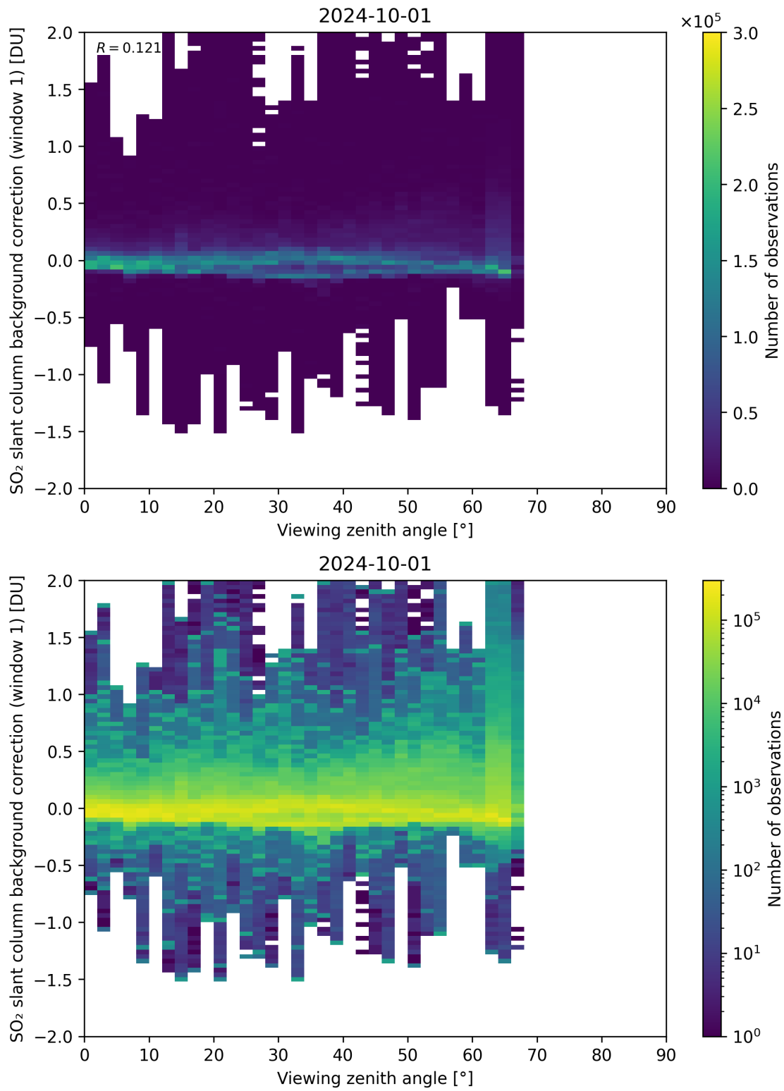
Figure 308: Scatter density plot of “Viewing zenith angle” against “SO 2 slant column background correction (window 1)” for 2024-09-30 to 2024-10-02.
