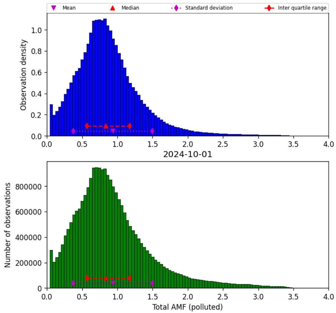
Figure 71: Histogram of “Total AMF (polluted)” for 2024-09-30 to 2024-10-02
