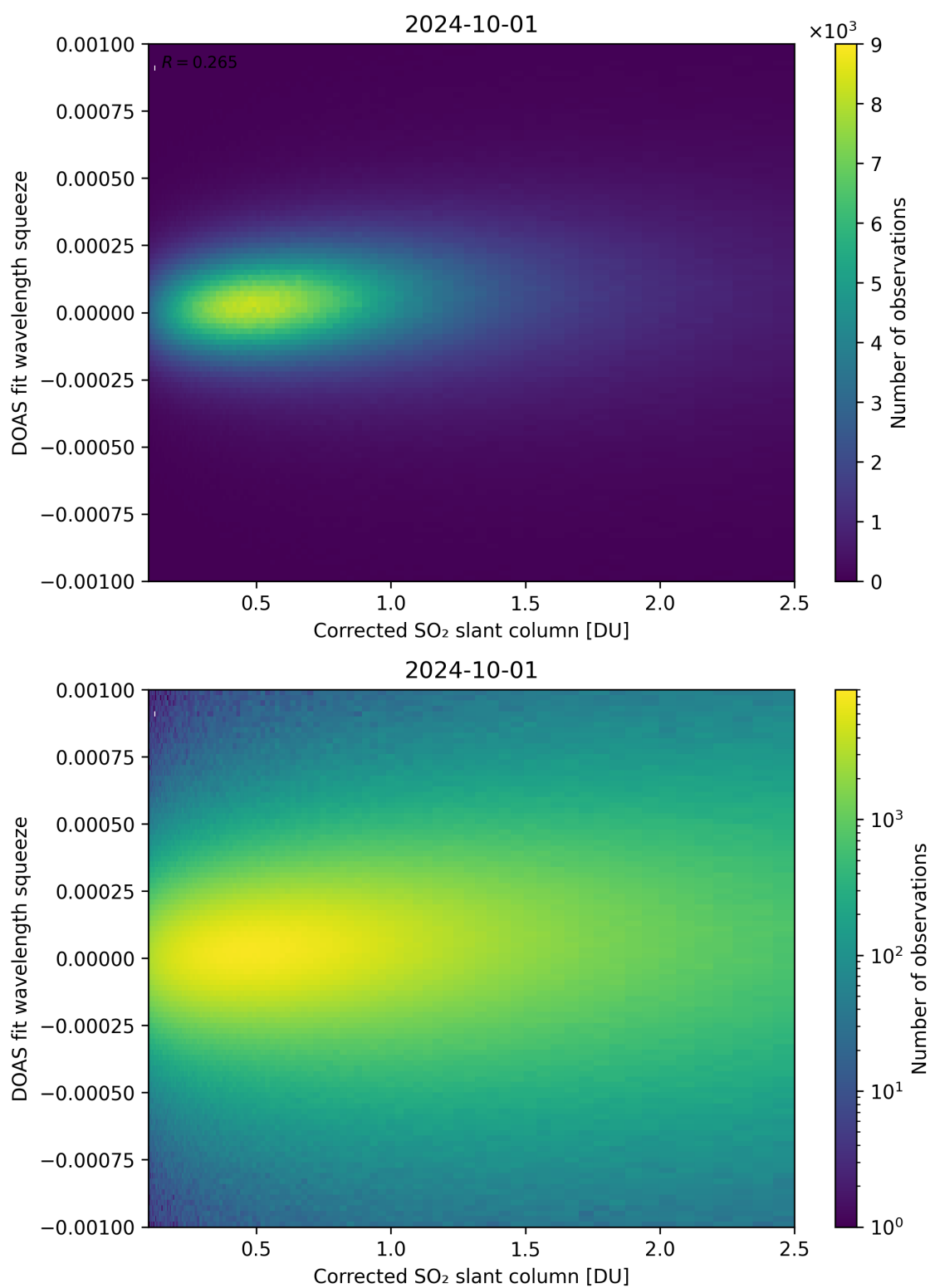
Figure 182: Scatter density plot of “Corrected SO 2 slant column” against “DOAS fit wavelength squeeze” for 2024-09-30 to 2024-10-02.
