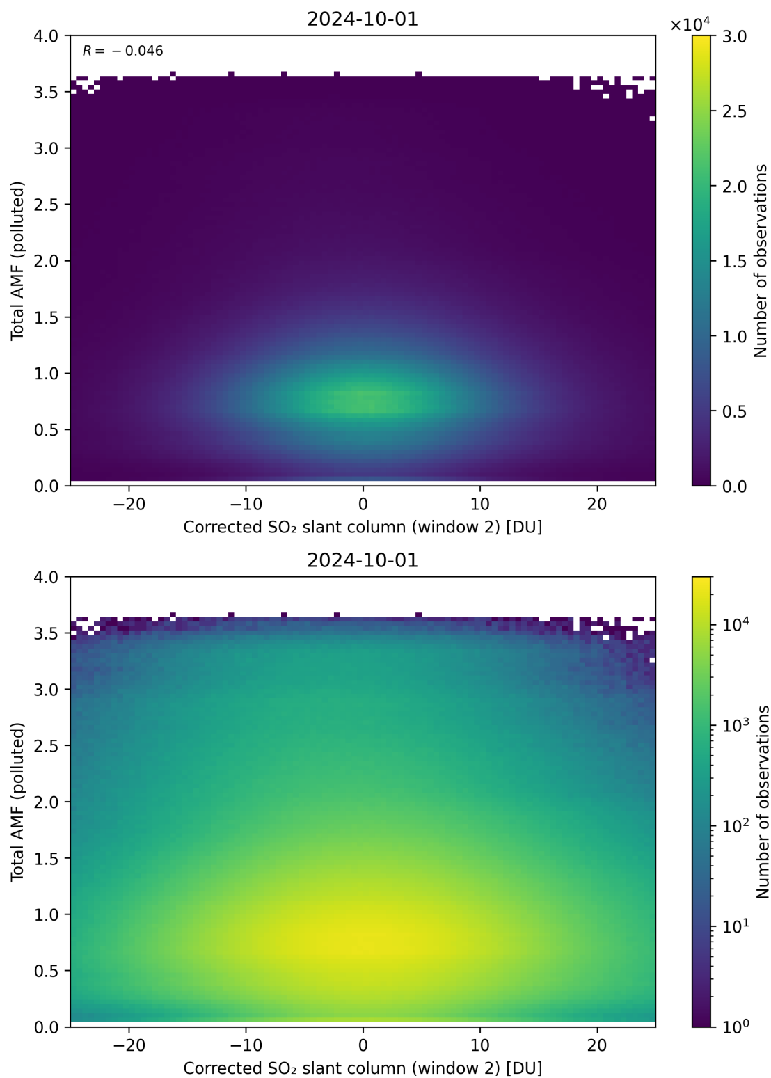
Figure 203: Scatter density plot of “Corrected SO 2 slant column (window 2)” against “Total AMF (polluted)” for 2024-09-30 to 2024-10-02.
