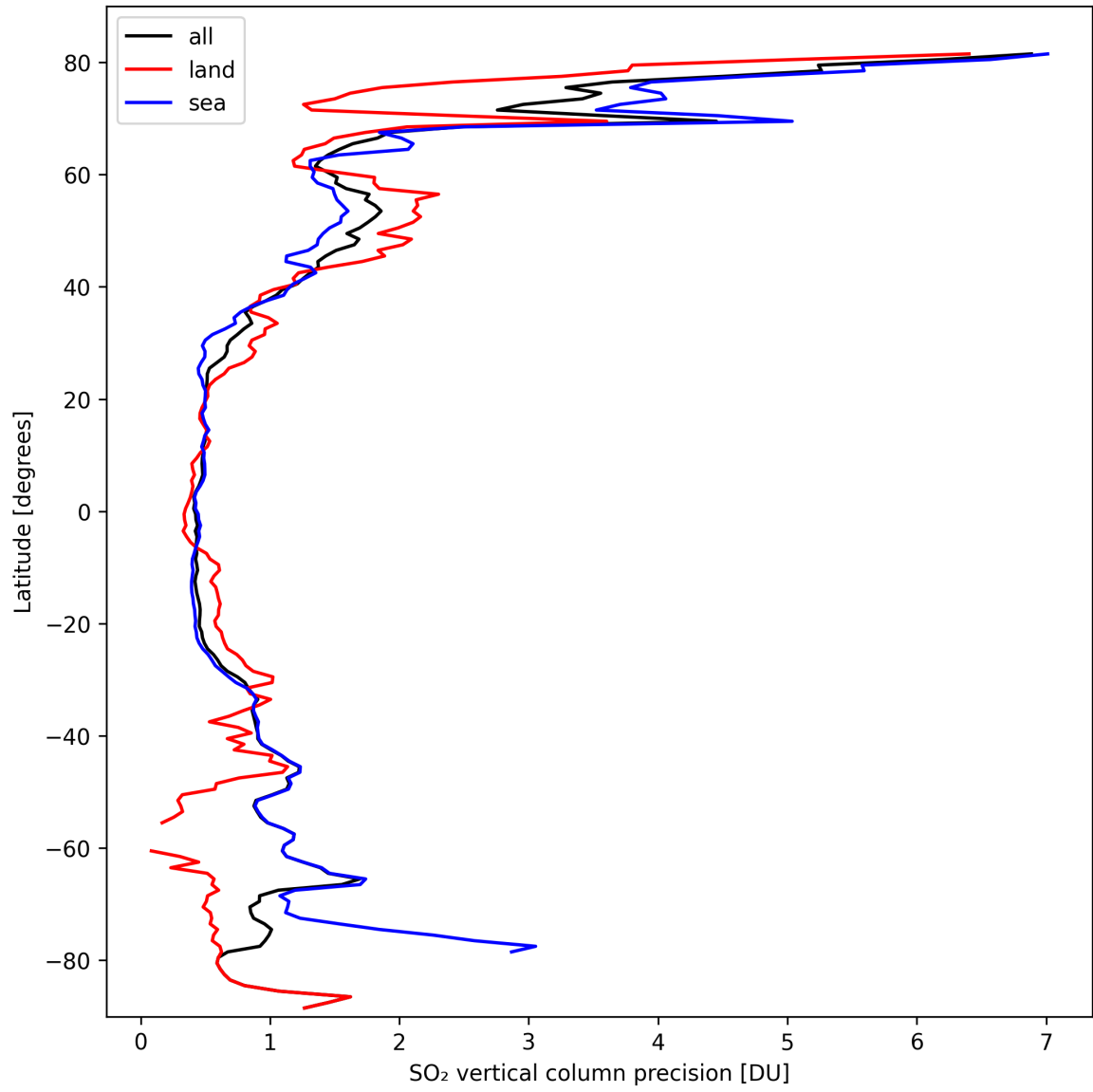
Figure 31: Zonal average of “SO 2 vertical column precision” for 2024-09-30 to 2024-10-02.
