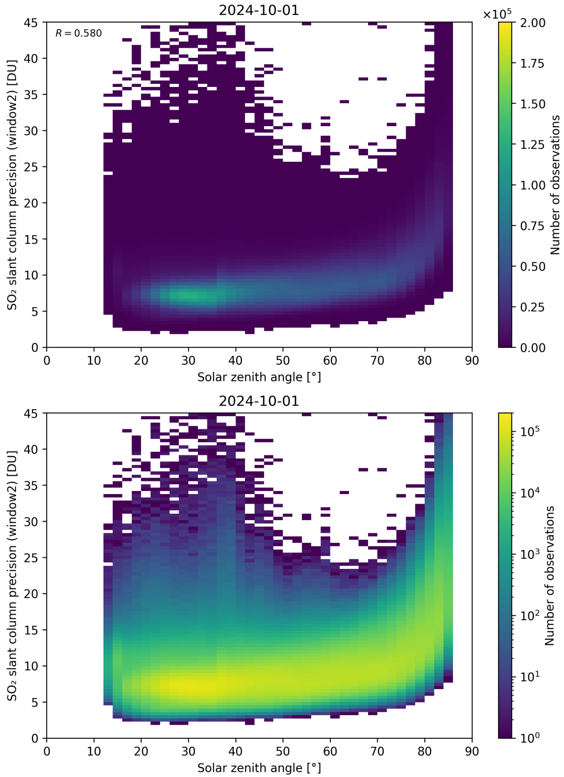
Figure 171: Scatter density plot of “Solar zenith angle” against “SO 2 slant column precision (window2)” for 2024-09-30 to 2024-10-02.
