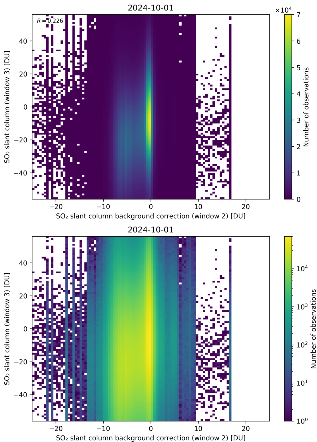
Figure 117: Scatter density plot of “SO 2 slant column background correction (window 2)” against “SO 2 slant column (window 3)” for 2024-09-30 to 2024-10-02.
