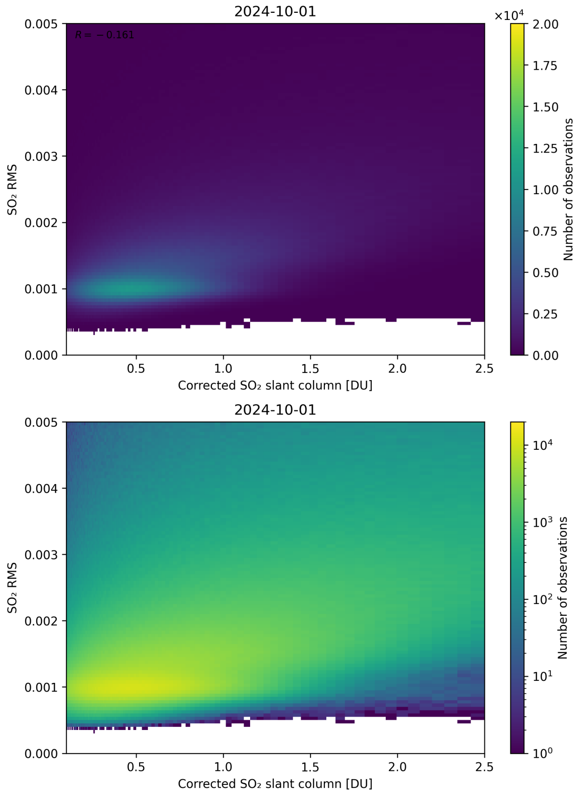
Figure 183: Scatter density plot of “Corrected SO 2 slant column” against “SO 2 RMS” for 2024-09-30 to 2024-10-02.
