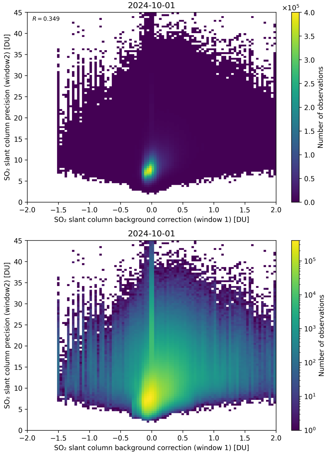
Figure 106: Scatter density plot of “SO 2 slant column background correction (window 1)” against “SO 2 slant column precision (window2)” for 2024-09-30 to 2024-10-02.
