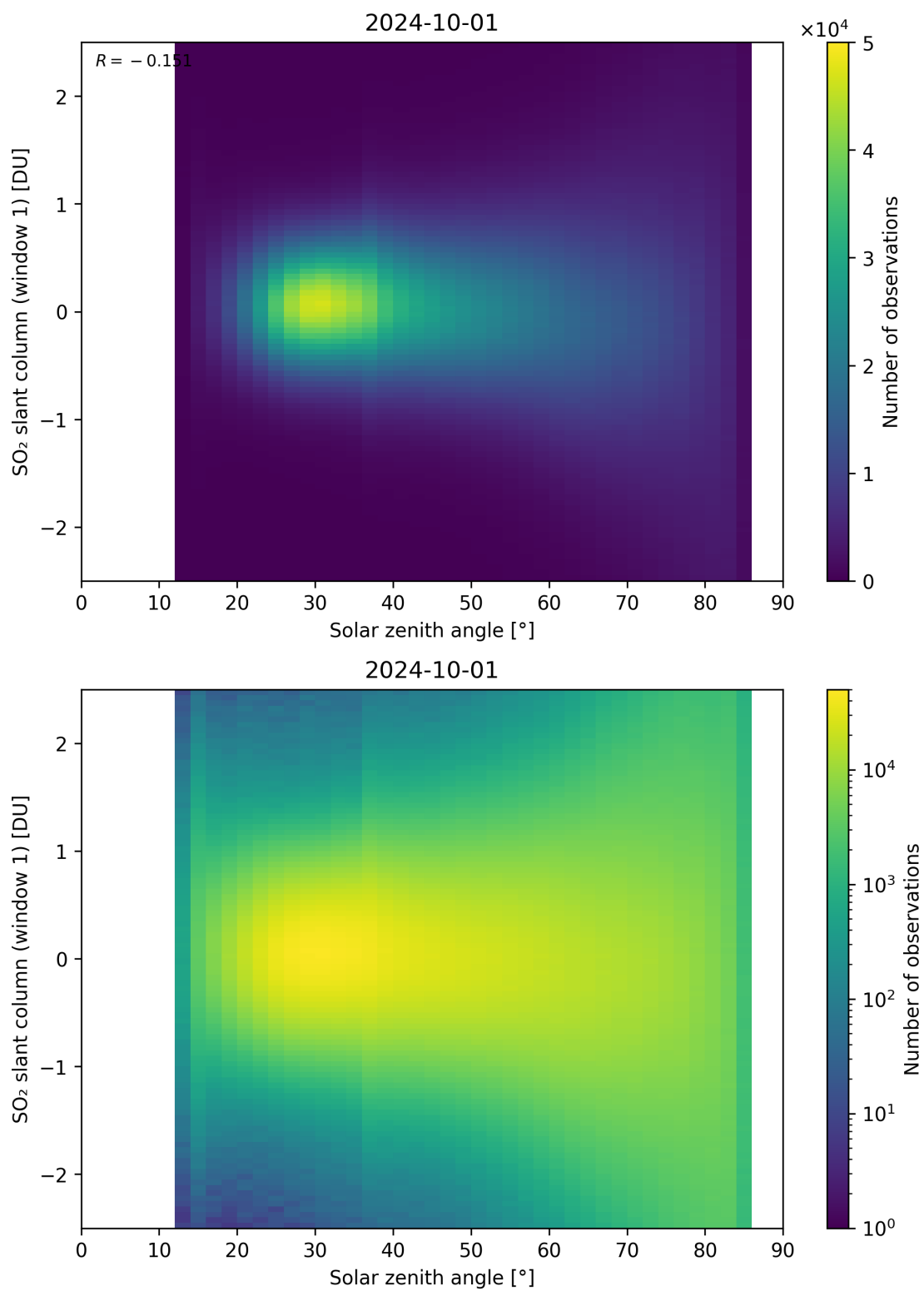
Figure 169: Scatter density plot of “Solar zenith angle” against “SO 2 slant column (window 1)” for 2024-09-30 to 2024-10-02.
