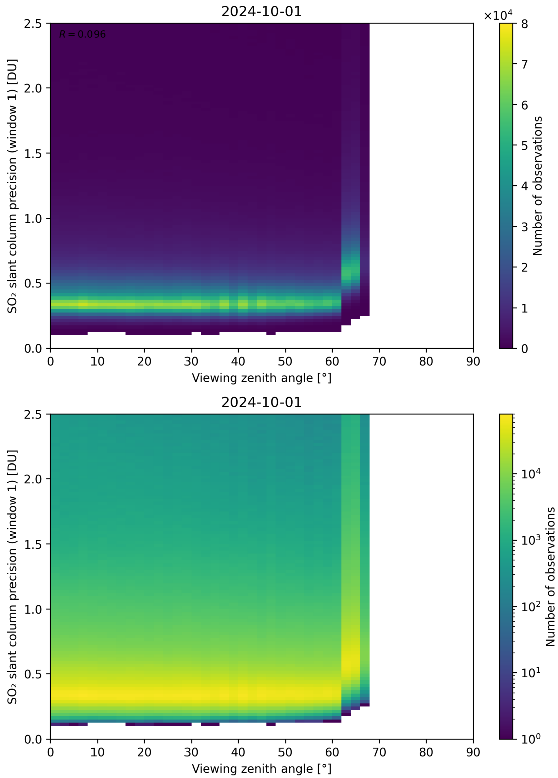
Figure 321: Scatter density plot of “Viewing zenith angle” against “SO 2 slant column precision (window 1)” for 2024-09-30 to 2024-10-02.
