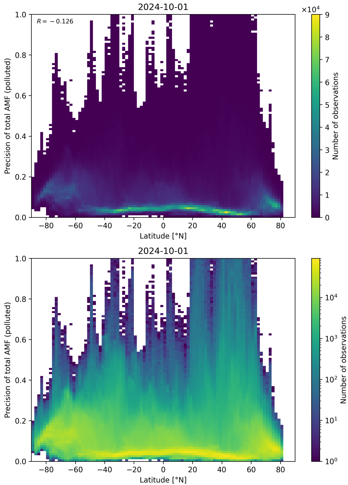
Figure 155: Scatter density plot of “Latitude” against “Precision of total AMF (polluted)” for 2024-09-30 to 2024-10-02.
