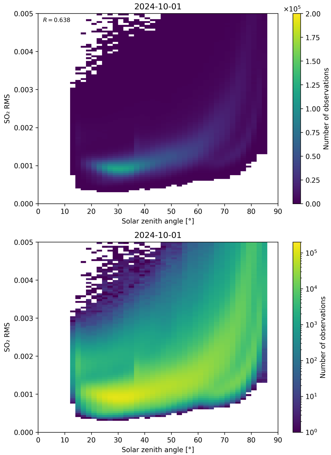
Figure 163: Scatter density plot of “Solar zenith angle” against “SO 2 RMS” for 2024-09-30 to 2024-10-02.
