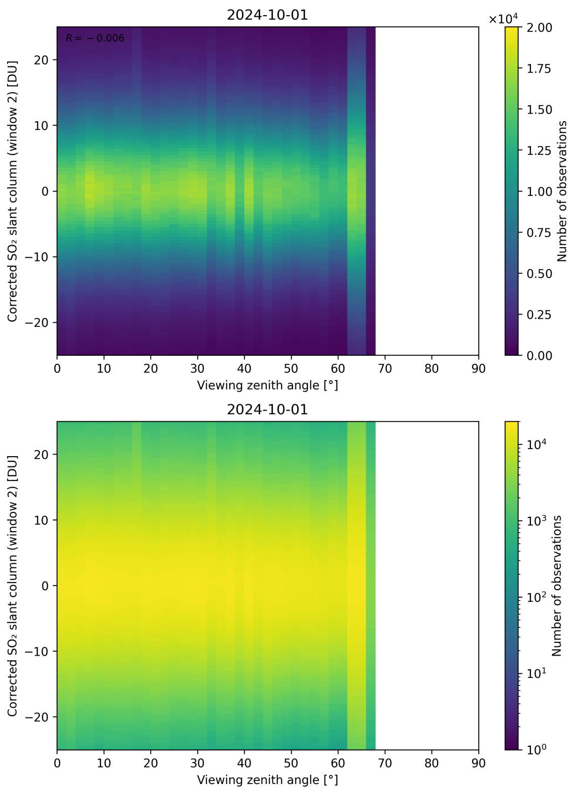
Figure 318: Scatter density plot of “Viewing zenith angle” against “Corrected SO 2 slant column (window 2)” for 2024-09-30 to 2024-10-02.
