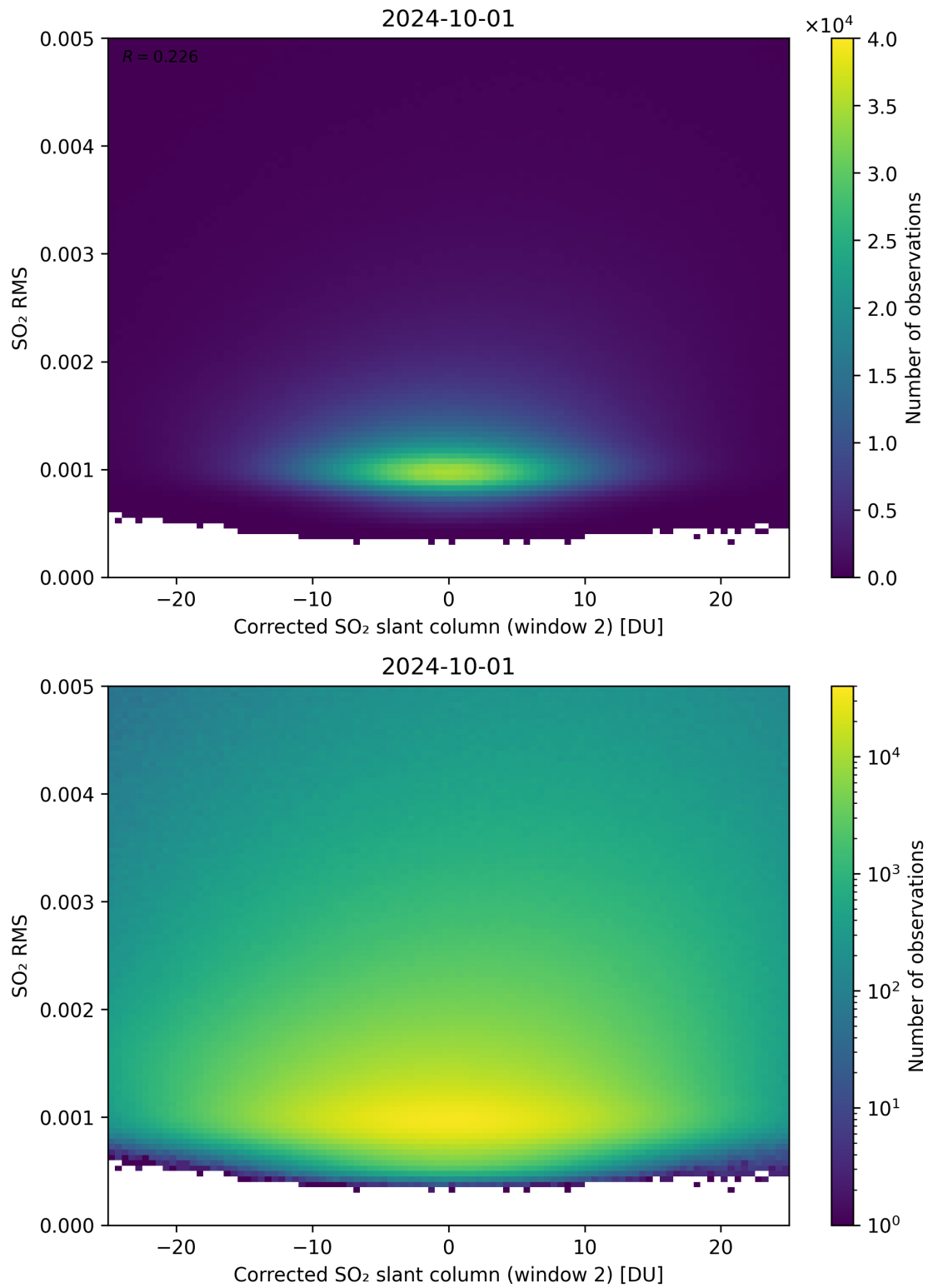
Figure 198: Scatter density plot of “Corrected SO 2 slant column (window 2)” against “SO 2 RMS” for 2024-09-30 to 2024-10-02.
