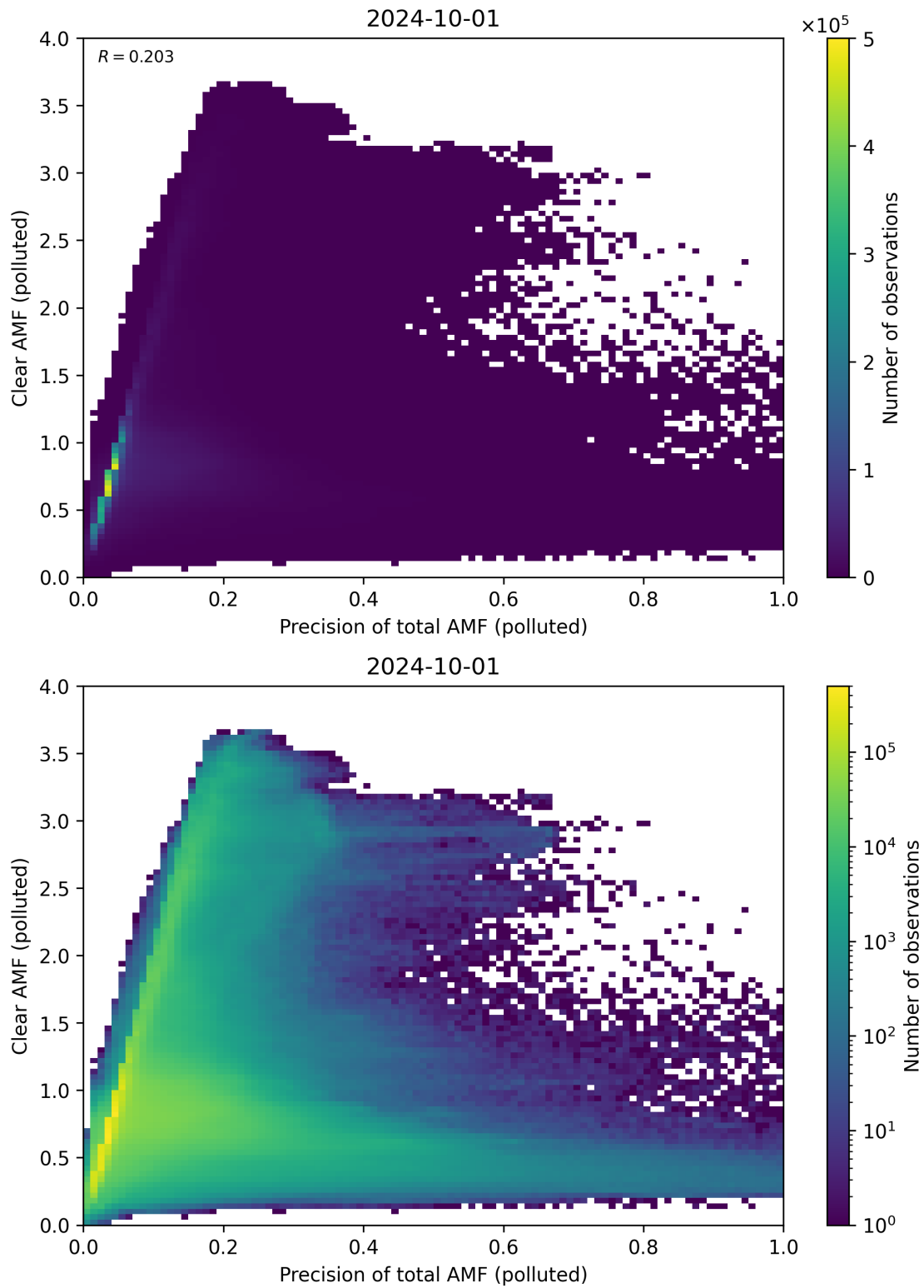
Figure 270: Scatter density plot of “Precision of total AMF (polluted)” against “Clear AMF (polluted)” for 2024-09-30 to 2024-10-02.
