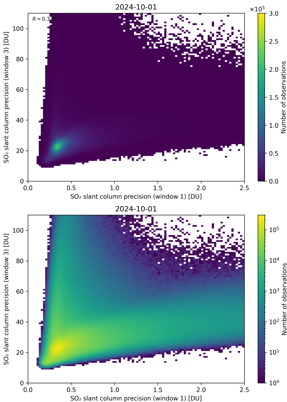
Figure 229: Scatter density plot of “SO 2 slant column precision (window 1)” against “SO 2 slant column precision (window 3)” for 2024-09-30 to 2024-10-02.
