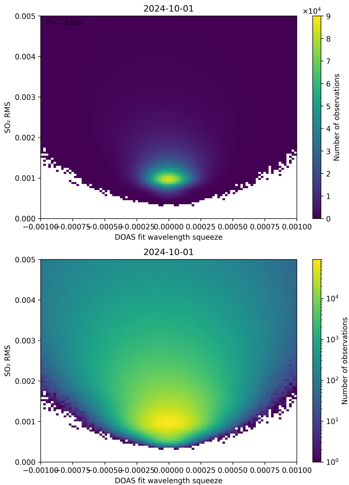
Figure 132: Scatter density plot of “DOAS fit wavelength squeeze” against “SO 2 RMS” for 2024-09-30 to 2024-10-02.
