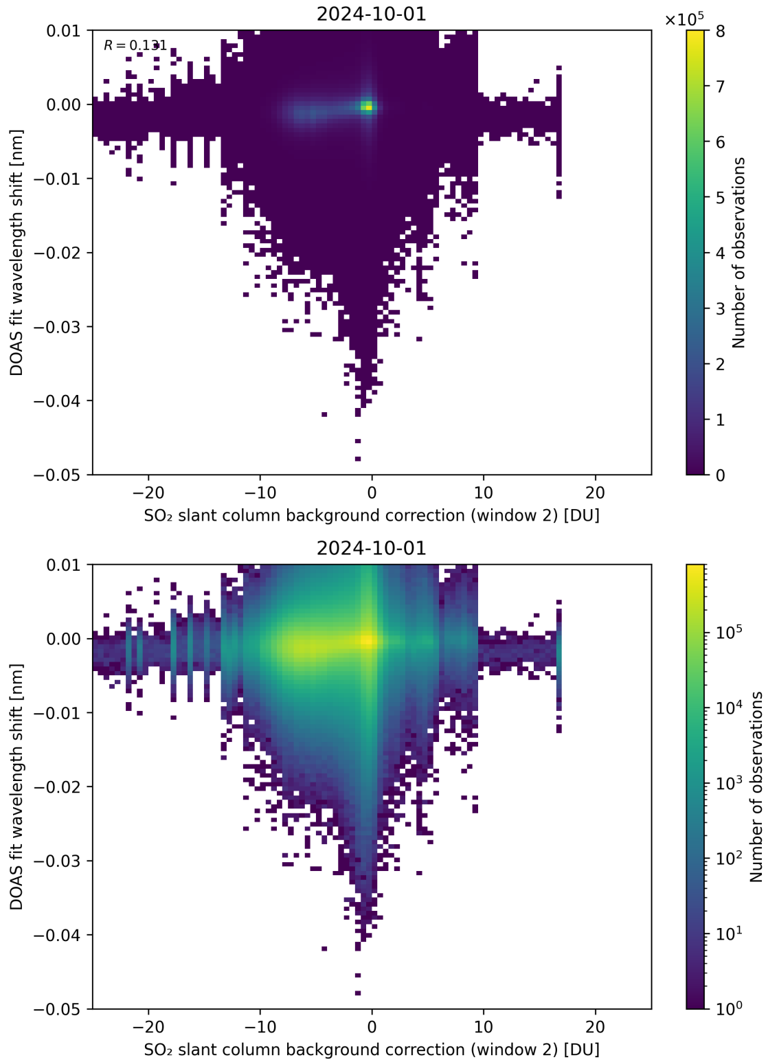
Figure 112: Scatter density plot of “SO 2 slant column background correction (window 2)” against “DOAS fit wavelength shift” for 2024-09-30 to 2024-10-02.
