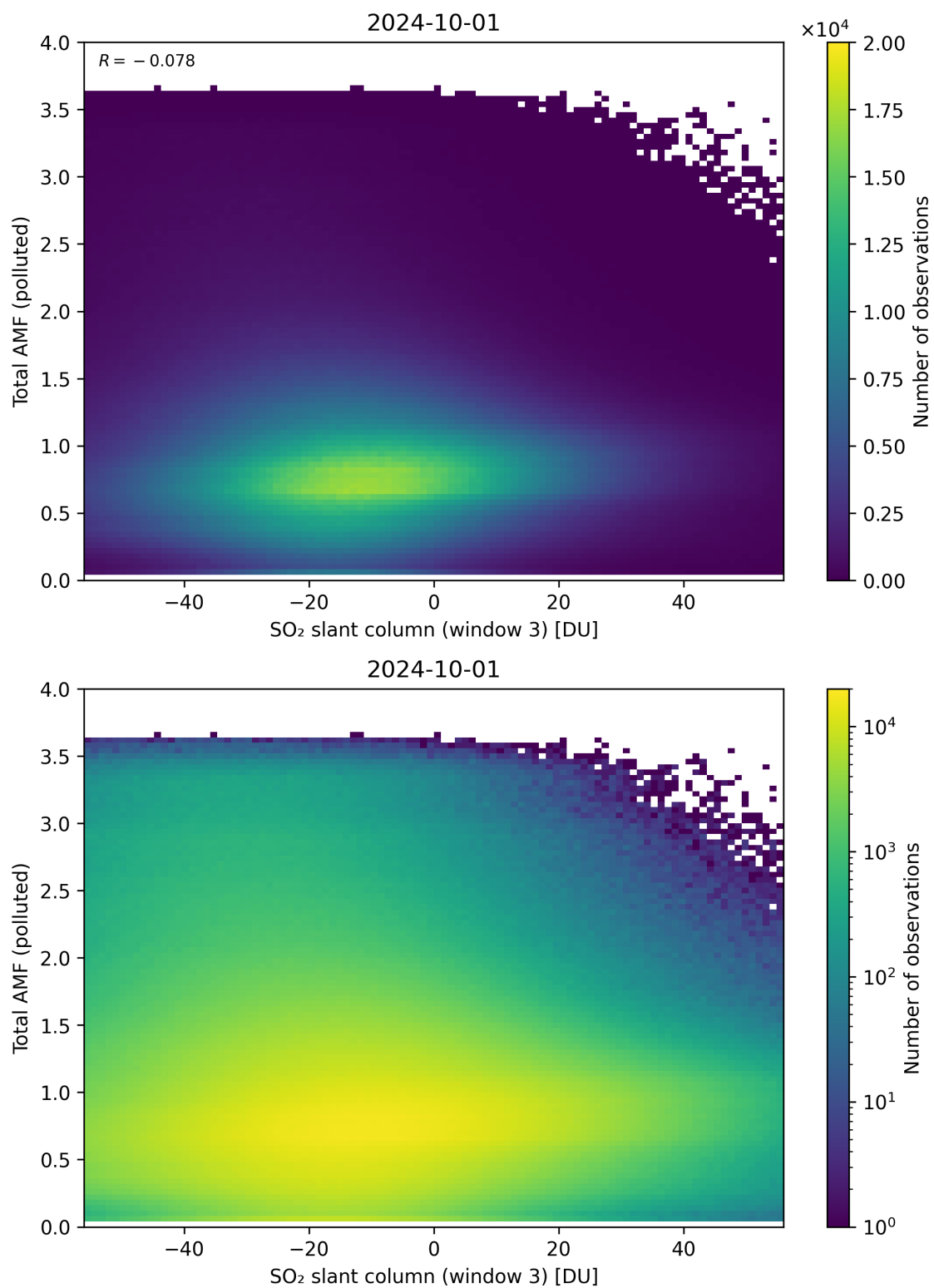
Figure 268: Scatter density plot of “SO 2 slant column (window 3)” against “Total AMF (polluted)” for 2024-09-30 to 2024-10-02.
