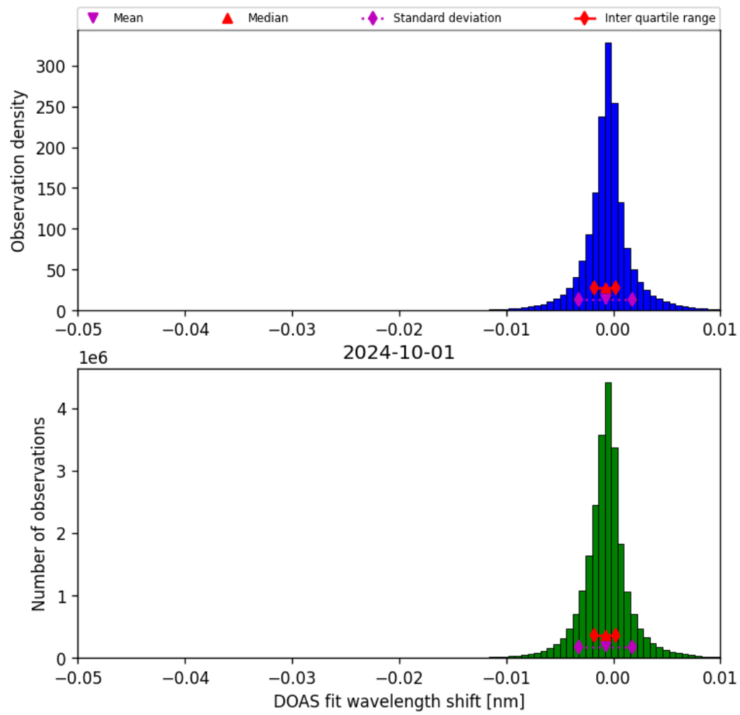
Figure 68: Histogram of “DOAS fit wavelength shift” for 2024-09-30 to 2024-10-02
