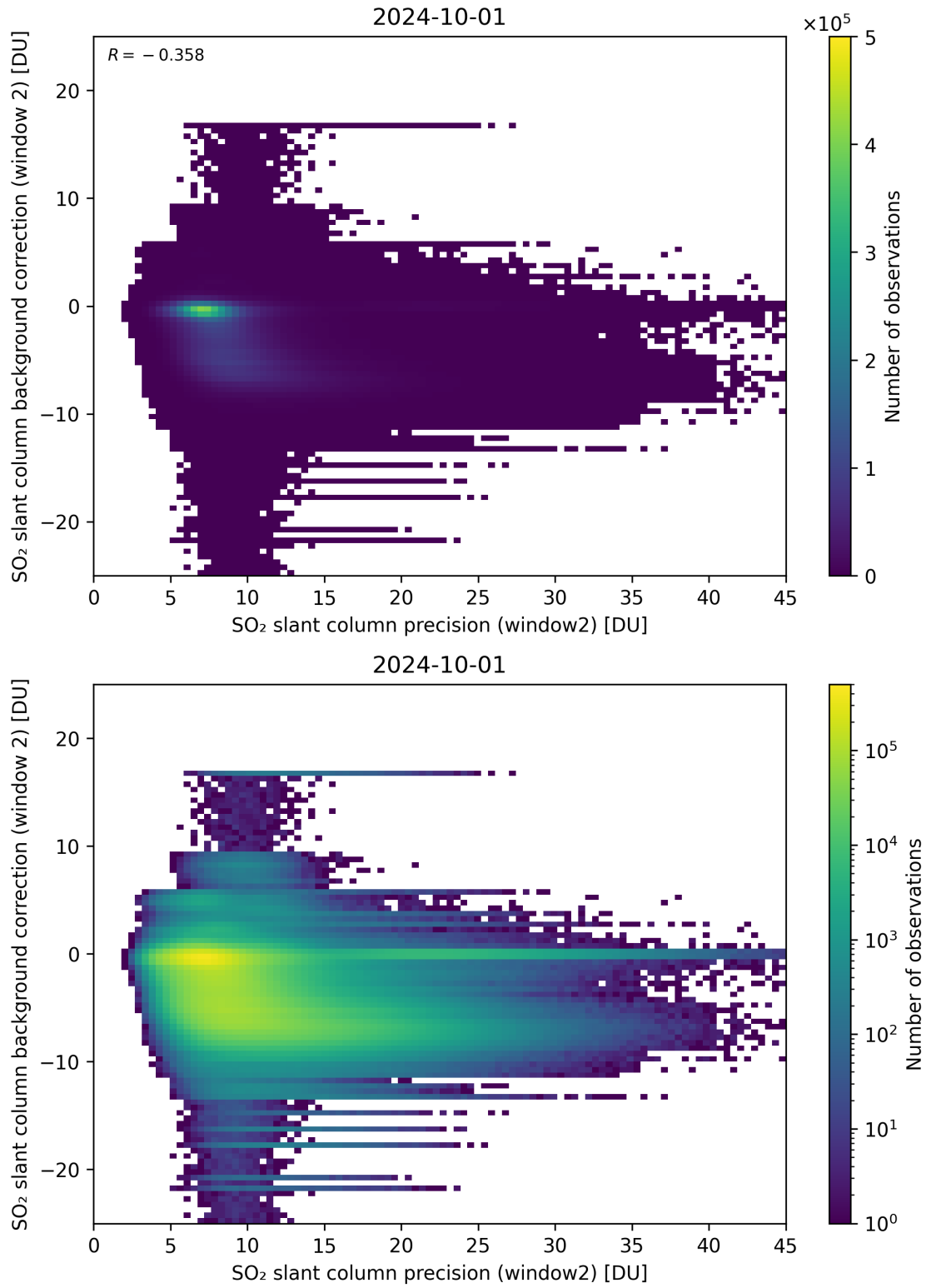
Figure 241: Scatter density plot of “SO 2 slant column precision (window2)” against “SO 2 slant column background correction (window 2)” for 2024-09-30 to 2024-10-02.
