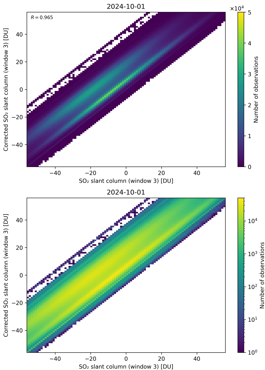
Figure 266: Scatter density plot of “SO 2 slant column (window 3)” against “Corrected SO 2 slant column (window 3)” for 2024-09-30 to 2024-10-02.
