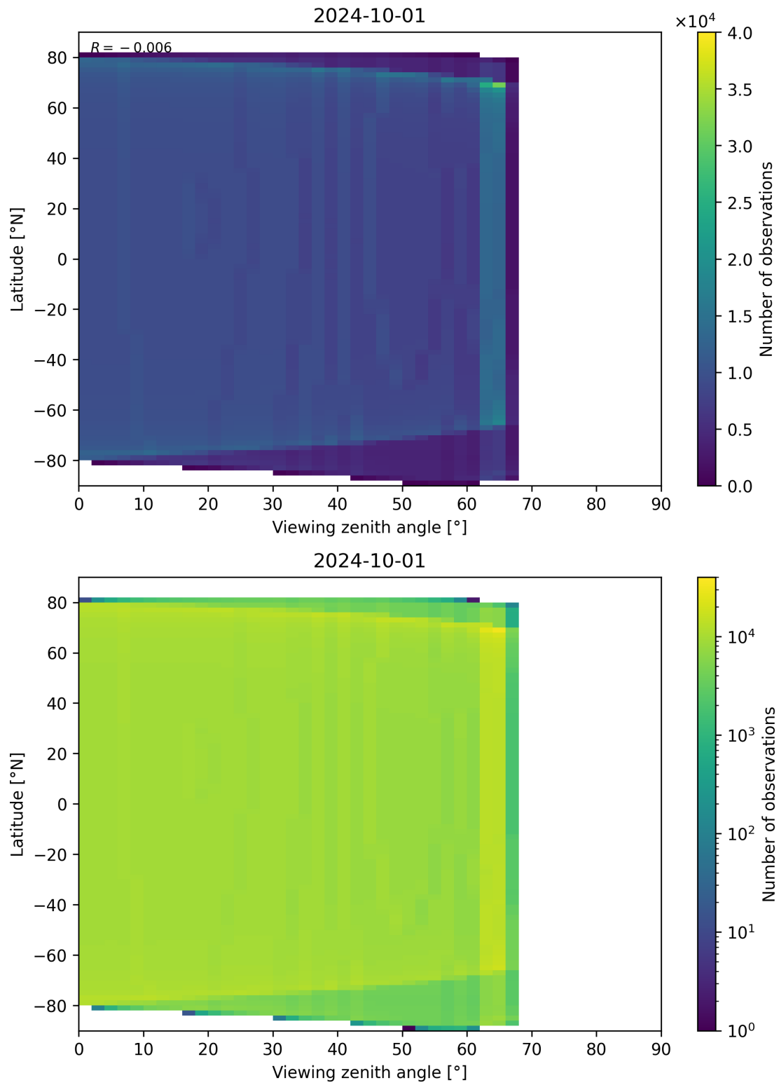
Figure 314: Scatter density plot of “Viewing zenith angle” against “Latitude” for 2024-09-30 to 2024-10-02.
