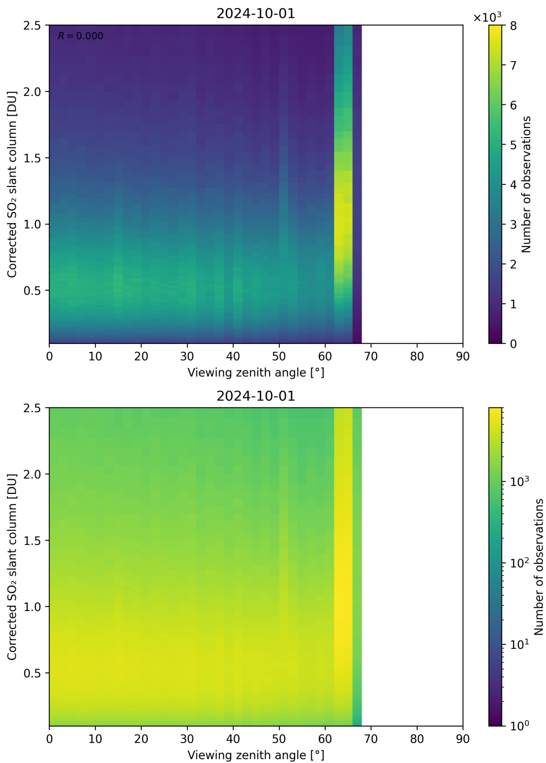
Figure 317: Scatter density plot of “Viewing zenith angle” against “Corrected SO 2 slant column” for 2024-09-30 to 2024-10-02.
