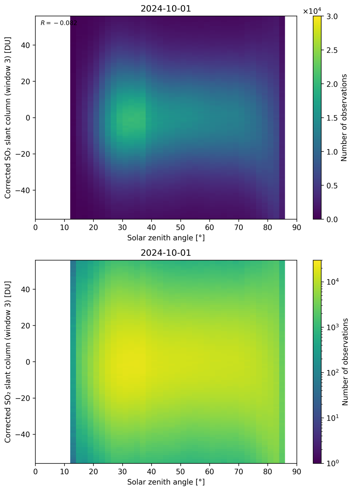
Figure 168: Scatter density plot of “Solar zenith angle” against “Corrected SO 2 slant column (window 3)” for 2024-09-30 to 2024-10-02.
