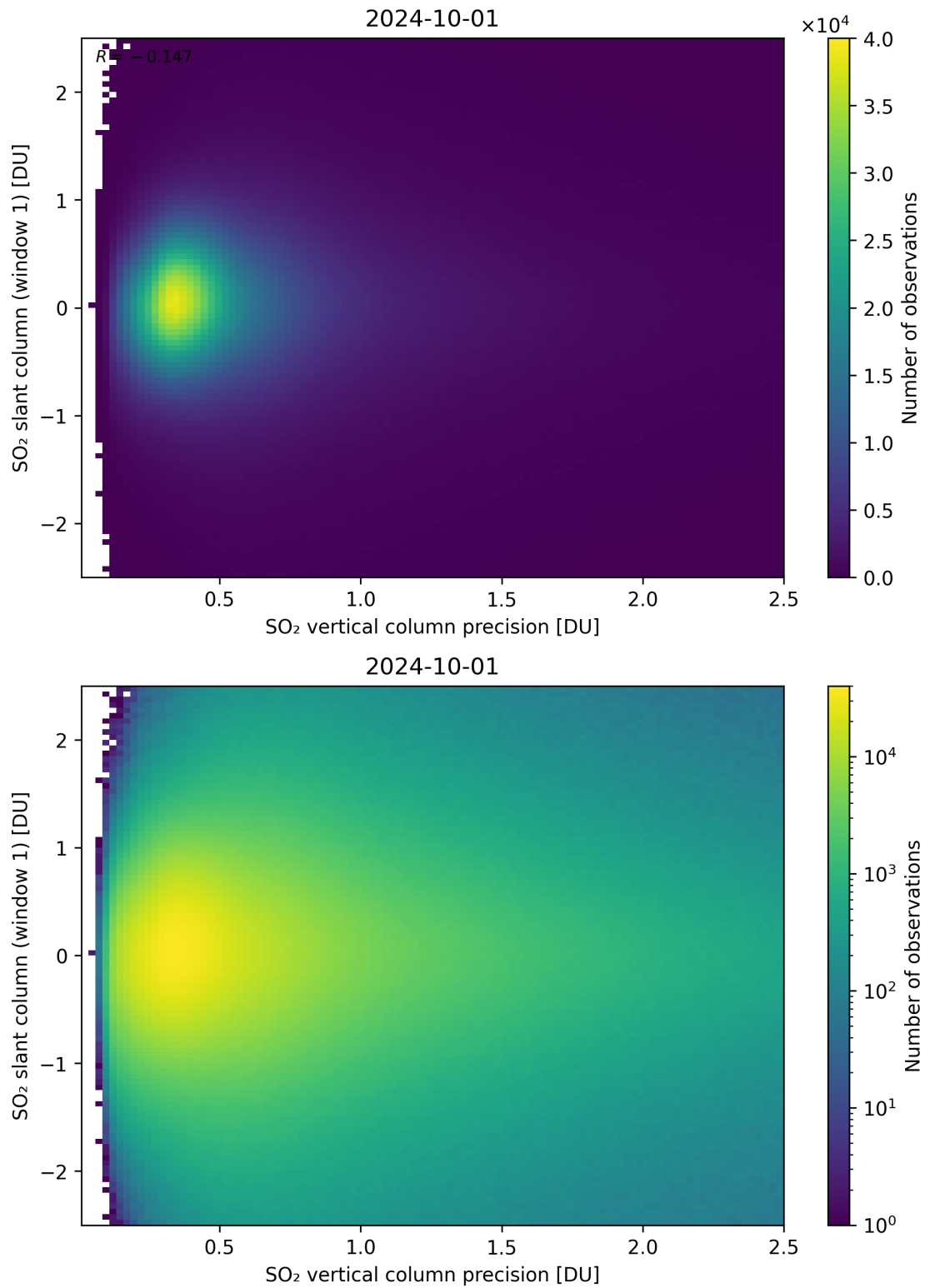
Figure 289: Scatter density plot of “SO 2 vertical column precision” against “SO 2 slant column (window 1)” for 2024-09-30 to 2024-10-02.
