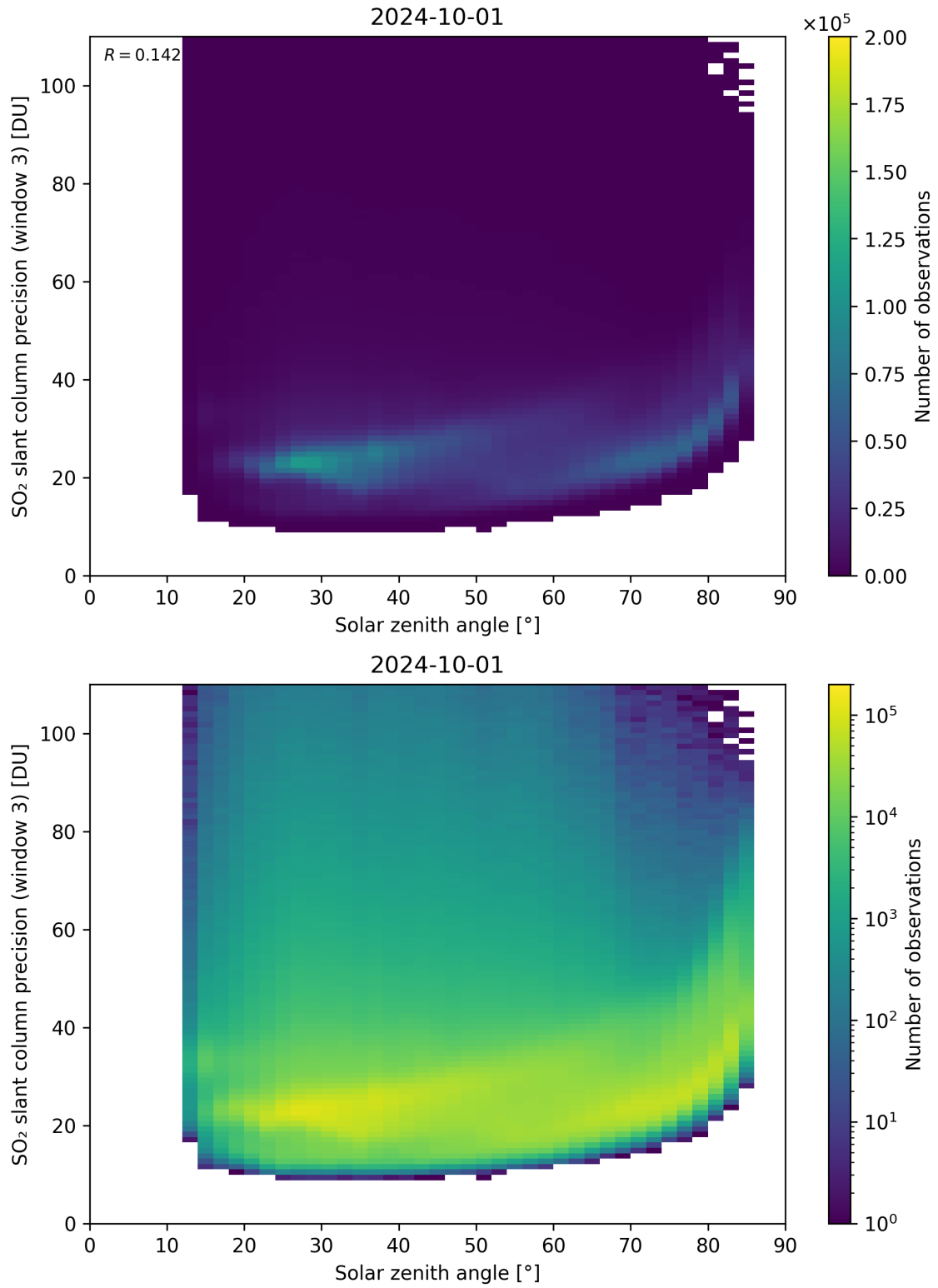
Figure 173: Scatter density plot of “Solar zenith angle” against “SO 2 slant column precision (window 3)” for 2024-09-30 to 2024-10-02.
