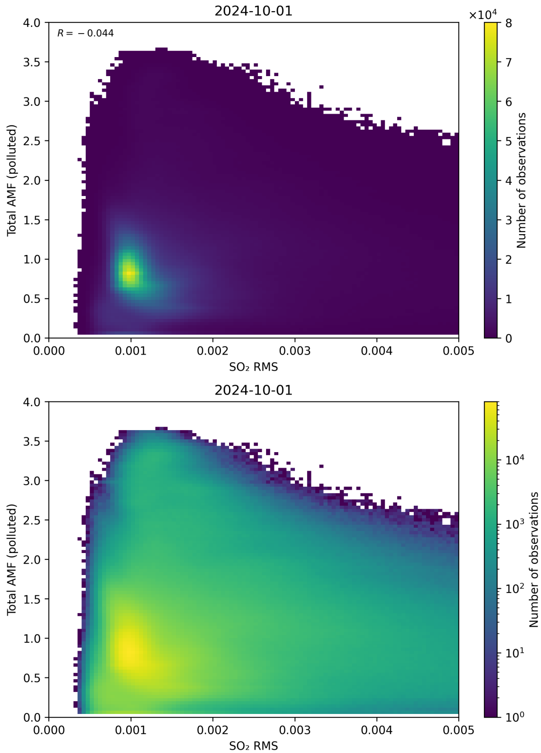
Figure 137: Scatter density plot of “SO 2 RMS” against “Total AMF (polluted)” for 2024-09-30 to 2024-10-02.
