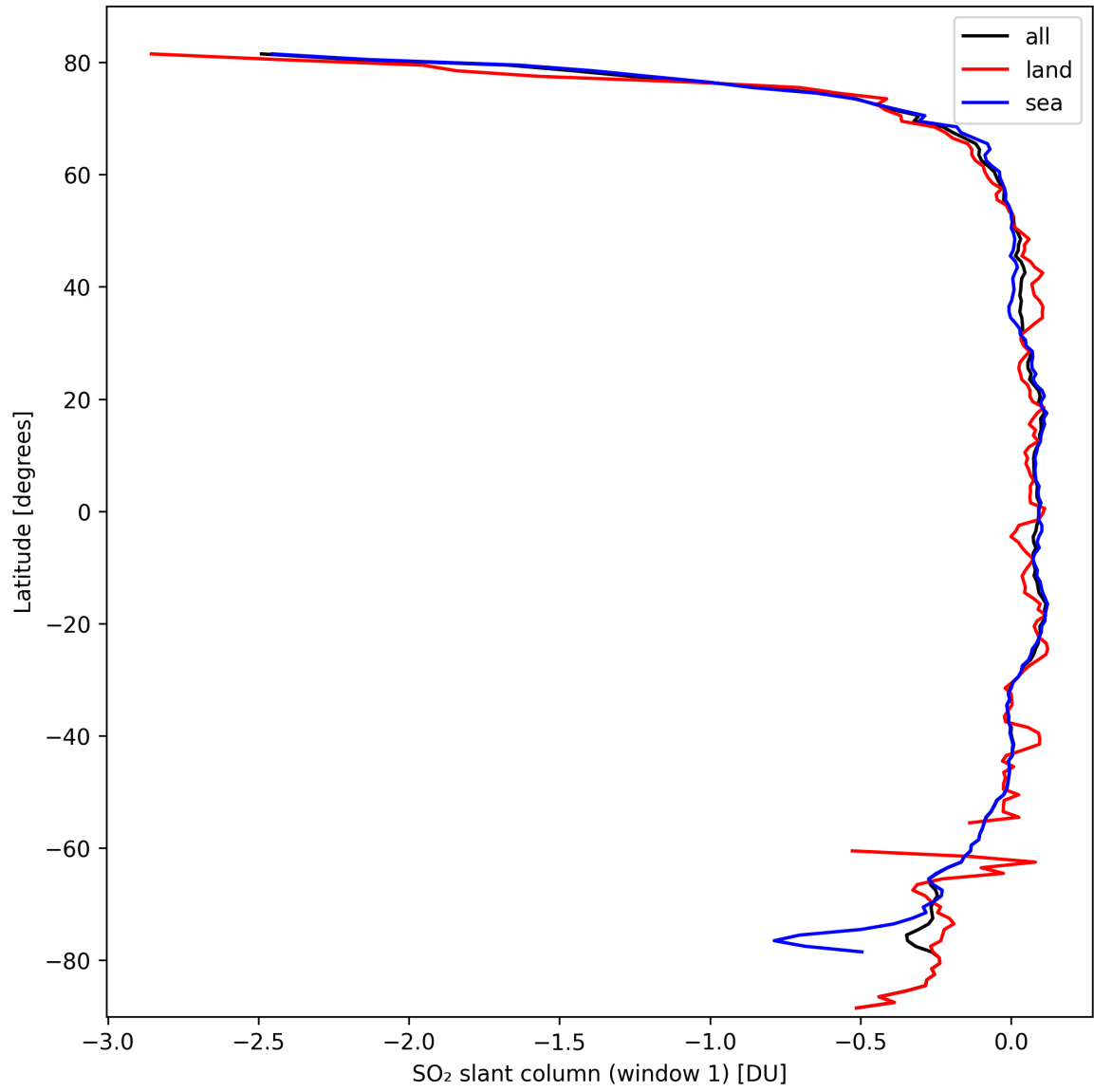
Figure 33: Zonal average of “SO 2 slant column (window 1)” for 2024-09-30 to 2024-10-02.
