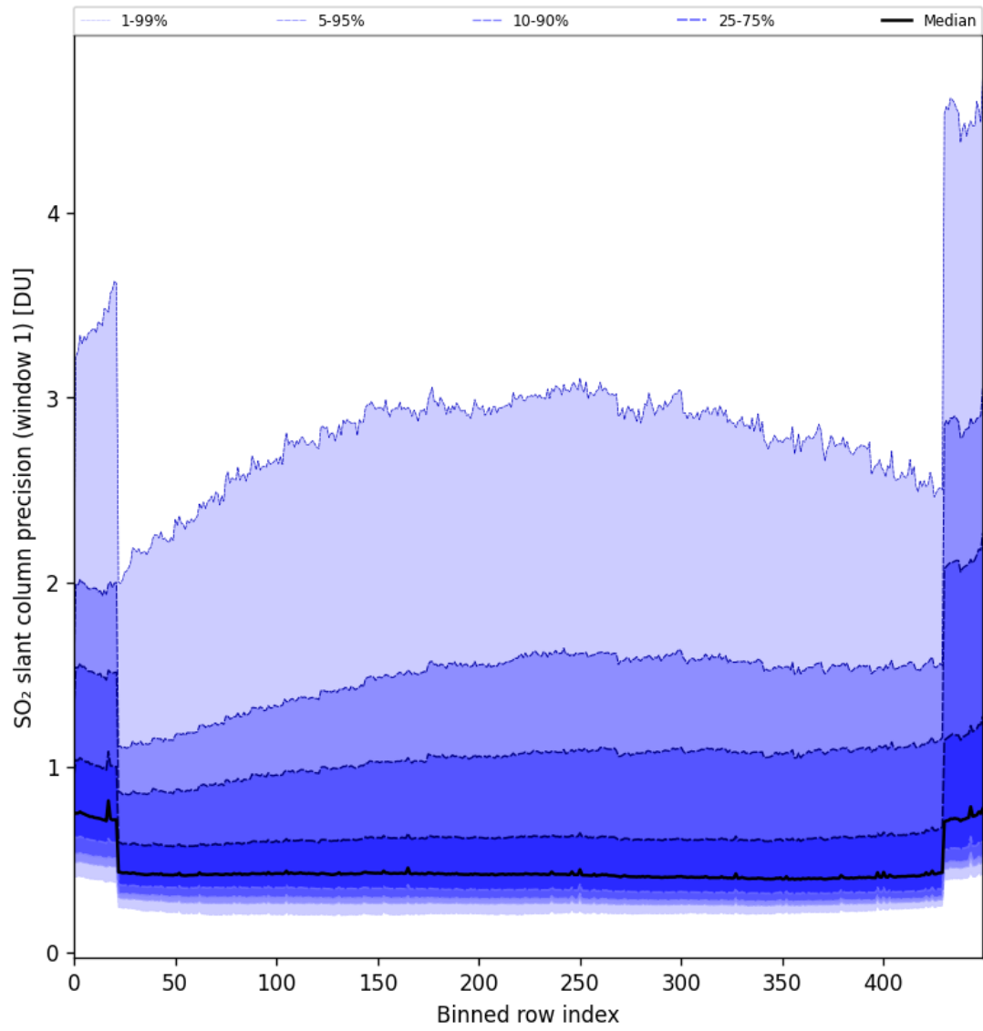
Figure 80: Along track statistics of “SO 2 slant column precision (window 1)” for 2024-09-30 to 2024-10-02
