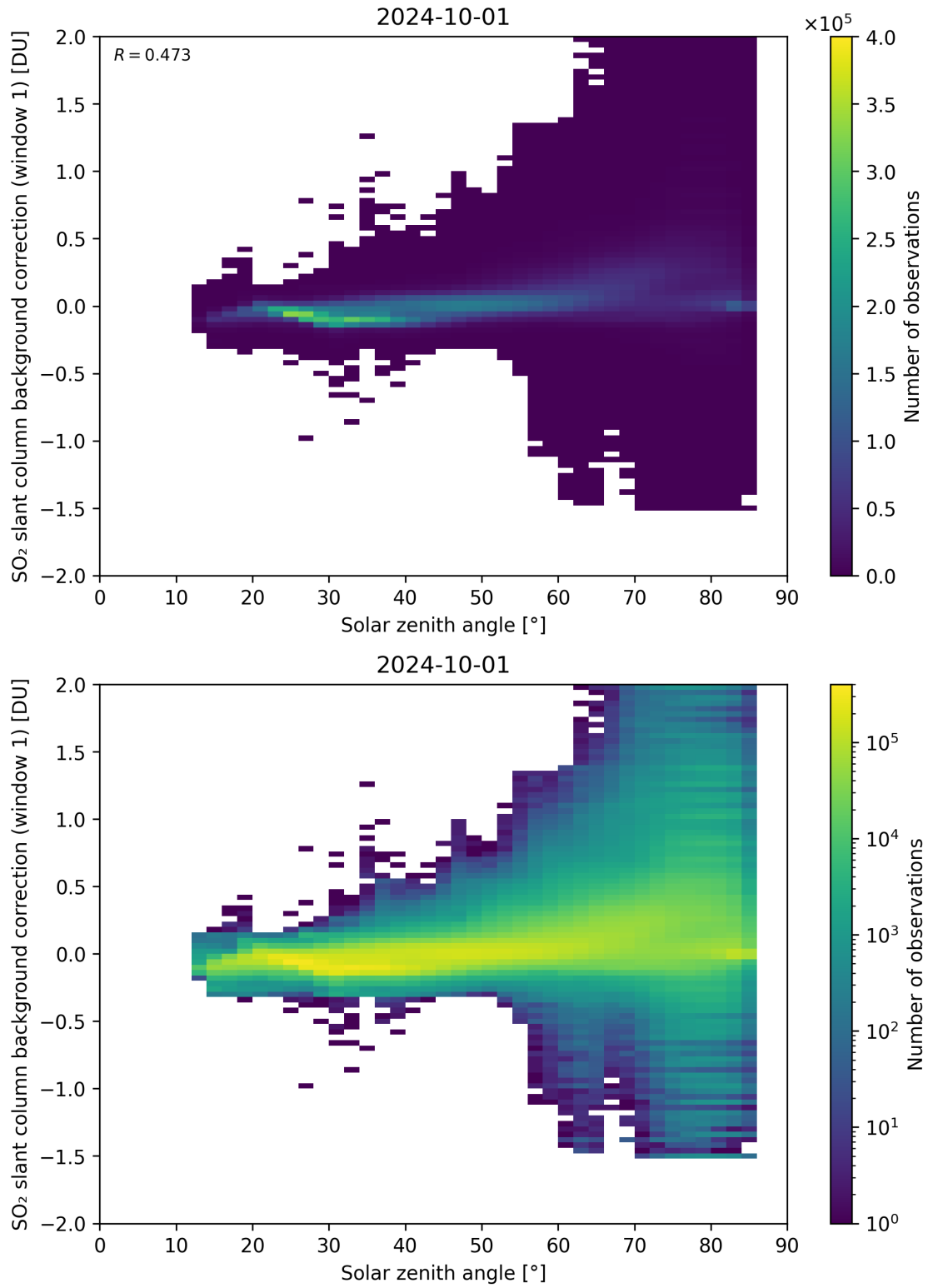
Figure 158: Scatter density plot of “Solar zenith angle” against “SO 2 slant column background correction (window 1)” for 2024-09-30 to 2024-10-02.
