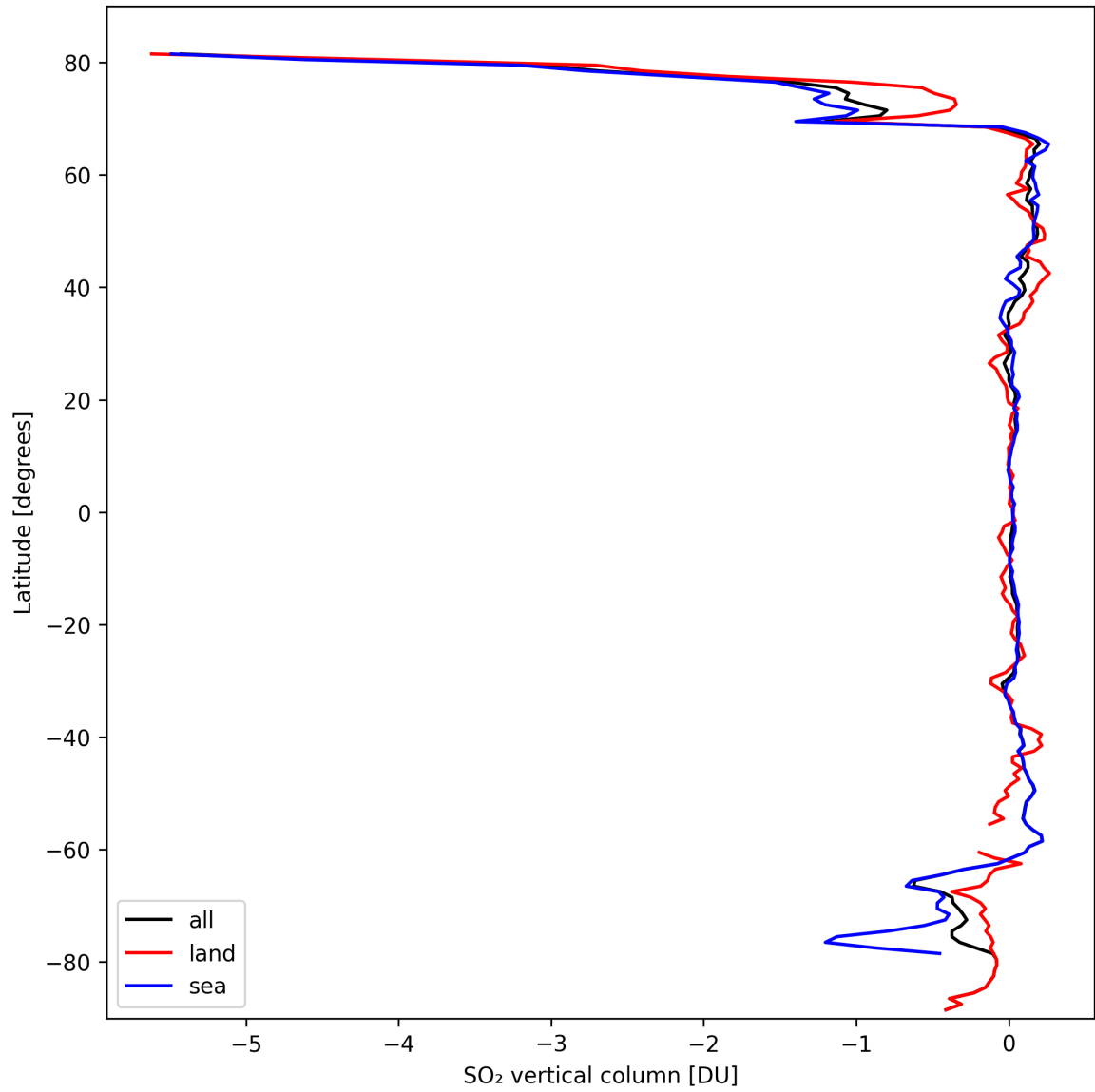
Figure 30: Zonal average of “SO 2 vertical column” for 2024-09-30 to 2024-10-02.
