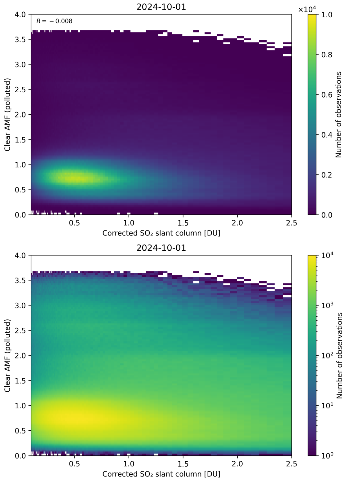
Figure 184: Scatter density plot of “Corrected SO 2 slant column” against “Clear AMF (polluted)” for 2024-09-30 to 2024-10-02.
