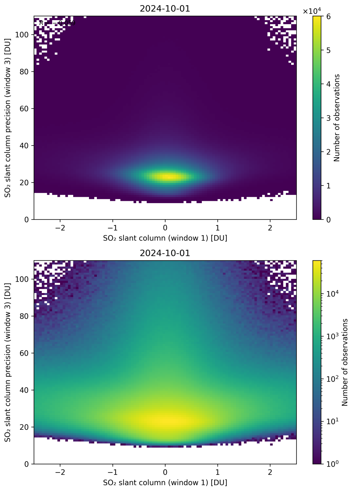
Figure 238: Scatter density plot of “SO 2 slant column (window 1)” against “SO 2 slant column precision (window 3)” for 2024-09-30 to 2024-10-02.
