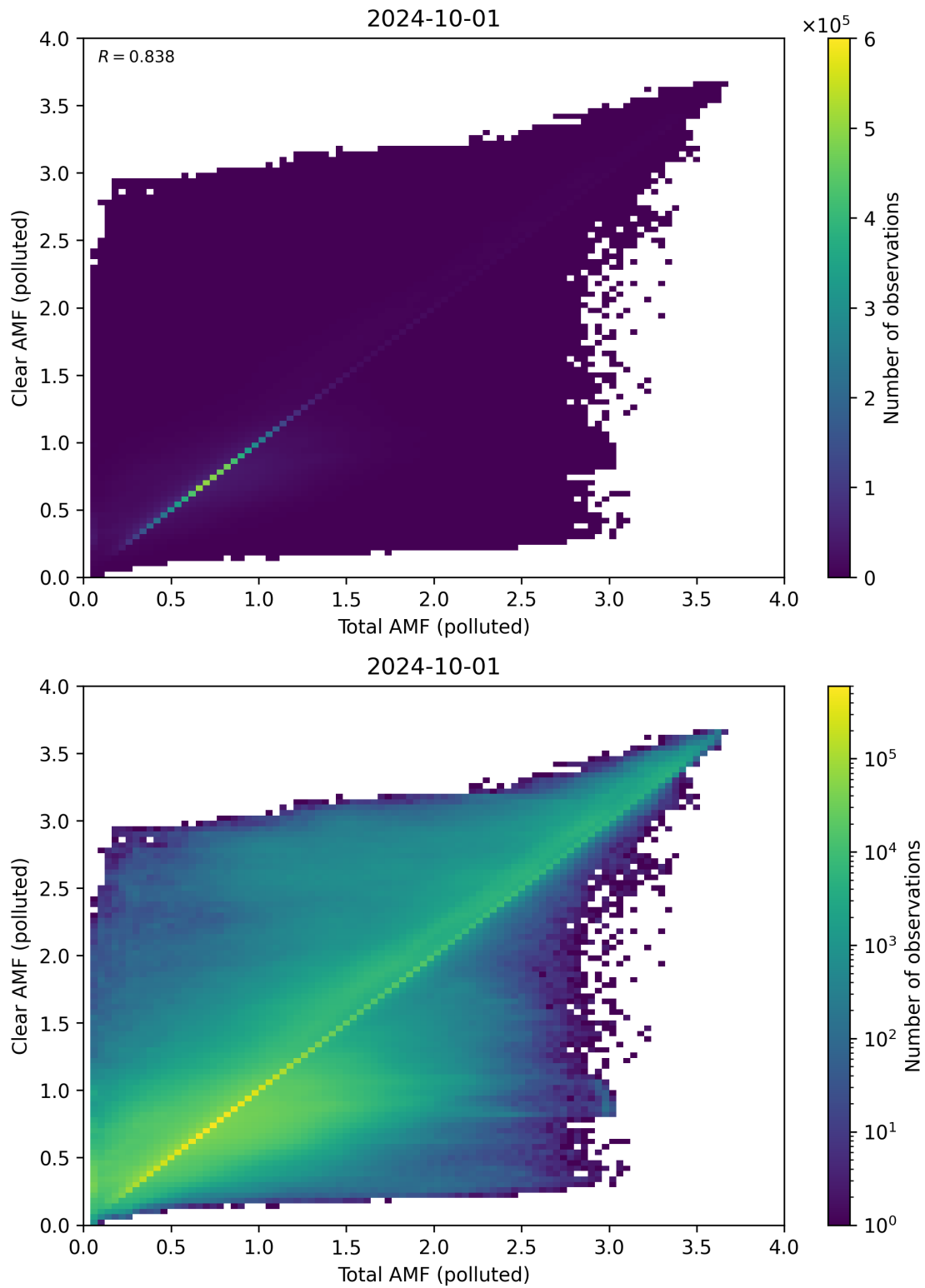
Figure 271: Scatter density plot of “Total AMF (polluted)” against “Clear AMF (polluted)” for 2024-09-30 to 2024-10-02.
