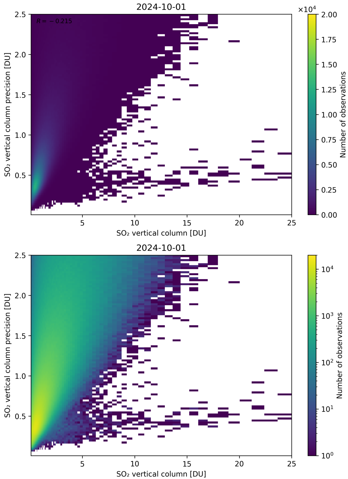
Figure 307: Scatter density plot of “SO 2 vertical column” against “SO 2 vertical column precision” for 2024-09-30 to 2024-10-02.
