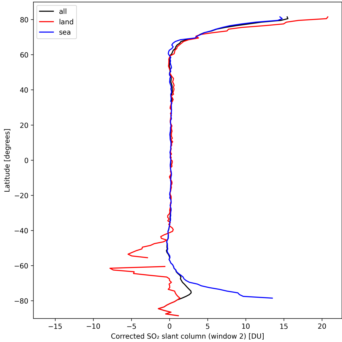
Figure 39: Zonal average of “Corrected SO 2 slant column (window 2)” for 2024-09-30 to 2024-10-02.
