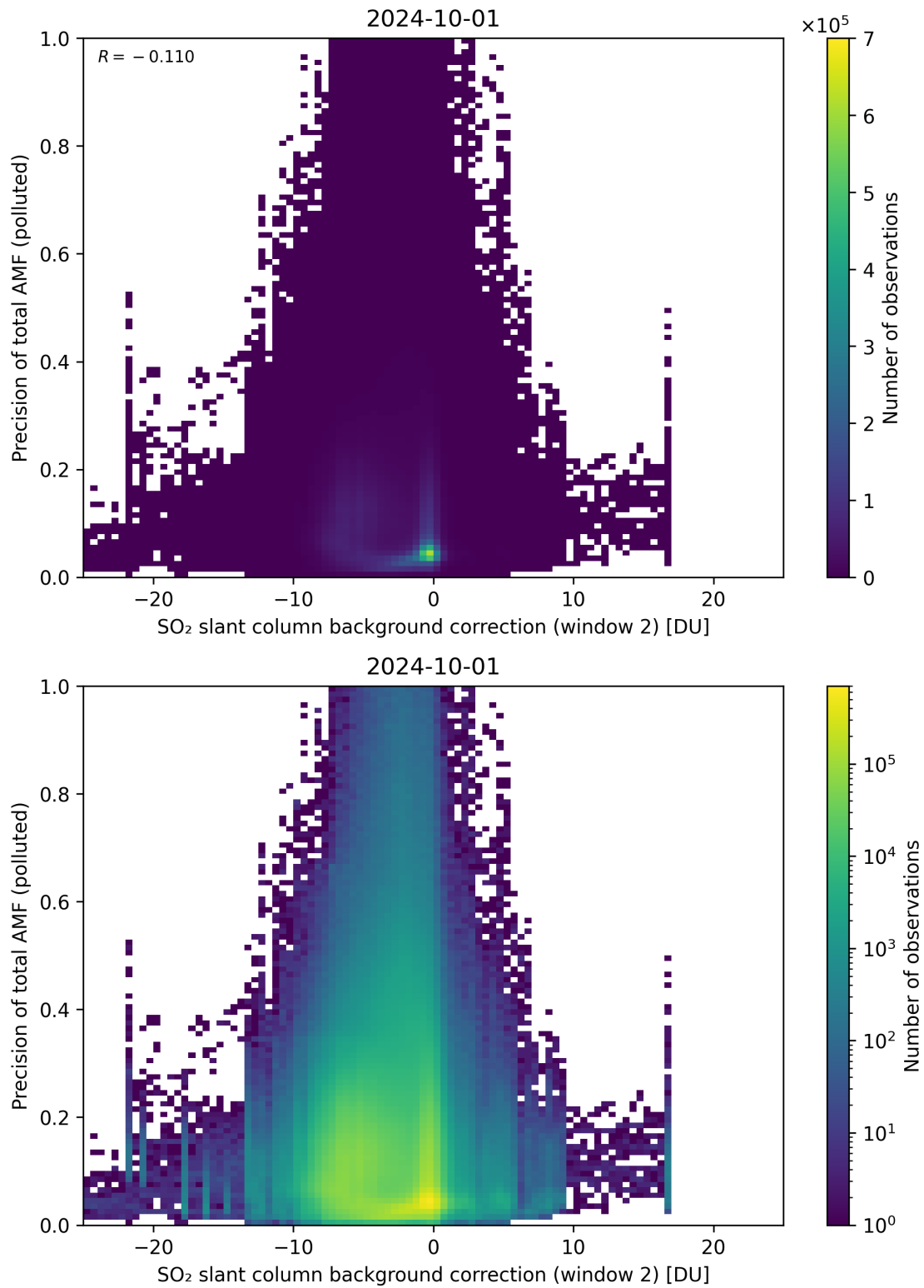
Figure 120: Scatter density plot of “SO 2 slant column background correction (window 2)” against “Precision of total AMF (polluted)” for 2024-09-30 to 2024-10-02.
