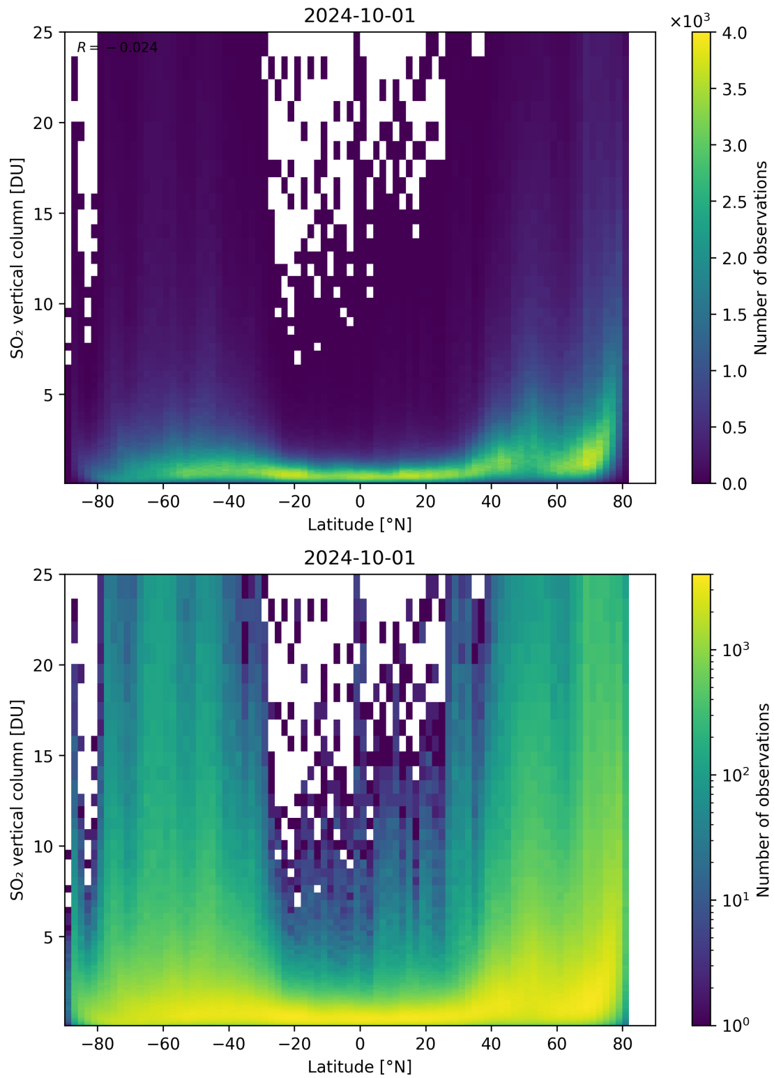
Figure 156: Scatter density plot of “Latitude” against “SO 2 vertical column” for 2024-09-30 to 2024-10-02.
