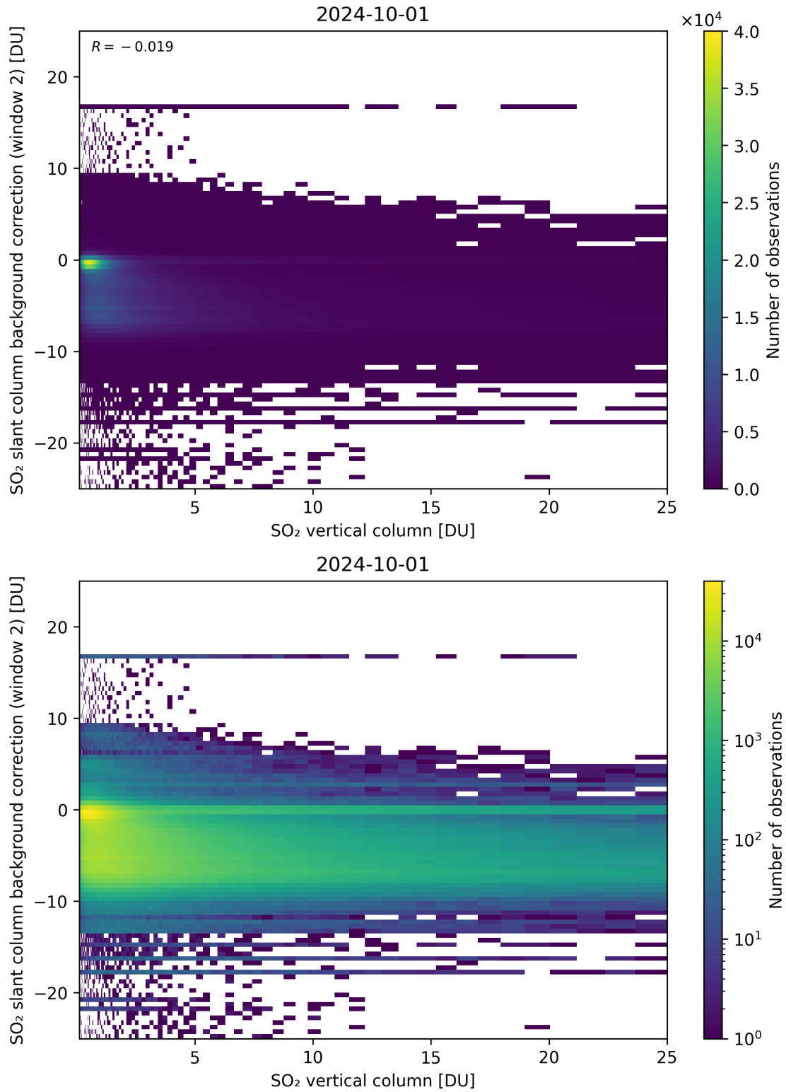
Figure 274: Scatter density plot of “SO 2 vertical column” against “SO 2 slant column background correction (window 2)” for 2024-09-30 to 2024-10-02.
