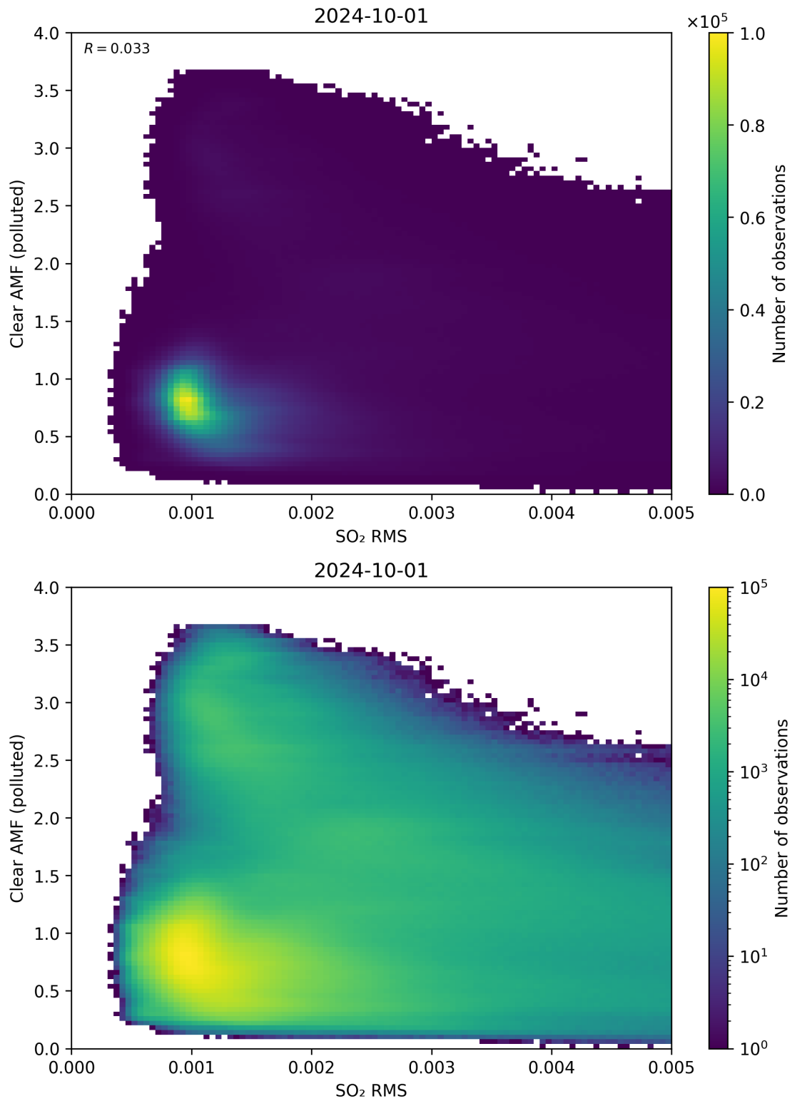
Figure 136: Scatter density plot of “SO 2 RMS” against “Clear AMF (polluted)” for 2024-09-30 to 2024-10-02.
