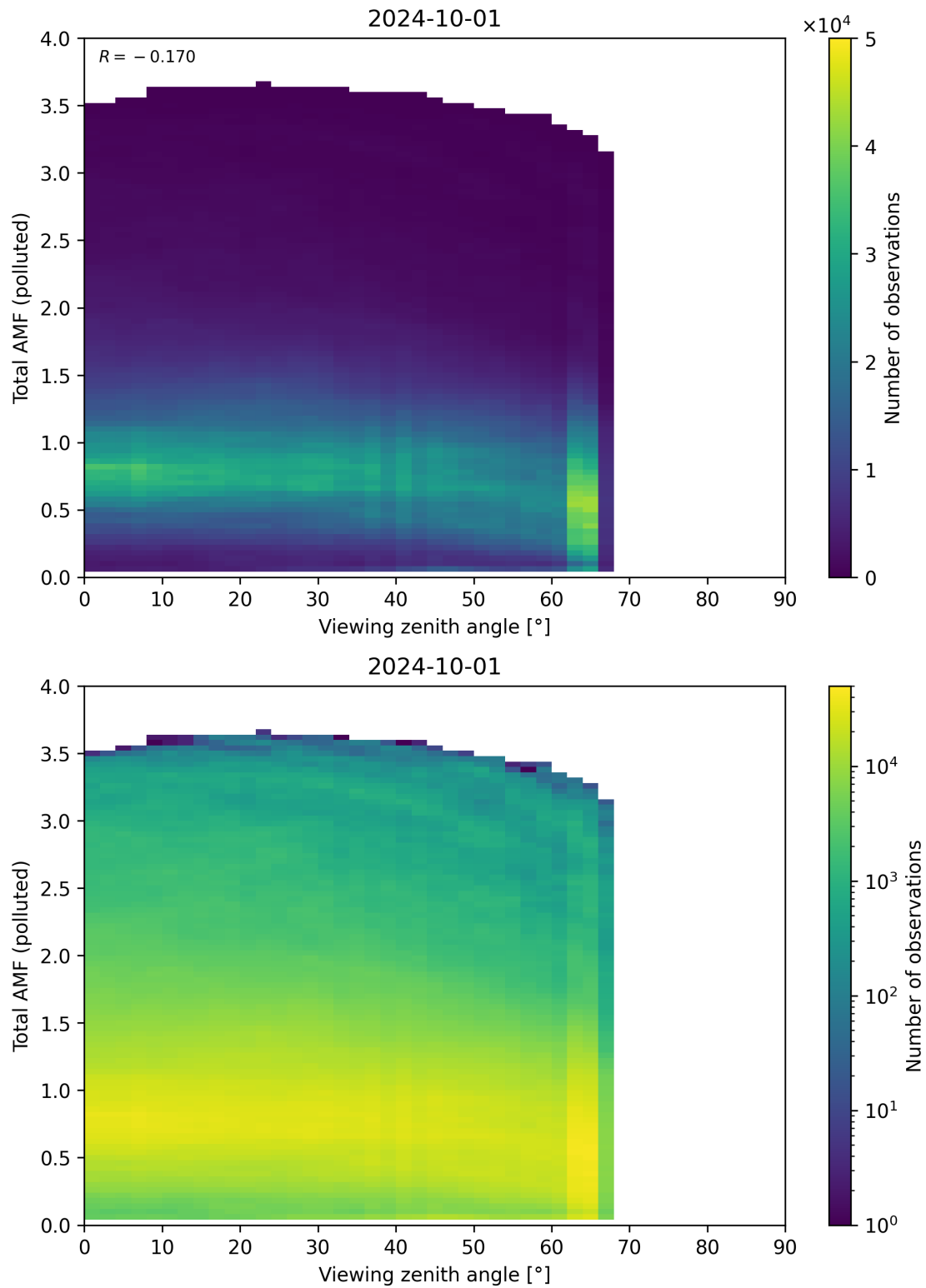
Figure 325: Scatter density plot of “Viewing zenith angle” against “Total AMF (polluted)” for 2024-09-30 to 2024-10-02.
