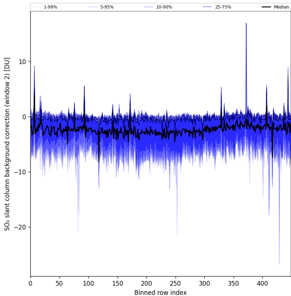
Figure 86: Along track statistics of “SO 2 slant column background correction (window 2)” for 2024-09-30 to 2024-10-02
