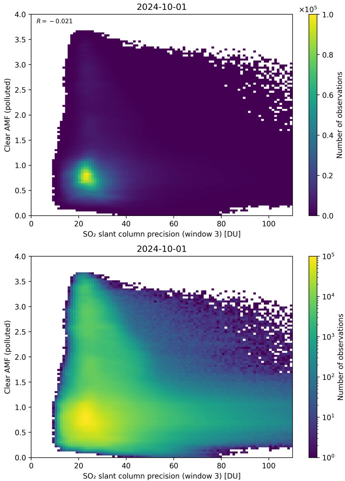
Figure 261: Scatter density plot of “SO 2 slant column precision (window 3)” against “Clear AMF (polluted)” for 2024-09-30 to 2024-10-02.
