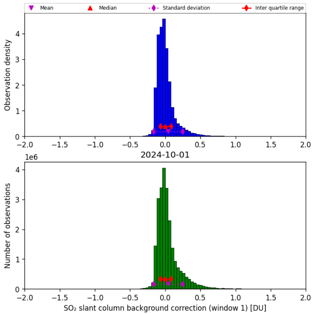
Figure 59: Histogram of “SO 2 slant column background correction (window 1)” for 2024-09-30 to 2024-10-02
