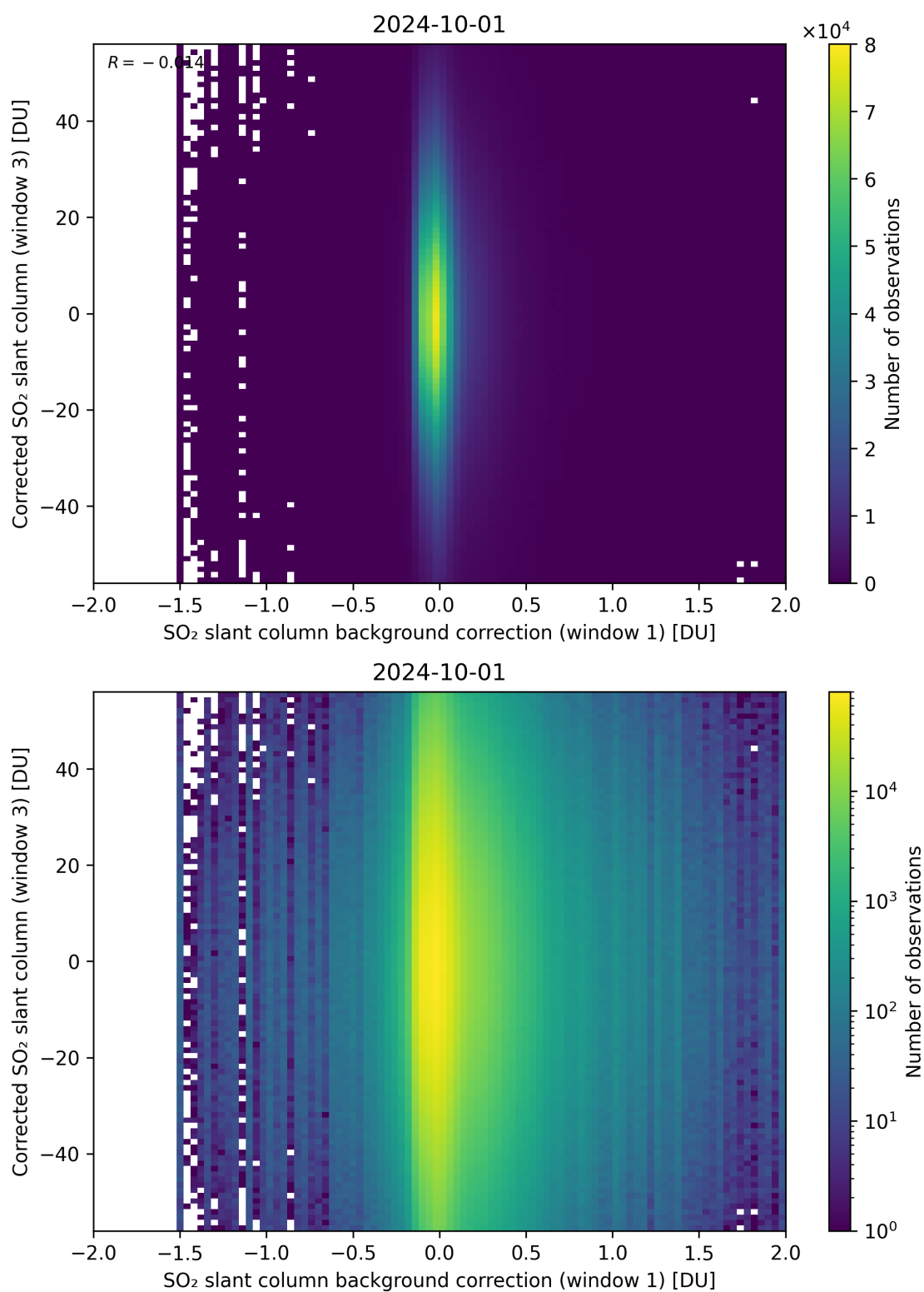
Figure 105: Scatter density plot of “SO 2 slant column background correction (window 1)” against “Corrected SO 2 slant column (window 3)” for 2024-09-30 to 2024-10-02.
