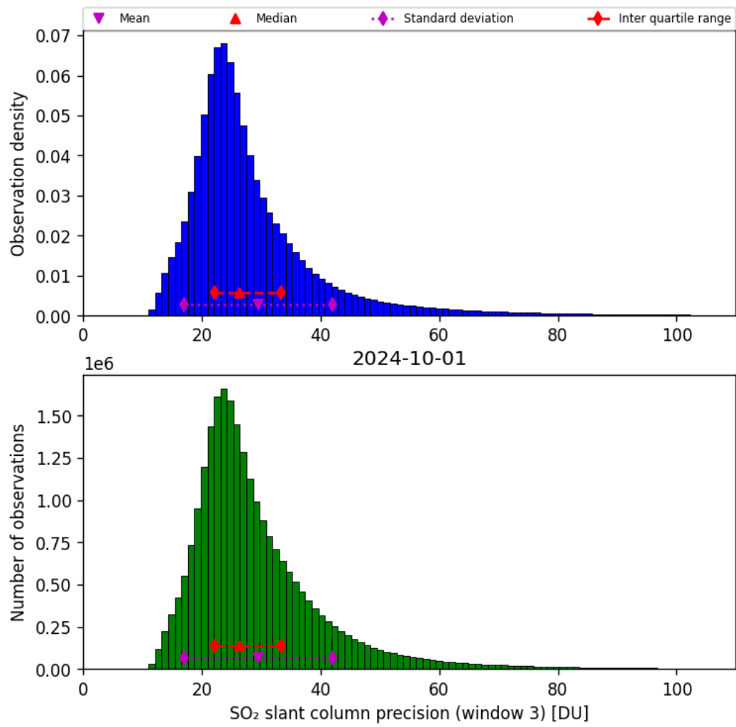
Figure 65: Histogram of “SO 2 slant column precision (window 3)” for 2024-09-30 to 2024-10-02
