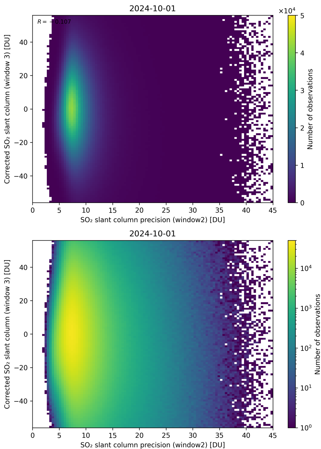
Figure 248: Scatter density plot of “SO 2 slant column precision (window2)” against “Corrected SO 2 slant column (window 3)” for 2024-09-30 to 2024-10-02.
