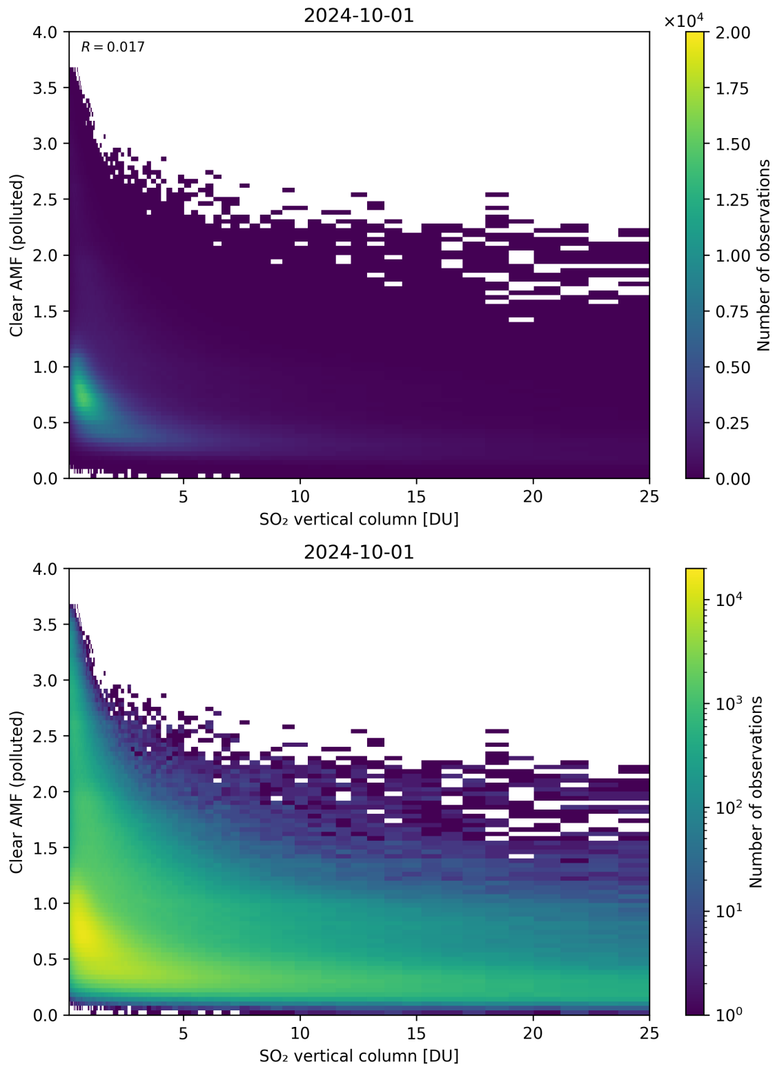
Figure 296: Scatter density plot of “SO 2 vertical column” against “Clear AMF (polluted)” for 2024-09-30 to 2024-10-02.
