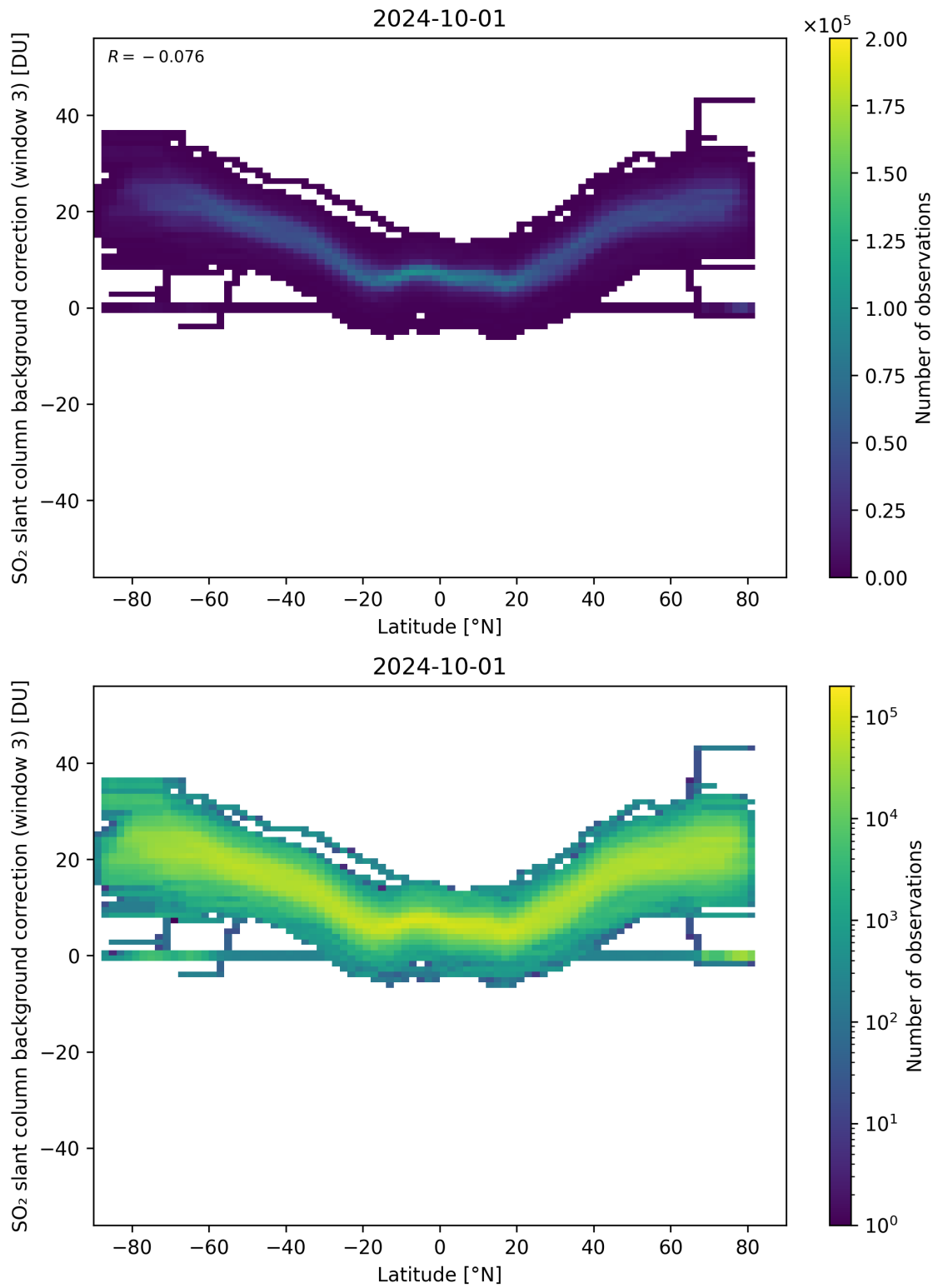
Figure 141: Scatter density plot of “Latitude” against “SO 2 slant column background correction (window 3)” for 2024-09-30 to 2024-10-02.
