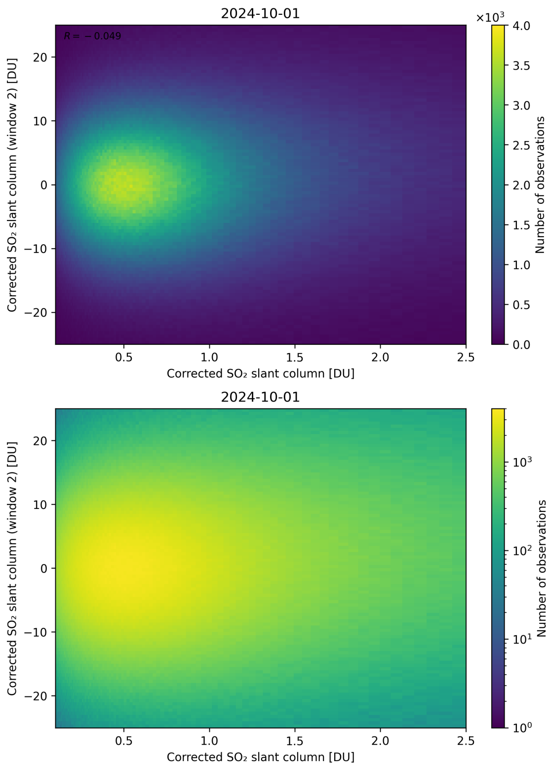
Figure 185: Scatter density plot of “Corrected SO 2 slant column” against “Corrected SO 2 slant column (window 2)” for 2024-09-30 to 2024-10-02.
