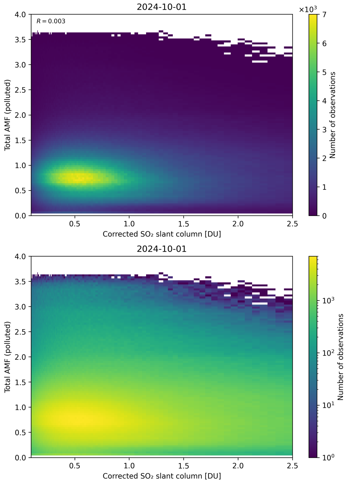
Figure 192: Scatter density plot of “Corrected SO 2 slant column” against “Total AMF (polluted)” for 2024-09-30 to 2024-10-02.
