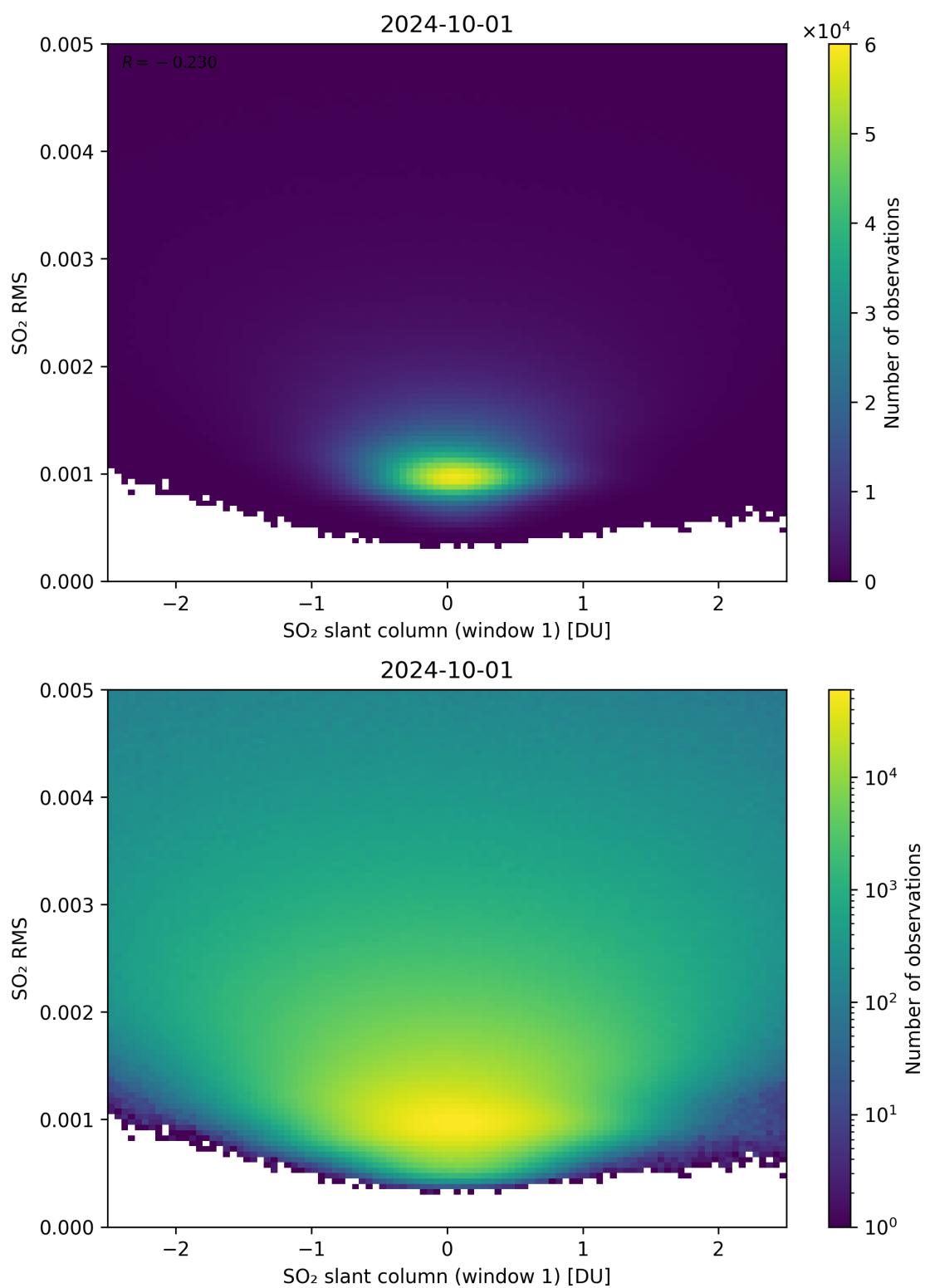
Figure 217: Scatter density plot of “SO 2 slant column (window 1)” against “SO 2 RMS” for 2024-09-30 to 2024-10-02.
