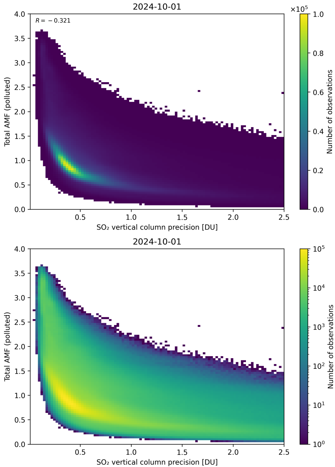
Figure 294: Scatter density plot of “SO 2 vertical column precision” against “Total AMF (polluted)” for 2024-09-30 to 2024-10-02.
