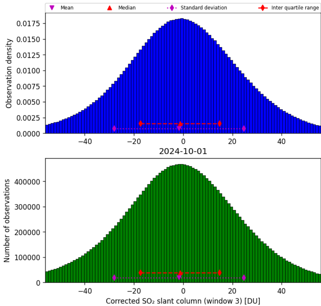
Figure 66: Histogram of “Corrected SO 2 slant column (window 3)” for 2024-09-30 to 2024-10-02
