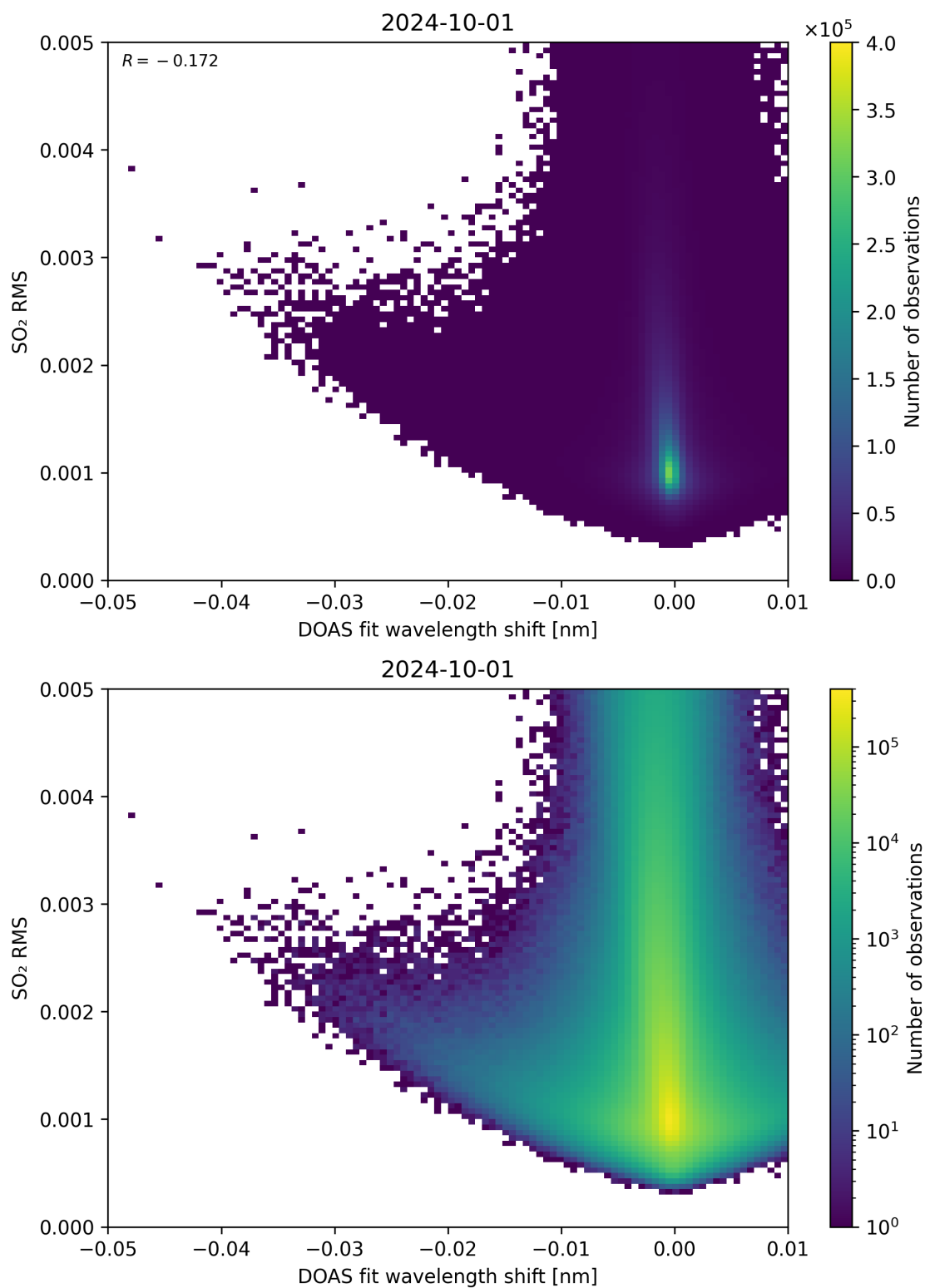
Figure 128: Scatter density plot of “DOAS fit wavelength shift” against “SO 2 RMS” for 2024-09-30 to 2024-10-02.
