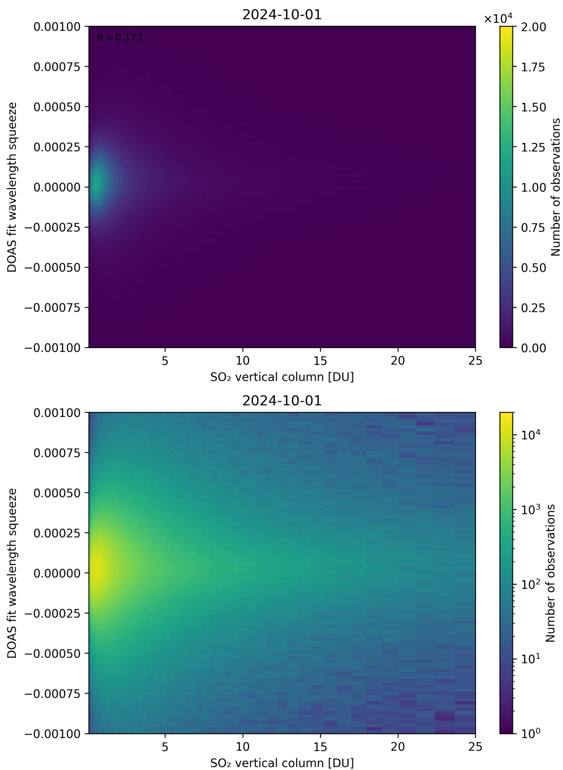
Figure 277: Scatter density plot of “SO 2 vertical column” against “DOAS fit wavelength squeeze” for 2024-09-30 to 2024-10-02.
