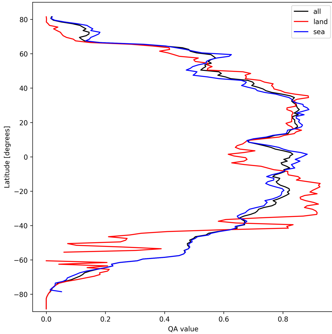
Figure 29: Zonal average of “QA value” for 2024-09-30 to 2024-10-02.
