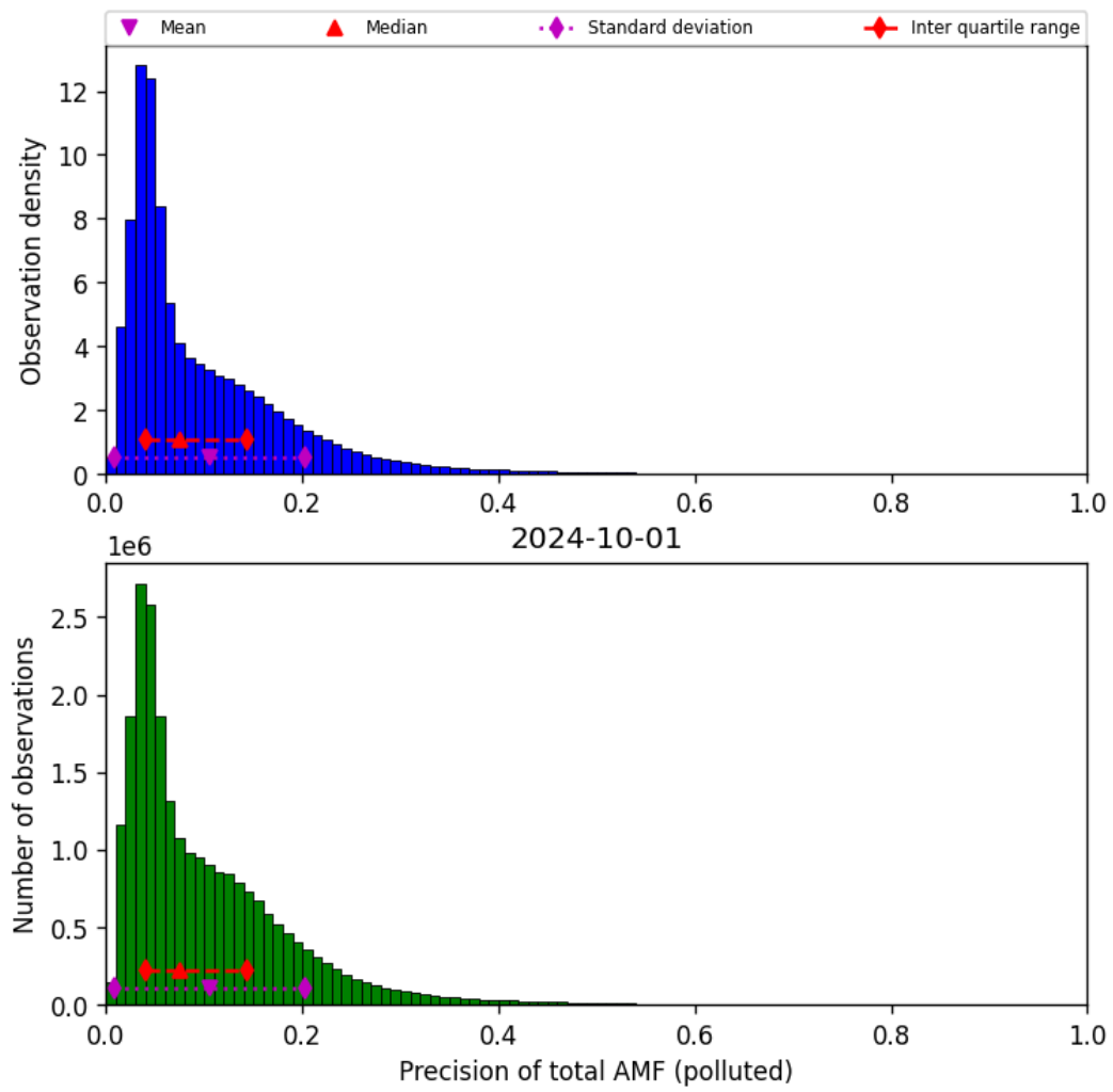
Figure 72: Histogram of “Precision of total AMF (polluted)” for 2024-09-30 to 2024-10-02
