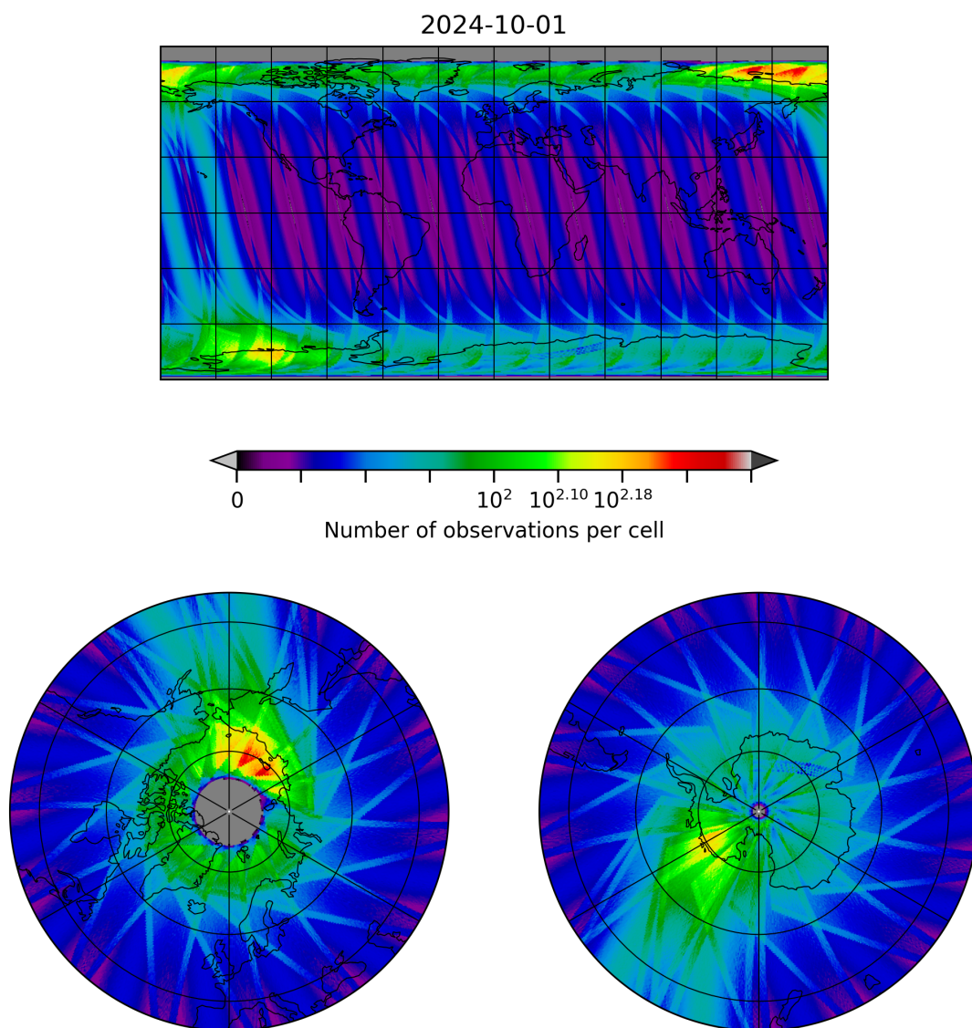
Figure 28: Map of the number of observations for 2024-09-30 to 2024-10-02
