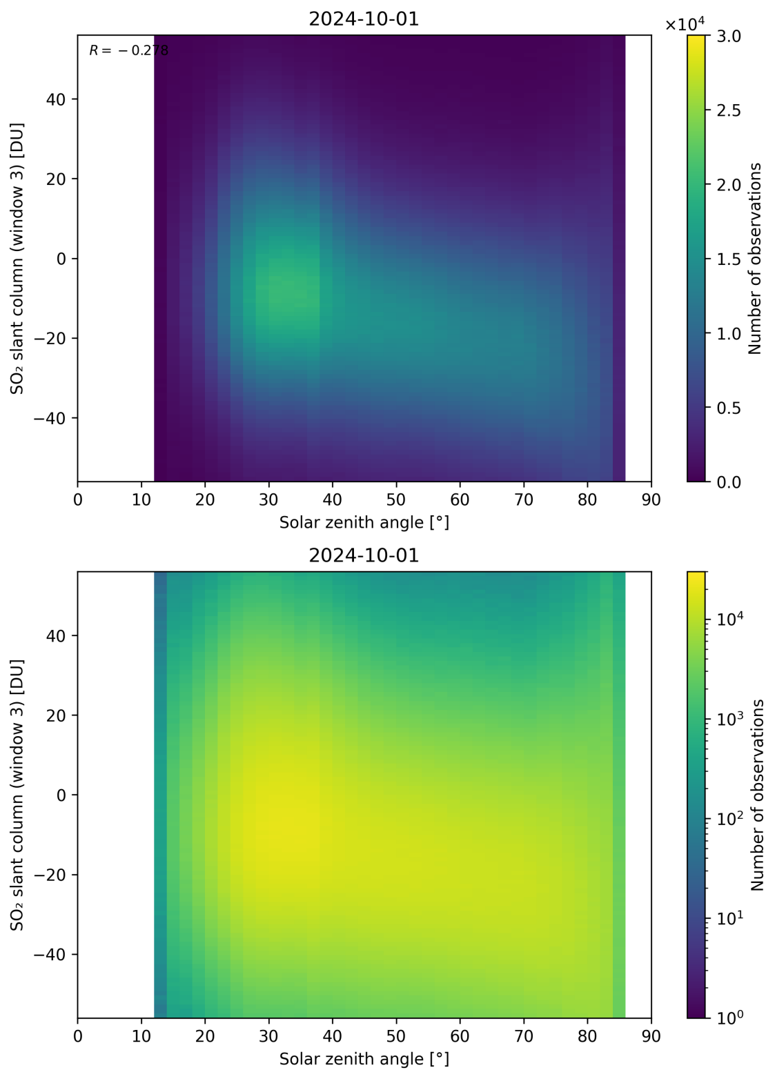
Figure 172: Scatter density plot of “Solar zenith angle” against “SO 2 slant column (window 3)” for 2024-09-30 to 2024-10-02.
