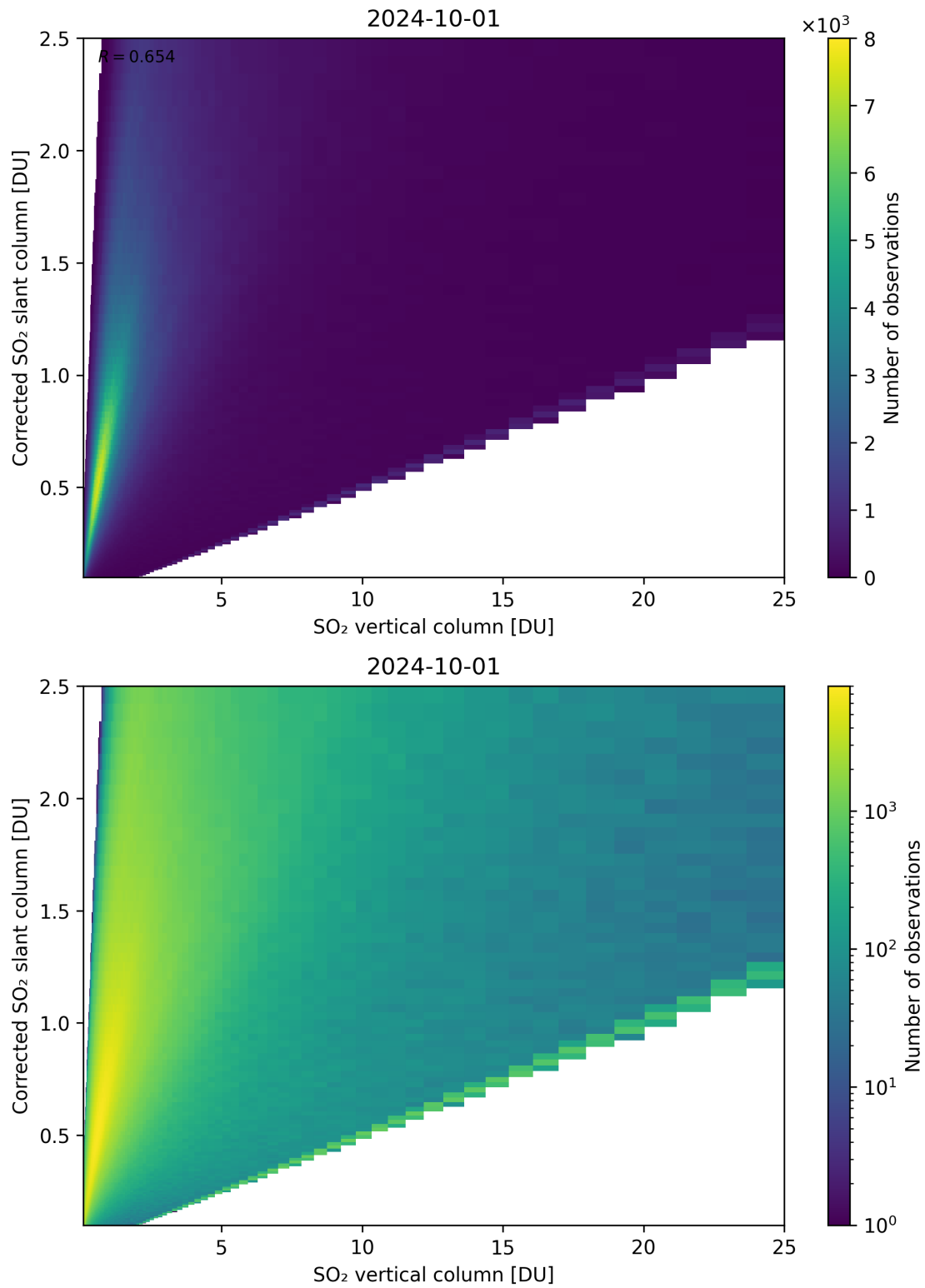
Figure 297: Scatter density plot of “SO 2 vertical column” against “Corrected SO 2 slant column” for 2024-09-30 to 2024-10-02.
