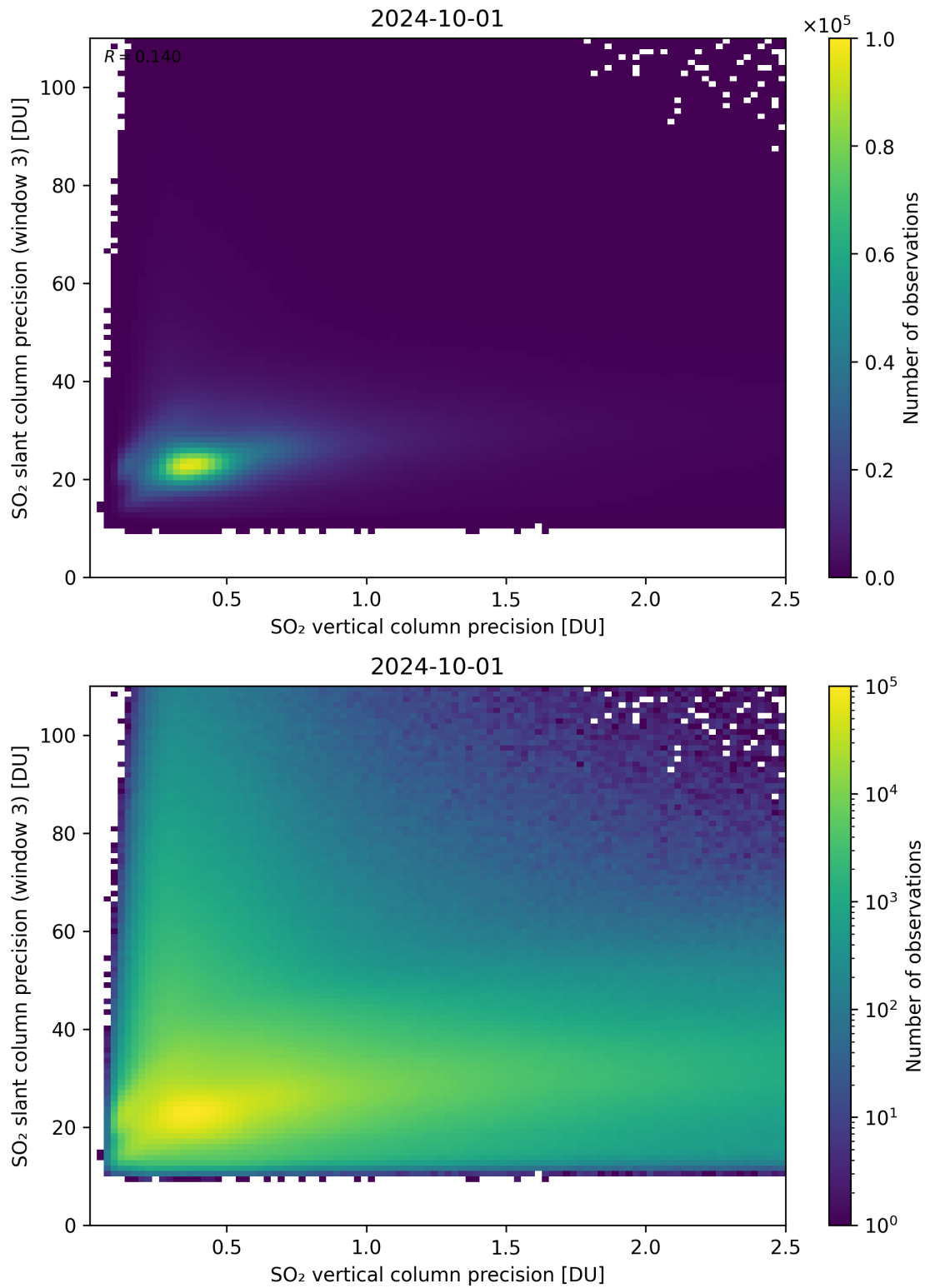
Figure 293: Scatter density plot of “SO 2 vertical column precision” against “SO 2 slant column precision (window 3)” for 2024-09-30 to 2024-10-02.
