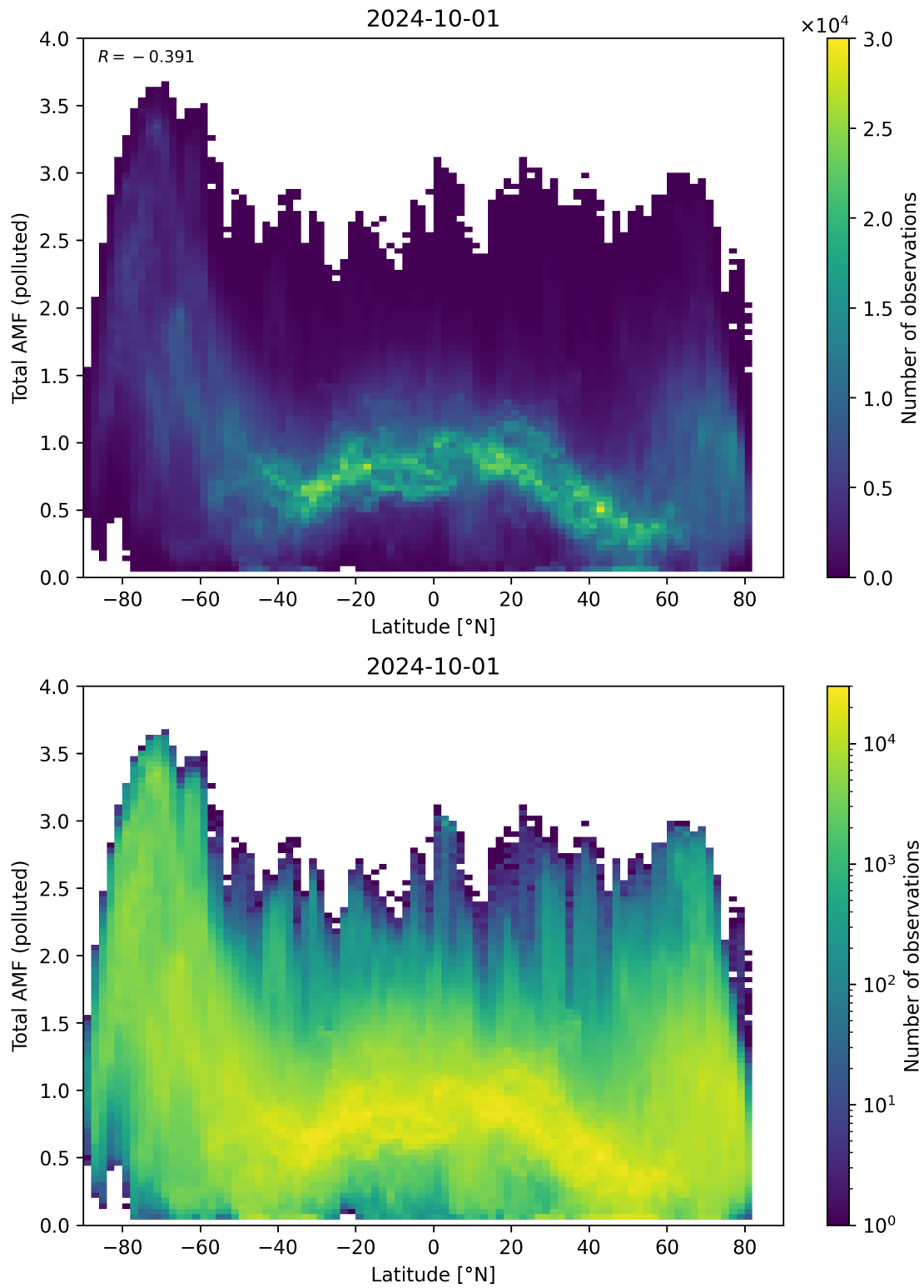
Figure 154: Scatter density plot of “Latitude” against “Total AMF (polluted)” for 2024-09-30 to 2024-10-02.
