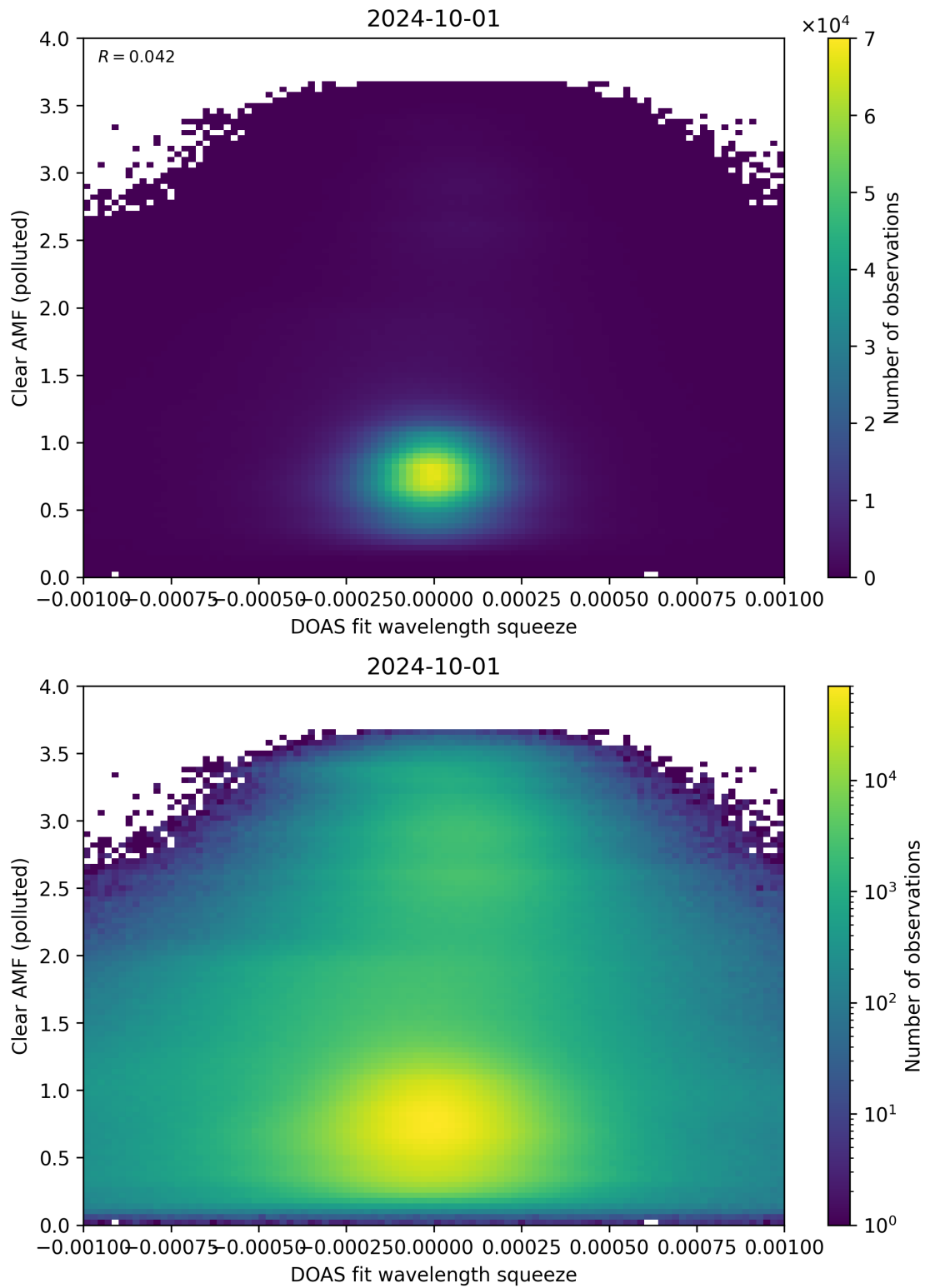
Figure 133: Scatter density plot of “DOAS fit wavelength squeeze” against “Clear AMF (polluted)” for 2024-09-30 to 2024-10-02.
