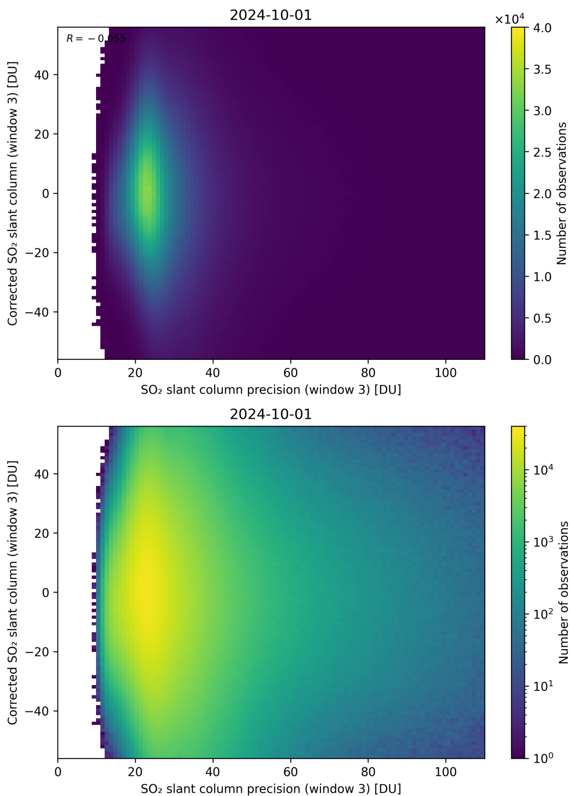
Figure 262: Scatter density plot of “SO 2 slant column precision (window 3)” against “Corrected SO 2 slant column (window 3)” for 2024-09-30 to 2024-10-02.
