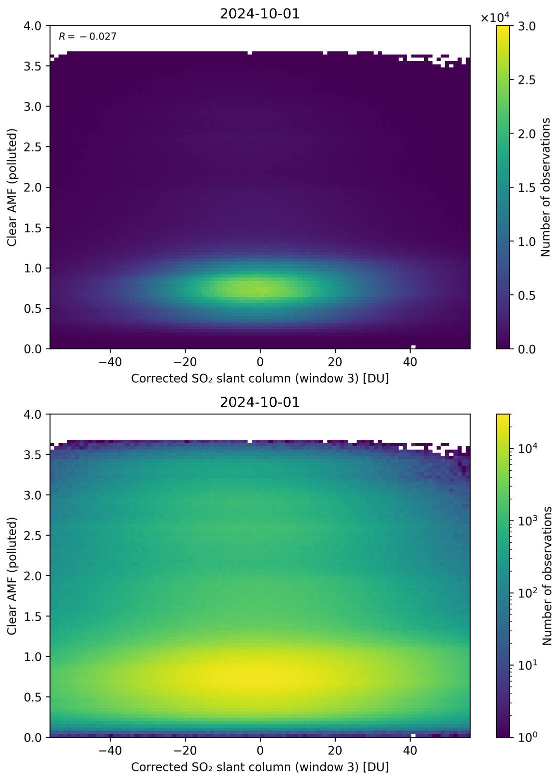
Figure 209: Scatter density plot of “Corrected SO 2 slant column (window 3)” against “Clear AMF (polluted)” for 2024-09-30 to 2024-10-02.
