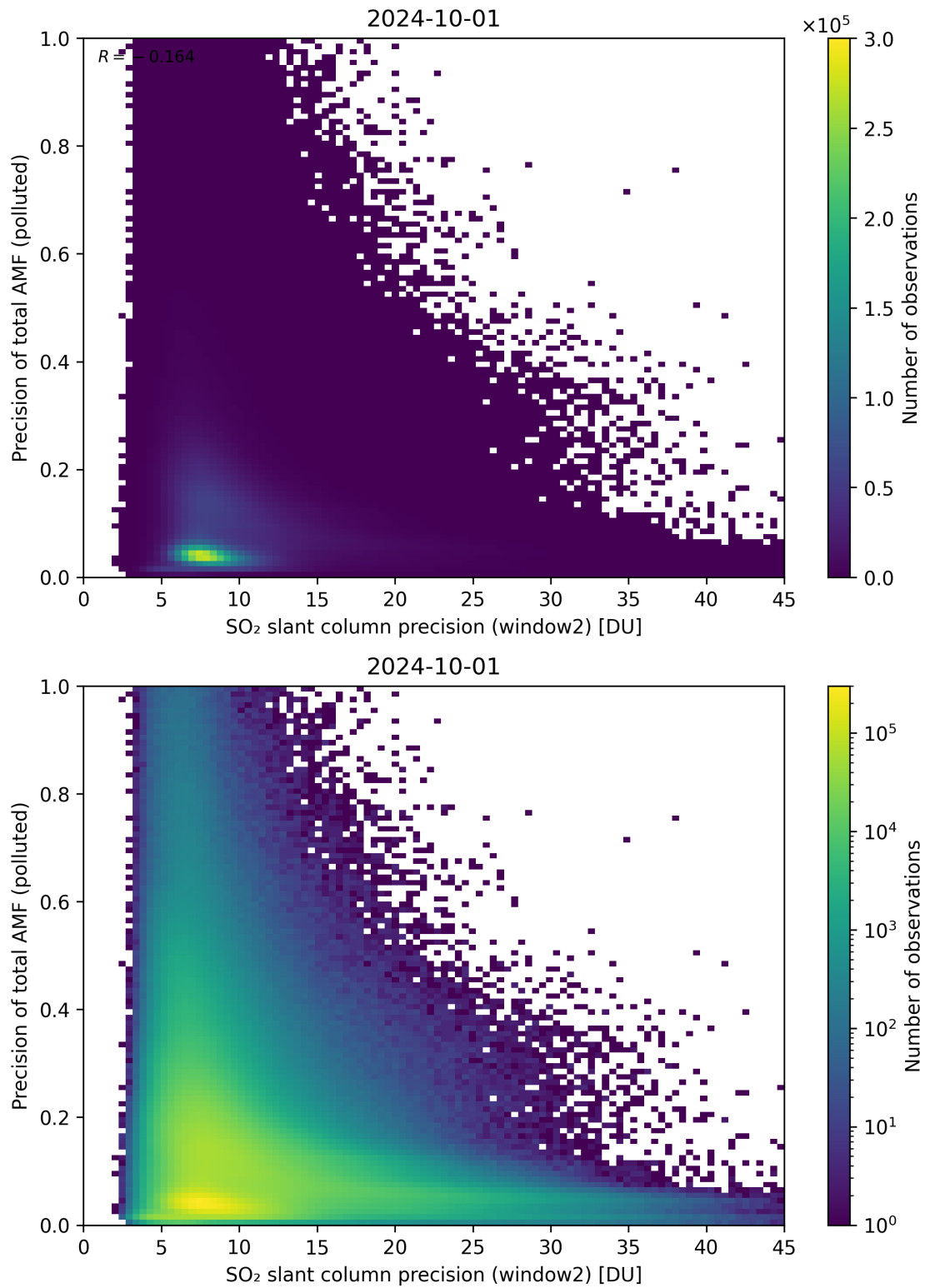
Figure 252: Scatter density plot of “SO 2 slant column precision (window2)” against “Precision of total AMF (polluted)” for 2024-09-30 to 2024-10-02.
