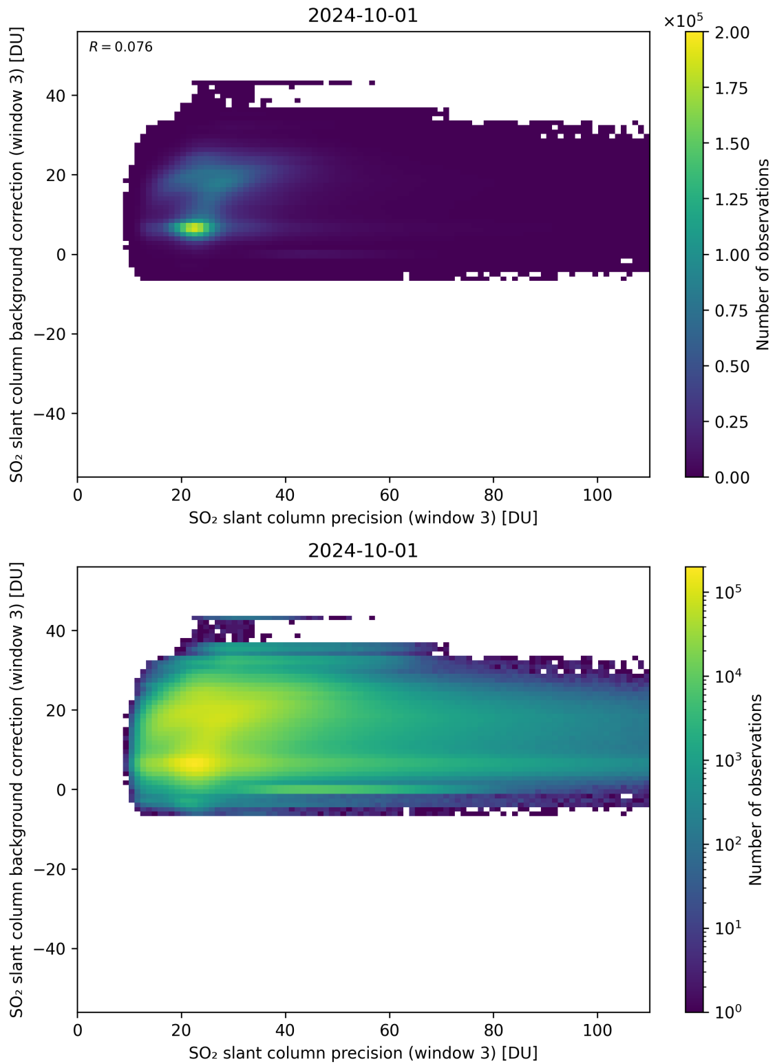
Figure 257: Scatter density plot of “SO 2 slant column precision (window 3)” against “SO 2 slant column background correction (window 3)” for 2024-09-30 to 2024-10-02.
