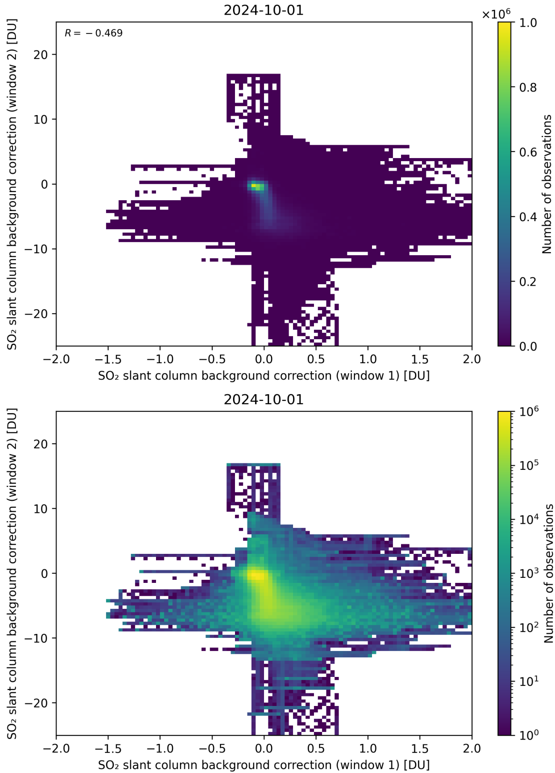
Figure 98: Scatter density plot of “SO 2 slant column background correction (window 1)” against “SO 2 slant column background correction (window 2)” for 2024-09-30 to 2024-10-02.
