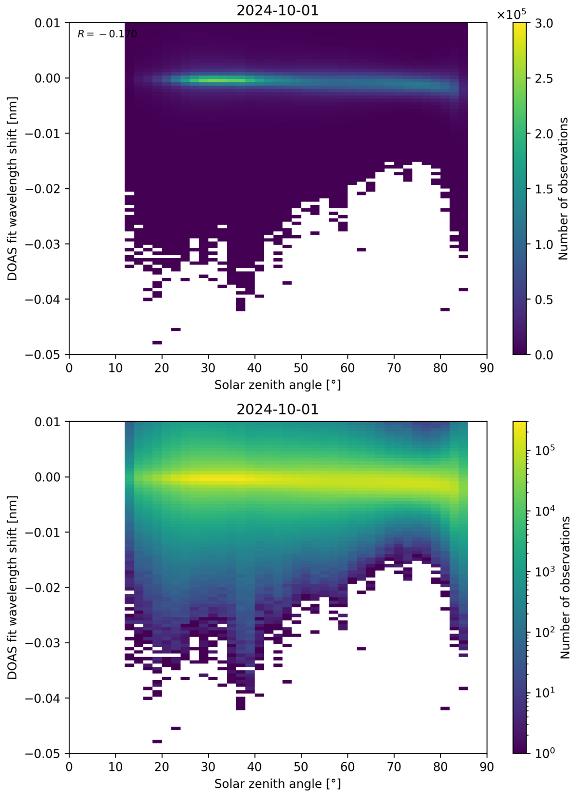
Figure 161: Scatter density plot of “Solar zenith angle” against “DOAS fit wavelength shift” for 2024-09-30 to 2024-10-02.
