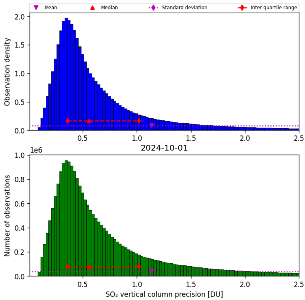
Figure 54: Histogram of “SO 2 vertical column precision” for 2024-09-30 to 2024-10-02
