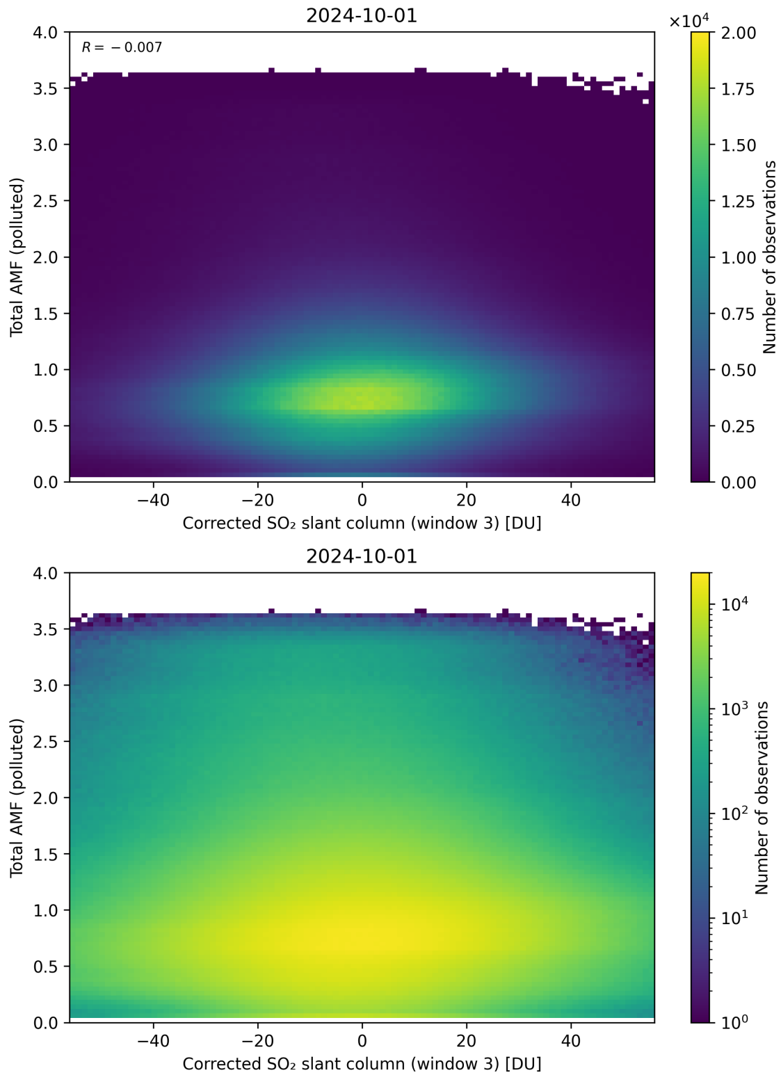
Figure 210: Scatter density plot of “Corrected SO 2 slant column (window 3)” against “Total AMF (polluted)” for 2024-09-30 to 2024-10-02.
