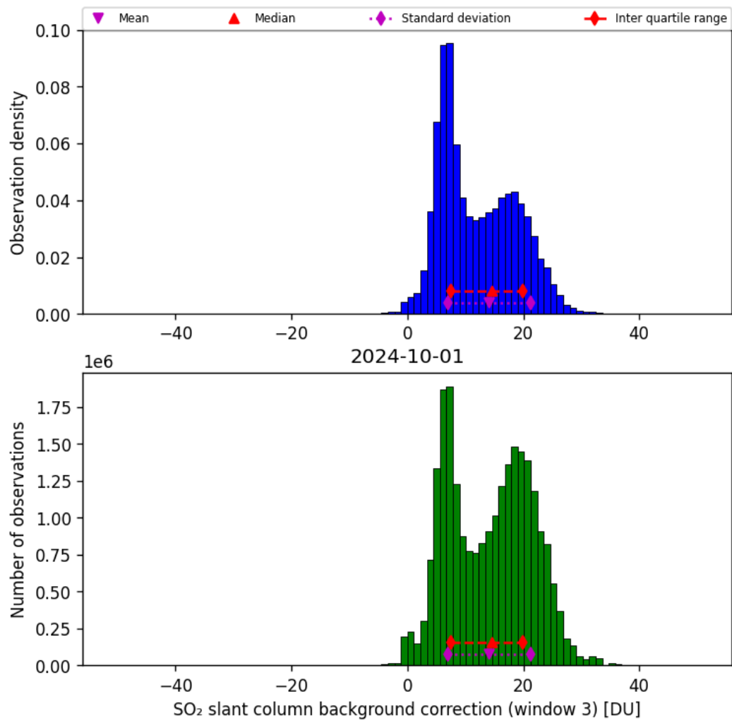
Figure 67: Histogram of “SO 2 slant column background correction (window 3)” for 2024-09-30 to 2024-10-02
