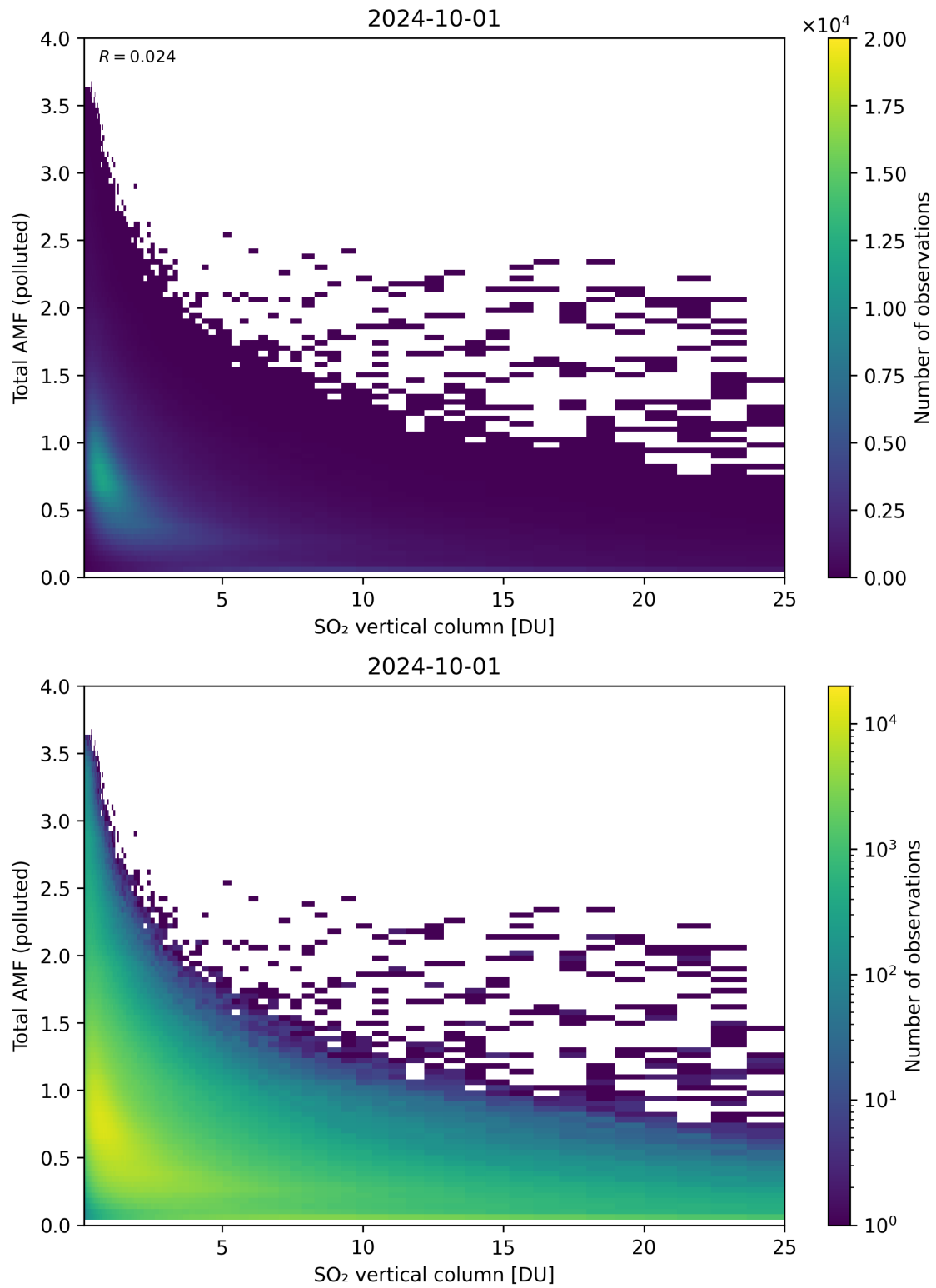
Figure 305: Scatter density plot of “SO 2 vertical column” against “Total AMF (polluted)” for 2024-09-30 to 2024-10-02.
