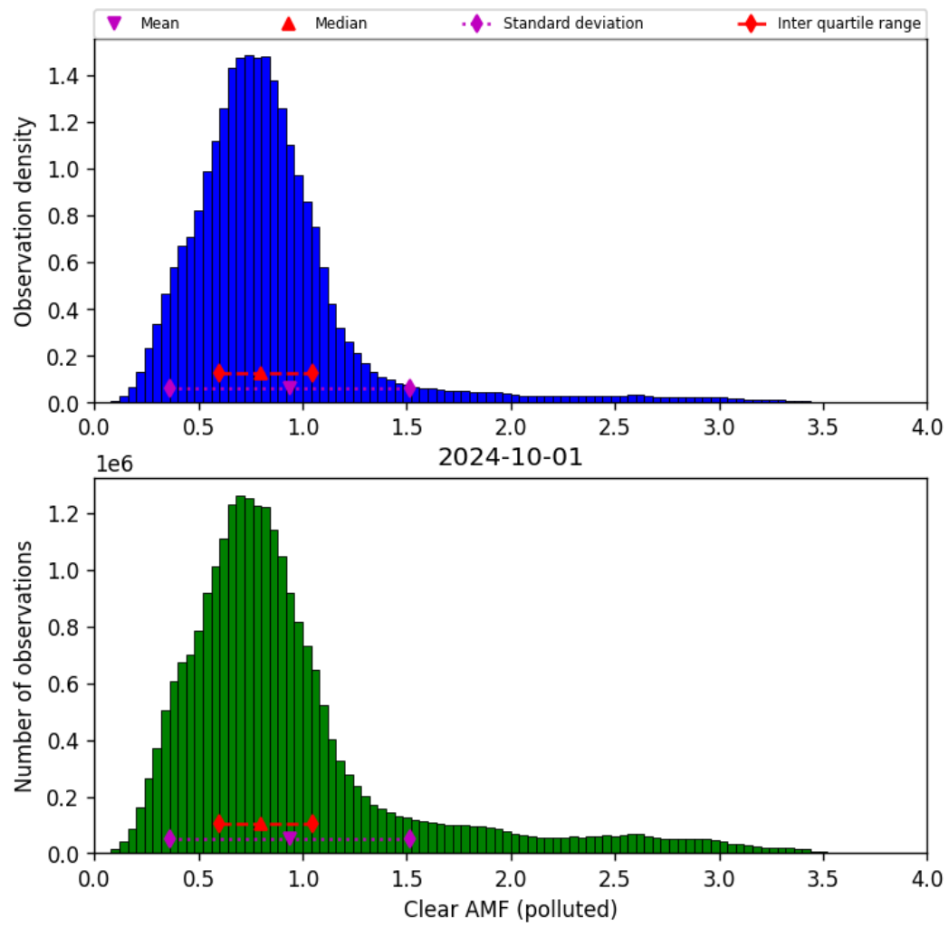
Figure 73: Histogram of “Clear AMF (polluted)” for 2024-09-30 to 2024-10-02
