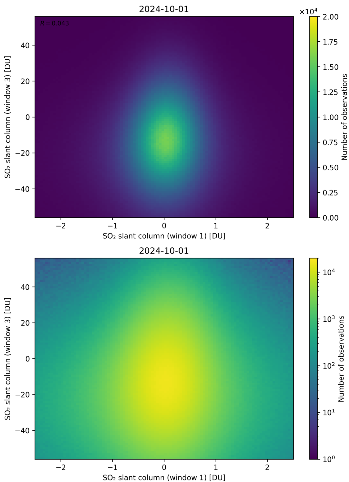
Figure 237: Scatter density plot of “SO 2 slant column (window 1)” against “SO 2 slant column (window 3)” for 2024-09-30 to 2024-10-02.
