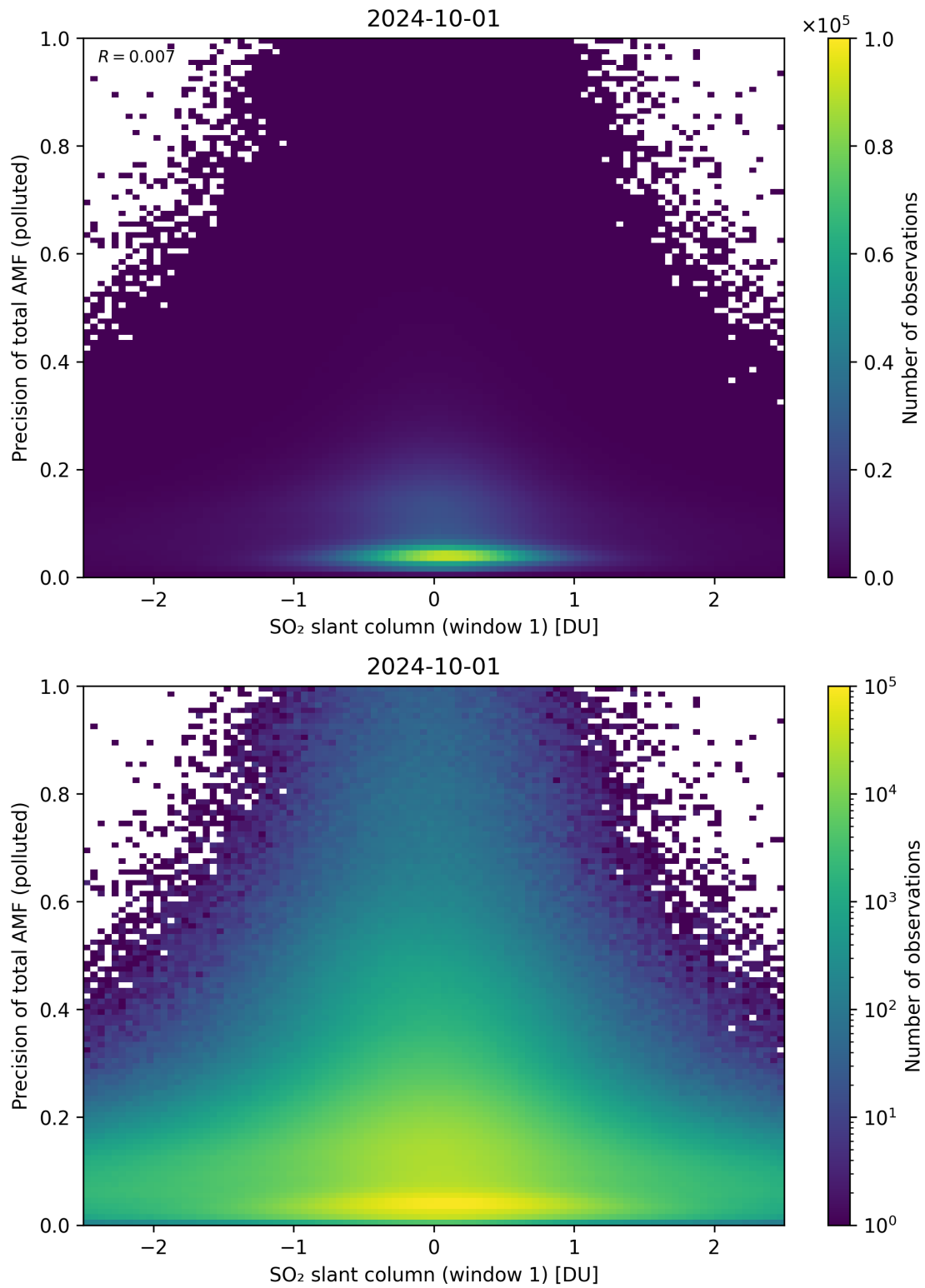
Figure 240: Scatter density plot of “SO 2 slant column (window 1)” against “Precision of total AMF (polluted)” for 2024-09-30 to 2024-10-02.
