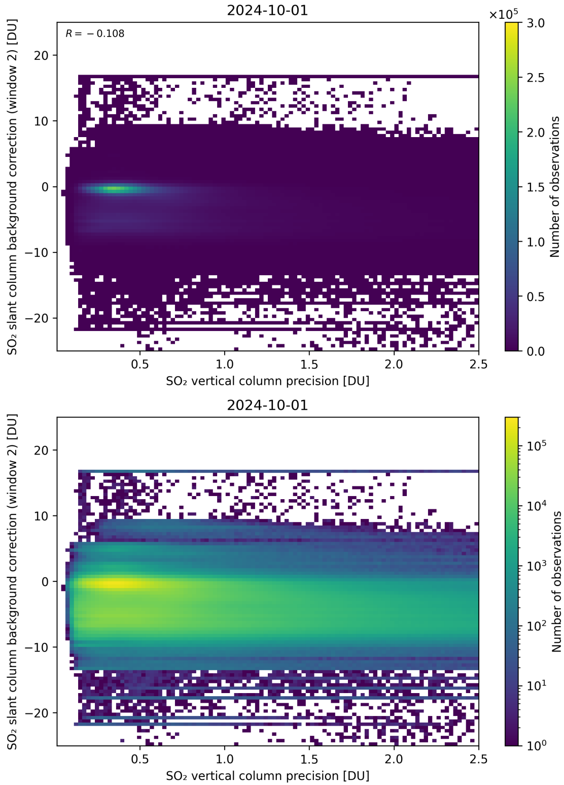
Figure 280: Scatter density plot of “SO 2 vertical column precision” against “SO 2 slant column background correction (window 2)” for 2024-09-30 to 2024-10-02.
