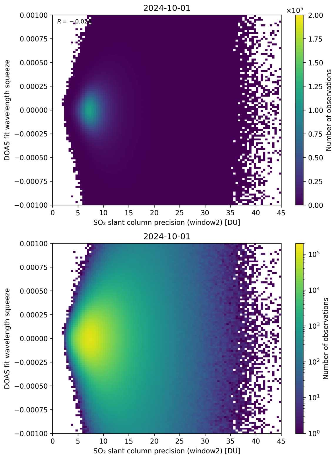
Figure 244: Scatter density plot of “SO 2 slant column precision (window2)” against “DOAS fit wavelength squeeze” for 2024-09-30 to 2024-10-02.
