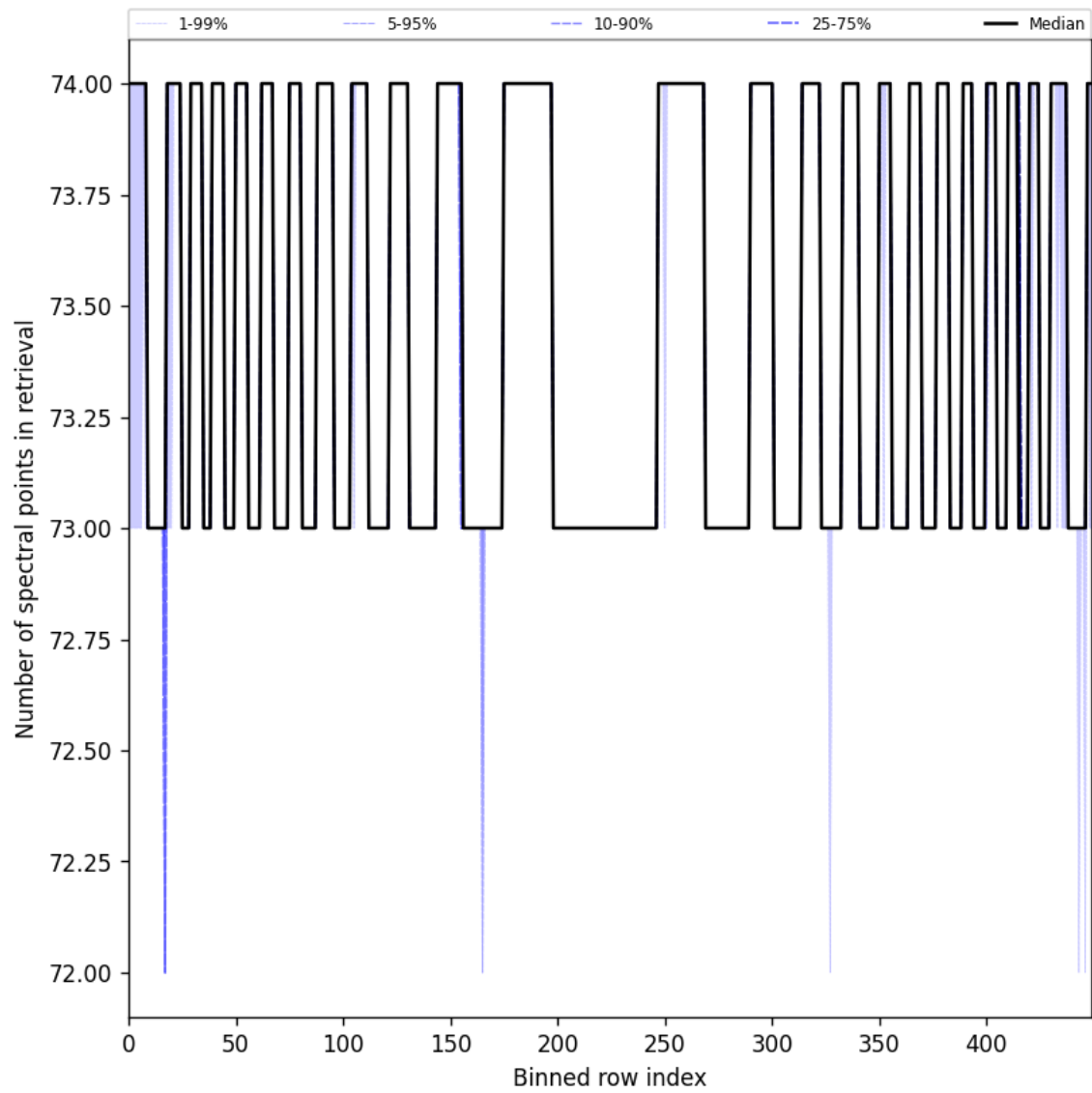
Figure 97: Along track statistics of “Number of spectral points in retrieval” for 2024-09-30 to 2024-10-02
