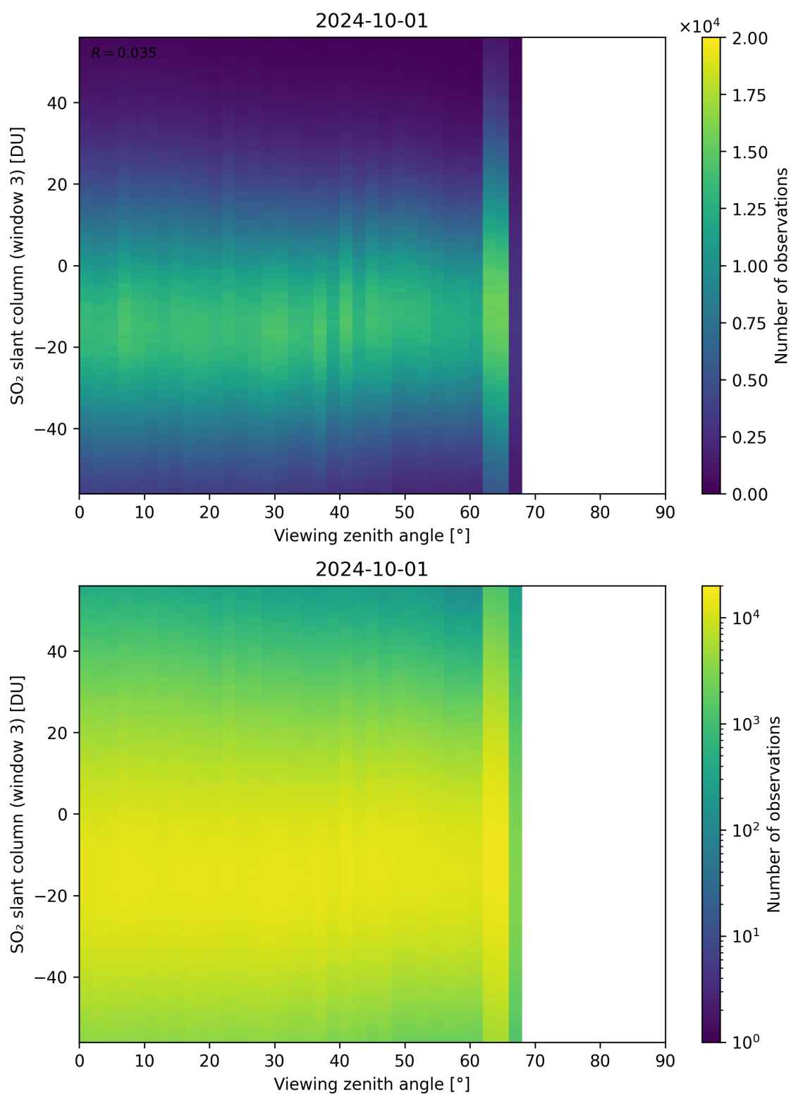
Figure 323: Scatter density plot of “Viewing zenith angle” against “SO 2 slant column (window 3)” for 2024-09-30 to 2024-10-02.
