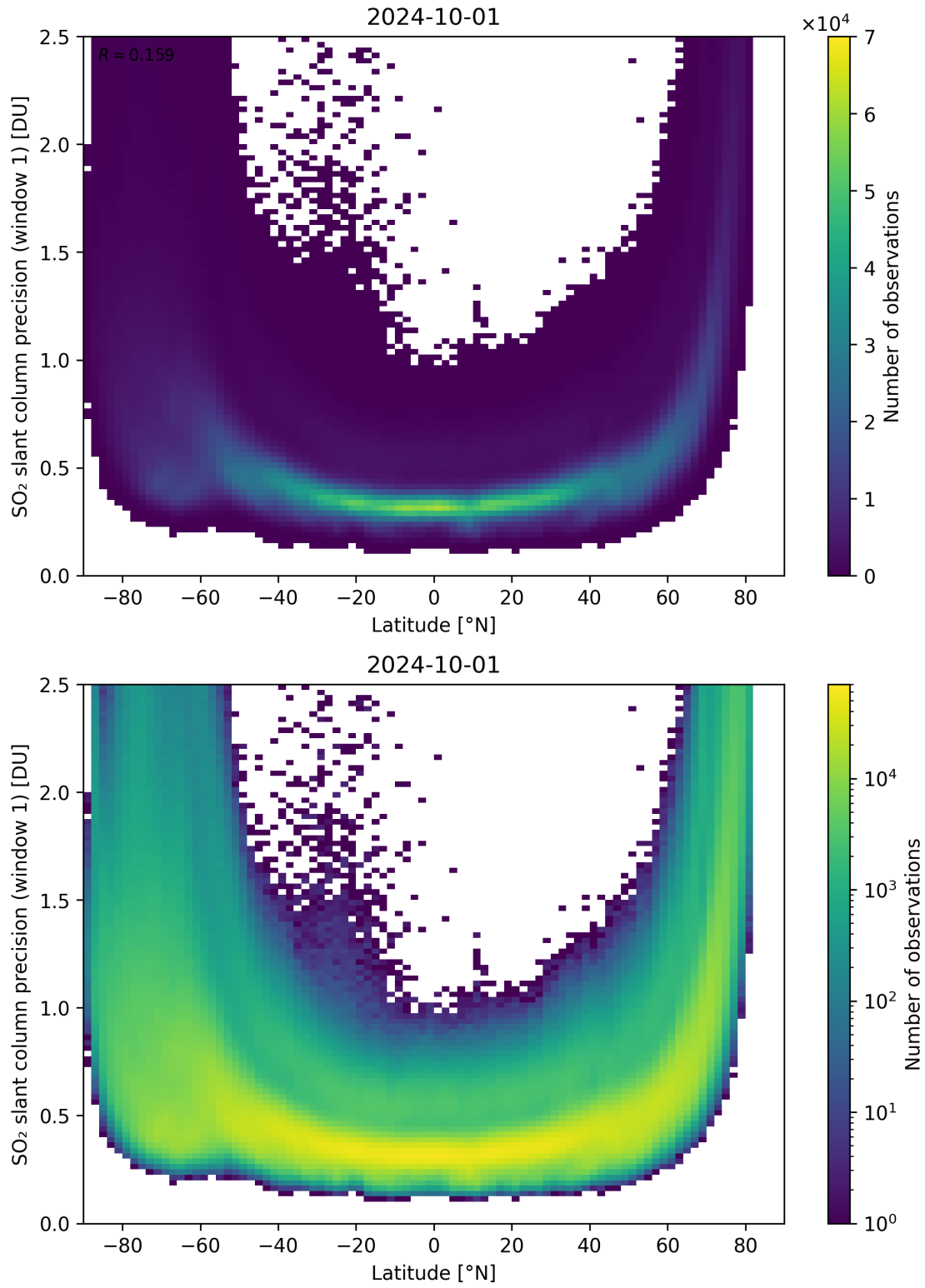
Figure 150: Scatter density plot of “Latitude” against “SO 2 slant column precision (window 1)” for 2024-09-30 to 2024-10-02.
