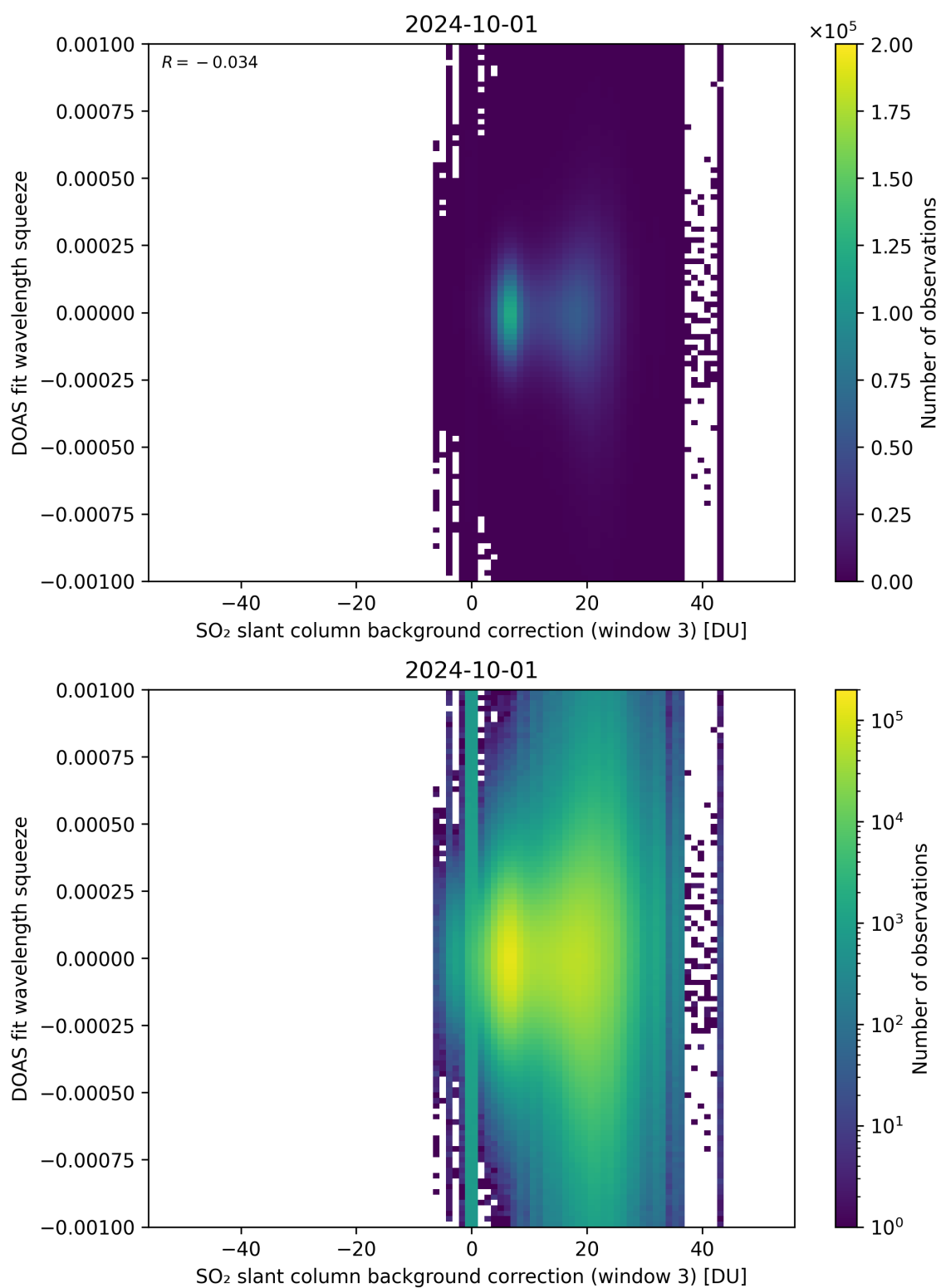
Figure 122: Scatter density plot of “SO 2 slant column background correction (window 3)” against “DOAS fit wavelength squeeze” for 2024-09-30 to 2024-10-02.
