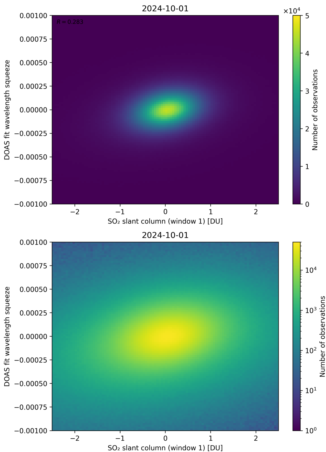
Figure 216: Scatter density plot of “SO 2 slant column (window 1)” against “DOAS fit wavelength squeeze” for 2024-09-30 to 2024-10-02.
