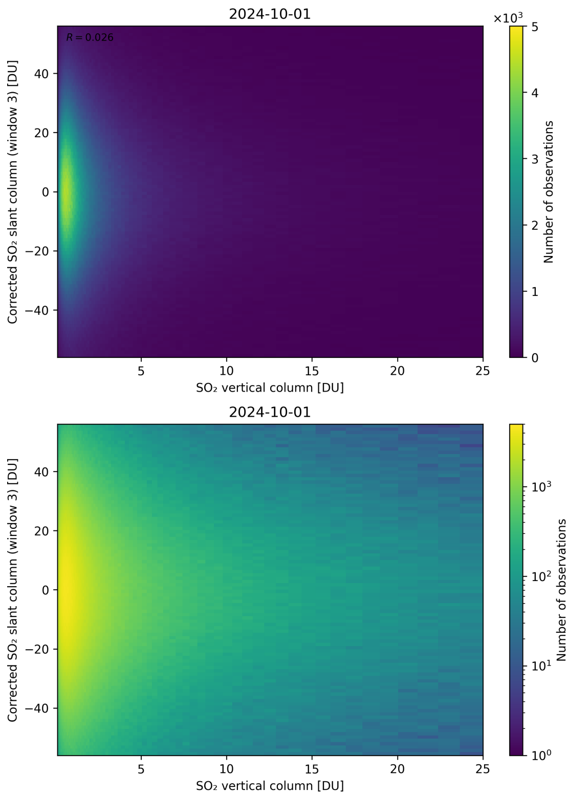
Figure 299: Scatter density plot of “SO 2 vertical column” against “Corrected SO 2 slant column (window 3)” for 2024-09-30 to 2024-10-02.
