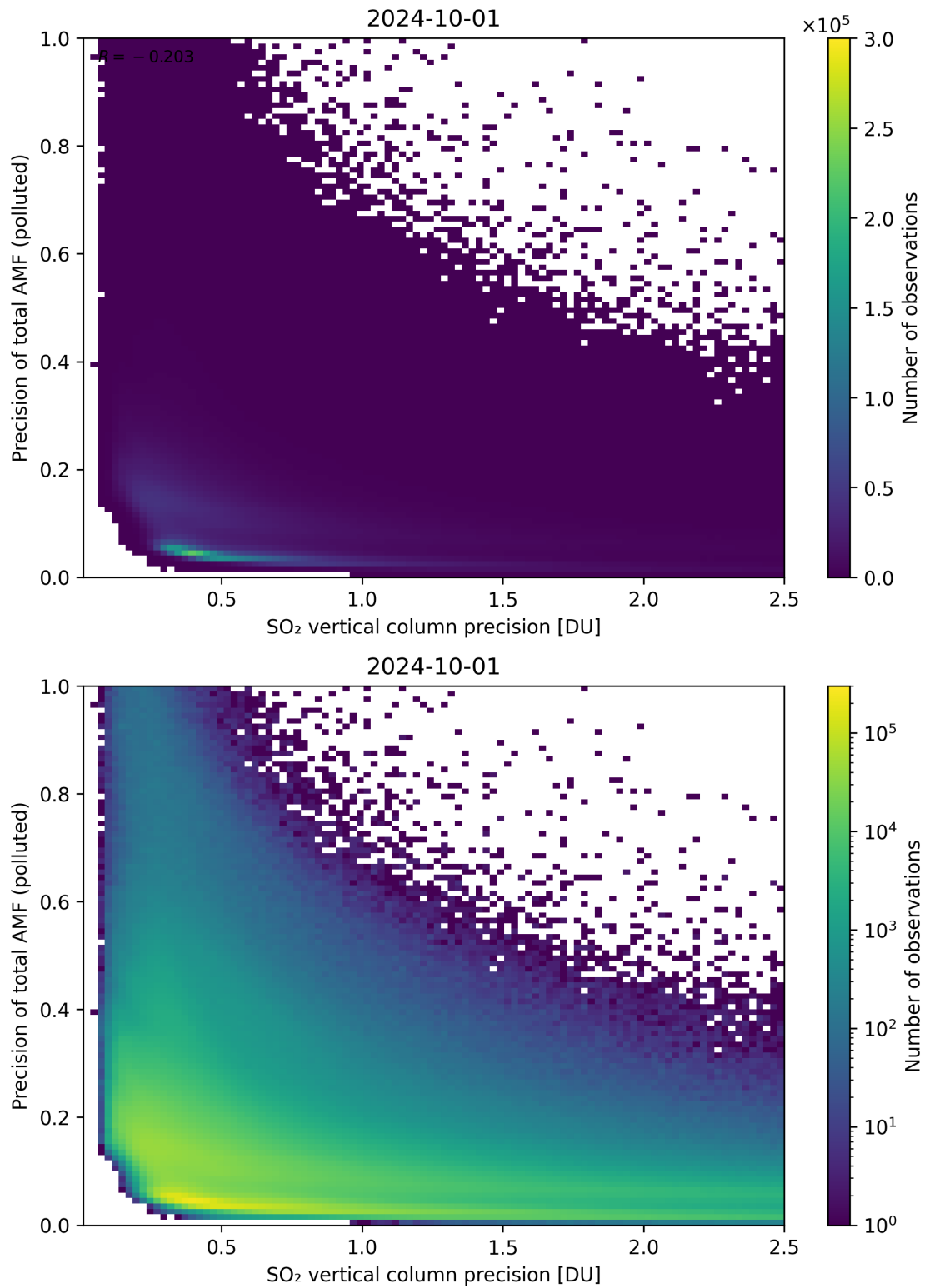
Figure 295: Scatter density plot of “SO 2 vertical column precision” against “Precision of total AMF (polluted)” for 2024-09-30 to 2024-10-02.
