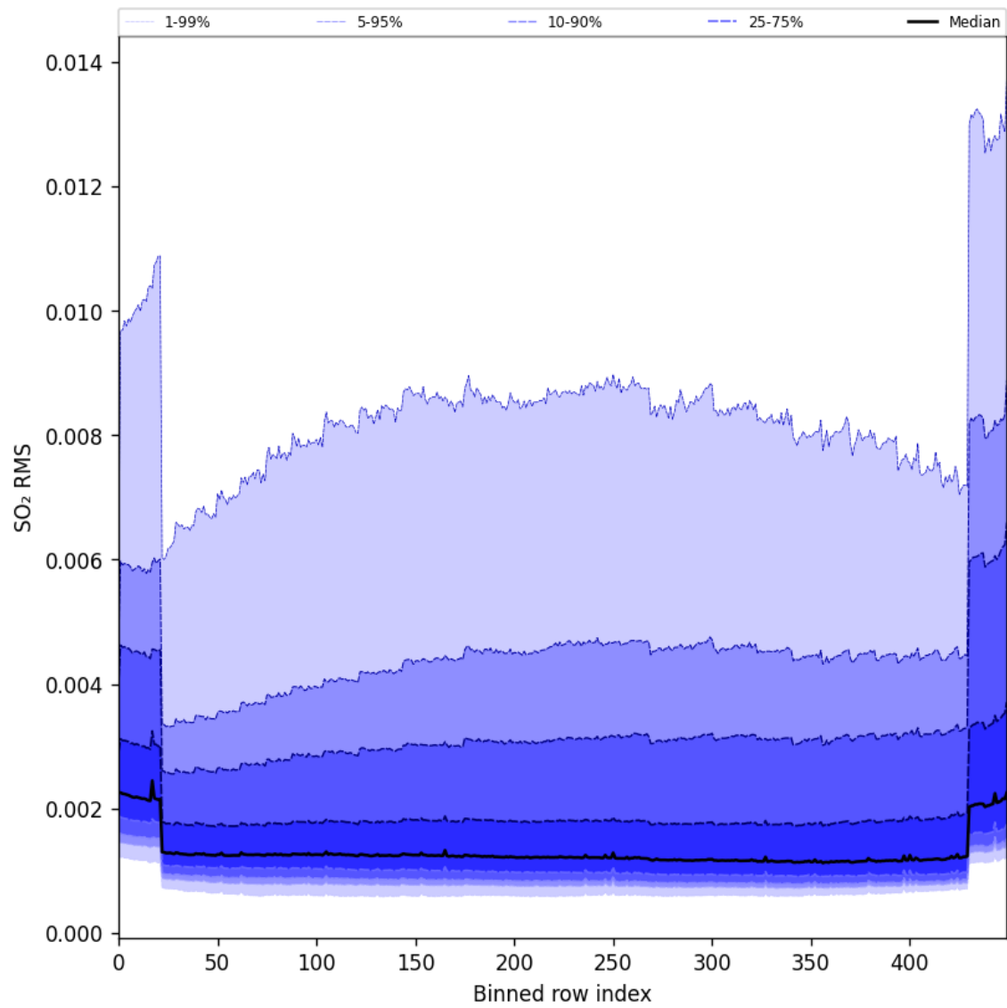
Figure 93: Along track statistics of “SO 2 RMS” for 2024-09-30 to 2024-10-02
