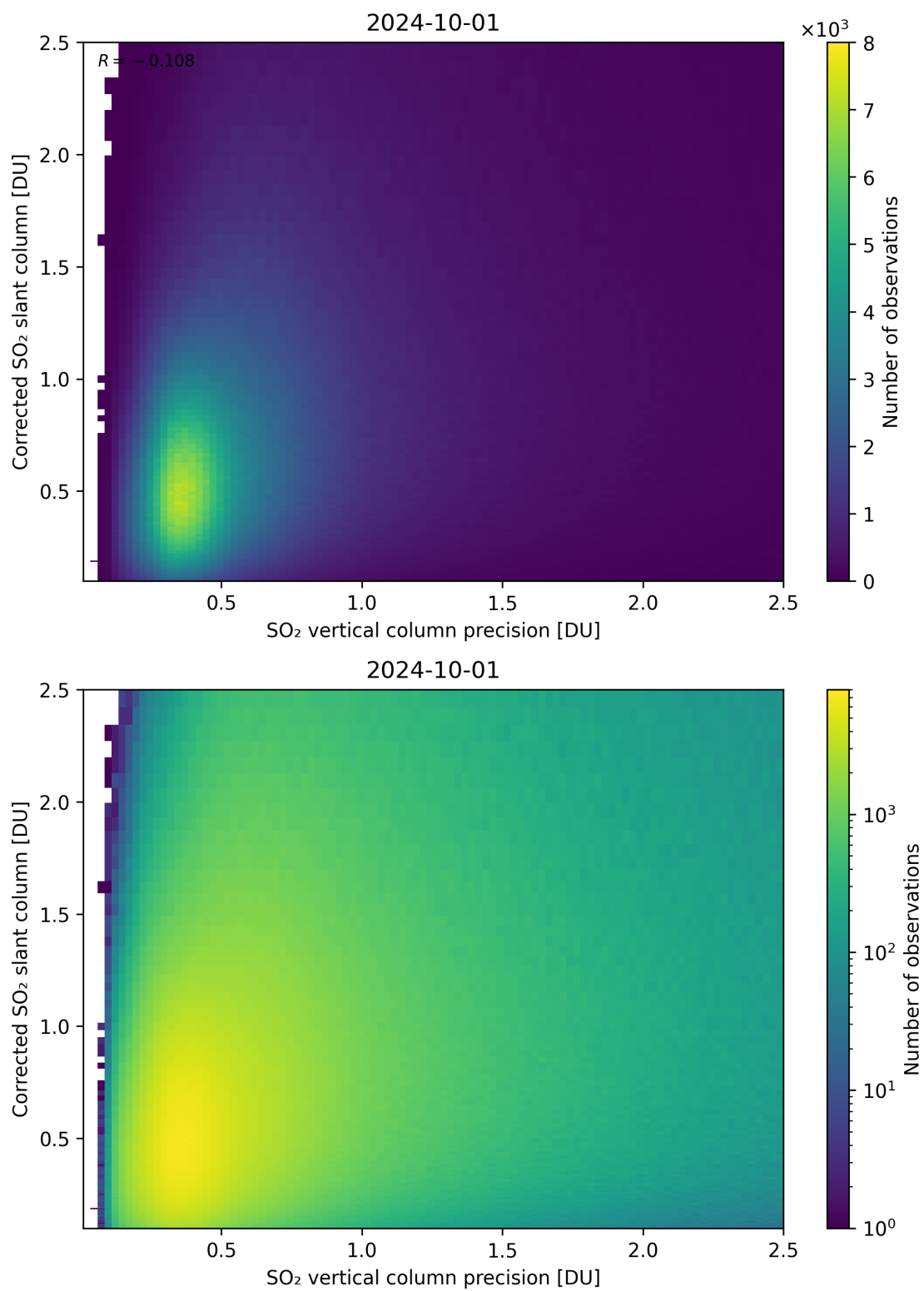
Figure 286: Scatter density plot of “SO 2 vertical column precision” against “Corrected SO 2 slant column” for 2024-09-30 to 2024-10-02.
