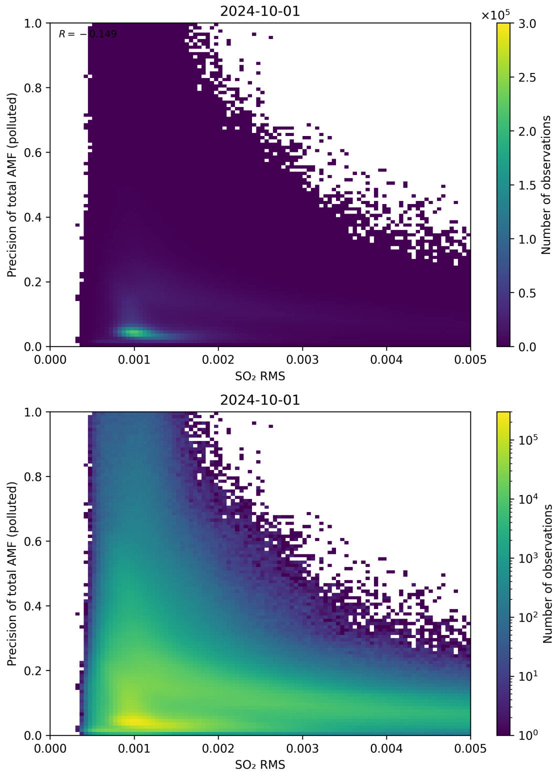
Figure 138: Scatter density plot of “SO 2 RMS” against “Precision of total AMF (polluted)” for 2024-09-30 to 2024-10-02.
