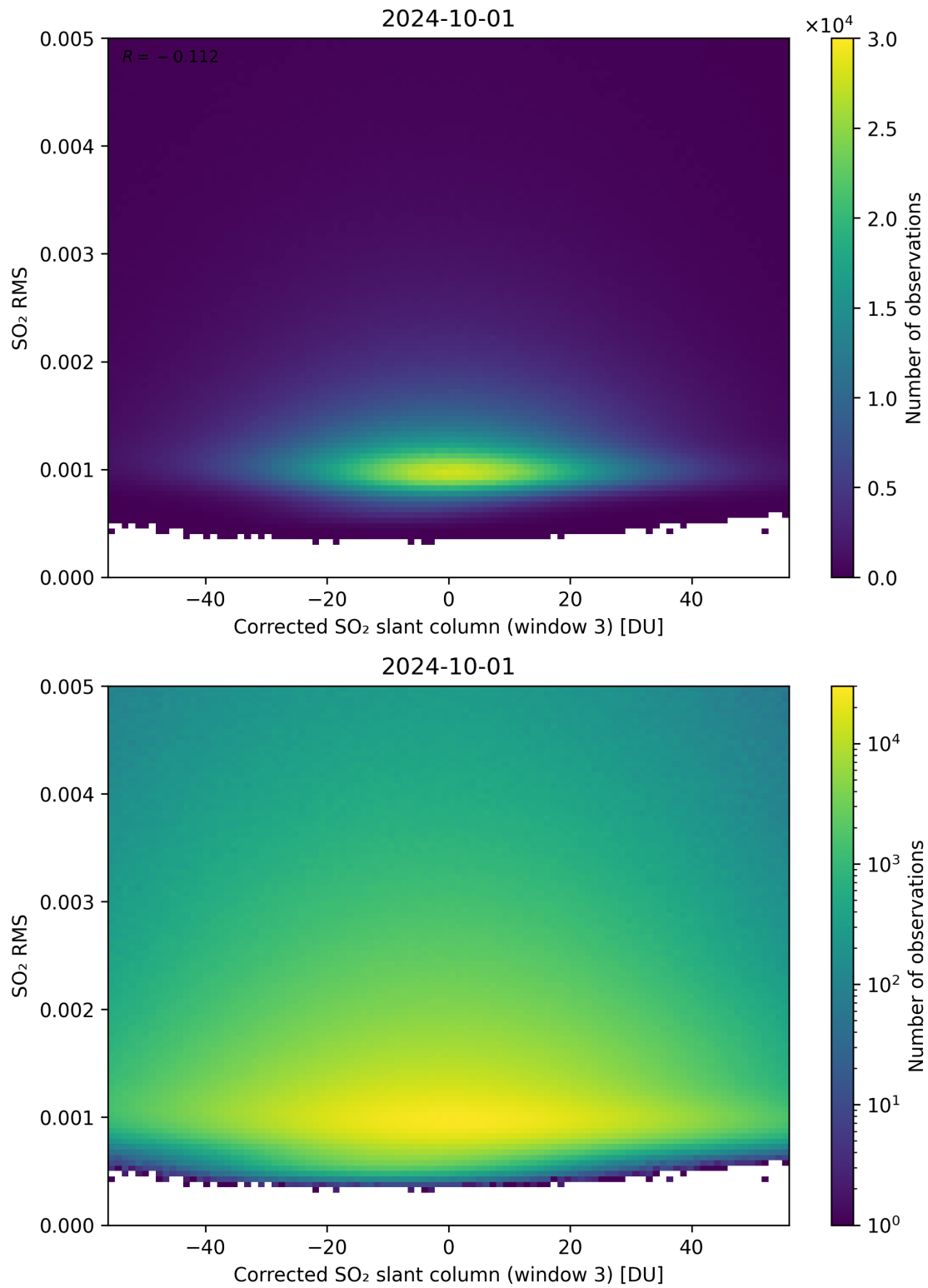
Figure 208: Scatter density plot of “Corrected SO 2 slant column (window 3)” against “SO 2 RMS” for 2024-09-30 to 2024-10-02.
