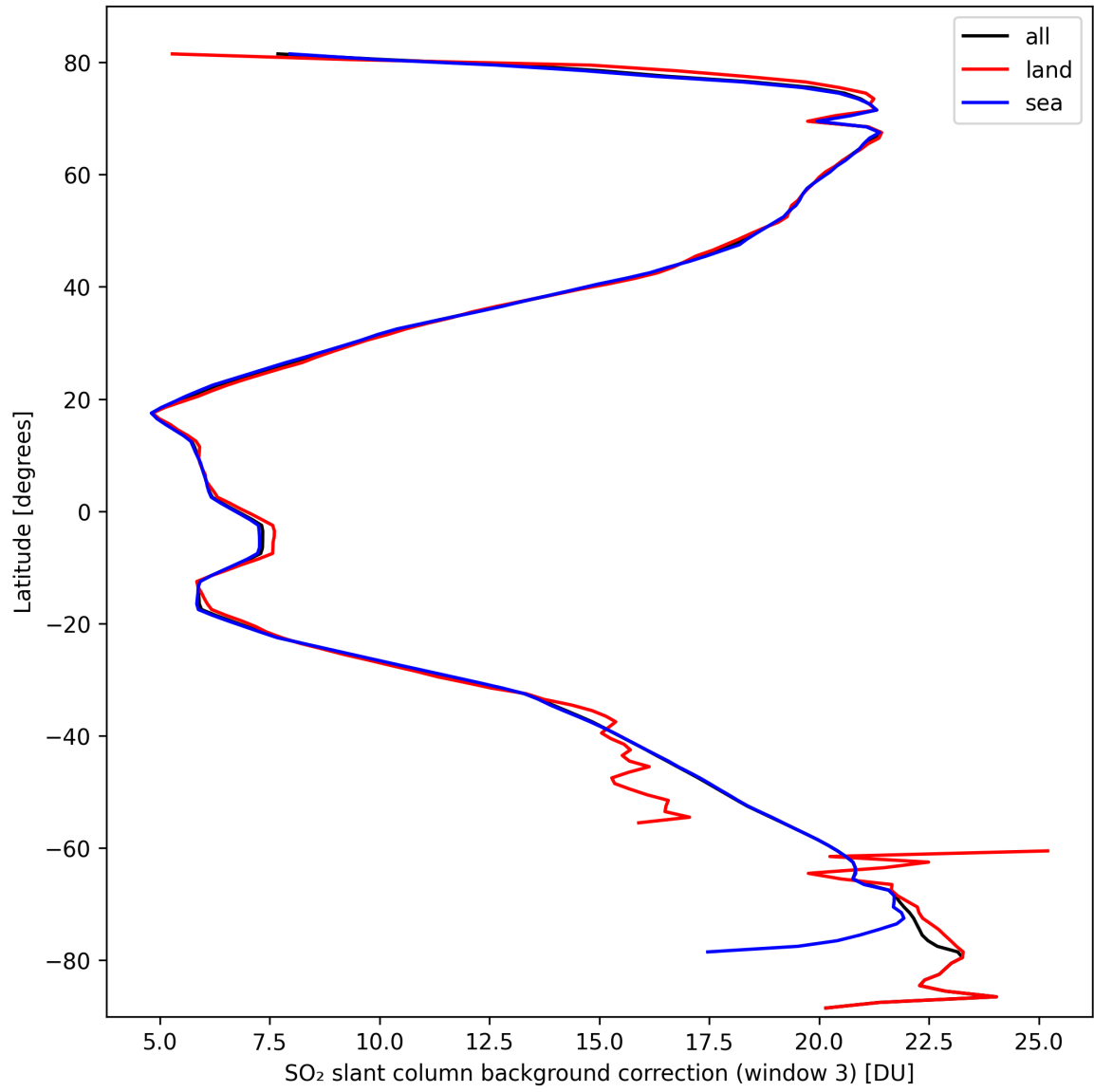
Figure 44: Zonal average of “SO 2 slant column background correction (window 3)” for 2024-09-30 to 2024-10-02.
