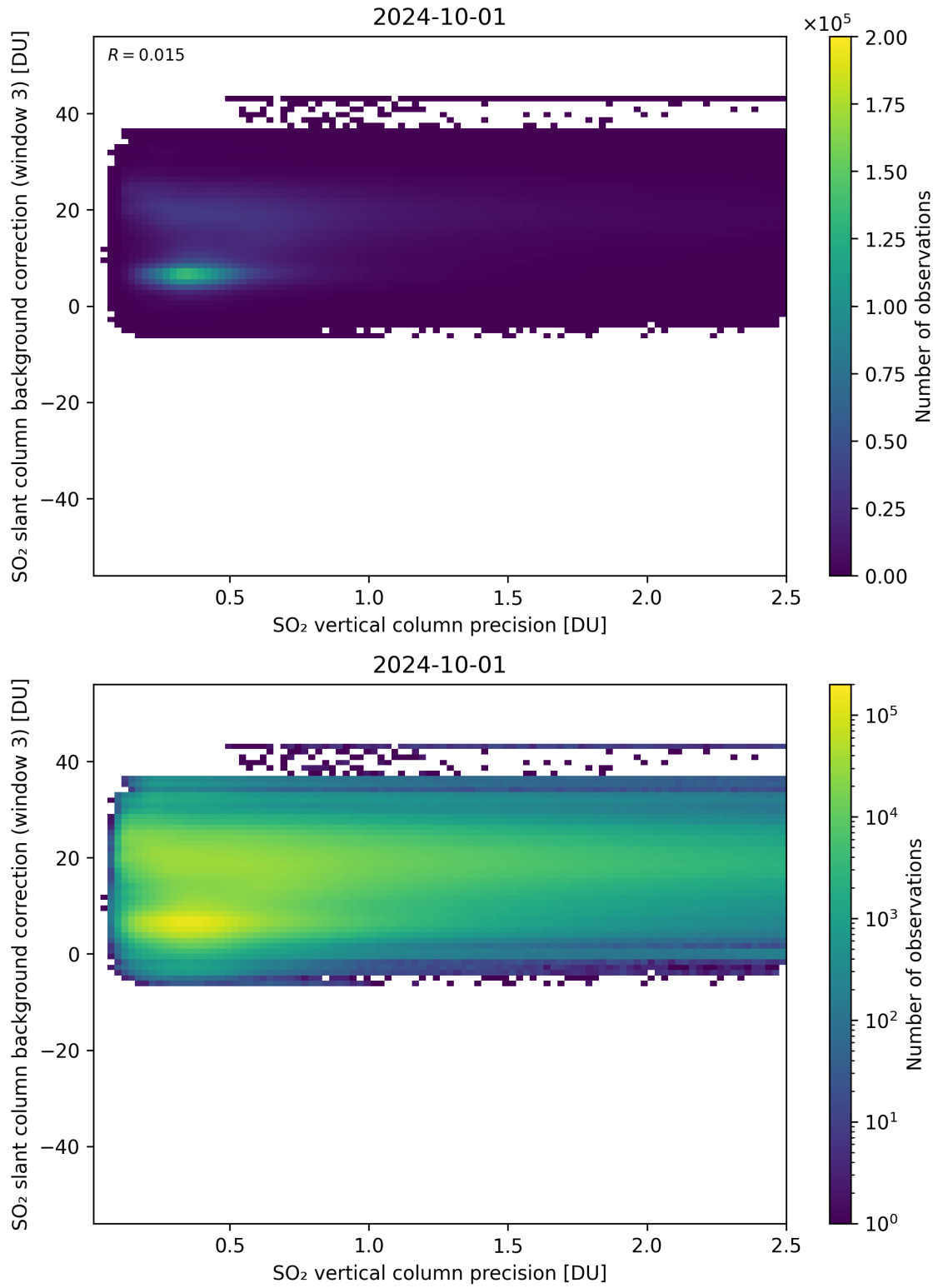
Figure 281: Scatter density plot of “SO 2 vertical column precision” against “SO 2 slant column background correction (window 3)” for 2024-09-30 to 2024-10-02.
