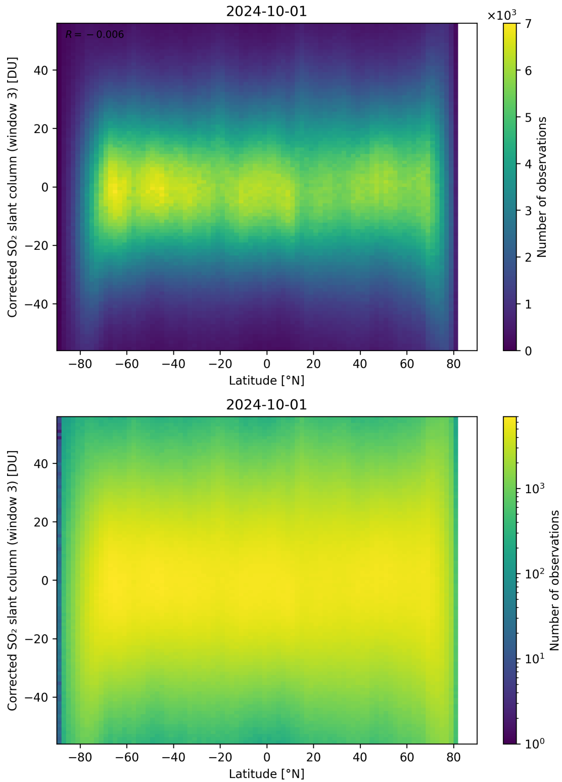
Figure 148: Scatter density plot of “Latitude” against “Corrected SO 2 slant column (window 3)” for 2024-09-30 to 2024-10-02.
