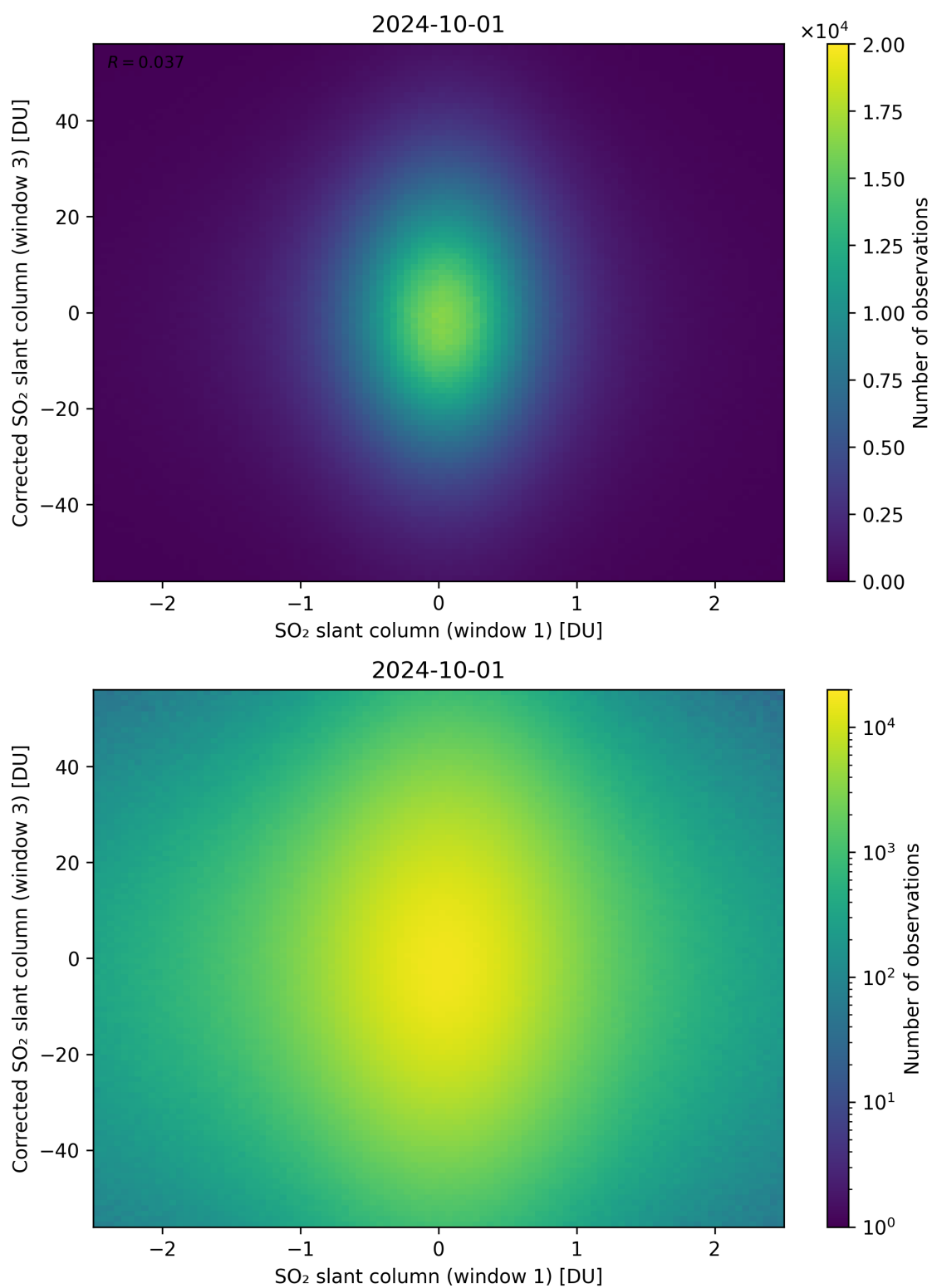
Figure 234: Scatter density plot of “SO 2 slant column (window 1)” against “Corrected SO 2 slant column (window 3)” for 2024-09-30 to 2024-10-02.
