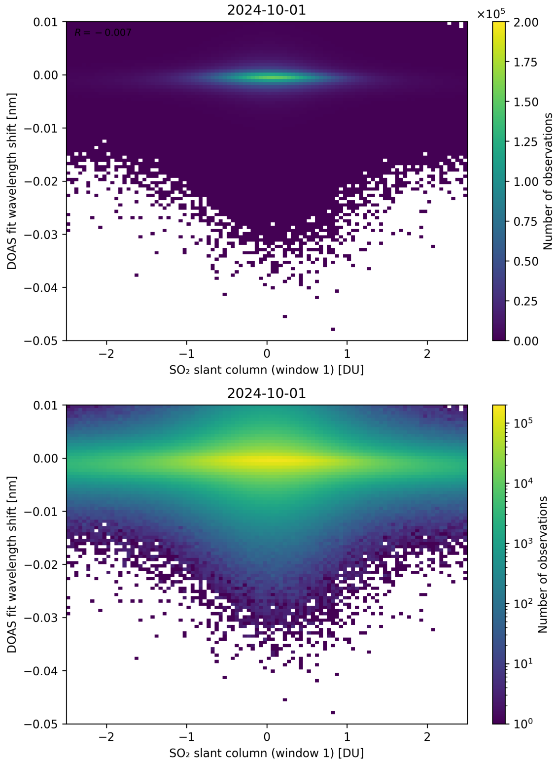
Figure 215: Scatter density plot of “SO 2 slant column (window 1)” against “DOAS fit wavelength shift” for 2024-09-30 to 2024-10-02.
