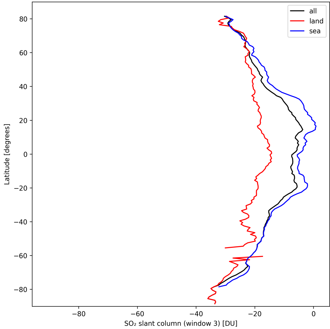
Figure 41: Zonal average of “SO 2 slant column (window 3)” for 2024-09-30 to 2024-10-02.
