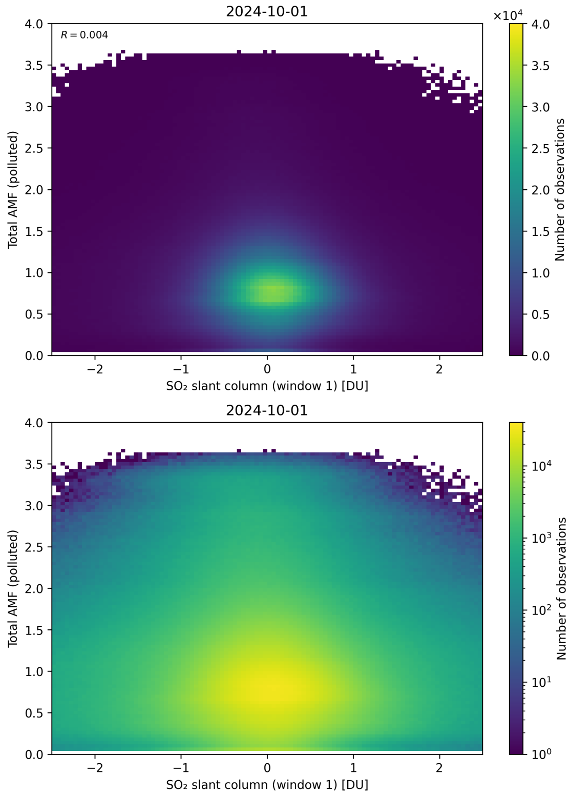
Figure 239: Scatter density plot of “SO 2 slant column (window 1)” against “Total AMF (polluted)” for 2024-09-30 to 2024-10-02.
