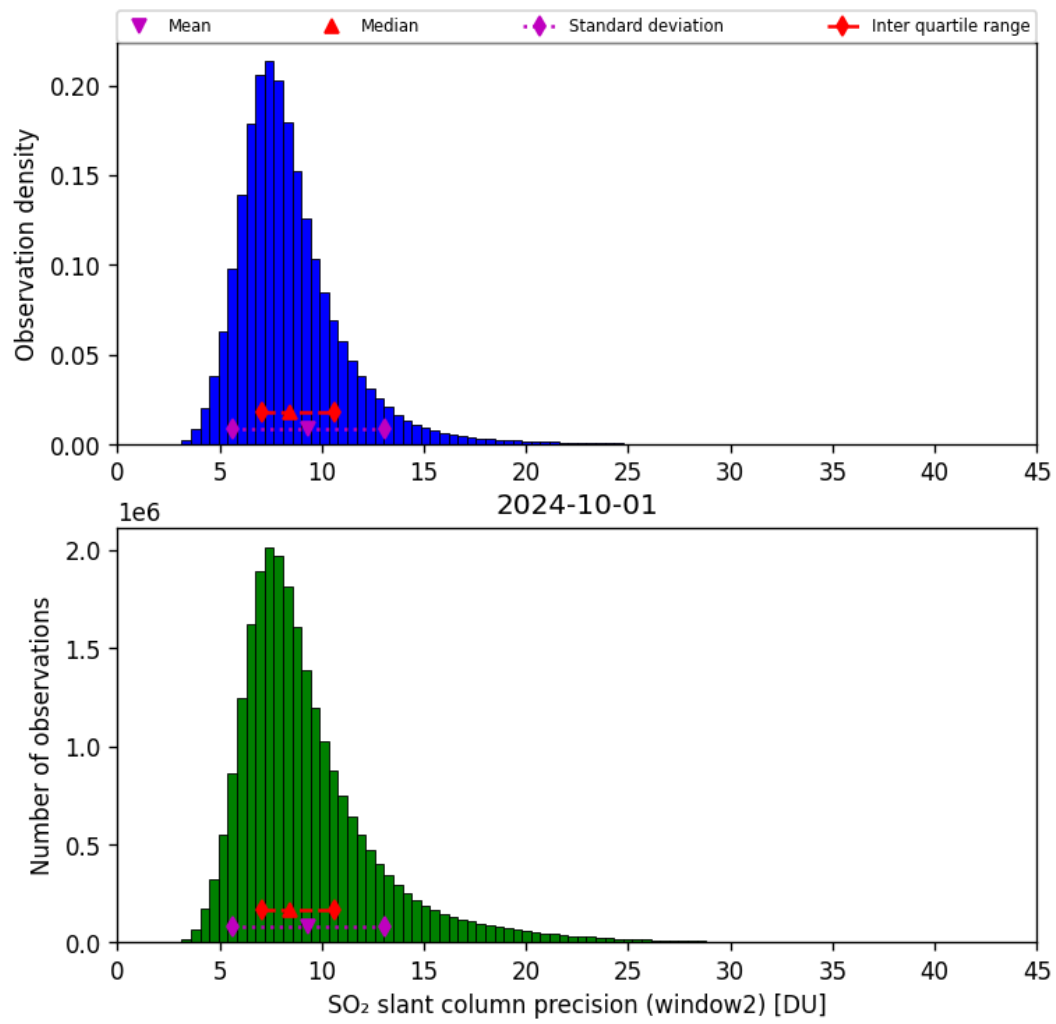
Figure 61: Histogram of “SO 2 slant column precision (window2)” for 2024-09-30 to 2024-10-02
