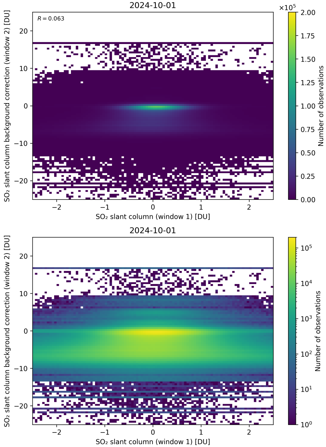
Figure 213: Scatter density plot of “SO 2 slant column (window 1)” against “SO 2 slant column background correction (window 2)” for 2024-09-30 to 2024-10-02.
