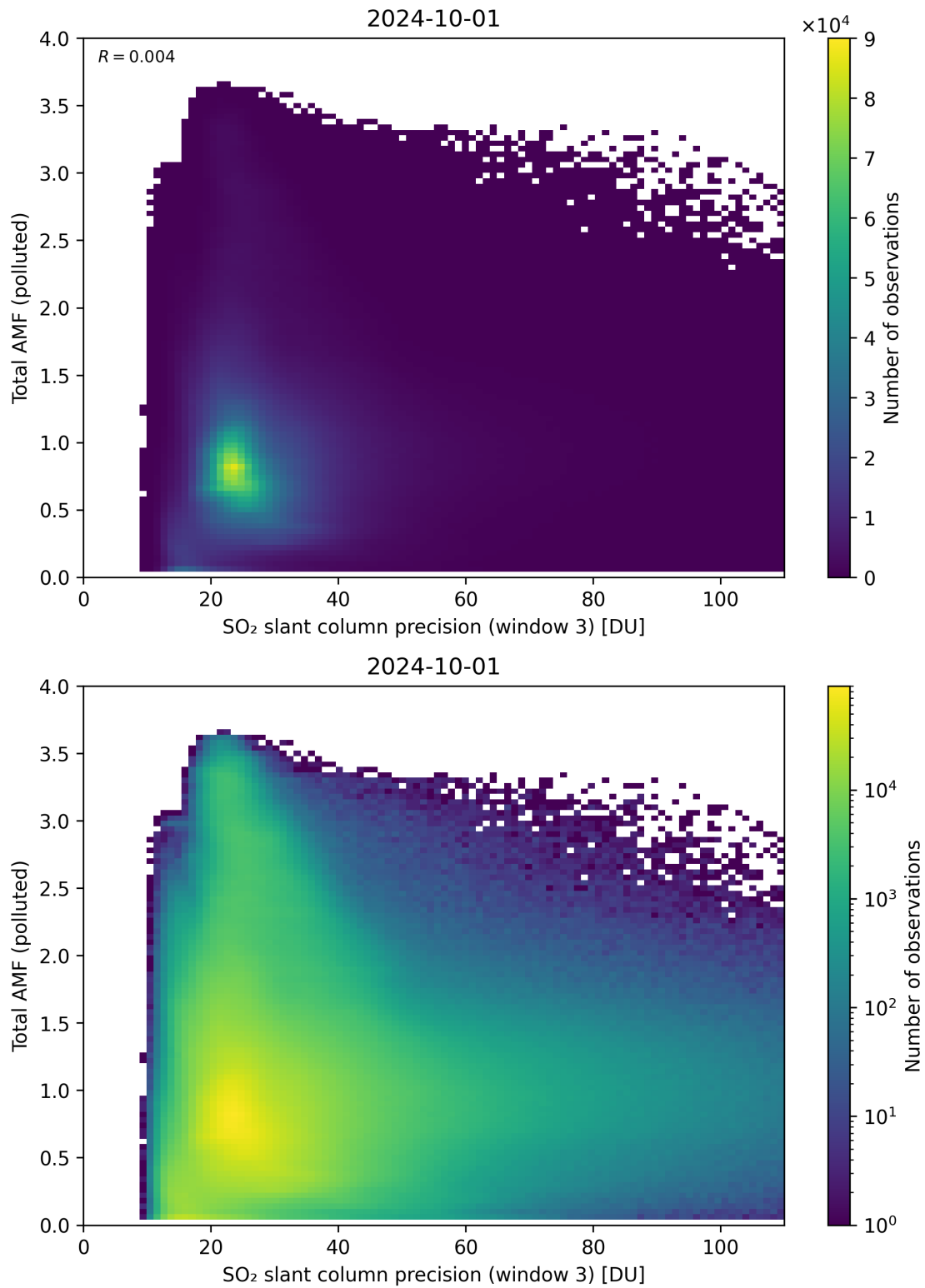
Figure 263: Scatter density plot of “SO 2 slant column precision (window 3)” against “Total AMF (polluted)” for 2024-09-30 to 2024-10-02.
