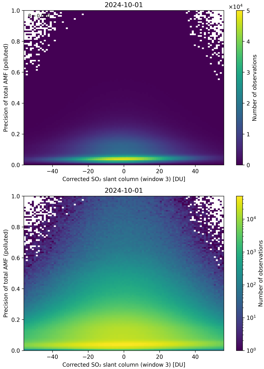
Figure 211: Scatter density plot of “Corrected SO 2 slant column (window 3)” against “Precision of total AMF (polluted)” for 2024-09-30 to 2024-10-02.
