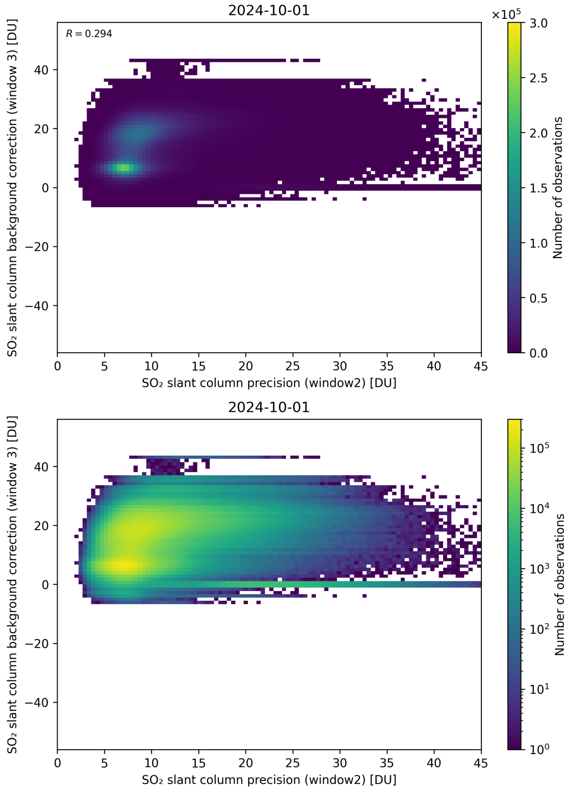
Figure 242: Scatter density plot of “SO 2 slant column precision (window2)” against “SO 2 slant column background correction (window 3)” for 2024-09-30 to 2024-10-02.
