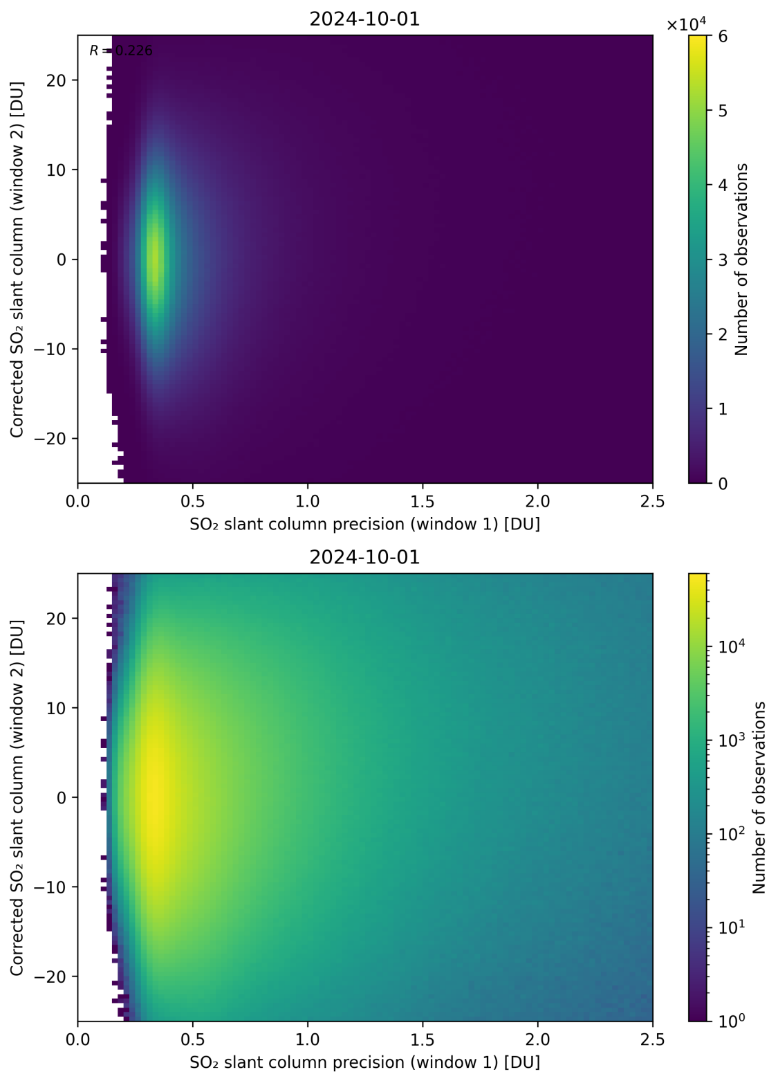
Figure 225: Scatter density plot of “SO 2 slant column precision (window 1)” against “Corrected SO 2 slant column (window 2)” for 2024-09-30 to 2024-10-02.
