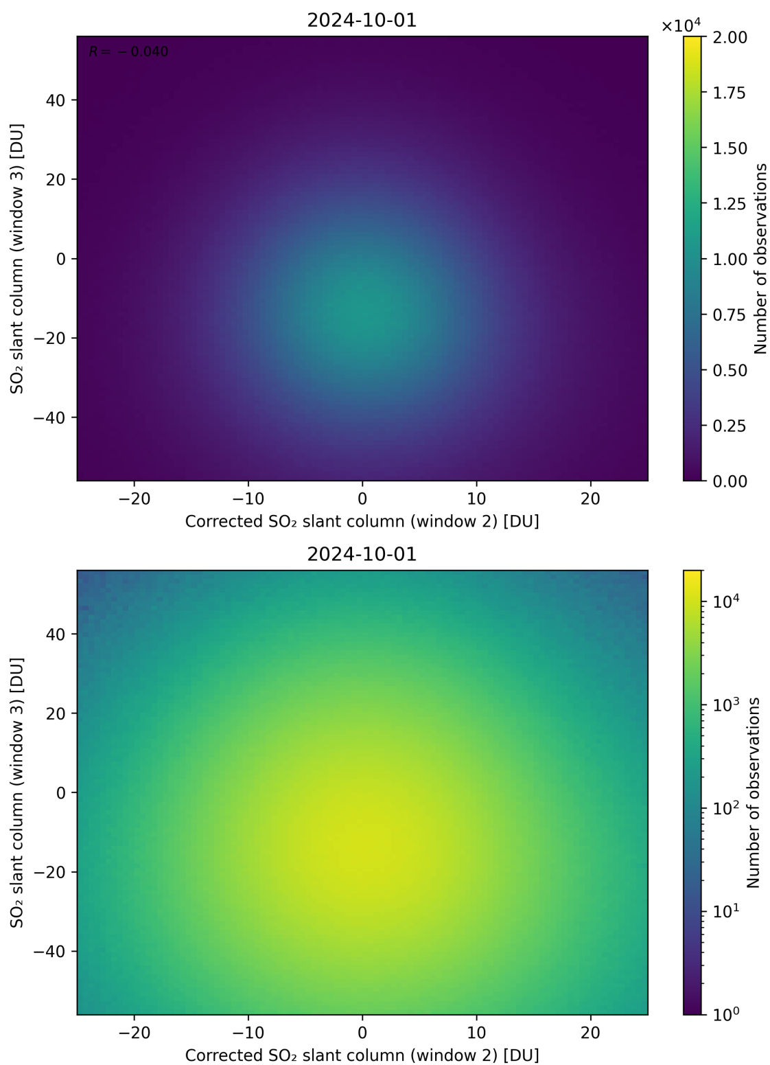
Figure 201: Scatter density plot of “Corrected SO 2 slant column (window 2)” against “SO 2 slant column (window 3)” for 2024-09-30 to 2024-10-02.
