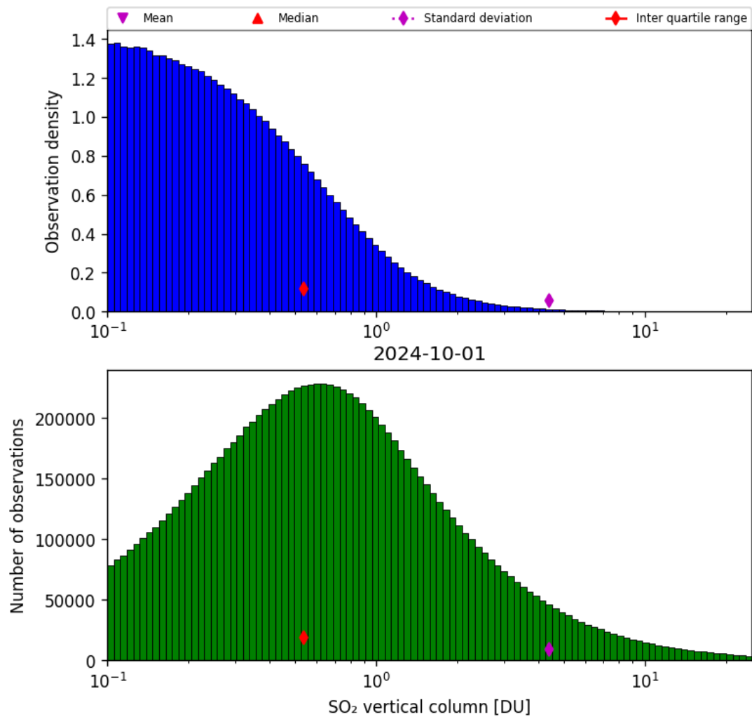
Figure 53: Histogram of “SO 2 vertical column” for 2024-09-30 to 2024-10-02
