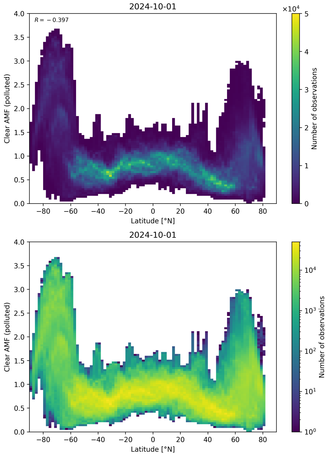
Figure 145: Scatter density plot of “Latitude” against “Clear AMF (polluted)” for 2024-09-30 to 2024-10-02.
