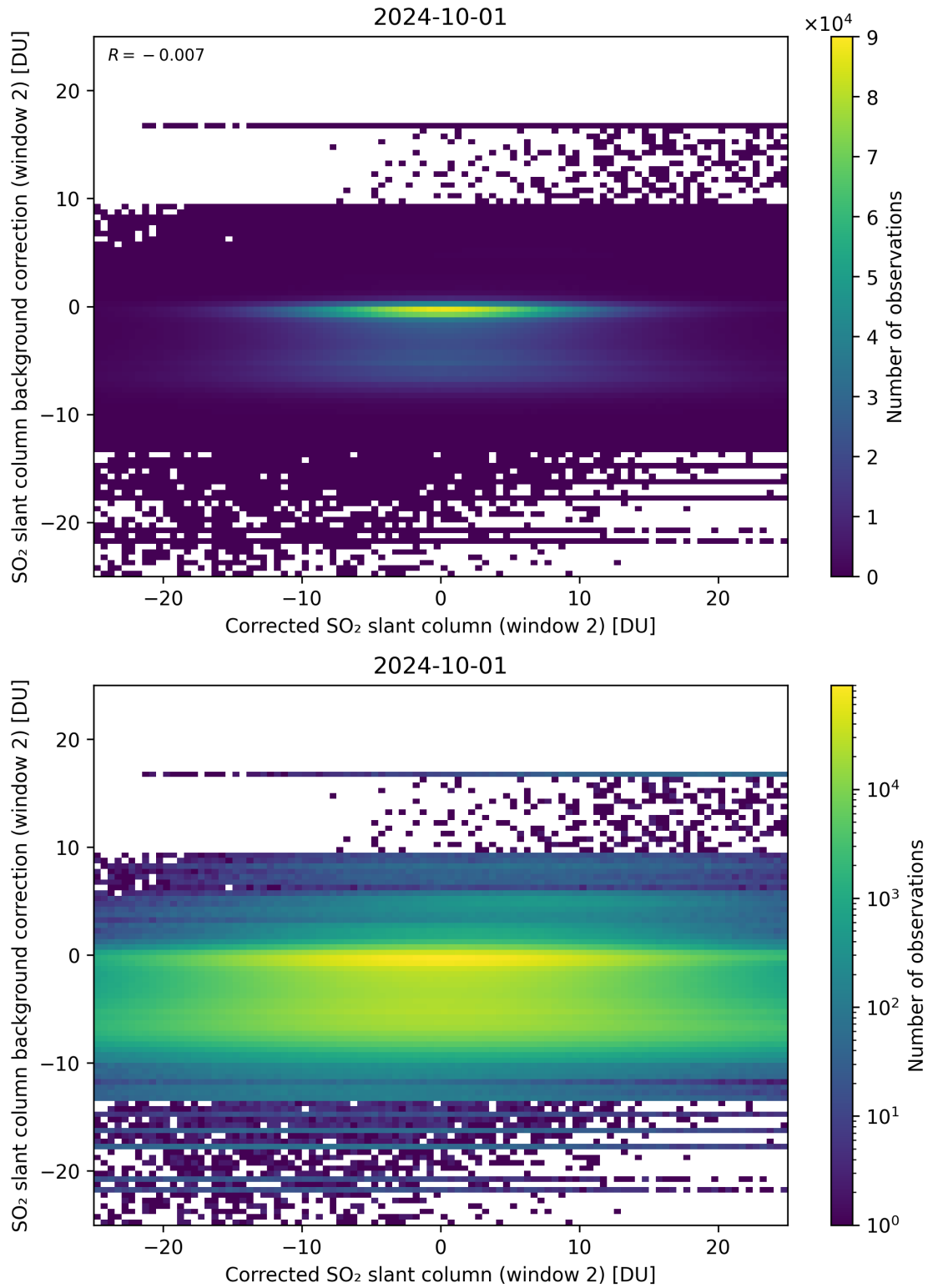
Figure 194: Scatter density plot of “Corrected SO 2 slant column (window 2)” against “SO 2 slant column background correction (window 2)” for 2024-09-30 to 2024-10-02.
