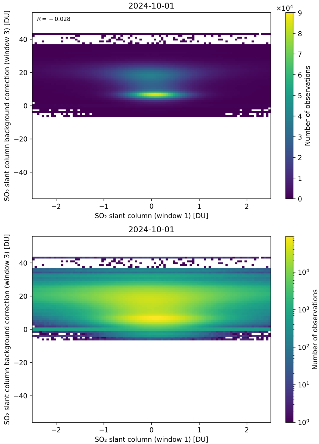
Figure 214: Scatter density plot of “SO 2 slant column (window 1)” against “SO 2 slant column background correction (window 3)” for 2024-09-30 to 2024-10-02.
