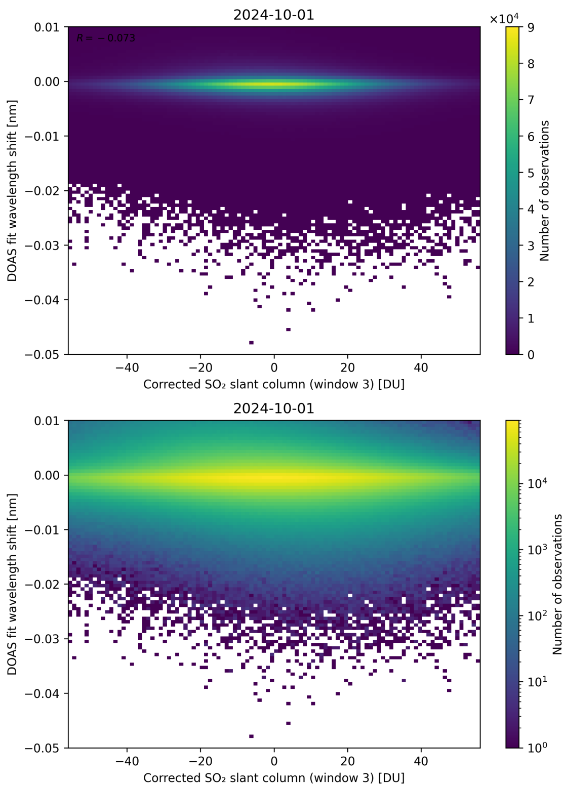
Figure 206: Scatter density plot of “Corrected SO 2 slant column (window 3)” against “DOAS fit wavelength shift” for 2024-09-30 to 2024-10-02.
