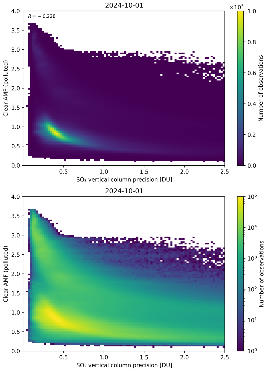
Figure 285: Scatter density plot of “SO 2 vertical column precision” against “Clear AMF (polluted)” for 2024-09-30 to 2024-10-02.
