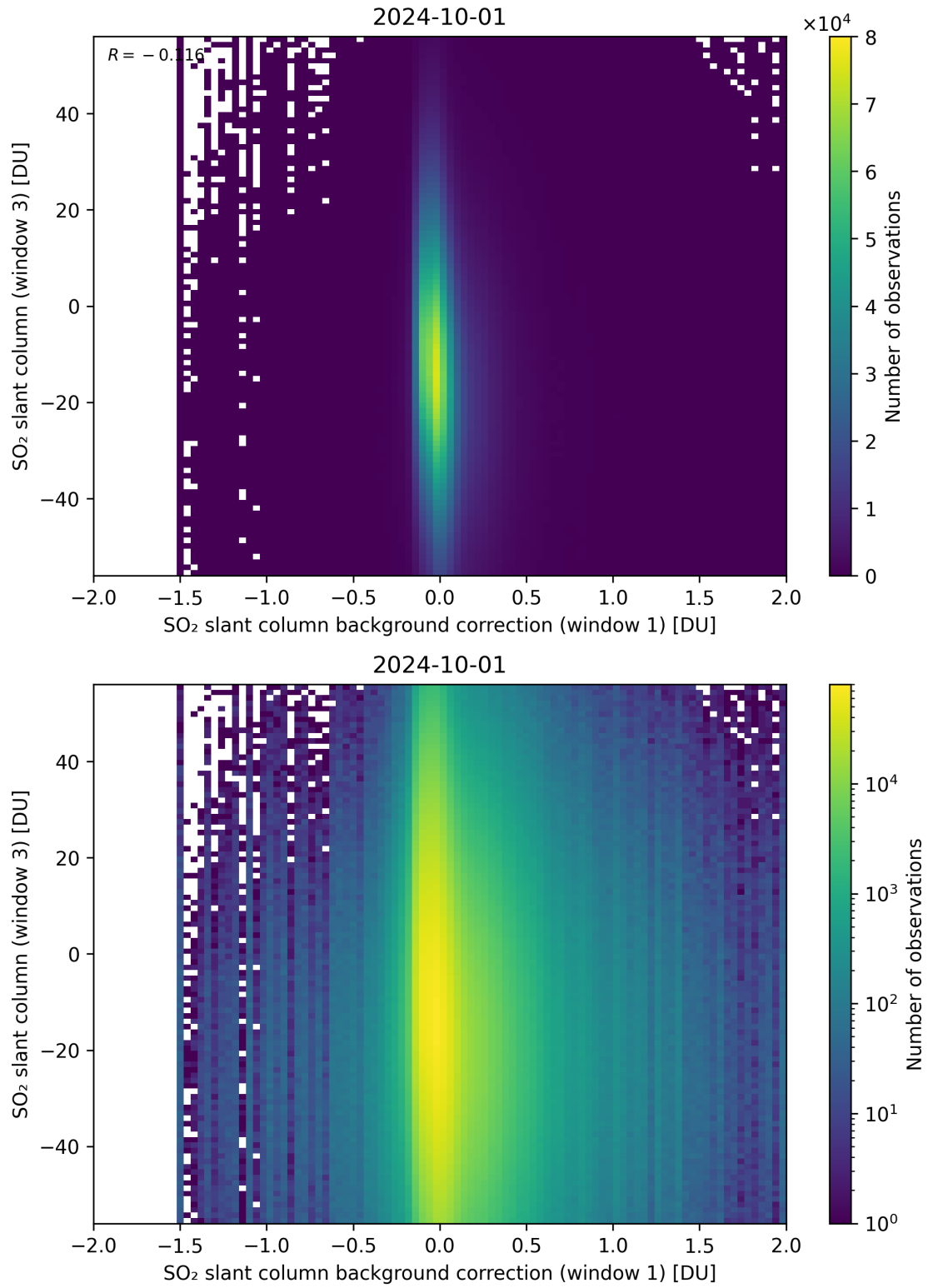
Figure 107: Scatter density plot of “SO 2 slant column background correction (window 1)” against “SO 2 slant column (window 3)” for 2024-09-30 to 2024-10-02.
