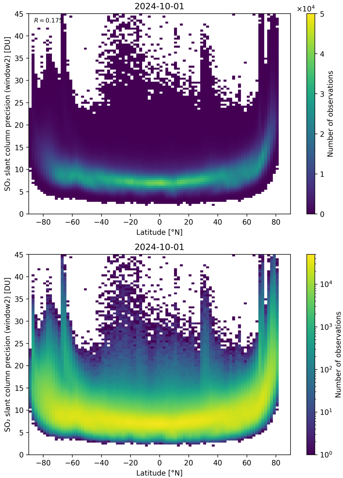
Figure 151: Scatter density plot of “Latitude” against “SO 2 slant column precision (window2)” for 2024-09-30 to 2024-10-02.
