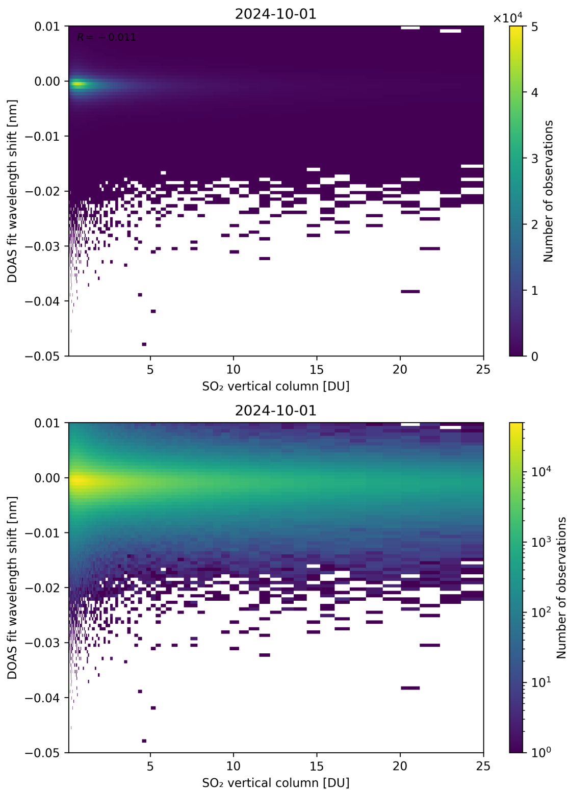
Figure 276: Scatter density plot of “SO 2 vertical column” against “DOAS fit wavelength shift” for 2024-09-30 to 2024-10-02.
