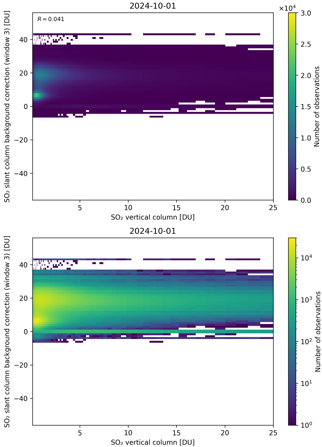
Figure 275: Scatter density plot of “SO 2 vertical column” against “SO 2 slant column background correction (window 3)” for 2024-09-30 to 2024-10-02.
