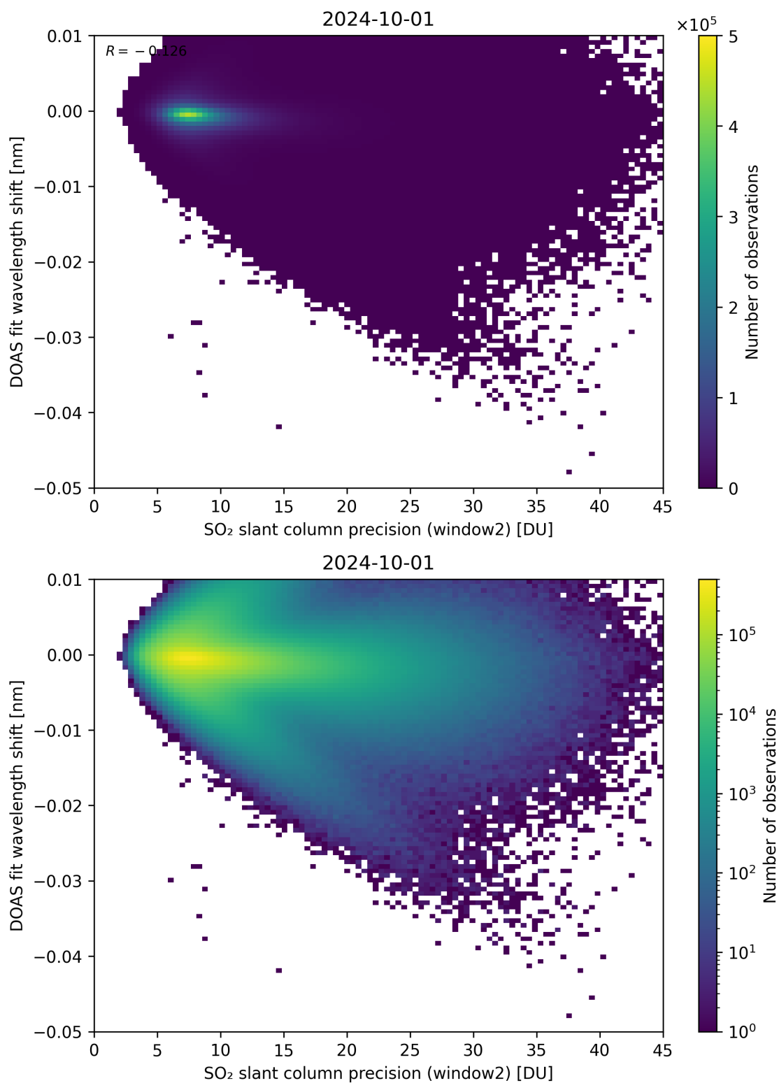
Figure 243: Scatter density plot of “SO 2 slant column precision (window2)” against “DOAS fit wavelength shift” for 2024-09-30 to 2024-10-02.
