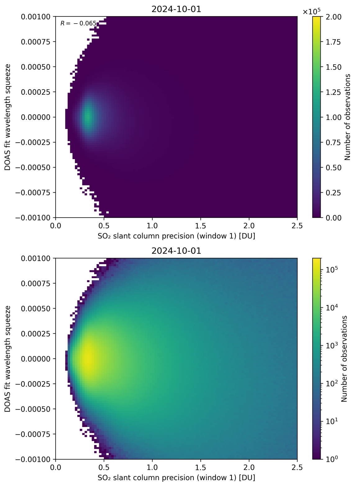
Figure 222: Scatter density plot of “SO 2 slant column precision (window 1)” against “DOAS fit wavelength squeeze” for 2024-09-30 to 2024-10-02.
