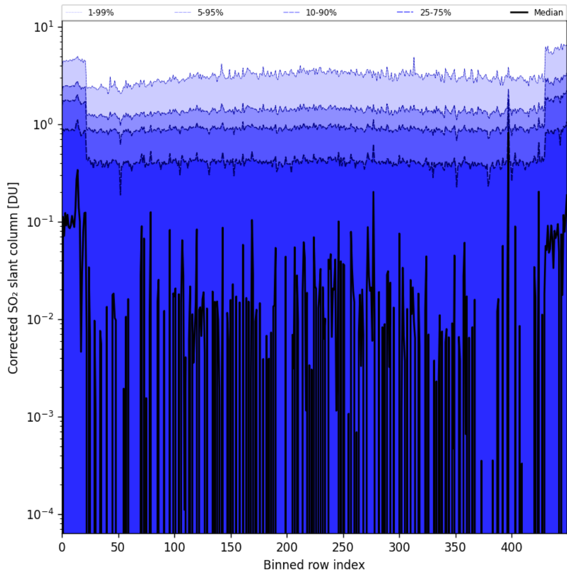
Figure 78: Along track statistics of “Corrected SO 2 slant column” for 2024-09-30 to 2024-10-02
