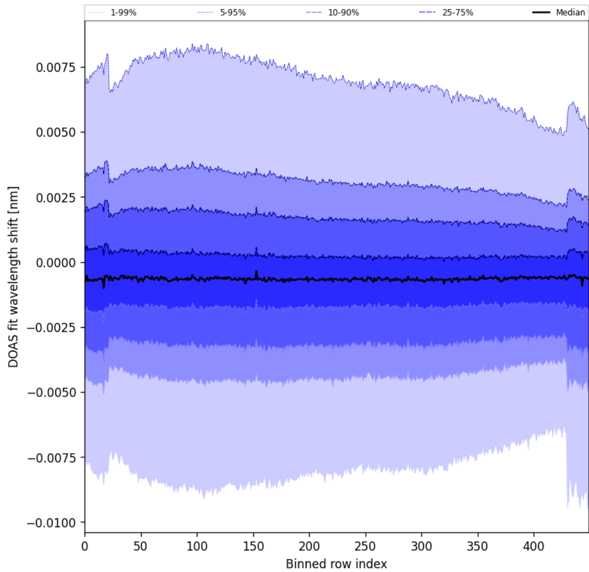
Figure 91: Along track statistics of “DOAS fit wavelength shift” for 2024-09-30 to 2024-10-02
