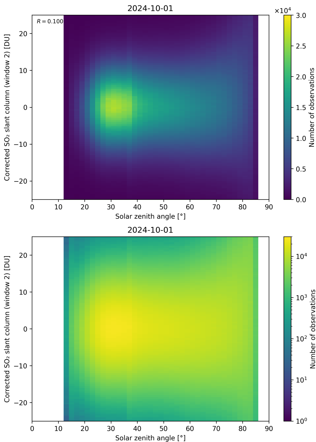
Figure 167: Scatter density plot of “Solar zenith angle” against “Corrected SO 2 slant column (window 2)” for 2024-09-30 to 2024-10-02.
