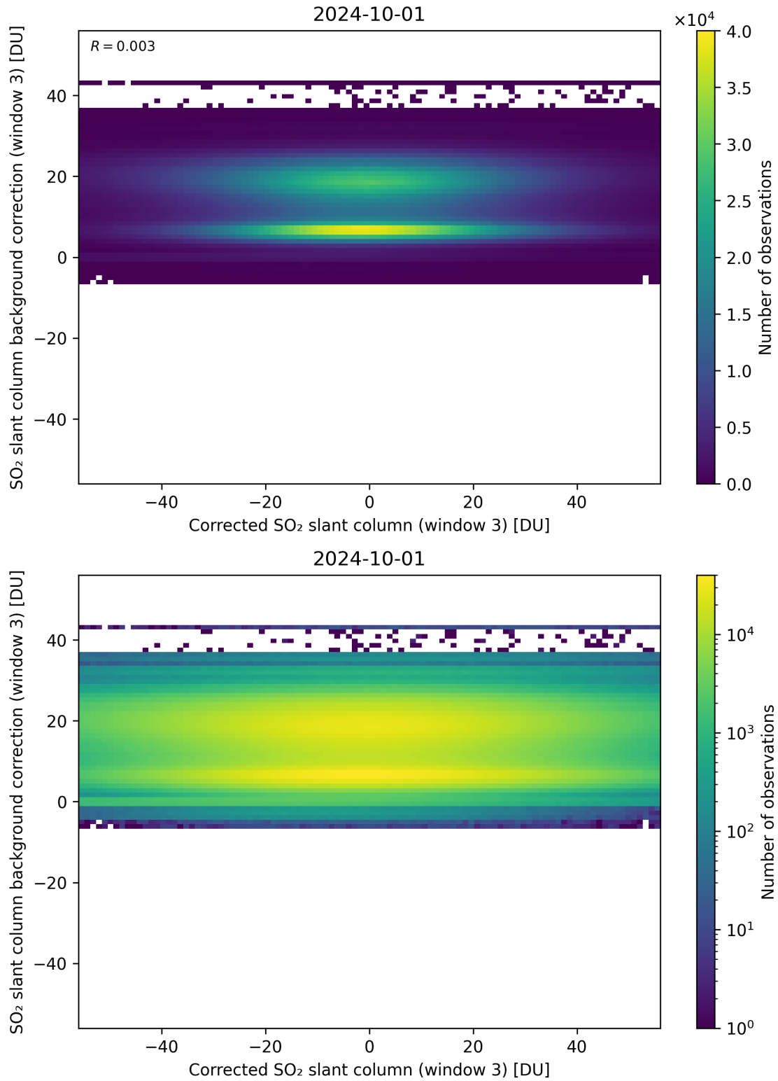
Figure 205: Scatter density plot of “Corrected SO 2 slant column (window 3)” against “SO 2 slant column background correction (window 3)” for 2024-09-30 to 2024-10-02.
