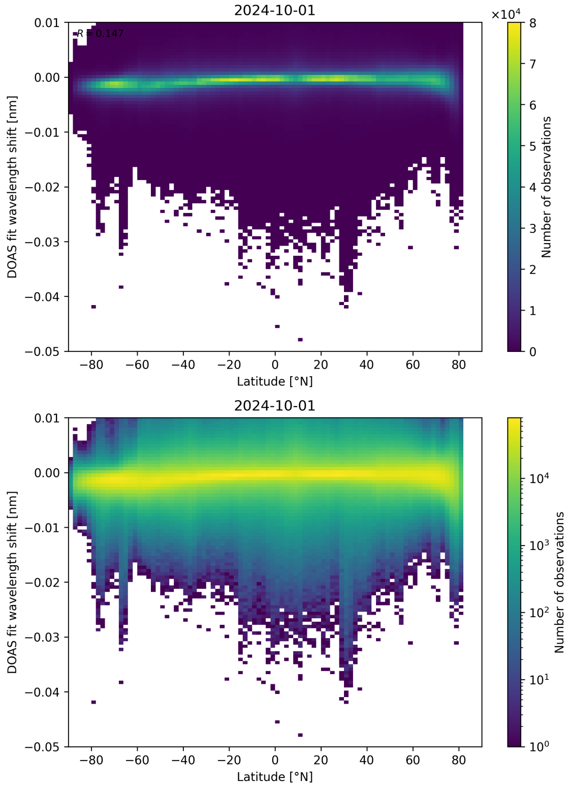
Figure 142: Scatter density plot of “Latitude” against “DOAS fit wavelength shift” for 2024-09-30 to 2024-10-02.
