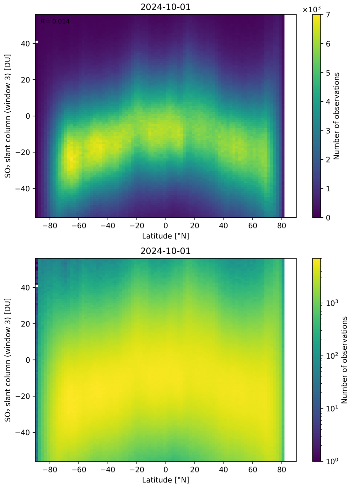
Figure 152: Scatter density plot of “Latitude” against “SO 2 slant column (window 3)” for 2024-09-30 to 2024-10-02.
