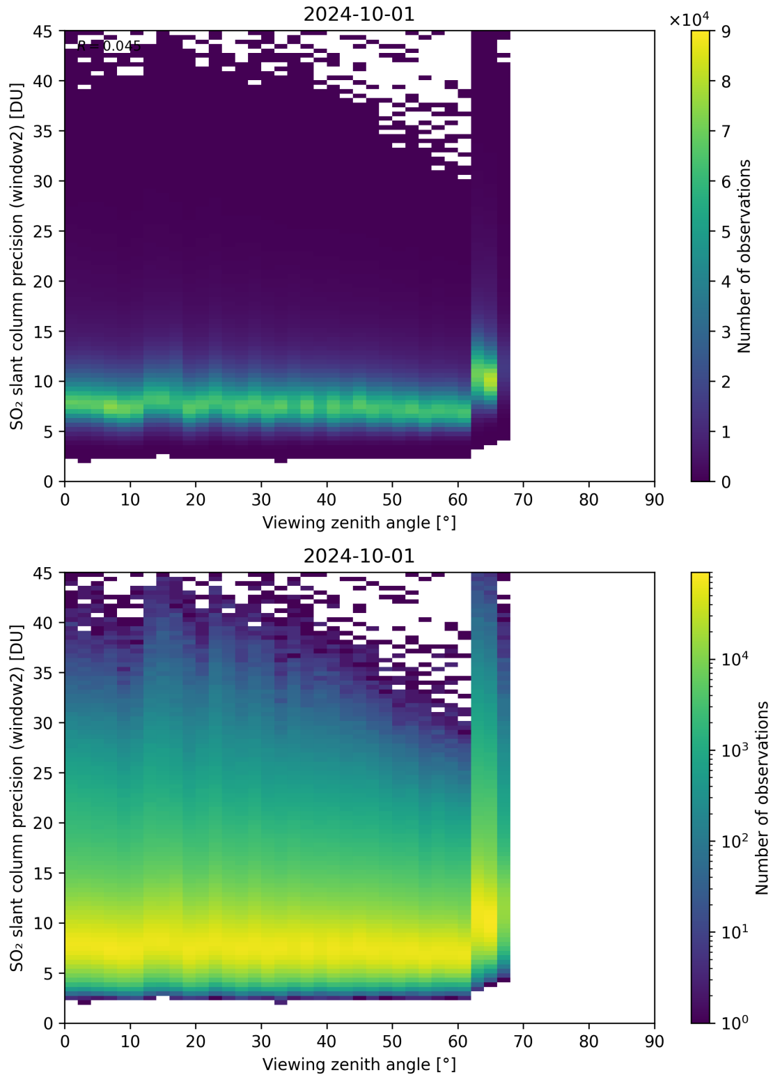
Figure 322: Scatter density plot of “Viewing zenith angle” against “SO 2 slant column precision (window2)” for 2024-09-30 to 2024-10-02.
