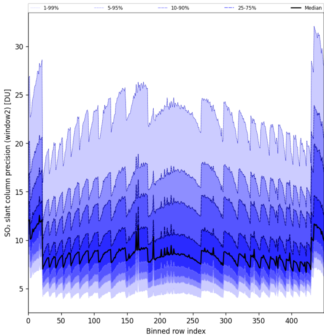
Figure 84: Along track statistics of “SO 2 slant column precision (window2)” for 2024-09-30 to 2024-10-02
