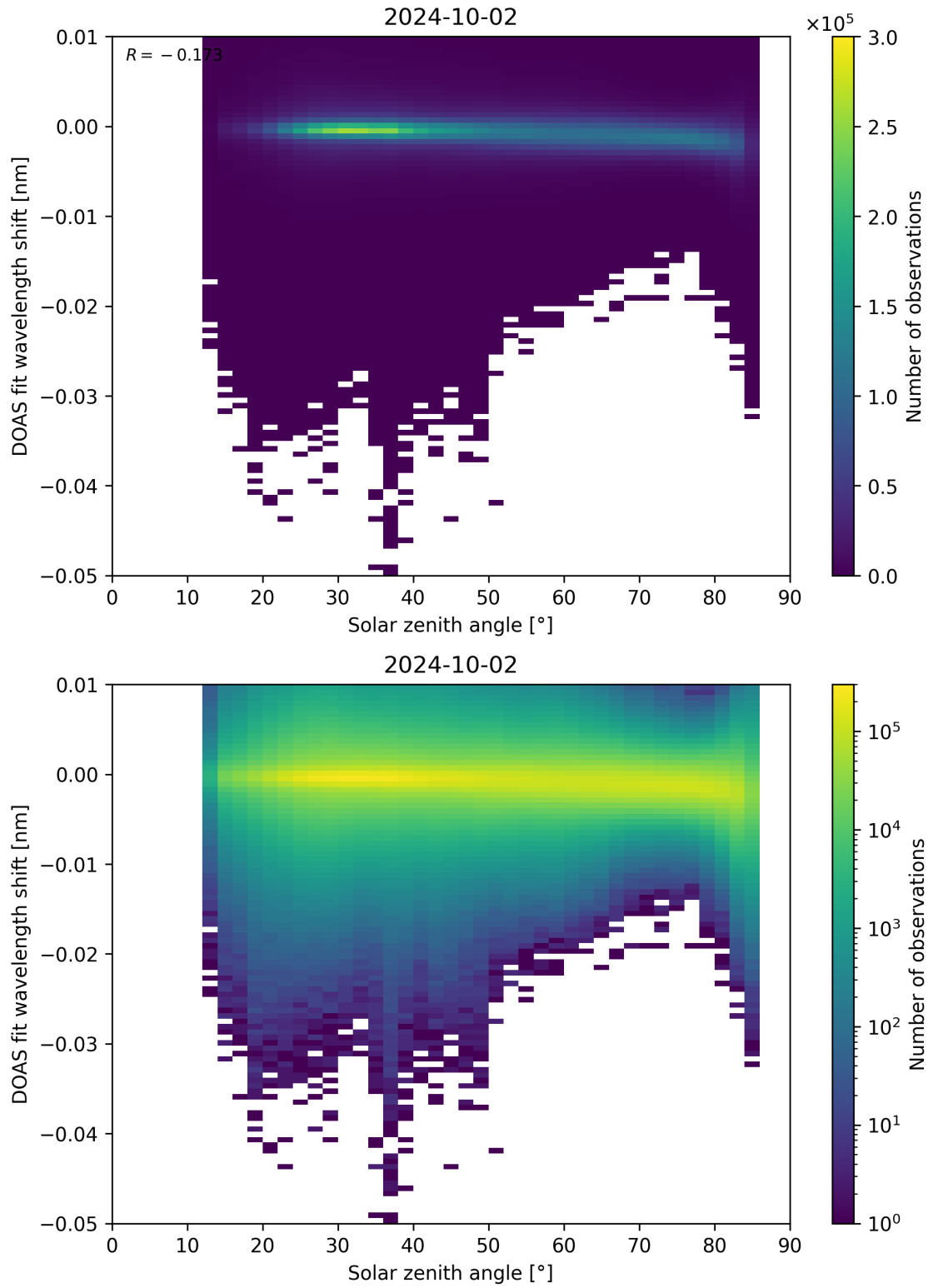
Figure 161: Scatter density plot of “Solar zenith angle” against “DOAS fit wavelength shift” for 2024-10-01 to 2024-10-03.
