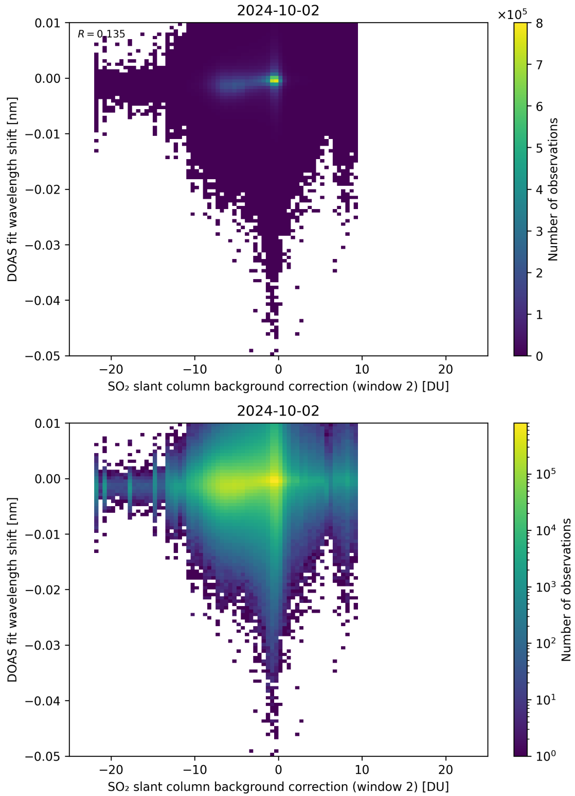
Figure 112: Scatter density plot of “SO 2 slant column background correction (window 2)” against “DOAS fit wavelength shift” for 2024-10-01 to 2024-10-03.
