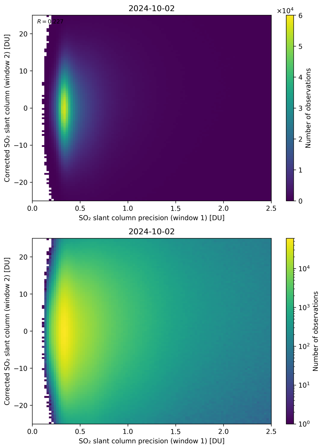
Figure 225: Scatter density plot of “SO 2 slant column precision (window 1)” against “Corrected SO 2 slant column (window 2)” for 2024-10-01 to 2024-10-03.
