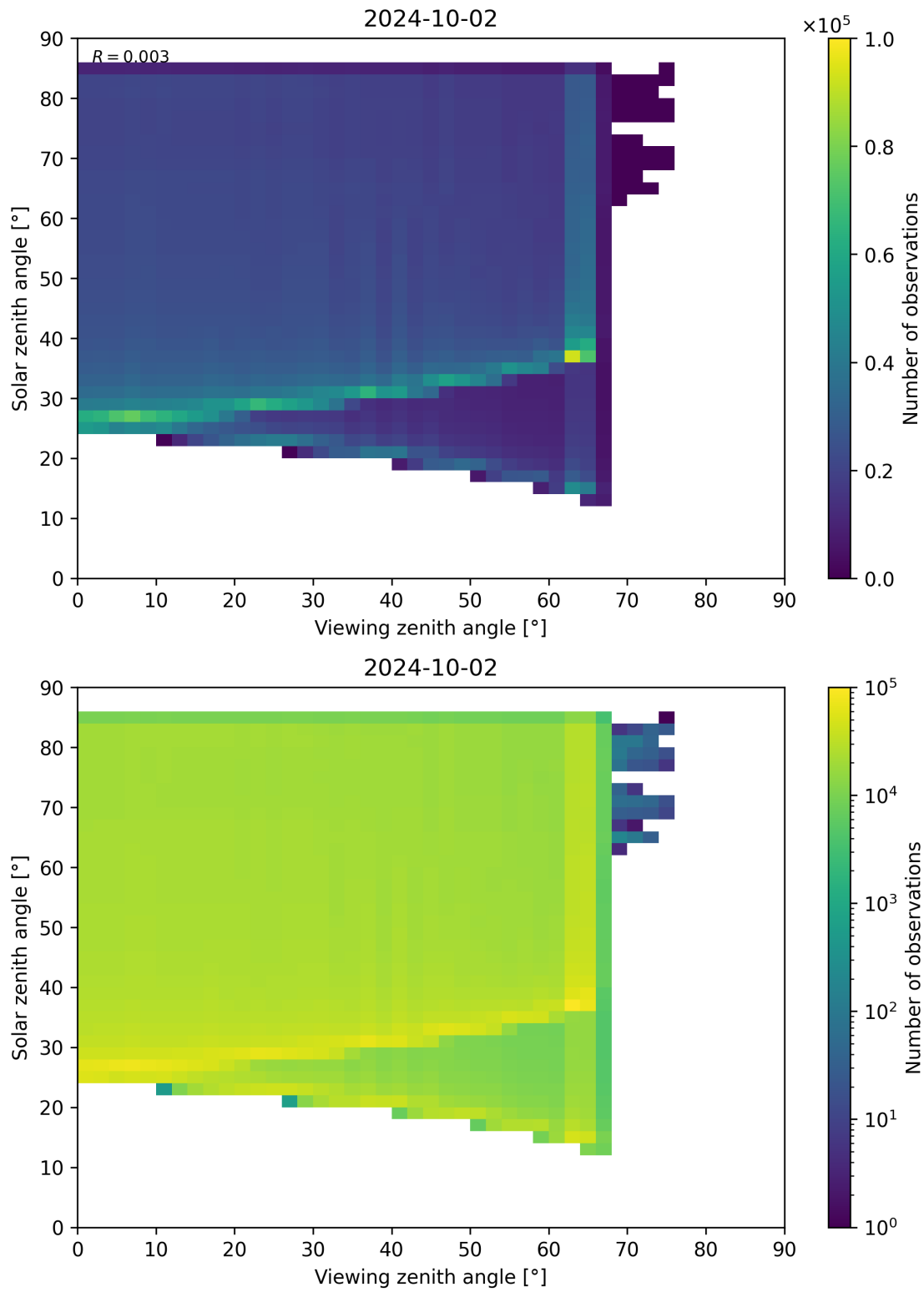
Figure 315: Scatter density plot of “Viewing zenith angle” against “Solar zenith angle” for 2024-10-01 to 2024-10-03.
