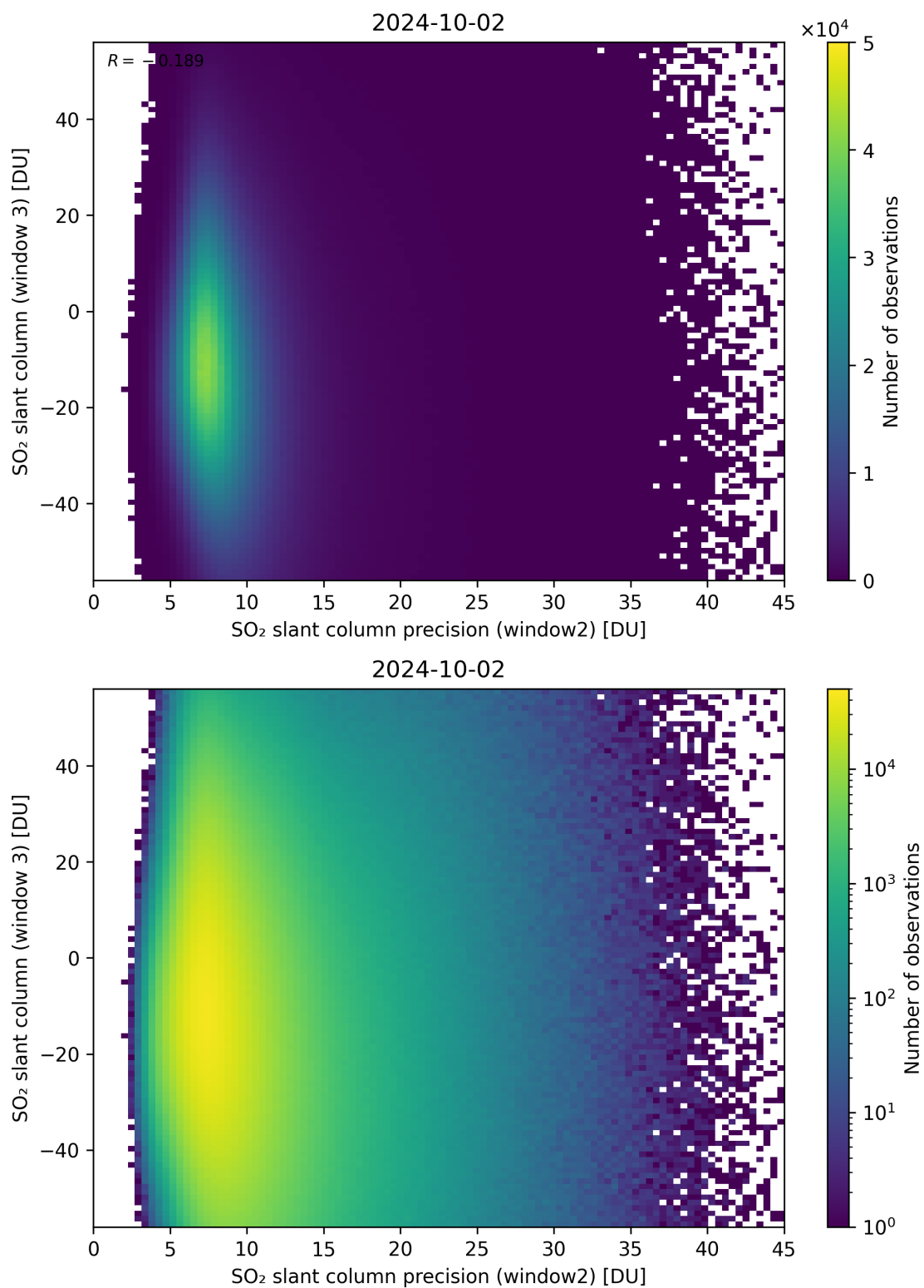
Figure 249: Scatter density plot of “SO 2 slant column precision (window2)” against “SO 2 slant column (window 3)” for 2024-10-01 to 2024-10-03.
