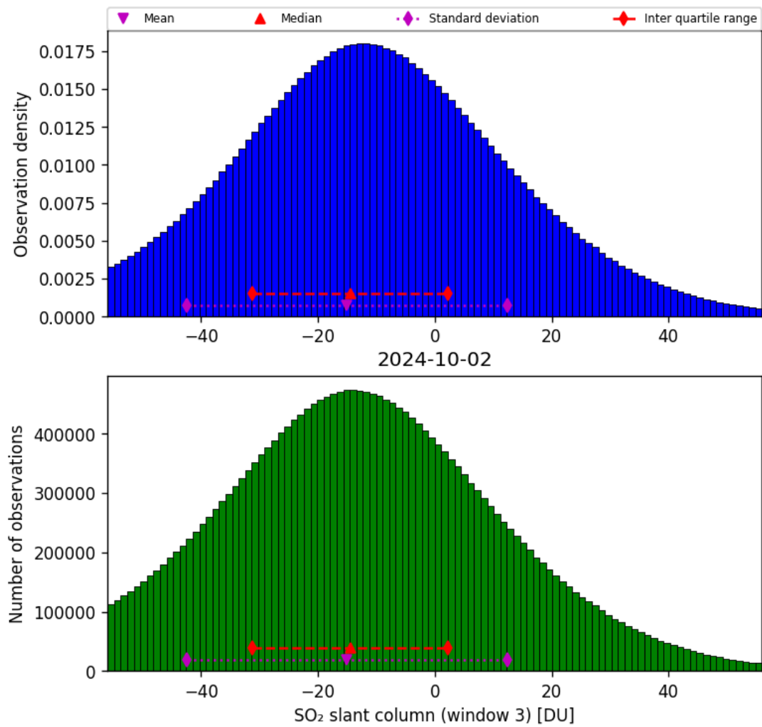
Figure 64: Histogram of “SO 2 slant column (window 3)” for 2024-10-01 to 2024-10-03
