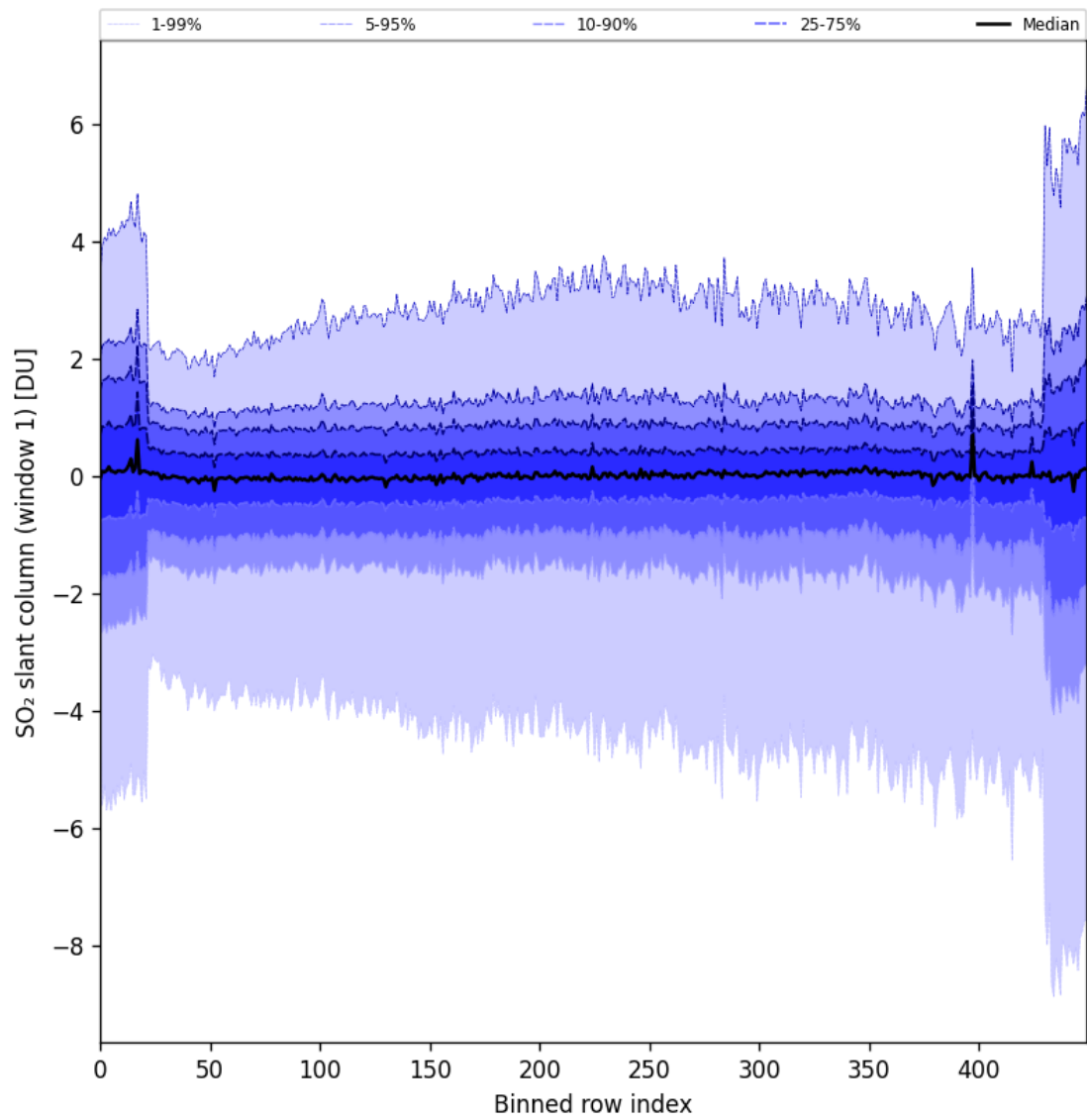
Figure 79: Along track statistics of “SO 2 slant column (window 1)” for 2024-10-01 to 2024-10-03
