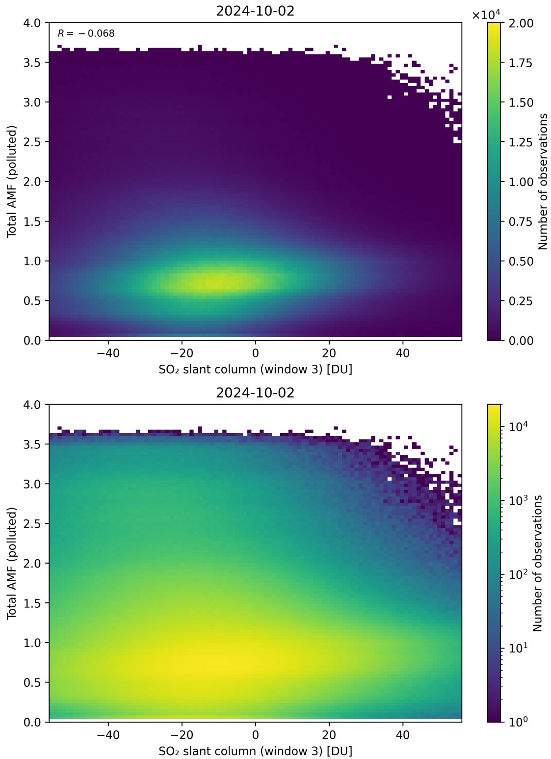
Figure 268: Scatter density plot of “SO 2 slant column (window 3)” against “Total AMF (polluted)” for 2024-10-01 to 2024-10-03.
