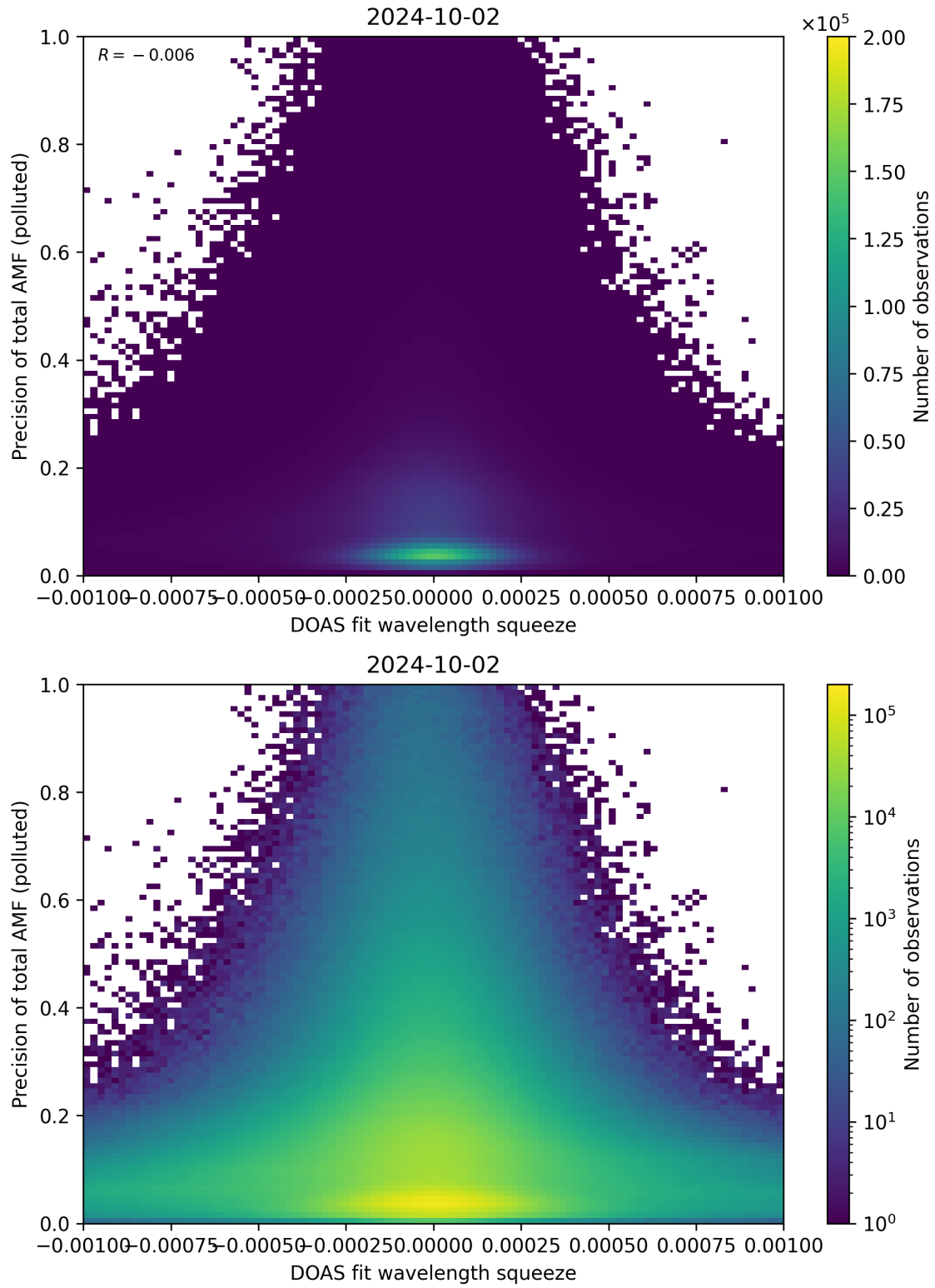
Figure 135: Scatter density plot of “DOAS fit wavelength squeeze” against “Precision of total AMF (polluted)” for 2024-10-01 to 2024-10-03.
