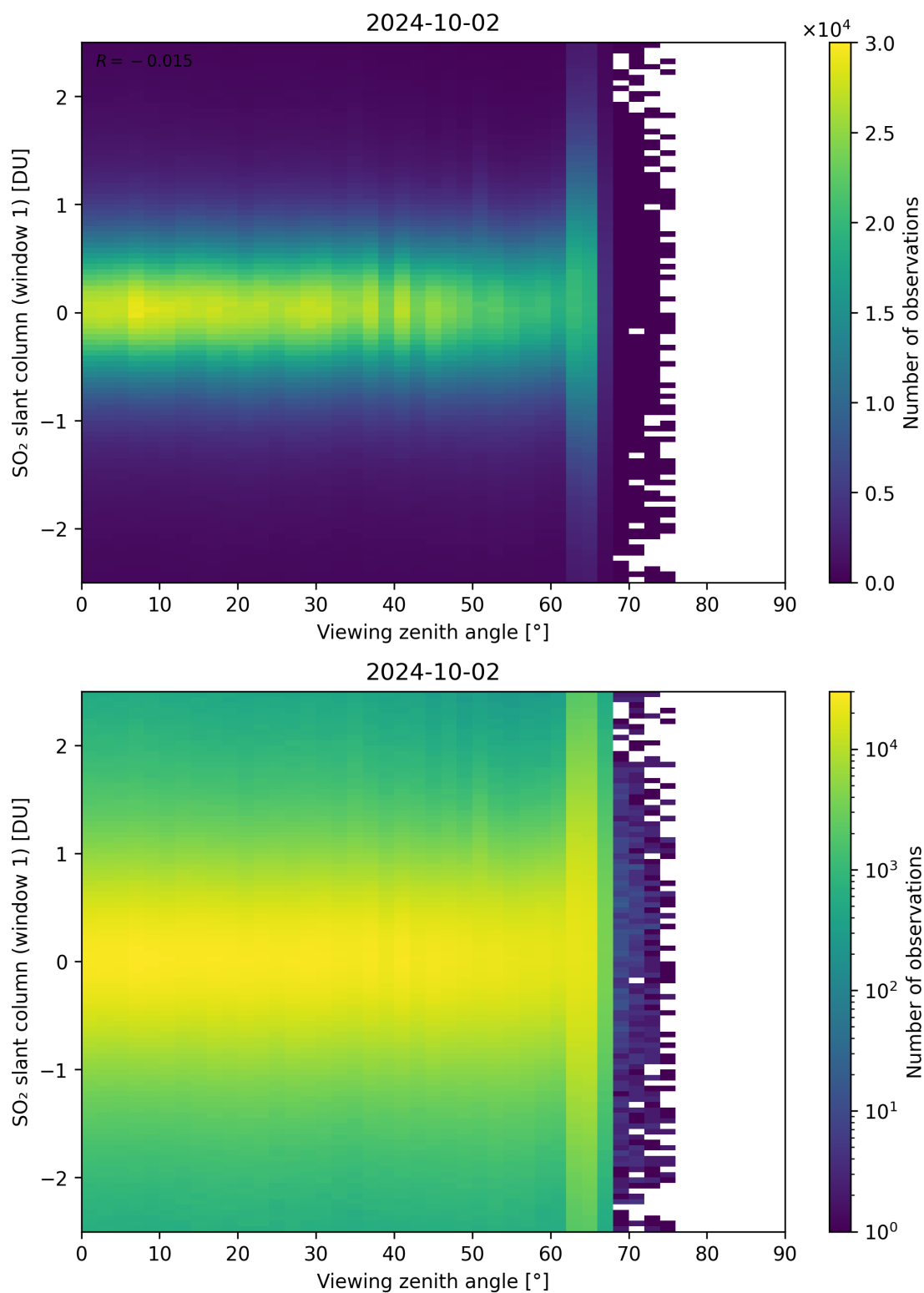
Figure 320: Scatter density plot of “Viewing zenith angle” against “SO 2 slant column (window 1)” for 2024-10-01 to 2024-10-03.
