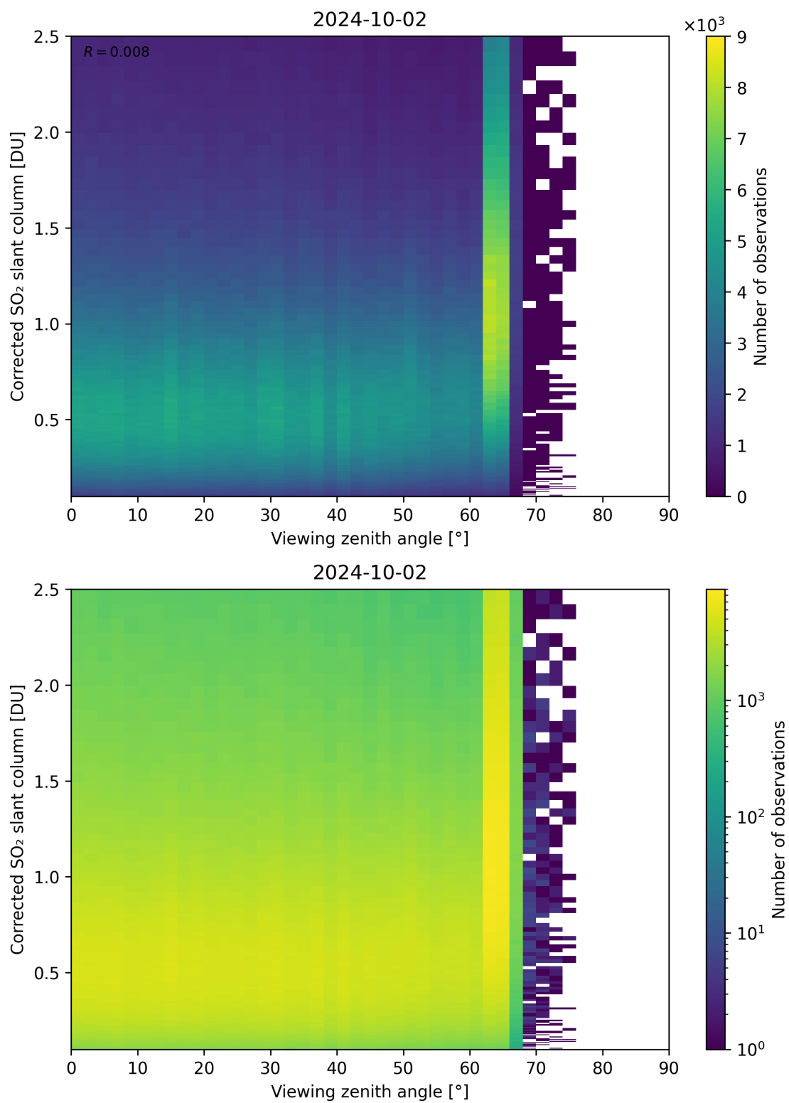
Figure 317: Scatter density plot of “Viewing zenith angle” against “Corrected SO 2 slant column” for 2024-10-01 to 2024-10-03.
