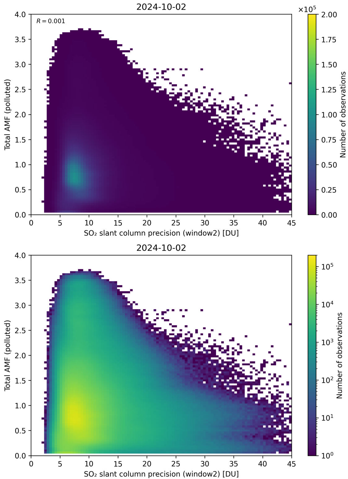
Figure 251: Scatter density plot of “SO 2 slant column precision (window2)” against “Total AMF (polluted)” for 2024-10-01 to 2024-10-03.
