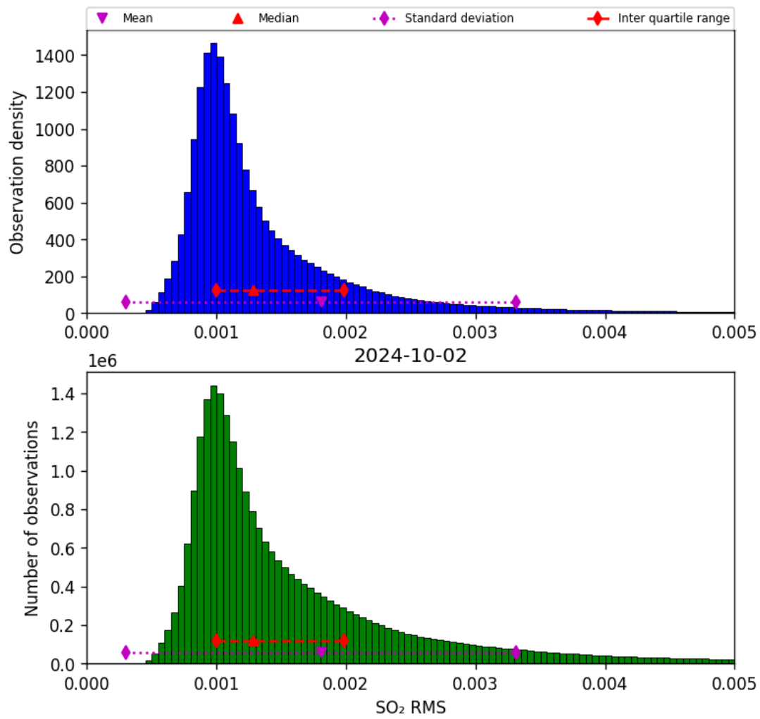
Figure 70: Histogram of “SO 2 RMS” for 2024-10-01 to 2024-10-03
