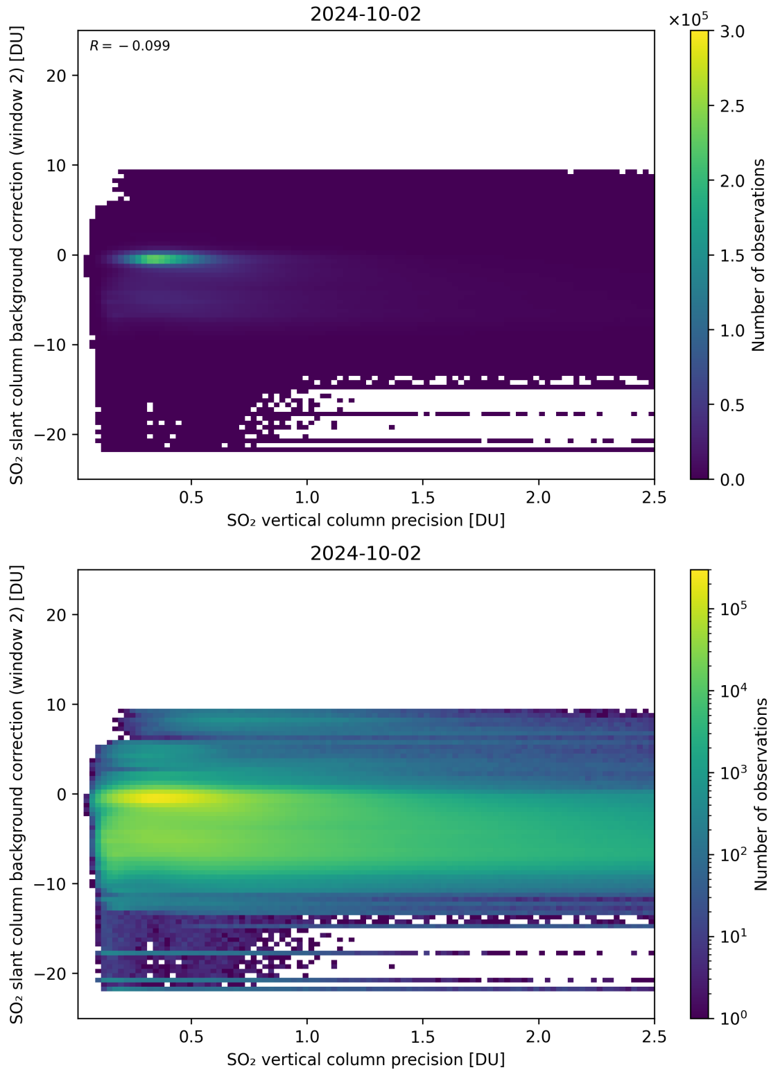
Figure 280: Scatter density plot of “SO 2 vertical column precision” against “SO 2 slant column background correction (window 2)” for 2024-10-01 to 2024-10-03.
