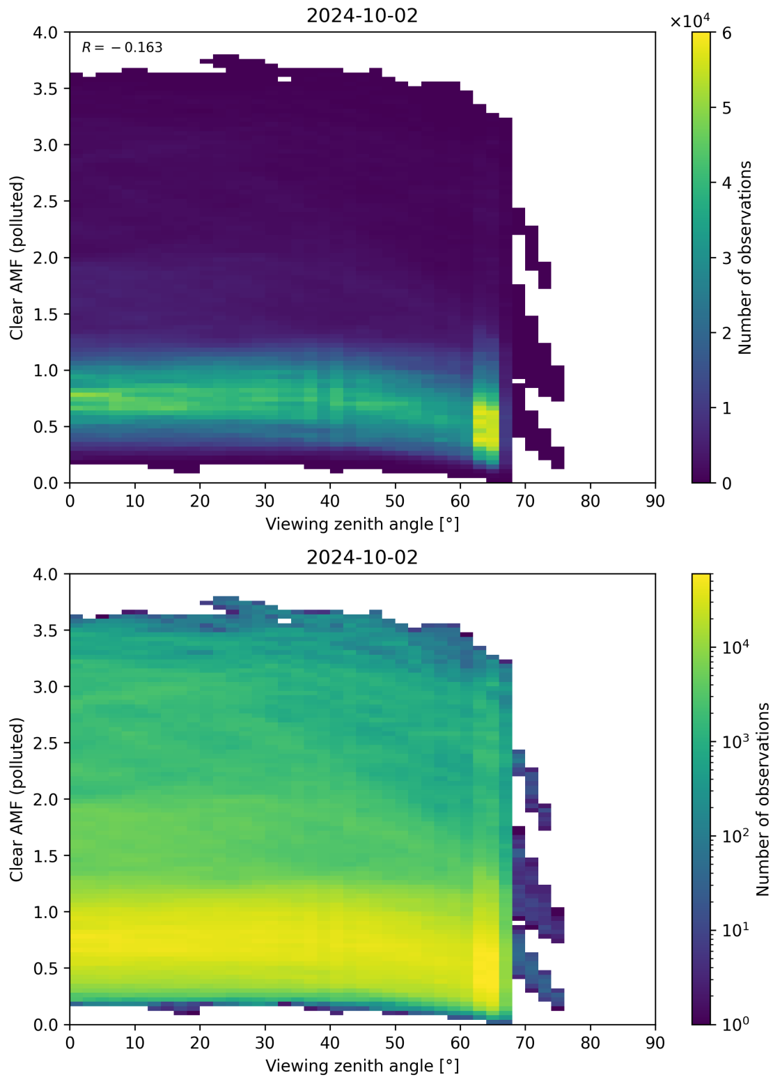
Figure 316: Scatter density plot of “Viewing zenith angle” against “Clear AMF (polluted)” for 2024-10-01 to 2024-10-03.
