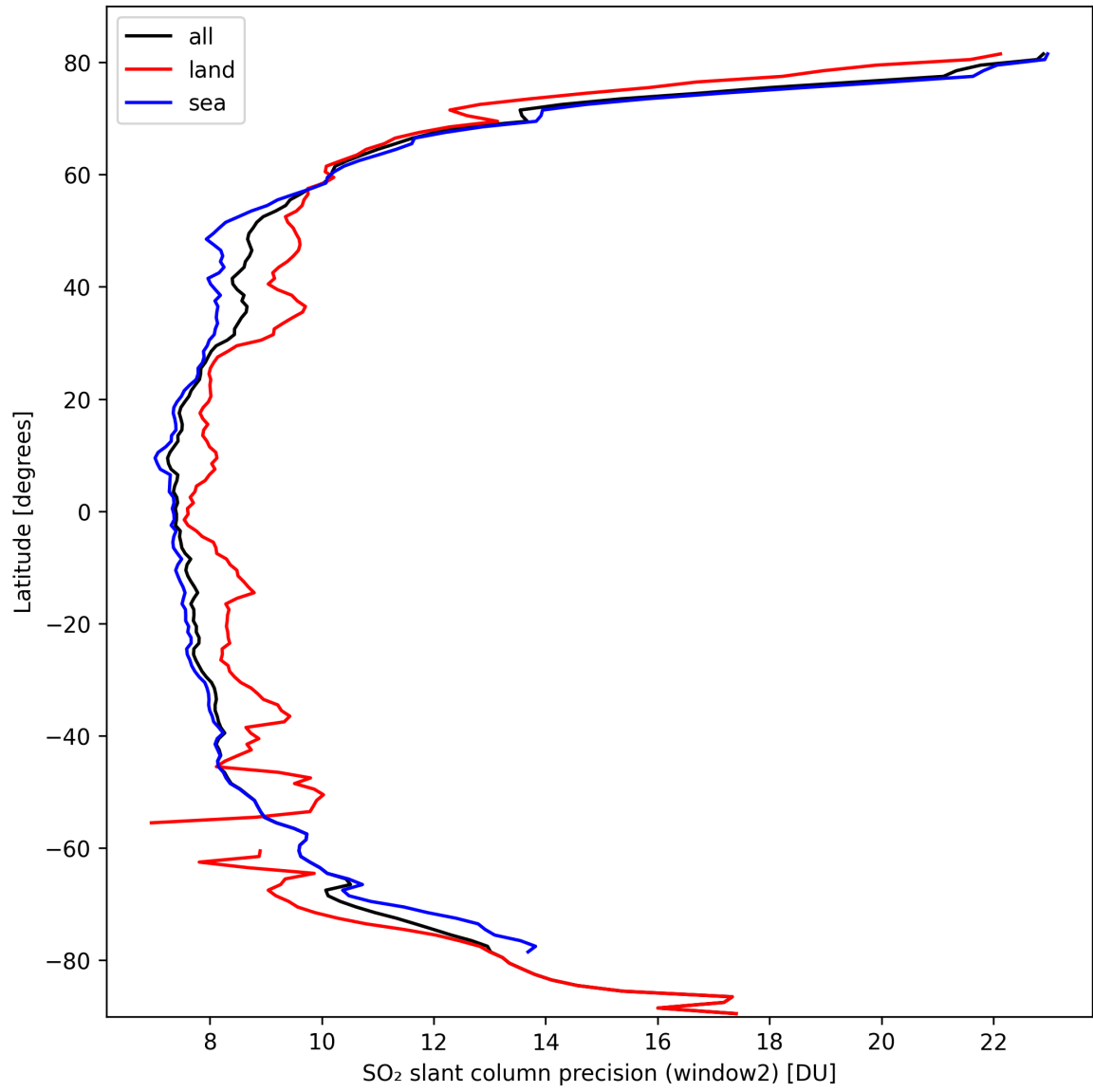
Figure 38: Zonal average of “SO 2 slant column precision (window2)” for 2024-10-01 to 2024-10-03.
