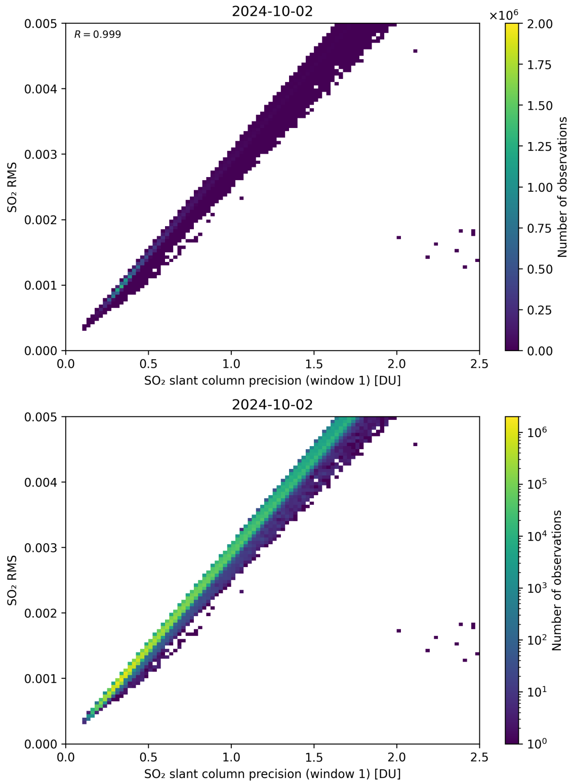
Figure 223: Scatter density plot of “SO 2 slant column precision (window 1)” against “SO 2 RMS” for 2024-10-01 to 2024-10-03.
