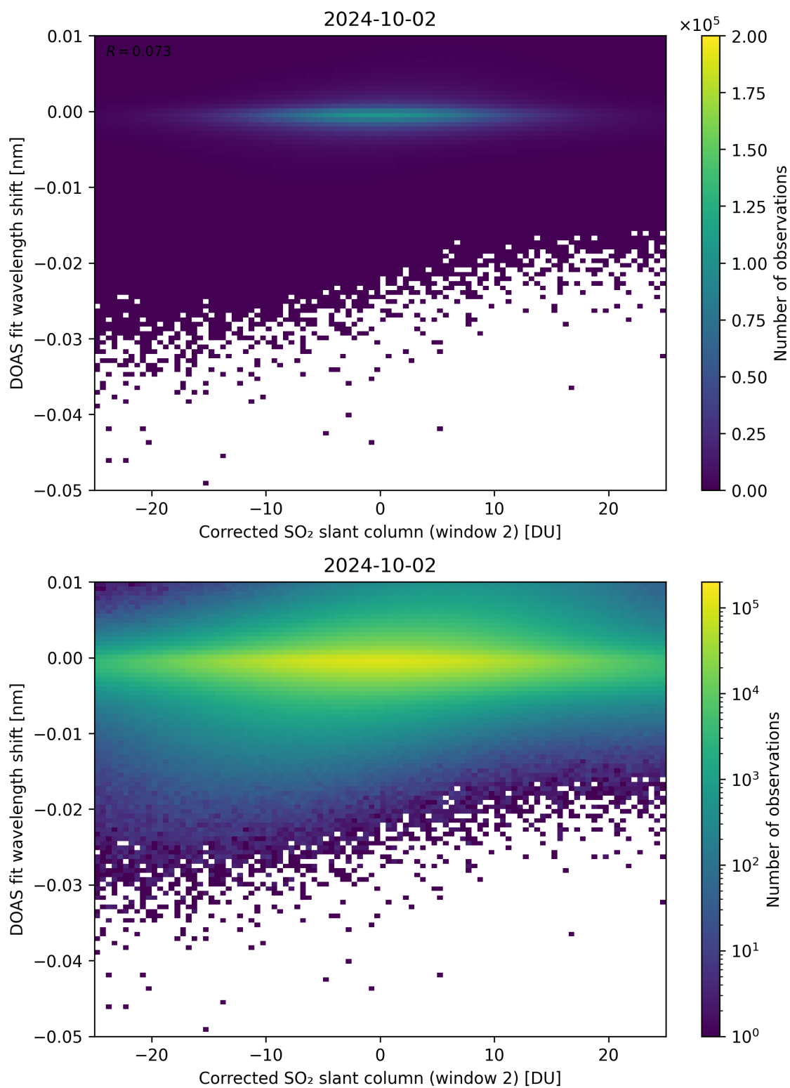
Figure 196: Scatter density plot of “Corrected SO 2 slant column (window 2)” against “DOAS fit wavelength shift” for 2024-10-01 to 2024-10-03.
