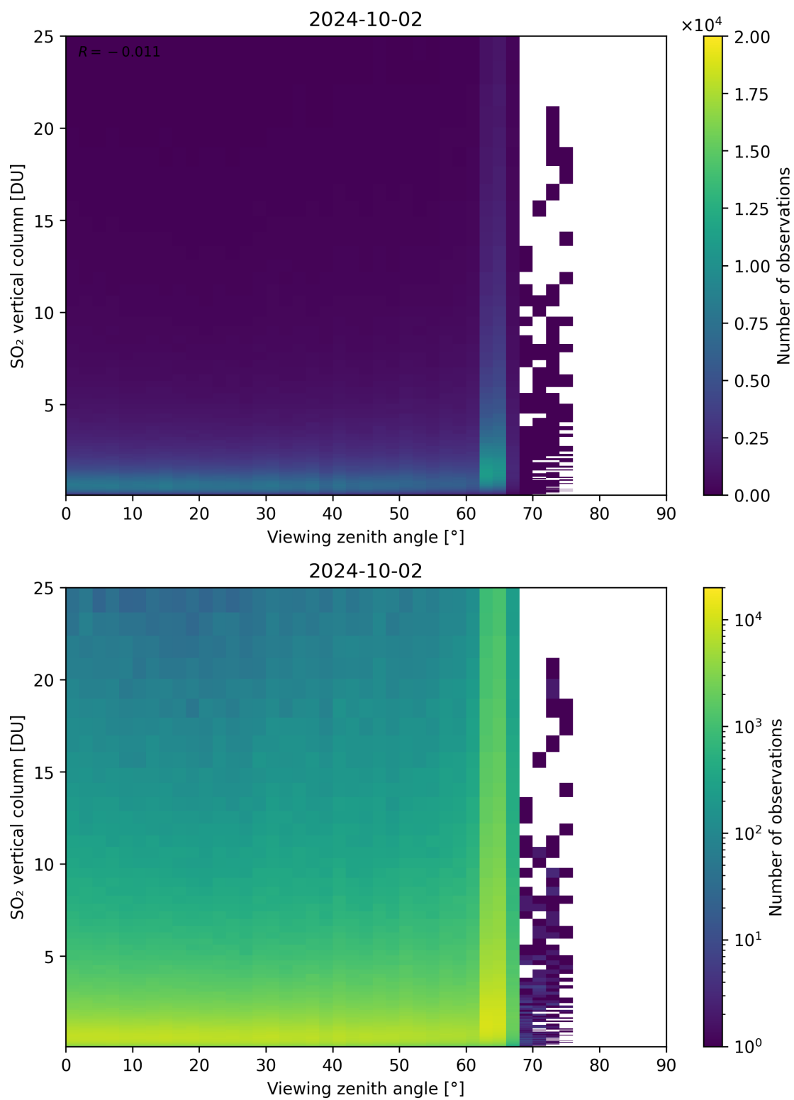
Figure 327: Scatter density plot of “Viewing zenith angle” against “SO 2 vertical column” for 2024-10-01 to 2024-10-03.
