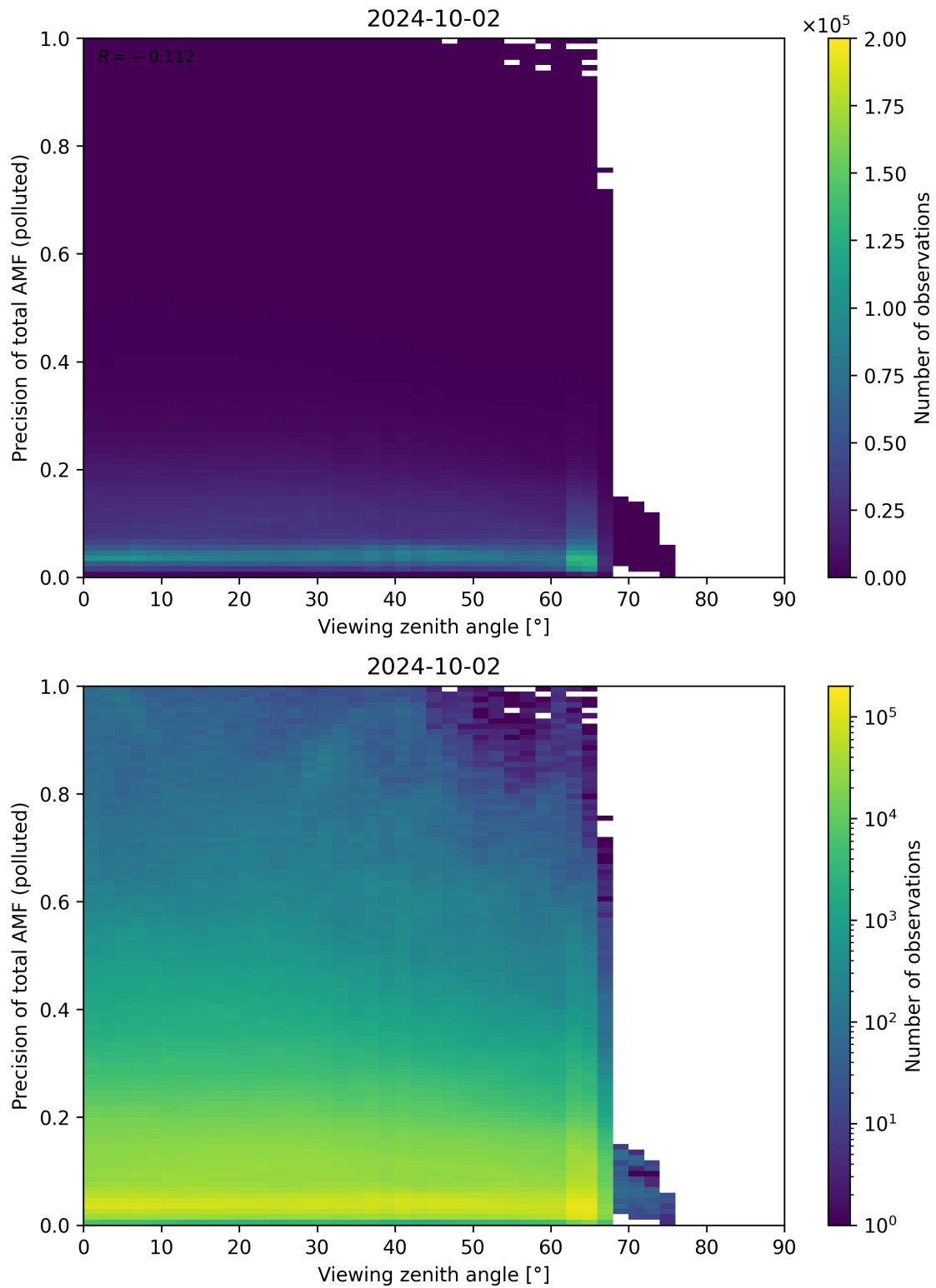
Figure 326: Scatter density plot of “Viewing zenith angle” against “Precision of total AMF (polluted)” for 2024-10-01 to 2024-10-03.
