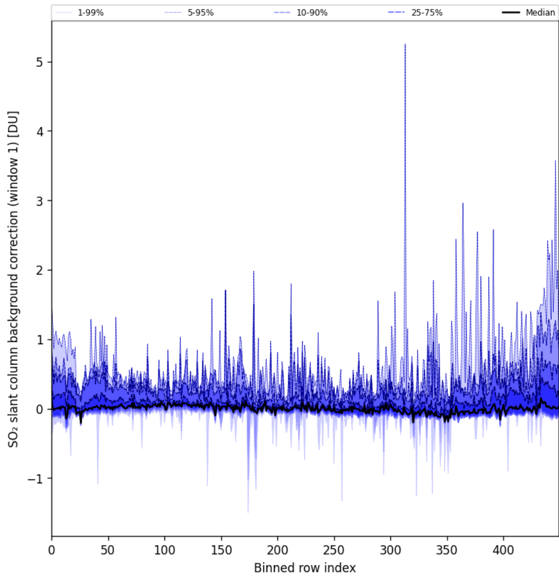
Figure 82: Along track statistics of “SO 2 slant column background correction (window 1)” for 2024-10-01 to 2024-10-03
