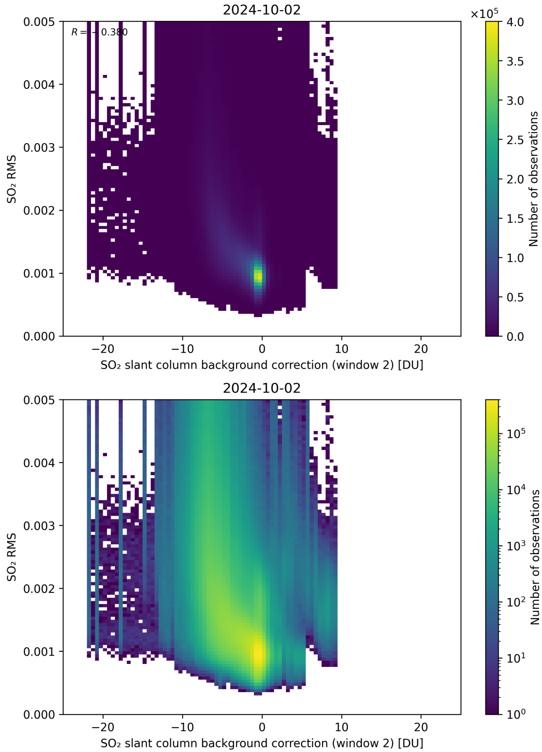
Figure 114: Scatter density plot of “SO 2 slant column background correction (window 2)” against “SO 2 RMS” for 2024-10-01 to 2024-10-03.
