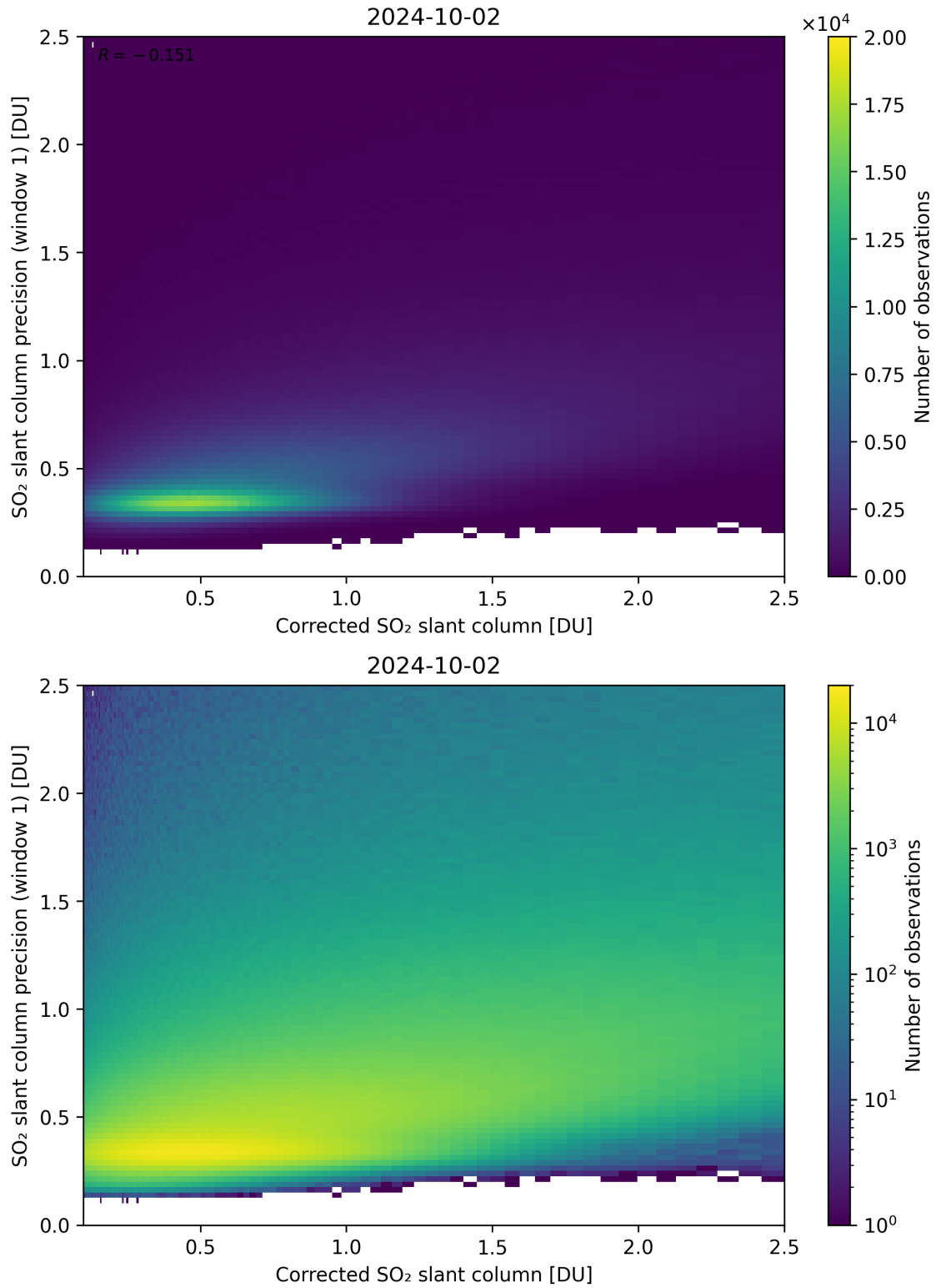
Figure 188: Scatter density plot of “Corrected SO 2 slant column” against “SO 2 slant column precision (window 1)” for 2024-10-01 to 2024-10-03.
