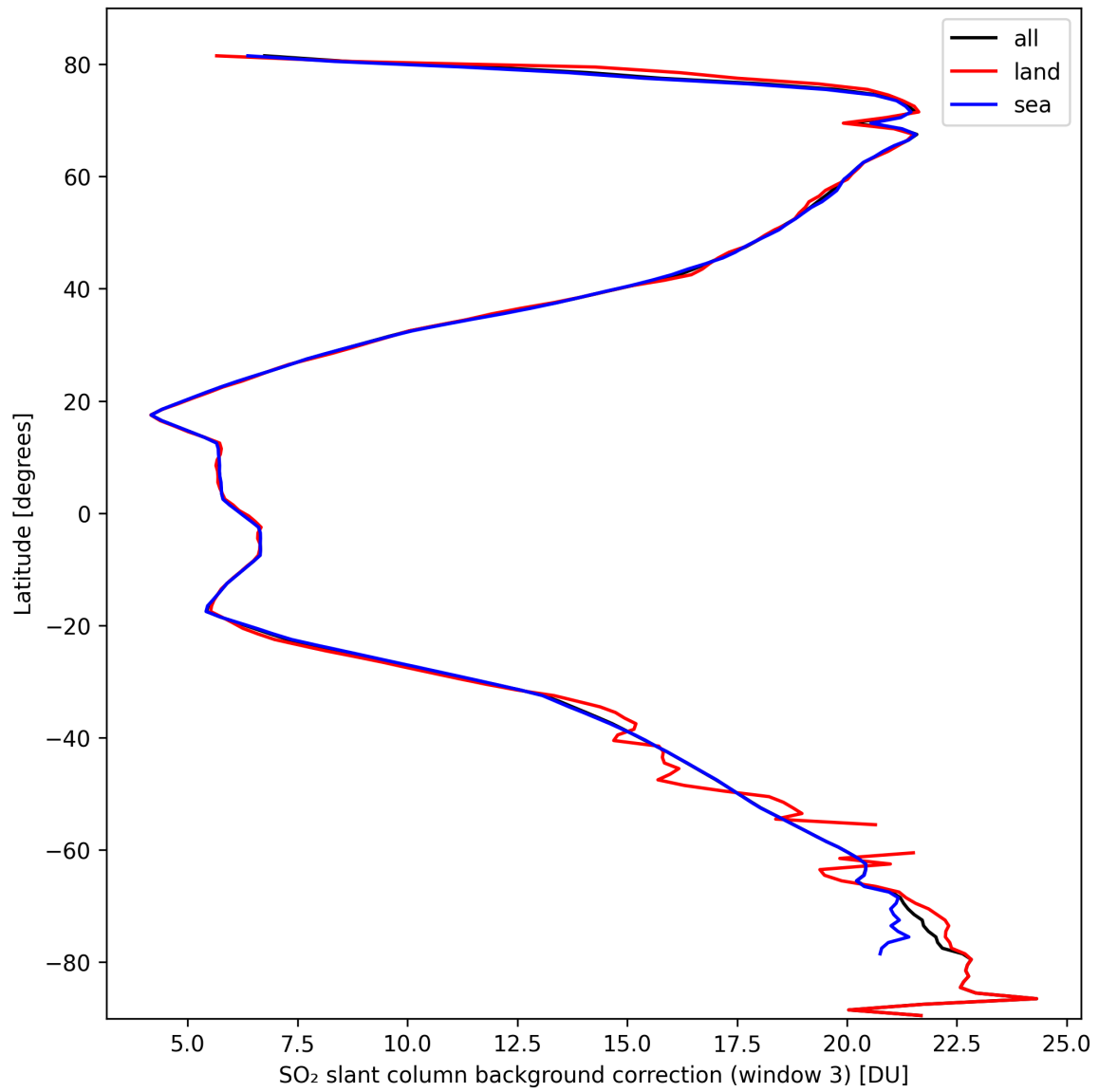
Figure 44: Zonal average of “SO 2 slant column background correction (window 3)” for 2024-10-01 to 2024-10-03.
