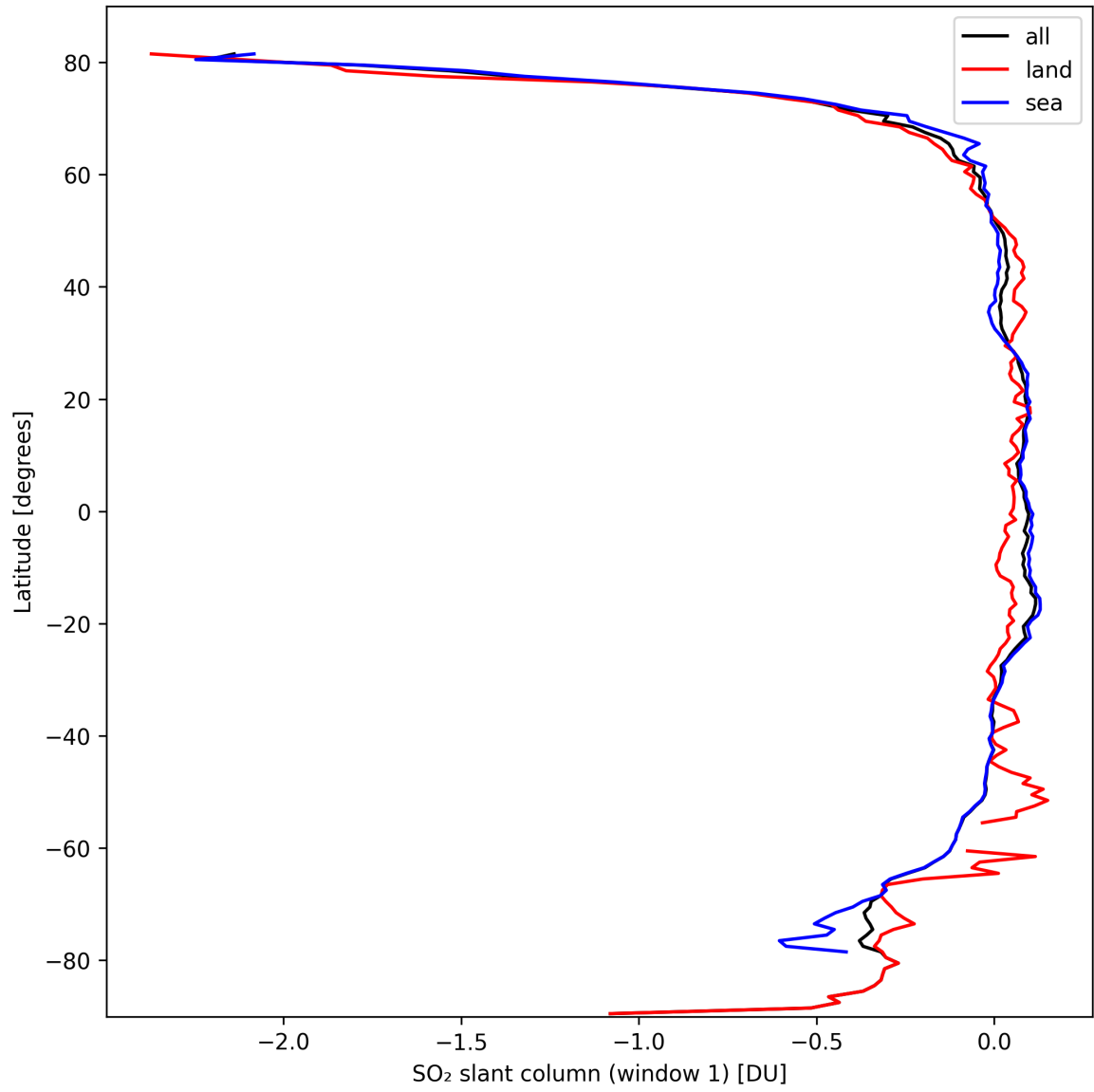
Figure 33: Zonal average of “SO 2 slant column (window 1)” for 2024-10-01 to 2024-10-03.
