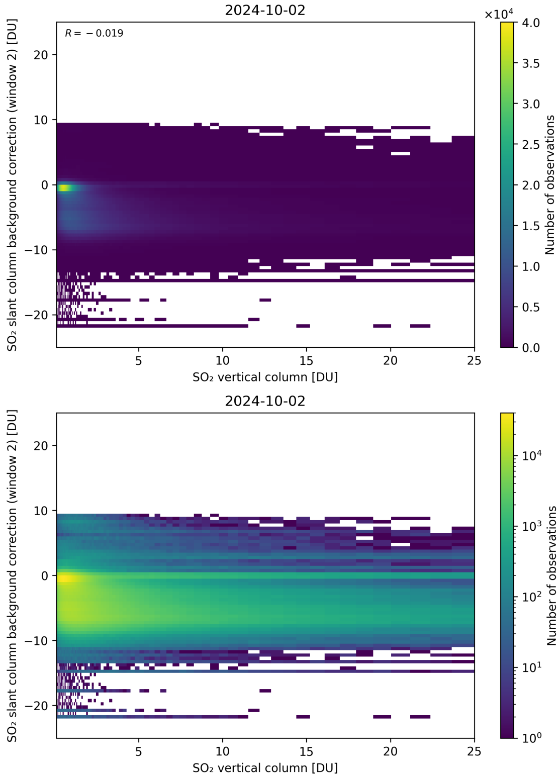
Figure 274: Scatter density plot of “SO 2 vertical column” against “SO 2 slant column background correction (window 2)” for 2024-10-01 to 2024-10-03.
