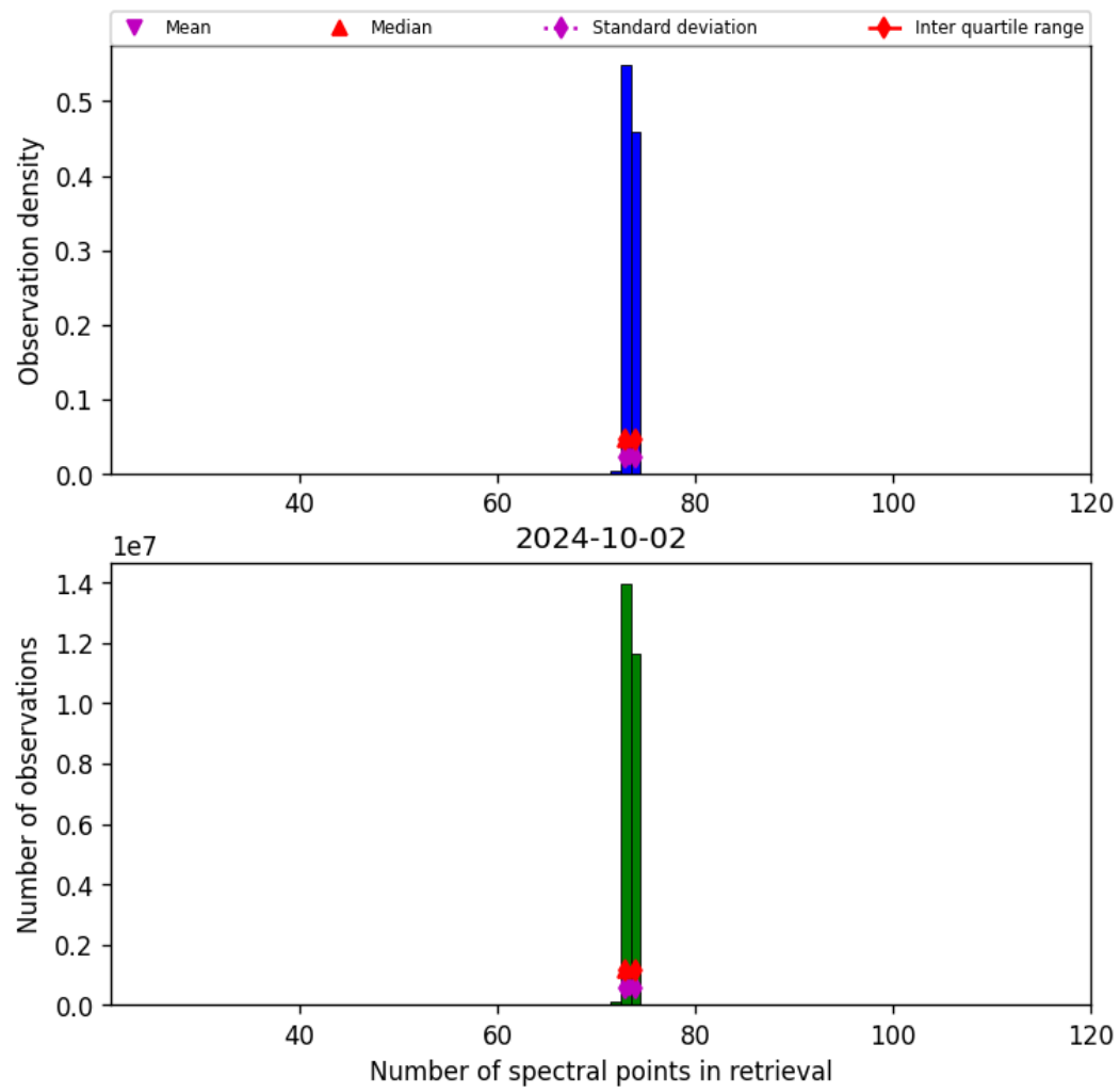
Figure 74: Histogram of “Number of spectral points in retrieval” for 2024-10-01 to 2024-10-03
