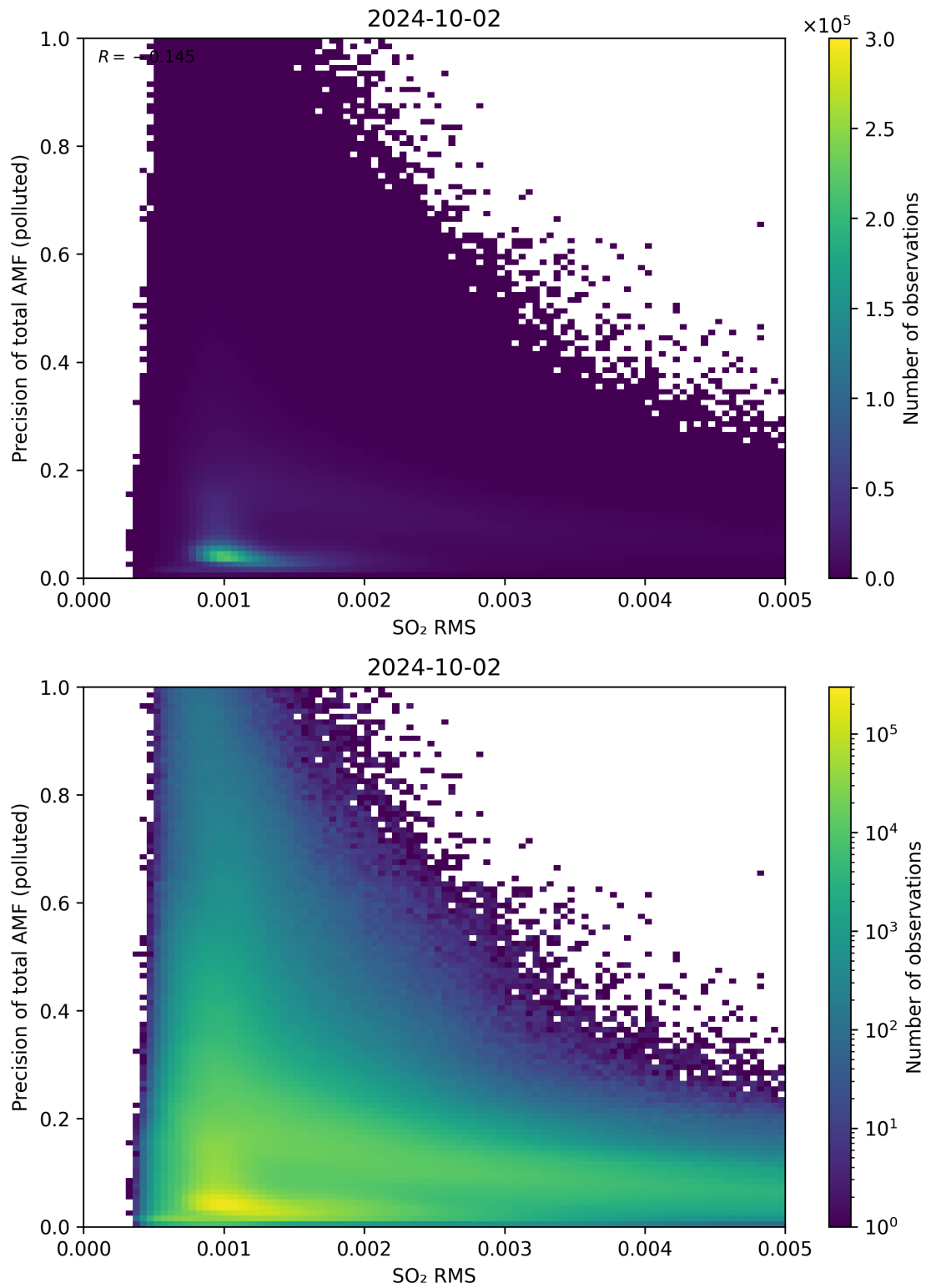
Figure 138: Scatter density plot of “SO 2 RMS” against “Precision of total AMF (polluted)” for 2024-10-01 to 2024-10-03.
