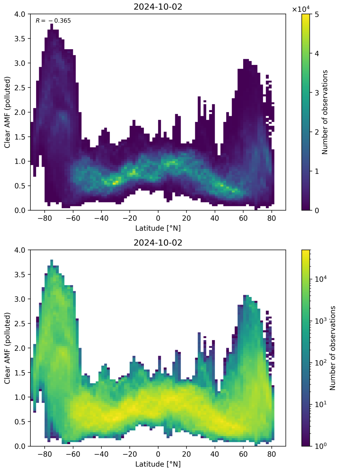
Figure 145: Scatter density plot of “Latitude” against “Clear AMF (polluted)” for 2024-10-01 to 2024-10-03.
