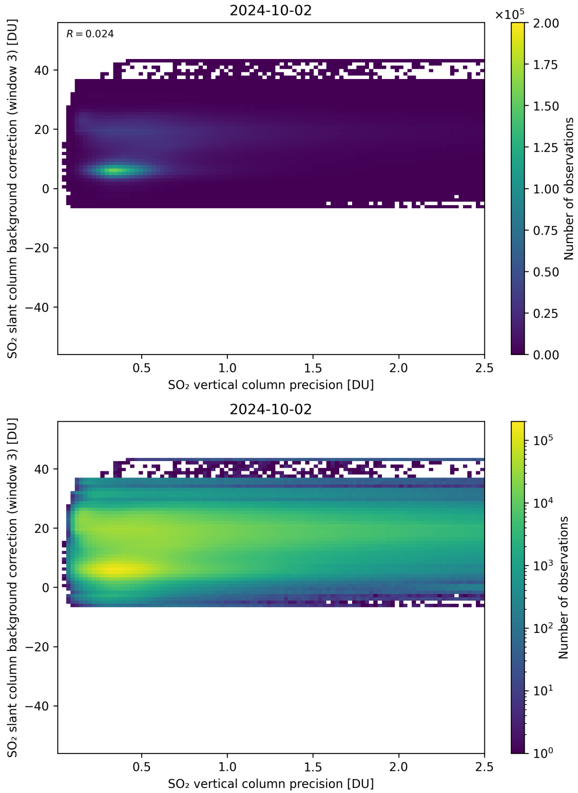
Figure 281: Scatter density plot of “SO 2 vertical column precision” against “SO 2 slant column background correction (window 3)” for 2024-10-01 to 2024-10-03.
