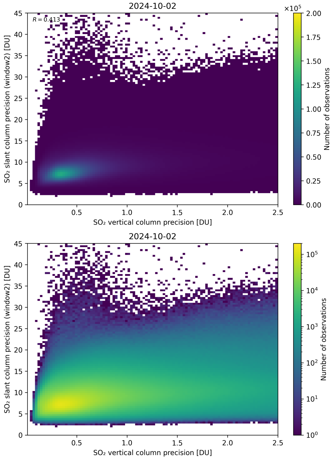
Figure 291: Scatter density plot of “SO 2 vertical column precision” against “SO 2 slant column precision (window2)” for 2024-10-01 to 2024-10-03.
