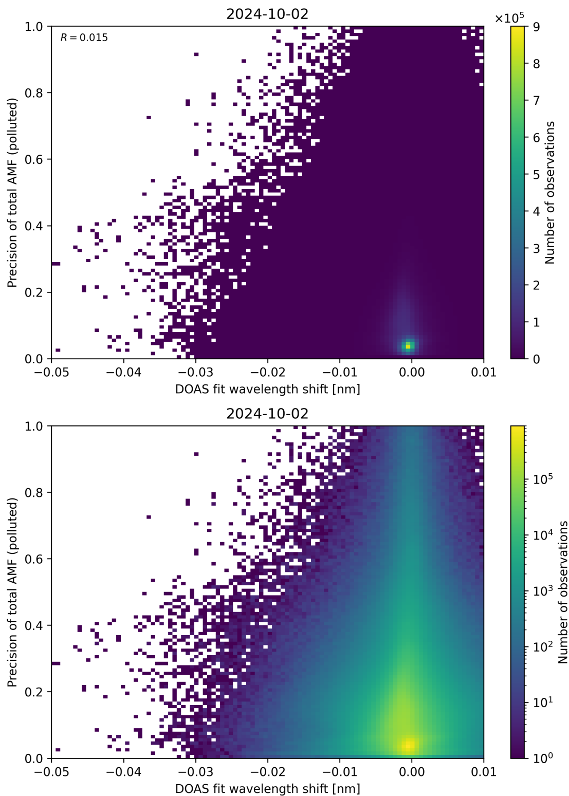
Figure 131: Scatter density plot of “DOAS fit wavelength shift” against “Precision of total AMF (polluted)” for 2024-10-01 to 2024-10-03.
