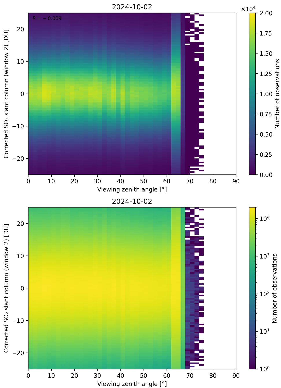
Figure 318: Scatter density plot of “Viewing zenith angle” against “Corrected SO 2 slant column (window 2)” for 2024-10-01 to 2024-10-03.
