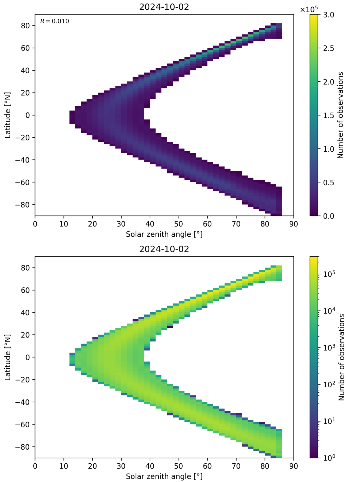
Figure 164: Scatter density plot of “Solar zenith angle” against “Latitude” for 2024-10-01 to 2024-10-03.
