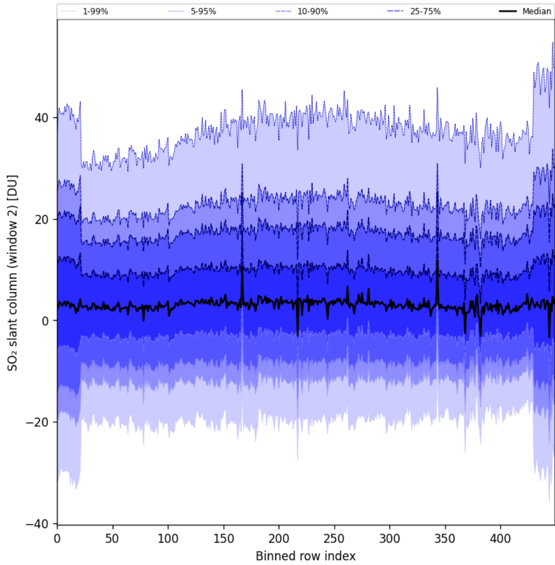
Figure 83: Along track statistics of “SO 2 slant column (window 2)” for 2024-10-01 to 2024-10-03
