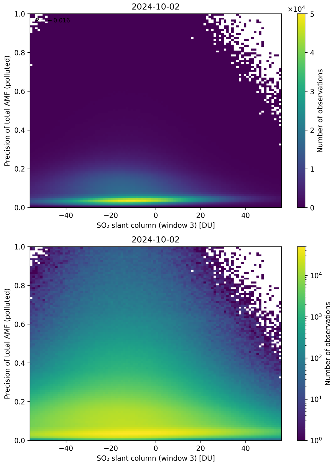
Figure 269: Scatter density plot of “SO 2 slant column (window 3)” against “Precision of total AMF (polluted)” for 2024-10-01 to 2024-10-03.
