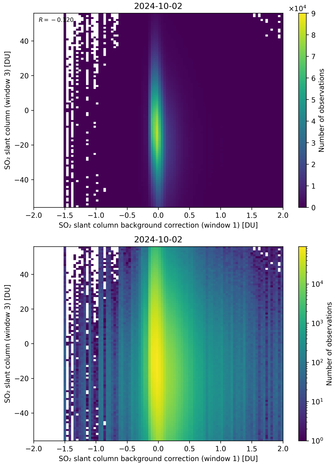
Figure 107: Scatter density plot of “SO 2 slant column background correction (window 1)” against “SO 2 slant column (window 3)” for 2024-10-01 to 2024-10-03.
