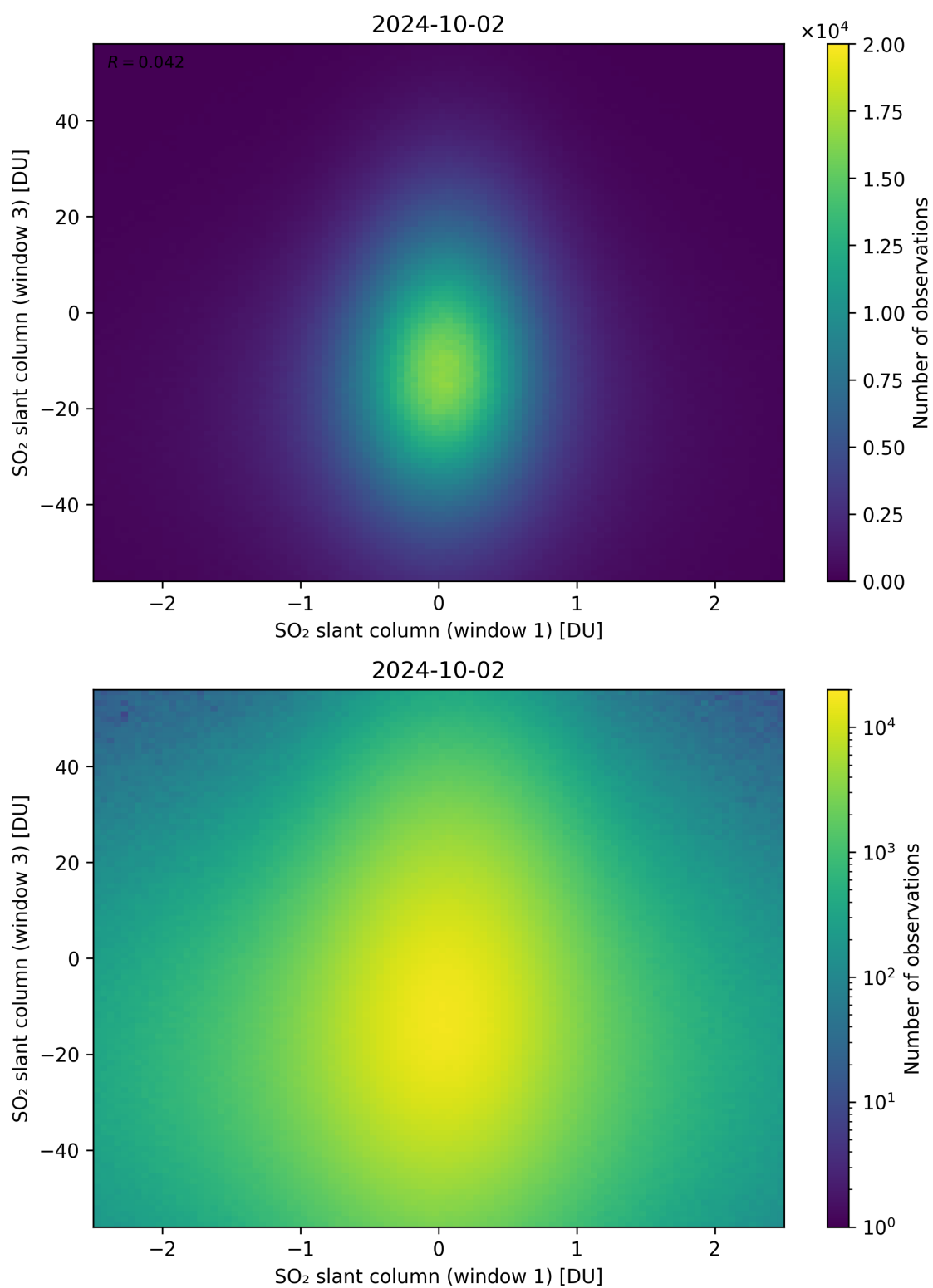
Figure 237: Scatter density plot of “SO 2 slant column (window 1)” against “SO 2 slant column (window 3)” for 2024-10-01 to 2024-10-03.
