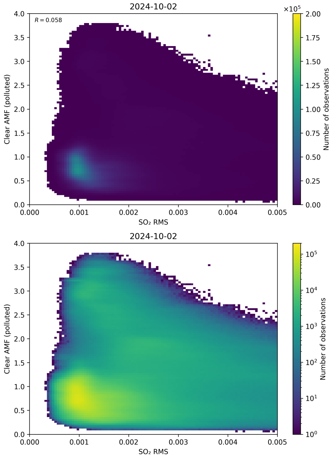
Figure 136: Scatter density plot of “SO 2 RMS” against “Clear AMF (polluted)” for 2024-10-01 to 2024-10-03.
