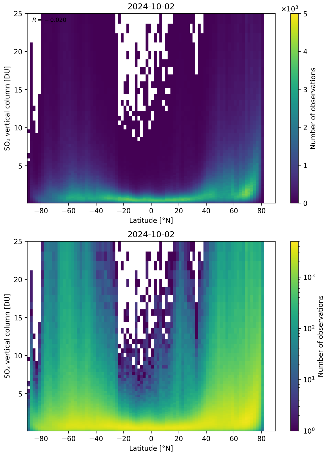
Figure 156: Scatter density plot of “Latitude” against “SO 2 vertical column” for 2024-10-01 to 2024-10-03.
