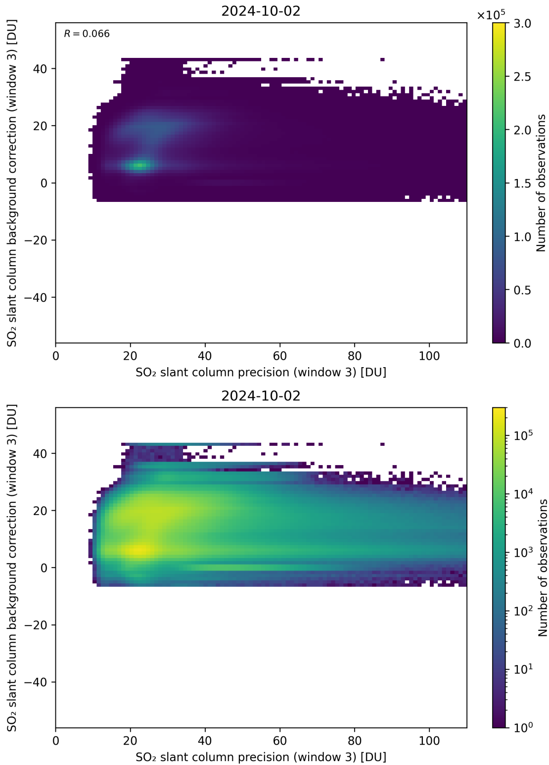
Figure 257: Scatter density plot of “SO 2 slant column precision (window 3)” against “SO 2 slant column background correction (window 3)” for 2024-10-01 to 2024-10-03.
