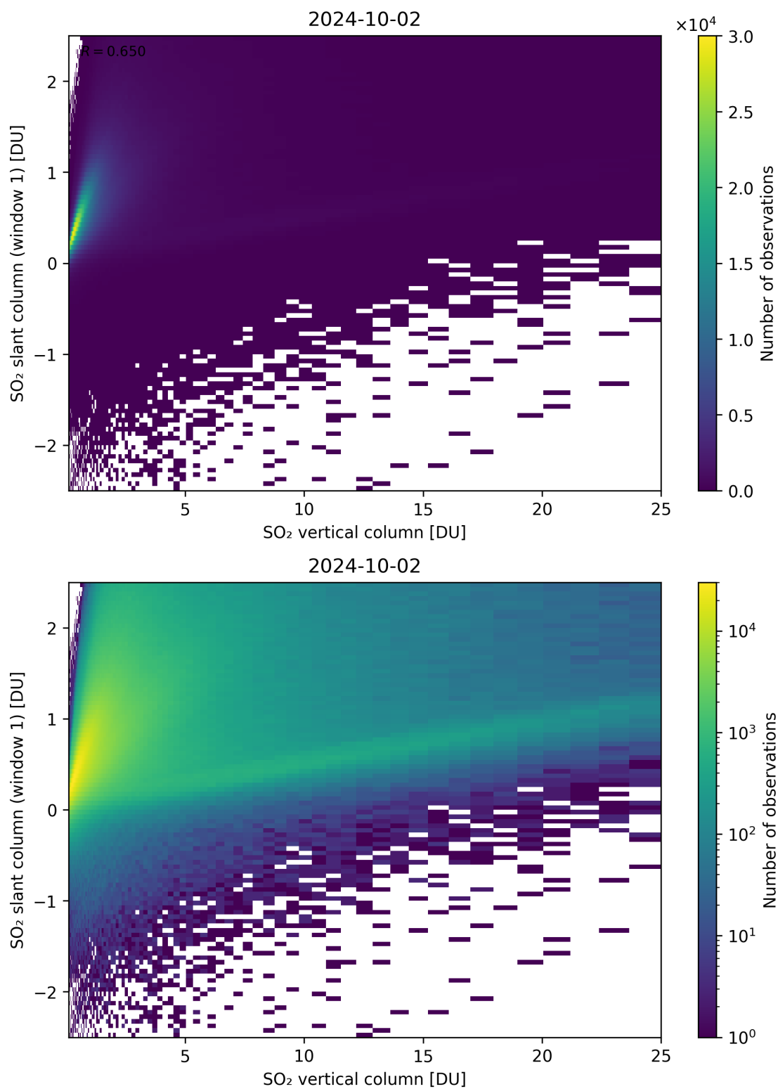
Figure 300: Scatter density plot of “SO 2 vertical column” against “SO 2 slant column (window 1)” for 2024-10-01 to 2024-10-03.
