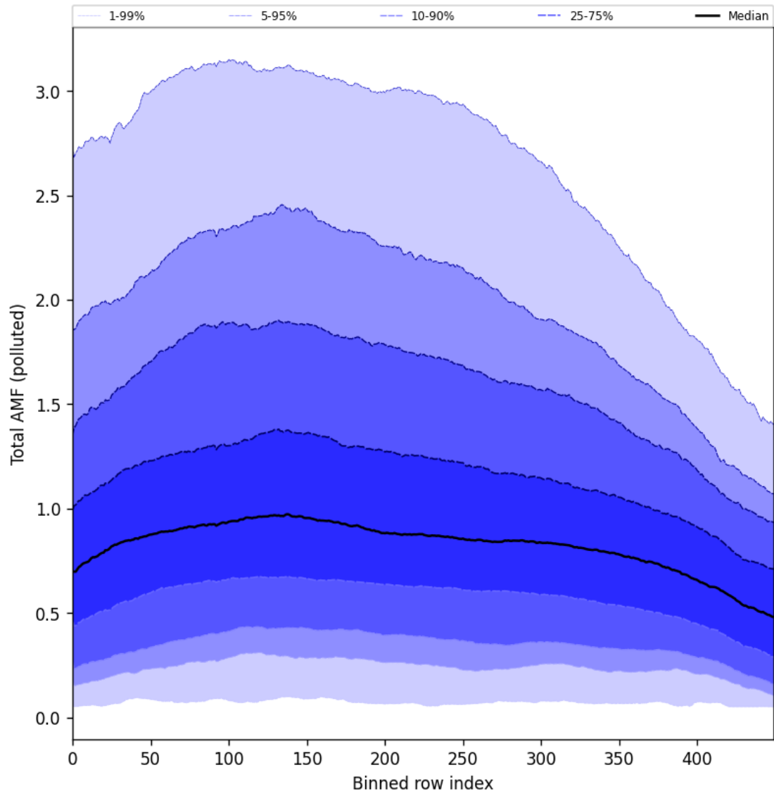
Figure 94: Along track statistics of “Total AMF (polluted)” for 2024-10-01 to 2024-10-03
