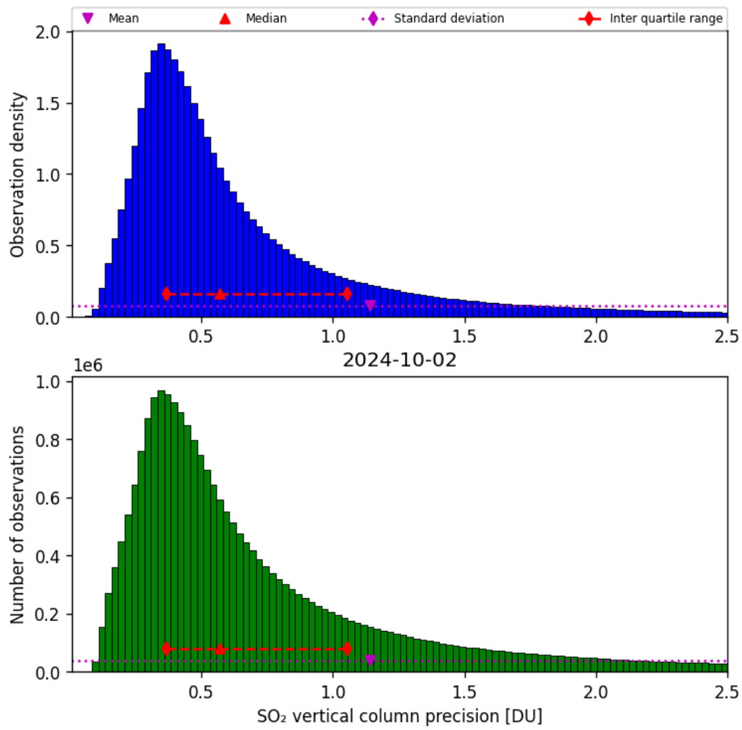
Figure 54: Histogram of “SO 2 vertical column precision” for 2024-10-01 to 2024-10-03
