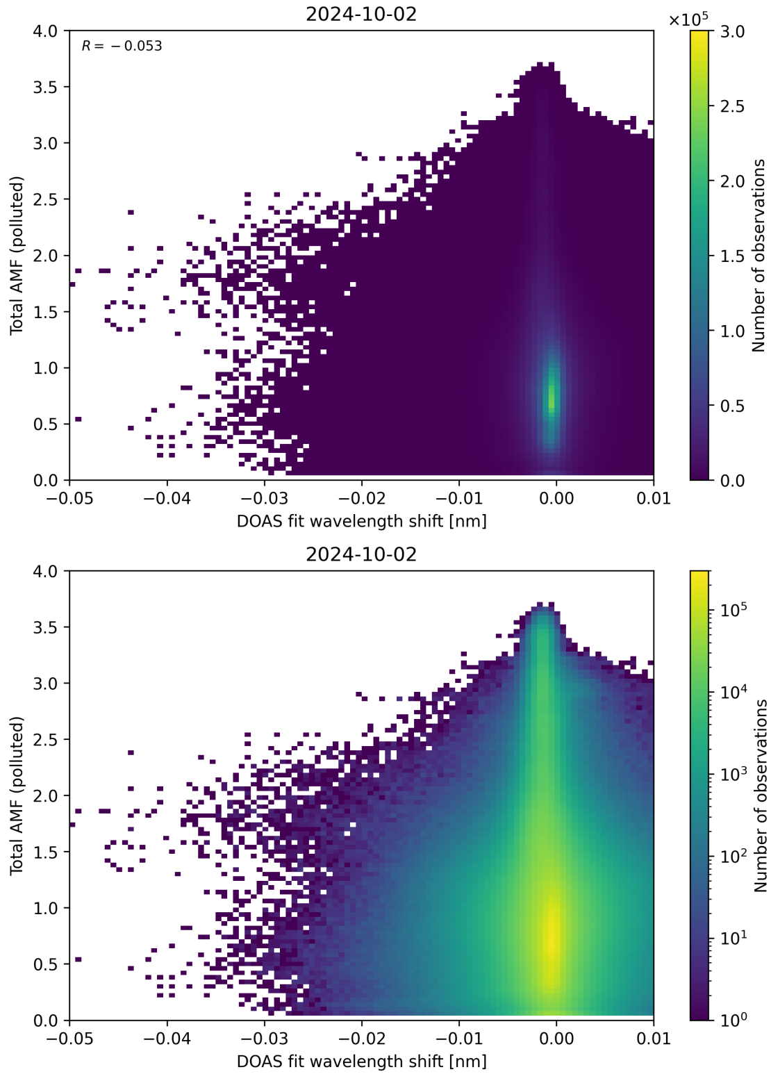
Figure 130: Scatter density plot of “DOAS fit wavelength shift” against “Total AMF (polluted)” for 2024-10-01 to 2024-10-03.
