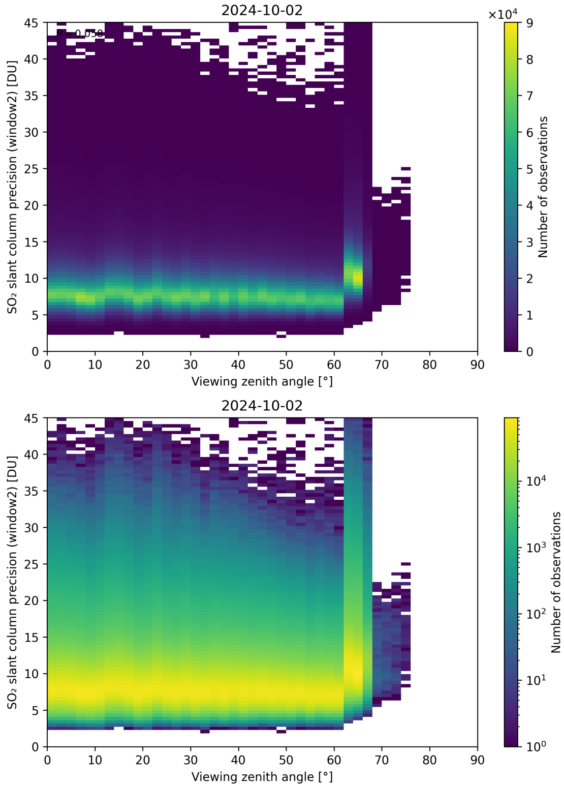
Figure 322: Scatter density plot of “Viewing zenith angle” against “SO 2 slant column precision (window2)” for 2024-10-01 to 2024-10-03.
