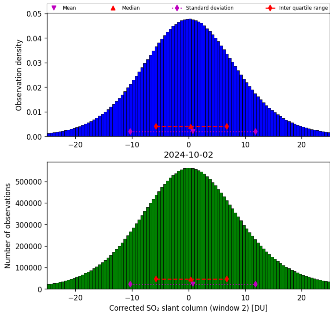
Figure 62: Histogram of “Corrected SO 2 slant column (window 2)” for 2024-10-01 to 2024-10-03
