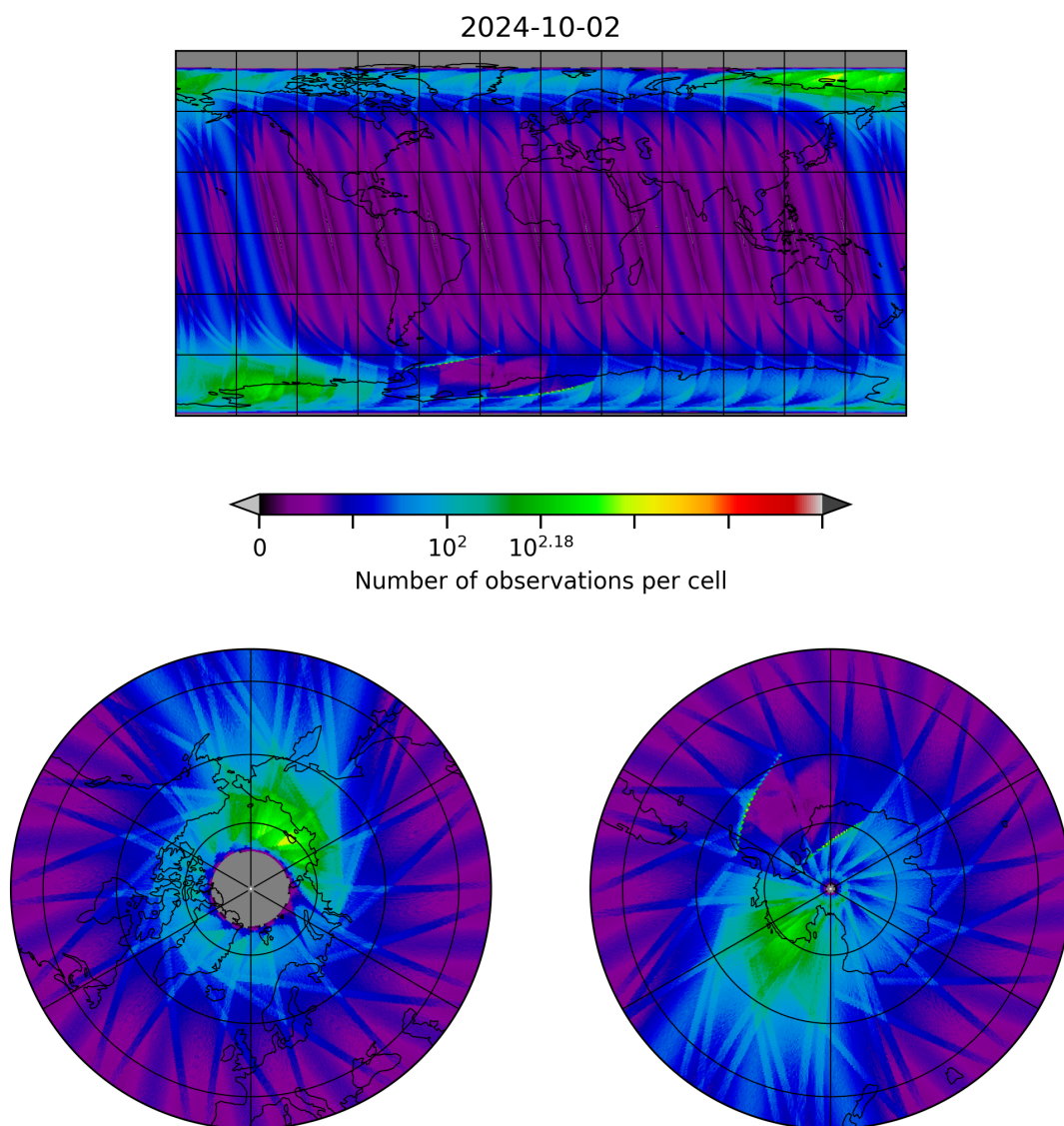
Figure 28: Map of the number of observations for 2024-10-01 to 2024-10-03
