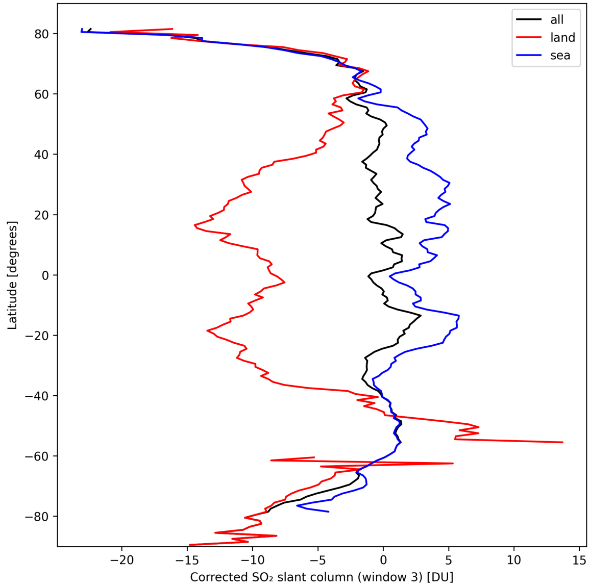
Figure 43: Zonal average of “Corrected SO 2 slant column (window 3)” for 2024-10-01 to 2024-10-03.
