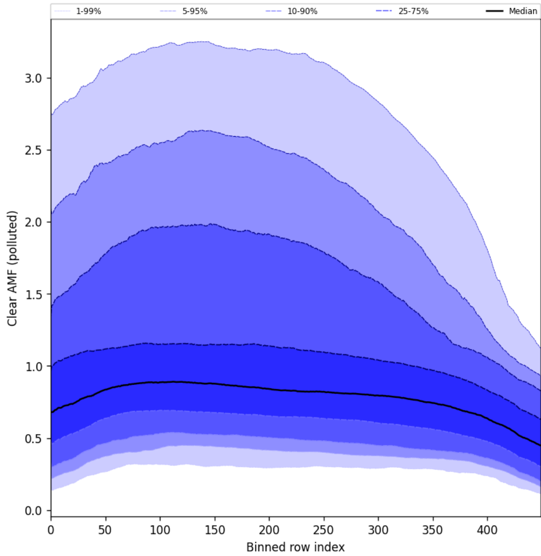
Figure 96: Along track statistics of “Clear AMF (polluted)” for 2024-10-01 to 2024-10-03
