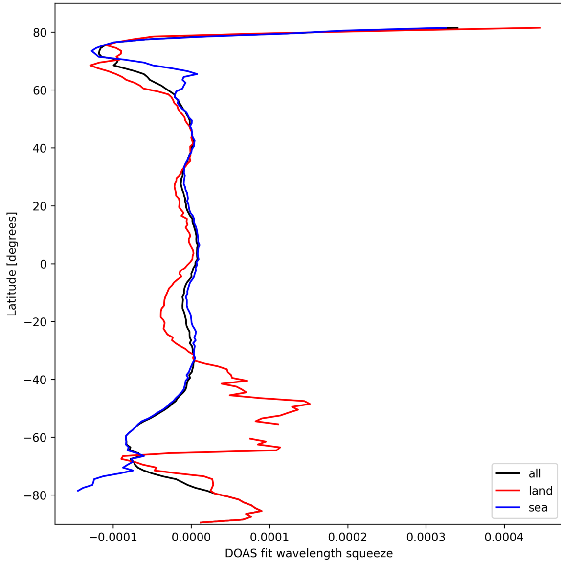
Figure 46: Zonal average of “DOAS fit wavelength squeeze” for 2024-10-01 to 2024-10-03.
