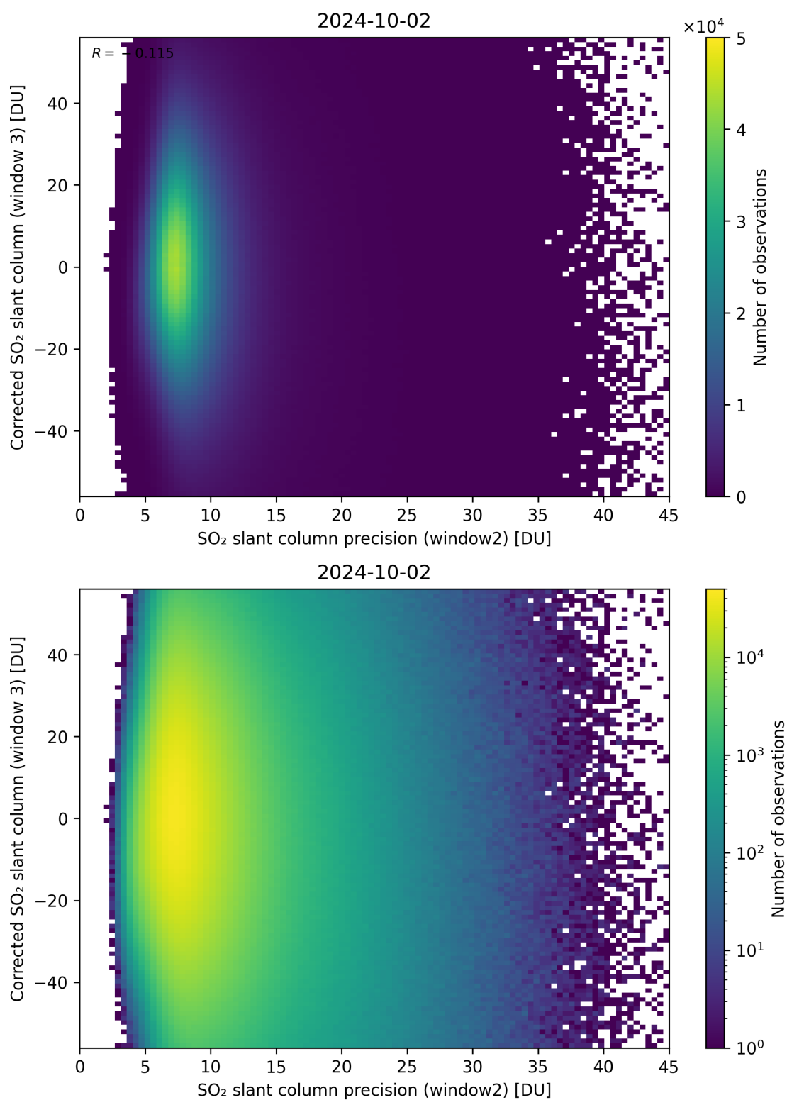
Figure 248: Scatter density plot of “SO 2 slant column precision (window2)” against “Corrected SO 2 slant column (window 3)” for 2024-10-01 to 2024-10-03.
