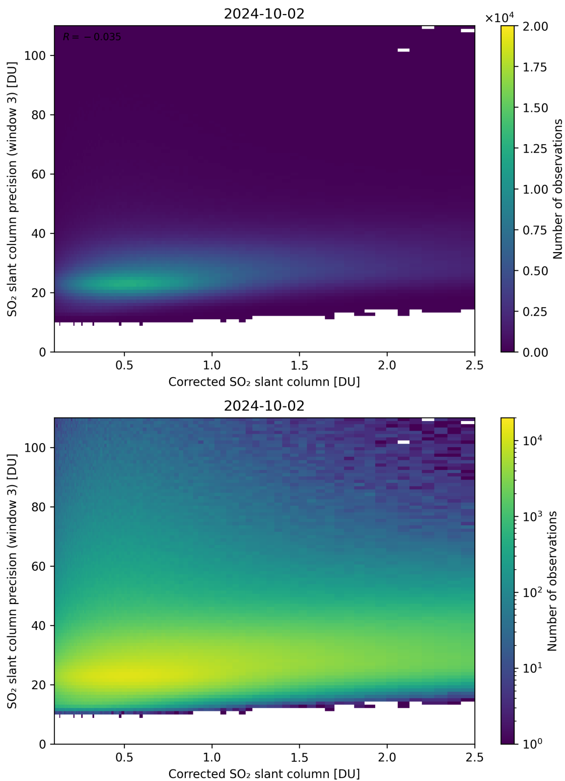
Figure 191: Scatter density plot of “Corrected SO 2 slant column” against “SO 2 slant column precision (window 3)” for 2024-10-01 to 2024-10-03.
