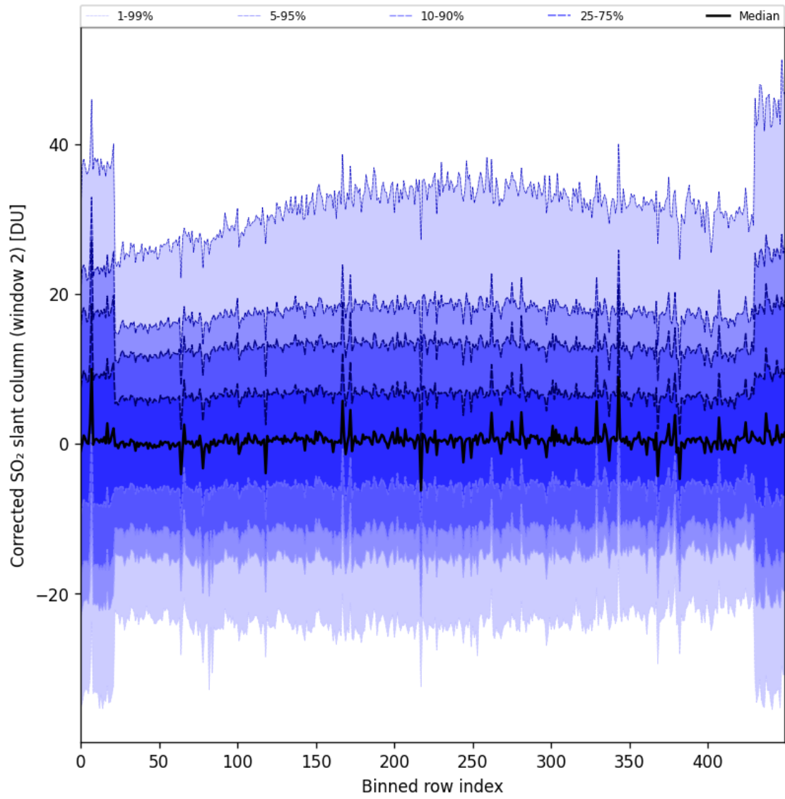
Figure 85: Along track statistics of “Corrected SO 2 slant column (window 2)” for 2024-10-01 to 2024-10-03
