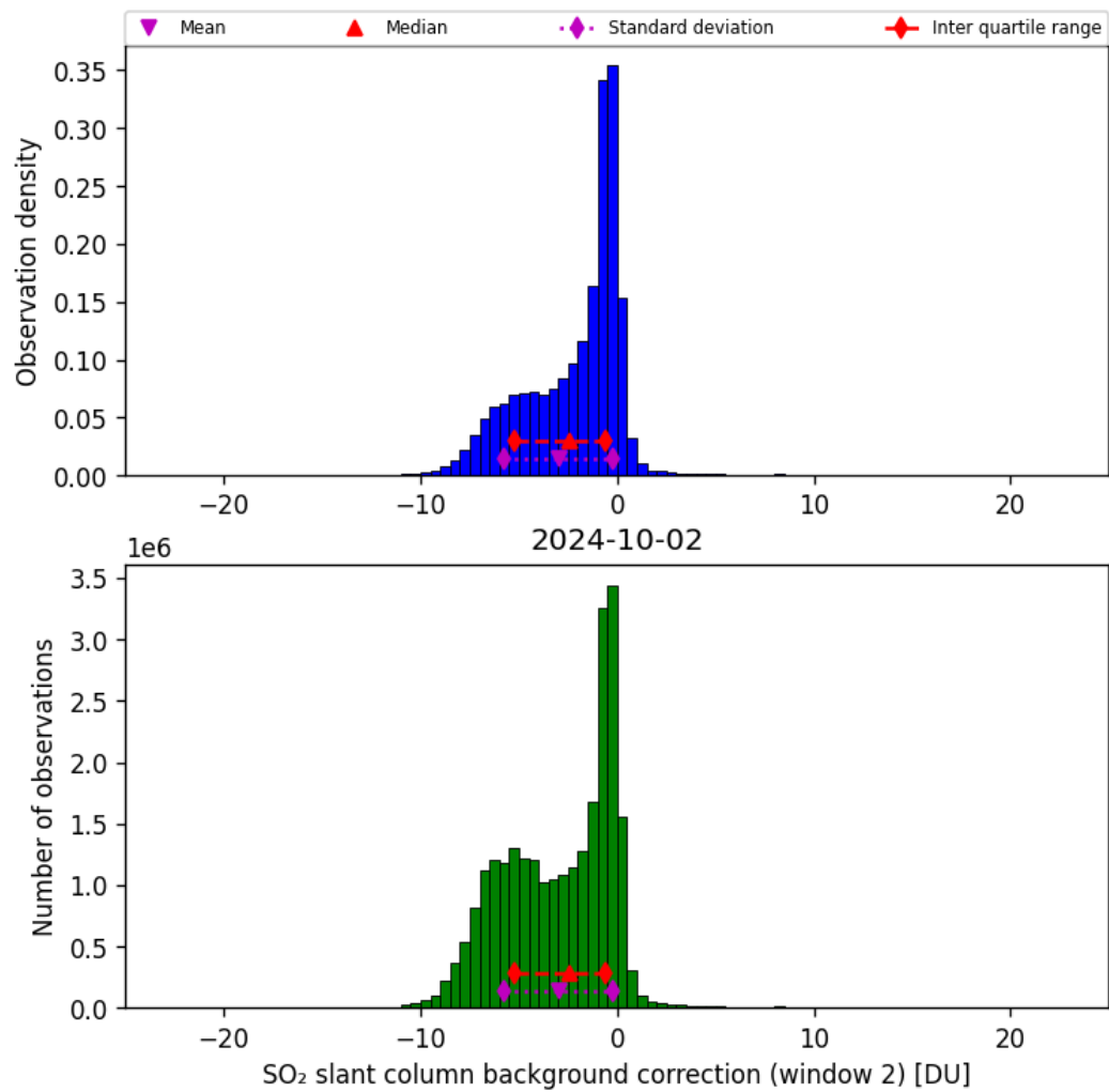
Figure 63: Histogram of “SO 2 slant column background correction (window 2)” for 2024-10-01 to 2024-10-03
