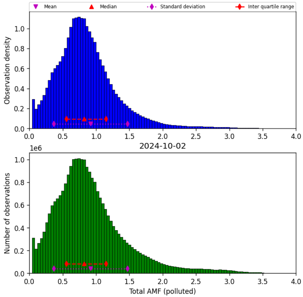
Figure 71: Histogram of “Total AMF (polluted)” for 2024-10-01 to 2024-10-03
