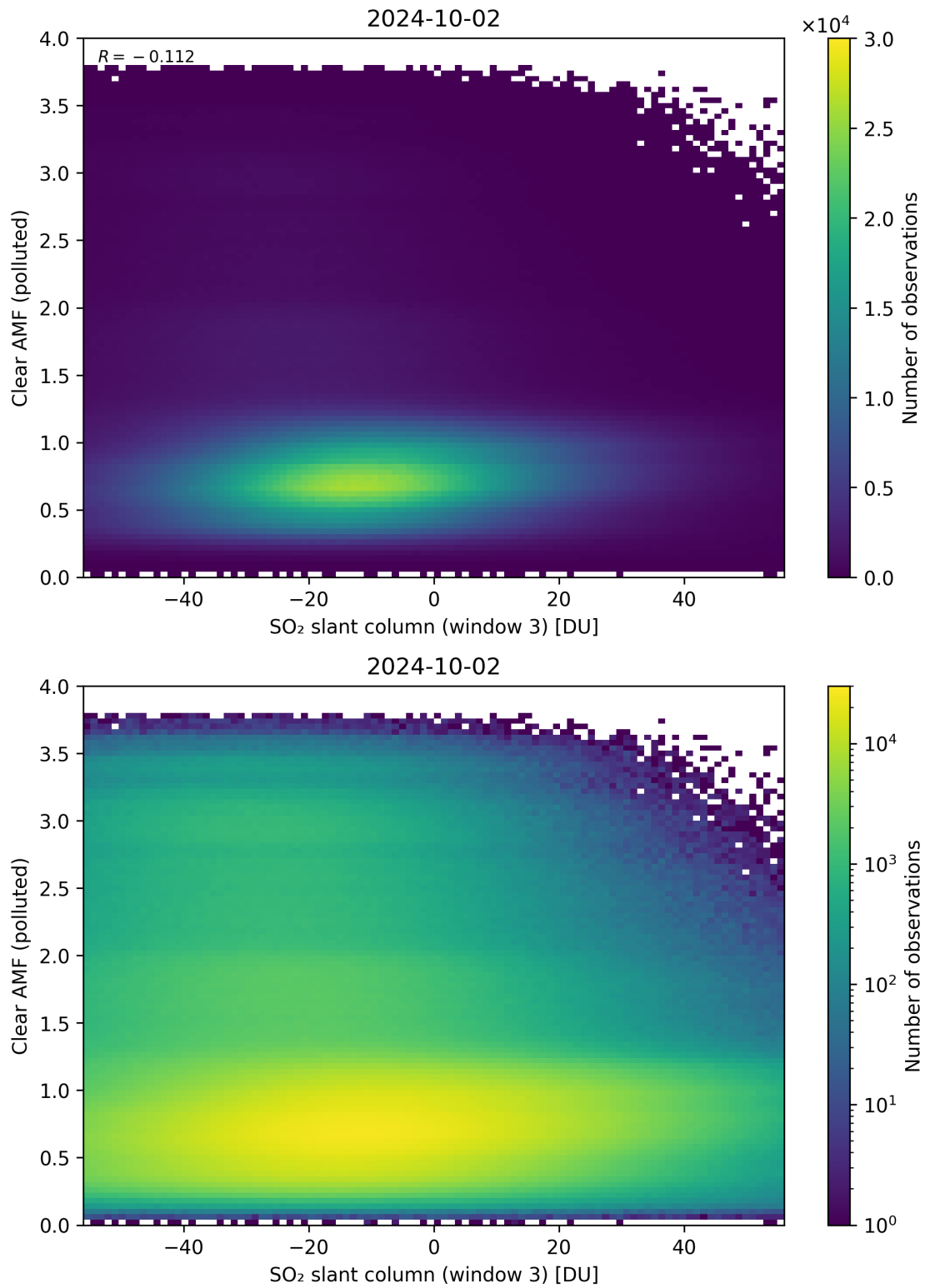
Figure 265: Scatter density plot of “SO 2 slant column (window 3)” against “Clear AMF (polluted)” for 2024-10-01 to 2024-10-03.
