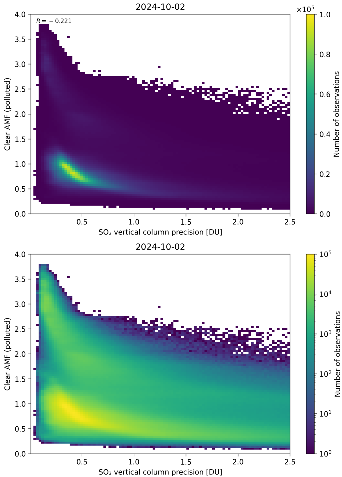
Figure 285: Scatter density plot of “SO 2 vertical column precision” against “Clear AMF (polluted)” for 2024-10-01 to 2024-10-03.
