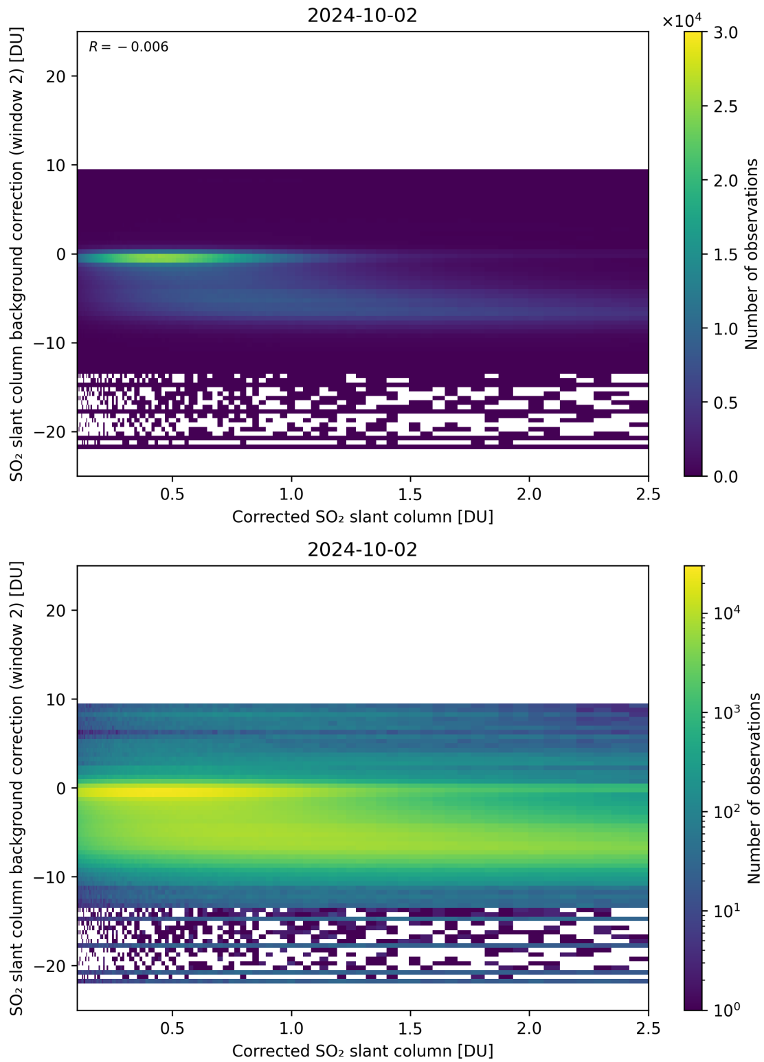
Figure 179: Scatter density plot of “Corrected SO 2 slant column” against “SO 2 slant column background correction (window 2)” for 2024-10-01 to 2024-10-03.
