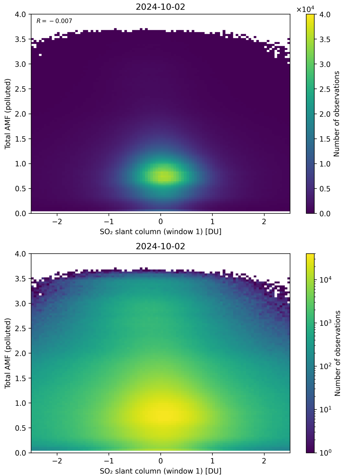
Figure 239: Scatter density plot of “SO 2 slant column (window 1)” against “Total AMF (polluted)” for 2024-10-01 to 2024-10-03.
