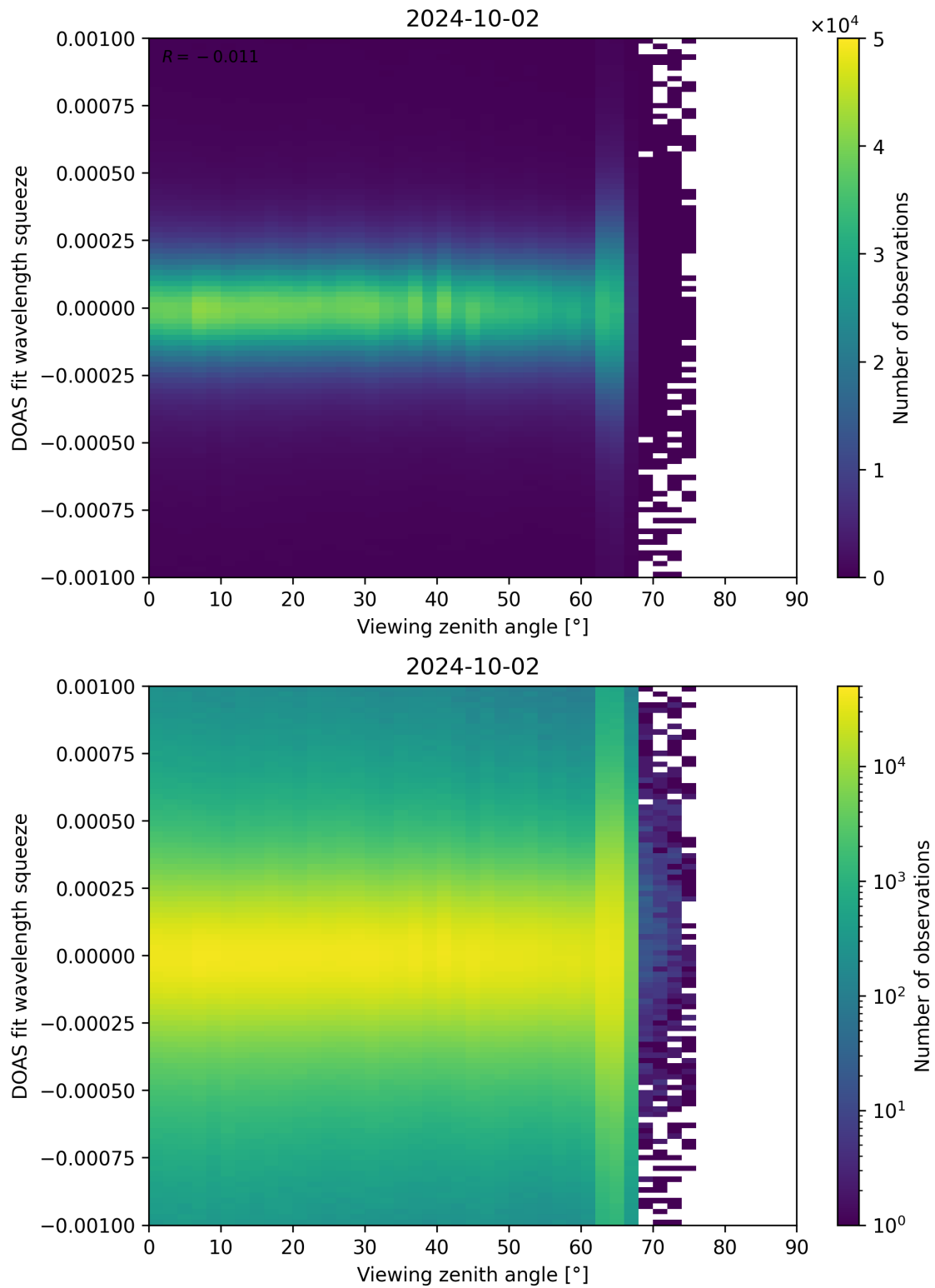
Figure 312: Scatter density plot of “Viewing zenith angle” against “DOAS fit wavelength squeeze” for 2024-10-01 to 2024-10-03.
