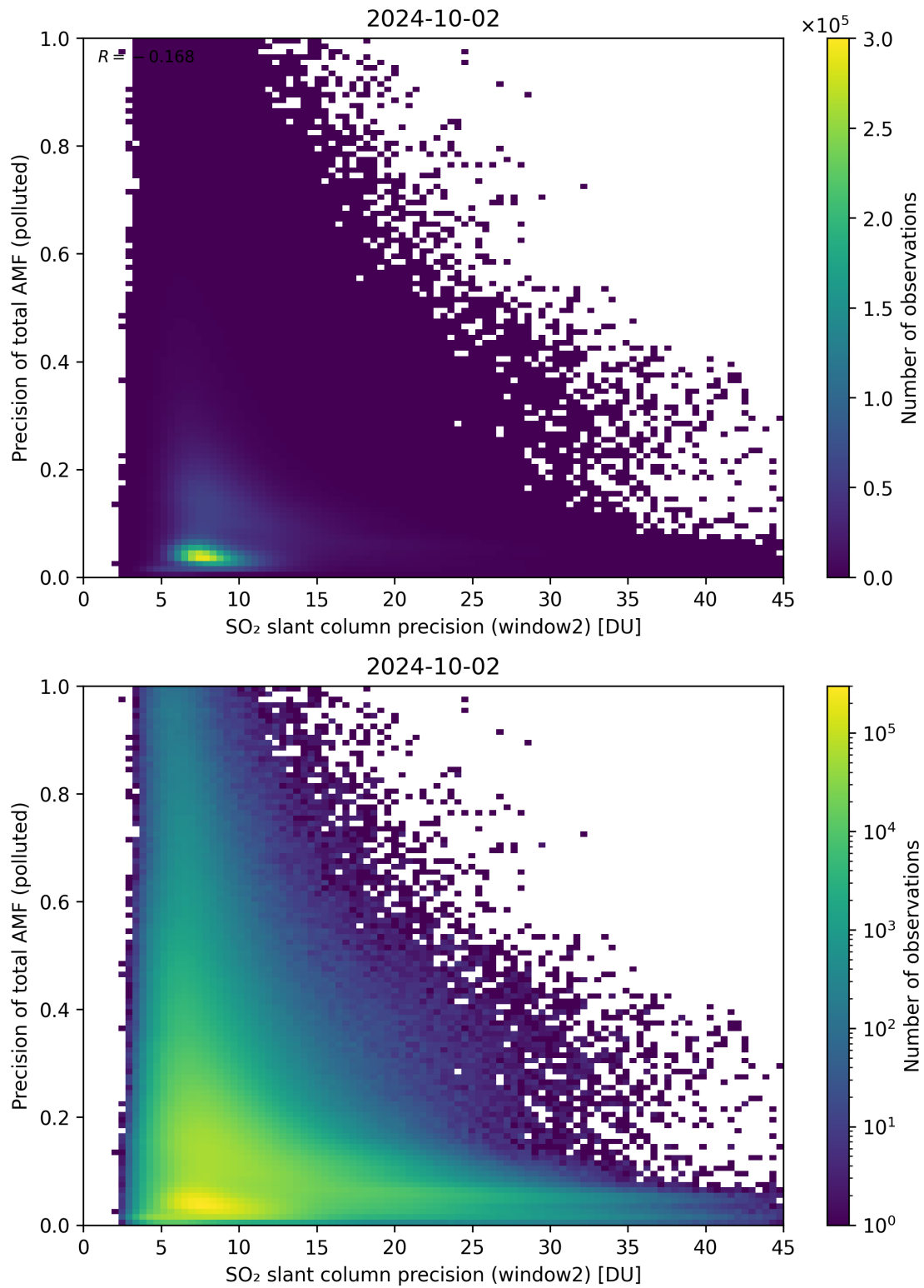
Figure 252: Scatter density plot of “SO 2 slant column precision (window2)” against “Precision of total AMF (polluted)” for 2024-10-01 to 2024-10-03.
