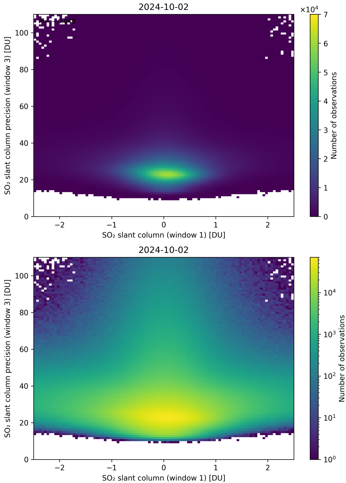
Figure 238: Scatter density plot of “SO 2 slant column (window 1)” against “SO 2 slant column precision (window 3)” for 2024-10-01 to 2024-10-03.
