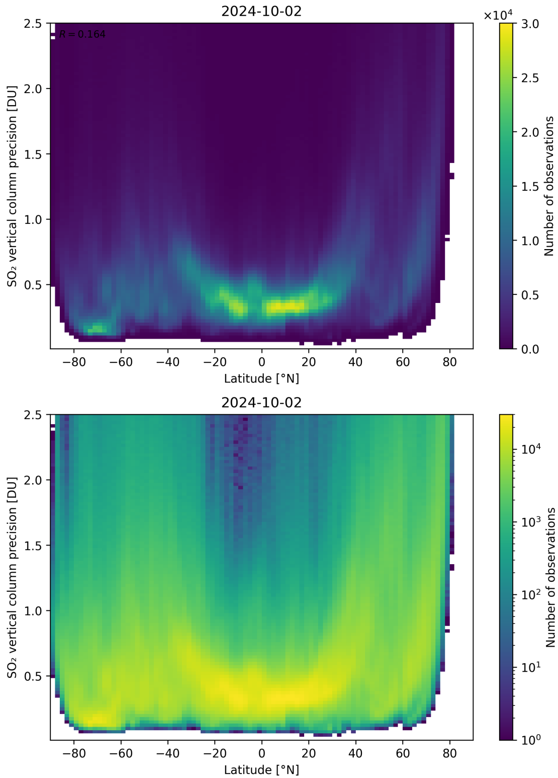
Figure 157: Scatter density plot of “Latitude” against “SO 2 vertical column precision” for 2024-10-01 to 2024-10-03.
