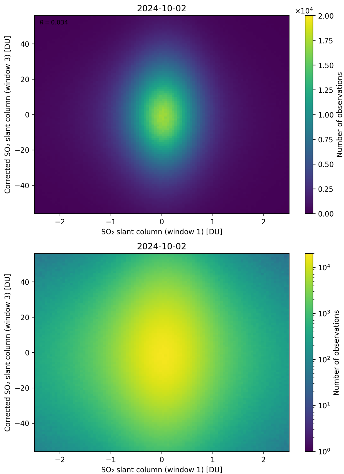
Figure 234: Scatter density plot of “SO 2 slant column (window 1)” against “Corrected SO 2 slant column (window 3)” for 2024-10-01 to 2024-10-03.
