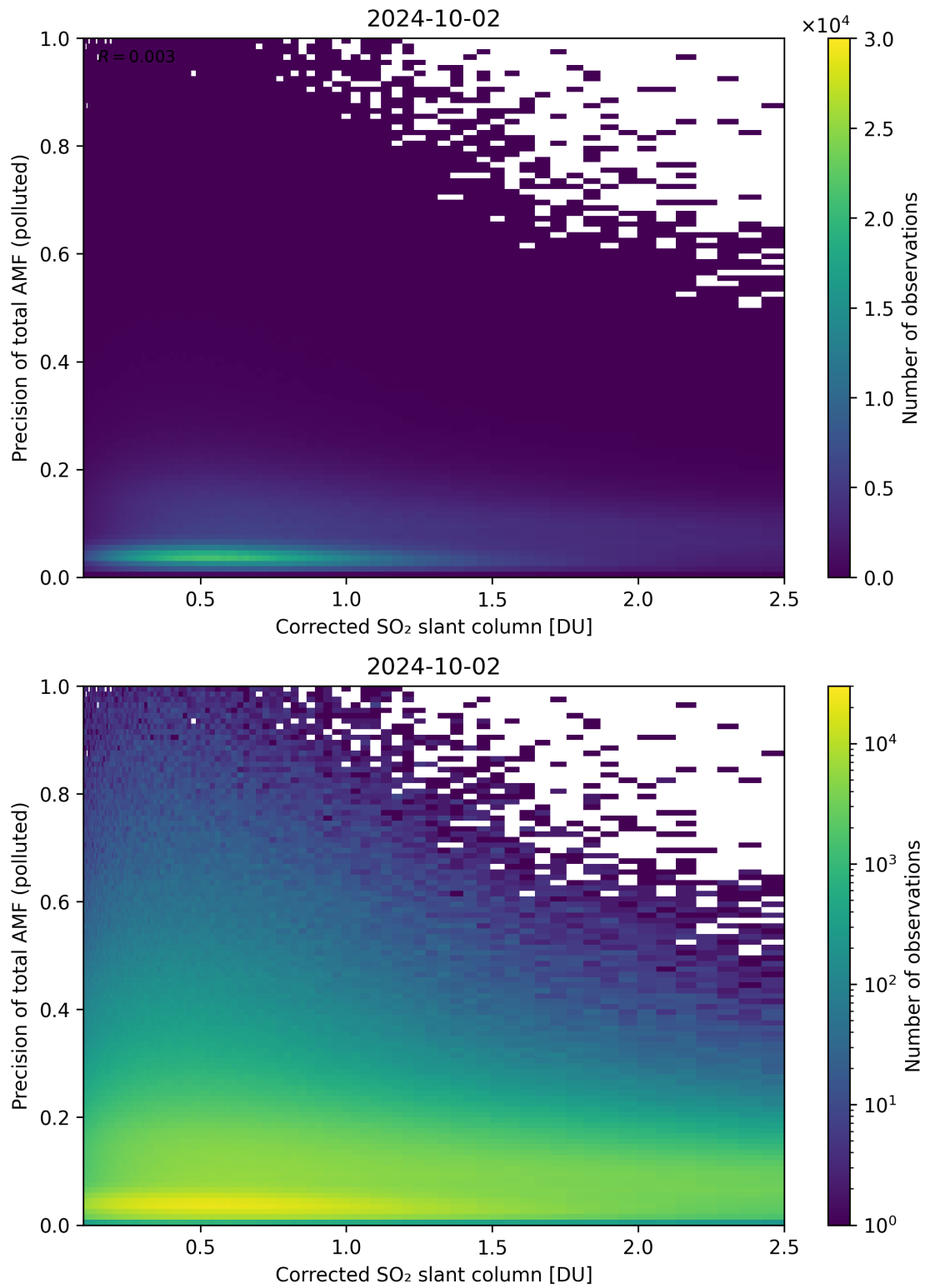
Figure 193: Scatter density plot of “Corrected SO 2 slant column” against “Precision of total AMF (polluted)” for 2024-10-01 to 2024-10-03.
