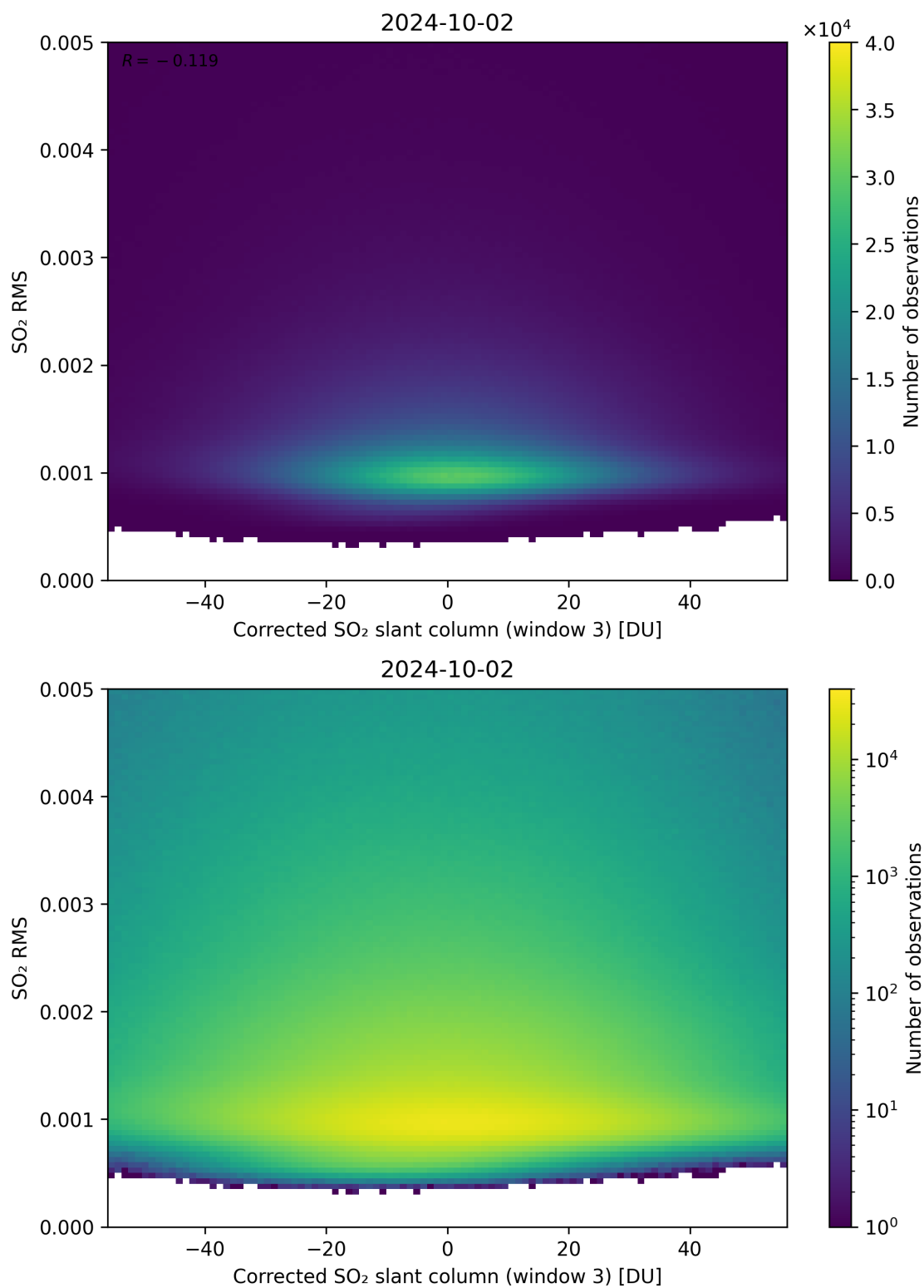
Figure 208: Scatter density plot of “Corrected SO 2 slant column (window 3)” against “SO 2 RMS” for 2024-10-01 to 2024-10-03.
