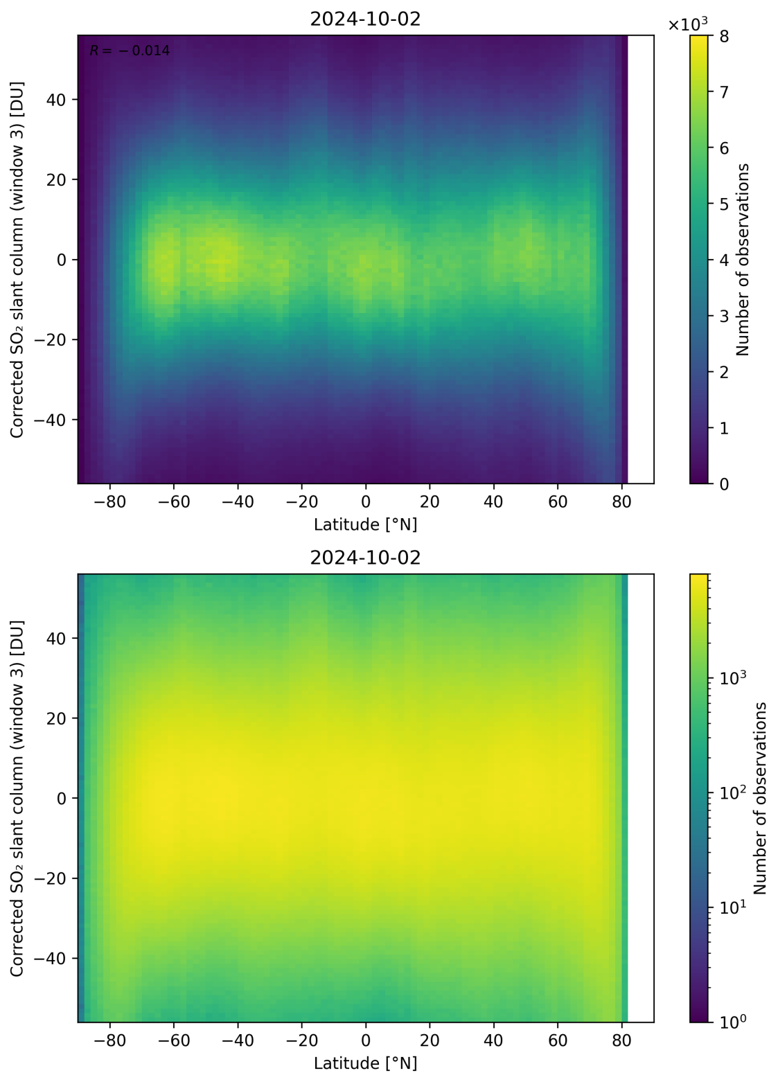
Figure 148: Scatter density plot of “Latitude” against “Corrected SO 2 slant column (window 3)” for 2024-10-01 to 2024-10-03.
