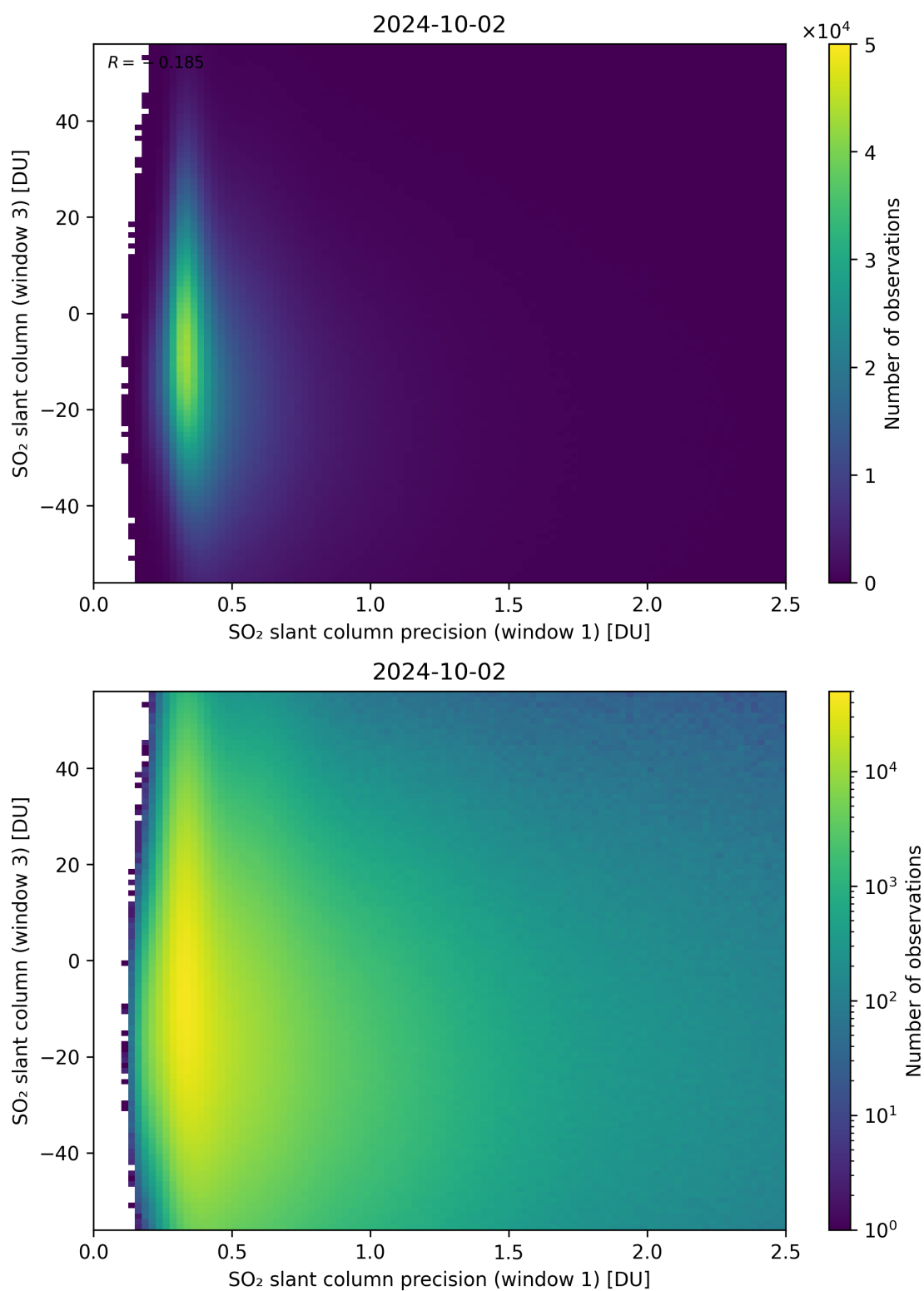
Figure 228: Scatter density plot of “SO 2 slant column precision (window 1)” against “SO 2 slant column (window 3)” for 2024-10-01 to 2024-10-03.
