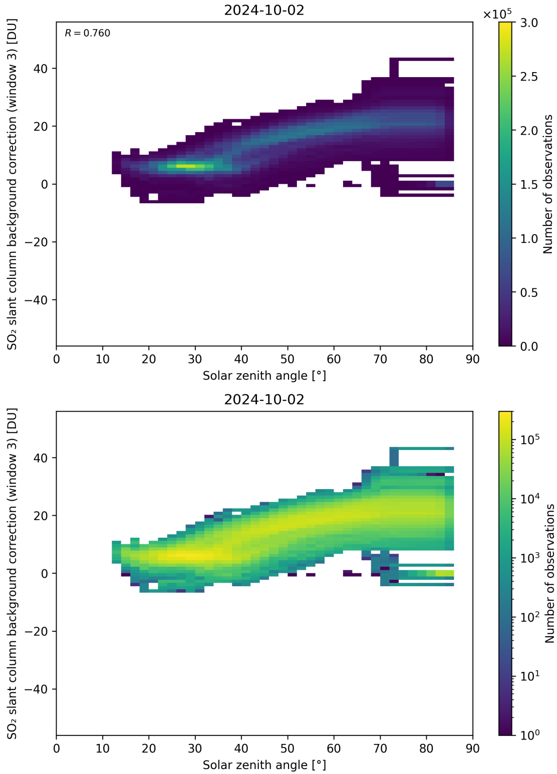
Figure 160: Scatter density plot of “Solar zenith angle” against “SO 2 slant column background correction (window 3)” for 2024-10-01 to 2024-10-03.
