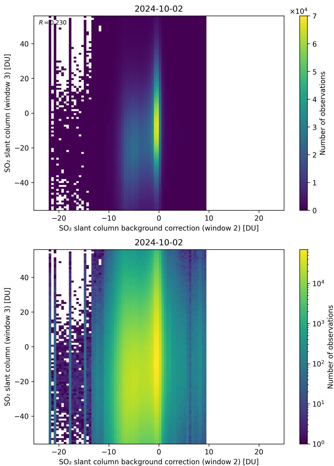
Figure 117: Scatter density plot of “SO 2 slant column background correction (window 2)” against “SO 2 slant column (window 3)” for 2024-10-01 to 2024-10-03.
