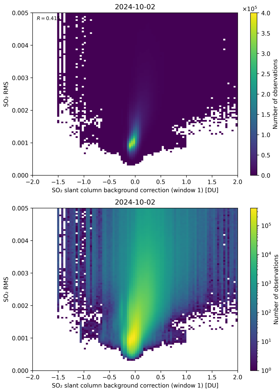
Figure 102: Scatter density plot of “SO 2 slant column background correction (window 1)” against “SO 2 RMS” for 2024-10-01 to 2024-10-03.
