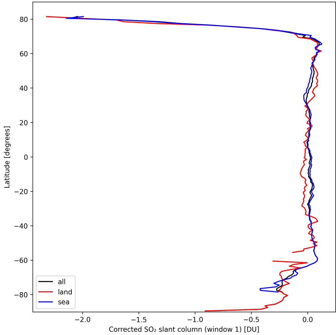
Figure 35: Zonal average of “Corrected SO 2 slant column (window 1)” for 2024-10-01 to 2024-10-03.
