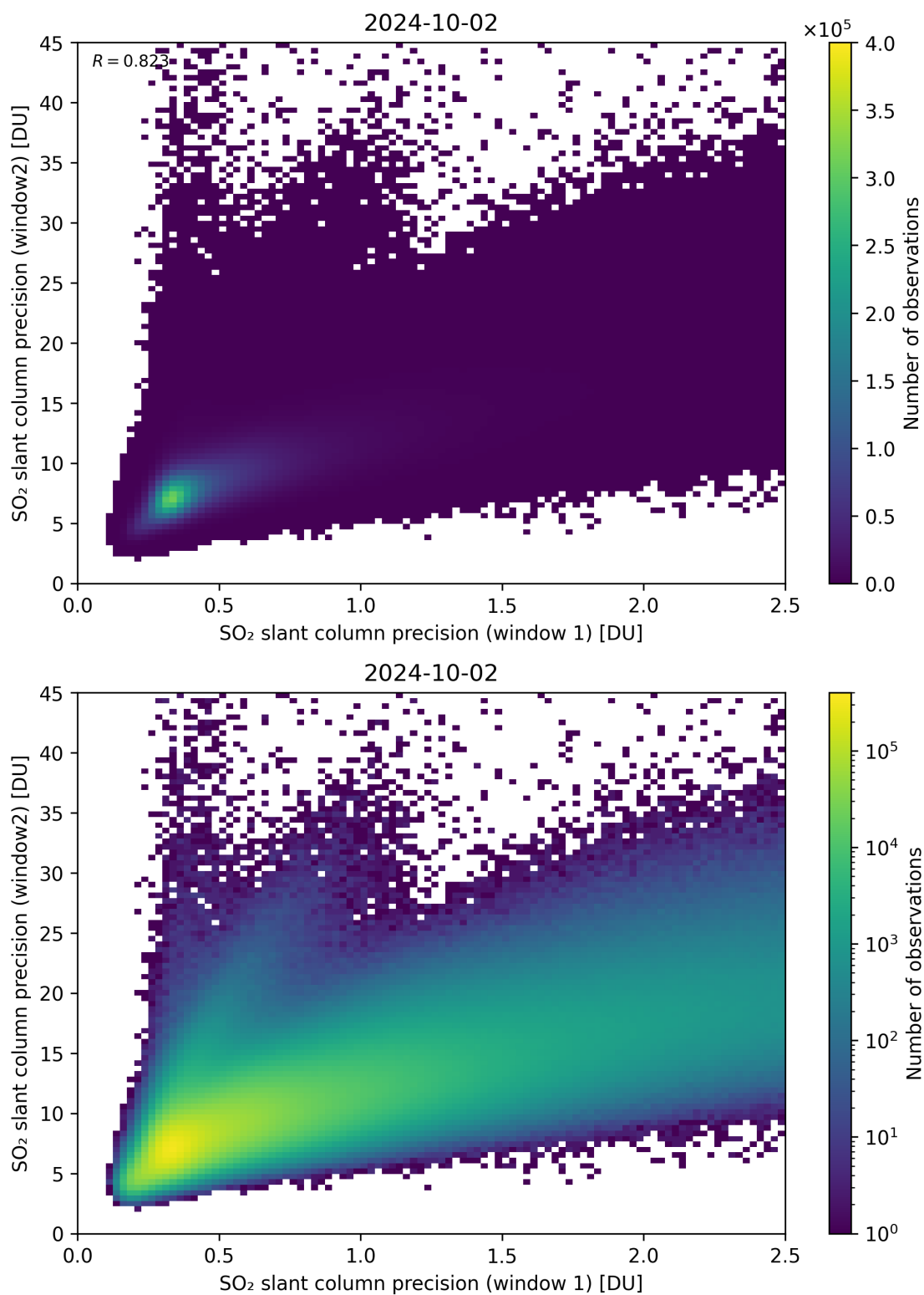
Figure 227: Scatter density plot of “SO 2 slant column precision (window 1)” against “SO 2 slant column precision (window 2)” for 2024-10-01 to 2024-10-03.
