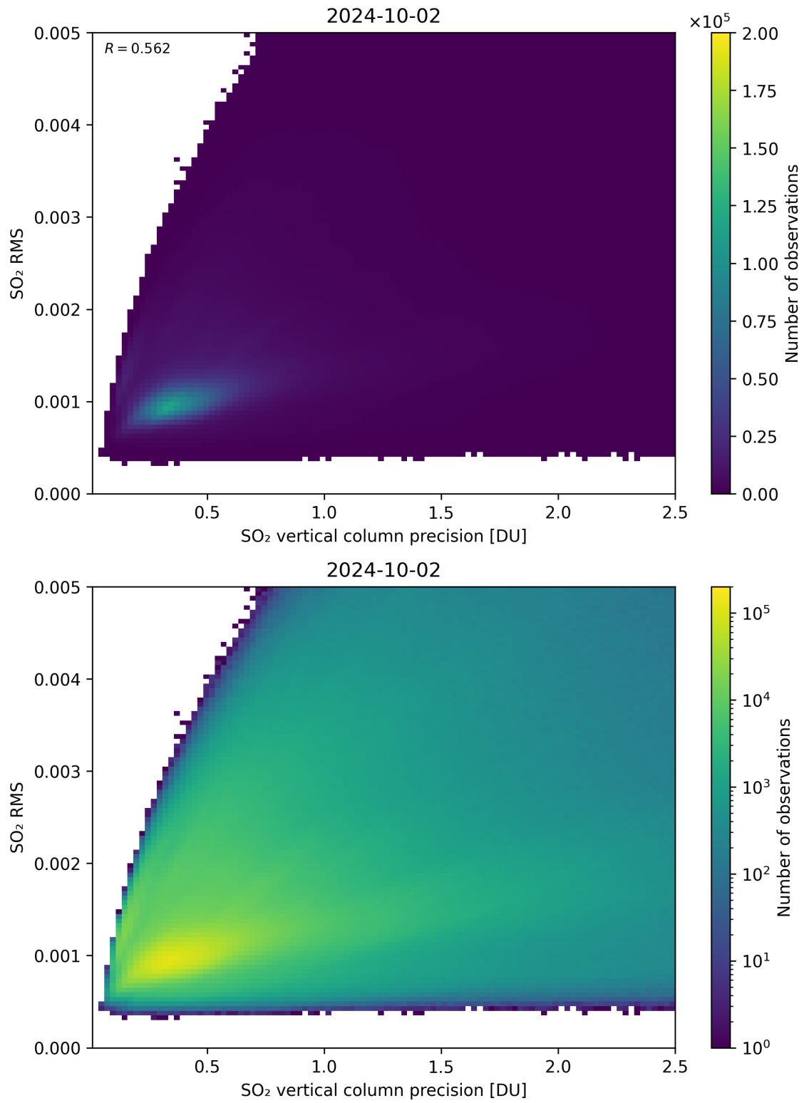
Figure 284: Scatter density plot of “SO 2 vertical column precision” against “SO 2 RMS” for 2024-10-01 to 2024-10-03.
