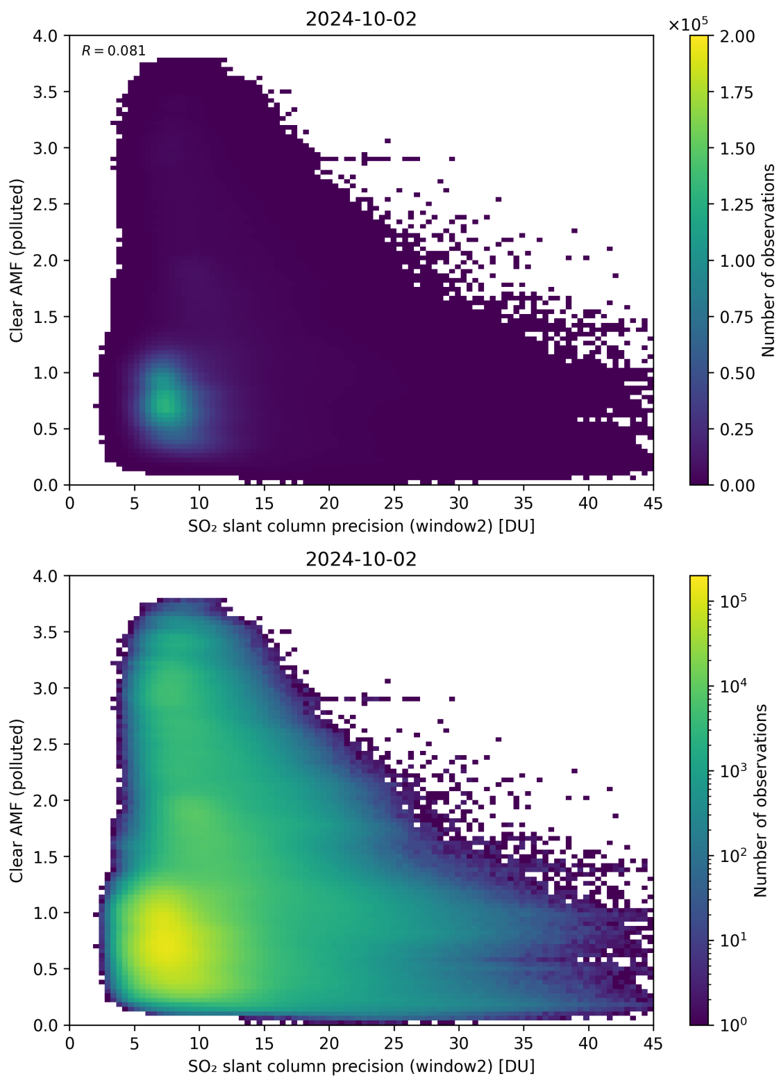
Figure 246: Scatter density plot of “SO 2 slant column precision (window2)” against “Clear AMF (polluted)” for 2024-10-01 to 2024-10-03.
