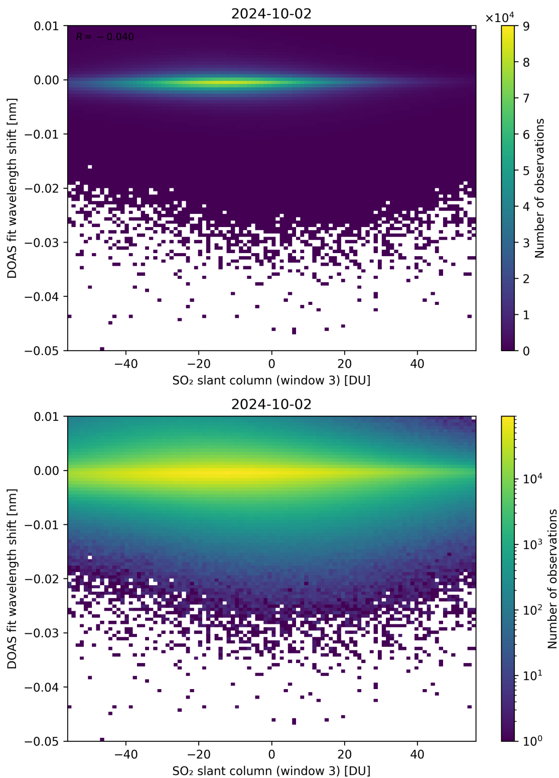
Figure 254: Scatter density plot of “SO 2 slant column (window 3)” against “DOAS fit wavelength shift” for 2024-10-01 to 2024-10-03.
