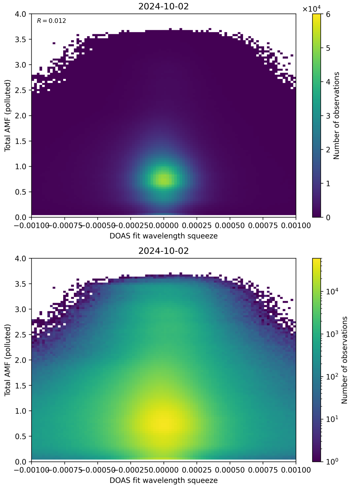
Figure 134: Scatter density plot of “DOAS fit wavelength squeeze” against “Total AMF (polluted)” for 2024-10-01 to 2024-10-03.
