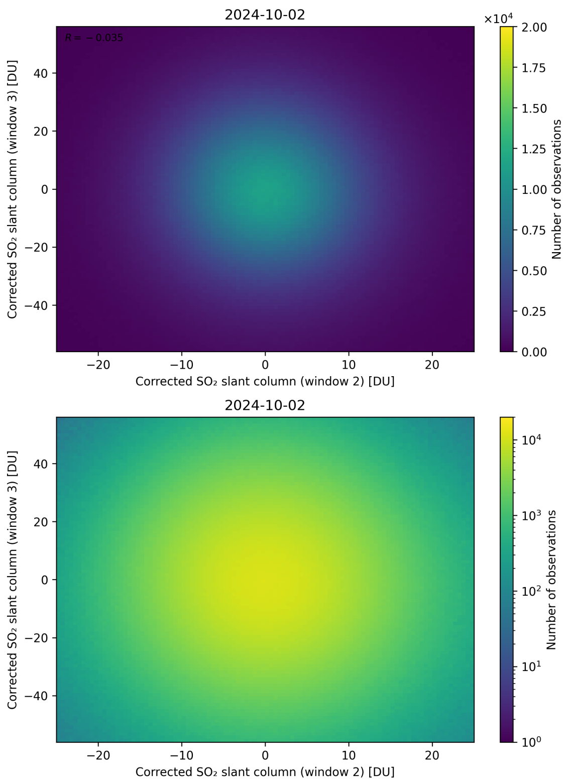
Figure 200: Scatter density plot of “Corrected SO 2 slant column (window 2)” against “Corrected SO 2 slant column (window 3)” for 2024-10-01 to 2024-10-03.
