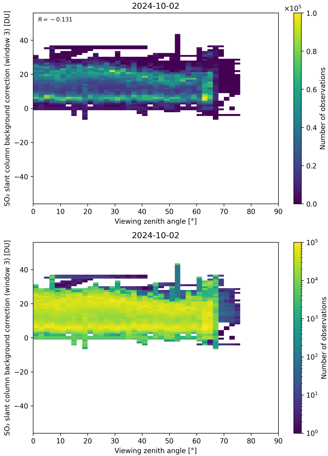
Figure 310: Scatter density plot of “Viewing zenith angle” against “SO 2 slant column background correction (window 3)” for 2024-10-01 to 2024-10-03.
