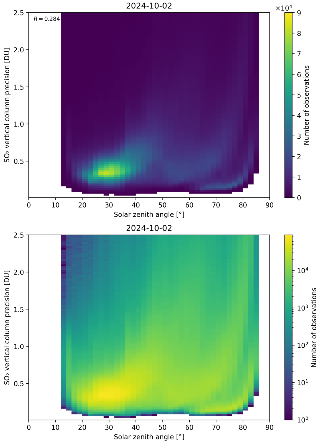
Figure 177: Scatter density plot of “Solar zenith angle” against “SO 2 vertical column precision” for 2024-10-01 to 2024-10-03.
