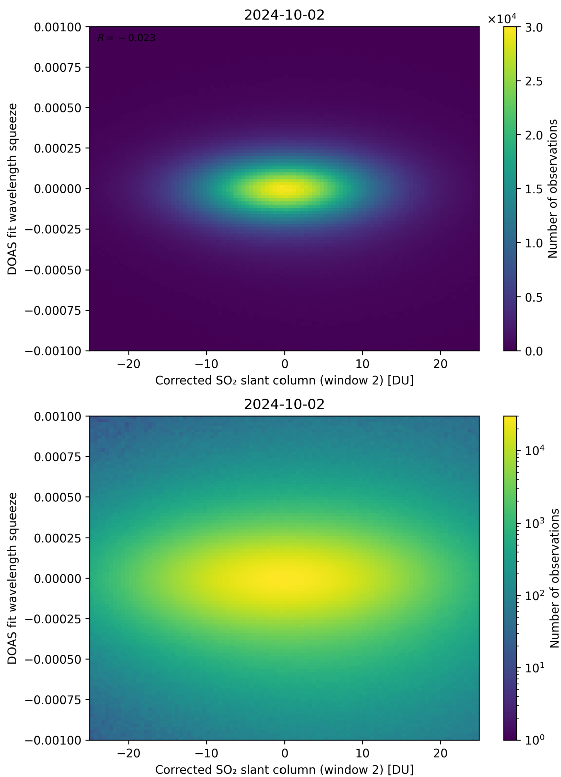
Figure 197: Scatter density plot of “Corrected SO 2 slant column (window 2)” against “DOAS fit wavelength squeeze” for 2024-10-01 to 2024-10-03.
