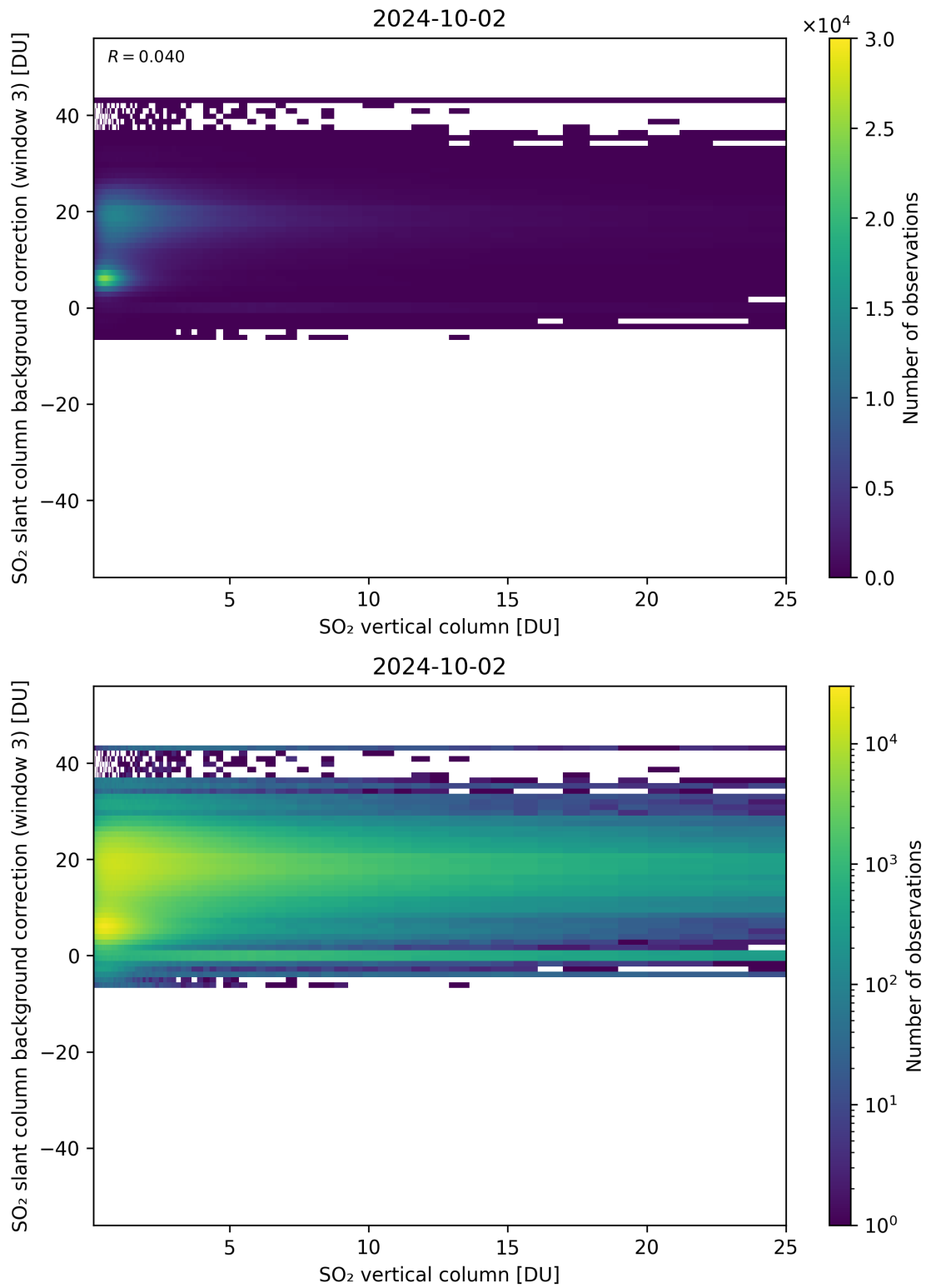
Figure 275: Scatter density plot of “SO 2 vertical column” against “SO 2 slant column background correction (window 3)” for 2024-10-01 to 2024-10-03.
