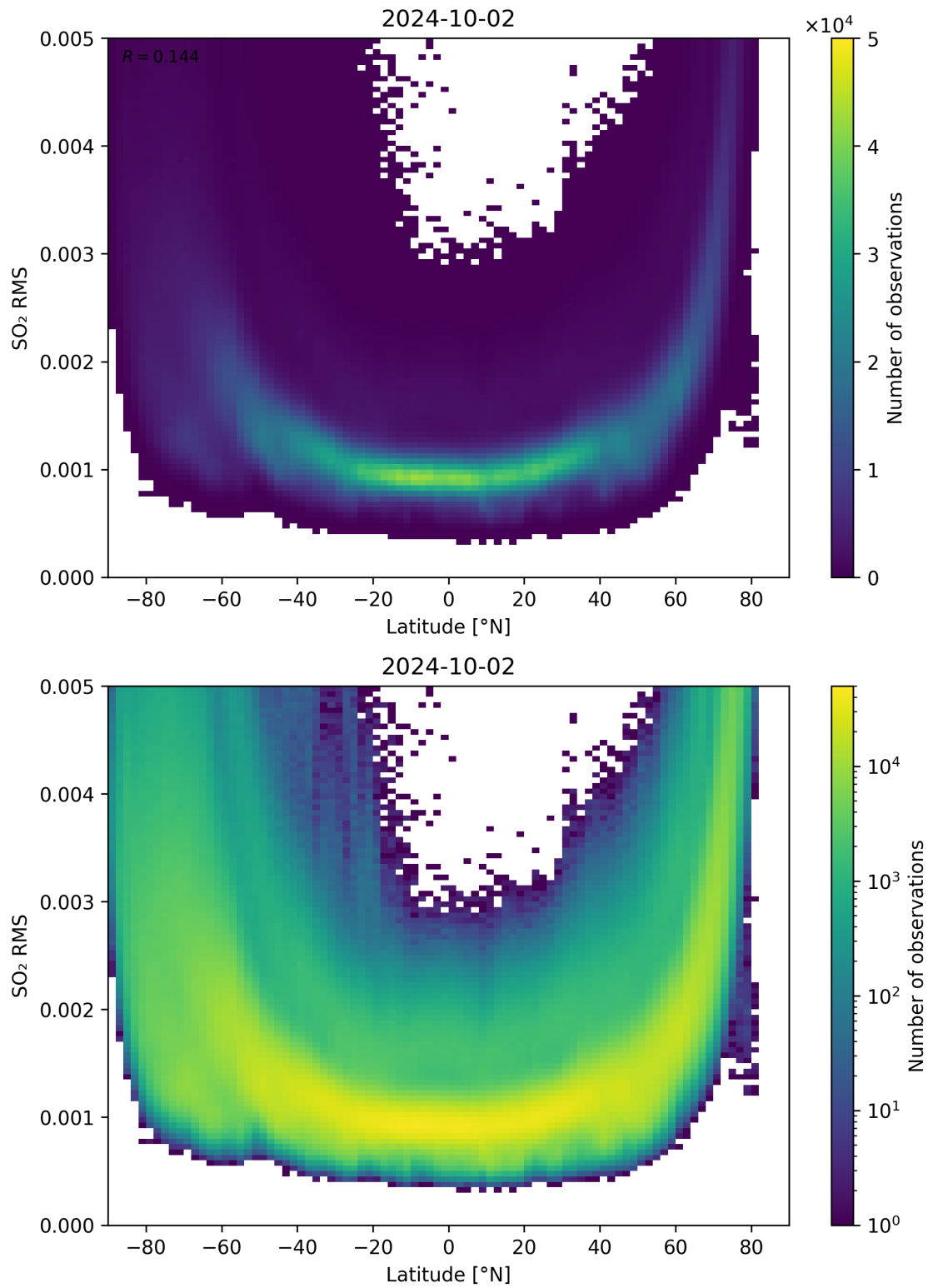
Figure 144: Scatter density plot of “Latitude” against “SO 2 RMS” for 2024-10-01 to 2024-10-03.
