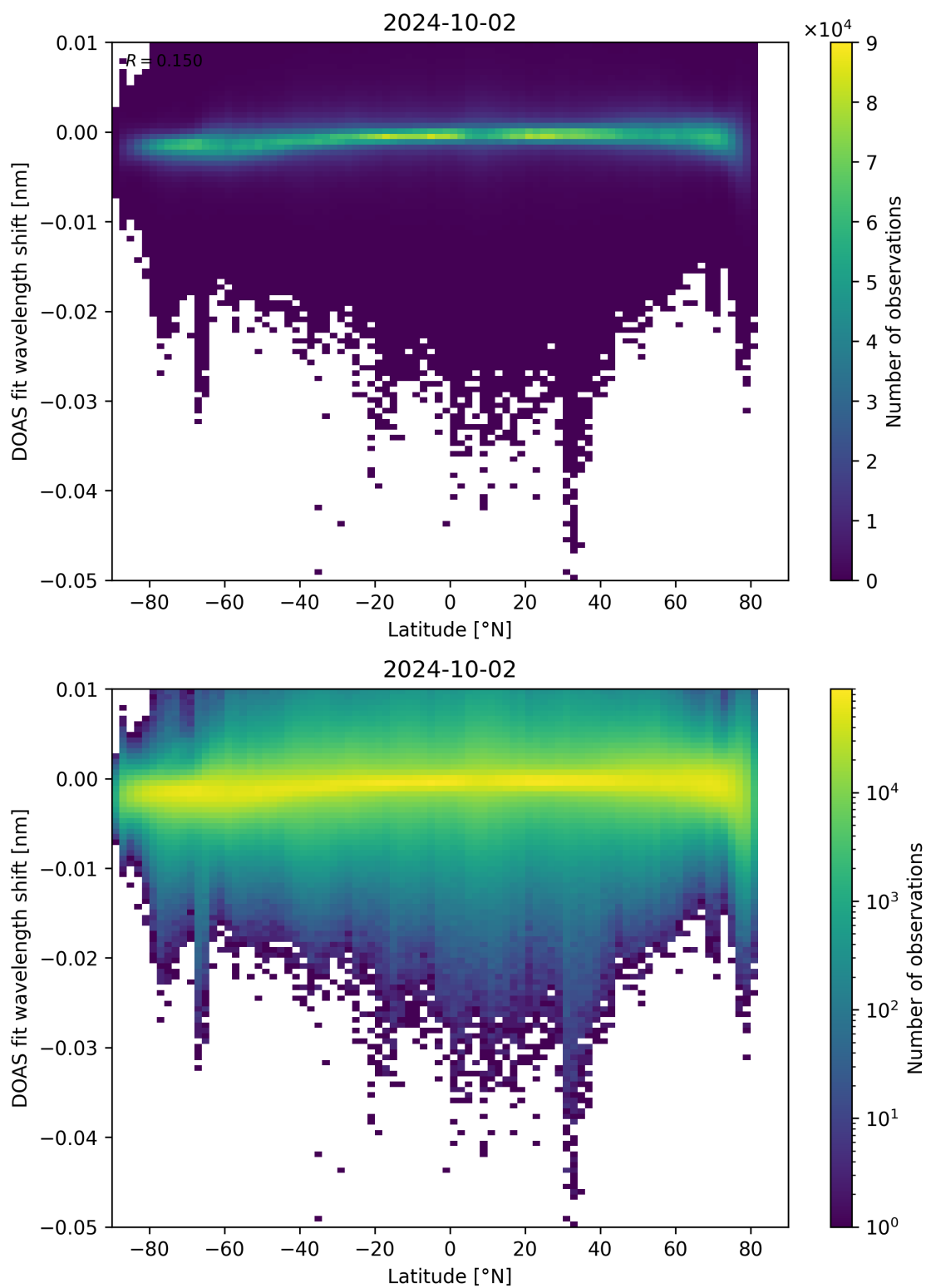
Figure 142: Scatter density plot of “Latitude” against “DOAS fit wavelength shift” for 2024-10-01 to 2024-10-03.
