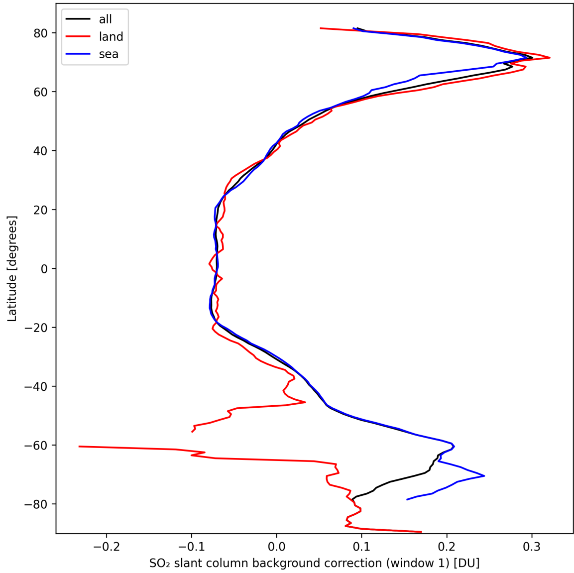
Figure 36: Zonal average of “SO 2 slant column background correction (window 1)” for 2024-10-01 to 2024-10-03.
