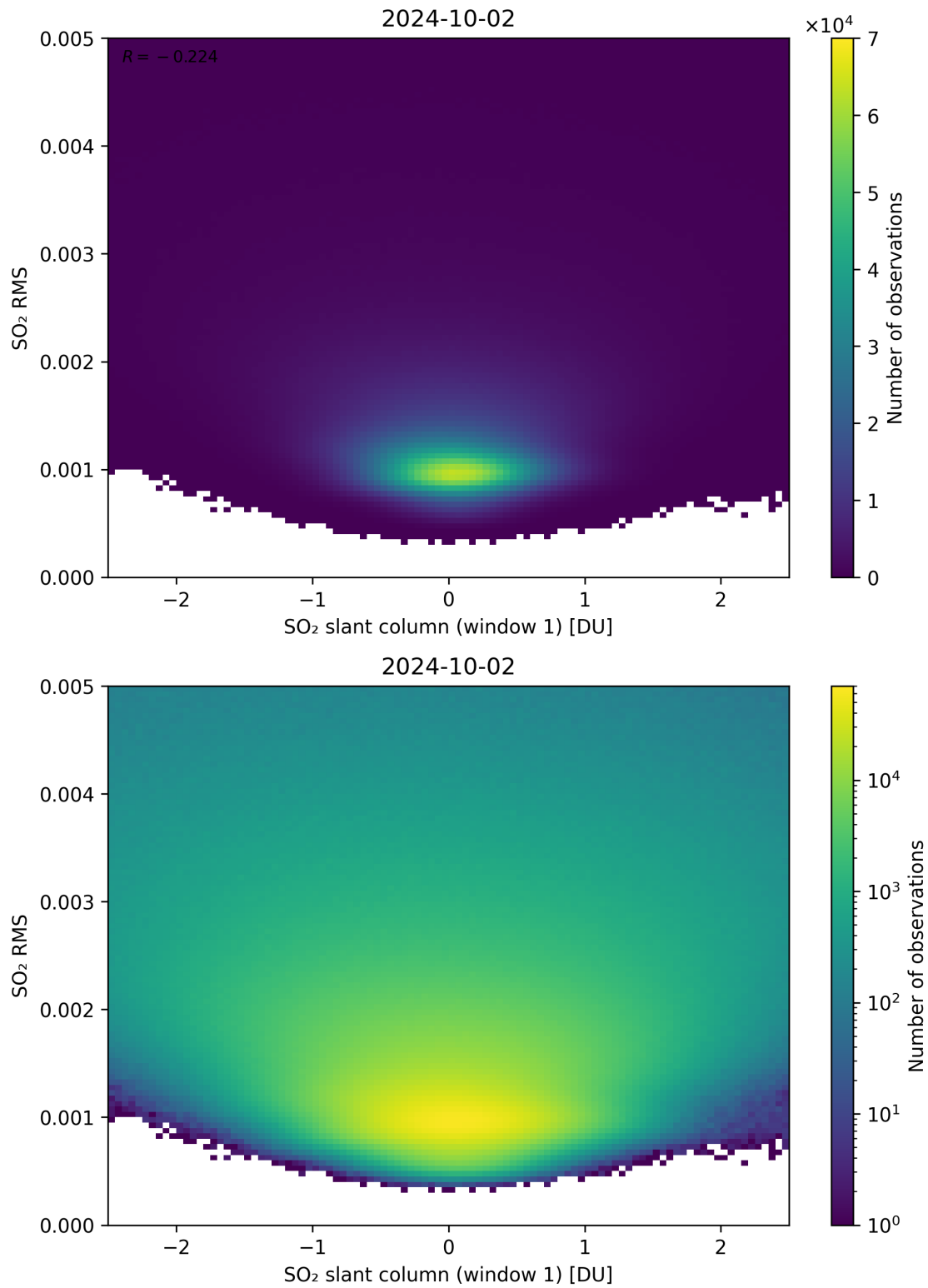
Figure 217: Scatter density plot of “SO 2 slant column (window 1)” against “SO 2 RMS” for 2024-10-01 to 2024-10-03.
