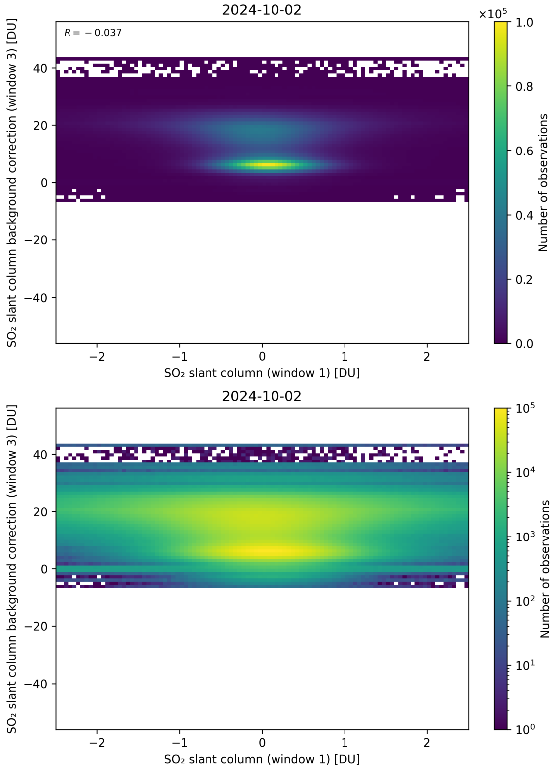
Figure 214: Scatter density plot of “SO 2 slant column (window 1)” against “SO 2 slant column background correction (window 3)” for 2024-10-01 to 2024-10-03.
