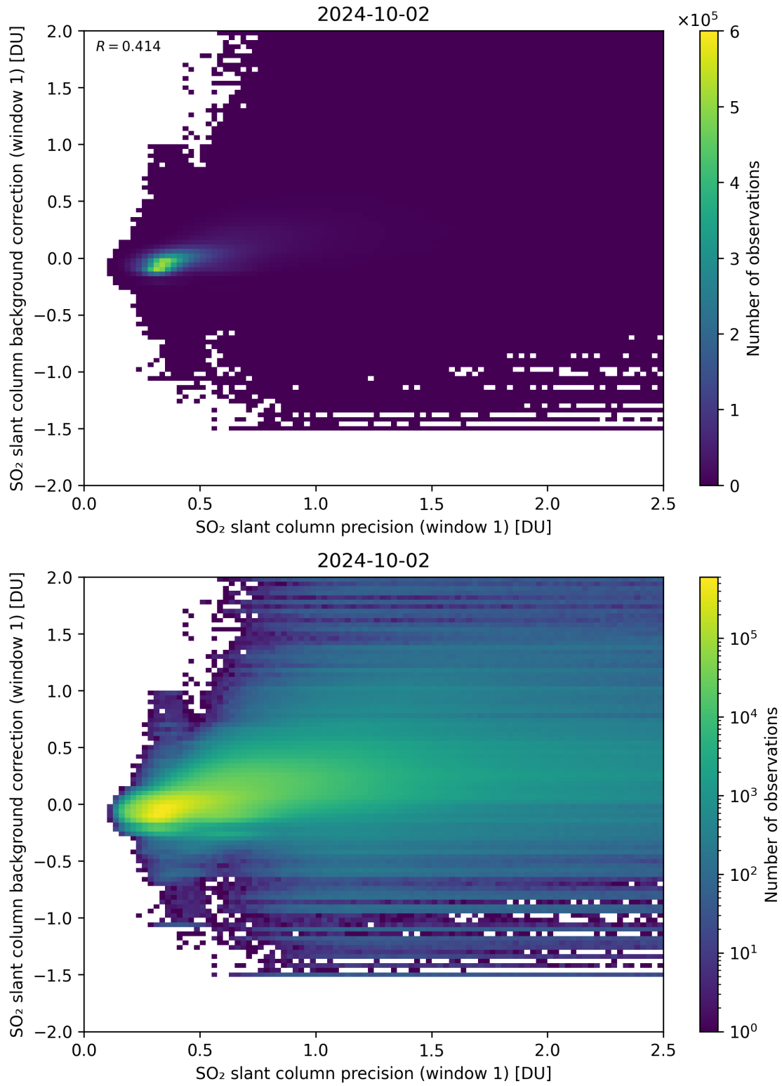
Figure 218: Scatter density plot of “SO 2 slant column precision (window 1)” against “SO 2 slant column background correction (window 1)” for 2024-10-01 to 2024-10-03.
