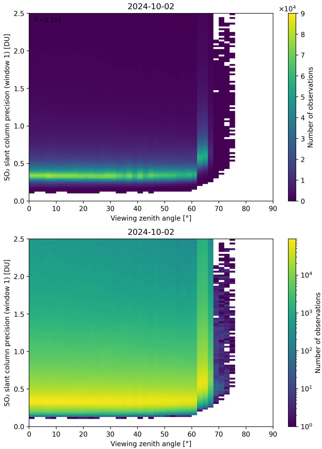
Figure 321: Scatter density plot of “Viewing zenith angle” against “SO 2 slant column precision (window 1)” for 2024-10-01 to 2024-10-03.
