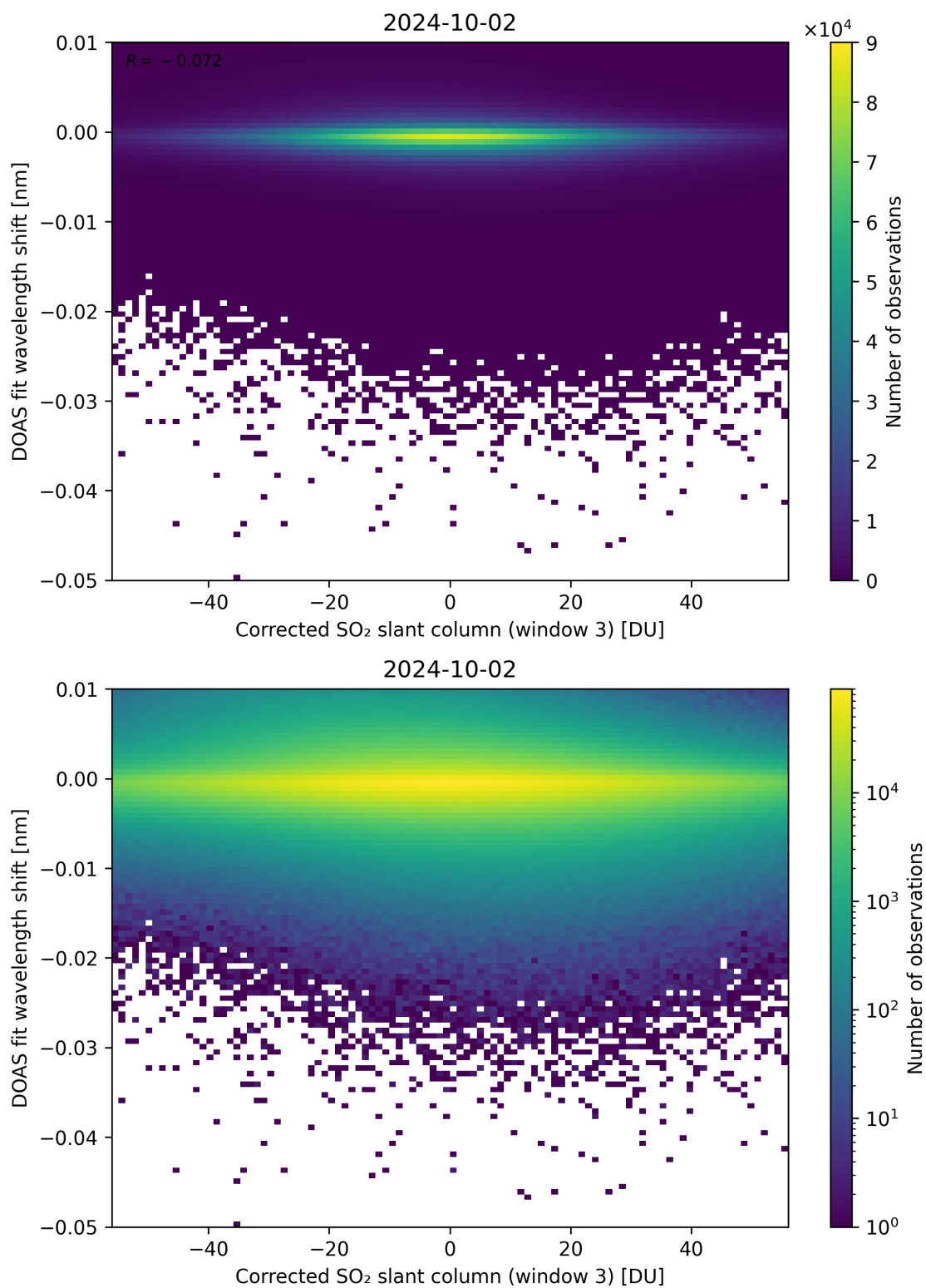
Figure 206: Scatter density plot of “Corrected SO 2 slant column (window 3)” against “DOAS fit wavelength shift” for 2024-10-01 to 2024-10-03.
