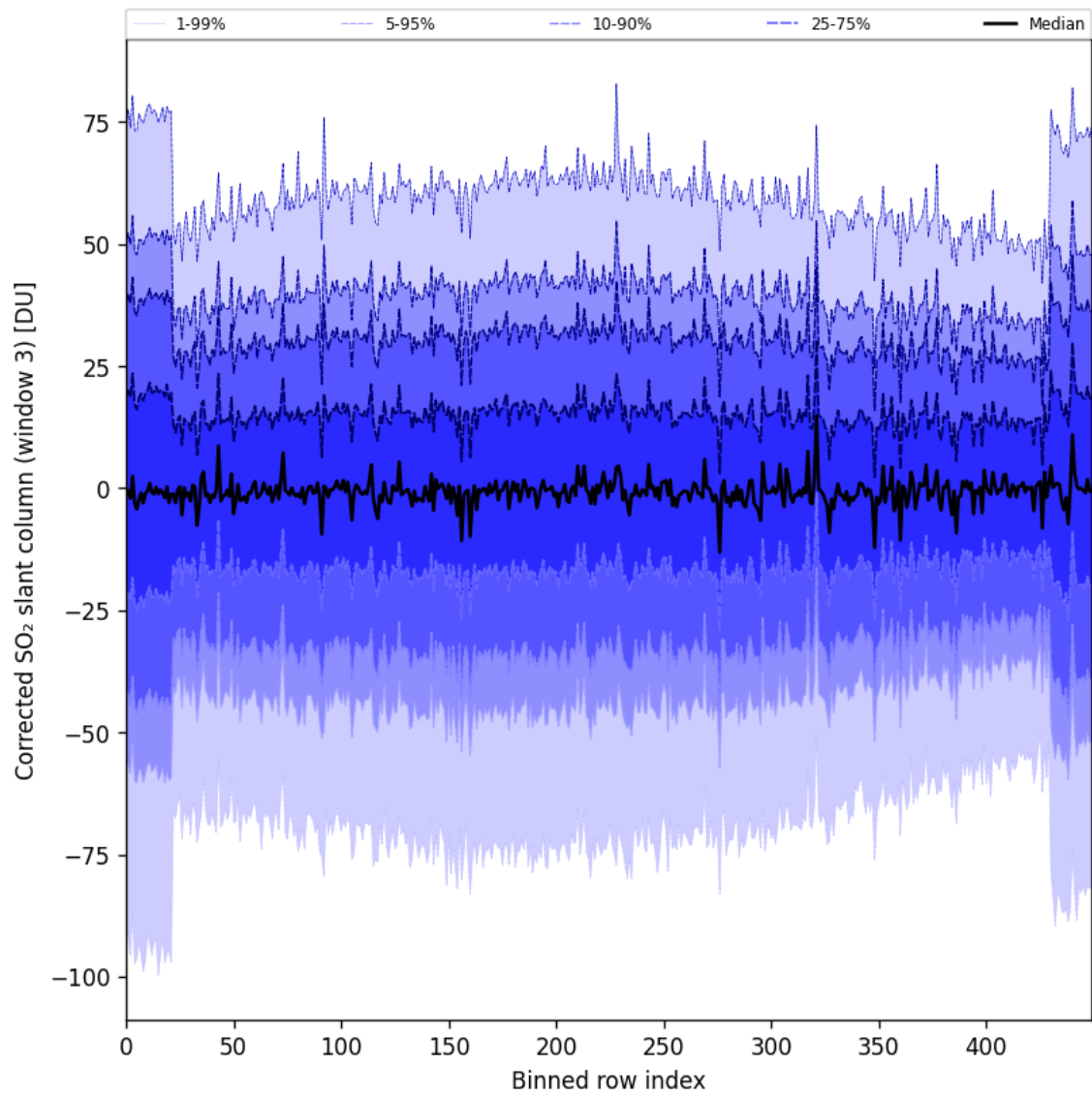
Figure 89: Along track statistics of “Corrected SO 2 slant column (window 3)” for 2024-10-01 to 2024-10-03
