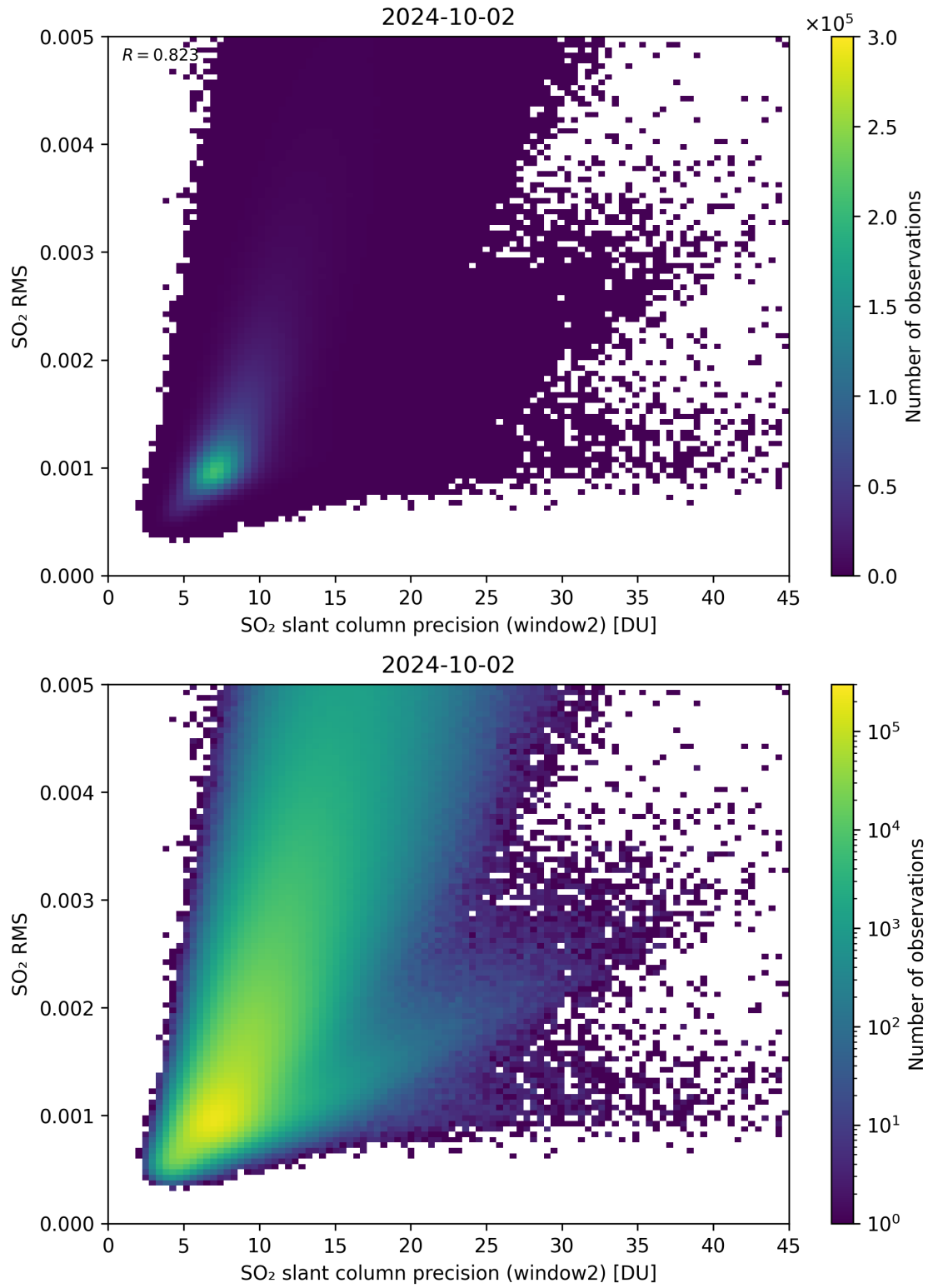
Figure 245: Scatter density plot of “SO 2 slant column precision (window2)” against “SO 2 RMS” for 2024-10-01 to 2024-10-03.
