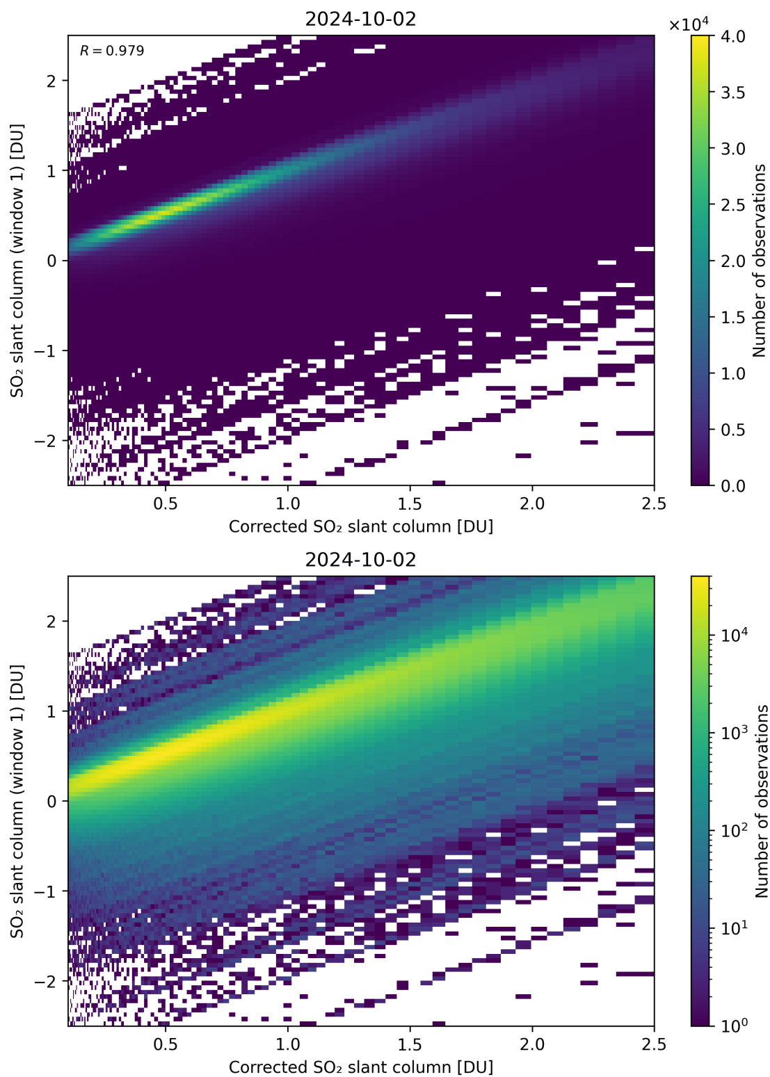
Figure 187: Scatter density plot of “Corrected SO 2 slant column” against “SO 2 slant column (window 1)” for 2024-10-01 to 2024-10-03.
