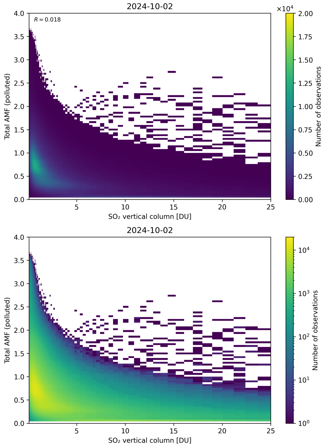
Figure 305: Scatter density plot of “SO 2 vertical column” against “Total AMF (polluted)” for 2024-10-01 to 2024-10-03.
