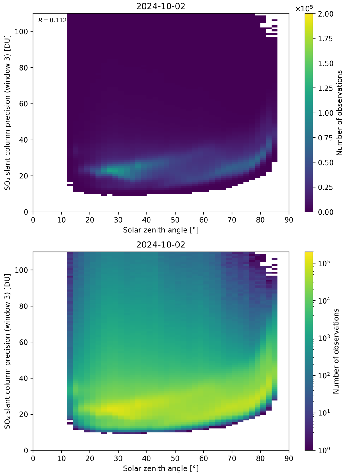
Figure 173: Scatter density plot of “Solar zenith angle” against “SO 2 slant column precision (window 3)” for 2024-10-01 to 2024-10-03.
