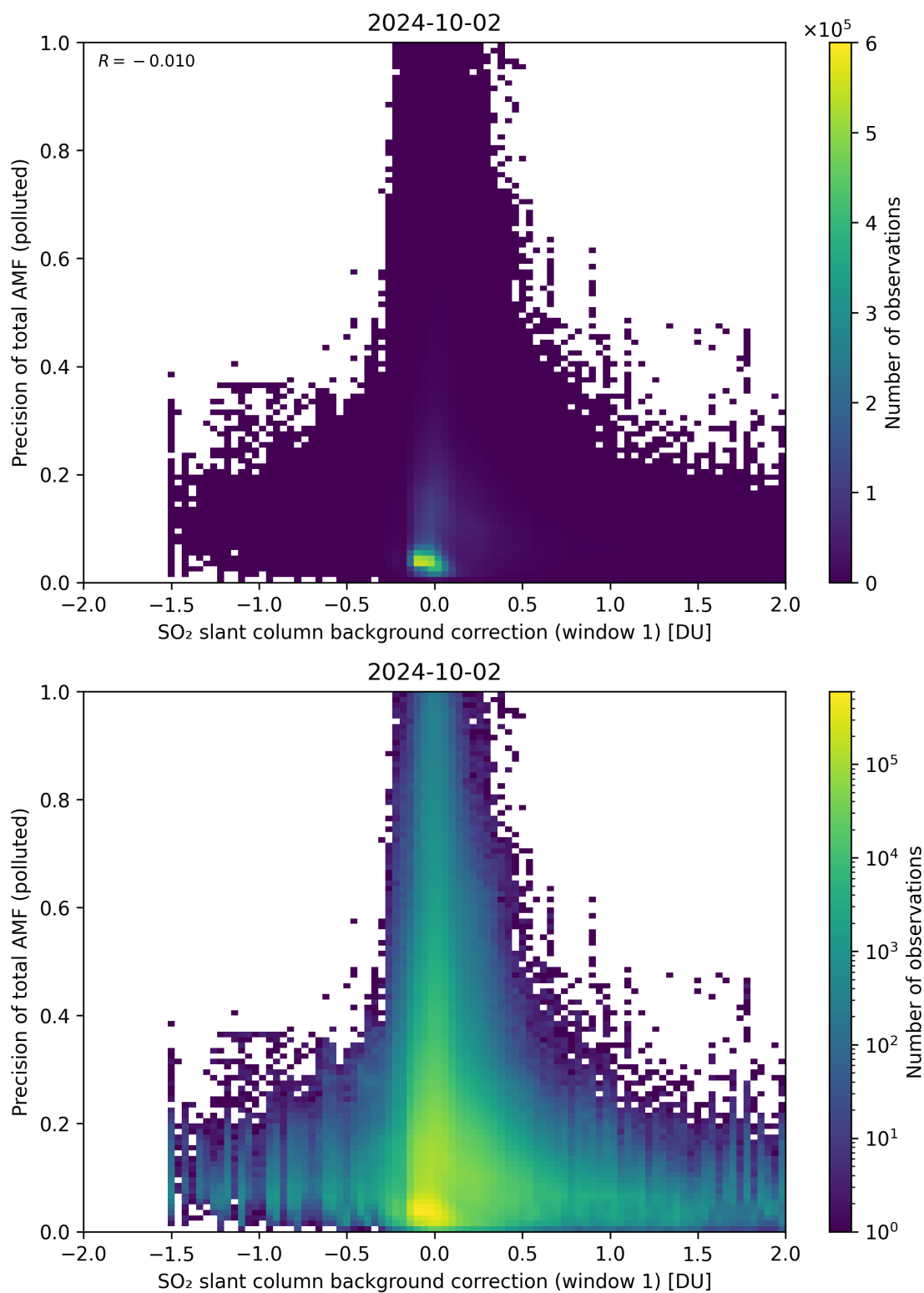
Figure 110: Scatter density plot of “SO 2 slant column background correction (window 1)” against “Precision of total AMF (polluted)” for 2024-10-01 to 2024-10-03.
