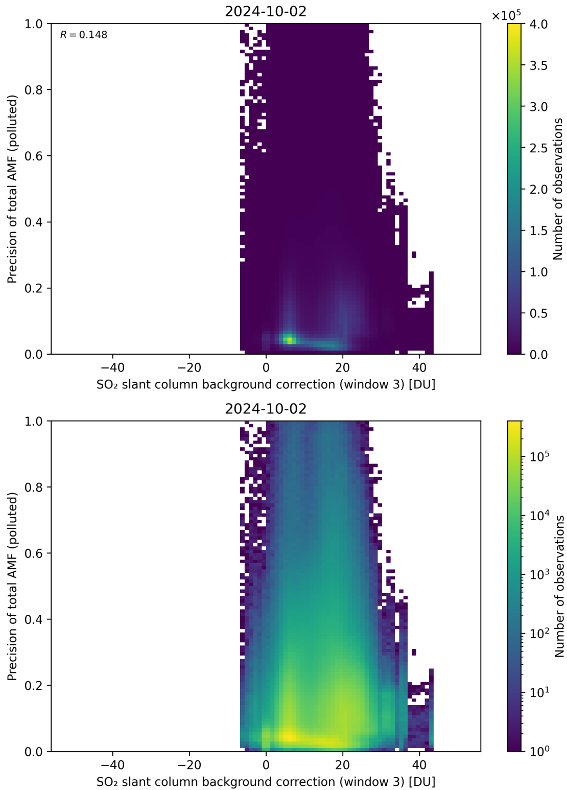
Figure 126: Scatter density plot of “SO 2 slant column background correction (window 3)” against “Precision of total AMF (polluted)” for 2024-10-01 to 2024-10-03.
