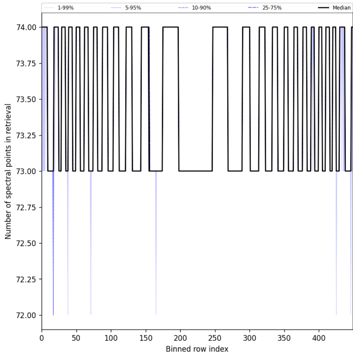
Figure 97: Along track statistics of “Number of spectral points in retrieval” for 2024-10-01 to 2024-10-03
