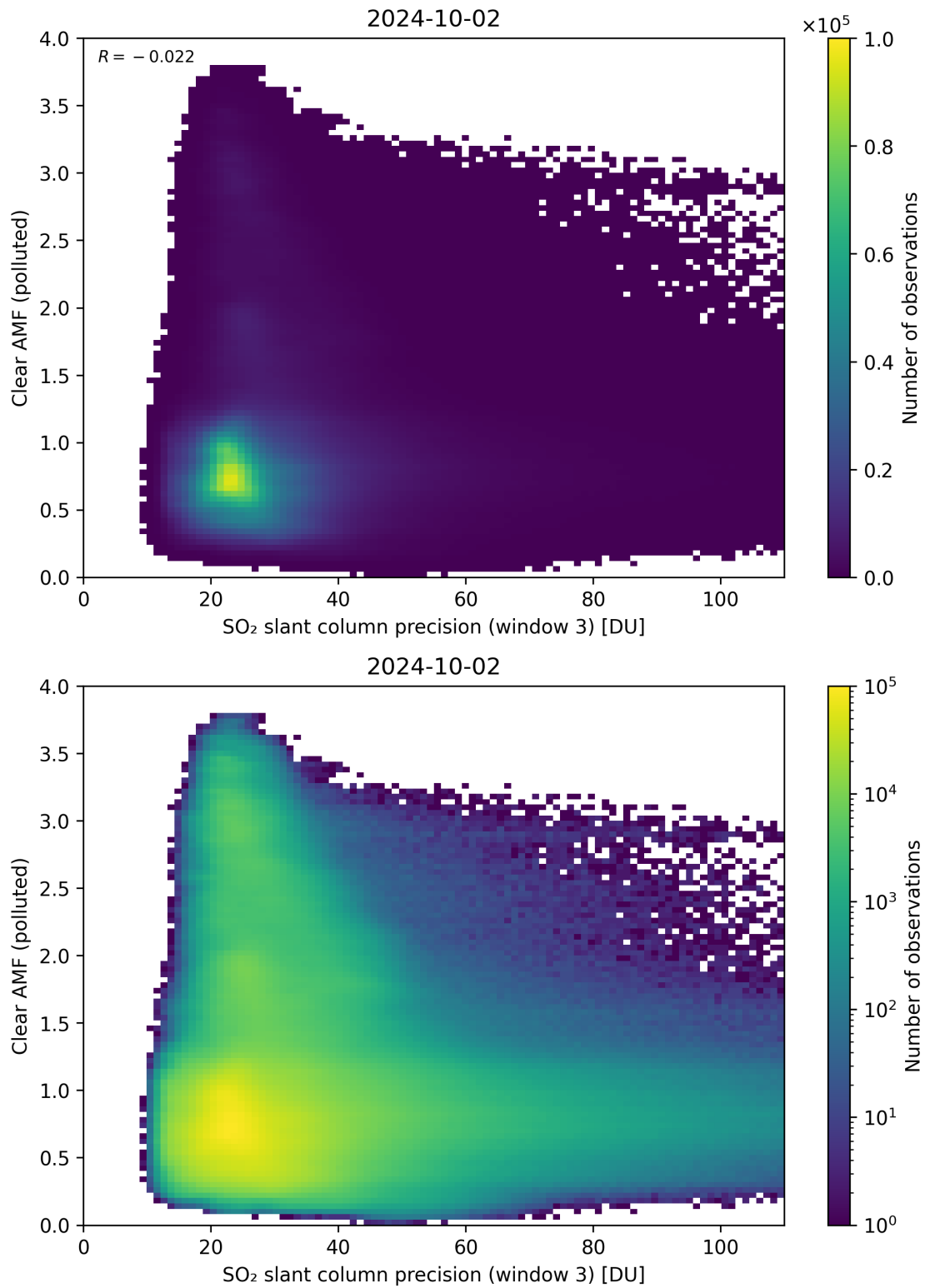
Figure 261: Scatter density plot of “SO 2 slant column precision (window 3)” against “Clear AMF (polluted)” for 2024-10-01 to 2024-10-03.
