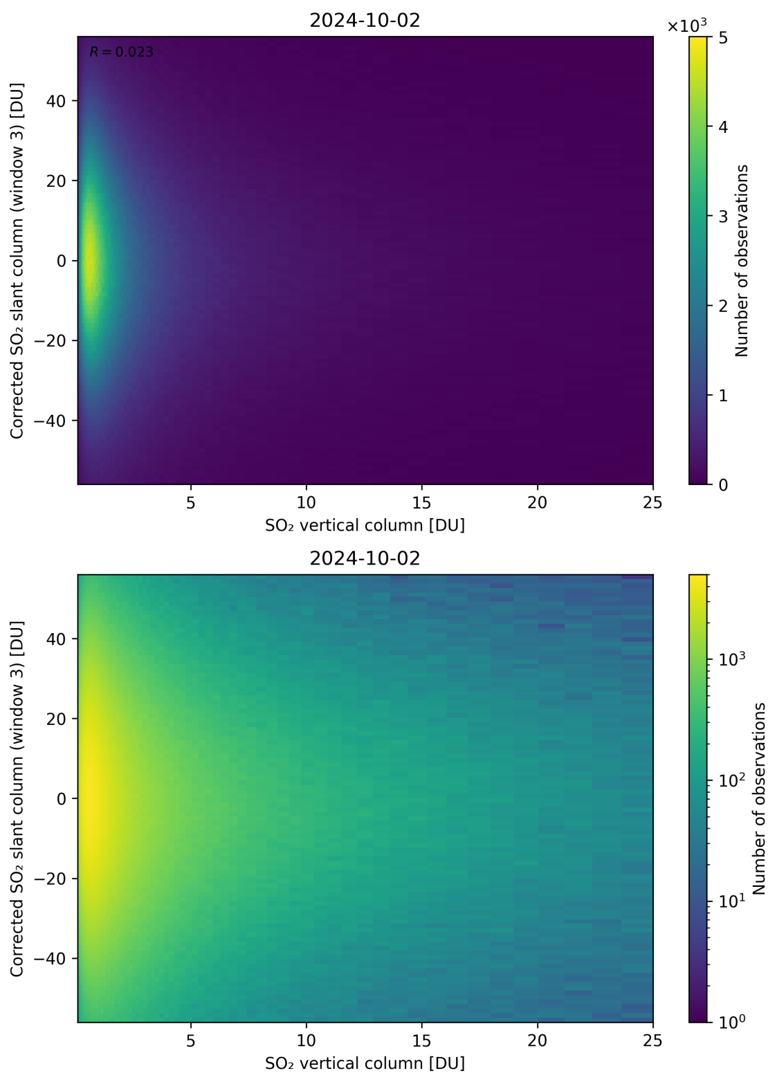
Figure 299: Scatter density plot of “SO 2 vertical column” against “Corrected SO 2 slant column (window 3)” for 2024-10-01 to 2024-10-03.
