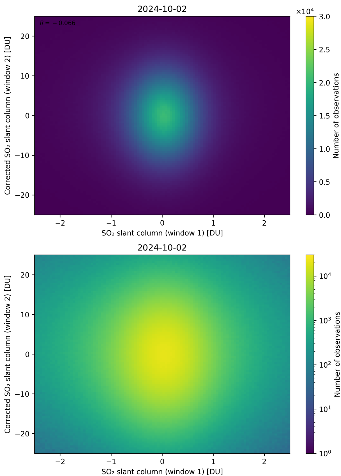
Figure 233: Scatter density plot of “SO 2 slant column (window 1)” against “Corrected SO 2 slant column (window 2)” for 2024-10-01 to 2024-10-03.
