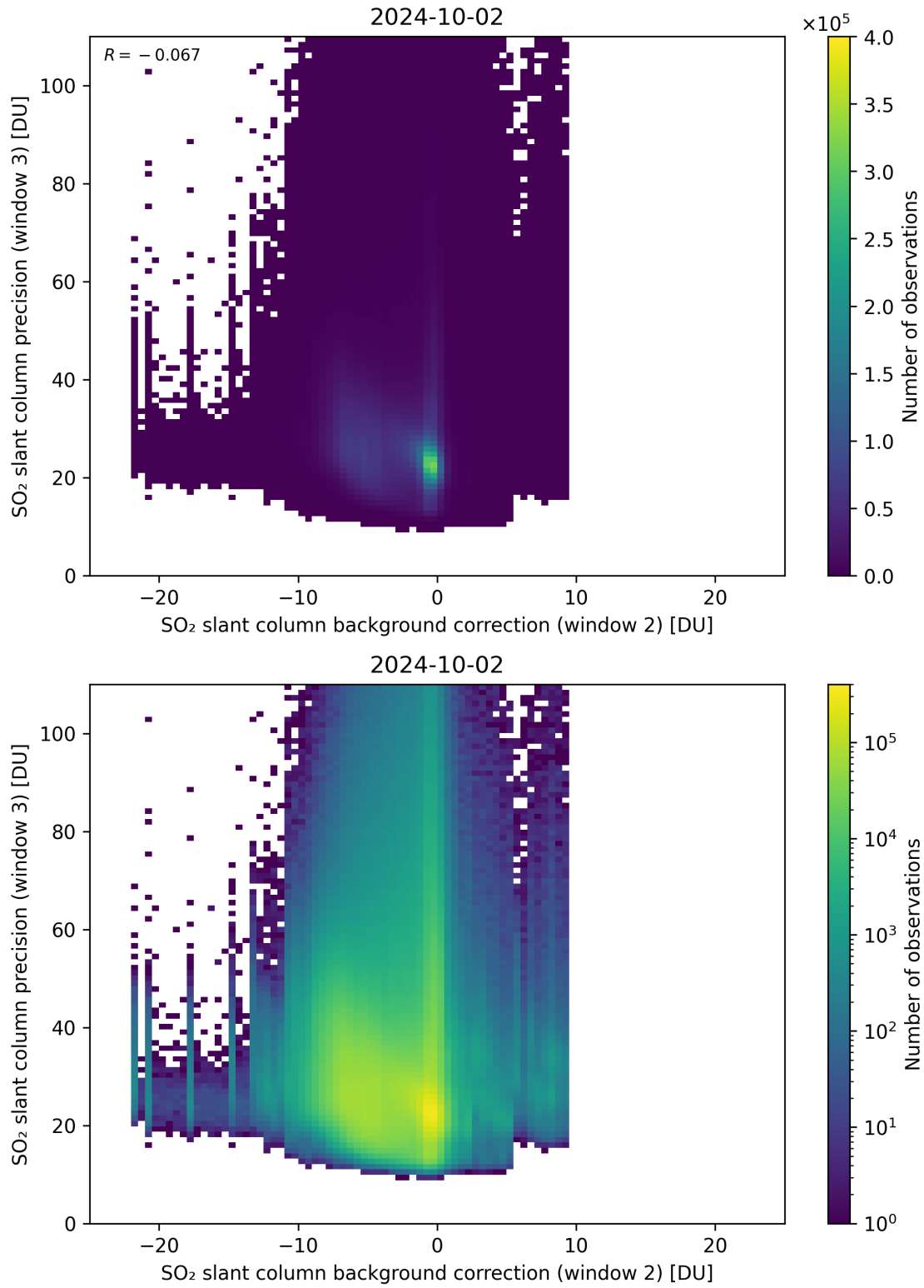
Figure 118: Scatter density plot of “SO 2 slant column background correction (window 2)” against “SO 2 slant column precision (window 3)” for 2024-10-01 to 2024-10-03.
