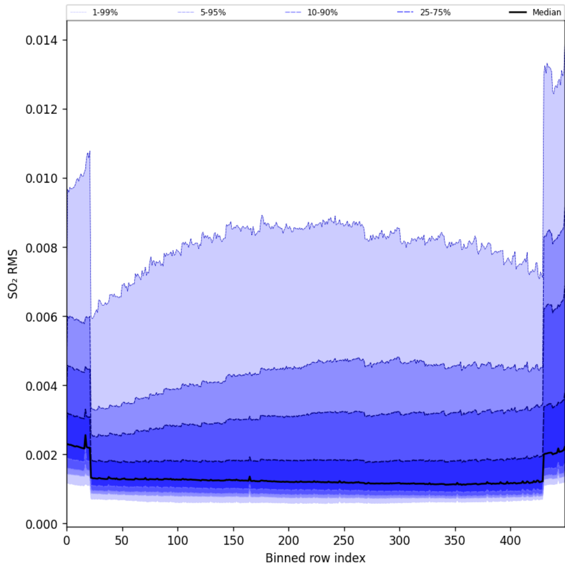
Figure 93: Along track statistics of “SO 2 RMS” for 2024-10-01 to 2024-10-03
