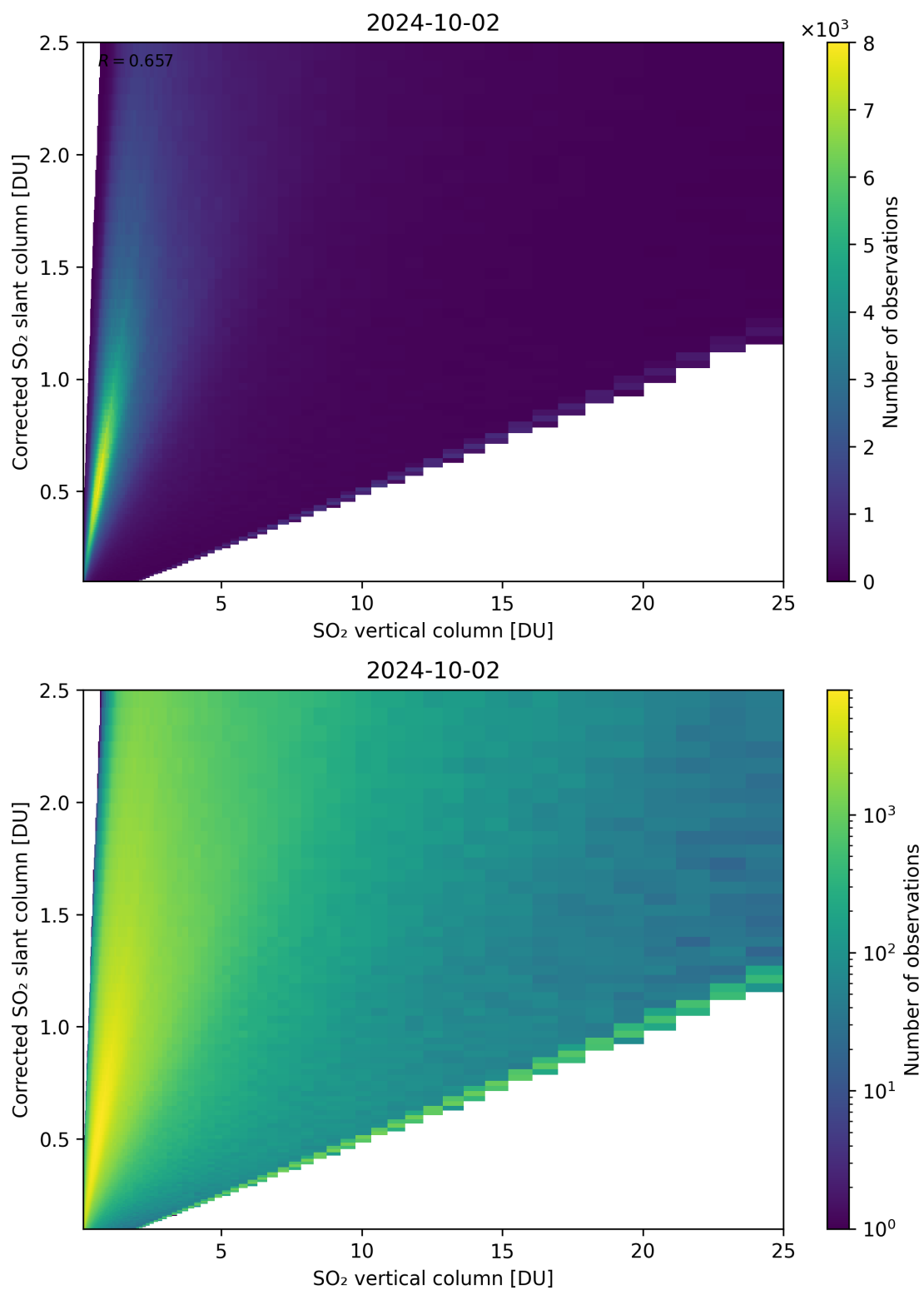
Figure 297: Scatter density plot of “SO 2 vertical column” against “Corrected SO 2 slant column” for 2024-10-01 to 2024-10-03.
