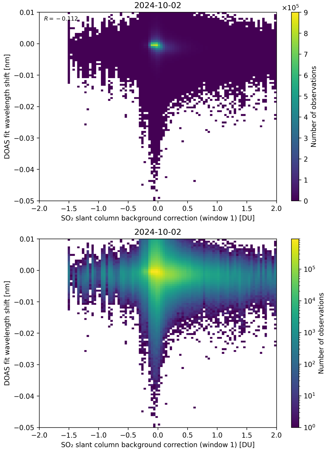
Figure 100: Scatter density plot of “SO 2 slant column background correction (window 1)” against “DOAS fit wavelength shift” for 2024-10-01 to 2024-10-03.
