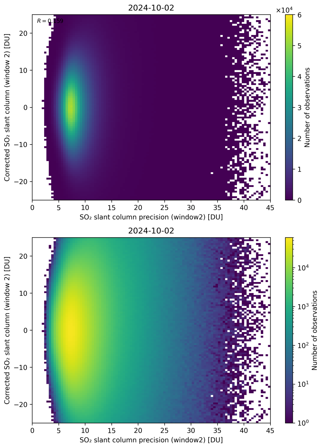
Figure 247: Scatter density plot of “SO 2 slant column precision (window2)” against “Corrected SO 2 slant column (window 2)” for 2024-10-01 to 2024-10-03.
