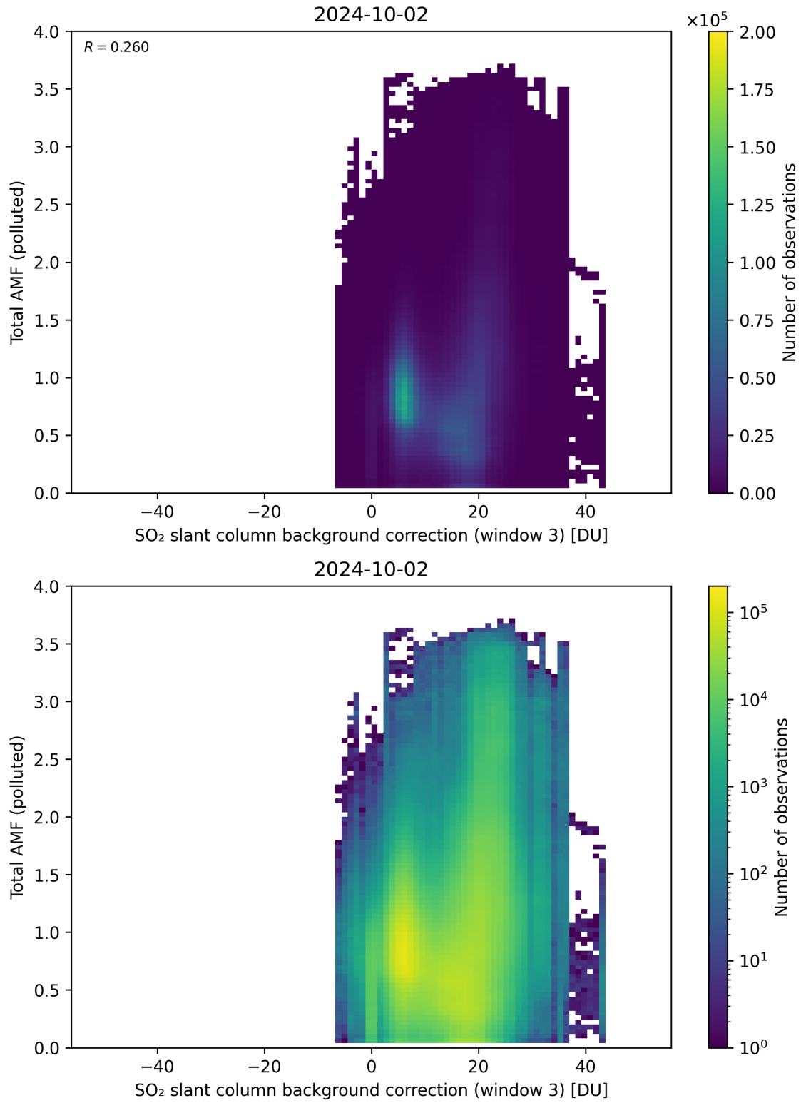
Figure 125: Scatter density plot of “SO 2 slant column background correction (window 3)” against “Total AMF (polluted)” for 2024-10-01 to 2024-10-03.
