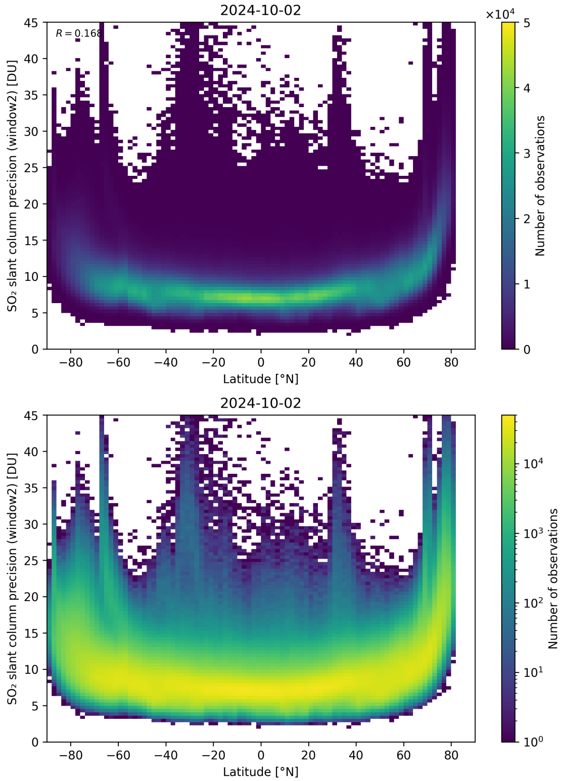
Figure 151: Scatter density plot of “Latitude” against “SO 2 slant column precision (window2)” for 2024-10-01 to 2024-10-03.
