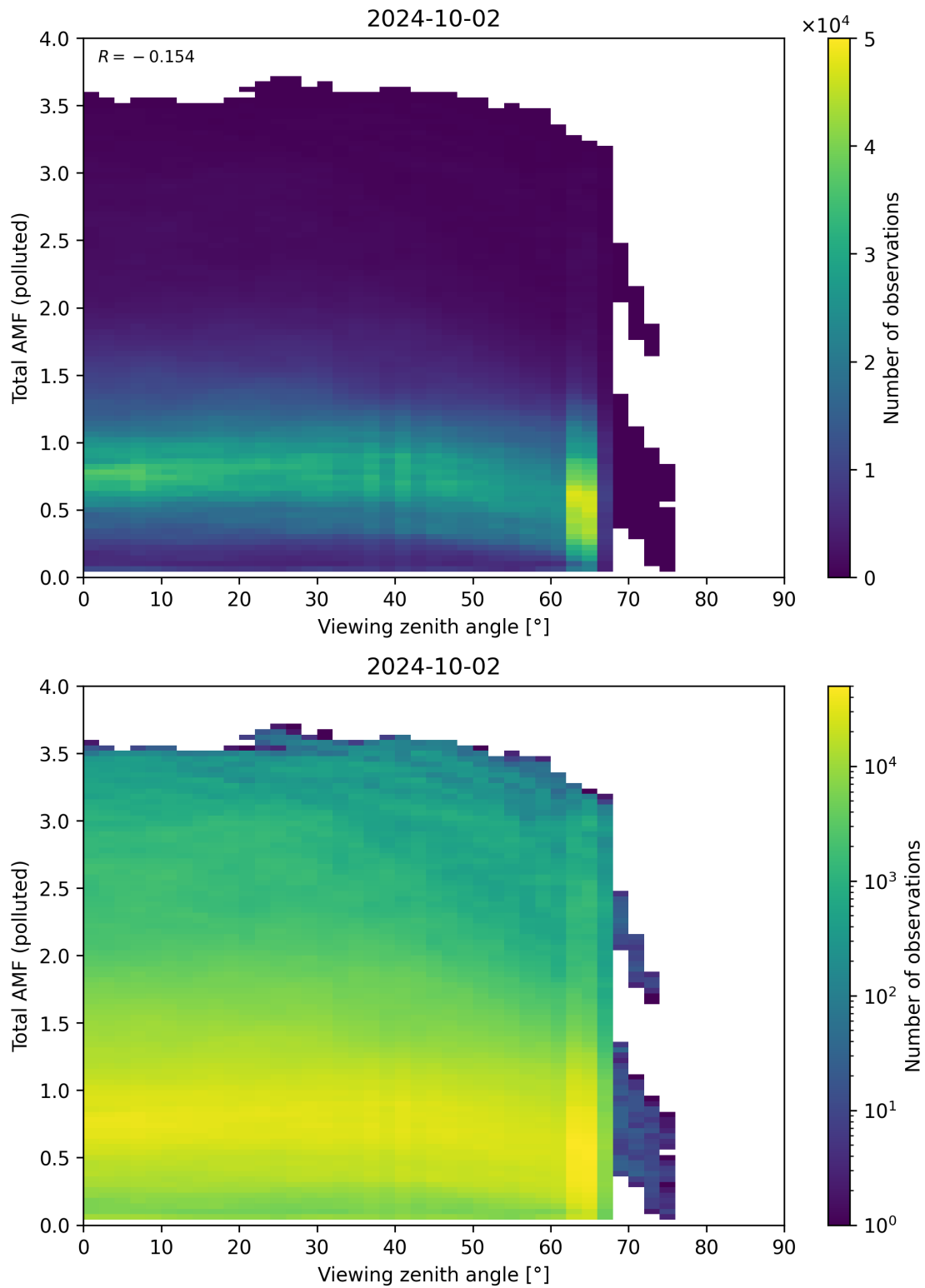
Figure 325: Scatter density plot of “Viewing zenith angle” against “Total AMF (polluted)” for 2024-10-01 to 2024-10-03.
