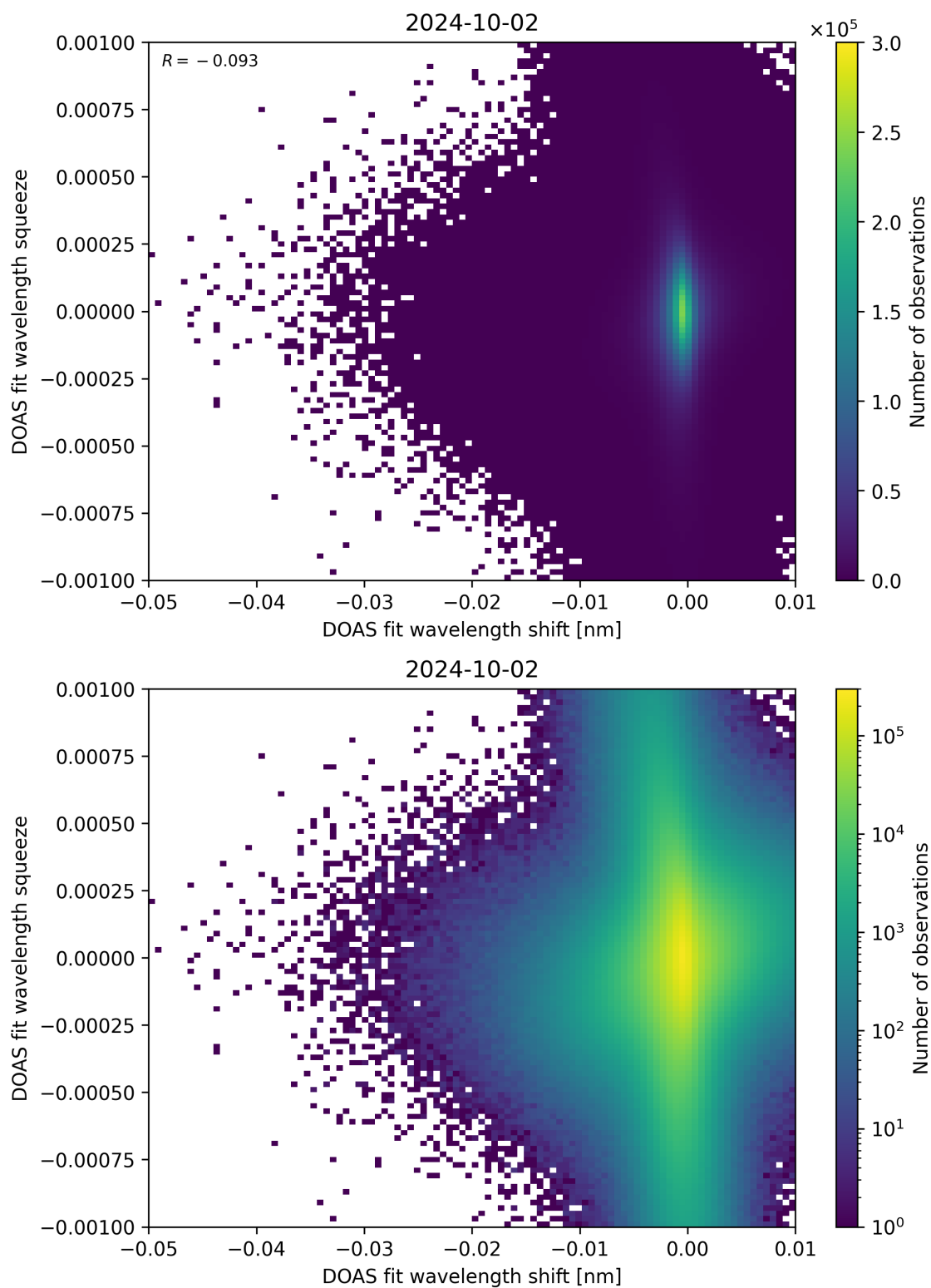
Figure 127: Scatter density plot of “DOAS fit wavelength shift” against “DOAS fit wavelength squeeze” for 2024-10-01 to 2024-10-03.
