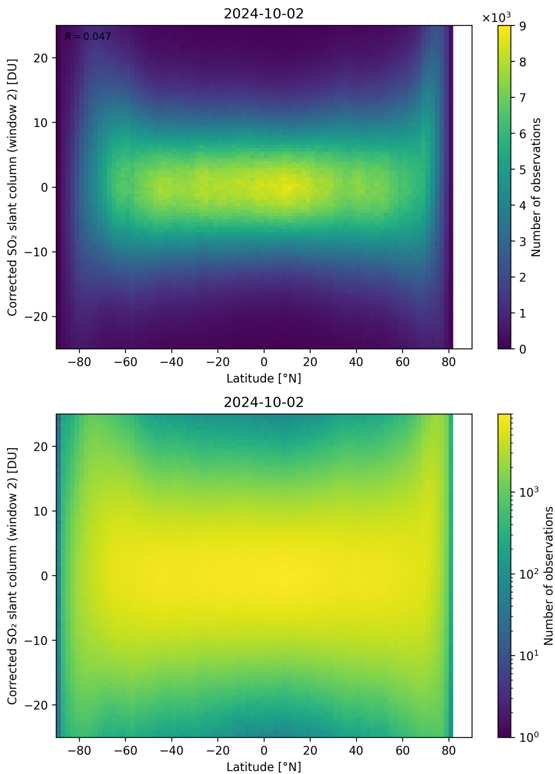
Figure 147: Scatter density plot of “Latitude” against “Corrected SO 2 slant column (window 2)” for 2024-10-01 to 2024-10-03.
