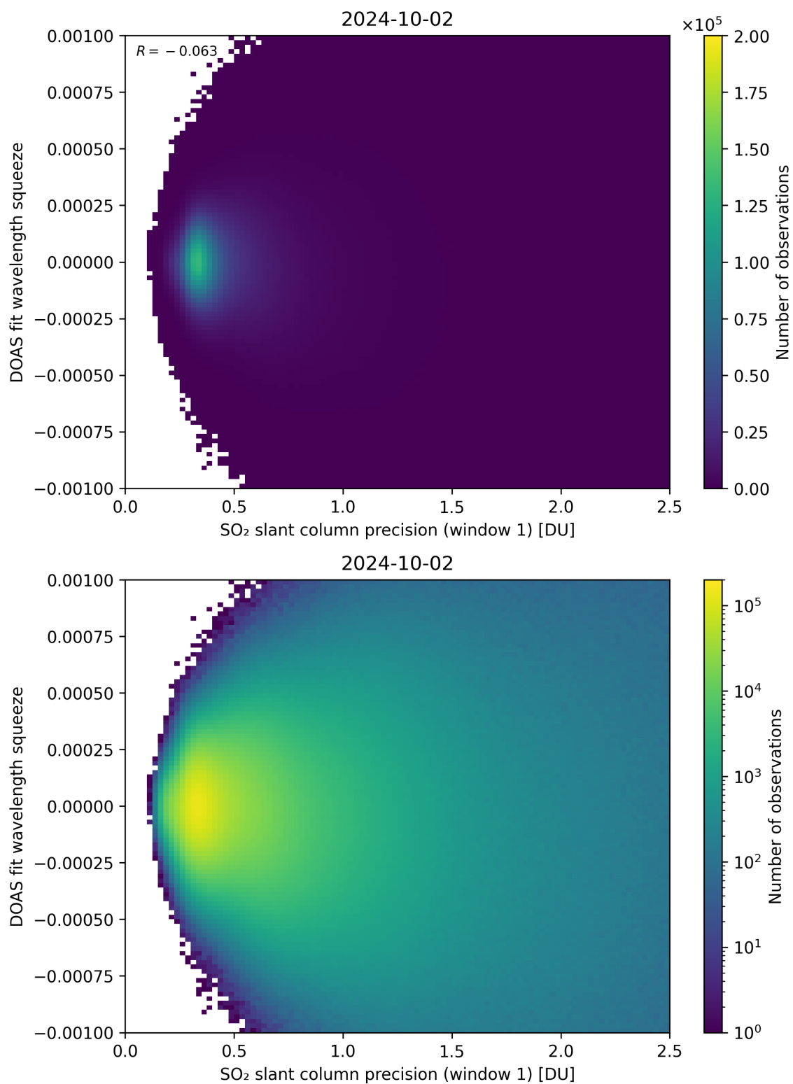
Figure 222: Scatter density plot of “SO 2 slant column precision (window 1)” against “DOAS fit wavelength squeeze” for 2024-10-01 to 2024-10-03.
