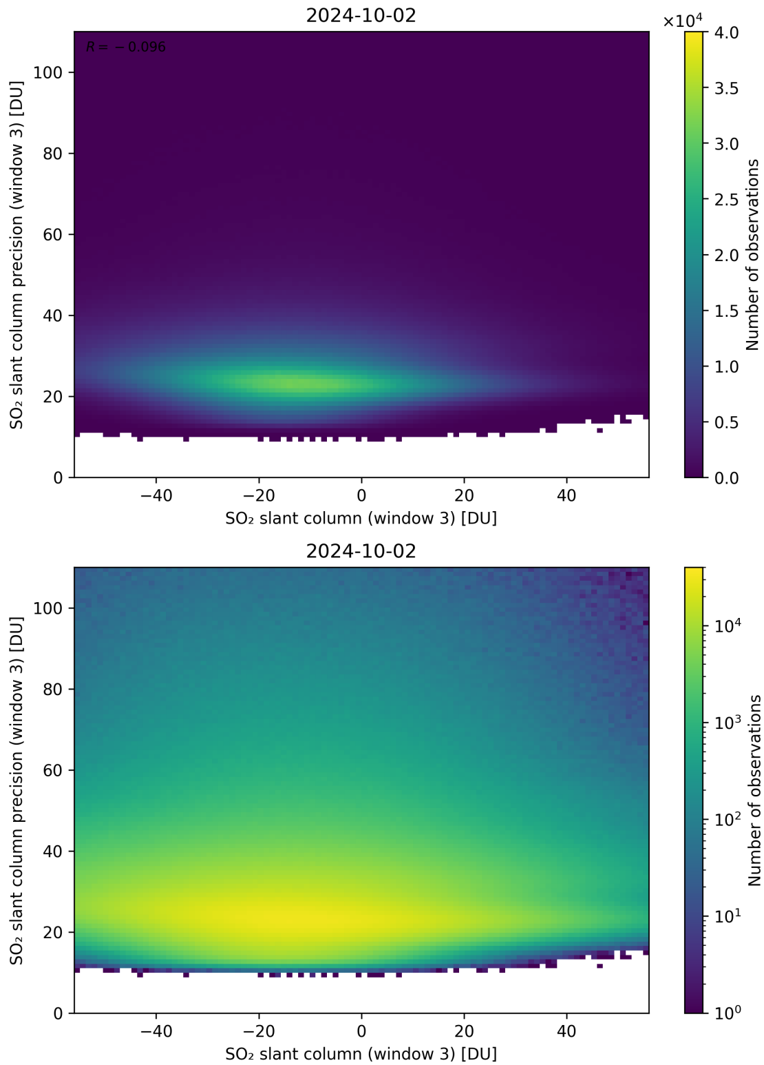
Figure 267: Scatter density plot of “SO 2 slant column (window 3)” against “SO 2 slant column precision (window 3)” for 2024-10-01 to 2024-10-03.
