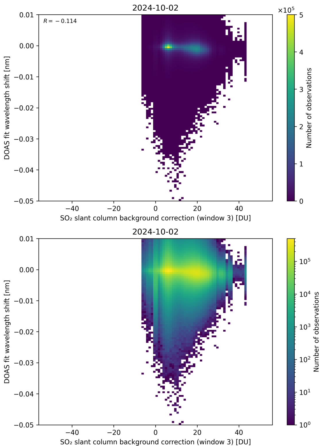
Figure 121: Scatter density plot of “SO 2 slant column background correction (window 3)” against “DOAS fit wavelength shift” for 2024-10-01 to 2024-10-03.
