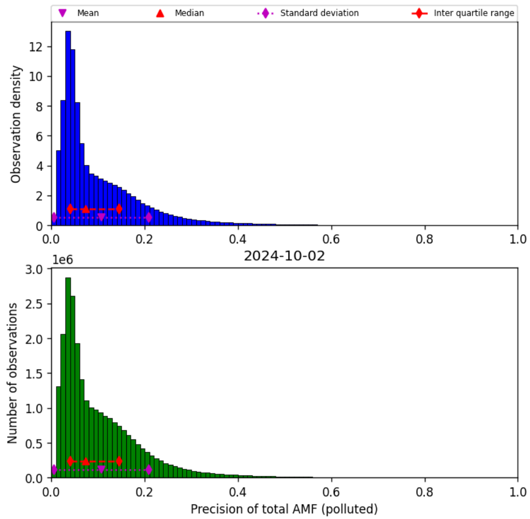
Figure 72: Histogram of “Precision of total AMF (polluted)” for 2024-10-01 to 2024-10-03
