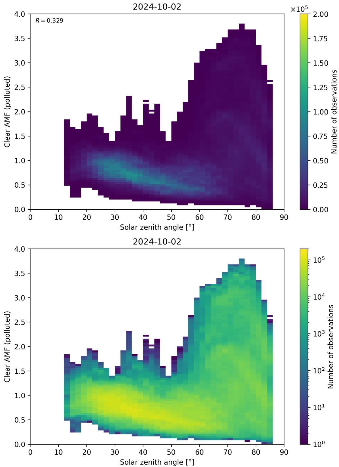
Figure 165: Scatter density plot of “Solar zenith angle” against “Clear AMF (polluted)” for 2024-10-01 to 2024-10-03.
