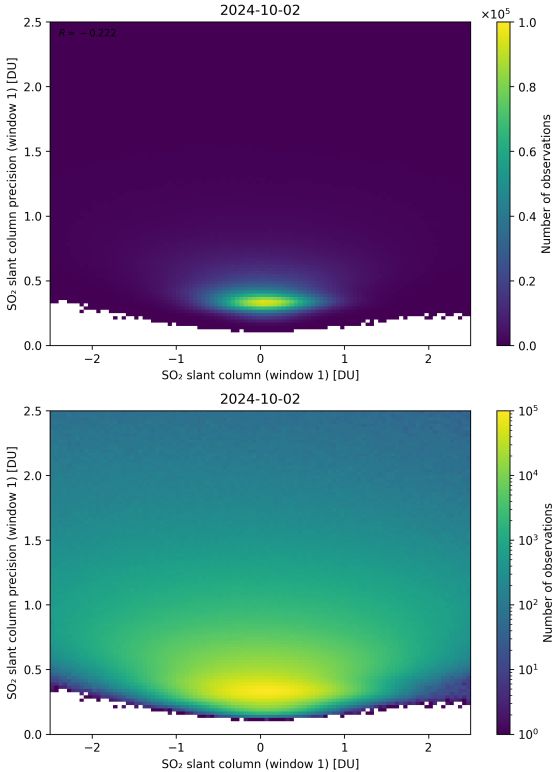
Figure 235: Scatter density plot of “SO 2 slant column (window 1)” against “SO 2 slant column precision (window 1)” for 2024-10-01 to 2024-10-03.
