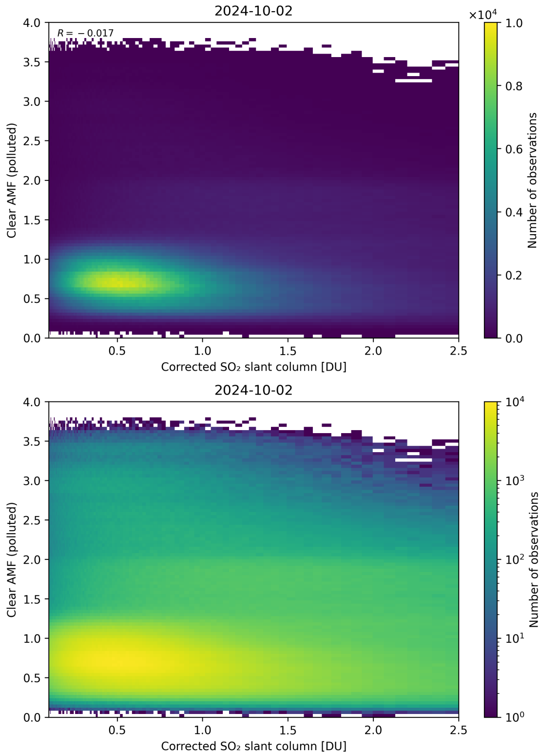
Figure 184: Scatter density plot of “Corrected SO 2 slant column” against “Clear AMF (polluted)” for 2024-10-01 to 2024-10-03.
