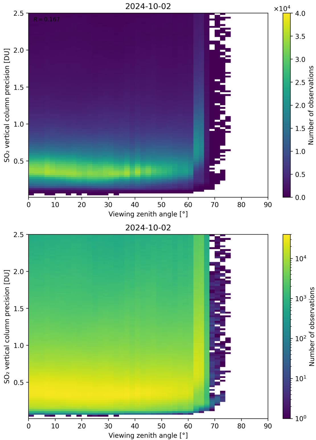
Figure 328: Scatter density plot of “Viewing zenith angle” against “SO 2 vertical column precision” for 2024-10-01 to 2024-10-03.
