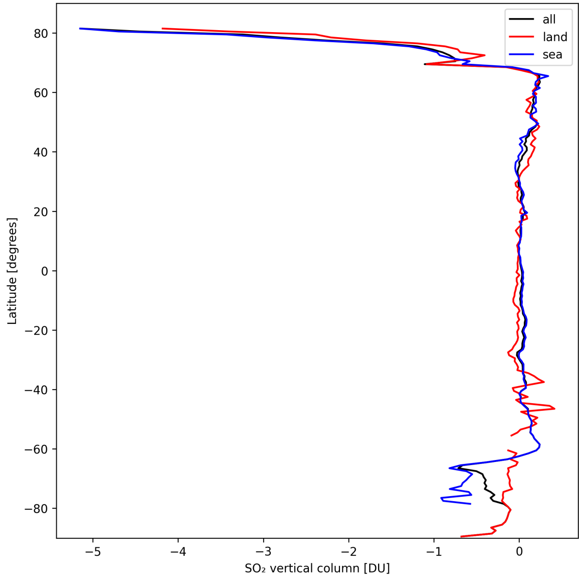
Figure 30: Zonal average of “SO 2 vertical column” for 2024-10-01 to 2024-10-03.
