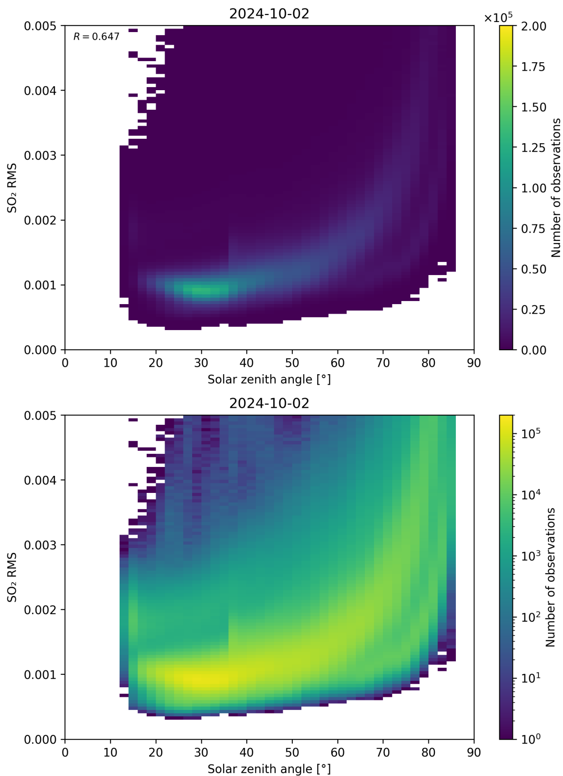
Figure 163: Scatter density plot of “Solar zenith angle” against “SO 2 RMS” for 2024-10-01 to 2024-10-03.
