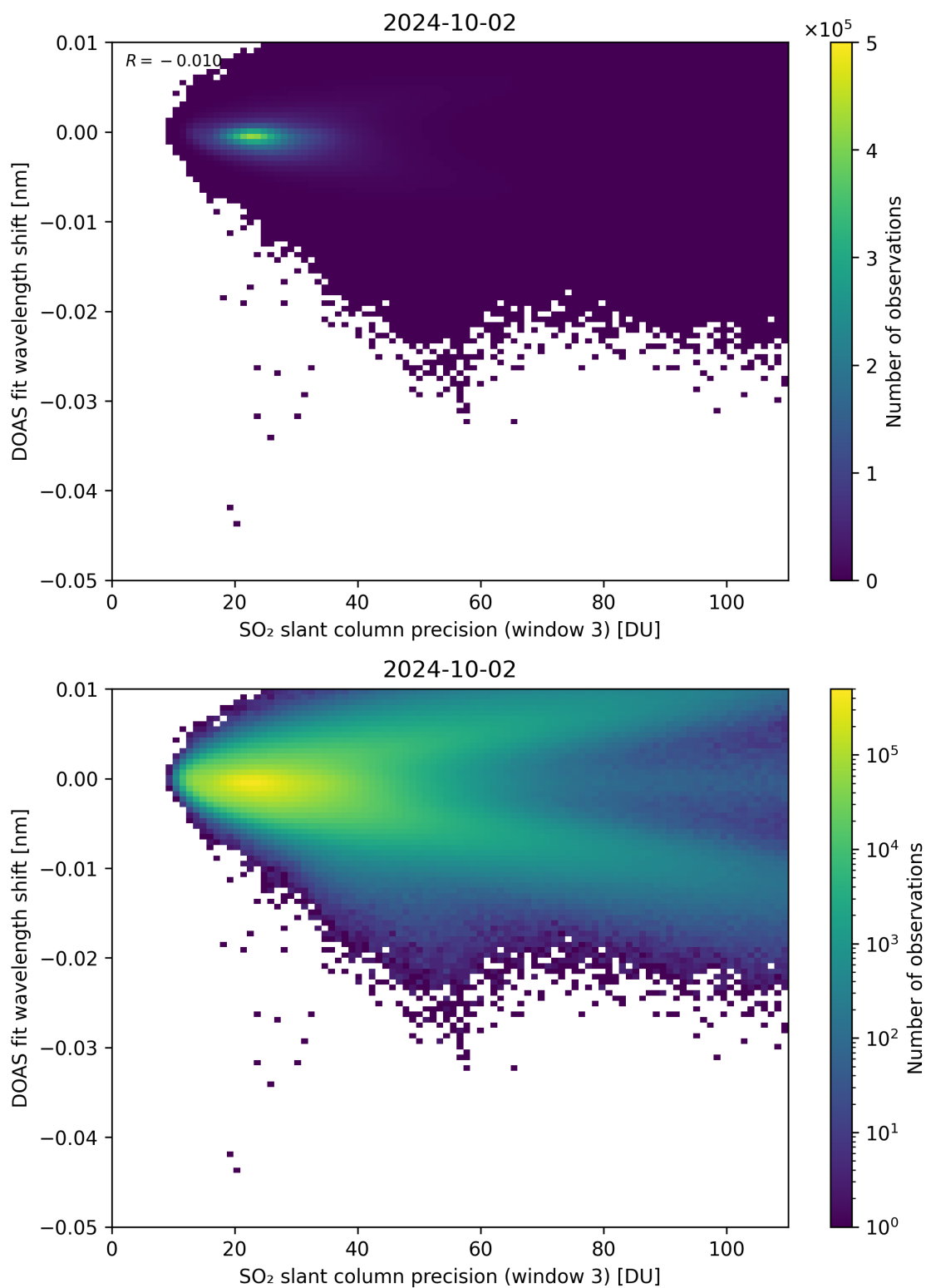
Figure 258: Scatter density plot of “SO 2 slant column precision (window 3)” against “DOAS fit wavelength shift” for 2024-10-01 to 2024-10-03.
