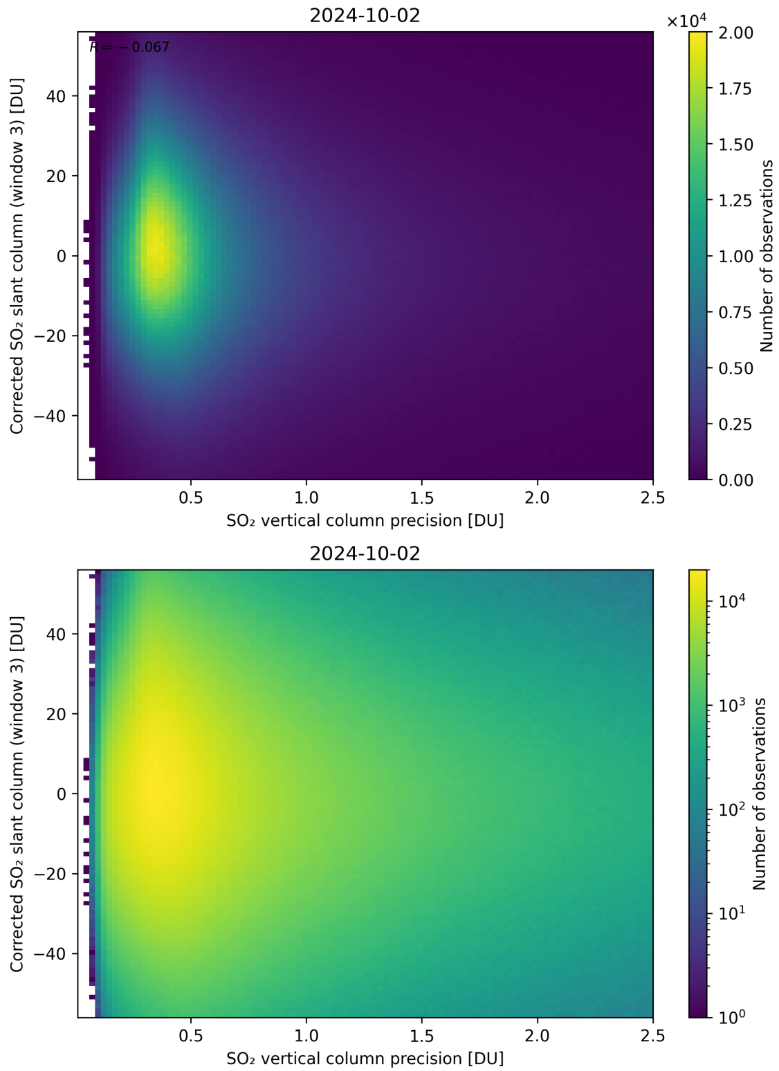
Figure 288: Scatter density plot of “SO 2 vertical column precision” against “Corrected SO 2 slant column (window 3)” for 2024-10-01 to 2024-10-03.
