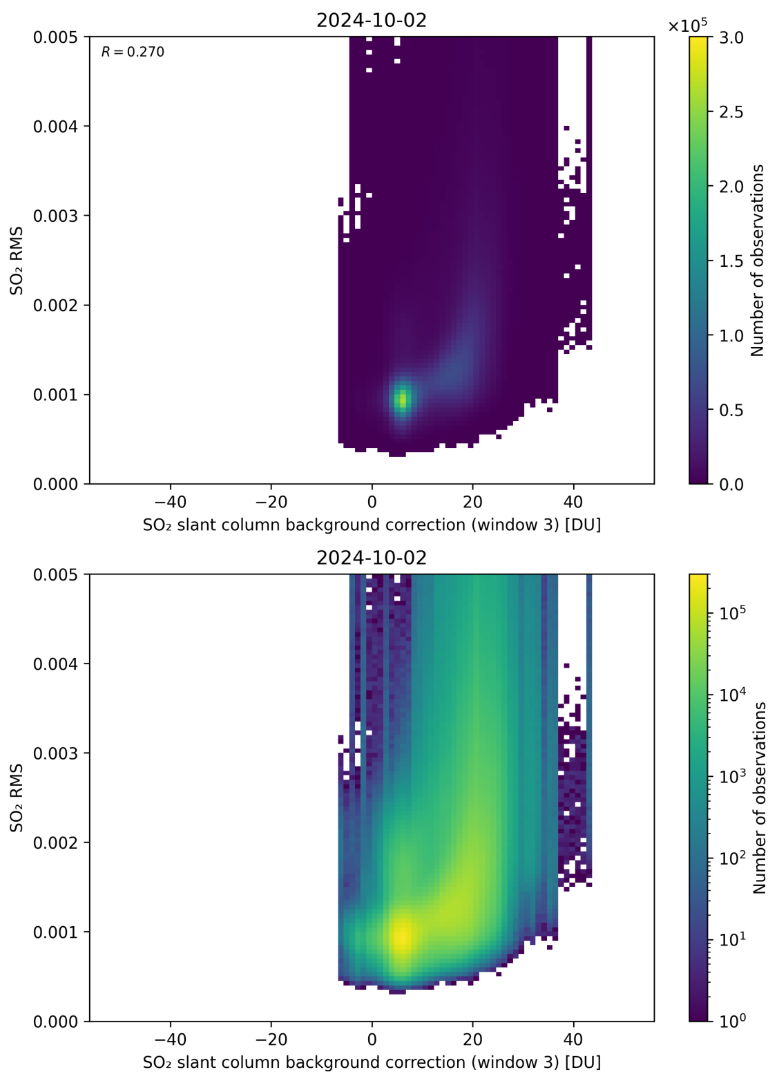
Figure 123: Scatter density plot of “SO 2 slant column background correction (window 3)” against “SO 2 RMS” for 2024-10-01 to 2024-10-03.
