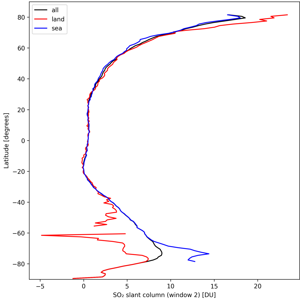
Figure 37: Zonal average of “SO 2 slant column (window 2)” for 2024-10-01 to 2024-10-03.
