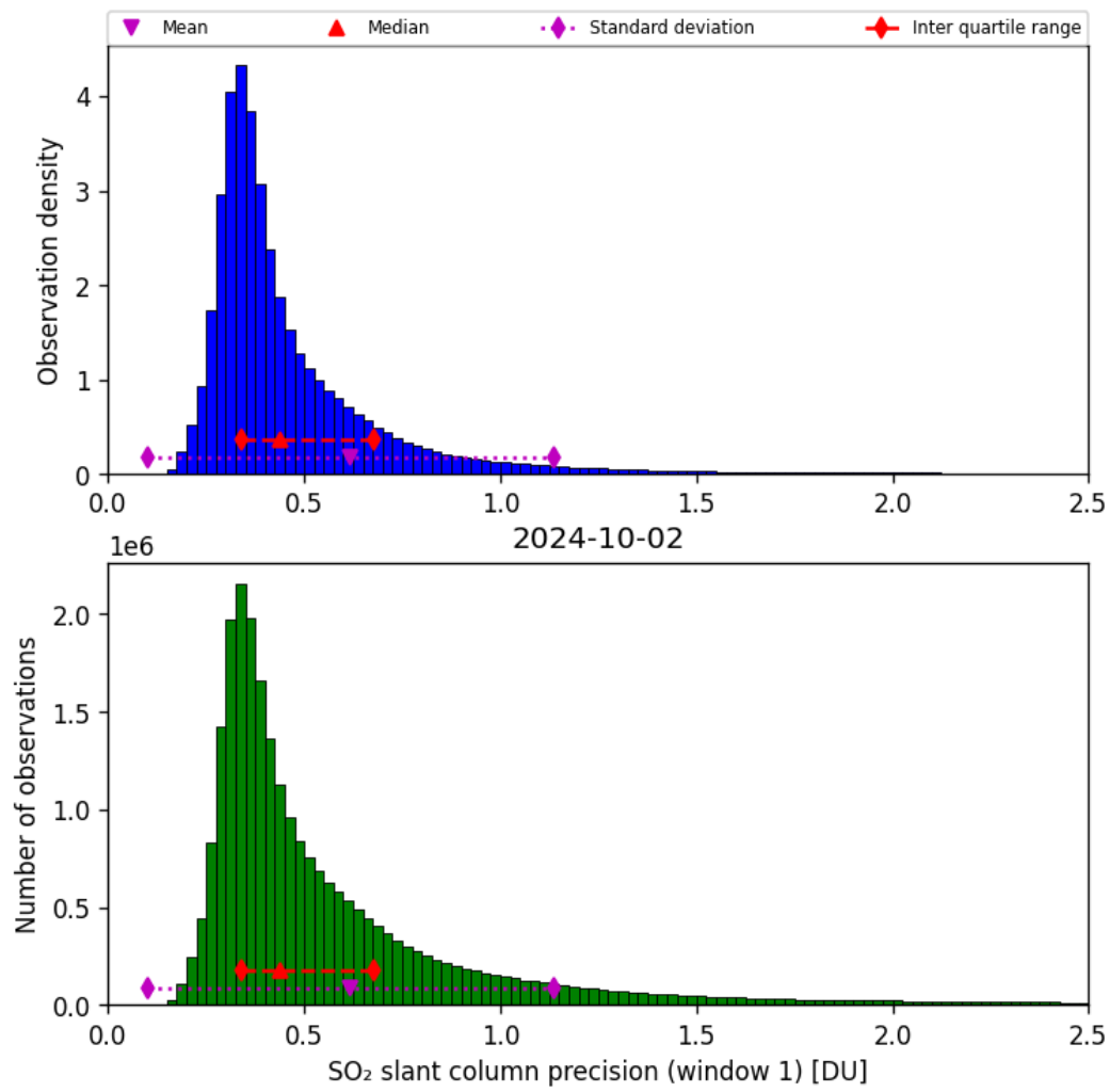
Figure 57: Histogram of “SO 2 slant column precision (window 1)” for 2024-10-01 to 2024-10-03
