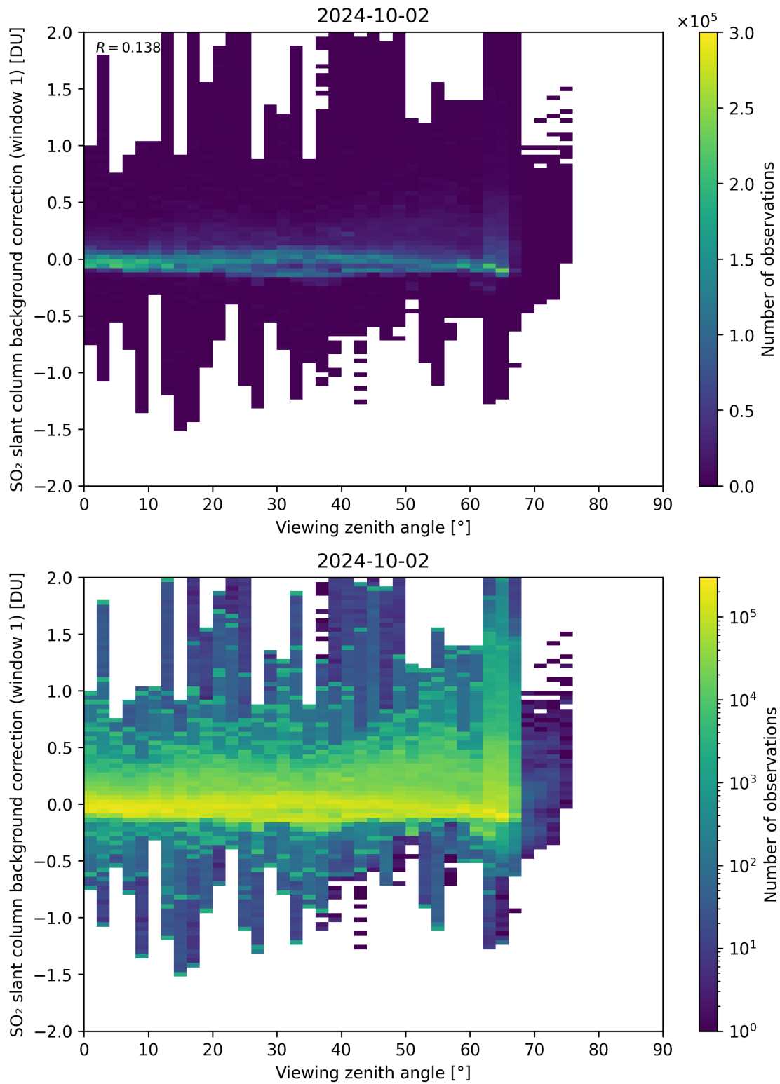
Figure 308: Scatter density plot of “Viewing zenith angle” against “SO 2 slant column background correction (window 1)” for 2024-10-01 to 2024-10-03.
