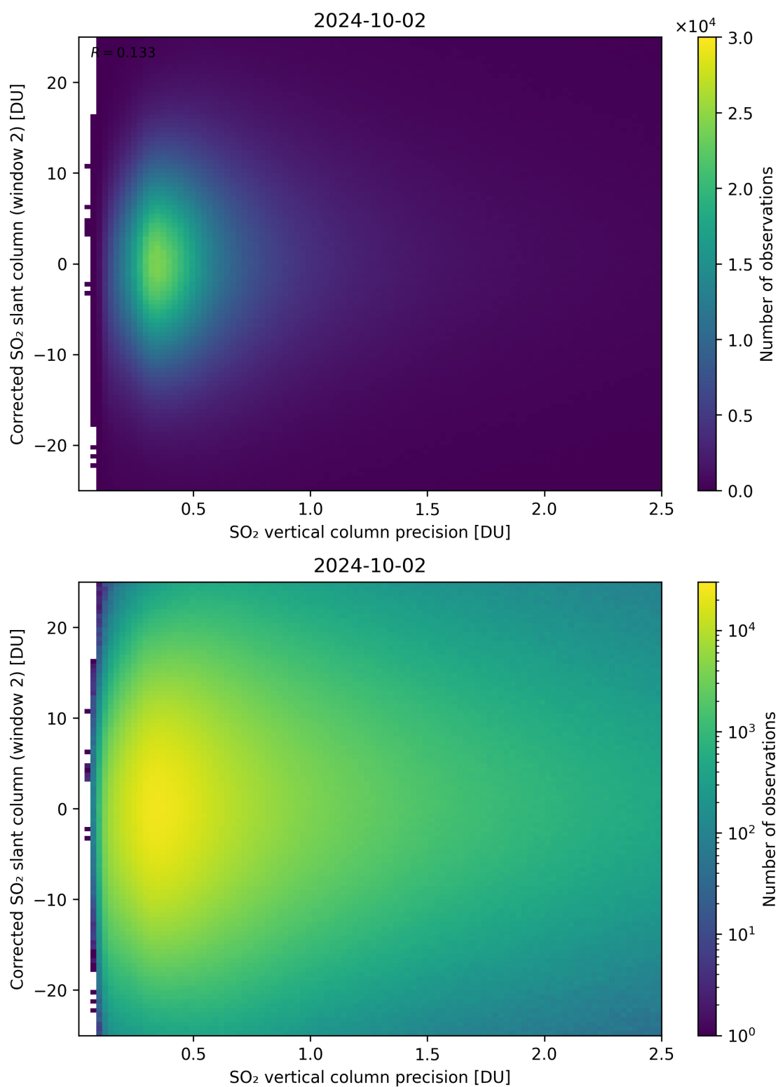
Figure 287: Scatter density plot of “SO 2 vertical column precision” against “Corrected SO 2 slant column (window 2)” for 2024-10-01 to 2024-10-03.
