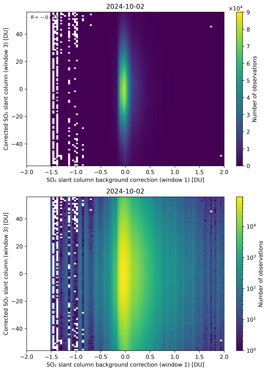
Figure 105: Scatter density plot of “SO 2 slant column background correction (window 1)” against “Corrected SO 2 slant column (window 3)” for 2024-10-01 to 2024-10-03.
