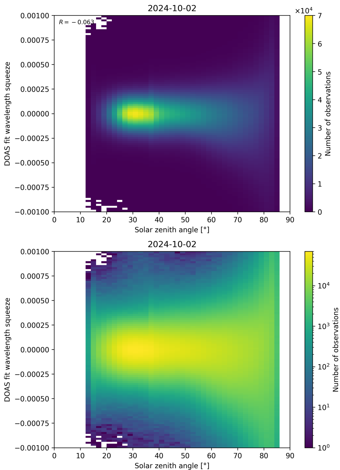
Figure 162: Scatter density plot of “Solar zenith angle” against “DOAS fit wavelength squeeze” for 2024-10-01 to 2024-10-03.
