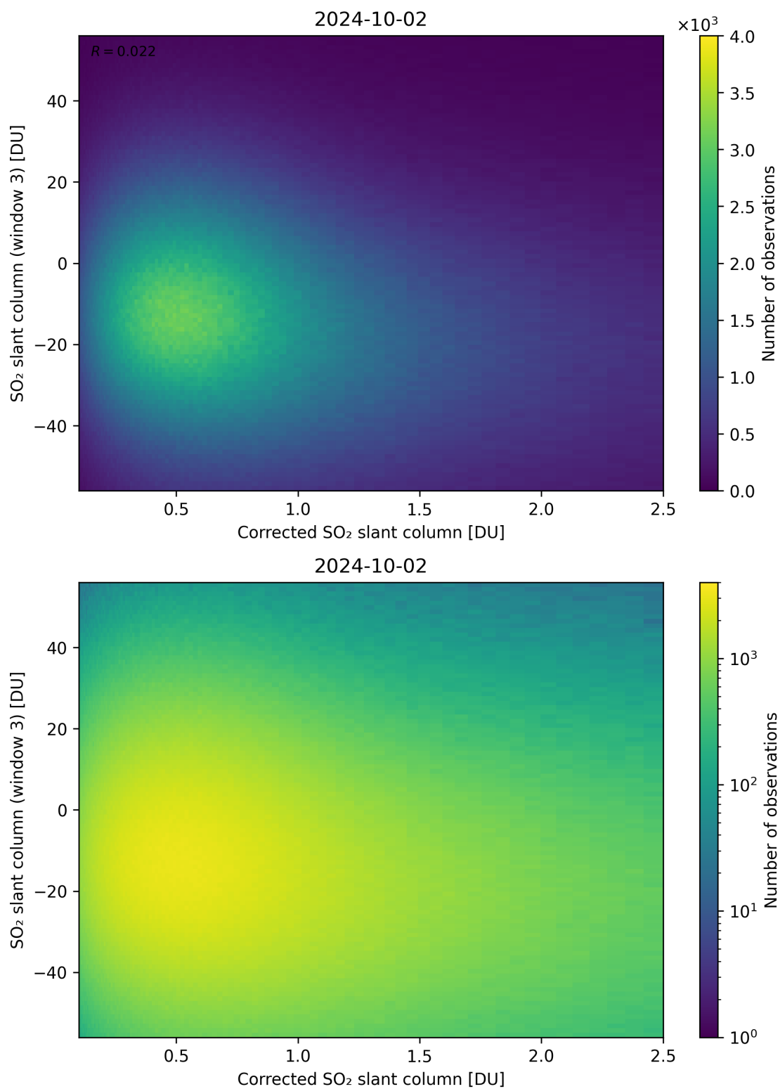
Figure 190: Scatter density plot of “Corrected SO 2 slant column” against “SO 2 slant column (window 3)” for 2024-10-01 to 2024-10-03.
