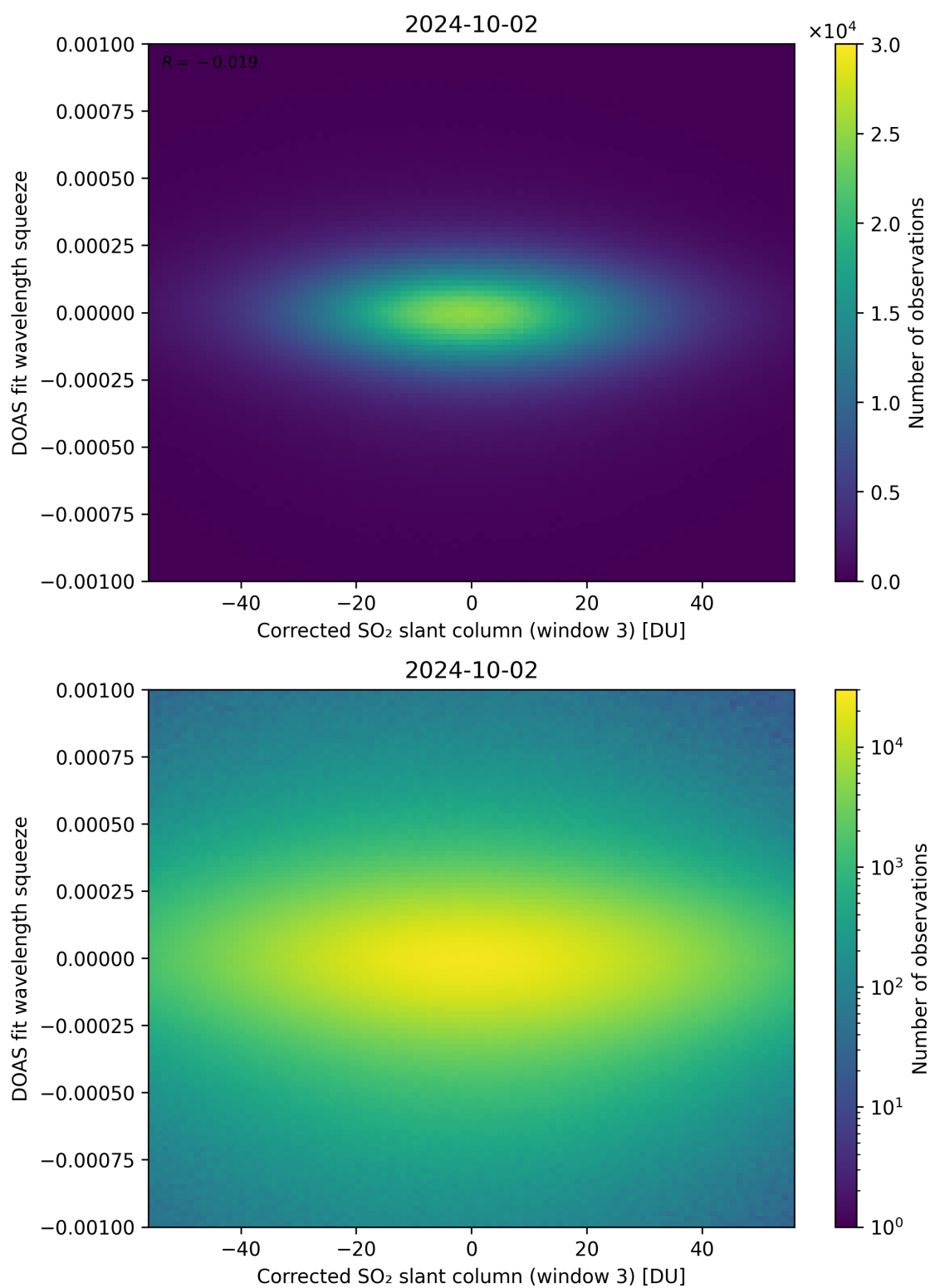
Figure 207: Scatter density plot of “Corrected SO 2 slant column (window 3)” against “DOAS fit wavelength squeeze” for 2024-10-01 to 2024-10-03.
