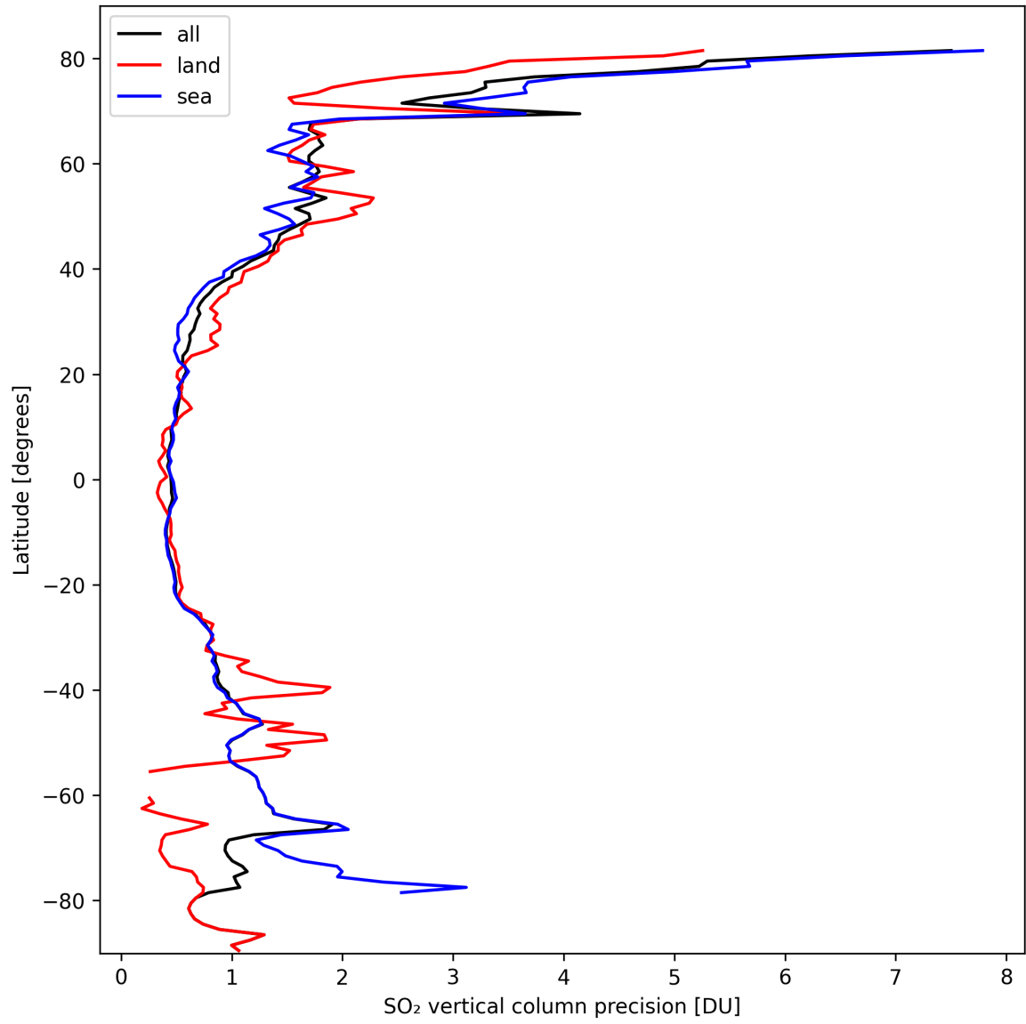
Figure 31: Zonal average of “SO 2 vertical column precision” for 2024-10-01 to 2024-10-03.
