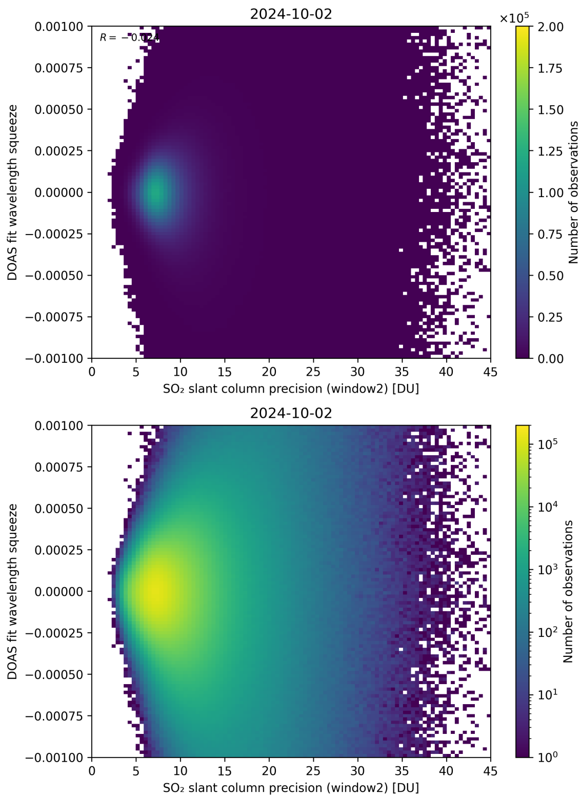
Figure 244: Scatter density plot of “SO 2 slant column precision (window2)” against “DOAS fit wavelength squeeze” for 2024-10-01 to 2024-10-03.
