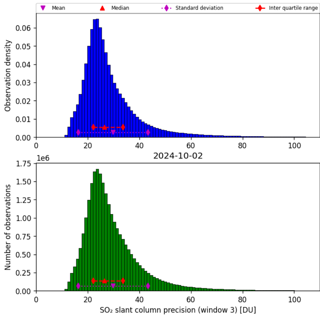
Figure 65: Histogram of “SO 2 slant column precision (window 3)” for 2024-10-01 to 2024-10-03
