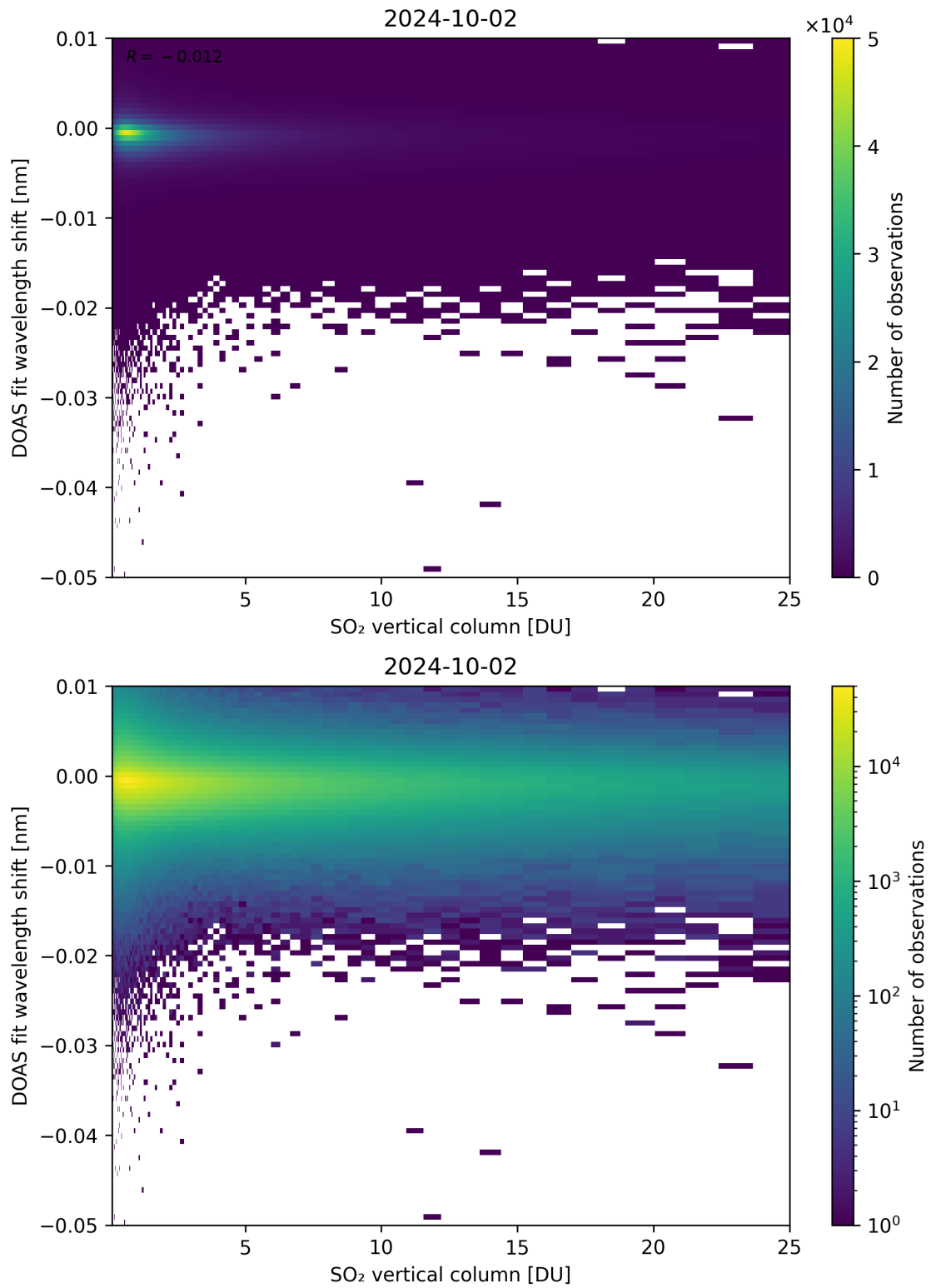
Figure 276: Scatter density plot of “SO 2 vertical column” against “DOAS fit wavelength shift” for 2024-10-01 to 2024-10-03.
