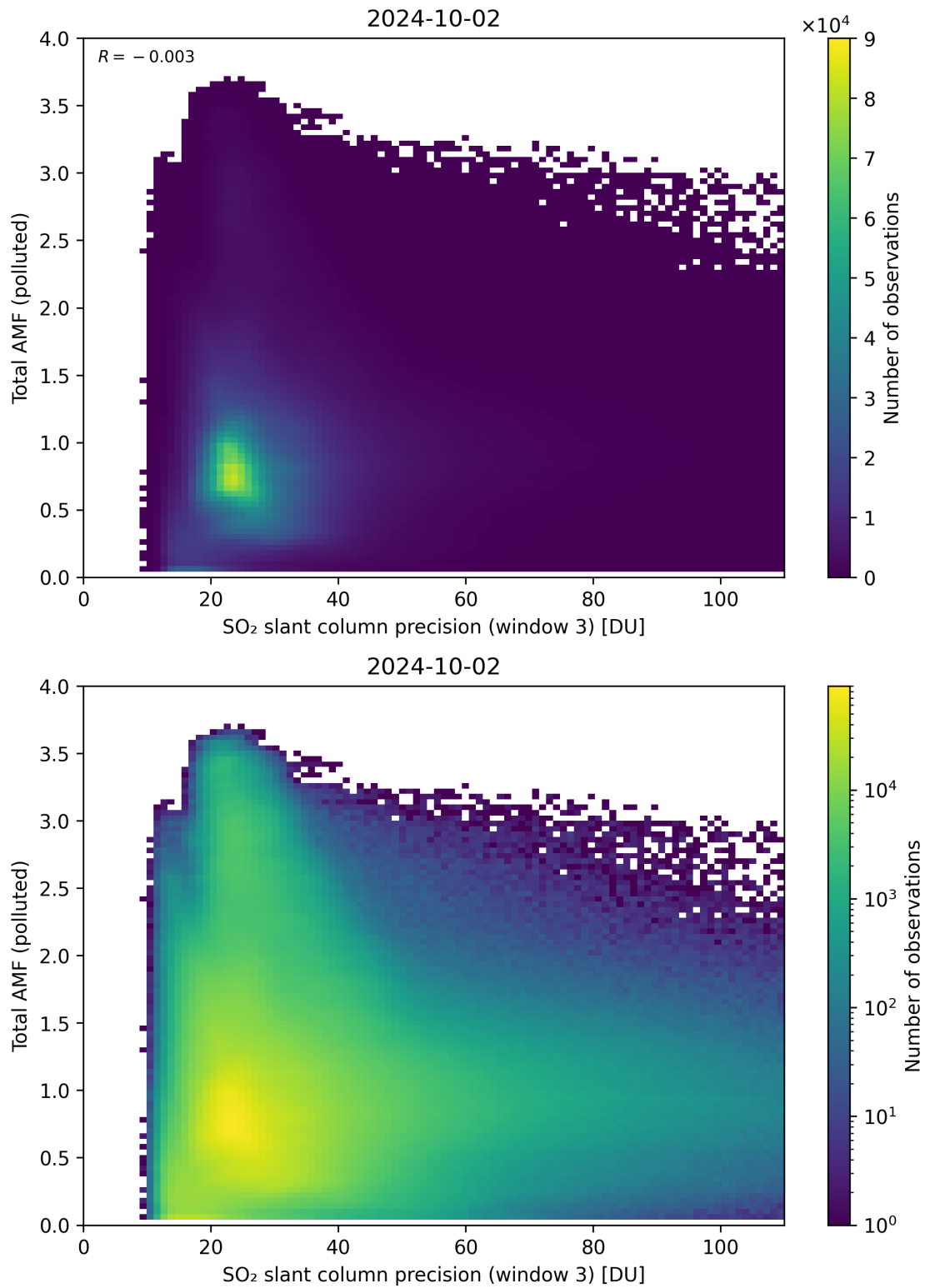
Figure 263: Scatter density plot of “SO 2 slant column precision (window 3)” against “Total AMF (polluted)” for 2024-10-01 to 2024-10-03.
