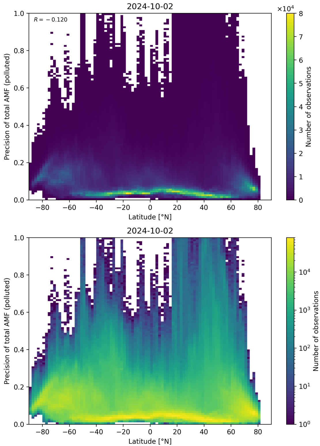
Figure 155: Scatter density plot of “Latitude” against “Precision of total AMF (polluted)” for 2024-10-01 to 2024-10-03.
