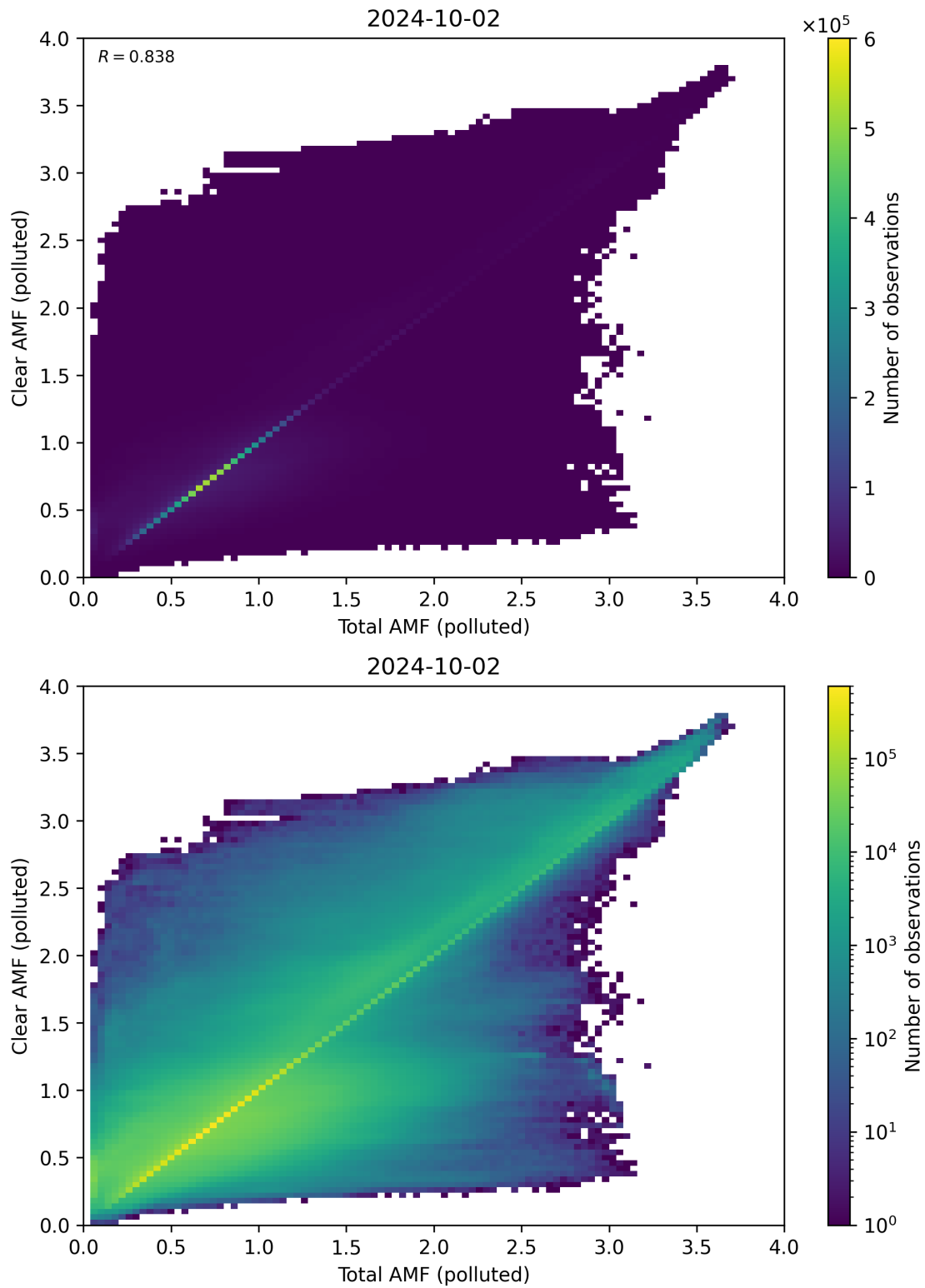
Figure 271: Scatter density plot of “Total AMF (polluted)” against “Clear AMF (polluted)” for 2024-10-01 to 2024-10-03.
