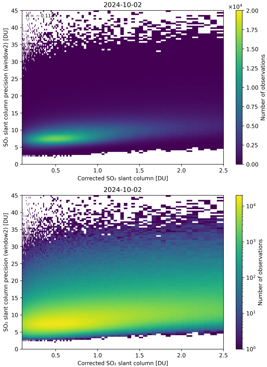
Figure 189: Scatter density plot of “Corrected SO 2 slant column” against “SO 2 slant column precision (window2)” for 2024-10-01 to 2024-10-03.
