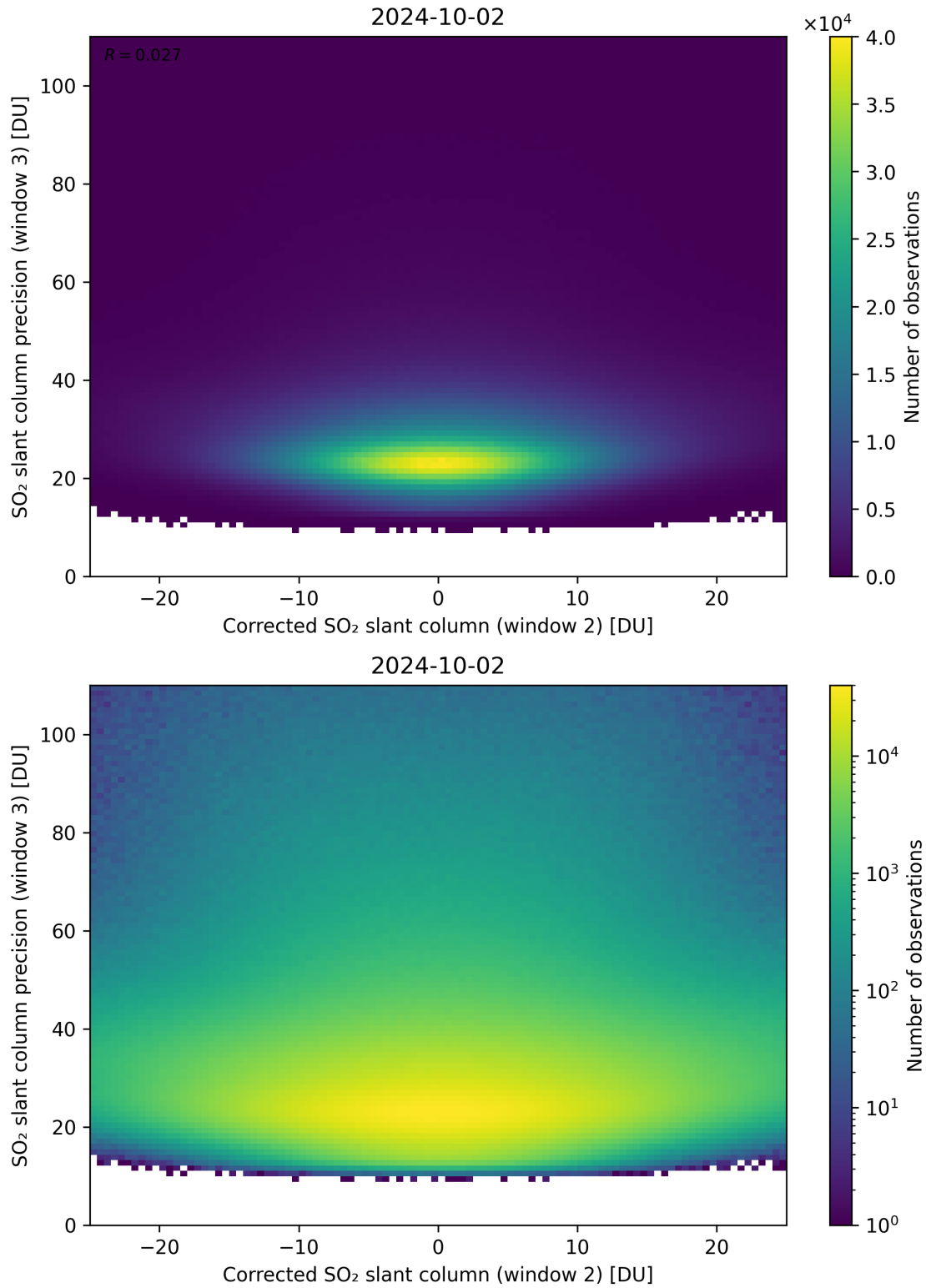
Figure 202: Scatter density plot of “Corrected SO 2 slant column (window 2)” against “SO 2 slant column precision (window 3)” for 2024-10-01 to 2024-10-03.
