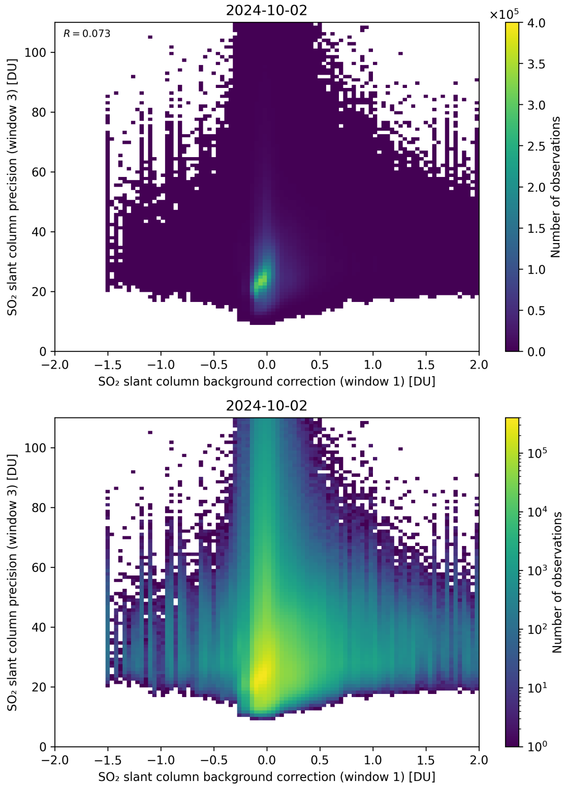
Figure 108: Scatter density plot of “SO 2 slant column background correction (window 1)” against “SO 2 slant column precision (window 3)” for 2024-10-01 to 2024-10-03.
