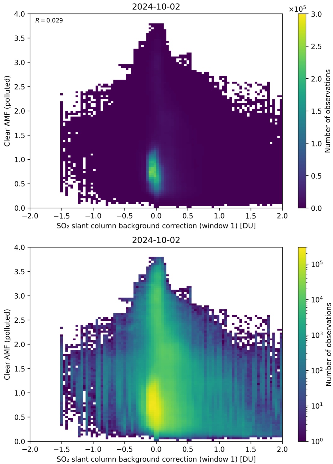
Figure 103: Scatter density plot of “SO 2 slant column background correction (window 1)” against “Clear AMF (polluted)” for 2024-10-01 to 2024-10-03.
