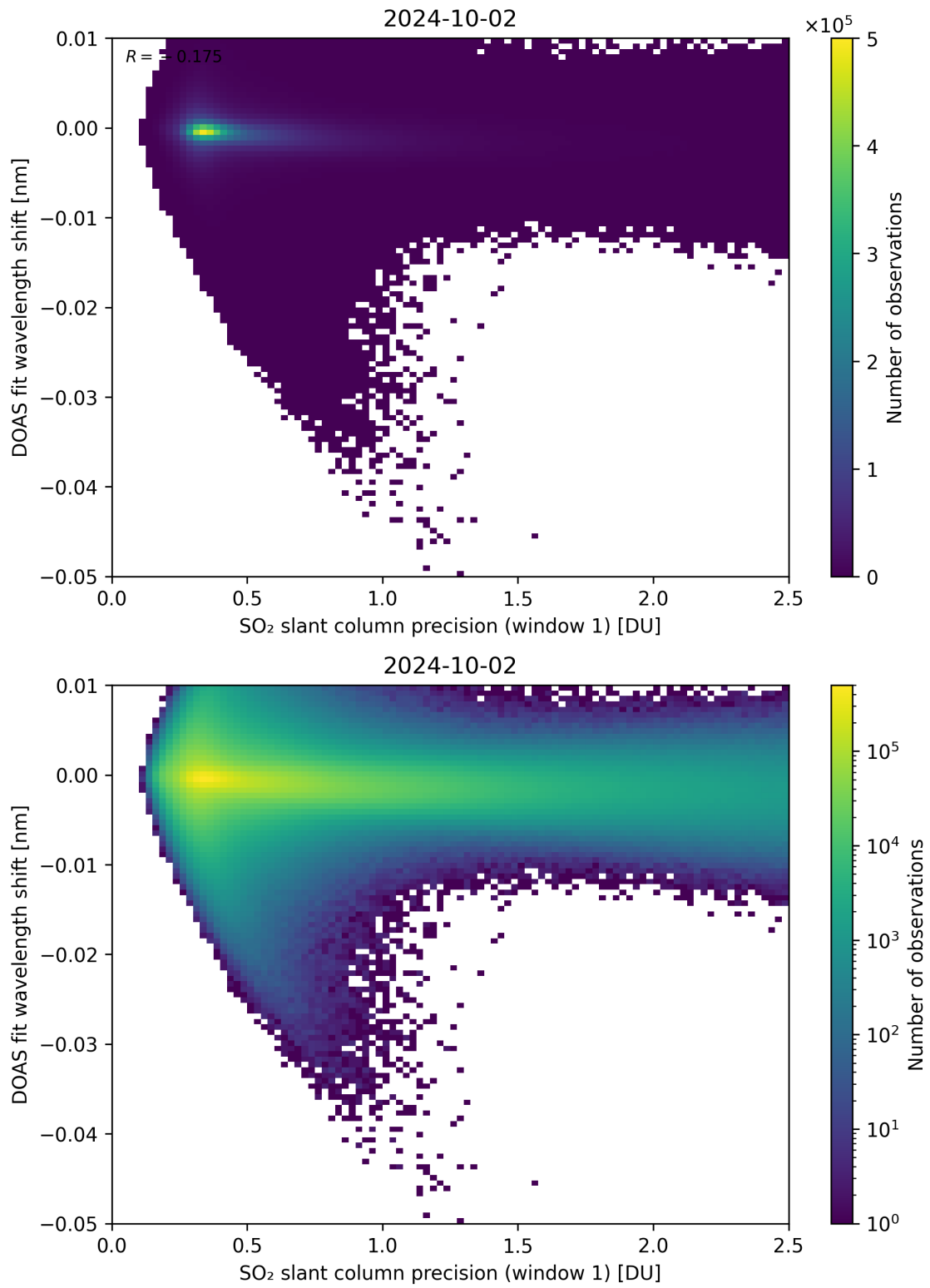
Figure 221: Scatter density plot of “SO 2 slant column precision (window 1)” against “DOAS fit wavelength shift” for 2024-10-01 to 2024-10-03.
