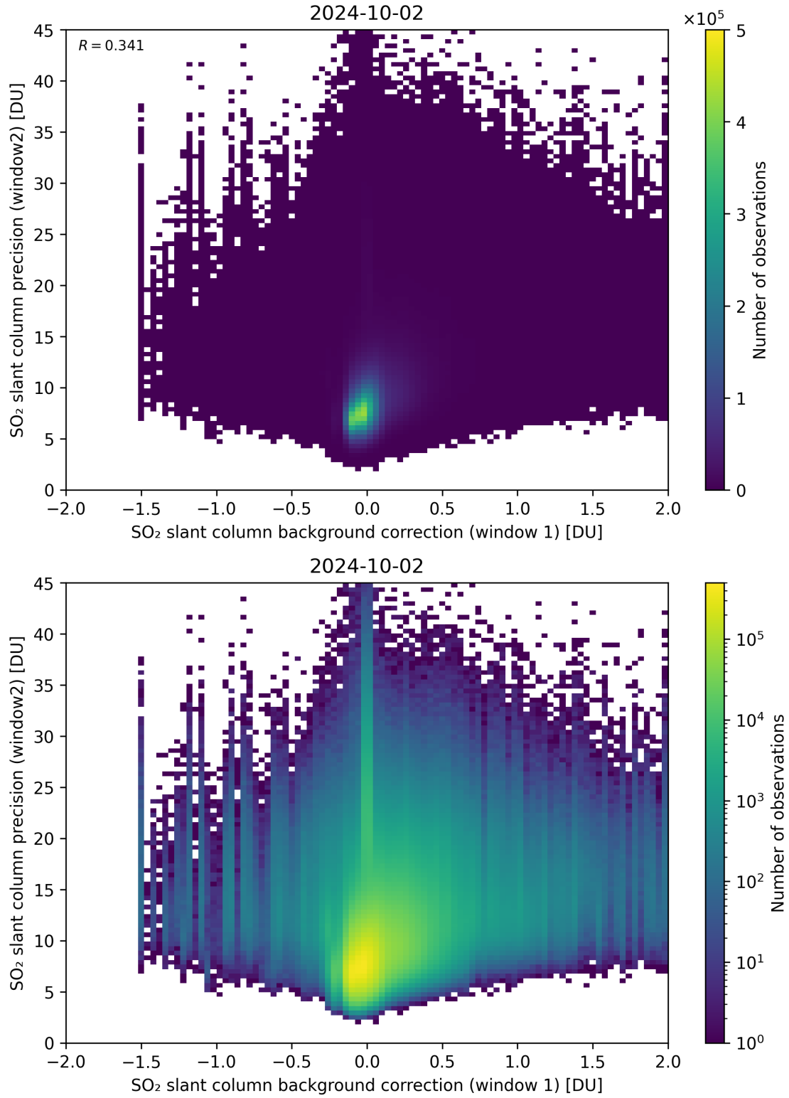
Figure 106: Scatter density plot of “SO 2 slant column background correction (window 1)” against “SO 2 slant column precision (window2)” for 2024-10-01 to 2024-10-03.
