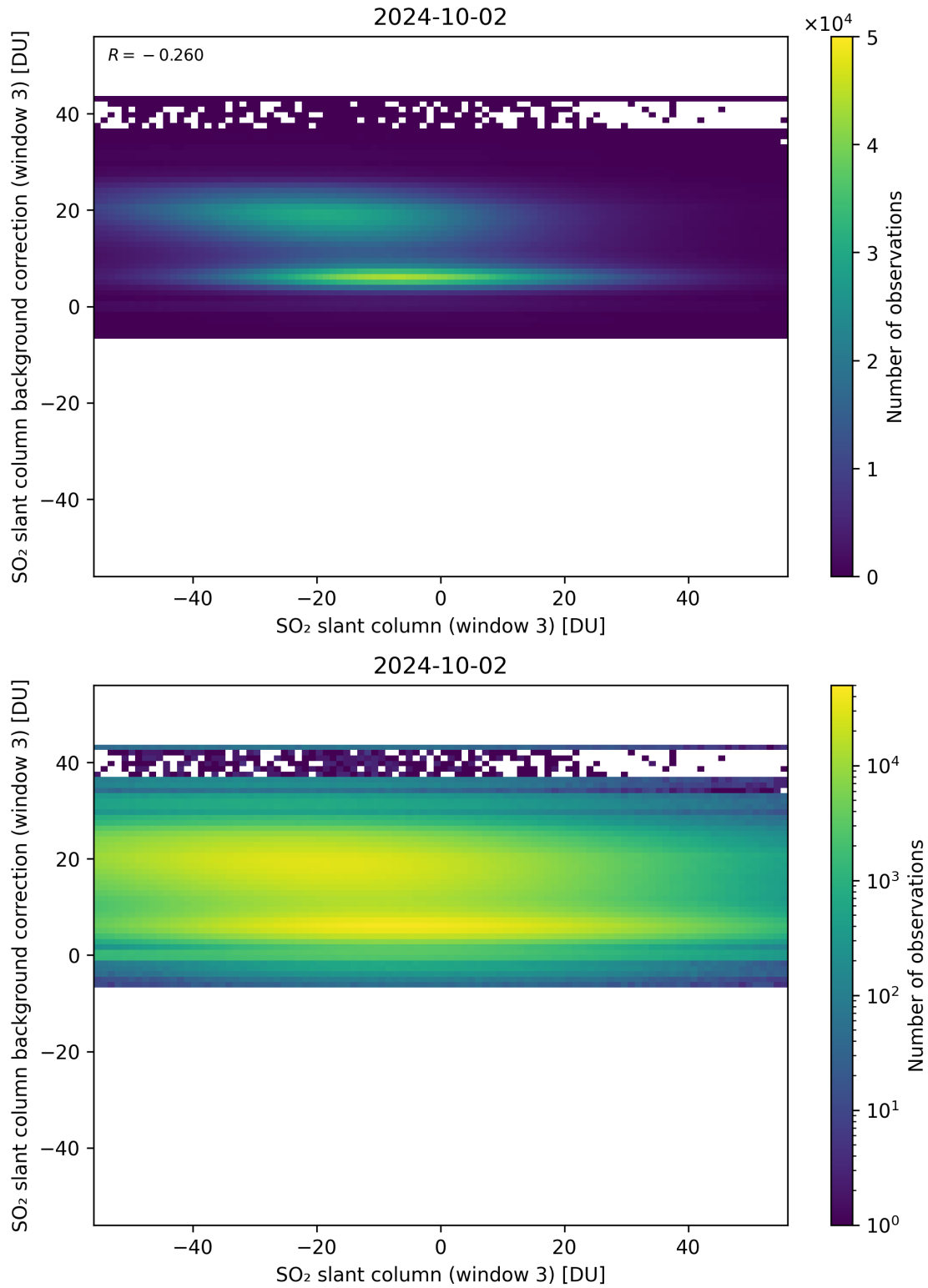
Figure 253: Scatter density plot of “SO 2 slant column (window 3)” against “SO 2 slant column background correction (window 3)” for 2024-10-01 to 2024-10-03.
