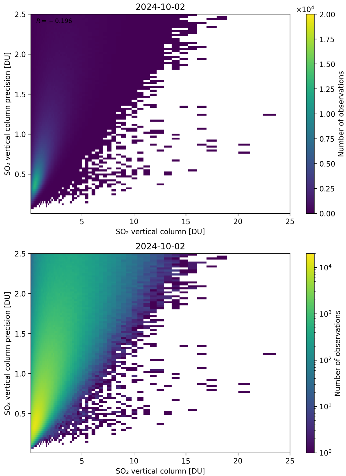
Figure 307: Scatter density plot of “SO 2 vertical column” against “SO 2 vertical column precision” for 2024-10-01 to 2024-10-03.
