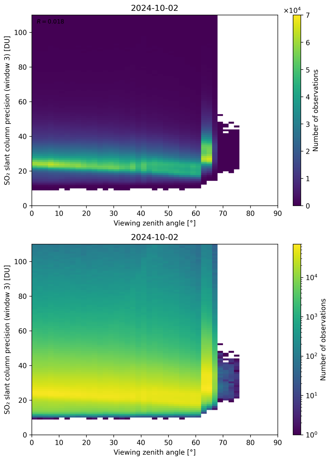
Figure 324: Scatter density plot of “Viewing zenith angle” against “SO 2 slant column precision (window 3)” for 2024-10-01 to 2024-10-03.
