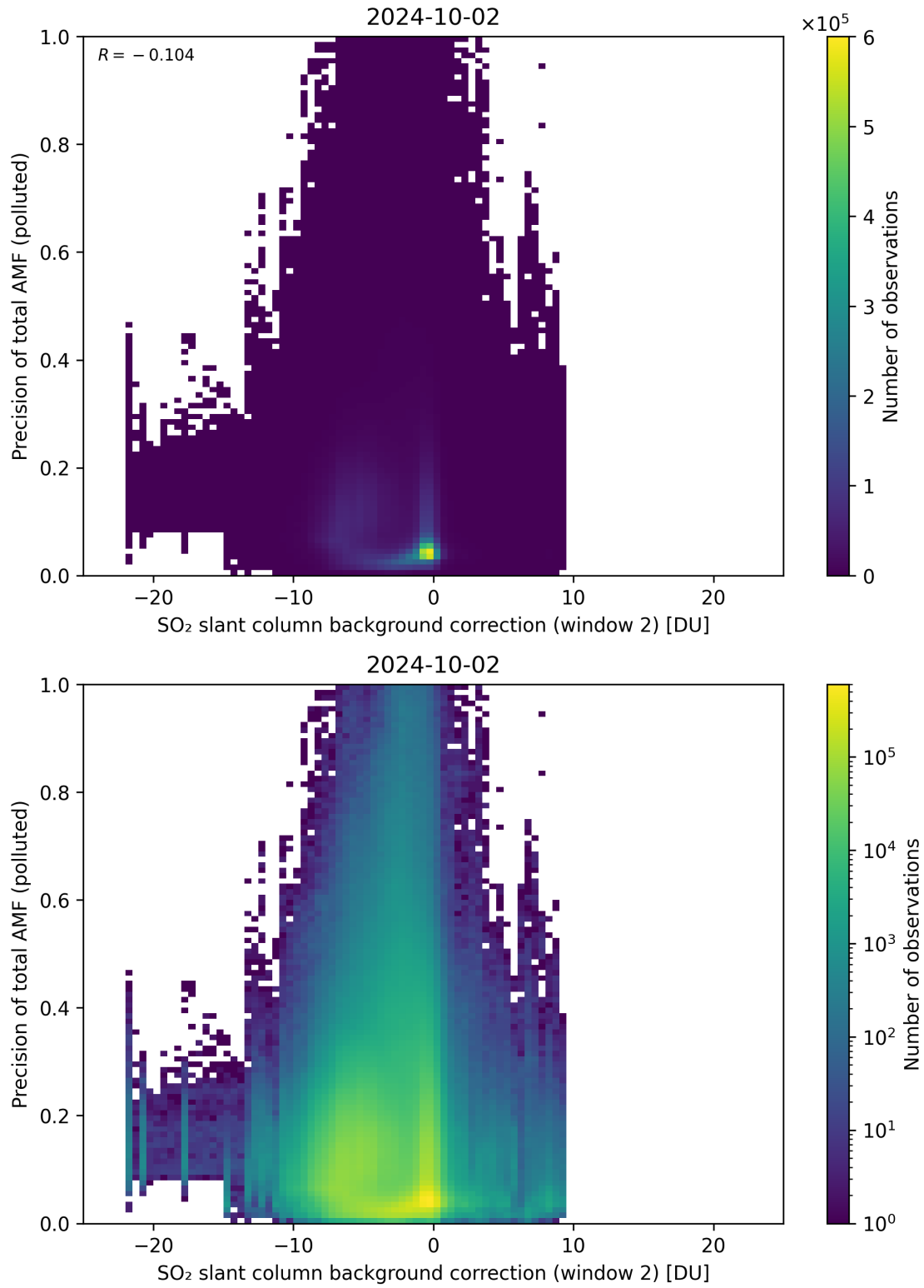
Figure 120: Scatter density plot of “SO 2 slant column background correction (window 2)” against “Precision of total AMF (polluted)” for 2024-10-01 to 2024-10-03.
