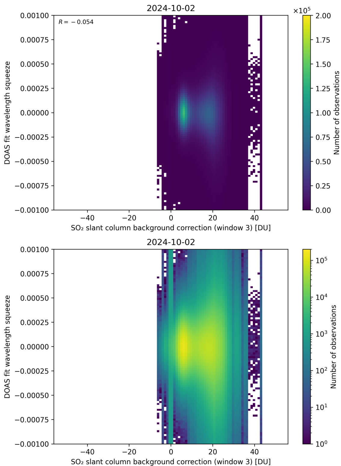
Figure 122: Scatter density plot of “SO 2 slant column background correction (window 3)” against “DOAS fit wavelength squeeze” for 2024-10-01 to 2024-10-03.
