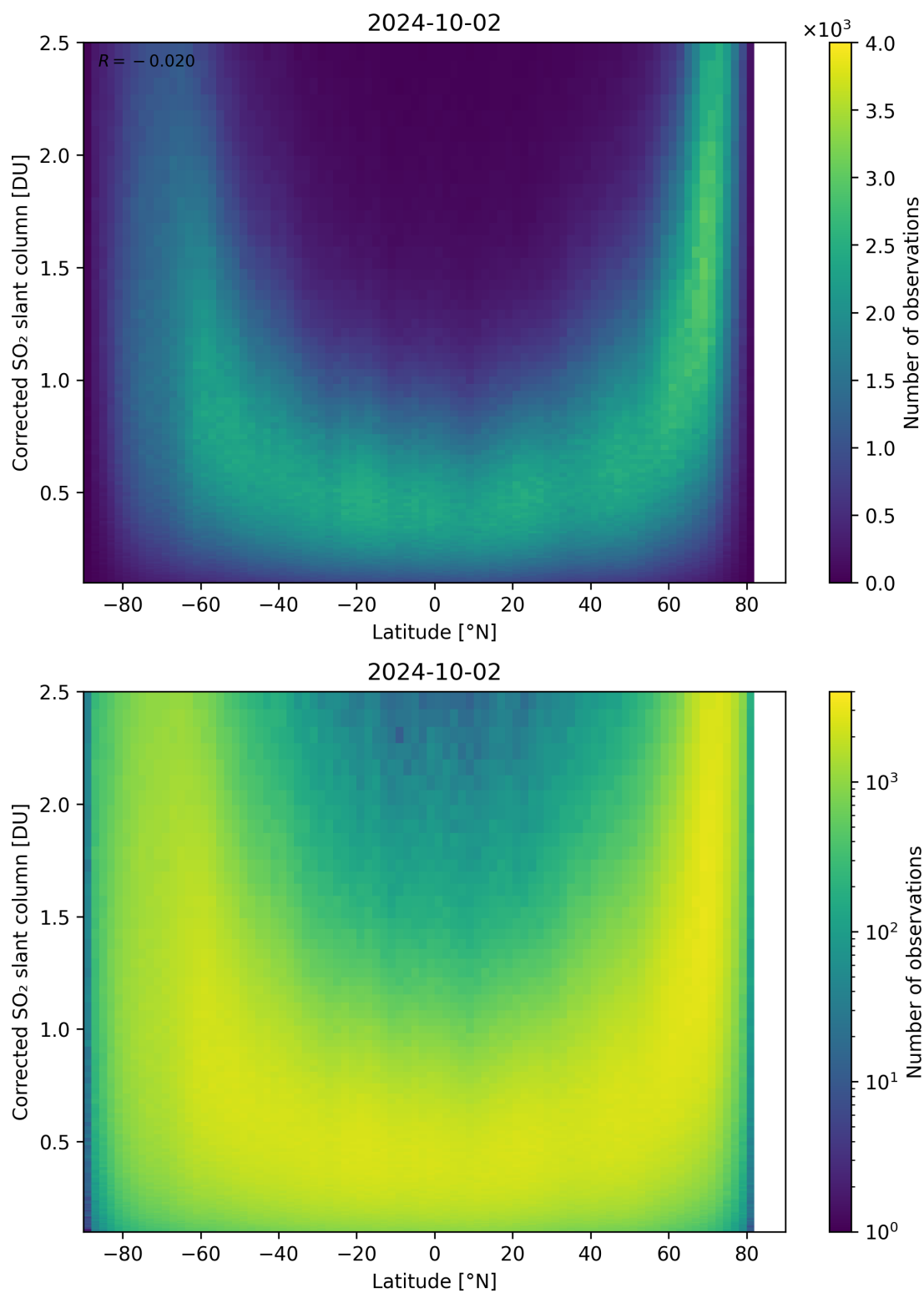
Figure 146: Scatter density plot of “Latitude” against “Corrected SO 2 slant column” for 2024-10-01 to 2024-10-03.
