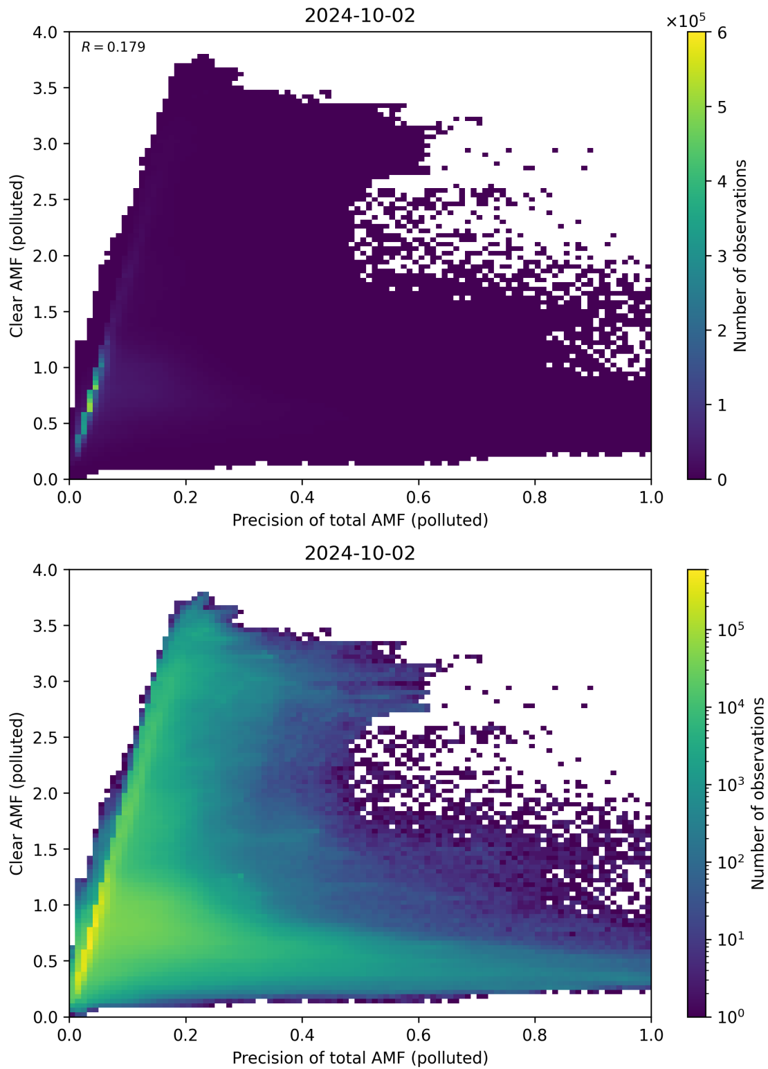
Figure 270: Scatter density plot of “Precision of total AMF (polluted)” against “Clear AMF (polluted)” for 2024-10-01 to 2024-10-03.
