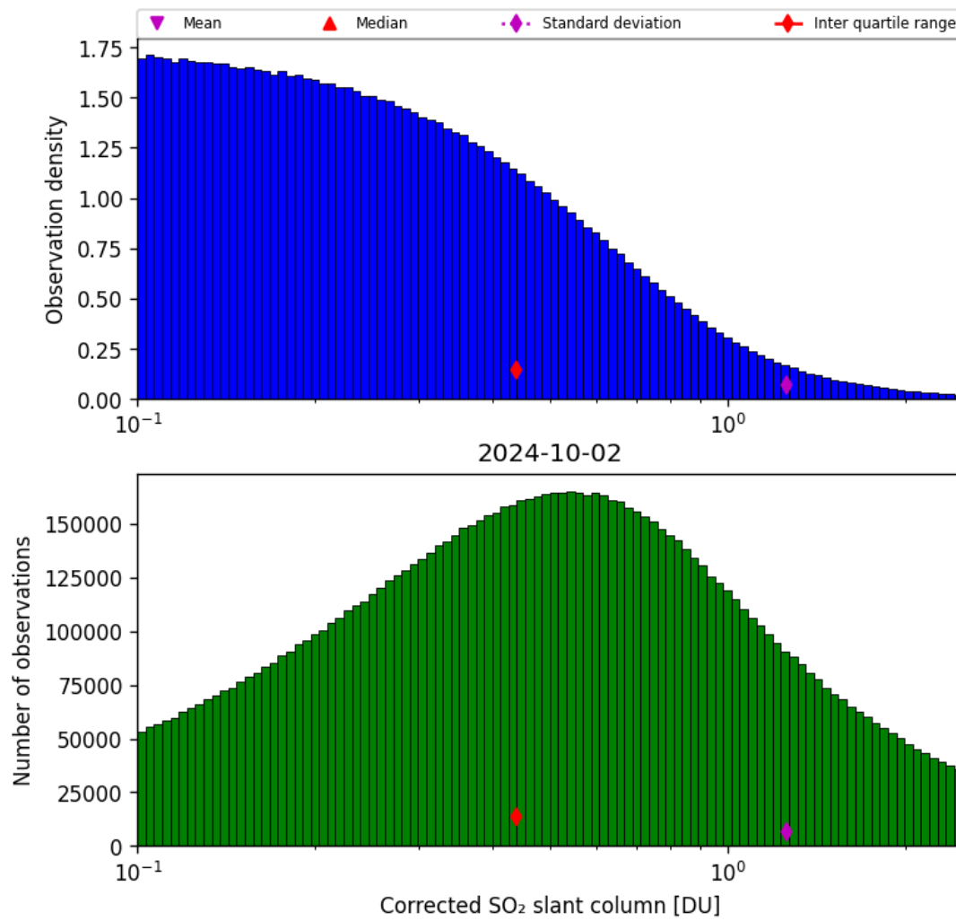
Figure 55: Histogram of “Corrected SO 2 slant column” for 2024-10-01 to 2024-10-03
