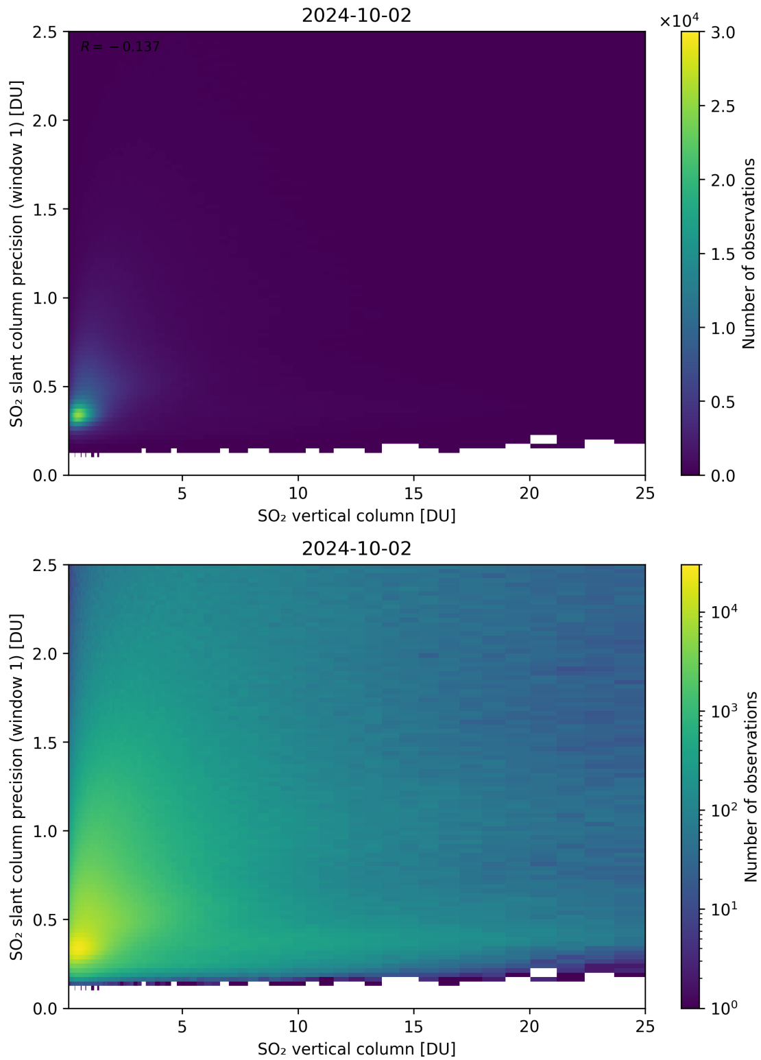
Figure 301: Scatter density plot of “SO 2 vertical column” against “SO 2 slant column precision (window 1)” for 2024-10-01 to 2024-10-03.
