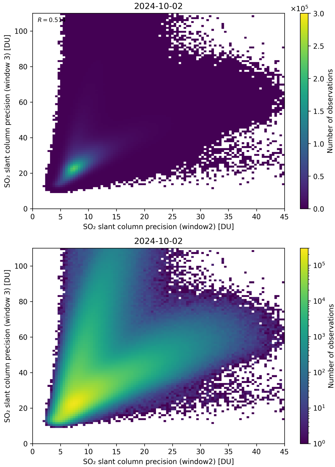
Figure 250: Scatter density plot of “SO 2 slant column precision (window2)” against “SO 2 slant column precision (window 3)” for 2024-10-01 to 2024-10-03.
