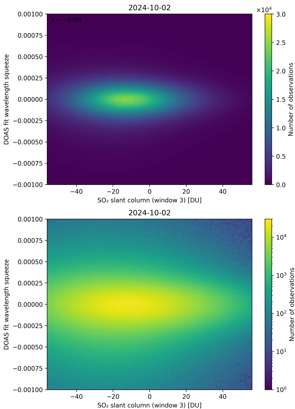
Figure 255: Scatter density plot of “SO 2 slant column (window 3)” against “DOAS fit wavelength squeeze” for 2024-10-01 to 2024-10-03.
