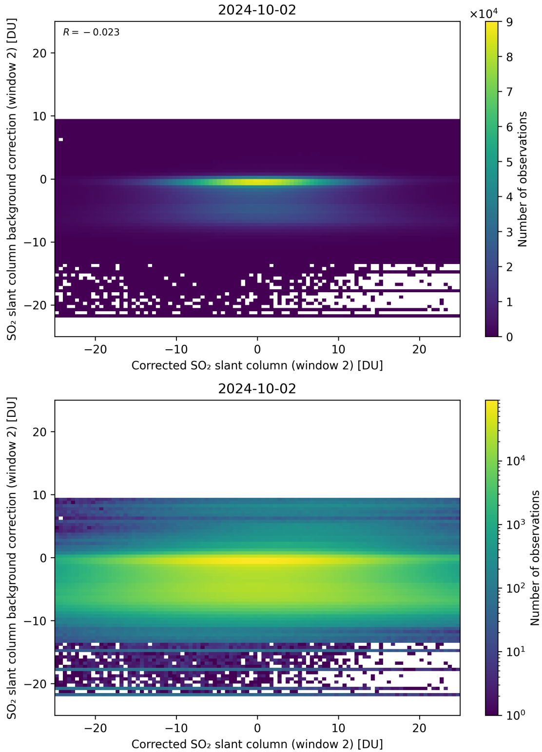
Figure 194: Scatter density plot of “Corrected SO 2 slant column (window 2)” against “SO 2 slant column background correction (window 2)” for 2024-10-01 to 2024-10-03.
