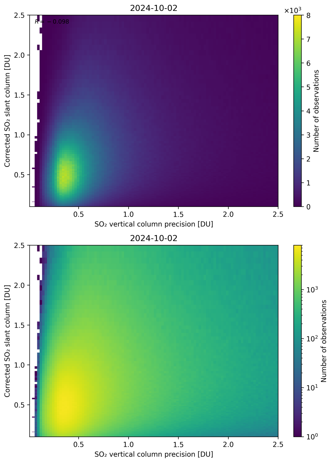
Figure 286: Scatter density plot of “SO 2 vertical column precision” against “Corrected SO 2 slant column” for 2024-10-01 to 2024-10-03.
