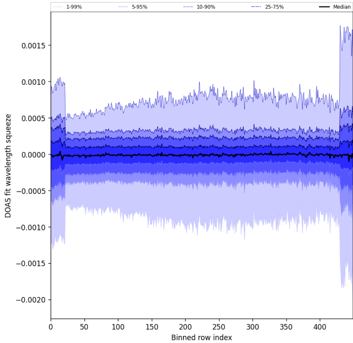
Figure 92: Along track statistics of “DOAS fit wavelength squeeze” for 2024-10-01 to 2024-10-03
