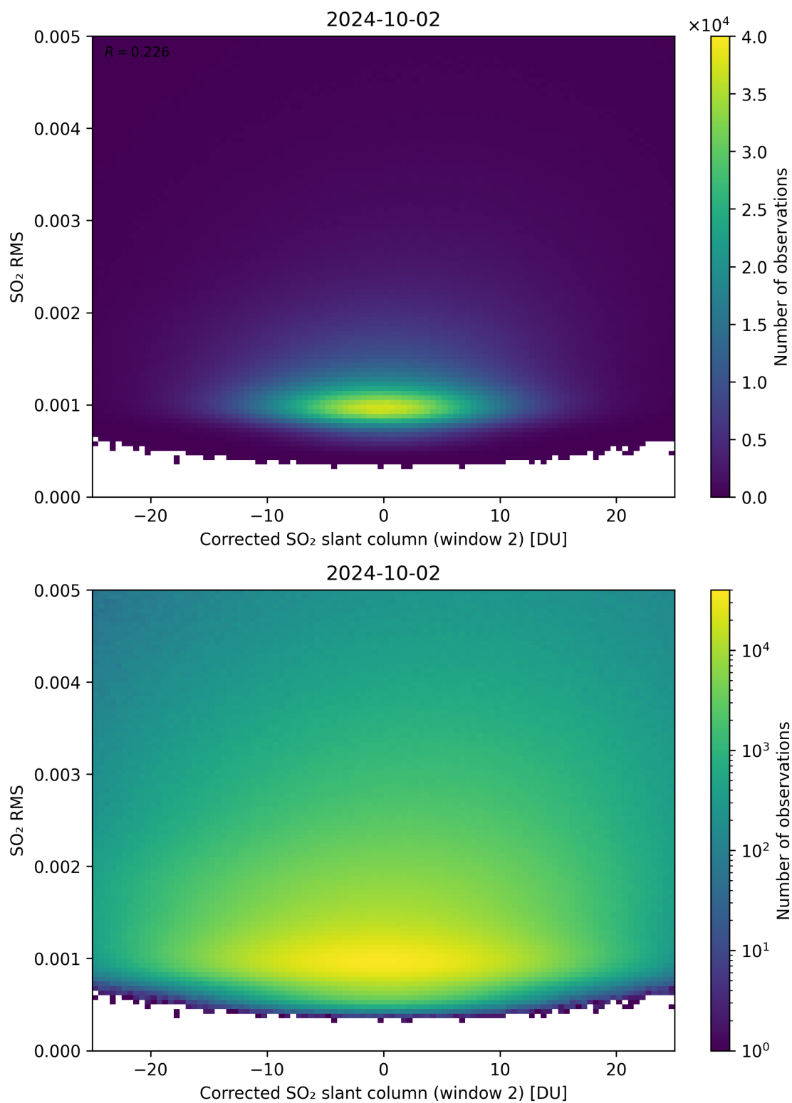
Figure 198: Scatter density plot of “Corrected SO 2 slant column (window 2)” against “SO 2 RMS” for 2024-10-01 to 2024-10-03.
