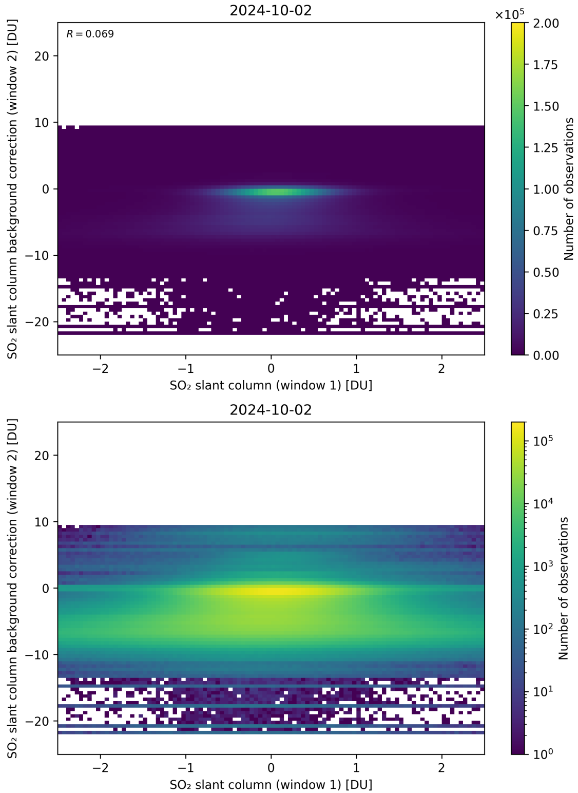
Figure 213: Scatter density plot of “SO 2 slant column (window 1)” against “SO 2 slant column background correction (window 2)” for 2024-10-01 to 2024-10-03.
