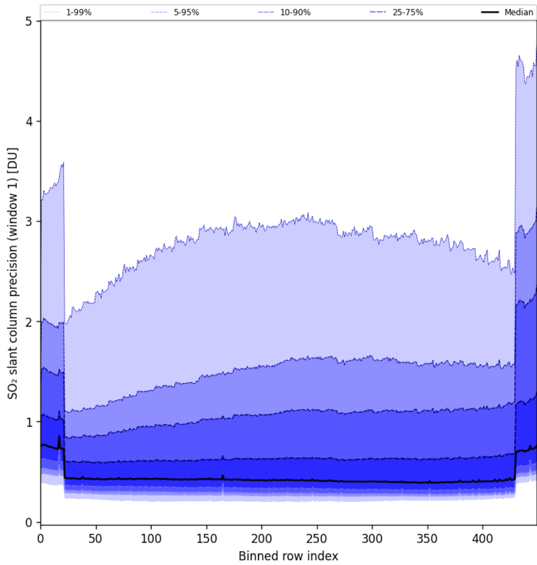
Figure 80: Along track statistics of “SO 2 slant column precision (window 1)” for 2024-10-01 to 2024-10-03
