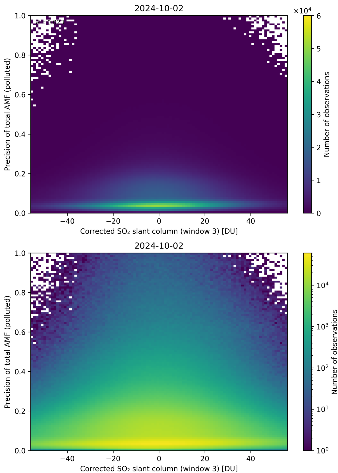
Figure 211: Scatter density plot of “Corrected SO 2 slant column (window 3)” against “Precision of total AMF (polluted)” for 2024-10-01 to 2024-10-03.
