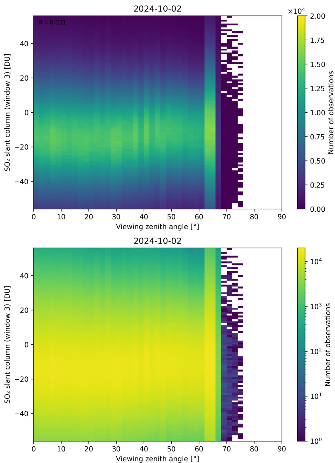
Figure 323: Scatter density plot of “Viewing zenith angle” against “SO 2 slant column (window 3)” for 2024-10-01 to 2024-10-03.
