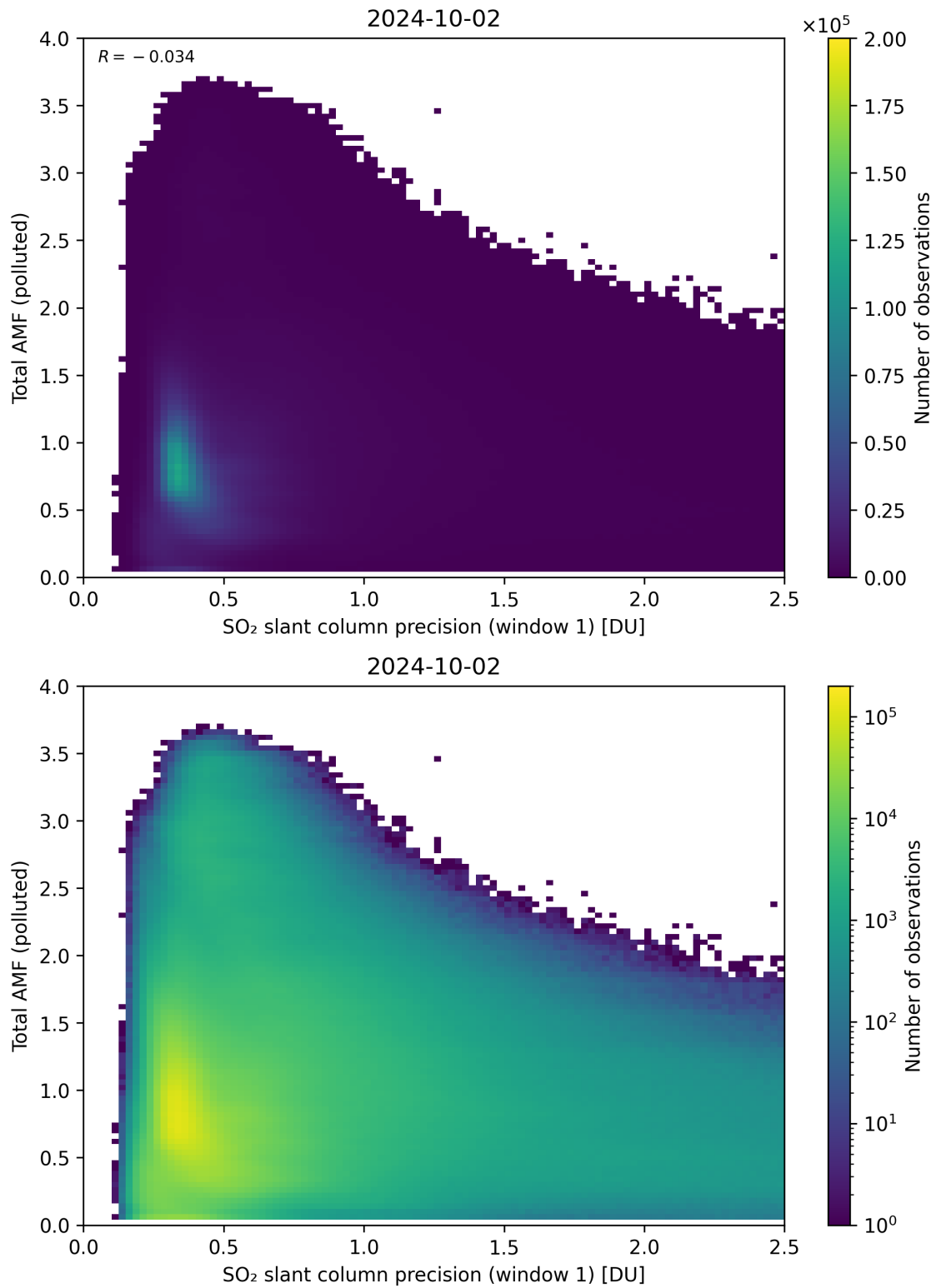
Figure 230: Scatter density plot of “SO 2 slant column precision (window 1)” against “Total AMF (polluted)” for 2024-10-01 to 2024-10-03.
