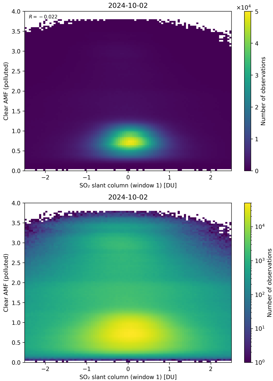
Figure 232: Scatter density plot of “SO 2 slant column (window 1)” against “Clear AMF (polluted)” for 2024-10-01 to 2024-10-03.
