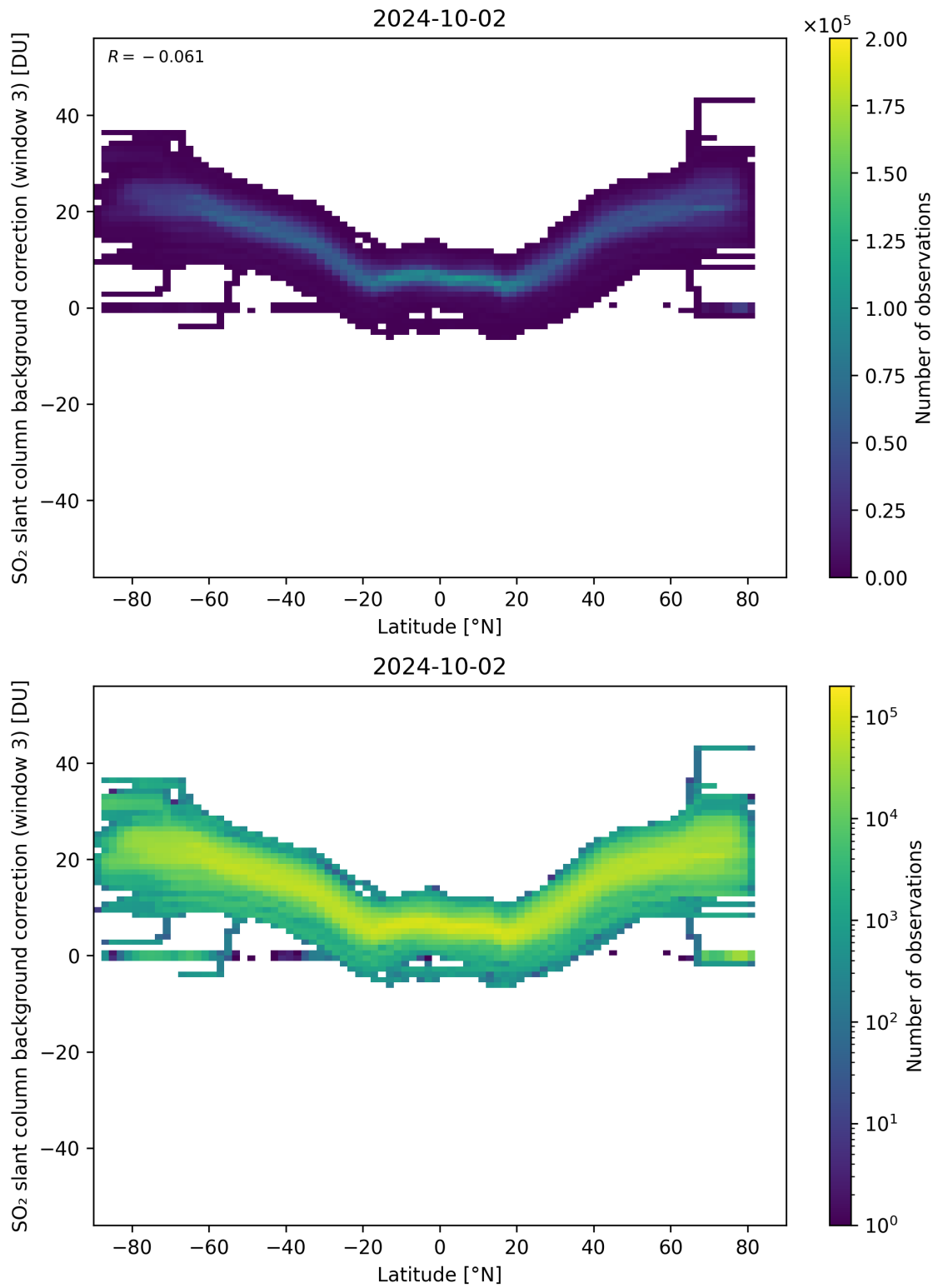
Figure 141: Scatter density plot of “Latitude” against “SO 2 slant column background correction (window 3)” for 2024-10-01 to 2024-10-03.
