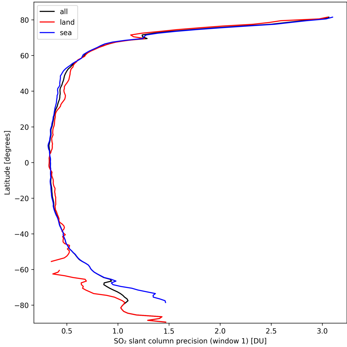
Figure 34: Zonal average of “SO 2 slant column precision (window 1)” for 2024-10-01 to 2024-10-03.
