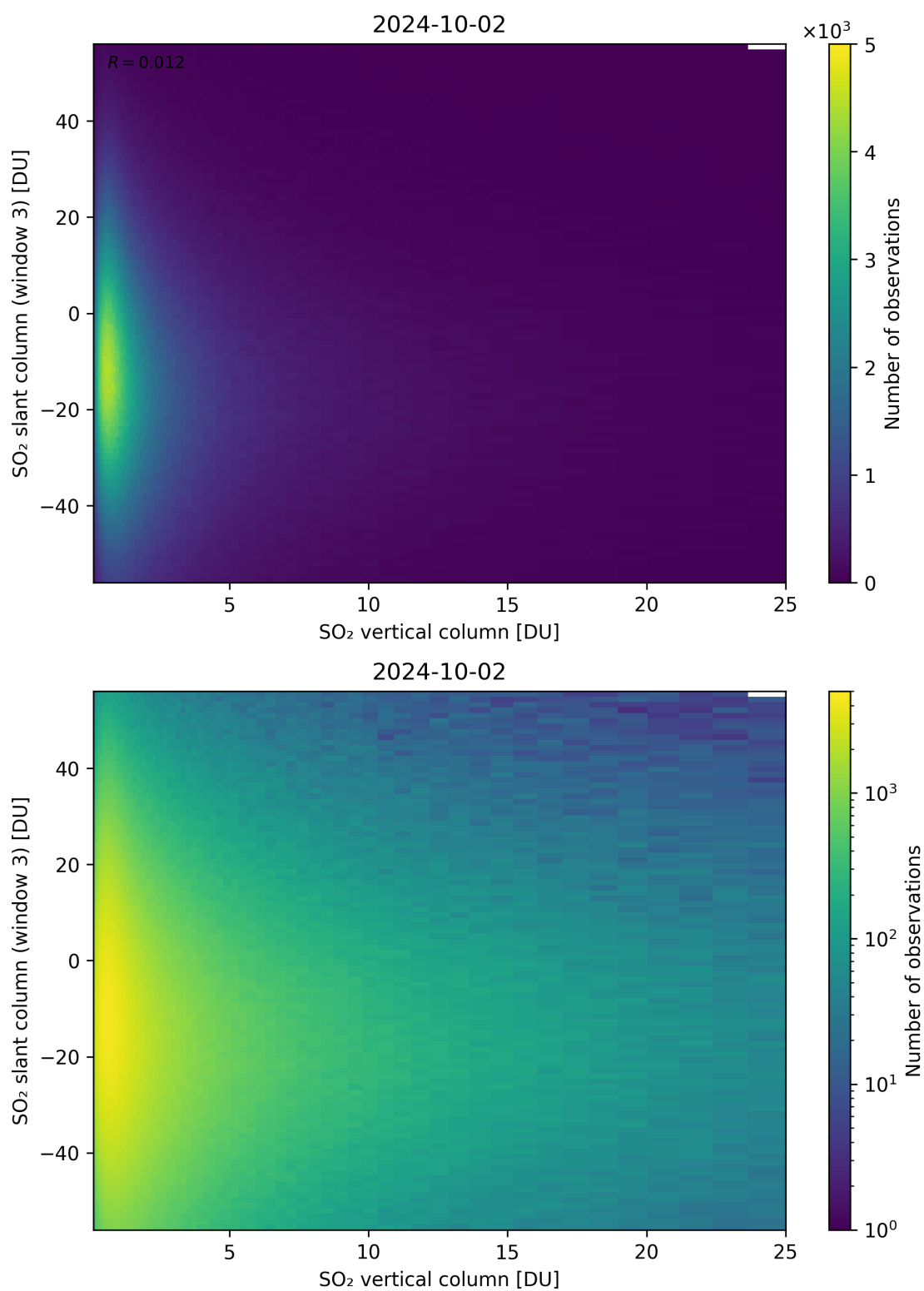
Figure 303: Scatter density plot of “SO 2 vertical column” against “SO 2 slant column (window 3)” for 2024-10-01 to 2024-10-03.
