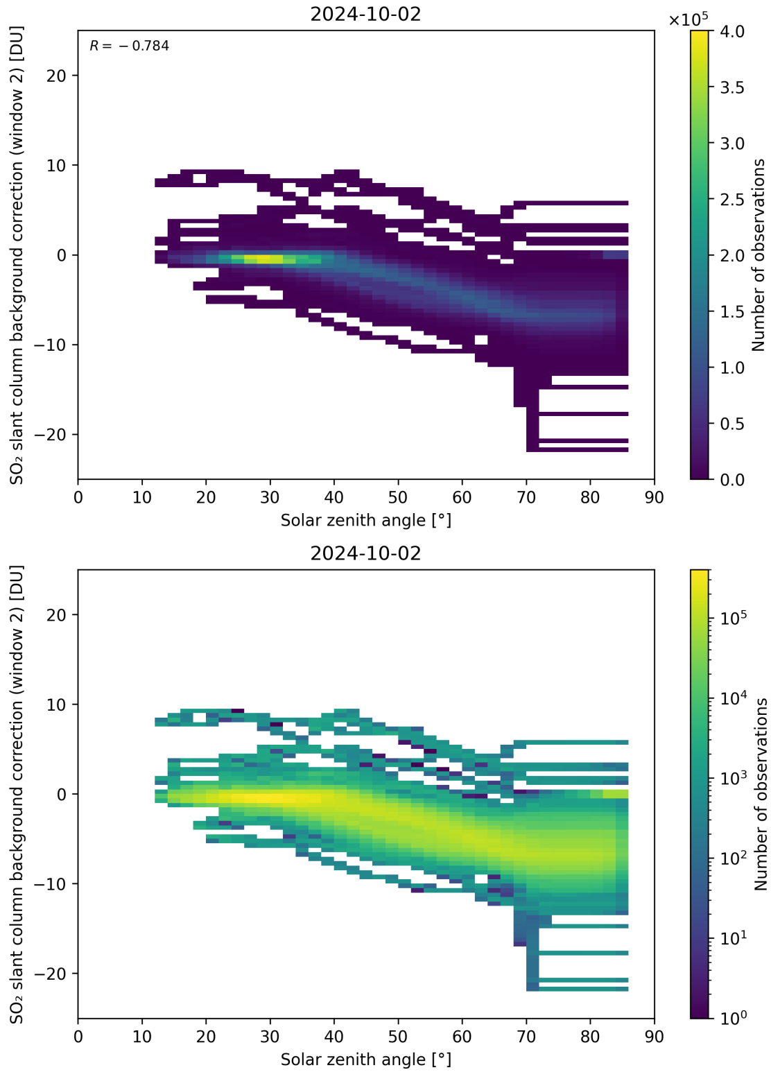
Figure 159: Scatter density plot of “Solar zenith angle” against “SO 2 slant column background correction (window 2)” for 2024-10-01 to 2024-10-03.
