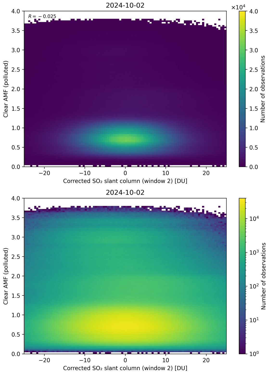
Figure 199: Scatter density plot of “Corrected SO 2 slant column (window 2)” against “Clear AMF (polluted)” for 2024-10-01 to 2024-10-03.
