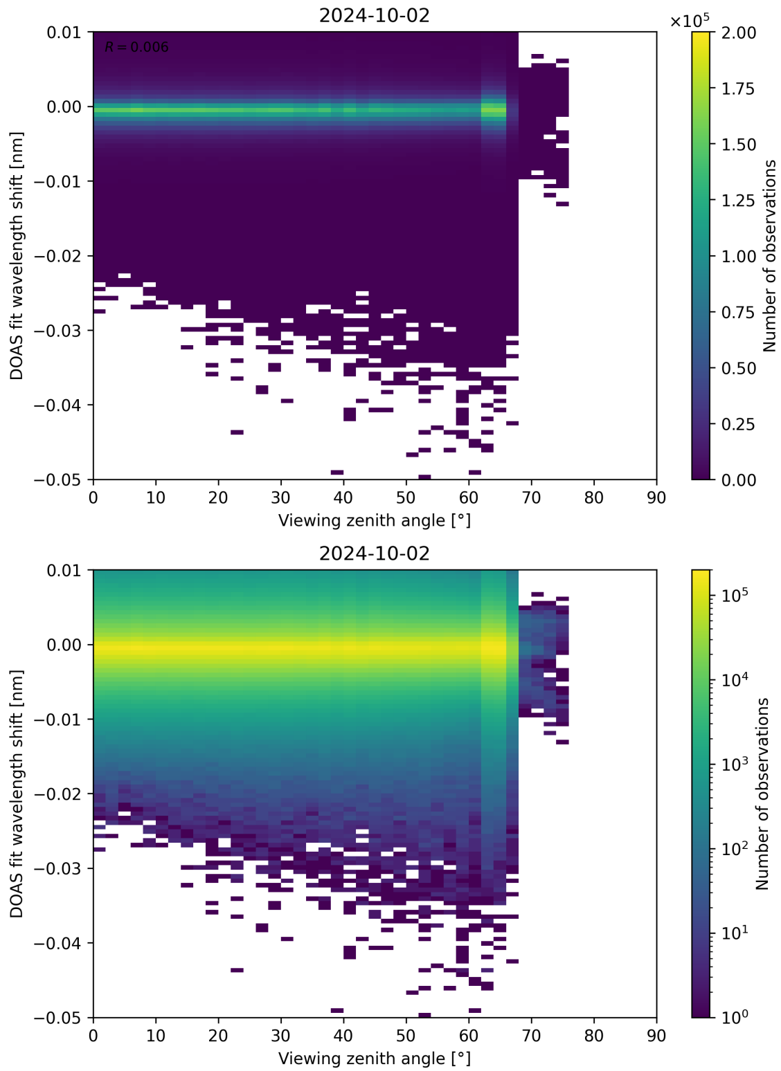
Figure 311: Scatter density plot of “Viewing zenith angle” against “DOAS fit wavelength shift” for 2024-10-01 to 2024-10-03.
