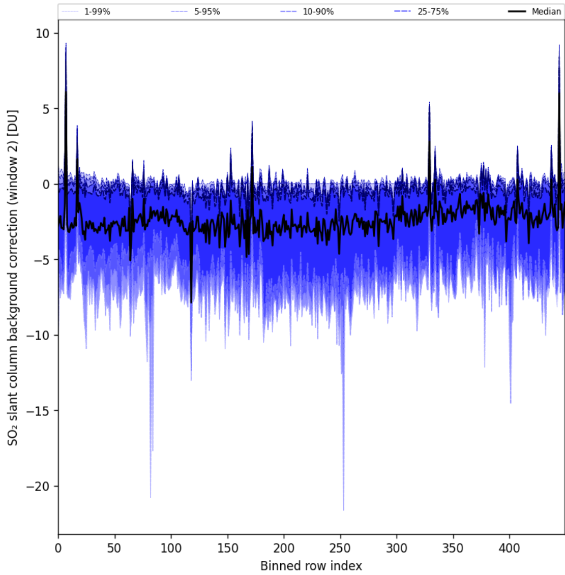
Figure 86: Along track statistics of “SO 2 slant column background correction (window 2)” for 2024-10-01 to 2024-10-03
