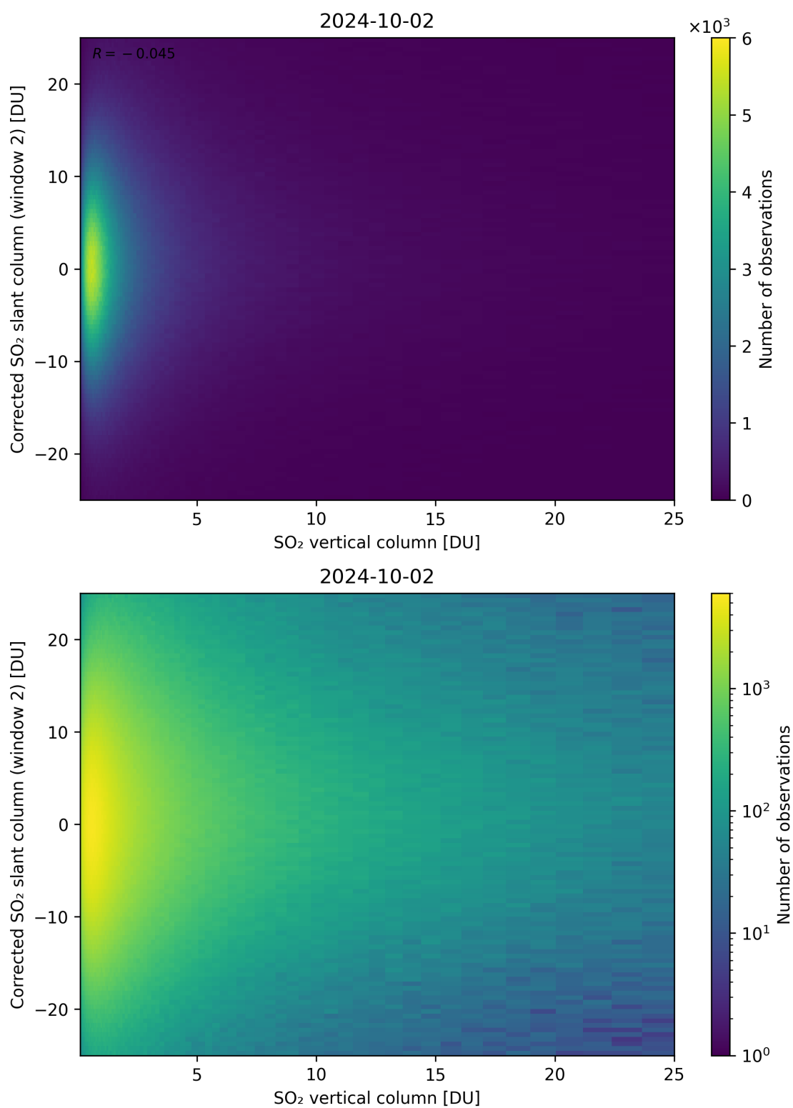
Figure 298: Scatter density plot of “SO 2 vertical column” against “Corrected SO 2 slant column (window 2)” for 2024-10-01 to 2024-10-03.
