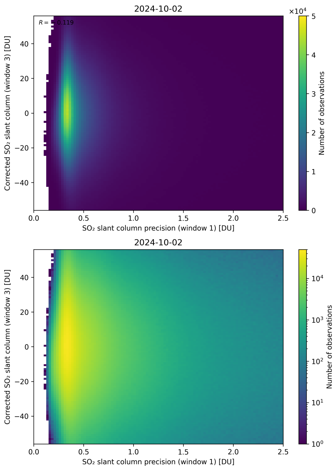
Figure 226: Scatter density plot of “SO 2 slant column precision (window 1)” against “Corrected SO 2 slant column (window 3)” for 2024-10-01 to 2024-10-03.
