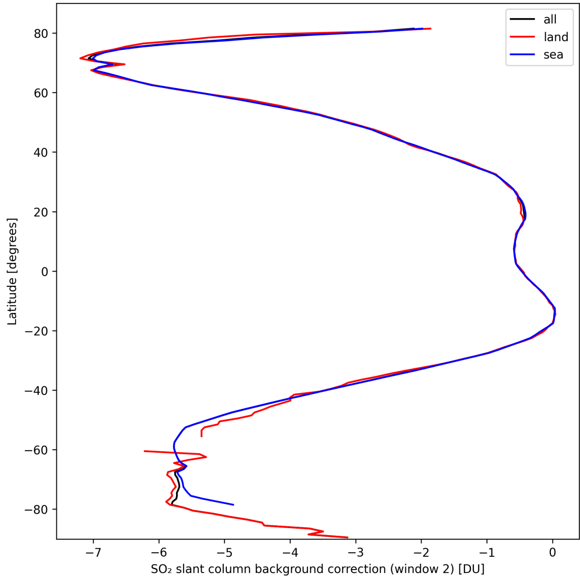
Figure 40: Zonal average of “SO 2 slant column background correction (window 2)” for 2024-10-01 to 2024-10-03.
