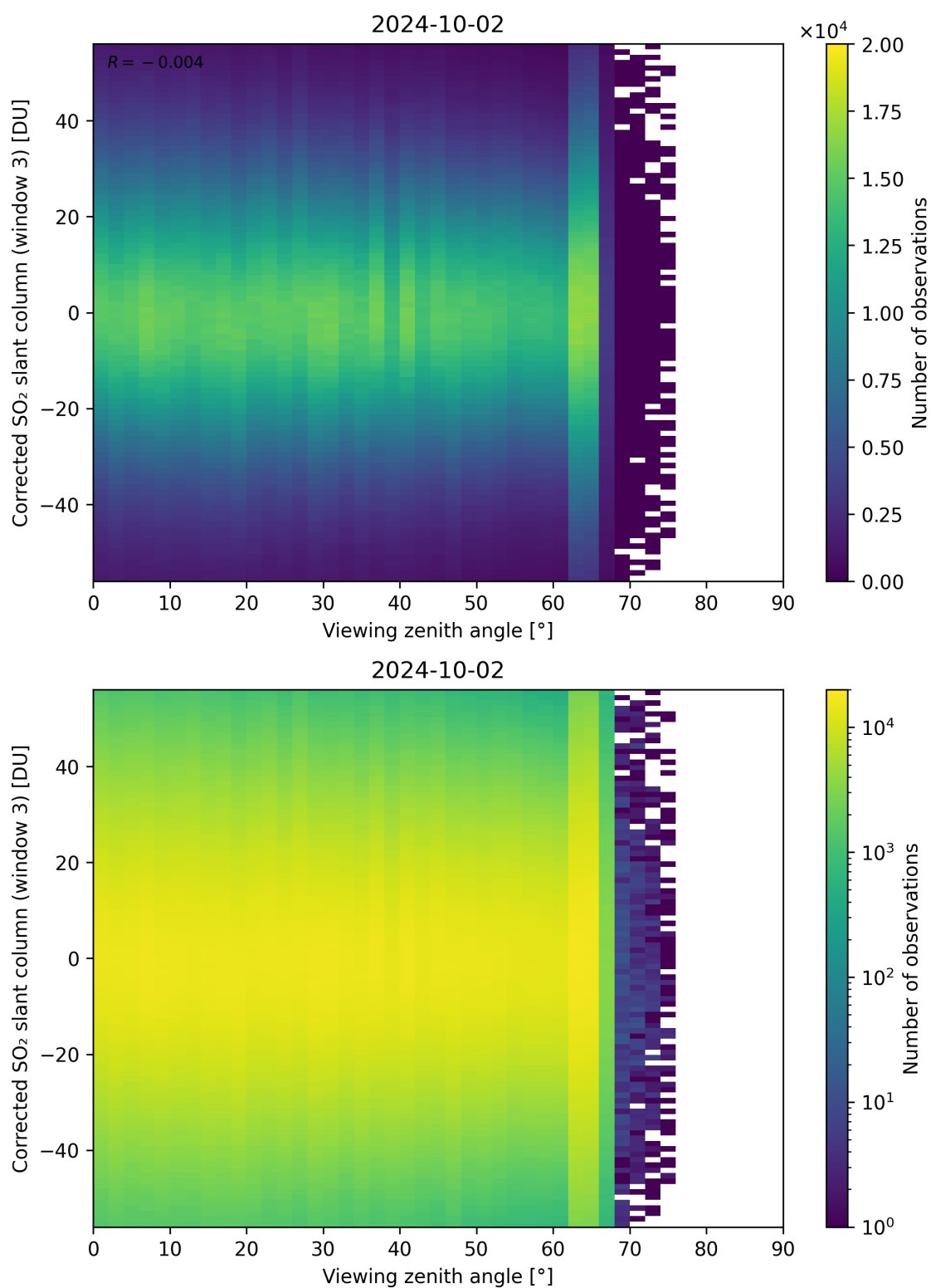
Figure 319: Scatter density plot of “Viewing zenith angle” against “Corrected SO 2 slant column (window 3)” for 2024-10-01 to 2024-10-03.
