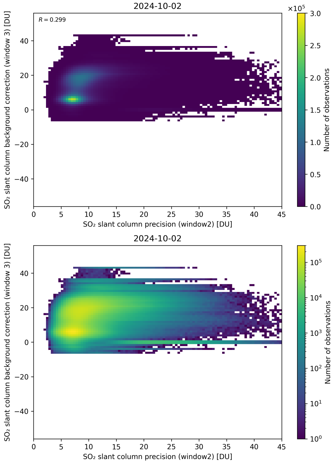
Figure 242: Scatter density plot of “SO 2 slant column precision (window2)” against “SO 2 slant column background correction (window 3)” for 2024-10-01 to 2024-10-03.
