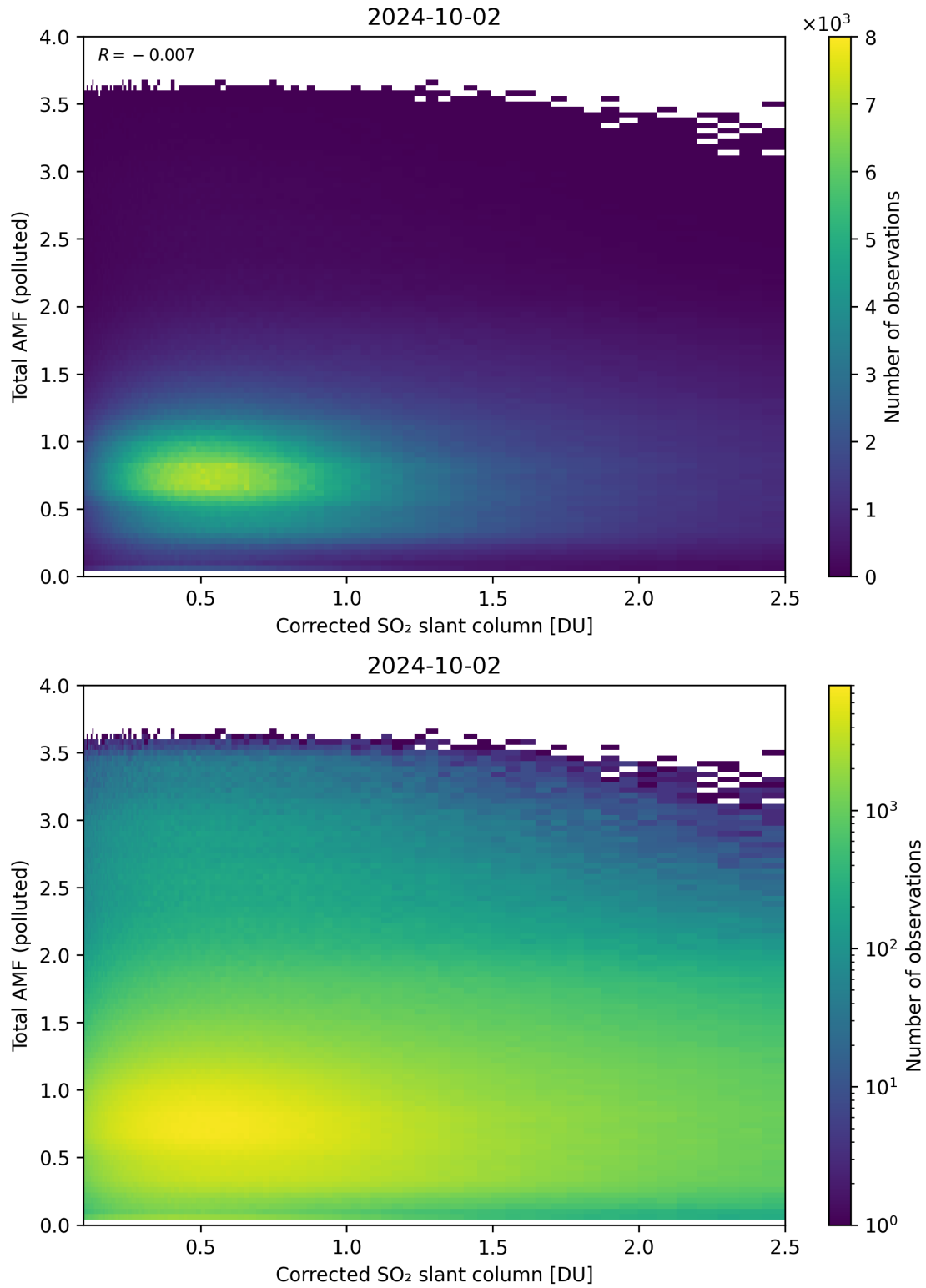
Figure 192: Scatter density plot of “Corrected SO 2 slant column” against “Total AMF (polluted)” for 2024-10-01 to 2024-10-03.
