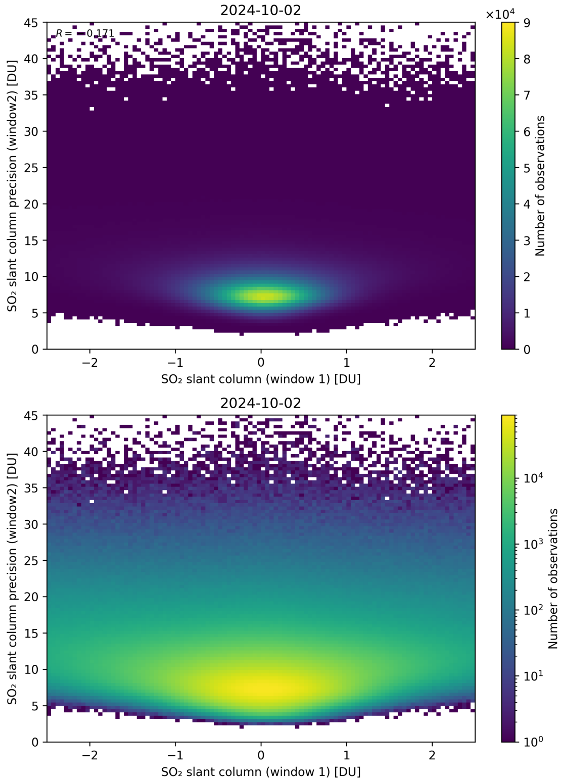
Figure 236: Scatter density plot of “SO 2 slant column (window 1)” against “SO 2 slant column precision (window2)” for 2024-10-01 to 2024-10-03.
