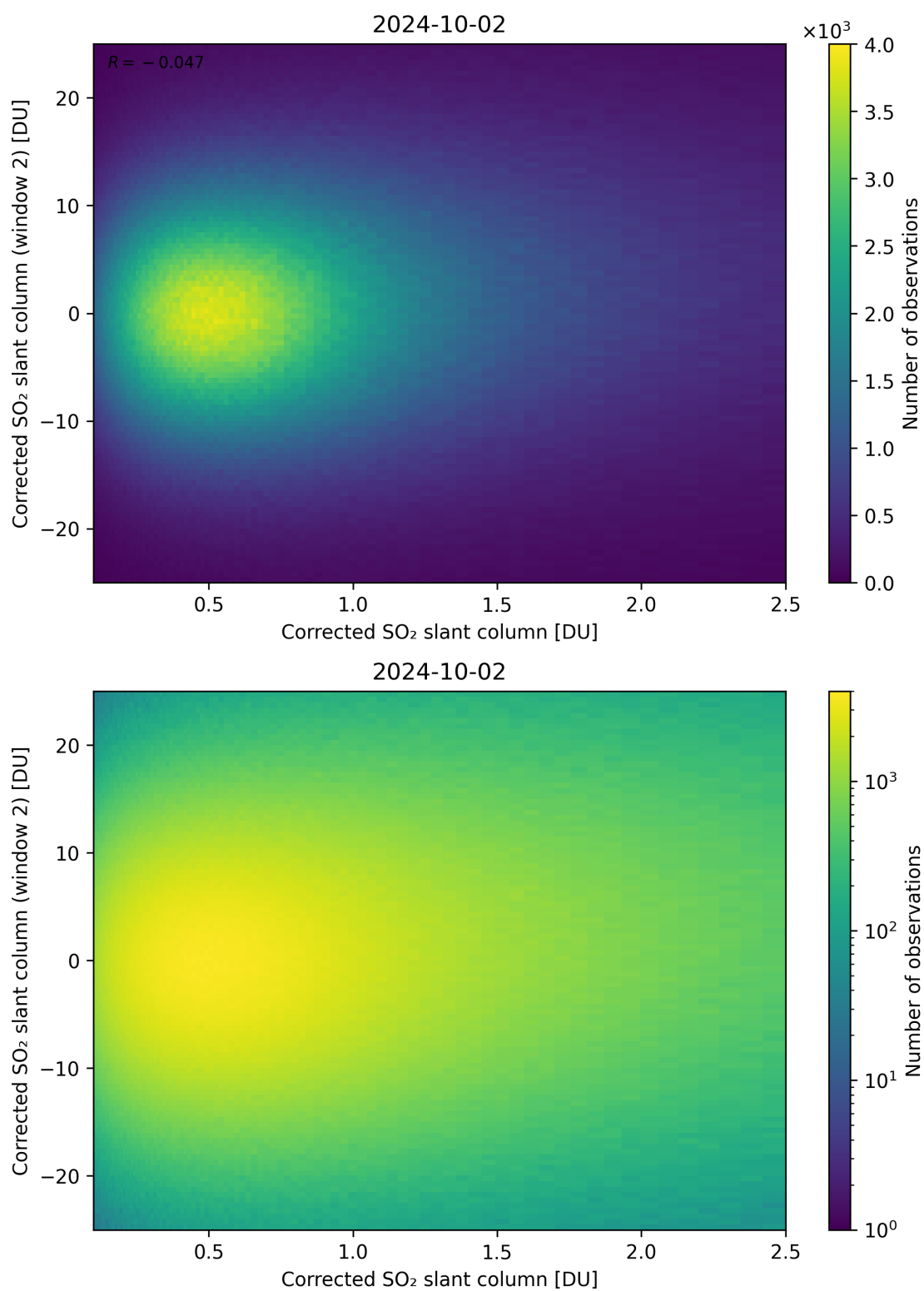
Figure 185: Scatter density plot of “Corrected SO 2 slant column” against “Corrected SO 2 slant column (window 2)” for 2024-10-01 to 2024-10-03.
