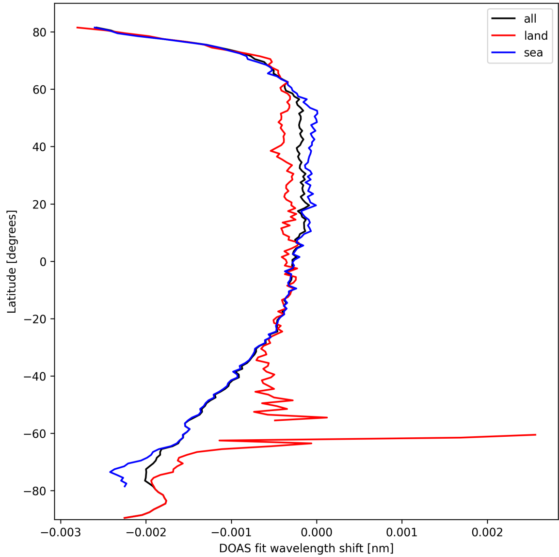
Figure 45: Zonal average of “DOAS fit wavelength shift” for 2024-10-01 to 2024-10-03.
