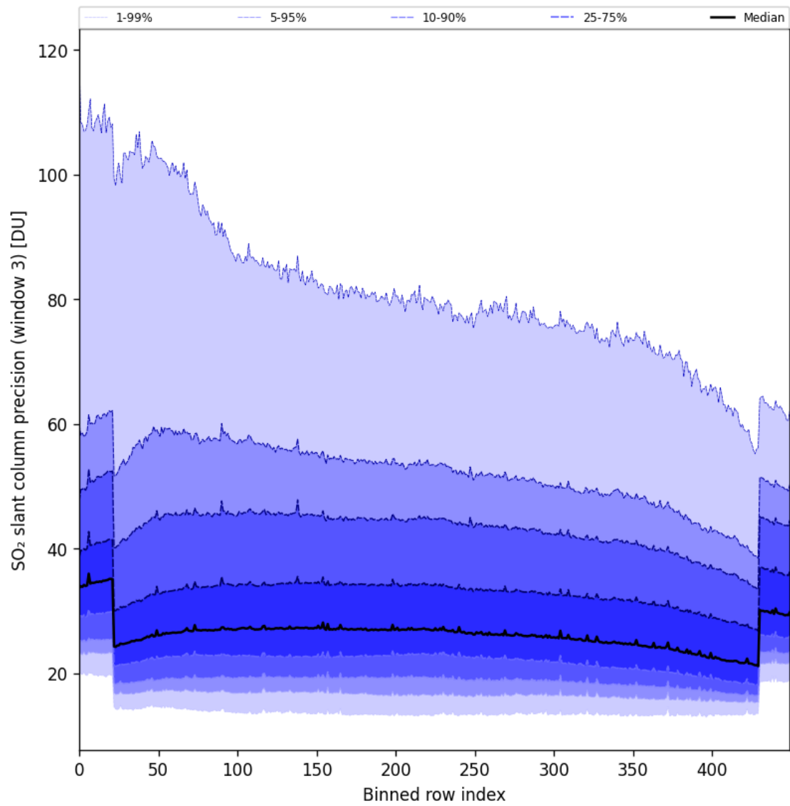
Figure 88: Along track statistics of “SO 2 slant column precision (window 3)” for 2024-10-01 to 2024-10-03
