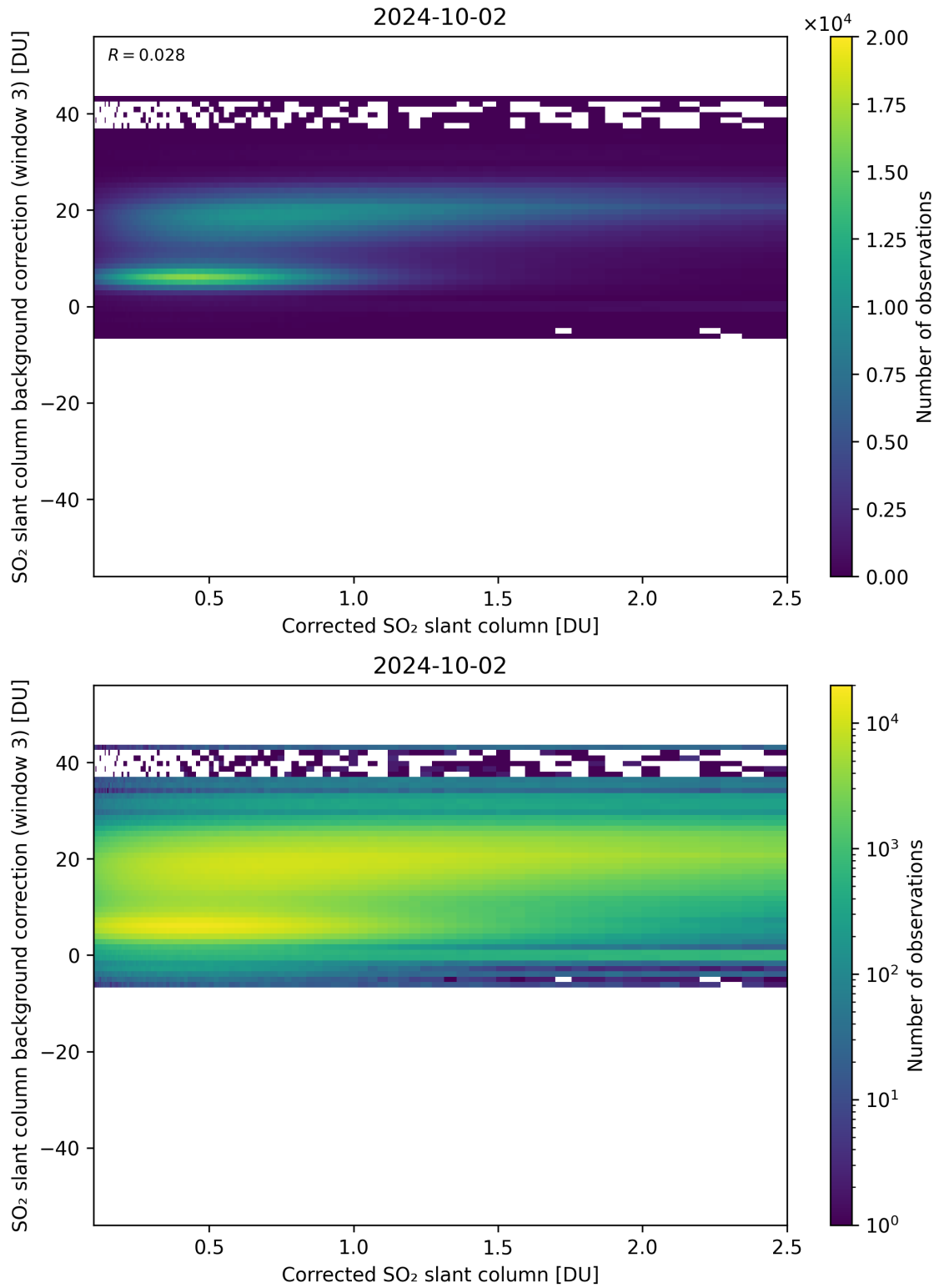
Figure 180: Scatter density plot of “Corrected SO 2 slant column” against “SO 2 slant column background correction (window 3)” for 2024-10-01 to 2024-10-03.
