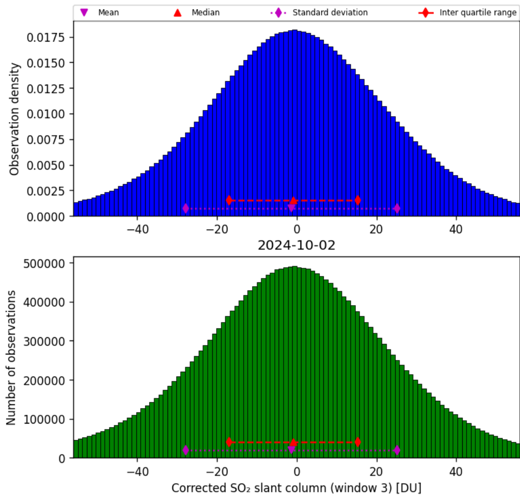
Figure 66: Histogram of “Corrected SO 2 slant column (window 3)” for 2024-10-01 to 2024-10-03
