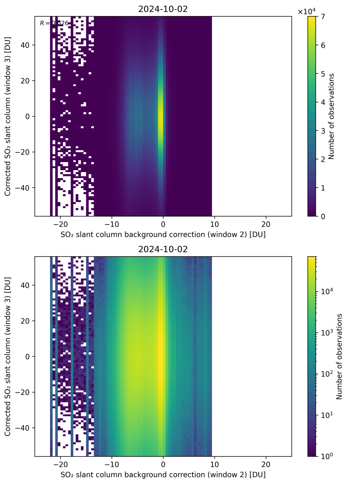
Figure 116: Scatter density plot of “SO 2 slant column background correction (window 2)” against “Corrected SO 2 slant column (window 3)” for 2024-10-01 to 2024-10-03.
