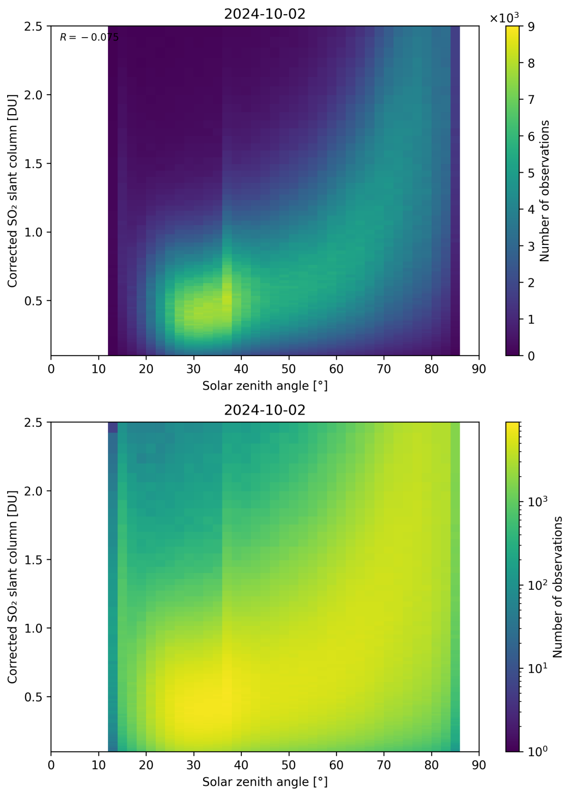
Figure 166: Scatter density plot of “Solar zenith angle” against “Corrected SO 2 slant column” for 2024-10-01 to 2024-10-03.
