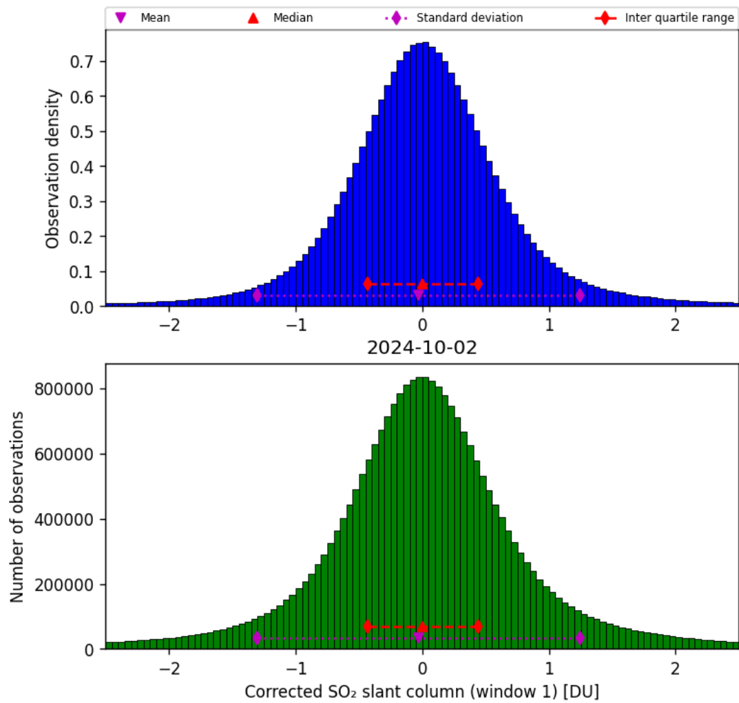
Figure 58: Histogram of “Corrected SO 2 slant column (window 1)” for 2024-10-01 to 2024-10-03
