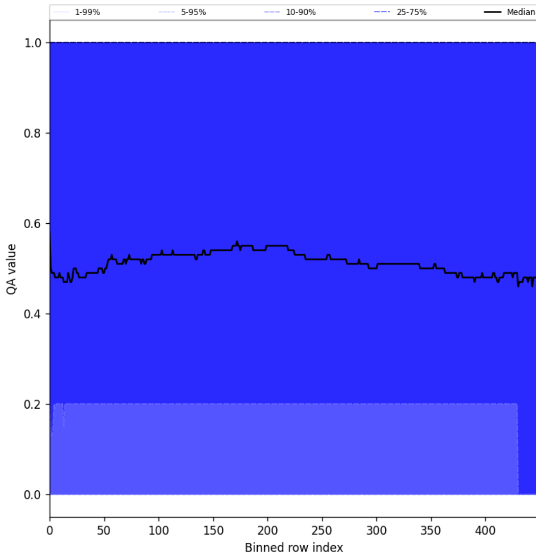
Figure 75: Along track statistics of “QA value” for 2024-10-01 to 2024-10-03
