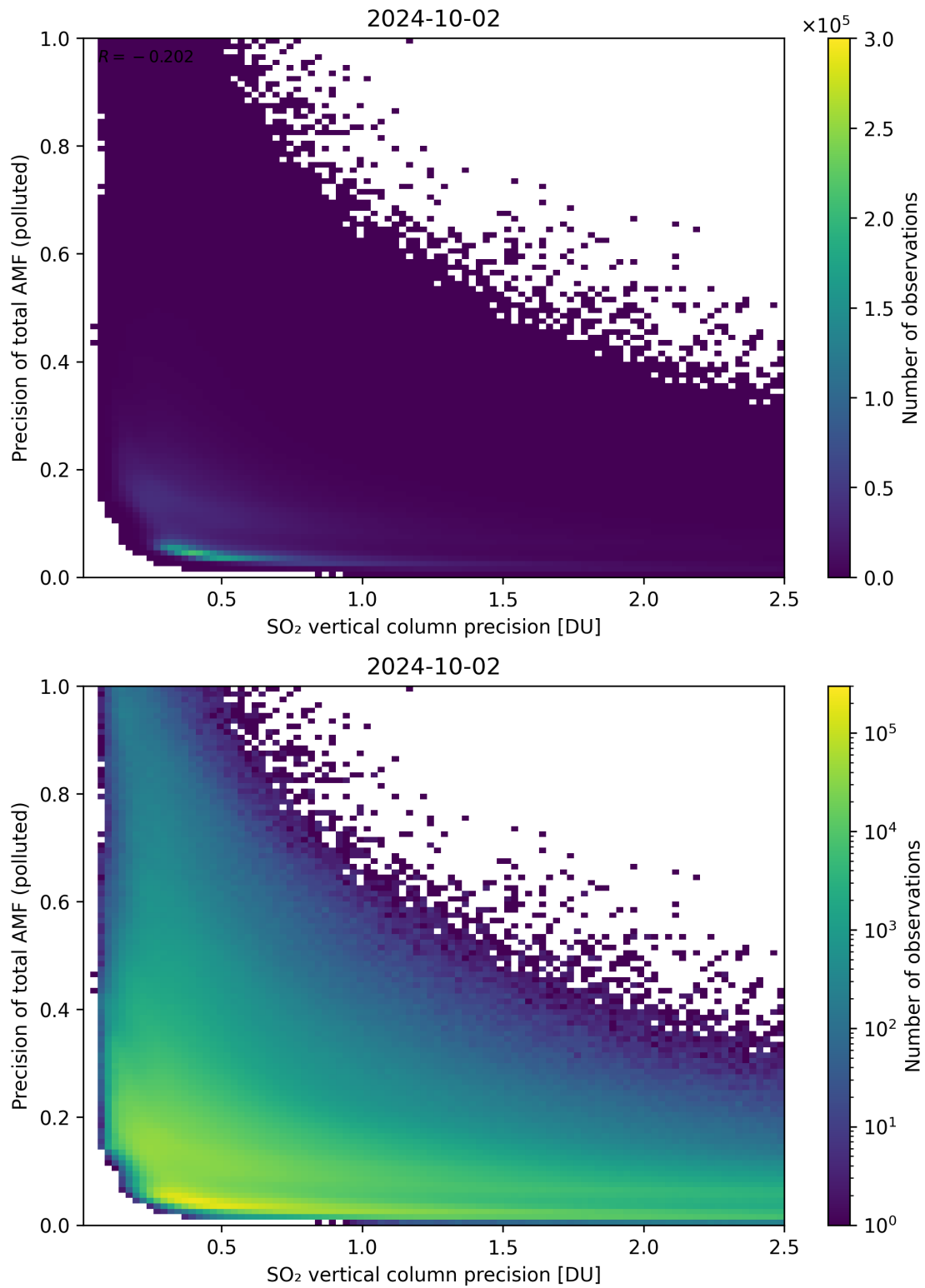
Figure 295: Scatter density plot of “SO 2 vertical column precision” against “Precision of total AMF (polluted)” for 2024-10-01 to 2024-10-03.
