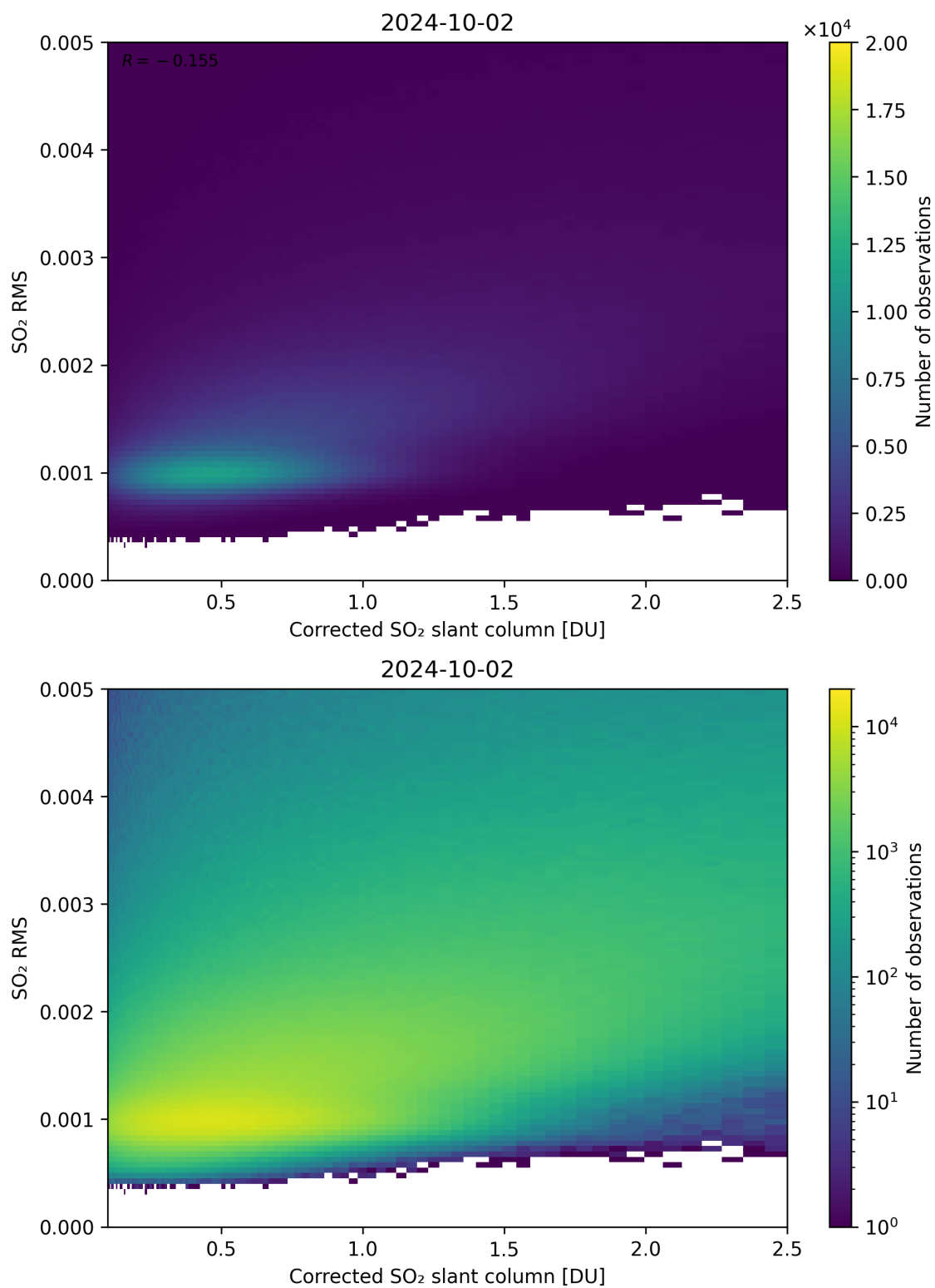
Figure 183: Scatter density plot of “Corrected SO 2 slant column” against “SO 2 RMS” for 2024-10-01 to 2024-10-03.
