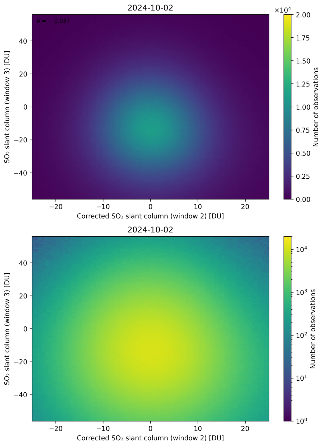
Figure 201: Scatter density plot of “Corrected SO 2 slant column (window 2)” against “SO 2 slant column (window 3)” for 2024-10-01 to 2024-10-03.
