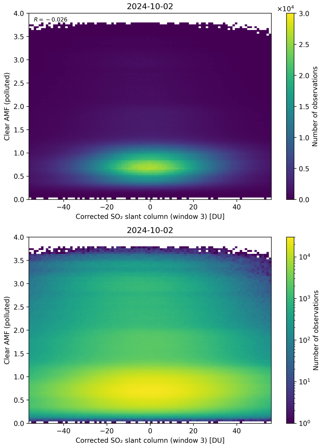
Figure 209: Scatter density plot of “Corrected SO 2 slant column (window 3)” against “Clear AMF (polluted)” for 2024-10-01 to 2024-10-03.
