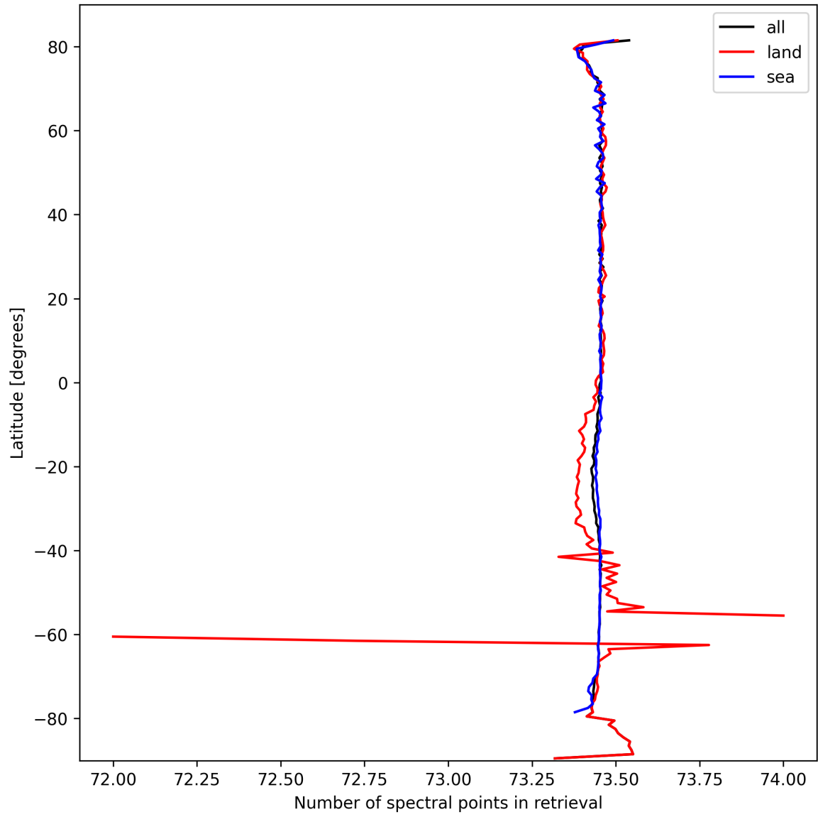
Figure 51: Zonal average of “Number of spectral points in retrieval” for 2024-10-01 to 2024-10-03.
