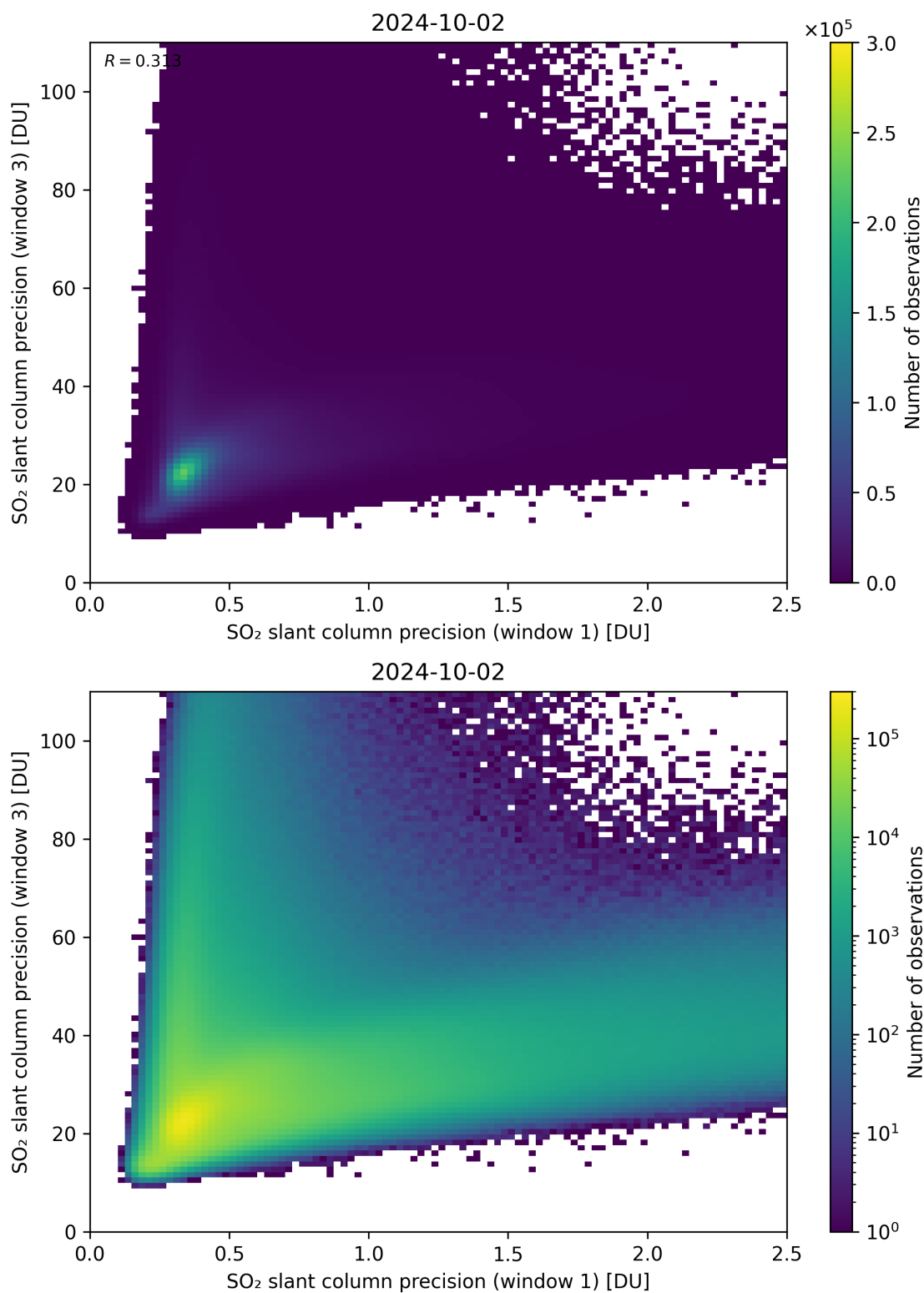
Figure 229: Scatter density plot of “SO 2 slant column precision (window 1)” against “SO 2 slant column precision (window 3)” for 2024-10-01 to 2024-10-03.
