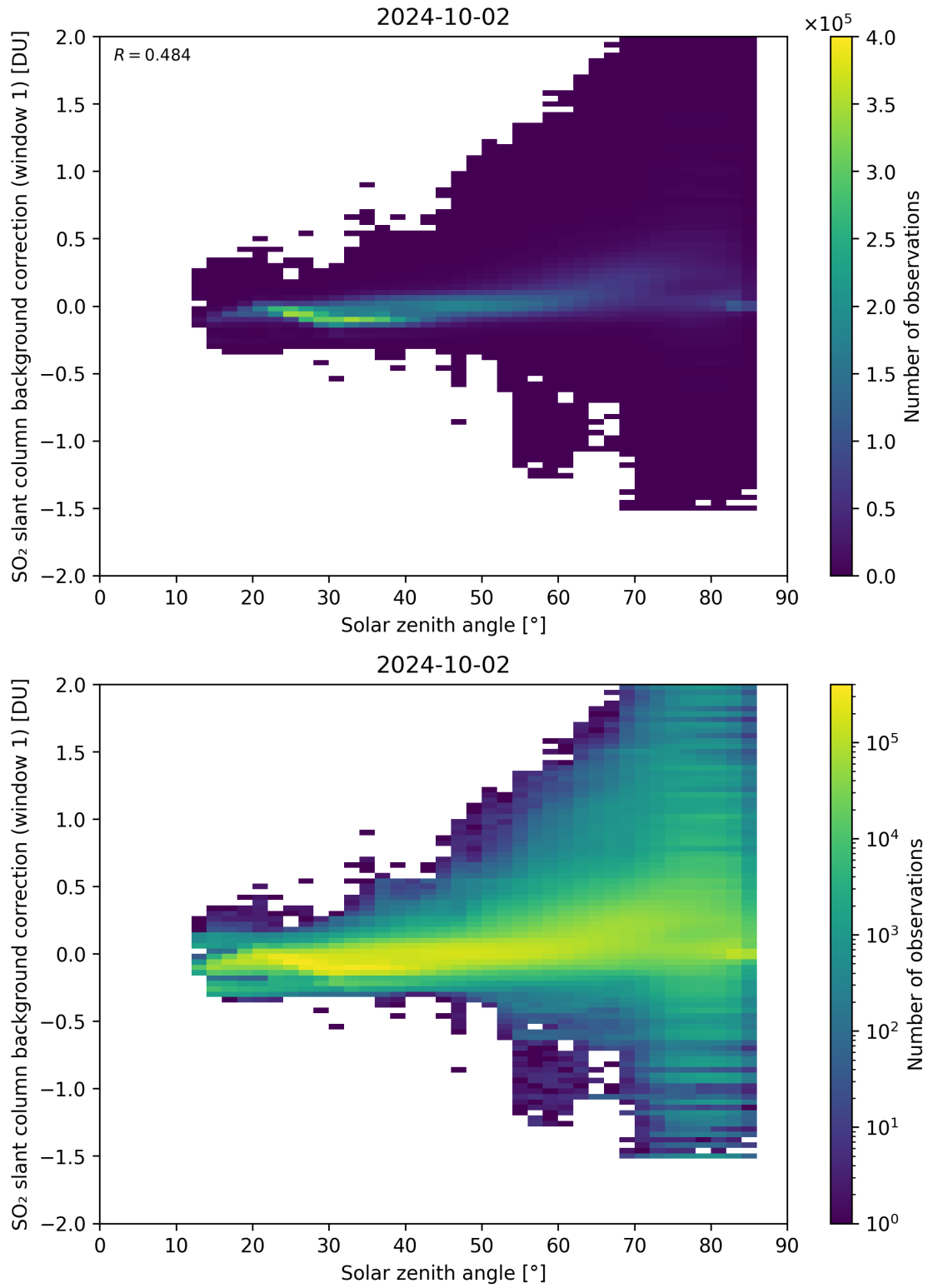
Figure 158: Scatter density plot of “Solar zenith angle” against “SO 2 slant column background correction (window 1)” for 2024-10-01 to 2024-10-03.
