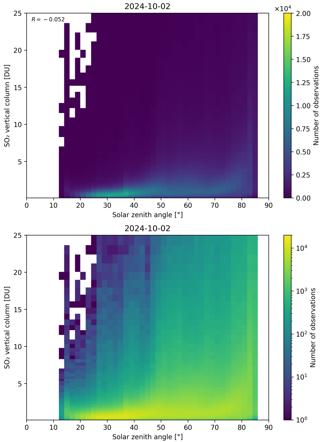
Figure 176: Scatter density plot of “Solar zenith angle” against “SO 2 vertical column” for 2024-10-01 to 2024-10-03.
