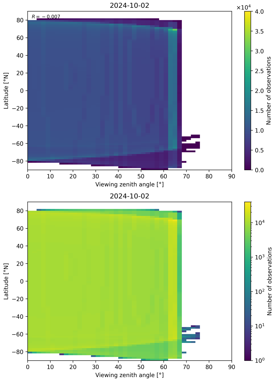
Figure 314: Scatter density plot of “Viewing zenith angle” against “Latitude” for 2024-10-01 to 2024-10-03.
