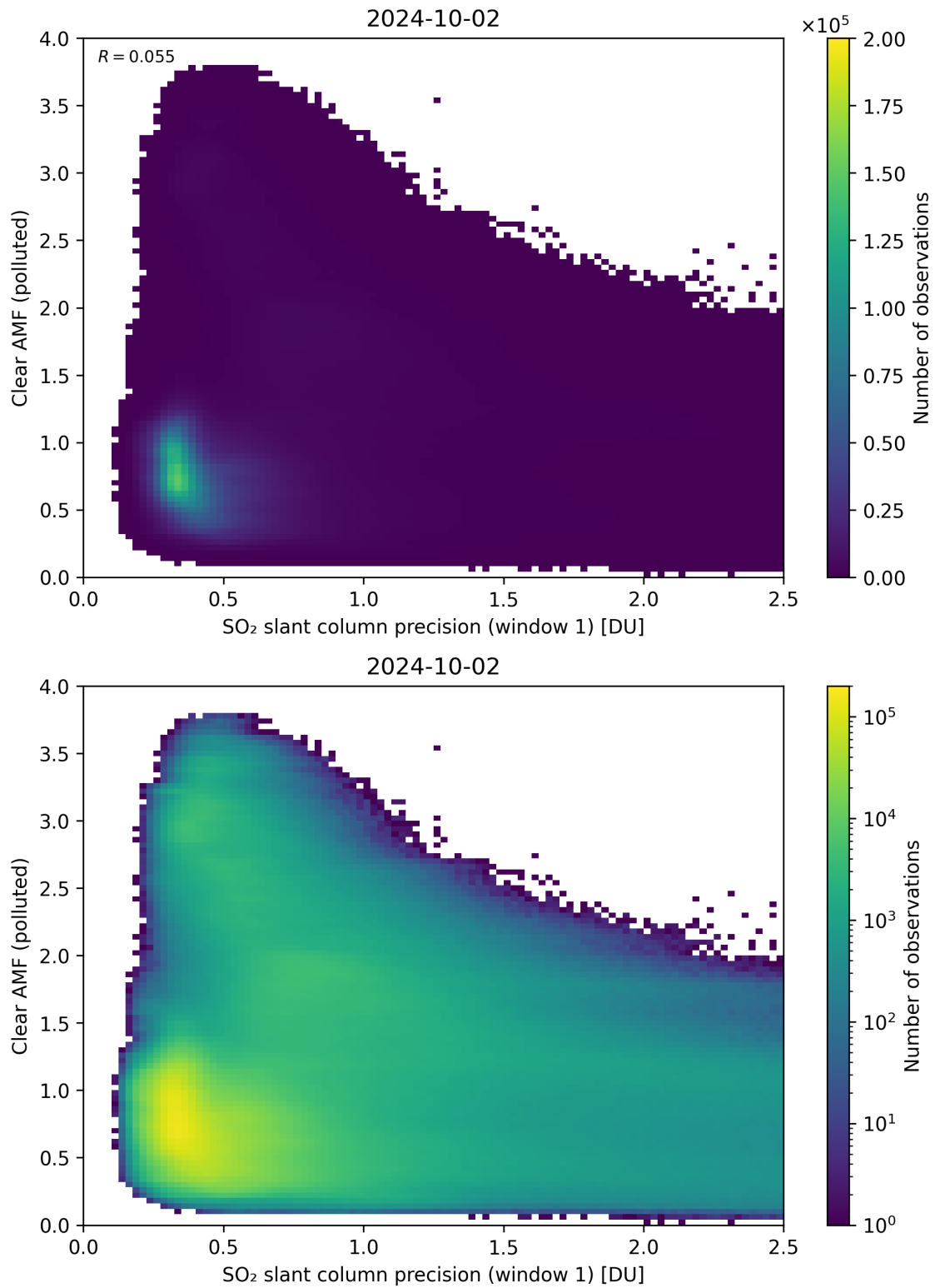
Figure 224: Scatter density plot of “SO 2 slant column precision (window 1)” against “Clear AMF (polluted)” for 2024-10-01 to 2024-10-03.
