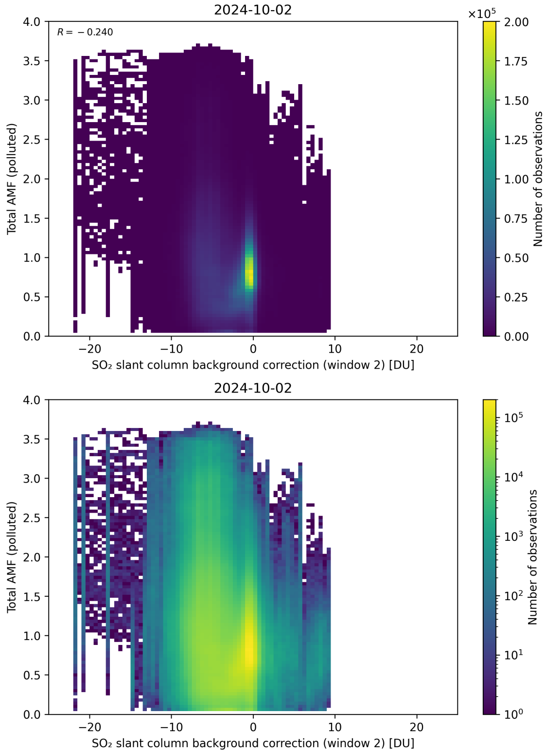
Figure 119: Scatter density plot of “SO 2 slant column background correction (window 2)” against “Total AMF (polluted)” for 2024-10-01 to 2024-10-03.
