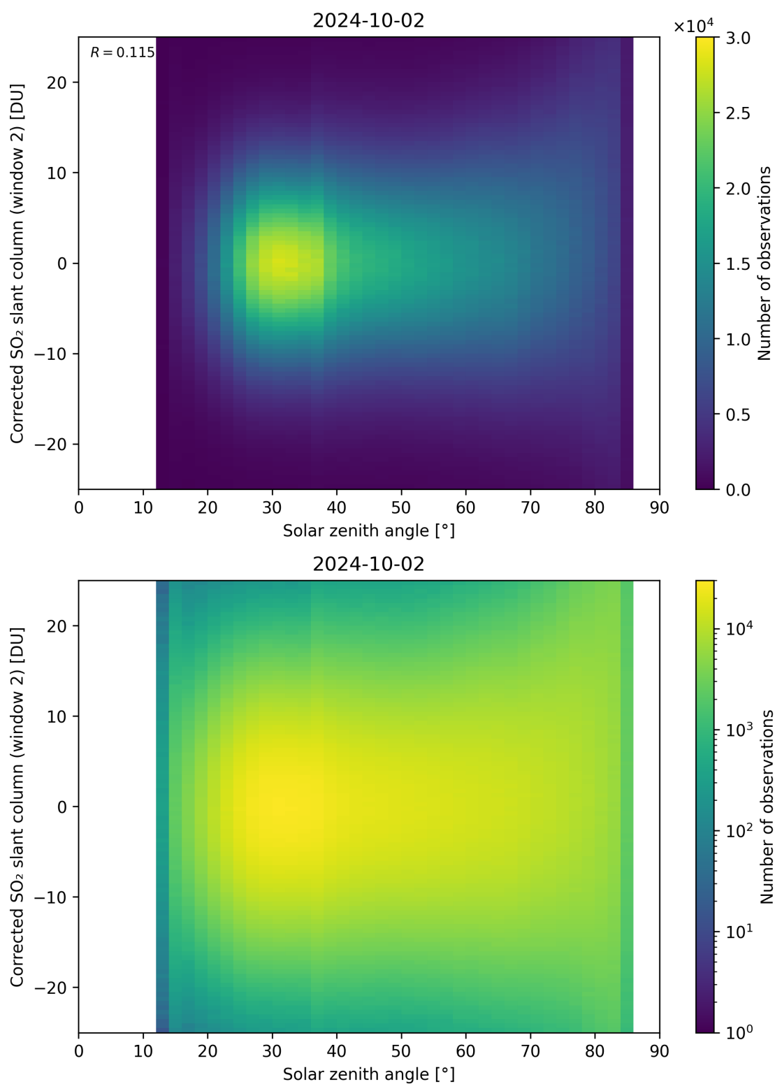
Figure 167: Scatter density plot of “Solar zenith angle” against “Corrected SO 2 slant column (window 2)” for 2024-10-01 to 2024-10-03.
