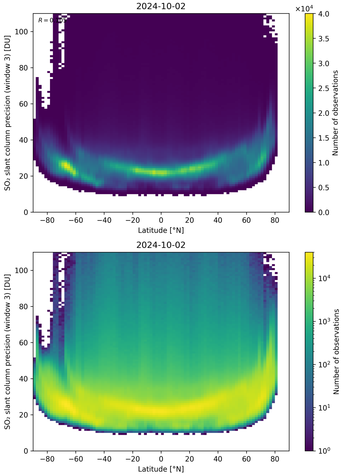
Figure 153: Scatter density plot of “Latitude” against “SO 2 slant column precision (window 3)” for 2024-10-01 to 2024-10-03.
