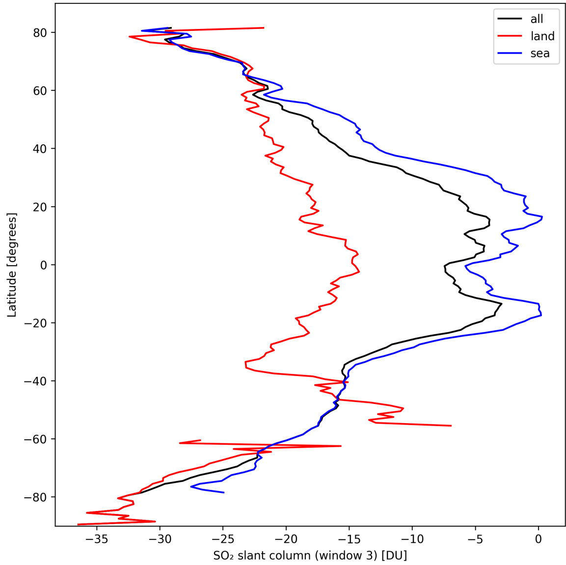
Figure 41: Zonal average of “SO 2 slant column (window 3)” for 2024-10-01 to 2024-10-03.
