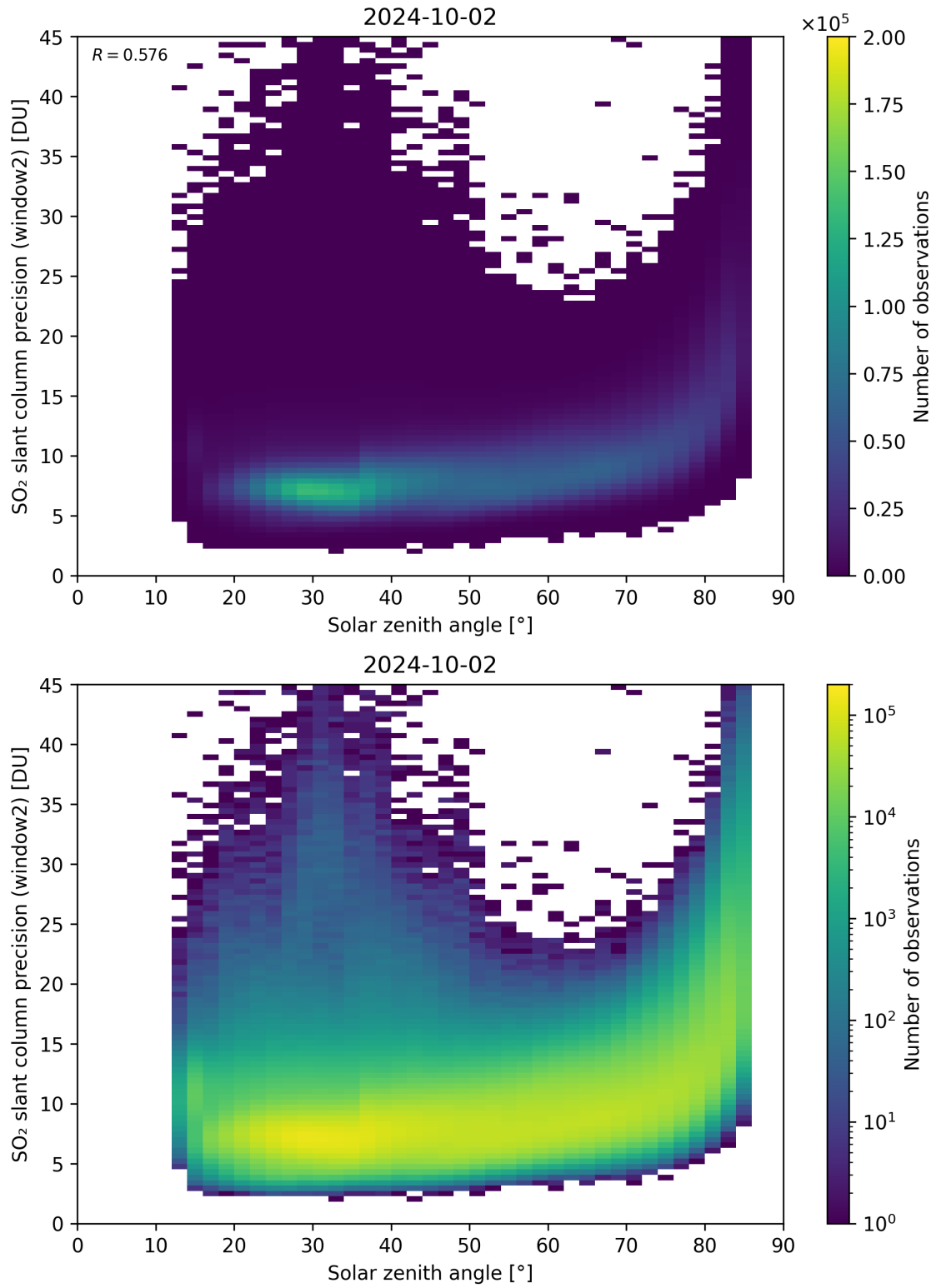
Figure 171: Scatter density plot of “Solar zenith angle” against “SO 2 slant column precision (window2)” for 2024-10-01 to 2024-10-03.
