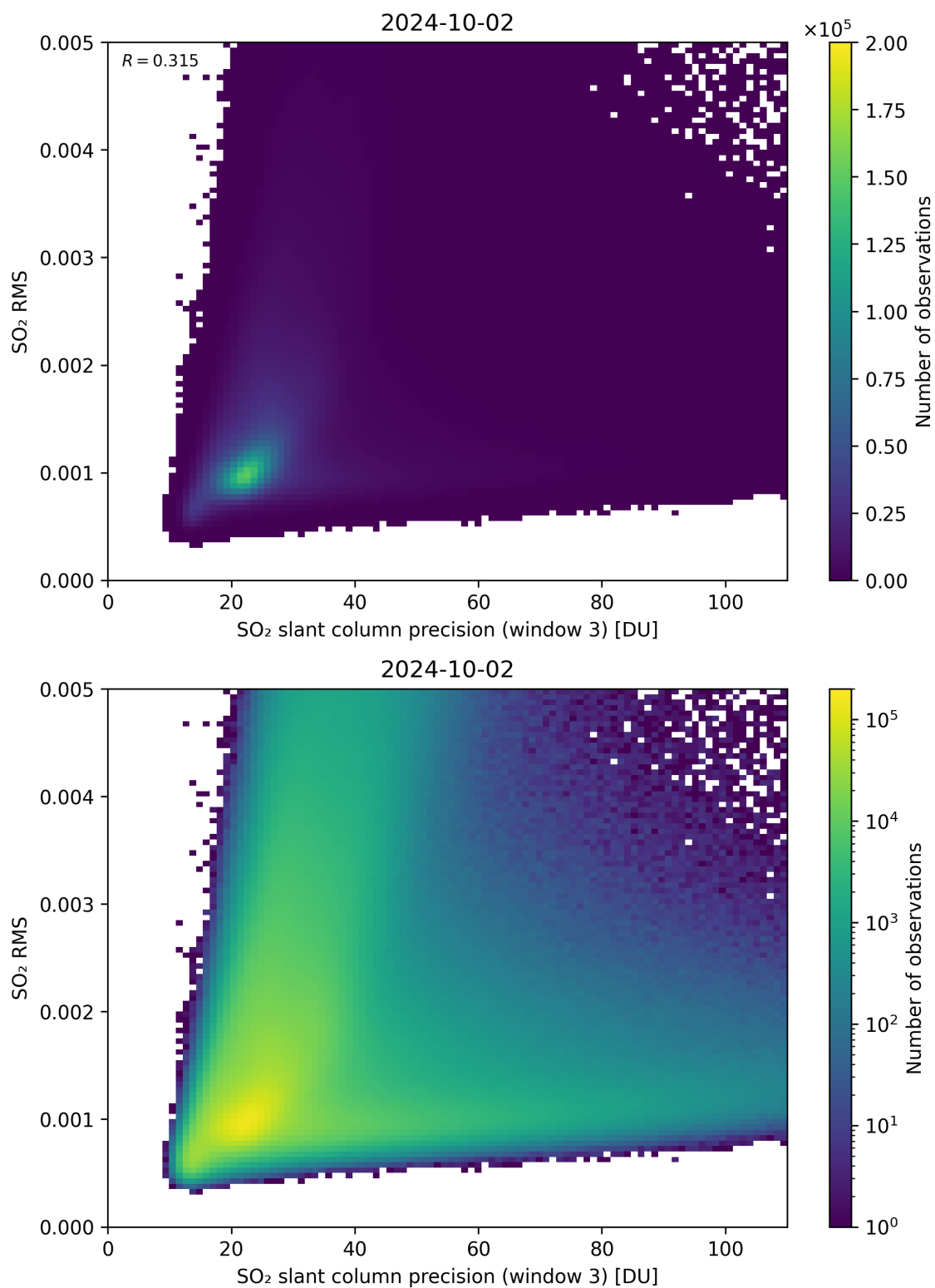
Figure 260: Scatter density plot of “SO 2 slant column precision (window 3)” against “SO 2 RMS” for 2024-10-01 to 2024-10-03.
