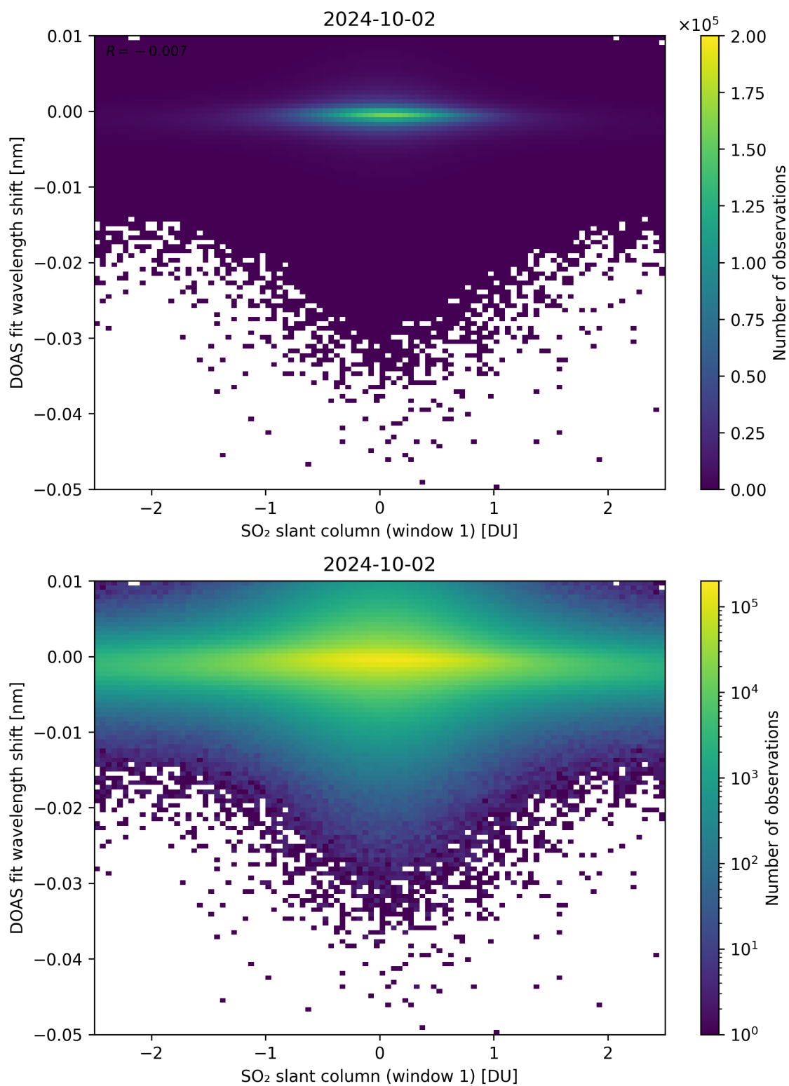
Figure 215: Scatter density plot of “SO 2 slant column (window 1)” against “DOAS fit wavelength shift” for 2024-10-01 to 2024-10-03.
