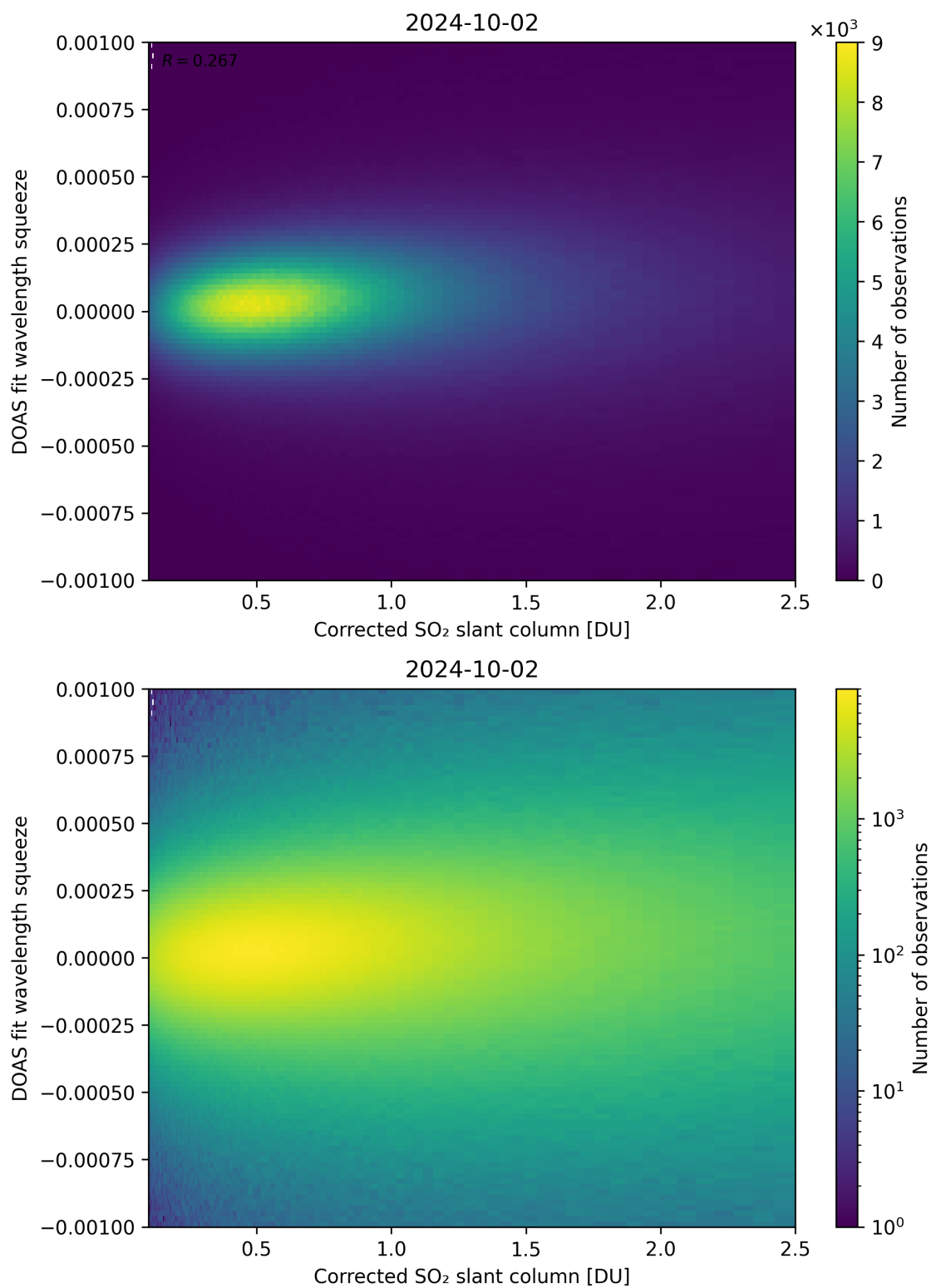
Figure 182: Scatter density plot of “Corrected SO 2 slant column” against “DOAS fit wavelength squeeze” for 2024-10-01 to 2024-10-03.
