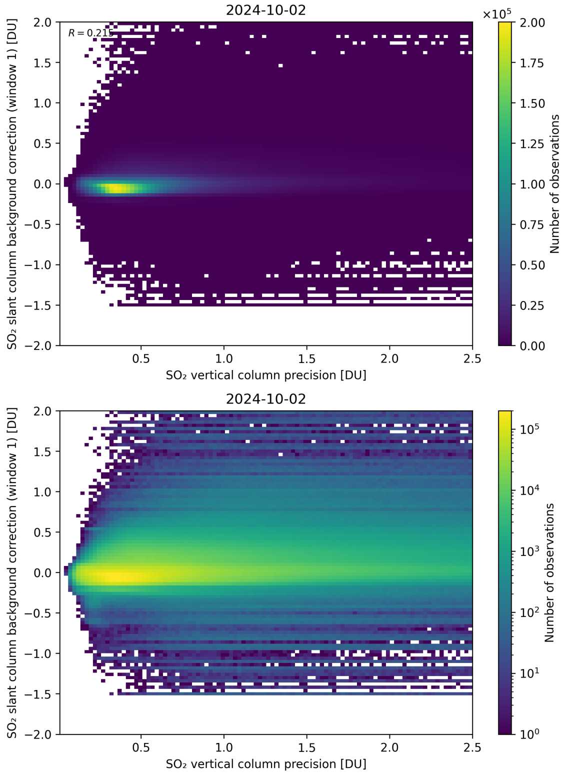
Figure 279: Scatter density plot of “SO 2 vertical column precision” against “SO 2 slant column background correction (window 1)” for 2024-10-01 to 2024-10-03.
