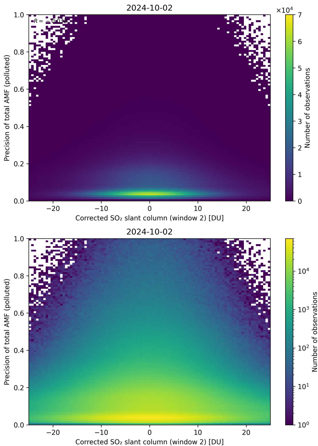
Figure 204: Scatter density plot of “Corrected SO 2 slant column (window 2)” against “Precision of total AMF (polluted)” for 2024-10-01 to 2024-10-03.
