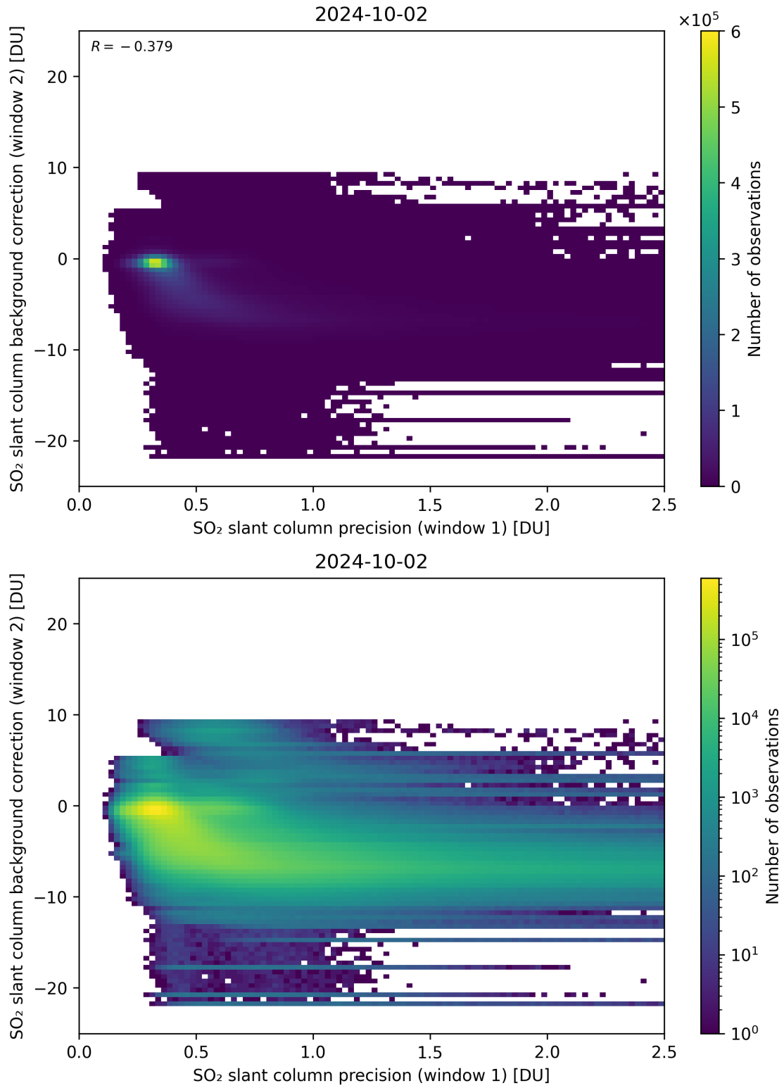
Figure 219: Scatter density plot of “SO 2 slant column precision (window 1)” against “SO 2 slant column background correction (window 2)” for 2024-10-01 to 2024-10-03.
