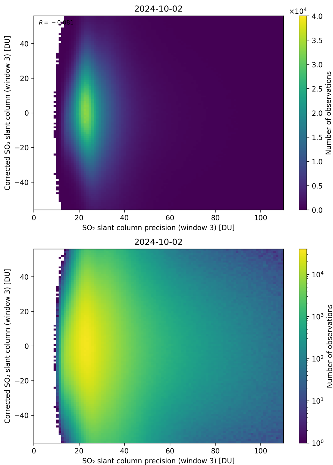
Figure 262: Scatter density plot of “SO 2 slant column precision (window 3)” against “Corrected SO 2 slant column (window 3)” for 2024-10-01 to 2024-10-03.
