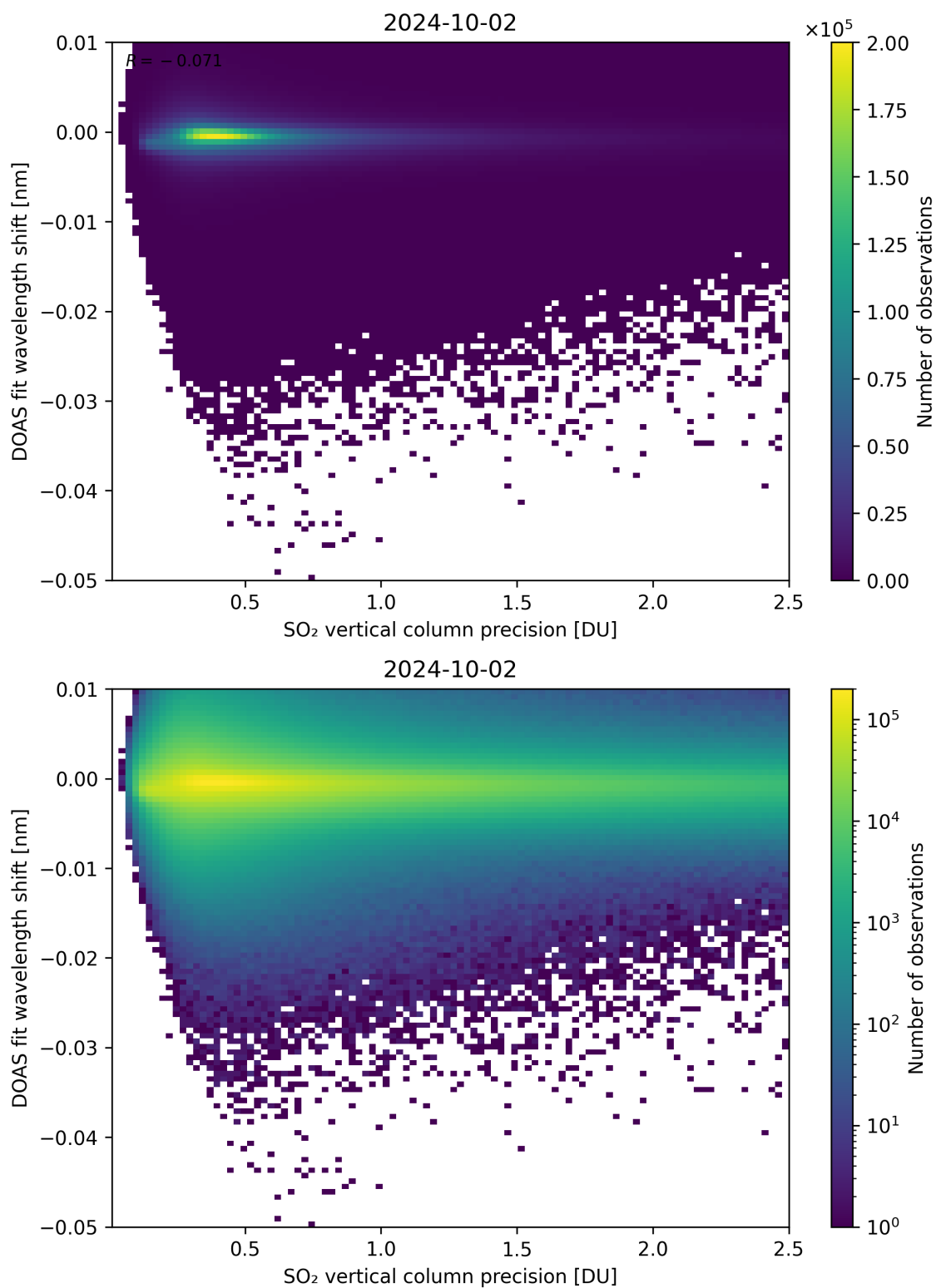
Figure 282: Scatter density plot of “SO 2 vertical column precision” against “DOAS fit wavelength shift” for 2024-10-01 to 2024-10-03.
