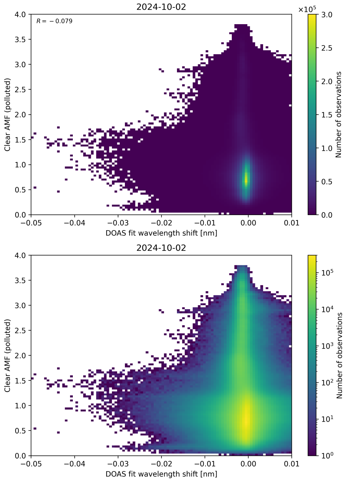
Figure 129: Scatter density plot of “DOAS fit wavelength shift” against “Clear AMF (polluted)” for 2024-10-01 to 2024-10-03.
