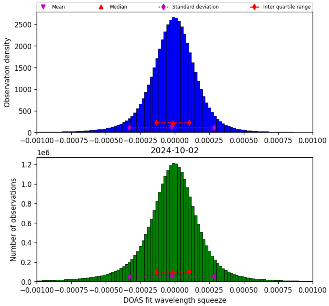
Figure 69: Histogram of “DOAS fit wavelength squeeze” for 2024-10-01 to 2024-10-03
