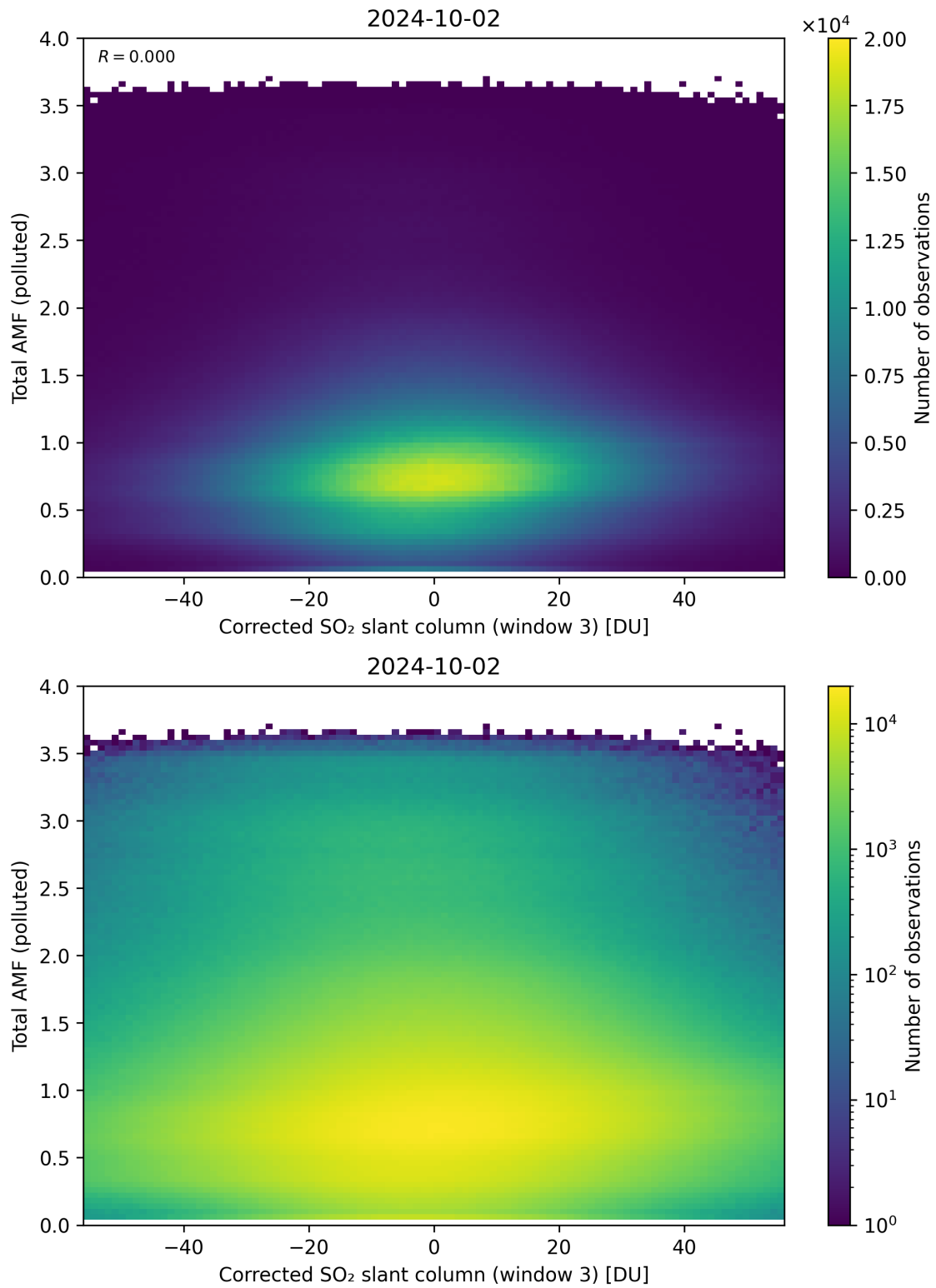
Figure 210: Scatter density plot of “Corrected SO 2 slant column (window 3)” against “Total AMF (polluted)” for 2024-10-01 to 2024-10-03.
