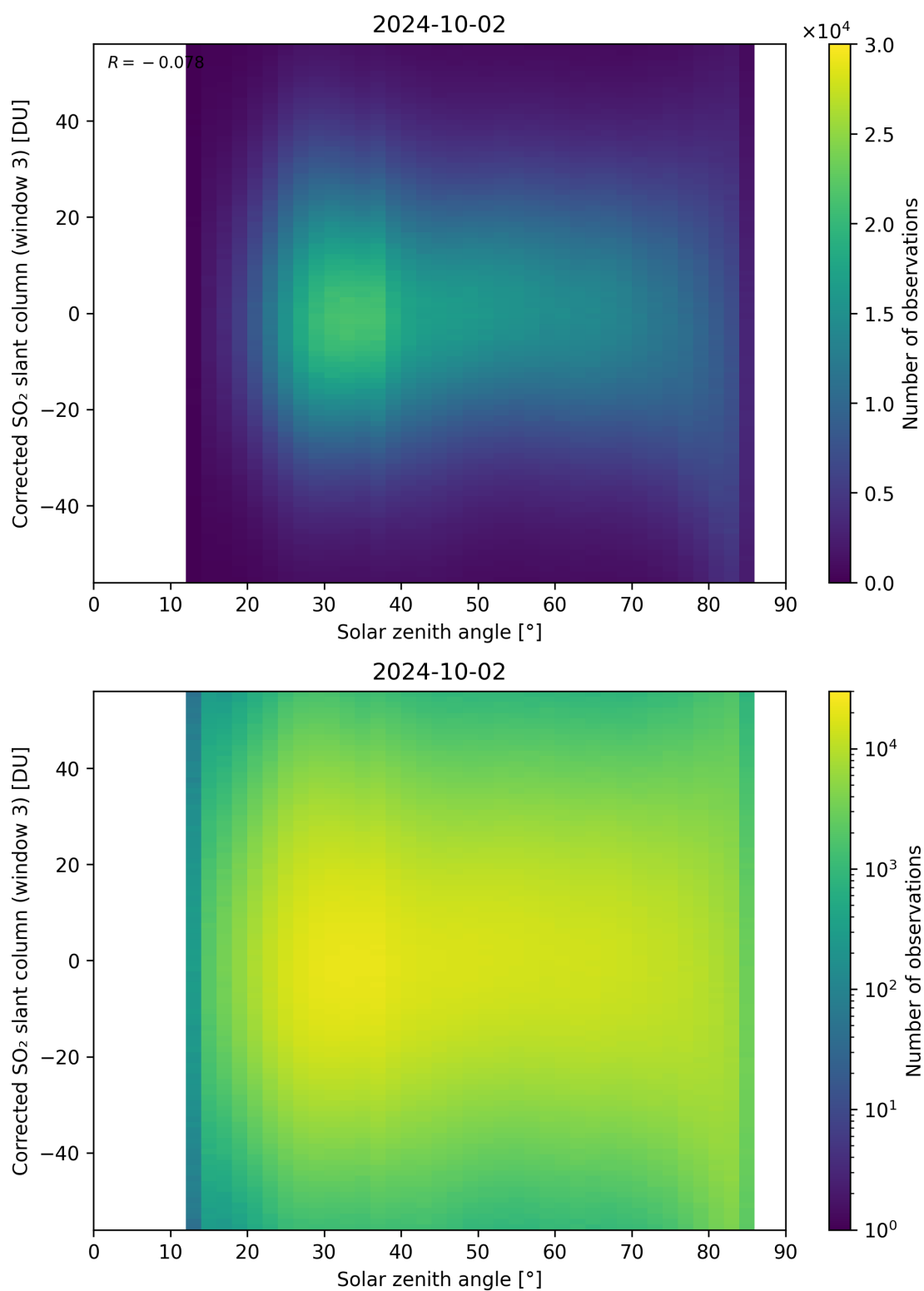
Figure 168: Scatter density plot of “Solar zenith angle” against “Corrected SO 2 slant column (window 3)” for 2024-10-01 to 2024-10-03.
