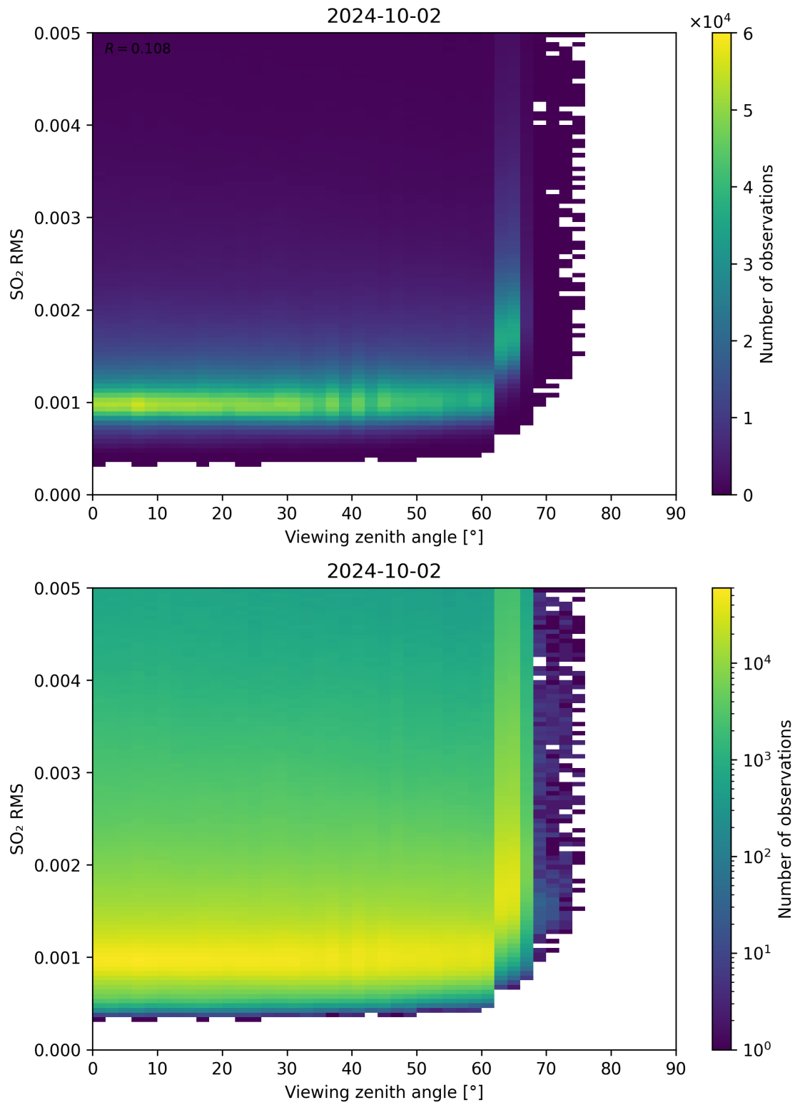
Figure 313: Scatter density plot of “Viewing zenith angle” against “SO 2 RMS” for 2024-10-01 to 2024-10-03.
