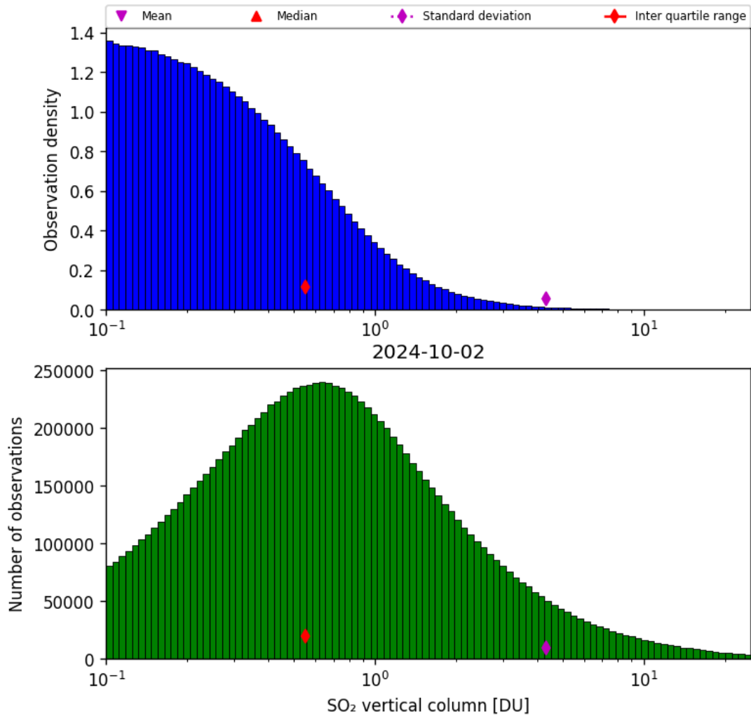
Figure 53: Histogram of “SO 2 vertical column” for 2024-10-01 to 2024-10-03
