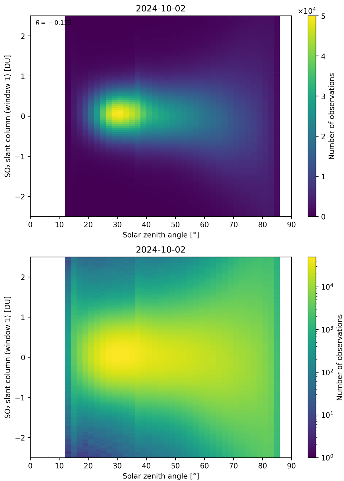
Figure 169: Scatter density plot of “Solar zenith angle” against “SO 2 slant column (window 1)” for 2024-10-01 to 2024-10-03.
