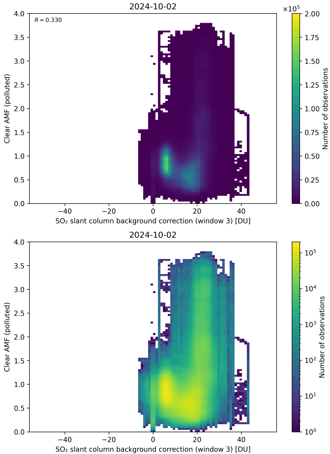
Figure 124: Scatter density plot of “SO 2 slant column background correction (window 3)” against “Clear AMF (polluted)” for 2024-10-01 to 2024-10-03.
