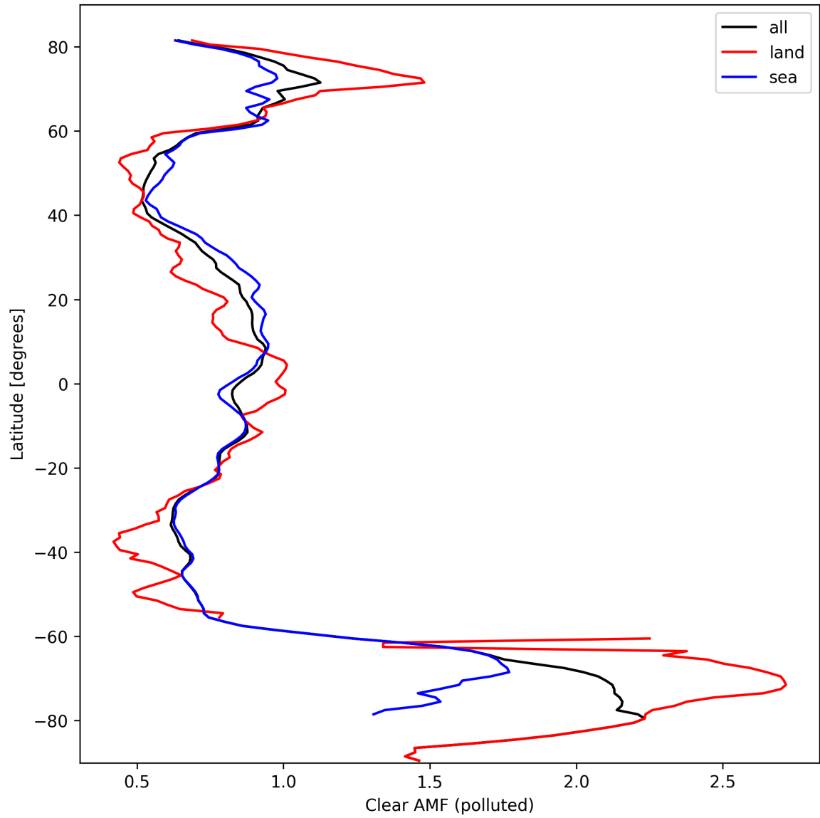
Figure 50: Zonal average of “Clear AMF (polluted)” for 2024-10-01 to 2024-10-03.
