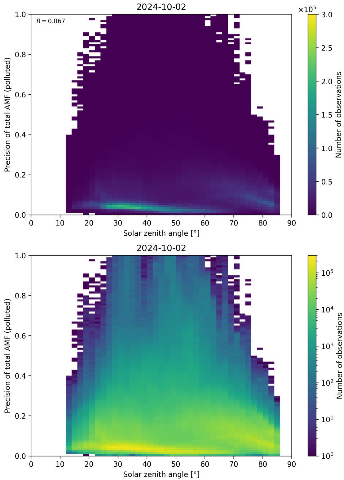
Figure 175: Scatter density plot of “Solar zenith angle” against “Precision of total AMF (polluted)” for 2024-10-01 to 2024-10-03.
