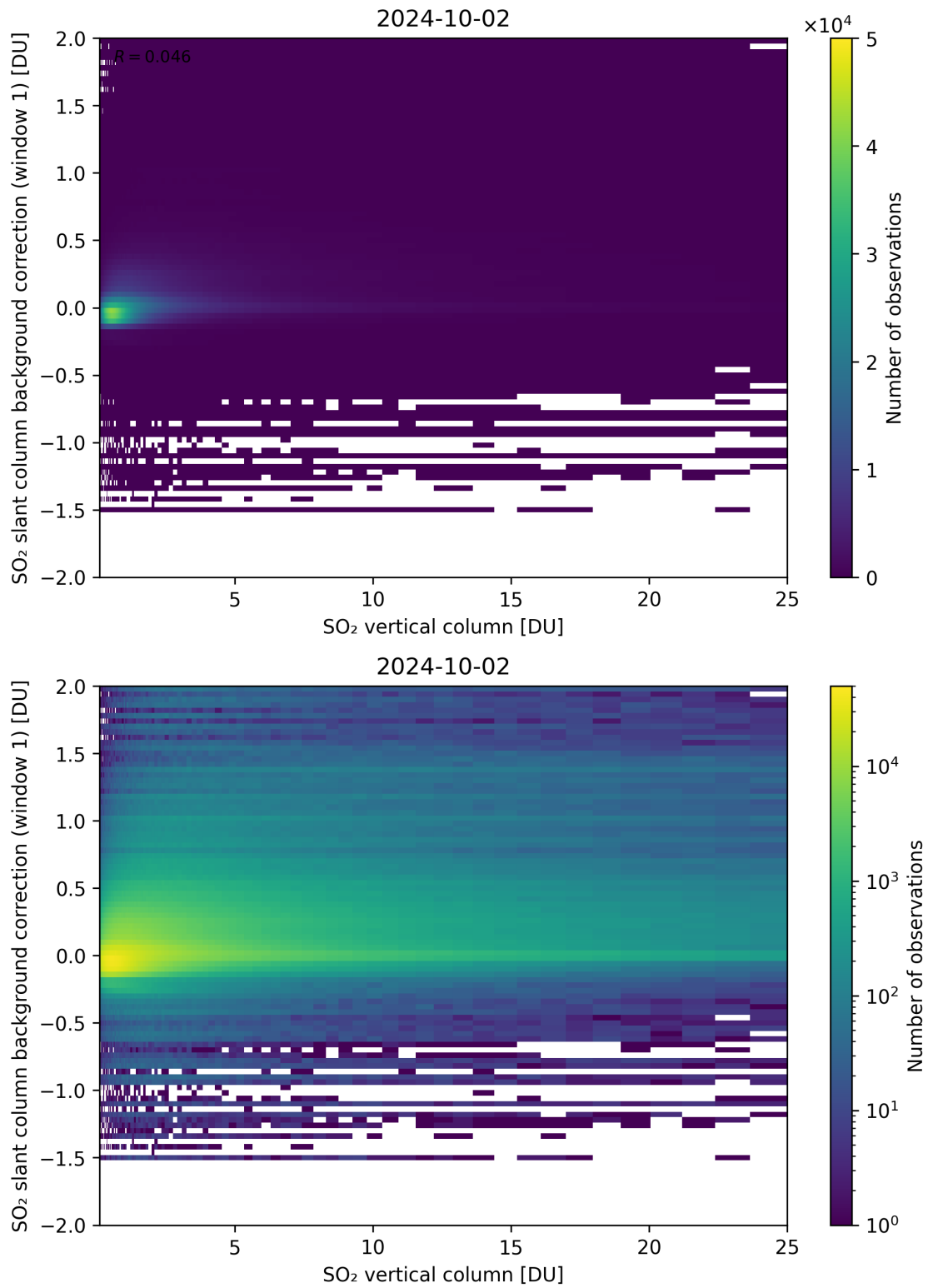
Figure 273: Scatter density plot of “SO 2 vertical column” against “SO 2 slant column background correction (window 1)” for 2024-10-01 to 2024-10-03.
