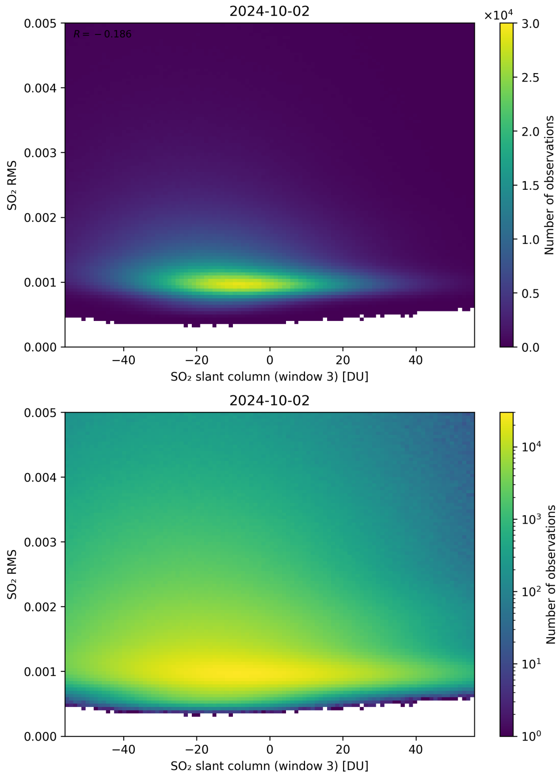
Figure 256: Scatter density plot of “SO 2 slant column (window 3)” against “SO 2 RMS” for 2024-10-01 to 2024-10-03.
