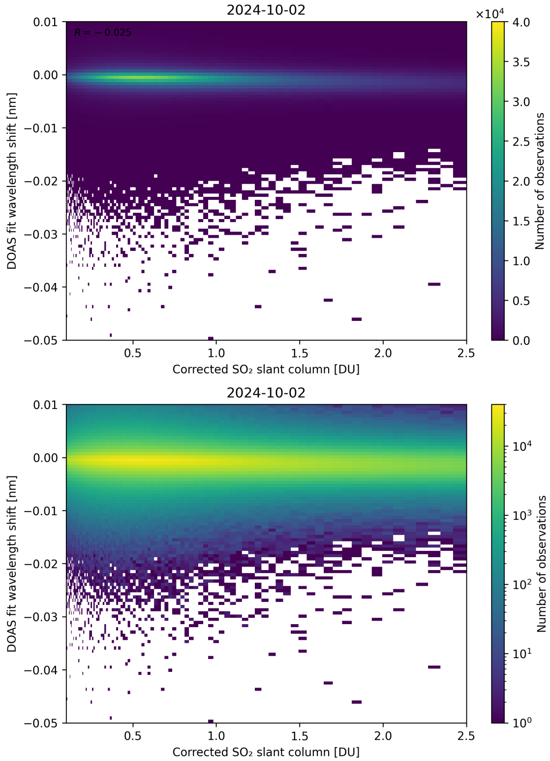
Figure 181: Scatter density plot of “Corrected SO 2 slant column” against “DOAS fit wavelength shift” for 2024-10-01 to 2024-10-03.
