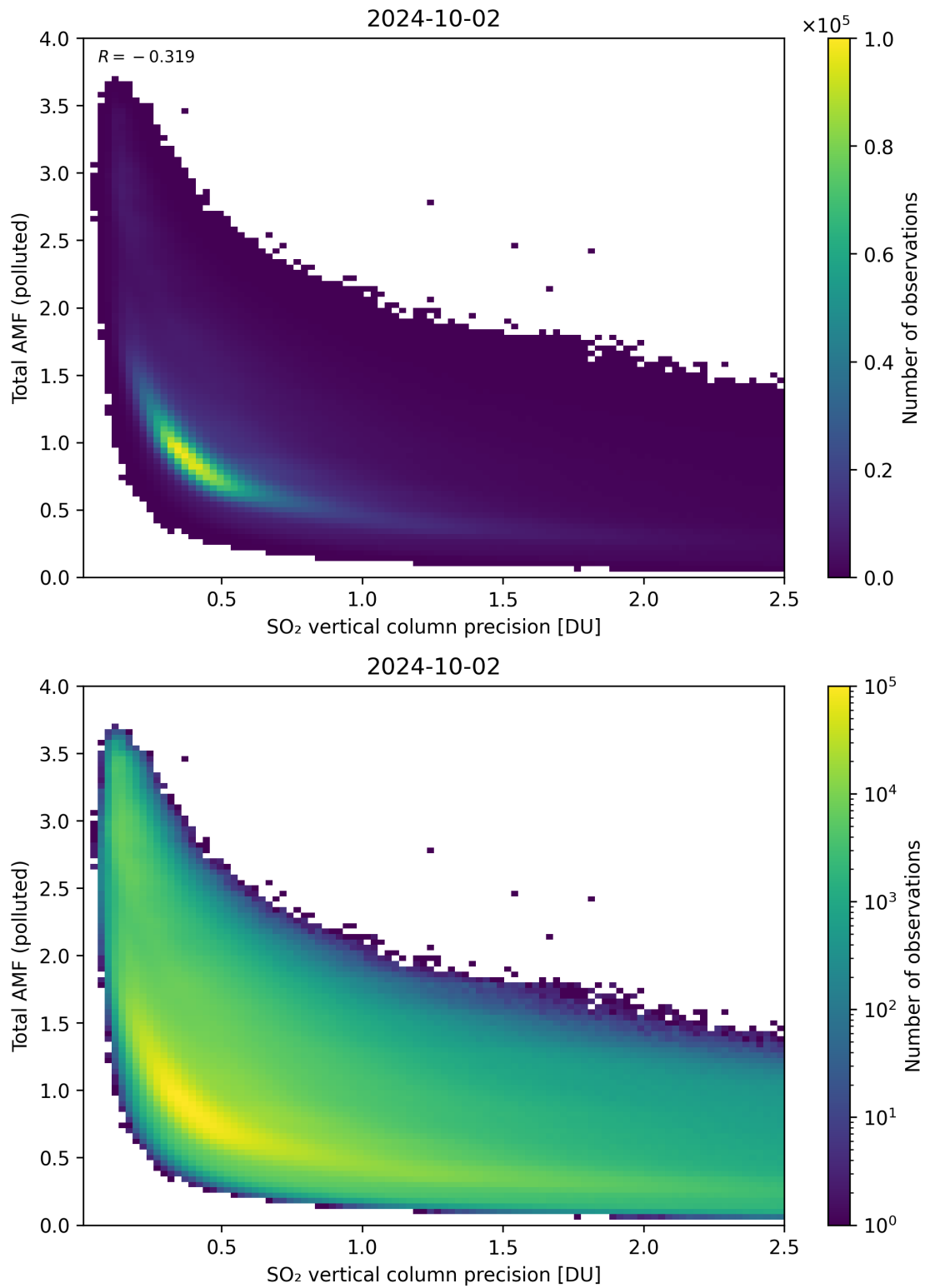
Figure 294: Scatter density plot of “SO 2 vertical column precision” against “Total AMF (polluted)” for 2024-10-01 to 2024-10-03.
