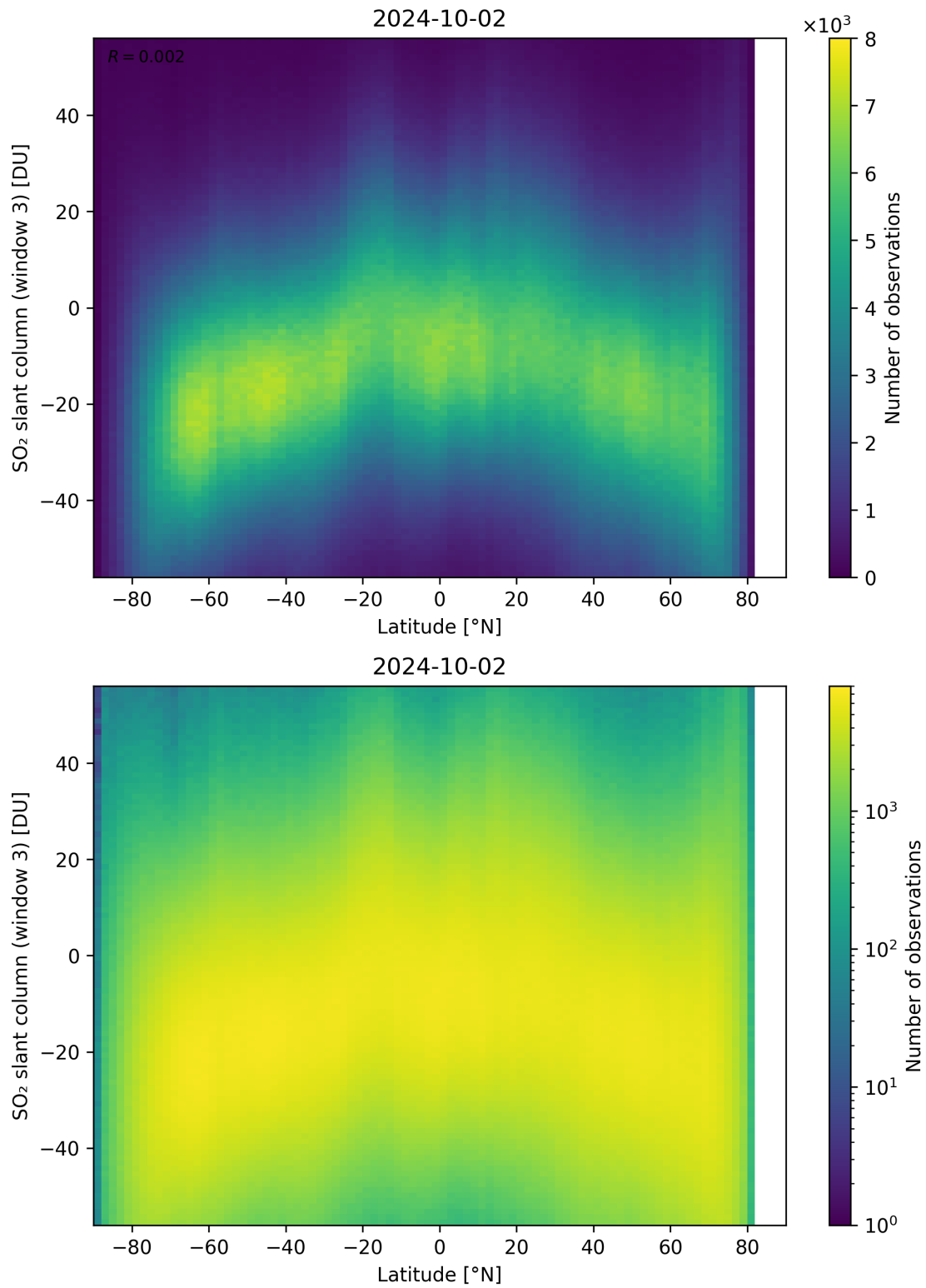
Figure 152: Scatter density plot of “Latitude” against “SO 2 slant column (window 3)” for 2024-10-01 to 2024-10-03.
