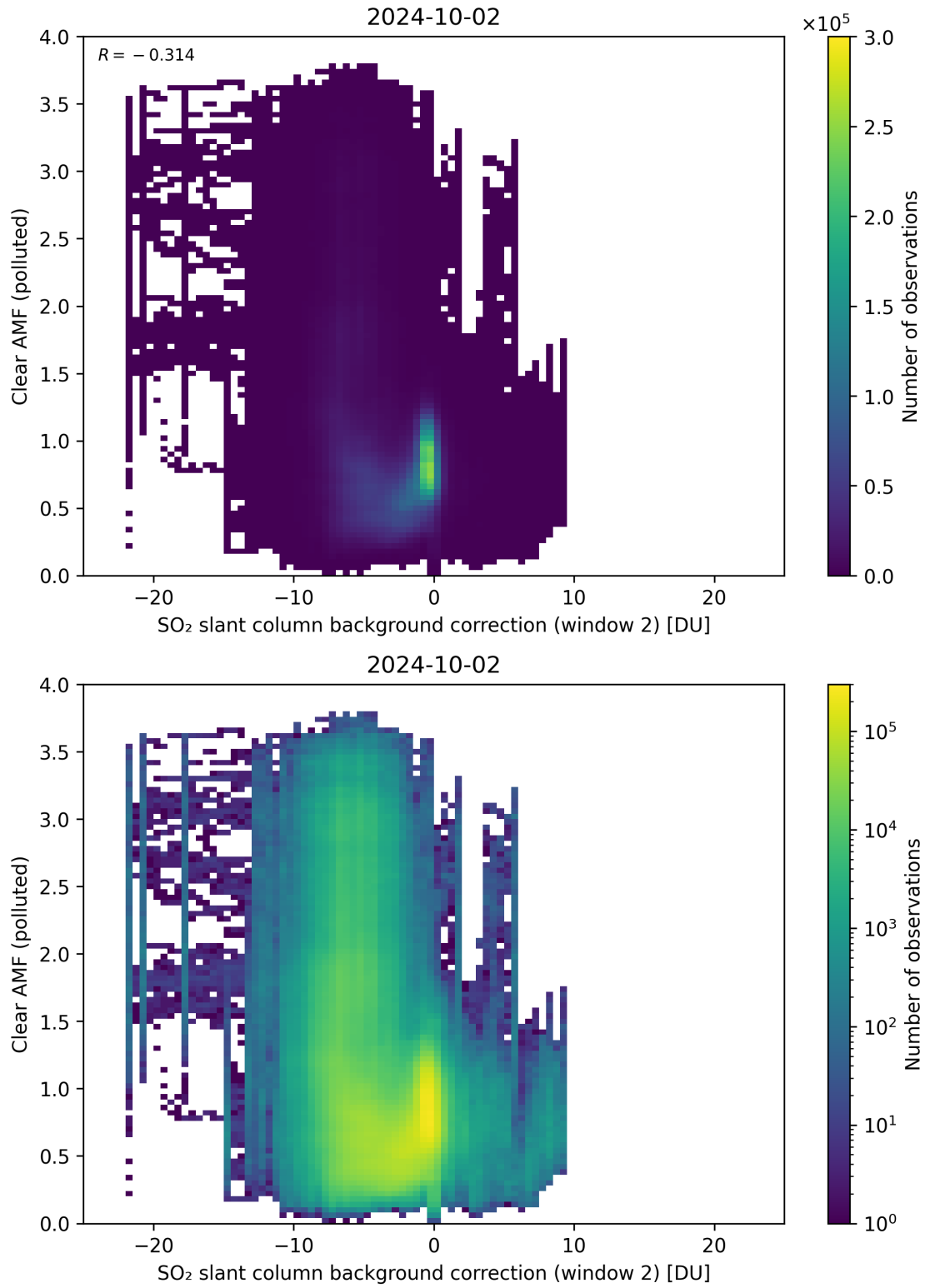
Figure 115: Scatter density plot of “SO 2 slant column background correction (window 2)” against “Clear AMF (polluted)” for 2024-10-01 to 2024-10-03.
