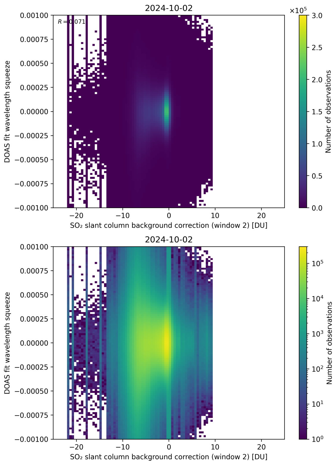
Figure 113: Scatter density plot of “SO 2 slant column background correction (window 2)” against “DOAS fit wavelength squeeze” for 2024-10-01 to 2024-10-03.
