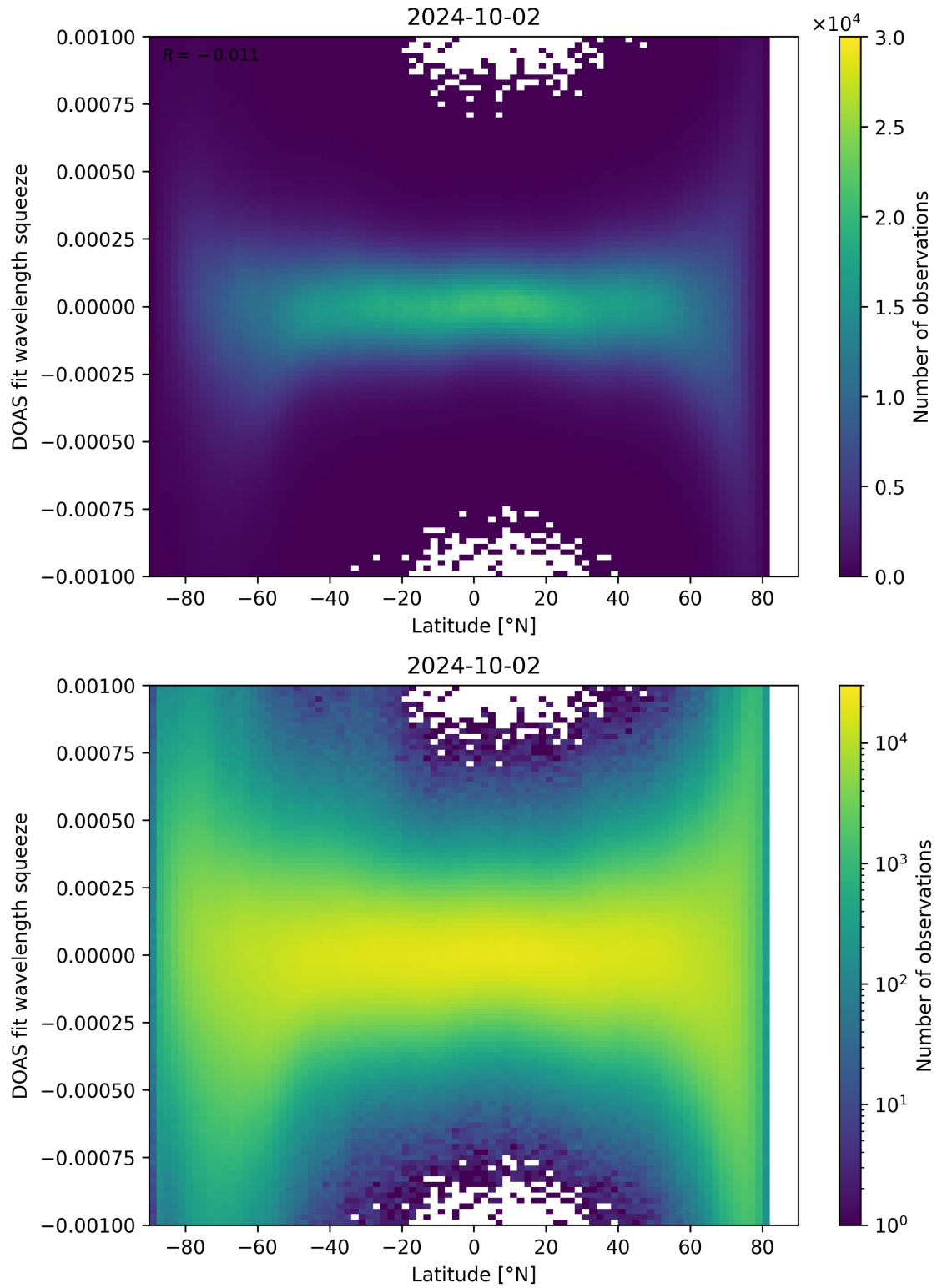
Figure 143: Scatter density plot of “Latitude” against “DOAS fit wavelength squeeze” for 2024-10-01 to 2024-10-03.
