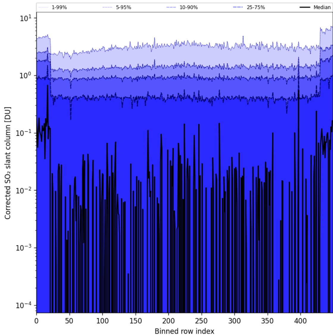
Figure 78: Along track statistics of “Corrected SO 2 slant column” for 2024-10-01 to 2024-10-03
