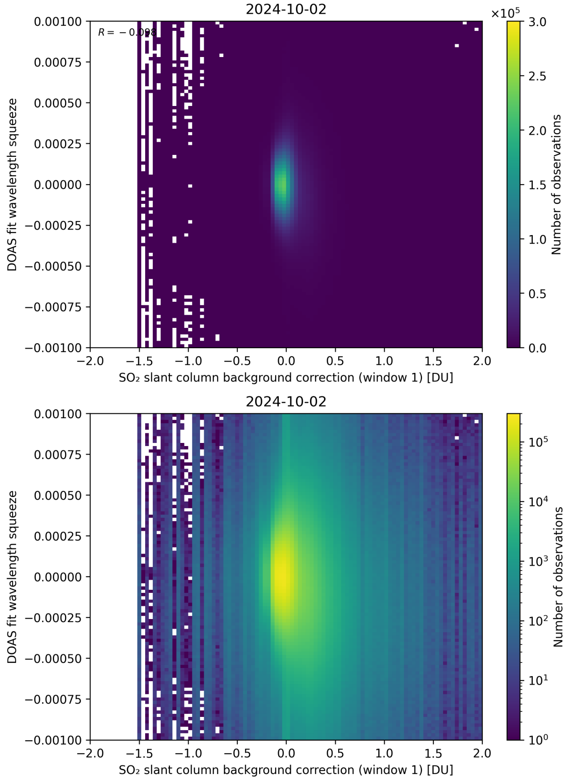
Figure 101: Scatter density plot of “SO 2 slant column background correction (window 1)” against “DOAS fit wavelength squeeze” for 2024-10-01 to 2024-10-03.
