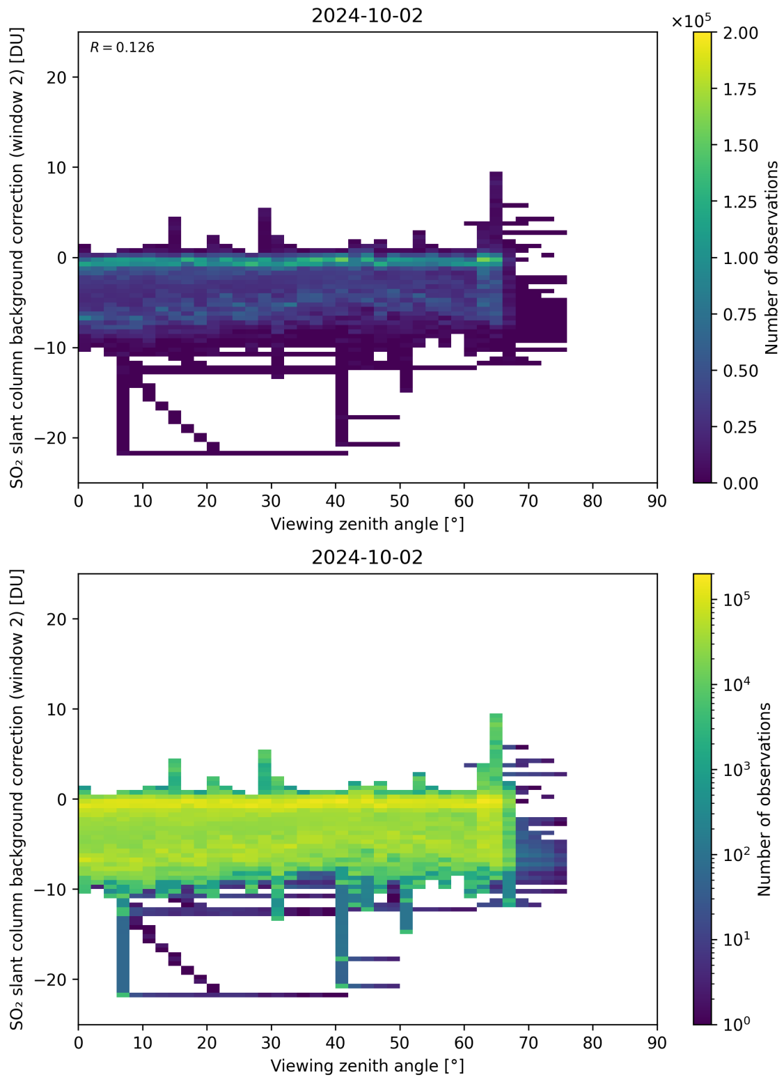
Figure 309: Scatter density plot of “Viewing zenith angle” against “SO 2 slant column background correction (window 2)” for 2024-10-01 to 2024-10-03.
