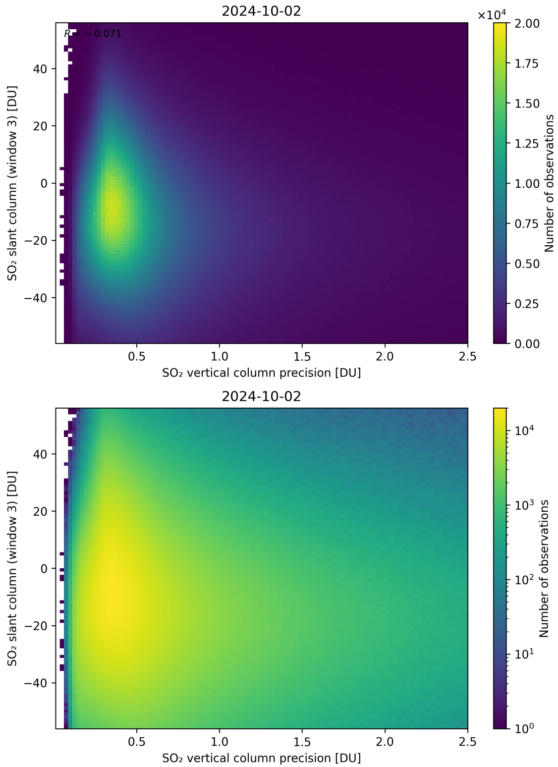
Figure 292: Scatter density plot of “SO 2 vertical column precision” against “SO 2 slant column (window 3)” for 2024-10-01 to 2024-10-03.
