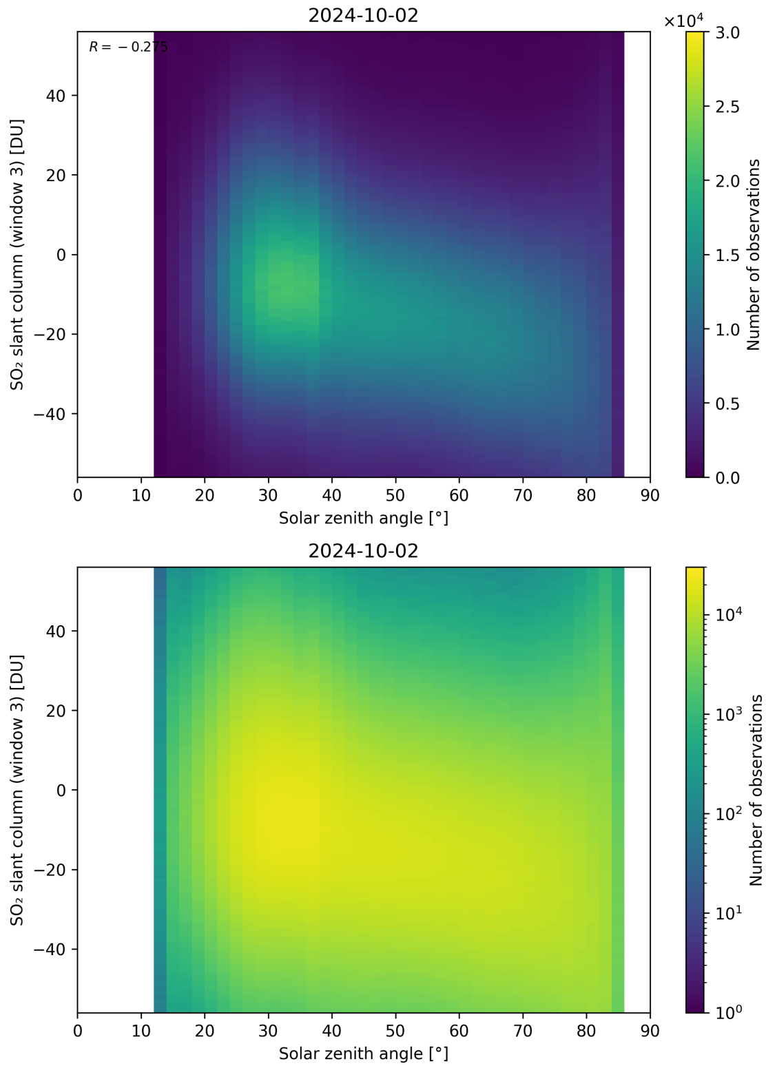
Figure 172: Scatter density plot of “Solar zenith angle” against “SO 2 slant column (window 3)” for 2024-10-01 to 2024-10-03.
