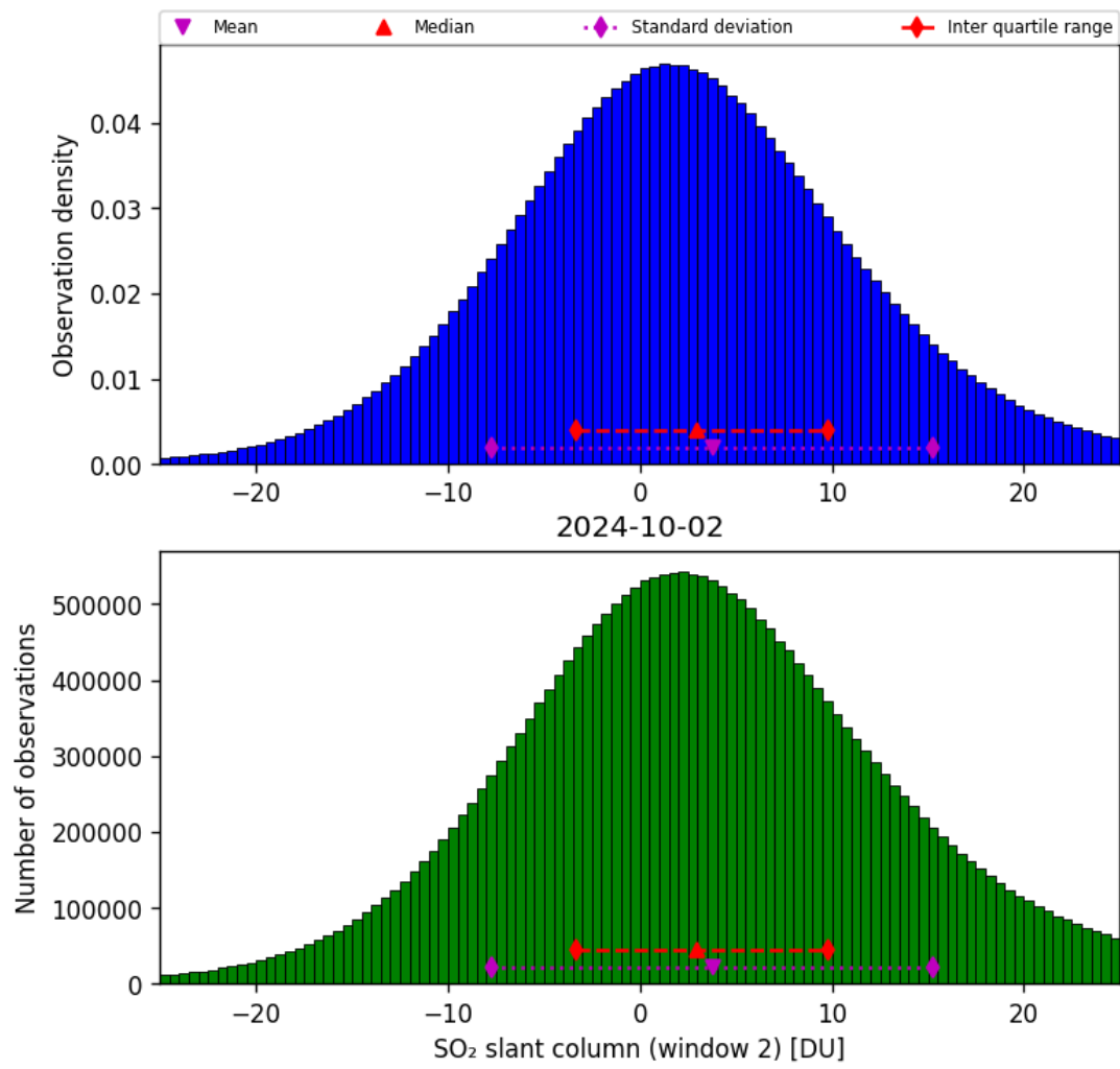
Figure 60: Histogram of “SO 2 slant column (window 2)” for 2024-10-01 to 2024-10-03
