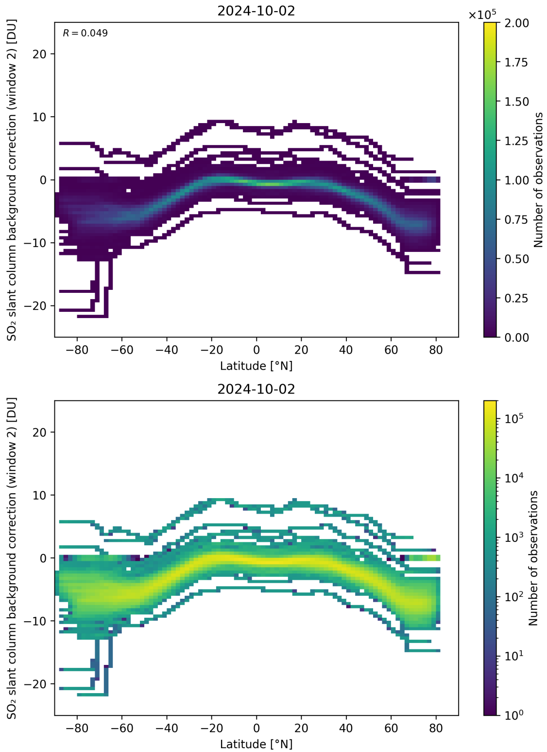
Figure 140: Scatter density plot of “Latitude” against “SO 2 slant column background correction (window 2)” for 2024-10-01 to 2024-10-03.
