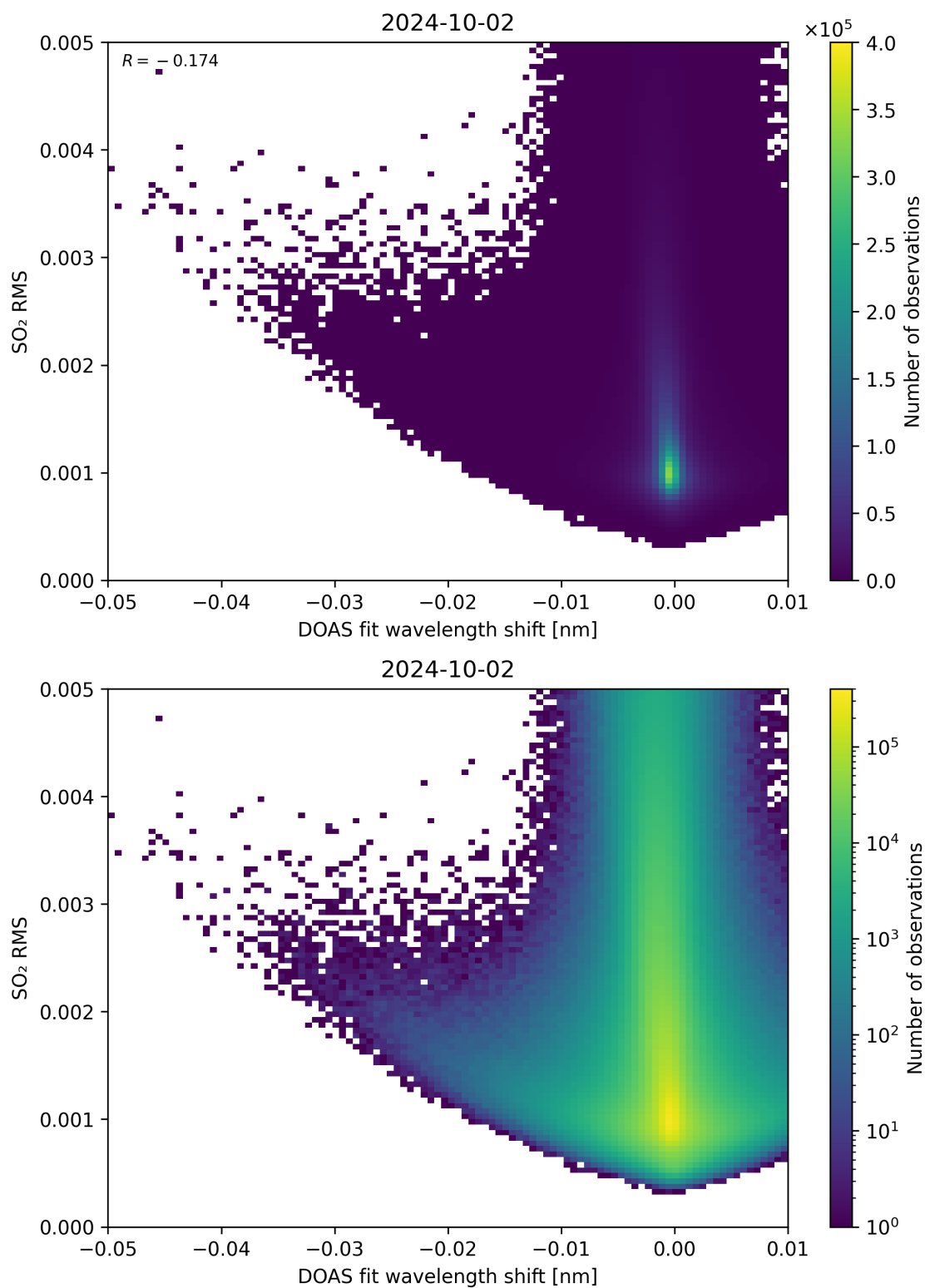
Figure 128: Scatter density plot of “DOAS fit wavelength shift” against “SO 2 RMS” for 2024-10-01 to 2024-10-03.
