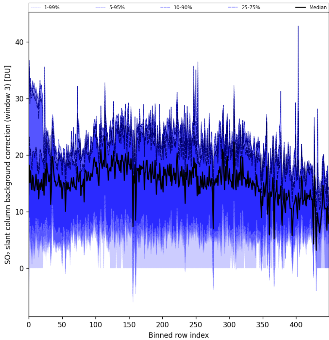
Figure 90: Along track statistics of “SO 2 slant column background correction (window 3)” for 2024-10-01 to 2024-10-03
