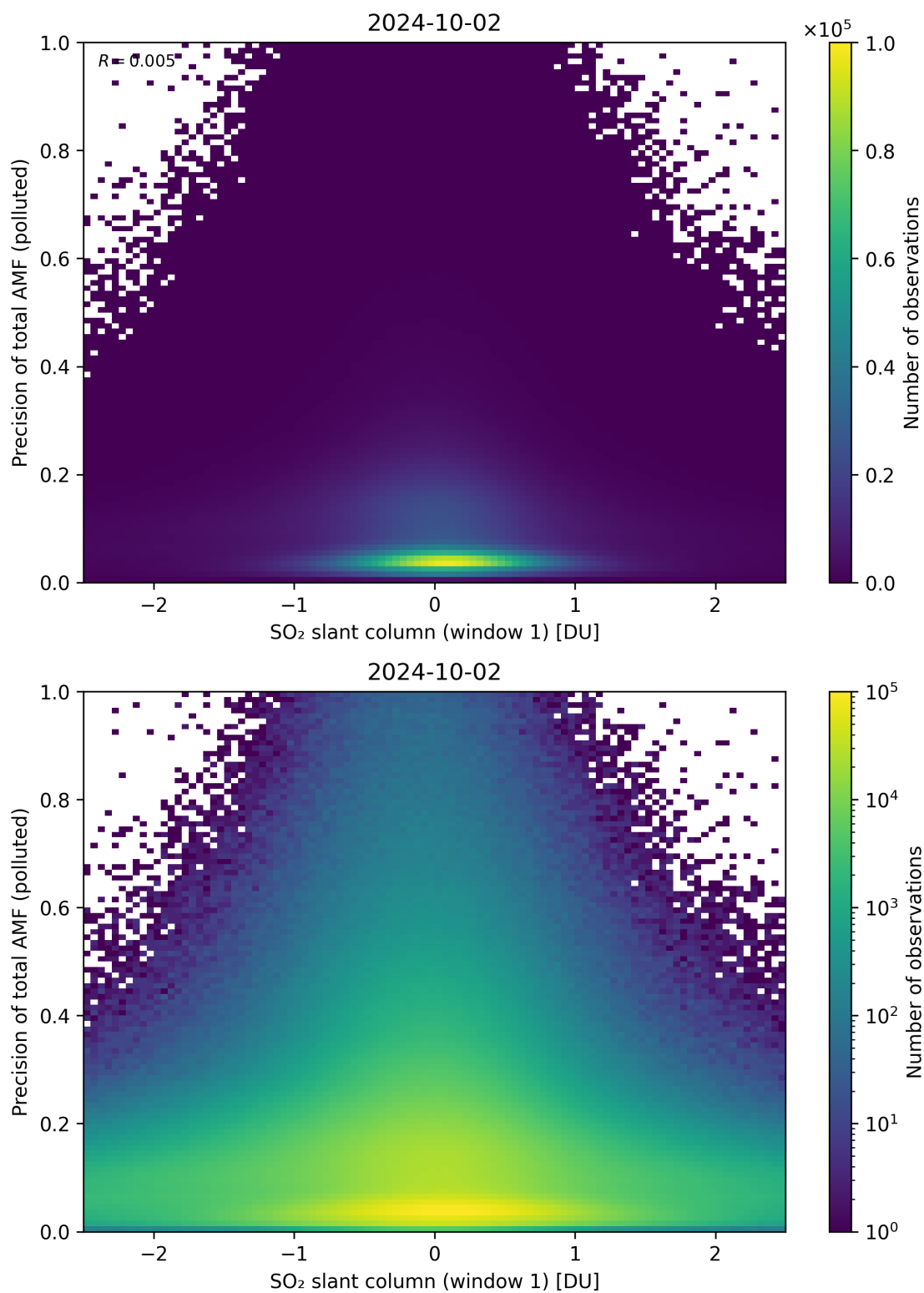
Figure 240: Scatter density plot of “SO 2 slant column (window 1)” against “Precision of total AMF (polluted)” for 2024-10-01 to 2024-10-03.
