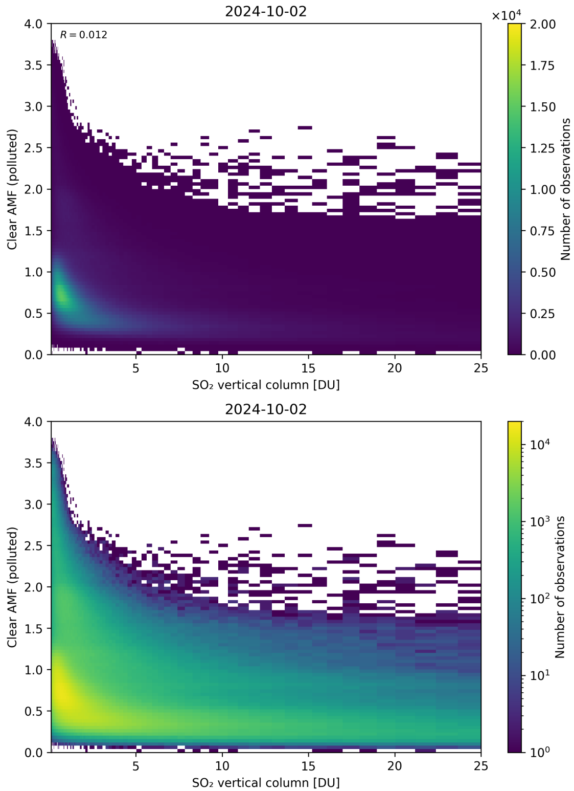
Figure 296: Scatter density plot of “SO 2 vertical column” against “Clear AMF (polluted)” for 2024-10-01 to 2024-10-03.
