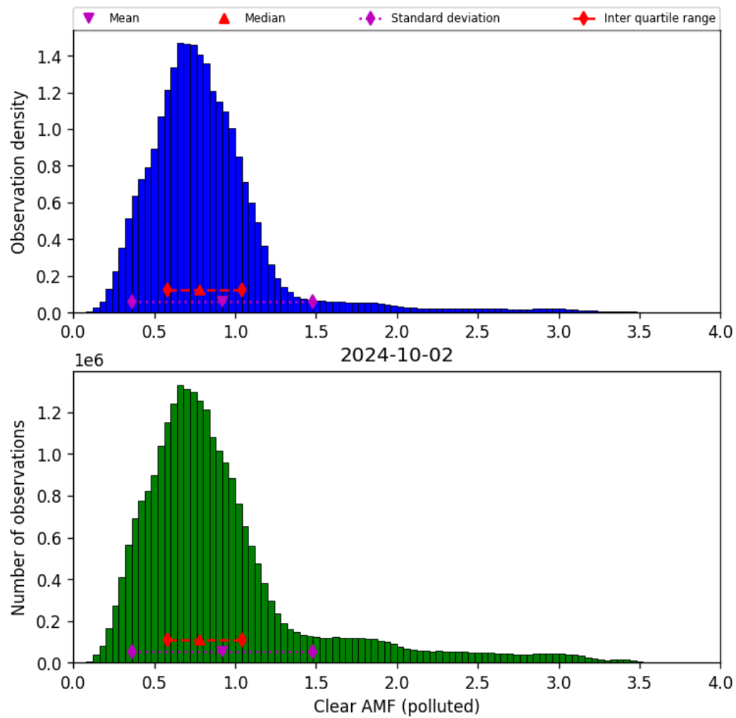
Figure 73: Histogram of “Clear AMF (polluted)” for 2024-10-01 to 2024-10-03
