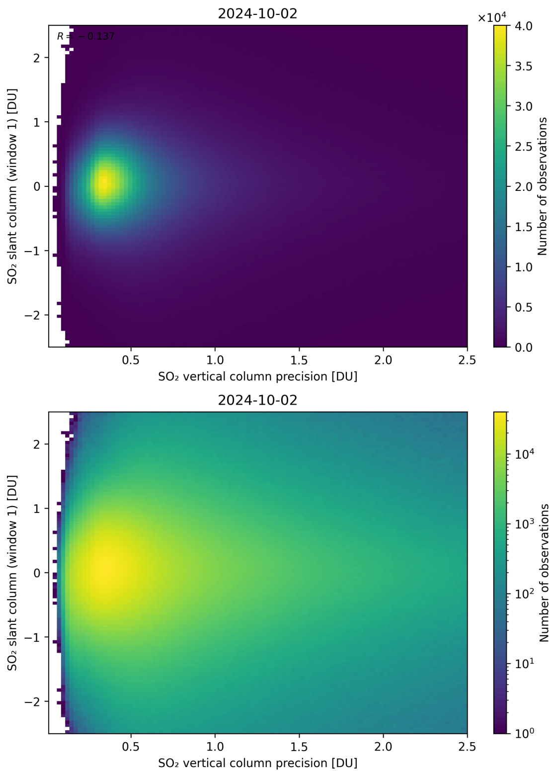
Figure 289: Scatter density plot of “SO 2 vertical column precision” against “SO 2 slant column (window 1)” for 2024-10-01 to 2024-10-03.
