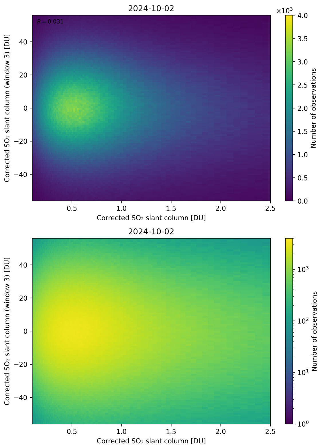
Figure 186: Scatter density plot of “Corrected SO 2 slant column” against “Corrected SO 2 slant column (window 3)” for 2024-10-01 to 2024-10-03.
