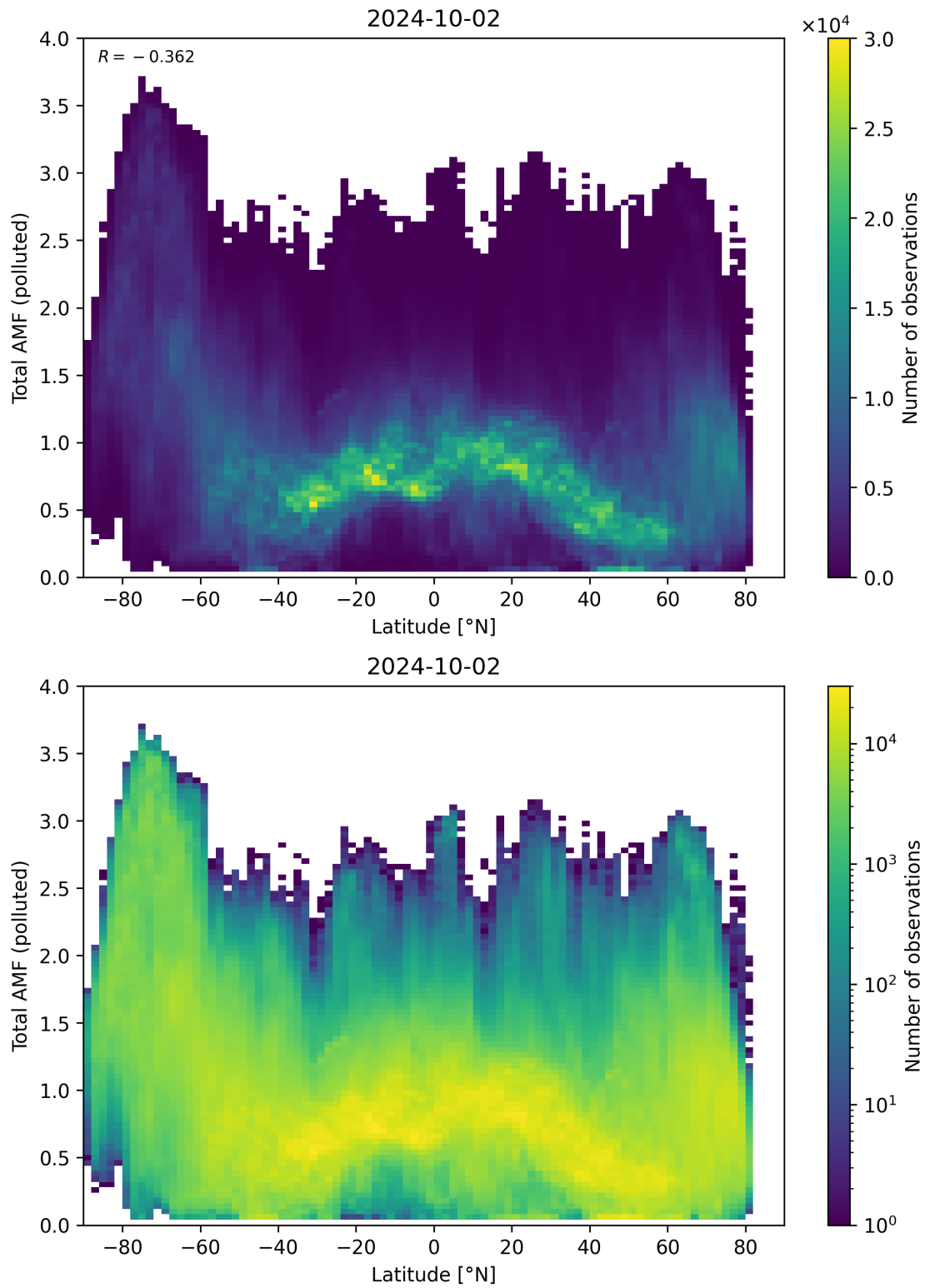
Figure 154: Scatter density plot of “Latitude” against “Total AMF (polluted)” for 2024-10-01 to 2024-10-03.
