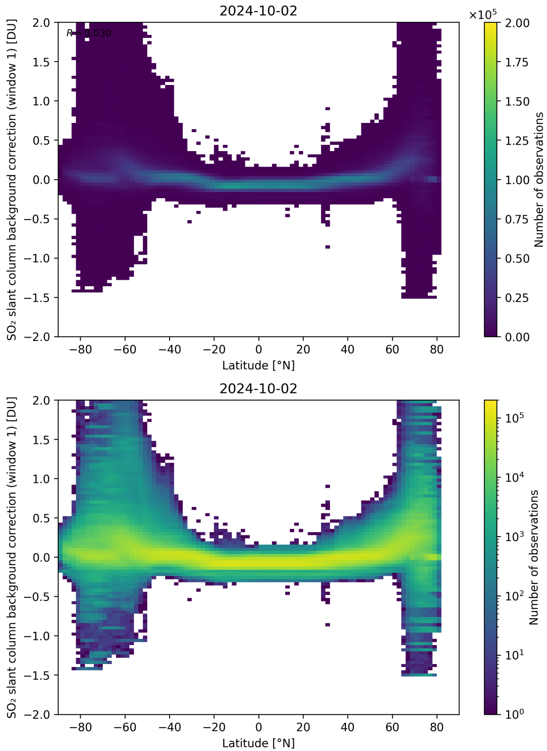
Figure 139: Scatter density plot of “Latitude” against “SO 2 slant column background correction (window 1)” for 2024-10-01 to 2024-10-03.
