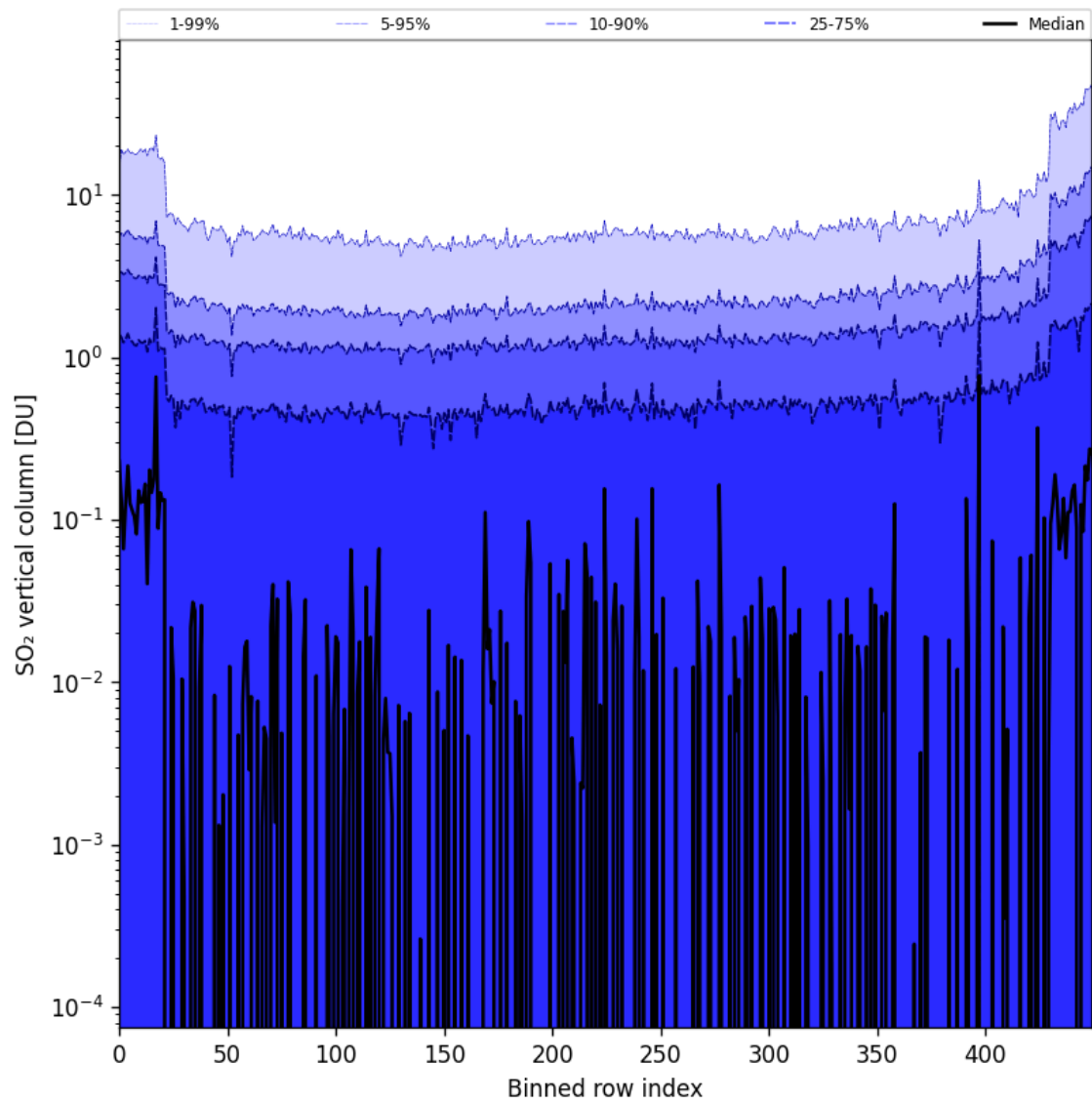
Figure 76: Along track statistics of “SO 2 vertical column” for 2024-10-01 to 2024-10-03
