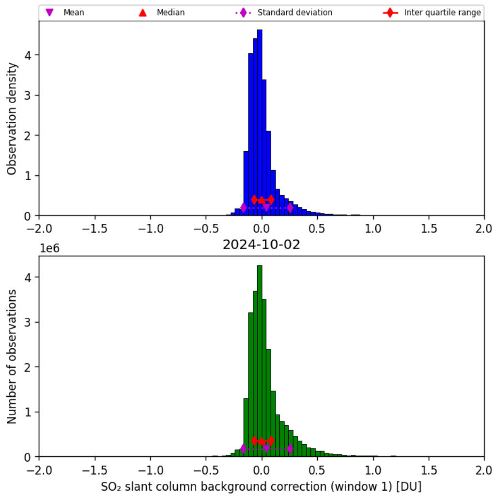
Figure 59: Histogram of “SO 2 slant column background correction (window 1)” for 2024-10-01 to 2024-10-03
