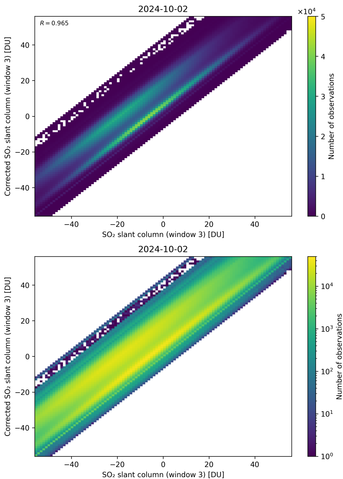
Figure 266: Scatter density plot of “SO 2 slant column (window 3)” against “Corrected SO 2 slant column (window 3)” for 2024-10-01 to 2024-10-03.
