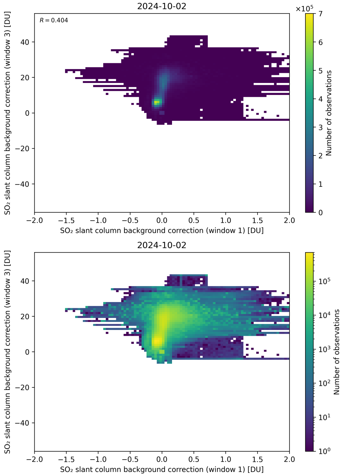
Figure 99: Scatter density plot of “SO 2 slant column background correction (window 1)” against “SO 2 slant column background correction (window 3)” for 2024-10-01 to 2024-10-03.
