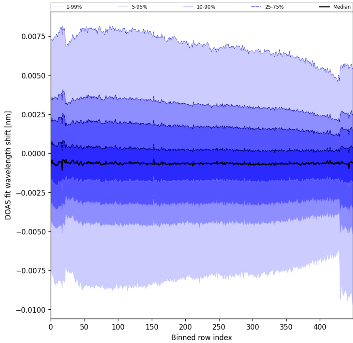
Figure 91: Along track statistics of “DOAS fit wavelength shift” for 2024-10-01 to 2024-10-03
