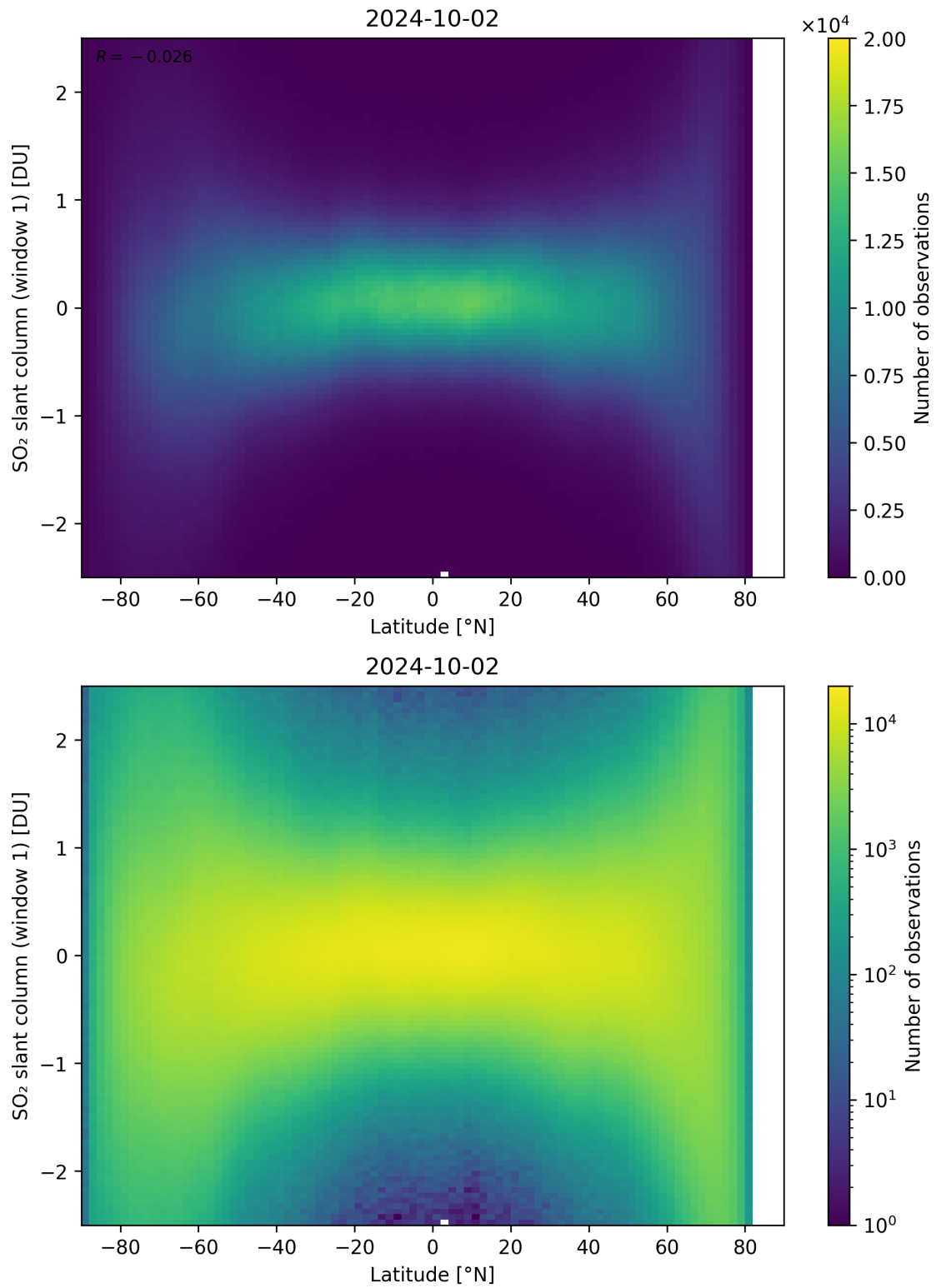
Figure 149: Scatter density plot of “Latitude” against “SO 2 slant column (window 1)” for 2024-10-01 to 2024-10-03.
