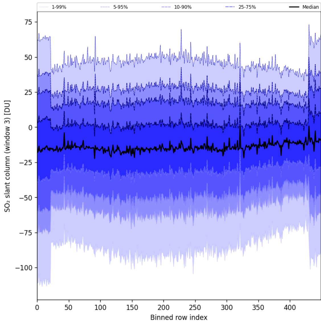
Figure 87: Along track statistics of “SO 2 slant column (window 3)” for 2024-10-01 to 2024-10-03
