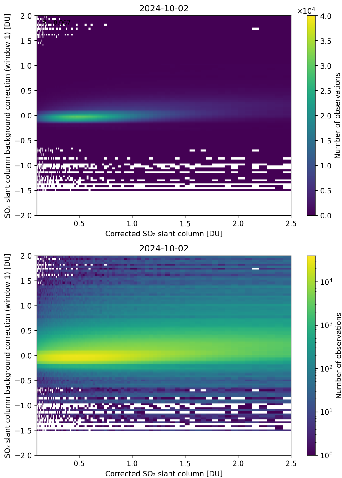
Figure 178: Scatter density plot of “Corrected SO 2 slant column” against “SO 2 slant column background correction (window 1)” for 2024-10-01 to 2024-10-03.
