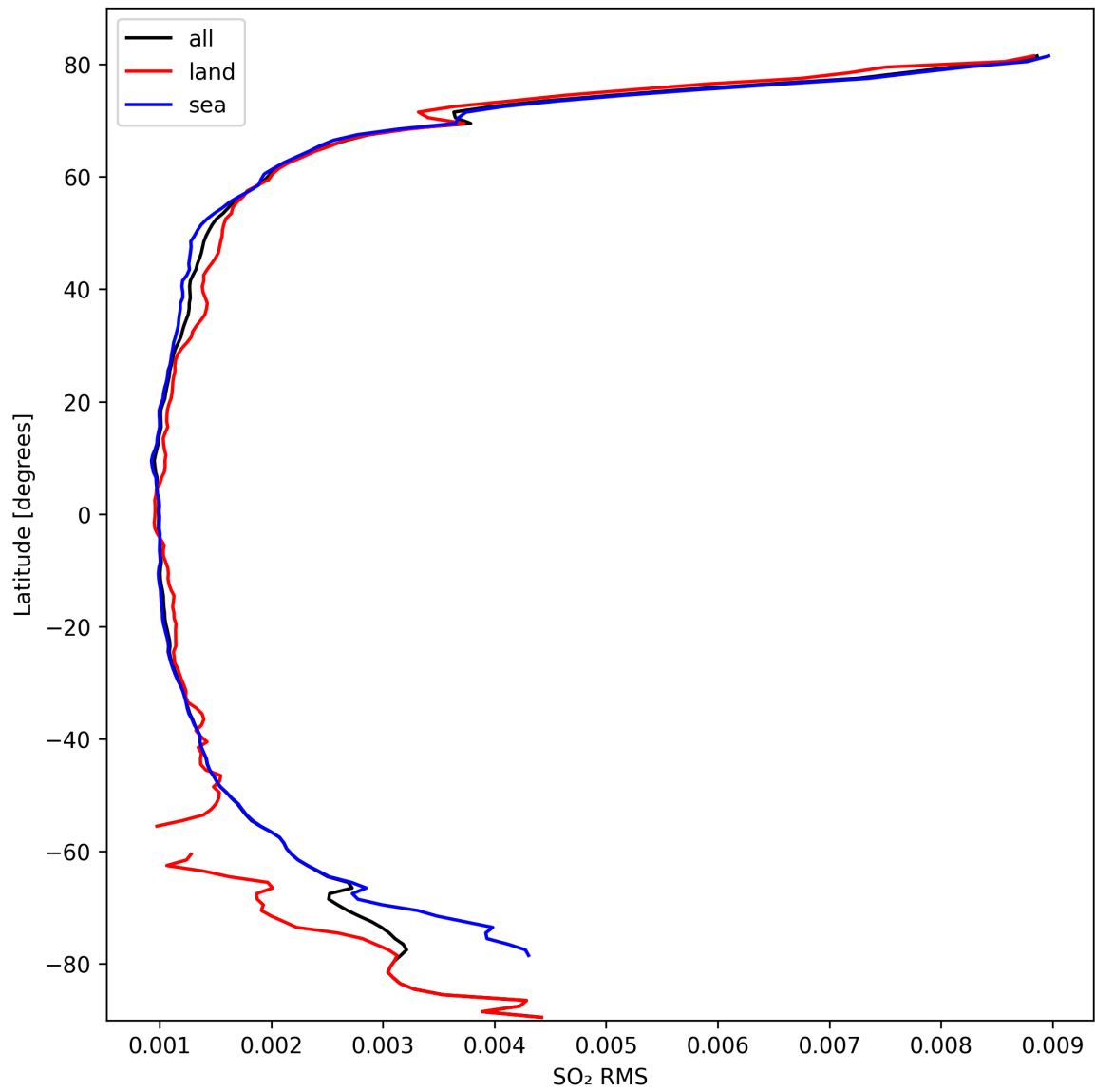
Figure 47: Zonal average of “SO 2 RMS” for 2024-10-01 to 2024-10-03.
