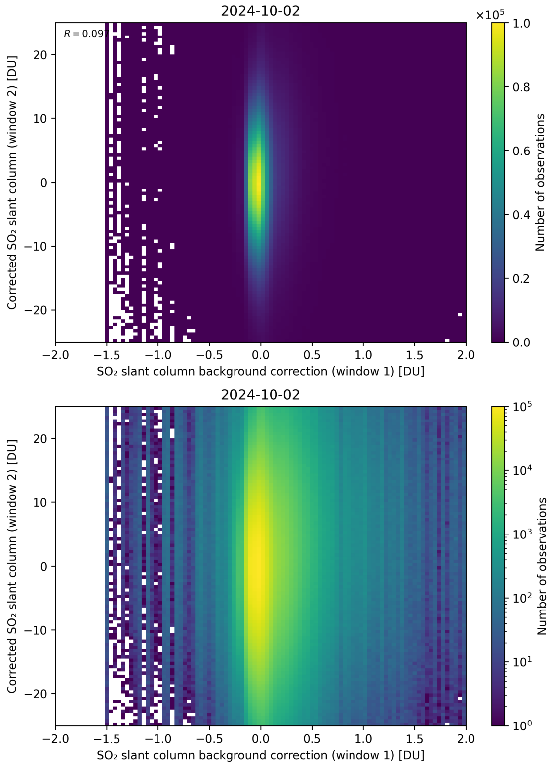
Figure 104: Scatter density plot of “SO 2 slant column background correction (window 1)” against “Corrected SO 2 slant column (window 2)” for 2024-10-01 to 2024-10-03.
