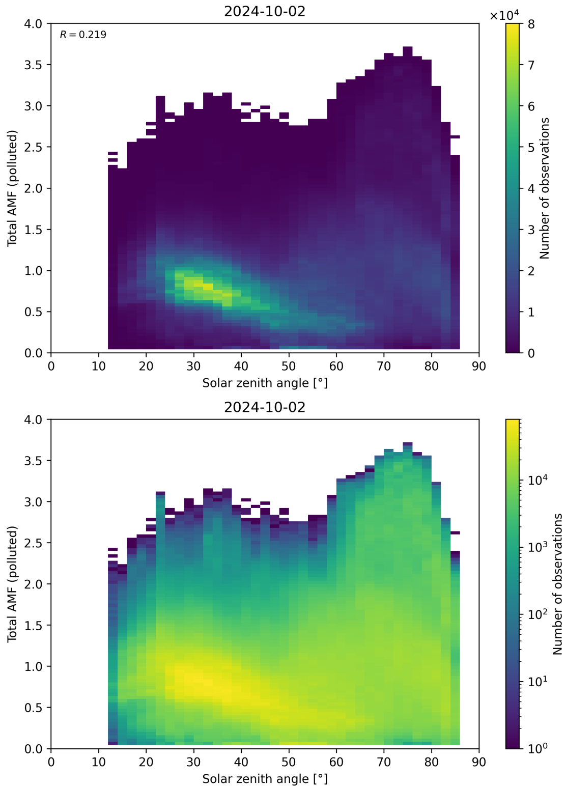
Figure 174: Scatter density plot of “Solar zenith angle” against “Total AMF (polluted)” for 2024-10-01 to 2024-10-03.
