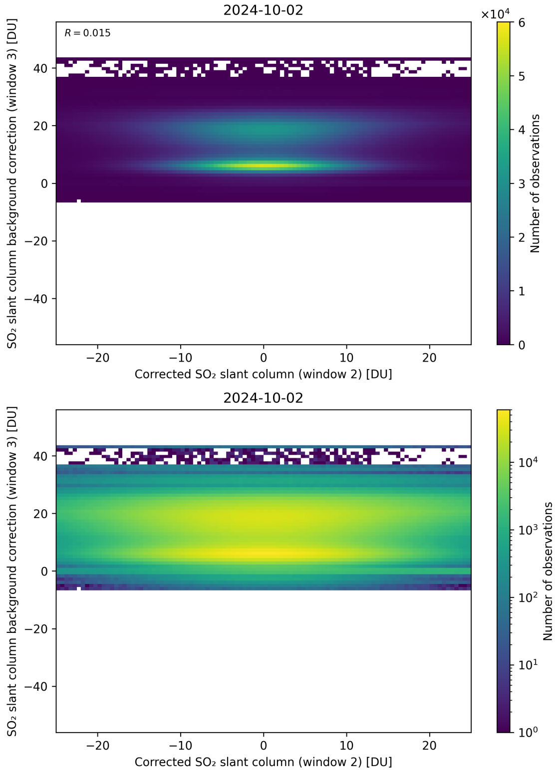
Figure 195: Scatter density plot of “Corrected SO 2 slant column (window 2)” against “SO 2 slant column background correction (window 3)” for 2024-10-01 to 2024-10-03.
