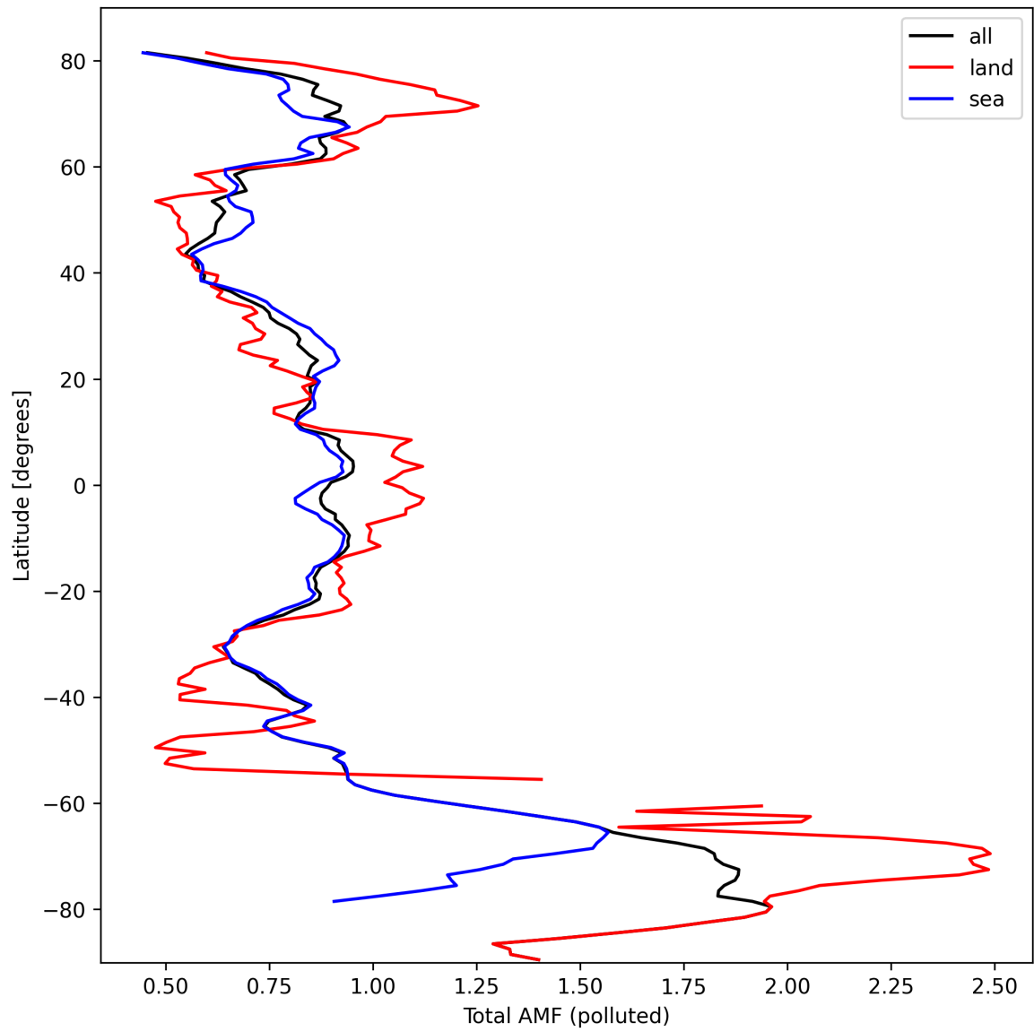
Figure 48: Zonal average of “Total AMF (polluted)” for 2024-10-01 to 2024-10-03.
