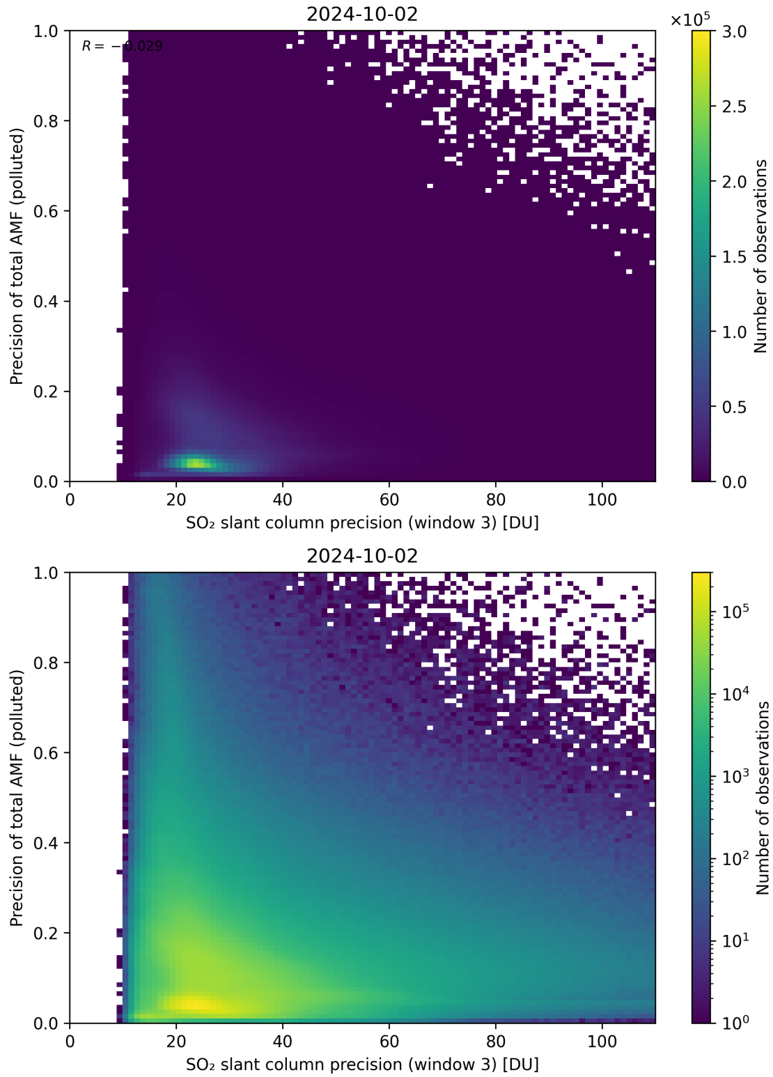
Figure 264: Scatter density plot of “SO 2 slant column precision (window 3)” against “Precision of total AMF (polluted)” for 2024-10-01 to 2024-10-03.
