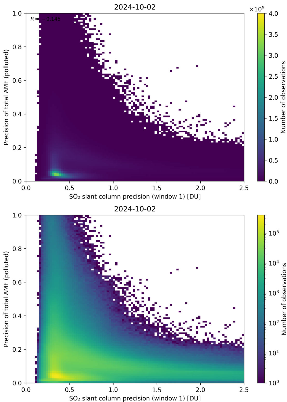
Figure 231: Scatter density plot of “SO 2 slant column precision (window 1)” against “Precision of total AMF (polluted)” for 2024-10-01 to 2024-10-03.
