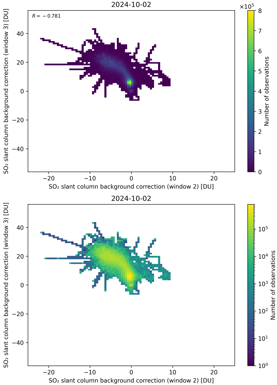
Figure 111: Scatter density plot of “SO 2 slant column background correction (window 2)” against “SO 2 slant column background correction (window 3)” for 2024-10-01 to 2024-10-03.
