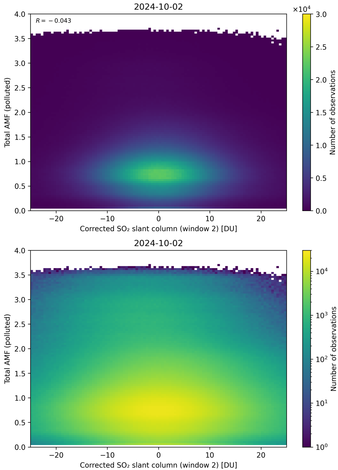
Figure 203: Scatter density plot of “Corrected SO 2 slant column (window 2)” against “Total AMF (polluted)” for 2024-10-01 to 2024-10-03.
