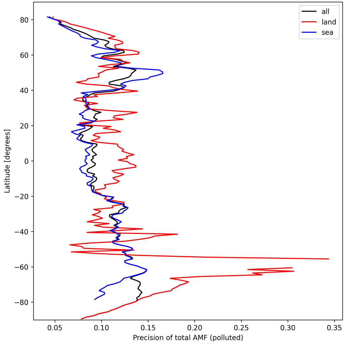
Figure 49: Zonal average of “Precision of total AMF (polluted)” for 2024-10-01 to 2024-10-03.
