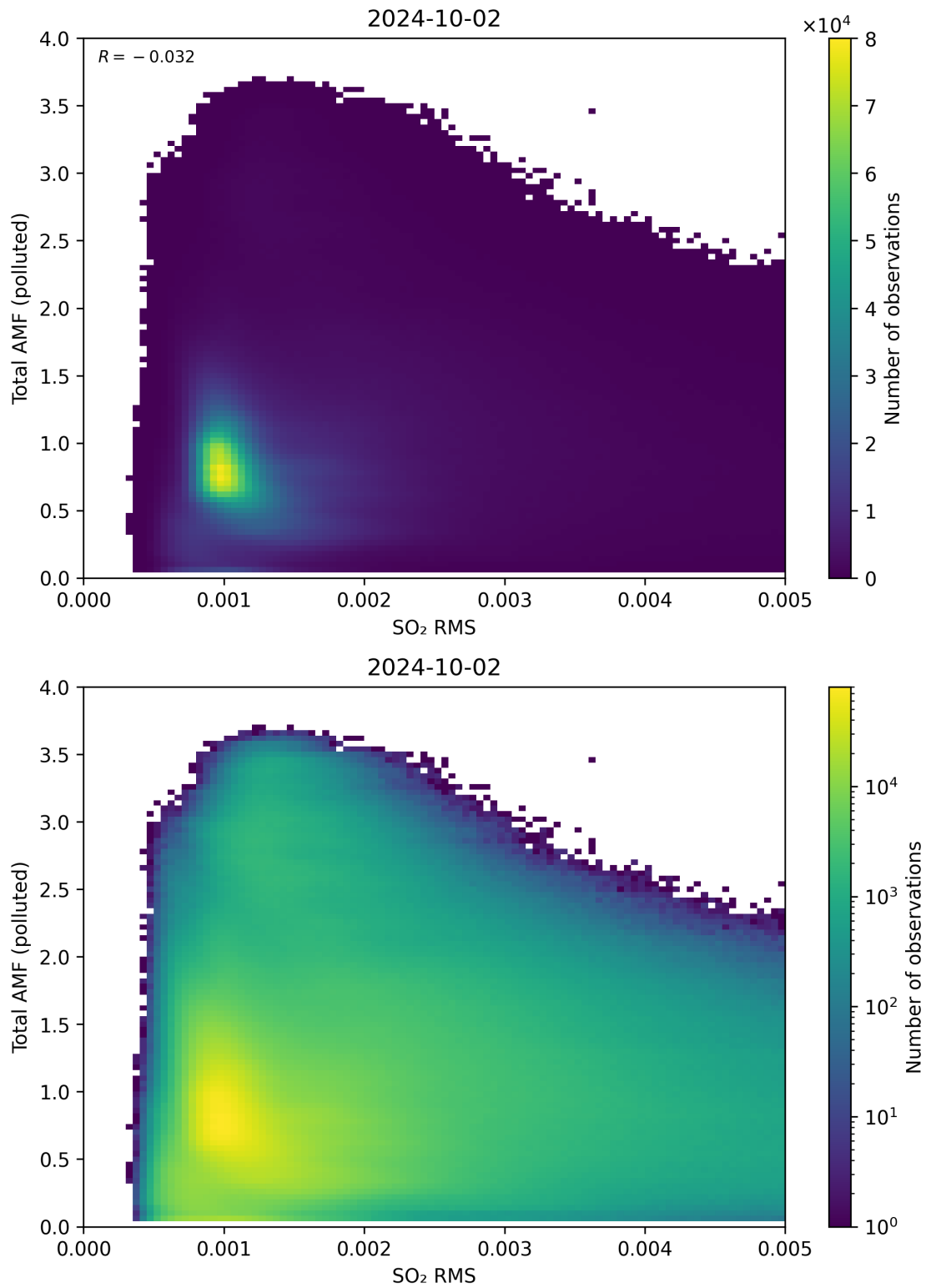
Figure 137: Scatter density plot of “SO 2 RMS” against “Total AMF (polluted)” for 2024-10-01 to 2024-10-03.
