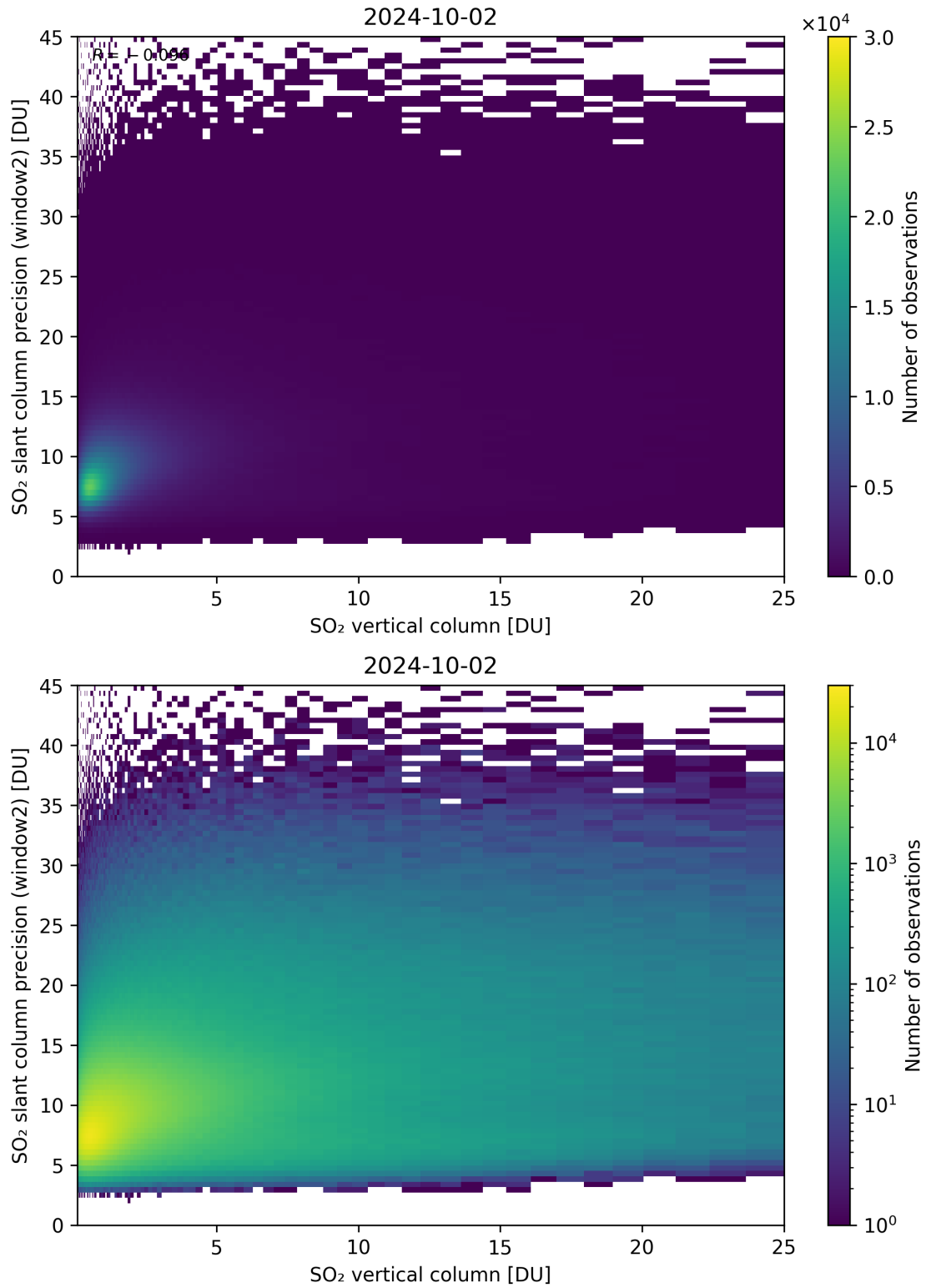
Figure 302: Scatter density plot of “SO 2 vertical column” against “SO 2 slant column precision (window2)” for 2024-10-01 to 2024-10-03.
