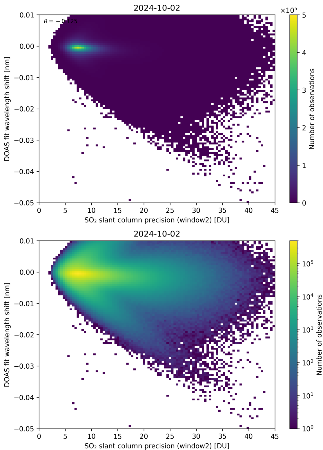
Figure 243: Scatter density plot of “SO 2 slant column precision (window2)” against “DOAS fit wavelength shift” for 2024-10-01 to 2024-10-03.
