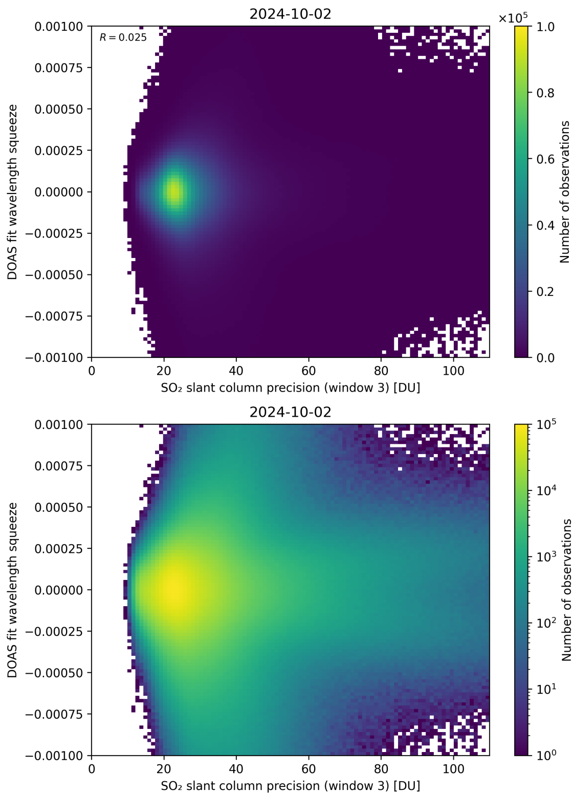
Figure 259: Scatter density plot of “SO 2 slant column precision (window 3)” against “DOAS fit wavelength squeeze” for 2024-10-01 to 2024-10-03.
