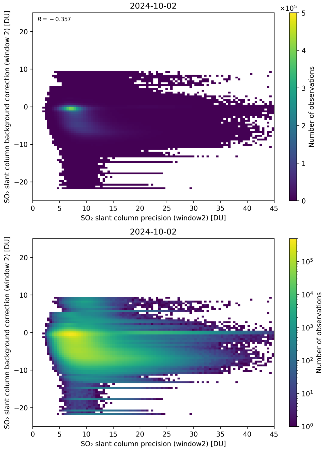
Figure 241: Scatter density plot of “SO 2 slant column precision (window2)” against “SO 2 slant column background correction (window 2)” for 2024-10-01 to 2024-10-03.
