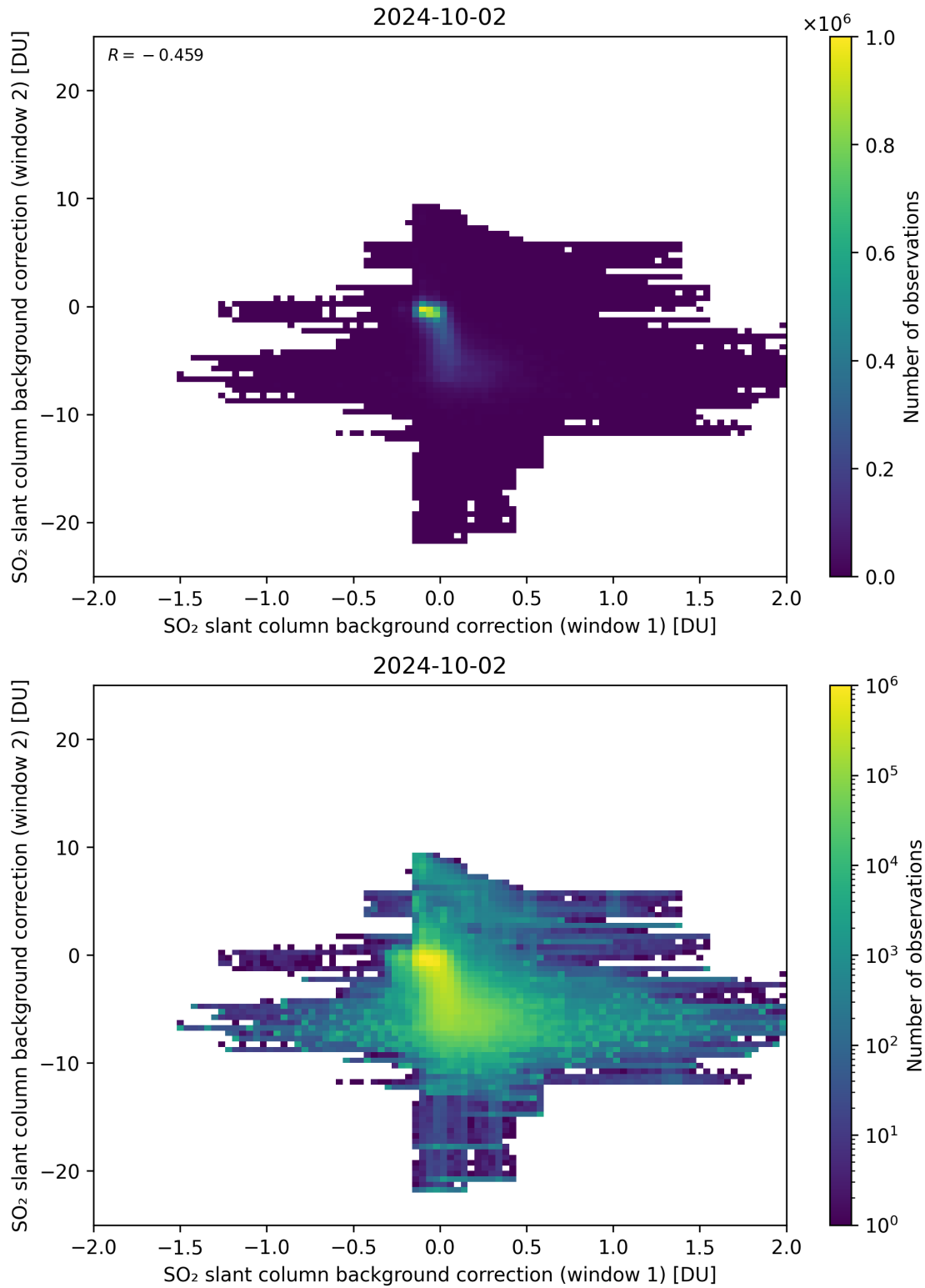
Figure 98: Scatter density plot of “SO 2 slant column background correction (window 1)” against “SO 2 slant column background correction (window 2)” for 2024-10-01 to 2024-10-03.
