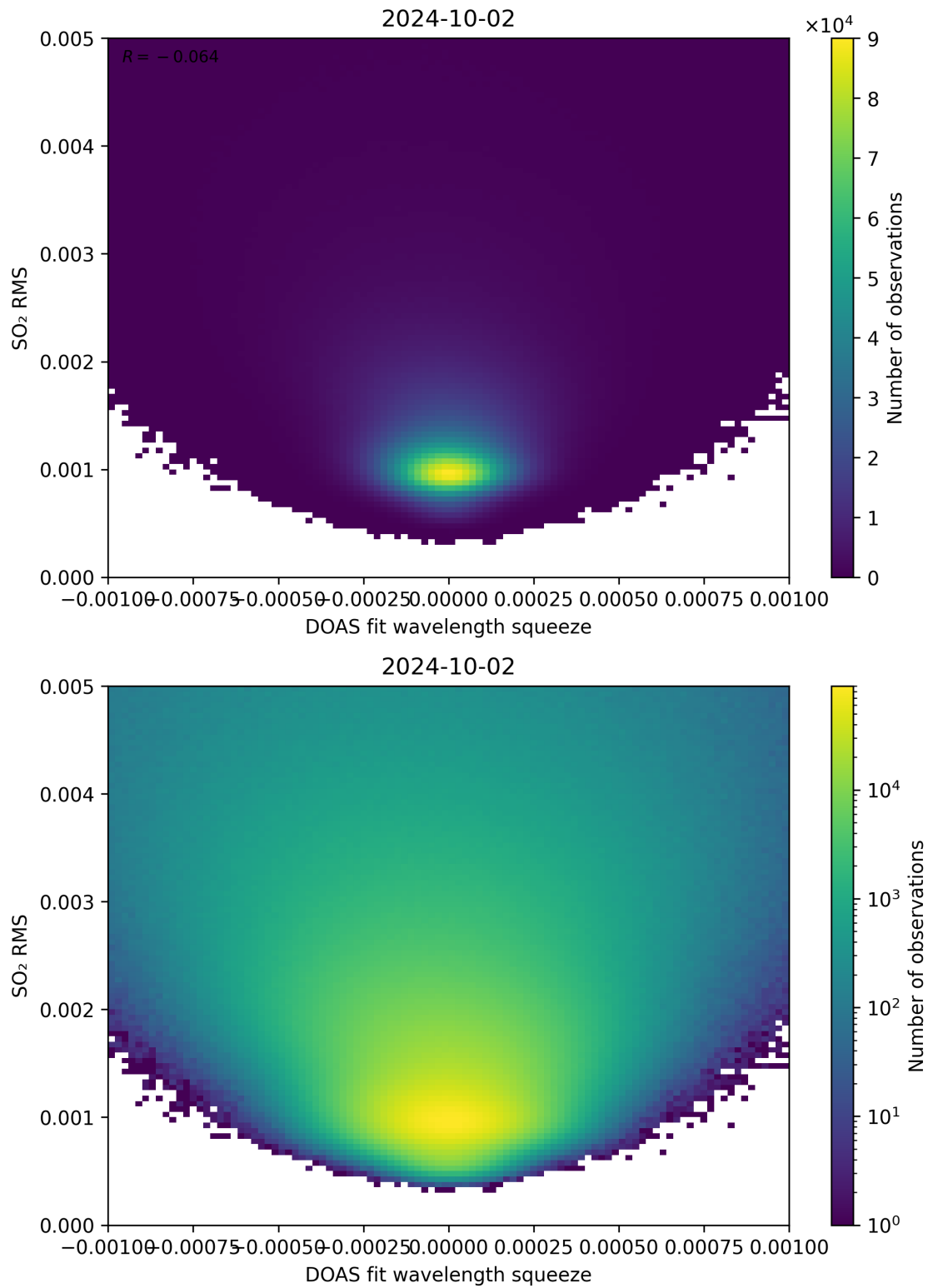
Figure 132: Scatter density plot of “DOAS fit wavelength squeeze” against “SO 2 RMS” for 2024-10-01 to 2024-10-03.
