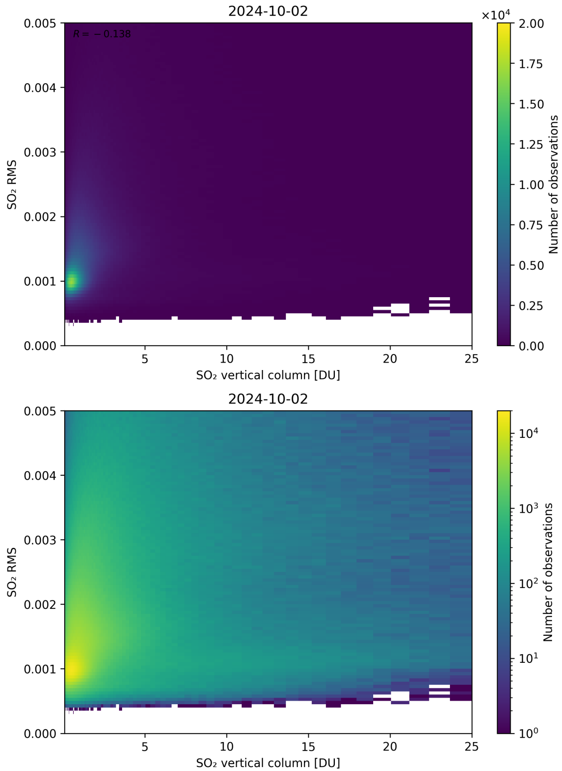
Figure 278: Scatter density plot of “SO 2 vertical column” against “SO 2 RMS” for 2024-10-01 to 2024-10-03.
