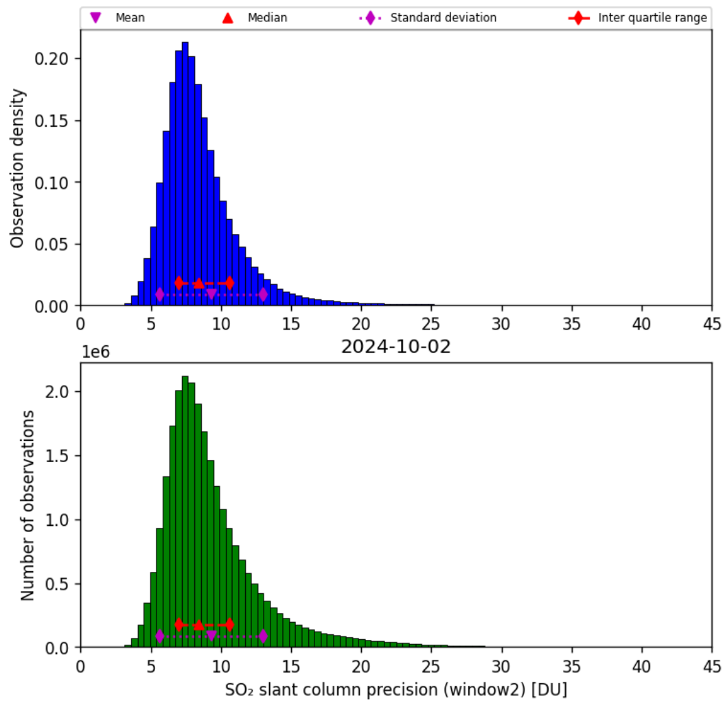
Figure 61: Histogram of “SO 2 slant column precision (window2)” for 2024-10-01 to 2024-10-03
