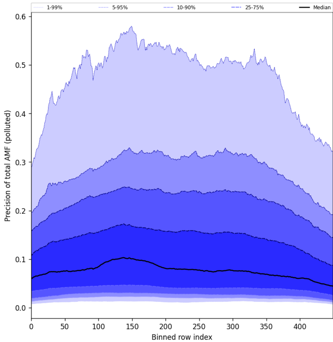
Figure 95: Along track statistics of “Precision of total AMF (polluted)” for 2024-10-01 to 2024-10-03
