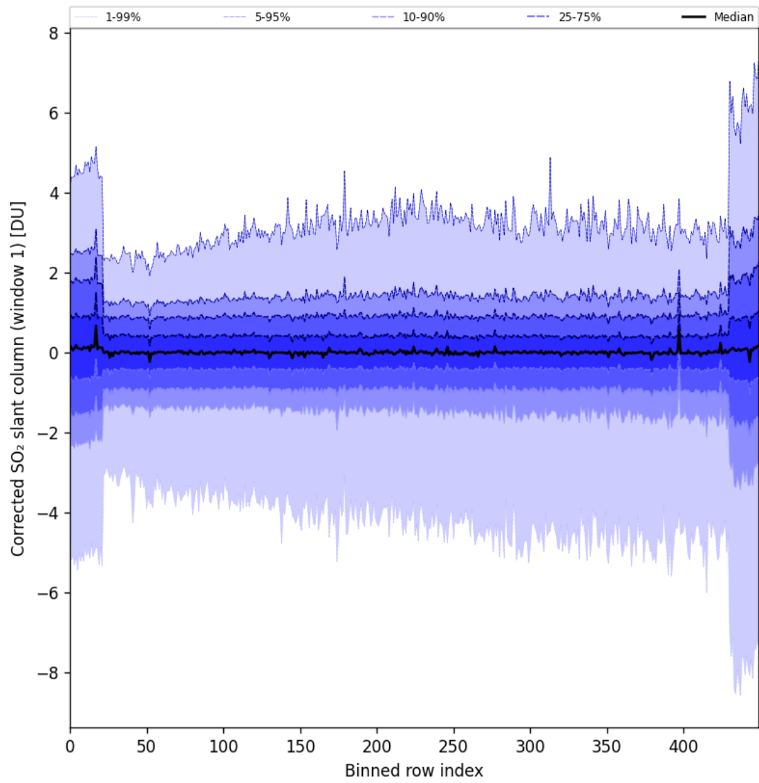
Figure 81: Along track statistics of “Corrected SO 2 slant column (window 1)” for 2024-10-01 to 2024-10-03
