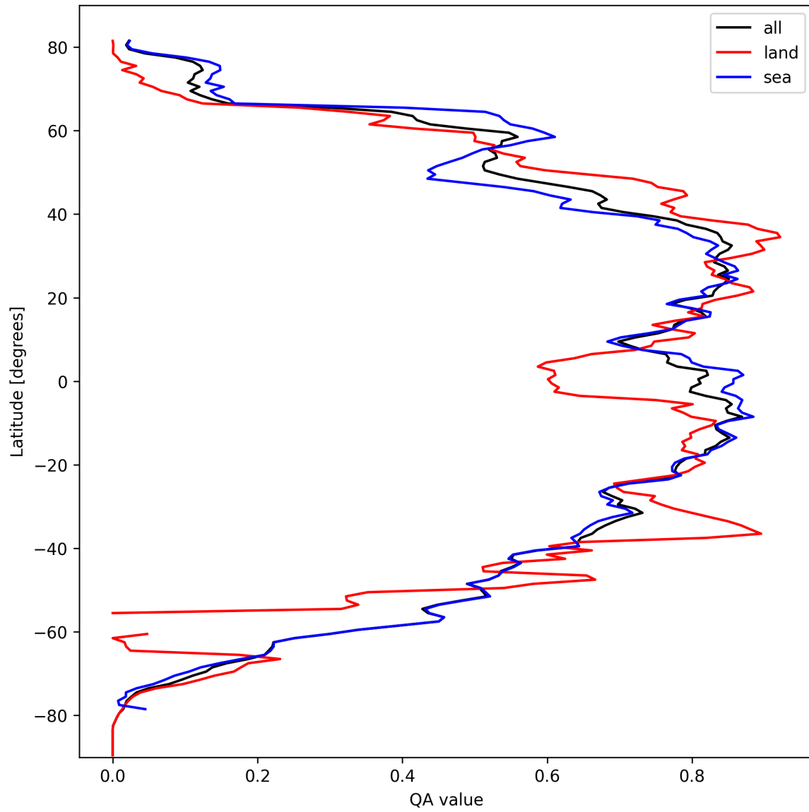
Figure 29: Zonal average of “QA value” for 2024-10-01 to 2024-10-03.
