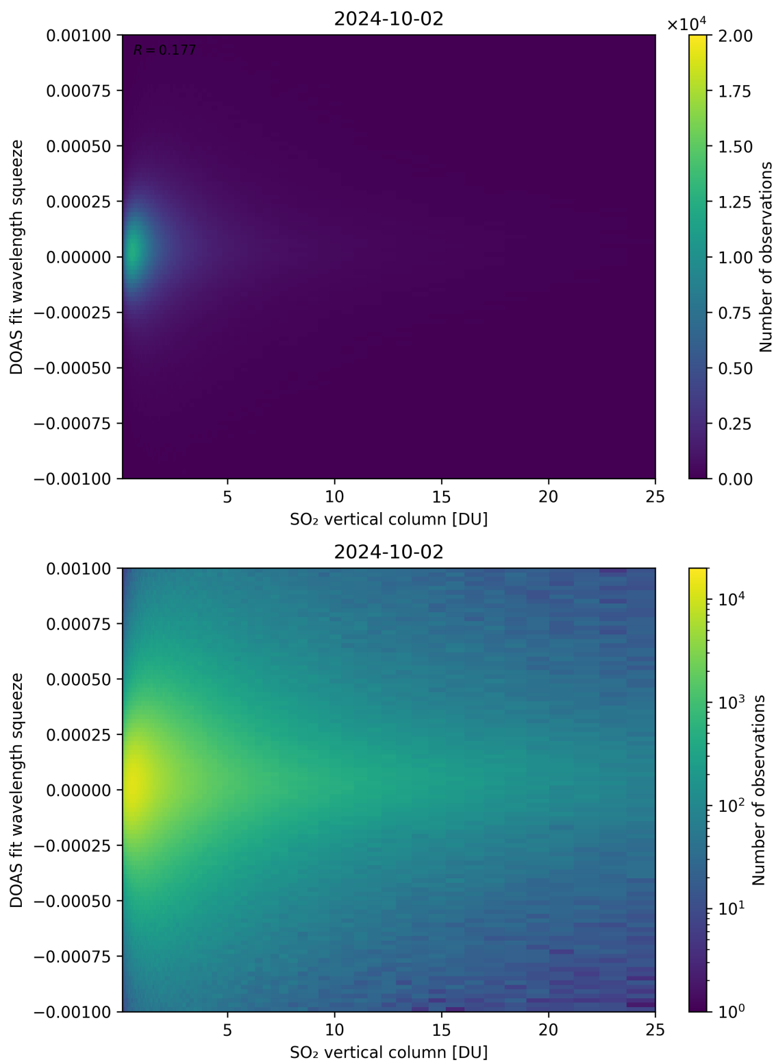
Figure 277: Scatter density plot of “SO 2 vertical column” against “DOAS fit wavelength squeeze” for 2024-10-01 to 2024-10-03.
