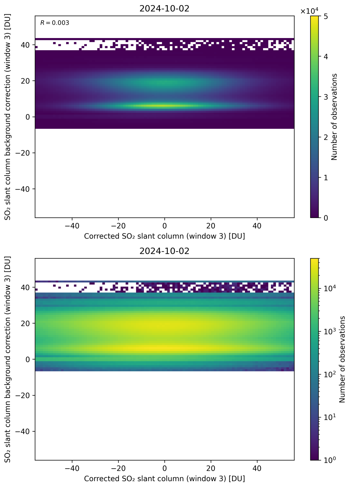
Figure 205: Scatter density plot of “Corrected SO 2 slant column (window 3)” against “SO 2 slant column background correction (window 3)” for 2024-10-01 to 2024-10-03.
