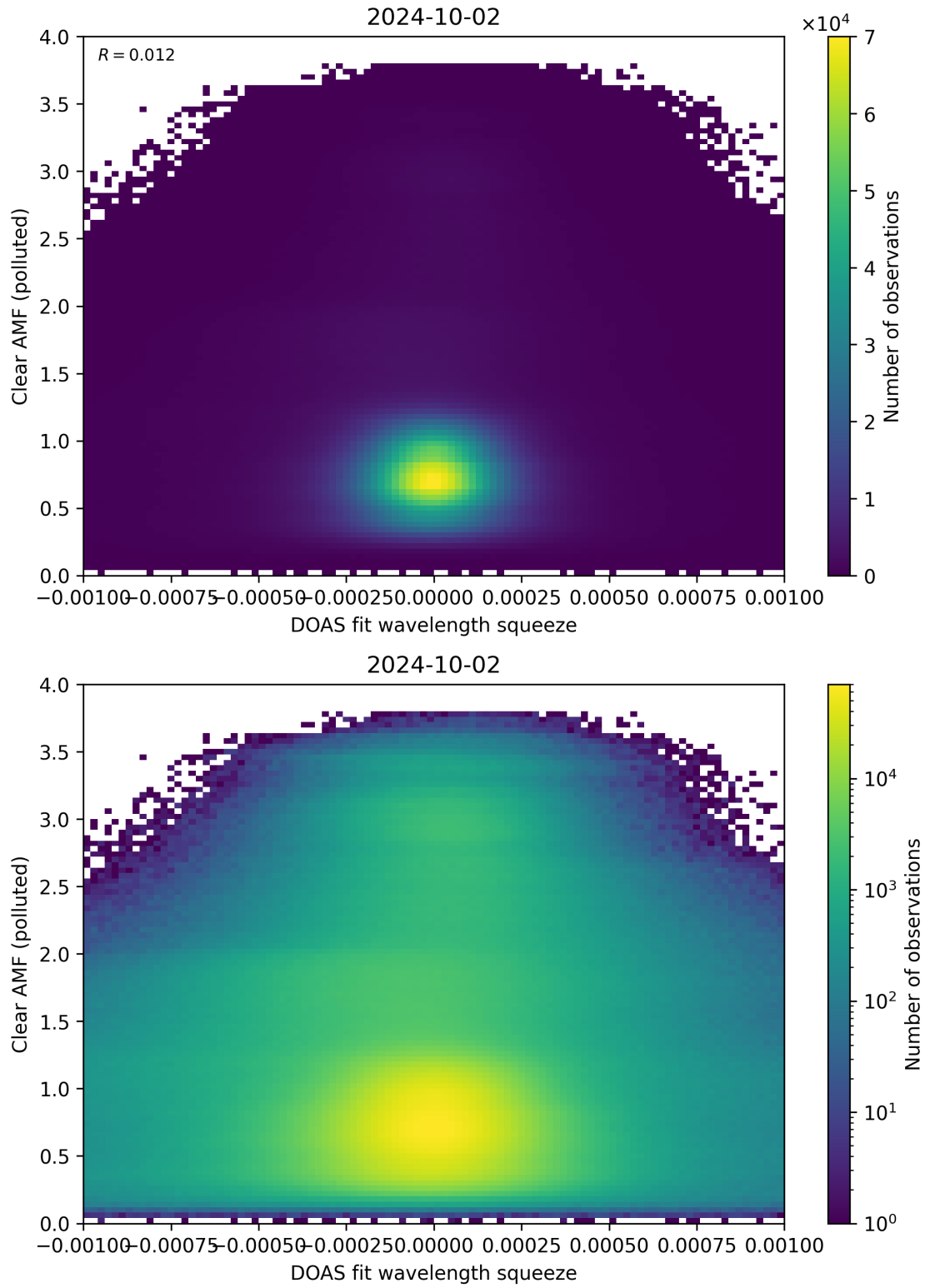
Figure 133: Scatter density plot of “DOAS fit wavelength squeeze” against “Clear AMF (polluted)” for 2024-10-01 to 2024-10-03.
