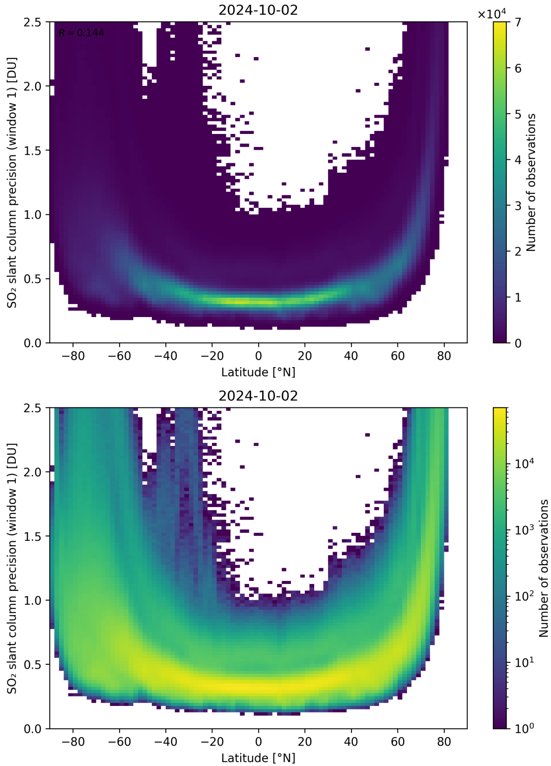
Figure 150: Scatter density plot of “Latitude” against “SO 2 slant column precision (window 1)” for 2024-10-01 to 2024-10-03.
