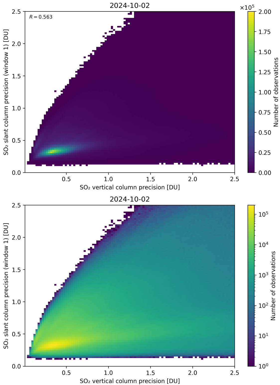
Figure 290: Scatter density plot of “SO 2 vertical column precision” against “SO 2 slant column precision (window 1)” for 2024-10-01 to 2024-10-03.
