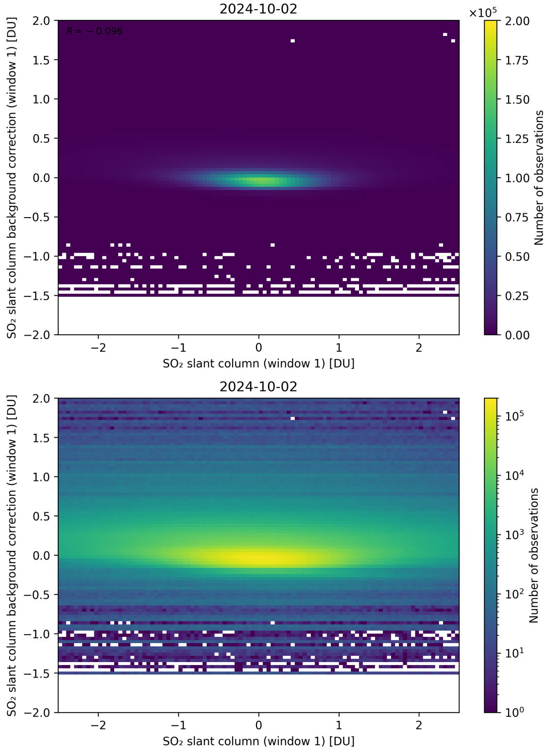
Figure 212: Scatter density plot of “SO 2 slant column (window 1)” against “SO 2 slant column background correction (window 1)” for 2024-10-01 to 2024-10-03.
