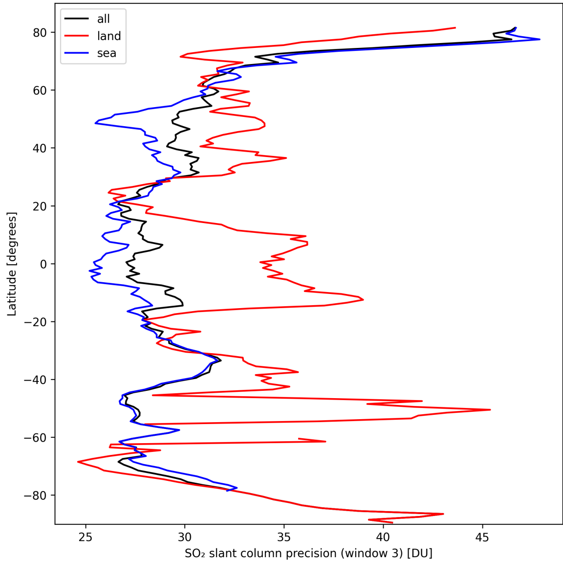
Figure 42: Zonal average of “SO 2 slant column precision (window 3)” for 2024-10-01 to 2024-10-03.
