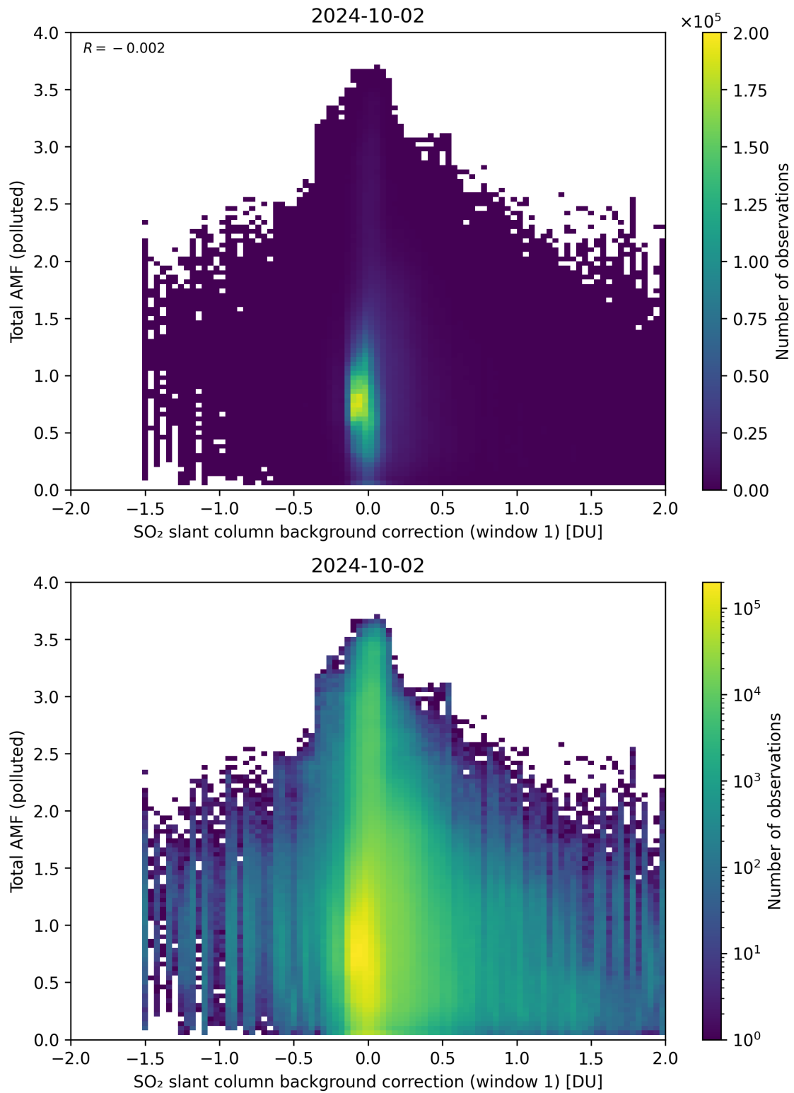
Figure 109: Scatter density plot of “SO 2 slant column background correction (window 1)” against “Total AMF (polluted)” for 2024-10-01 to 2024-10-03.
