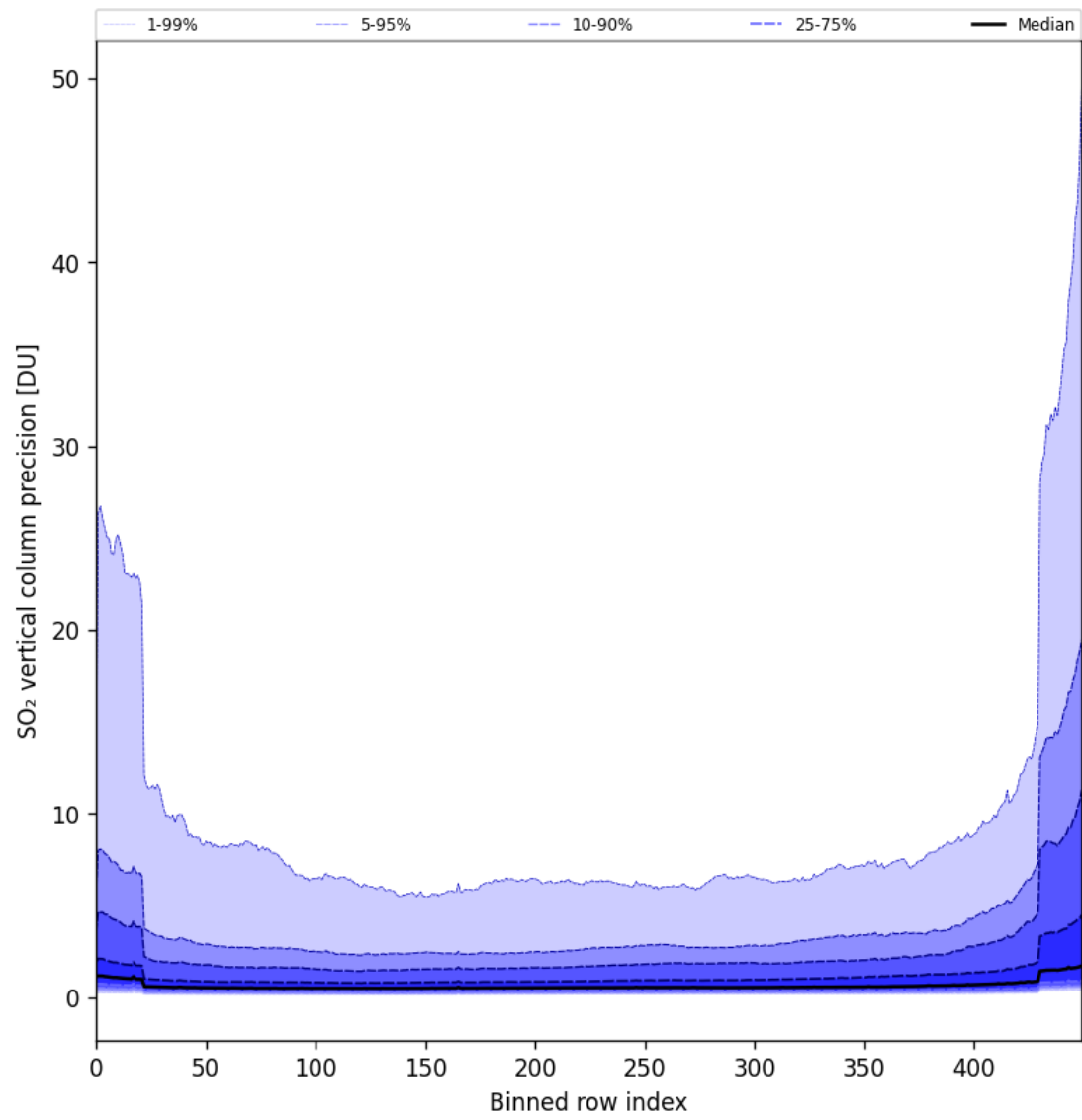
Figure 77: Along track statistics of “SO 2 vertical column precision” for 2024-10-01 to 2024-10-03
