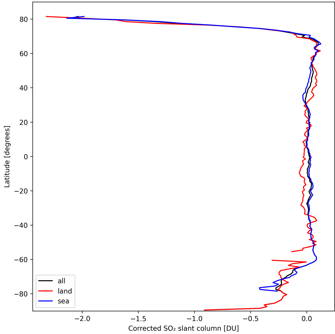
Figure 32: Zonal average of “Corrected SO 2 slant column” for 2024-10-01 to 2024-10-03.
