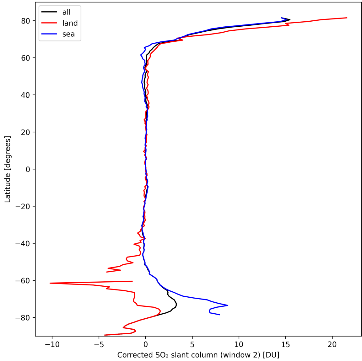
Figure 39: Zonal average of “Corrected SO 2 slant column (window 2)” for 2024-10-01 to 2024-10-03.
