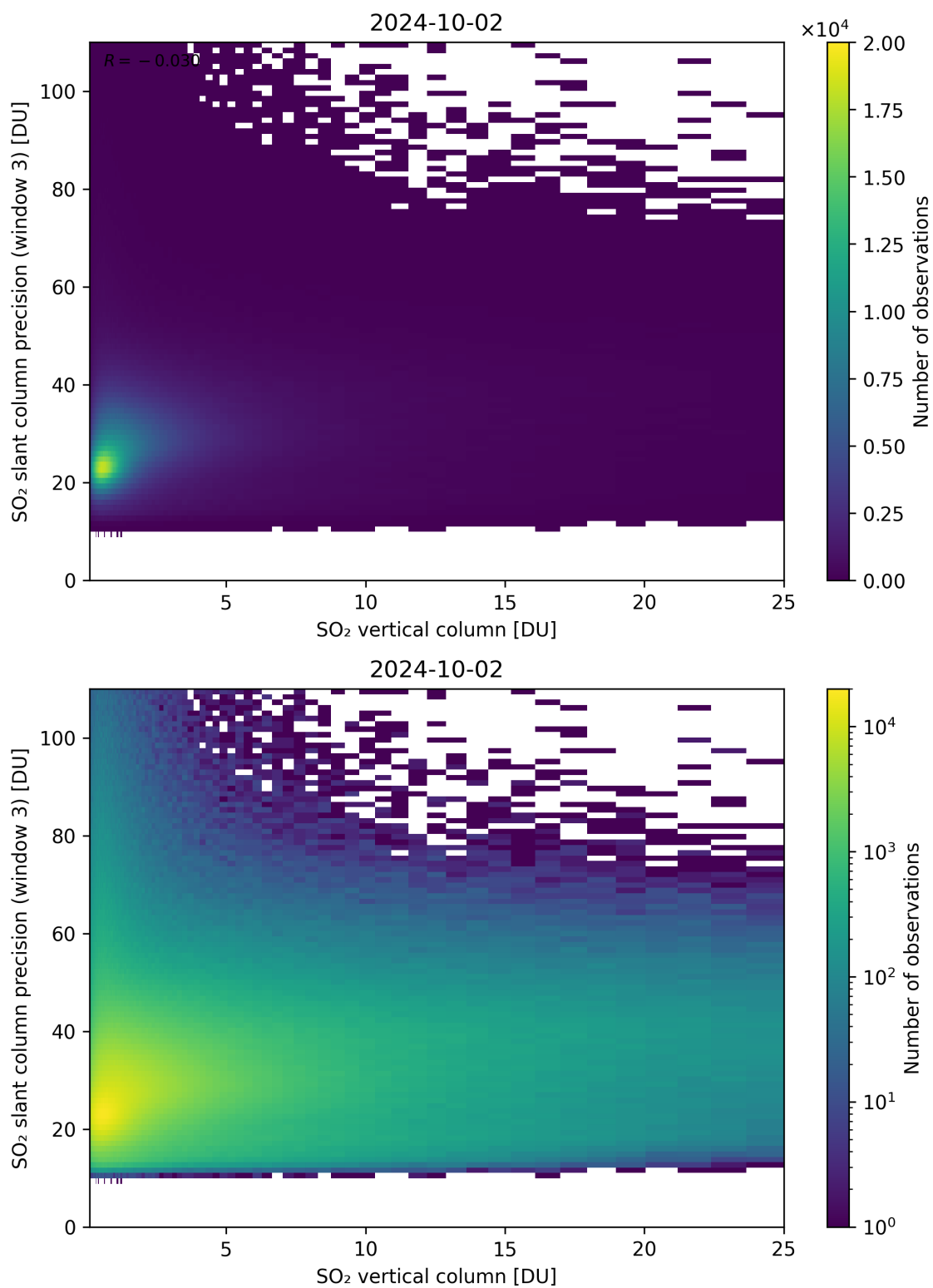
Figure 304: Scatter density plot of “SO 2 vertical column” against “SO 2 slant column precision (window 3)” for 2024-10-01 to 2024-10-03.
