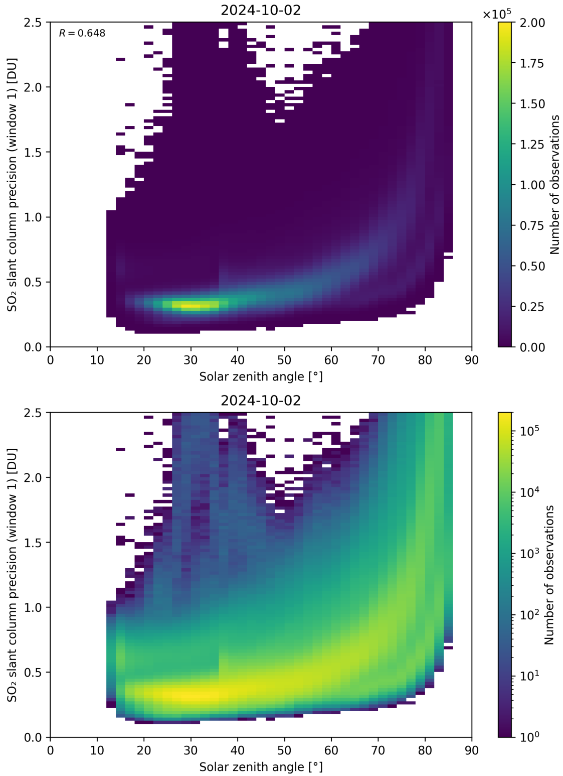
Figure 170: Scatter density plot of “Solar zenith angle” against “SO 2 slant column precision (window 1)” for 2024-10-01 to 2024-10-03.
