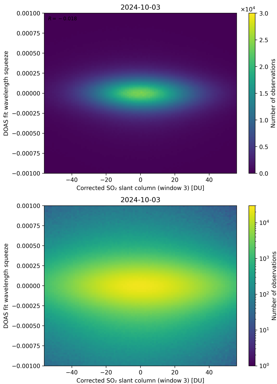
Figure 207: Scatter density plot of “Corrected SO 2 slant column (window 3)” against “DOAS fit wavelength squeeze” for 2024-10-03 to 2024-10-04.
