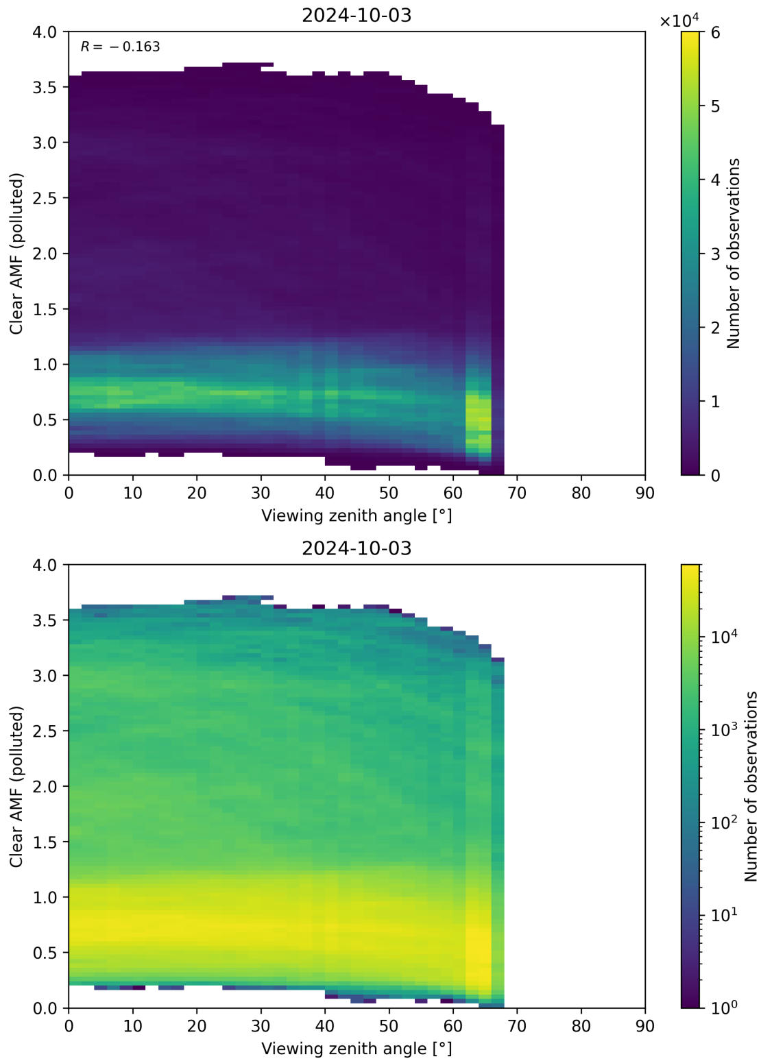
Figure 316: Scatter density plot of “Viewing zenith angle” against “Clear AMF (polluted)” for 2024-10-03 to 2024-10-04.
