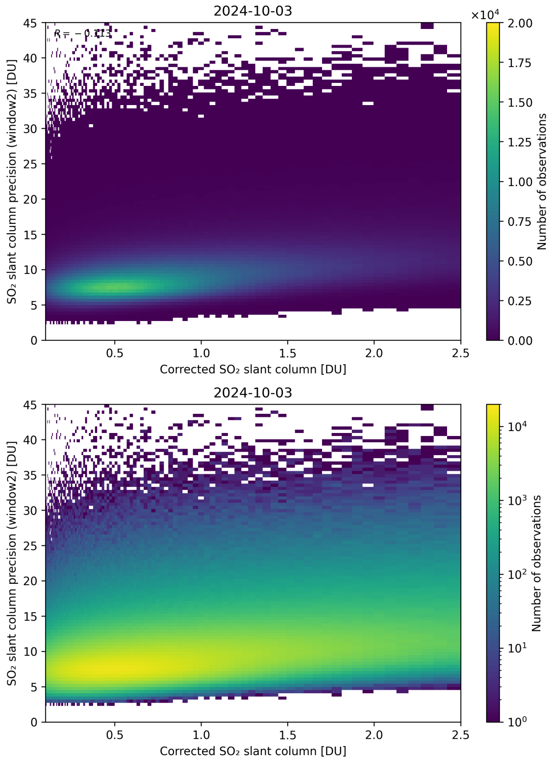
Figure 189: Scatter density plot of “Corrected SO 2 slant column” against “SO 2 slant column precision (window2)” for 2024-10-03 to 2024-10-04.
