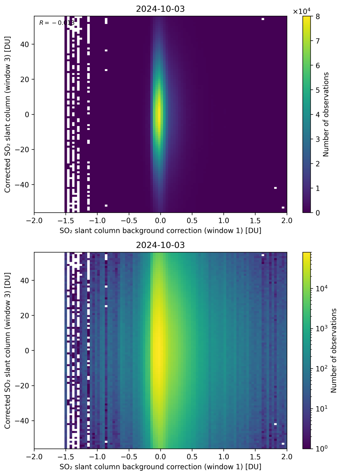
Figure 105: Scatter density plot of “SO 2 slant column background correction (window 1)” against “Corrected SO 2 slant column (window 3)” for 2024-10-03 to 2024-10-04.
