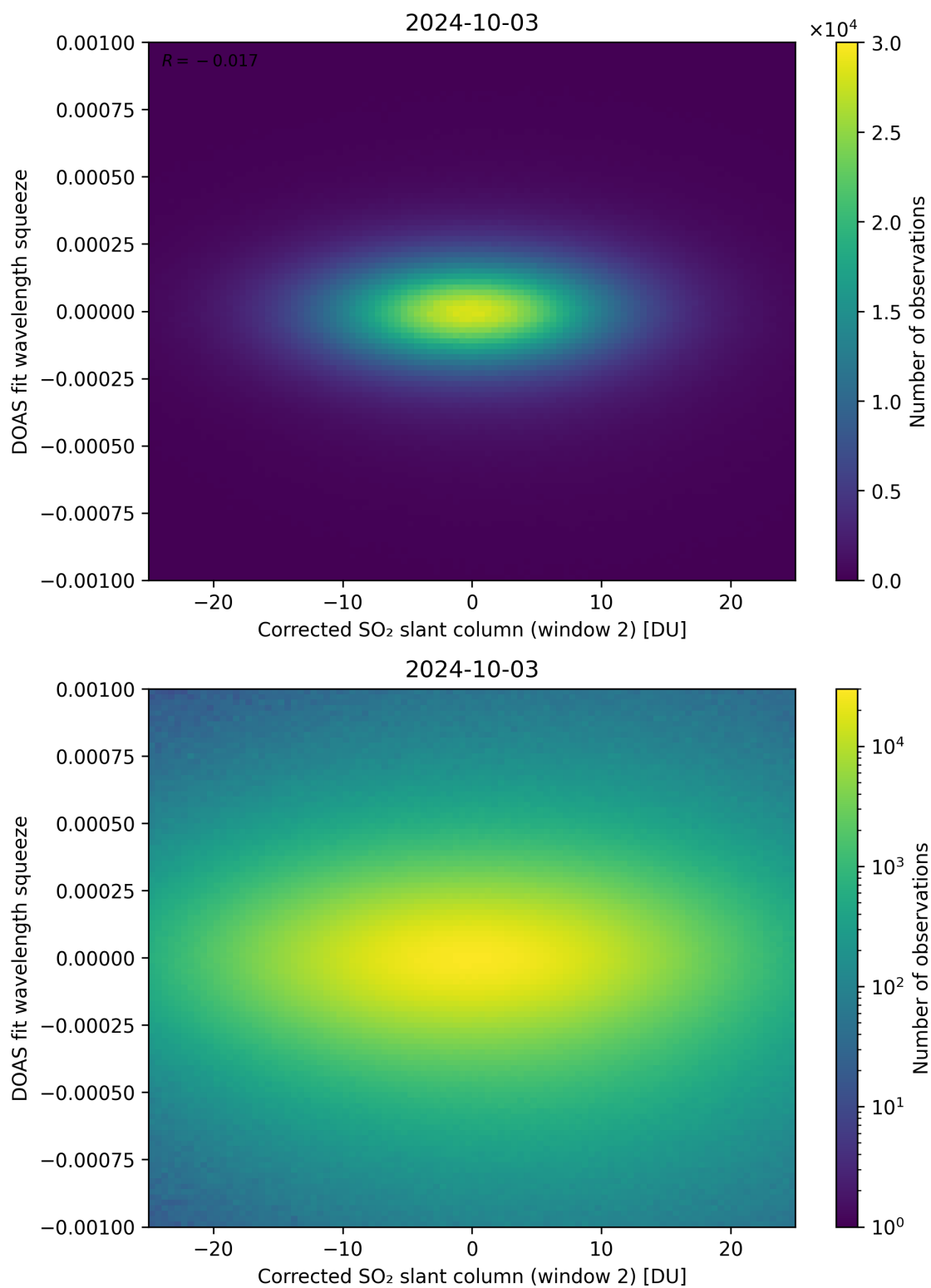
Figure 197: Scatter density plot of “Corrected SO 2 slant column (window 2)” against “DOAS fit wavelength squeeze” for 2024-10-03 to 2024-10-04.
