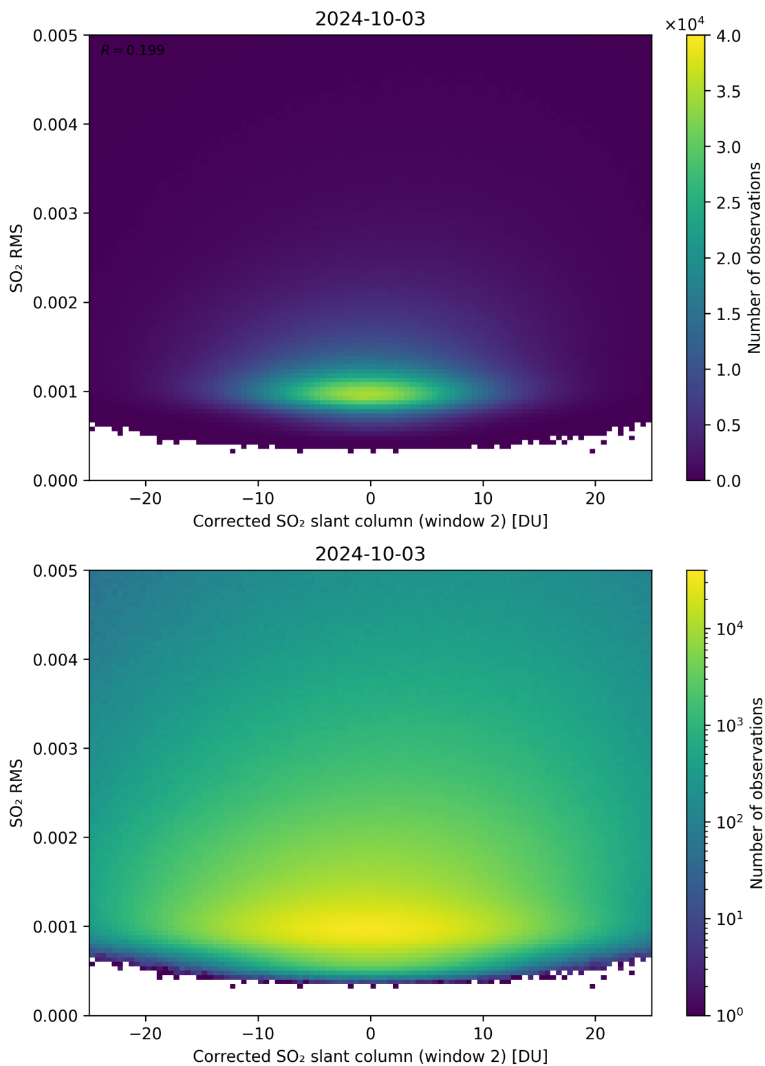
Figure 198: Scatter density plot of “Corrected SO 2 slant column (window 2)” against “SO 2 RMS” for 2024-10-03 to 2024-10-04.
