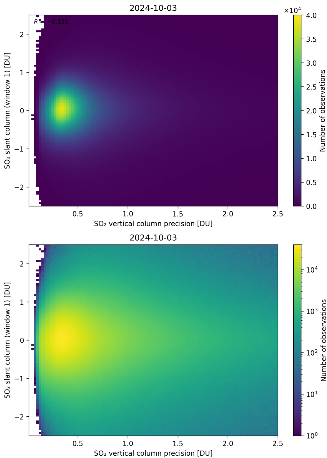
Figure 289: Scatter density plot of “SO 2 vertical column precision” against “SO 2 slant column (window 1)” for 2024-10-03 to 2024-10-04.
