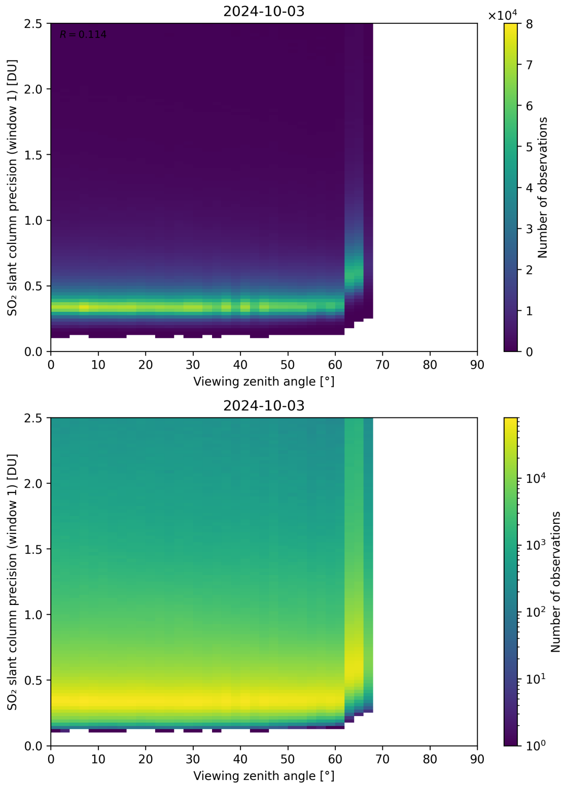
Figure 321: Scatter density plot of “Viewing zenith angle” against “SO 2 slant column precision (window 1)” for 2024-10-03 to 2024-10-04.
