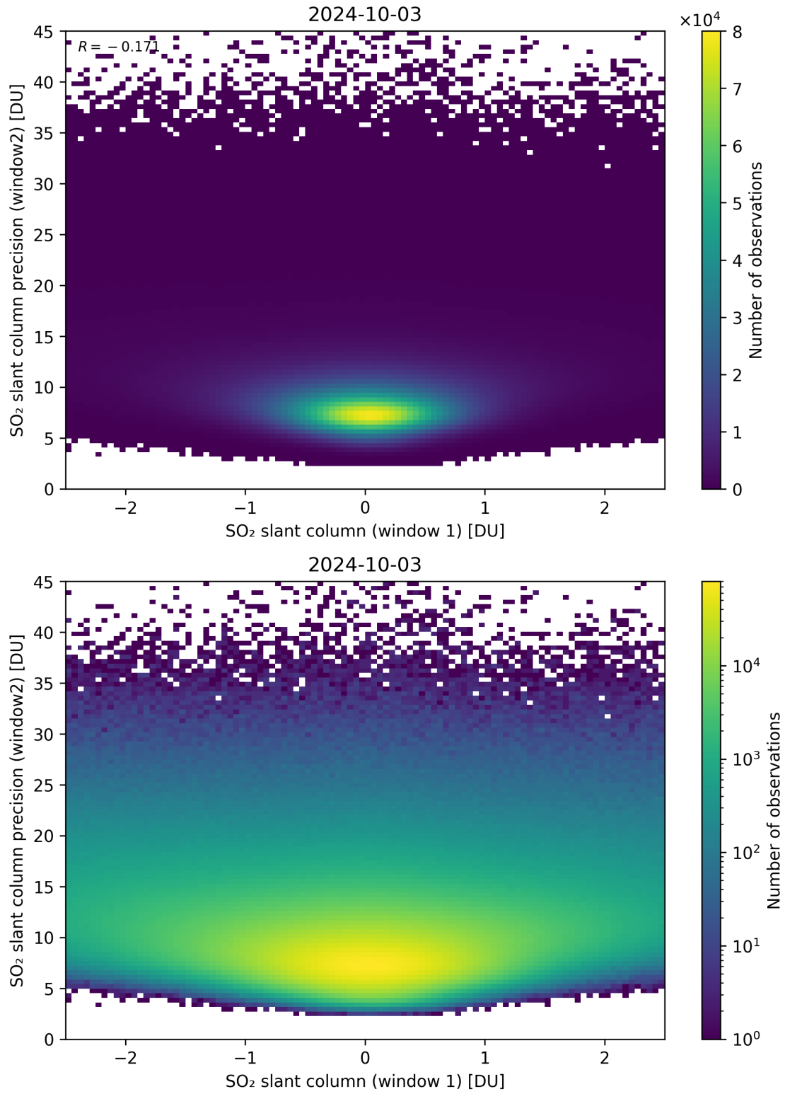
Figure 236: Scatter density plot of “SO 2 slant column (window 1)” against “SO 2 slant column precision (window2)” for 2024-10-03 to 2024-10-04.
