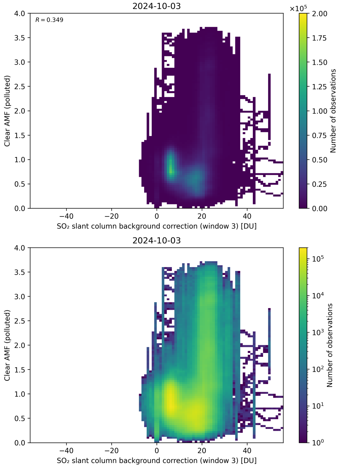
Figure 124: Scatter density plot of “SO 2 slant column background correction (window 3)” against “Clear AMF (polluted)” for 2024-10-03 to 2024-10-04.
