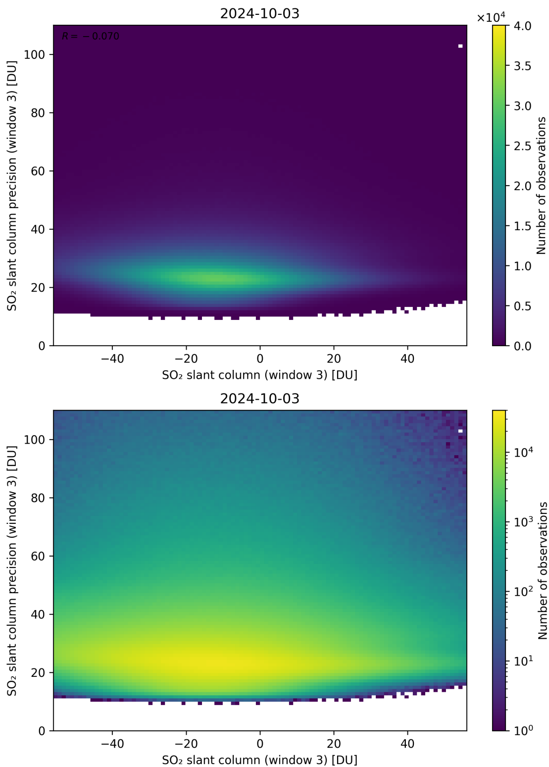
Figure 267: Scatter density plot of “SO 2 slant column (window 3)” against “SO 2 slant column precision (window 3)” for 2024-10-03 to 2024-10-04.
