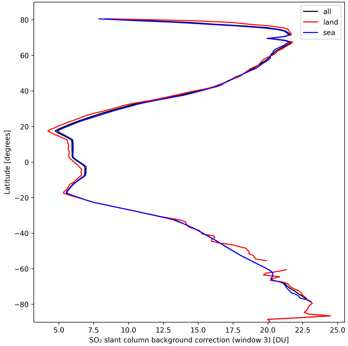
Figure 44: Zonal average of “SO 2 slant column background correction (window 3)” for 2024-10-03 to 2024-10-04.
