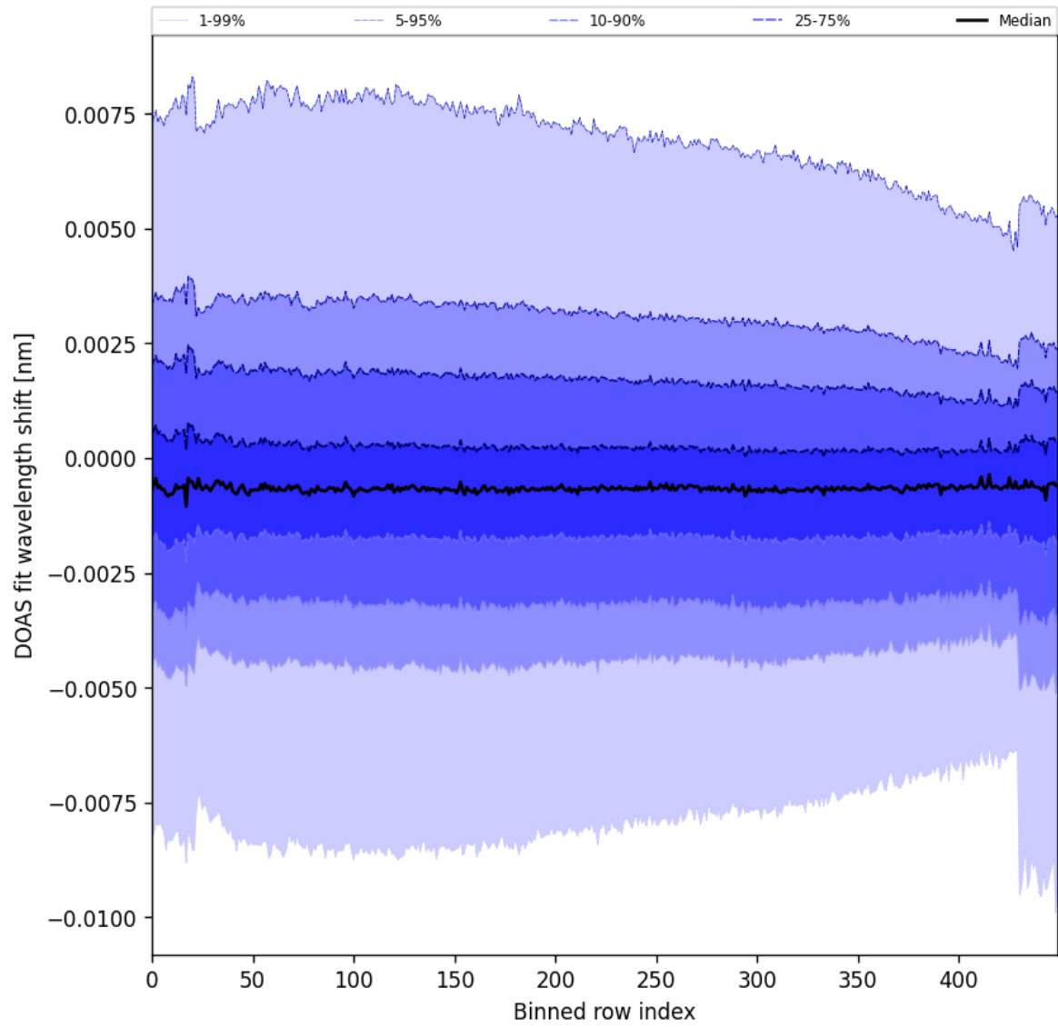
Figure 91: Along track statistics of “DOAS fit wavelength shift” for 2024-10-03 to 2024-10-04
