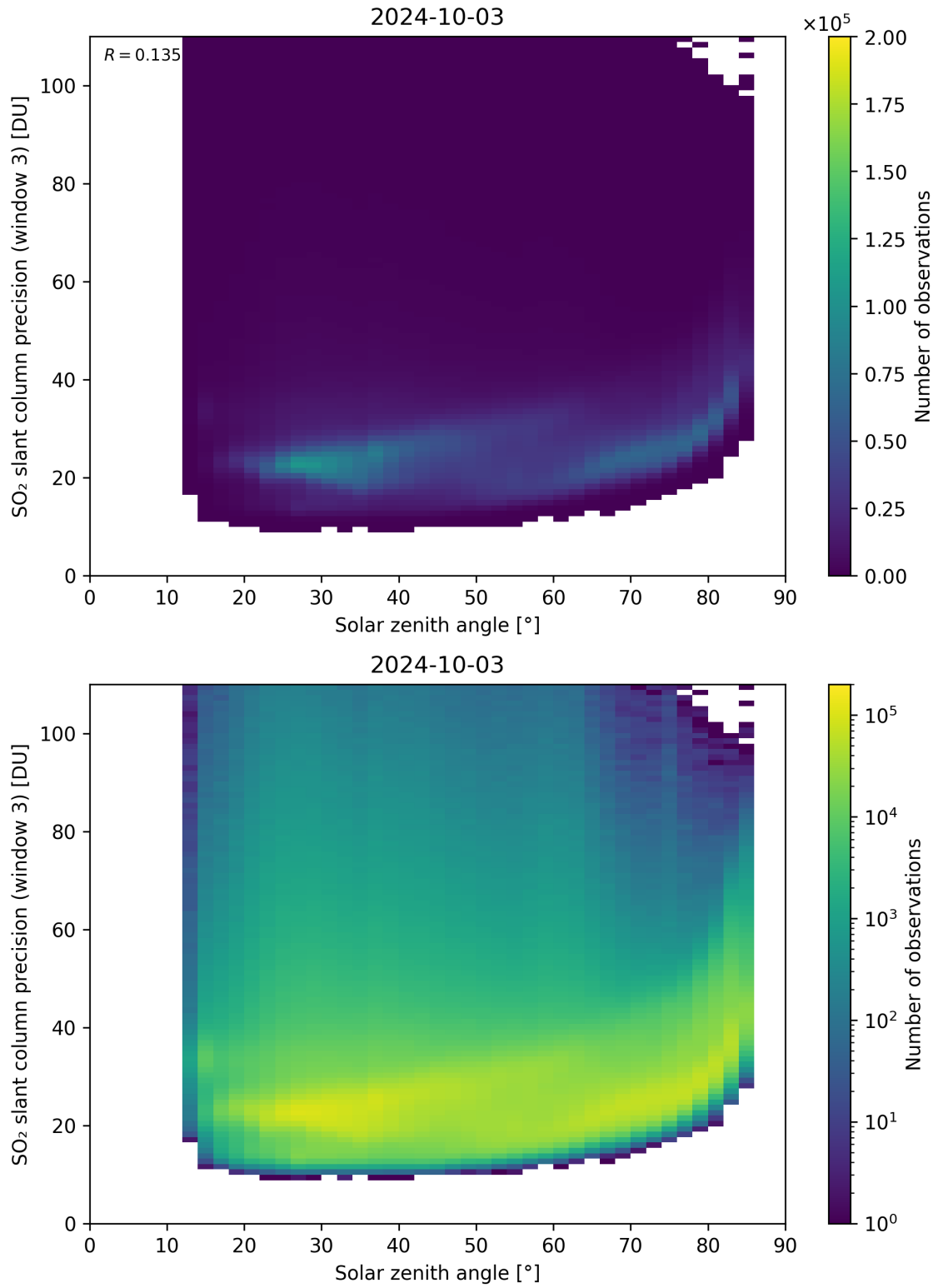
Figure 173: Scatter density plot of “Solar zenith angle” against “SO 2 slant column precision (window 3)” for 2024-10-03 to 2024-10-04.
