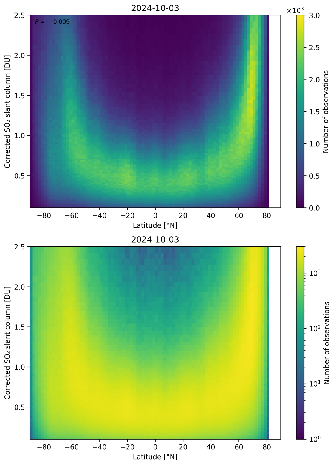
Figure 146: Scatter density plot of “Latitude” against “Corrected SO 2 slant column” for 2024-10-03 to 2024-10-04.
