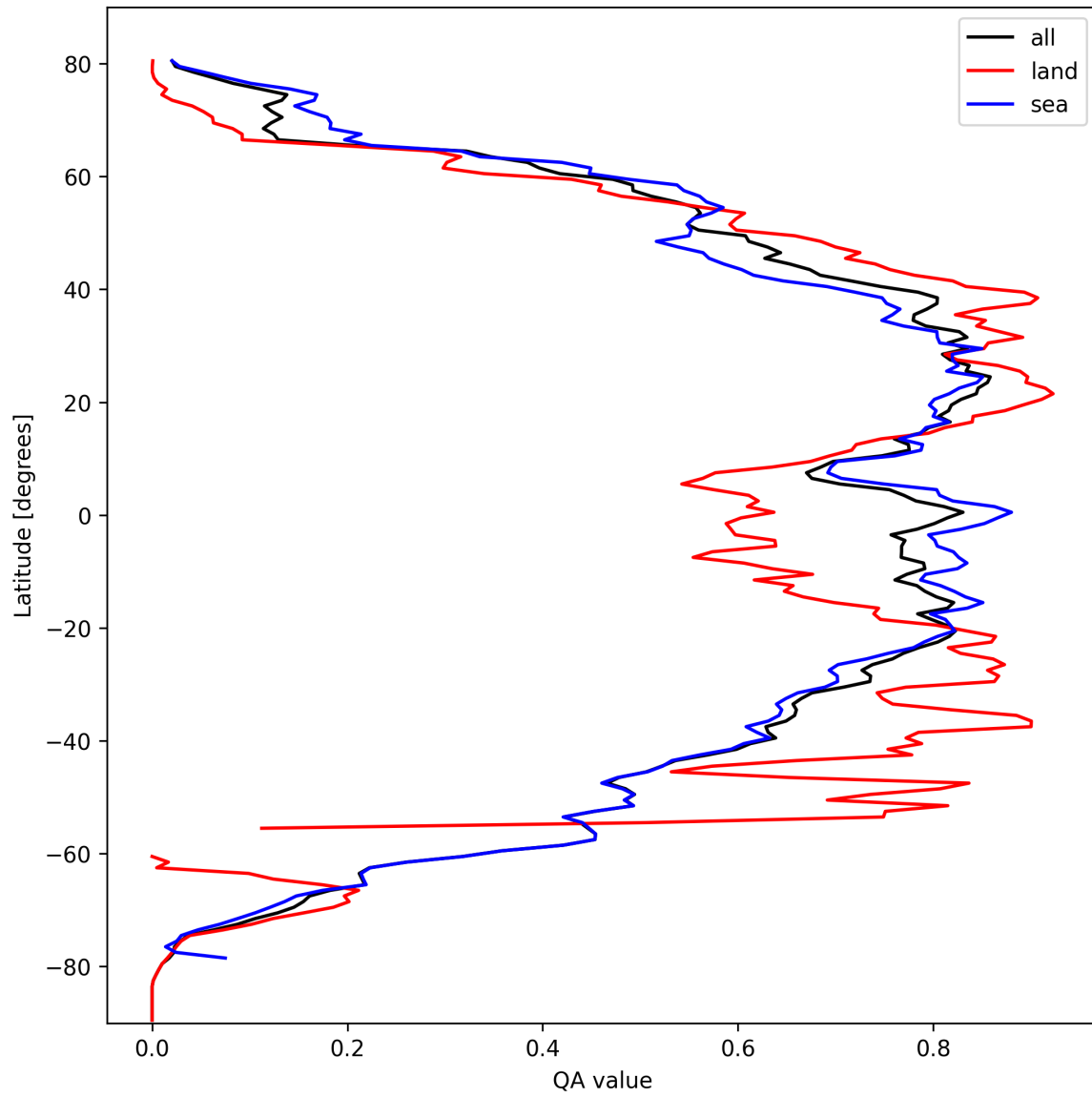
Figure 29: Zonal average of “QA value” for 2024-10-03 to 2024-10-04.
