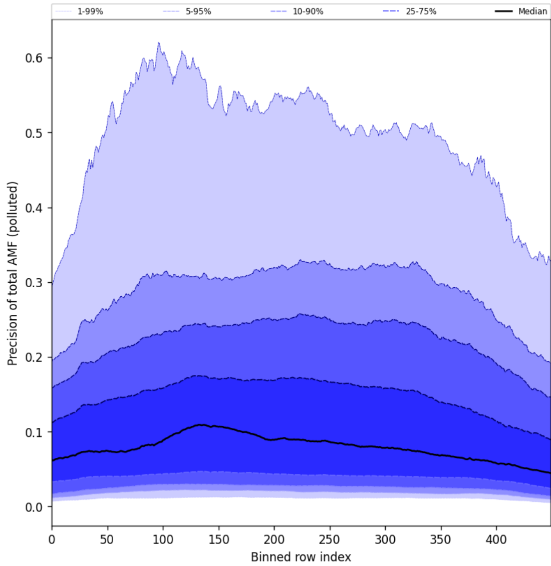
Figure 95: Along track statistics of “Precision of total AMF (polluted)” for 2024-10-03 to 2024-10-04
