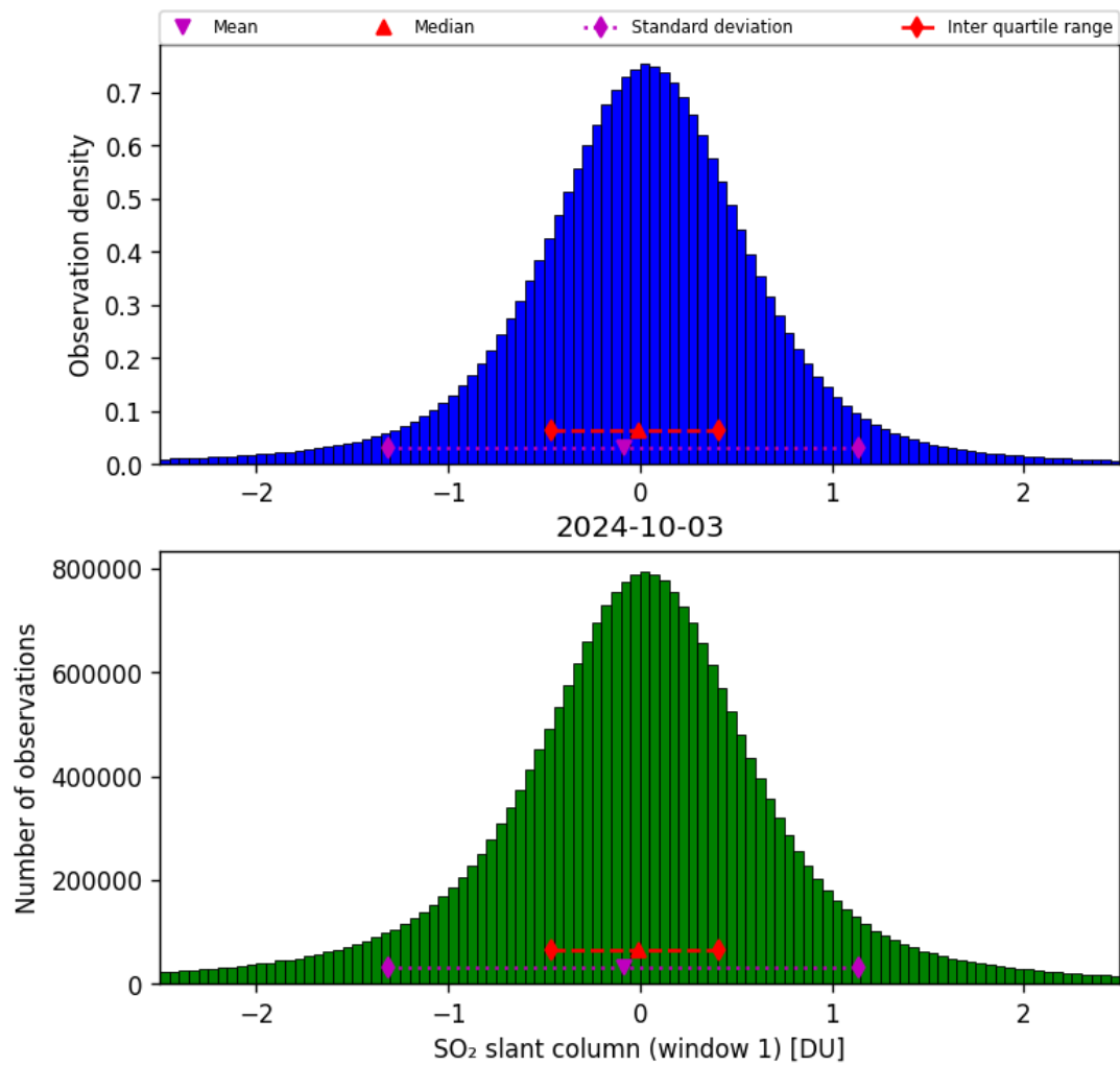
Figure 56: Histogram of “SO 2 slant column (window 1)” for 2024-10-03 to 2024-10-04
