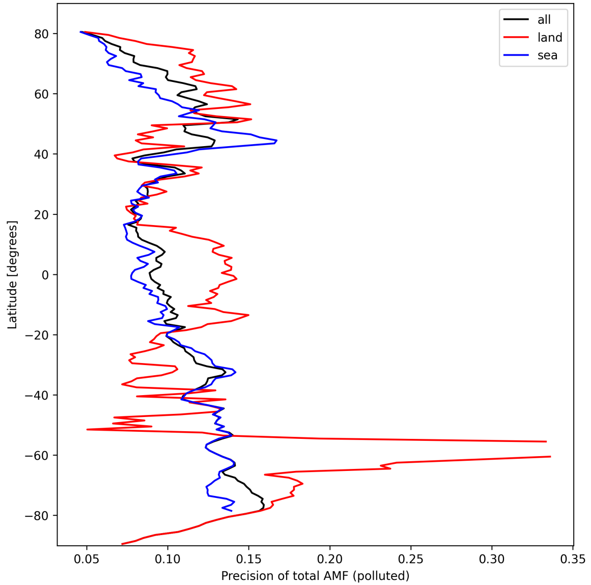
Figure 49: Zonal average of “Precision of total AMF (polluted)” for 2024-10-03 to 2024-10-04.
