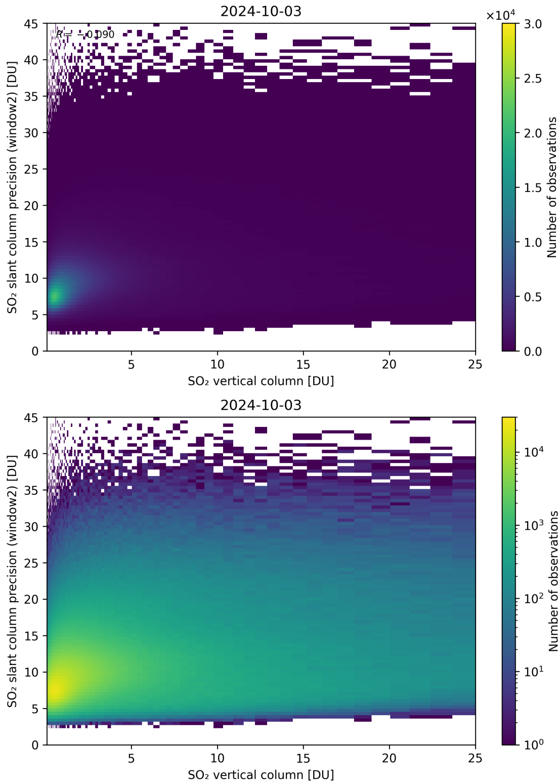
Figure 302: Scatter density plot of “SO 2 vertical column” against “SO 2 slant column precision (window2)” for 2024-10-03 to 2024-10-04.
