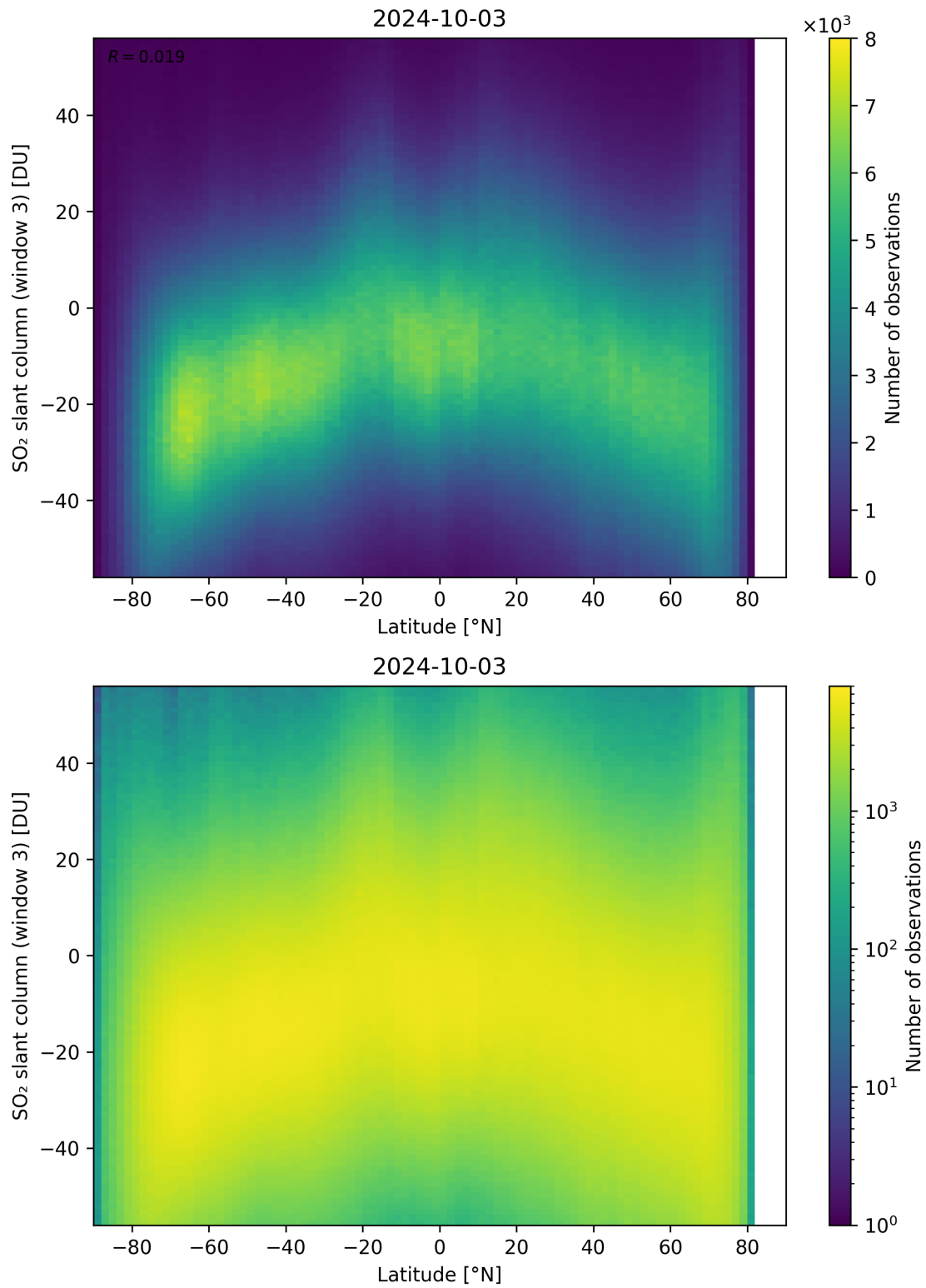
Figure 152: Scatter density plot of “Latitude” against “SO 2 slant column (window 3)” for 2024-10-03 to 2024-10-04.
