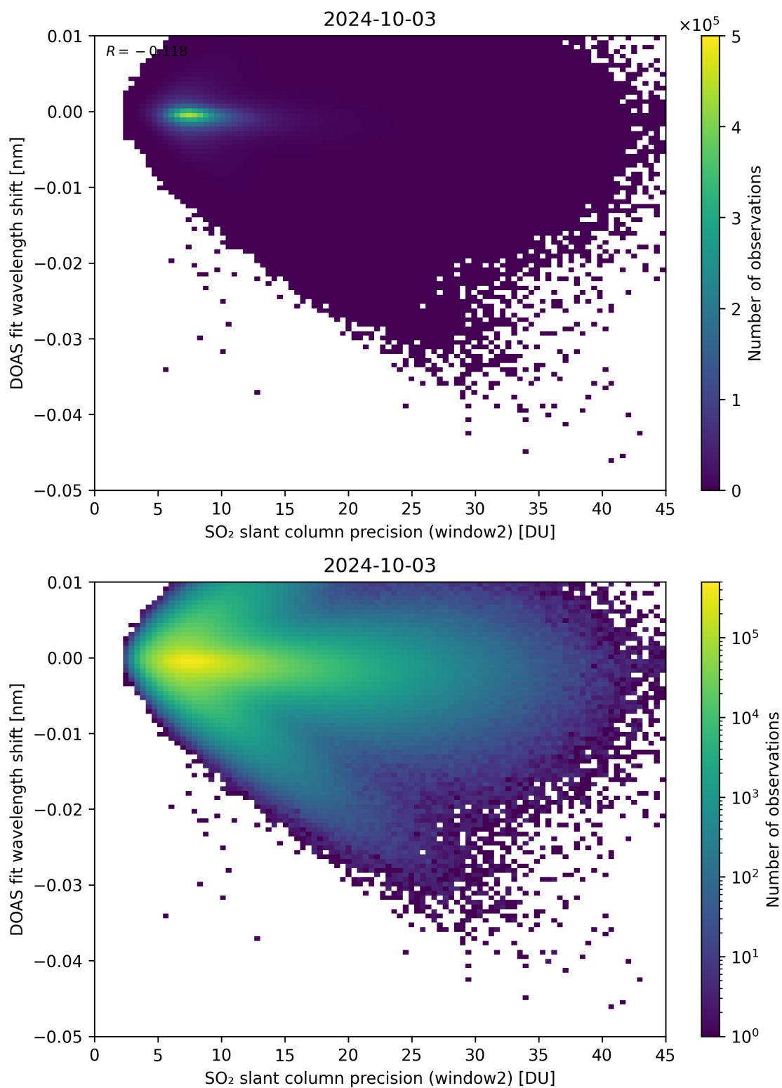
Figure 243: Scatter density plot of “SO 2 slant column precision (window2)” against “DOAS fit wavelength shift” for 2024-10-03 to 2024-10-04.
