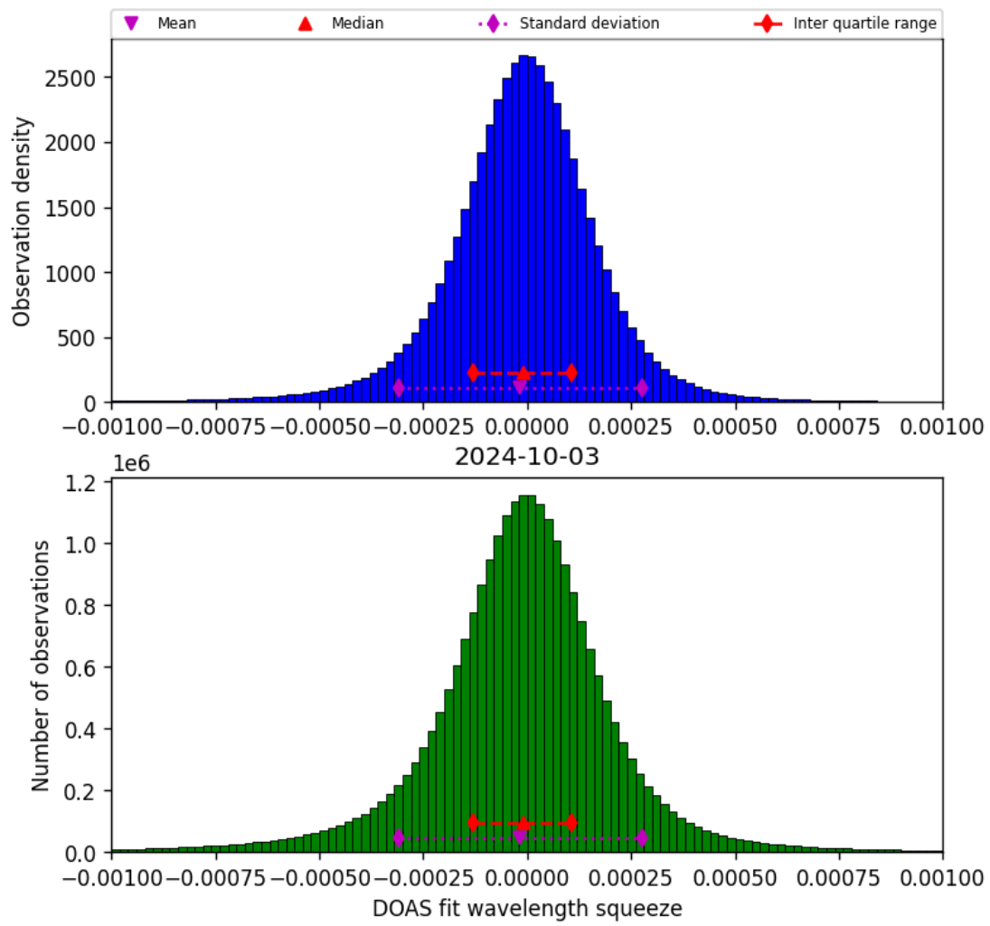
Figure 69: Histogram of “DOAS fit wavelength squeeze” for 2024-10-03 to 2024-10-04
