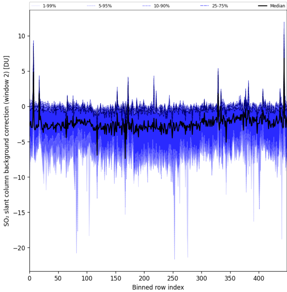
Figure 86: Along track statistics of “SO 2 slant column background correction (window 2)” for 2024-10-03 to 2024-10-04
