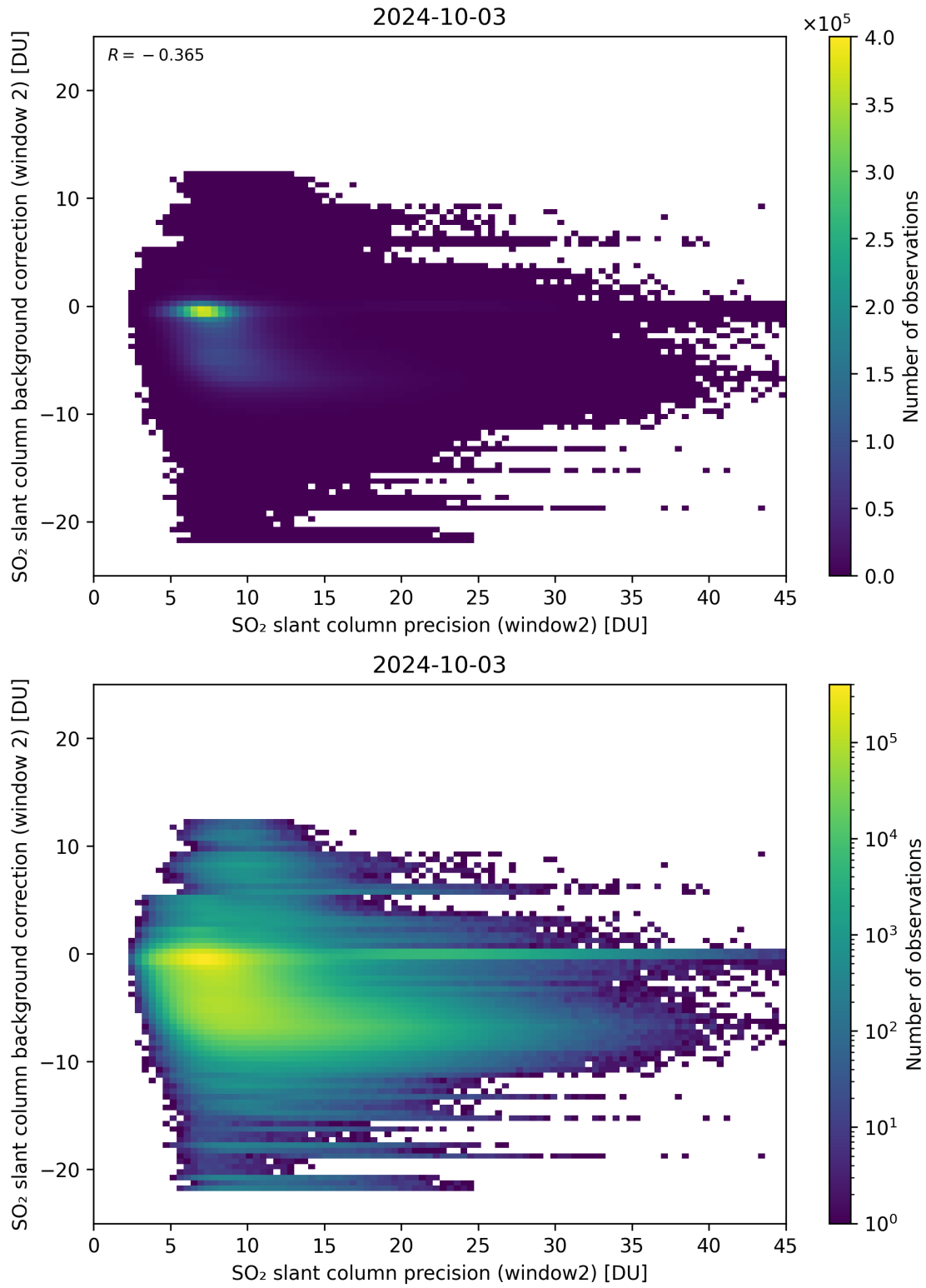
Figure 241: Scatter density plot of “SO 2 slant column precision (window2)” against “SO 2 slant column background correction (window 2)” for 2024-10-03 to 2024-10-04.
