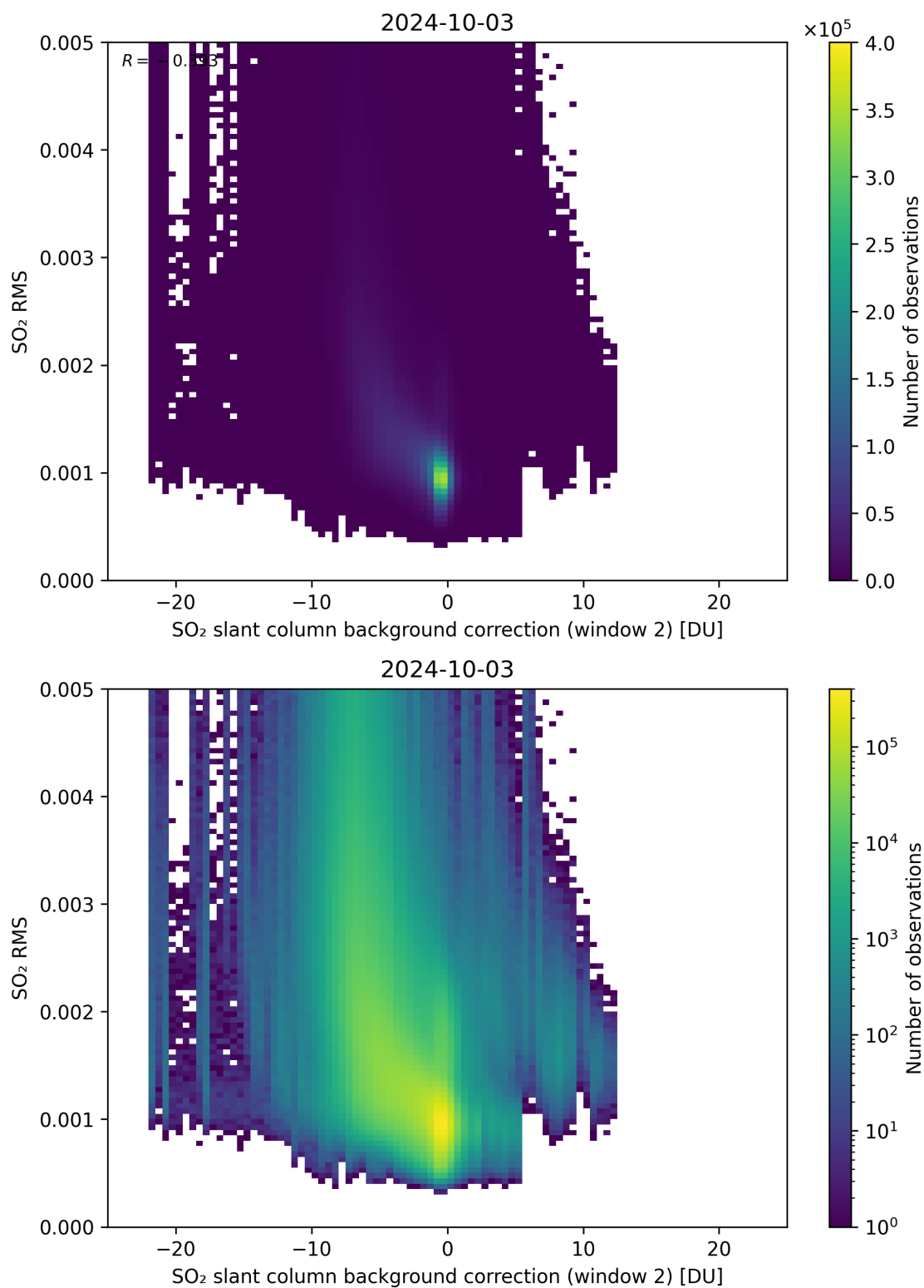
Figure 114: Scatter density plot of “SO 2 slant column background correction (window 2)” against “SO 2 RMS” for 2024-10-03 to 2024-10-04.
