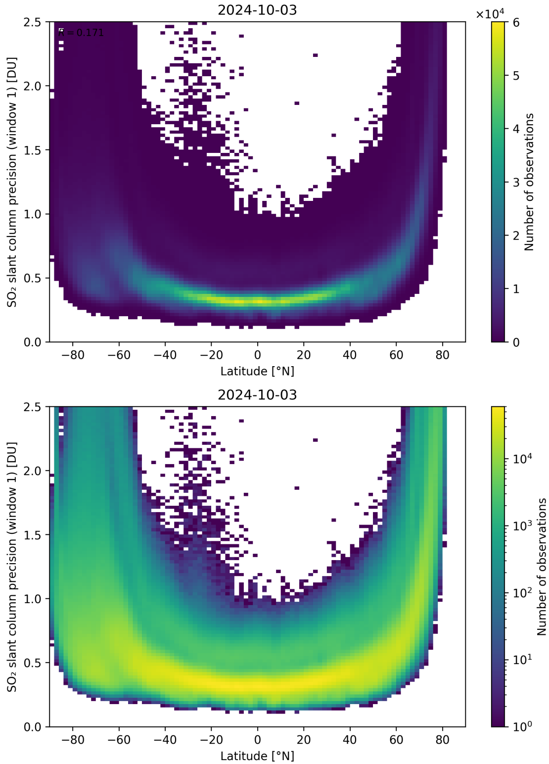
Figure 150: Scatter density plot of “Latitude” against “SO 2 slant column precision (window 1)” for 2024-10-03 to 2024-10-04.
