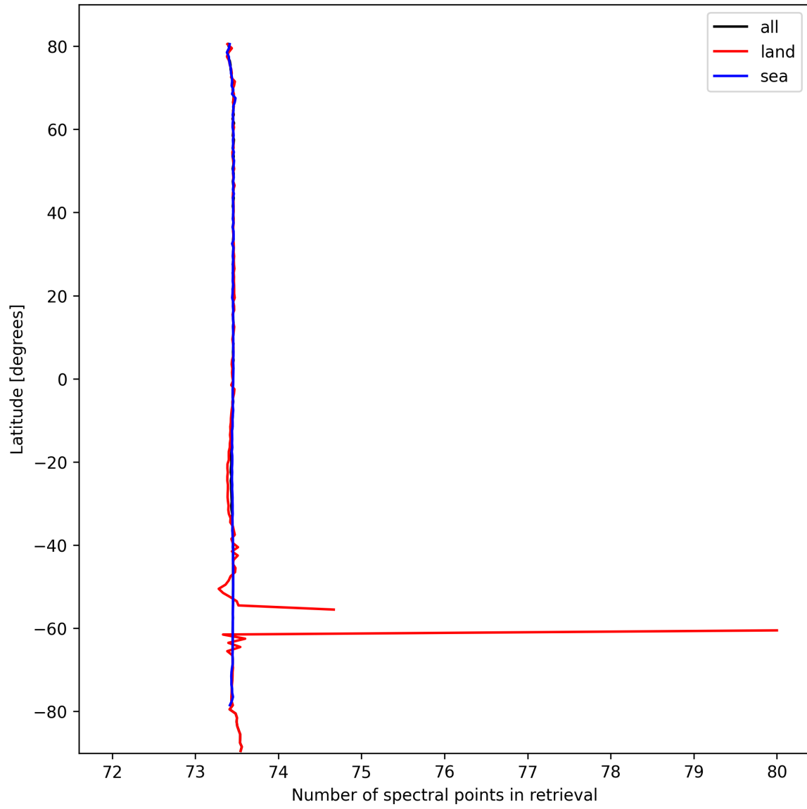
Figure 51: Zonal average of “Number of spectral points in retrieval” for 2024-10-03 to 2024-10-04.
