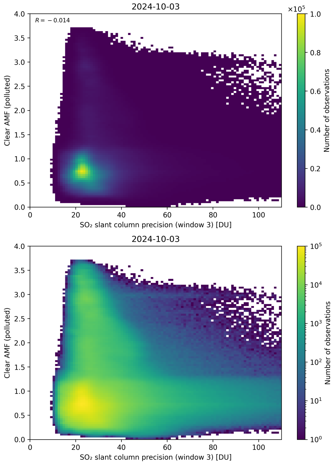
Figure 261: Scatter density plot of “SO 2 slant column precision (window 3)” against “Clear AMF (polluted)” for 2024-10-03 to 2024-10-04.
