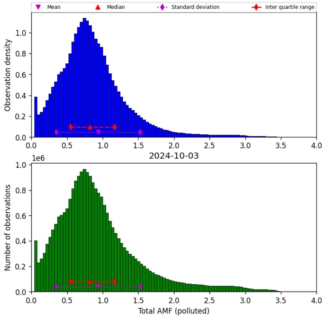
Figure 71: Histogram of “Total AMF (polluted)” for 2024-10-03 to 2024-10-04
