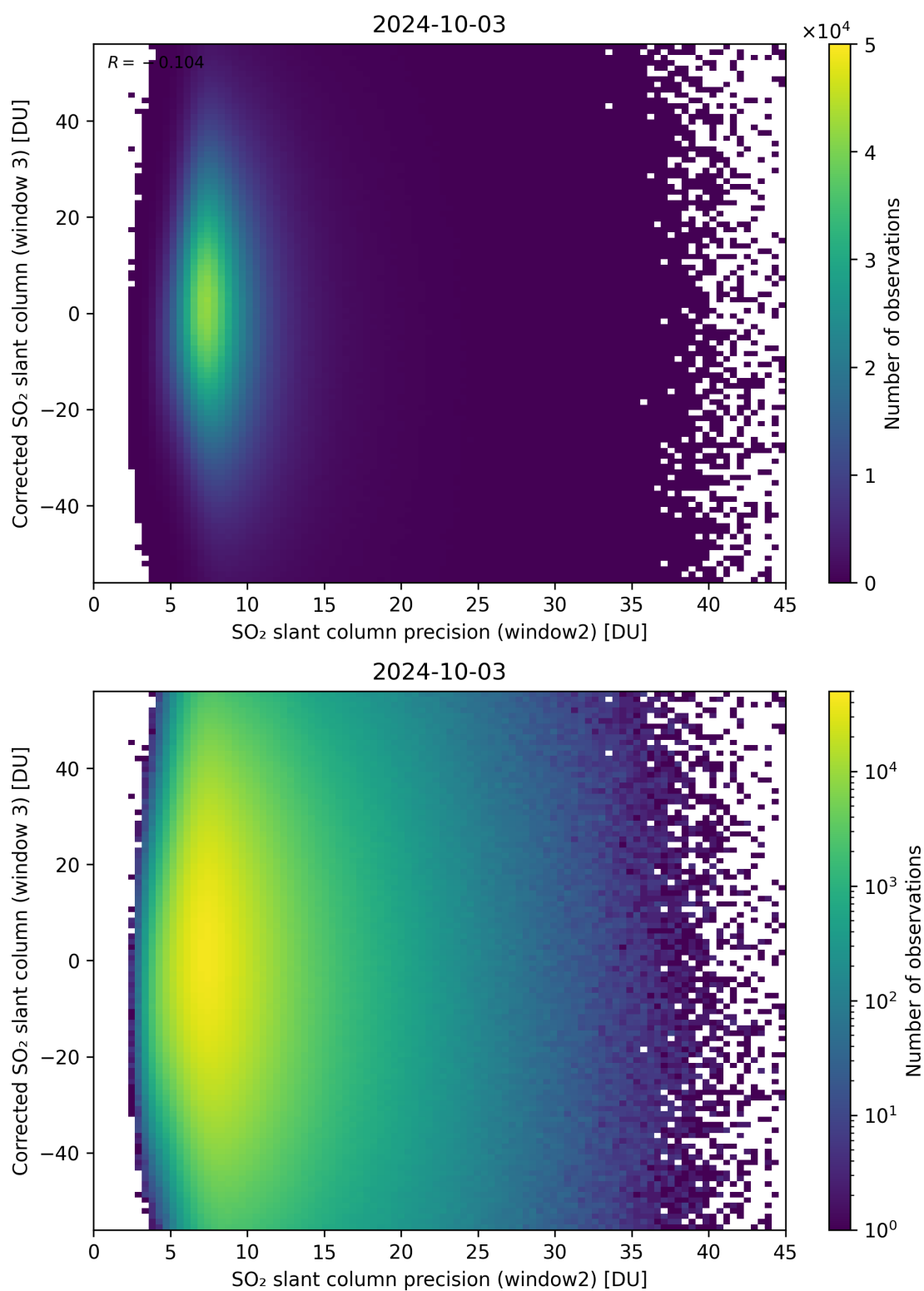
Figure 248: Scatter density plot of “SO 2 slant column precision (window2)” against “Corrected SO 2 slant column (window 3)” for 2024-10-03 to 2024-10-04.
