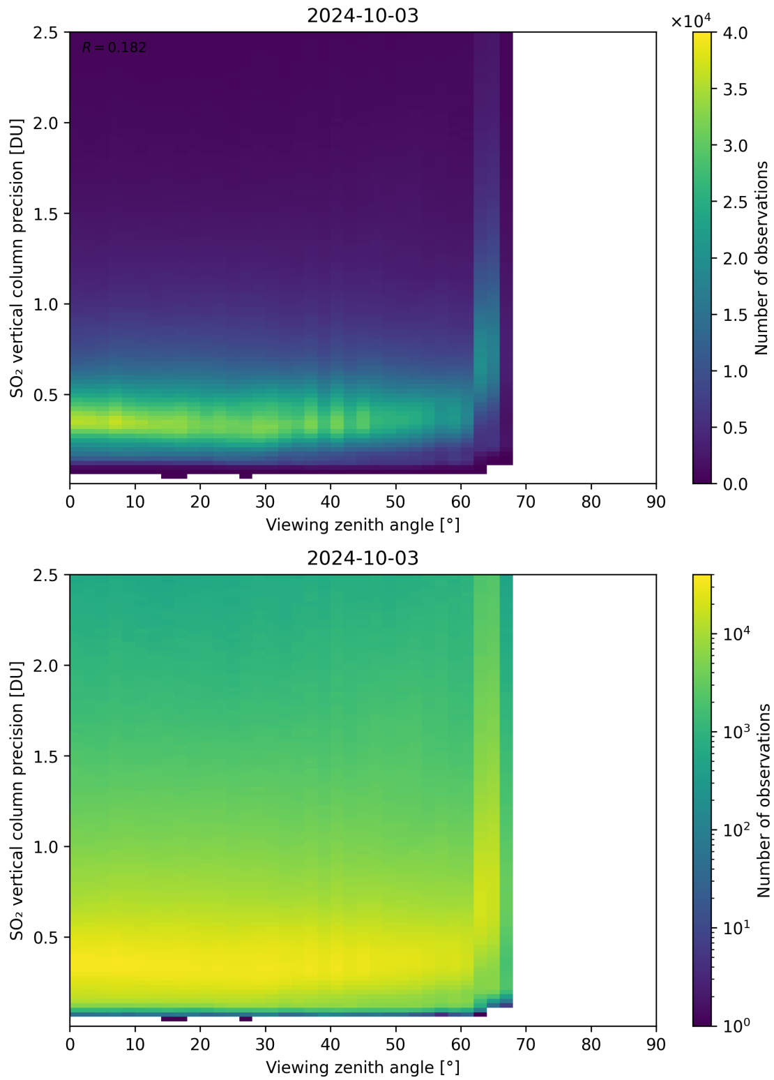
Figure 328: Scatter density plot of “Viewing zenith angle” against “SO 2 vertical column precision” for 2024-10-03 to 2024-10-04.
