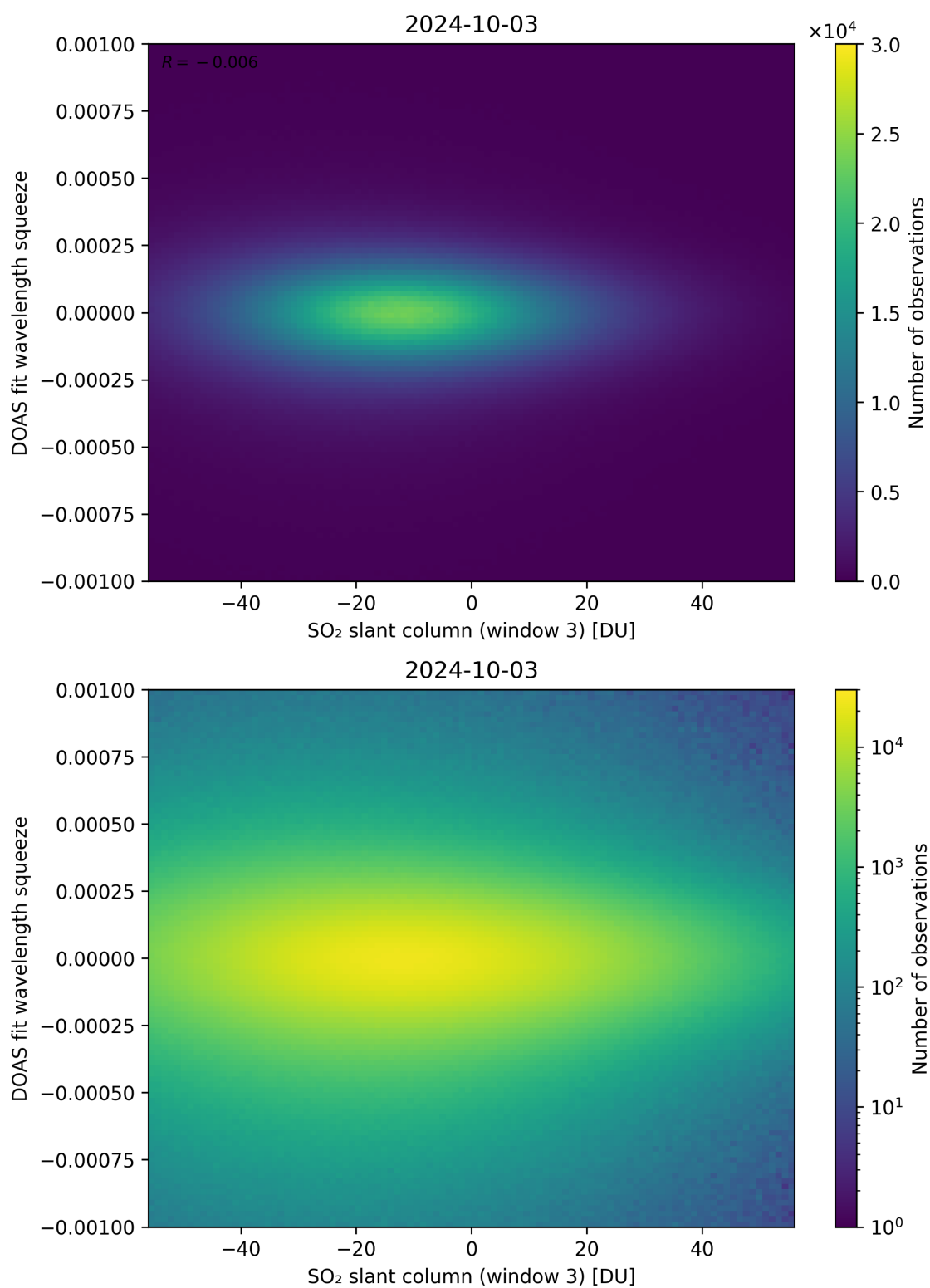
Figure 255: Scatter density plot of “SO 2 slant column (window 3)” against “DOAS fit wavelength squeeze” for 2024-10-03 to 2024-10-04.
