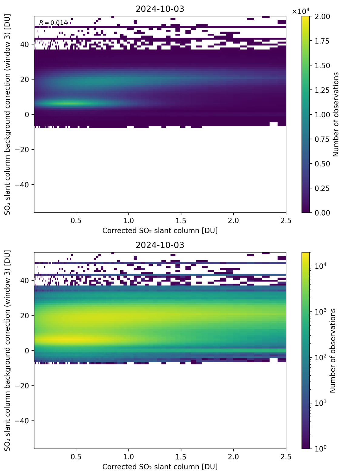
Figure 180: Scatter density plot of “Corrected SO 2 slant column” against “SO 2 slant column background correction (window 3)” for 2024-10-03 to 2024-10-04.
