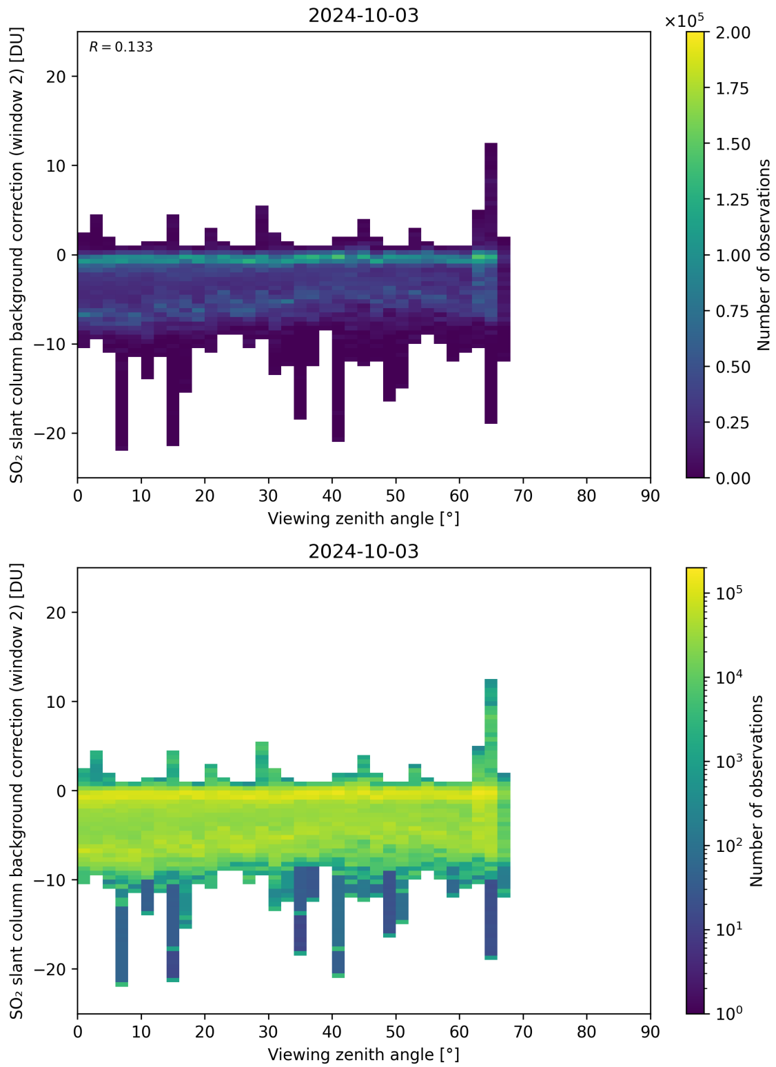
Figure 309: Scatter density plot of “Viewing zenith angle” against “SO 2 slant column background correction (window 2)” for 2024-10-03 to 2024-10-04.
