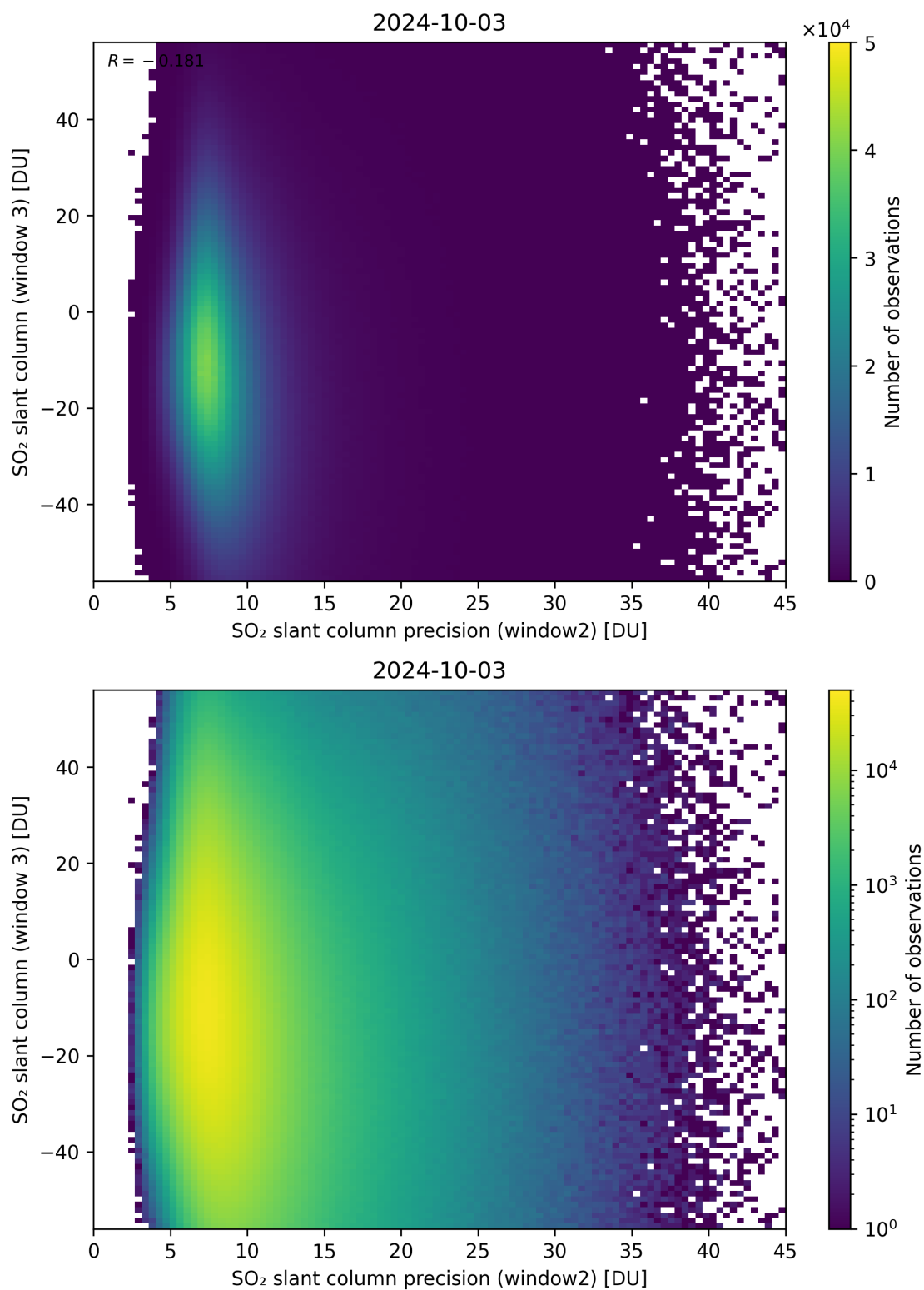
Figure 249: Scatter density plot of “SO 2 slant column precision (window2)” against “SO 2 slant column (window 3)” for 2024-10-03 to 2024-10-04.
