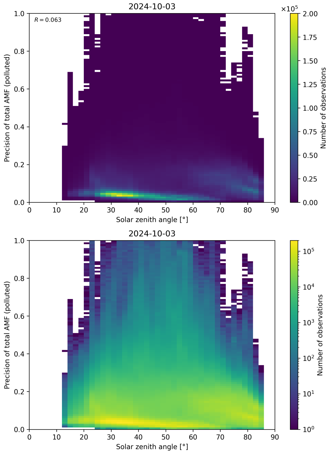
Figure 175: Scatter density plot of “Solar zenith angle” against “Precision of total AMF (polluted)” for 2024-10-03 to 2024-10-04.
