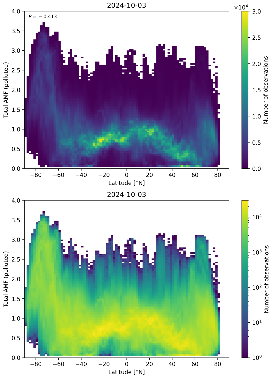
Figure 154: Scatter density plot of “Latitude” against “Total AMF (polluted)” for 2024-10-03 to 2024-10-04.
