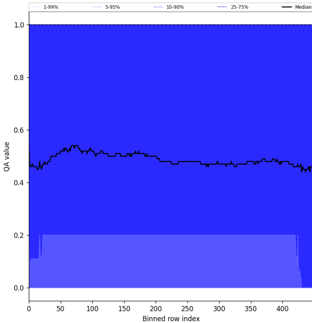
Figure 75: Along track statistics of “QA value” for 2024-10-03 to 2024-10-04
