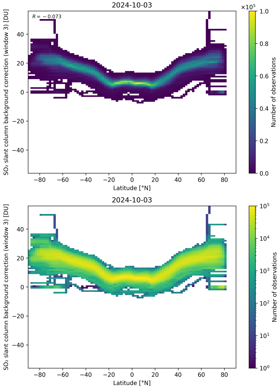
Figure 141: Scatter density plot of “Latitude” against “SO 2 slant column background correction (window 3)” for 2024-10-03 to 2024-10-04.
