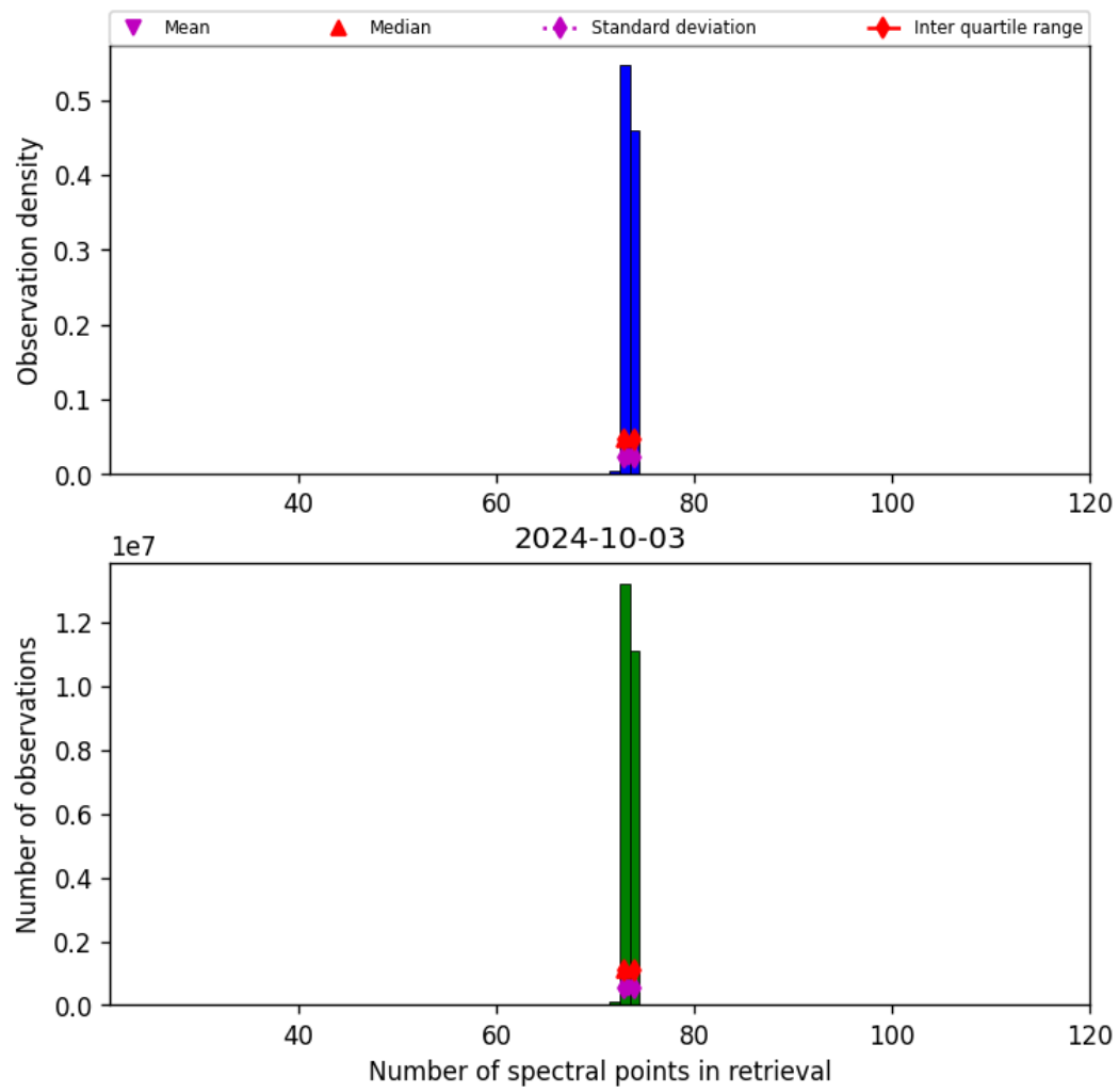
Figure 74: Histogram of “Number of spectral points in retrieval” for 2024-10-03 to 2024-10-04
