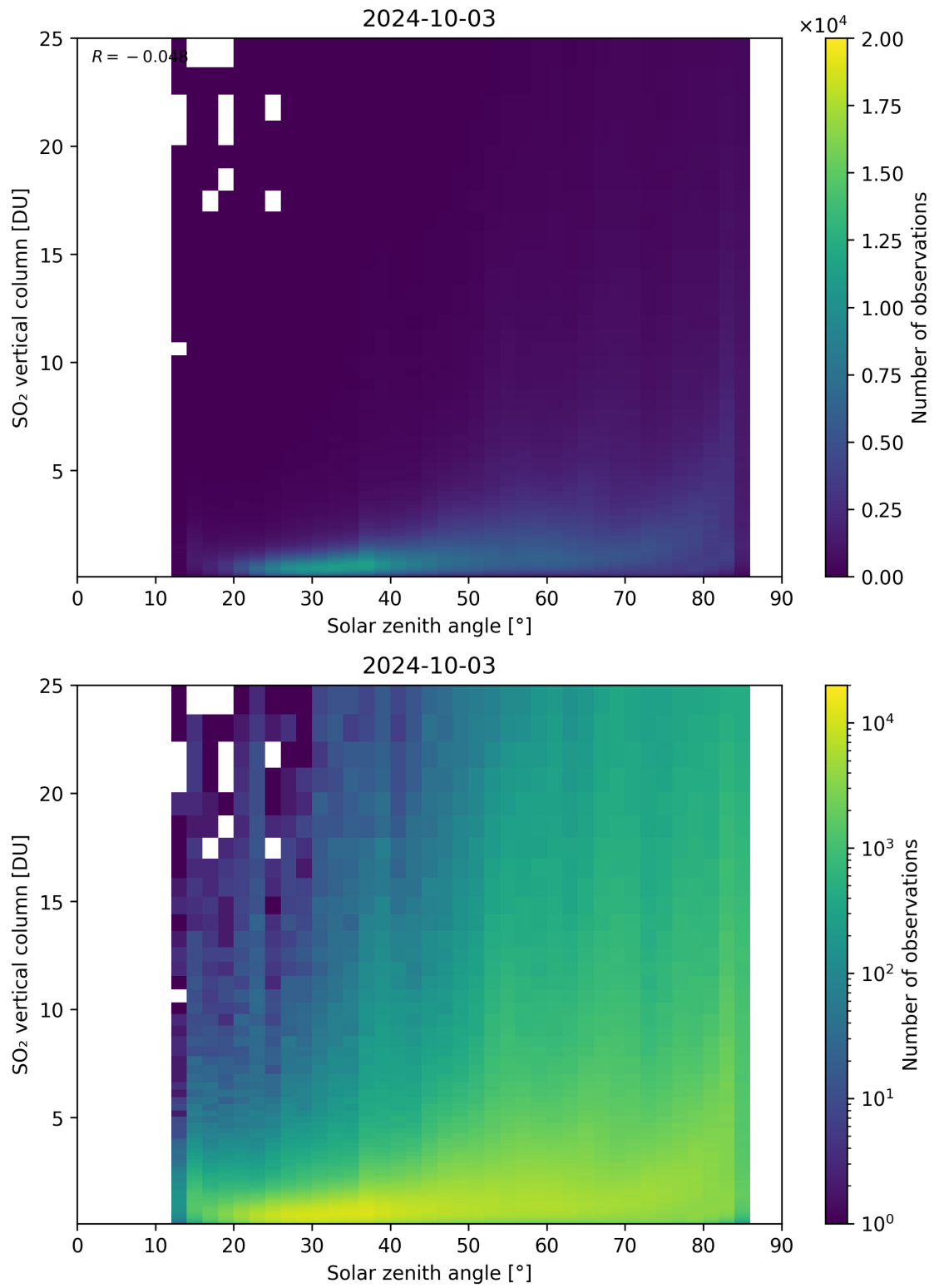
Figure 176: Scatter density plot of “Solar zenith angle” against “SO 2 vertical column” for 2024-10-03 to 2024-10-04.
