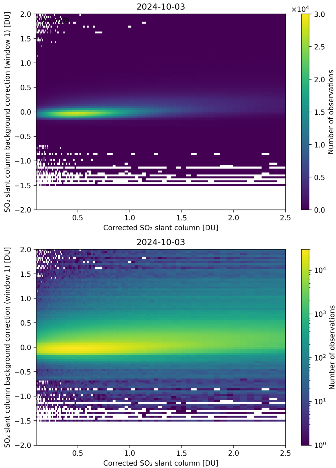
Figure 178: Scatter density plot of “Corrected SO 2 slant column” against “SO 2 slant column background correction (window 1)” for 2024-10-03 to 2024-10-04.
