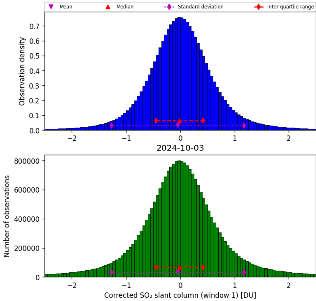
Figure 58: Histogram of “Corrected SO 2 slant column (window 1)” for 2024-10-03 to 2024-10-04
