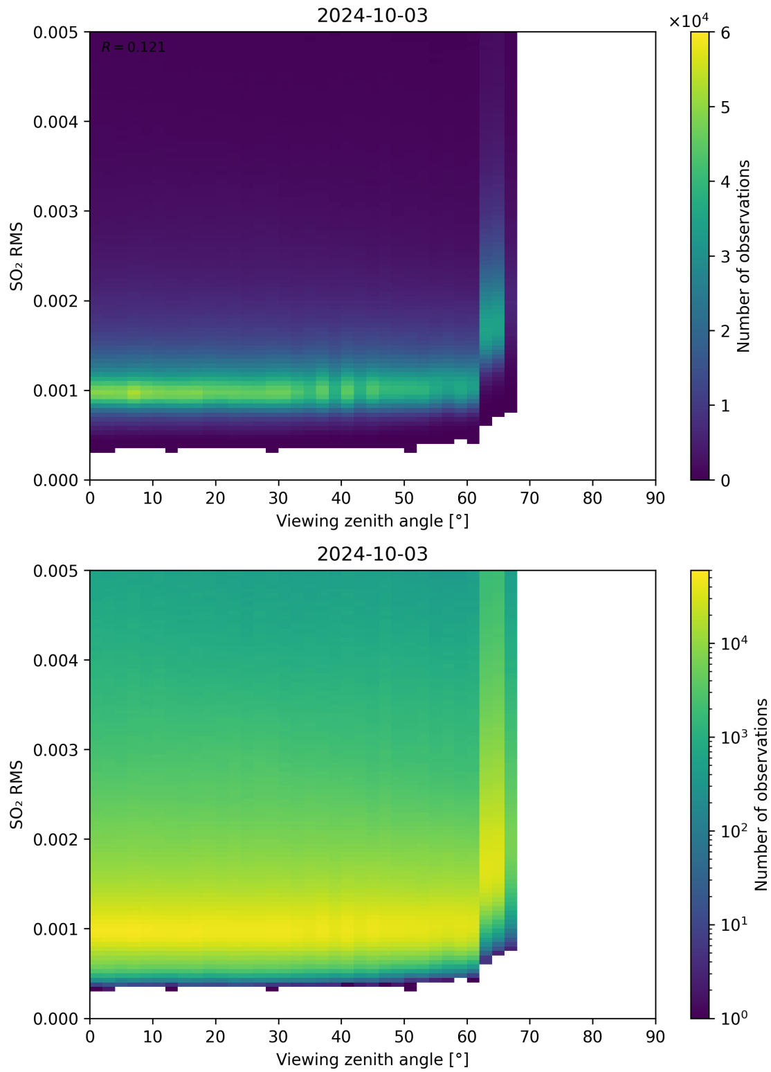
Figure 313: Scatter density plot of “Viewing zenith angle” against “SO 2 RMS” for 2024-10-03 to 2024-10-04.
