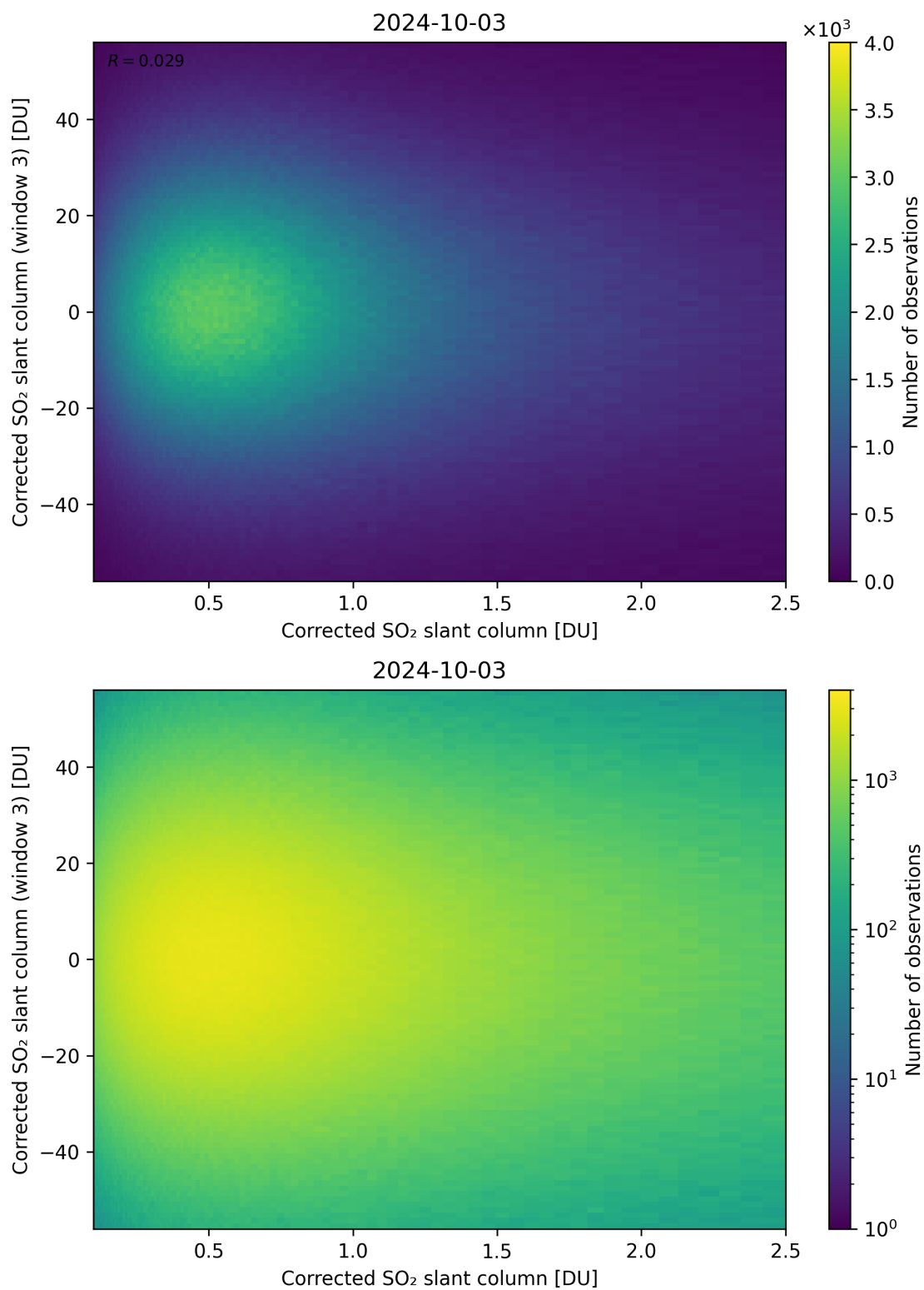
Figure 186: Scatter density plot of “Corrected SO 2 slant column” against “Corrected SO 2 slant column (window 3)” for 2024-10-03 to 2024-10-04.
