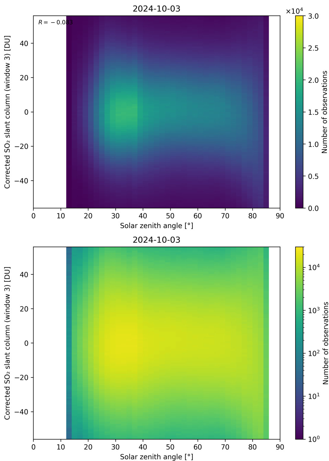
Figure 168: Scatter density plot of “Solar zenith angle” against “Corrected SO 2 slant column (window 3)” for 2024-10-03 to 2024-10-04.
