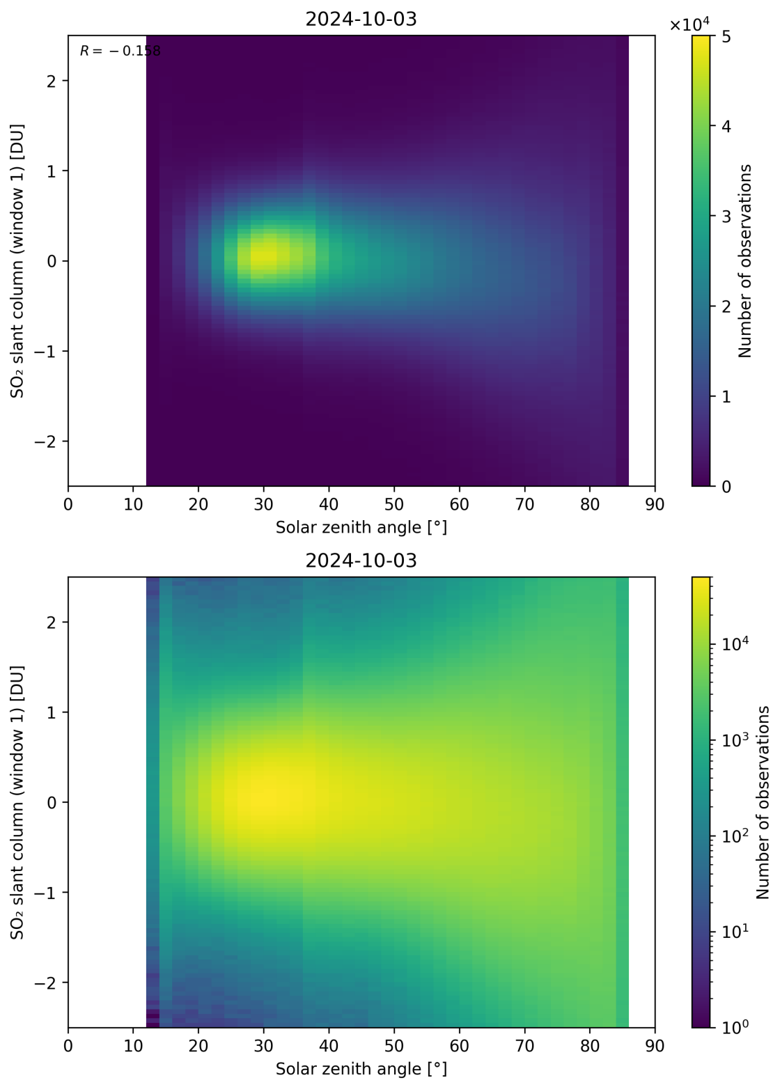
Figure 169: Scatter density plot of “Solar zenith angle” against “SO 2 slant column (window 1)” for 2024-10-03 to 2024-10-04.
