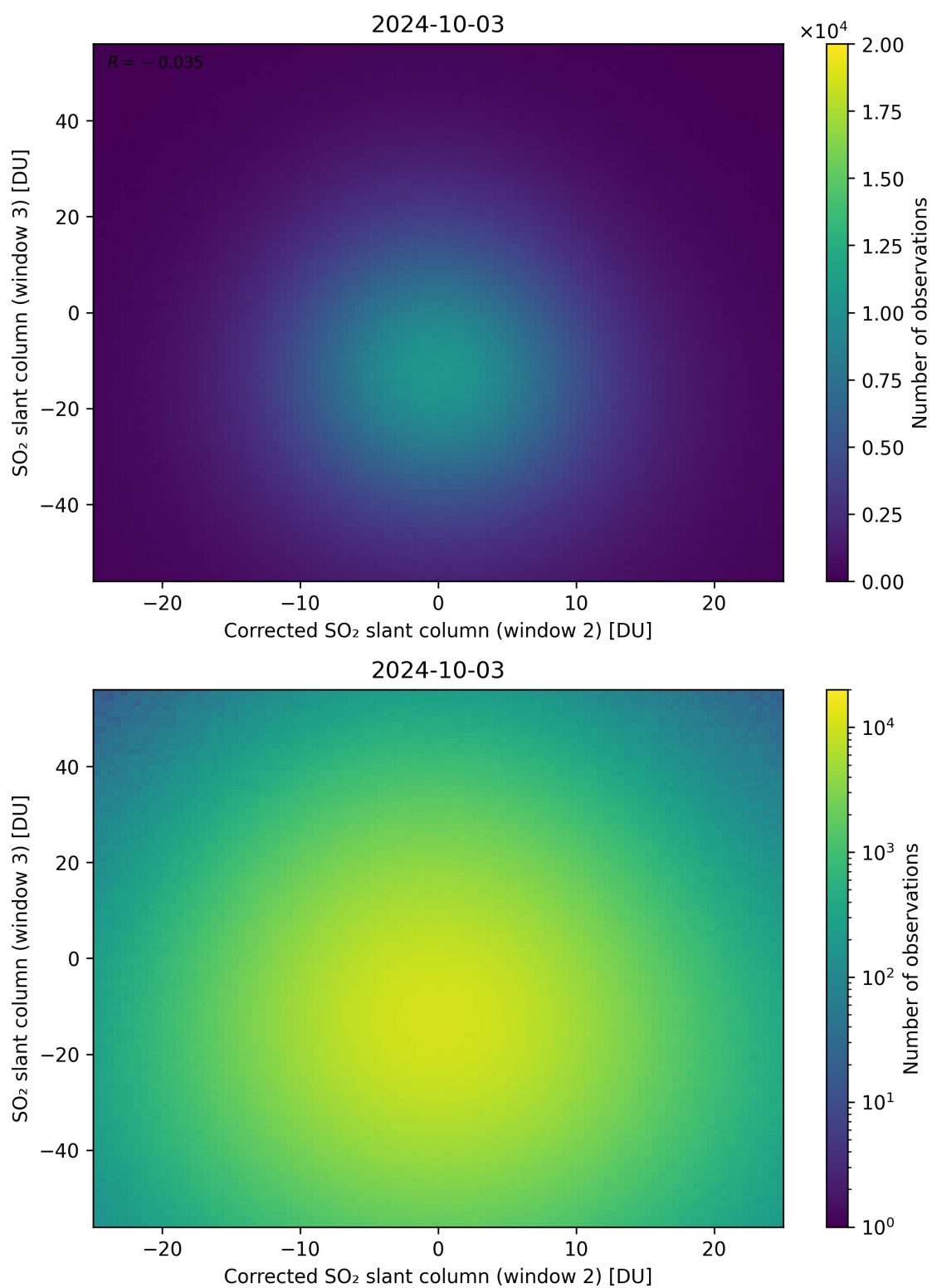
Figure 201: Scatter density plot of “Corrected SO 2 slant column (window 2)” against “SO 2 slant column (window 3)” for 2024-10-03 to 2024-10-04.
