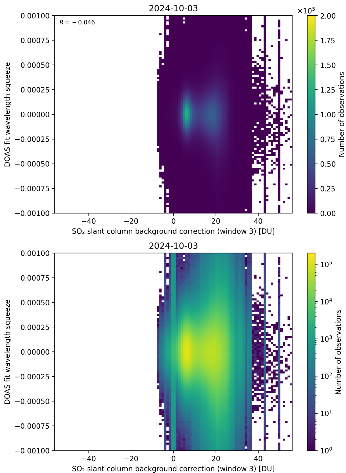
Figure 122: Scatter density plot of “SO 2 slant column background correction (window 3)” against “DOAS fit wavelength squeeze” for 2024-10-03 to 2024-10-04.
