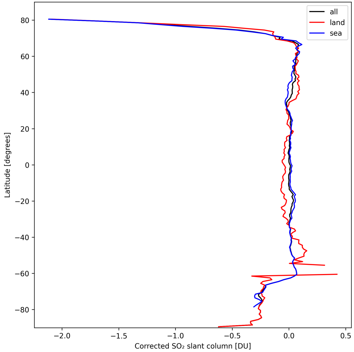
Figure 32: Zonal average of “Corrected SO 2 slant column” for 2024-10-03 to 2024-10-04.
