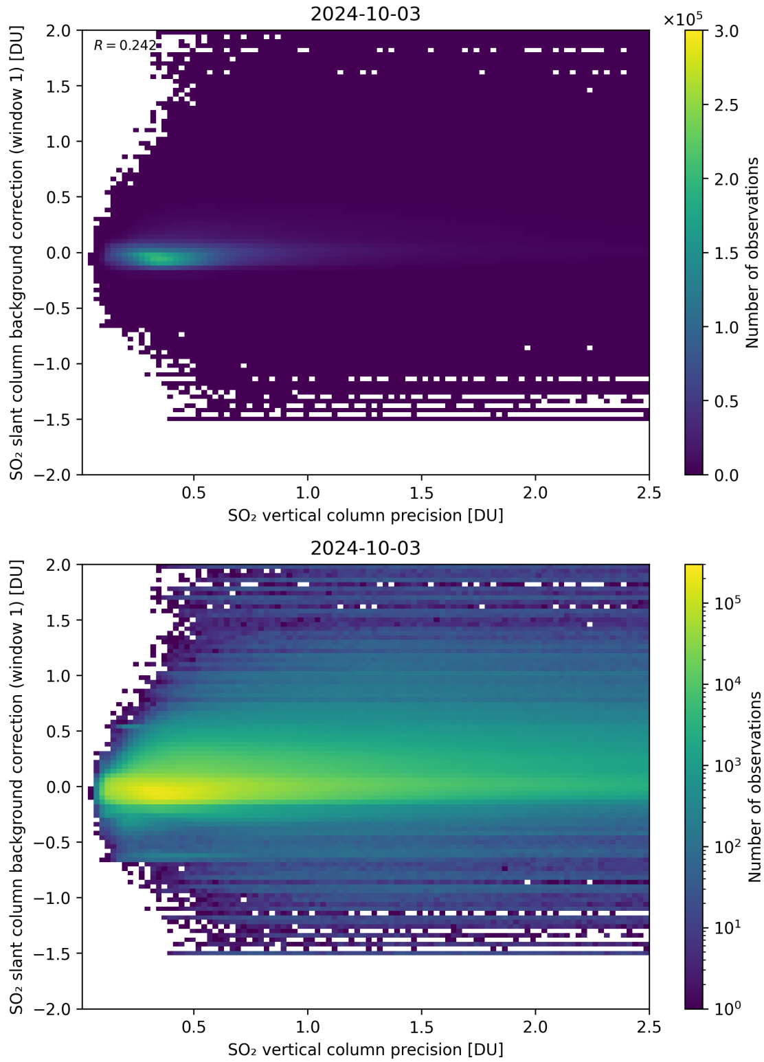
Figure 279: Scatter density plot of “SO 2 vertical column precision” against “SO 2 slant column background correction (window 1)” for 2024-10-03 to 2024-10-04.
