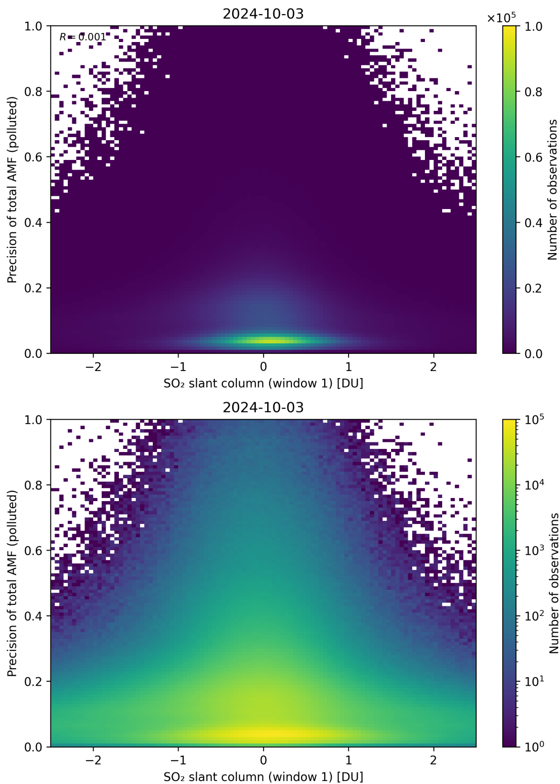
Figure 240: Scatter density plot of “SO 2 slant column (window 1)” against “Precision of total AMF (polluted)” for 2024-10-03 to 2024-10-04.
