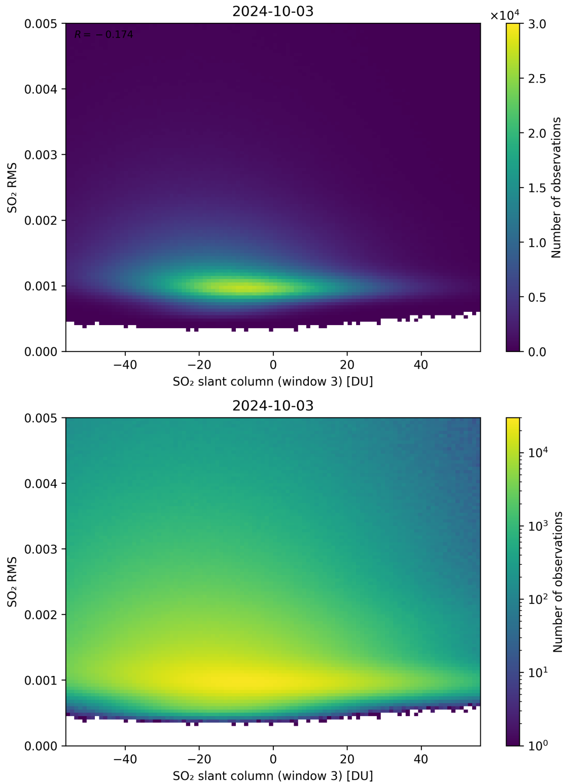
Figure 256: Scatter density plot of “SO 2 slant column (window 3)” against “SO 2 RMS” for 2024-10-03 to 2024-10-04.
