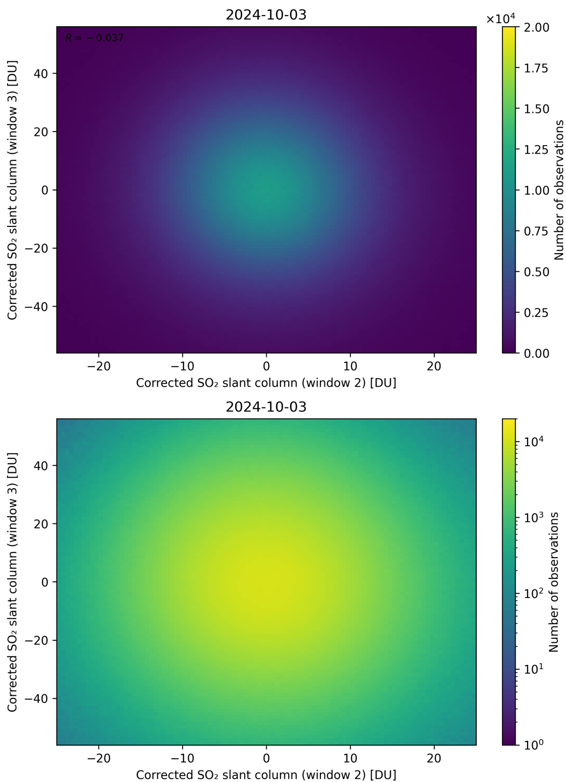
Figure 200: Scatter density plot of “Corrected SO 2 slant column (window 2)” against “Corrected SO 2 slant column (window 3)” for 2024-10-03 to 2024-10-04.
