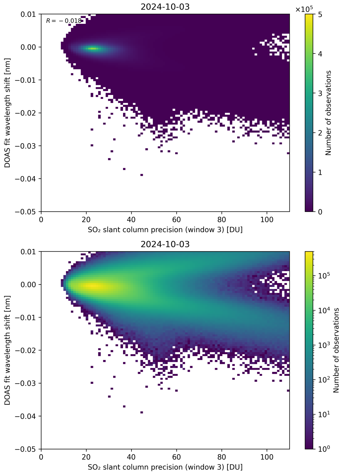
Figure 258: Scatter density plot of “SO 2 slant column precision (window 3)” against “DOAS fit wavelength shift” for 2024-10-03 to 2024-10-04.
