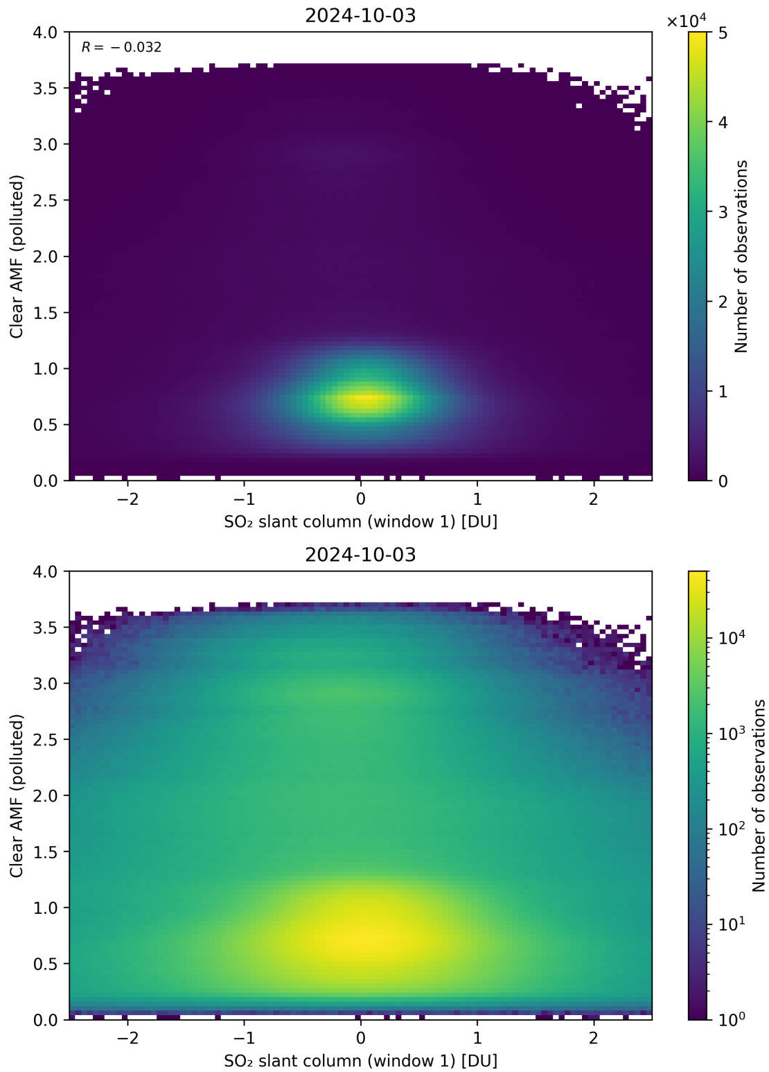
Figure 232: Scatter density plot of “SO 2 slant column (window 1)” against “Clear AMF (polluted)” for 2024-10-03 to 2024-10-04.
