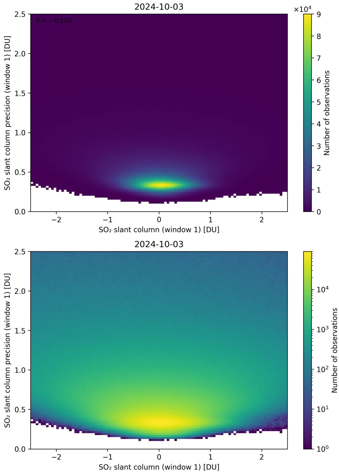
Figure 235: Scatter density plot of “SO 2 slant column (window 1)” against “SO 2 slant column precision (window 1)” for 2024-10-03 to 2024-10-04.
