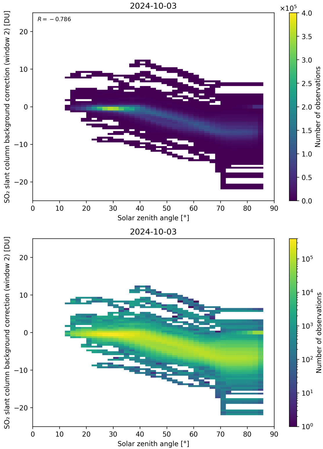
Figure 159: Scatter density plot of “Solar zenith angle” against “SO 2 slant column background correction (window 2)” for 2024-10-03 to 2024-10-04.
