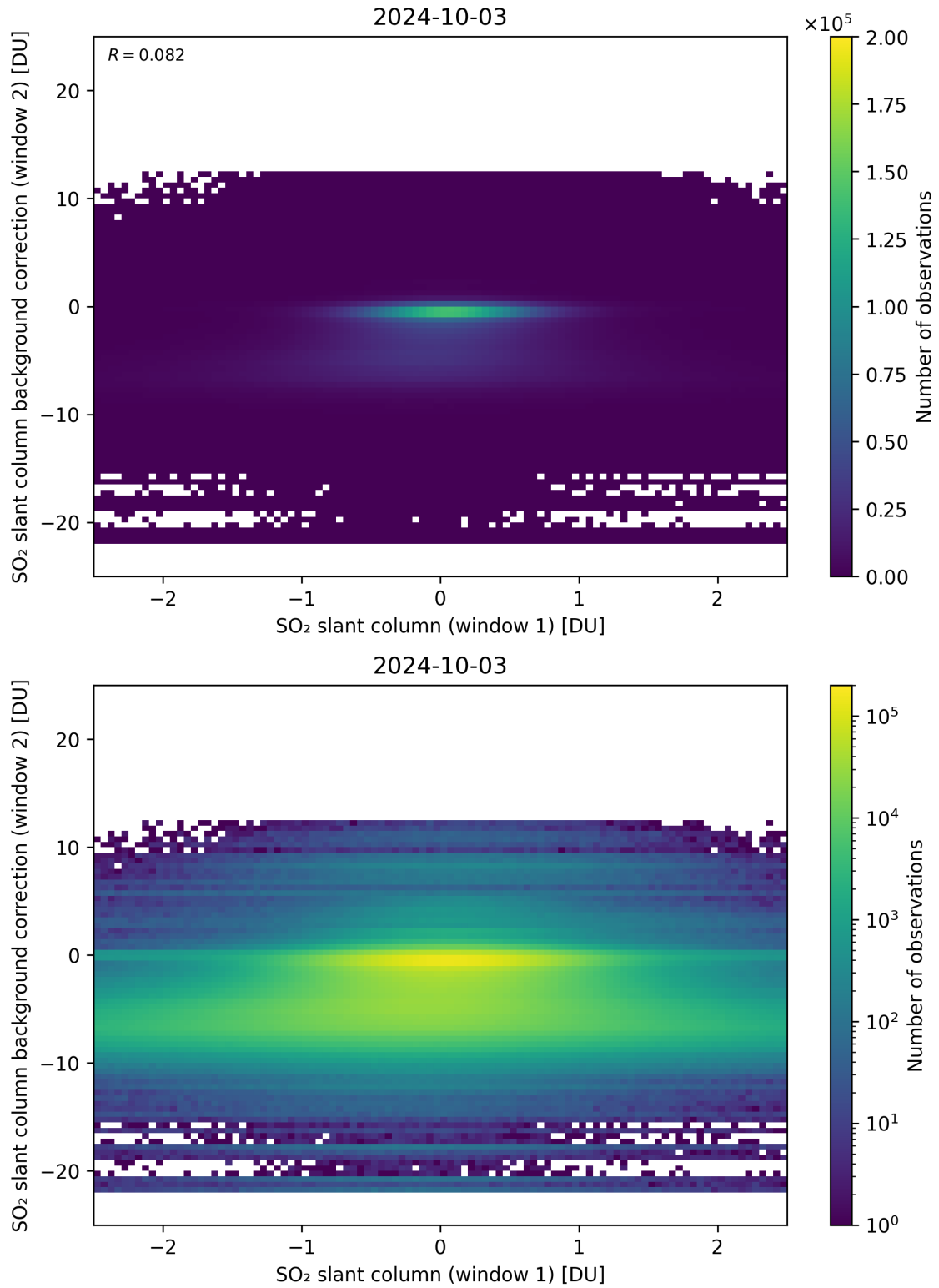
Figure 213: Scatter density plot of “SO 2 slant column (window 1)” against “SO 2 slant column background correction (window 2)” for 2024-10-03 to 2024-10-04.
