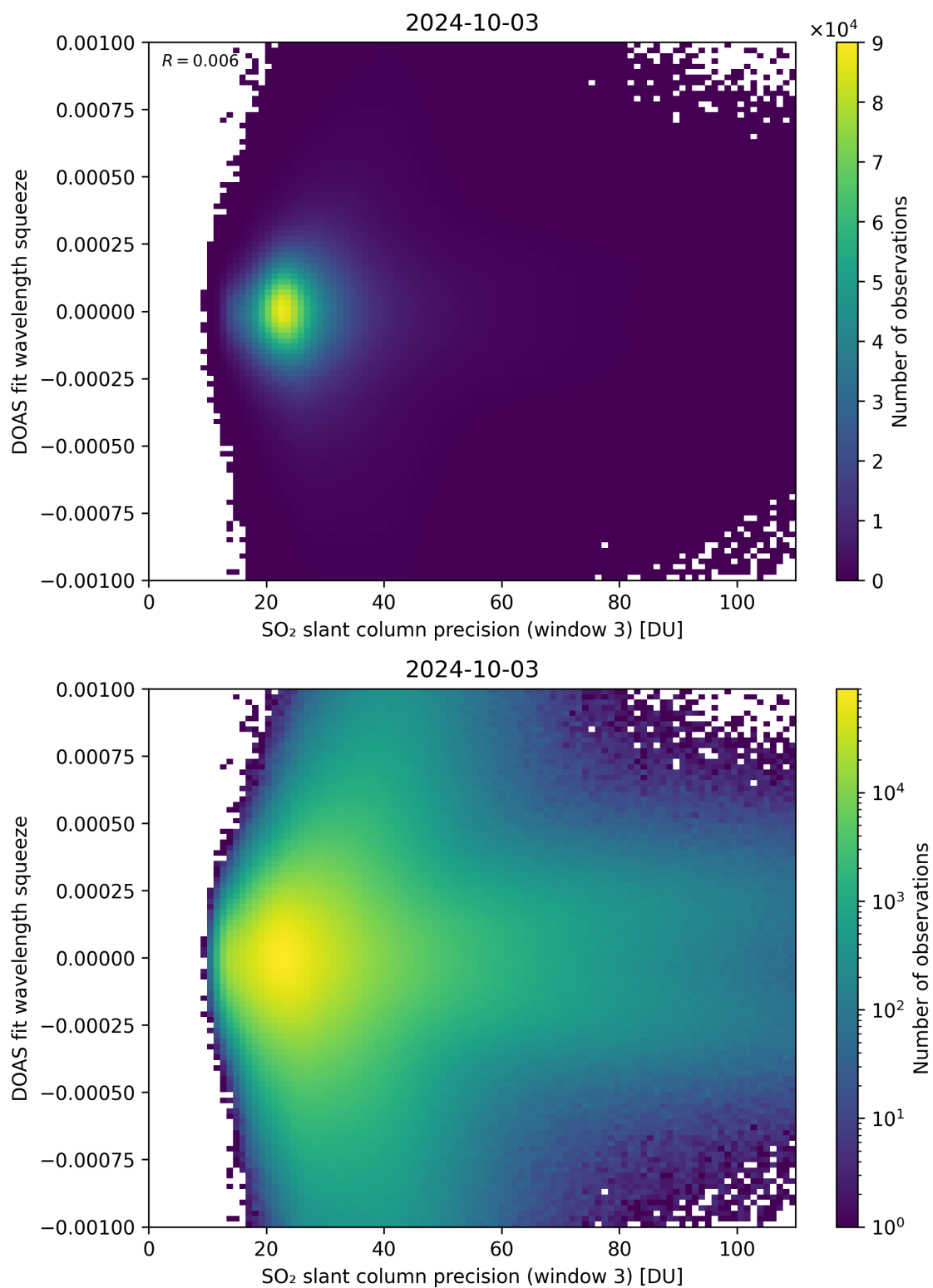
Figure 259: Scatter density plot of “SO 2 slant column precision (window 3)” against “DOAS fit wavelength squeeze” for 2024-10-03 to 2024-10-04.
