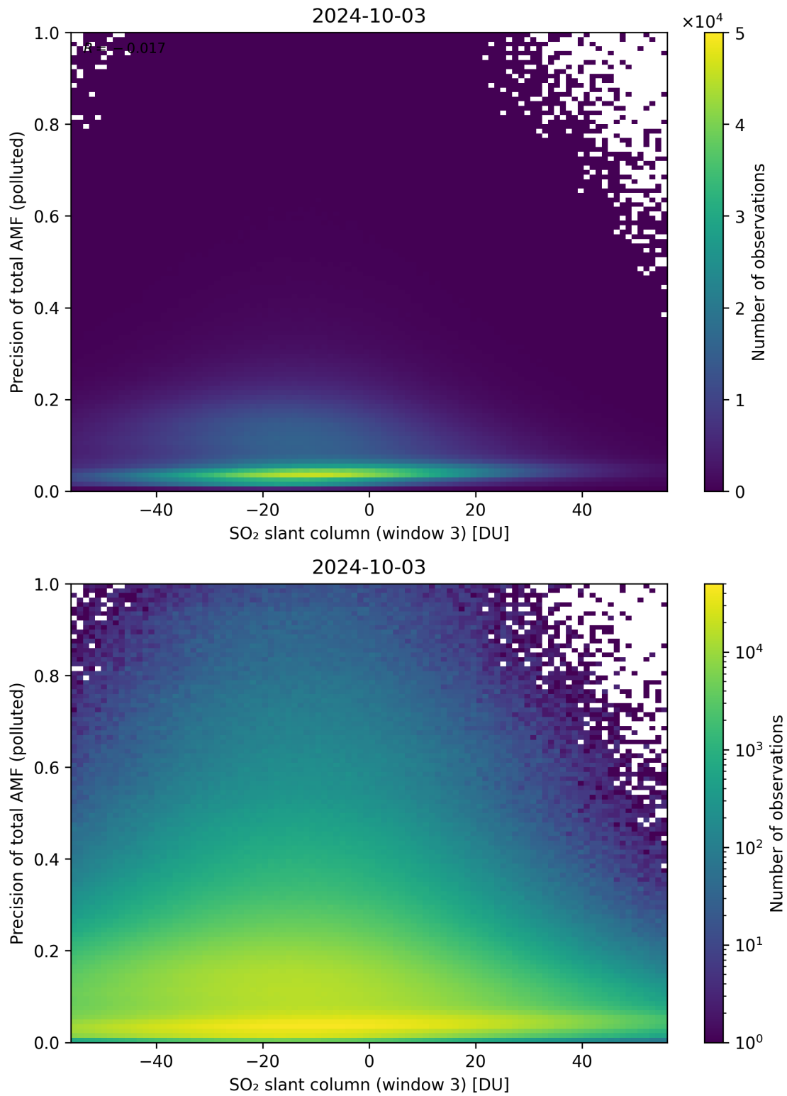
Figure 269: Scatter density plot of “SO 2 slant column (window 3)” against “Precision of total AMF (polluted)” for 2024-10-03 to 2024-10-04.
