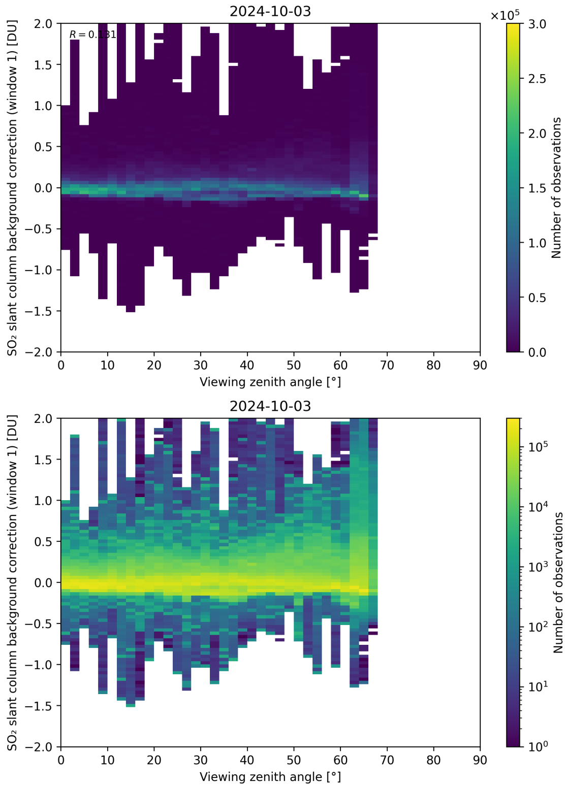
Figure 308: Scatter density plot of “Viewing zenith angle” against “SO 2 slant column background correction (window 1)” for 2024-10-03 to 2024-10-04.
