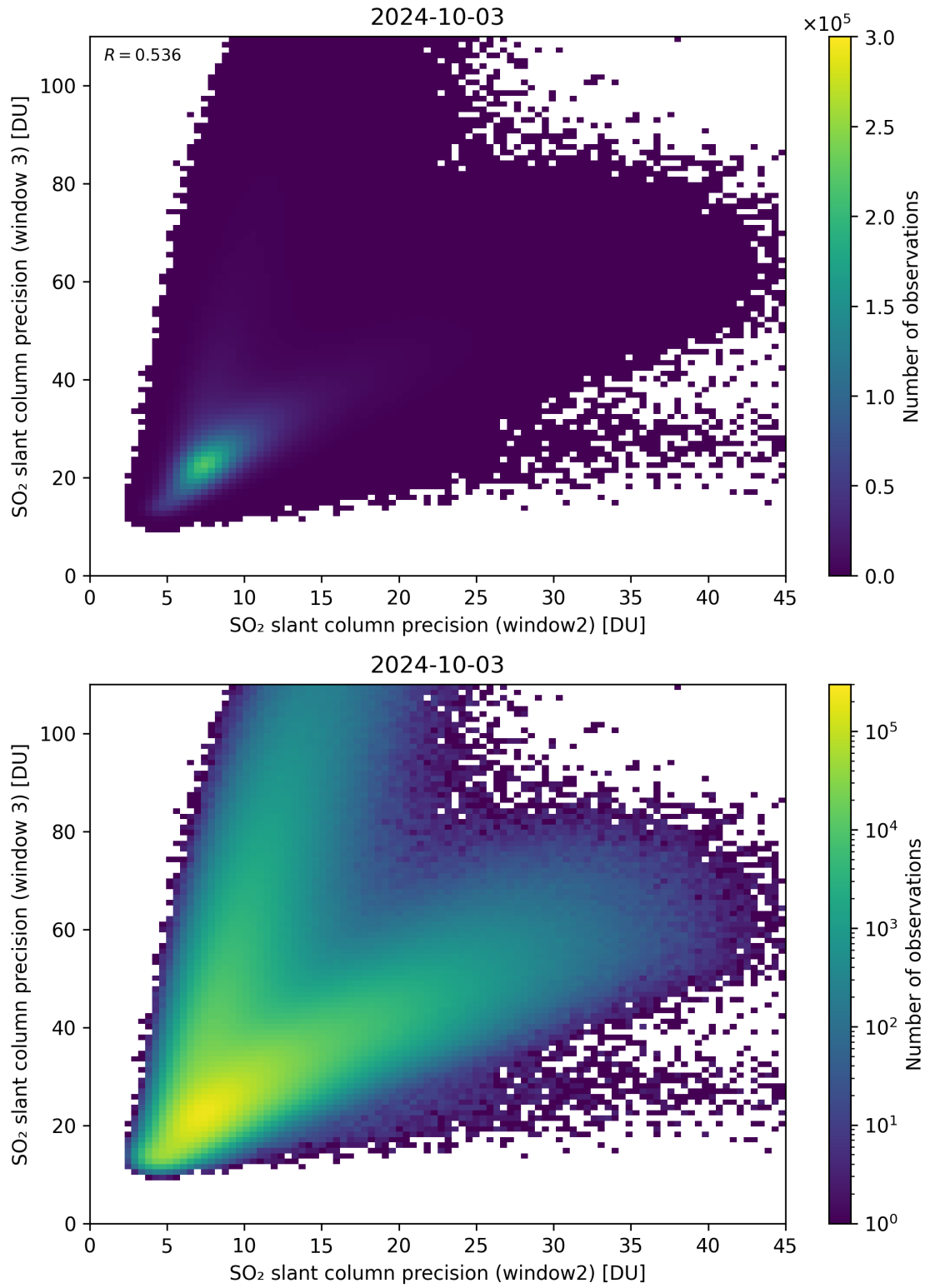
Figure 250: Scatter density plot of “SO 2 slant column precision (window2)” against “SO 2 slant column precision (window 3)” for 2024-10-03 to 2024-10-04.
