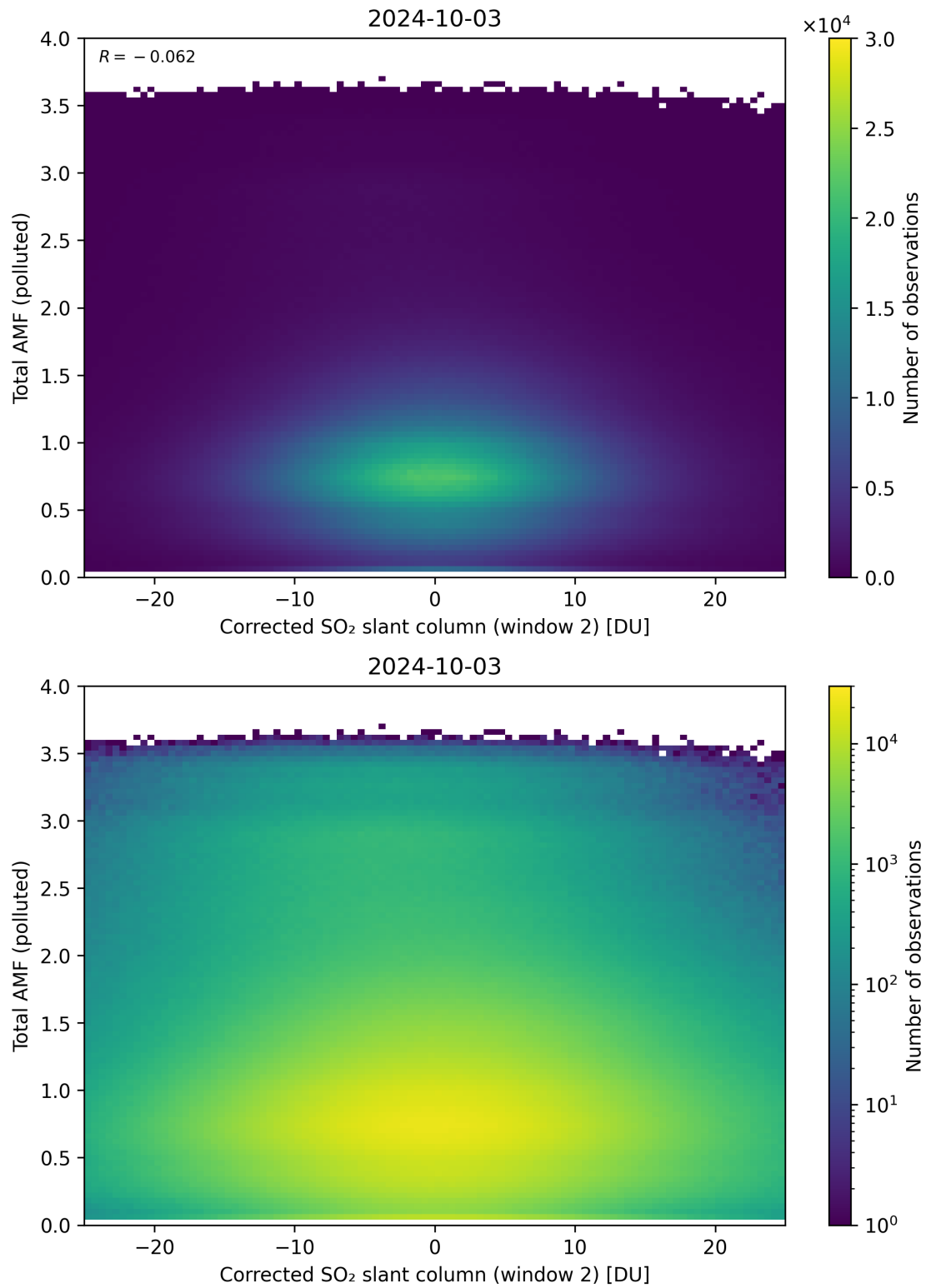
Figure 203: Scatter density plot of “Corrected SO 2 slant column (window 2)” against “Total AMF (polluted)” for 2024-10-03 to 2024-10-04.
