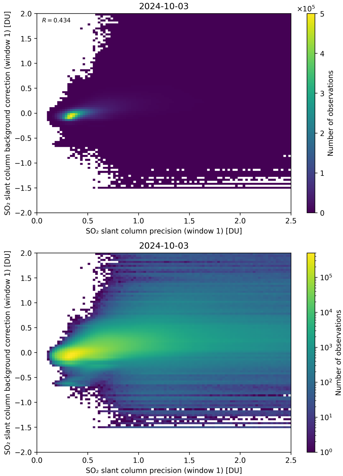
Figure 218: Scatter density plot of “SO 2 slant column precision (window 1)” against “SO 2 slant column background correction (window 1)” for 2024-10-03 to 2024-10-04.
