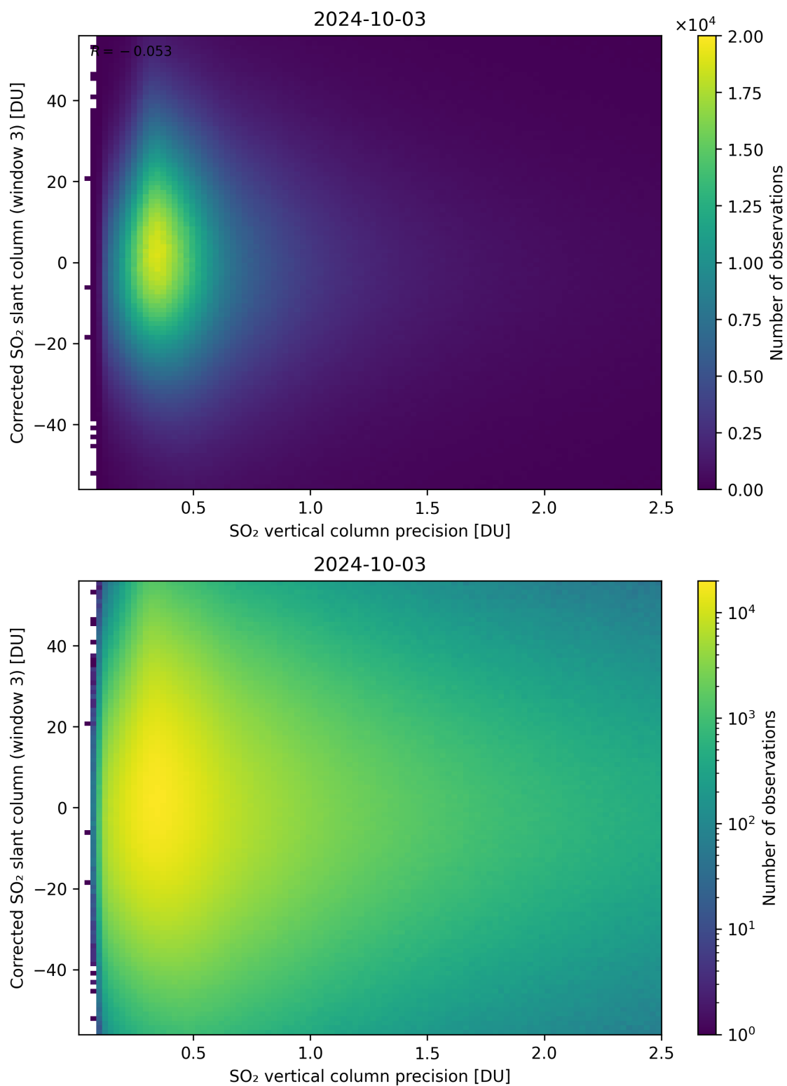
Figure 288: Scatter density plot of “SO 2 vertical column precision” against “Corrected SO 2 slant column (window 3)” for 2024-10-03 to 2024-10-04.
