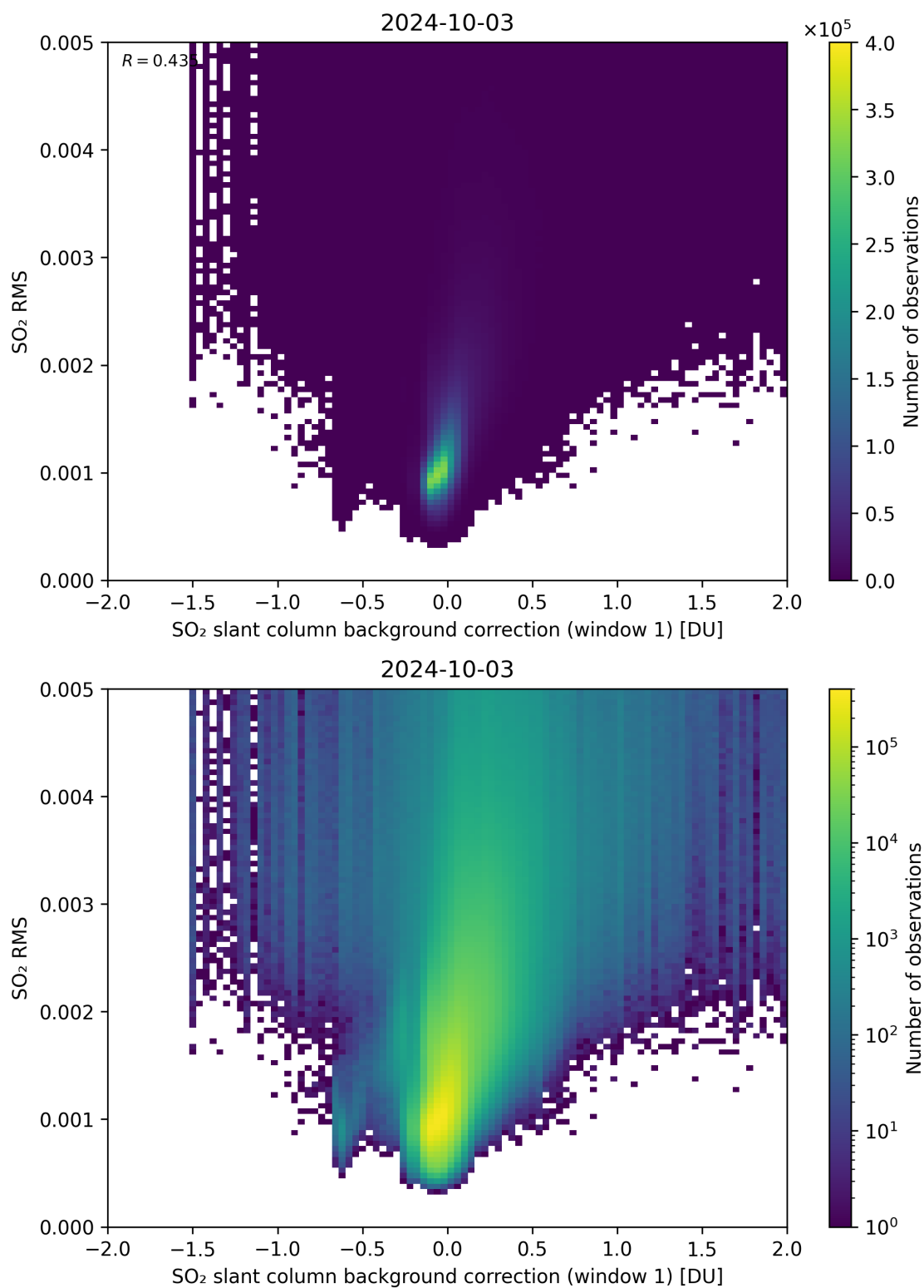
Figure 102: Scatter density plot of “SO 2 slant column background correction (window 1)” against “SO 2 RMS” for 2024-10-03 to 2024-10-04.
