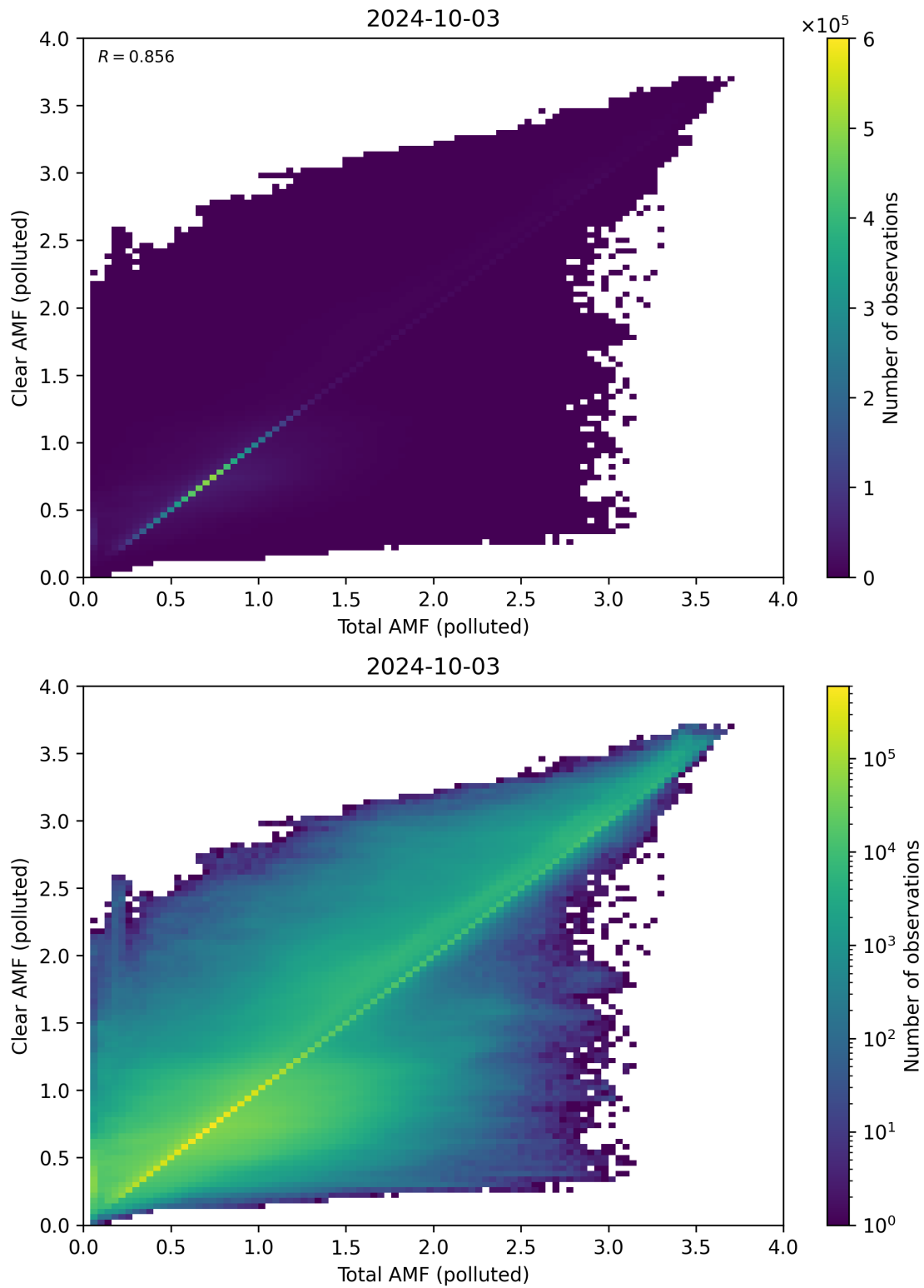
Figure 271: Scatter density plot of “Total AMF (polluted)” against “Clear AMF (polluted)” for 2024-10-03 to 2024-10-04.
