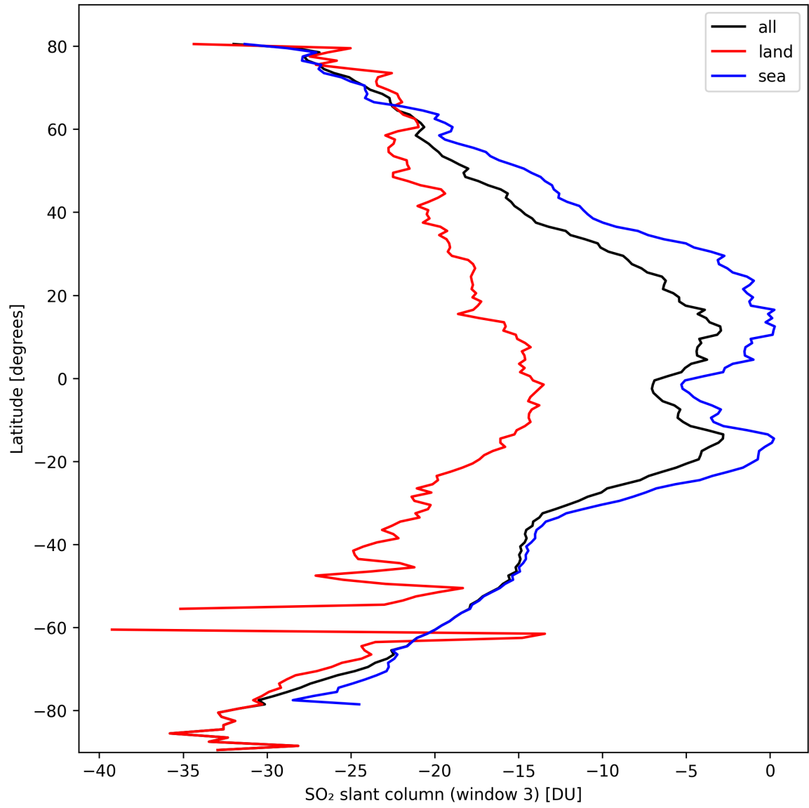
Figure 41: Zonal average of “SO 2 slant column (window 3)” for 2024-10-03 to 2024-10-04.
