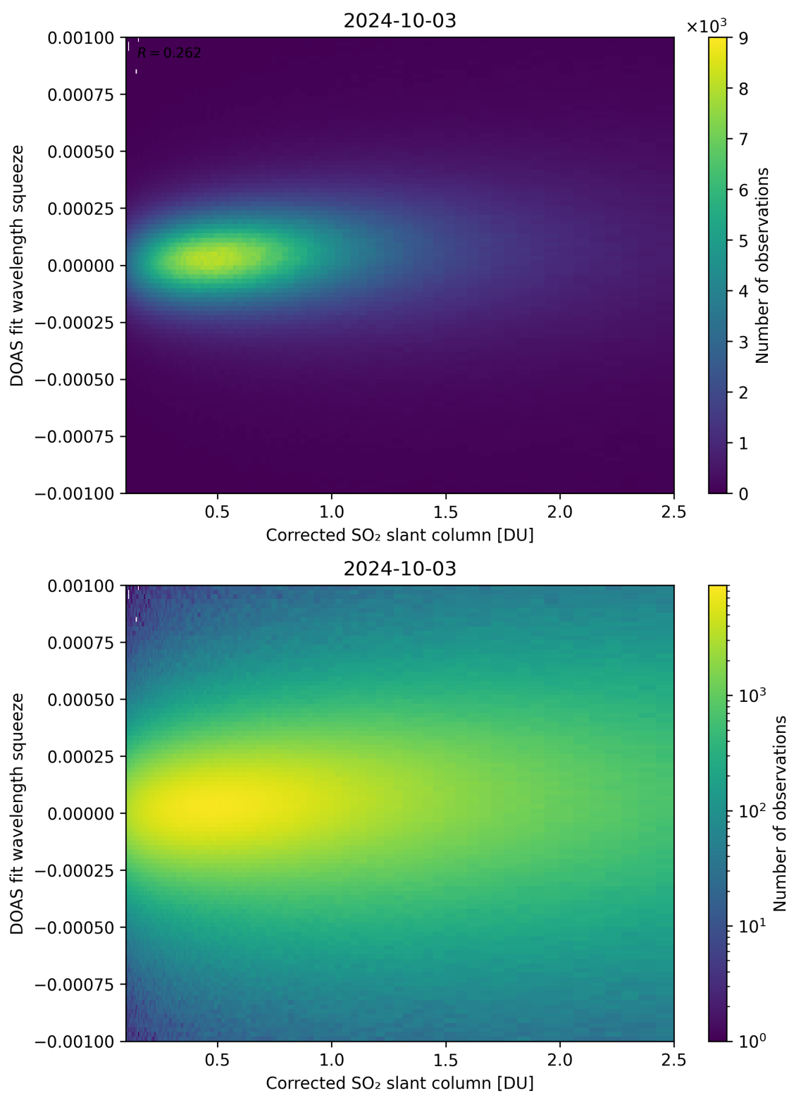
Figure 182: Scatter density plot of “Corrected SO 2 slant column” against “DOAS fit wavelength squeeze” for 2024-10-03 to 2024-10-04.
