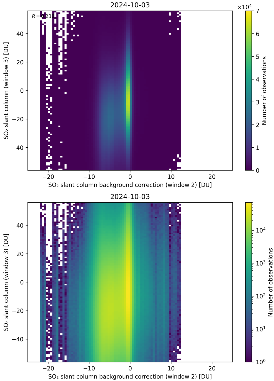
Figure 117: Scatter density plot of “SO 2 slant column background correction (window 2)” against “SO 2 slant column (window 3)” for 2024-10-03 to 2024-10-04.
