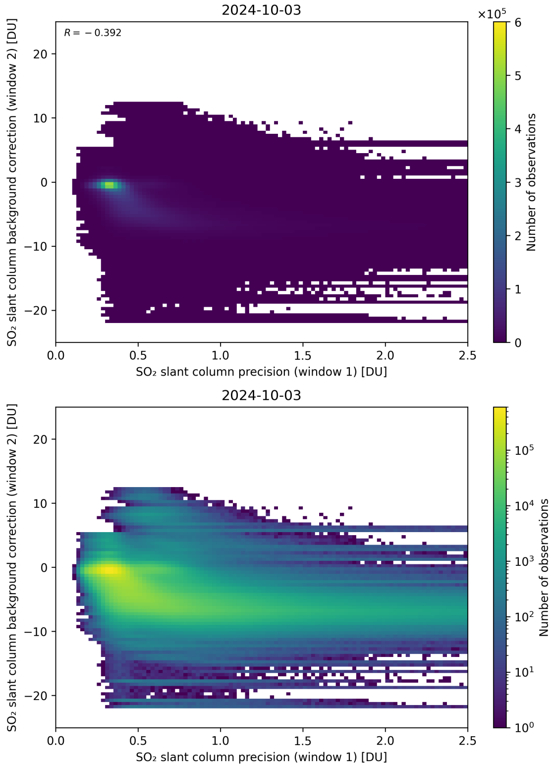
Figure 219: Scatter density plot of “SO 2 slant column precision (window 1)” against “SO 2 slant column background correction (window 2)” for 2024-10-03 to 2024-10-04.
