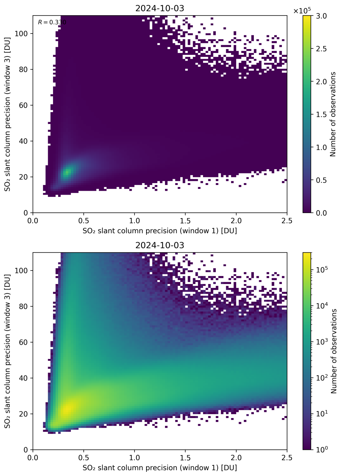
Figure 229: Scatter density plot of “SO 2 slant column precision (window 1)” against “SO 2 slant column precision (window 3)” for 2024-10-03 to 2024-10-04.
