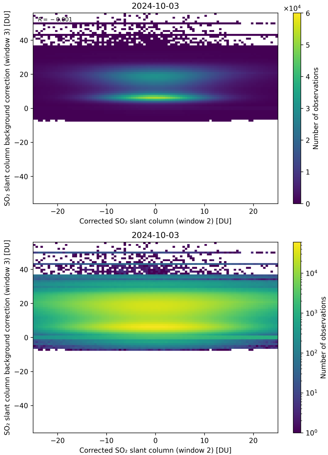
Figure 195: Scatter density plot of “Corrected SO 2 slant column (window 2)” against “SO 2 slant column background correction (window 3)” for 2024-10-03 to 2024-10-04.
