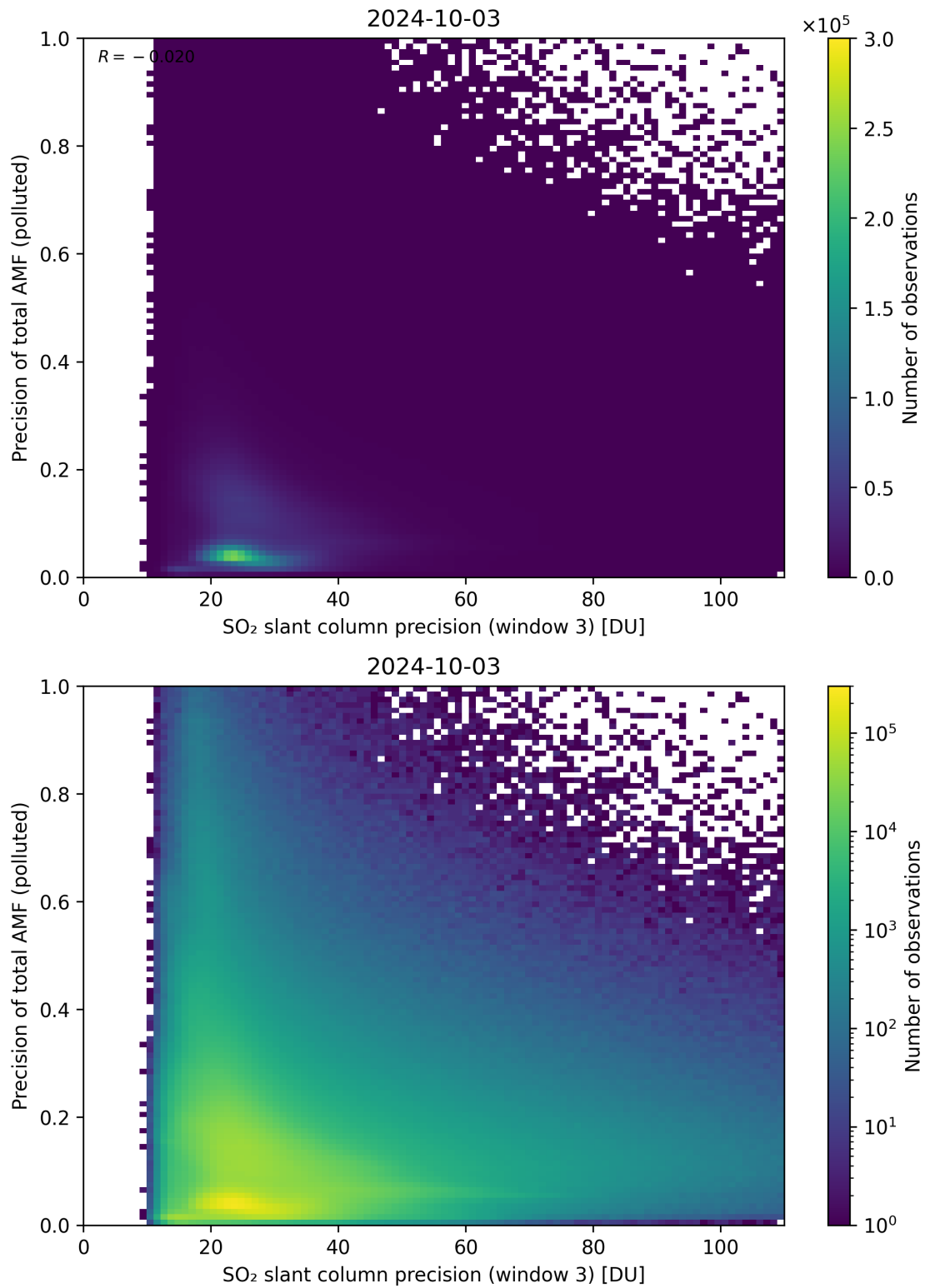
Figure 264: Scatter density plot of “SO 2 slant column precision (window 3)” against “Precision of total AMF (polluted)” for 2024-10-03 to 2024-10-04.
