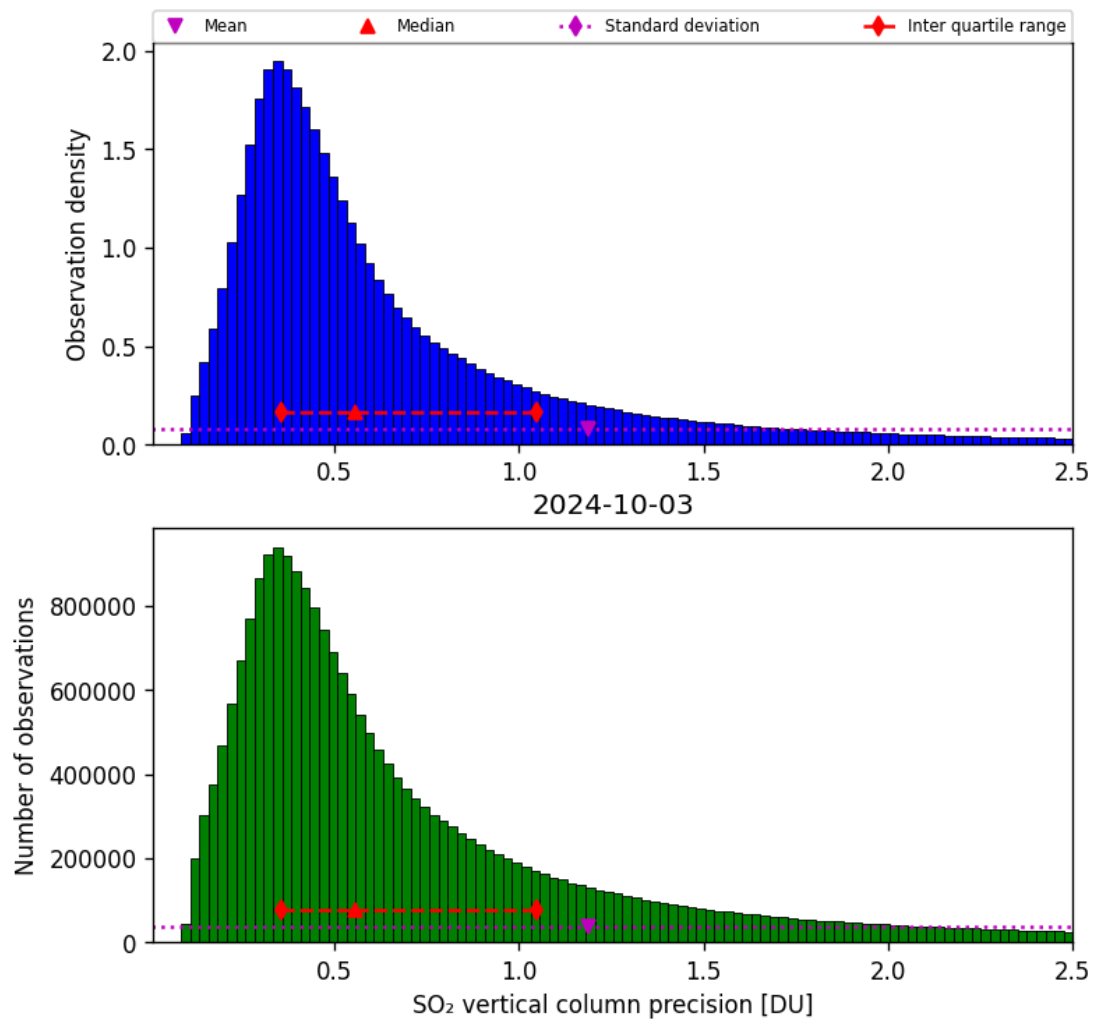
Figure 54: Histogram of “SO 2 vertical column precision” for 2024-10-03 to 2024-10-04
