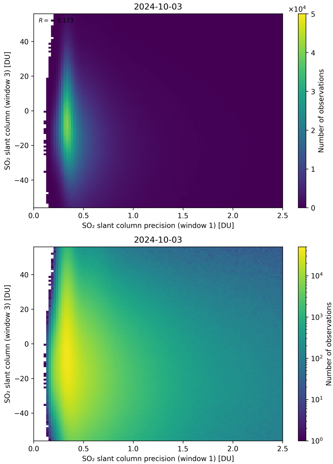
Figure 228: Scatter density plot of “SO 2 slant column precision (window 1)” against “SO 2 slant column (window 3)” for 2024-10-03 to 2024-10-04.
