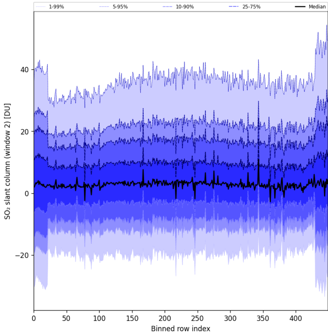
Figure 83: Along track statistics of “SO 2 slant column (window 2)” for 2024-10-03 to 2024-10-04
