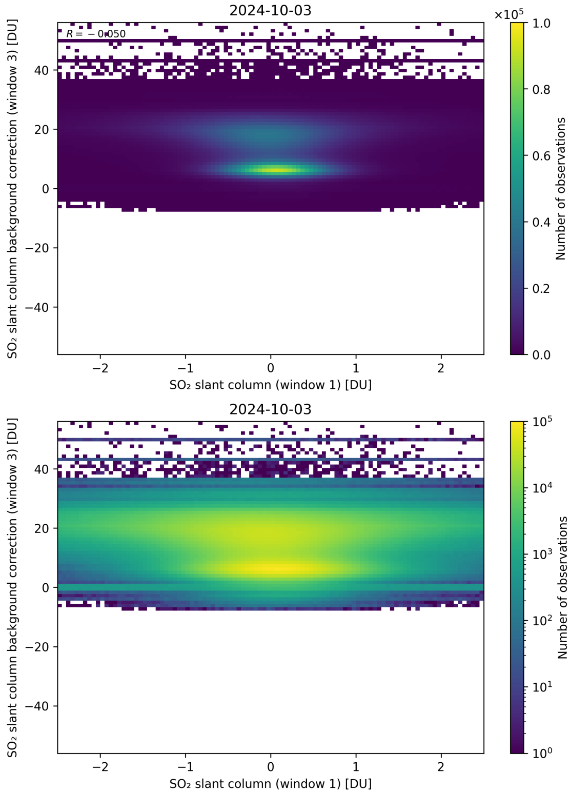
Figure 214: Scatter density plot of “SO 2 slant column (window 1)” against “SO 2 slant column background correction (window 3)” for 2024-10-03 to 2024-10-04.
