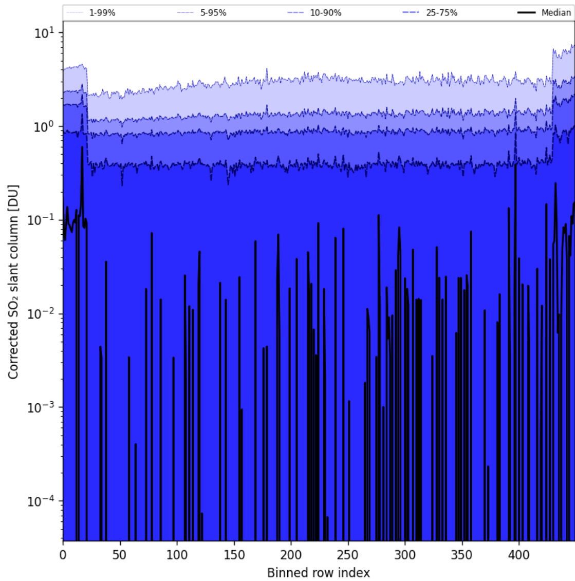
Figure 78: Along track statistics of “Corrected SO 2 slant column” for 2024-10-03 to 2024-10-04
