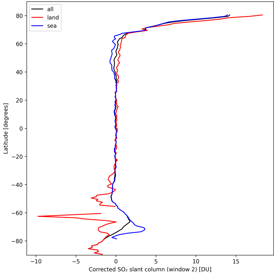
Figure 39: Zonal average of “Corrected SO 2 slant column (window 2)” for 2024-10-03 to 2024-10-04.
