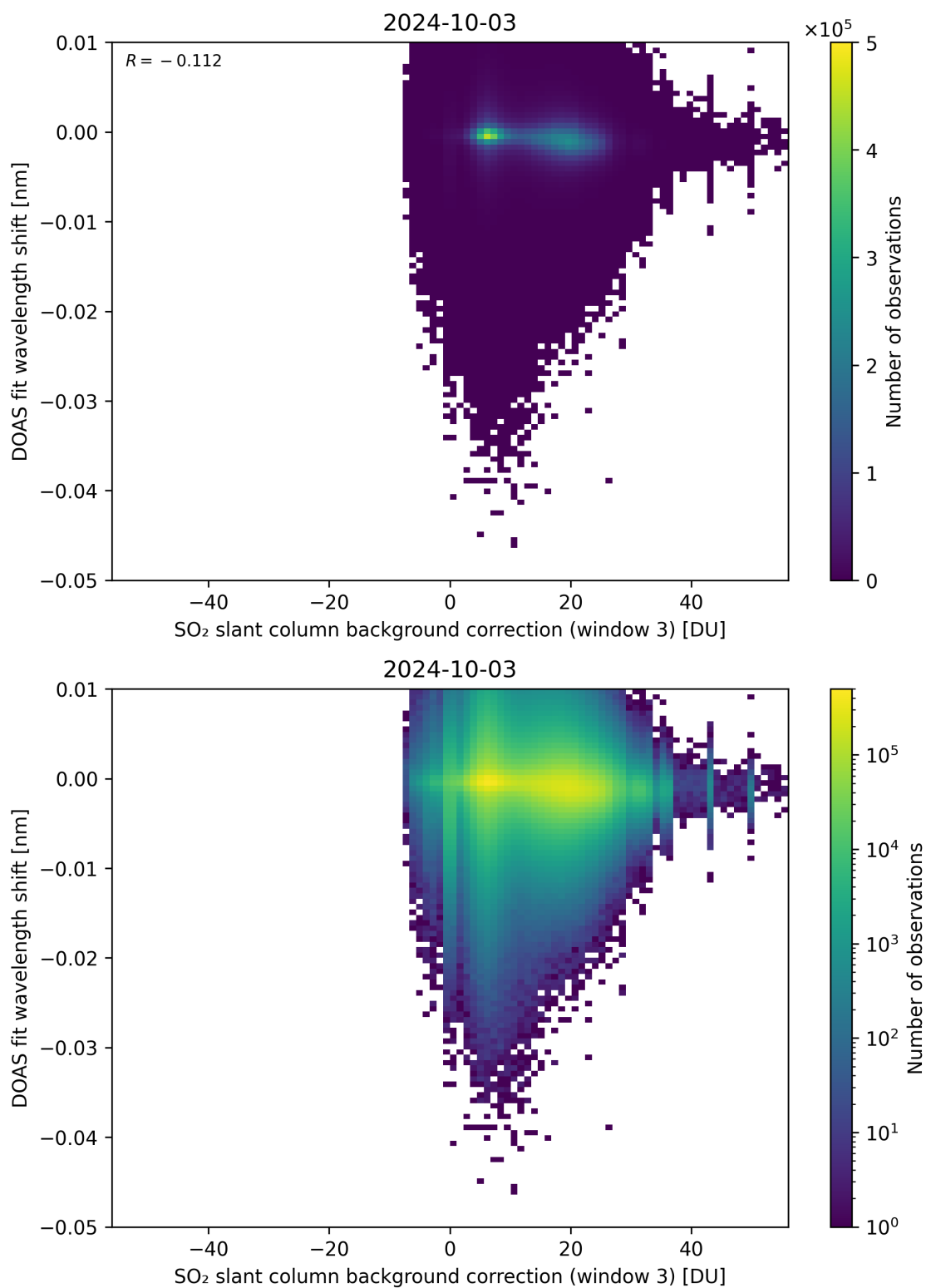
Figure 121: Scatter density plot of “SO 2 slant column background correction (window 3)” against “DOAS fit wavelength shift” for 2024-10-03 to 2024-10-04.
