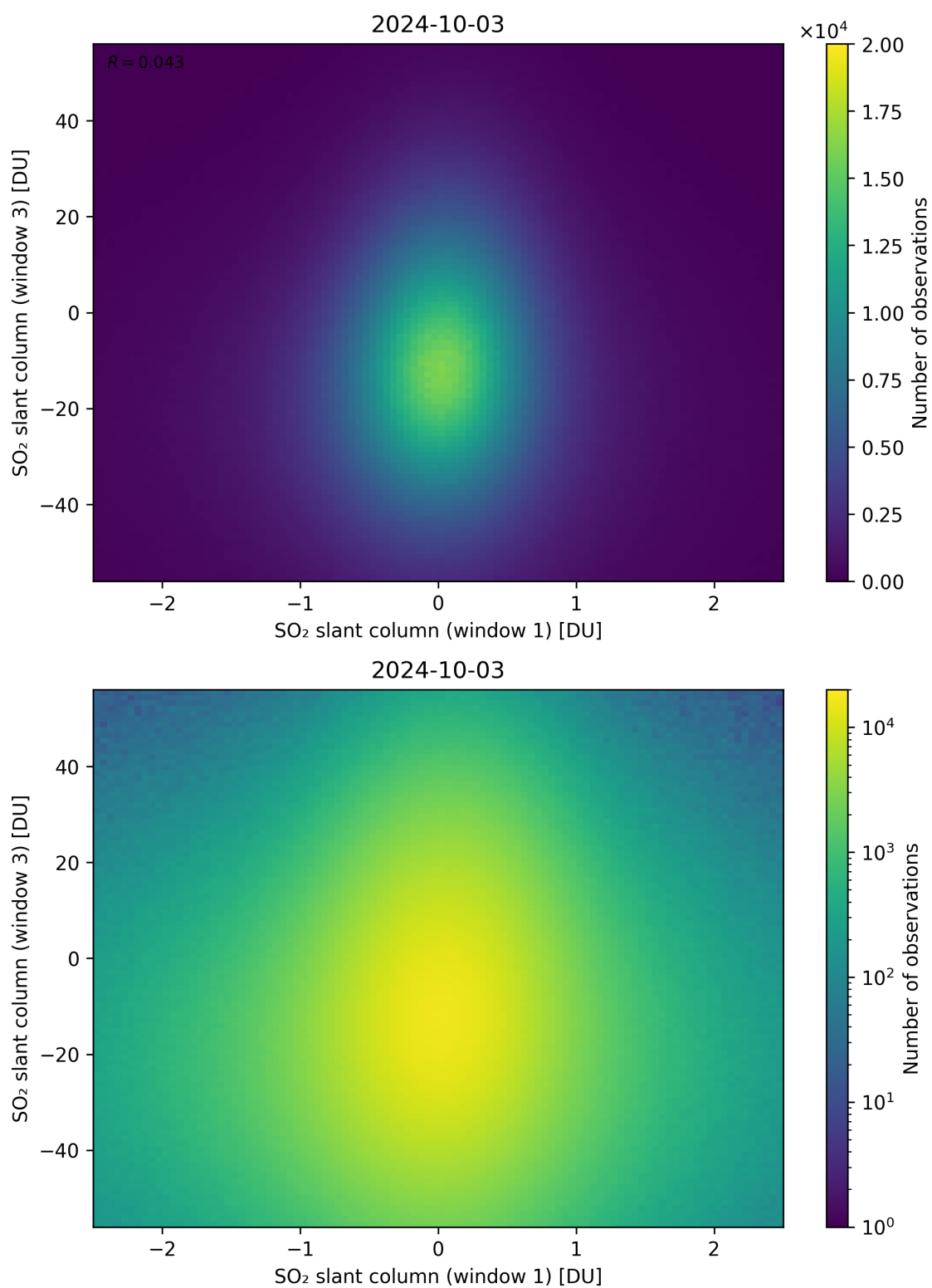
Figure 237: Scatter density plot of “SO 2 slant column (window 1)” against “SO 2 slant column (window 3)” for 2024-10-03 to 2024-10-04.
