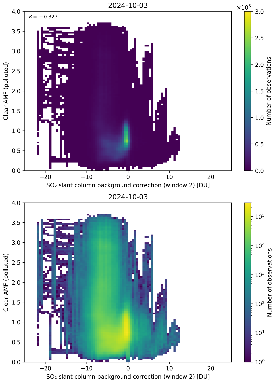
Figure 115: Scatter density plot of “SO 2 slant column background correction (window 2)” against “Clear AMF (polluted)” for 2024-10-03 to 2024-10-04.
