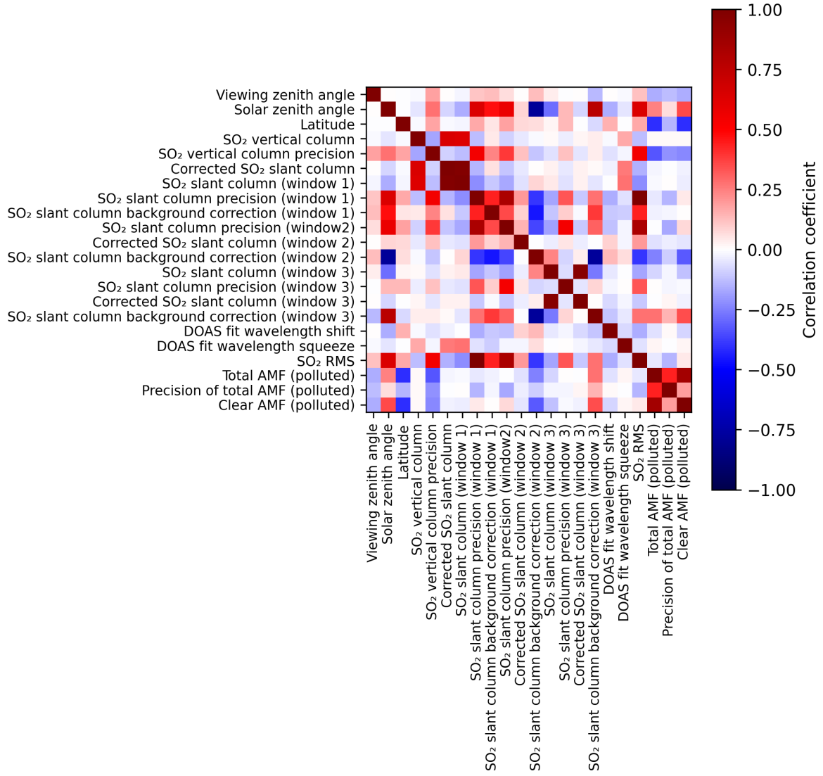
Figure 2: Map of correlation matrix for 2024-10-03 to 2024-10-04.
