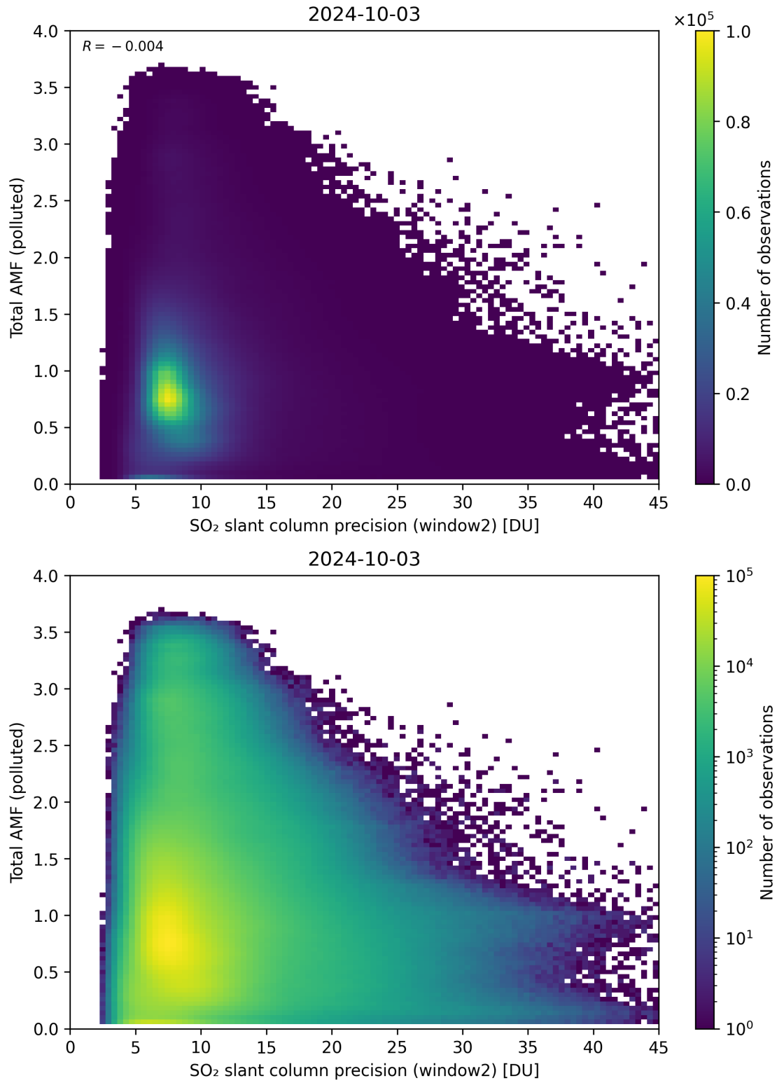
Figure 251: Scatter density plot of “SO 2 slant column precision (window2)” against “Total AMF (polluted)” for 2024-10-03 to 2024-10-04.
