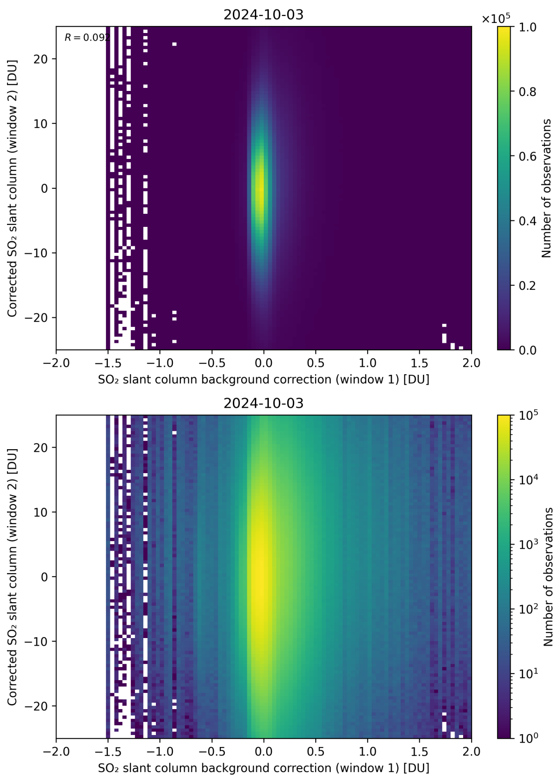
Figure 104: Scatter density plot of “SO 2 slant column background correction (window 1)” against “Corrected SO 2 slant column (window 2)” for 2024-10-03 to 2024-10-04.
