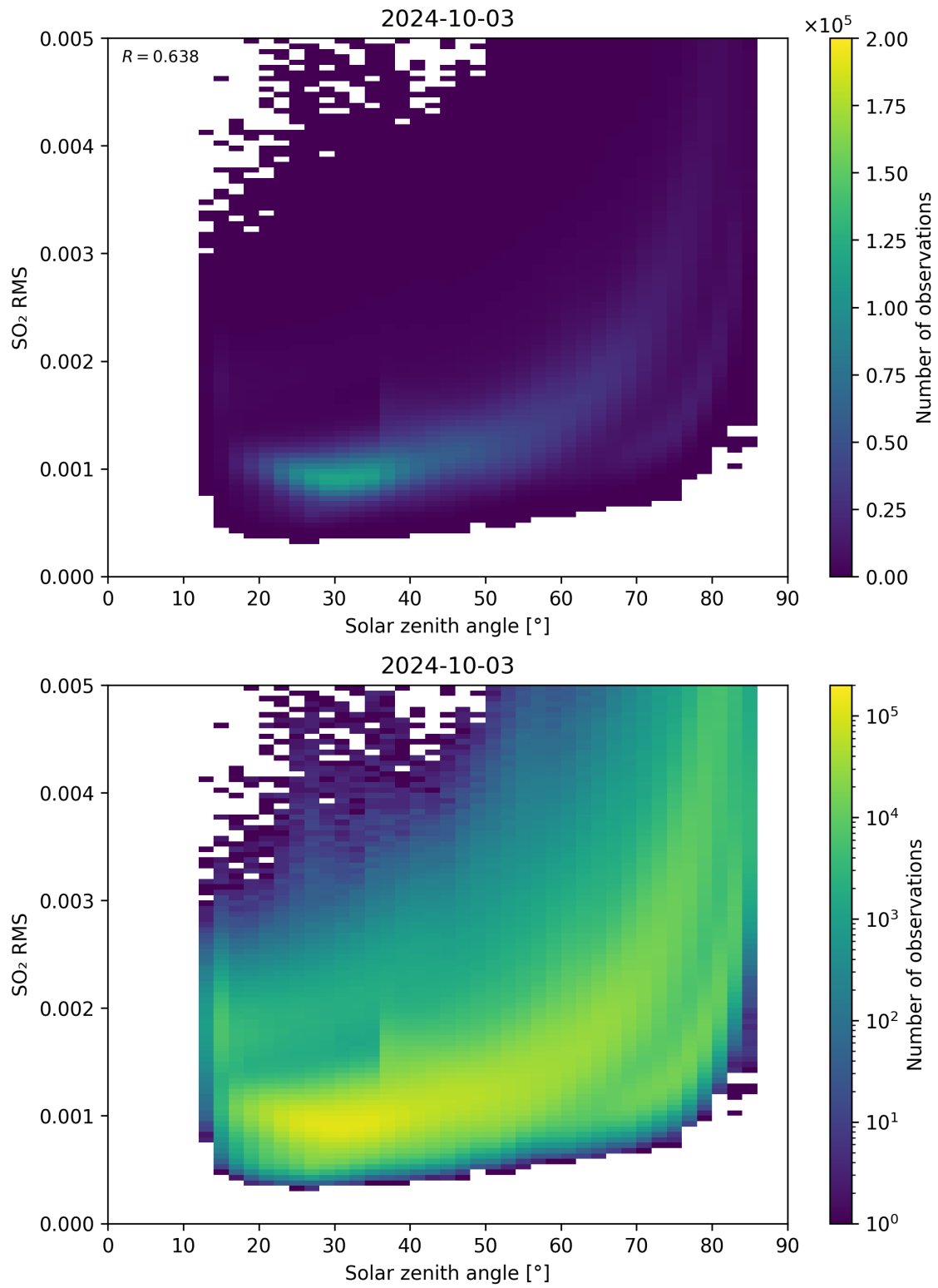
Figure 163: Scatter density plot of “Solar zenith angle” against “SO 2 RMS” for 2024-10-03 to 2024-10-04.
