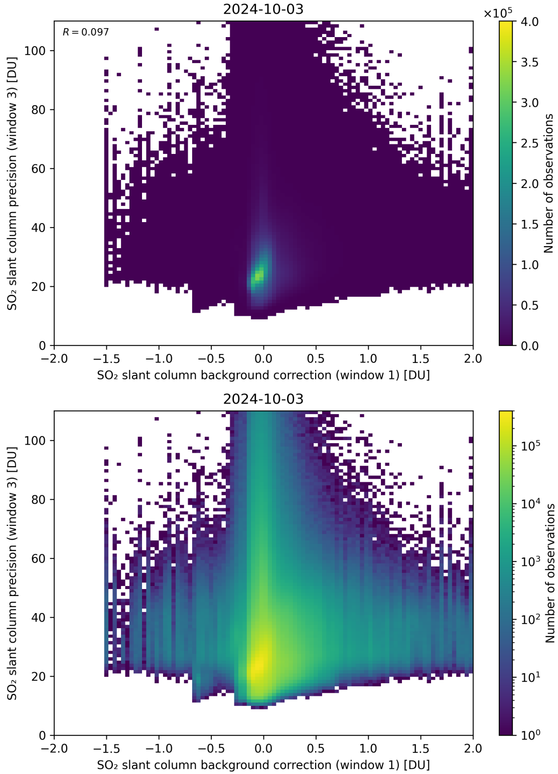
Figure 108: Scatter density plot of “SO 2 slant column background correction (window 1)” against “SO 2 slant column precision (window 3)” for 2024-10-03 to 2024-10-04.
