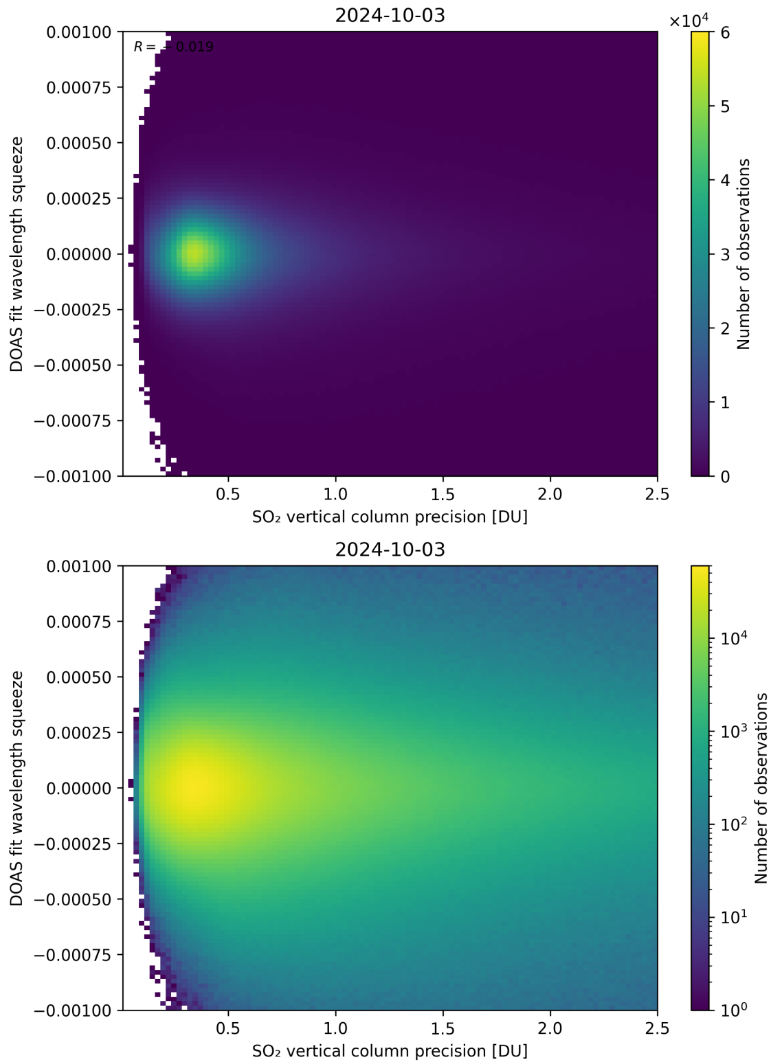
Figure 283: Scatter density plot of “SO 2 vertical column precision” against “DOAS fit wavelength squeeze” for 2024-10-03 to 2024-10-04.
