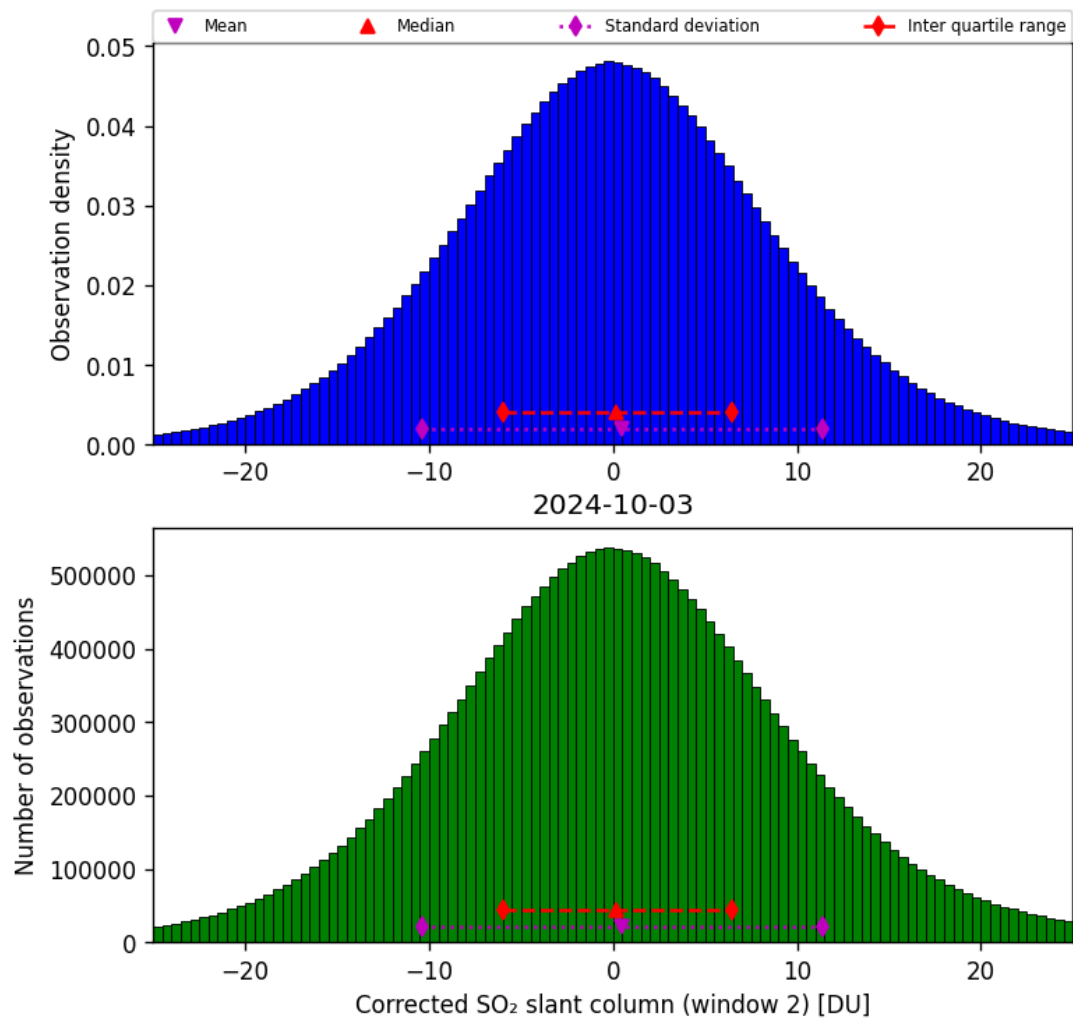
Figure 62: Histogram of “Corrected SO 2 slant column (window 2)” for 2024-10-03 to 2024-10-04
