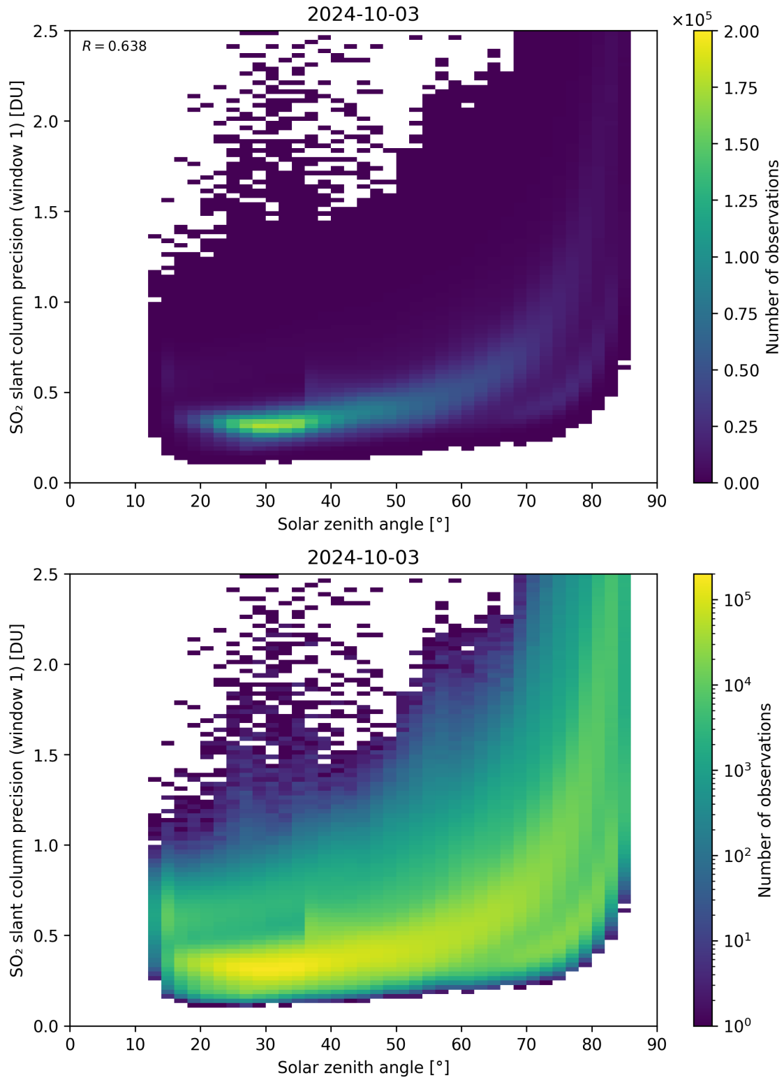
Figure 170: Scatter density plot of “Solar zenith angle” against “SO 2 slant column precision (window 1)” for 2024-10-03 to 2024-10-04.
