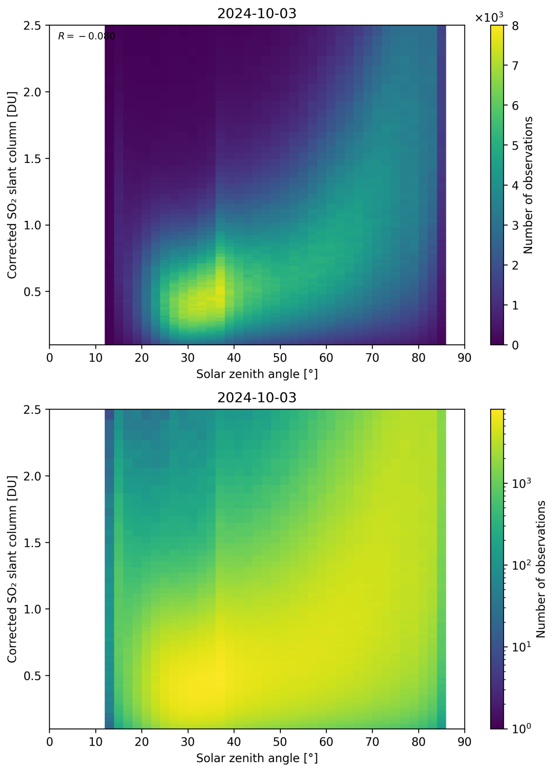
Figure 166: Scatter density plot of “Solar zenith angle” against “Corrected SO 2 slant column” for 2024-10-03 to 2024-10-04.
