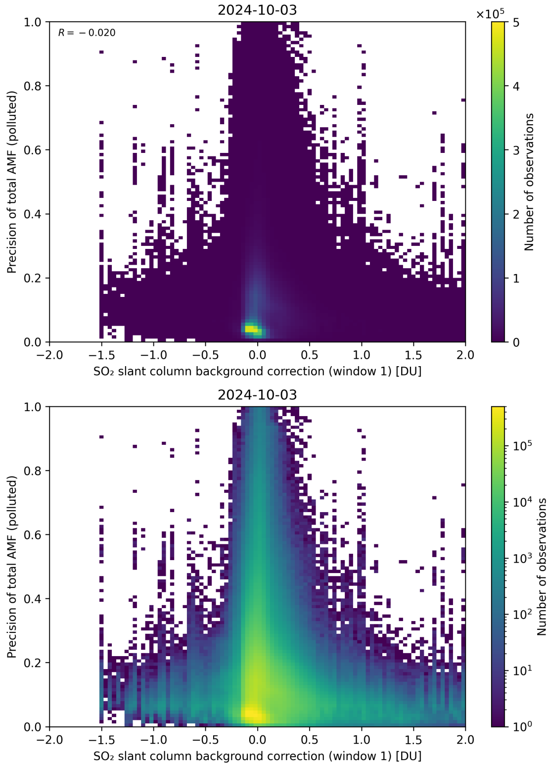
Figure 110: Scatter density plot of “SO 2 slant column background correction (window 1)” against “Precision of total AMF (polluted)” for 2024-10-03 to 2024-10-04.
