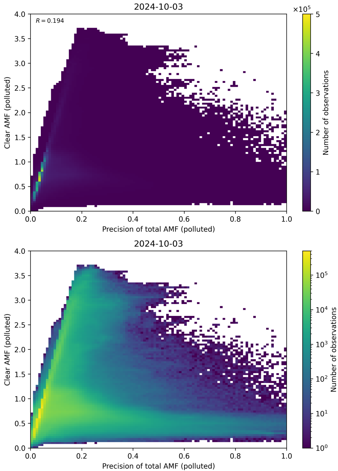
Figure 270: Scatter density plot of “Precision of total AMF (polluted)” against “Clear AMF (polluted)” for 2024-10-03 to 2024-10-04.
