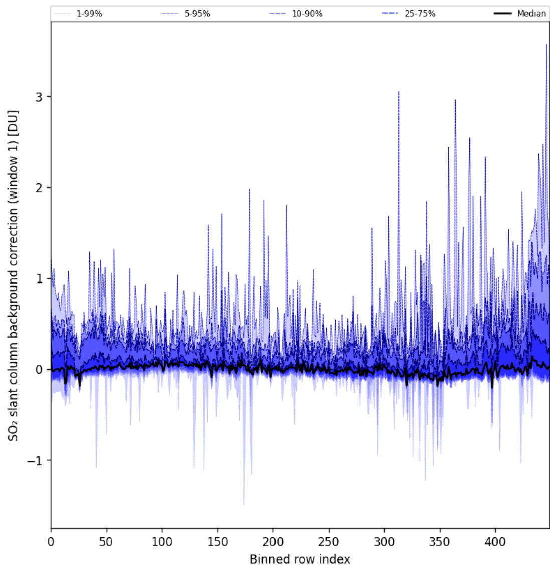
Figure 82: Along track statistics of “SO 2 slant column background correction (window 1)” for 2024-10-03 to 2024-10-04
