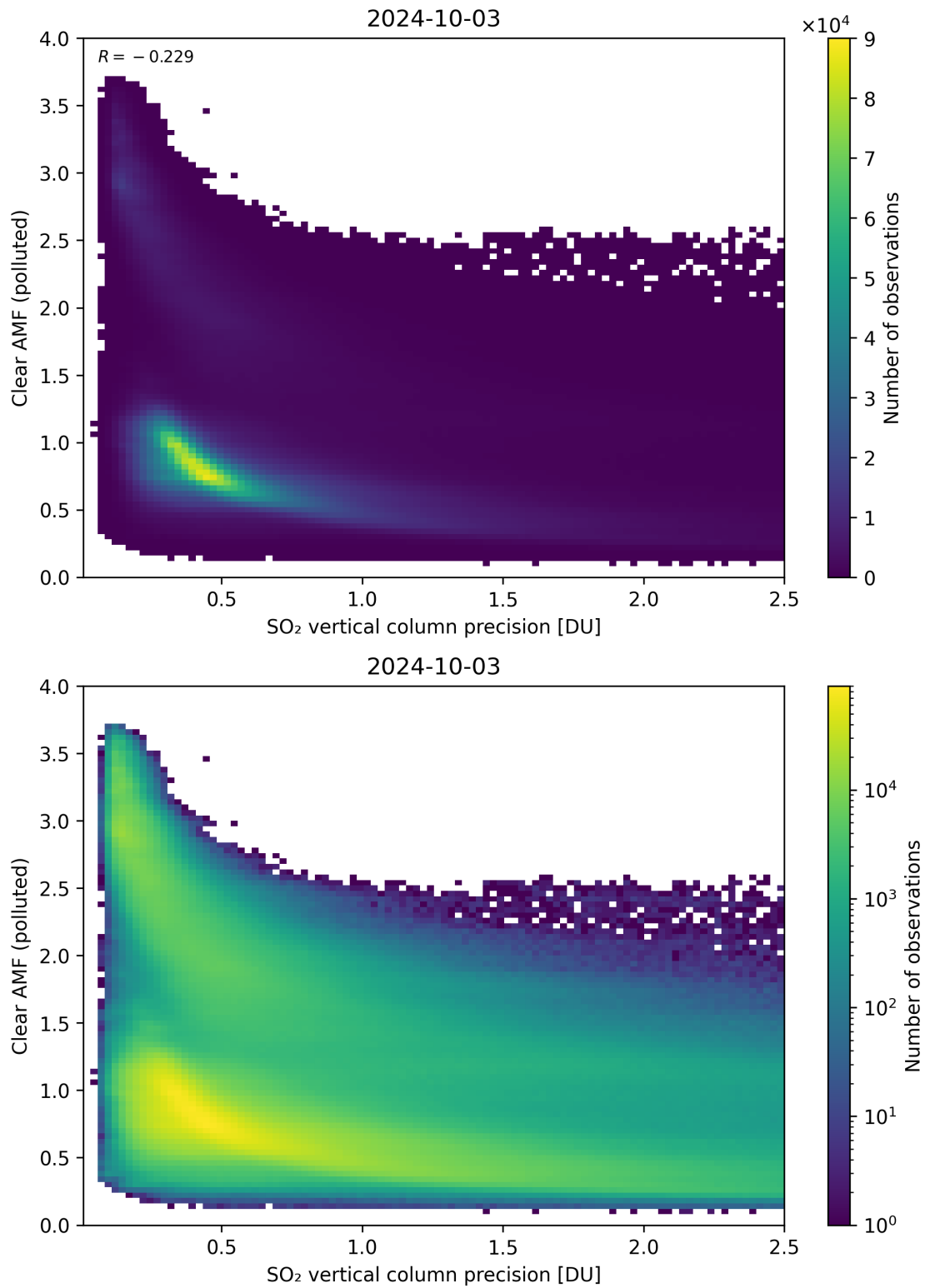
Figure 285: Scatter density plot of “SO 2 vertical column precision” against “Clear AMF (polluted)” for 2024-10-03 to 2024-10-04.
