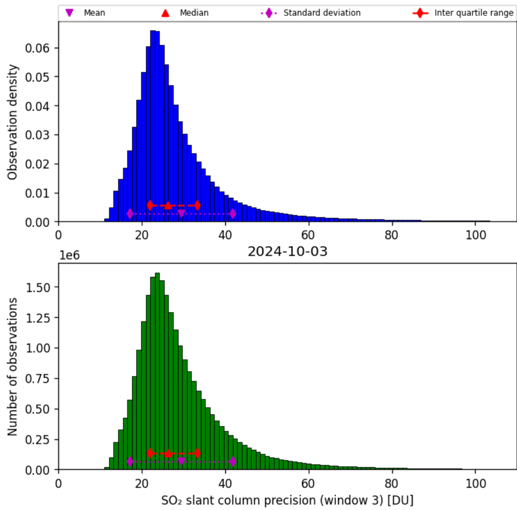
Figure 65: Histogram of “SO 2 slant column precision (window 3)” for 2024-10-03 to 2024-10-04
