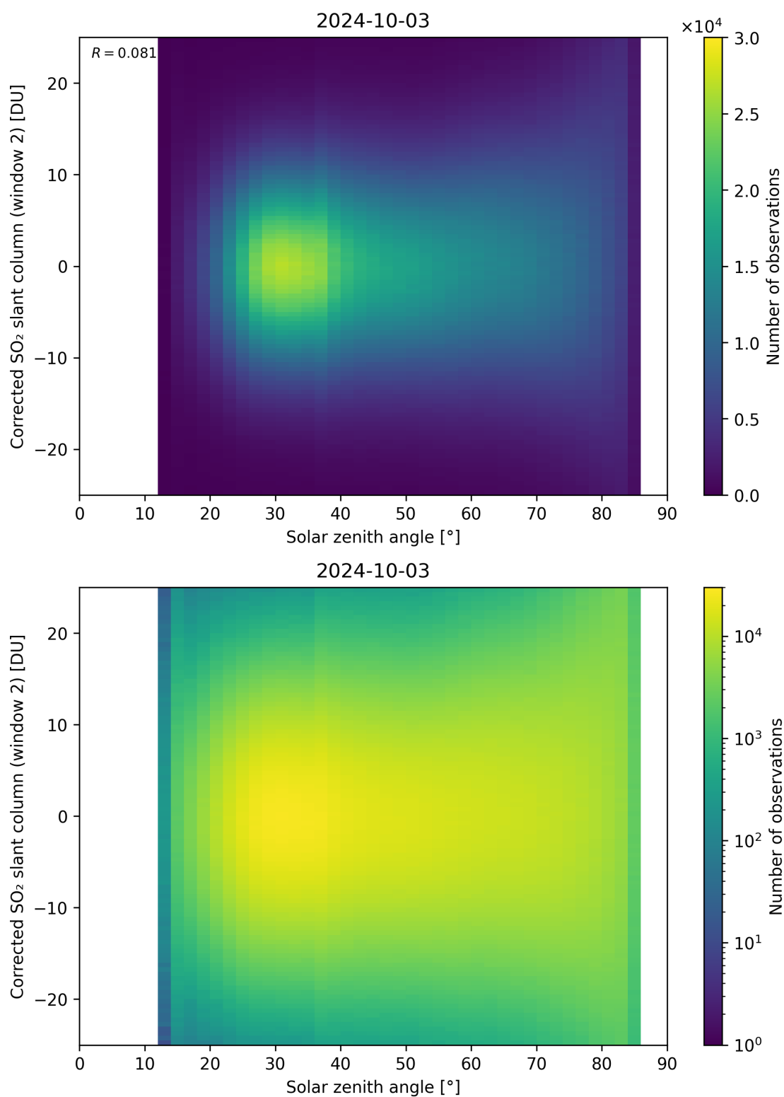
Figure 167: Scatter density plot of “Solar zenith angle” against “Corrected SO 2 slant column (window 2)” for 2024-10-03 to 2024-10-04.
