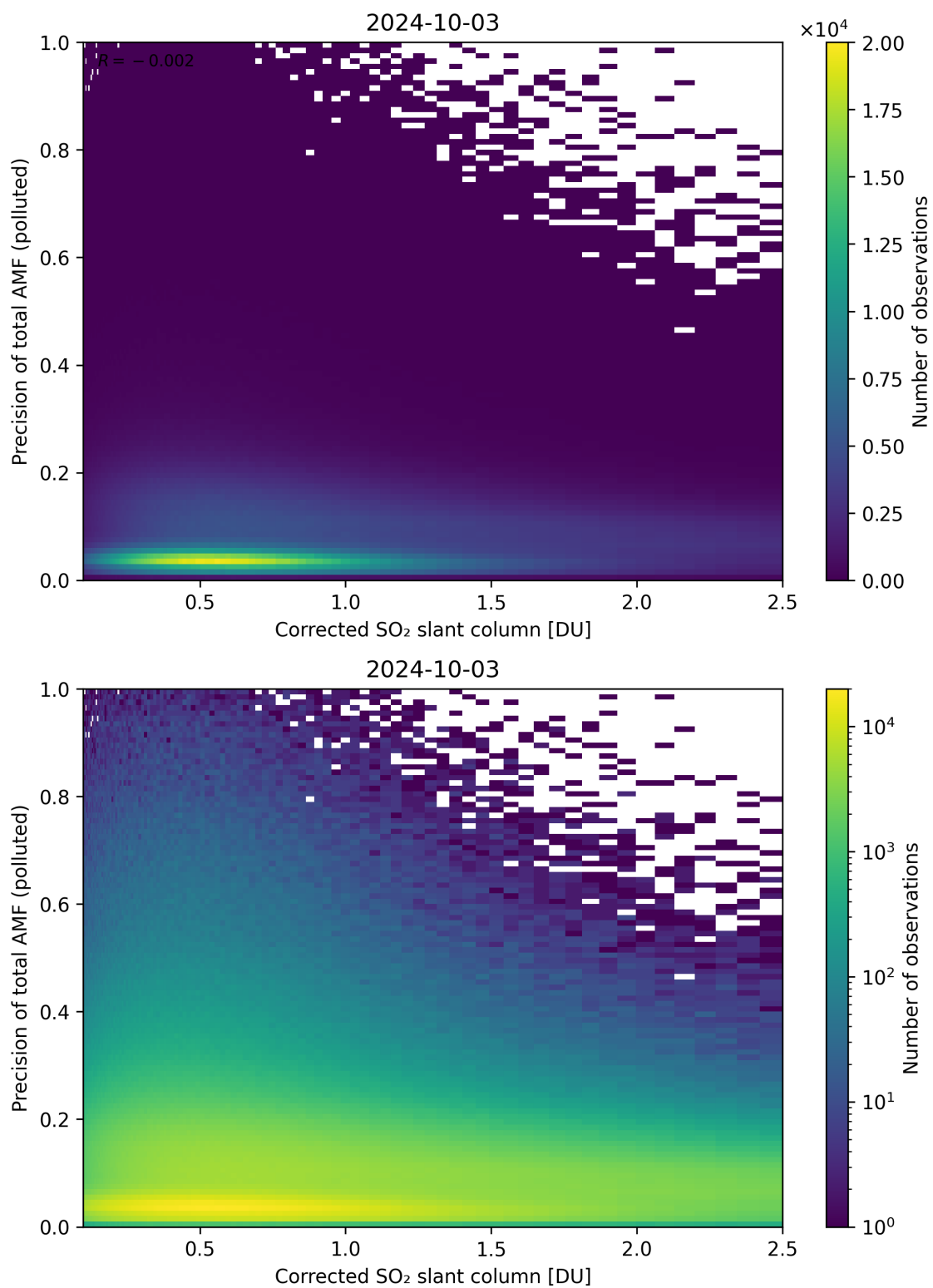
Figure 193: Scatter density plot of “Corrected SO 2 slant column” against “Precision of total AMF (polluted)” for 2024-10-03 to 2024-10-04.
