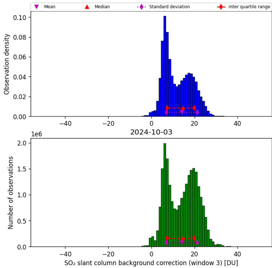
Figure 67: Histogram of “SO 2 slant column background correction (window 3)” for 2024-10-03 to 2024-10-04
