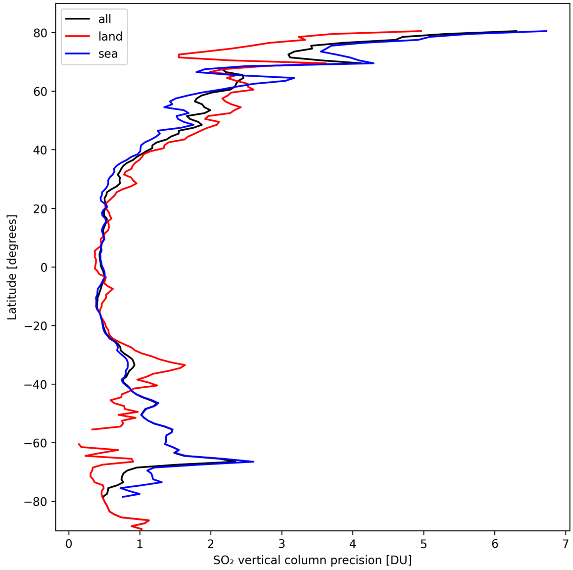
Figure 31: Zonal average of “SO 2 vertical column precision” for 2024-10-03 to 2024-10-04.
