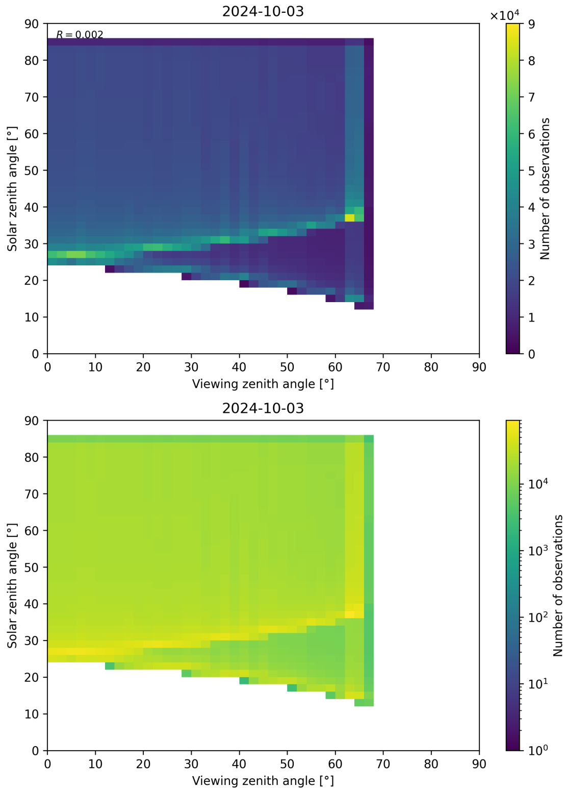
Figure 315: Scatter density plot of “Viewing zenith angle” against “Solar zenith angle” for 2024-10-03 to 2024-10-04.
