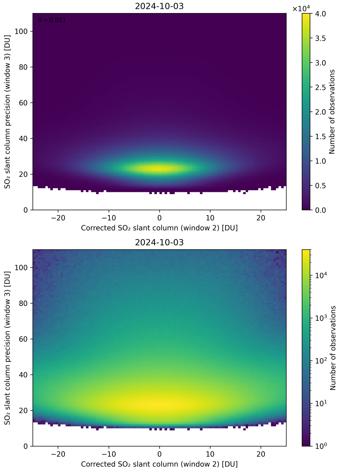
Figure 202: Scatter density plot of “Corrected SO 2 slant column (window 2)” against “SO 2 slant column precision (window 3)” for 2024-10-03 to 2024-10-04.
