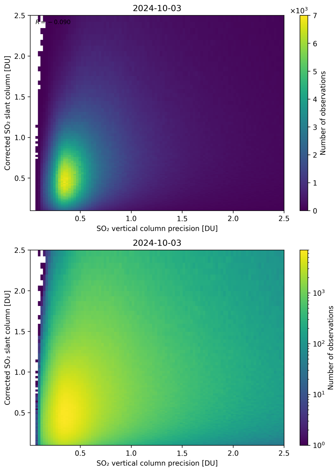
Figure 286: Scatter density plot of “SO 2 vertical column precision” against “Corrected SO 2 slant column” for 2024-10-03 to 2024-10-04.
