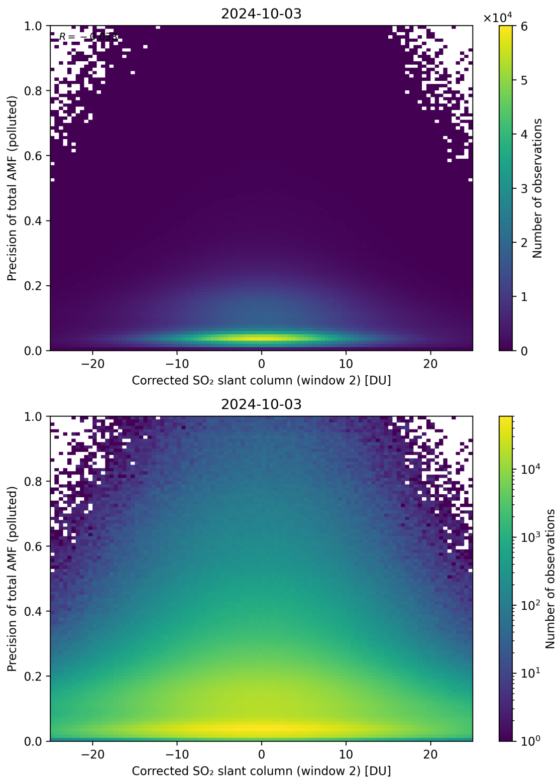
Figure 204: Scatter density plot of “Corrected SO 2 slant column (window 2)” against “Precision of total AMF (polluted)” for 2024-10-03 to 2024-10-04.
