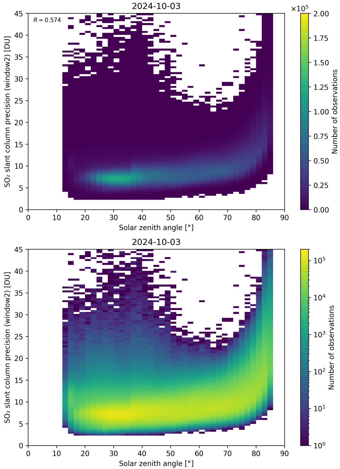
Figure 171: Scatter density plot of “Solar zenith angle” against “SO 2 slant column precision (window2)” for 2024-10-03 to 2024-10-04.
