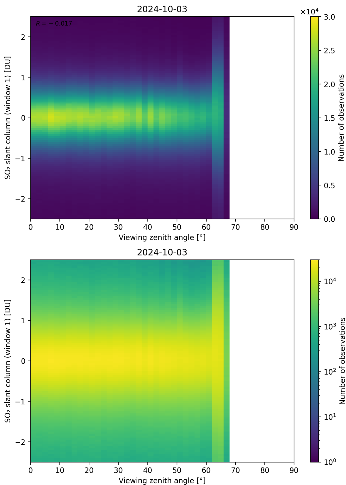
Figure 320: Scatter density plot of “Viewing zenith angle” against “SO 2 slant column (window 1)” for 2024-10-03 to 2024-10-04.
