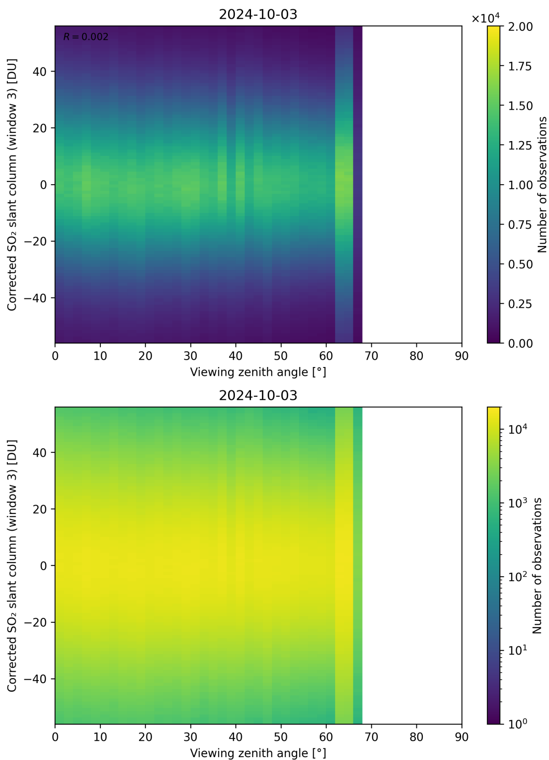
Figure 319: Scatter density plot of “Viewing zenith angle” against “Corrected SO 2 slant column (window 3)” for 2024-10-03 to 2024-10-04.
