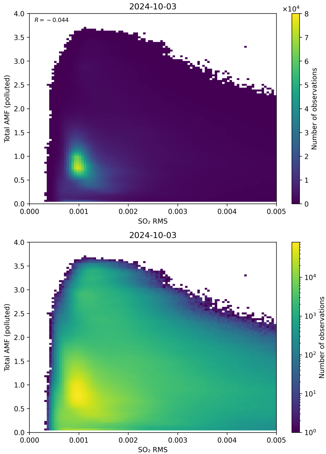
Figure 137: Scatter density plot of “SO 2 RMS” against “Total AMF (polluted)” for 2024-10-03 to 2024-10-04.
