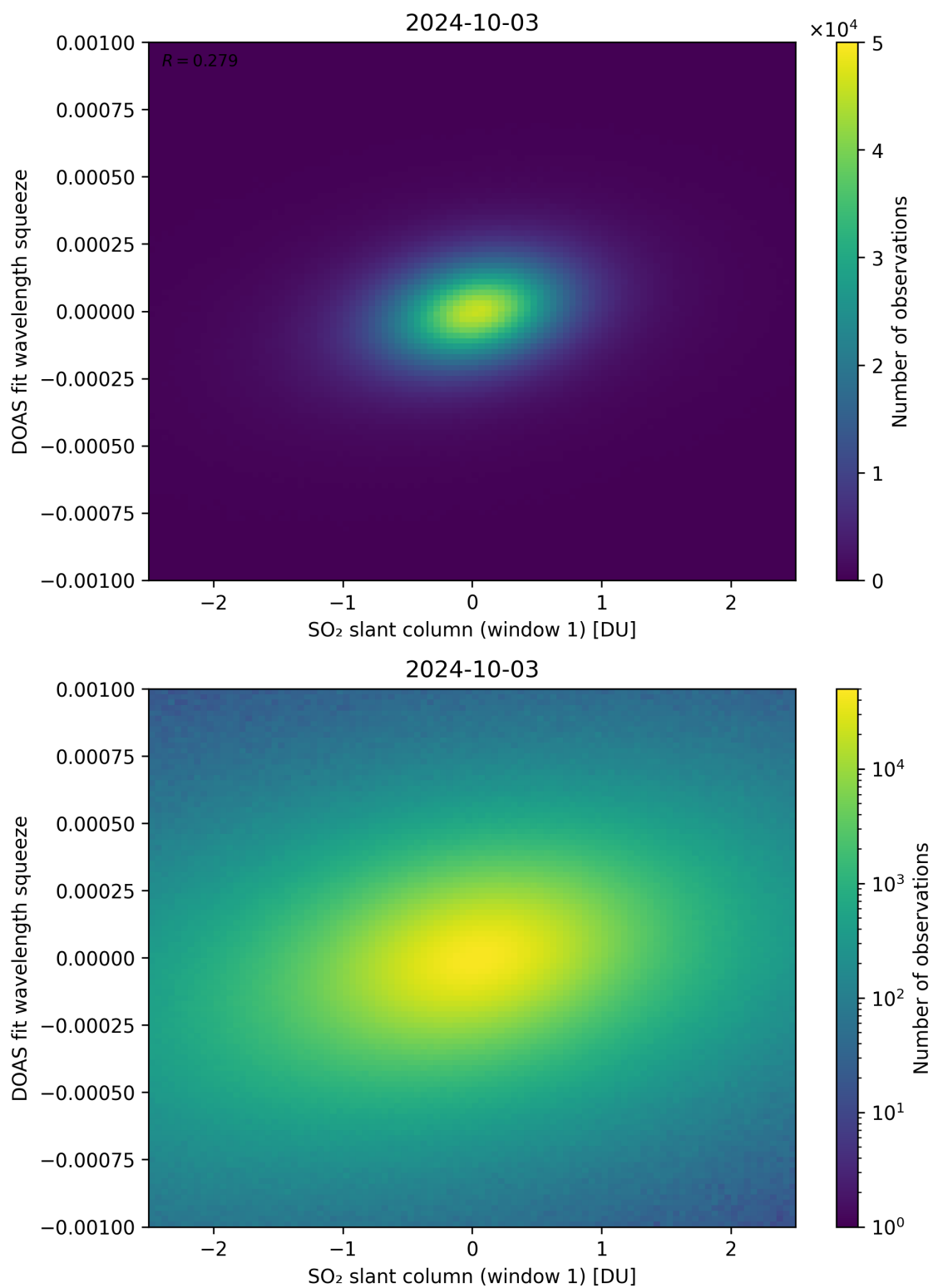
Figure 216: Scatter density plot of “SO 2 slant column (window 1)” against “DOAS fit wavelength squeeze” for 2024-10-03 to 2024-10-04.
