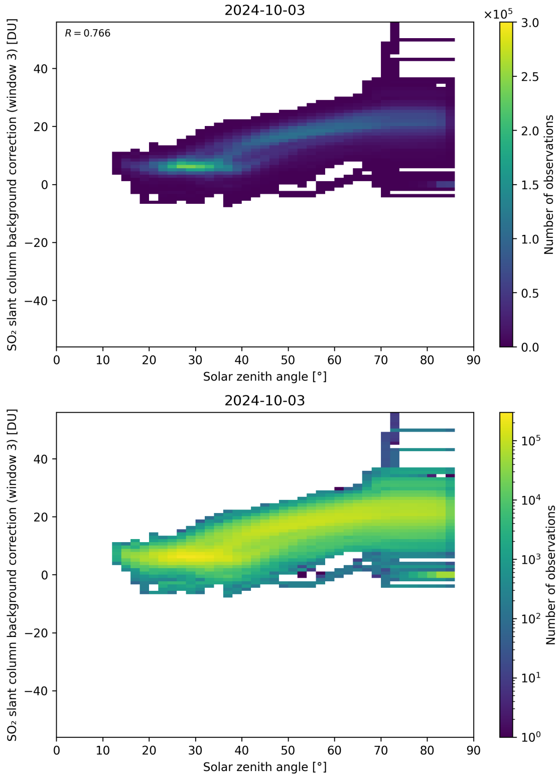
Figure 160: Scatter density plot of “Solar zenith angle” against “SO 2 slant column background correction (window 3)” for 2024-10-03 to 2024-10-04.
