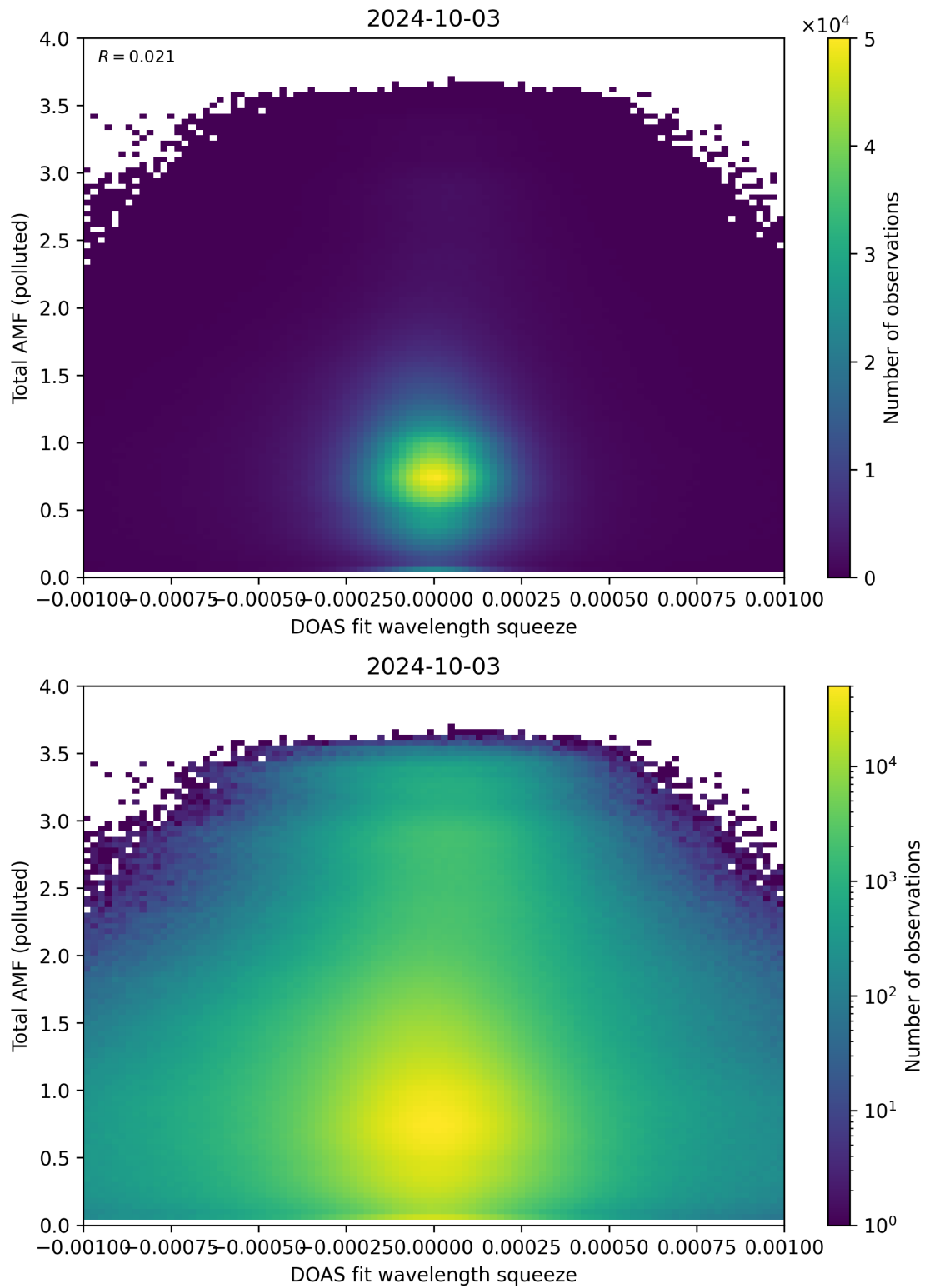
Figure 134: Scatter density plot of “DOAS fit wavelength squeeze” against “Total AMF (polluted)” for 2024-10-03 to 2024-10-04.
