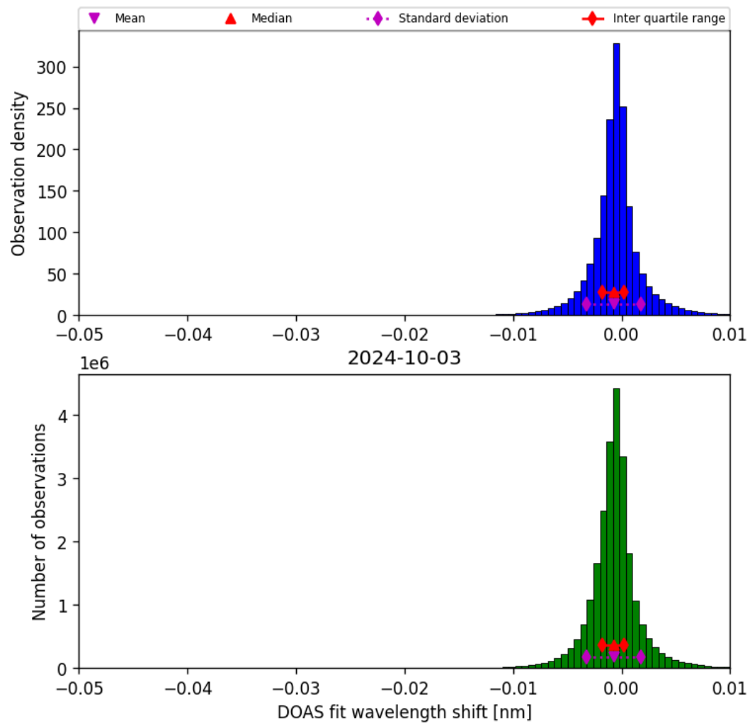
Figure 68: Histogram of “DOAS fit wavelength shift” for 2024-10-03 to 2024-10-04
