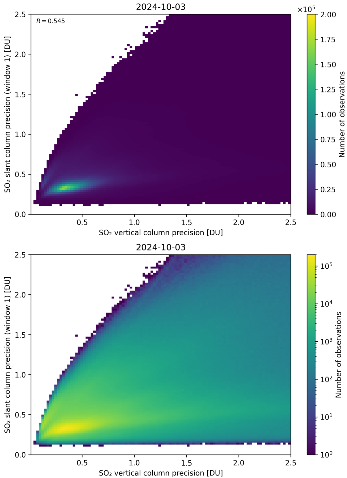
Figure 290: Scatter density plot of “SO 2 vertical column precision” against “SO 2 slant column precision (window 1)” for 2024-10-03 to 2024-10-04.
