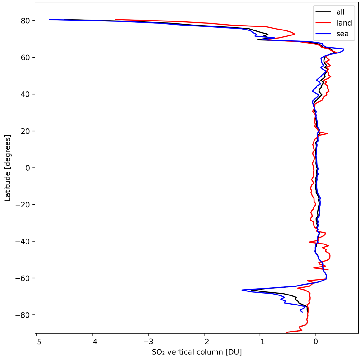
Figure 30: Zonal average of “SO 2 vertical column” for 2024-10-03 to 2024-10-04.
