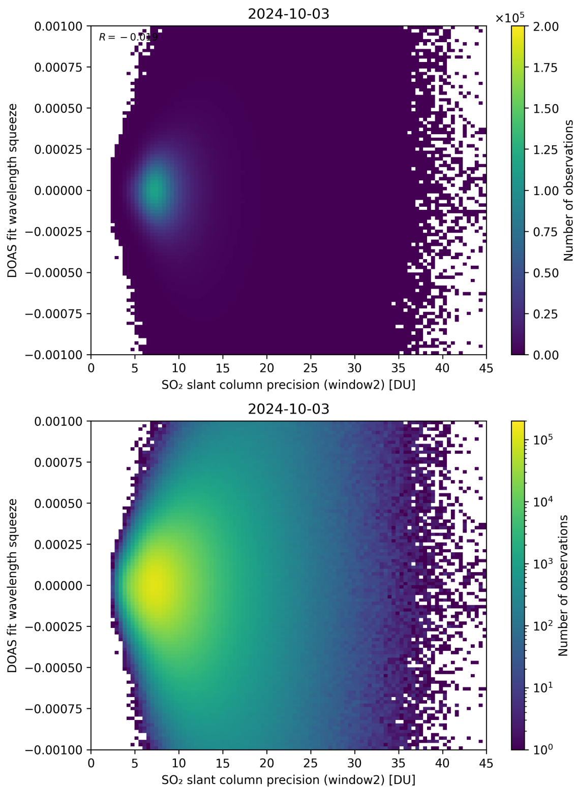
Figure 244: Scatter density plot of “SO 2 slant column precision (window2)” against “DOAS fit wavelength squeeze” for 2024-10-03 to 2024-10-04.
