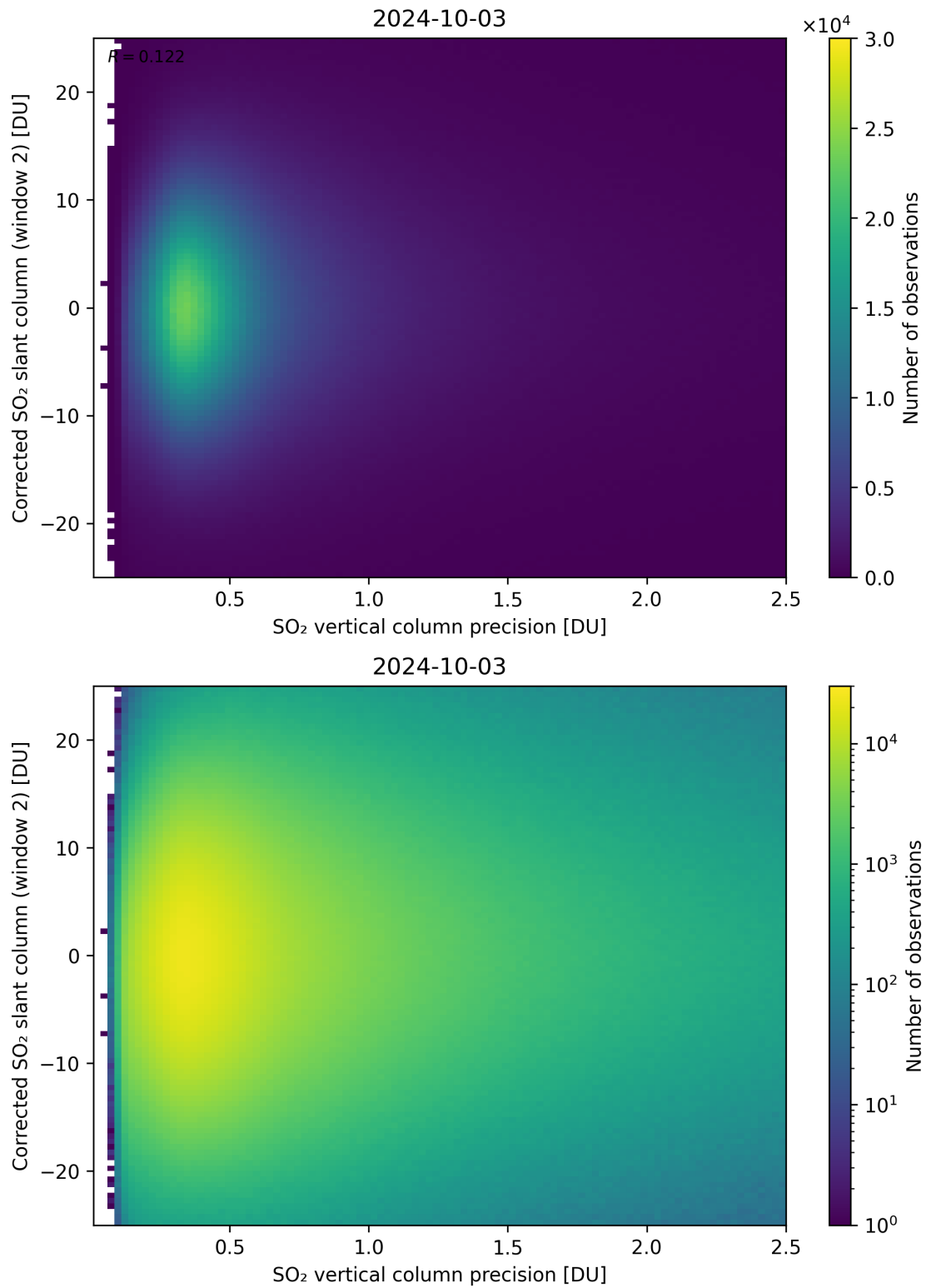
Figure 287: Scatter density plot of “SO 2 vertical column precision” against “Corrected SO 2 slant column (window 2)” for 2024-10-03 to 2024-10-04.
