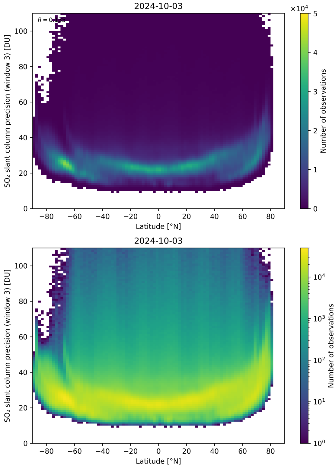
Figure 153: Scatter density plot of “Latitude” against “SO 2 slant column precision (window 3)” for 2024-10-03 to 2024-10-04.
