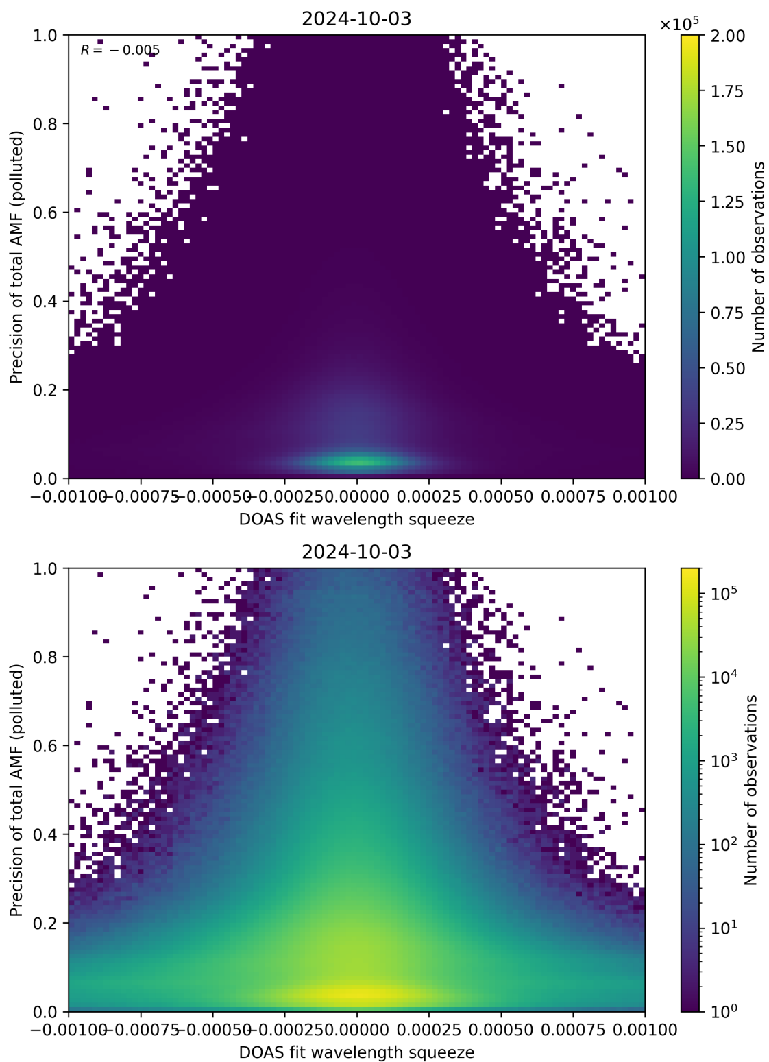
Figure 135: Scatter density plot of “DOAS fit wavelength squeeze” against “Precision of total AMF (polluted)” for 2024-10-03 to 2024-10-04.
