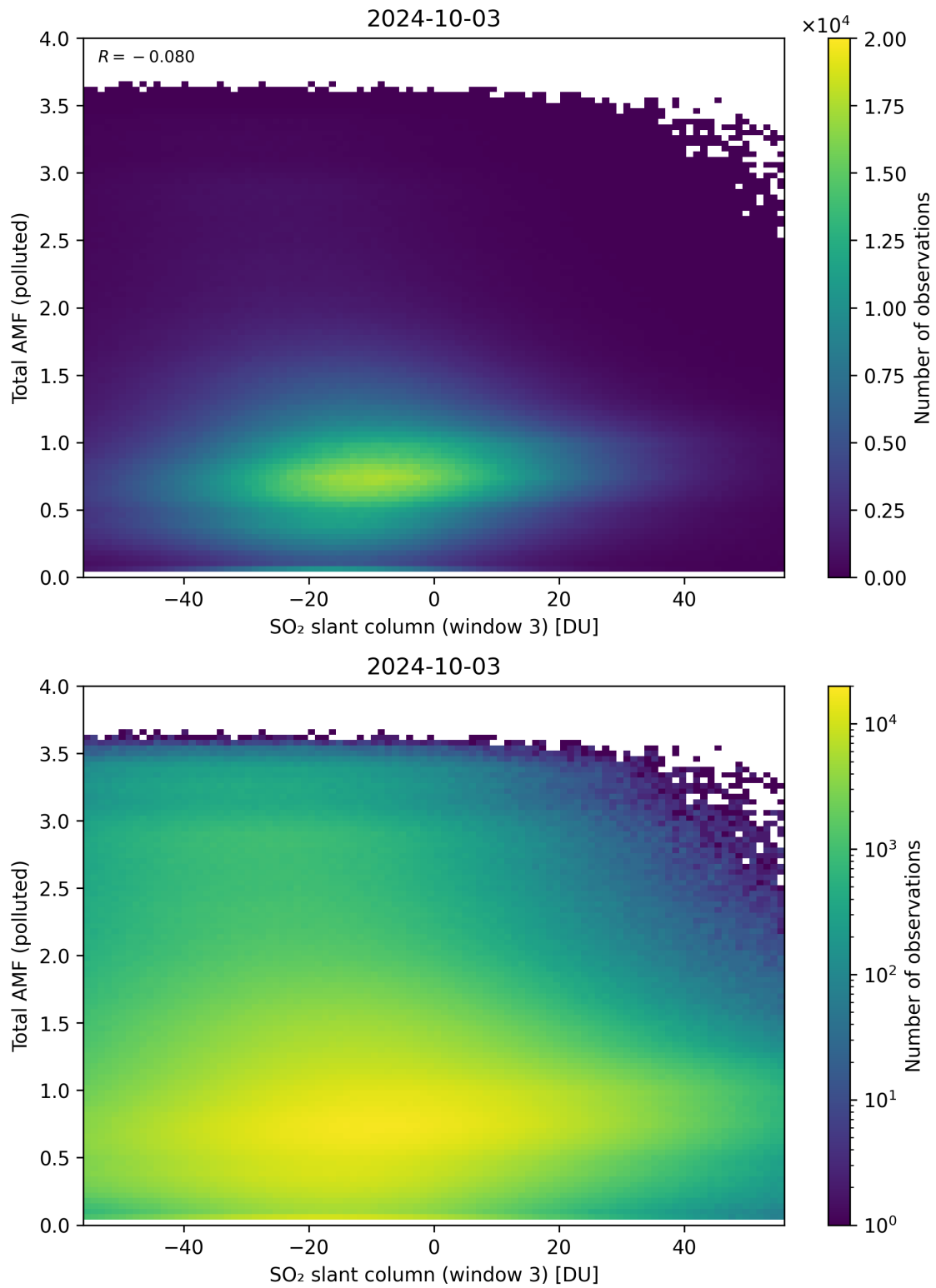
Figure 268: Scatter density plot of “SO 2 slant column (window 3)” against “Total AMF (polluted)” for 2024-10-03 to 2024-10-04.
