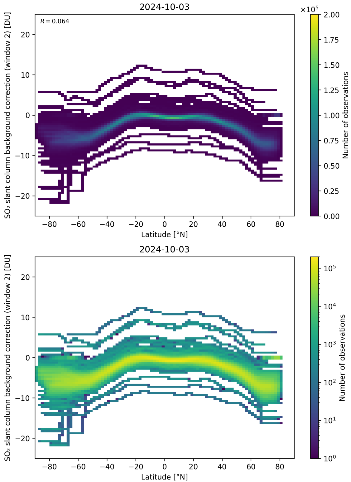
Figure 140: Scatter density plot of “Latitude” against “SO 2 slant column background correction (window 2)” for 2024-10-03 to 2024-10-04.
