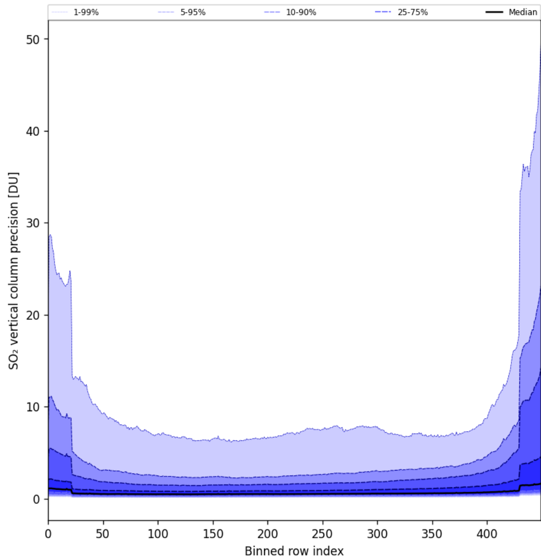
Figure 77: Along track statistics of “SO 2 vertical column precision” for 2024-10-03 to 2024-10-04
