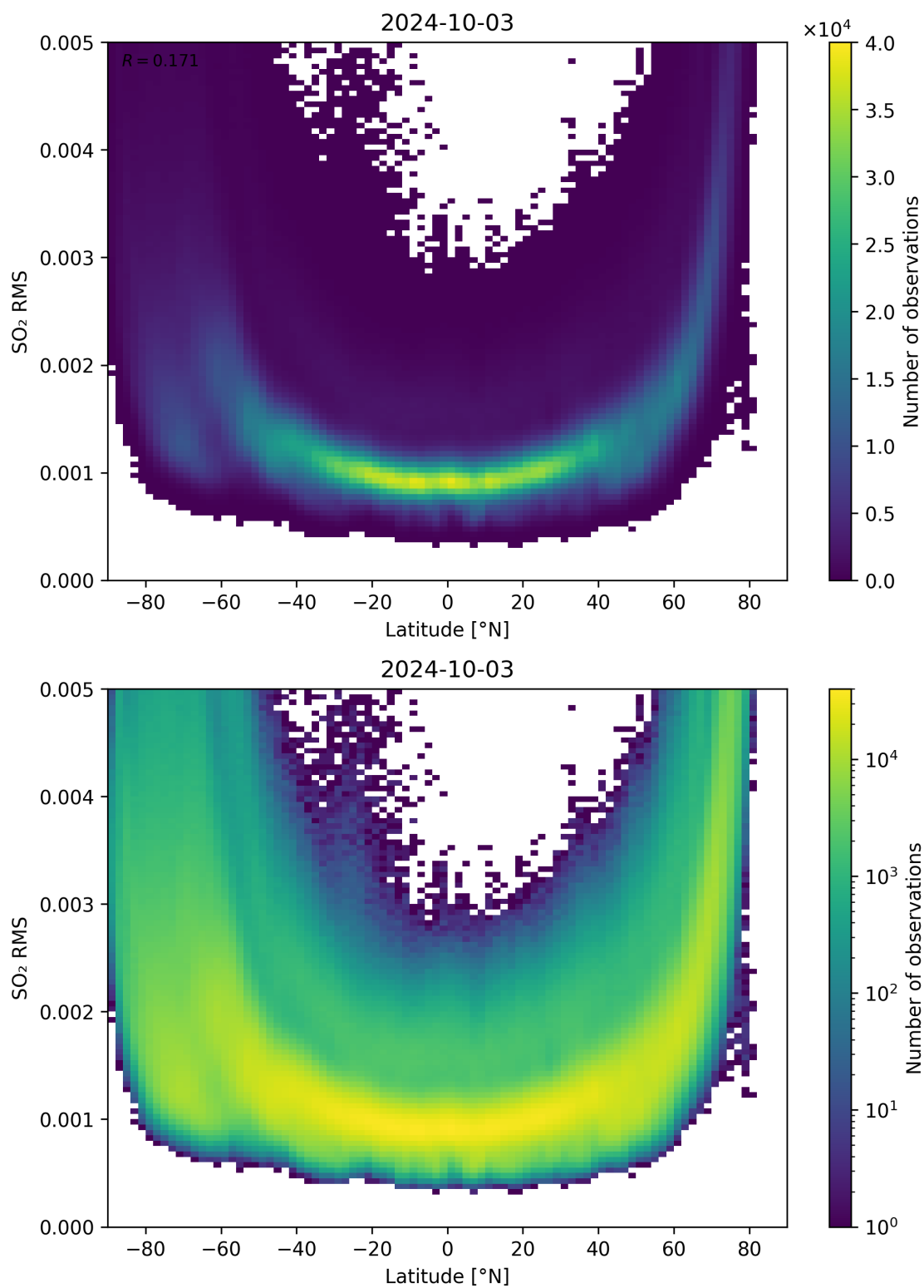
Figure 144: Scatter density plot of “Latitude” against “SO 2 RMS” for 2024-10-03 to 2024-10-04.
