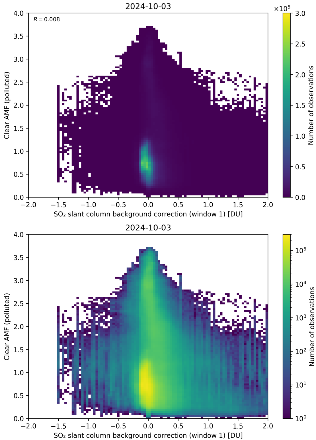
Figure 103: Scatter density plot of “SO 2 slant column background correction (window 1)” against “Clear AMF (polluted)” for 2024-10-03 to 2024-10-04.
