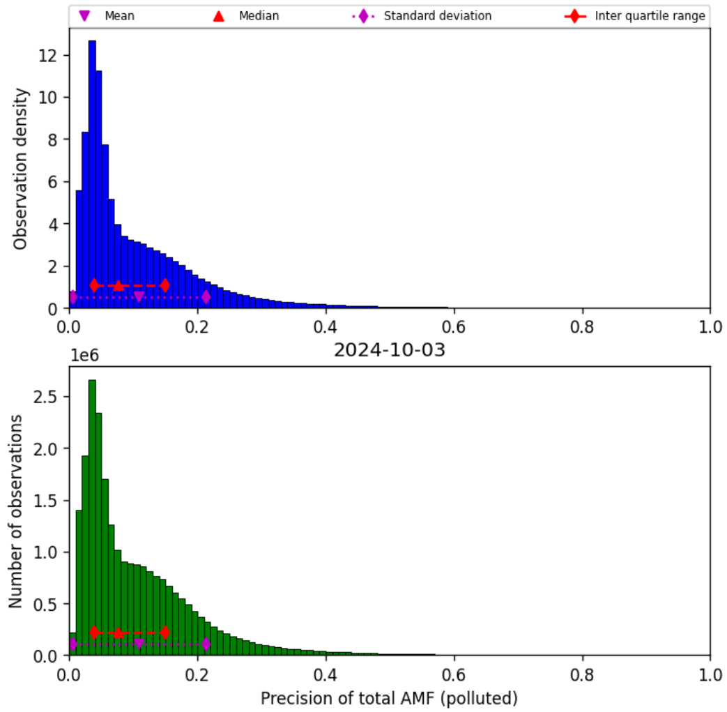
Figure 72: Histogram of “Precision of total AMF (polluted)” for 2024-10-03 to 2024-10-04
