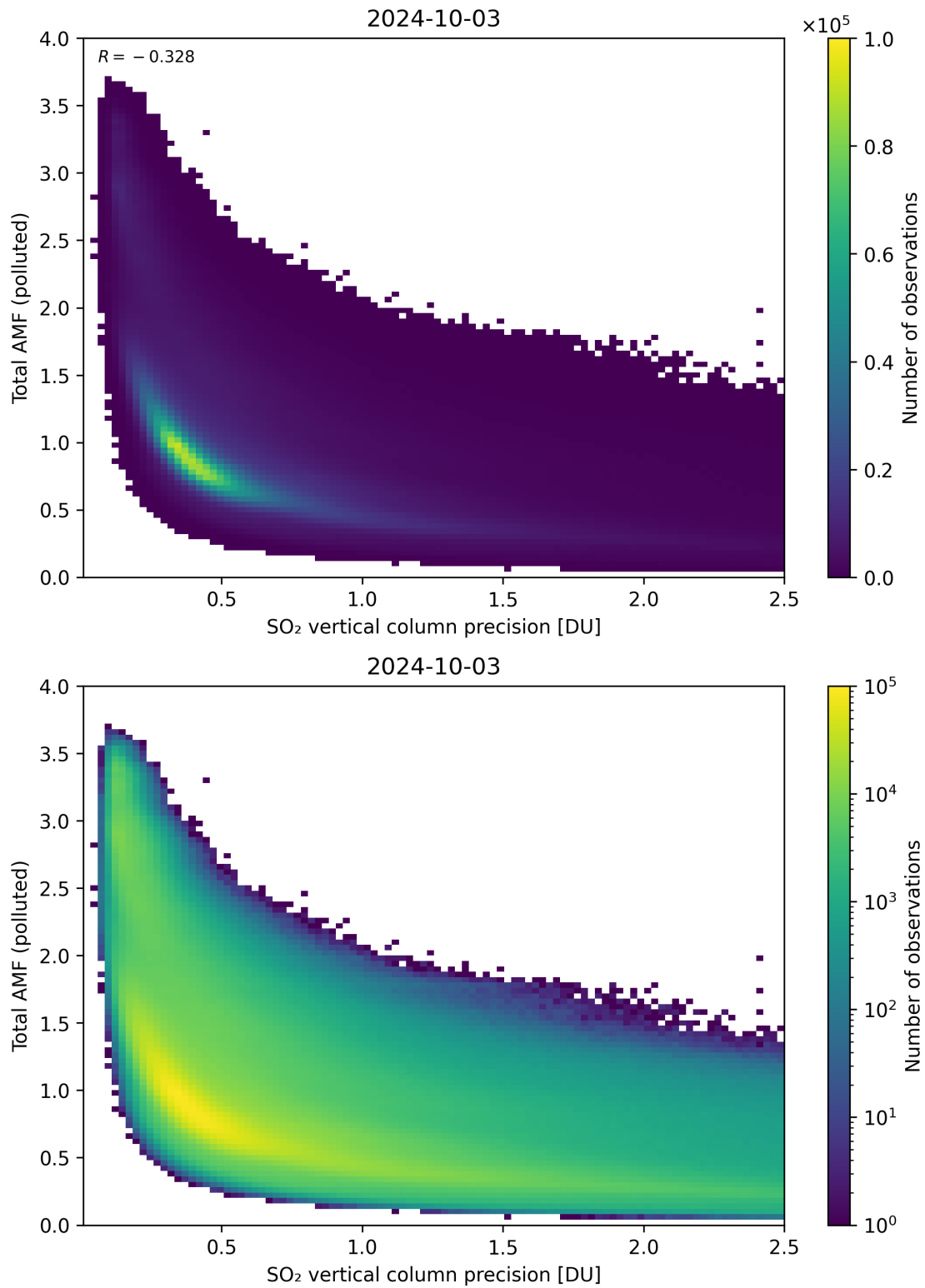
Figure 294: Scatter density plot of “SO 2 vertical column precision” against “Total AMF (polluted)” for 2024-10-03 to 2024-10-04.
