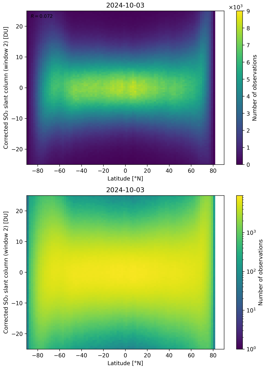
Figure 147: Scatter density plot of “Latitude” against “Corrected SO 2 slant column (window 2)” for 2024-10-03 to 2024-10-04.
