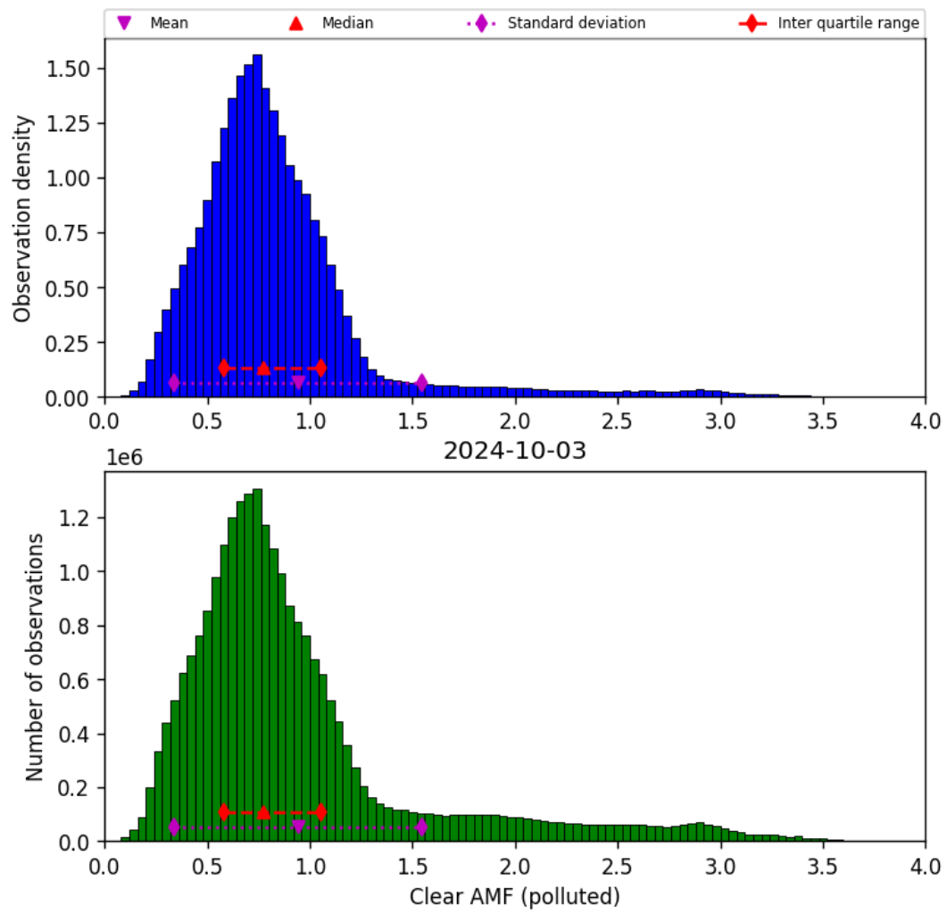
Figure 73: Histogram of “Clear AMF (polluted)” for 2024-10-03 to 2024-10-04
