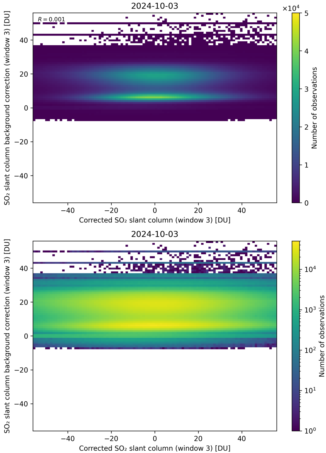
Figure 205: Scatter density plot of “Corrected SO 2 slant column (window 3)” against “SO 2 slant column background correction (window 3)” for 2024-10-03 to 2024-10-04.
