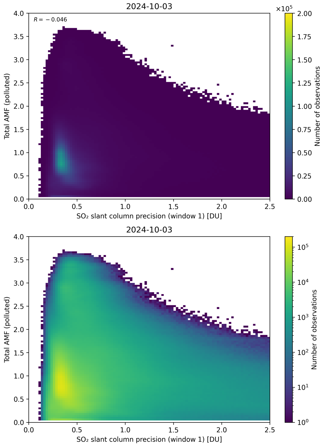
Figure 230: Scatter density plot of “SO 2 slant column precision (window 1)” against “Total AMF (polluted)” for 2024-10-03 to 2024-10-04.
