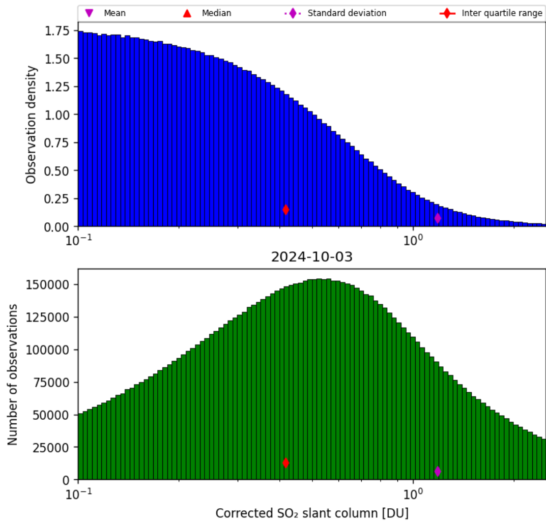
Figure 55: Histogram of “Corrected SO 2 slant column” for 2024-10-03 to 2024-10-04
