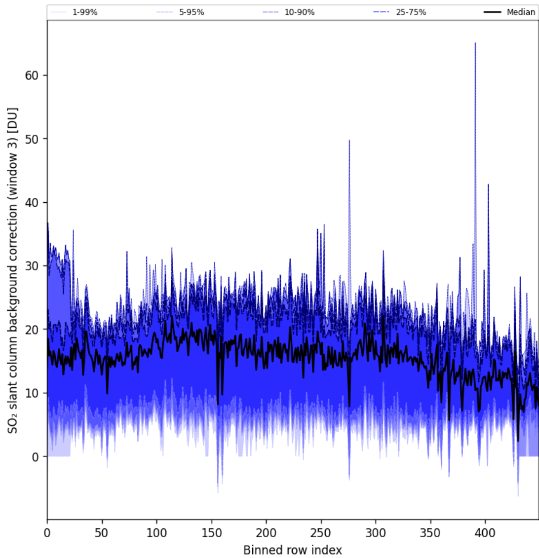
Figure 90: Along track statistics of “SO 2 slant column background correction (window 3)” for 2024-10-03 to 2024-10-04
