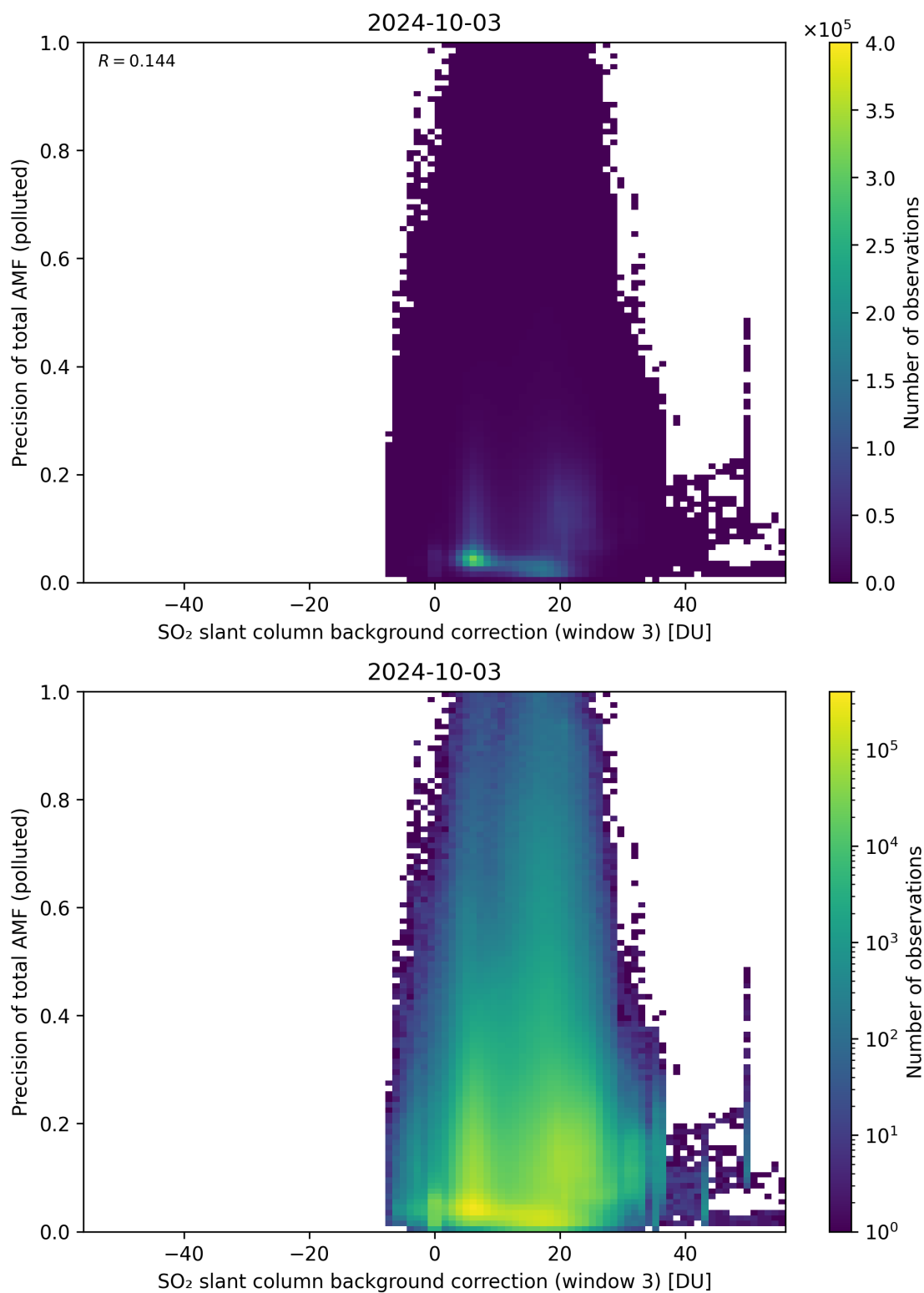
Figure 126: Scatter density plot of “SO 2 slant column background correction (window 3)” against “Precision of total AMF (polluted)” for 2024-10-03 to 2024-10-04.
