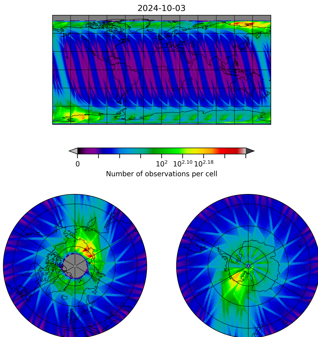
Figure 28: Map of the number of observations for 2024-10-03 to 2024-10-04
