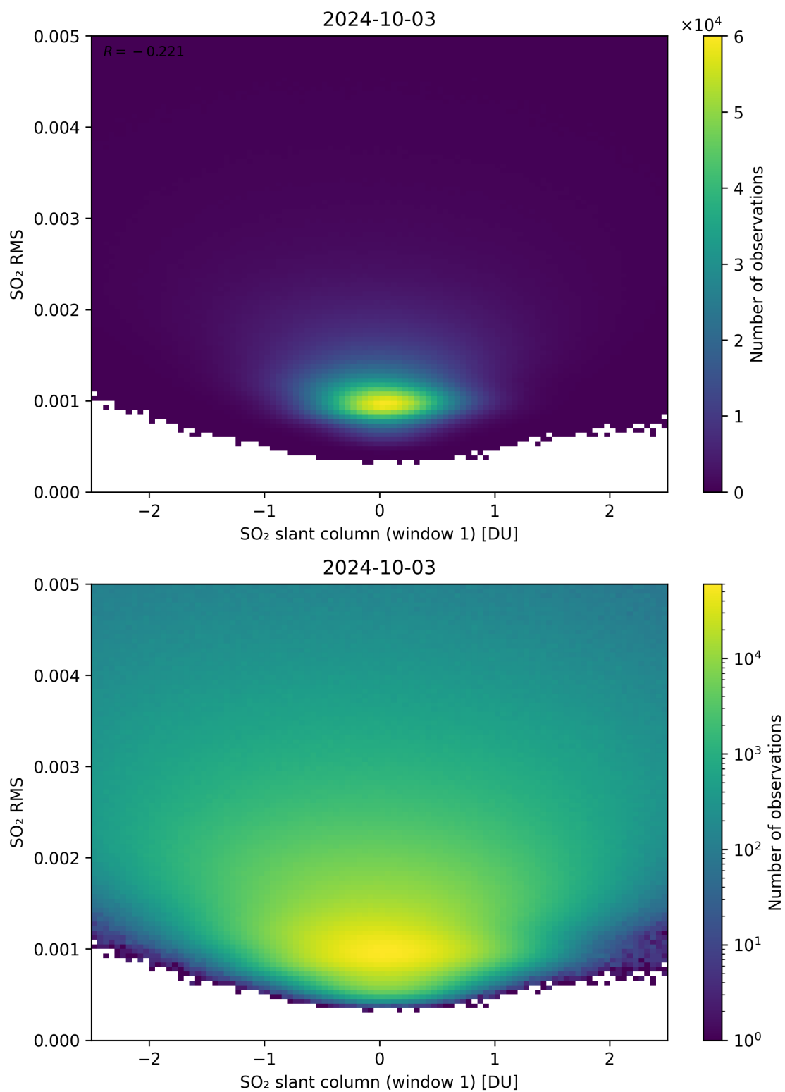
Figure 217: Scatter density plot of “SO 2 slant column (window 1)” against “SO 2 RMS” for 2024-10-03 to 2024-10-04.
