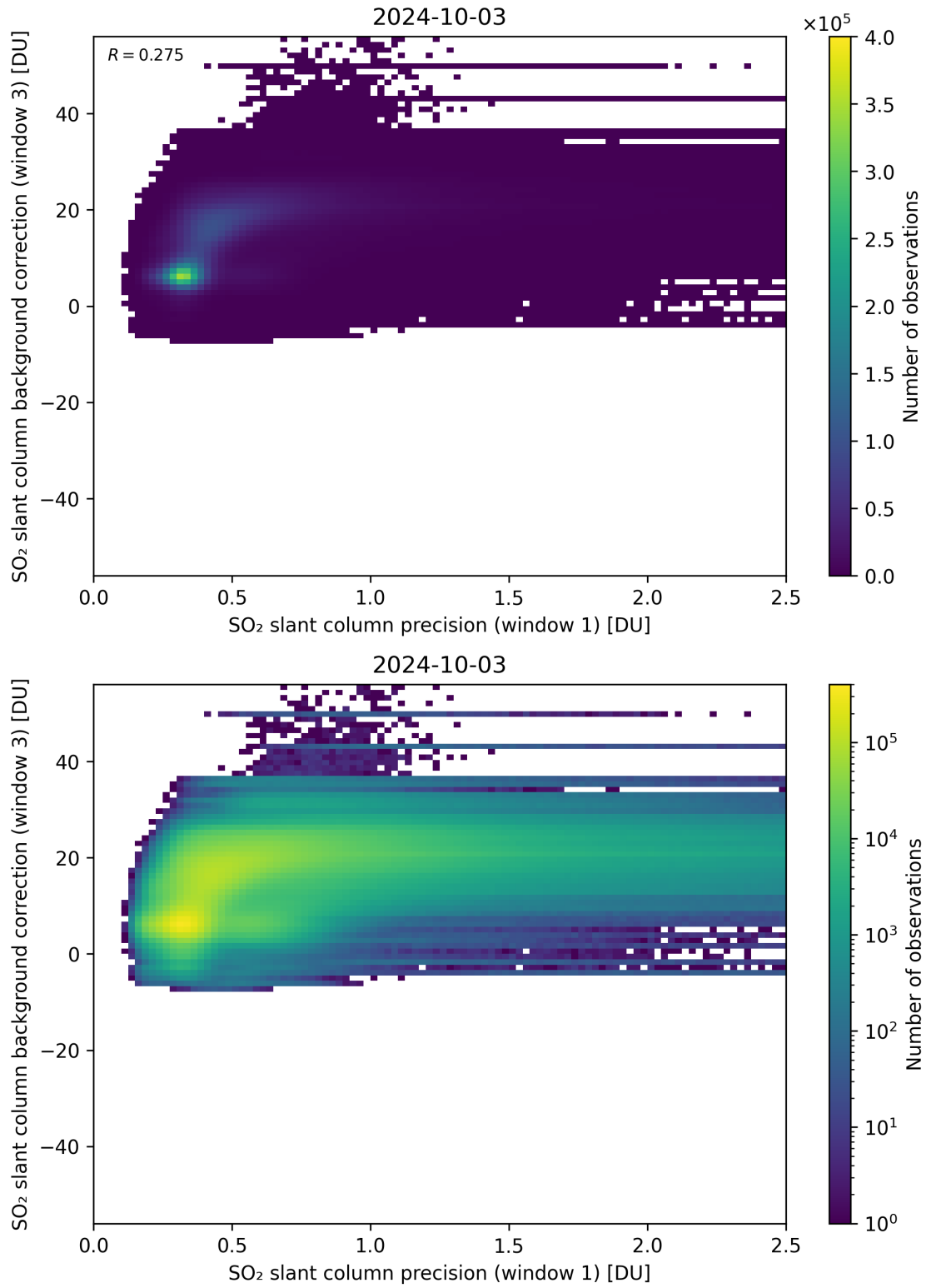
Figure 220: Scatter density plot of “SO 2 slant column precision (window 1)” against “SO 2 slant column background correction (window 3)” for 2024-10-03 to 2024-10-04.
