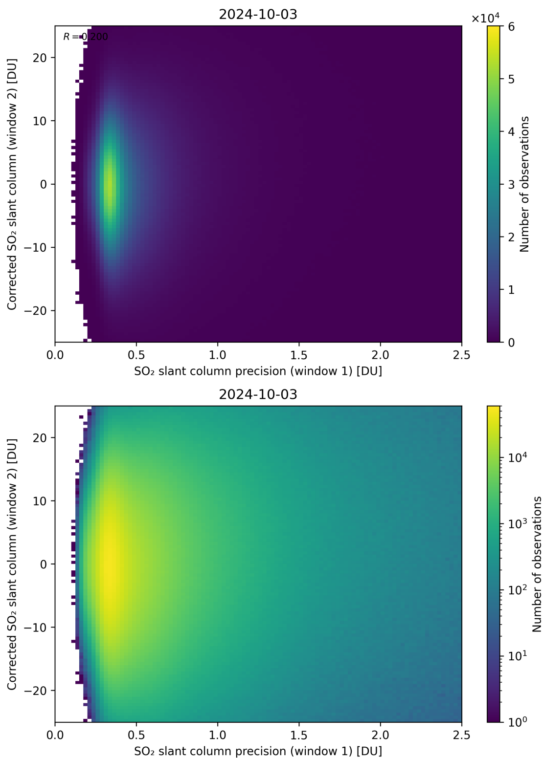
Figure 225: Scatter density plot of “SO 2 slant column precision (window 1)” against “Corrected SO 2 slant column (window 2)” for 2024-10-03 to 2024-10-04.
