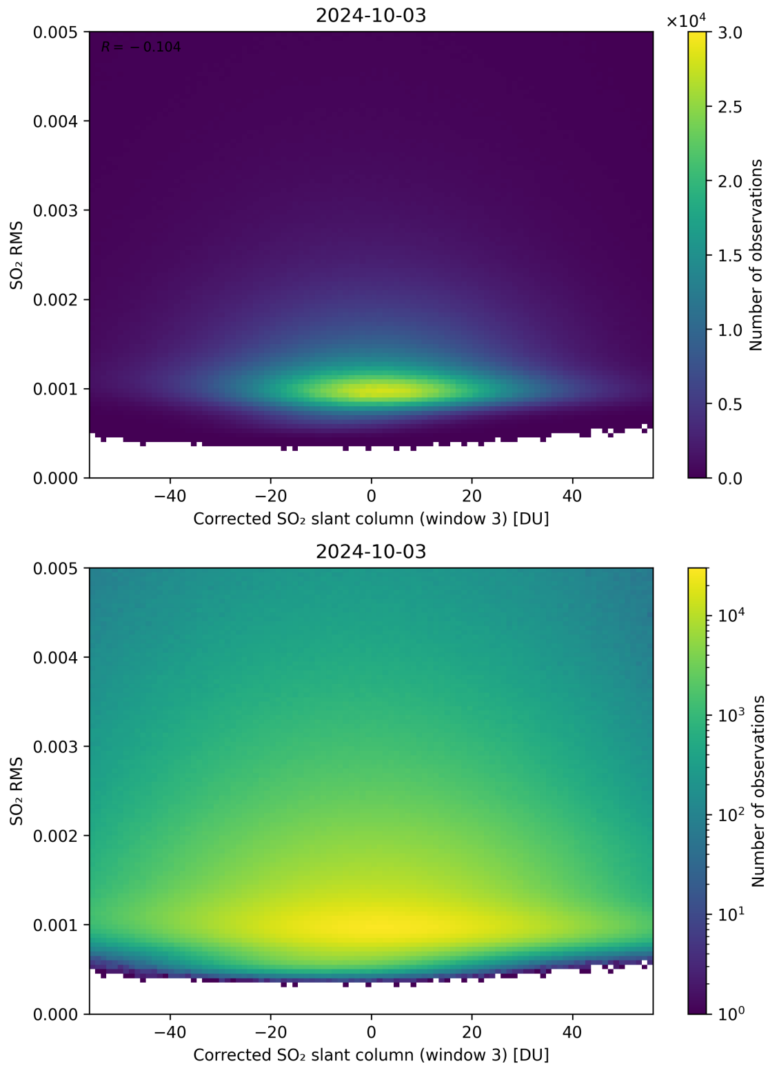
Figure 208: Scatter density plot of “Corrected SO 2 slant column (window 3)” against “SO 2 RMS” for 2024-10-03 to 2024-10-04.
