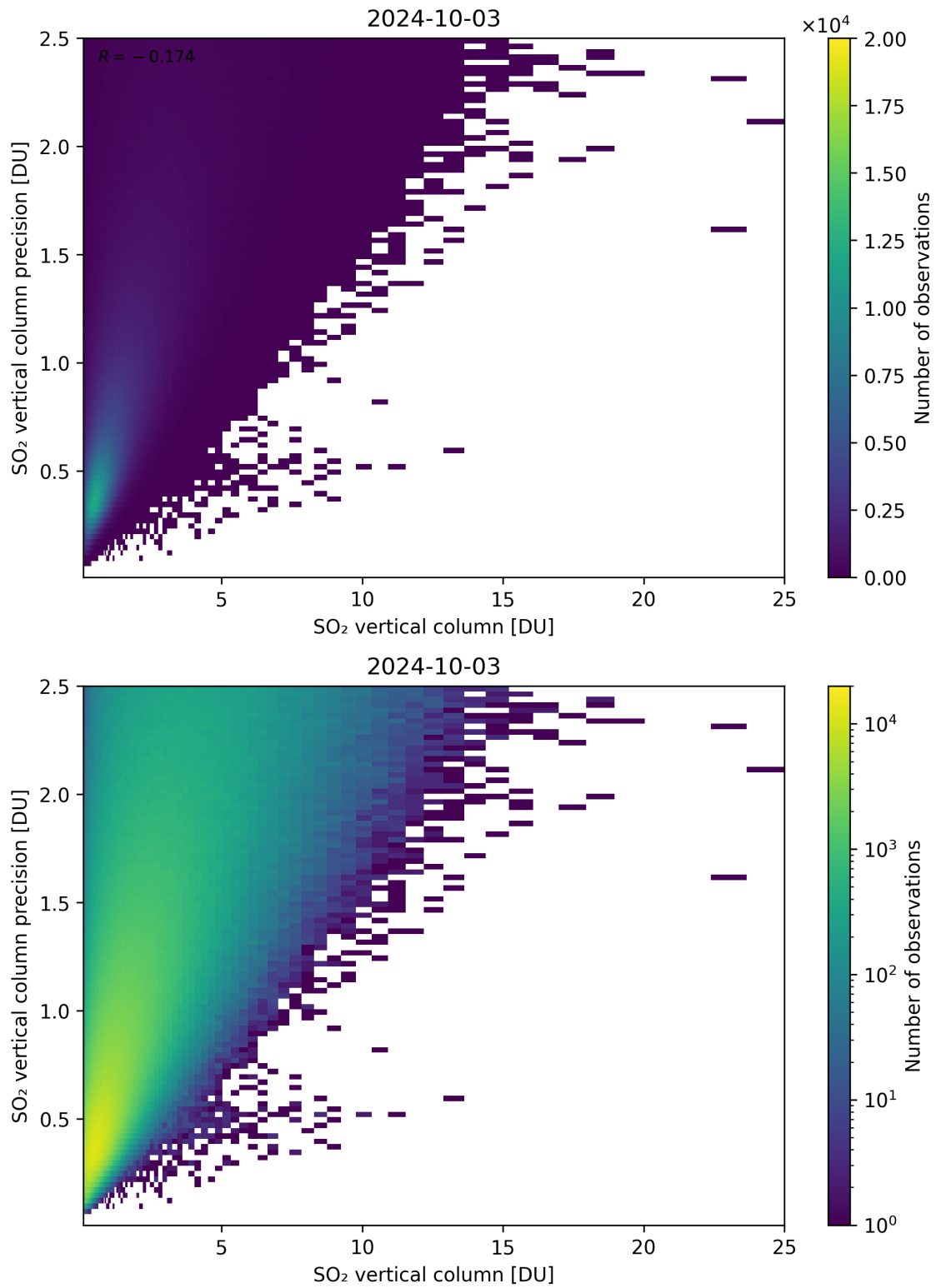
Figure 307: Scatter density plot of “SO 2 vertical column” against “SO 2 vertical column precision” for 2024-10-03 to 2024-10-04.
