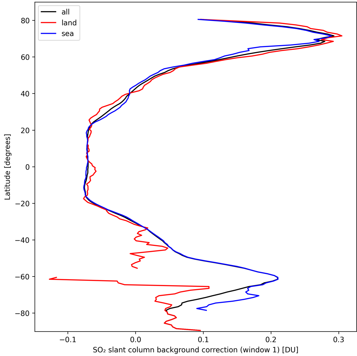
Figure 36: Zonal average of “SO 2 slant column background correction (window 1)” for 2024-10-03 to 2024-10-04.
