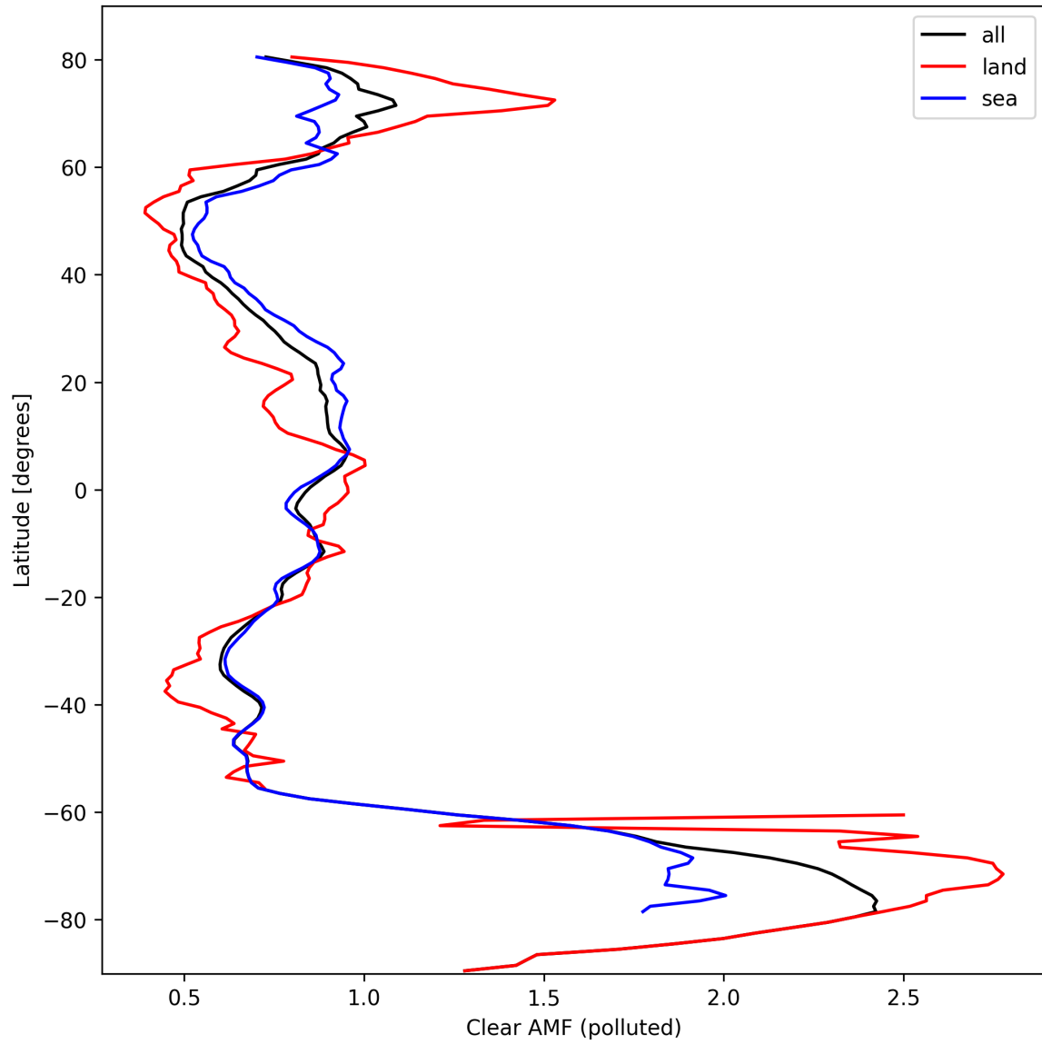
Figure 50: Zonal average of “Clear AMF (polluted)” for 2024-10-03 to 2024-10-04.
