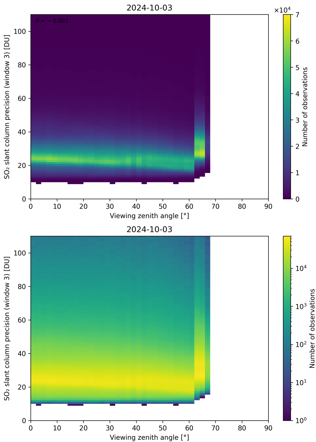
Figure 324: Scatter density plot of “Viewing zenith angle” against “SO 2 slant column precision (window 3)” for 2024-10-03 to 2024-10-04.
