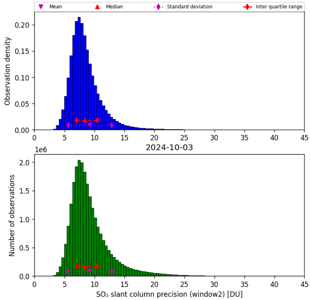
Figure 61: Histogram of “SO 2 slant column precision (window2)” for 2024-10-03 to 2024-10-04
