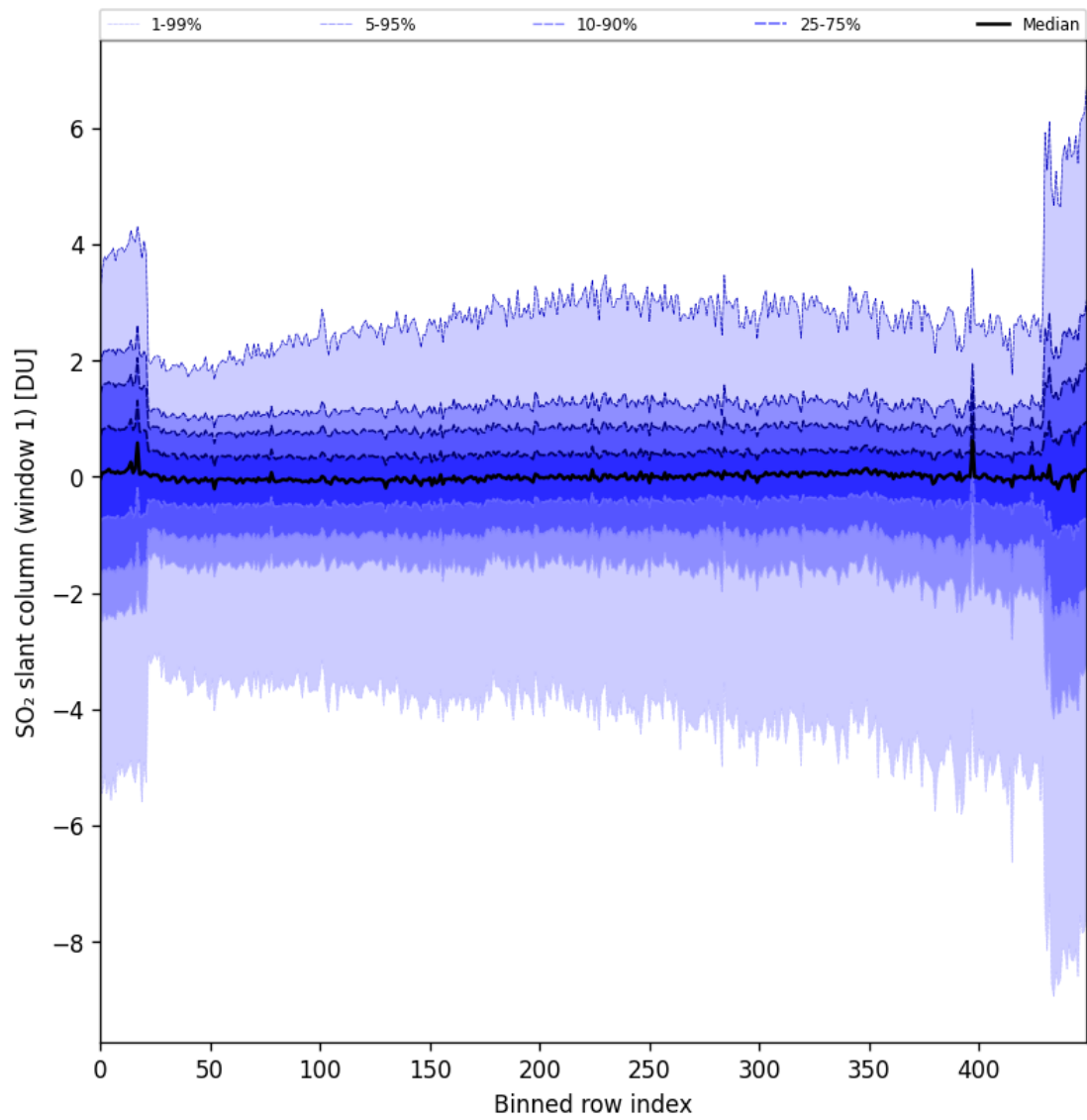
Figure 79: Along track statistics of “SO 2 slant column (window 1)” for 2024-10-03 to 2024-10-04
