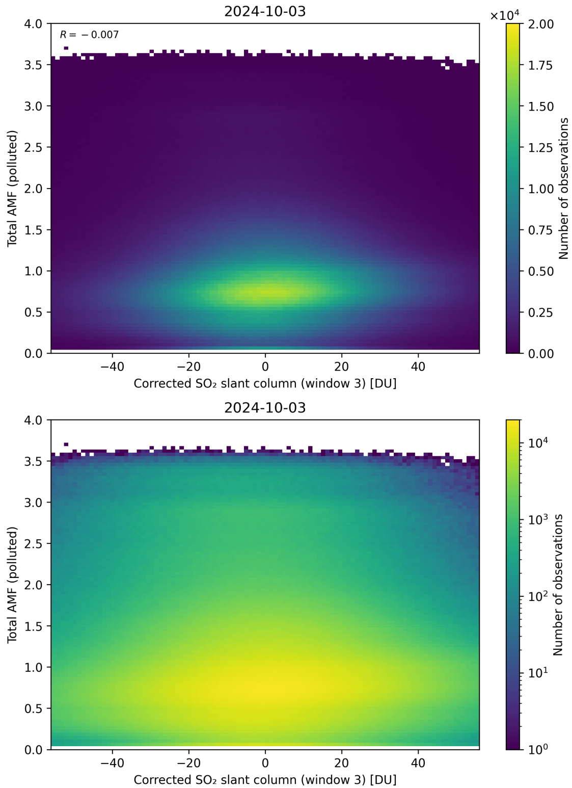
Figure 210: Scatter density plot of “Corrected SO 2 slant column (window 3)” against “Total AMF (polluted)” for 2024-10-03 to 2024-10-04.
