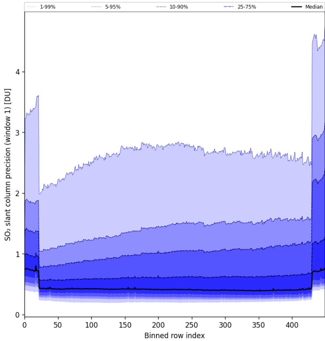
Figure 80: Along track statistics of “SO 2 slant column precision (window 1)” for 2024-10-03 to 2024-10-04
