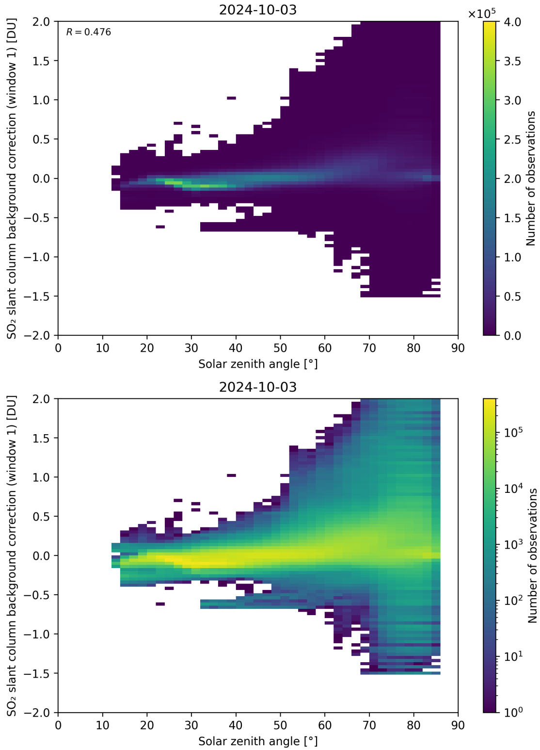
Figure 158: Scatter density plot of “Solar zenith angle” against “SO 2 slant column background correction (window 1)” for 2024-10-03 to 2024-10-04.
