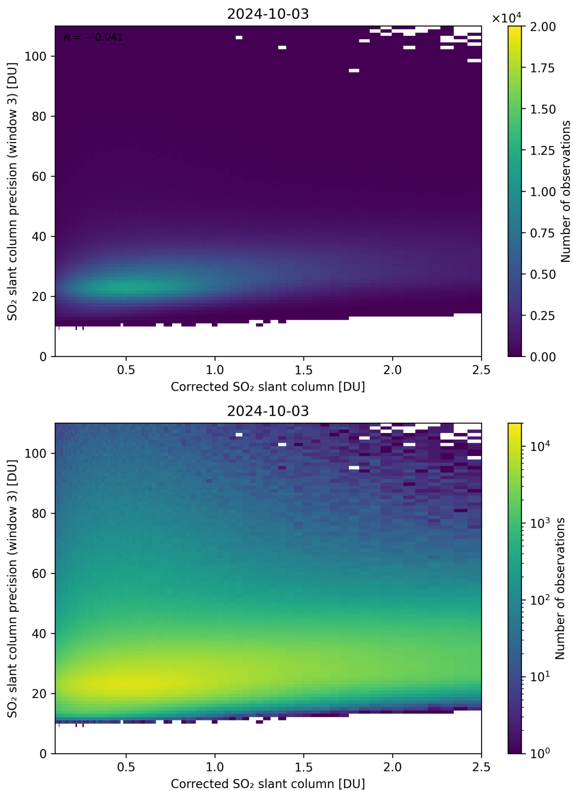
Figure 191: Scatter density plot of “Corrected SO 2 slant column” against “SO 2 slant column precision (window 3)” for 2024-10-03 to 2024-10-04.
