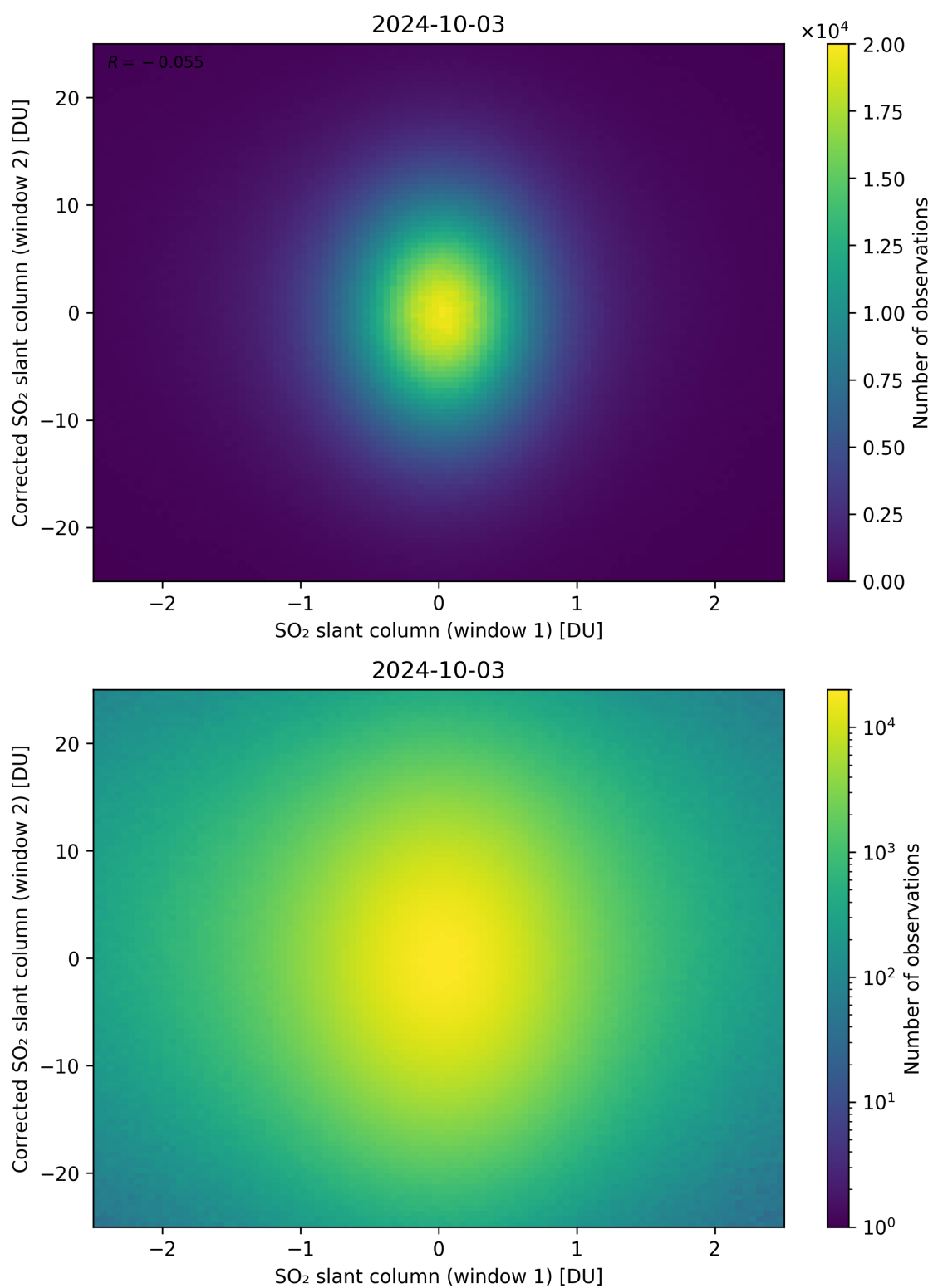
Figure 233: Scatter density plot of “SO 2 slant column (window 1)” against “Corrected SO 2 slant column (window 2)” for 2024-10-03 to 2024-10-04.
