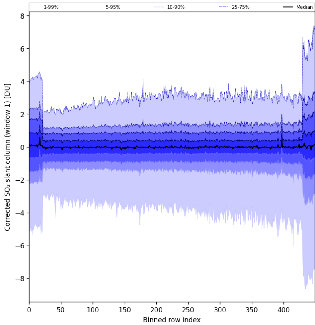
Figure 81: Along track statistics of “Corrected SO 2 slant column (window 1)” for 2024-10-03 to 2024-10-04
