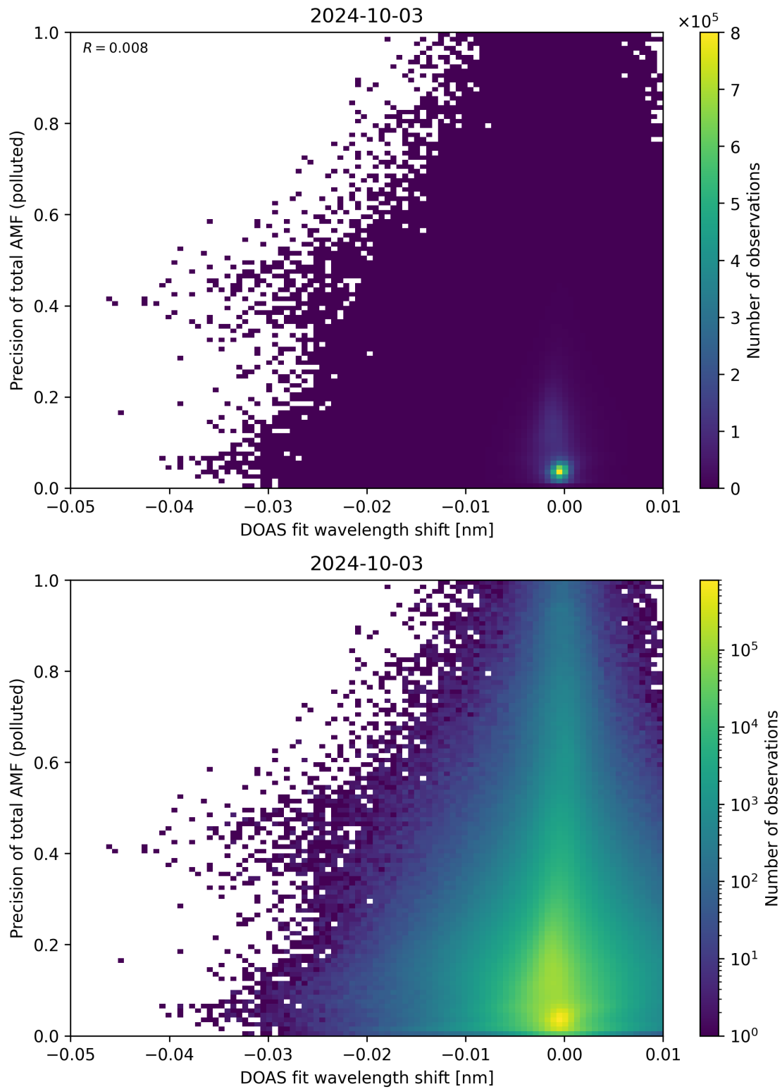
Figure 131: Scatter density plot of “DOAS fit wavelength shift” against “Precision of total AMF (polluted)” for 2024-10-03 to 2024-10-04.
