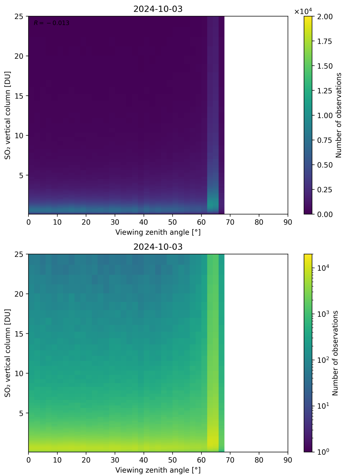
Figure 327: Scatter density plot of “Viewing zenith angle” against “SO 2 vertical column” for 2024-10-03 to 2024-10-04.
