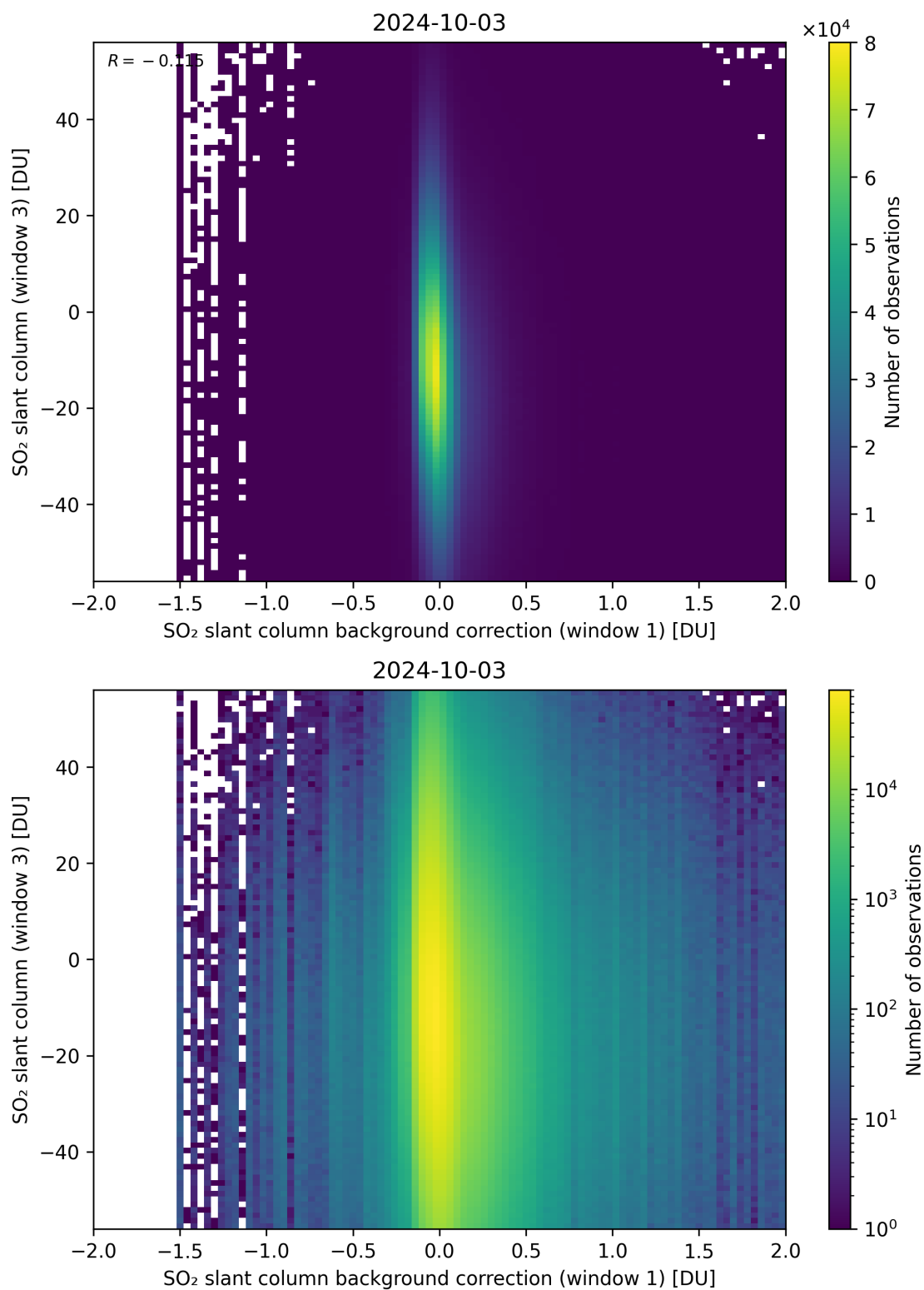
Figure 107: Scatter density plot of “SO 2 slant column background correction (window 1)” against “SO 2 slant column (window 3)” for 2024-10-03 to 2024-10-04.
