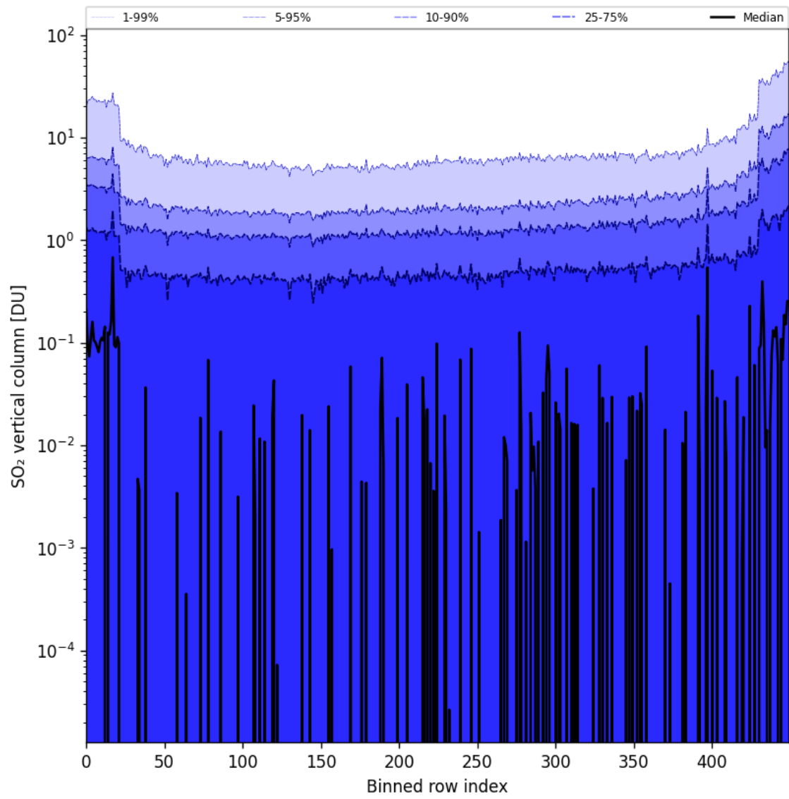
Figure 76: Along track statistics of "SO 2 vertical column" for 2024-10-03 to 2024-10-04
