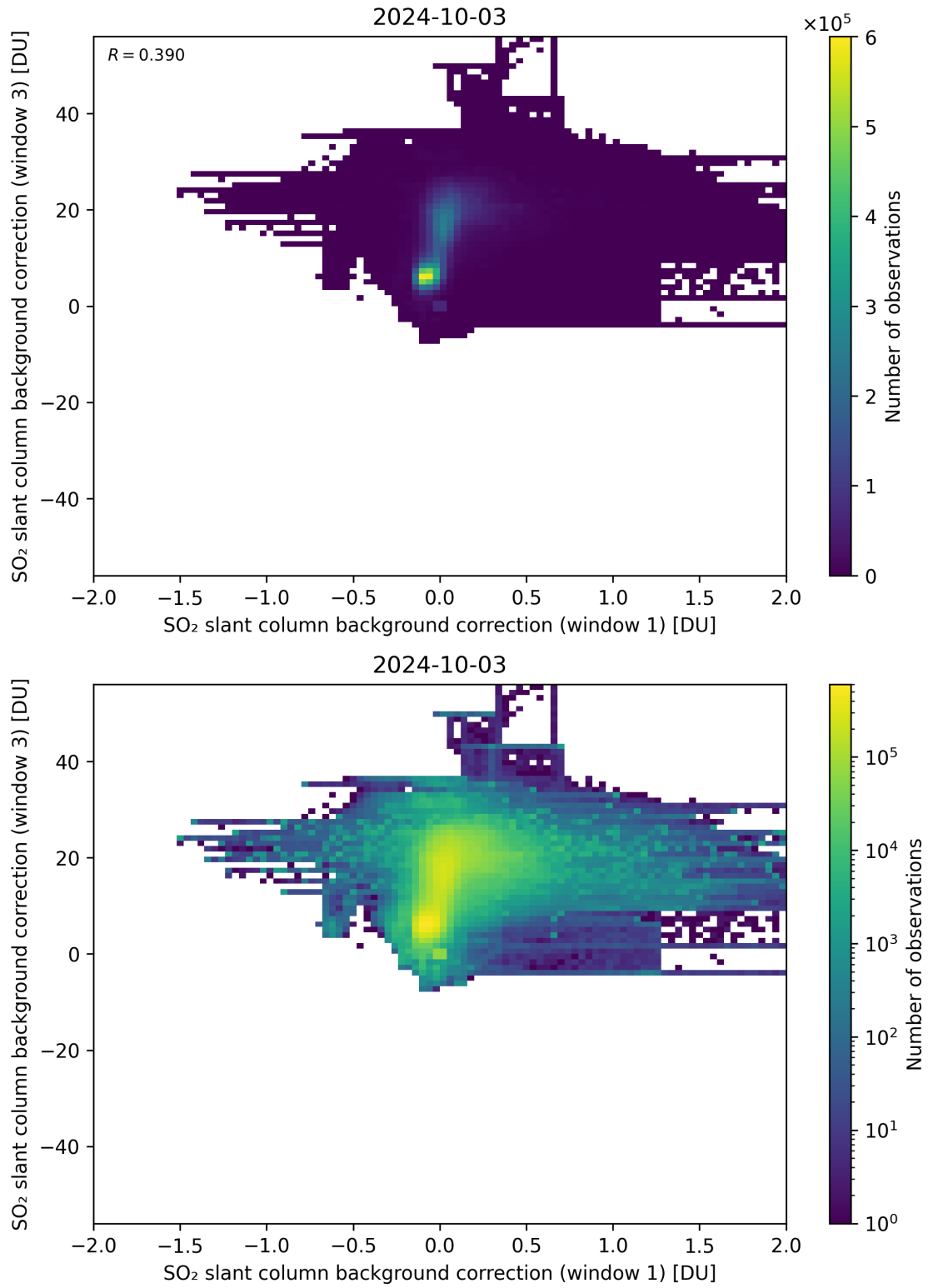
Figure 99: Scatter density plot of “SO 2 slant column background correction (window 1)” against “SO 2 slant column background correction (window 3)” for 2024-10-03 to 2024-10-04.
