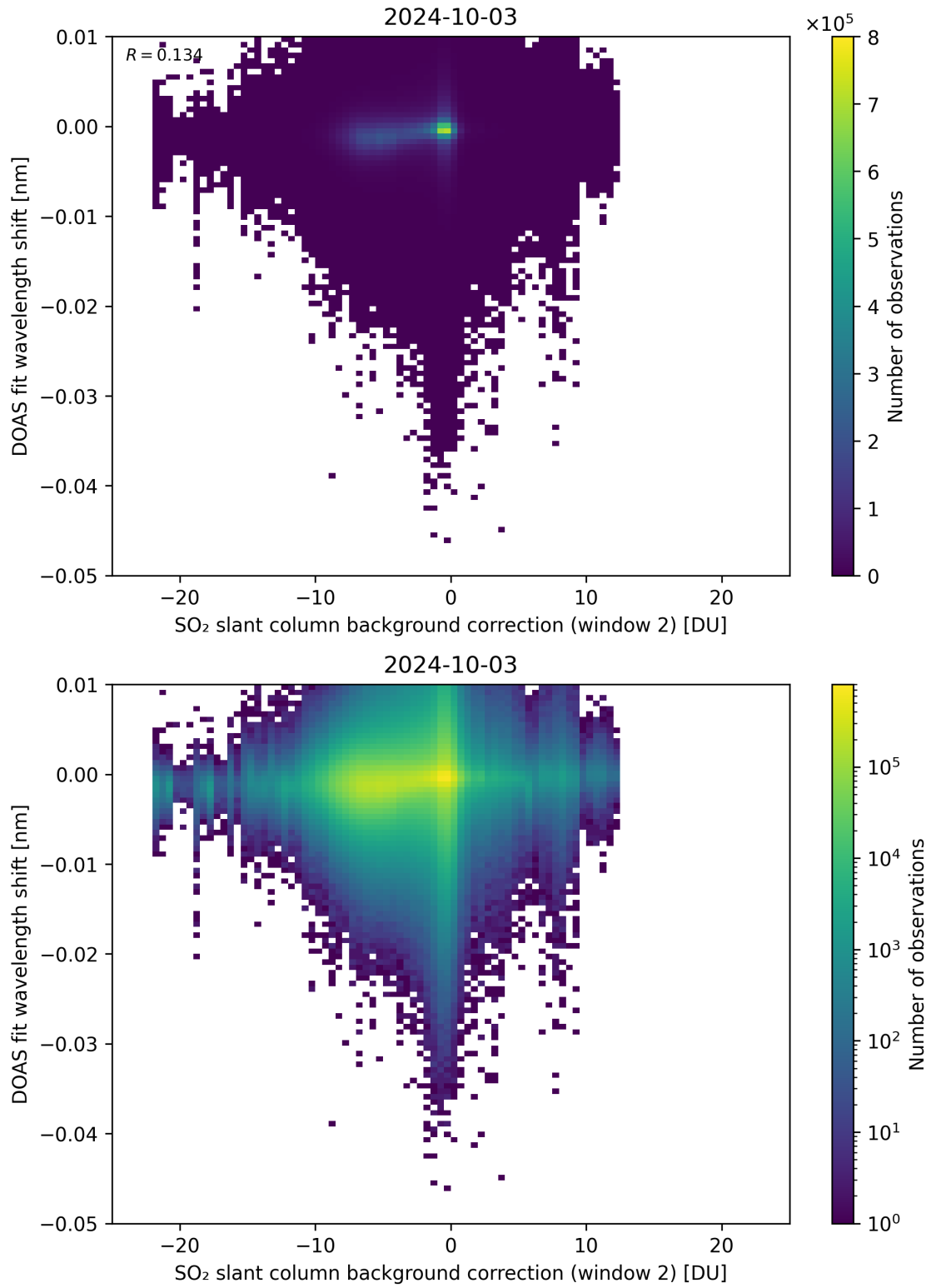
Figure 112: Scatter density plot of “SO 2 slant column background correction (window 2)” against “DOAS fit wavelength shift” for 2024-10-03 to 2024-10-04.
