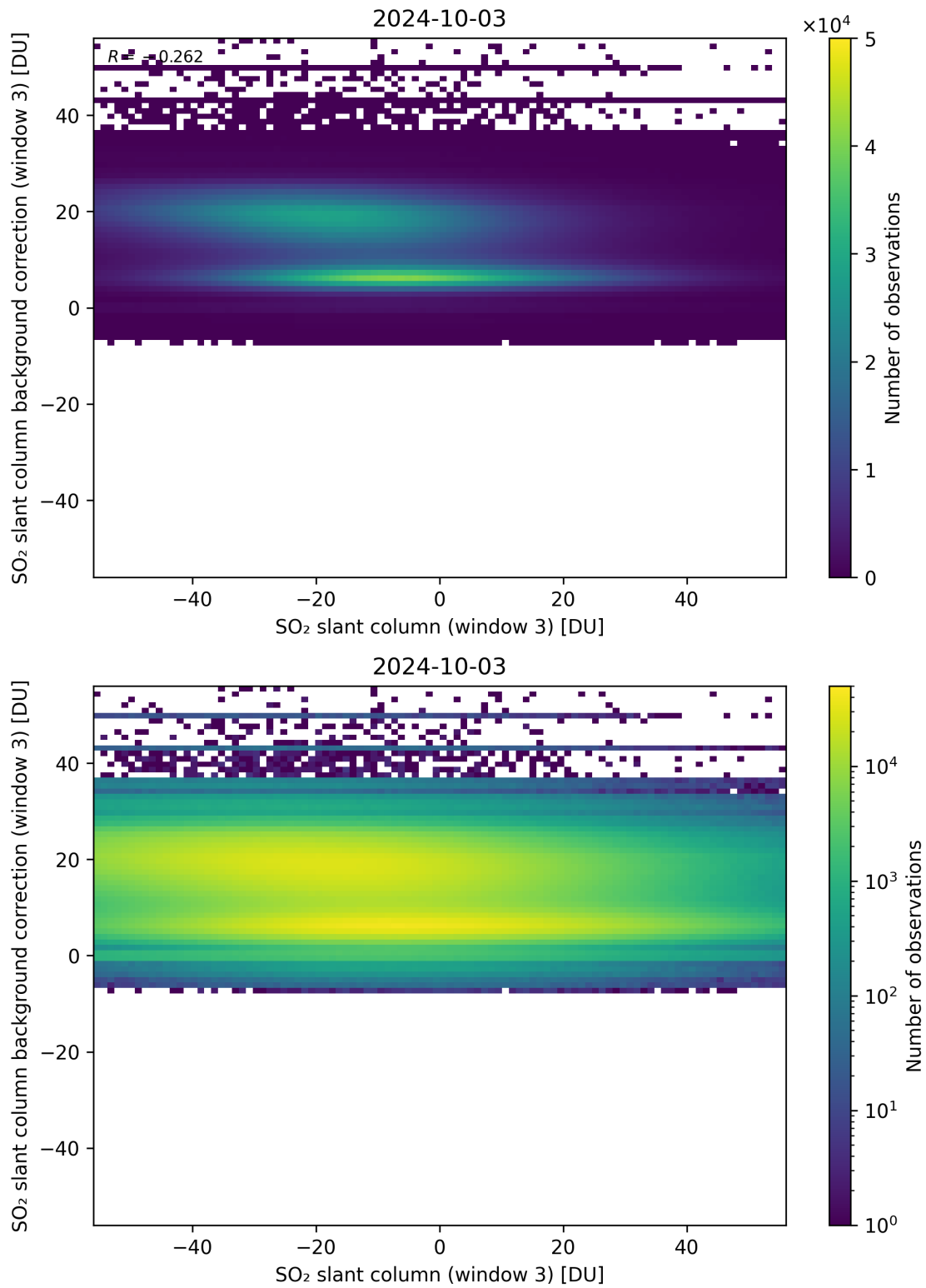
Figure 253: Scatter density plot of “SO 2 slant column (window 3)” against “SO 2 slant column background correction (window 3)” for 2024-10-03 to 2024-10-04.
