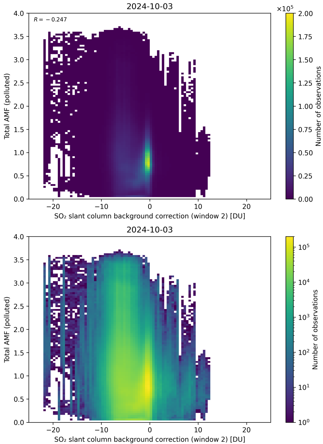
Figure 119: Scatter density plot of “SO 2 slant column background correction (window 2)” against “Total AMF (polluted)” for 2024-10-03 to 2024-10-04.
