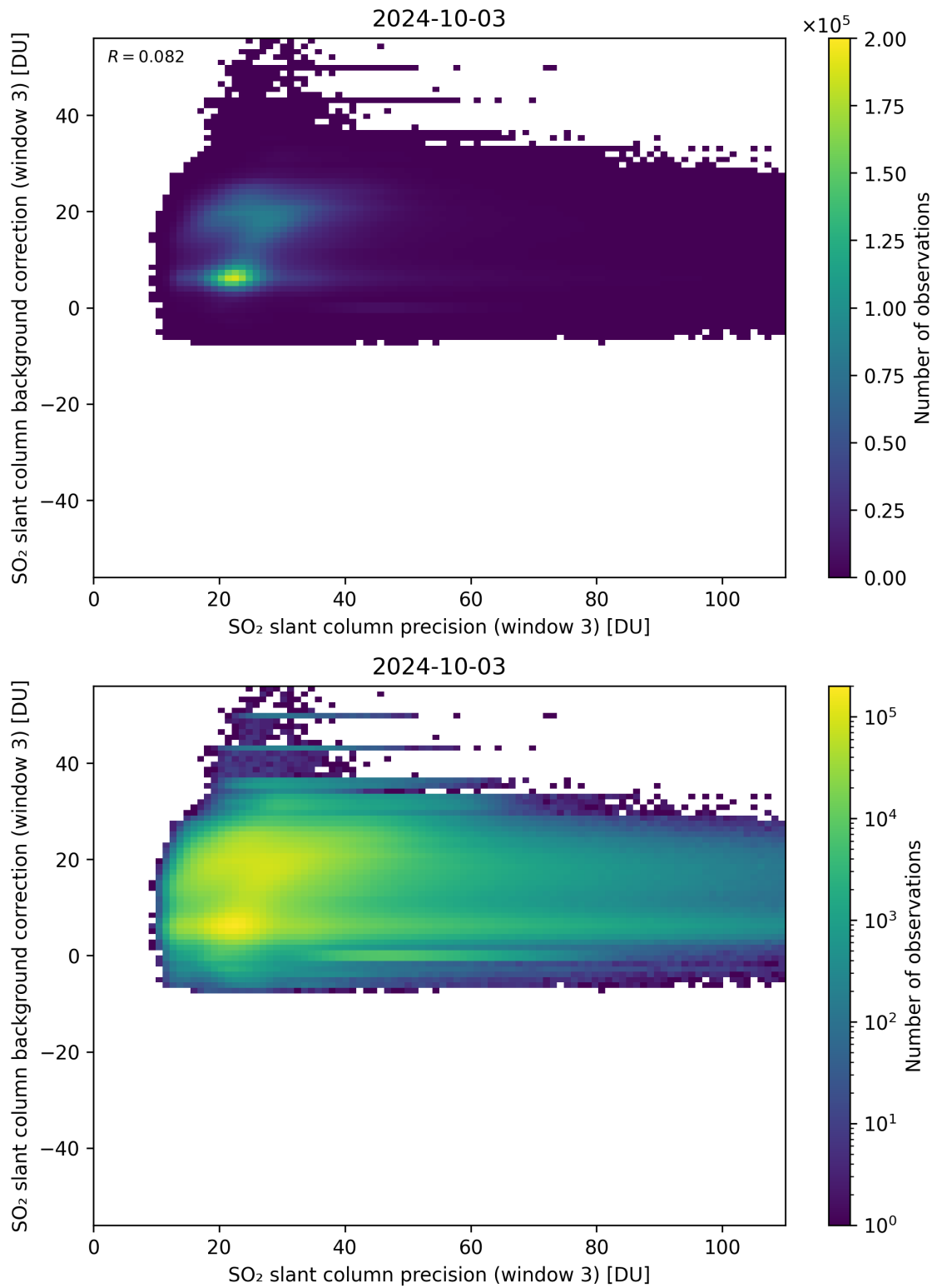
Figure 257: Scatter density plot of “SO 2 slant column precision (window 3)” against “SO 2 slant column background correction (window 3)” for 2024-10-03 to 2024-10-04.
