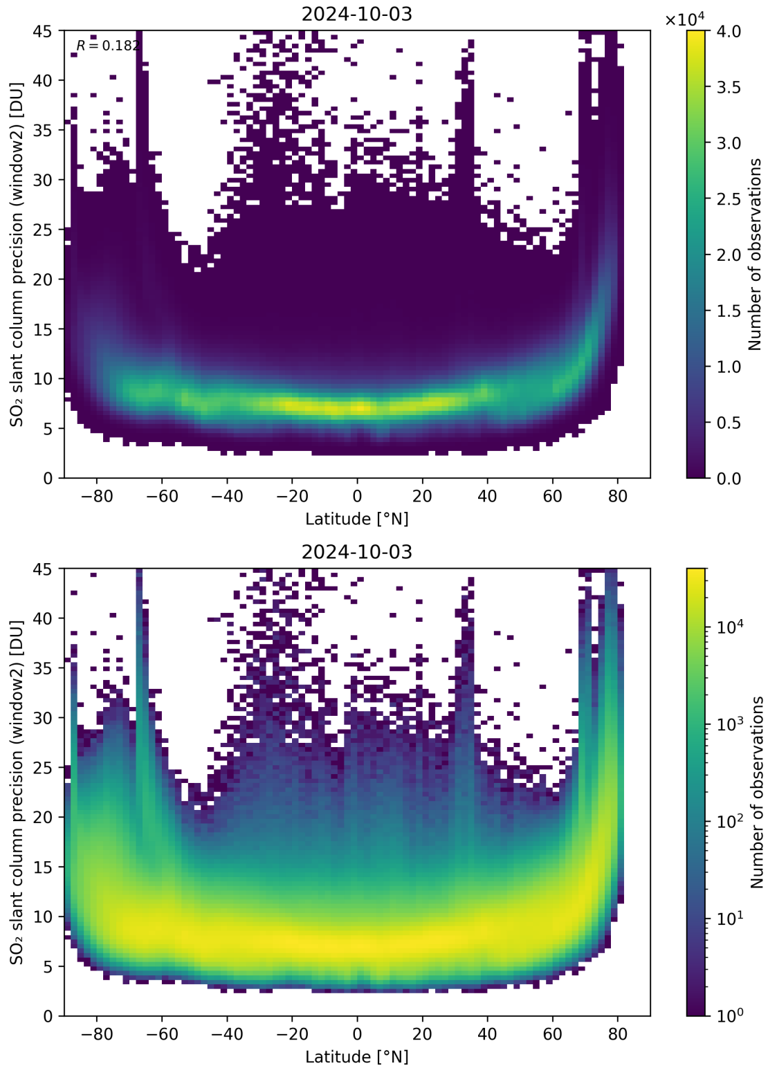
Figure 151: Scatter density plot of “Latitude” against “SO 2 slant column precision (window2)” for 2024-10-03 to 2024-10-04.
