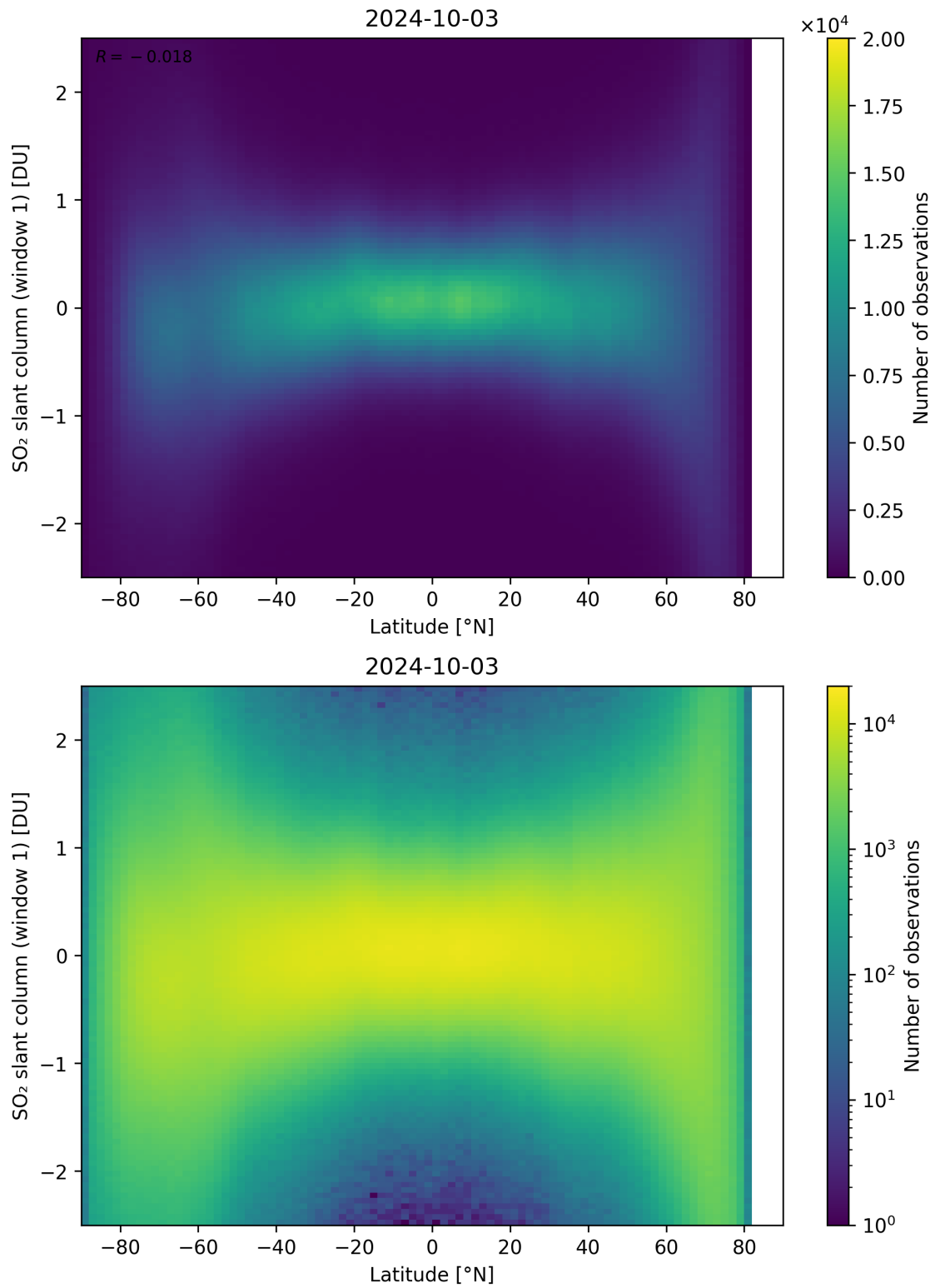
Figure 149: Scatter density plot of “Latitude” against “SO 2 slant column (window 1)” for 2024-10-03 to 2024-10-04.
