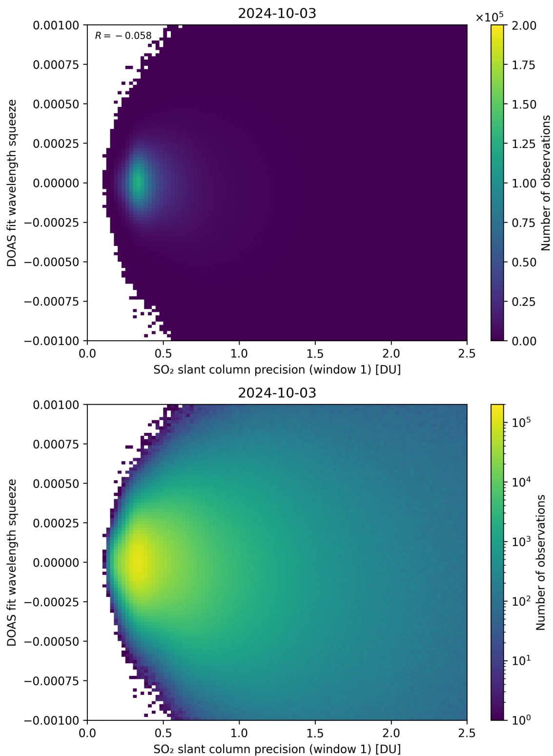
Figure 222: Scatter density plot of “SO 2 slant column precision (window 1)” against “DOAS fit wavelength squeeze” for 2024-10-03 to 2024-10-04.
