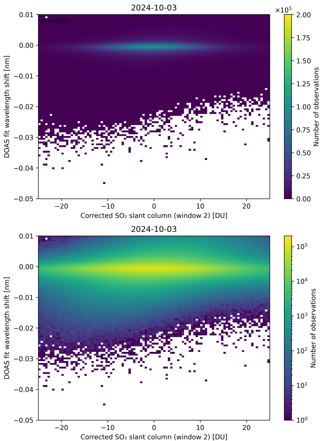
Figure 196: Scatter density plot of “Corrected SO 2 slant column (window 2)” against “DOAS fit wavelength shift” for 2024-10-03 to 2024-10-04.
