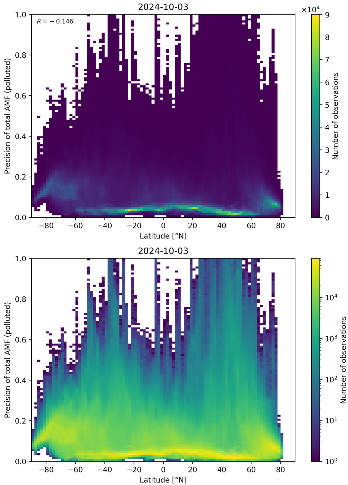
Figure 155: Scatter density plot of “Latitude” against “Precision of total AMF (polluted)” for 2024-10-03 to 2024-10-04.
