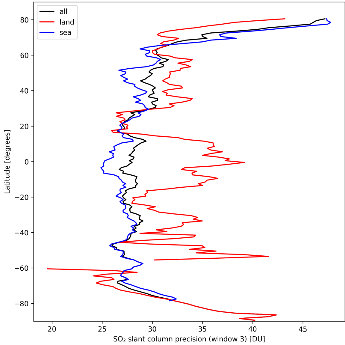
Figure 42: Zonal average of “SO 2 slant column precision (window 3)” for 2024-10-03 to 2024-10-04.
