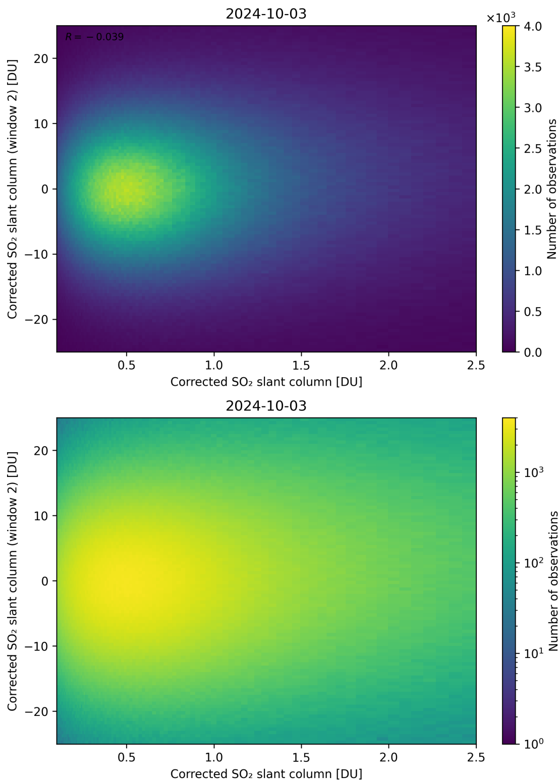
Figure 185: Scatter density plot of “Corrected SO 2 slant column” against “Corrected SO 2 slant column (window 2)” for 2024-10-03 to 2024-10-04.
