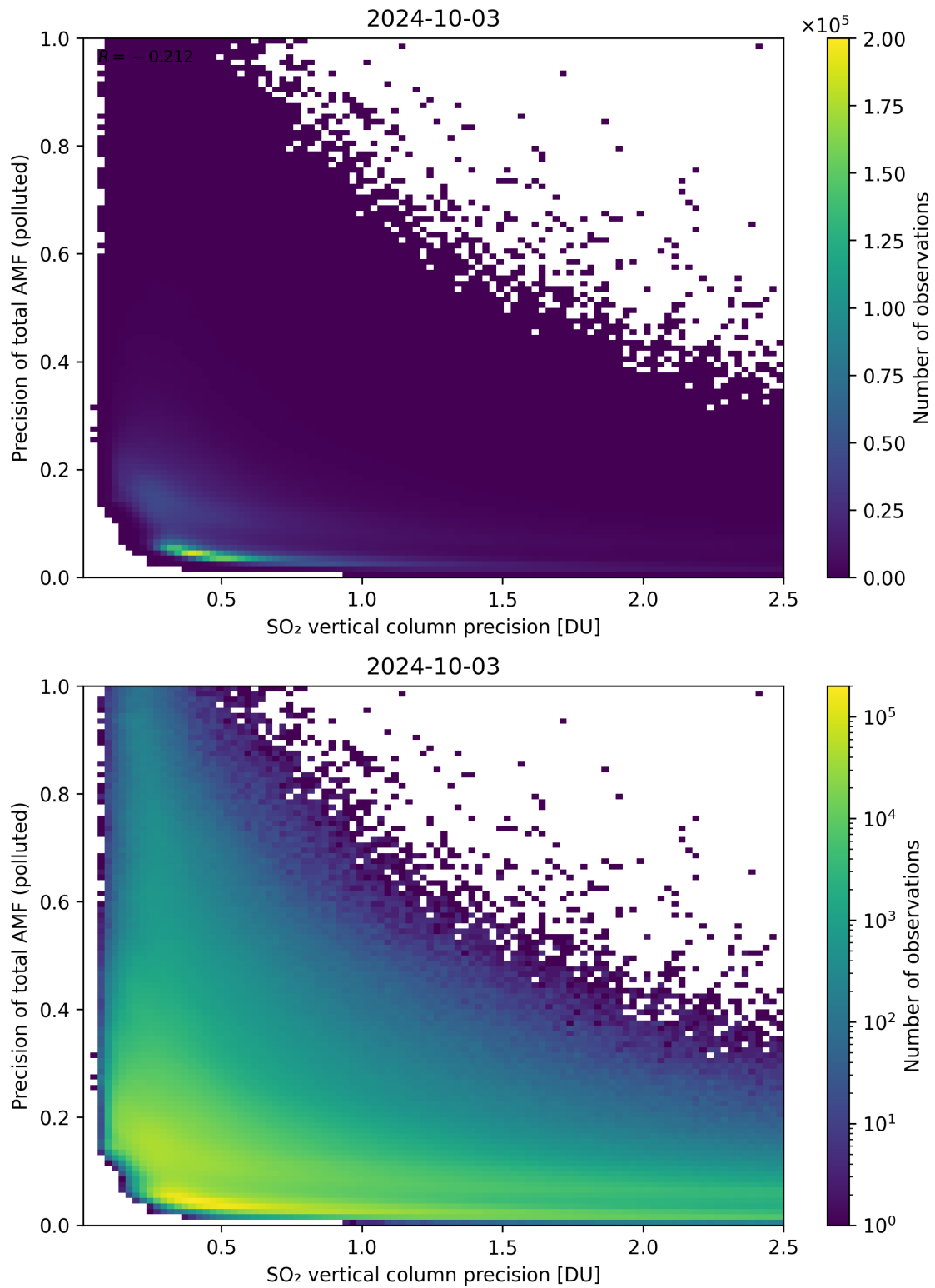
Figure 295: Scatter density plot of “SO 2 vertical column precision” against “Precision of total AMF (polluted)” for 2024-10-03 to 2024-10-04.
