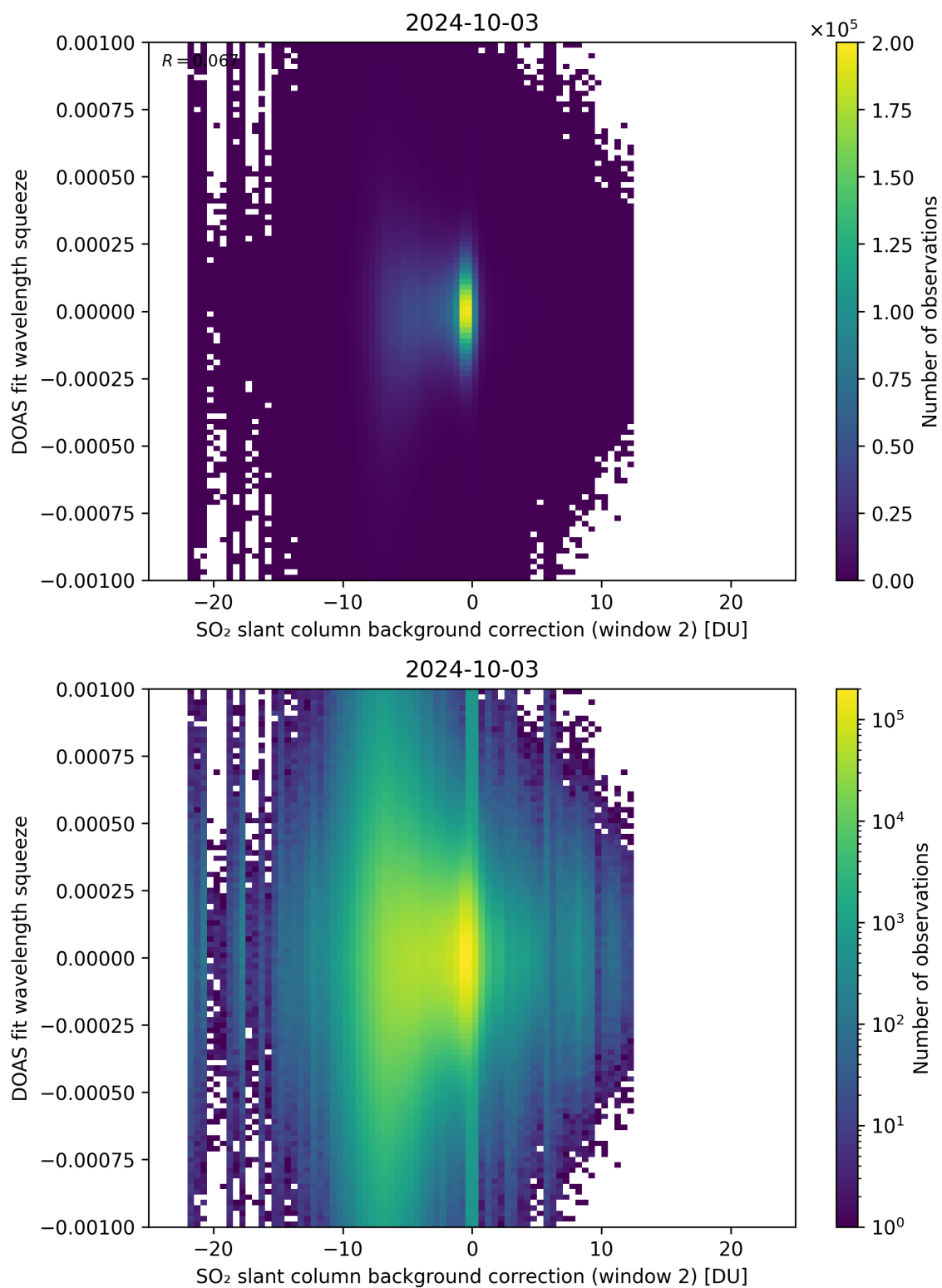
Figure 113: Scatter density plot of “SO 2 slant column background correction (window 2)” against “DOAS fit wavelength squeeze” for 2024-10-03 to 2024-10-04.
