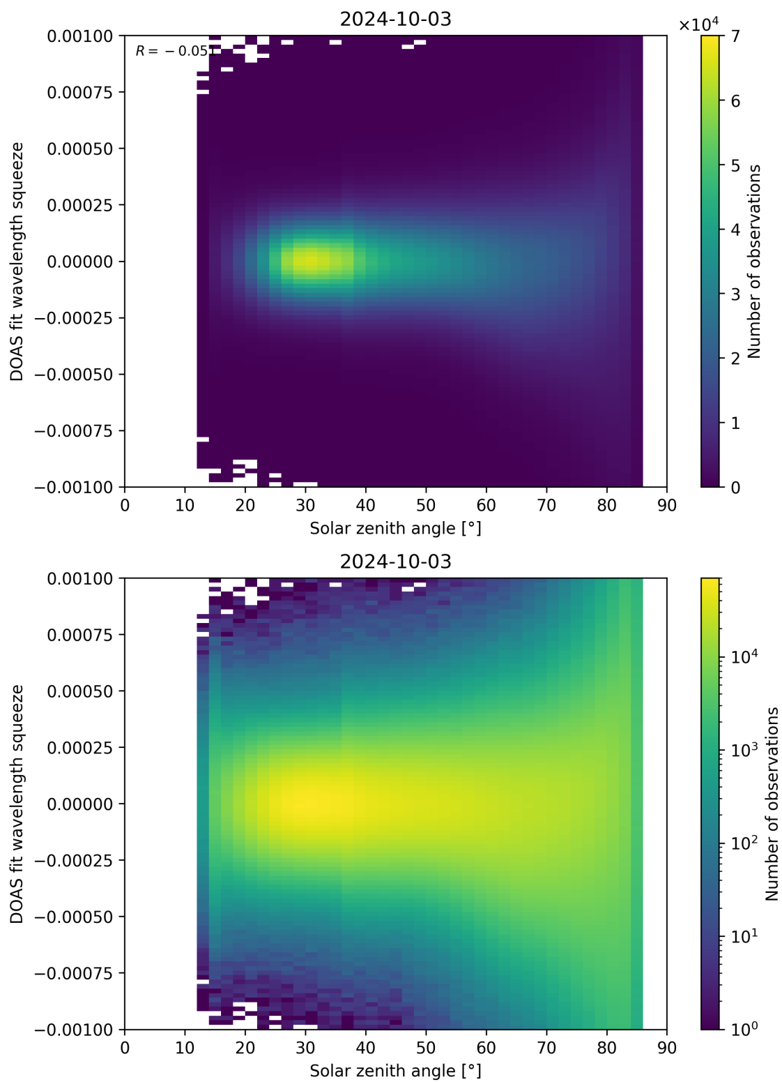
Figure 162: Scatter density plot of “Solar zenith angle” against “DOAS fit wavelength squeeze” for 2024-10-03 to 2024-10-04.
