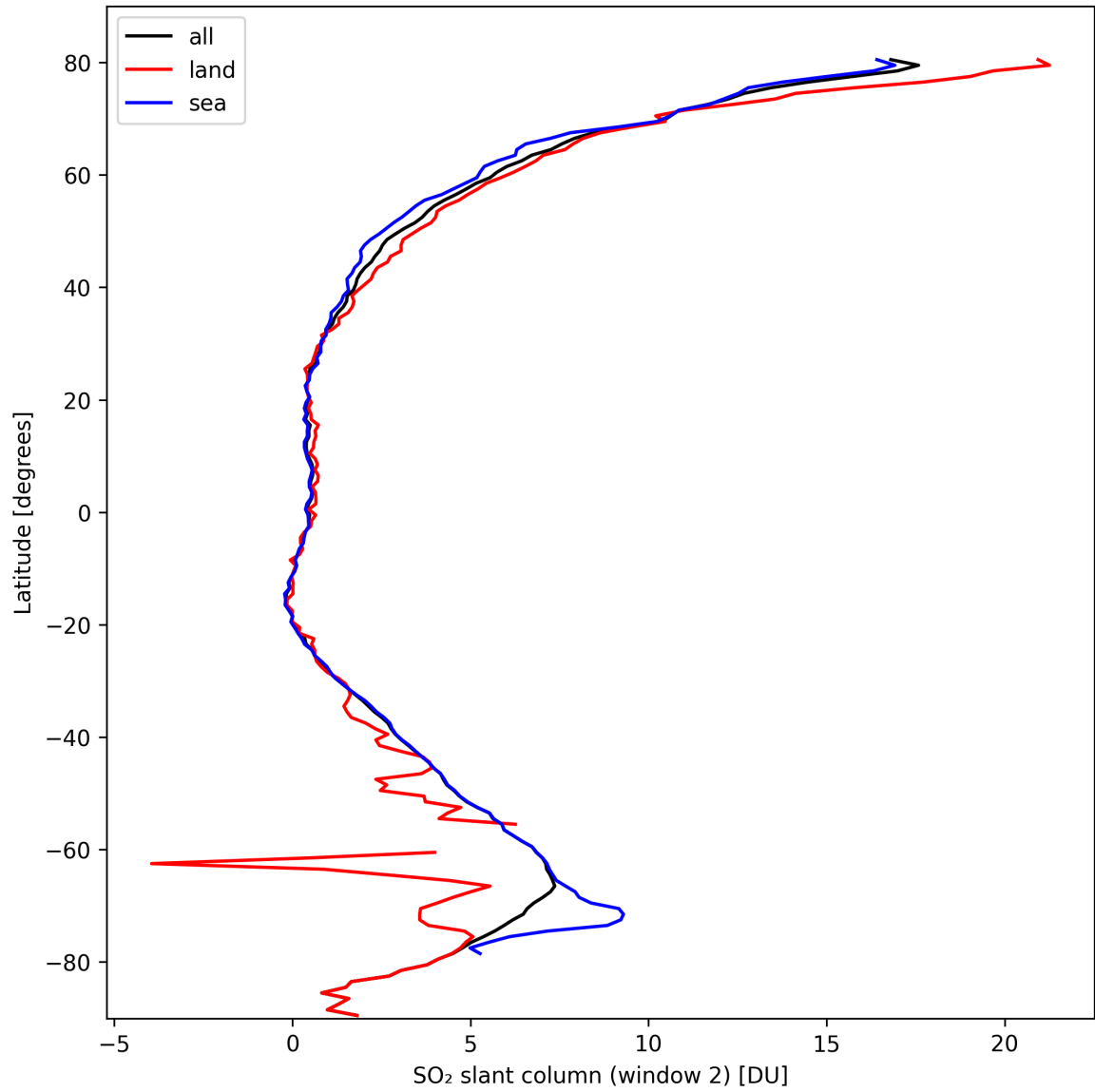
Figure 37: Zonal average of “SO 2 slant column (window 2)” for 2024-10-03 to 2024-10-04.
