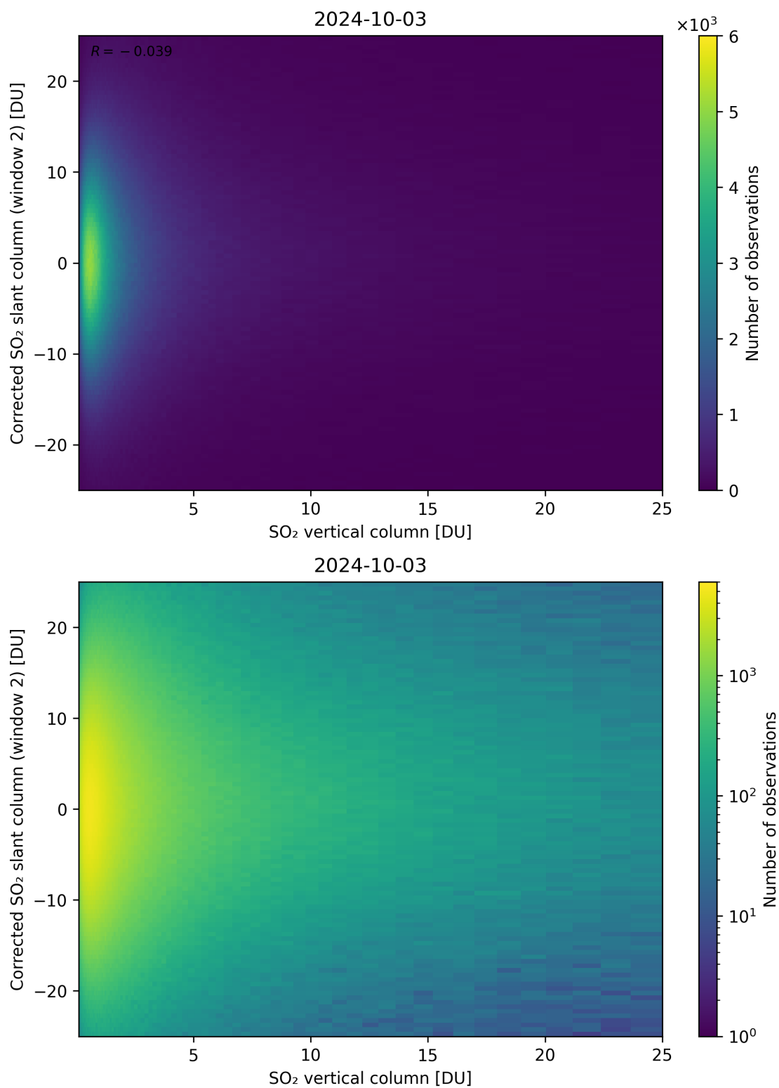
Figure 298: Scatter density plot of “SO 2 vertical column” against “Corrected SO 2 slant column (window 2)” for 2024-10-03 to 2024-10-04.
