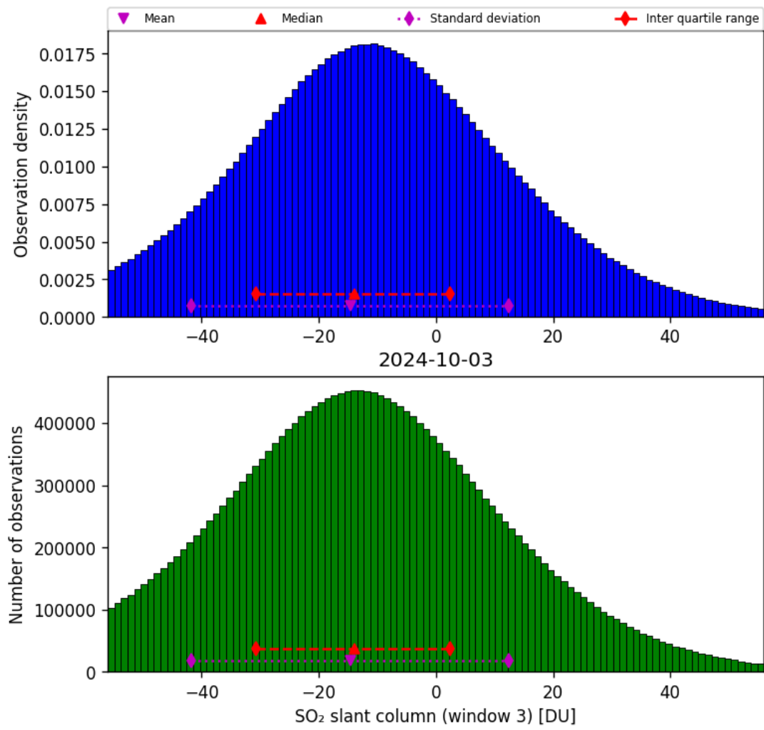
Figure 64: Histogram of “SO 2 slant column (window 3)” for 2024-10-03 to 2024-10-04
