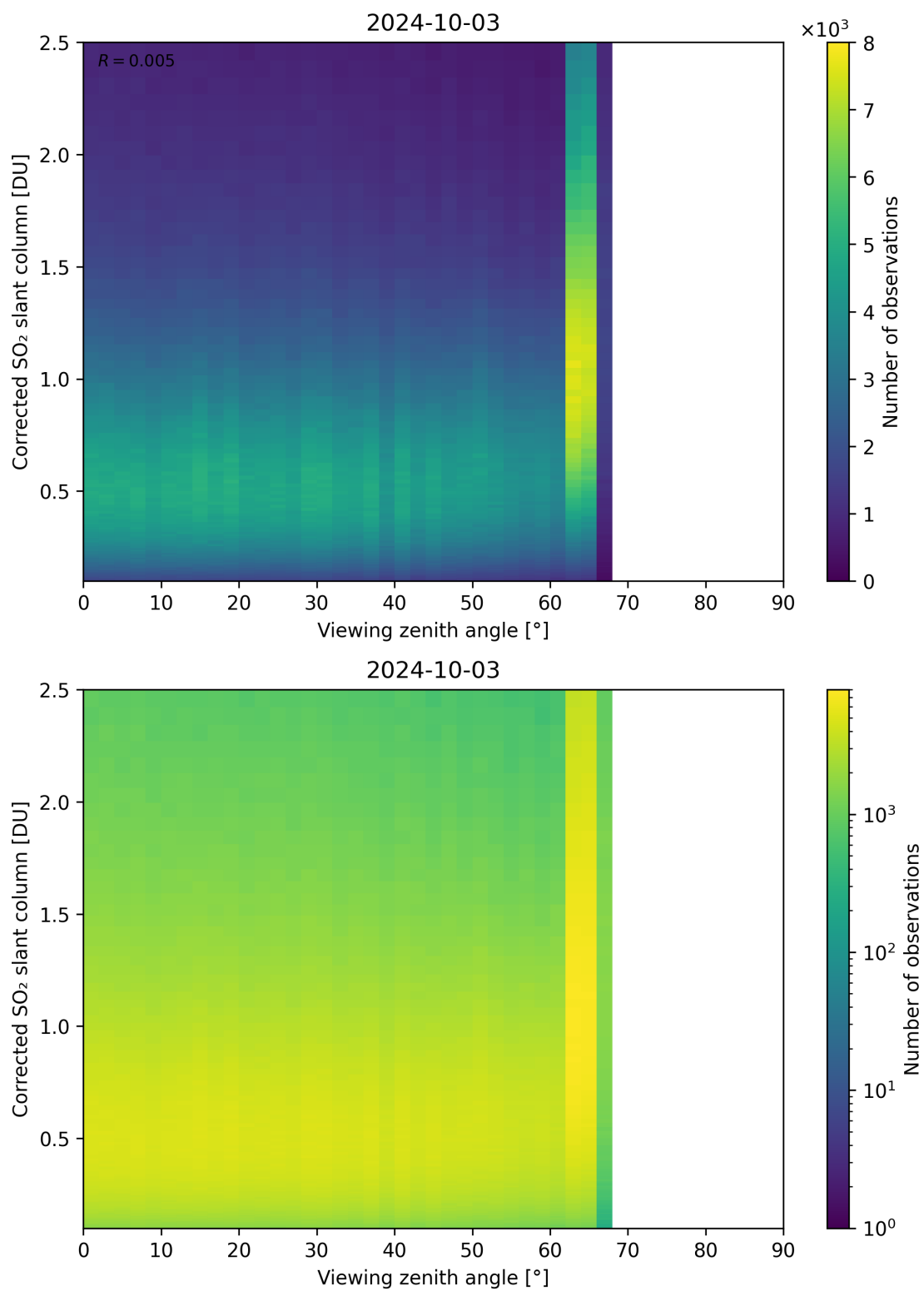
Figure 317: Scatter density plot of “Viewing zenith angle” against “Corrected SO 2 slant column” for 2024-10-03 to 2024-10-04.
