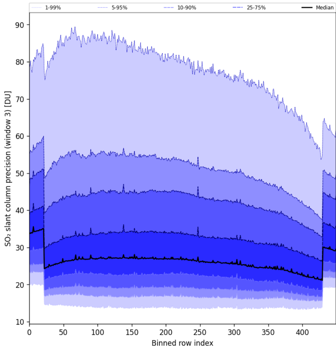
Figure 88: Along track statistics of “SO 2 slant column precision (window 3)” for 2024-10-03 to 2024-10-04
