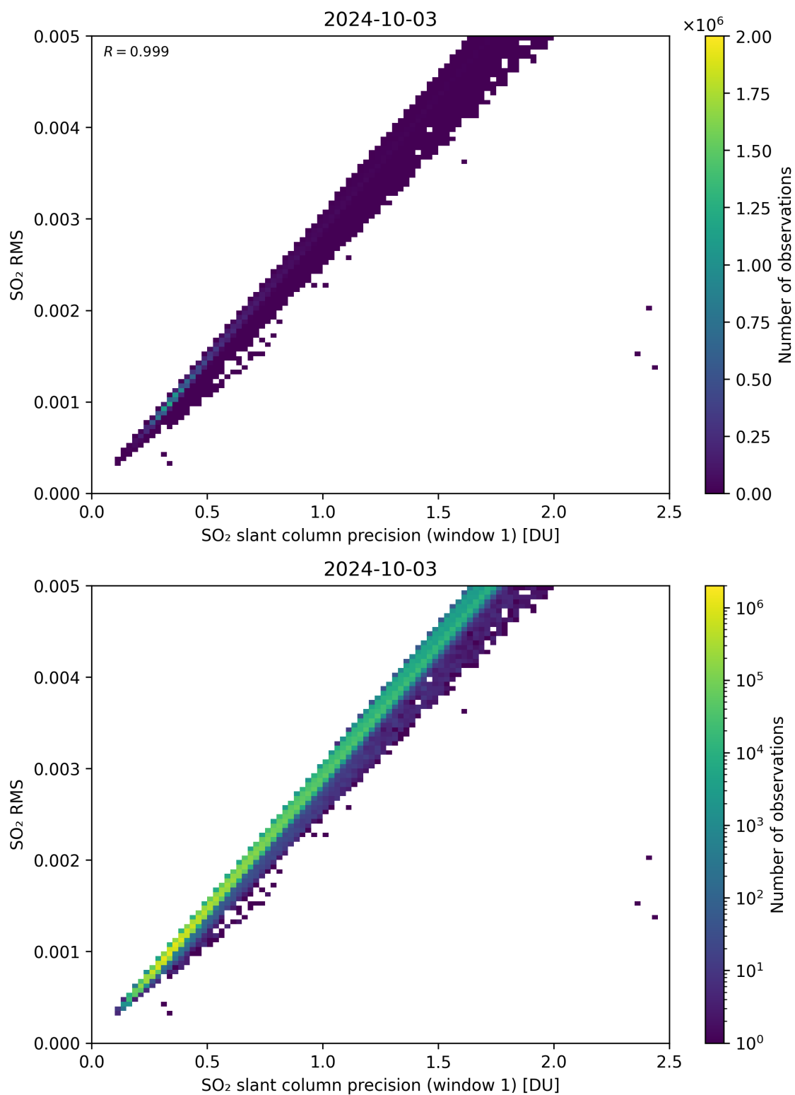
Figure 223: Scatter density plot of “SO 2 slant column precision (window 1)” against “SO 2 RMS” for 2024-10-03 to 2024-10-04.
