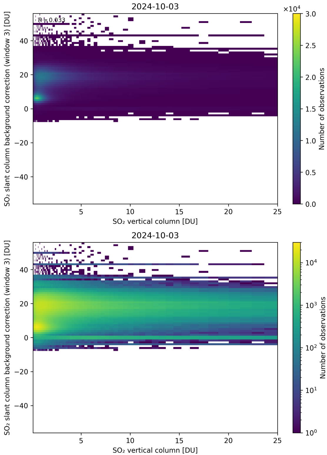
Figure 275: Scatter density plot of “SO 2 vertical column” against “SO 2 slant column background correction (window 3)” for 2024-10-03 to 2024-10-04.
