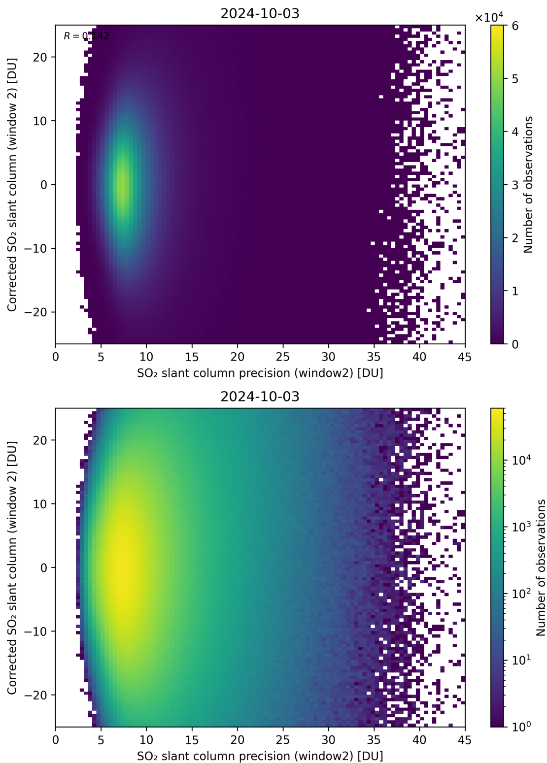
Figure 247: Scatter density plot of “SO 2 slant column precision (window2)” against “Corrected SO 2 slant column (window 2)” for 2024-10-03 to 2024-10-04.
