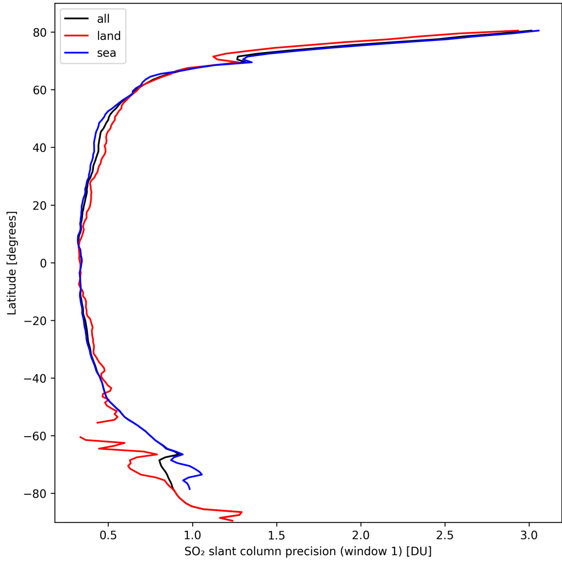
Figure 34: Zonal average of “SO 2 slant column precision (window 1)” for 2024-10-03 to 2024-10-04.
