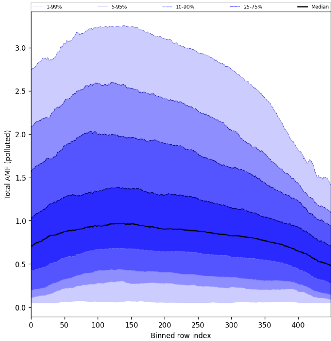
Figure 94: Along track statistics of “Total AMF (polluted)” for 2024-10-03 to 2024-10-04
