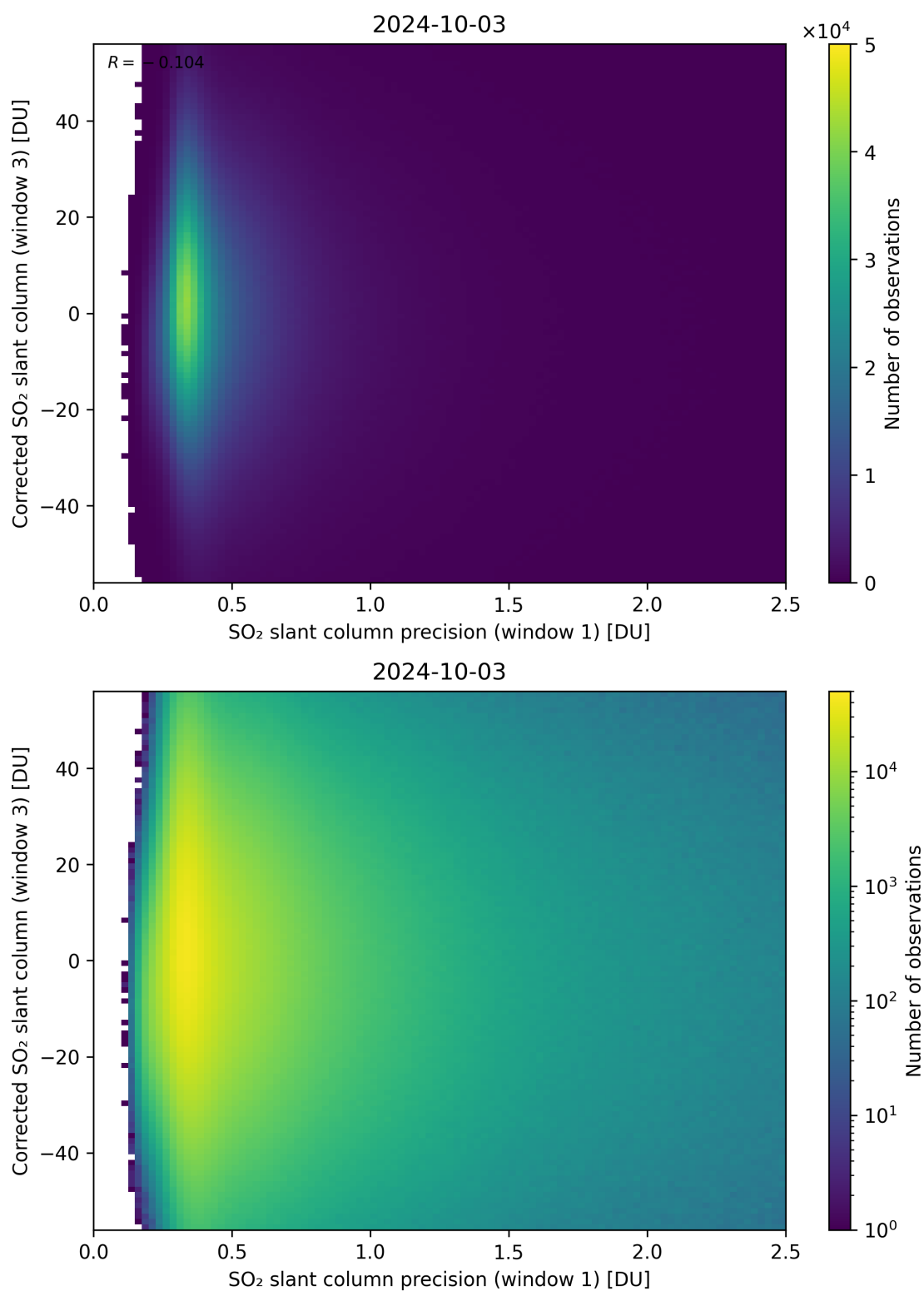
Figure 226: Scatter density plot of “SO 2 slant column precision (window 1)” against “Corrected SO 2 slant column (window 3)” for 2024-10-03 to 2024-10-04.
