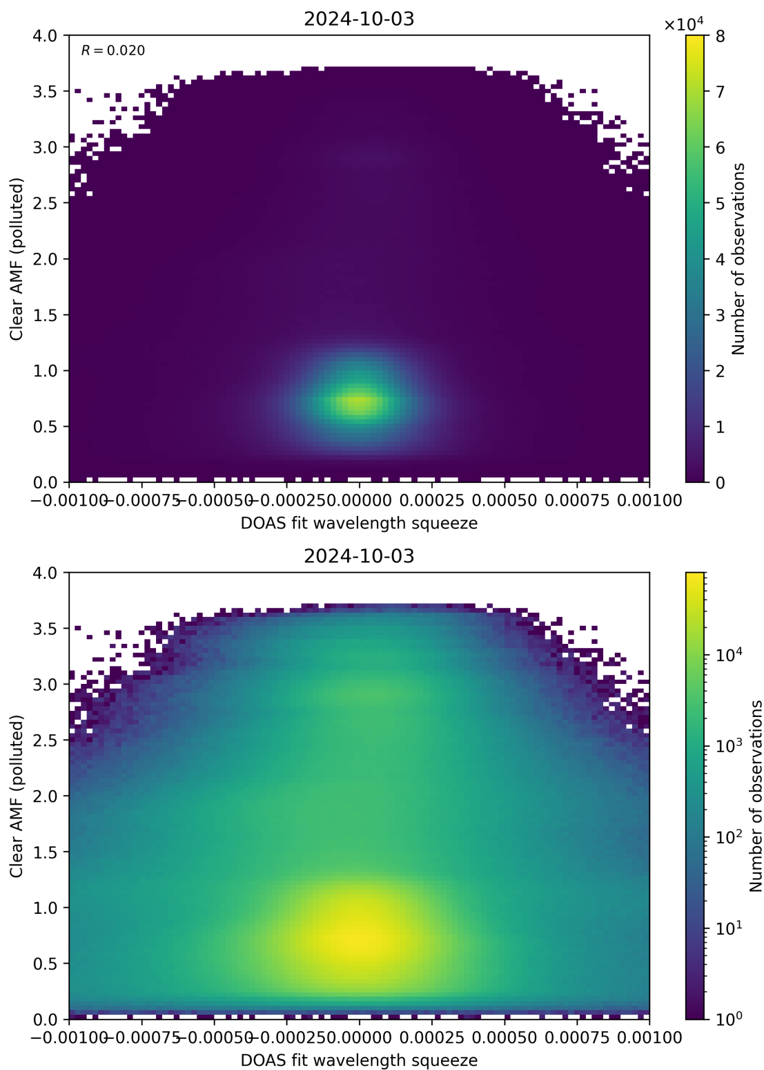
Figure 133: Scatter density plot of “DOAS fit wavelength squeeze” against “Clear AMF (polluted)” for 2024-10-03 to 2024-10-04.
