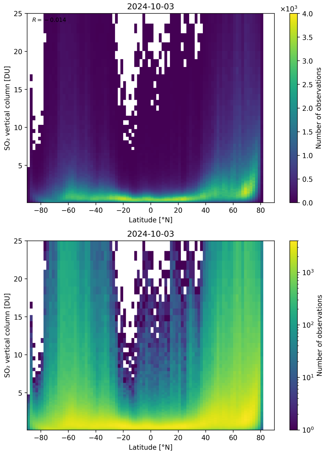
Figure 156: Scatter density plot of “Latitude” against “SO 2 vertical column” for 2024-10-03 to 2024-10-04.
