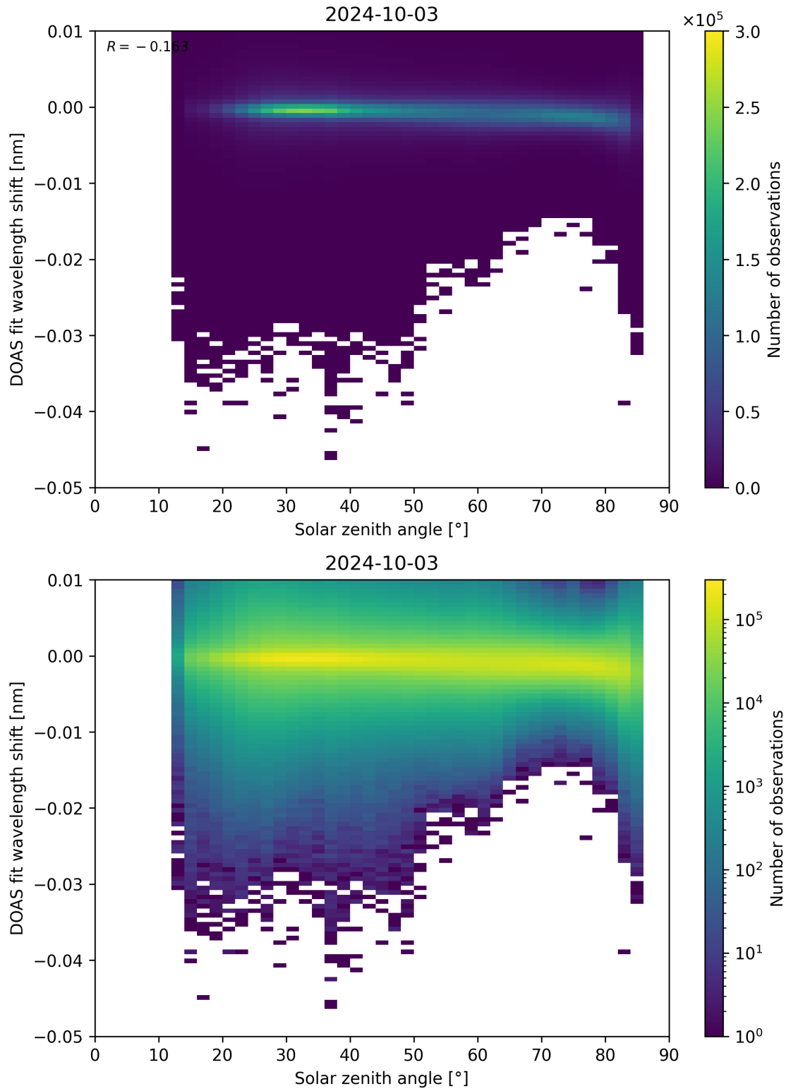
Figure 161: Scatter density plot of “Solar zenith angle” against “DOAS fit wavelength shift” for 2024-10-03 to 2024-10-04.
