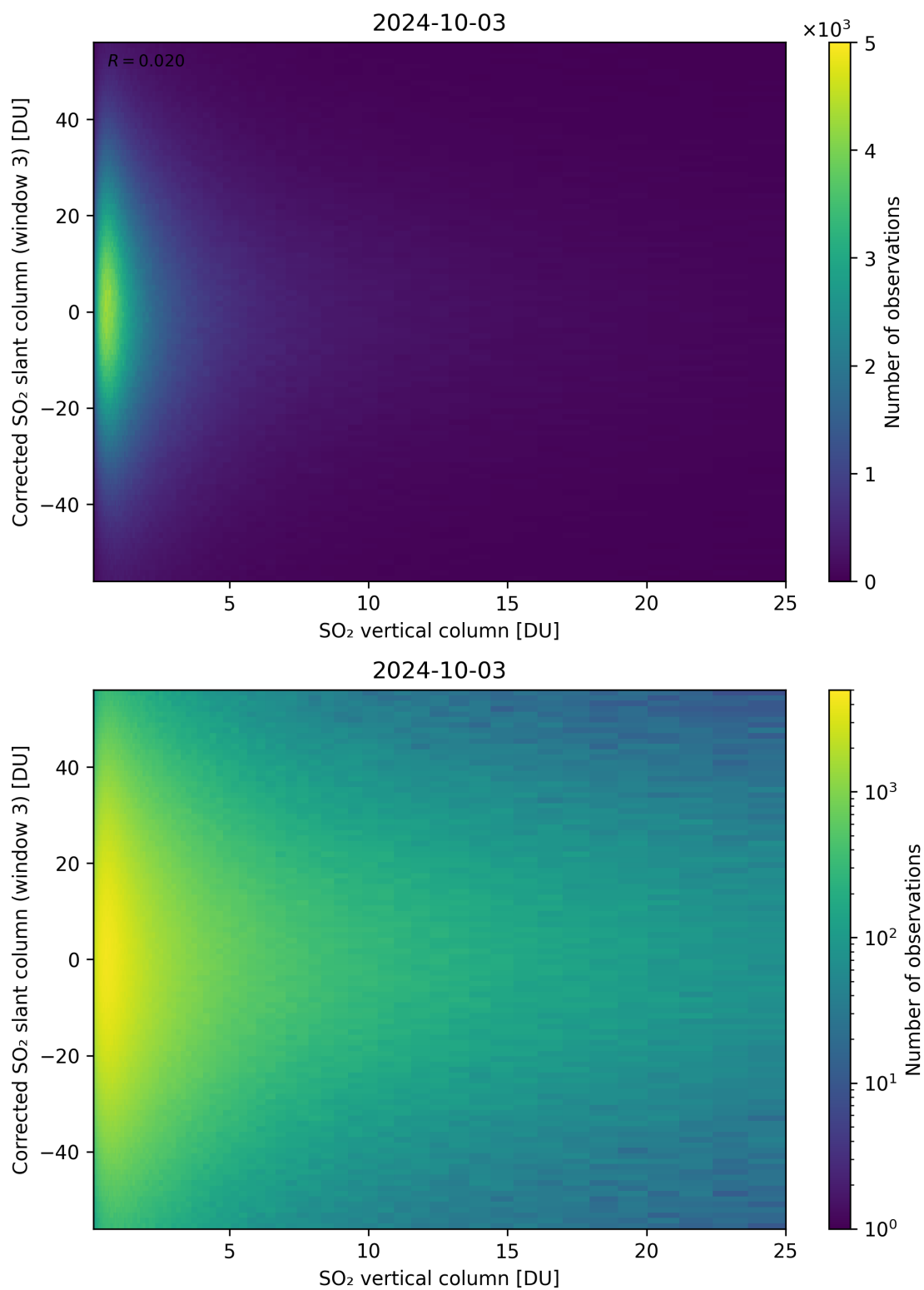
Figure 299: Scatter density plot of “SO 2 vertical column” against “Corrected SO 2 slant column (window 3)” for 2024-10-03 to 2024-10-04.
