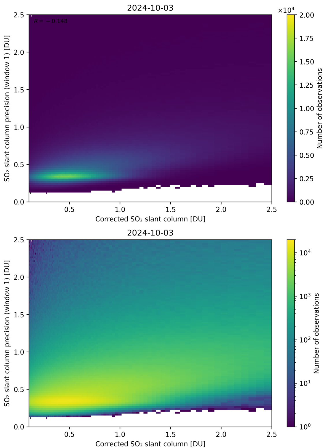
Figure 188: Scatter density plot of “Corrected SO 2 slant column” against “SO 2 slant column precision (window 1)” for 2024-10-03 to 2024-10-04.
