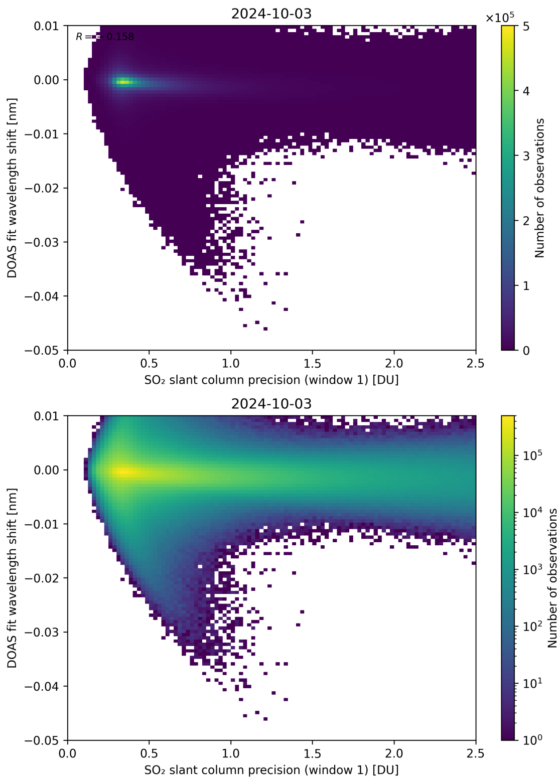
Figure 221: Scatter density plot of “SO 2 slant column precision (window 1)” against “DOAS fit wavelength shift” for 2024-10-03 to 2024-10-04.
