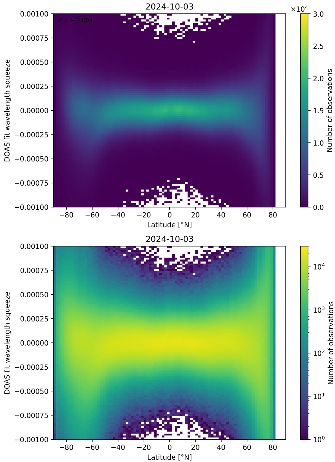
Figure 143: Scatter density plot of “Latitude” against “DOAS fit wavelength squeeze” for 2024-10-03 to 2024-10-04.
