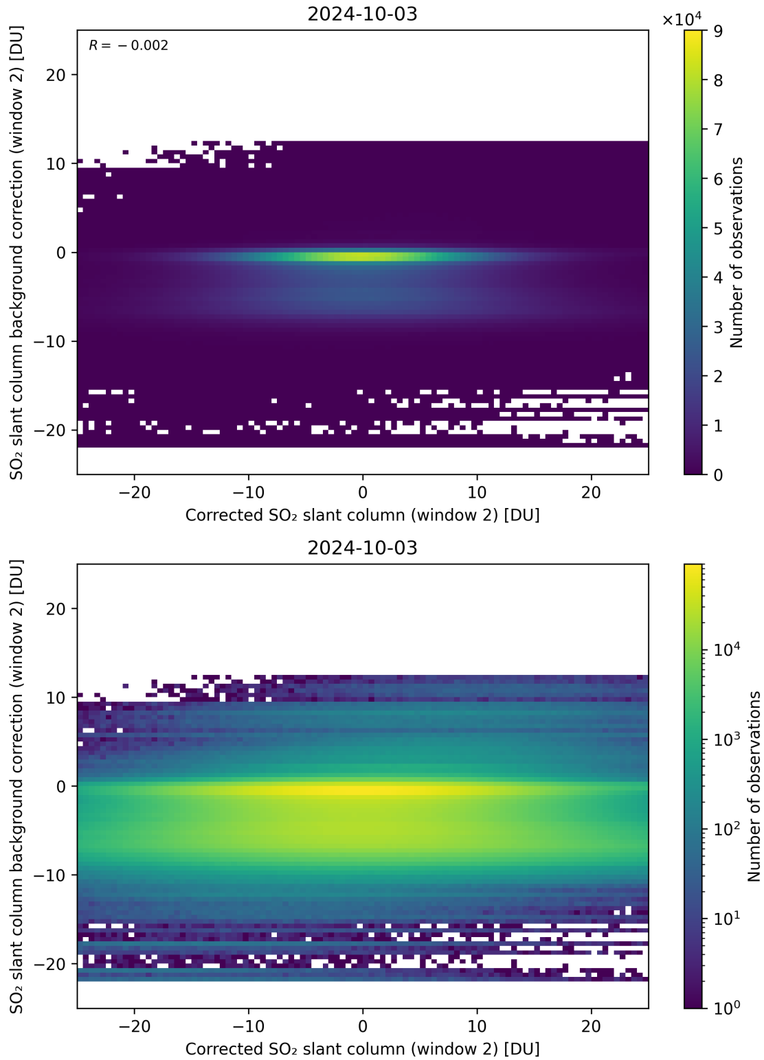
Figure 194: Scatter density plot of “Corrected SO 2 slant column (window 2)” against “SO 2 slant column background correction (window 2)” for 2024-10-03 to 2024-10-04.
