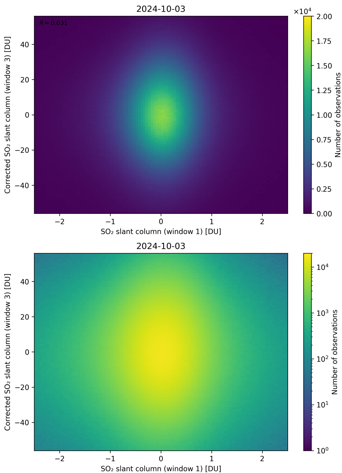
Figure 234: Scatter density plot of “SO 2 slant column (window 1)” against “Corrected SO 2 slant column (window 3)” for 2024-10-03 to 2024-10-04.
