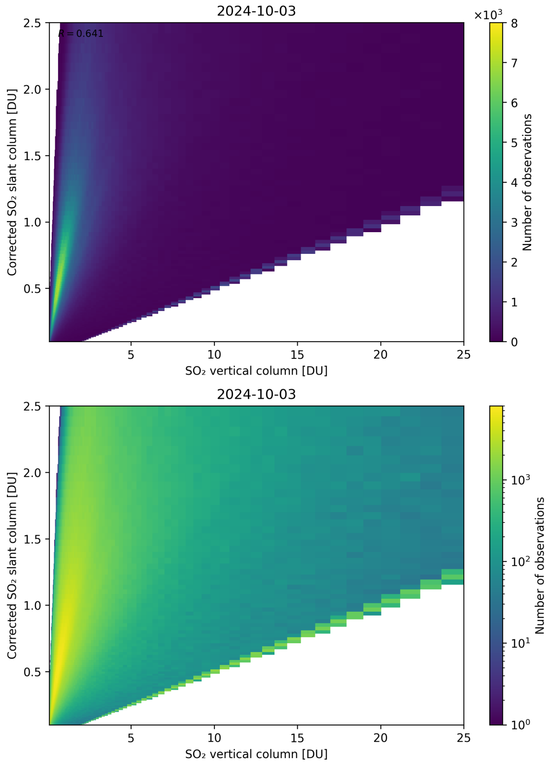
Figure 297: Scatter density plot of “SO 2 vertical column” against “Corrected SO 2 slant column” for 2024-10-03 to 2024-10-04.
