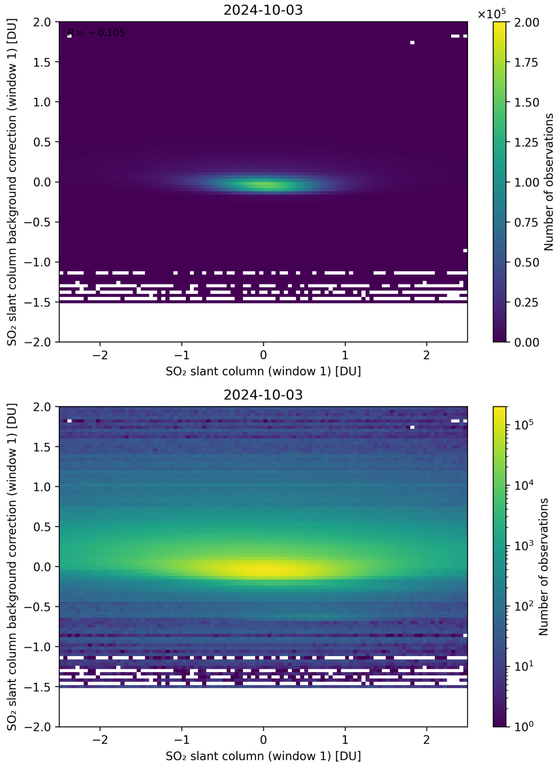
Figure 212: Scatter density plot of “SO 2 slant column (window 1)” against “SO 2 slant column background correction (window 1)” for 2024-10-03 to 2024-10-04.
