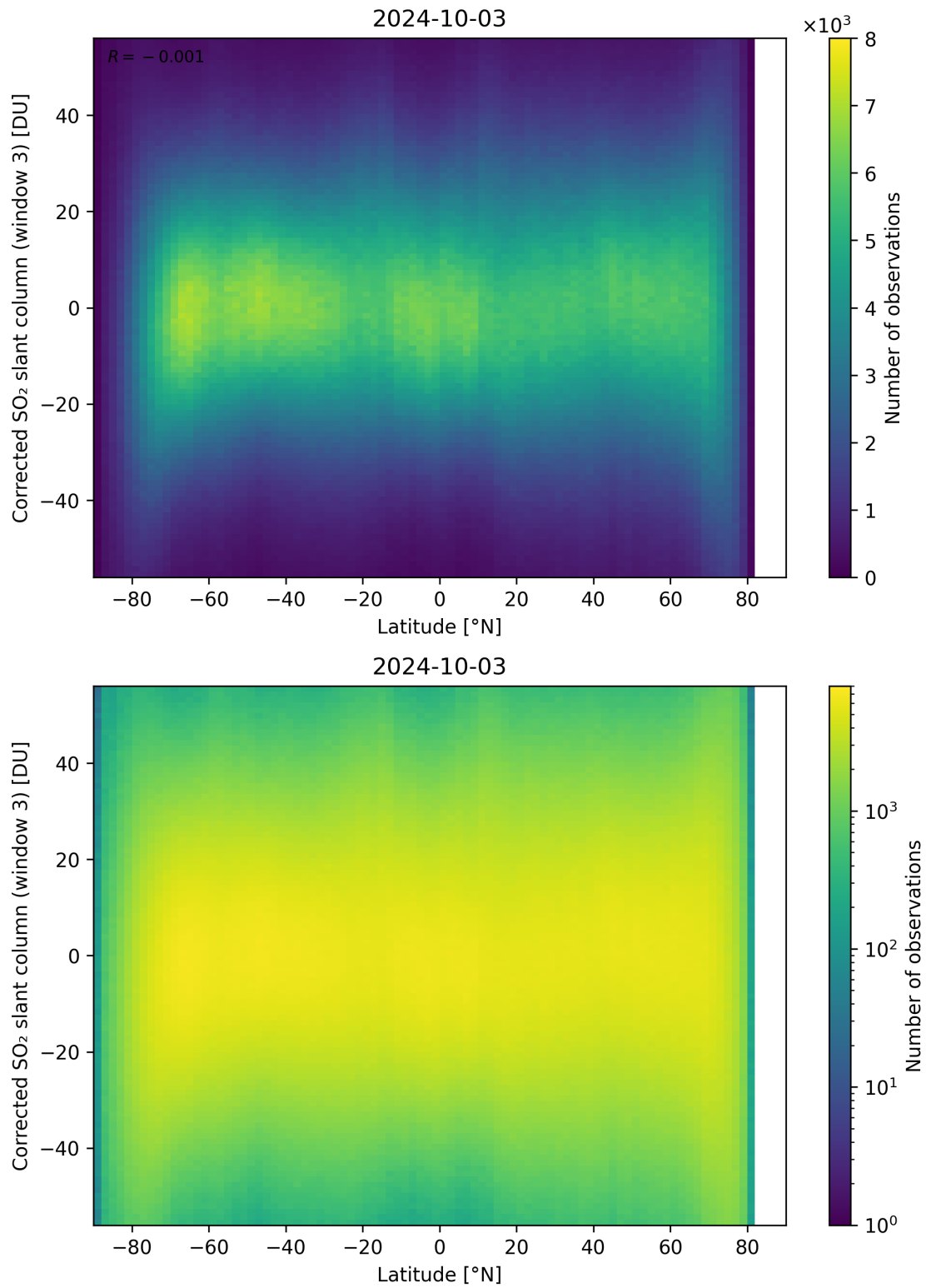
Figure 148: Scatter density plot of “Latitude” against “Corrected SO 2 slant column (window 3)” for 2024-10-03 to 2024-10-04.
