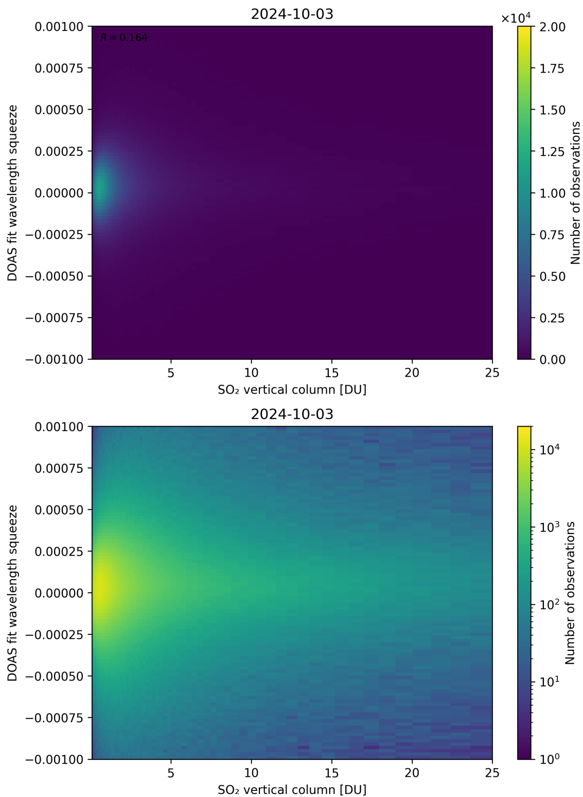
Figure 277: Scatter density plot of “SO 2 vertical column” against “DOAS fit wavelength squeeze” for 2024-10-03 to 2024-10-04.
