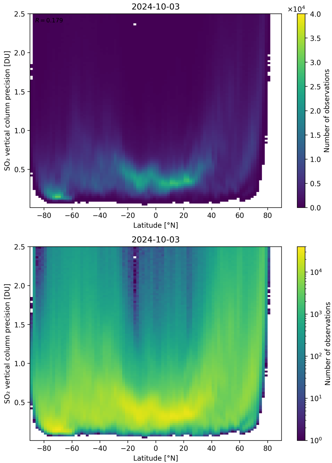
Figure 157: Scatter density plot of “Latitude” against “SO 2 vertical column precision” for 2024-10-03 to 2024-10-04.
