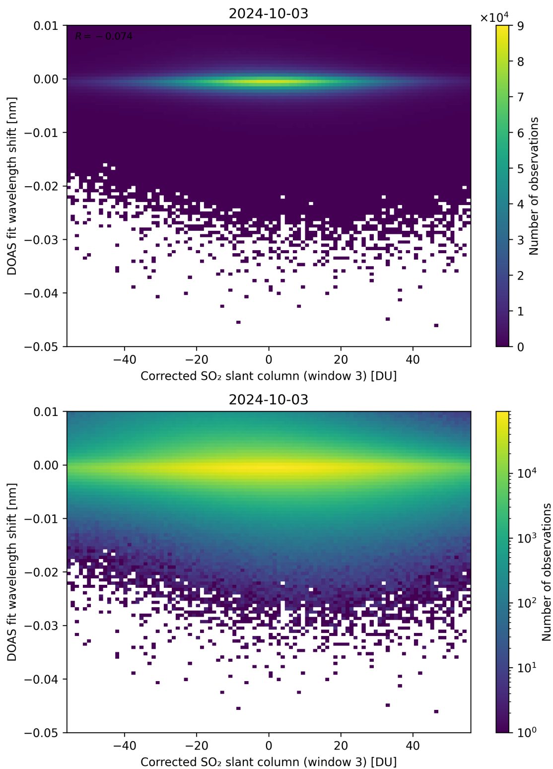
Figure 206: Scatter density plot of “Corrected SO 2 slant column (window 3)” against “DOAS fit wavelength shift” for 2024-10-03 to 2024-10-04.
