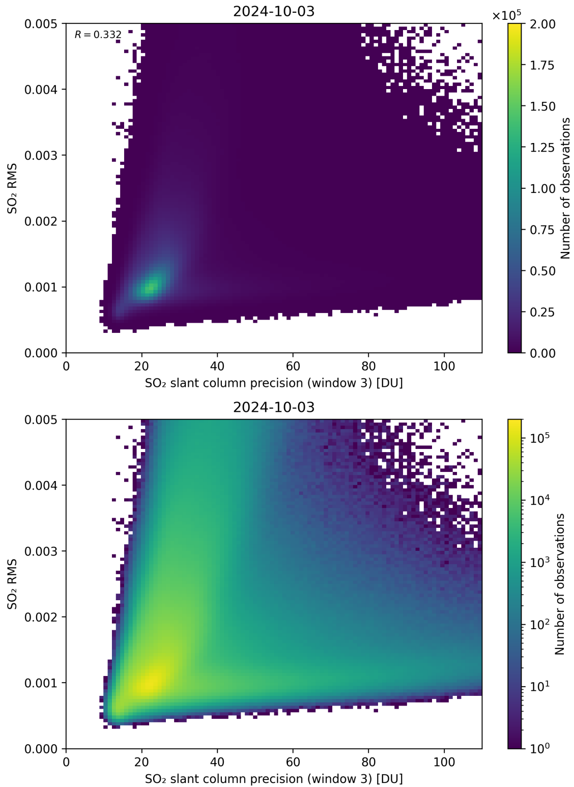
Figure 260: Scatter density plot of “SO 2 slant column precision (window 3)” against “SO 2 RMS” for 2024-10-03 to 2024-10-04.
