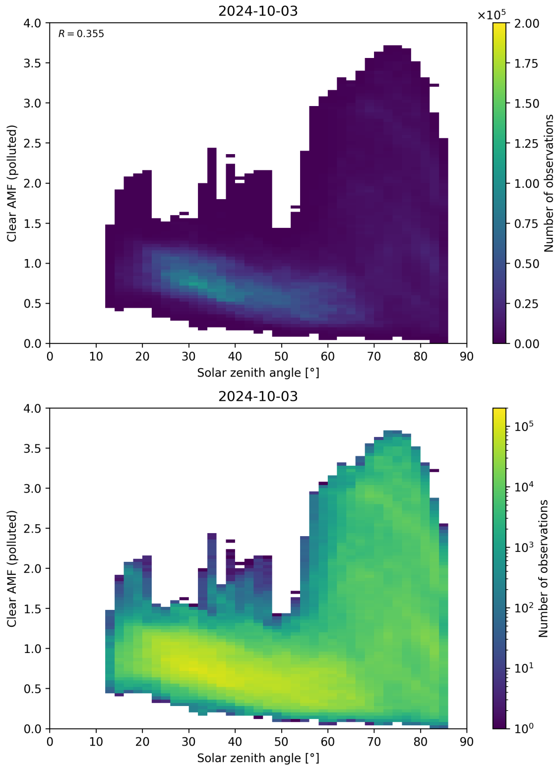
Figure 165: Scatter density plot of “Solar zenith angle” against “Clear AMF (polluted)” for 2024-10-03 to 2024-10-04.
