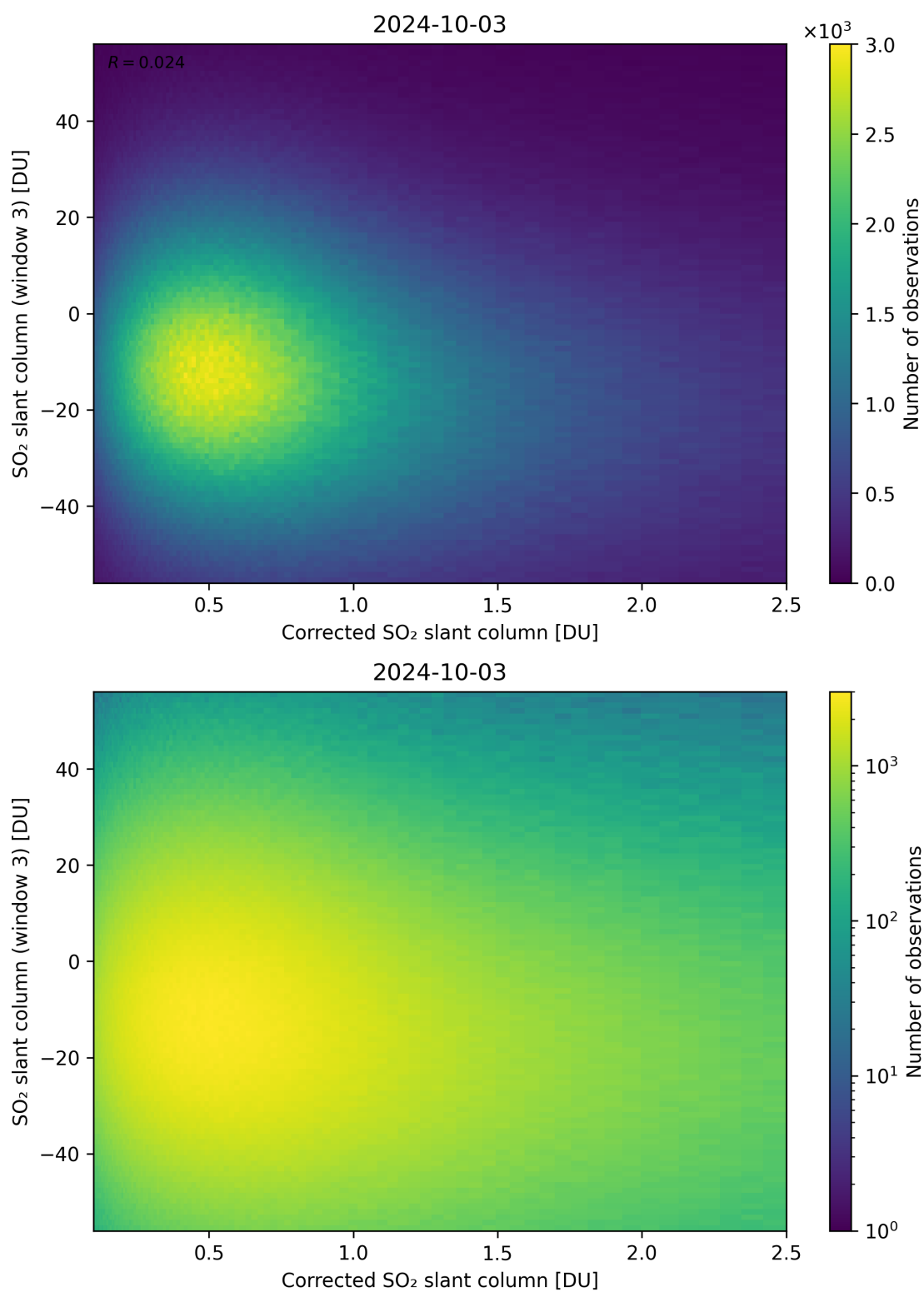
Figure 190: Scatter density plot of “Corrected SO 2 slant column” against “SO 2 slant column (window 3)” for 2024-10-03 to 2024-10-04.
