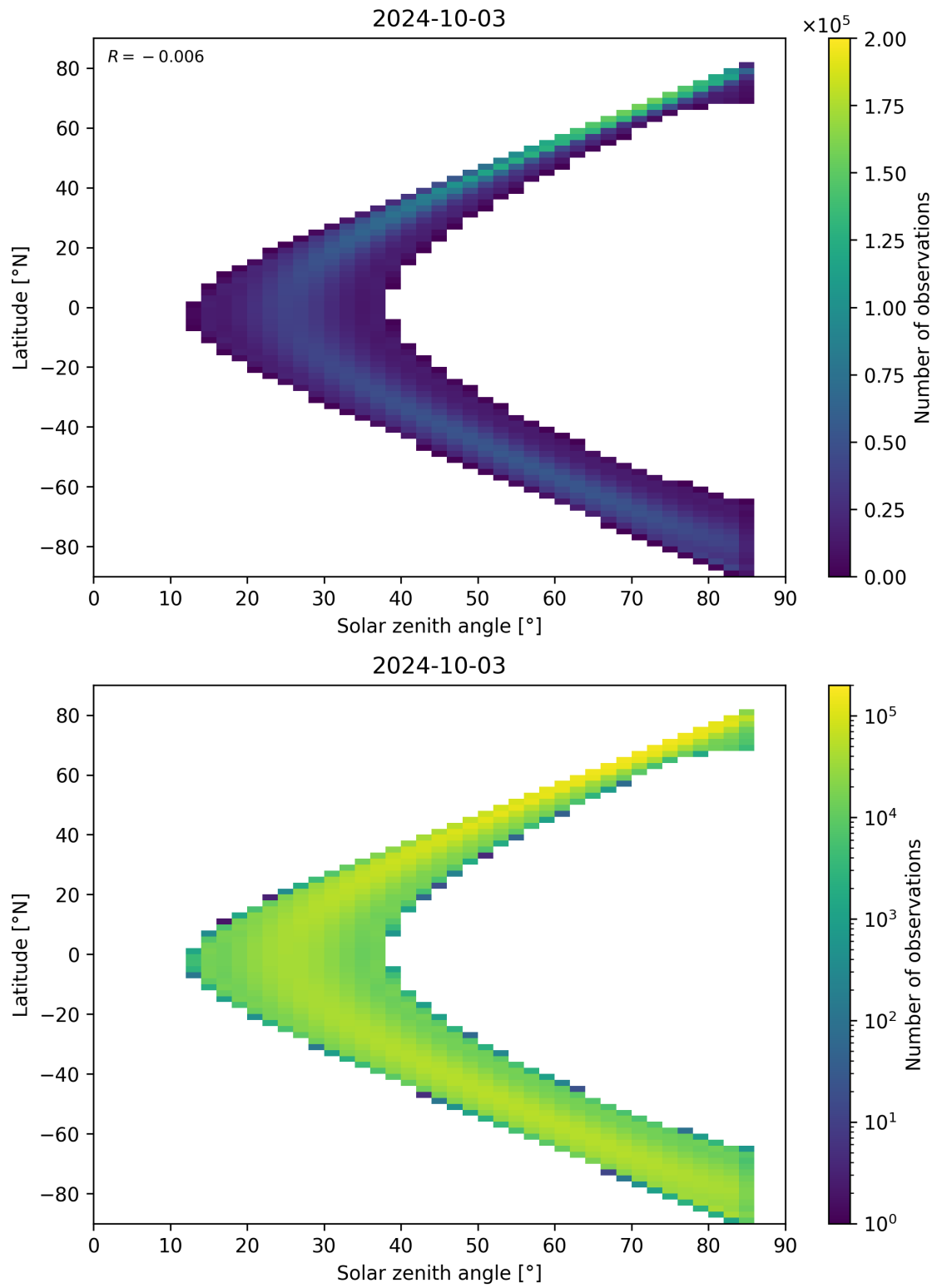
Figure 164: Scatter density plot of “Solar zenith angle” against “Latitude” for 2024-10-03 to 2024-10-04.
