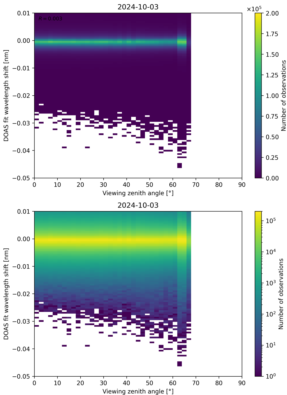
Figure 311: Scatter density plot of “Viewing zenith angle” against “DOAS fit wavelength shift” for 2024-10-03 to 2024-10-04.
