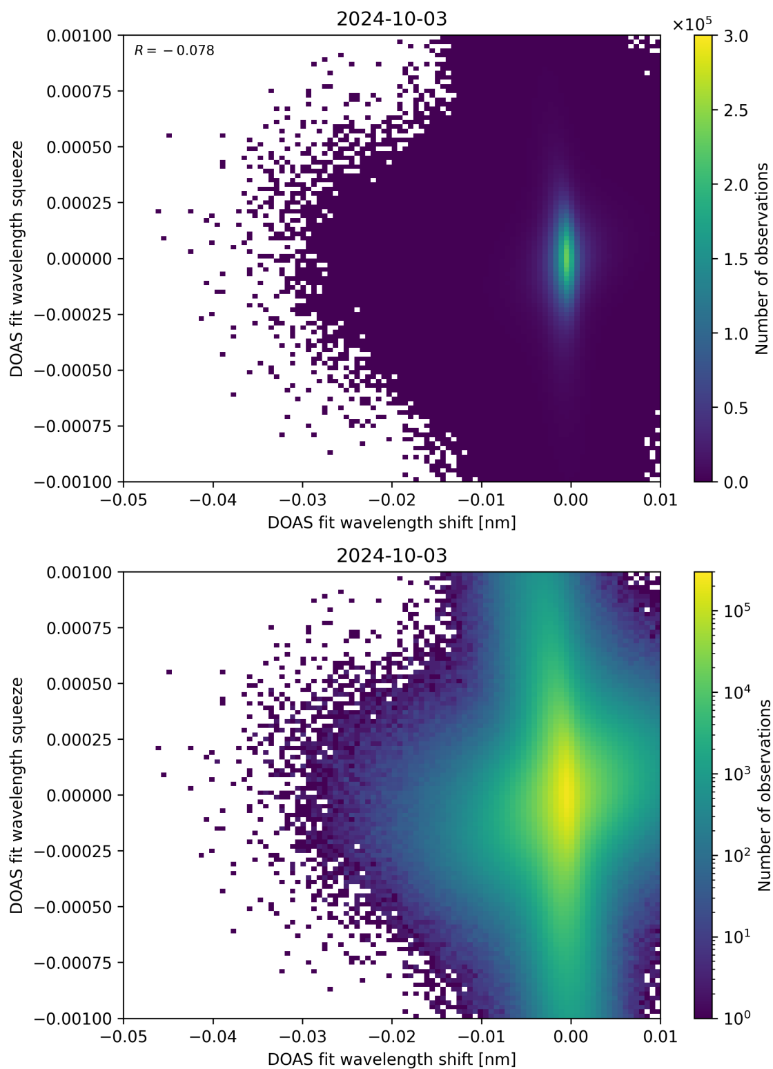
Figure 127: Scatter density plot of “DOAS fit wavelength shift” against “DOAS fit wavelength squeeze” for 2024-10-03 to 2024-10-04.
