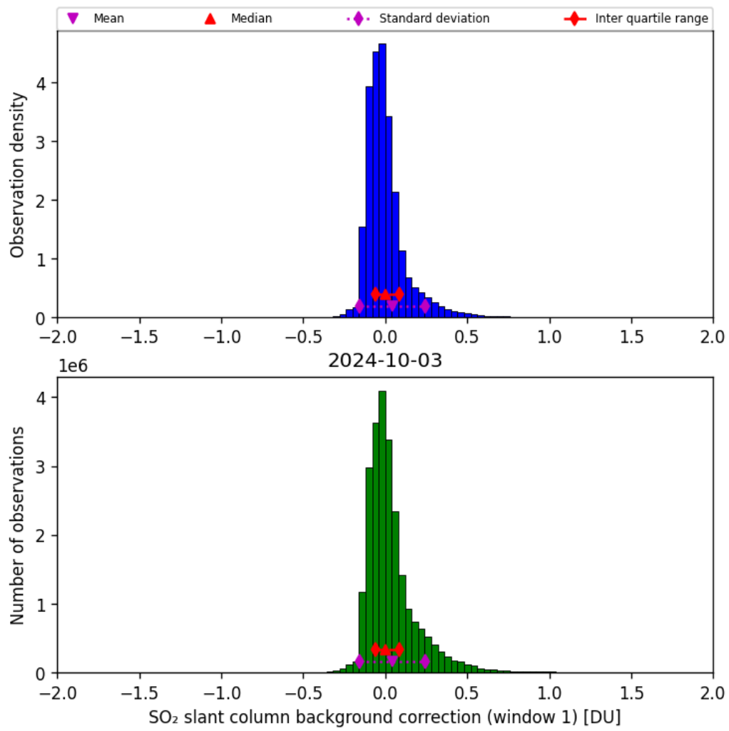
Figure 59: Histogram of “SO 2 slant column background correction (window 1)” for 2024-10-03 to 2024-10-04
