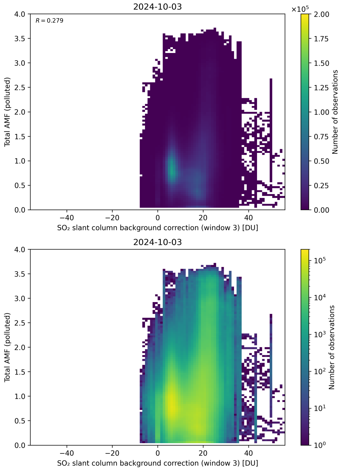
Figure 125: Scatter density plot of “SO 2 slant column background correction (window 3)” against “Total AMF (polluted)” for 2024-10-03 to 2024-10-04.
