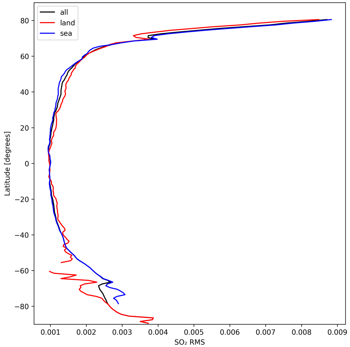
Figure 47: Zonal average of “SO 2 RMS” for 2024-10-03 to 2024-10-04.
