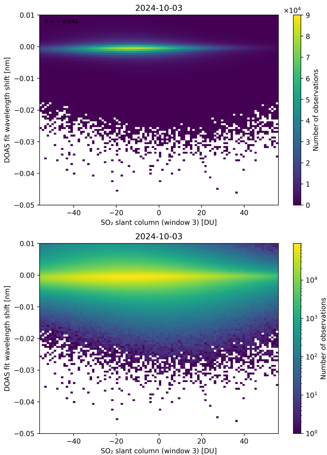
Figure 254: Scatter density plot of “SO 2 slant column (window 3)” against “DOAS fit wavelength shift” for 2024-10-03 to 2024-10-04.
