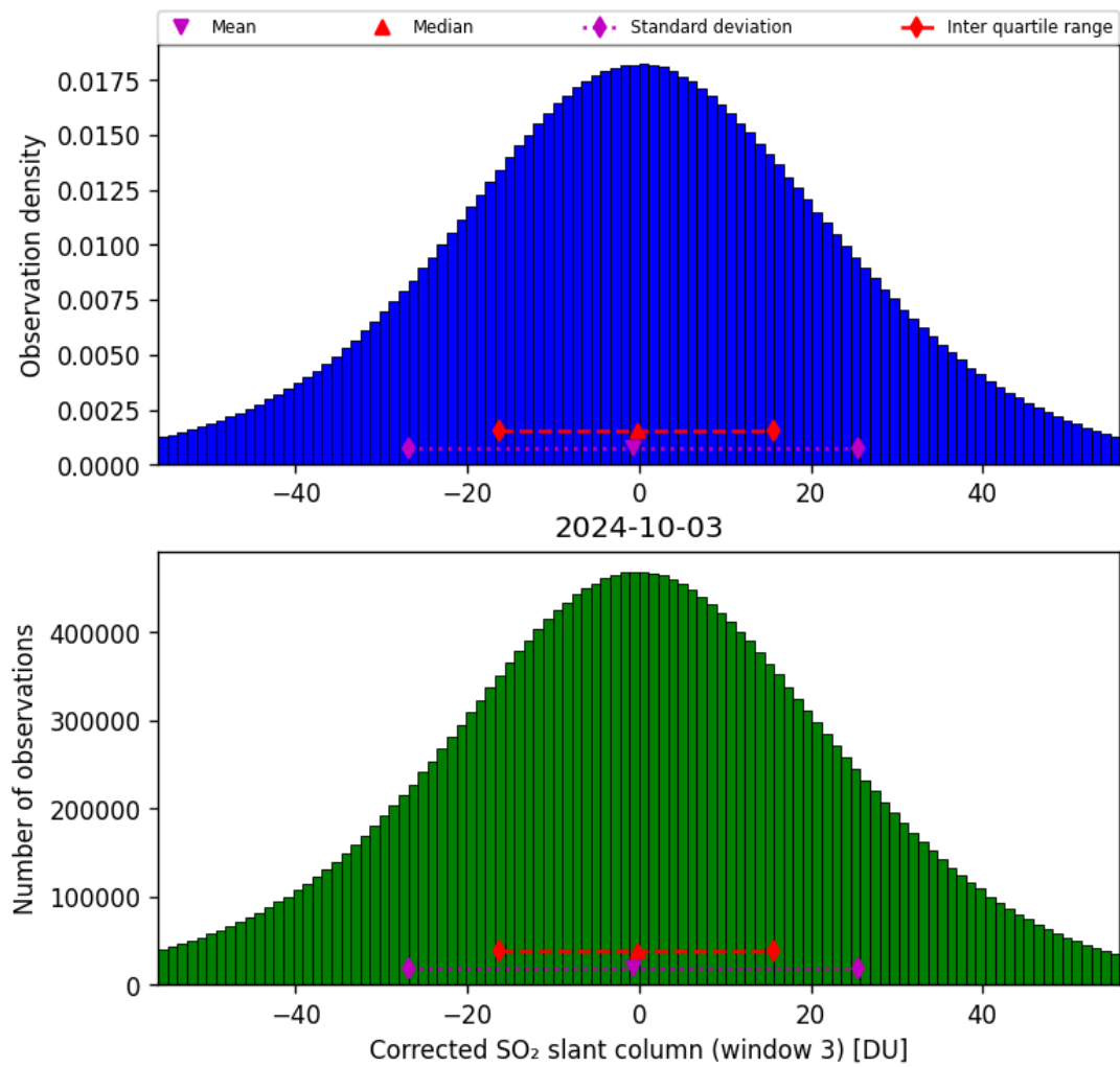
Figure 66: Histogram of “Corrected SO 2 slant column (window 3)” for 2024-10-03 to 2024-10-04
