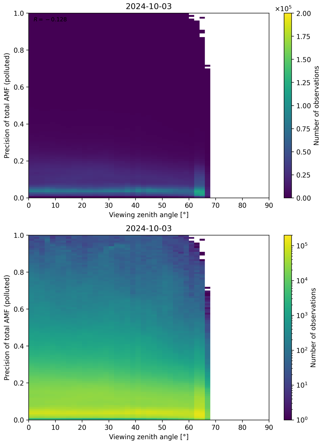
Figure 326: Scatter density plot of “Viewing zenith angle” against “Precision of total AMF (polluted)” for 2024-10-03 to 2024-10-04.
