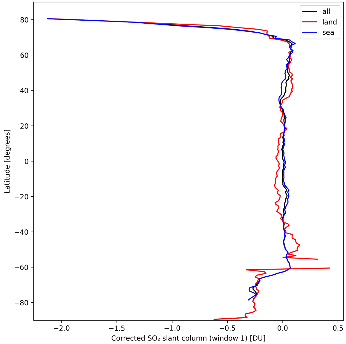
Figure 35: Zonal average of “Corrected SO 2 slant column (window 1)” for 2024-10-03 to 2024-10-04.
