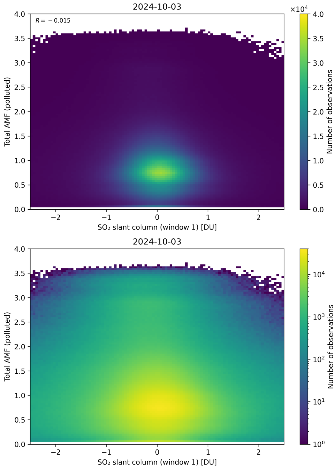
Figure 239: Scatter density plot of “SO 2 slant column (window 1)” against “Total AMF (polluted)” for 2024-10-03 to 2024-10-04.
