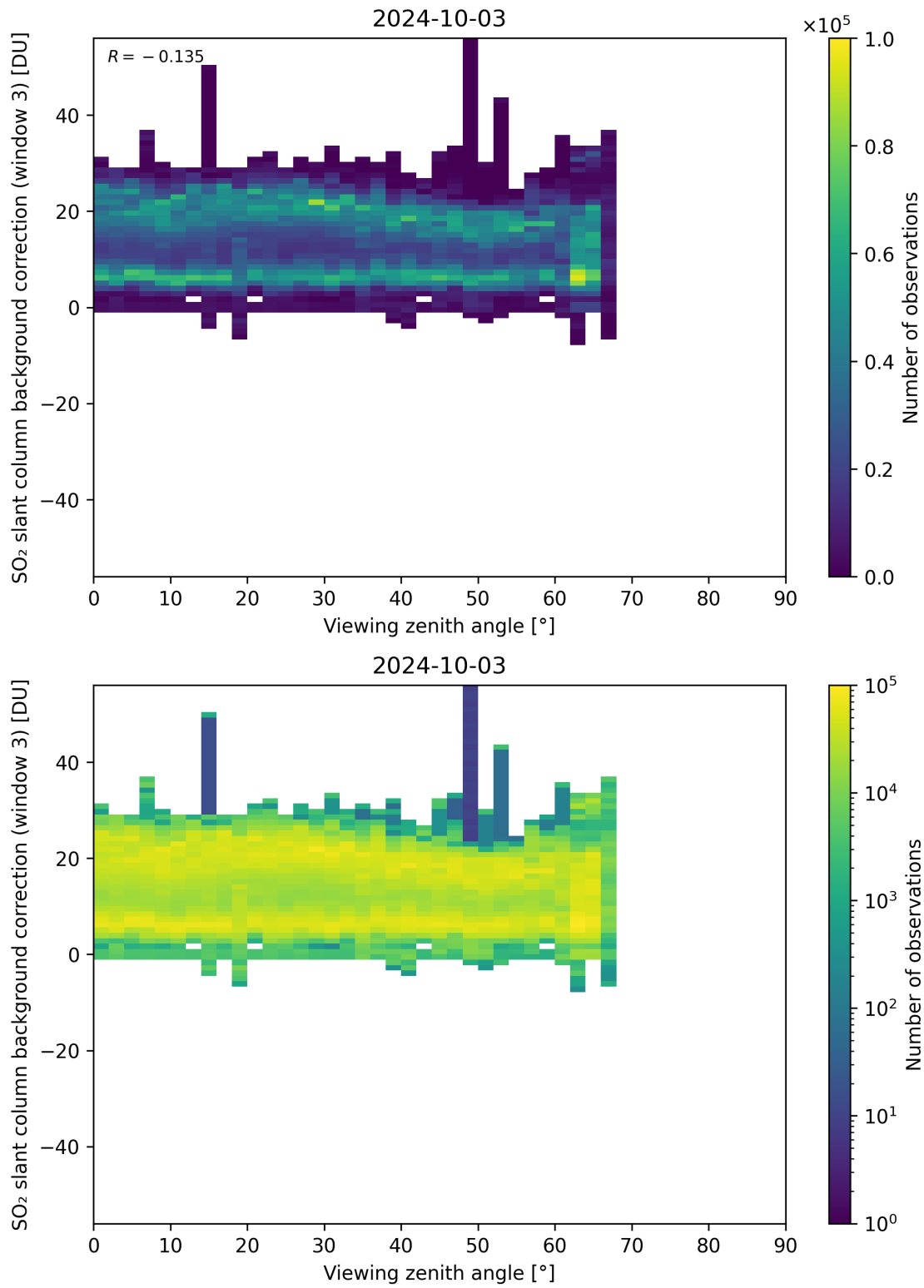
Figure 310: Scatter density plot of “Viewing zenith angle” against “SO 2 slant column background correction (window 3)” for 2024-10-03 to 2024-10-04.
