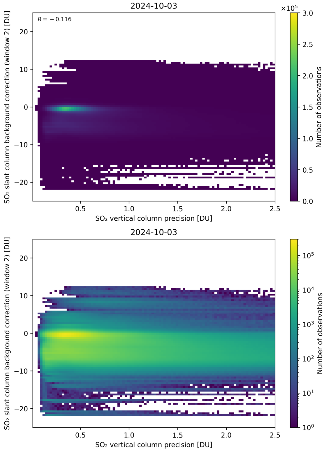
Figure 280: Scatter density plot of “SO 2 vertical column precision” against “SO 2 slant column background correction (window 2)” for 2024-10-03 to 2024-10-04.
