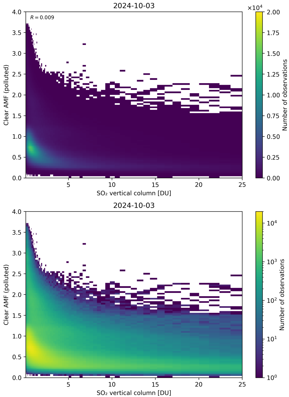
Figure 296: Scatter density plot of “SO 2 vertical column” against “Clear AMF (polluted)” for 2024-10-03 to 2024-10-04.
