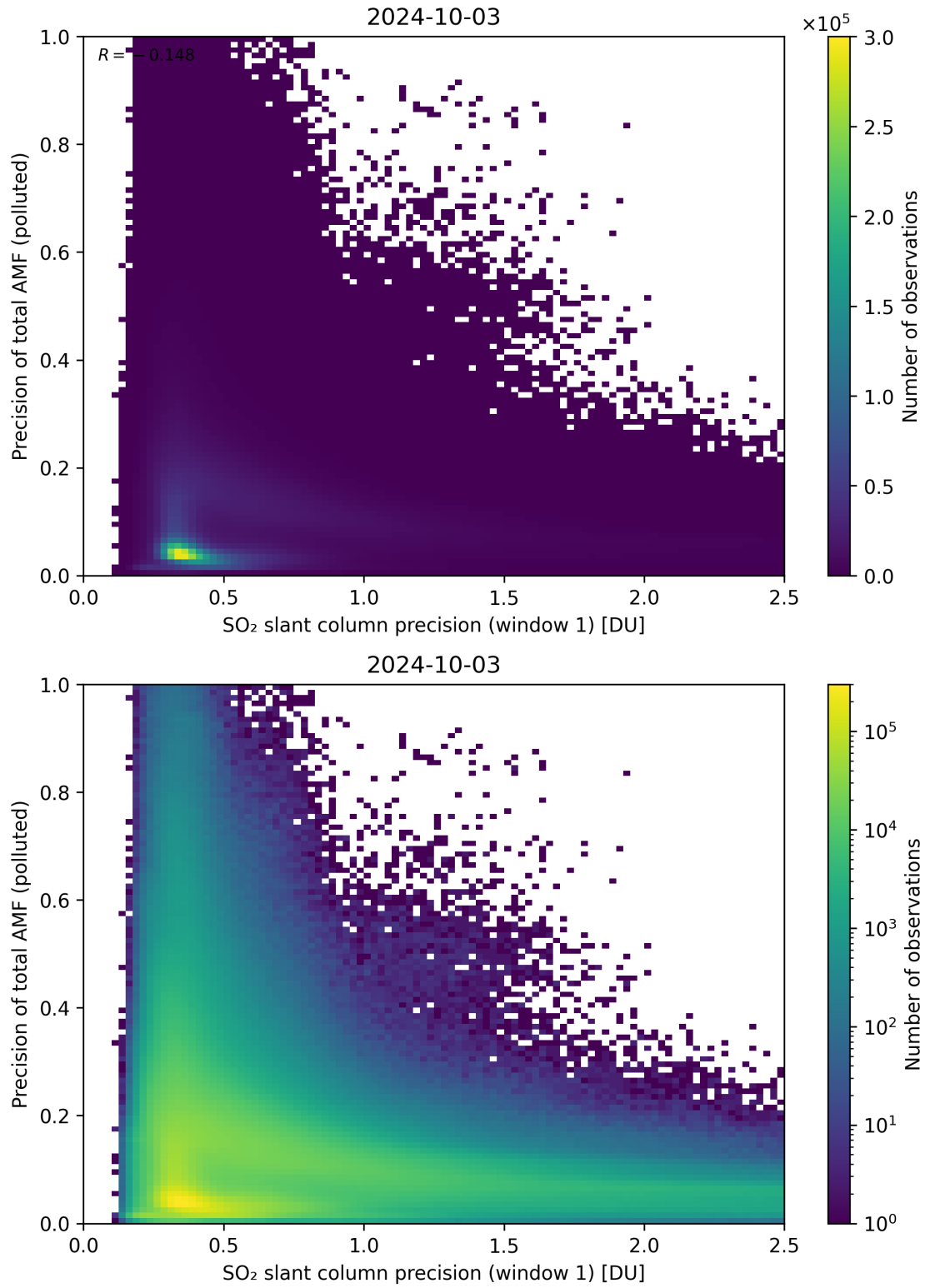
Figure 231: Scatter density plot of “SO 2 slant column precision (window 1)” against “Precision of total AMF (polluted)” for 2024-10-03 to 2024-10-04.
