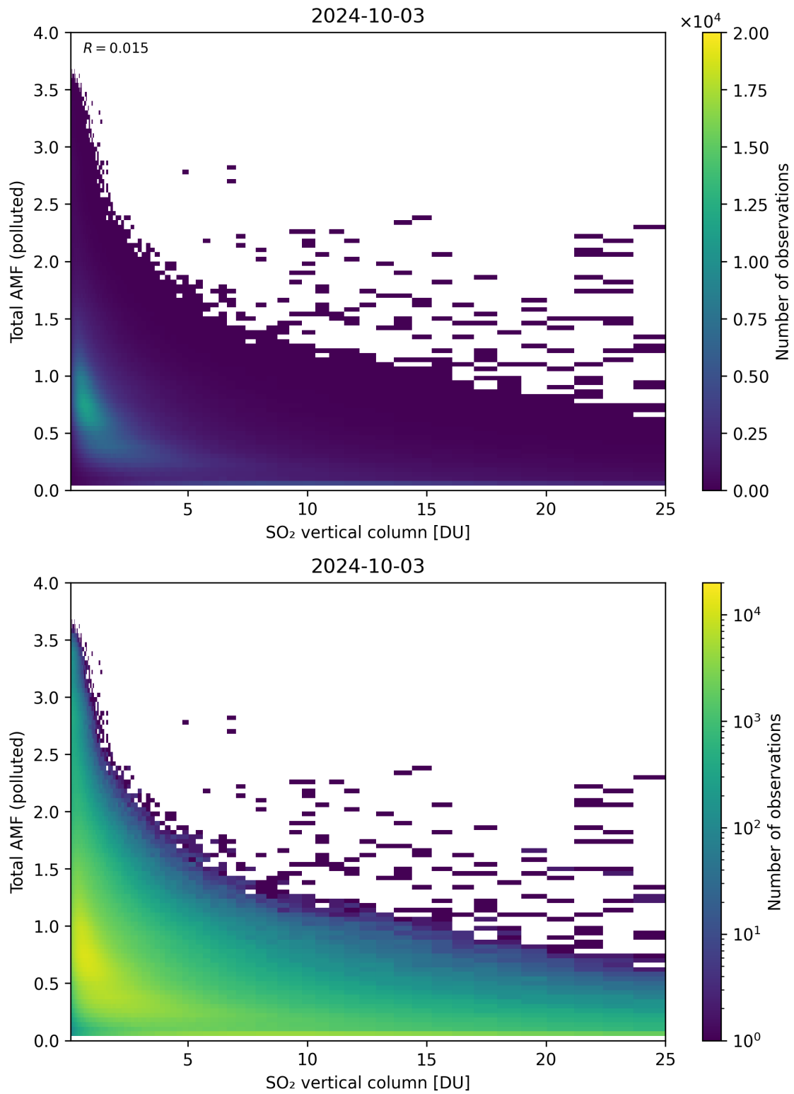
Figure 305: Scatter density plot of “SO 2 vertical column” against “Total AMF (polluted)” for 2024-10-03 to 2024-10-04.
