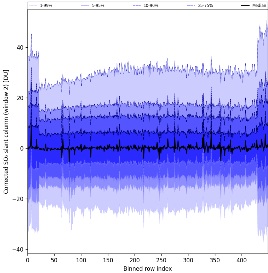
Figure 85: Along track statistics of “Corrected SO 2 slant column (window 2)” for 2024-10-03 to 2024-10-04
