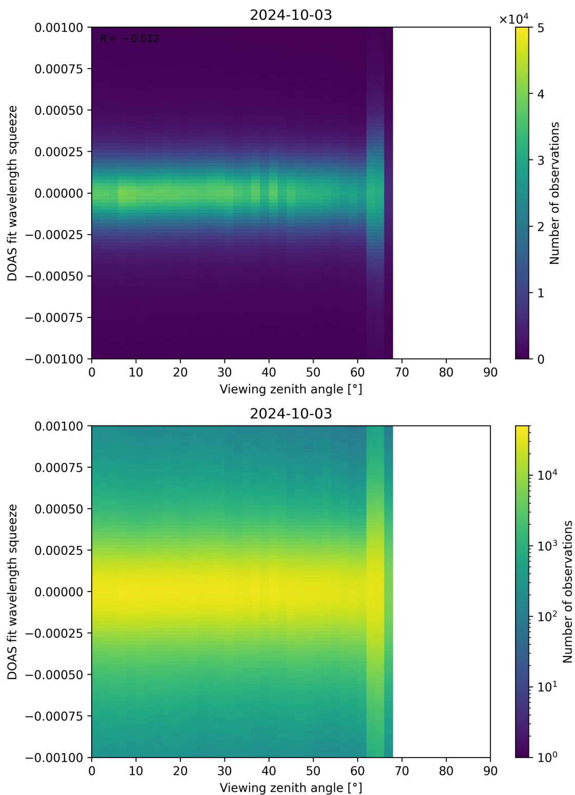
Figure 312: Scatter density plot of “Viewing zenith angle” against “DOAS fit wavelength squeeze” for 2024-10-03 to 2024-10-04.
