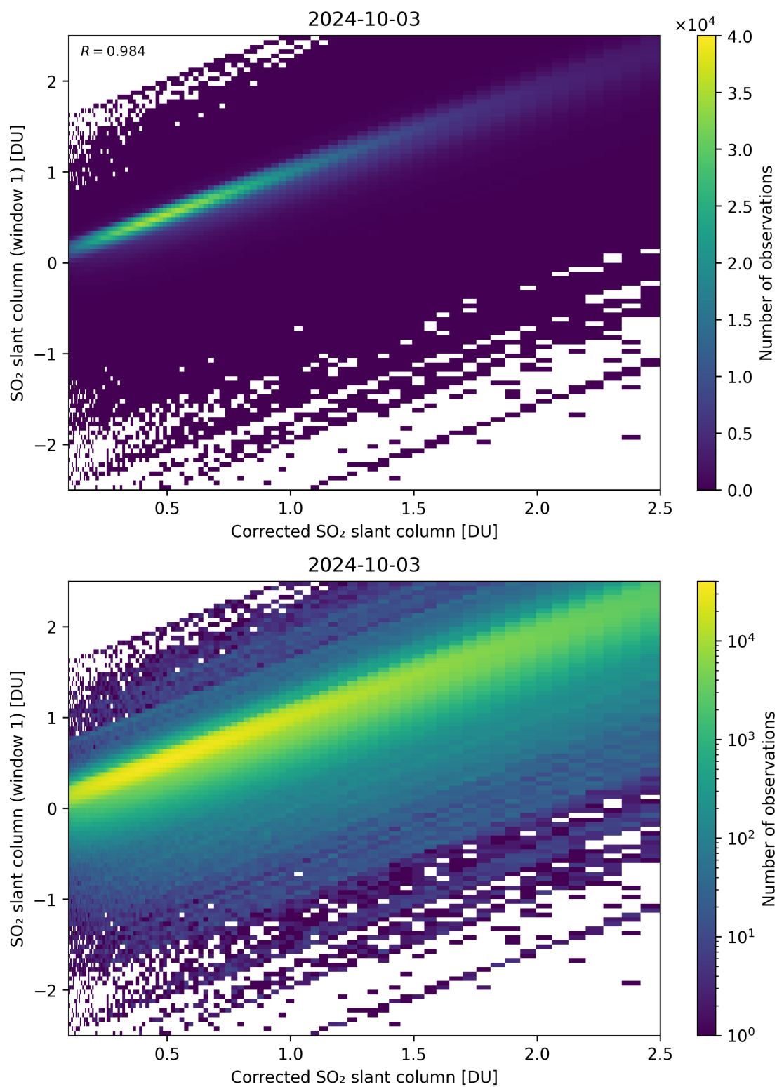
Figure 187: Scatter density plot of “Corrected SO 2 slant column” against “SO 2 slant column (window 1)” for 2024-10-03 to 2024-10-04.
