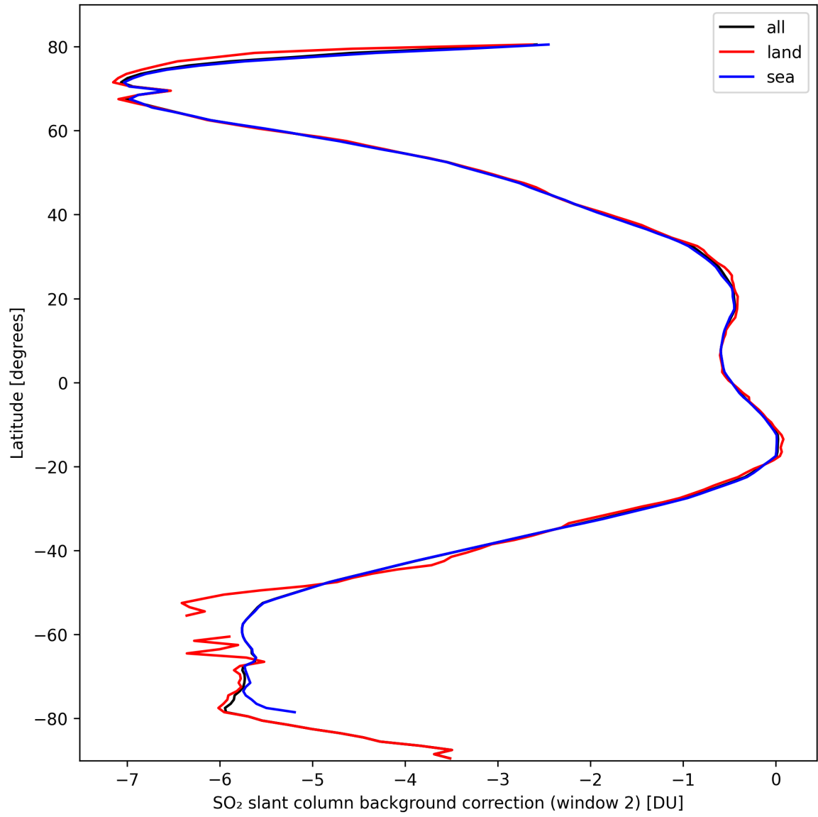
Figure 40: Zonal average of “SO 2 slant column background correction (window 2)” for 2024-10-03 to 2024-10-04.
