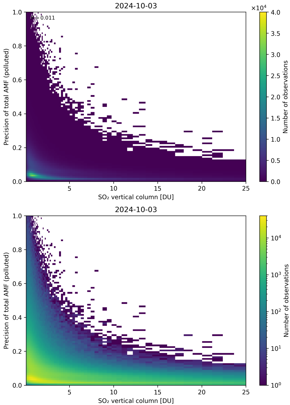
Figure 306: Scatter density plot of “SO 2 vertical column” against “Precision of total AMF (polluted)” for 2024-10-03 to 2024-10-04.
