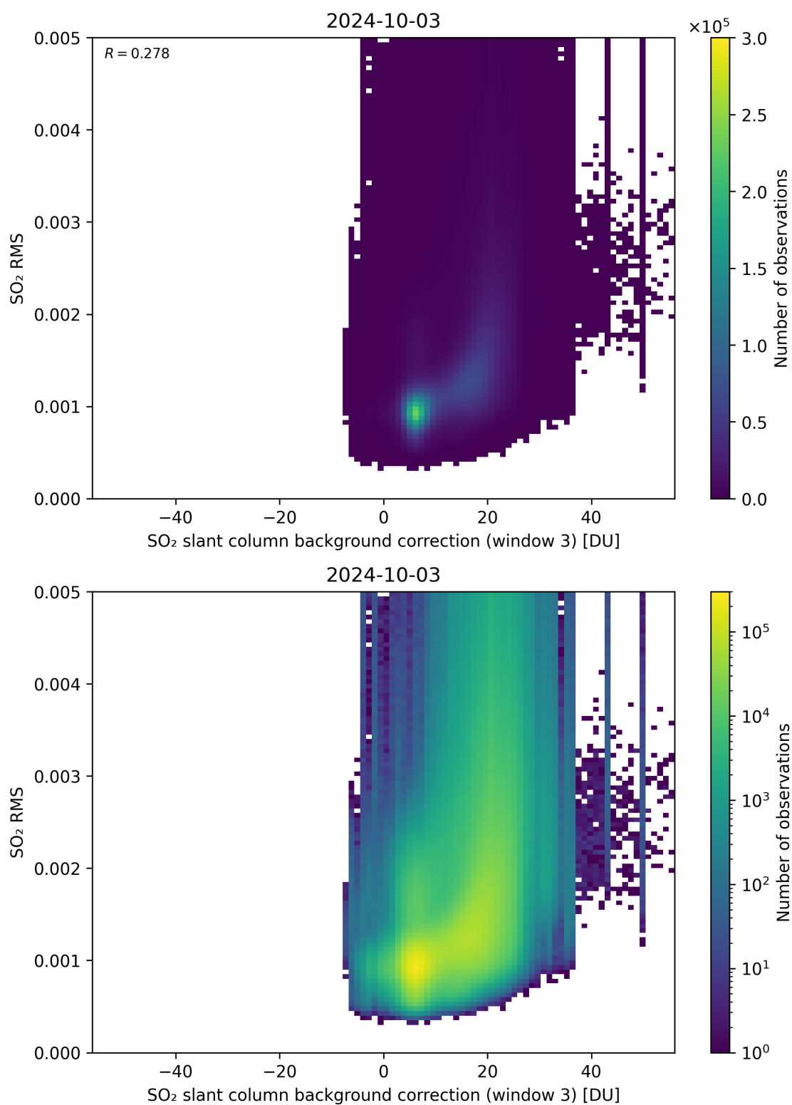
Figure 123: Scatter density plot of “SO 2 slant column background correction (window 3)” against “SO 2 RMS” for 2024-10-03 to 2024-10-04.
