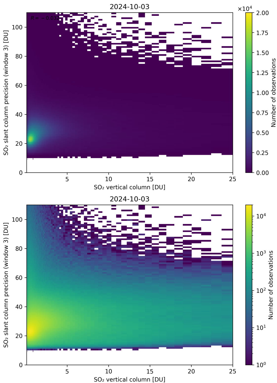
Figure 304: Scatter density plot of “SO 2 vertical column” against “SO 2 slant column precision (window 3)” for 2024-10-03 to 2024-10-04.
