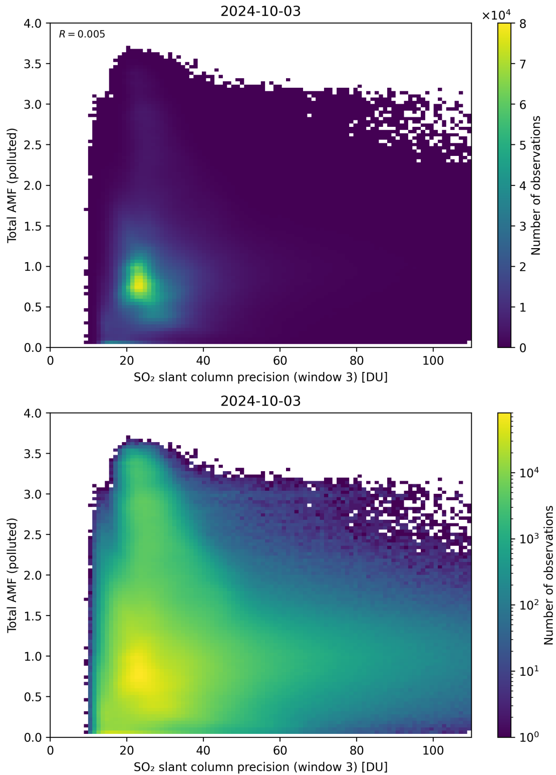
Figure 263: Scatter density plot of “SO 2 slant column precision (window 3)” against “Total AMF (polluted)” for 2024-10-03 to 2024-10-04.
