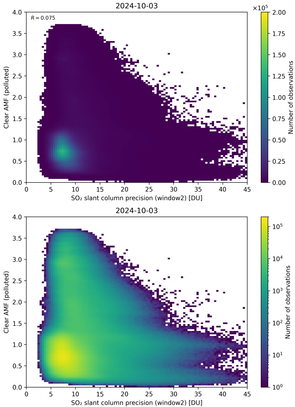
Figure 246: Scatter density plot of “SO 2 slant column precision (window2)” against “Clear AMF (polluted)” for 2024-10-03 to 2024-10-04.
