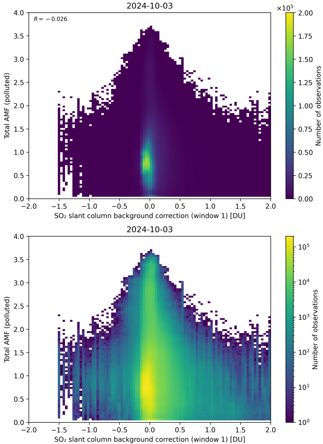
Figure 109: Scatter density plot of “SO 2 slant column background correction (window 1)” against “Total AMF (polluted)” for 2024-10-03 to 2024-10-04.
