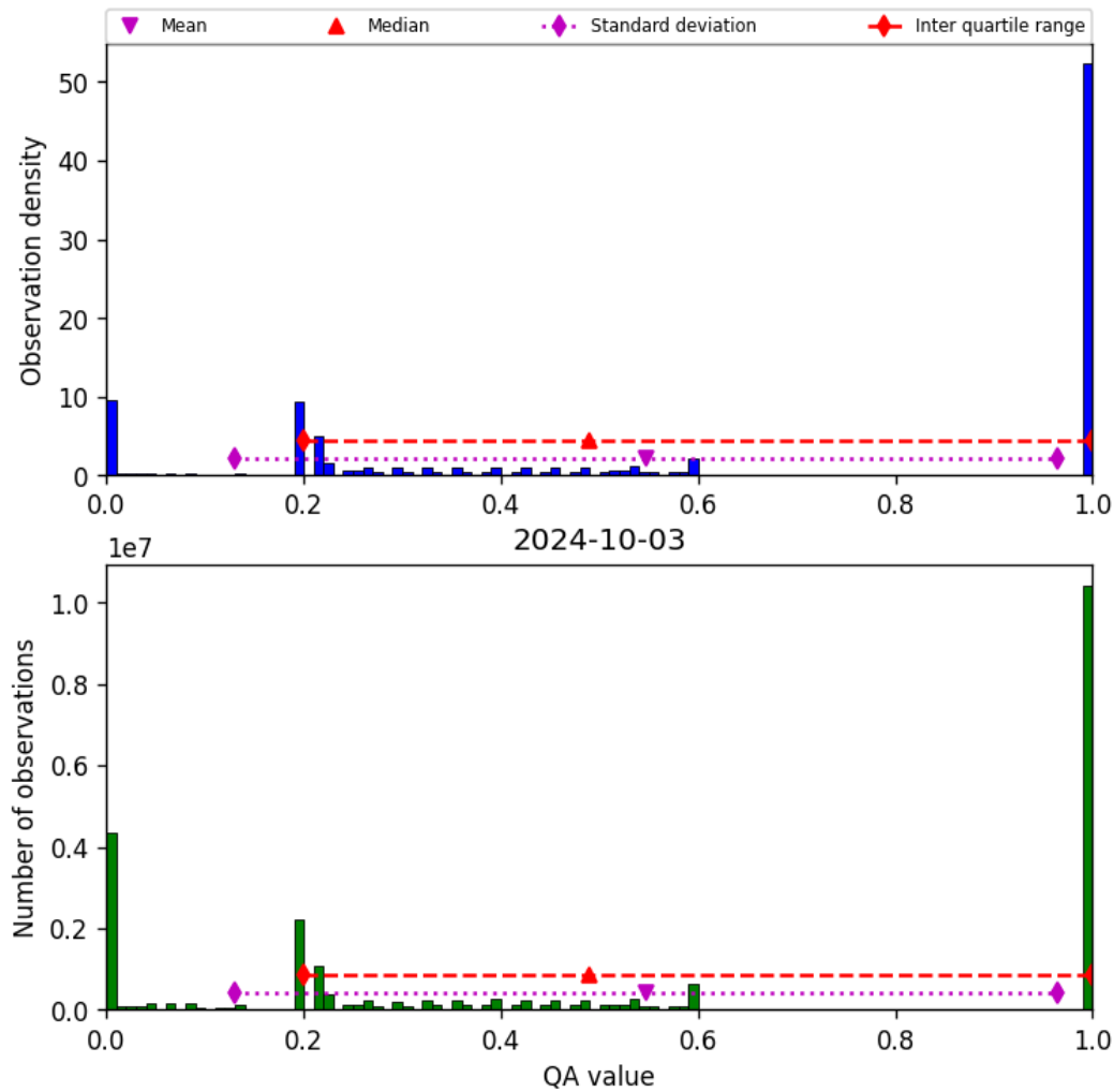
Figure 52: Histogram of “QA value” for 2024-10-03 to 2024-10-04
