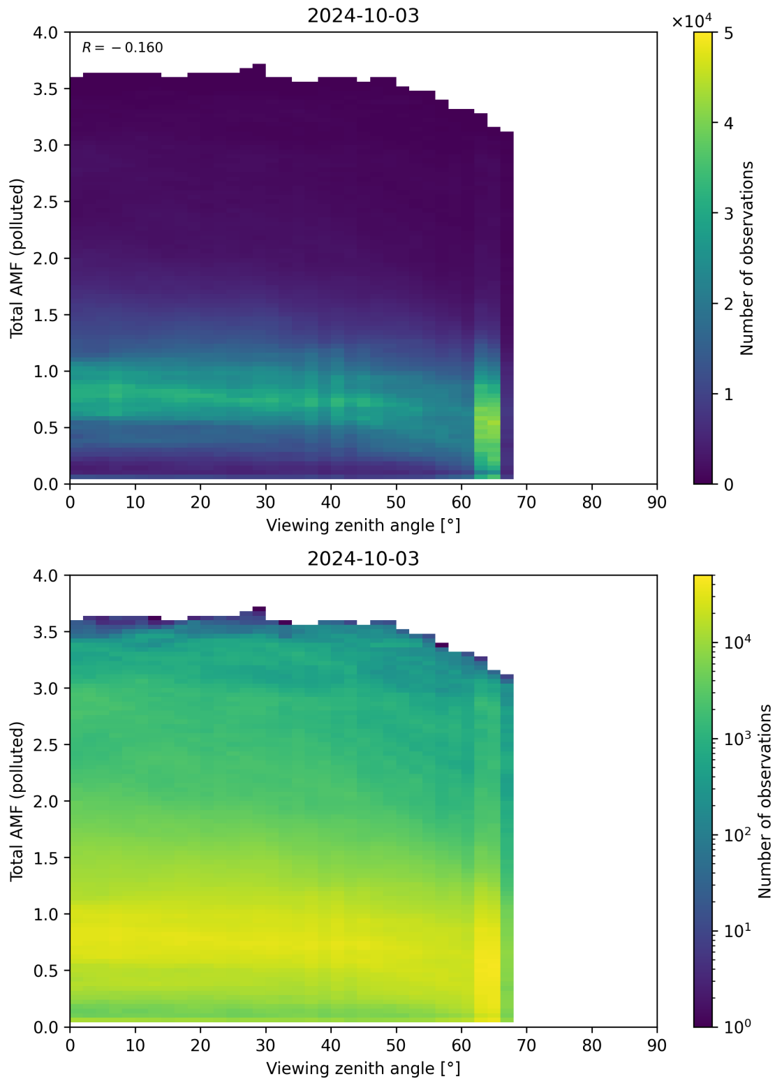
Figure 325: Scatter density plot of “Viewing zenith angle” against “Total AMF (polluted)” for 2024-10-03 to 2024-10-04.
