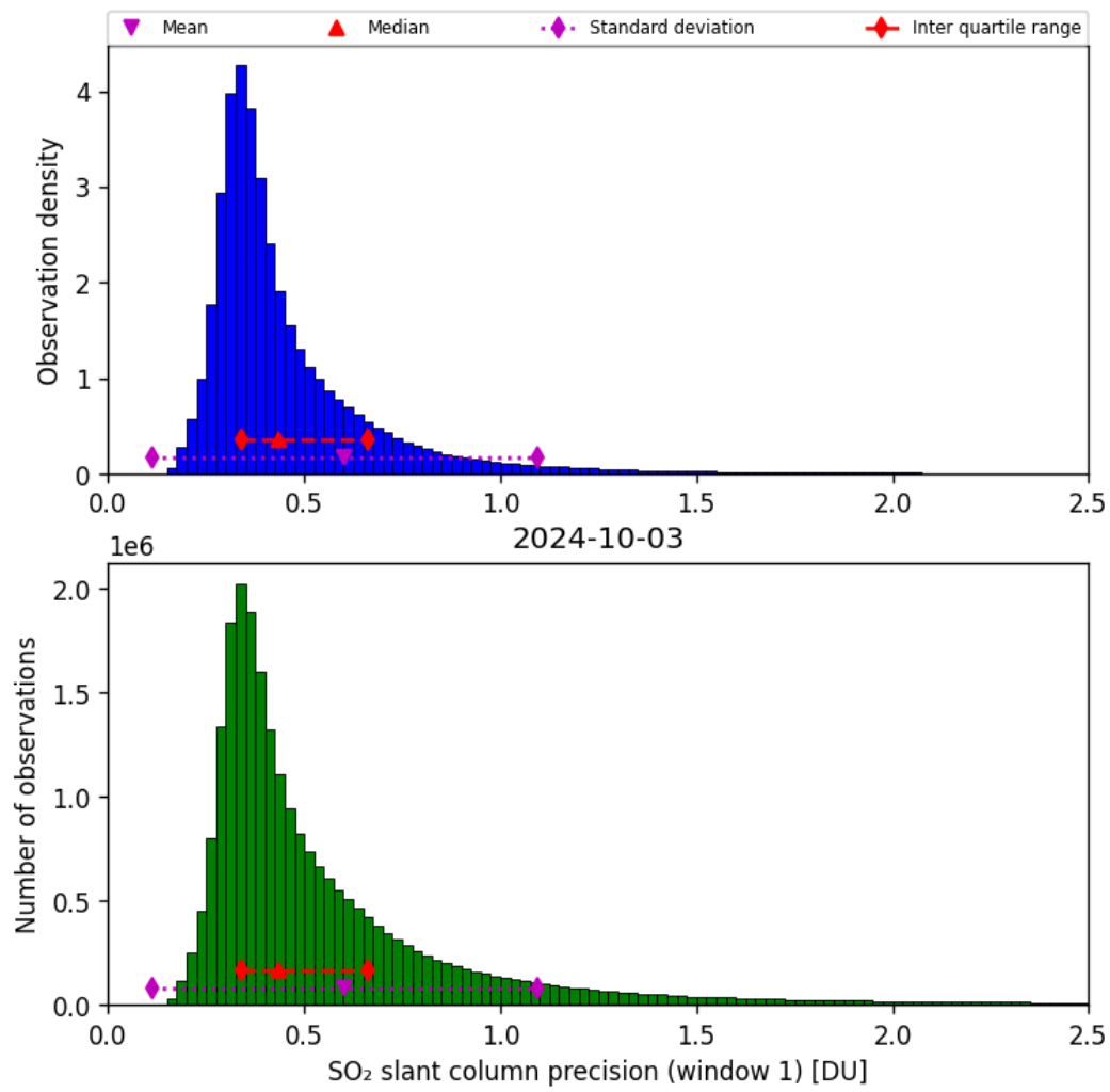
Figure 57: Histogram of “SO 2 slant column precision (window 1)” for 2024-10-03 to 2024-10-04
