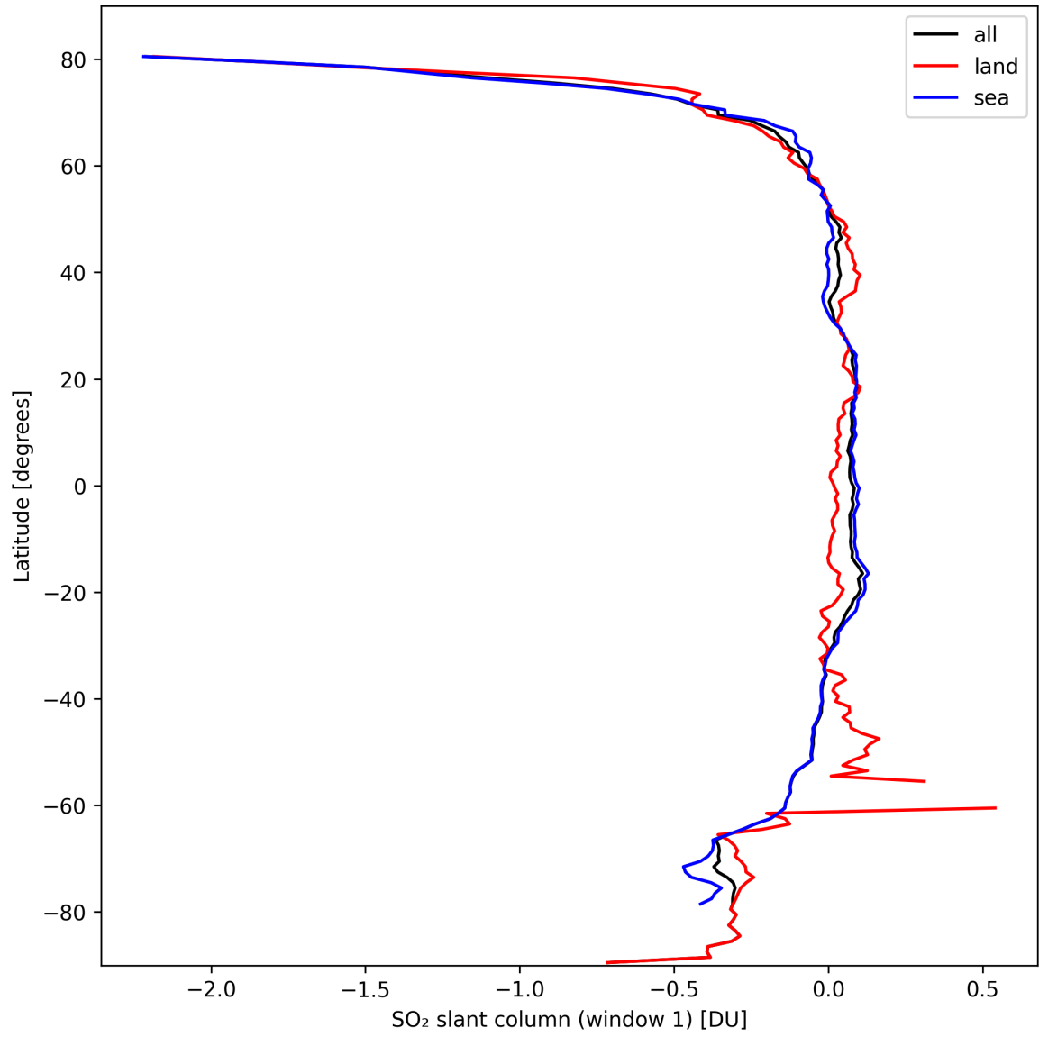
Figure 33: Zonal average of “SO 2 slant column (window 1)” for 2024-10-03 to 2024-10-04.
