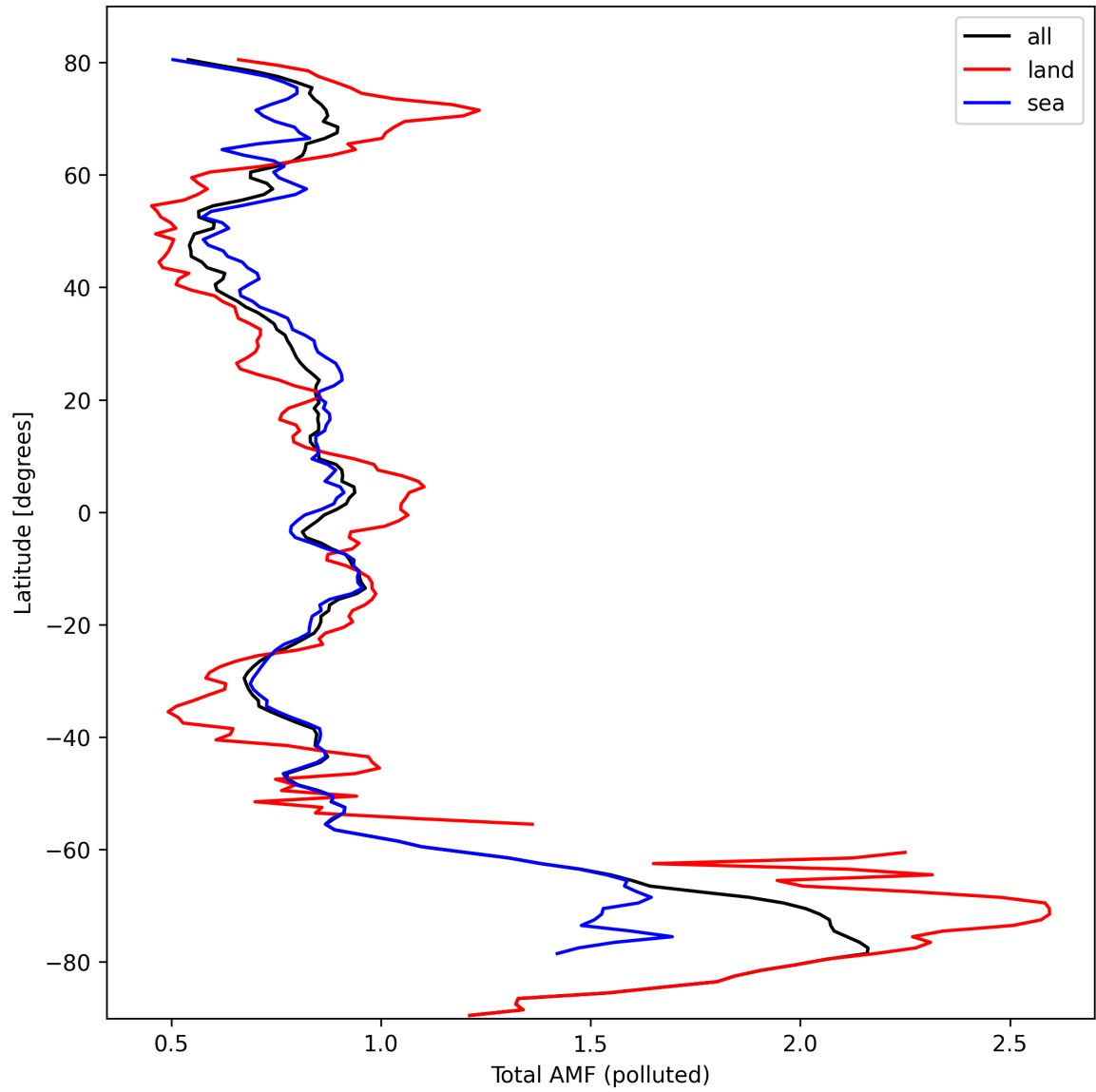
Figure 48: Zonal average of “Total AMF (polluted)” for 2024-10-03 to 2024-10-04.
