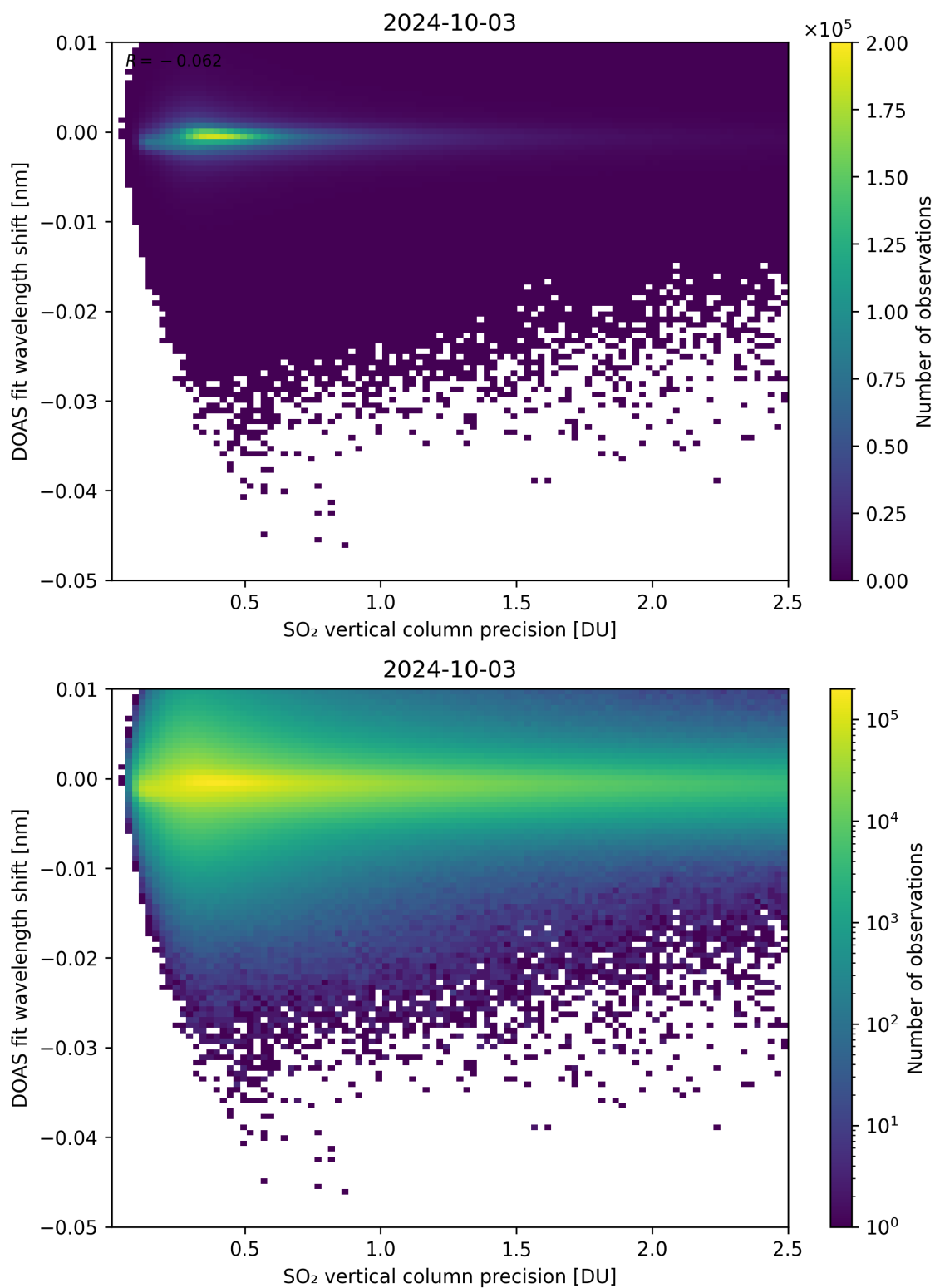
Figure 282: Scatter density plot of “SO 2 vertical column precision” against “DOAS fit wavelength shift” for 2024-10-03 to 2024-10-04.
