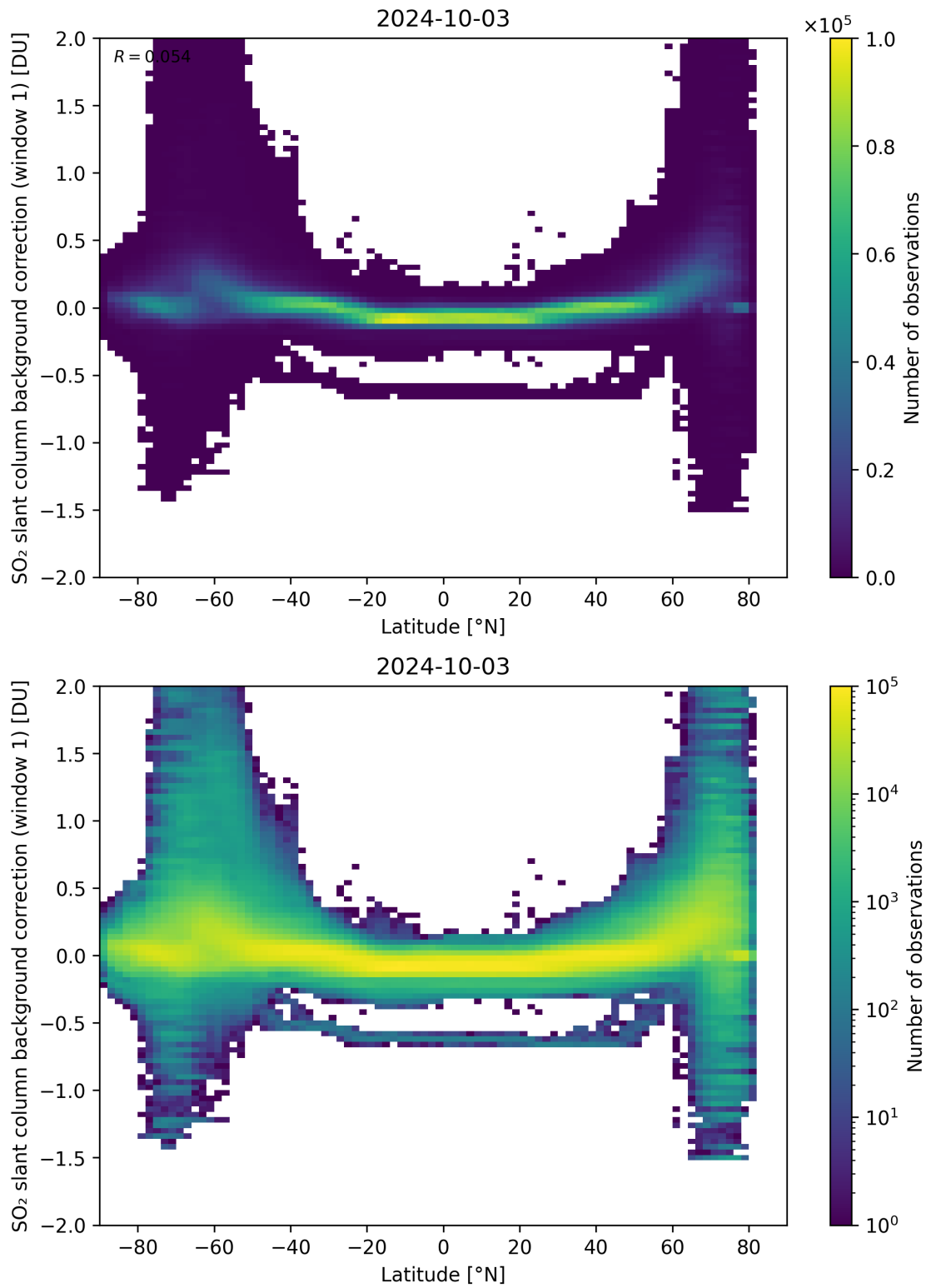
Figure 139: Scatter density plot of “Latitude” against “SO 2 slant column background correction (window 1)” for 2024-10-03 to 2024-10-04.
