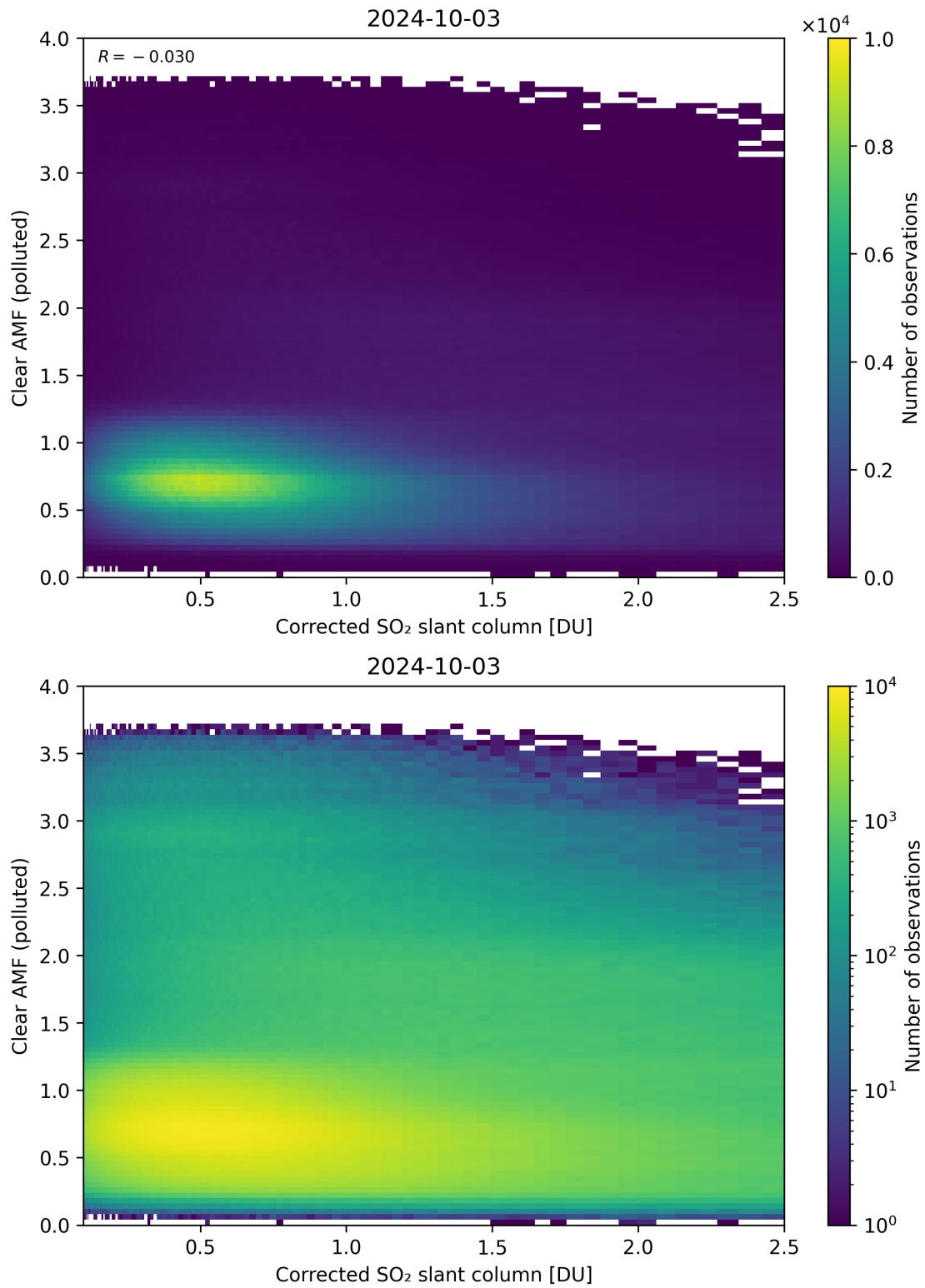
Figure 184: Scatter density plot of “Corrected SO 2 slant column” against “Clear AMF (polluted)” for 2024-10-03 to 2024-10-04.
