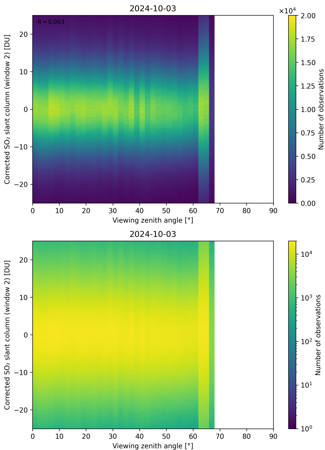
Figure 318: Scatter density plot of “Viewing zenith angle” against “Corrected SO 2 slant column (window 2)” for 2024-10-03 to 2024-10-04.
