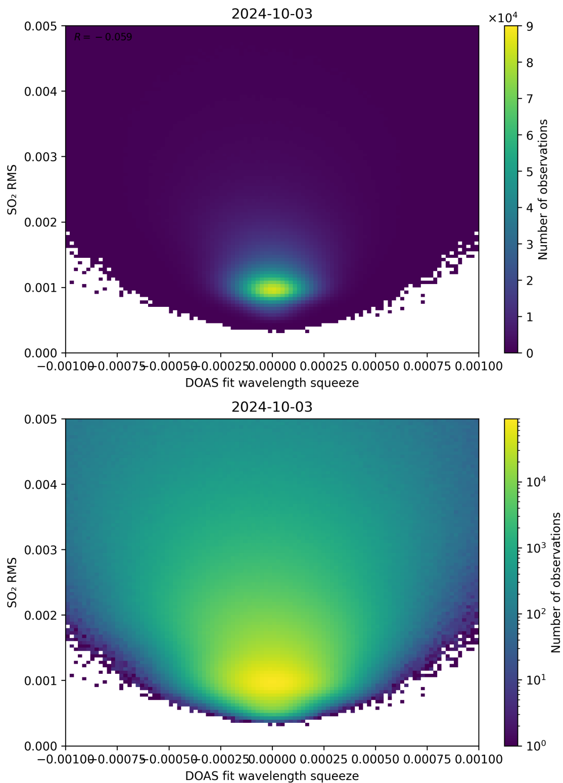
Figure 132: Scatter density plot of “DOAS fit wavelength squeeze” against “SO 2 RMS” for 2024-10-03 to 2024-10-04.
