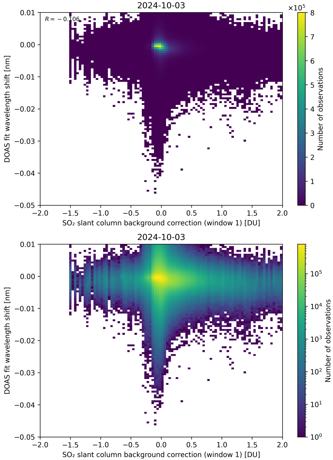
Figure 100: Scatter density plot of “SO 2 slant column background correction (window 1)” against “DOAS fit wavelength shift” for 2024-10-03 to 2024-10-04.
