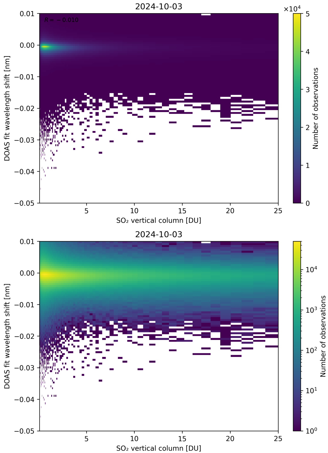
Figure 276: Scatter density plot of “SO 2 vertical column” against “DOAS fit wavelength shift” for 2024-10-03 to 2024-10-04.
