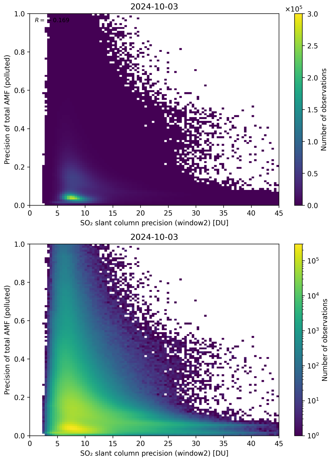
Figure 252: Scatter density plot of “SO 2 slant column precision (window2)” against “Precision of total AMF (polluted)” for 2024-10-03 to 2024-10-04.
