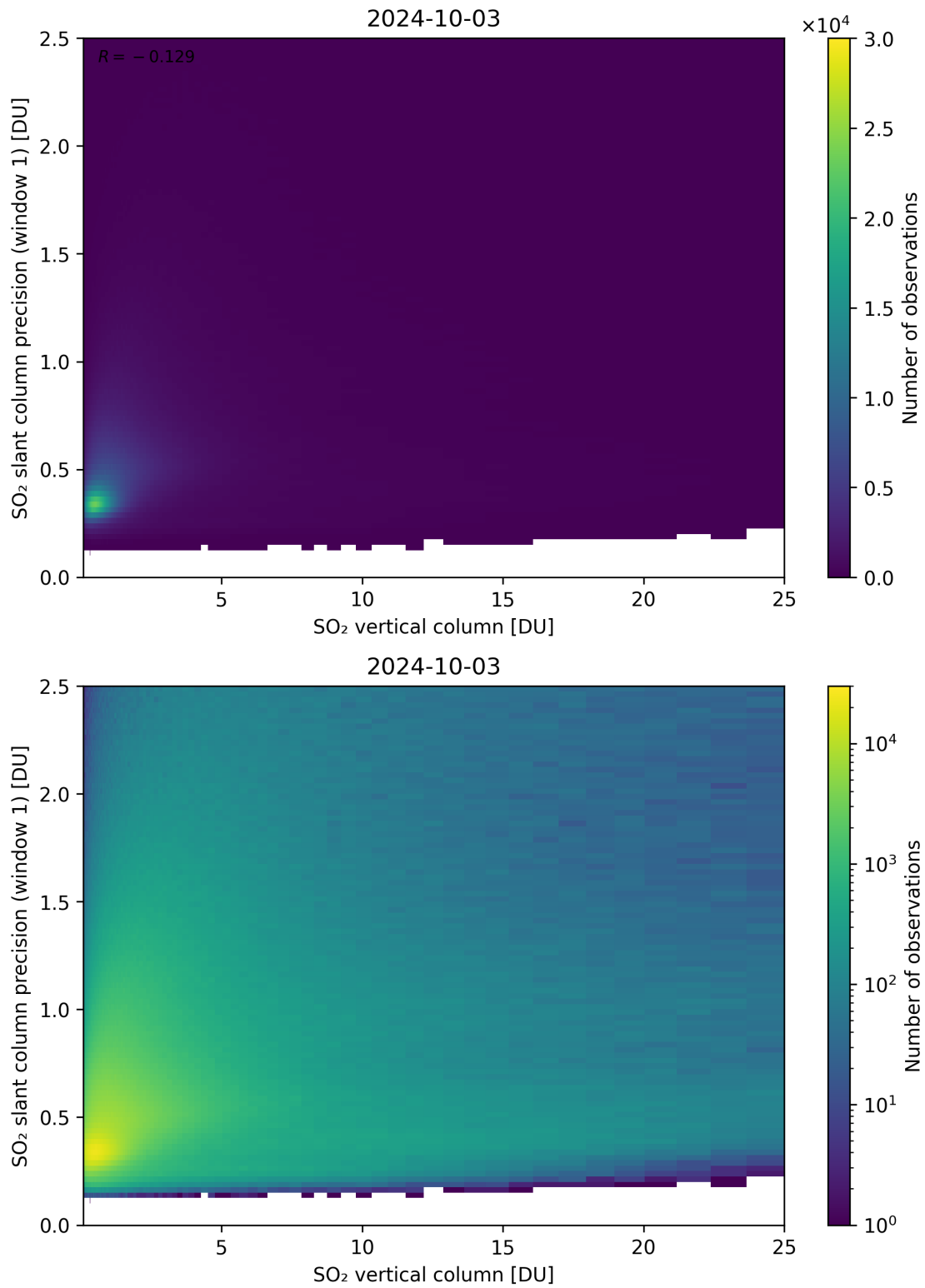
Figure 301: Scatter density plot of “SO 2 vertical column” against “SO 2 slant column precision (window 1)” for 2024-10-03 to 2024-10-04.
