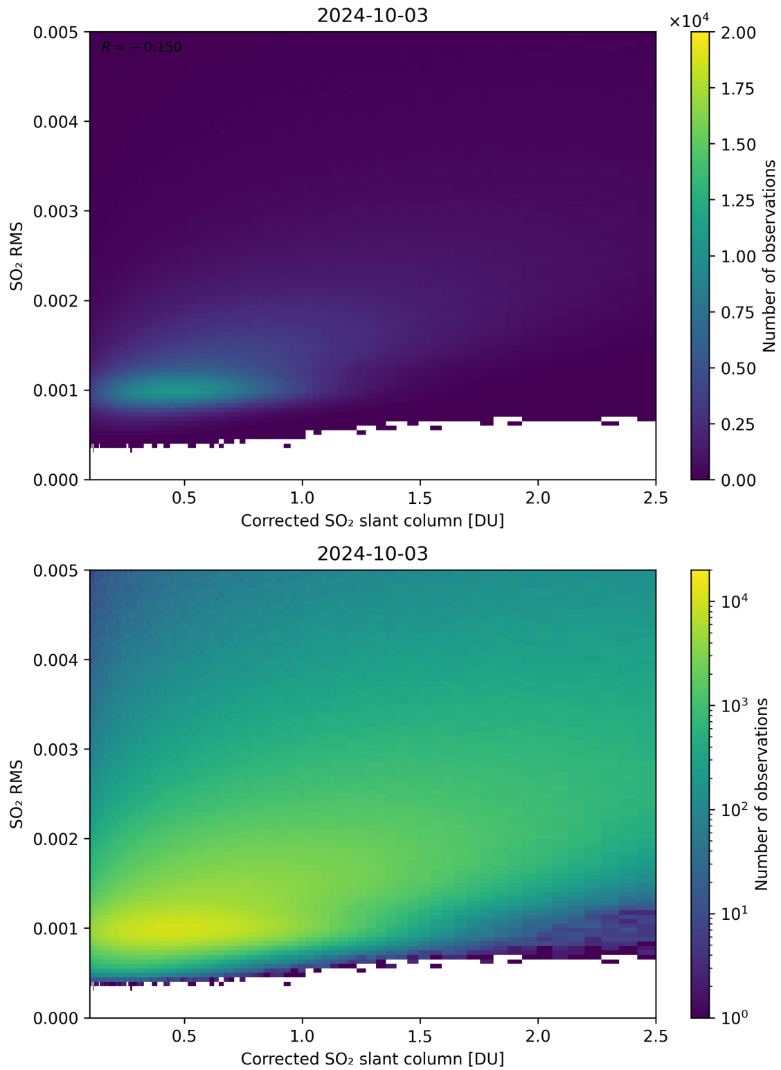
Figure 183: Scatter density plot of “Corrected SO 2 slant column” against “SO 2 RMS” for 2024-10-03 to 2024-10-04.
