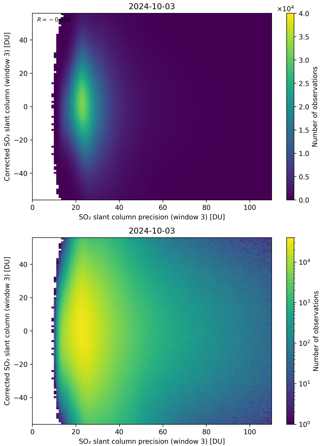
Figure 262: Scatter density plot of “SO 2 slant column precision (window 3)” against “Corrected SO 2 slant column (window 3)” for 2024-10-03 to 2024-10-04.
