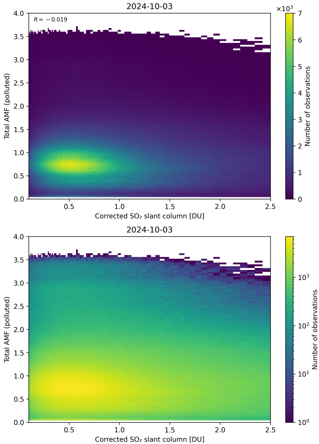
Figure 192: Scatter density plot of “Corrected SO 2 slant column” against “Total AMF (polluted)” for 2024-10-03 to 2024-10-04.
