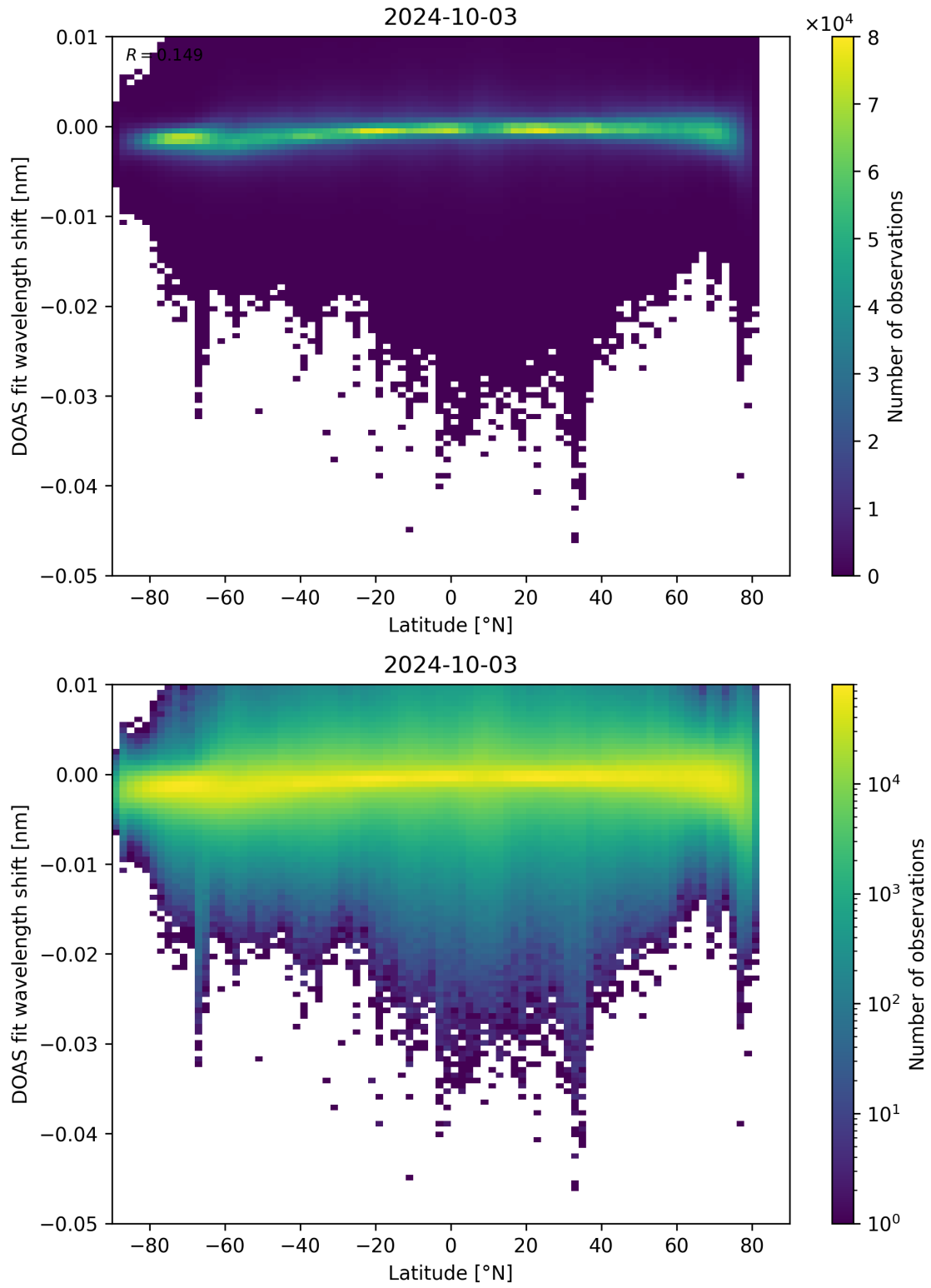
Figure 142: Scatter density plot of “Latitude” against “DOAS fit wavelength shift” for 2024-10-03 to 2024-10-04.
