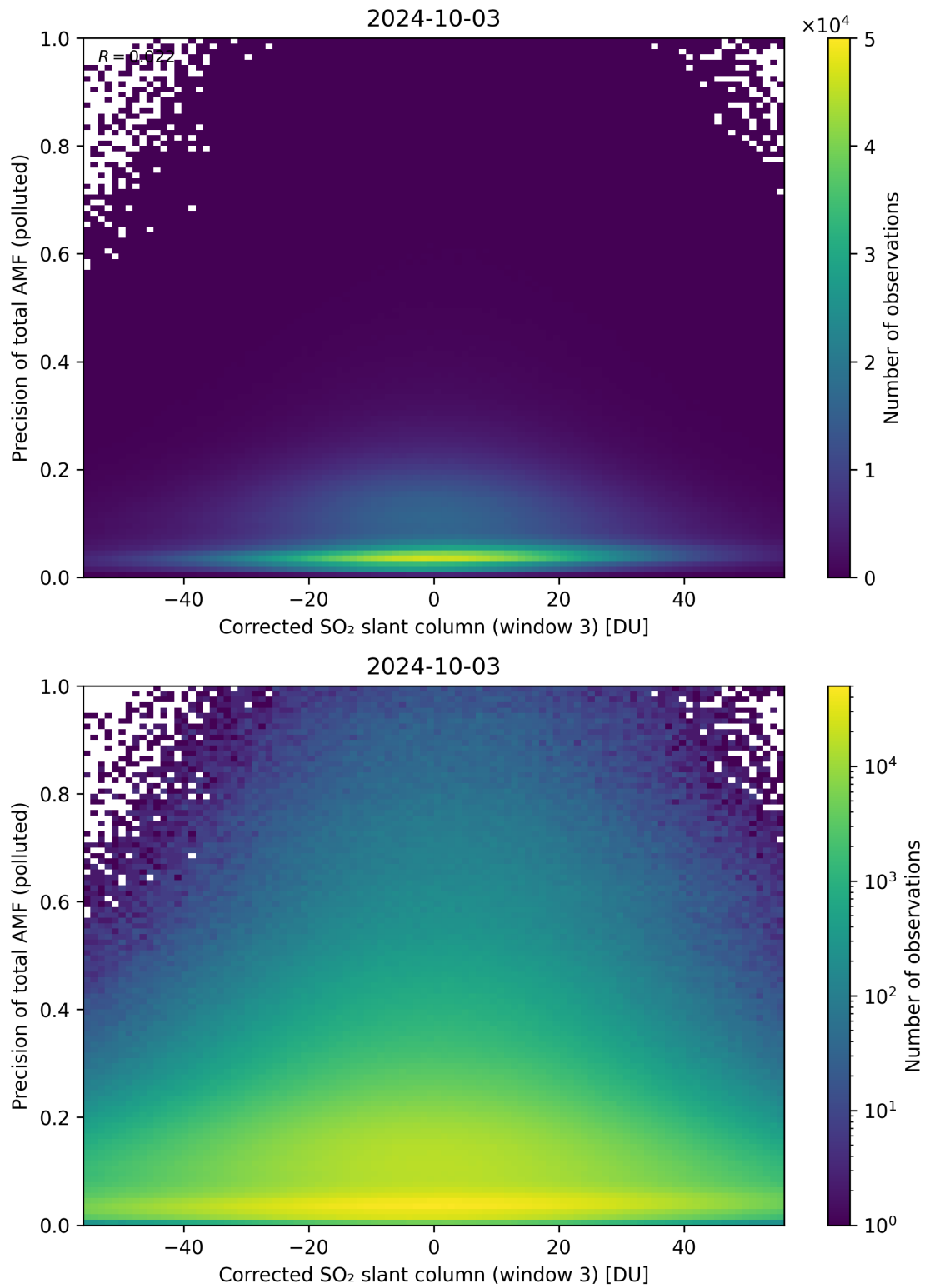
Figure 211: Scatter density plot of “Corrected SO 2 slant column (window 3)” against “Precision of total AMF (polluted)” for 2024-10-03 to 2024-10-04.
