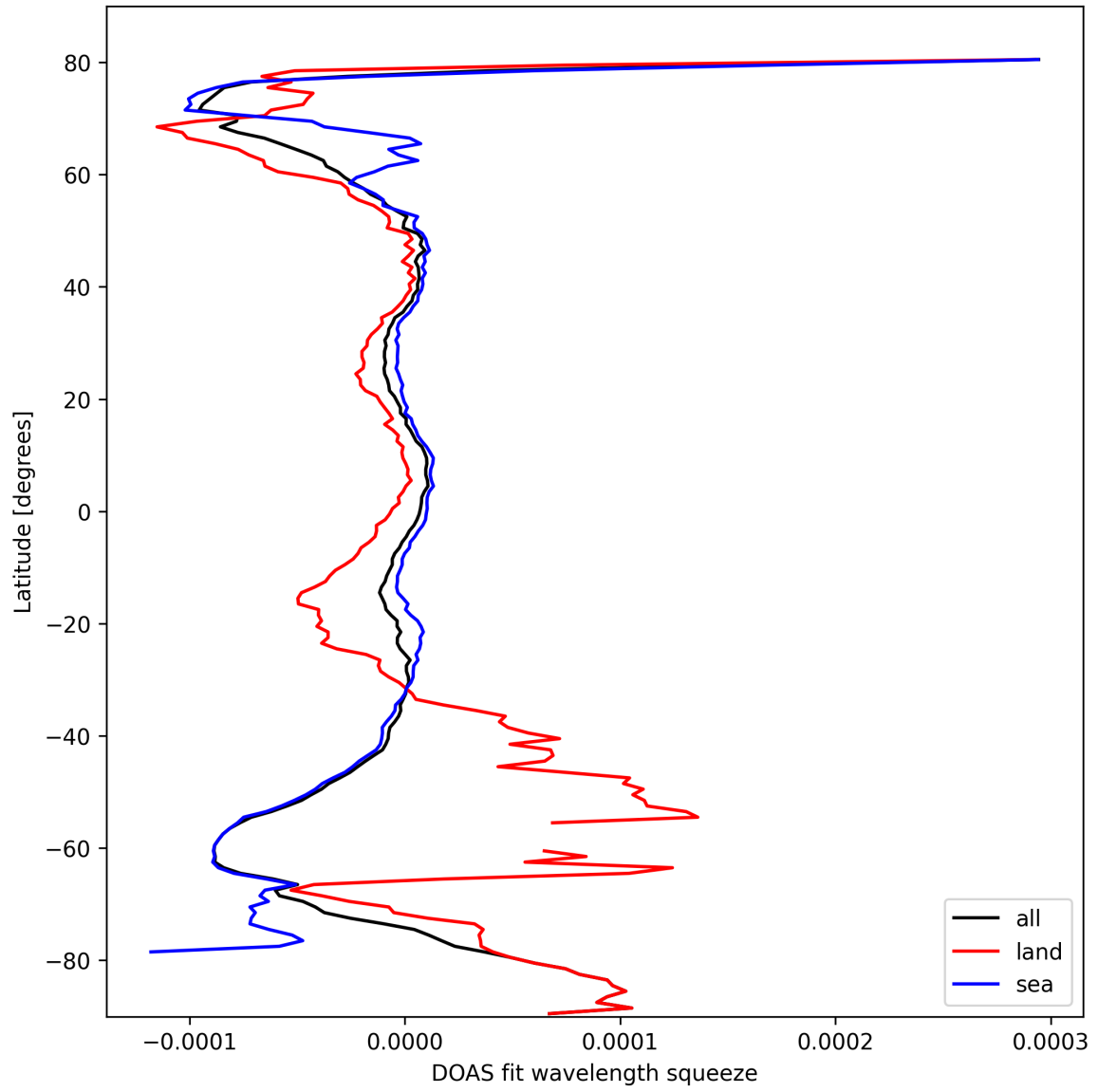
Figure 46: Zonal average of “DOAS fit wavelength squeeze” for 2024-10-03 to 2024-10-04.
