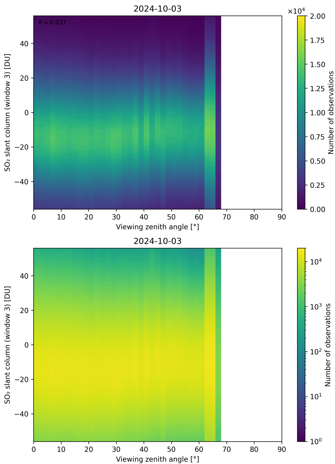
Figure 323: Scatter density plot of “Viewing zenith angle” against “SO 2 slant column (window 3)” for 2024-10-03 to 2024-10-04.
