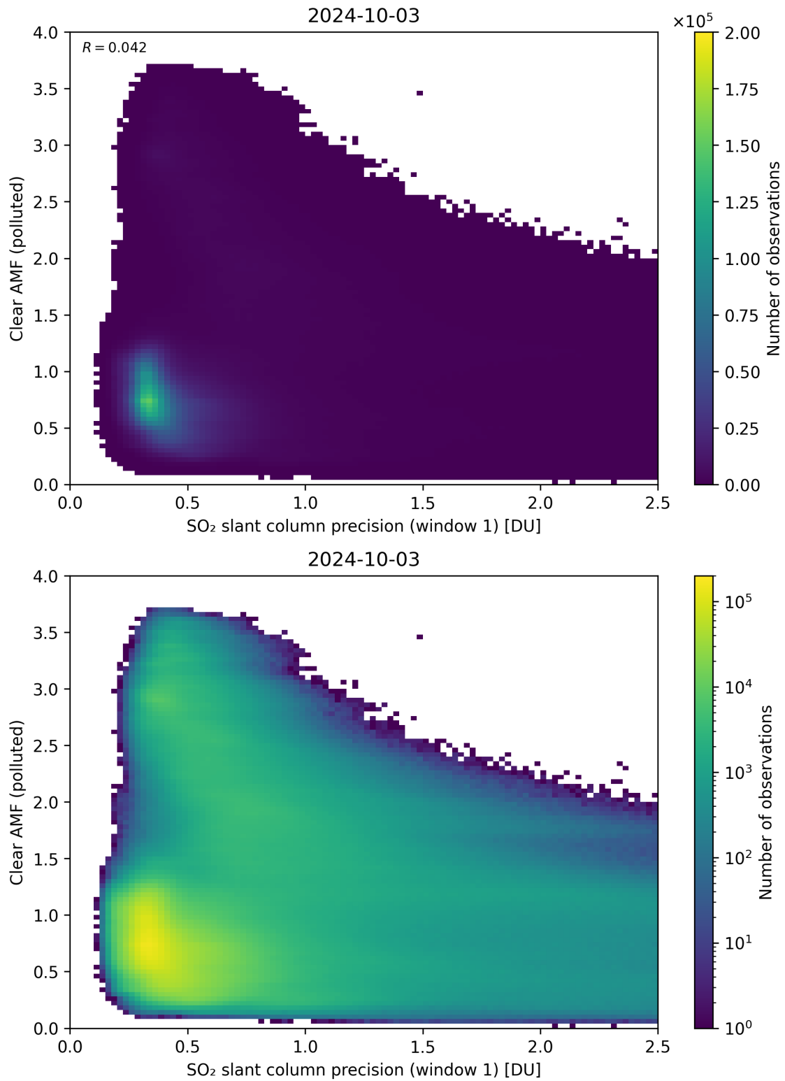
Figure 224: Scatter density plot of “SO 2 slant column precision (window 1)” against “Clear AMF (polluted)” for 2024-10-03 to 2024-10-04.
