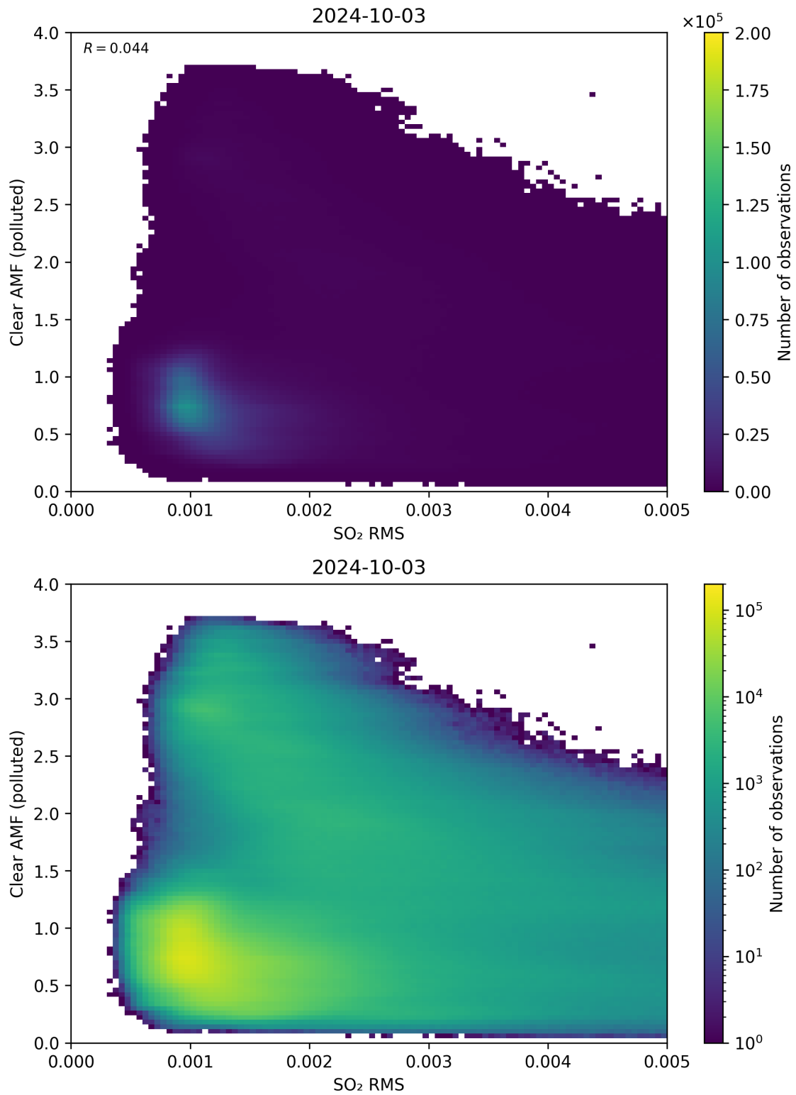
Figure 136: Scatter density plot of “SO 2 RMS” against “Clear AMF (polluted)” for 2024-10-03 to 2024-10-04.
