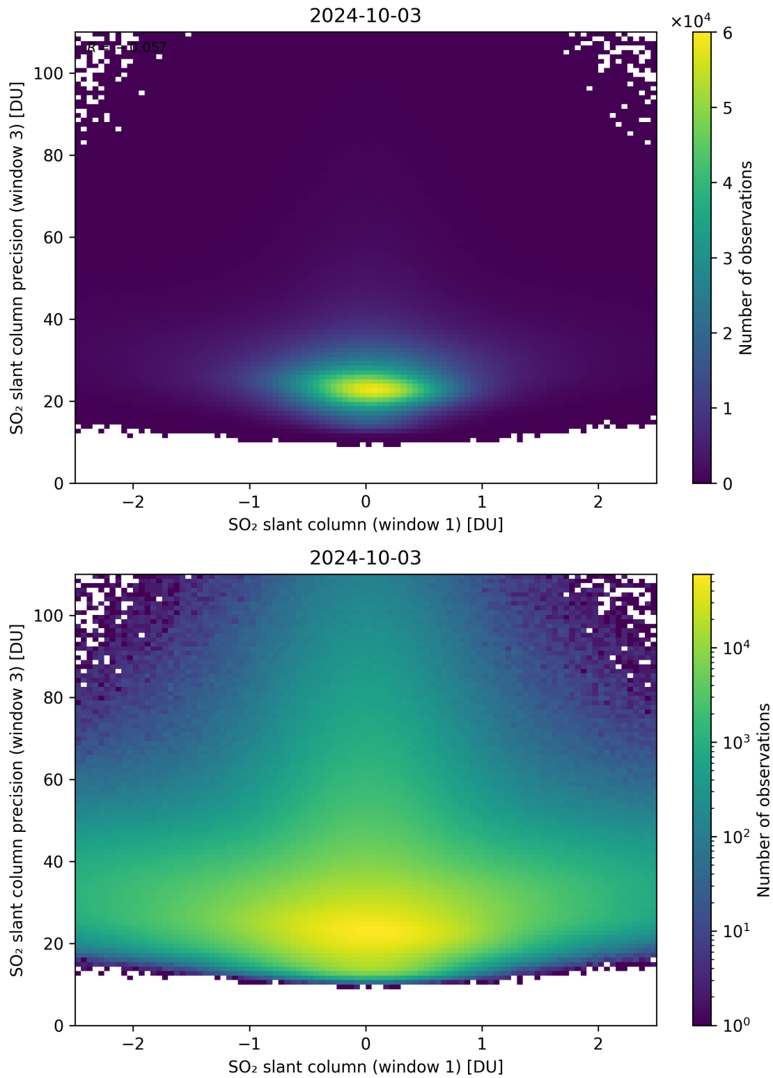
Figure 238: Scatter density plot of “SO 2 slant column (window 1)” against “SO 2 slant column precision (window 3)” for 2024-10-03 to 2024-10-04.
