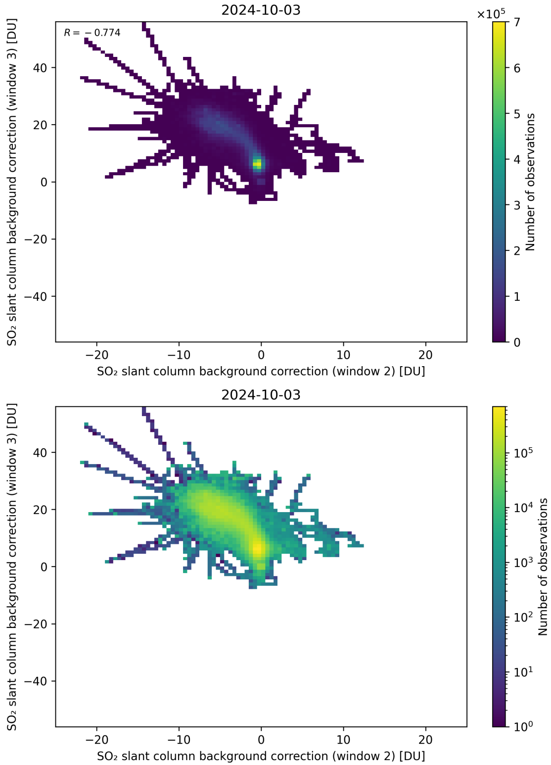
Figure 111: Scatter density plot of “SO 2 slant column background correction (window 2)” against “SO 2 slant column background correction (window 3)” for 2024-10-03 to 2024-10-04.
