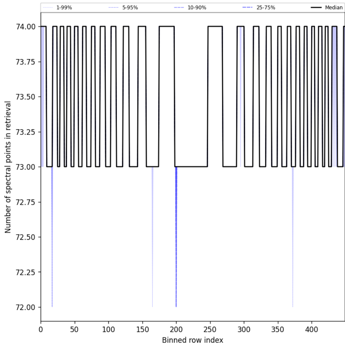
Figure 97: Along track statistics of “Number of spectral points in retrieval” for 2024-10-03 to 2024-10-04
