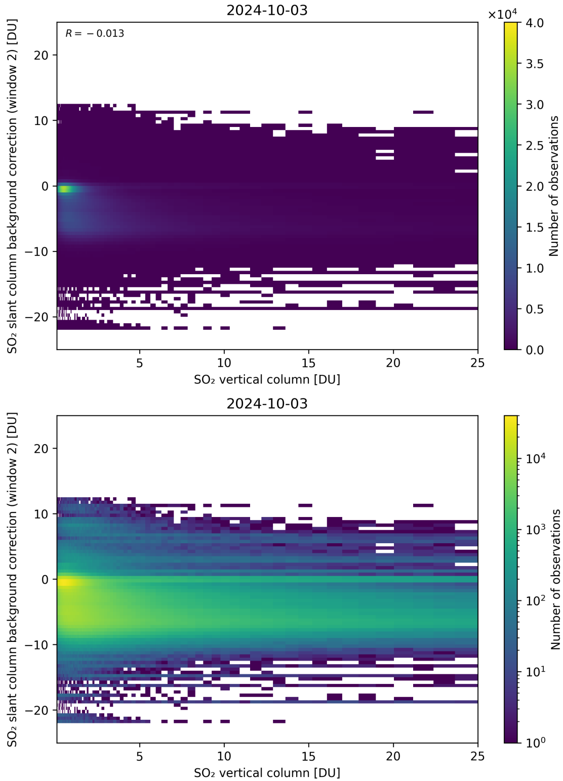
Figure 274: Scatter density plot of “SO 2 vertical column” against “SO 2 slant column background correction (window 2)” for 2024-10-03 to 2024-10-04.
