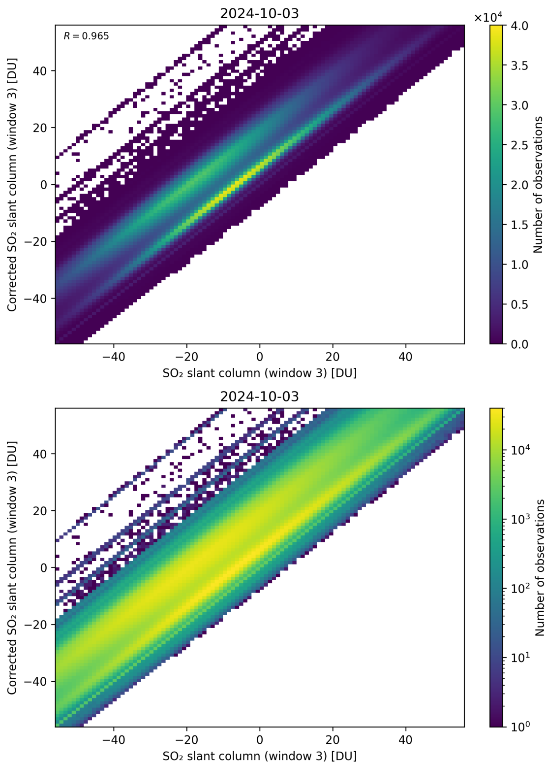
Figure 266: Scatter density plot of “SO 2 slant column (window 3)” against “Corrected SO 2 slant column (window 3)” for 2024-10-03 to 2024-10-04.
