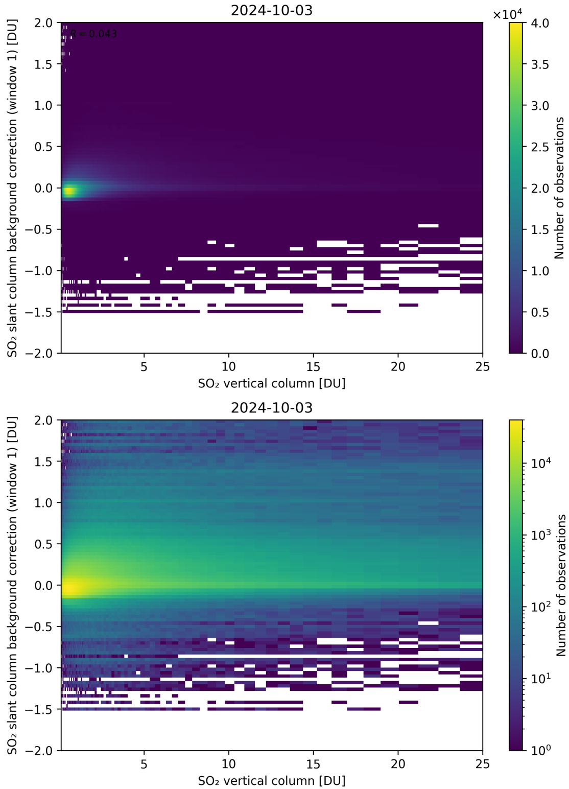
Figure 273: Scatter density plot of “SO 2 vertical column” against “SO 2 slant column background correction (window 1)” for 2024-10-03 to 2024-10-04.
