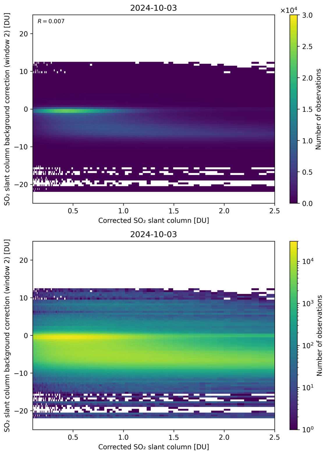
Figure 179: Scatter density plot of “Corrected SO 2 slant column” against “SO 2 slant column background correction (window 2)” for 2024-10-03 to 2024-10-04.
