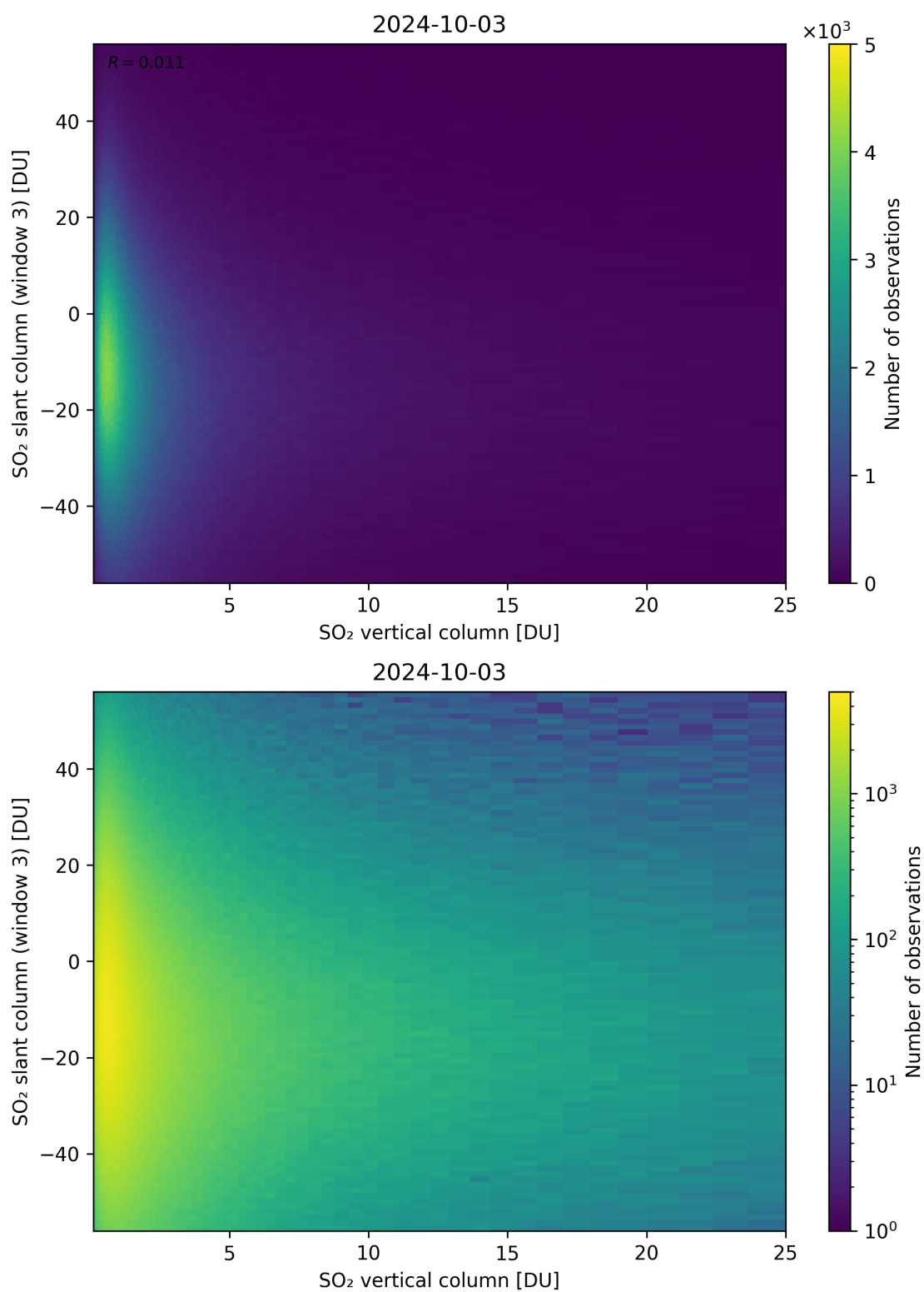
Figure 303: Scatter density plot of “SO 2 vertical column” against “SO 2 slant column (window 3)” for 2024-10-03 to 2024-10-04.
