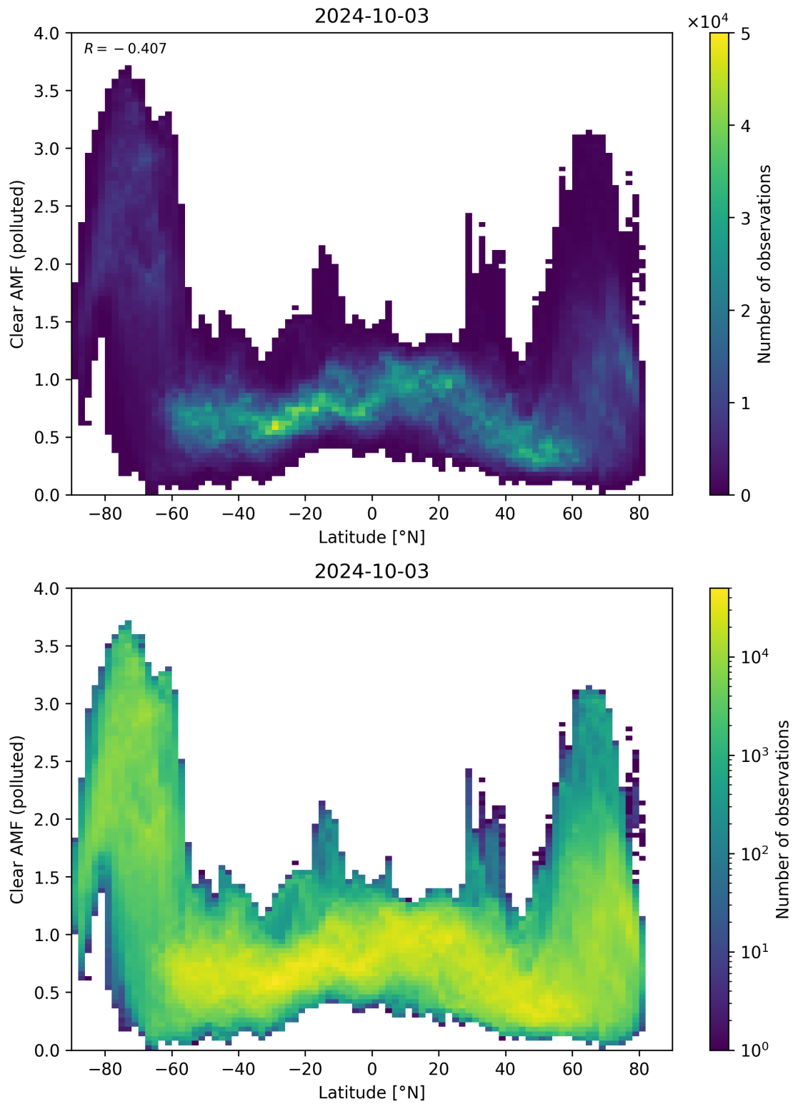
Figure 145: Scatter density plot of “Latitude” against “Clear AMF (polluted)” for 2024-10-03 to 2024-10-04.
