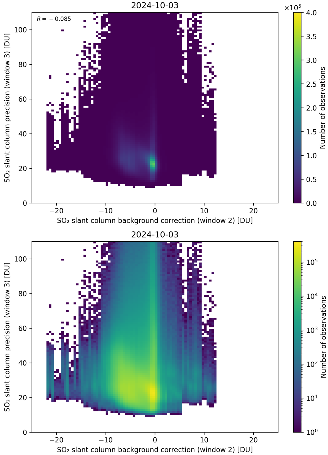
Figure 118: Scatter density plot of “SO 2 slant column background correction (window 2)” against “SO 2 slant column precision (window 3)” for 2024-10-03 to 2024-10-04.
