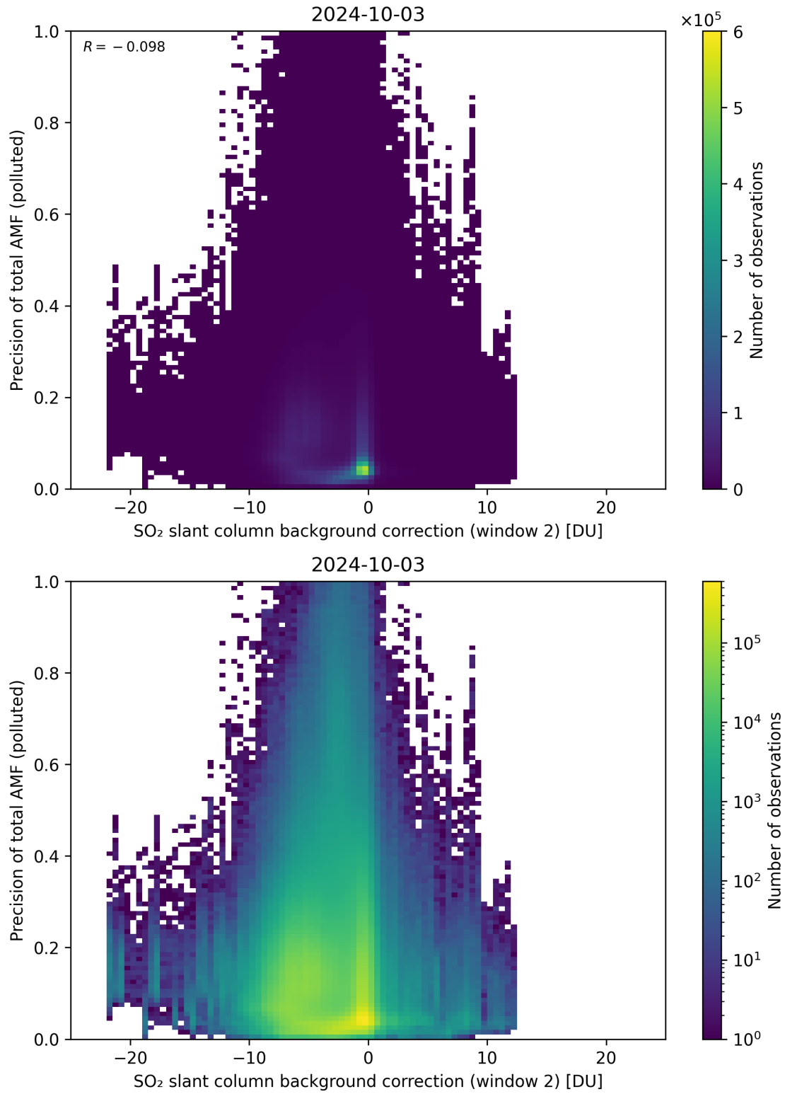
Figure 120: Scatter density plot of “SO 2 slant column background correction (window 2)” against “Precision of total AMF (polluted)” for 2024-10-03 to 2024-10-04.
