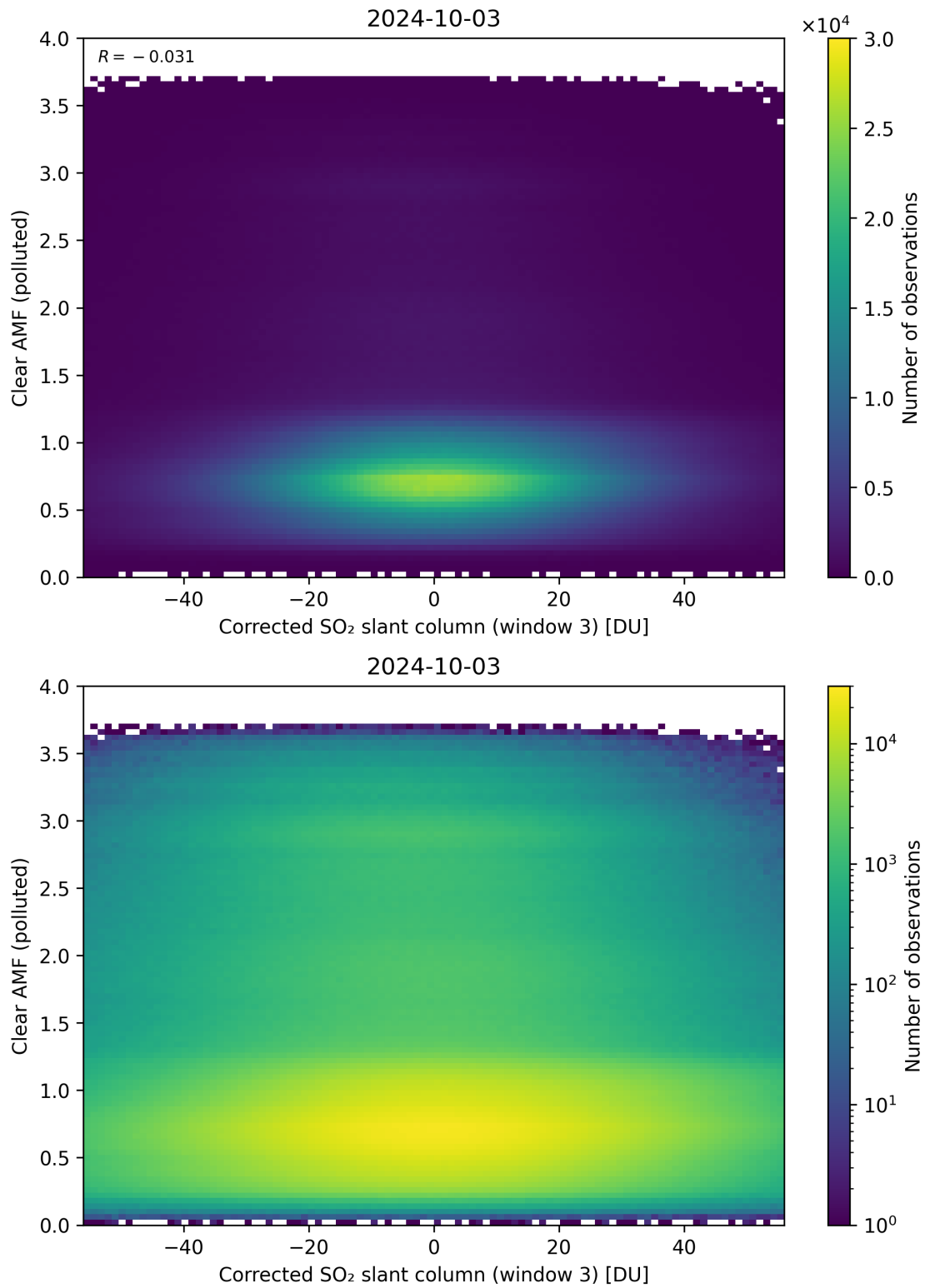
Figure 209: Scatter density plot of “Corrected SO 2 slant column (window 3)” against “Clear AMF (polluted)” for 2024-10-03 to 2024-10-04.
