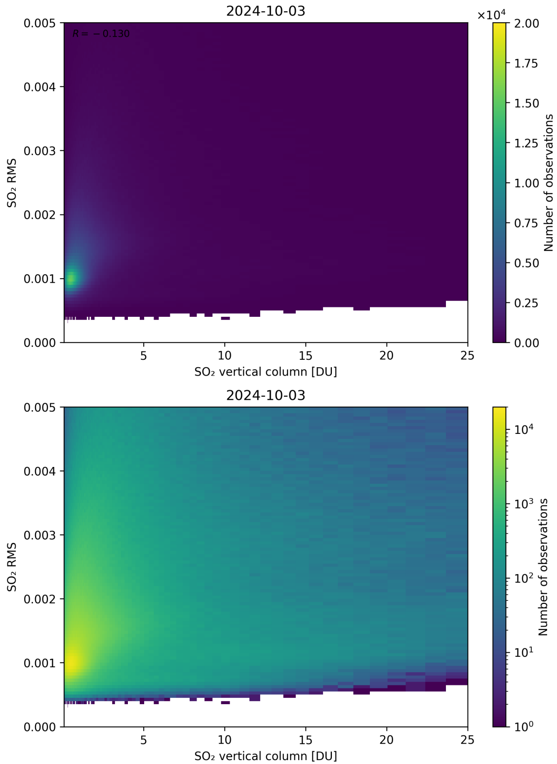
Figure 278: Scatter density plot of “SO 2 vertical column” against “SO 2 RMS” for 2024-10-03 to 2024-10-04.
