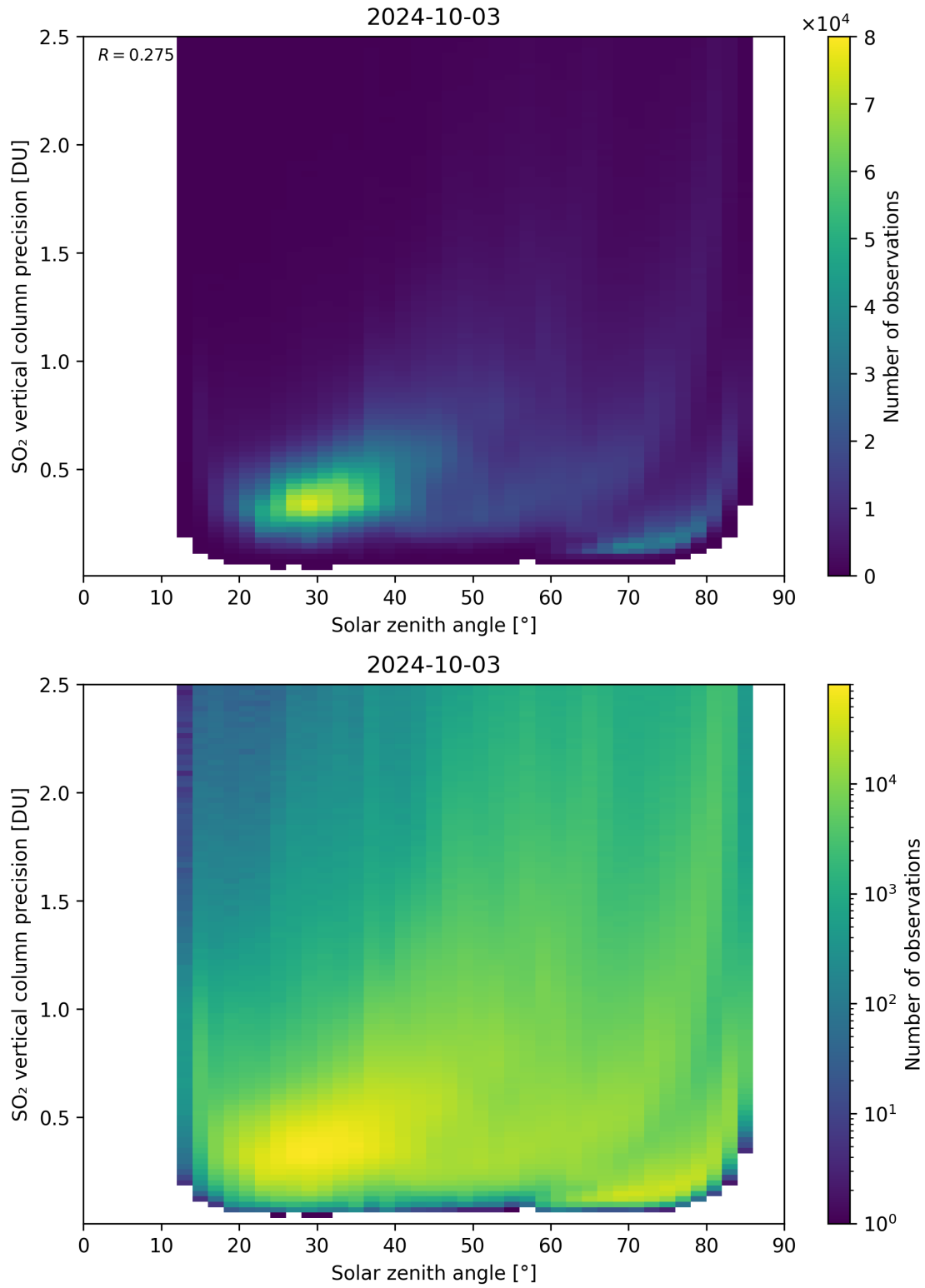
Figure 177: Scatter density plot of “Solar zenith angle” against “SO 2 vertical column precision” for 2024-10-03 to 2024-10-04.
