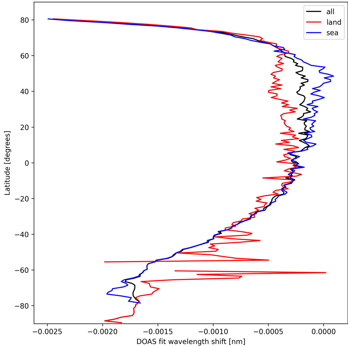
Figure 45: Zonal average of “DOAS fit wavelength shift” for 2024-10-03 to 2024-10-04.
