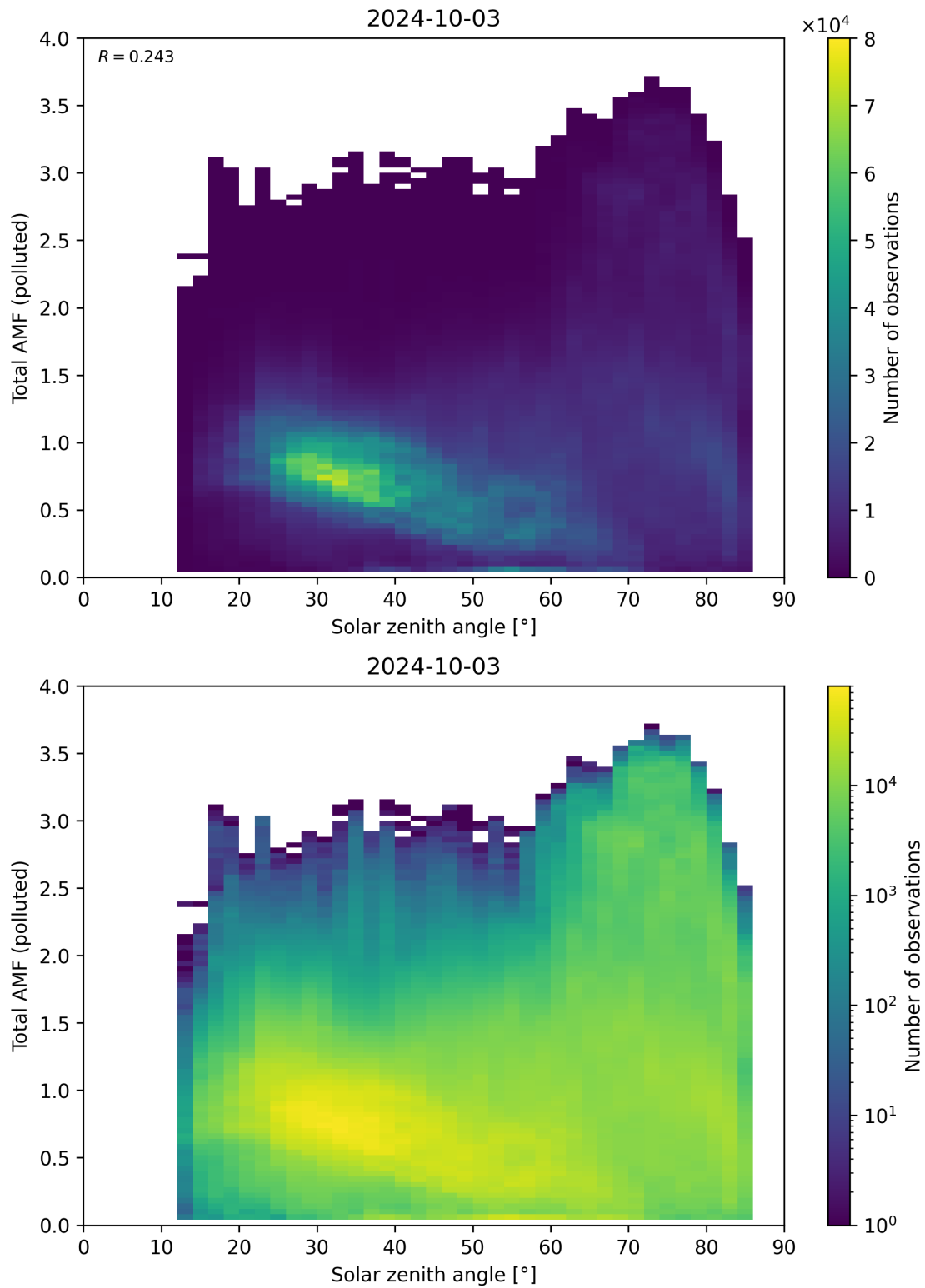
Figure 174: Scatter density plot of “Solar zenith angle” against “Total AMF (polluted)” for 2024-10-03 to 2024-10-04.
