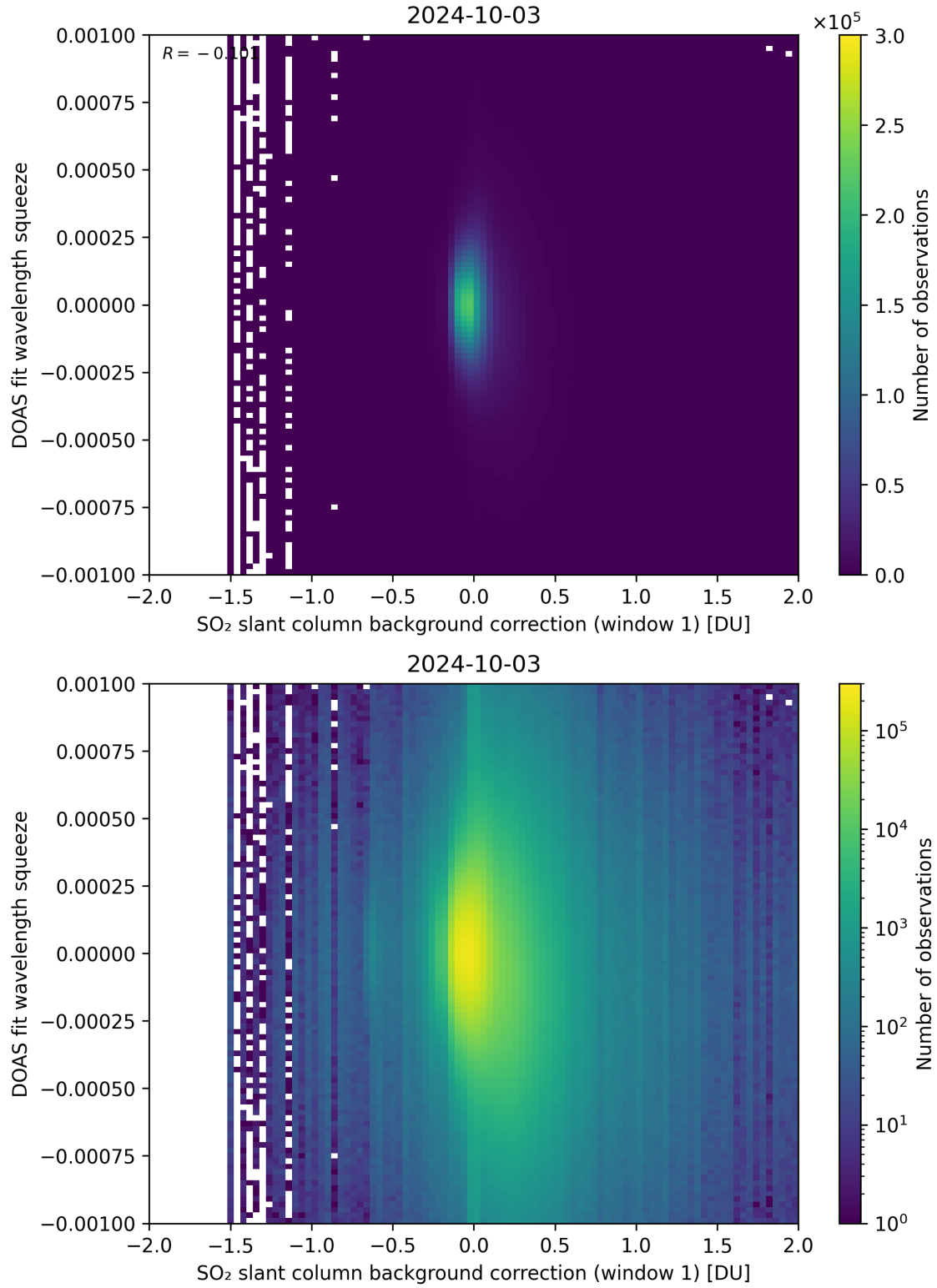
Figure 101: Scatter density plot of “SO 2 slant column background correction (window 1)” against “DOAS fit wavelength squeeze” for 2024-10-03 to 2024-10-04.
