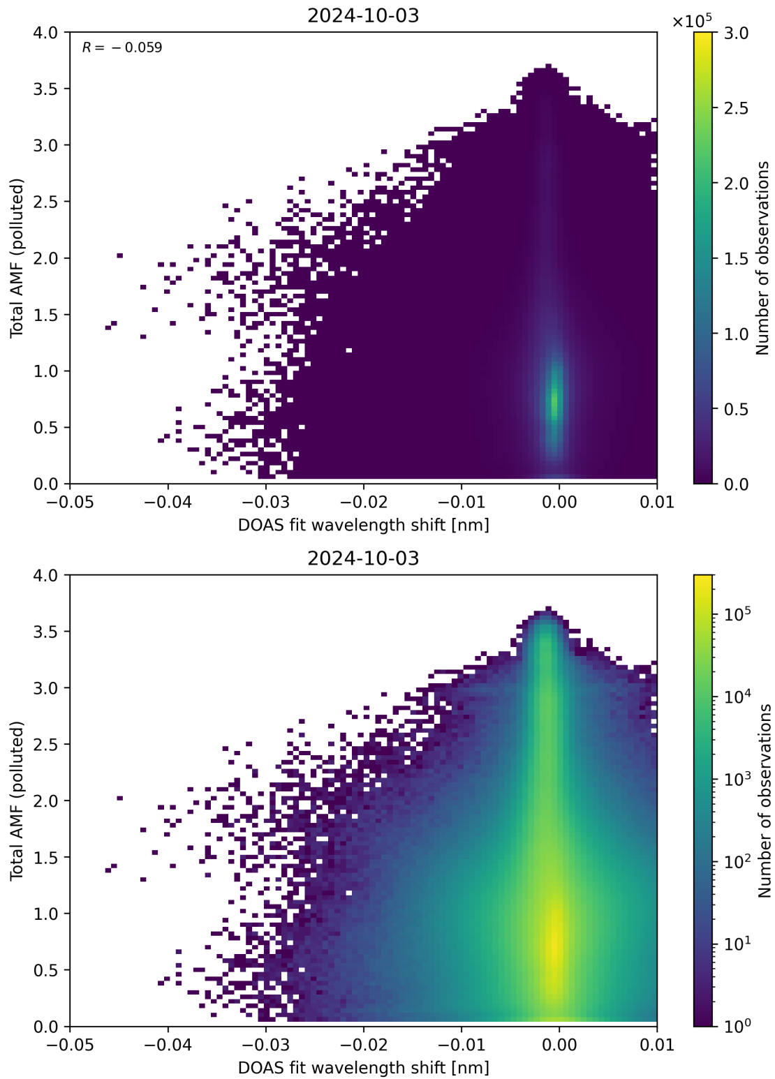
Figure 130: Scatter density plot of “DOAS fit wavelength shift” against “Total AMF (polluted)” for 2024-10-03 to 2024-10-04.
