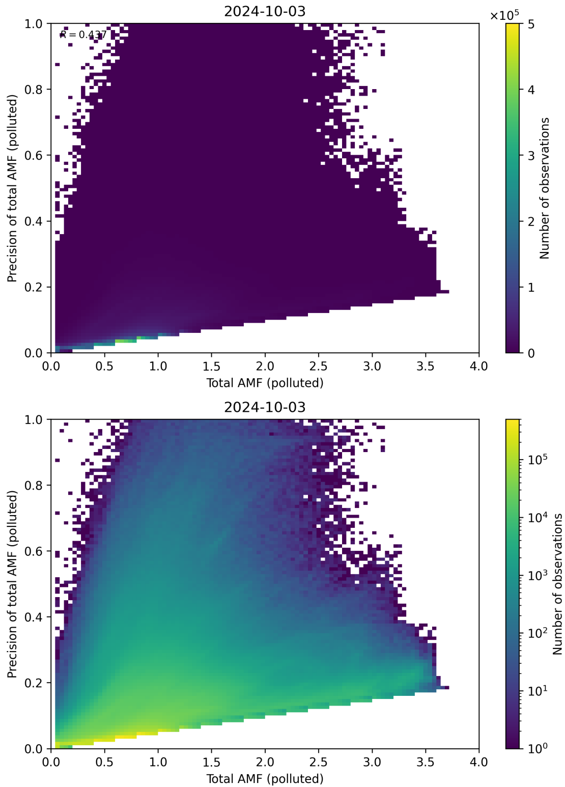
Figure 272: Scatter density plot of “Total AMF (polluted)” against “Precision of total AMF (polluted)” for 2024-10-03 to 2024-10-04.
