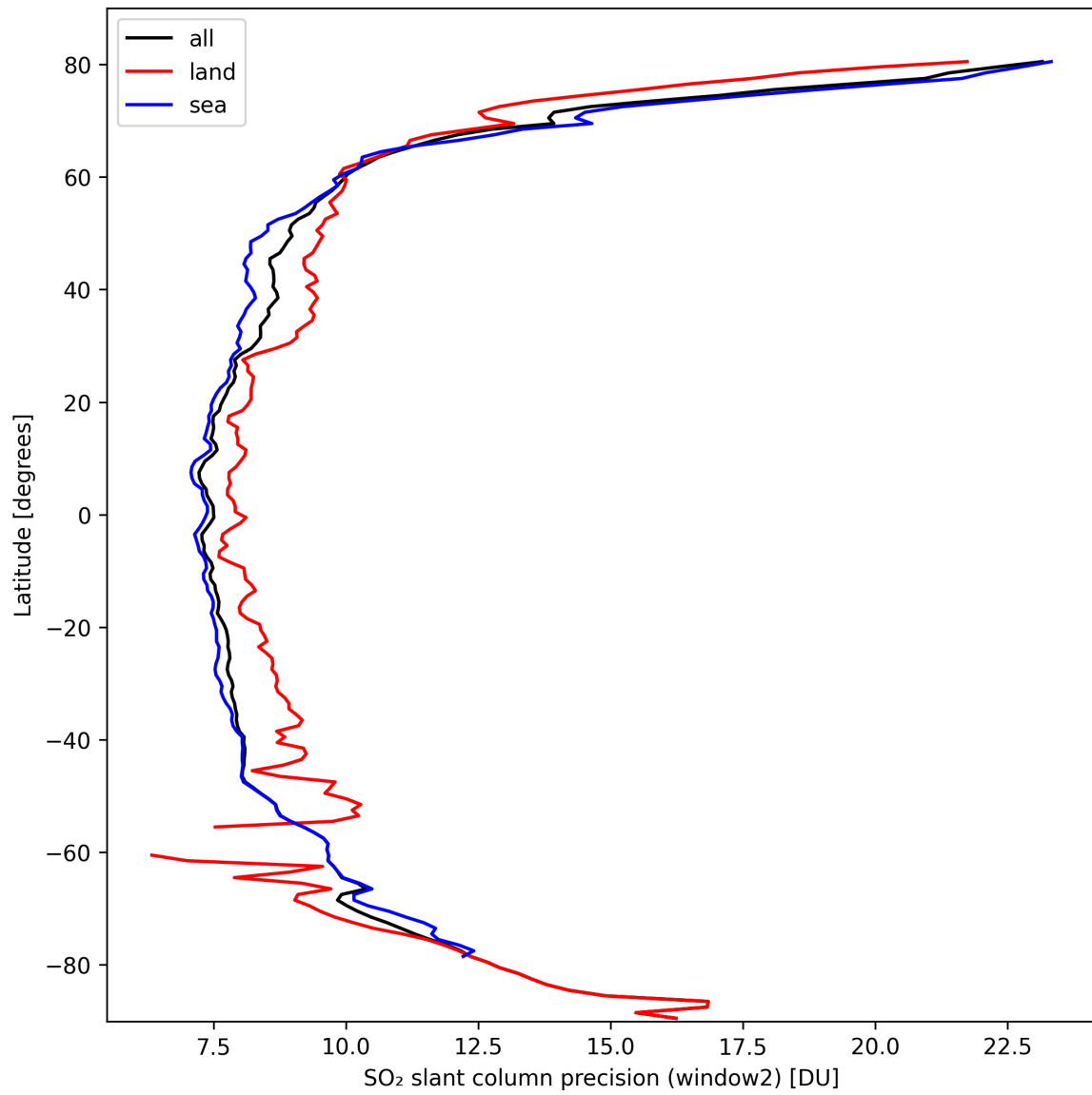
Figure 38: Zonal average of “SO 2 slant column precision (window2)” for 2024-10-03 to 2024-10-04.
