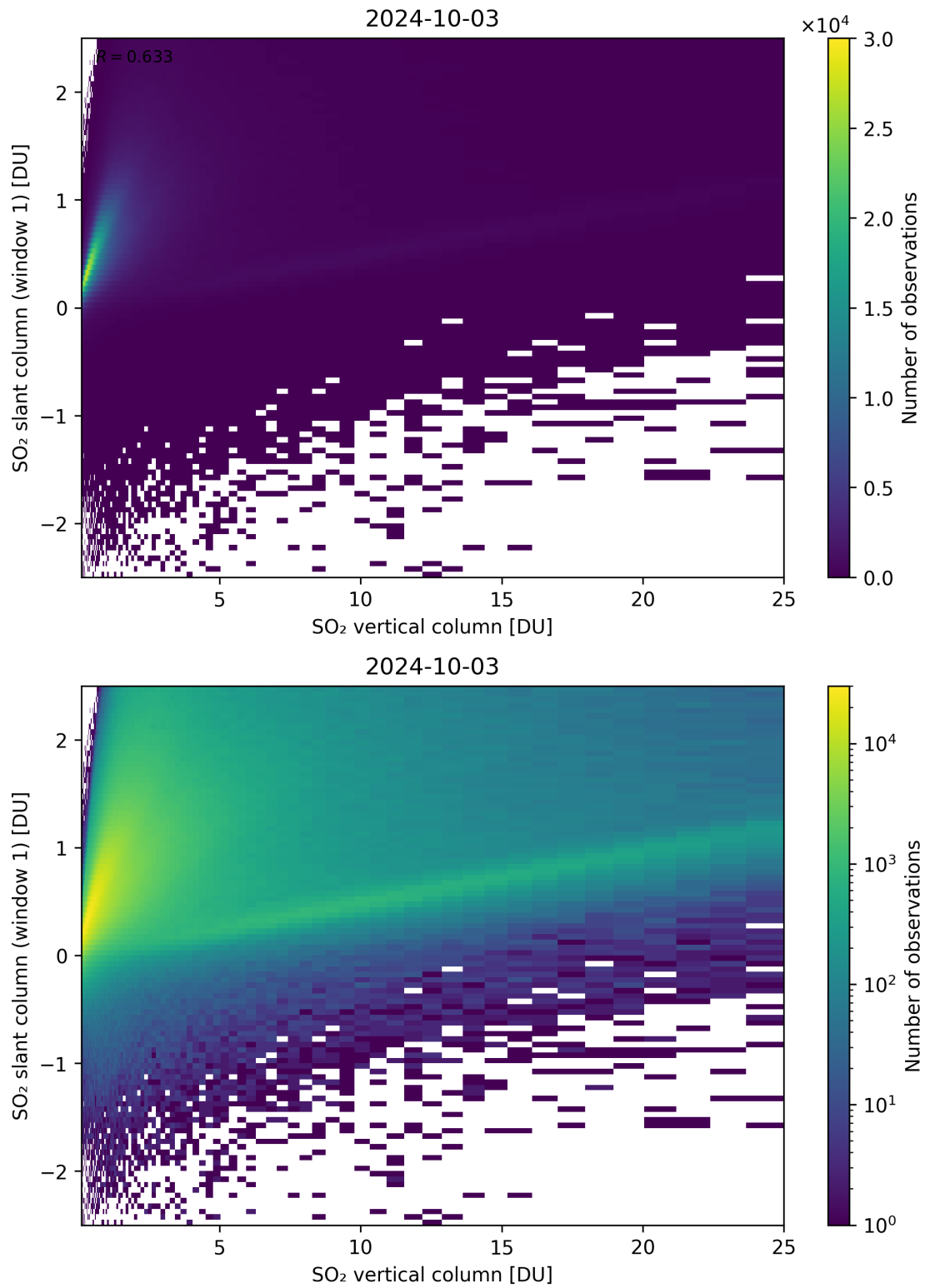
Figure 300: Scatter density plot of “SO 2 vertical column” against “SO 2 slant column (window 1)” for 2024-10-03 to 2024-10-04.
