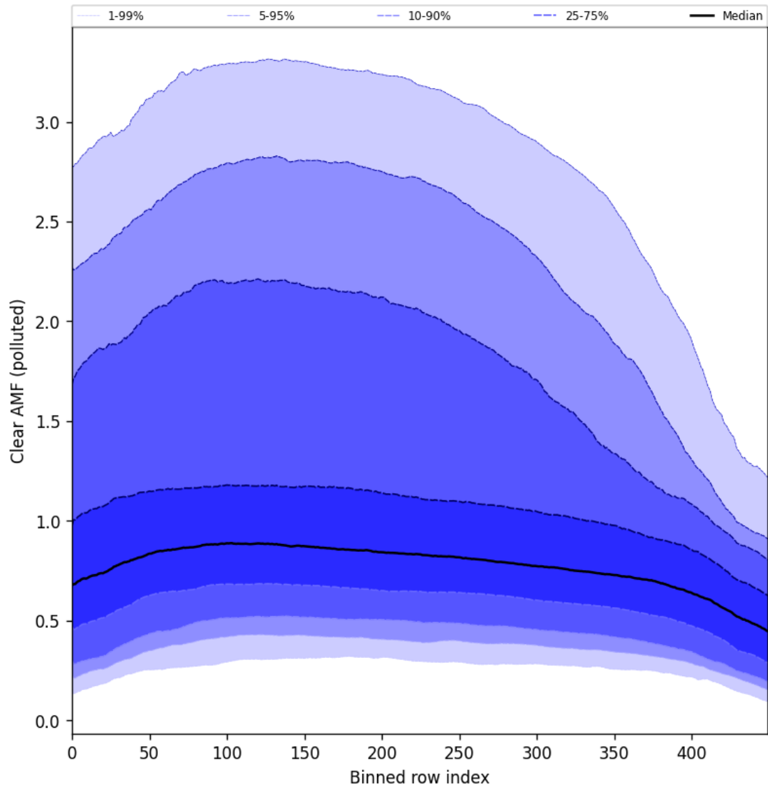
Figure 96: Along track statistics of “Clear AMF (polluted)” for 2024-10-03 to 2024-10-04
