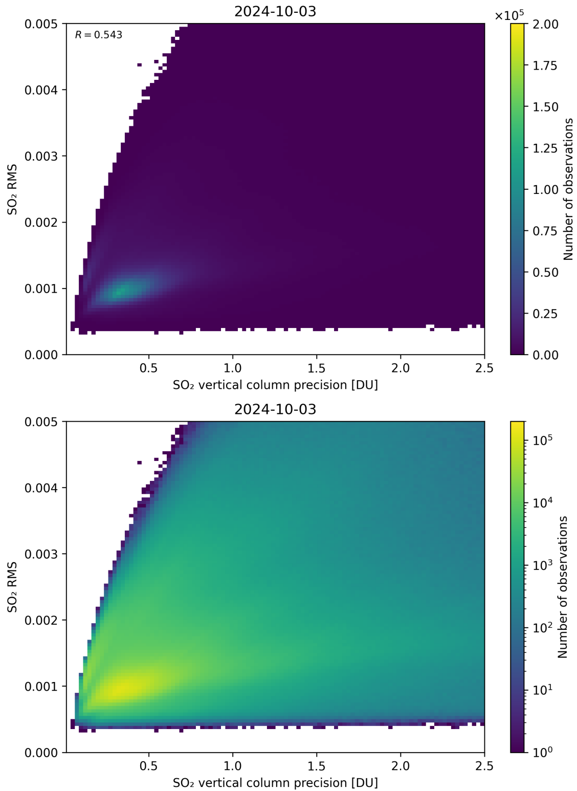
Figure 284: Scatter density plot of “SO 2 vertical column precision” against “SO 2 RMS” for 2024-10-03 to 2024-10-04.
