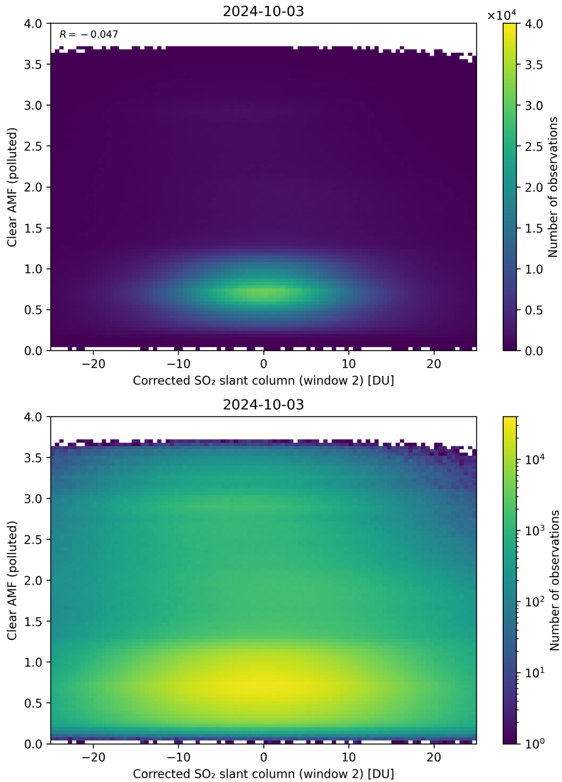
Figure 199: Scatter density plot of “Corrected SO 2 slant column (window 2)” against “Clear AMF (polluted)” for 2024-10-03 to 2024-10-04.
