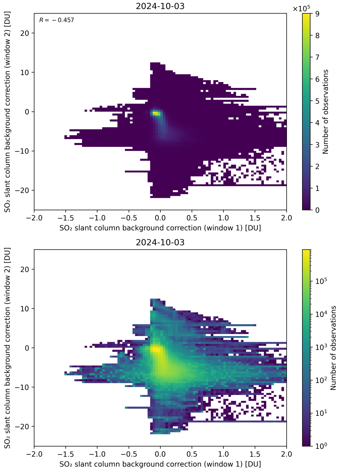
Figure 98: Scatter density plot of “SO 2 slant column background correction (window 1)” against “SO 2 slant column background correction (window 2)” for 2024-10-03 to 2024-10-04.
