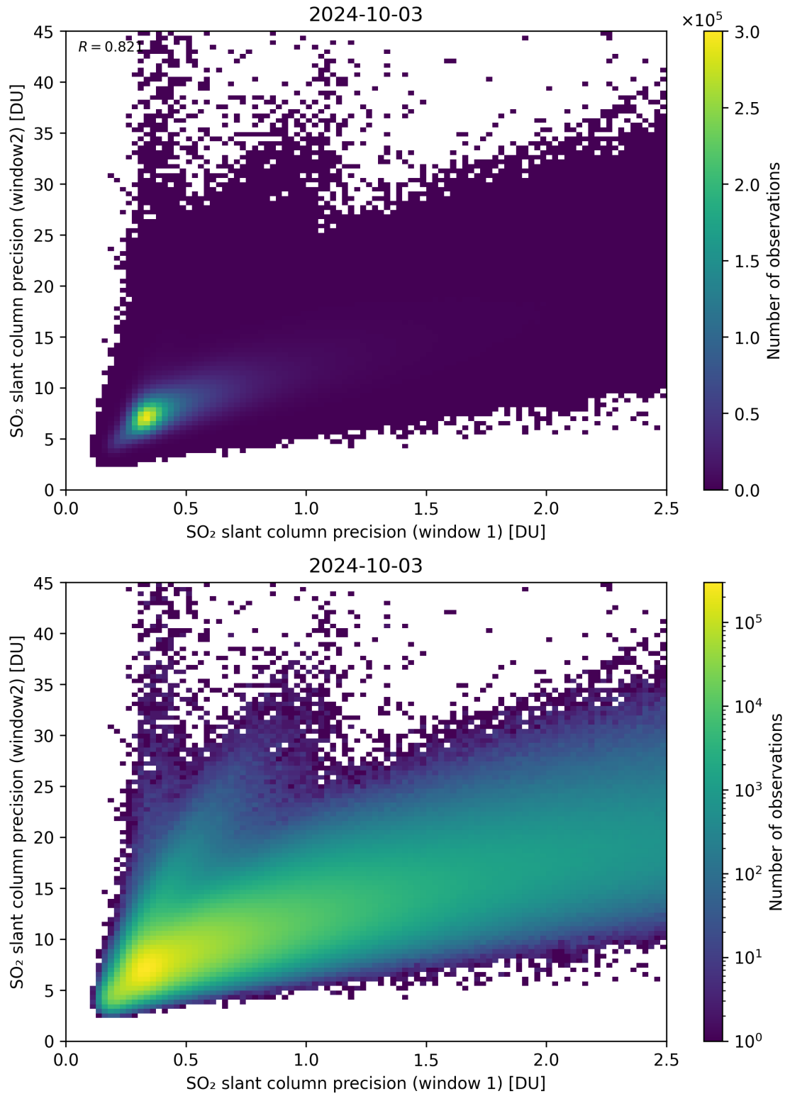
Figure 227: Scatter density plot of “SO 2 slant column precision (window 1)” against “SO 2 slant column precision (window2)” for 2024-10-03 to 2024-10-04.
