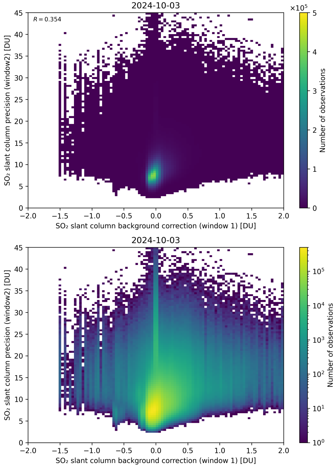
Figure 106: Scatter density plot of “SO 2 slant column background correction (window 1)” against “SO 2 slant column precision (window2)” for 2024-10-03 to 2024-10-04.
