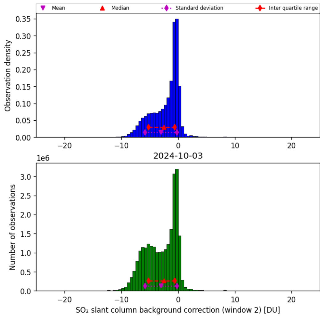
Figure 63: Histogram of “SO 2 slant column background correction (window 2)” for 2024-10-03 to 2024-10-04
