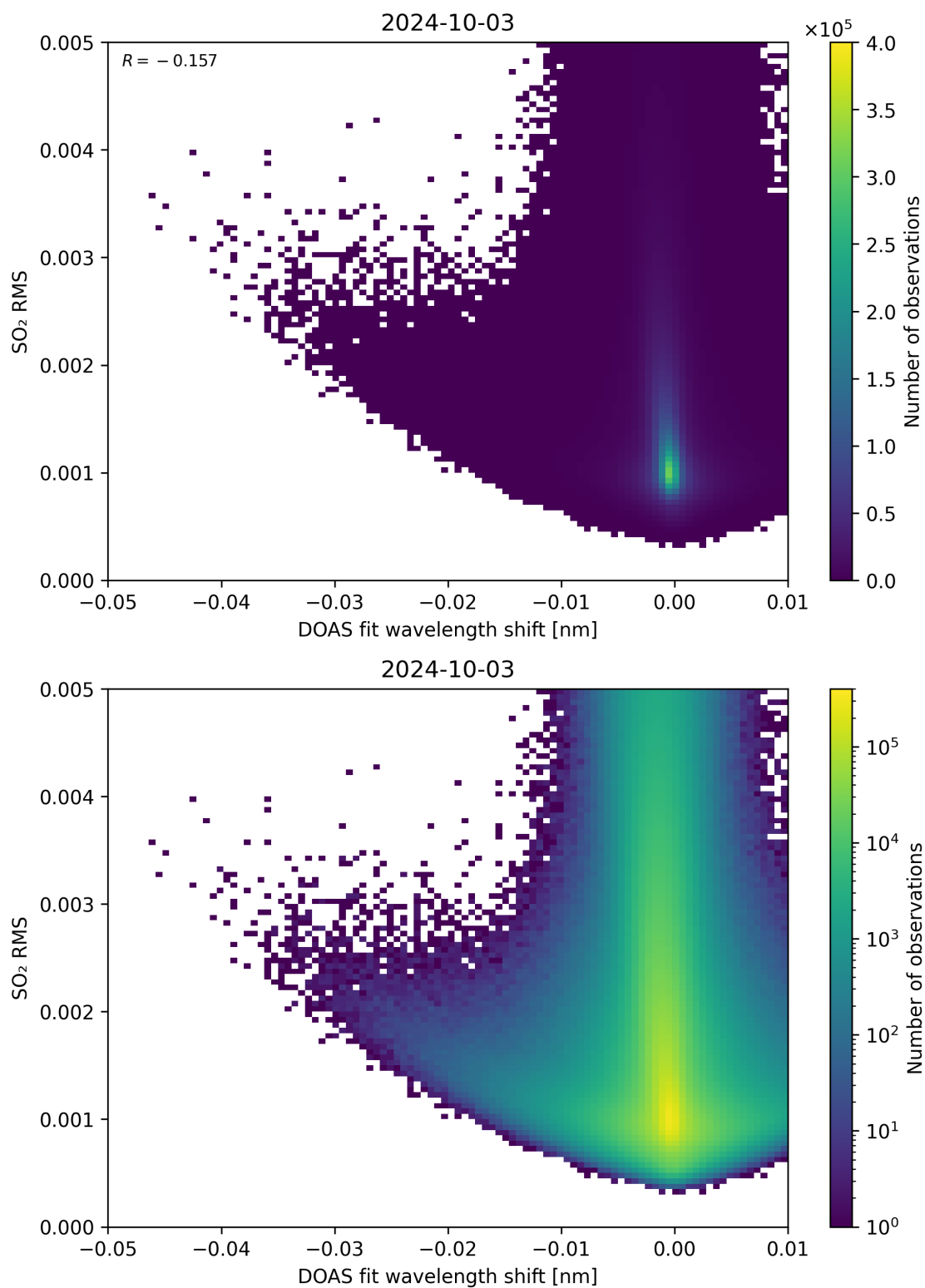
Figure 128: Scatter density plot of “DOAS fit wavelength shift” against “SO 2 RMS” for 2024-10-03 to 2024-10-04.
