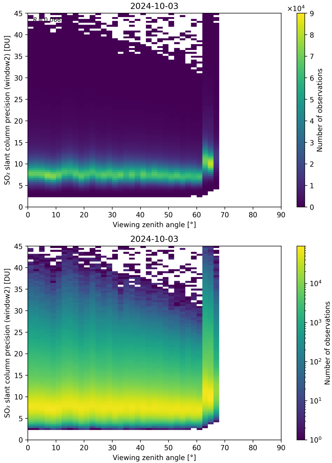
Figure 322: Scatter density plot of “Viewing zenith angle” against “SO 2 slant column precision (window2)” for 2024-10-03 to 2024-10-04.
