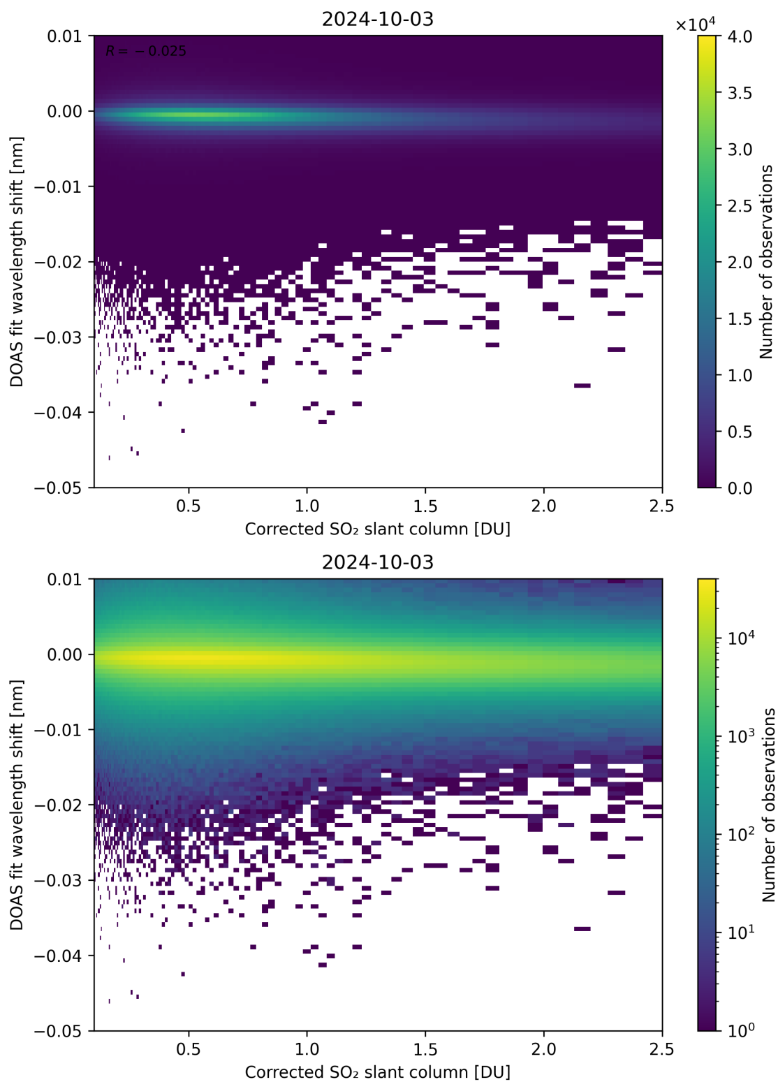
Figure 181: Scatter density plot of “Corrected SO 2 slant column” against “DOAS fit wavelength shift” for 2024-10-03 to 2024-10-04.
