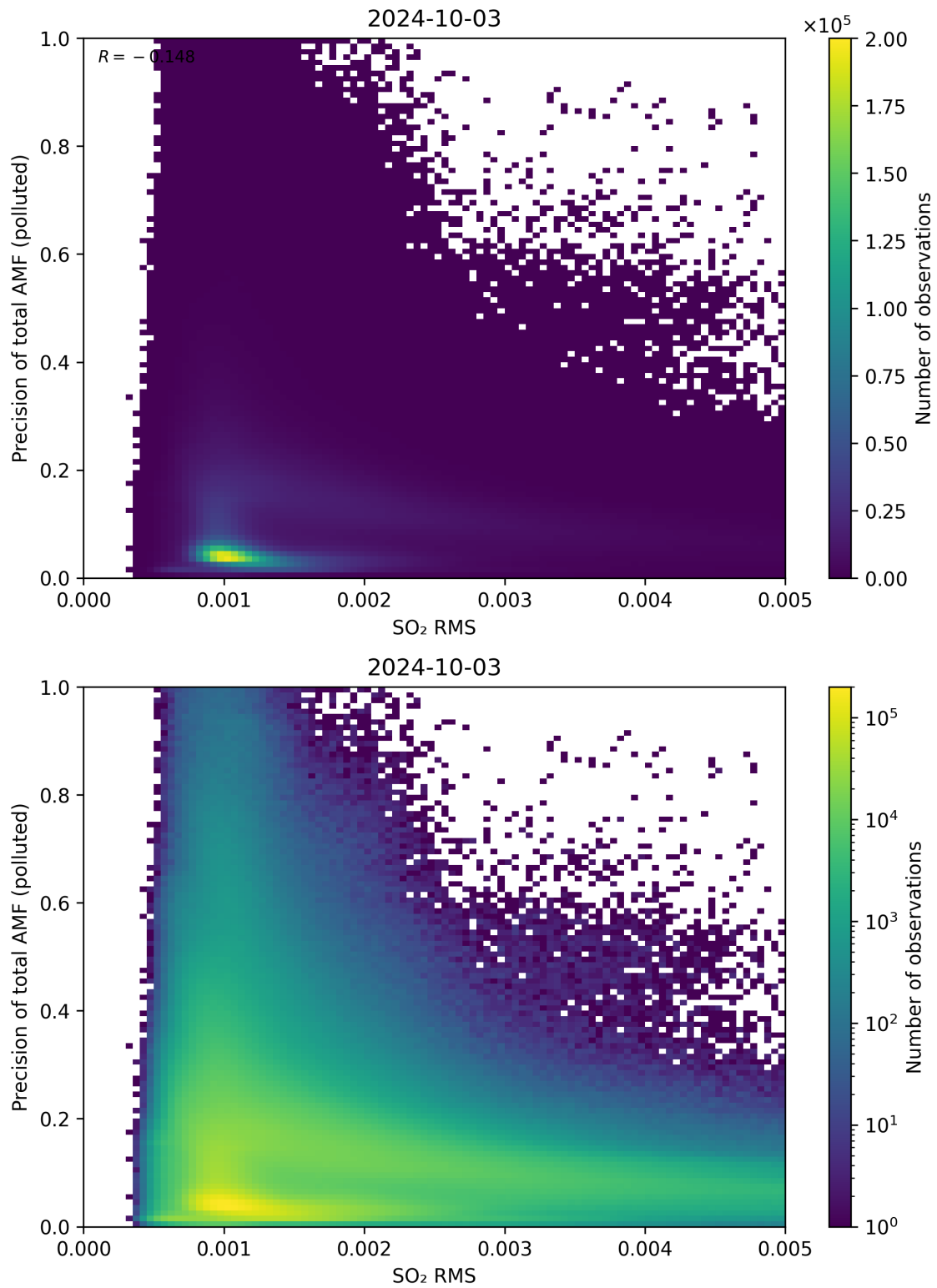
Figure 138: Scatter density plot of “SO 2 RMS” against “Precision of total AMF (polluted)” for 2024-10-03 to 2024-10-04.
