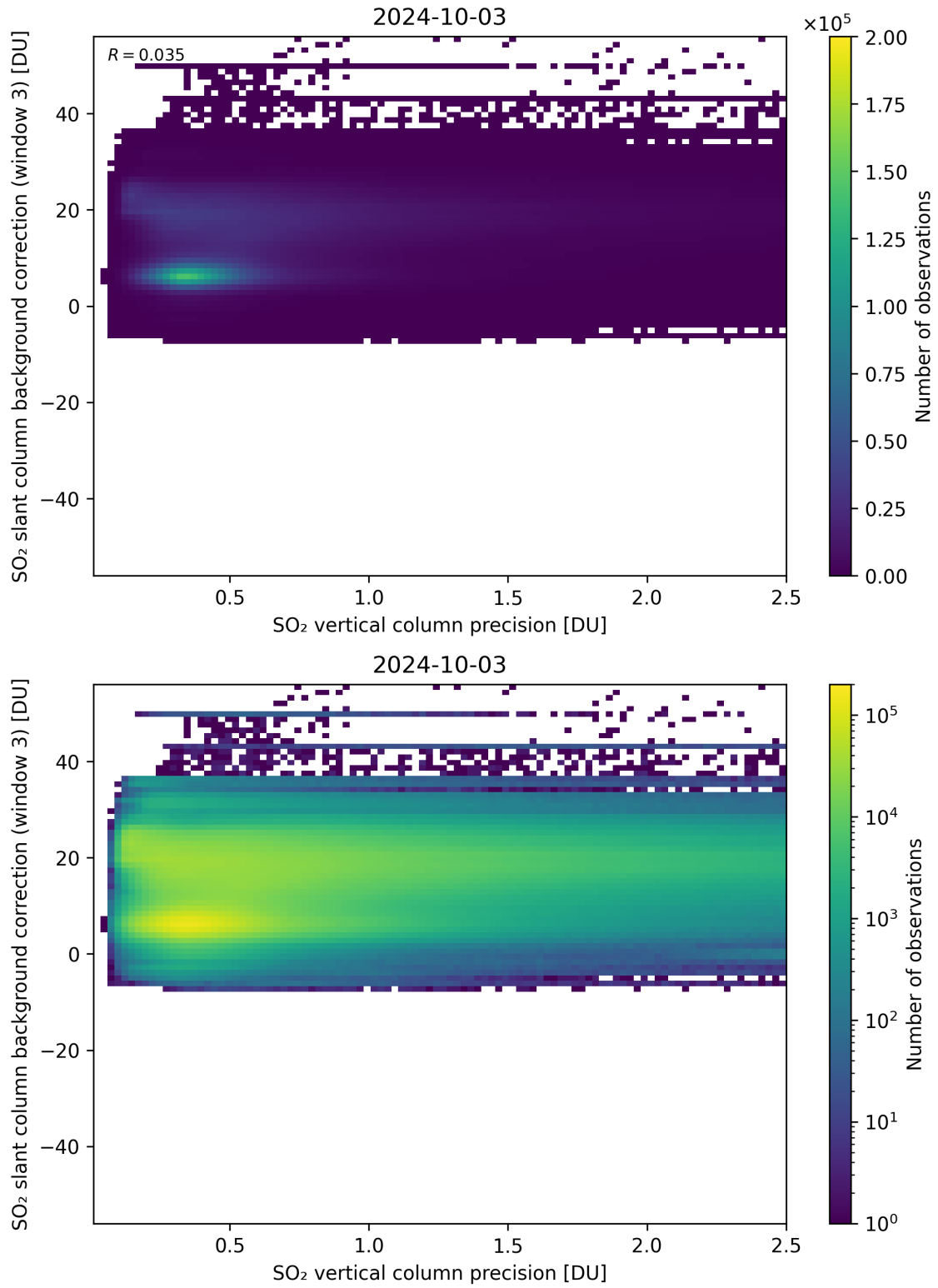
Figure 281: Scatter density plot of “SO 2 vertical column precision” against “SO 2 slant column background correction (window 3)” for 2024-10-03 to 2024-10-04.
