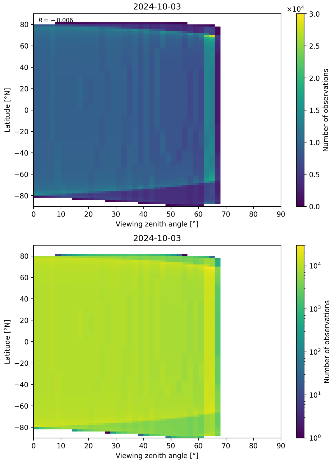
Figure 314: Scatter density plot of “Viewing zenith angle” against “Latitude” for 2024-10-03 to 2024-10-04.
