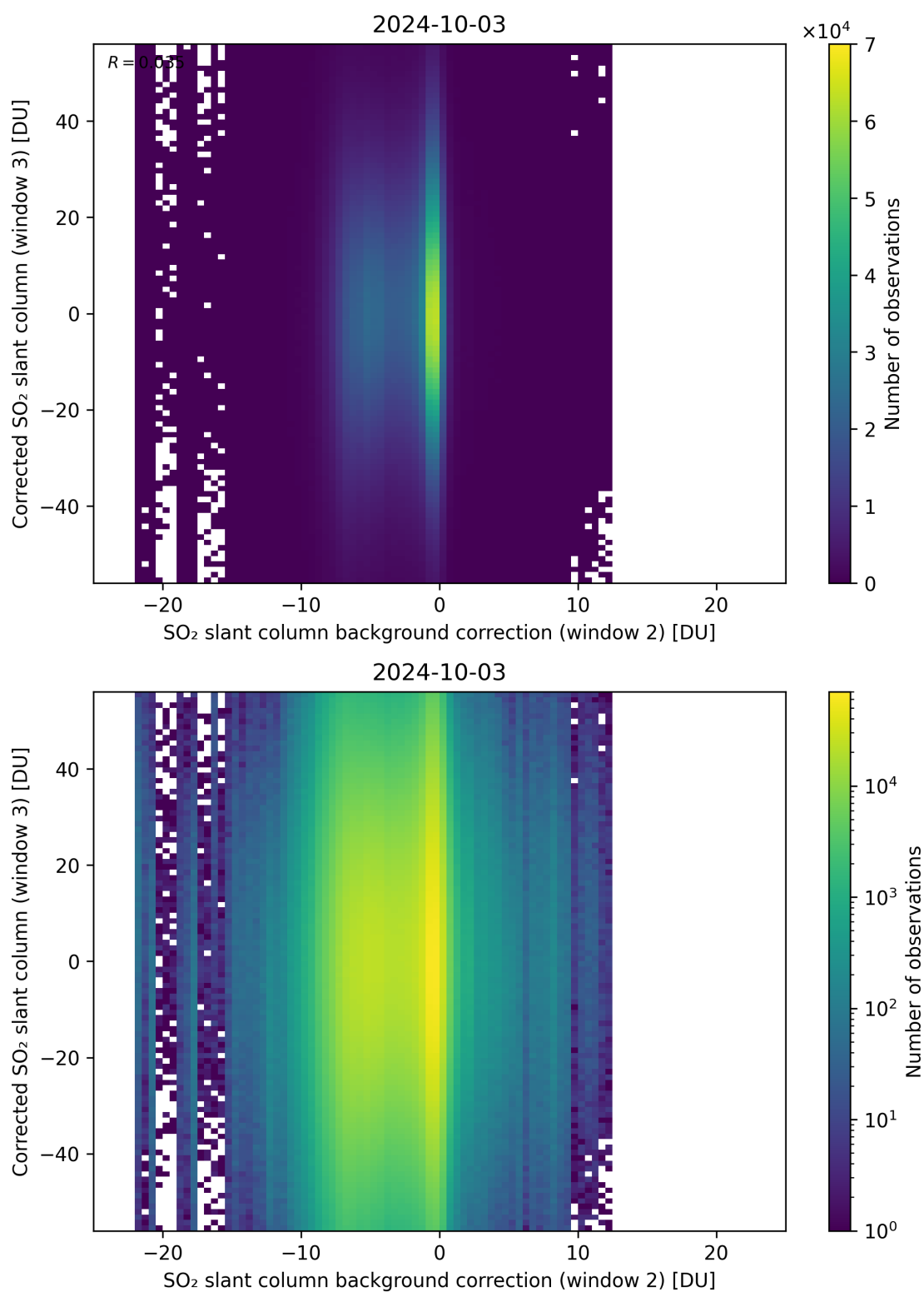
Figure 116: Scatter density plot of “SO 2 slant column background correction (window 2)” against “Corrected SO 2 slant column (window 3)” for 2024-10-03 to 2024-10-04.
