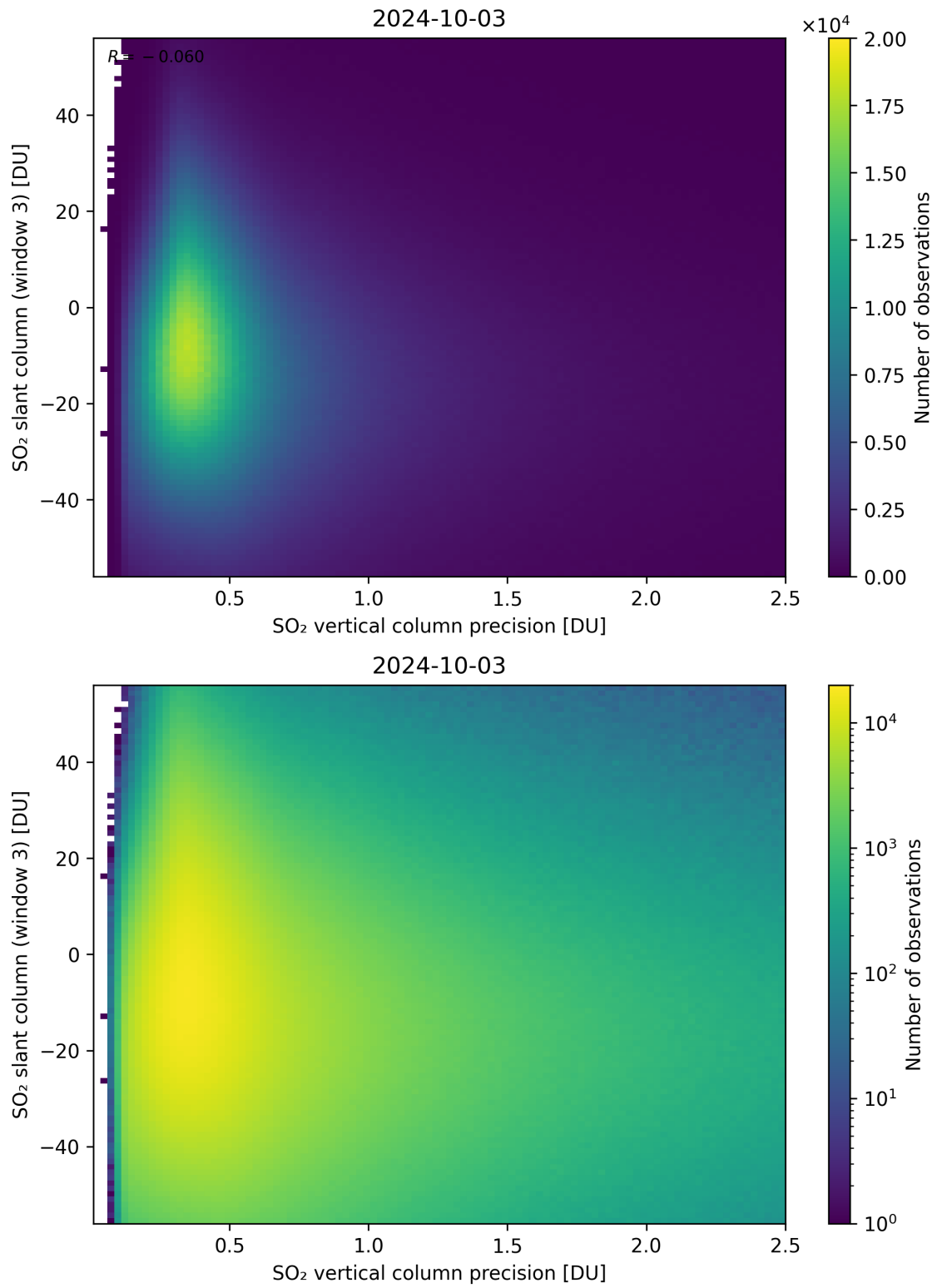
Figure 292: Scatter density plot of “SO 2 vertical column precision” against “SO 2 slant column (window 3)” for 2024-10-03 to 2024-10-04.
