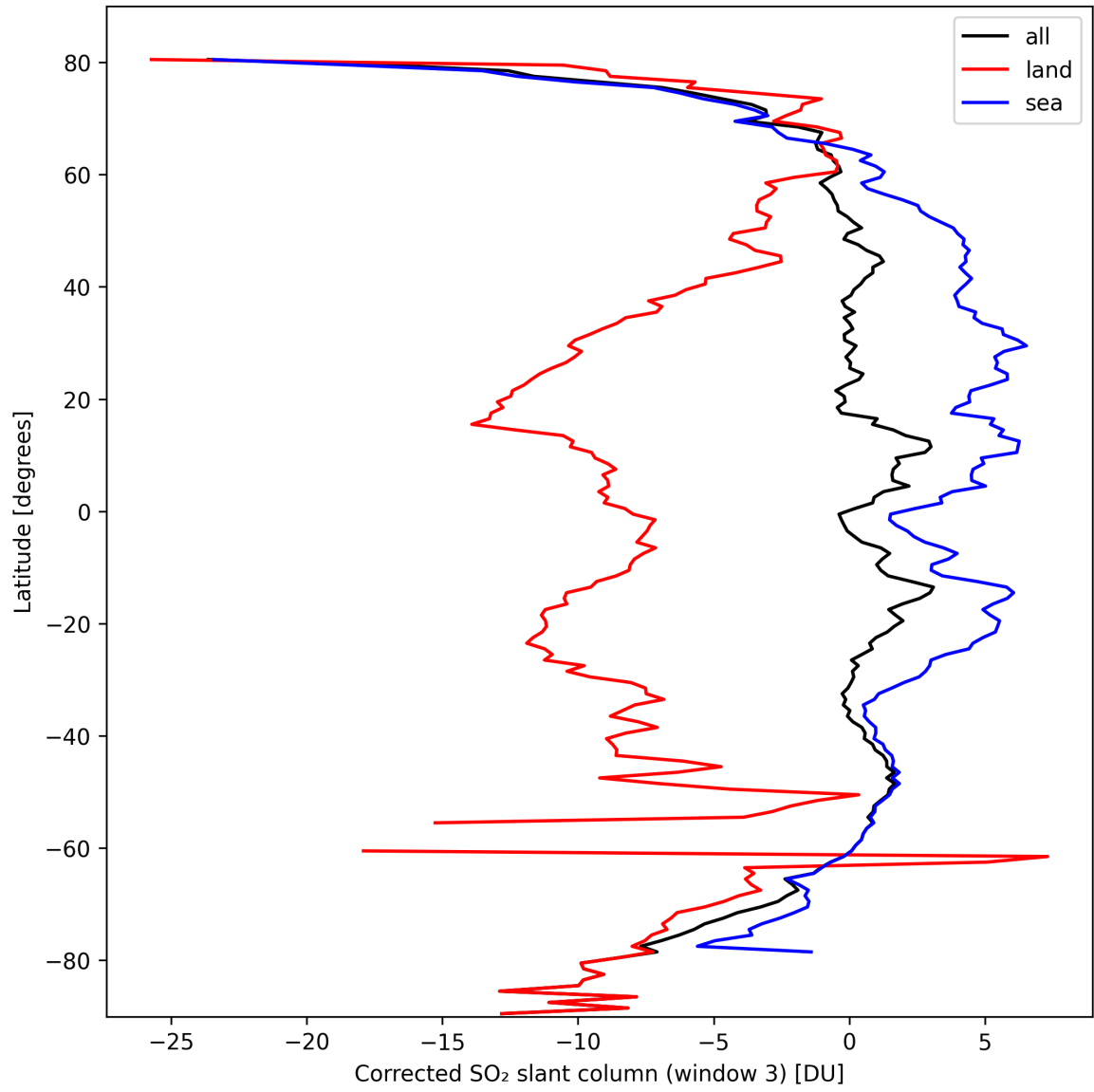
Figure 43: Zonal average of “Corrected SO 2 slant column (window 3)” for 2024-10-03 to 2024-10-04.
