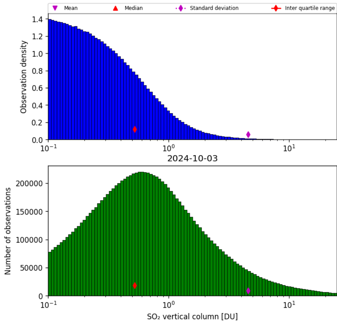
Figure 53: Histogram of “SO 2 vertical column” for 2024-10-03 to 2024-10-04
