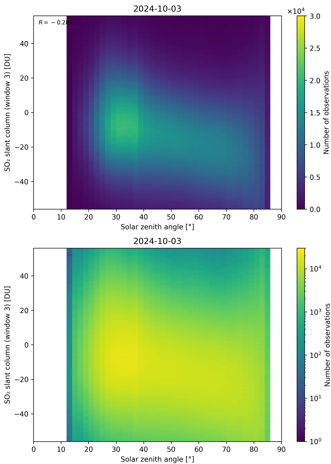
Figure 172: Scatter density plot of “Solar zenith angle” against “SO 2 slant column (window 3)” for 2024-10-03 to 2024-10-04.
