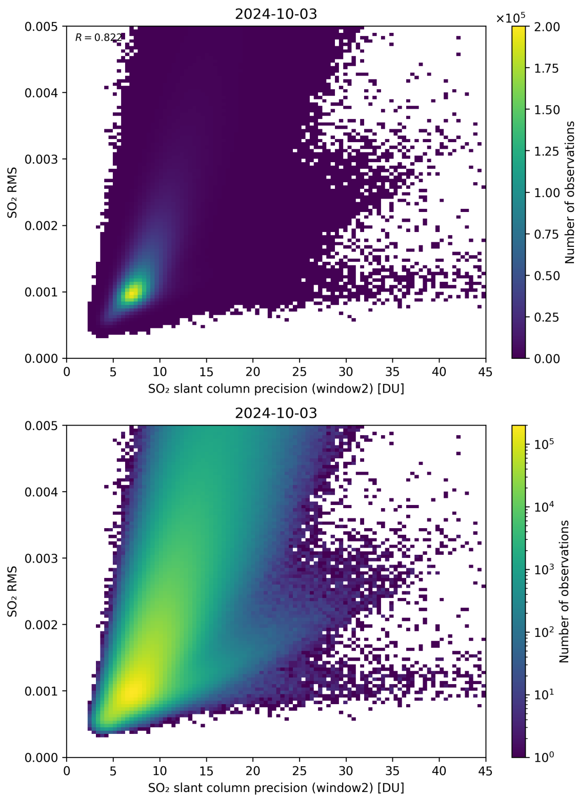
Figure 245: Scatter density plot of “SO 2 slant column precision (window2)” against “SO 2 RMS” for 2024-10-03 to 2024-10-04.
