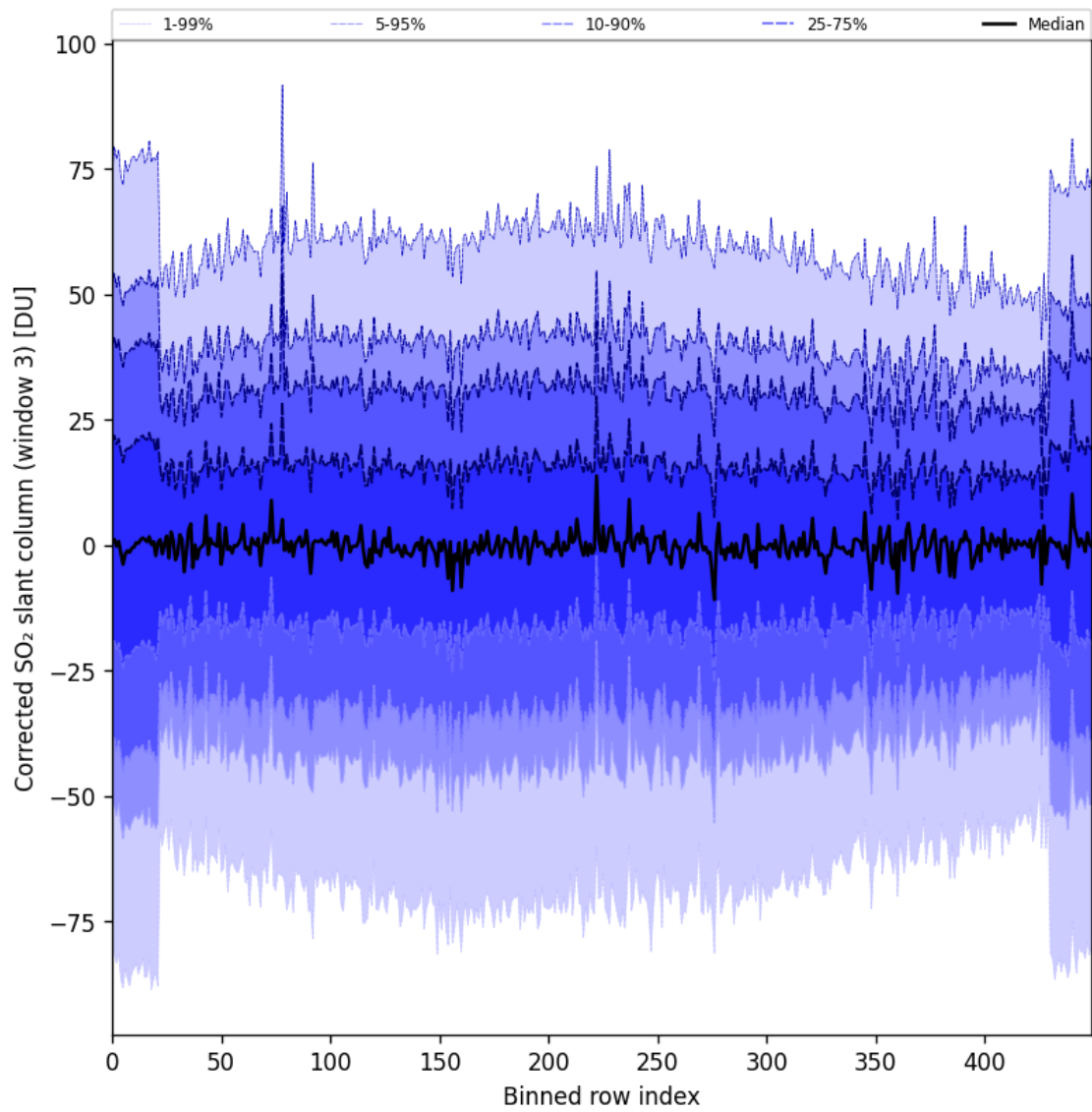
Figure 89: Along track statistics of “Corrected SO 2 slant column (window 3)” for 2024-10-03 to 2024-10-04
