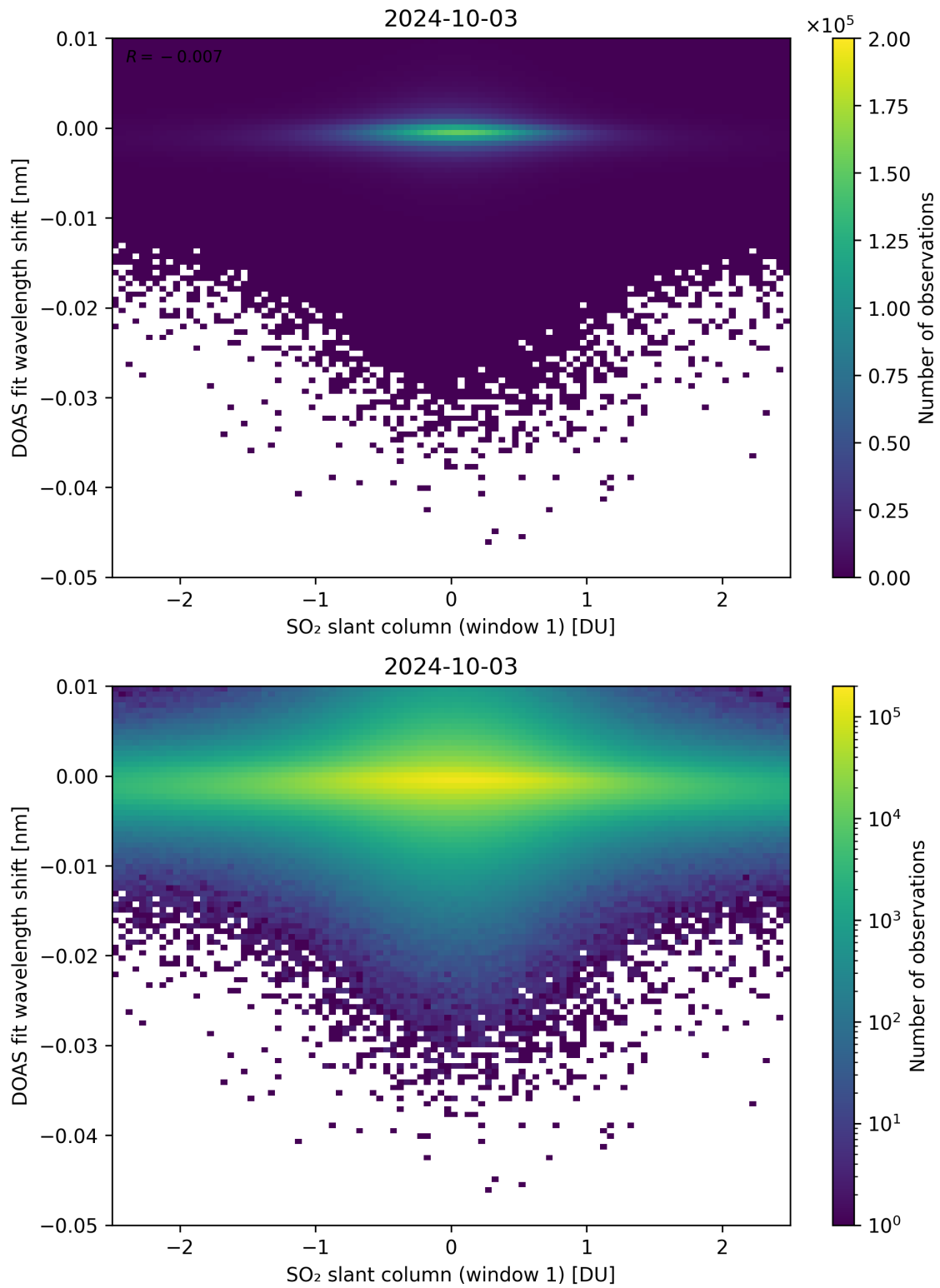
Figure 215: Scatter density plot of “SO 2 slant column (window 1)” against “DOAS fit wavelength shift” for 2024-10-03 to 2024-10-04.
