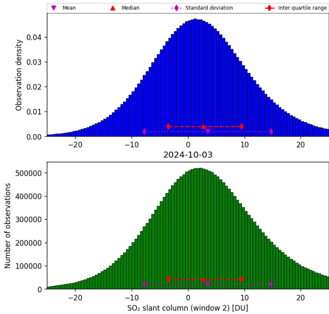
Figure 60: Histogram of “SO 2 slant column (window 2)” for 2024-10-03 to 2024-10-04
