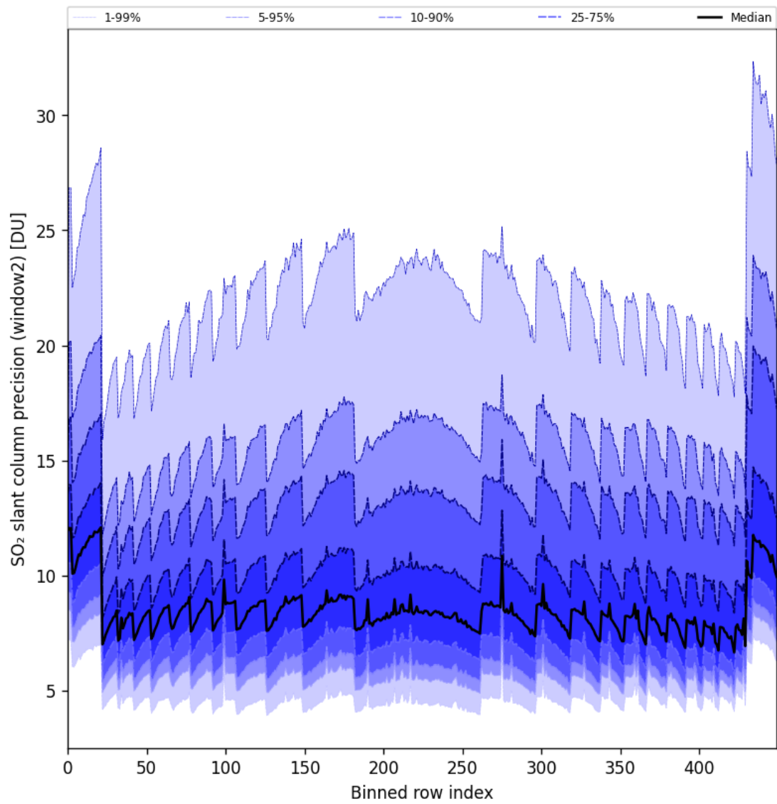
Figure 84: Along track statistics of “SO 2 slant column precision (window2)” for 2024-10-03 to 2024-10-04
