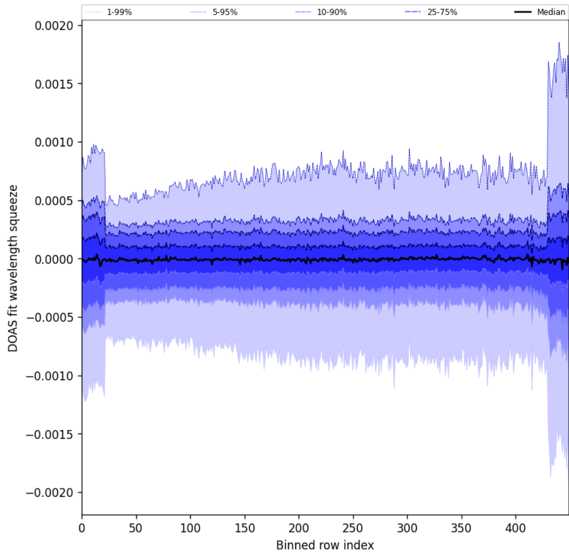
Figure 92: Along track statistics of “DOAS fit wavelength squeeze” for 2024-10-03 to 2024-10-04
