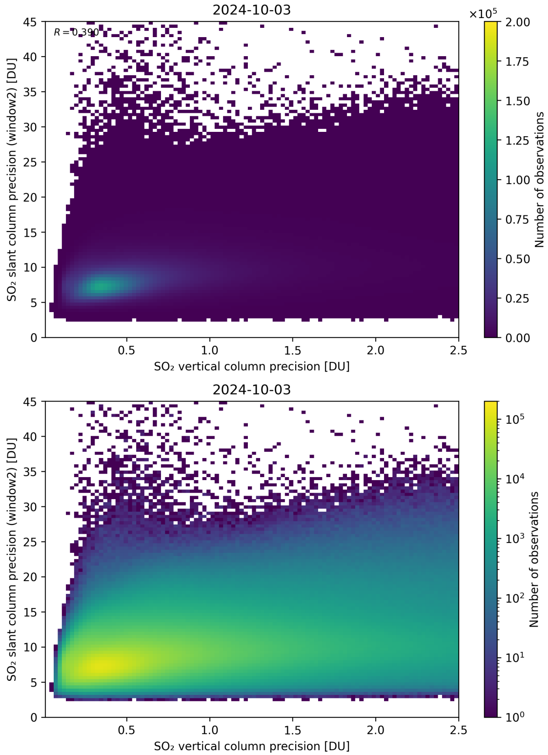
Figure 291: Scatter density plot of “SO 2 vertical column precision” against “SO 2 slant column precision (window2)” for 2024-10-03 to 2024-10-04.
