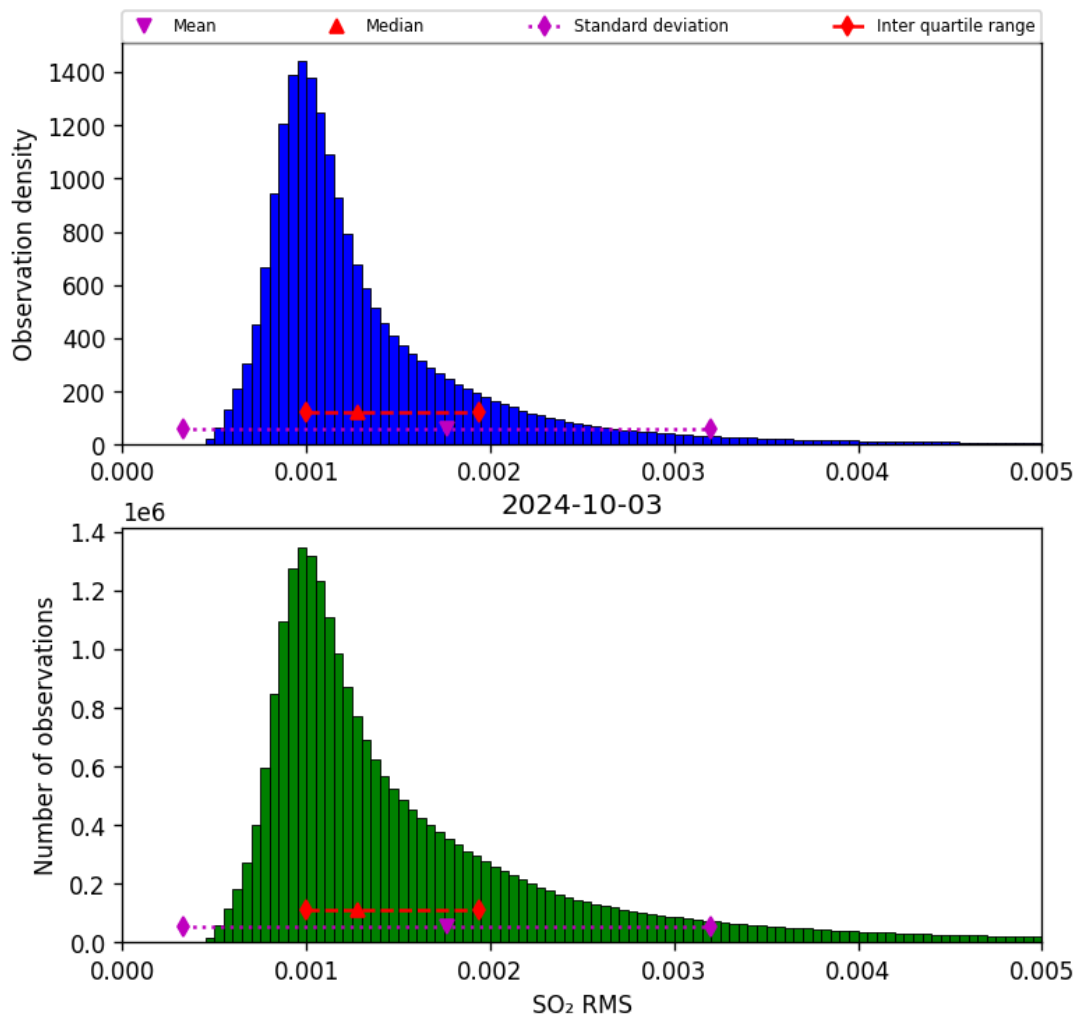
Figure 70: Histogram of “SO 2 RMS” for 2024-10-03 to 2024-10-04
