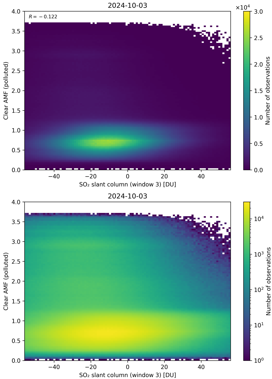
Figure 265: Scatter density plot of “SO 2 slant column (window 3)” against “Clear AMF (polluted)” for 2024-10-03 to 2024-10-04.
