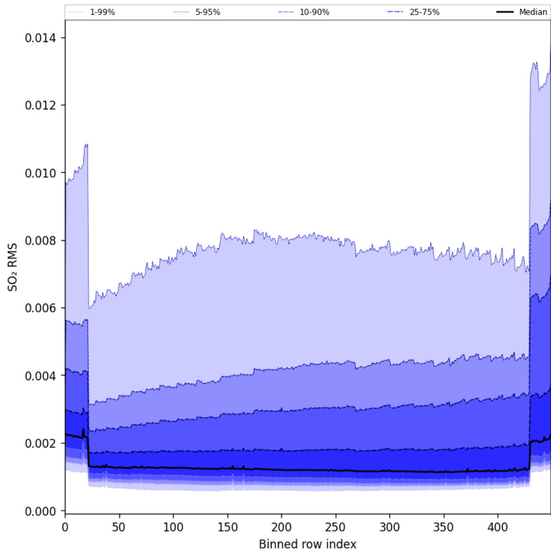
Figure 93: Along track statistics of “SO 2 RMS” for 2024-10-03 to 2024-10-04
