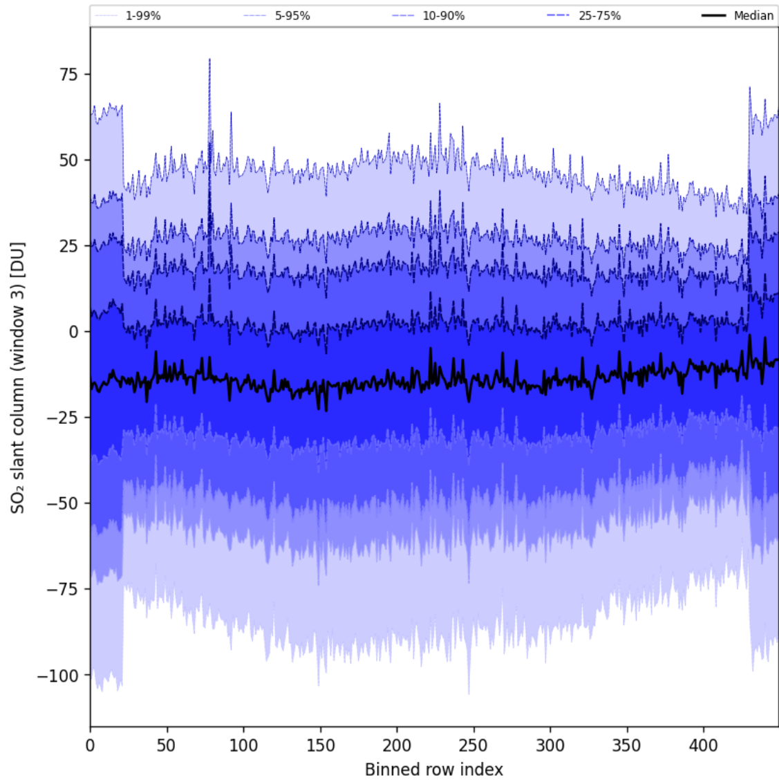
Figure 87: Along track statistics of “SO 2 slant column (window 3)” for 2024-10-03 to 2024-10-04
