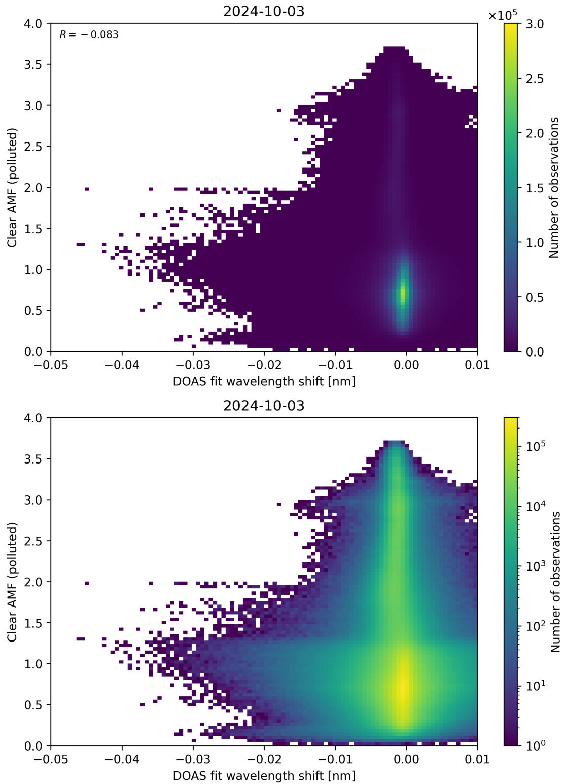
Figure 129: Scatter density plot of “DOAS fit wavelength shift” against “Clear AMF (polluted)” for 2024-10-03 to 2024-10-04.
