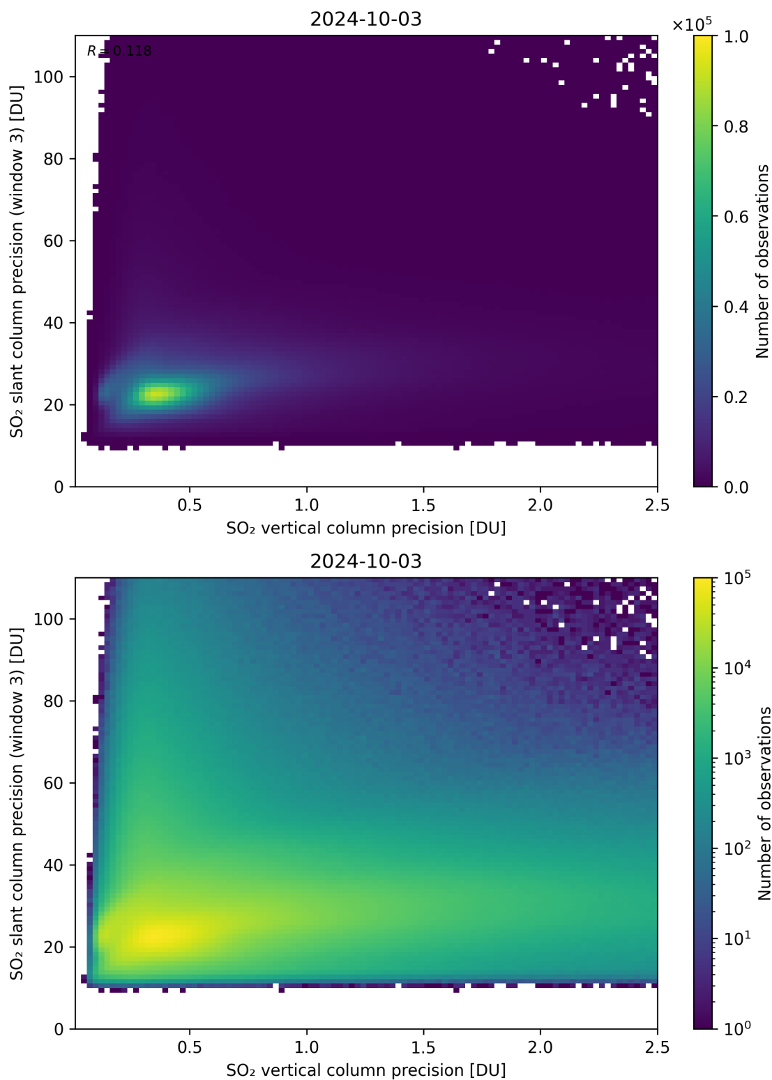
Figure 293: Scatter density plot of “SO 2 vertical column precision” against “SO 2 slant column precision (window 3)” for 2024-10-03 to 2024-10-04.
