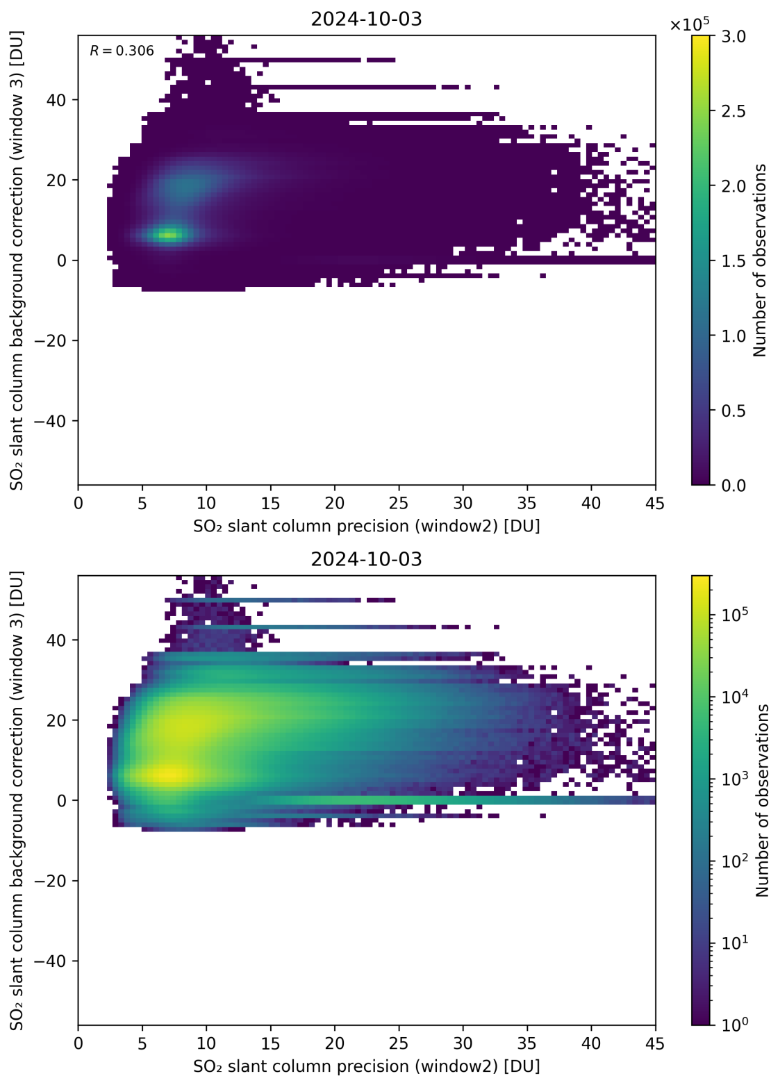
Figure 242: Scatter density plot of “SO 2 slant column precision (window2)” against “SO 2 slant column background correction (window 3)” for 2024-10-03 to 2024-10-04.
