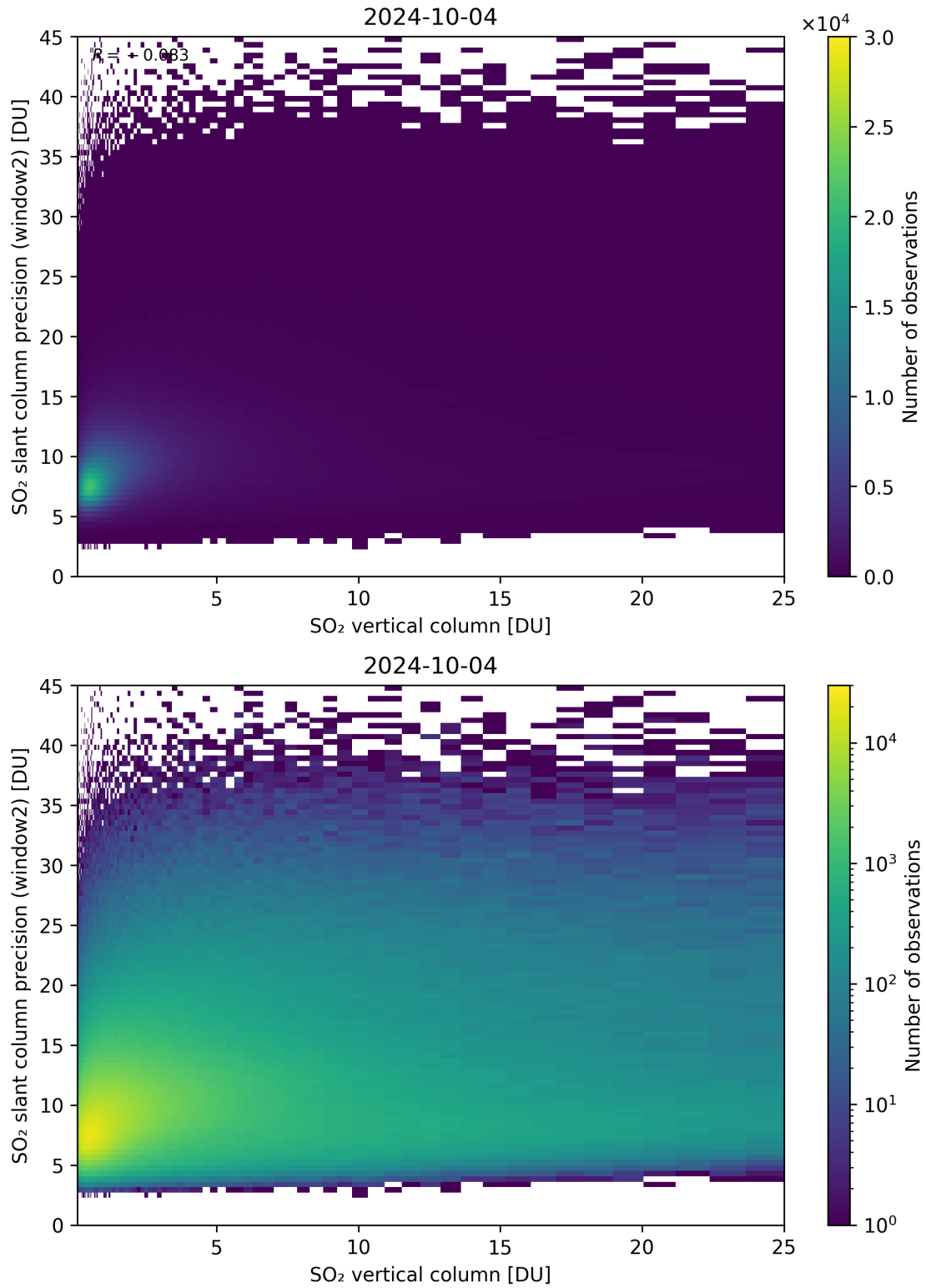
Figure 302: Scatter density plot of “SO 2 vertical column” against “SO 2 slant column precision (window2)” for 2024-10-03 to 2024-10-05.
