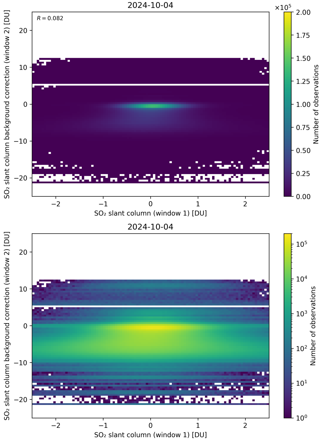
Figure 213: Scatter density plot of “SO 2 slant column (window 1)” against “SO 2 slant column background correction (window 2)” for 2024-10-03 to 2024-10-05.
