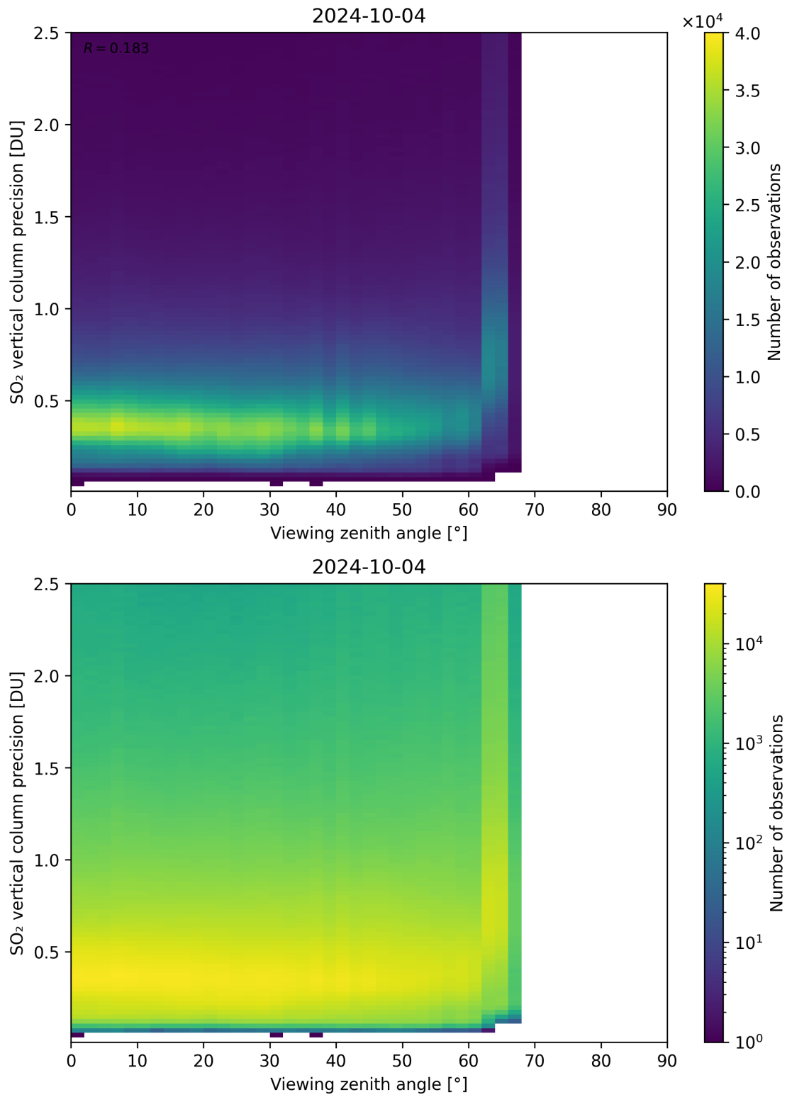
Figure 328: Scatter density plot of “Viewing zenith angle” against “SO 2 vertical column precision” for 2024-10-03 to 2024-10-05.
