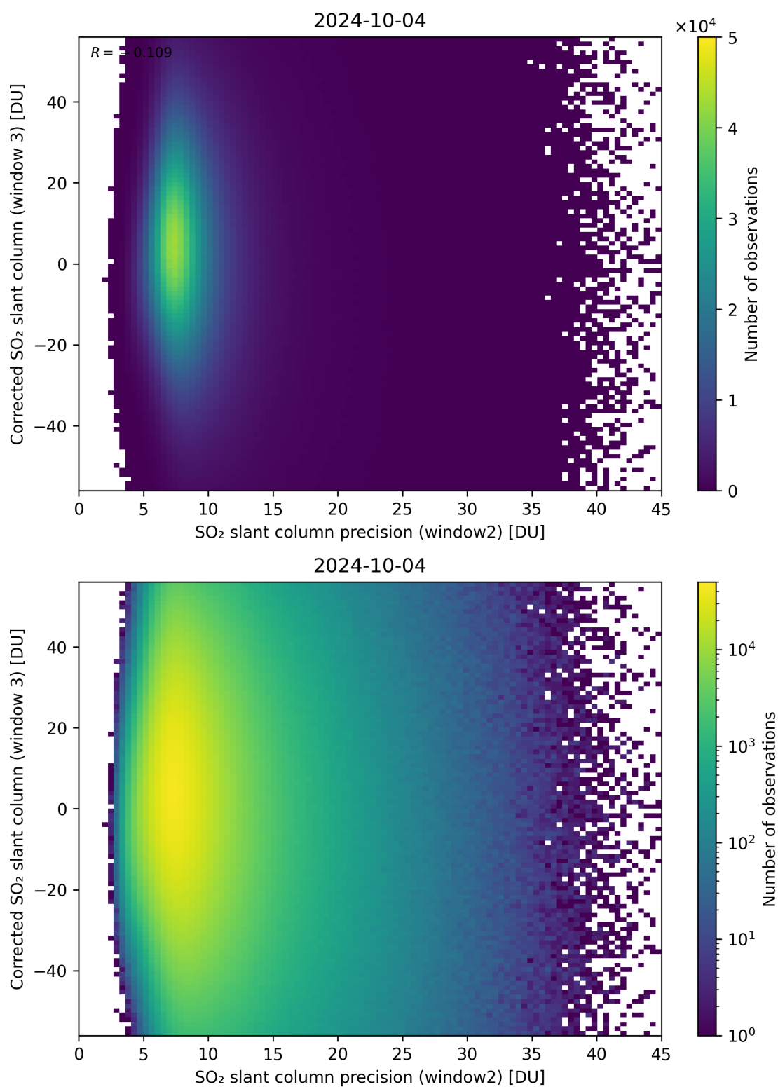
Figure 248: Scatter density plot of “SO 2 slant column precision (window2)” against “Corrected SO 2 slant column (window 3)” for 2024-10-03 to 2024-10-05.
