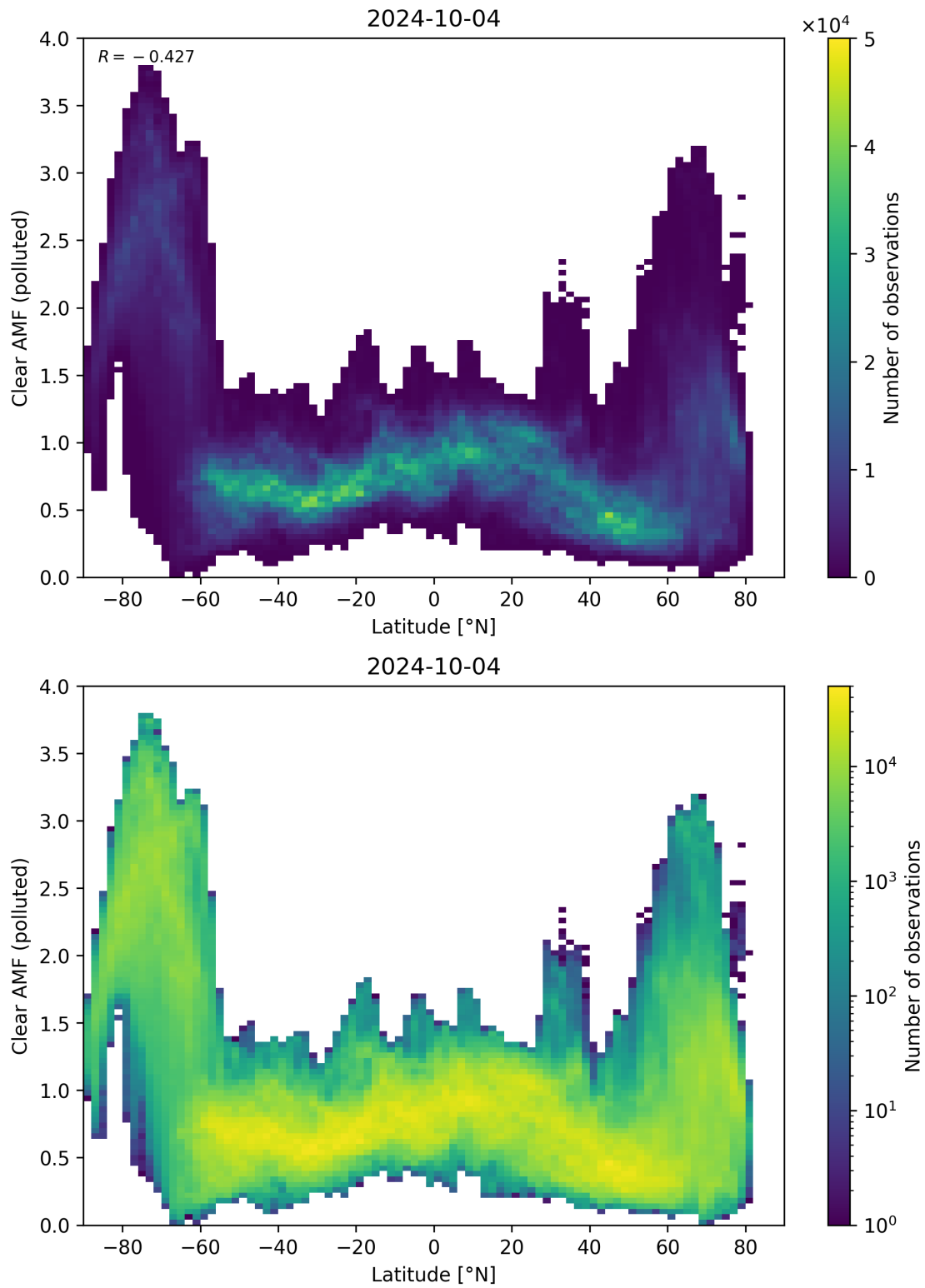
Figure 145: Scatter density plot of “Latitude” against “Clear AMF (polluted)” for 2024-10-03 to 2024-10-05.
