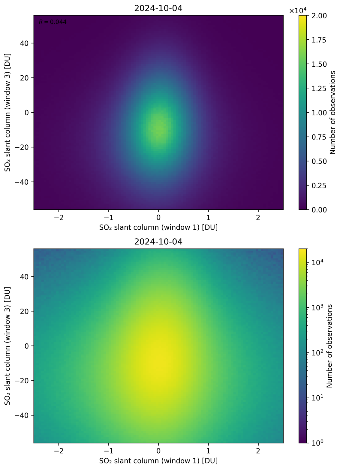
Figure 237: Scatter density plot of “SO 2 slant column (window 1)” against “SO 2 slant column (window 3)” for 2024-10-03 to 2024-10-05.
