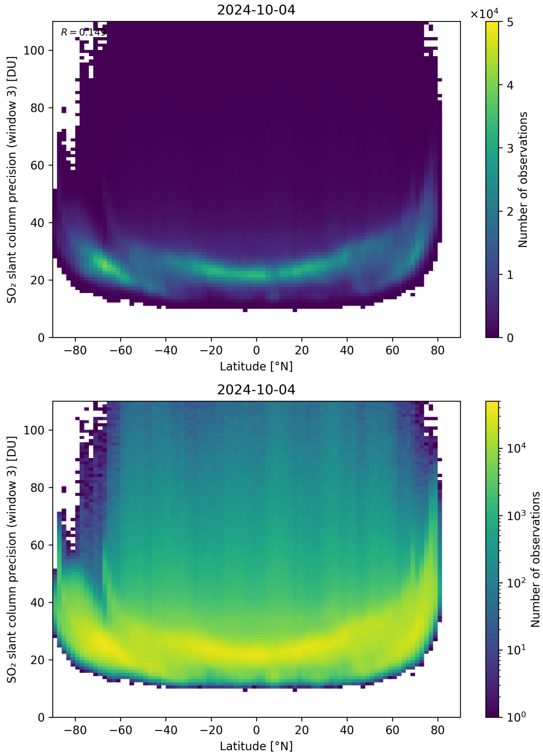
Figure 153: Scatter density plot of “Latitude” against “SO 2 slant column precision (window 3)” for 2024-10-03 to 2024-10-05.
