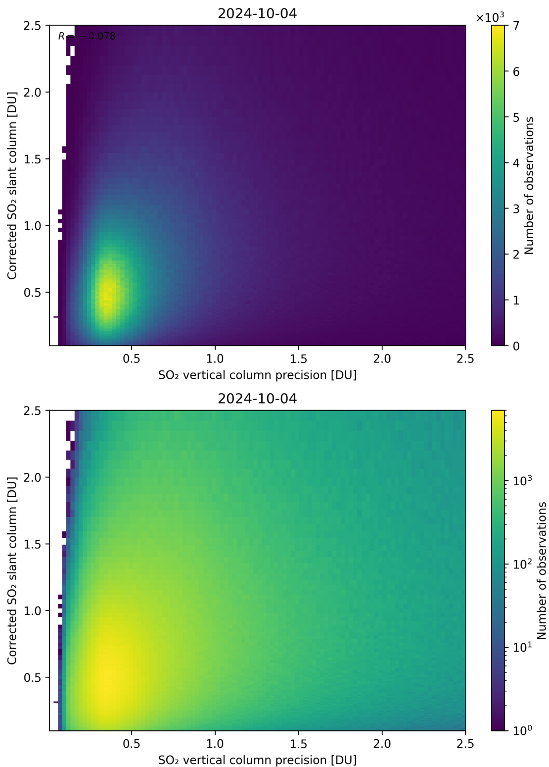
Figure 286: Scatter density plot of “SO 2 vertical column precision” against “Corrected SO 2 slant column” for 2024-10-03 to 2024-10-05.
