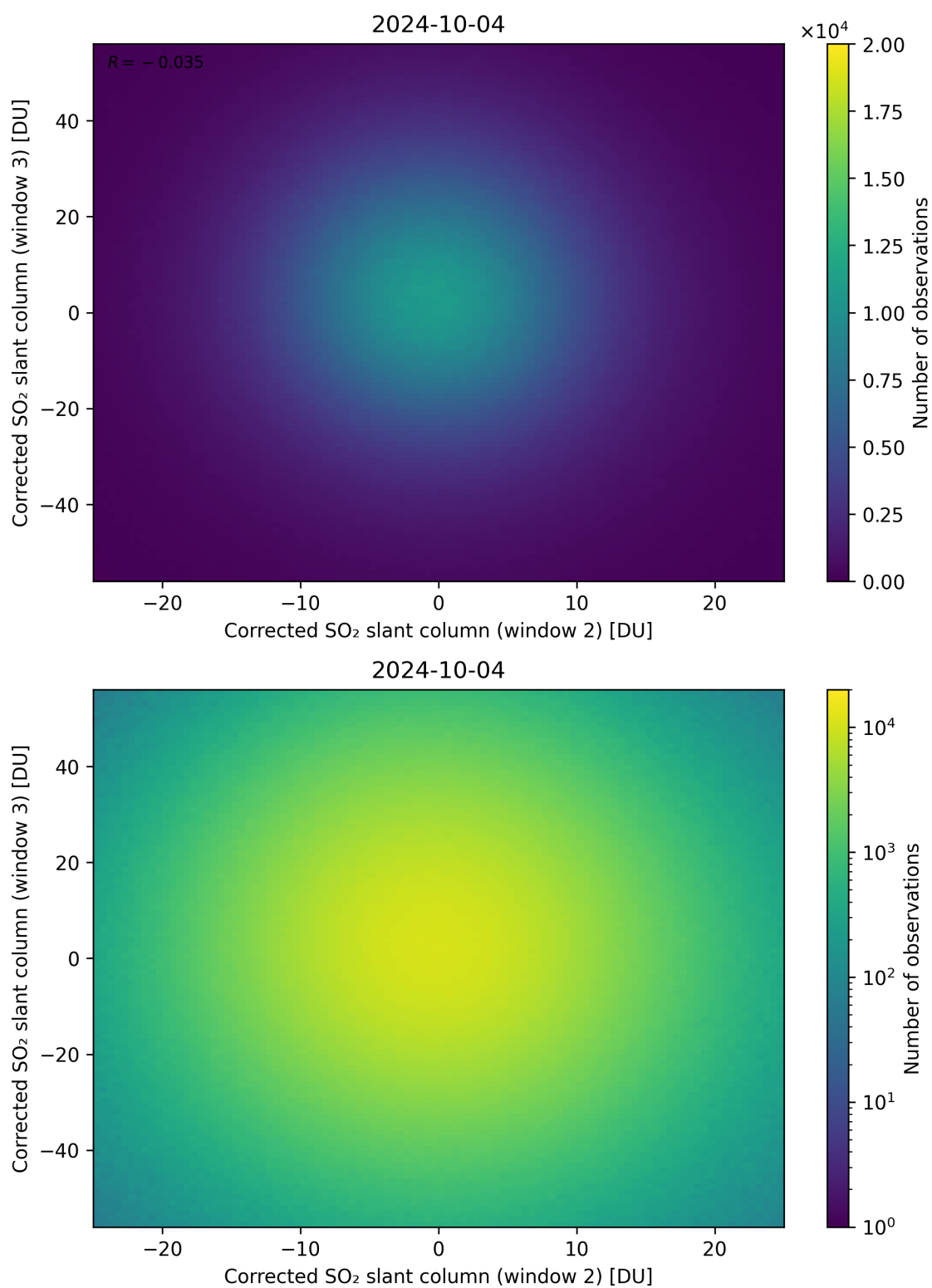
Figure 200: Scatter density plot of “Corrected SO 2 slant column (window 2)” against “Corrected SO 2 slant column (window 3)” for 2024-10-03 to 2024-10-05.
