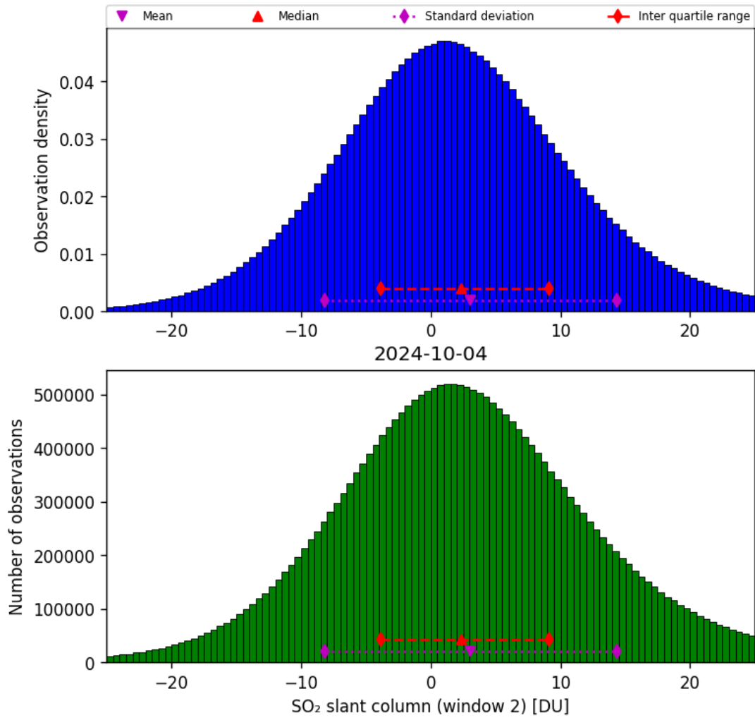
Figure 60: Histogram of “SO 2 slant column (window 2)” for 2024-10-03 to 2024-10-05
