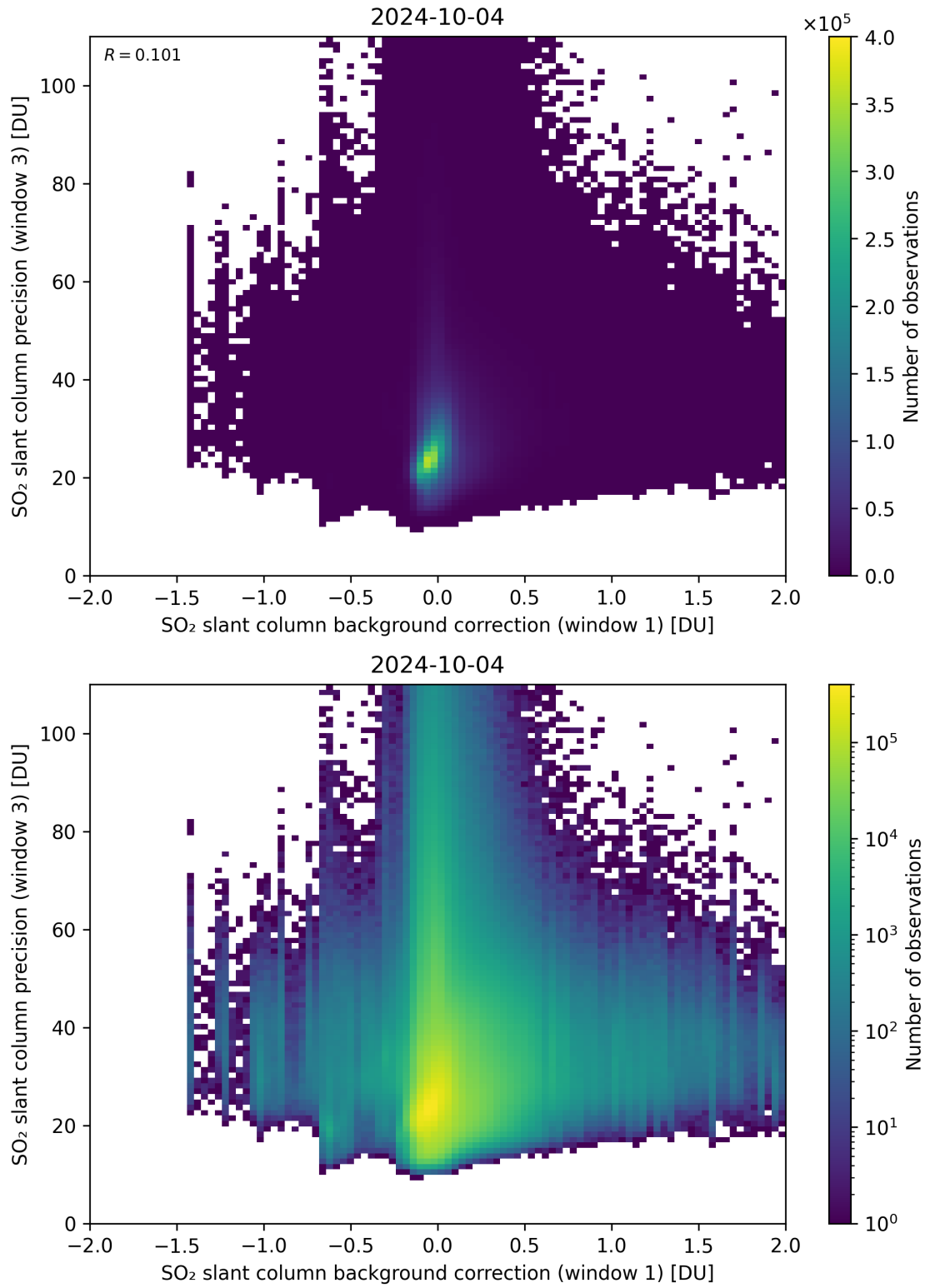
Figure 108: Scatter density plot of “SO 2 slant column background correction (window 1)” against “SO 2 slant column precision (window 3)” for 2024-10-03 to 2024-10-05.
