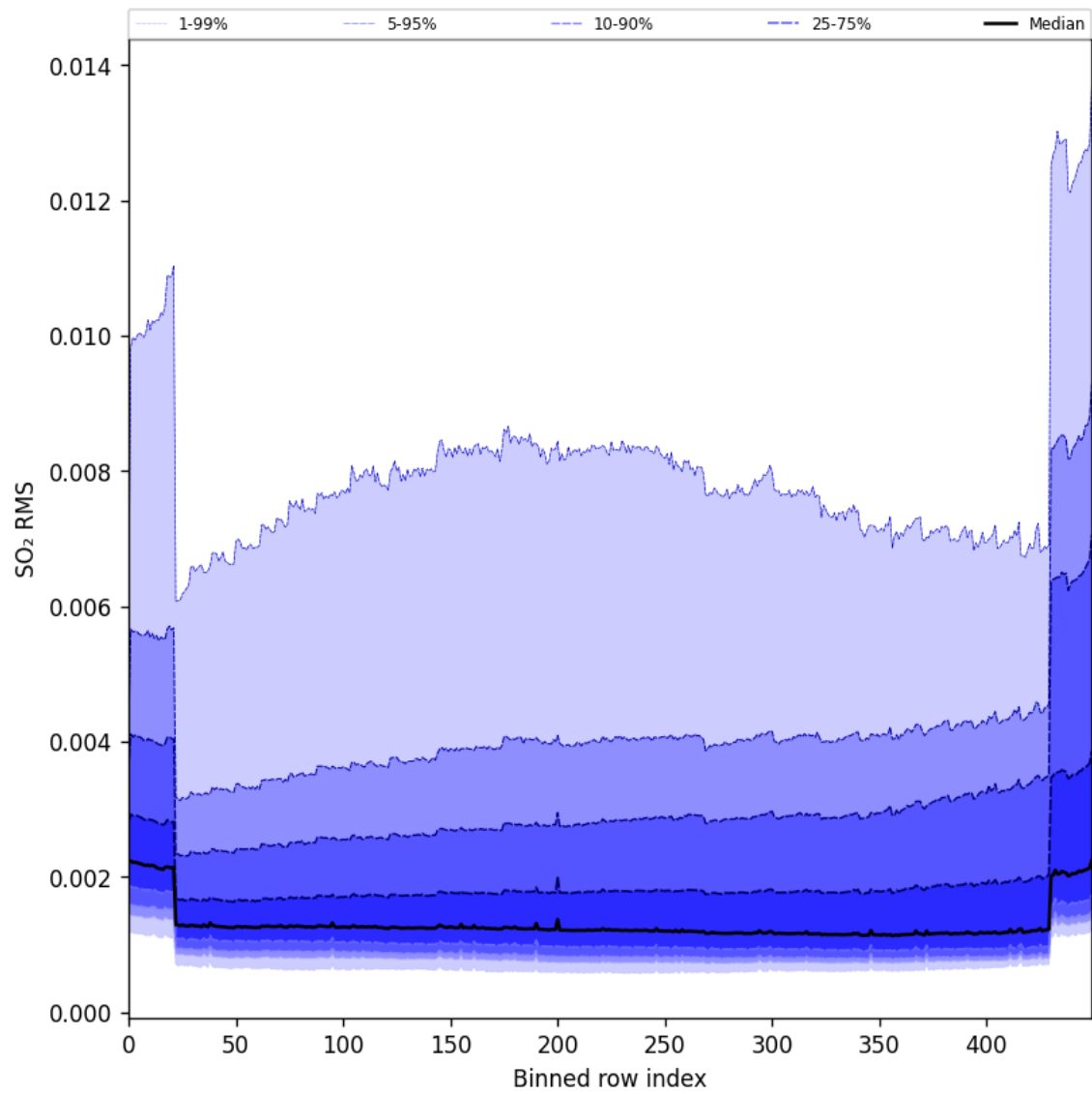
Figure 93: Along track statistics of “SO 2 RMS” for 2024-10-03 to 2024-10-05
