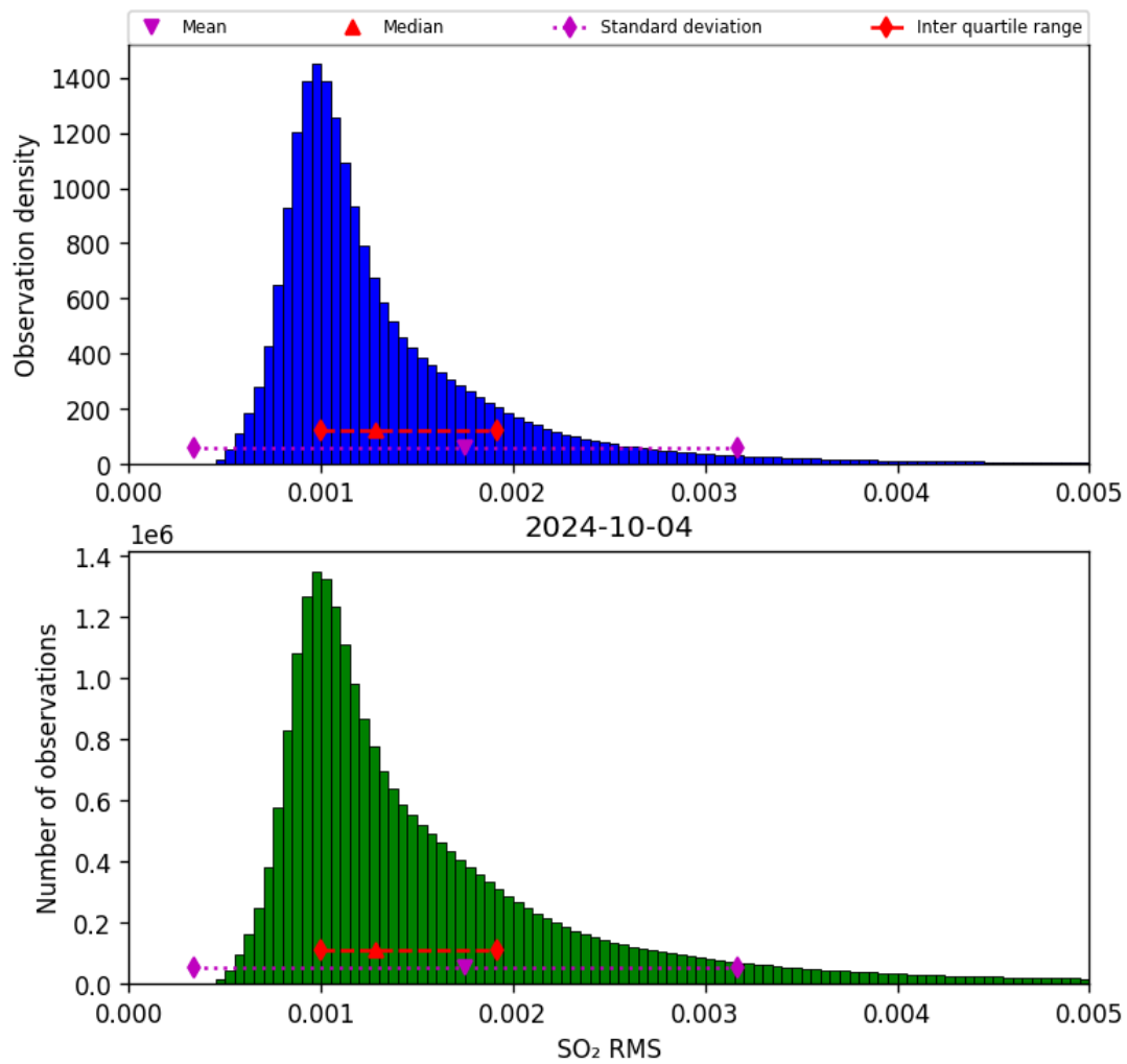
Figure 70: Histogram of “SO 2 RMS” for 2024-10-03 to 2024-10-05
