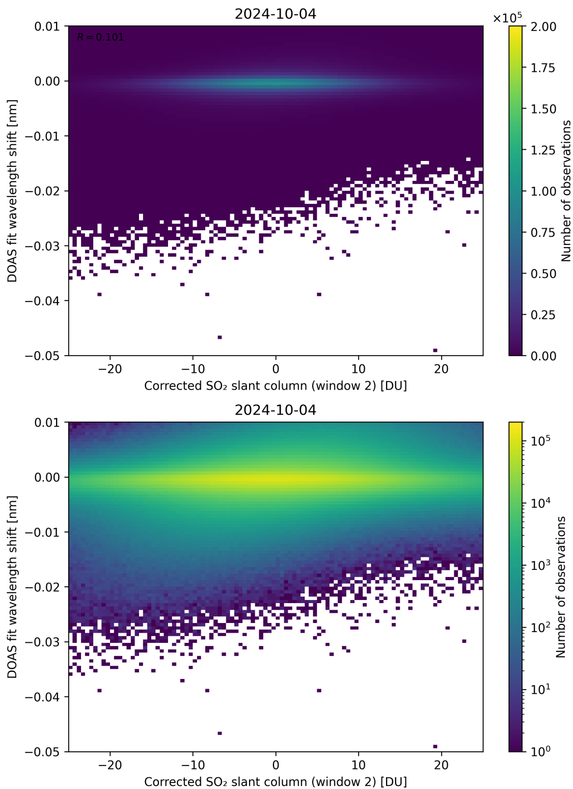
Figure 196: Scatter density plot of “Corrected SO 2 slant column (window 2)” against “DOAS fit wavelength shift” for 2024-10-03 to 2024-10-05.
