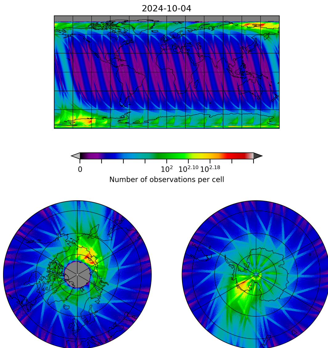
Figure 28: Map of the number of observations for 2024-10-03 to 2024-10-05
