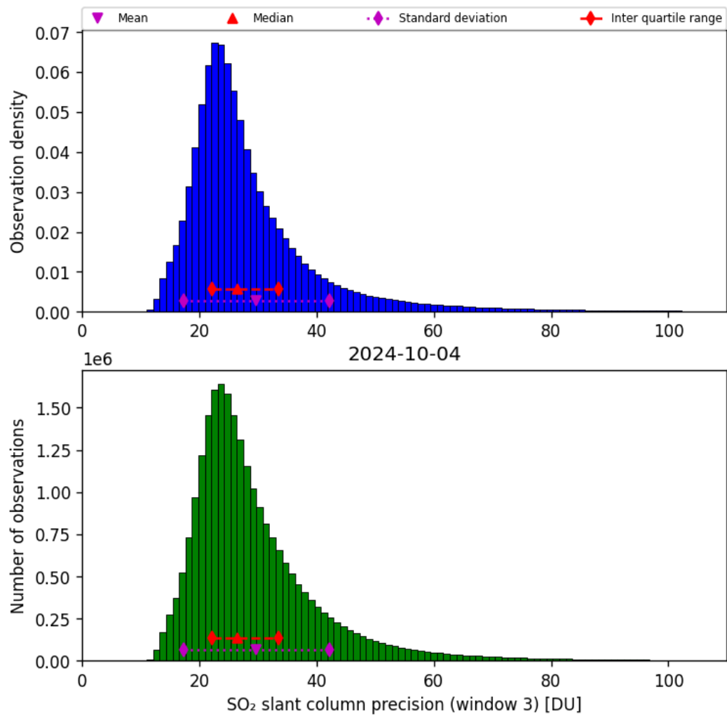
Figure 65: Histogram of “SO 2 slant column precision (window 3)” for 2024-10-03 to 2024-10-05
