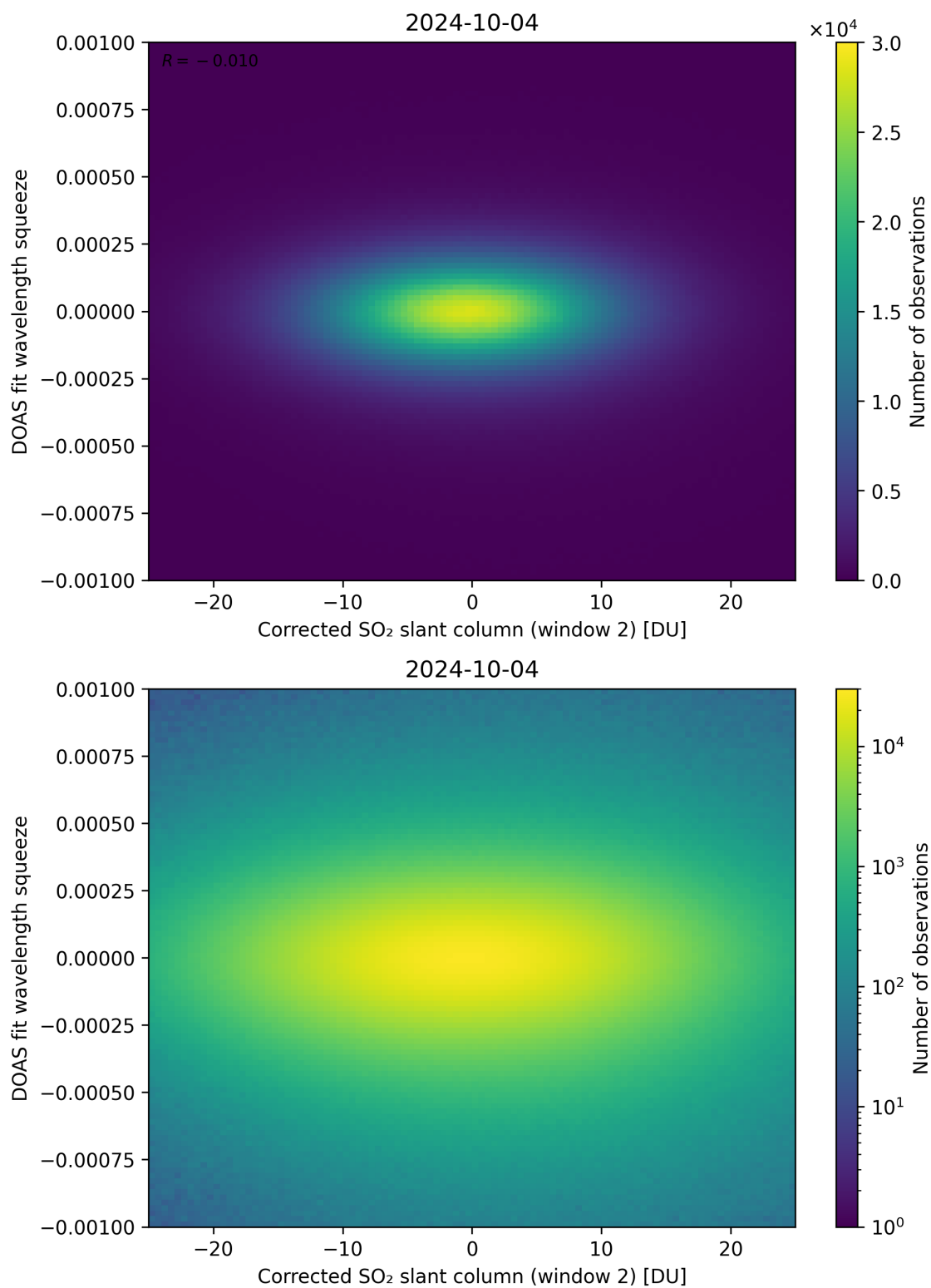
Figure 197: Scatter density plot of “Corrected SO 2 slant column (window 2)” against “DOAS fit wavelength squeeze” for 2024-10-03 to 2024-10-05.
