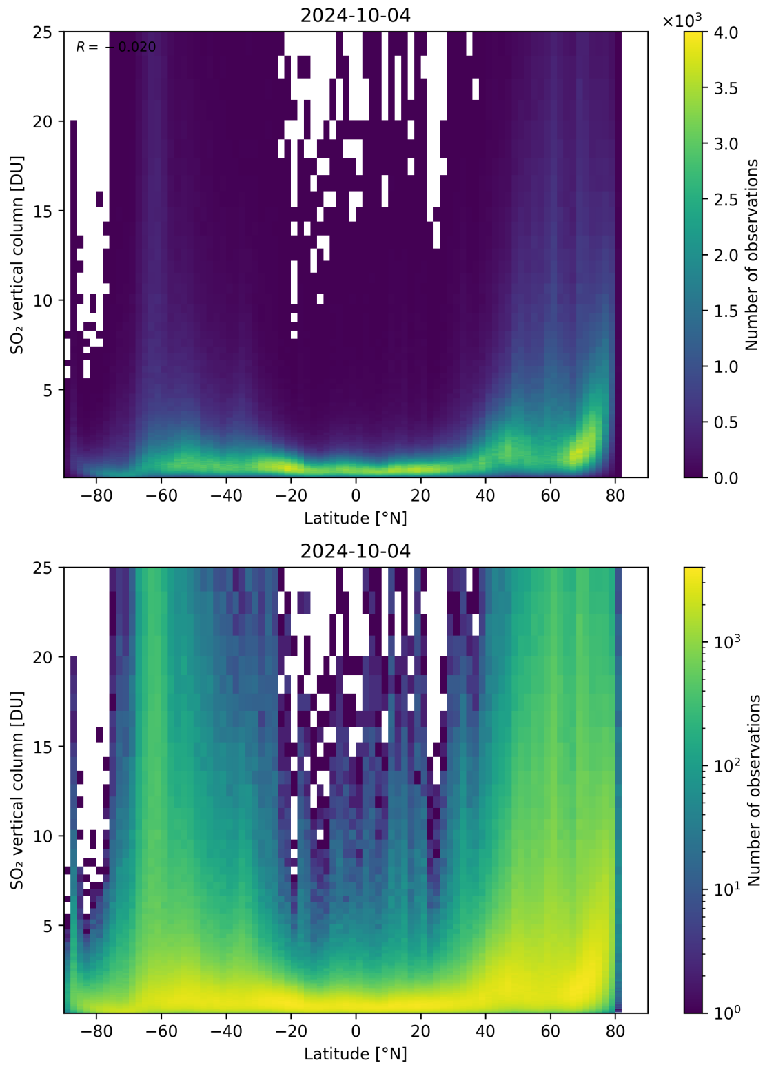
Figure 156: Scatter density plot of “Latitude” against “SO 2 vertical column” for 2024-10-03 to 2024-10-05.
