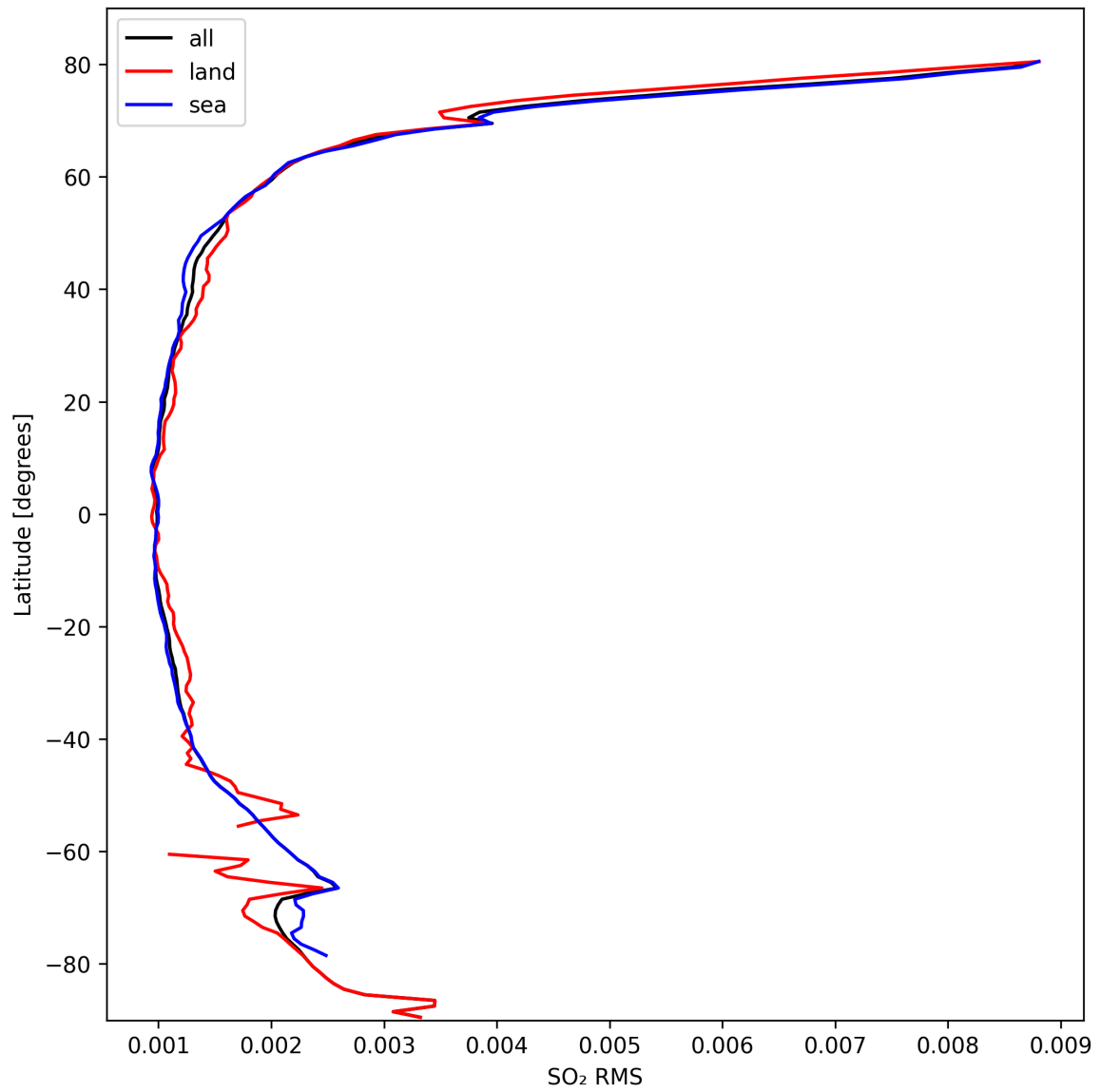
Figure 47: Zonal average of “SO 2 RMS” for 2024-10-03 to 2024-10-05.
