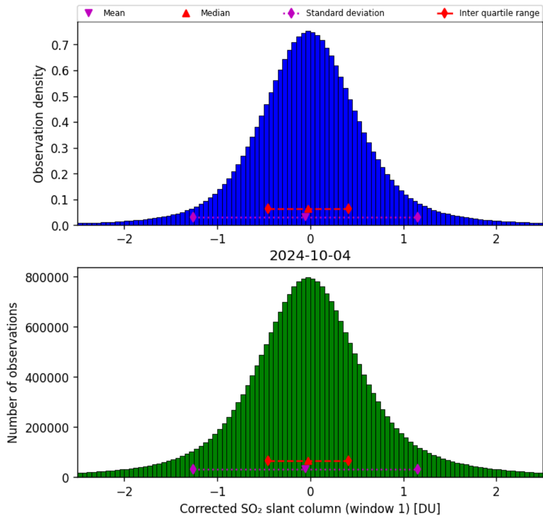
Figure 58: Histogram of “Corrected SO 2 slant column (window 1)” for 2024-10-03 to 2024-10-05
