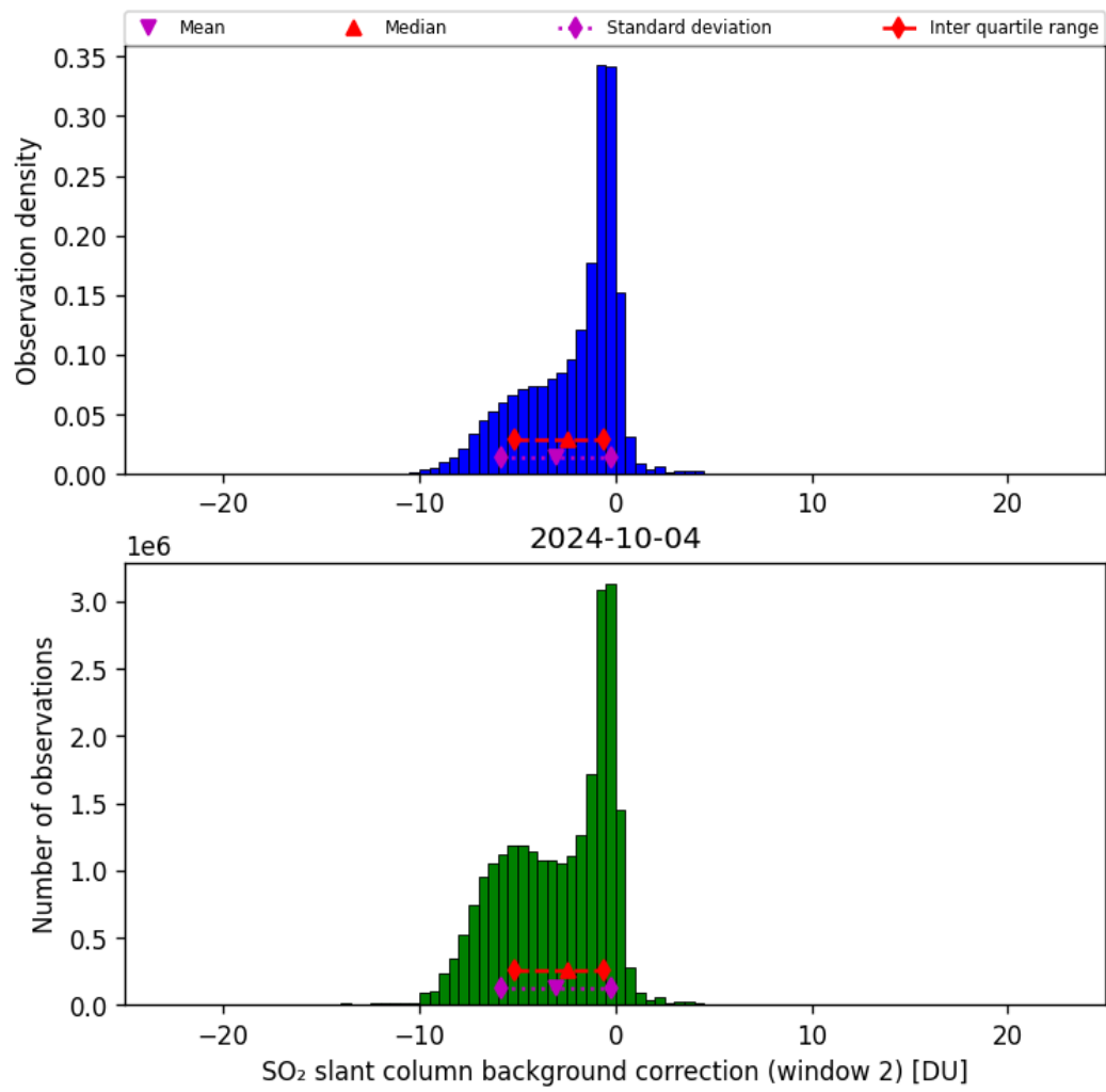
Figure 63: Histogram of “SO 2 slant column background correction (window 2)” for 2024-10-03 to 2024-10-05
