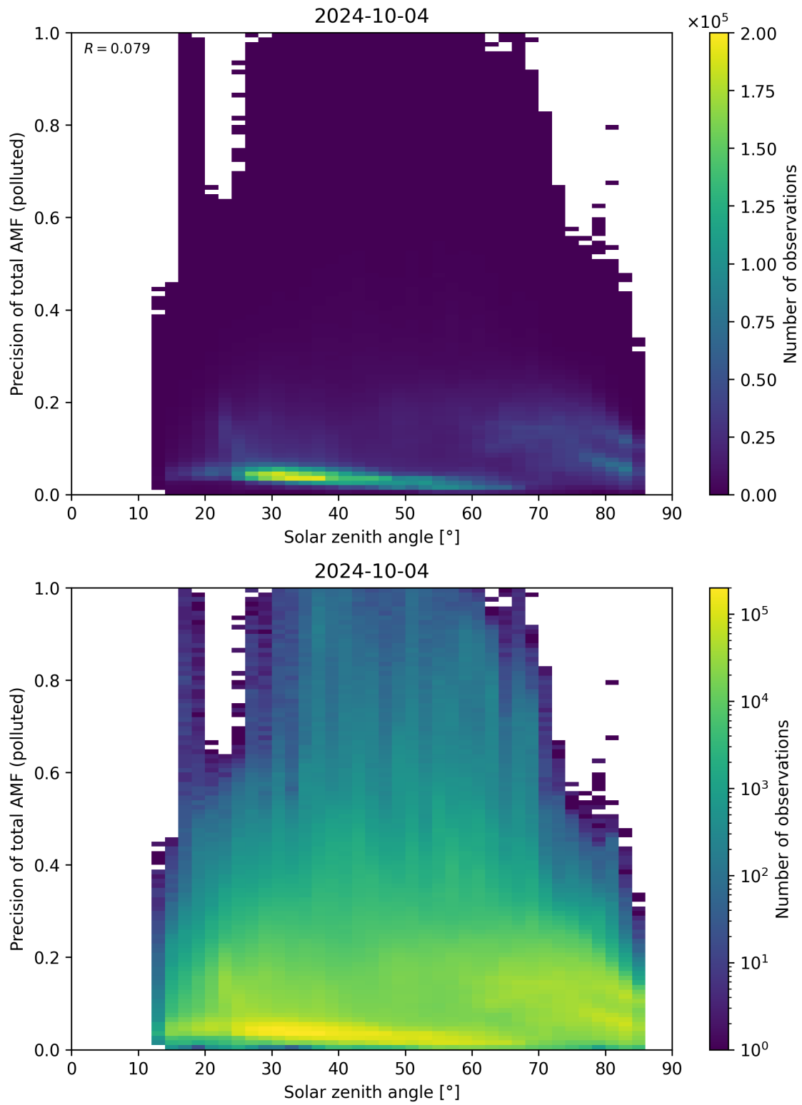
Figure 175: Scatter density plot of “Solar zenith angle” against “Precision of total AMF (polluted)” for 2024-10-03 to 2024-10-05.
