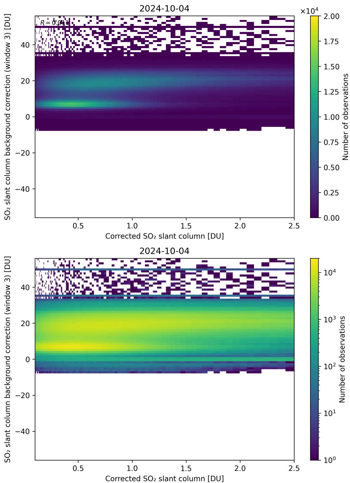
Figure 180: Scatter density plot of “Corrected SO 2 slant column” against “SO 2 slant column background correction (window 3)” for 2024-10-03 to 2024-10-05.
