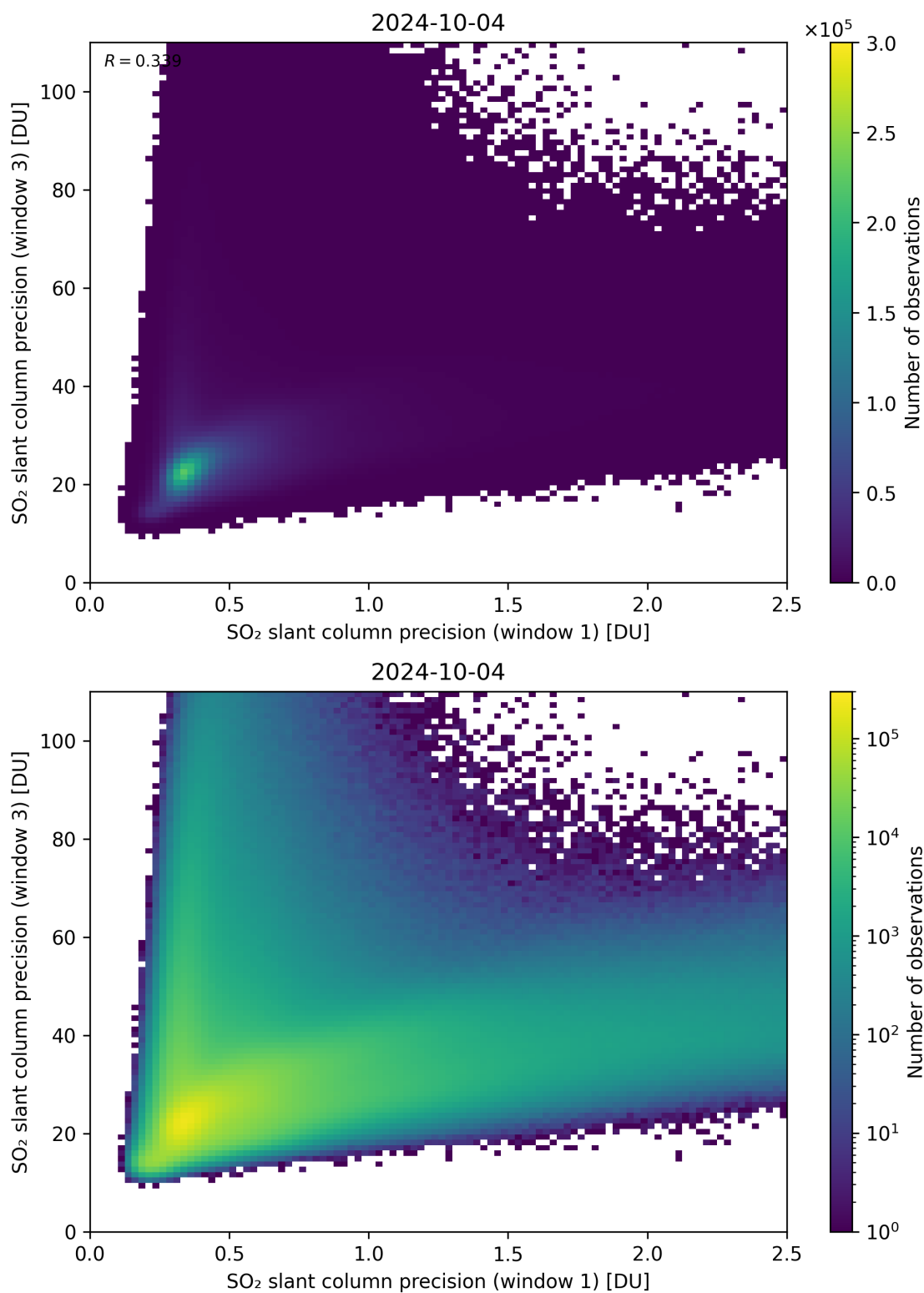
Figure 229: Scatter density plot of “SO 2 slant column precision (window 1)” against “SO 2 slant column precision (window 3)” for 2024-10-03 to 2024-10-05.
