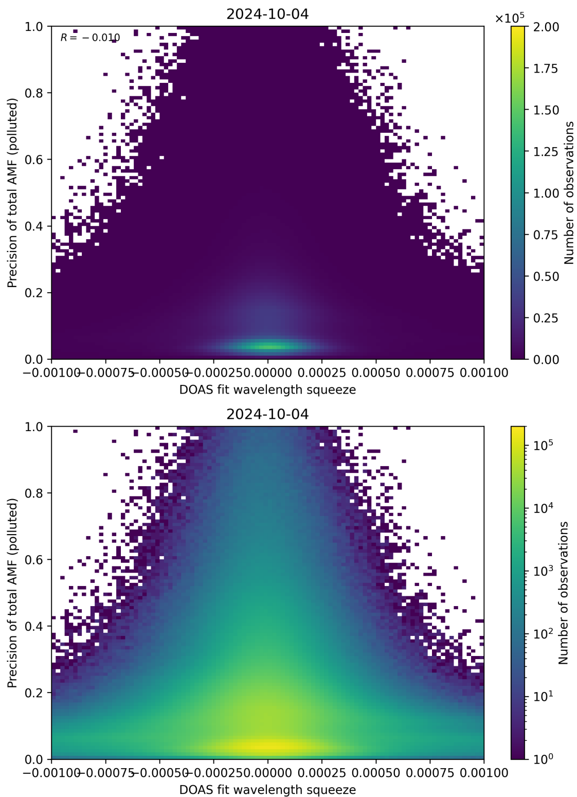
Figure 135: Scatter density plot of “DOAS fit wavelength squeeze” against “Precision of total AMF (polluted)” for 2024-10-03 to 2024-10-05.
