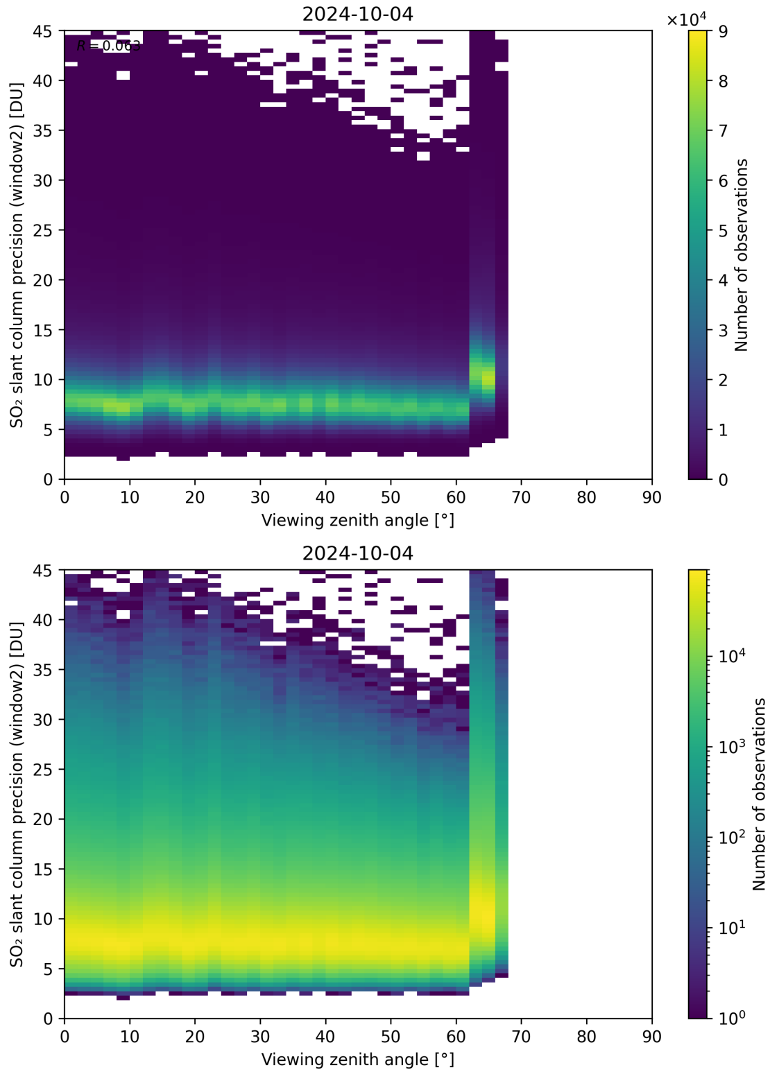
Figure 322: Scatter density plot of “Viewing zenith angle” against “SO 2 slant column precision (window2)” for 2024-10-03 to 2024-10-05.
