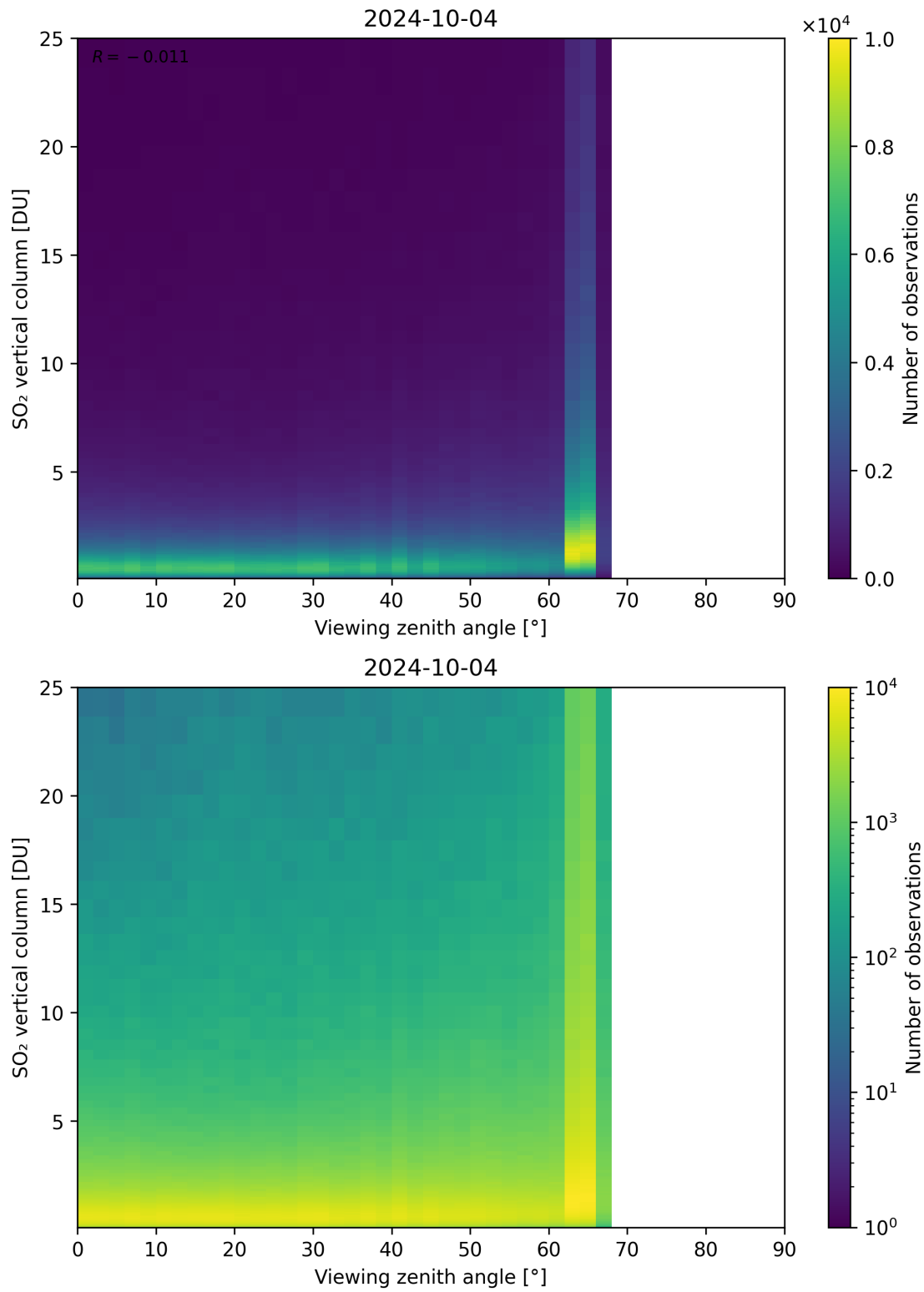
Figure 327: Scatter density plot of “Viewing zenith angle” against “SO 2 vertical column” for 2024-10-03 to 2024-10-05.
