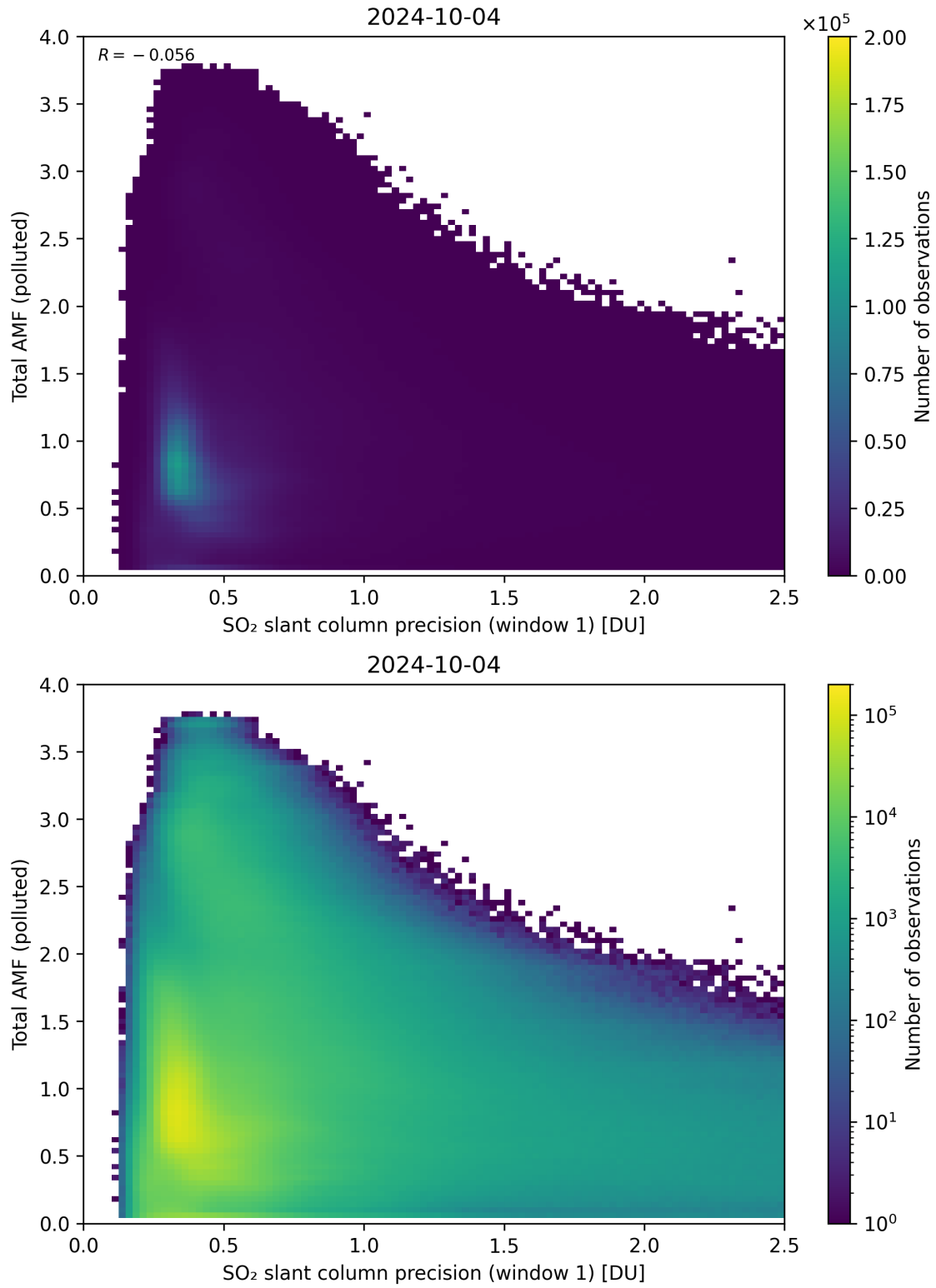
Figure 230: Scatter density plot of “SO 2 slant column precision (window 1)” against “Total AMF (polluted)” for 2024-10-03 to 2024-10-05.
