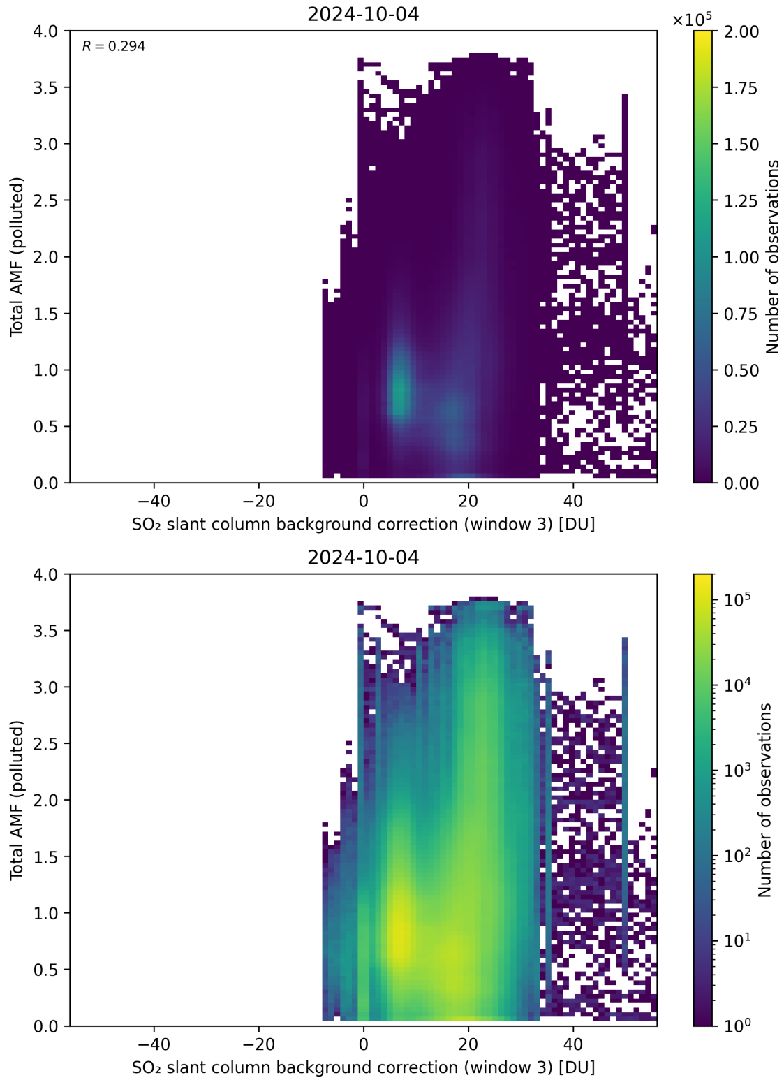
Figure 125: Scatter density plot of “SO 2 slant column background correction (window 3)” against “Total AMF (polluted)” for 2024-10-03 to 2024-10-05.
