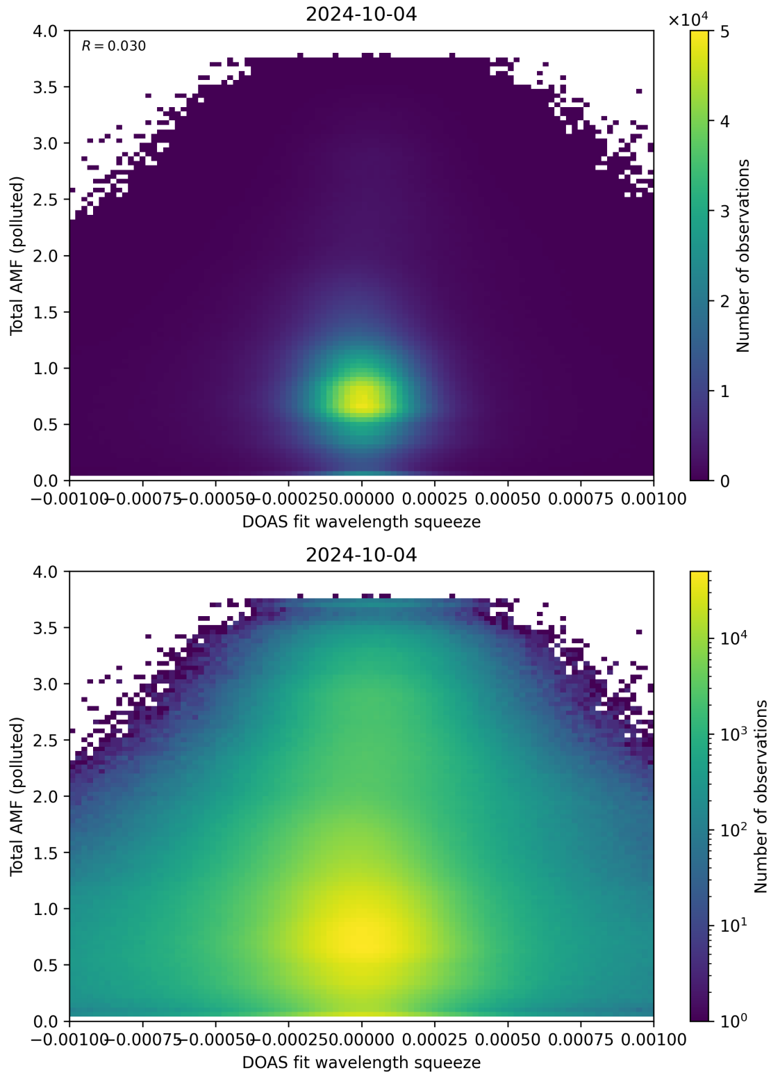
Figure 134: Scatter density plot of “DOAS fit wavelength squeeze” against “Total AMF (polluted)” for 2024-10-03 to 2024-10-05.
