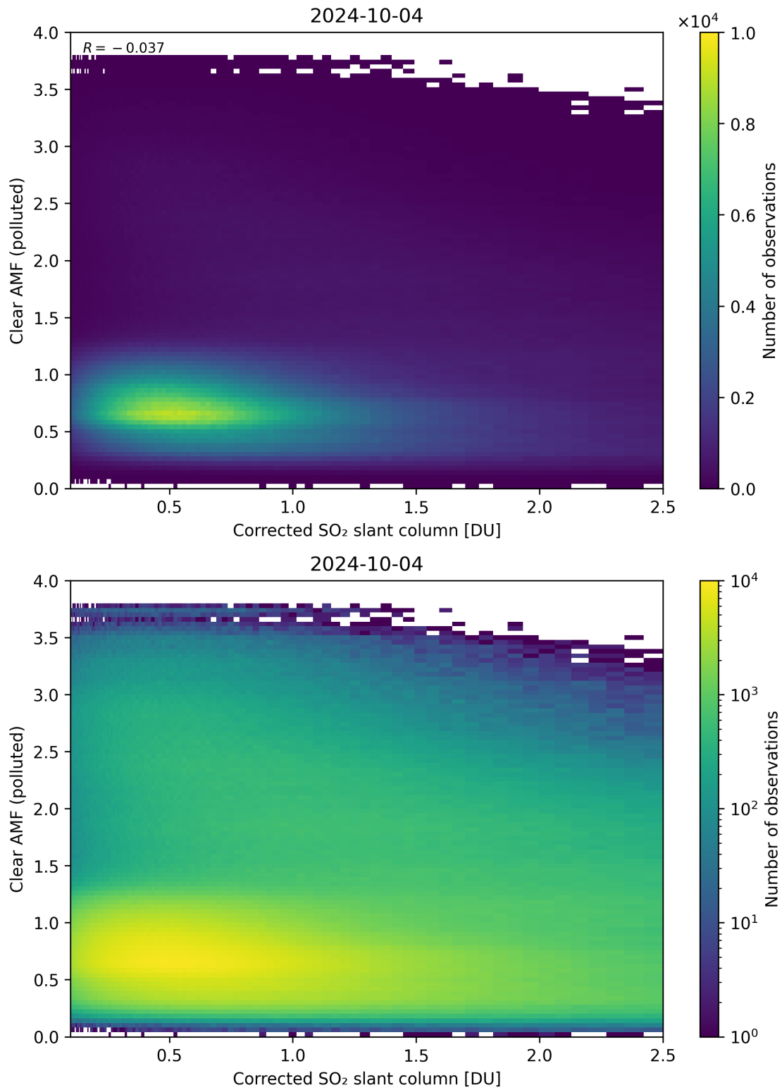
Figure 184: Scatter density plot of “Corrected SO 2 slant column” against “Clear AMF (polluted)” for 2024-10-03 to 2024-10-05.
