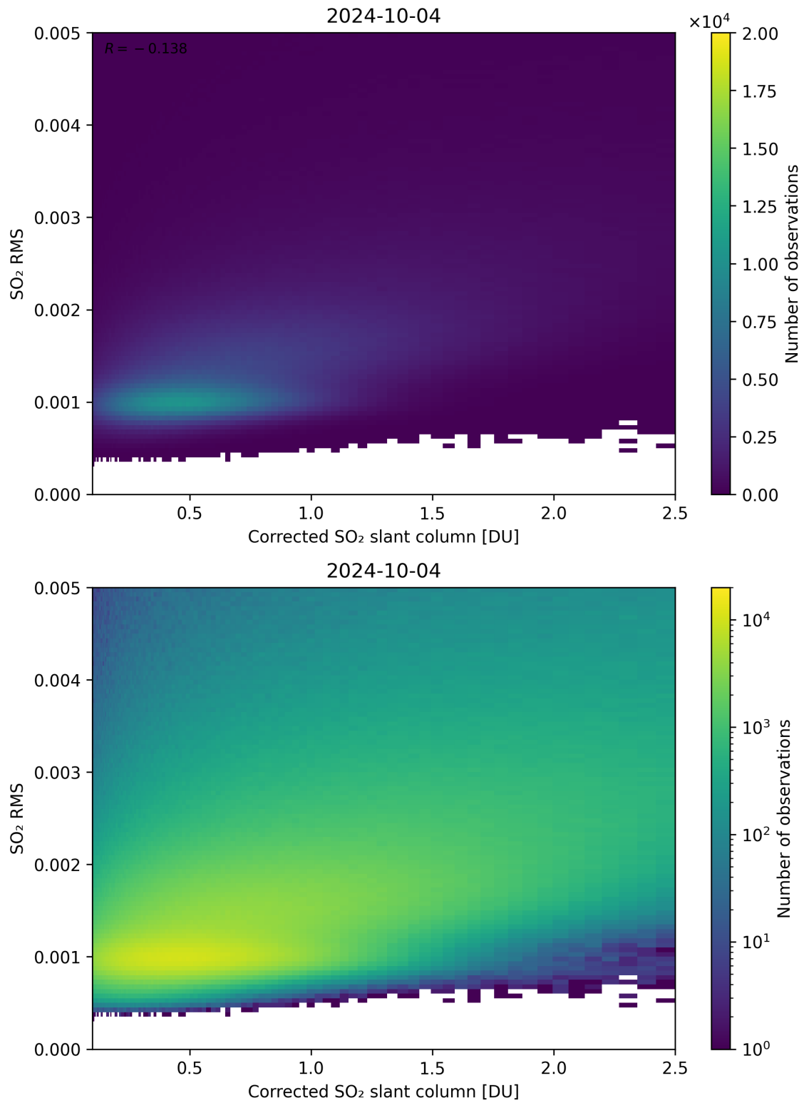
Figure 183: Scatter density plot of “Corrected SO 2 slant column” against “SO 2 RMS” for 2024-10-03 to 2024-10-05.
