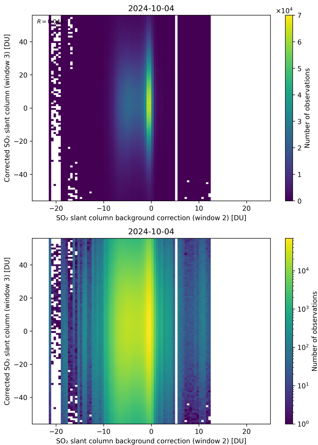
Figure 116: Scatter density plot of “SO 2 slant column background correction (window 2)” against “Corrected SO 2 slant column (window 3)” for 2024-10-03 to 2024-10-05.
