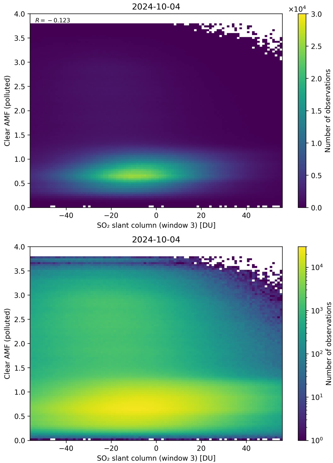
Figure 265: Scatter density plot of “SO 2 slant column (window 3)” against “Clear AMF (polluted)” for 2024-10-03 to 2024-10-05.
