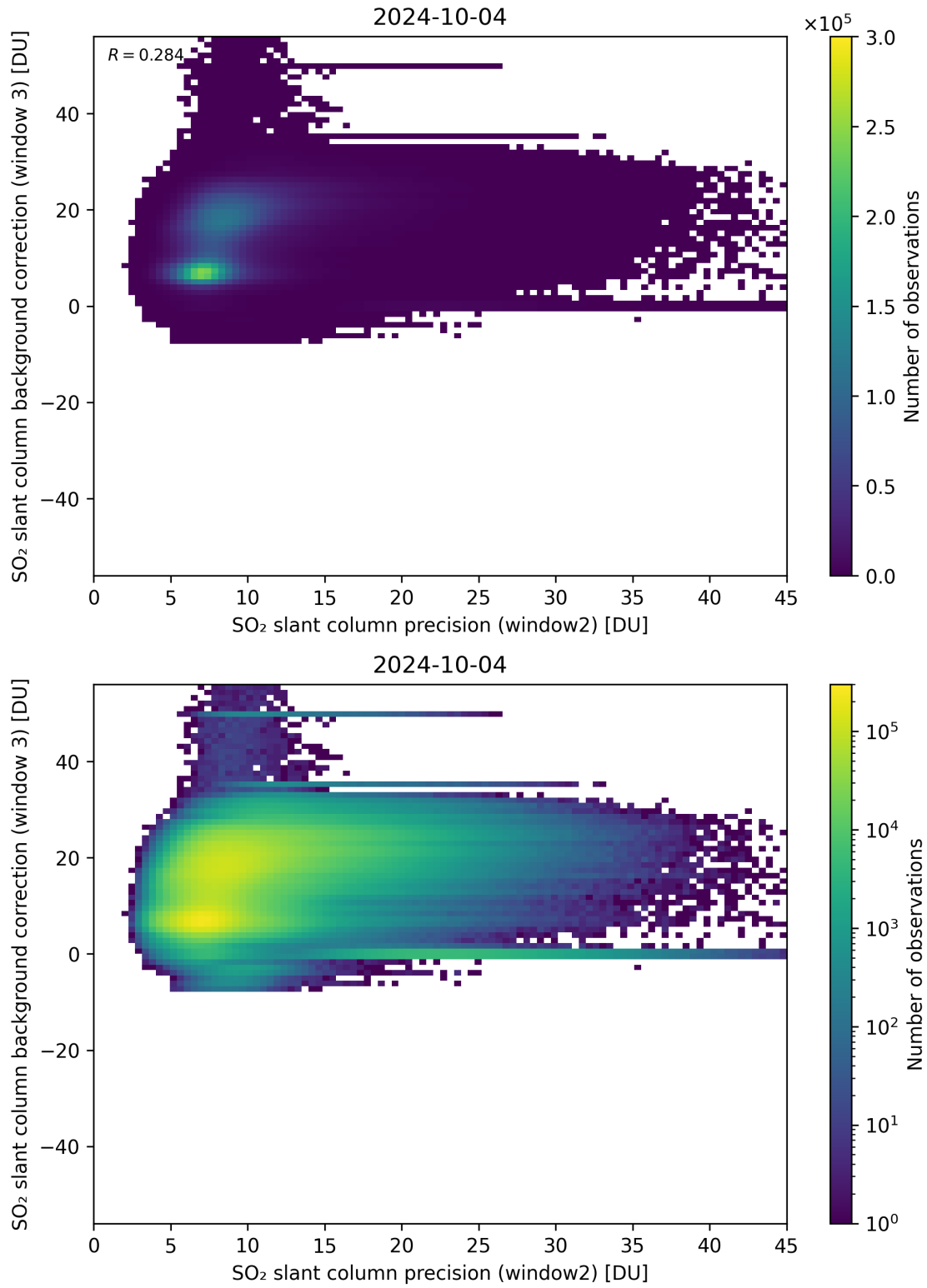
Figure 242: Scatter density plot of “SO 2 slant column precision (window2)” against “SO 2 slant column background correction (window 3)” for 2024-10-03 to 2024-10-05.
