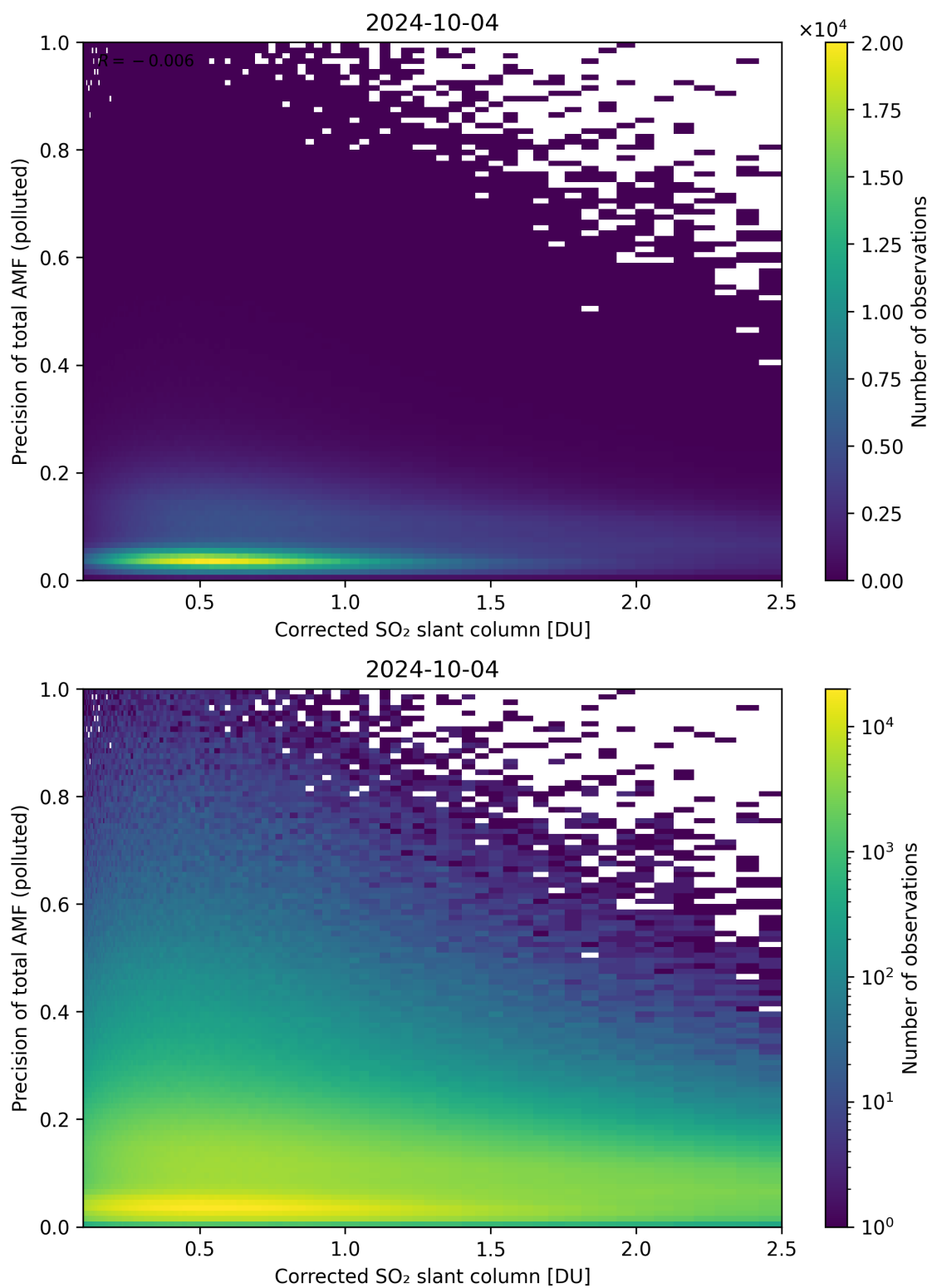
Figure 193: Scatter density plot of “Corrected SO 2 slant column” against “Precision of total AMF (polluted)” for 2024-10-03 to 2024-10-05.
