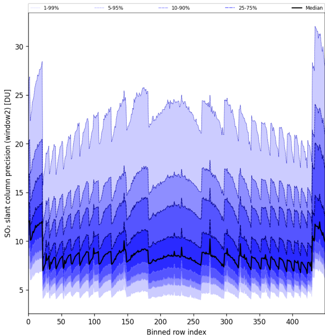
Figure 84: Along track statistics of “SO 2 slant column precision (window2)” for 2024-10-03 to 2024-10-05
