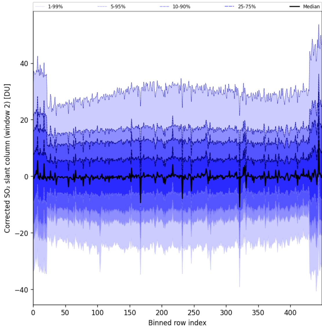
Figure 85: Along track statistics of “Corrected SO 2 slant column (window 2)” for 2024-10-03 to 2024-10-05
