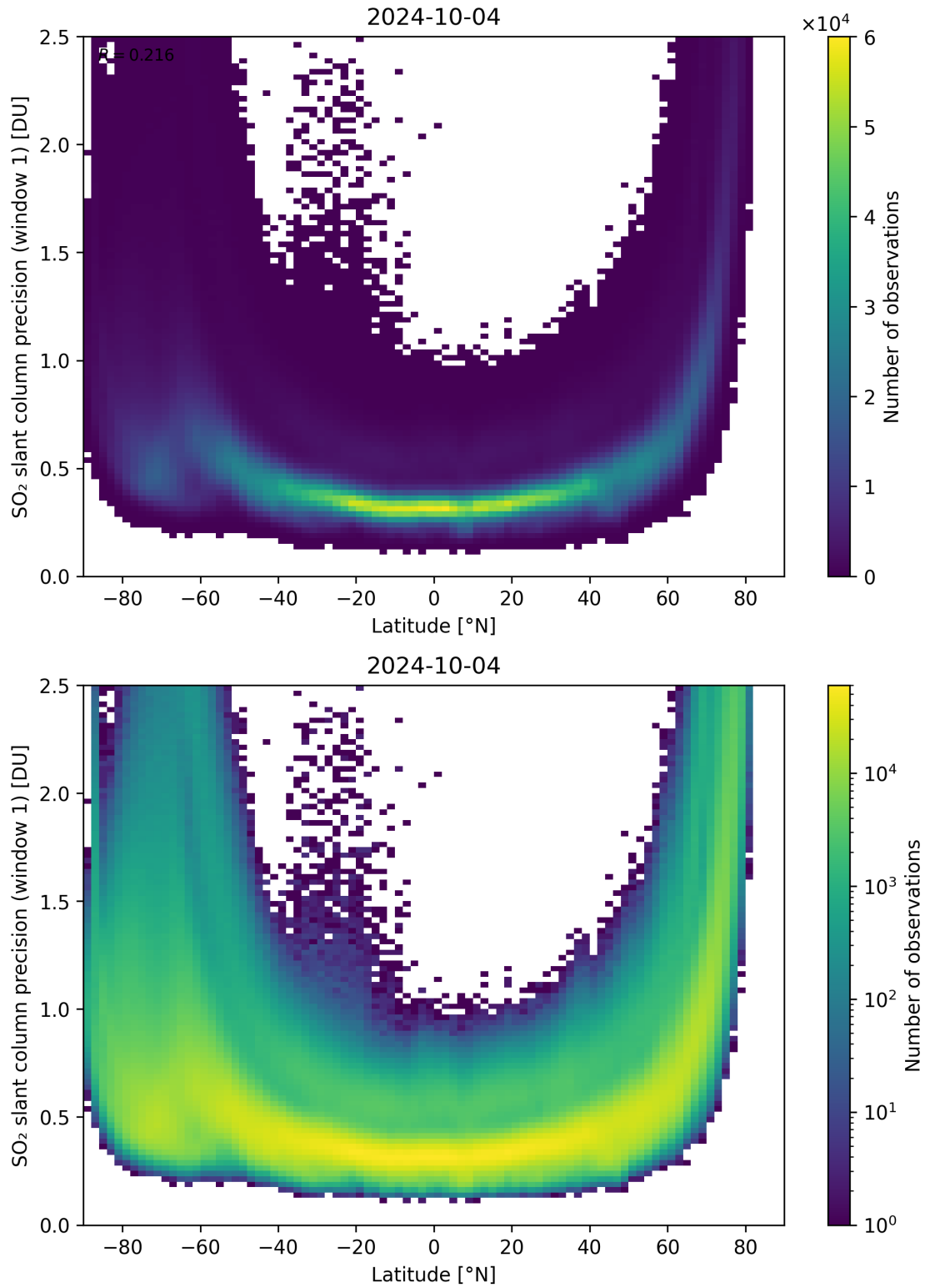
Figure 150: Scatter density plot of “Latitude” against “SO 2 slant column precision (window 1)” for 2024-10-03 to 2024-10-05.
