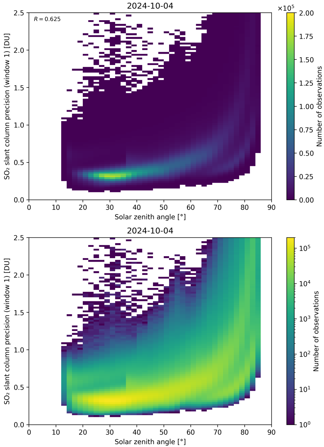
Figure 170: Scatter density plot of “Solar zenith angle” against “SO 2 slant column precision (window 1)” for 2024-10-03 to 2024-10-05.
