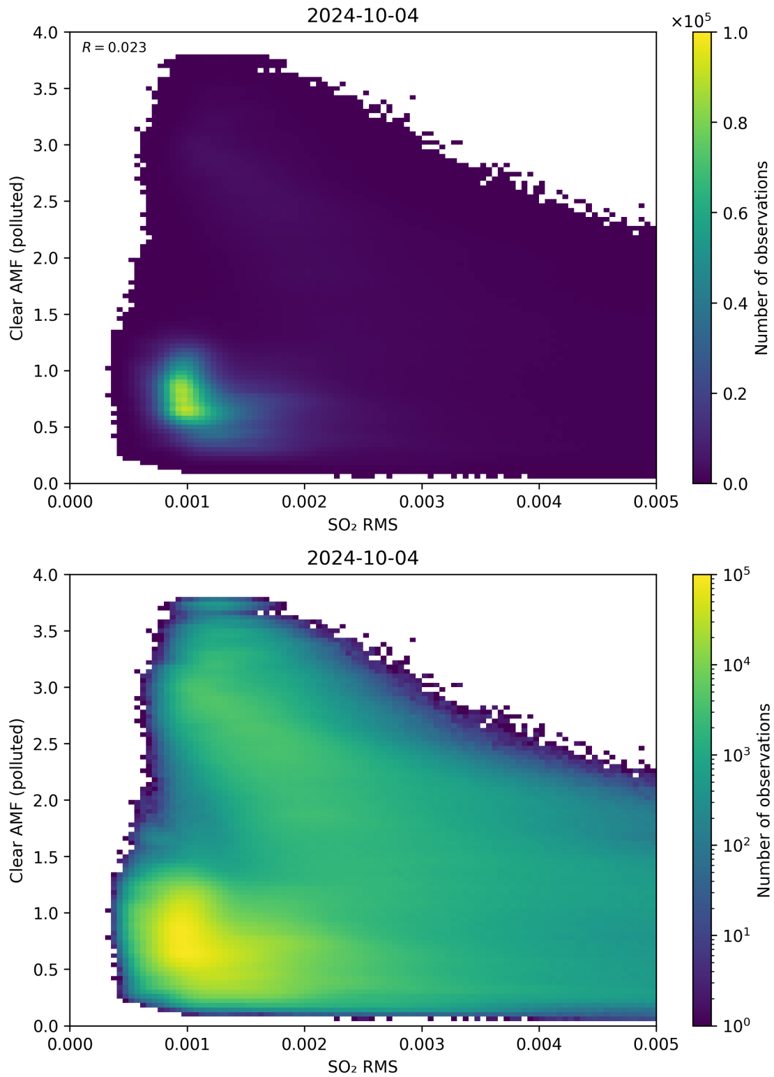
Figure 136: Scatter density plot of “SO 2 RMS” against “Clear AMF (polluted)” for 2024-10-03 to 2024-10-05.
