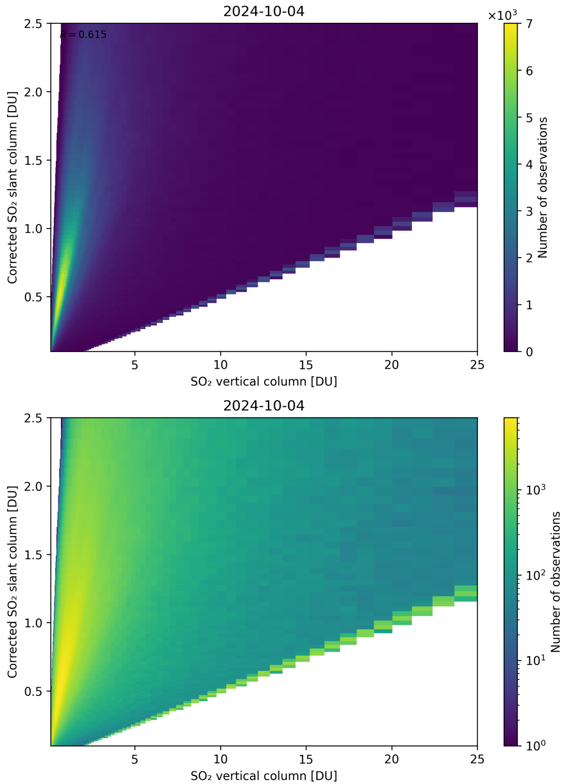
Figure 297: Scatter density plot of “SO 2 vertical column” against “Corrected SO 2 slant column” for 2024-10-03 to 2024-10-05.
