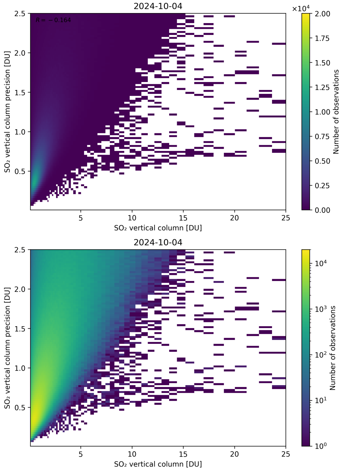
Figure 307: Scatter density plot of “SO 2 vertical column” against “SO 2 vertical column precision” for 2024-10-03 to 2024-10-05.
