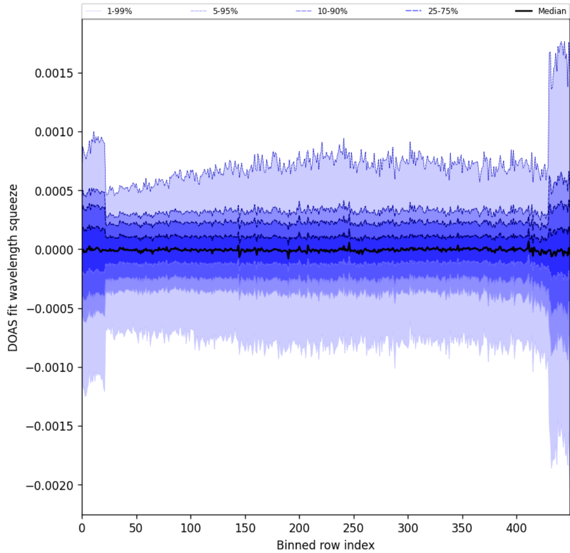
Figure 92: Along track statistics of “DOAS fit wavelength squeeze” for 2024-10-03 to 2024-10-05
