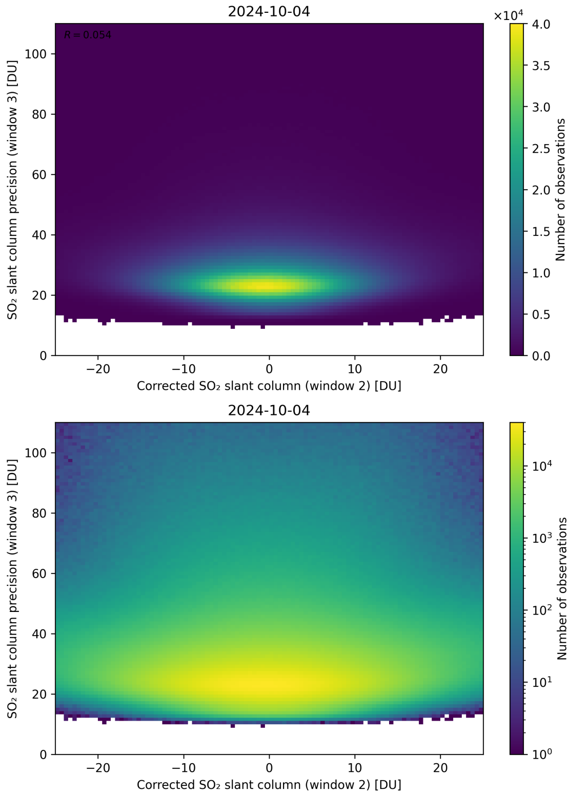
Figure 202: Scatter density plot of “Corrected SO 2 slant column (window 2)” against “SO 2 slant column precision (window 3)” for 2024-10-03 to 2024-10-05.
