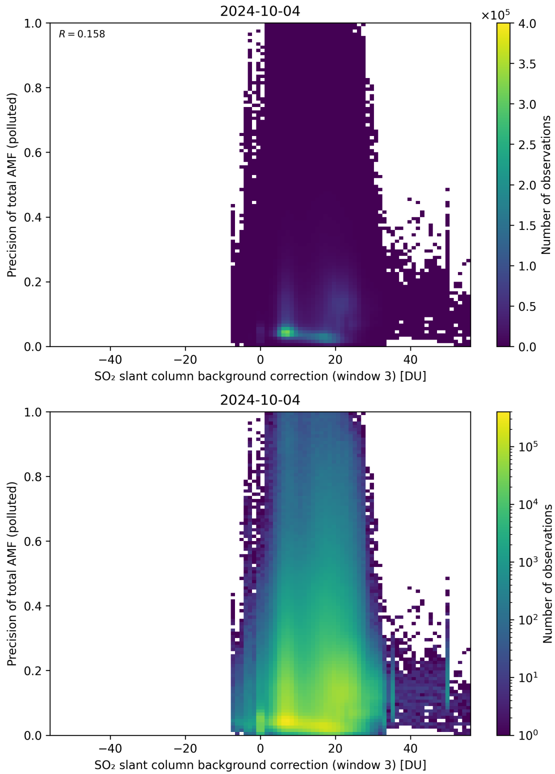
Figure 126: Scatter density plot of “SO 2 slant column background correction (window 3)” against “Precision of total AMF (polluted)” for 2024-10-03 to 2024-10-05.
