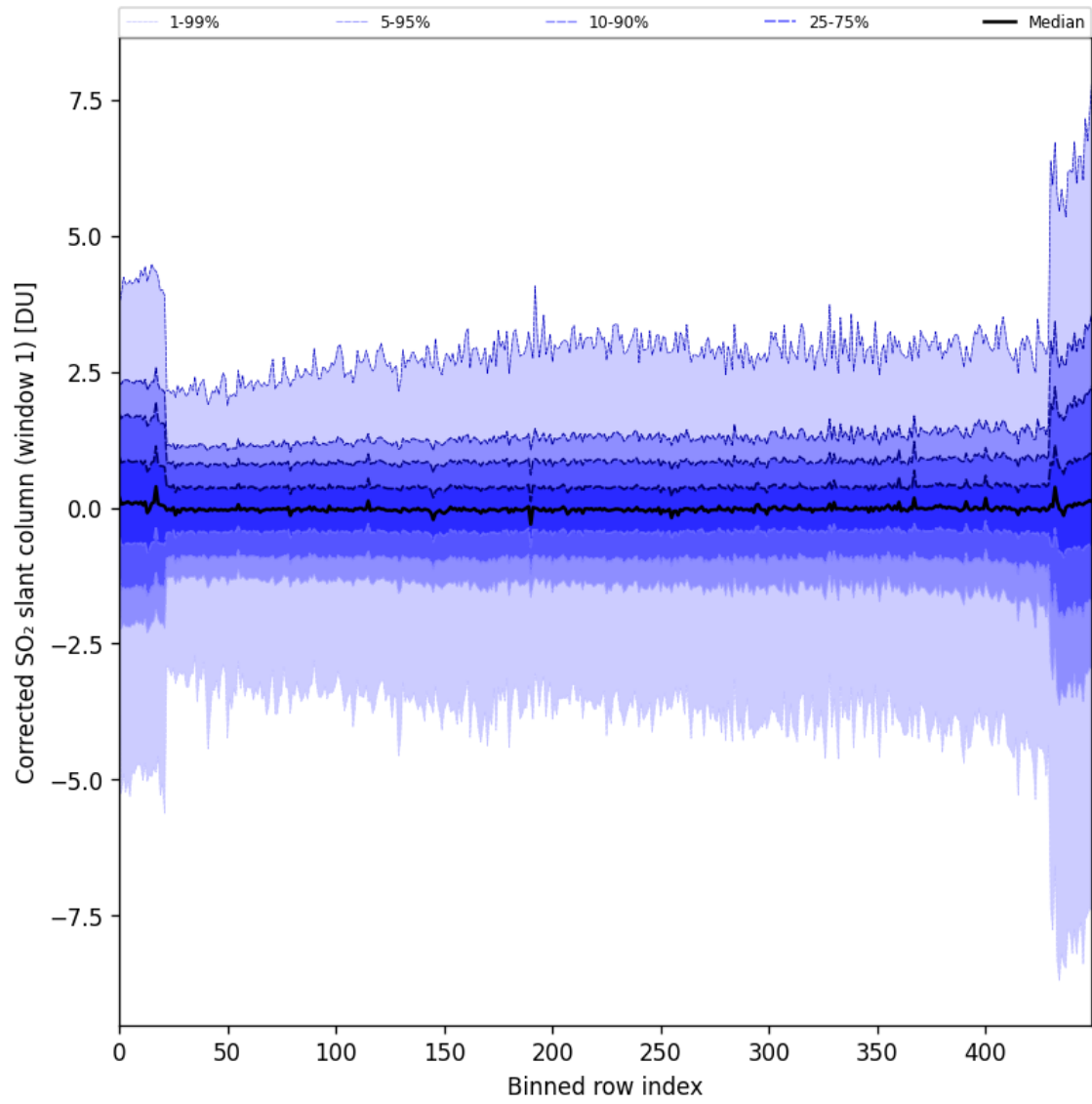
Figure 81: Along track statistics of “Corrected SO 2 slant column (window 1)” for 2024-10-03 to 2024-10-05
