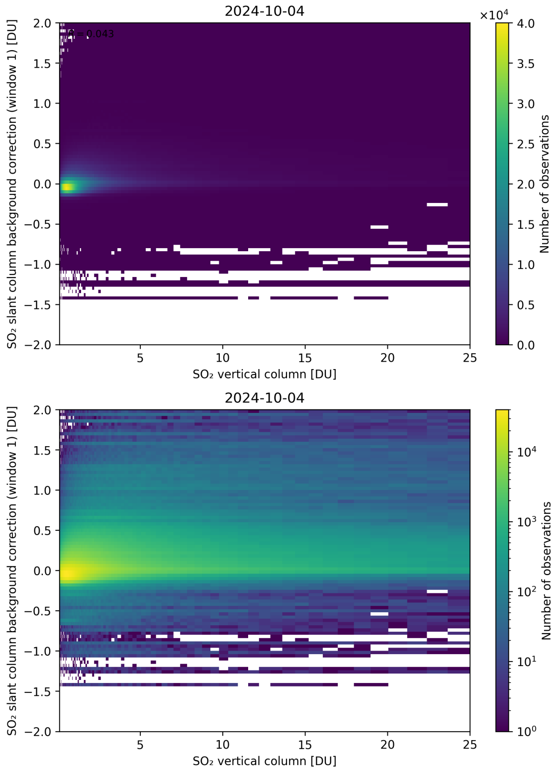
Figure 273: Scatter density plot of “SO 2 vertical column” against “SO 2 slant column background correction (window 1)” for 2024-10-03 to 2024-10-05.
