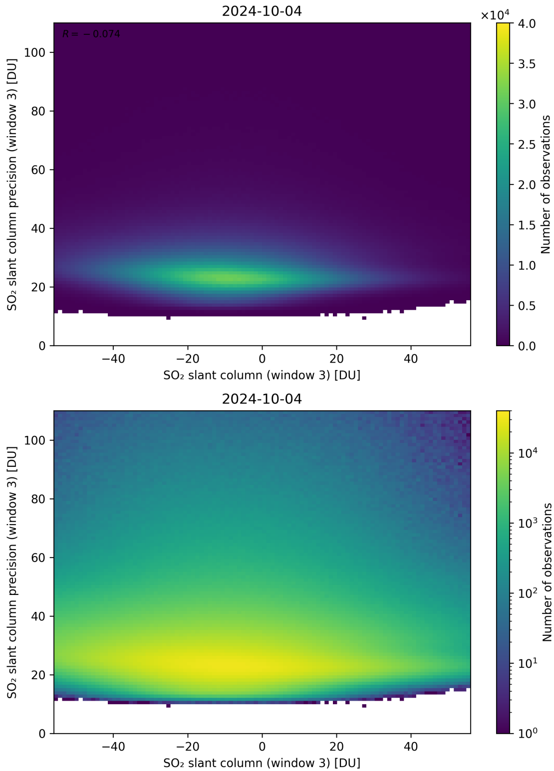
Figure 267: Scatter density plot of “SO 2 slant column (window 3)” against “SO 2 slant column precision (window 3)” for 2024-10-03 to 2024-10-05.
