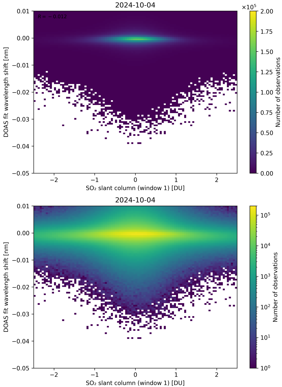
Figure 215: Scatter density plot of “SO 2 slant column (window 1)” against “DOAS fit wavelength shift” for 2024-10-03 to 2024-10-05.
