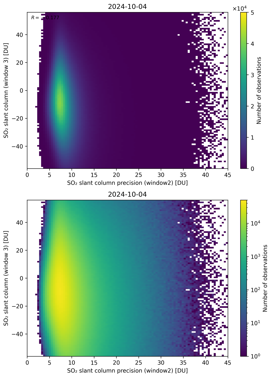
Figure 249: Scatter density plot of “SO 2 slant column precision (window2)” against “SO 2 slant column (window 3)” for 2024-10-03 to 2024-10-05.
