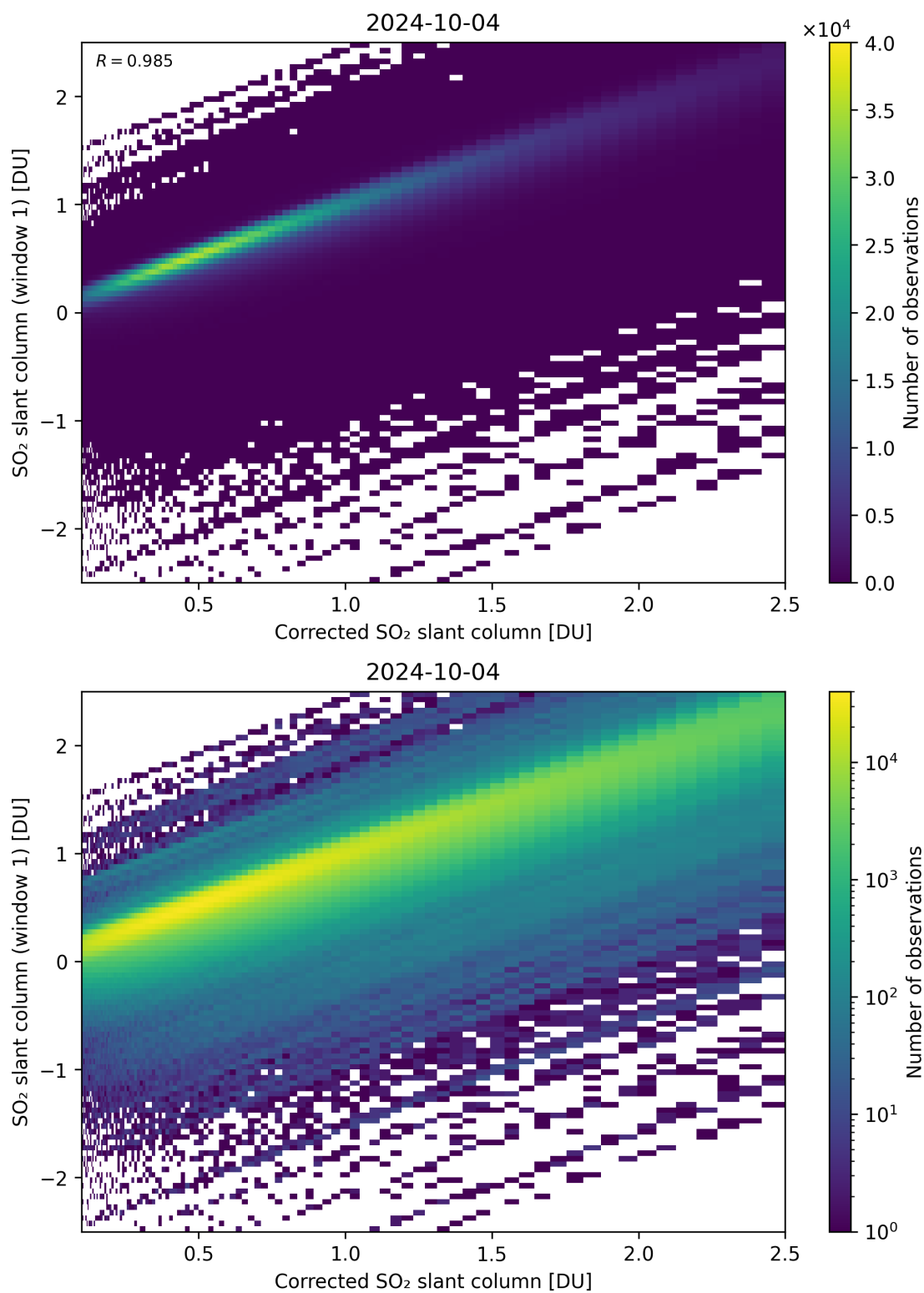
Figure 187: Scatter density plot of “Corrected SO 2 slant column” against “SO 2 slant column (window 1)” for 2024-10-03 to 2024-10-05.
