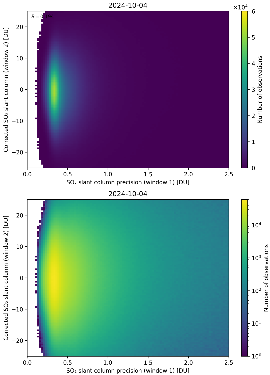
Figure 225: Scatter density plot of “SO 2 slant column precision (window 1)” against “Corrected SO 2 slant column (window 2)” for 2024-10-03 to 2024-10-05.
