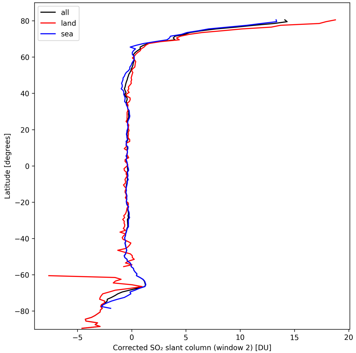
Figure 39: Zonal average of “Corrected SO 2 slant column (window 2)” for 2024-10-03 to 2024-10-05.
