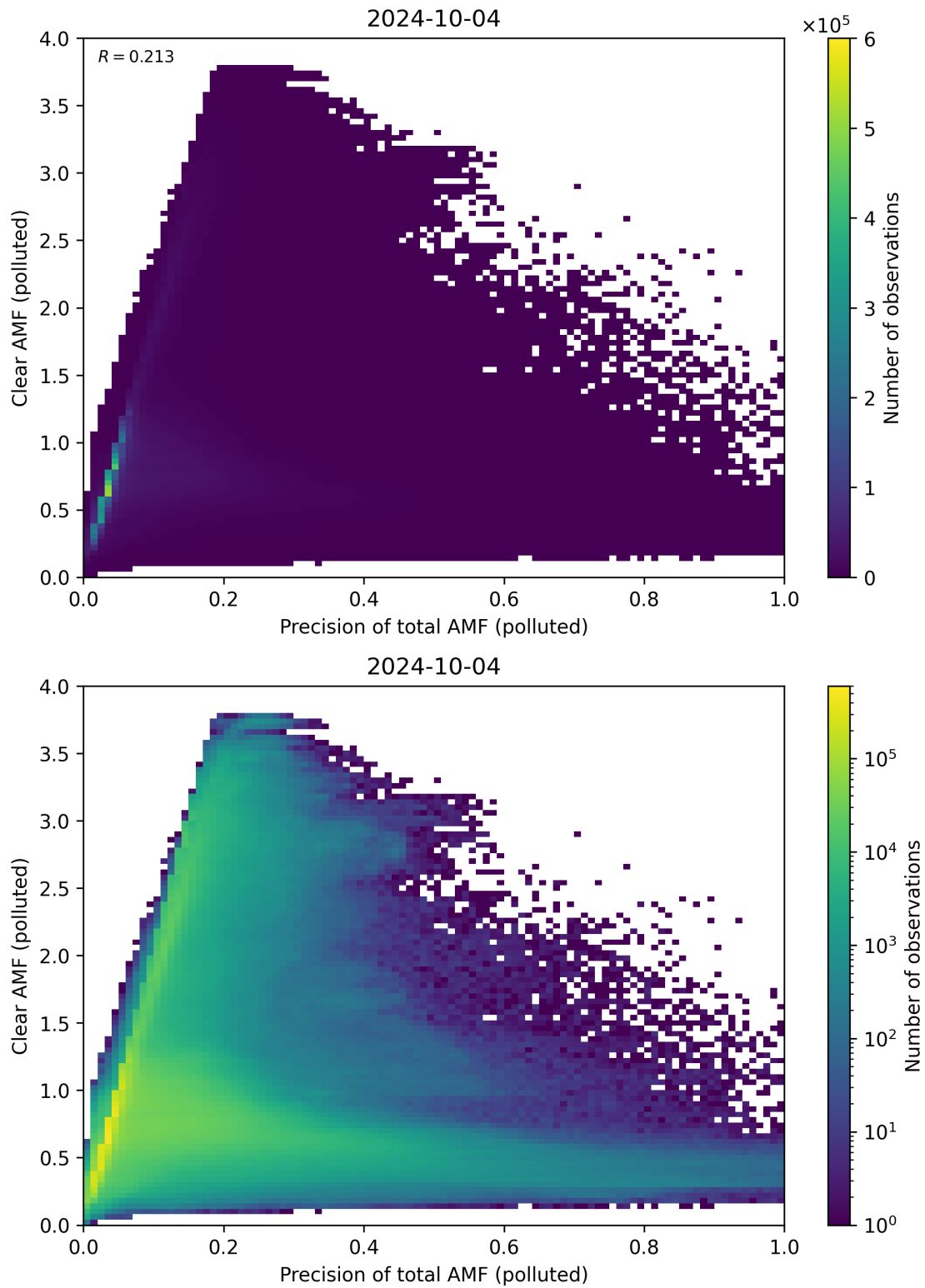
Figure 270: Scatter density plot of “Precision of total AMF (polluted)” against “Clear AMF (polluted)” for 2024-10-03 to 2024-10-05.
