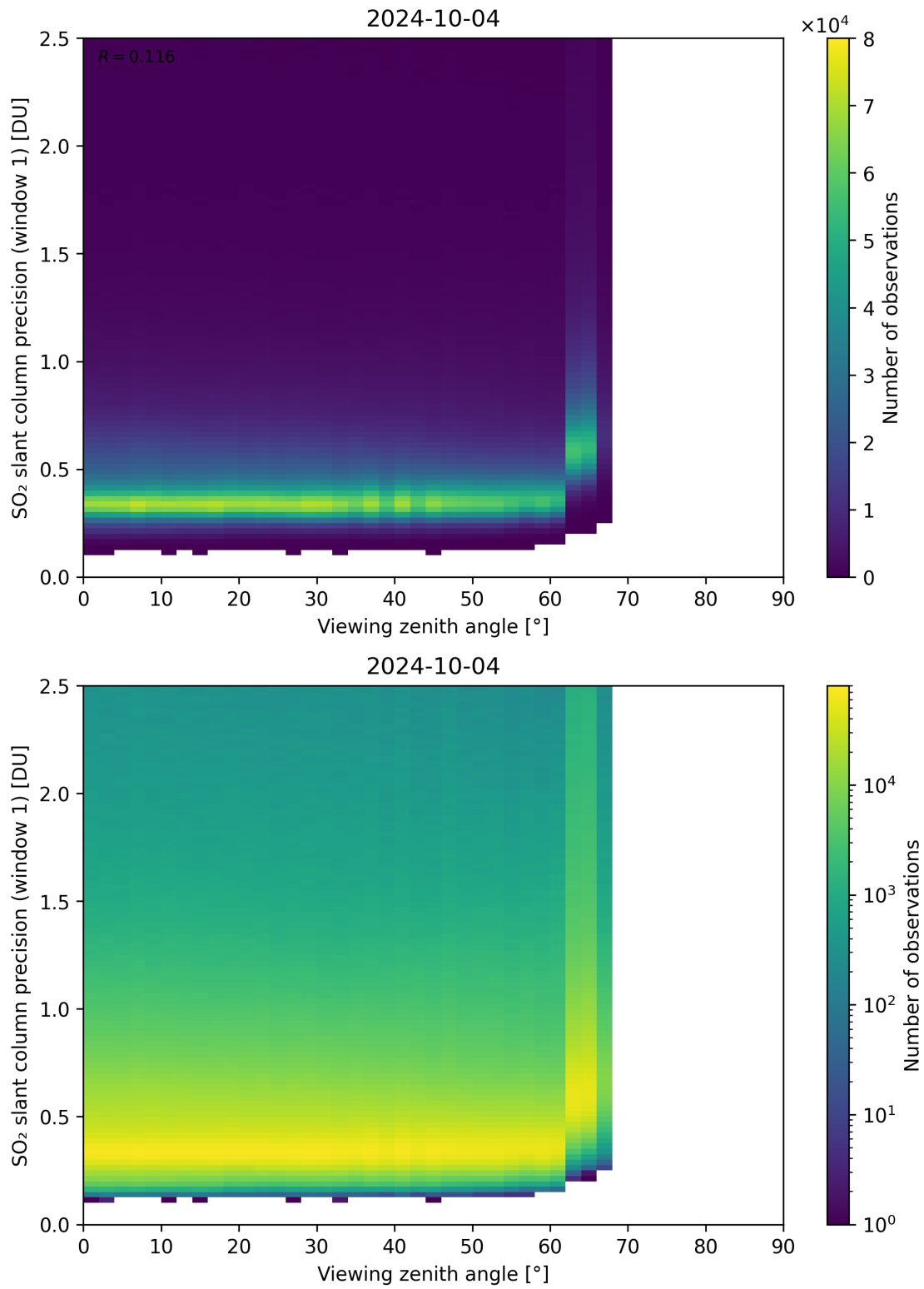
Figure 321: Scatter density plot of “Viewing zenith angle” against “SO 2 slant column precision (window 1)” for 2024-10-03 to 2024-10-05.
