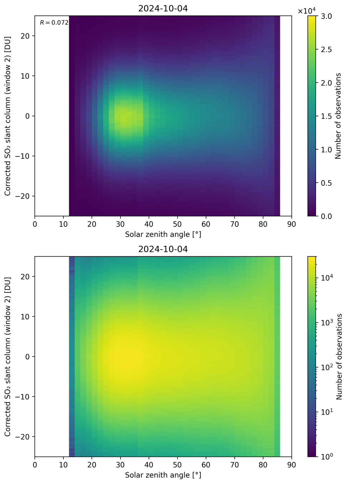
Figure 167: Scatter density plot of “Solar zenith angle” against “Corrected SO 2 slant column (window 2)” for 2024-10-03 to 2024-10-05.
