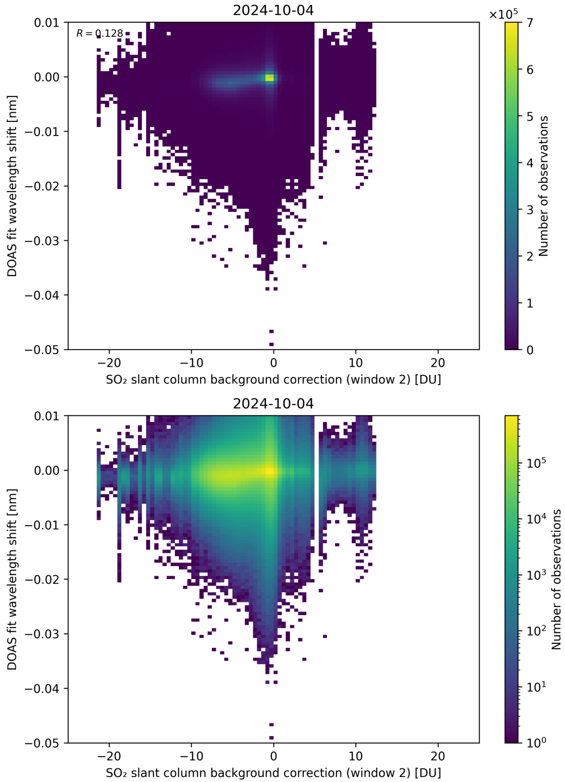
Figure 112: Scatter density plot of “SO 2 slant column background correction (window 2)” against “DOAS fit wavelength shift” for 2024-10-03 to 2024-10-05.
