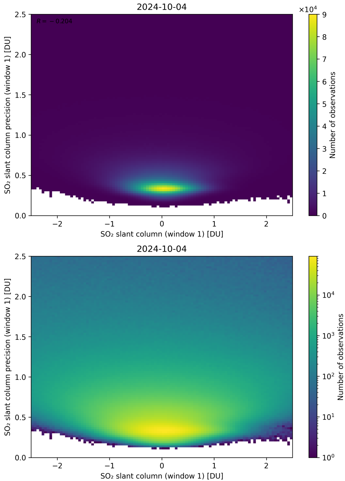
Figure 235: Scatter density plot of “SO 2 slant column (window 1)” against “SO 2 slant column precision (window 1)” for 2024-10-03 to 2024-10-05.
