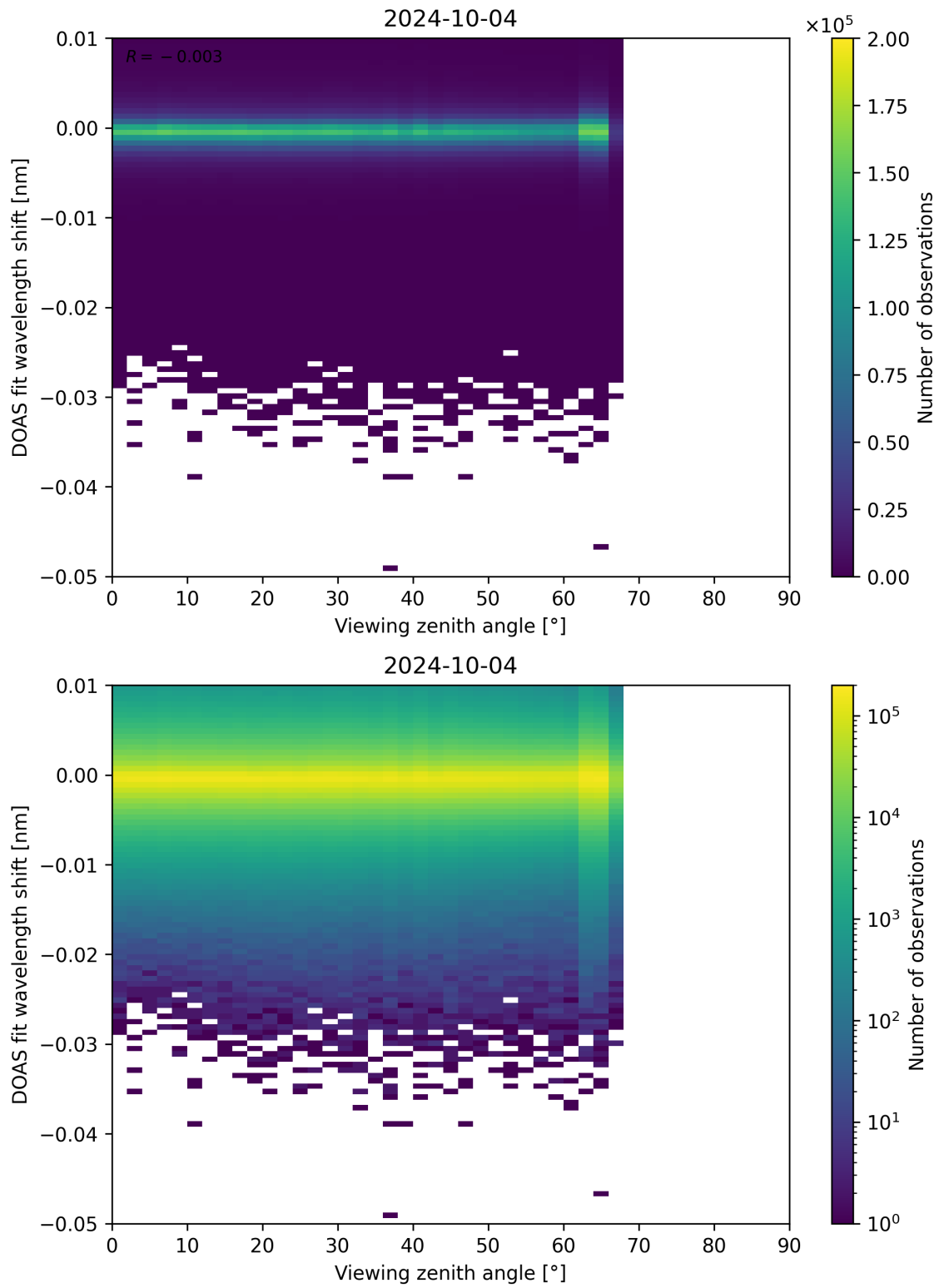
Figure 311: Scatter density plot of “Viewing zenith angle” against “DOAS fit wavelength shift” for 2024-10-03 to 2024-10-05.
