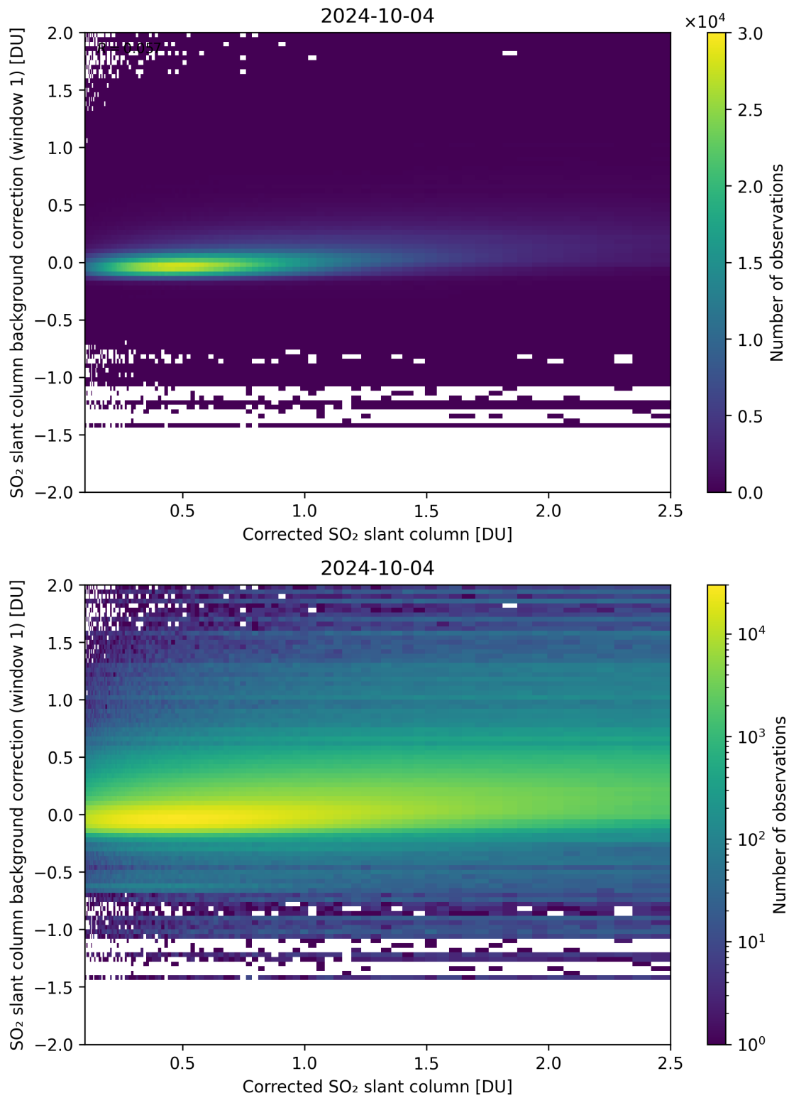
Figure 178: Scatter density plot of “Corrected SO 2 slant column” against “SO 2 slant column background correction (window 1)” for 2024-10-03 to 2024-10-05.
