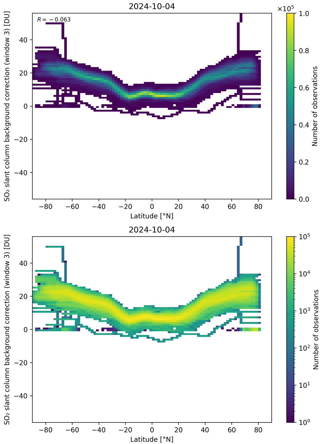
Figure 141: Scatter density plot of “Latitude” against “SO 2 slant column background correction (window 3)” for 2024-10-03 to 2024-10-05.
