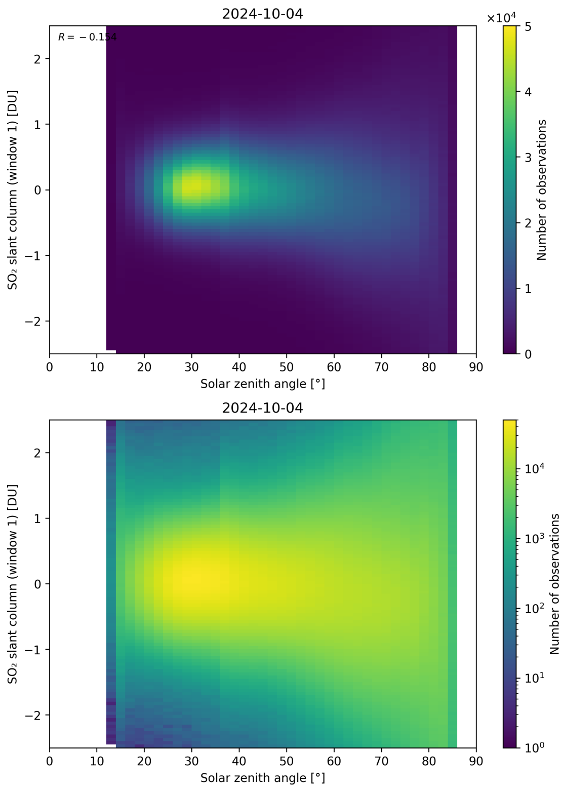
Figure 169: Scatter density plot of “Solar zenith angle” against “SO 2 slant column (window 1)” for 2024-10-03 to 2024-10-05.
