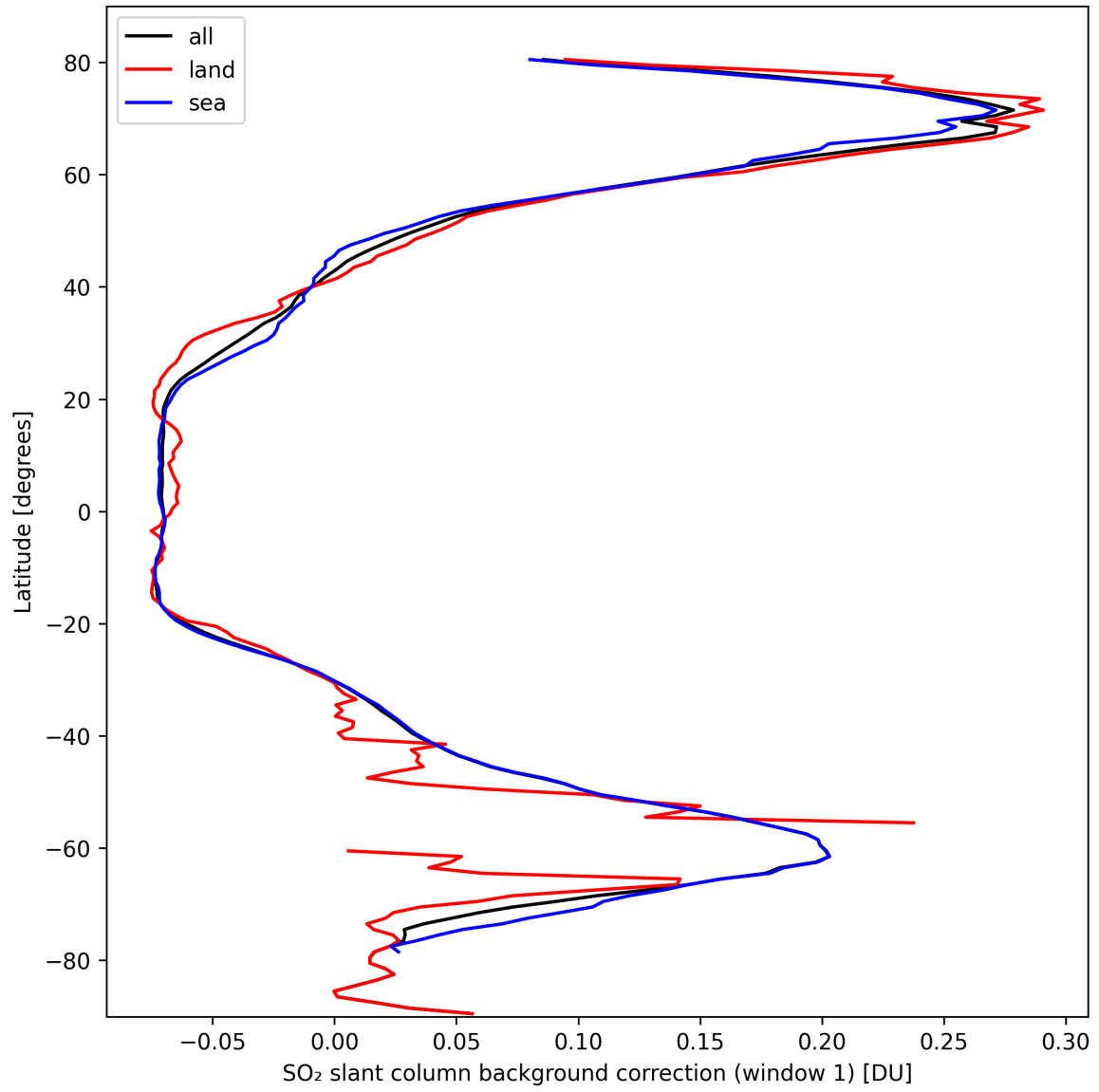
Figure 36: Zonal average of “SO 2 slant column background correction (window 1)” for 2024-10-03 to 2024-10-05.
