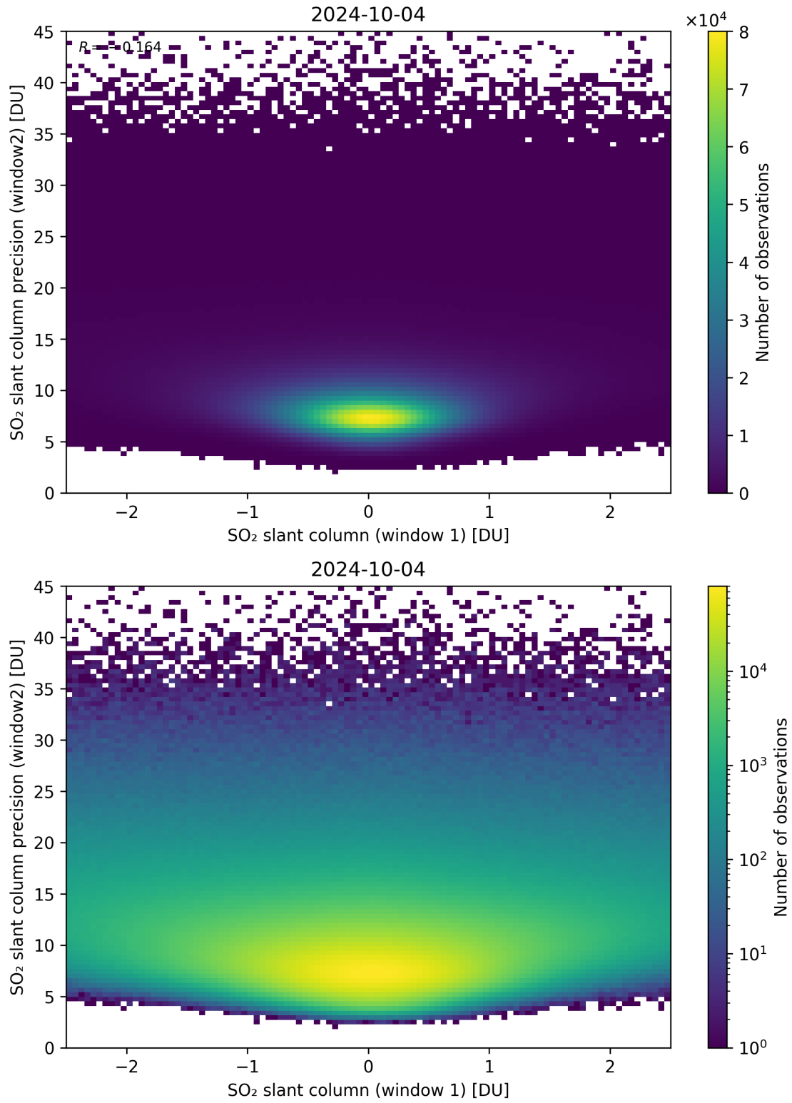
Figure 236: Scatter density plot of “SO 2 slant column (window 1)” against “SO 2 slant column precision (window2)” for 2024-10-03 to 2024-10-05.
