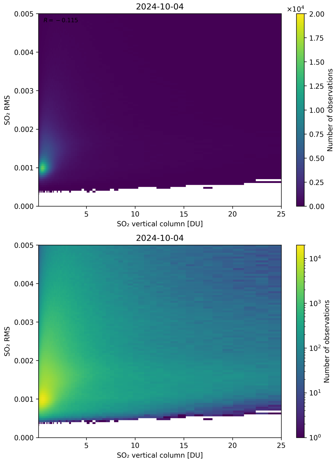
Figure 278: Scatter density plot of “SO 2 vertical column” against “SO 2 RMS” for 2024-10-03 to 2024-10-05.
