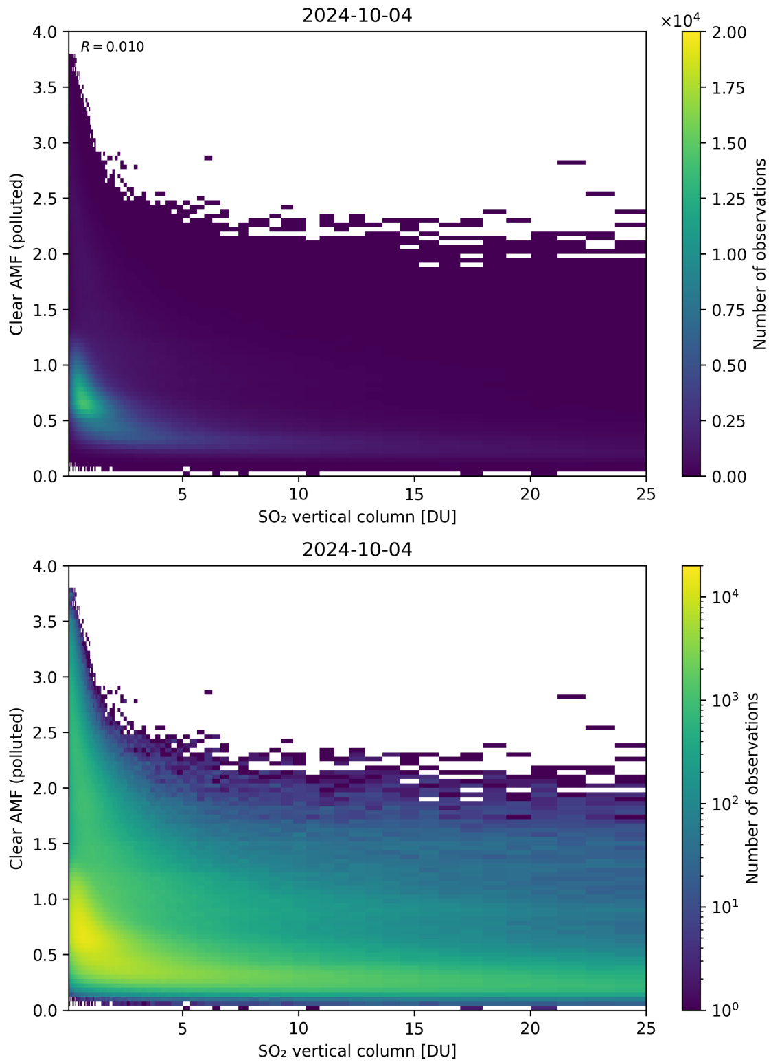
Figure 296: Scatter density plot of “SO 2 vertical column” against “Clear AMF (polluted)” for 2024-10-03 to 2024-10-05.
