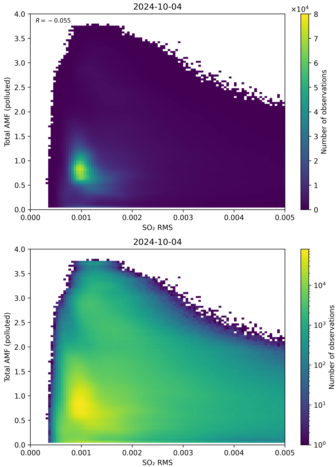
Figure 137: Scatter density plot of “SO 2 RMS” against “Total AMF (polluted)” for 2024-10-03 to 2024-10-05.
