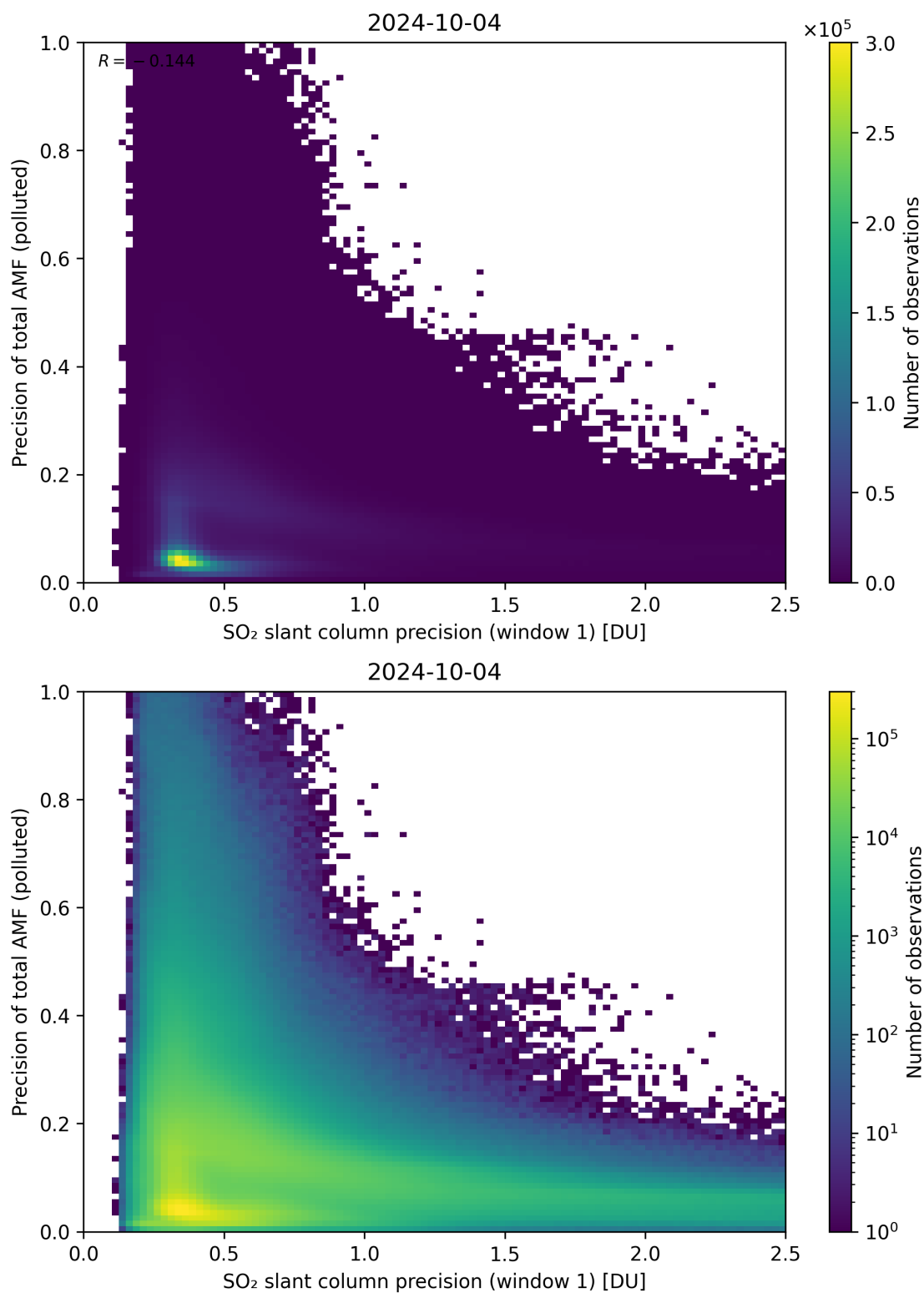
Figure 231: Scatter density plot of “SO 2 slant column precision (window 1)” against “Precision of total AMF (polluted)” for 2024-10-03 to 2024-10-05.
