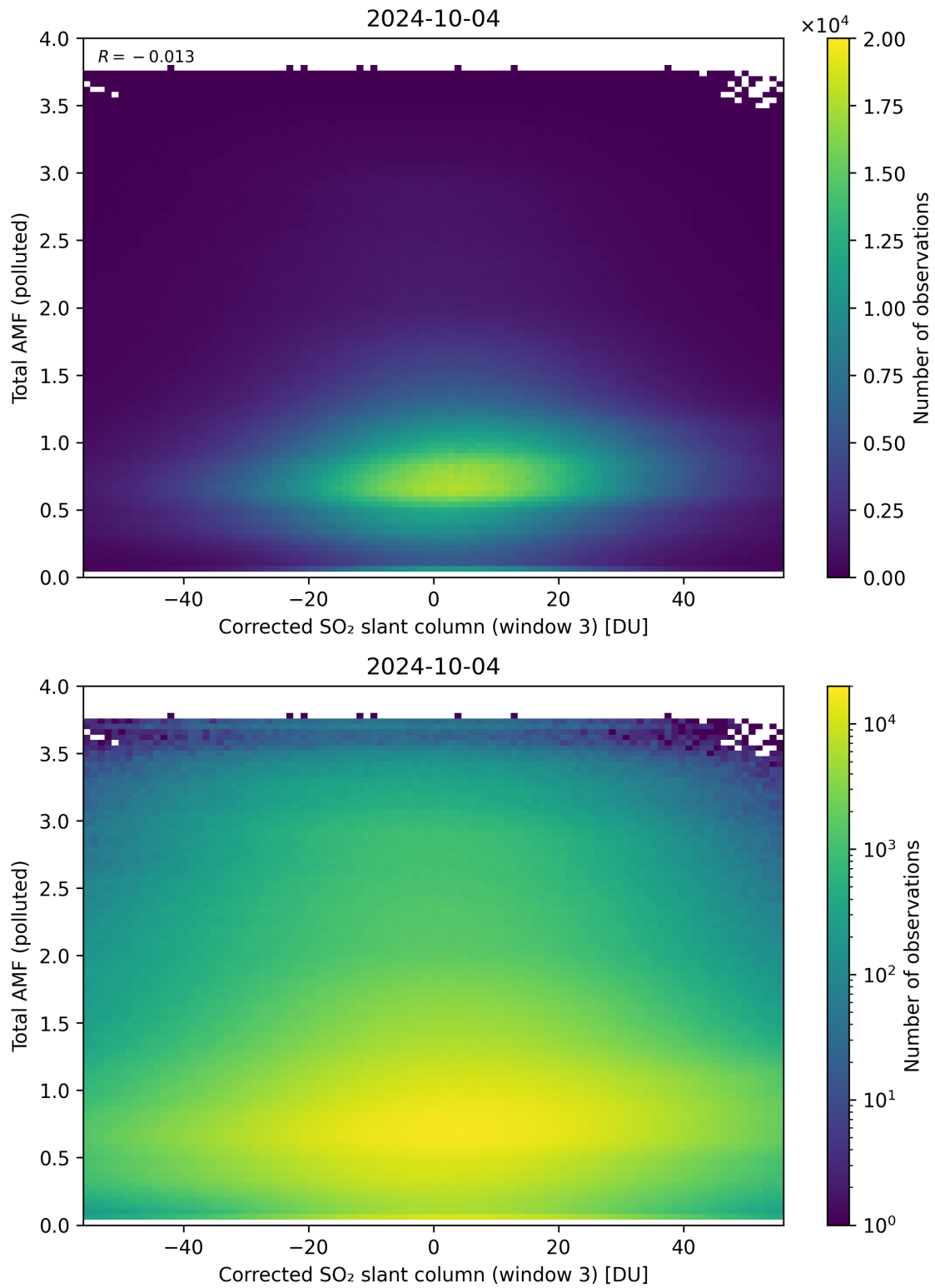
Figure 210: Scatter density plot of “Corrected SO 2 slant column (window 3)” against “Total AMF (polluted)” for 2024-10-03 to 2024-10-05.
