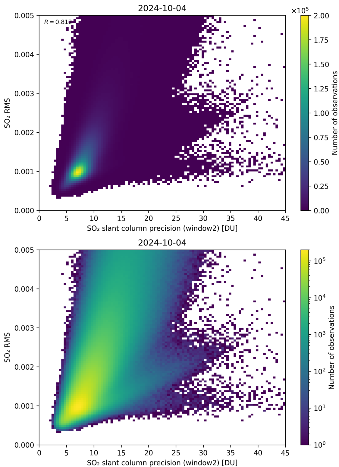
Figure 245: Scatter density plot of “SO 2 slant column precision (window2)” against “SO 2 RMS” for 2024-10-03 to 2024-10-05.
