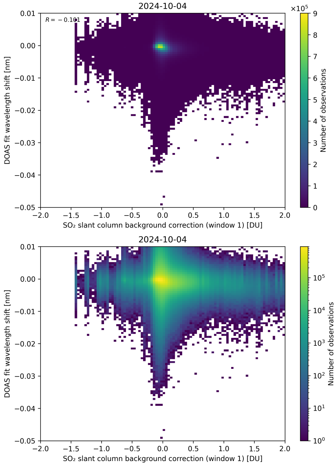
Figure 100: Scatter density plot of “SO 2 slant column background correction (window 1)” against “DOAS fit wavelength shift” for 2024-10-03 to 2024-10-05.
