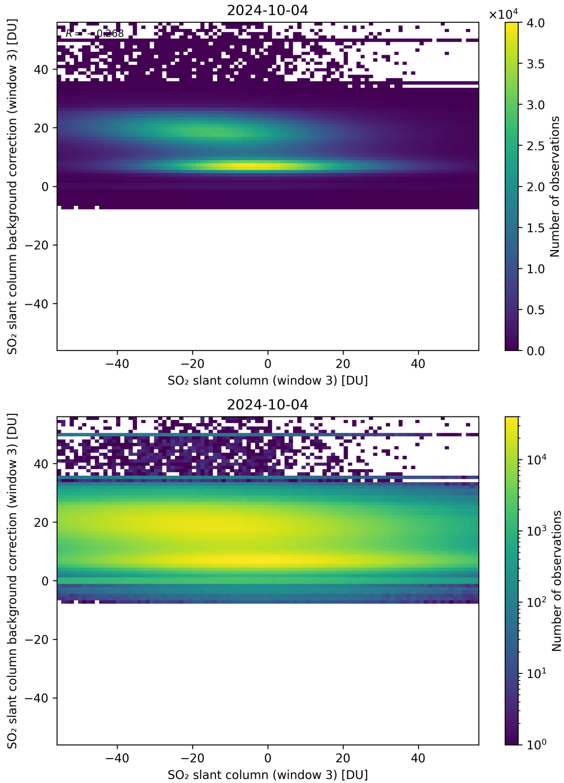
Figure 253: Scatter density plot of “SO 2 slant column (window 3)” against “SO 2 slant column background correction (window 3)” for 2024-10-03 to 2024-10-05.
