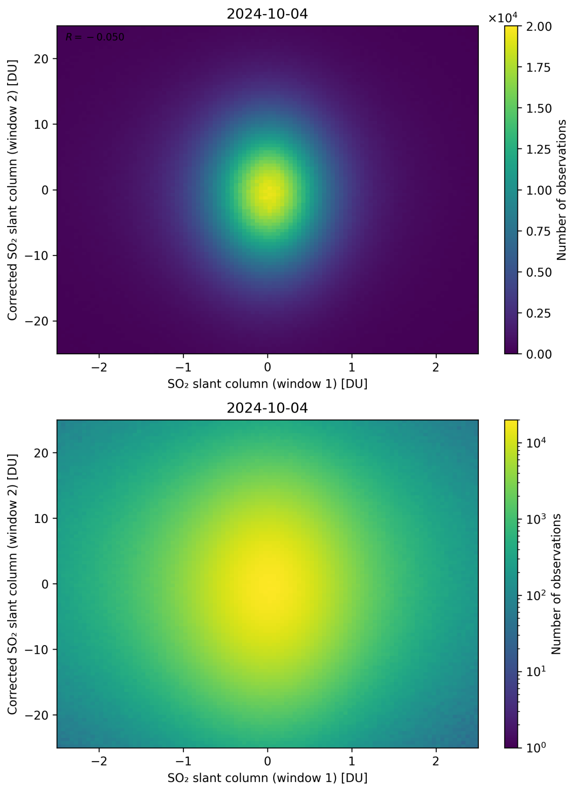
Figure 233: Scatter density plot of “SO 2 slant column (window 1)” against “Corrected SO 2 slant column (window 2)” for 2024-10-03 to 2024-10-05.
