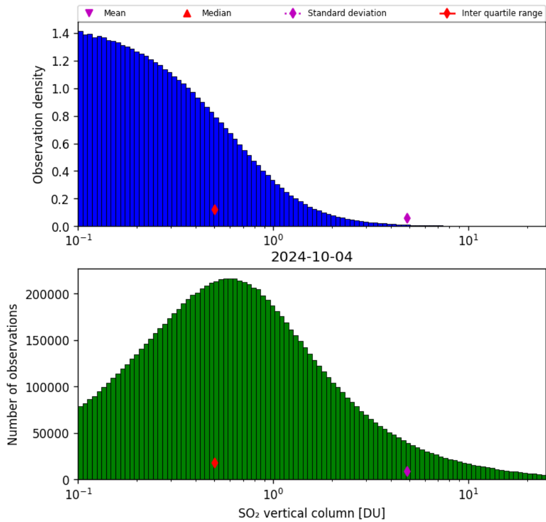
Figure 53: Histogram of “SO 2 vertical column” for 2024-10-03 to 2024-10-05
