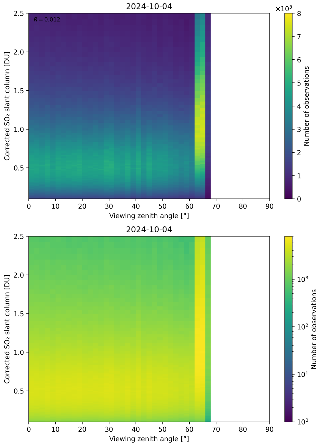
Figure 317: Scatter density plot of “Viewing zenith angle” against “Corrected SO 2 slant column” for 2024-10-03 to 2024-10-05.
