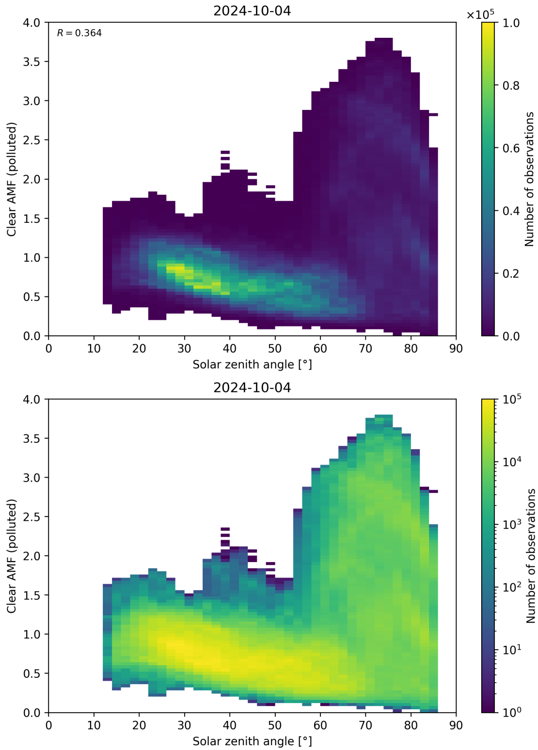
Figure 165: Scatter density plot of “Solar zenith angle” against “Clear AMF (polluted)” for 2024-10-03 to 2024-10-05.
