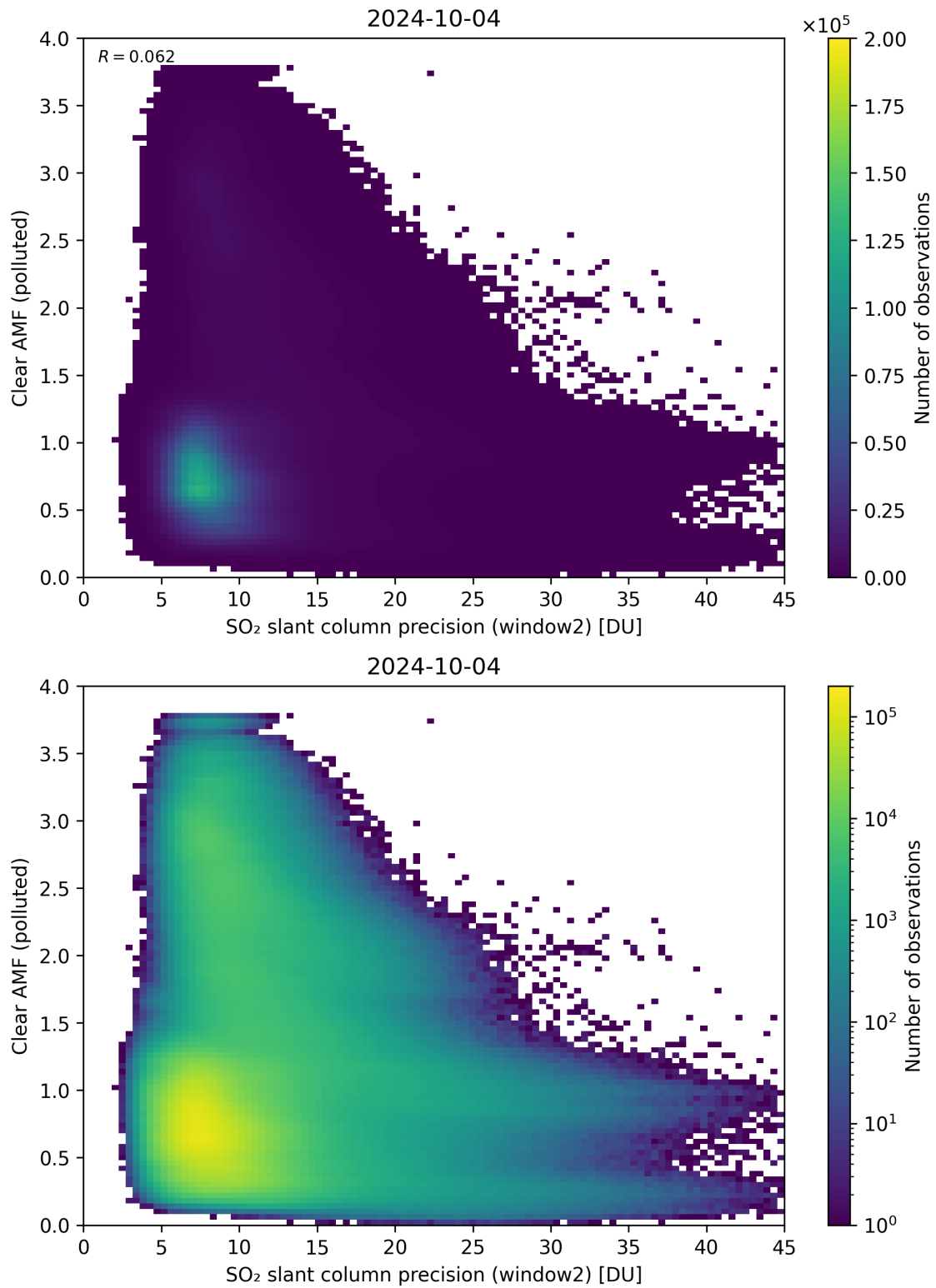
Figure 246: Scatter density plot of “SO 2 slant column precision (window2)” against “Clear AMF (polluted)” for 2024-10-03 to 2024-10-05.
