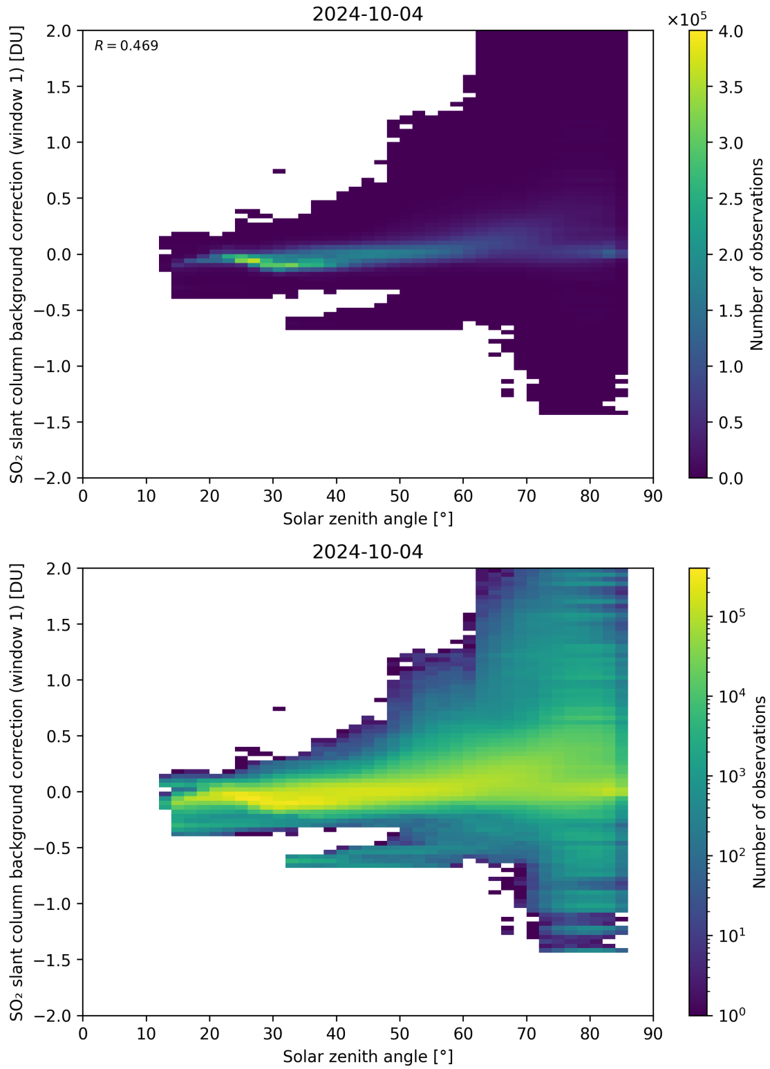
Figure 158: Scatter density plot of “Solar zenith angle” against “SO 2 slant column background correction (window 1)” for 2024-10-03 to 2024-10-05.
