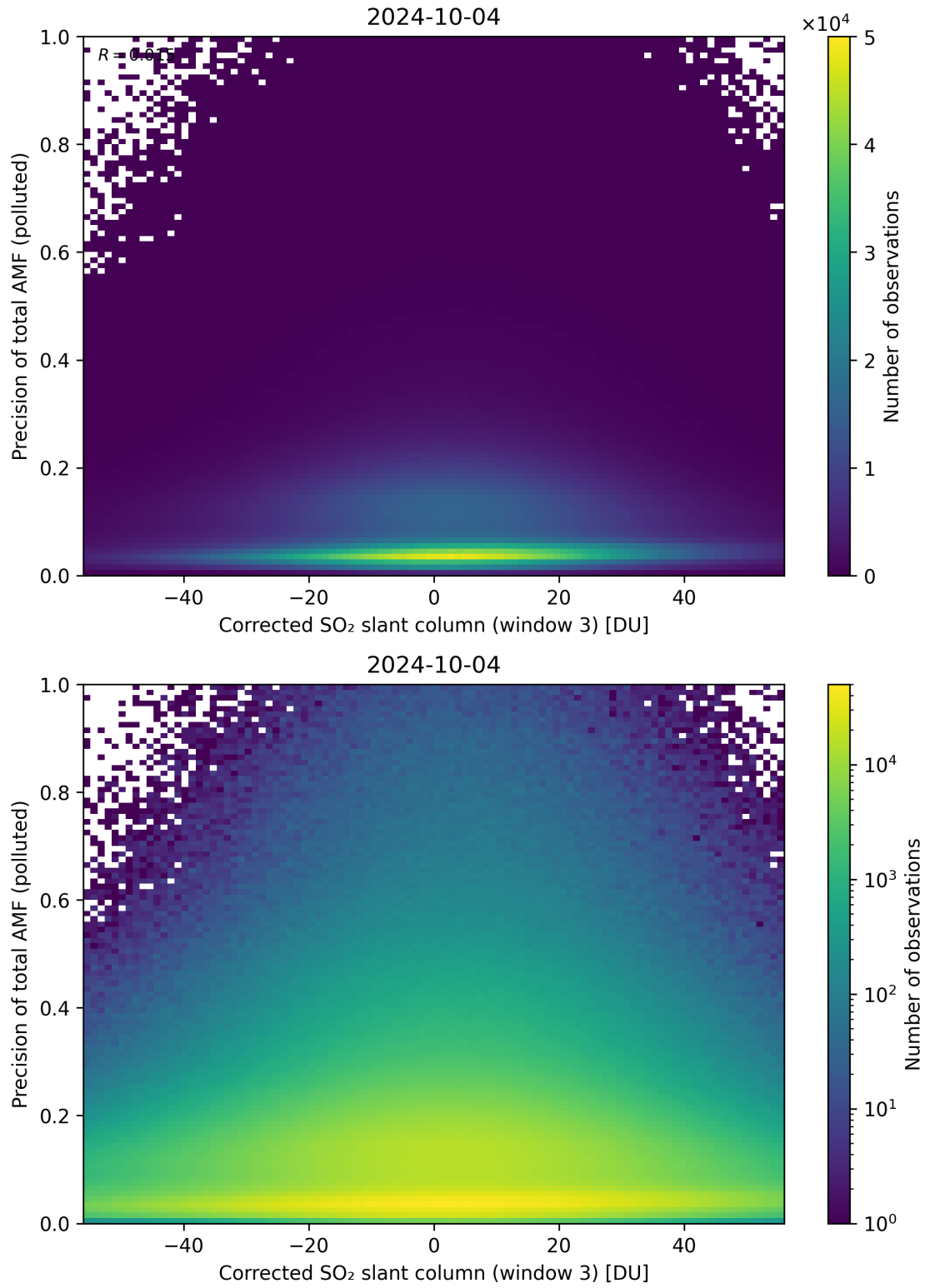
Figure 211: Scatter density plot of “Corrected SO 2 slant column (window 3)” against “Precision of total AMF (polluted)” for 2024-10-03 to 2024-10-05.
