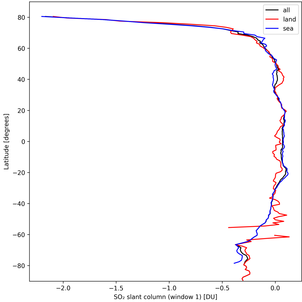
Figure 33: Zonal average of “SO 2 slant column (window 1)” for 2024-10-03 to 2024-10-05.
