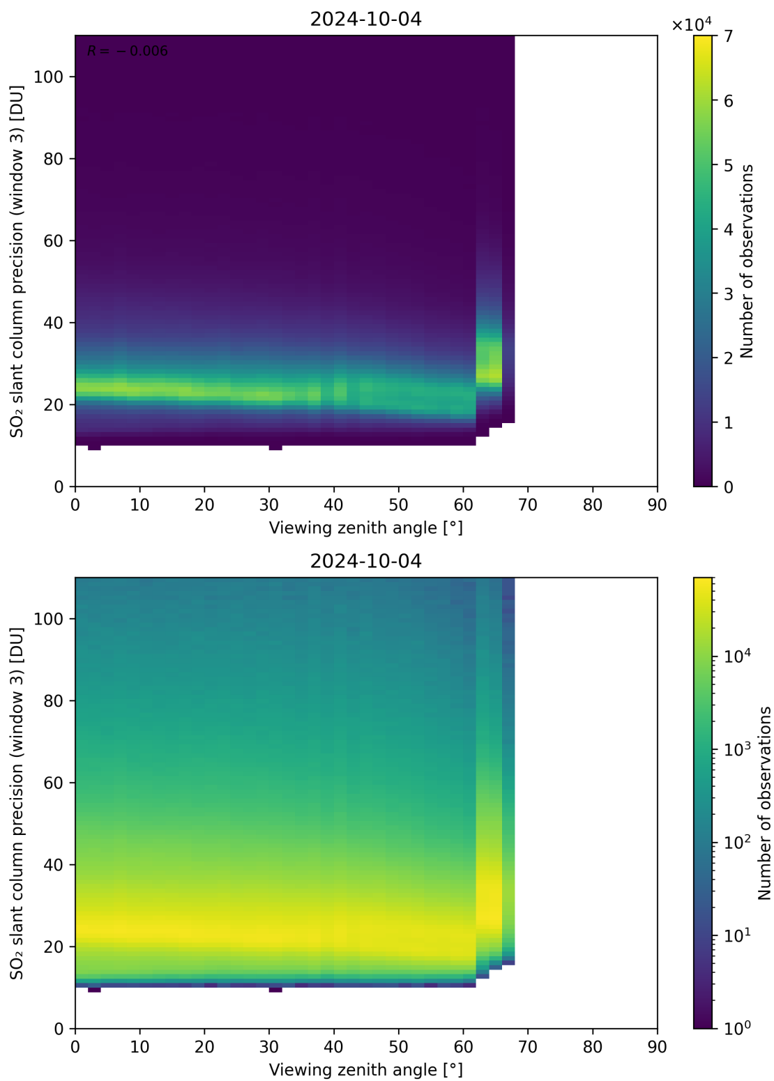
Figure 324: Scatter density plot of “Viewing zenith angle” against “SO 2 slant column precision (window 3)” for 2024-10-03 to 2024-10-05.
