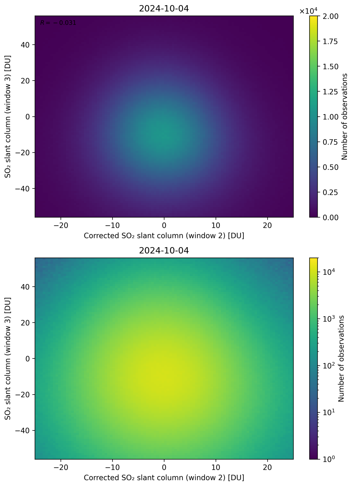
Figure 201: Scatter density plot of “Corrected SO 2 slant column (window 2)” against “SO 2 slant column (window 3)” for 2024-10-03 to 2024-10-05.
