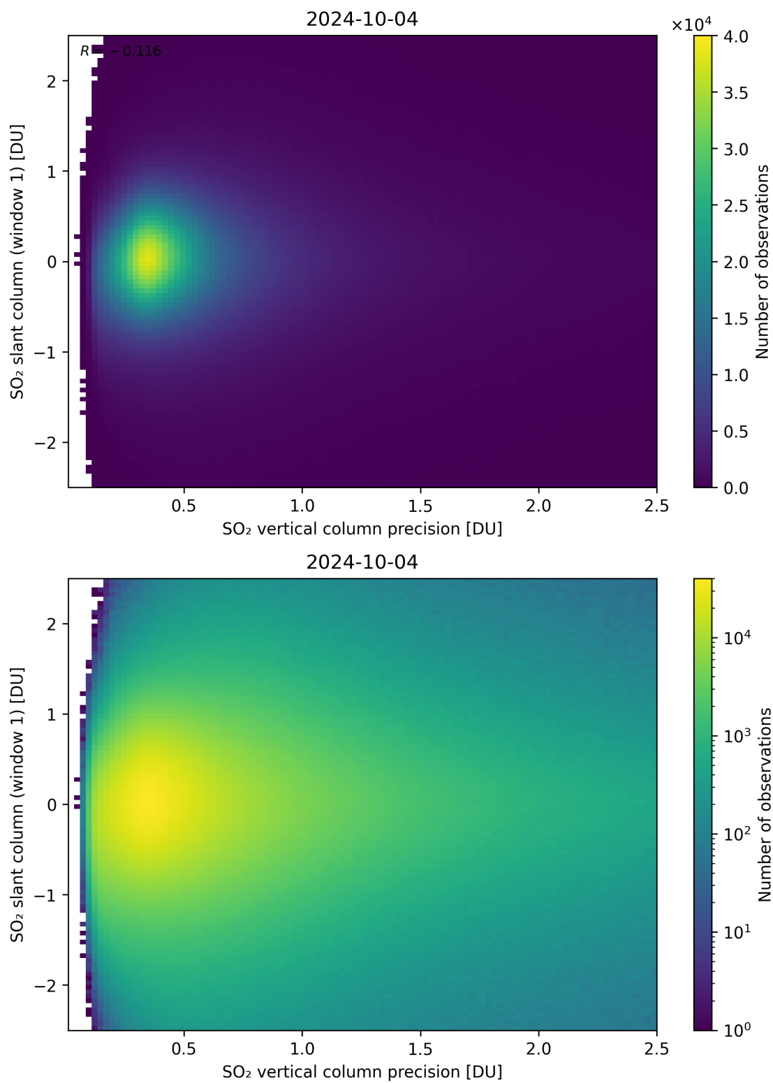
Figure 289: Scatter density plot of “SO 2 vertical column precision” against “SO 2 slant column (window 1)” for 2024-10-03 to 2024-10-05.
