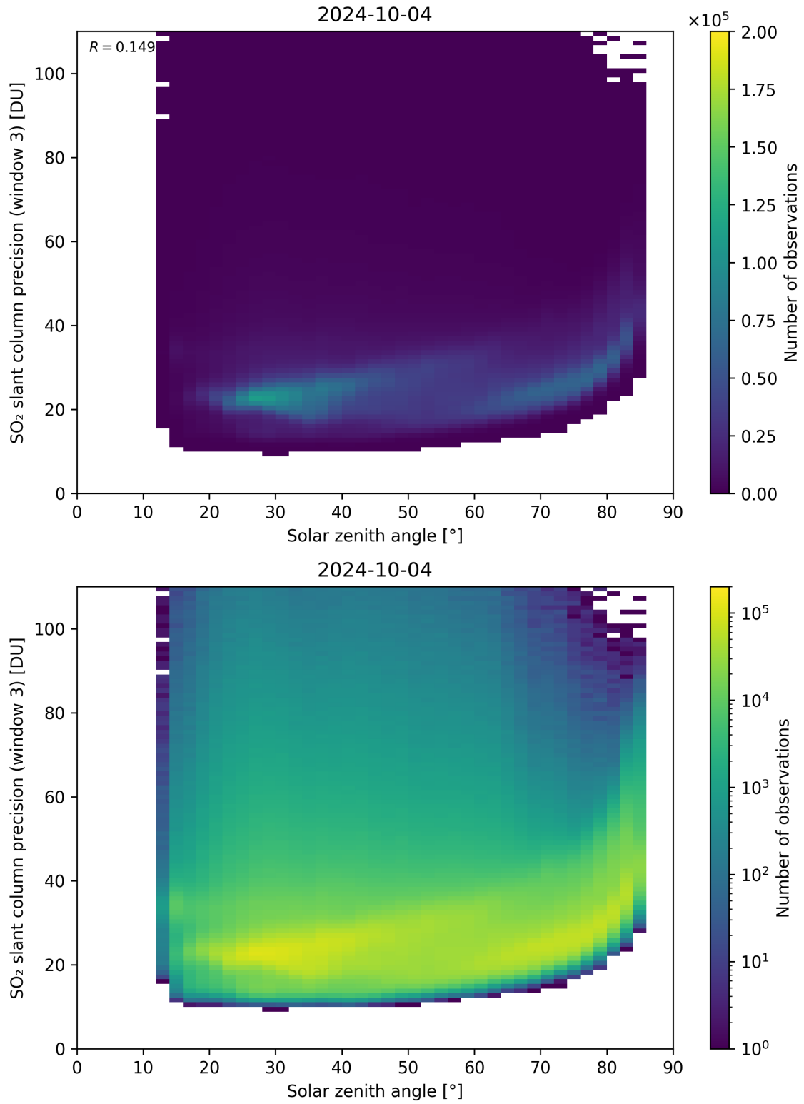
Figure 173: Scatter density plot of “Solar zenith angle” against “SO 2 slant column precision (window 3)” for 2024-10-03 to 2024-10-05.
