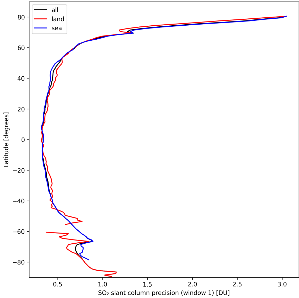
Figure 34: Zonal average of “SO 2 slant column precision (window 1)” for 2024-10-03 to 2024-10-05.
