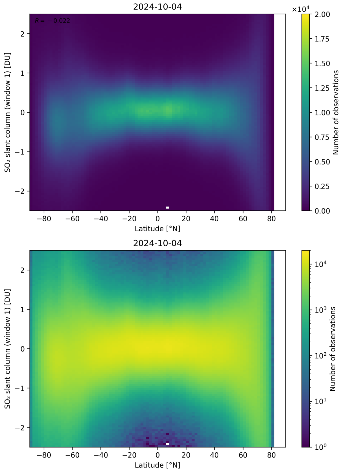
Figure 149: Scatter density plot of “Latitude” against “SO 2 slant column (window 1)” for 2024-10-03 to 2024-10-05.
