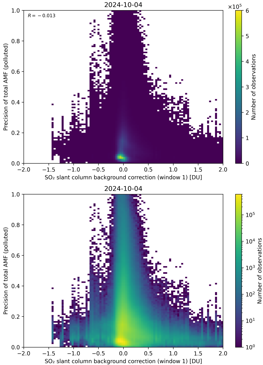
Figure 110: Scatter density plot of “SO 2 slant column background correction (window 1)” against “Precision of total AMF (polluted)” for 2024-10-03 to 2024-10-05.
