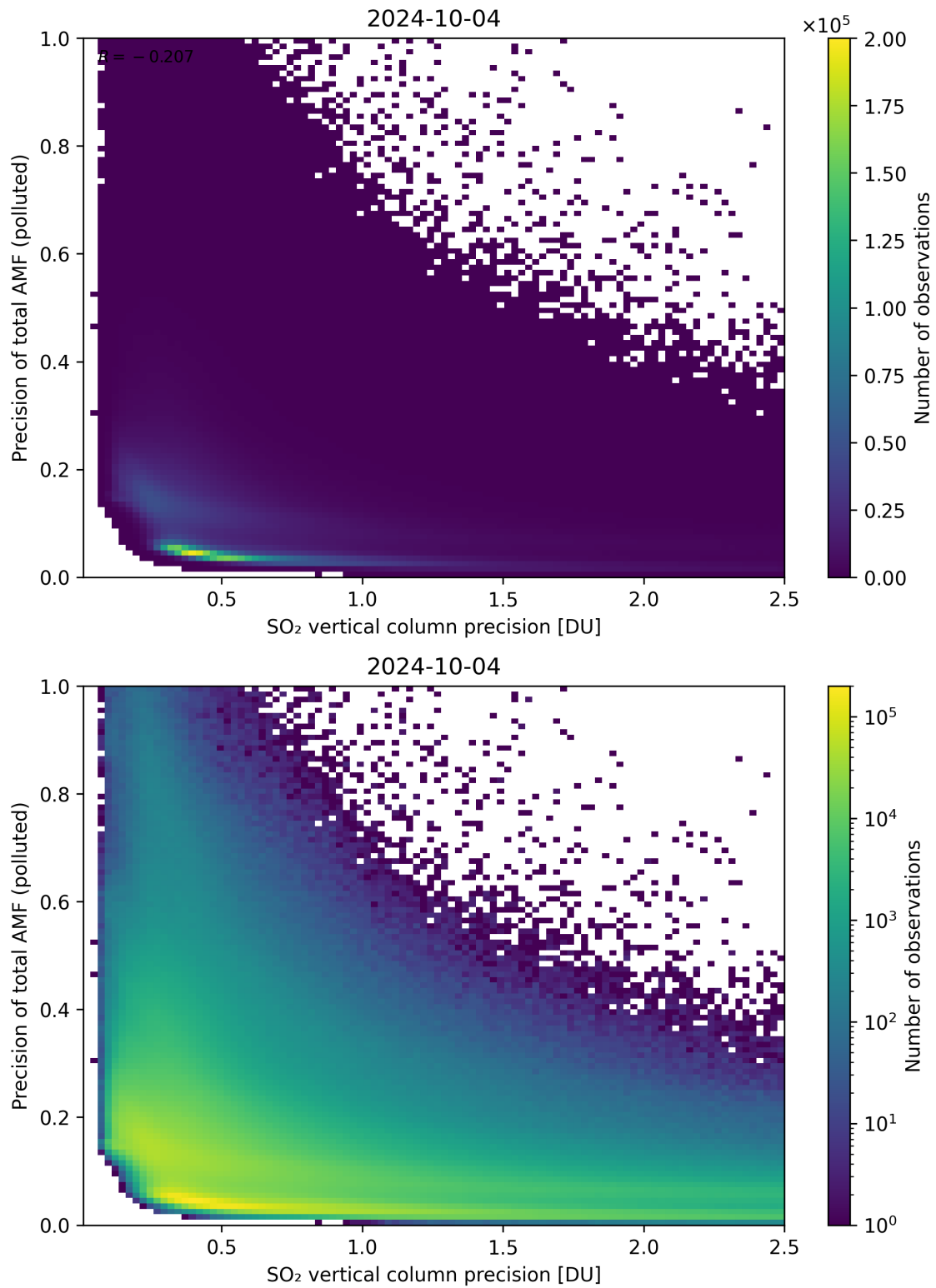
Figure 295: Scatter density plot of “SO 2 vertical column precision” against “Precision of total AMF (polluted)” for 2024-10-03 to 2024-10-05.
