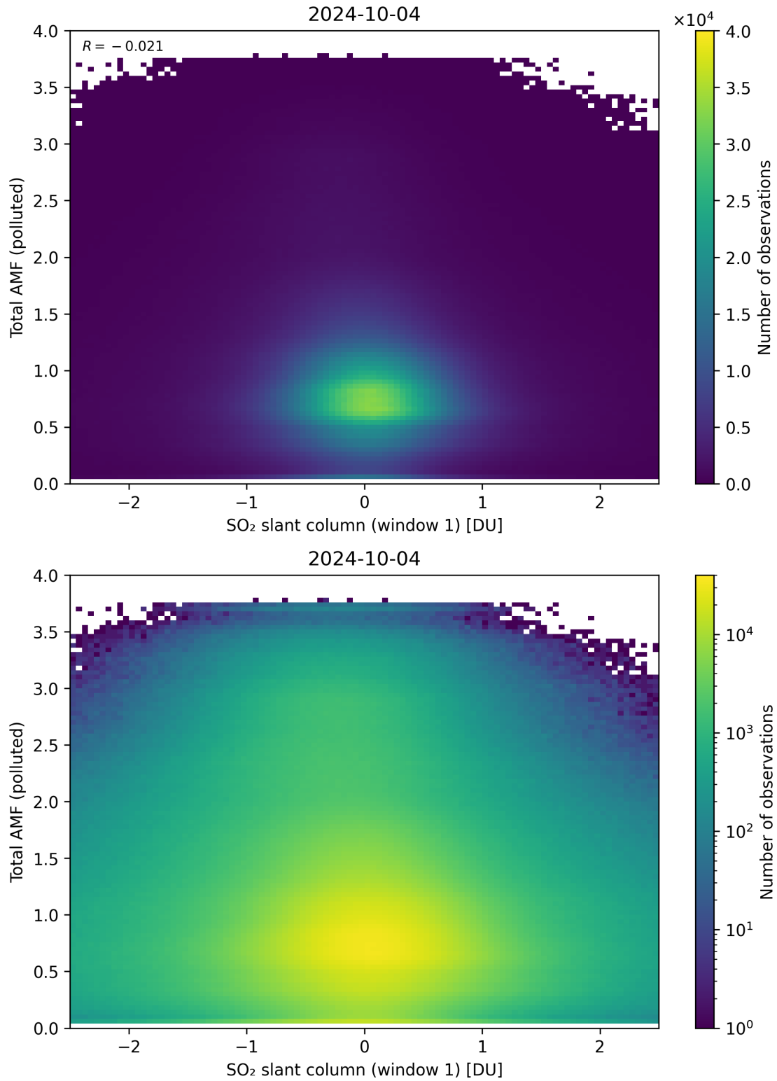
Figure 239: Scatter density plot of “SO 2 slant column (window 1)” against “Total AMF (polluted)” for 2024-10-03 to 2024-10-05.
