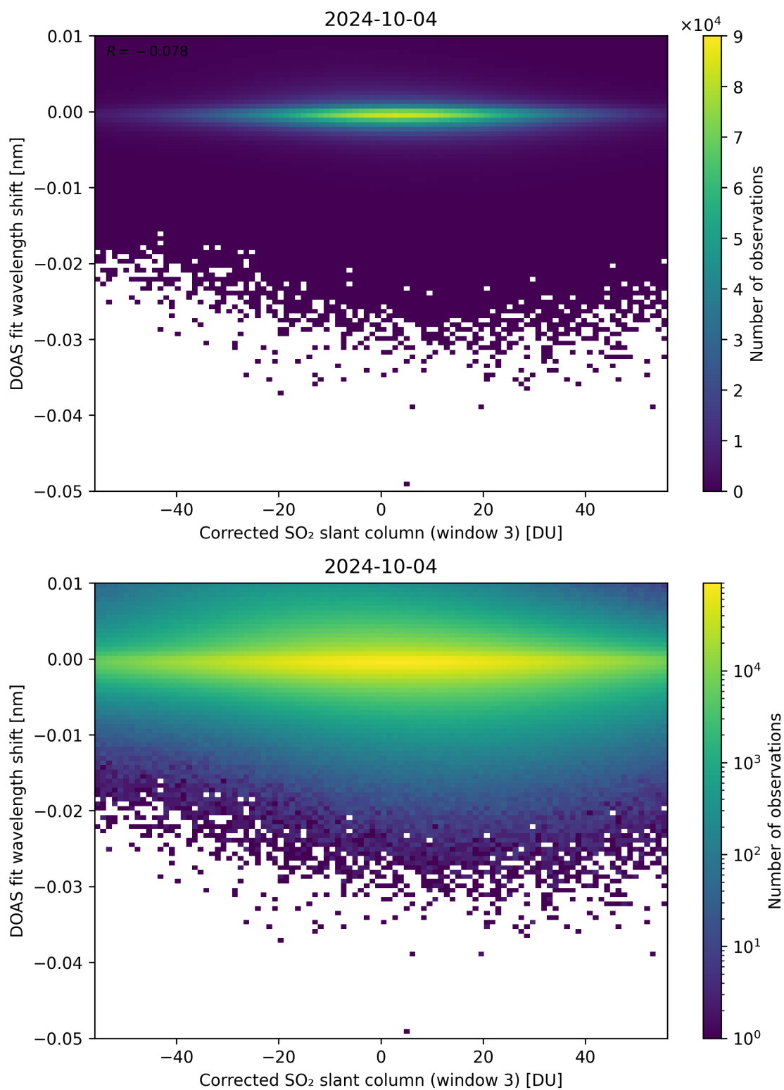
Figure 206: Scatter density plot of “Corrected SO 2 slant column (window 3)” against “DOAS fit wavelength shift” for 2024-10-03 to 2024-10-05.
