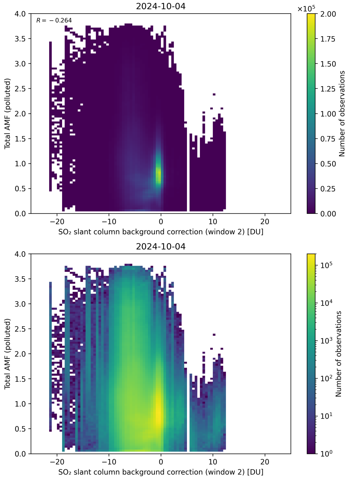
Figure 119: Scatter density plot of “SO 2 slant column background correction (window 2)” against “Total AMF (polluted)” for 2024-10-03 to 2024-10-05.
