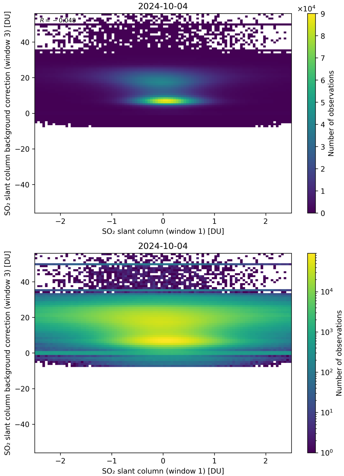
Figure 214: Scatter density plot of “SO 2 slant column (window 1)” against “SO 2 slant column background correction (window 3)” for 2024-10-03 to 2024-10-05.
