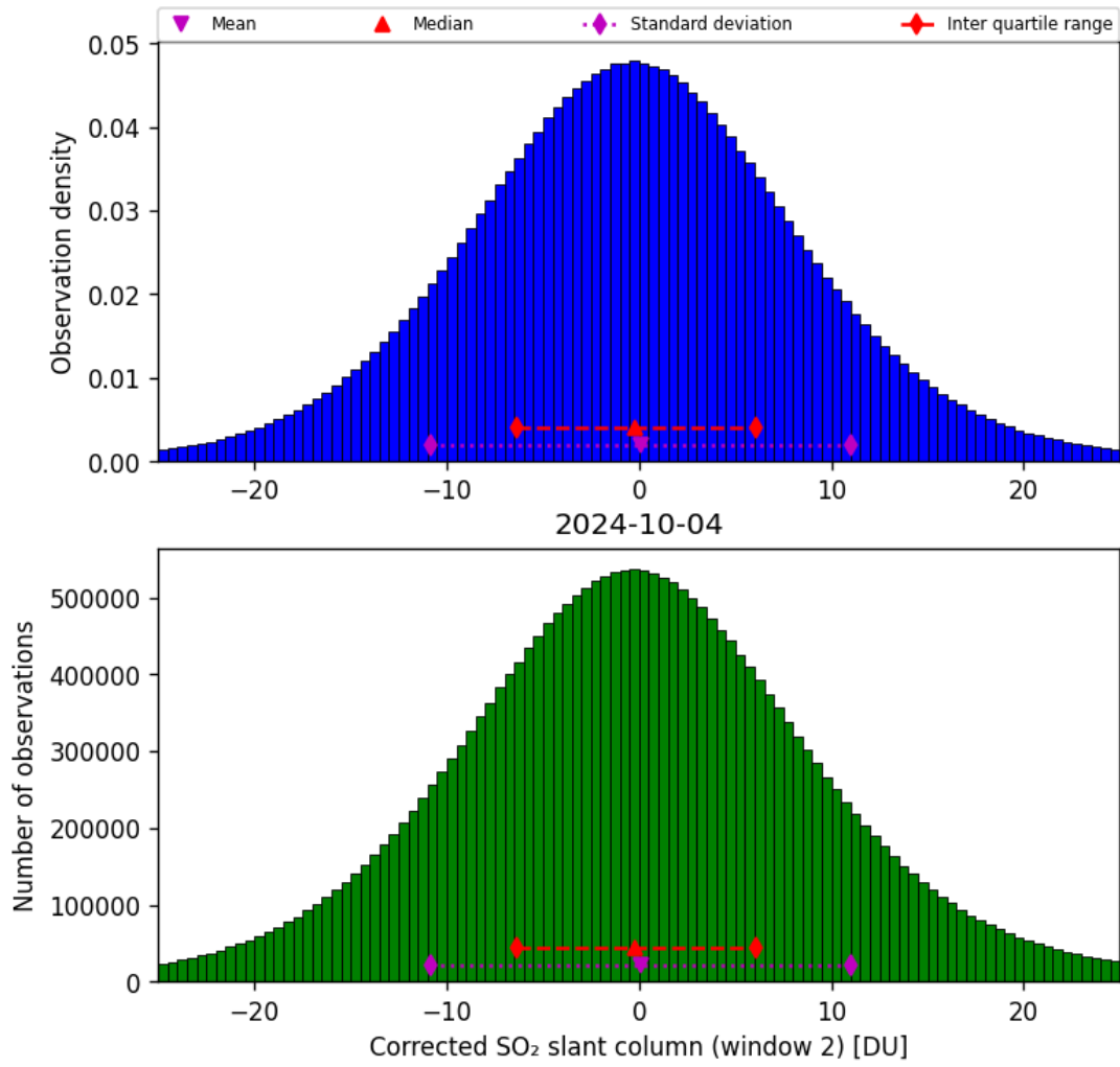
Figure 62: Histogram of “Corrected SO 2 slant column (window 2)” for 2024-10-03 to 2024-10-05
