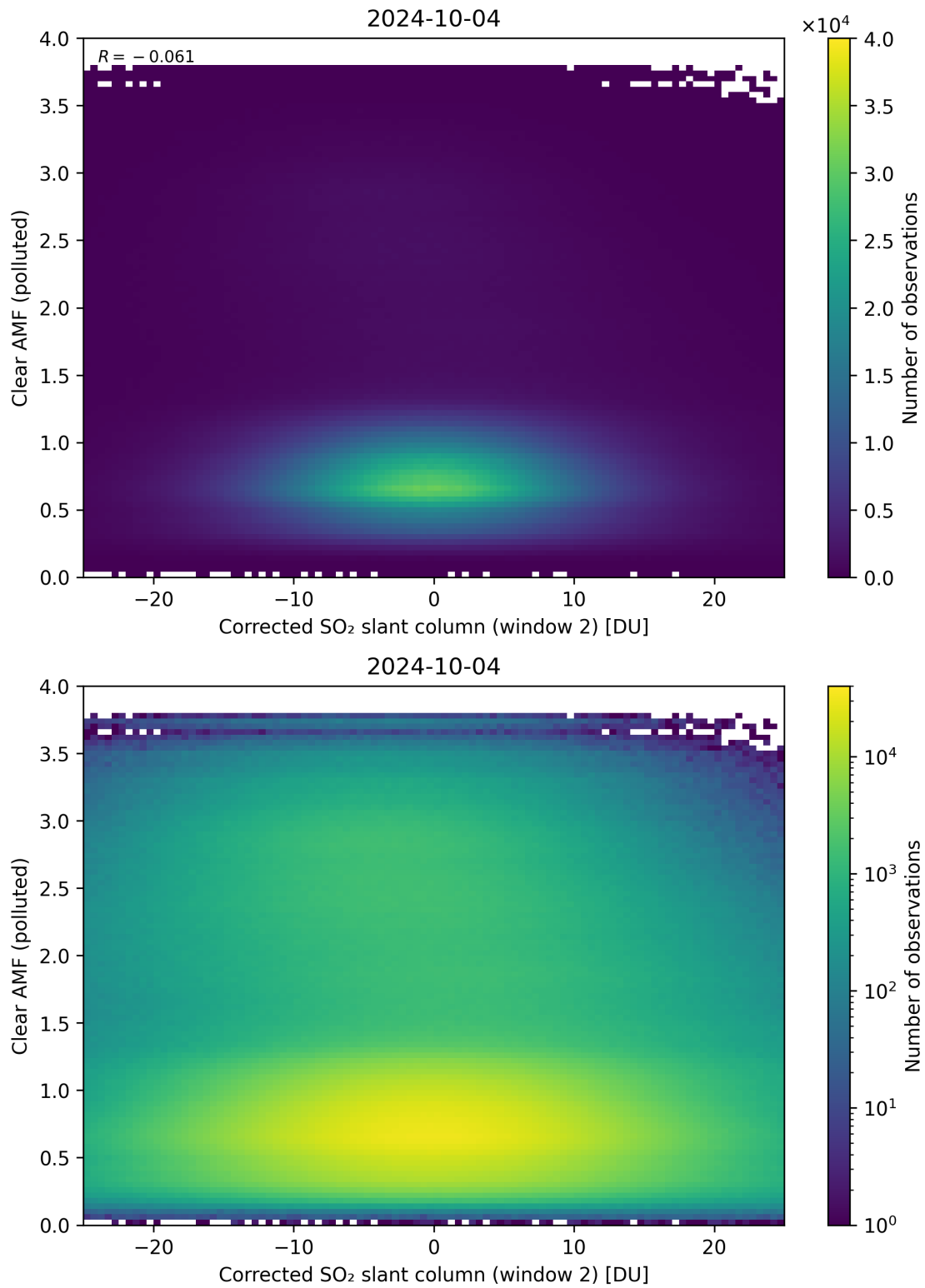
Figure 199: Scatter density plot of “Corrected SO 2 slant column (window 2)” against “Clear AMF (polluted)” for 2024-10-03 to 2024-10-05.
