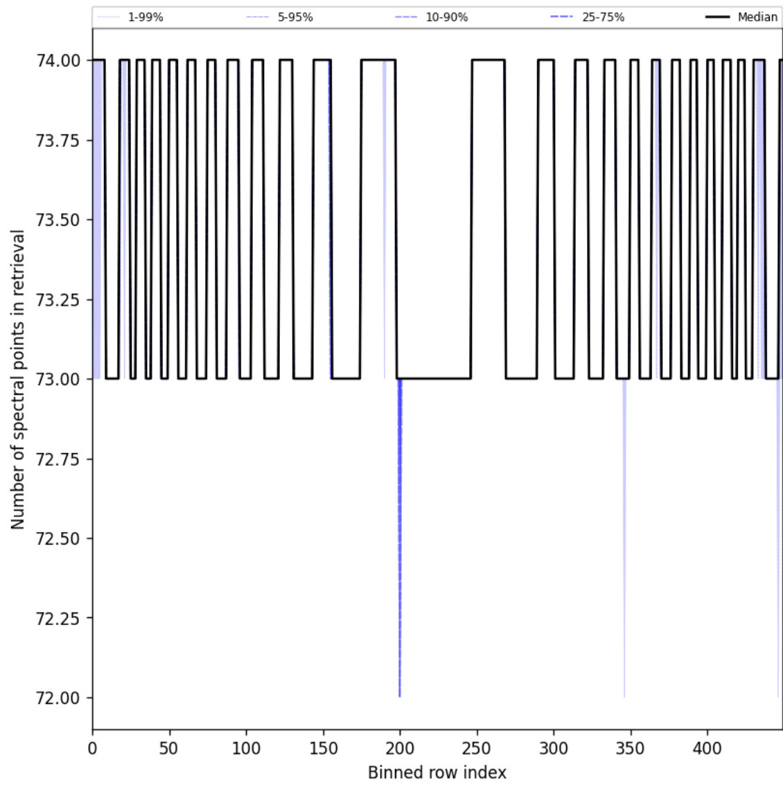
Figure 97: Along track statistics of “Number of spectral points in retrieval” for 2024-10-03 to 2024-10-05
