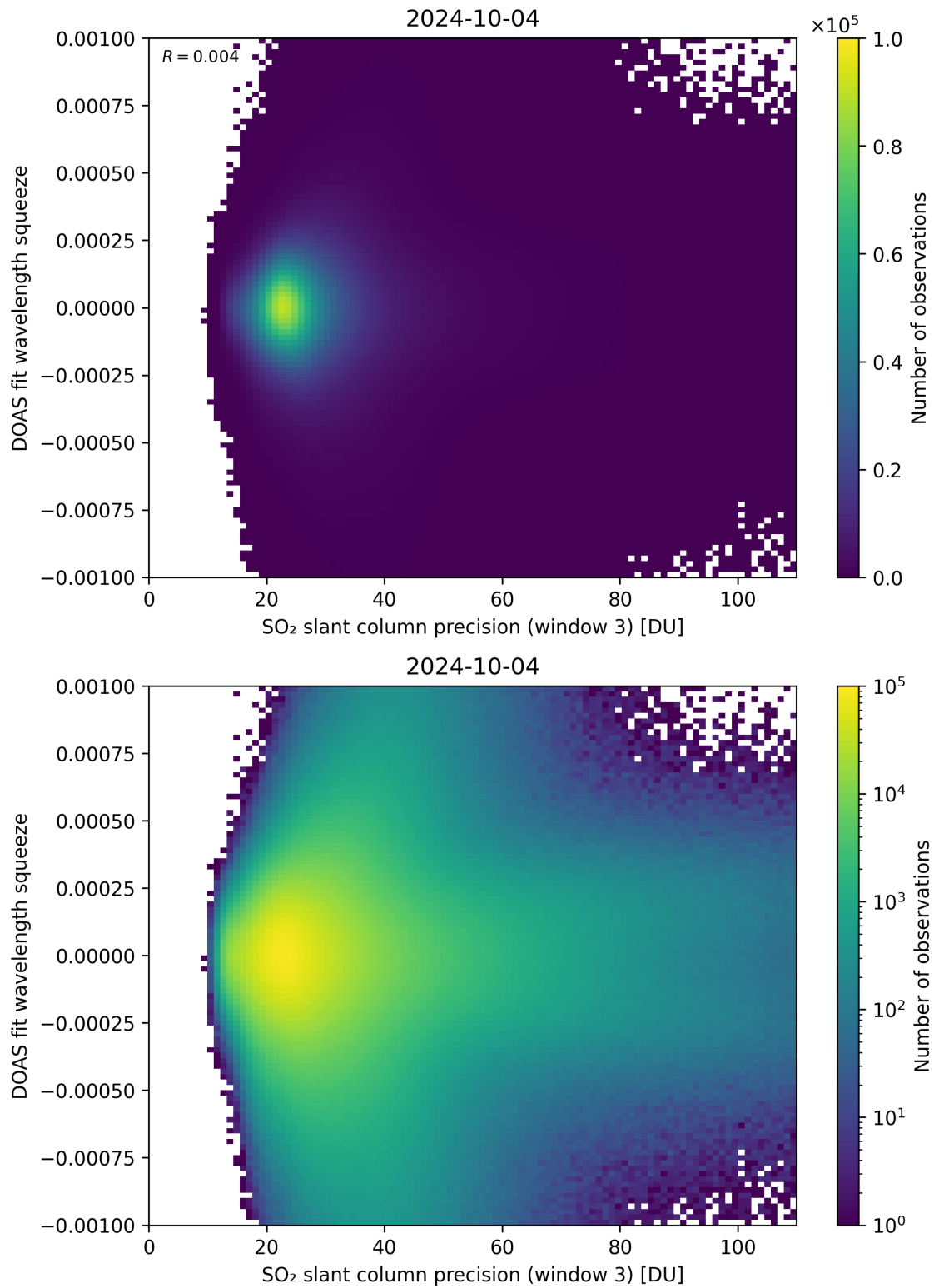
Figure 259: Scatter density plot of “SO 2 slant column precision (window 3)” against “DOAS fit wavelength squeeze” for 2024-10-03 to 2024-10-05.
