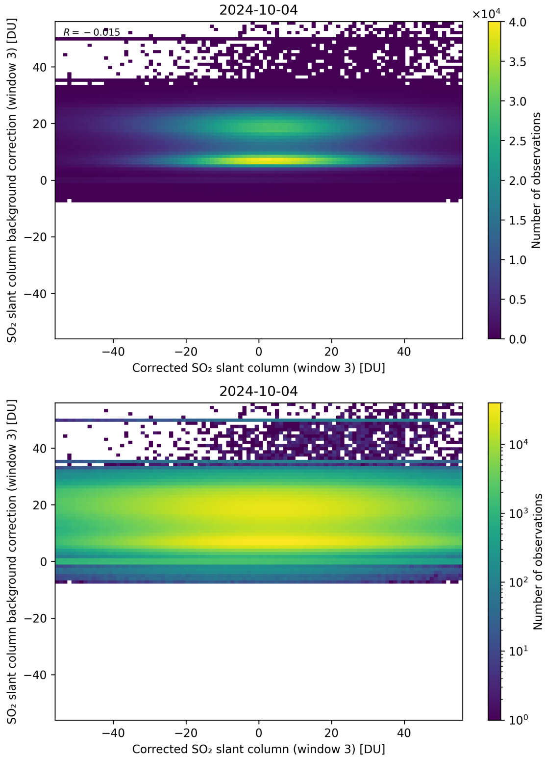
Figure 205: Scatter density plot of “Corrected SO 2 slant column (window 3)” against “SO 2 slant column background correction (window 3)” for 2024-10-03 to 2024-10-05.
