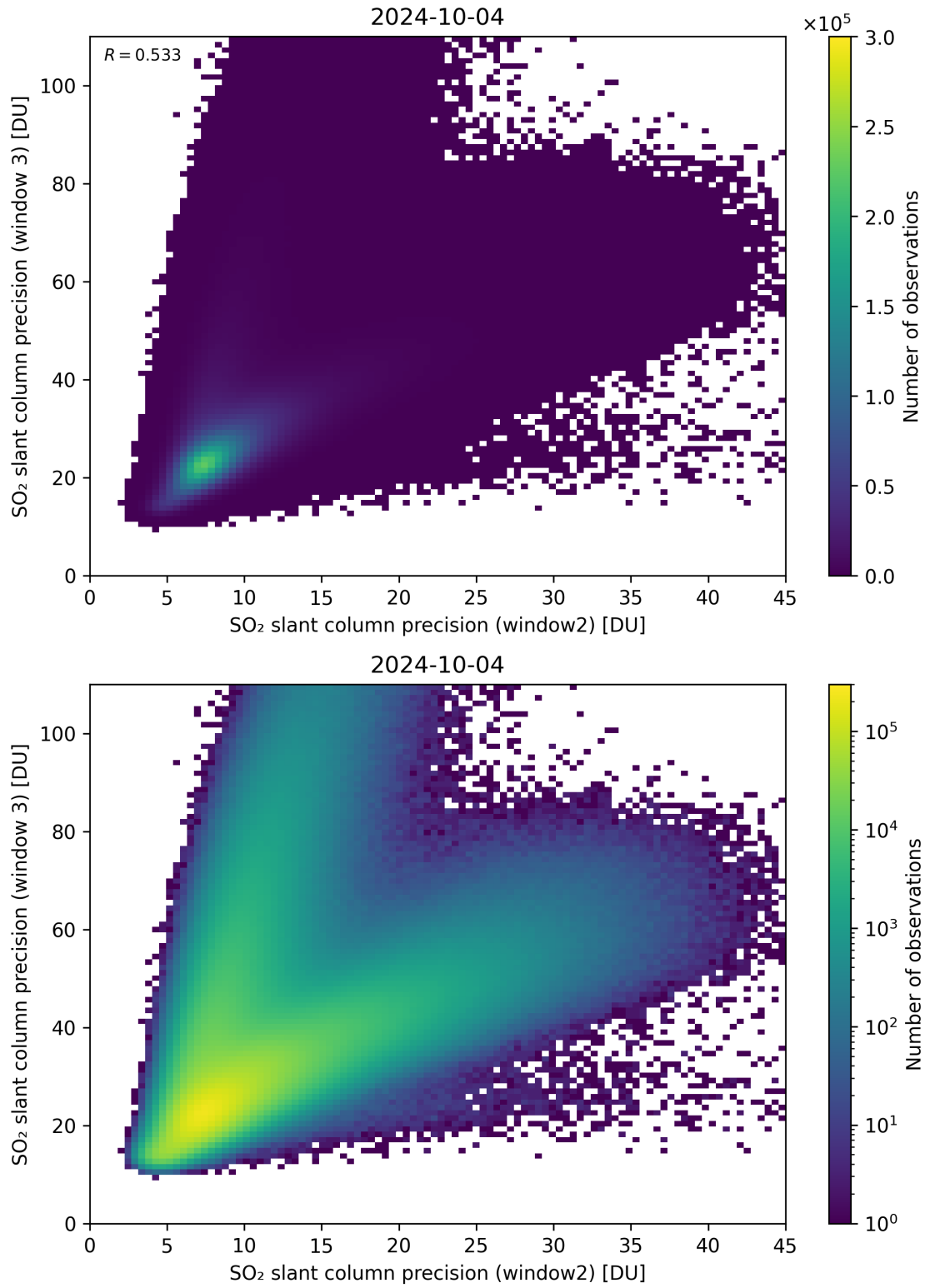
Figure 250: Scatter density plot of “SO 2 slant column precision (window2)” against “SO 2 slant column precision (window 3)” for 2024-10-03 to 2024-10-05.
