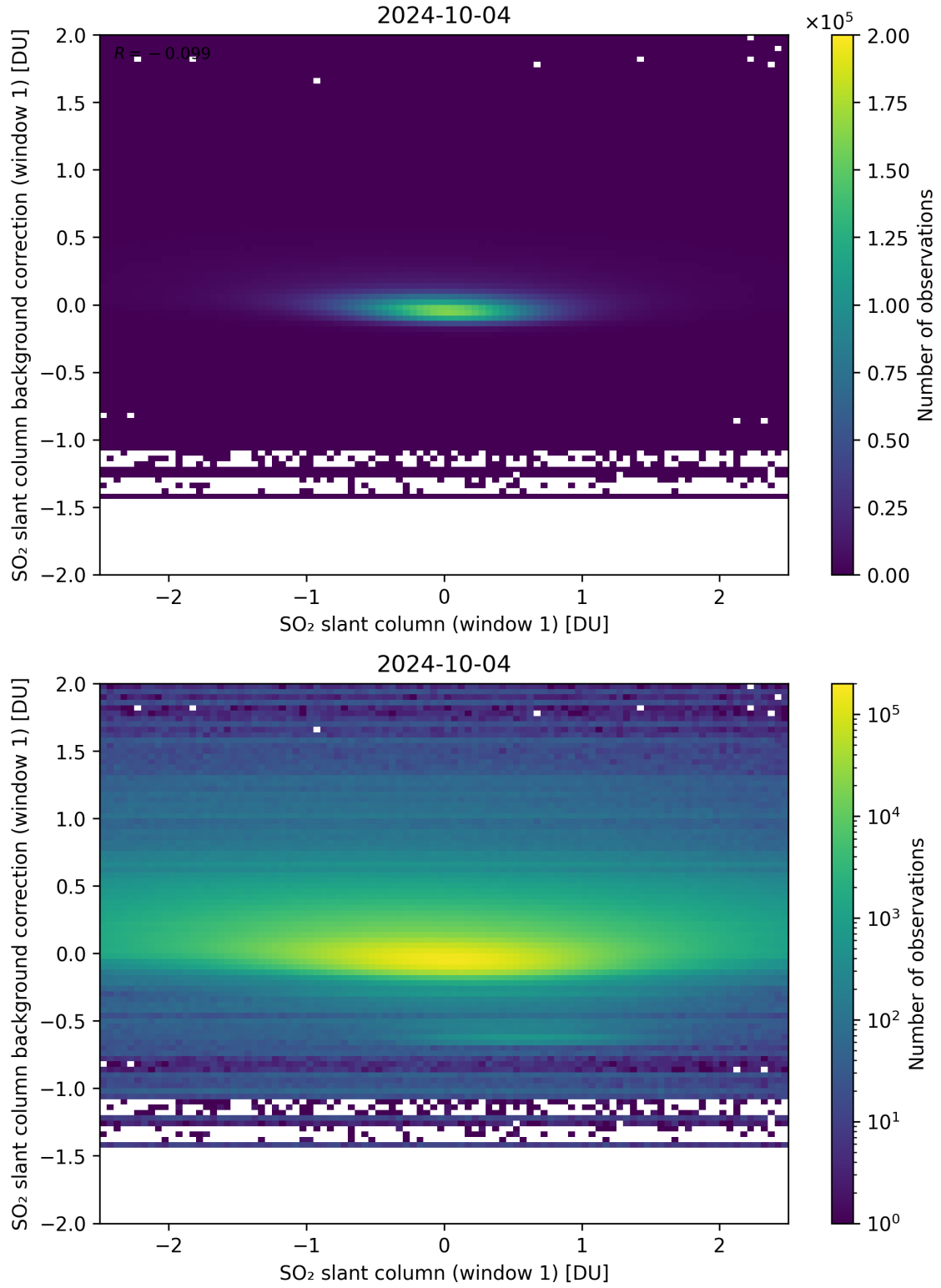
Figure 212: Scatter density plot of “SO 2 slant column (window 1)” against “SO 2 slant column background correction (window 1)” for 2024-10-03 to 2024-10-05.
