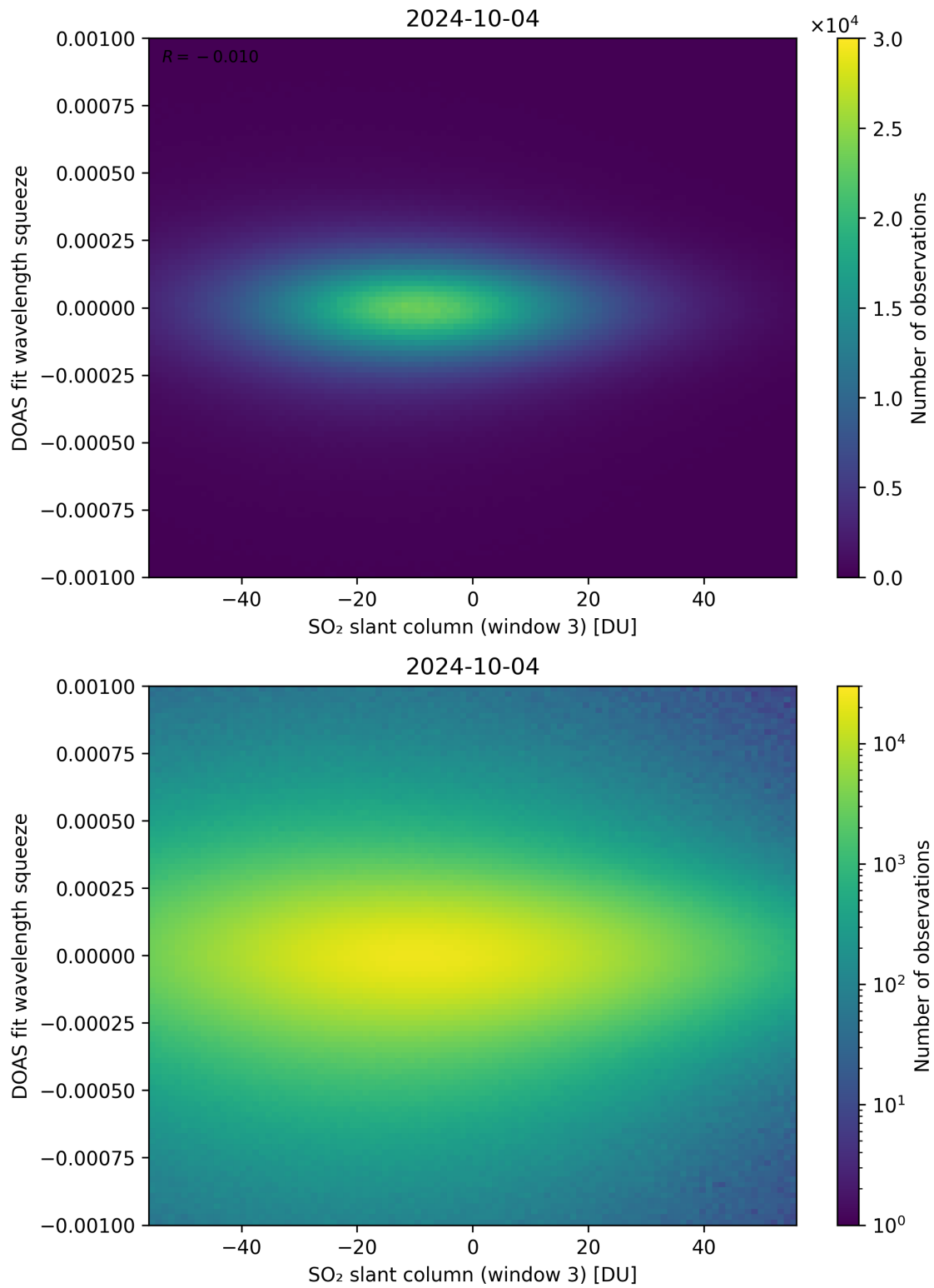
Figure 255: Scatter density plot of “SO 2 slant column (window 3)” against “DOAS fit wavelength squeeze” for 2024-10-03 to 2024-10-05.
