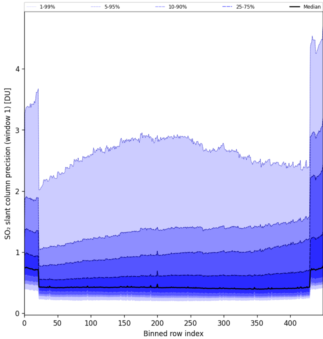
Figure 80: Along track statistics of “SO 2 slant column precision (window 1)” for 2024-10-03 to 2024-10-05
