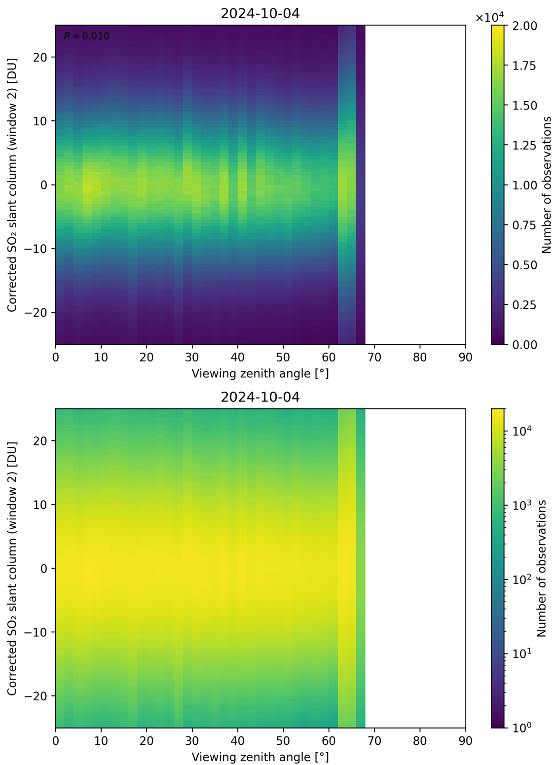
Figure 318: Scatter density plot of “Viewing zenith angle” against “Corrected SO 2 slant column (window 2)” for 2024-10-03 to 2024-10-05.
