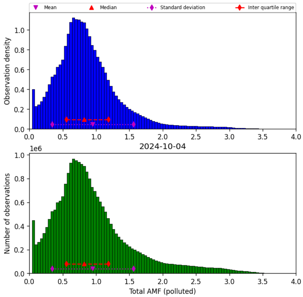
Figure 71: Histogram of “Total AMF (polluted)” for 2024-10-03 to 2024-10-05
