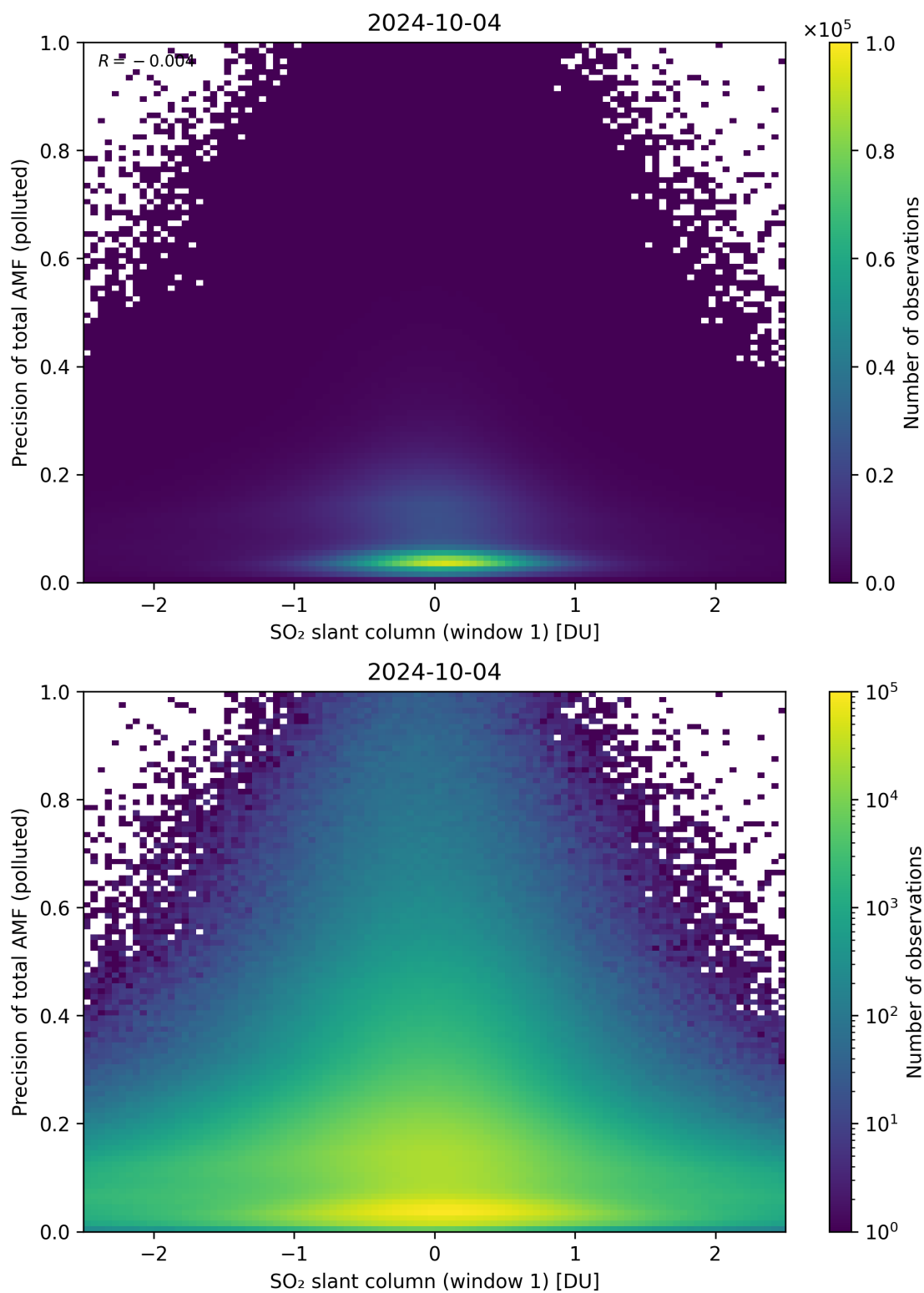
Figure 240: Scatter density plot of “SO 2 slant column (window 1)” against “Precision of total AMF (polluted)” for 2024-10-03 to 2024-10-05.
