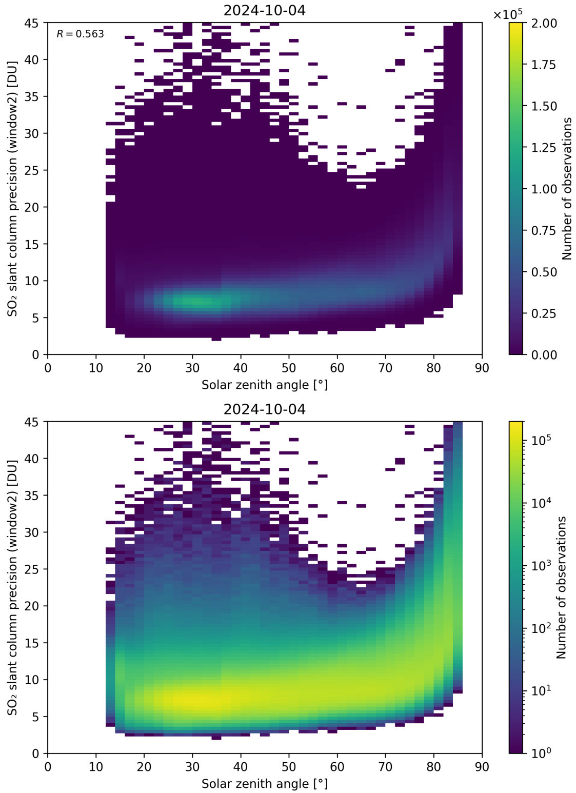
Figure 171: Scatter density plot of “Solar zenith angle” against “SO 2 slant column precision (window2)” for 2024-10-03 to 2024-10-05.
