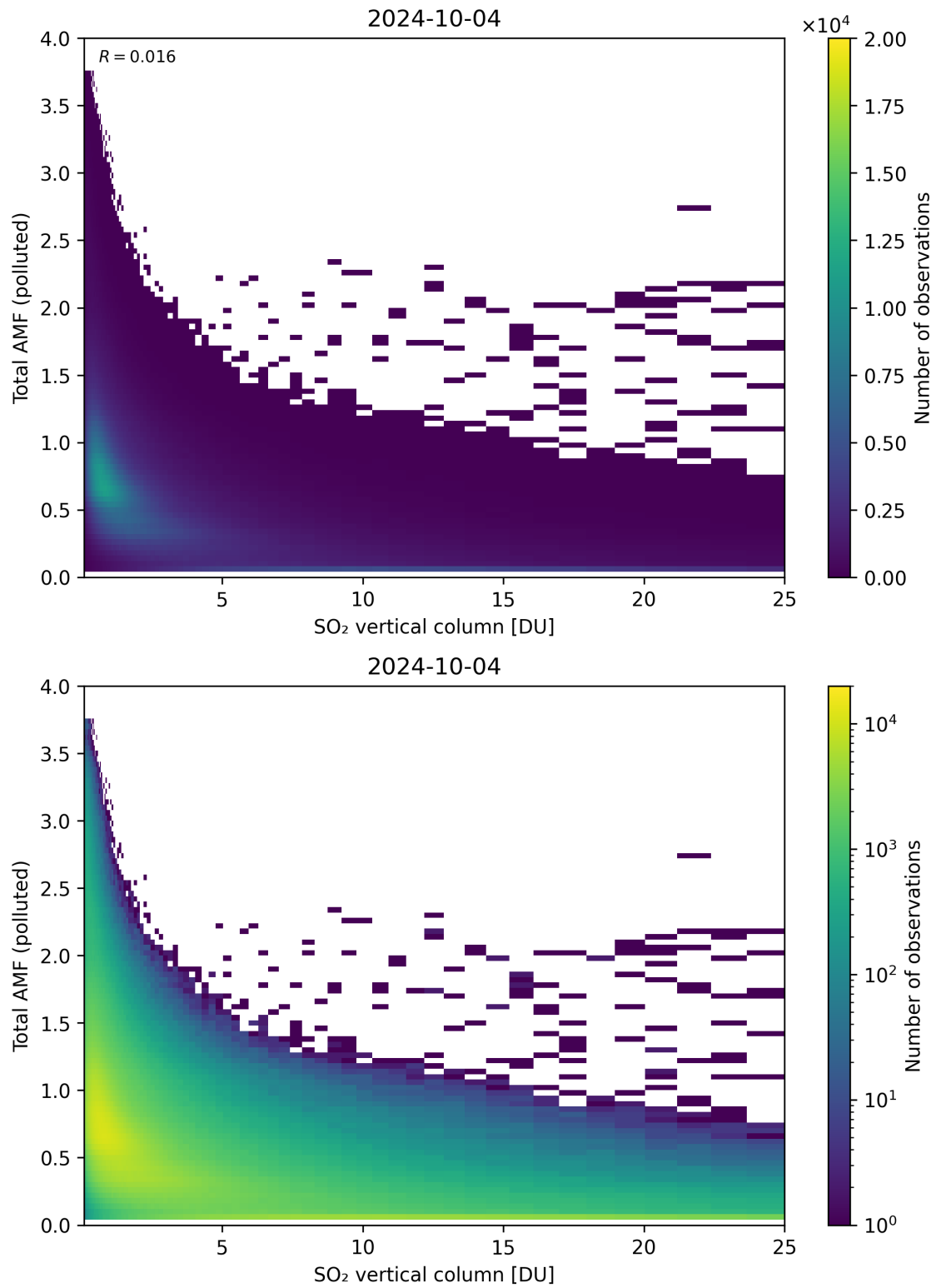
Figure 305: Scatter density plot of “SO 2 vertical column” against “Total AMF (polluted)” for 2024-10-03 to 2024-10-05.
