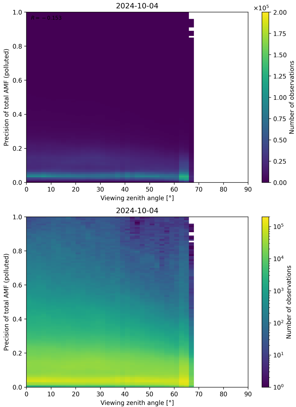
Figure 326: Scatter density plot of “Viewing zenith angle” against “Precision of total AMF (polluted)” for 2024-10-03 to 2024-10-05.
