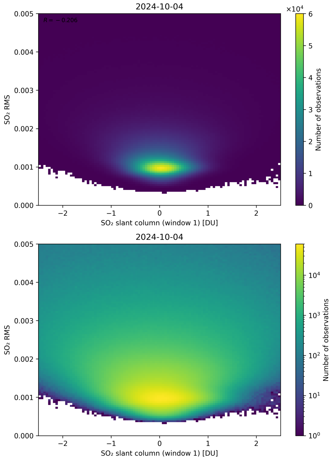
Figure 217: Scatter density plot of “SO 2 slant column (window 1)” against “SO 2 RMS” for 2024-10-03 to 2024-10-05.
