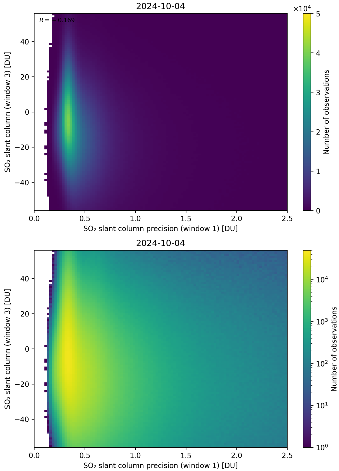
Figure 228: Scatter density plot of “SO 2 slant column precision (window 1)” against “SO 2 slant column (window 3)” for 2024-10-03 to 2024-10-05.
