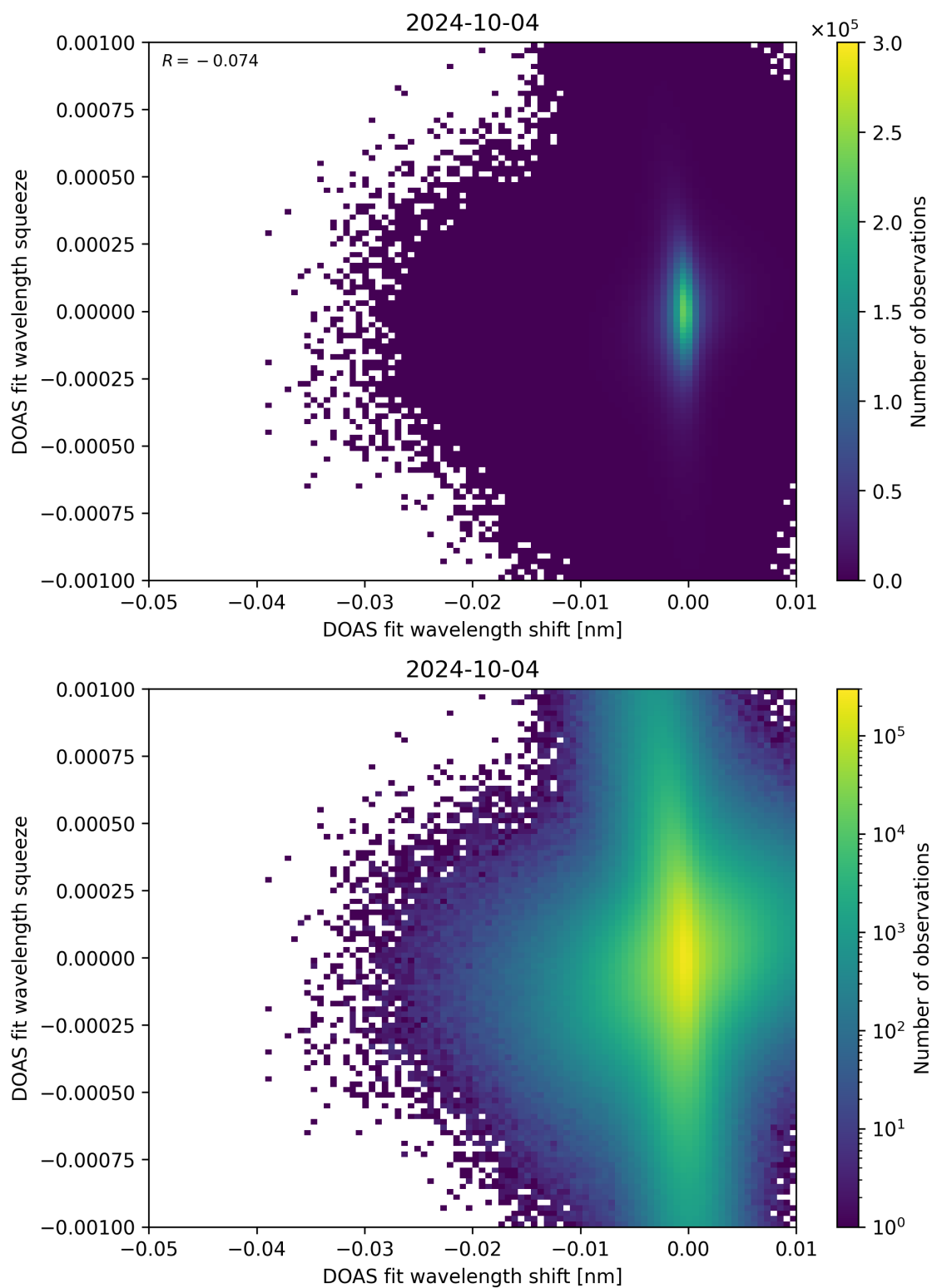
Figure 127: Scatter density plot of “DOAS fit wavelength shift” against “DOAS fit wavelength squeeze” for 2024-10-03 to 2024-10-05.
