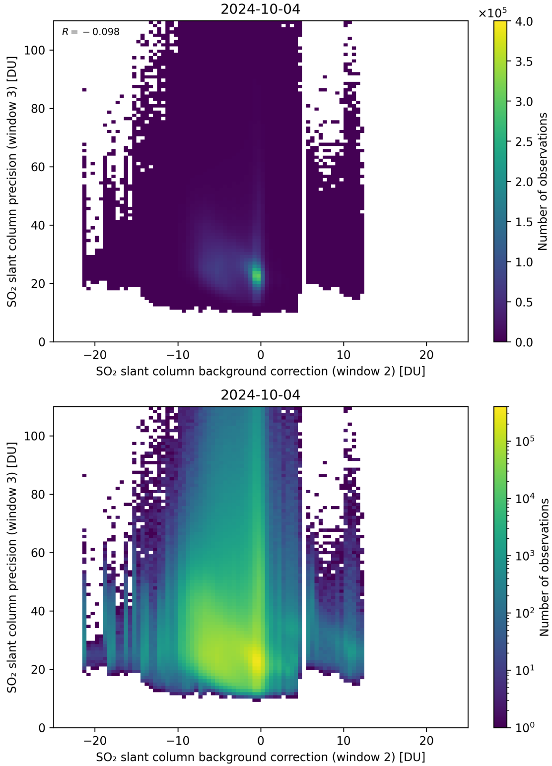
Figure 118: Scatter density plot of “SO 2 slant column background correction (window 2)” against “SO 2 slant column precision (window 3)” for 2024-10-03 to 2024-10-05.
