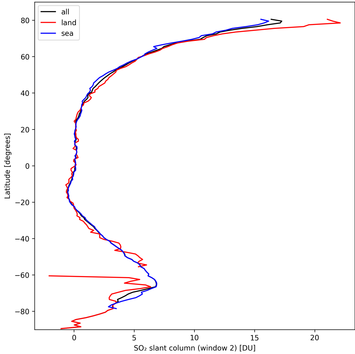
Figure 37: Zonal average of “SO 2 slant column (window 2)” for 2024-10-03 to 2024-10-05.
