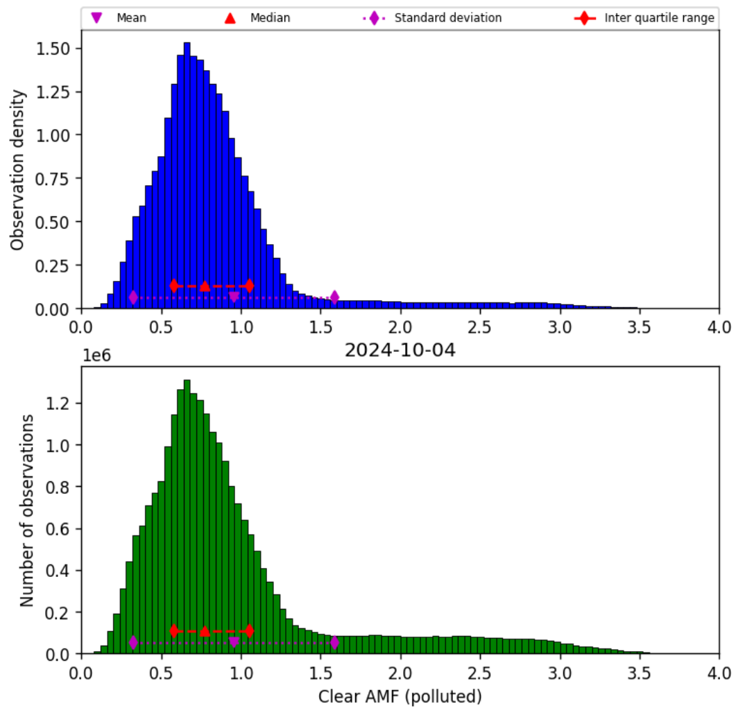
Figure 73: Histogram of “Clear AMF (polluted)” for 2024-10-03 to 2024-10-05
