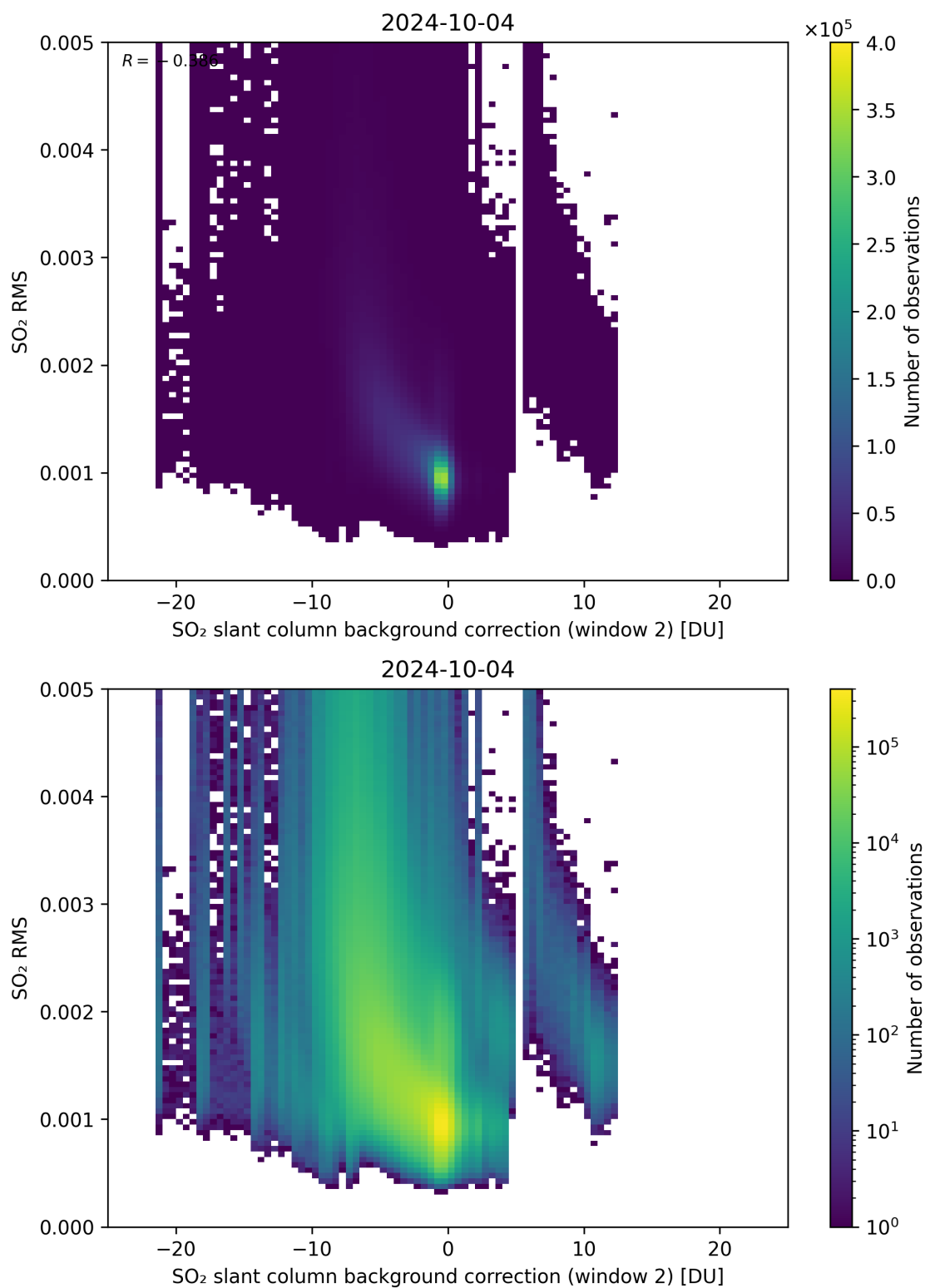
Figure 114: Scatter density plot of “SO 2 slant column background correction (window 2)” against “SO 2 RMS” for 2024-10-03 to 2024-10-05.
