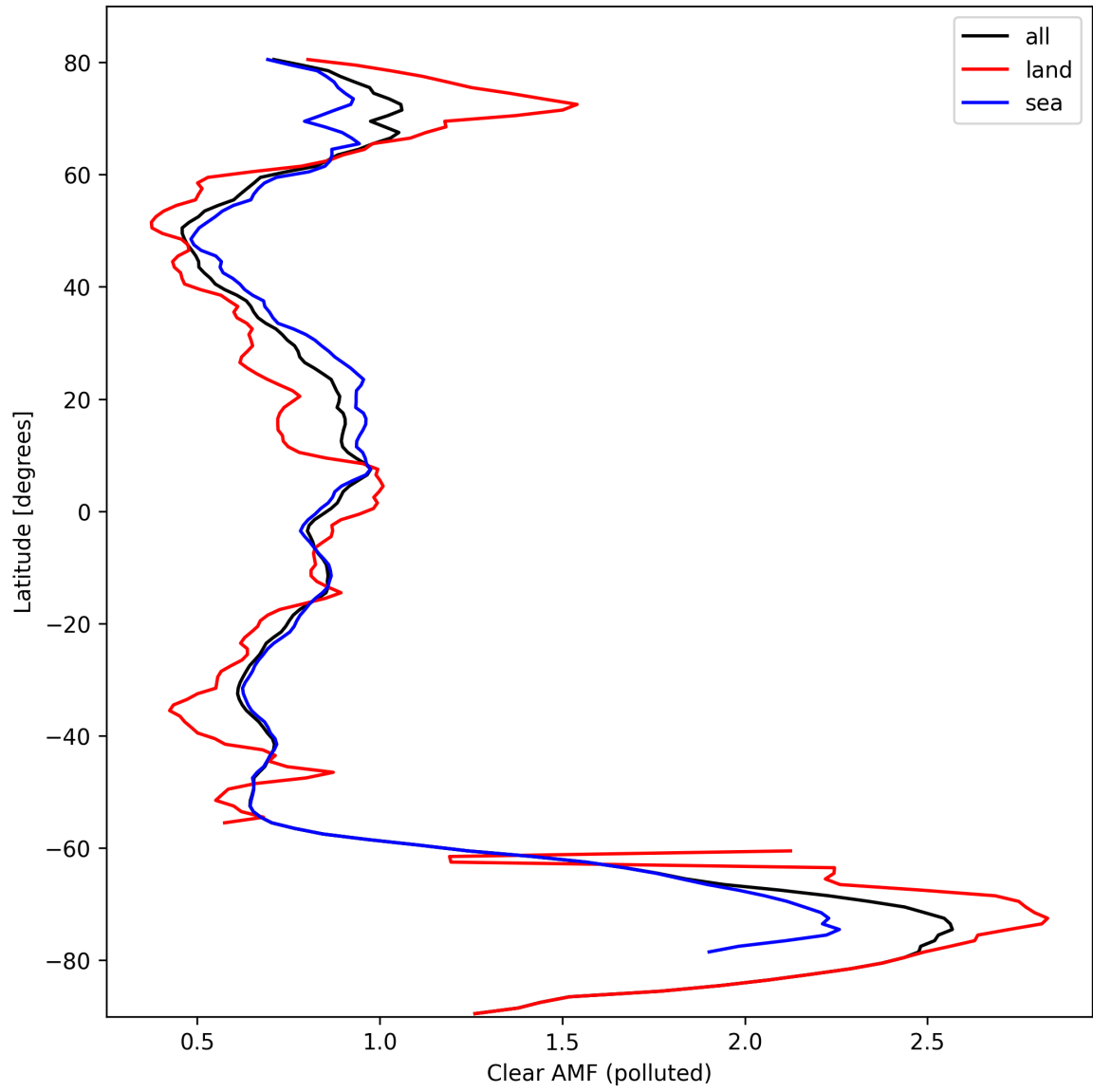
Figure 50: Zonal average of “Clear AMF (polluted)” for 2024-10-03 to 2024-10-05.
