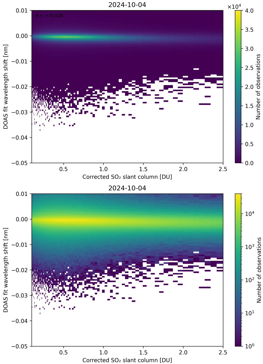
Figure 181: Scatter density plot of “Corrected SO 2 slant column” against “DOAS fit wavelength shift” for 2024-10-03 to 2024-10-05.
