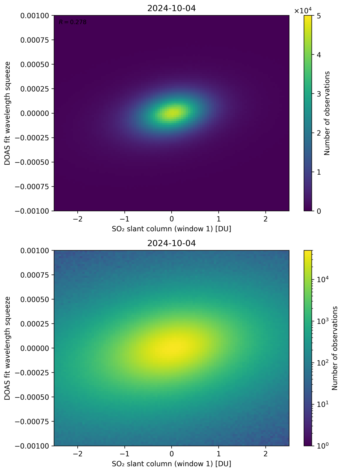
Figure 216: Scatter density plot of “SO 2 slant column (window 1)” against “DOAS fit wavelength squeeze” for 2024-10-03 to 2024-10-05.
