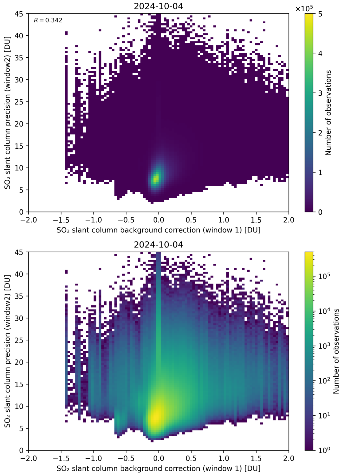
Figure 106: Scatter density plot of “SO 2 slant column background correction (window 1)” against “SO 2 slant column precision (window2)” for 2024-10-03 to 2024-10-05.
