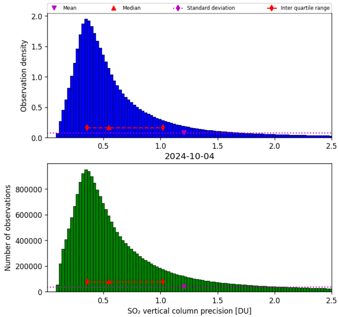
Figure 54: Histogram of “SO 2 vertical column precision” for 2024-10-03 to 2024-10-05
