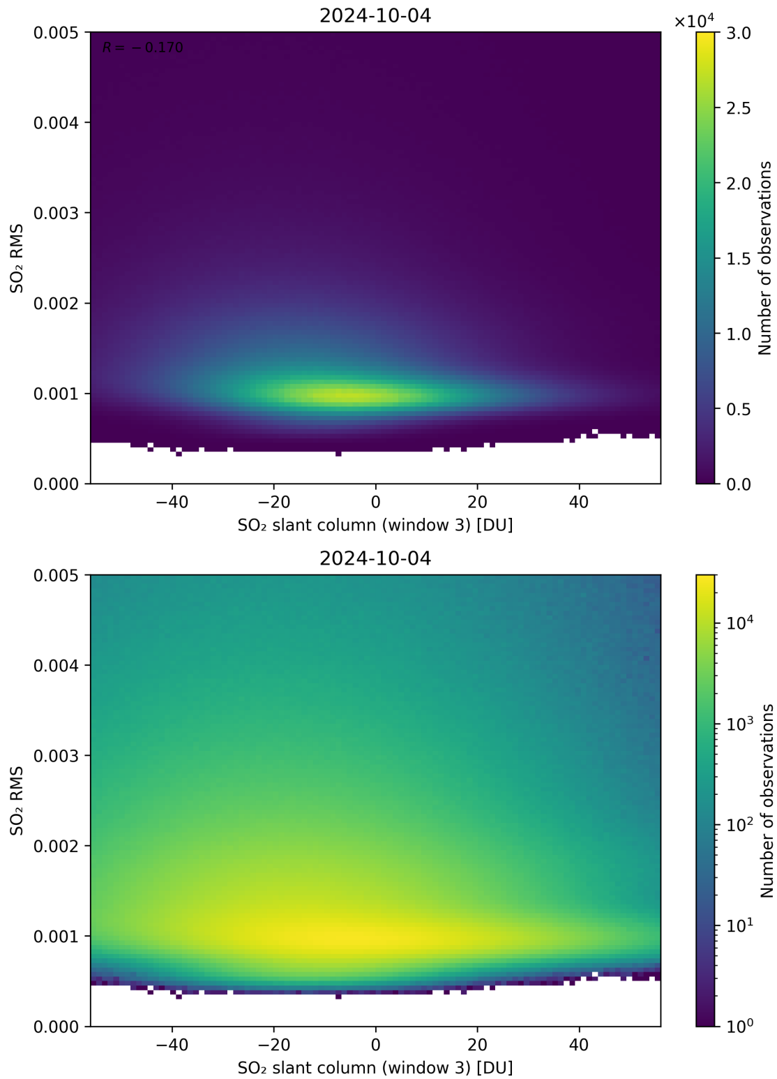
Figure 256: Scatter density plot of “SO 2 slant column (window 3)” against “SO 2 RMS” for 2024-10-03 to 2024-10-05.
