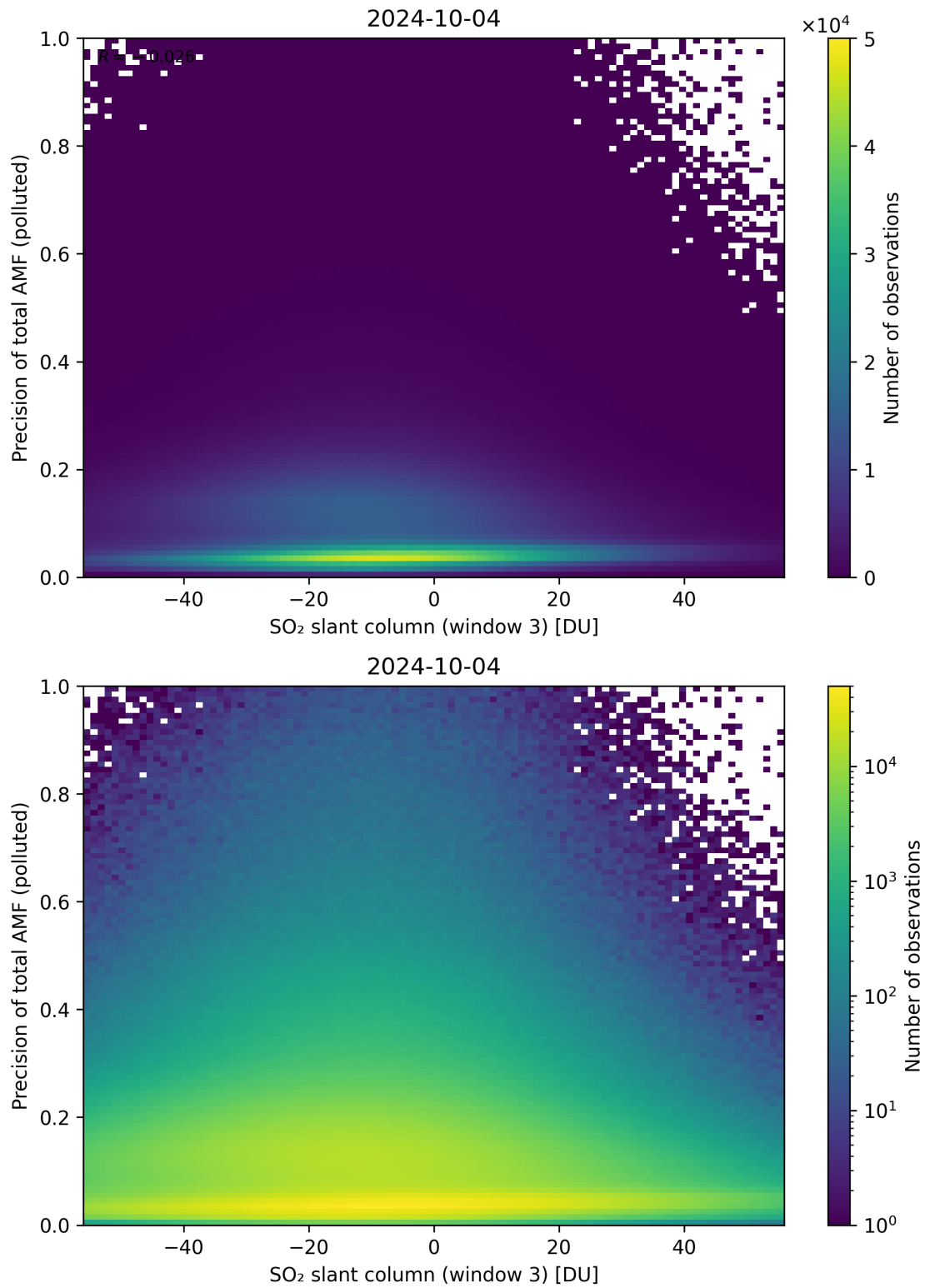
Figure 269: Scatter density plot of “SO 2 slant column (window 3)” against “Precision of total AMF (polluted)” for 2024-10-03 to 2024-10-05.
