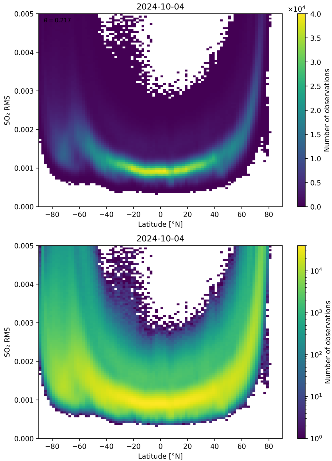
Figure 144: Scatter density plot of “Latitude” against “SO 2 RMS” for 2024-10-03 to 2024-10-05.
