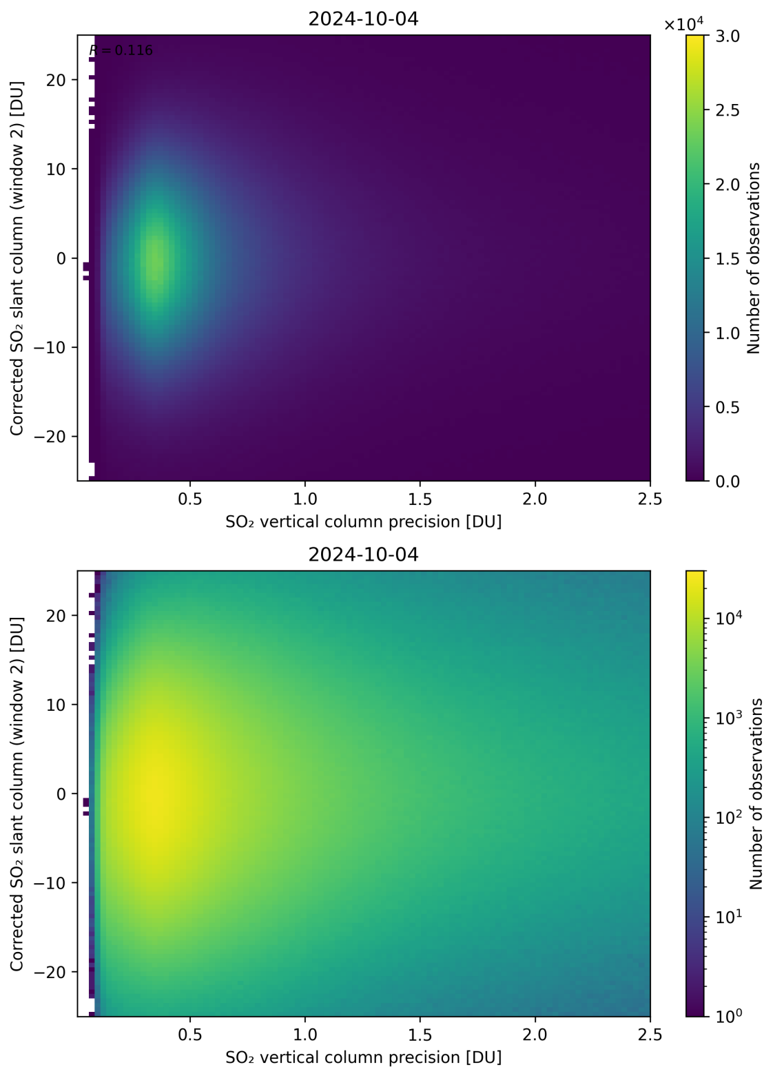
Figure 287: Scatter density plot of “SO 2 vertical column precision” against “Corrected SO 2 slant column (window 2)” for 2024-10-03 to 2024-10-05.
