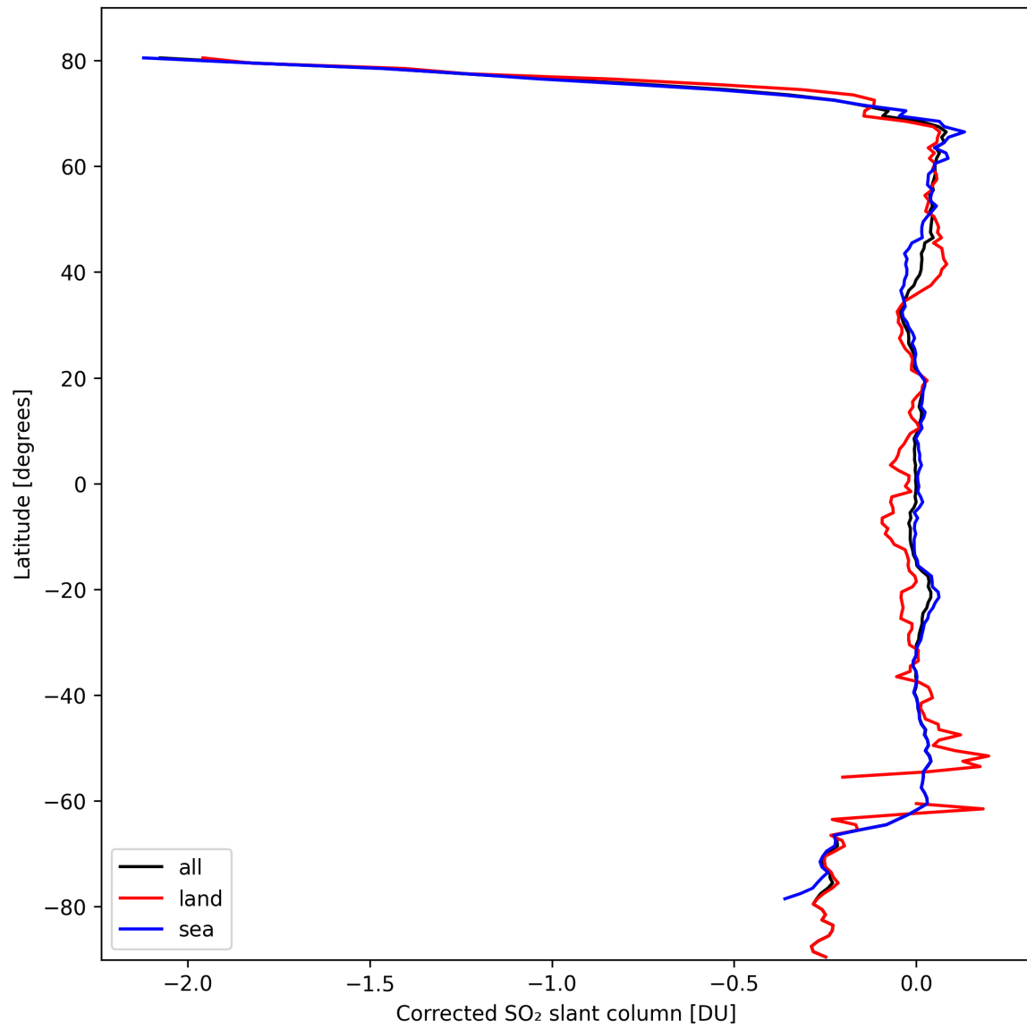
Figure 32: Zonal average of “Corrected SO 2 slant column” for 2024-10-03 to 2024-10-05.
