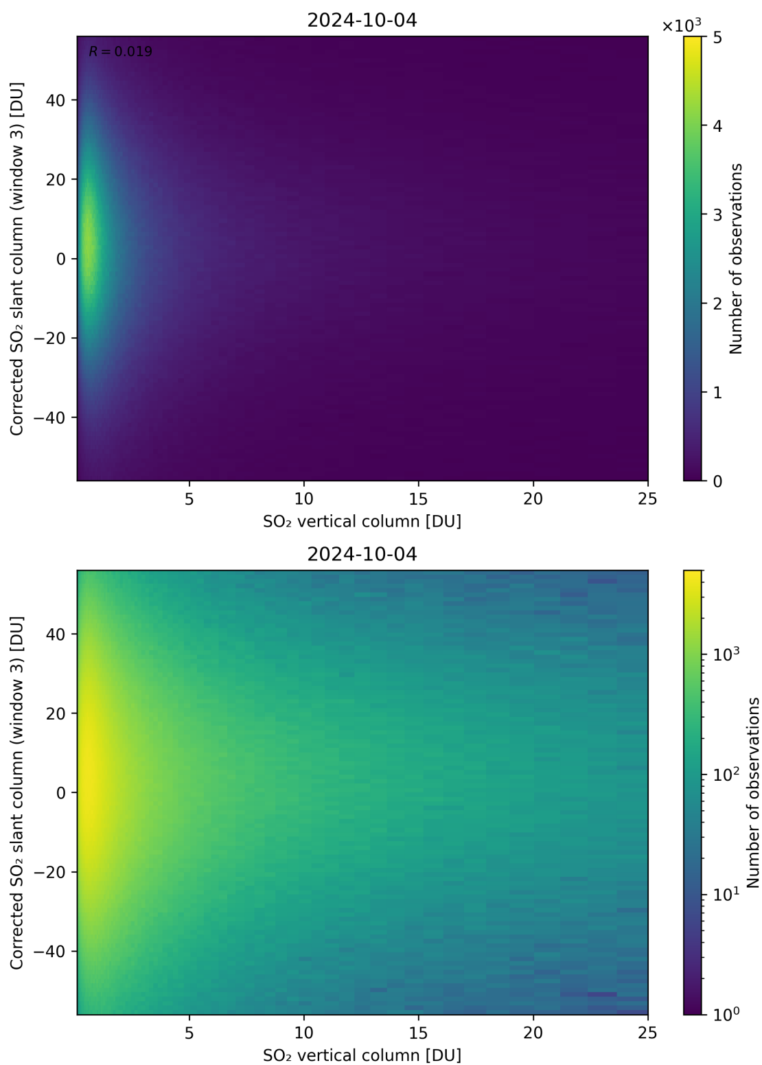
Figure 299: Scatter density plot of “SO 2 vertical column” against “Corrected SO 2 slant column (window 3)” for 2024-10-03 to 2024-10-05.
