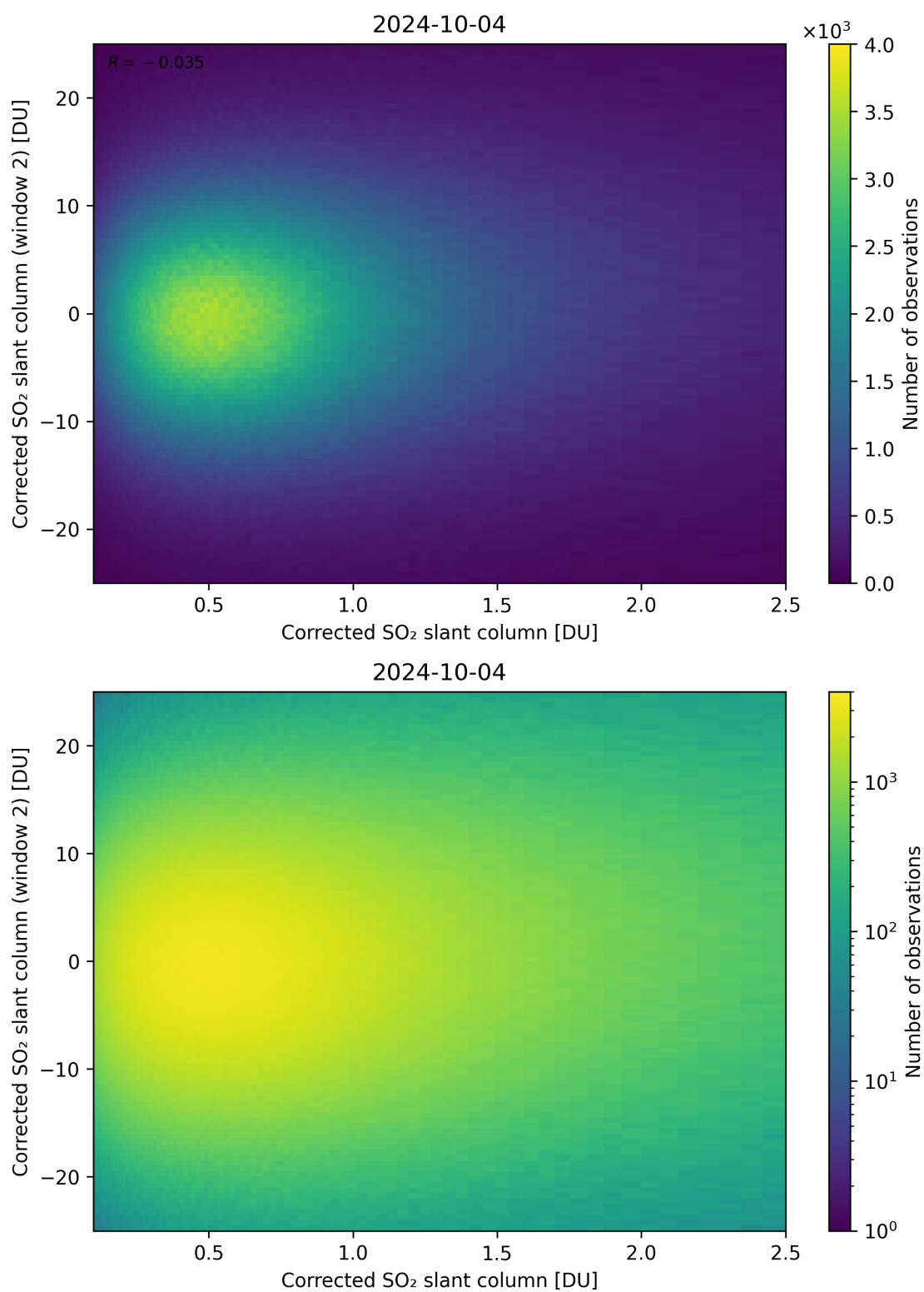
Figure 185: Scatter density plot of “Corrected SO 2 slant column” against “Corrected SO 2 slant column (window 2)” for 2024-10-03 to 2024-10-05.
