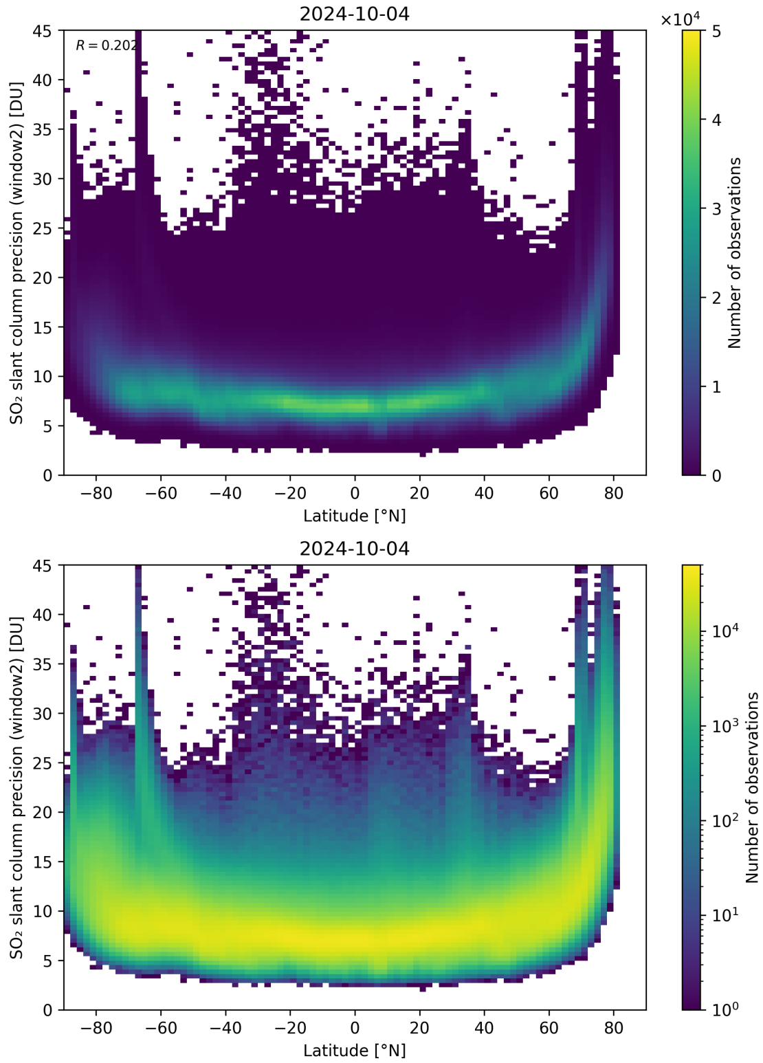
Figure 151: Scatter density plot of “Latitude” against “SO 2 slant column precision (window2)” for 2024-10-03 to 2024-10-05.
