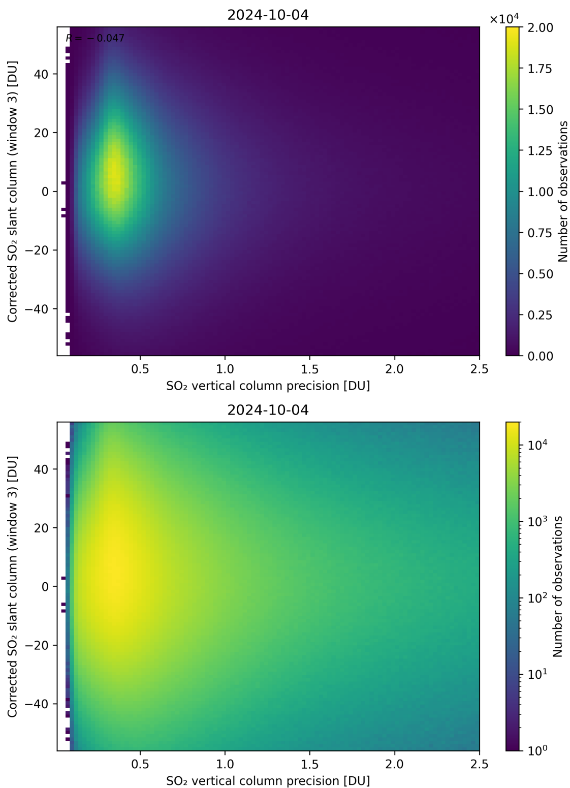
Figure 288: Scatter density plot of “SO 2 vertical column precision” against “Corrected SO 2 slant column (window 3)” for 2024-10-03 to 2024-10-05.
