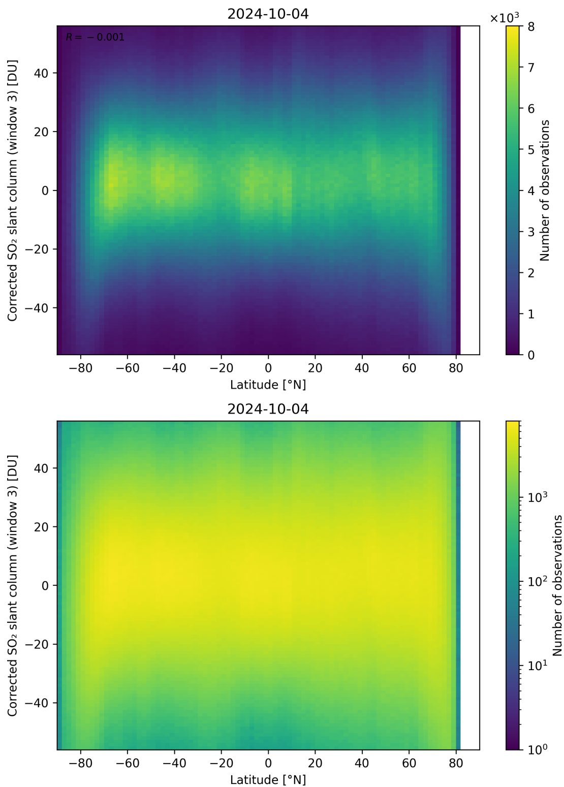
Figure 148: Scatter density plot of “Latitude” against “Corrected SO 2 slant column (window 3)” for 2024-10-03 to 2024-10-05.
