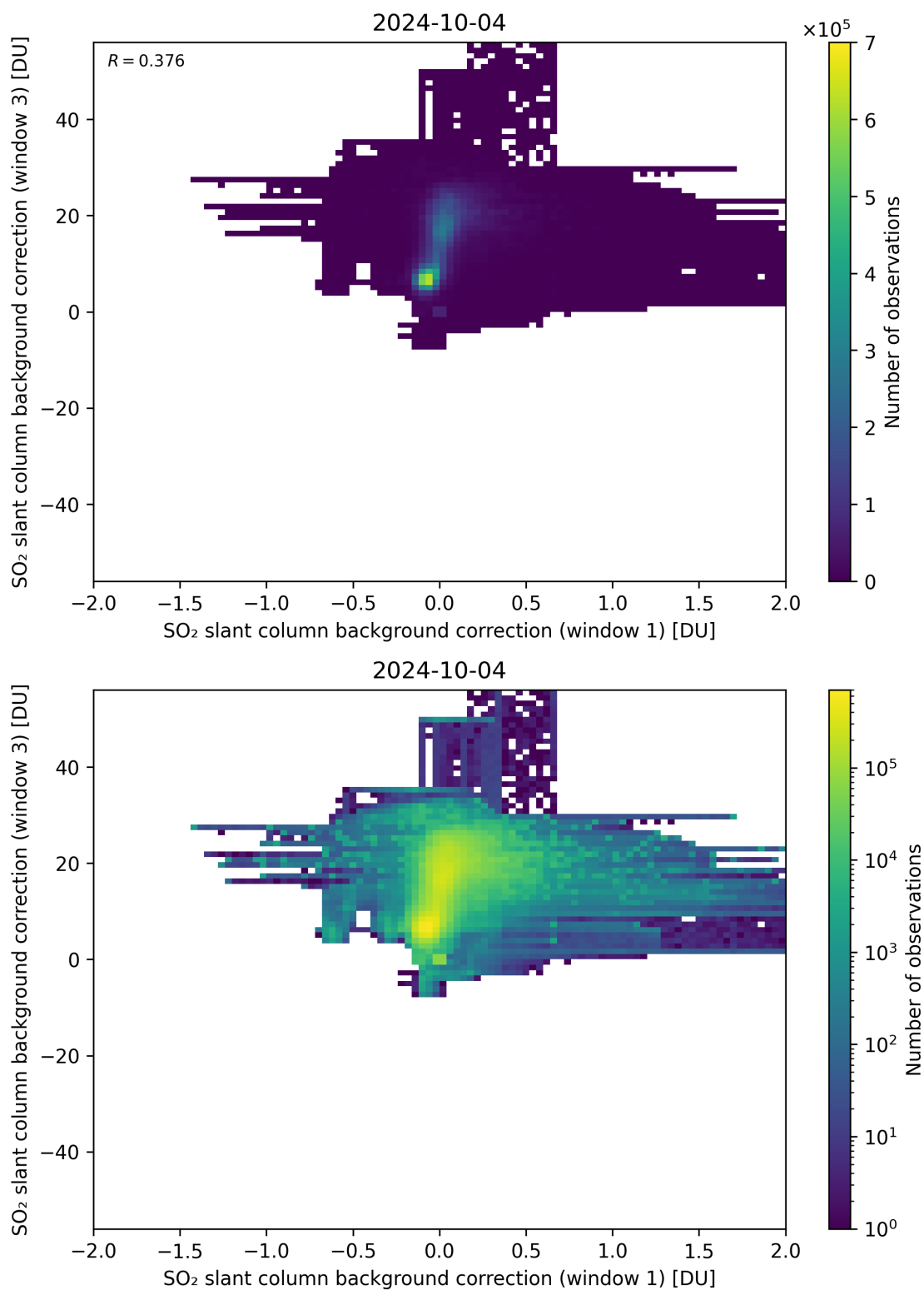
Figure 99: Scatter density plot of “SO 2 slant column background correction (window 1)” against “SO 2 slant column background correction (window 3)” for 2024-10-03 to 2024-10-05.
