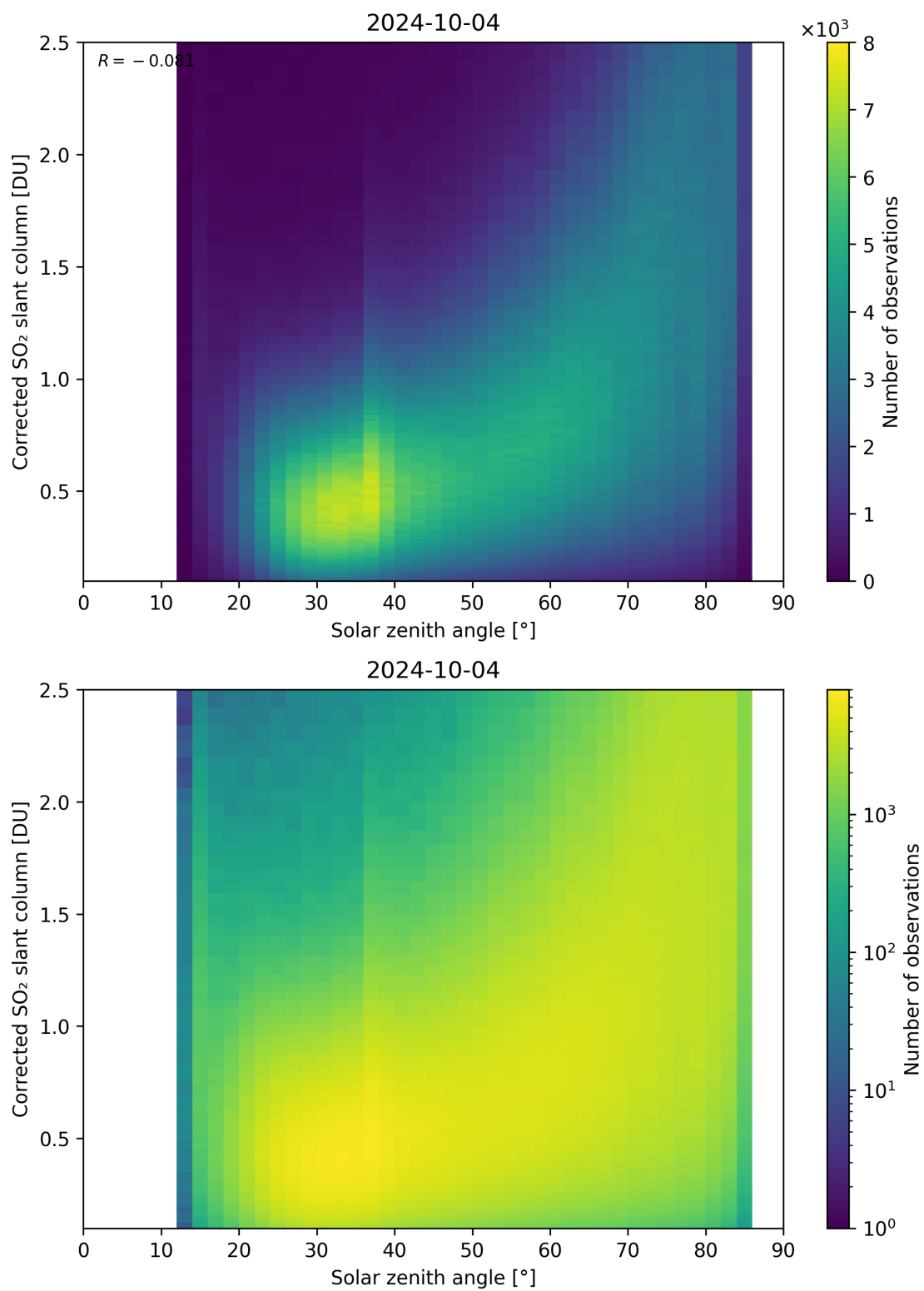
Figure 166: Scatter density plot of “Solar zenith angle” against “Corrected SO 2 slant column” for 2024-10-03 to 2024-10-05.
