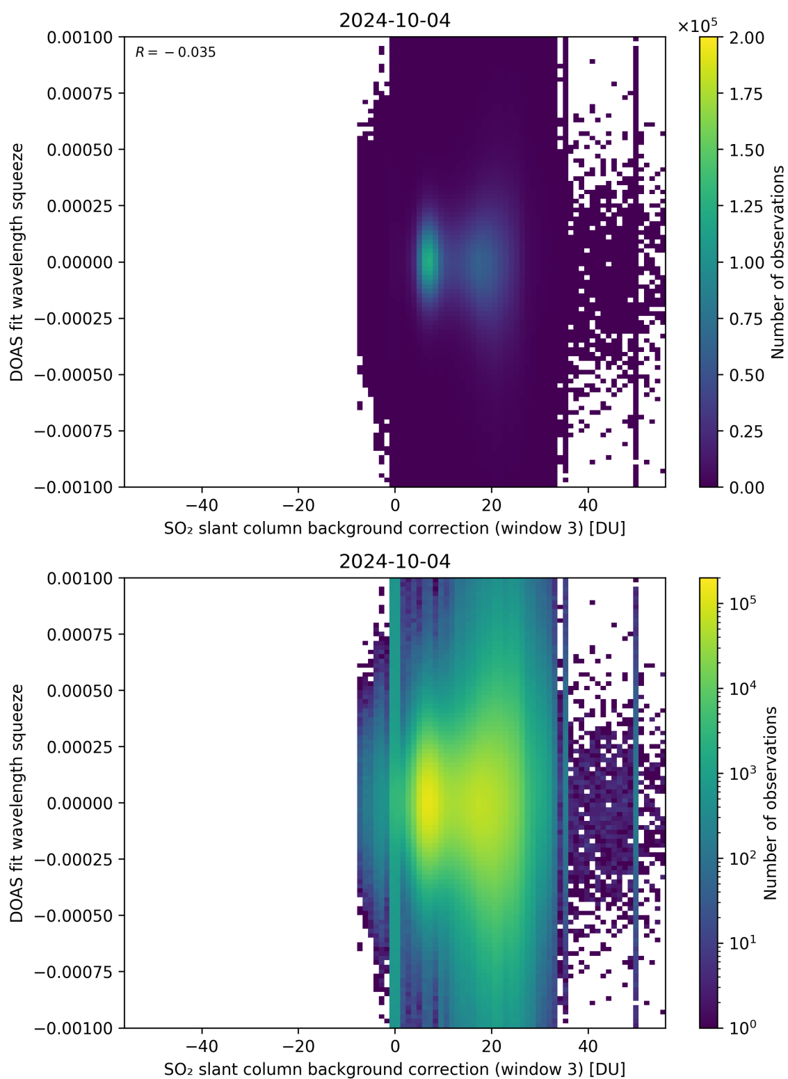
Figure 122: Scatter density plot of “SO 2 slant column background correction (window 3)” against “DOAS fit wavelength squeeze” for 2024-10-03 to 2024-10-05.
