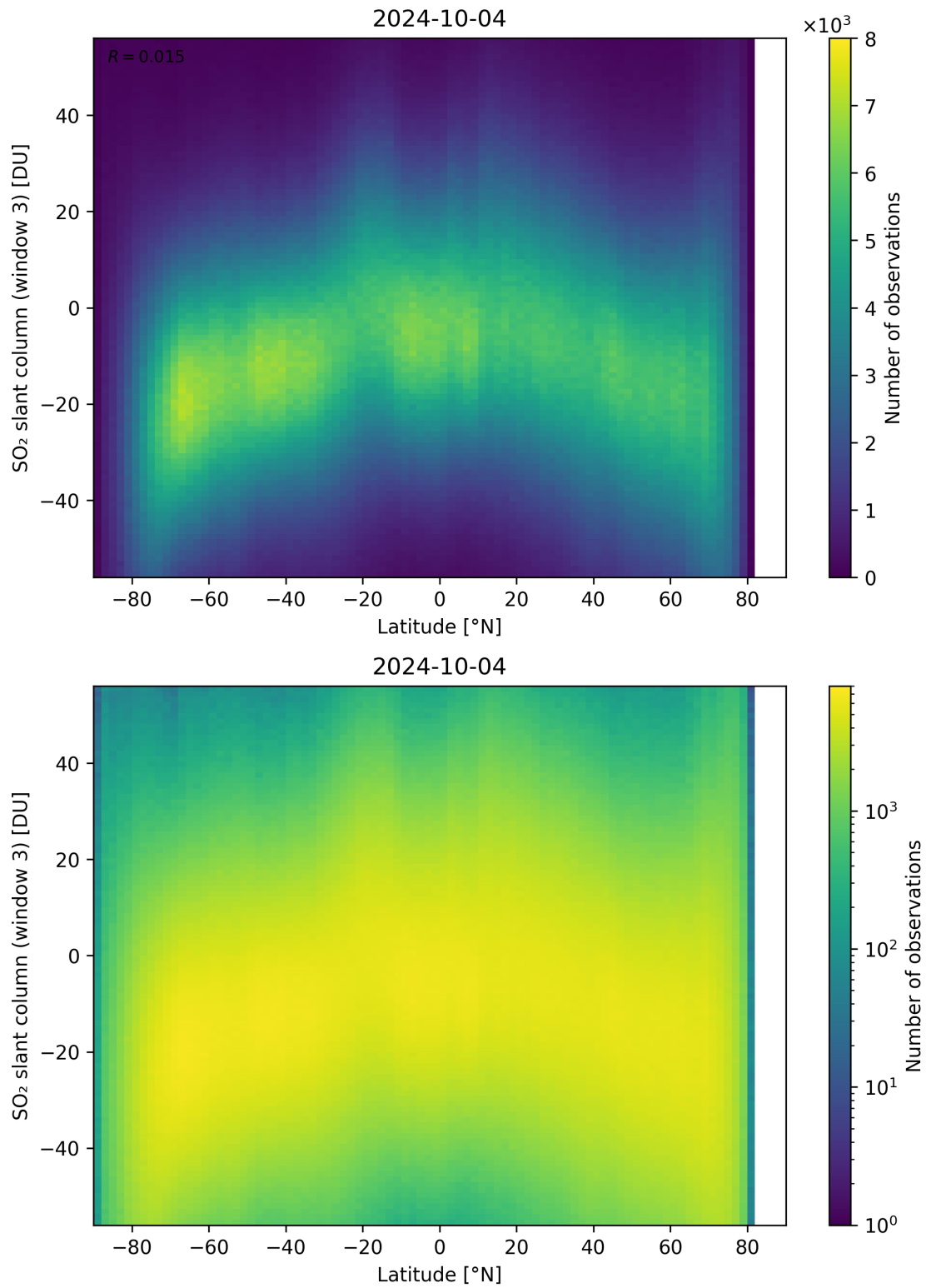
Figure 152: Scatter density plot of “Latitude” against “SO 2 slant column (window 3)” for 2024-10-03 to 2024-10-05.
