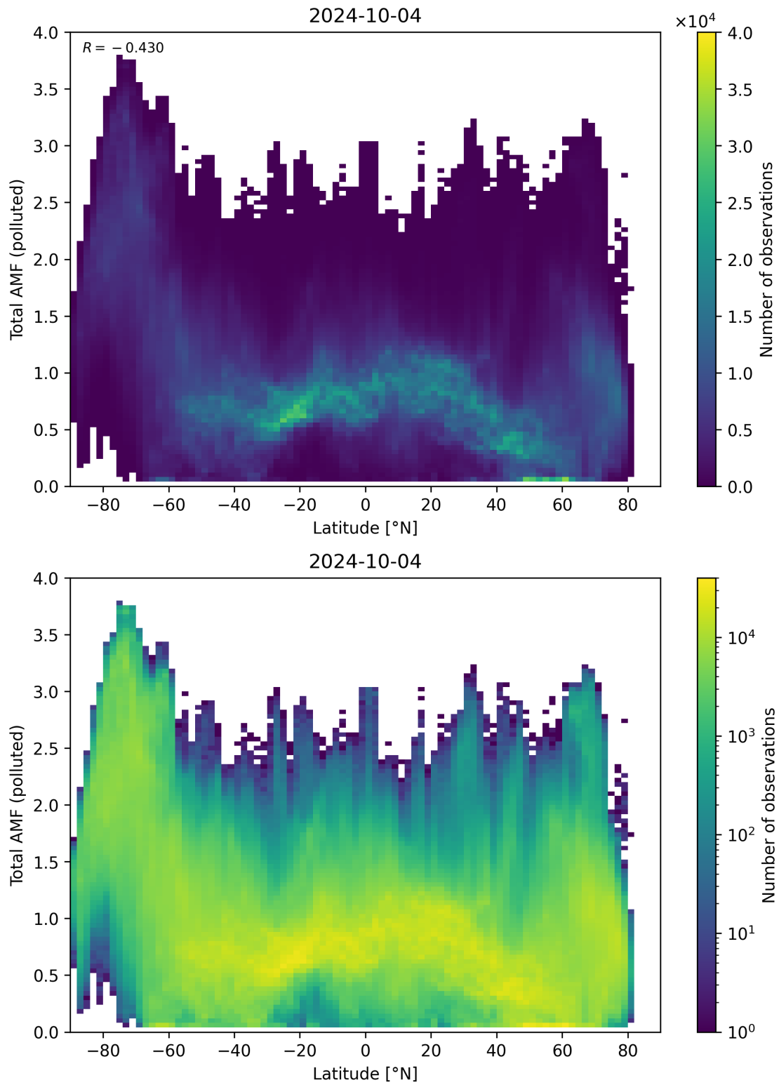
Figure 154: Scatter density plot of “Latitude” against “Total AMF (polluted)” for 2024-10-03 to 2024-10-05.
