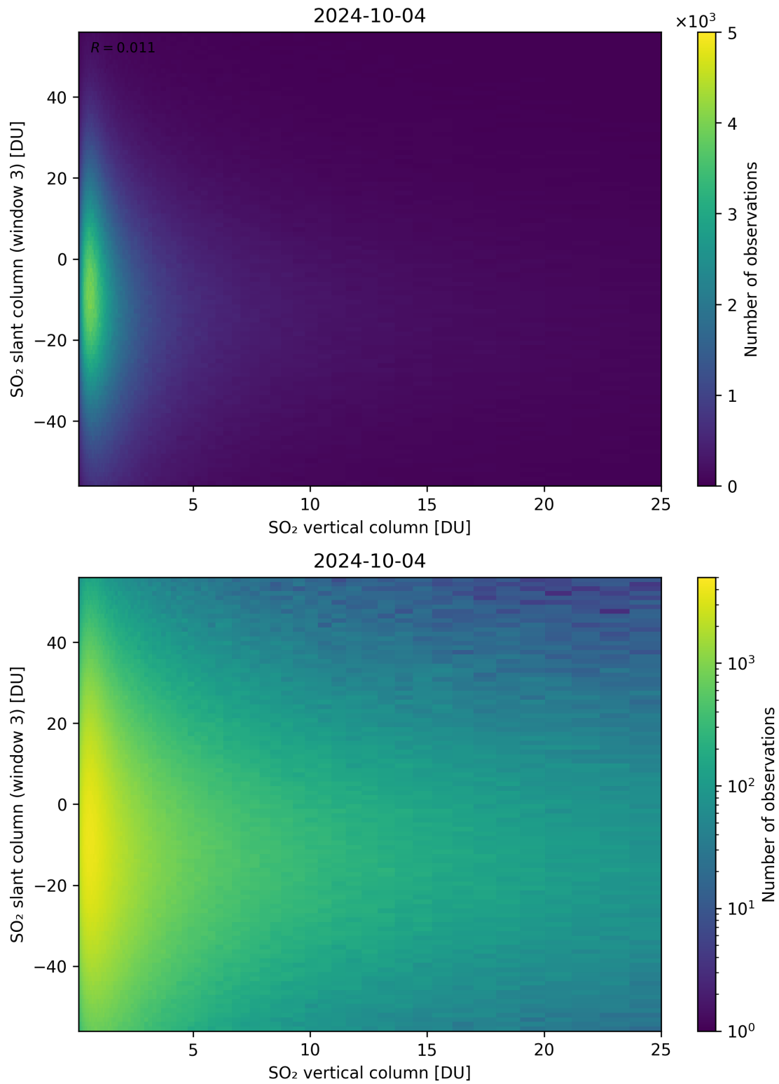
Figure 303: Scatter density plot of “SO 2 vertical column” against “SO 2 slant column (window 3)” for 2024-10-03 to 2024-10-05.
