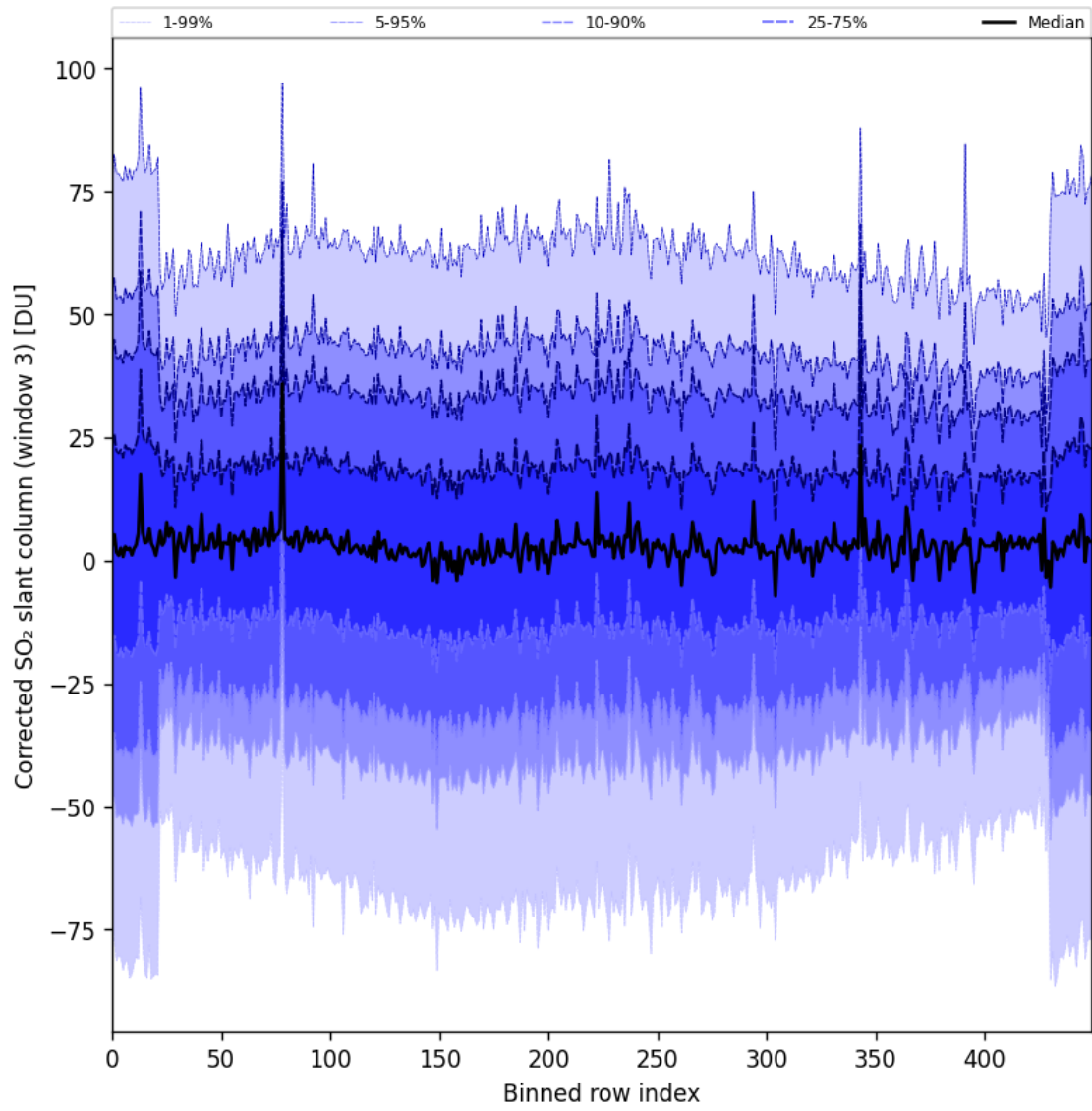
Figure 89: Along track statistics of “Corrected SO 2 slant column (window 3)” for 2024-10-03 to 2024-10-05
