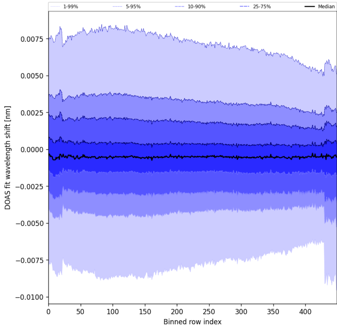
Figure 91: Along track statistics of “DOAS fit wavelength shift” for 2024-10-03 to 2024-10-05
