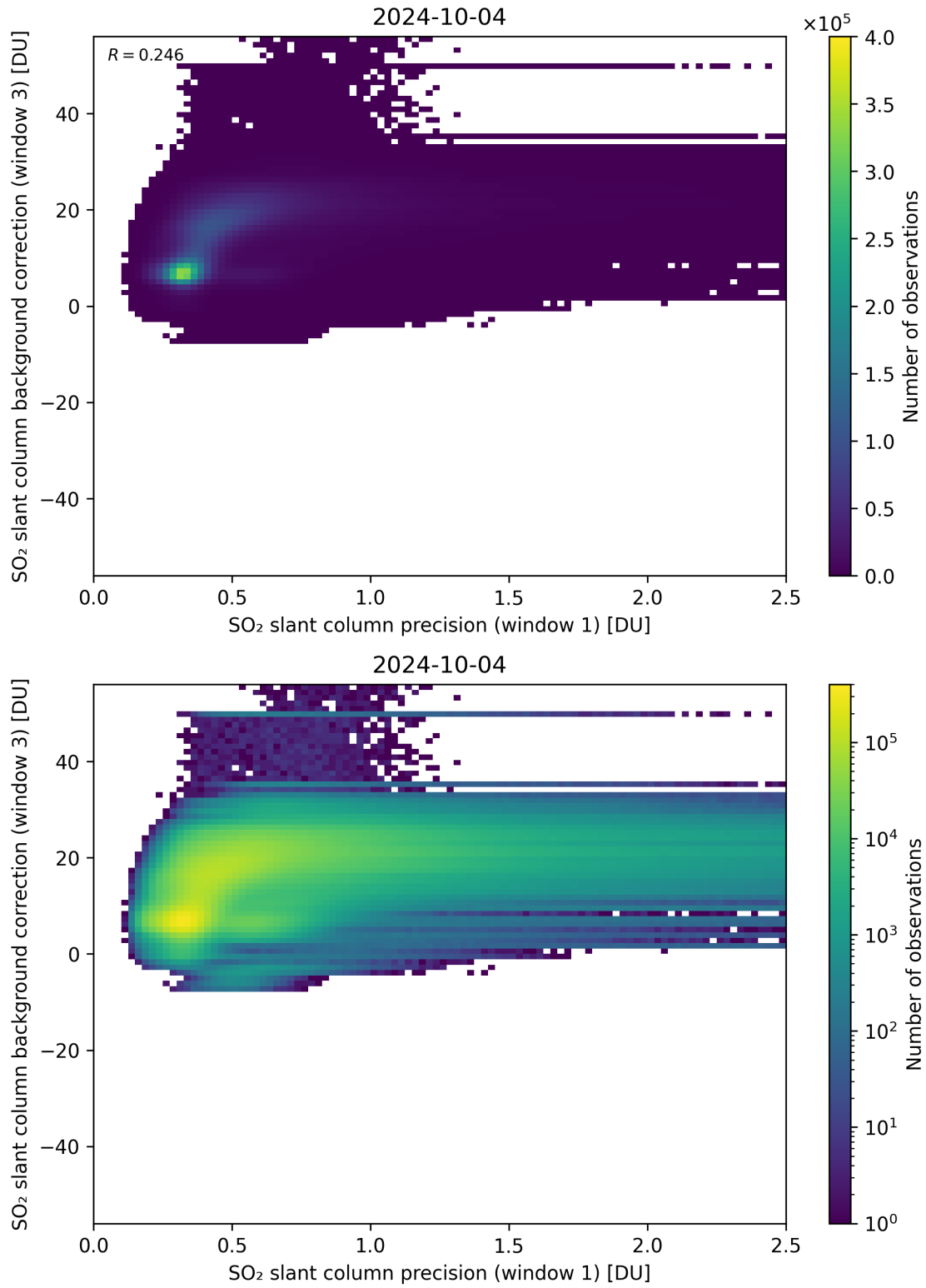
Figure 220: Scatter density plot of “SO 2 slant column precision (window 1)” against “SO 2 slant column background correction (window 3)” for 2024-10-03 to 2024-10-05.
