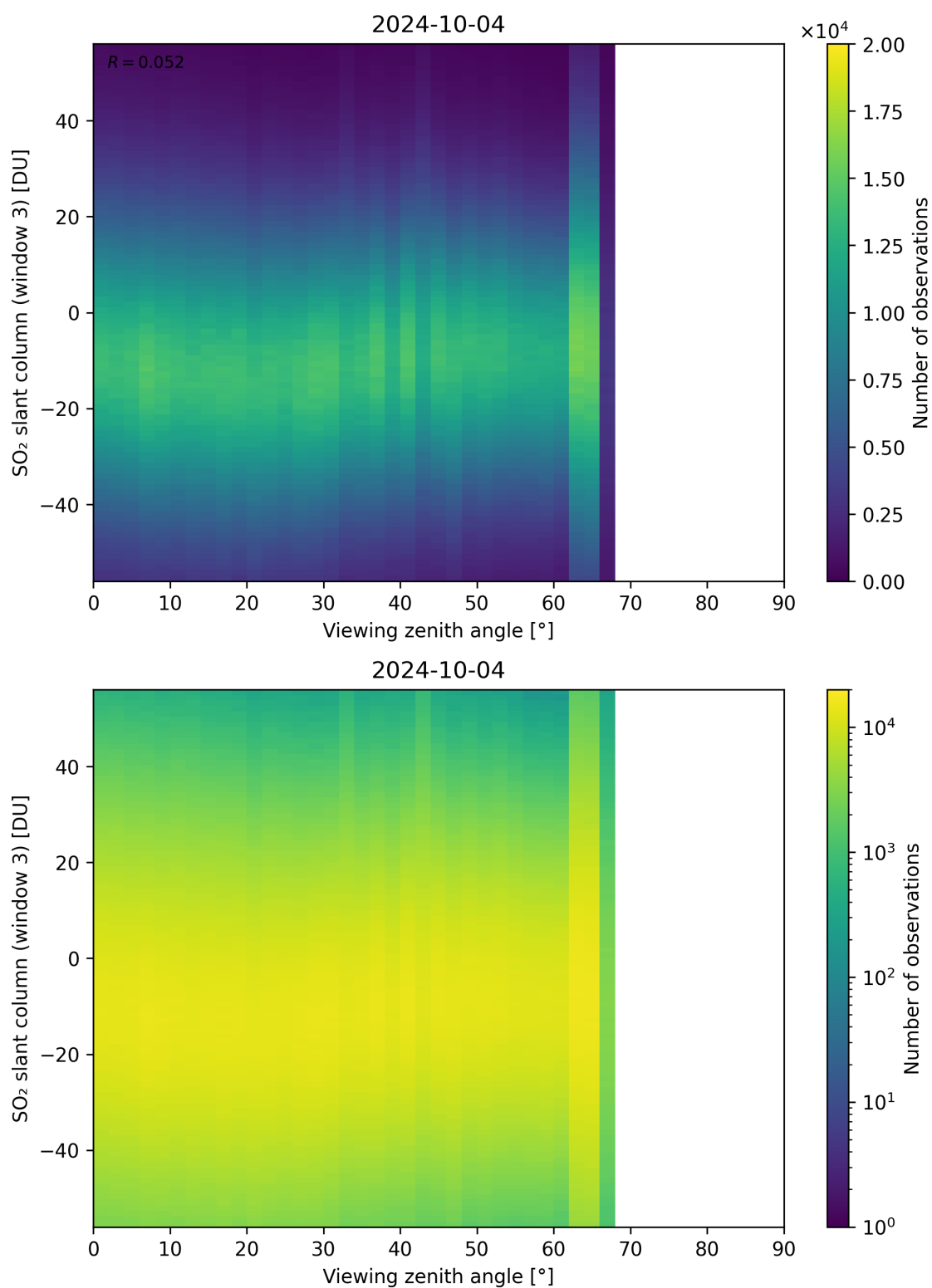
Figure 323: Scatter density plot of “Viewing zenith angle” against “SO 2 slant column (window 3)” for 2024-10-03 to 2024-10-05.
