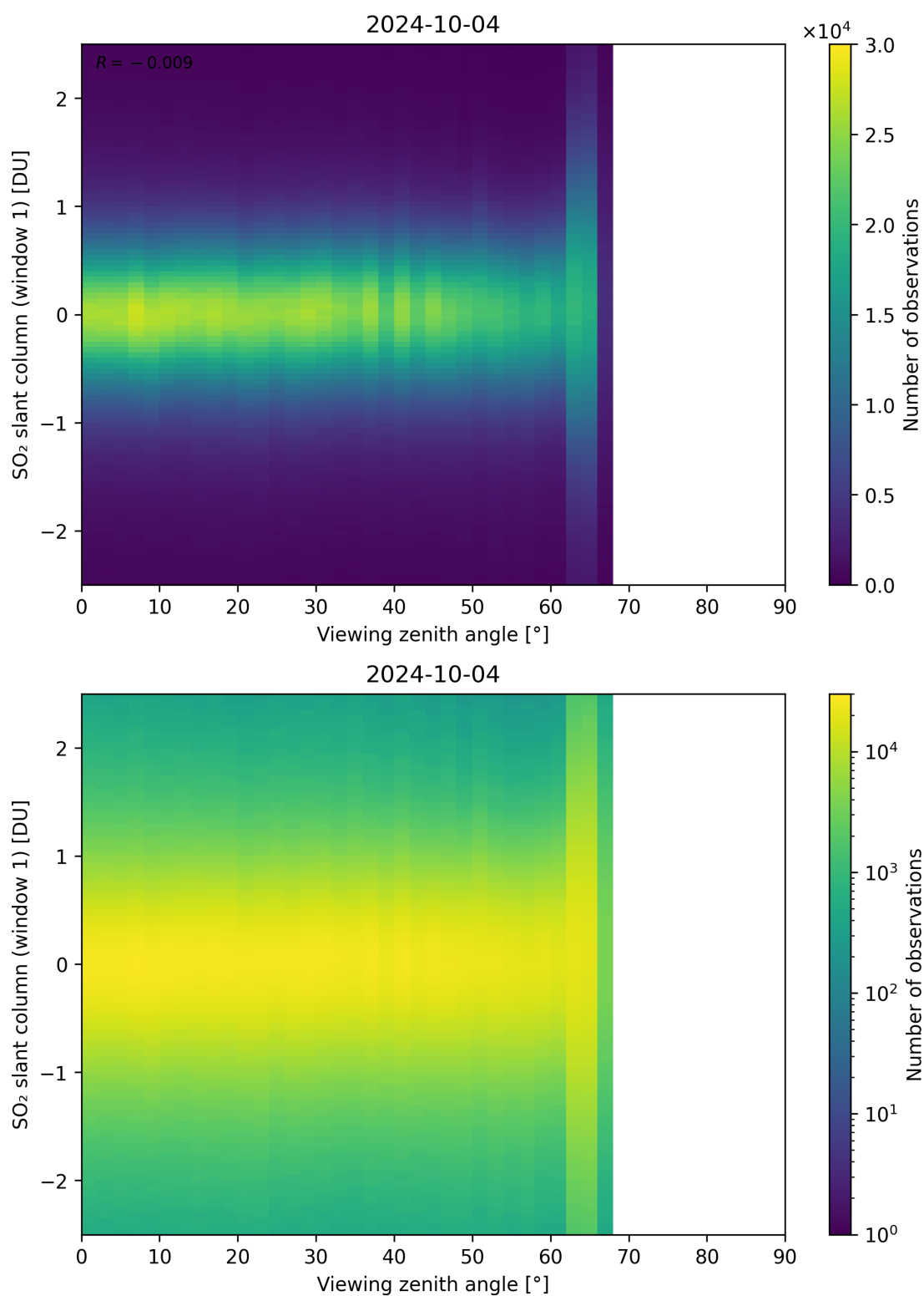
Figure 320: Scatter density plot of “Viewing zenith angle” against “SO 2 slant column (window 1)” for 2024-10-03 to 2024-10-05.
