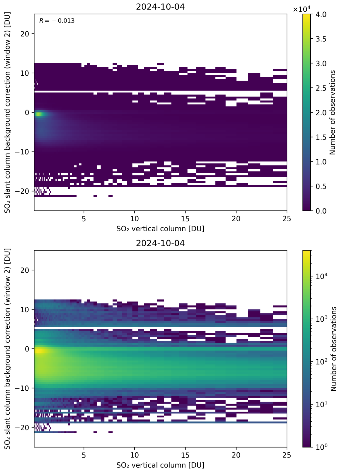
Figure 274: Scatter density plot of “SO 2 vertical column” against “SO 2 slant column background correction (window 2)” for 2024-10-03 to 2024-10-05.
