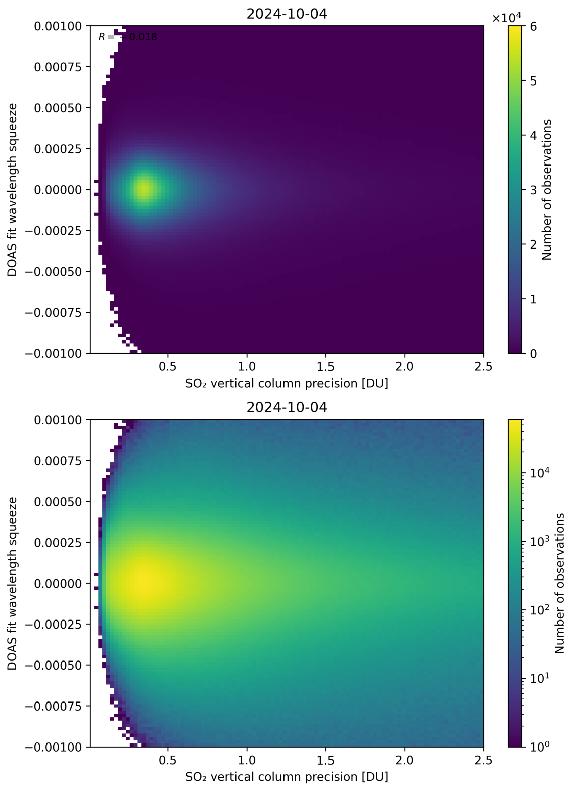
Figure 283: Scatter density plot of “SO 2 vertical column precision” against “DOAS fit wavelength squeeze” for 2024-10-03 to 2024-10-05.
