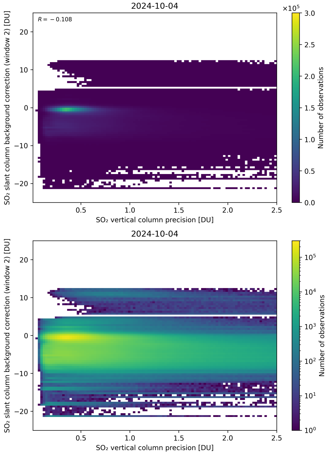
Figure 280: Scatter density plot of “SO 2 vertical column precision” against “SO 2 slant column background correction (window 2)” for 2024-10-03 to 2024-10-05.
