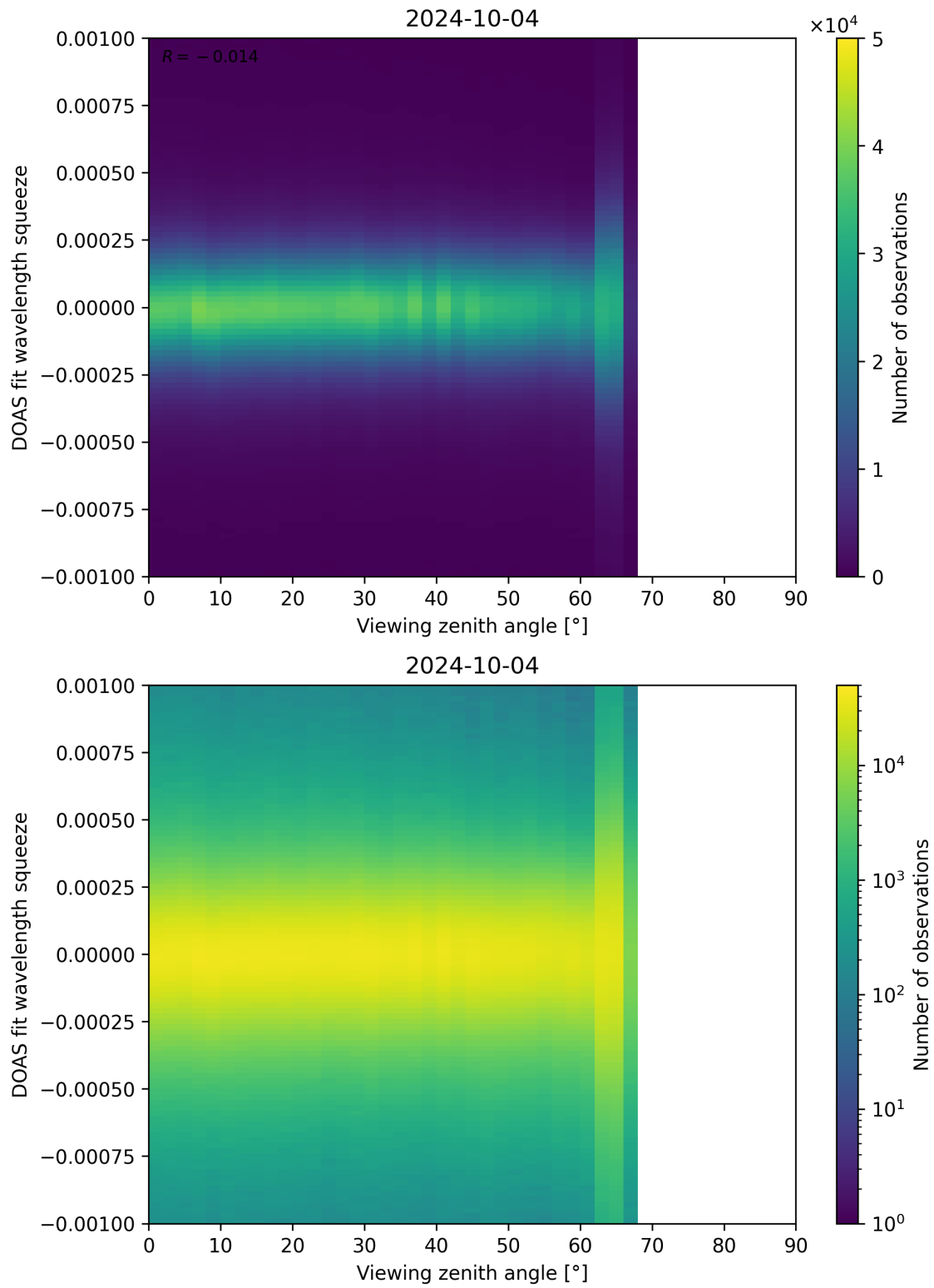
Figure 312: Scatter density plot of “Viewing zenith angle” against “DOAS fit wavelength squeeze” for 2024-10-03 to 2024-10-05.
