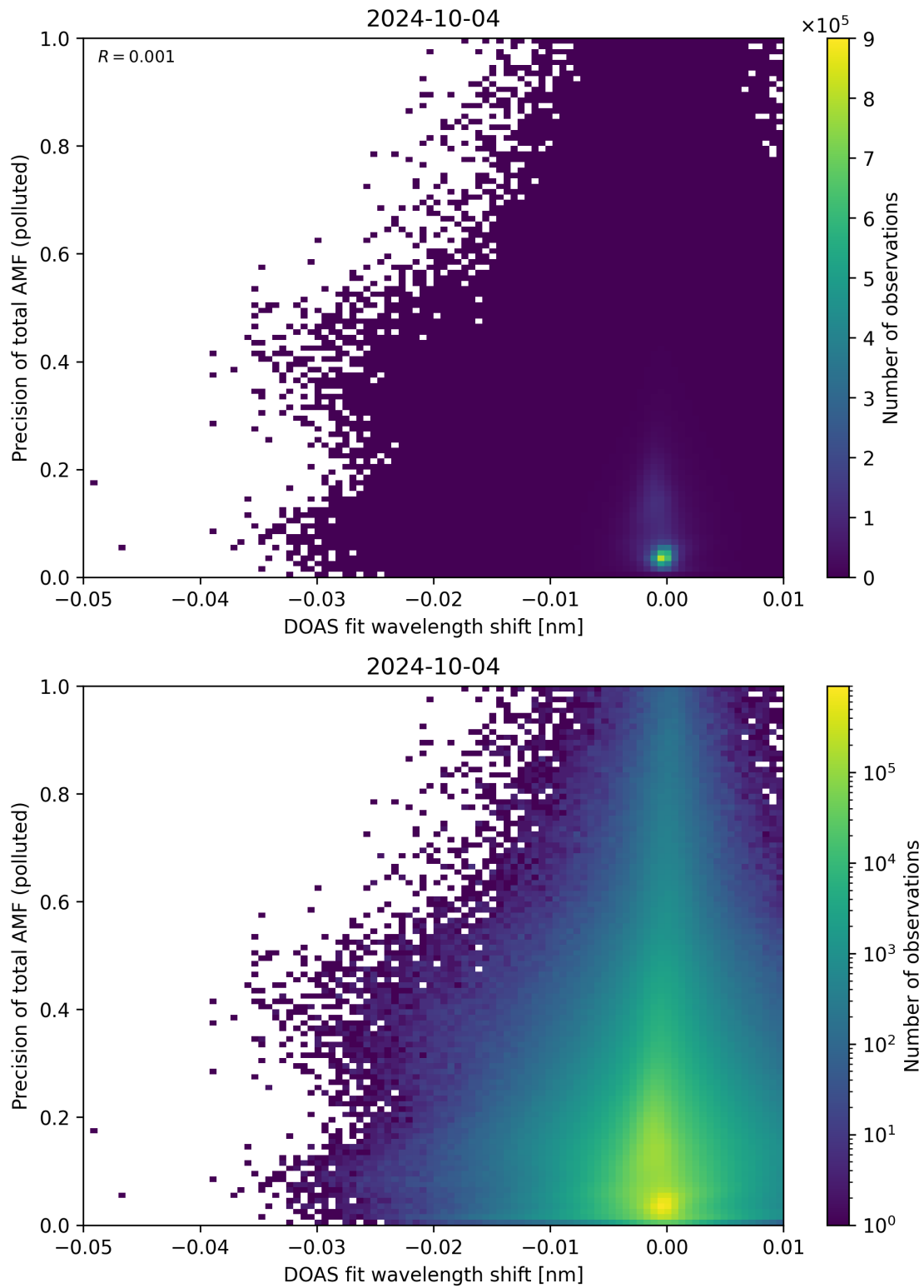
Figure 131: Scatter density plot of “DOAS fit wavelength shift” against “Precision of total AMF (polluted)” for 2024-10-03 to 2024-10-05.
