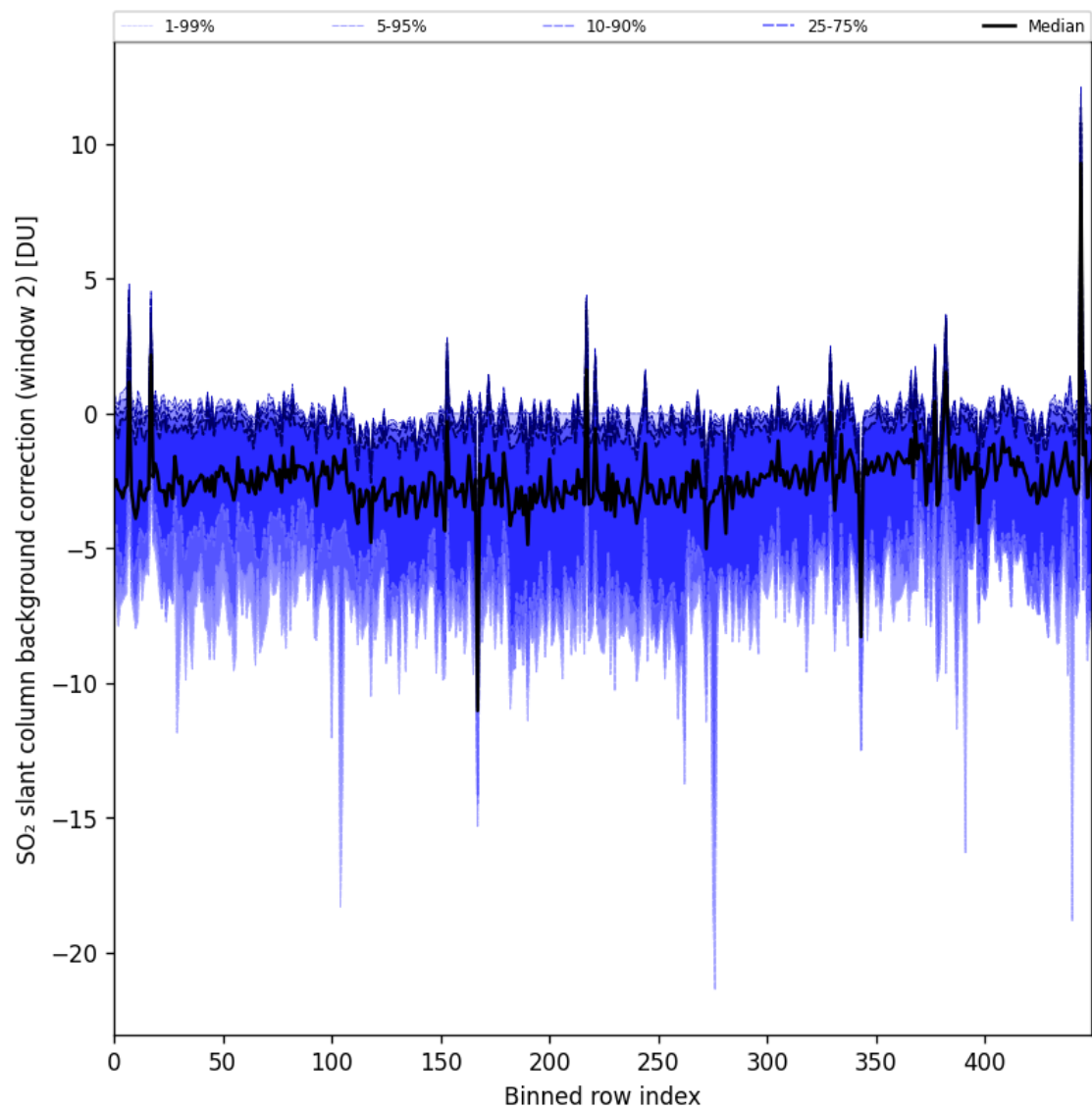
Figure 86: Along track statistics of “SO 2 slant column background correction (window 2)” for 2024-10-03 to 2024-10-05
