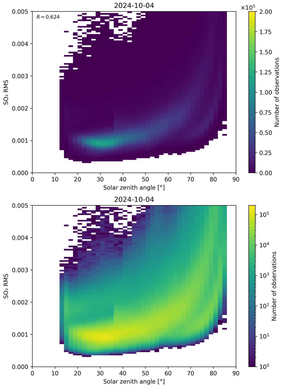
Figure 163: Scatter density plot of “Solar zenith angle” against “SO 2 RMS” for 2024-10-03 to 2024-10-05.
