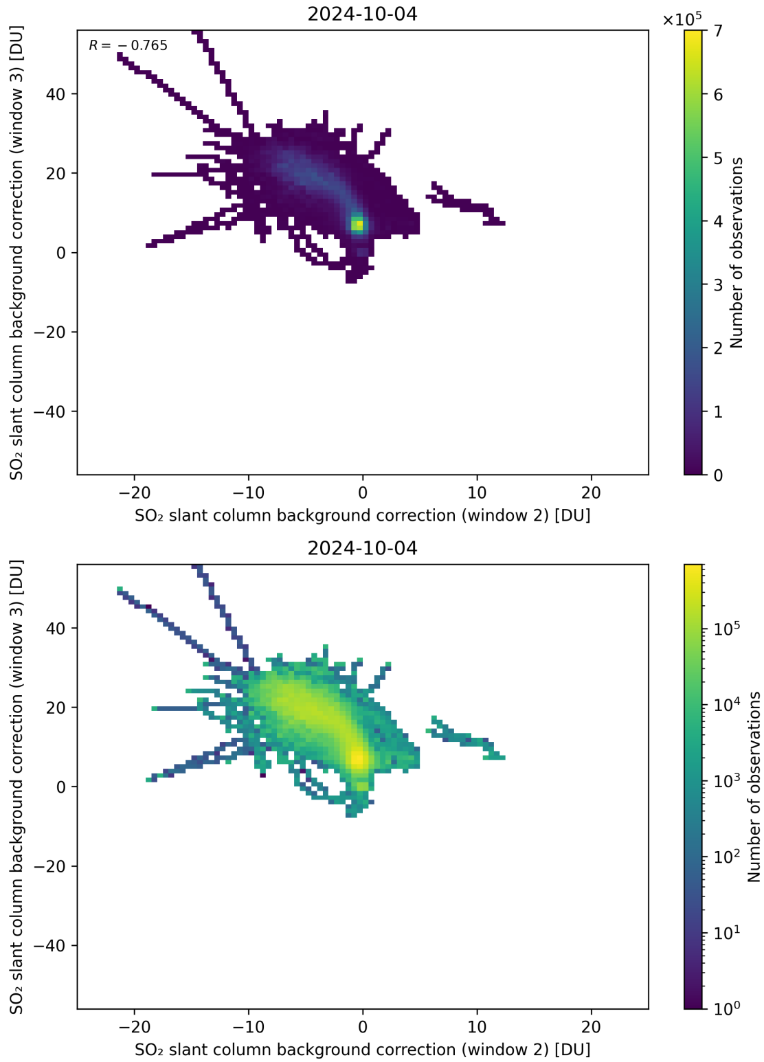
Figure 111: Scatter density plot of “SO 2 slant column background correction (window 2)” against “SO 2 slant column background correction (window 3)” for 2024-10-03 to 2024-10-05.
