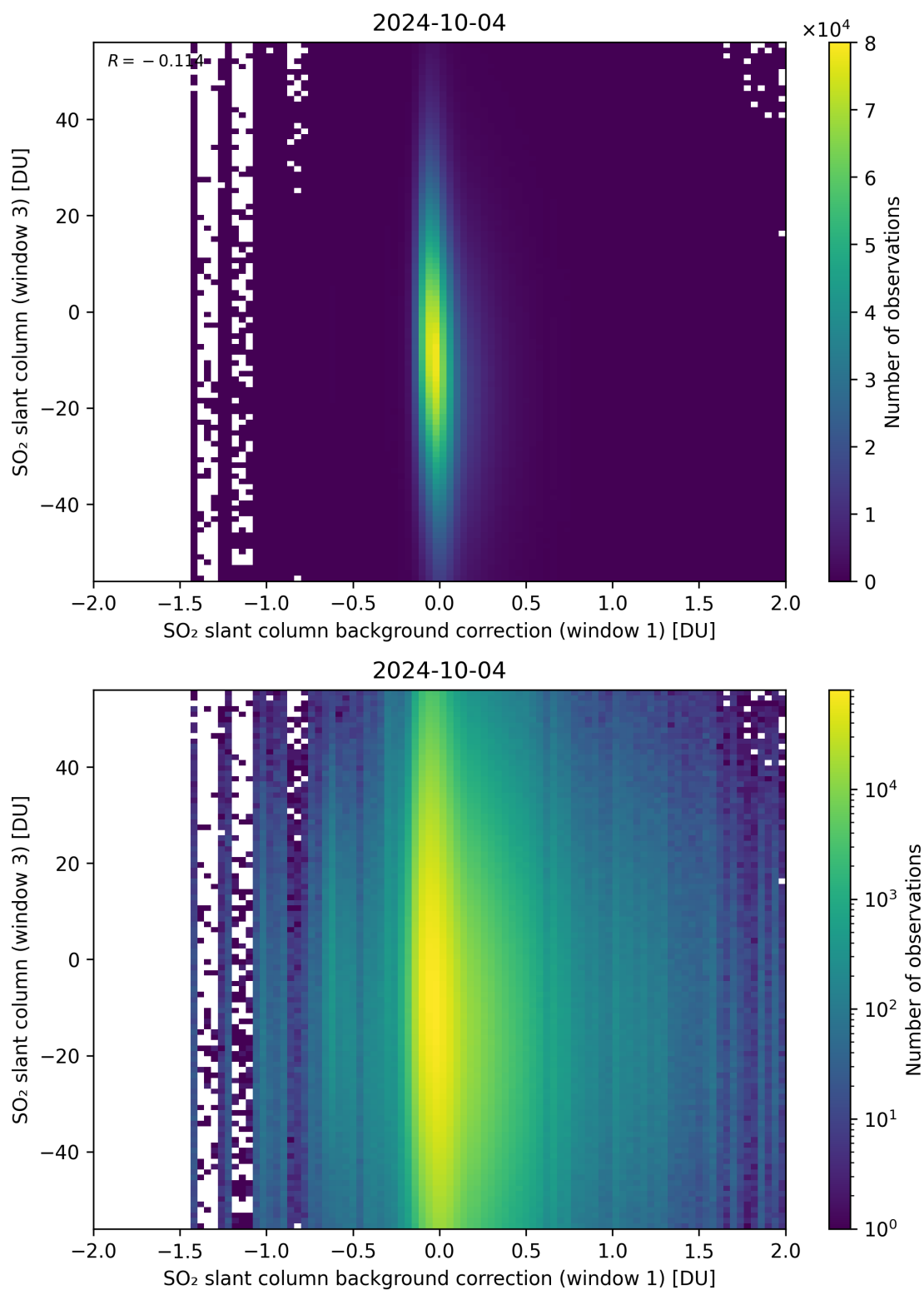
Figure 107: Scatter density plot of “SO 2 slant column background correction (window 1)” against “SO 2 slant column (window 3)” for 2024-10-03 to 2024-10-05.
