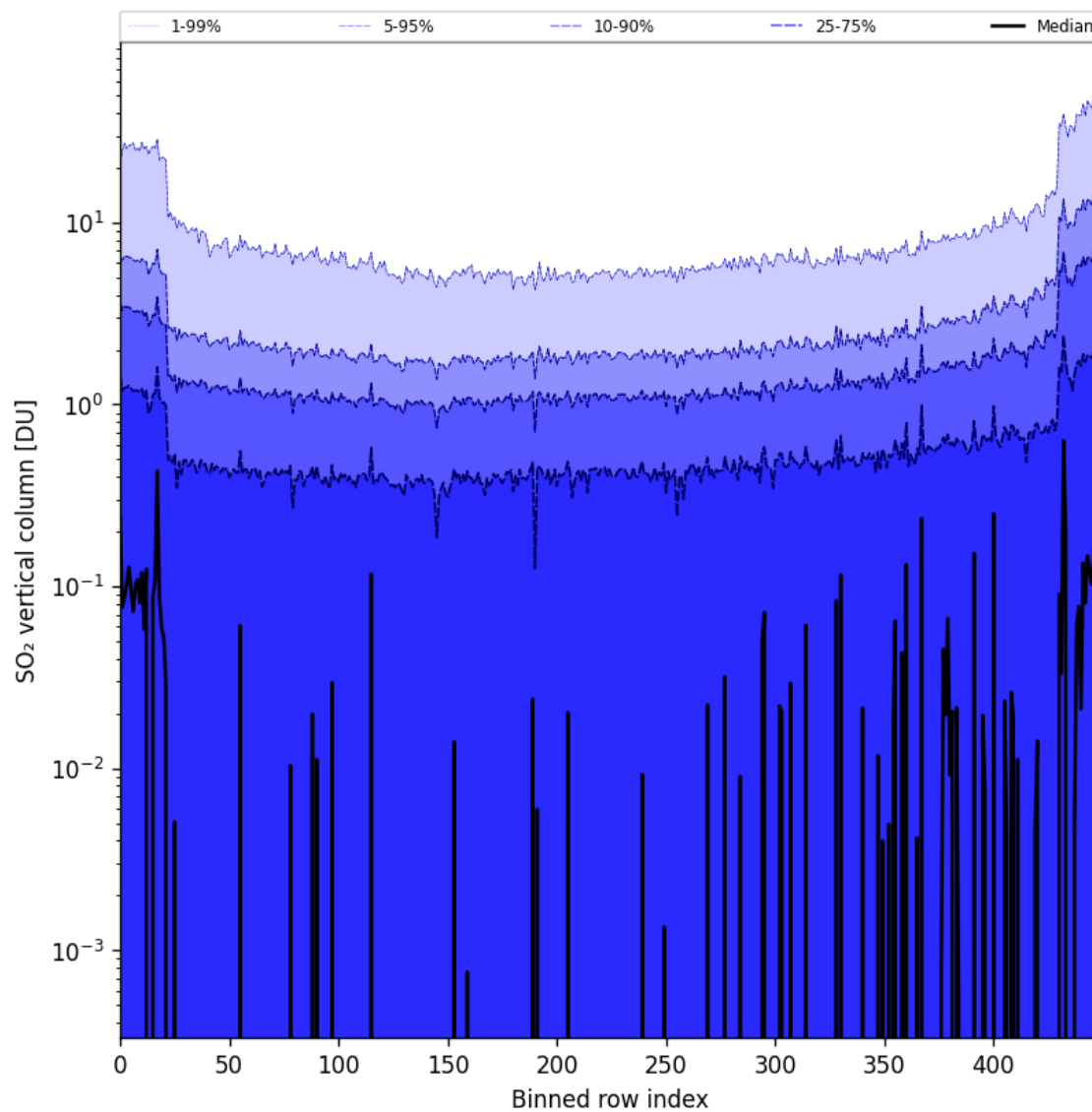
Figure 76: Along track statistics of “SO 2 vertical column” for 2024-10-03 to 2024-10-05
