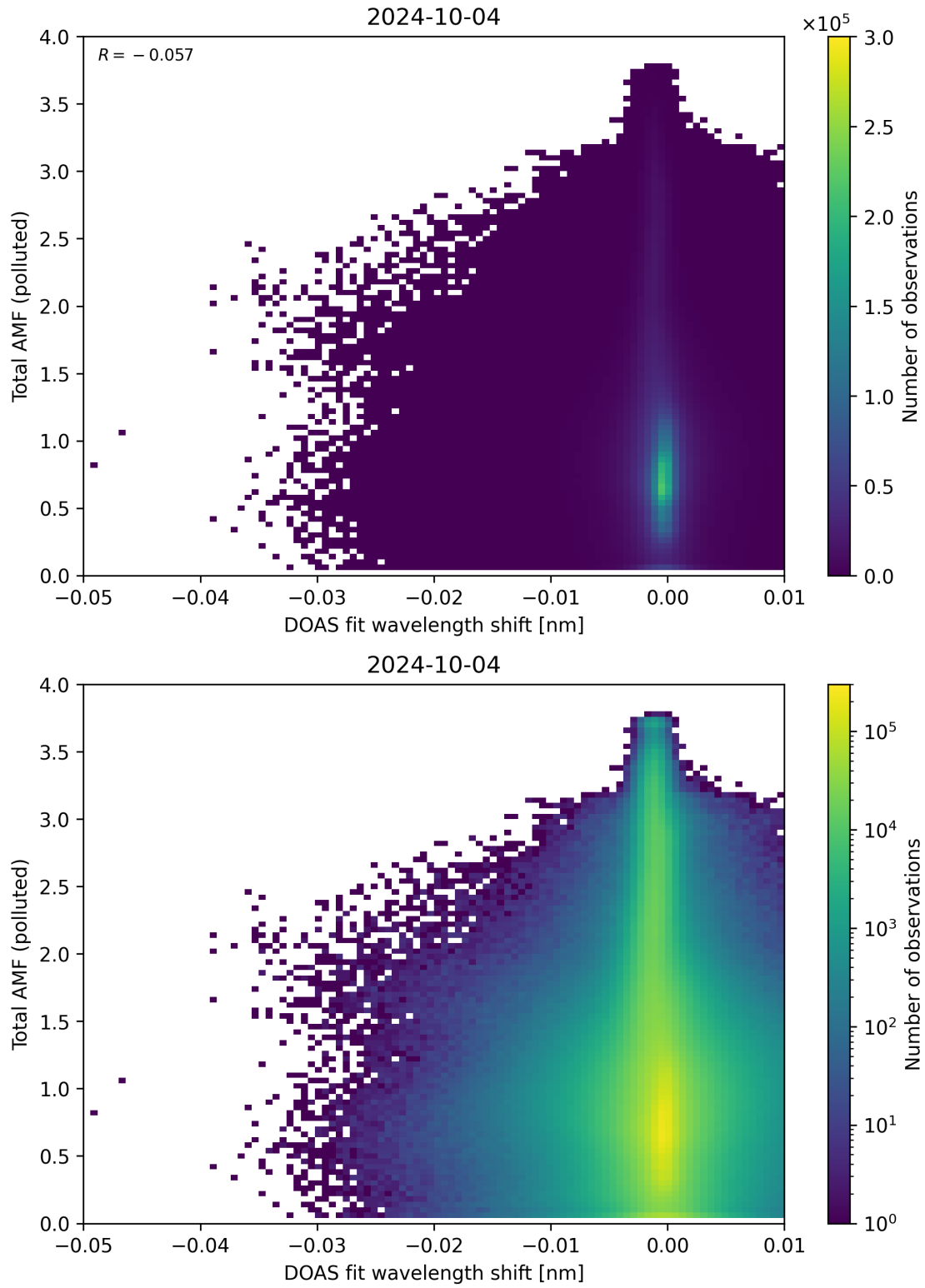
Figure 130: Scatter density plot of “DOAS fit wavelength shift” against “Total AMF (polluted)” for 2024-10-03 to 2024-10-05.
