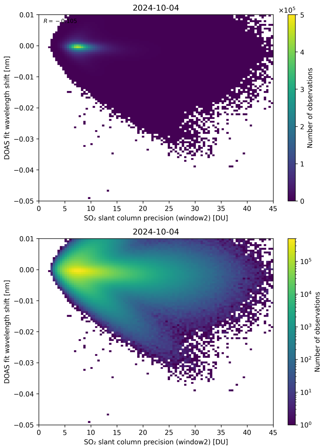
Figure 243: Scatter density plot of “SO 2 slant column precision (window2)” against “DOAS fit wavelength shift” for 2024-10-03 to 2024-10-05.
