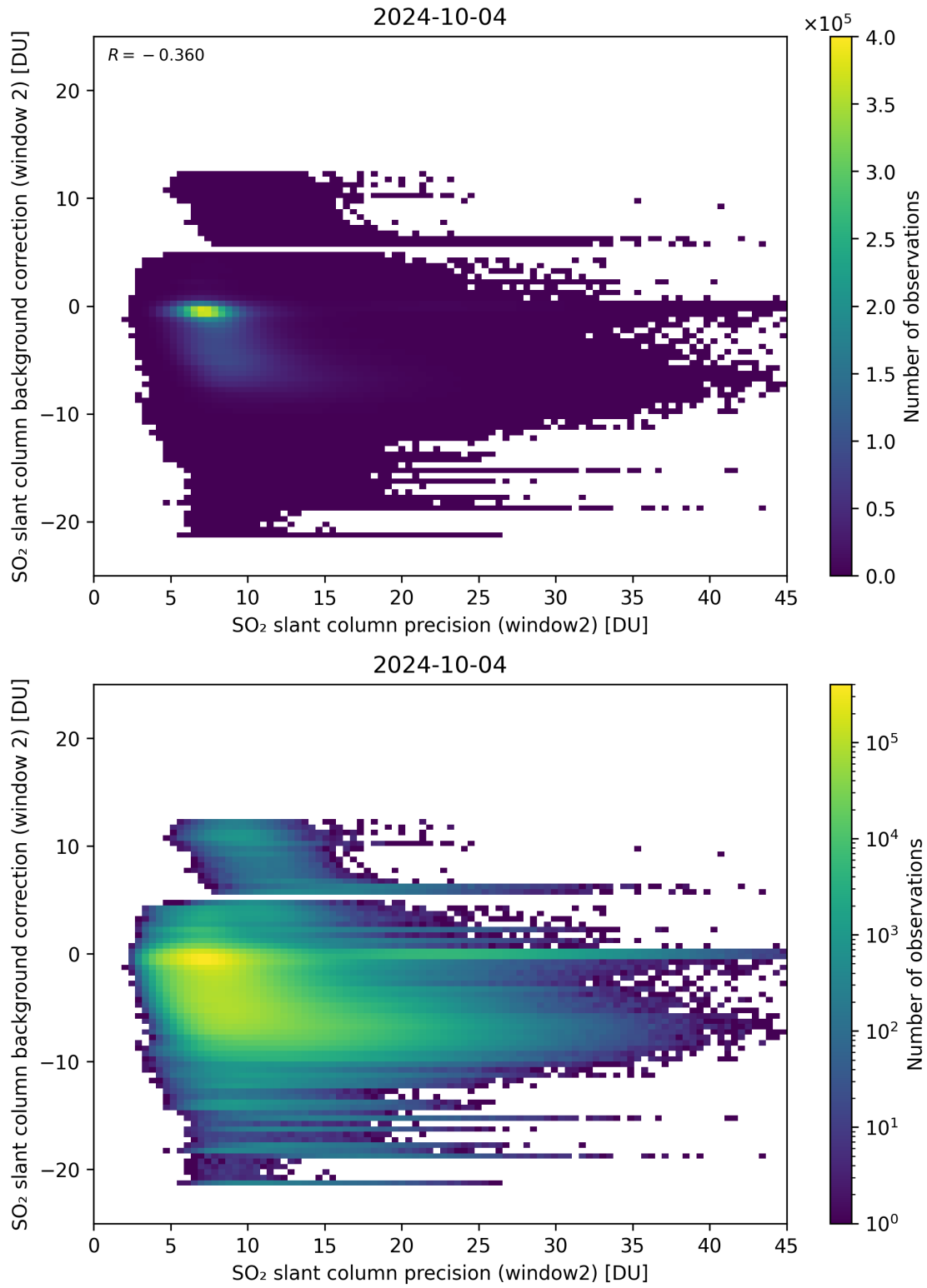
Figure 241: Scatter density plot of “SO 2 slant column precision (window2)” against “SO 2 slant column background correction (window 2)” for 2024-10-03 to 2024-10-05.
