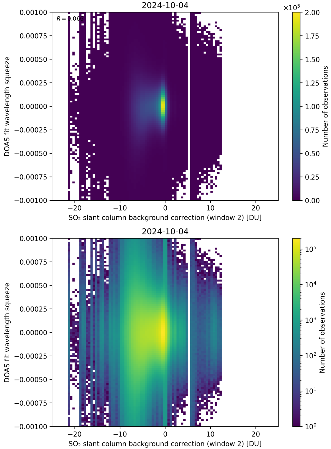
Figure 113: Scatter density plot of “SO 2 slant column background correction (window 2)” against “DOAS fit wavelength squeeze” for 2024-10-03 to 2024-10-05.
