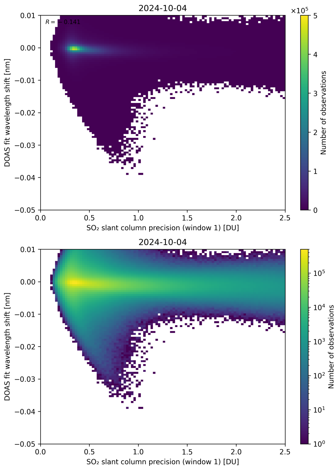
Figure 221: Scatter density plot of “SO 2 slant column precision (window 1)” against “DOAS fit wavelength shift” for 2024-10-03 to 2024-10-05.
