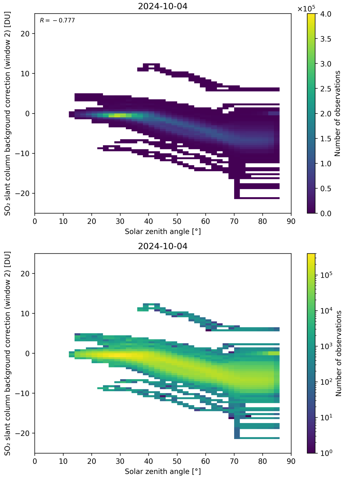
Figure 159: Scatter density plot of “Solar zenith angle” against “SO 2 slant column background correction (window 2)” for 2024-10-03 to 2024-10-05.
