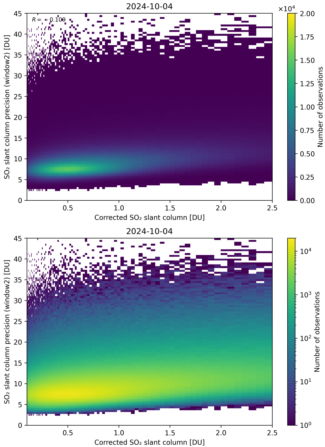
Figure 189: Scatter density plot of “Corrected SO 2 slant column” against “SO 2 slant column precision (window2)” for 2024-10-03 to 2024-10-05.
