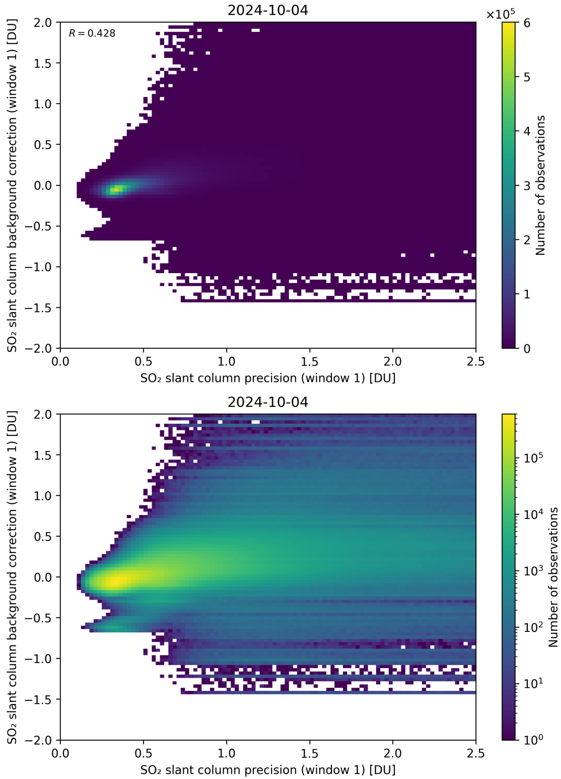
Figure 218: Scatter density plot of “SO 2 slant column precision (window 1)” against “SO 2 slant column background correction (window 1)” for 2024-10-03 to 2024-10-05.
