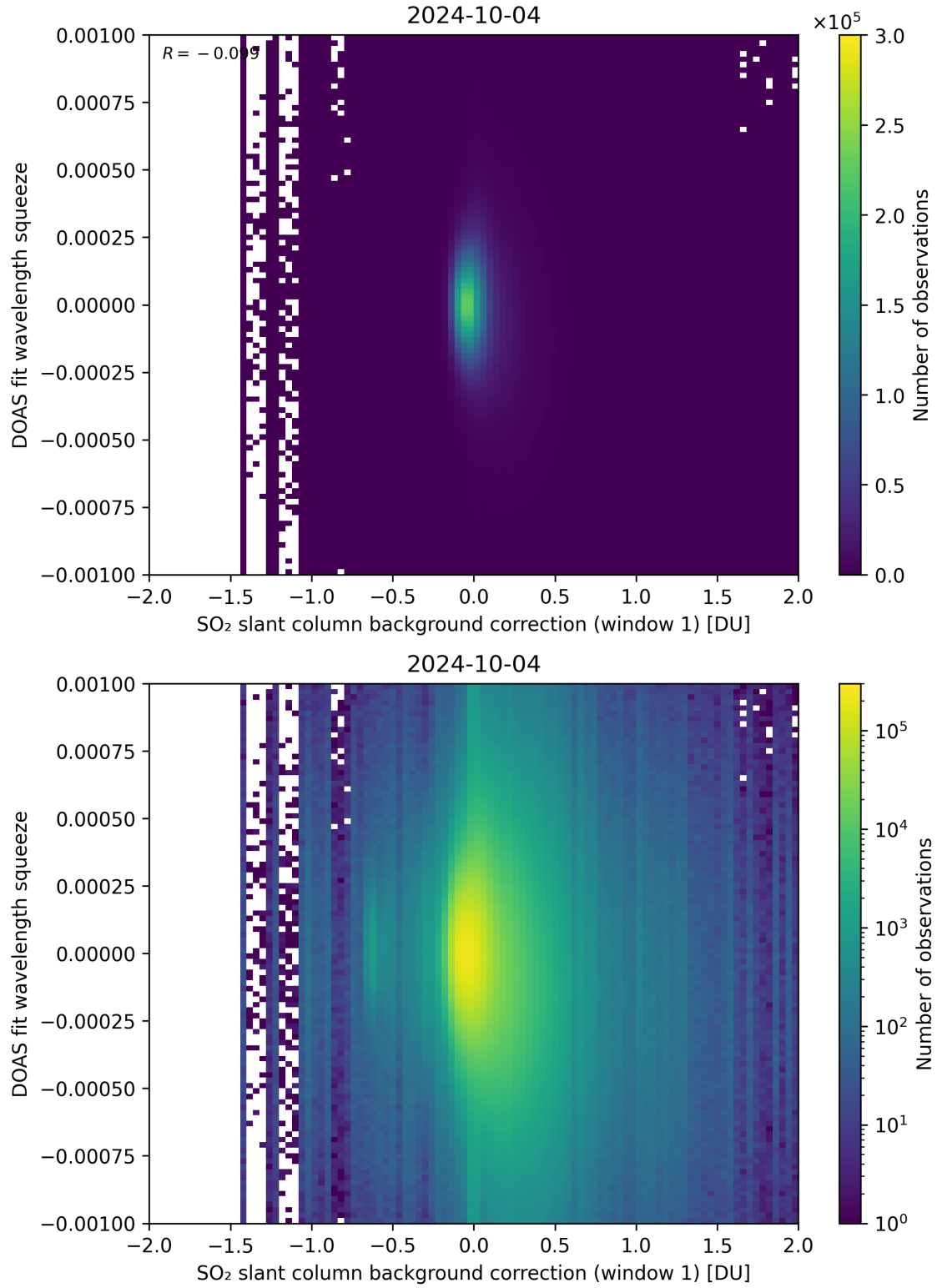
Figure 101: Scatter density plot of “SO 2 slant column background correction (window 1)” against “DOAS fit wavelength squeeze” for 2024-10-03 to 2024-10-05.
