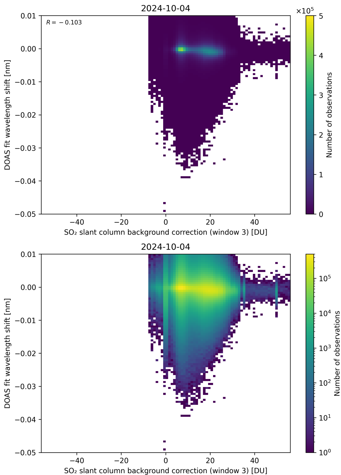
Figure 121: Scatter density plot of “SO 2 slant column background correction (window 3)” against “DOAS fit wavelength shift” for 2024-10-03 to 2024-10-05.
