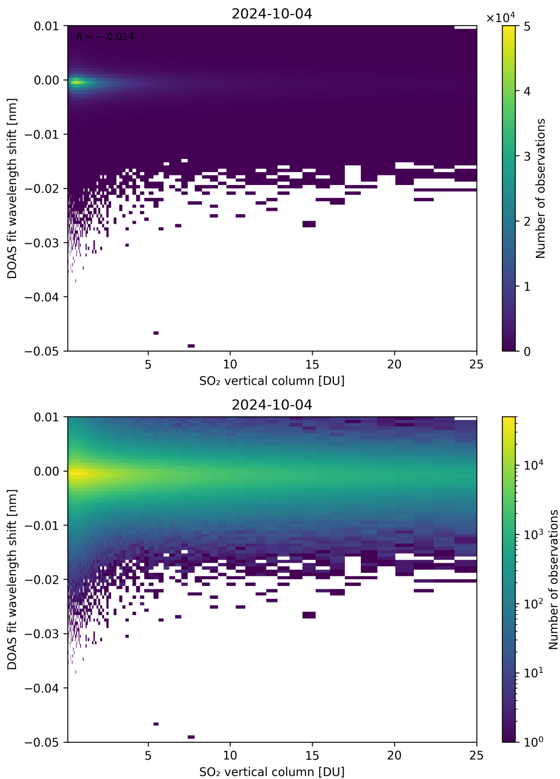
Figure 276: Scatter density plot of “SO 2 vertical column” against “DOAS fit wavelength shift” for 2024-10-03 to 2024-10-05.
