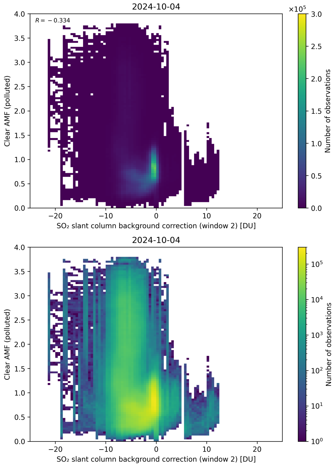
Figure 115: Scatter density plot of “SO 2 slant column background correction (window 2)” against “Clear AMF (polluted)” for 2024-10-03 to 2024-10-05.
