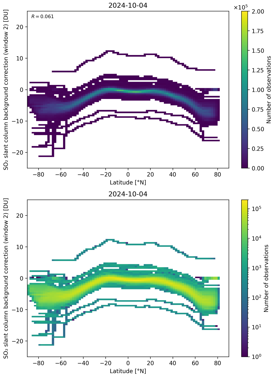
Figure 140: Scatter density plot of “Latitude” against “SO 2 slant column background correction (window 2)” for 2024-10-03 to 2024-10-05.
