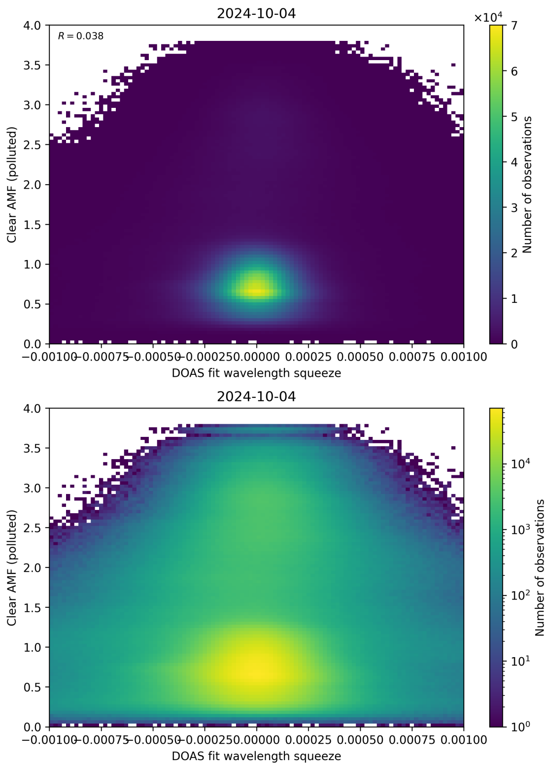
Figure 133: Scatter density plot of “DOAS fit wavelength squeeze” against “Clear AMF (polluted)” for 2024-10-03 to 2024-10-05.
