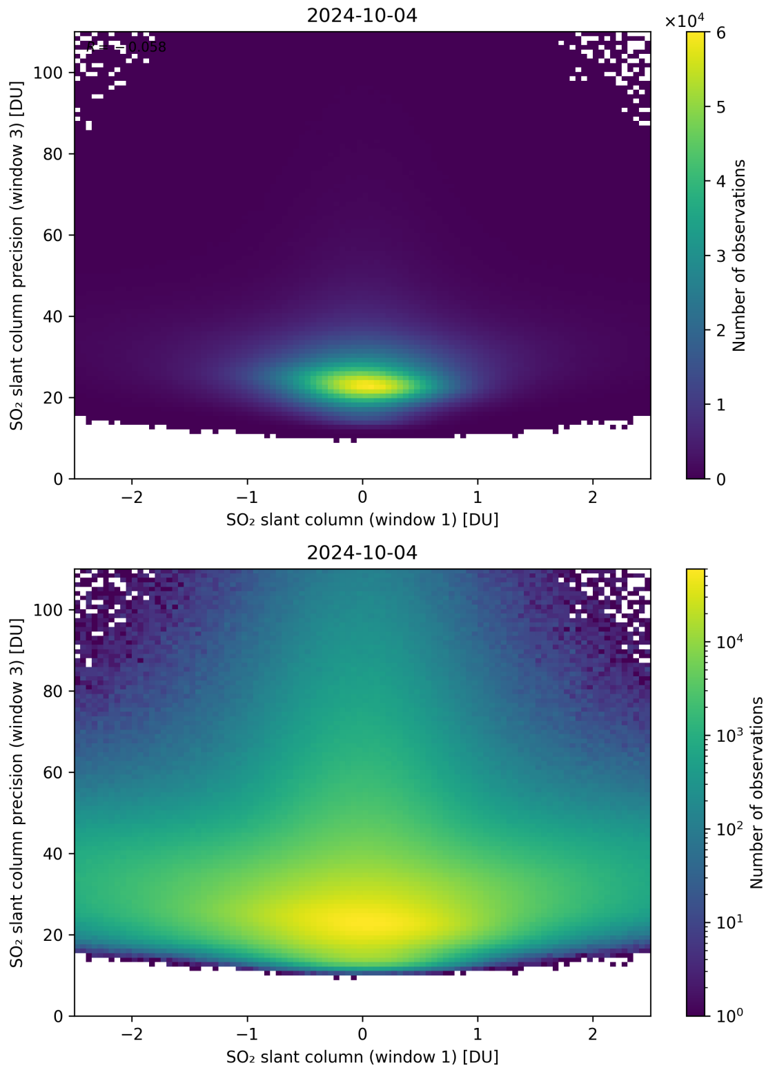
Figure 238: Scatter density plot of “SO 2 slant column (window 1)” against “SO 2 slant column precision (window 3)” for 2024-10-03 to 2024-10-05.
