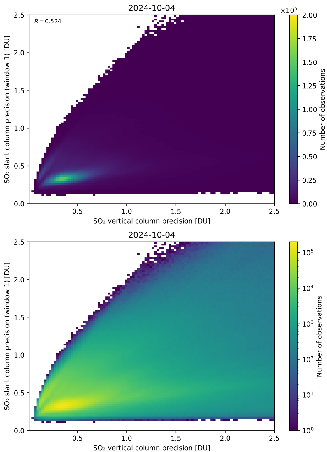
Figure 290: Scatter density plot of “SO 2 vertical column precision” against “SO 2 slant column precision (window 1)” for 2024-10-03 to 2024-10-05.
