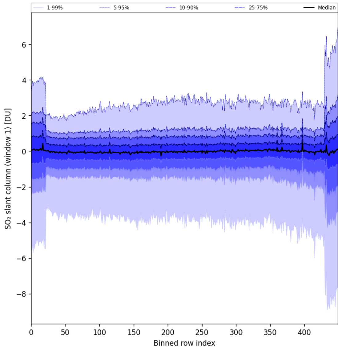
Figure 79: Along track statistics of “SO 2 slant column (window 1)” for 2024-10-03 to 2024-10-05
