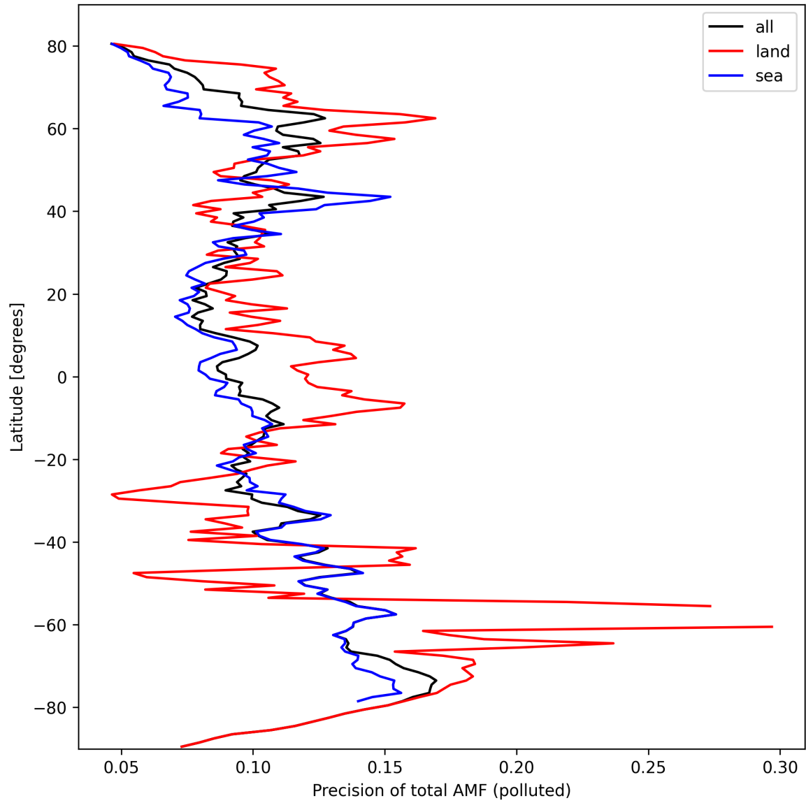
Figure 49: Zonal average of “Precision of total AMF (polluted)” for 2024-10-03 to 2024-10-05.
