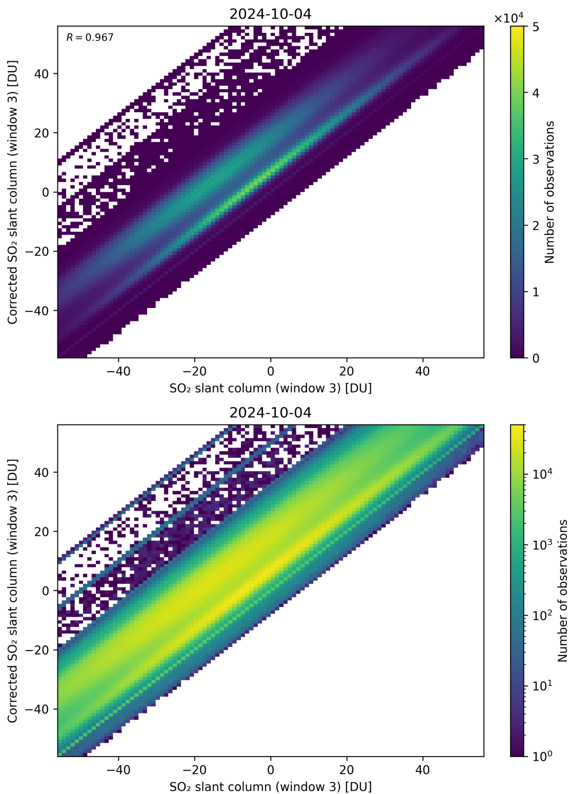
Figure 266: Scatter density plot of “SO 2 slant column (window 3)” against “Corrected SO 2 slant column (window 3)” for 2024-10-03 to 2024-10-05.
