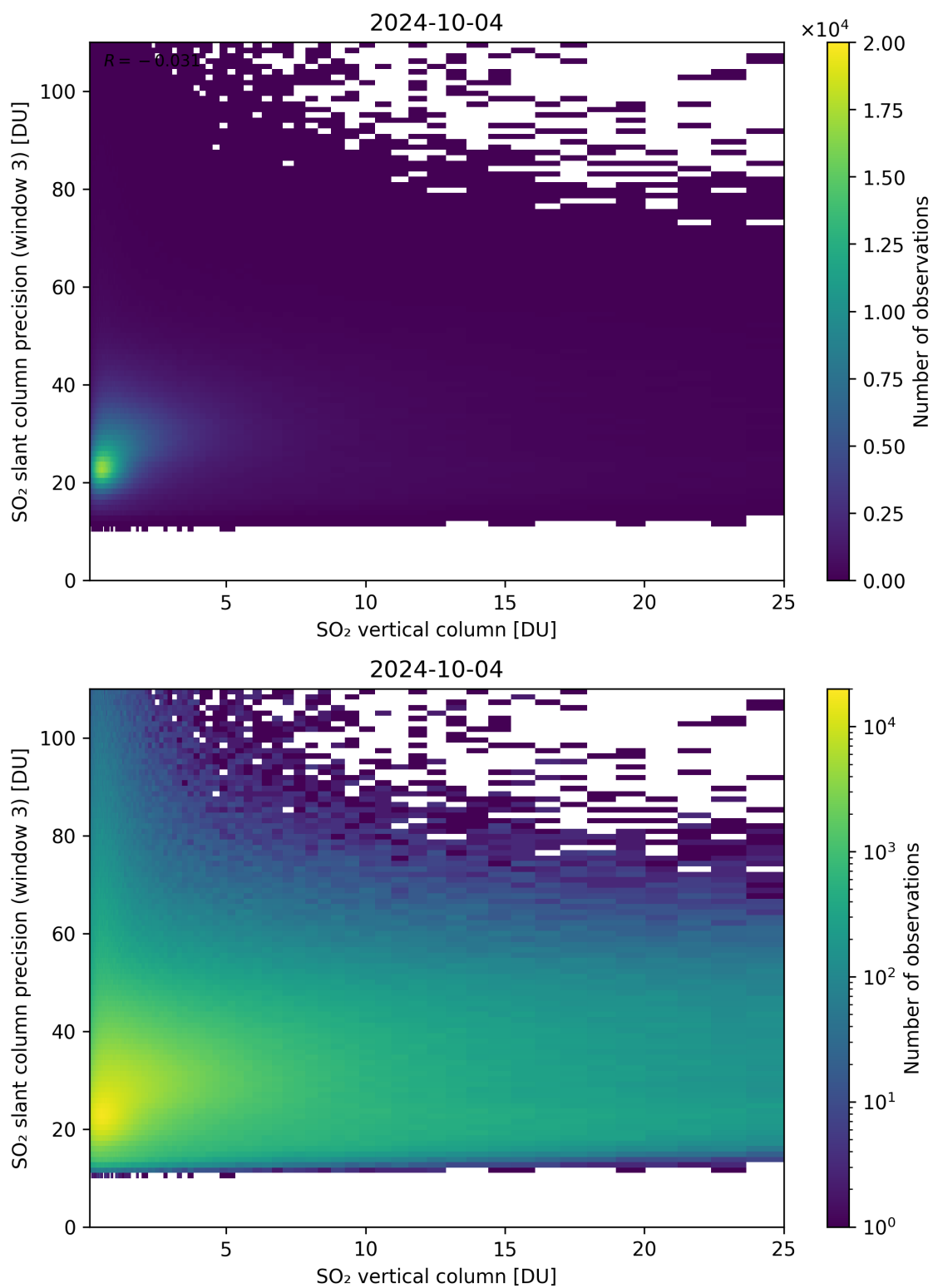
Figure 304: Scatter density plot of “SO 2 vertical column” against “SO 2 slant column precision (window 3)” for 2024-10-03 to 2024-10-05.
