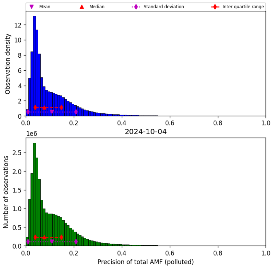
Figure 72: Histogram of “Precision of total AMF (polluted)” for 2024-10-03 to 2024-10-05
