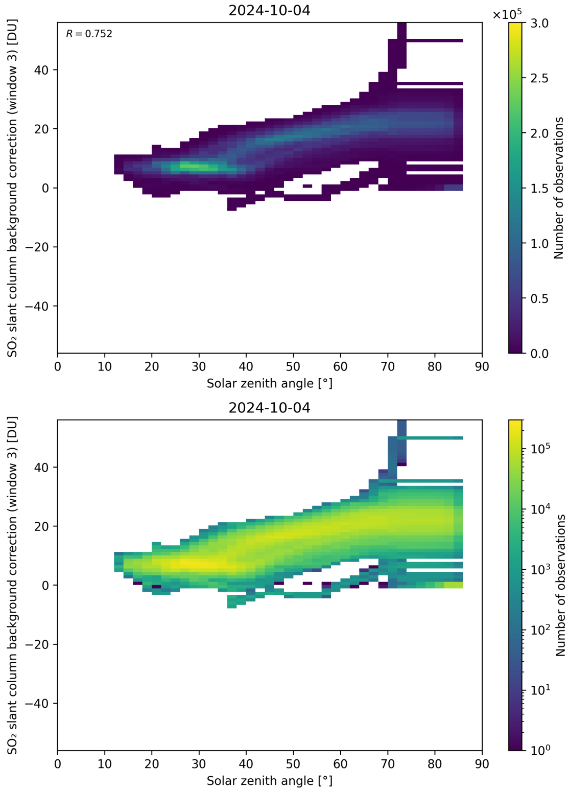
Figure 160: Scatter density plot of “Solar zenith angle” against “SO 2 slant column background correction (window 3)” for 2024-10-03 to 2024-10-05.
