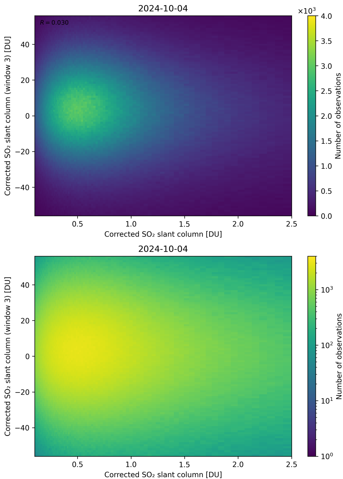
Figure 186: Scatter density plot of “Corrected SO 2 slant column” against “Corrected SO 2 slant column (window 3)” for 2024-10-03 to 2024-10-05.
