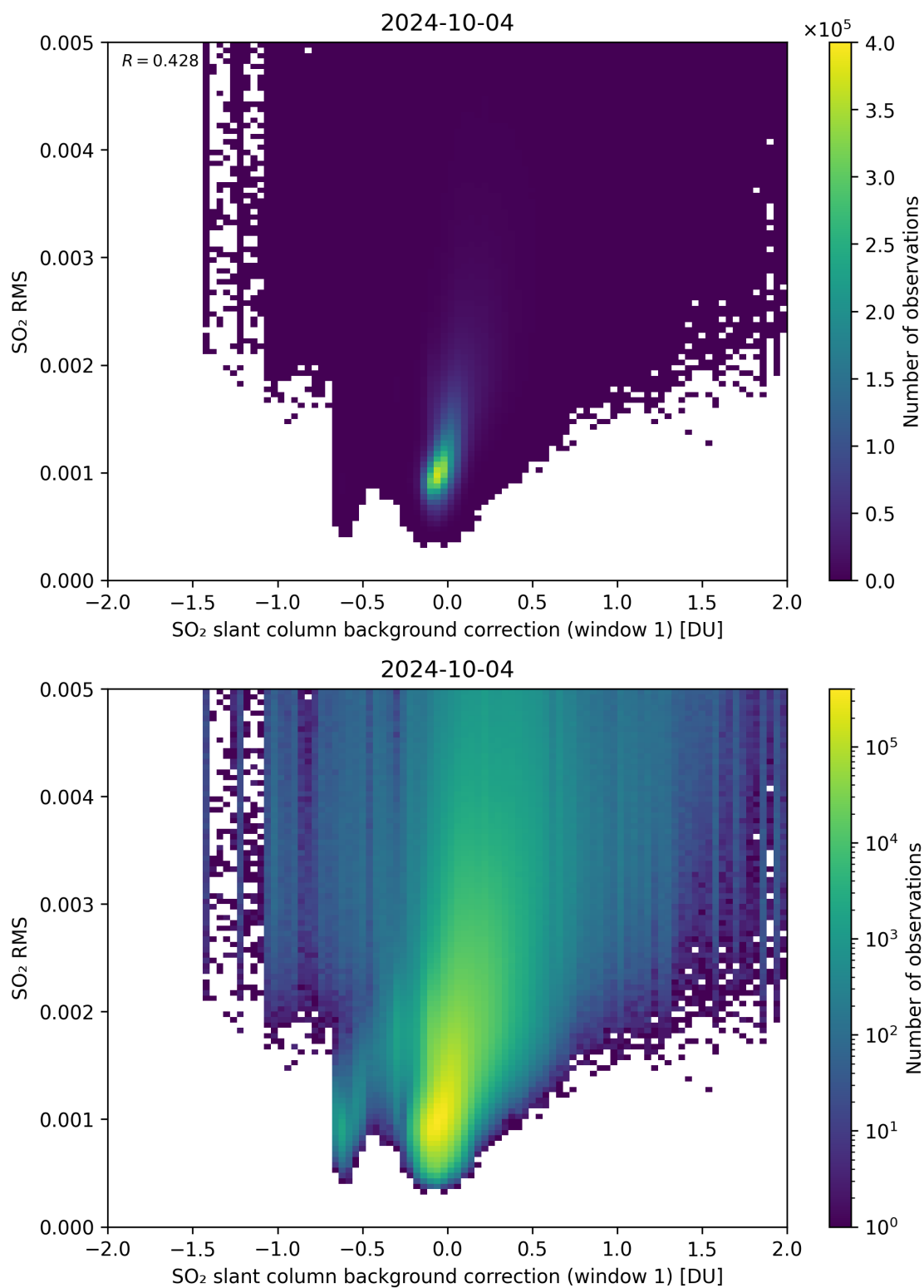
Figure 102: Scatter density plot of “SO 2 slant column background correction (window 1)” against “SO 2 RMS” for 2024-10-03 to 2024-10-05.
