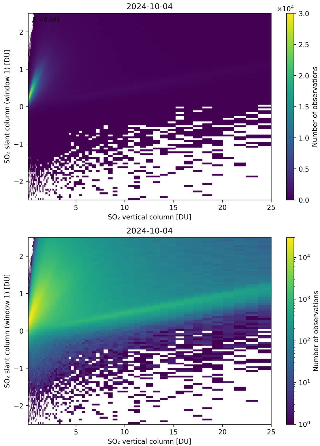
Figure 300: Scatter density plot of “SO 2 vertical column” against “SO 2 slant column (window 1)” for 2024-10-03 to 2024-10-05.
