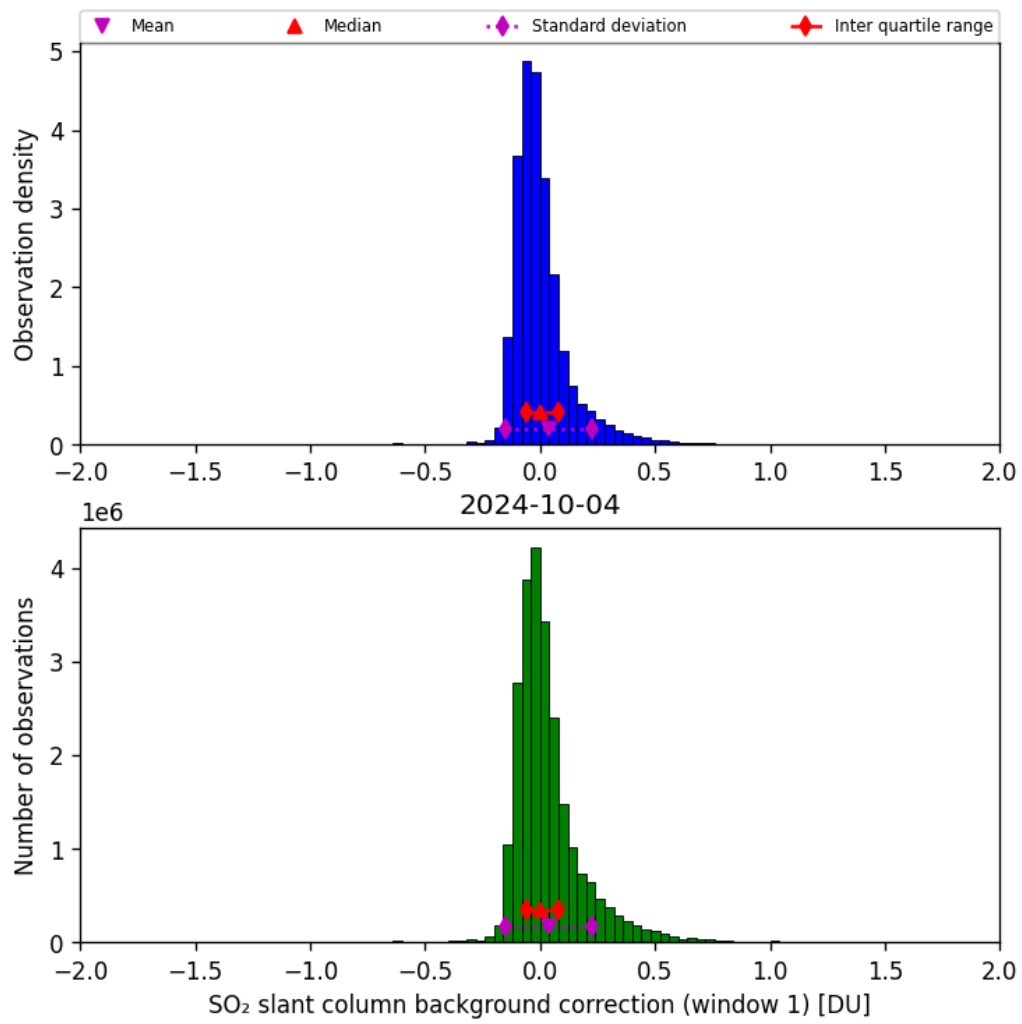
Figure 59: Histogram of “SO 2 slant column background correction (window 1)” for 2024-10-03 to 2024-10-05
