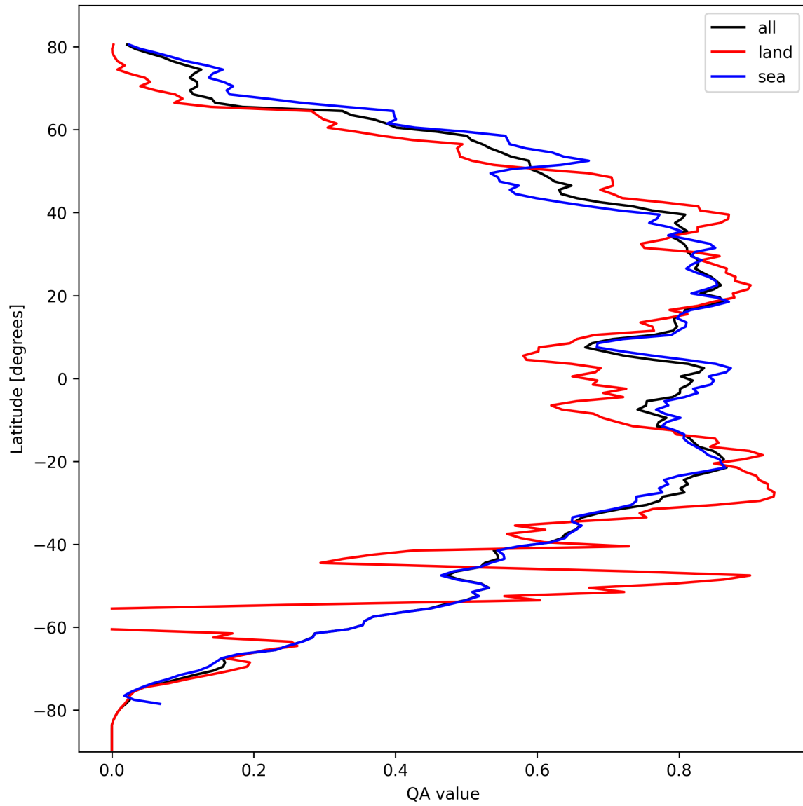
Figure 29: Zonal average of “QA value” for 2024-10-03 to 2024-10-05.
