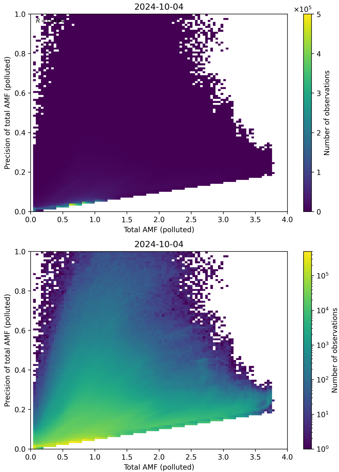
Figure 272: Scatter density plot of “Total AMF (polluted)” against “Precision of total AMF (polluted)” for 2024-10-03 to 2024-10-05.
