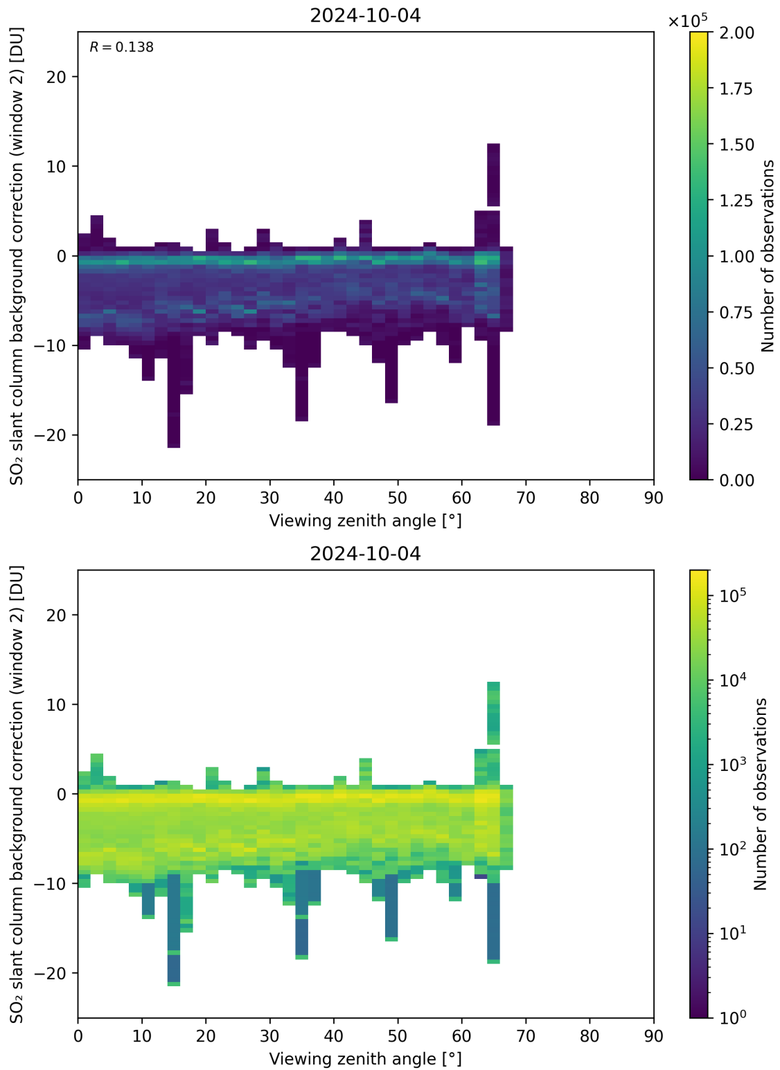
Figure 309: Scatter density plot of “Viewing zenith angle” against “SO 2 slant column background correction (window 2)” for 2024-10-03 to 2024-10-05.
