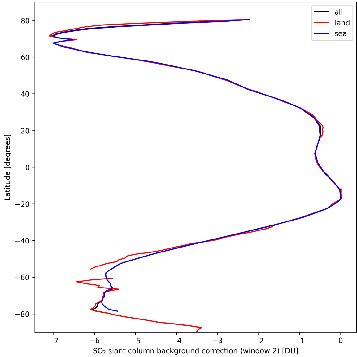
Figure 40: Zonal average of “SO 2 slant column background correction (window 2)” for 2024-10-03 to 2024-10-05.
