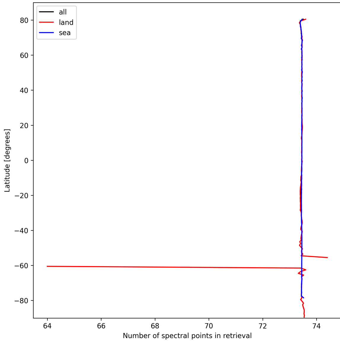
Figure 51: Zonal average of “Number of spectral points in retrieval” for 2024-10-03 to 2024-10-05.
