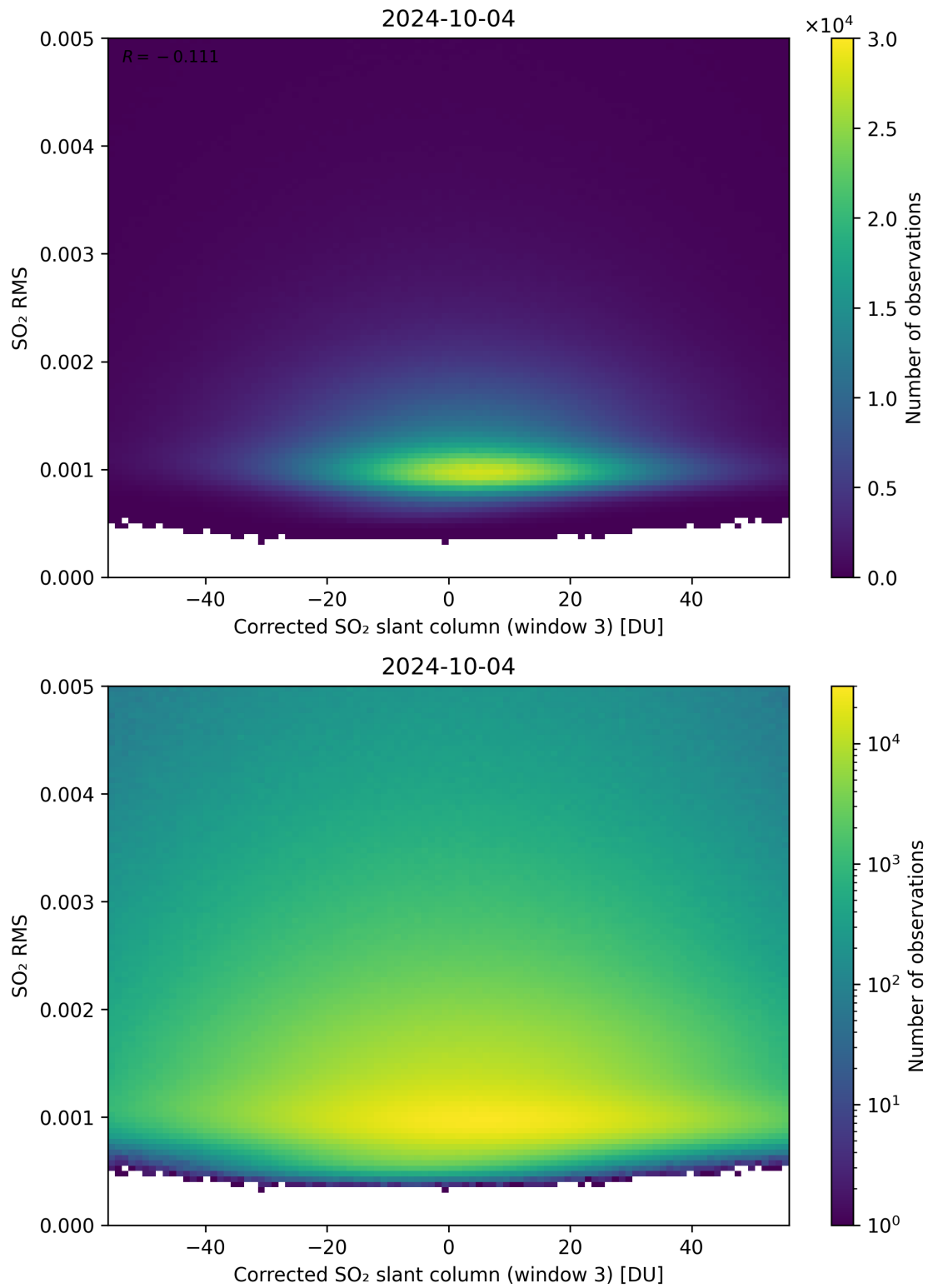
Figure 208: Scatter density plot of “Corrected SO 2 slant column (window 3)” against “SO 2 RMS” for 2024-10-03 to 2024-10-05.
