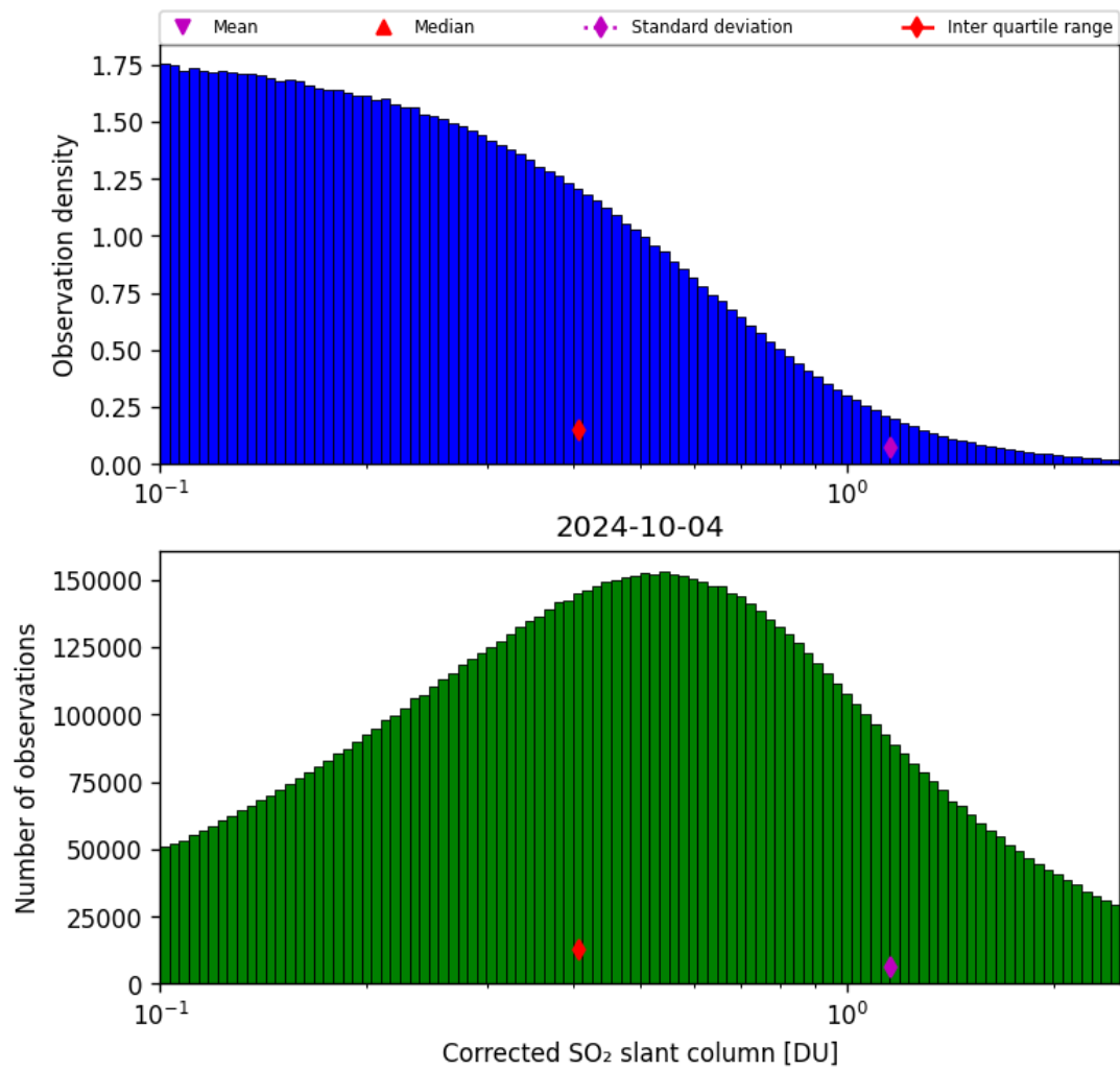
Figure 55: Histogram of “Corrected SO 2 slant column” for 2024-10-03 to 2024-10-05
