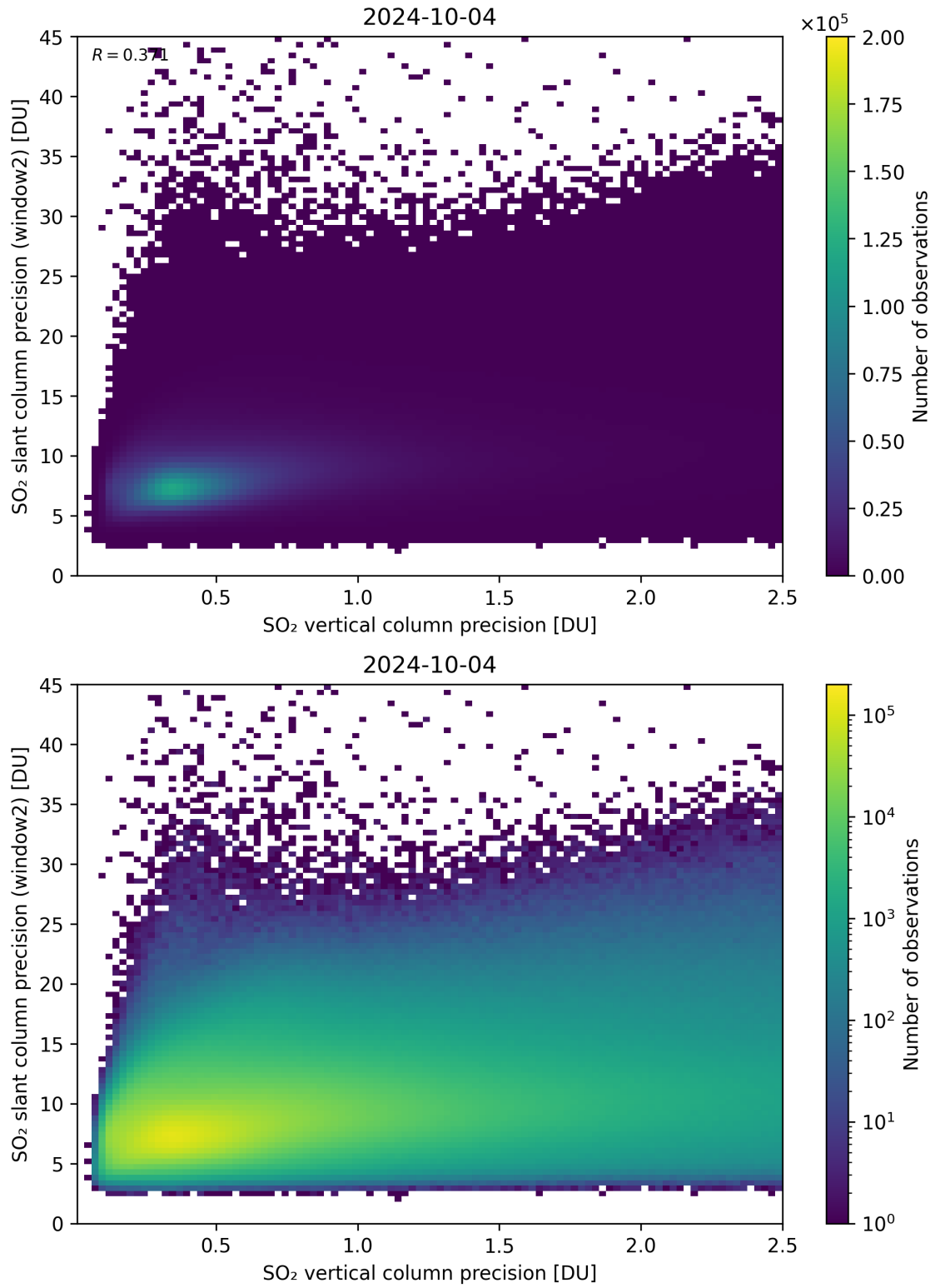
Figure 291: Scatter density plot of “SO 2 vertical column precision” against “SO 2 slant column precision (window2)” for 2024-10-03 to 2024-10-05.
