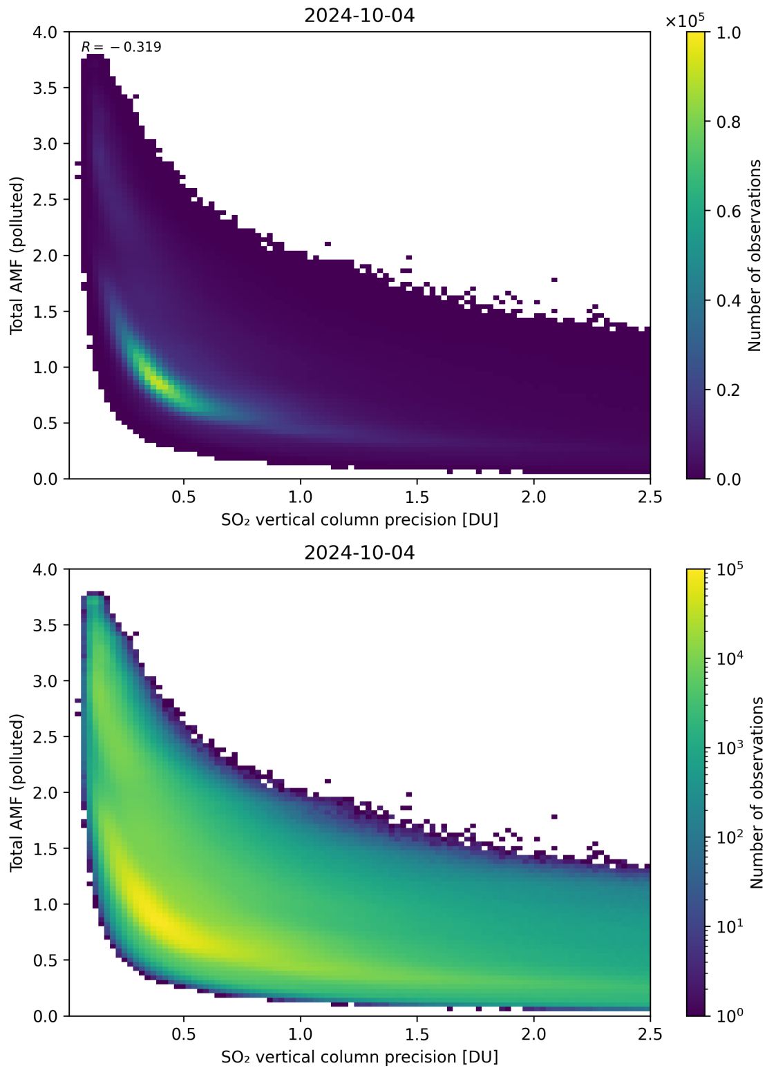
Figure 294: Scatter density plot of “SO 2 vertical column precision” against “Total AMF (polluted)” for 2024-10-03 to 2024-10-05.
