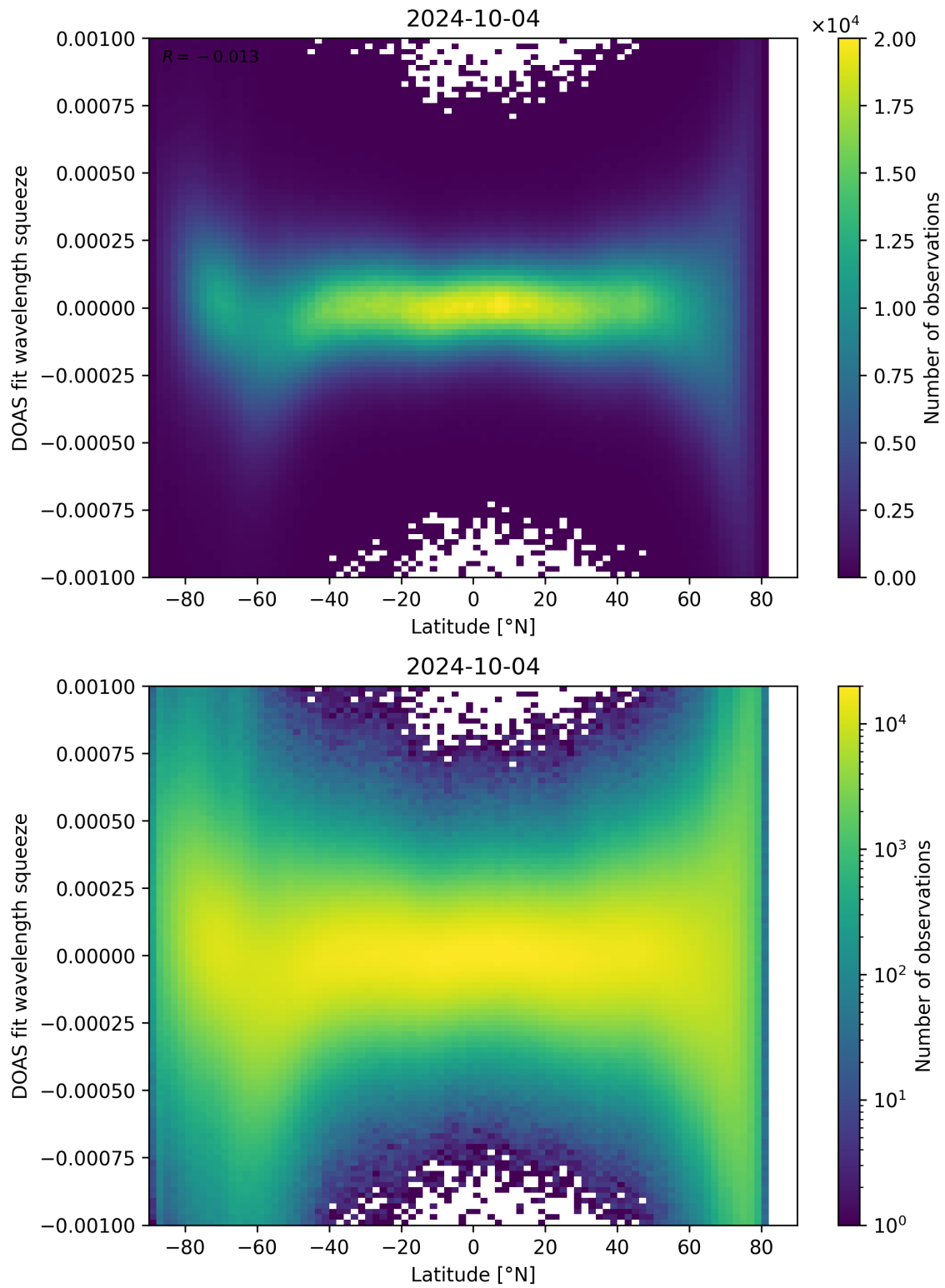
Figure 143: Scatter density plot of “Latitude” against “DOAS fit wavelength squeeze” for 2024-10-03 to 2024-10-05.
