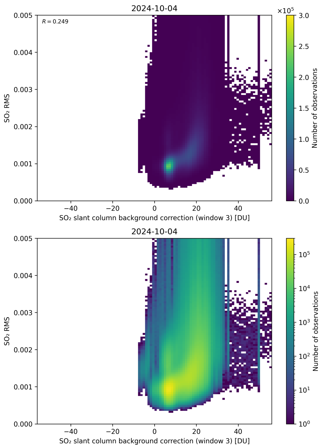
Figure 123: Scatter density plot of “SO 2 slant column background correction (window 3)” against “SO 2 RMS” for 2024-10-03 to 2024-10-05.
