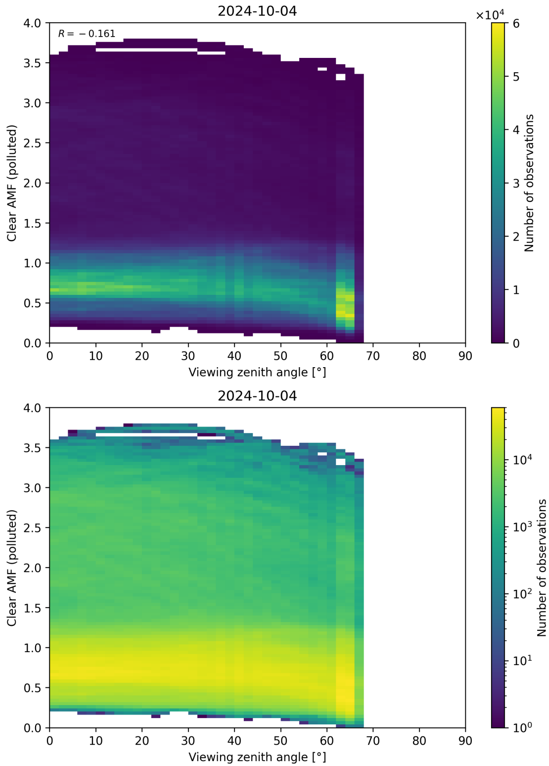
Figure 316: Scatter density plot of “Viewing zenith angle” against “Clear AMF (polluted)” for 2024-10-03 to 2024-10-05.
