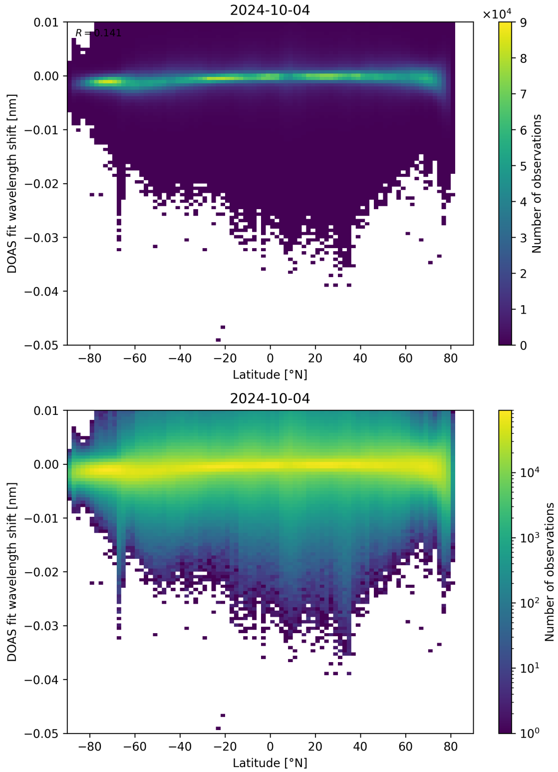
Figure 142: Scatter density plot of “Latitude” against “DOAS fit wavelength shift” for 2024-10-03 to 2024-10-05.
