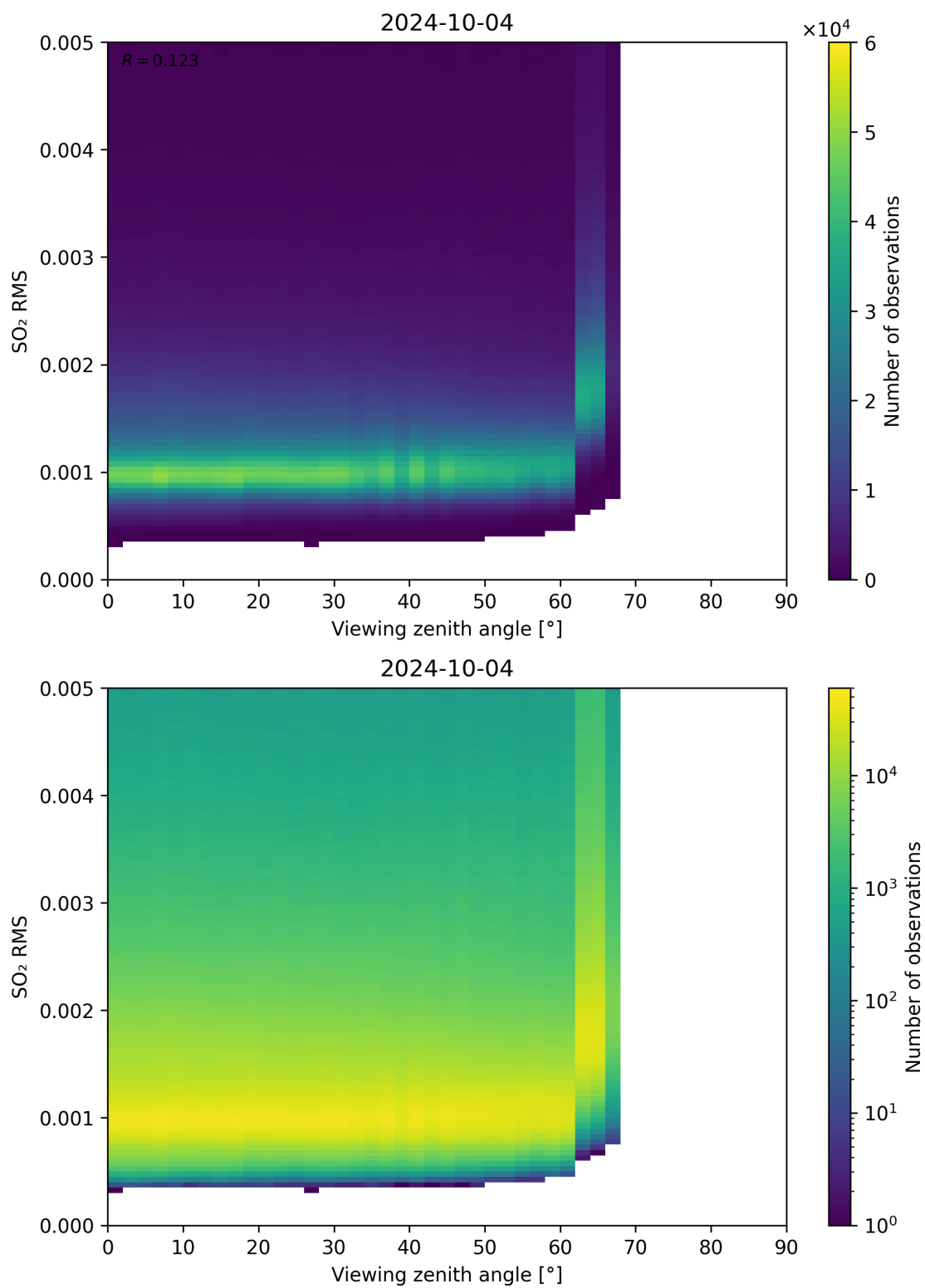
Figure 313: Scatter density plot of “Viewing zenith angle” against “SO 2 RMS” for 2024-10-03 to 2024-10-05.
