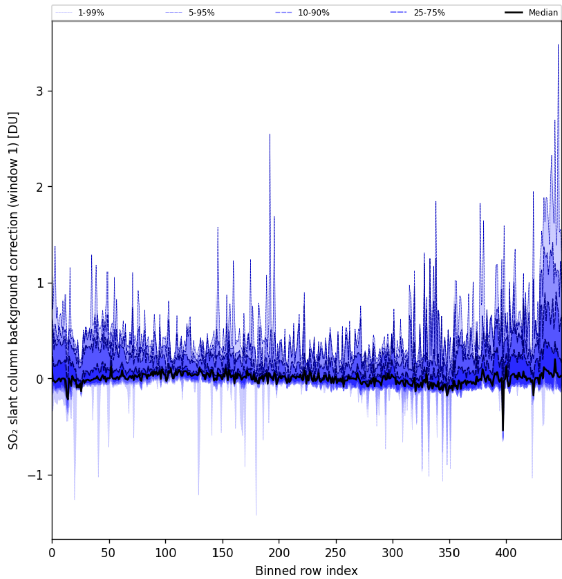
Figure 82: Along track statistics of “SO 2 slant column background correction (window 1)” for 2024-10-03 to 2024-10-05
