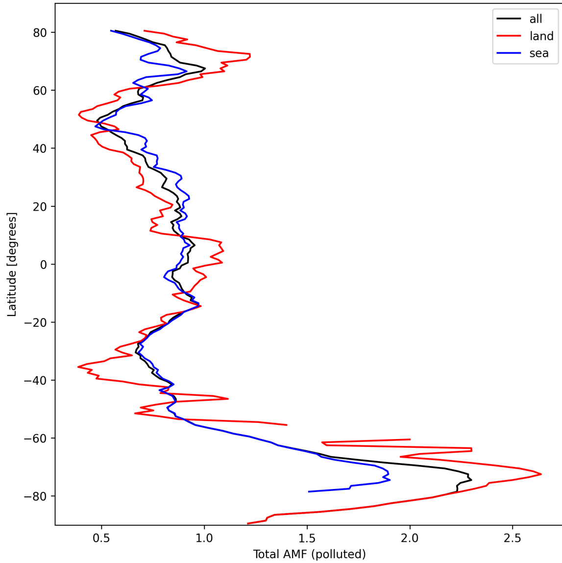
Figure 48: Zonal average of “Total AMF (polluted)” for 2024-10-03 to 2024-10-05.
