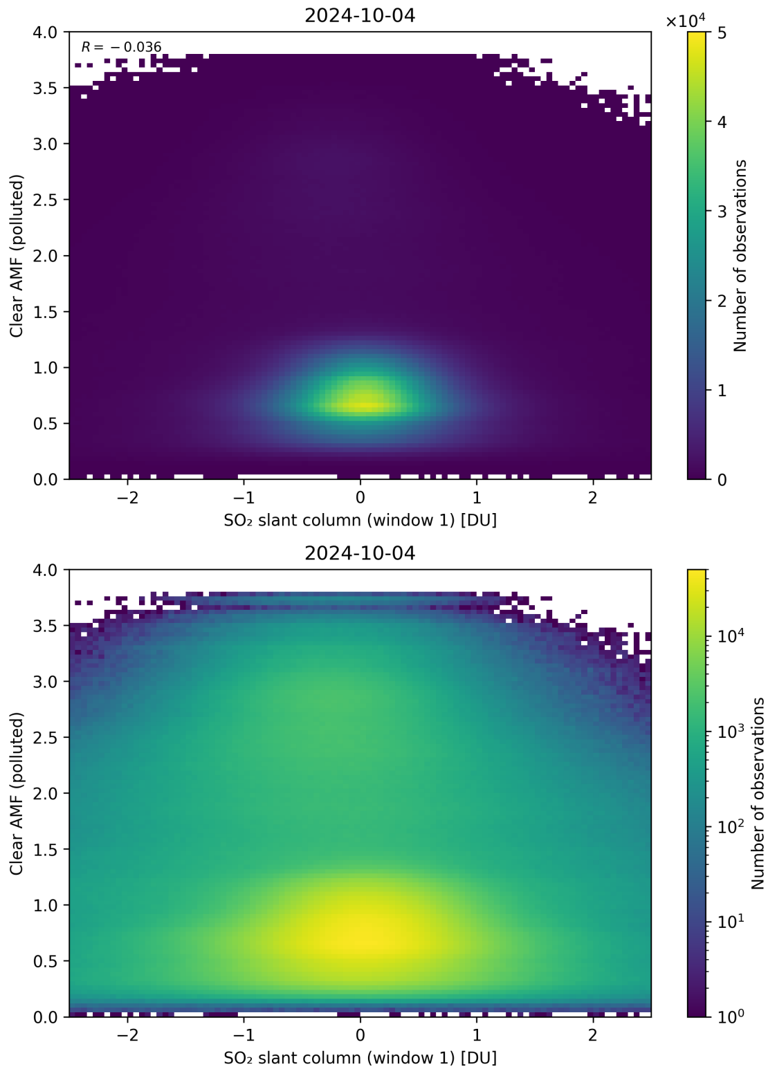
Figure 232: Scatter density plot of “SO 2 slant column (window 1)” against “Clear AMF (polluted)” for 2024-10-03 to 2024-10-05.
