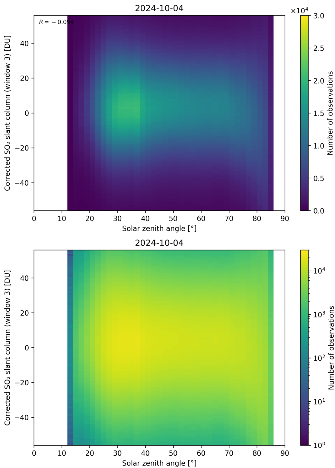
Figure 168: Scatter density plot of “Solar zenith angle” against “Corrected SO 2 slant column (window 3)” for 2024-10-03 to 2024-10-05.
