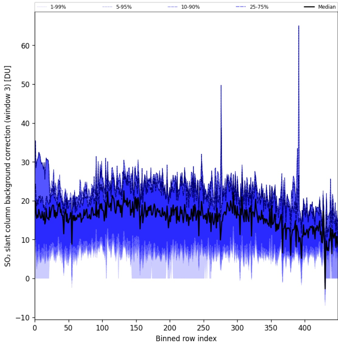
Figure 90: Along track statistics of “SO 2 slant column background correction (window 3)” for 2024-10-03 to 2024-10-05
