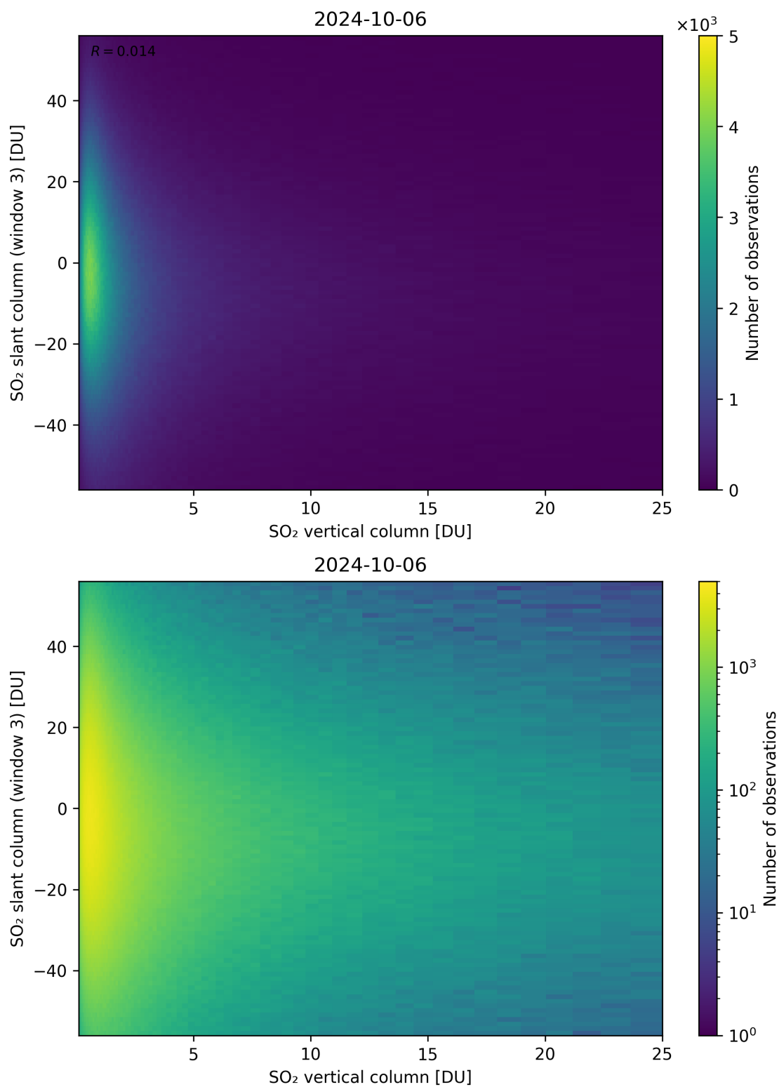
Figure 303: Scatter density plot of “SO 2 vertical column” against “SO 2 slant column (window 3)” for 2024-10-05 to 2024-10-07.
