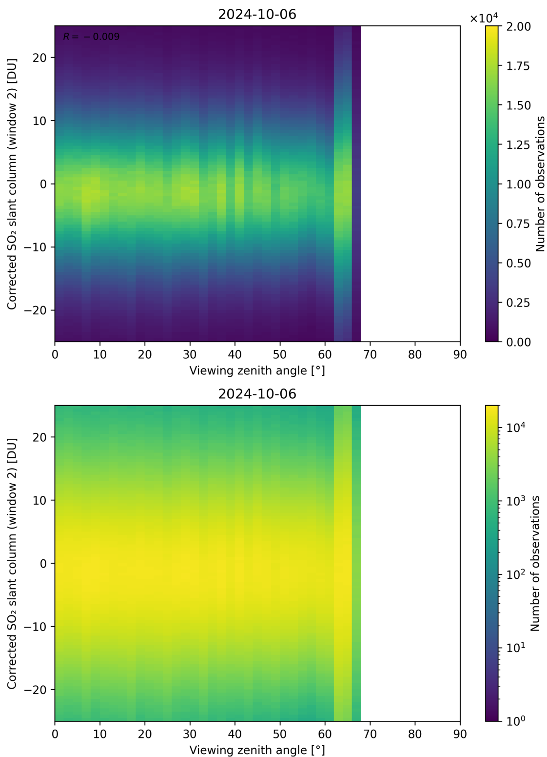
Figure 318: Scatter density plot of “Viewing zenith angle” against “Corrected SO 2 slant column (window 2)” for 2024-10-05 to 2024-10-07.
