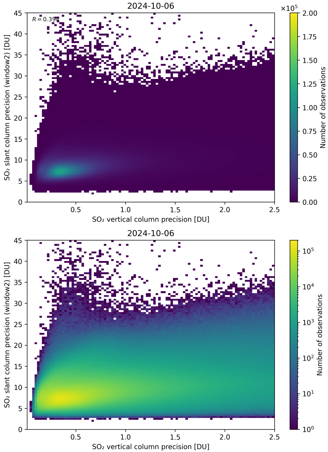
Figure 291: Scatter density plot of “SO 2 vertical column precision” against “SO 2 slant column precision (window2)” for 2024-10-05 to 2024-10-07.
