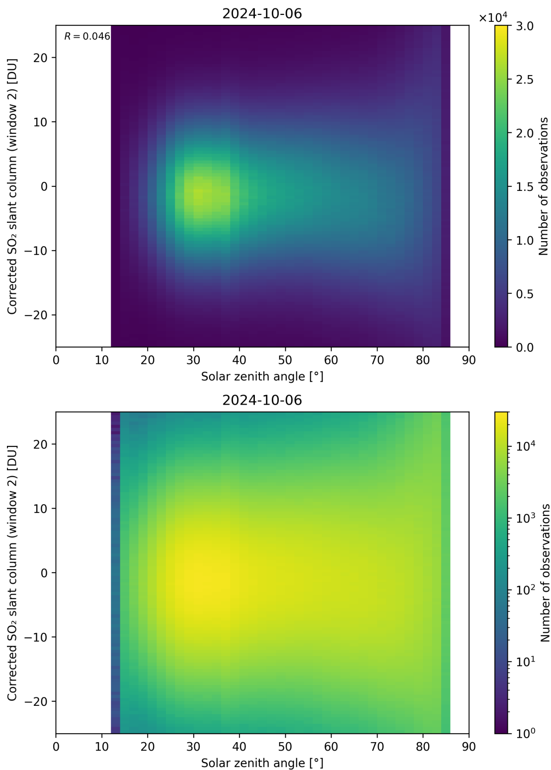
Figure 167: Scatter density plot of “Solar zenith angle” against “Corrected SO 2 slant column (window 2)” for 2024-10-05 to 2024-10-07.
