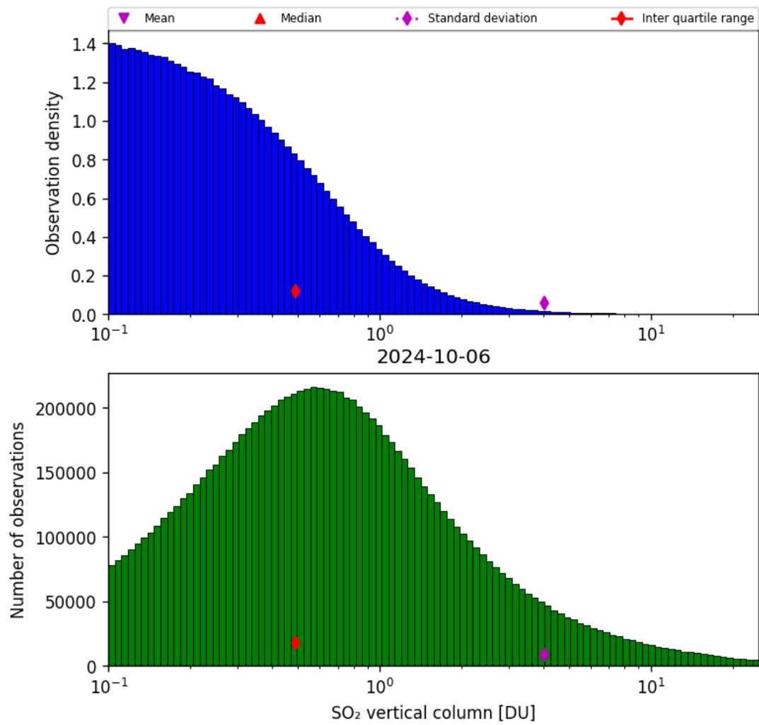
Figure 53: Histogram of “SO 2 vertical column” for 2024-10-05 to 2024-10-07
