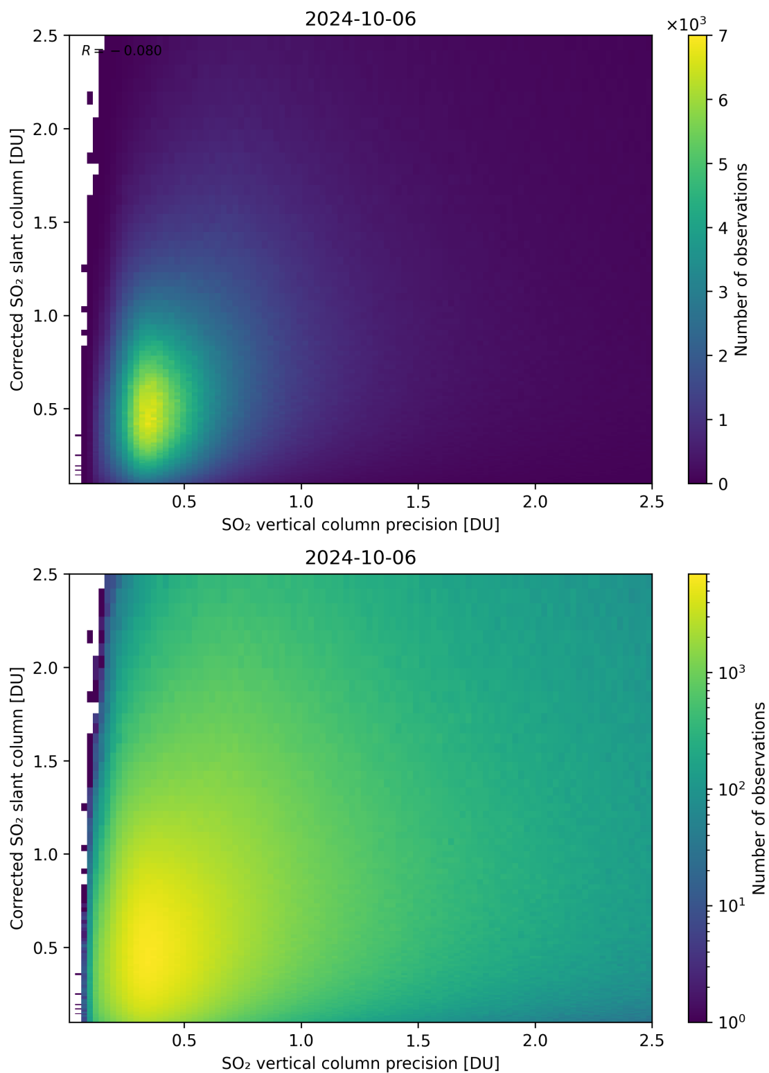
Figure 286: Scatter density plot of “SO 2 vertical column precision” against “Corrected SO 2 slant column” for 2024-10-05 to 2024-10-07.
