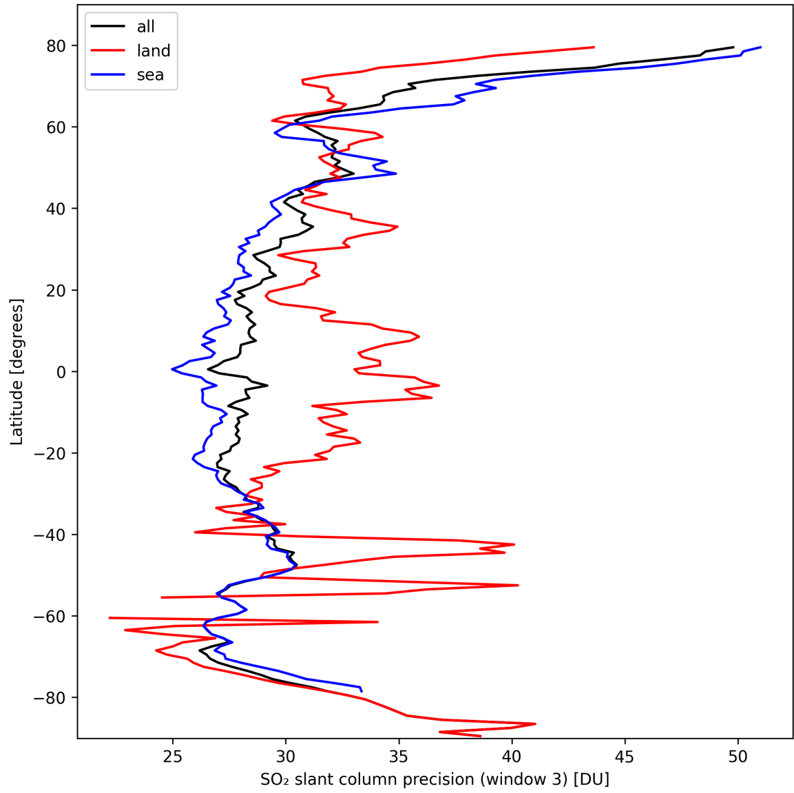
Figure 42: Zonal average of “SO 2 slant column precision (window 3)” for 2024-10-05 to 2024-10-07.
