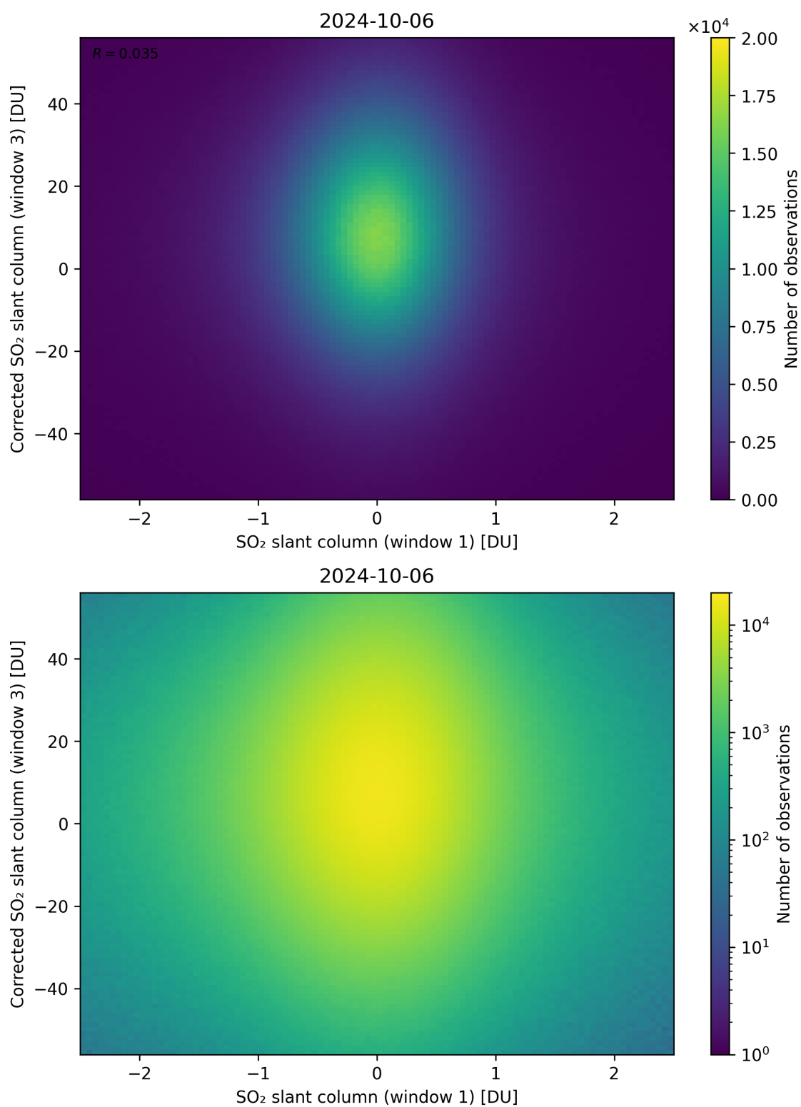
Figure 234: Scatter density plot of “SO 2 slant column (window 1)” against “Corrected SO 2 slant column (window 3)” for 2024-10-05 to 2024-10-07.
