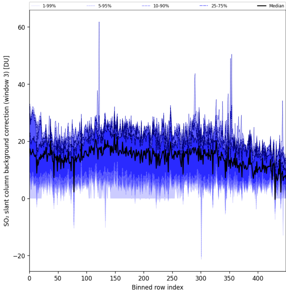
Figure 90: Along track statistics of “SO 2 slant column background correction (window 3)” for 2024-10-05 to 2024-10-07
