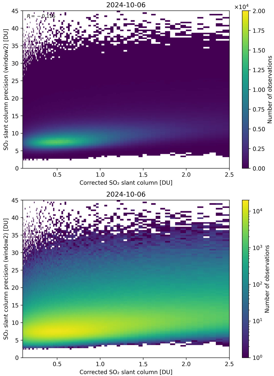
Figure 189: Scatter density plot of “Corrected SO 2 slant column” against “SO 2 slant column precision (window2)” for 2024-10-05 to 2024-10-07.
