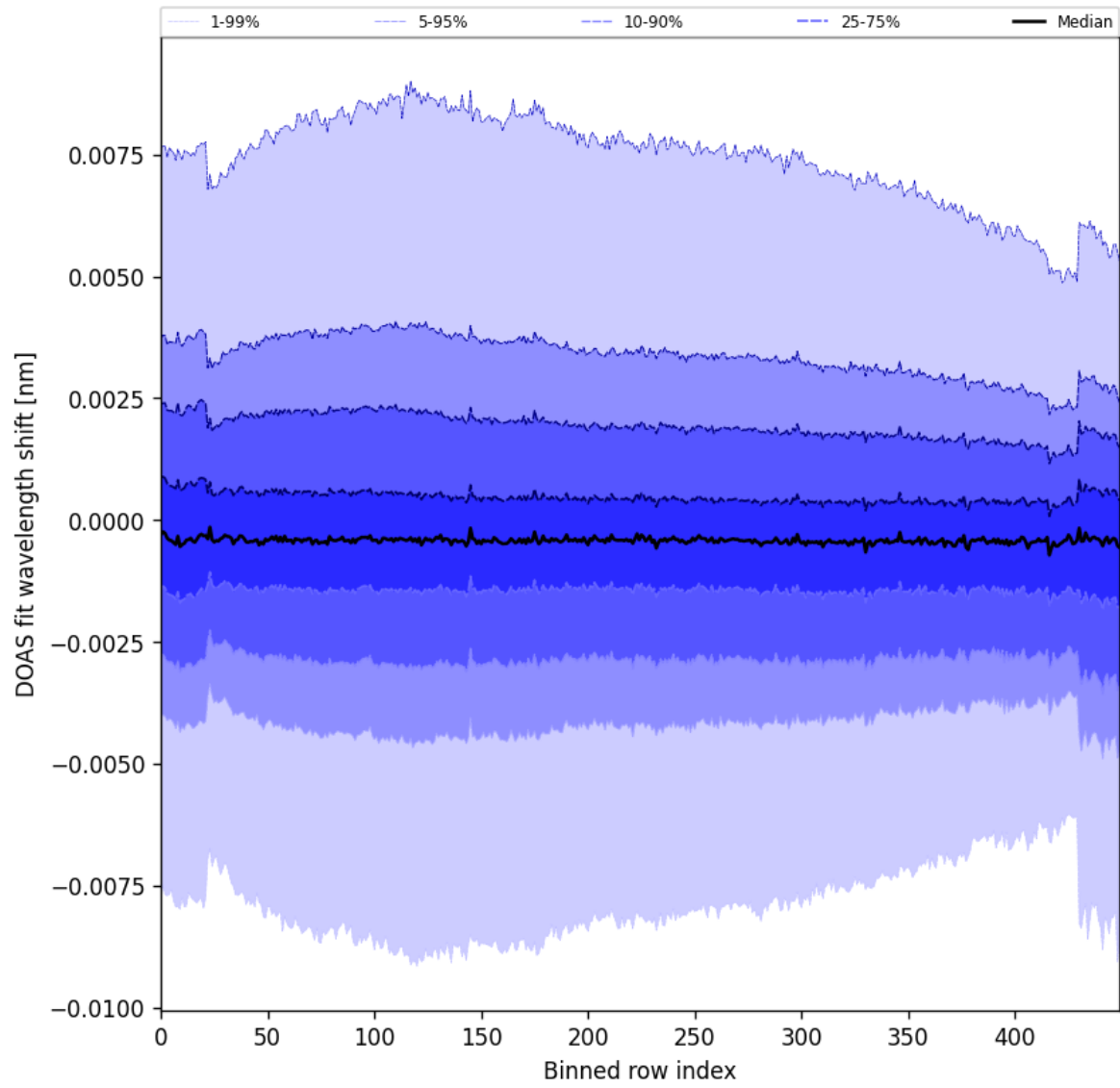
Figure 91: Along track statistics of “DOAS fit wavelength shift” for 2024-10-05 to 2024-10-07
