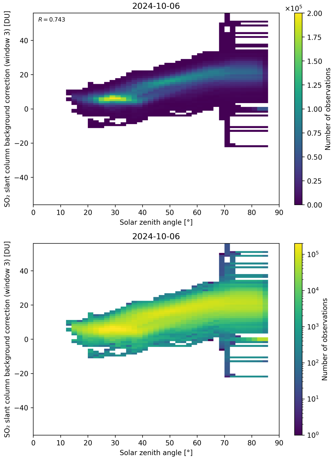
Figure 160: Scatter density plot of “Solar zenith angle” against “SO 2 slant column background correction (window 3)” for 2024-10-05 to 2024-10-07.
