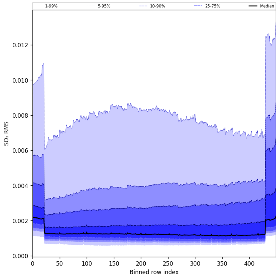
Figure 93: Along track statistics of “SO 2 RMS” for 2024-10-05 to 2024-10-07
