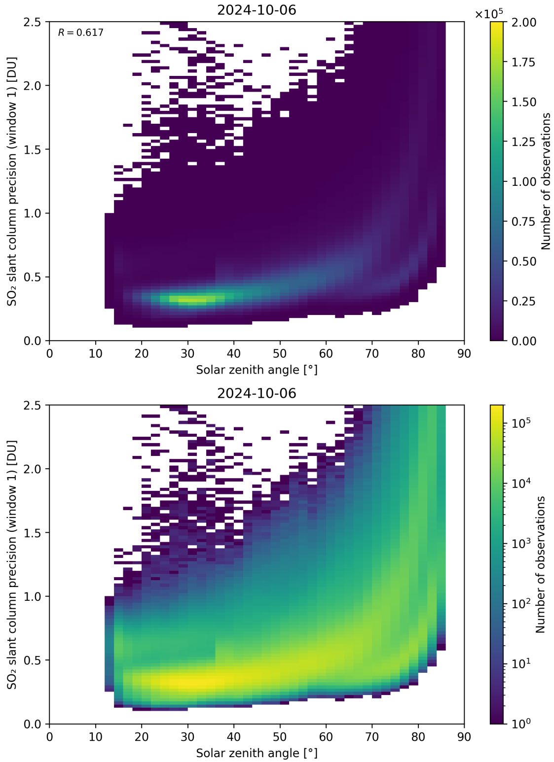
Figure 170: Scatter density plot of “Solar zenith angle” against “SO 2 slant column precision (window 1)” for 2024-10-05 to 2024-10-07.
