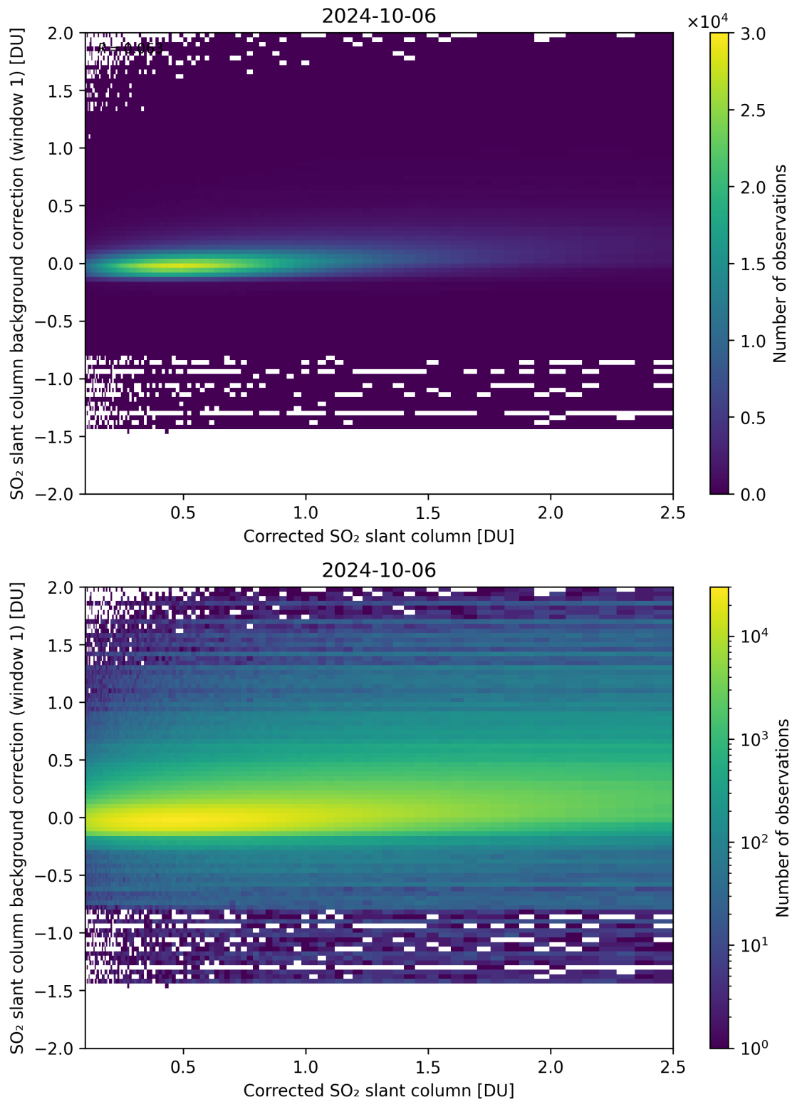
Figure 178: Scatter density plot of “Corrected SO 2 slant column” against “SO 2 slant column background correction (window 1)” for 2024-10-05 to 2024-10-07.
