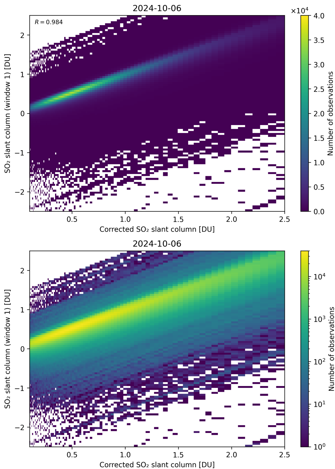
Figure 187: Scatter density plot of “Corrected SO 2 slant column” against “SO 2 slant column (window 1)” for 2024-10-05 to 2024-10-07.
