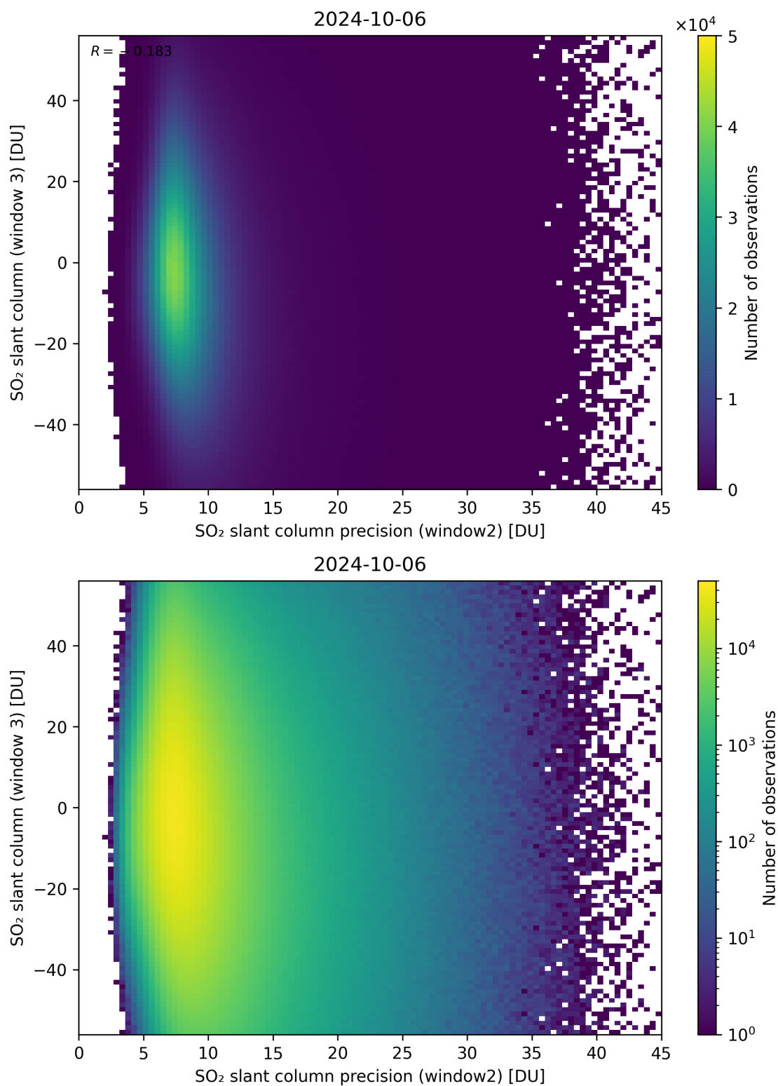
Figure 249: Scatter density plot of “SO 2 slant column precision (window2)” against “SO 2 slant column (window 3)” for 2024-10-05 to 2024-10-07.
