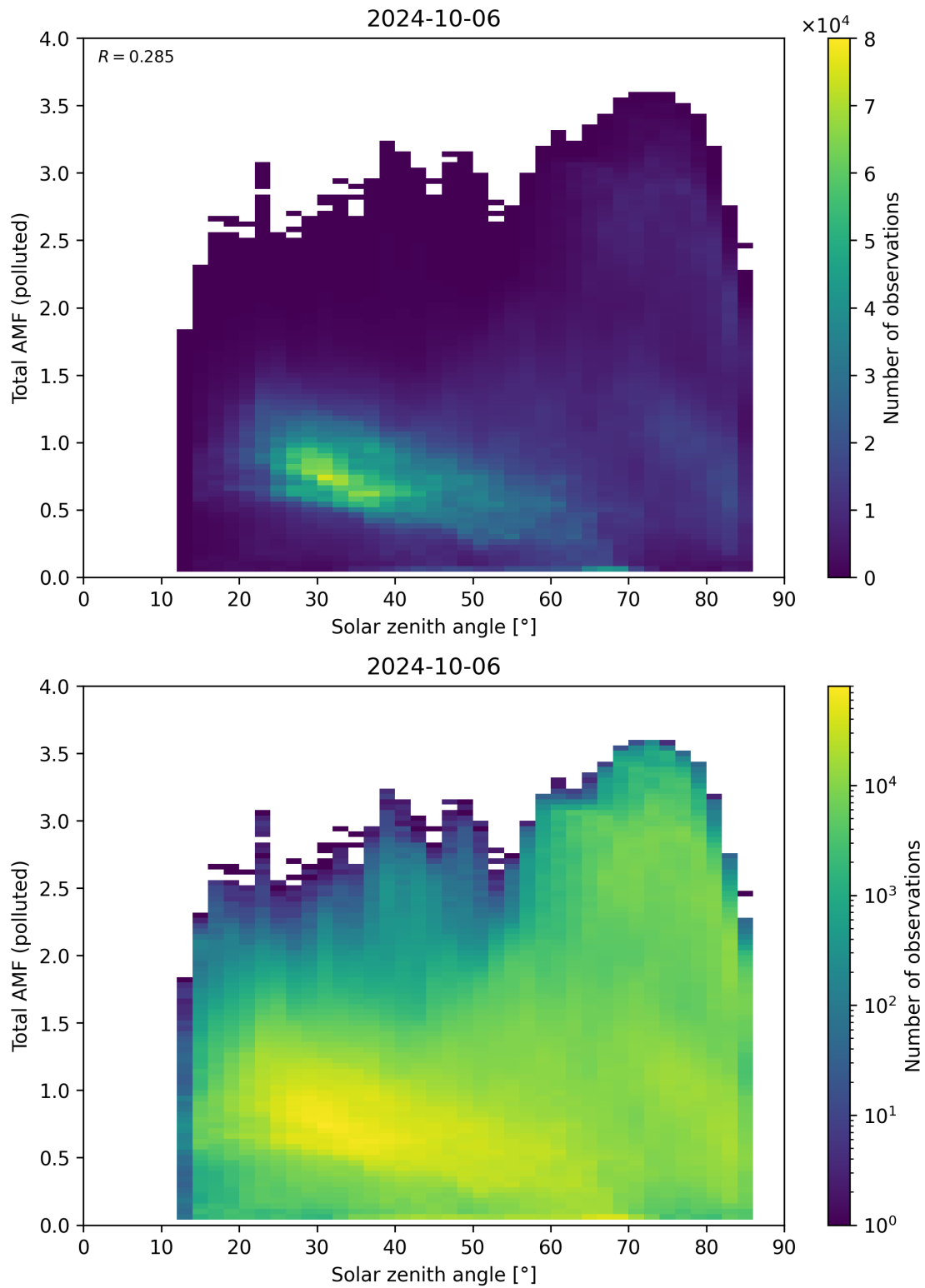
Figure 174: Scatter density plot of “Solar zenith angle” against “Total AMF (polluted)” for 2024-10-05 to 2024-10-07.
