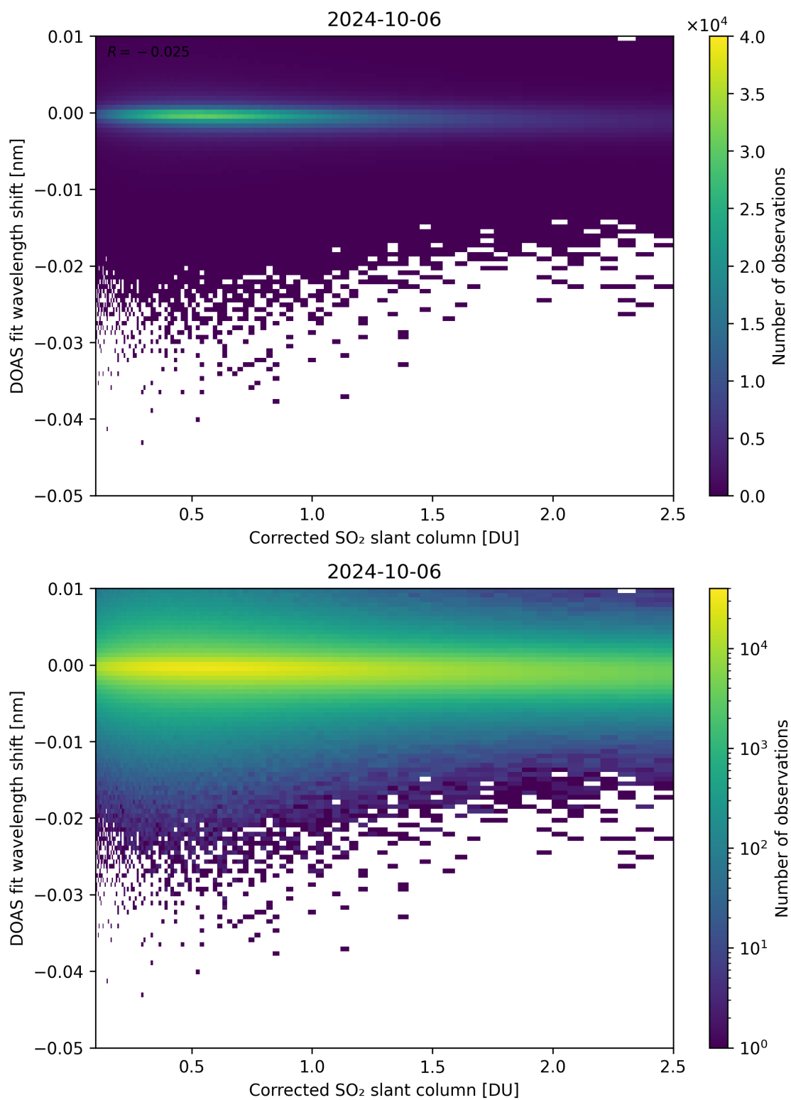
Figure 181: Scatter density plot of “Corrected SO 2 slant column” against “DOAS fit wavelength shift” for 2024-10-05 to 2024-10-07.
