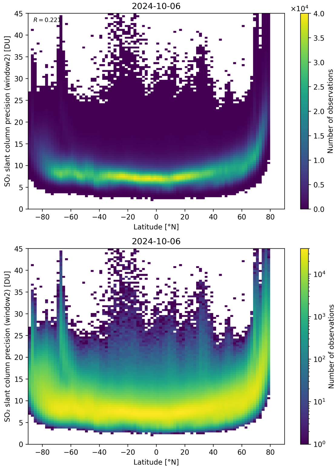
Figure 151: Scatter density plot of “Latitude” against “SO 2 slant column precision (window2)” for 2024-10-05 to 2024-10-07.
