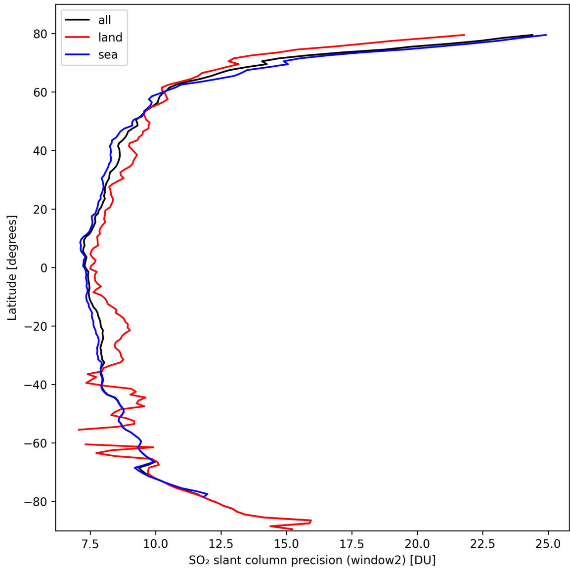
Figure 38: Zonal average of "SO 2 slant column precision (window2)" for 2024-10-05 to 2024-10-07.
