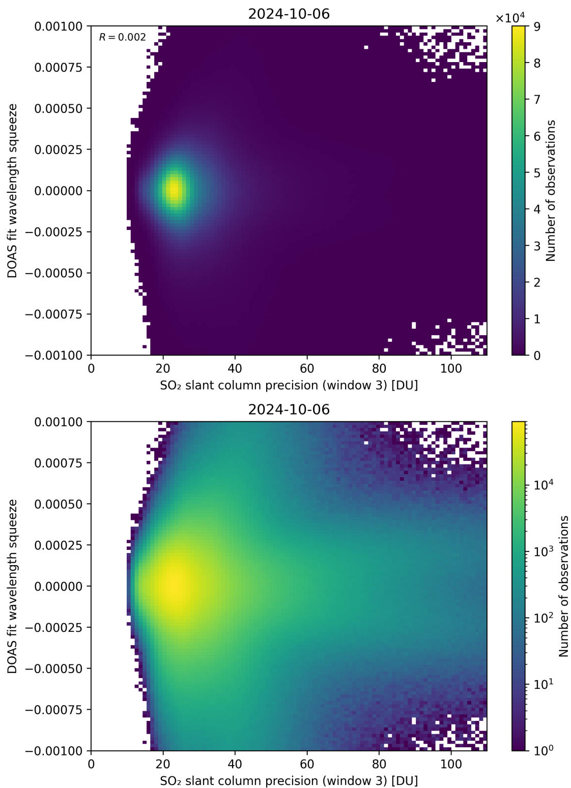
Figure 259: Scatter density plot of “SO 2 slant column precision (window 3)” against “DOAS fit wavelength squeeze” for 2024-10-05 to 2024-10-07.
