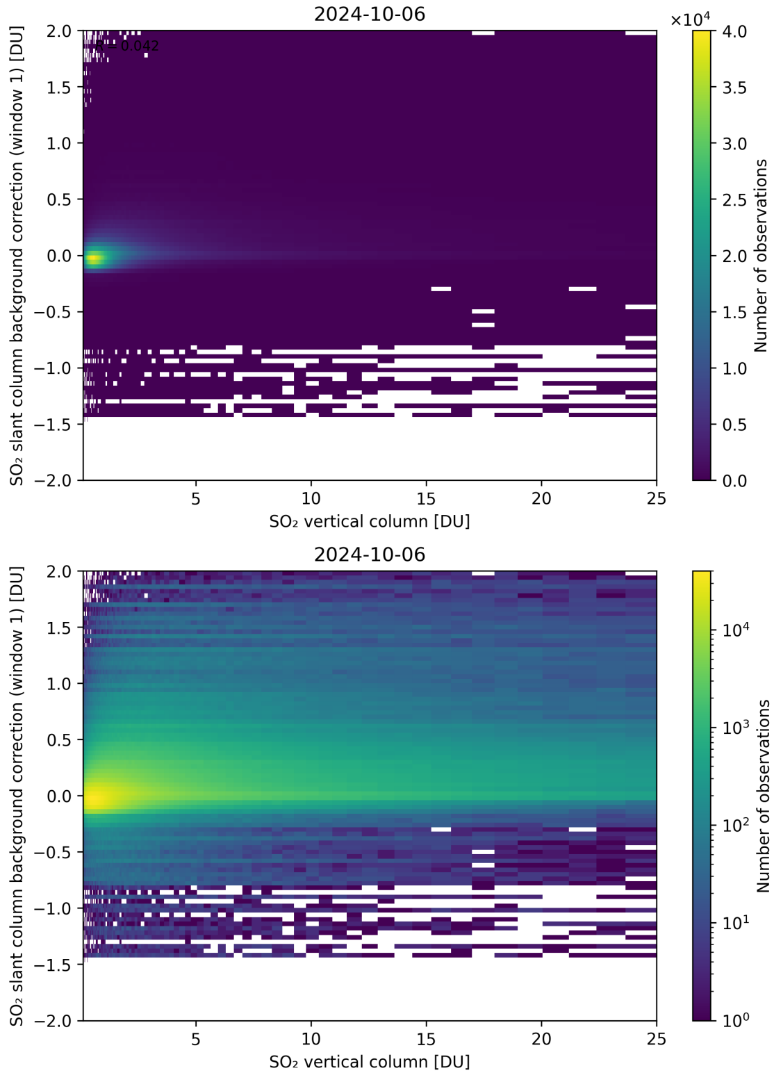
Figure 273: Scatter density plot of “SO 2 vertical column” against “SO 2 slant column background correction (window 1)” for 2024-10-05 to 2024-10-07.
