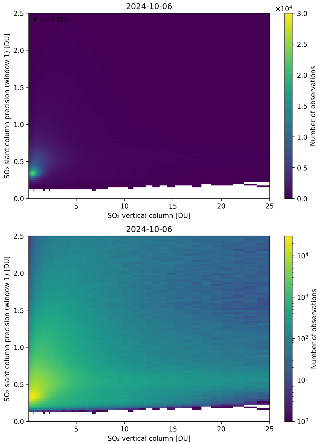
Figure 301: Scatter density plot of “SO 2 vertical column” against “SO 2 slant column precision (window 1)” for 2024-10-05 to 2024-10-07.
