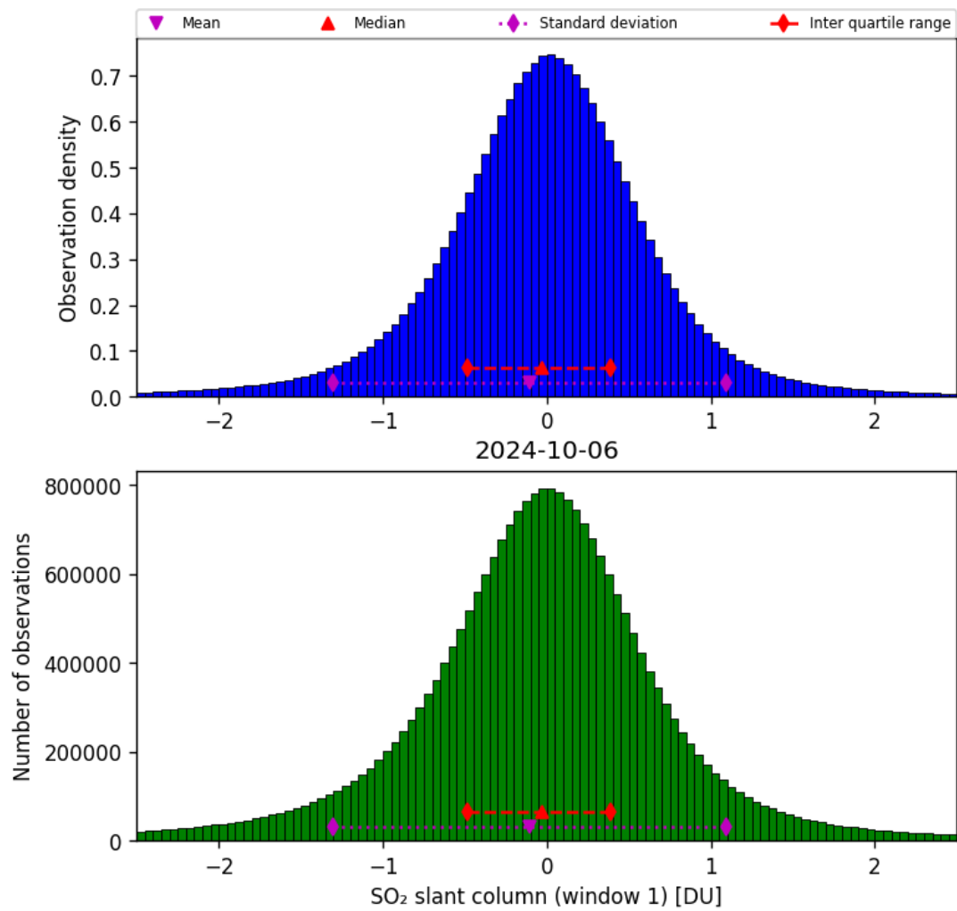
Figure 56: Histogram of “SO 2 slant column (window 1)” for 2024-10-05 to 2024-10-07
