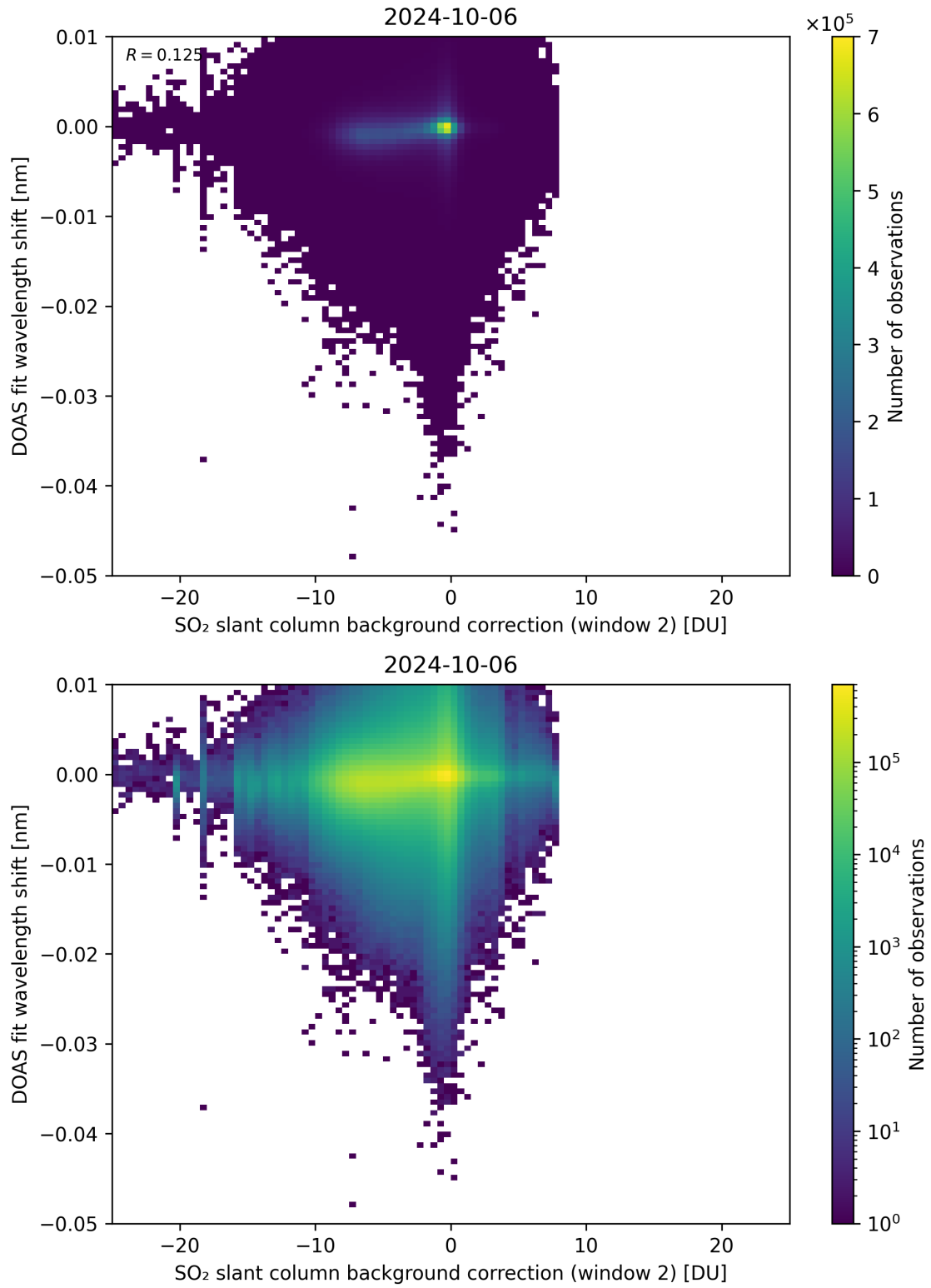
Figure 112: Scatter density plot of “SO 2 slant column background correction (window 2)” against “DOAS fit wavelength shift” for 2024-10-05 to 2024-10-07.
