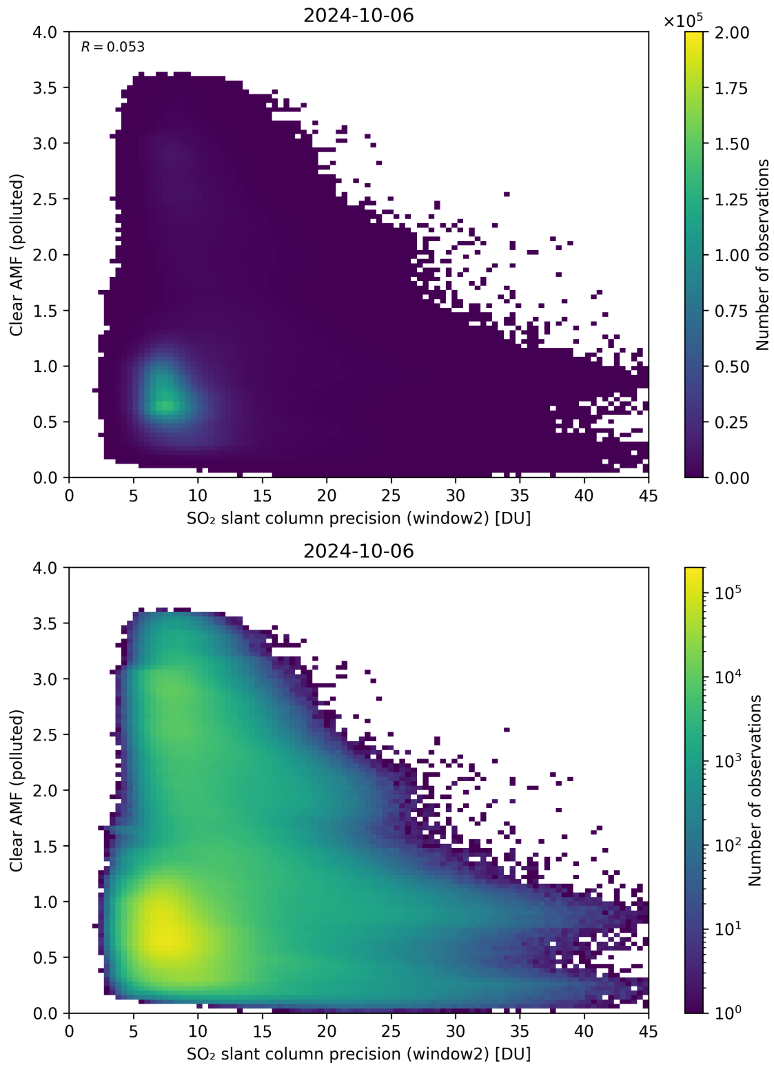
Figure 246: Scatter density plot of “SO 2 slant column precision (window2)” against “Clear AMF (polluted)” for 2024-10-05 to 2024-10-07.
