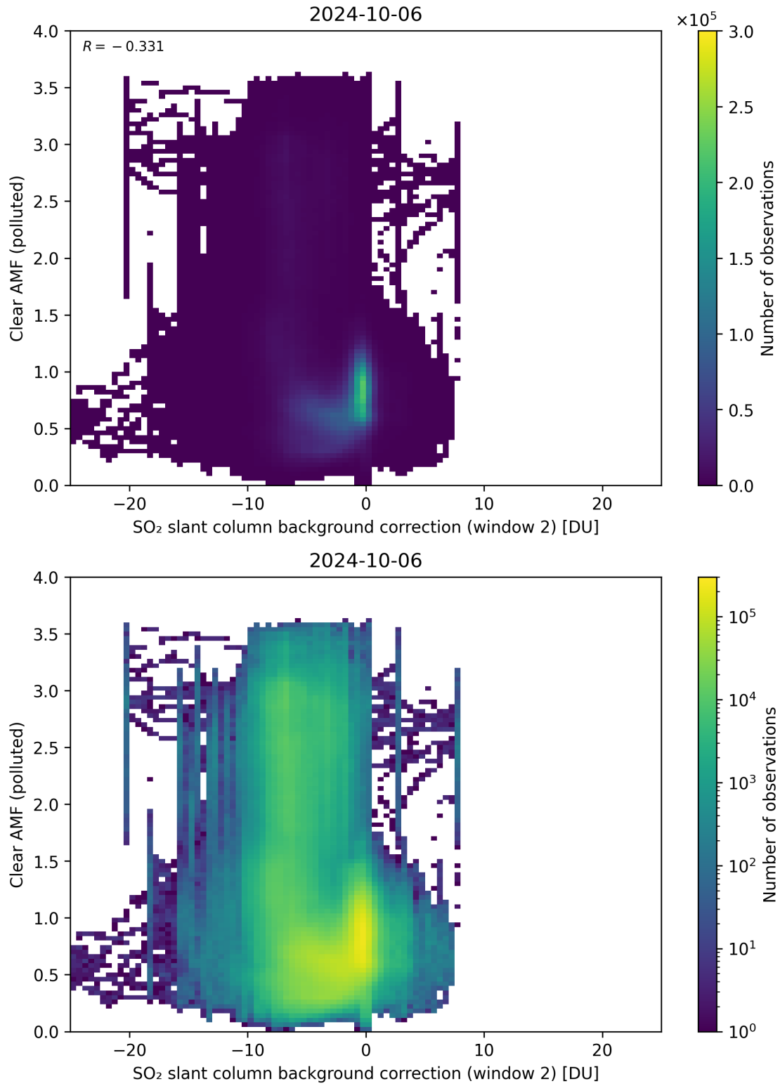
Figure 115: Scatter density plot of “SO 2 slant column background correction (window 2)” against “Clear AMF (polluted)” for 2024-10-05 to 2024-10-07.
