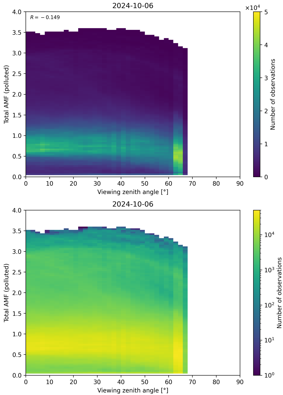
Figure 325: Scatter density plot of “Viewing zenith angle” against “Total AMF (polluted)” for 2024-10-05 to 2024-10-07.
