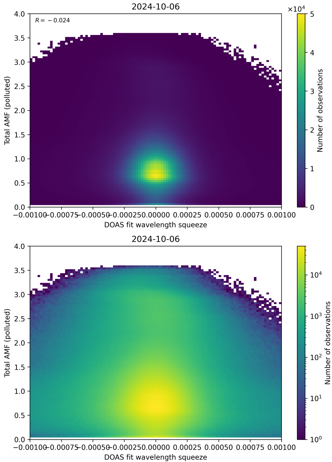
Figure 134: Scatter density plot of “DOAS fit wavelength squeeze” against “Total AMF (polluted)” for 2024-10-05 to 2024-10-07.
