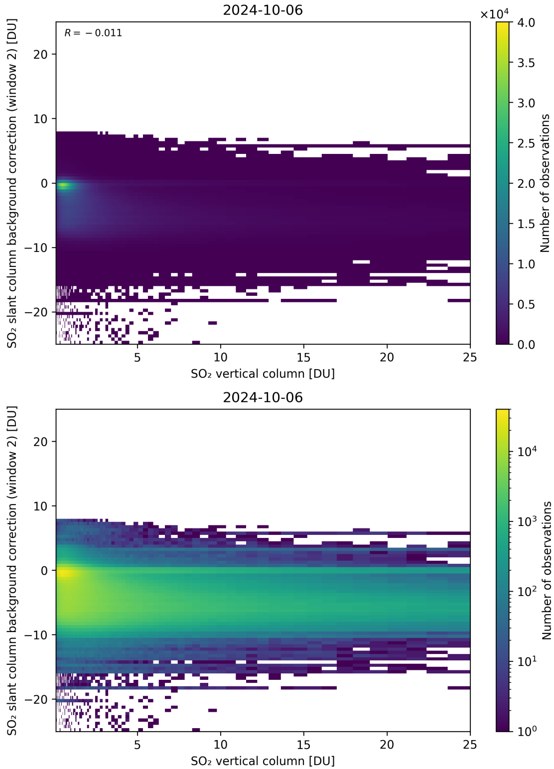
Figure 274: Scatter density plot of “SO 2 vertical column” against “SO 2 slant column background correction (window 2)” for 2024-10-05 to 2024-10-07.
