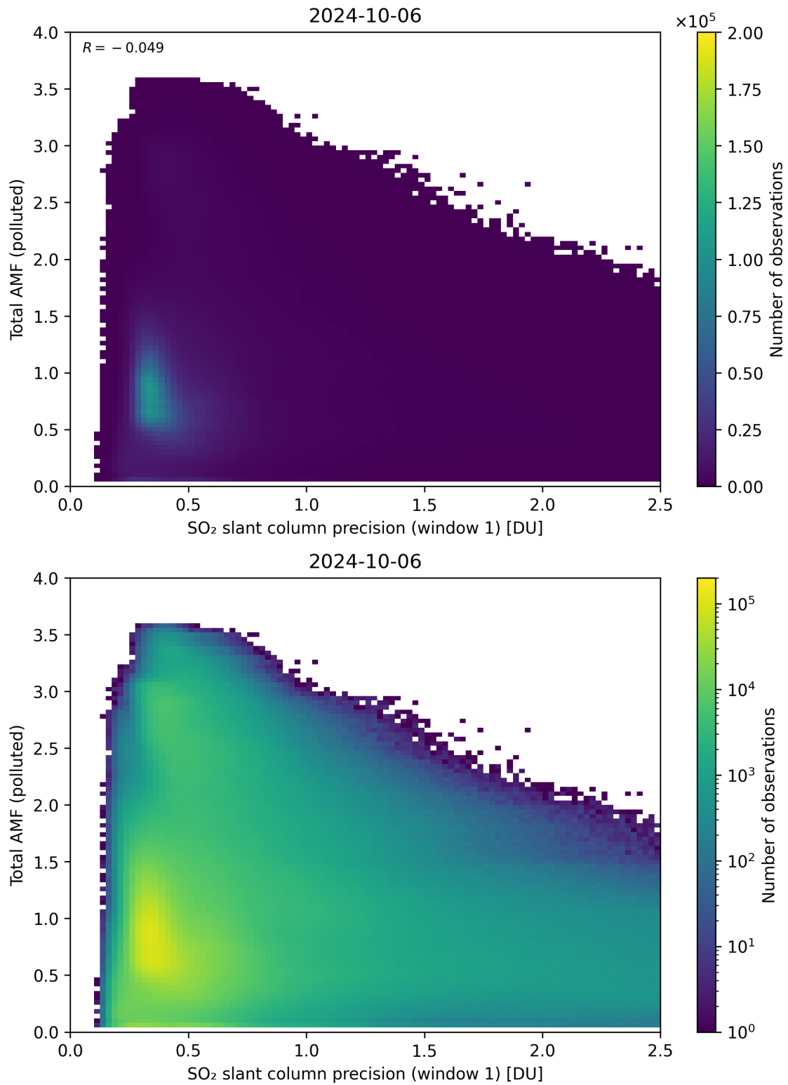
Figure 230: Scatter density plot of “SO 2 slant column precision (window 1)” against “Total AMF (polluted)” for 2024-10-05 to 2024-10-07.
