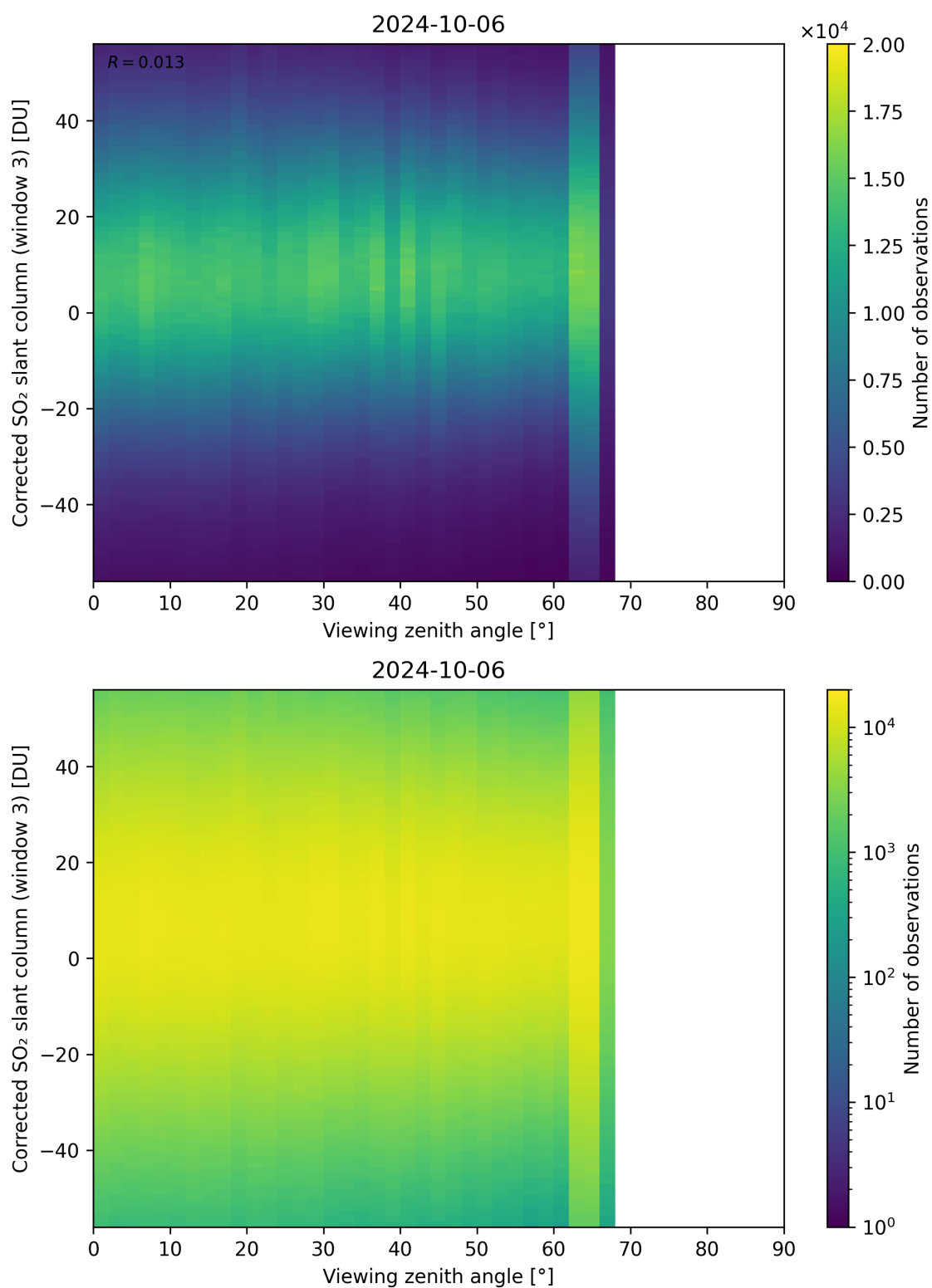
Figure 319: Scatter density plot of “Viewing zenith angle” against “Corrected SO 2 slant column (window 3)” for 2024-10-05 to 2024-10-07.
