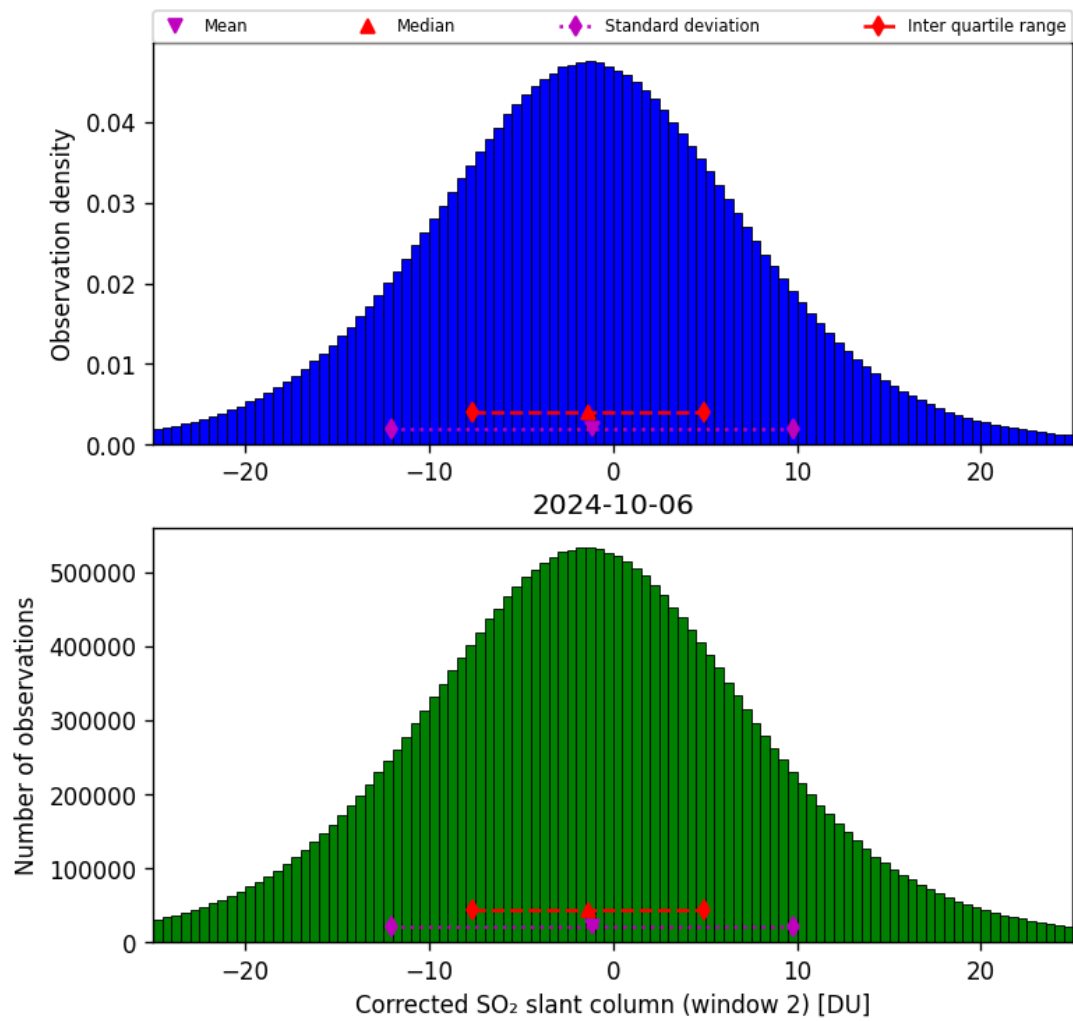
Figure 62: Histogram of “Corrected SO 2 slant column (window 2)” for 2024-10-05 to 2024-10-07
