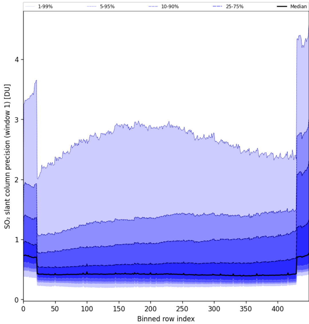
Figure 80: Along track statistics of “SO 2 slant column precision (window 1)” for 2024-10-05 to 2024-10-07
