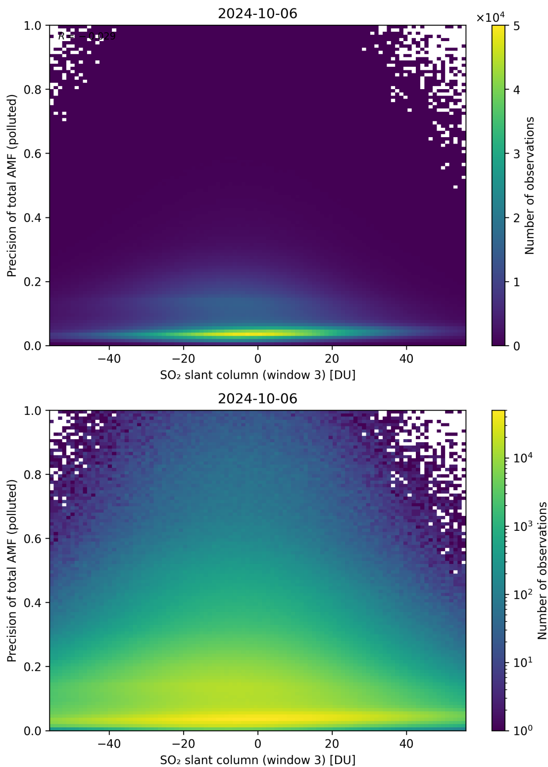
Figure 269: Scatter density plot of “SO 2 slant column (window 3)” against “Precision of total AMF (polluted)” for 2024-10-05 to 2024-10-07.
