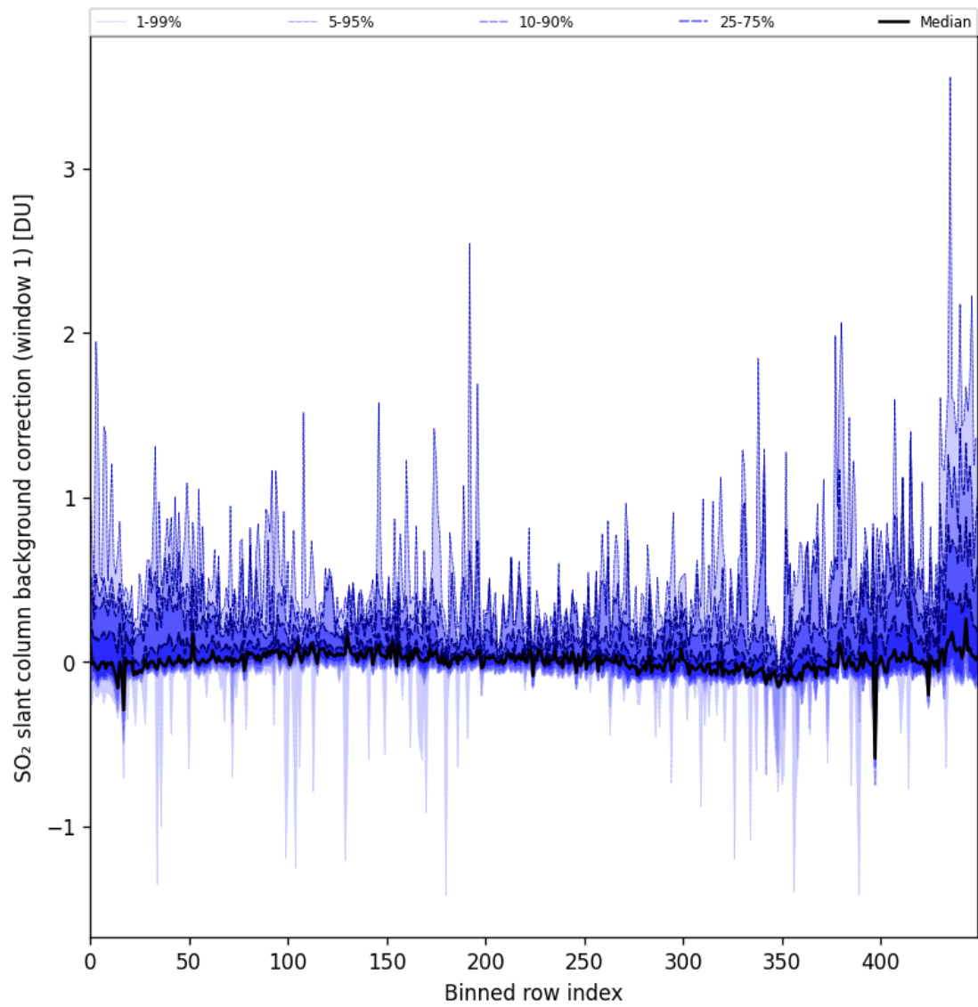
Figure 82: Along track statistics of “SO 2 slant column background correction (window 1)” for 2024-10-05 to 2024-10-07
