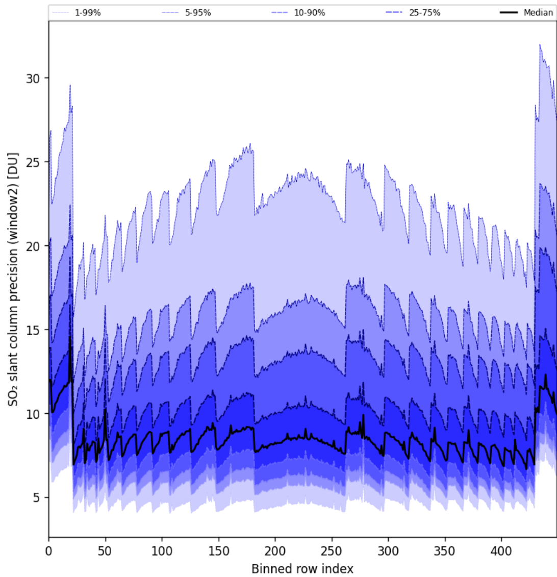
Figure 84: Along track statistics of “SO 2 slant column precision (window2)” for 2024-10-05 to 2024-10-07
