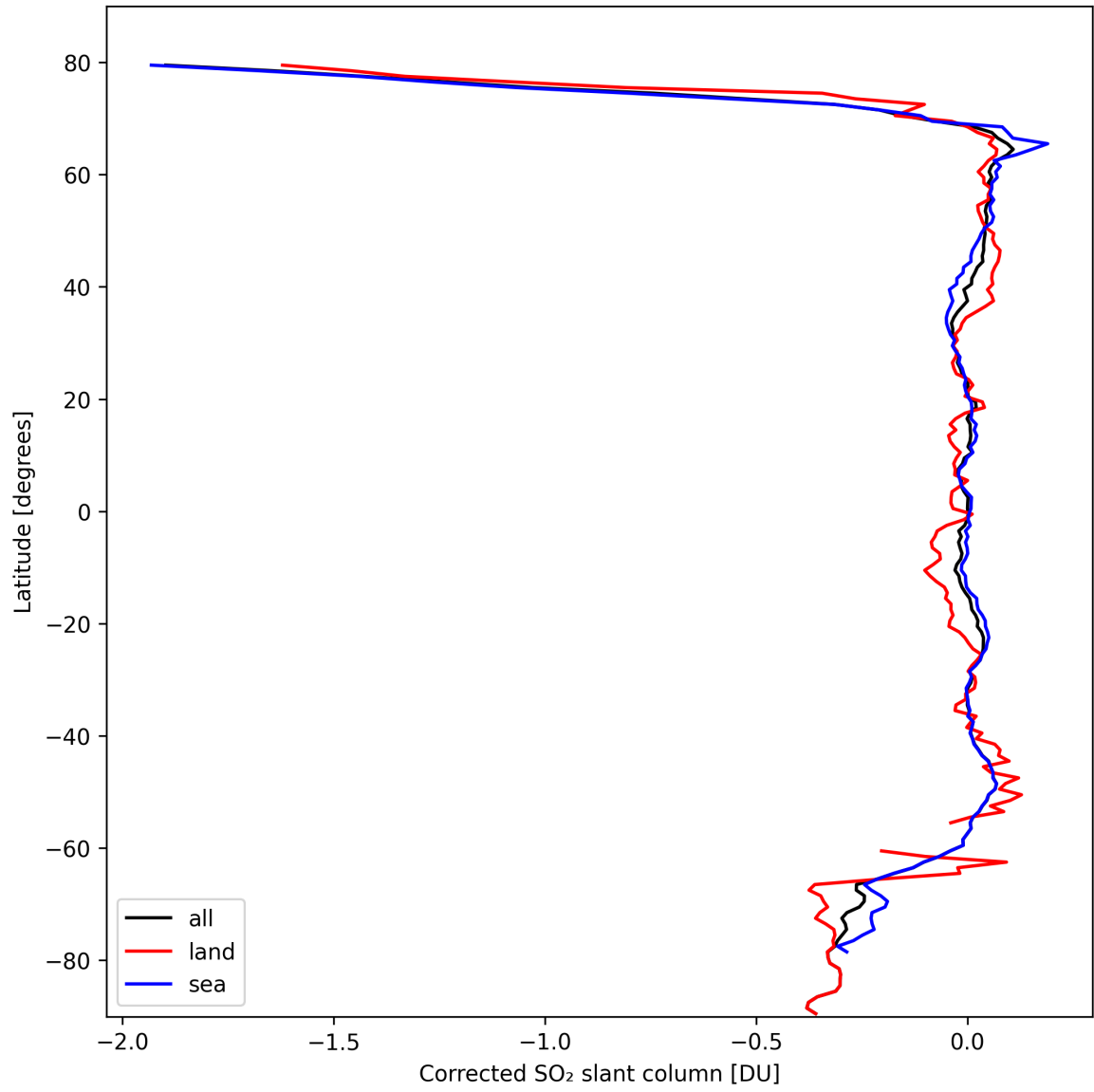
Figure 32: Zonal average of “Corrected SO 2 slant column” for 2024-10-05 to 2024-10-07.
