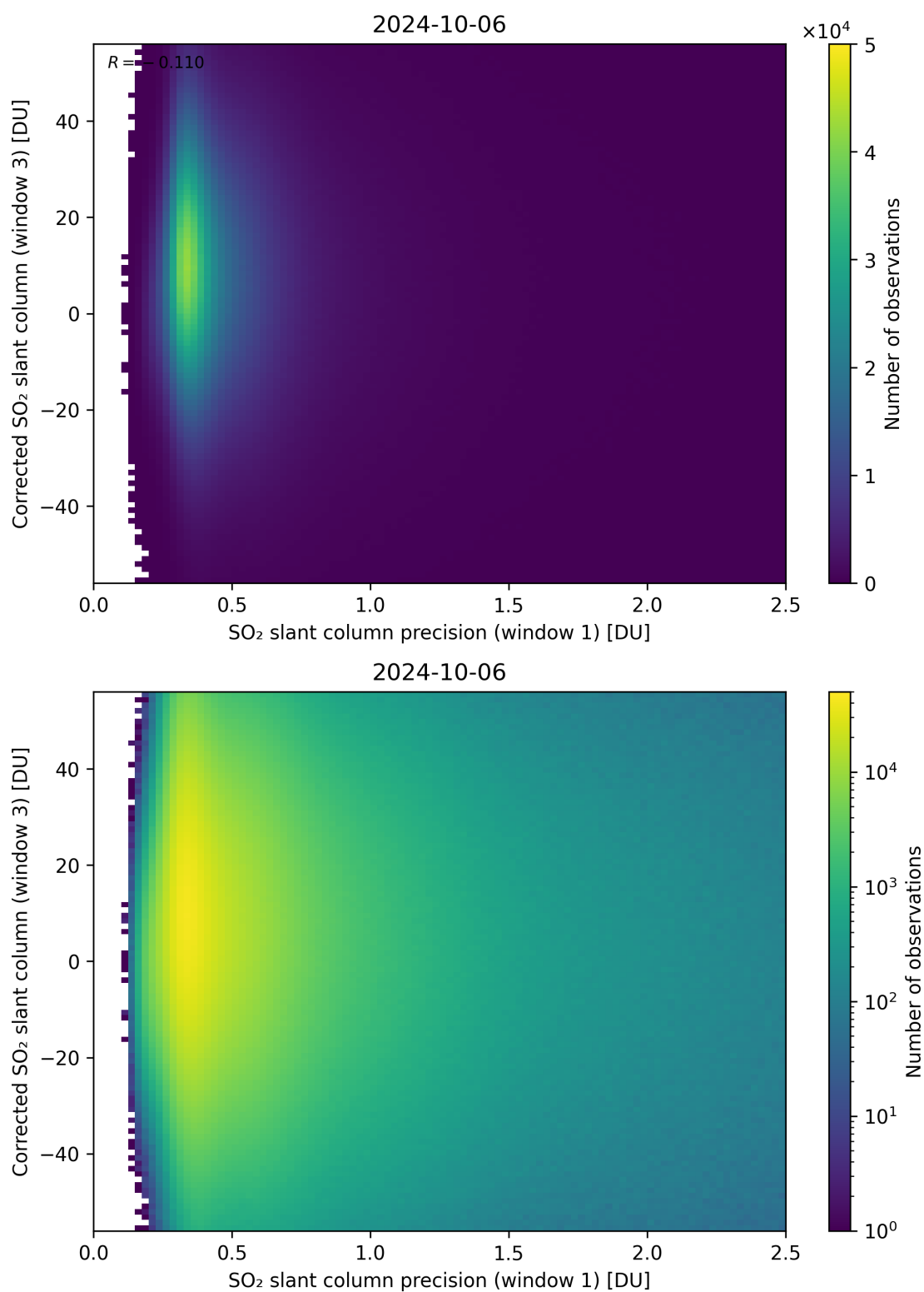
Figure 226: Scatter density plot of “SO 2 slant column precision (window 1)” against “Corrected SO 2 slant column (window 3)” for 2024-10-05 to 2024-10-07.
