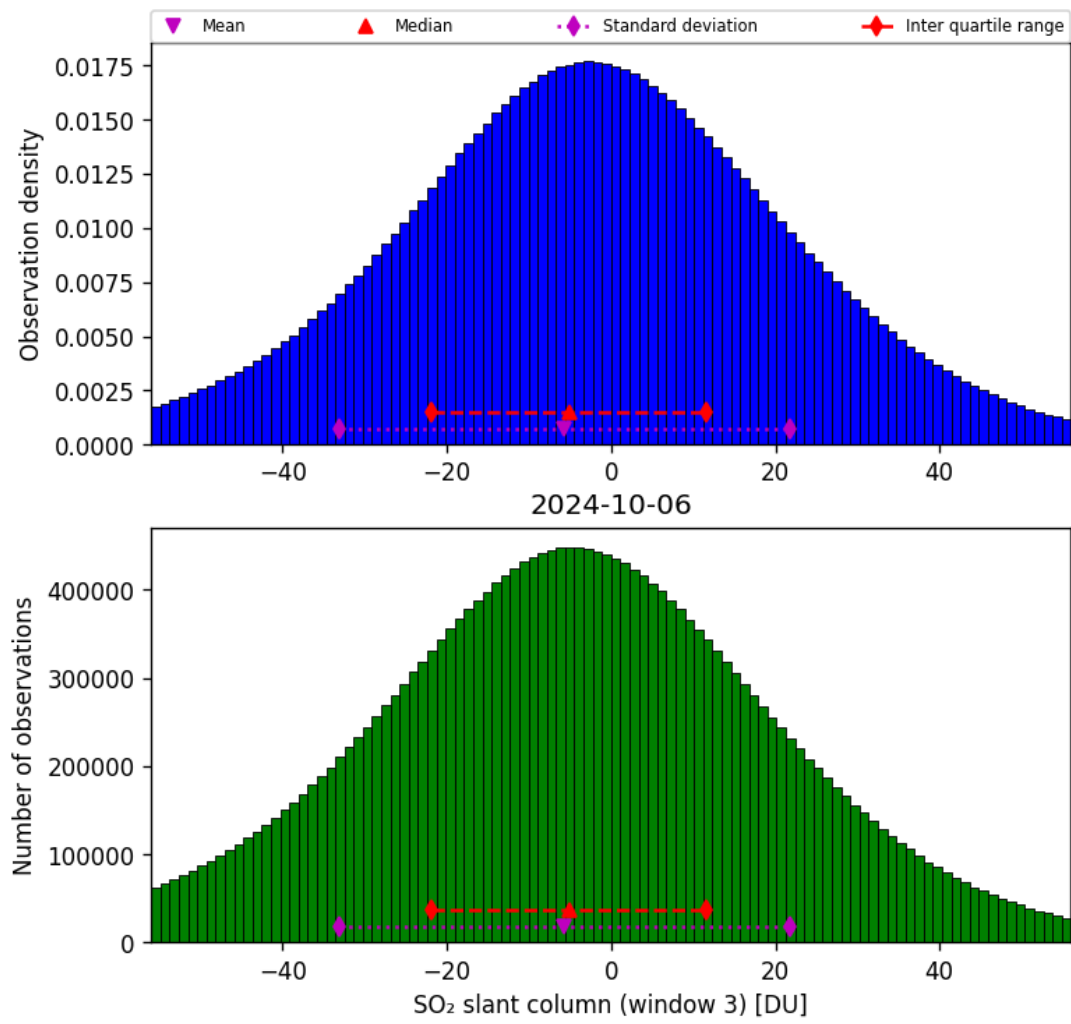
Figure 64: Histogram of “SO 2 slant column (window 3)” for 2024-10-05 to 2024-10-07
