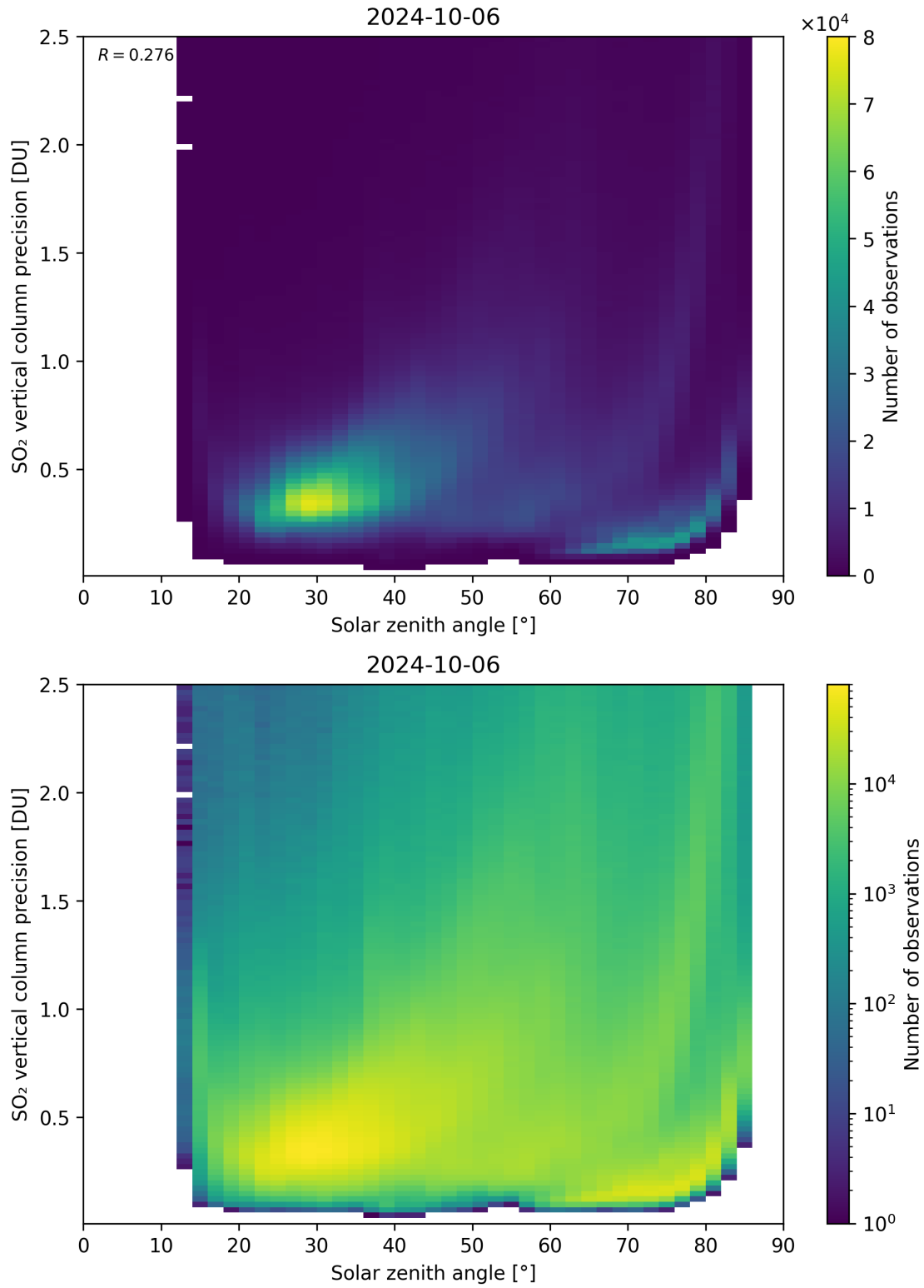
Figure 177: Scatter density plot of “Solar zenith angle” against “SO 2 vertical column precision” for 2024-10-05 to 2024-10-07.
