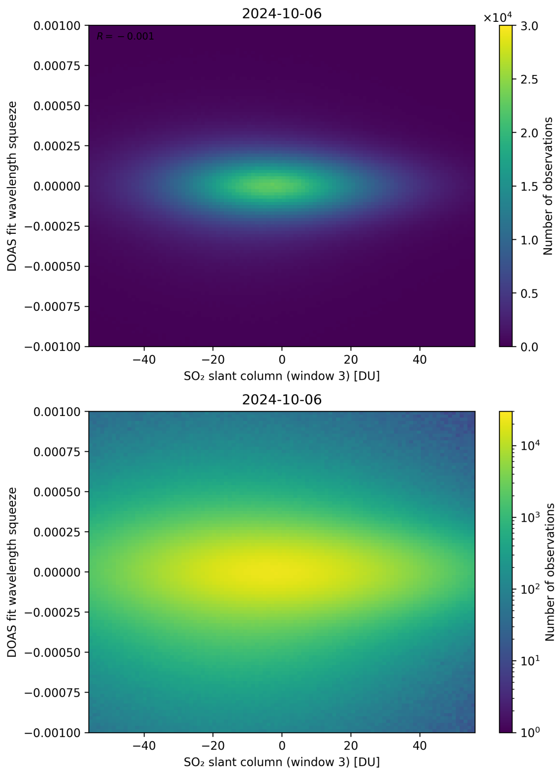
Figure 255: Scatter density plot of “SO 2 slant column (window 3)” against “DOAS fit wavelength squeeze” for 2024-10-05 to 2024-10-07.
