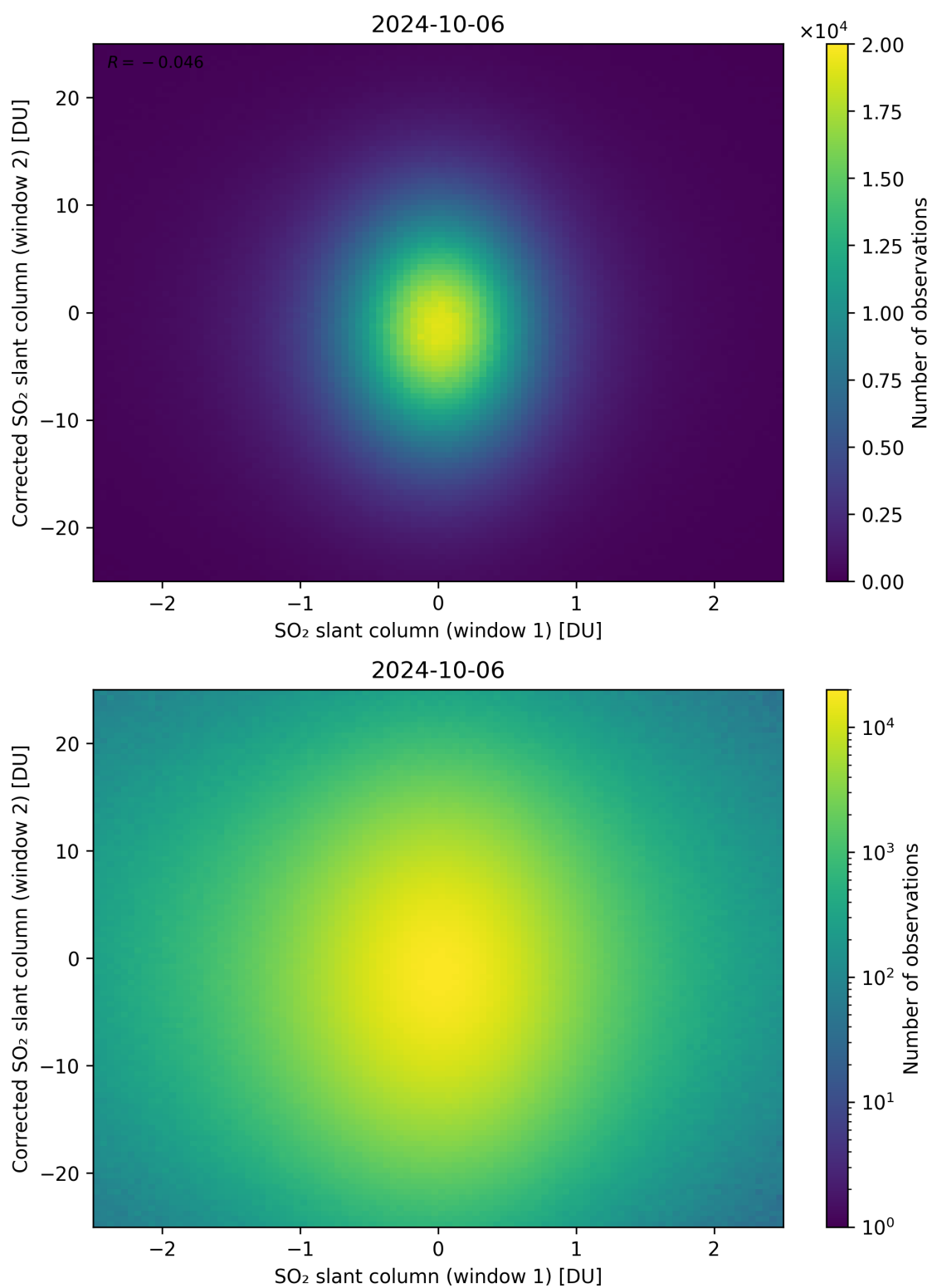
Figure 233: Scatter density plot of “SO 2 slant column (window 1)” against “Corrected SO 2 slant column (window 2)” for 2024-10-05 to 2024-10-07.
