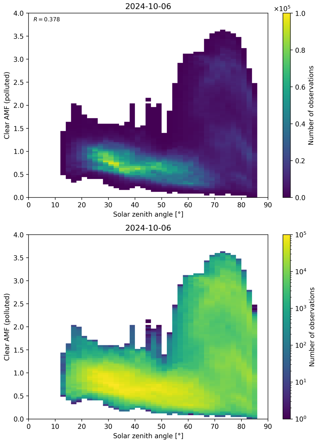
Figure 165: Scatter density plot of “Solar zenith angle” against “Clear AMF (polluted)” for 2024-10-05 to 2024-10-07.
