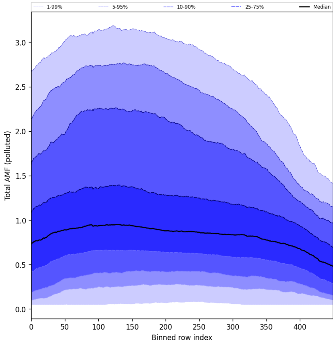
Figure 94: Along track statistics of “Total AMF (polluted)” for 2024-10-05 to 2024-10-07
