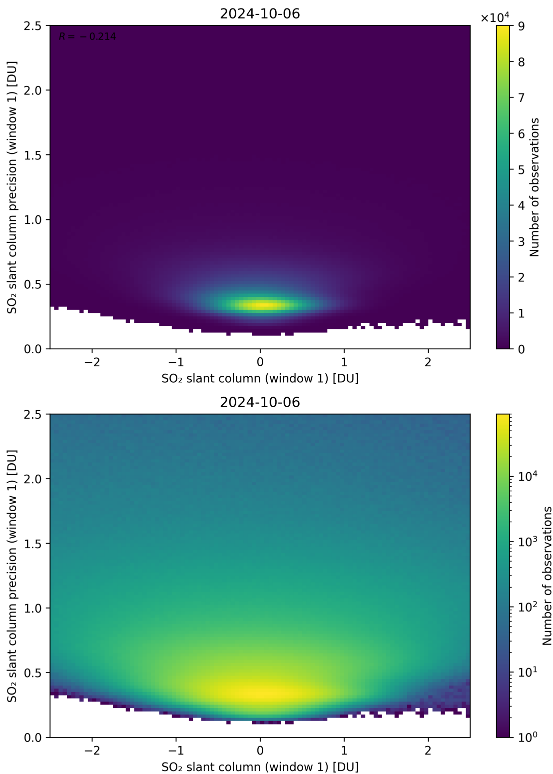
Figure 235: Scatter density plot of “SO 2 slant column (window 1)” against “SO 2 slant column precision (window 1)” for 2024-10-05 to 2024-10-07.
