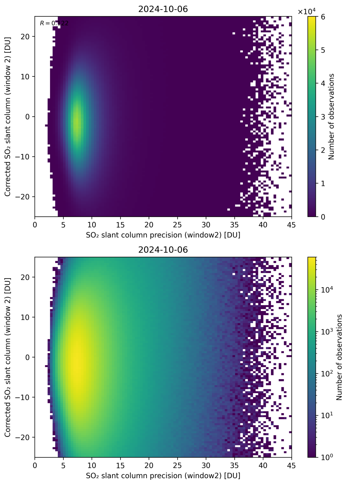
Figure 247: Scatter density plot of “SO 2 slant column precision (window2)” against “Corrected SO 2 slant column (window 2)” for 2024-10-05 to 2024-10-07.
