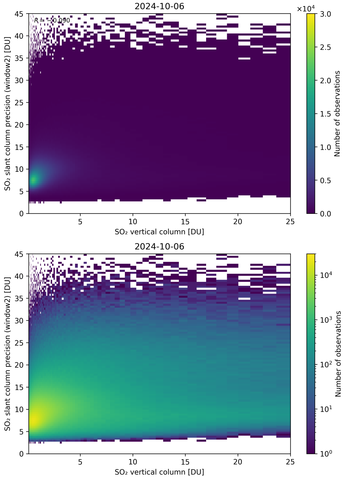
Figure 302: Scatter density plot of “SO 2 vertical column” against “SO 2 slant column precision (window2)” for 2024-10-05 to 2024-10-07.
