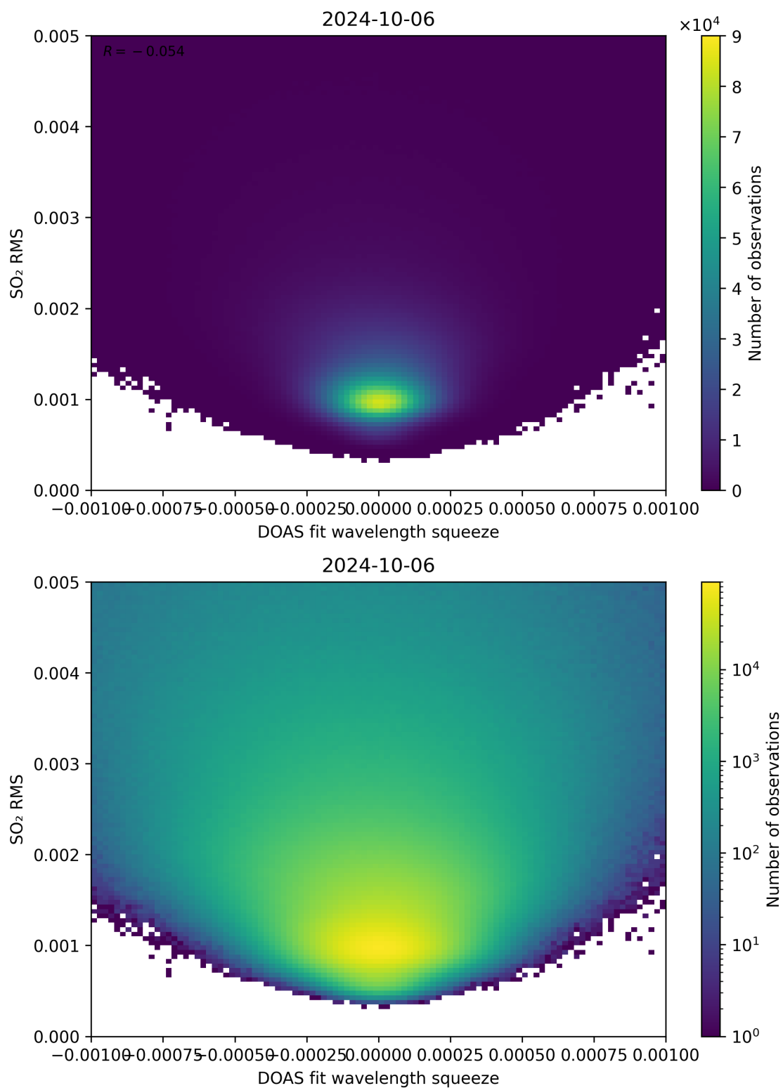
Figure 132: Scatter density plot of “DOAS fit wavelength squeeze” against “SO 2 RMS” for 2024-10-05 to 2024-10-07.
