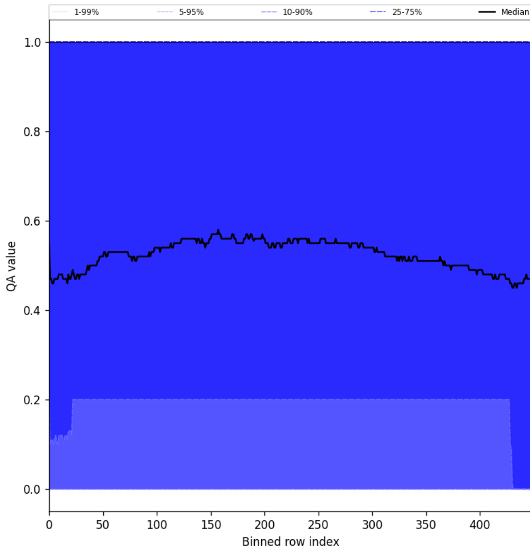
Figure 75: Along track statistics of “QA value” for 2024-10-05 to 2024-10-07
