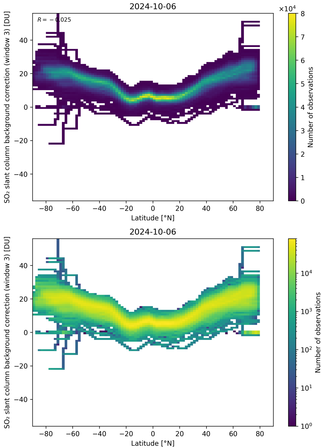
Figure 141: Scatter density plot of “Latitude” against “SO 2 slant column background correction (window 3)” for 2024-10-05 to 2024-10-07.
