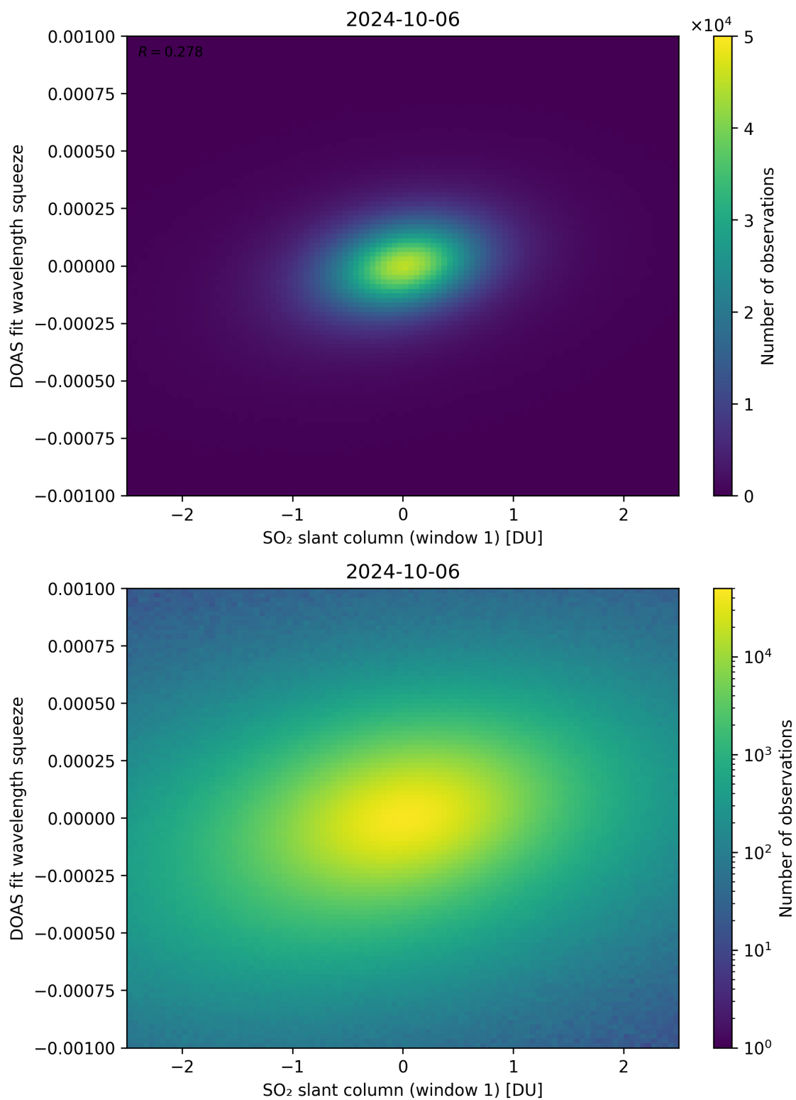
Figure 216: Scatter density plot of “SO 2 slant column (window 1)” against “DOAS fit wavelength squeeze” for 2024-10-05 to 2024-10-07.
