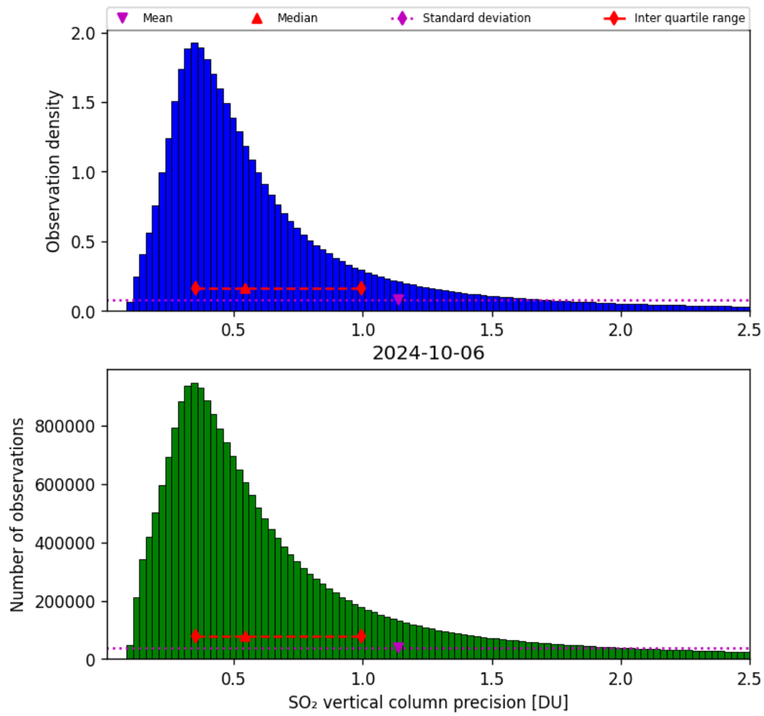
Figure 54: Histogram of “SO 2 vertical column precision” for 2024-10-05 to 2024-10-07
