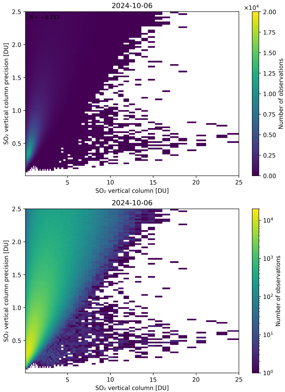
Figure 307: Scatter density plot of “SO 2 vertical column” against “SO 2 vertical column precision” for 2024-10-05 to 2024-10-07.
