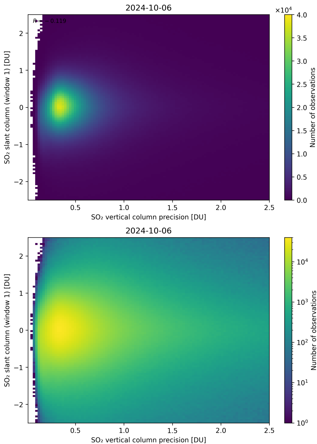
Figure 289: Scatter density plot of “SO 2 vertical column precision” against “SO 2 slant column (window 1)” for 2024-10-05 to 2024-10-07.
