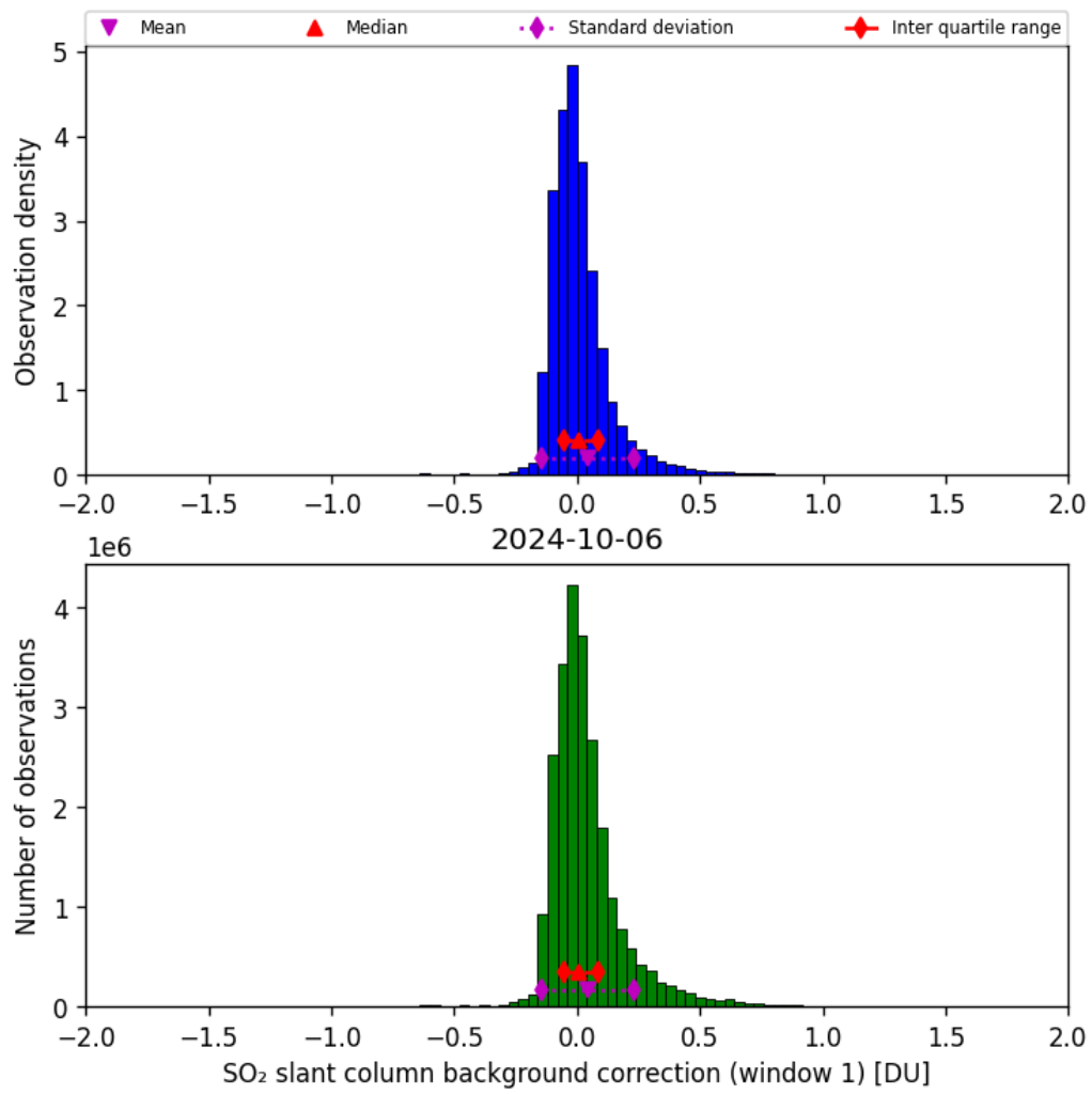
Figure 59: Histogram of “SO 2 slant column background correction (window 1)” for 2024-10-05 to 2024-10-07
