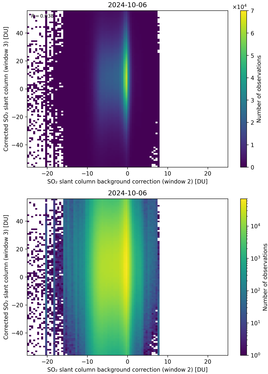
Figure 116: Scatter density plot of “SO 2 slant column background correction (window 2)” against “Corrected SO 2 slant column (window 3)” for 2024-10-05 to 2024-10-07.
