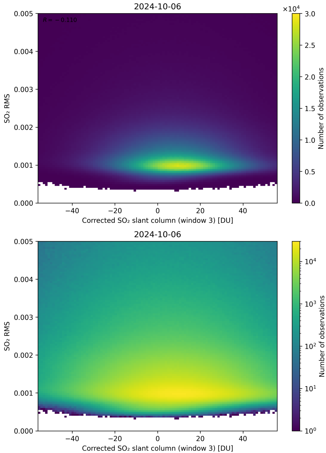
Figure 208: Scatter density plot of “Corrected SO 2 slant column (window 3)” against “SO 2 RMS” for 2024-10-05 to 2024-10-07.
