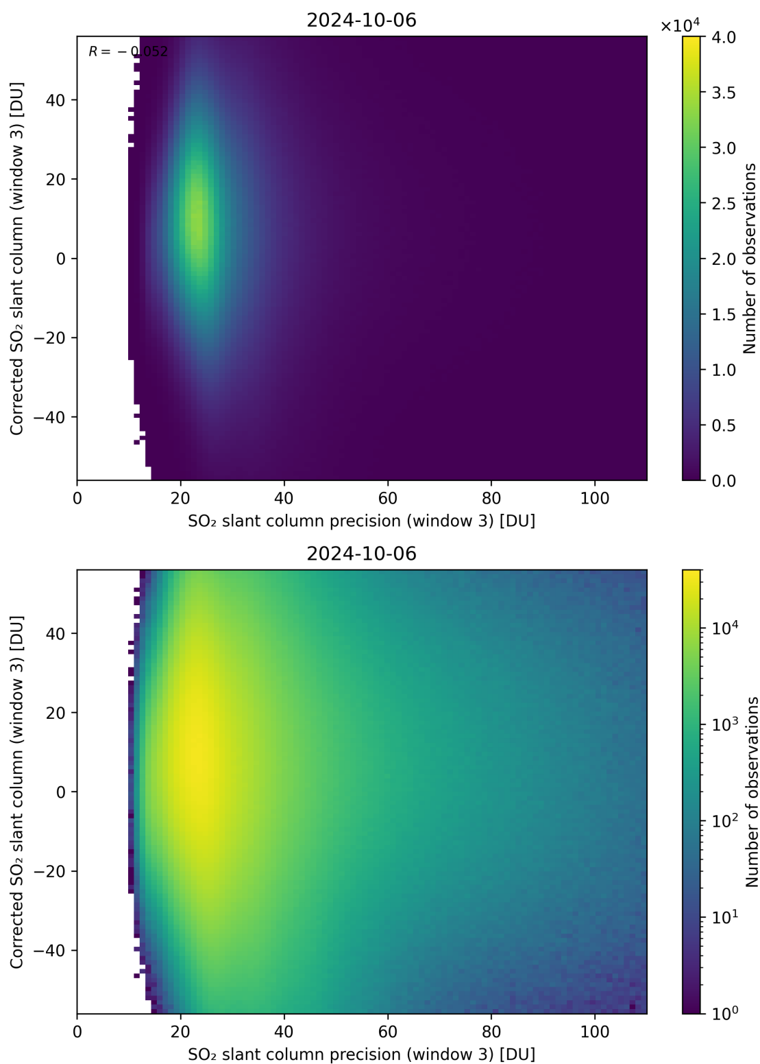
Figure 262: Scatter density plot of “SO 2 slant column precision (window 3)” against “Corrected SO 2 slant column (window 3)” for 2024-10-05 to 2024-10-07.
