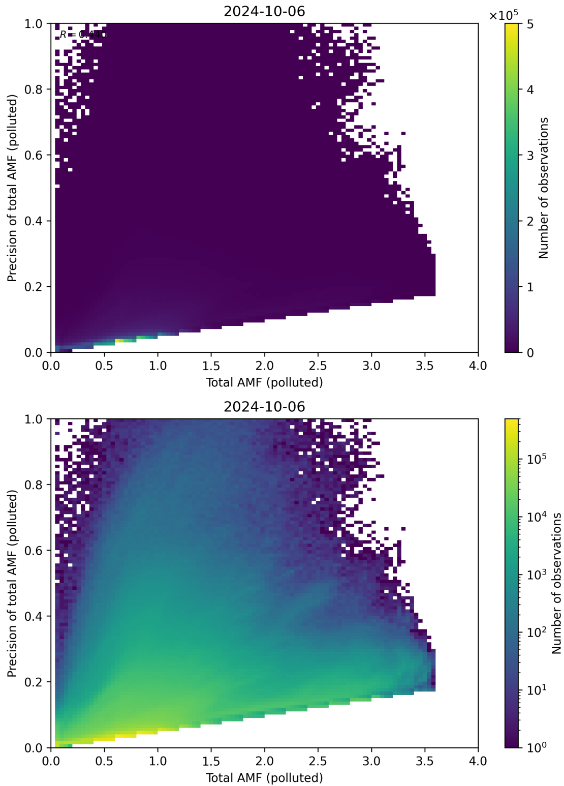
Figure 272: Scatter density plot of “Total AMF (polluted)” against “Precision of total AMF (polluted)” for 2024-10-05 to 2024-10-07.
