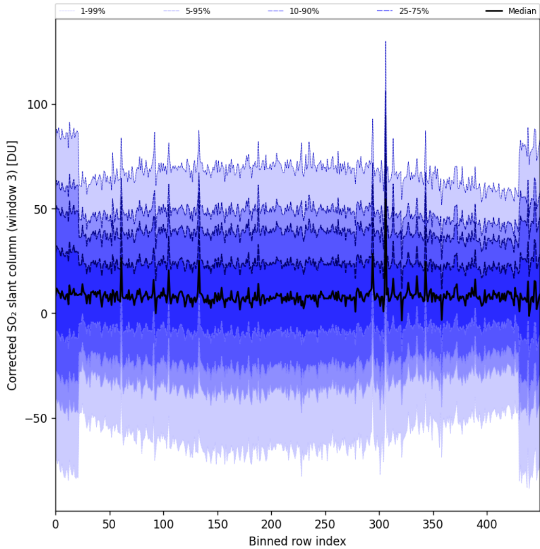
Figure 89: Along track statistics of “Corrected SO 2 slant column (window 3)” for 2024-10-05 to 2024-10-07
