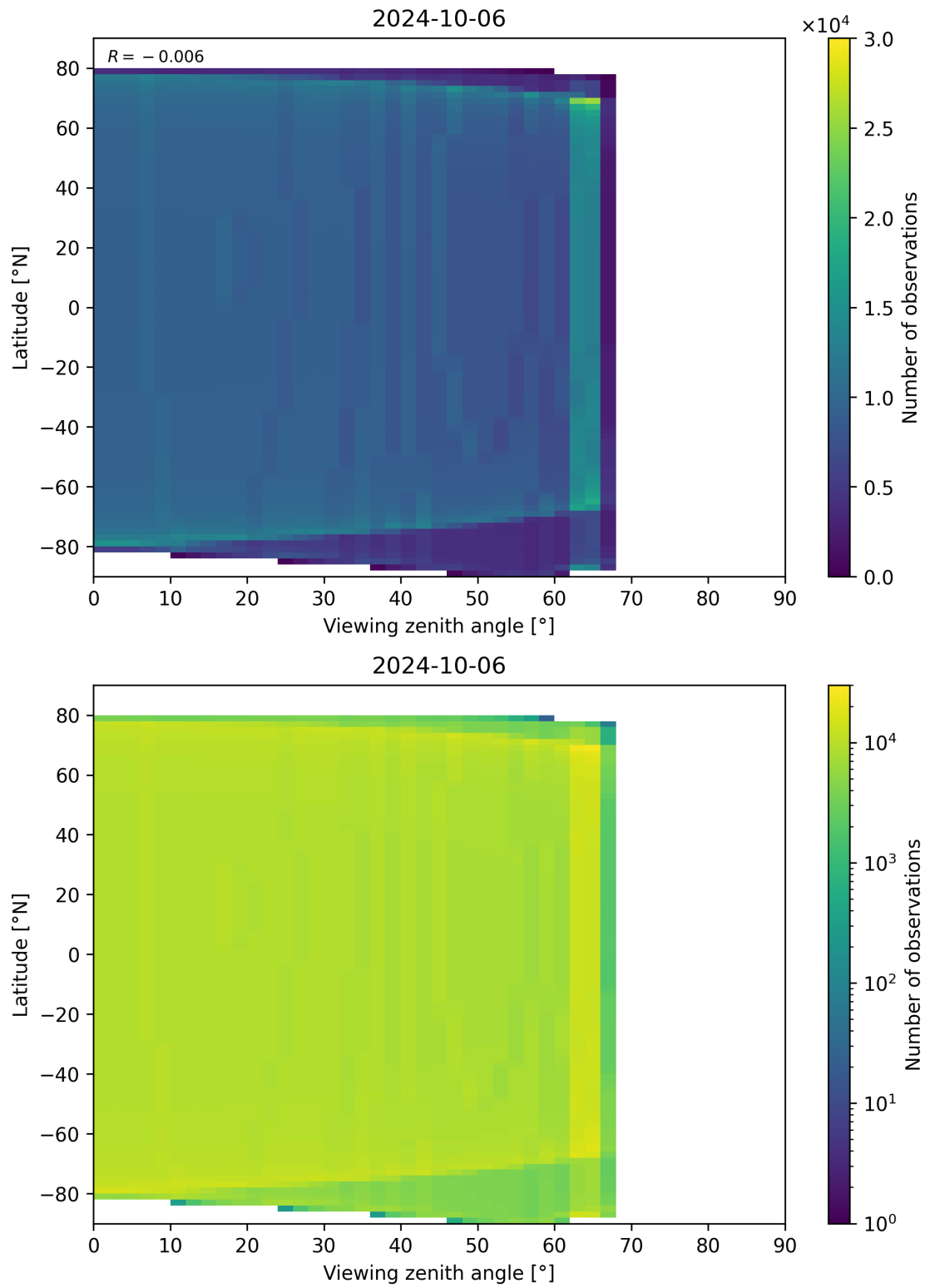
Figure 314: Scatter density plot of “Viewing zenith angle” against “Latitude” for 2024-10-05 to 2024-10-07.
