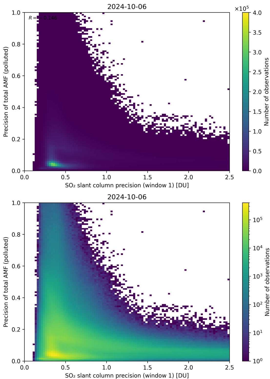
Figure 231: Scatter density plot of “SO 2 slant column precision (window 1)” against “Precision of total AMF (polluted)” for 2024-10-05 to 2024-10-07.
