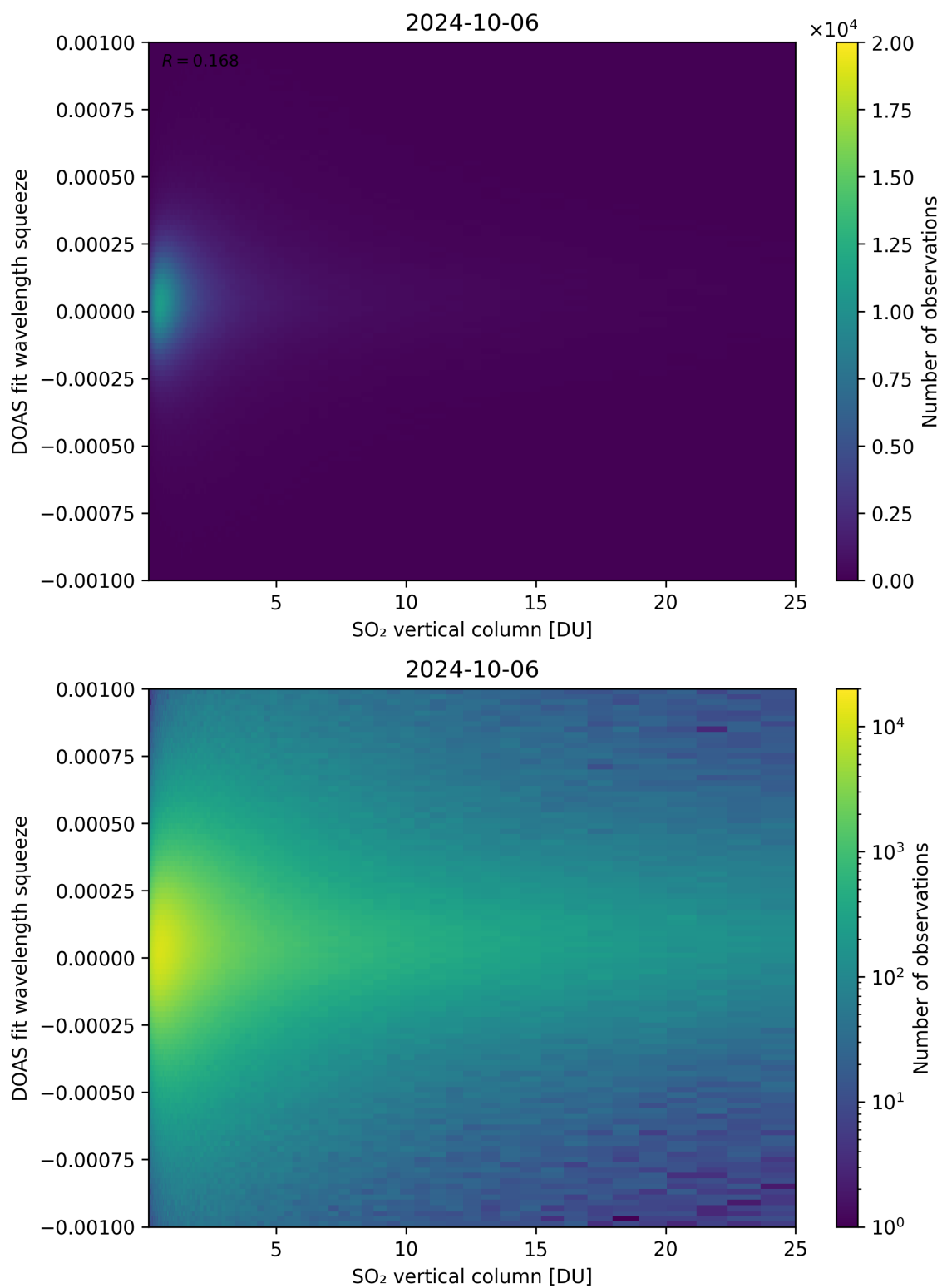
Figure 277: Scatter density plot of “SO 2 vertical column” against “DOAS fit wavelength squeeze” for 2024-10-05 to 2024-10-07.
