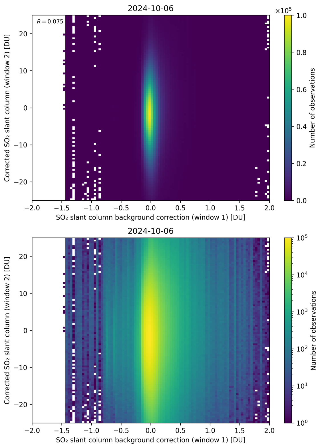
Figure 104: Scatter density plot of “SO 2 slant column background correction (window 1)” against “Corrected SO 2 slant column (window 2)” for 2024-10-05 to 2024-10-07.
