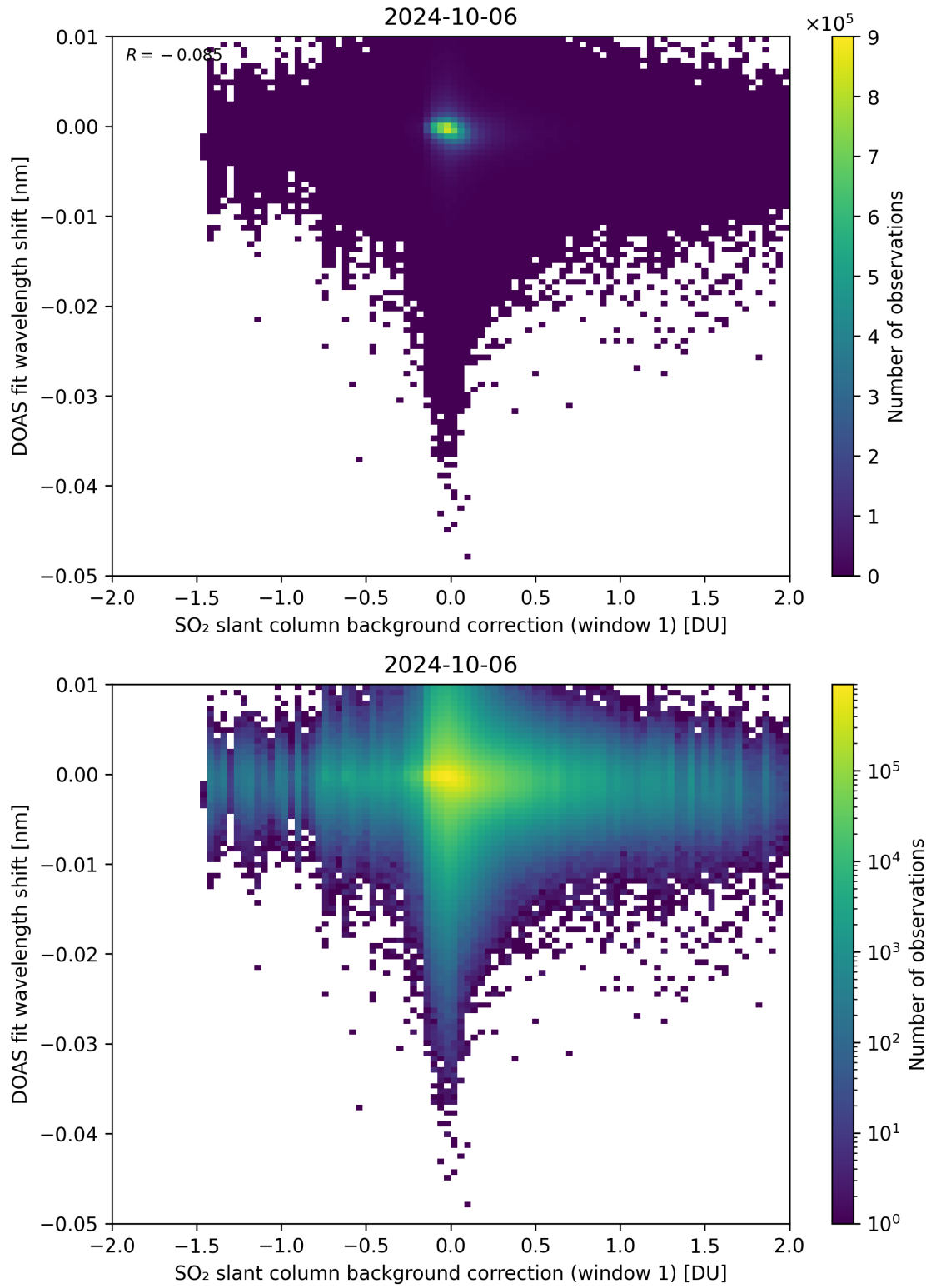
Figure 100: Scatter density plot of “SO 2 slant column background correction (window 1)” against “DOAS fit wavelength shift” for 2024-10-05 to 2024-10-07.
