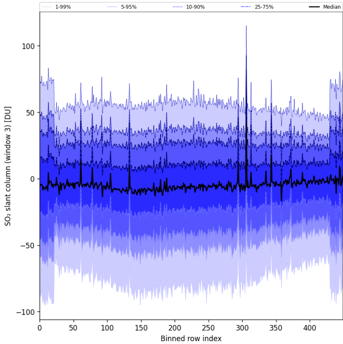
Figure 87: Along track statistics of “SO 2 slant column (window 3)” for 2024-10-05 to 2024-10-07
