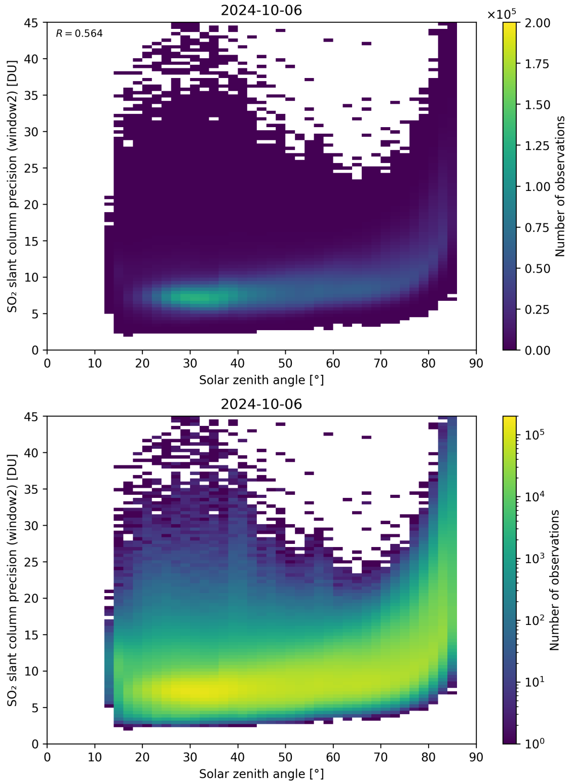
Figure 171: Scatter density plot of “Solar zenith angle” against “SO 2 slant column precision (window2)” for 2024-10-05 to 2024-10-07.
