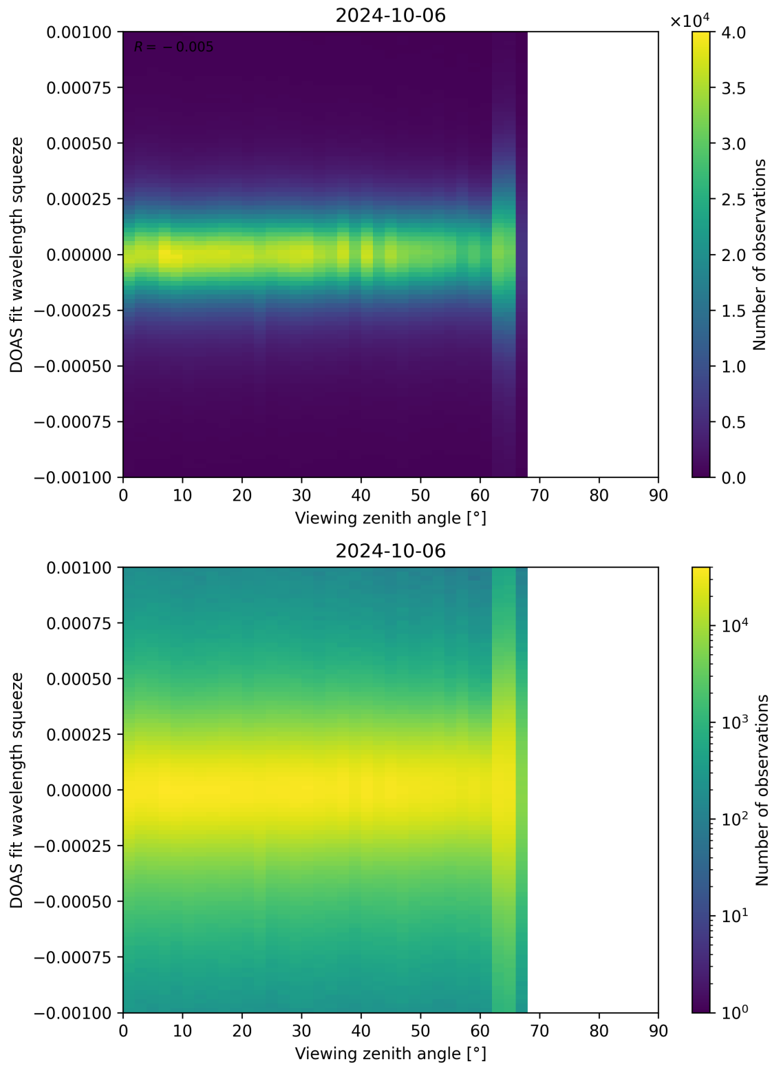
Figure 312: Scatter density plot of “Viewing zenith angle” against “DOAS fit wavelength squeeze” for 2024-10-05 to 2024-10-07.
