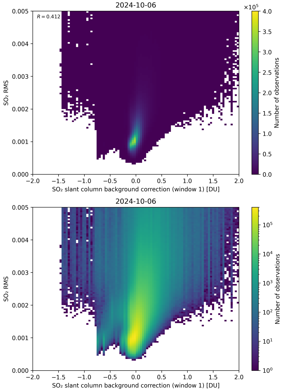
Figure 102: Scatter density plot of “SO 2 slant column background correction (window 1)” against “SO 2 RMS” for 2024-10-05 to 2024-10-07.
