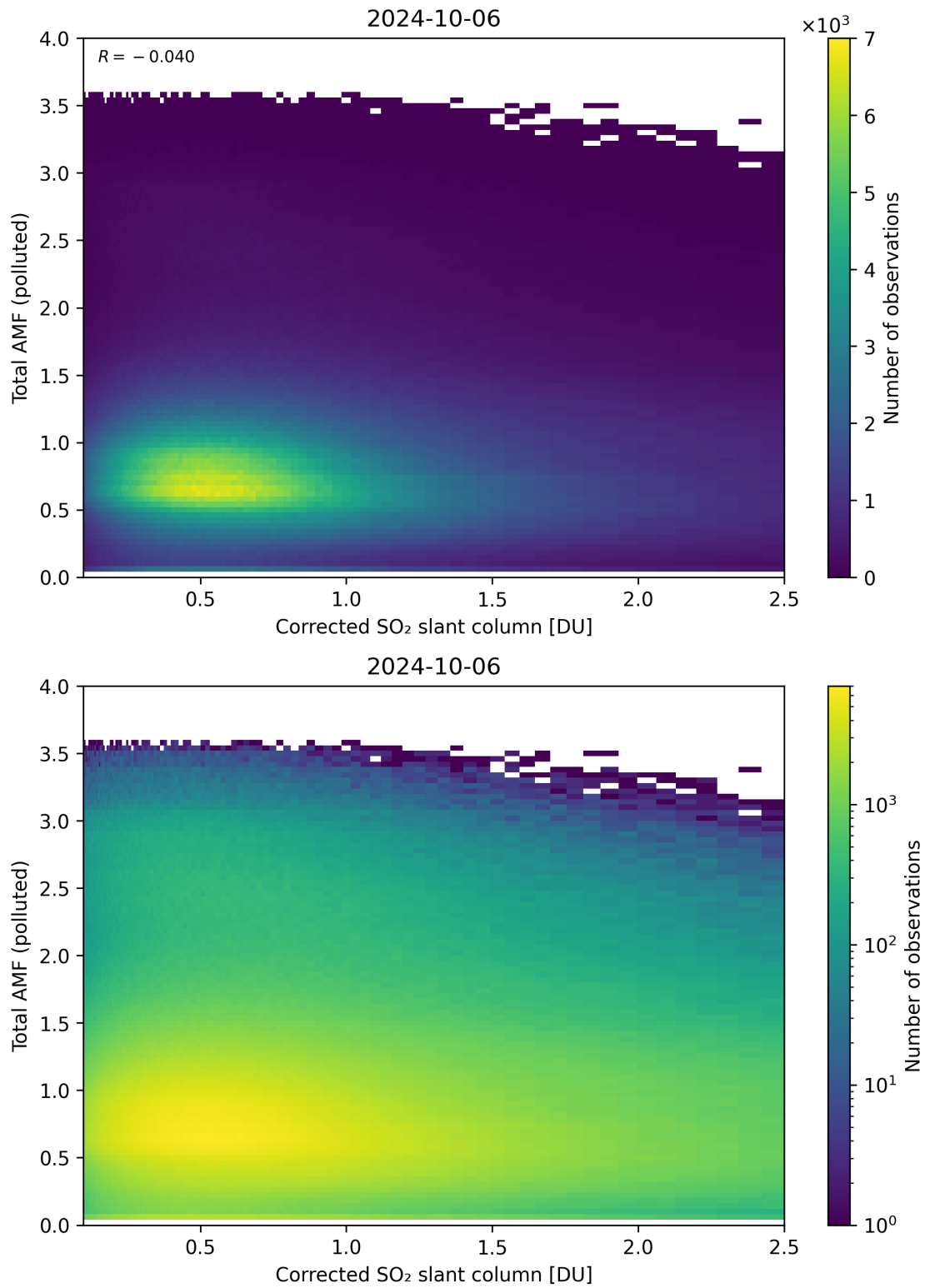
Figure 192: Scatter density plot of “Corrected SO 2 slant column” against “Total AMF (polluted)” for 2024-10-05 to 2024-10-07.
