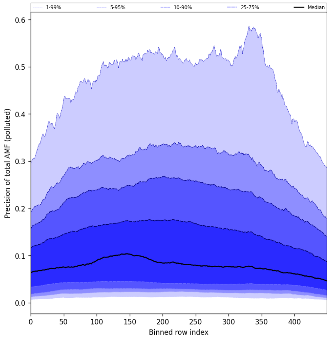
Figure 95: Along track statistics of “Precision of total AMF (polluted)” for 2024-10-05 to 2024-10-07
