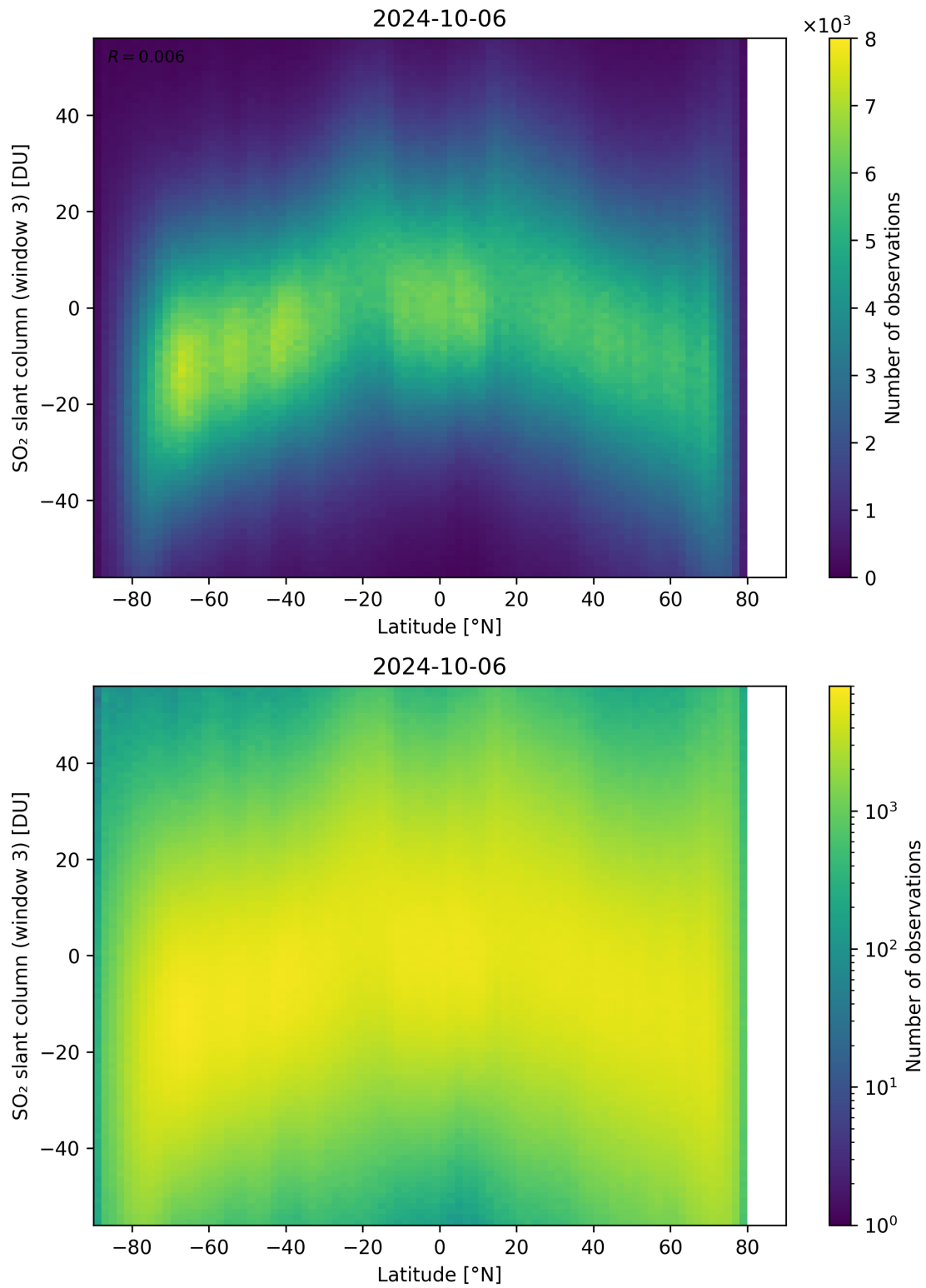
Figure 152: Scatter density plot of “Latitude” against “SO 2 slant column (window 3)” for 2024-10-05 to 2024-10-07.
