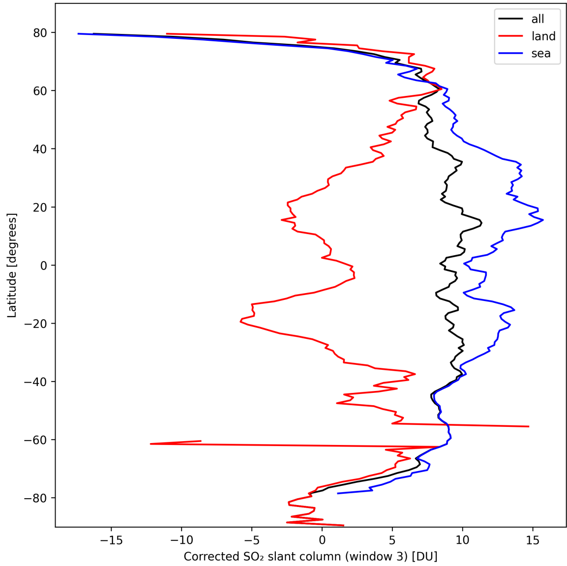
Figure 43: Zonal average of “Corrected SO 2 slant column (window 3)” for 2024-10-05 to 2024-10-07.
