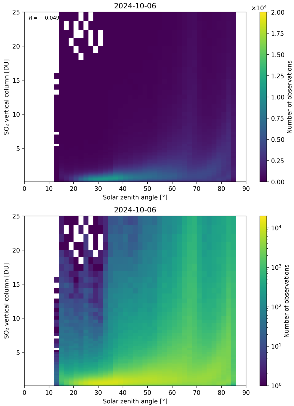
Figure 176: Scatter density plot of “Solar zenith angle” against “SO 2 vertical column” for 2024-10-05 to 2024-10-07.
