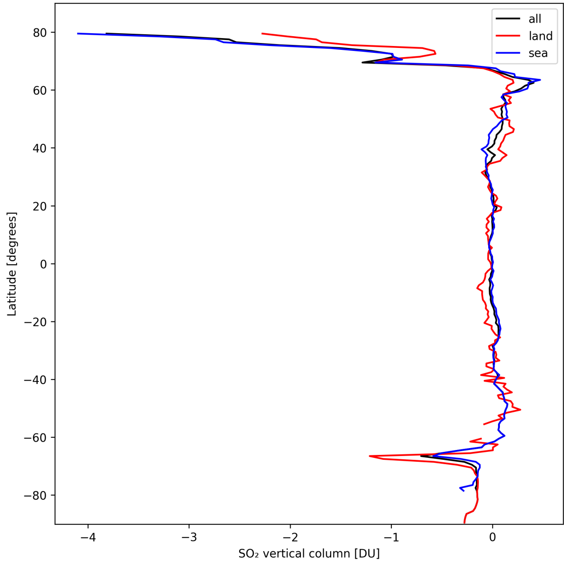
Figure 30: Zonal average of “SO 2 vertical column” for 2024-10-05 to 2024-10-07.
