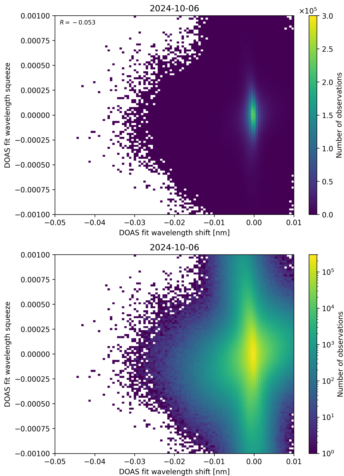
Figure 127: Scatter density plot of “DOAS fit wavelength shift” against “DOAS fit wavelength squeeze” for 2024-10-05 to 2024-10-07.
