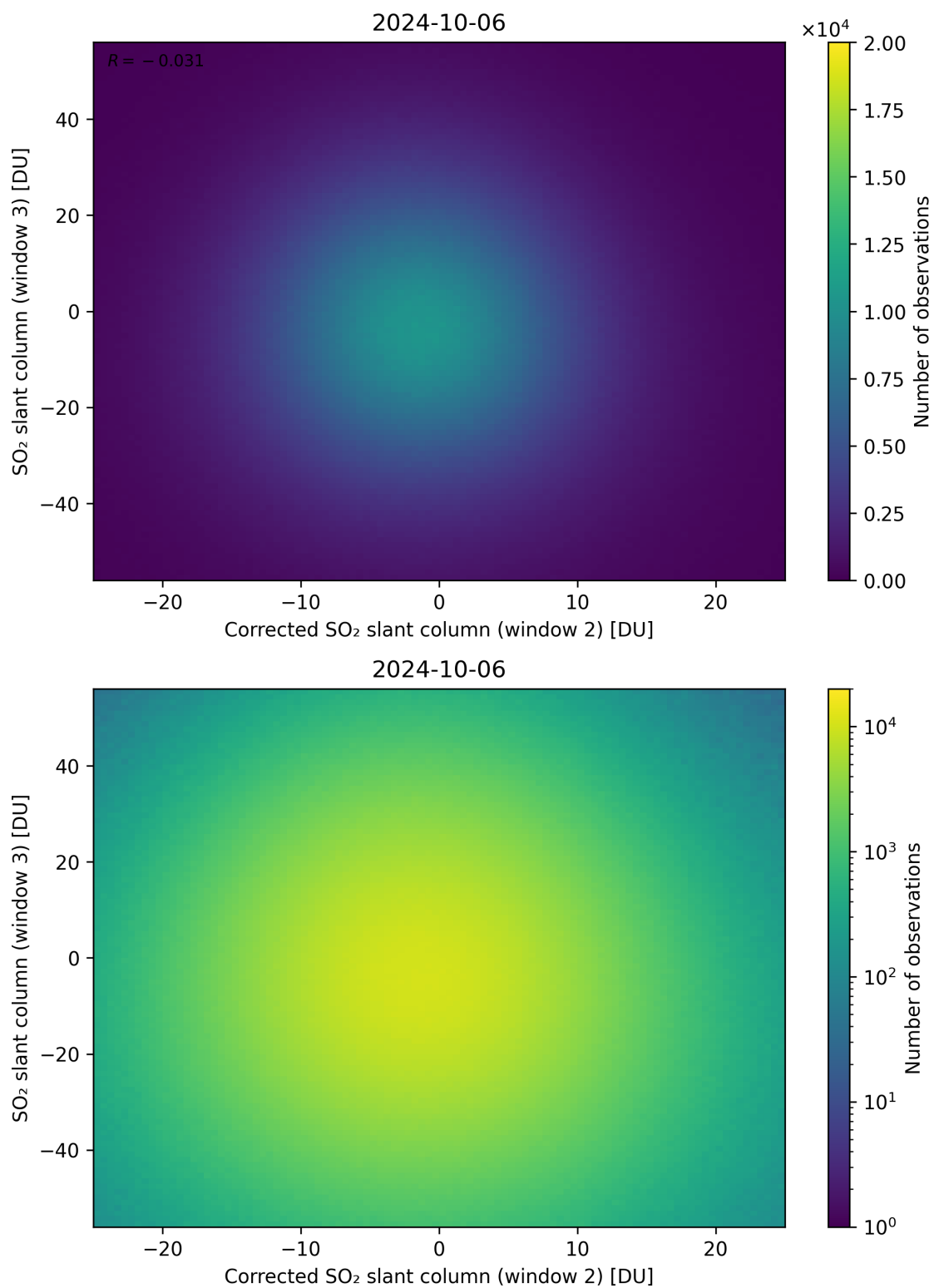
Figure 201: Scatter density plot of “Corrected SO 2 slant column (window 2)” against “SO 2 slant column (window 3)” for 2024-10-05 to 2024-10-07.
