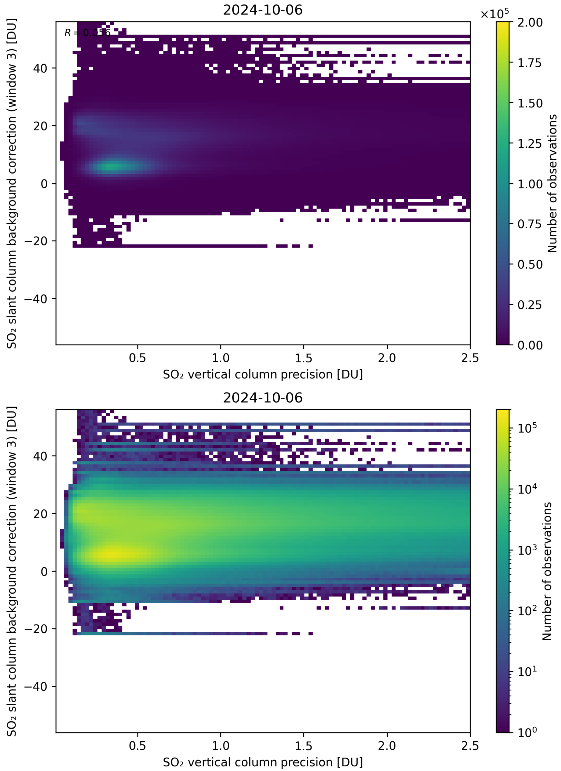
Figure 281: Scatter density plot of “SO 2 vertical column precision” against “SO 2 slant column background correction (window 3)” for 2024-10-05 to 2024-10-07.
