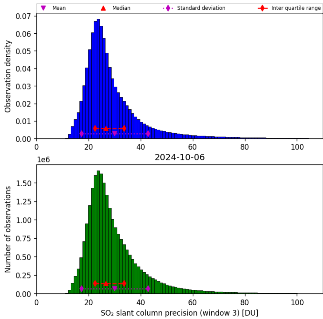
Figure 65: Histogram of “SO 2 slant column precision (window 3)” for 2024-10-05 to 2024-10-07
