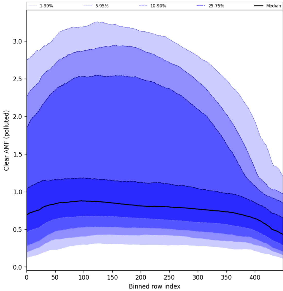
Figure 96: Along track statistics of “Clear AMF (polluted)” for 2024-10-05 to 2024-10-07
