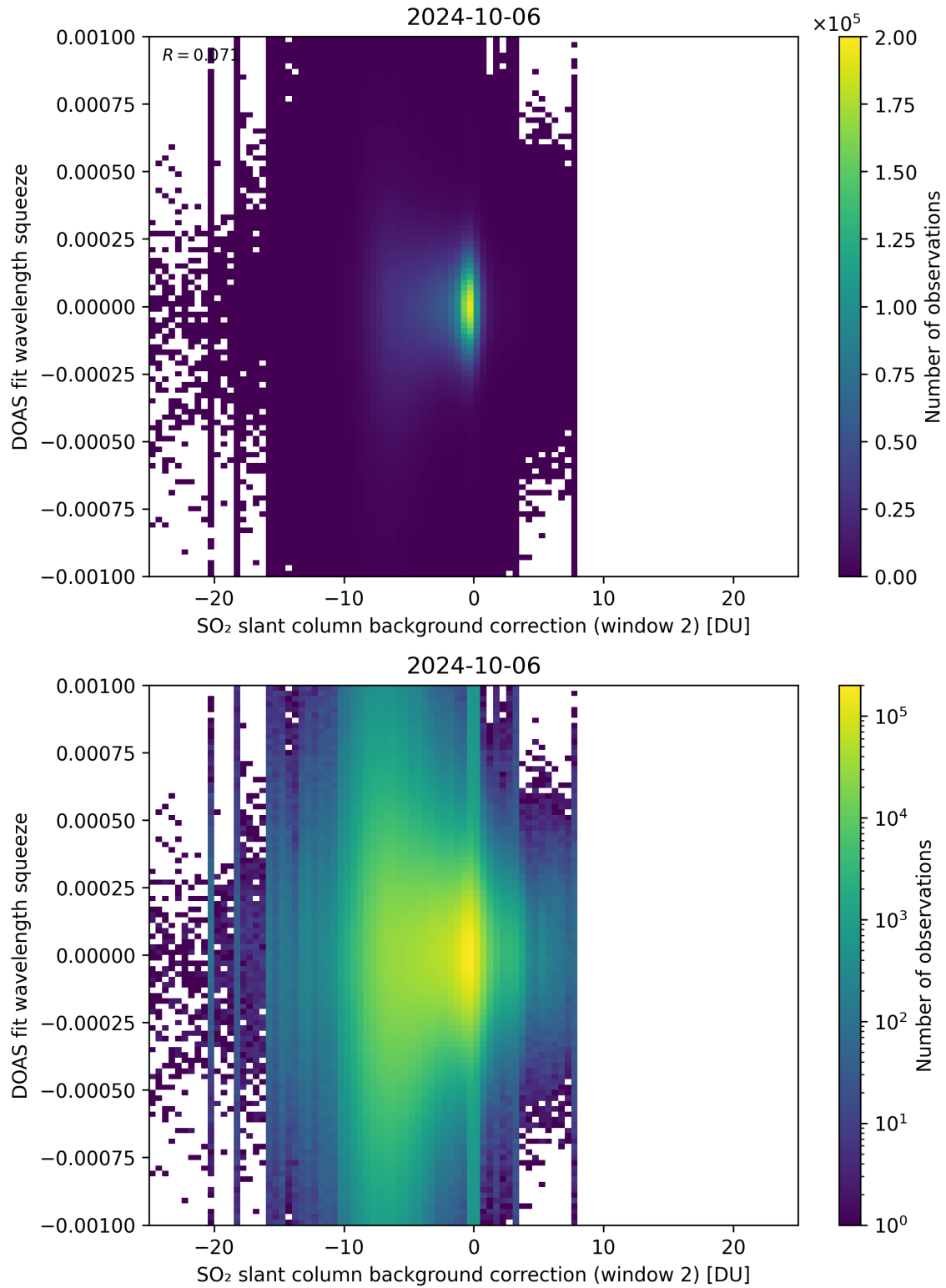
Figure 113: Scatter density plot of “SO 2 slant column background correction (window 2)” against “DOAS fit wavelength squeeze” for 2024-10-05 to 2024-10-07.
