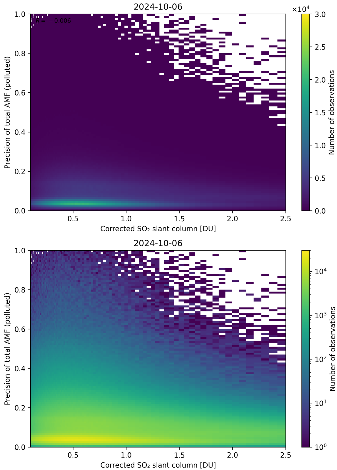
Figure 193: Scatter density plot of “Corrected SO 2 slant column” against “Precision of total AMF (polluted)” for 2024-10-05 to 2024-10-07.
