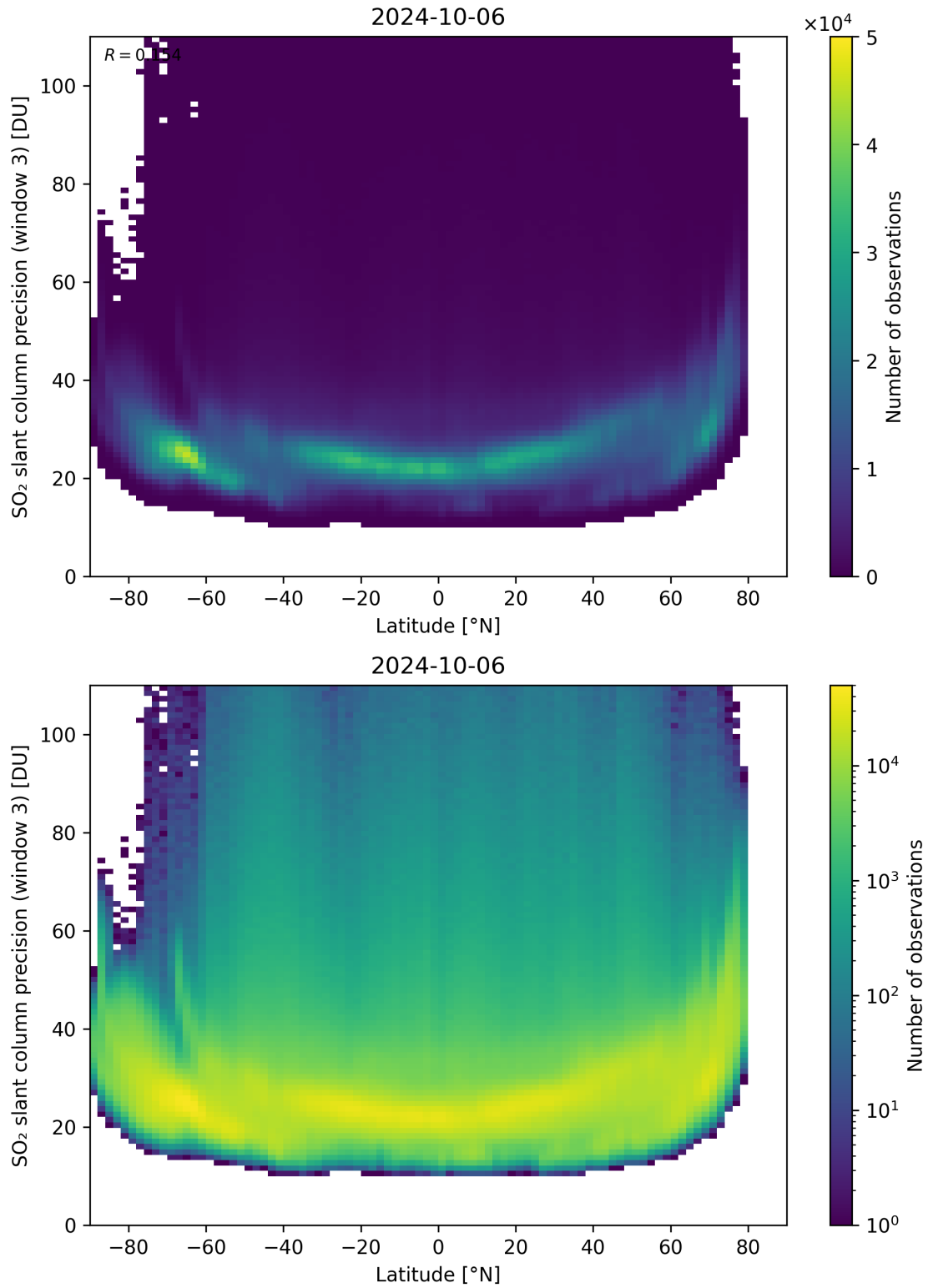
Figure 153: Scatter density plot of “Latitude” against “SO 2 slant column precision (window 3)” for 2024-10-05 to 2024-10-07.
