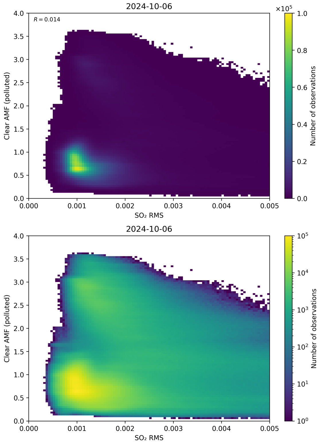
Figure 136: Scatter density plot of “SO 2 RMS” against “Clear AMF (polluted)” for 2024-10-05 to 2024-10-07.
