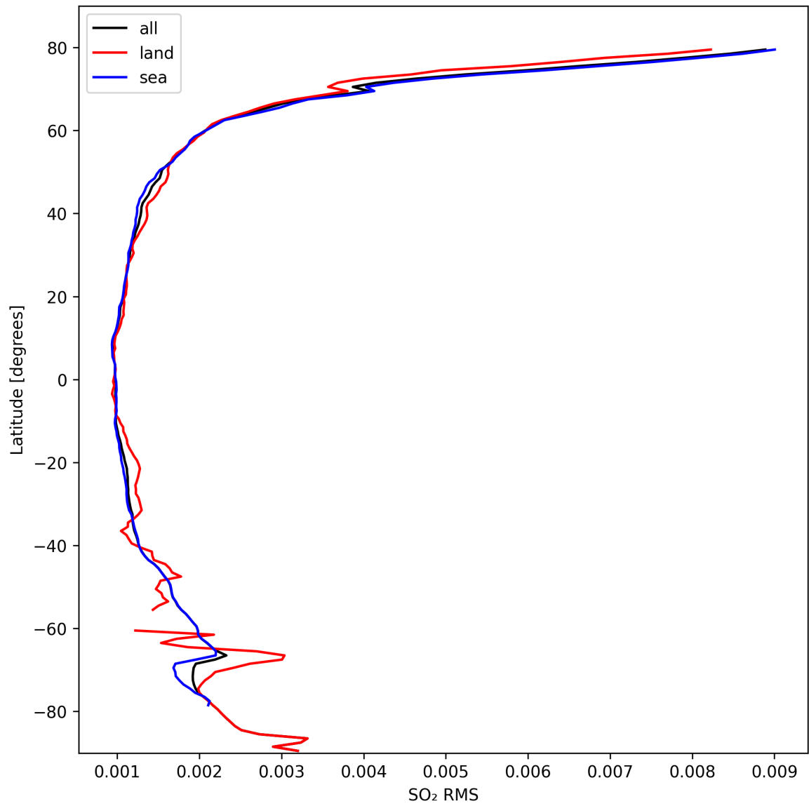
Figure 47: Zonal average of “SO 2 RMS” for 2024-10-05 to 2024-10-07.
