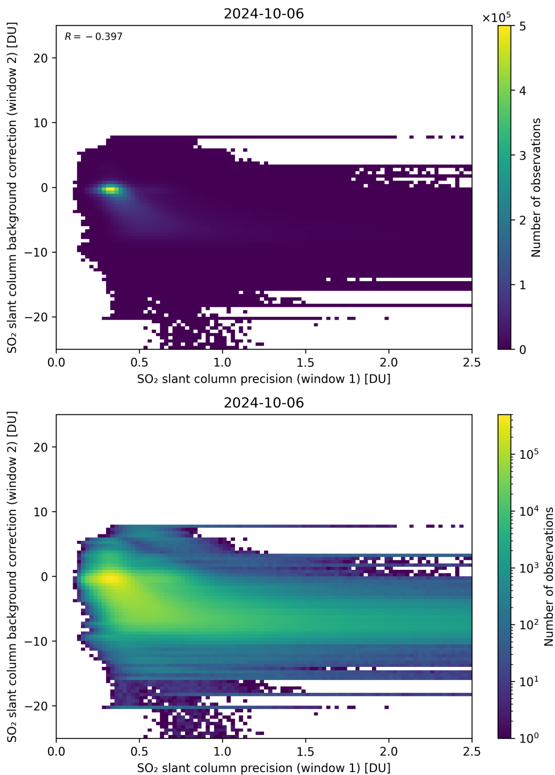
Figure 219: Scatter density plot of “SO 2 slant column precision (window 1)” against “SO 2 slant column background correction (window 2)” for 2024-10-05 to 2024-10-07.
