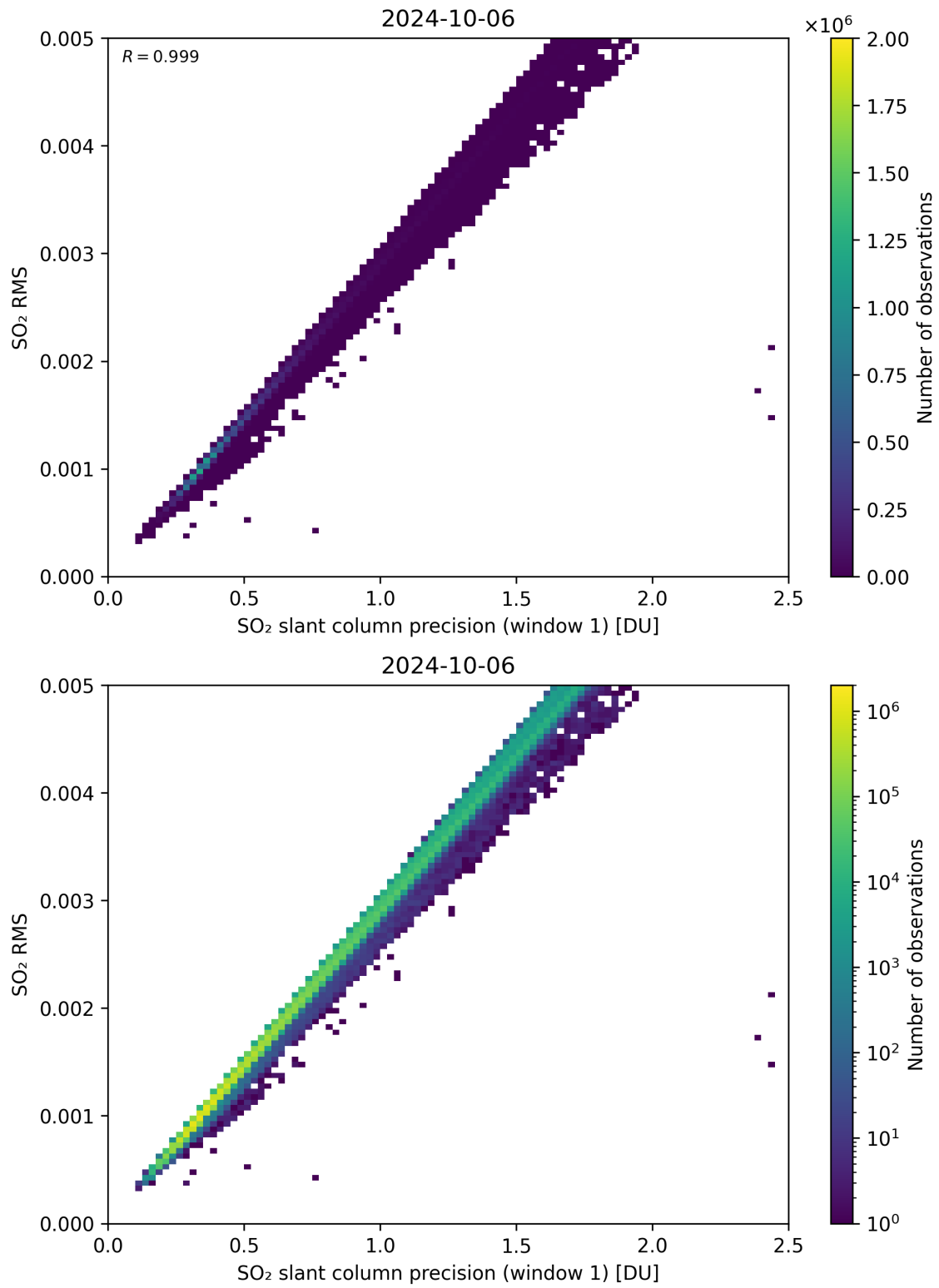
Figure 223: Scatter density plot of “SO 2 slant column precision (window 1)” against “SO 2 RMS” for 2024-10-05 to 2024-10-07.
