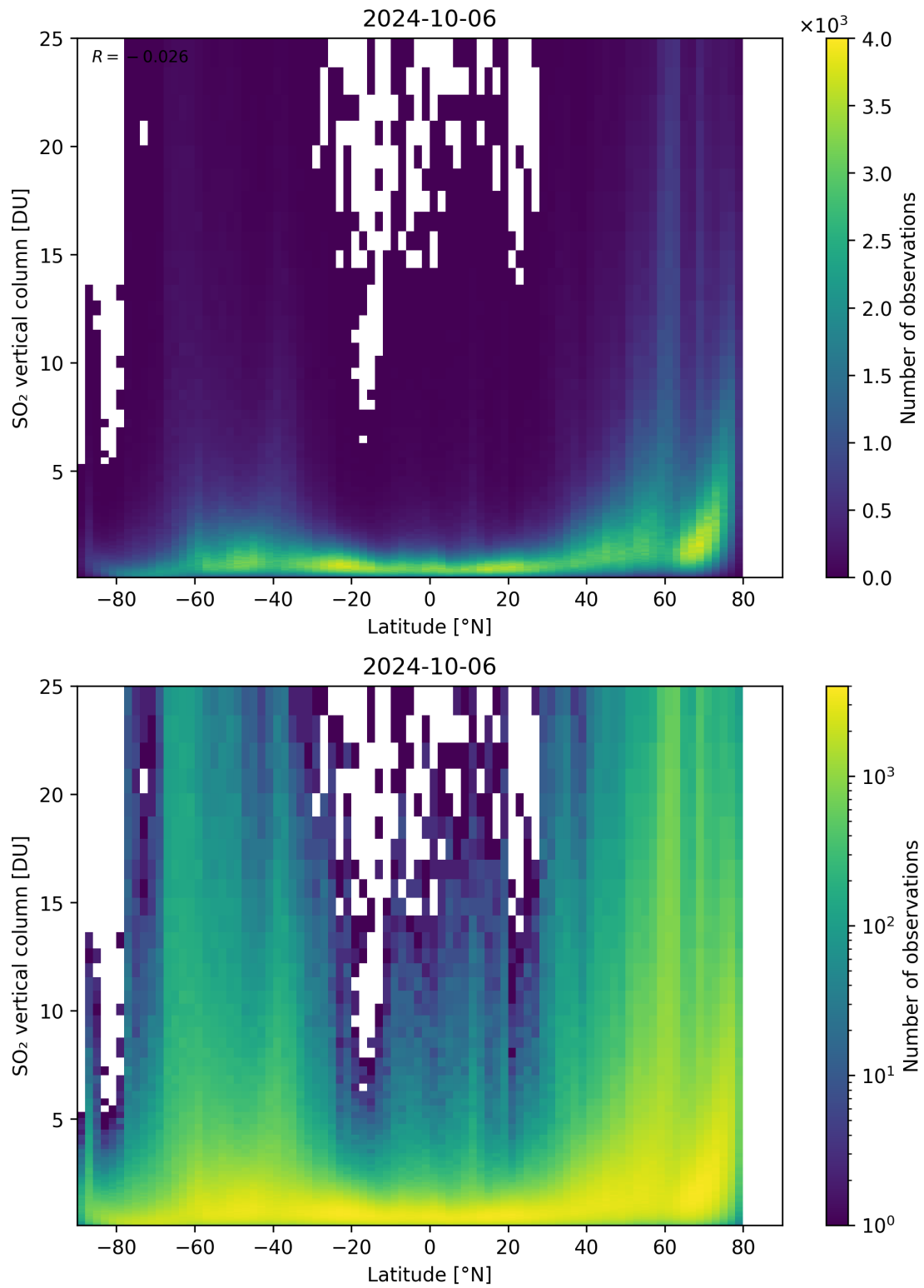
Figure 156: Scatter density plot of “Latitude” against “SO 2 vertical column” for 2024-10-05 to 2024-10-07.
