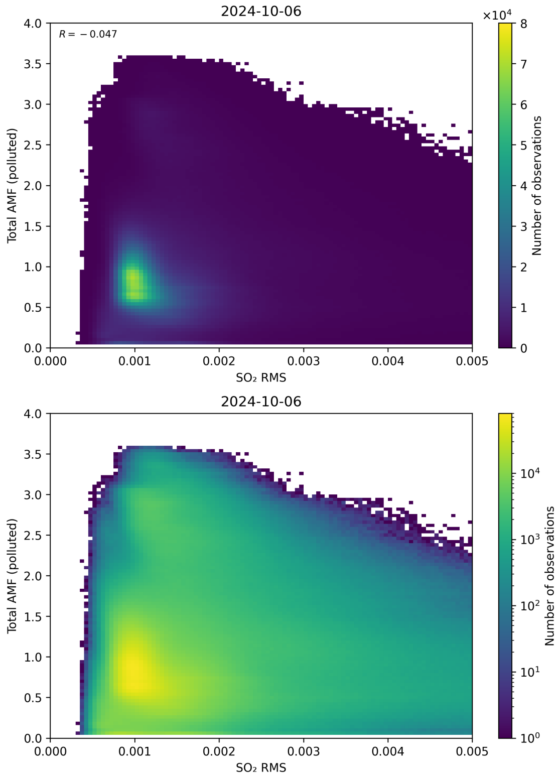
Figure 137: Scatter density plot of “SO 2 RMS” against “Total AMF (polluted)” for 2024-10-05 to 2024-10-07.
