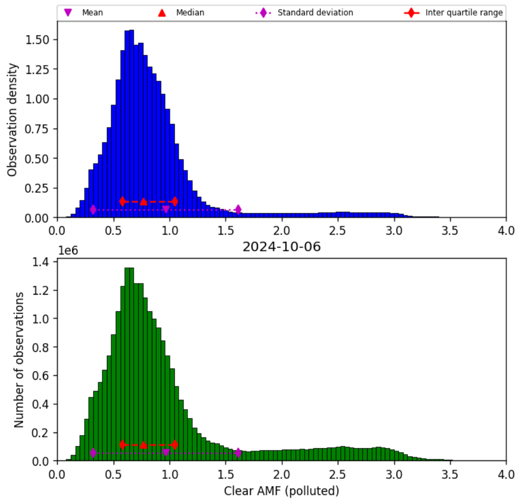
Figure 73: Histogram of “Clear AMF (polluted)” for 2024-10-05 to 2024-10-07
