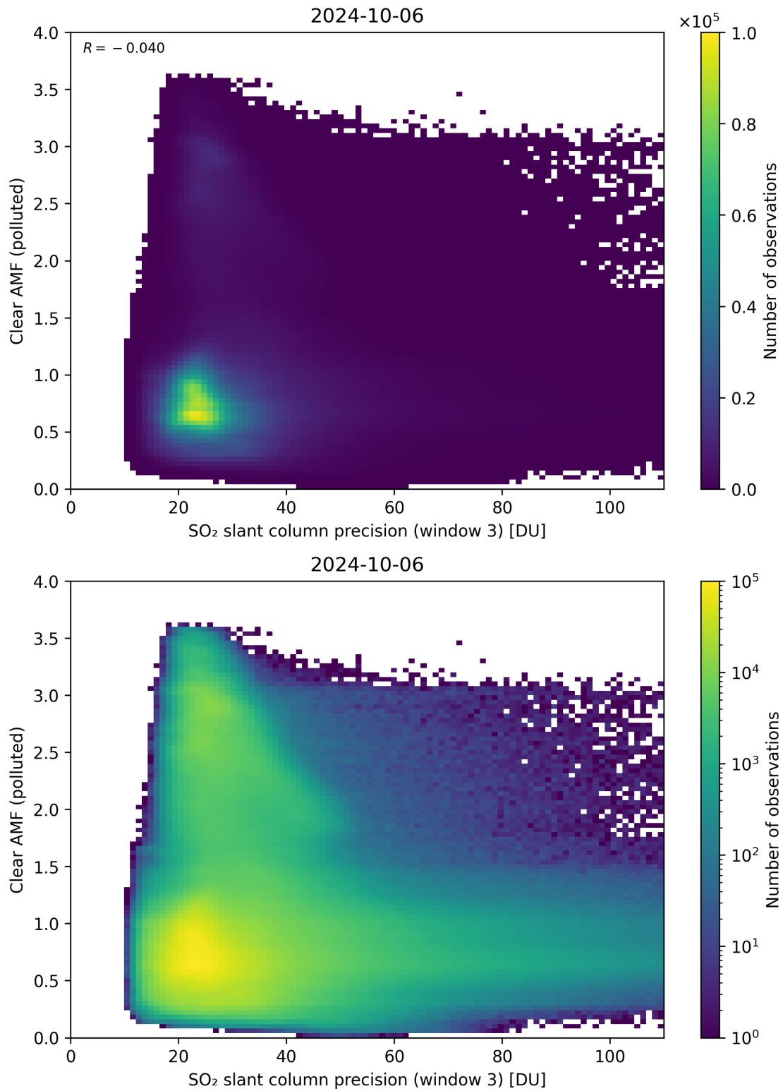
Figure 261: Scatter density plot of “SO 2 slant column precision (window 3)” against “Clear AMF (polluted)” for 2024-10-05 to 2024-10-07.
