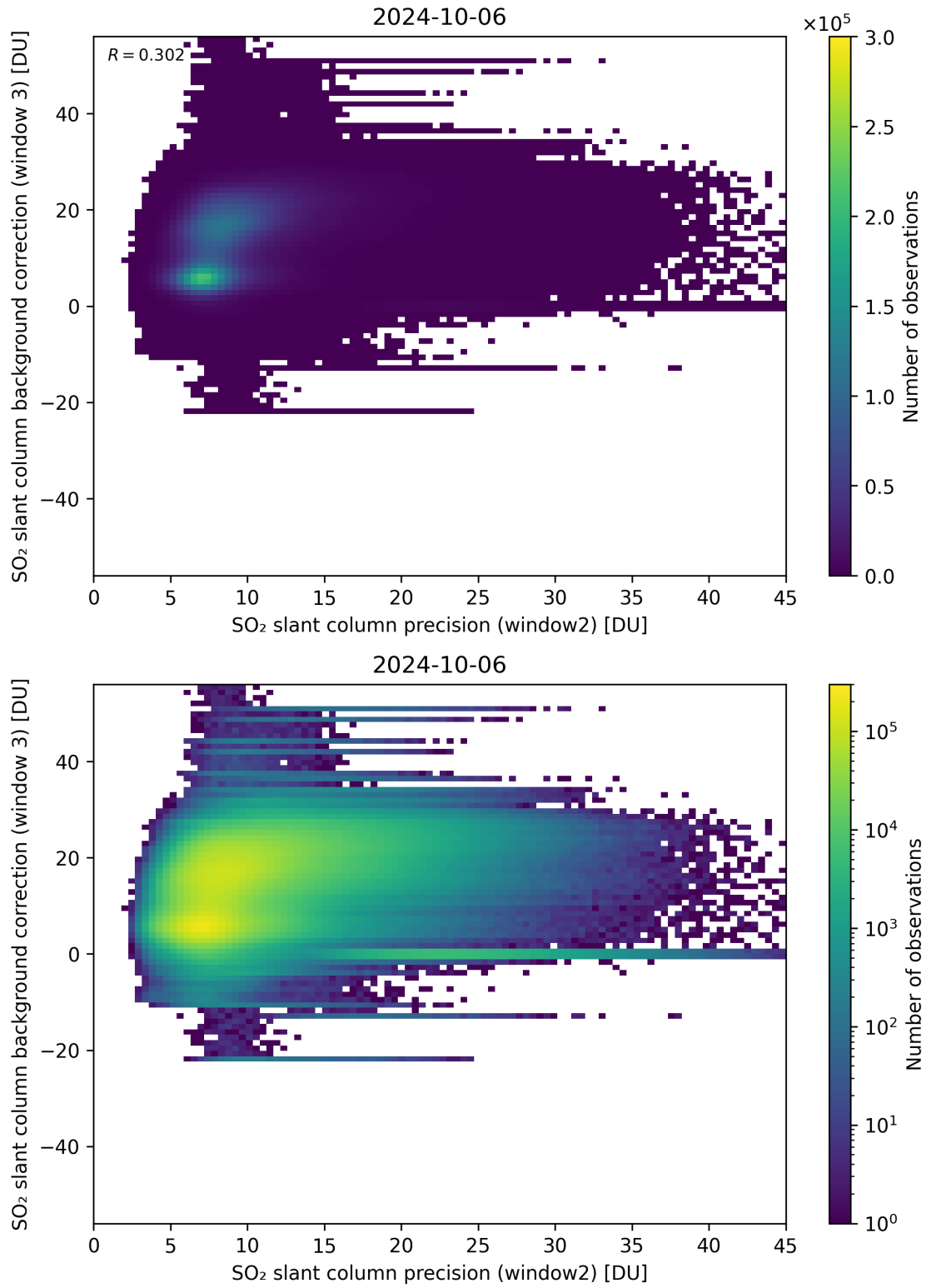
Figure 242: Scatter density plot of “SO 2 slant column precision (window2)” against “SO 2 slant column background correction (window 3)” for 2024-10-05 to 2024-10-07.
