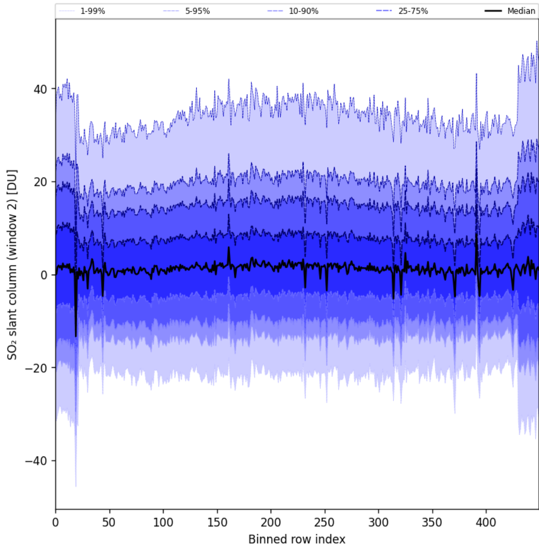
Figure 83: Along track statistics of “SO 2 slant column (window 2)” for 2024-10-05 to 2024-10-07
