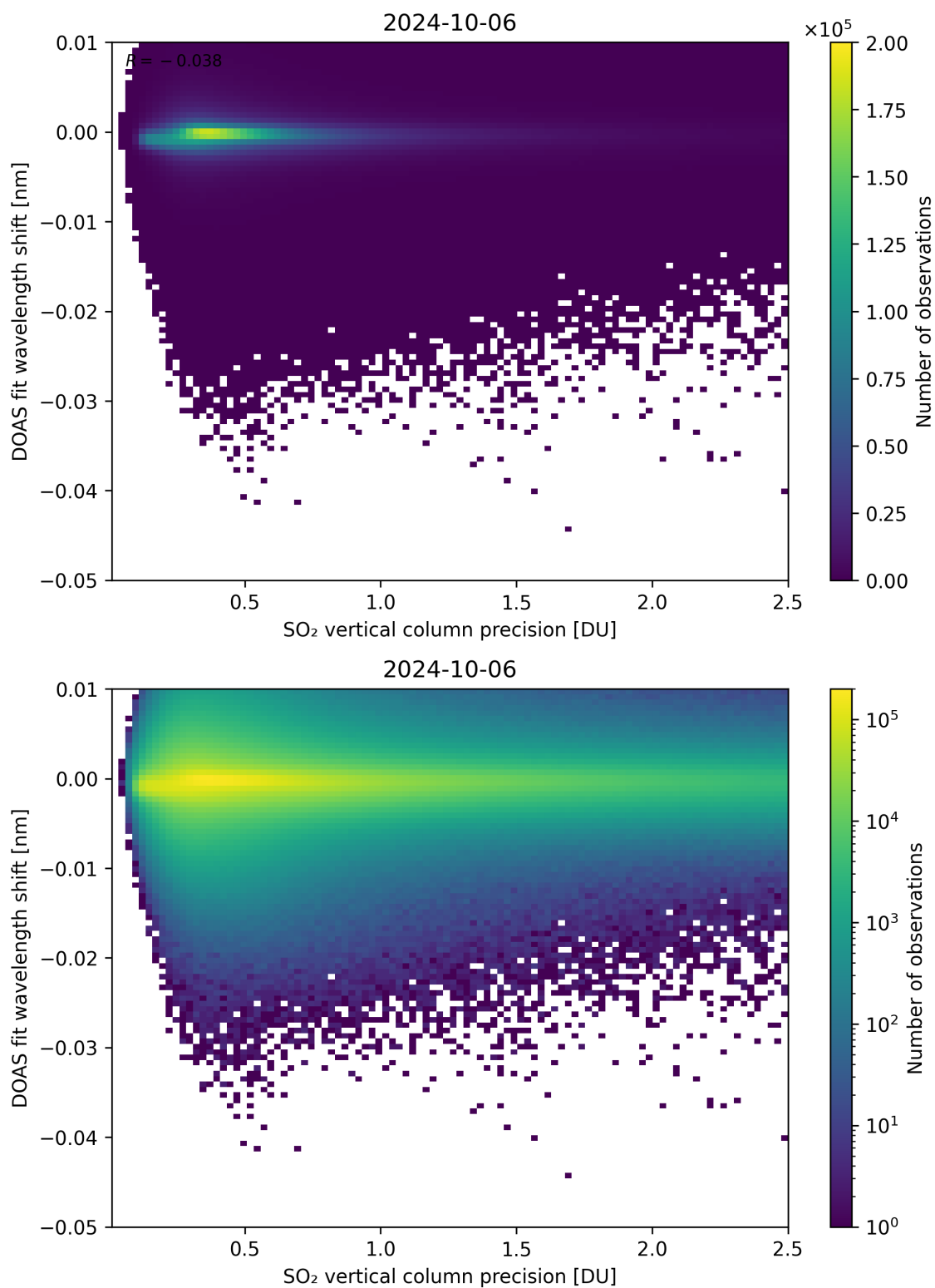
Figure 282: Scatter density plot of “SO 2 vertical column precision” against “DOAS fit wavelength shift” for 2024-10-05 to 2024-10-07.
