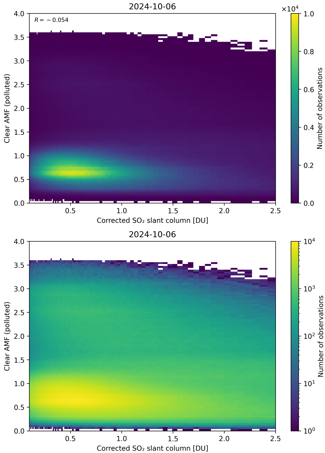
Figure 184: Scatter density plot of “Corrected SO 2 slant column” against “Clear AMF (polluted)” for 2024-10-05 to 2024-10-07.
