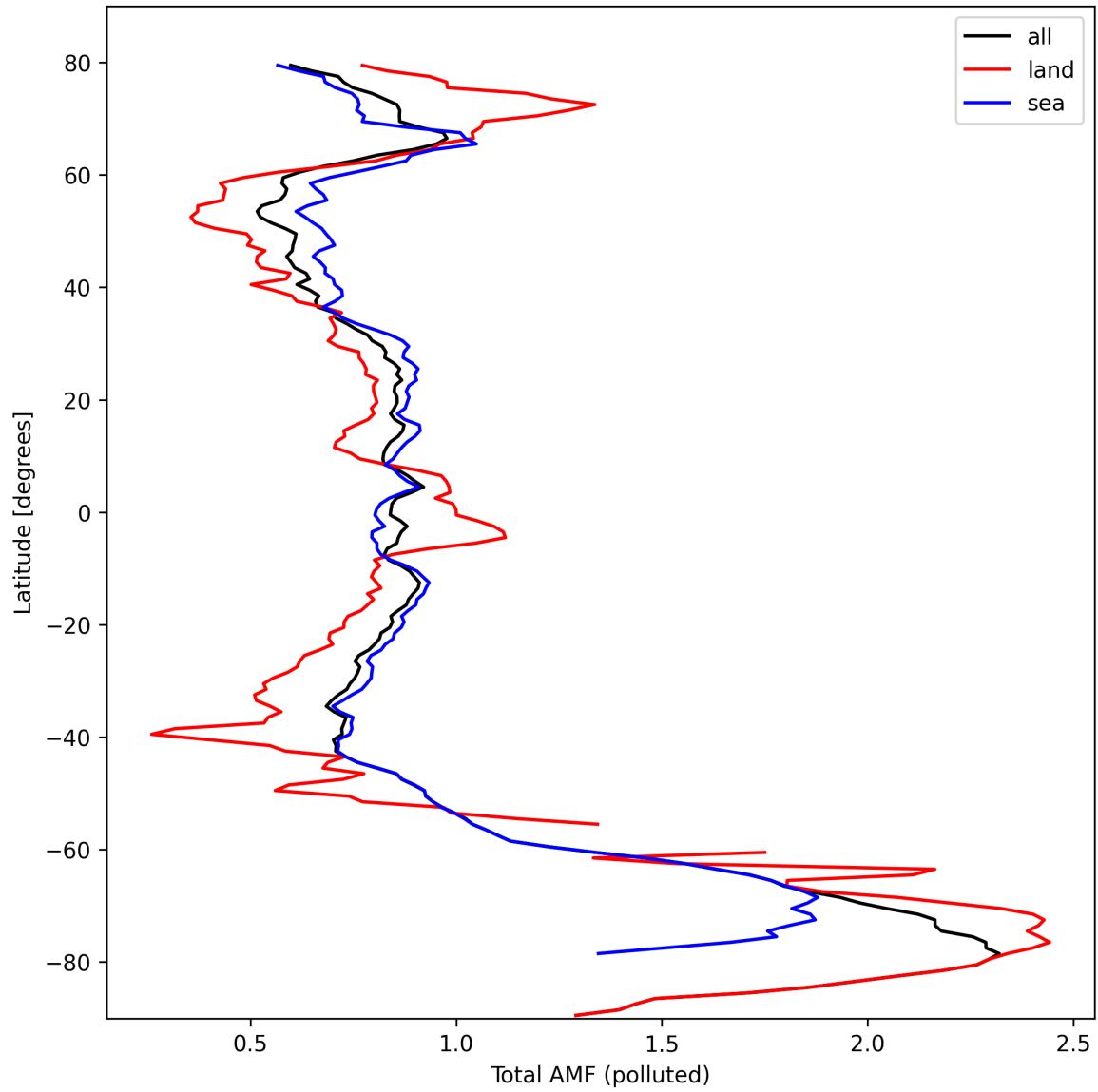
Figure 48: Zonal average of “Total AMF (polluted)” for 2024-10-05 to 2024-10-07.
