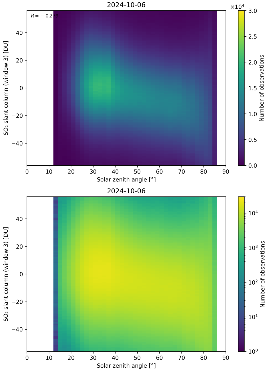
Figure 172: Scatter density plot of “Solar zenith angle” against “SO 2 slant column (window 3)” for 2024-10-05 to 2024-10-07.
