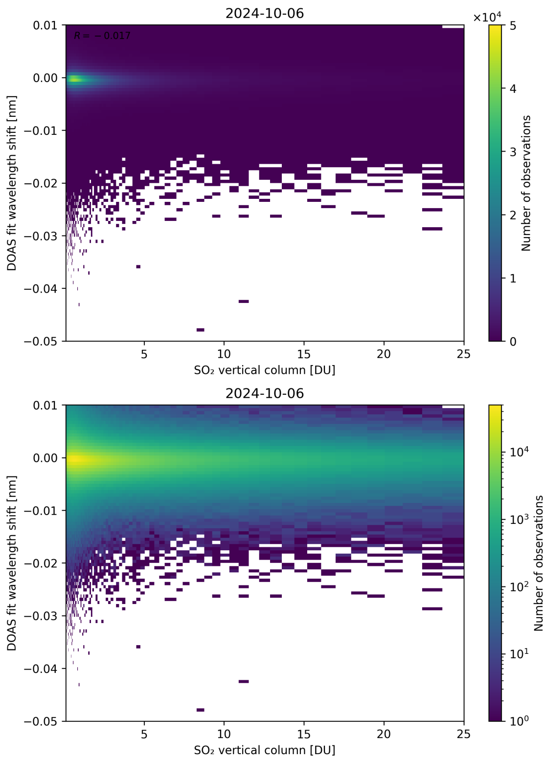
Figure 276: Scatter density plot of “SO 2 vertical column” against “DOAS fit wavelength shift” for 2024-10-05 to 2024-10-07.
