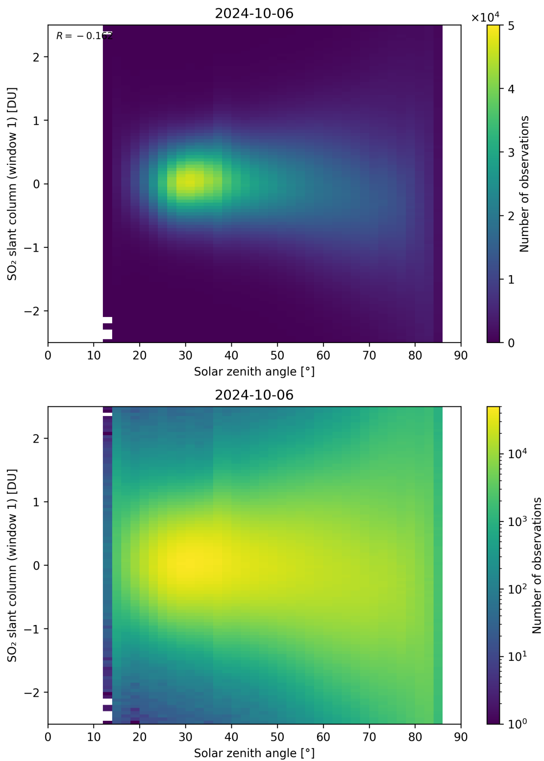
Figure 169: Scatter density plot of “Solar zenith angle” against “SO 2 slant column (window 1)” for 2024-10-05 to 2024-10-07.
