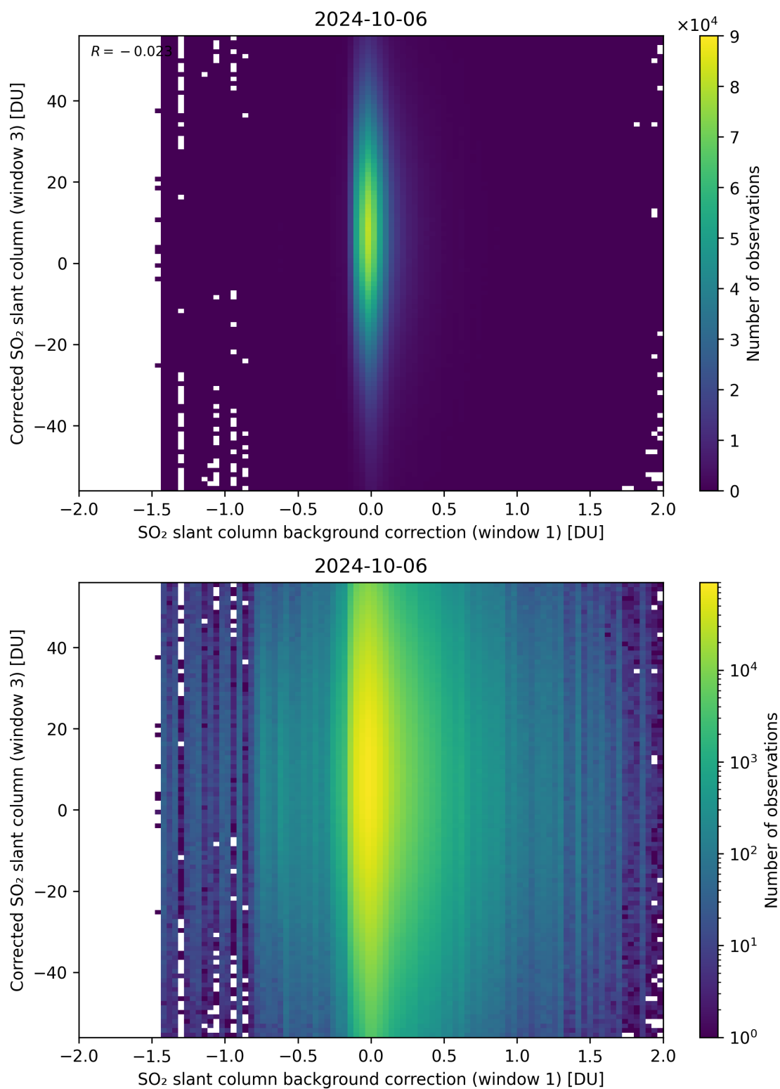
Figure 105: Scatter density plot of “SO 2 slant column background correction (window 1)” against “Corrected SO 2 slant column (window 3)” for 2024-10-05 to 2024-10-07.
