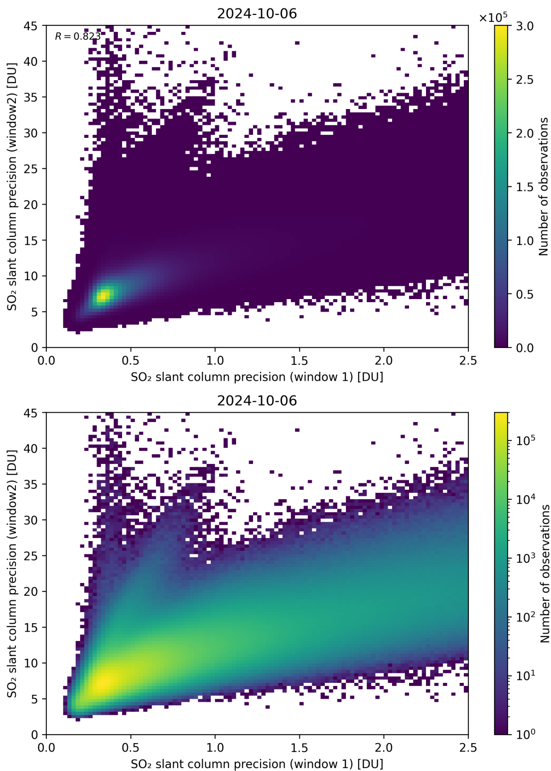
Figure 227: Scatter density plot of “SO 2 slant column precision (window 1)” against “SO 2 slant column precision (window2)” for 2024-10-05 to 2024-10-07.
