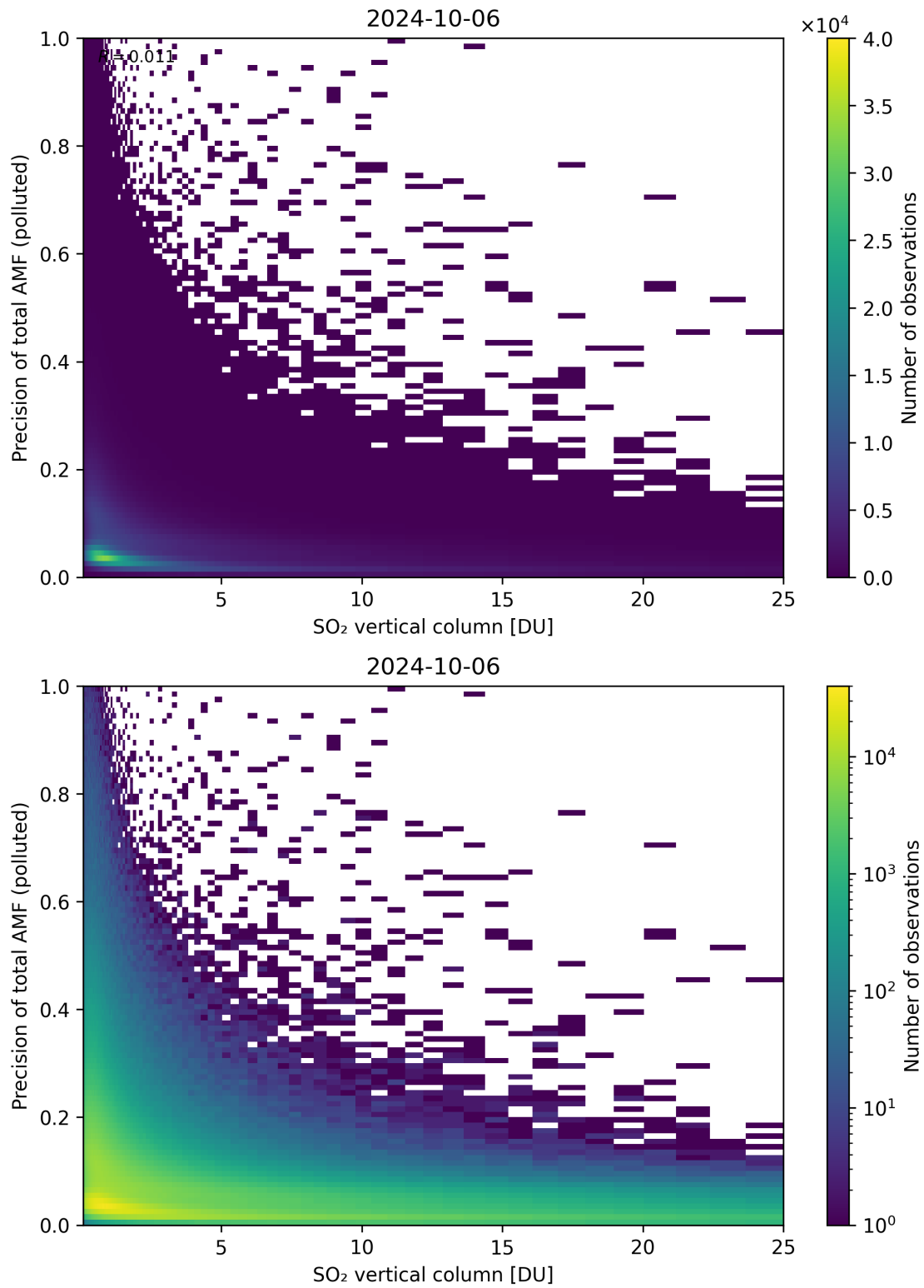
Figure 306: Scatter density plot of “SO 2 vertical column” against “Precision of total AMF (polluted)” for 2024-10-05 to 2024-10-07.
