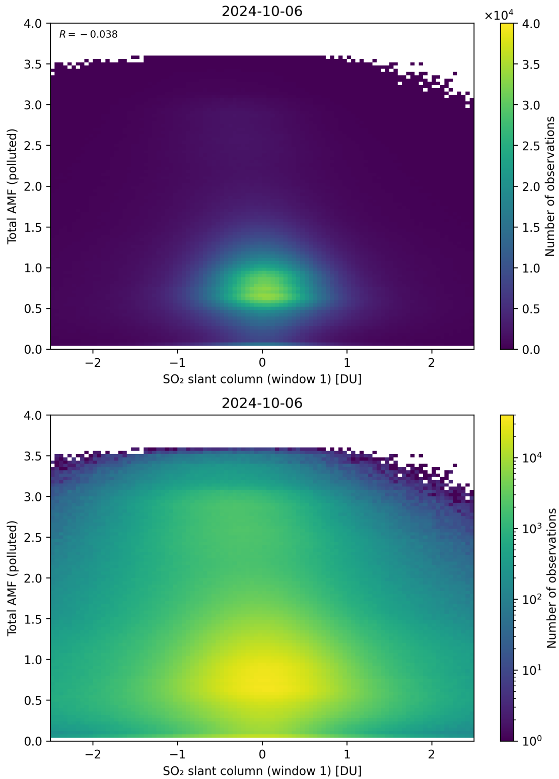
Figure 239: Scatter density plot of “SO 2 slant column (window 1)” against “Total AMF (polluted)” for 2024-10-05 to 2024-10-07.
