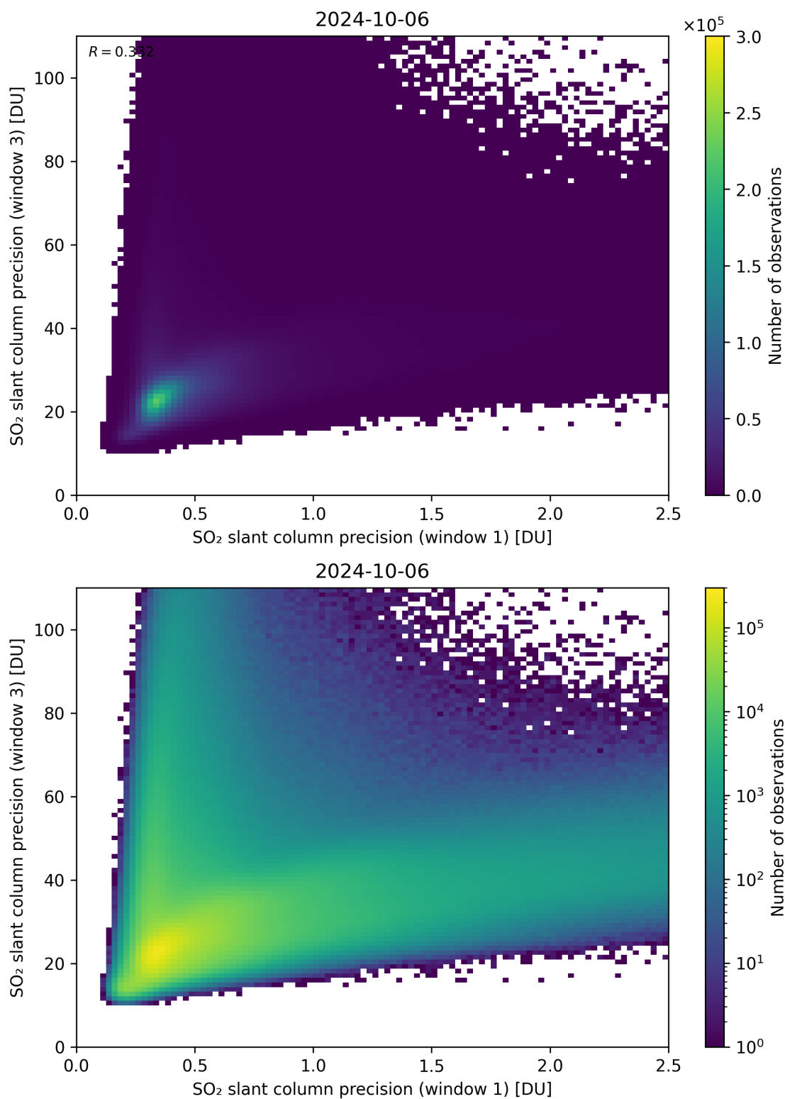
Figure 229: Scatter density plot of “SO 2 slant column precision (window 1)” against “SO 2 slant column precision (window 3)” for 2024-10-05 to 2024-10-07.
