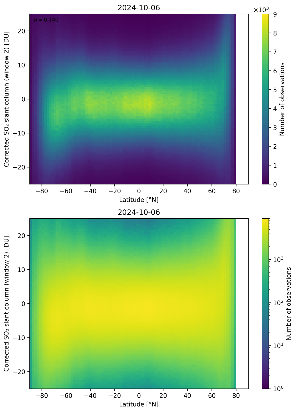
Figure 147: Scatter density plot of “Latitude” against “Corrected SO 2 slant column (window 2)” for 2024-10-05 to 2024-10-07.
