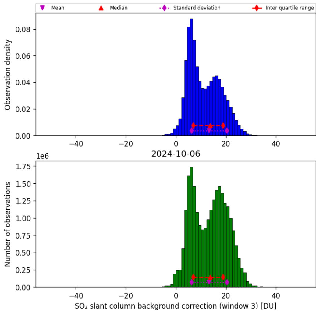
Figure 67: Histogram of “SO 2 slant column background correction (window 3)” for 2024-10-05 to 2024-10-07
