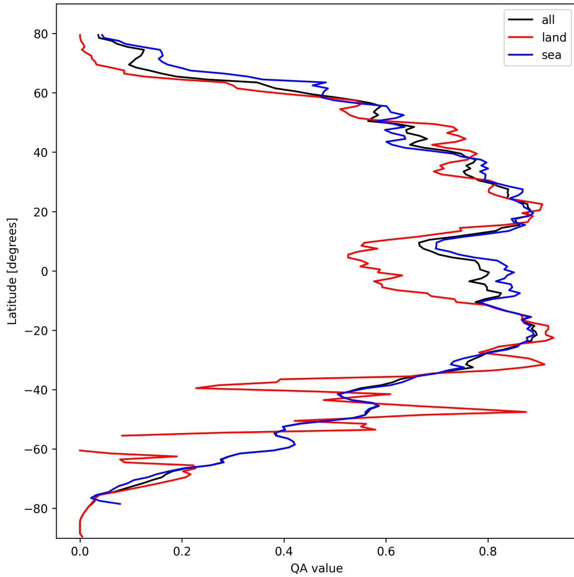
Figure 29: Zonal average of “QA value” for 2024-10-05 to 2024-10-07.
