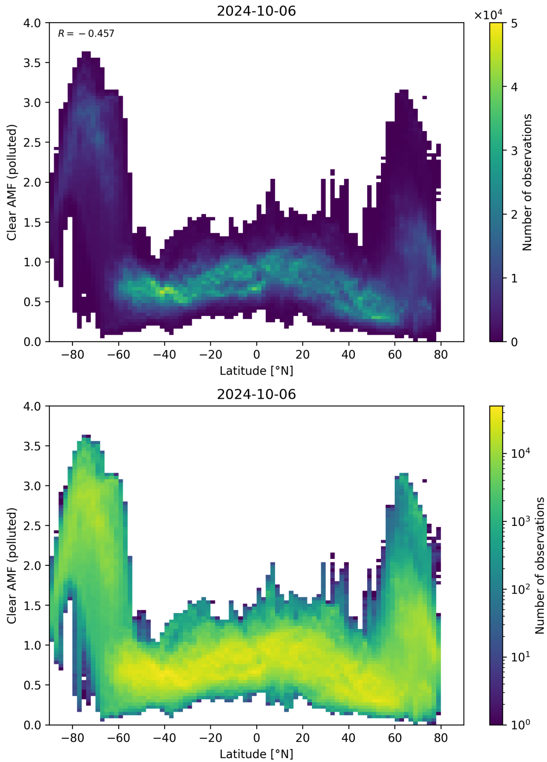
Figure 145: Scatter density plot of “Latitude” against “Clear AMF (polluted)” for 2024-10-05 to 2024-10-07.
