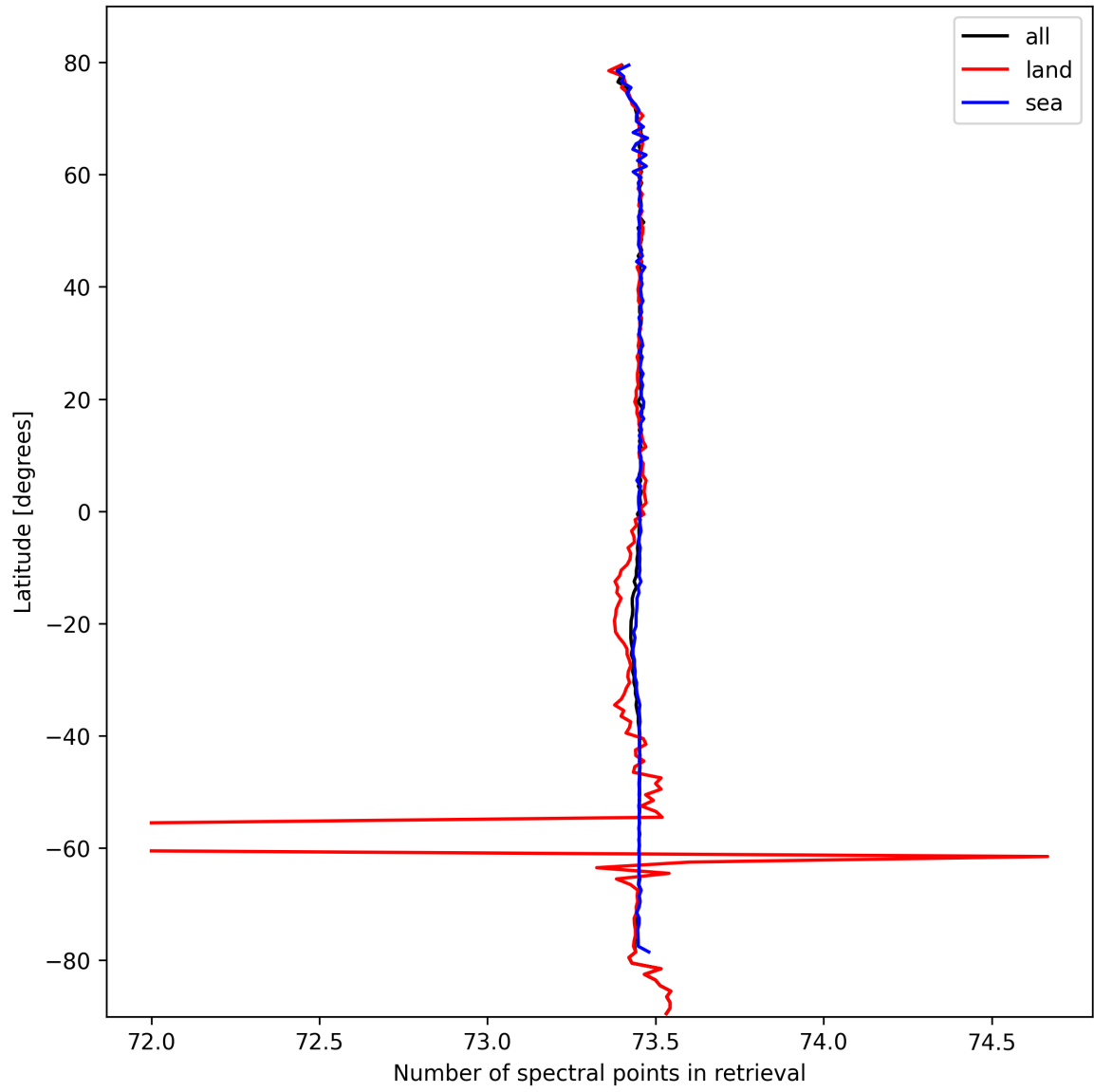
Figure 51: Zonal average of “Number of spectral points in retrieval” for 2024-10-05 to 2024-10-07.
