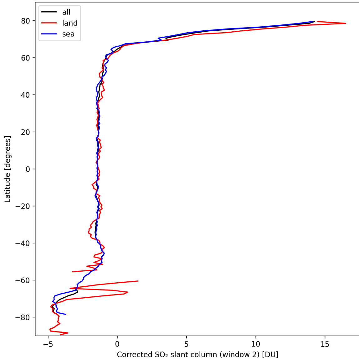
Figure 39: Zonal average of “Corrected SO 2 slant column (window 2)” for 2024-10-05 to 2024-10-07.
