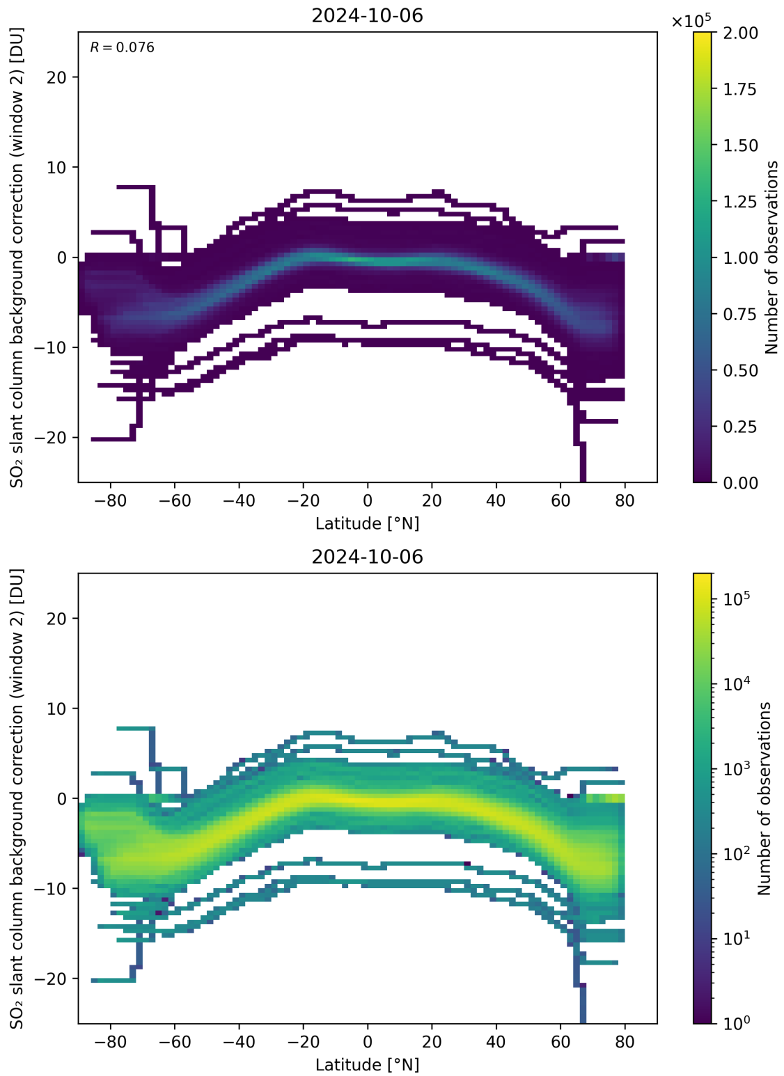
Figure 140: Scatter density plot of “Latitude” against “SO 2 slant column background correction (window 2)” for 2024-10-05 to 2024-10-07.
