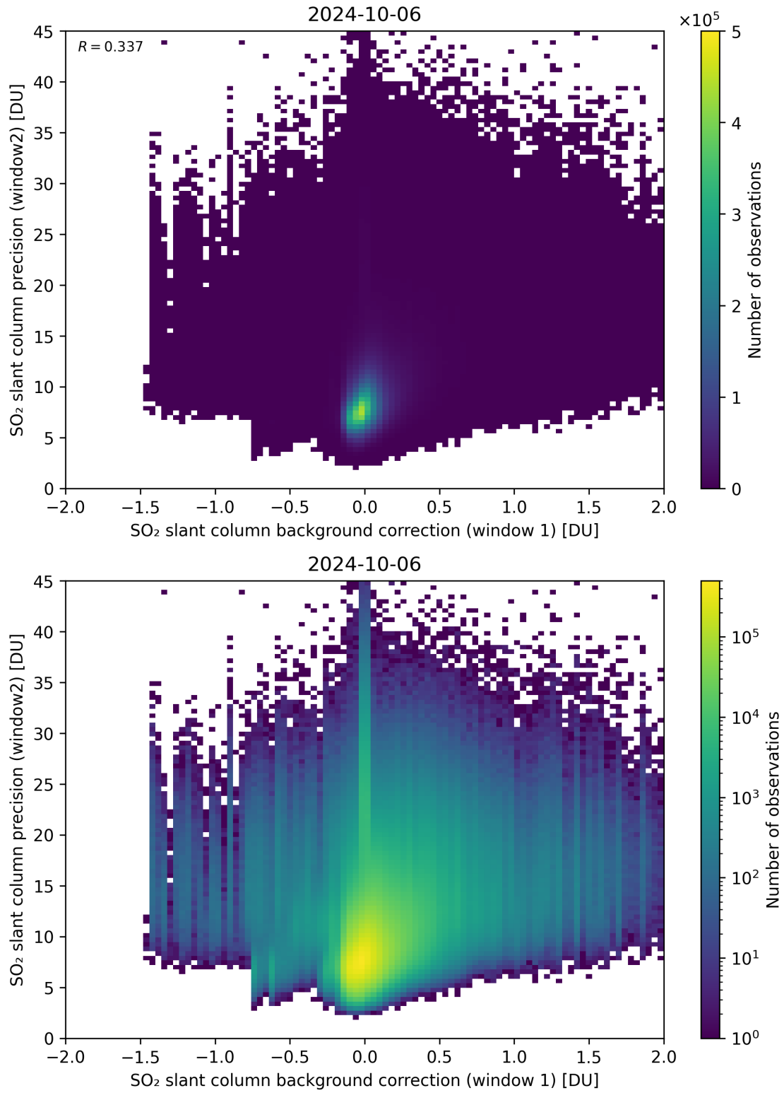
Figure 106: Scatter density plot of “SO 2 slant column background correction (window 1)” against “SO 2 slant column precision (window2)” for 2024-10-05 to 2024-10-07.
