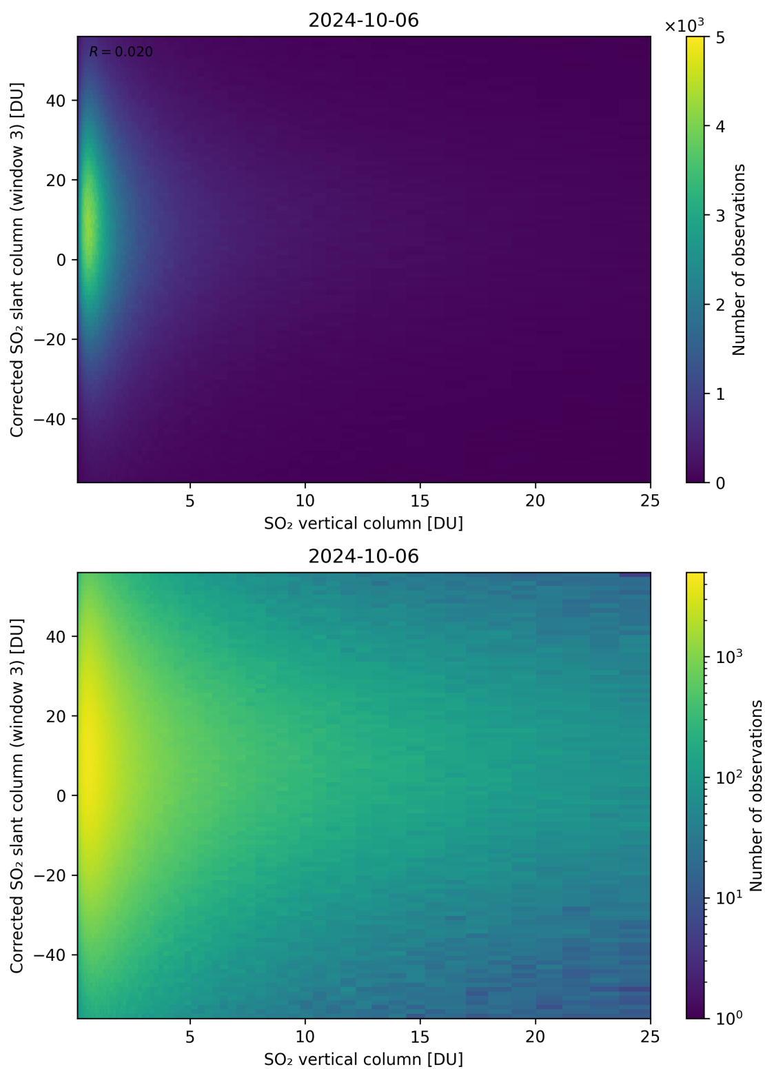
Figure 299: Scatter density plot of “SO 2 vertical column” against “Corrected SO 2 slant column (window 3)” for 2024-10-05 to 2024-10-07.
