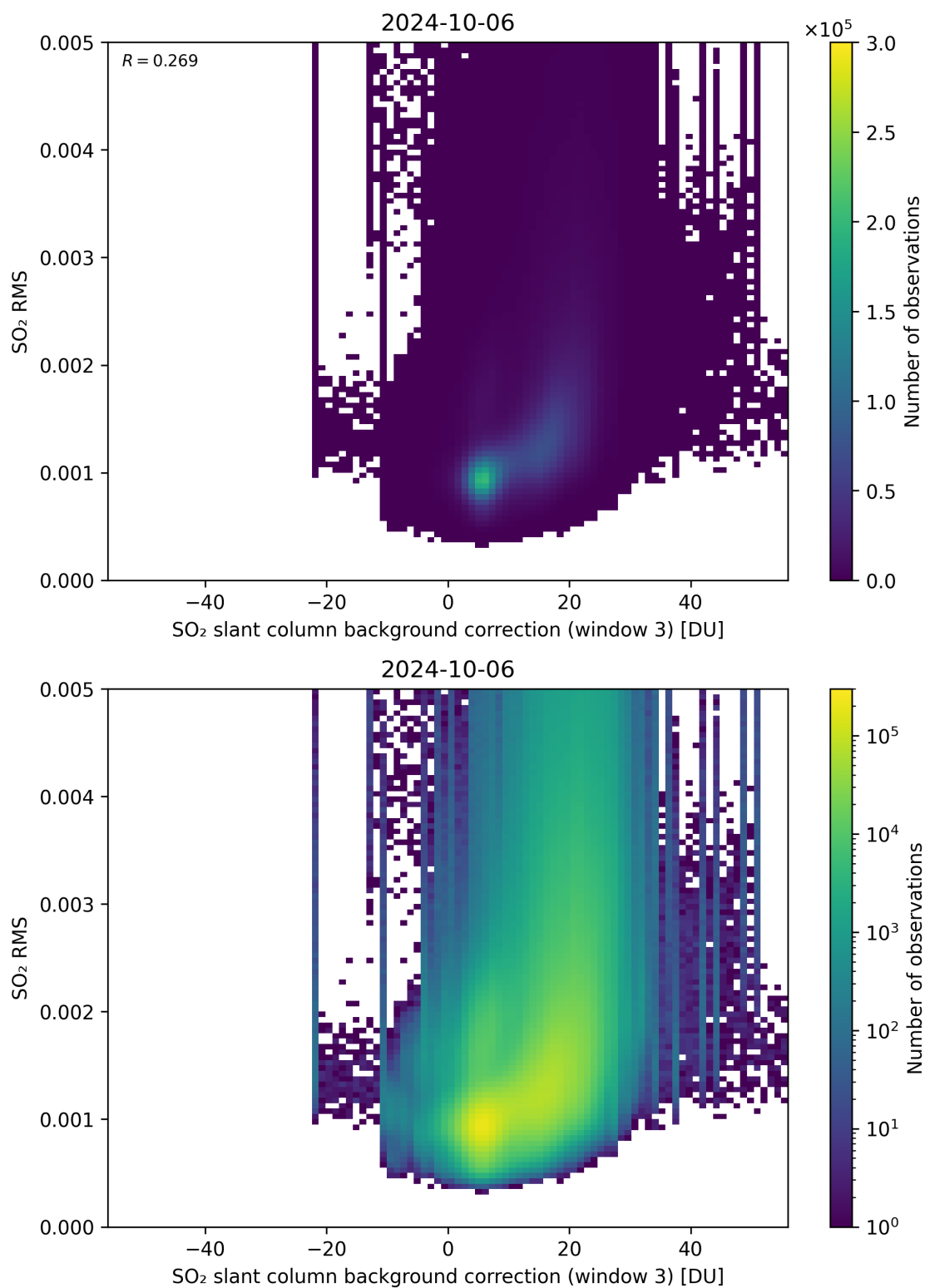
Figure 123: Scatter density plot of “SO 2 slant column background correction (window 3)” against “SO 2 RMS” for 2024-10-05 to 2024-10-07.
