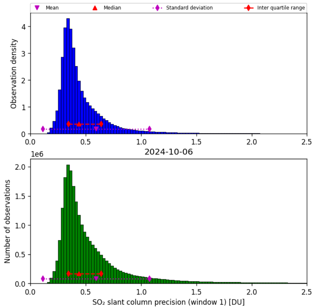
Figure 57: Histogram of “SO 2 slant column precision (window 1)” for 2024-10-05 to 2024-10-07
