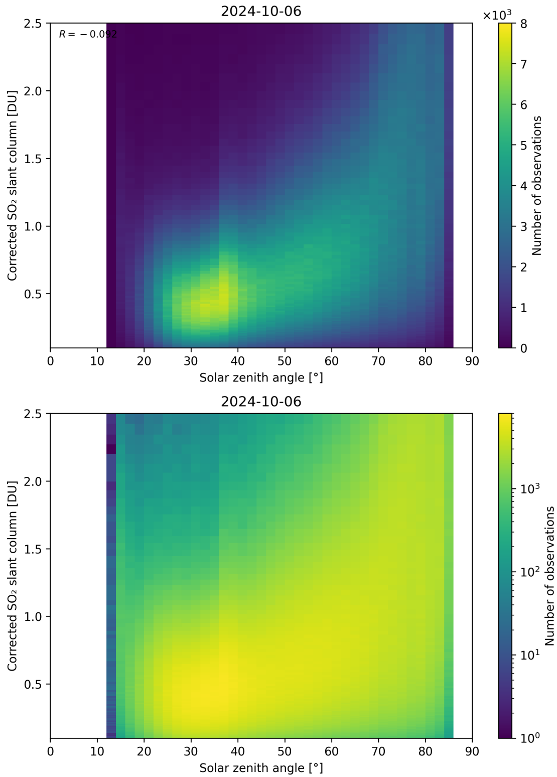
Figure 166: Scatter density plot of “Solar zenith angle” against “Corrected SO 2 slant column” for 2024-10-05 to 2024-10-07.
