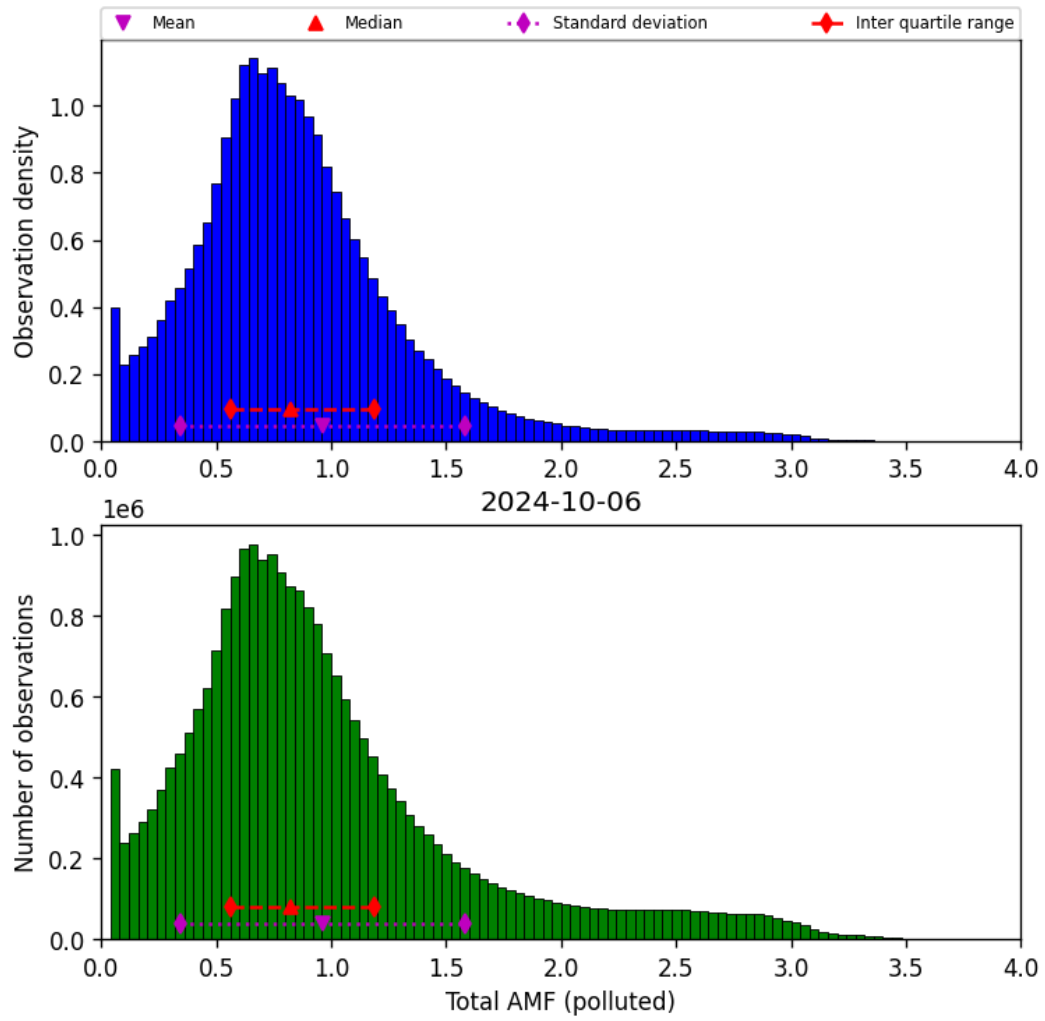
Figure 71: Histogram of “Total AMF (polluted)” for 2024-10-05 to 2024-10-07
