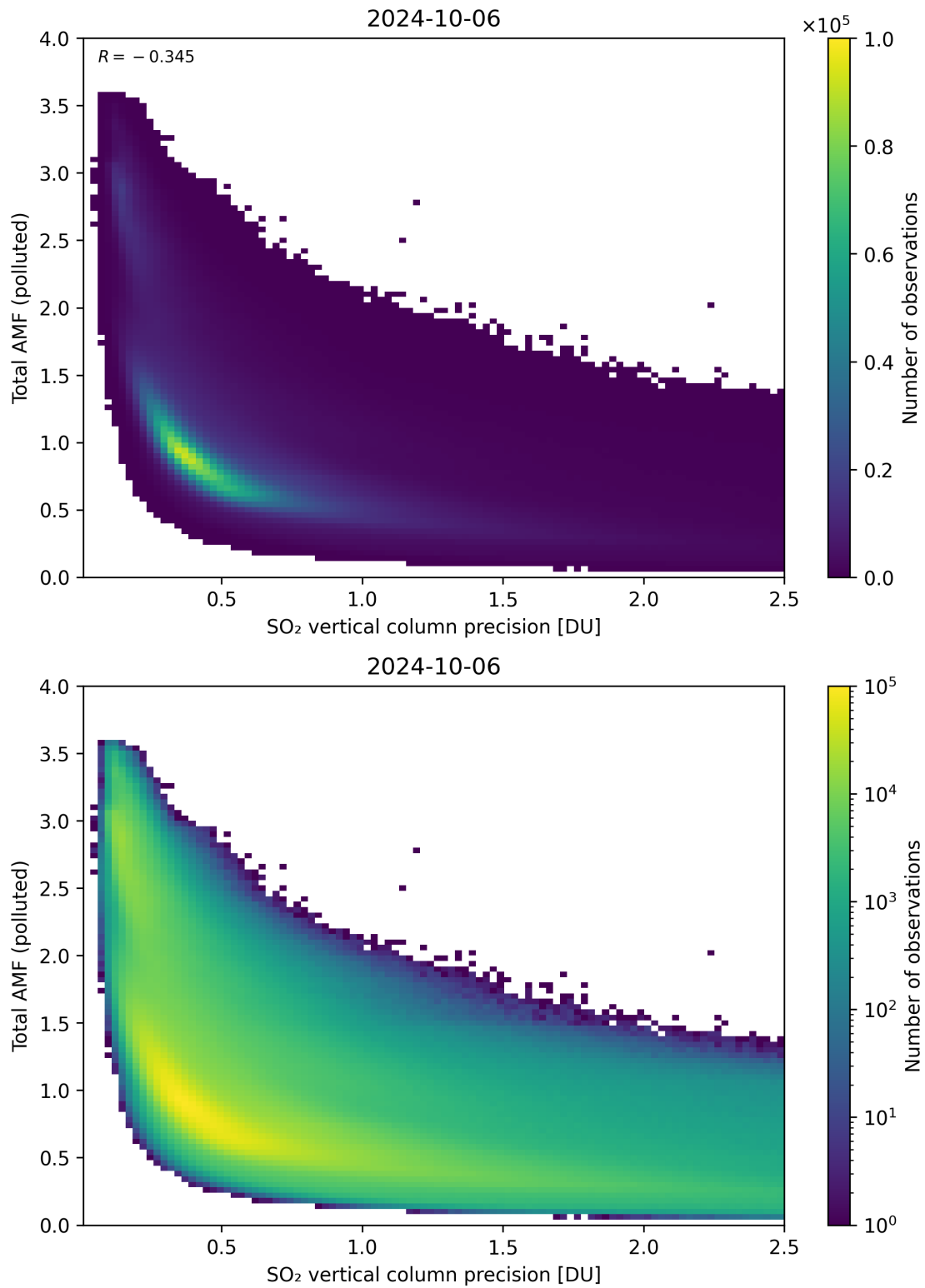
Figure 294: Scatter density plot of “SO 2 vertical column precision” against “Total AMF (polluted)” for 2024-10-05 to 2024-10-07.
