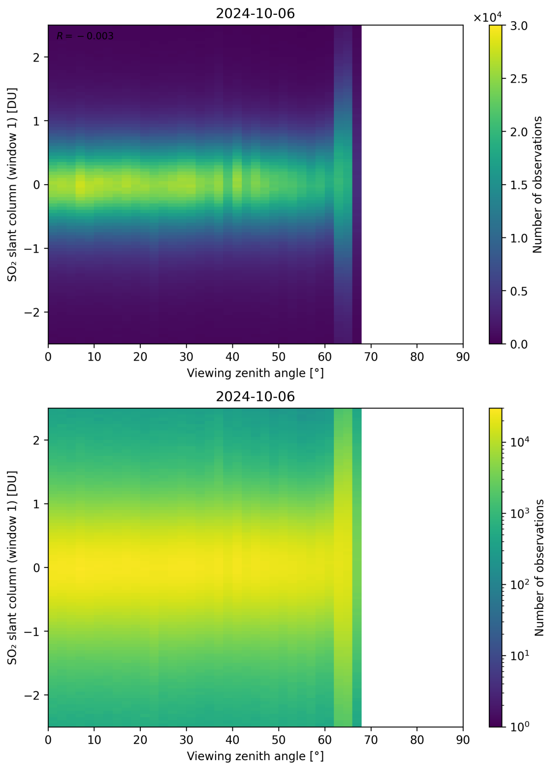
Figure 320: Scatter density plot of “Viewing zenith angle” against “SO 2 slant column (window 1)” for 2024-10-05 to 2024-10-07.
