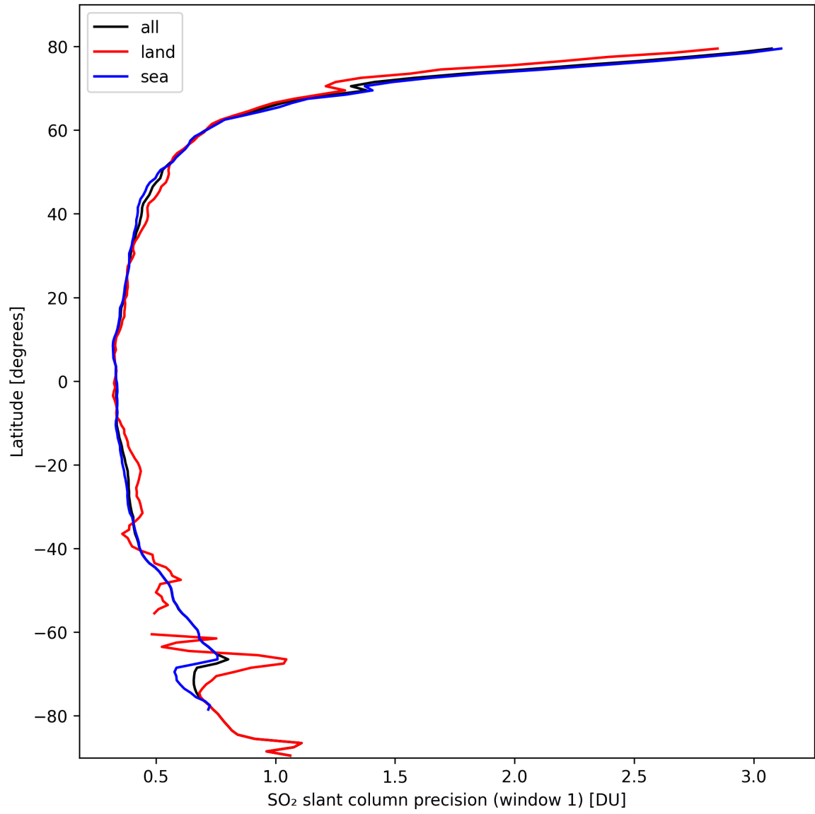
Figure 34: Zonal average of “SO 2 slant column precision (window 1)” for 2024-10-05 to 2024-10-07.
