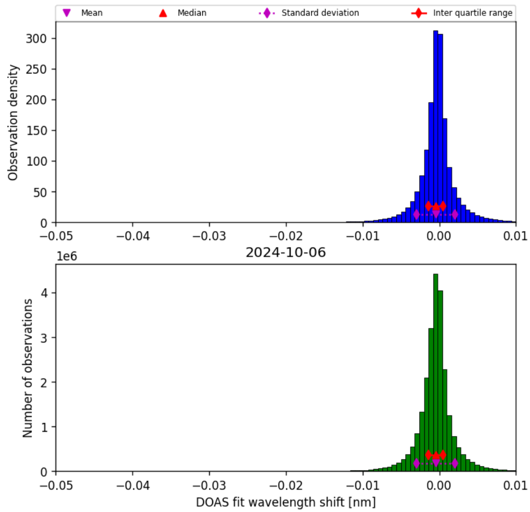
Figure 68: Histogram of “DOAS fit wavelength shift” for 2024-10-05 to 2024-10-07
