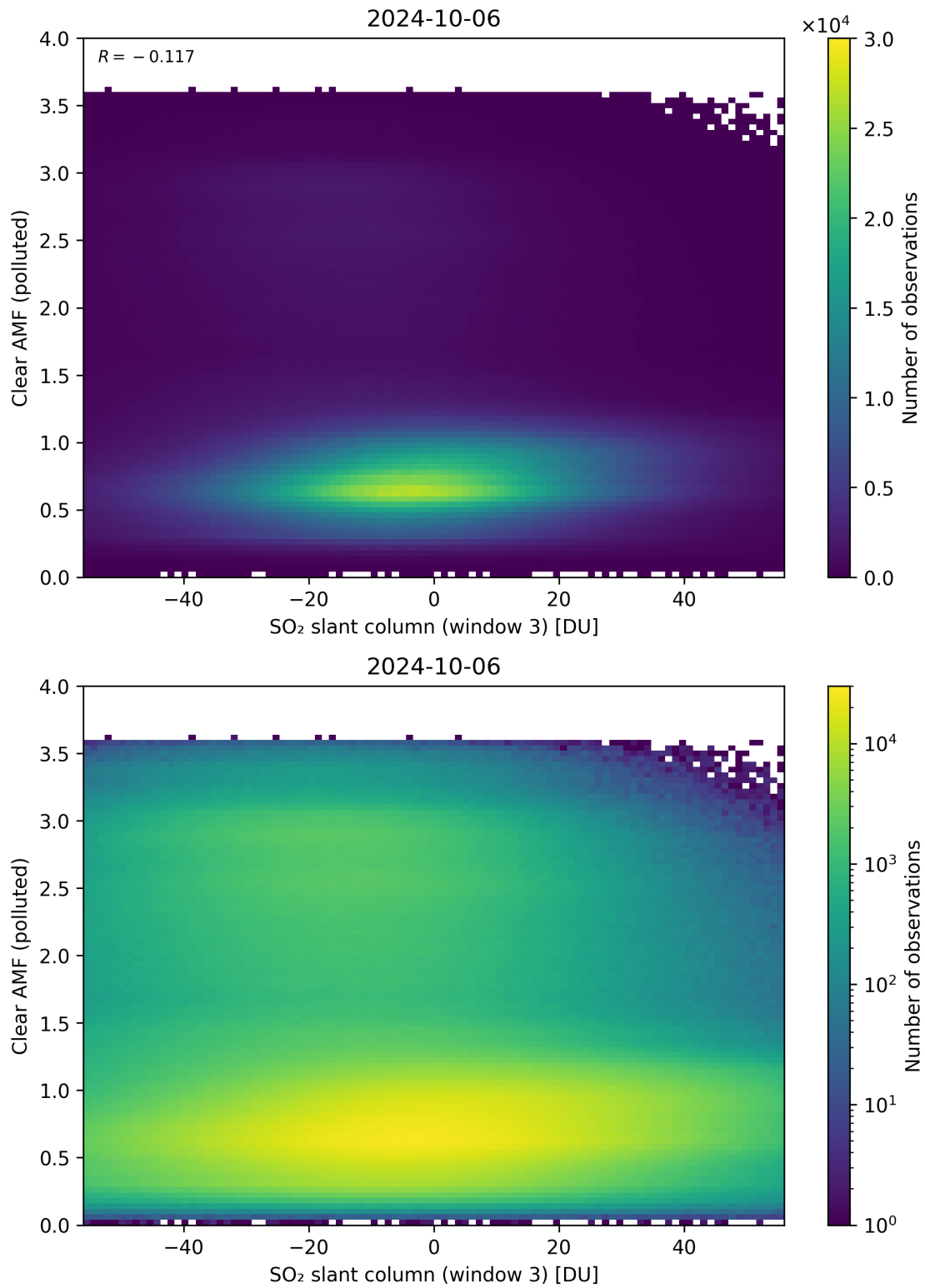
Figure 265: Scatter density plot of “SO 2 slant column (window 3)” against “Clear AMF (polluted)” for 2024-10-05 to 2024-10-07.
