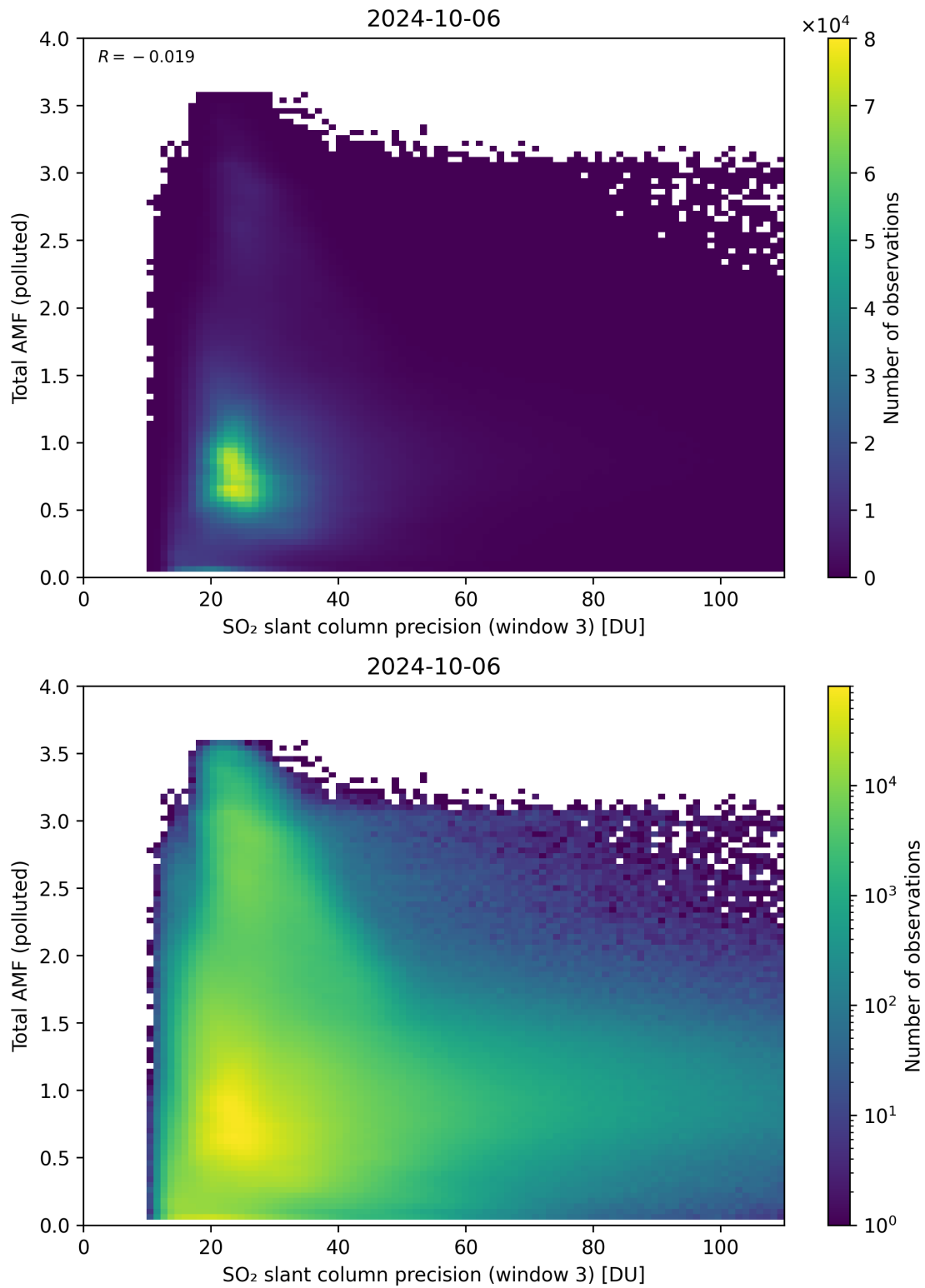
Figure 263: Scatter density plot of “SO 2 slant column precision (window 3)” against “Total AMF (polluted)” for 2024-10-05 to 2024-10-07.
