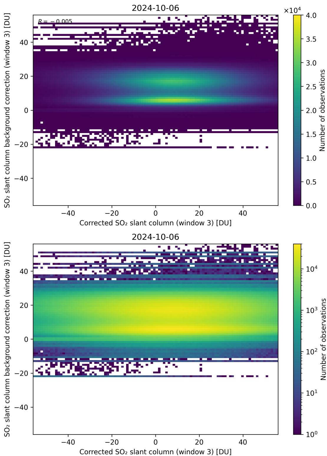
Figure 205: Scatter density plot of “Corrected SO 2 slant column (window 3)” against “SO 2 slant column background correction (window 3)” for 2024-10-05 to 2024-10-07.
