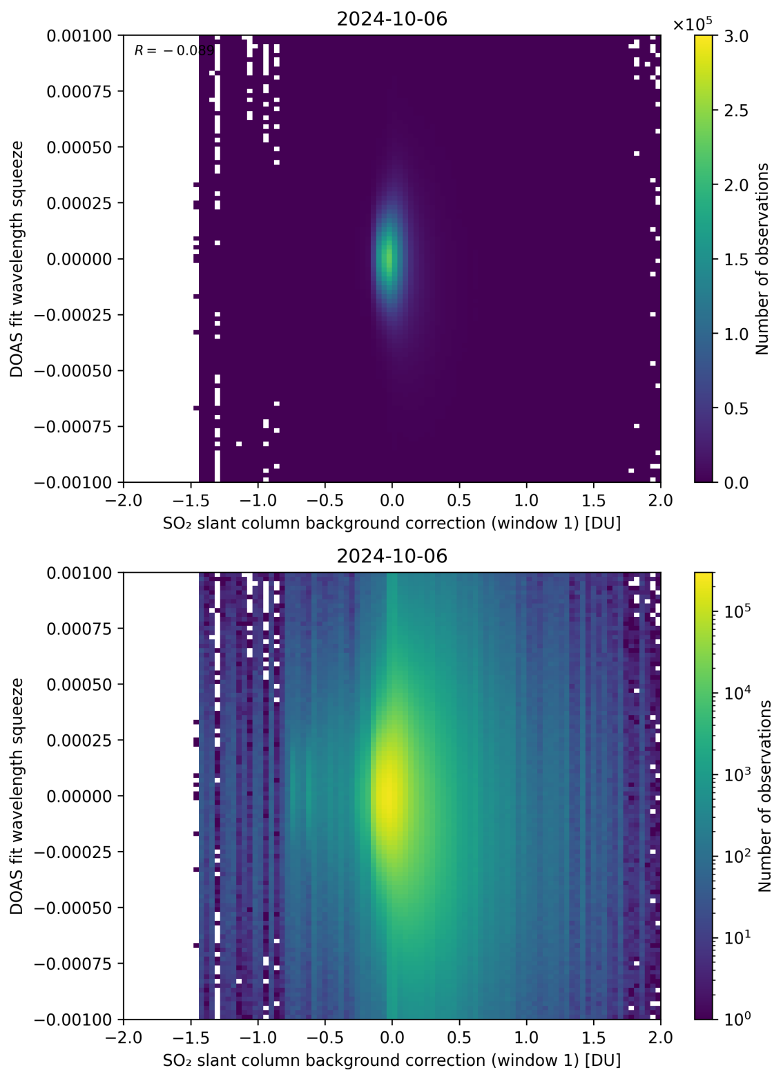
Figure 101: Scatter density plot of “SO 2 slant column background correction (window 1)” against “DOAS fit wavelength squeeze” for 2024-10-05 to 2024-10-07.
