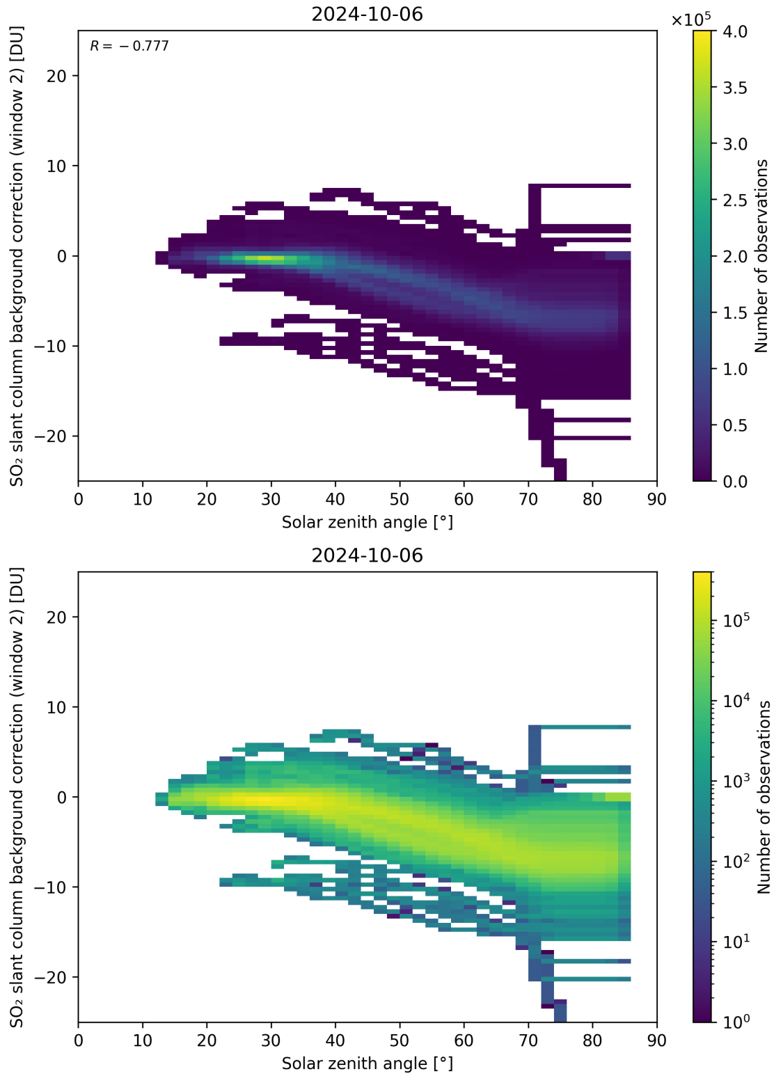
Figure 159: Scatter density plot of “Solar zenith angle” against “SO 2 slant column background correction (window 2)” for 2024-10-05 to 2024-10-07.
