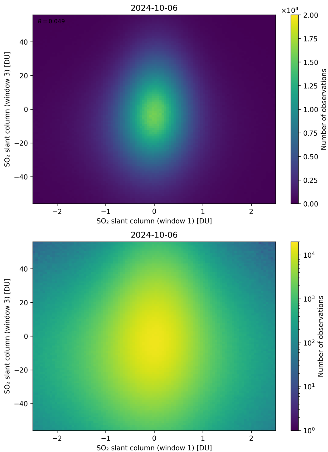
Figure 237: Scatter density plot of “SO 2 slant column (window 1)” against “SO 2 slant column (window 3)” for 2024-10-05 to 2024-10-07.
