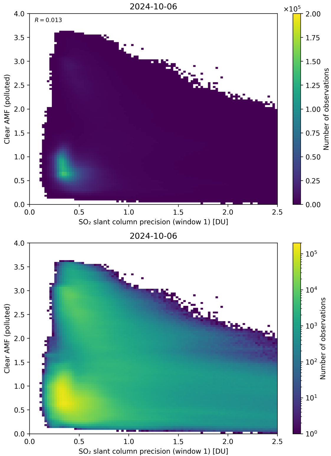
Figure 224: Scatter density plot of “SO 2 slant column precision (window 1)” against “Clear AMF (polluted)” for 2024-10-05 to 2024-10-07.
