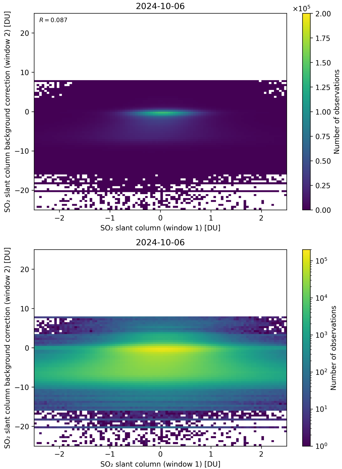
Figure 213: Scatter density plot of “SO 2 slant column (window 1)” against “SO 2 slant column background correction (window 2)” for 2024-10-05 to 2024-10-07.
