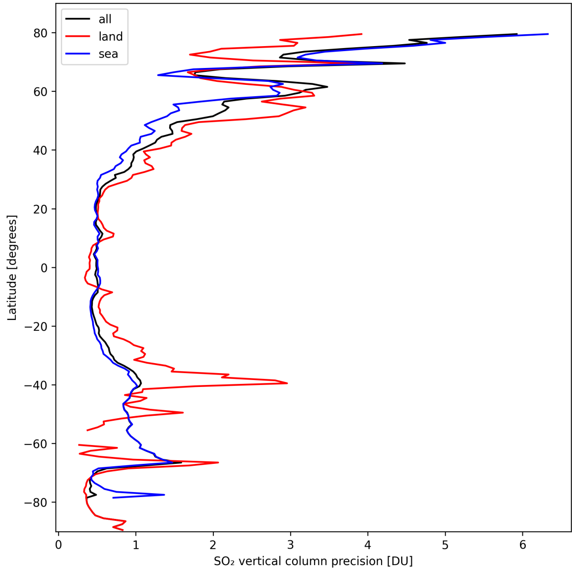
Figure 31: Zonal average of “SO 2 vertical column precision” for 2024-10-05 to 2024-10-07.
