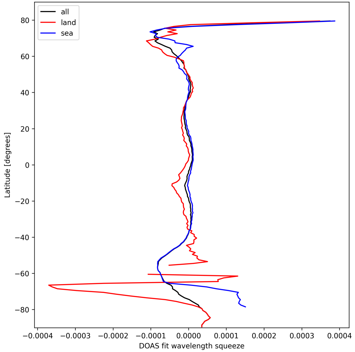
Figure 46: Zonal average of “DOAS fit wavelength squeeze” for 2024-10-05 to 2024-10-07.
