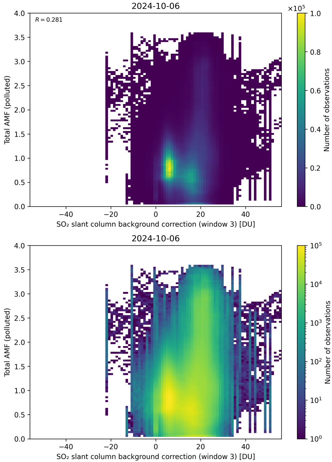
Figure 125: Scatter density plot of “SO 2 slant column background correction (window 3)” against “Total AMF (polluted)” for 2024-10-05 to 2024-10-07.
