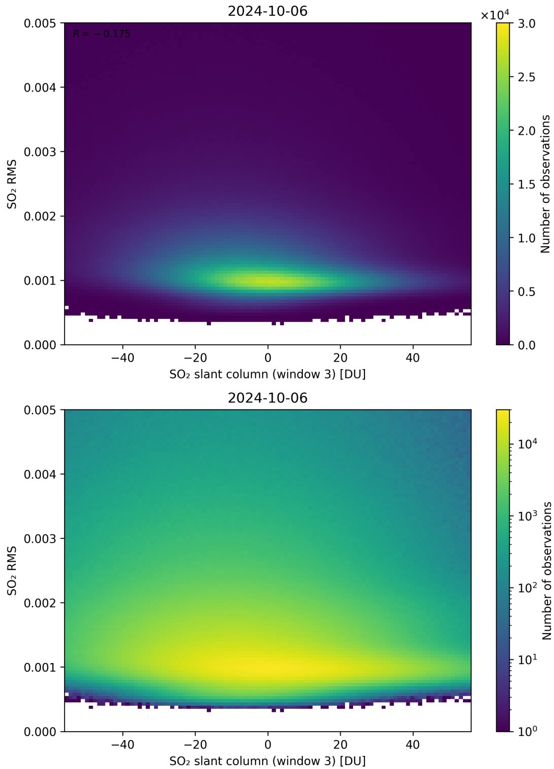
Figure 256: Scatter density plot of “SO 2 slant column (window 3)” against “SO 2 RMS” for 2024-10-05 to 2024-10-07.
