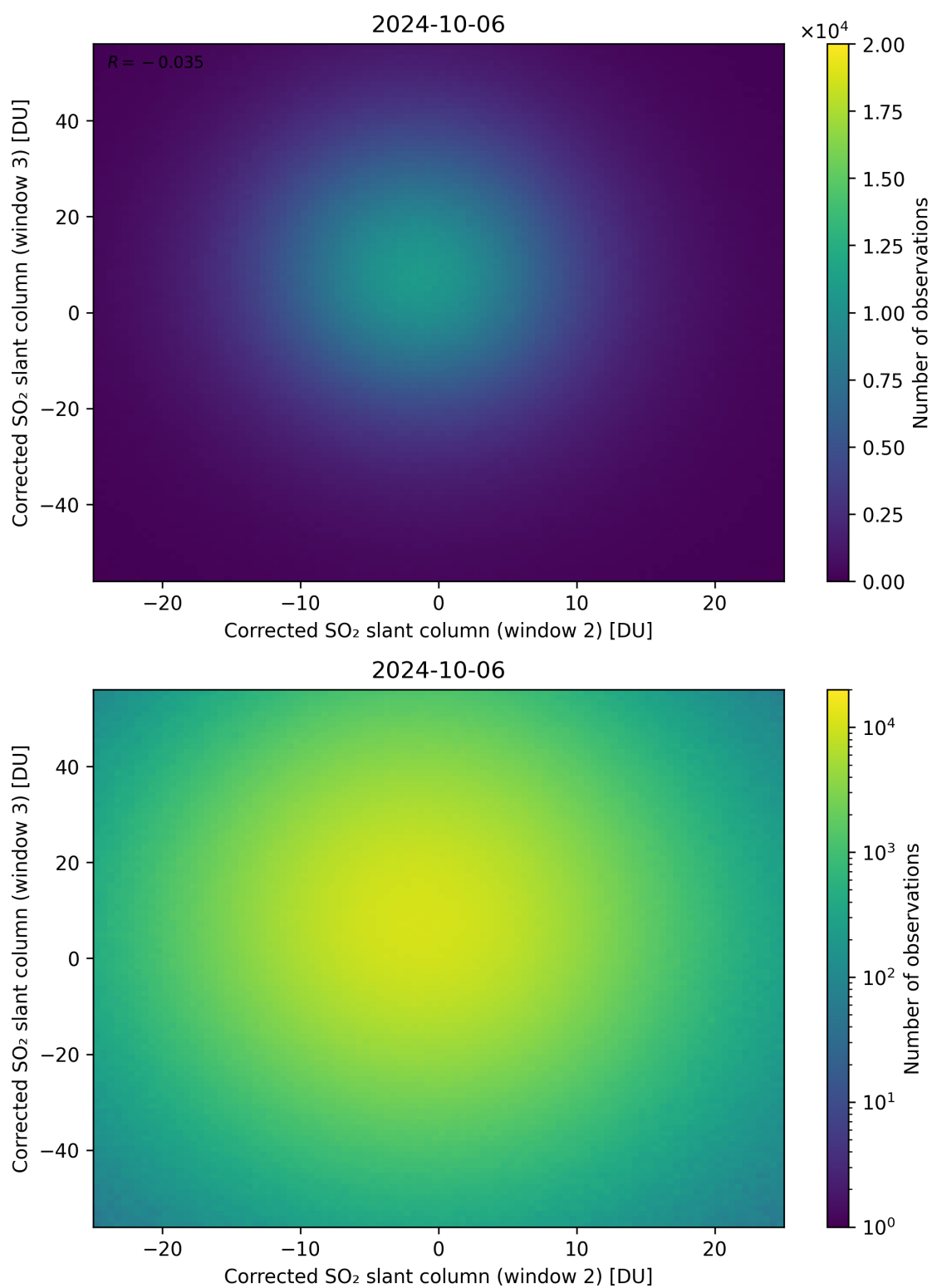
Figure 200: Scatter density plot of “Corrected SO 2 slant column (window 2)” against “Corrected SO 2 slant column (window 3)” for 2024-10-05 to 2024-10-07.
