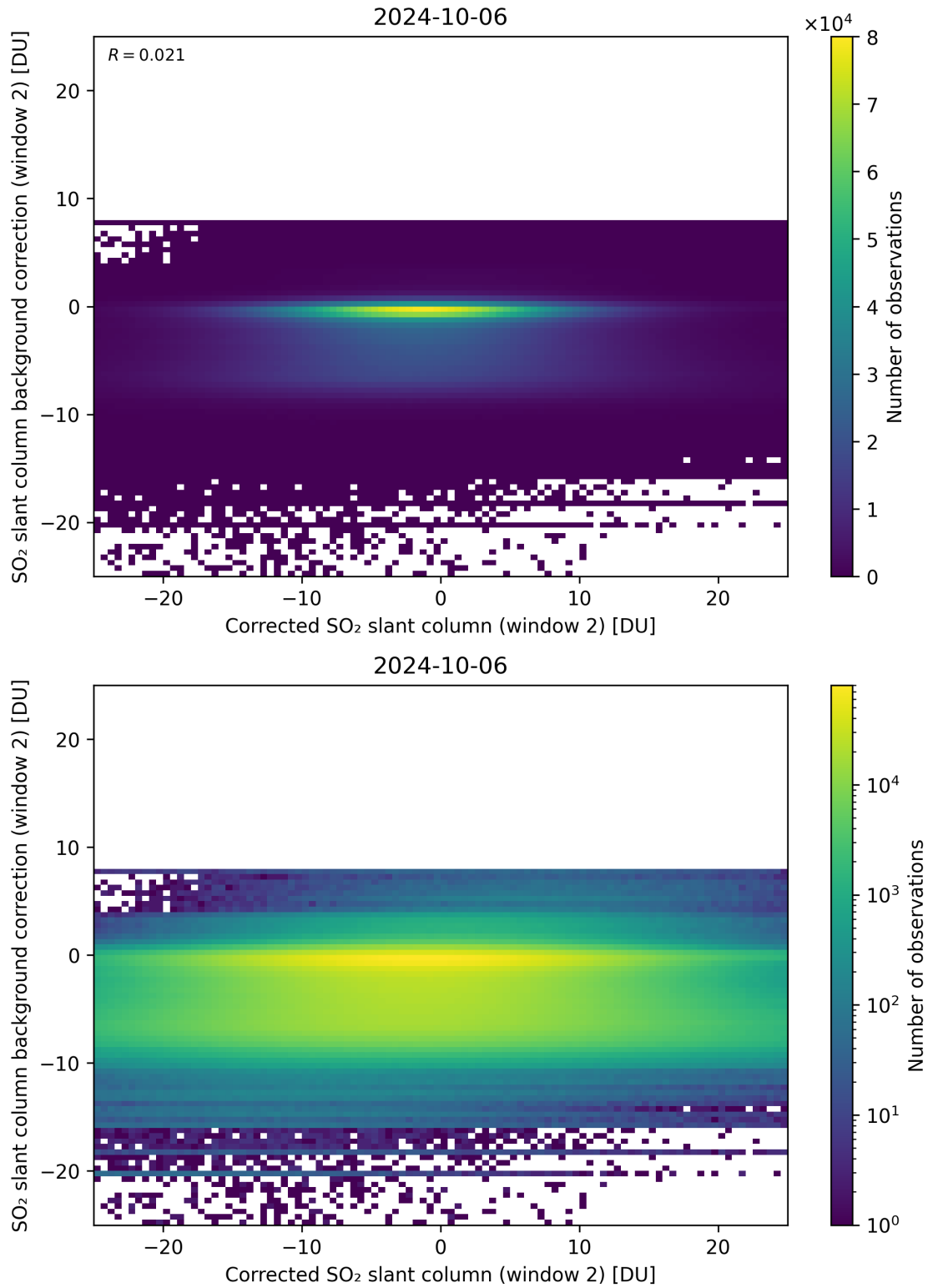
Figure 194: Scatter density plot of “Corrected SO 2 slant column (window 2)” against “SO 2 slant column background correction (window 2)” for 2024-10-05 to 2024-10-07.
