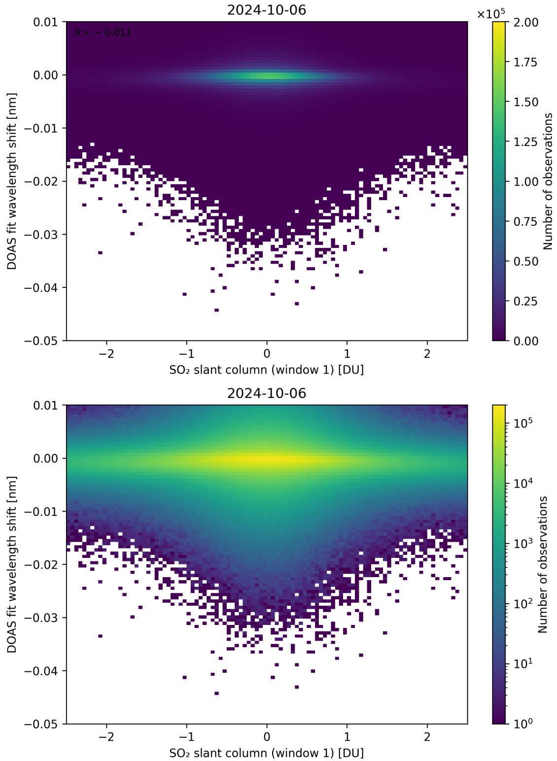
Figure 215: Scatter density plot of “SO 2 slant column (window 1)” against “DOAS fit wavelength shift” for 2024-10-05 to 2024-10-07.
