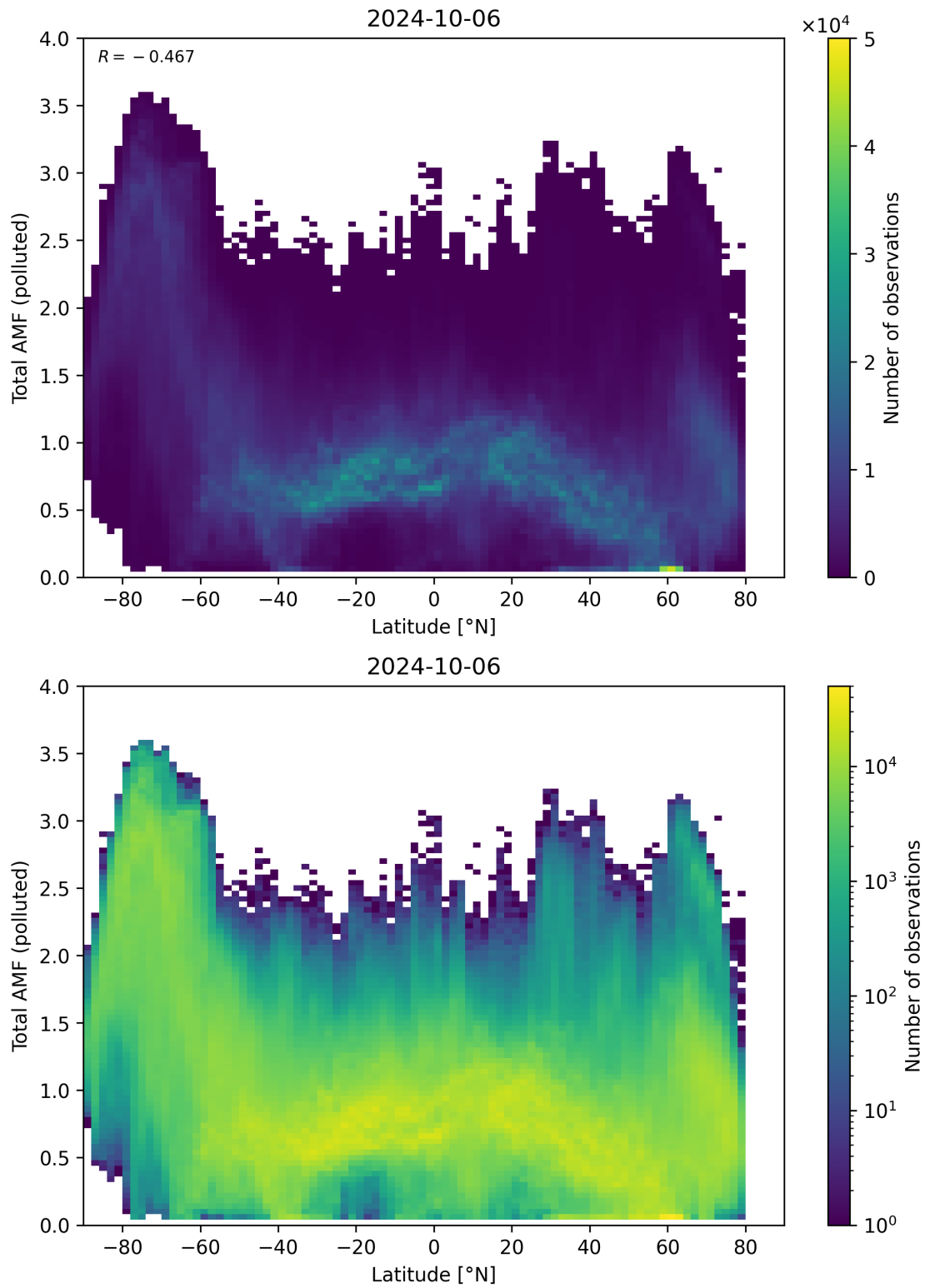
Figure 154: Scatter density plot of “Latitude” against “Total AMF (polluted)” for 2024-10-05 to 2024-10-07.
