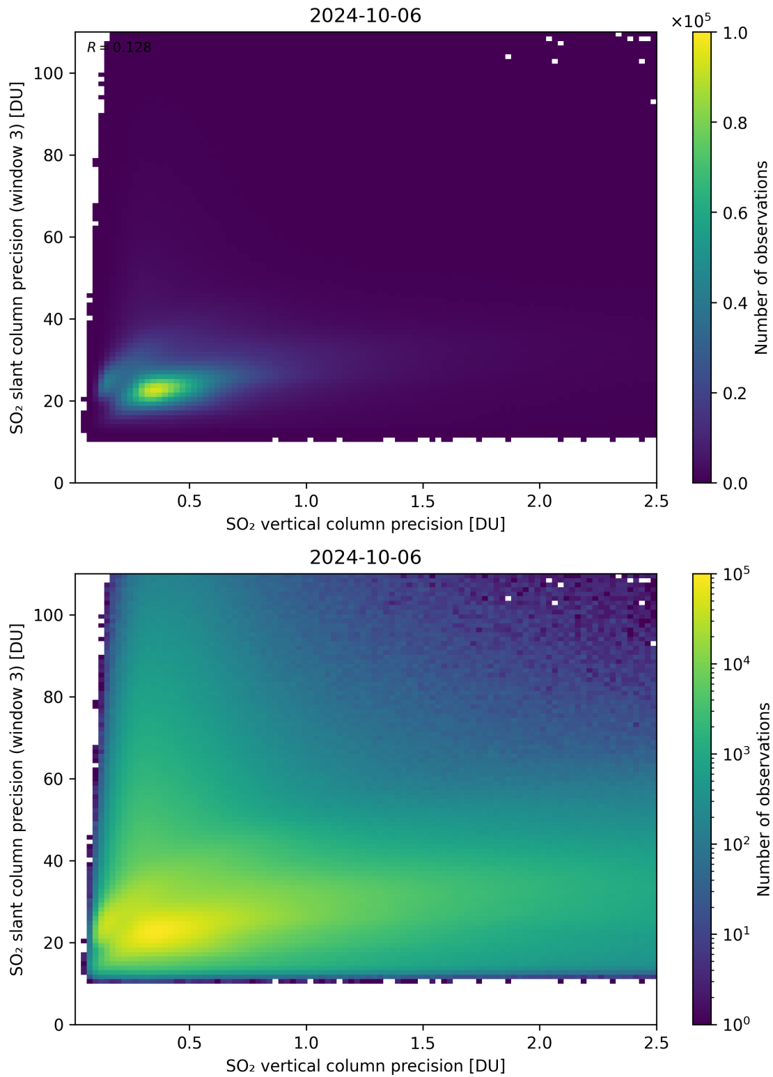
Figure 293: Scatter density plot of “SO 2 vertical column precision” against “SO 2 slant column precision (window 3)” for 2024-10-05 to 2024-10-07.
