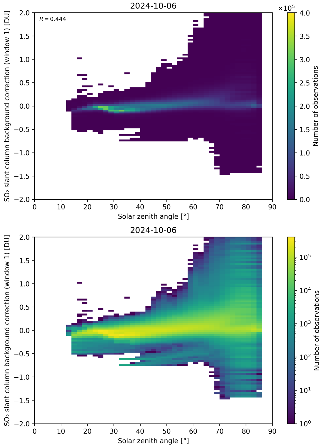
Figure 158: Scatter density plot of “Solar zenith angle” against “SO 2 slant column background correction (window 1)” for 2024-10-05 to 2024-10-07.
