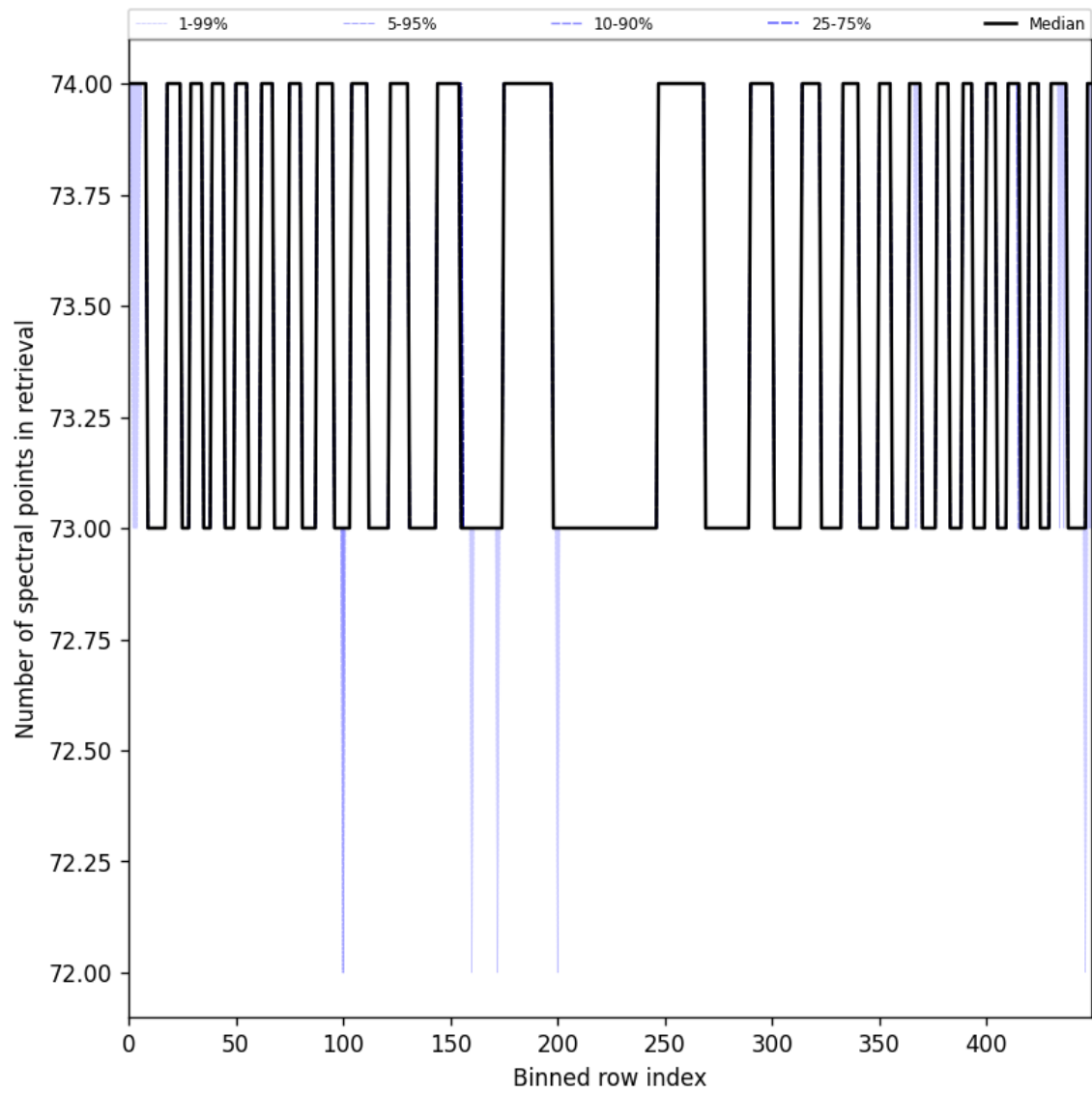
Figure 97: Along track statistics of “Number of spectral points in retrieval” for 2024-10-05 to 2024-10-07
