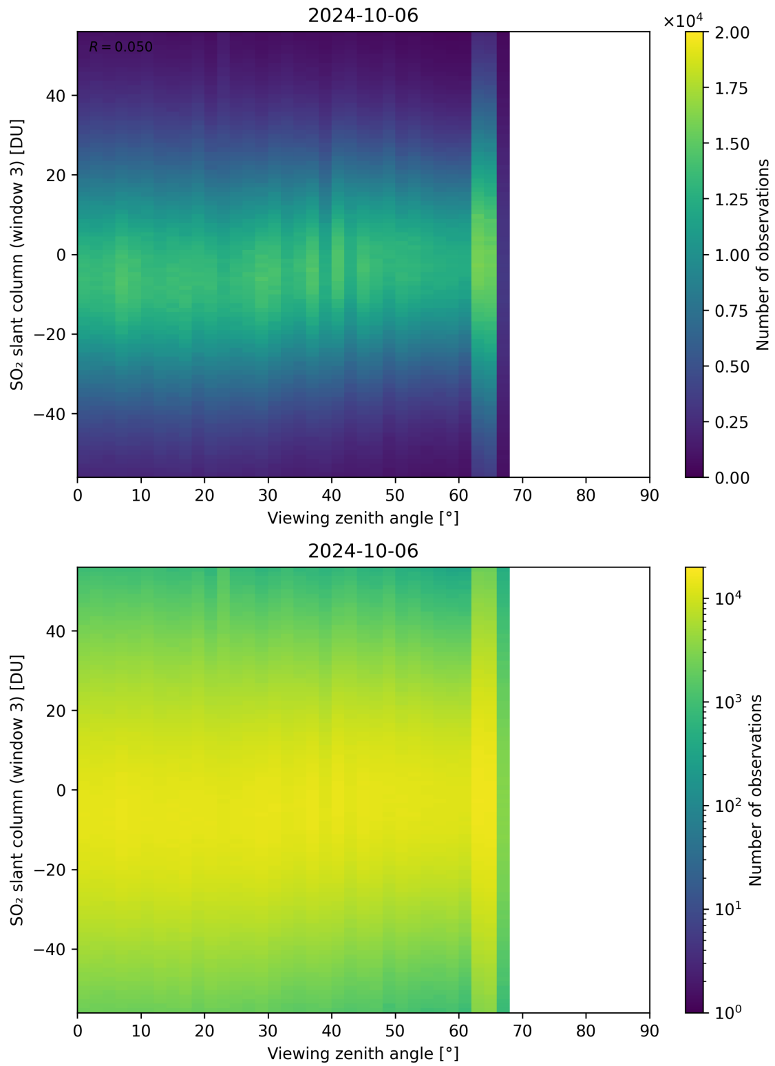
Figure 323: Scatter density plot of “Viewing zenith angle” against “SO 2 slant column (window 3)” for 2024-10-05 to 2024-10-07.
