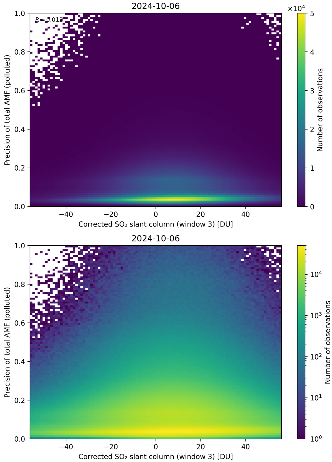
Figure 211: Scatter density plot of “Corrected SO 2 slant column (window 3)” against “Precision of total AMF (polluted)” for 2024-10-05 to 2024-10-07.
