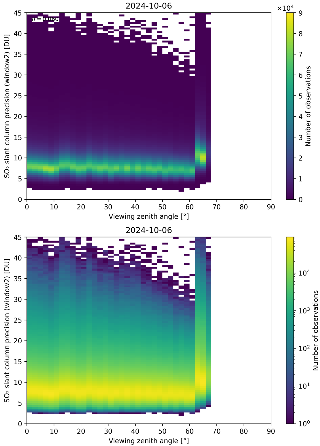
Figure 322: Scatter density plot of “Viewing zenith angle” against “SO 2 slant column precision (window2)” for 2024-10-05 to 2024-10-07.
