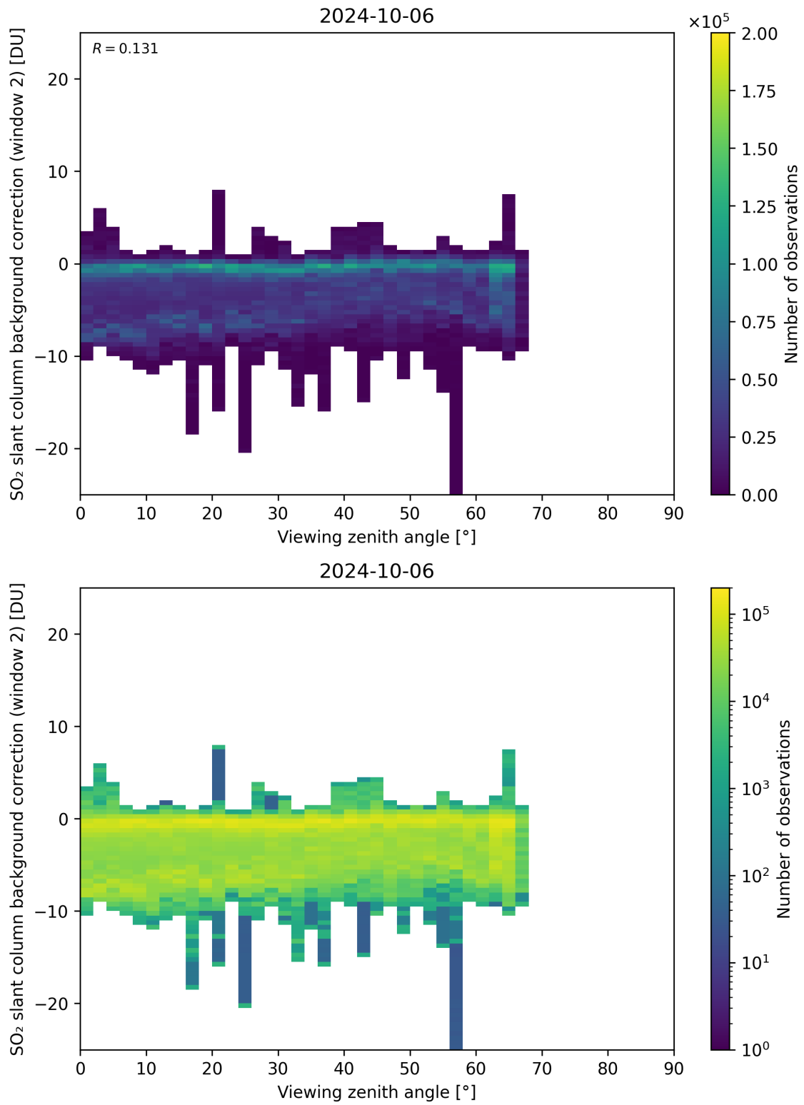
Figure 309: Scatter density plot of “Viewing zenith angle” against “SO 2 slant column background correction (window 2)” for 2024-10-05 to 2024-10-07.
