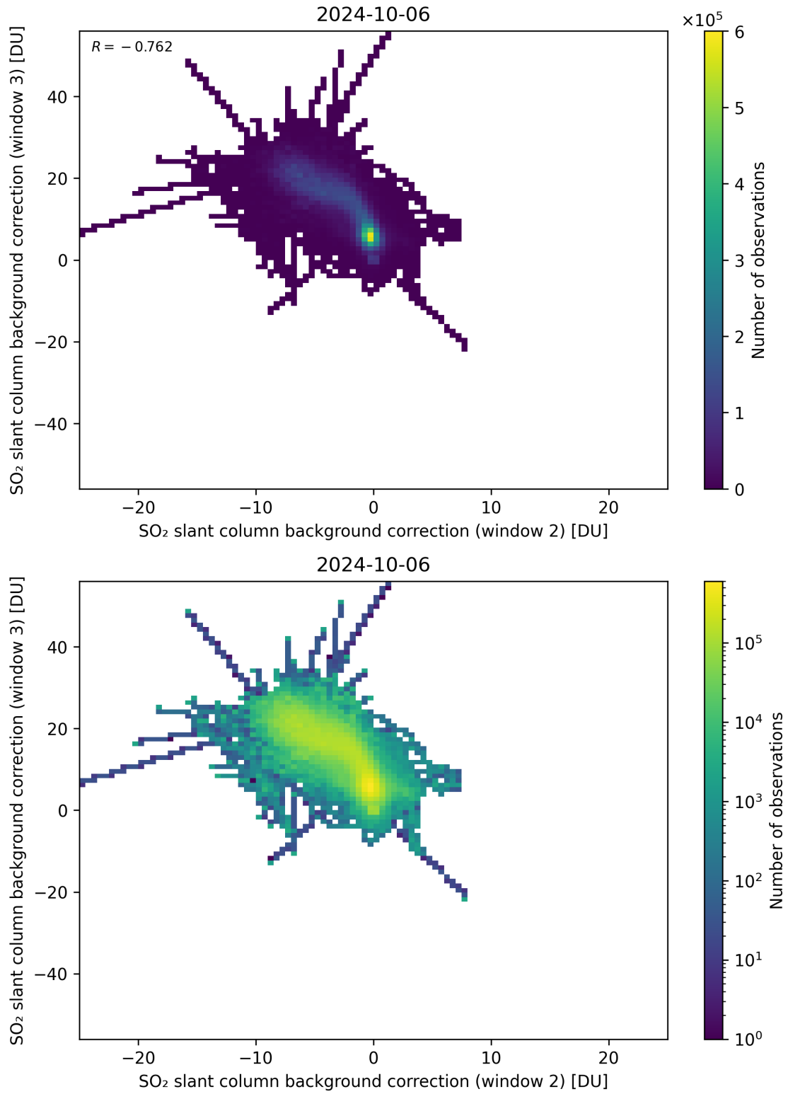
Figure 111: Scatter density plot of “SO 2 slant column background correction (window 2)” against “SO 2 slant column background correction (window 3)” for 2024-10-05 to 2024-10-07.
