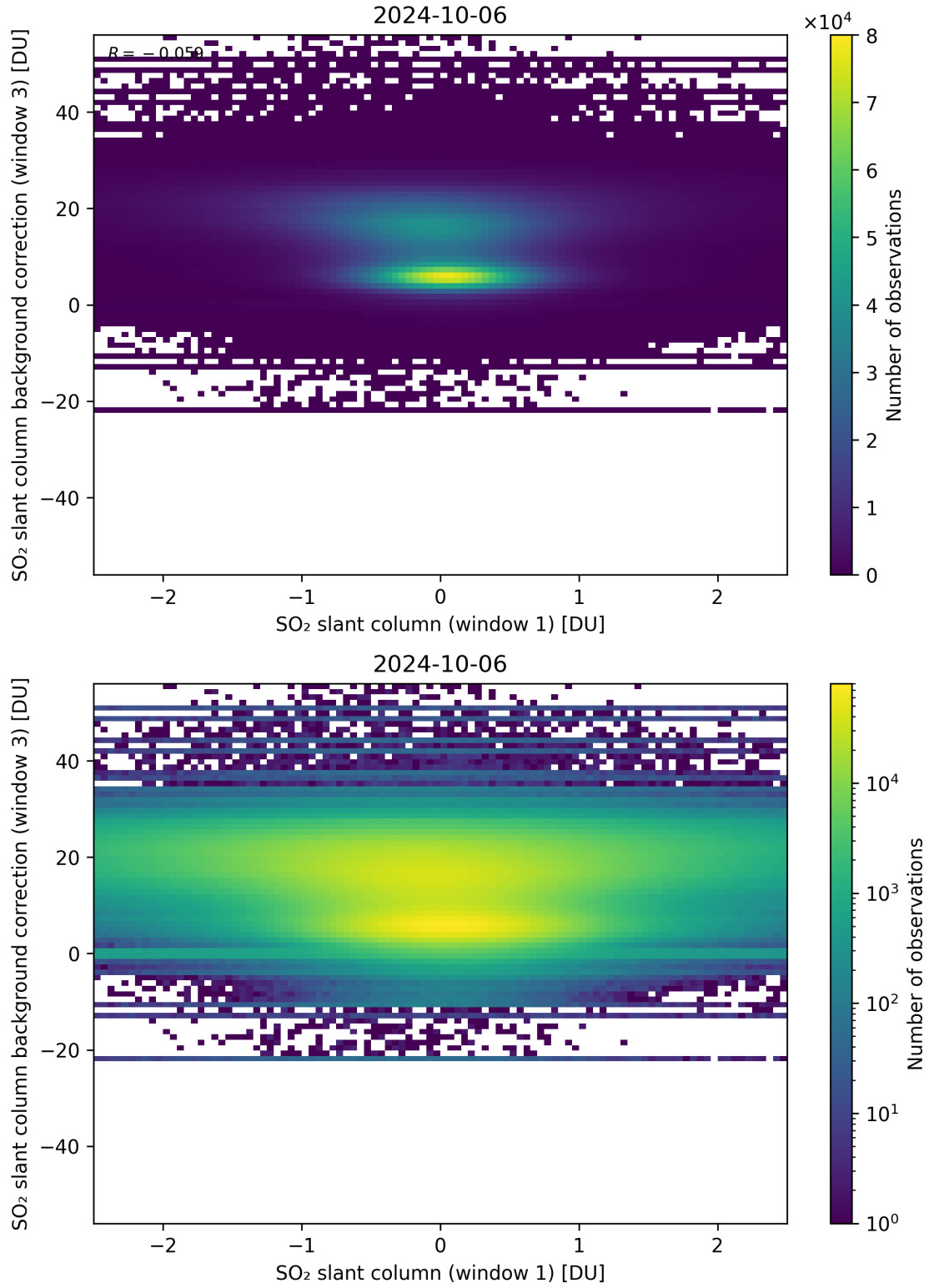
Figure 214: Scatter density plot of “SO 2 slant column (window 1)” against “SO 2 slant column background correction (window 3)” for 2024-10-05 to 2024-10-07.
