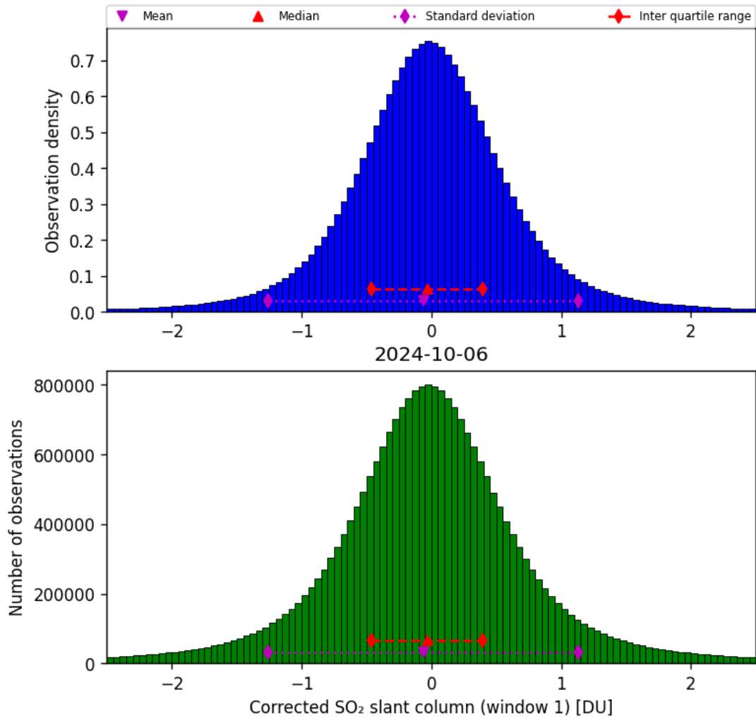
Figure 58: Histogram of “Corrected SO 2 slant column (window 1)” for 2024-10-05 to 2024-10-07
