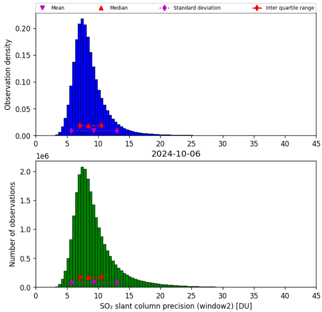
Figure 61: Histogram of “SO 2 slant column precision (window2)” for 2024-10-05 to 2024-10-07
