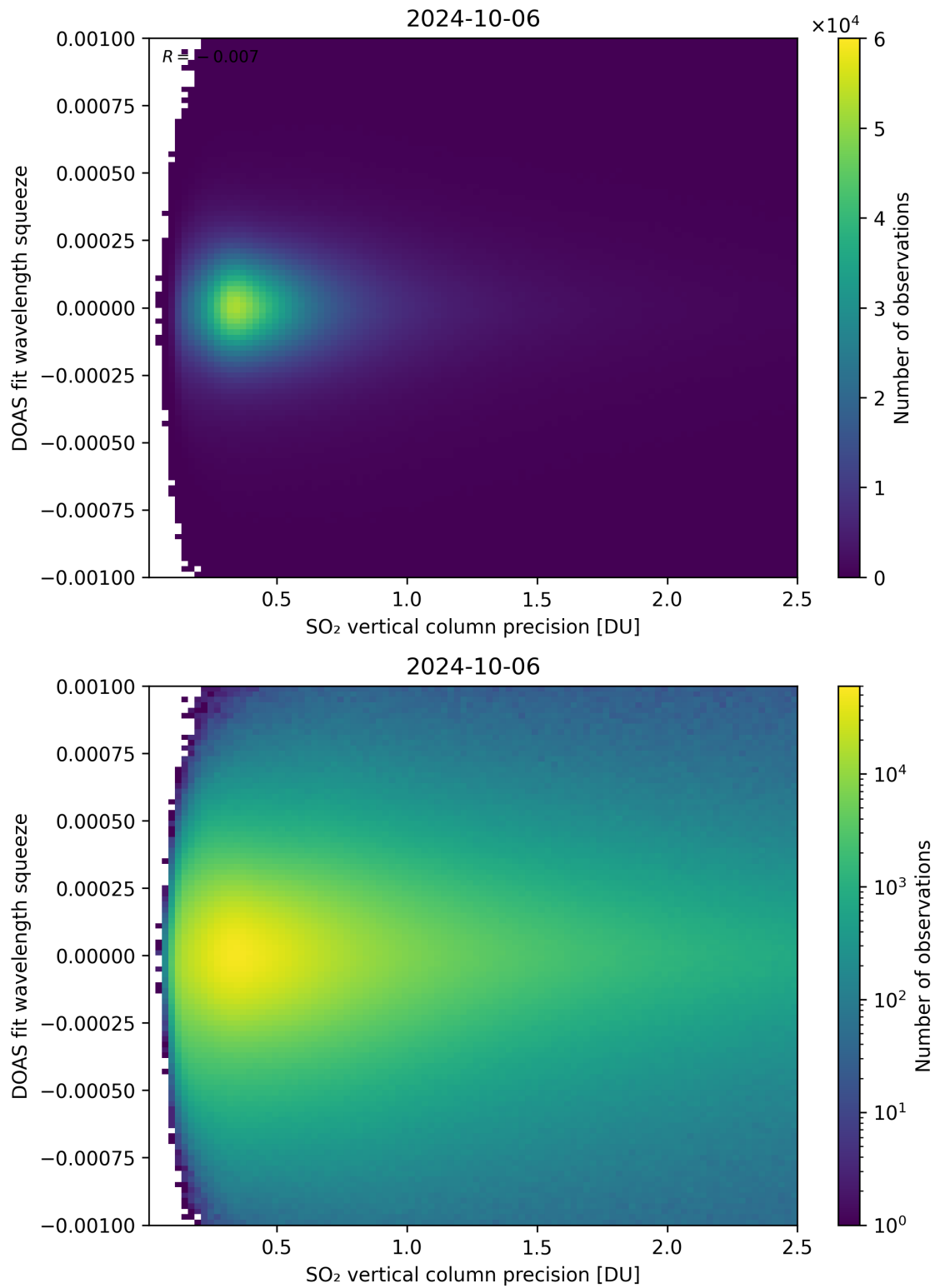
Figure 283: Scatter density plot of “SO 2 vertical column precision” against “DOAS fit wavelength squeeze” for 2024-10-05 to 2024-10-07.
