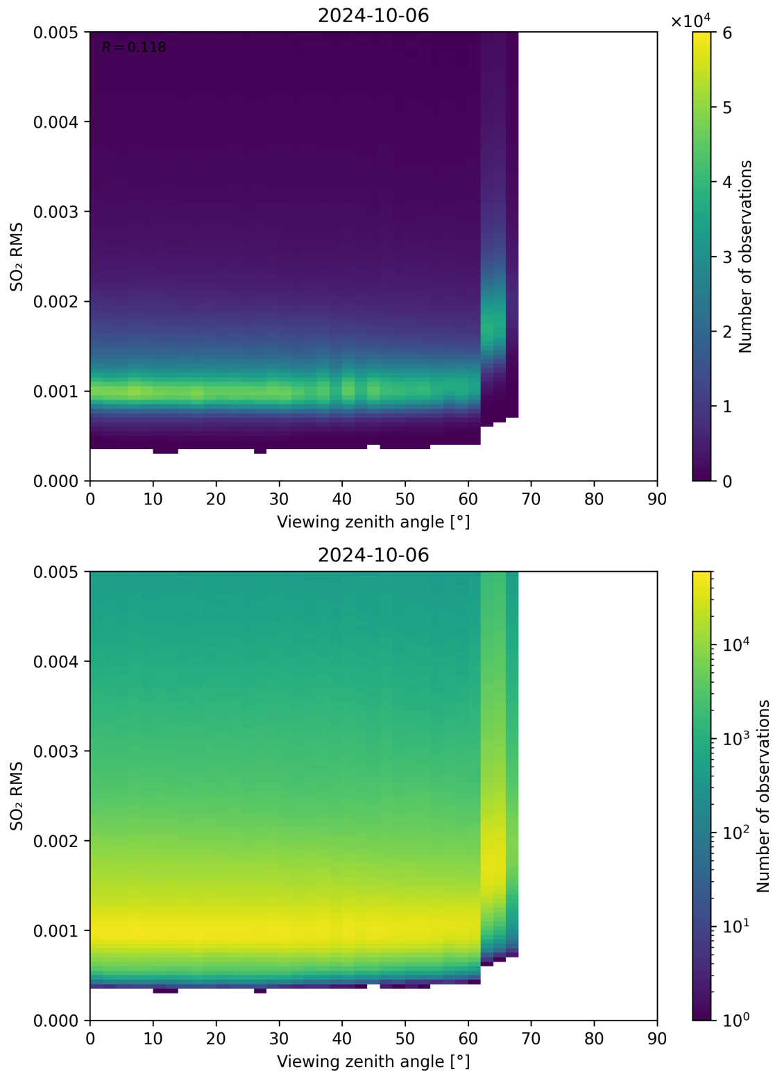
Figure 313: Scatter density plot of “Viewing zenith angle” against “SO 2 RMS” for 2024-10-05 to 2024-10-07.
