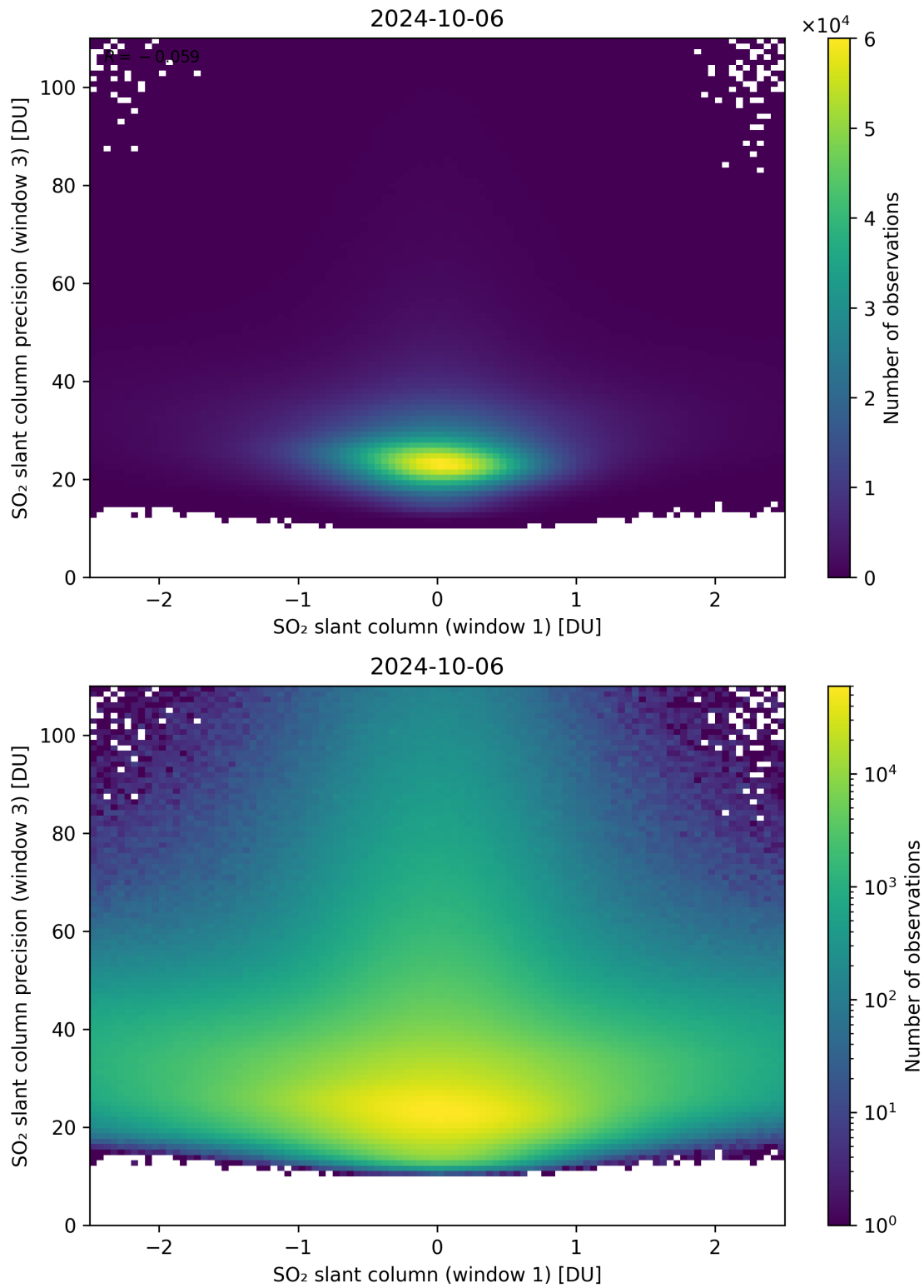
Figure 238: Scatter density plot of “SO 2 slant column (window 1)” against “SO 2 slant column precision (window 3)” for 2024-10-05 to 2024-10-07.
