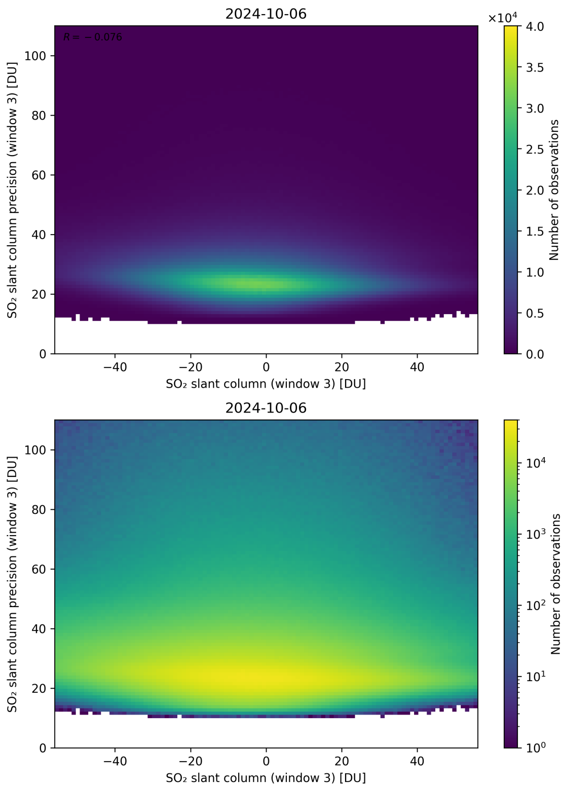
Figure 267: Scatter density plot of “SO 2 slant column (window 3)” against “SO 2 slant column precision (window 3)” for 2024-10-05 to 2024-10-07.
