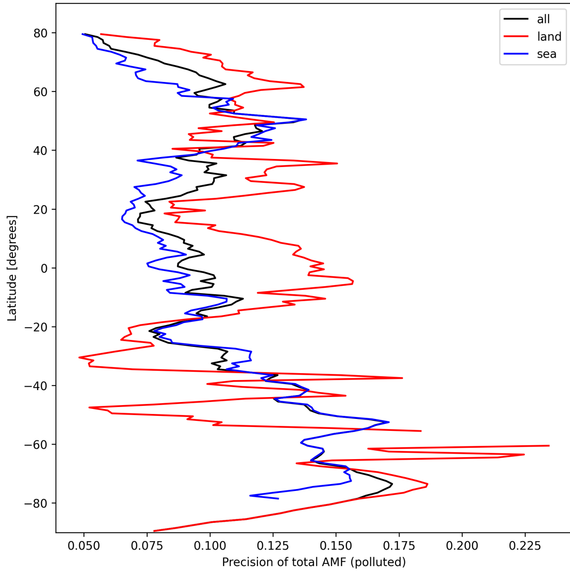
Figure 49: Zonal average of “Precision of total AMF (polluted)” for 2024-10-05 to 2024-10-07.
