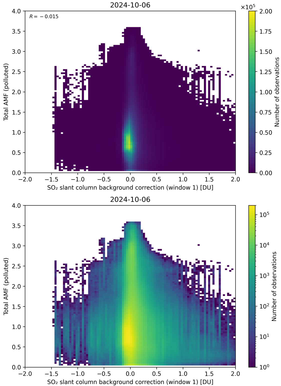
Figure 109: Scatter density plot of “SO 2 slant column background correction (window 1)” against “Total AMF (polluted)” for 2024-10-05 to 2024-10-07.
