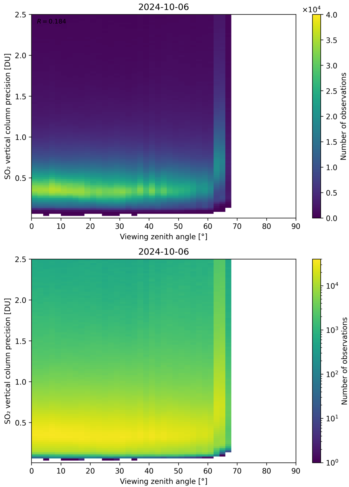
Figure 328: Scatter density plot of “Viewing zenith angle” against “SO 2 vertical column precision” for 2024-10-05 to 2024-10-07.
