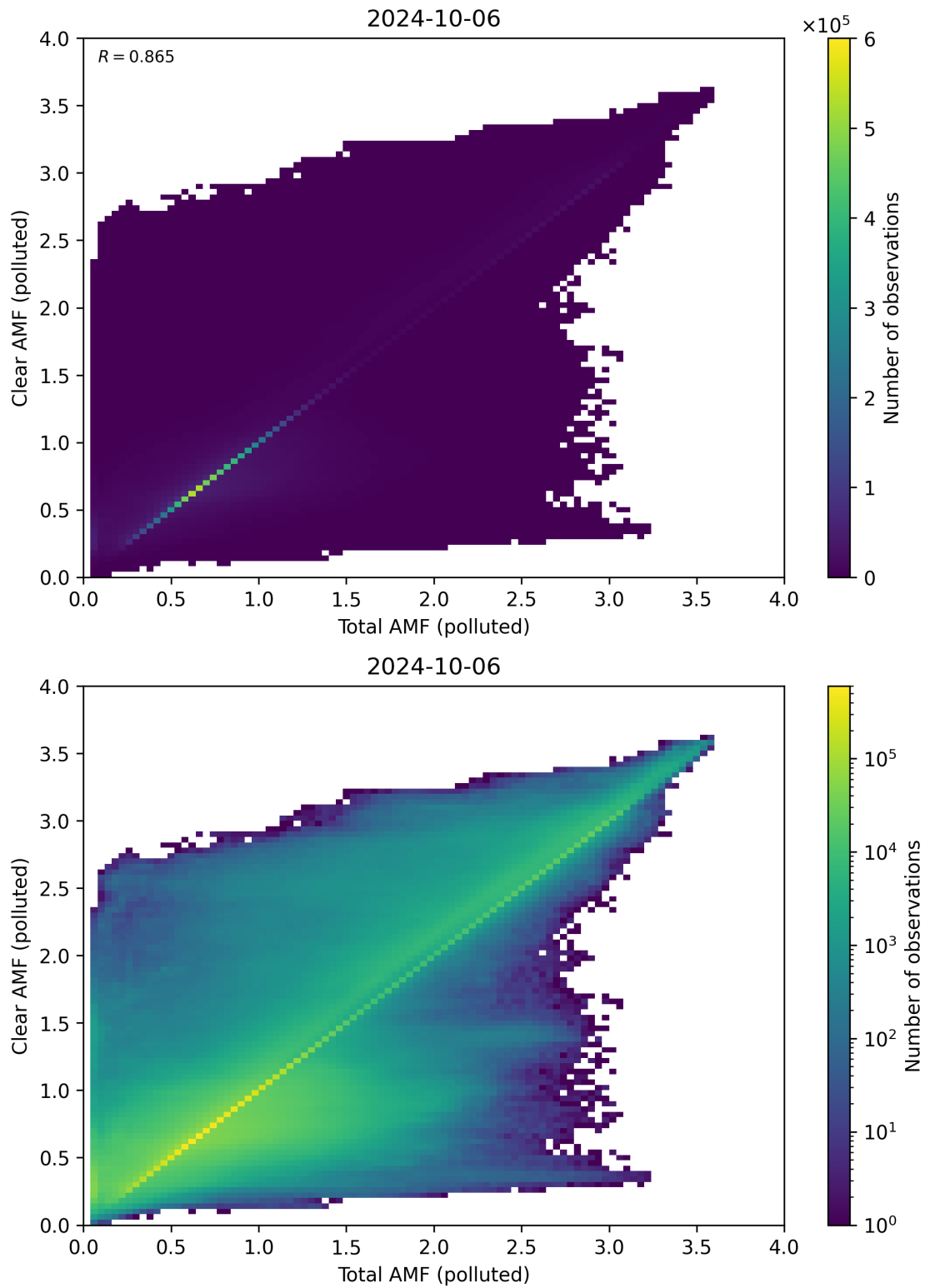
Figure 271: Scatter density plot of “Total AMF (polluted)” against “Clear AMF (polluted)” for 2024-10-05 to 2024-10-07.
