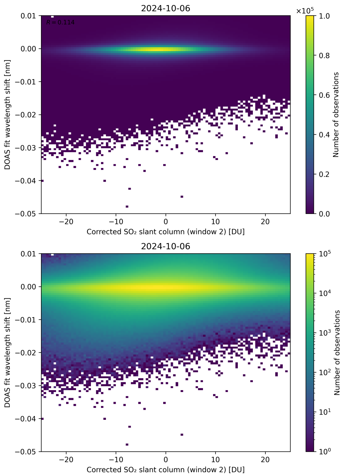
Figure 196: Scatter density plot of “Corrected SO 2 slant column (window 2)” against “DOAS fit wavelength shift” for 2024-10-05 to 2024-10-07.
