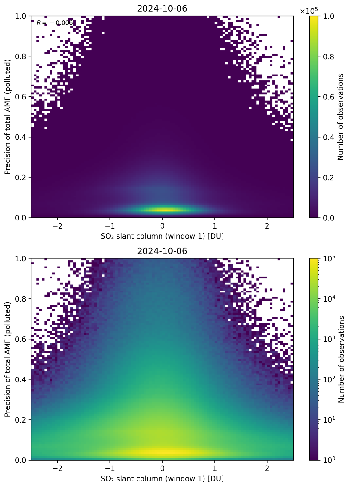
Figure 240: Scatter density plot of “SO 2 slant column (window 1)” against “Precision of total AMF (polluted)” for 2024-10-05 to 2024-10-07.
