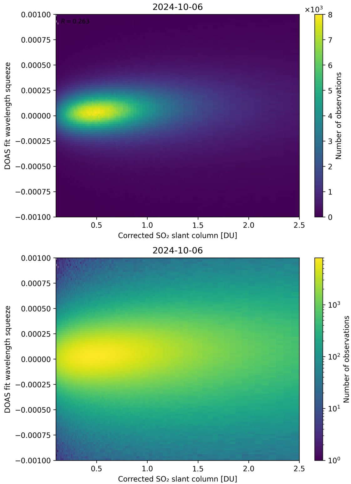
Figure 182: Scatter density plot of “Corrected SO 2 slant column” against “DOAS fit wavelength squeeze” for 2024-10-05 to 2024-10-07.
