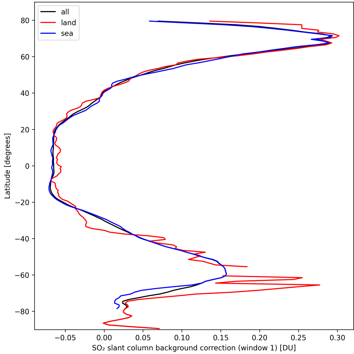
Figure 36: Zonal average of “SO 2 slant column background correction (window 1)” for 2024-10-05 to 2024-10-07.
