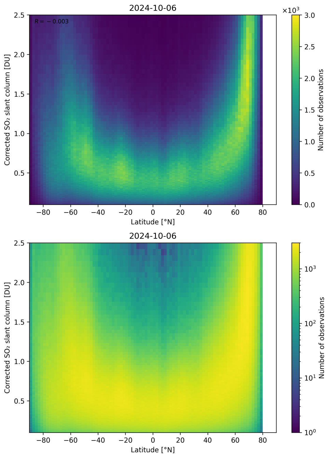
Figure 146: Scatter density plot of “Latitude” against “Corrected SO 2 slant column” for 2024-10-05 to 2024-10-07.
