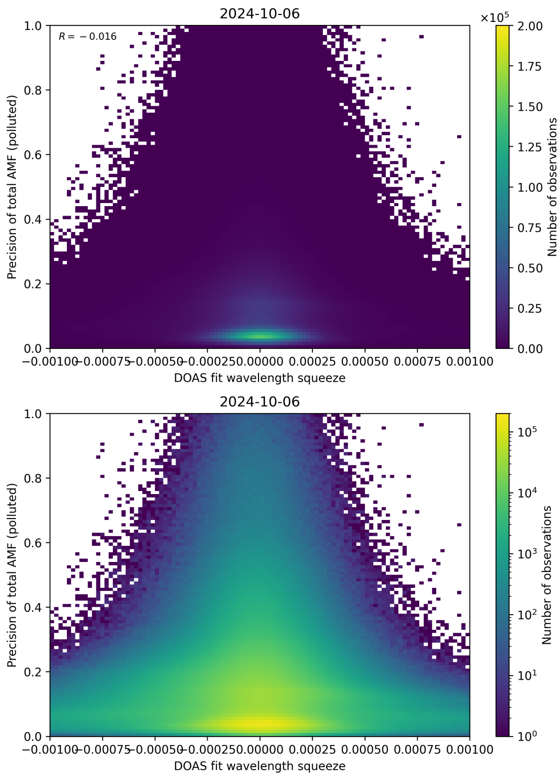
Figure 135: Scatter density plot of “DOAS fit wavelength squeeze” against “Precision of total AMF (polluted)” for 2024-10-05 to 2024-10-07.
