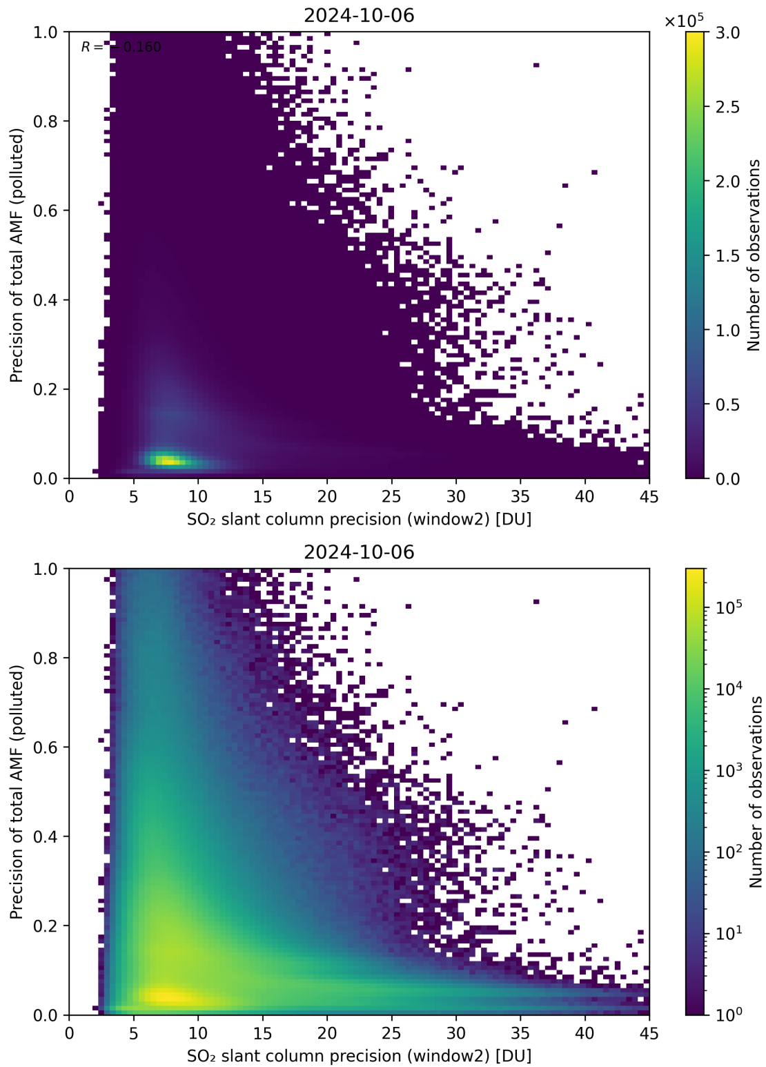
Figure 252: Scatter density plot of “SO 2 slant column precision (window2)” against “Precision of total AMF (polluted)” for 2024-10-05 to 2024-10-07.
