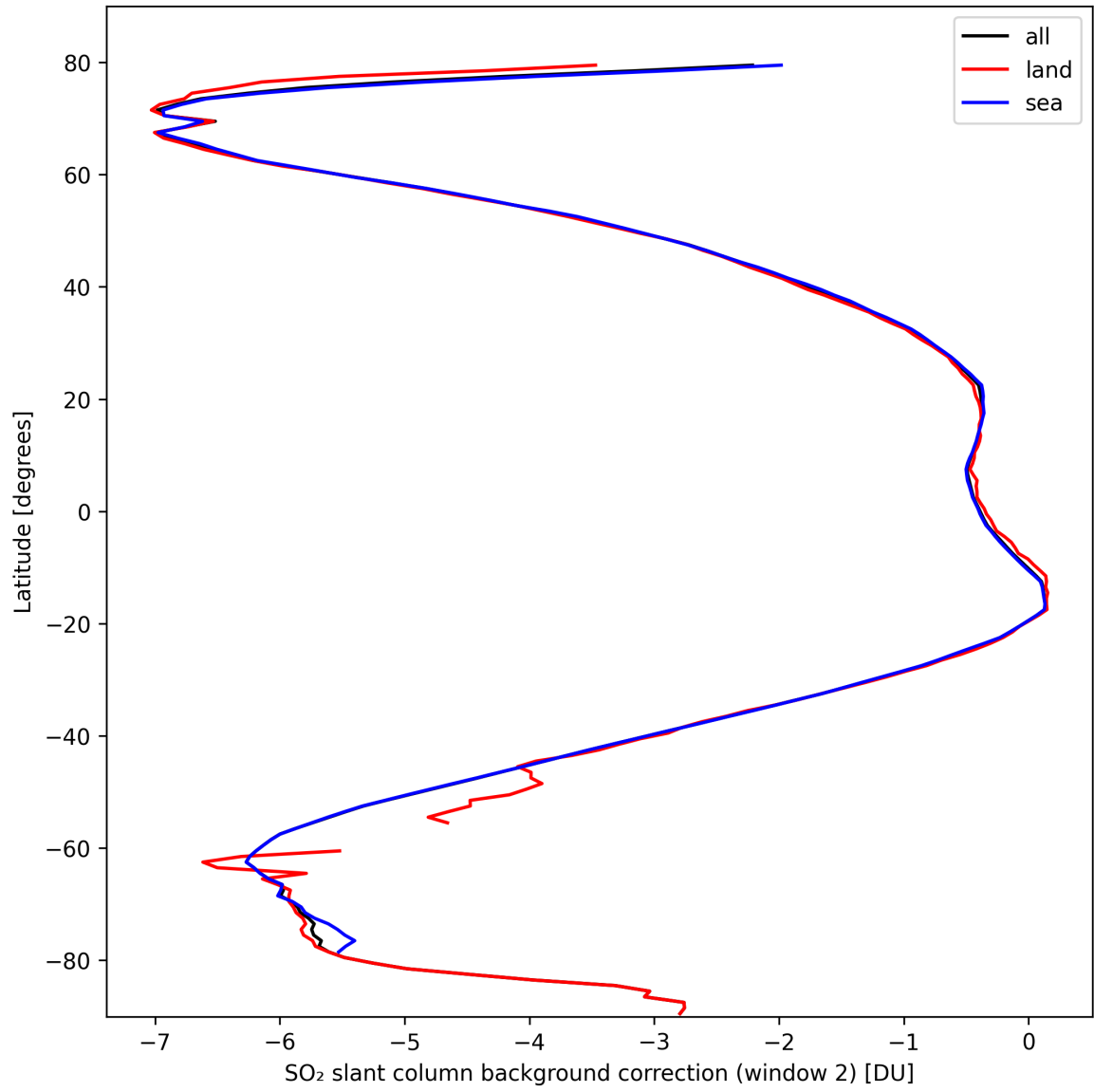
Figure 40: Zonal average of “SO 2 slant column background correction (window 2)” for 2024-10-05 to 2024-10-07.
