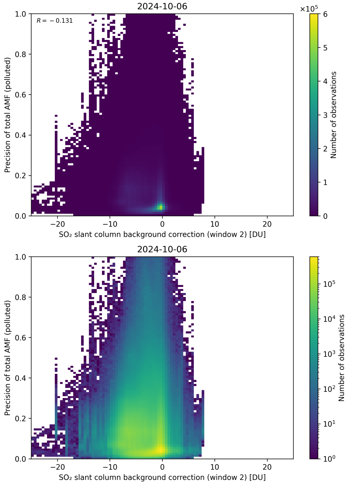
Figure 120: Scatter density plot of “SO 2 slant column background correction (window 2)” against “Precision of total AMF (polluted)” for 2024-10-05 to 2024-10-07.
