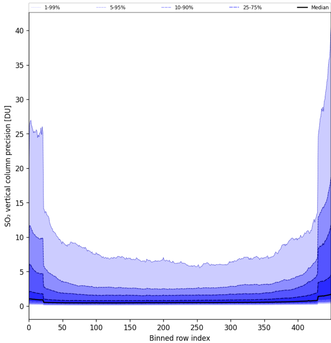
Figure 77: Along track statistics of “SO 2 vertical column precision” for 2024-10-05 to 2024-10-07
