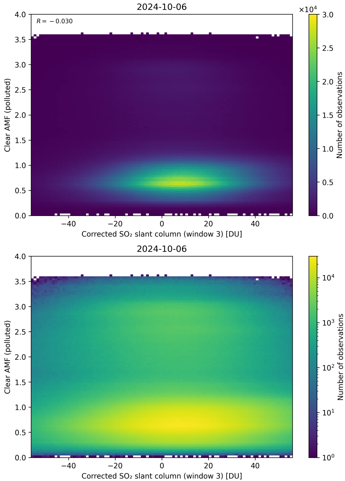
Figure 209: Scatter density plot of “Corrected SO 2 slant column (window 3)” against “Clear AMF (polluted)” for 2024-10-05 to 2024-10-07.
