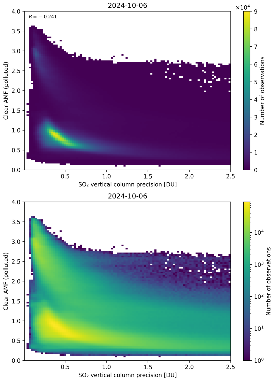
Figure 285: Scatter density plot of “SO 2 vertical column precision” against “Clear AMF (polluted)” for 2024-10-05 to 2024-10-07.
