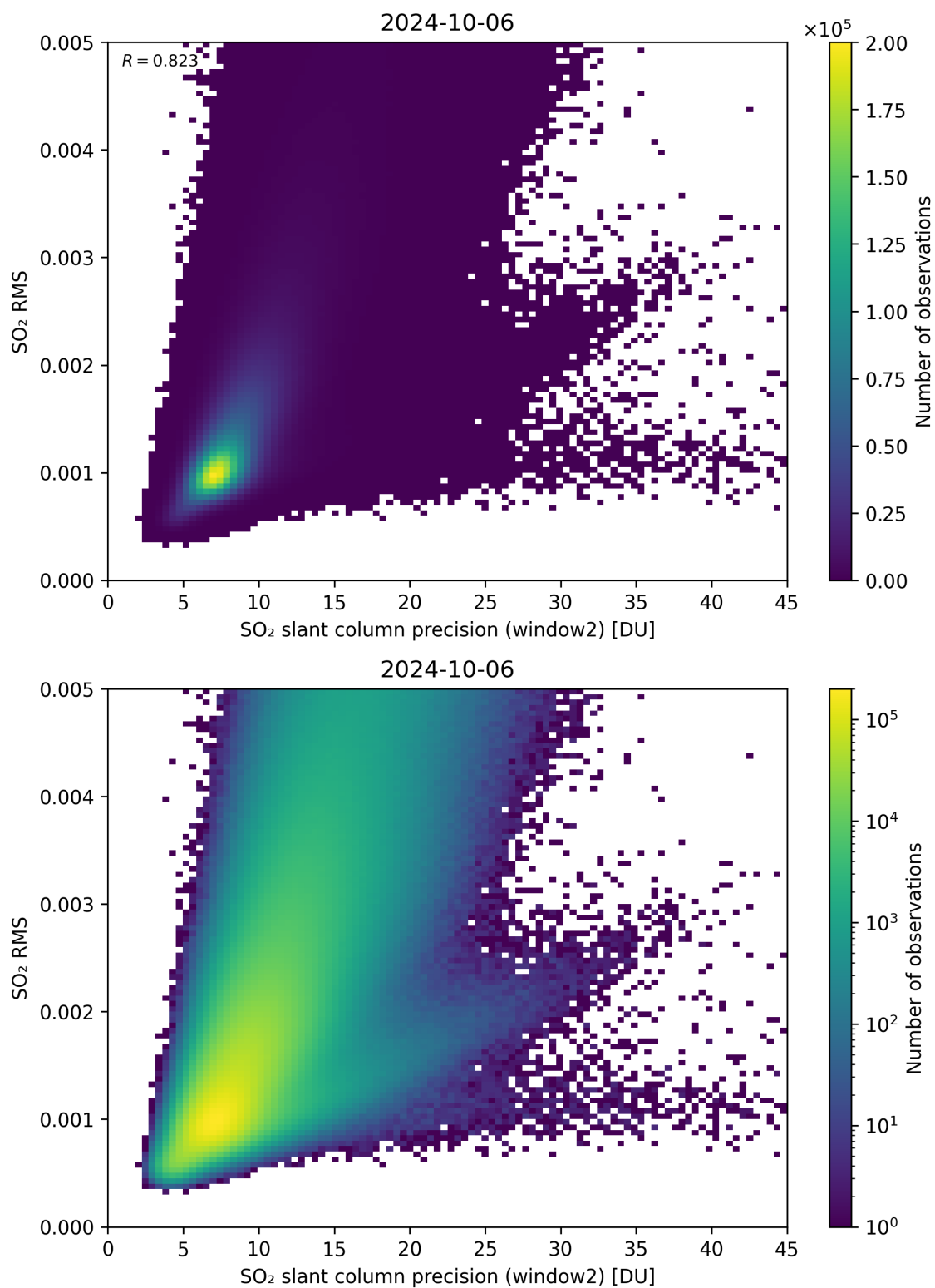
Figure 245: Scatter density plot of “SO 2 slant column precision (window2)” against “SO 2 RMS” for 2024-10-05 to 2024-10-07.
