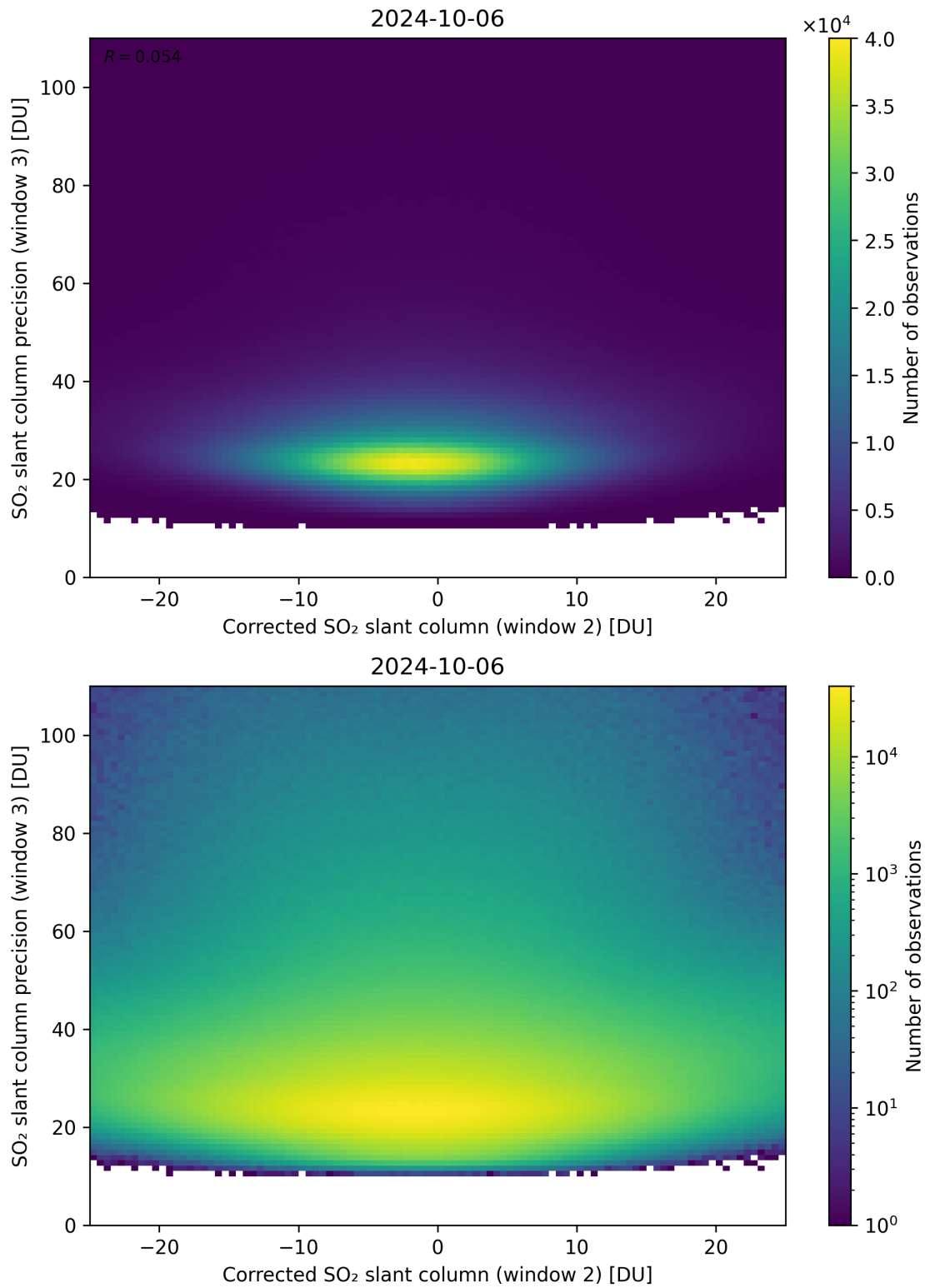
Figure 202: Scatter density plot of “Corrected SO 2 slant column (window 2)” against “SO 2 slant column precision (window 3)” for 2024-10-05 to 2024-10-07.
