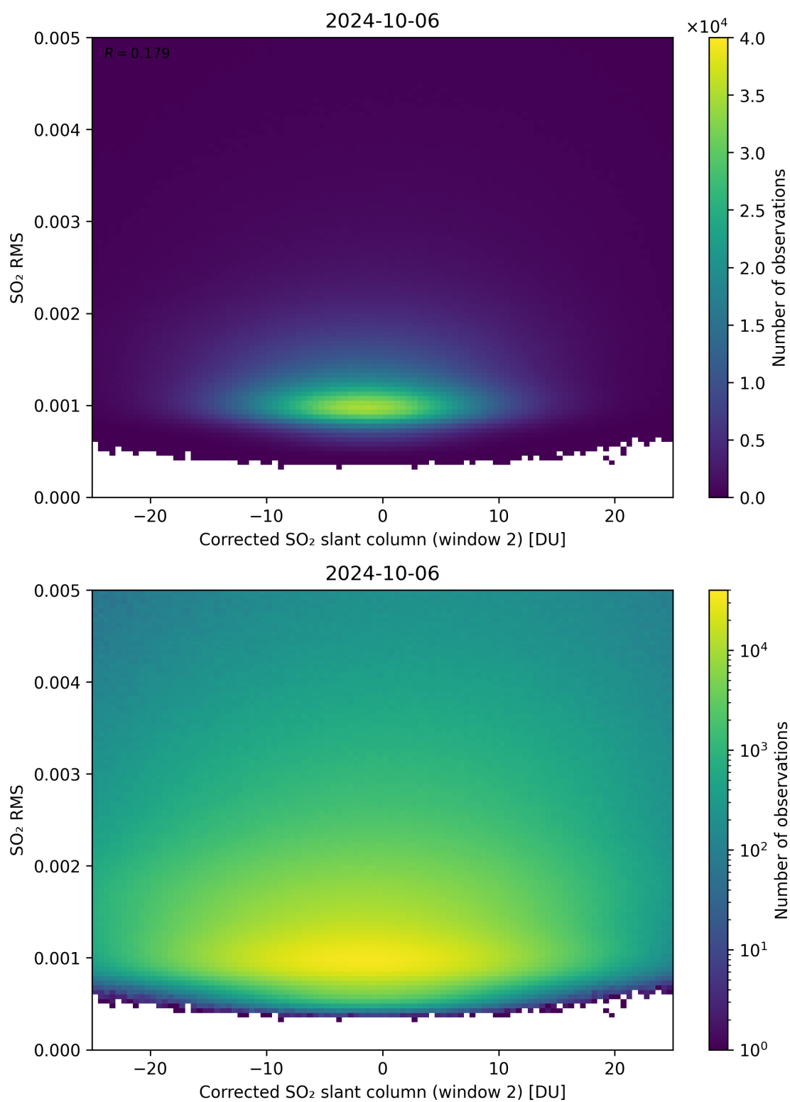
Figure 198: Scatter density plot of “Corrected SO 2 slant column (window 2)” against “SO 2 RMS” for 2024-10-05 to 2024-10-07.
