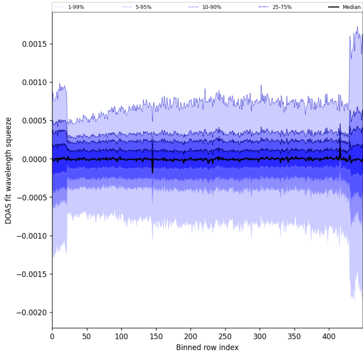
Figure 92: Along track statistics of “DOAS fit wavelength squeeze” for 2024-10-05 to 2024-10-07
