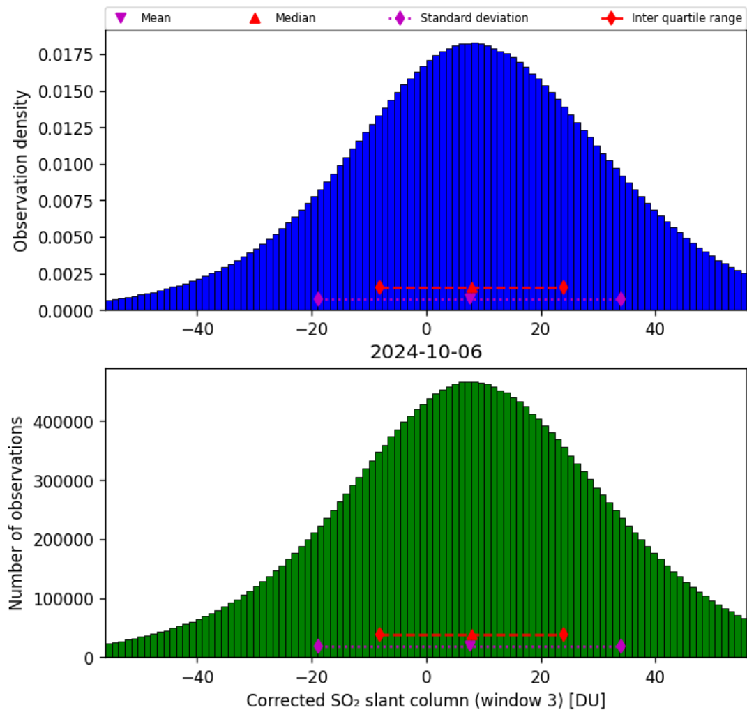
Figure 66: Histogram of “Corrected SO 2 slant column (window 3)” for 2024-10-05 to 2024-10-07
