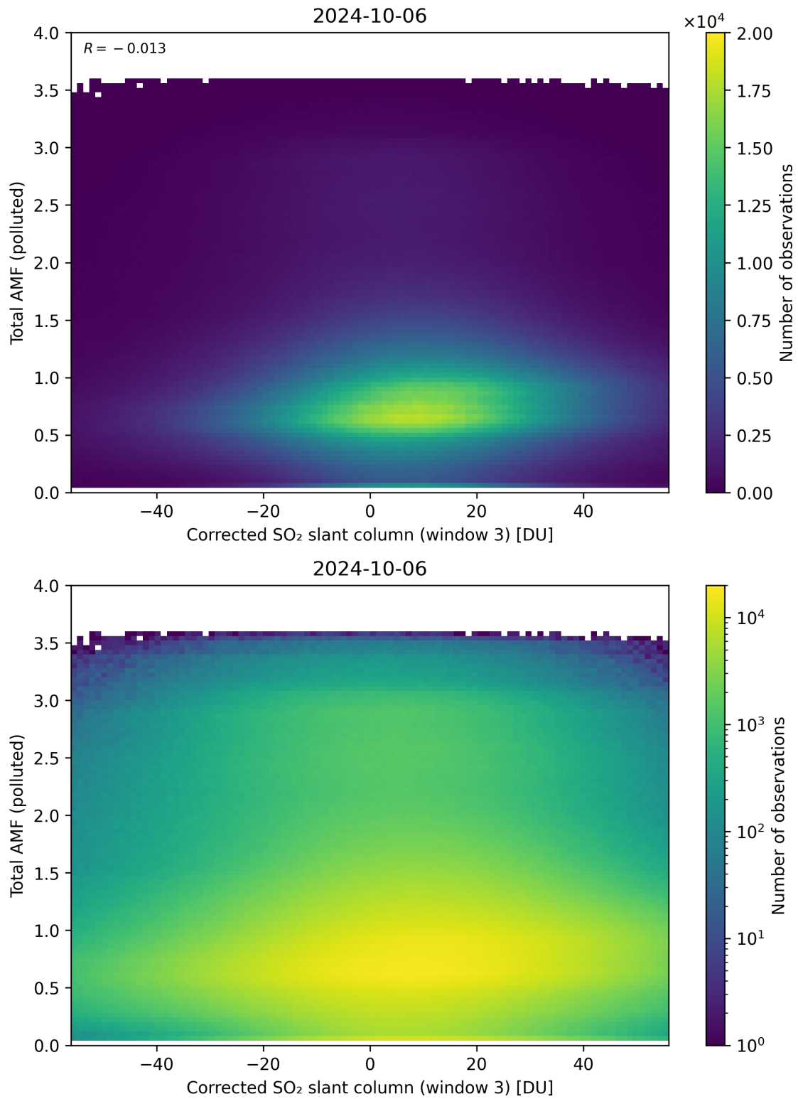
Figure 210: Scatter density plot of “Corrected SO 2 slant column (window 3)” against “Total AMF (polluted)” for 2024-10-05 to 2024-10-07.
