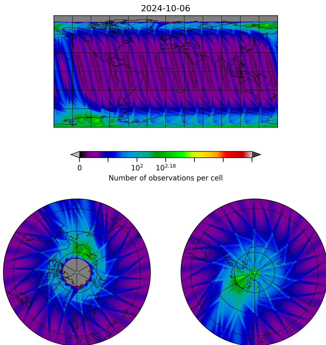
Figure 28: Map of the number of observations for 2024-10-05 to 2024-10-07
