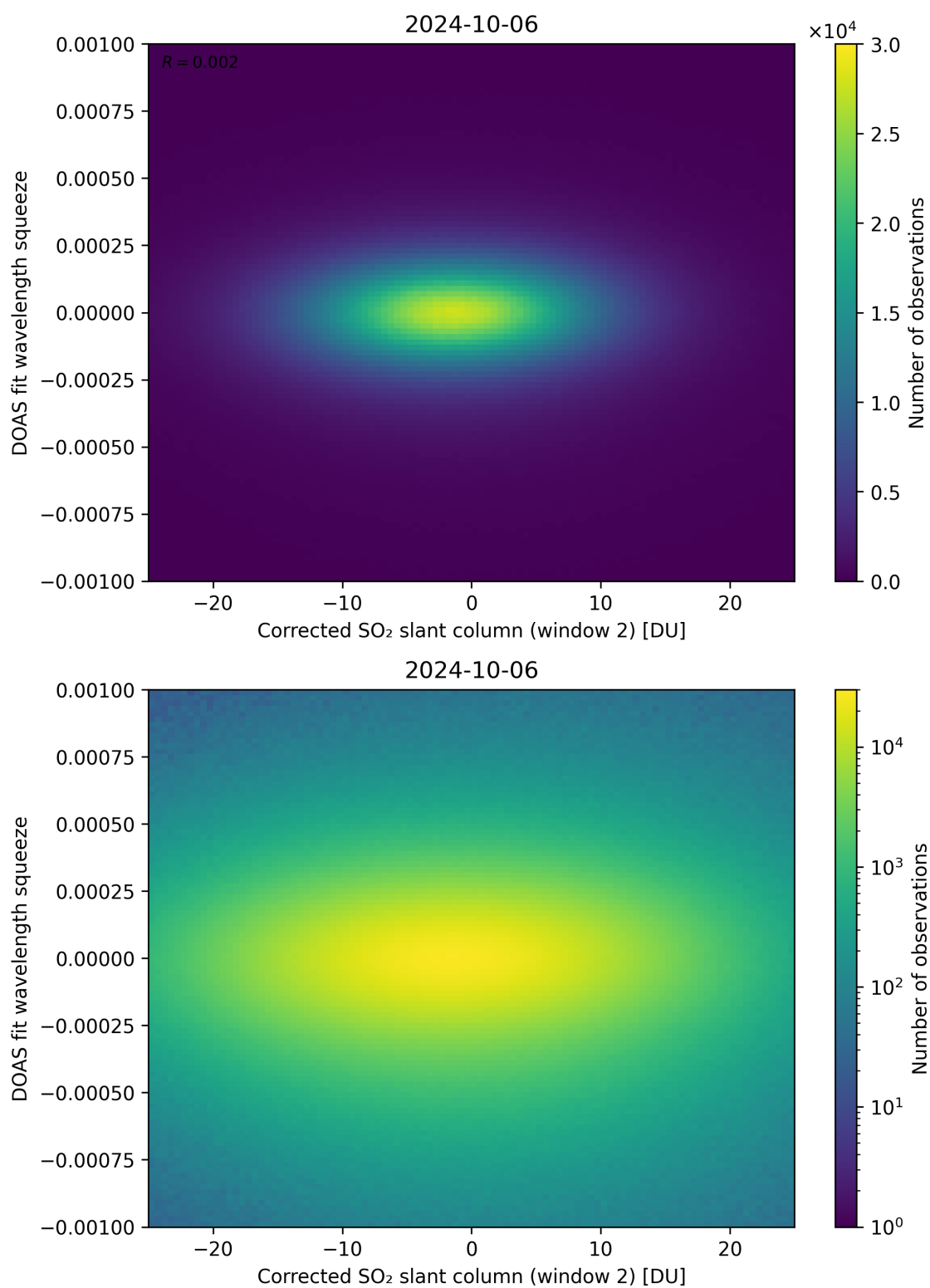
Figure 197: Scatter density plot of “Corrected SO 2 slant column (window 2)” against “DOAS fit wavelength squeeze” for 2024-10-05 to 2024-10-07.
