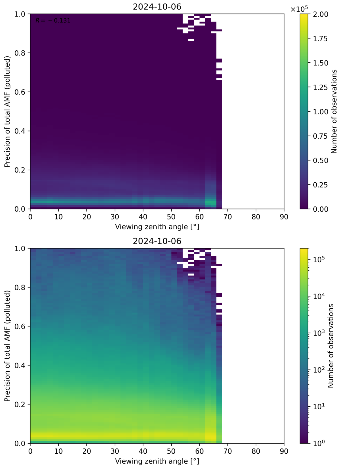
Figure 326: Scatter density plot of “Viewing zenith angle” against “Precision of total AMF (polluted)” for 2024-10-05 to 2024-10-07.
