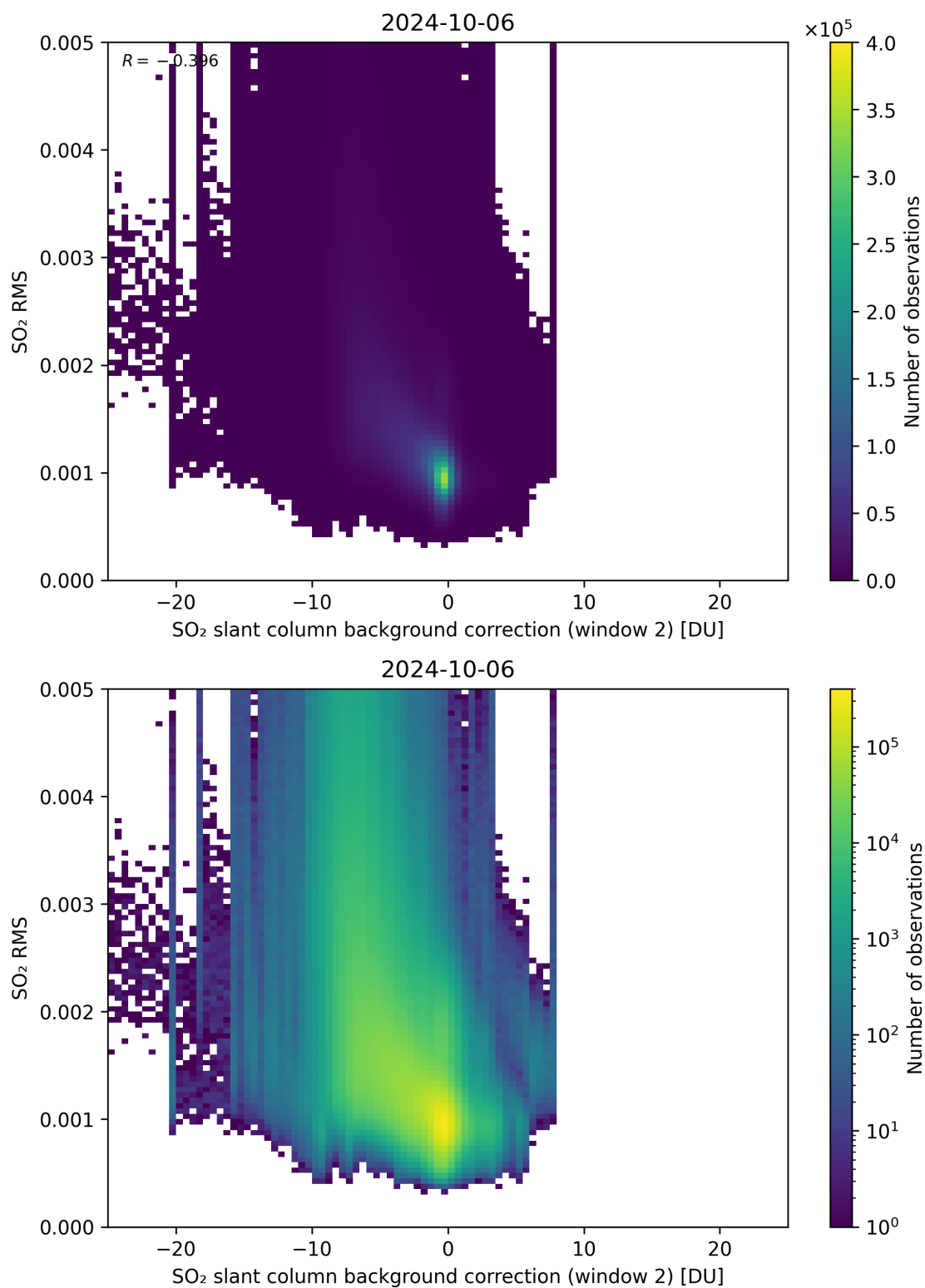
Figure 114: Scatter density plot of “SO 2 slant column background correction (window 2)” against “SO 2 RMS” for 2024-10-05 to 2024-10-07.
