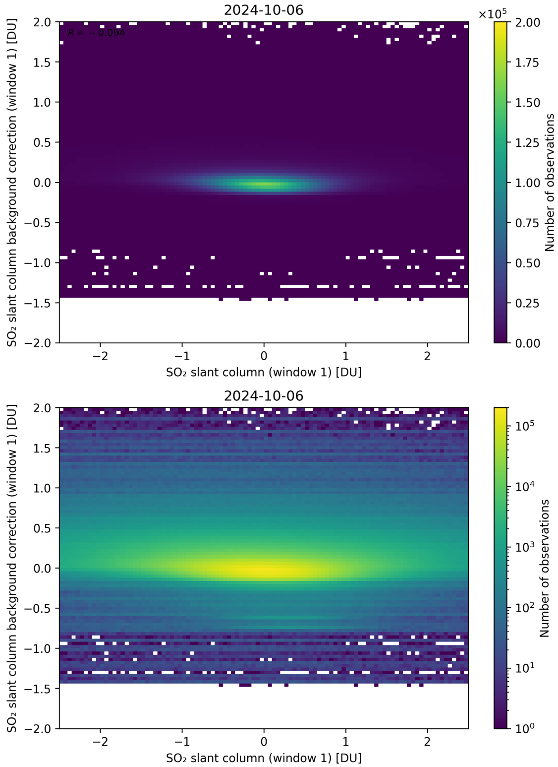
Figure 212: Scatter density plot of “SO 2 slant column (window 1)” against “SO 2 slant column background correction (window 1)” for 2024-10-05 to 2024-10-07.
