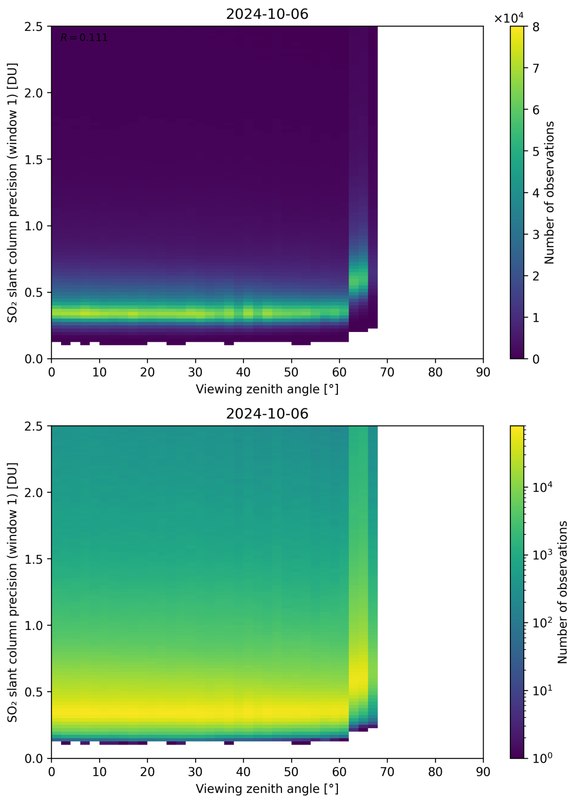
Figure 321: Scatter density plot of “Viewing zenith angle” against “SO 2 slant column precision (window 1)” for 2024-10-05 to 2024-10-07.
