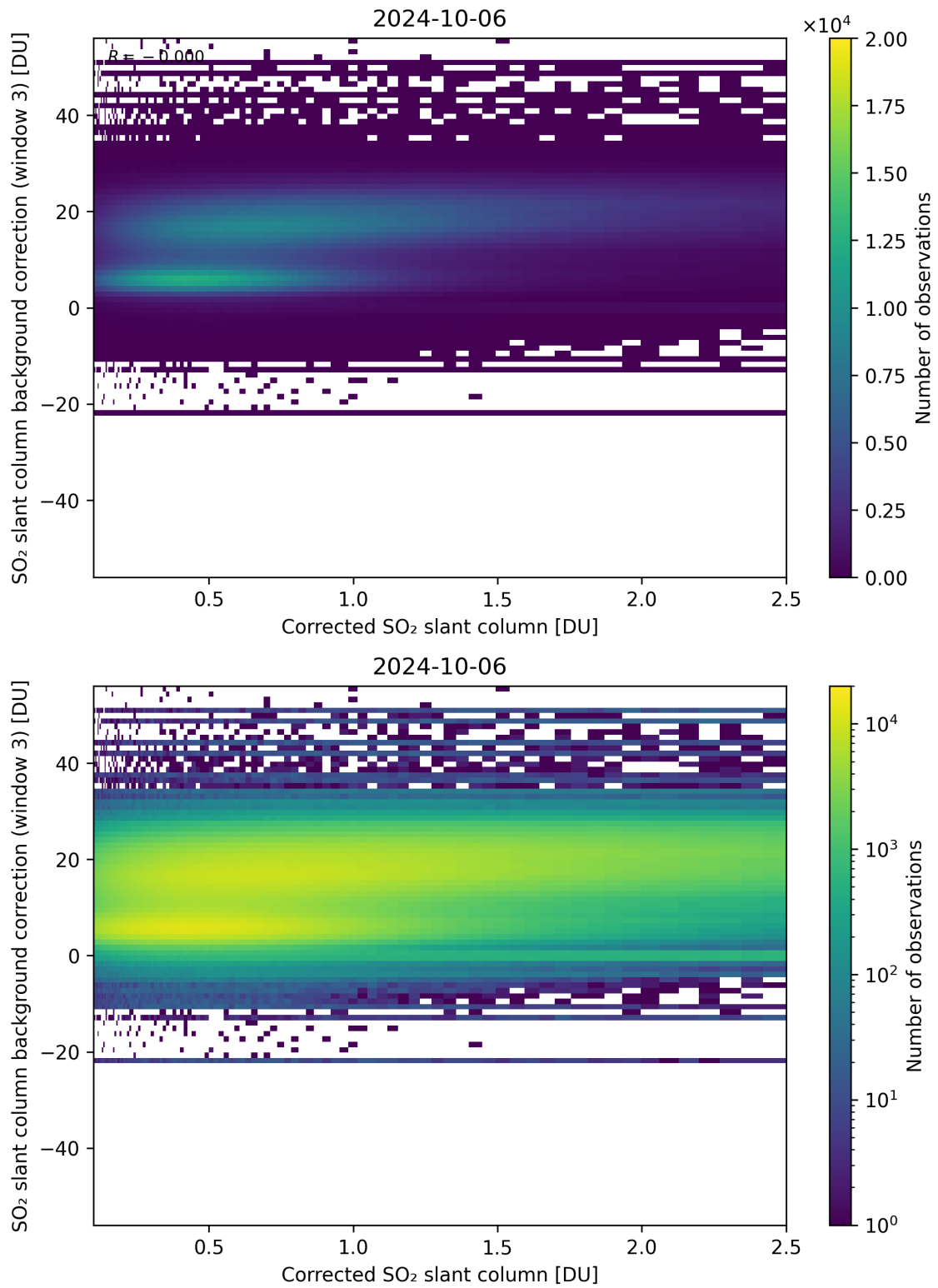
Figure 180: Scatter density plot of “Corrected SO 2 slant column” against “SO 2 slant column background correction (window 3)” for 2024-10-05 to 2024-10-07.
