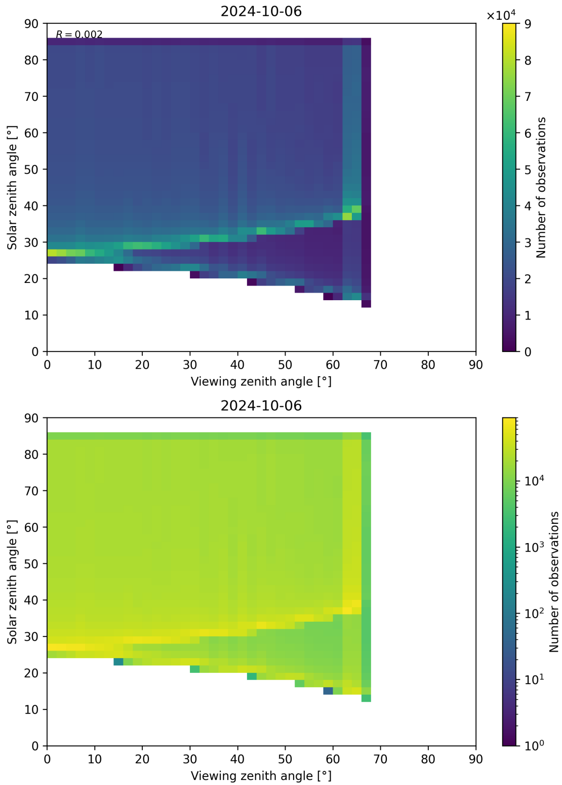
Figure 315: Scatter density plot of “Viewing zenith angle” against “Solar zenith angle” for 2024-10-05 to 2024-10-07.
