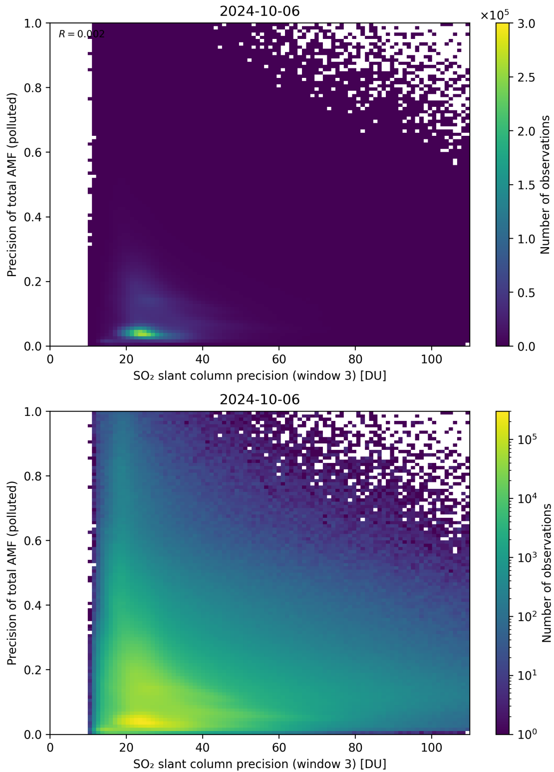
Figure 264: Scatter density plot of “SO 2 slant column precision (window 3)” against “Precision of total AMF (polluted)” for 2024-10-05 to 2024-10-07.
