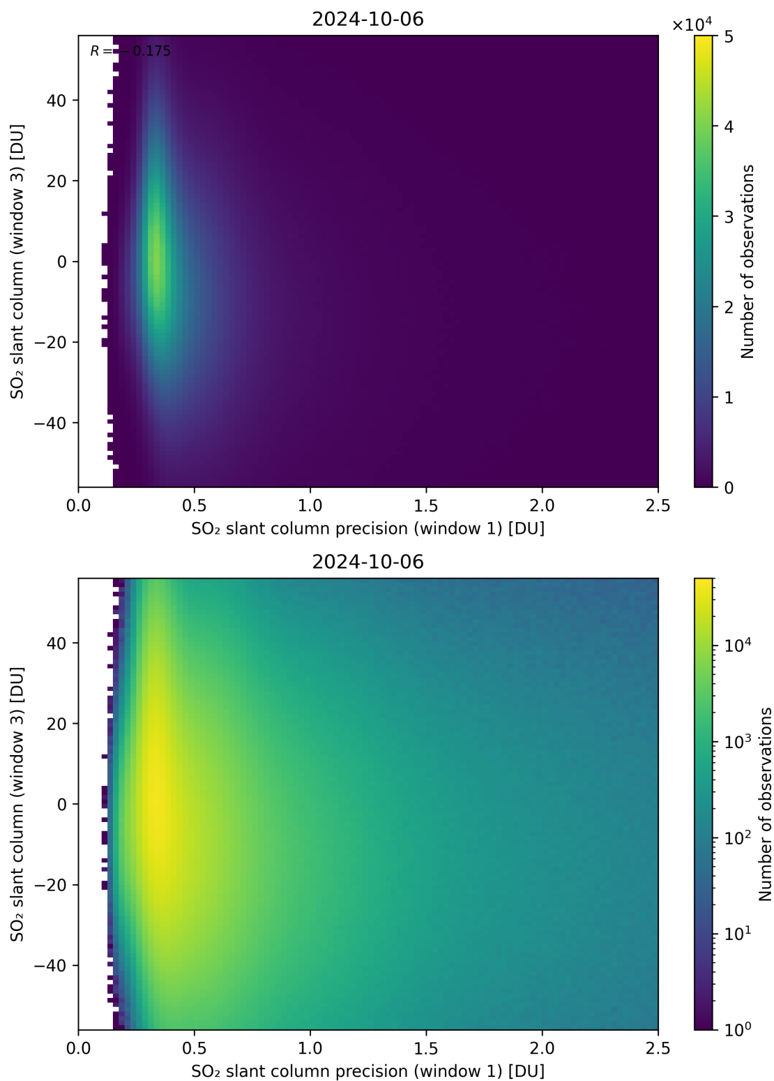
Figure 228: Scatter density plot of “SO 2 slant column precision (window 1)” against “SO 2 slant column (window 3)” for 2024-10-05 to 2024-10-07.
