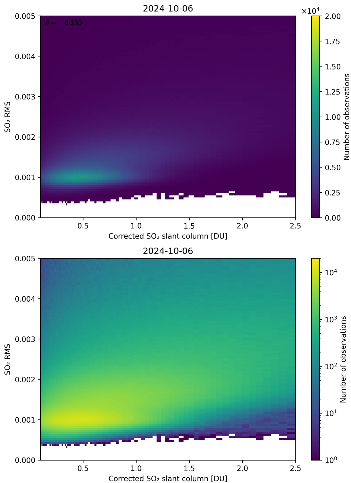
Figure 183: Scatter density plot of “Corrected SO 2 slant column” against “SO 2 RMS” for 2024-10-05 to 2024-10-07.
