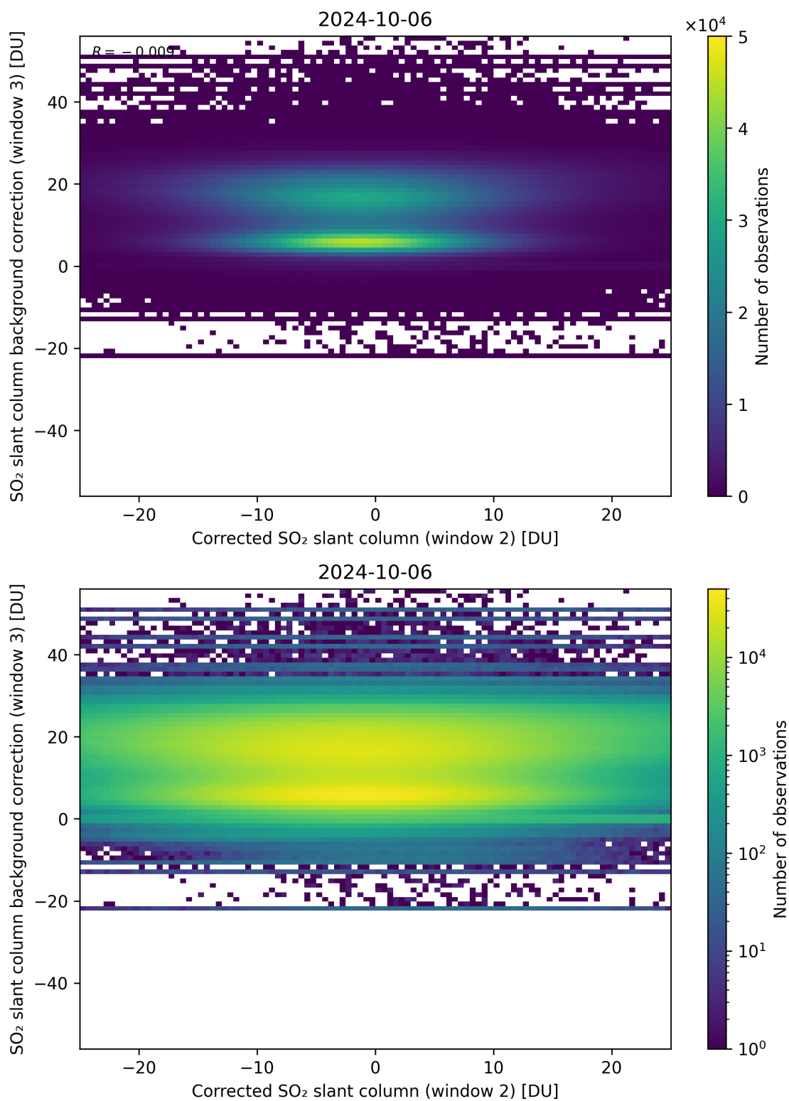
Figure 195: Scatter density plot of “Corrected SO 2 slant column (window 2)” against “SO 2 slant column background correction (window 3)” for 2024-10-05 to 2024-10-07.
