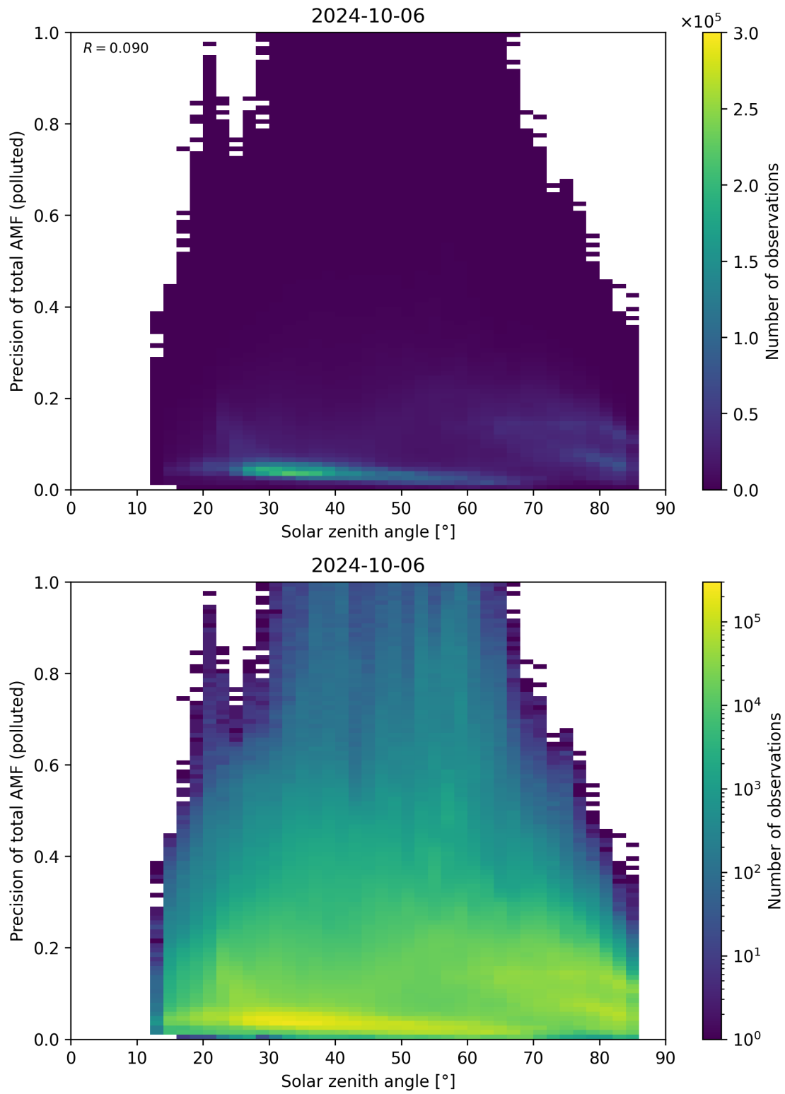
Figure 175: Scatter density plot of “Solar zenith angle” against “Precision of total AMF (polluted)” for 2024-10-05 to 2024-10-07.
