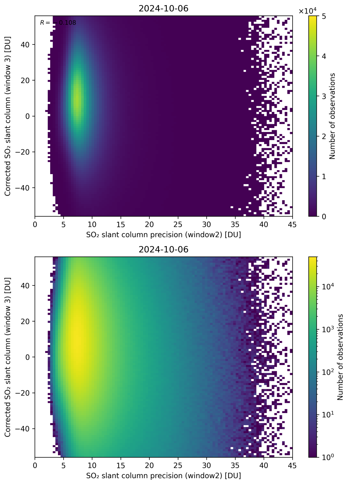
Figure 248: Scatter density plot of “SO 2 slant column precision (window2)” against “Corrected SO 2 slant column (window 3)” for 2024-10-05 to 2024-10-07.
