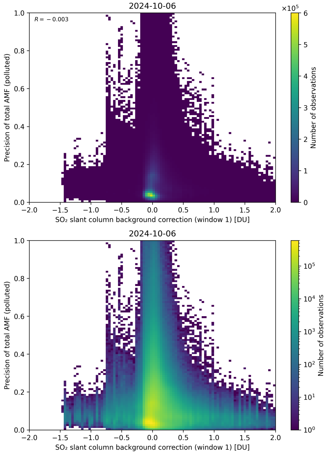
Figure 110: Scatter density plot of “SO 2 slant column background correction (window 1)” against “Precision of total AMF (polluted)” for 2024-10-05 to 2024-10-07.
