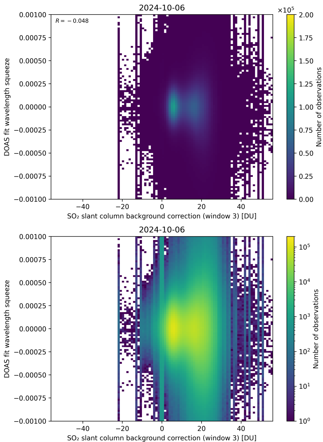
Figure 122: Scatter density plot of “SO 2 slant column background correction (window 3)” against “DOAS fit wavelength squeeze” for 2024-10-05 to 2024-10-07.
