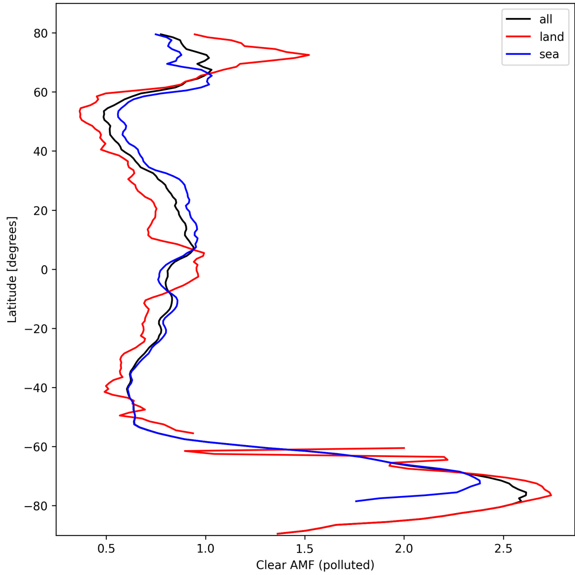
Figure 50: Zonal average of “Clear AMF (polluted)” for 2024-10-05 to 2024-10-07.
