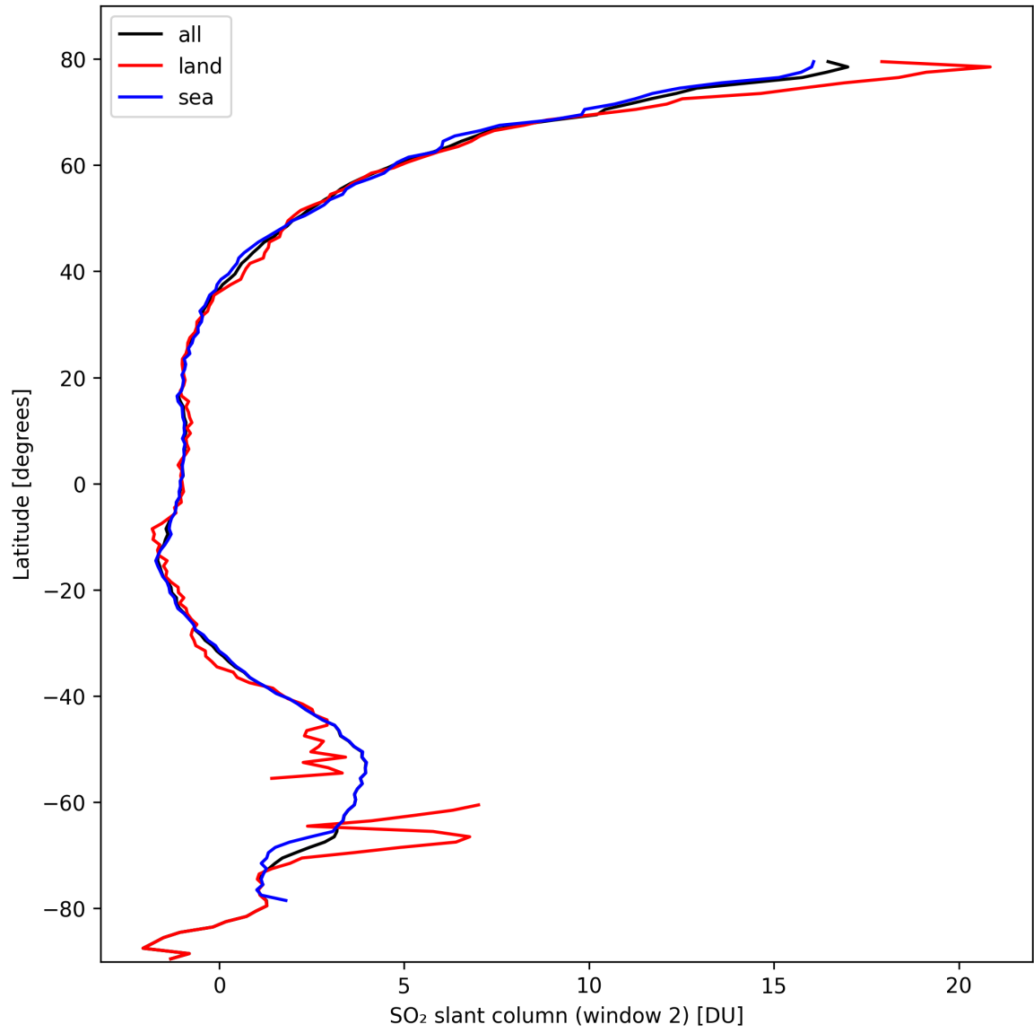
Figure 37: Zonal average of “SO 2 slant column (window 2)” for 2024-10-05 to 2024-10-07.
