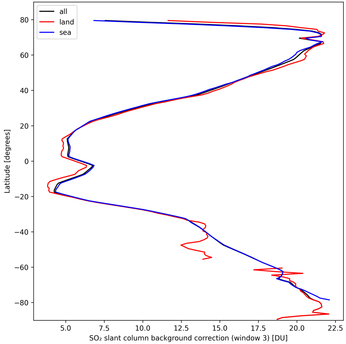
Figure 44: Zonal average of “SO 2 slant column background correction (window 3)” for 2024-10-05 to 2024-10-07.
