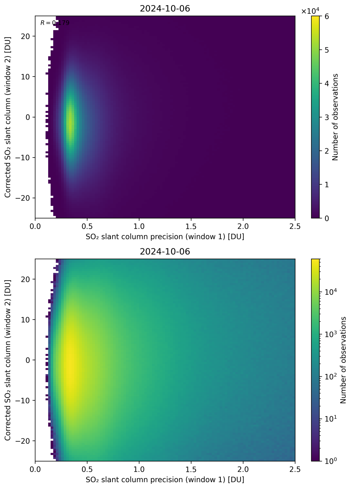
Figure 225: Scatter density plot of “SO 2 slant column precision (window 1)” against “Corrected SO 2 slant column (window 2)” for 2024-10-05 to 2024-10-07.
