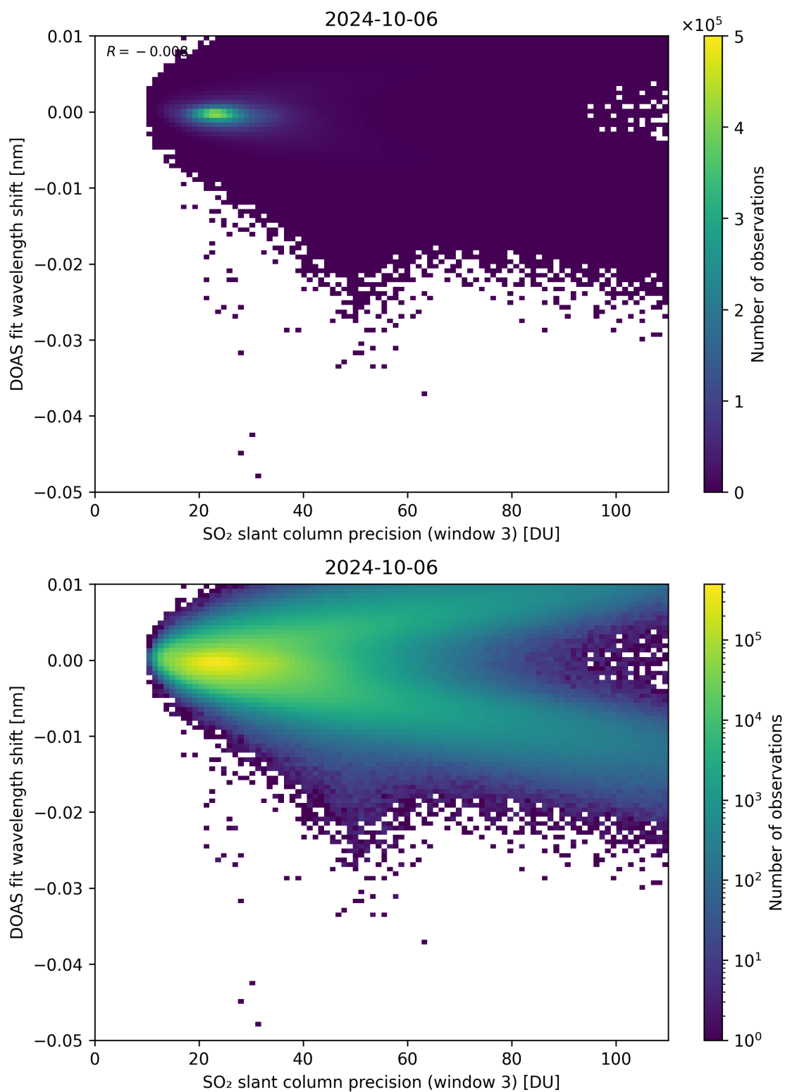
Figure 258: Scatter density plot of “SO 2 slant column precision (window 3)” against “DOAS fit wavelength shift” for 2024-10-05 to 2024-10-07.
