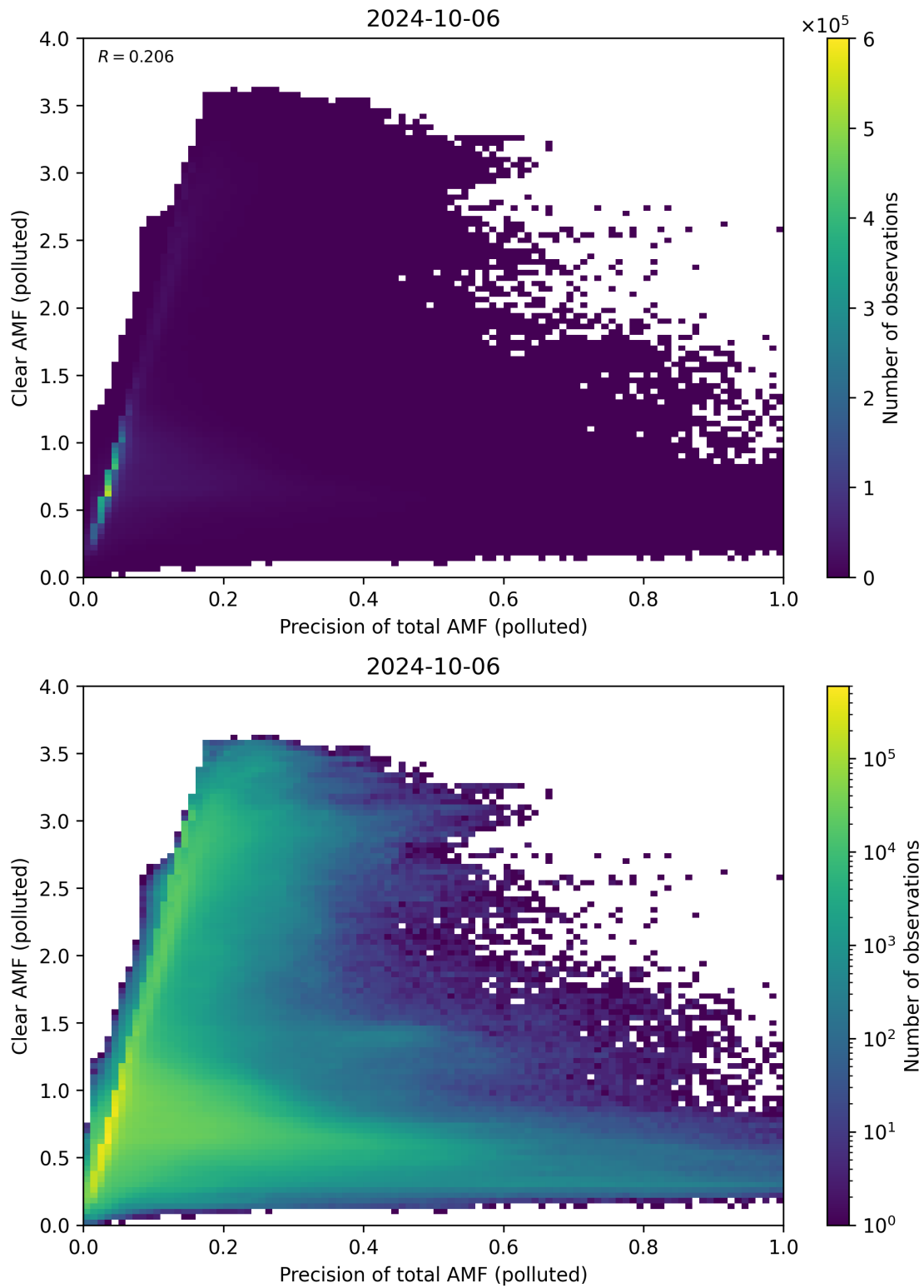
Figure 270: Scatter density plot of “Precision of total AMF (polluted)” against “Clear AMF (polluted)” for 2024-10-05 to 2024-10-07.
