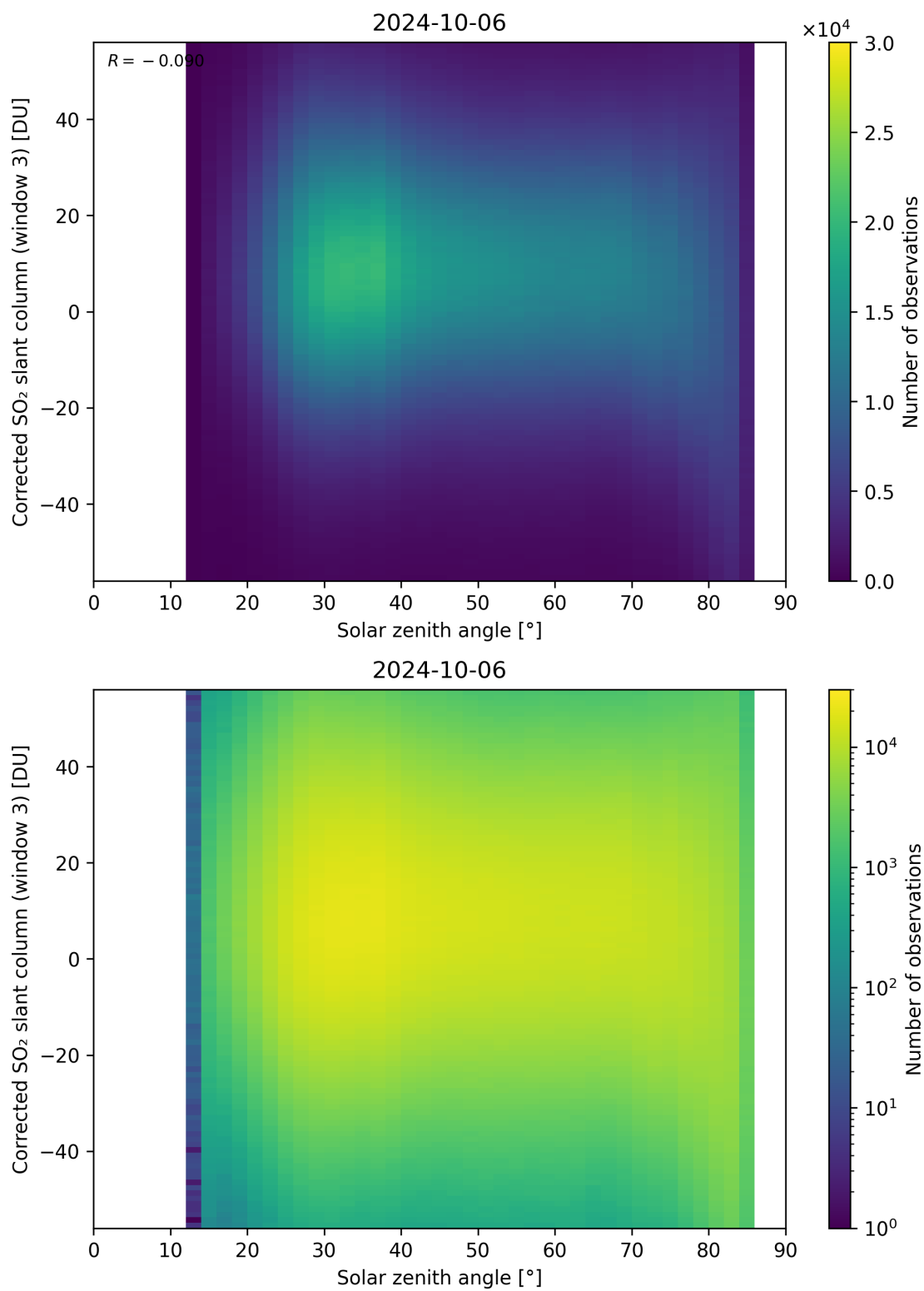
Figure 168: Scatter density plot of “Solar zenith angle” against “Corrected SO 2 slant column (window 3)” for 2024-10-05 to 2024-10-07.
