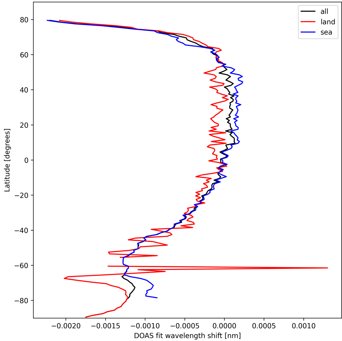
Figure 45: Zonal average of “DOAS fit wavelength shift” for 2024-10-05 to 2024-10-07.
