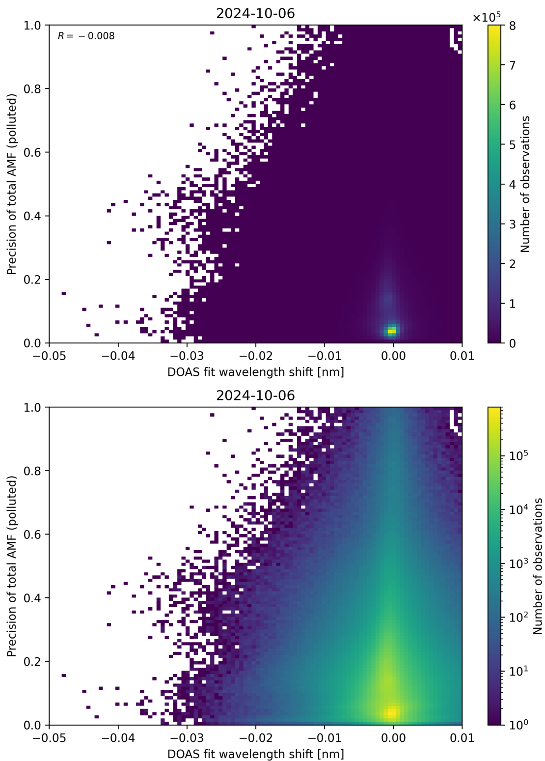
Figure 131: Scatter density plot of “DOAS fit wavelength shift” against “Precision of total AMF (polluted)” for 2024-10-05 to 2024-10-07.
