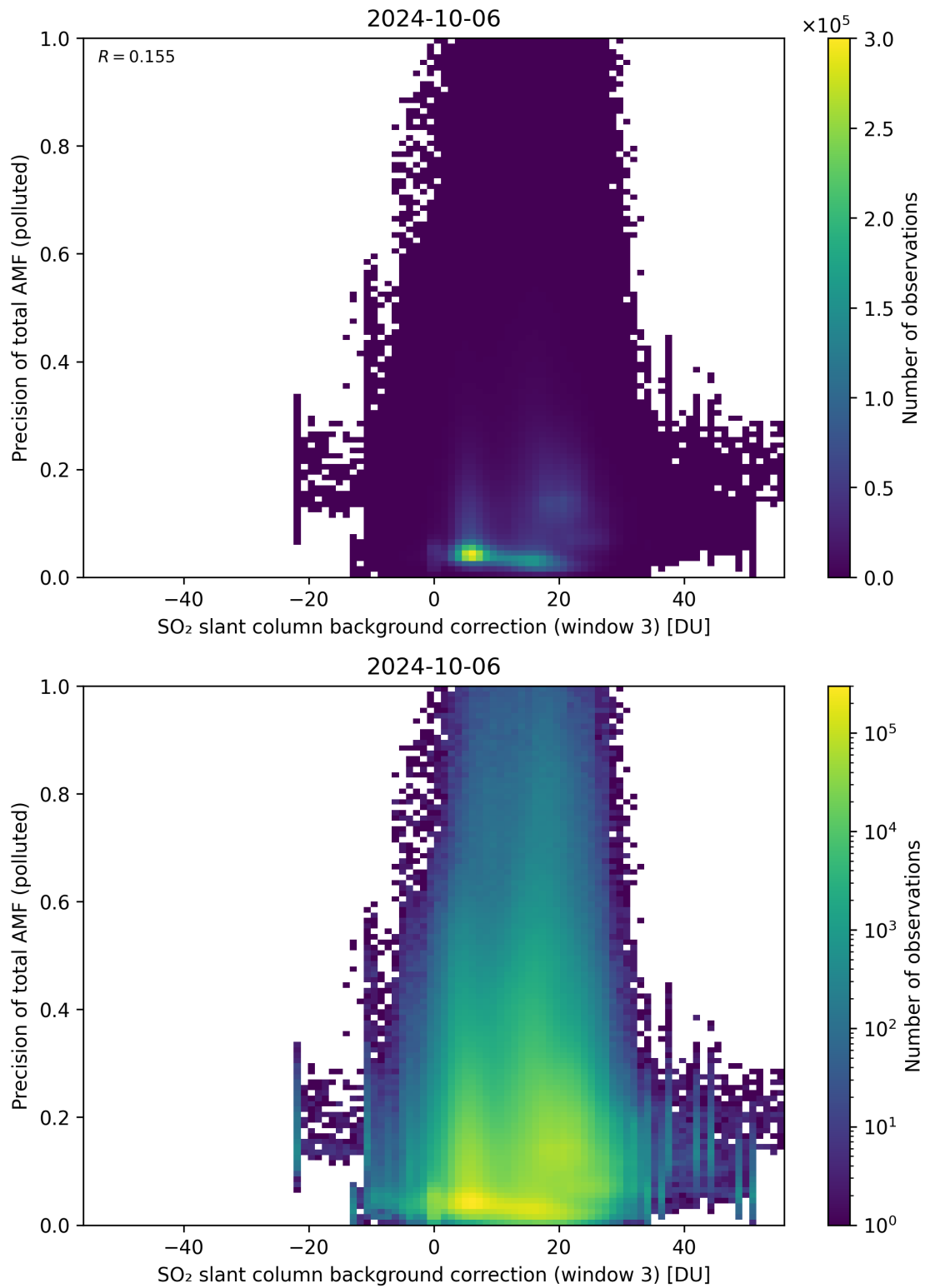
Figure 126: Scatter density plot of “SO 2 slant column background correction (window 3)” against “Precision of total AMF (polluted)” for 2024-10-05 to 2024-10-07.
