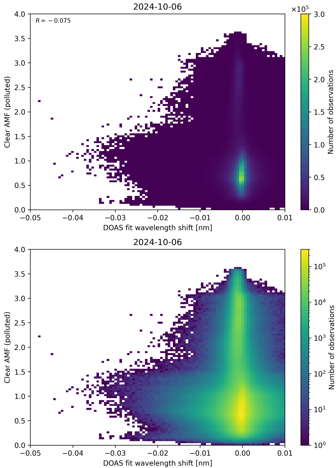
Figure 129: Scatter density plot of “DOAS fit wavelength shift” against “Clear AMF (polluted)” for 2024-10-05 to 2024-10-07.
