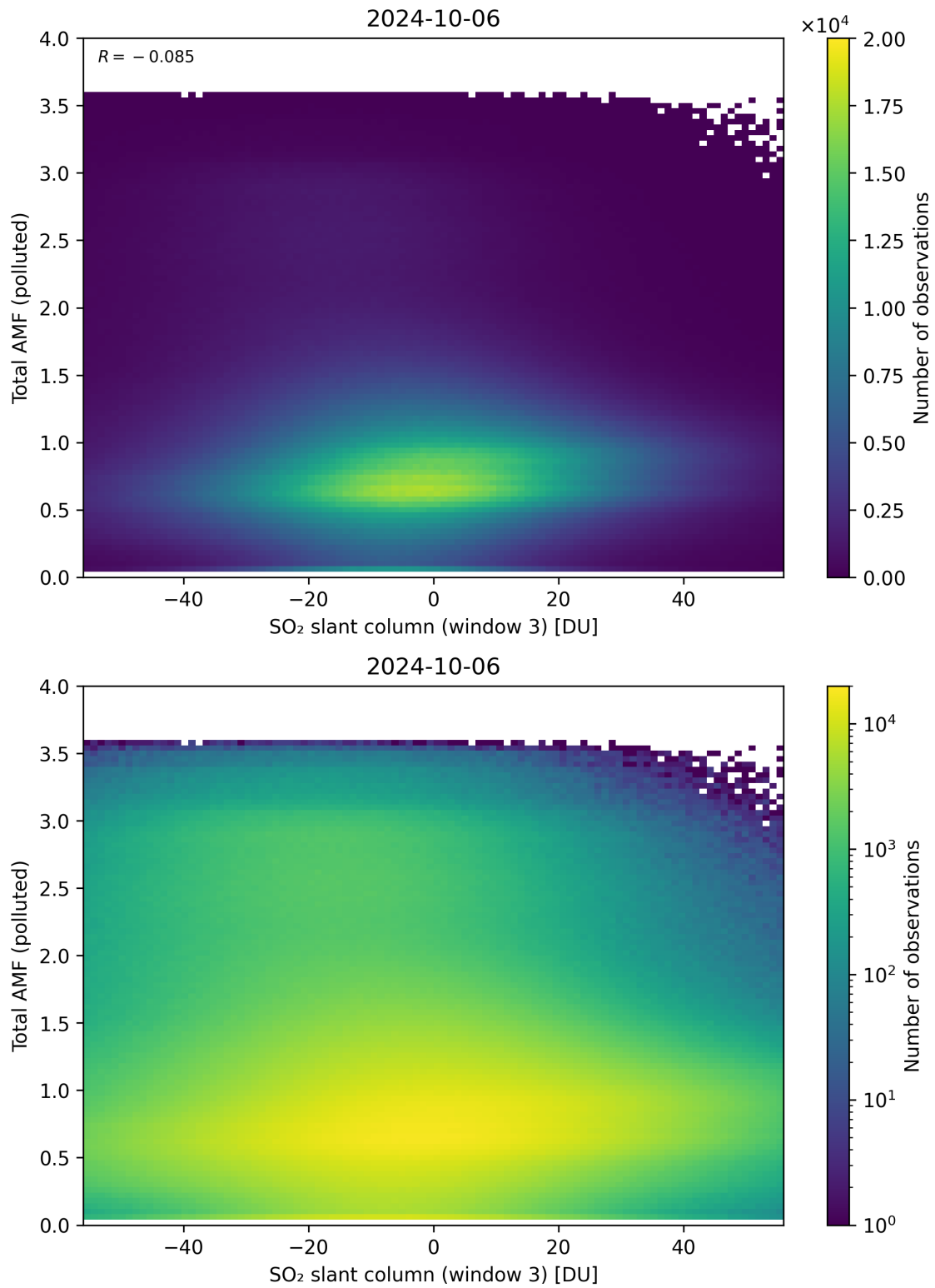
Figure 268: Scatter density plot of “SO 2 slant column (window 3)” against “Total AMF (polluted)” for 2024-10-05 to 2024-10-07.
