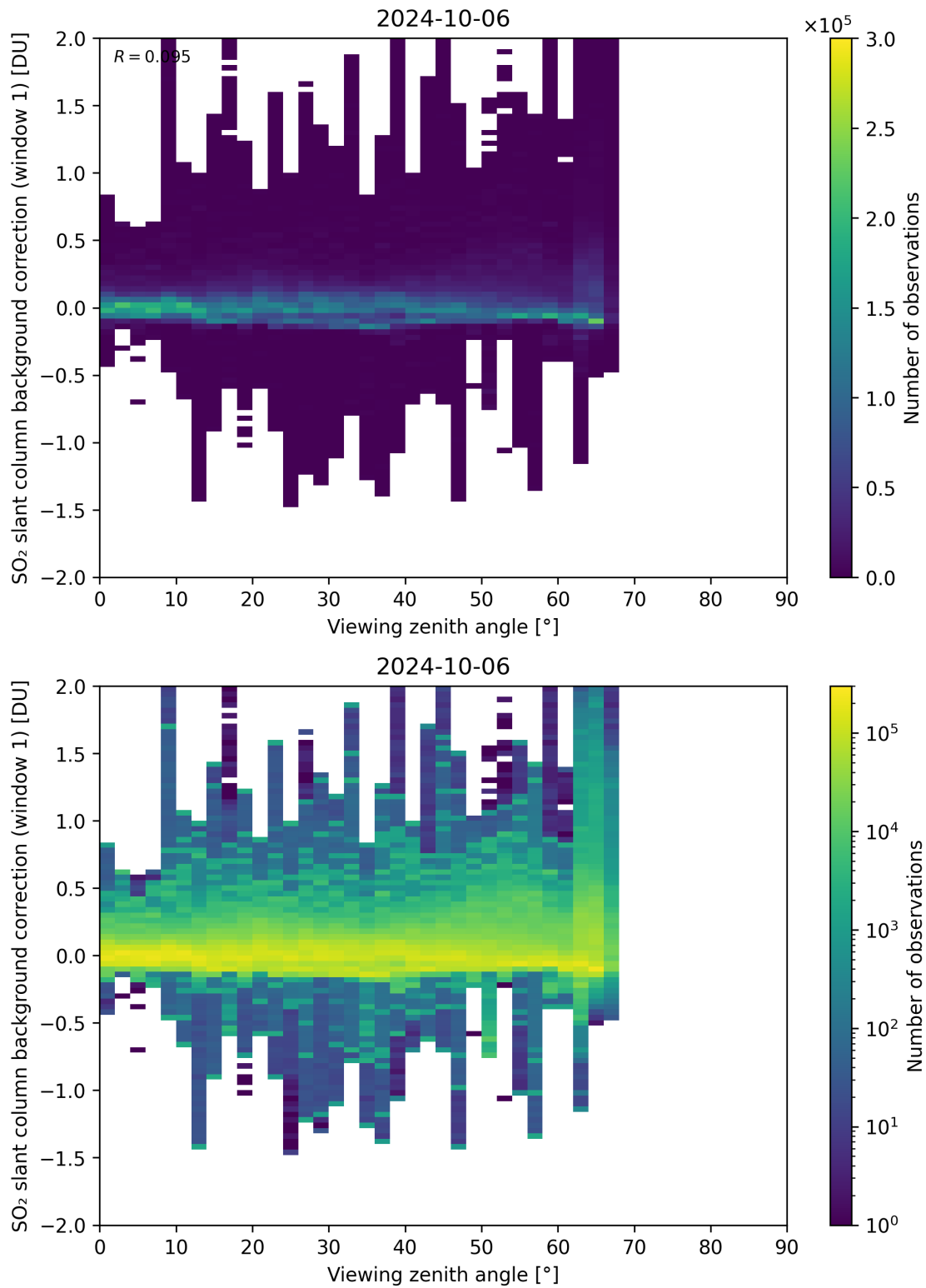
Figure 308: Scatter density plot of “Viewing zenith angle” against “SO 2 slant column background correction (window 1)” for 2024-10-05 to 2024-10-07.
