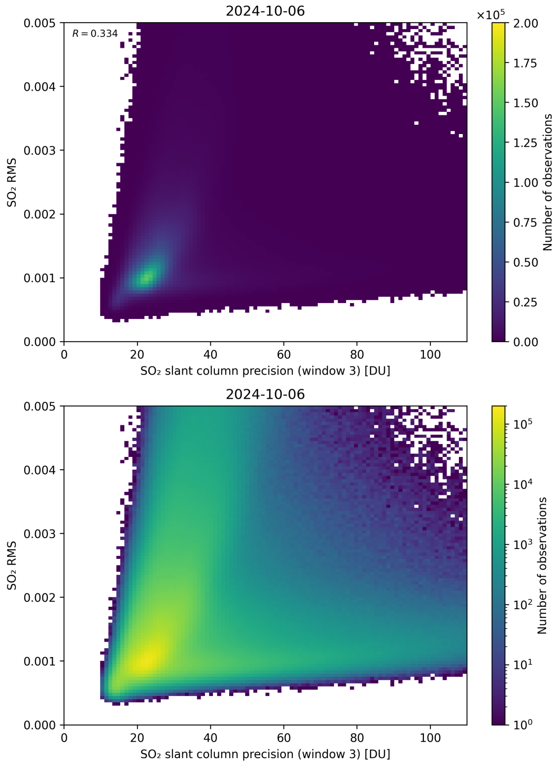
Figure 260: Scatter density plot of “SO 2 slant column precision (window 3)” against “SO 2 RMS” for 2024-10-05 to 2024-10-07.
