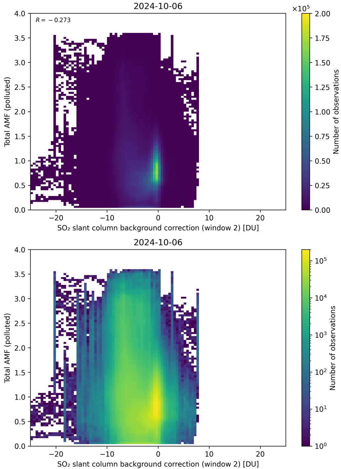
Figure 119: Scatter density plot of “SO 2 slant column background correction (window 2)” against “Total AMF (polluted)” for 2024-10-05 to 2024-10-07.
