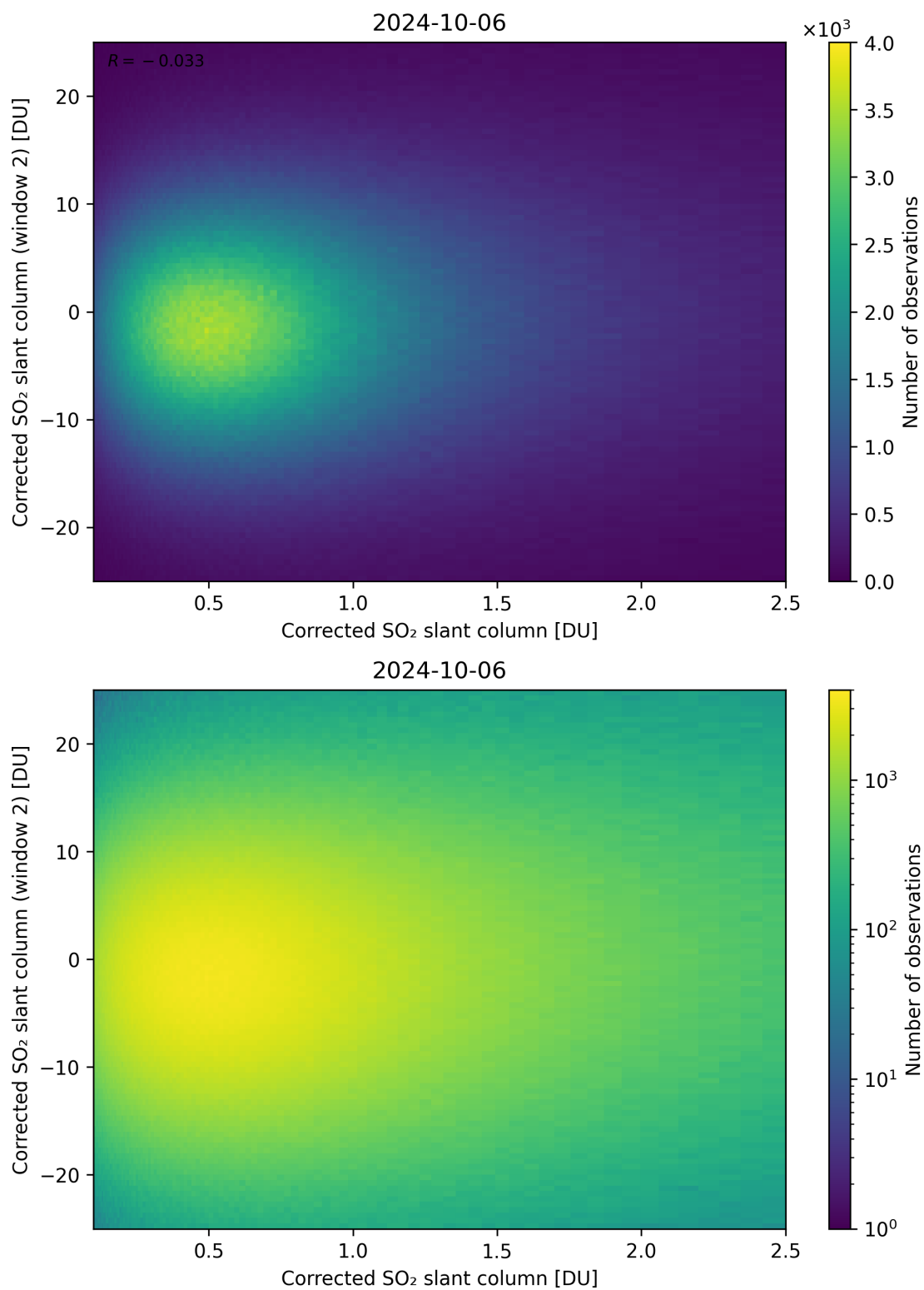
Figure 185: Scatter density plot of “Corrected SO 2 slant column” against “Corrected SO 2 slant column (window 2)” for 2024-10-05 to 2024-10-07.
