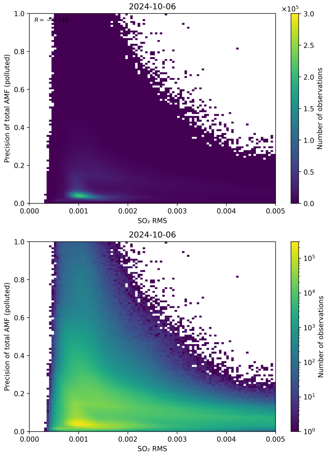
Figure 138: Scatter density plot of “SO 2 RMS” against “Precision of total AMF (polluted)” for 2024-10-05 to 2024-10-07.
