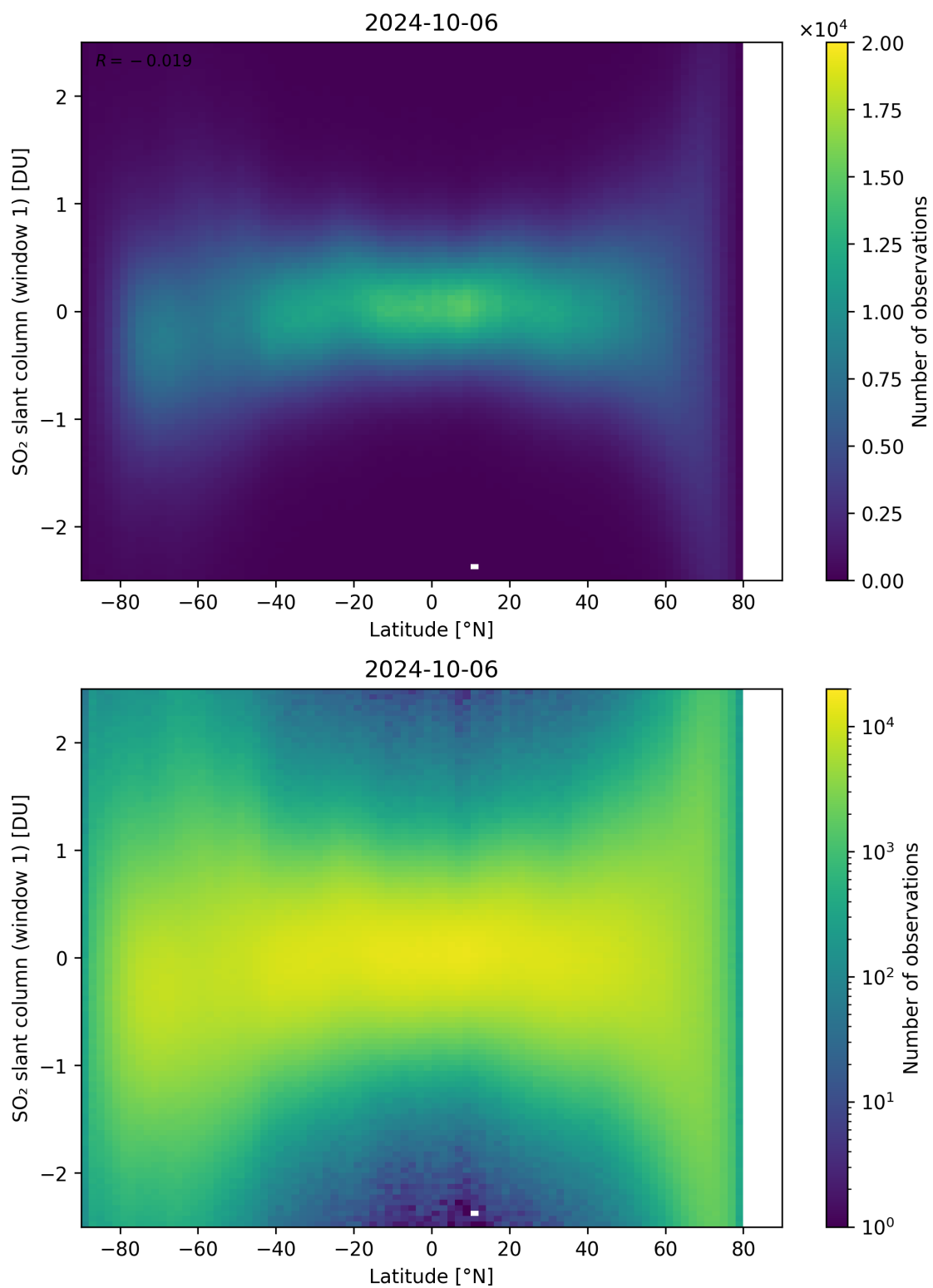
Figure 149: Scatter density plot of “Latitude” against “SO 2 slant column (window 1)” for 2024-10-05 to 2024-10-07.
