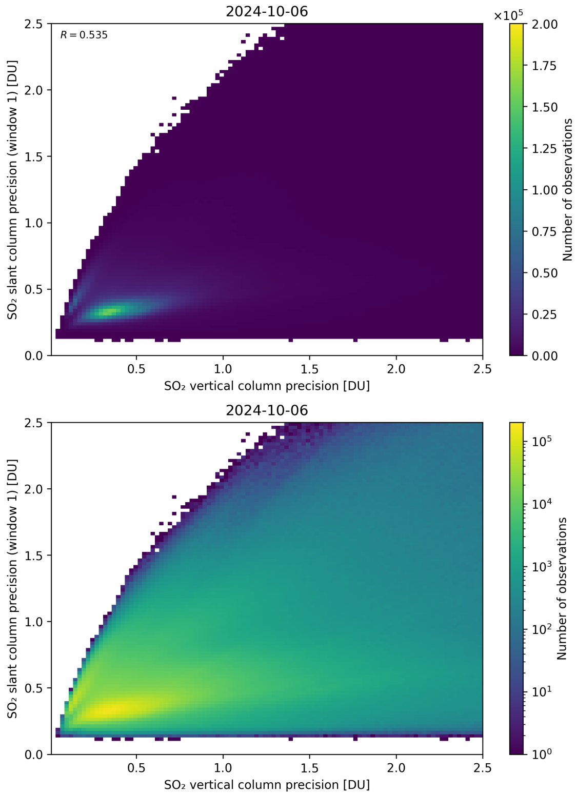
Figure 290: Scatter density plot of “SO 2 vertical column precision” against “SO 2 slant column precision (window 1)” for 2024-10-05 to 2024-10-07.
