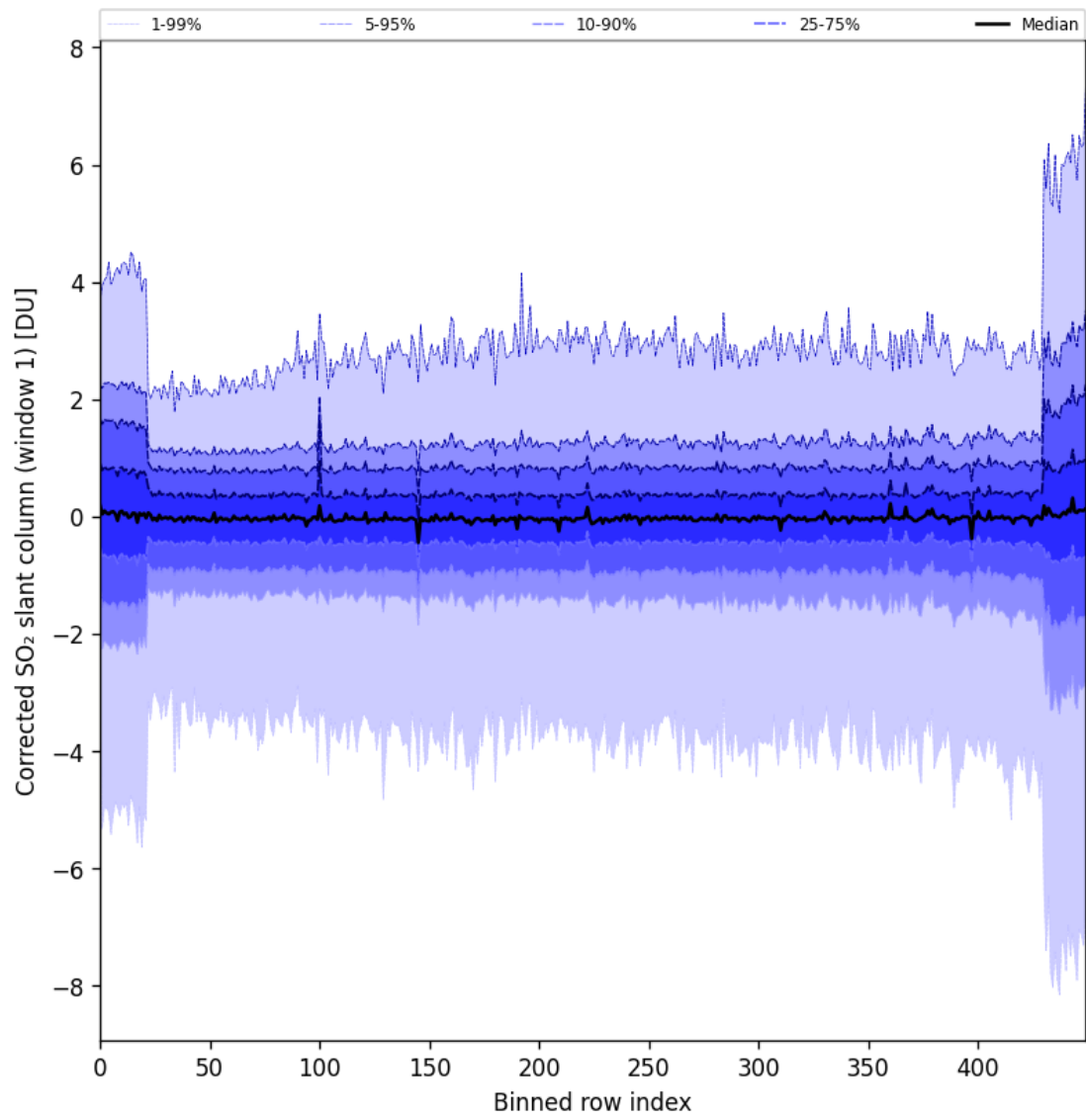
Figure 81: Along track statistics of "Corrected SO 2 slant column (window 1)" for 2024-10-05 to 2024-10-07
