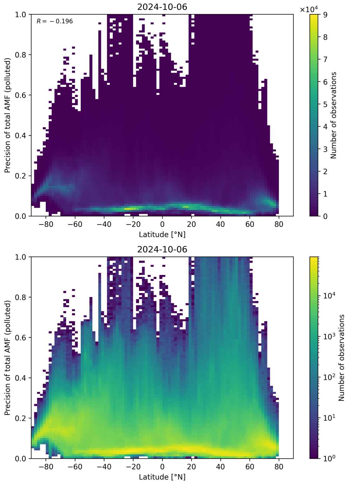
Figure 155: Scatter density plot of “Latitude” against “Precision of total AMF (polluted)” for 2024-10-05 to 2024-10-07.
