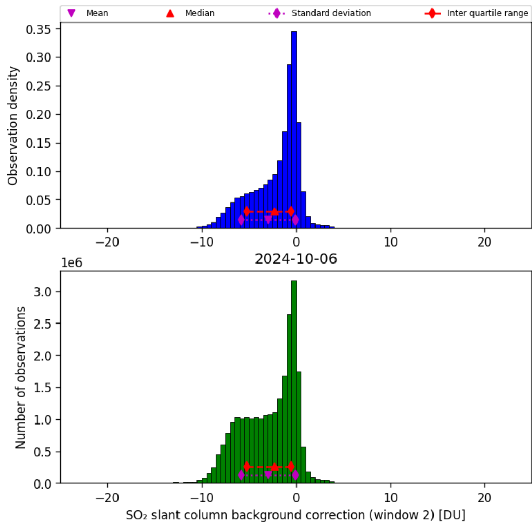
Figure 63: Histogram of “SO 2 slant column background correction (window 2)” for 2024-10-05 to 2024-10-07
