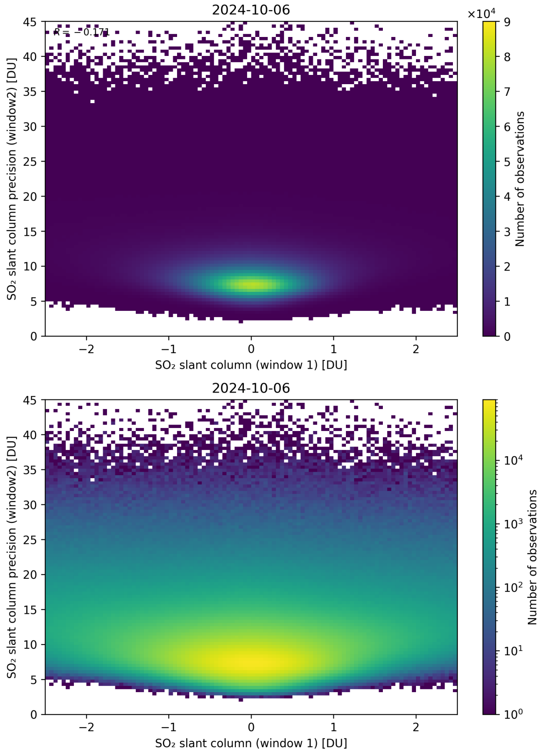
Figure 236: Scatter density plot of “SO 2 slant column (window 1)” against “SO 2 slant column precision (window2)” for 2024-10-05 to 2024-10-07.
