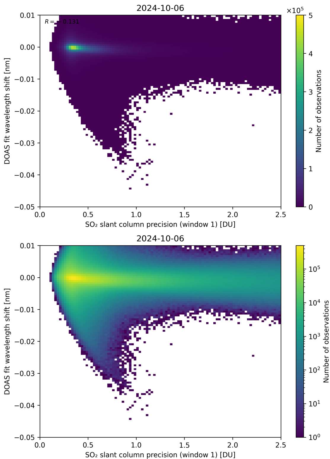
Figure 221: Scatter density plot of “SO 2 slant column precision (window 1)” against “DOAS fit wavelength shift” for 2024-10-05 to 2024-10-07.
