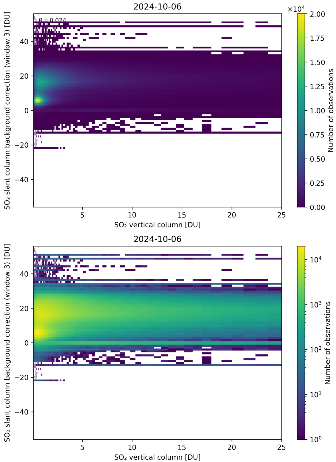
Figure 275: Scatter density plot of “SO 2 vertical column” against “SO 2 slant column background correction (window 3)” for 2024-10-05 to 2024-10-07.
