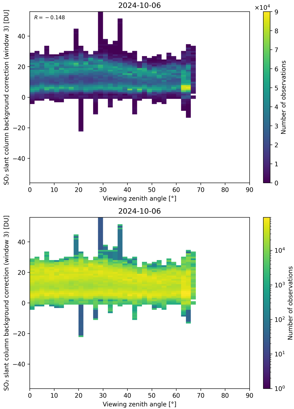
Figure 310: Scatter density plot of “Viewing zenith angle” against “SO 2 slant column background correction (window 3)” for 2024-10-05 to 2024-10-07.
