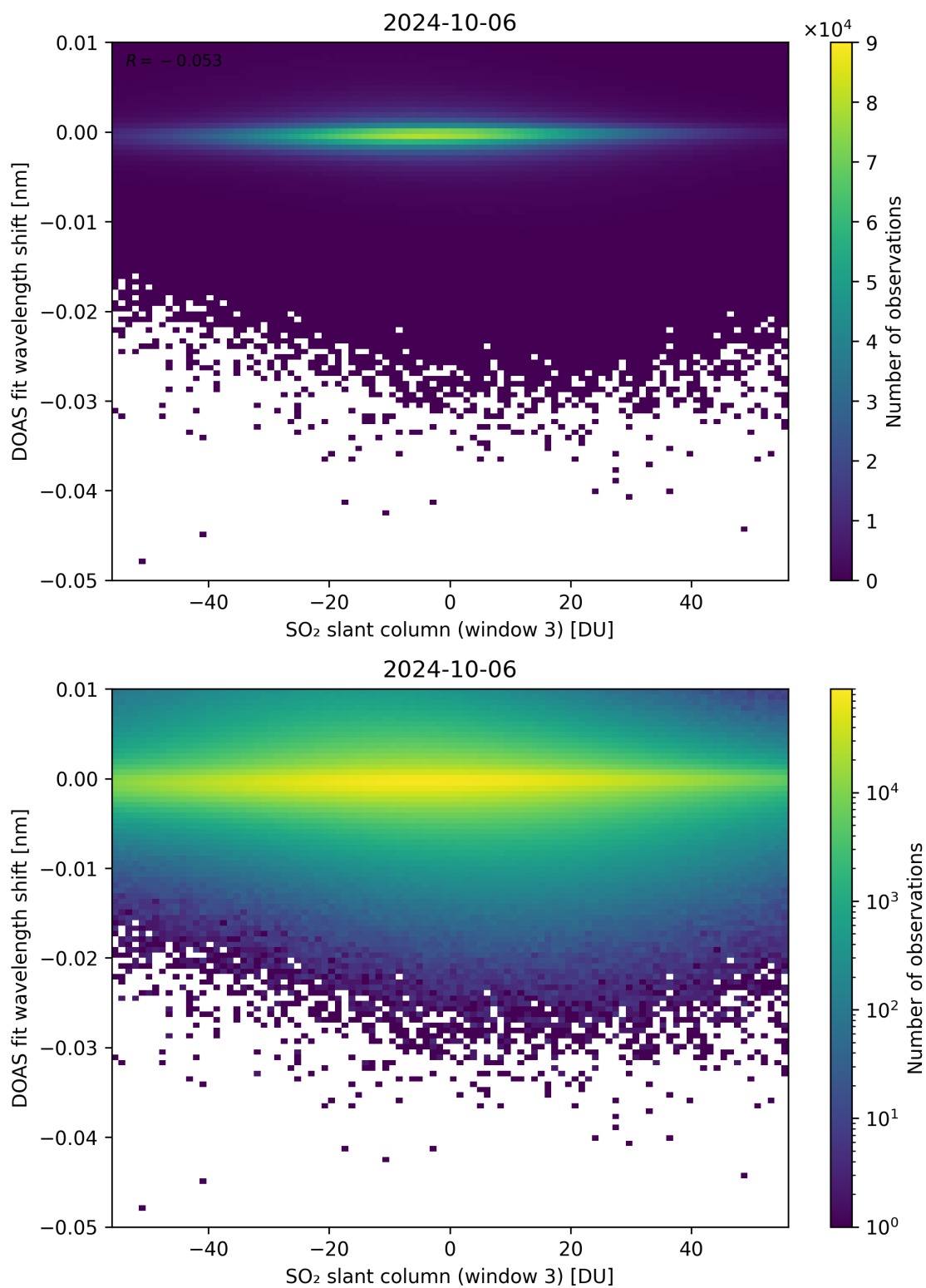
Figure 254: Scatter density plot of “SO 2 slant column (window 3)” against “DOAS fit wavelength shift” for 2024-10-05 to 2024-10-07.
