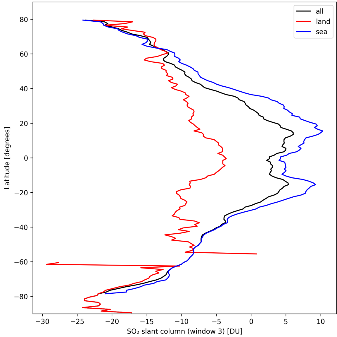
Figure 41: Zonal average of “SO 2 slant column (window 3)” for 2024-10-05 to 2024-10-07.
