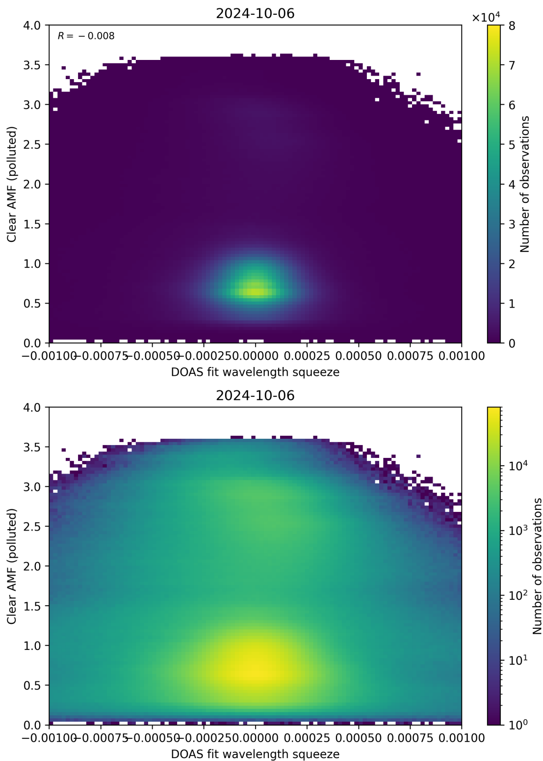
Figure 133: Scatter density plot of “DOAS fit wavelength squeeze” against “Clear AMF (polluted)” for 2024-10-05 to 2024-10-07.
