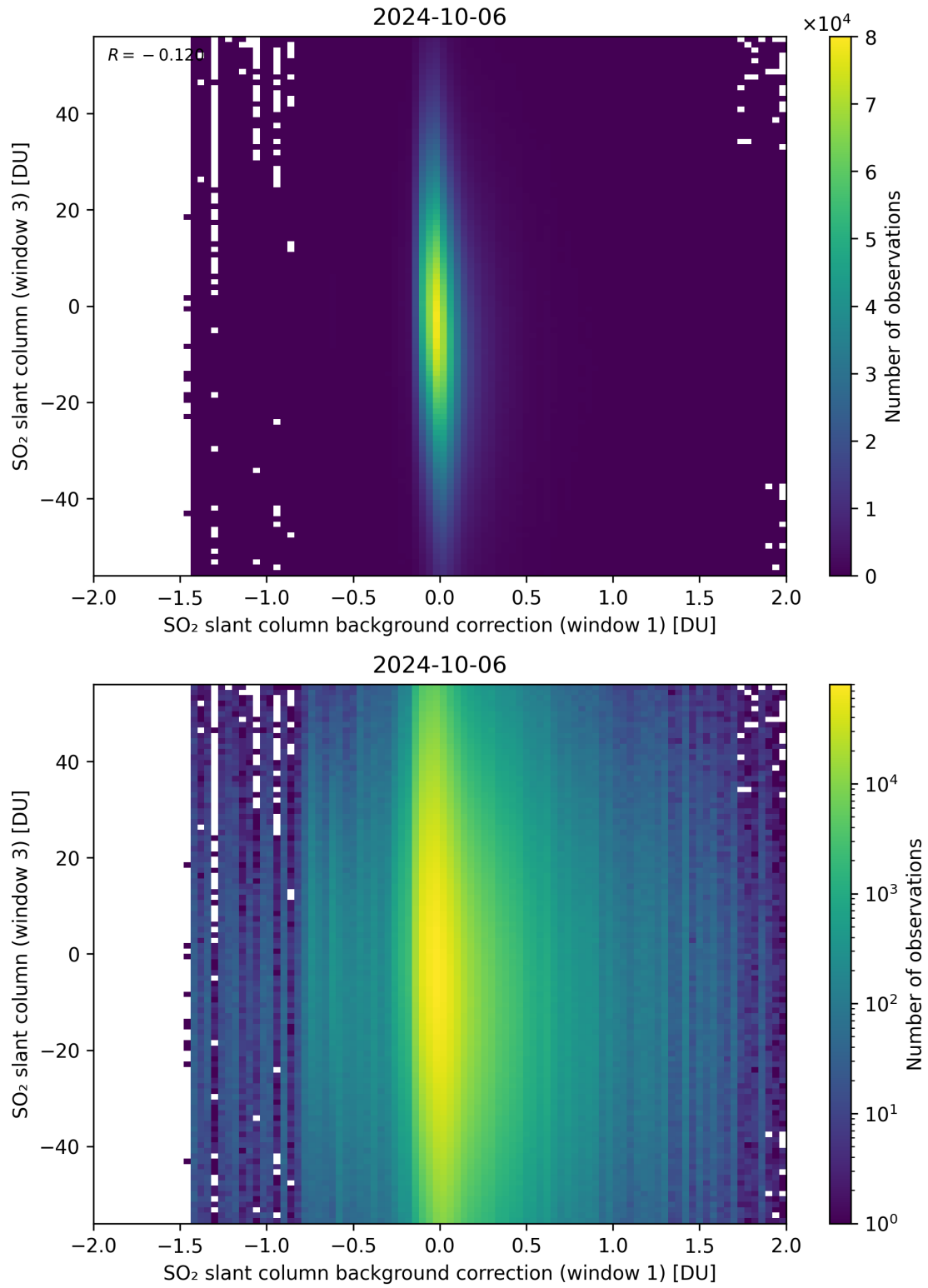
Figure 107: Scatter density plot of “SO 2 slant column background correction (window 1)” against “SO 2 slant column (window 3)” for 2024-10-05 to 2024-10-07.
