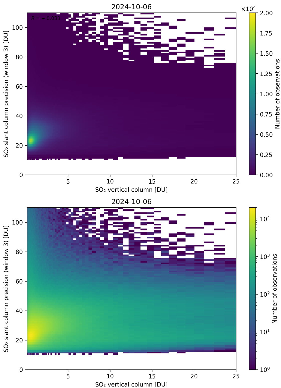
Figure 304: Scatter density plot of “SO 2 vertical column” against “SO 2 slant column precision (window 3)” for 2024-10-05 to 2024-10-07.
