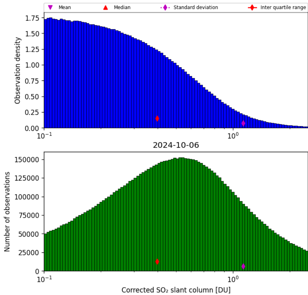
Figure 55: Histogram of “Corrected SO 2 slant column” for 2024-10-05 to 2024-10-07
