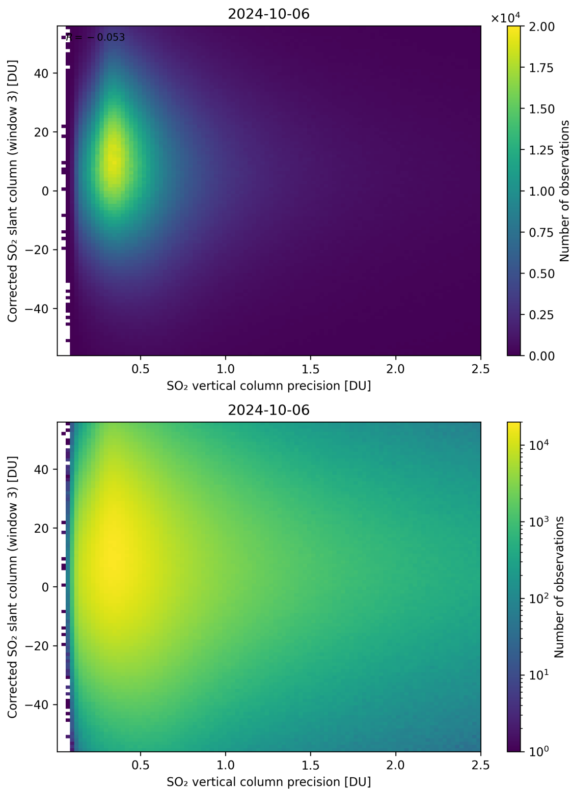
Figure 288: Scatter density plot of “SO 2 vertical column precision” against “Corrected SO 2 slant column (window 3)” for 2024-10-05 to 2024-10-07.
