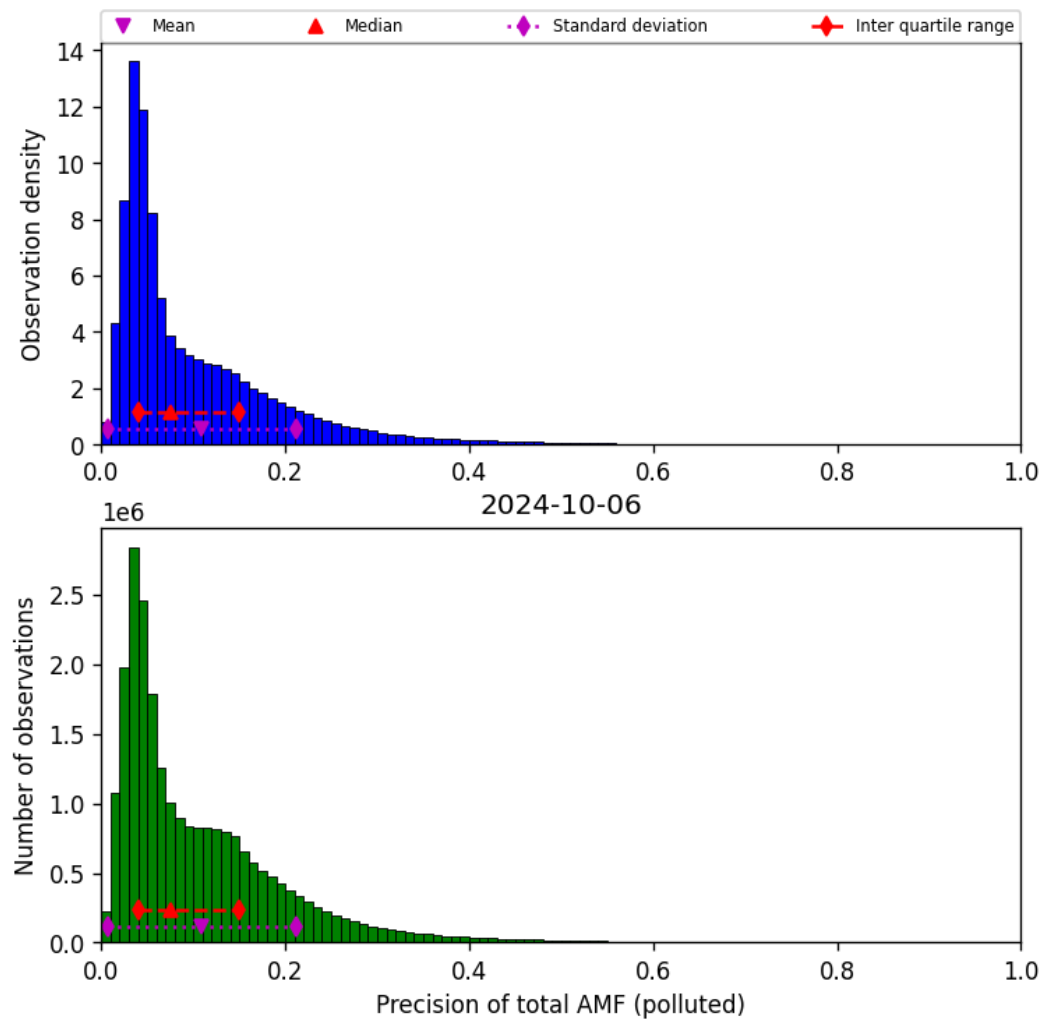
Figure 72: Histogram of “Precision of total AMF (polluted)” for 2024-10-05 to 2024-10-07
