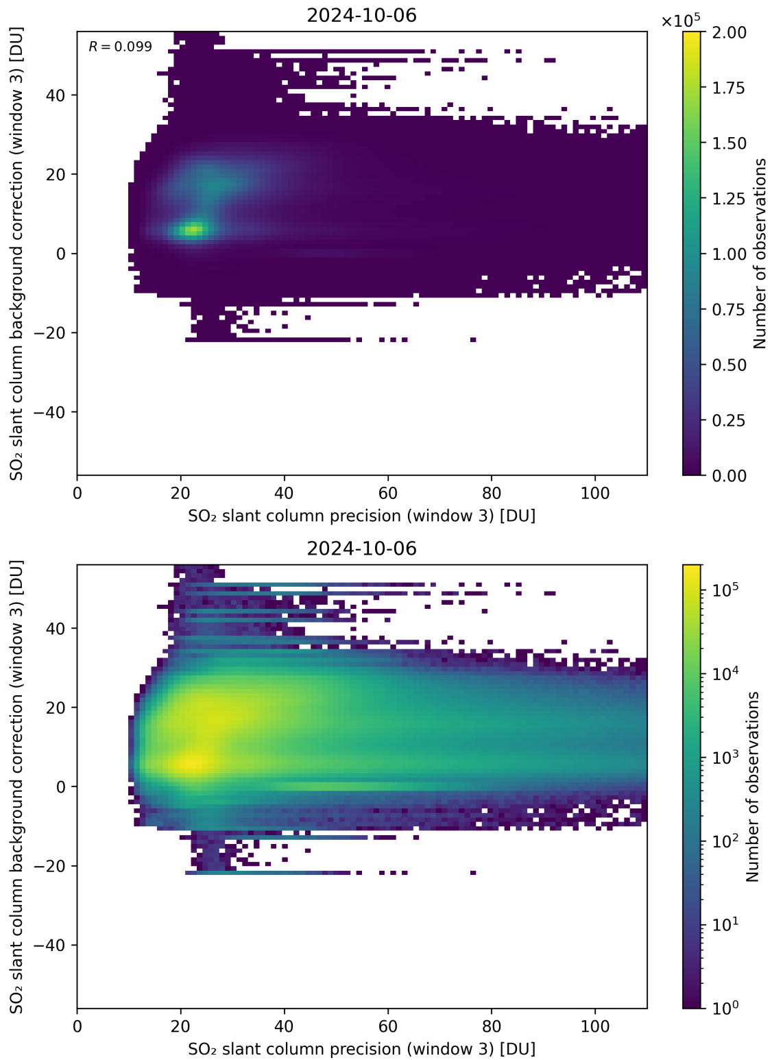
Figure 257: Scatter density plot of “SO 2 slant column precision (window 3)” against “SO 2 slant column background correction (window 3)” for 2024-10-05 to 2024-10-07.
