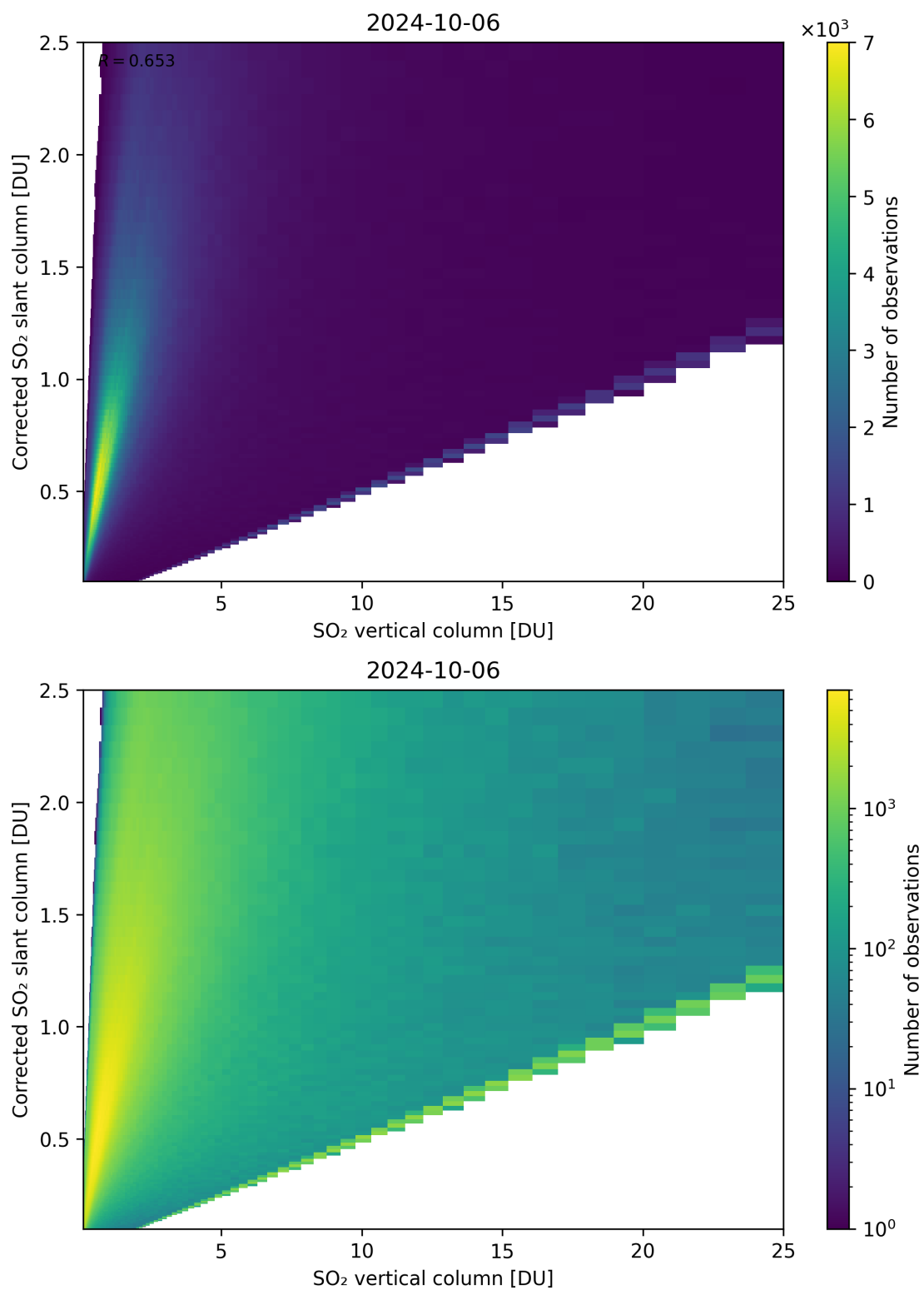
Figure 297: Scatter density plot of “SO 2 vertical column” against “Corrected SO 2 slant column” for 2024-10-05 to 2024-10-07.
