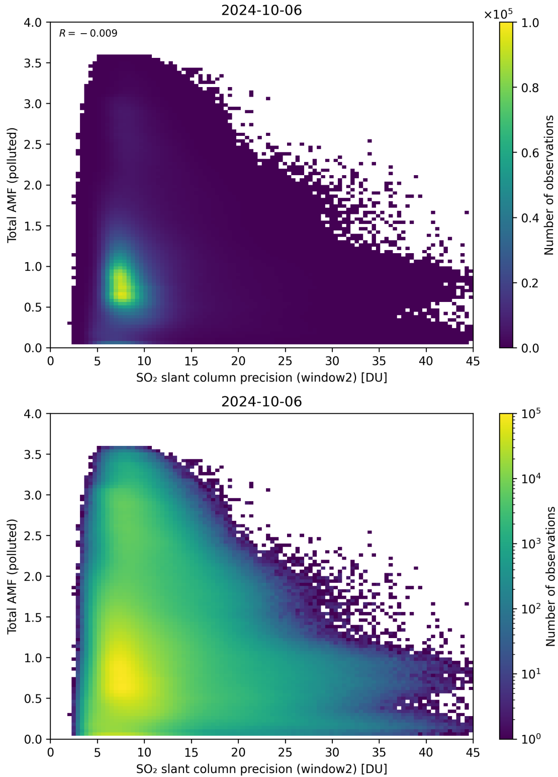
Figure 251: Scatter density plot of “SO 2 slant column precision (window2)” against “Total AMF (polluted)” for 2024-10-05 to 2024-10-07.
