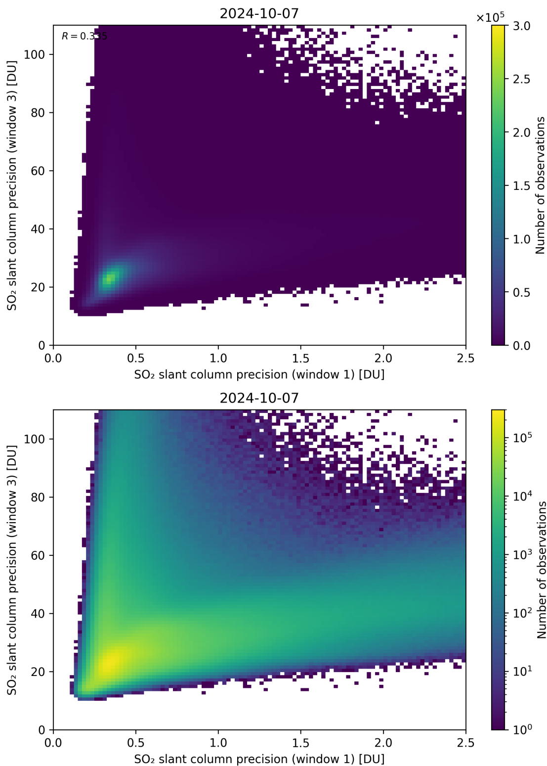
Figure 229: Scatter density plot of “SO 2 slant column precision (window 1)” against “SO 2 slant column precision (window 3)” for 2024-10-06 to 2024-10-08.
