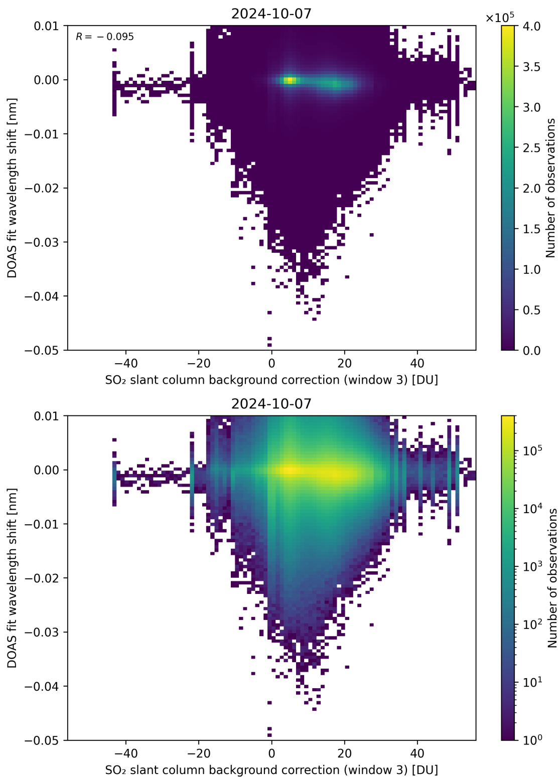
Figure 121: Scatter density plot of “SO 2 slant column background correction (window 3)” against “DOAS fit wavelength shift” for 2024-10-06 to 2024-10-08.
