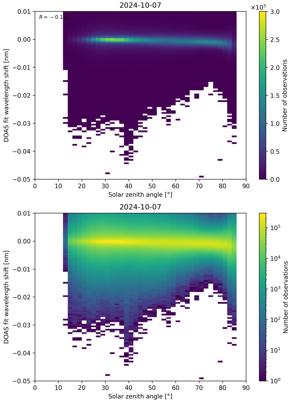
Figure 161: Scatter density plot of “Solar zenith angle” against “DOAS fit wavelength shift” for 2024-10-06 to 2024-10-08.
