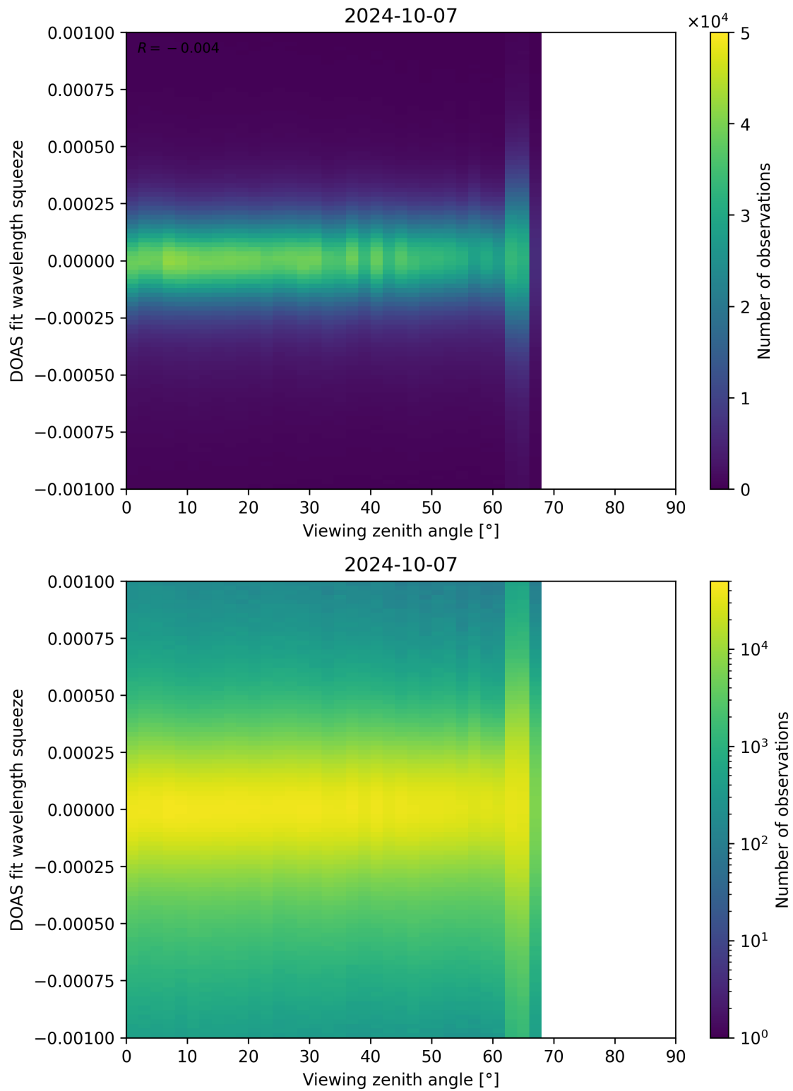
Figure 312: Scatter density plot of “Viewing zenith angle” against “DOAS fit wavelength squeeze” for 2024-10-06 to 2024-10-08.
