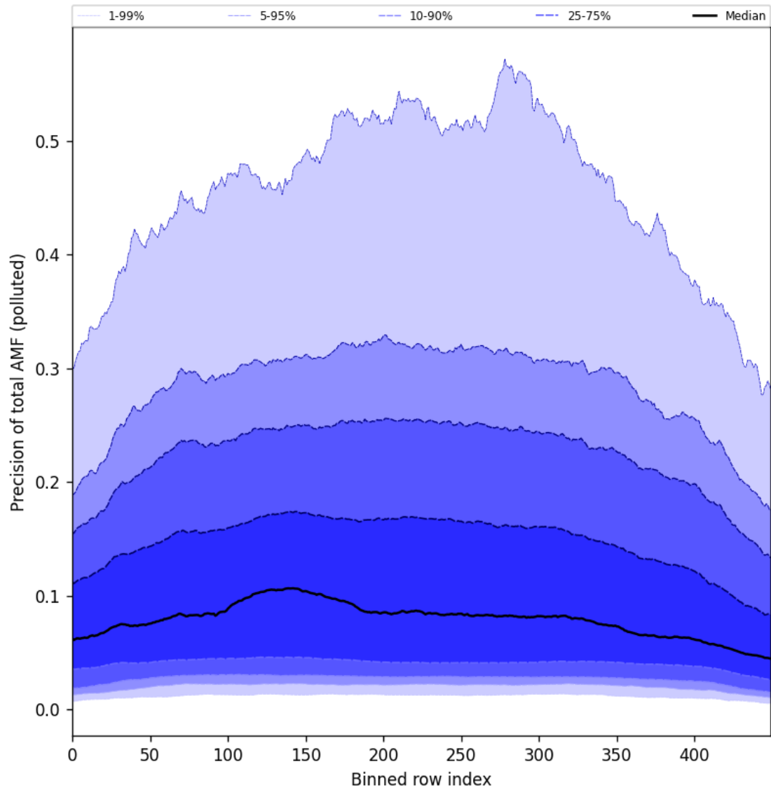
Figure 95: Along track statistics of “Precision of total AMF (polluted)” for 2024-10-06 to 2024-10-08
