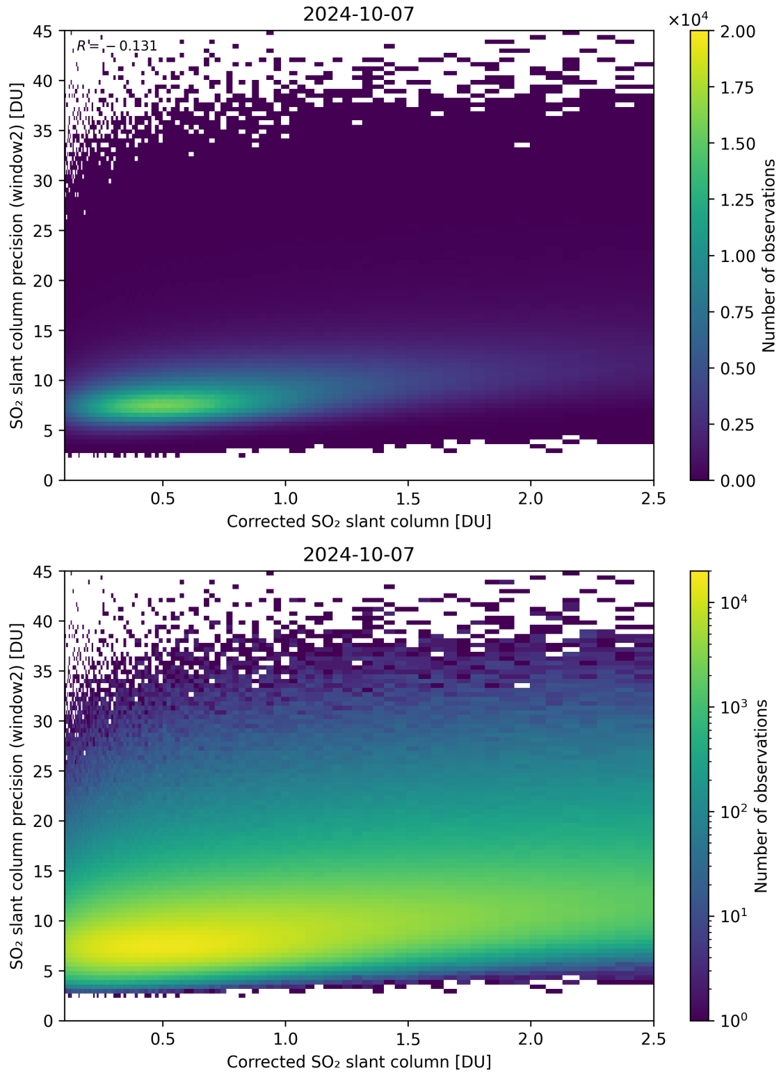
Figure 189: Scatter density plot of “Corrected SO 2 slant column” against “SO 2 slant column precision (window2)” for 2024-10-06 to 2024-10-08.
