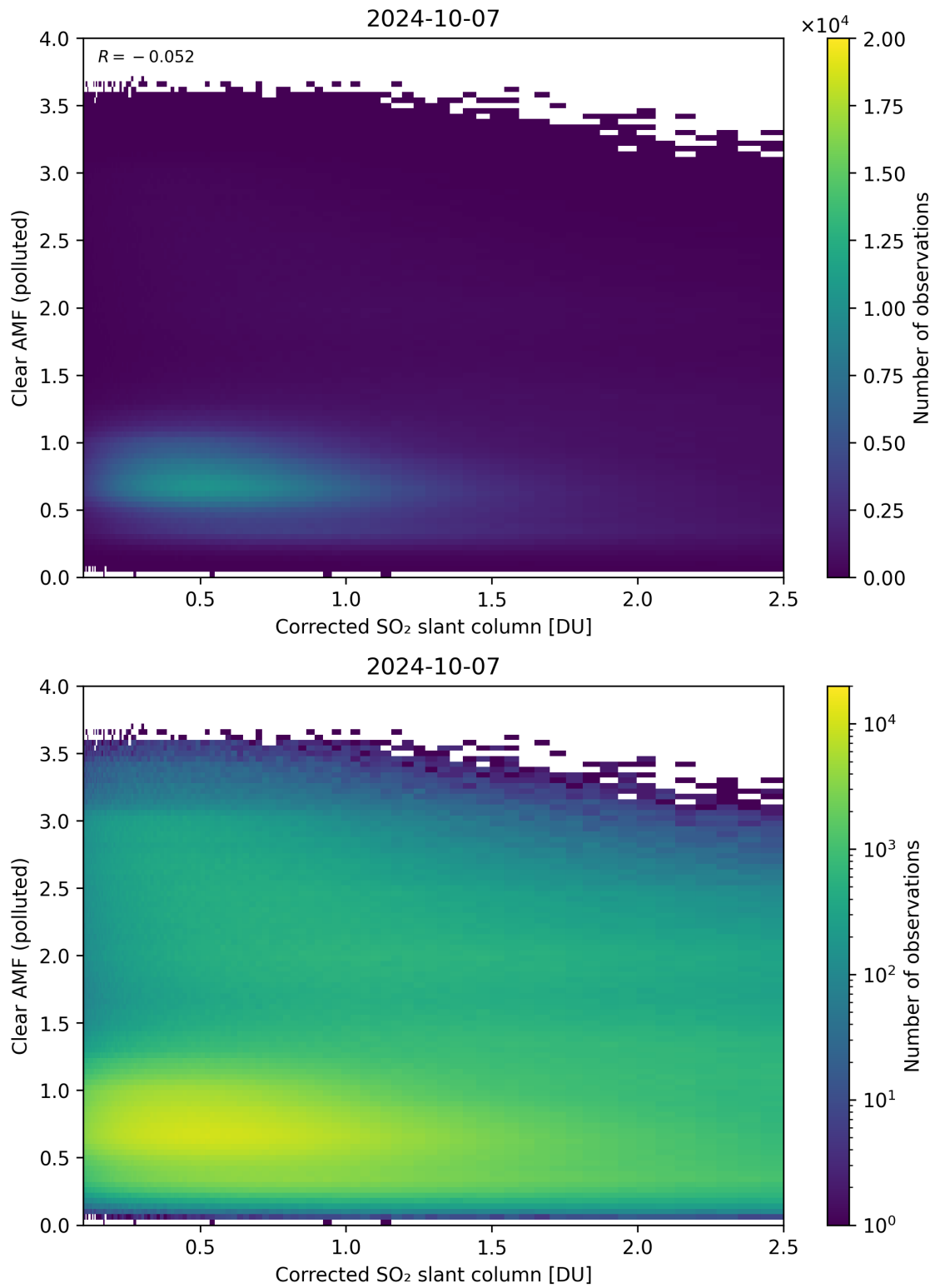
Figure 184: Scatter density plot of “Corrected SO 2 slant column” against “Clear AMF (polluted)” for 2024-10-06 to 2024-10-08.
