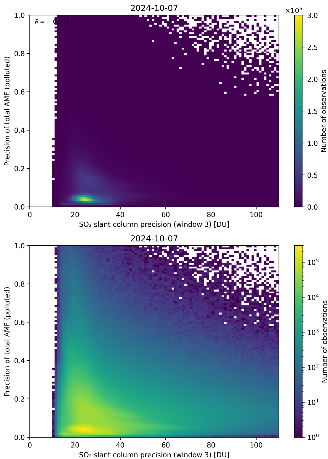
Figure 264: Scatter density plot of “SO 2 slant column precision (window 3)” against “Precision of total AMF (polluted)” for 2024-10-06 to 2024-10-08.
