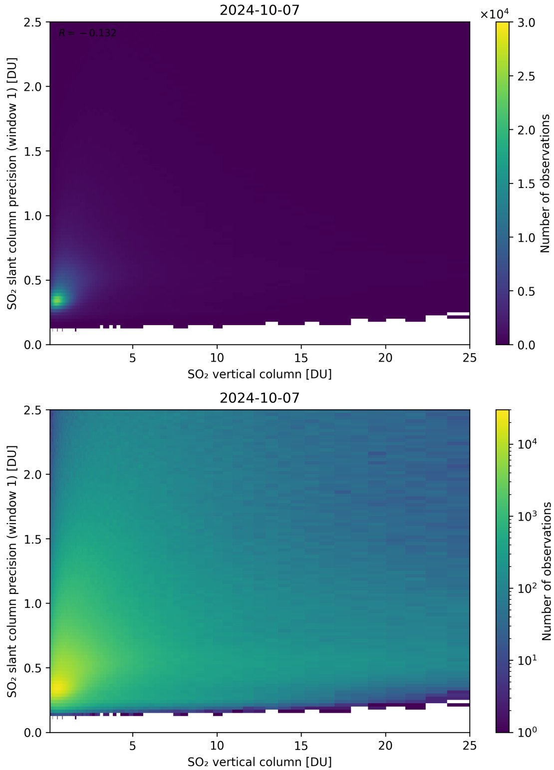
Figure 301: Scatter density plot of “SO 2 vertical column” against “SO 2 slant column precision (window 1)” for 2024-10-06 to 2024-10-08.
