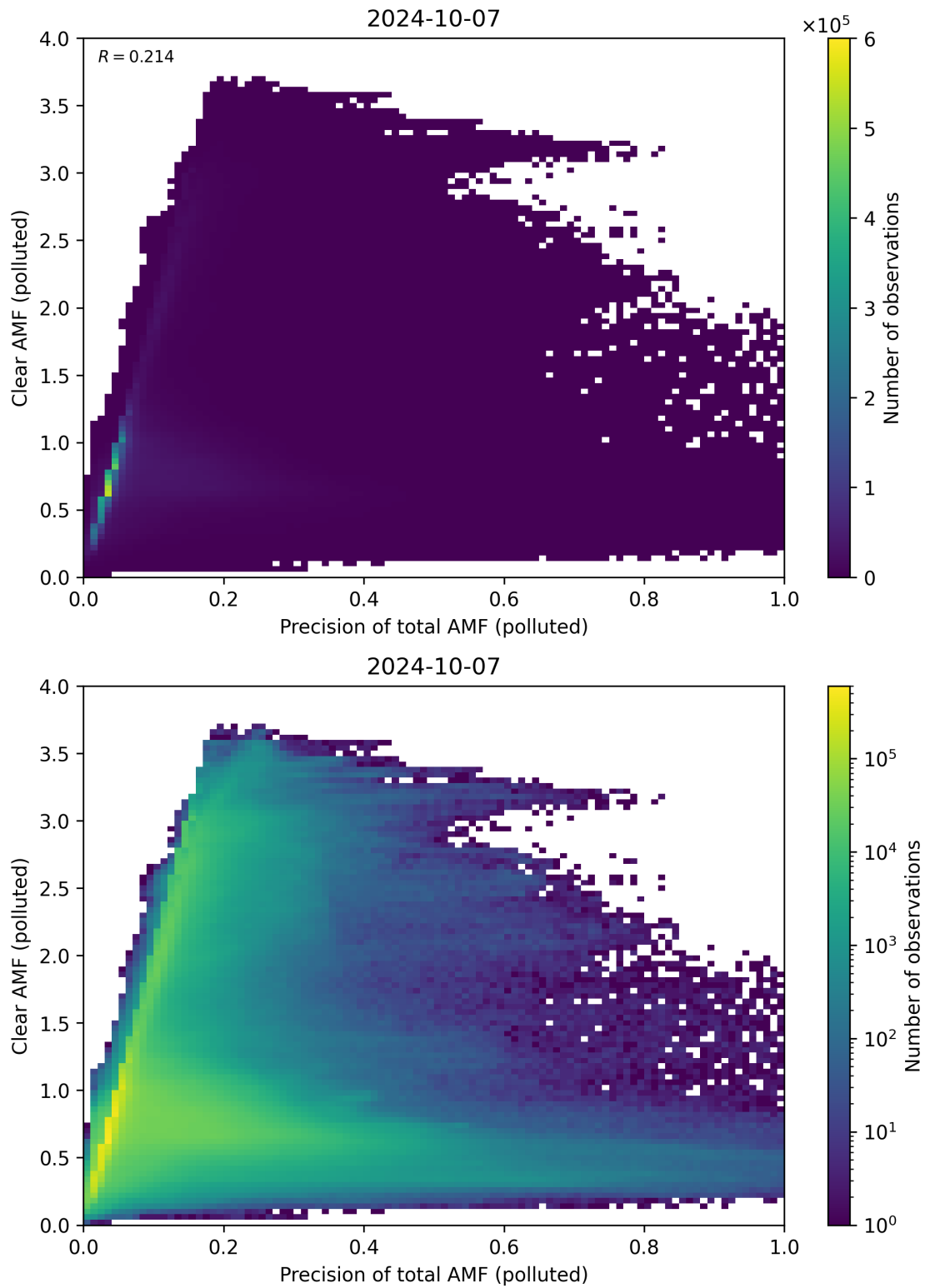
Figure 270: Scatter density plot of “Precision of total AMF (polluted)” against “Clear AMF (polluted)” for 2024-10-06 to 2024-10-08.
