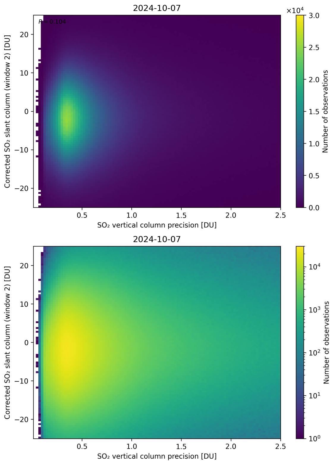
Figure 287: Scatter density plot of “SO 2 vertical column precision” against “Corrected SO 2 slant column (window 2)” for 2024-10-06 to 2024-10-08.
