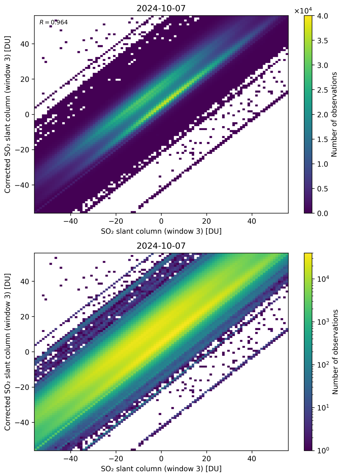
Figure 266: Scatter density plot of “SO 2 slant column (window 3)” against “Corrected SO 2 slant column (window 3)” for 2024-10-06 to 2024-10-08.
