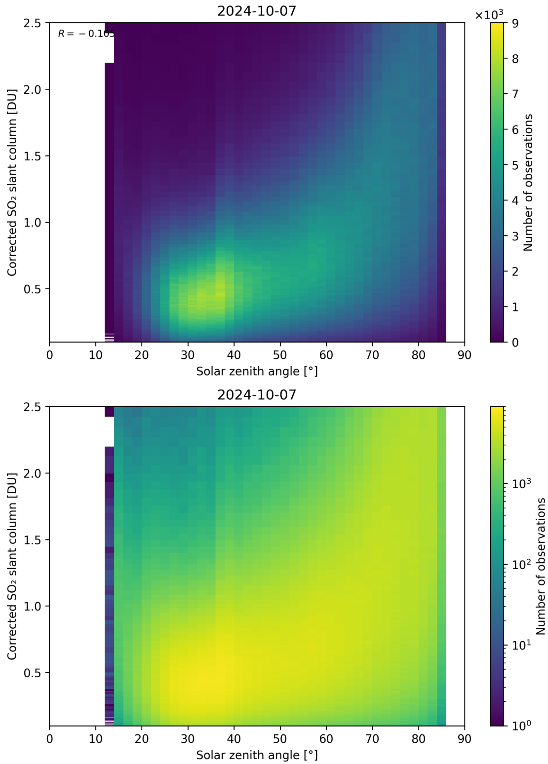
Figure 166: Scatter density plot of “Solar zenith angle” against “Corrected SO 2 slant column” for 2024-10-06 to 2024-10-08.
