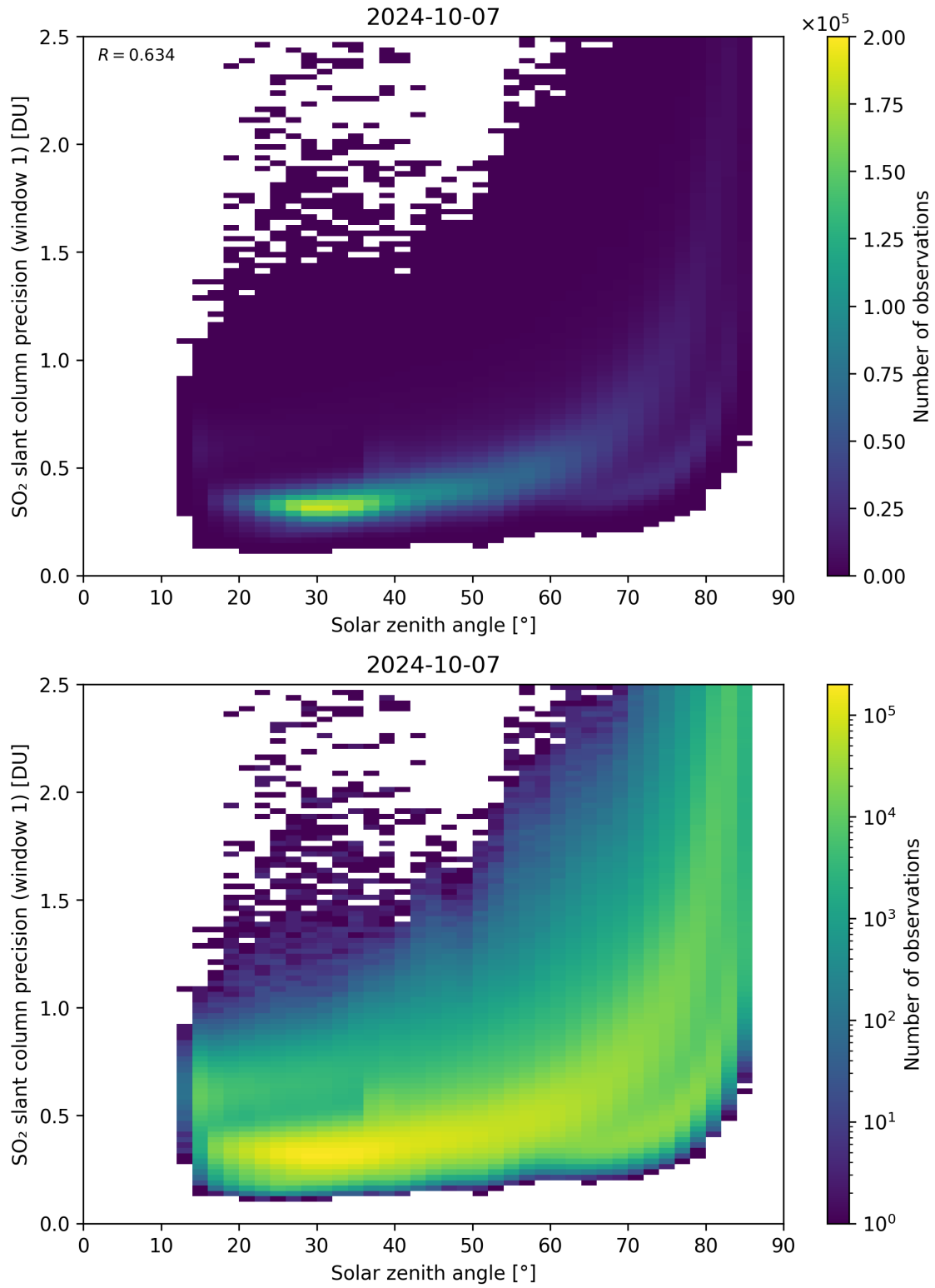
Figure 170: Scatter density plot of “Solar zenith angle” against “SO 2 slant column precision (window 1)” for 2024-10-06 to 2024-10-08.
