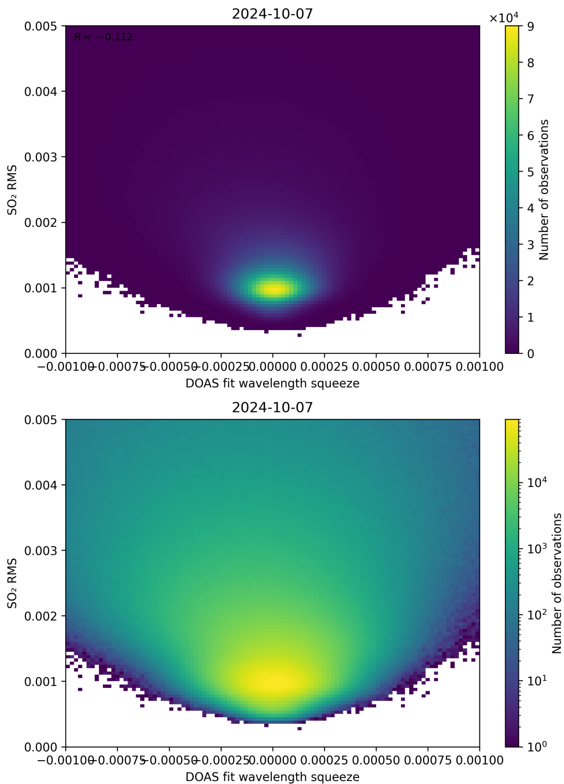
Figure 132: Scatter density plot of “DOAS fit wavelength squeeze” against “SO 2 RMS” for 2024-10-06 to 2024-10-08.
