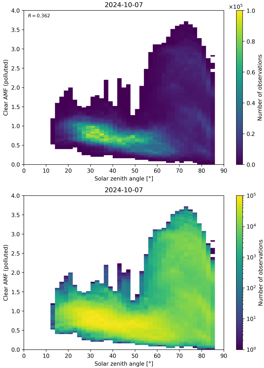
Figure 165: Scatter density plot of “Solar zenith angle” against “Clear AMF (polluted)” for 2024-10-06 to 2024-10-08.
