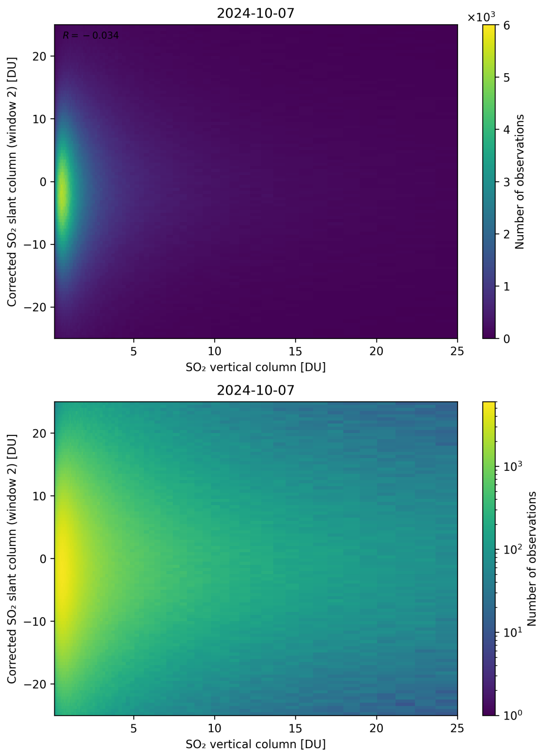
Figure 298: Scatter density plot of “SO 2 vertical column” against “Corrected SO 2 slant column (window 2)” for 2024-10-06 to 2024-10-08.
