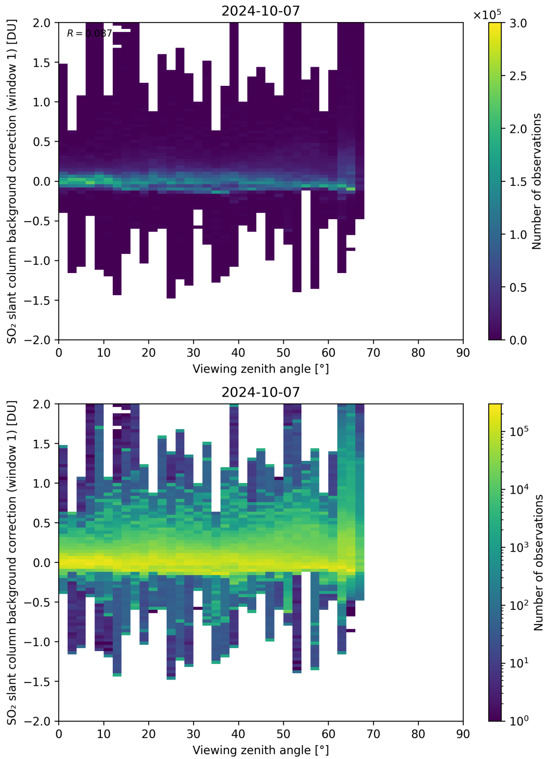
Figure 308: Scatter density plot of “Viewing zenith angle” against “SO 2 slant column background correction (window 1)” for 2024-10-06 to 2024-10-08.
