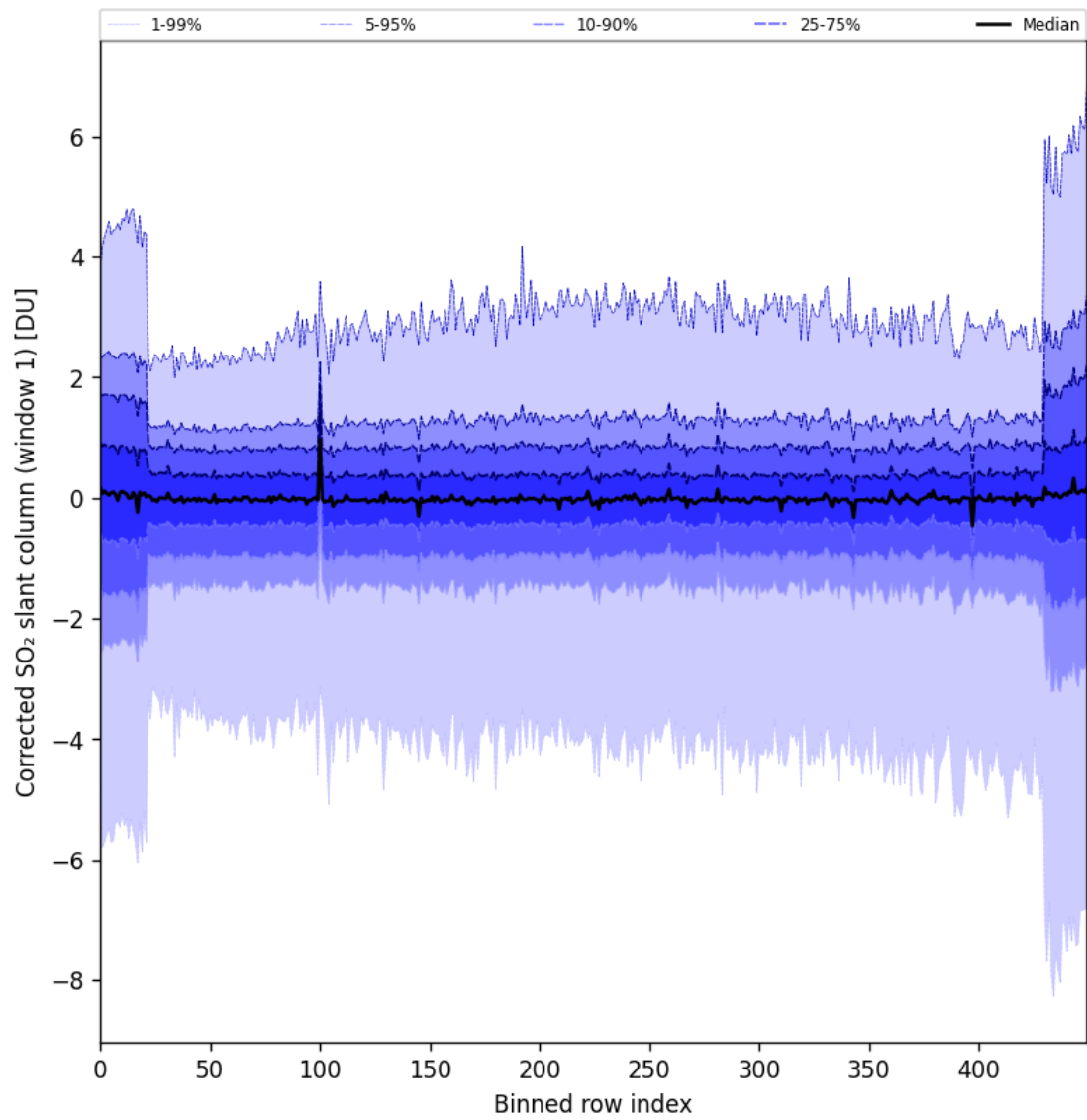
Figure 81: Along track statistics of “Corrected SO 2 slant column (window 1)” for 2024-10-06 to 2024-10-08
