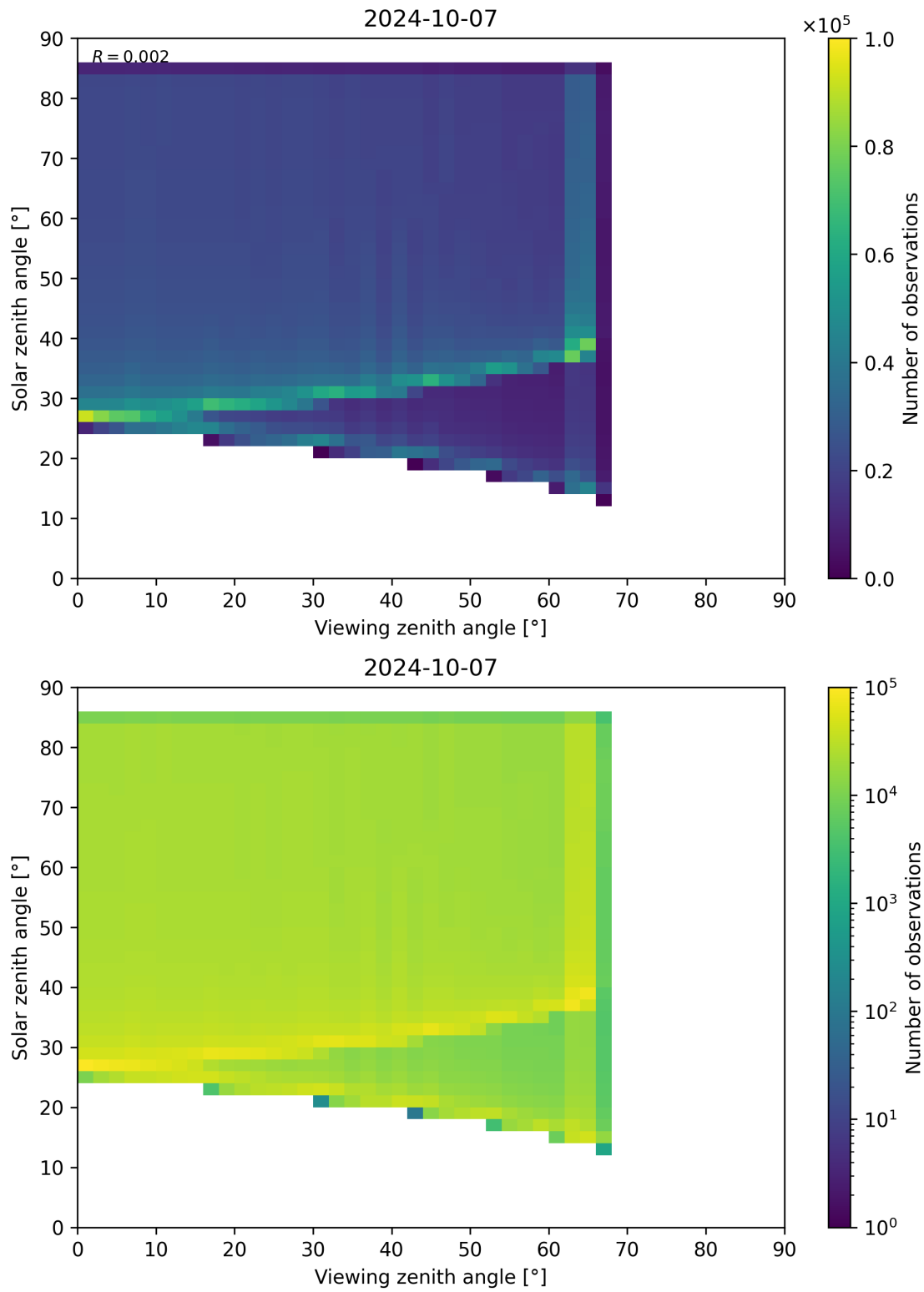
Figure 315: Scatter density plot of “Viewing zenith angle” against “Solar zenith angle” for 2024-10-06 to 2024-10-08.
