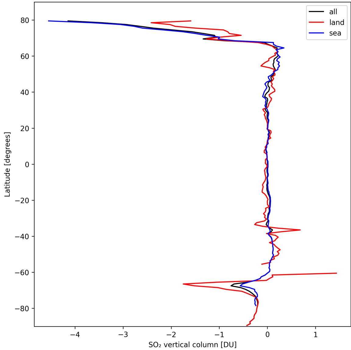
Figure 30: Zonal average of “SO 2 vertical column” for 2024-10-06 to 2024-10-08.
