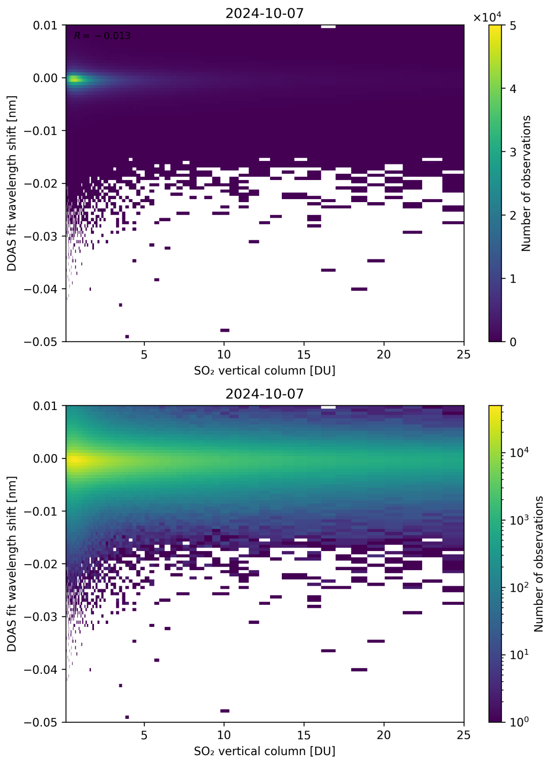
Figure 276: Scatter density plot of “SO 2 vertical column” against “DOAS fit wavelength shift” for 2024-10-06 to 2024-10-08.
