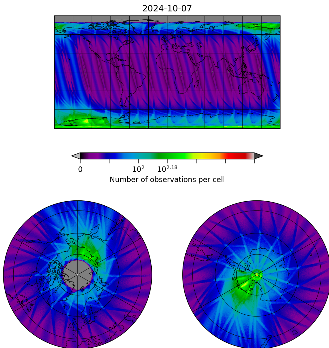
Figure 28: Map of the number of observations for 2024-10-06 to 2024-10-08
