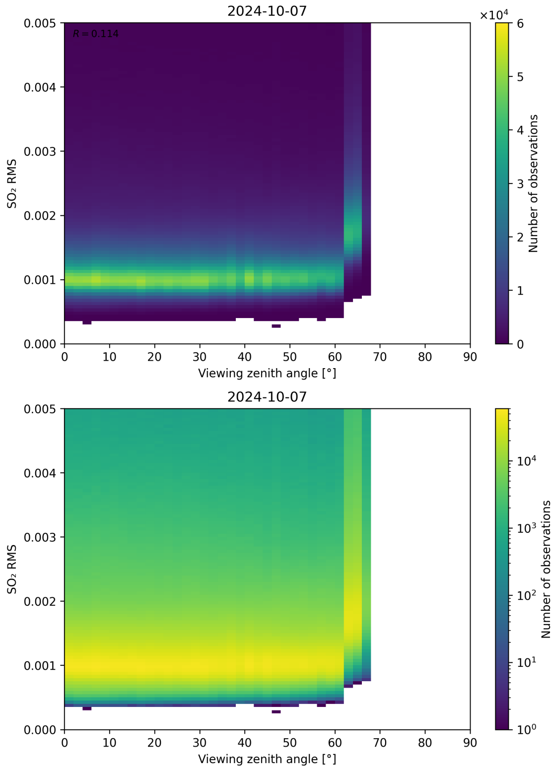
Figure 313: Scatter density plot of “Viewing zenith angle” against “SO 2 RMS” for 2024-10-06 to 2024-10-08.
