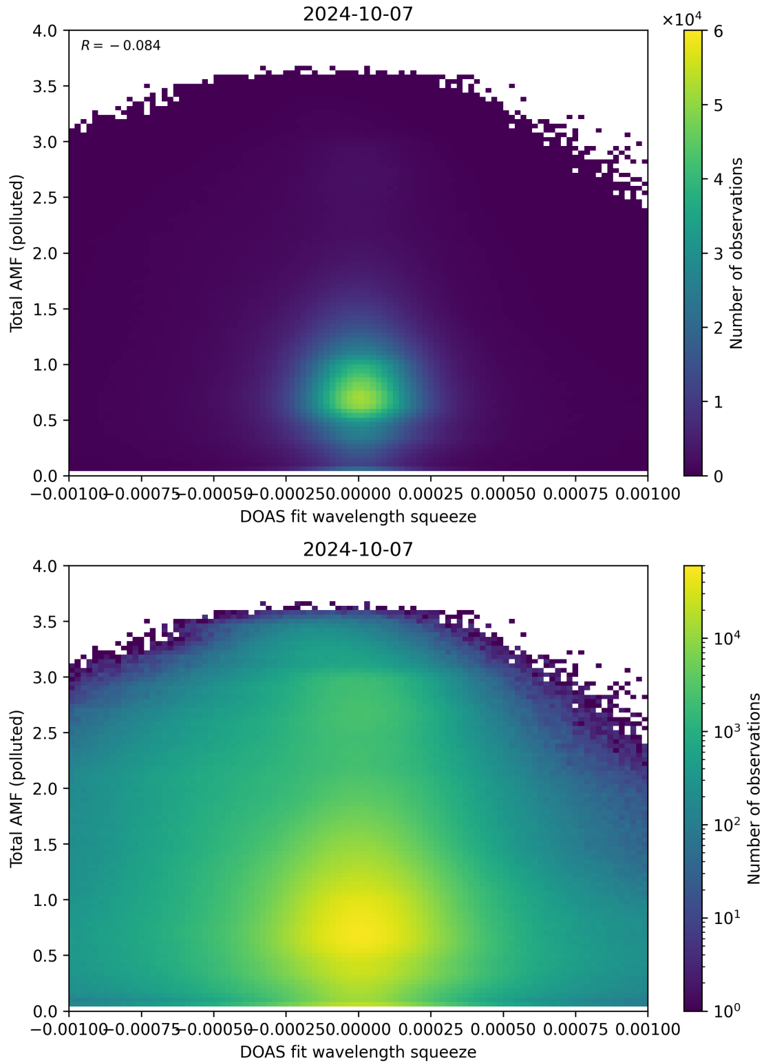
Figure 134: Scatter density plot of “DOAS fit wavelength squeeze” against “Total AMF (polluted)” for 2024-10-06 to 2024-10-08.
