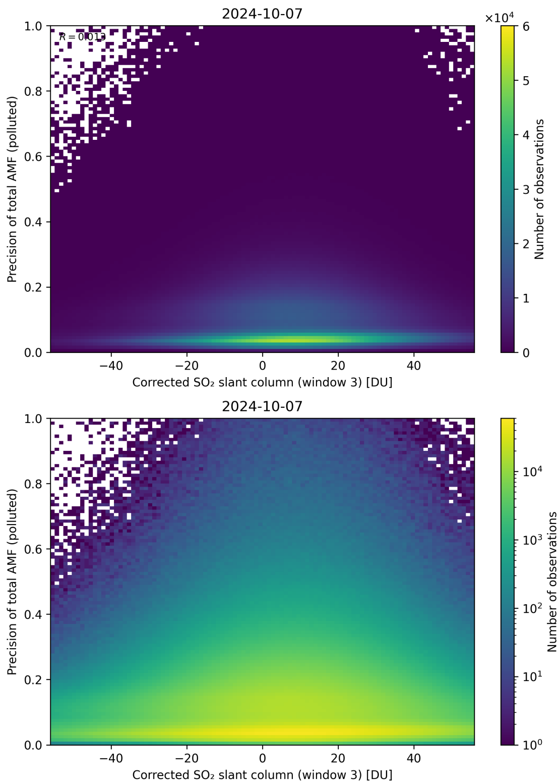
Figure 211: Scatter density plot of “Corrected SO 2 slant column (window 3)” against “Precision of total AMF (polluted)” for 2024-10-06 to 2024-10-08.
