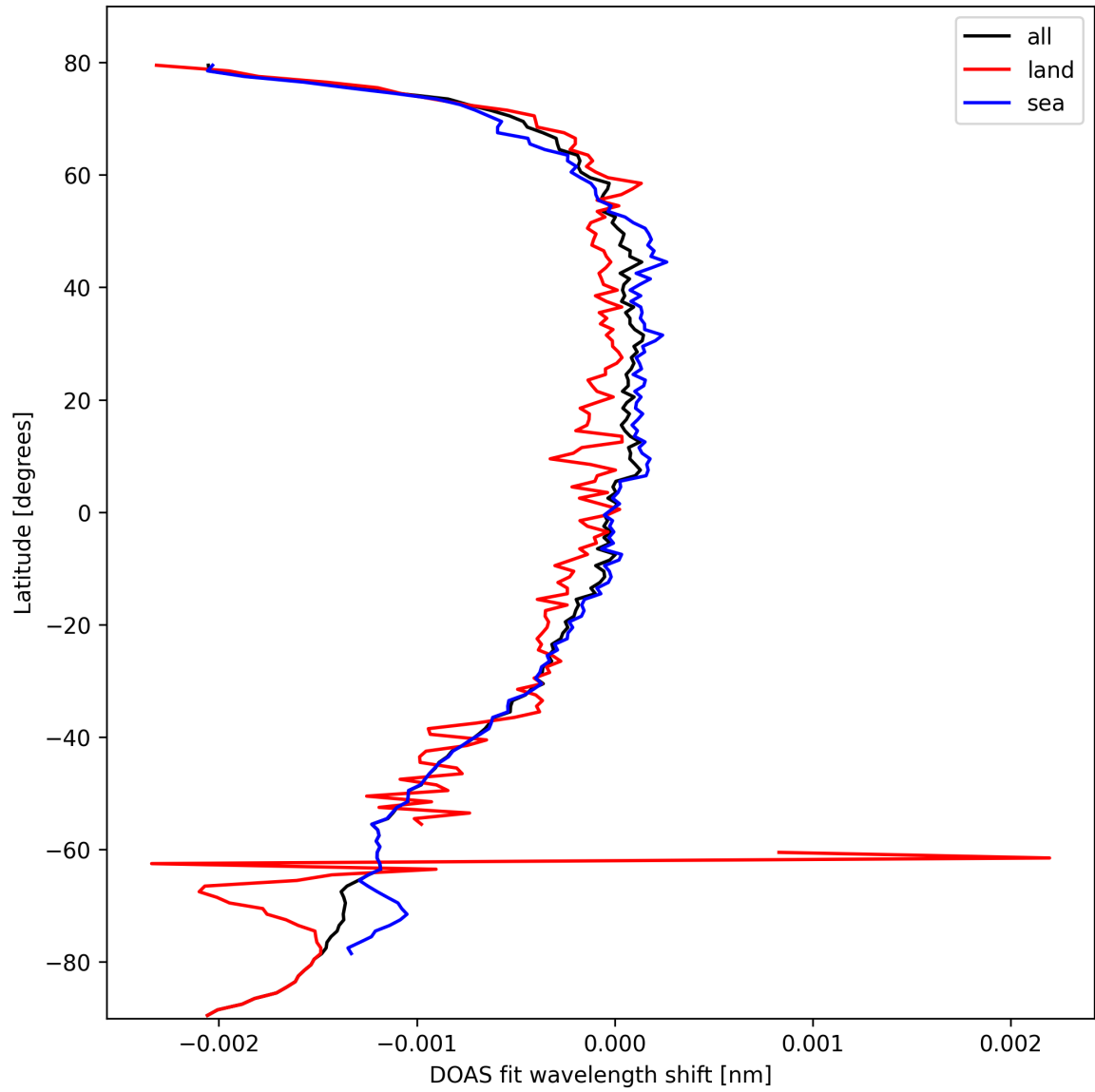
Figure 45: Zonal average of “DOAS fit wavelength shift” for 2024-10-06 to 2024-10-08.
