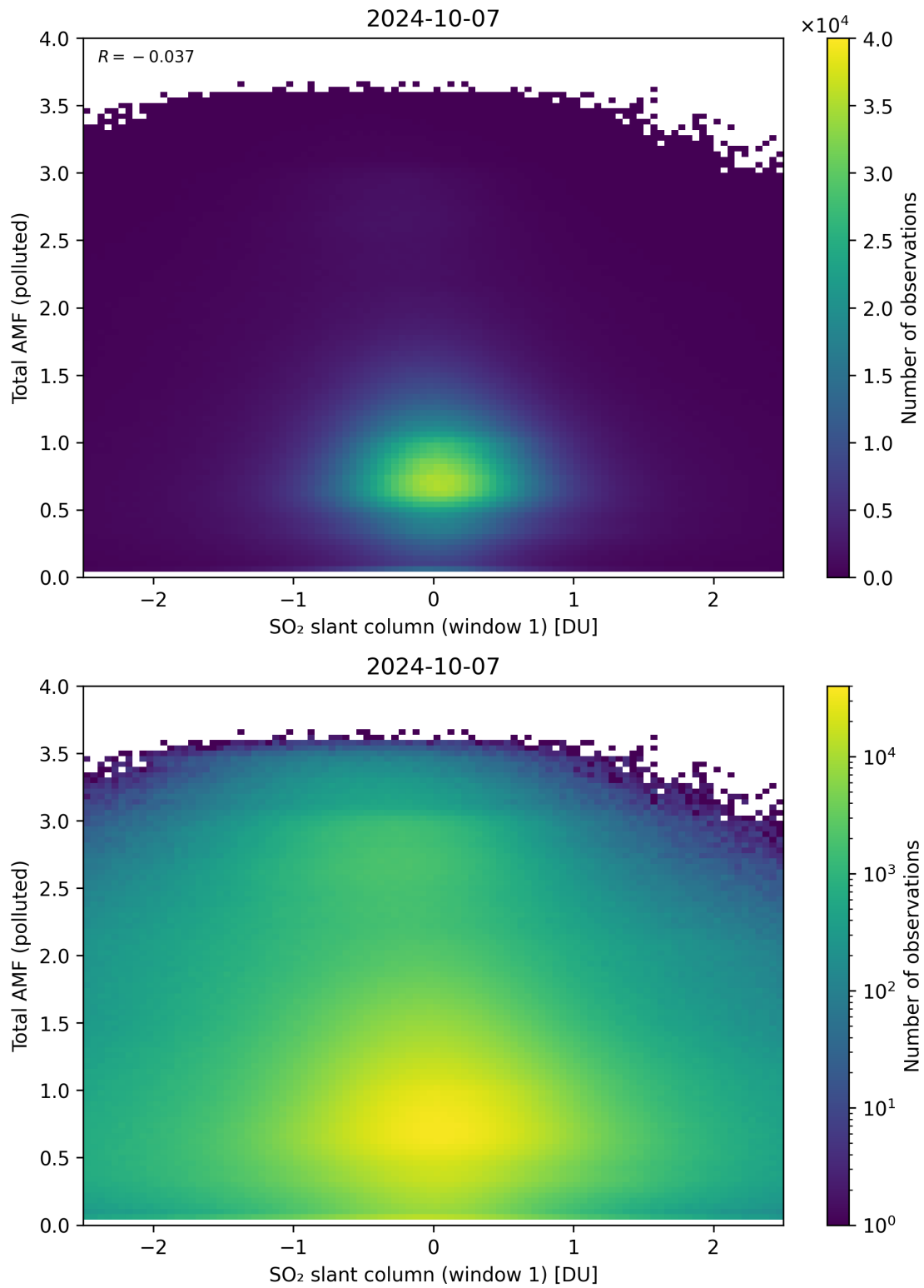
Figure 239: Scatter density plot of “SO 2 slant column (window 1)” against “Total AMF (polluted)” for 2024-10-06 to 2024-10-08.
