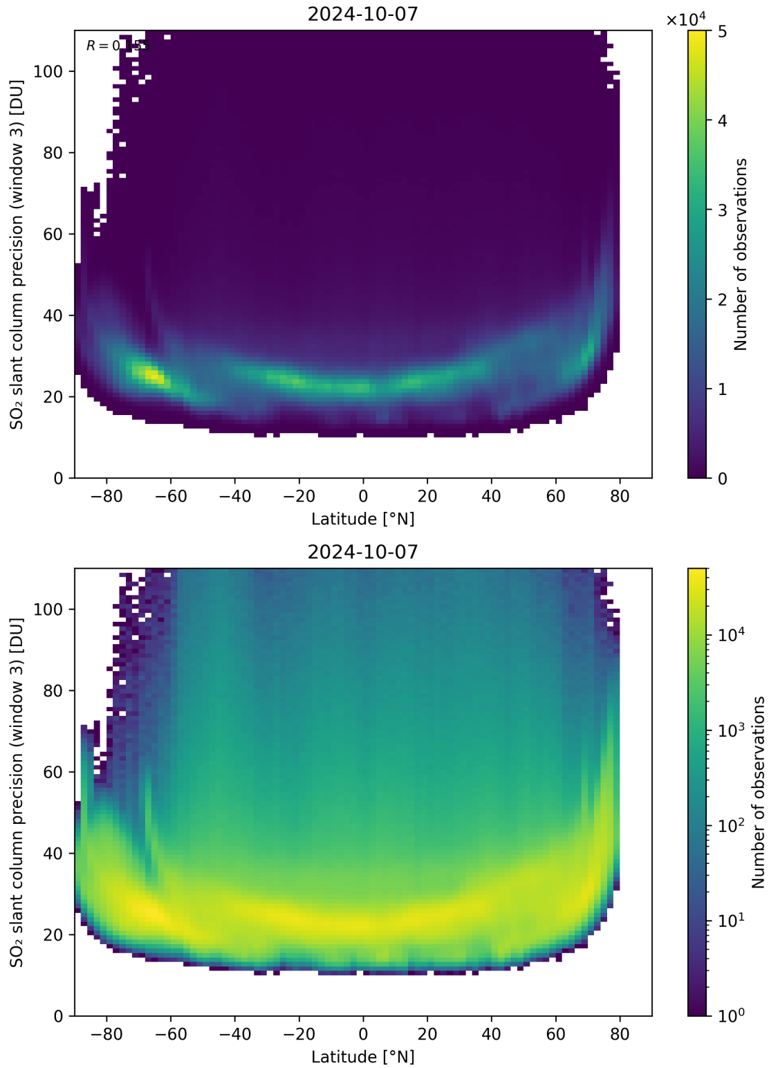
Figure 153: Scatter density plot of “Latitude” against “SO 2 slant column precision (window 3)” for 2024-10-06 to 2024-10-08.
