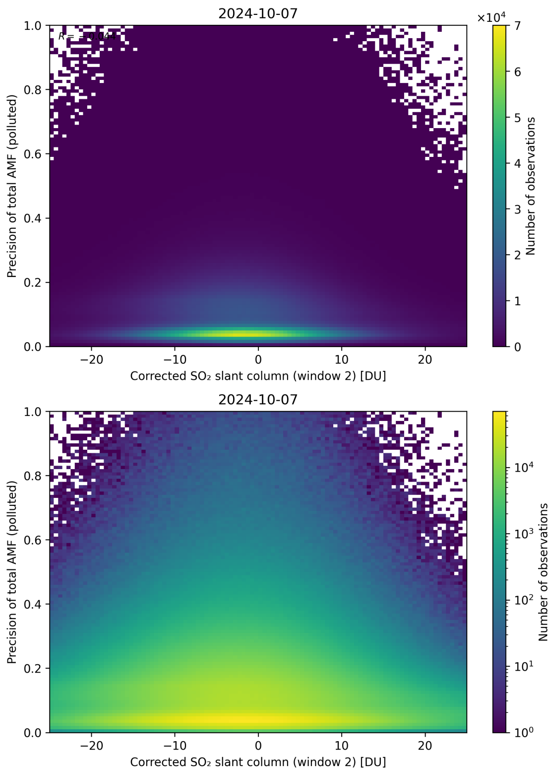
Figure 204: Scatter density plot of “Corrected SO 2 slant column (window 2)” against “Precision of total AMF (polluted)” for 2024-10-06 to 2024-10-08.
