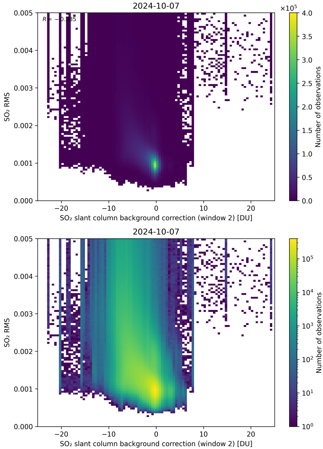
Figure 114: Scatter density plot of “SO 2 slant column background correction (window 2)” against “SO 2 RMS” for 2024-10-06 to 2024-10-08.
