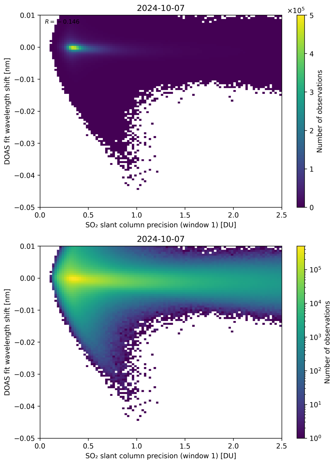
Figure 221: Scatter density plot of “SO 2 slant column precision (window 1)” against “DOAS fit wavelength shift” for 2024-10-06 to 2024-10-08.
