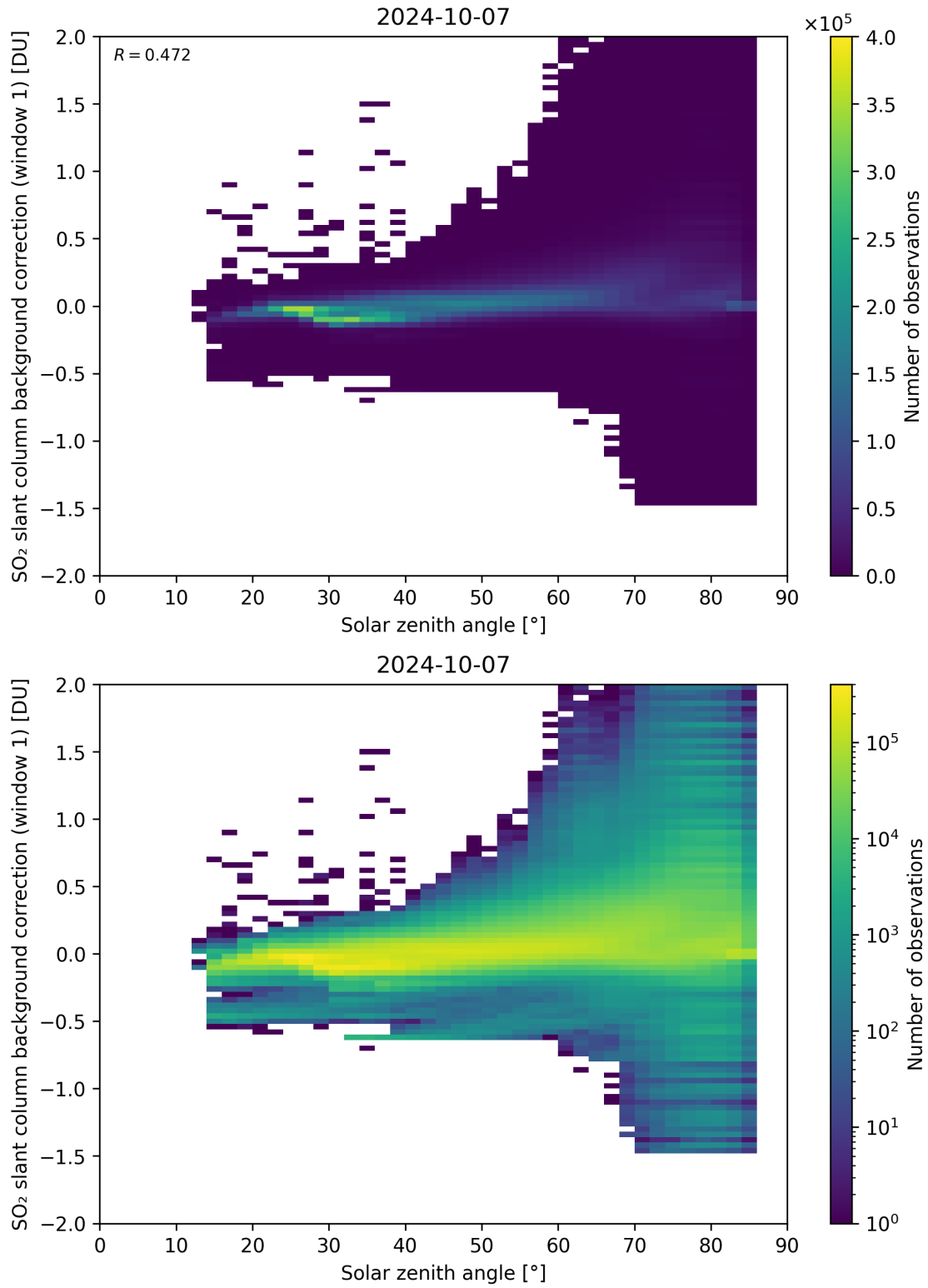
Figure 158: Scatter density plot of “Solar zenith angle” against “SO 2 slant column background correction (window 1)” for 2024-10-06 to 2024-10-08.
