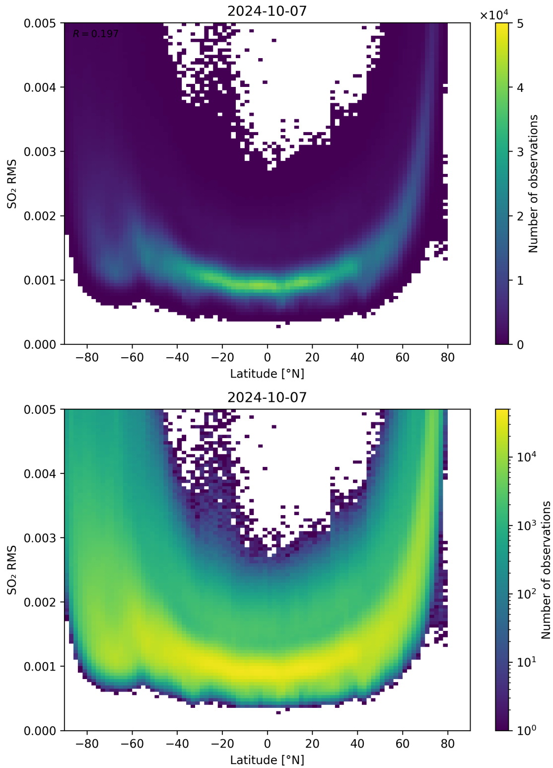
Figure 144: Scatter density plot of “Latitude” against “SO 2 RMS” for 2024-10-06 to 2024-10-08.
