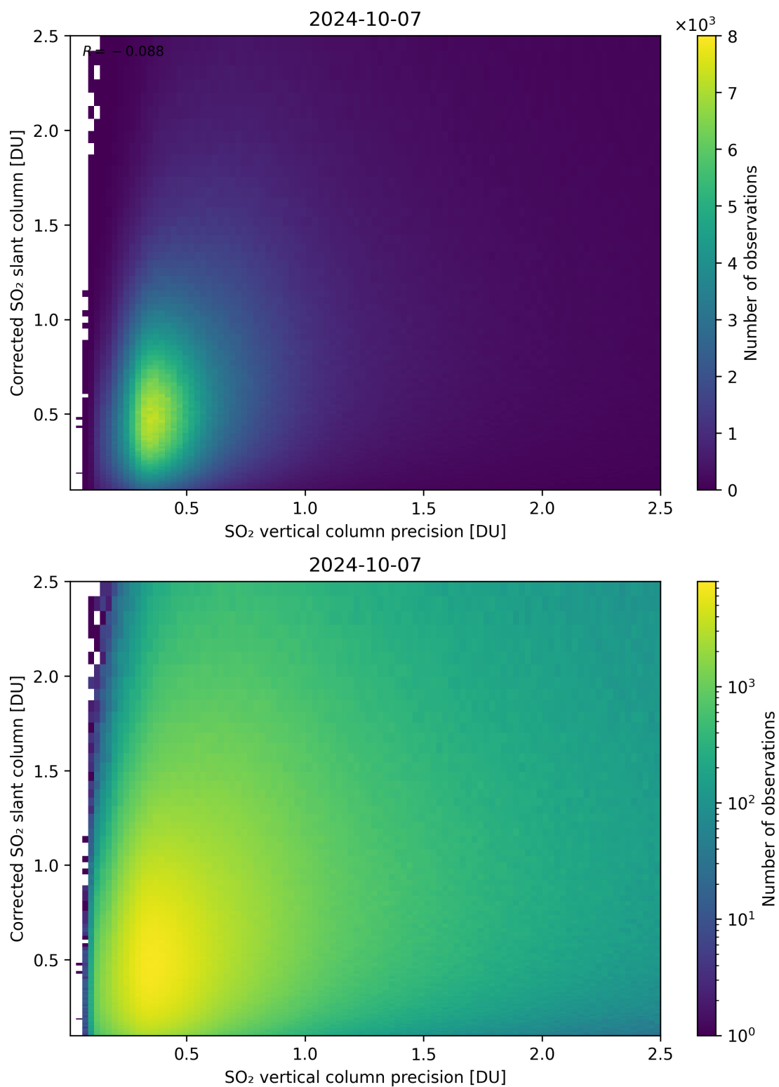
Figure 286: Scatter density plot of “SO 2 vertical column precision” against “Corrected SO 2 slant column” for 2024-10-06 to 2024-10-08.
