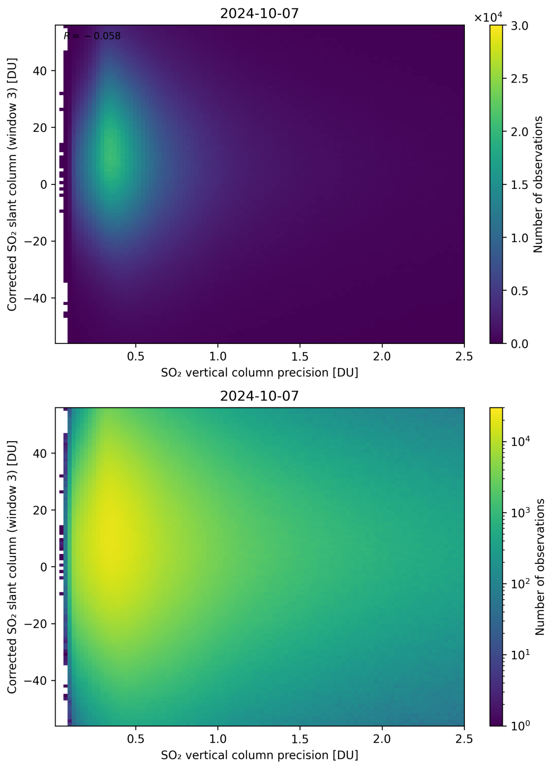
Figure 288: Scatter density plot of “SO 2 vertical column precision” against “Corrected SO 2 slant column (window 3)” for 2024-10-06 to 2024-10-08.
