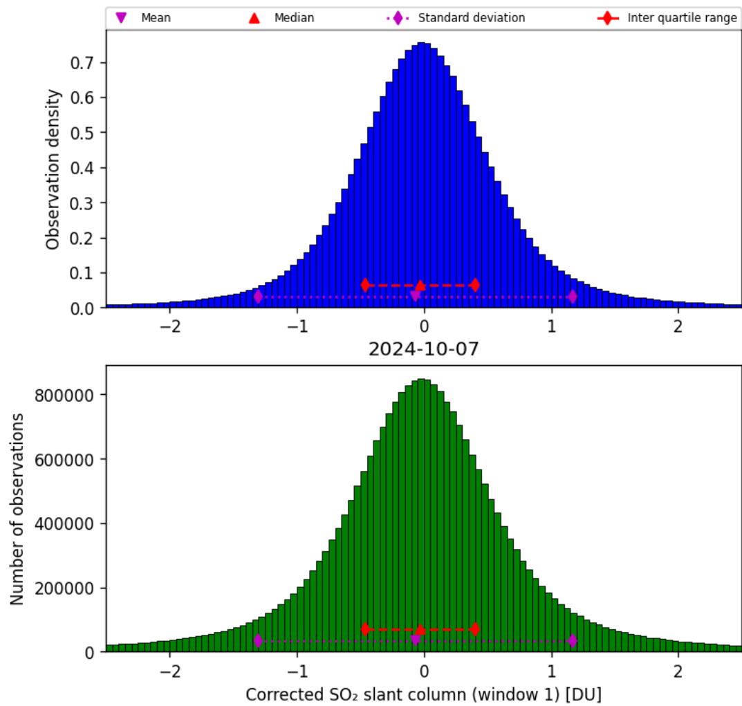
Figure 58: Histogram of “Corrected SO 2 slant column (window 1)” for 2024-10-06 to 2024-10-08
