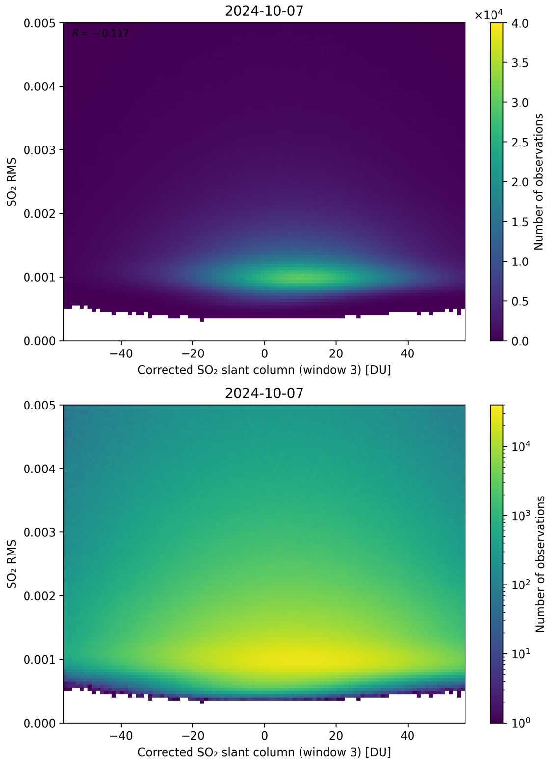
Figure 208: Scatter density plot of “Corrected SO 2 slant column (window 3)” against “SO 2 RMS” for 2024-10-06 to 2024-10-08.
