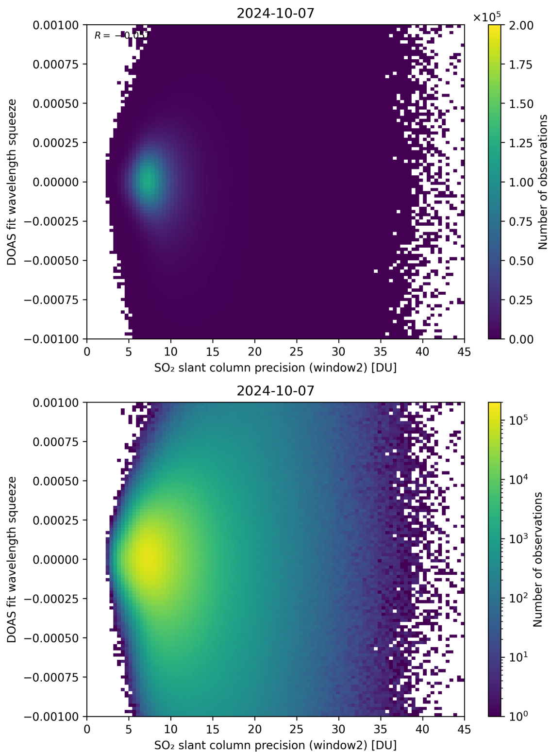
Figure 244: Scatter density plot of “SO 2 slant column precision (window2)” against “DOAS fit wavelength squeeze” for 2024-10-06 to 2024-10-08.
