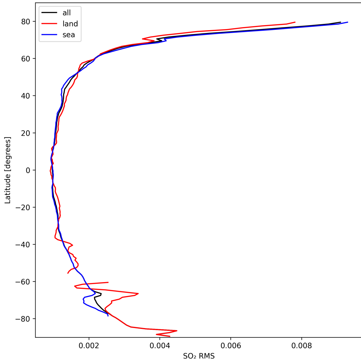
Figure 47: Zonal average of “SO 2 RMS” for 2024-10-06 to 2024-10-08.
