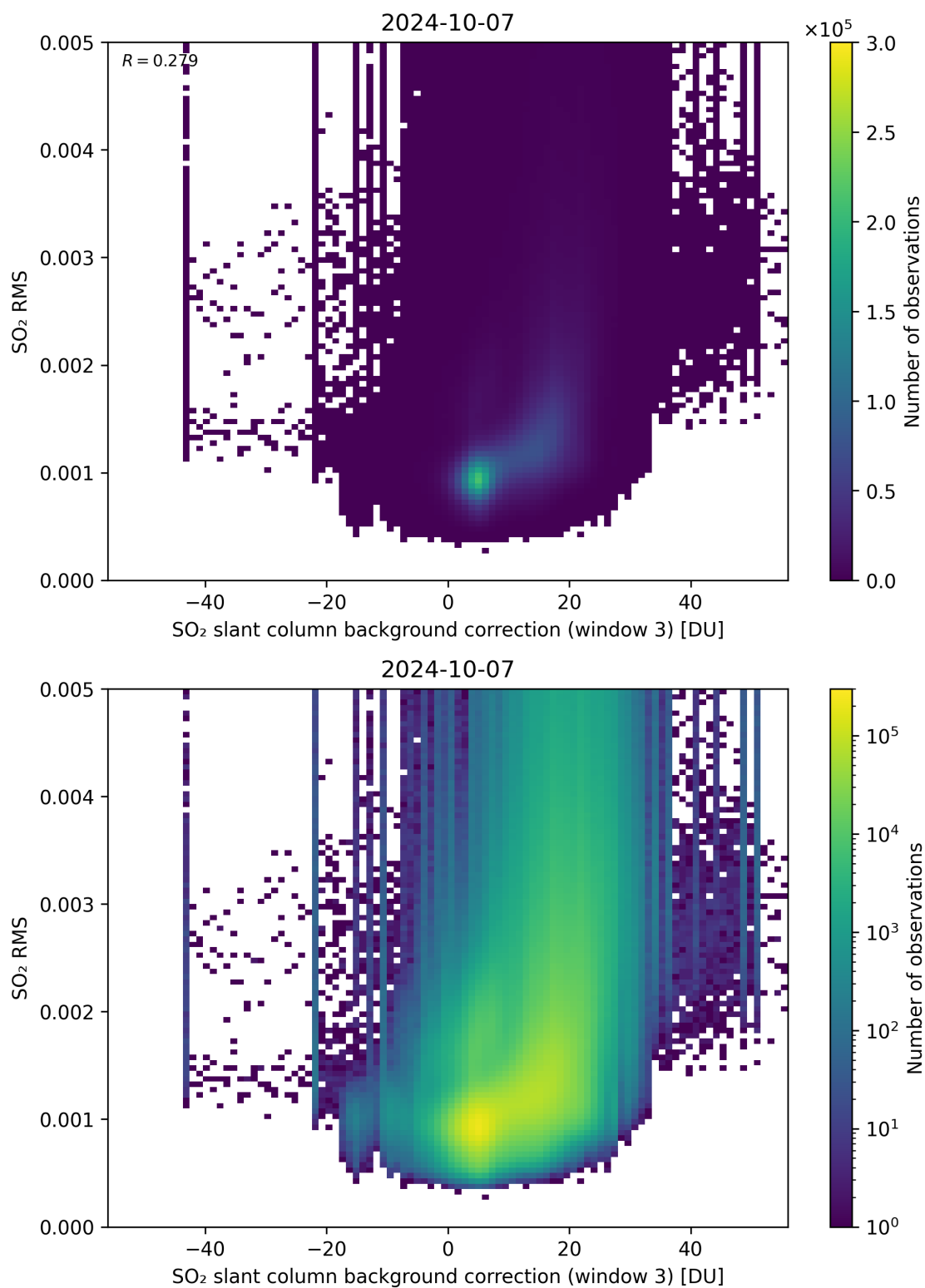
Figure 123: Scatter density plot of “SO 2 slant column background correction (window 3)” against “SO 2 RMS” for 2024-10-06 to 2024-10-08.
