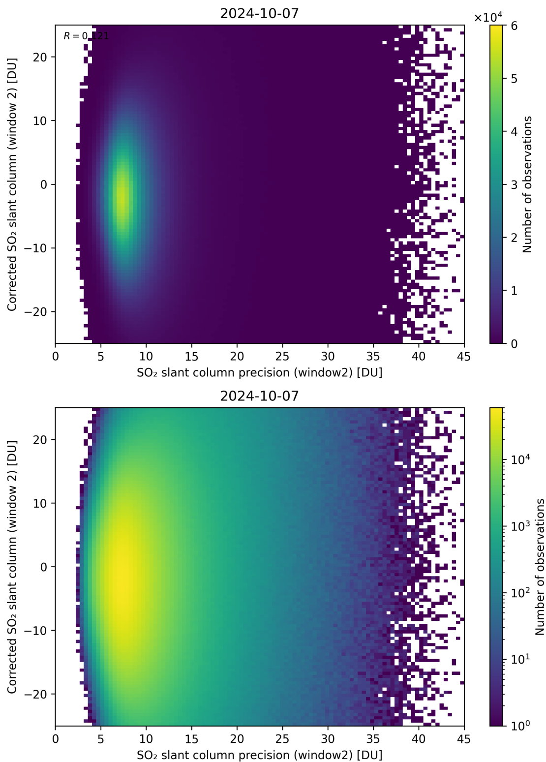
Figure 247: Scatter density plot of “SO 2 slant column precision (window2)” against “Corrected SO 2 slant column (window 2)” for 2024-10-06 to 2024-10-08.
