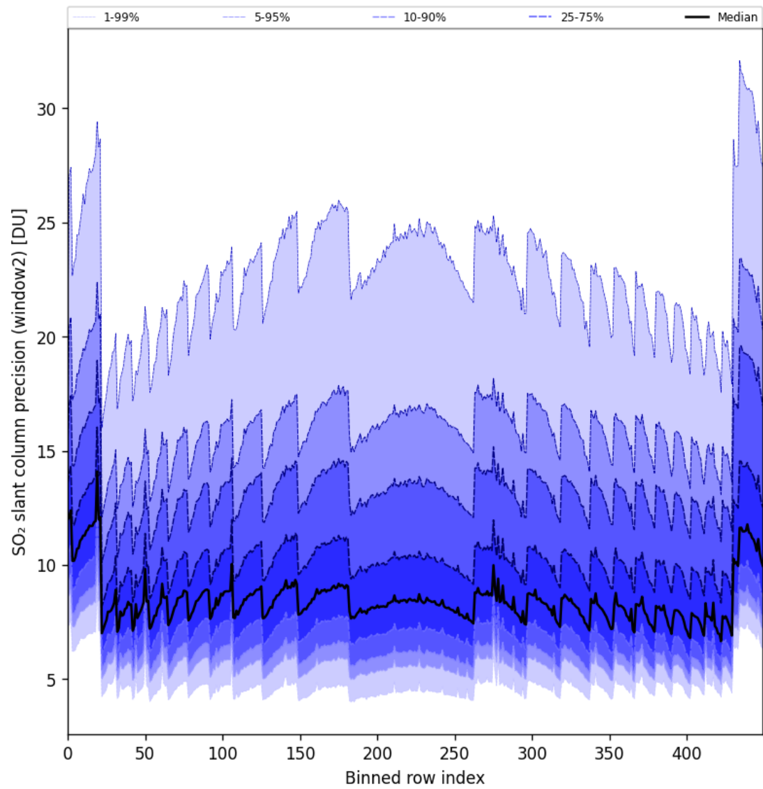
Figure 84: Along track statistics of “SO 2 slant column precision (window2)” for 2024-10-06 to 2024-10-08
