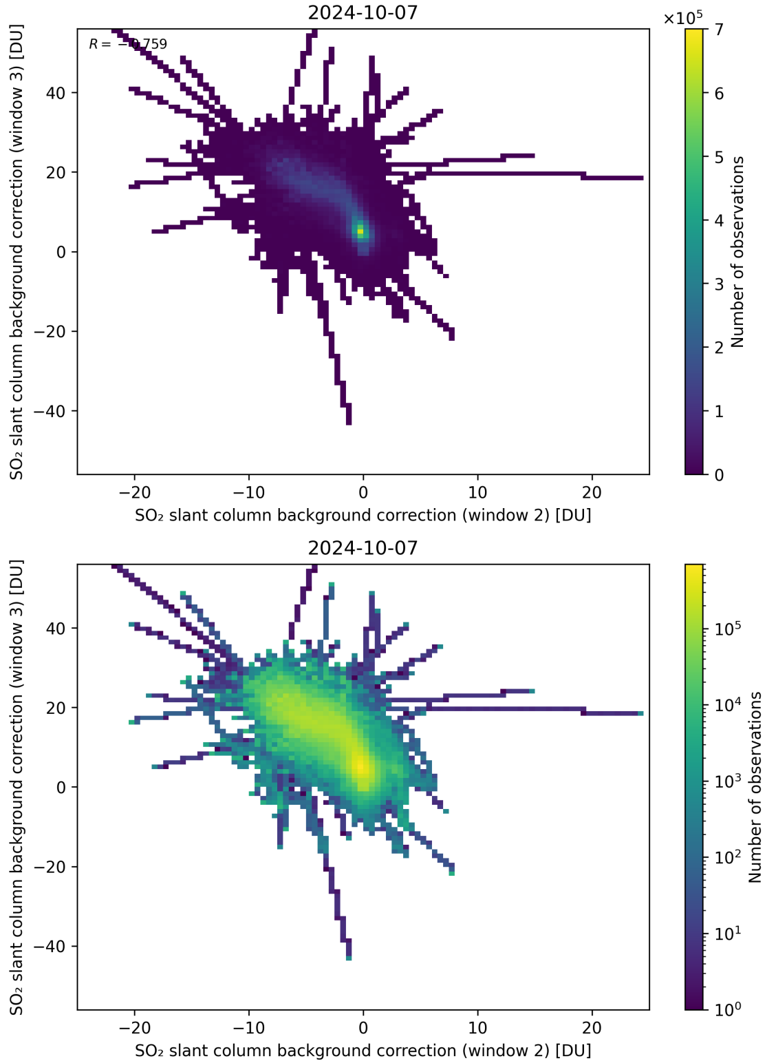
Figure 111: Scatter density plot of “SO 2 slant column background correction (window 2)” against “SO 2 slant column background correction (window 3)” for 2024-10-06 to 2024-10-08.
