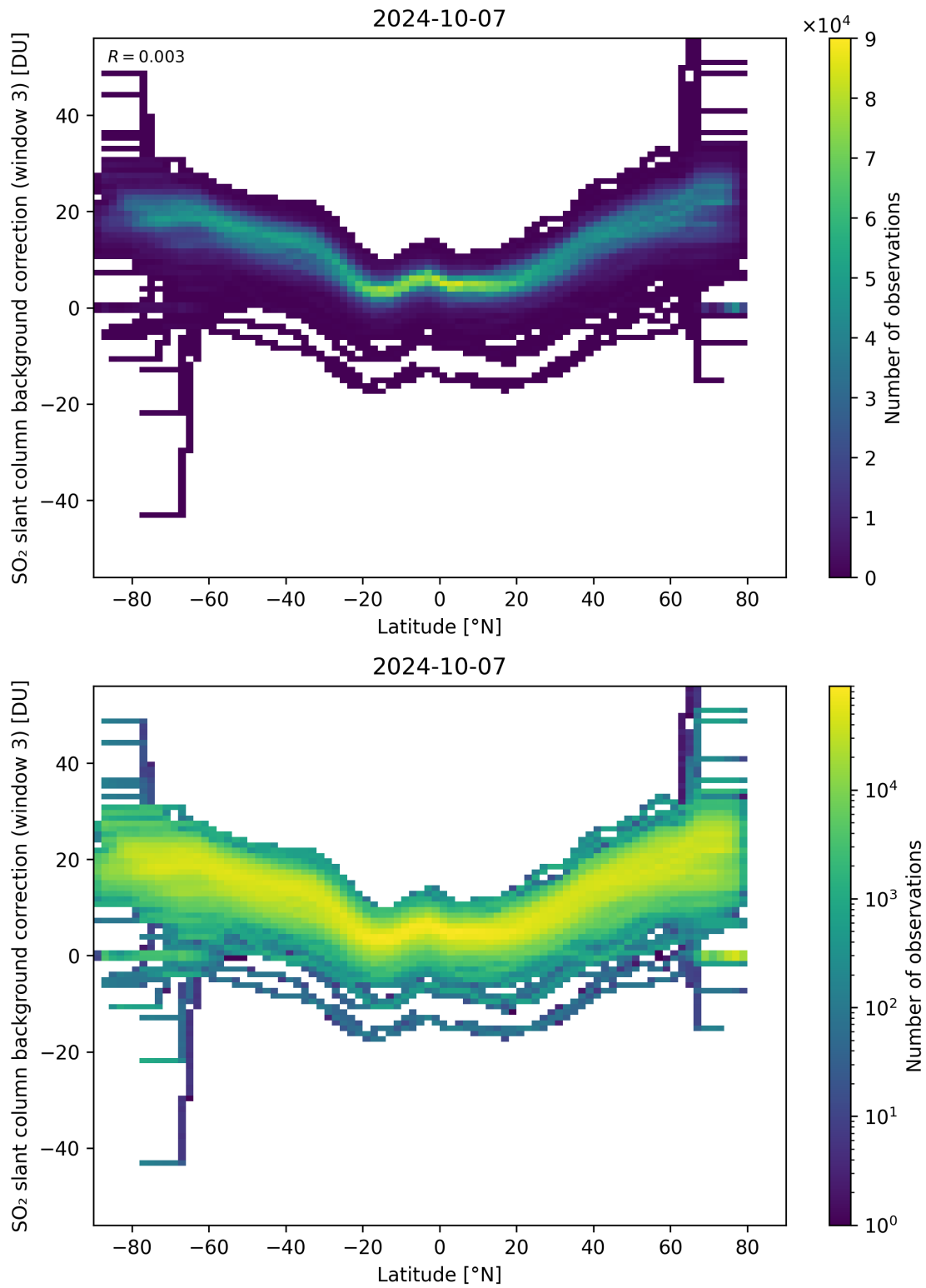
Figure 141: Scatter density plot of “Latitude” against “SO 2 slant column background correction (window 3)” for 2024-10-06 to 2024-10-08.
