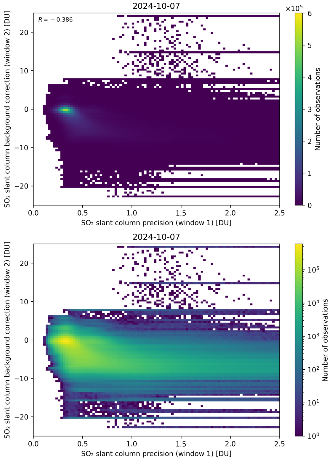
Figure 219: Scatter density plot of “SO 2 slant column precision (window 1)” against “SO 2 slant column background correction (window 2)” for 2024-10-06 to 2024-10-08.
