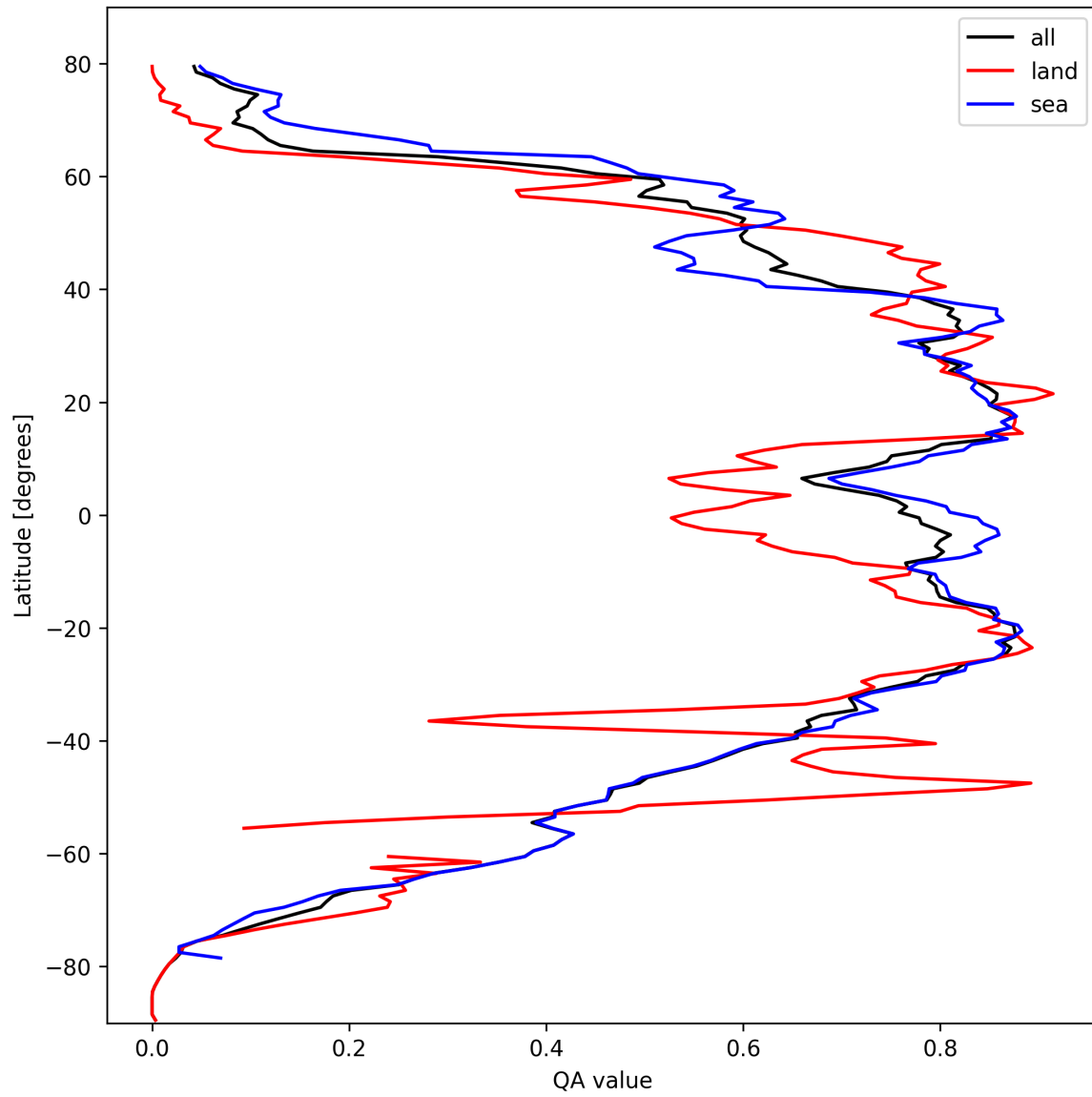
Figure 29: Zonal average of “QA value” for 2024-10-06 to 2024-10-08.
