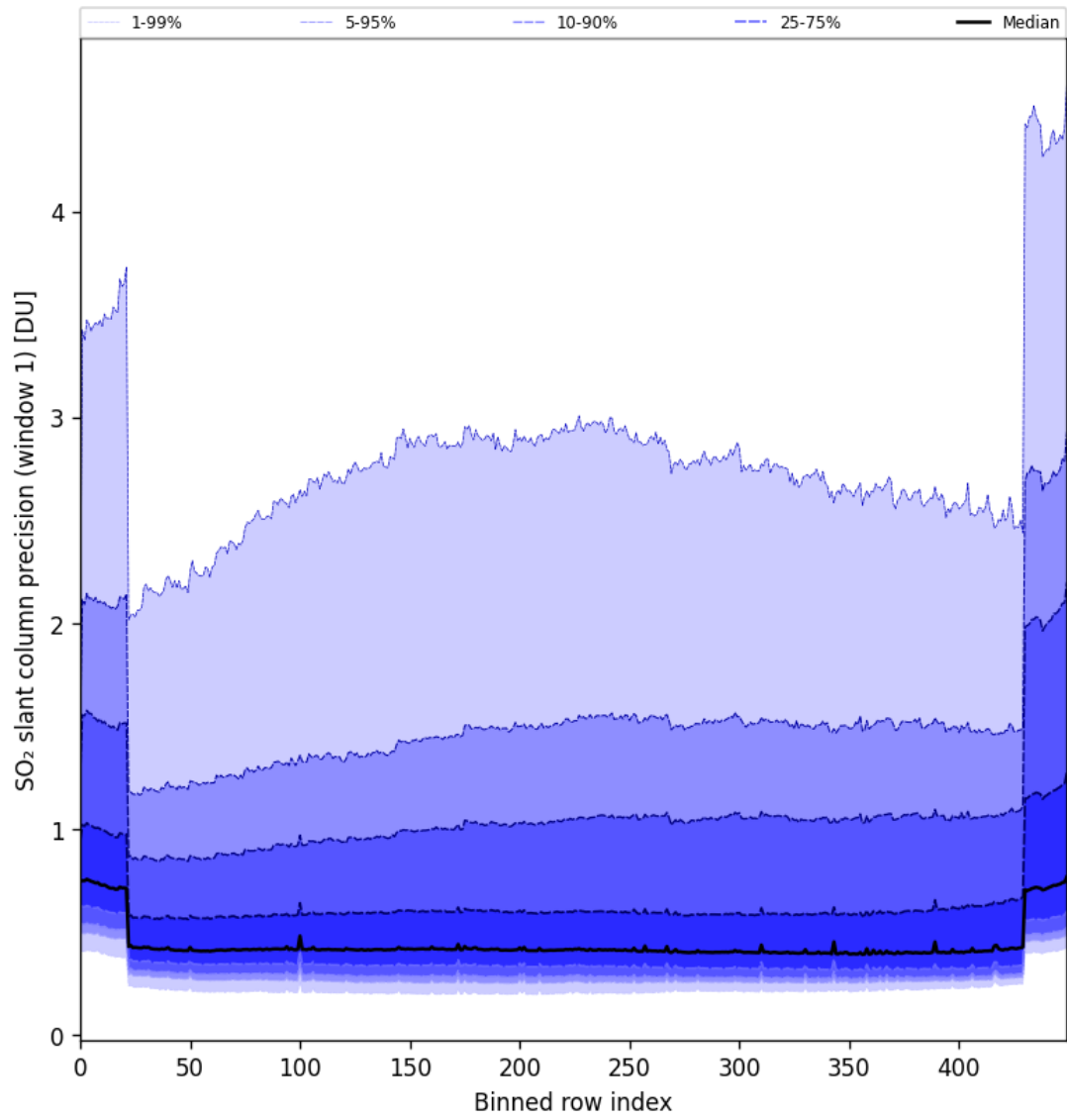
Figure 80: Along track statistics of “SO 2 slant column precision (window 1)” for 2024-10-06 to 2024-10-08
