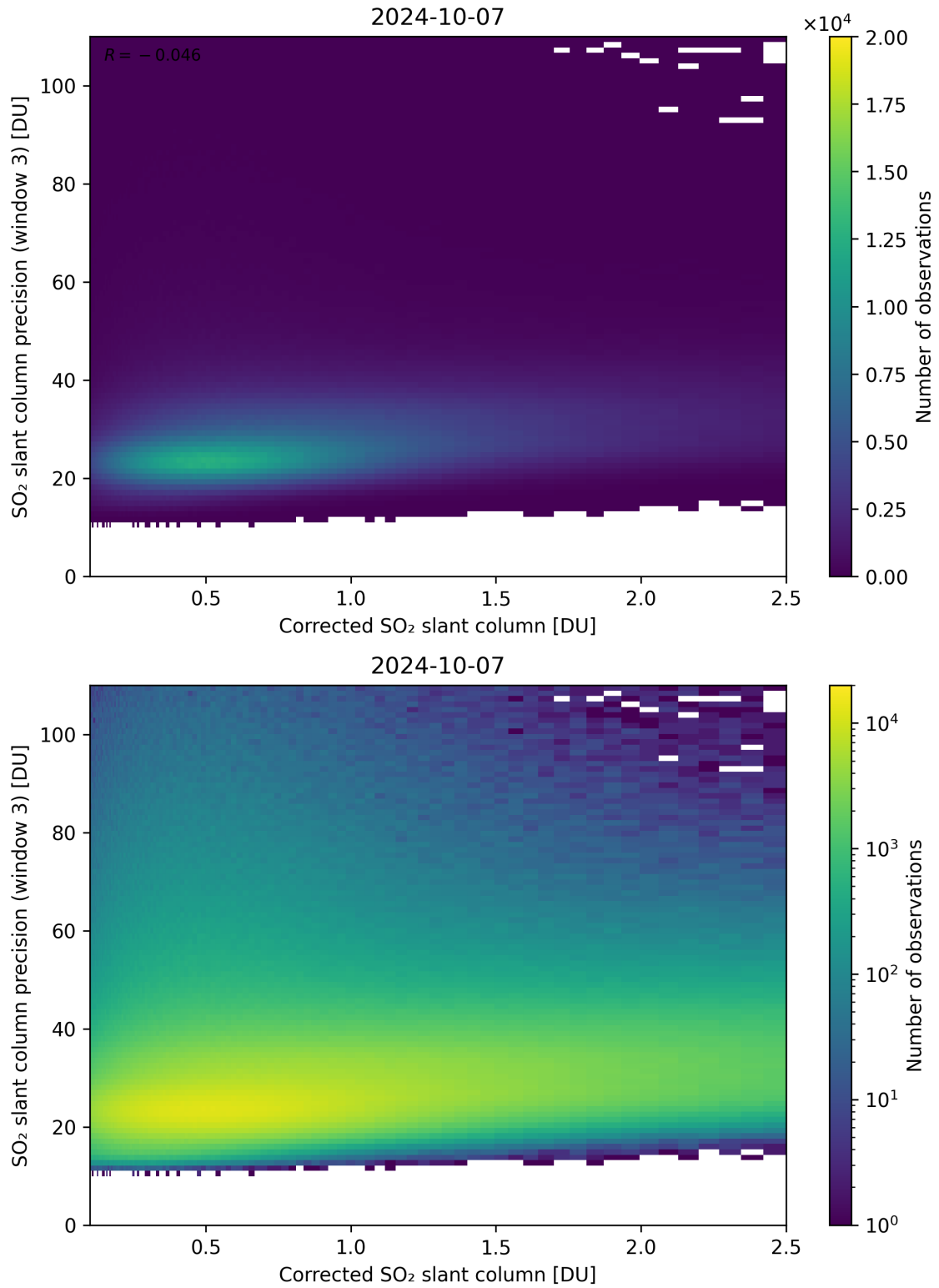
Figure 191: Scatter density plot of “Corrected SO 2 slant column” against “SO 2 slant column precision (window 3)” for 2024-10-06 to 2024-10-08.
