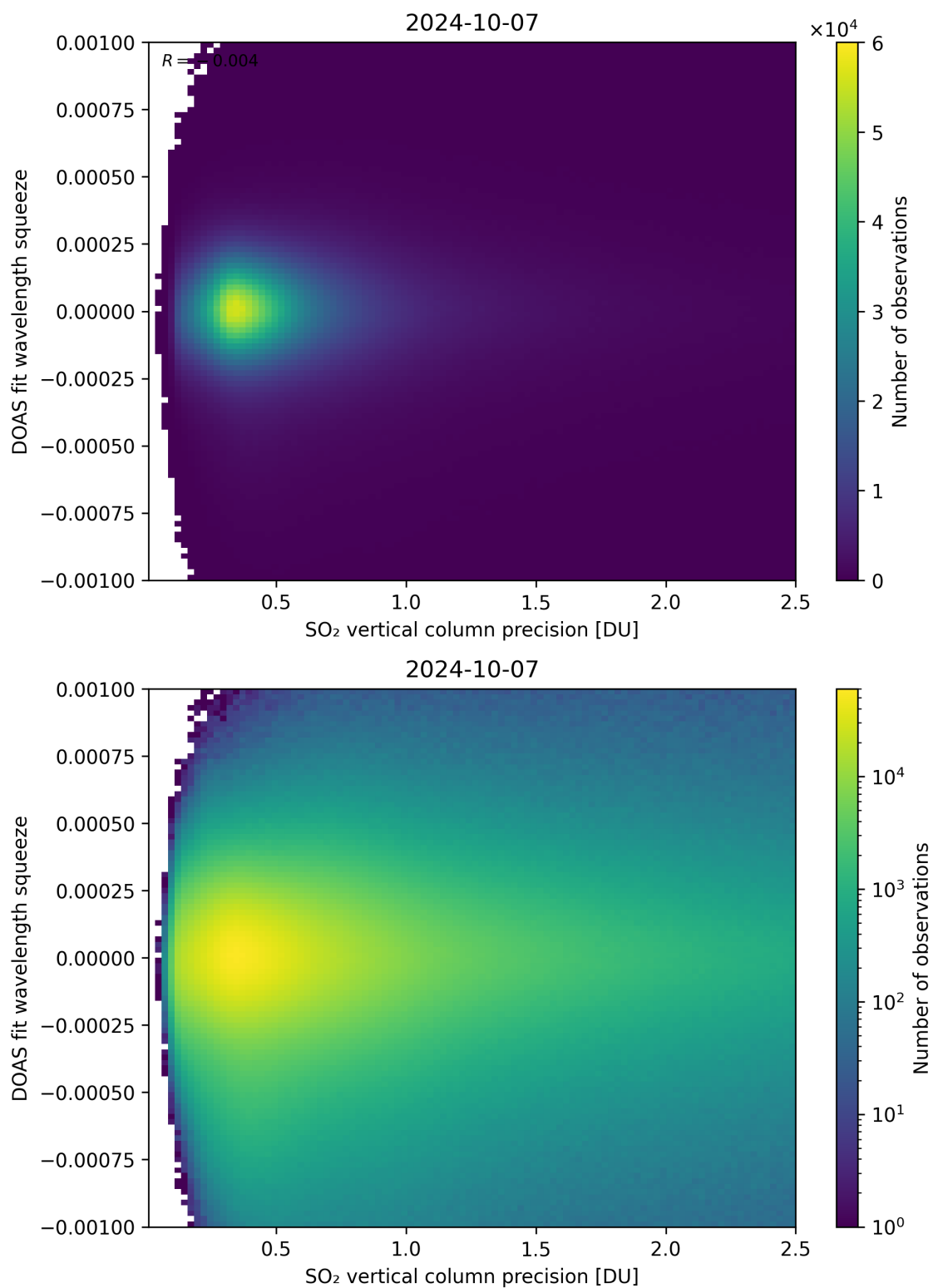
Figure 283: Scatter density plot of “SO 2 vertical column precision” against “DOAS fit wavelength squeeze” for 2024-10-06 to 2024-10-08.
