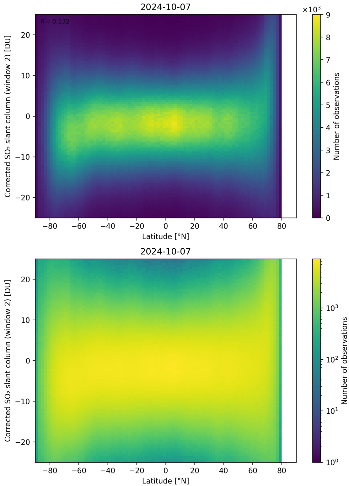
Figure 147: Scatter density plot of “Latitude” against “Corrected SO 2 slant column (window 2)” for 2024-10-06 to 2024-10-08.
