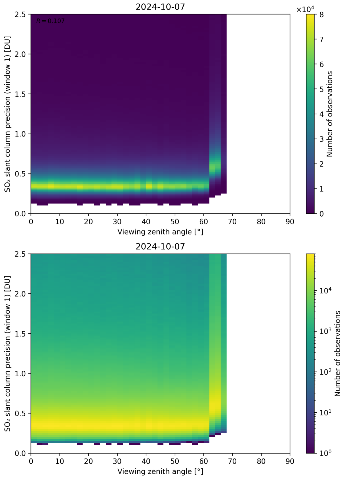
Figure 321: Scatter density plot of “Viewing zenith angle” against “SO 2 slant column precision (window 1)” for 2024-10-06 to 2024-10-08.
