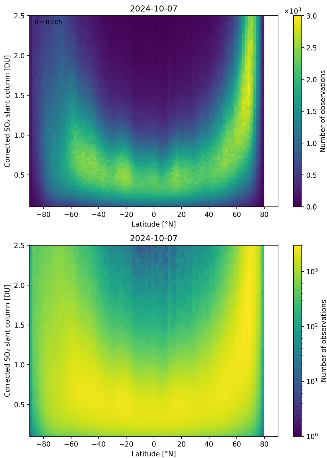
Figure 146: Scatter density plot of “Latitude” against “Corrected SO 2 slant column” for 2024-10-06 to 2024-10-08.
