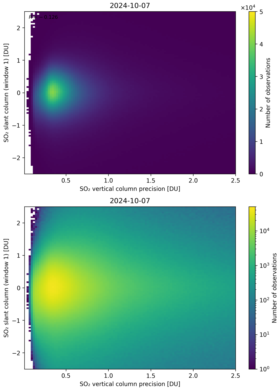
Figure 289: Scatter density plot of “SO 2 vertical column precision” against “SO 2 slant column (window 1)” for 2024-10-06 to 2024-10-08.
