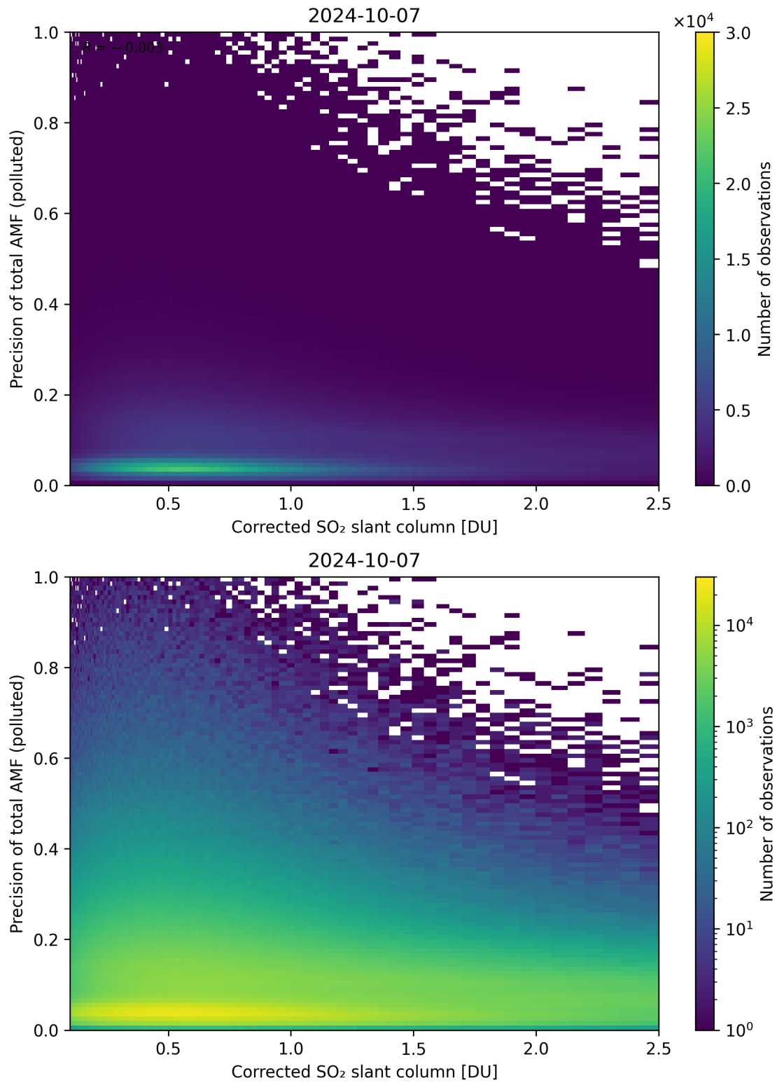
Figure 193: Scatter density plot of “Corrected SO 2 slant column” against “Precision of total AMF (polluted)” for 2024-10-06 to 2024-10-08.
