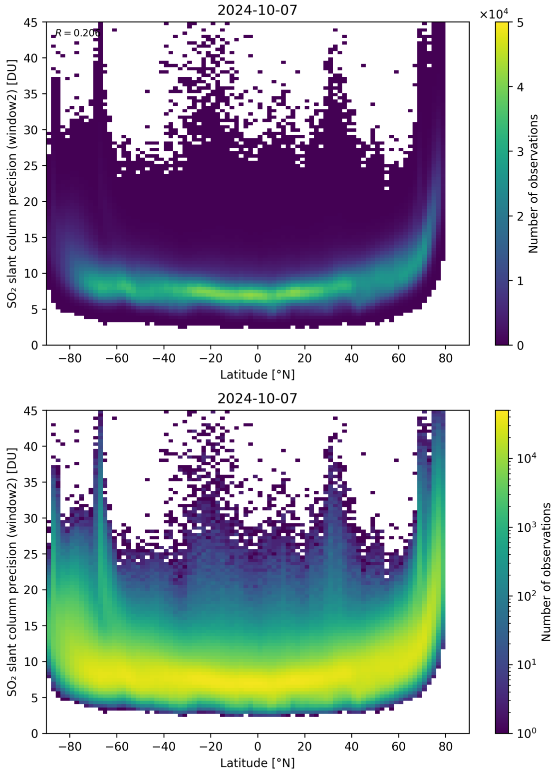
Figure 151: Scatter density plot of “Latitude” against “SO 2 slant column precision (window2)” for 2024-10-06 to 2024-10-08.
