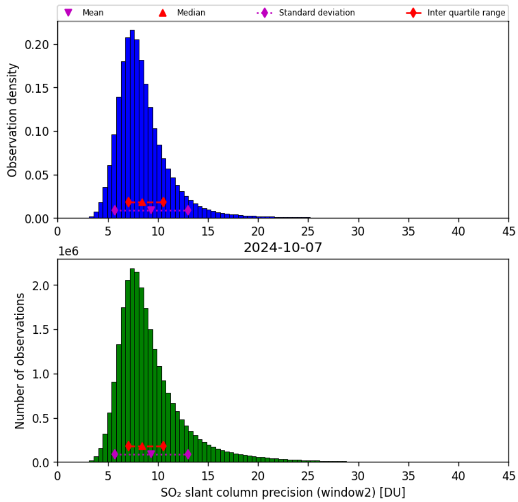
Figure 61: Histogram of “SO 2 slant column precision (window2)” for 2024-10-06 to 2024-10-08
