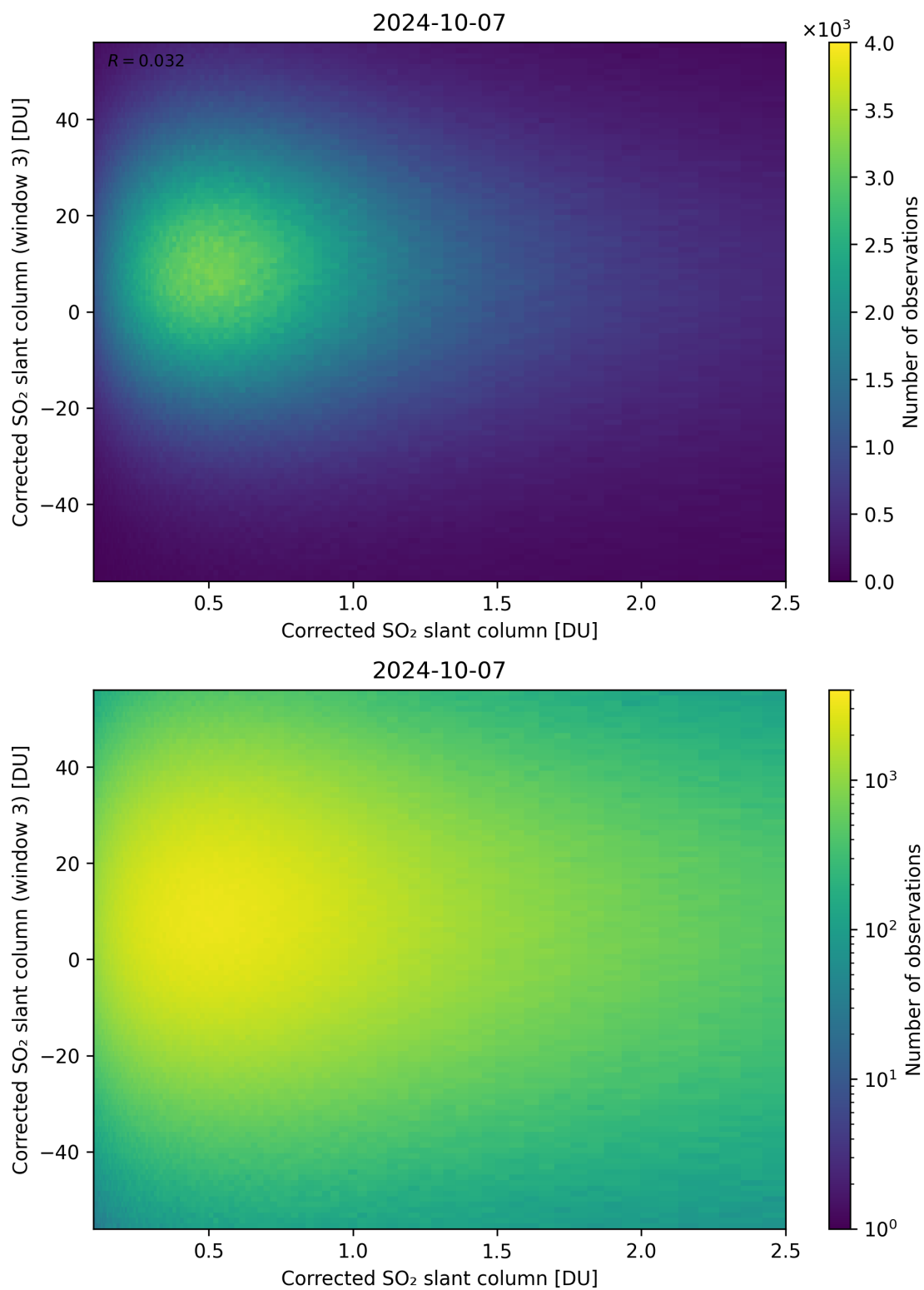
Figure 186: Scatter density plot of “Corrected SO 2 slant column” against “Corrected SO 2 slant column (window 3)” for 2024-10-06 to 2024-10-08.
