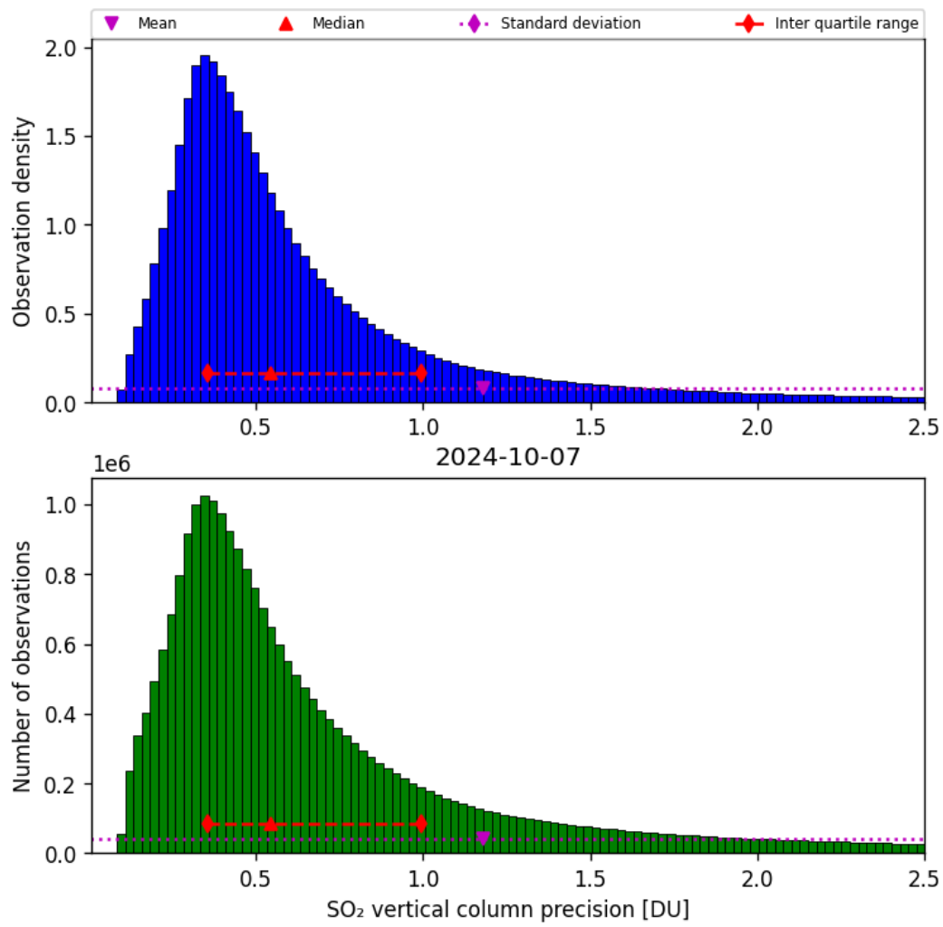
Figure 54: Histogram of “SO 2 vertical column precision” for 2024-10-06 to 2024-10-08
