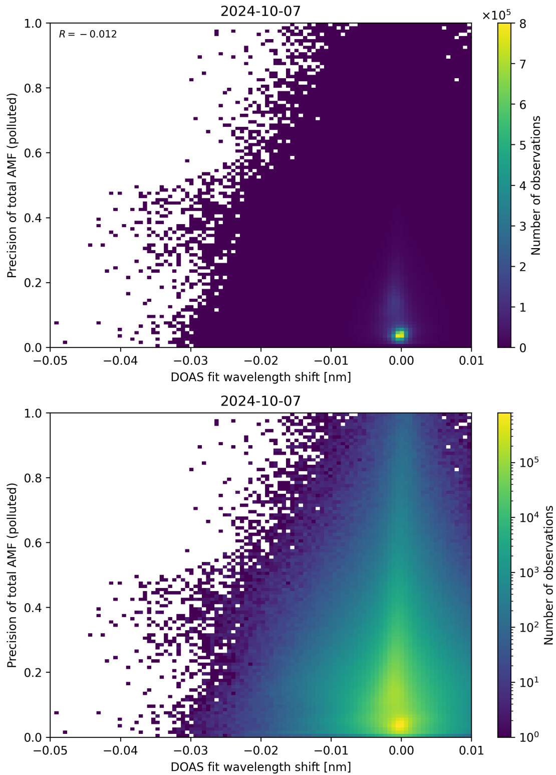
Figure 131: Scatter density plot of “DOAS fit wavelength shift” against “Precision of total AMF (polluted)” for 2024-10-06 to 2024-10-08.
