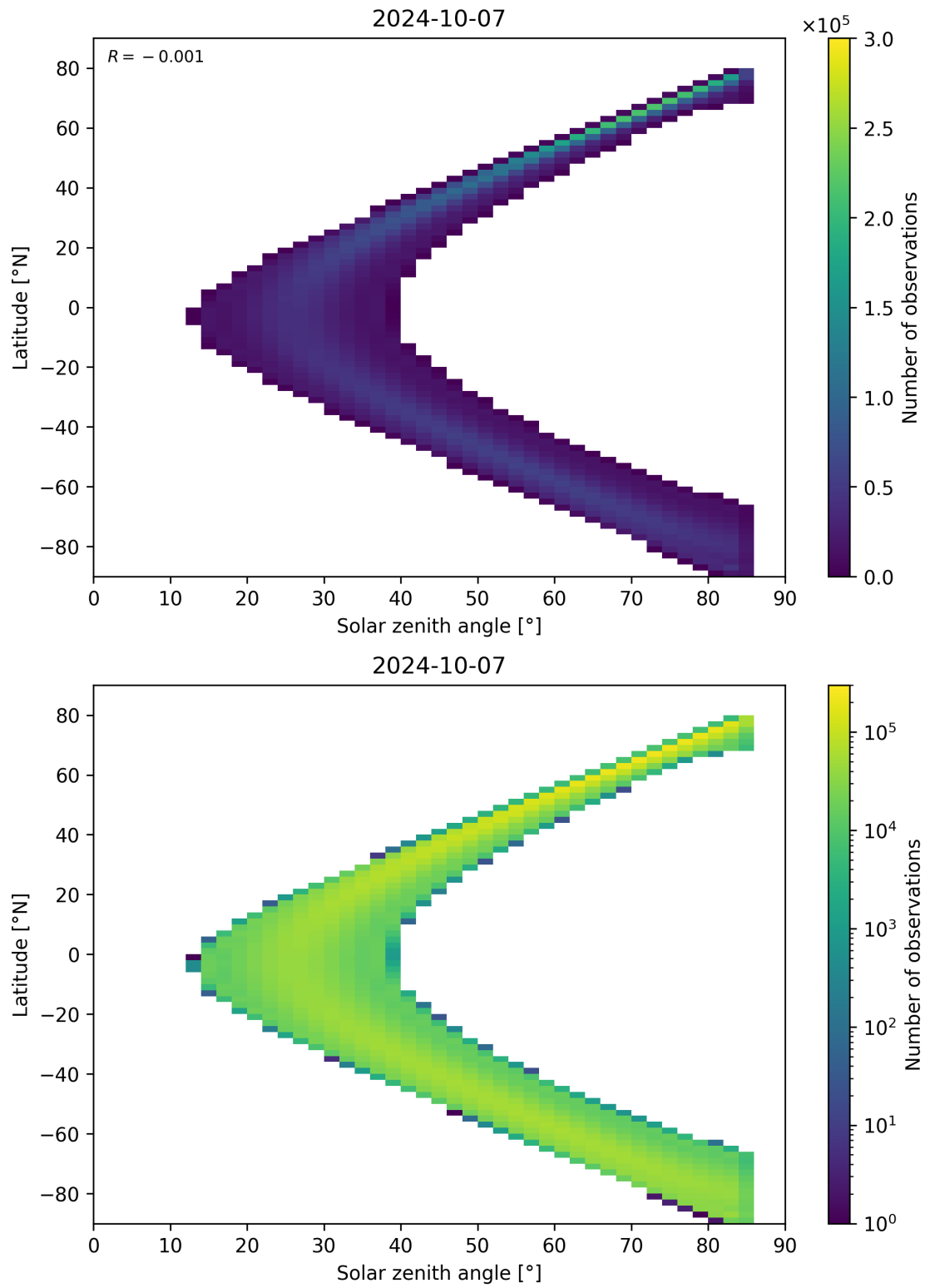
Figure 164: Scatter density plot of “Solar zenith angle” against “Latitude” for 2024-10-06 to 2024-10-08.
