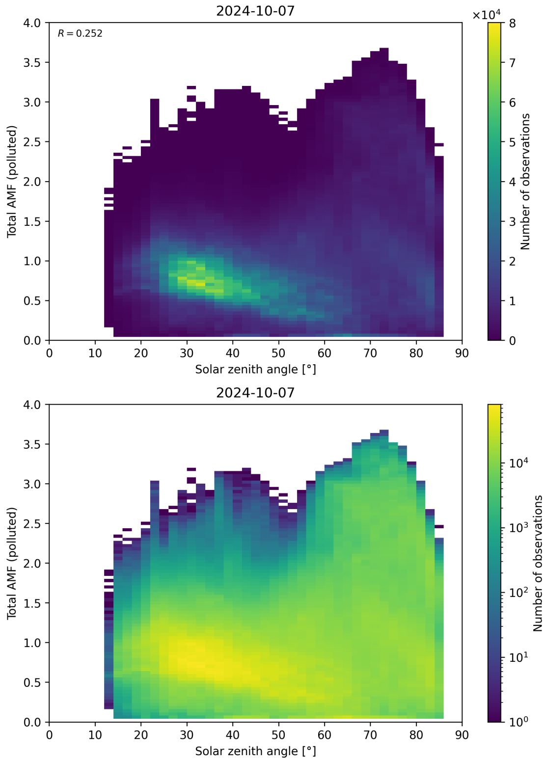
Figure 174: Scatter density plot of “Solar zenith angle” against “Total AMF (polluted)” for 2024-10-06 to 2024-10-08.
