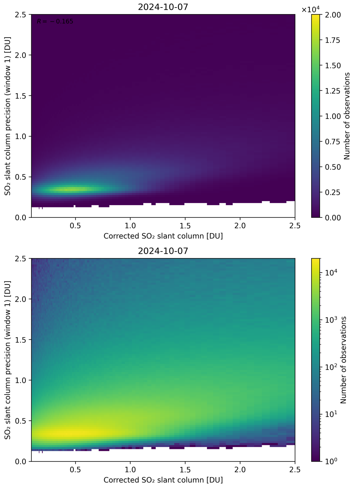
Figure 188: Scatter density plot of “Corrected SO 2 slant column” against “SO 2 slant column precision (window 1)” for 2024-10-06 to 2024-10-08.
