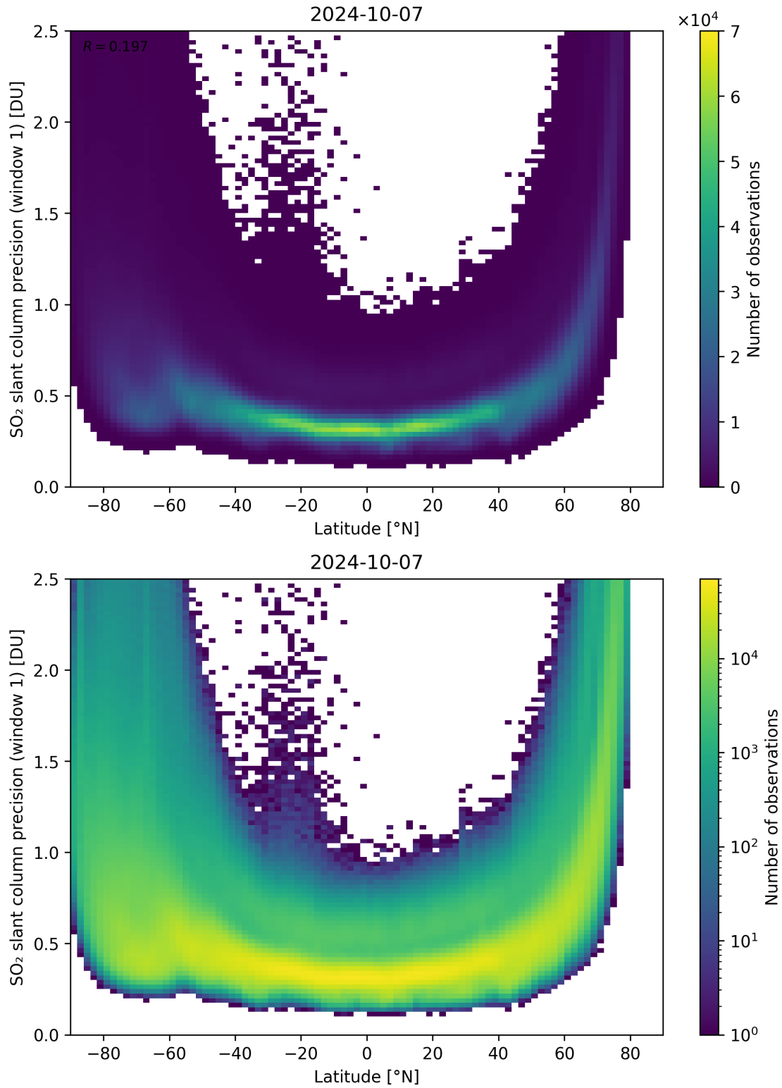
Figure 150: Scatter density plot of “Latitude” against “SO 2 slant column precision (window 1)” for 2024-10-06 to 2024-10-08.
