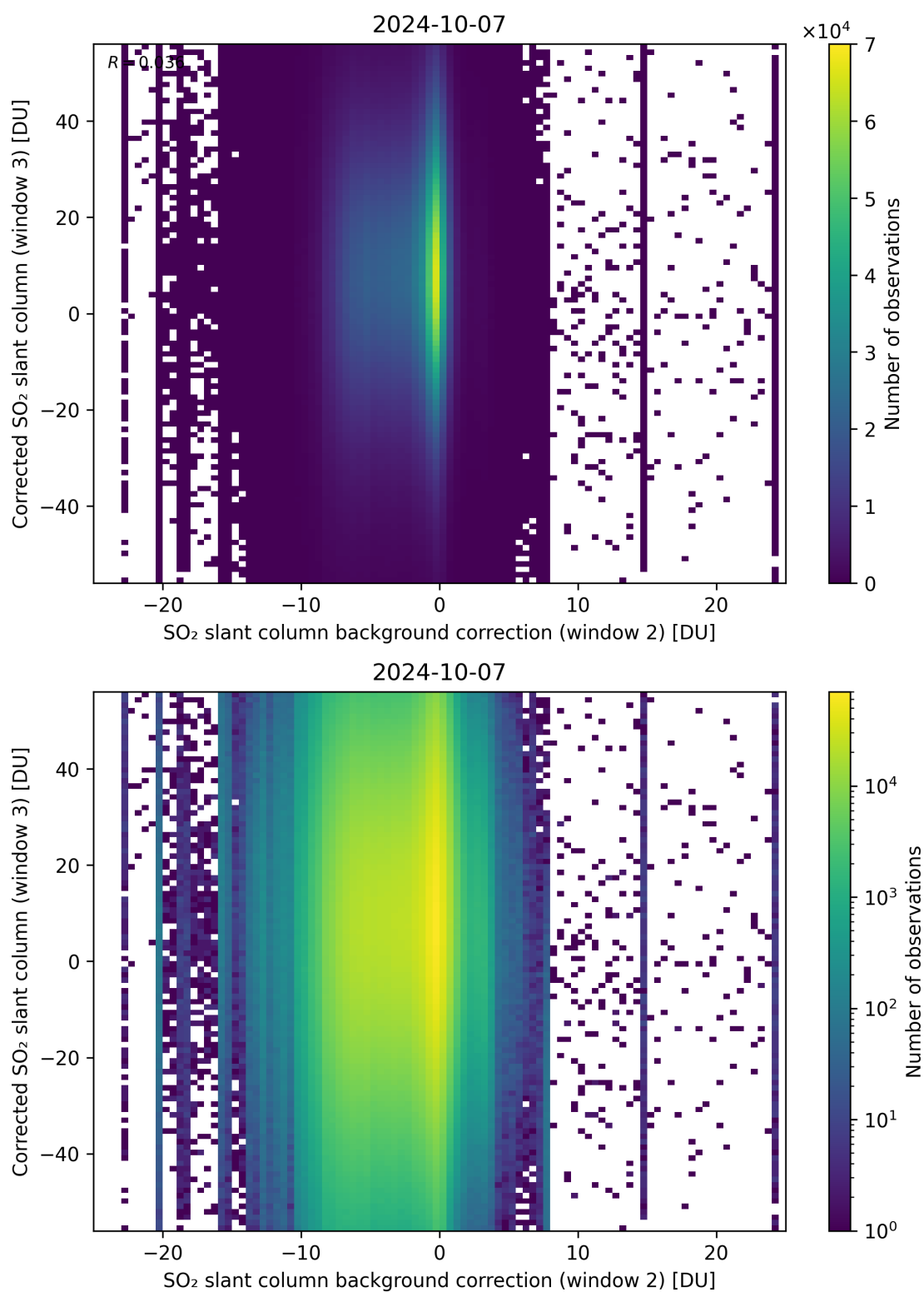
Figure 116: Scatter density plot of “SO 2 slant column background correction (window 2)” against “Corrected SO 2 slant column (window 3)” for 2024-10-06 to 2024-10-08.
