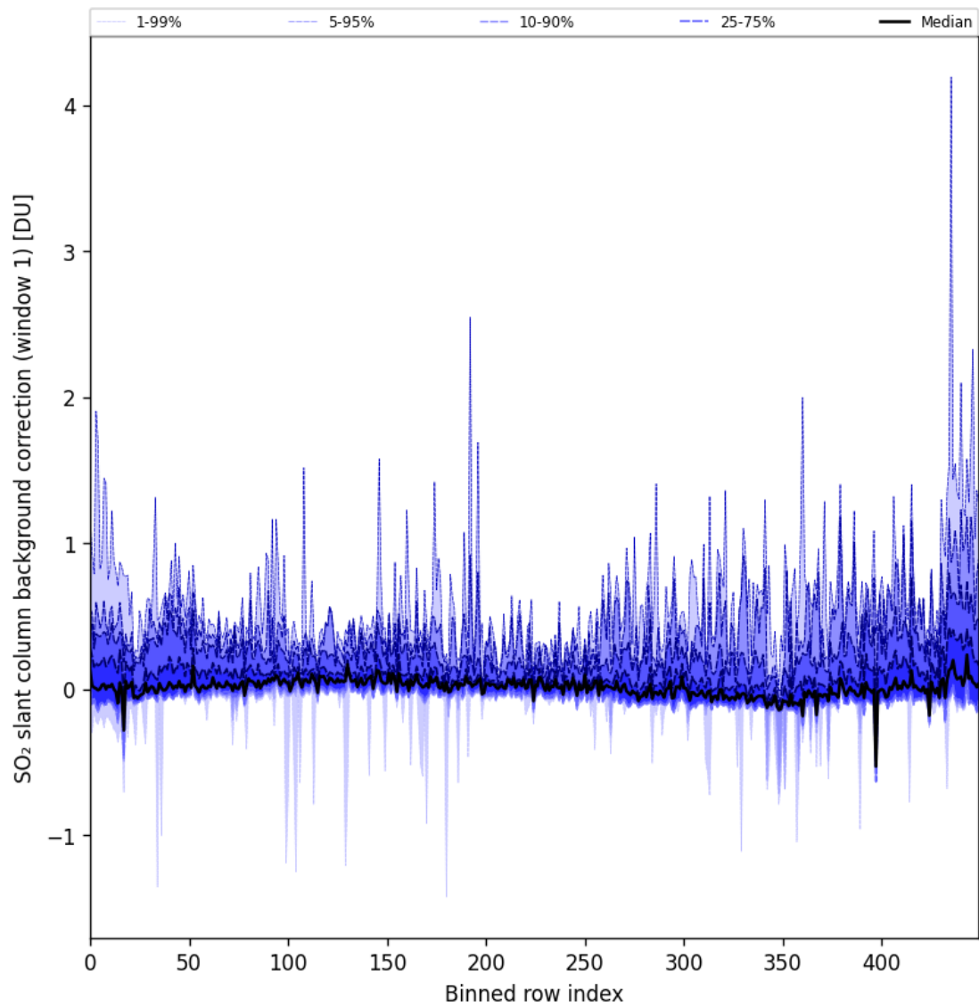
Figure 82: Along track statistics of “SO 2 slant column background correction (window 1)” for 2024-10-06 to 2024-10-08
