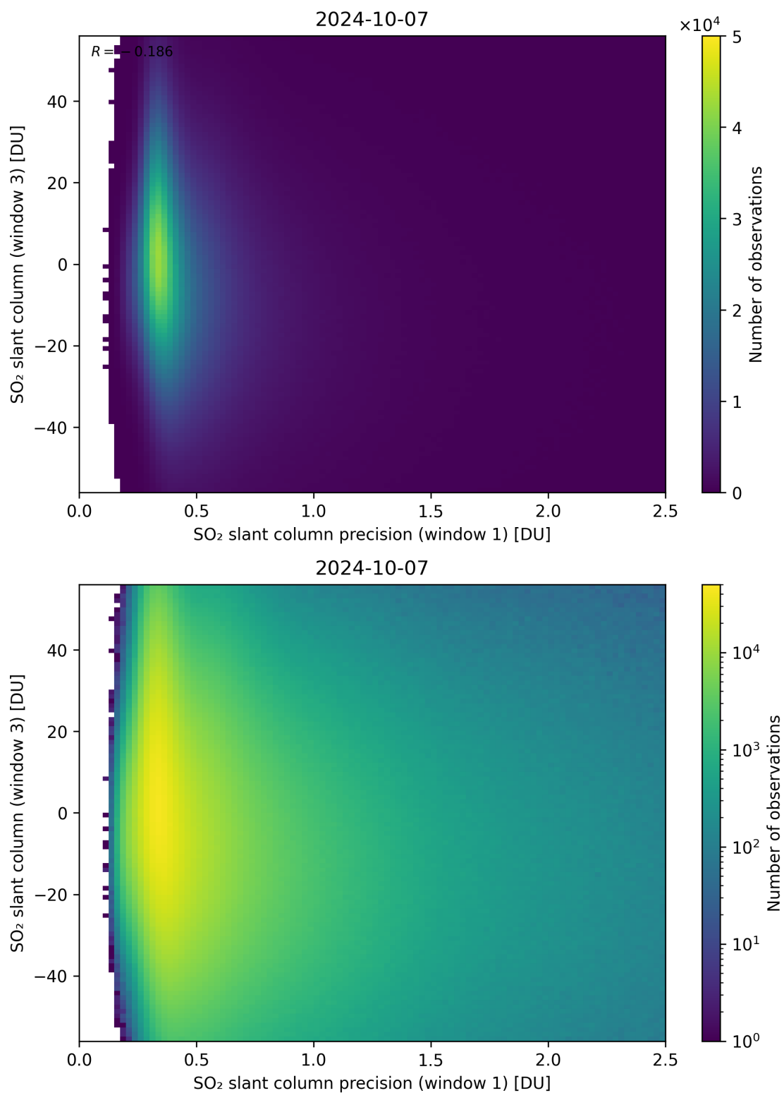
Figure 228: Scatter density plot of “SO 2 slant column precision (window 1)” against “SO 2 slant column (window 3)” for 2024-10-06 to 2024-10-08.
