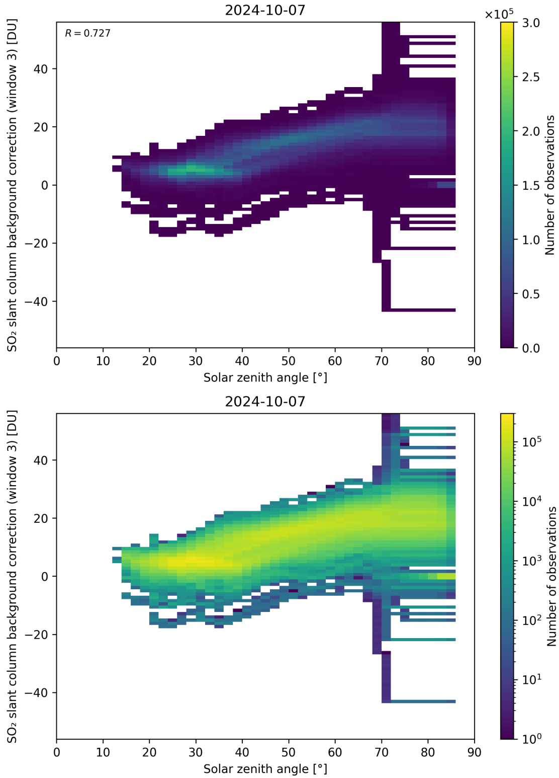
Figure 160: Scatter density plot of “Solar zenith angle” against “SO 2 slant column background correction (window 3)” for 2024-10-06 to 2024-10-08.
