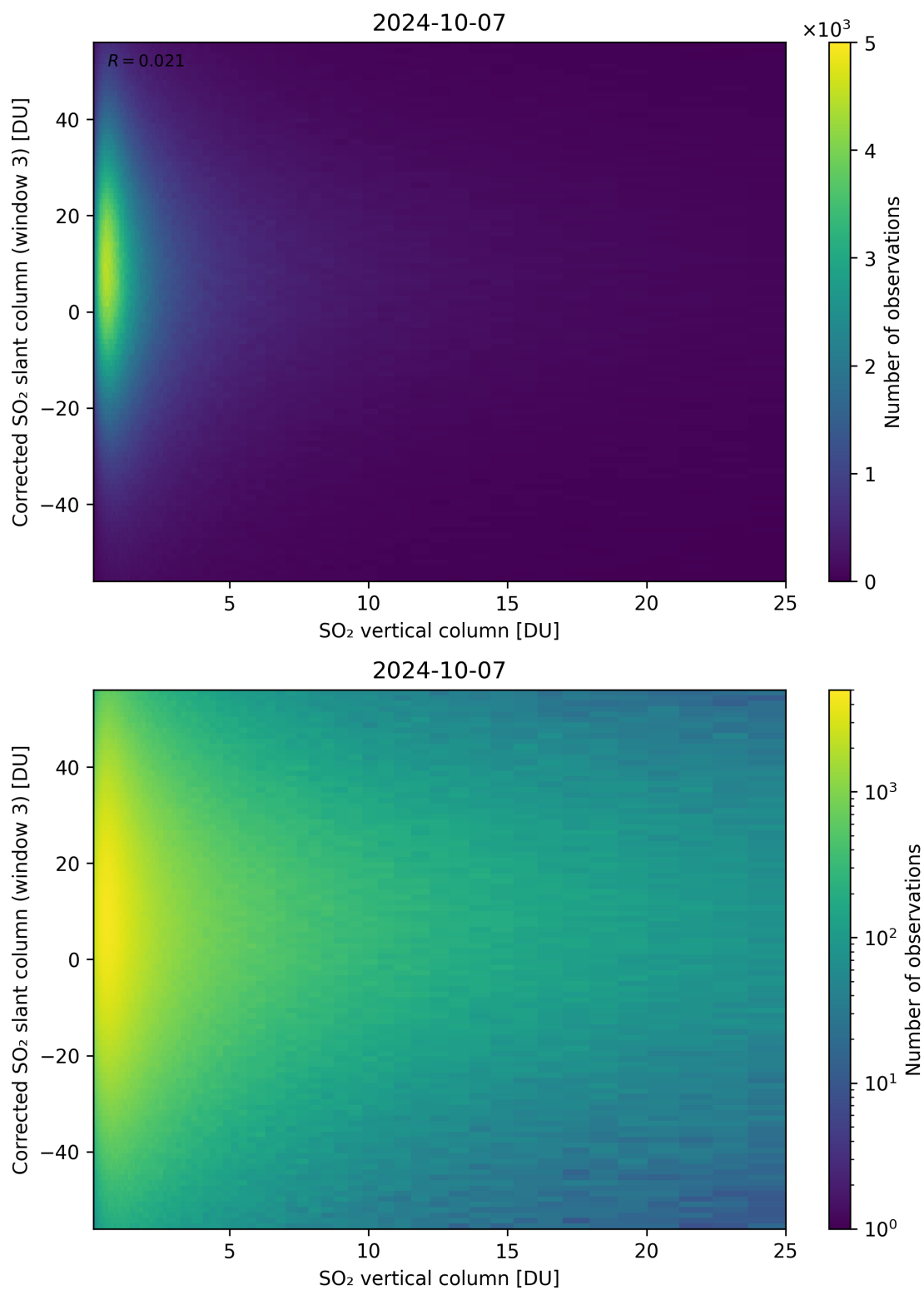
Figure 299: Scatter density plot of “SO 2 vertical column” against “Corrected SO 2 slant column (window 3)” for 2024-10-06 to 2024-10-08.
