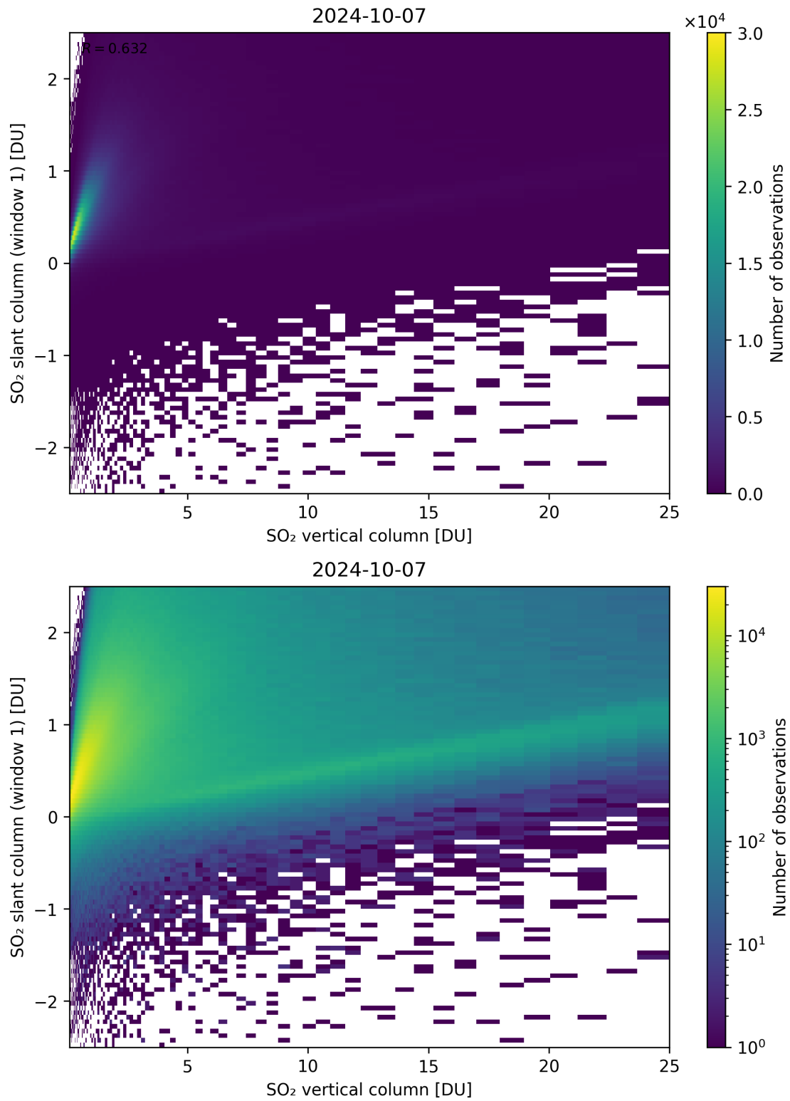
Figure 300: Scatter density plot of “SO 2 vertical column” against “SO 2 slant column (window 1)” for 2024-10-06 to 2024-10-08.
