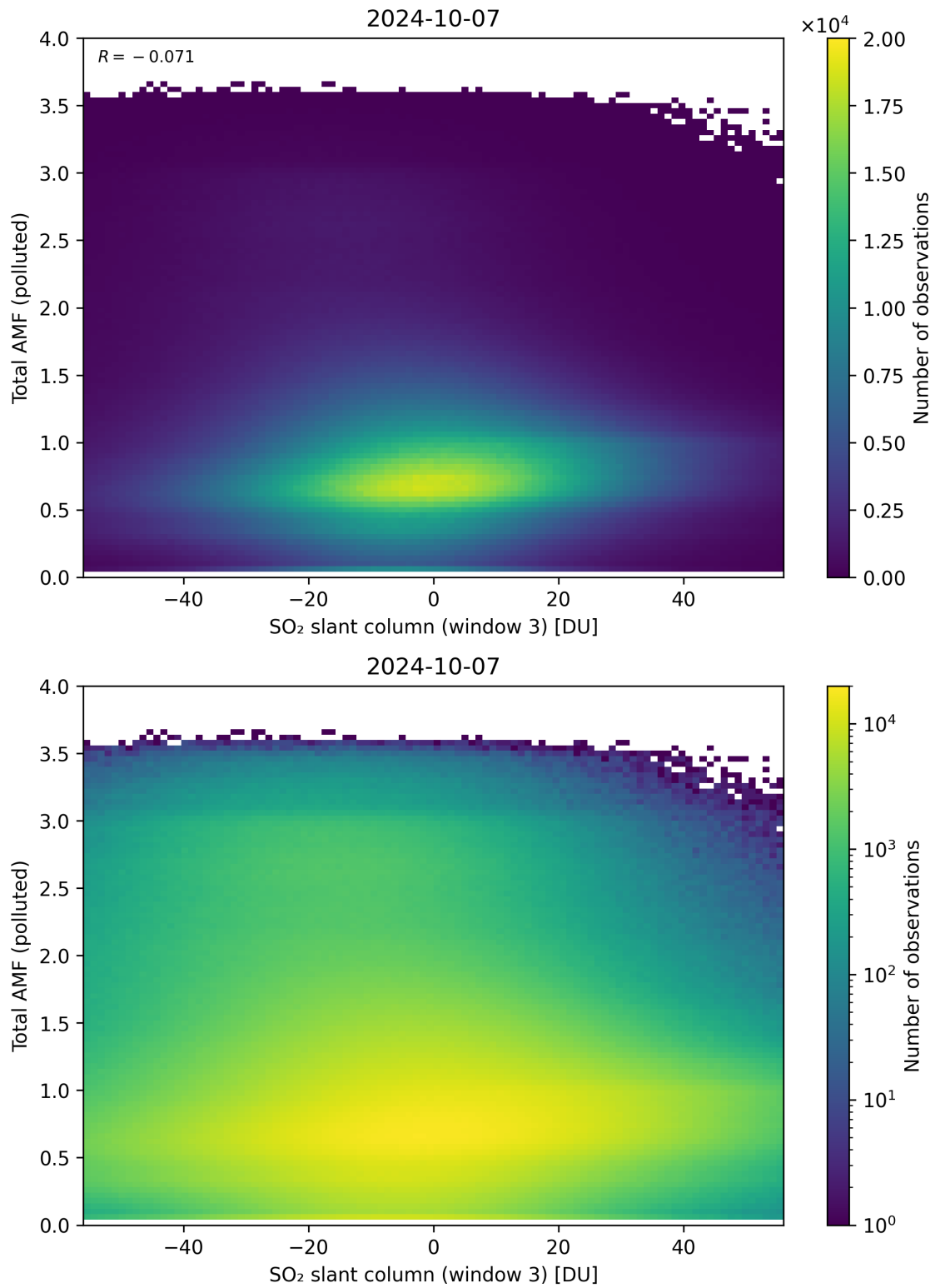
Figure 268: Scatter density plot of “SO 2 slant column (window 3)” against “Total AMF (polluted)” for 2024-10-06 to 2024-10-08.
