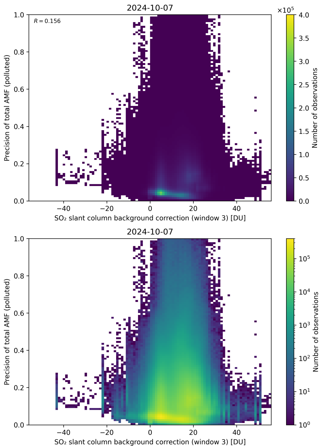
Figure 126: Scatter density plot of “SO 2 slant column background correction (window 3)” against “Precision of total AMF (polluted)” for 2024-10-06 to 2024-10-08.
