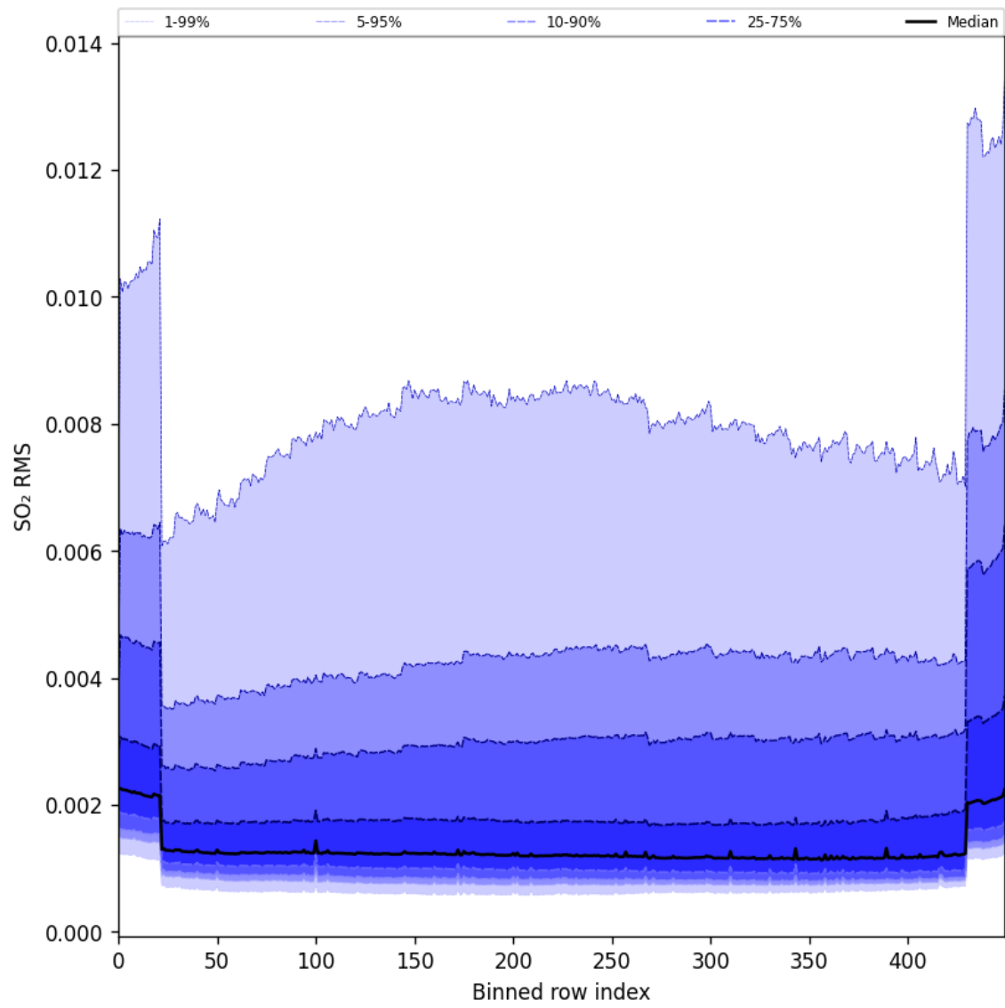
Figure 93: Along track statistics of “SO 2 RMS” for 2024-10-06 to 2024-10-08
