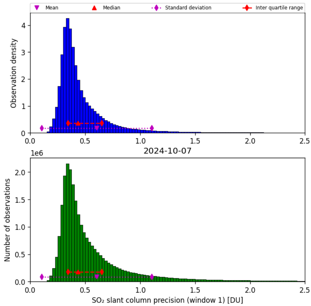
Figure 57: Histogram of “SO 2 slant column precision (window 1)” for 2024-10-06 to 2024-10-08
