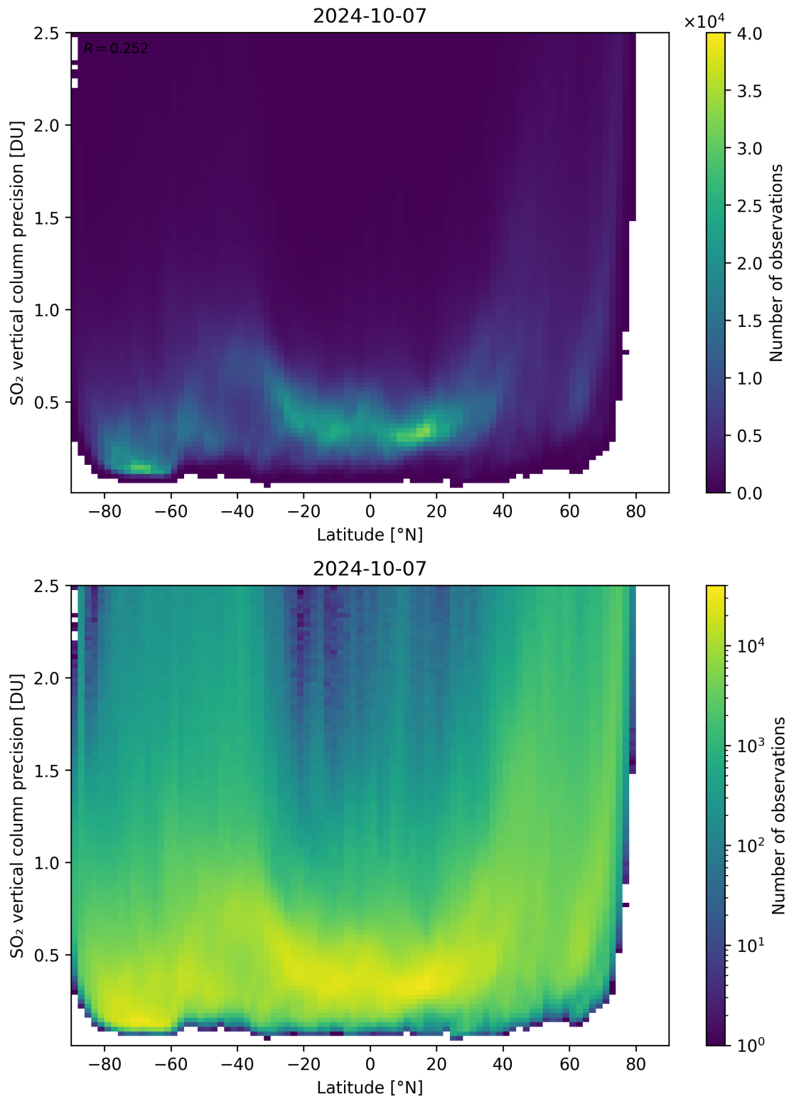
Figure 157: Scatter density plot of “Latitude” against “SO 2 vertical column precision” for 2024-10-06 to 2024-10-08.
