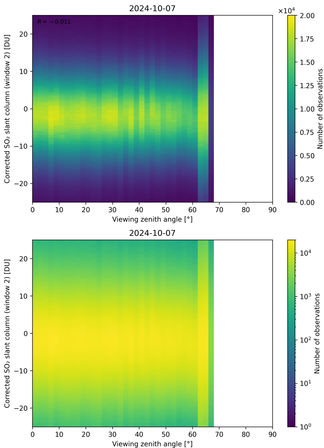
Figure 318: Scatter density plot of “Viewing zenith angle” against “Corrected SO 2 slant column (window 2)” for 2024-10-06 to 2024-10-08.
