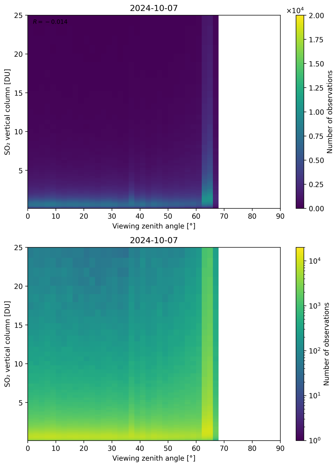
Figure 327: Scatter density plot of “Viewing zenith angle” against “SO 2 vertical column” for 2024-10-06 to 2024-10-08.
