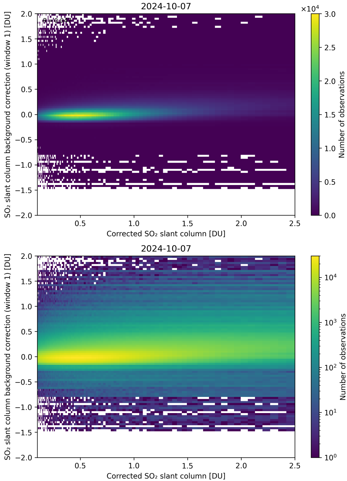
Figure 178: Scatter density plot of “Corrected SO 2 slant column” against “SO 2 slant column background correction (window 1)” for 2024-10-06 to 2024-10-08.
