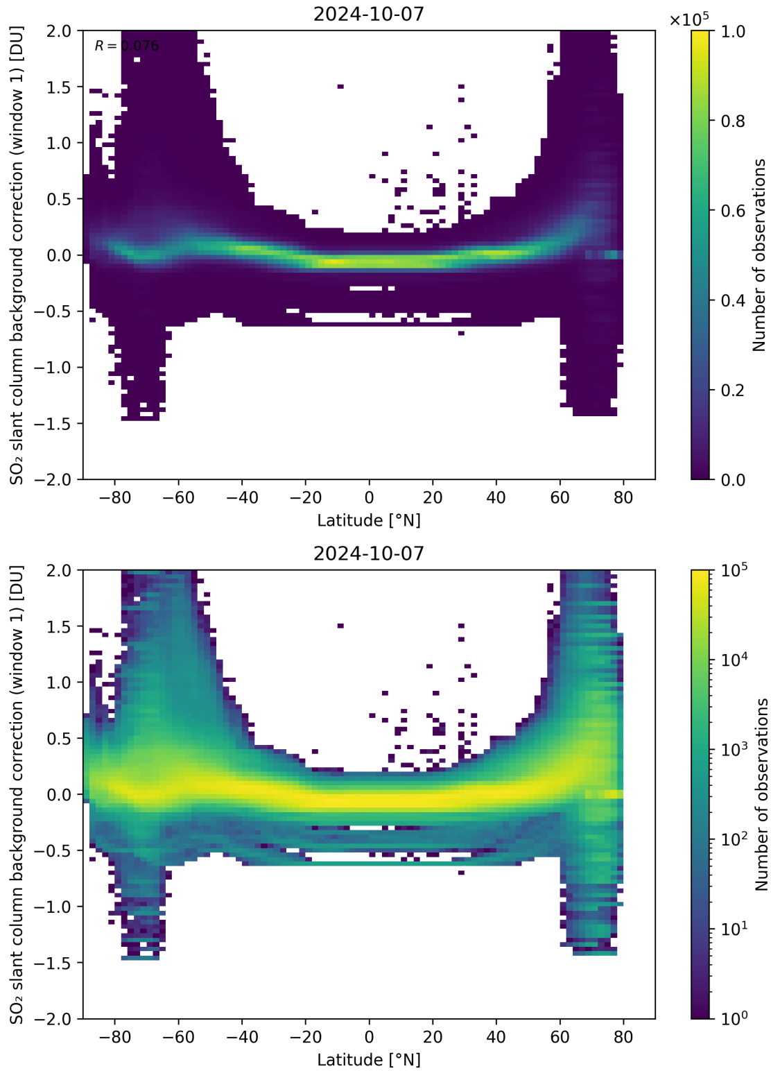
Figure 139: Scatter density plot of “Latitude” against “SO 2 slant column background correction (window 1)” for 2024-10-06 to 2024-10-08.
