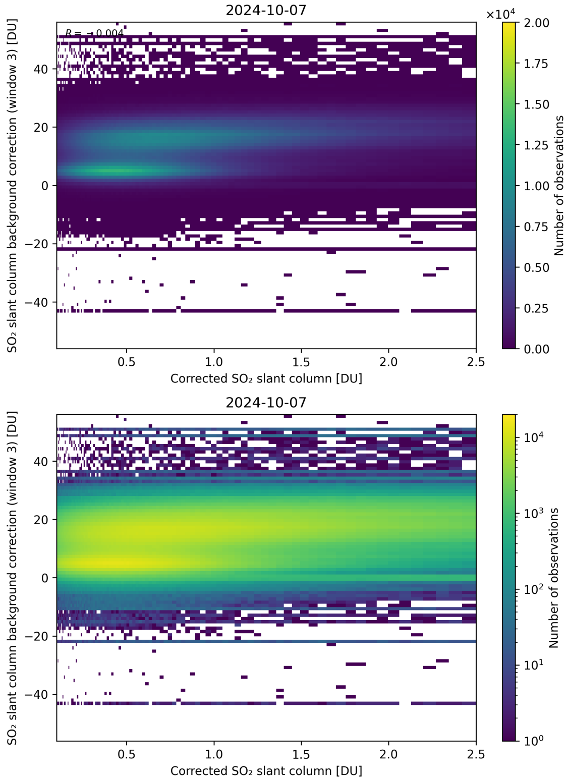
Figure 180: Scatter density plot of “Corrected SO 2 slant column” against “SO 2 slant column background correction (window 3)” for 2024-10-06 to 2024-10-08.
