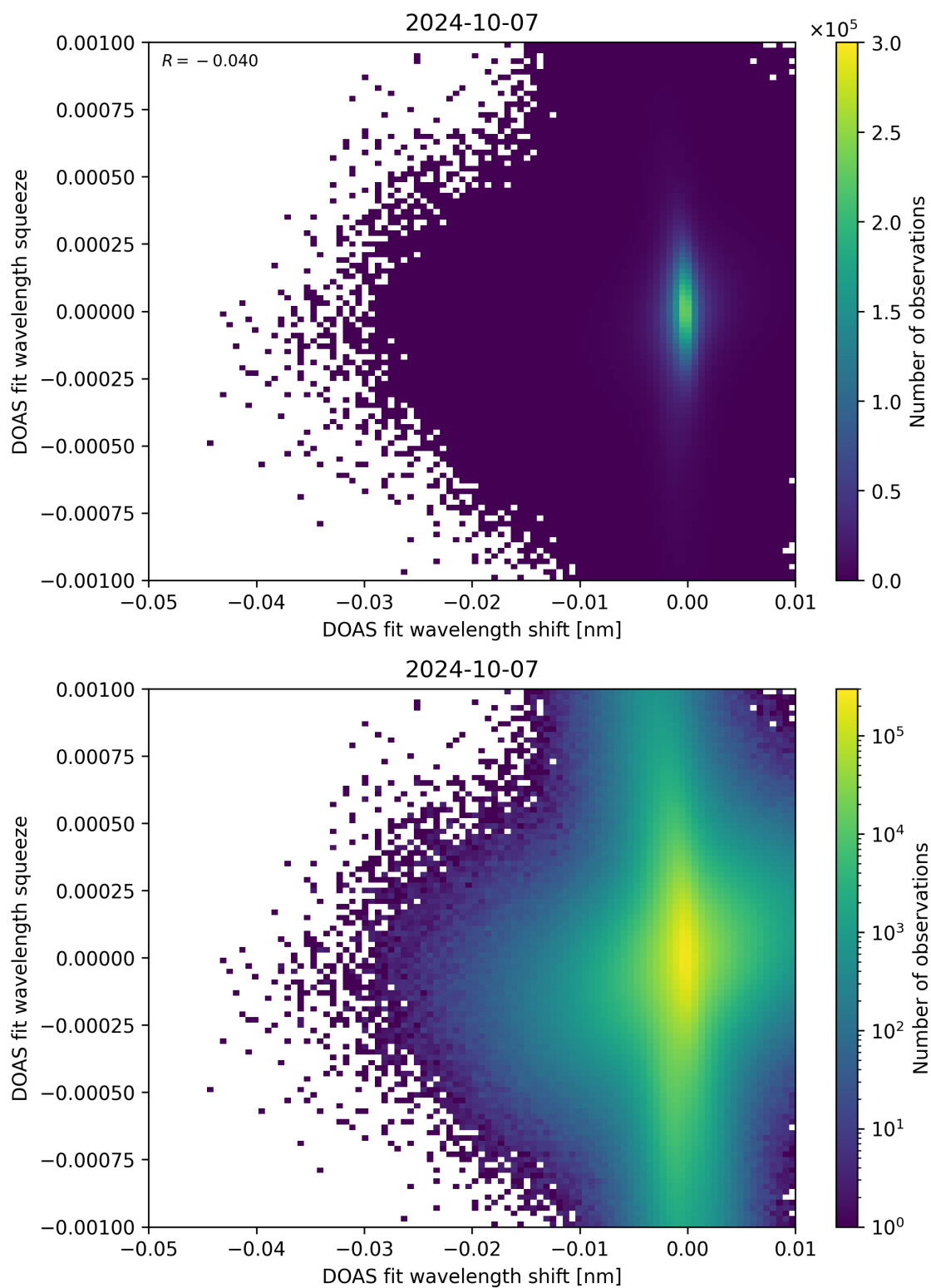
Figure 127: Scatter density plot of “DOAS fit wavelength shift” against “DOAS fit wavelength squeeze” for 2024-10-06 to 2024-10-08.
