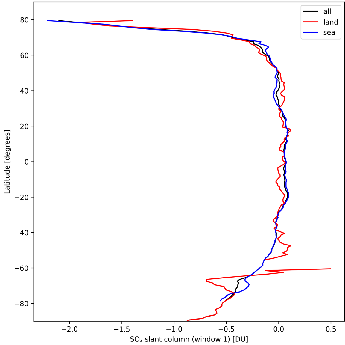
Figure 33: Zonal average of “SO 2 slant column (window 1)” for 2024-10-06 to 2024-10-08.
