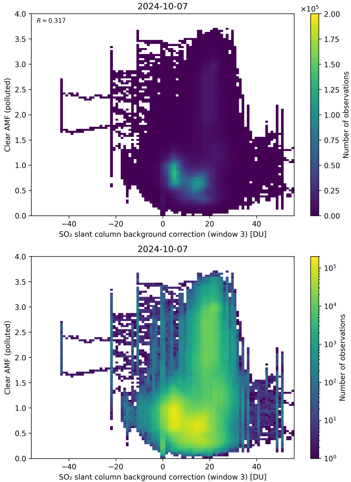
Figure 124: Scatter density plot of “SO 2 slant column background correction (window 3)” against “Clear AMF (polluted)” for 2024-10-06 to 2024-10-08.
