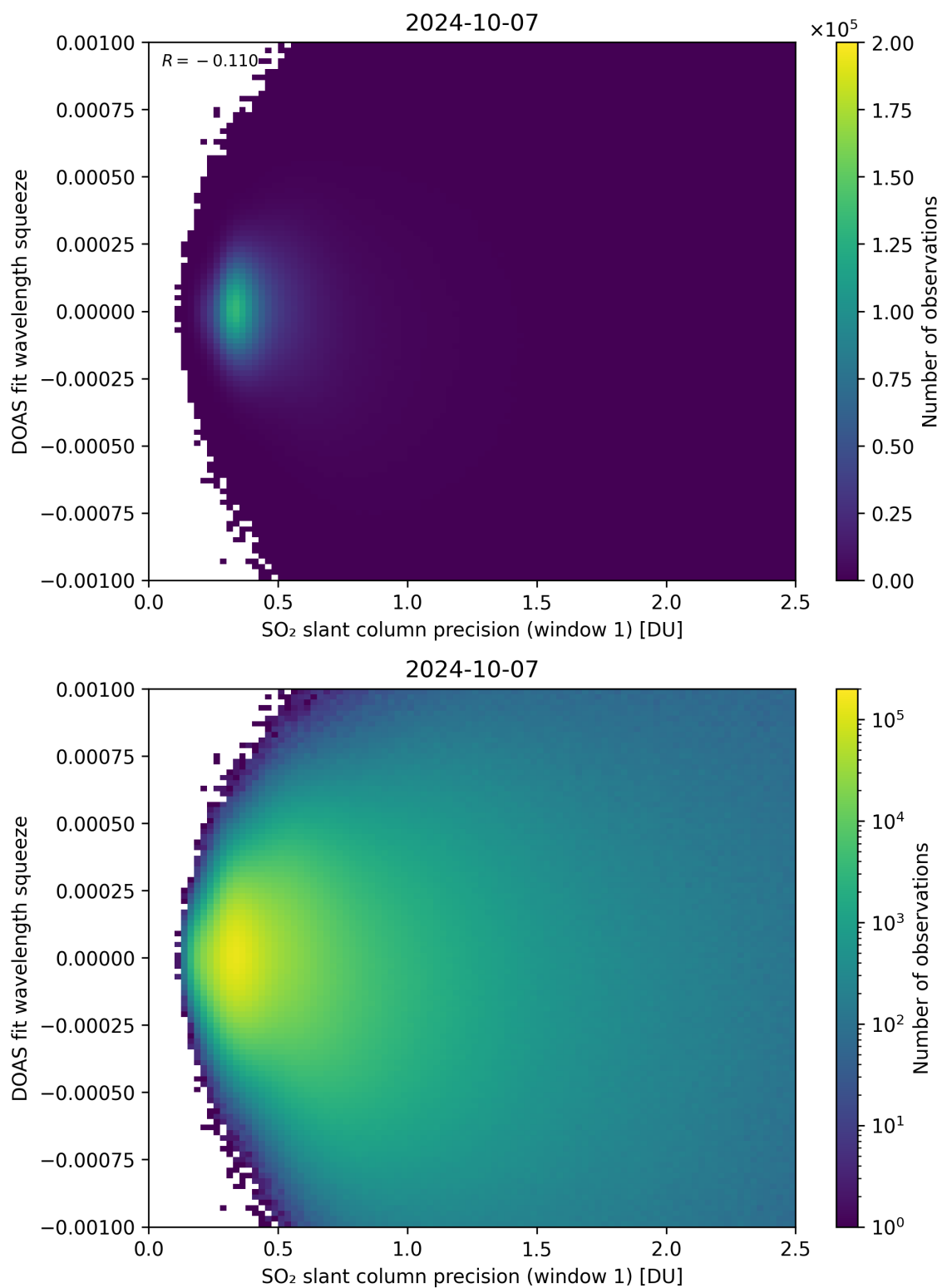
Figure 222: Scatter density plot of “SO 2 slant column precision (window 1)” against “DOAS fit wavelength squeeze” for 2024-10-06 to 2024-10-08.
