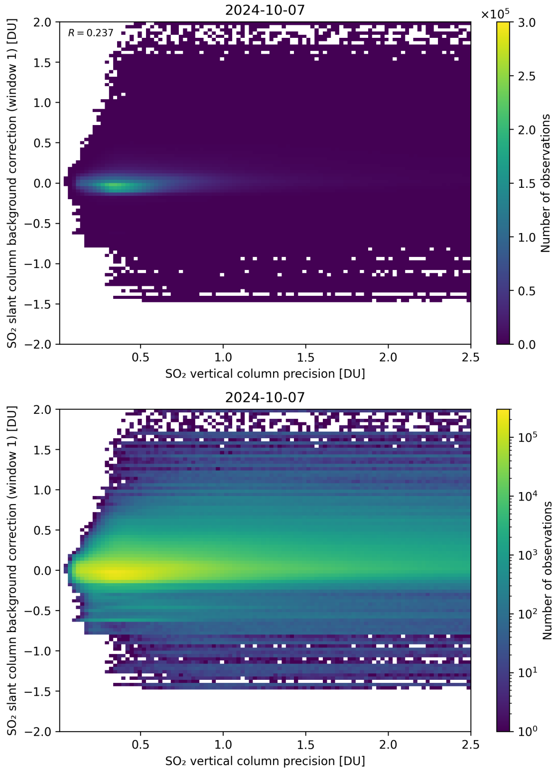
Figure 279: Scatter density plot of “SO 2 vertical column precision” against “SO 2 slant column background correction (window 1)” for 2024-10-06 to 2024-10-08.
