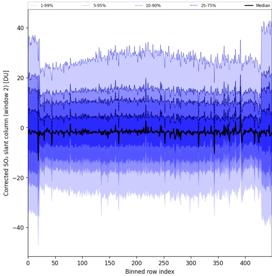
Figure 85: Along track statistics of “Corrected SO 2 slant column (window 2)” for 2024-10-06 to 2024-10-08
