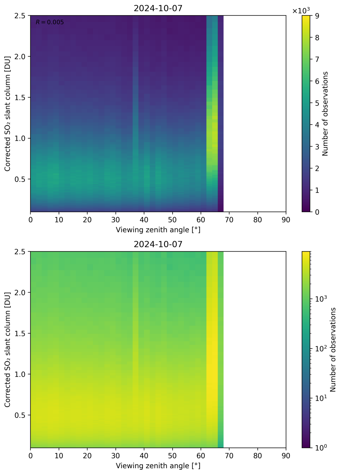
Figure 317: Scatter density plot of “Viewing zenith angle” against “Corrected SO 2 slant column” for 2024-10-06 to 2024-10-08.
