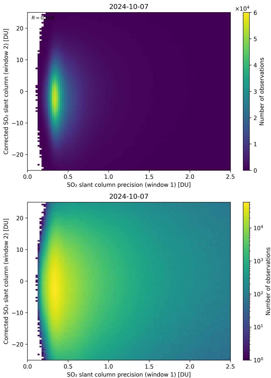
Figure 225: Scatter density plot of “SO 2 slant column precision (window 1)” against “Corrected SO 2 slant column (window 2)” for 2024-10-06 to 2024-10-08.
