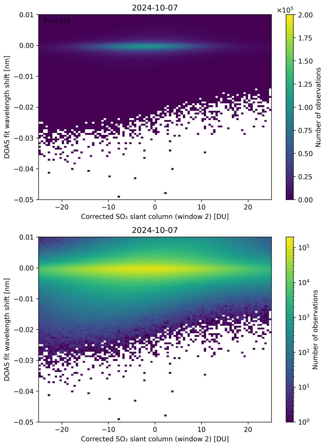
Figure 196: Scatter density plot of “Corrected SO 2 slant column (window 2)” against “DOAS fit wavelength shift” for 2024-10-06 to 2024-10-08.
