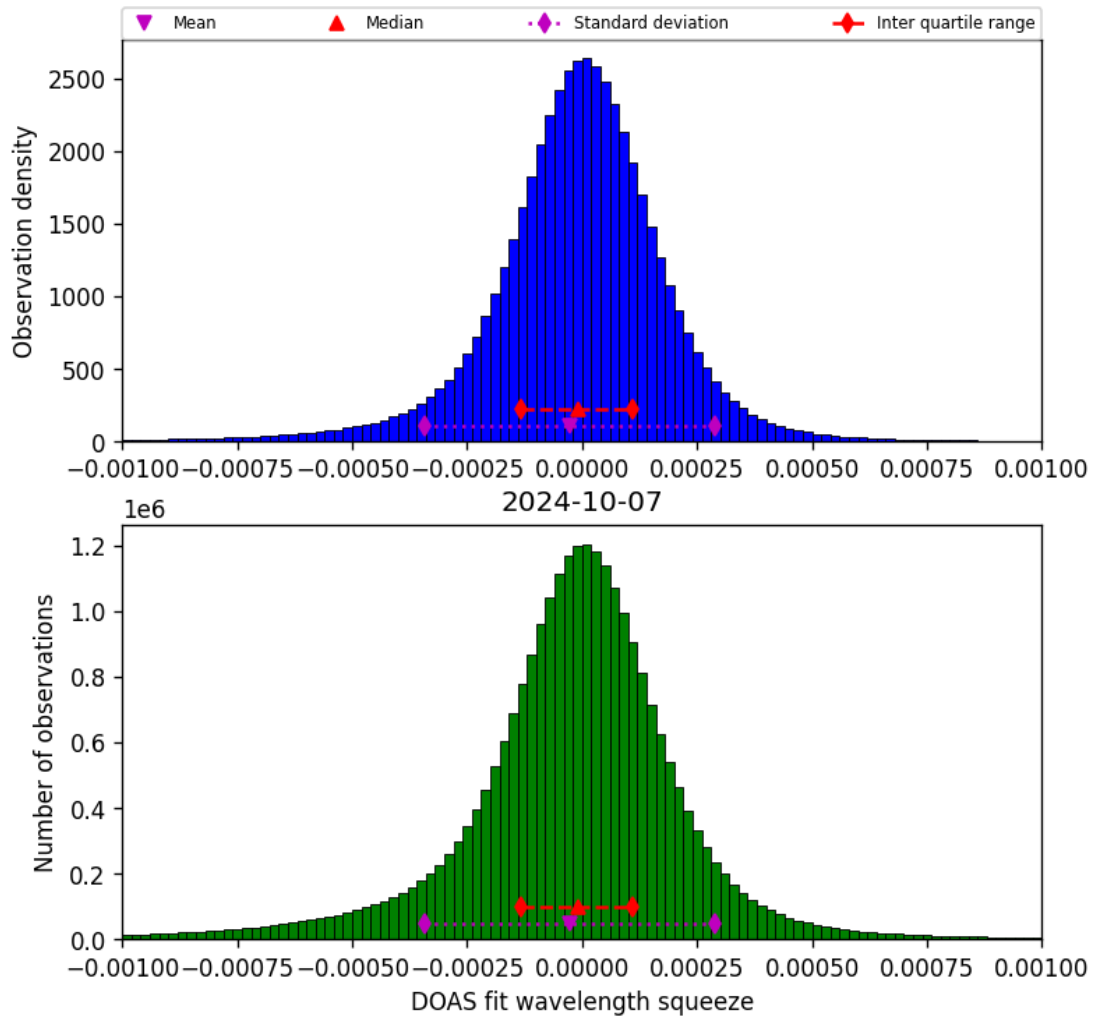
Figure 69: Histogram of “DOAS fit wavelength squeeze” for 2024-10-06 to 2024-10-08
