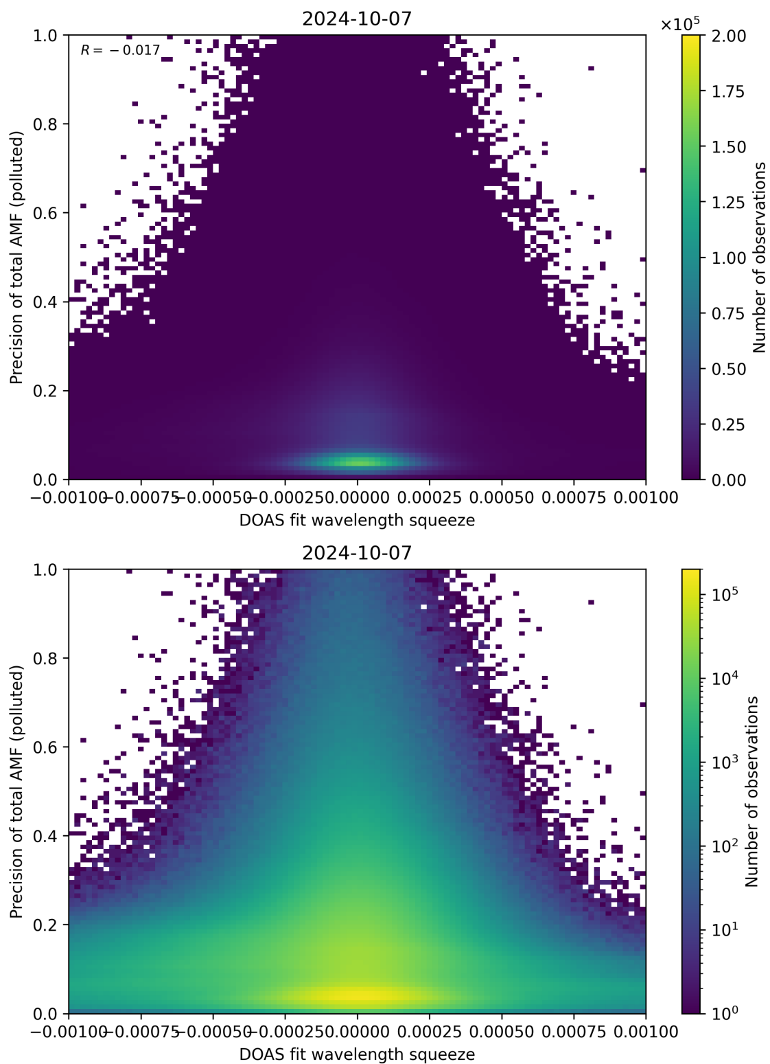
Figure 135: Scatter density plot of “DOAS fit wavelength squeeze” against “Precision of total AMF (polluted)” for 2024-10-06 to 2024-10-08.
