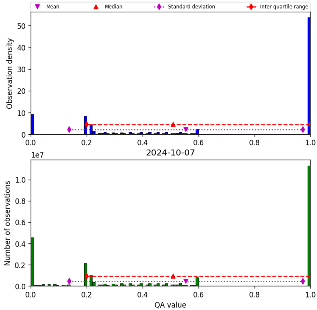
Figure 52: Histogram of “QA value” for 2024-10-06 to 2024-10-08
