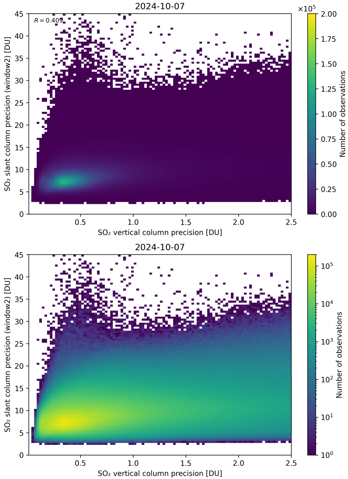
Figure 291: Scatter density plot of “SO 2 vertical column precision” against “SO 2 slant column precision (window2)” for 2024-10-06 to 2024-10-08.
