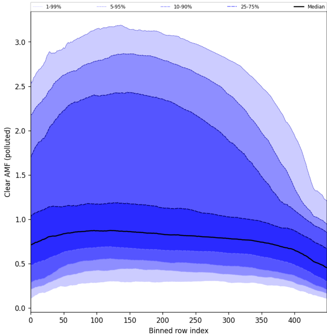
Figure 96: Along track statistics of “Clear AMF (polluted)” for 2024-10-06 to 2024-10-08
