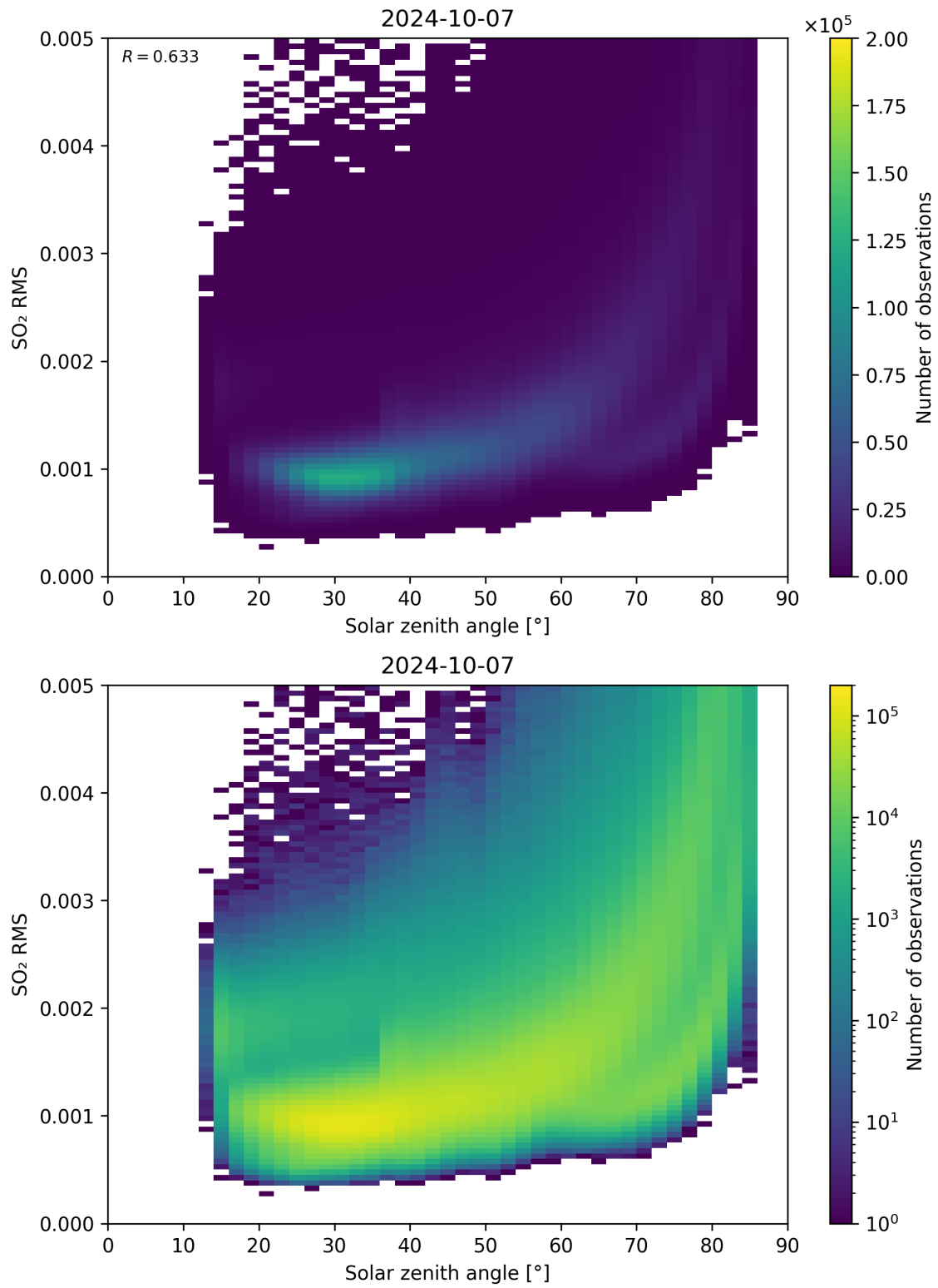
Figure 163: Scatter density plot of “Solar zenith angle” against “SO 2 RMS” for 2024-10-06 to 2024-10-08.
