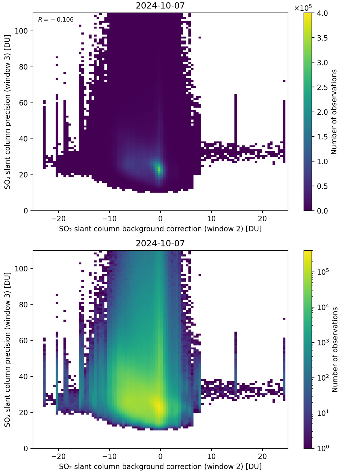
Figure 118: Scatter density plot of “SO 2 slant column background correction (window 2)” against “SO 2 slant column precision (window 3)” for 2024-10-06 to 2024-10-08.
