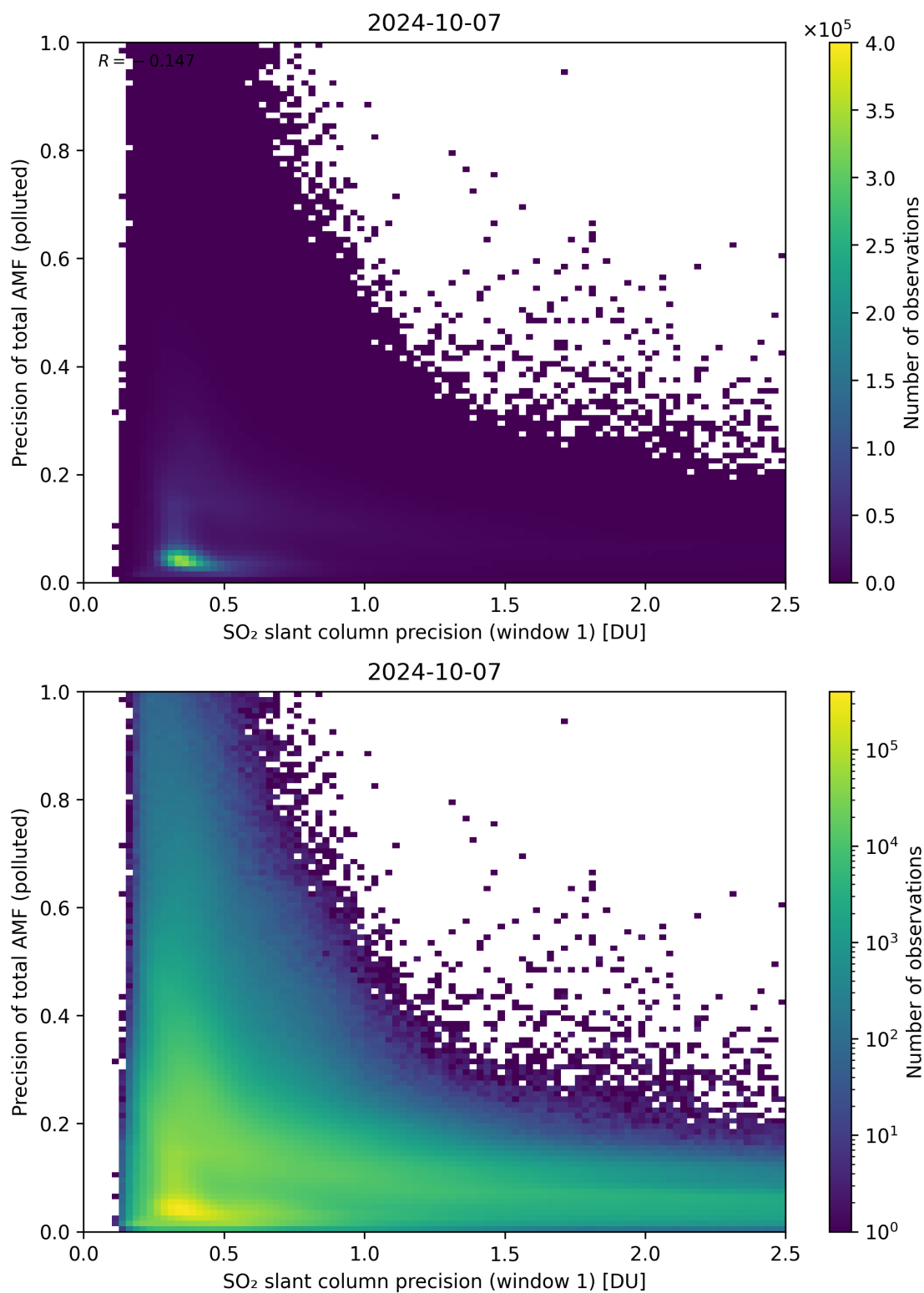
Figure 231: Scatter density plot of “SO 2 slant column precision (window 1)” against “Precision of total AMF (polluted)” for 2024-10-06 to 2024-10-08.
