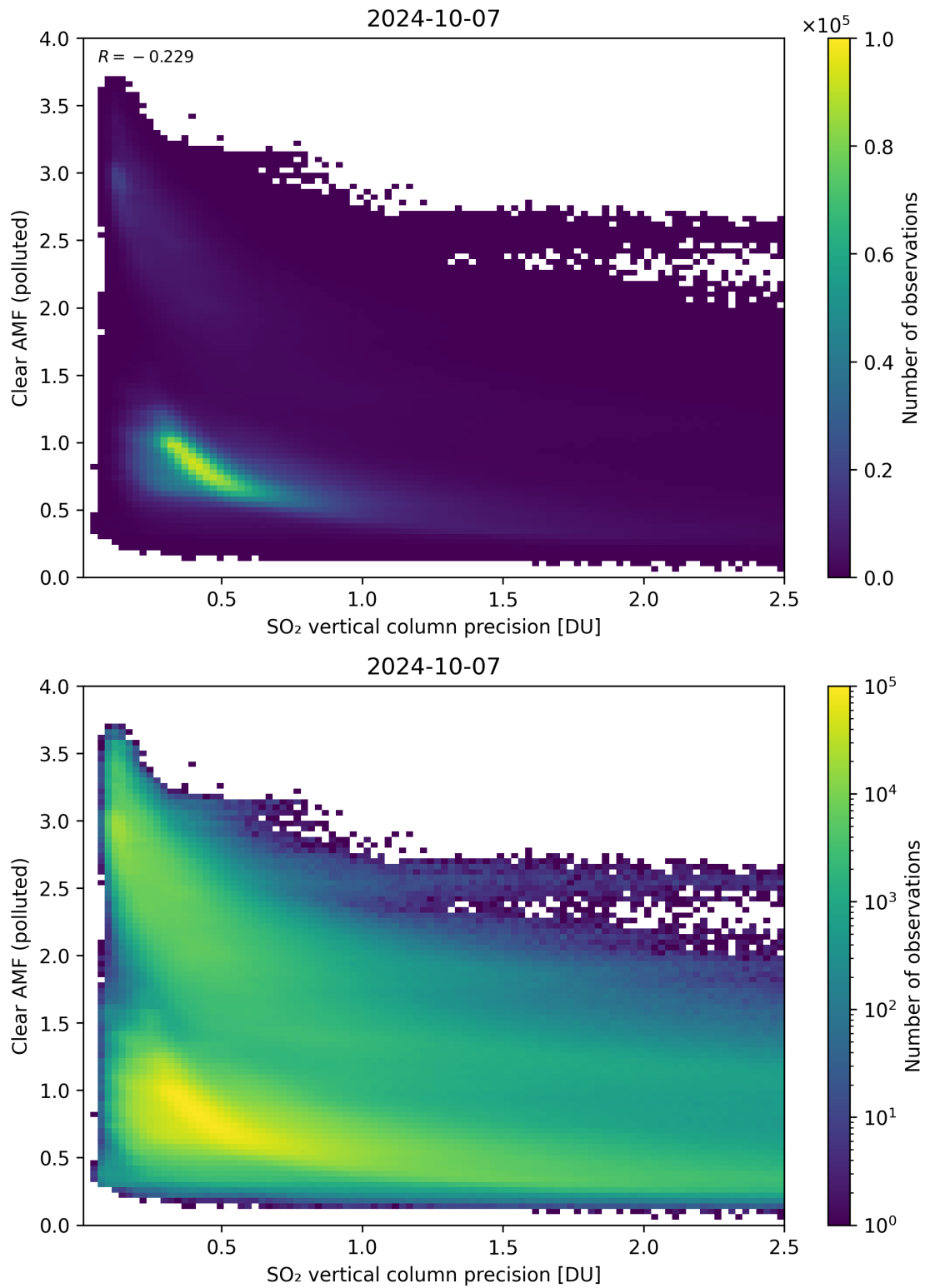
Figure 285: Scatter density plot of “SO 2 vertical column precision” against “Clear AMF (polluted)” for 2024-10-06 to 2024-10-08.
