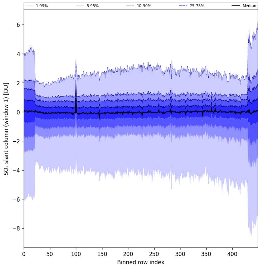
Figure 79: Along track statistics of “SO 2 slant column (window 1)” for 2024-10-06 to 2024-10-08
