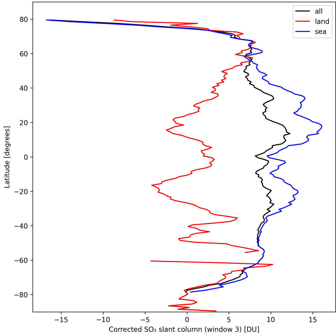
Figure 43: Zonal average of “Corrected SO 2 slant column (window 3)” for 2024-10-06 to 2024-10-08.
