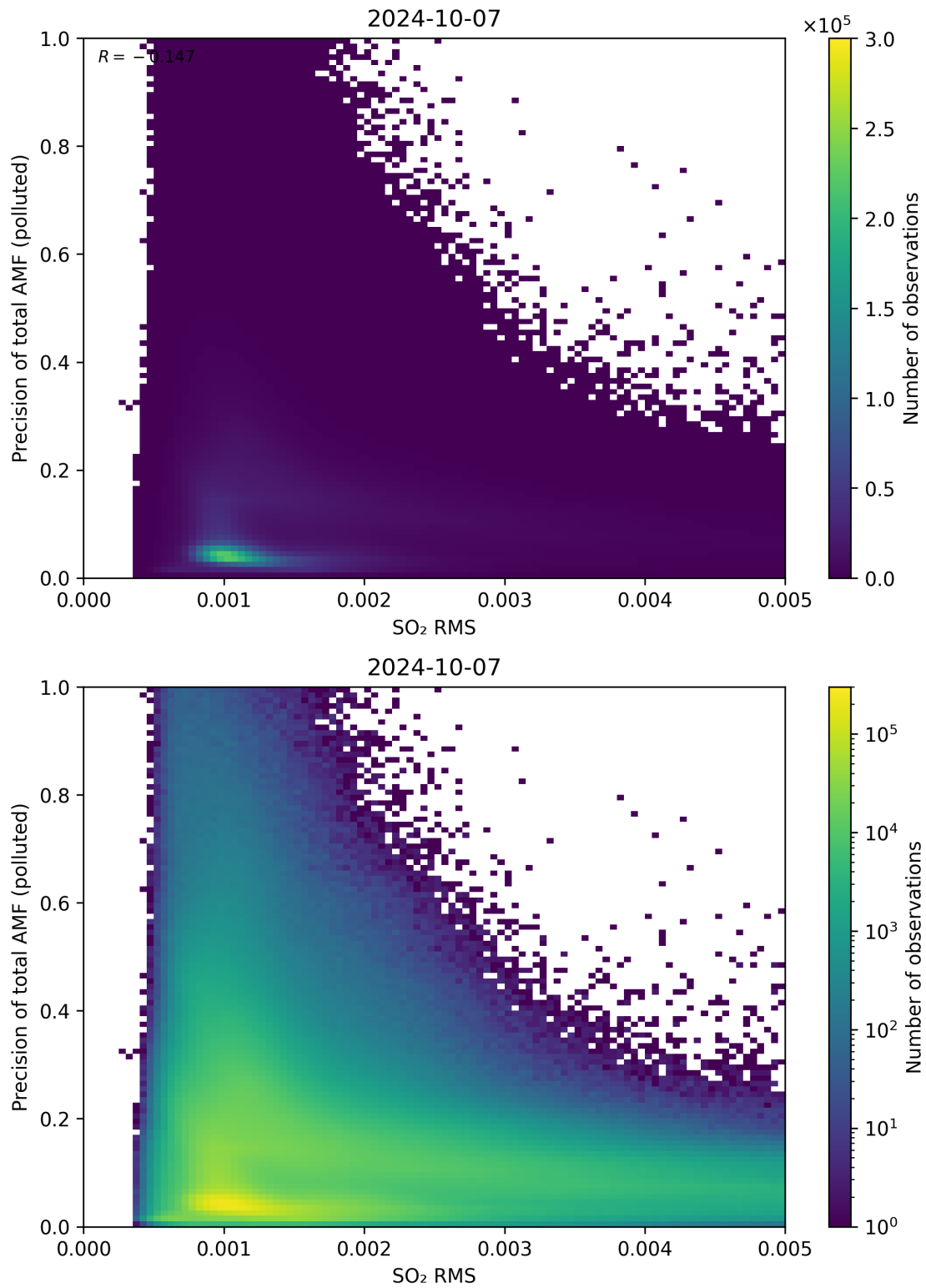
Figure 138: Scatter density plot of “SO 2 RMS” against “Precision of total AMF (polluted)” for 2024-10-06 to 2024-10-08.
