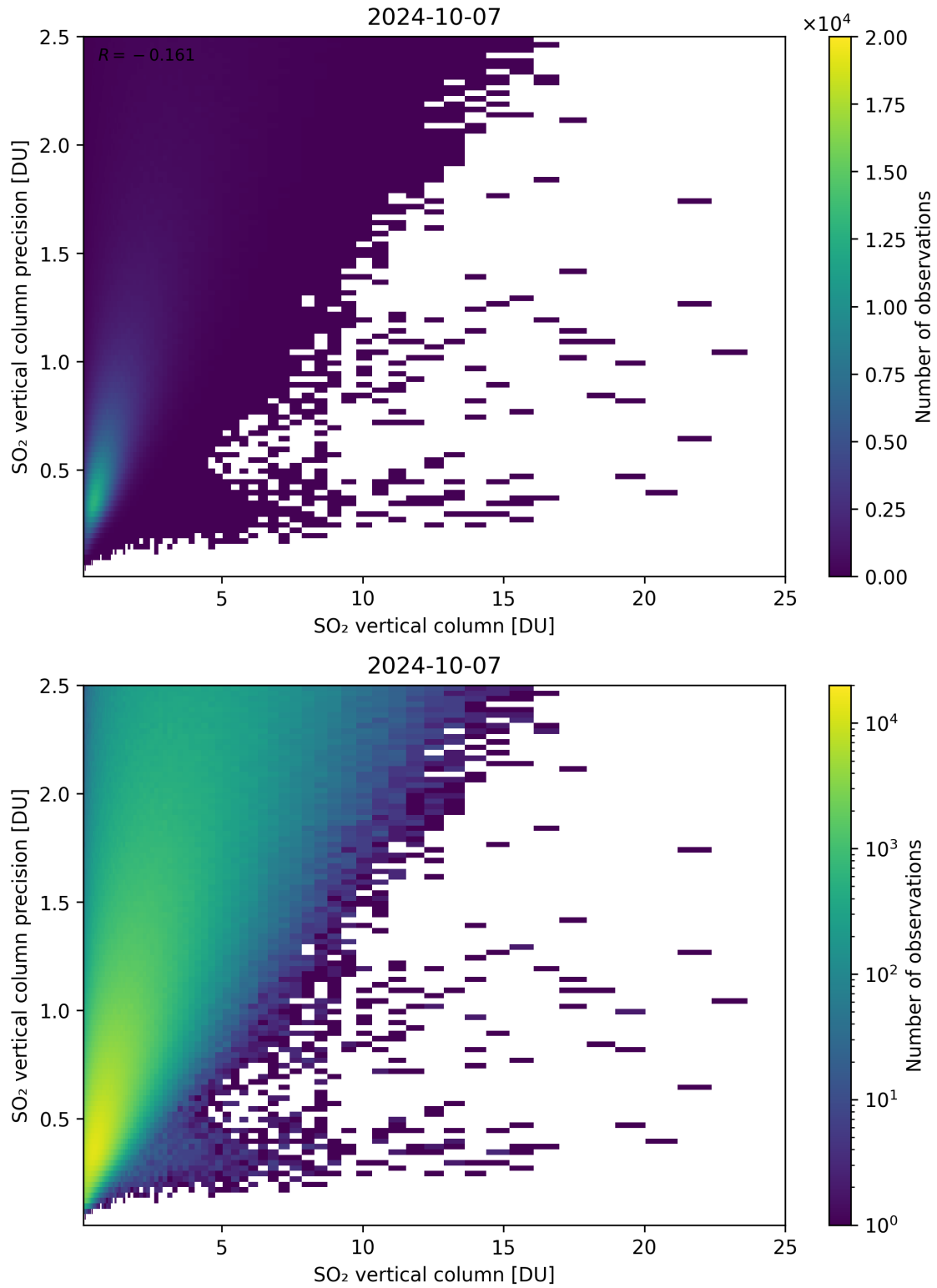
Figure 307: Scatter density plot of “SO 2 vertical column” against “SO 2 vertical column precision” for 2024-10-06 to 2024-10-08.
