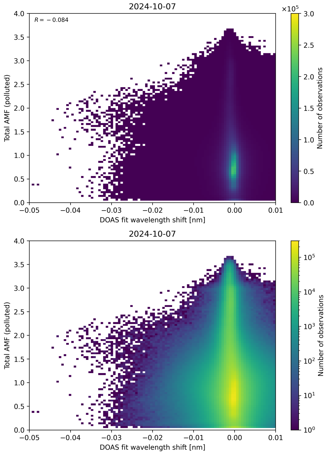
Figure 130: Scatter density plot of “DOAS fit wavelength shift” against “Total AMF (polluted)” for 2024-10-06 to 2024-10-08.
