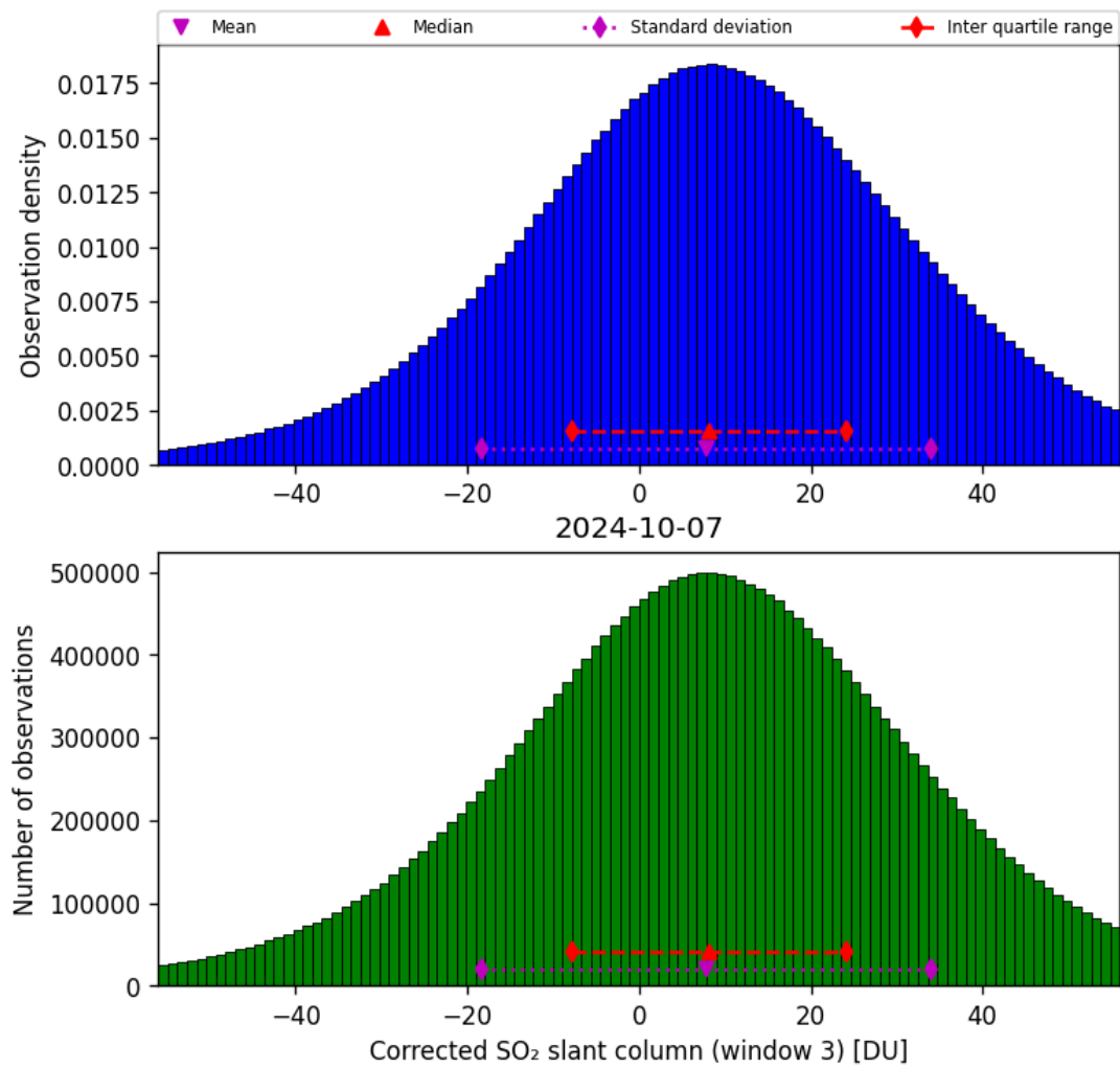
Figure 66: Histogram of “Corrected SO 2 slant column (window 3)” for 2024-10-06 to 2024-10-08
