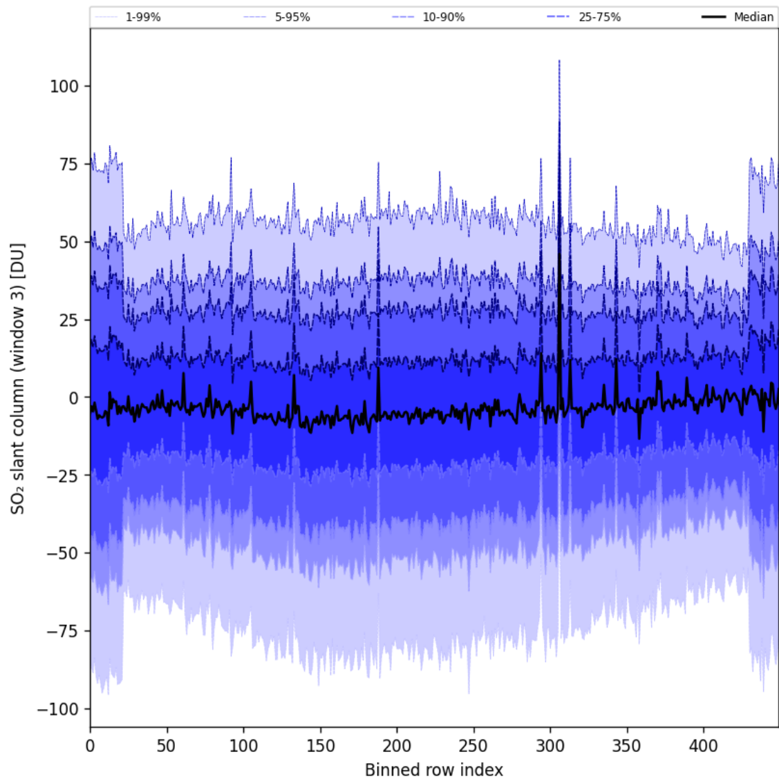
Figure 87: Along track statistics of “SO 2 slant column (window 3)” for 2024-10-06 to 2024-10-08
