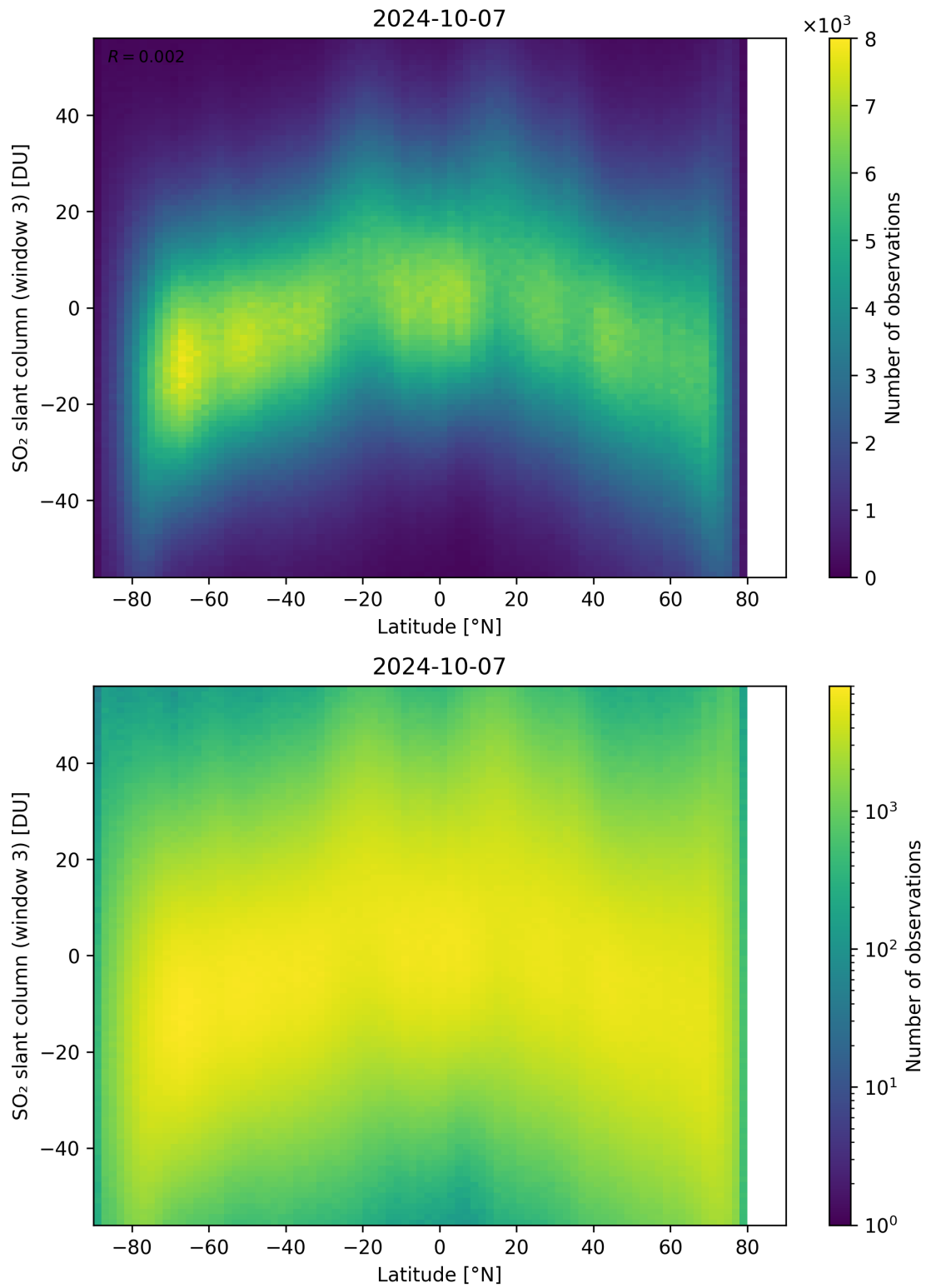
Figure 152: Scatter density plot of “Latitude” against “SO 2 slant column (window 3)” for 2024-10-06 to 2024-10-08.
