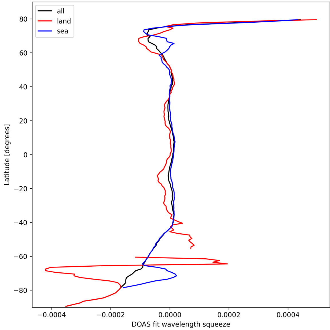
Figure 46: Zonal average of “DOAS fit wavelength squeeze” for 2024-10-06 to 2024-10-08.
