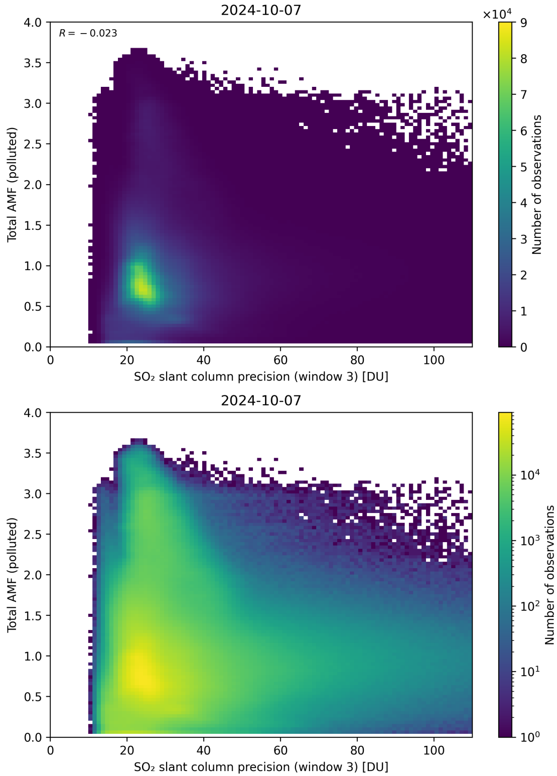
Figure 263: Scatter density plot of “SO 2 slant column precision (window 3)” against “Total AMF (polluted)” for 2024-10-06 to 2024-10-08.
