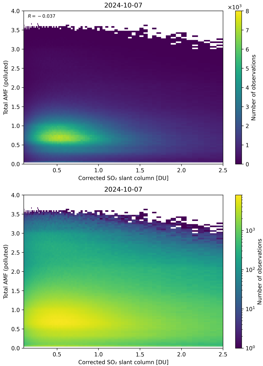
Figure 192: Scatter density plot of “Corrected SO 2 slant column” against “Total AMF (polluted)” for 2024-10-06 to 2024-10-08.
