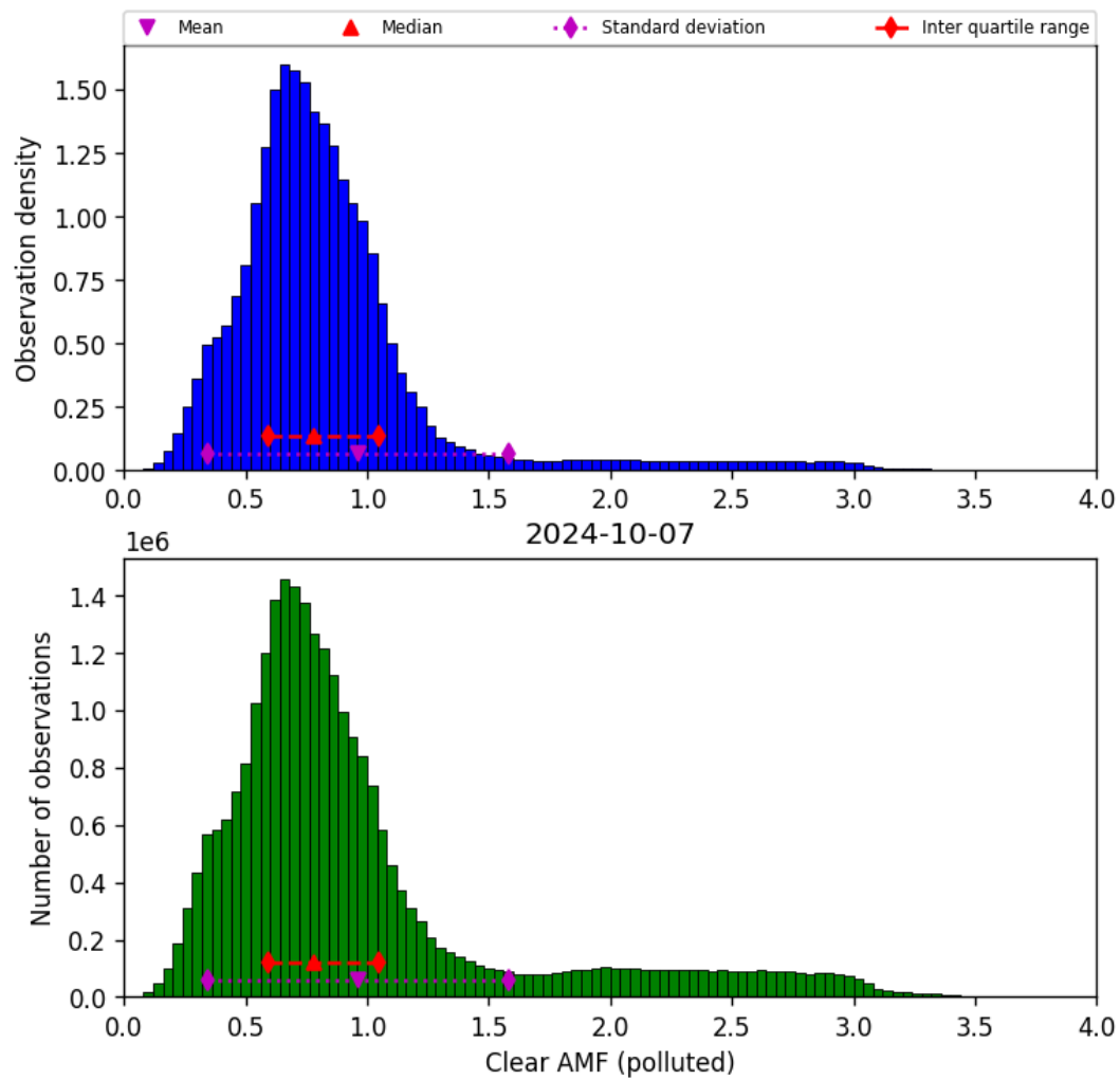
Figure 73: Histogram of “Clear AMF (polluted)” for 2024-10-06 to 2024-10-08
