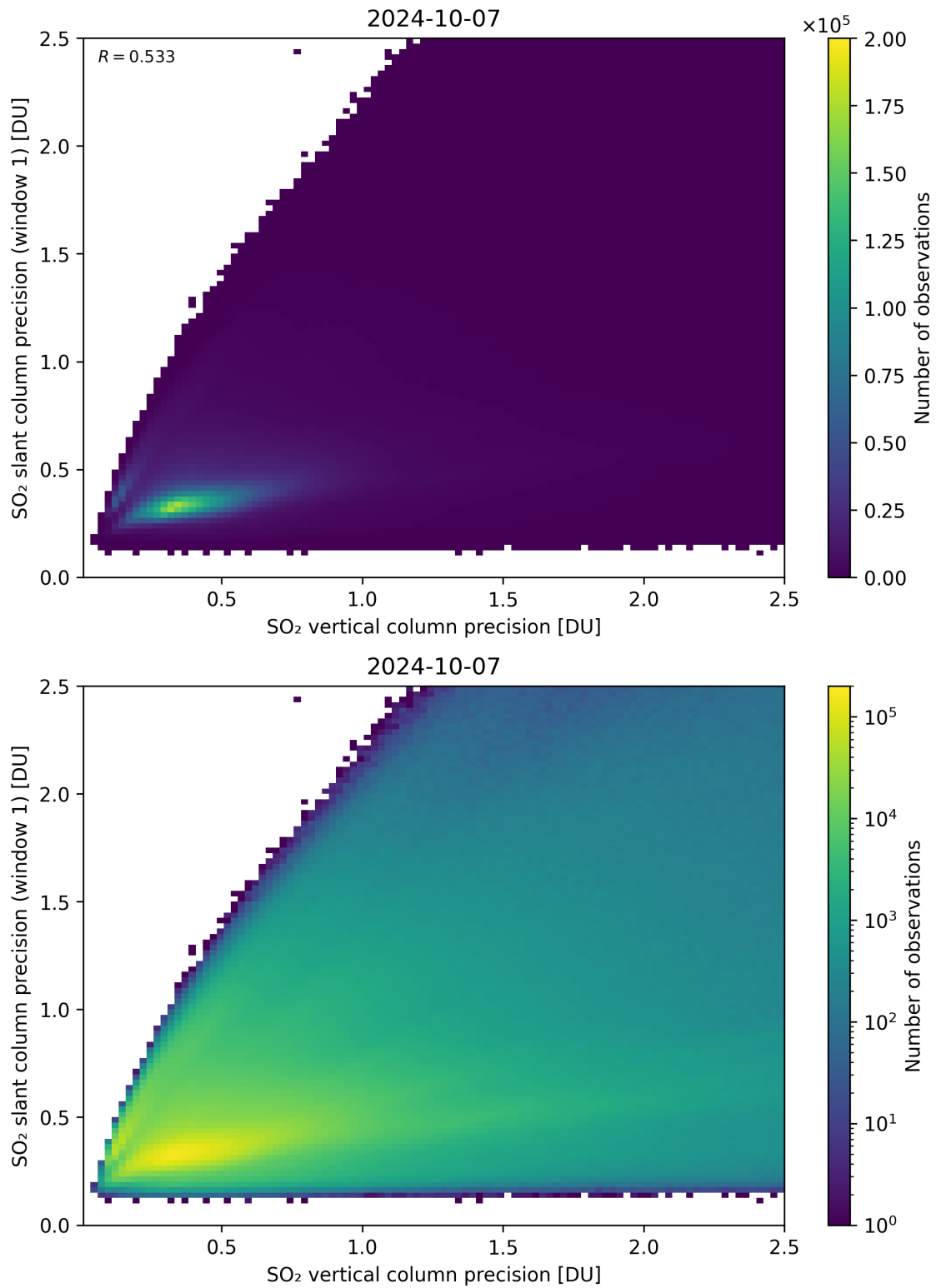
Figure 290: Scatter density plot of “SO 2 vertical column precision” against “SO 2 slant column precision (window 1)” for 2024-10-06 to 2024-10-08.
