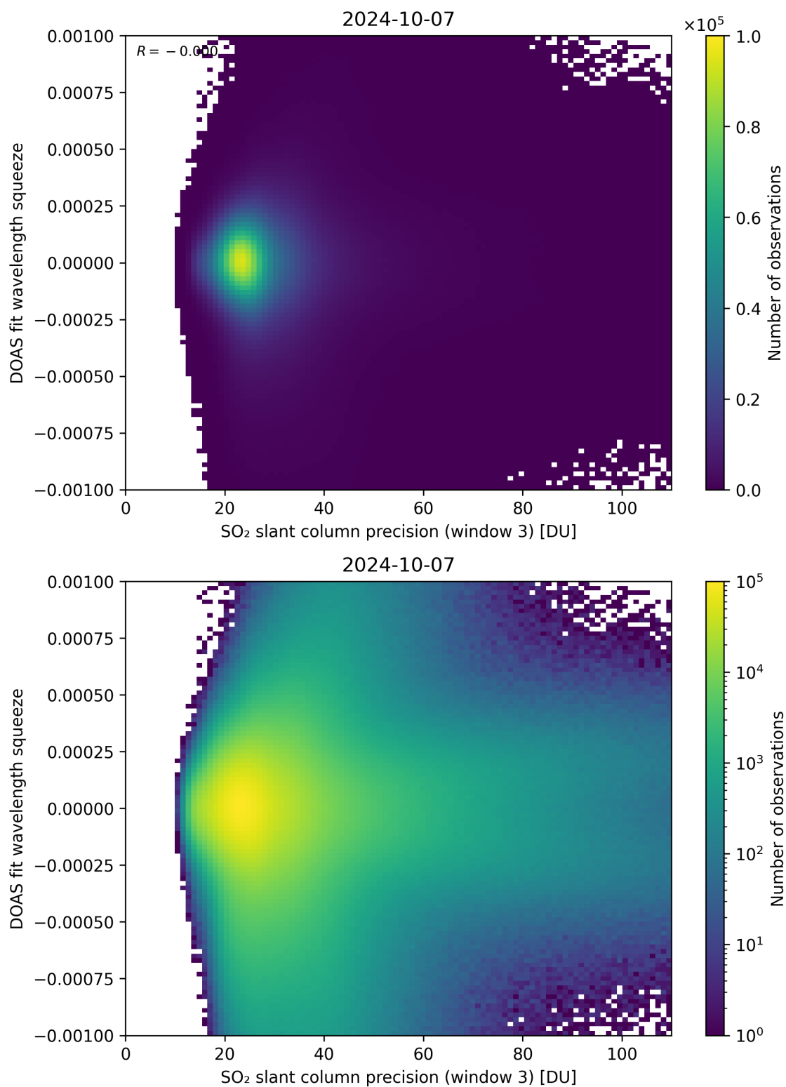
Figure 259: Scatter density plot of “SO 2 slant column precision (window 3)” against “DOAS fit wavelength squeeze” for 2024-10-06 to 2024-10-08.
