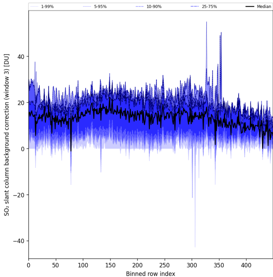
Figure 90: Along track statistics of “SO 2 slant column background correction (window 3)” for 2024-10-06 to 2024-10-08
