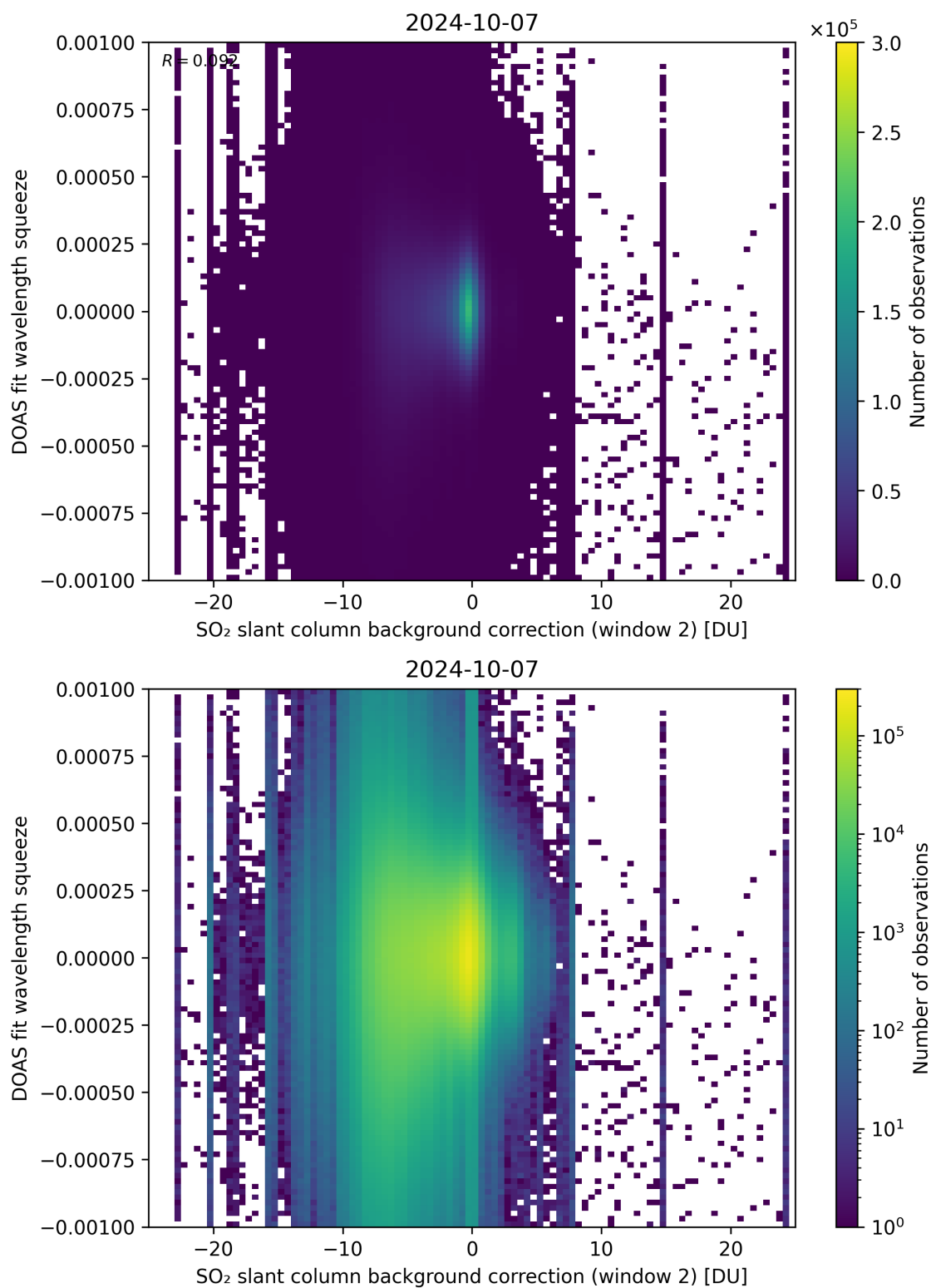
Figure 113: Scatter density plot of “SO 2 slant column background correction (window 2)” against “DOAS fit wavelength squeeze” for 2024-10-06 to 2024-10-08.
