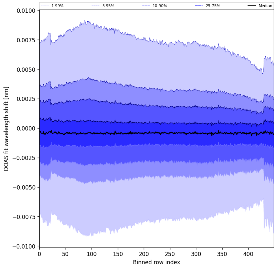
Figure 91: Along track statistics of “DOAS fit wavelength shift” for 2024-10-06 to 2024-10-08
