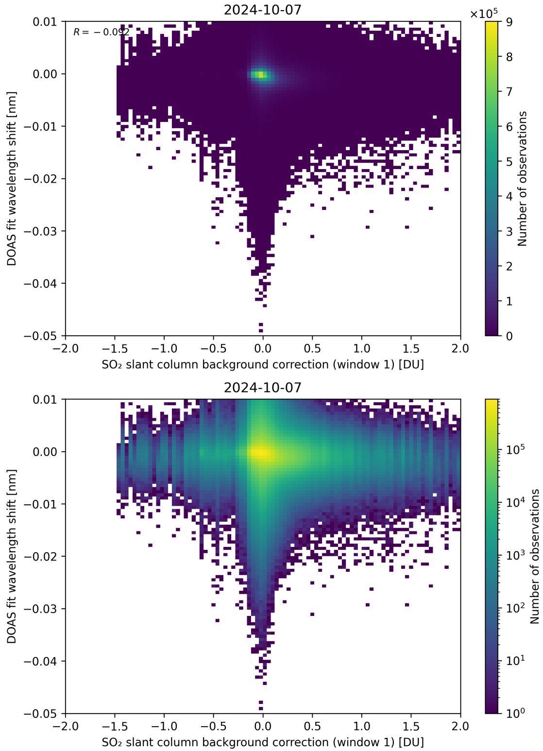
Figure 100: Scatter density plot of “SO 2 slant column background correction (window 1)” against “DOAS fit wavelength shift” for 2024-10-06 to 2024-10-08.
