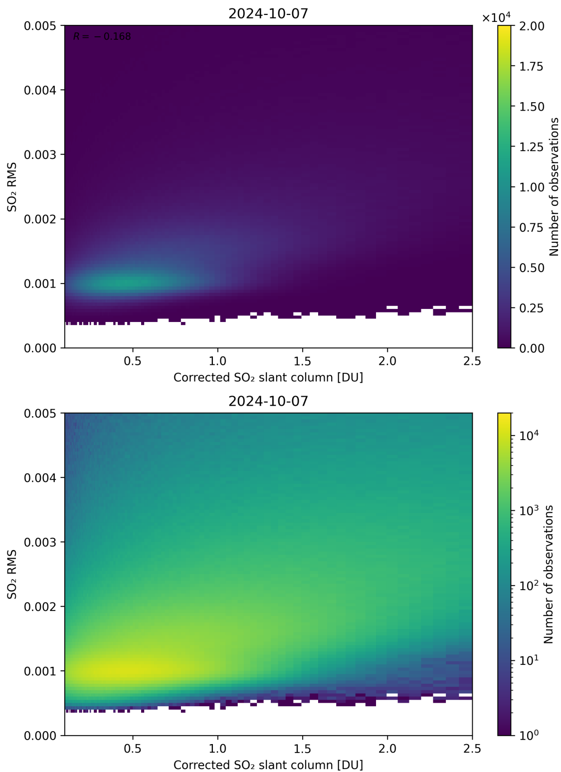
Figure 183: Scatter density plot of “Corrected SO 2 slant column” against “SO 2 RMS” for 2024-10-06 to 2024-10-08.
