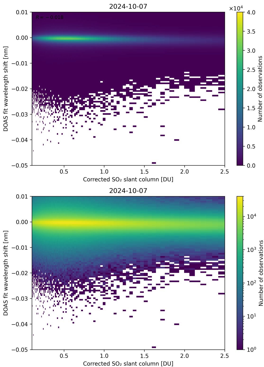
Figure 181: Scatter density plot of “Corrected SO 2 slant column” against “DOAS fit wavelength shift” for 2024-10-06 to 2024-10-08.
