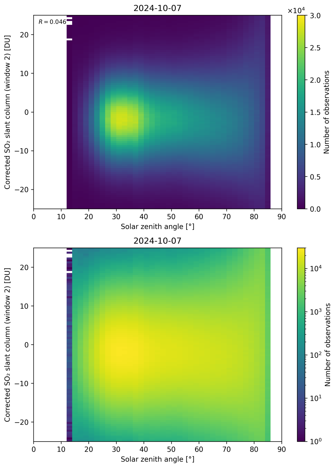
Figure 167: Scatter density plot of “Solar zenith angle” against “Corrected SO 2 slant column (window 2)” for 2024-10-06 to 2024-10-08.
