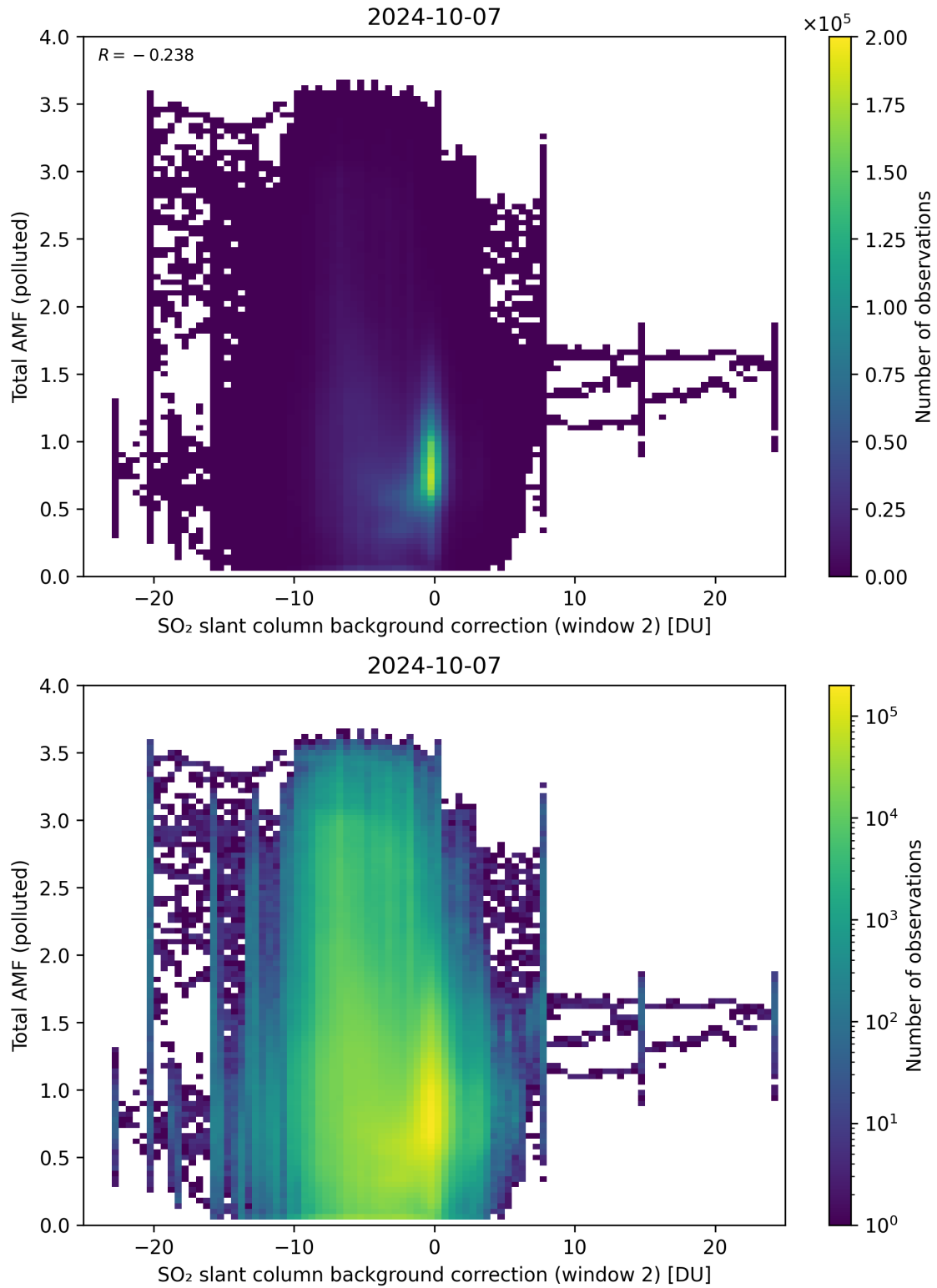
Figure 119: Scatter density plot of “SO 2 slant column background correction (window 2)” against “Total AMF (polluted)” for 2024-10-06 to 2024-10-08.
