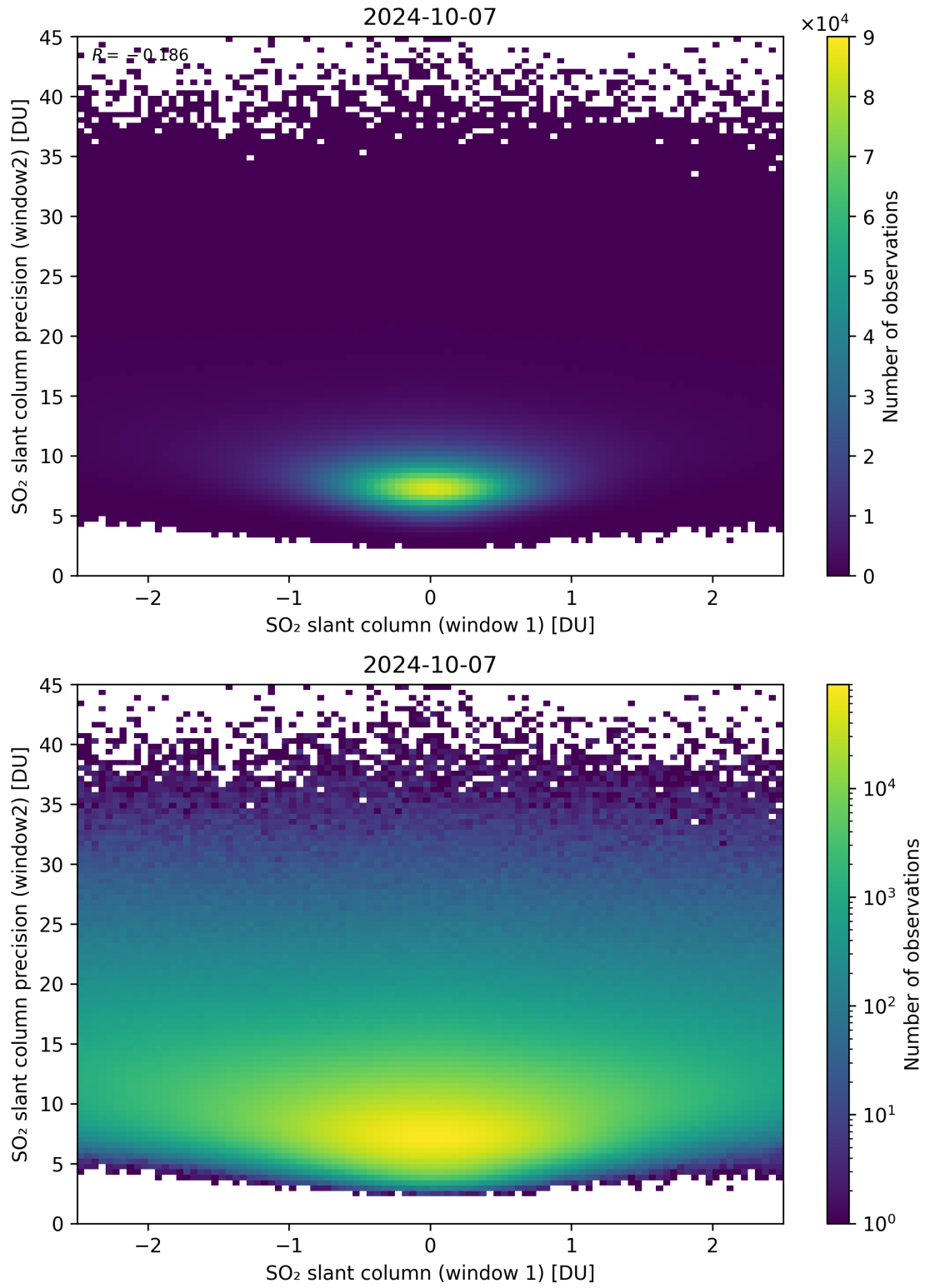
Figure 236: Scatter density plot of “SO 2 slant column (window 1)” against “SO 2 slant column precision (window2)” for 2024-10-06 to 2024-10-08.
