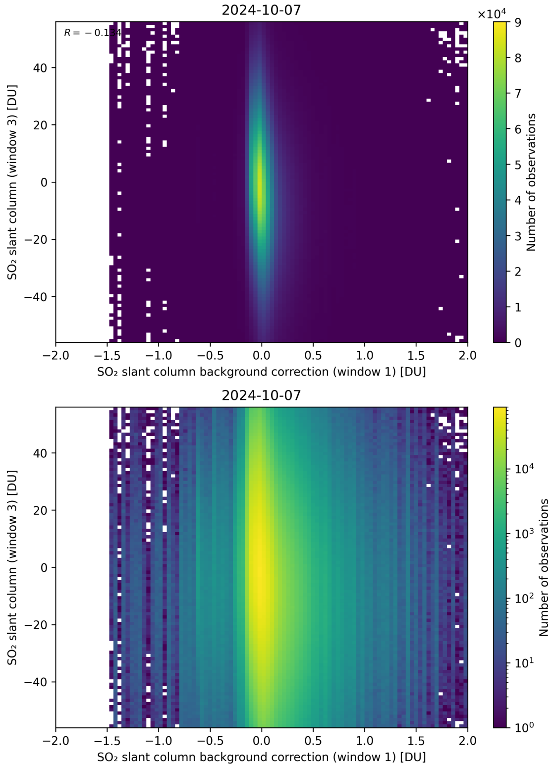
Figure 107: Scatter density plot of “SO 2 slant column background correction (window 1)” against “SO 2 slant column (window 3)” for 2024-10-06 to 2024-10-08.
