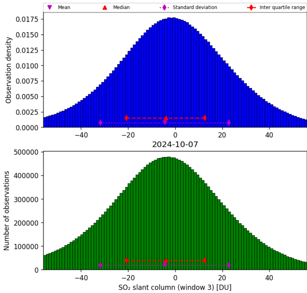
Figure 64: Histogram of “SO 2 slant column (window 3)” for 2024-10-06 to 2024-10-08
