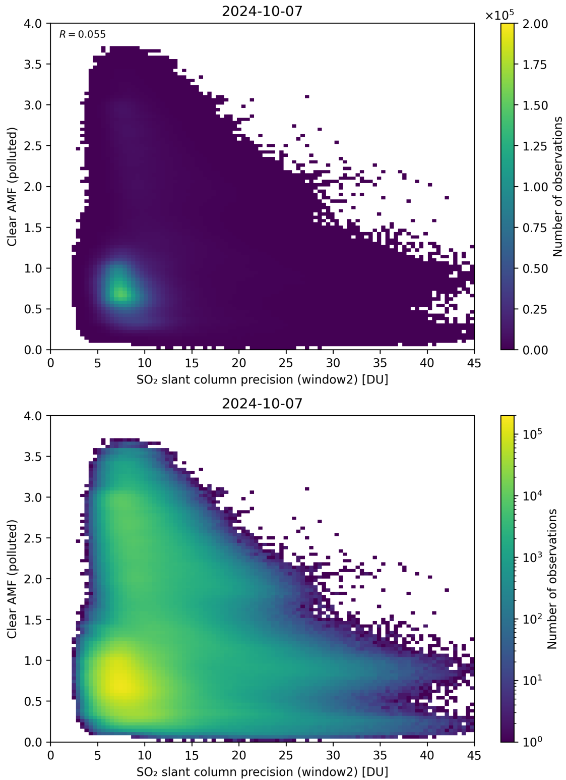
Figure 246: Scatter density plot of “SO 2 slant column precision (window2)” against “Clear AMF (polluted)” for 2024-10-06 to 2024-10-08.
