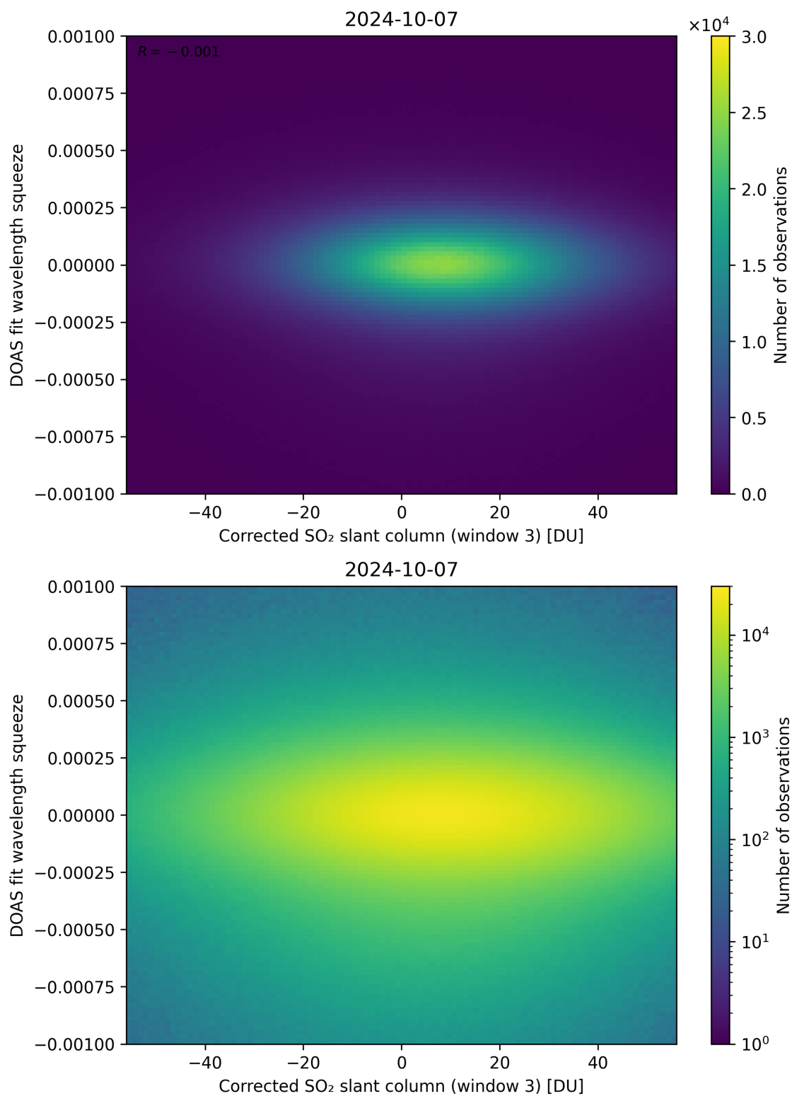
Figure 207: Scatter density plot of “Corrected SO 2 slant column (window 3)” against “DOAS fit wavelength squeeze” for 2024-10-06 to 2024-10-08.
