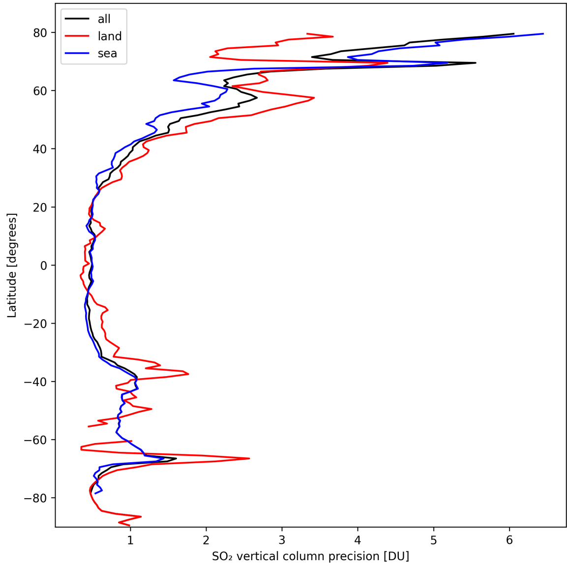
Figure 31: Zonal average of “SO 2 vertical column precision” for 2024-10-06 to 2024-10-08.
