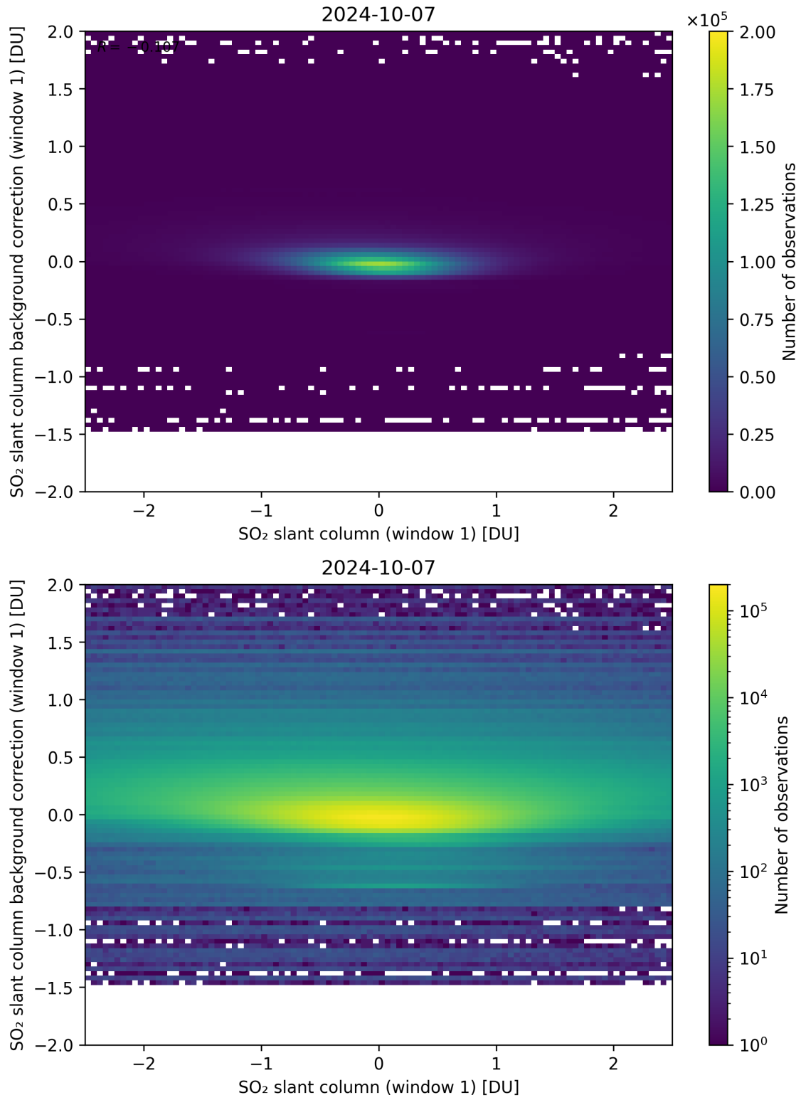
Figure 212: Scatter density plot of “SO 2 slant column (window 1)” against “SO 2 slant column background correction (window 1)” for 2024-10-06 to 2024-10-08.
