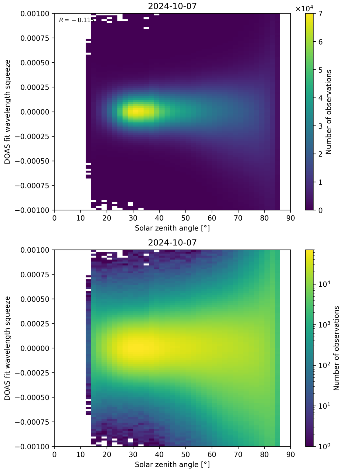
Figure 162: Scatter density plot of “Solar zenith angle” against “DOAS fit wavelength squeeze” for 2024-10-06 to 2024-10-08.
