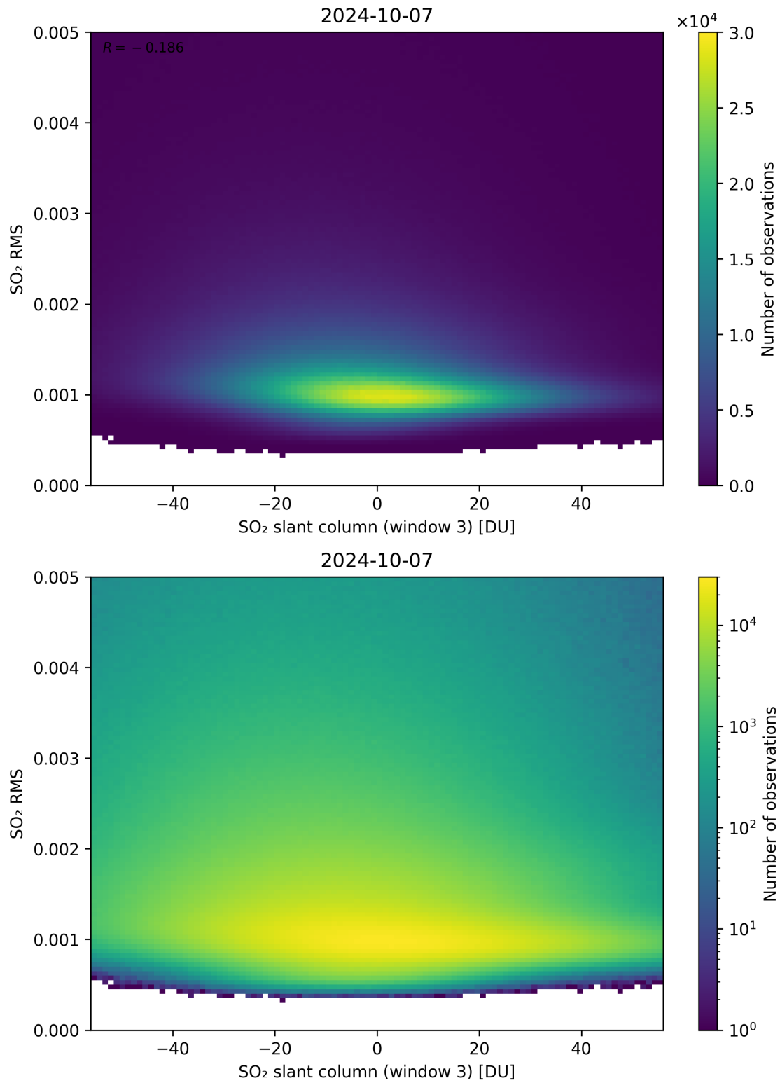
Figure 256: Scatter density plot of “SO 2 slant column (window 3)” against “SO 2 RMS” for 2024-10-06 to 2024-10-08.
