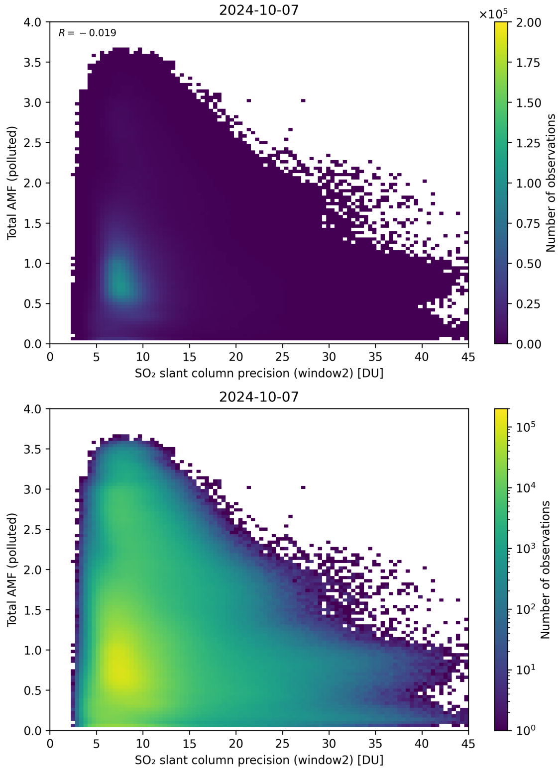
Figure 251: Scatter density plot of “SO 2 slant column precision (window2)” against “Total AMF (polluted)” for 2024-10-06 to 2024-10-08.
