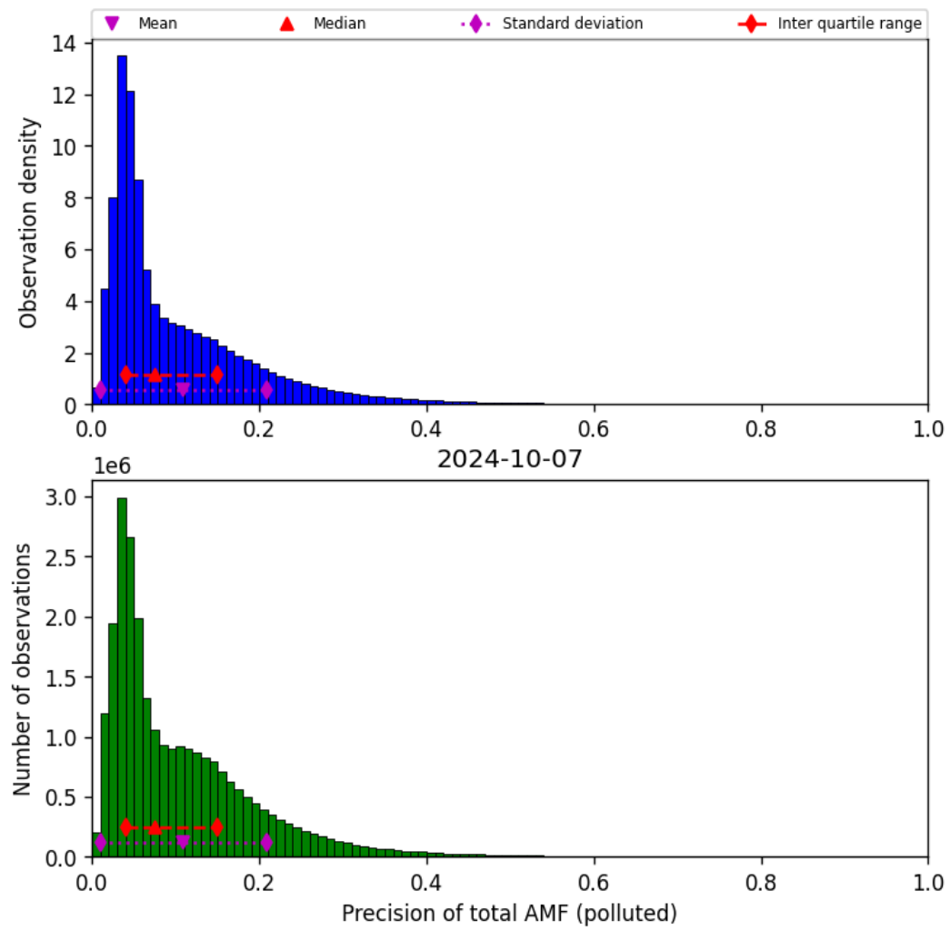
Figure 72: Histogram of “Precision of total AMF (polluted)” for 2024-10-06 to 2024-10-08
