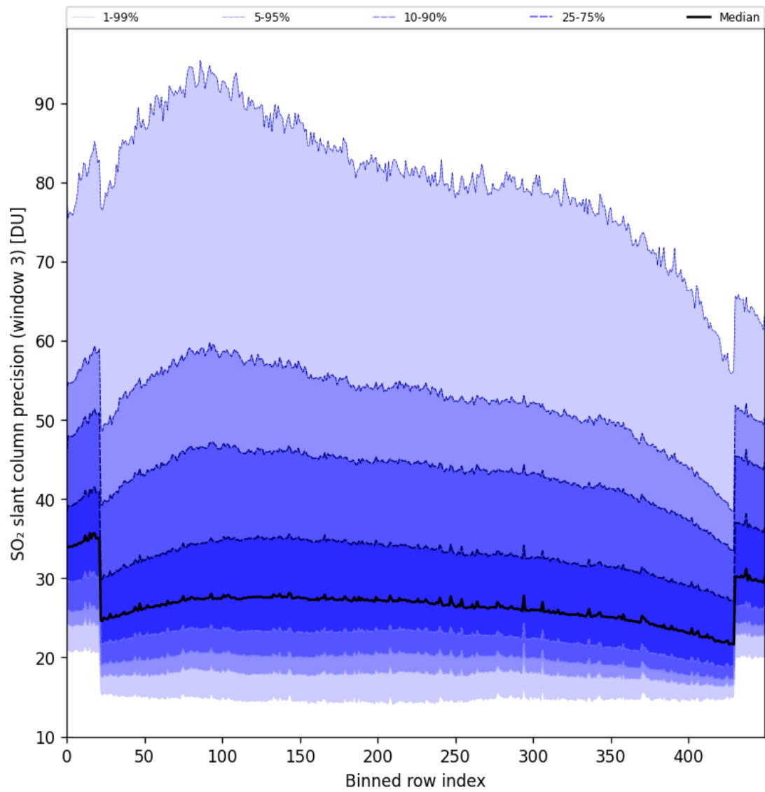
Figure 88: Along track statistics of “SO 2 slant column precision (window 3)” for 2024-10-06 to 2024-10-08
