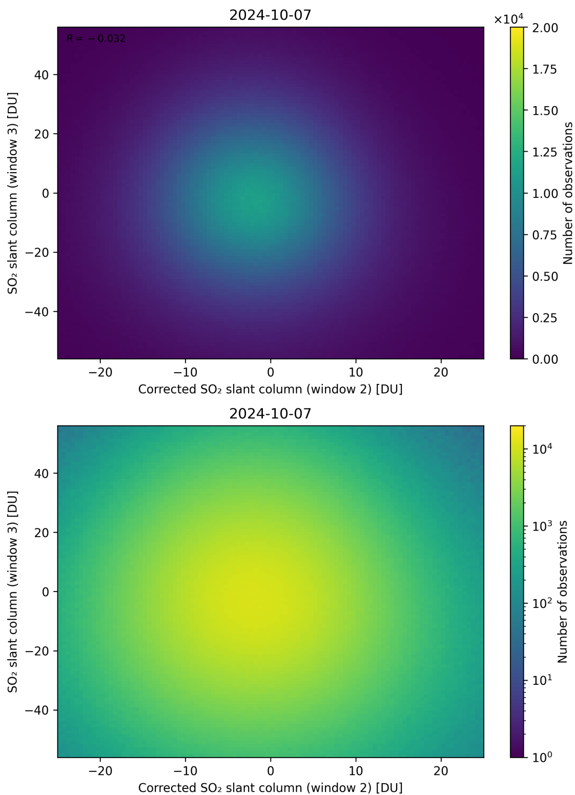
Figure 201: Scatter density plot of “Corrected SO 2 slant column (window 2)” against “SO 2 slant column (window 3)” for 2024-10-06 to 2024-10-08.
