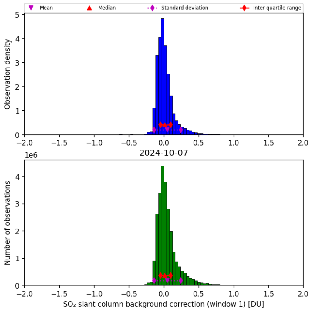
Figure 59: Histogram of “SO 2 slant column background correction (window 1)” for 2024-10-06 to 2024-10-08
