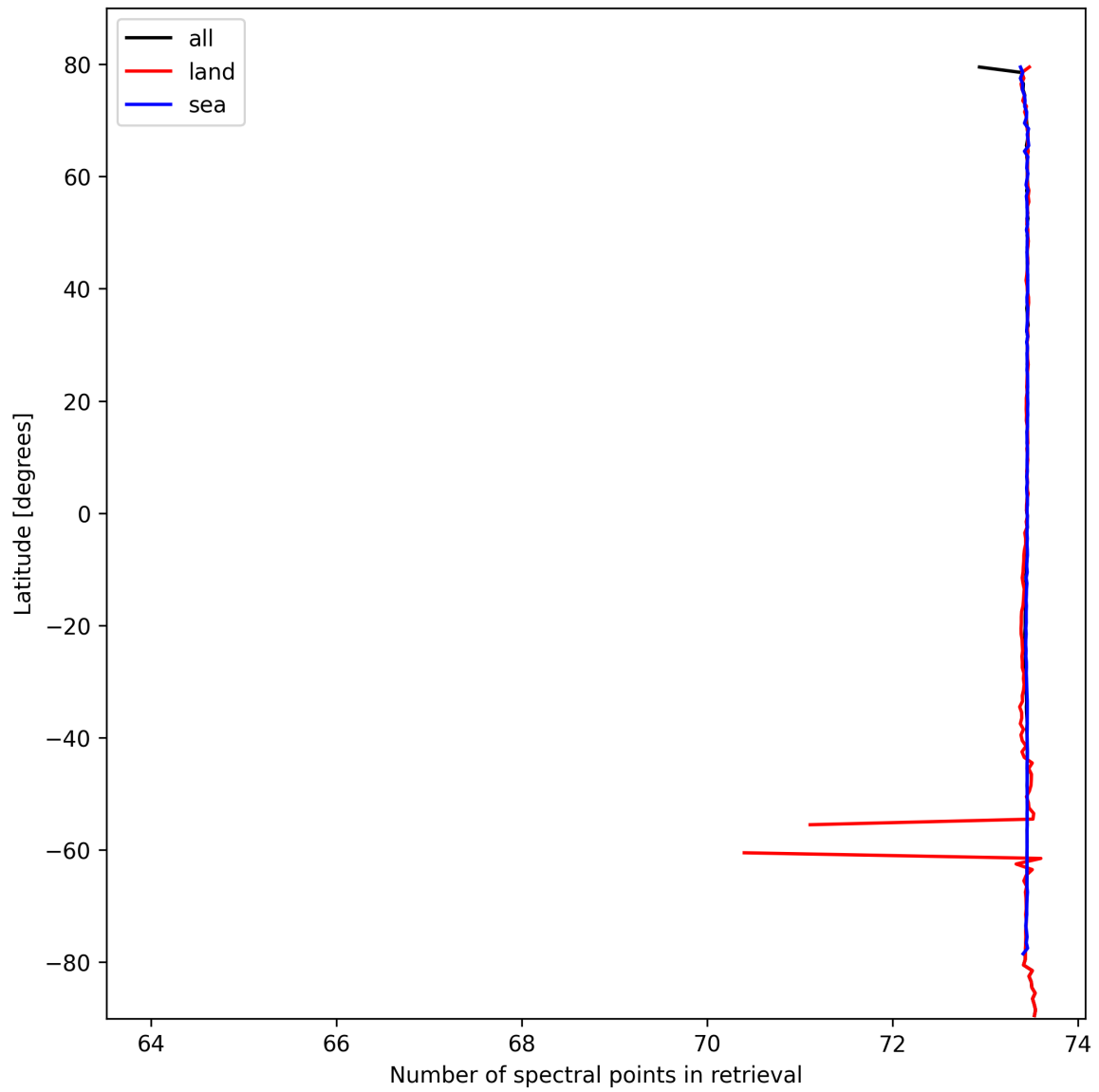
Figure 51: Zonal average of “Number of spectral points in retrieval” for 2024-10-06 to 2024-10-08.
