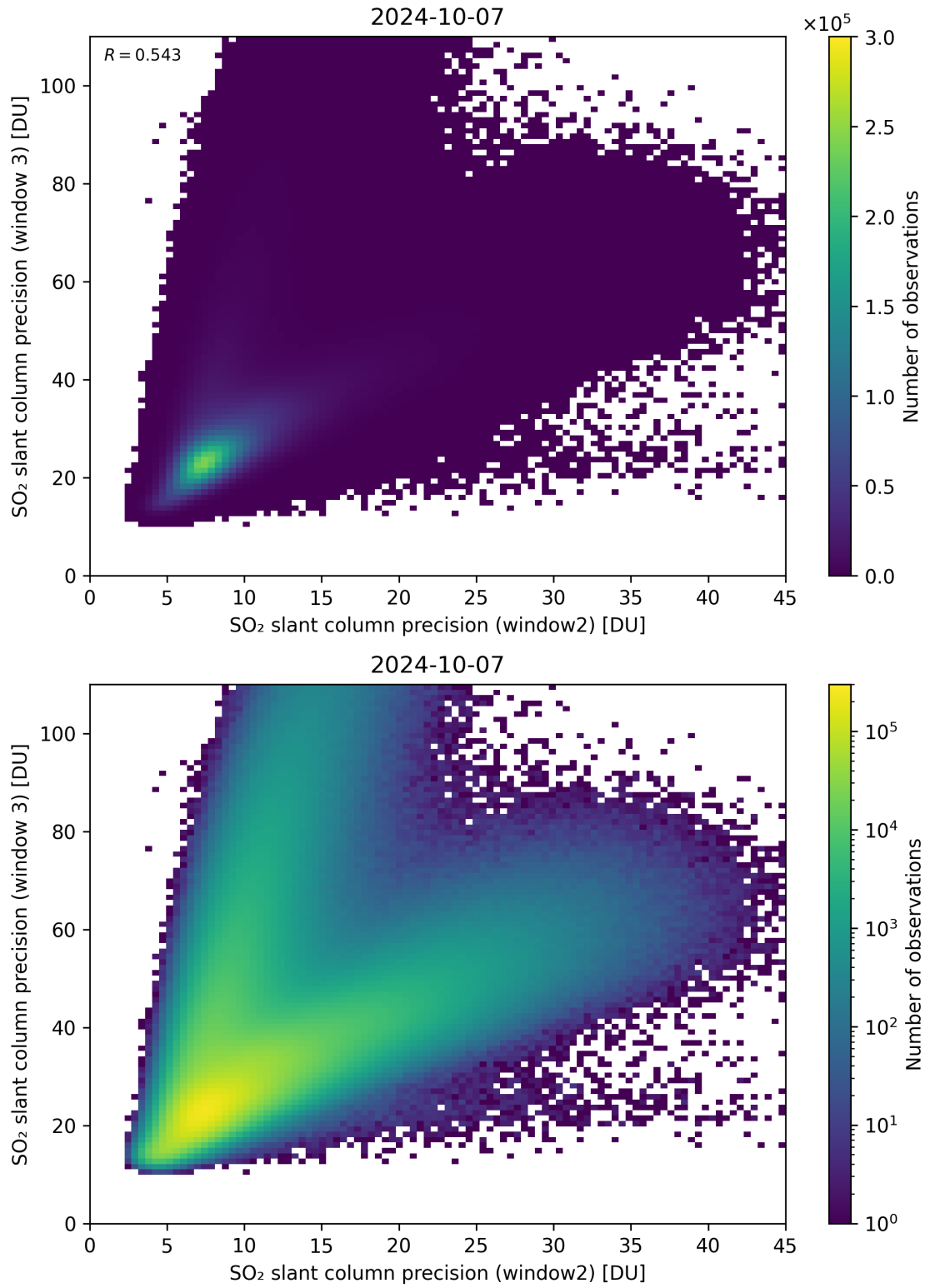
Figure 250: Scatter density plot of “SO 2 slant column precision (window2)” against “SO 2 slant column precision (window 3)” for 2024-10-06 to 2024-10-08.
