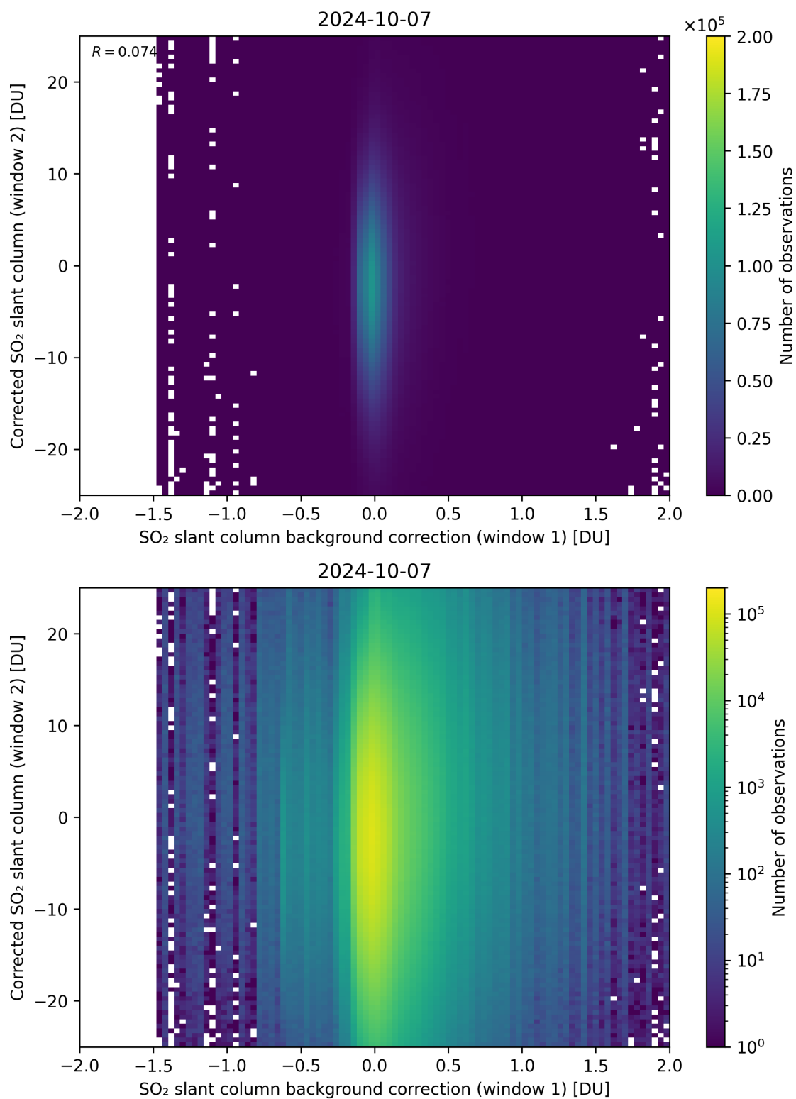
Figure 104: Scatter density plot of “SO 2 slant column background correction (window 1)” against “Corrected SO 2 slant column (window 2)” for 2024-10-06 to 2024-10-08.
