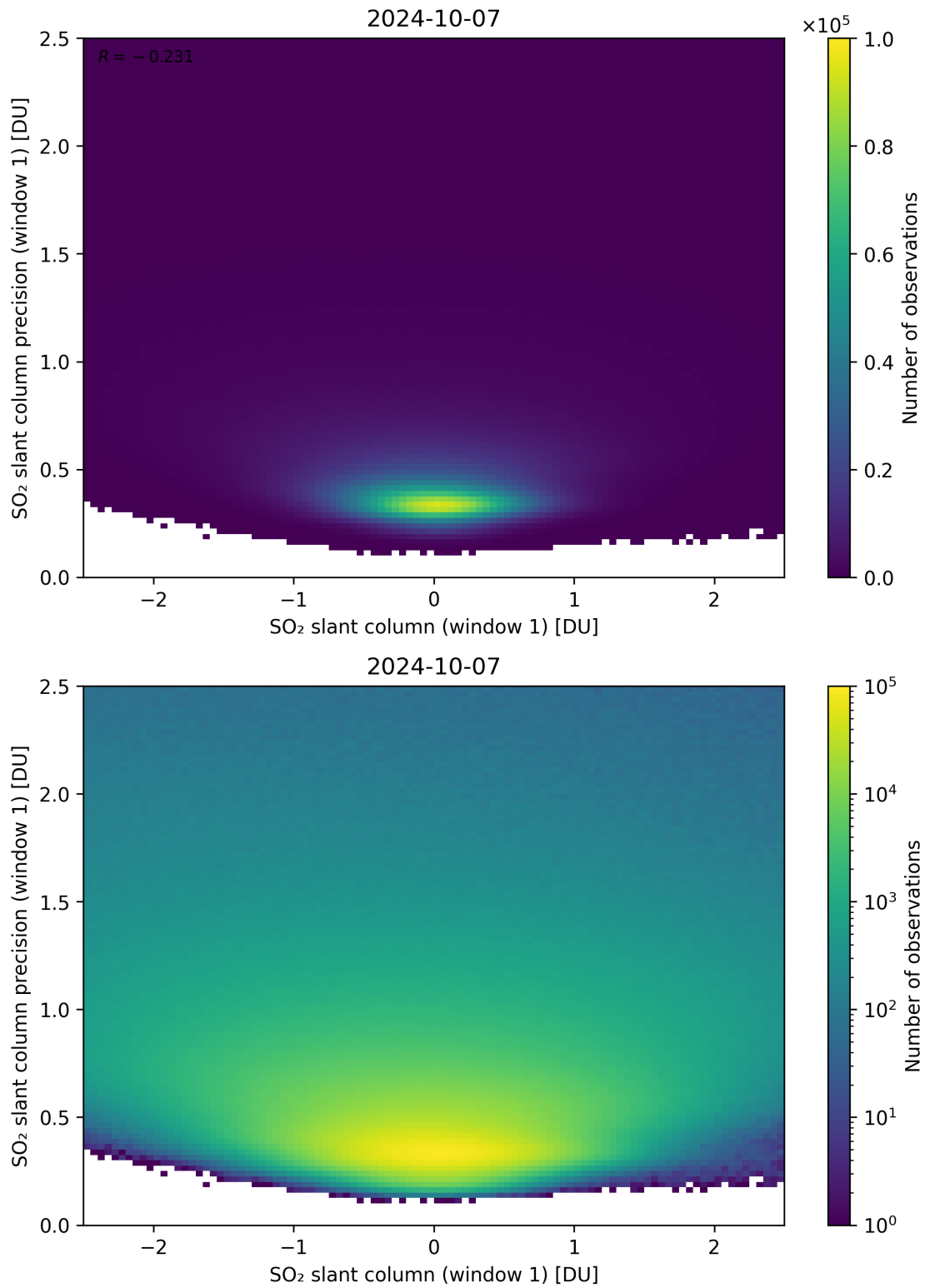
Figure 235: Scatter density plot of “SO 2 slant column (window 1)” against “SO 2 slant column precision (window 1)” for 2024-10-06 to 2024-10-08.
