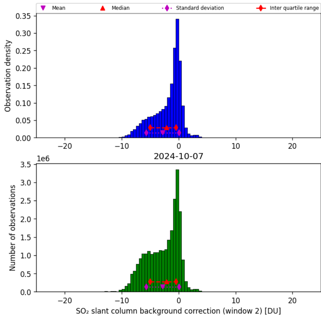
Figure 63: Histogram of “SO 2 slant column background correction (window 2)” for 2024-10-06 to 2024-10-08
