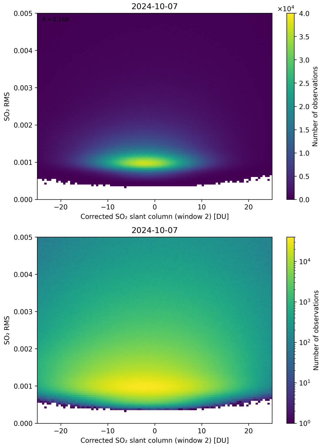
Figure 198: Scatter density plot of “Corrected SO 2 slant column (window 2)” against “SO 2 RMS” for 2024-10-06 to 2024-10-08.
