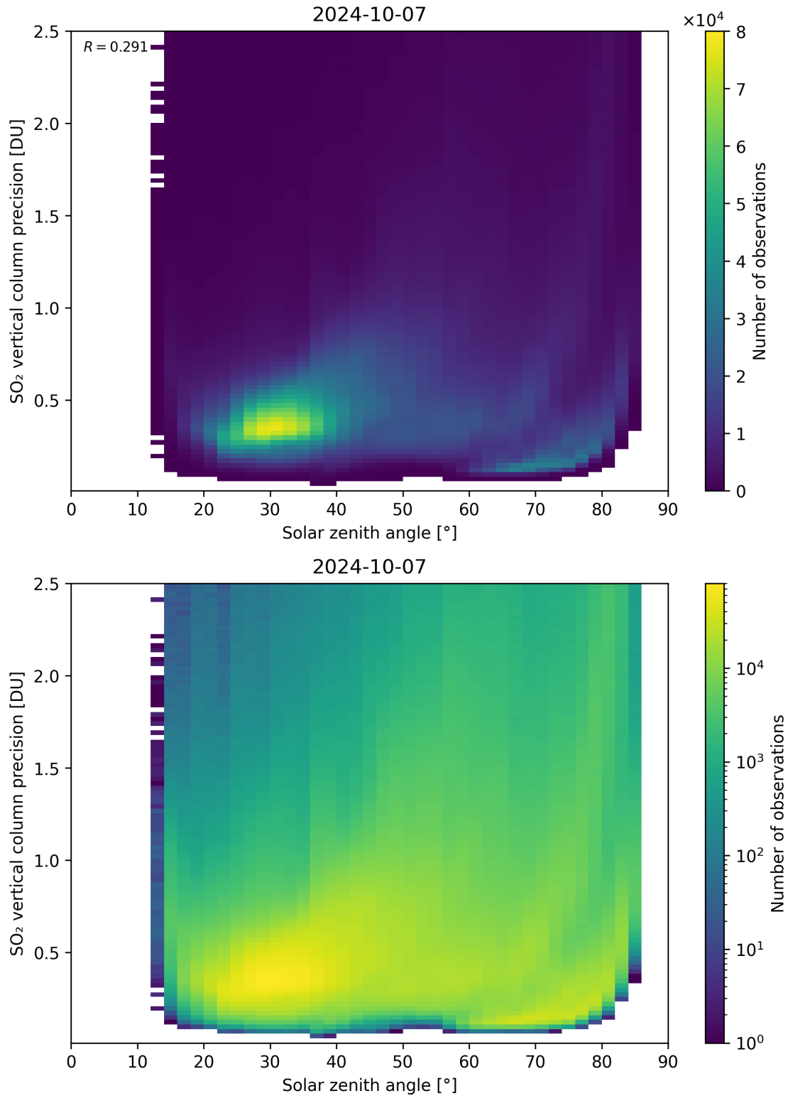
Figure 177: Scatter density plot of “Solar zenith angle” against “SO 2 vertical column precision” for 2024-10-06 to 2024-10-08.
