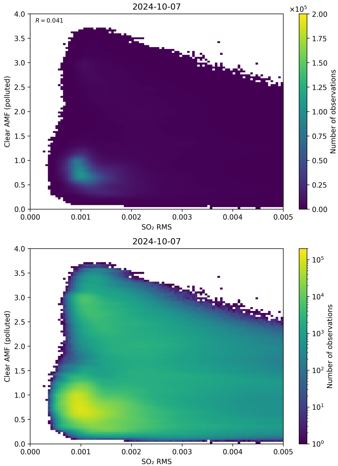
Figure 136: Scatter density plot of “SO 2 RMS” against “Clear AMF (polluted)” for 2024-10-06 to 2024-10-08.
