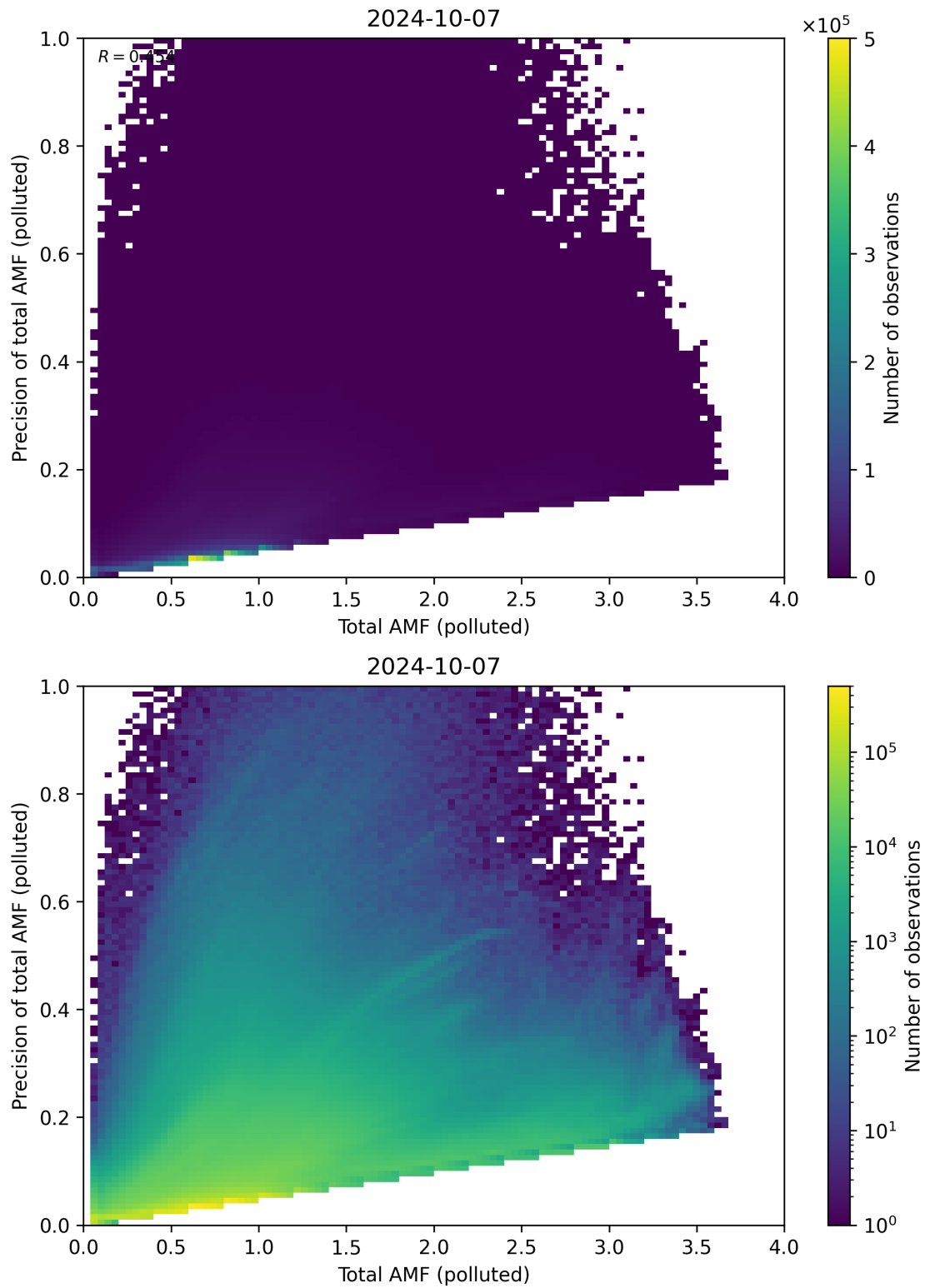
Figure 272: Scatter density plot of “Total AMF (polluted)” against “Precision of total AMF (polluted)” for 2024-10-06 to 2024-10-08.
