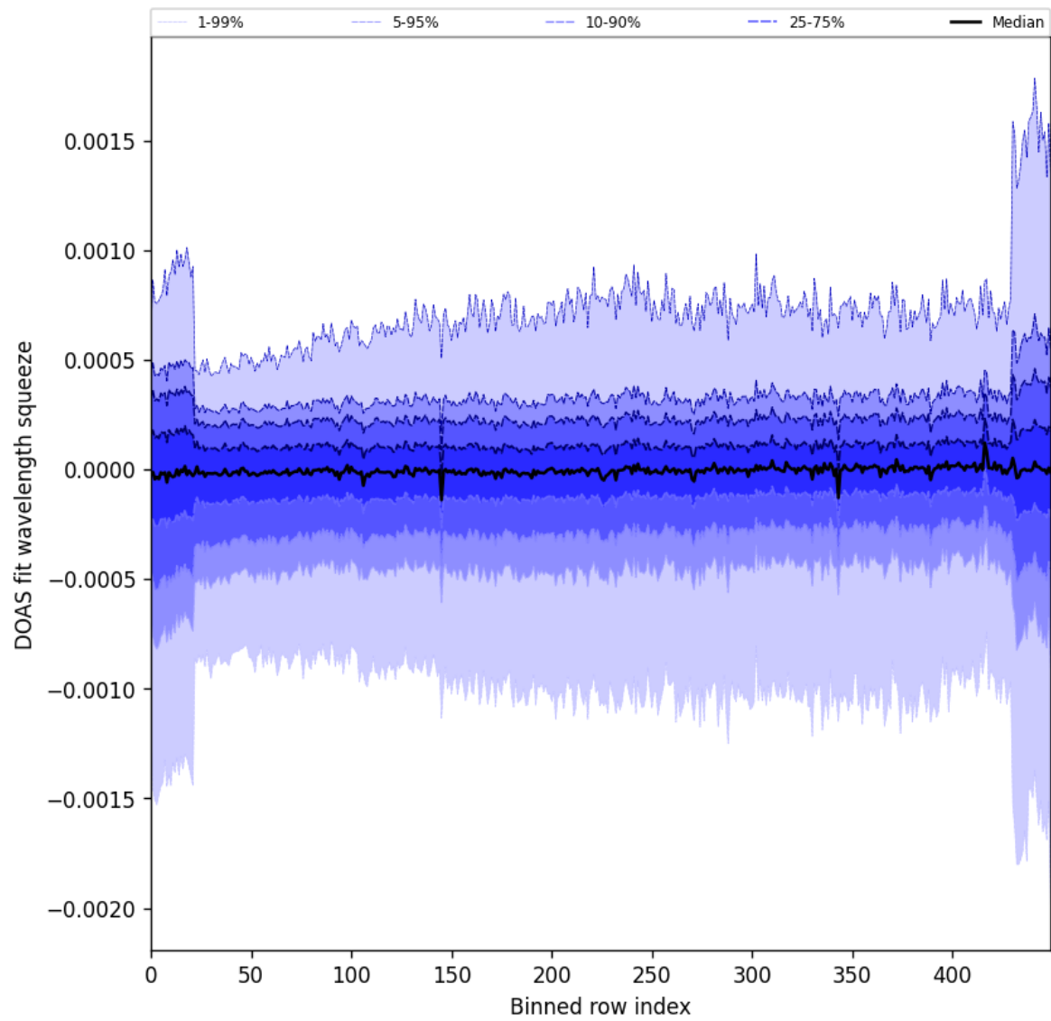
Figure 92: Along track statistics of “DOAS fit wavelength squeeze” for 2024-10-06 to 2024-10-08
