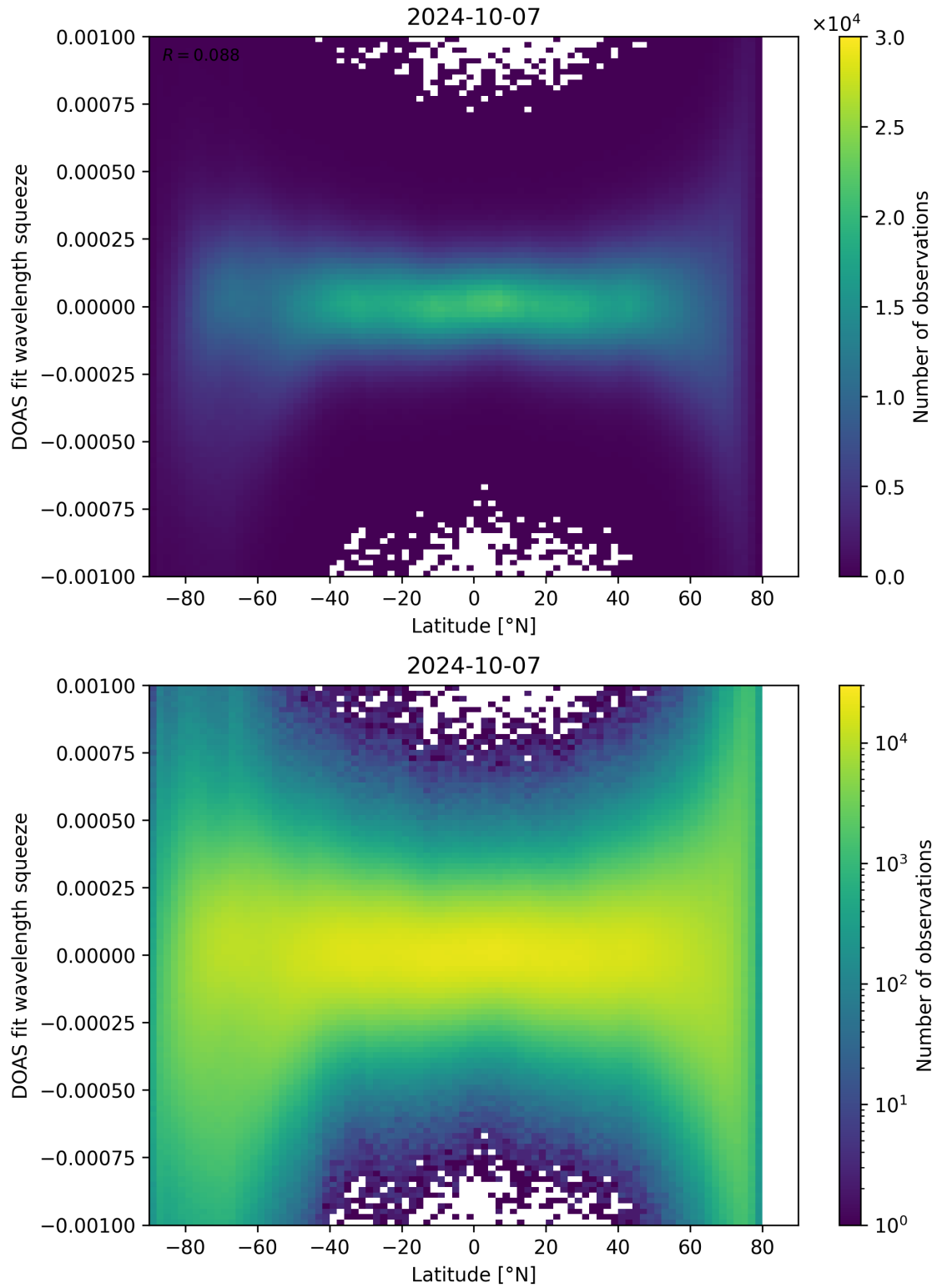
Figure 143: Scatter density plot of “Latitude” against “DOAS fit wavelength squeeze” for 2024-10-06 to 2024-10-08.
