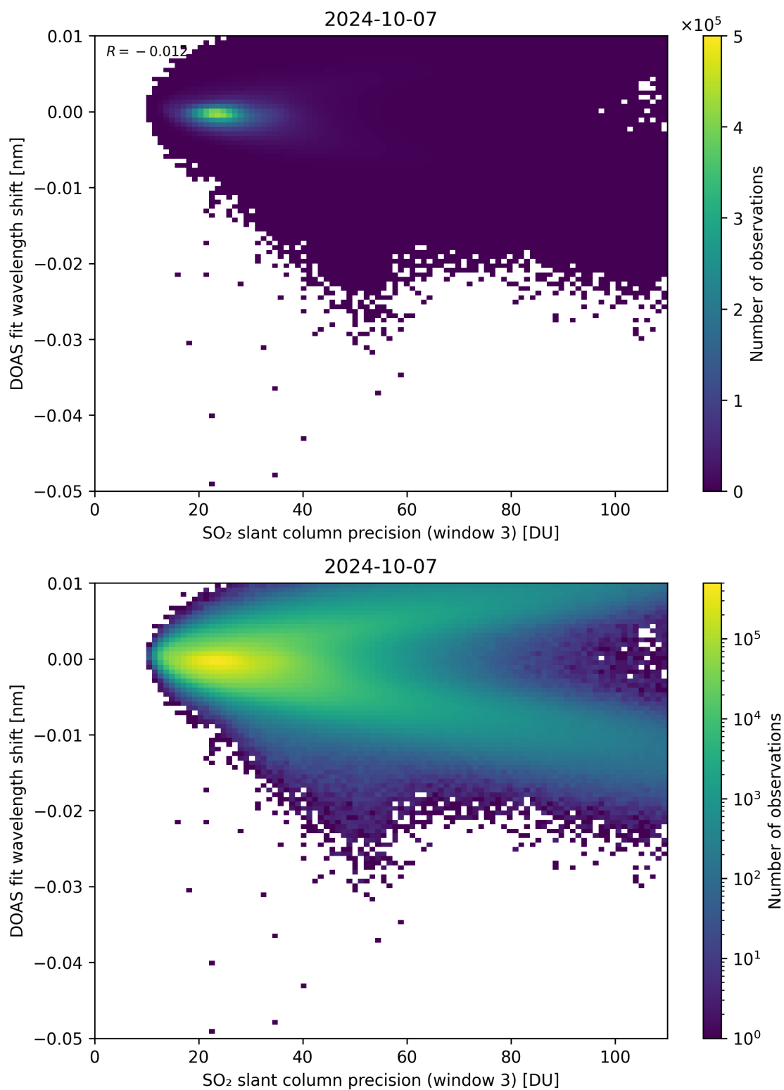
Figure 258: Scatter density plot of “SO 2 slant column precision (window 3)” against “DOAS fit wavelength shift” for 2024-10-06 to 2024-10-08.
