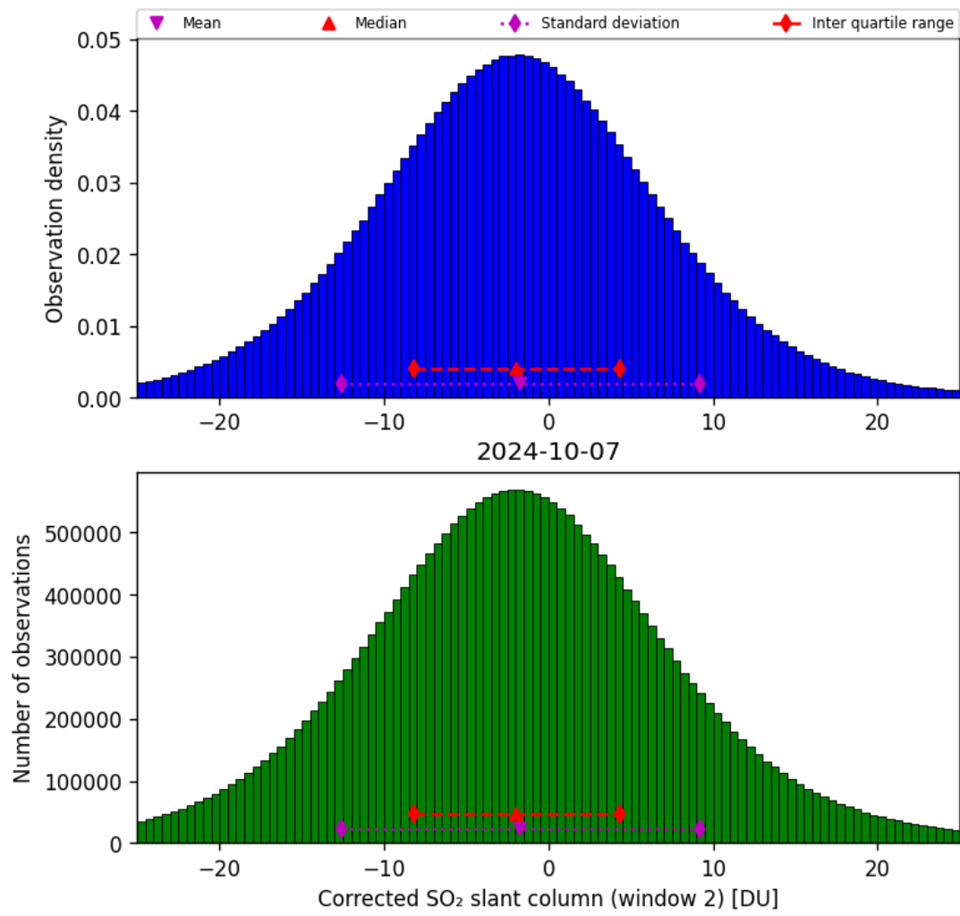
Figure 62: Histogram of “Corrected SO 2 slant column (window 2)” for 2024-10-06 to 2024-10-08
