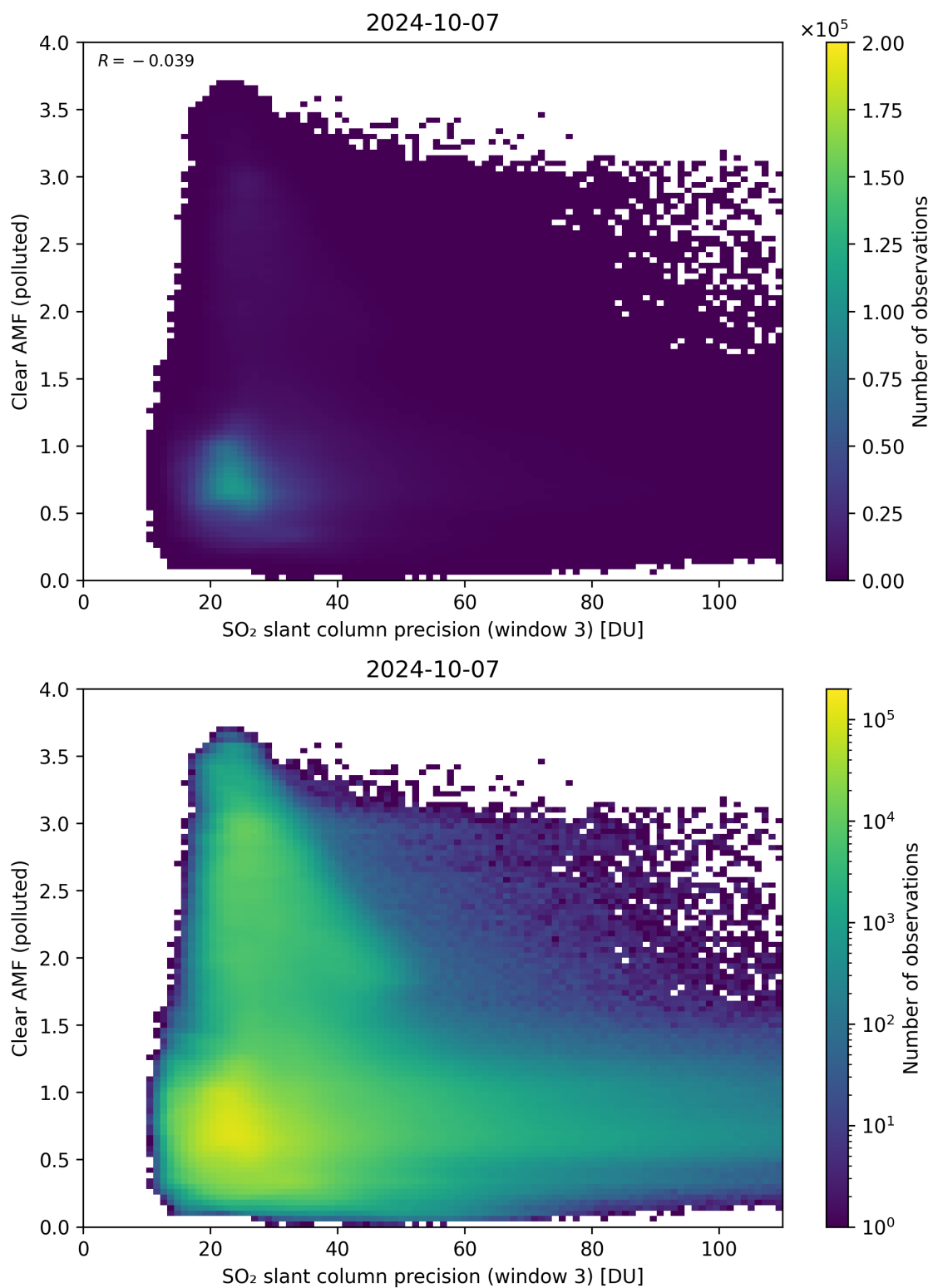
Figure 261: Scatter density plot of “SO 2 slant column precision (window 3)” against “Clear AMF (polluted)” for 2024-10-06 to 2024-10-08.
