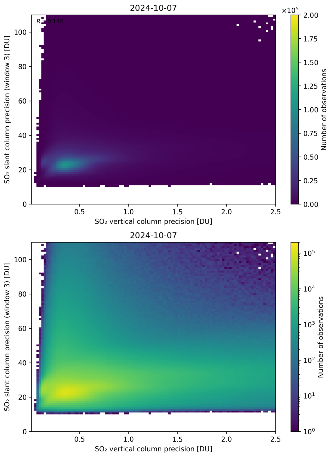
Figure 293: Scatter density plot of “SO 2 vertical column precision” against “SO 2 slant column precision (window 3)” for 2024-10-06 to 2024-10-08.
