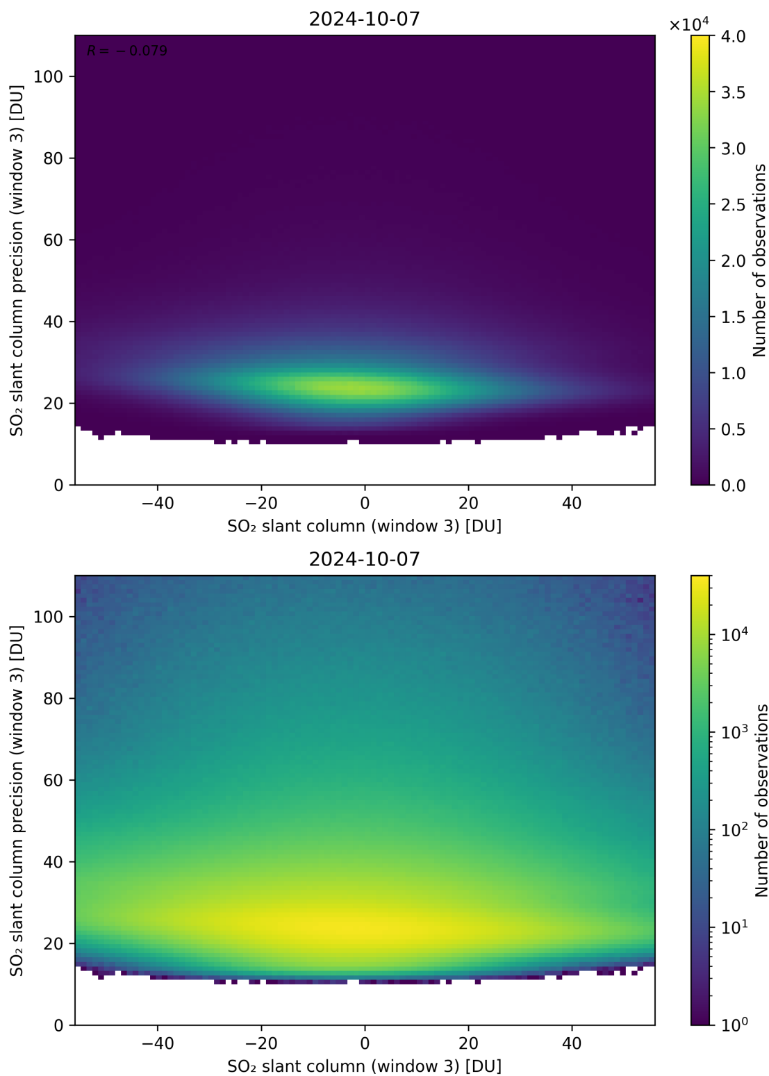
Figure 267: Scatter density plot of “SO 2 slant column (window 3)” against “SO 2 slant column precision (window 3)” for 2024-10-06 to 2024-10-08.
