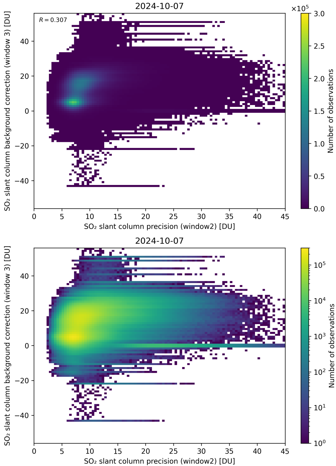
Figure 242: Scatter density plot of “SO 2 slant column precision (window2)” against “SO 2 slant column background correction (window 3)” for 2024-10-06 to 2024-10-08.
