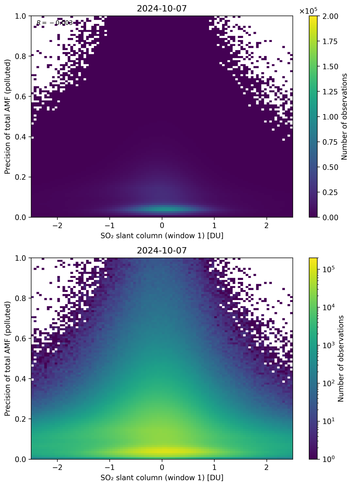
Figure 240: Scatter density plot of “SO 2 slant column (window 1)” against “Precision of total AMF (polluted)” for 2024-10-06 to 2024-10-08.
