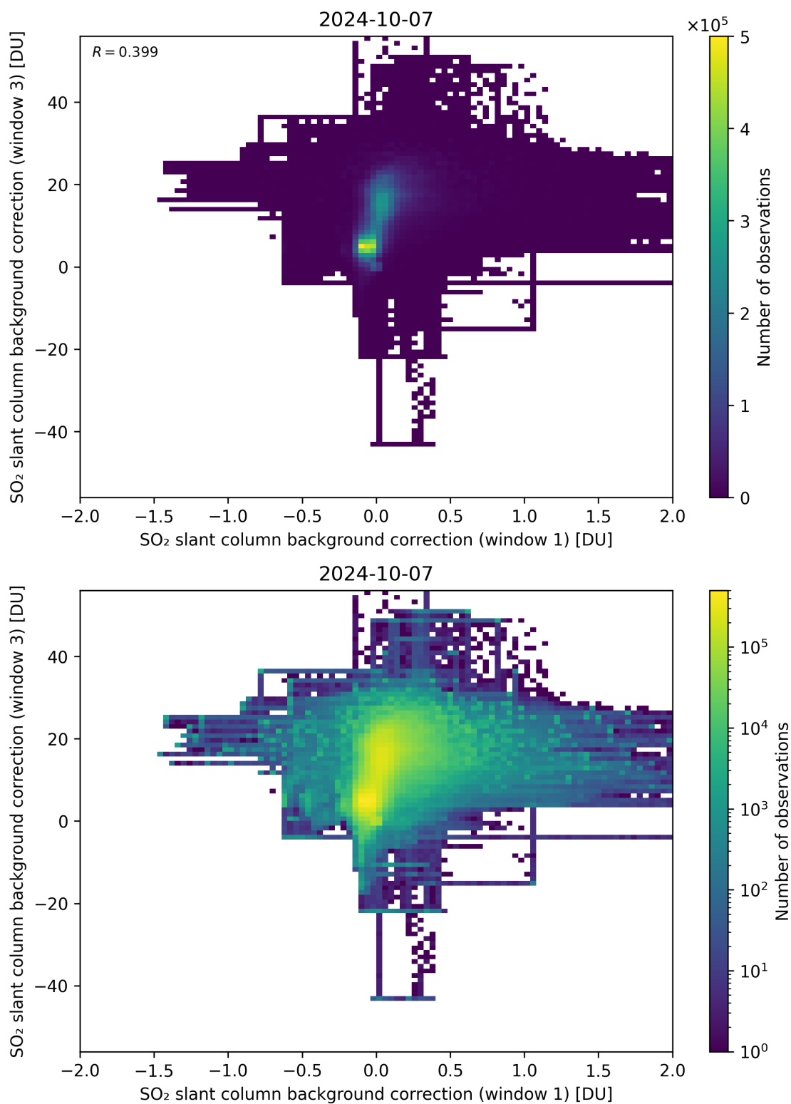
Figure 99: Scatter density plot of “SO 2 slant column background correction (window 1)” against “SO 2 slant column background correction (window 3)” for 2024-10-06 to 2024-10-08.
