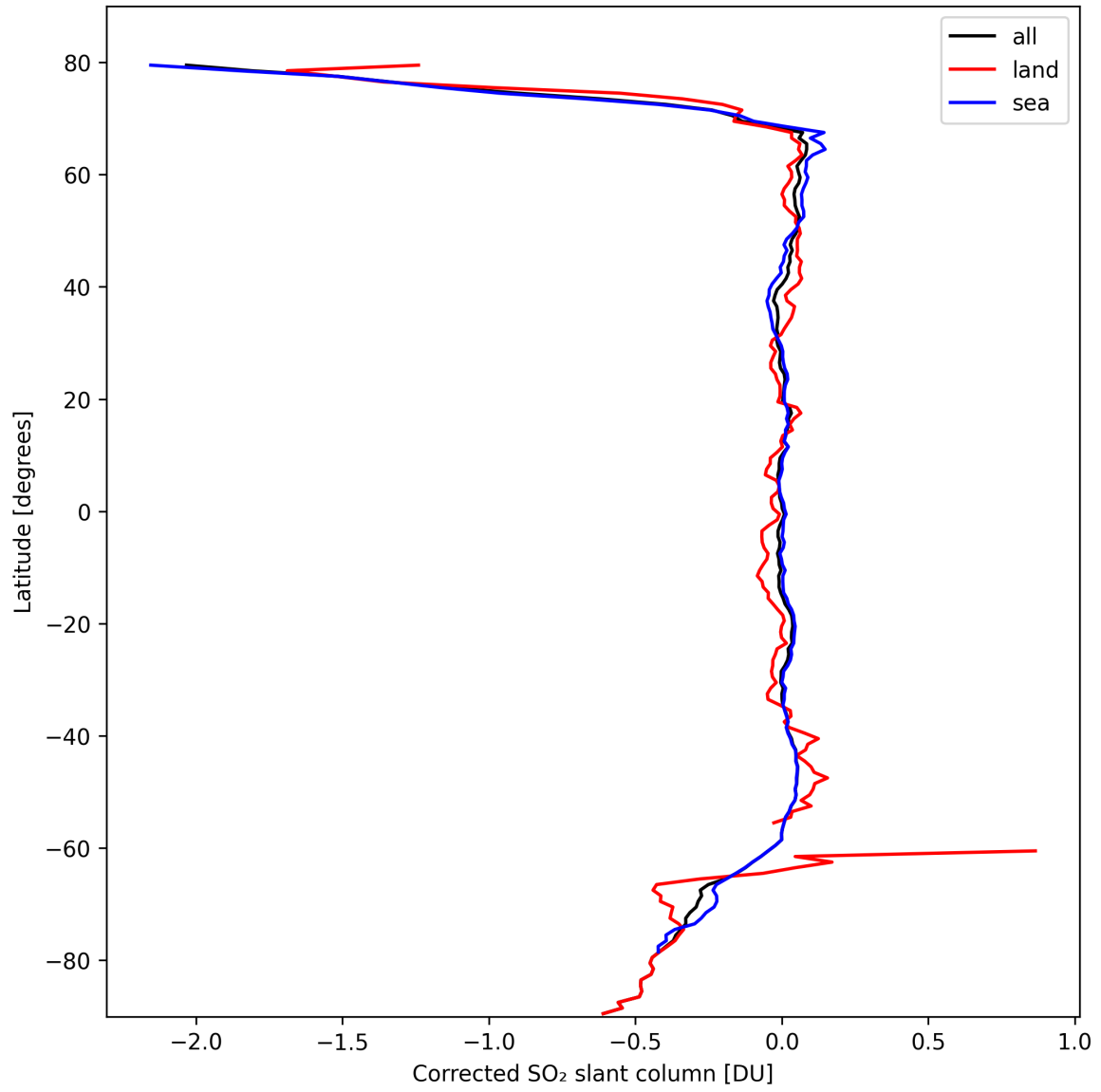
Figure 32: Zonal average of “Corrected SO 2 slant column” for 2024-10-06 to 2024-10-08.
