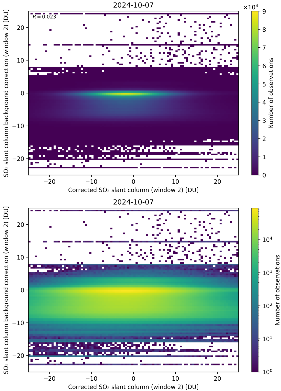
Figure 194: Scatter density plot of “Corrected SO 2 slant column (window 2)” against “SO 2 slant column background correction (window 2)” for 2024-10-06 to 2024-10-08.
