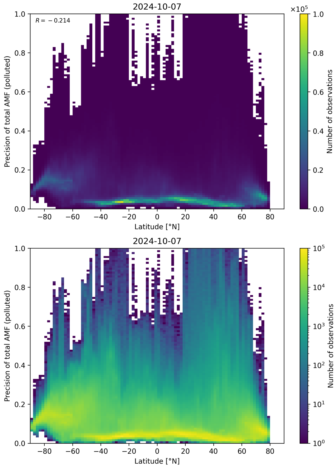
Figure 155: Scatter density plot of “Latitude” against “Precision of total AMF (polluted)” for 2024-10-06 to 2024-10-08.
