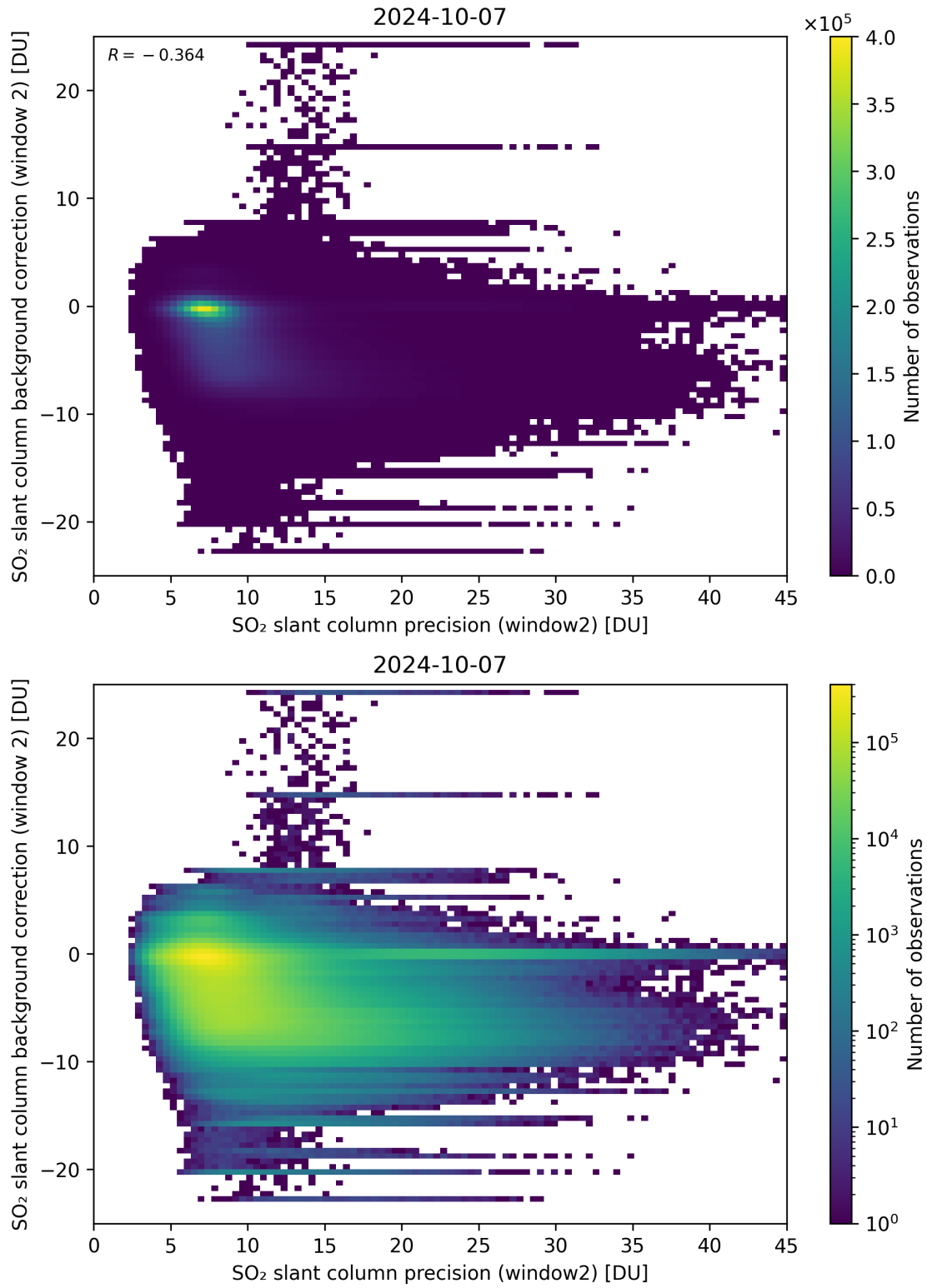
Figure 241: Scatter density plot of “SO 2 slant column precision (window2)” against “SO 2 slant column background correction (window 2)” for 2024-10-06 to 2024-10-08.
