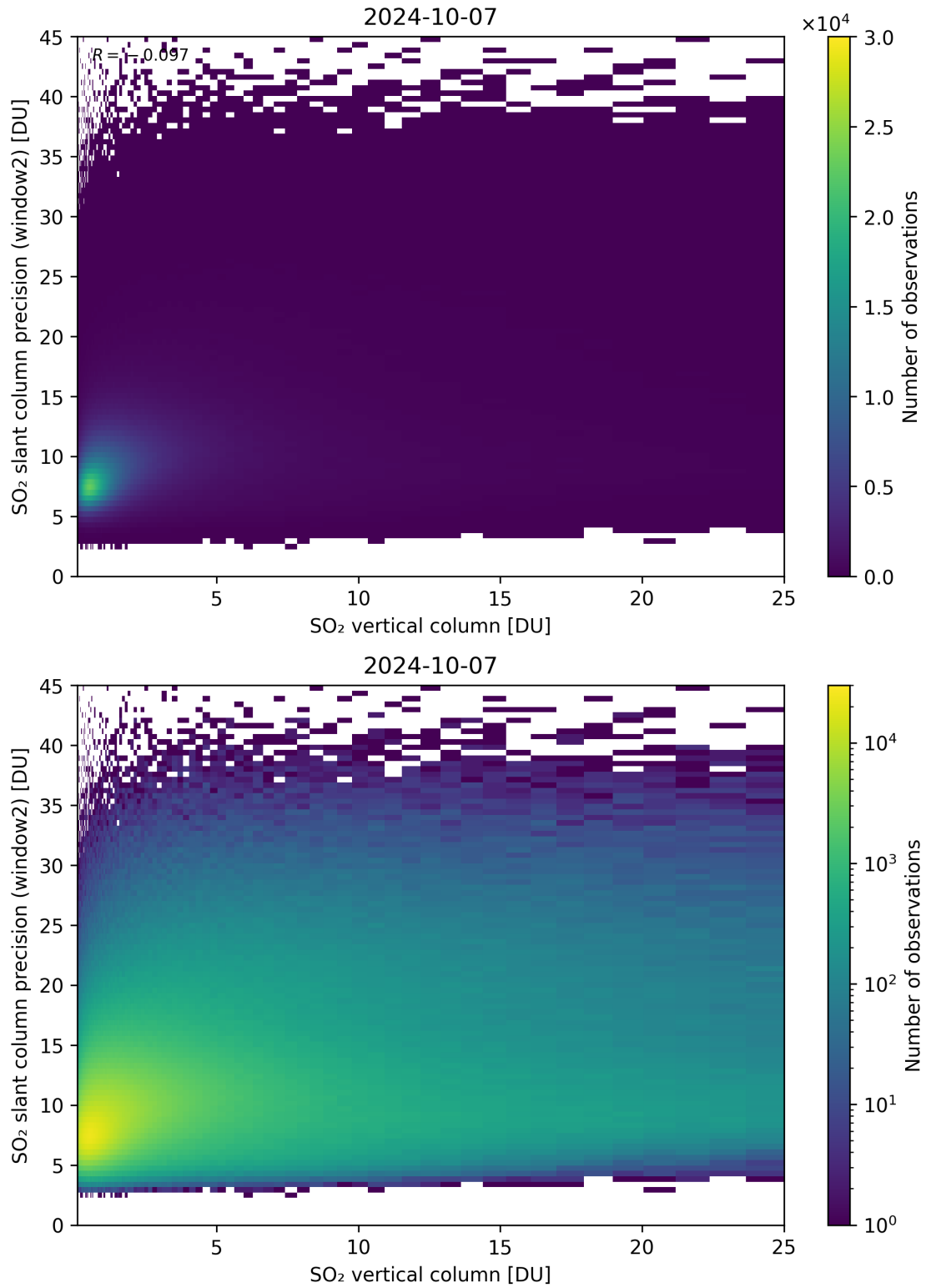
Figure 302: Scatter density plot of “SO 2 vertical column” against “SO 2 slant column precision (window2)” for 2024-10-06 to 2024-10-08.
