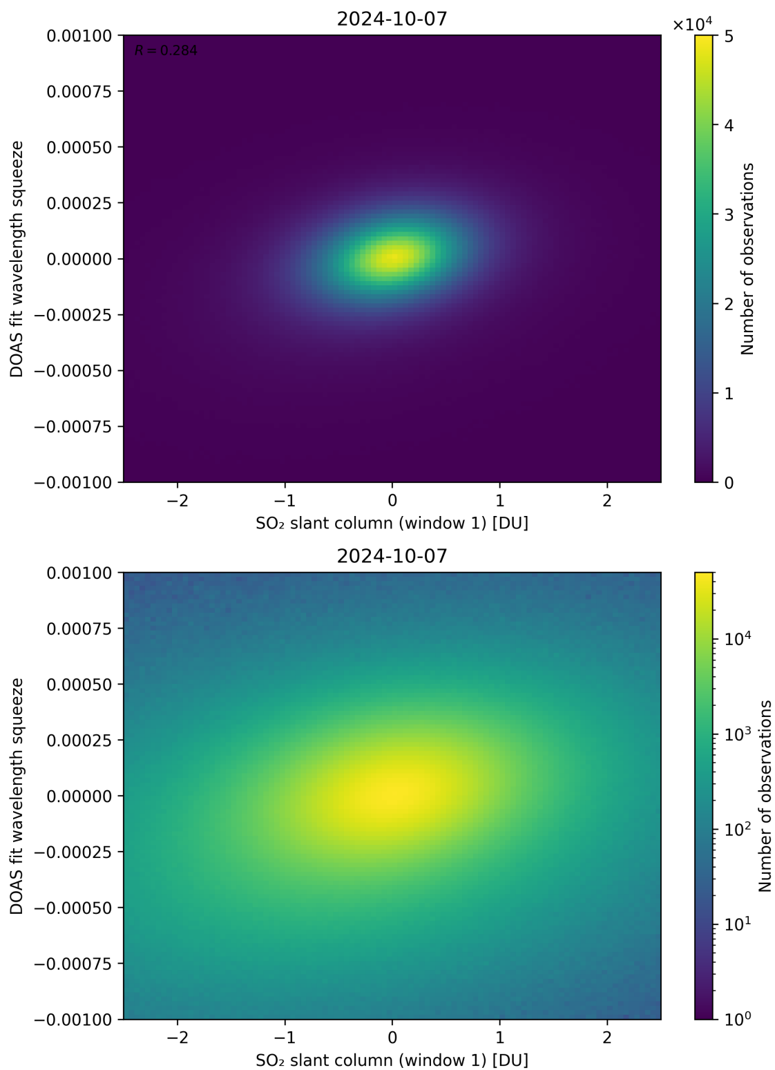
Figure 216: Scatter density plot of “SO 2 slant column (window 1)” against “DOAS fit wavelength squeeze” for 2024-10-06 to 2024-10-08.
