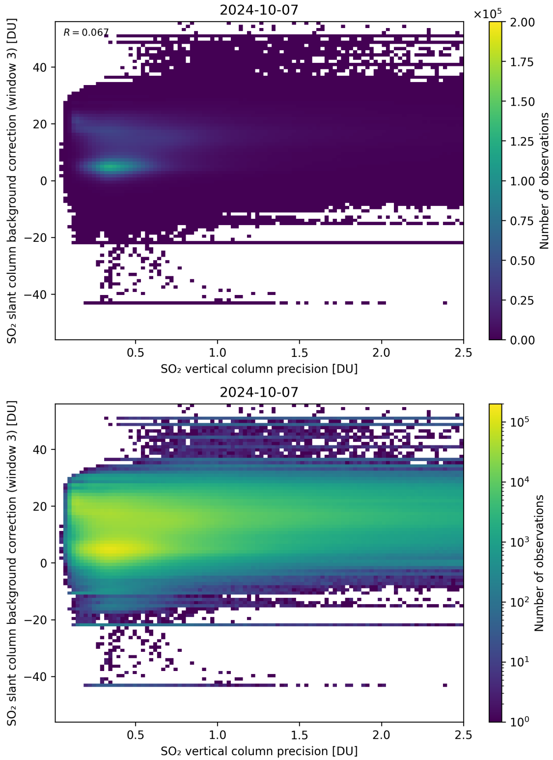
Figure 281: Scatter density plot of “SO 2 vertical column precision” against “SO 2 slant column background correction (window 3)” for 2024-10-06 to 2024-10-08.
