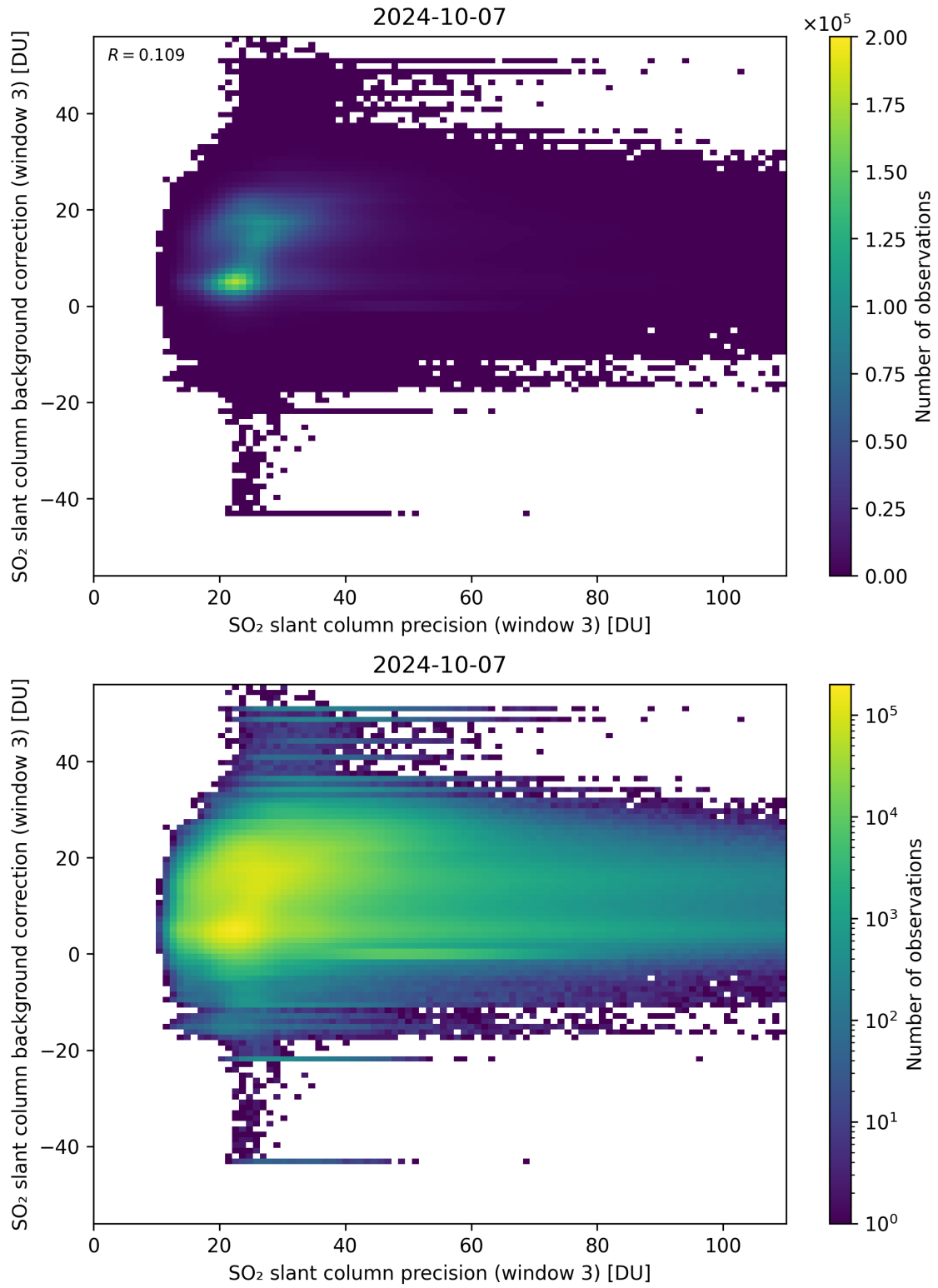
Figure 257: Scatter density plot of “SO 2 slant column precision (window 3)” against “SO 2 slant column background correction (window 3)” for 2024-10-06 to 2024-10-08.
