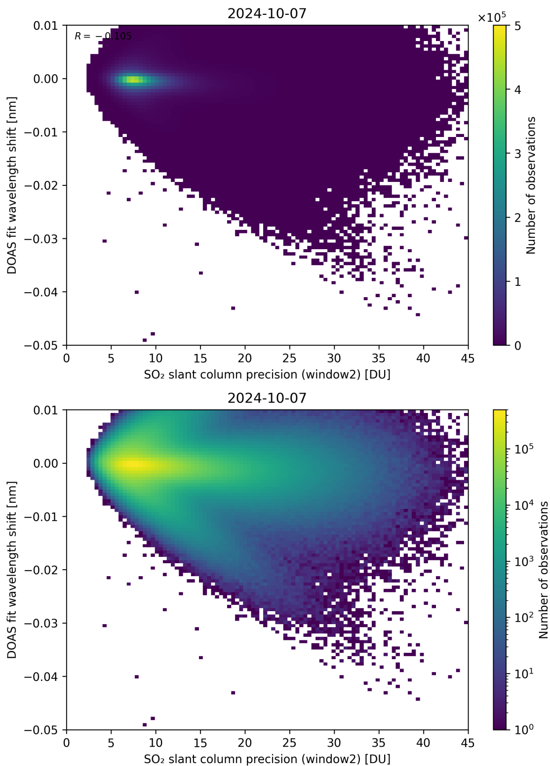
Figure 243: Scatter density plot of “SO 2 slant column precision (window2)” against “DOAS fit wavelength shift” for 2024-10-06 to 2024-10-08.
