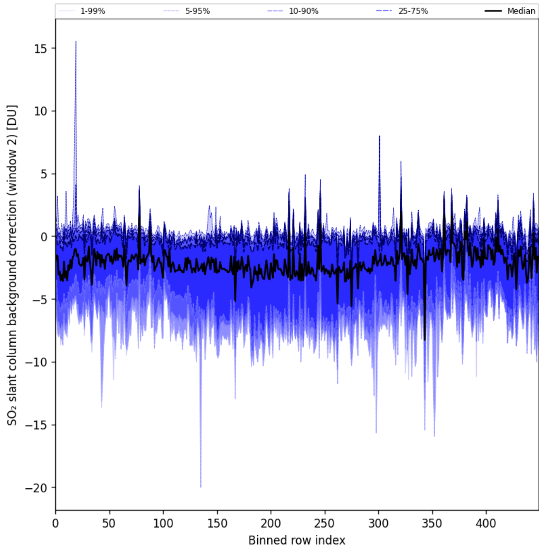
Figure 86: Along track statistics of “SO 2 slant column background correction (window 2)” for 2024-10-06 to 2024-10-08
