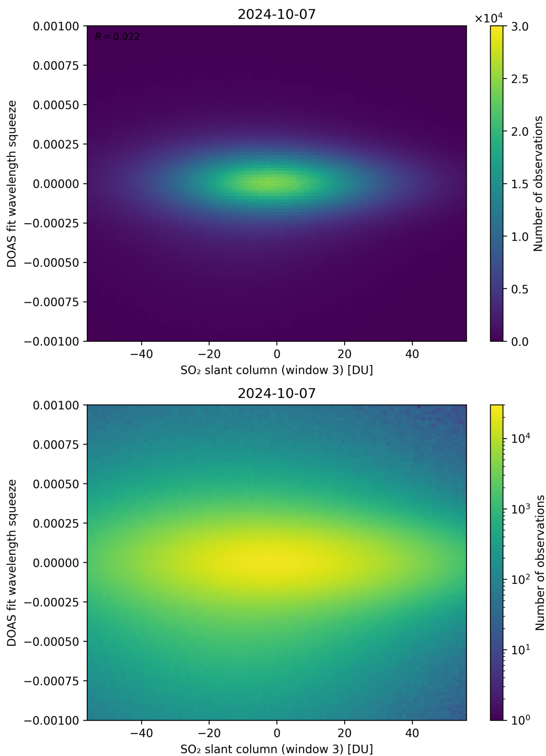
Figure 255: Scatter density plot of “SO 2 slant column (window 3)” against “DOAS fit wavelength squeeze” for 2024-10-06 to 2024-10-08.
