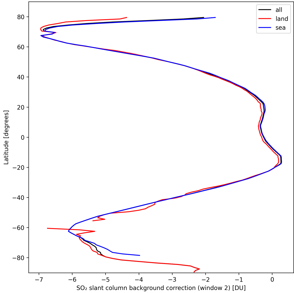
Figure 40: Zonal average of “SO 2 slant column background correction (window 2)” for 2024-10-06 to 2024-10-08.
