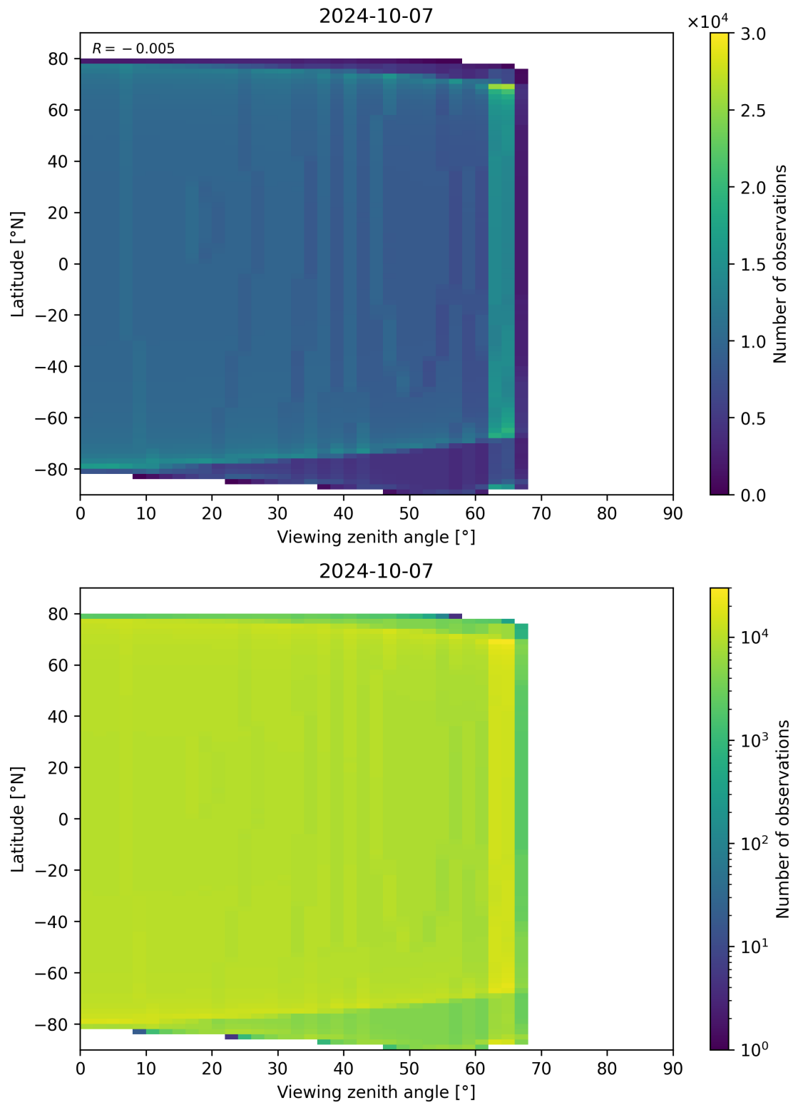
Figure 314: Scatter density plot of “Viewing zenith angle” against “Latitude” for 2024-10-06 to 2024-10-08.
