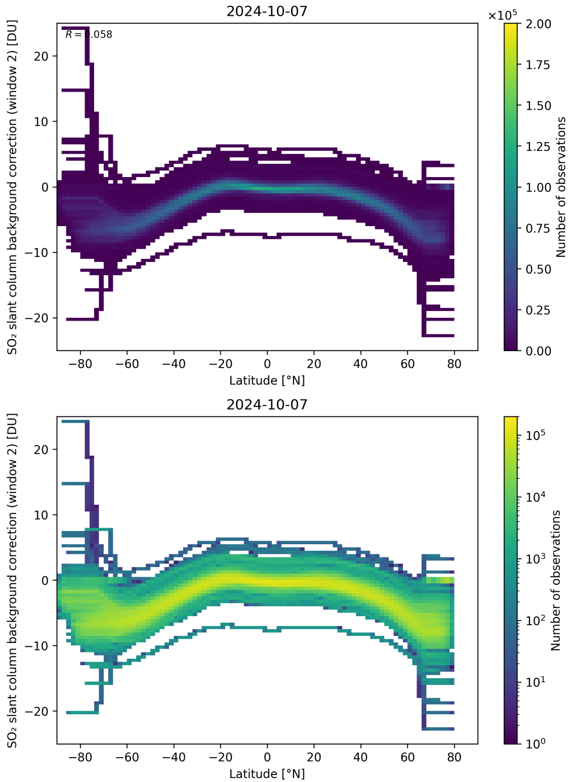
Figure 140: Scatter density plot of “Latitude” against “SO 2 slant column background correction (window 2)” for 2024-10-06 to 2024-10-08.
