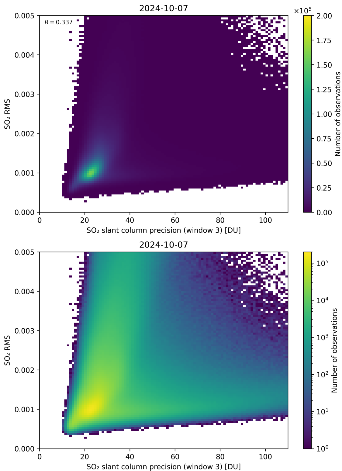
Figure 260: Scatter density plot of “SO 2 slant column precision (window 3)” against “SO 2 RMS” for 2024-10-06 to 2024-10-08.
