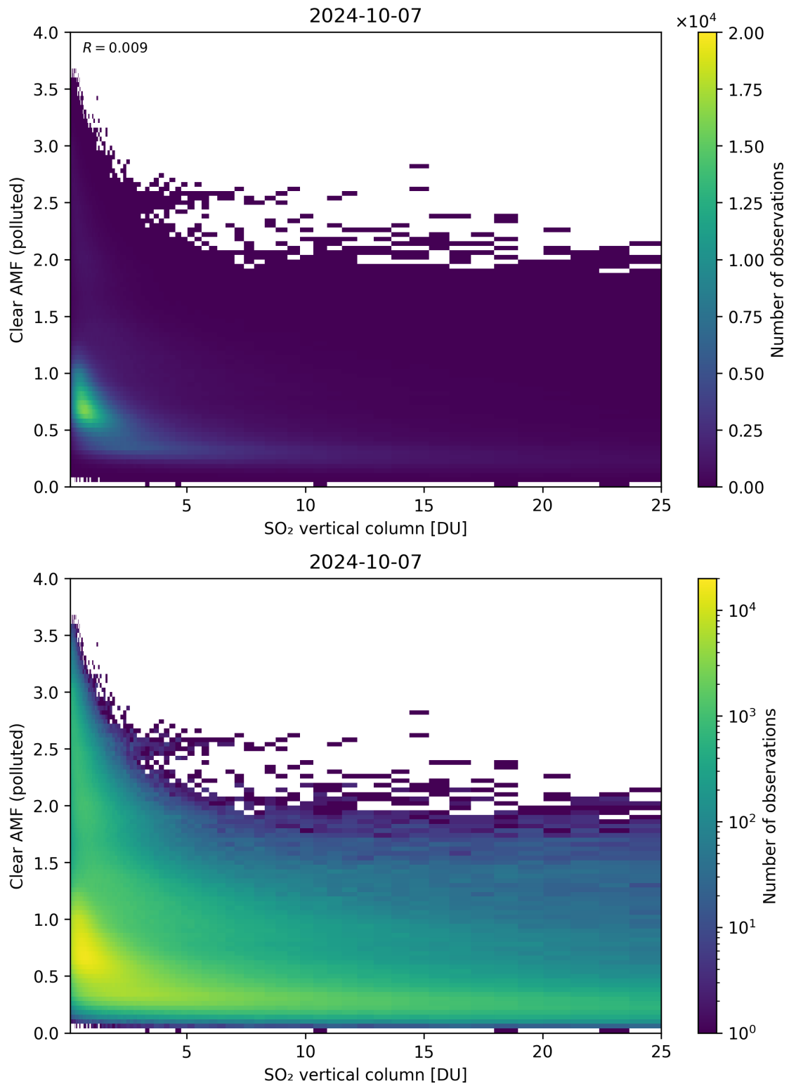
Figure 296: Scatter density plot of “SO 2 vertical column” against “Clear AMF (polluted)” for 2024-10-06 to 2024-10-08.
