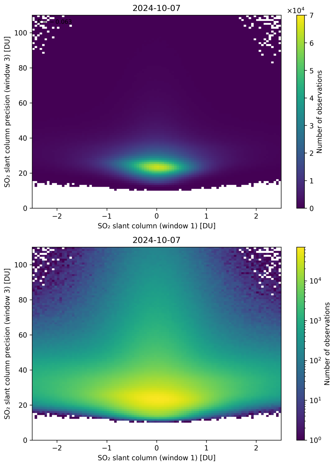
Figure 238: Scatter density plot of “SO 2 slant column (window 1)” against “SO 2 slant column precision (window 3)” for 2024-10-06 to 2024-10-08.
