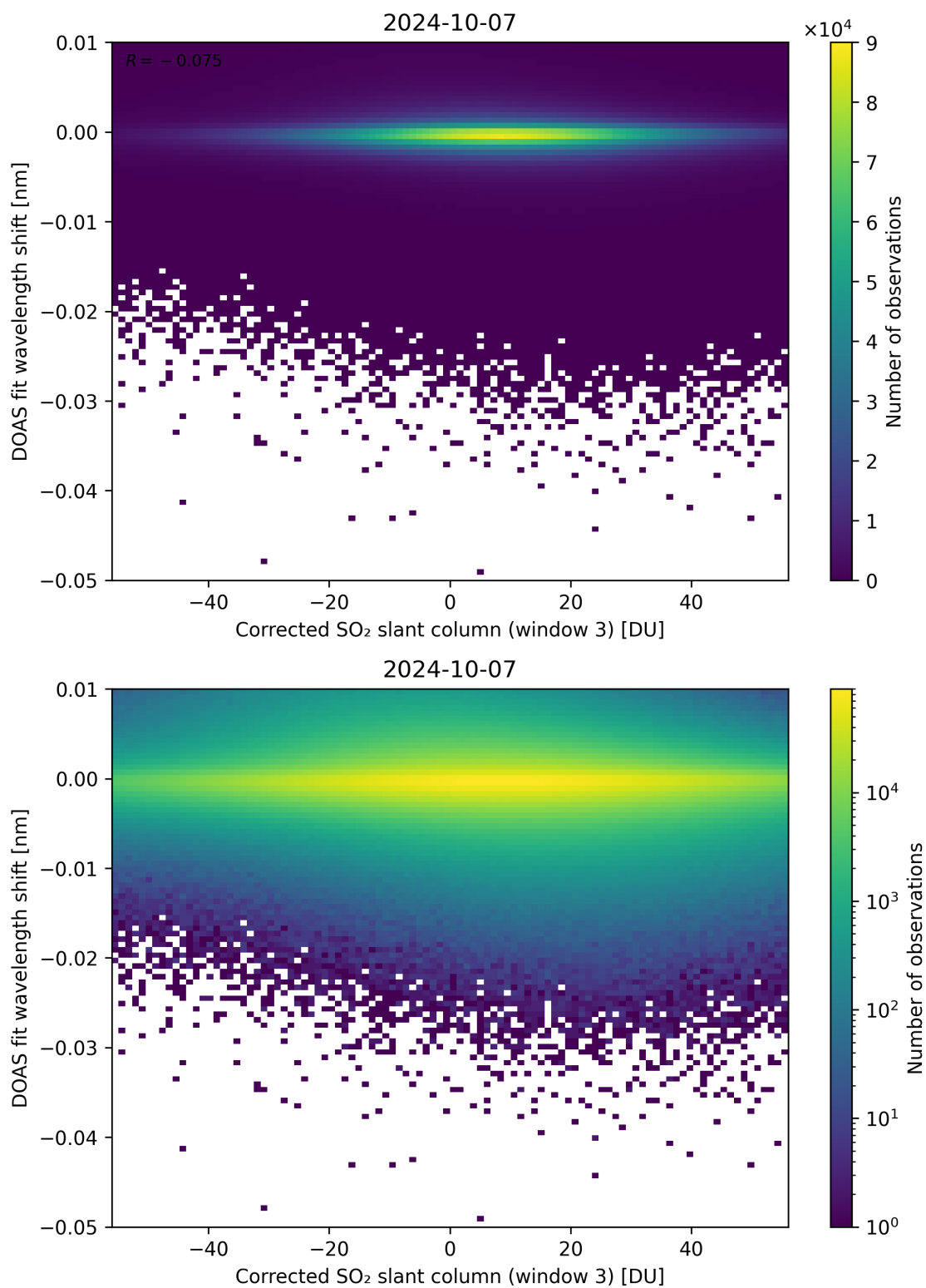
Figure 206: Scatter density plot of “Corrected SO 2 slant column (window 3)” against “DOAS fit wavelength shift” for 2024-10-06 to 2024-10-08.
