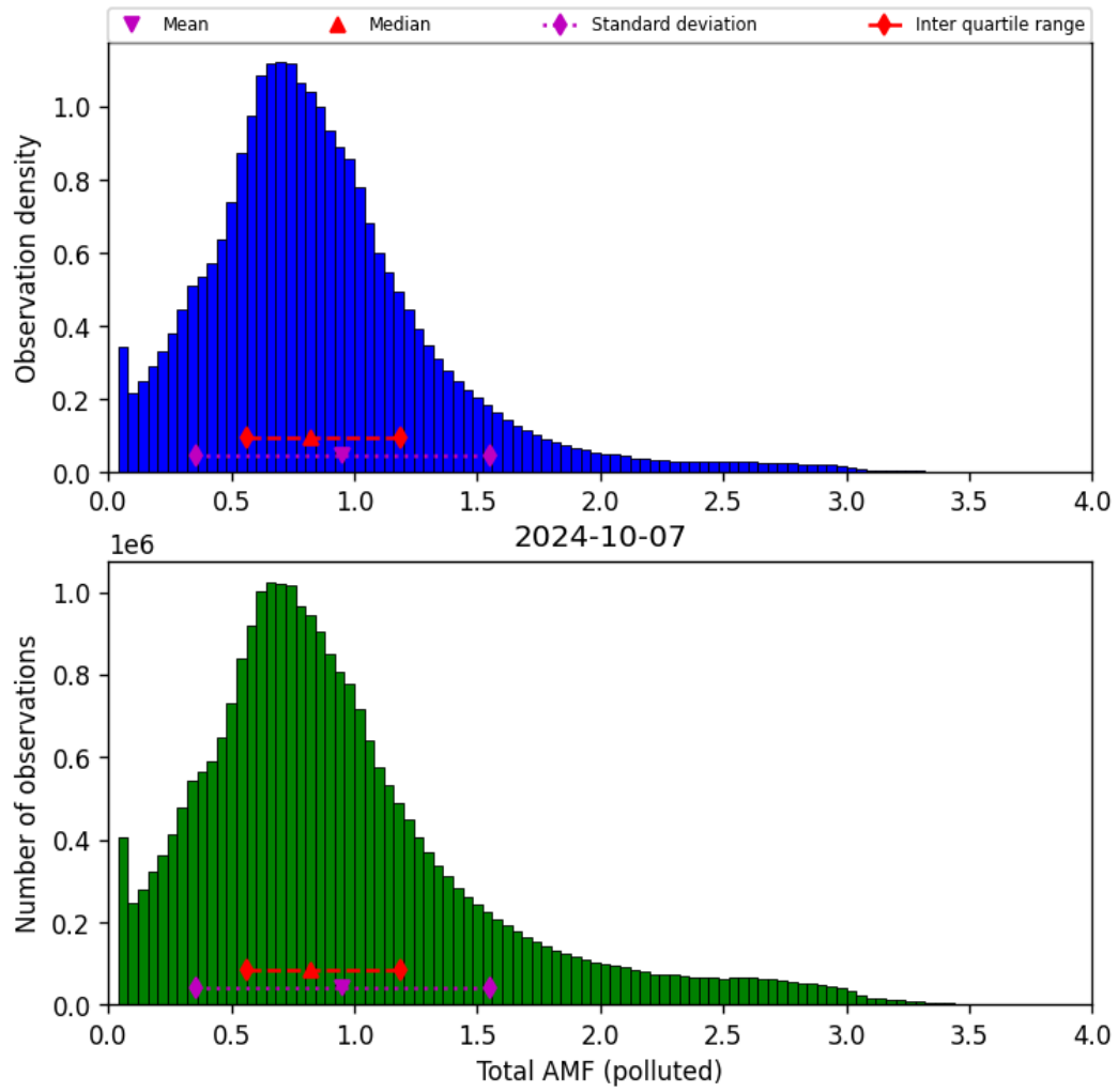
Figure 71: Histogram of “Total AMF (polluted)” for 2024-10-06 to 2024-10-08
