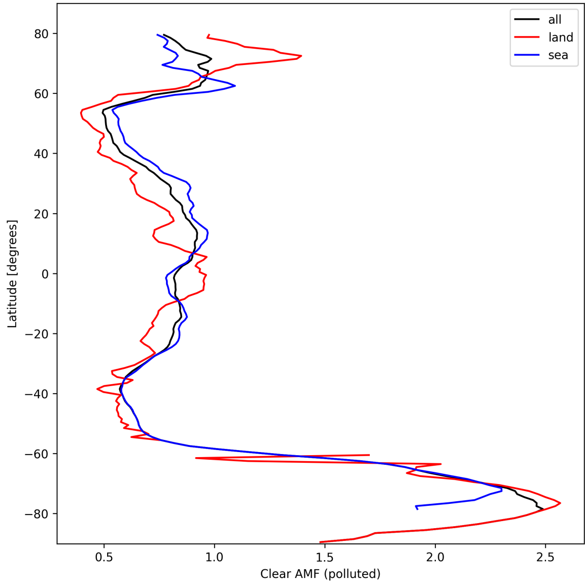
Figure 50: Zonal average of “Clear AMF (polluted)” for 2024-10-06 to 2024-10-08.
