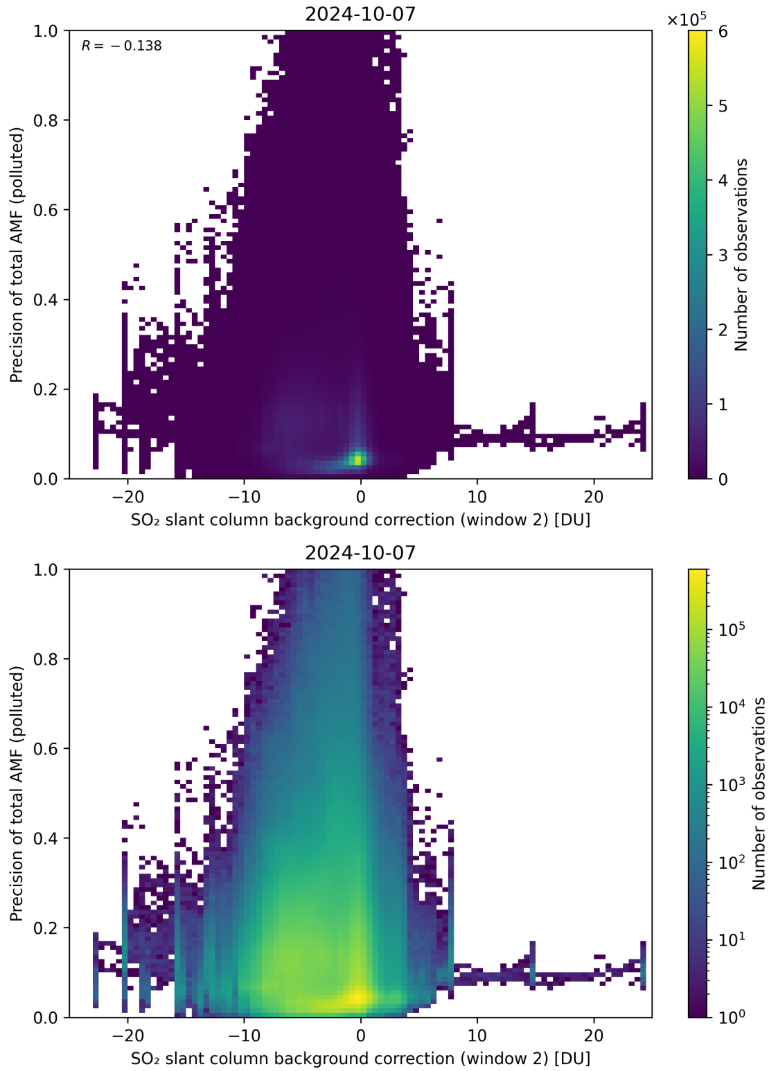
Figure 120: Scatter density plot of “SO 2 slant column background correction (window 2)” against “Precision of total AMF (polluted)” for 2024-10-06 to 2024-10-08.
