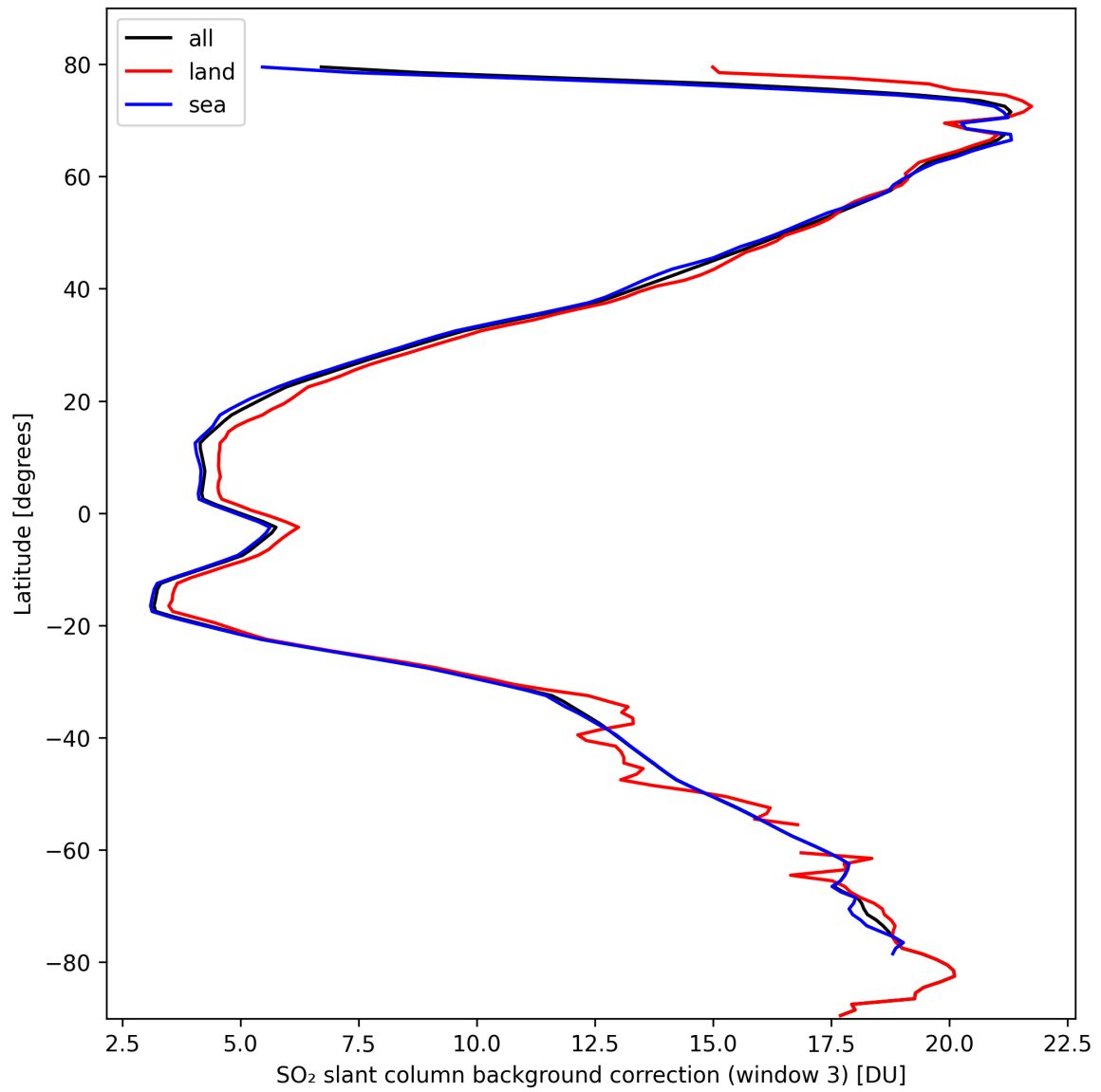
Figure 44: Zonal average of “SO 2 slant column background correction (window 3)” for 2024-10-06 to 2024-10-08.
