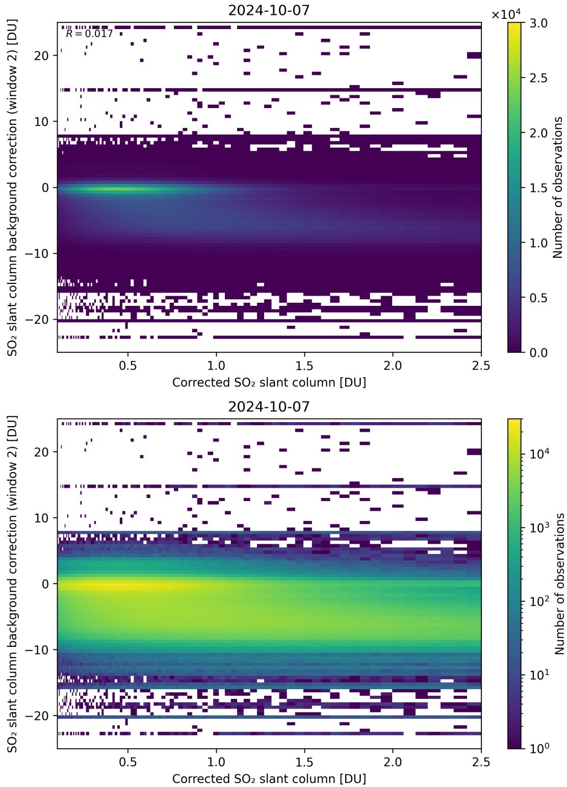
Figure 179: Scatter density plot of “Corrected SO 2 slant column” against “SO 2 slant column background correction (window 2)” for 2024-10-06 to 2024-10-08.
