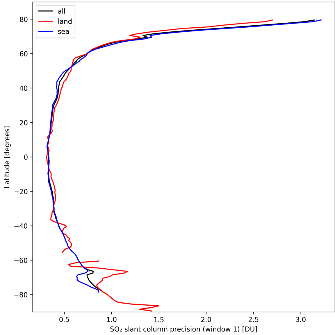
Figure 34: Zonal average of “SO 2 slant column precision (window 1)” for 2024-10-06 to 2024-10-08.
