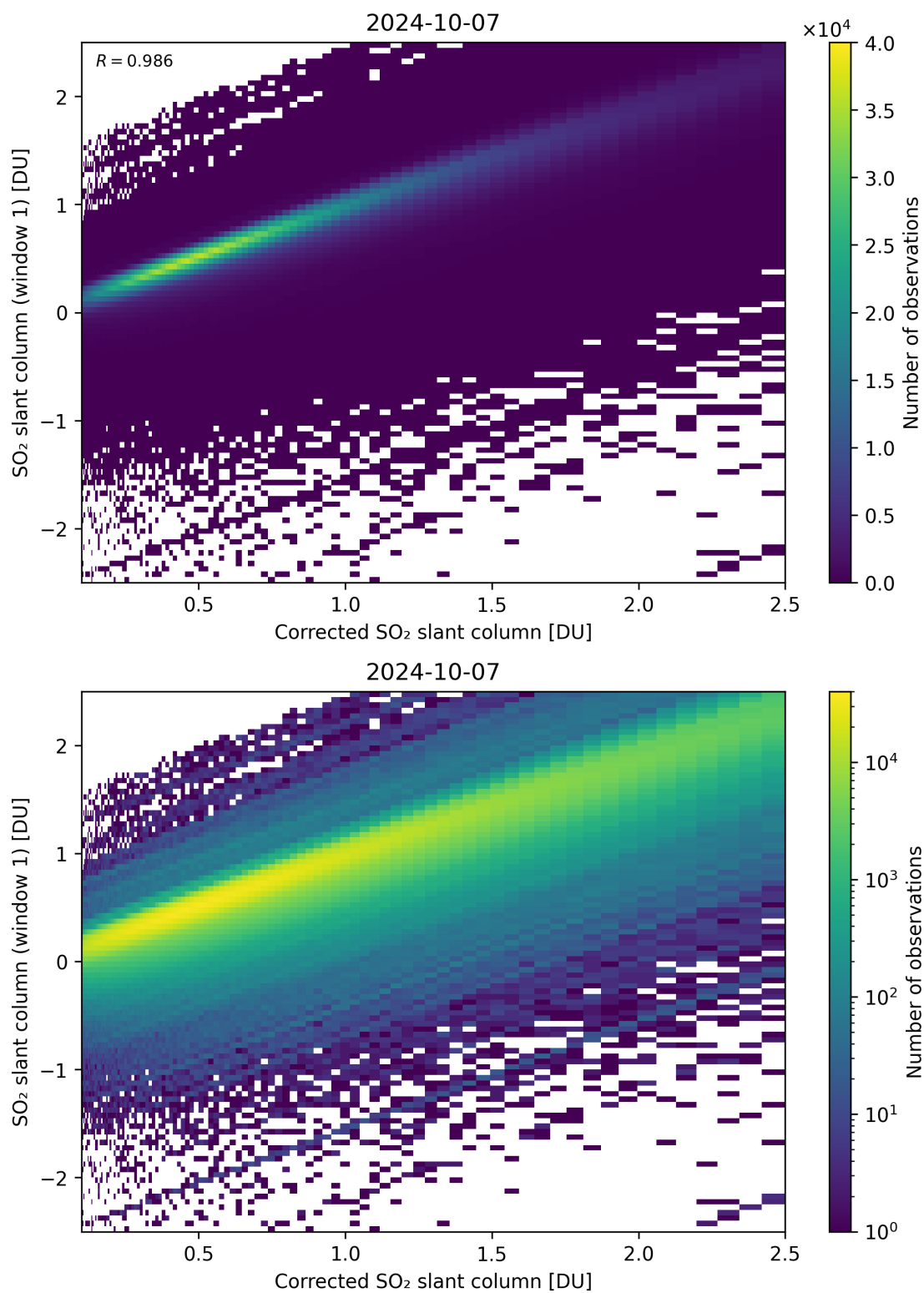
Figure 187: Scatter density plot of “Corrected SO 2 slant column” against “SO 2 slant column (window 1)” for 2024-10-06 to 2024-10-08.
