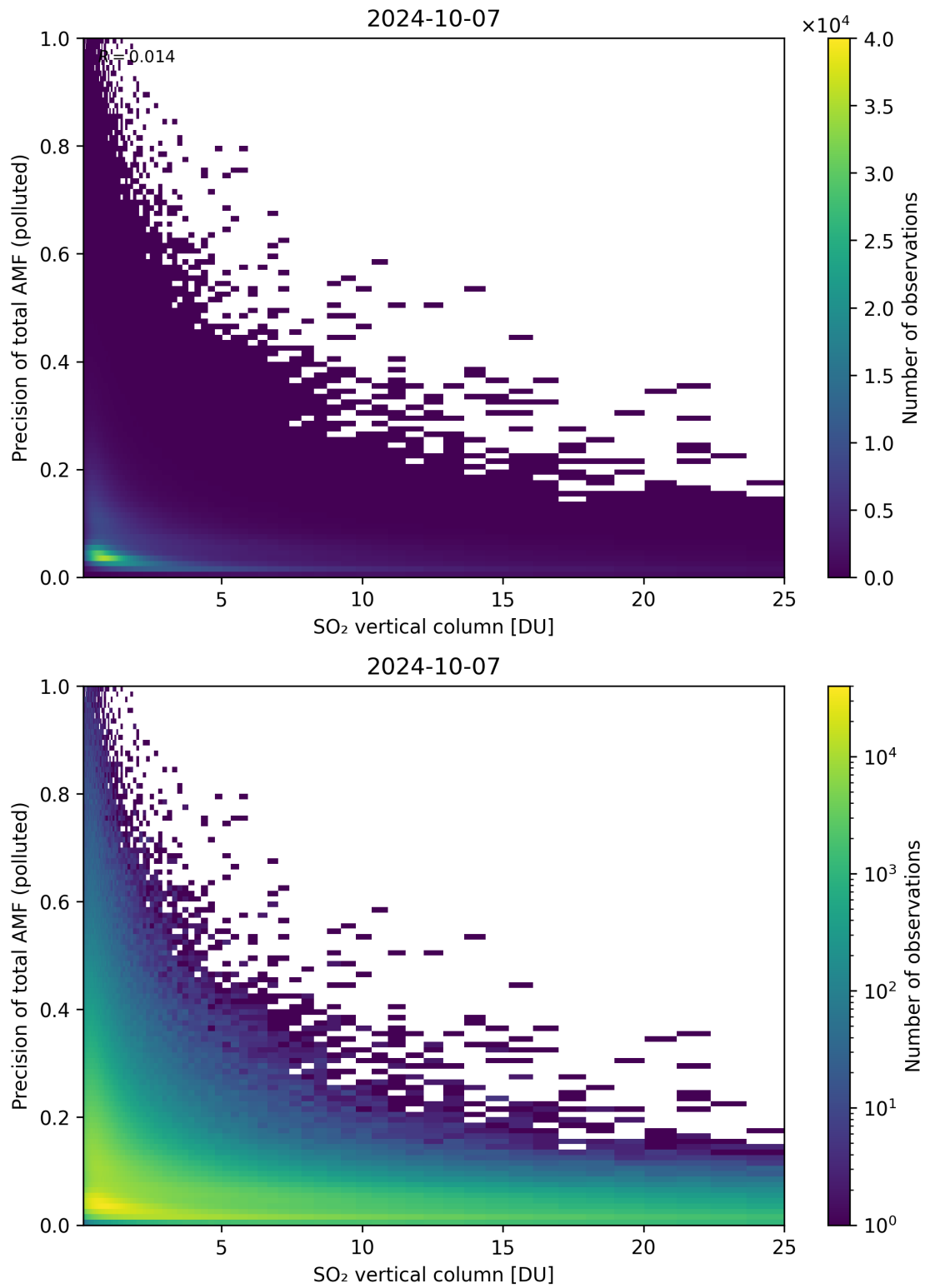
Figure 306: Scatter density plot of “SO 2 vertical column” against “Precision of total AMF (polluted)” for 2024-10-06 to 2024-10-08.
