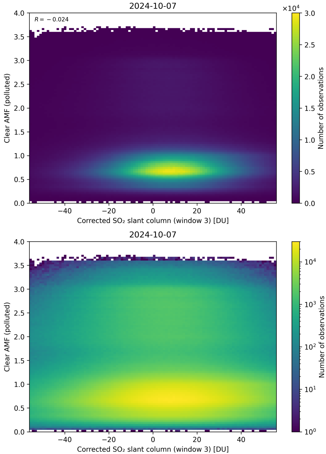
Figure 209: Scatter density plot of “Corrected SO 2 slant column (window 3)” against “Clear AMF (polluted)” for 2024-10-06 to 2024-10-08.
