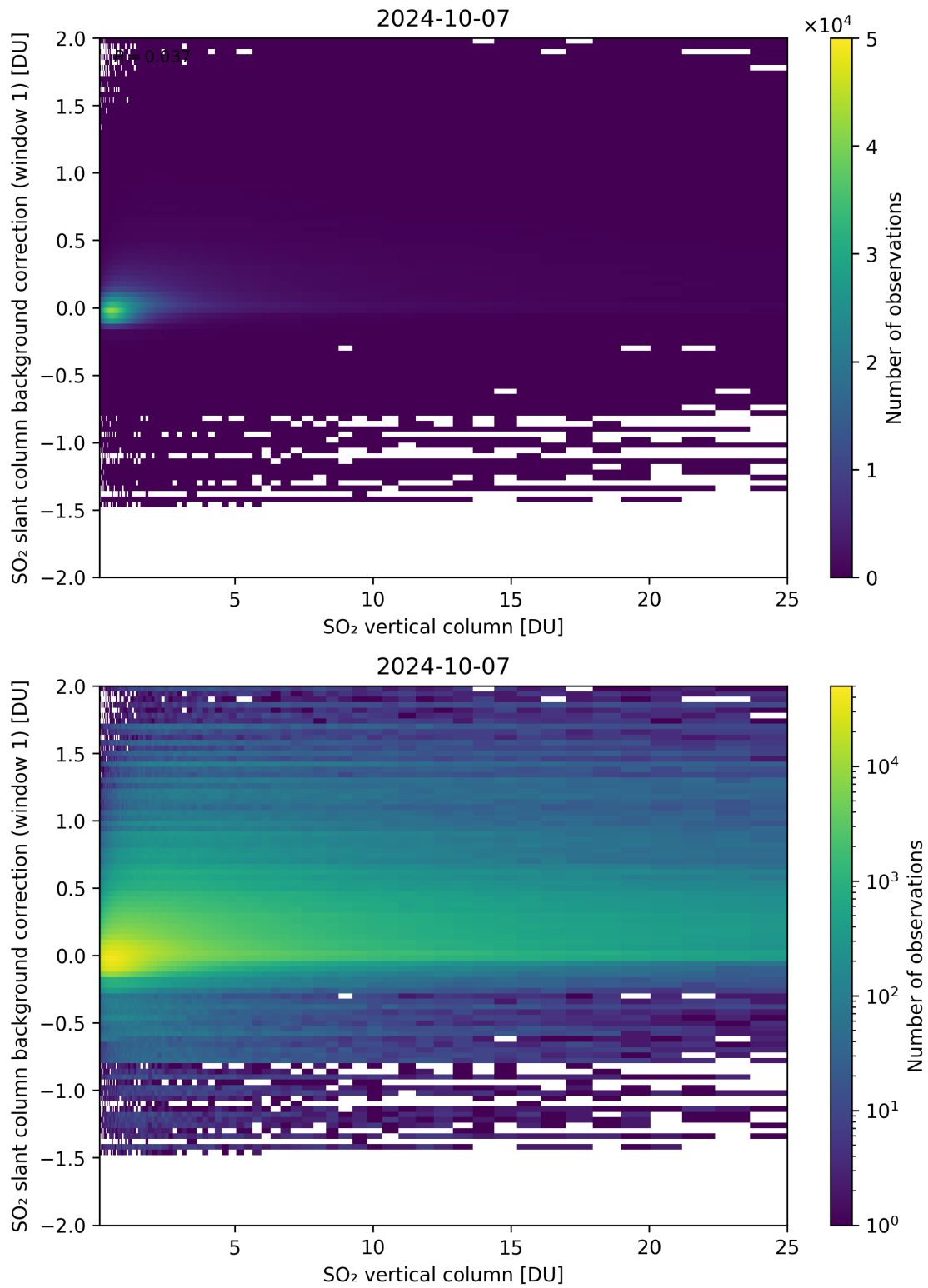
Figure 273: Scatter density plot of “SO 2 vertical column” against “SO 2 slant column background correction (window 1)” for 2024-10-06 to 2024-10-08.
