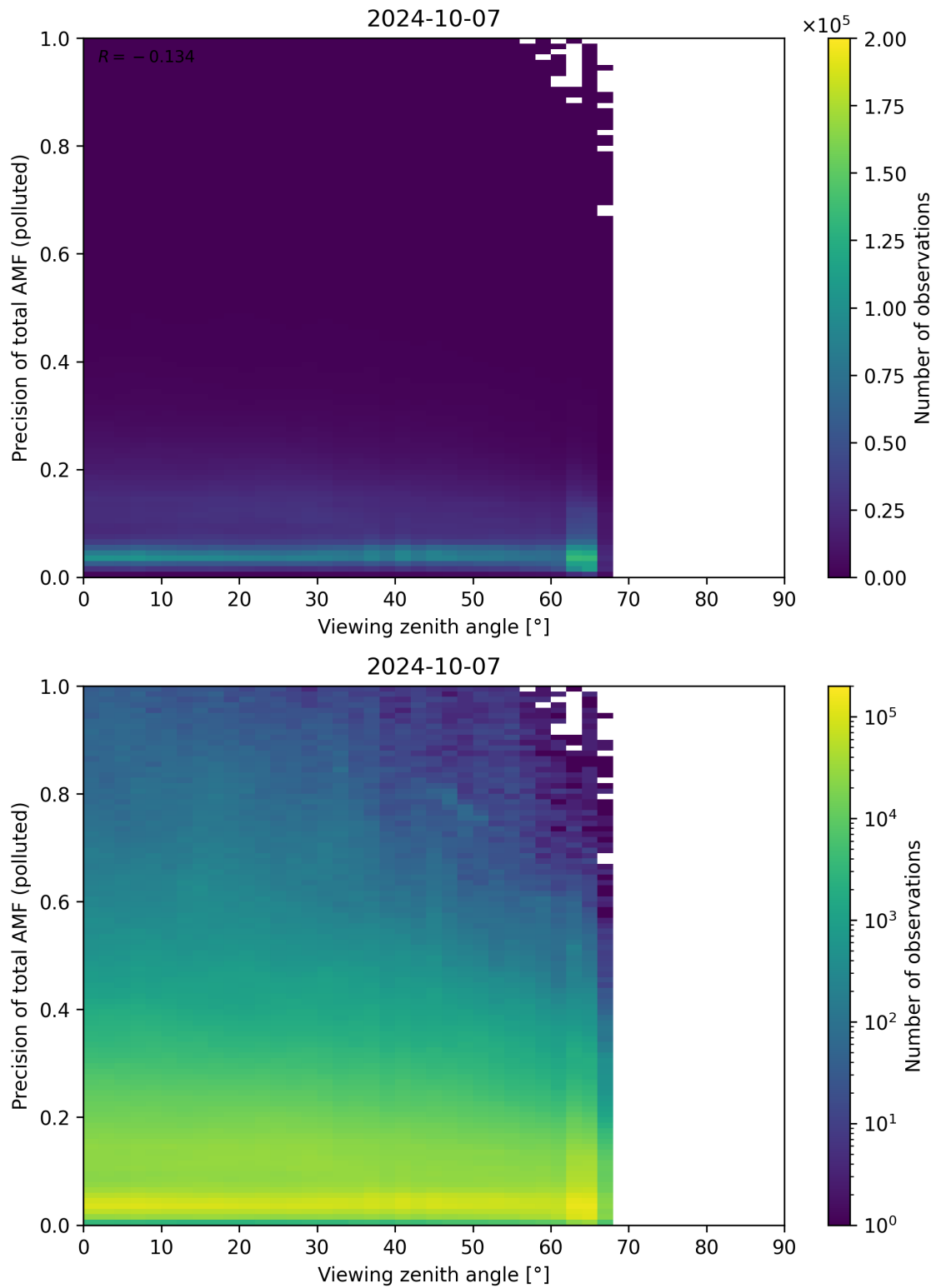
Figure 326: Scatter density plot of “Viewing zenith angle” against “Precision of total AMF (polluted)” for 2024-10-06 to 2024-10-08.
