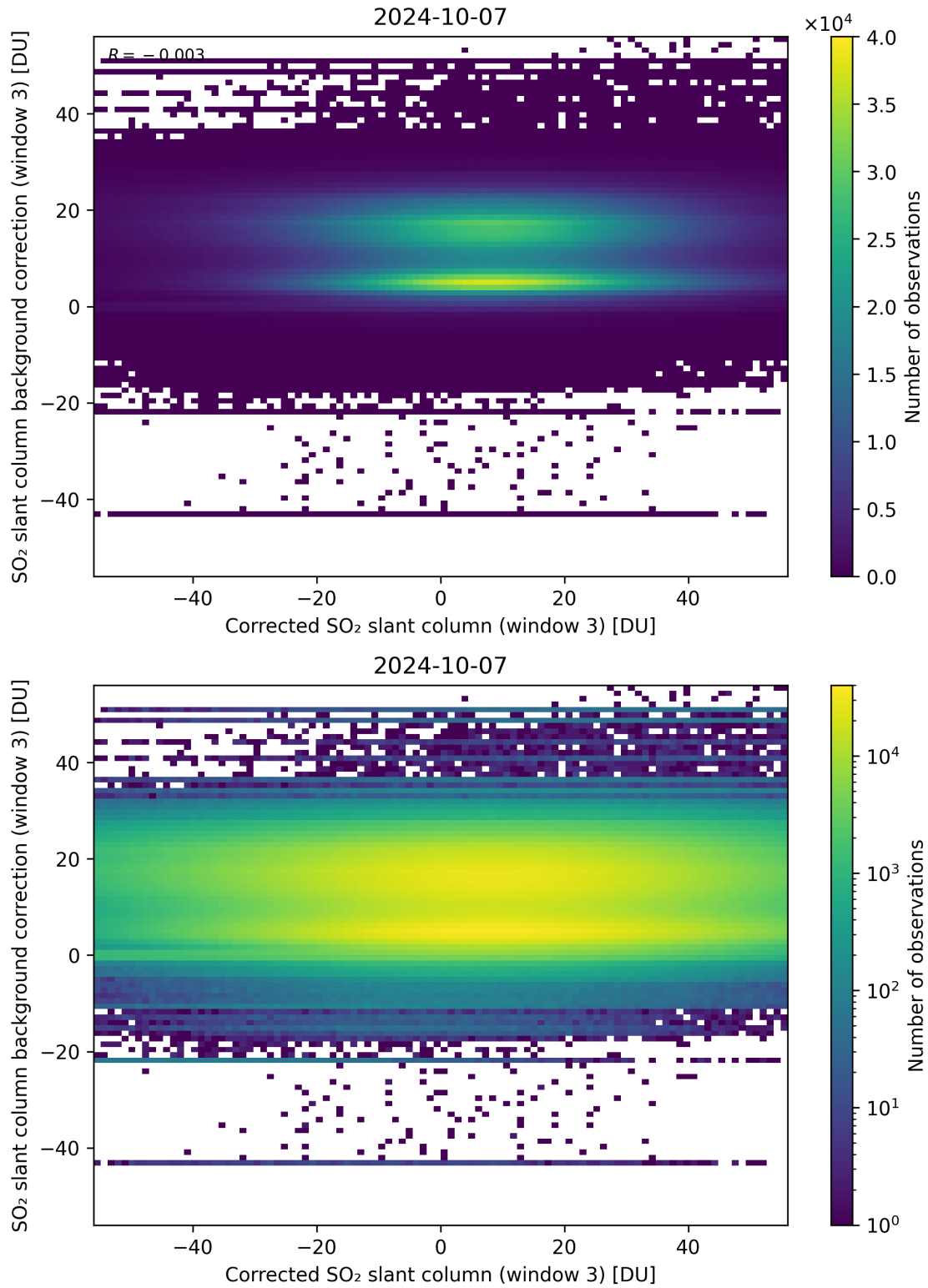
Figure 205: Scatter density plot of “Corrected SO 2 slant column (window 3)” against “SO 2 slant column background correction (window 3)” for 2024-10-06 to 2024-10-08.
