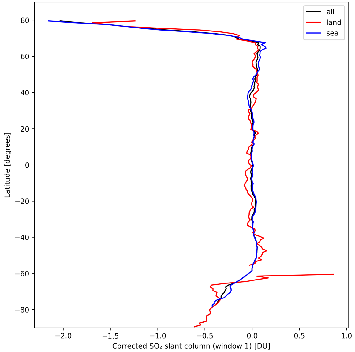
Figure 35: Zonal average of “Corrected SO 2 slant column (window 1)” for 2024-10-06 to 2024-10-08.
