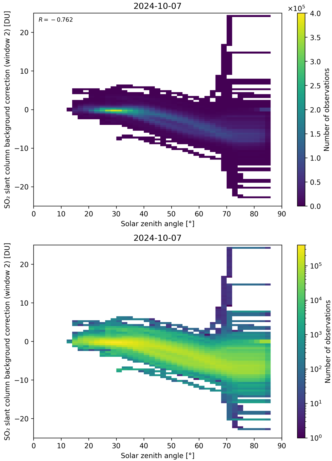
Figure 159: Scatter density plot of “Solar zenith angle” against “SO 2 slant column background correction (window 2)” for 2024-10-06 to 2024-10-08.
