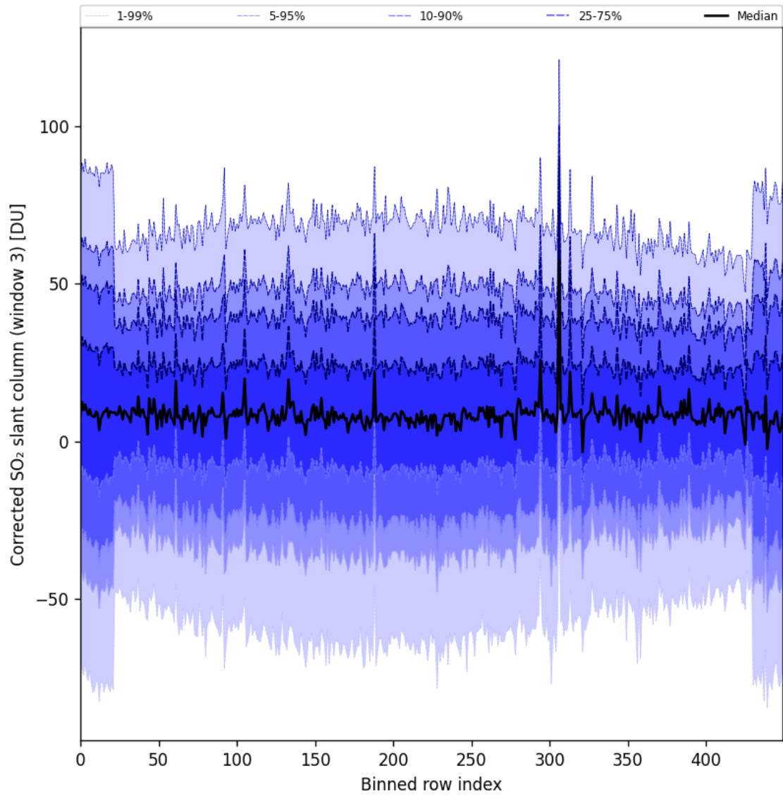
Figure 89: Along track statistics of “Corrected SO 2 slant column (window 3)” for 2024-10-06 to 2024-10-08
