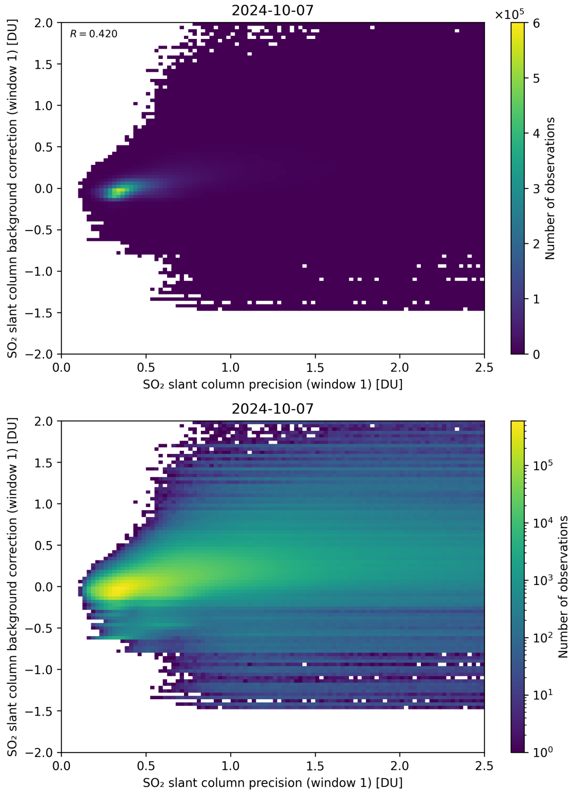
Figure 218: Scatter density plot of “SO 2 slant column precision (window 1)” against “SO 2 slant column background correction (window 1)” for 2024-10-06 to 2024-10-08.
