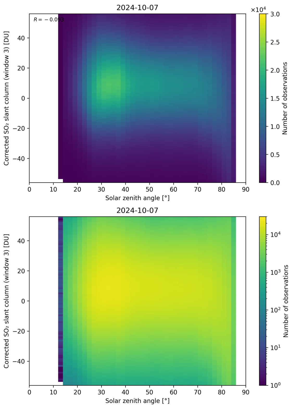
Figure 168: Scatter density plot of “Solar zenith angle” against “Corrected SO 2 slant column (window 3)” for 2024-10-06 to 2024-10-08.
