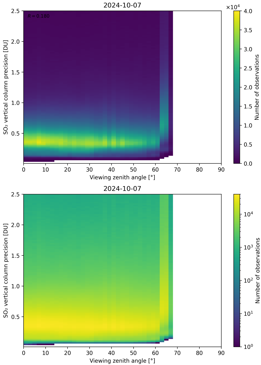
Figure 328: Scatter density plot of “Viewing zenith angle” against “SO 2 vertical column precision” for 2024-10-06 to 2024-10-08.
