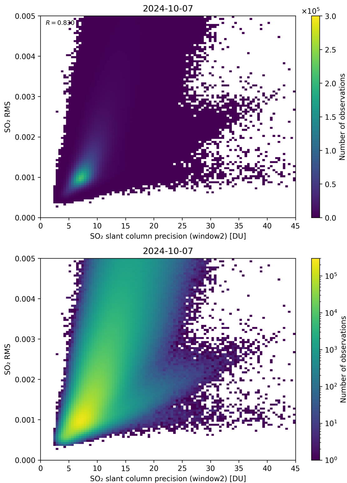
Figure 245: Scatter density plot of “SO 2 slant column precision (window2)” against “SO 2 RMS” for 2024-10-06 to 2024-10-08.
