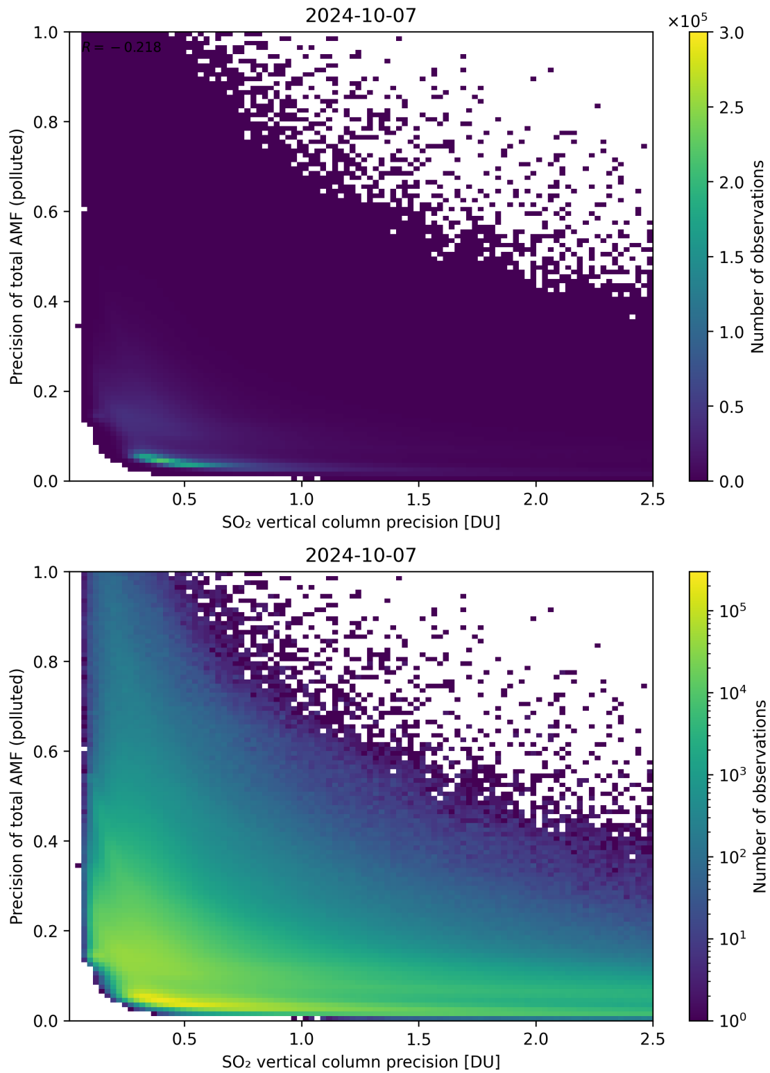
Figure 295: Scatter density plot of “SO 2 vertical column precision” against “Precision of total AMF (polluted)” for 2024-10-06 to 2024-10-08.
