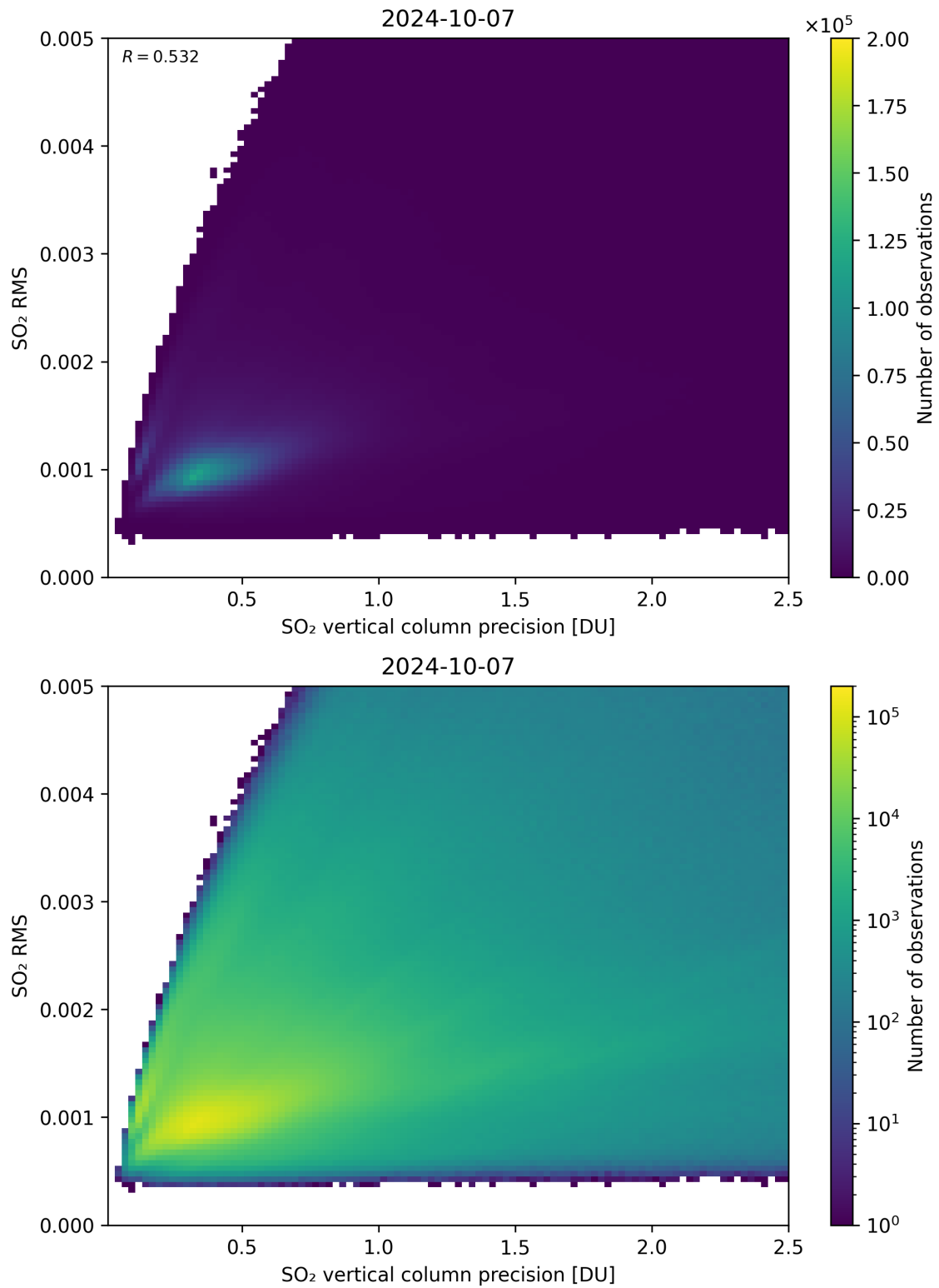
Figure 284: Scatter density plot of “SO 2 vertical column precision” against “SO 2 RMS” for 2024-10-06 to 2024-10-08.
