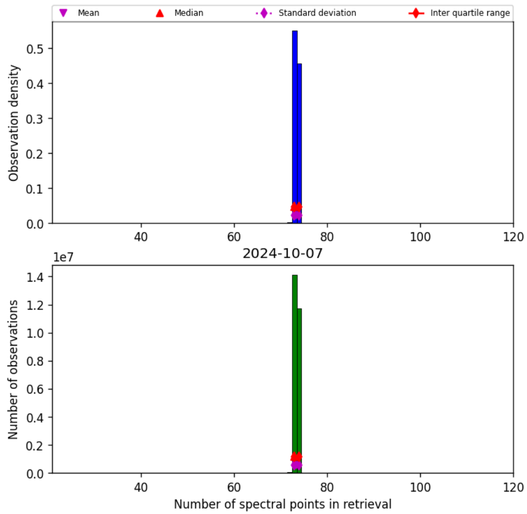
Figure 74: Histogram of “Number of spectral points in retrieval” for 2024-10-06 to 2024-10-08
