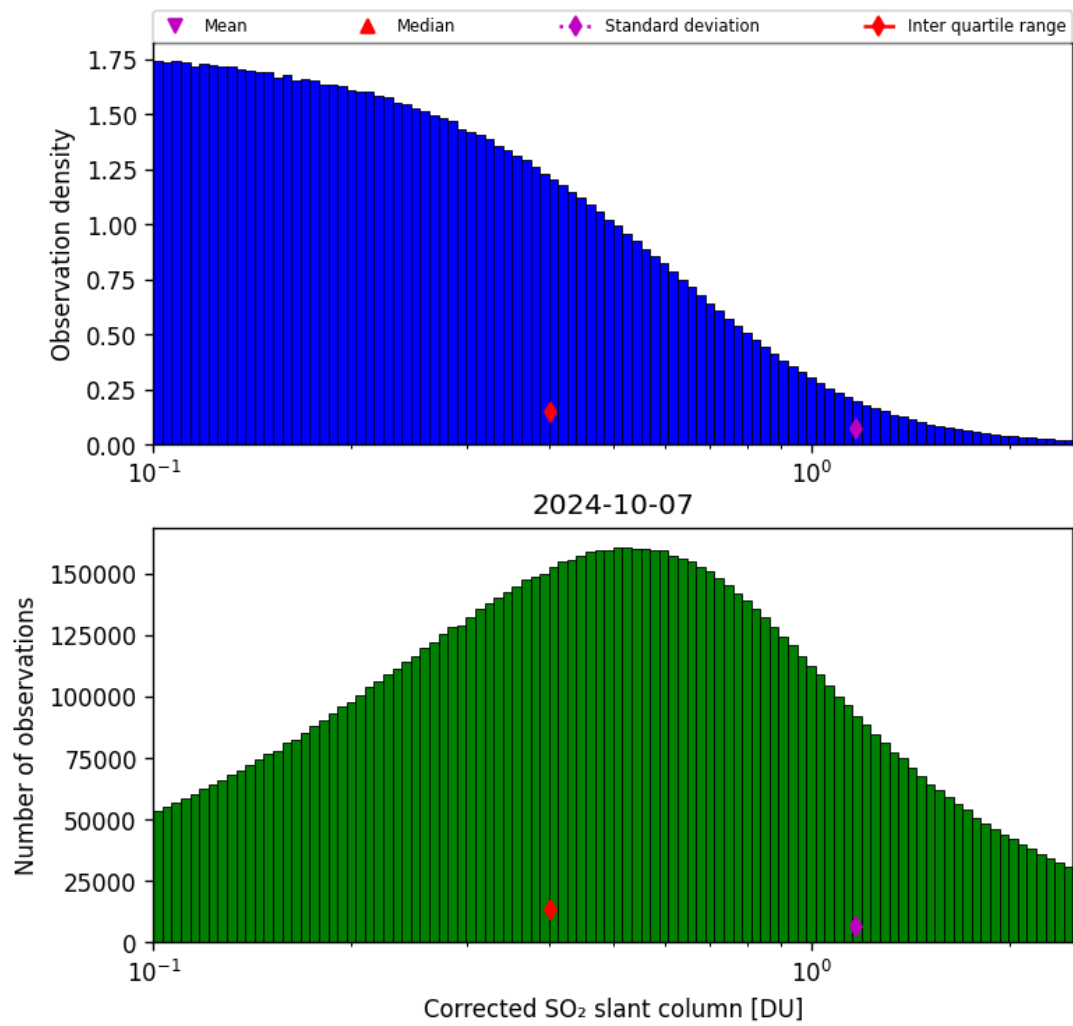
Figure 55: Histogram of “Corrected SO 2 slant column” for 2024-10-06 to 2024-10-08
