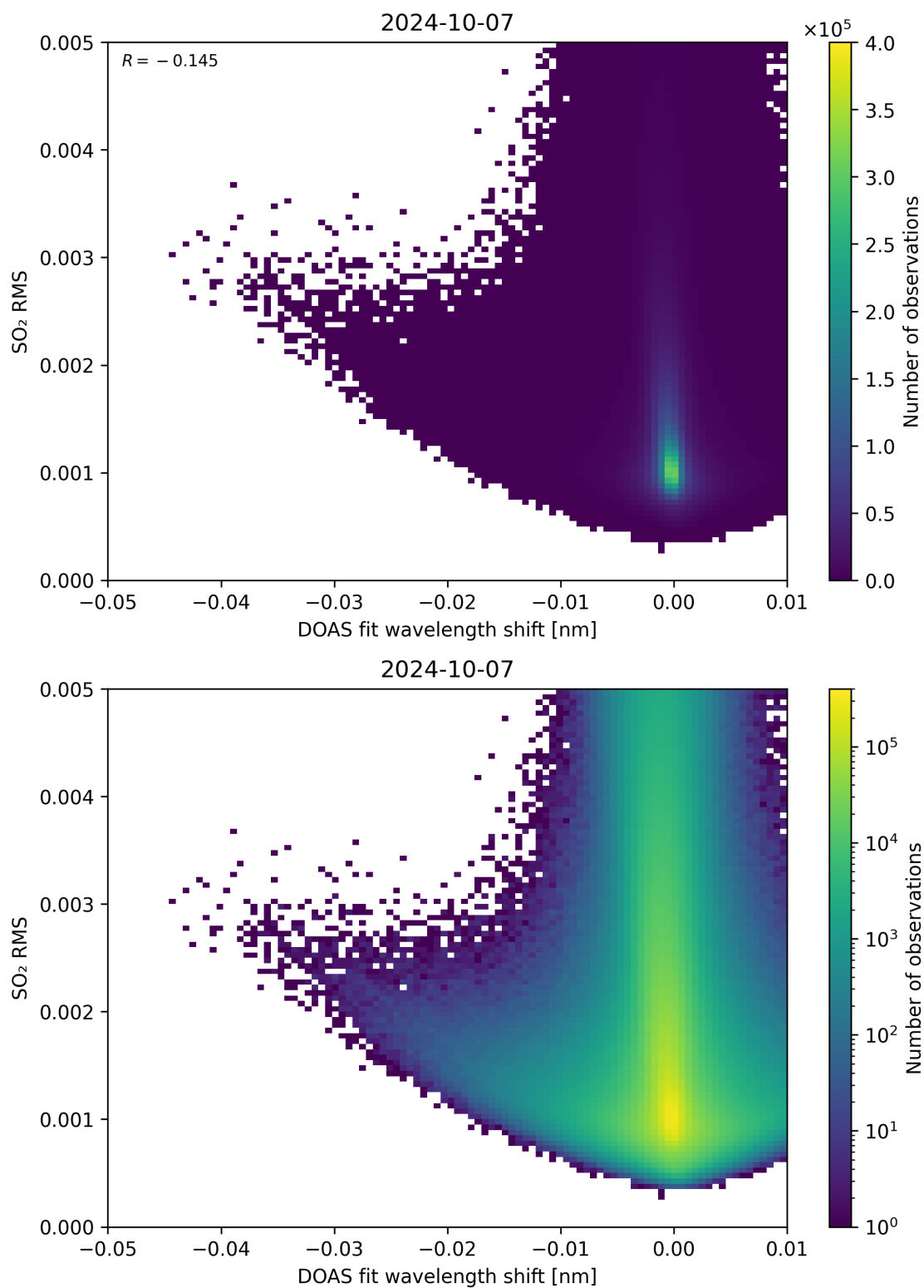
Figure 128: Scatter density plot of “DOAS fit wavelength shift” against “SO 2 RMS” for 2024-10-06 to 2024-10-08.
