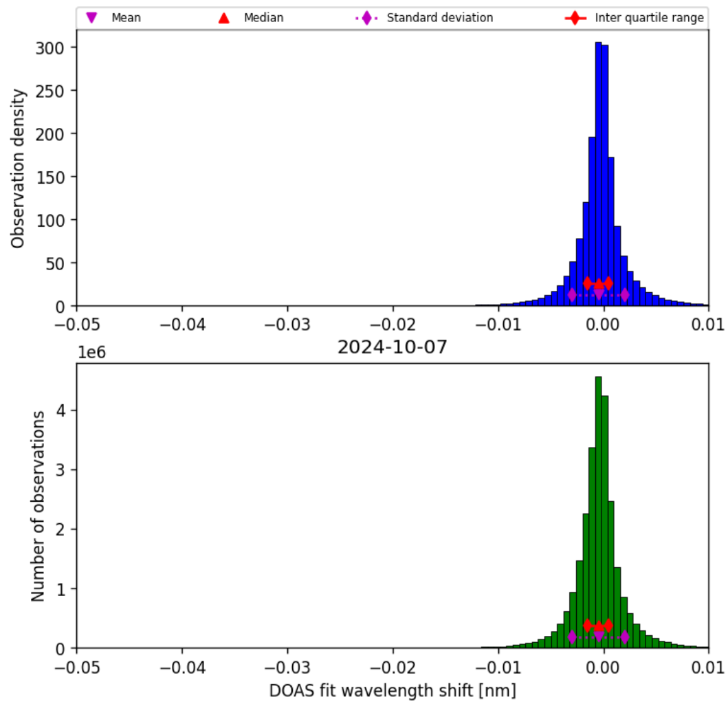
Figure 68: Histogram of “DOAS fit wavelength shift” for 2024-10-06 to 2024-10-08
