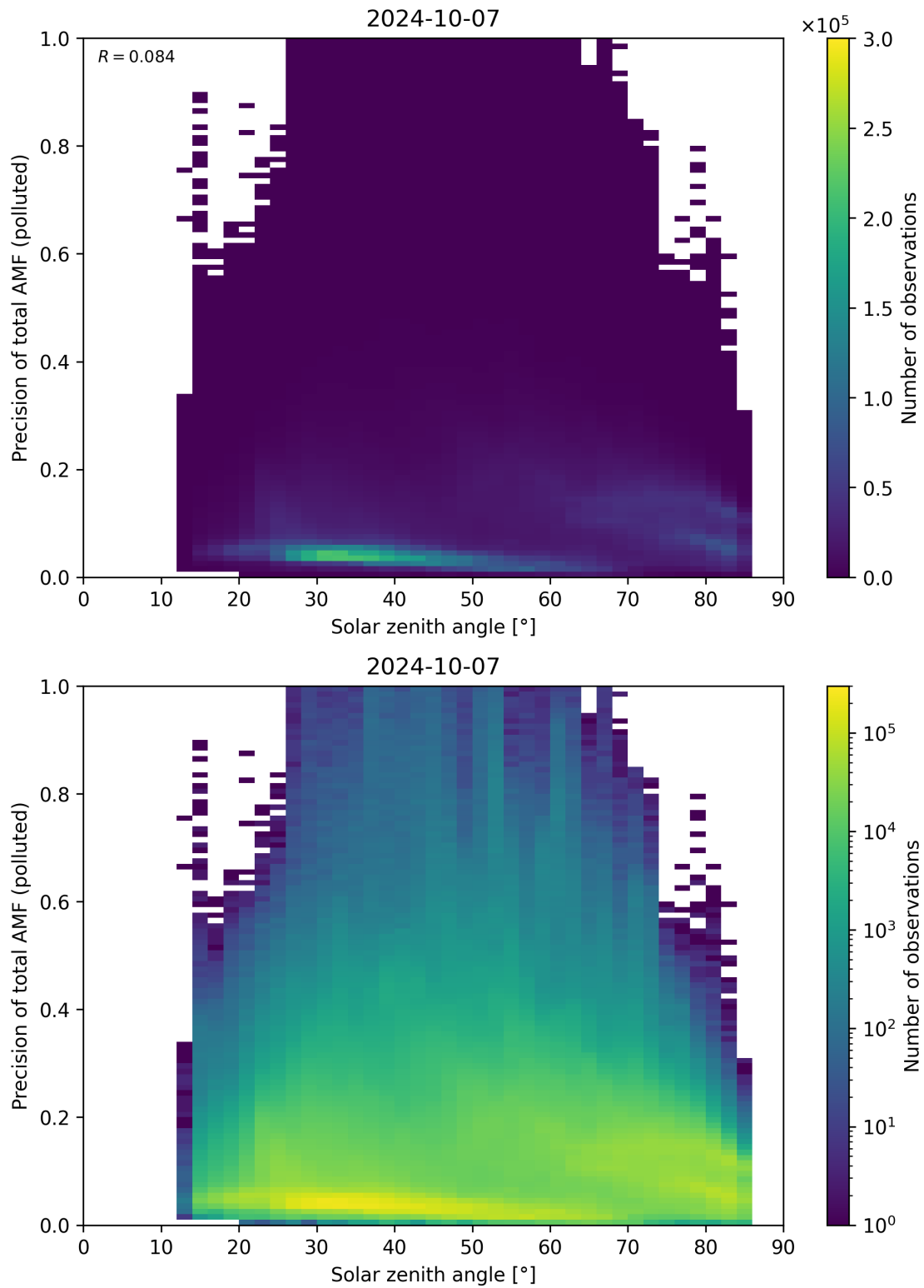
Figure 175: Scatter density plot of “Solar zenith angle” against “Precision of total AMF (polluted)” for 2024-10-06 to 2024-10-08.
