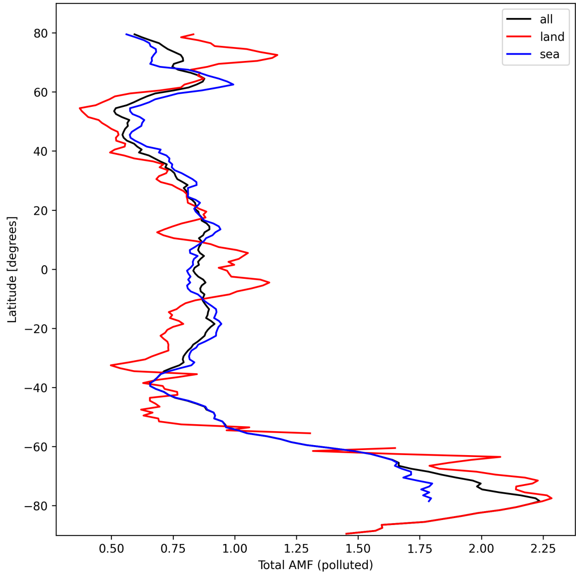
Figure 48: Zonal average of “Total AMF (polluted)” for 2024-10-06 to 2024-10-08.
