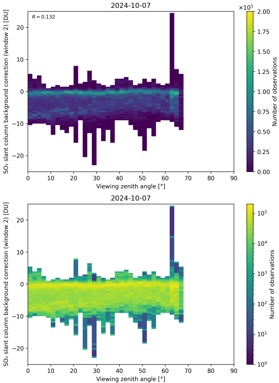
Figure 309: Scatter density plot of “Viewing zenith angle” against “SO 2 slant column background correction (window 2)” for 2024-10-06 to 2024-10-08.
