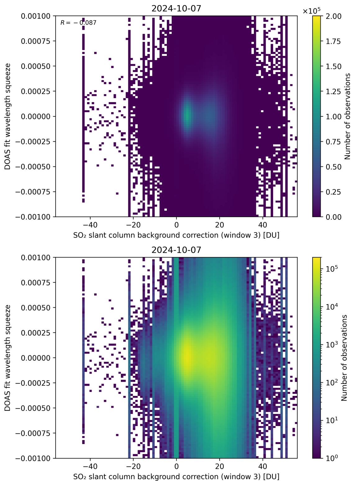
Figure 122: Scatter density plot of “SO 2 slant column background correction (window 3)” against “DOAS fit wavelength squeeze” for 2024-10-06 to 2024-10-08.
