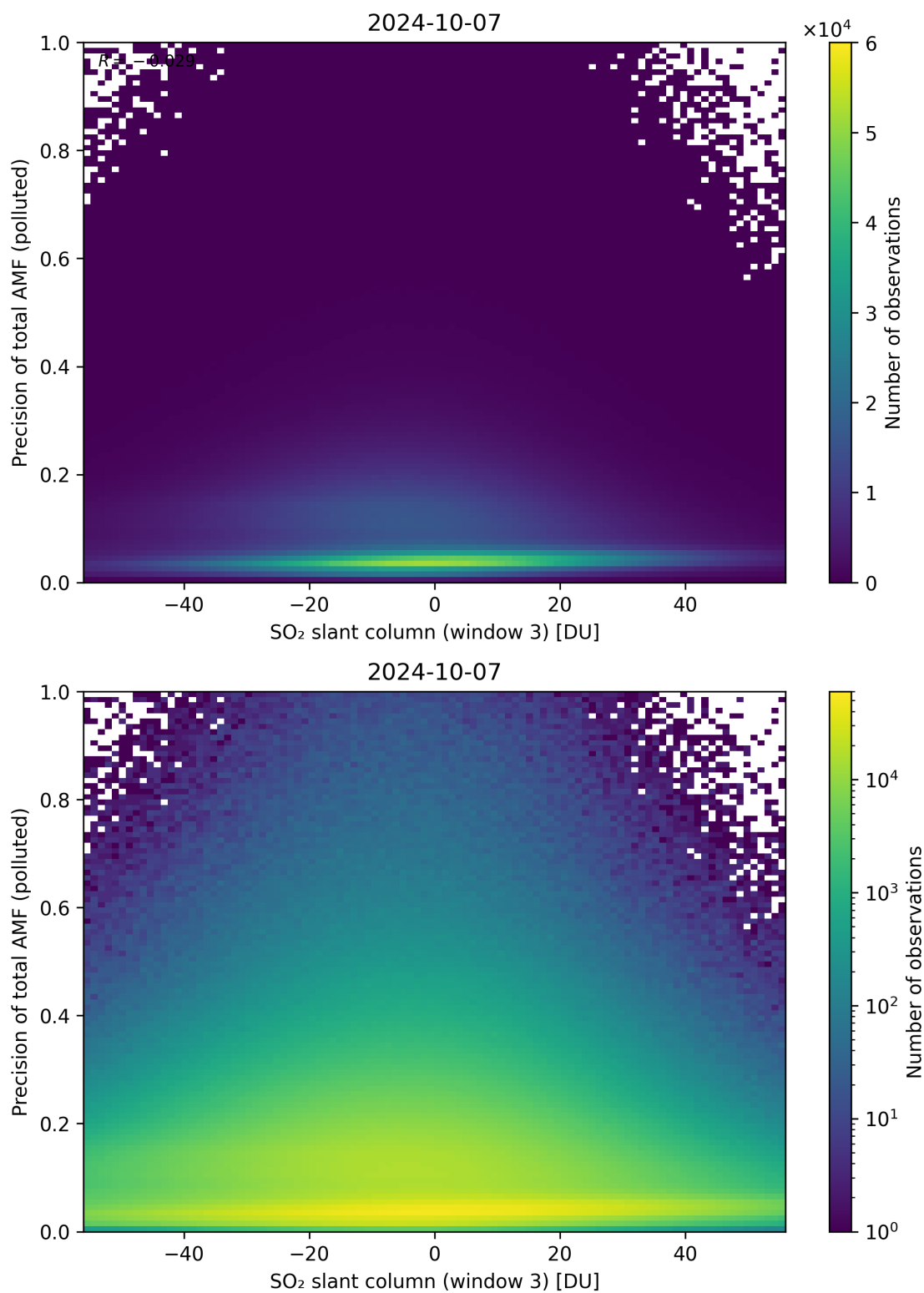
Figure 269: Scatter density plot of “SO 2 slant column (window 3)” against “Precision of total AMF (polluted)” for 2024-10-06 to 2024-10-08.
