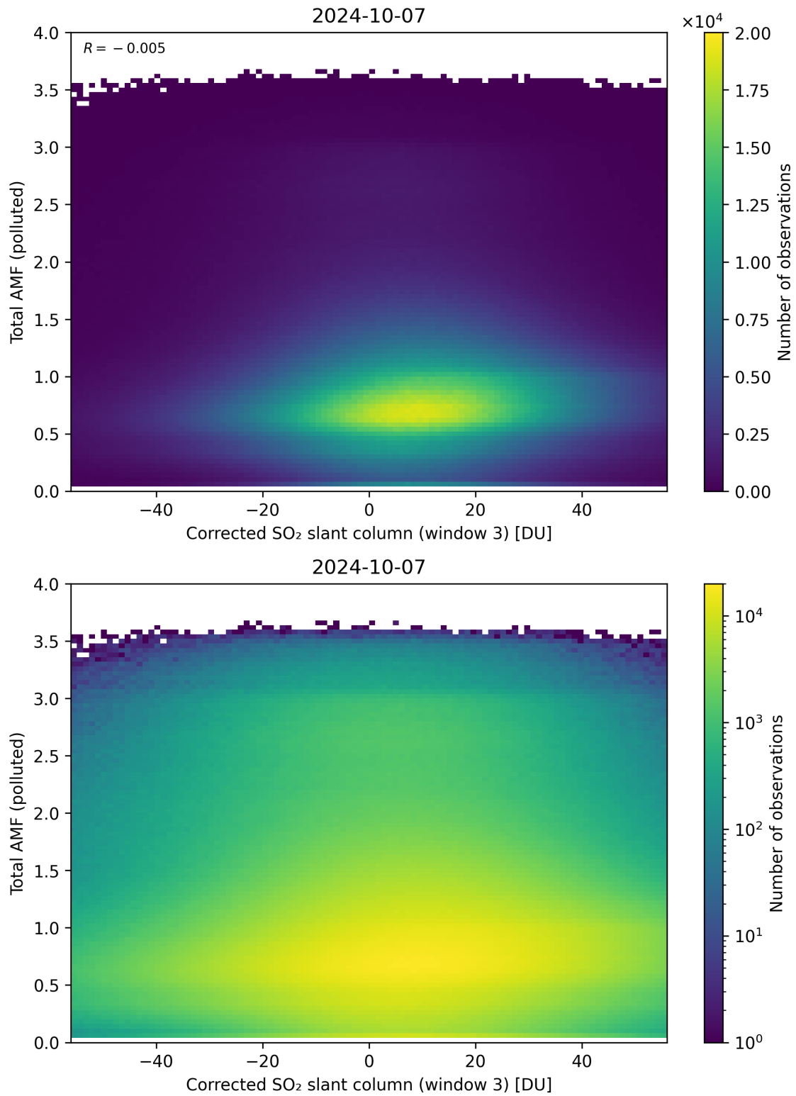
Figure 210: Scatter density plot of “Corrected SO 2 slant column (window 3)” against “Total AMF (polluted)” for 2024-10-06 to 2024-10-08.
