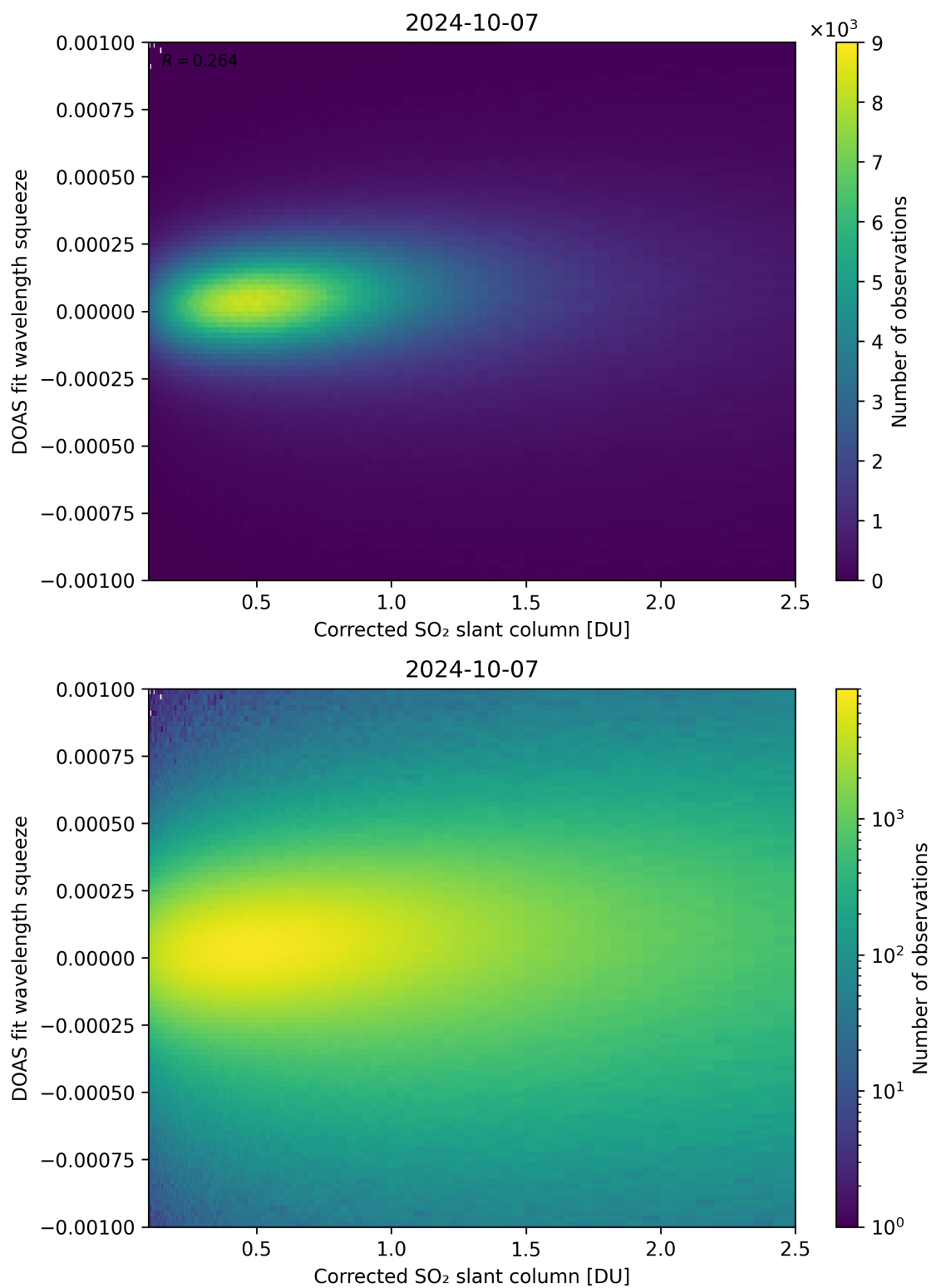
Figure 182: Scatter density plot of “Corrected SO 2 slant column” against “DOAS fit wavelength squeeze” for 2024-10-06 to 2024-10-08.
