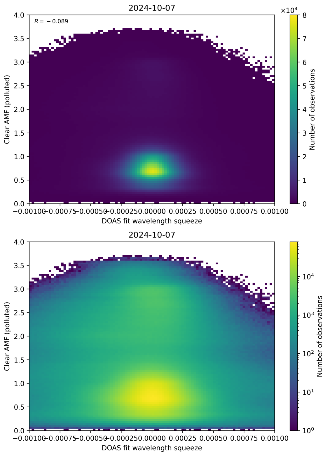
Figure 133: Scatter density plot of “DOAS fit wavelength squeeze” against “Clear AMF (polluted)” for 2024-10-06 to 2024-10-08.
