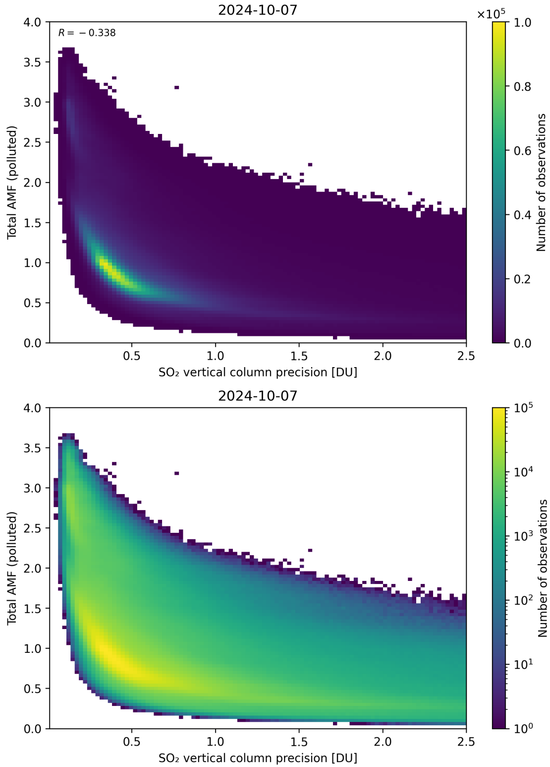
Figure 294: Scatter density plot of “SO 2 vertical column precision” against “Total AMF (polluted)” for 2024-10-06 to 2024-10-08.
