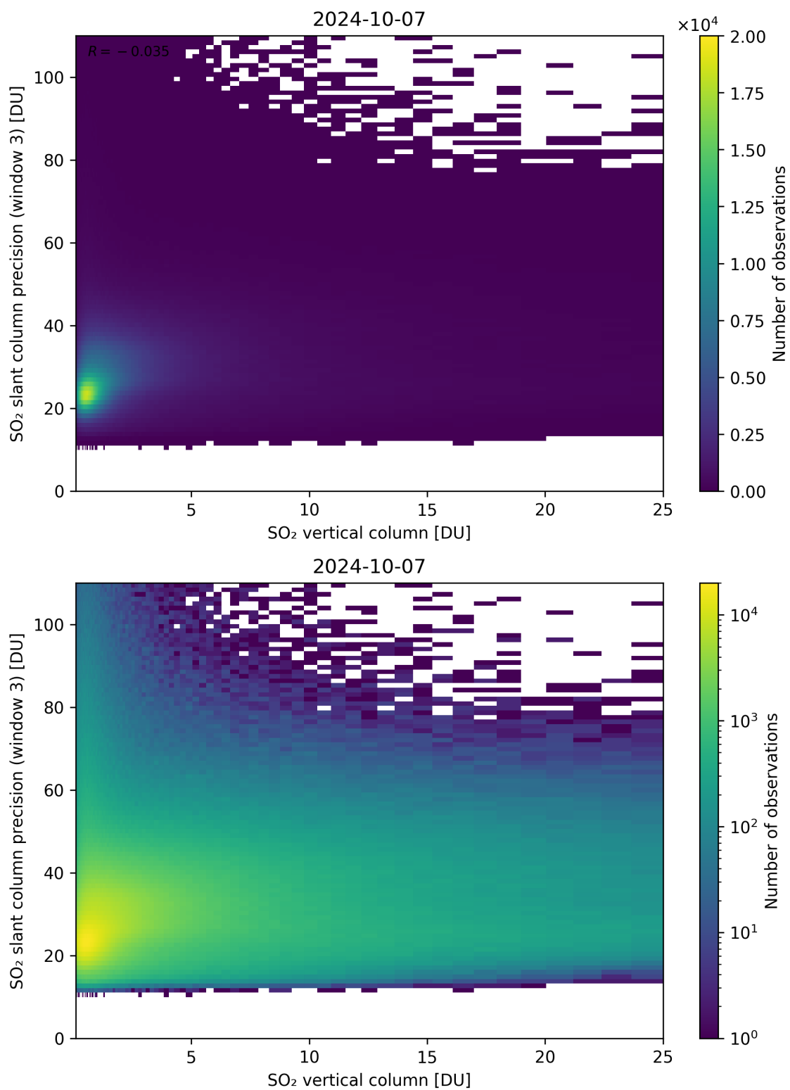
Figure 304: Scatter density plot of “SO 2 vertical column” against “SO 2 slant column precision (window 3)” for 2024-10-06 to 2024-10-08.
