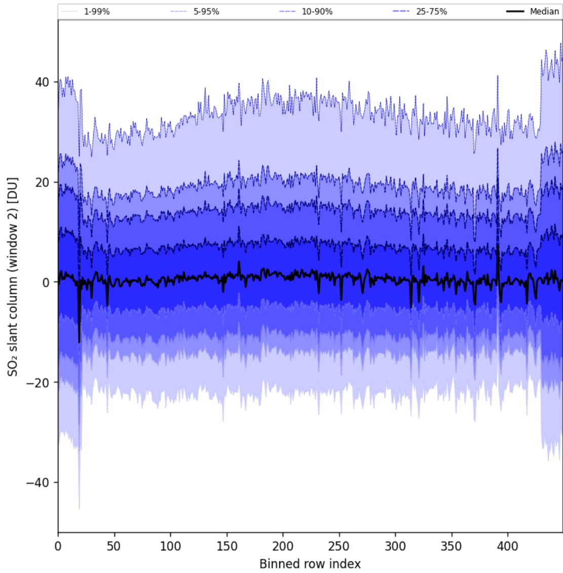
Figure 83: Along track statistics of “SO 2 slant column (window 2)” for 2024-10-06 to 2024-10-08
