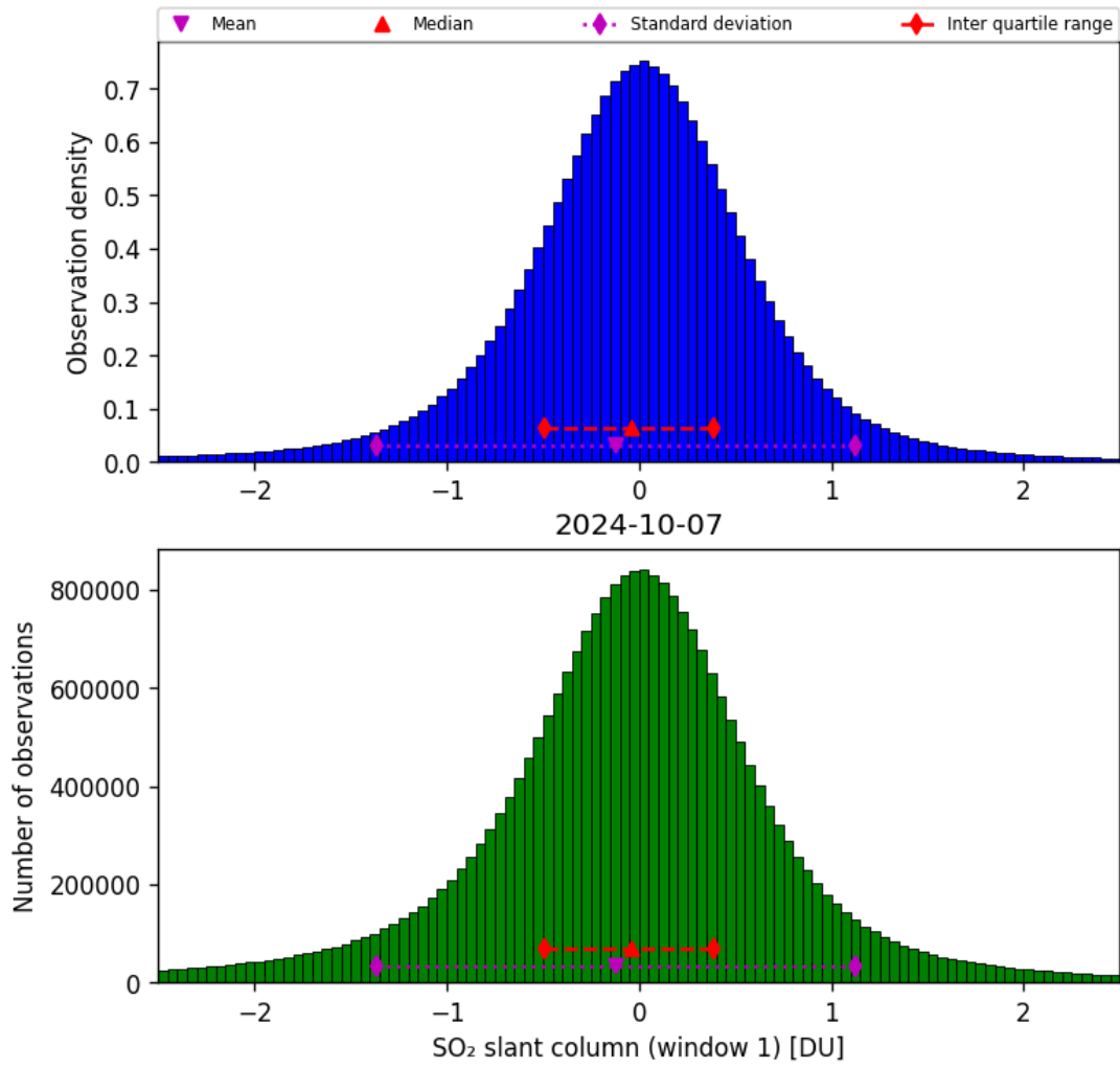
Figure 56: Histogram of “SO 2 slant column (window 1)” for 2024-10-06 to 2024-10-08
