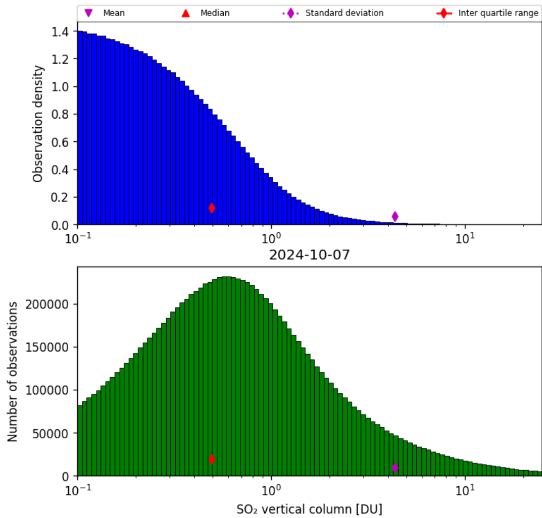
Figure 53: Histogram of “SO 2 vertical column” for 2024-10-06 to 2024-10-08
