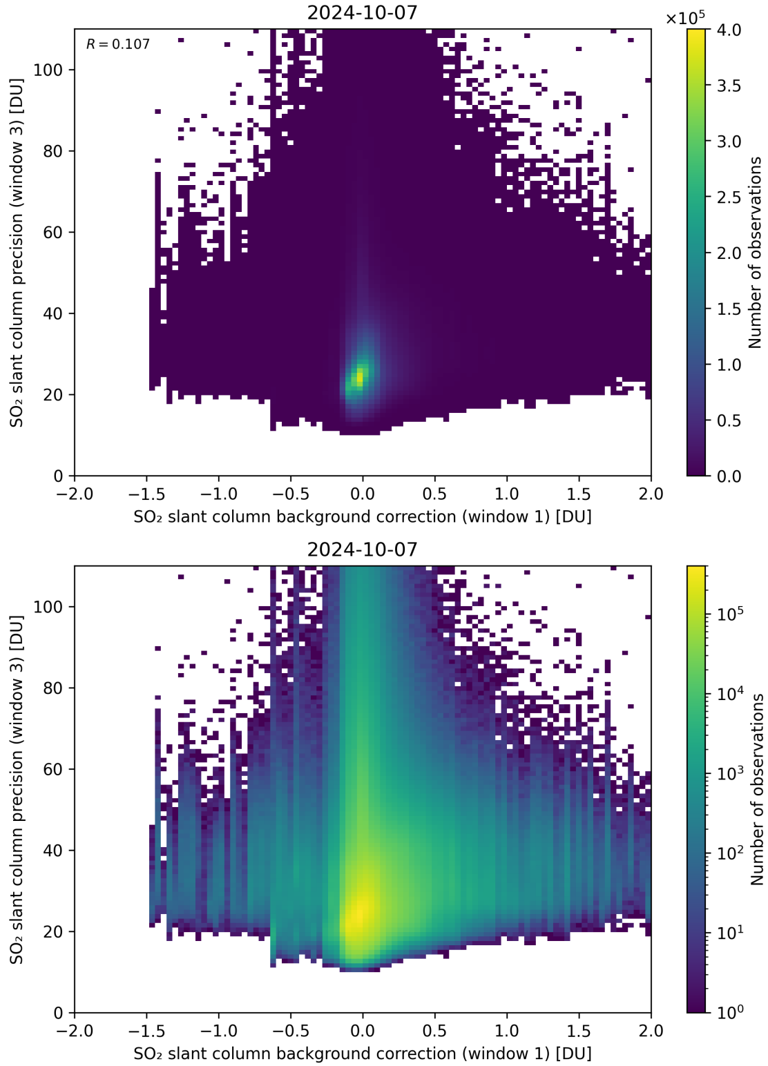
Figure 108: Scatter density plot of “SO 2 slant column background correction (window 1)” against “SO 2 slant column precision (window 3)” for 2024-10-06 to 2024-10-08.
