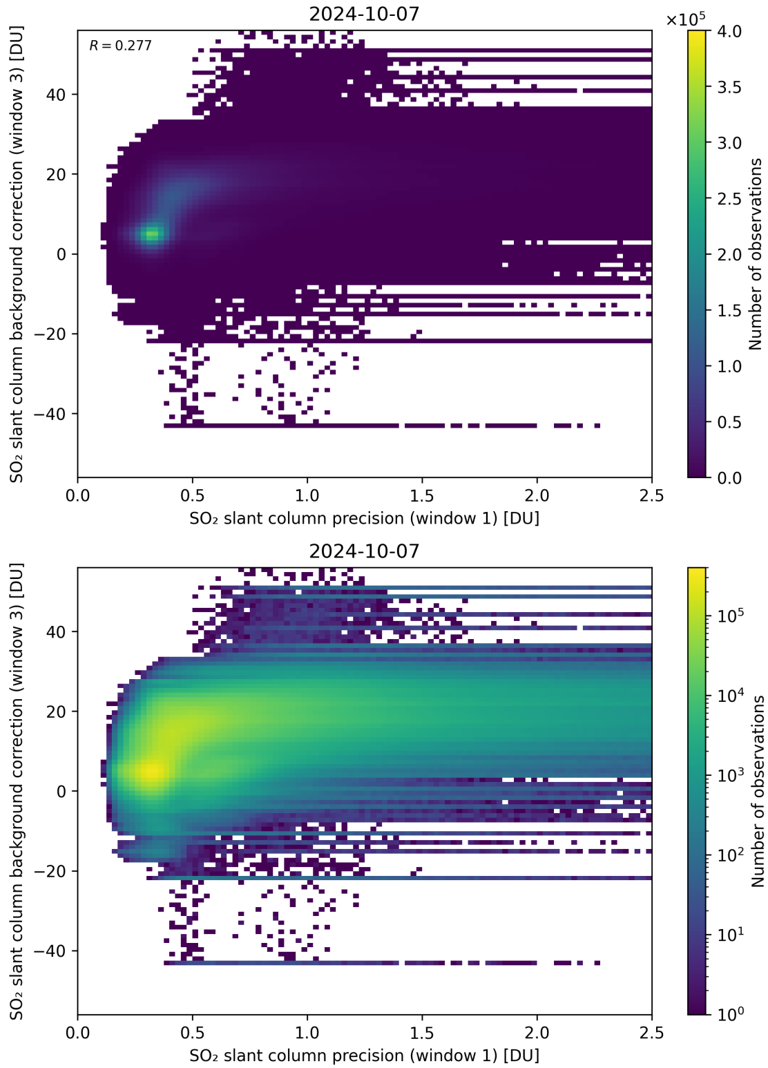
Figure 220: Scatter density plot of “SO 2 slant column precision (window 1)” against “SO 2 slant column background correction (window 3)” for 2024-10-06 to 2024-10-08.
