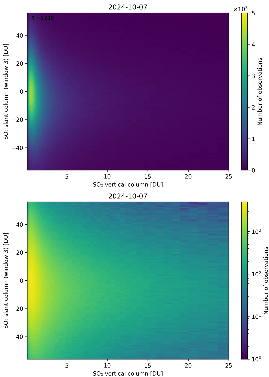
Figure 303: Scatter density plot of “SO 2 vertical column” against “SO 2 slant column (window 3)” for 2024-10-06 to 2024-10-08.
