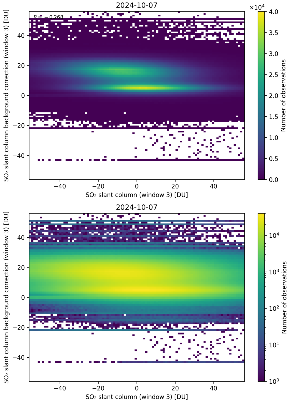
Figure 253: Scatter density plot of “SO 2 slant column (window 3)” against “SO 2 slant column background correction (window 3)” for 2024-10-06 to 2024-10-08.
