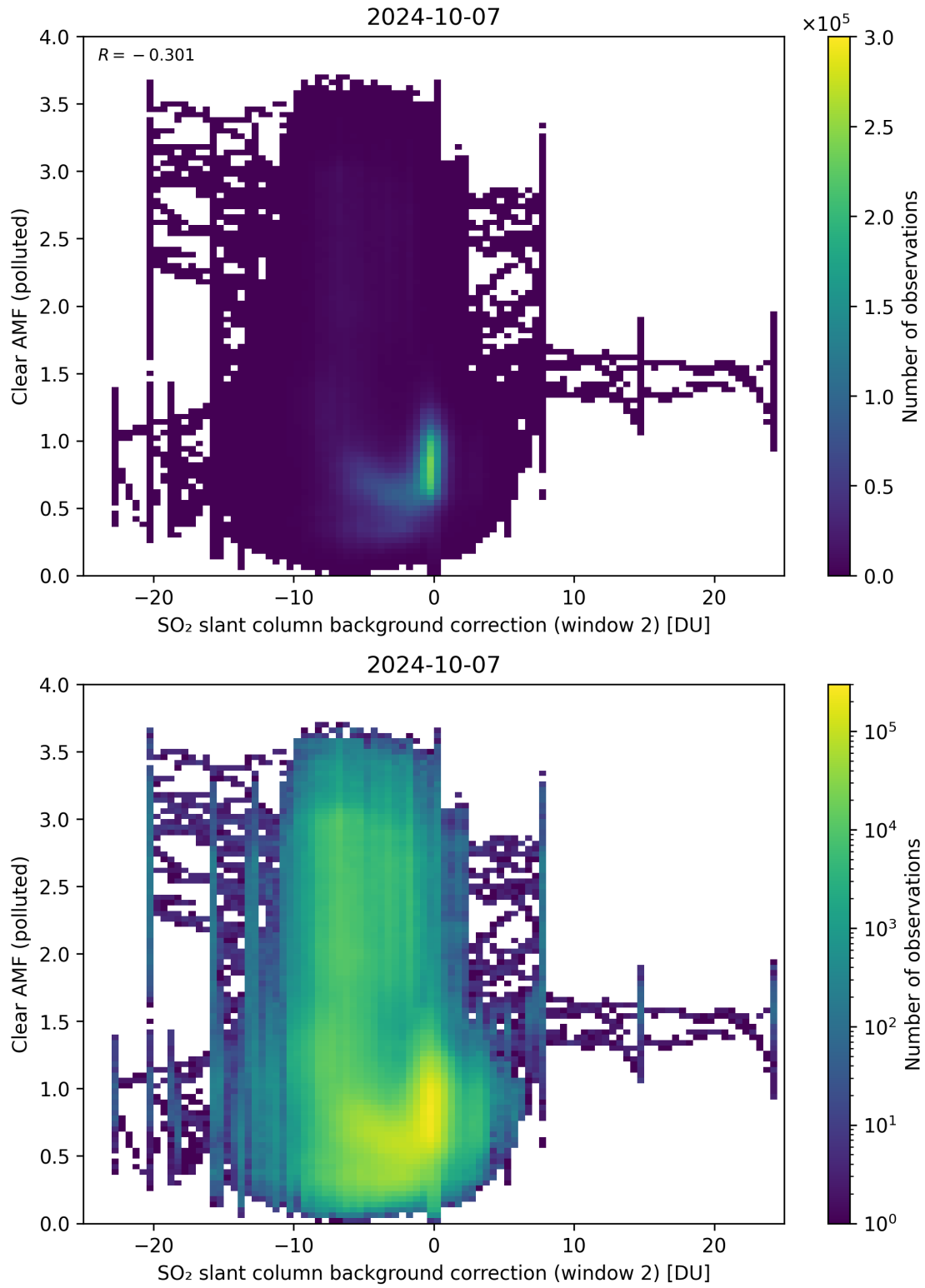
Figure 115: Scatter density plot of “SO 2 slant column background correction (window 2)” against “Clear AMF (polluted)” for 2024-10-06 to 2024-10-08.
