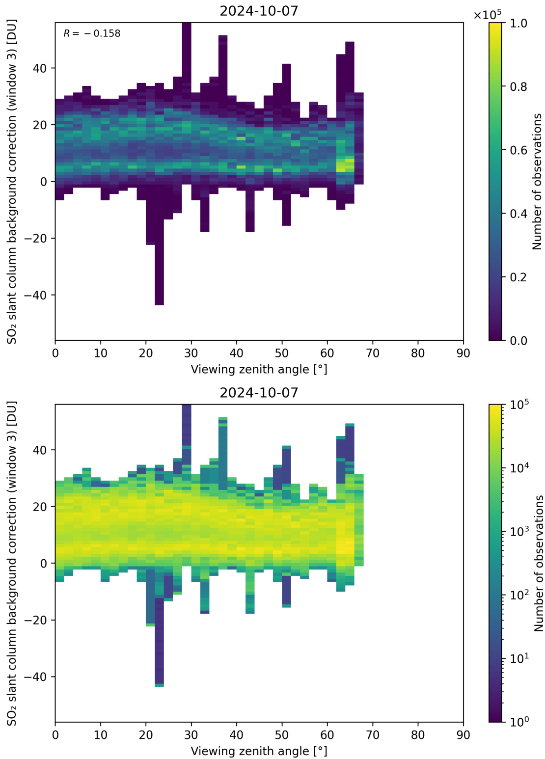
Figure 310: Scatter density plot of “Viewing zenith angle” against “SO 2 slant column background correction (window 3)” for 2024-10-06 to 2024-10-08.
