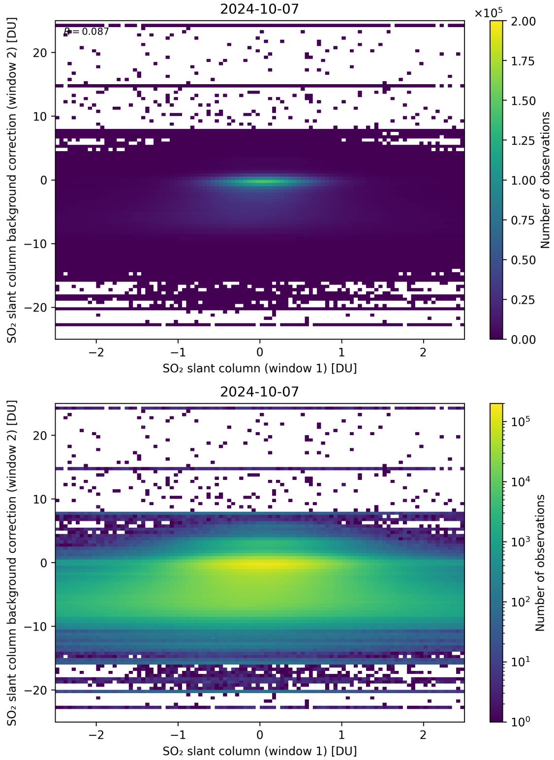
Figure 213: Scatter density plot of “SO 2 slant column (window 1)” against “SO 2 slant column background correction (window 2)” for 2024-10-06 to 2024-10-08.
