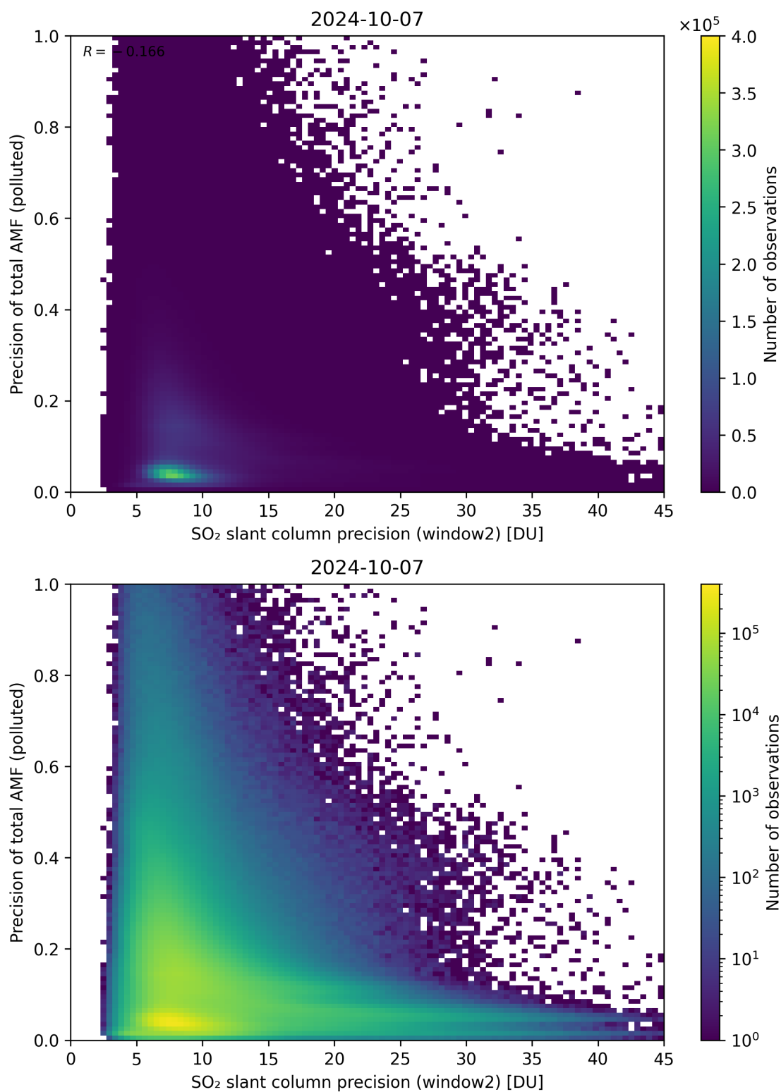
Figure 252: Scatter density plot of “SO 2 slant column precision (window2)” against “Precision of total AMF (polluted)” for 2024-10-06 to 2024-10-08.
