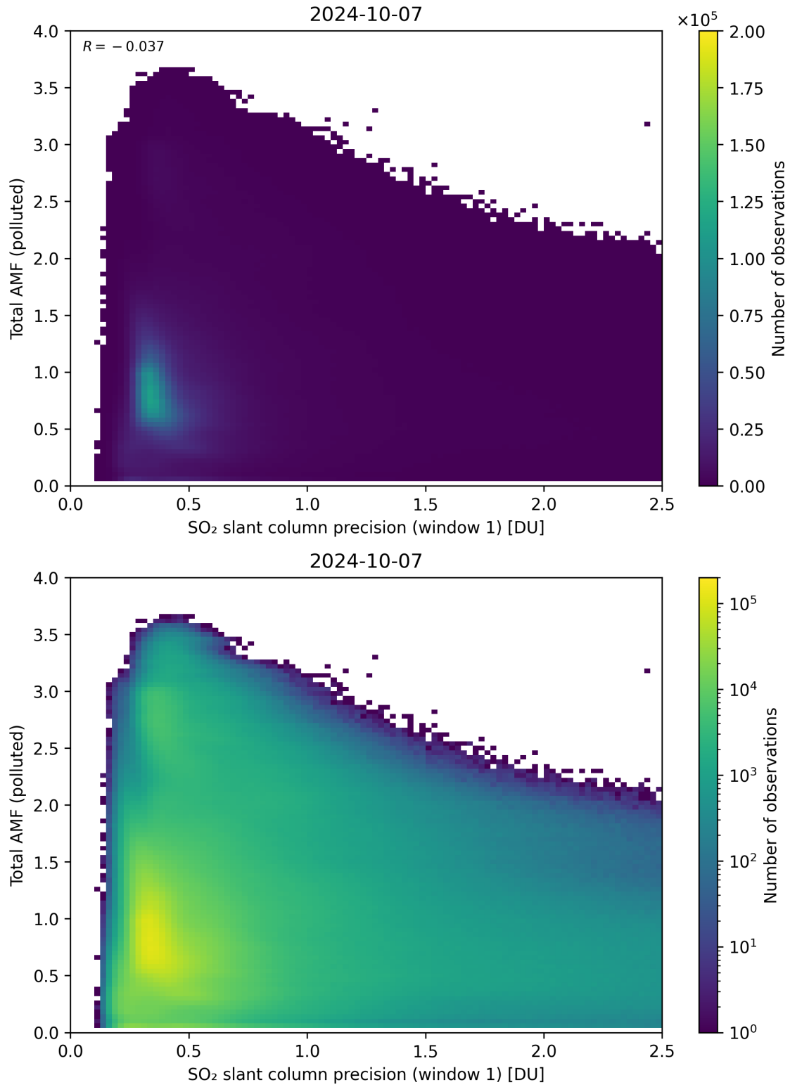
Figure 230: Scatter density plot of “SO 2 slant column precision (window 1)” against “Total AMF (polluted)” for 2024-10-06 to 2024-10-08.
