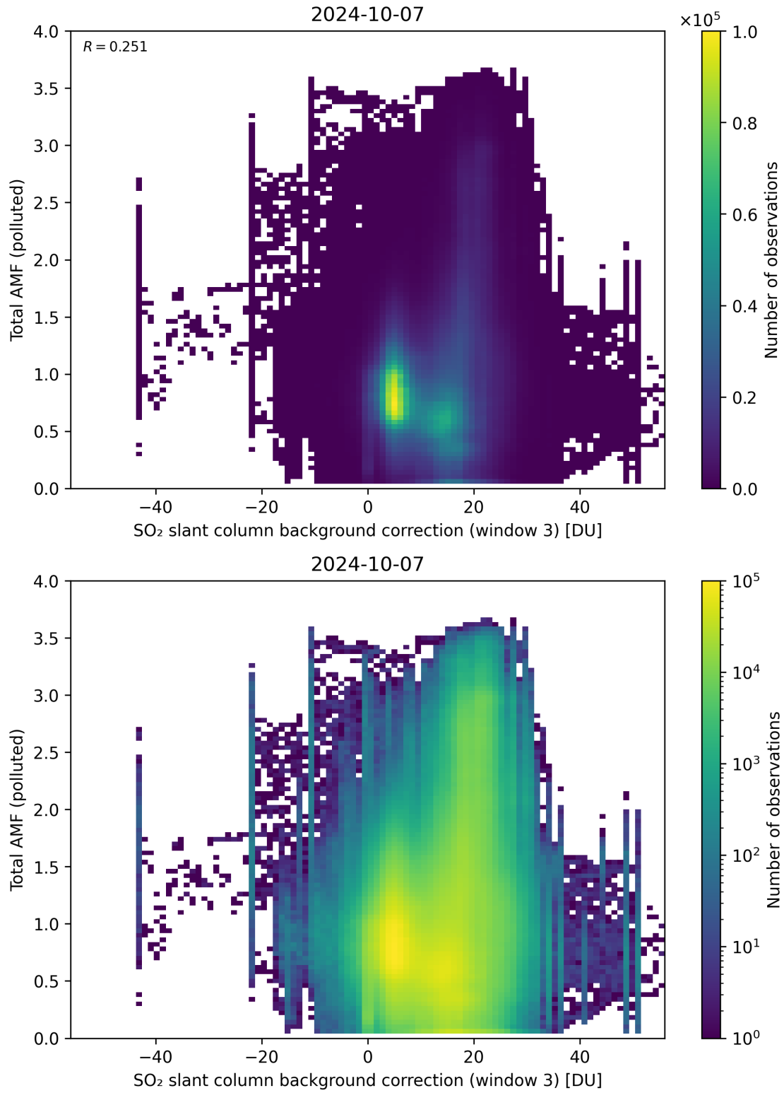
Figure 125: Scatter density plot of “SO 2 slant column background correction (window 3)” against “Total AMF (polluted)” for 2024-10-06 to 2024-10-08.
