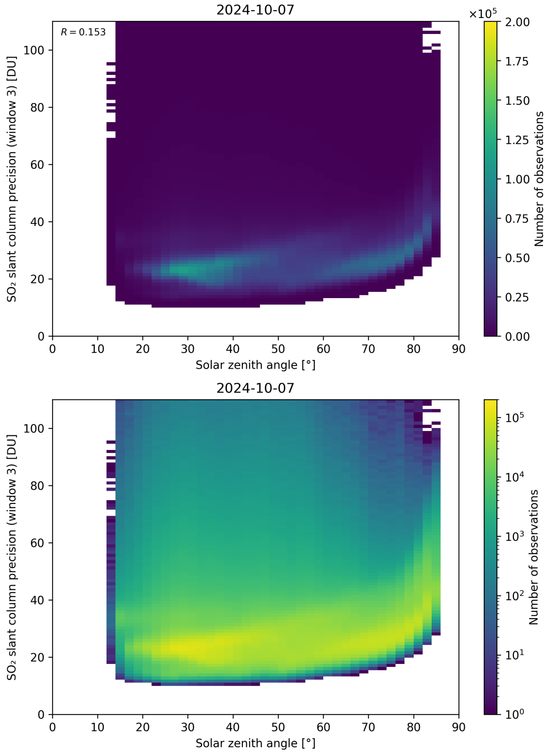
Figure 173: Scatter density plot of “Solar zenith angle” against “SO 2 slant column precision (window 3)” for 2024-10-06 to 2024-10-08.
