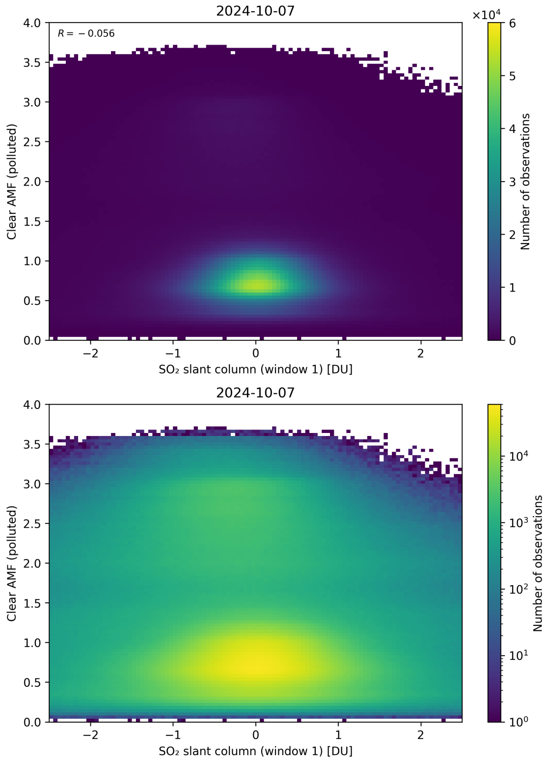
Figure 232: Scatter density plot of “SO 2 slant column (window 1)” against “Clear AMF (polluted)” for 2024-10-06 to 2024-10-08.
