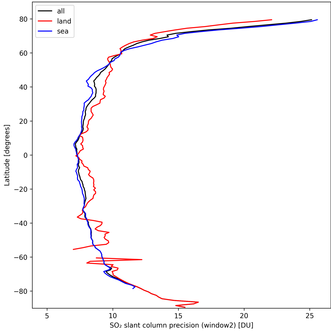
Figure 38: Zonal average of "SO 2 slant column precision (window2)" for 2024-10-06 to 2024-10-08.
