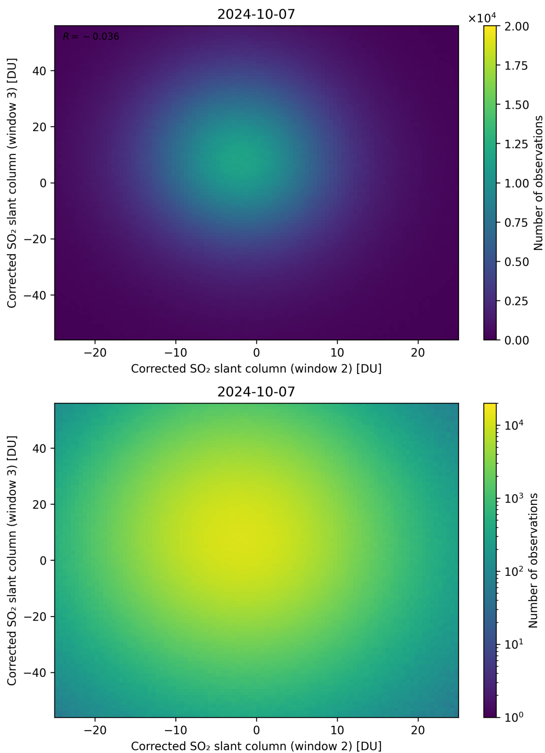
Figure 200: Scatter density plot of “Corrected SO 2 slant column (window 2)” against “Corrected SO 2 slant column (window 3)” for 2024-10-06 to 2024-10-08.
