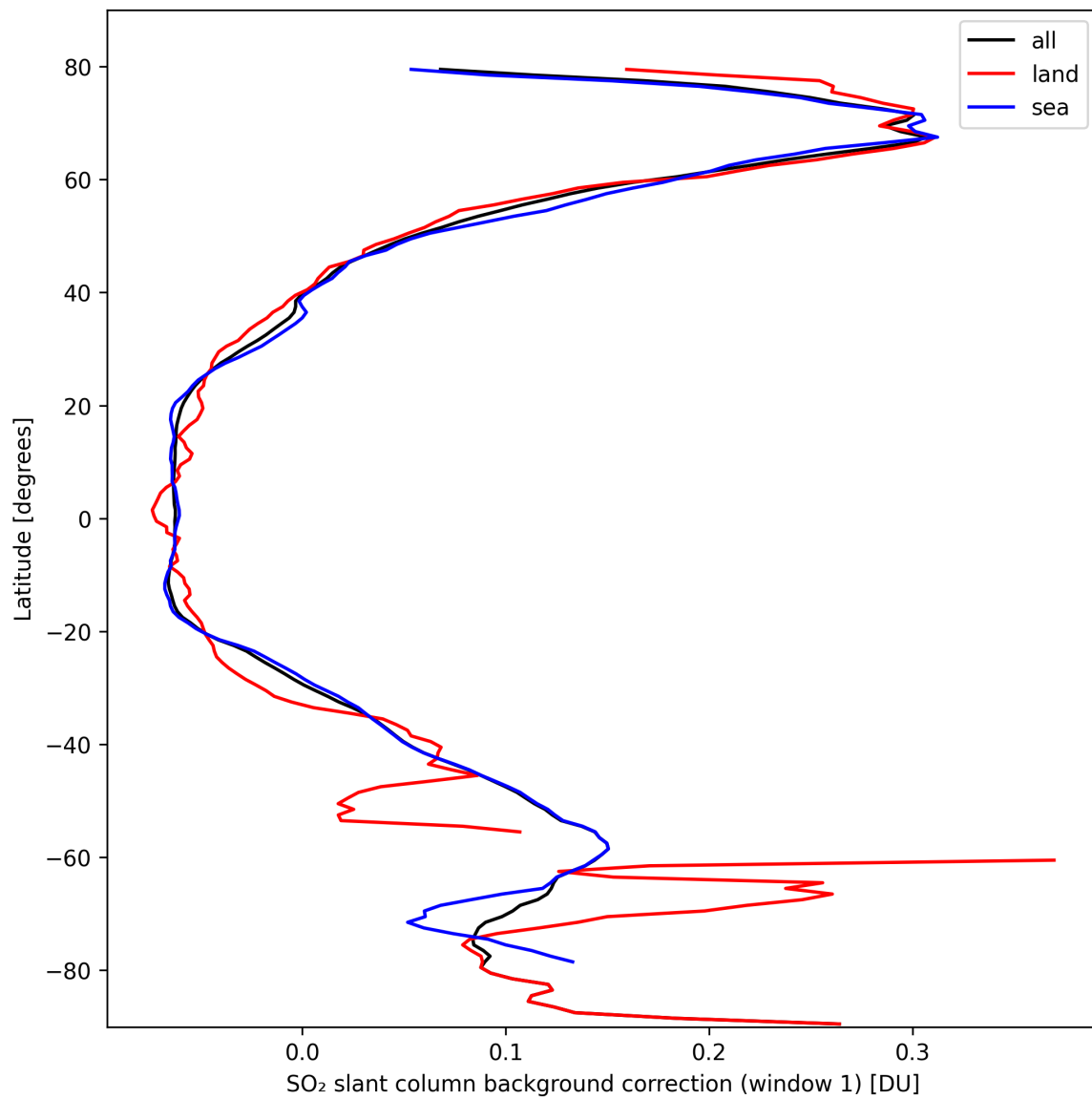
Figure 36: Zonal average of “SO 2 slant column background correction (window 1)” for 2024-10-06 to 2024-10-08.
