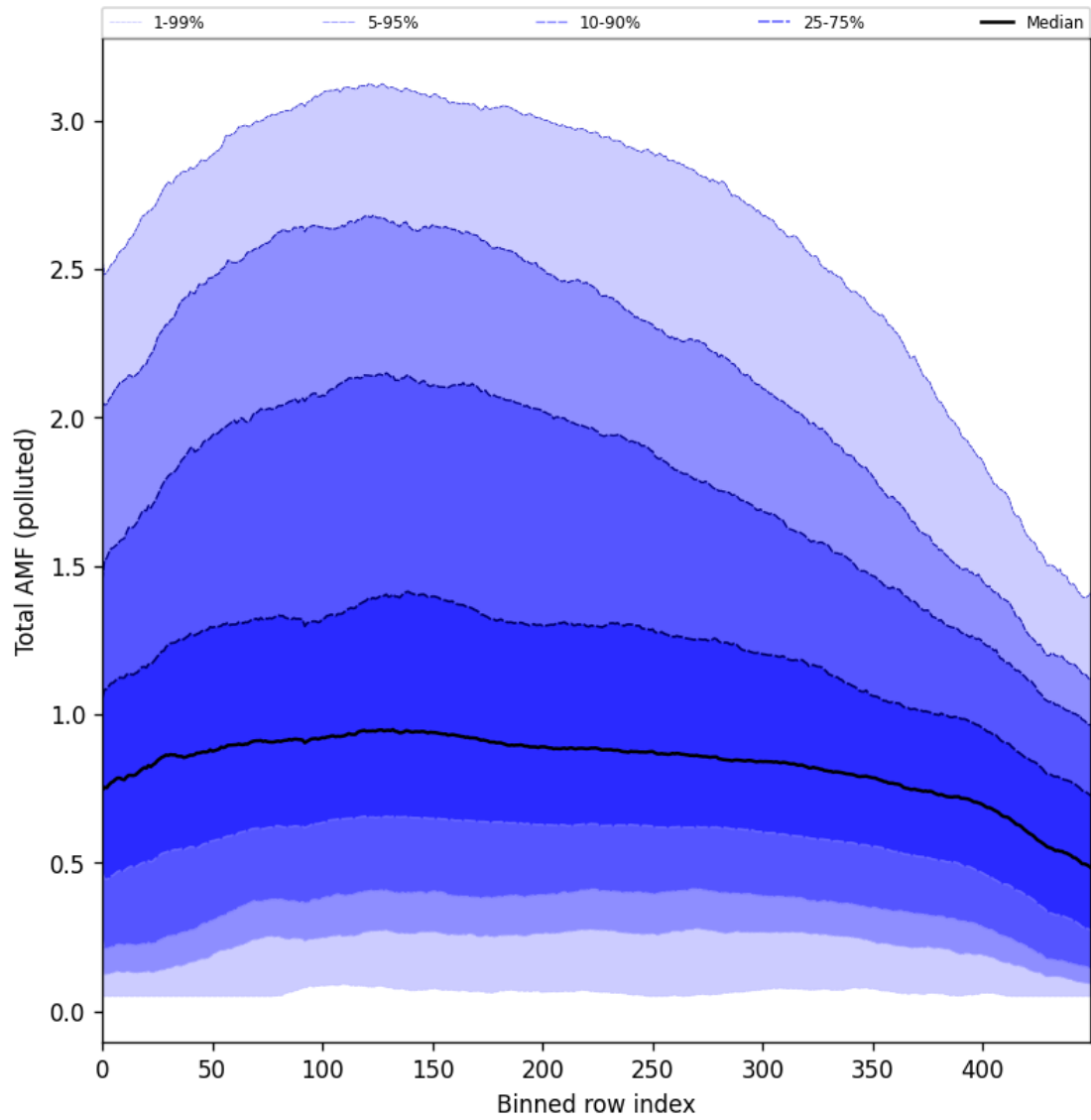
Figure 94: Along track statistics of “Total AMF (polluted)” for 2024-10-06 to 2024-10-08
