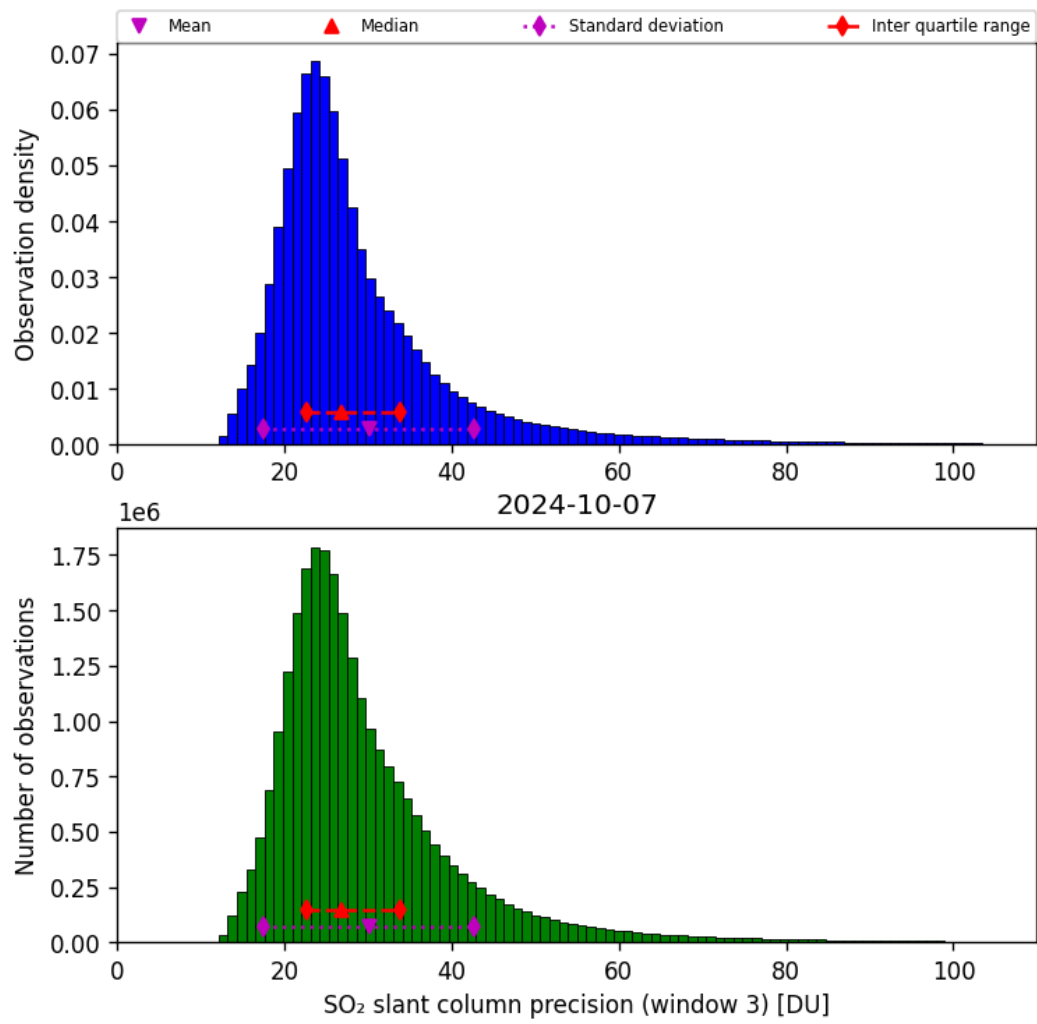
Figure 65: Histogram of “SO 2 slant column precision (window 3)” for 2024-10-06 to 2024-10-08
