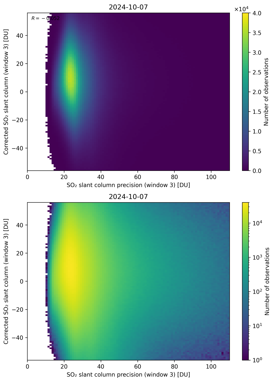
Figure 262: Scatter density plot of “SO 2 slant column precision (window 3)” against “Corrected SO 2 slant column (window 3)” for 2024-10-06 to 2024-10-08.
