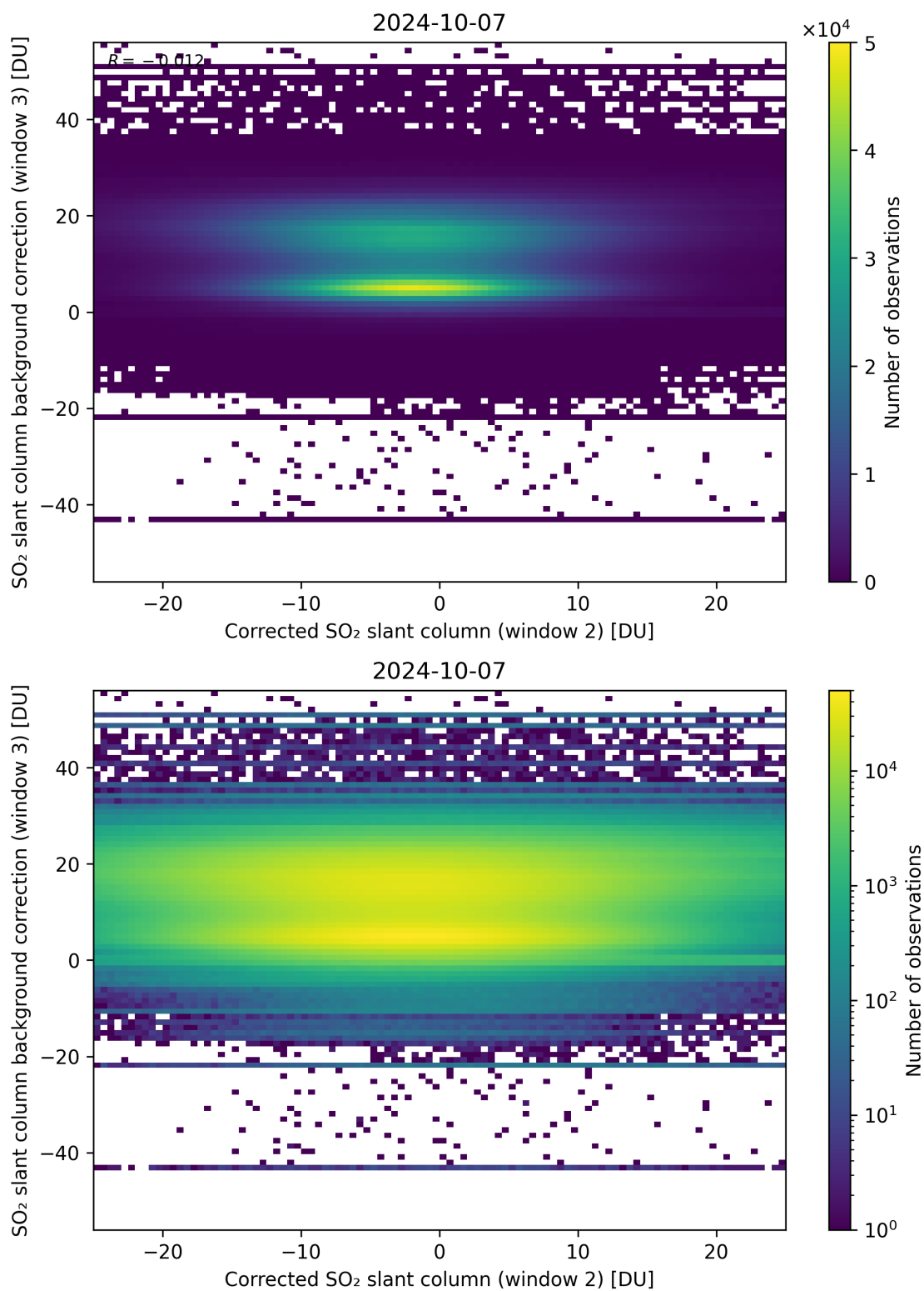
Figure 195: Scatter density plot of “Corrected SO 2 slant column (window 2)” against “SO 2 slant column background correction (window 3)” for 2024-10-06 to 2024-10-08.
