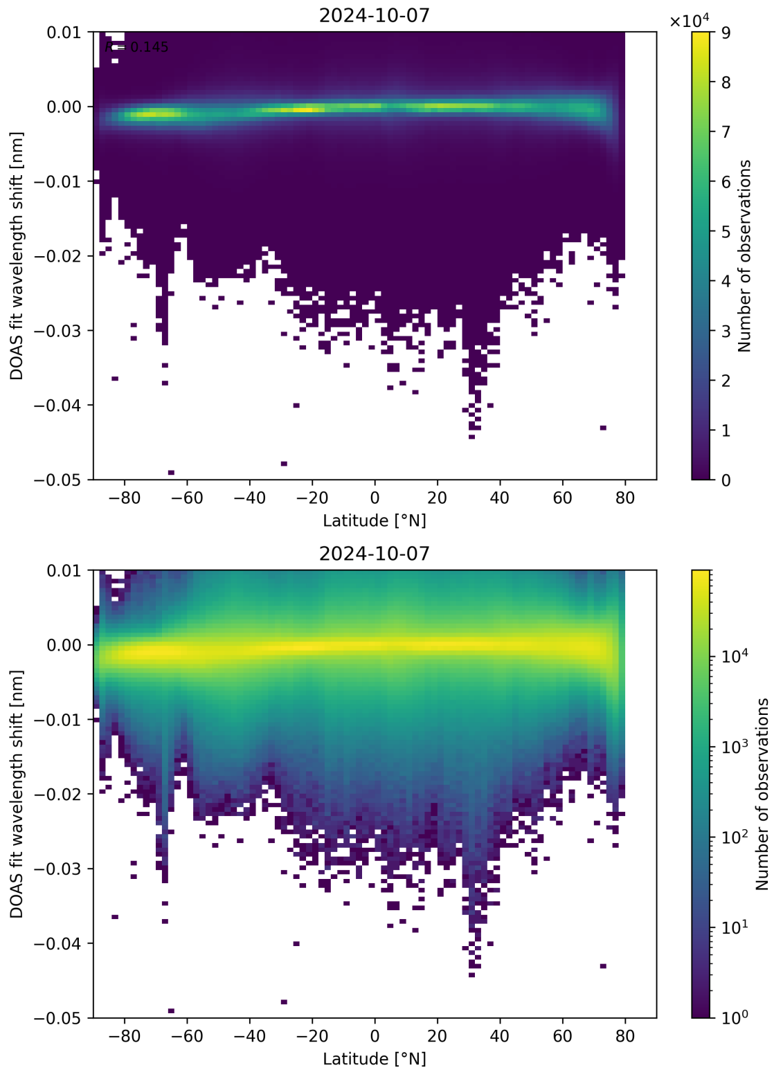
Figure 142: Scatter density plot of “Latitude” against “DOAS fit wavelength shift” for 2024-10-06 to 2024-10-08.
