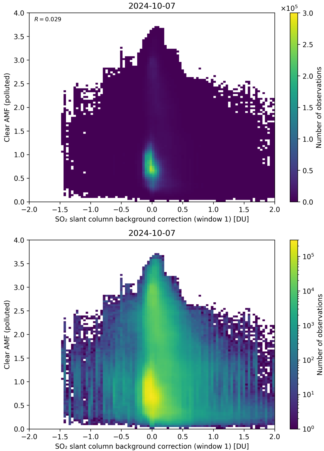
Figure 103: Scatter density plot of “SO 2 slant column background correction (window 1)” against “Clear AMF (polluted)” for 2024-10-06 to 2024-10-08.
