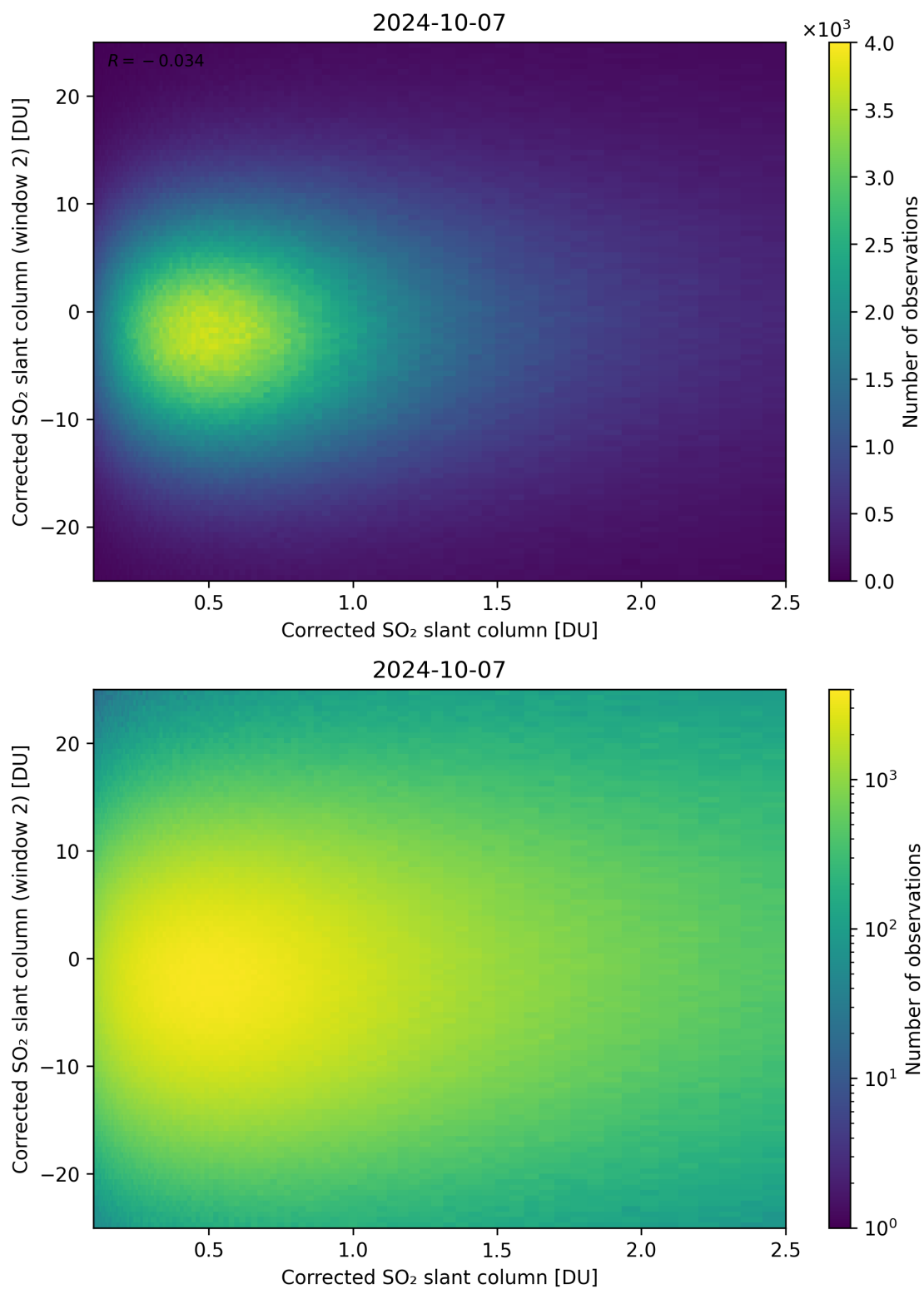
Figure 185: Scatter density plot of “Corrected SO 2 slant column” against “Corrected SO 2 slant column (window 2)” for 2024-10-06 to 2024-10-08.
