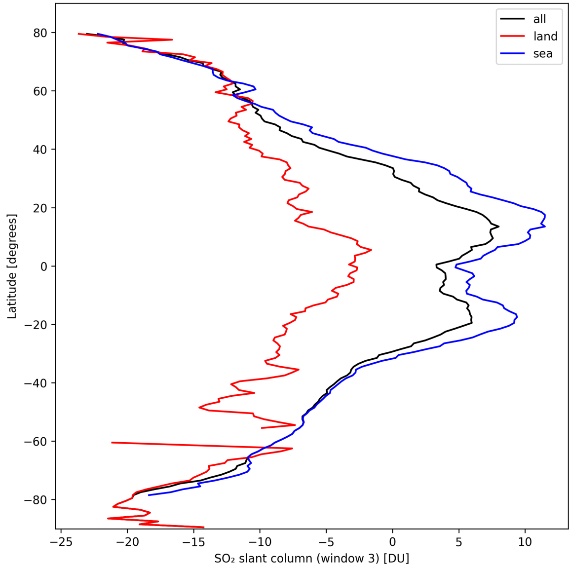
Figure 41: Zonal average of “SO 2 slant column (window 3)” for 2024-10-06 to 2024-10-08.
