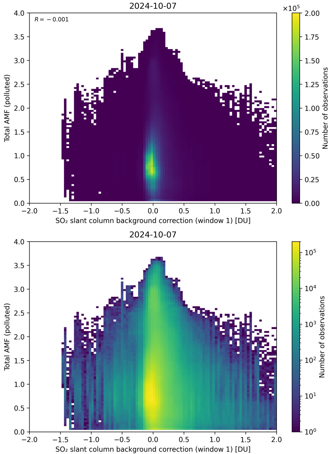
Figure 109: Scatter density plot of “SO 2 slant column background correction (window 1)” against “Total AMF (polluted)” for 2024-10-06 to 2024-10-08.
