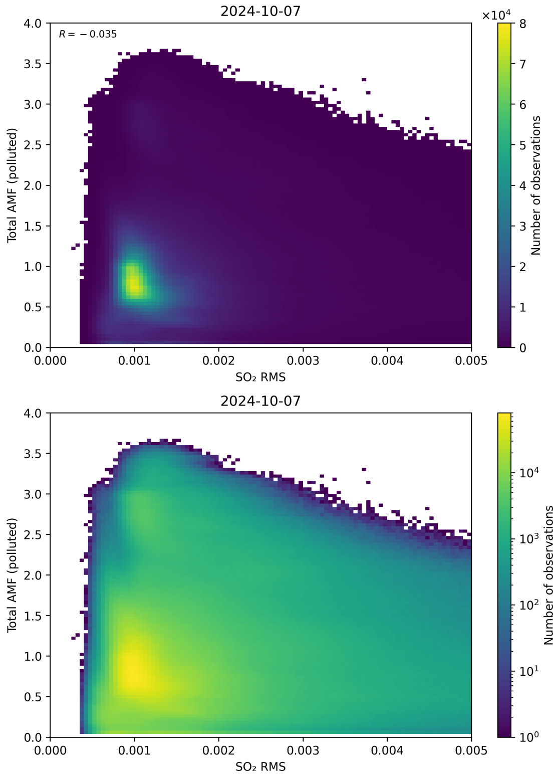
Figure 137: Scatter density plot of “SO 2 RMS” against “Total AMF (polluted)” for 2024-10-06 to 2024-10-08.
