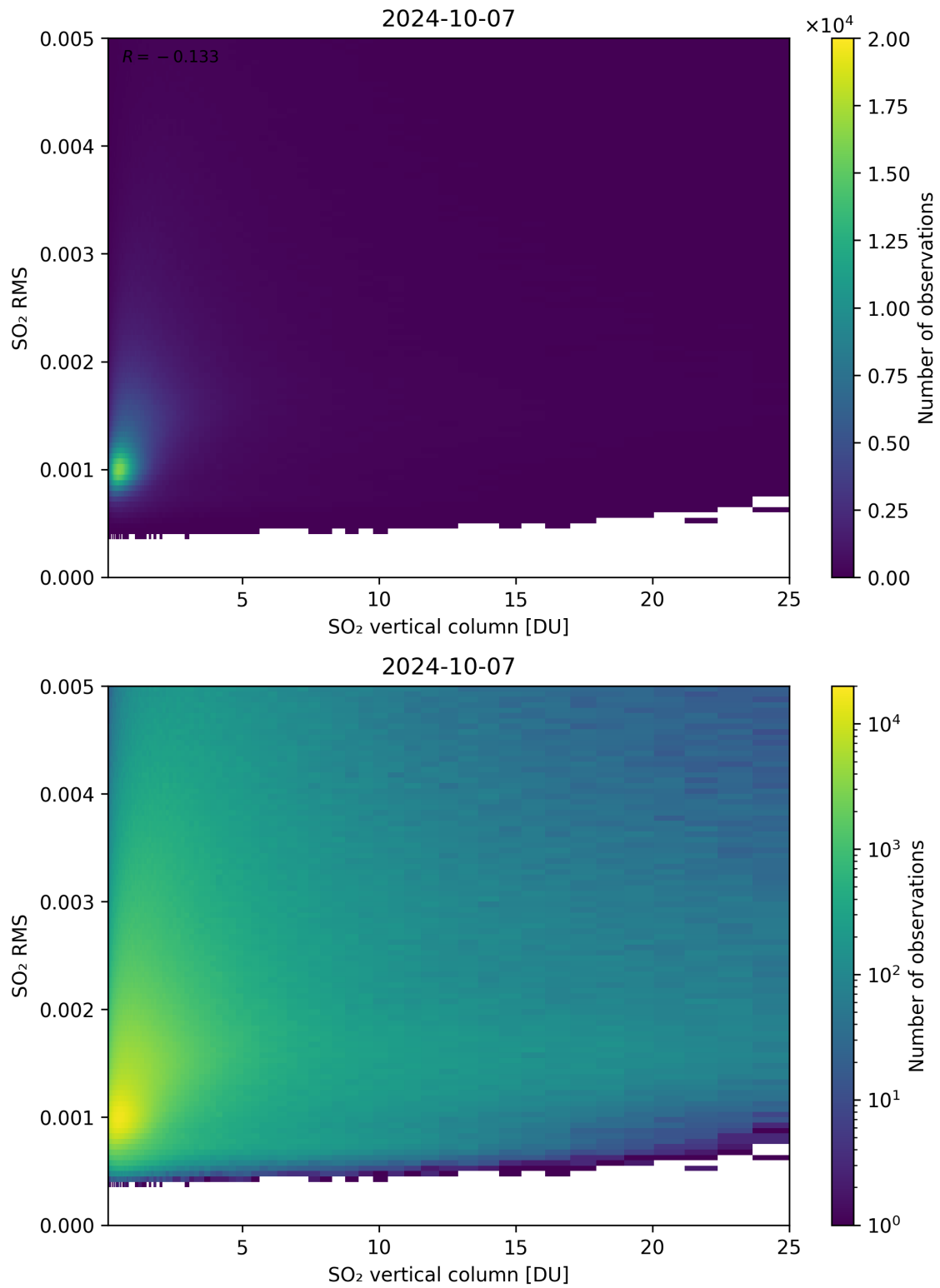
Figure 278: Scatter density plot of “SO 2 vertical column” against “SO 2 RMS” for 2024-10-06 to 2024-10-08.
