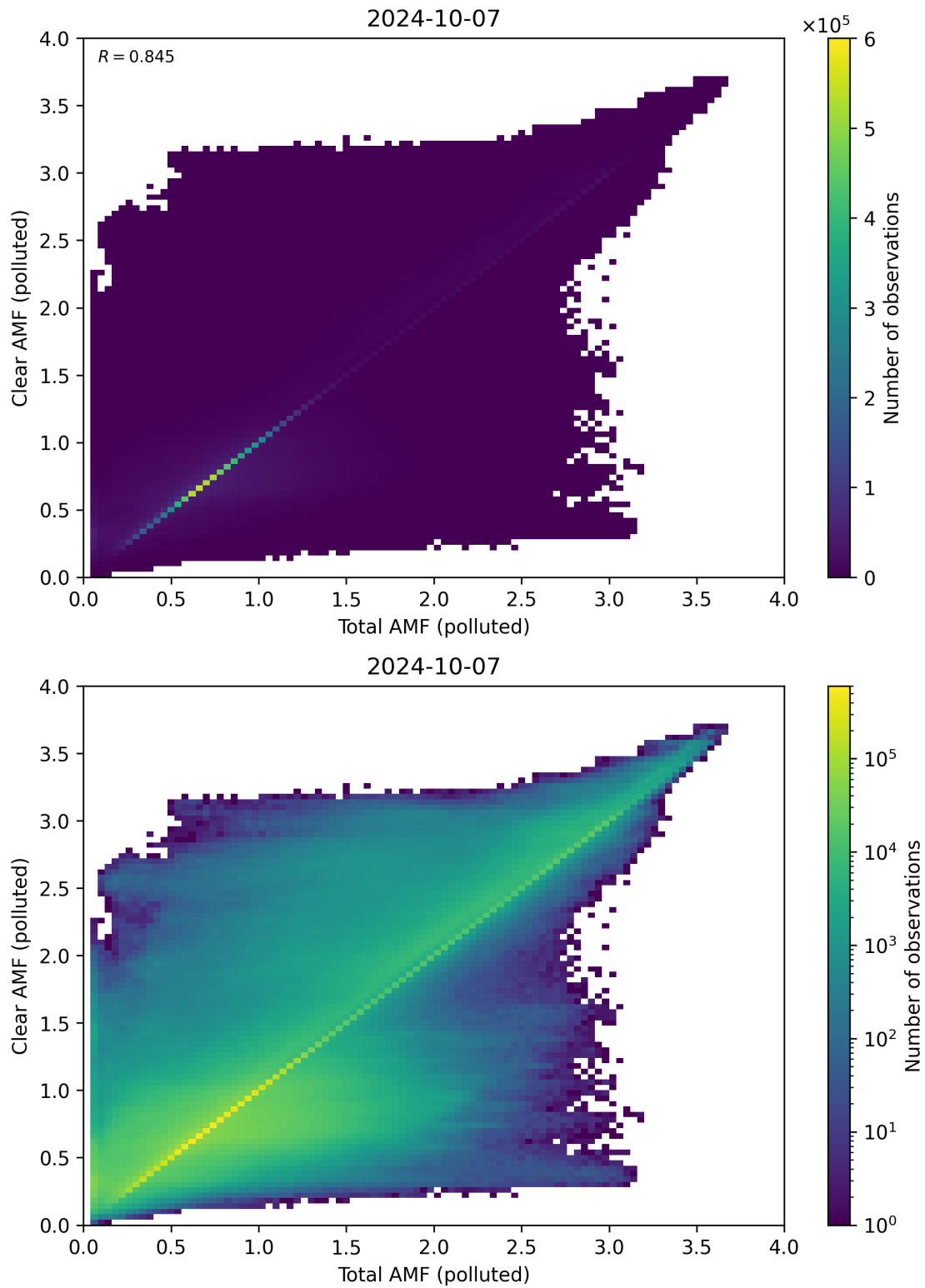
Figure 271: Scatter density plot of “Total AMF (polluted)” against “Clear AMF (polluted)” for 2024-10-06 to 2024-10-08.
