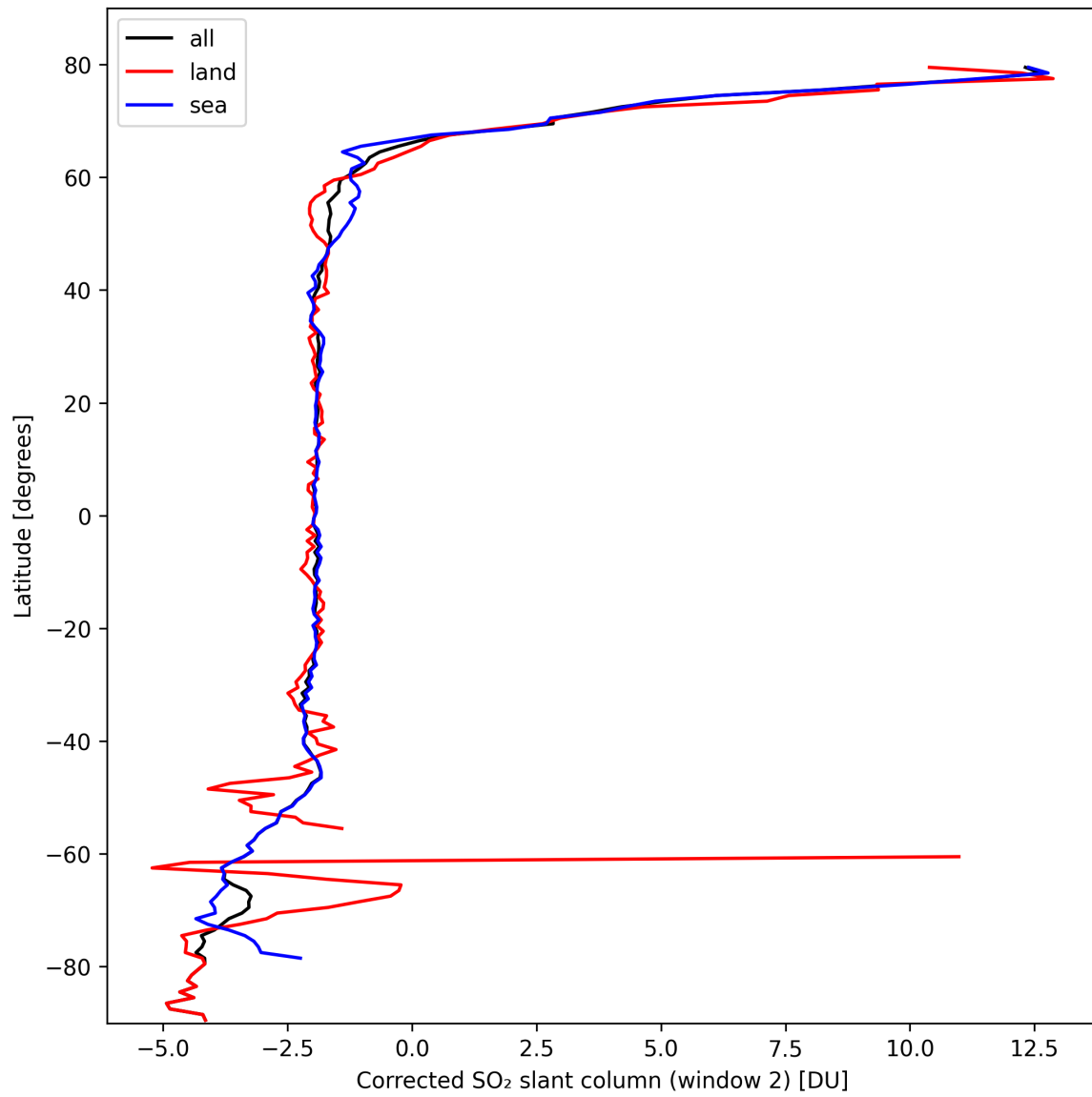
Figure 39: Zonal average of “Corrected SO 2 slant column (window 2)” for 2024-10-06 to 2024-10-08.
