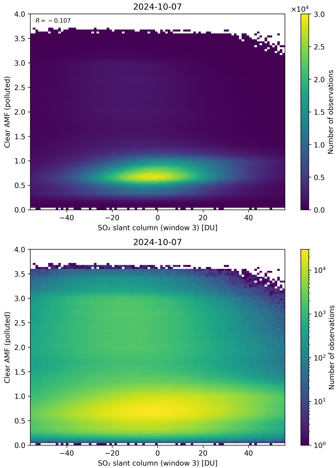
Figure 265: Scatter density plot of “SO 2 slant column (window 3)” against “Clear AMF (polluted)” for 2024-10-06 to 2024-10-08.
