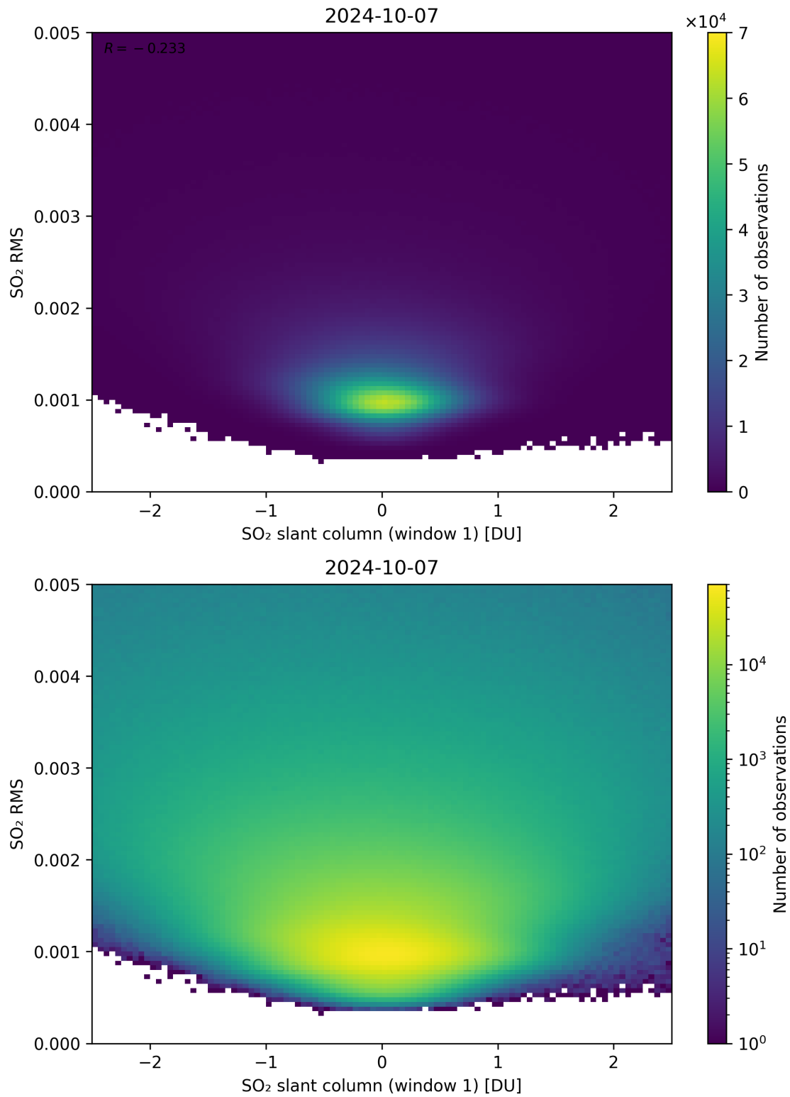
Figure 217: Scatter density plot of “SO 2 slant column (window 1)” against “SO 2 RMS” for 2024-10-06 to 2024-10-08.
