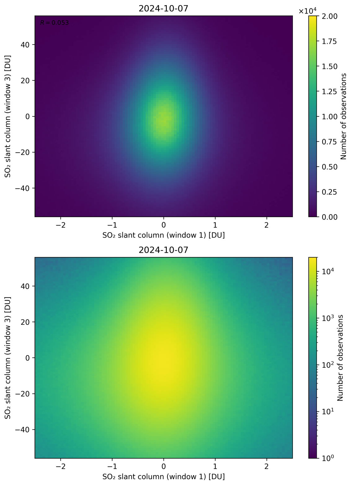
Figure 237: Scatter density plot of “SO 2 slant column (window 1)” against “SO 2 slant column (window 3)” for 2024-10-06 to 2024-10-08.
