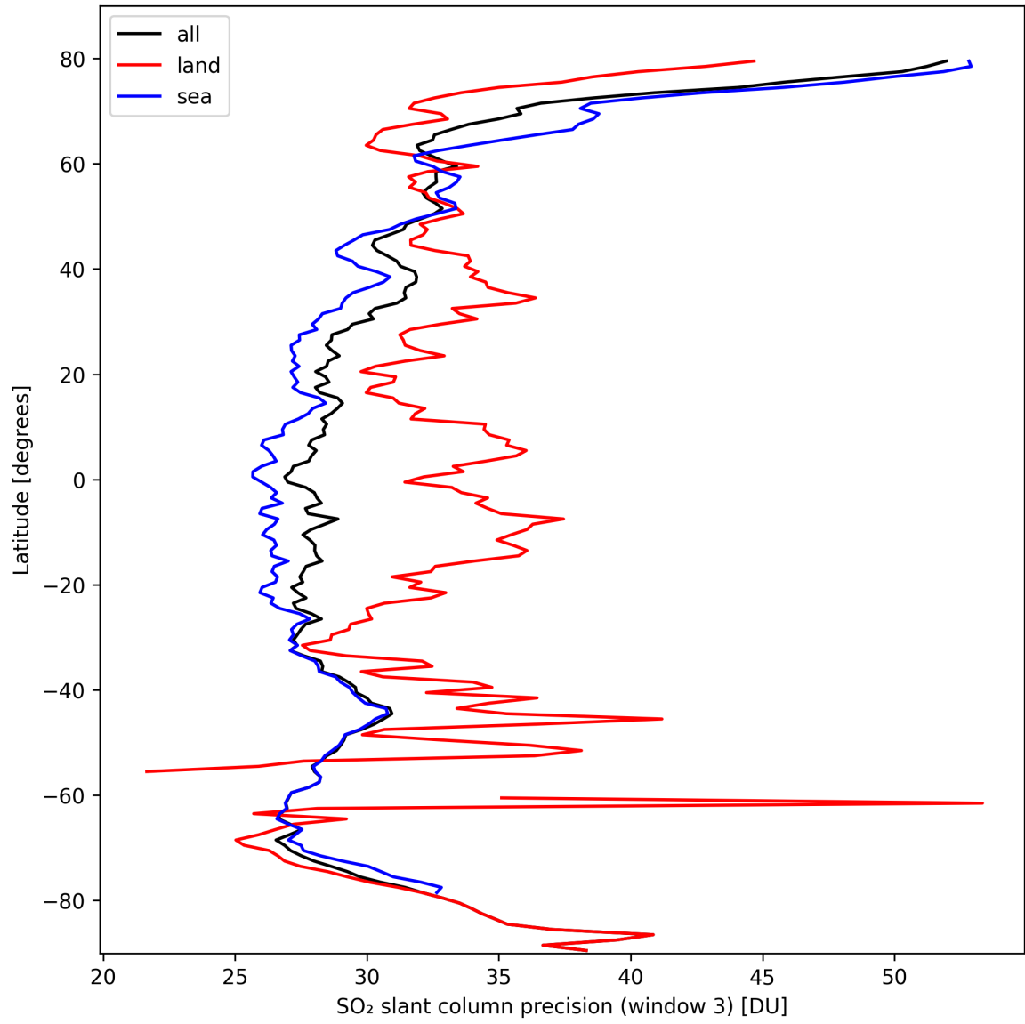
Figure 42: Zonal average of “SO 2 slant column precision (window 3)” for 2024-10-06 to 2024-10-08.
