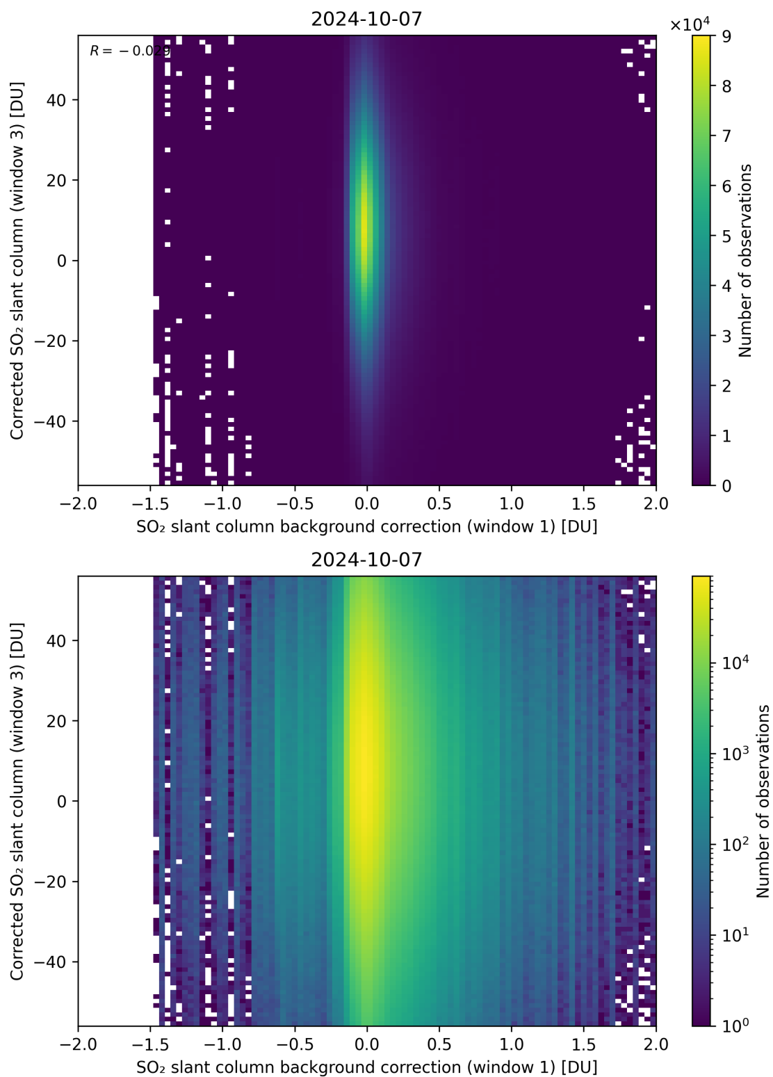
Figure 105: Scatter density plot of “SO 2 slant column background correction (window 1)” against “Corrected SO 2 slant column (window 3)” for 2024-10-06 to 2024-10-08.
