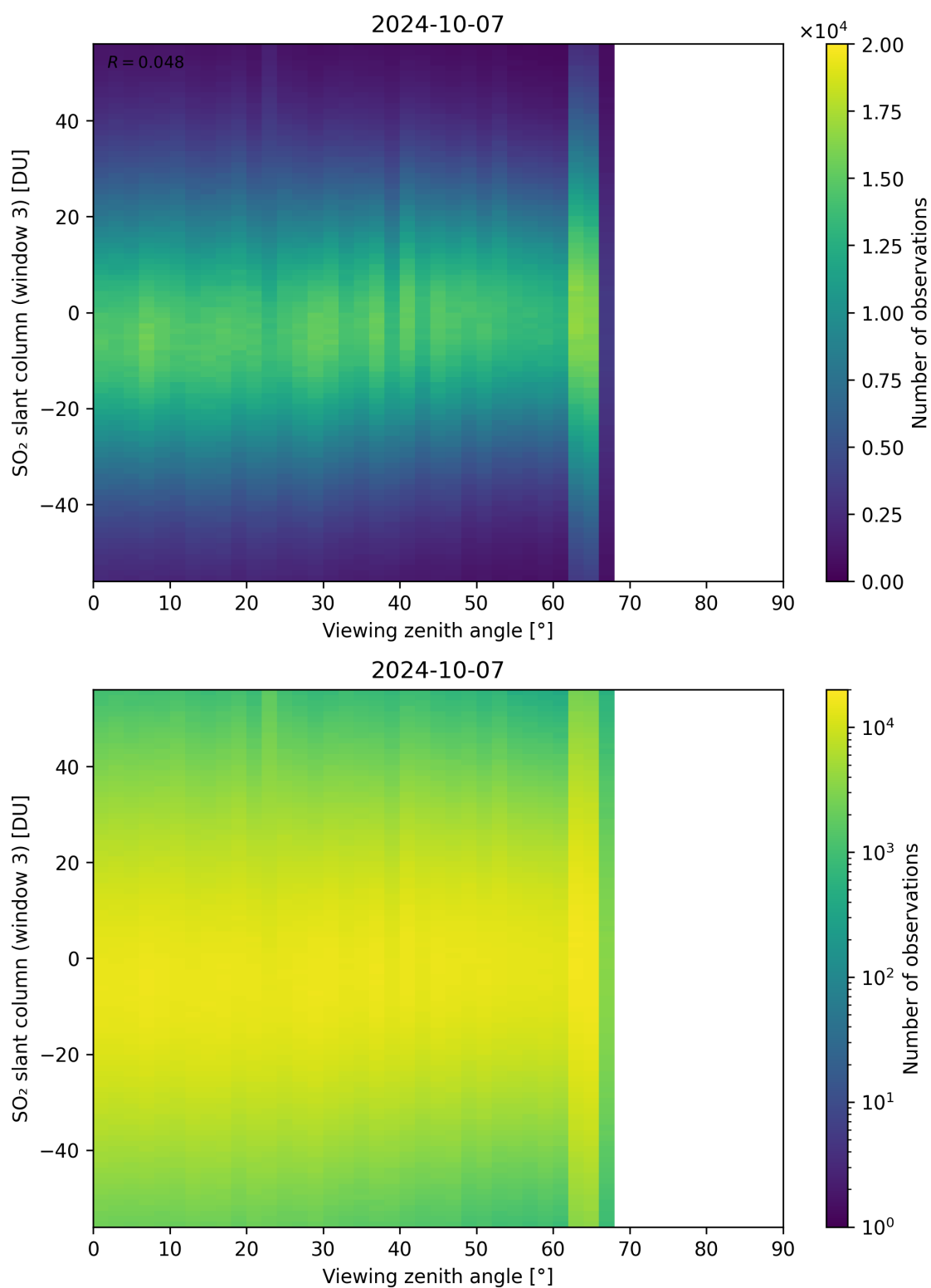
Figure 323: Scatter density plot of “Viewing zenith angle” against “SO 2 slant column (window 3)” for 2024-10-06 to 2024-10-08.
