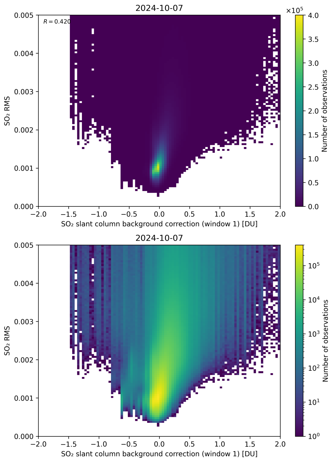
Figure 102: Scatter density plot of “SO 2 slant column background correction (window 1)” against “SO 2 RMS” for 2024-10-06 to 2024-10-08.
