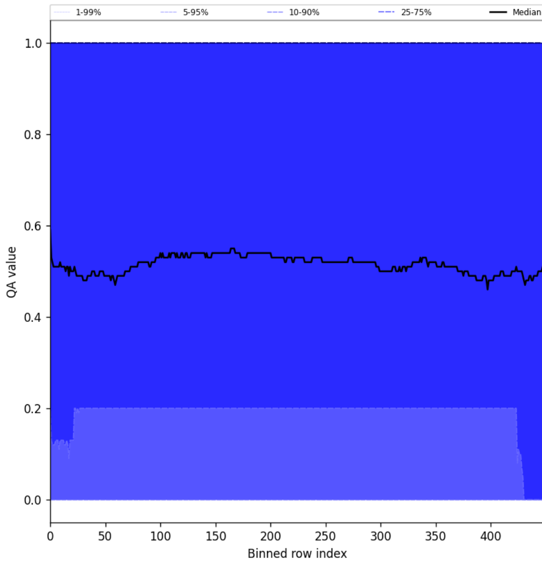
Figure 75: Along track statistics of “QA value” for 2024-10-06 to 2024-10-08
