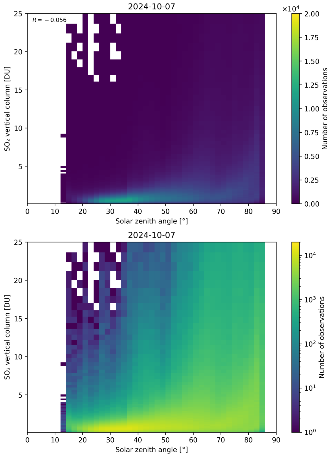
Figure 176: Scatter density plot of “Solar zenith angle” against “SO 2 vertical column” for 2024-10-06 to 2024-10-08.
