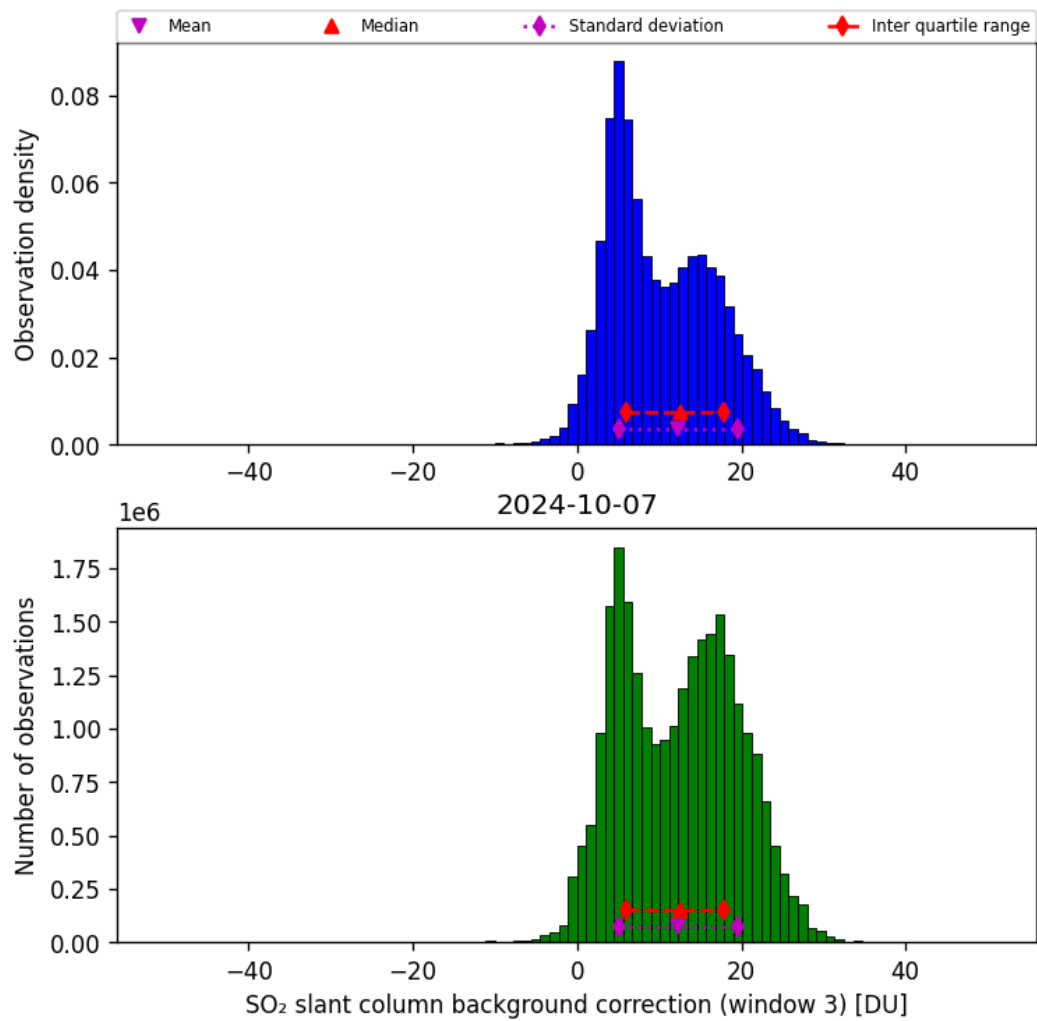
Figure 67: Histogram of “SO 2 slant column background correction (window 3)” for 2024-10-06 to 2024-10-08
