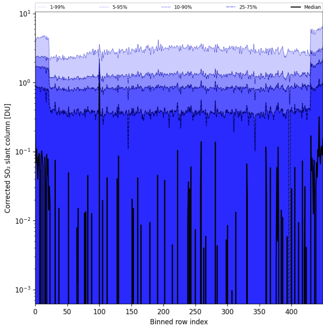
Figure 78: Along track statistics of “Corrected SO 2 slant column” for 2024-10-06 to 2024-10-08
