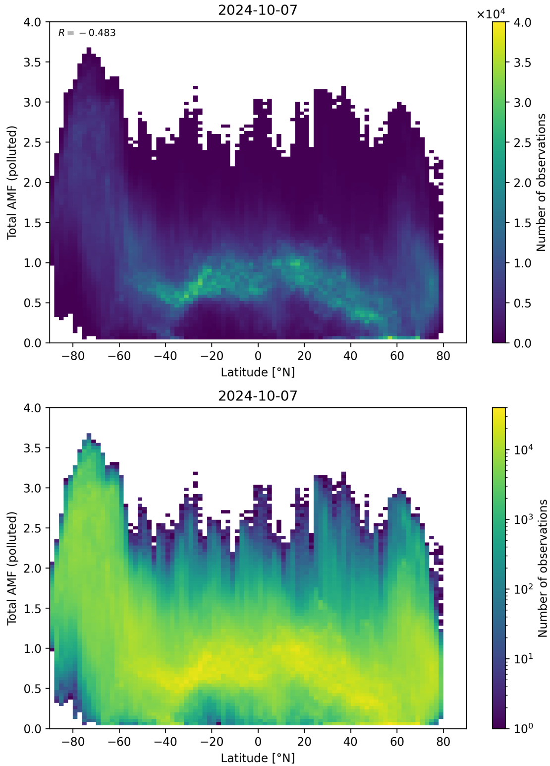
Figure 154: Scatter density plot of “Latitude” against “Total AMF (polluted)” for 2024-10-06 to 2024-10-08.
