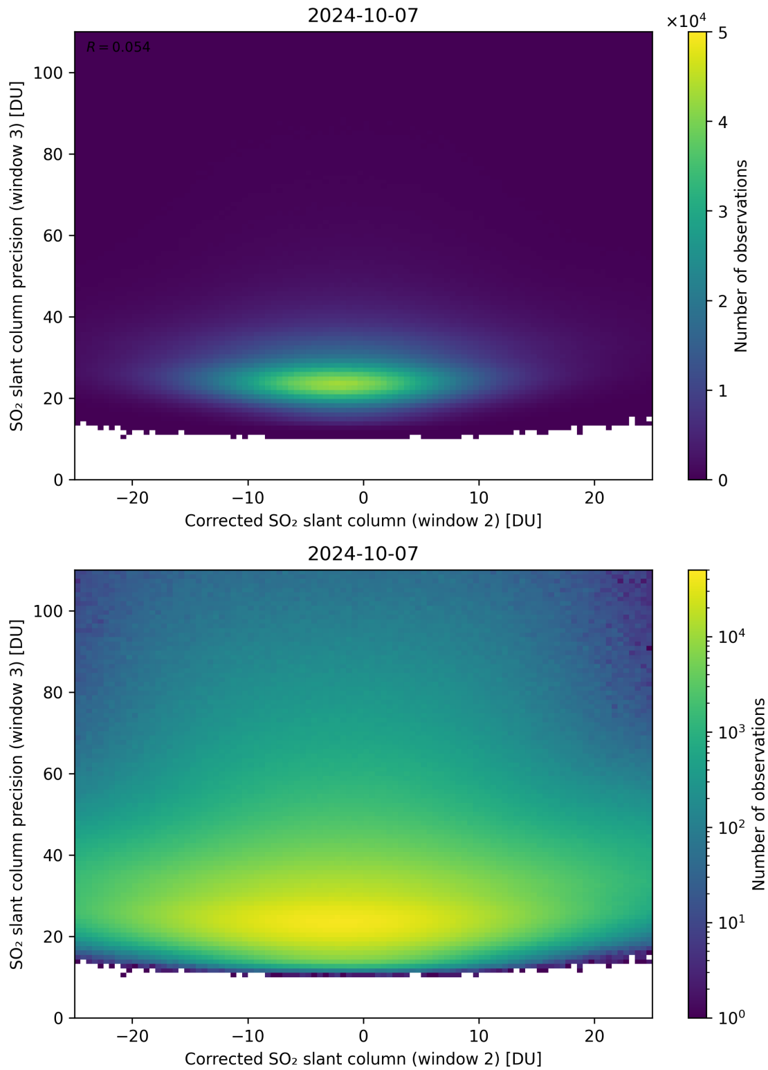
Figure 202: Scatter density plot of “Corrected SO 2 slant column (window 2)” against “SO 2 slant column precision (window 3)” for 2024-10-06 to 2024-10-08.
