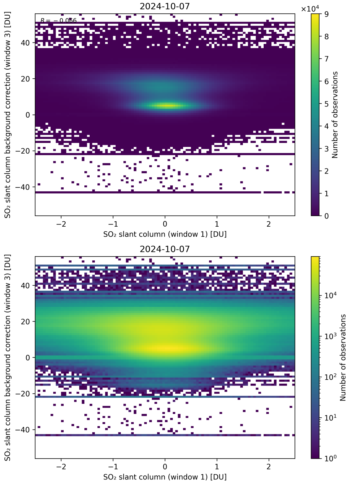
Figure 214: Scatter density plot of “SO 2 slant column (window 1)” against “SO 2 slant column background correction (window 3)” for 2024-10-06 to 2024-10-08.
