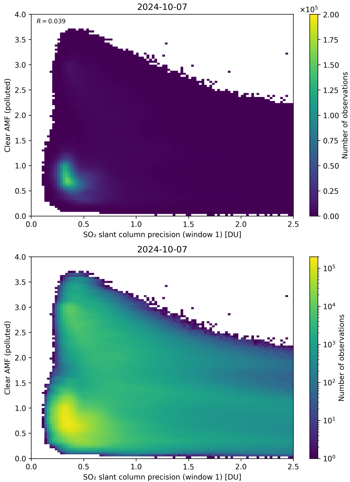
Figure 224: Scatter density plot of “SO 2 slant column precision (window 1)” against “Clear AMF (polluted)” for 2024-10-06 to 2024-10-08.
