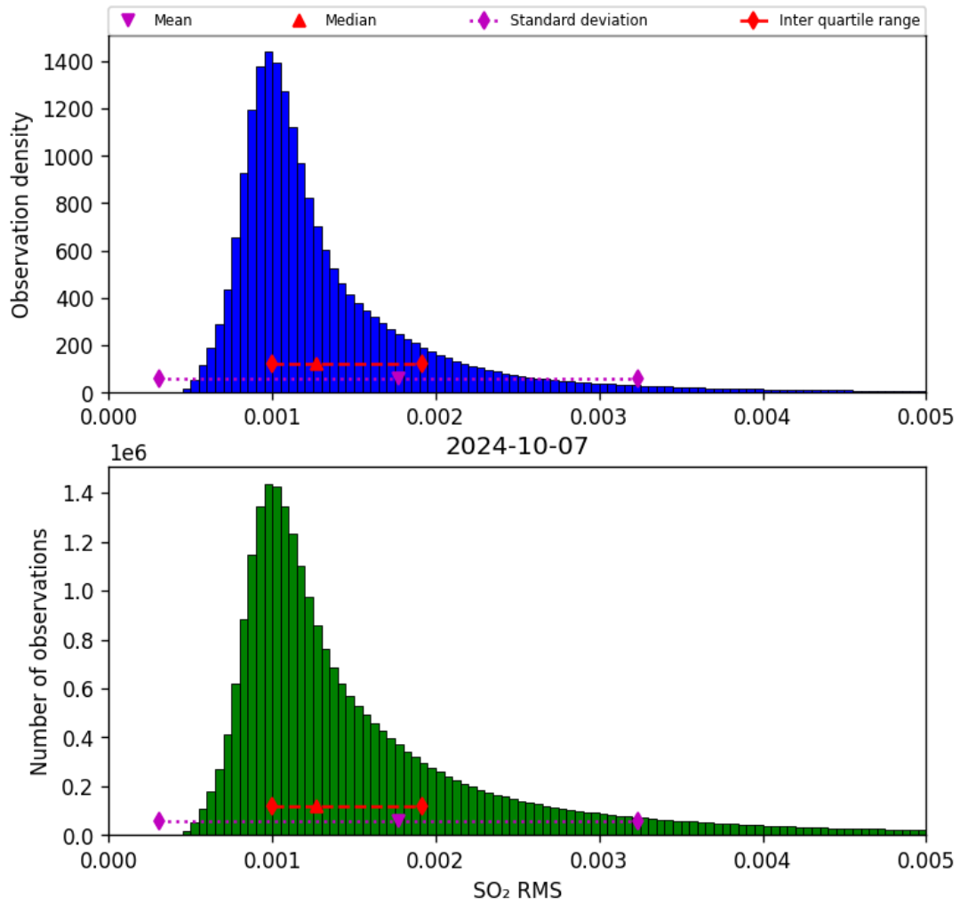
Figure 70: Histogram of “SO 2 RMS” for 2024-10-06 to 2024-10-08
