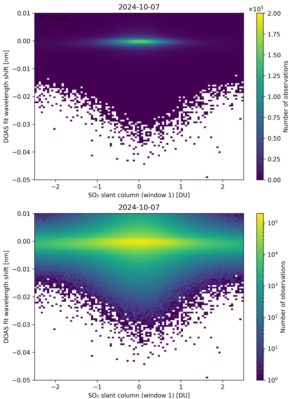
Figure 215: Scatter density plot of “SO 2 slant column (window 1)” against “DOAS fit wavelength shift” for 2024-10-06 to 2024-10-08.
