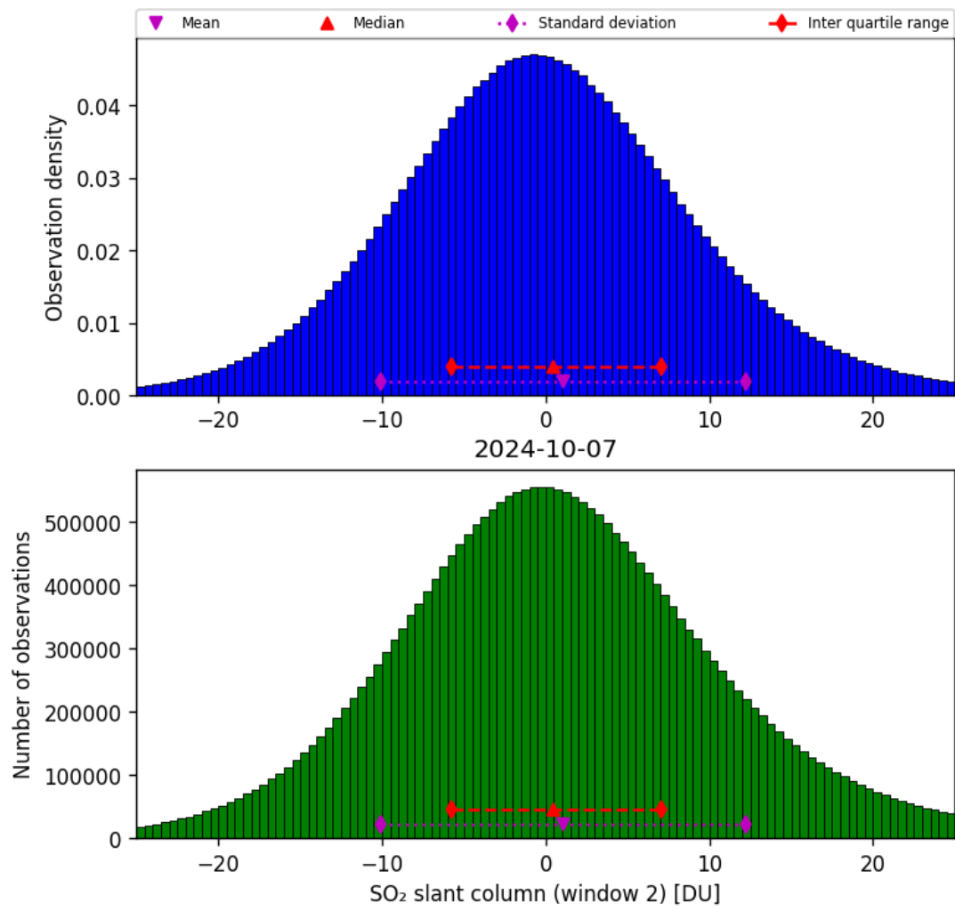
Figure 60: Histogram of “SO 2 slant column (window 2)” for 2024-10-06 to 2024-10-08
