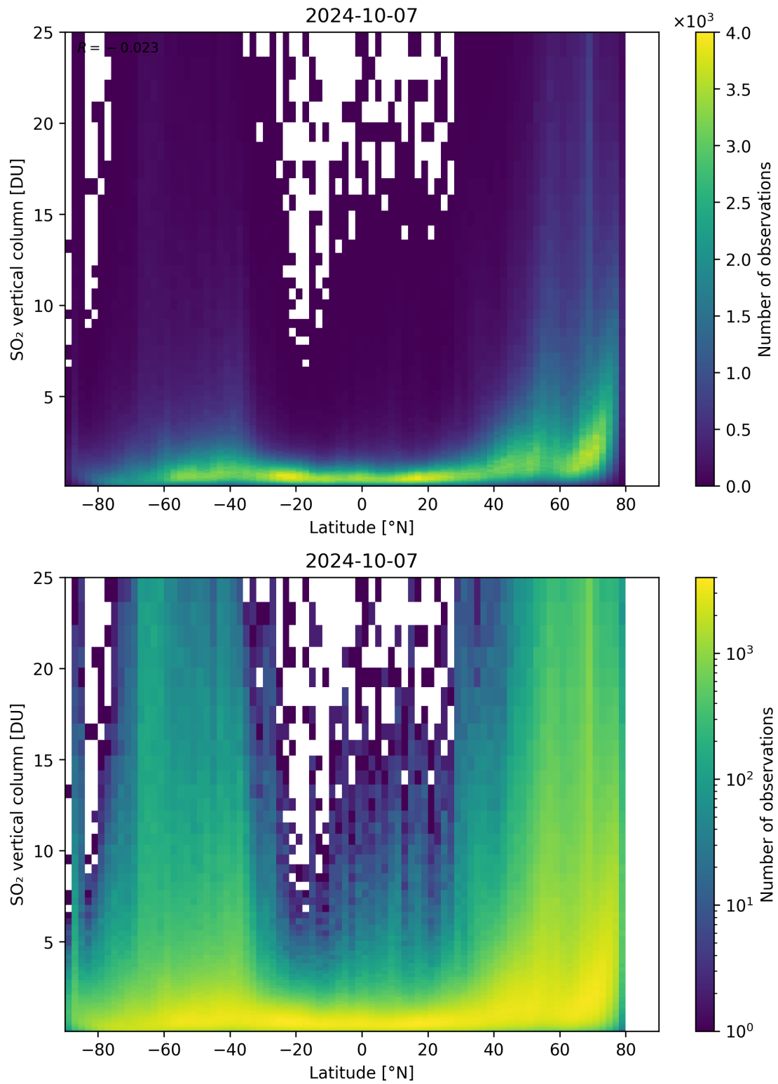
Figure 156: Scatter density plot of “Latitude” against “SO 2 vertical column” for 2024-10-06 to 2024-10-08.
