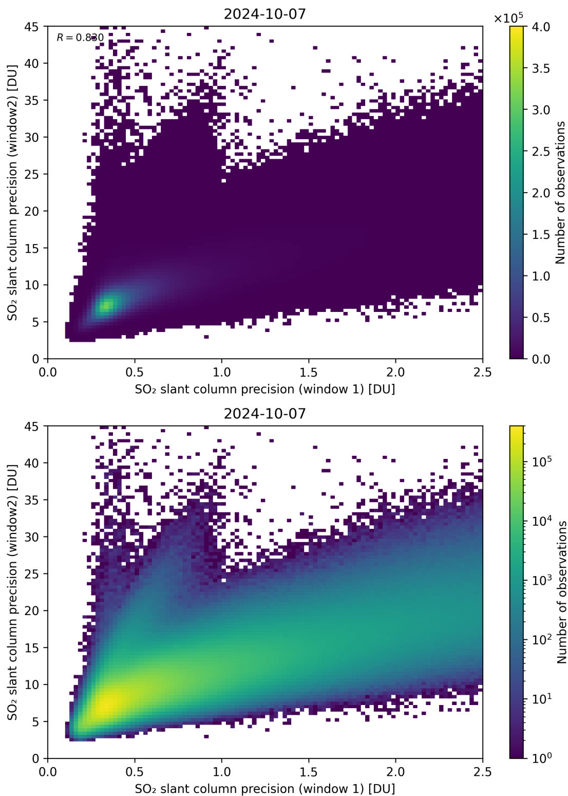
Figure 227: Scatter density plot of “SO 2 slant column precision (window 1)” against “SO 2 slant column precision (window2)” for 2024-10-06 to 2024-10-08.
