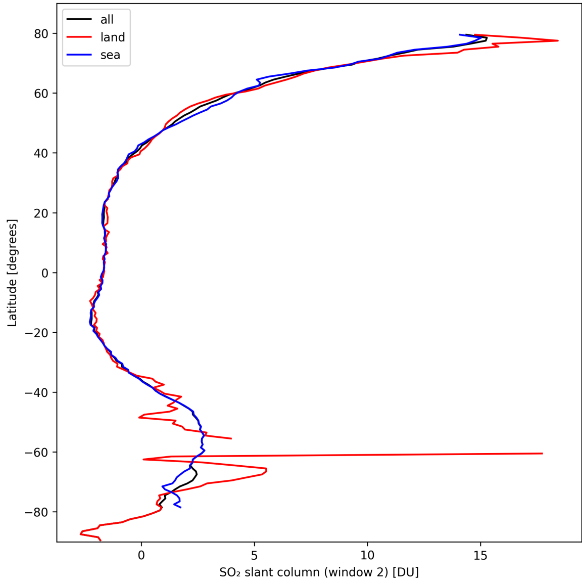
Figure 37: Zonal average of “SO 2 slant column (window 2)” for 2024-10-06 to 2024-10-08.
