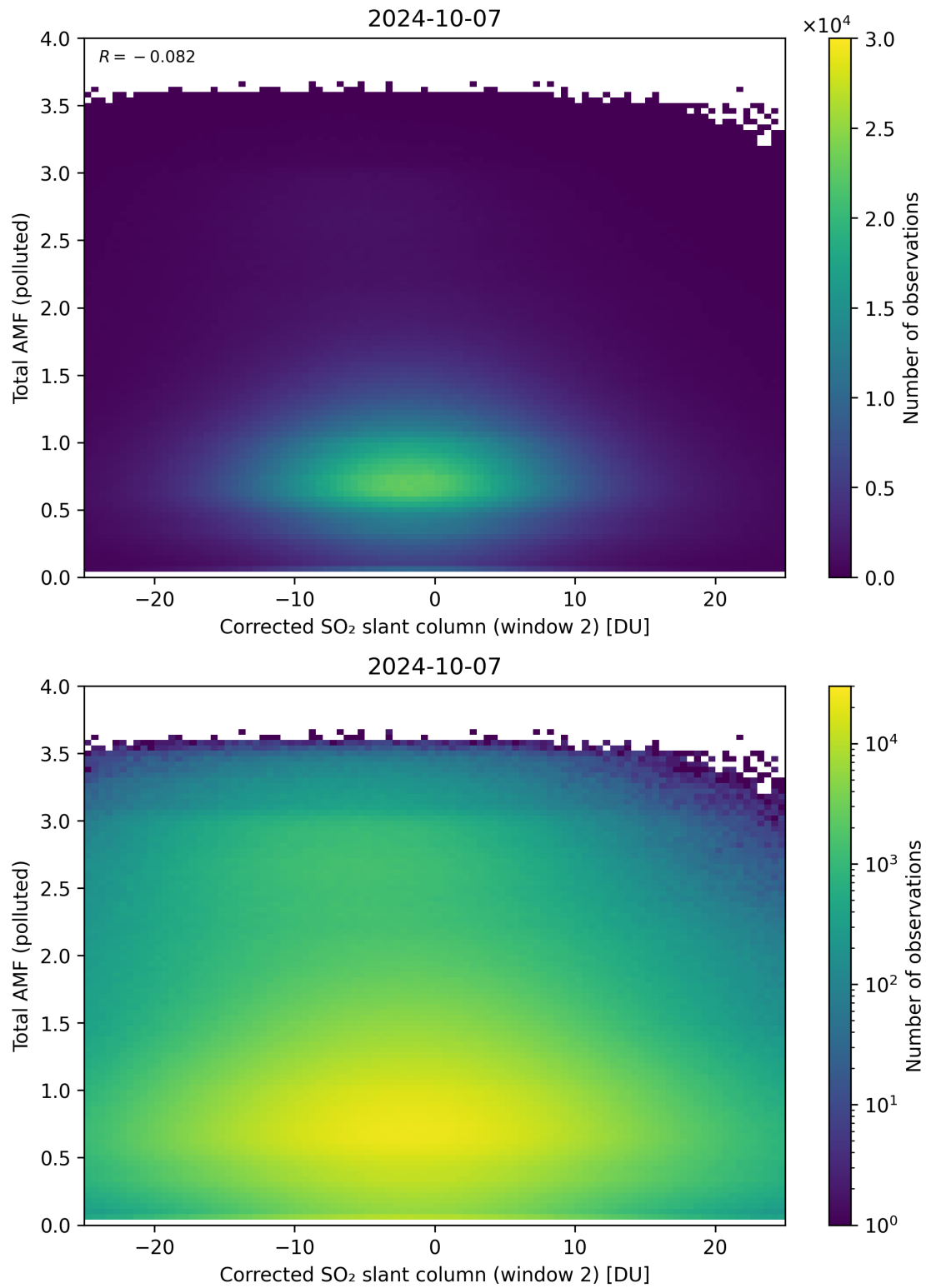
Figure 203: Scatter density plot of “Corrected SO 2 slant column (window 2)” against “Total AMF (polluted)” for 2024-10-06 to 2024-10-08.
