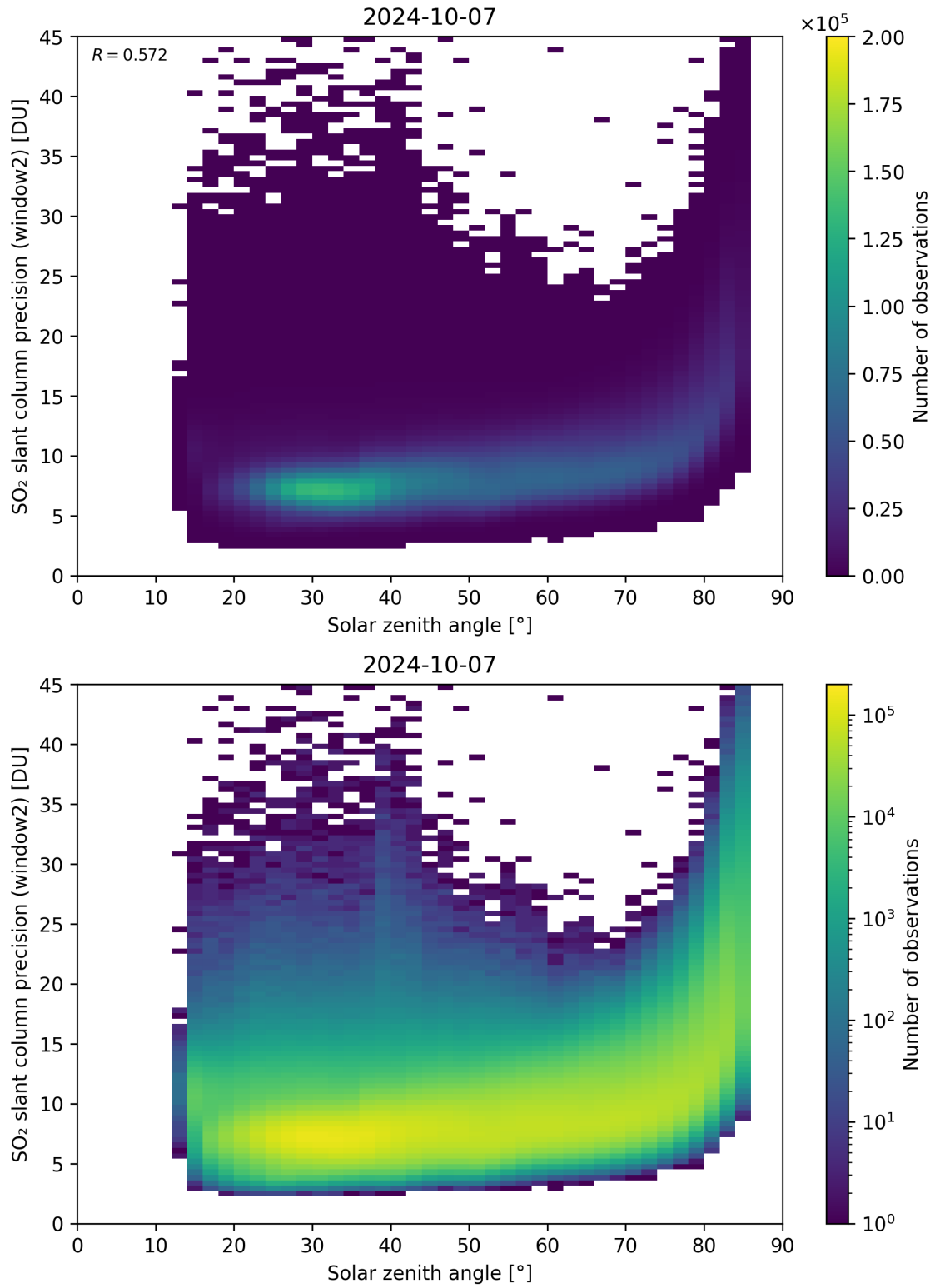
Figure 171: Scatter density plot of “Solar zenith angle” against “SO 2 slant column precision (window2)” for 2024-10-06 to 2024-10-08.
