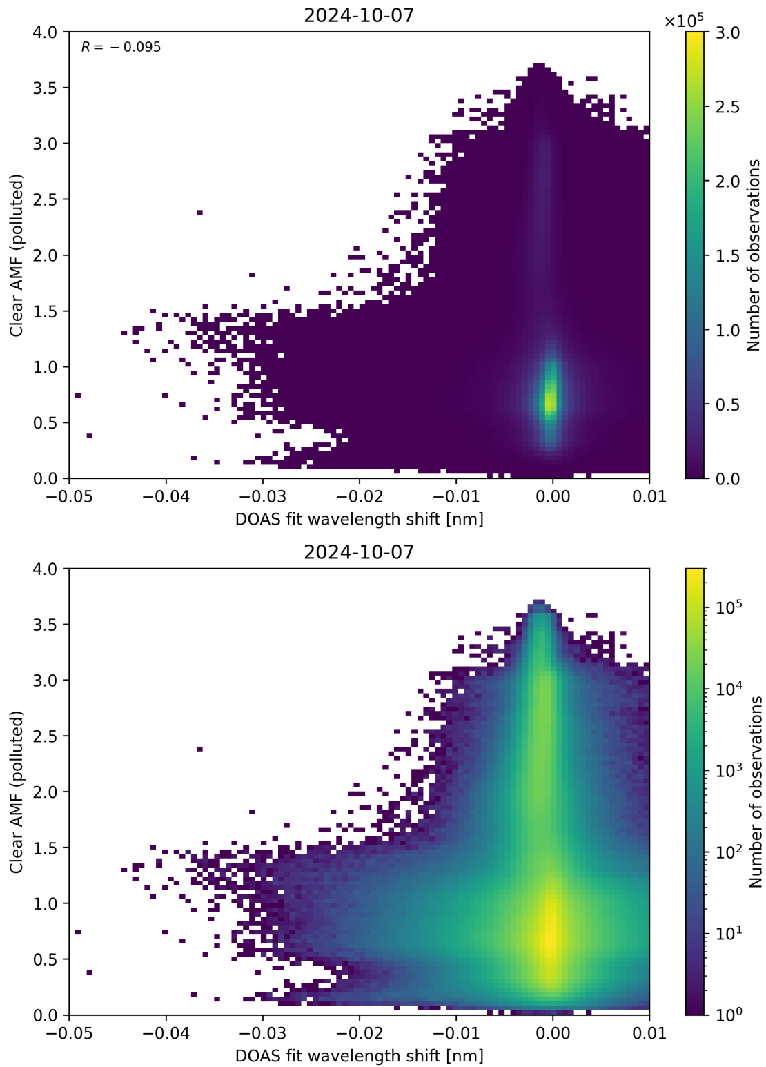
Figure 129: Scatter density plot of “DOAS fit wavelength shift” against “Clear AMF (polluted)” for 2024-10-06 to 2024-10-08.
