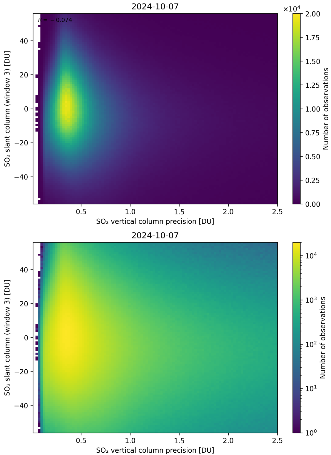
Figure 292: Scatter density plot of “SO 2 vertical column precision” against “SO 2 slant column (window 3)” for 2024-10-06 to 2024-10-08.
