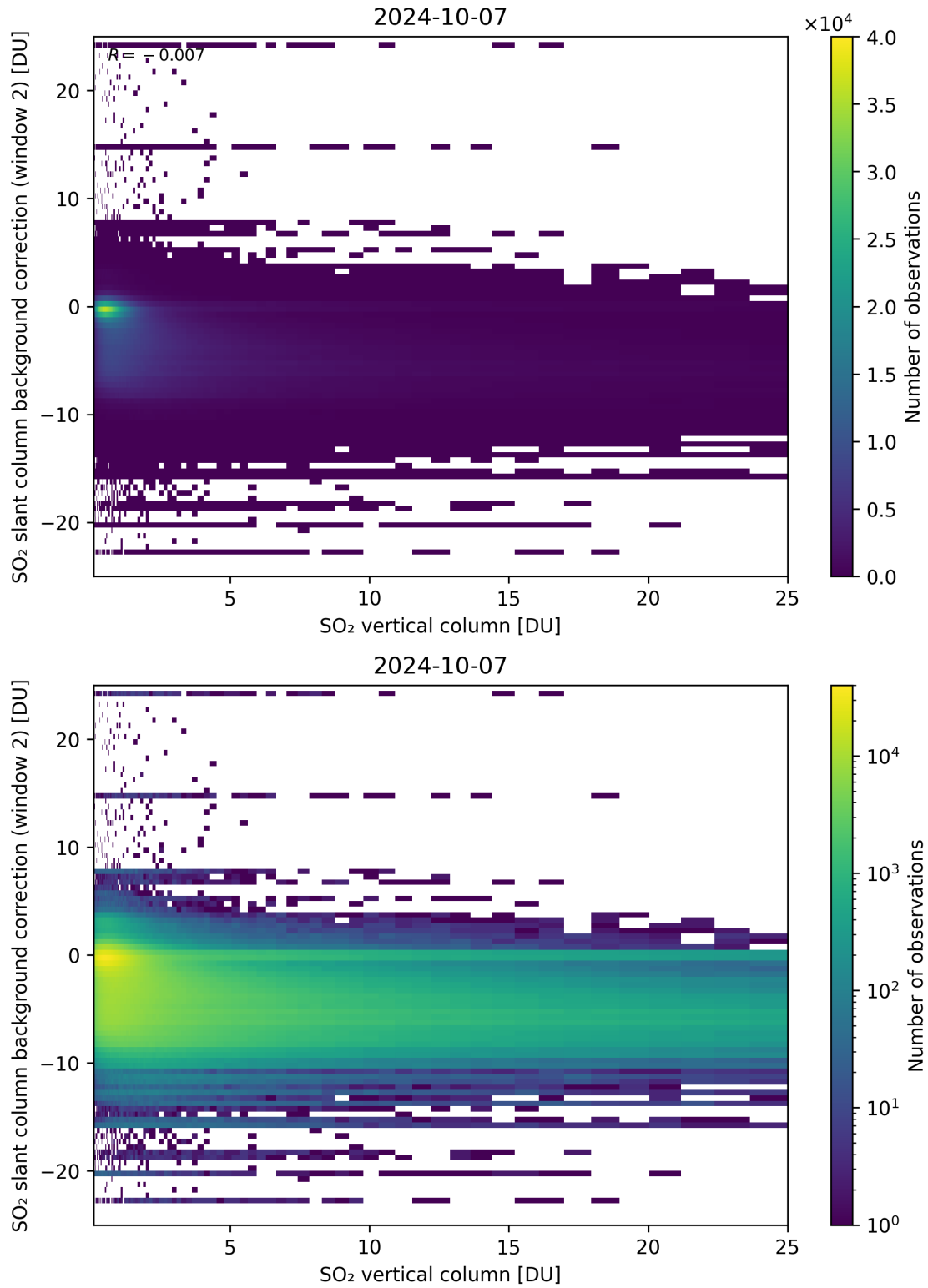
Figure 274: Scatter density plot of “SO 2 vertical column” against “SO 2 slant column background correction (window 2)” for 2024-10-06 to 2024-10-08.
