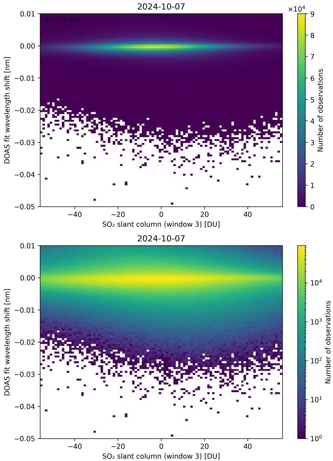
Figure 254: Scatter density plot of “SO 2 slant column (window 3)” against “DOAS fit wavelength shift” for 2024-10-06 to 2024-10-08.
