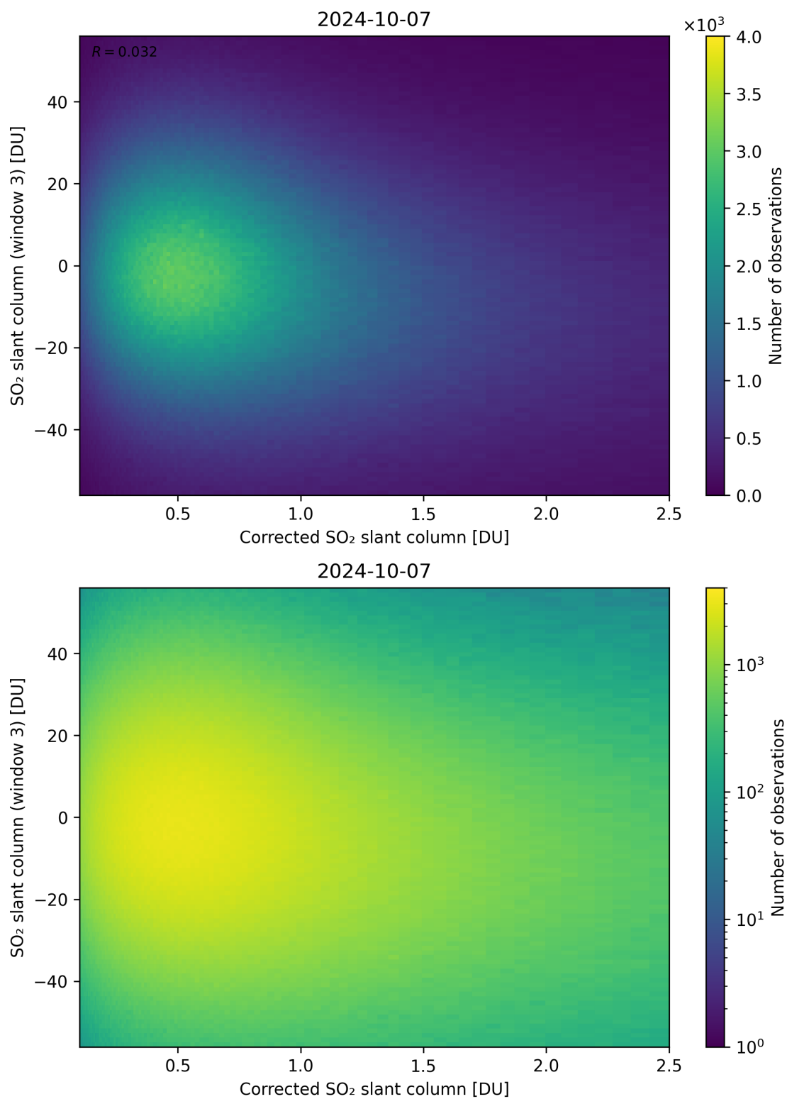
Figure 190: Scatter density plot of “Corrected SO 2 slant column” against “SO 2 slant column (window 3)” for 2024-10-06 to 2024-10-08.
