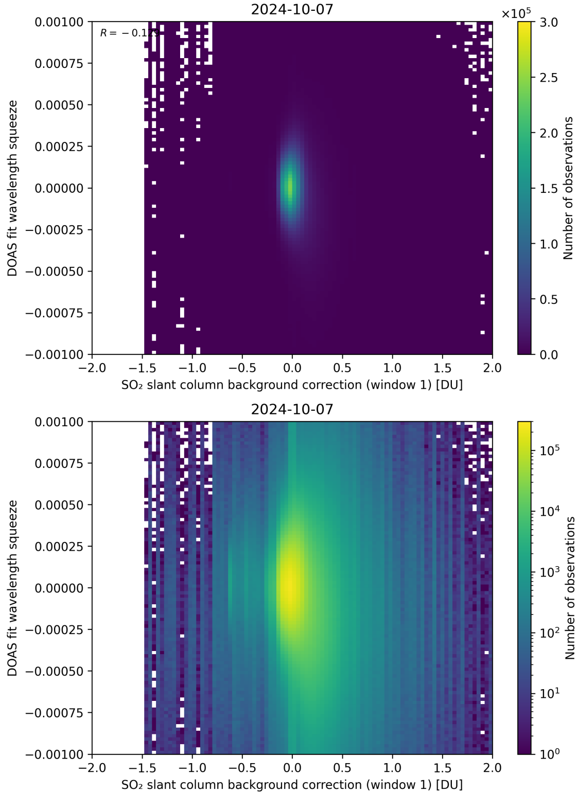
Figure 101: Scatter density plot of “SO 2 slant column background correction (window 1)” against “DOAS fit wavelength squeeze” for 2024-10-06 to 2024-10-08.
