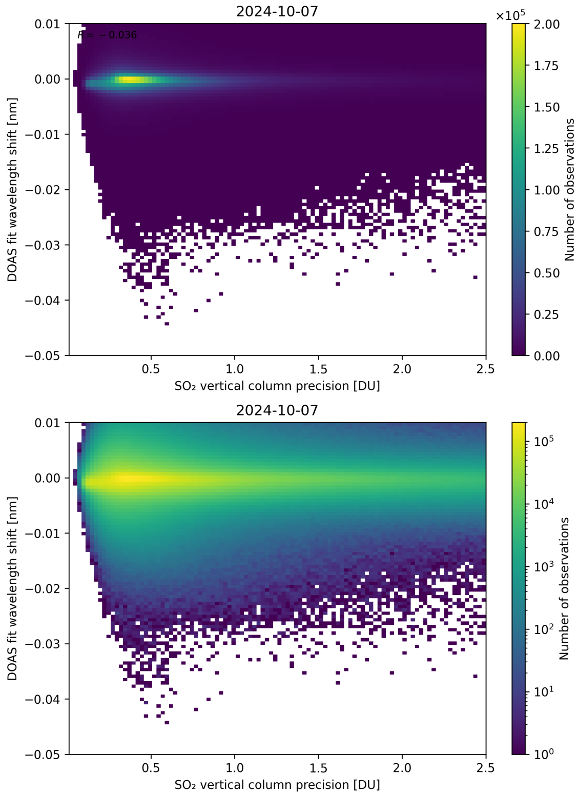
Figure 282: Scatter density plot of “SO 2 vertical column precision” against “DOAS fit wavelength shift” for 2024-10-06 to 2024-10-08.
