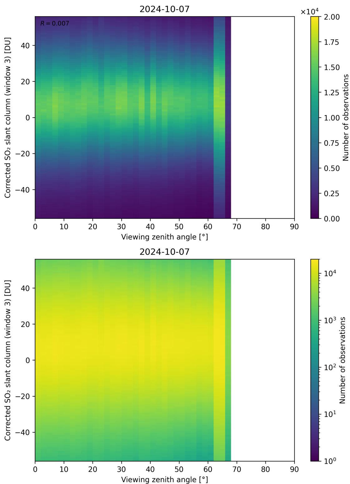
Figure 319: Scatter density plot of “Viewing zenith angle” against “Corrected SO 2 slant column (window 3)” for 2024-10-06 to 2024-10-08.
