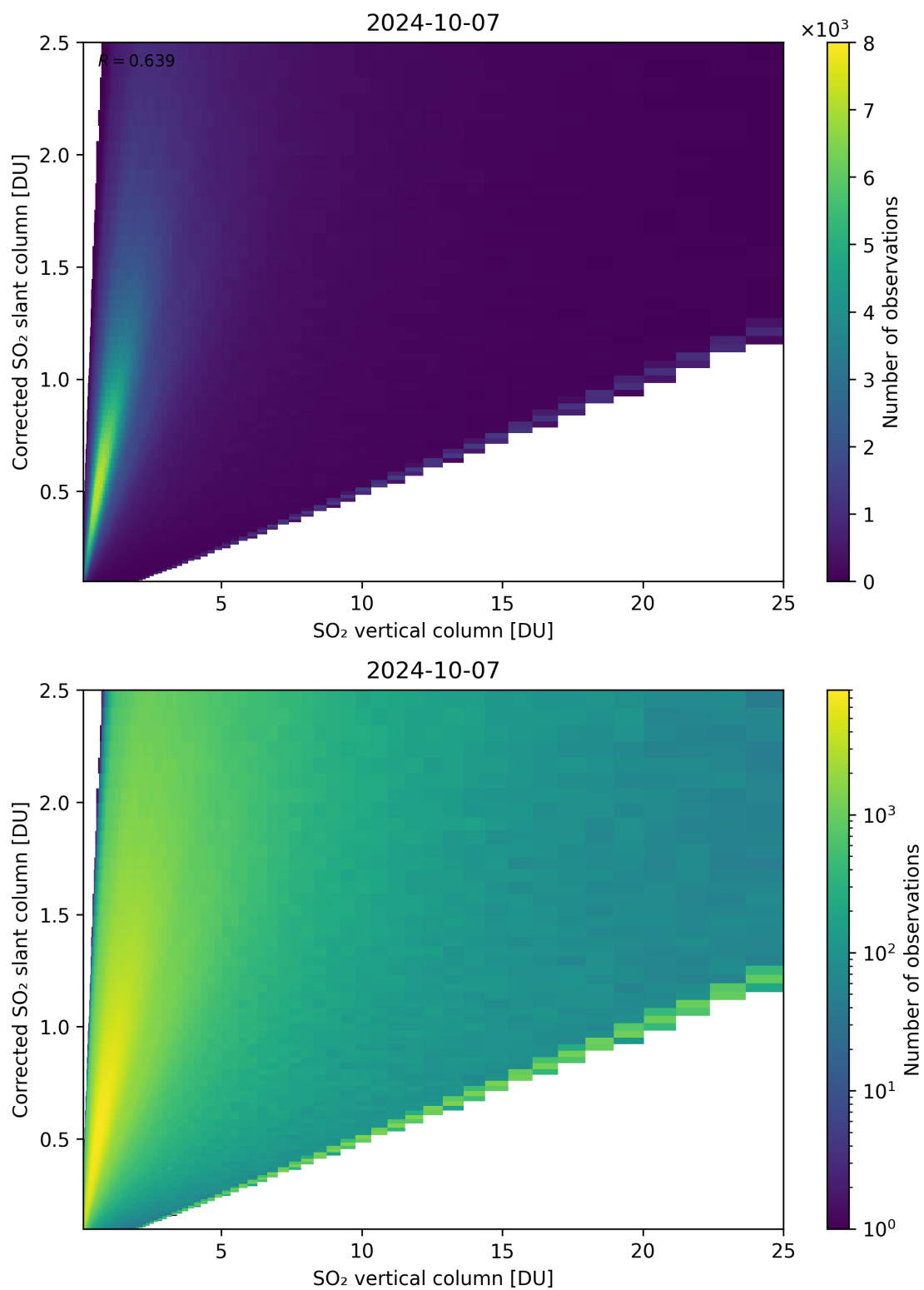
Figure 297: Scatter density plot of “SO 2 vertical column” against “Corrected SO 2 slant column” for 2024-10-06 to 2024-10-08.
