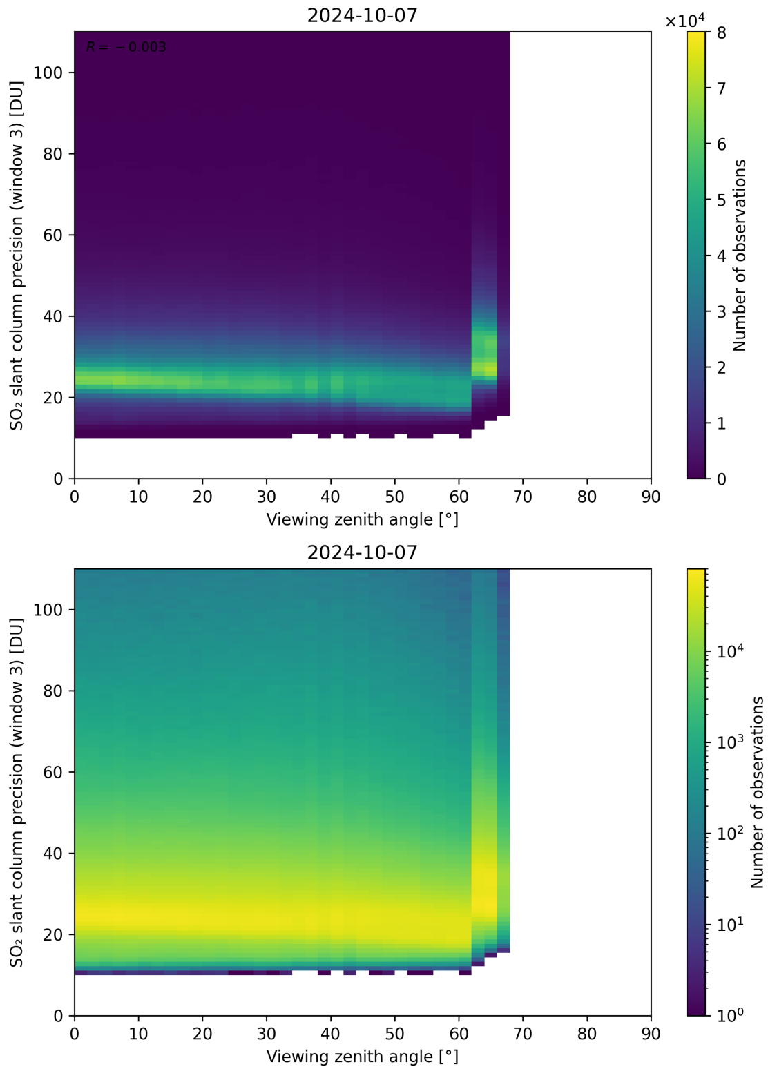
Figure 324: Scatter density plot of “Viewing zenith angle” against “SO 2 slant column precision (window 3)” for 2024-10-06 to 2024-10-08.
