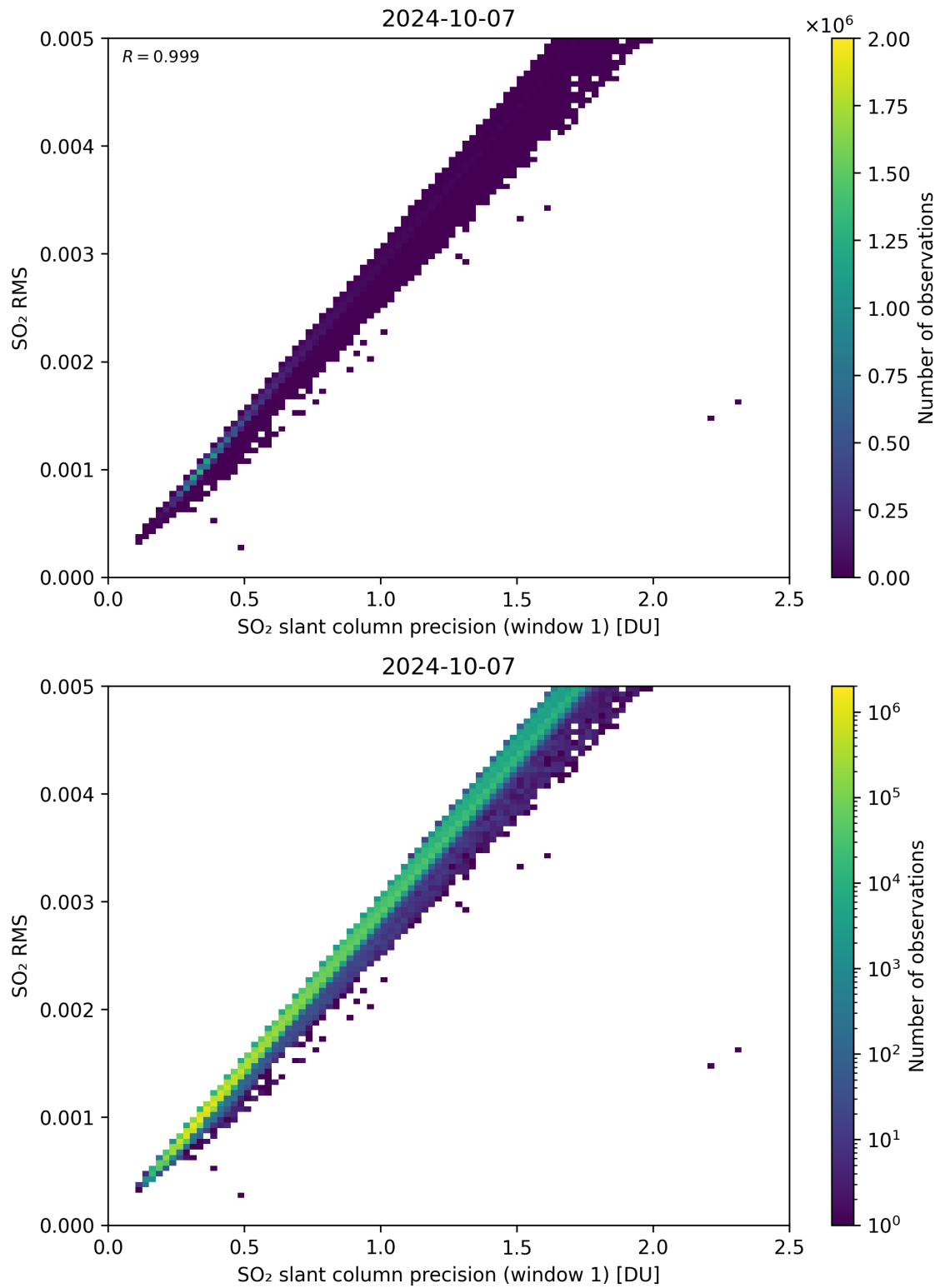
Figure 223: Scatter density plot of “SO 2 slant column precision (window 1)” against “SO 2 RMS” for 2024-10-06 to 2024-10-08.
