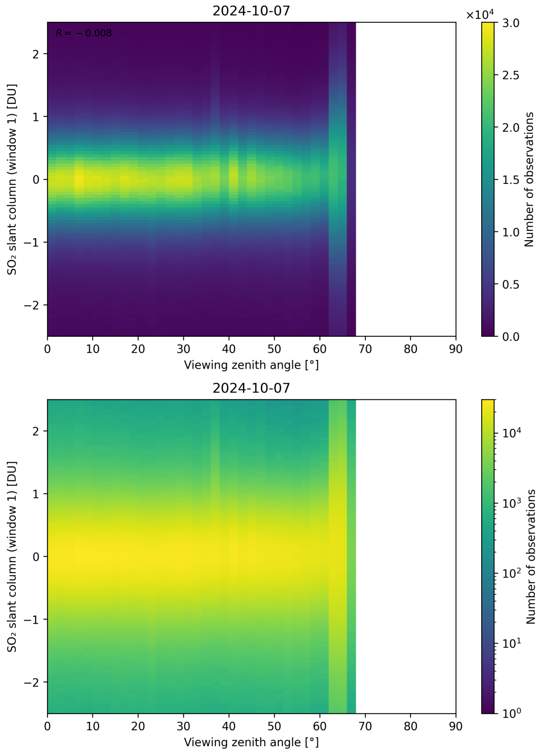
Figure 320: Scatter density plot of “Viewing zenith angle” against “SO 2 slant column (window 1)” for 2024-10-06 to 2024-10-08.
