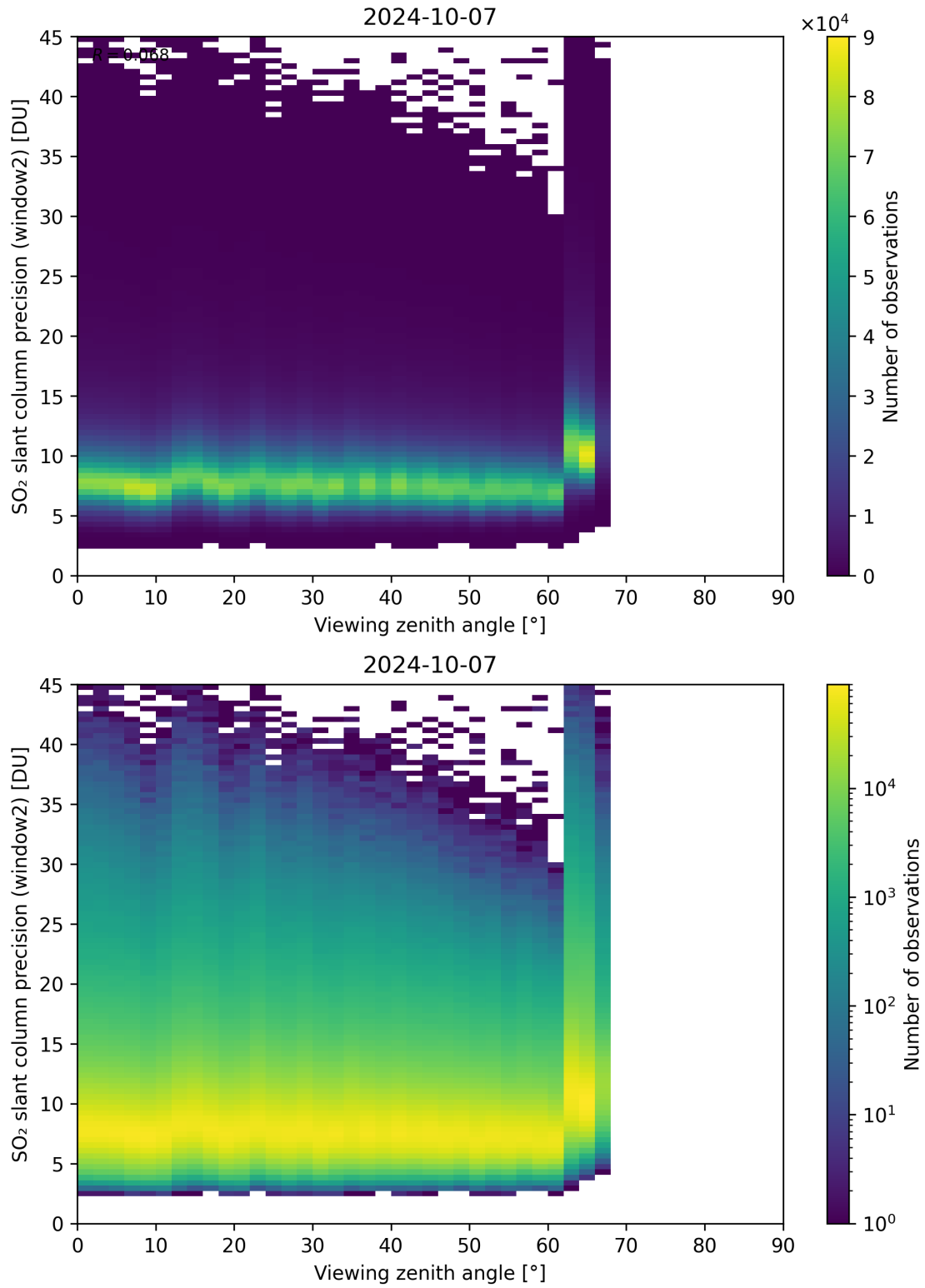
Figure 322: Scatter density plot of “Viewing zenith angle” against “SO 2 slant column precision (window2)” for 2024-10-06 to 2024-10-08.
