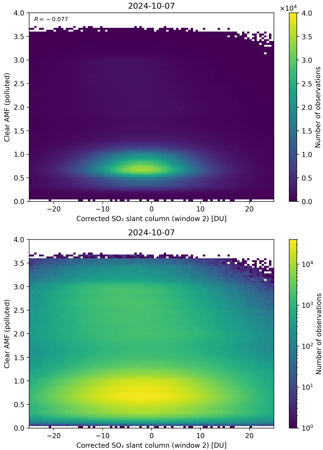
Figure 199: Scatter density plot of “Corrected SO 2 slant column (window 2)” against “Clear AMF (polluted)” for 2024-10-06 to 2024-10-08.
