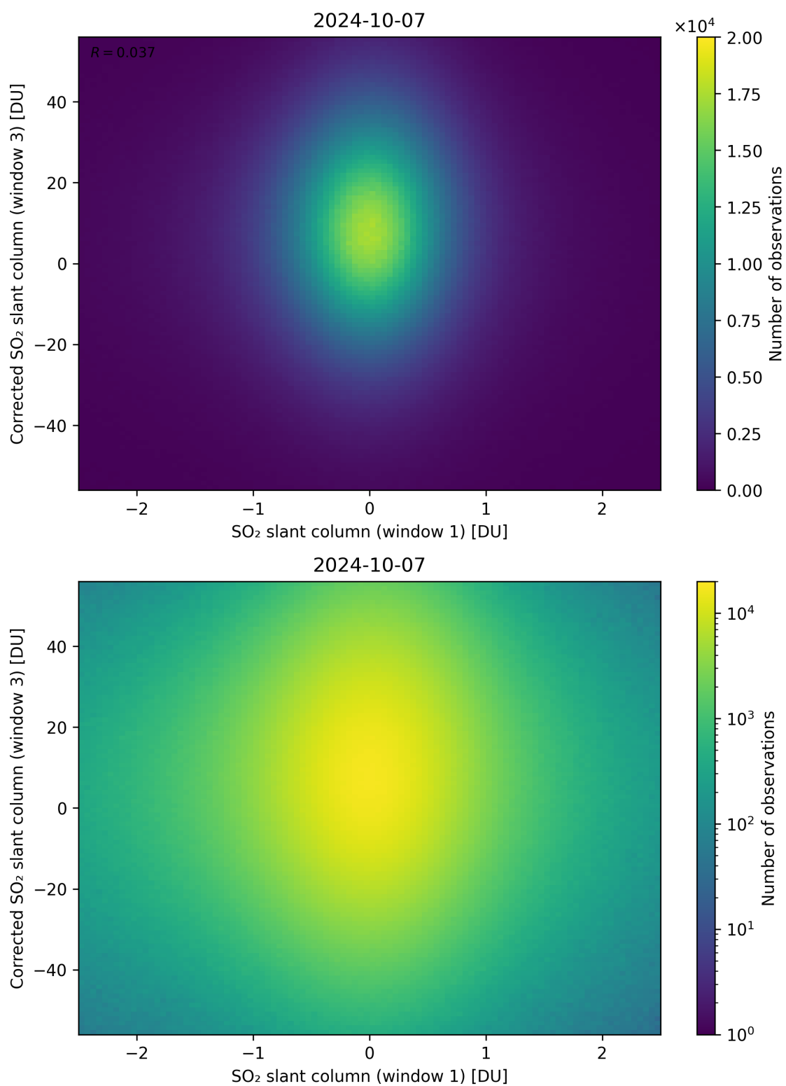
Figure 234: Scatter density plot of “SO 2 slant column (window 1)” against “Corrected SO 2 slant column (window 3)” for 2024-10-06 to 2024-10-08.
