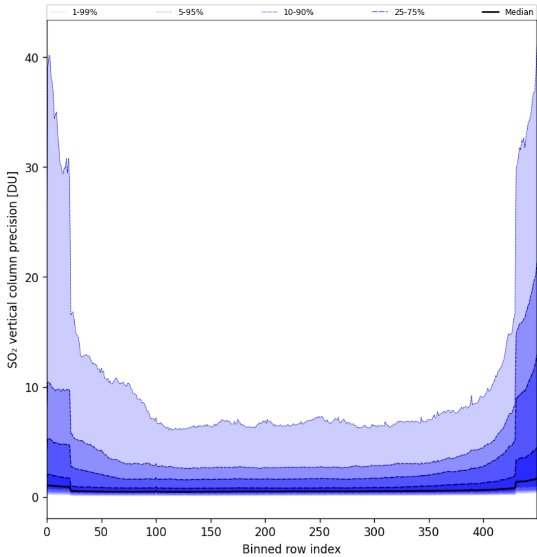
Figure 77: Along track statistics of “SO 2 vertical column precision” for 2024-10-06 to 2024-10-08
