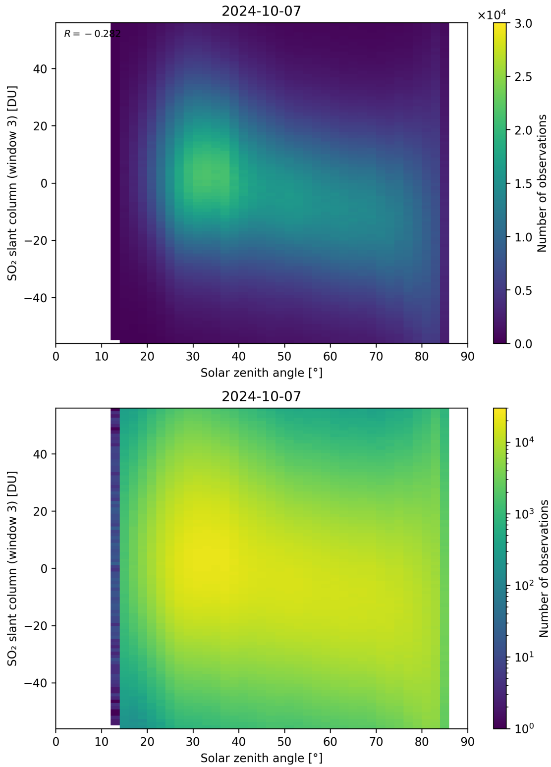
Figure 172: Scatter density plot of “Solar zenith angle” against “SO 2 slant column (window 3)” for 2024-10-06 to 2024-10-08.
