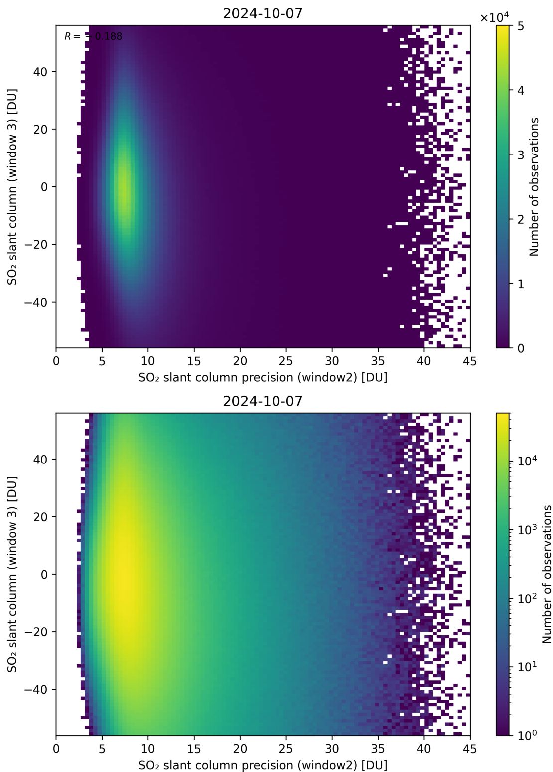
Figure 249: Scatter density plot of “SO 2 slant column precision (window2)” against “SO 2 slant column (window 3)” for 2024-10-06 to 2024-10-08.
