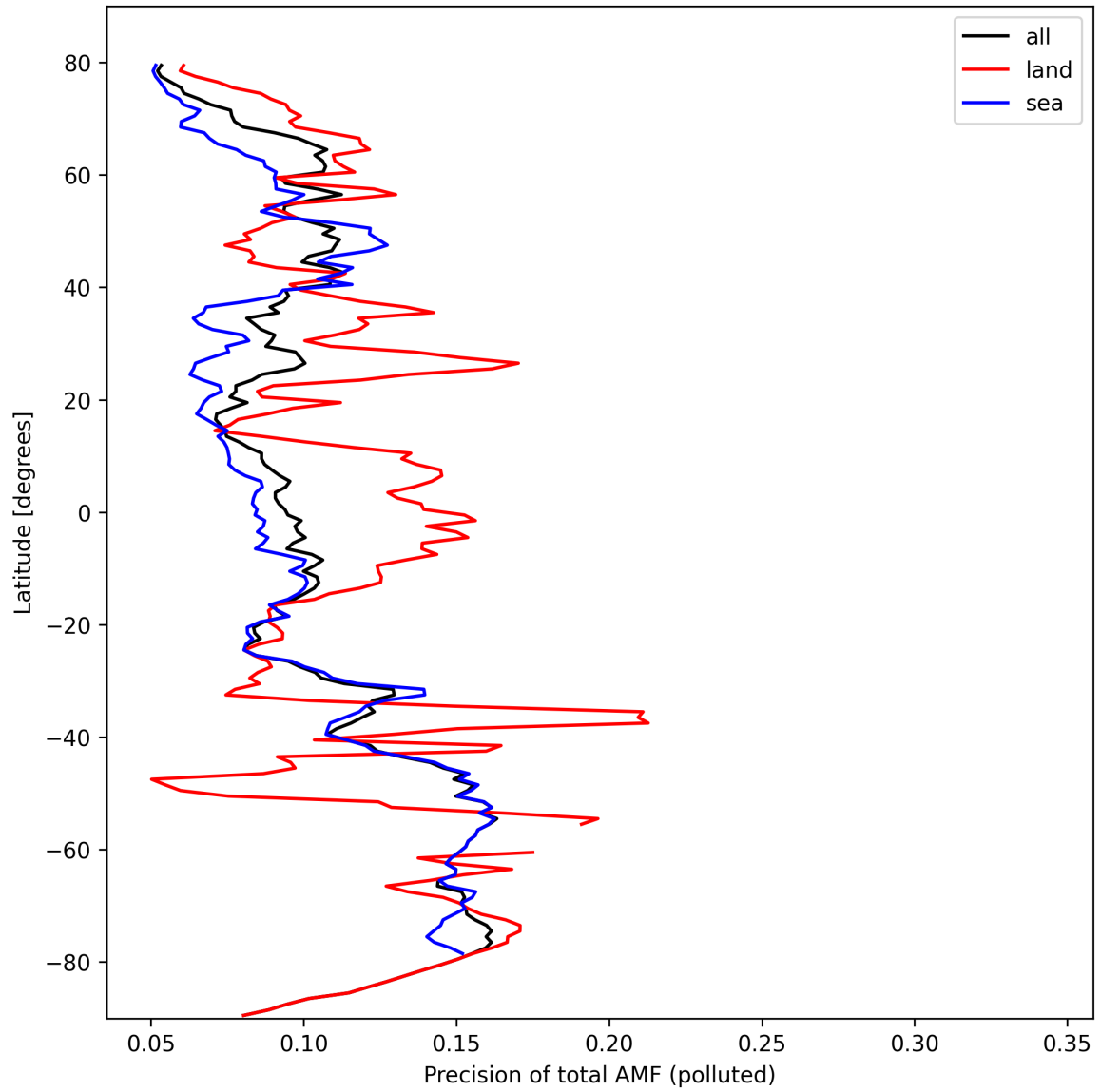
Figure 49: Zonal average of “Precision of total AMF (polluted)” for 2024-10-06 to 2024-10-08.
