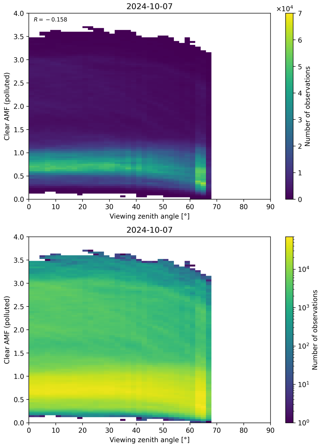
Figure 316: Scatter density plot of “Viewing zenith angle” against “Clear AMF (polluted)” for 2024-10-06 to 2024-10-08.
