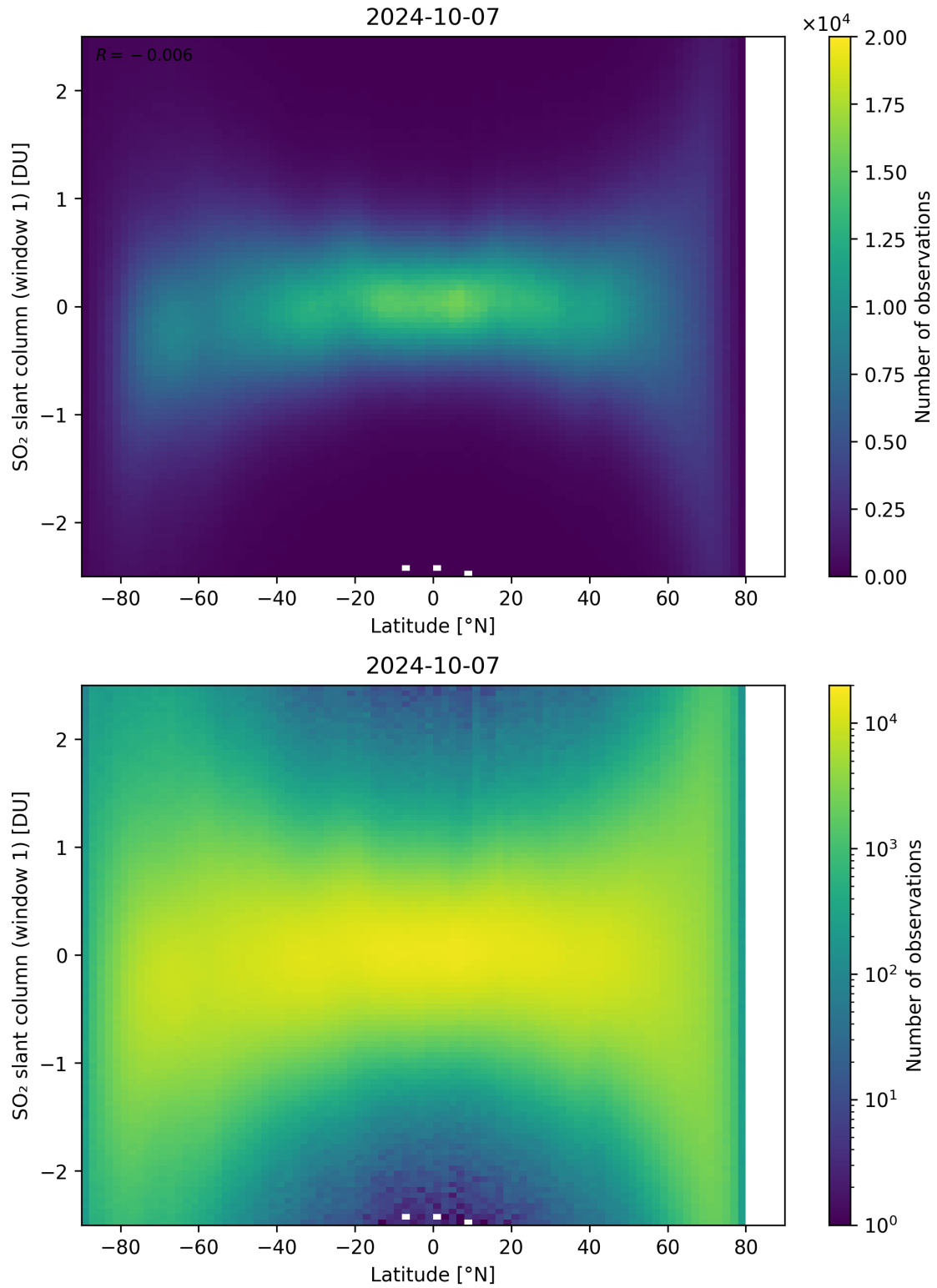
Figure 149: Scatter density plot of “Latitude” against “SO 2 slant column (window 1)” for 2024-10-06 to 2024-10-08.
