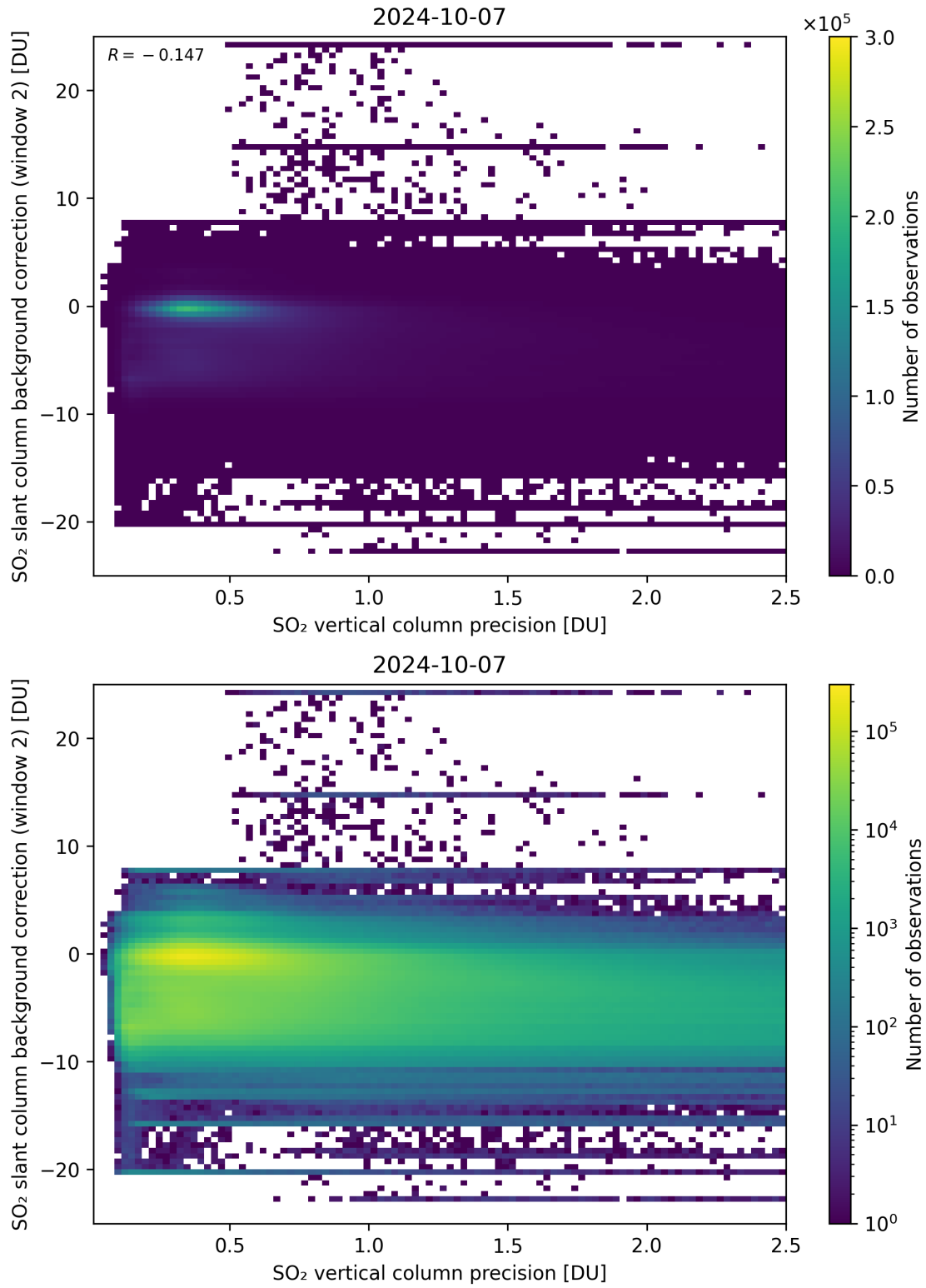
Figure 280: Scatter density plot of “SO 2 vertical column precision” against “SO 2 slant column background correction (window 2)” for 2024-10-06 to 2024-10-08.
