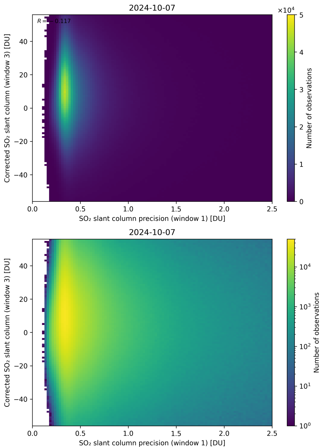
Figure 226: Scatter density plot of “SO 2 slant column precision (window 1)” against “Corrected SO 2 slant column (window 3)” for 2024-10-06 to 2024-10-08.
