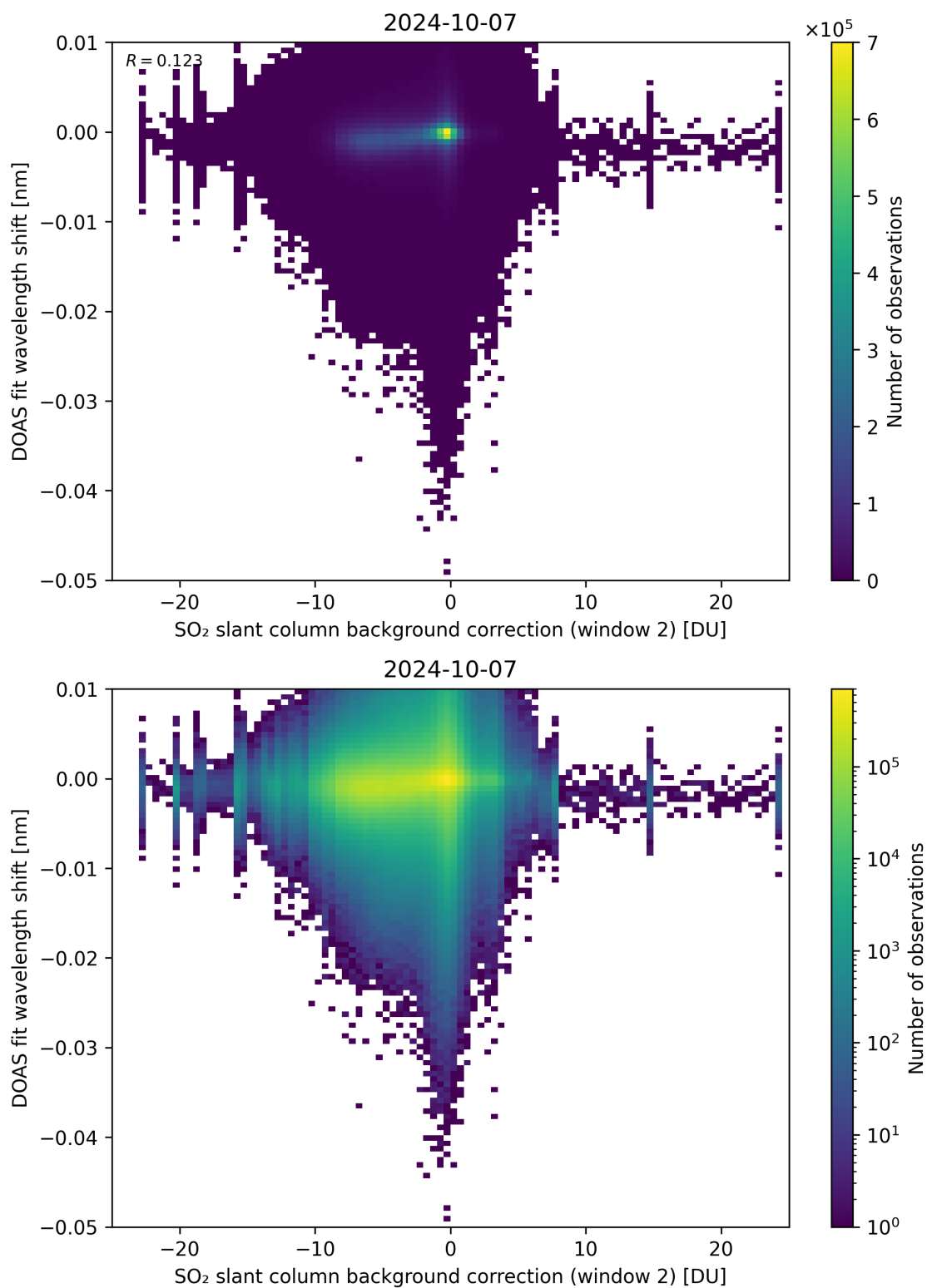
Figure 112: Scatter density plot of “SO 2 slant column background correction (window 2)” against “DOAS fit wavelength shift” for 2024-10-06 to 2024-10-08.
