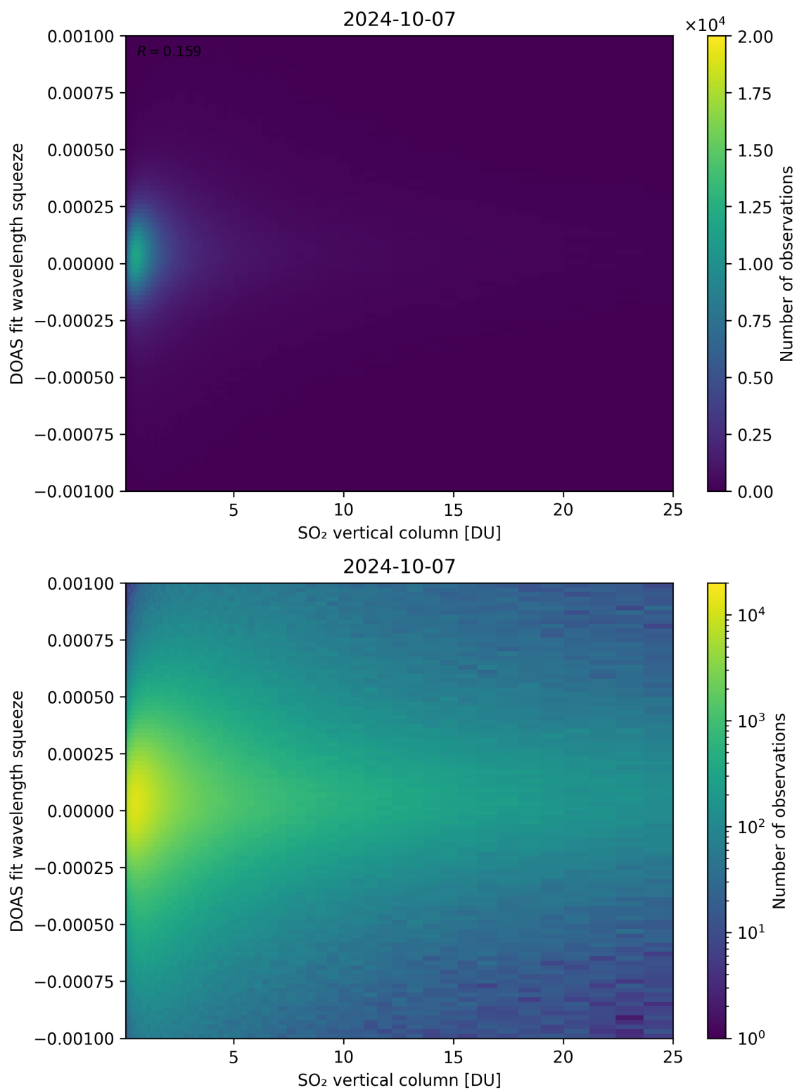
Figure 277: Scatter density plot of “SO 2 vertical column” against “DOAS fit wavelength squeeze” for 2024-10-06 to 2024-10-08.
