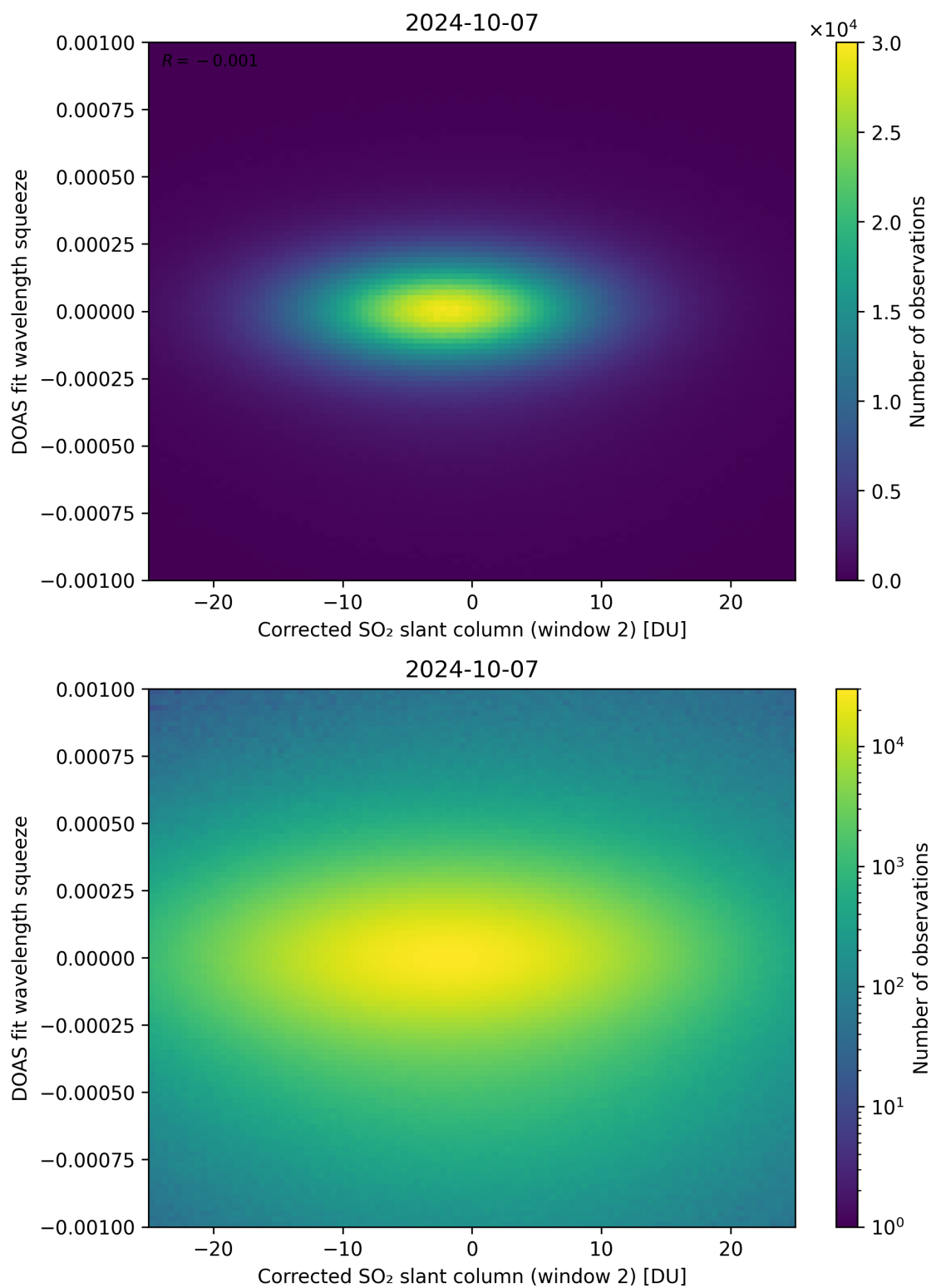
Figure 197: Scatter density plot of “Corrected SO 2 slant column (window 2)” against “DOAS fit wavelength squeeze” for 2024-10-06 to 2024-10-08.
