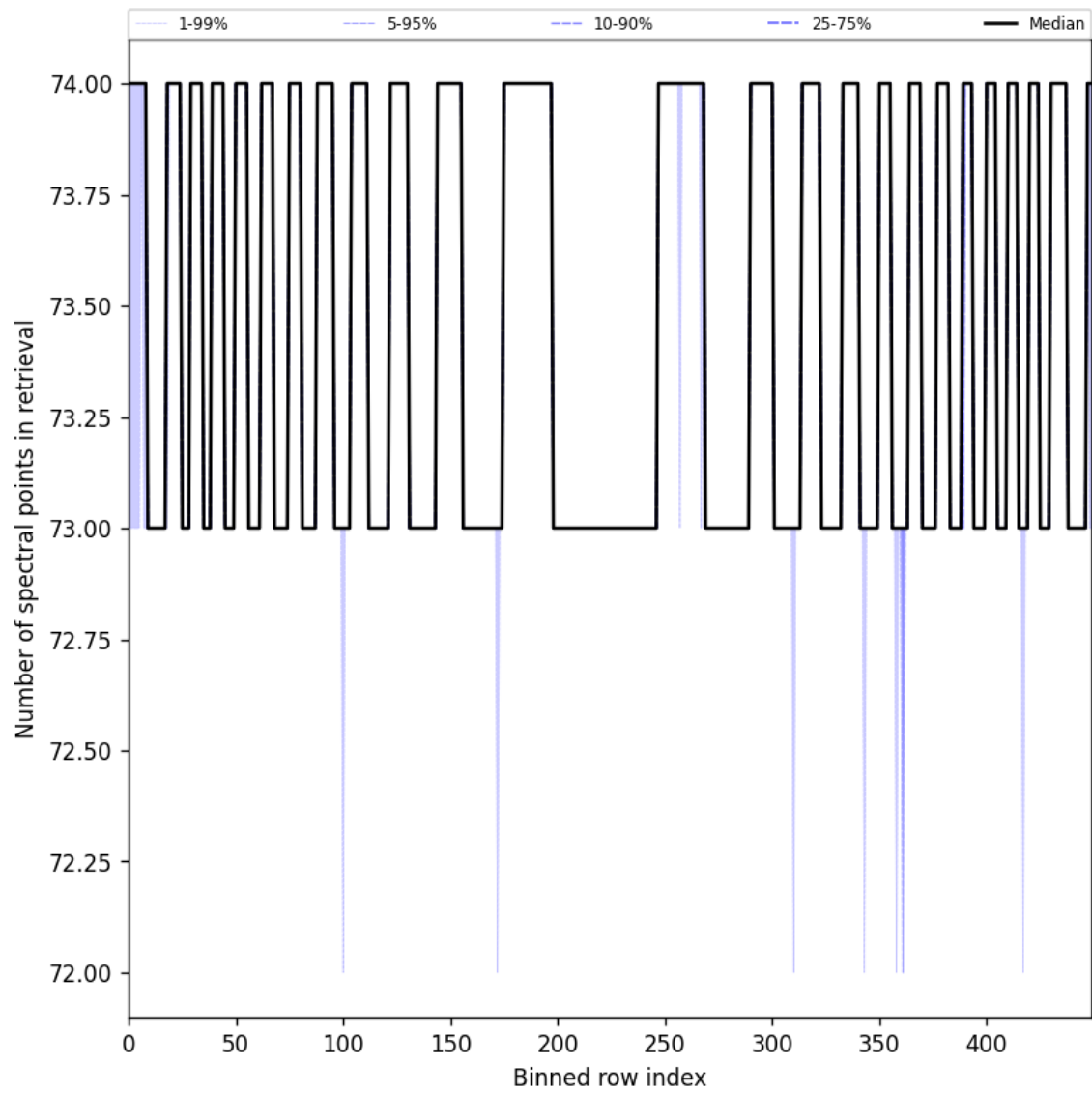
Figure 97: Along track statistics of “Number of spectral points in retrieval” for 2024-10-06 to 2024-10-08
