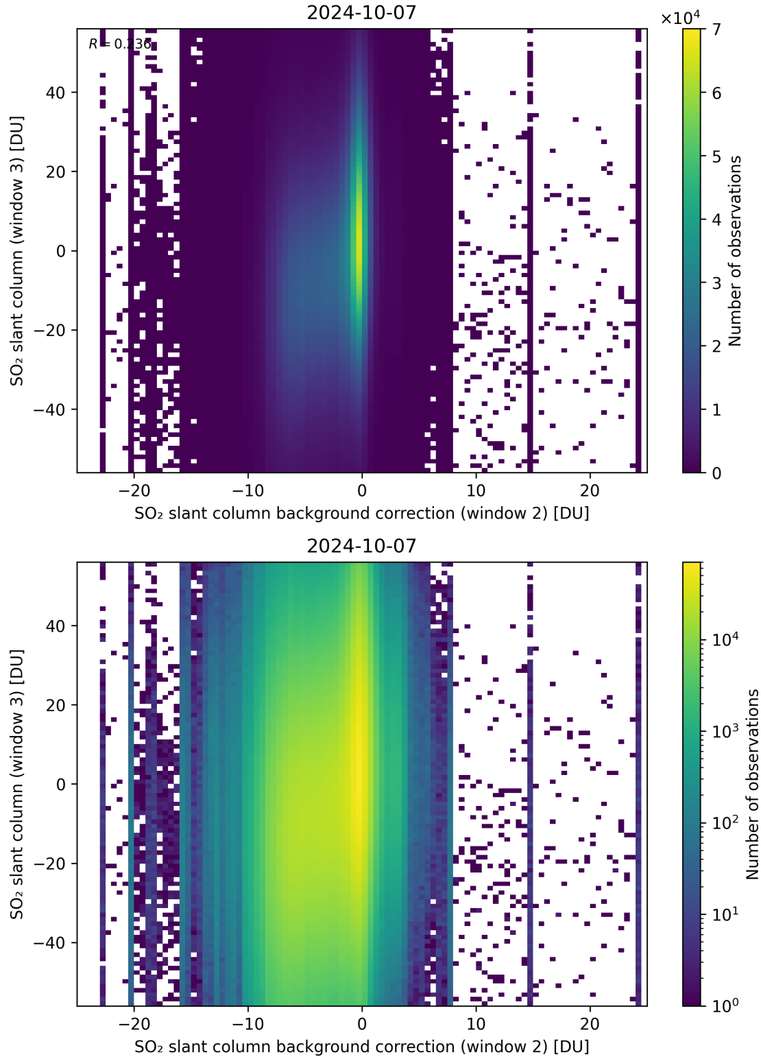
Figure 117: Scatter density plot of “SO 2 slant column background correction (window 2)” against “SO 2 slant column (window 3)” for 2024-10-06 to 2024-10-08.
