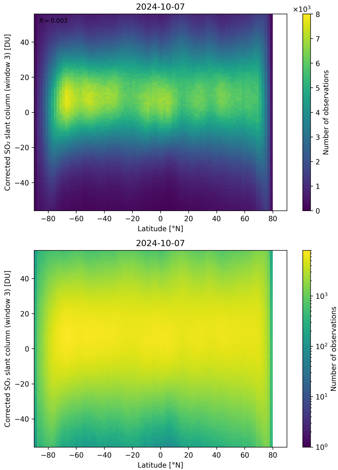
Figure 148: Scatter density plot of “Latitude” against “Corrected SO 2 slant column (window 3)” for 2024-10-06 to 2024-10-08.
