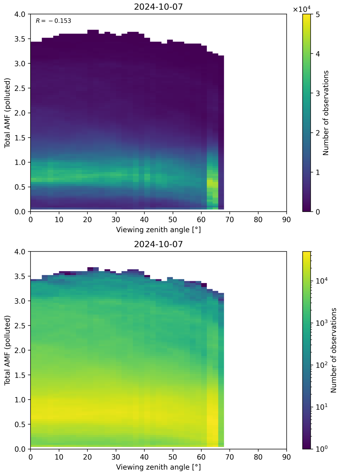
Figure 325: Scatter density plot of “Viewing zenith angle” against “Total AMF (polluted)” for 2024-10-06 to 2024-10-08.
