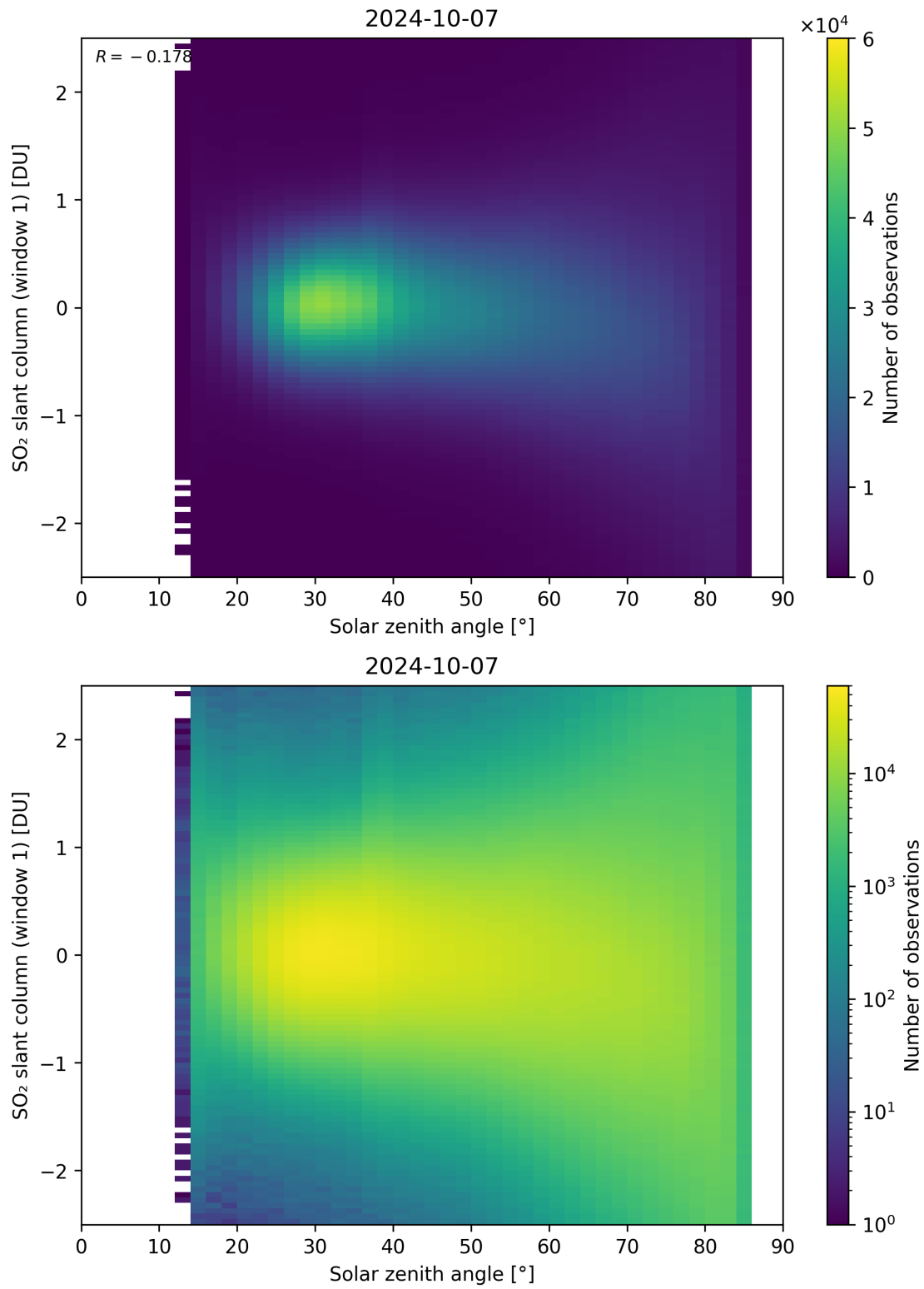
Figure 169: Scatter density plot of “Solar zenith angle” against “SO 2 slant column (window 1)” for 2024-10-06 to 2024-10-08.
