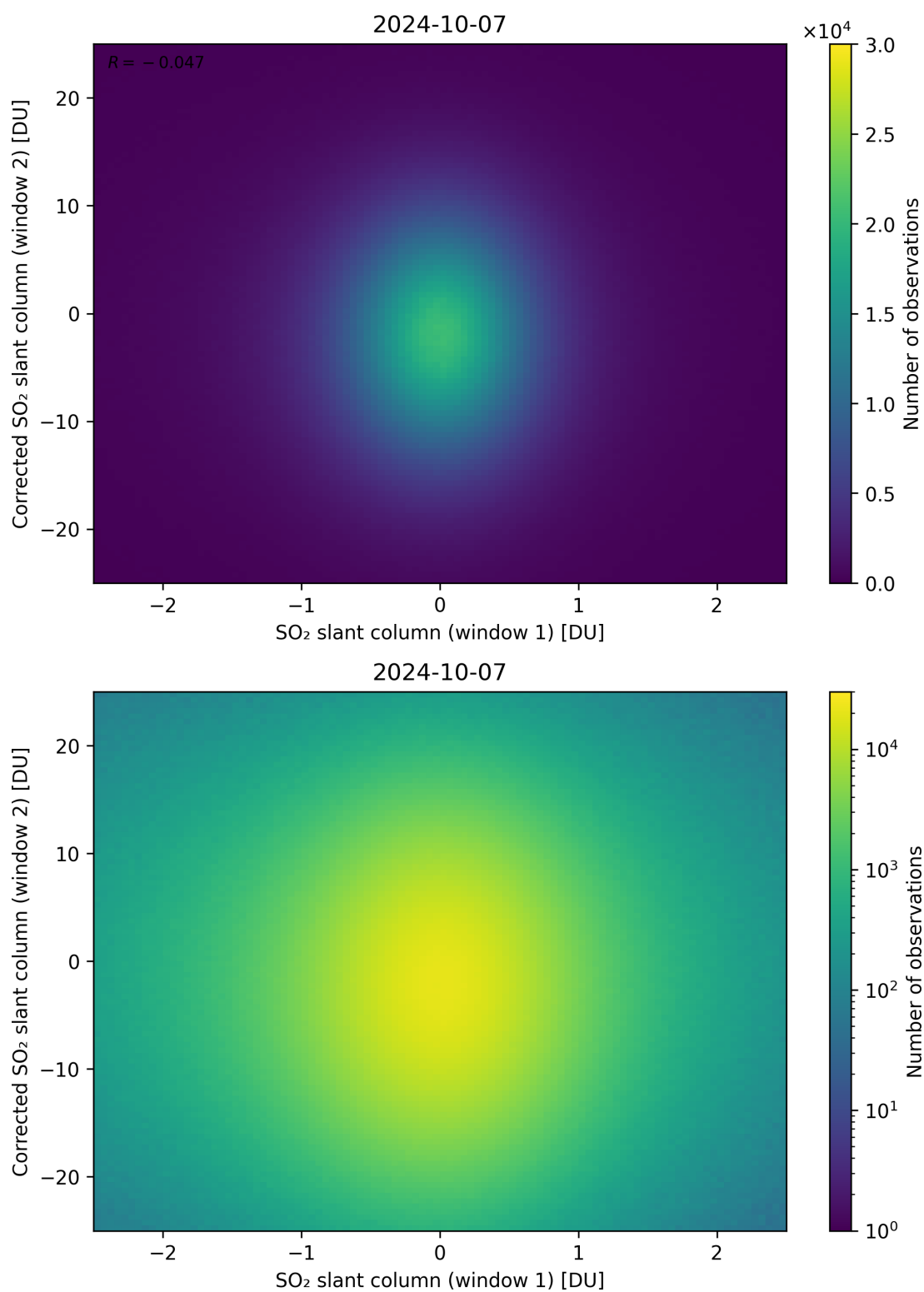
Figure 233: Scatter density plot of “SO 2 slant column (window 1)” against “Corrected SO 2 slant column (window 2)” for 2024-10-06 to 2024-10-08.
