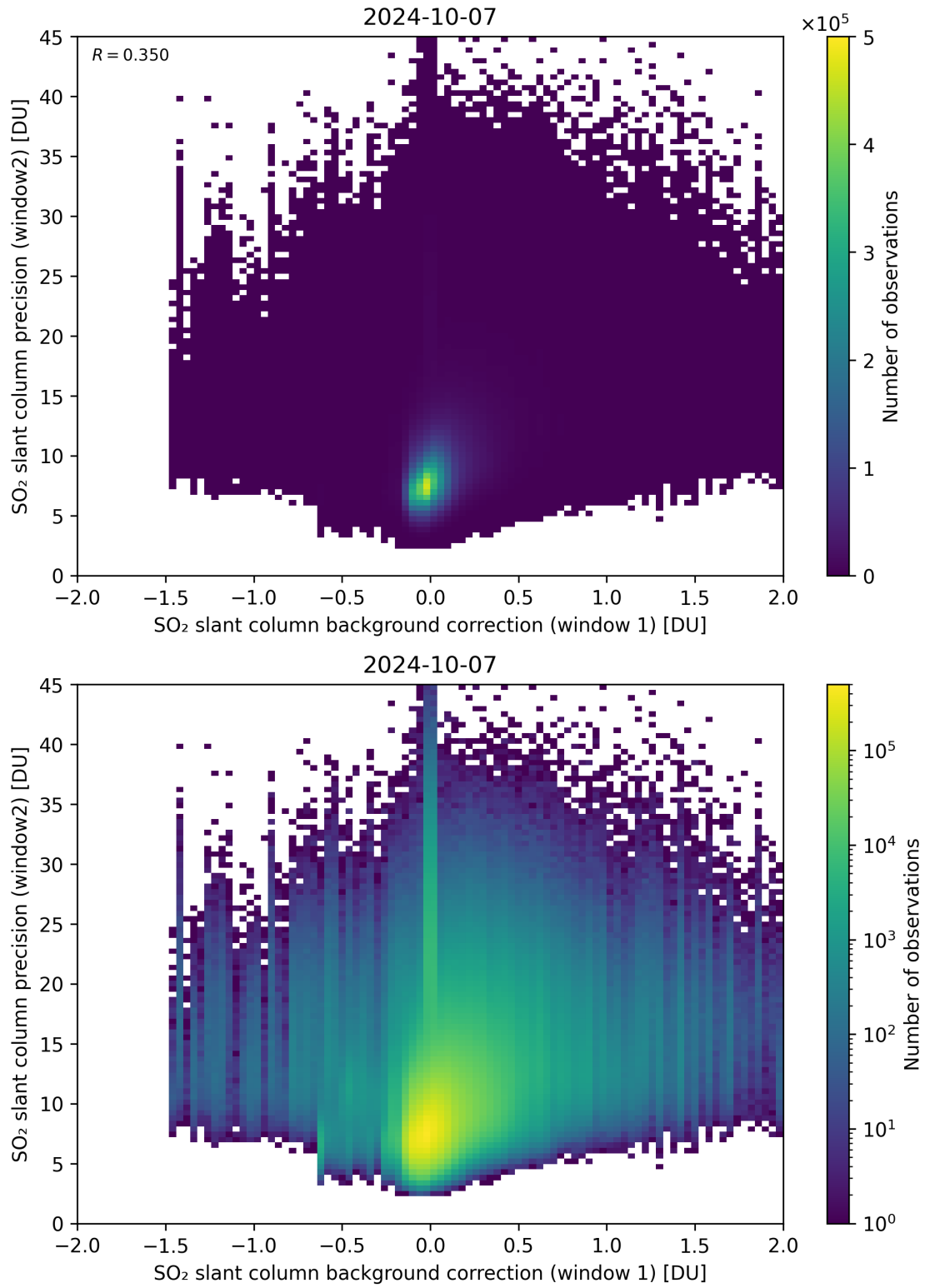
Figure 106: Scatter density plot of “SO 2 slant column background correction (window 1)” against “SO 2 slant column precision (window2)” for 2024-10-06 to 2024-10-08.
