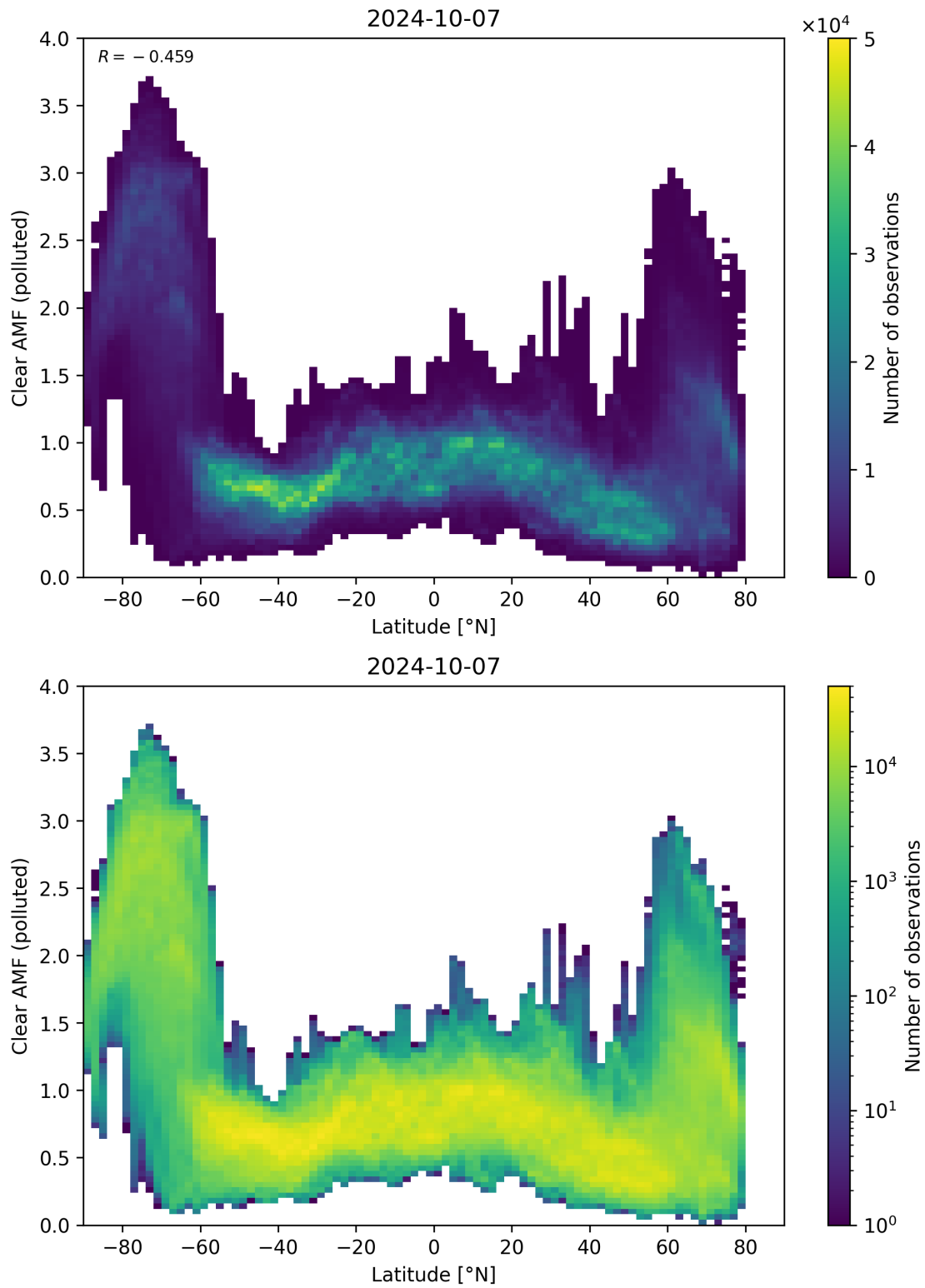
Figure 145: Scatter density plot of “Latitude” against “Clear AMF (polluted)” for 2024-10-06 to 2024-10-08.
