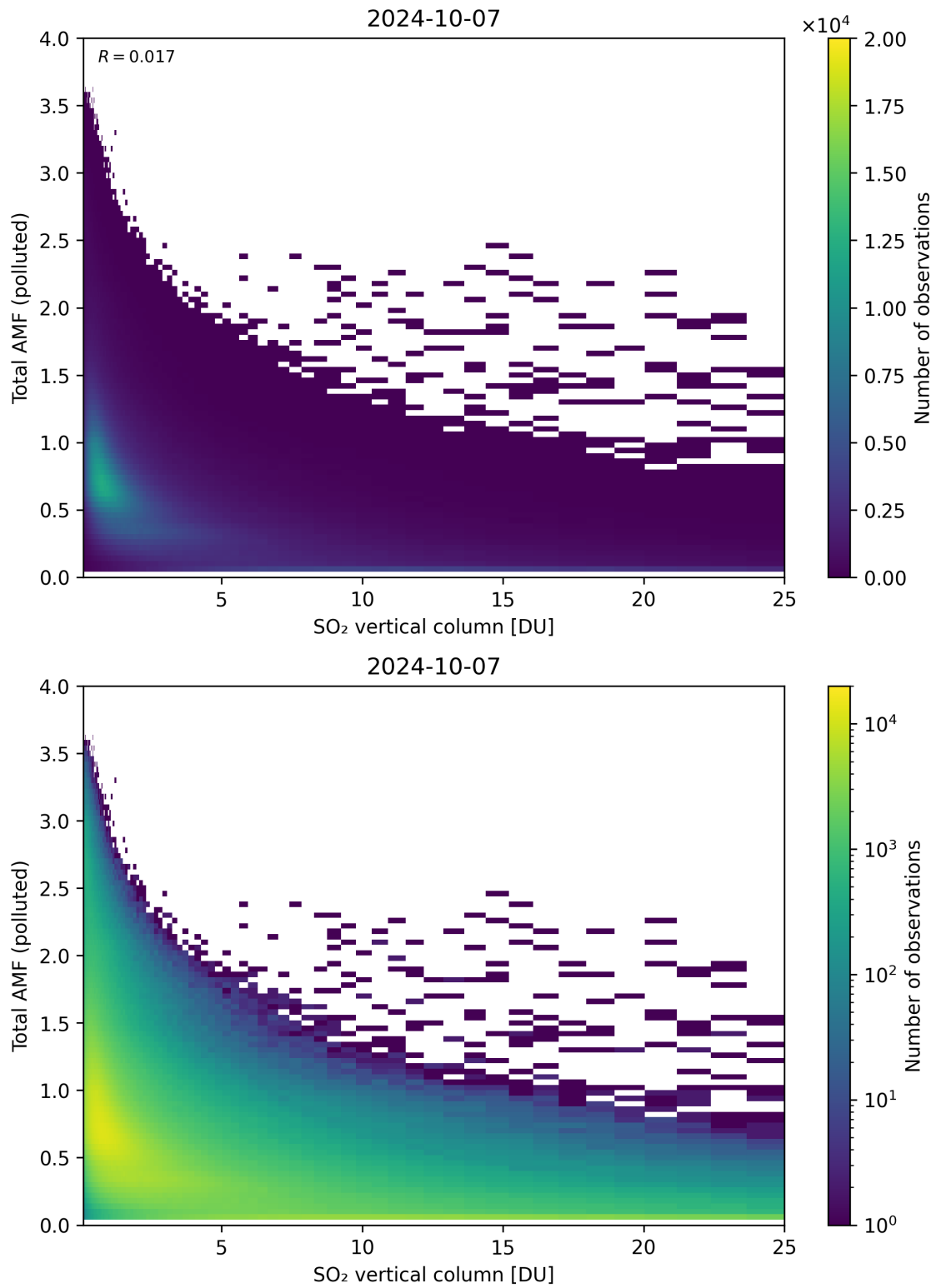
Figure 305: Scatter density plot of “SO 2 vertical column” against “Total AMF (polluted)” for 2024-10-06 to 2024-10-08.
