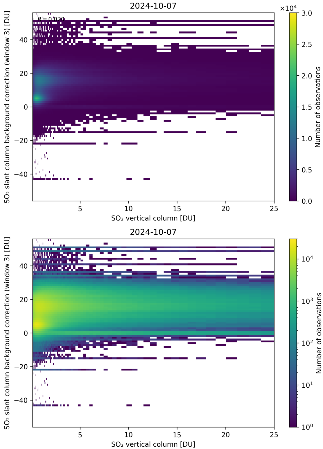
Figure 275: Scatter density plot of “SO 2 vertical column” against “SO 2 slant column background correction (window 3)” for 2024-10-06 to 2024-10-08.
