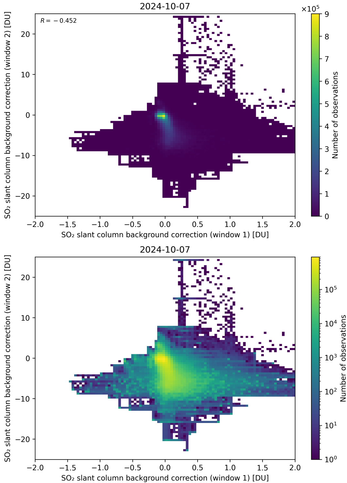
Figure 98: Scatter density plot of “SO 2 slant column background correction (window 1)” against “SO 2 slant column background correction (window 2)” for 2024-10-06 to 2024-10-08.
