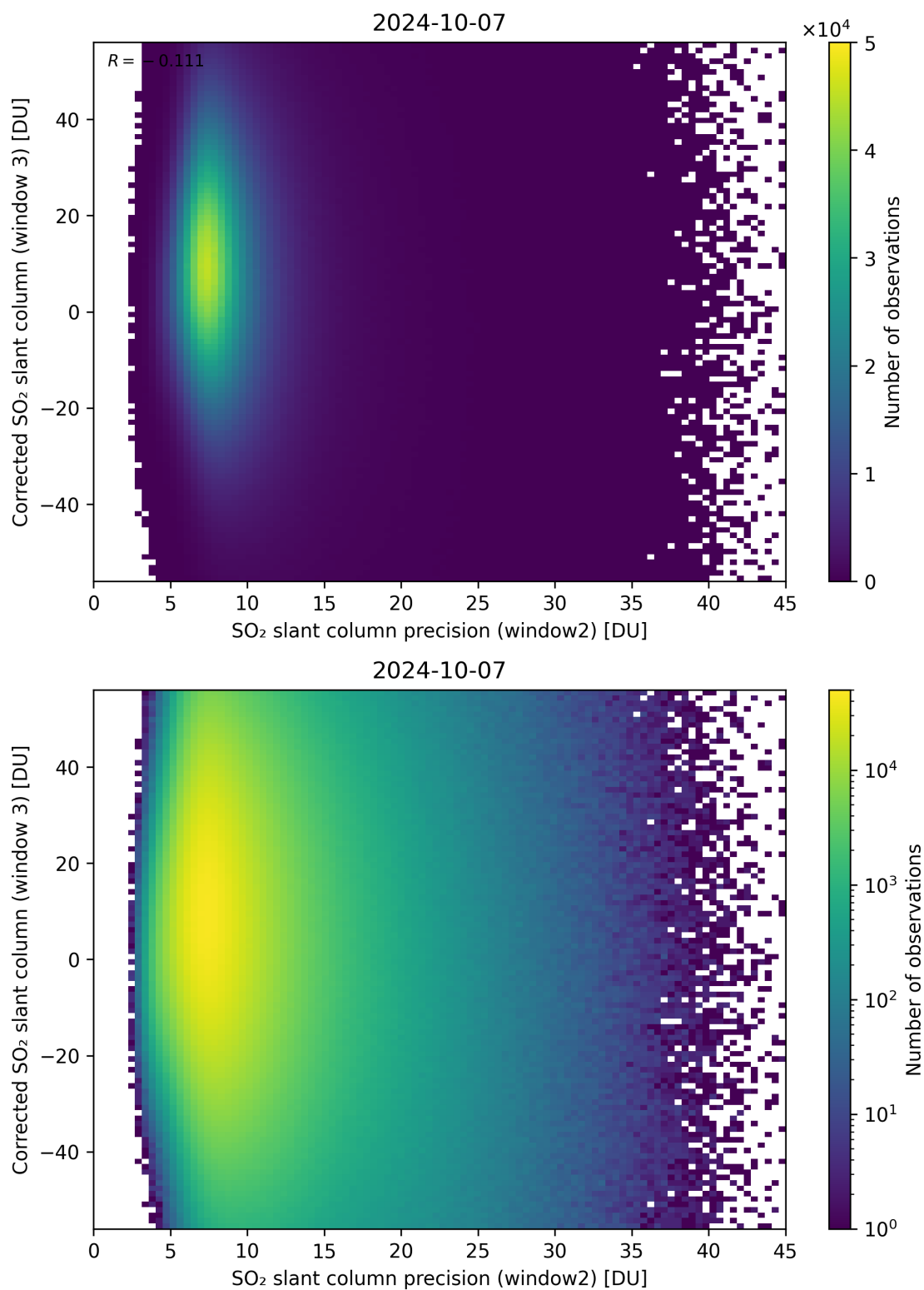
Figure 248: Scatter density plot of “SO 2 slant column precision (window2)” against “Corrected SO 2 slant column (window 3)” for 2024-10-06 to 2024-10-08.
