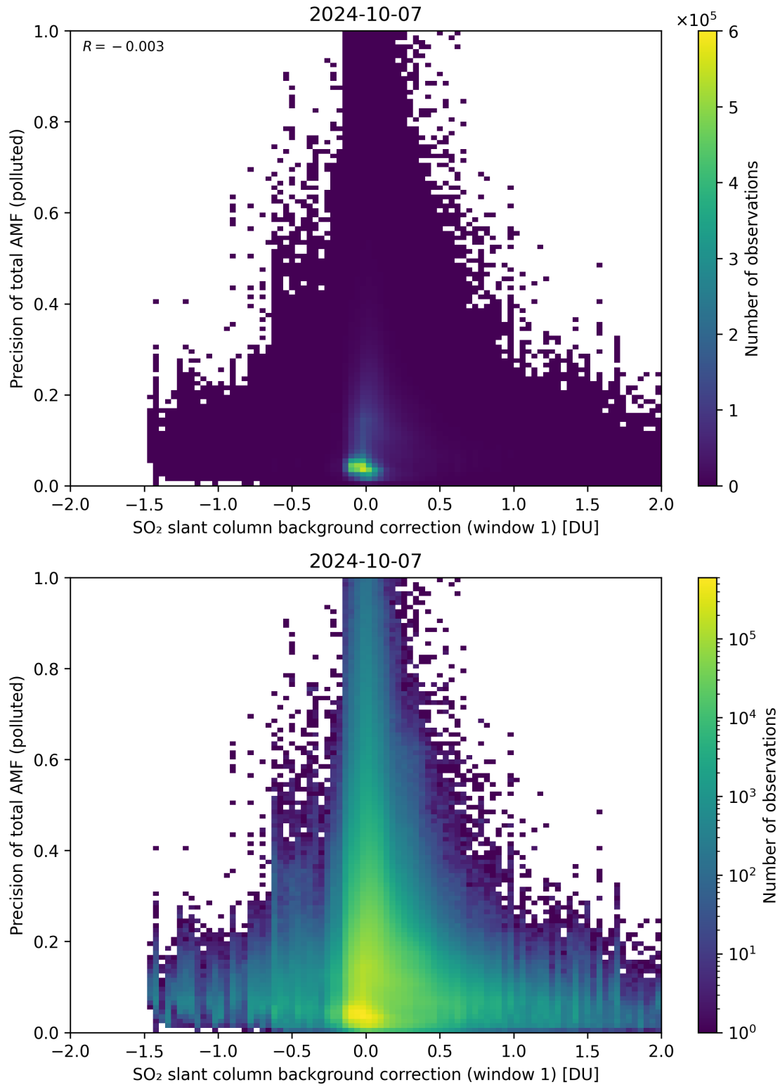
Figure 110: Scatter density plot of “SO 2 slant column background correction (window 1)” against “Precision of total AMF (polluted)” for 2024-10-06 to 2024-10-08.
