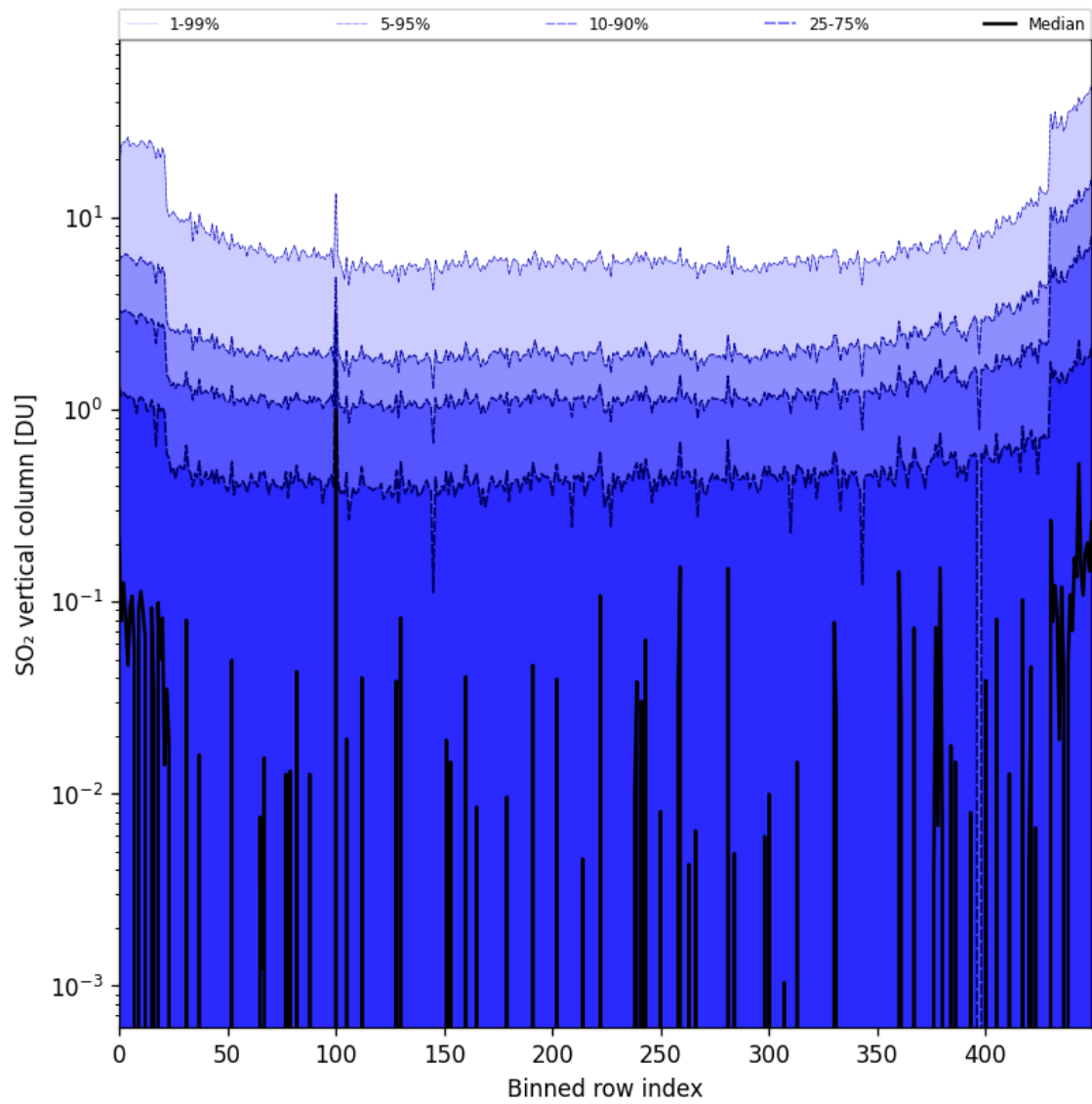
Figure 76: Along track statistics of “SO 2 vertical column” for 2024-10-06 to 2024-10-08
