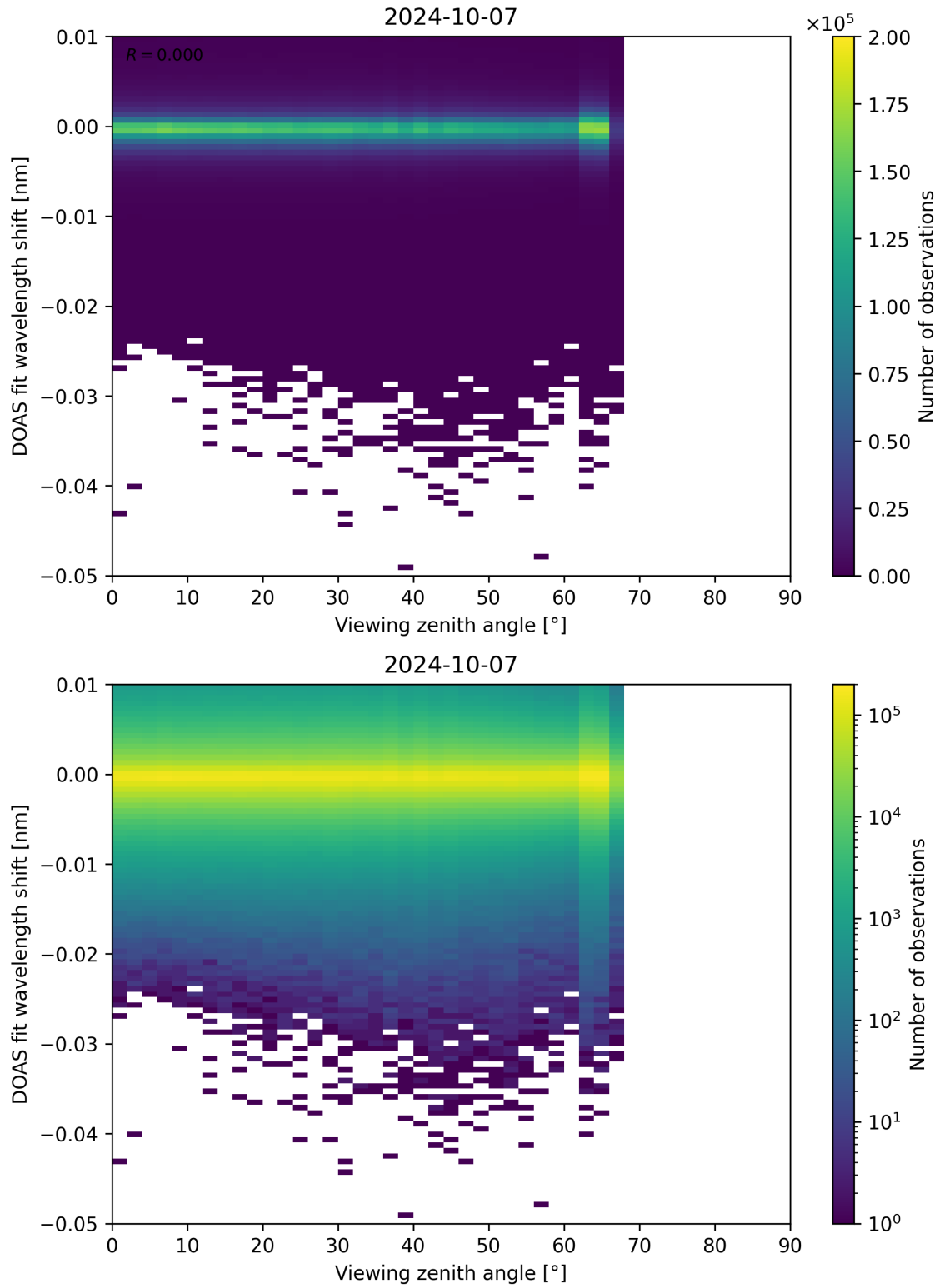
Figure 311: Scatter density plot of “Viewing zenith angle” against “DOAS fit wavelength shift” for 2024-10-06 to 2024-10-08.
