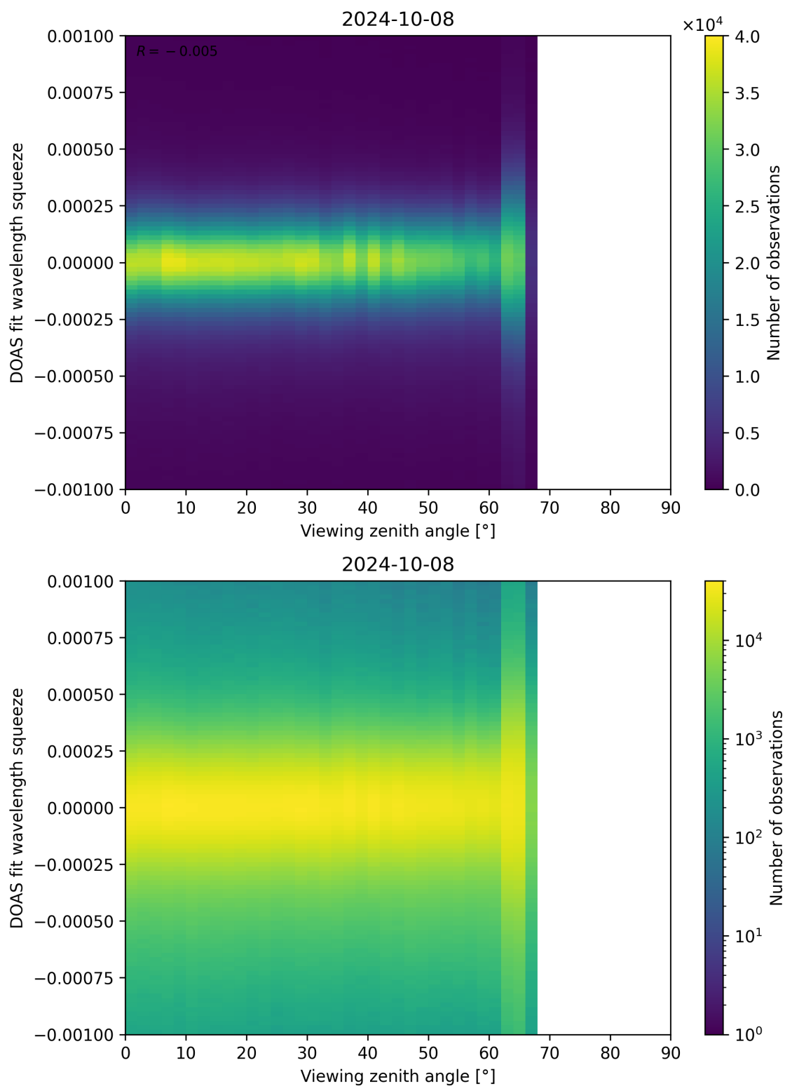
Figure 312: Scatter density plot of “Viewing zenith angle” against “DOAS fit wavelength squeeze” for 2024-10-08 to 2024-10-09.
