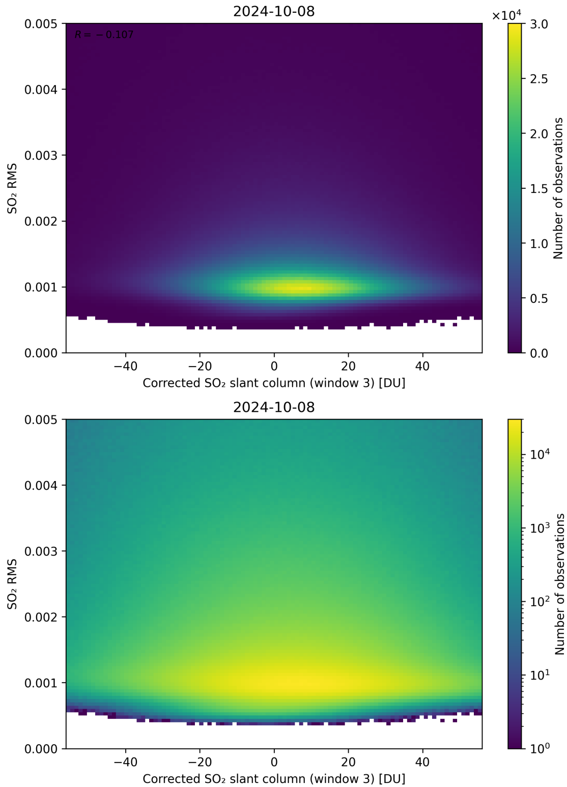
Figure 208: Scatter density plot of “Corrected SO 2 slant column (window 3)” against “SO 2 RMS” for 2024-10-08 to 2024-10-09.
