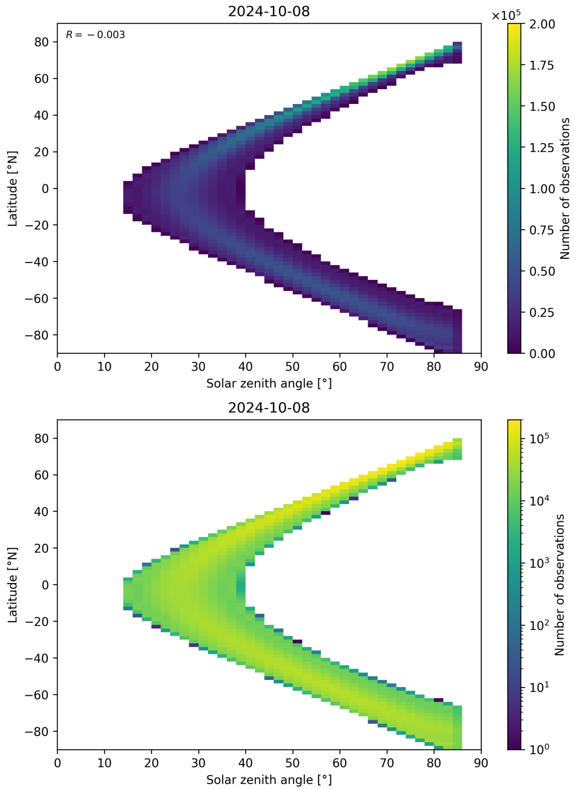
Figure 164: Scatter density plot of “Solar zenith angle” against “Latitude” for 2024-10-08 to 2024-10-09.
