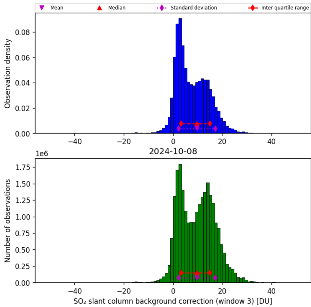
Figure 67: Histogram of “SO 2 slant column background correction (window 3)” for 2024-10-08 to 2024-10-09
