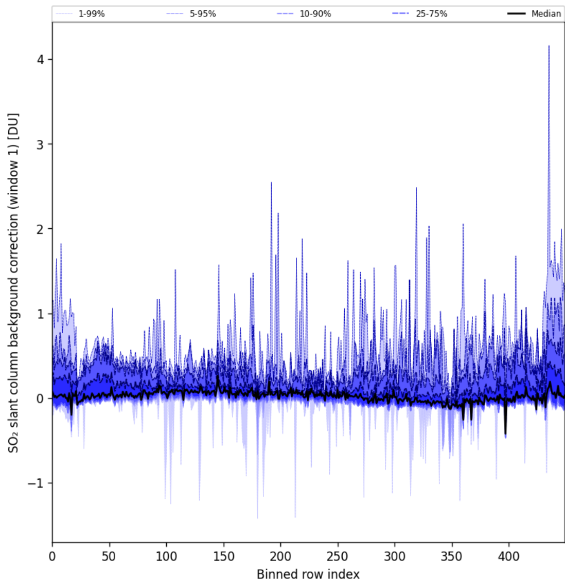
Figure 82: Along track statistics of “SO 2 slant column background correction (window 1)” for 2024-10-08 to 2024-10-09
