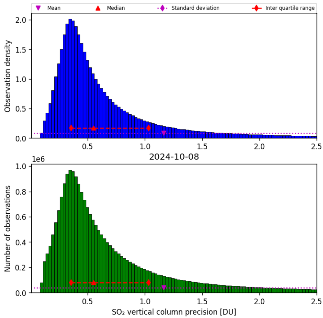
Figure 54: Histogram of “SO 2 vertical column precision” for 2024-10-08 to 2024-10-09
