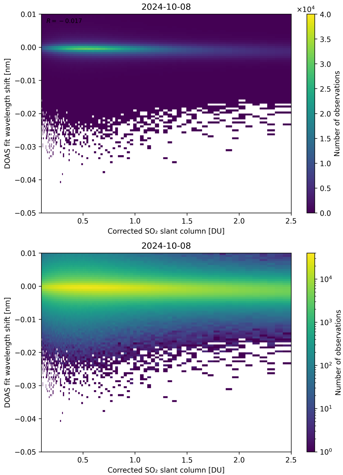
Figure 181: Scatter density plot of “Corrected SO 2 slant column” against “DOAS fit wavelength shift” for 2024-10-08 to 2024-10-09.
