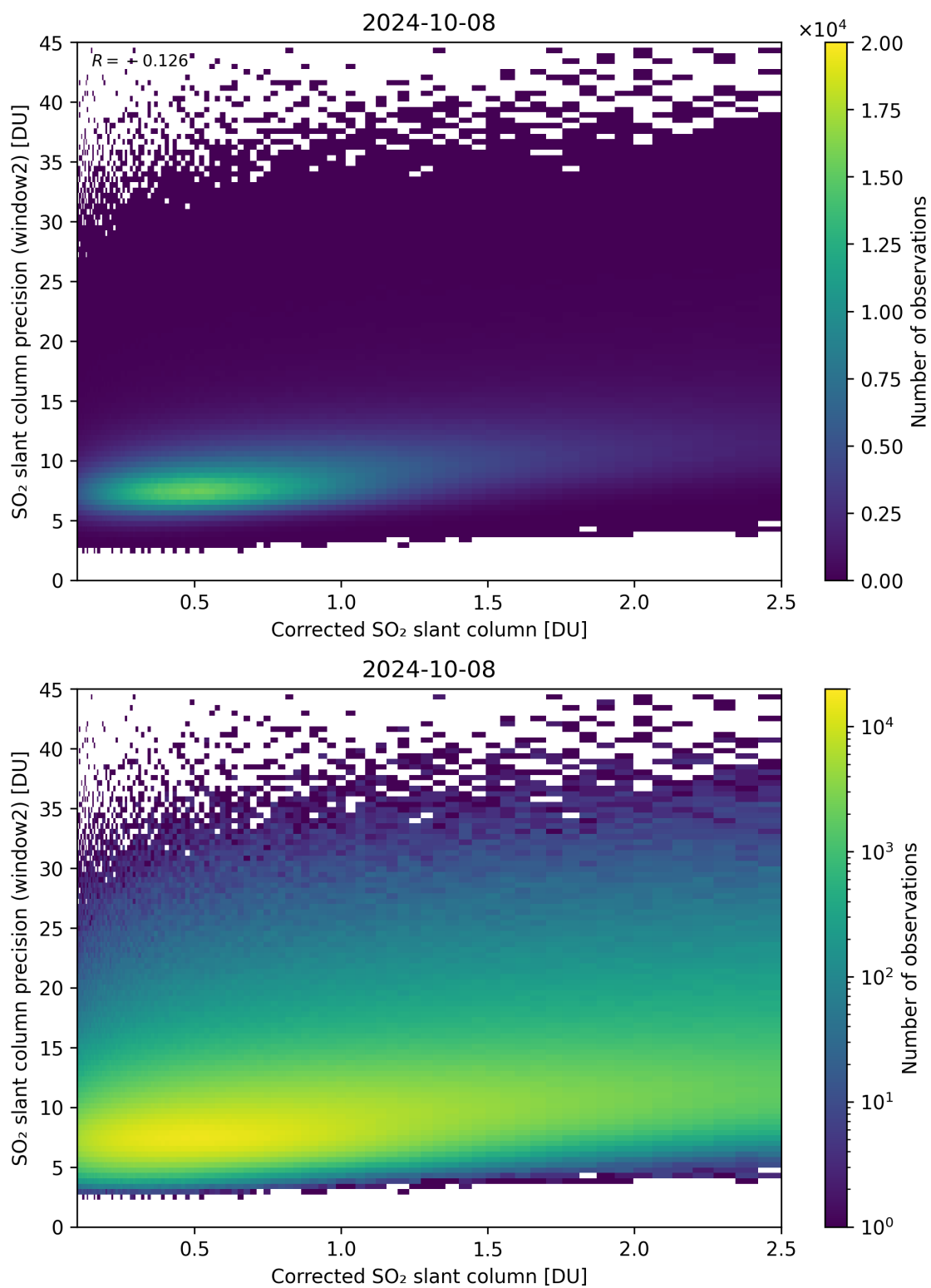
Figure 189: Scatter density plot of “Corrected SO 2 slant column” against “SO 2 slant column precision (window2)” for 2024-10-08 to 2024-10-09.
