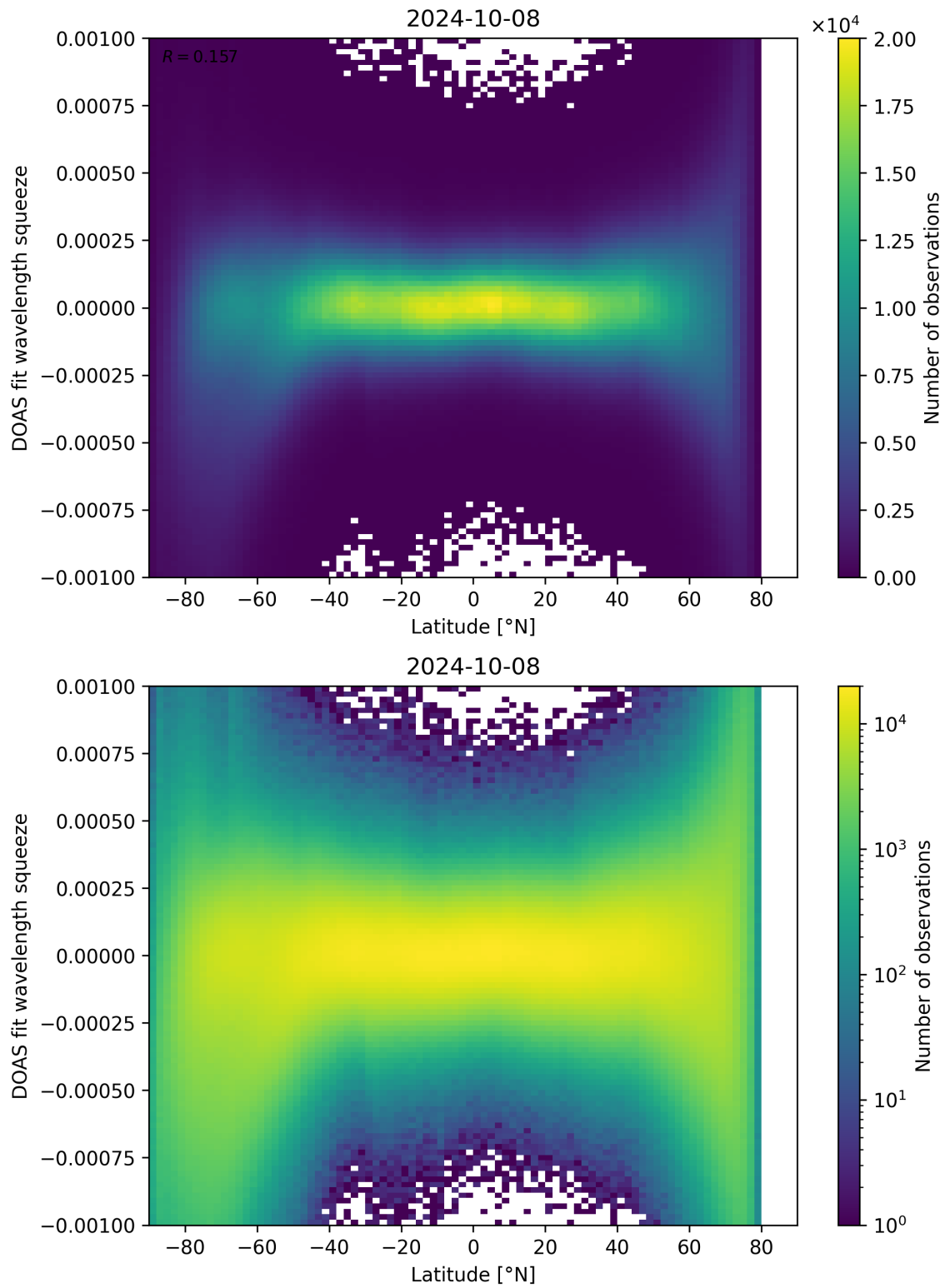
Figure 143: Scatter density plot of “Latitude” against “DOAS fit wavelength squeeze” for 2024-10-08 to 2024-10-09.
