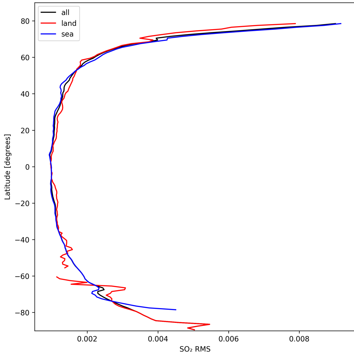
Figure 47: Zonal average of “SO 2 RMS” for 2024-10-08 to 2024-10-09.
