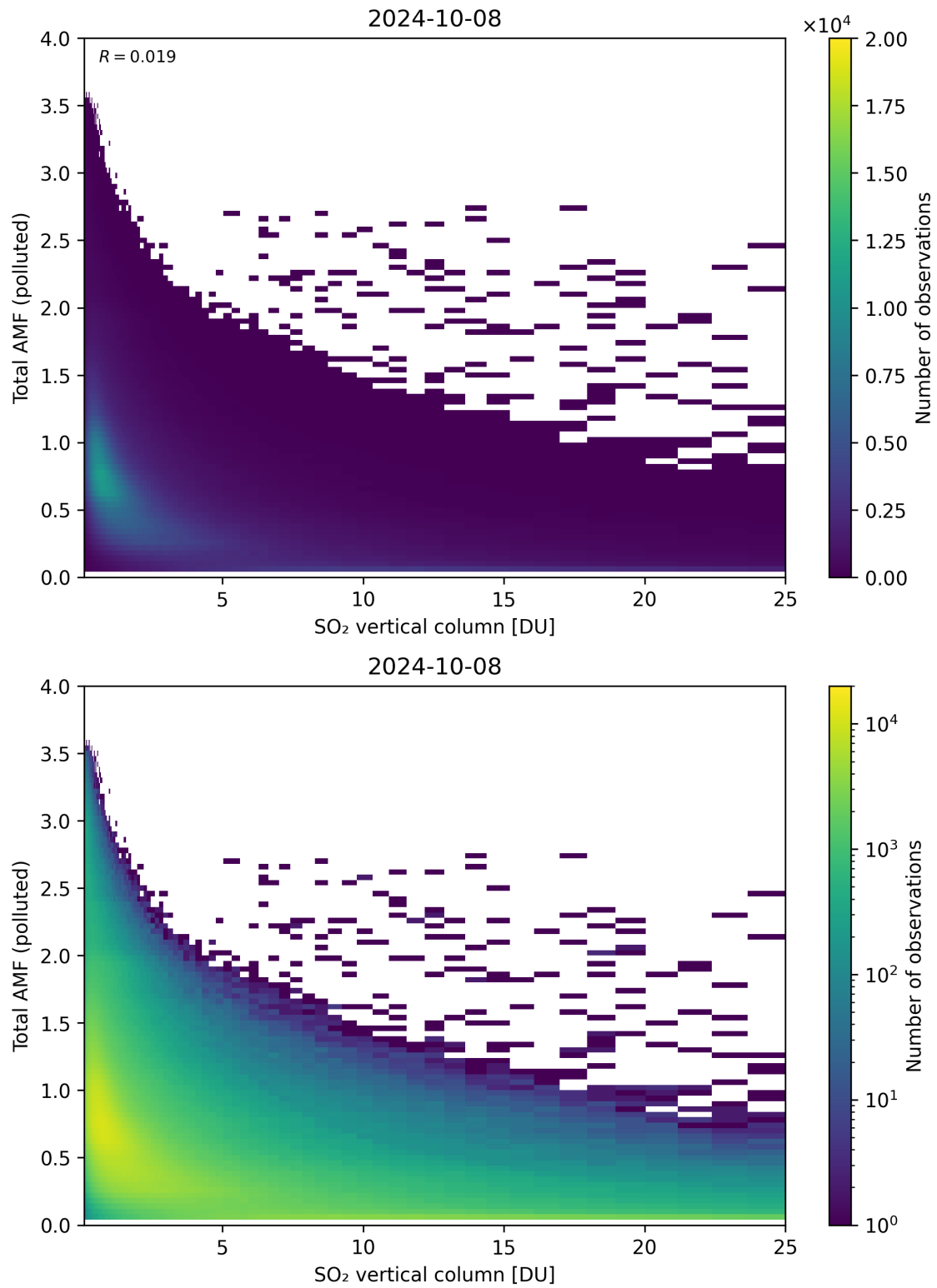
Figure 305: Scatter density plot of “SO 2 vertical column” against “Total AMF (polluted)” for 2024-10-08 to 2024-10-09.
