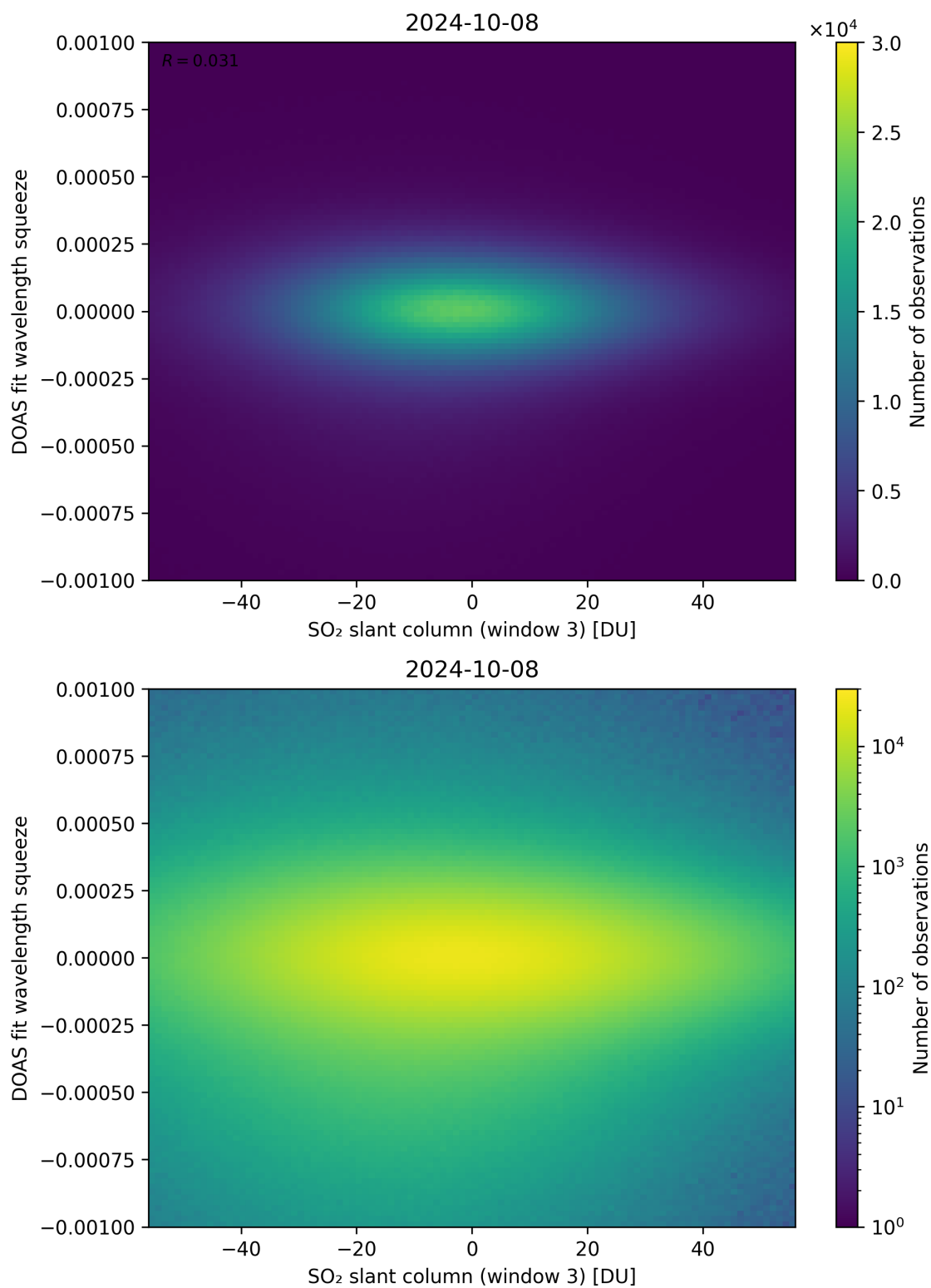
Figure 255: Scatter density plot of “SO 2 slant column (window 3)” against “DOAS fit wavelength squeeze” for 2024-10-08 to 2024-10-09.
