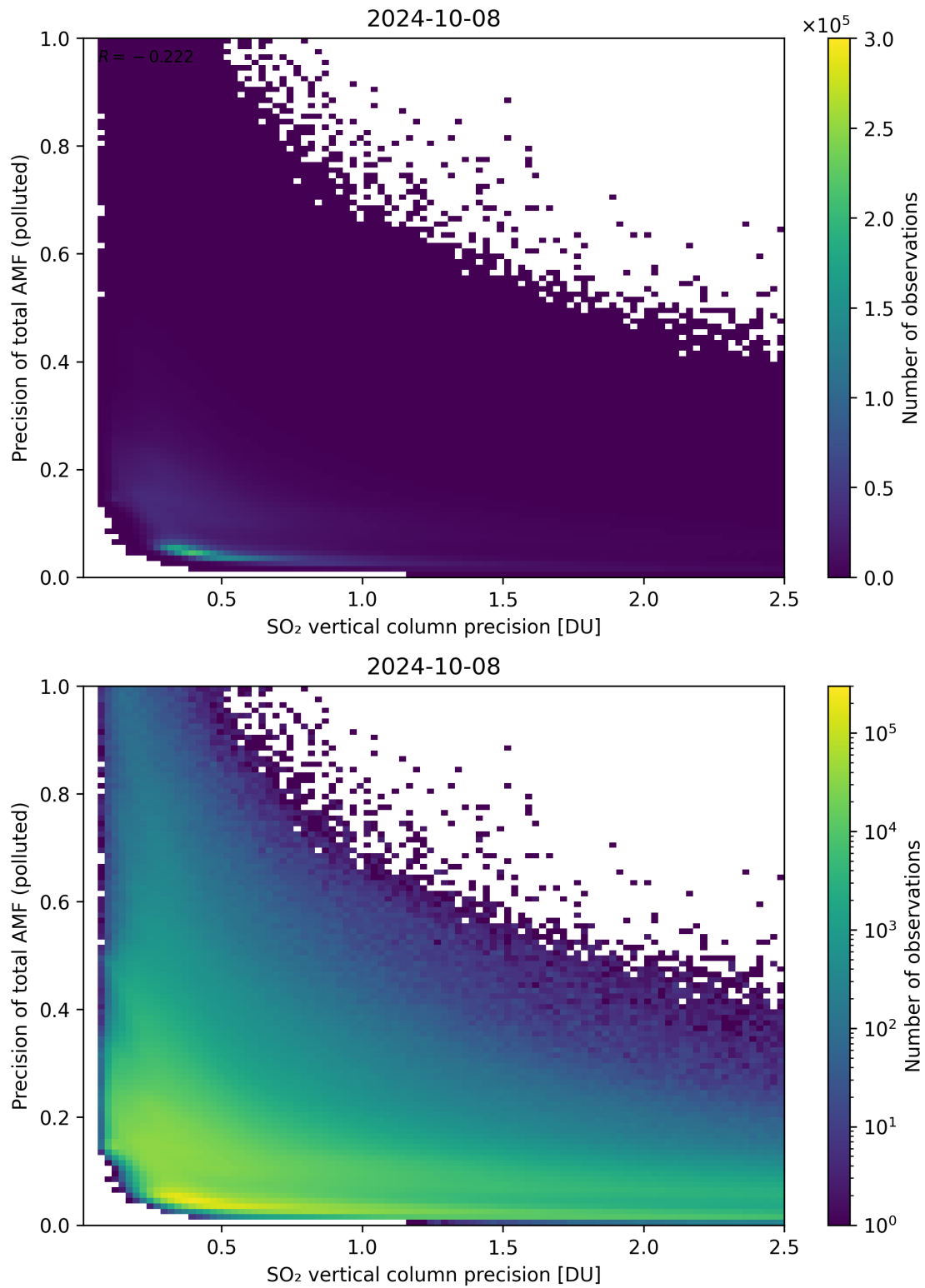
Figure 295: Scatter density plot of “SO 2 vertical column precision” against “Precision of total AMF (polluted)” for 2024-10-08 to 2024-10-09.
