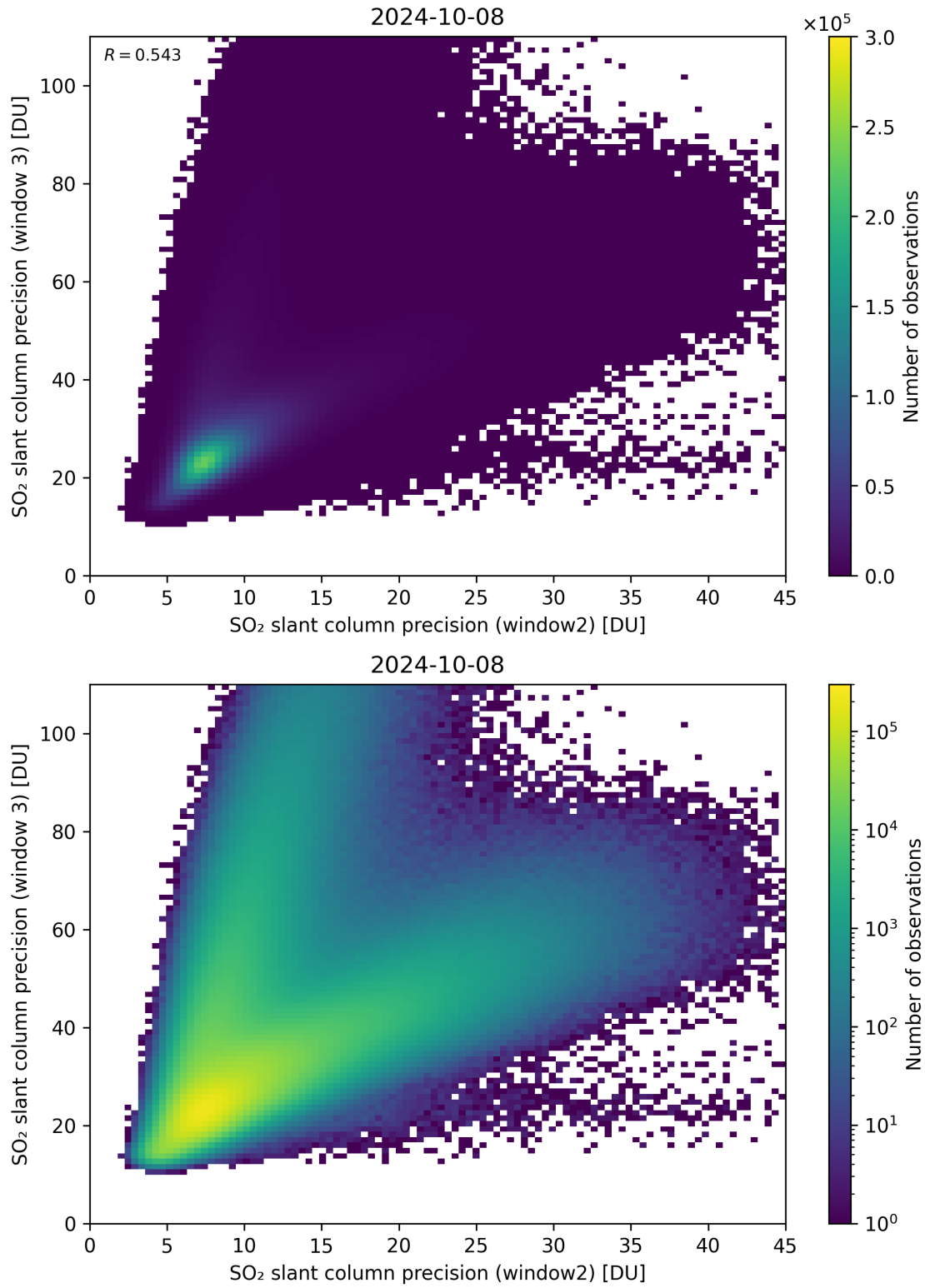
Figure 250: Scatter density plot of “SO 2 slant column precision (window2)” against “SO 2 slant column precision (window 3)” for 2024-10-08 to 2024-10-09.
