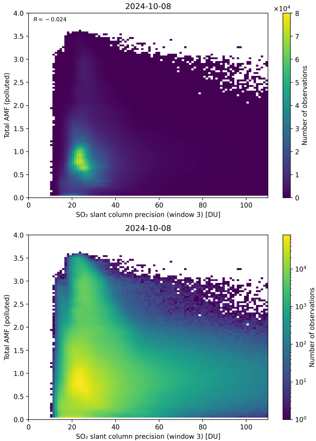
Figure 263: Scatter density plot of “SO 2 slant column precision (window 3)” against “Total AMF (polluted)” for 2024-10-08 to 2024-10-09.
