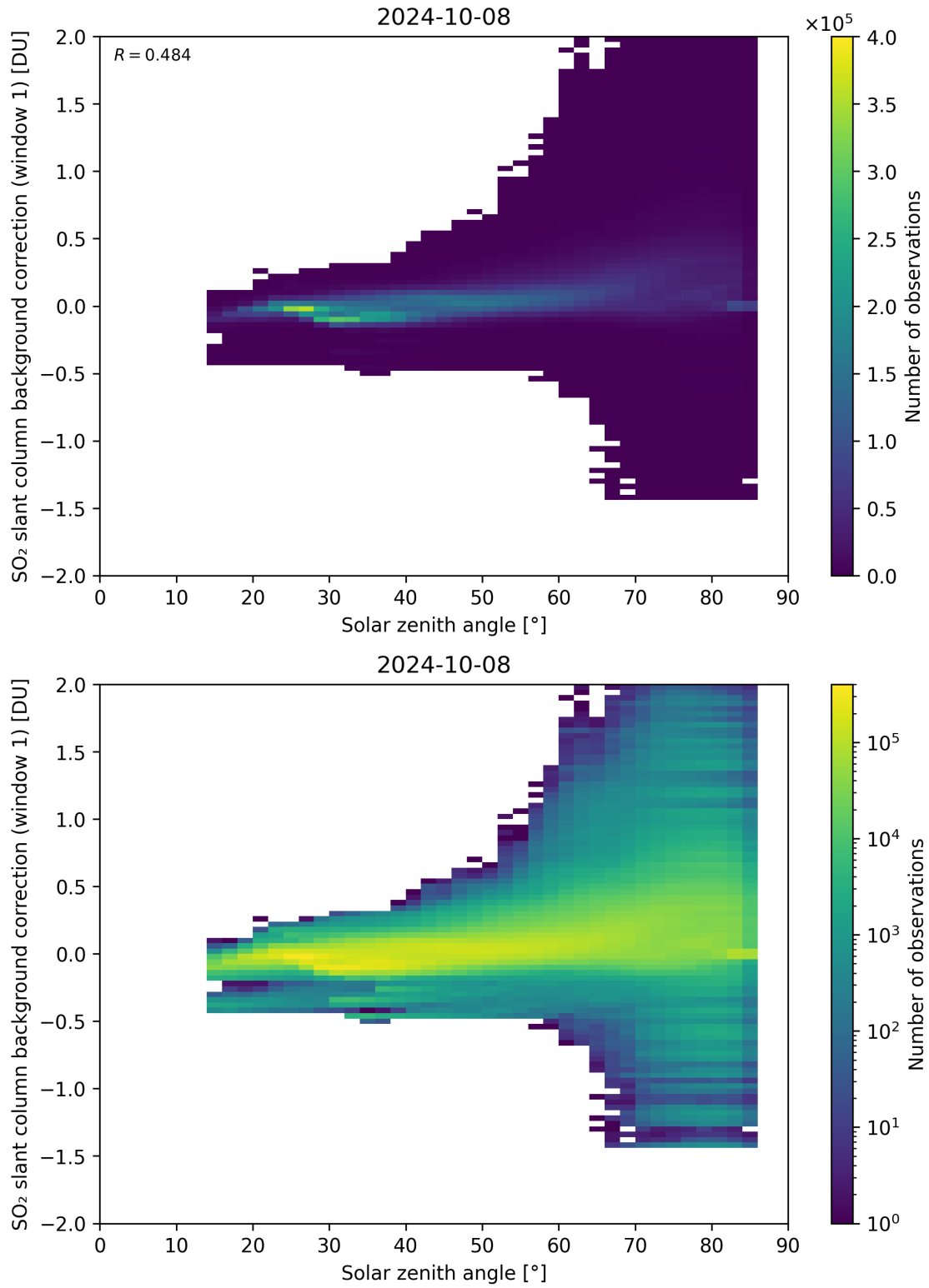
Figure 158: Scatter density plot of “Solar zenith angle” against “SO 2 slant column background correction (window 1)” for 2024-10-08 to 2024-10-09.
