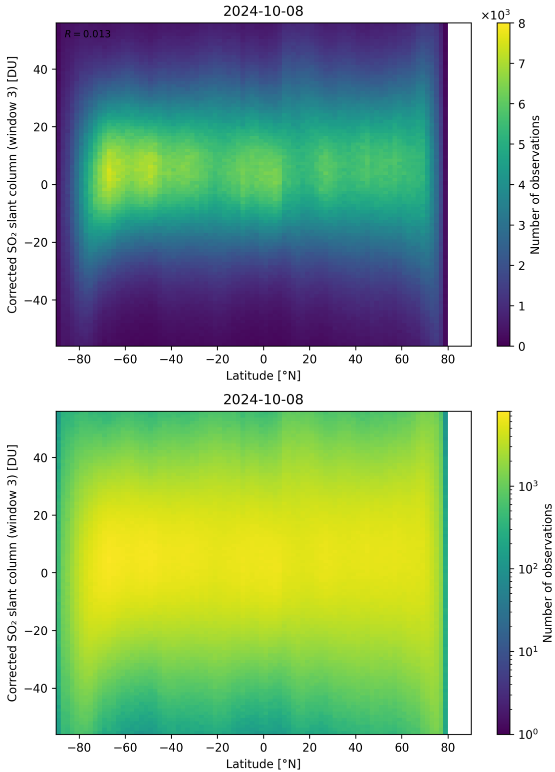
Figure 148: Scatter density plot of “Latitude” against “Corrected SO 2 slant column (window 3)” for 2024-10-08 to 2024-10-09.
