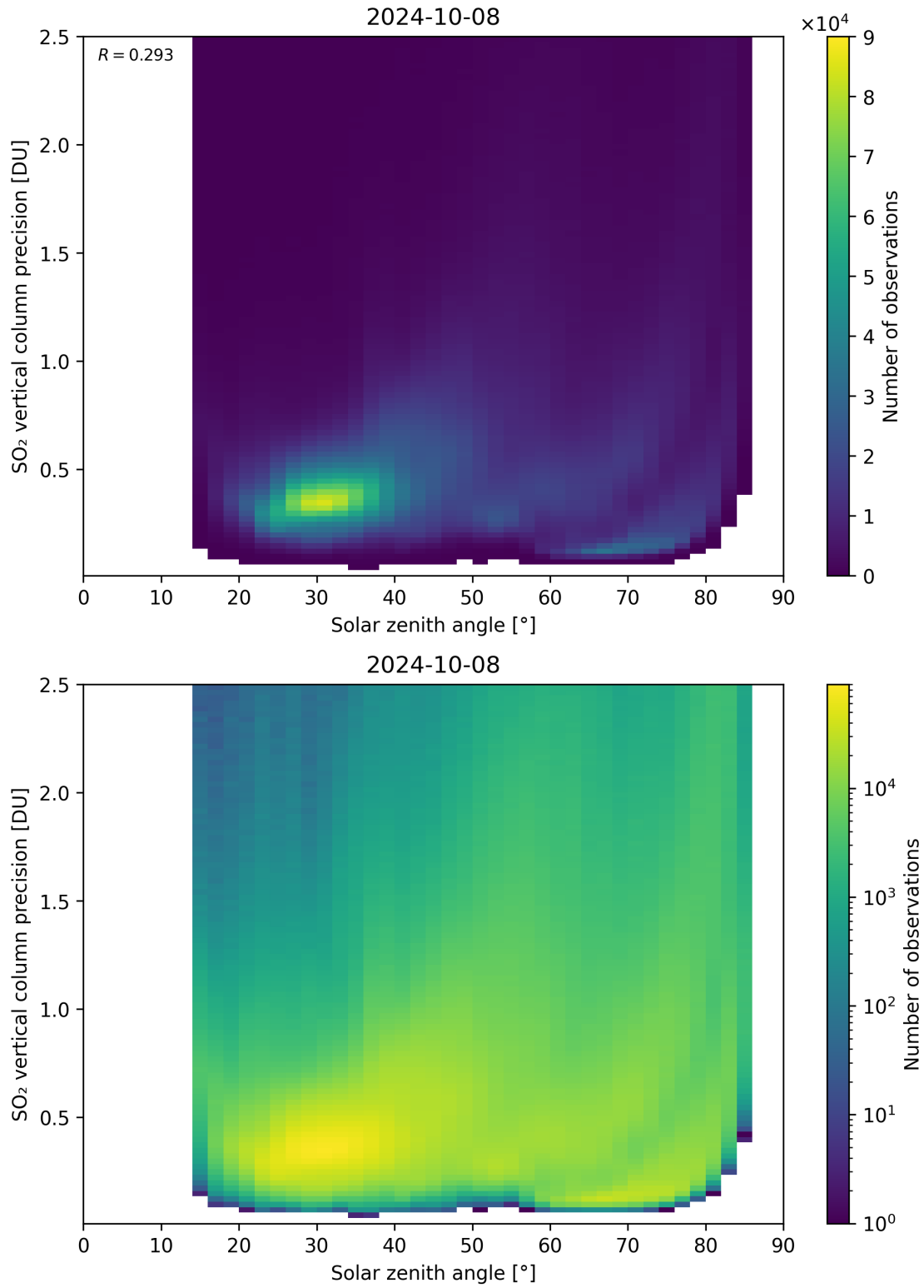
Figure 177: Scatter density plot of “Solar zenith angle” against “SO 2 vertical column precision” for 2024-10-08 to 2024-10-09.
