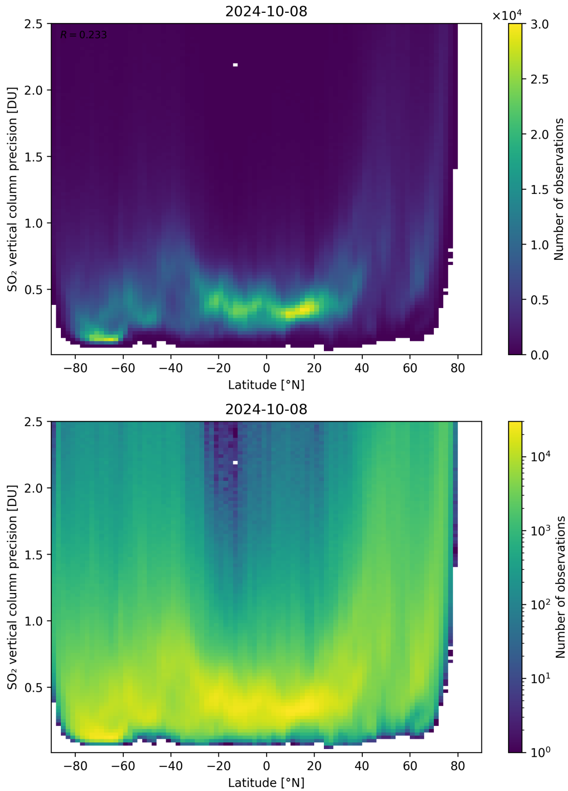
Figure 157: Scatter density plot of “Latitude” against “SO 2 vertical column precision” for 2024-10-08 to 2024-10-09.
