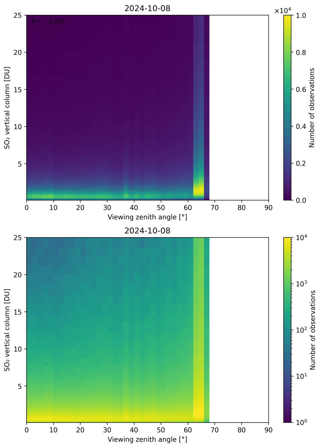
Figure 327: Scatter density plot of “Viewing zenith angle” against “SO 2 vertical column” for 2024-10-08 to 2024-10-09.
