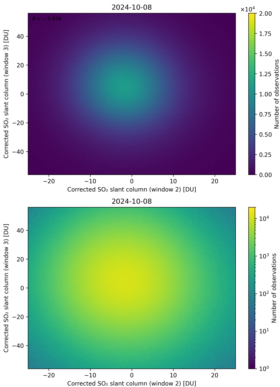
Figure 200: Scatter density plot of “Corrected SO 2 slant column (window 2)” against “Corrected SO 2 slant column (window 3)” for 2024-10-08 to 2024-10-09.
