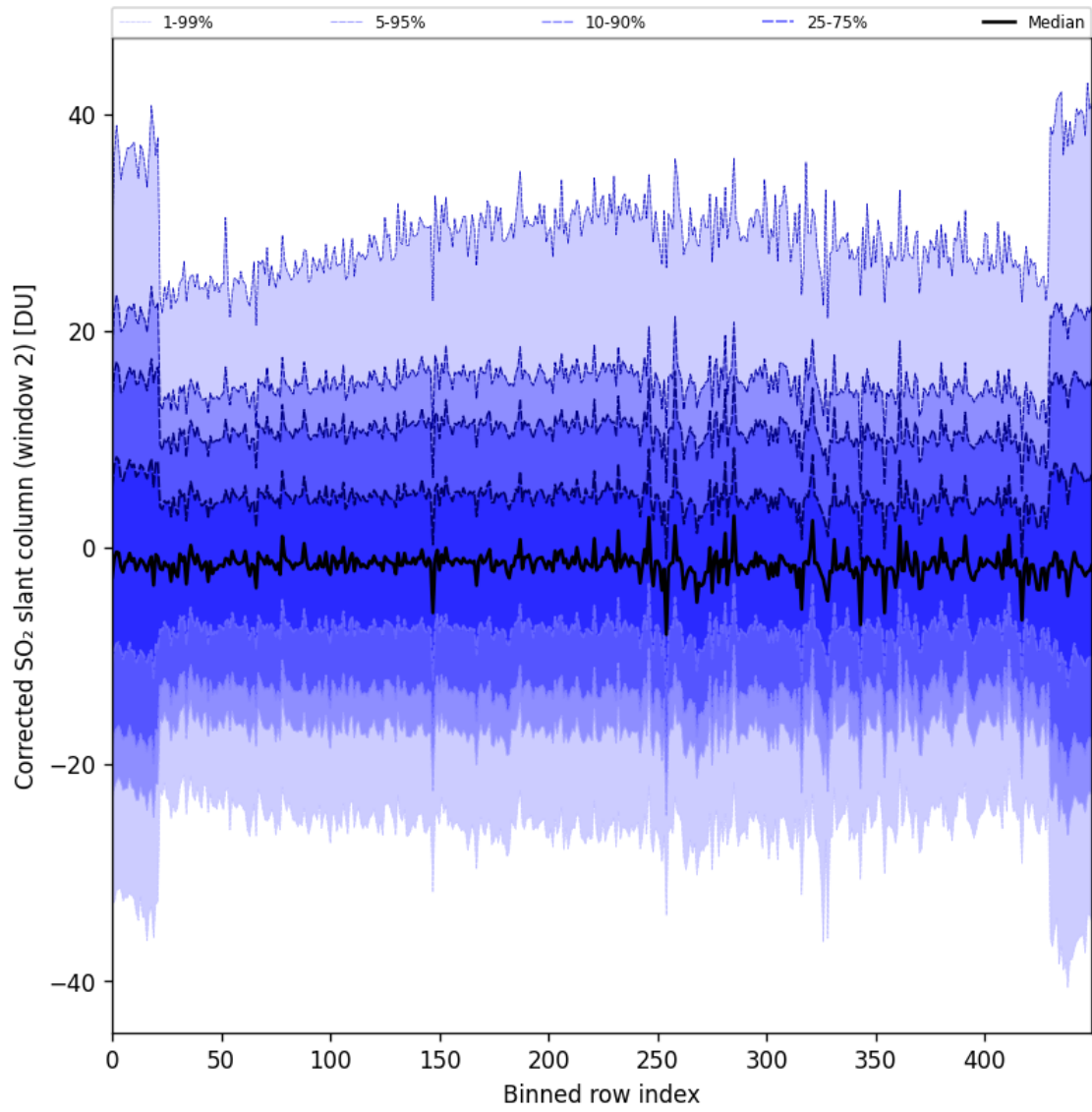
Figure 85: Along track statistics of “Corrected SO 2 slant column (window 2)” for 2024-10-08 to 2024-10-09
