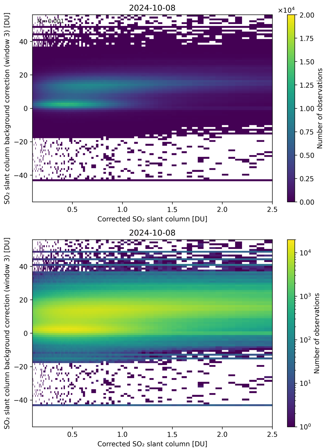
Figure 180: Scatter density plot of “Corrected SO 2 slant column” against “SO 2 slant column background correction (window 3)” for 2024-10-08 to 2024-10-09.
