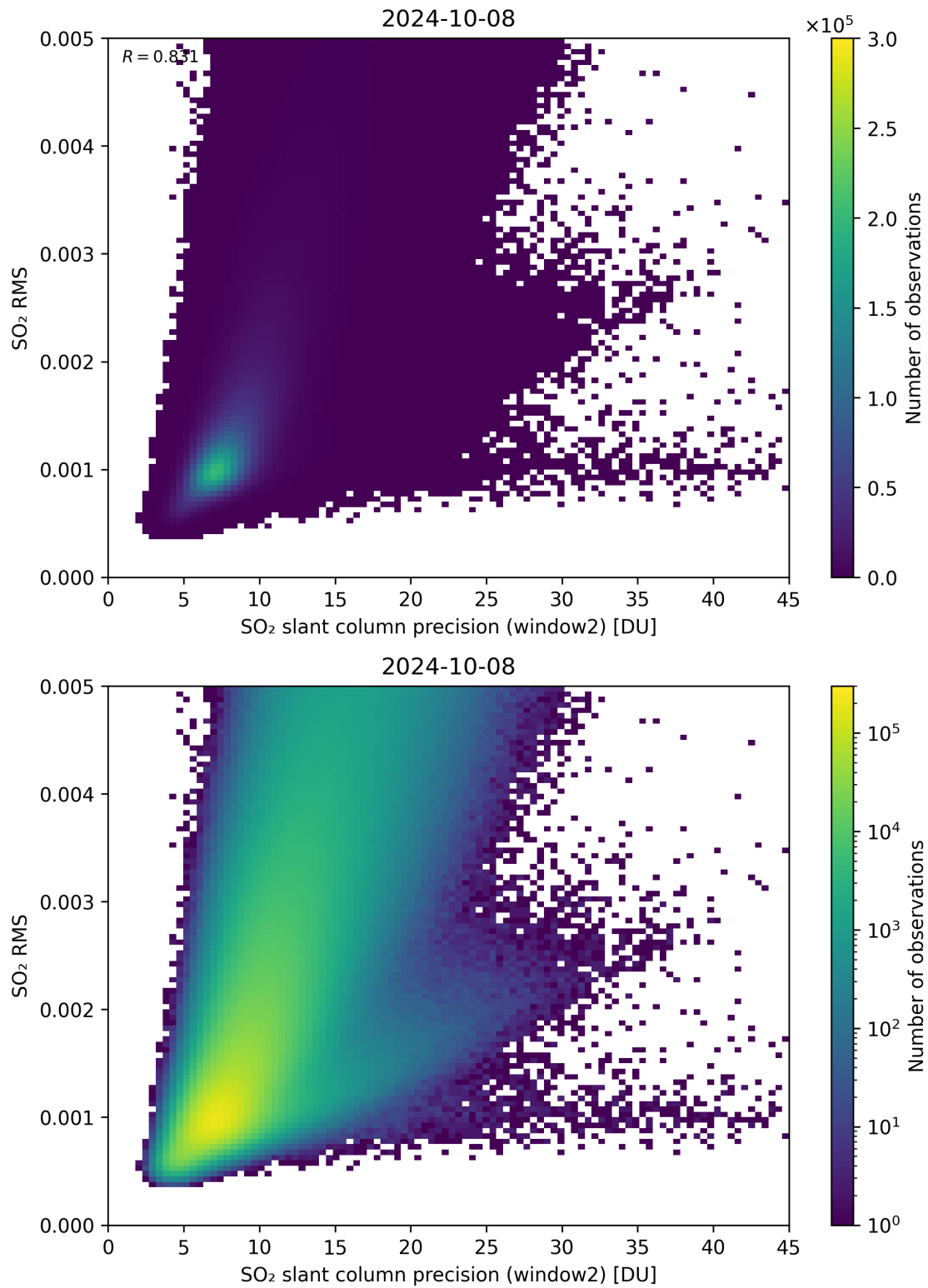
Figure 245: Scatter density plot of “SO 2 slant column precision (window2)” against “SO 2 RMS” for 2024-10-08 to 2024-10-09.
