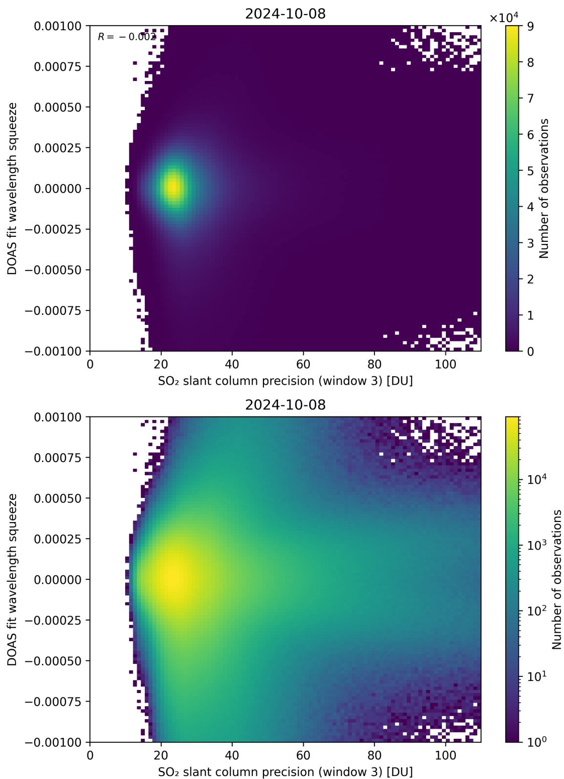
Figure 259: Scatter density plot of “SO 2 slant column precision (window 3)” against “DOAS fit wavelength squeeze” for 2024-10-08 to 2024-10-09.
