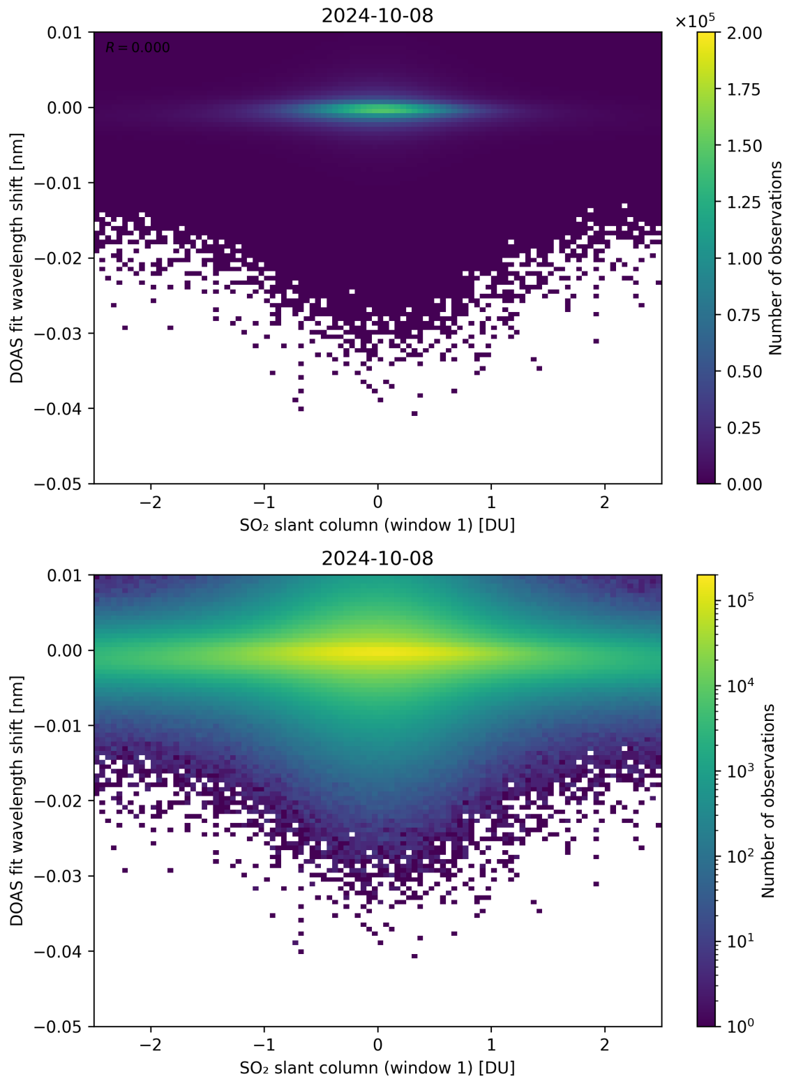
Figure 215: Scatter density plot of “SO 2 slant column (window 1)” against “DOAS fit wavelength shift” for 2024-10-08 to 2024-10-09.
