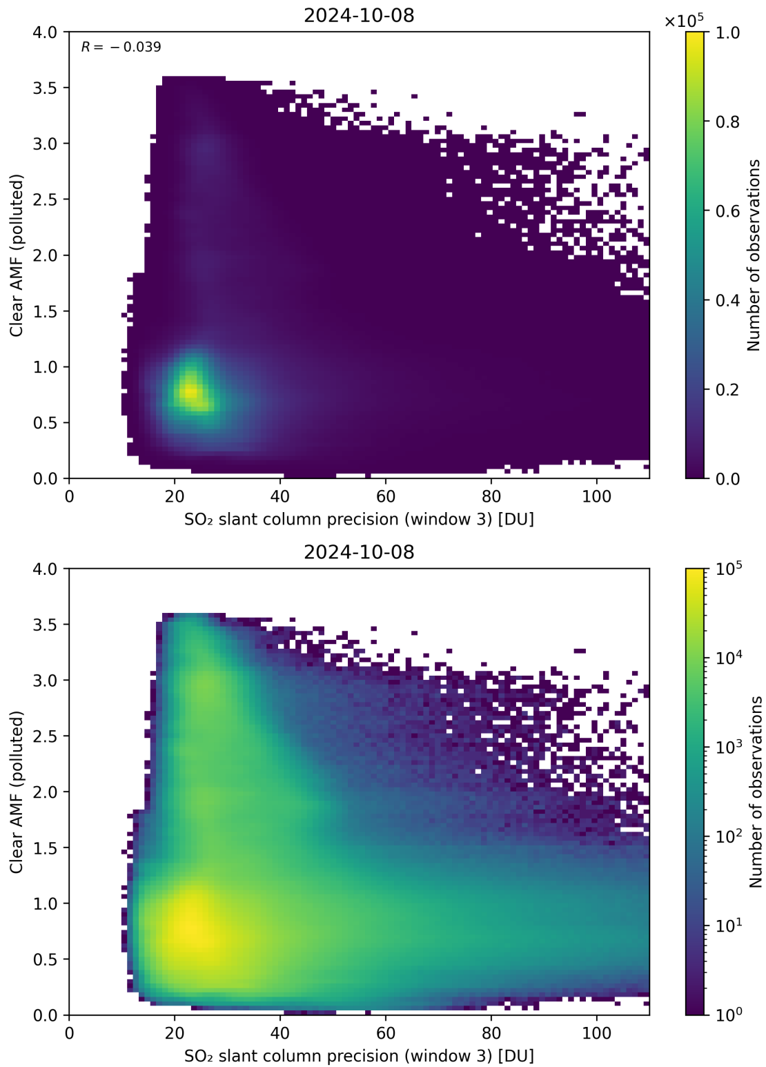
Figure 261: Scatter density plot of “SO 2 slant column precision (window 3)” against “Clear AMF (polluted)” for 2024-10-08 to 2024-10-09.
