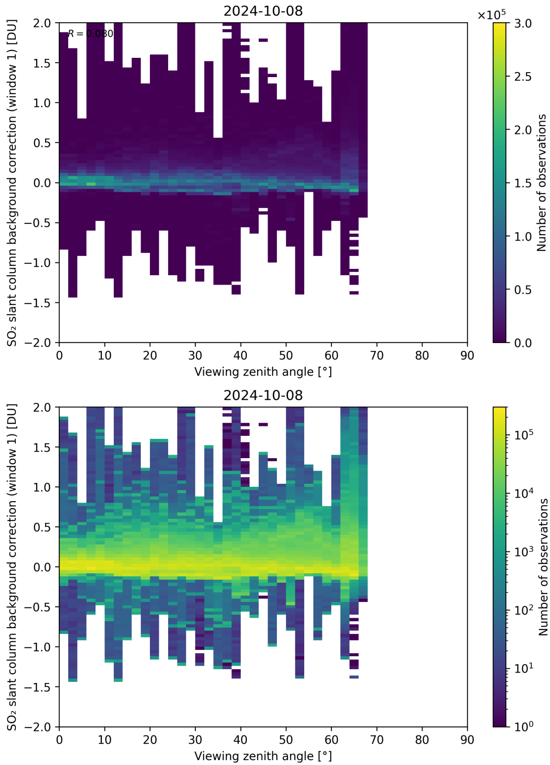
Figure 308: Scatter density plot of “Viewing zenith angle” against “SO 2 slant column background correction (window 1)” for 2024-10-08 to 2024-10-09.
