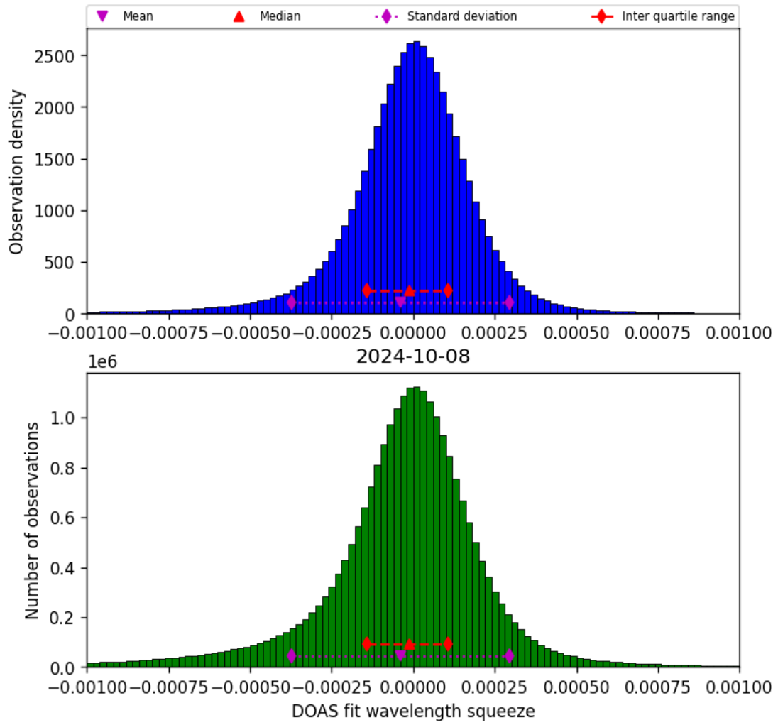
Figure 69: Histogram of “DOAS fit wavelength squeeze” for 2024-10-08 to 2024-10-09
