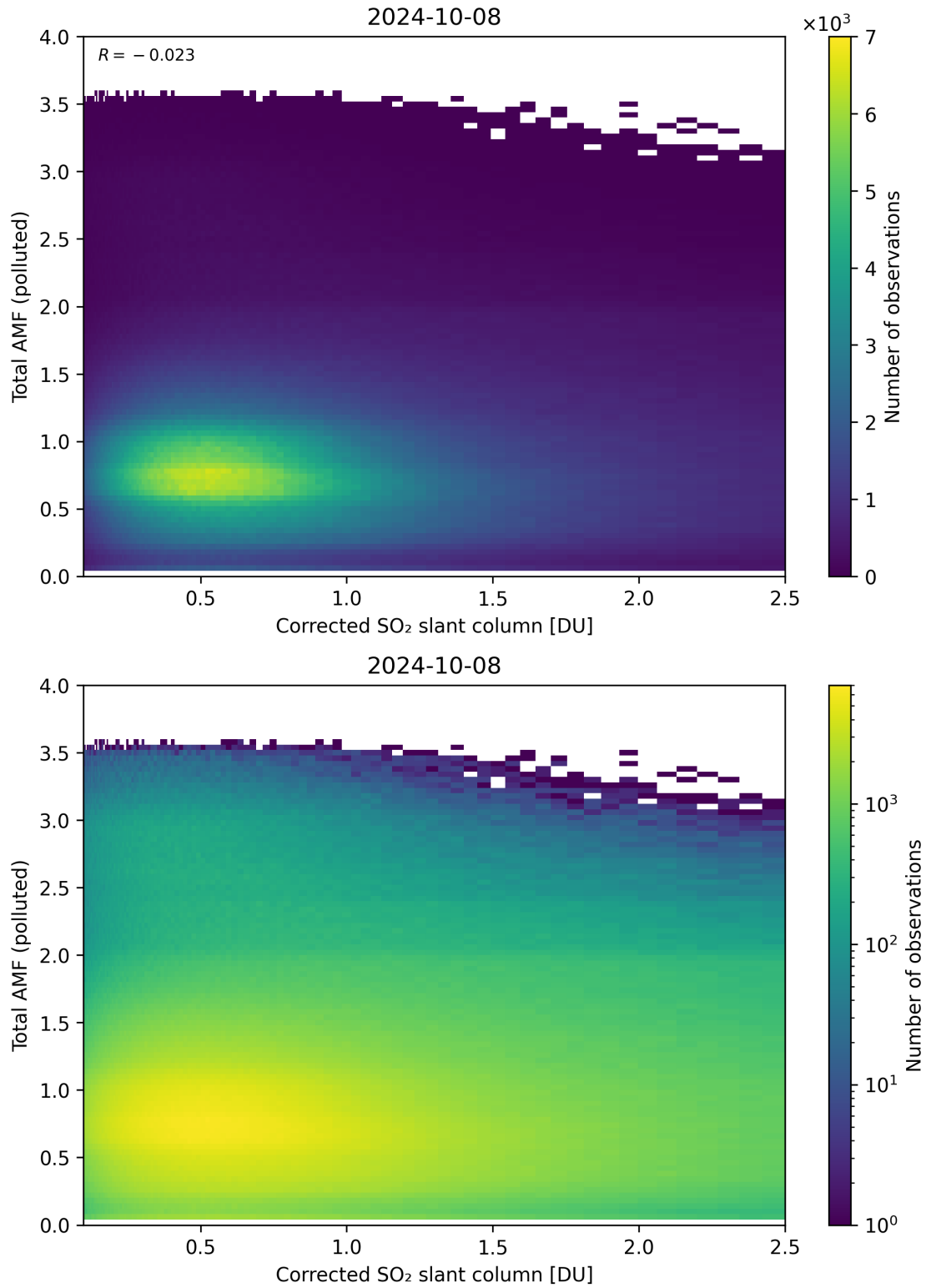
Figure 192: Scatter density plot of “Corrected SO 2 slant column” against “Total AMF (polluted)” for 2024-10-08 to 2024-10-09.
