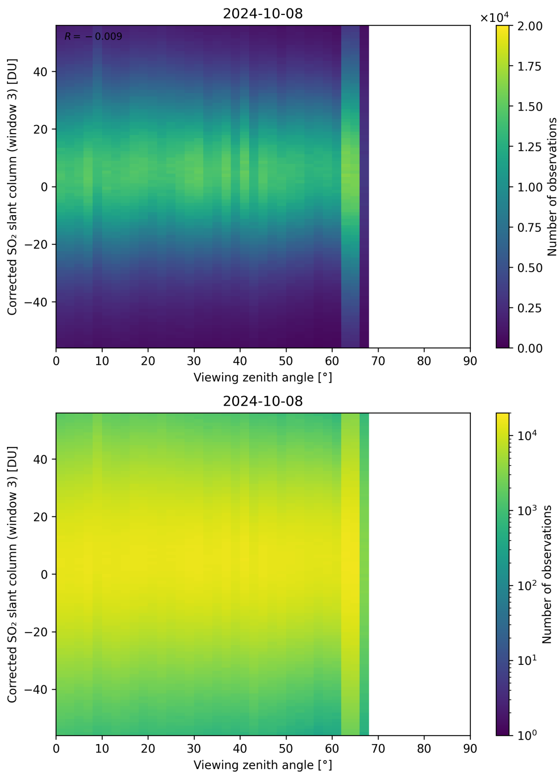
Figure 319: Scatter density plot of “Viewing zenith angle” against “Corrected SO 2 slant column (window 3)” for 2024-10-08 to 2024-10-09.
