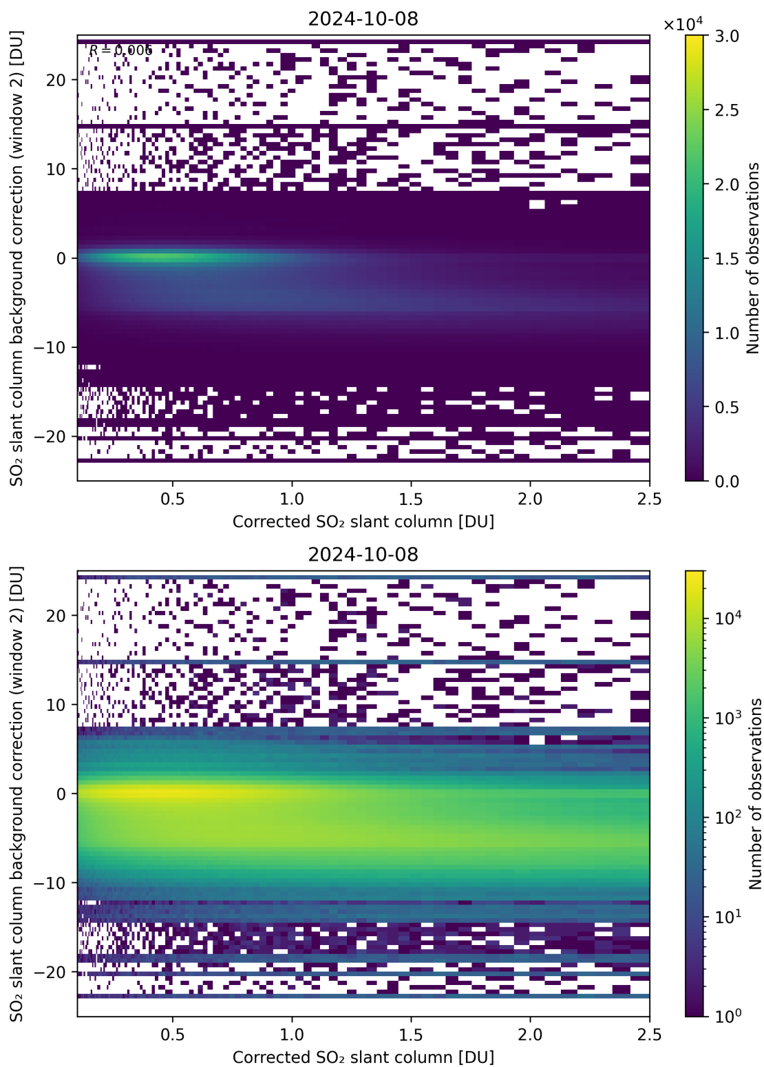
Figure 179: Scatter density plot of “Corrected SO 2 slant column” against “SO 2 slant column background correction (window 2)” for 2024-10-08 to 2024-10-09.
