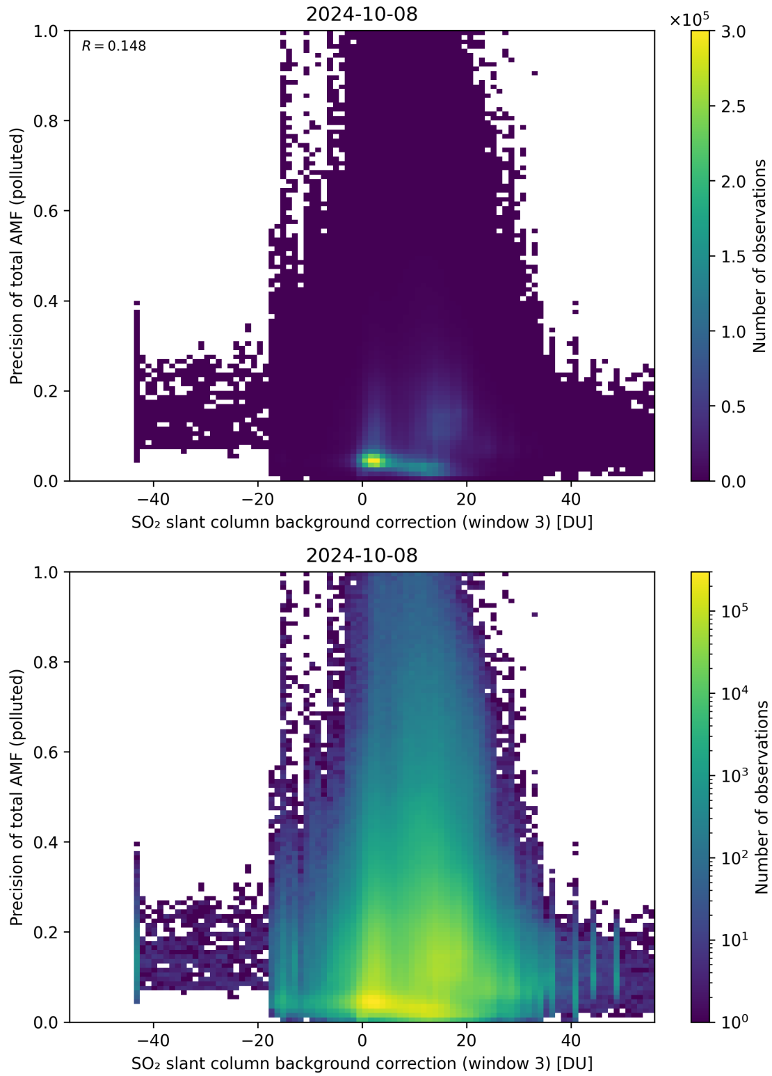
Figure 126: Scatter density plot of “SO 2 slant column background correction (window 3)” against “Precision of total AMF (polluted)” for 2024-10-08 to 2024-10-09.
