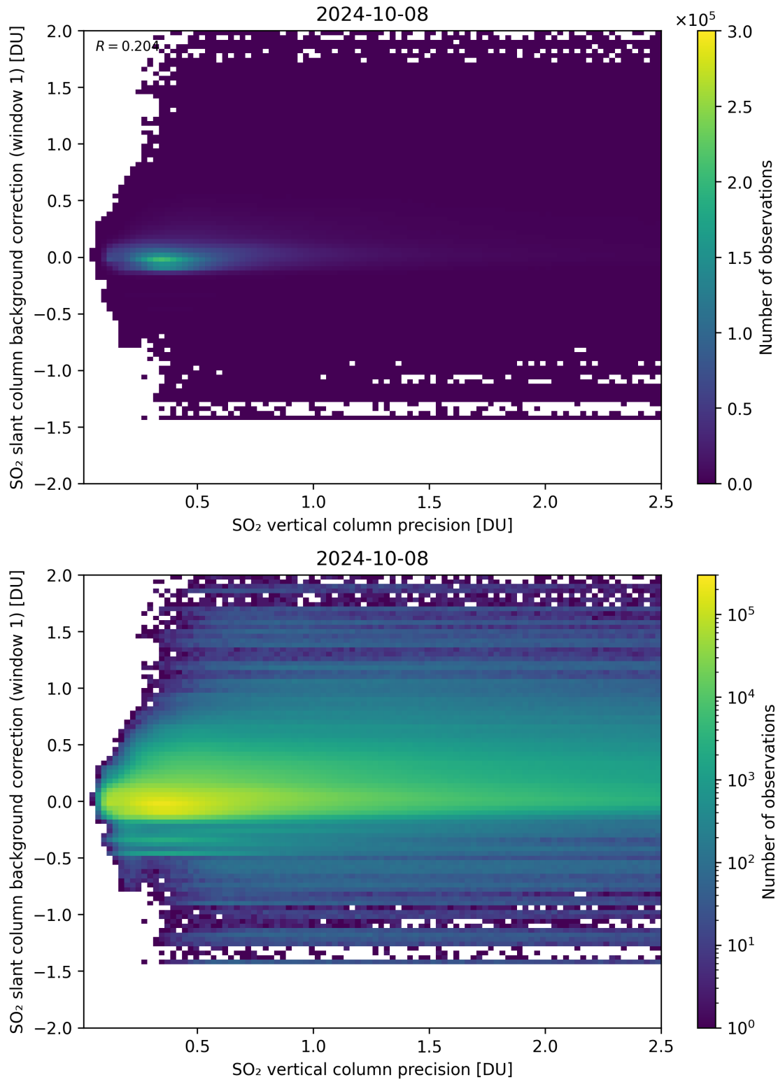
Figure 279: Scatter density plot of “SO 2 vertical column precision” against “SO 2 slant column background correction (window 1)” for 2024-10-08 to 2024-10-09.
