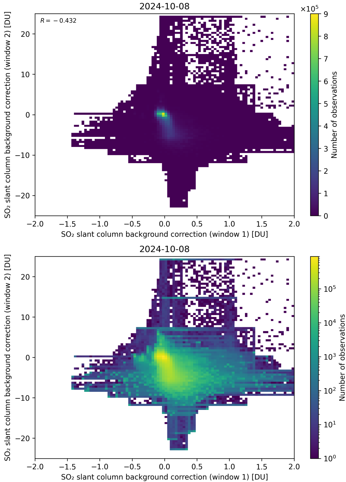
Figure 98: Scatter density plot of “SO 2 slant column background correction (window 1)” against “SO 2 slant column background correction (window 2)” for 2024-10-08 to 2024-10-09.
