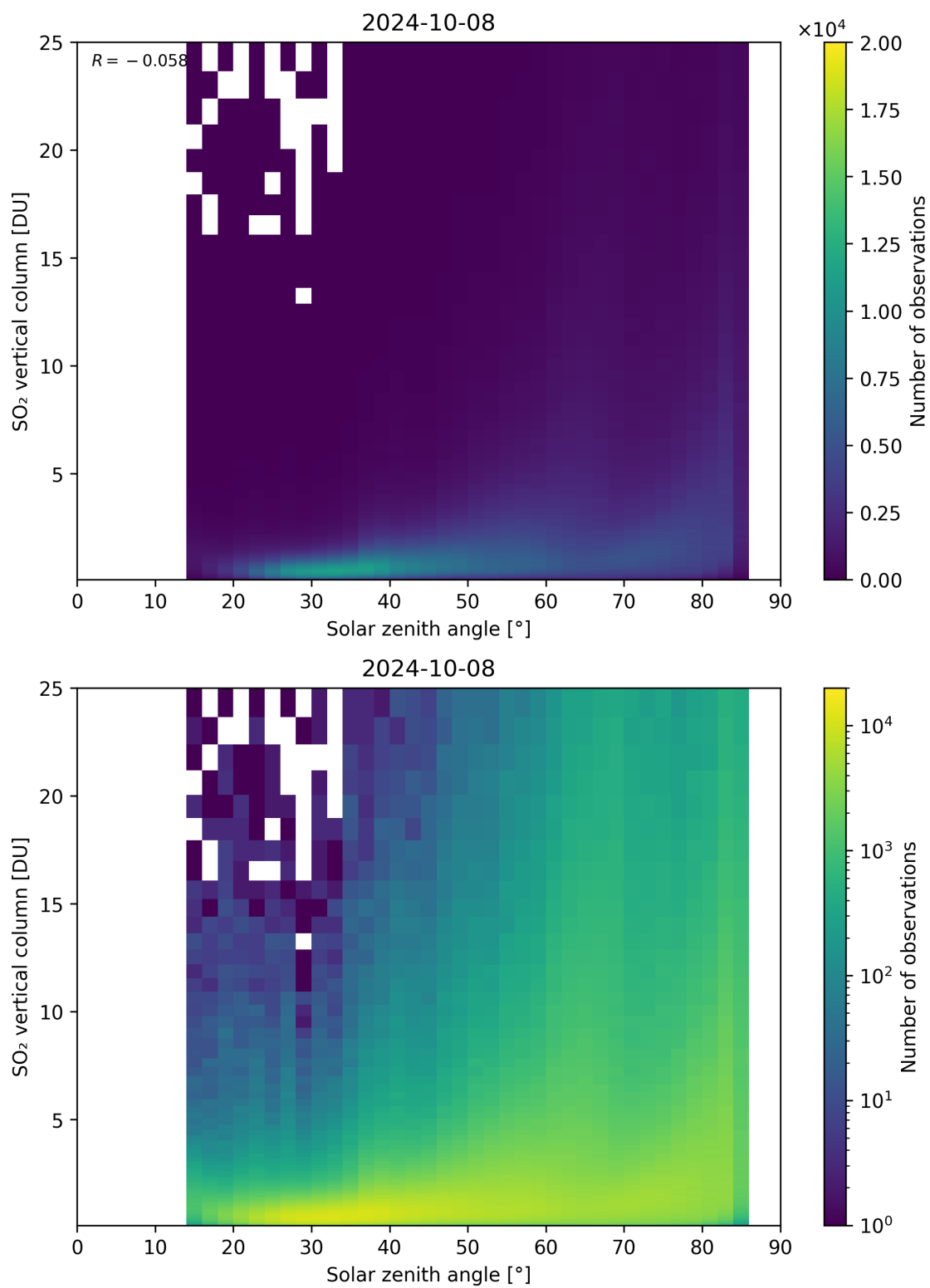
Figure 176: Scatter density plot of “Solar zenith angle” against “SO 2 vertical column” for 2024-10-08 to 2024-10-09.
