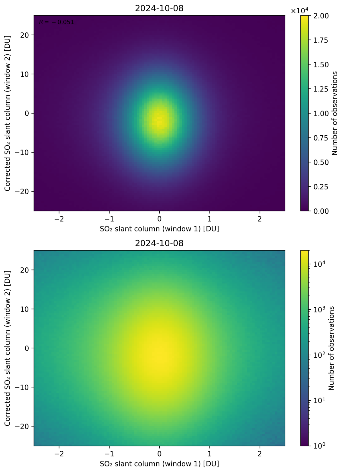
Figure 233: Scatter density plot of “SO 2 slant column (window 1)” against “Corrected SO 2 slant column (window 2)” for 2024-10-08 to 2024-10-09.
