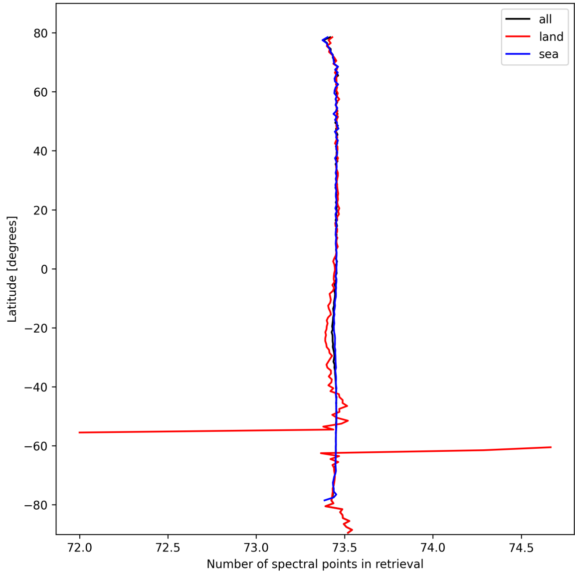
Figure 51: Zonal average of “Number of spectral points in retrieval” for 2024-10-08 to 2024-10-09.
