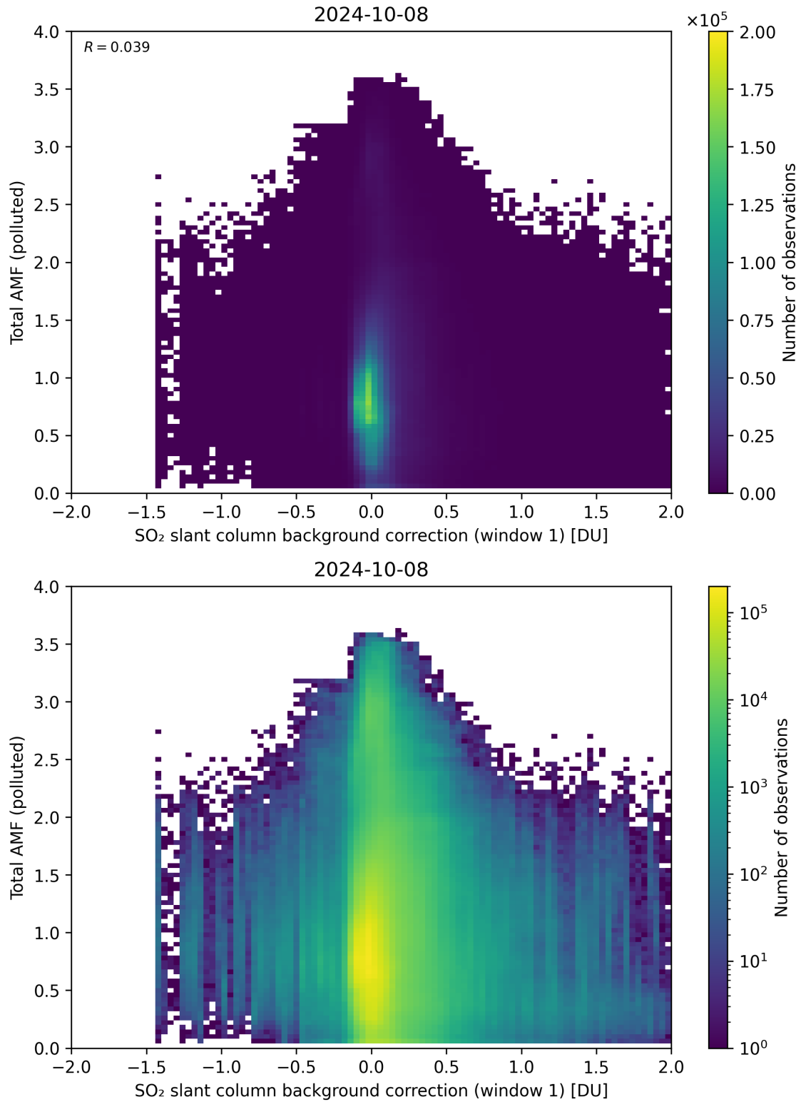
Figure 109: Scatter density plot of “SO 2 slant column background correction (window 1)” against “Total AMF (polluted)” for 2024-10-08 to 2024-10-09.
