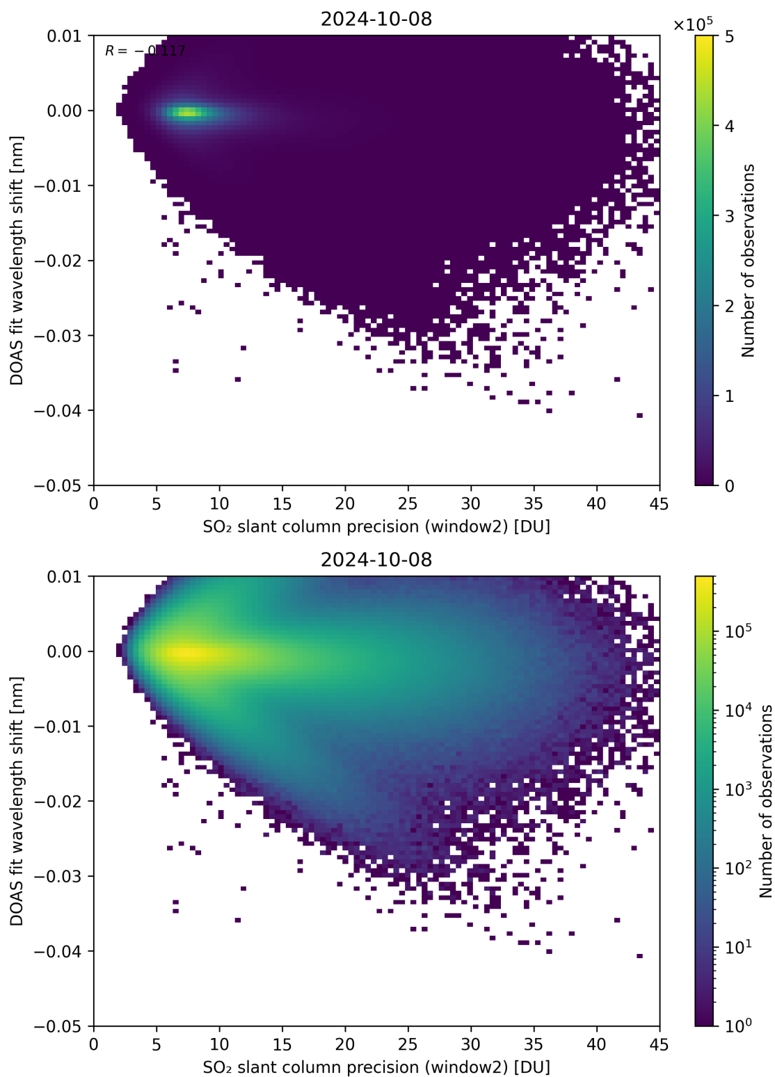
Figure 243: Scatter density plot of “SO 2 slant column precision (window2)” against “DOAS fit wavelength shift” for 2024-10-08 to 2024-10-09.
