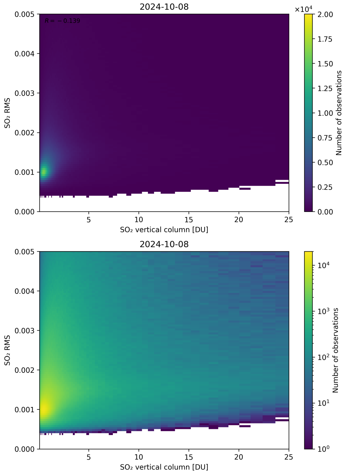
Figure 278: Scatter density plot of “SO 2 vertical column” against “SO 2 RMS” for 2024-10-08 to 2024-10-09.
