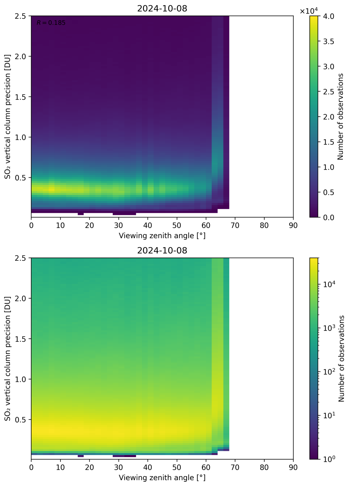
Figure 328: Scatter density plot of “Viewing zenith angle” against “SO 2 vertical column precision” for 2024-10-08 to 2024-10-09.
