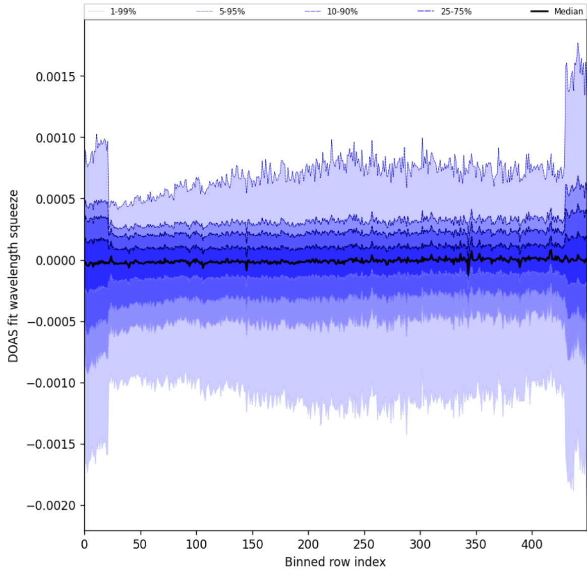
Figure 92: Along track statistics of “DOAS fit wavelength squeeze” for 2024-10-08 to 2024-10-09
