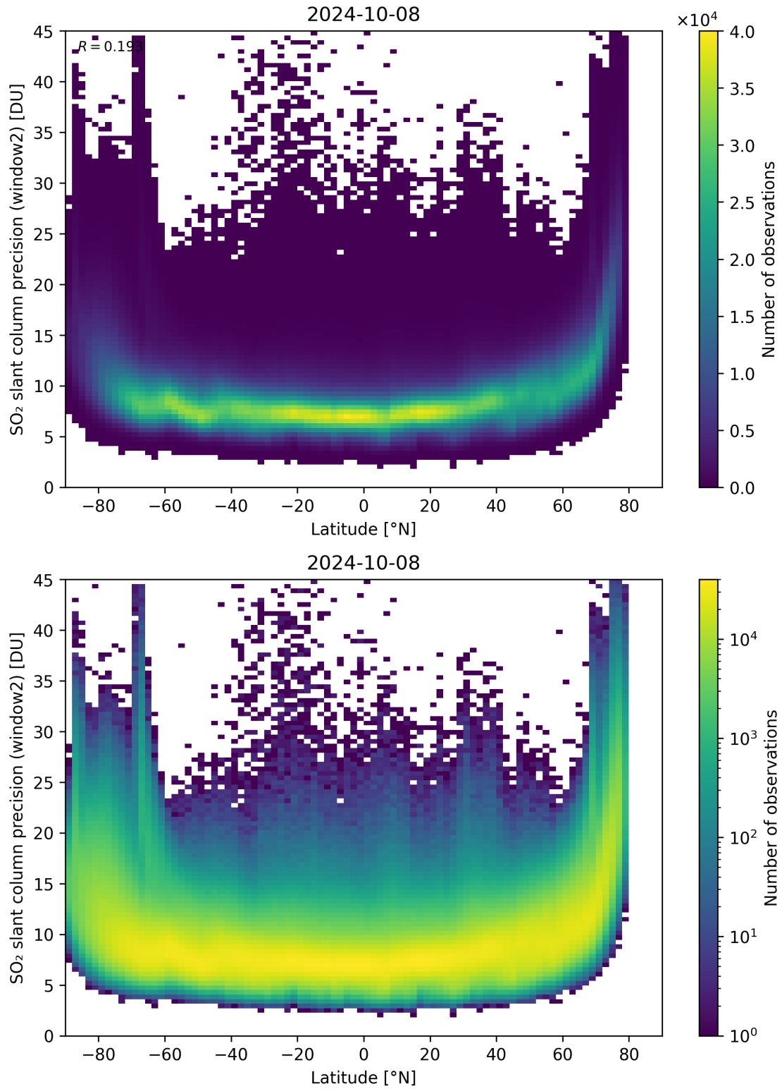
Figure 151: Scatter density plot of “Latitude” against “SO 2 slant column precision (window2)” for 2024-10-08 to 2024-10-09.
