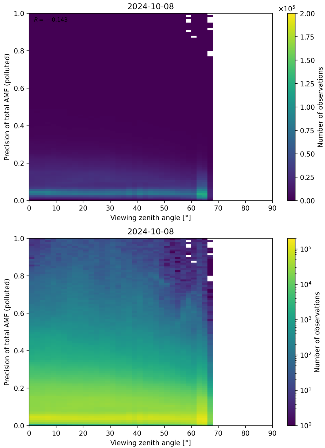
Figure 326: Scatter density plot of “Viewing zenith angle” against “Precision of total AMF (polluted)” for 2024-10-08 to 2024-10-09.
