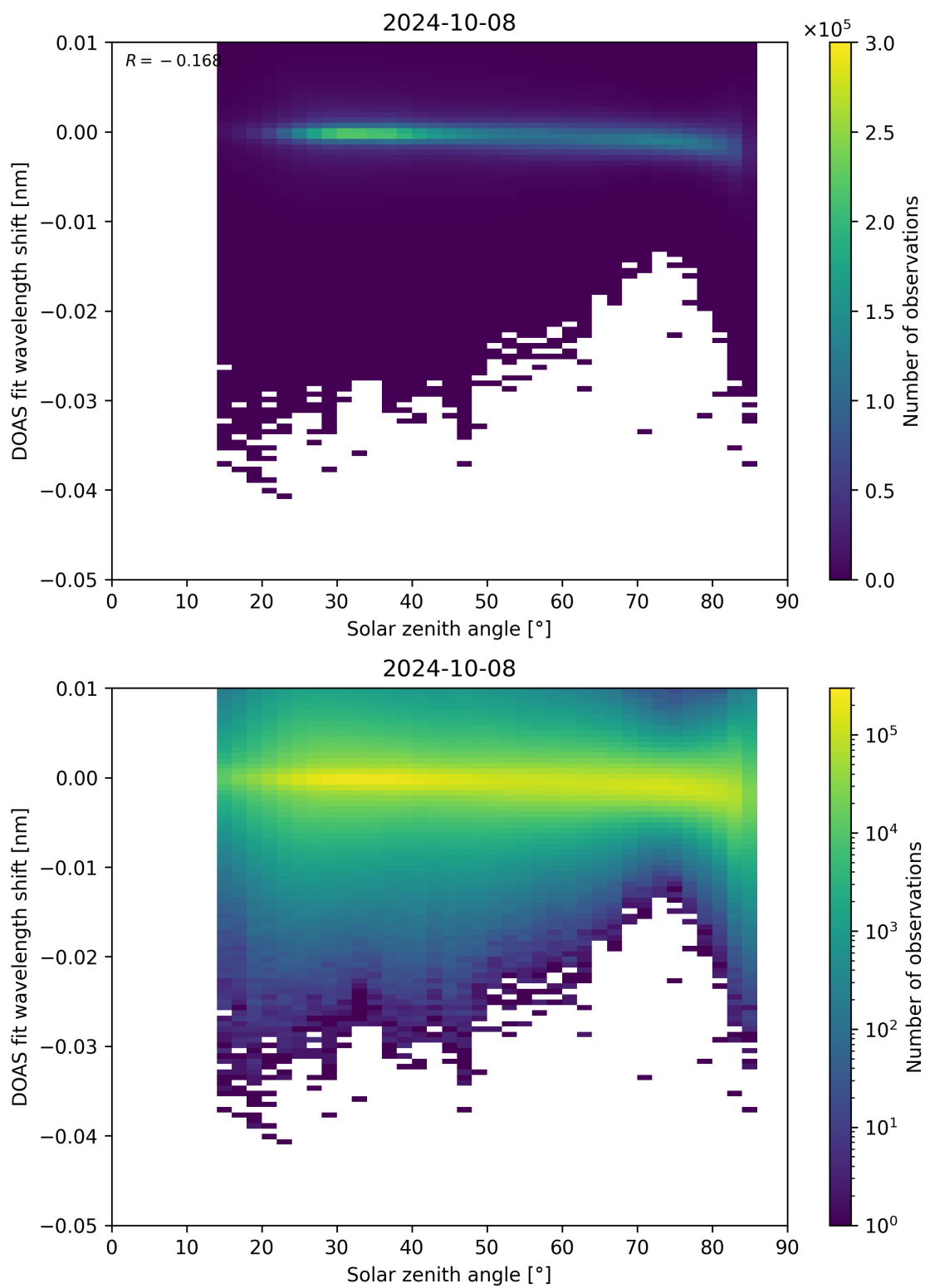
Figure 161: Scatter density plot of “Solar zenith angle” against “DOAS fit wavelength shift” for 2024-10-08 to 2024-10-09.
