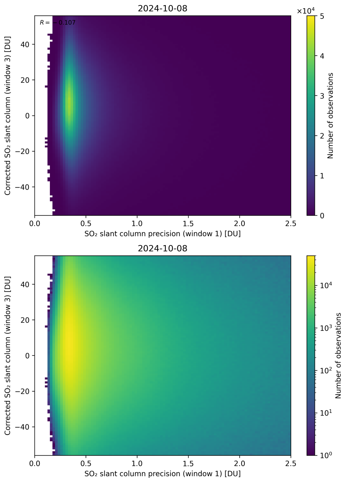
Figure 226: Scatter density plot of “SO 2 slant column precision (window 1)” against “Corrected SO 2 slant column (window 3)” for 2024-10-08 to 2024-10-09.
