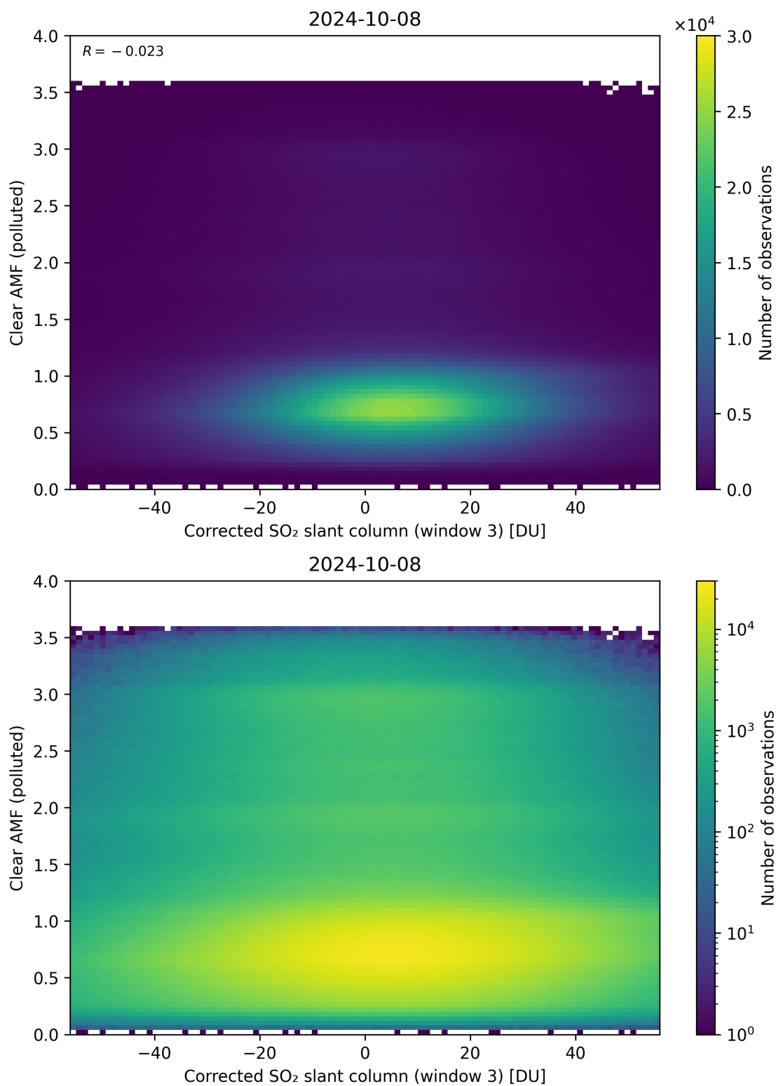
Figure 209: Scatter density plot of “Corrected SO 2 slant column (window 3)” against “Clear AMF (polluted)” for 2024-10-08 to 2024-10-09.
