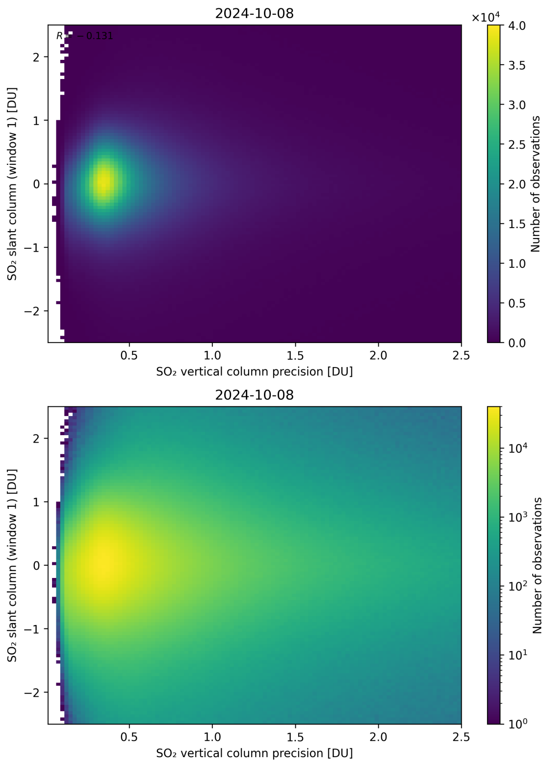
Figure 289: Scatter density plot of “SO 2 vertical column precision” against “SO 2 slant column (window 1)” for 2024-10-08 to 2024-10-09.
