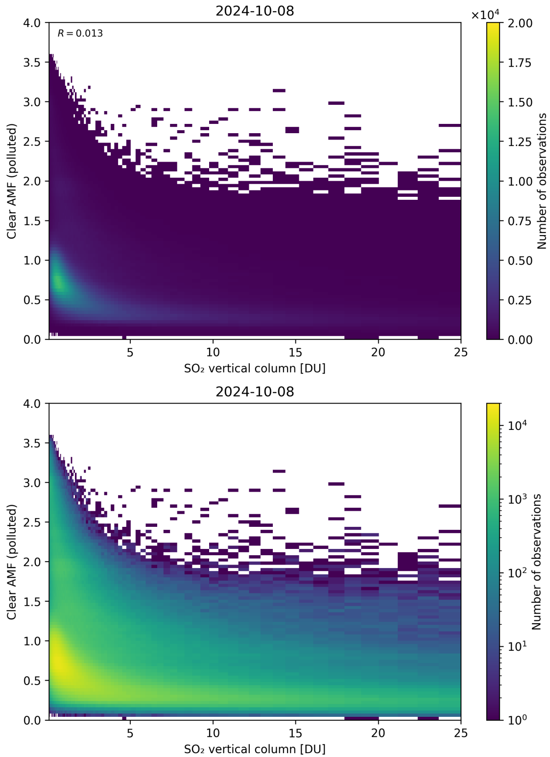
Figure 296: Scatter density plot of “SO 2 vertical column” against “Clear AMF (polluted)” for 2024-10-08 to 2024-10-09.
