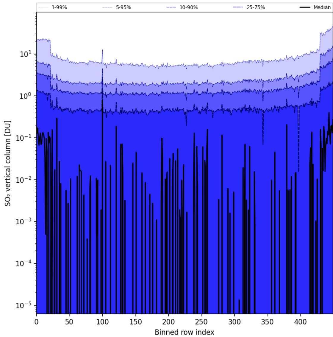
Figure 76: Along track statistics of “SO 2 vertical column” for 2024-10-08 to 2024-10-09
