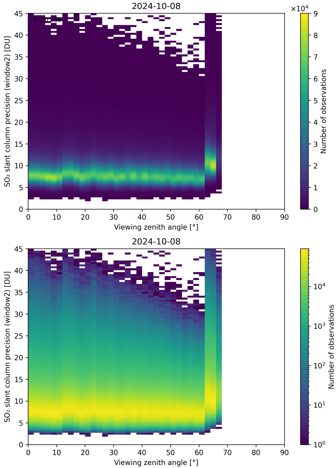
Figure 322: Scatter density plot of “Viewing zenith angle” against “SO 2 slant column precision (window2)” for 2024-10-08 to 2024-10-09.
