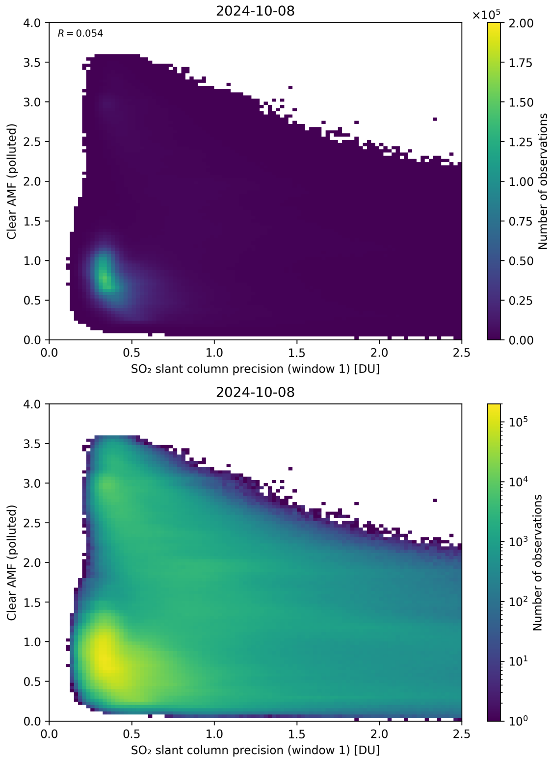
Figure 224: Scatter density plot of “SO 2 slant column precision (window 1)” against “Clear AMF (polluted)” for 2024-10-08 to 2024-10-09.
