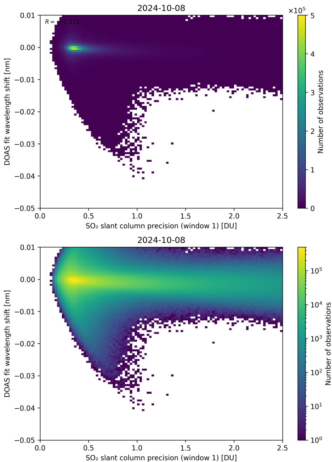
Figure 221: Scatter density plot of “SO 2 slant column precision (window 1)” against “DOAS fit wavelength shift” for 2024-10-08 to 2024-10-09.
