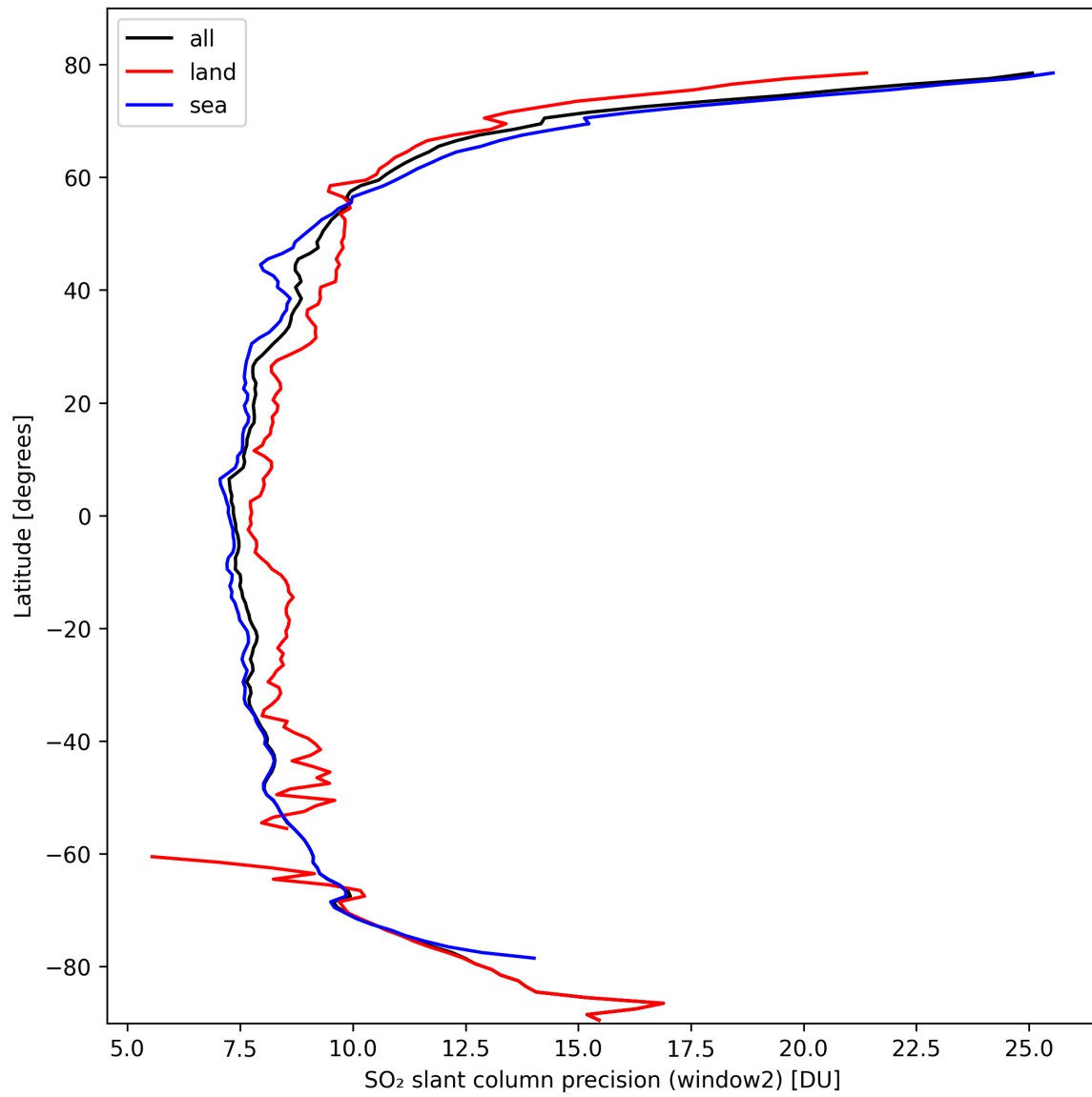
Figure 38: Zonal average of “SO 2 slant column precision (window2)” for 2024-10-08 to 2024-10-09.
