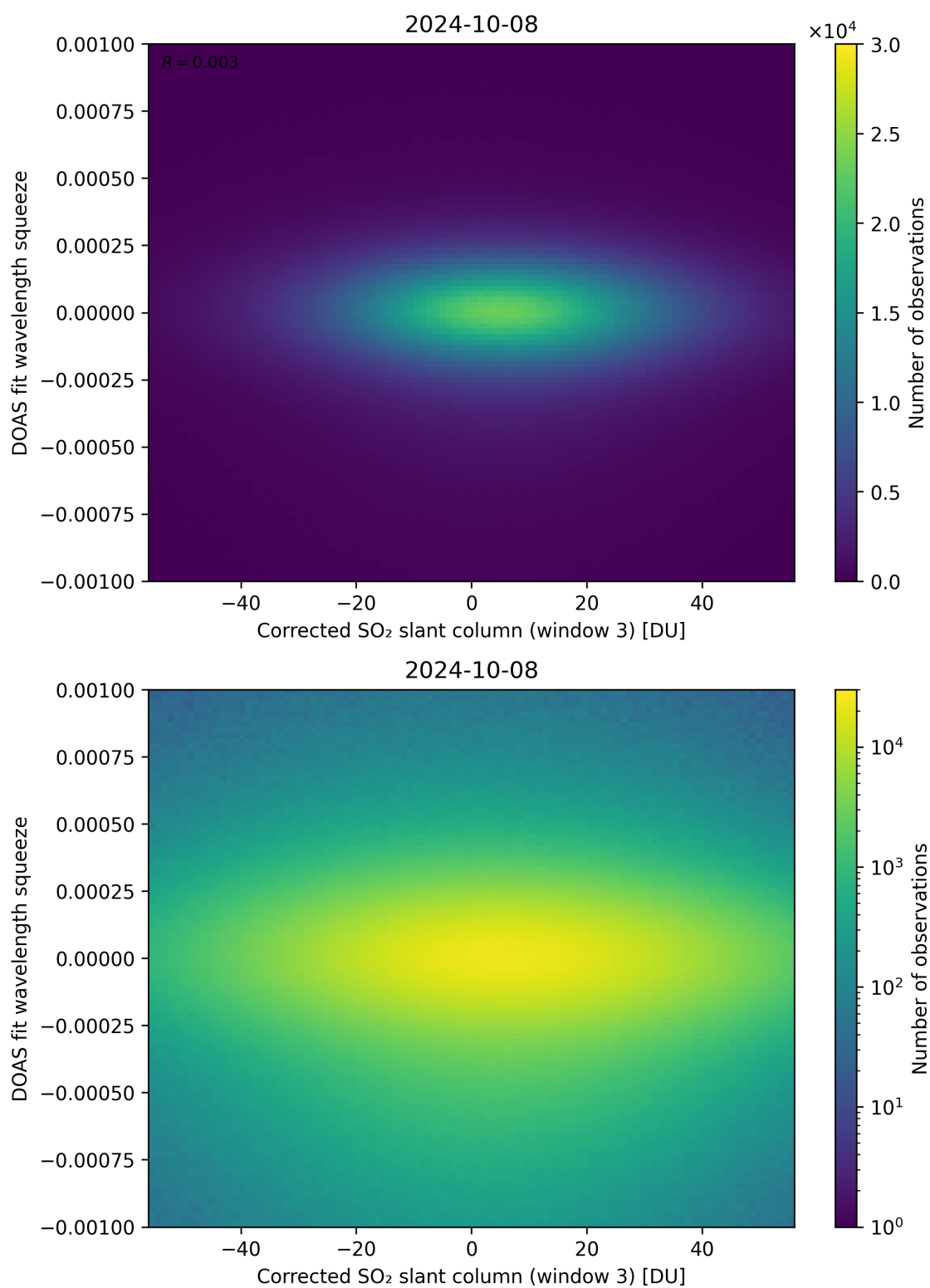
Figure 207: Scatter density plot of “Corrected SO 2 slant column (window 3)” against “DOAS fit wavelength squeeze” for 2024-10-08 to 2024-10-09.
