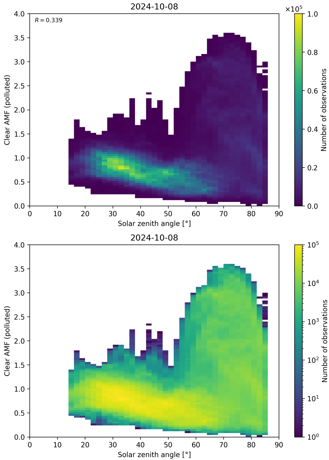
Figure 165: Scatter density plot of “Solar zenith angle” against “Clear AMF (polluted)” for 2024-10-08 to 2024-10-09.
