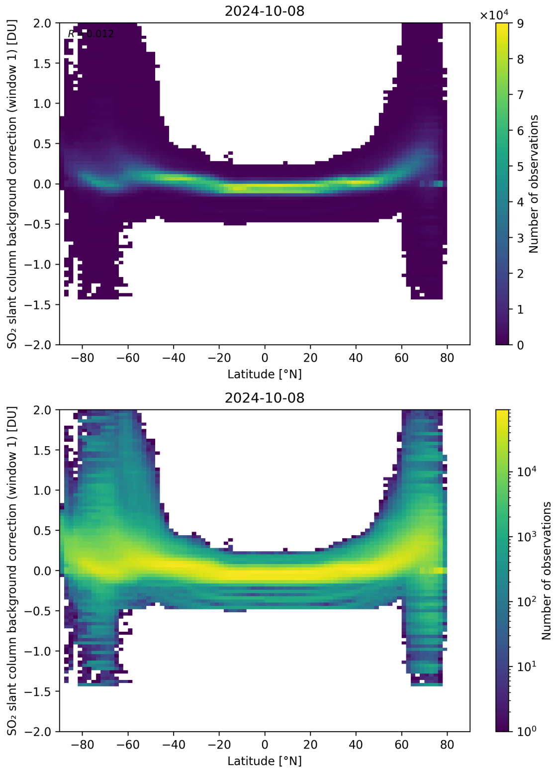
Figure 139: Scatter density plot of “Latitude” against “SO 2 slant column background correction (window 1)” for 2024-10-08 to 2024-10-09.
