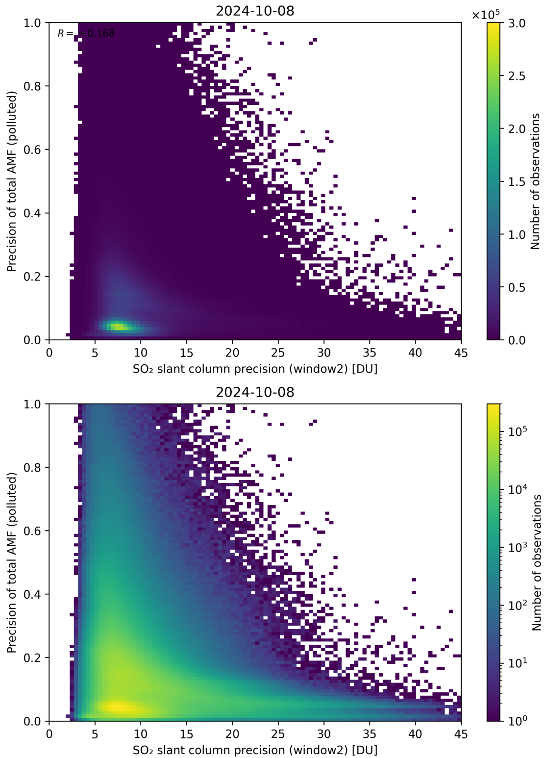
Figure 252: Scatter density plot of “SO 2 slant column precision (window2)” against “Precision of total AMF (polluted)” for 2024-10-08 to 2024-10-09.
