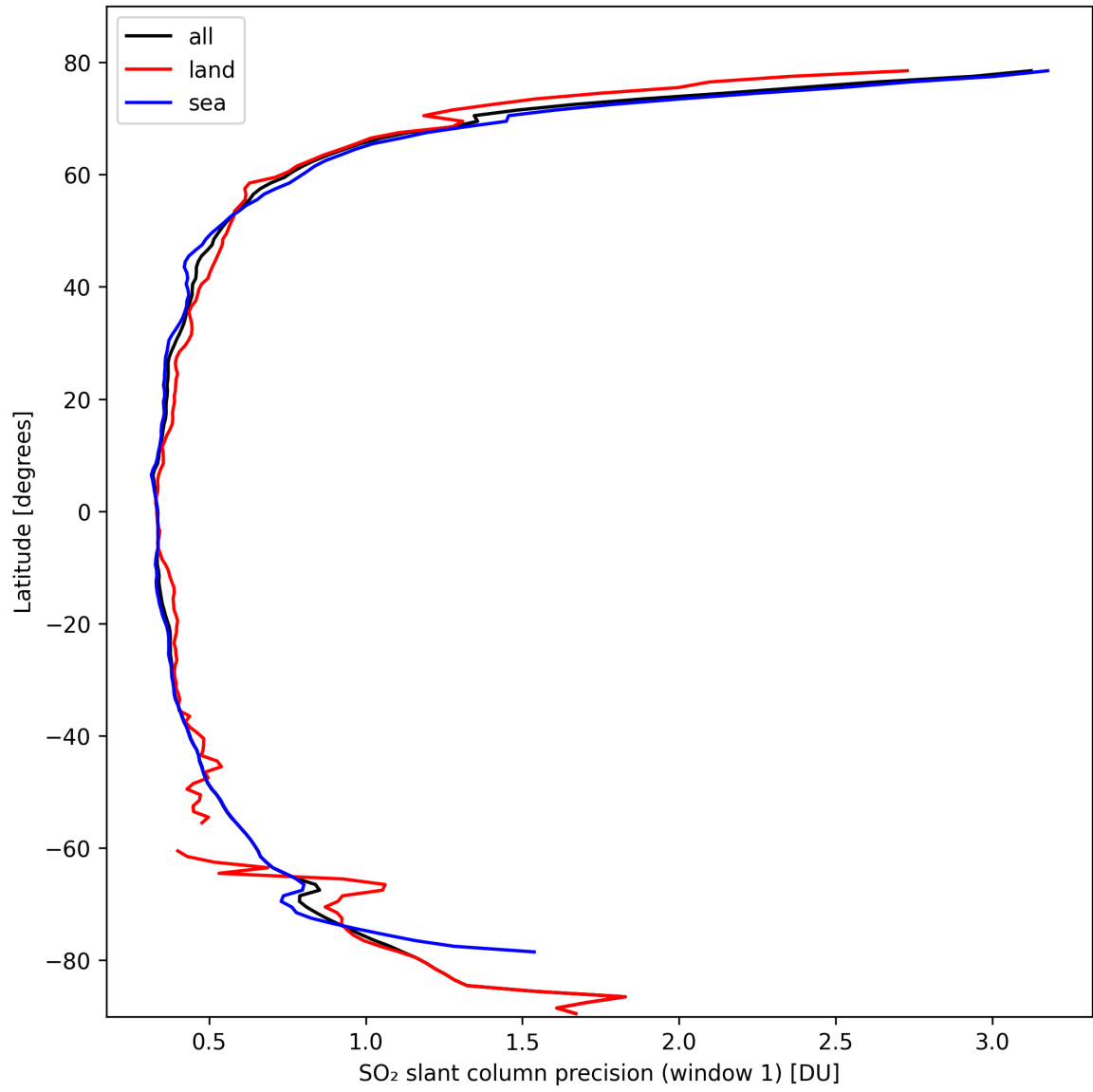
Figure 34: Zonal average of “SO 2 slant column precision (window 1)” for 2024-10-08 to 2024-10-09.
