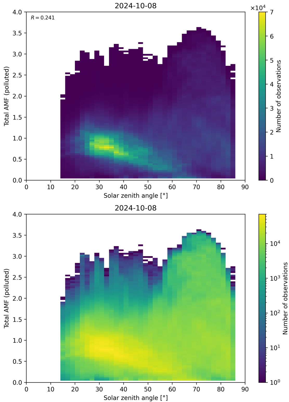
Figure 174: Scatter density plot of “Solar zenith angle” against “Total AMF (polluted)” for 2024-10-08 to 2024-10-09.
