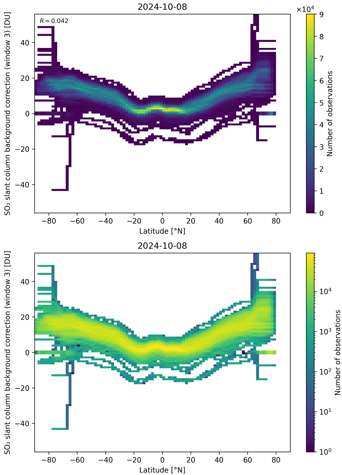
Figure 141: Scatter density plot of “Latitude” against “SO 2 slant column background correction (window 3)” for 2024-10-08 to 2024-10-09.
