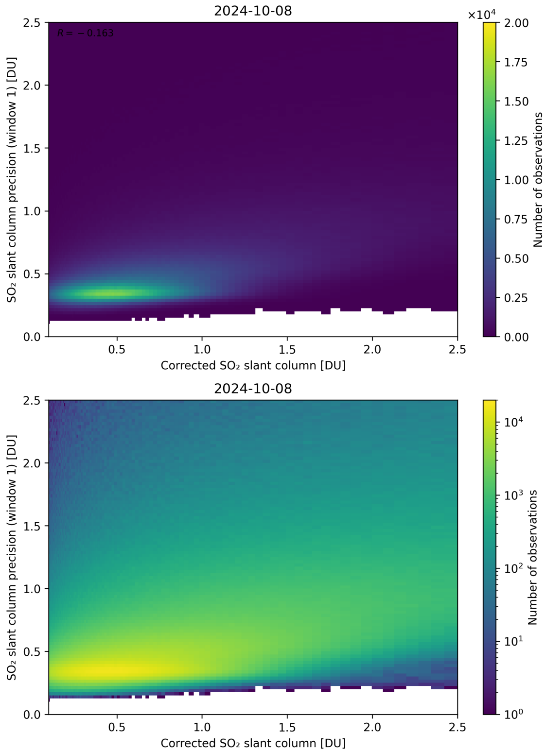
Figure 188: Scatter density plot of “Corrected SO 2 slant column” against “SO 2 slant column precision (window 1)” for 2024-10-08 to 2024-10-09.
