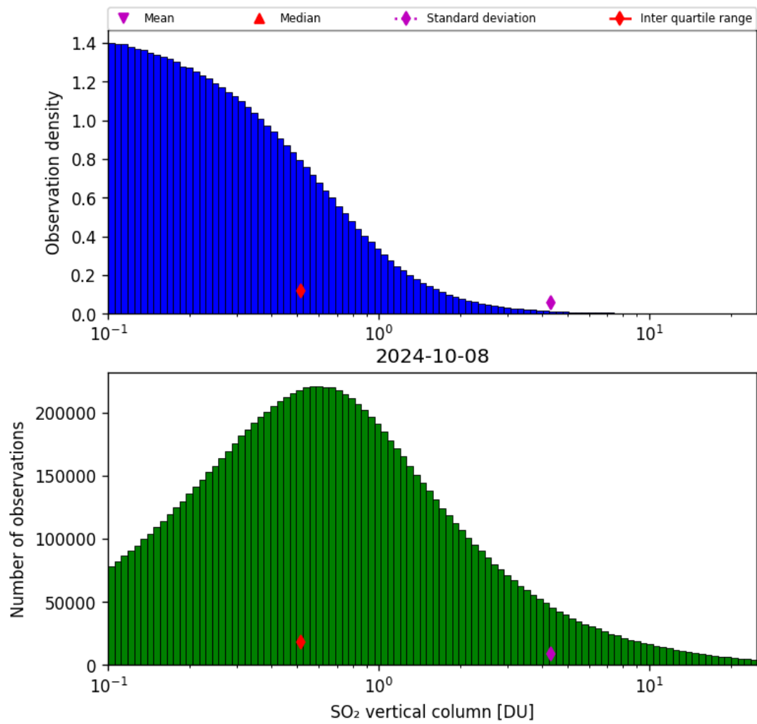
Figure 53: Histogram of “SO 2 vertical column” for 2024-10-08 to 2024-10-09
