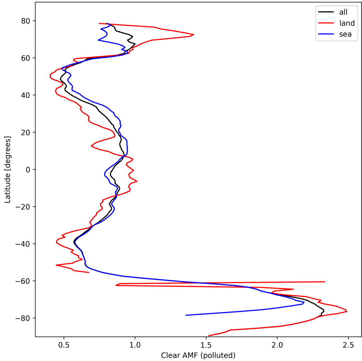
Figure 50: Zonal average of “Clear AMF (polluted)” for 2024-10-08 to 2024-10-09.
