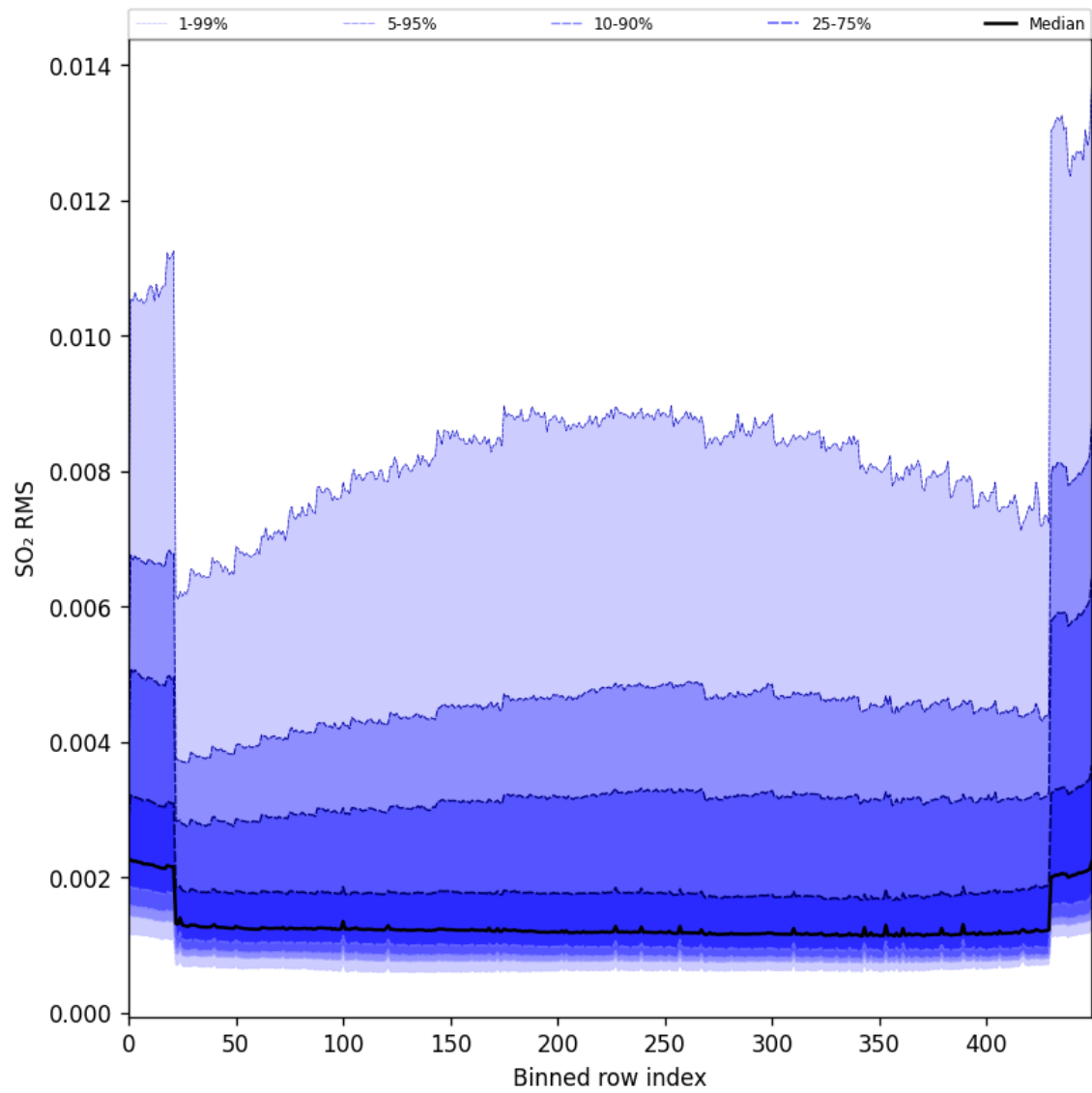
Figure 93: Along track statistics of “SO 2 RMS” for 2024-10-08 to 2024-10-09
