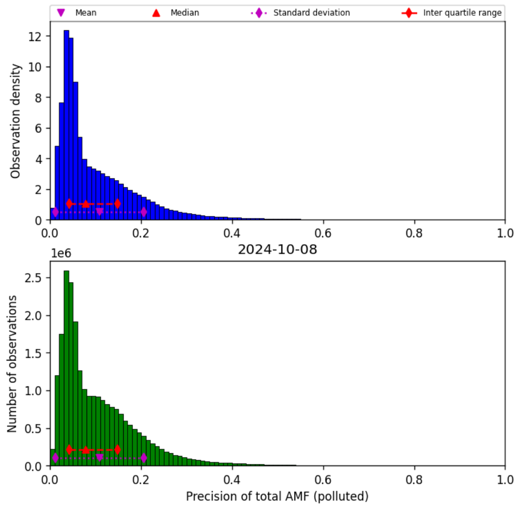
Figure 72: Histogram of “Precision of total AMF (polluted)” for 2024-10-08 to 2024-10-09
