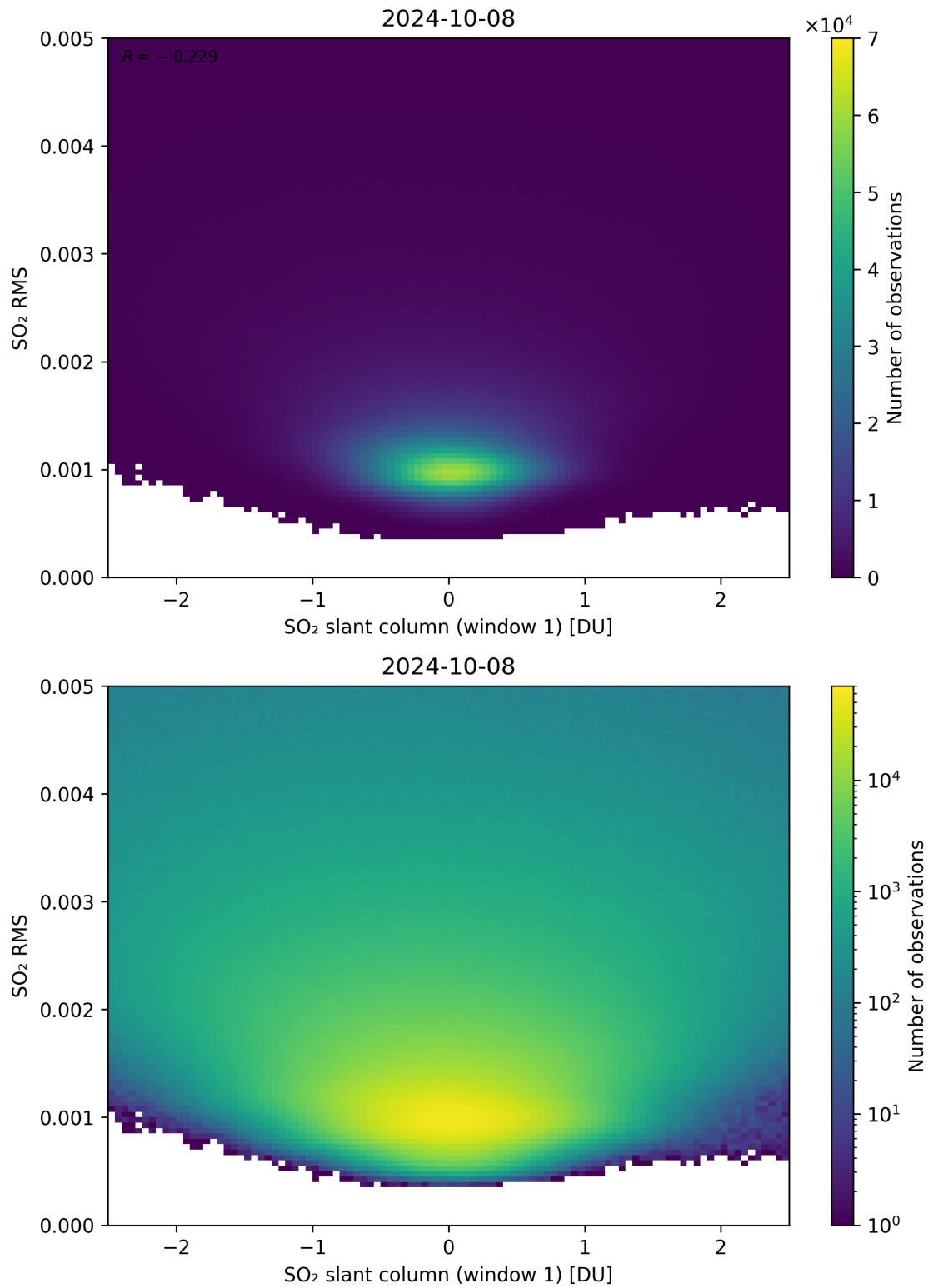
Figure 217: Scatter density plot of “SO 2 slant column (window 1)” against “SO 2 RMS” for 2024-10-08 to 2024-10-09.
