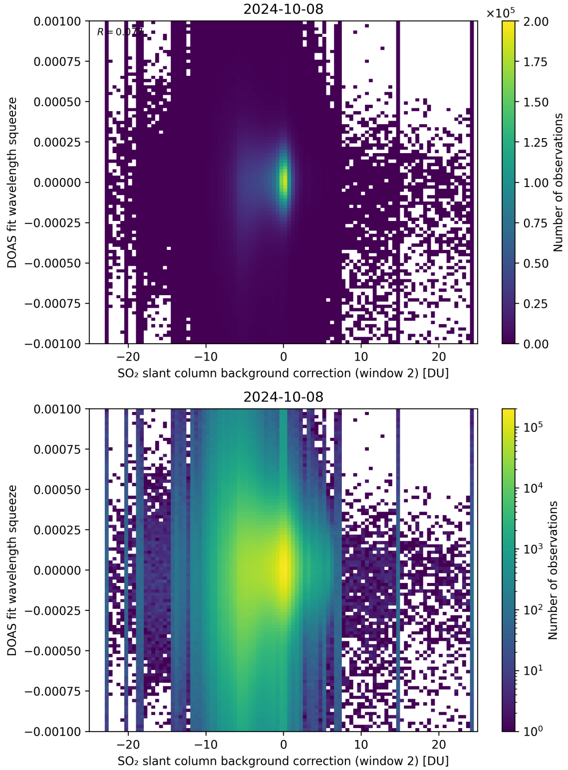
Figure 113: Scatter density plot of “SO 2 slant column background correction (window 2)” against “DOAS fit wavelength squeeze” for 2024-10-08 to 2024-10-09.
