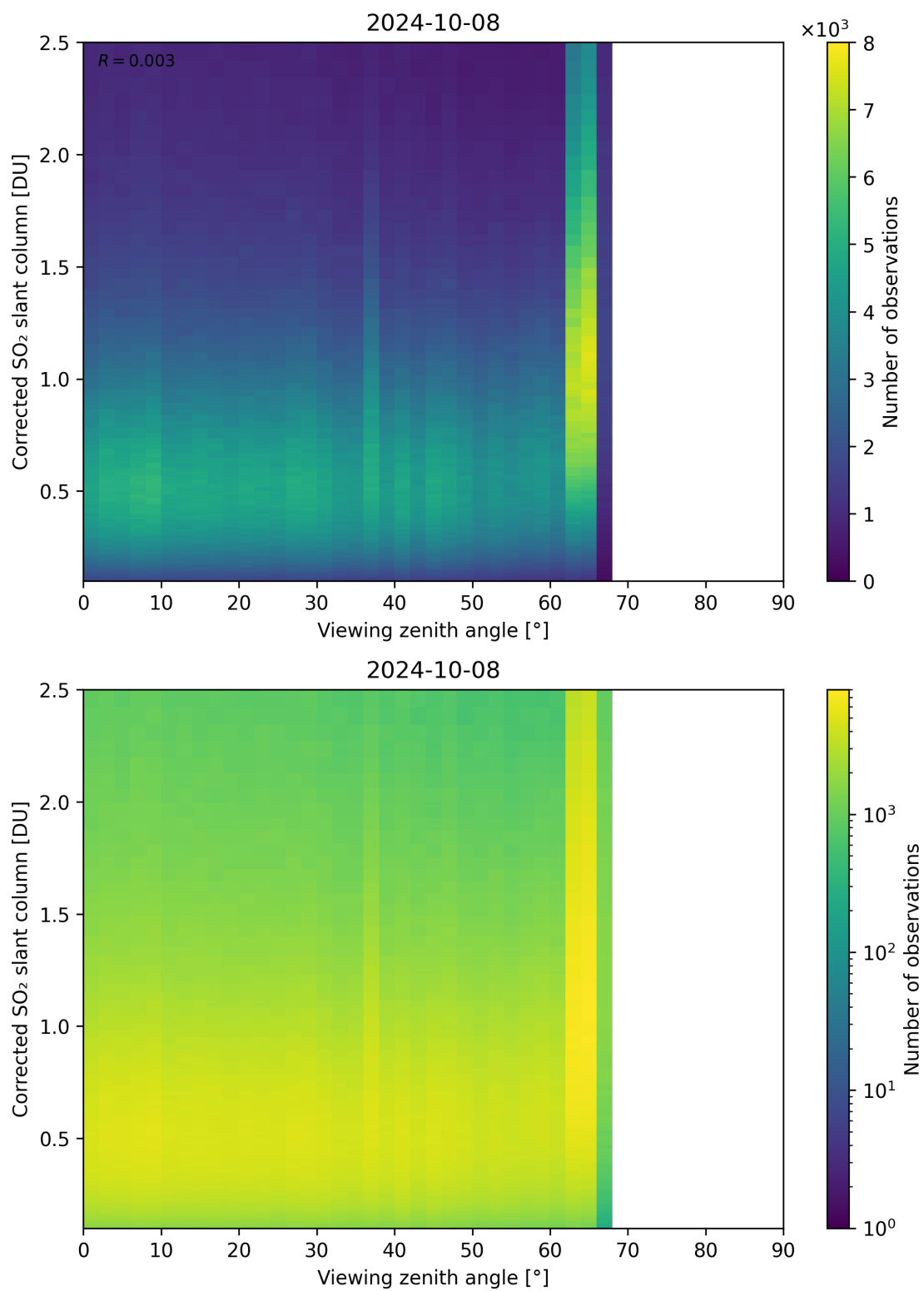
Figure 317: Scatter density plot of “Viewing zenith angle” against “Corrected SO 2 slant column” for 2024-10-08 to 2024-10-09.
