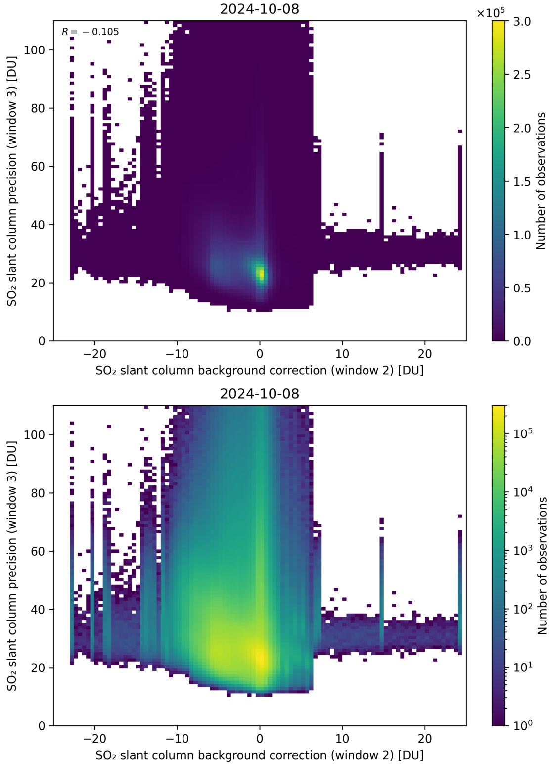
Figure 118: Scatter density plot of “SO 2 slant column background correction (window 2)” against “SO 2 slant column precision (window 3)” for 2024-10-08 to 2024-10-09.
