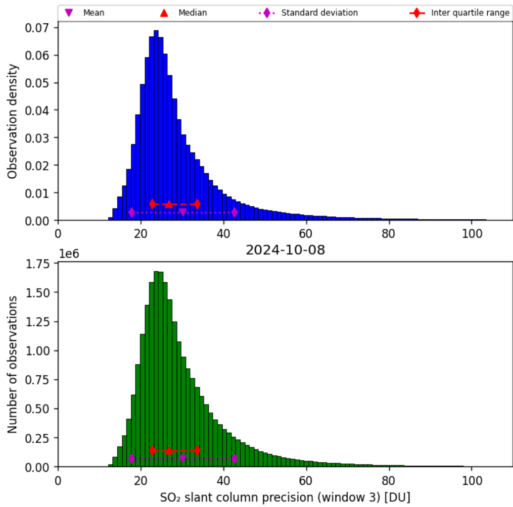
Figure 65: Histogram of “SO 2 slant column precision (window 3)” for 2024-10-08 to 2024-10-09
