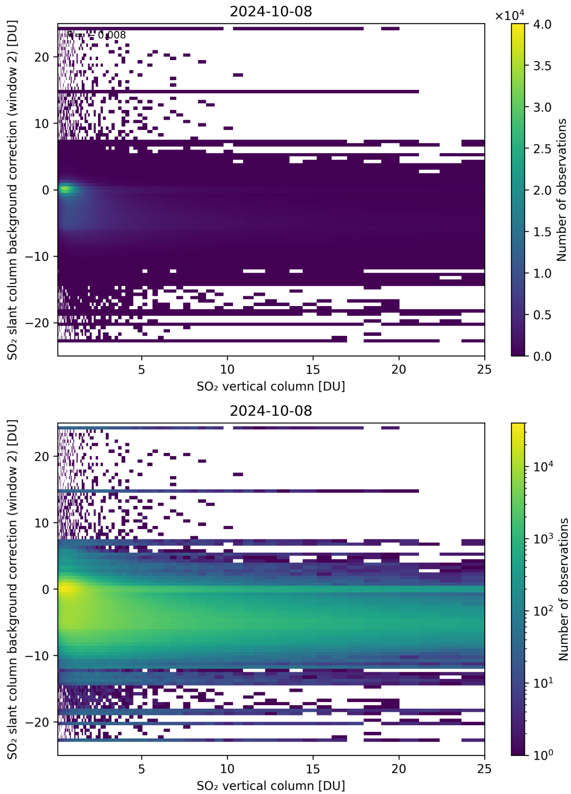
Figure 274: Scatter density plot of “SO 2 vertical column” against “SO 2 slant column background correction (window 2)” for 2024-10-08 to 2024-10-09.
