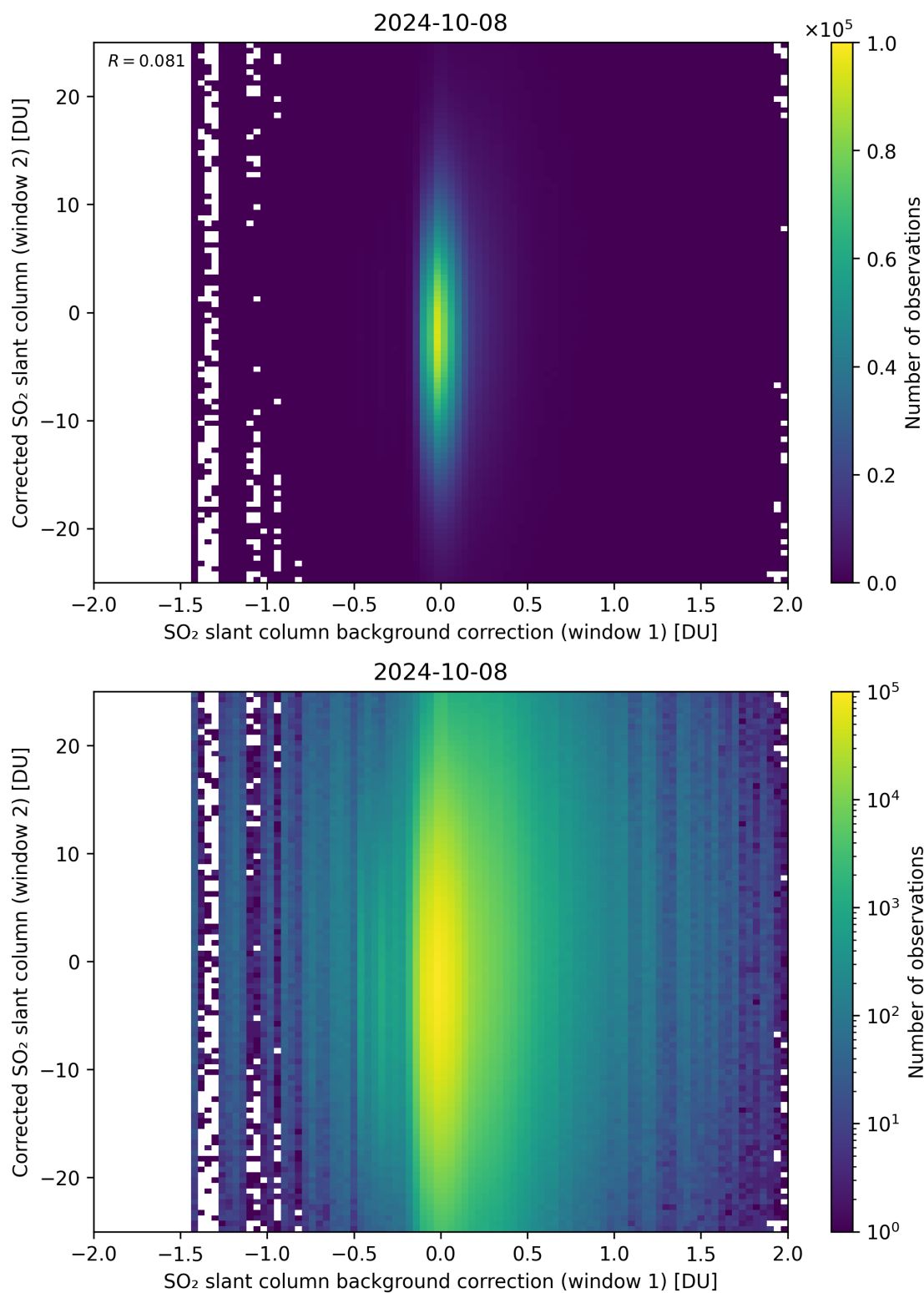
Figure 104: Scatter density plot of “SO 2 slant column background correction (window 1)” against “Corrected SO 2 slant column (window 2)” for 2024-10-08 to 2024-10-09.
