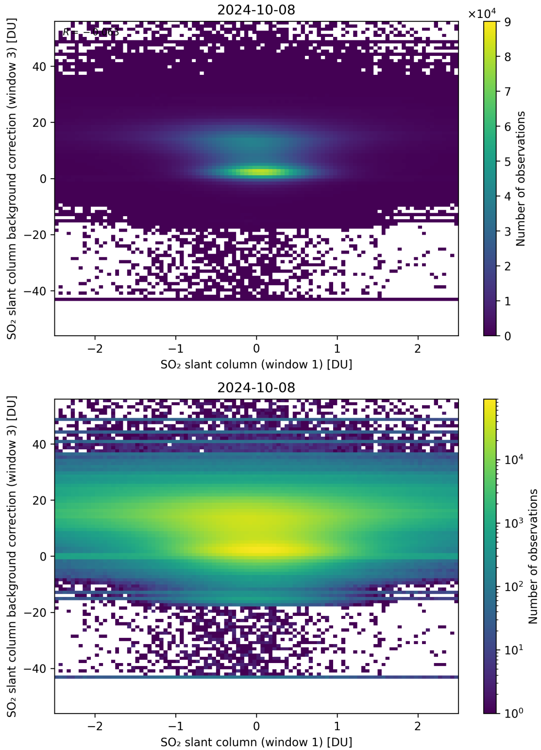
Figure 214: Scatter density plot of “SO 2 slant column (window 1)” against “SO 2 slant column background correction (window 3)” for 2024-10-08 to 2024-10-09.
