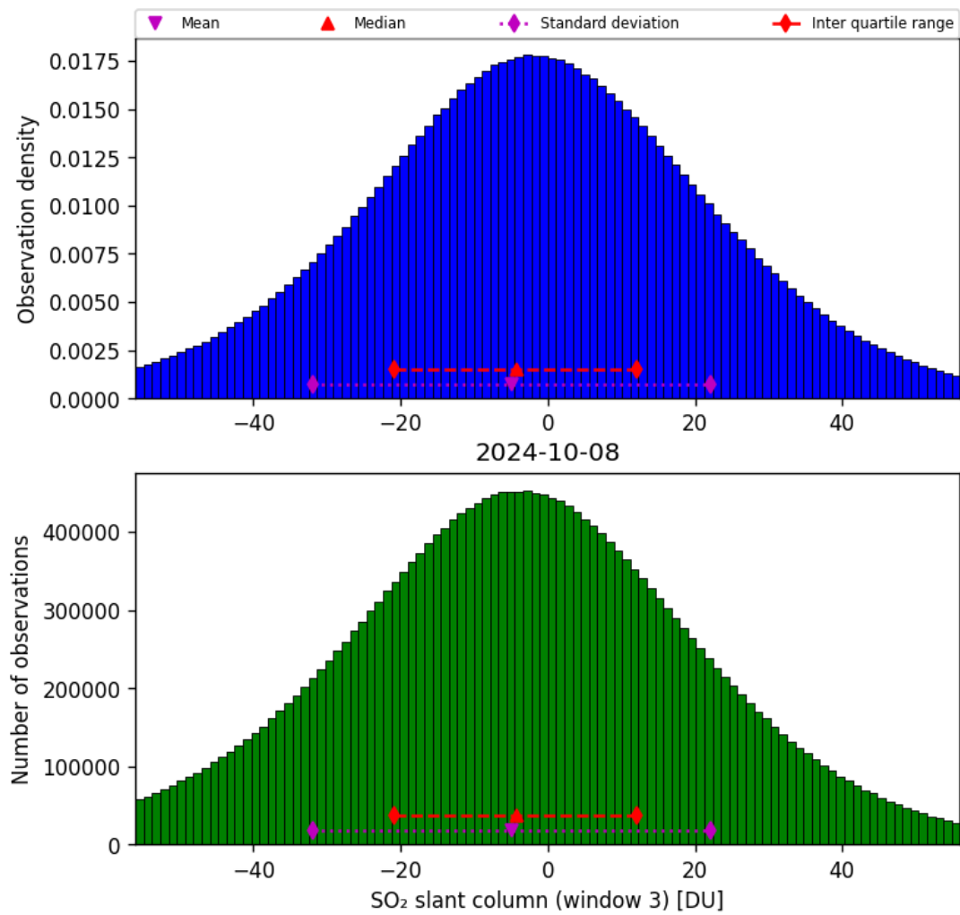
Figure 64: Histogram of “SO 2 slant column (window 3)” for 2024-10-08 to 2024-10-09
