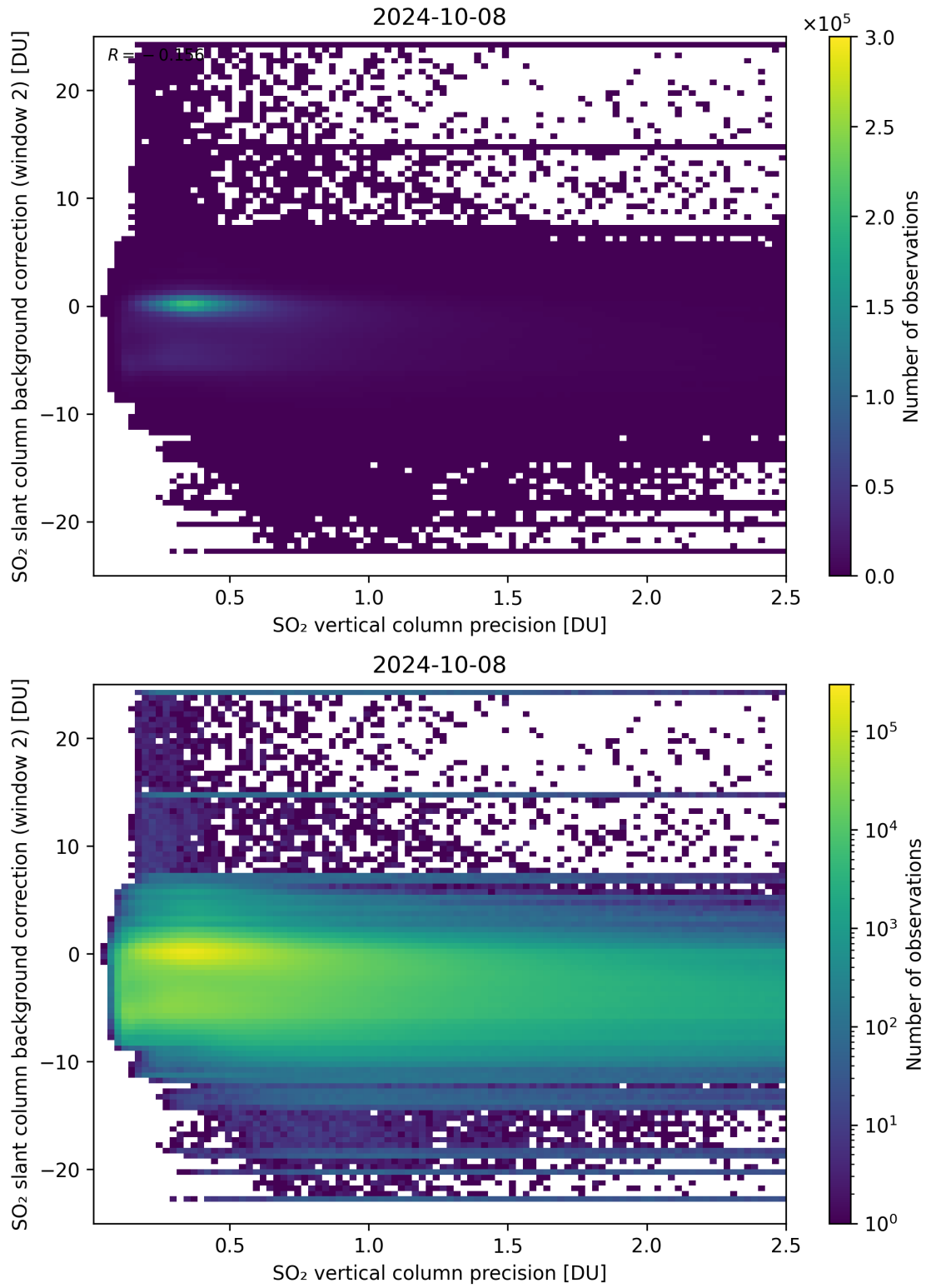
Figure 280: Scatter density plot of “SO 2 vertical column precision” against “SO 2 slant column background correction (window 2)” for 2024-10-08 to 2024-10-09.
