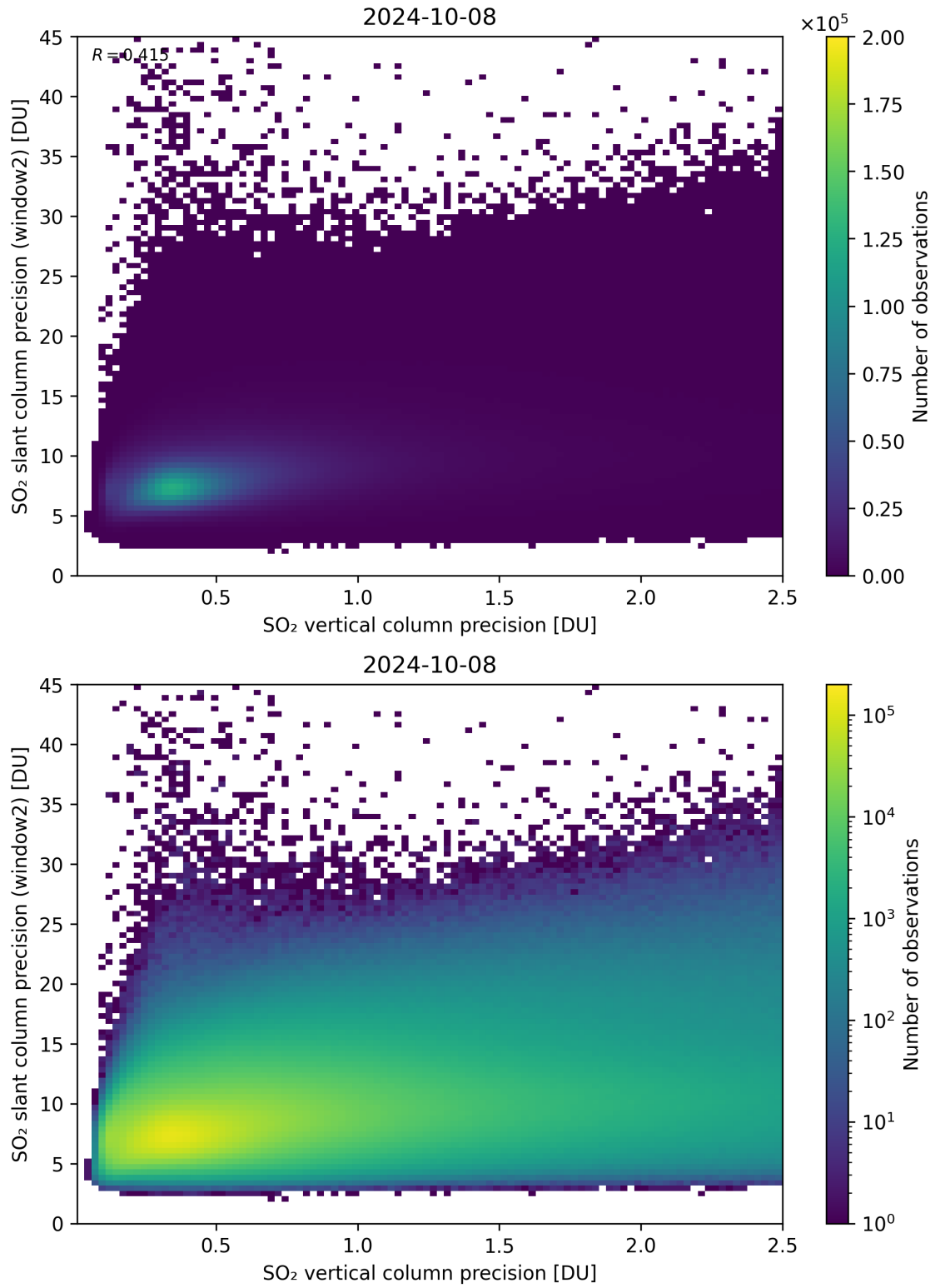
Figure 291: Scatter density plot of “SO 2 vertical column precision” against “SO 2 slant column precision (window2)” for 2024-10-08 to 2024-10-09.
