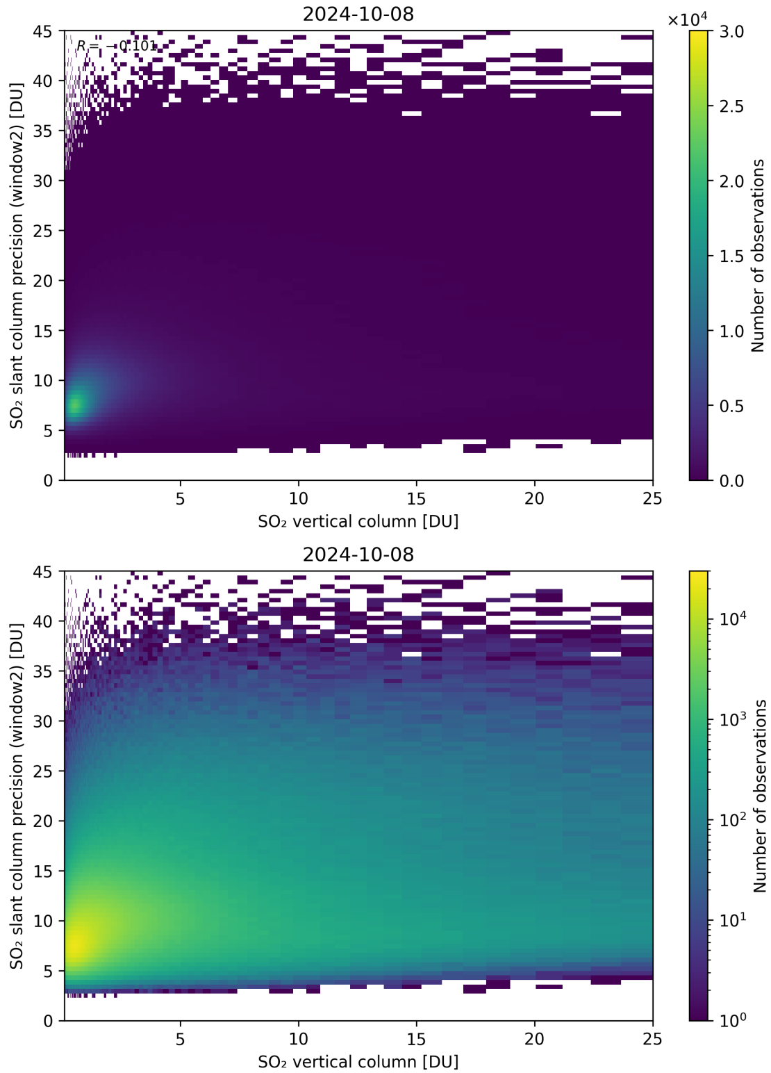
Figure 302: Scatter density plot of “SO 2 vertical column” against “SO 2 slant column precision (window2)” for 2024-10-08 to 2024-10-09.
