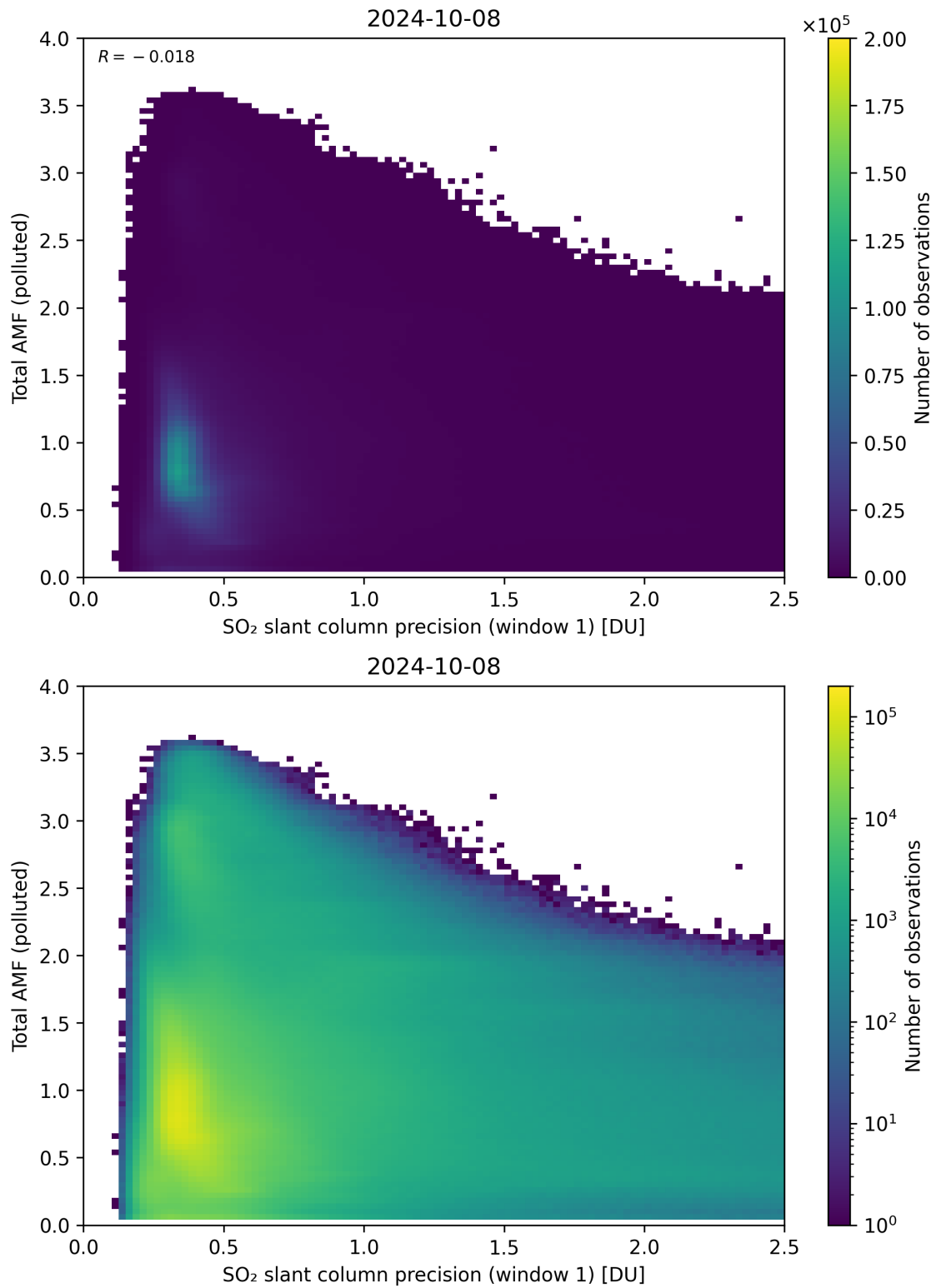
Figure 230: Scatter density plot of “SO 2 slant column precision (window 1)” against “Total AMF (polluted)” for 2024-10-08 to 2024-10-09.
