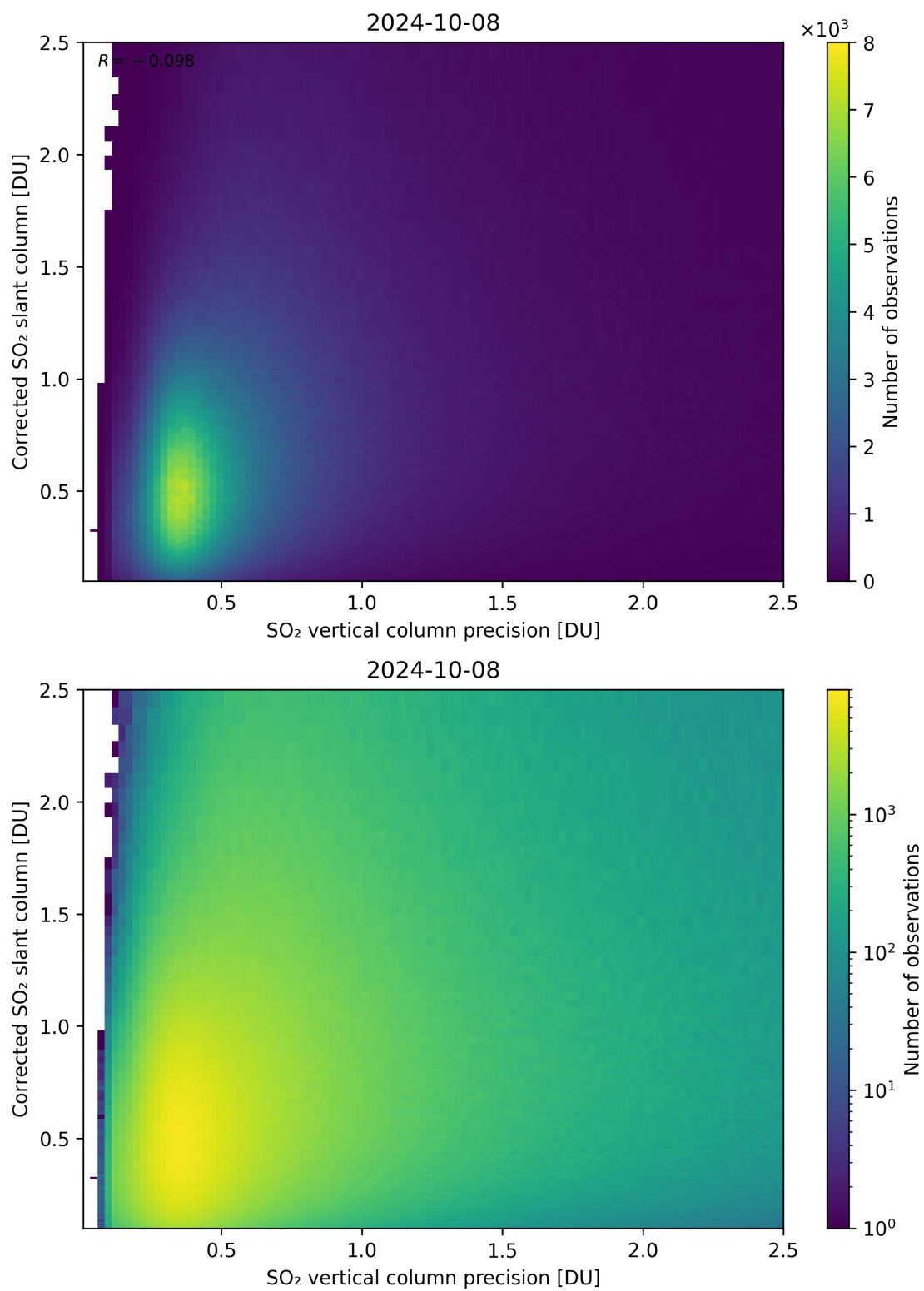
Figure 286: Scatter density plot of “SO 2 vertical column precision” against “Corrected SO 2 slant column” for 2024-10-08 to 2024-10-09.
