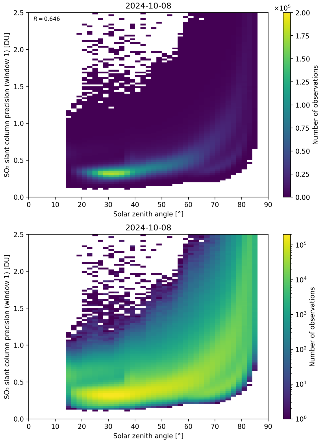
Figure 170: Scatter density plot of “Solar zenith angle” against “SO 2 slant column precision (window 1)” for 2024-10-08 to 2024-10-09.
