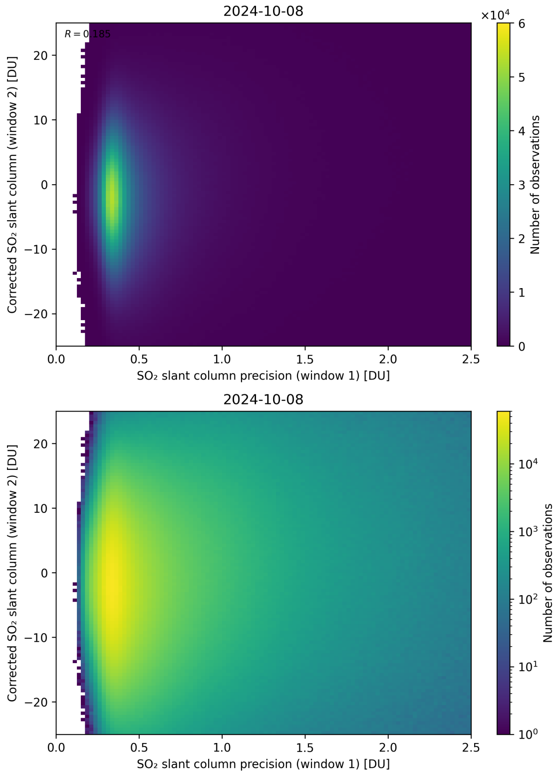
Figure 225: Scatter density plot of “SO 2 slant column precision (window 1)” against “Corrected SO 2 slant column (window 2)” for 2024-10-08 to 2024-10-09.
