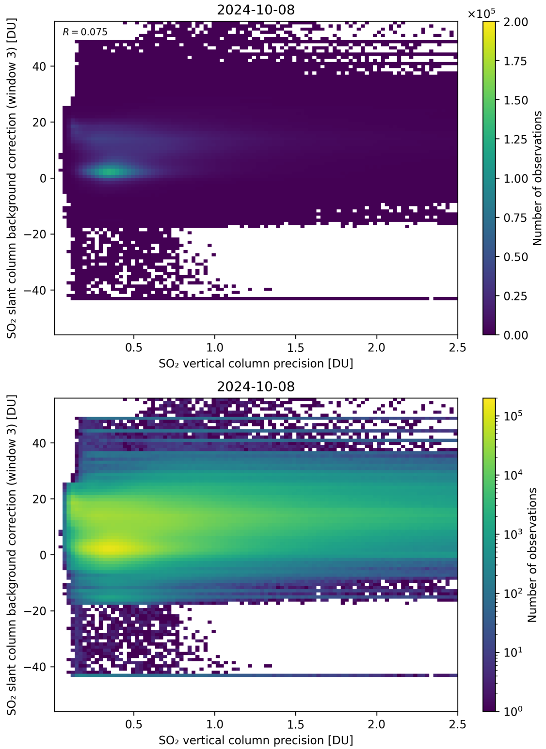
Figure 281: Scatter density plot of “SO 2 vertical column precision” against “SO 2 slant column background correction (window 3)” for 2024-10-08 to 2024-10-09.
