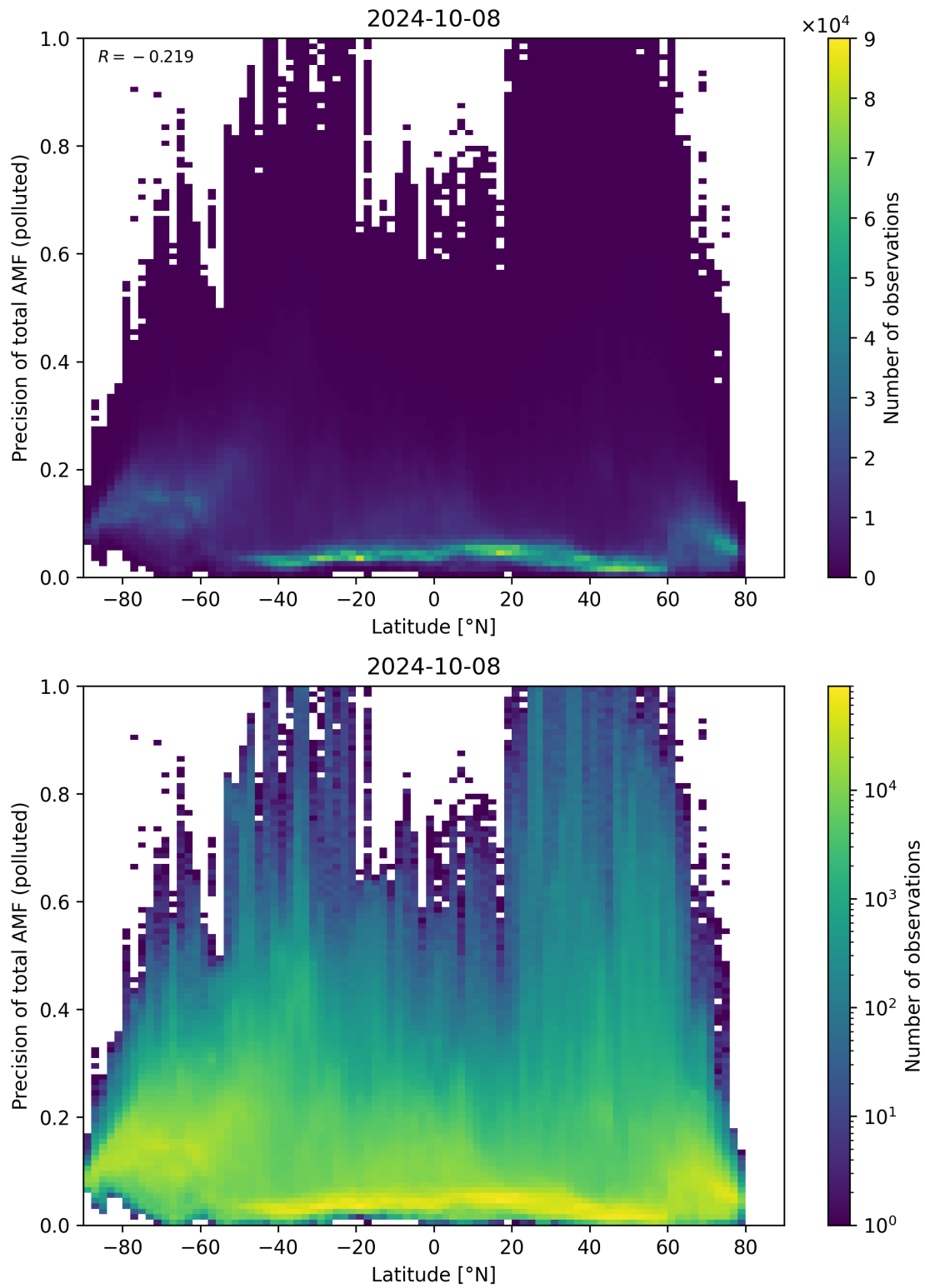
Figure 155: Scatter density plot of “Latitude” against “Precision of total AMF (polluted)” for 2024-10-08 to 2024-10-09.
