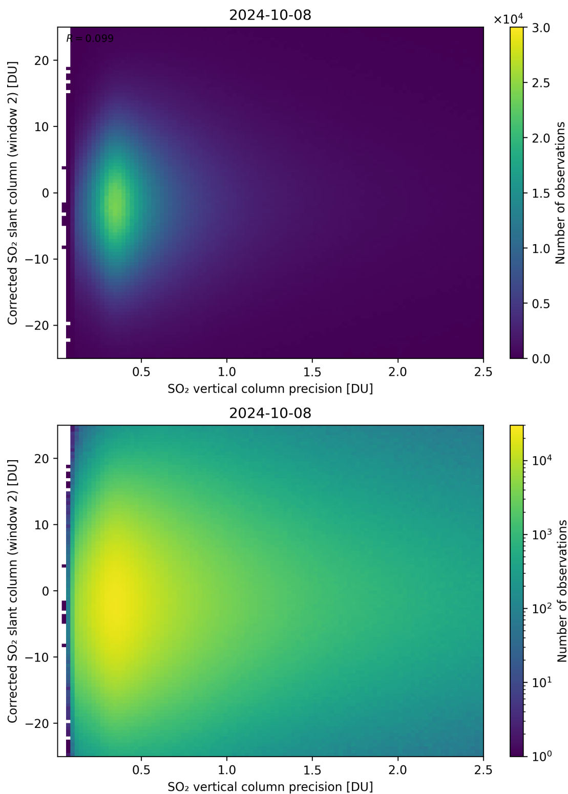
Figure 287: Scatter density plot of “SO 2 vertical column precision” against “Corrected SO 2 slant column (window 2)” for 2024-10-08 to 2024-10-09.
