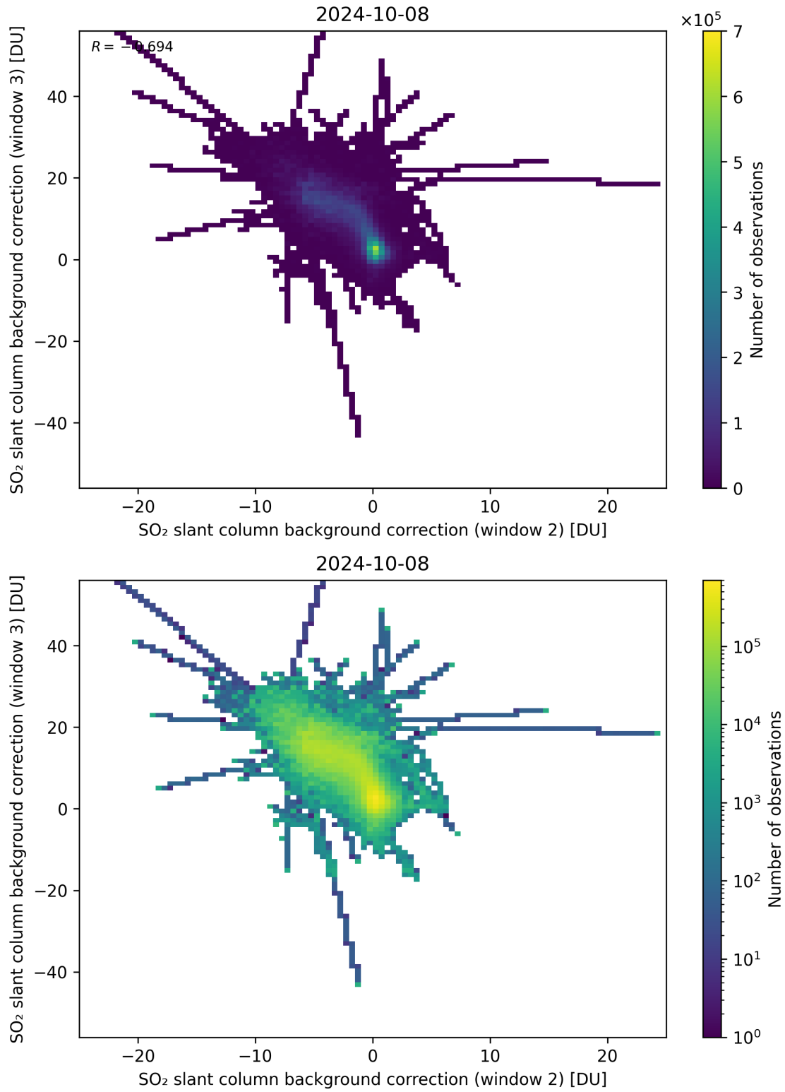
Figure 111: Scatter density plot of “SO 2 slant column background correction (window 2)” against “SO 2 slant column background correction (window 3)” for 2024-10-08 to 2024-10-09.
