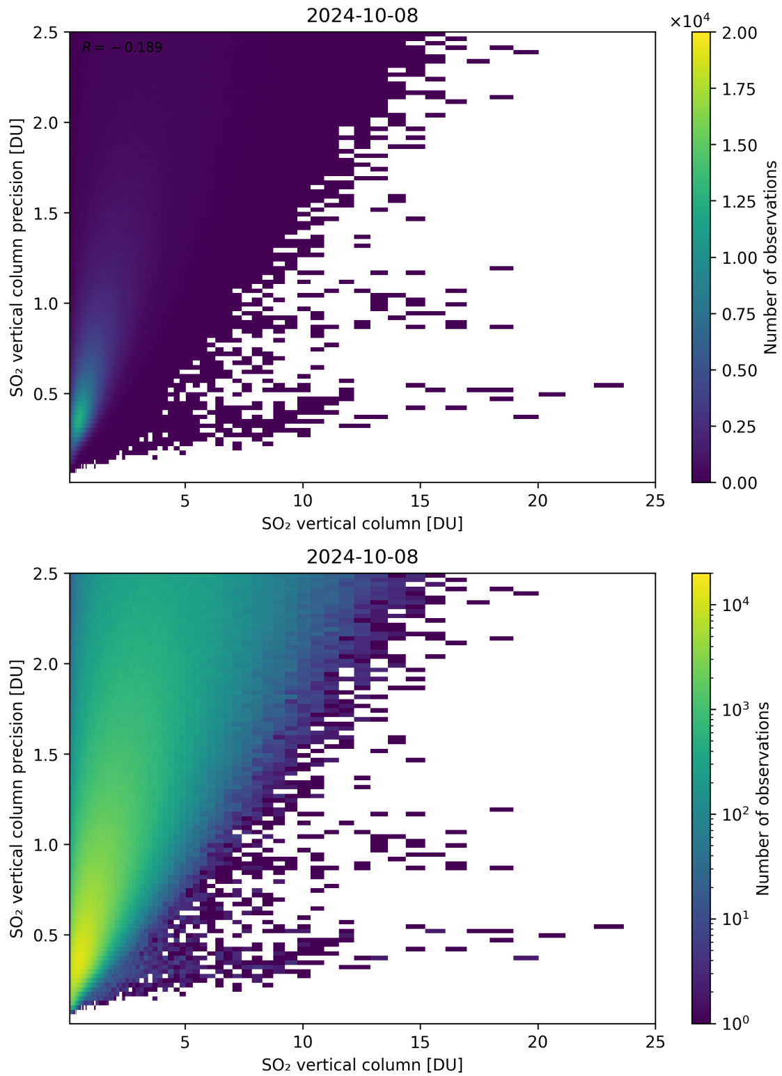
Figure 307: Scatter density plot of “SO 2 vertical column” against “SO 2 vertical column precision” for 2024-10-08 to 2024-10-09.
