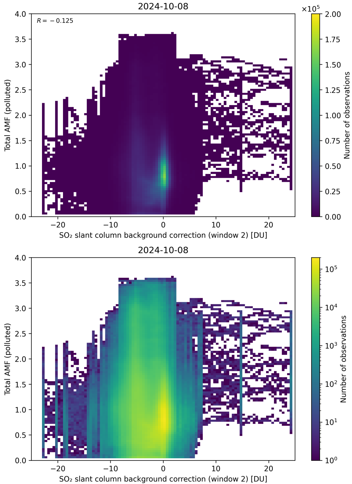
Figure 119: Scatter density plot of “SO 2 slant column background correction (window 2)” against “Total AMF (polluted)” for 2024-10-08 to 2024-10-09.
