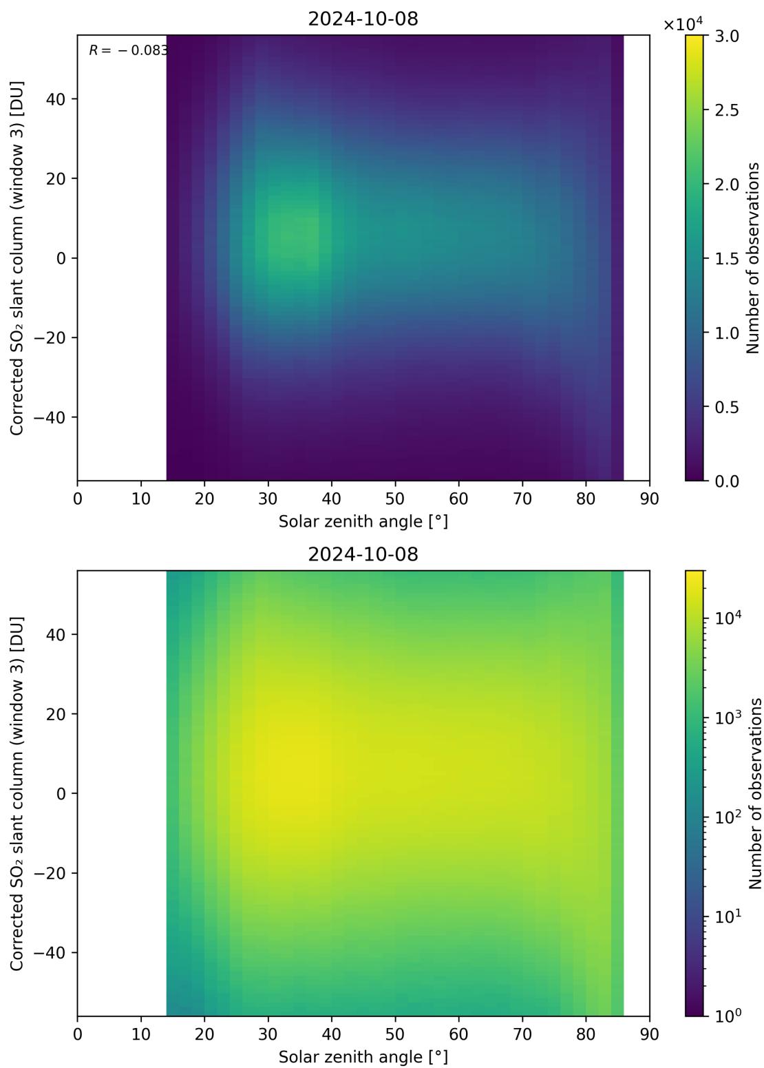
Figure 168: Scatter density plot of “Solar zenith angle” against “Corrected SO 2 slant column (window 3)” for 2024-10-08 to 2024-10-09.
