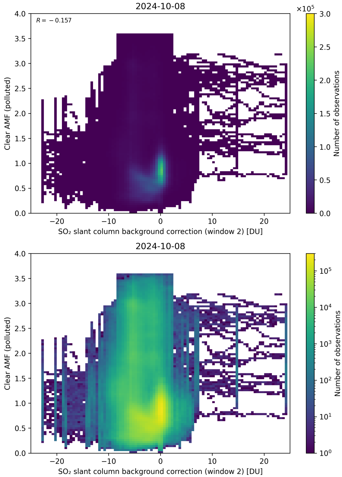
Figure 115: Scatter density plot of “SO 2 slant column background correction (window 2)” against “Clear AMF (polluted)” for 2024-10-08 to 2024-10-09.
