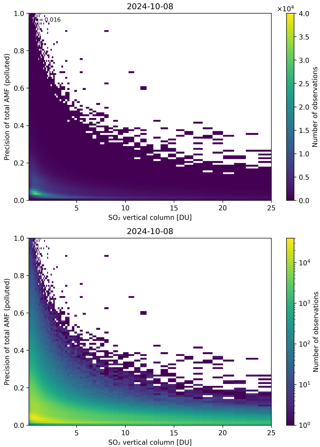
Figure 306: Scatter density plot of “SO 2 vertical column” against “Precision of total AMF (polluted)” for 2024-10-08 to 2024-10-09.
