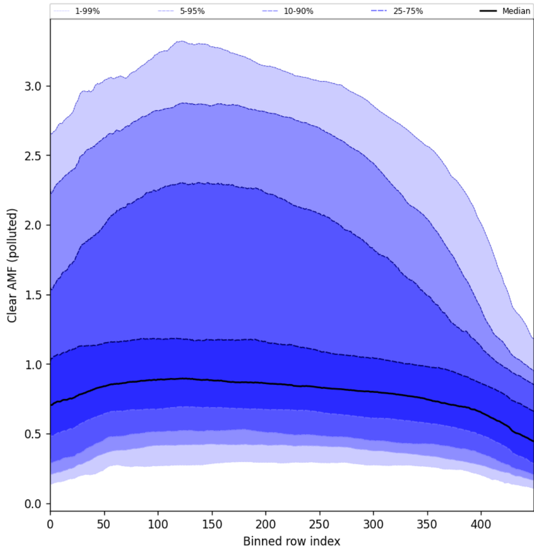
Figure 96: Along track statistics of “Clear AMF (polluted)” for 2024-10-08 to 2024-10-09
