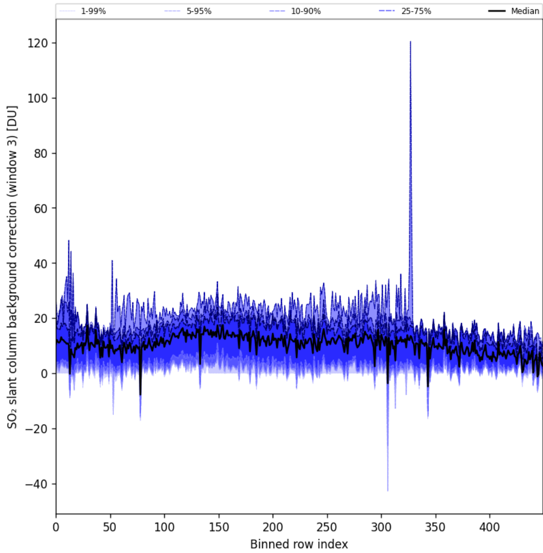
Figure 90: Along track statistics of “SO 2 slant column background correction (window 3)” for 2024-10-08 to 2024-10-09
