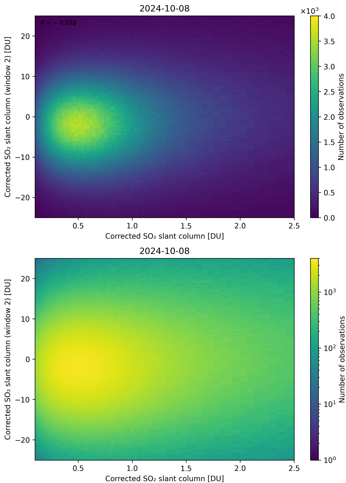
Figure 185: Scatter density plot of “Corrected SO 2 slant column” against “Corrected SO 2 slant column (window 2)” for 2024-10-08 to 2024-10-09.
