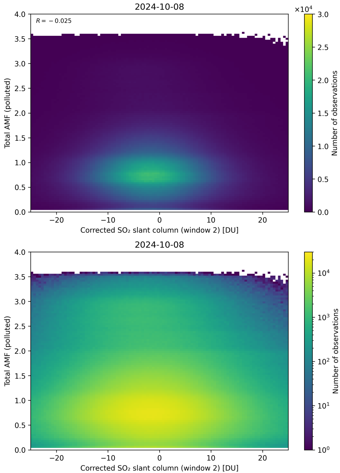
Figure 203: Scatter density plot of “Corrected SO 2 slant column (window 2)” against “Total AMF (polluted)” for 2024-10-08 to 2024-10-09.
