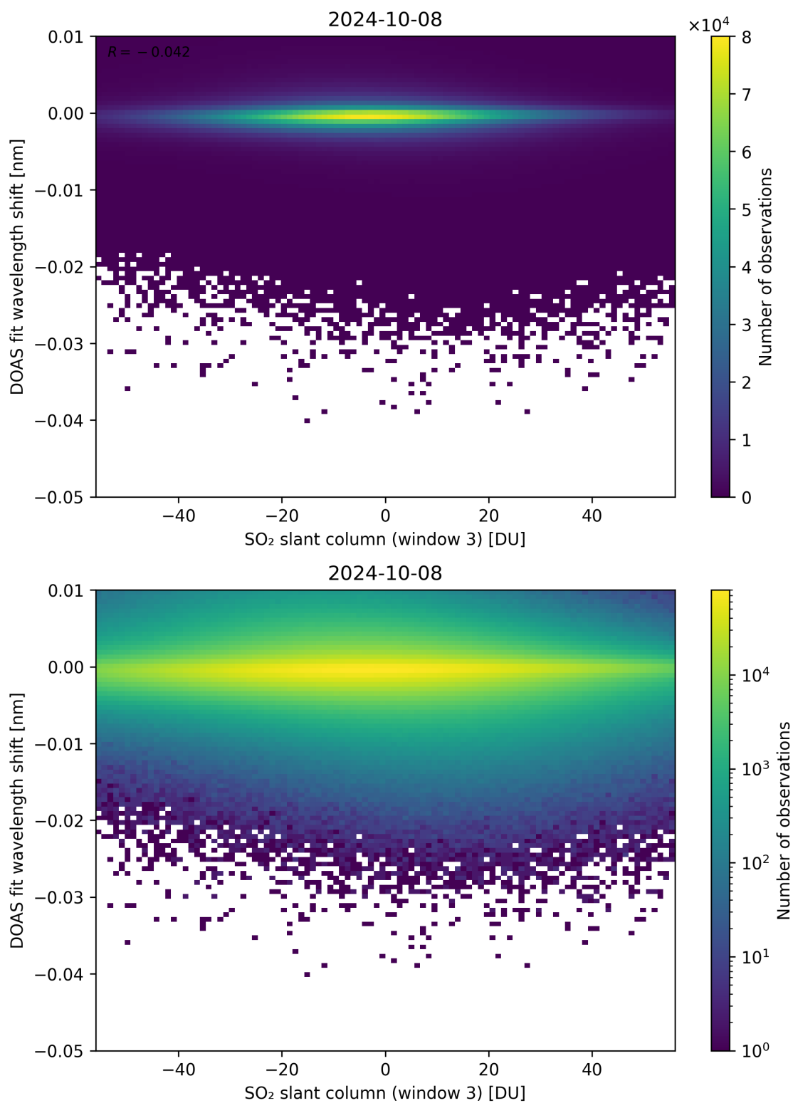
Figure 254: Scatter density plot of “SO 2 slant column (window 3)” against “DOAS fit wavelength shift” for 2024-10-08 to 2024-10-09.
