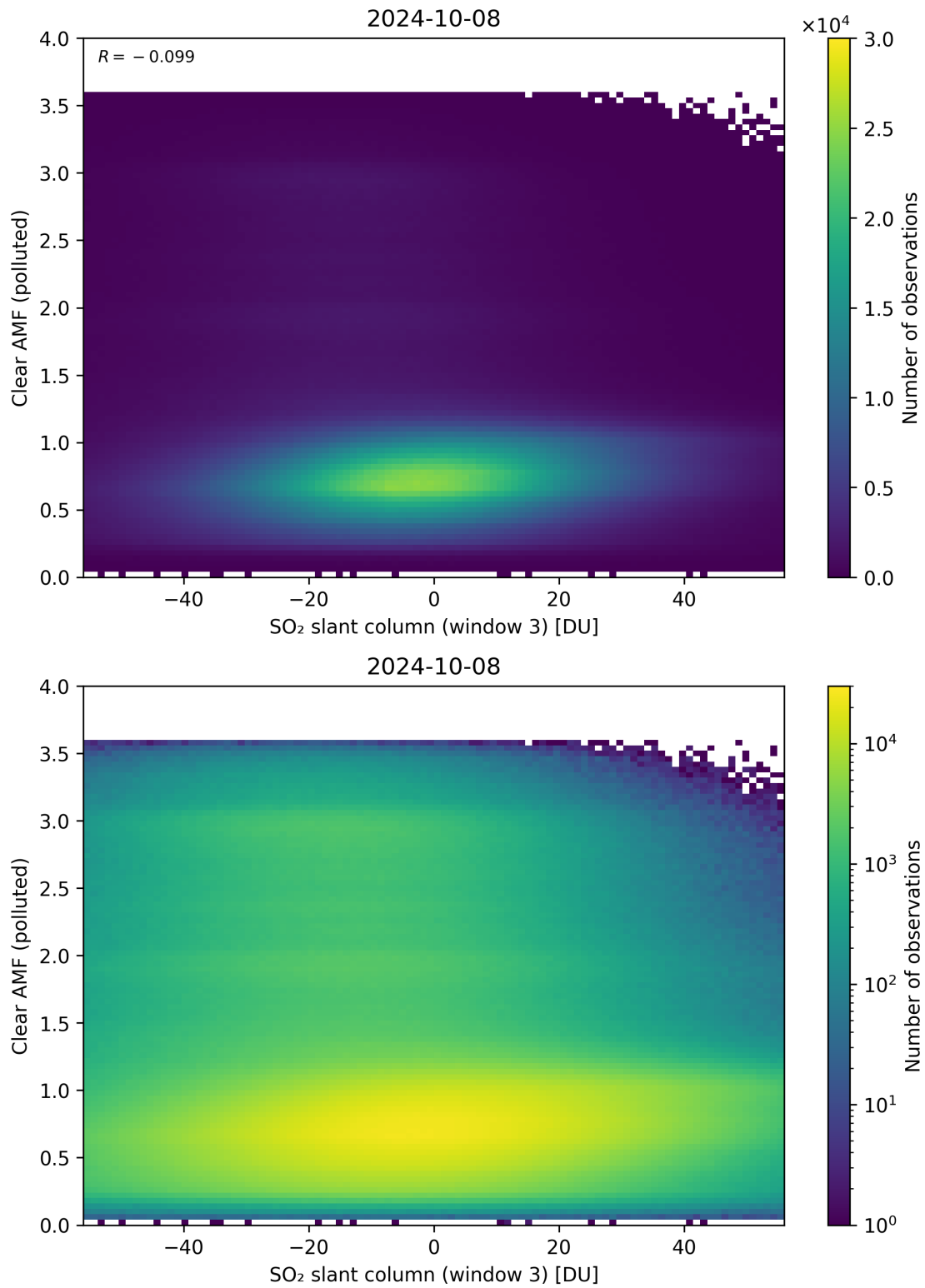
Figure 265: Scatter density plot of “SO 2 slant column (window 3)” against “Clear AMF (polluted)” for 2024-10-08 to 2024-10-09.
