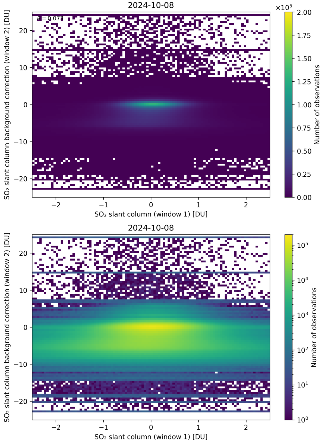
Figure 213: Scatter density plot of “SO 2 slant column (window 1)” against “SO 2 slant column background correction (window 2)” for 2024-10-08 to 2024-10-09.
