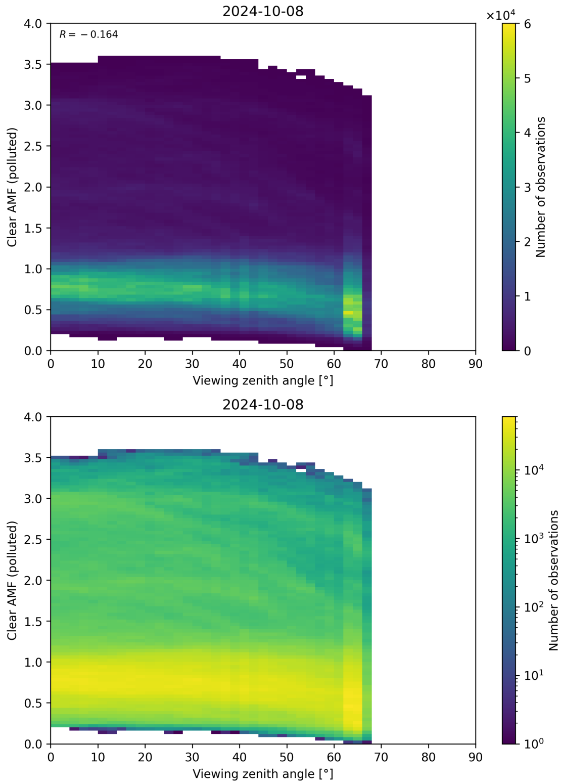
Figure 316: Scatter density plot of “Viewing zenith angle” against “Clear AMF (polluted)” for 2024-10-08 to 2024-10-09.
