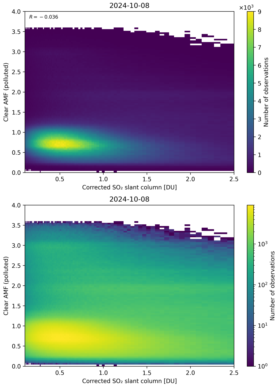
Figure 184: Scatter density plot of “Corrected SO 2 slant column” against “Clear AMF (polluted)” for 2024-10-08 to 2024-10-09.
