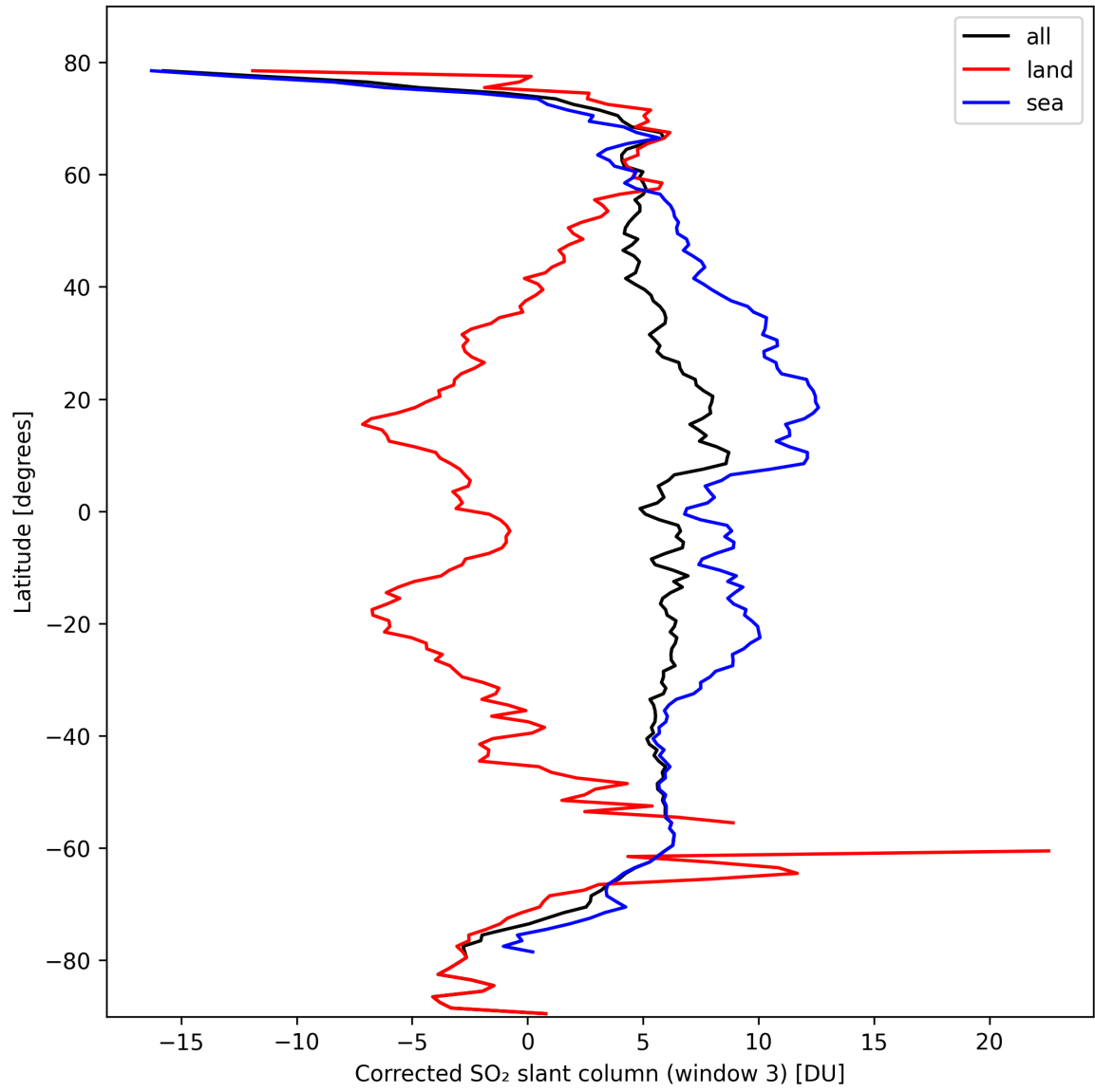
Figure 43: Zonal average of “Corrected SO 2 slant column (window 3)” for 2024-10-08 to 2024-10-09.
