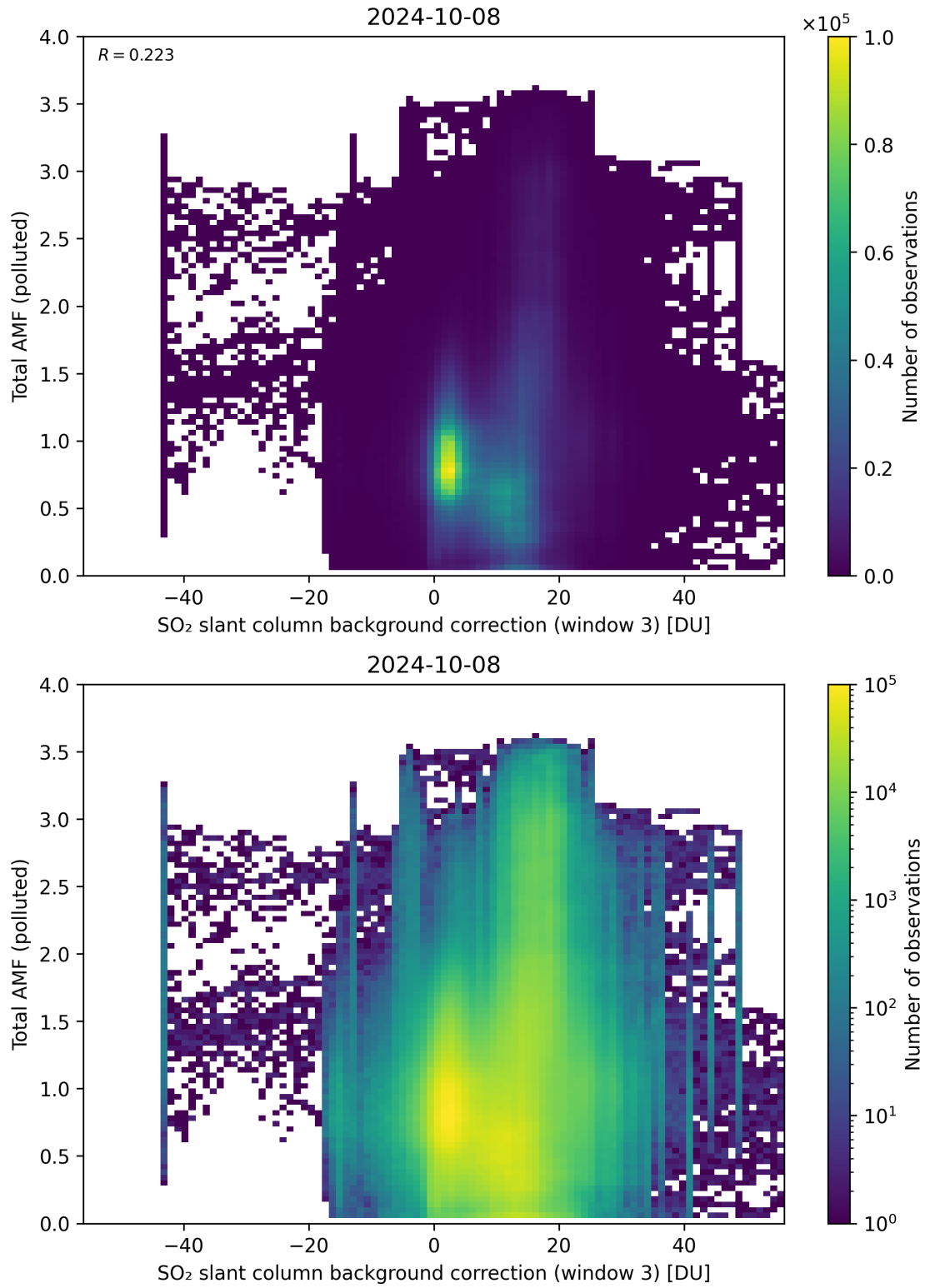
Figure 125: Scatter density plot of “SO 2 slant column background correction (window 3)” against “Total AMF (polluted)” for 2024-10-08 to 2024-10-09.
