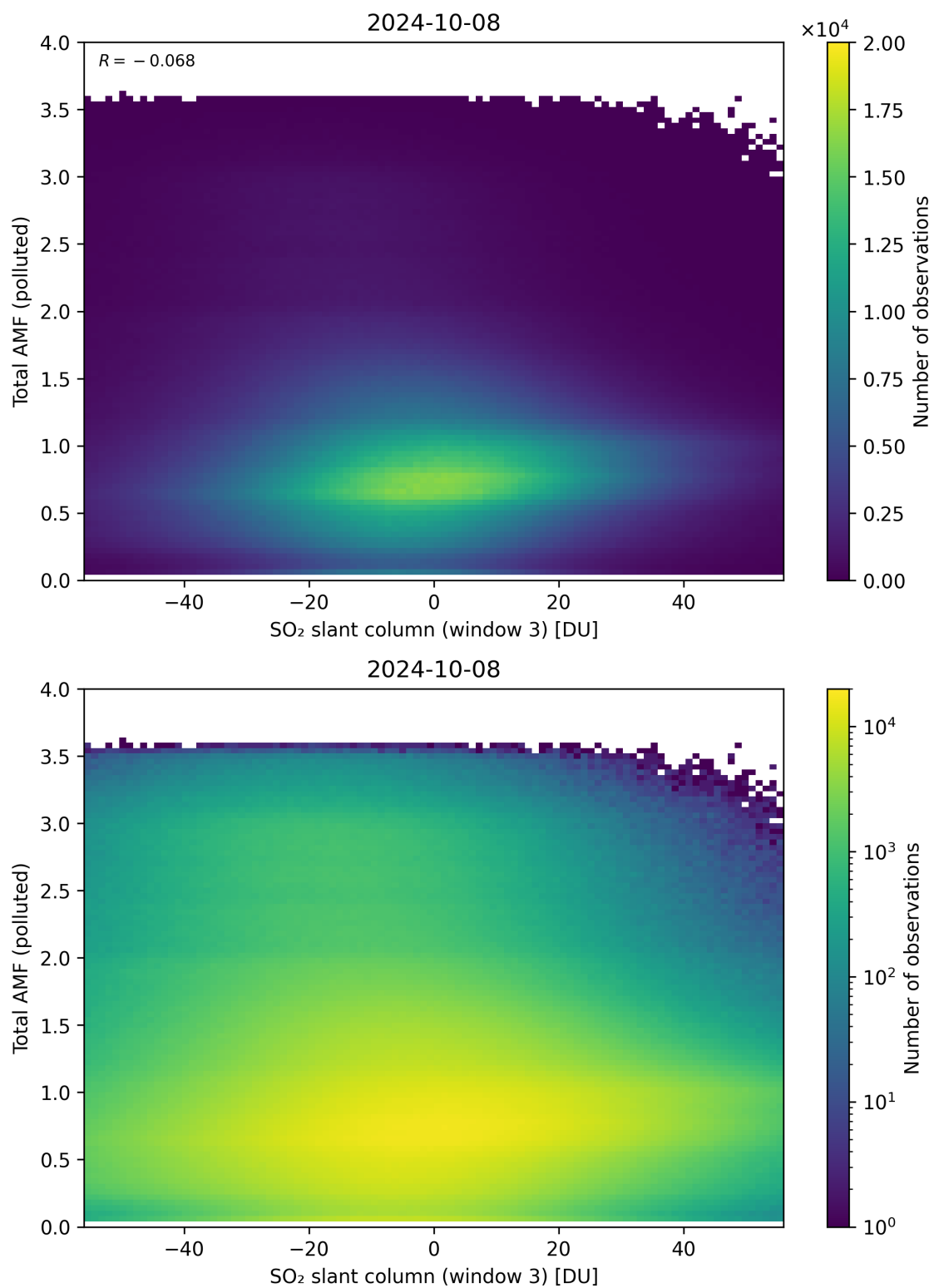
Figure 268: Scatter density plot of “SO 2 slant column (window 3)” against “Total AMF (polluted)” for 2024-10-08 to 2024-10-09.
