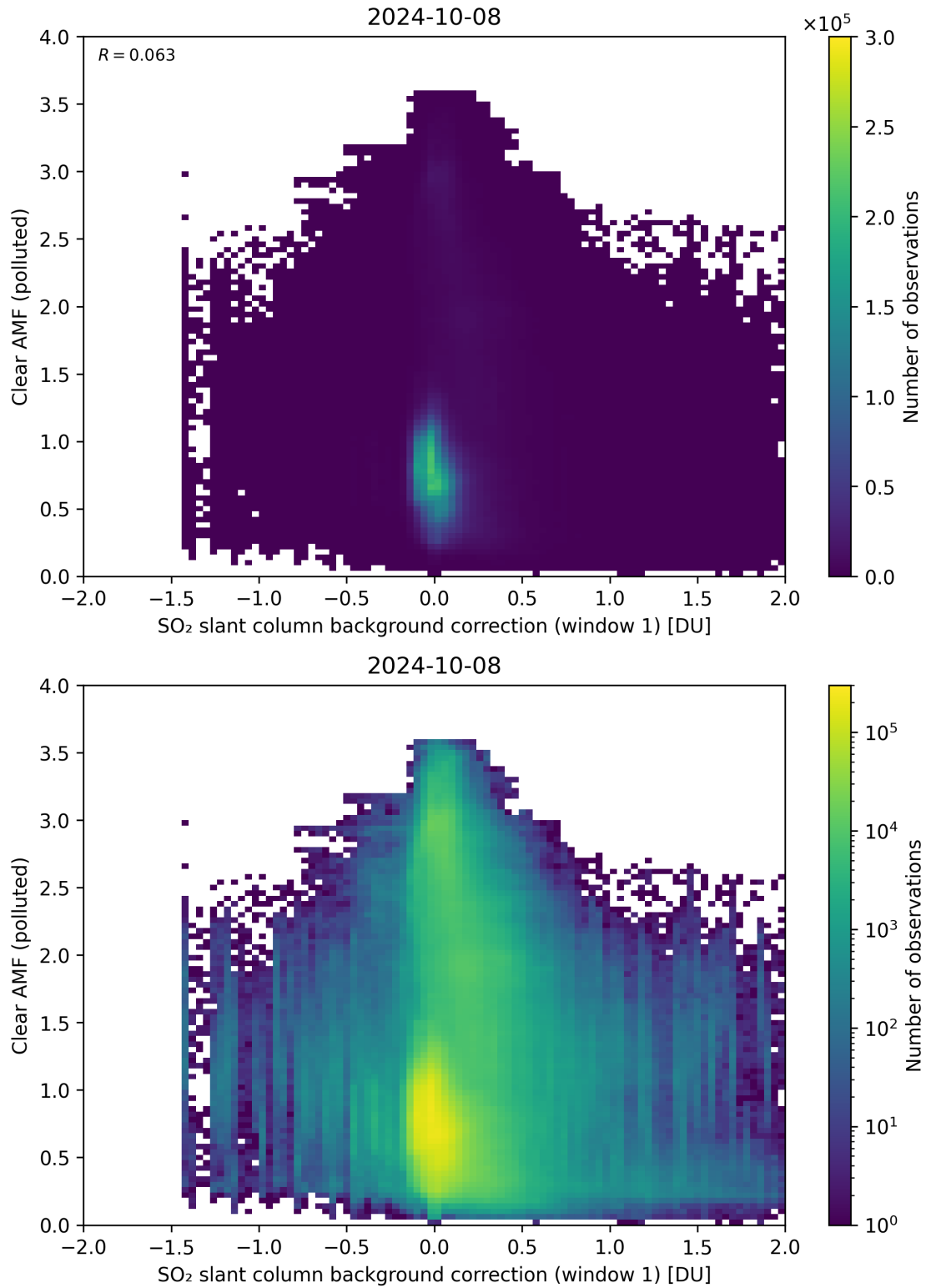
Figure 103: Scatter density plot of “SO 2 slant column background correction (window 1)” against “Clear AMF (polluted)” for 2024-10-08 to 2024-10-09.
