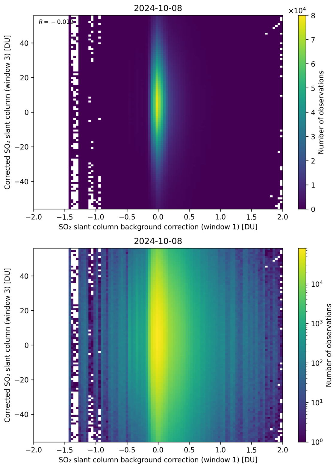
Figure 105: Scatter density plot of “SO 2 slant column background correction (window 1)” against “Corrected SO 2 slant column (window 3)” for 2024-10-08 to 2024-10-09.
