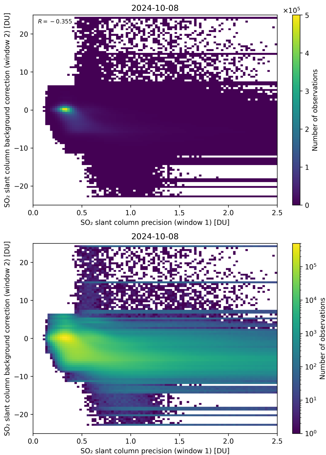
Figure 219: Scatter density plot of “SO 2 slant column precision (window 1)” against “SO 2 slant column background correction (window 2)” for 2024-10-08 to 2024-10-09.
