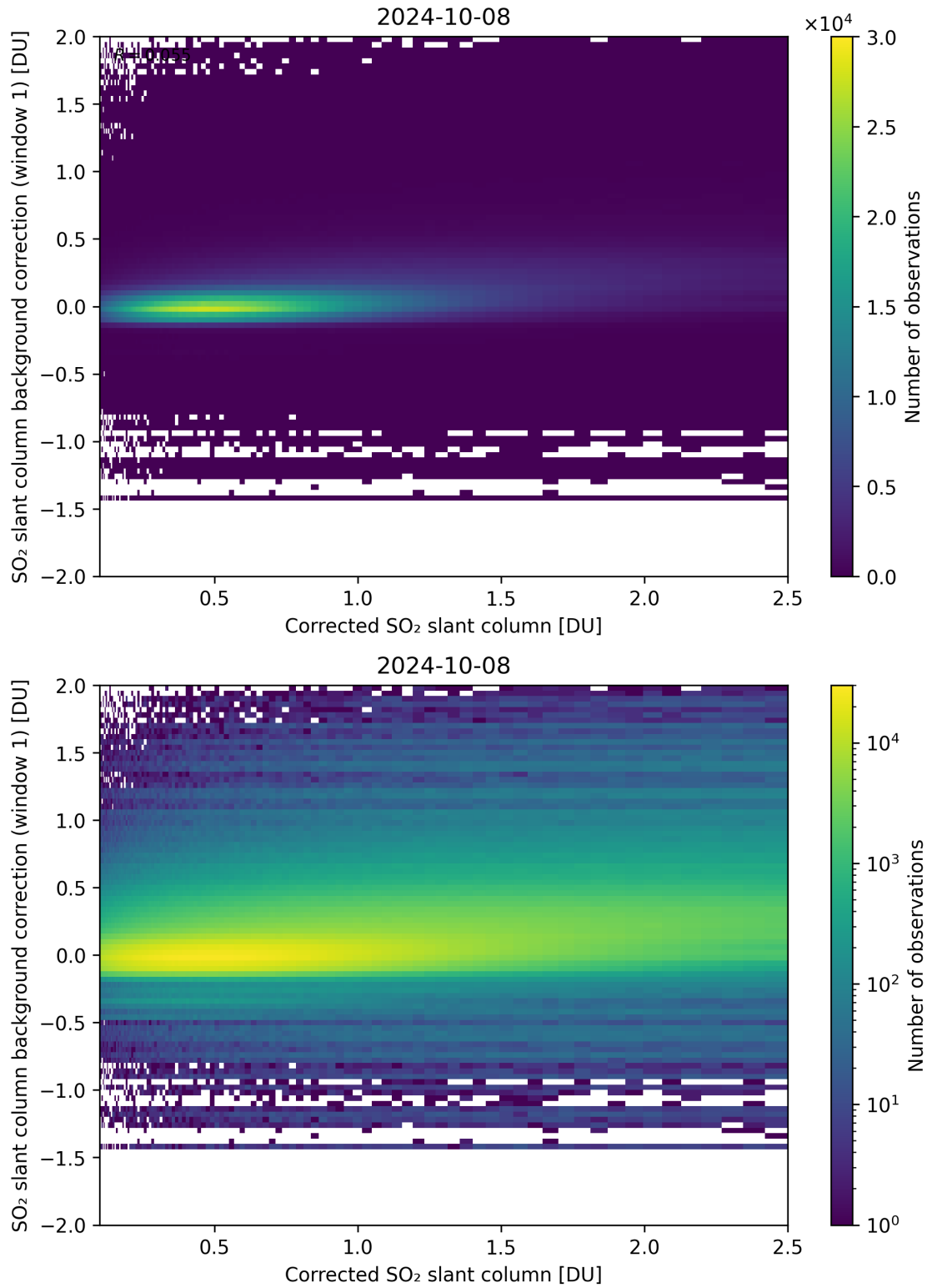
Figure 178: Scatter density plot of “Corrected SO 2 slant column” against “SO 2 slant column background correction (window 1)” for 2024-10-08 to 2024-10-09.
