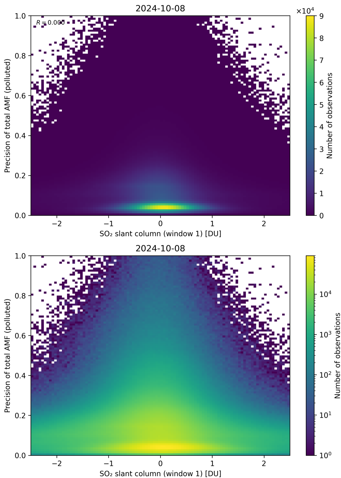
Figure 240: Scatter density plot of “SO 2 slant column (window 1)” against “Precision of total AMF (polluted)” for 2024-10-08 to 2024-10-09.
