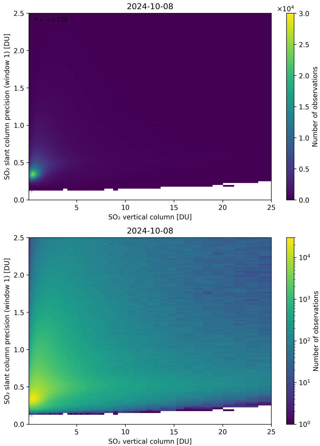
Figure 301: Scatter density plot of “SO 2 vertical column” against “SO 2 slant column precision (window 1)” for 2024-10-08 to 2024-10-09.
