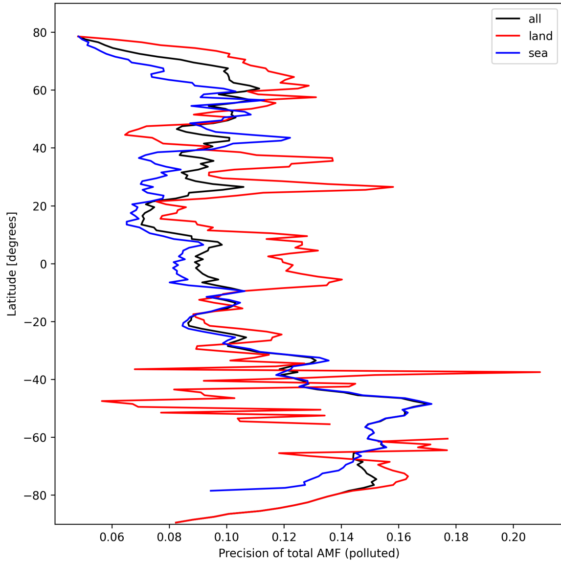
Figure 49: Zonal average of “Precision of total AMF (polluted)” for 2024-10-08 to 2024-10-09.
