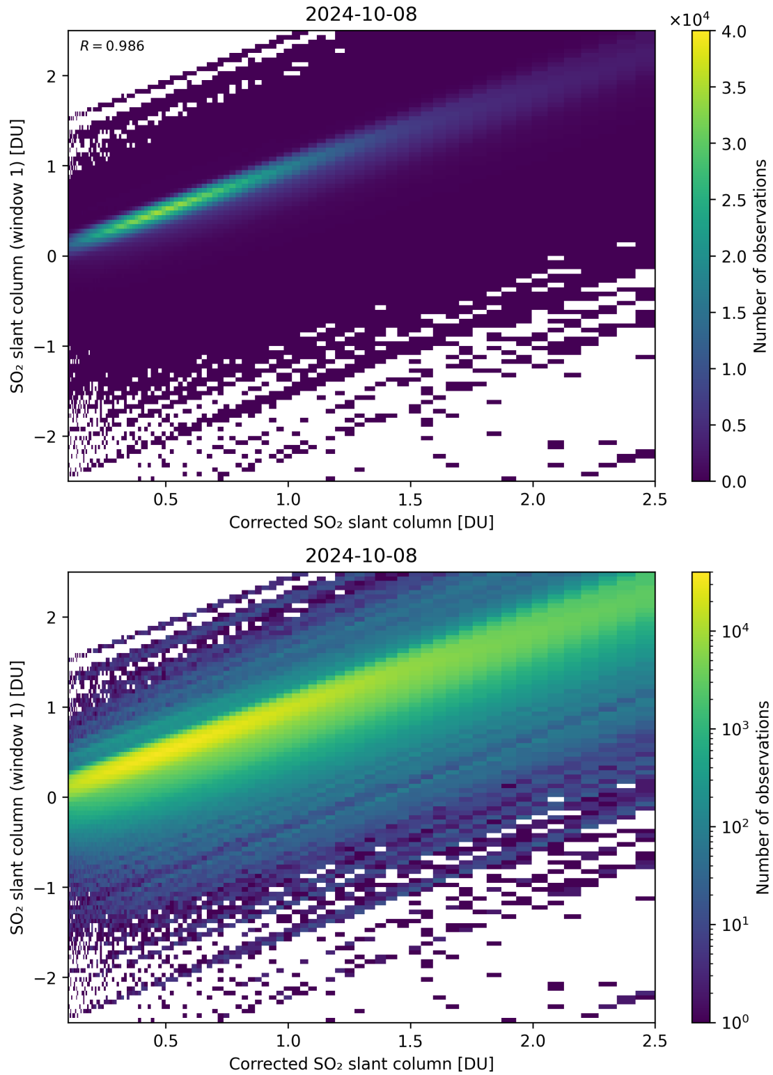
Figure 187: Scatter density plot of “Corrected SO 2 slant column” against “SO 2 slant column (window 1)” for 2024-10-08 to 2024-10-09.
