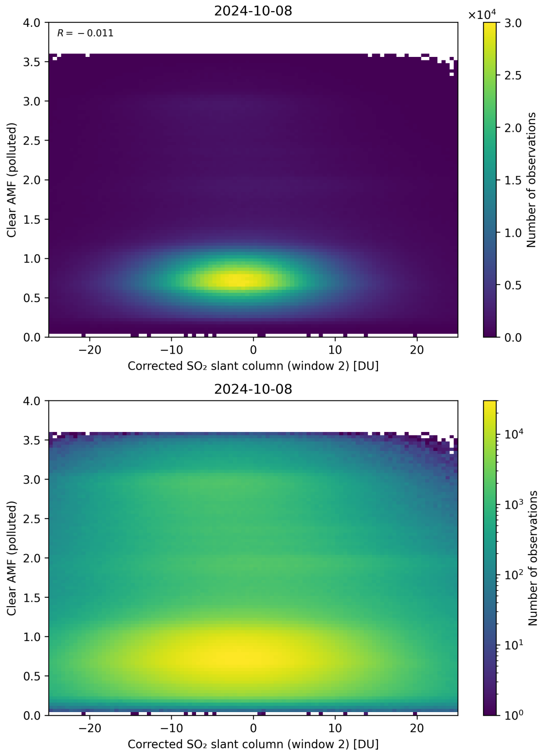
Figure 199: Scatter density plot of “Corrected SO 2 slant column (window 2)” against “Clear AMF (polluted)” for 2024-10-08 to 2024-10-09.
