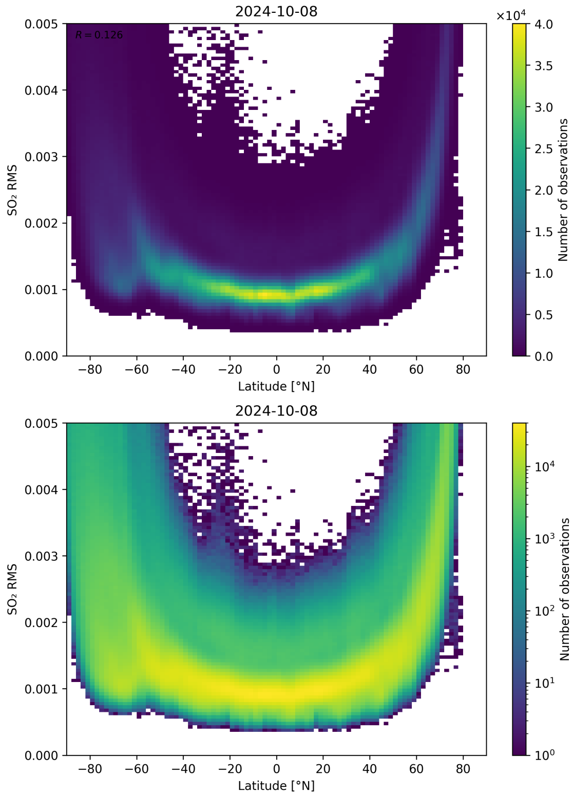
Figure 144: Scatter density plot of “Latitude” against “SO 2 RMS” for 2024-10-08 to 2024-10-09.
