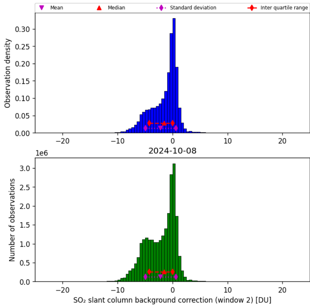
Figure 63: Histogram of “SO 2 slant column background correction (window 2)” for 2024-10-08 to 2024-10-09
