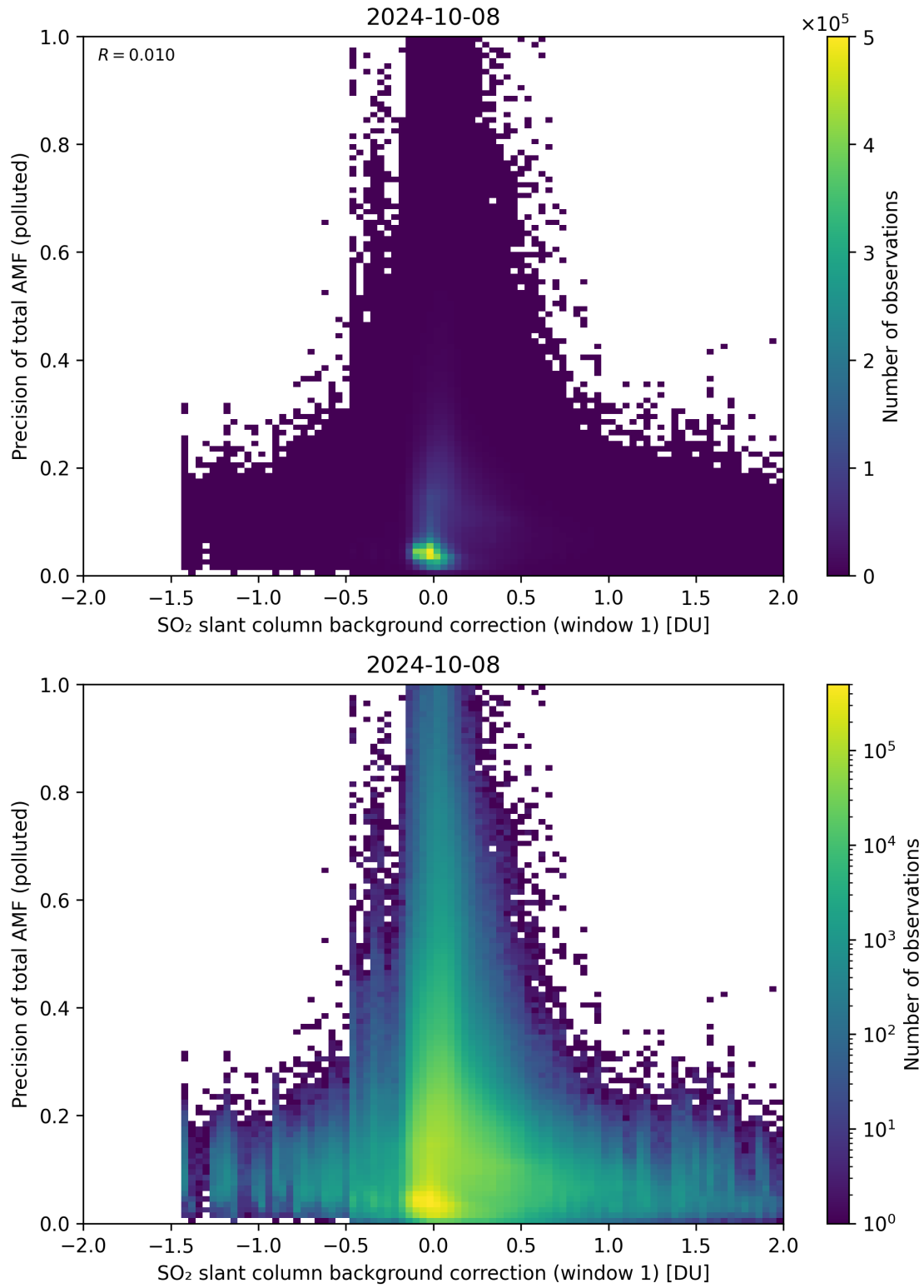
Figure 110: Scatter density plot of “SO 2 slant column background correction (window 1)” against “Precision of total AMF (polluted)” for 2024-10-08 to 2024-10-09.
