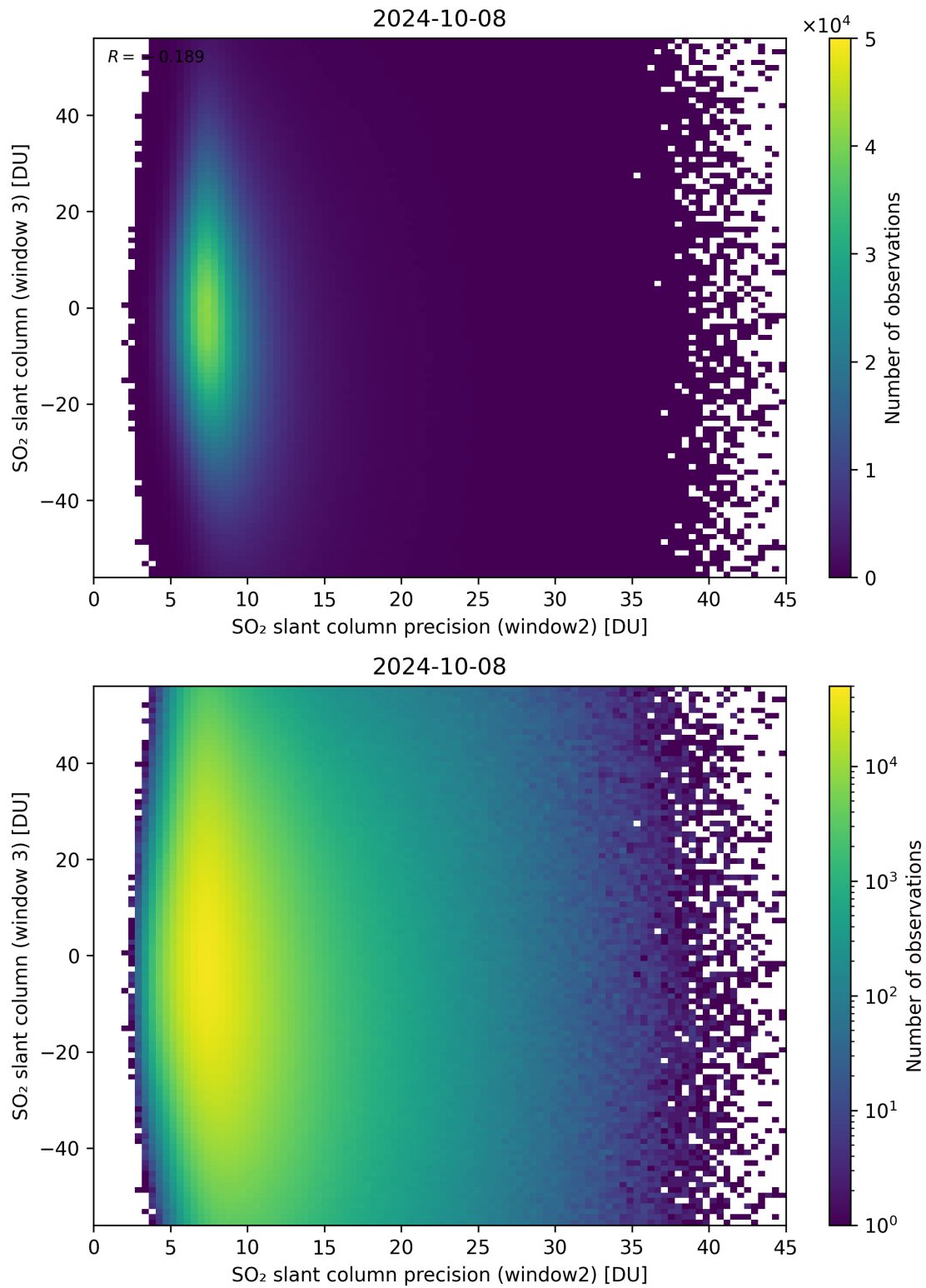
Figure 249: Scatter density plot of “SO 2 slant column precision (window2)” against “SO 2 slant column (window 3)” for 2024-10-08 to 2024-10-09.
