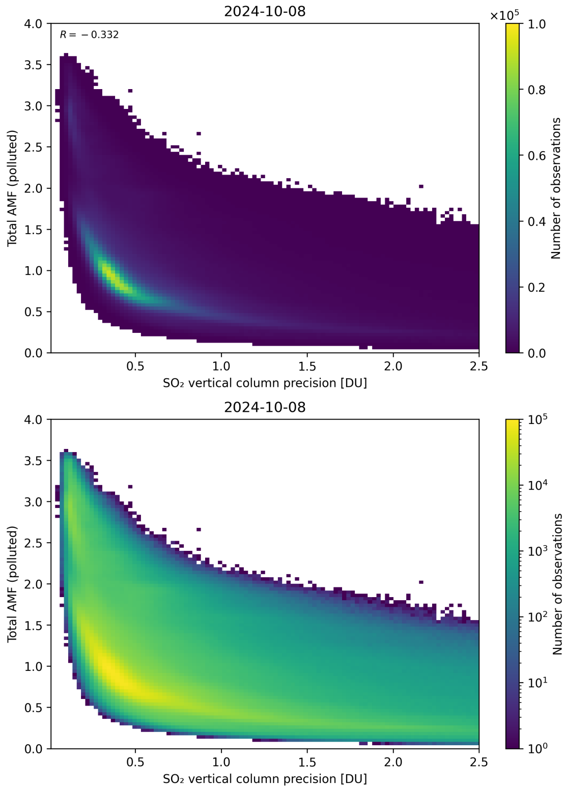
Figure 294: Scatter density plot of “SO 2 vertical column precision” against “Total AMF (polluted)” for 2024-10-08 to 2024-10-09.
