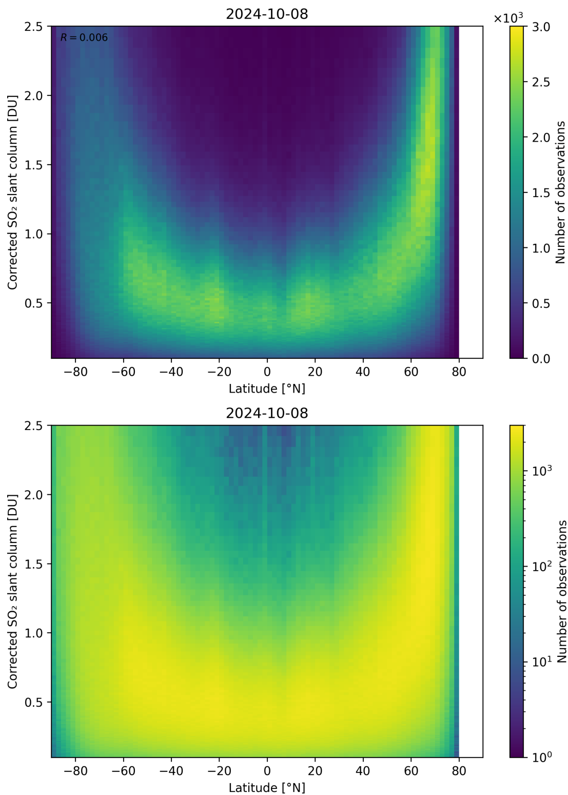
Figure 146: Scatter density plot of “Latitude” against “Corrected SO 2 slant column” for 2024-10-08 to 2024-10-09.
