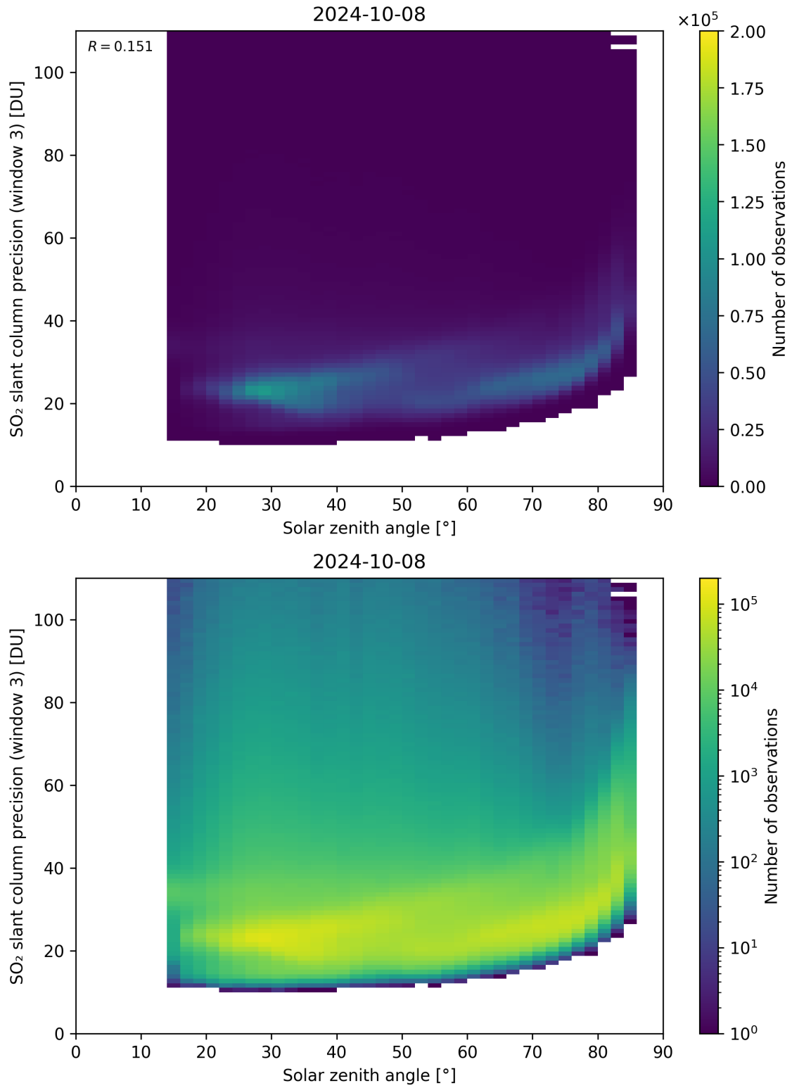
Figure 173: Scatter density plot of “Solar zenith angle” against “SO 2 slant column precision (window 3)” for 2024-10-08 to 2024-10-09.
