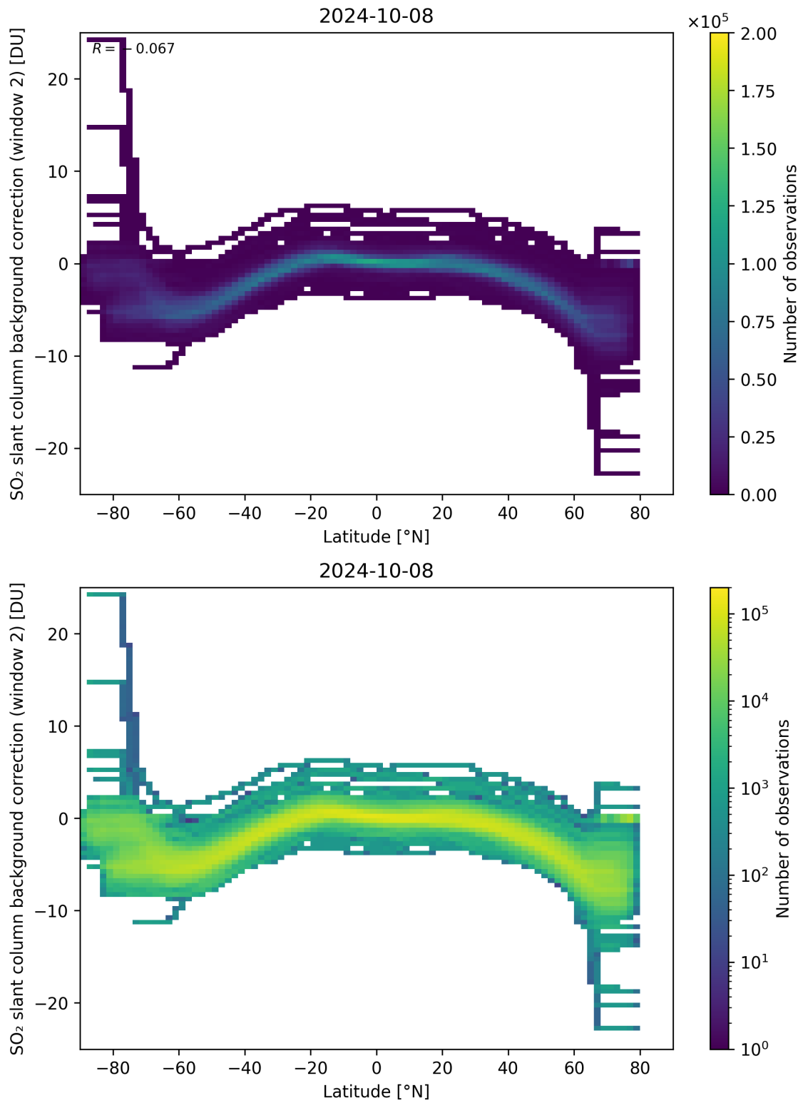
Figure 140: Scatter density plot of “Latitude” against “SO 2 slant column background correction (window 2)” for 2024-10-08 to 2024-10-09.
