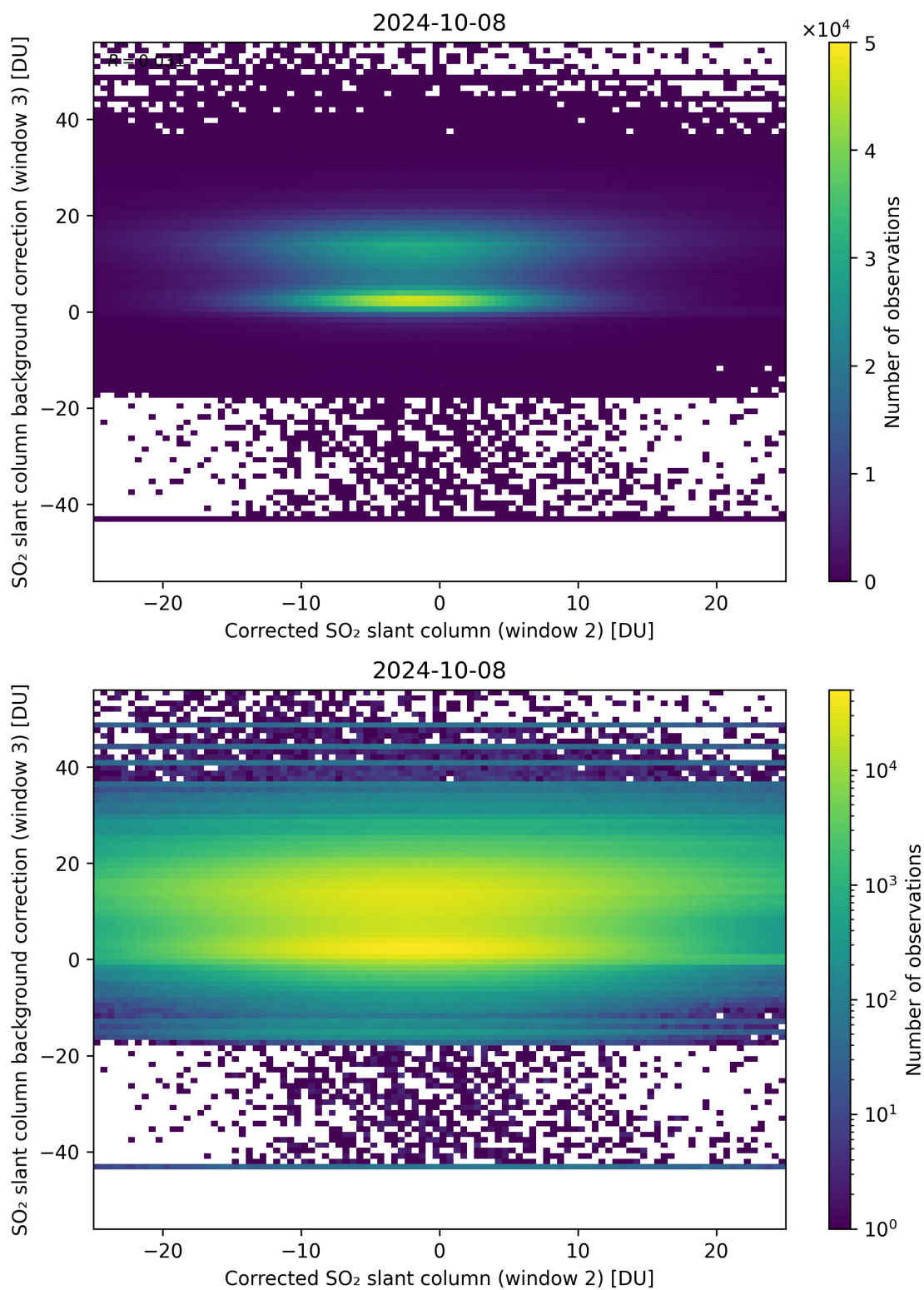
Figure 195: Scatter density plot of “Corrected SO 2 slant column (window 2)” against “SO 2 slant column background correction (window 3)” for 2024-10-08 to 2024-10-09.
