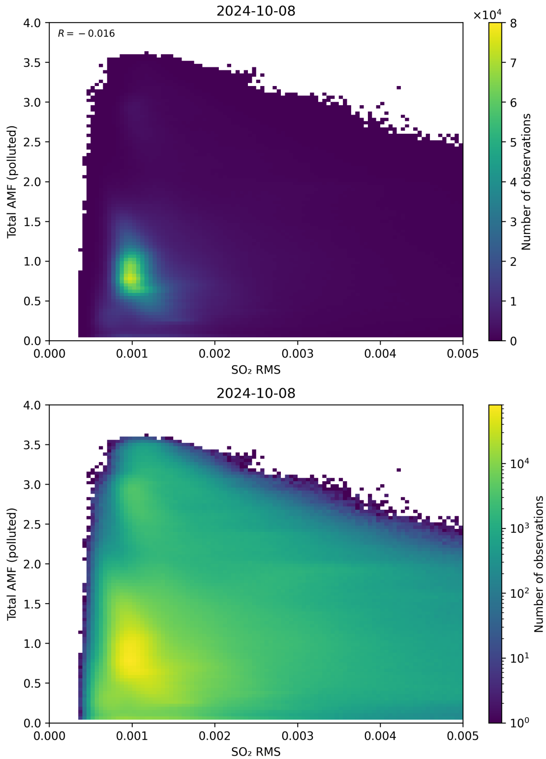
Figure 137: Scatter density plot of “SO 2 RMS” against “Total AMF (polluted)” for 2024-10-08 to 2024-10-09.
