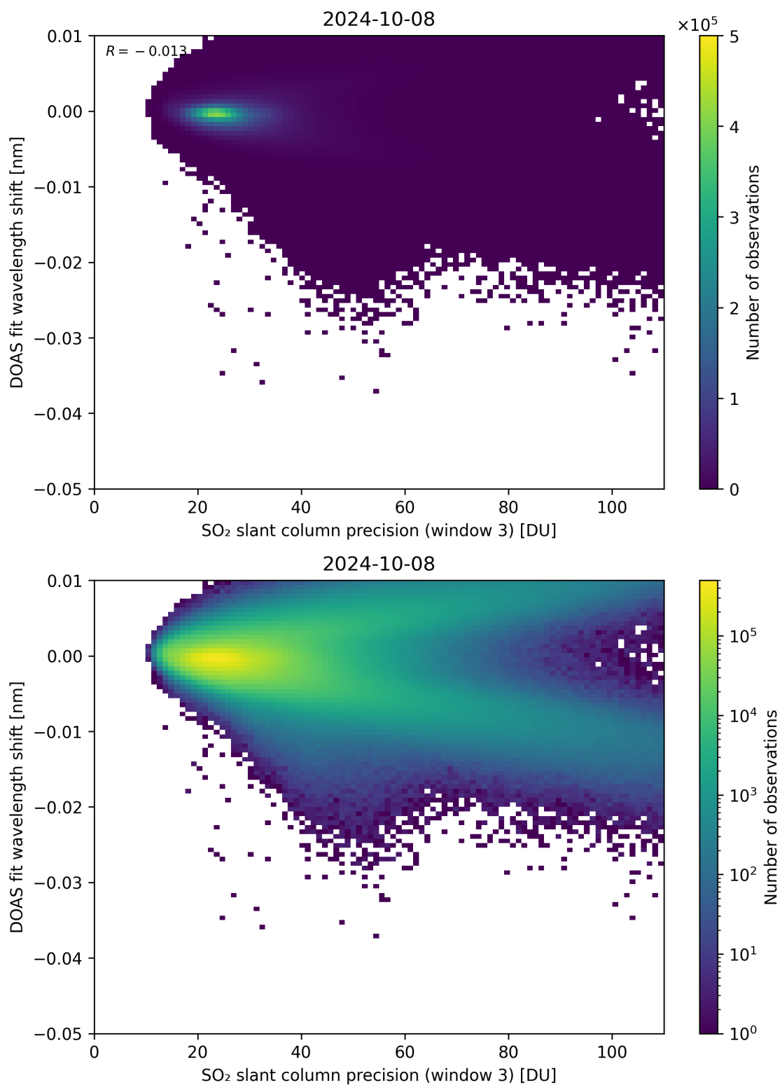
Figure 258: Scatter density plot of “SO 2 slant column precision (window 3)” against “DOAS fit wavelength shift” for 2024-10-08 to 2024-10-09.
