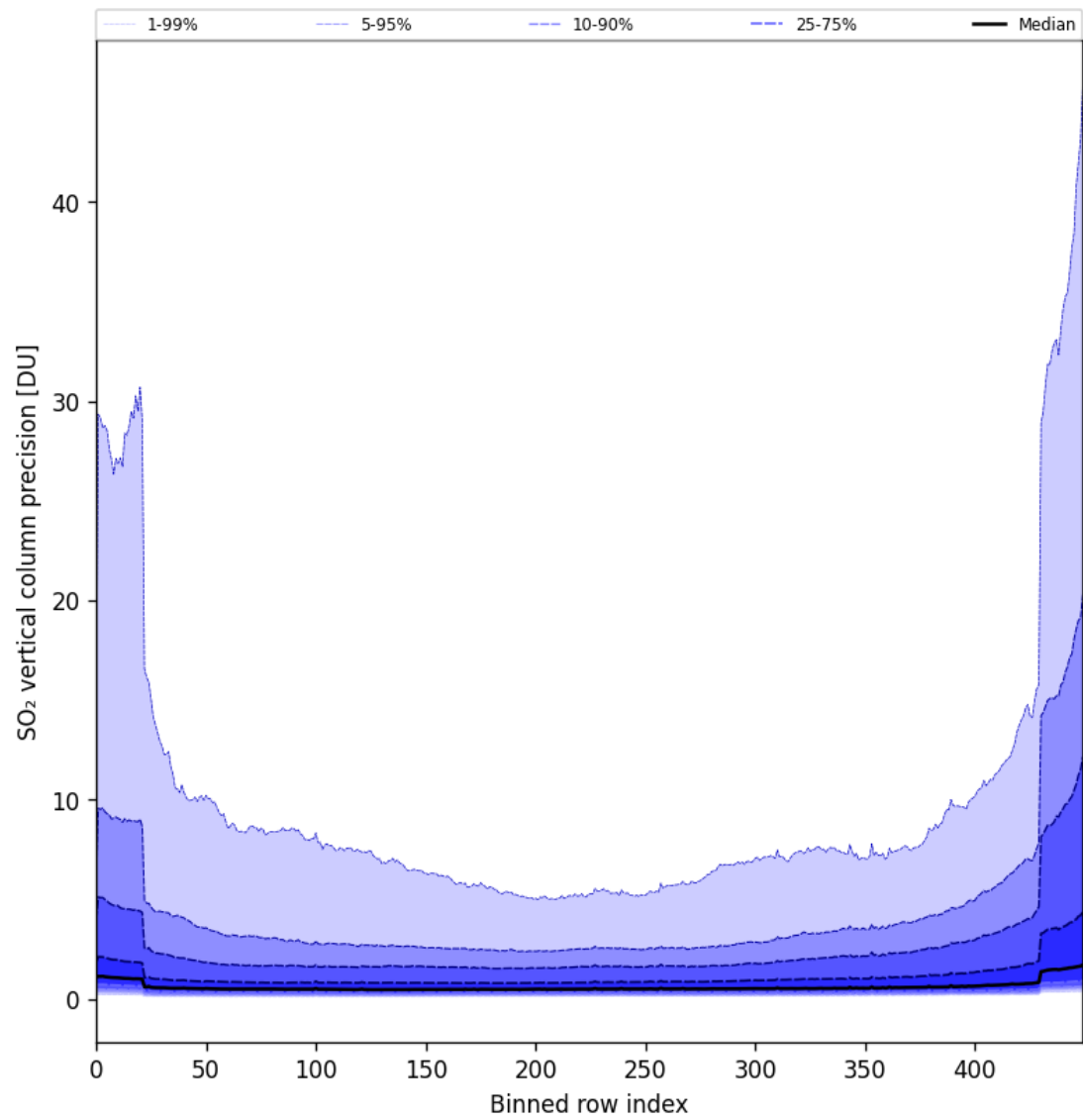
Figure 77: Along track statistics of “SO 2 vertical column precision” for 2024-10-08 to 2024-10-09
