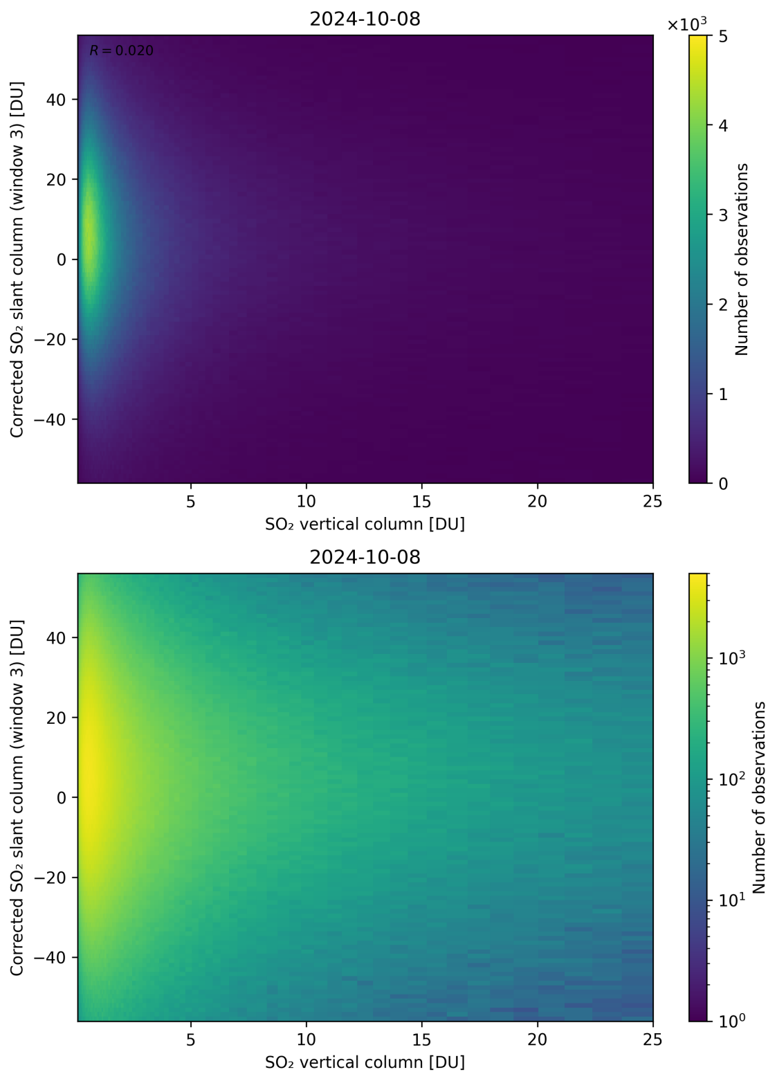
Figure 299: Scatter density plot of “SO 2 vertical column” against “Corrected SO 2 slant column (window 3)” for 2024-10-08 to 2024-10-09.
