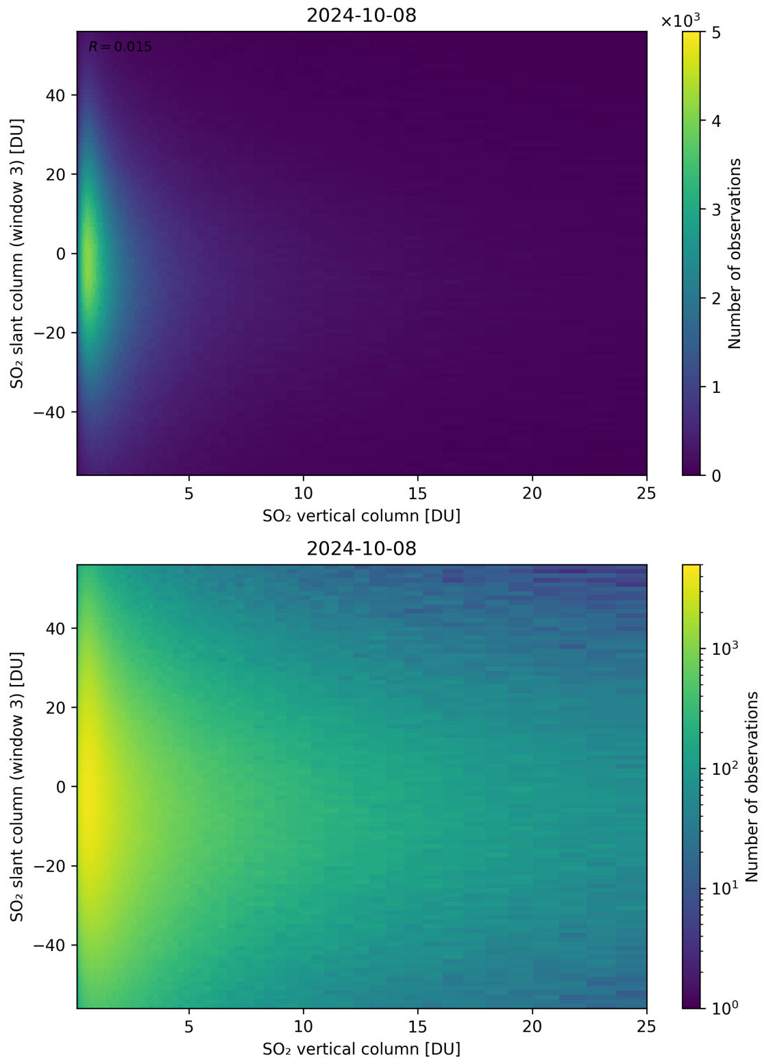
Figure 303: Scatter density plot of “SO 2 vertical column” against “SO 2 slant column (window 3)” for 2024-10-08 to 2024-10-09.
