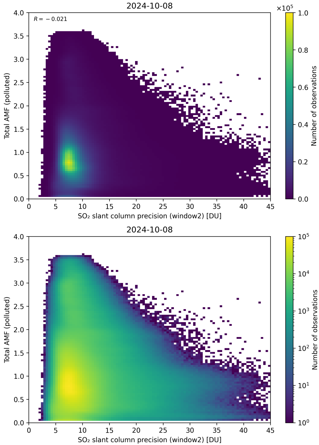
Figure 251: Scatter density plot of “SO 2 slant column precision (window2)” against “Total AMF (polluted)” for 2024-10-08 to 2024-10-09.
