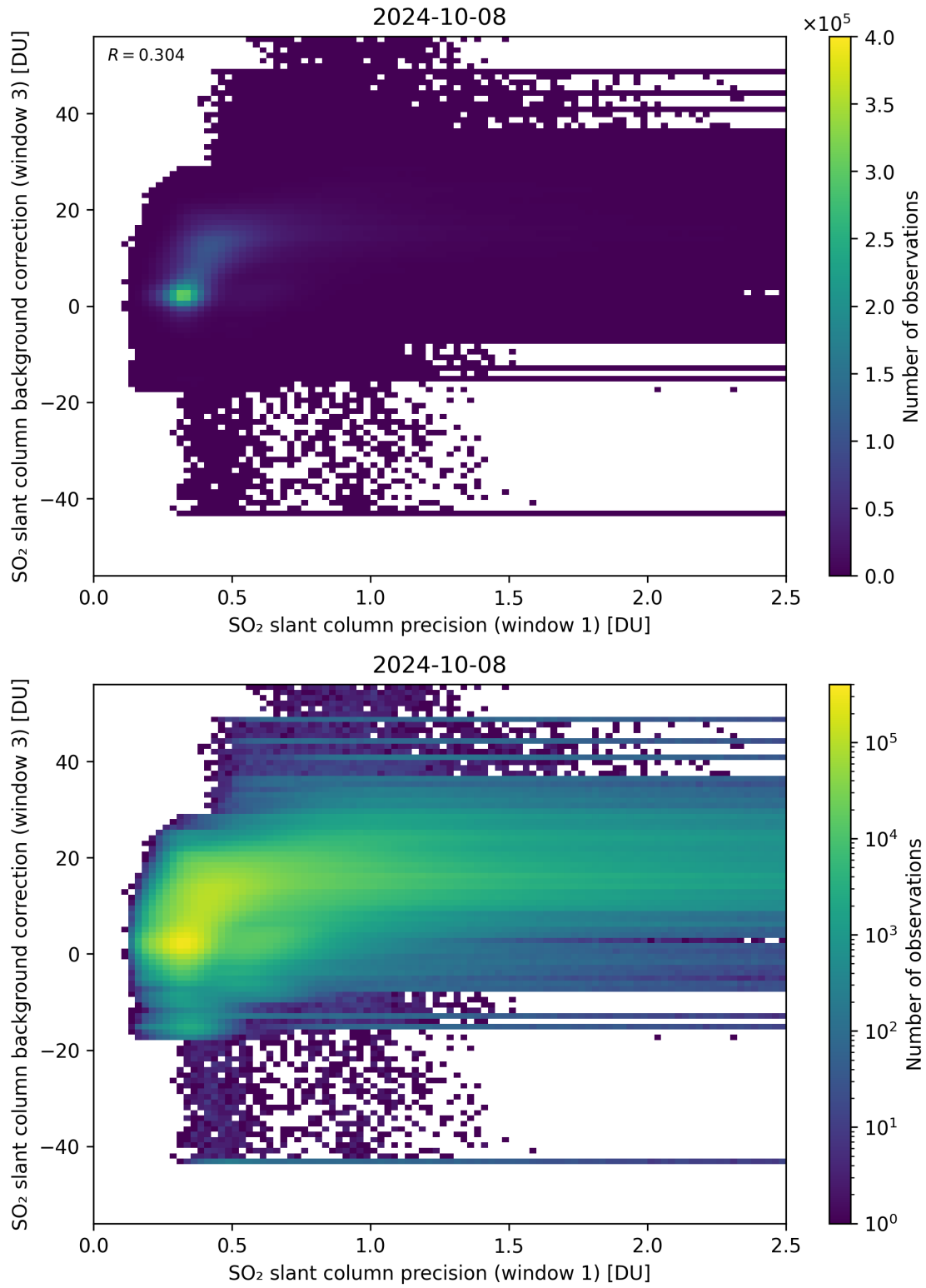
Figure 220: Scatter density plot of “SO 2 slant column precision (window 1)” against “SO 2 slant column background correction (window 3)” for 2024-10-08 to 2024-10-09.
