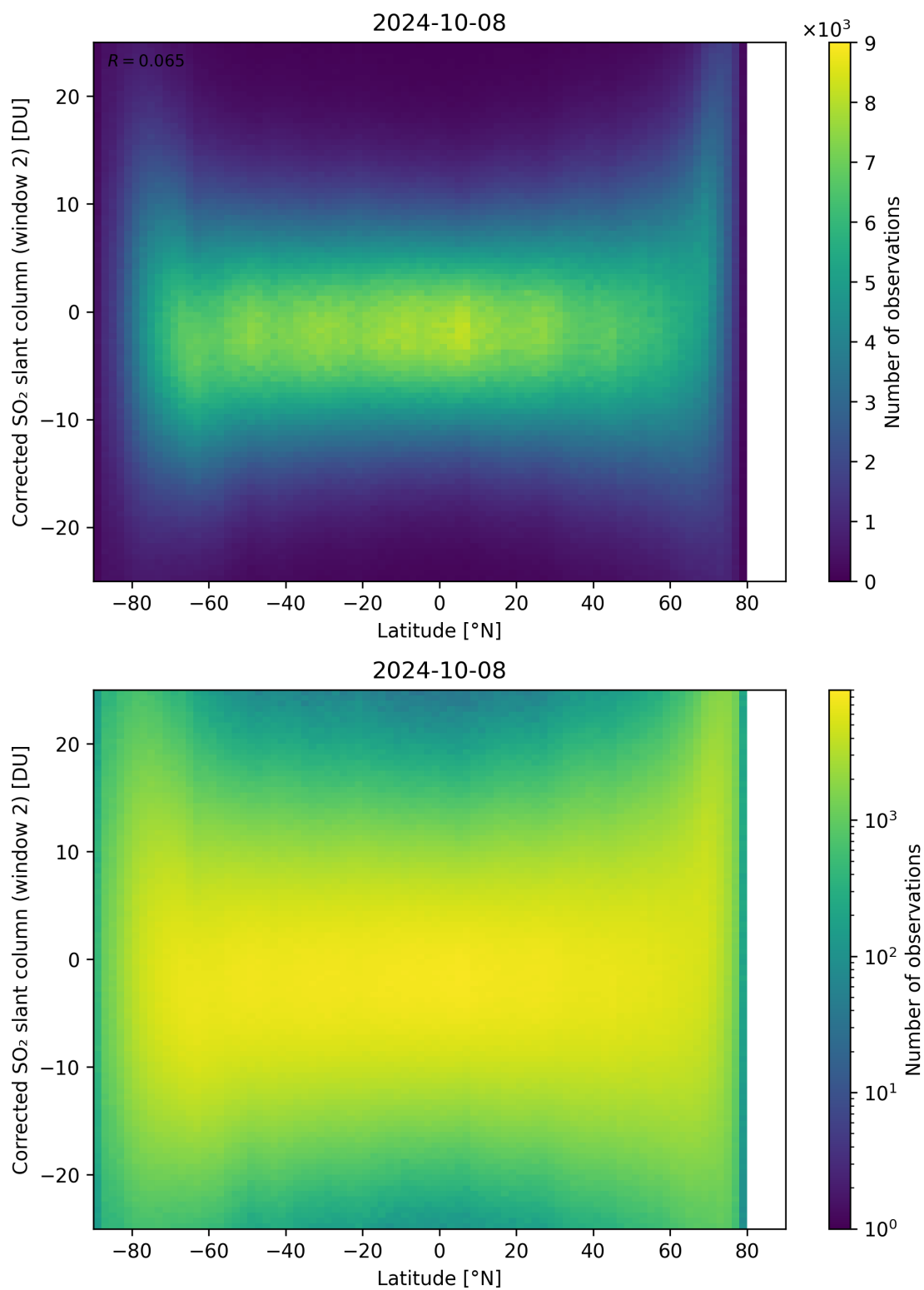
Figure 147: Scatter density plot of “Latitude” against “Corrected SO 2 slant column (window 2)” for 2024-10-08 to 2024-10-09.
