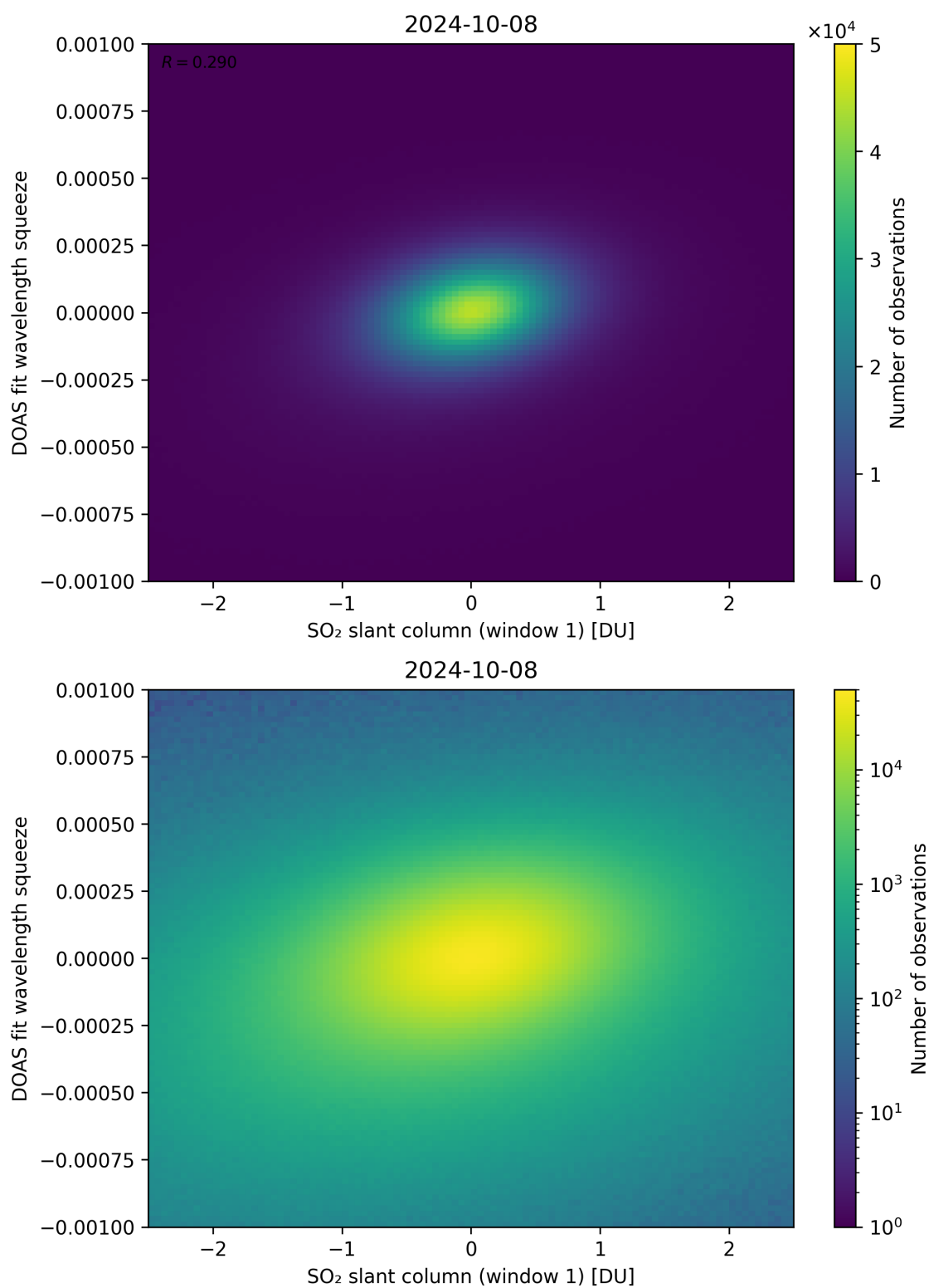
Figure 216: Scatter density plot of “SO 2 slant column (window 1)” against “DOAS fit wavelength squeeze” for 2024-10-08 to 2024-10-09.
