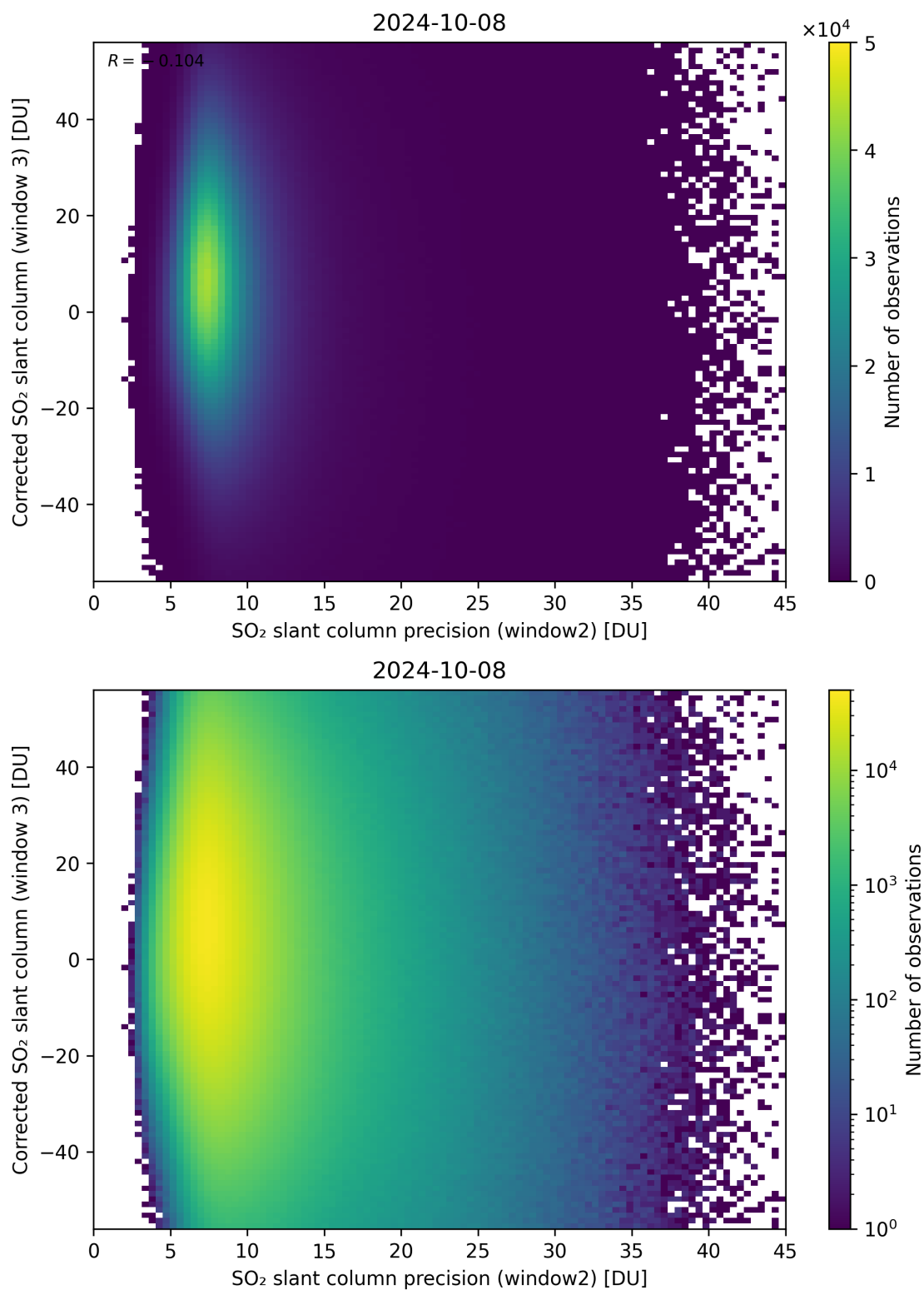
Figure 248: Scatter density plot of “SO 2 slant column precision (window2)” against “Corrected SO 2 slant column (window 3)” for 2024-10-08 to 2024-10-09.
