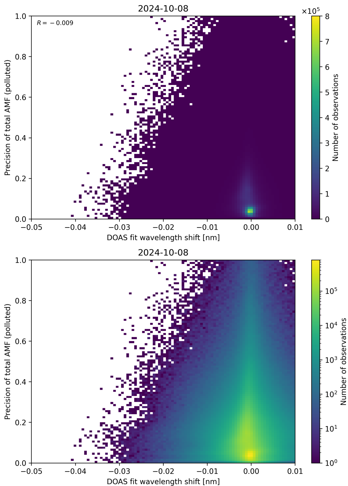
Figure 131: Scatter density plot of “DOAS fit wavelength shift” against “Precision of total AMF (polluted)” for 2024-10-08 to 2024-10-09.
