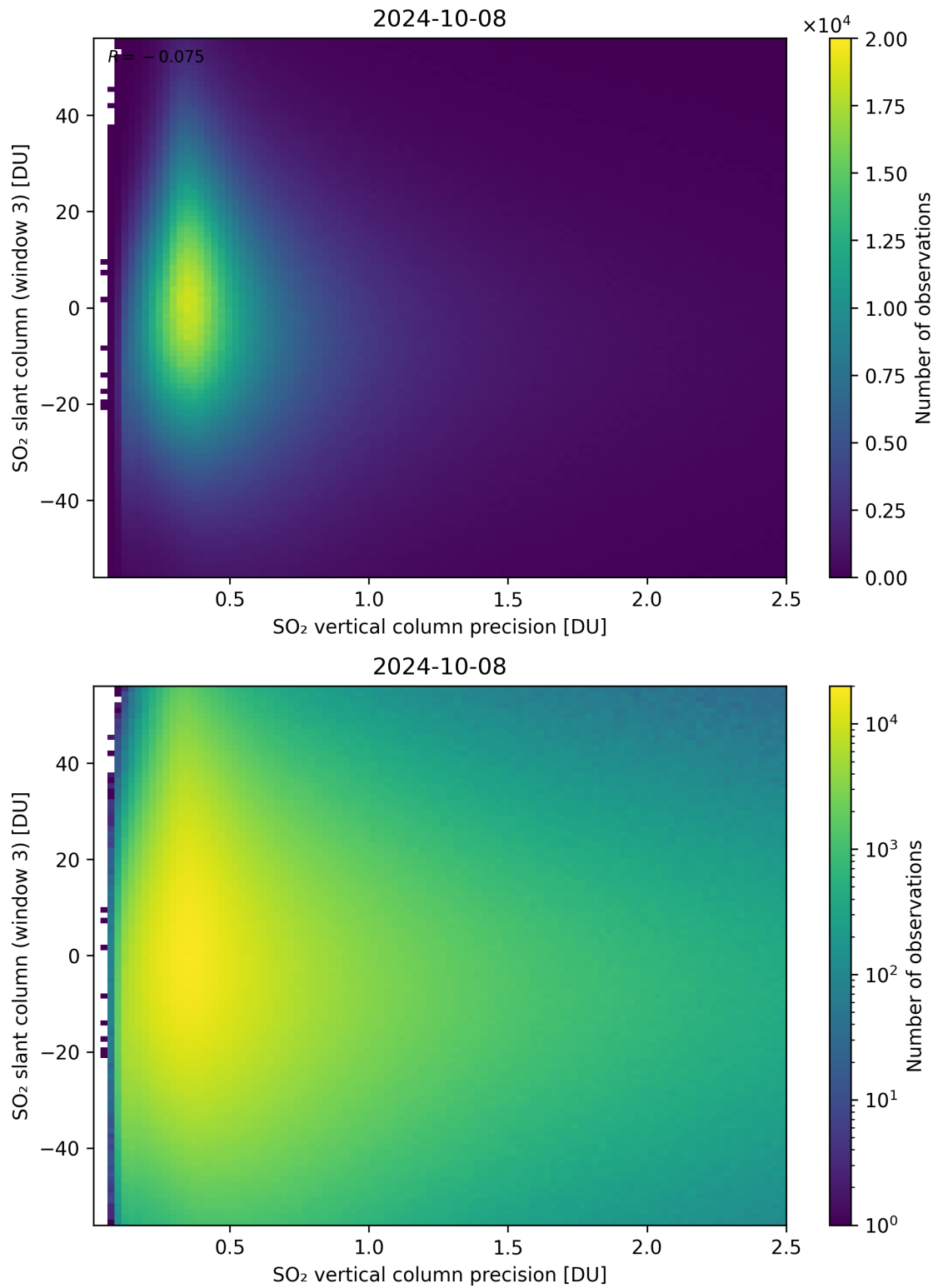
Figure 292: Scatter density plot of “SO 2 vertical column precision” against “SO 2 slant column (window 3)” for 2024-10-08 to 2024-10-09.
