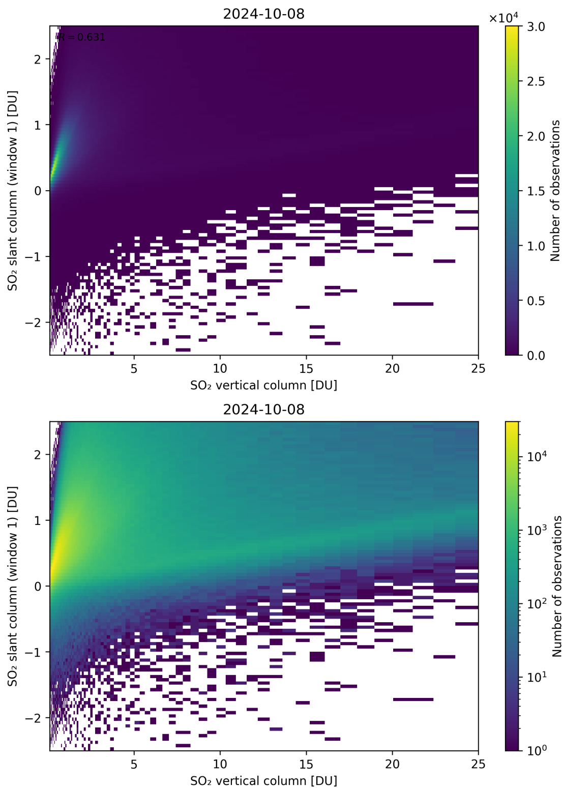
Figure 300: Scatter density plot of “SO 2 vertical column” against “SO 2 slant column (window 1)” for 2024-10-08 to 2024-10-09.
