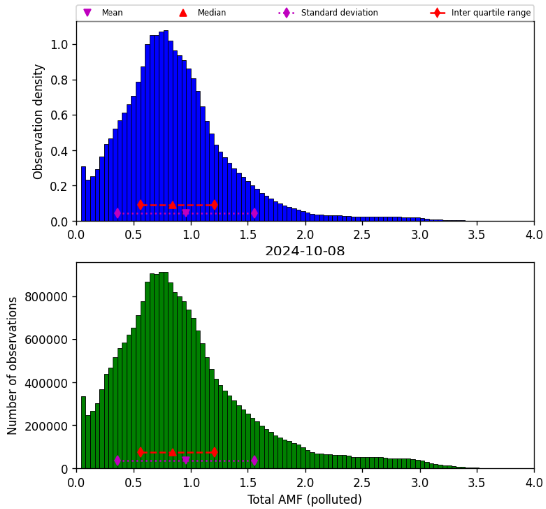
Figure 71: Histogram of “Total AMF (polluted)” for 2024-10-08 to 2024-10-09
