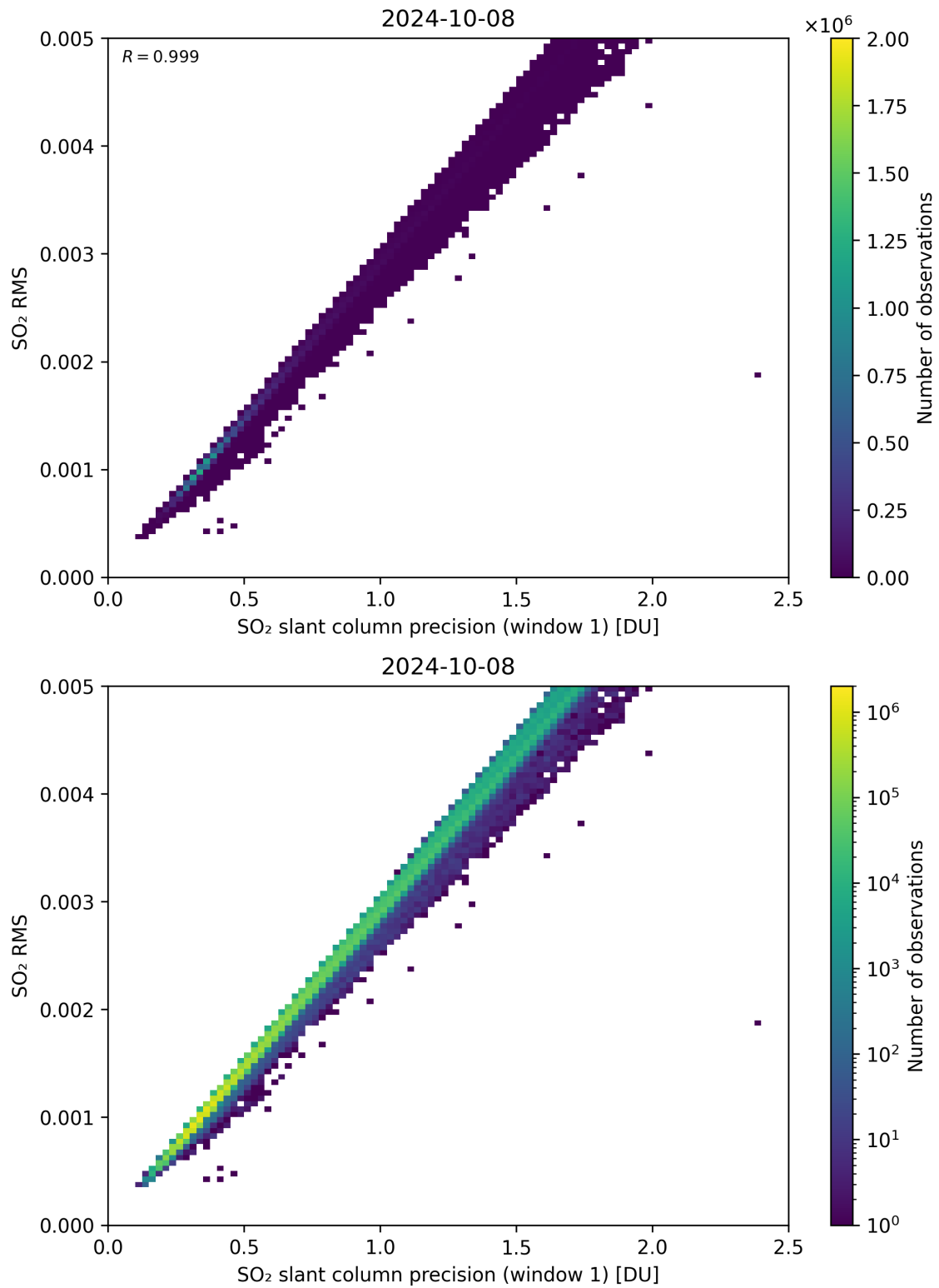
Figure 223: Scatter density plot of “SO 2 slant column precision (window 1)” against “SO 2 RMS” for 2024-10-08 to 2024-10-09.
