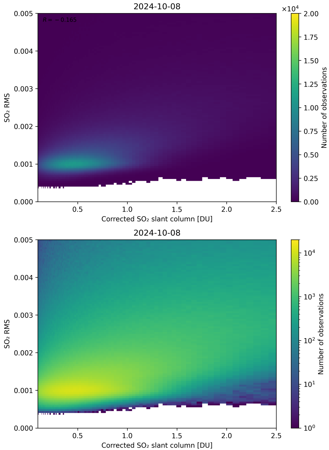
Figure 183: Scatter density plot of “Corrected SO 2 slant column” against “SO 2 RMS” for 2024-10-08 to 2024-10-09.
