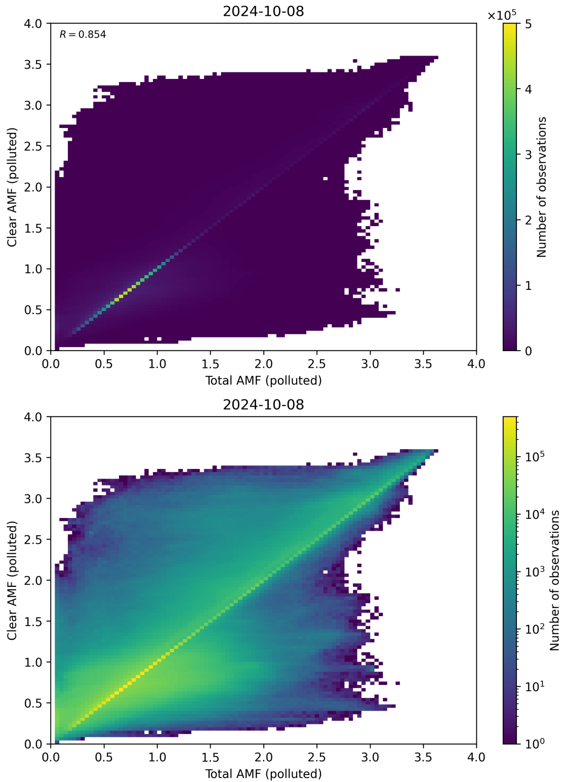
Figure 271: Scatter density plot of “Total AMF (polluted)” against “Clear AMF (polluted)” for 2024-10-08 to 2024-10-09.
