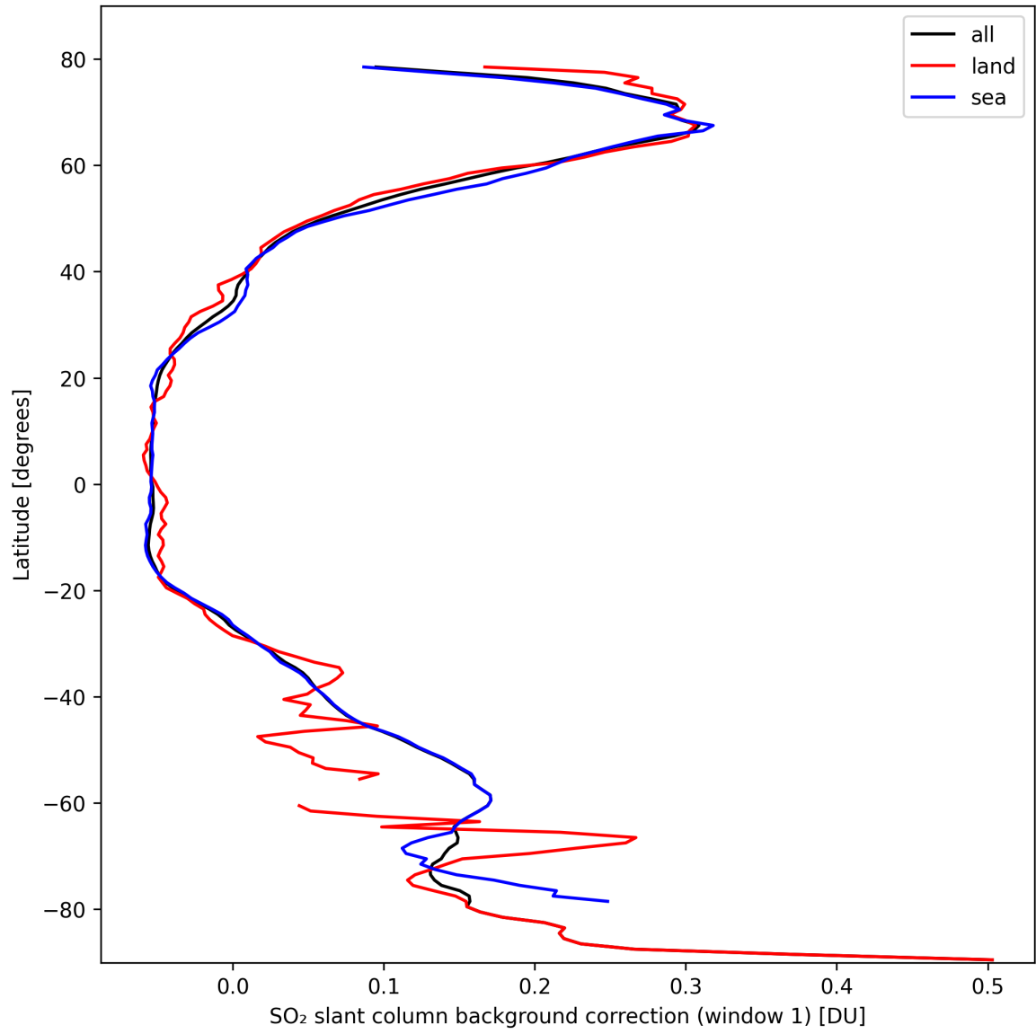
Figure 36: Zonal average of “SO 2 slant column background correction (window 1)” for 2024-10-08 to 2024-10-09.
