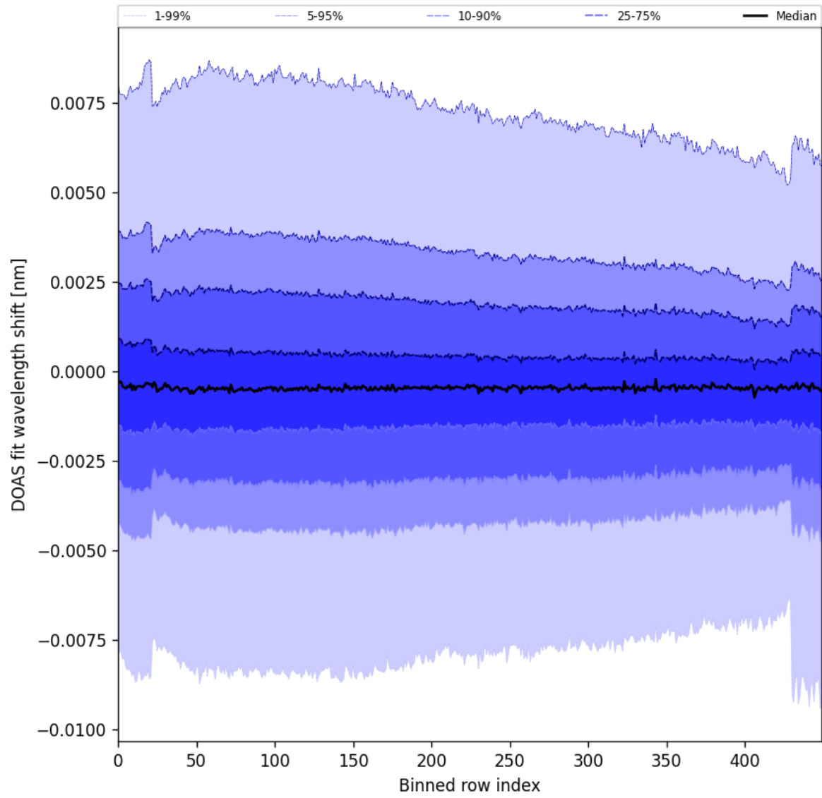
Figure 91: Along track statistics of “DOAS fit wavelength shift” for 2024-10-08 to 2024-10-09
