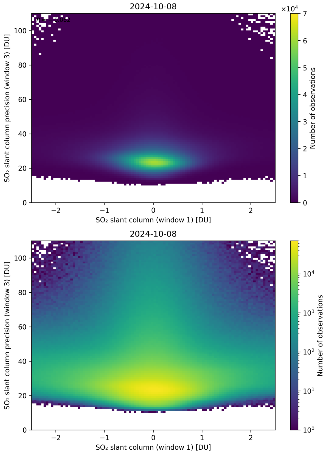
Figure 238: Scatter density plot of “SO 2 slant column (window 1)” against “SO 2 slant column precision (window 3)” for 2024-10-08 to 2024-10-09.
