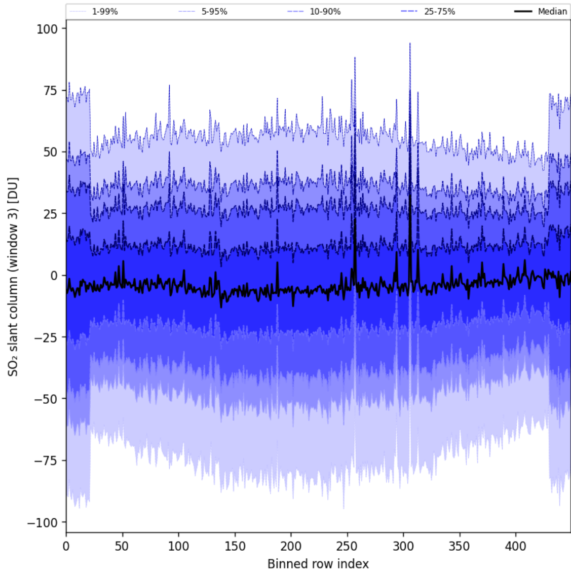
Figure 87: Along track statistics of “SO 2 slant column (window 3)” for 2024-10-08 to 2024-10-09
