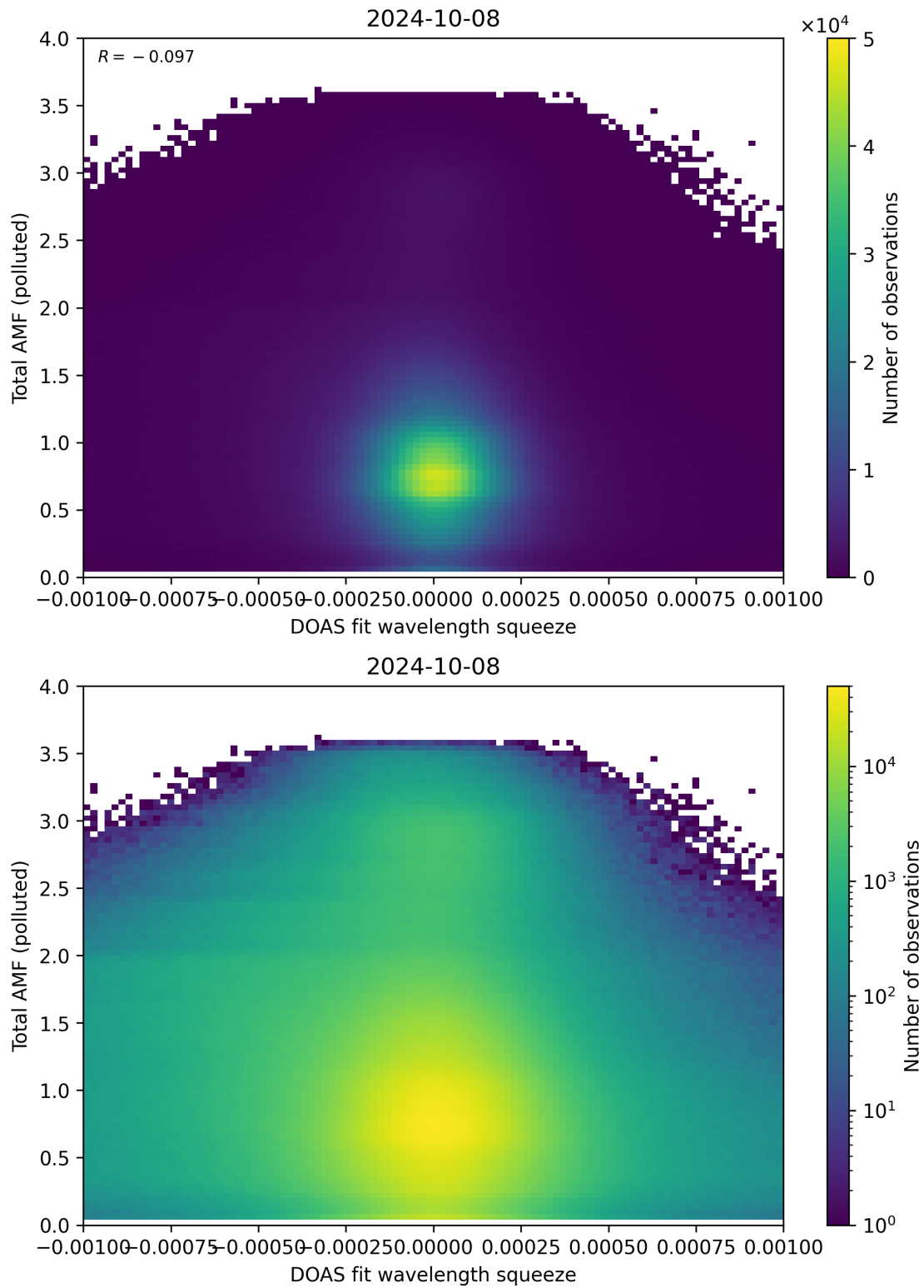
Figure 134: Scatter density plot of “DOAS fit wavelength squeeze” against “Total AMF (polluted)” for 2024-10-08 to 2024-10-09.
