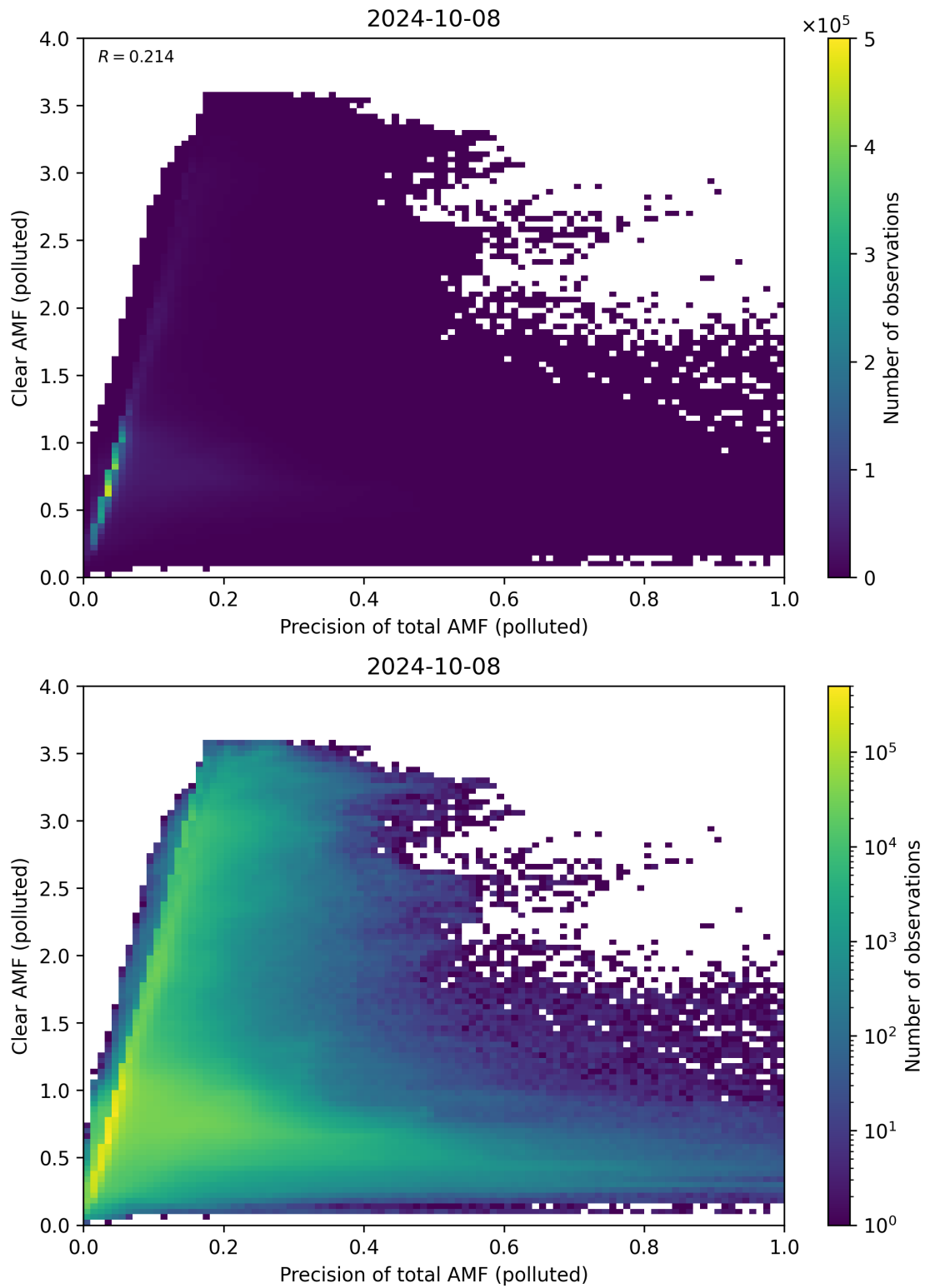
Figure 270: Scatter density plot of “Precision of total AMF (polluted)” against “Clear AMF (polluted)” for 2024-10-08 to 2024-10-09.
