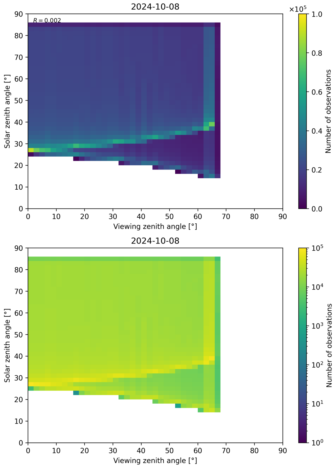
Figure 315: Scatter density plot of “Viewing zenith angle” against “Solar zenith angle” for 2024-10-08 to 2024-10-09.
