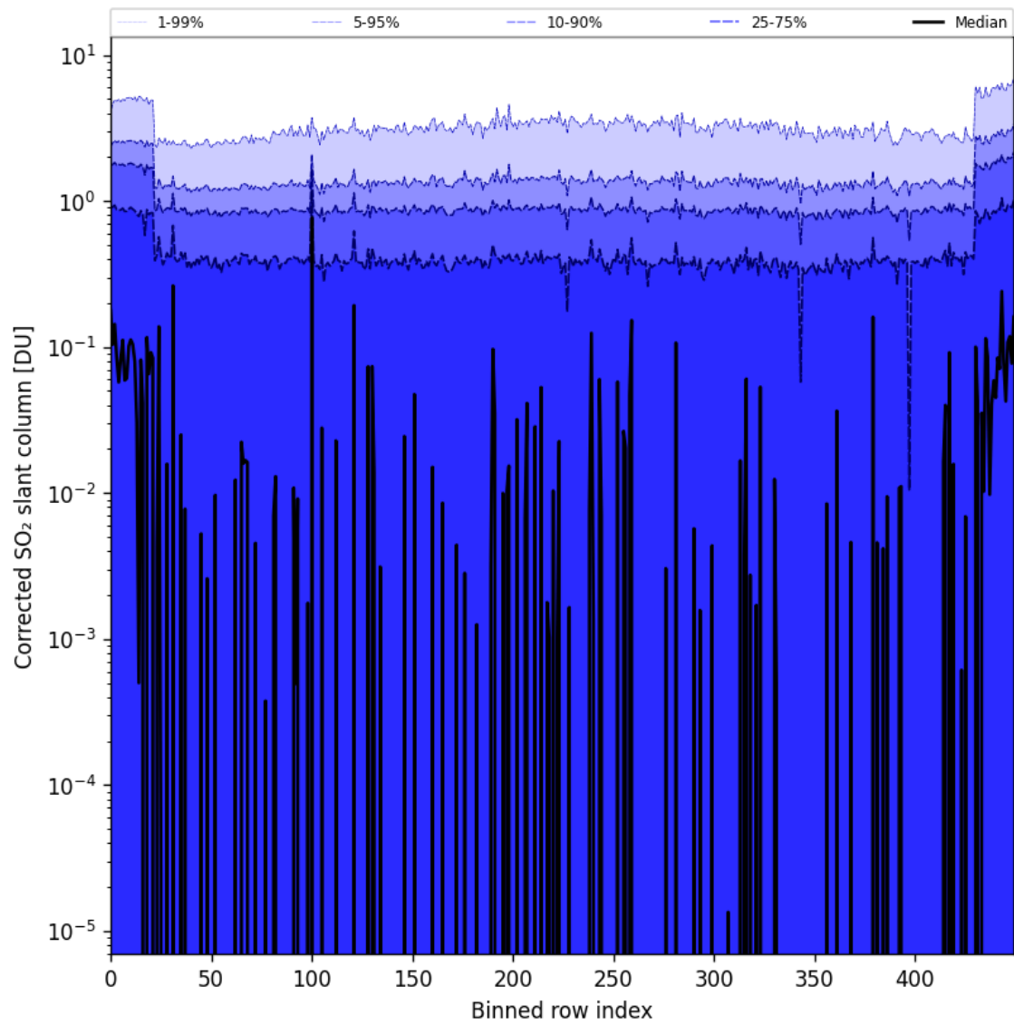
Figure 78: Along track statistics of “Corrected SO 2 slant column” for 2024-10-08 to 2024-10-09
