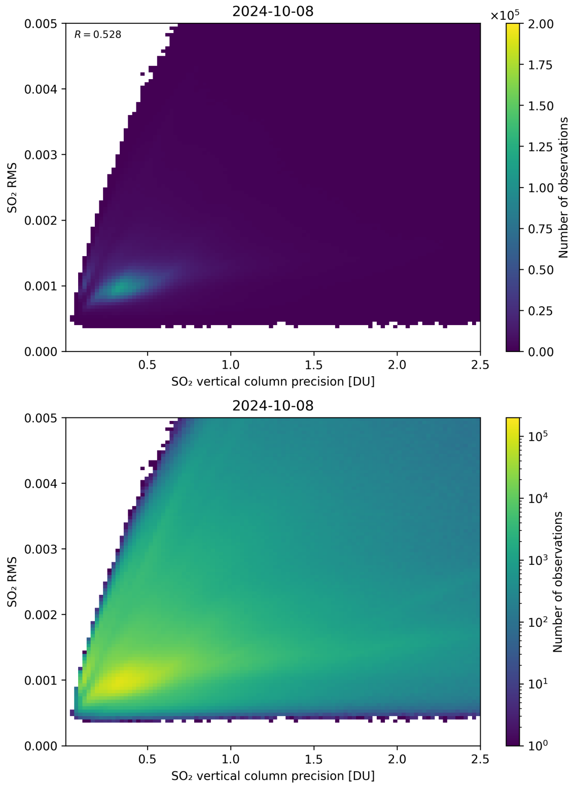
Figure 284: Scatter density plot of “SO 2 vertical column precision” against “SO 2 RMS” for 2024-10-08 to 2024-10-09.
