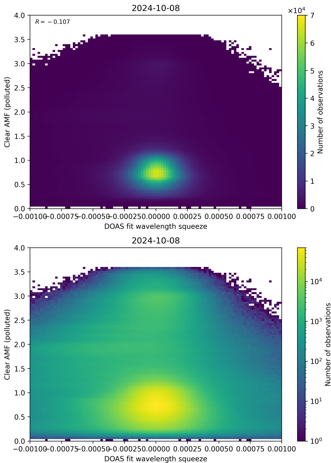
Figure 133: Scatter density plot of “DOAS fit wavelength squeeze” against “Clear AMF (polluted)” for 2024-10-08 to 2024-10-09.
