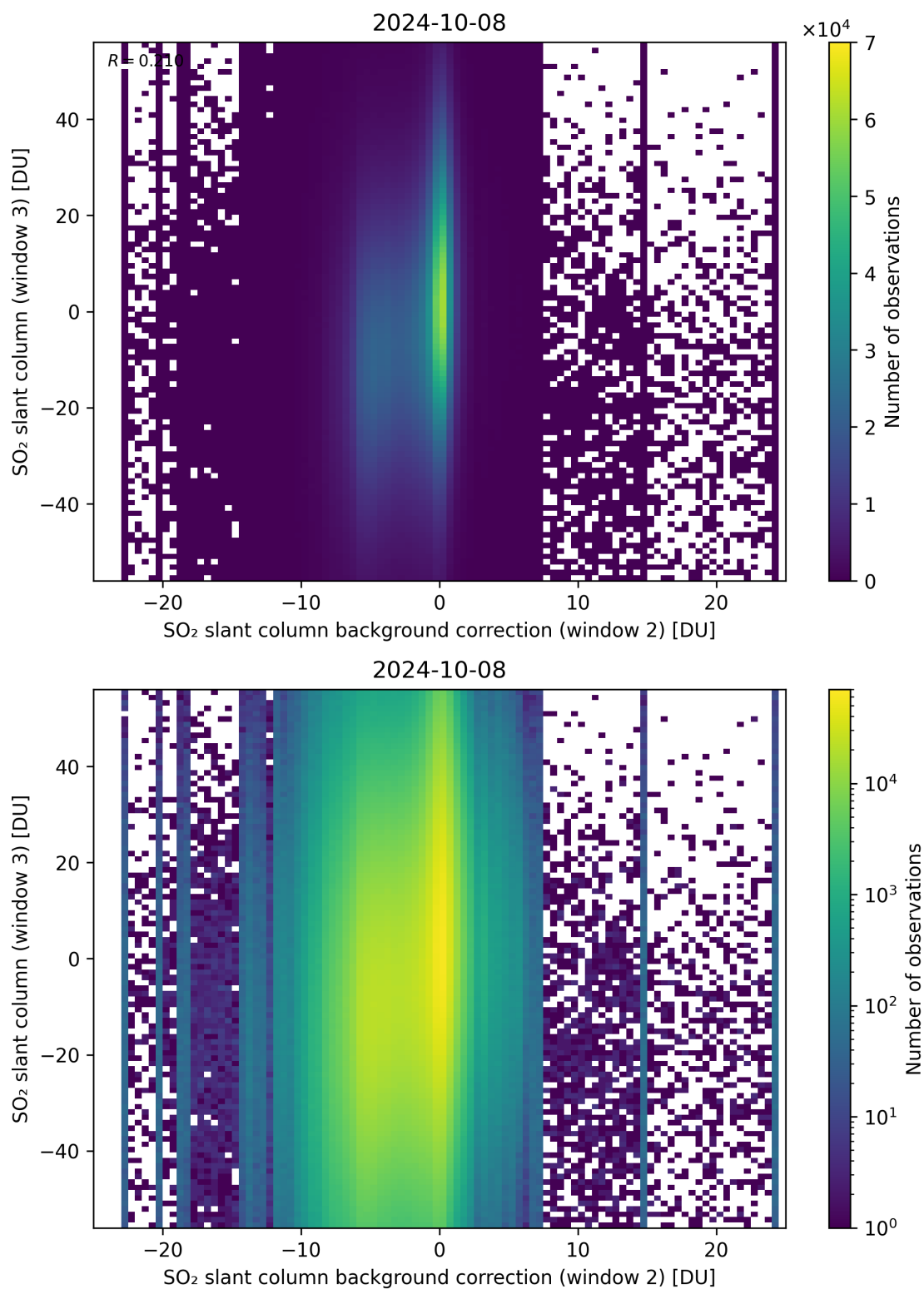
Figure 117: Scatter density plot of “SO 2 slant column background correction (window 2)” against “SO 2 slant column (window 3)” for 2024-10-08 to 2024-10-09.
