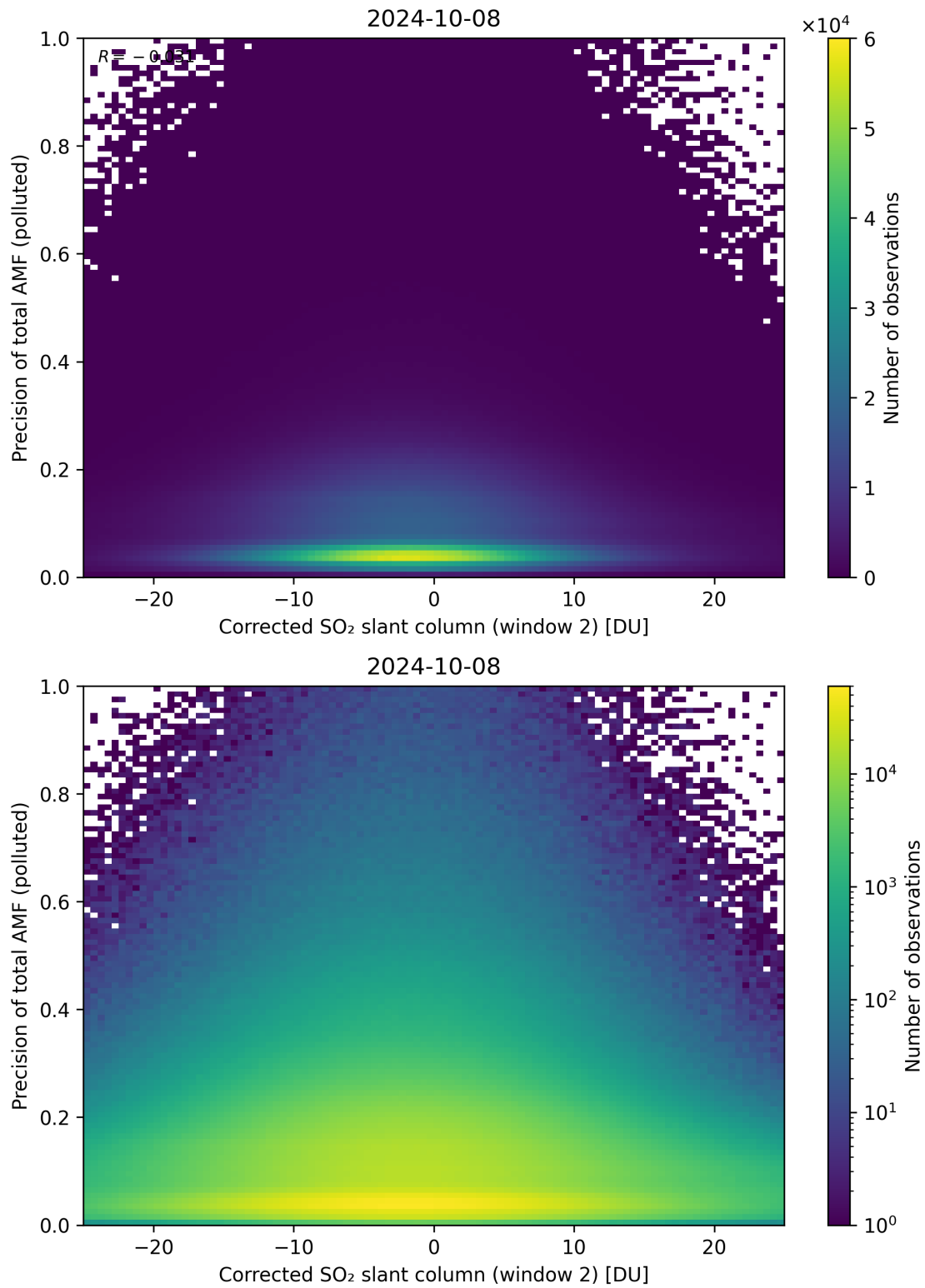
Figure 204: Scatter density plot of “Corrected SO 2 slant column (window 2)” against “Precision of total AMF (polluted)” for 2024-10-08 to 2024-10-09.
