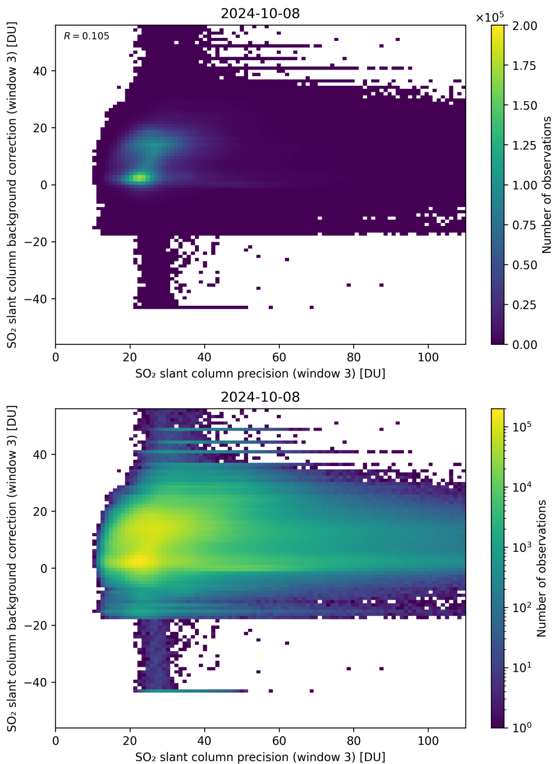
Figure 257: Scatter density plot of “SO 2 slant column precision (window 3)” against “SO 2 slant column background correction (window 3)” for 2024-10-08 to 2024-10-09.
