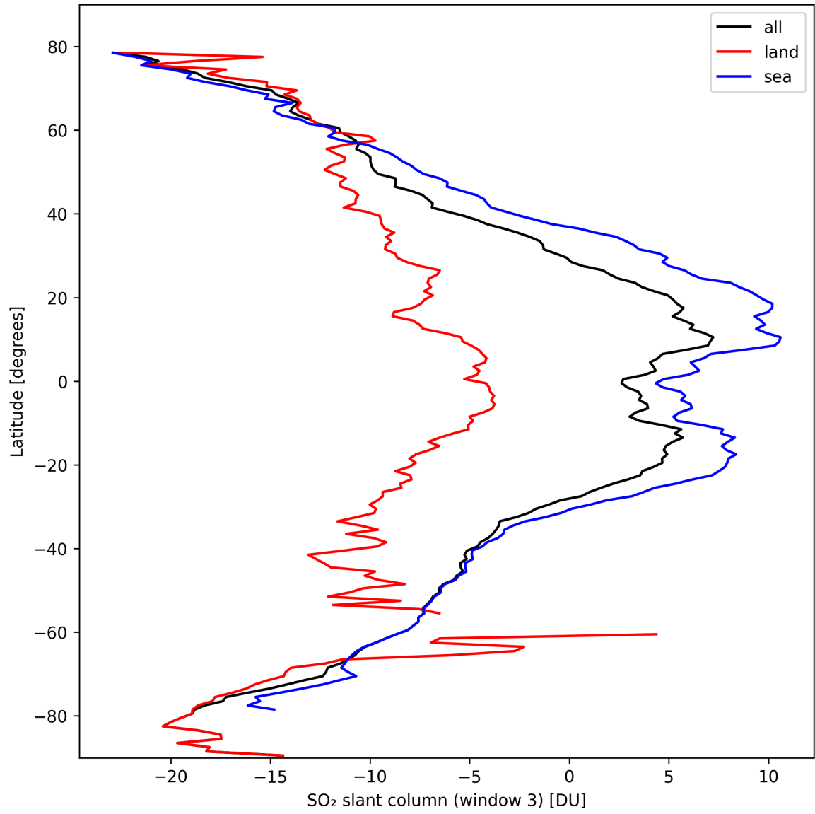
Figure 41: Zonal average of “SO 2 slant column (window 3)” for 2024-10-08 to 2024-10-09.
