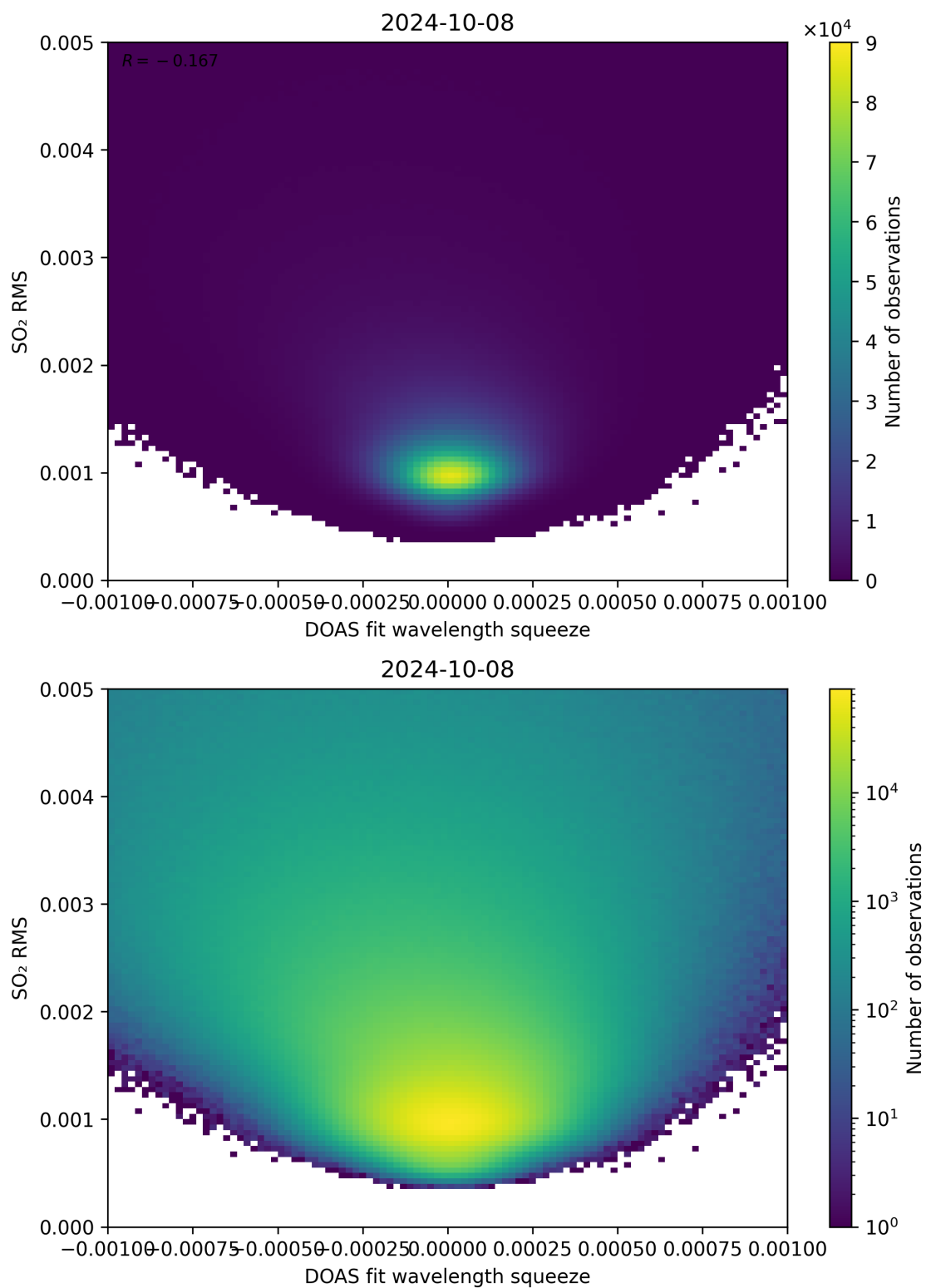
Figure 132: Scatter density plot of “DOAS fit wavelength squeeze” against “SO 2 RMS” for 2024-10-08 to 2024-10-09.
