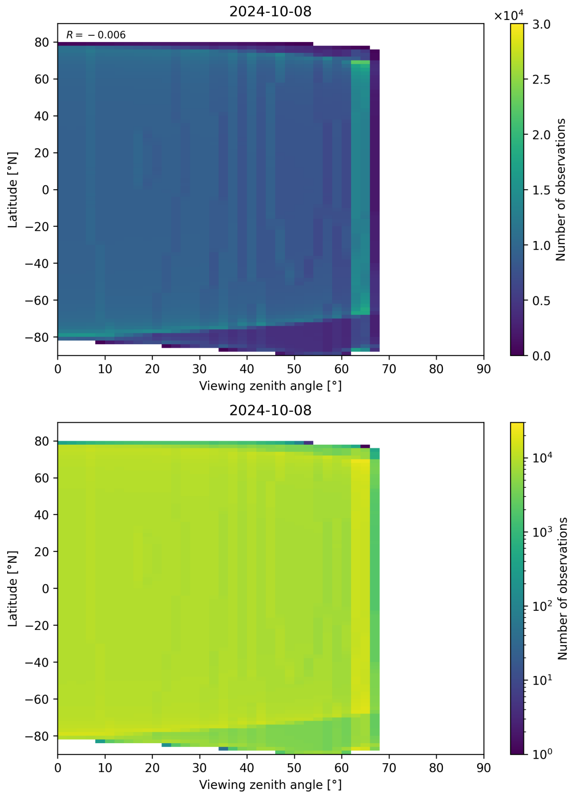
Figure 314: Scatter density plot of “Viewing zenith angle” against “Latitude” for 2024-10-08 to 2024-10-09.
