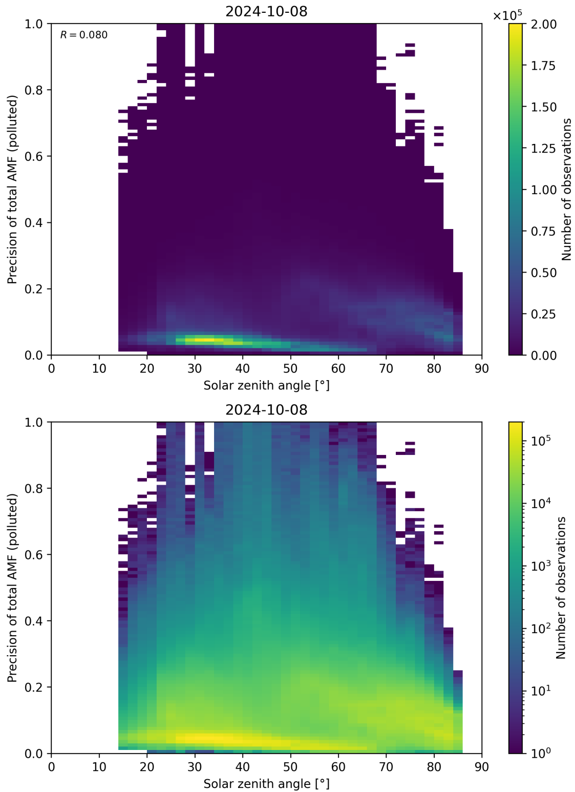
Figure 175: Scatter density plot of “Solar zenith angle” against “Precision of total AMF (polluted)” for 2024-10-08 to 2024-10-09.
