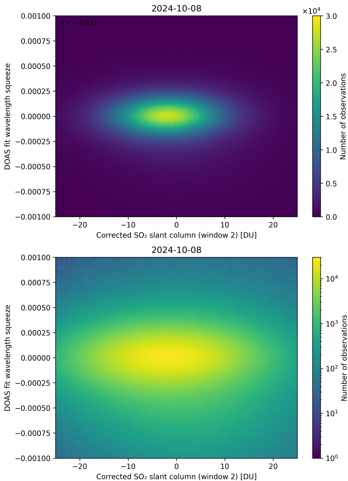
Figure 197: Scatter density plot of “Corrected SO 2 slant column (window 2)” against “DOAS fit wavelength squeeze” for 2024-10-08 to 2024-10-09.
