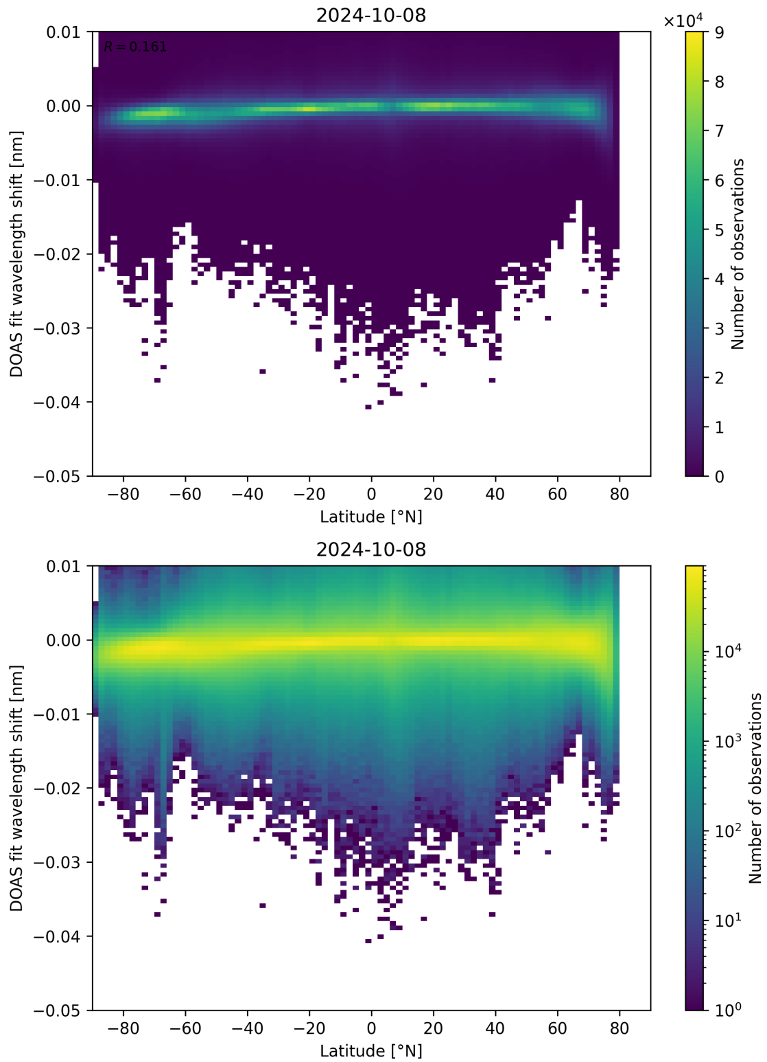
Figure 142: Scatter density plot of “Latitude” against “DOAS fit wavelength shift” for 2024-10-08 to 2024-10-09.
