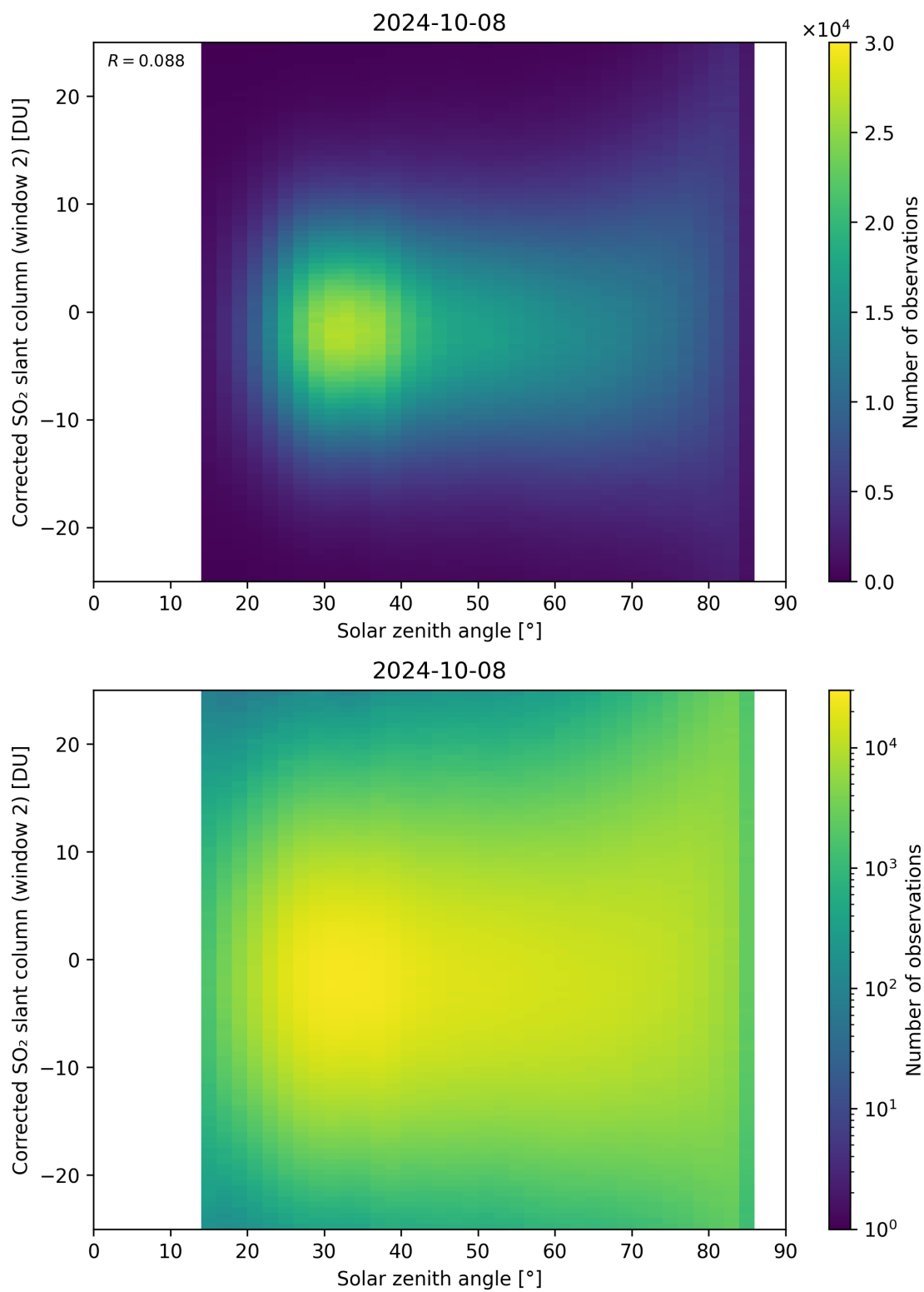
Figure 167: Scatter density plot of “Solar zenith angle” against “Corrected SO 2 slant column (window 2)” for 2024-10-08 to 2024-10-09.
