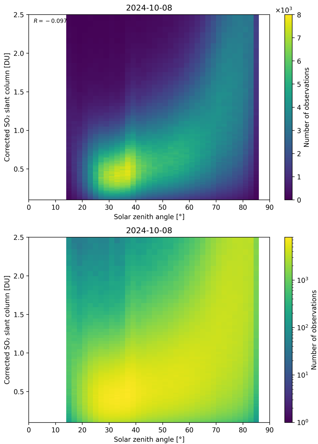
Figure 166: Scatter density plot of “Solar zenith angle” against “Corrected SO 2 slant column” for 2024-10-08 to 2024-10-09.
