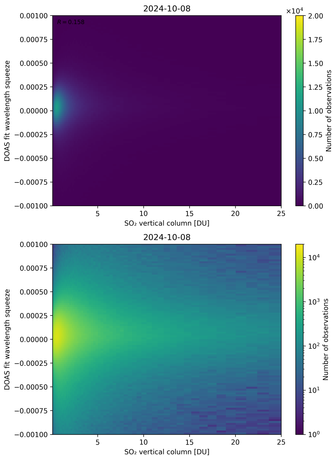
Figure 277: Scatter density plot of “SO 2 vertical column” against “DOAS fit wavelength squeeze” for 2024-10-08 to 2024-10-09.
