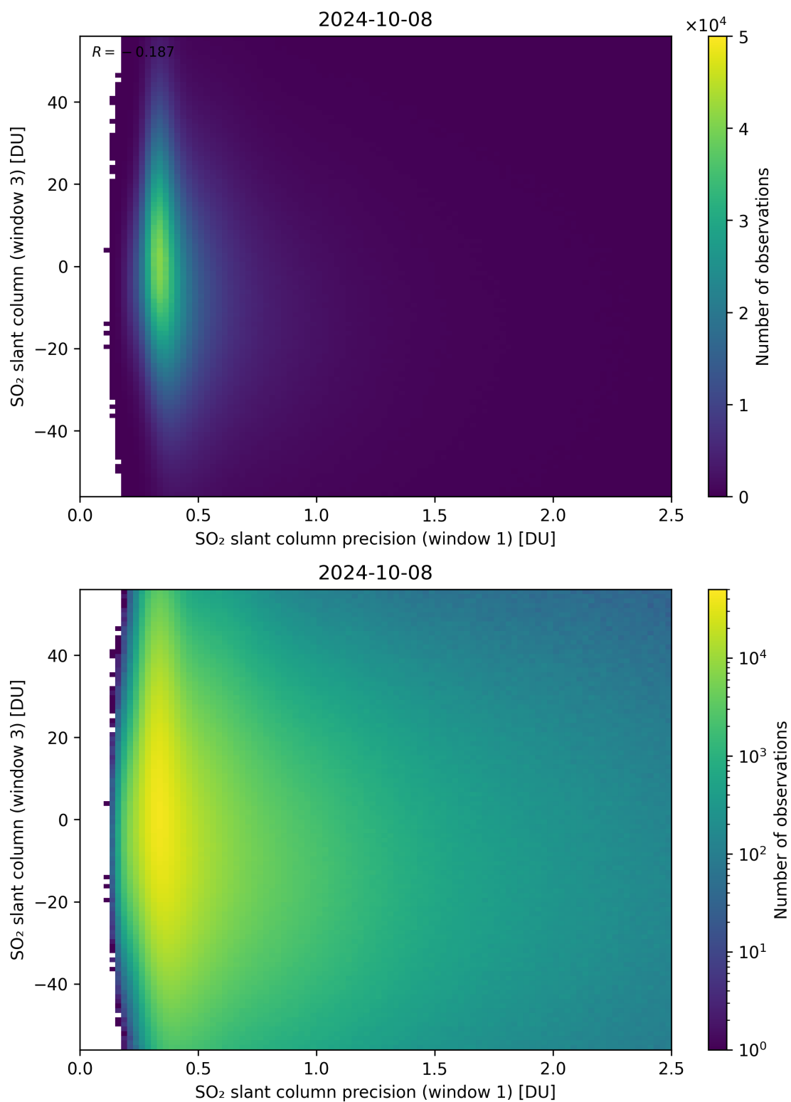
Figure 228: Scatter density plot of “SO 2 slant column precision (window 1)” against “SO 2 slant column (window 3)” for 2024-10-08 to 2024-10-09.
