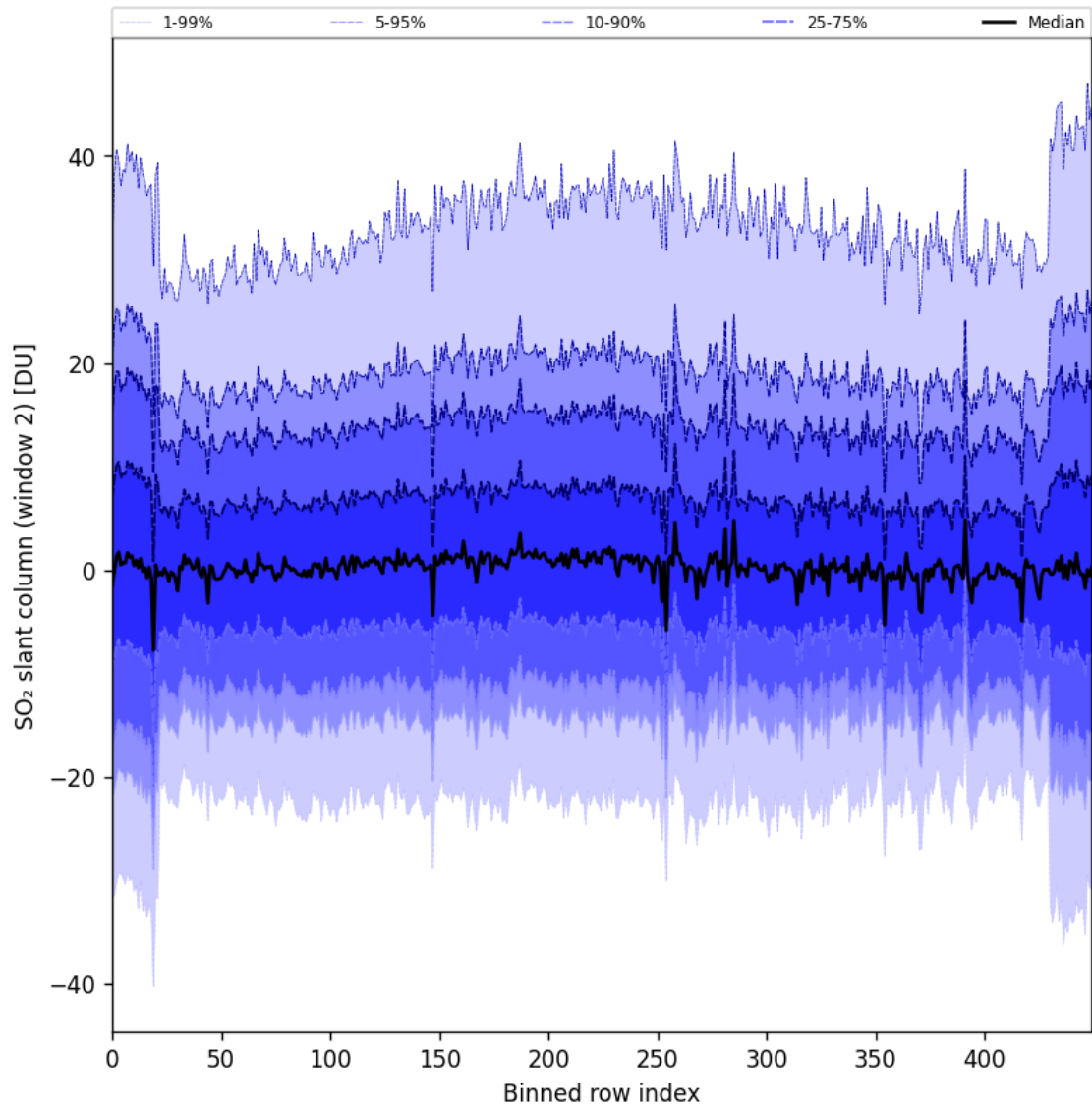
Figure 83: Along track statistics of “SO 2 slant column (window 2)” for 2024-10-08 to 2024-10-09
