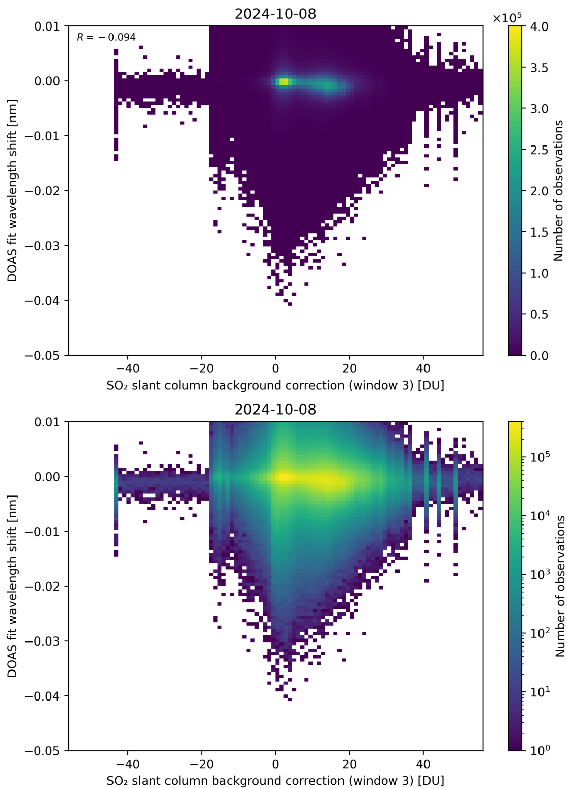
Figure 121: Scatter density plot of “SO 2 slant column background correction (window 3)” against “DOAS fit wavelength shift” for 2024-10-08 to 2024-10-09.
