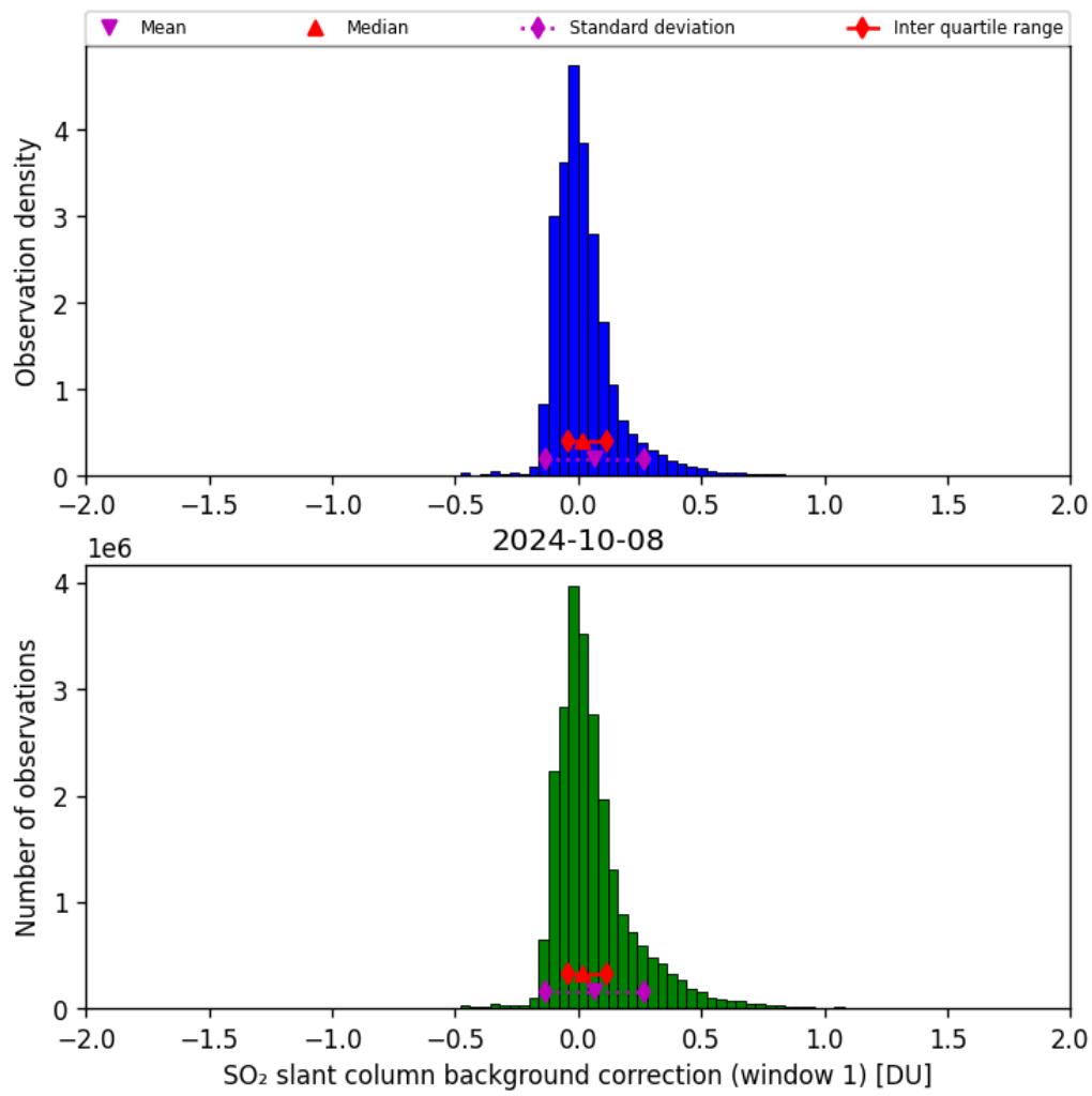
Figure 59: Histogram of “SO 2 slant column background correction (window 1)” for 2024-10-08 to 2024-10-09
