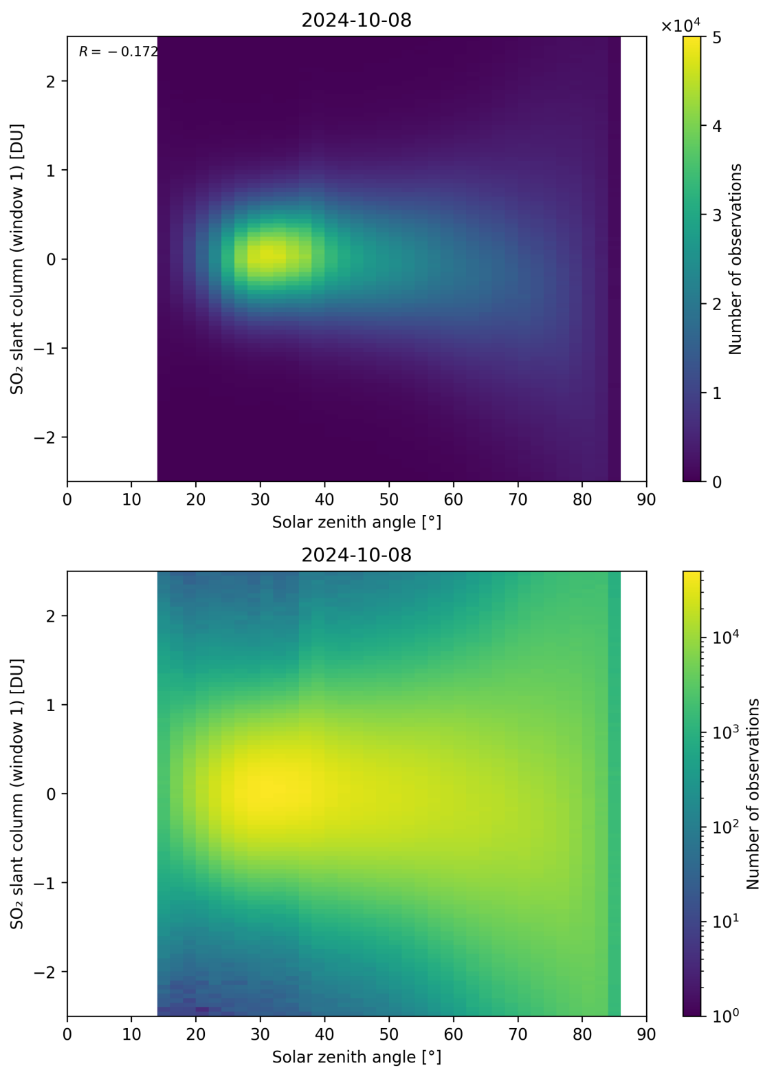
Figure 169: Scatter density plot of “Solar zenith angle” against “SO 2 slant column (window 1)” for 2024-10-08 to 2024-10-09.
