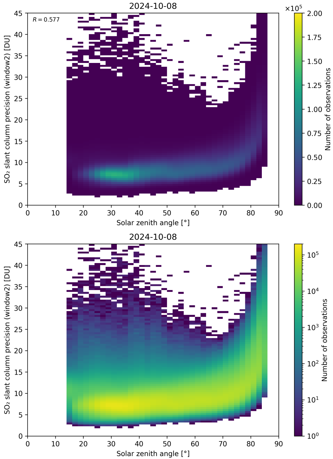
Figure 171: Scatter density plot of “Solar zenith angle” against “SO 2 slant column precision (window2)” for 2024-10-08 to 2024-10-09.
