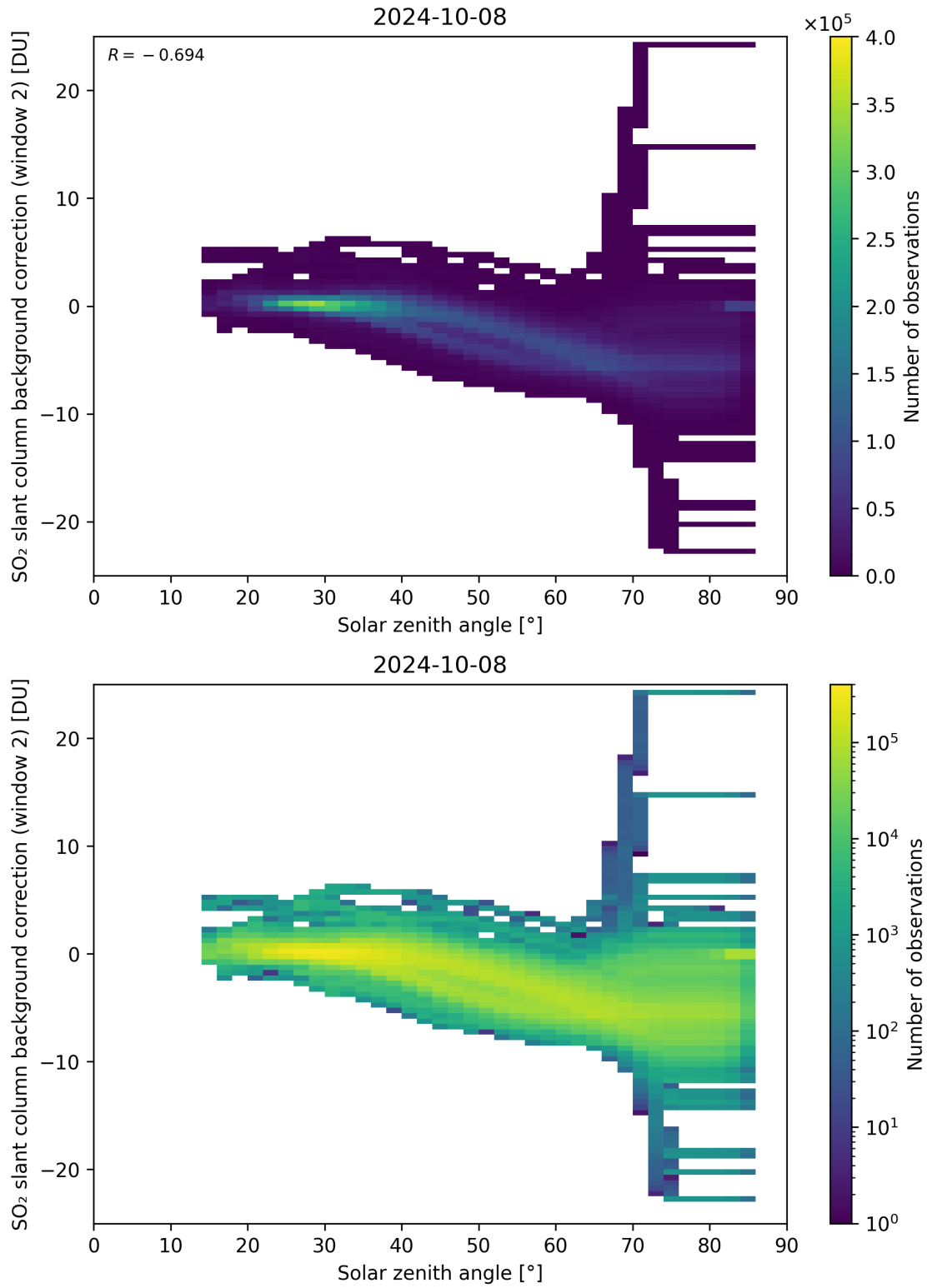
Figure 159: Scatter density plot of “Solar zenith angle” against “SO 2 slant column background correction (window 2)” for 2024-10-08 to 2024-10-09.
