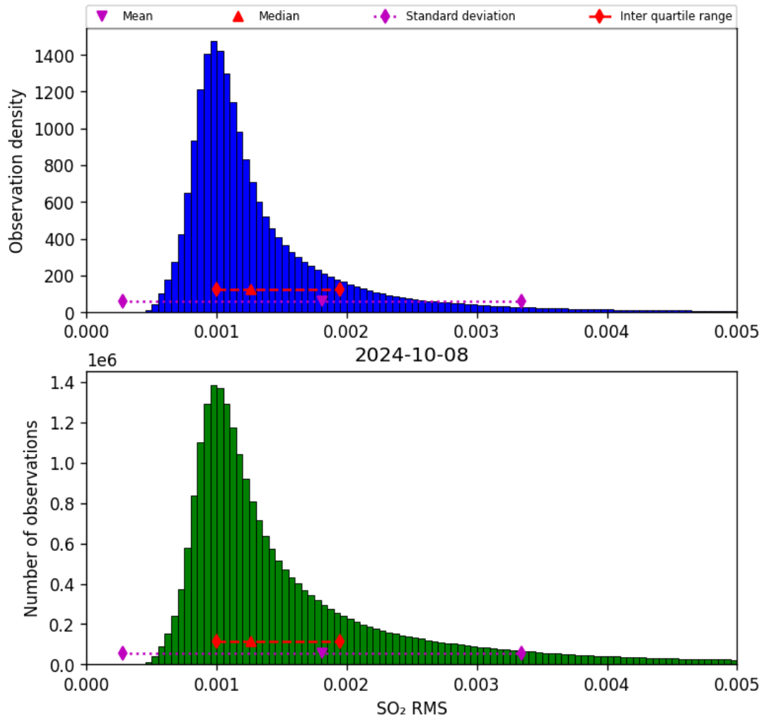
Figure 70: Histogram of “SO 2 RMS” for 2024-10-08 to 2024-10-09
