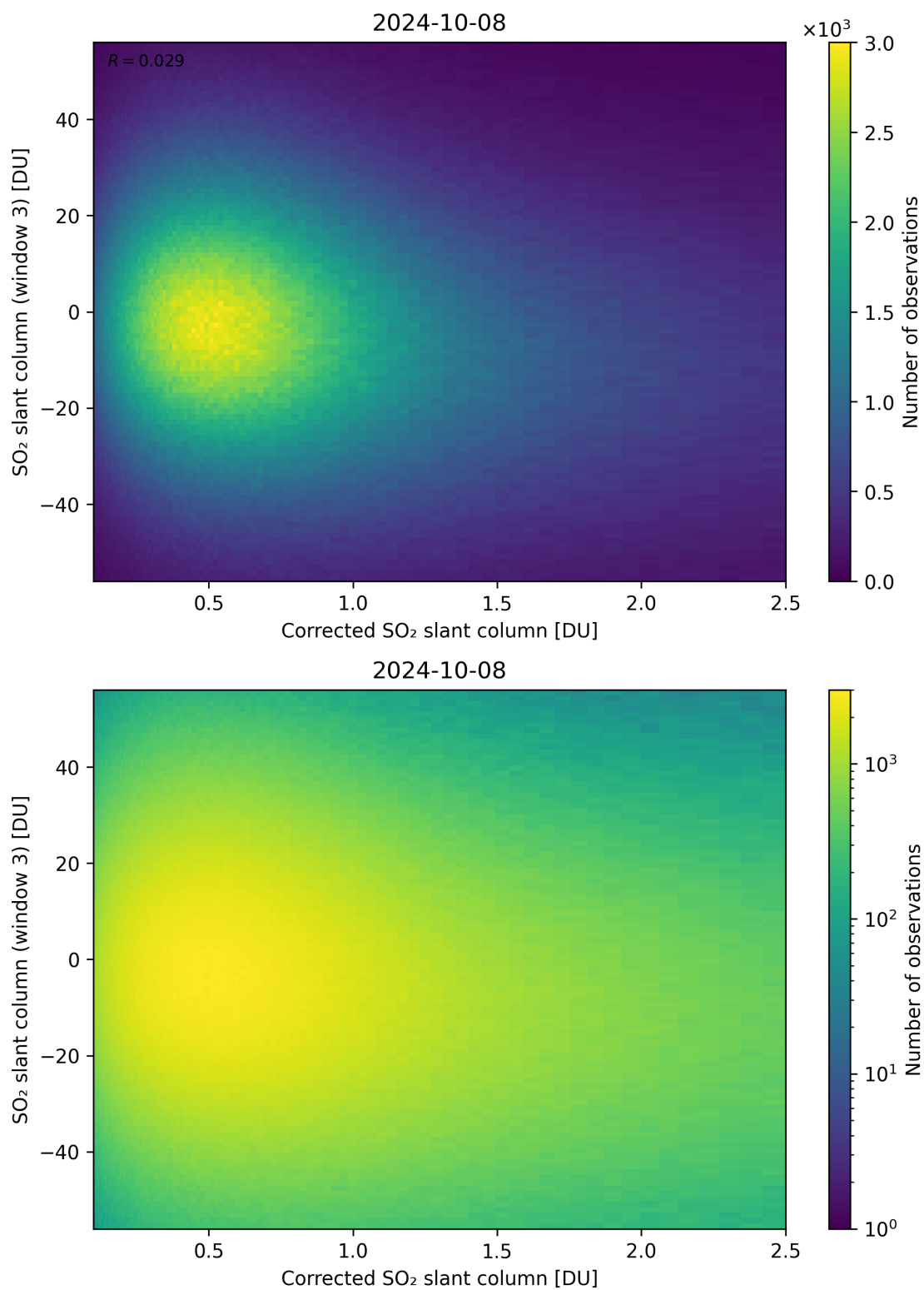
Figure 190: Scatter density plot of “Corrected SO 2 slant column” against “SO 2 slant column (window 3)” for 2024-10-08 to 2024-10-09.
