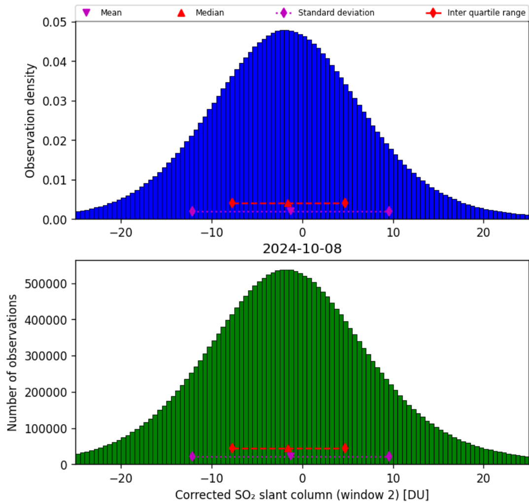
Figure 62: Histogram of “Corrected SO 2 slant column (window 2)” for 2024-10-08 to 2024-10-09
