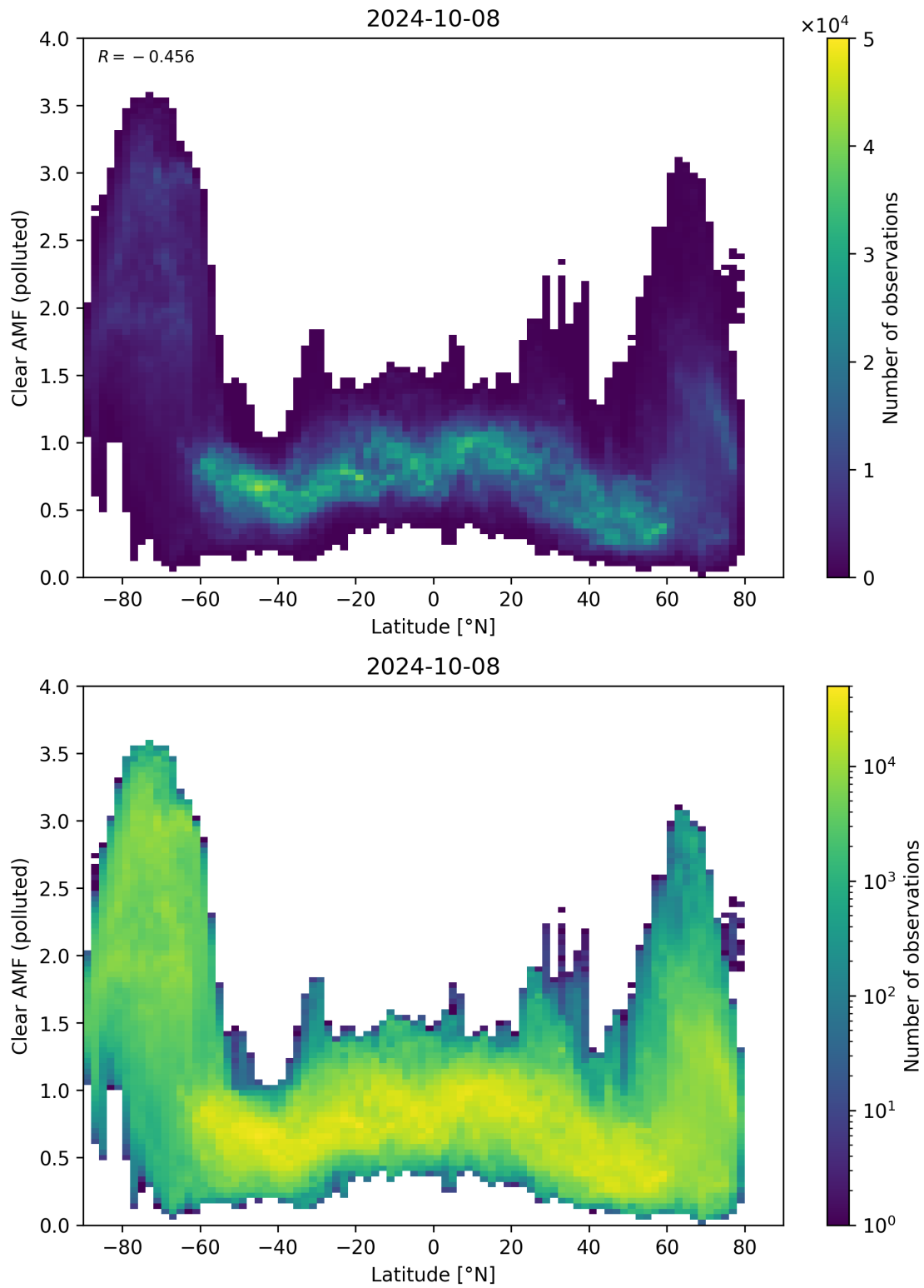
Figure 145: Scatter density plot of “Latitude” against “Clear AMF (polluted)” for 2024-10-08 to 2024-10-09.
