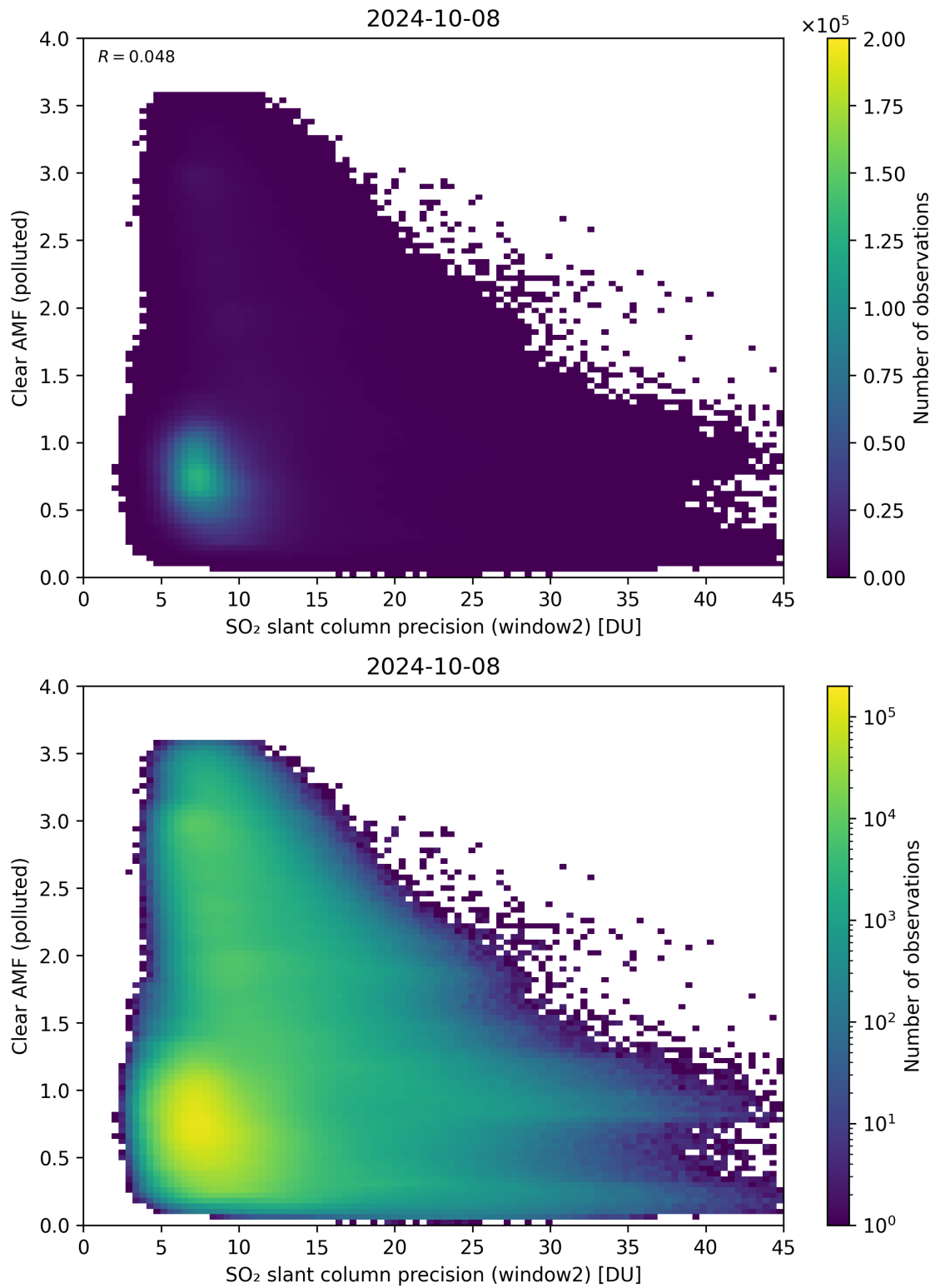
Figure 246: Scatter density plot of “SO 2 slant column precision (window2)” against “Clear AMF (polluted)” for 2024-10-08 to 2024-10-09.
