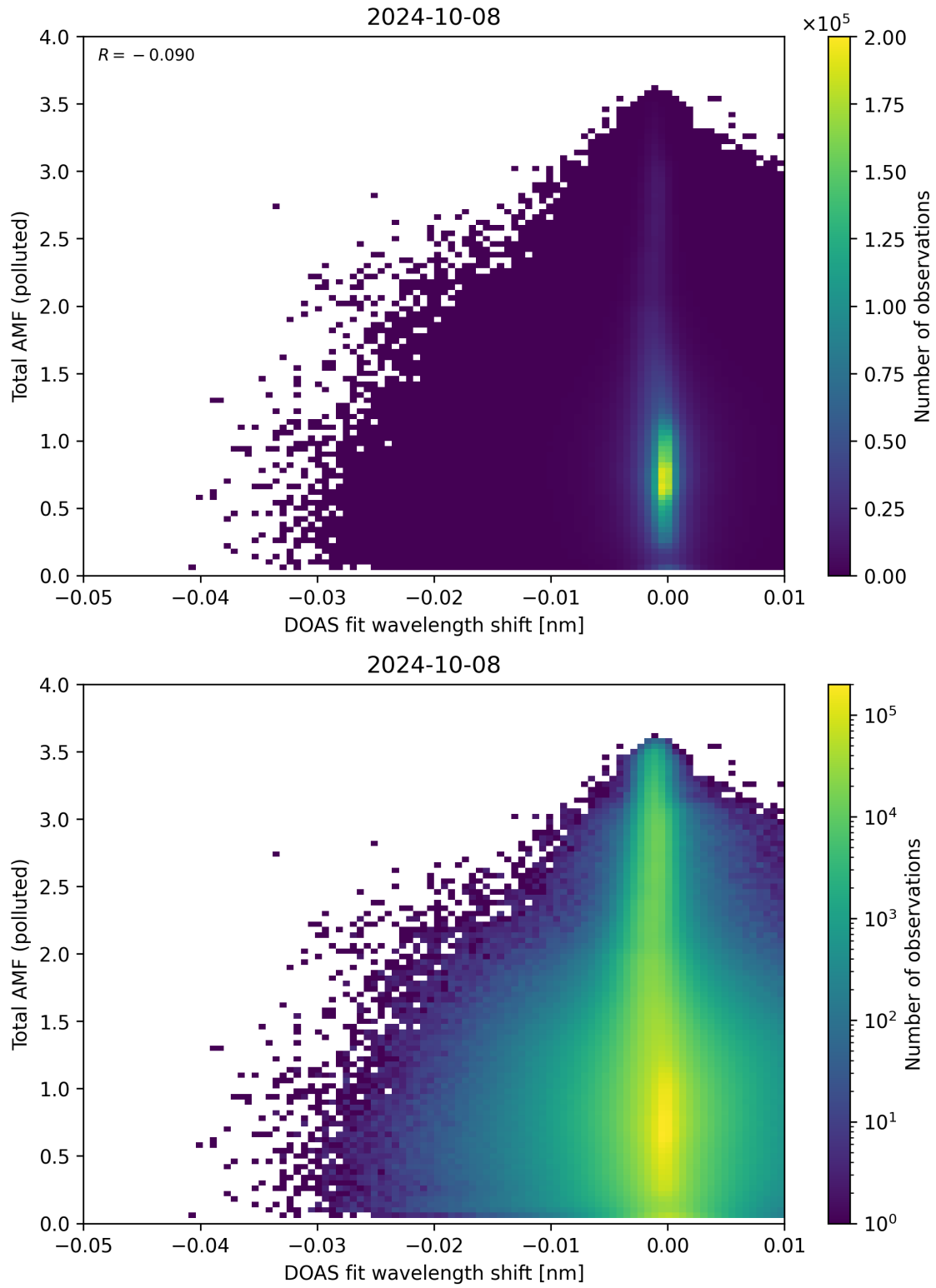
Figure 130: Scatter density plot of “DOAS fit wavelength shift” against “Total AMF (polluted)” for 2024-10-08 to 2024-10-09.
