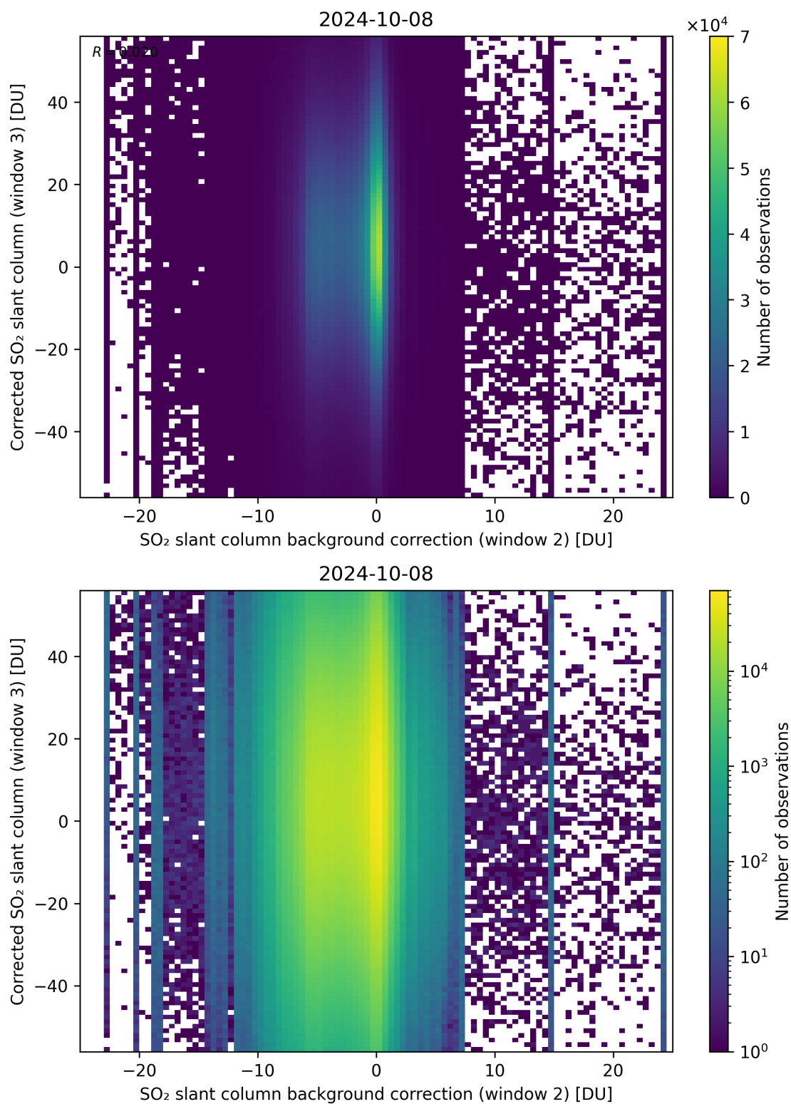
Figure 116: Scatter density plot of “SO 2 slant column background correction (window 2)” against “Corrected SO 2 slant column (window 3)” for 2024-10-08 to 2024-10-09.
