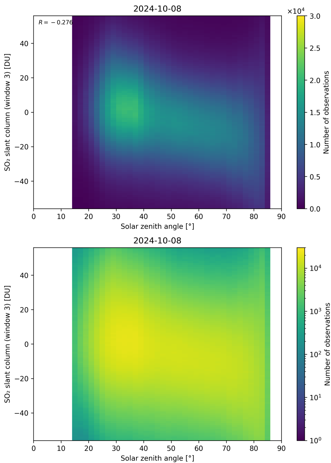
Figure 172: Scatter density plot of “Solar zenith angle” against “SO 2 slant column (window 3)” for 2024-10-08 to 2024-10-09.
