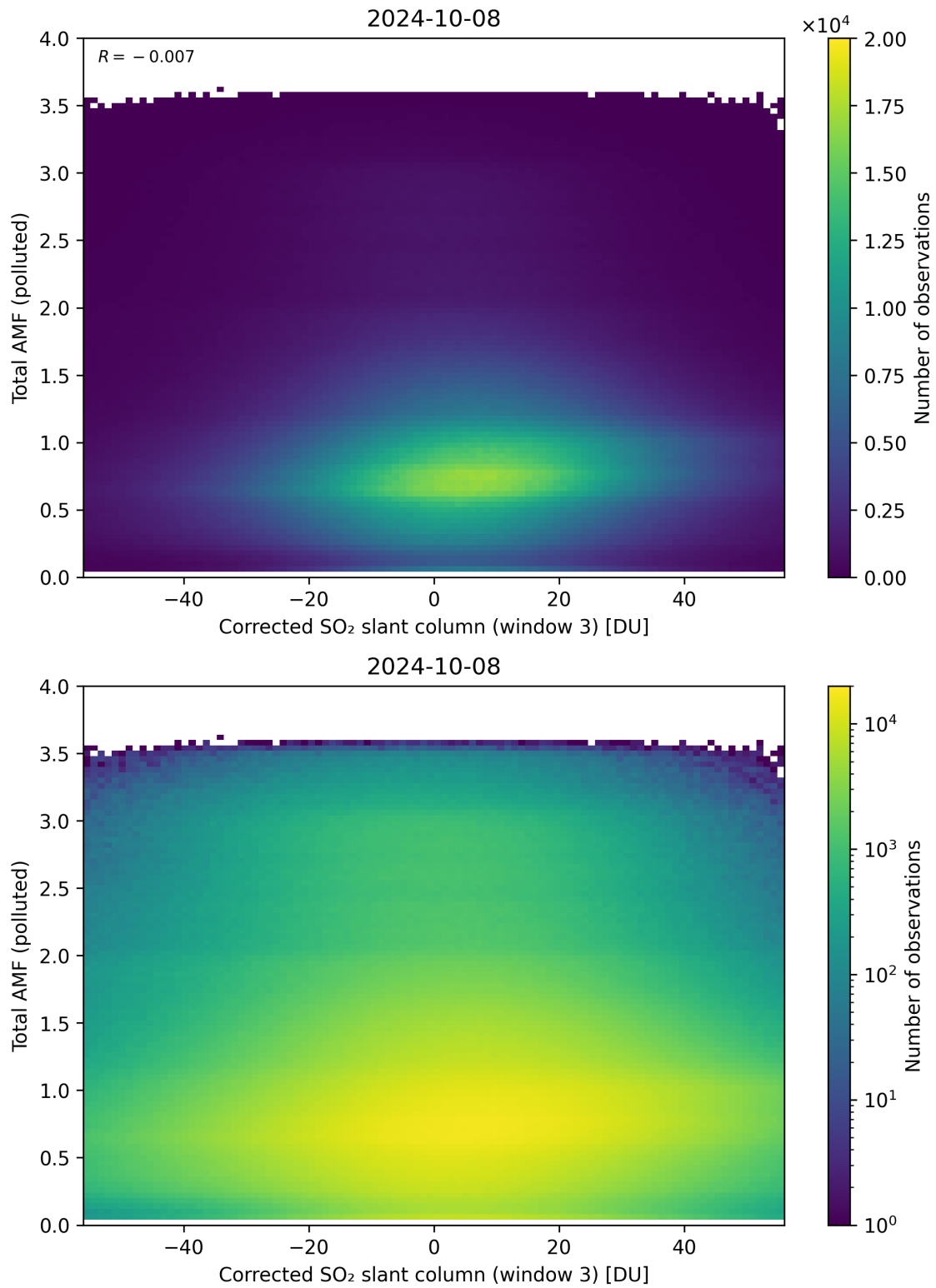
Figure 210: Scatter density plot of “Corrected SO 2 slant column (window 3)” against “Total AMF (polluted)” for 2024-10-08 to 2024-10-09.
