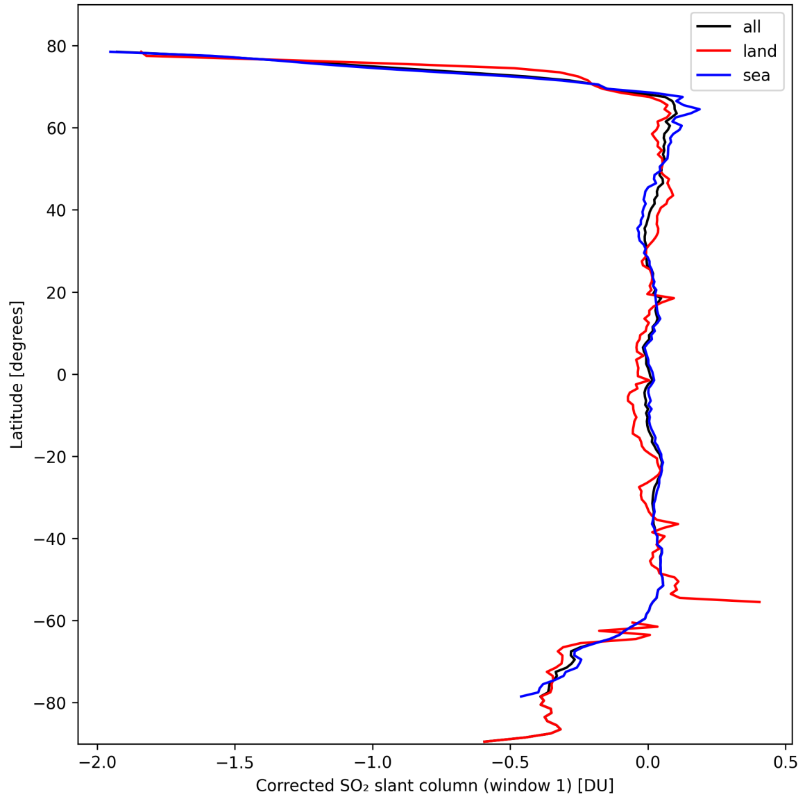
Figure 35: Zonal average of “Corrected SO 2 slant column (window 1)” for 2024-10-08 to 2024-10-09.
