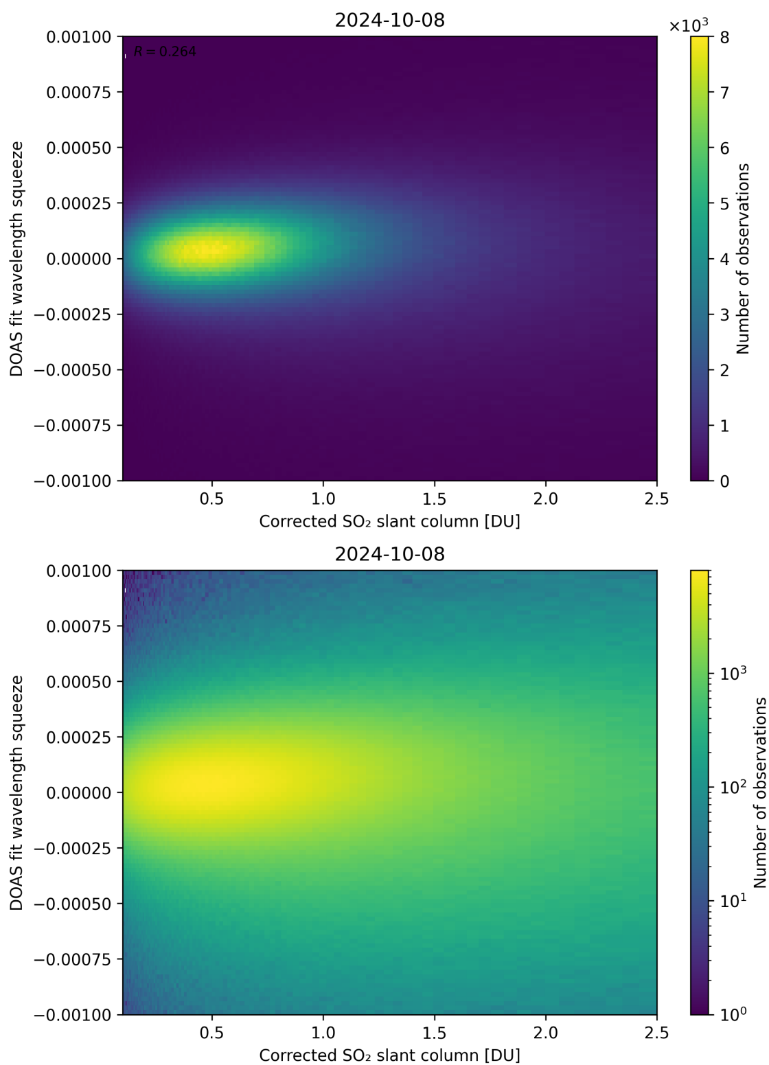
Figure 182: Scatter density plot of “Corrected SO 2 slant column” against “DOAS fit wavelength squeeze” for 2024-10-08 to 2024-10-09.
