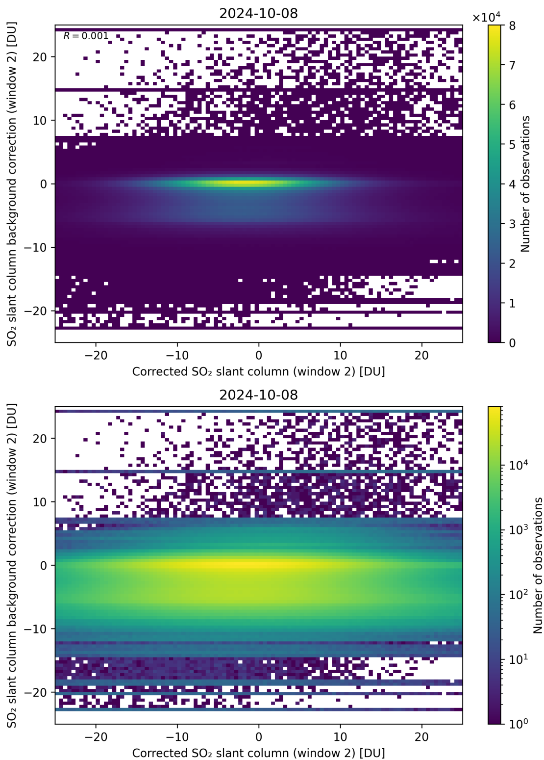
Figure 194: Scatter density plot of “Corrected SO 2 slant column (window 2)” against “SO 2 slant column background correction (window 2)” for 2024-10-08 to 2024-10-09.
