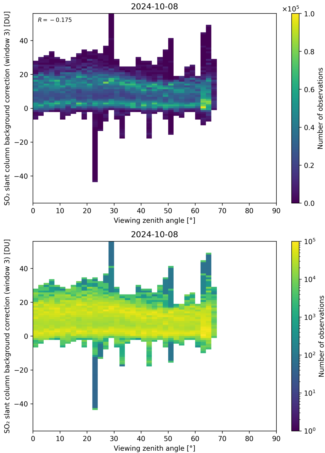
Figure 310: Scatter density plot of “Viewing zenith angle” against “SO 2 slant column background correction (window 3)” for 2024-10-08 to 2024-10-09.
