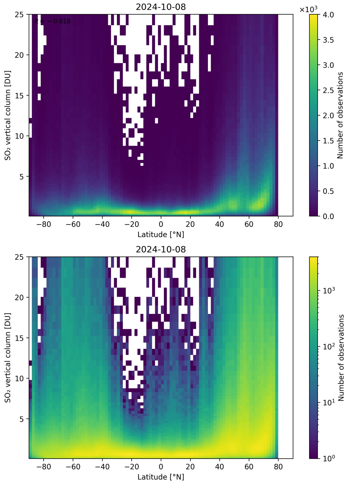
Figure 156: Scatter density plot of “Latitude” against “SO 2 vertical column” for 2024-10-08 to 2024-10-09.
