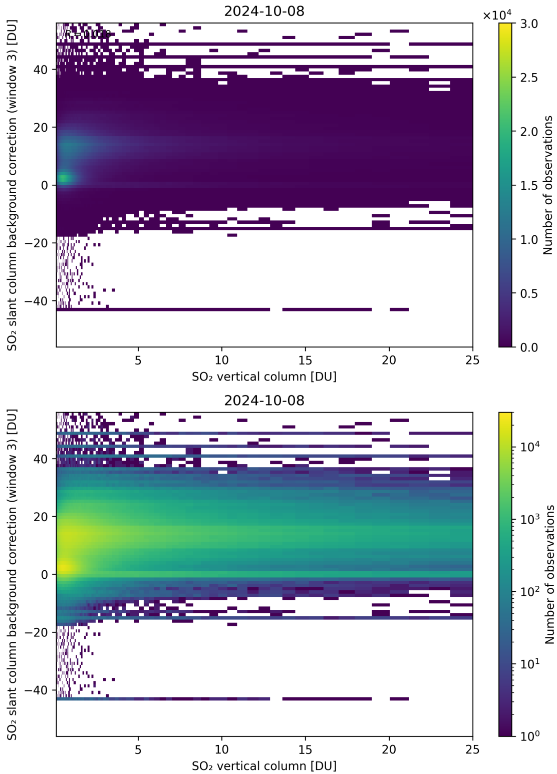
Figure 275: Scatter density plot of “SO 2 vertical column” against “SO 2 slant column background correction (window 3)” for 2024-10-08 to 2024-10-09.
