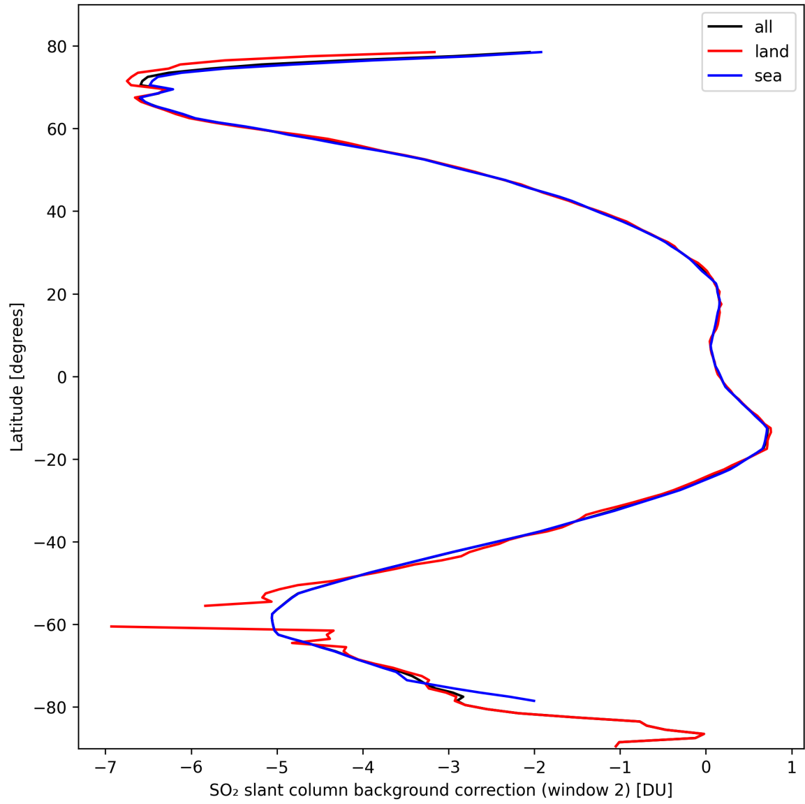
Figure 40: Zonal average of “SO 2 slant column background correction (window 2)” for 2024-10-08 to 2024-10-09.
