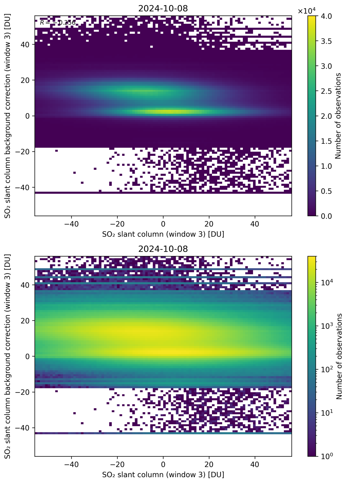
Figure 253: Scatter density plot of “SO 2 slant column (window 3)” against “SO 2 slant column background correction (window 3)” for 2024-10-08 to 2024-10-09.
