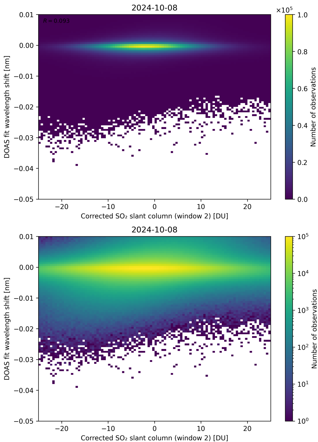
Figure 196: Scatter density plot of “Corrected SO 2 slant column (window 2)” against “DOAS fit wavelength shift” for 2024-10-08 to 2024-10-09.
