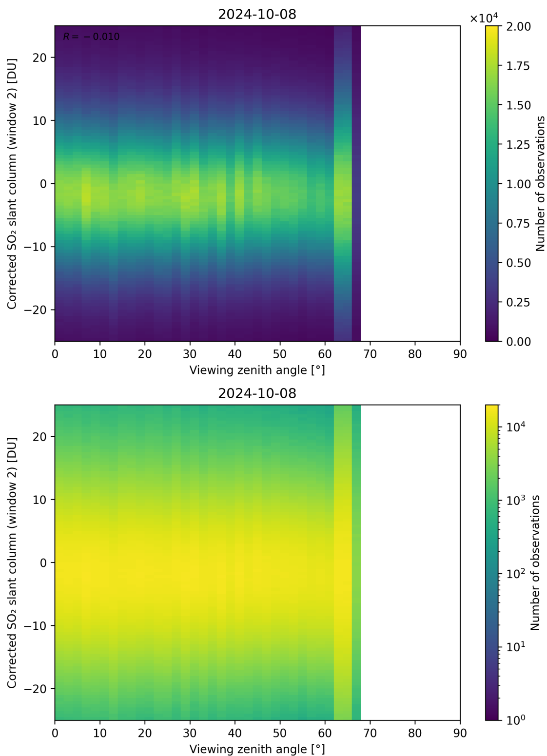
Figure 318: Scatter density plot of “Viewing zenith angle” against “Corrected SO 2 slant column (window 2)” for 2024-10-08 to 2024-10-09.
