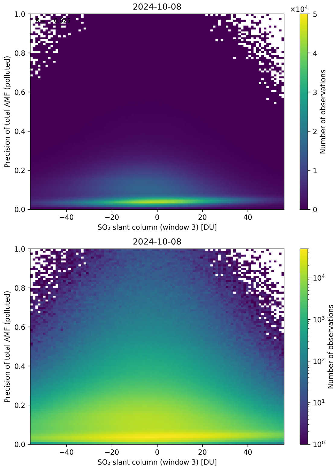
Figure 269: Scatter density plot of “SO 2 slant column (window 3)” against “Precision of total AMF (polluted)” for 2024-10-08 to 2024-10-09.
