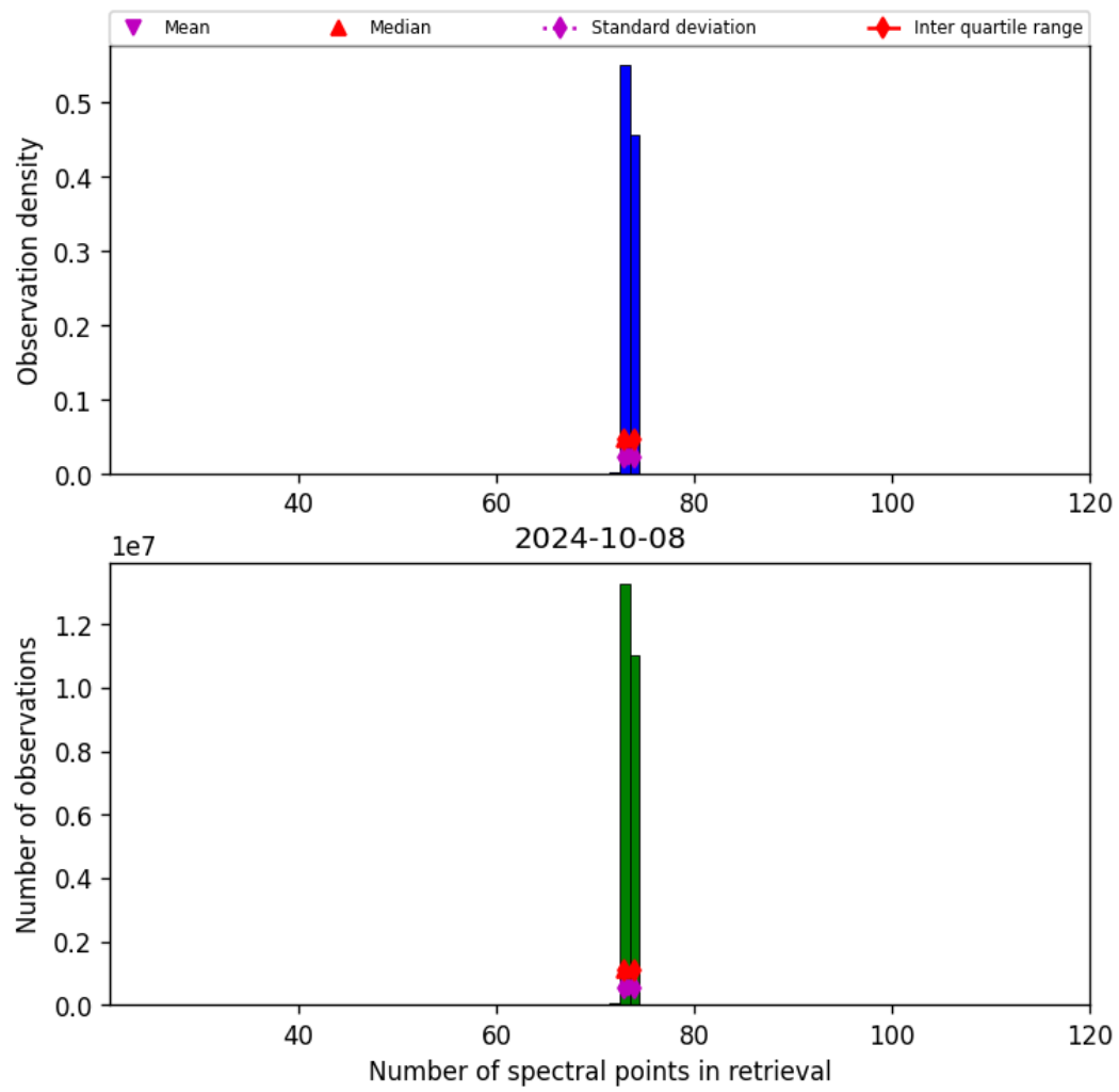
Figure 74: Histogram of “Number of spectral points in retrieval” for 2024-10-08 to 2024-10-09
