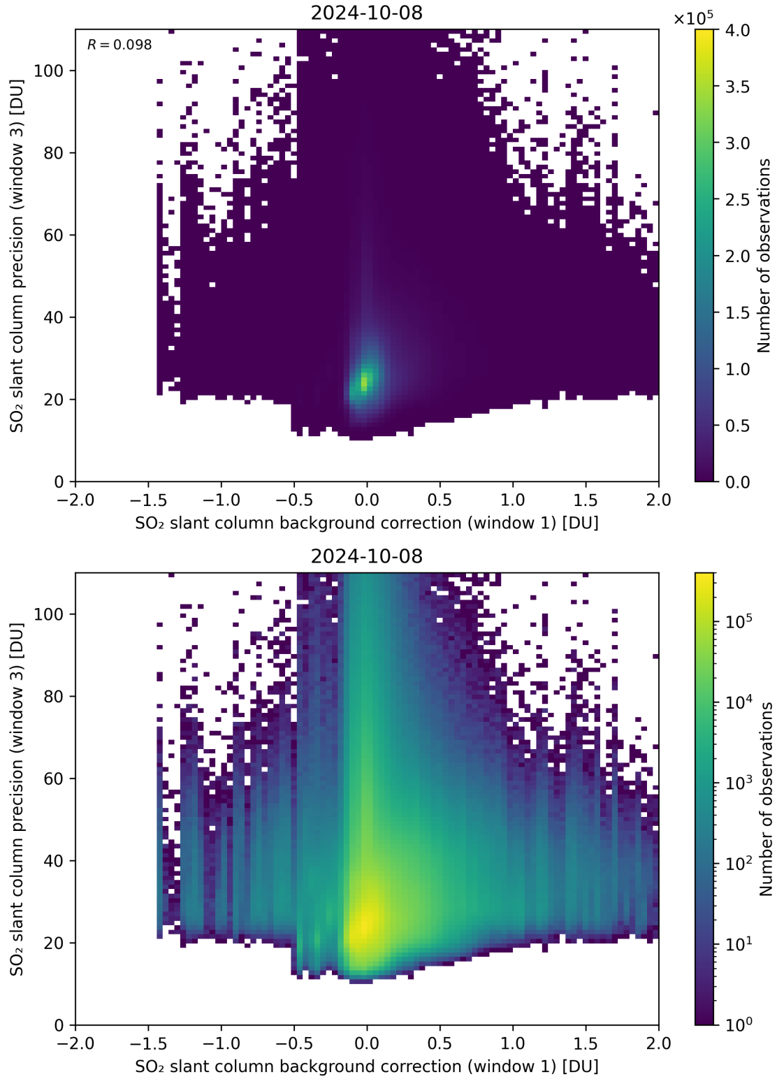
Figure 108: Scatter density plot of “SO 2 slant column background correction (window 1)” against “SO 2 slant column precision (window 3)” for 2024-10-08 to 2024-10-09.
