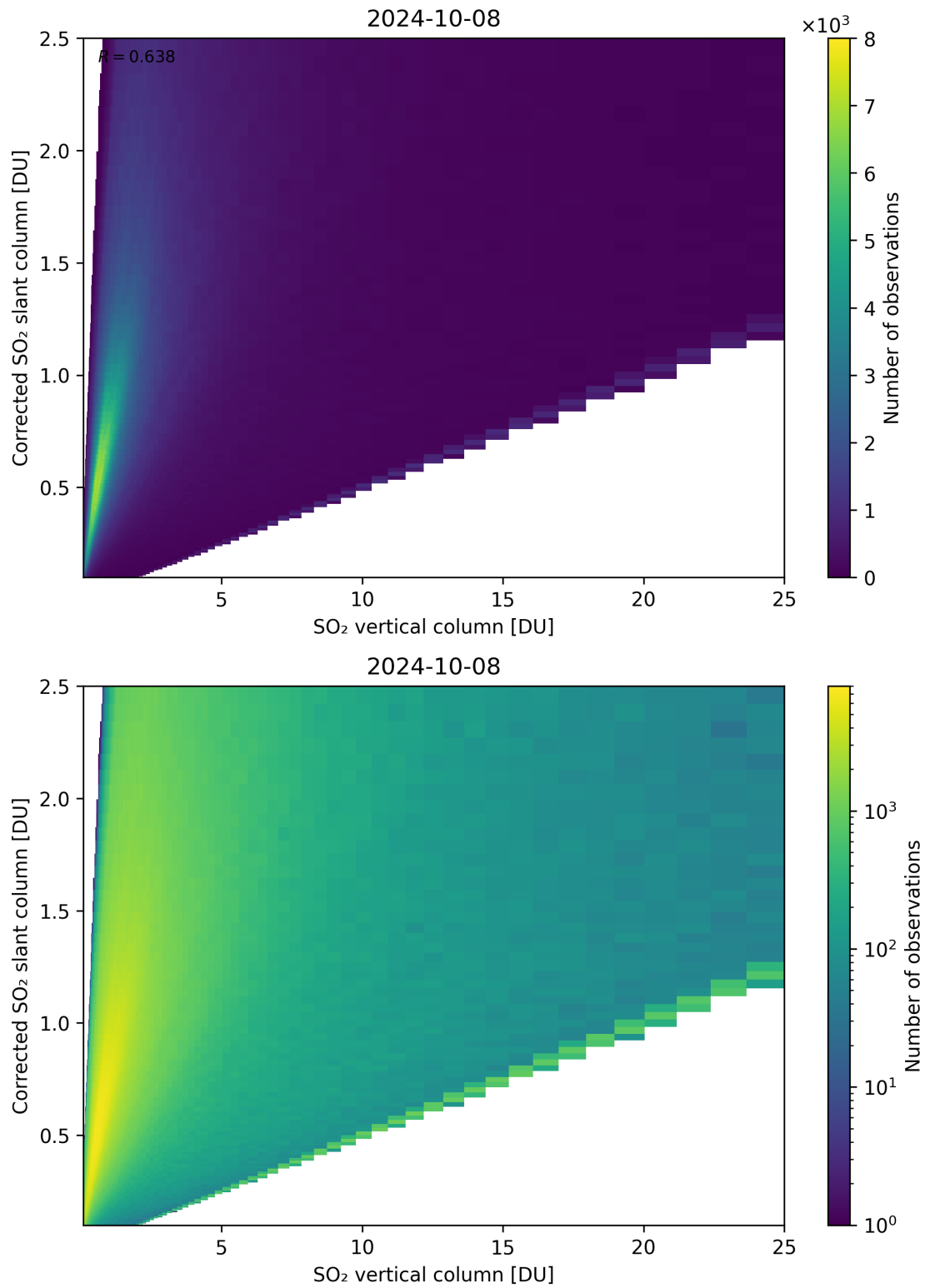
Figure 297: Scatter density plot of “SO 2 vertical column” against “Corrected SO 2 slant column” for 2024-10-08 to 2024-10-09.
