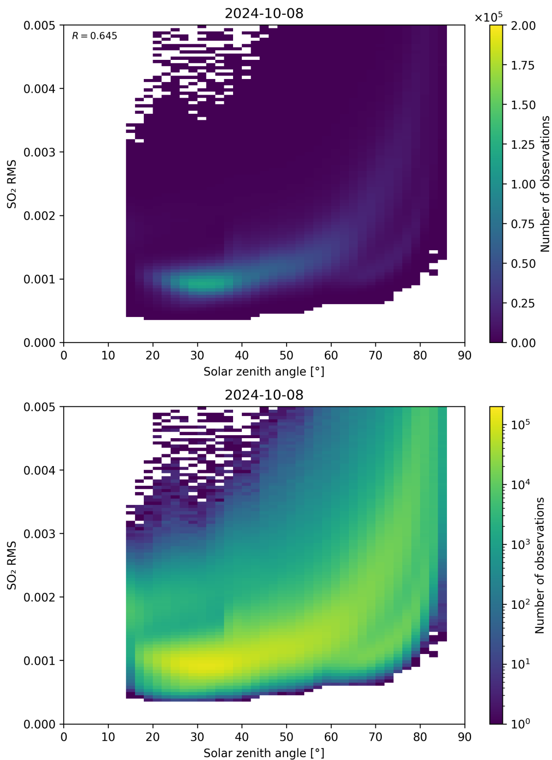
Figure 163: Scatter density plot of “Solar zenith angle” against “SO 2 RMS” for 2024-10-08 to 2024-10-09.
