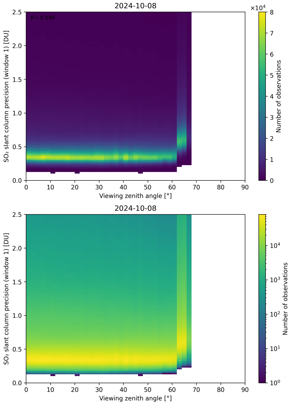
Figure 321: Scatter density plot of “Viewing zenith angle” against “SO 2 slant column precision (window 1)” for 2024-10-08 to 2024-10-09.
