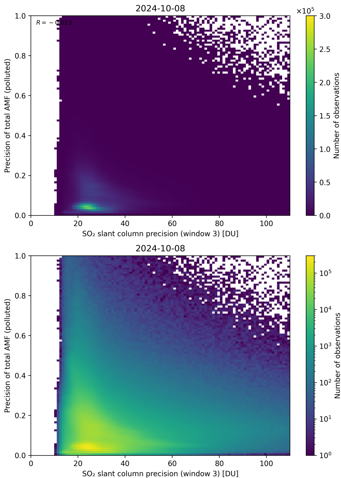
Figure 264: Scatter density plot of “SO 2 slant column precision (window 3)” against “Precision of total AMF (polluted)” for 2024-10-08 to 2024-10-09.
