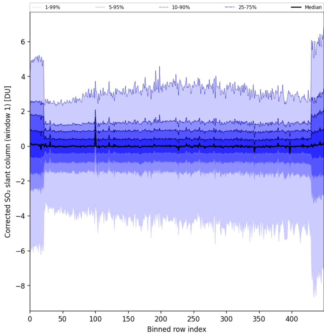
Figure 81: Along track statistics of “Corrected SO 2 slant column (window 1)” for 2024-10-08 to 2024-10-09
