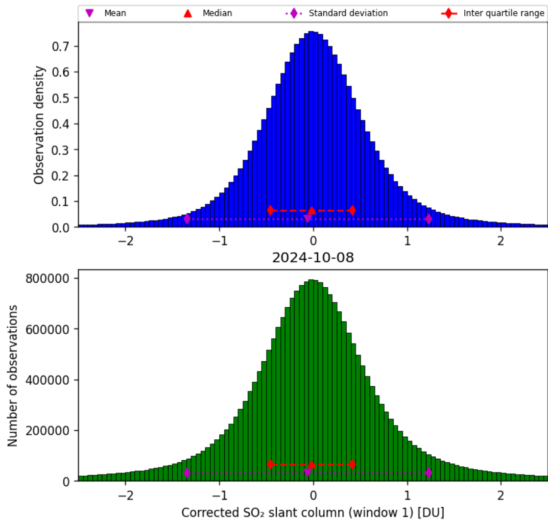
Figure 58: Histogram of “Corrected SO 2 slant column (window 1)” for 2024-10-08 to 2024-10-09
