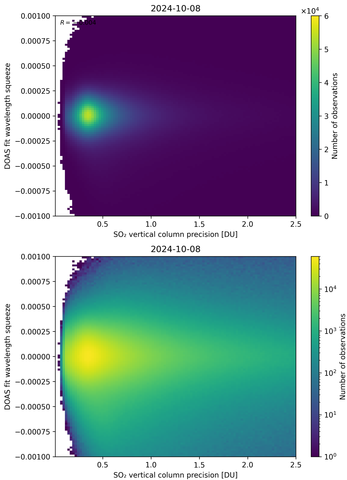
Figure 283: Scatter density plot of “SO 2 vertical column precision” against “DOAS fit wavelength squeeze” for 2024-10-08 to 2024-10-09.
