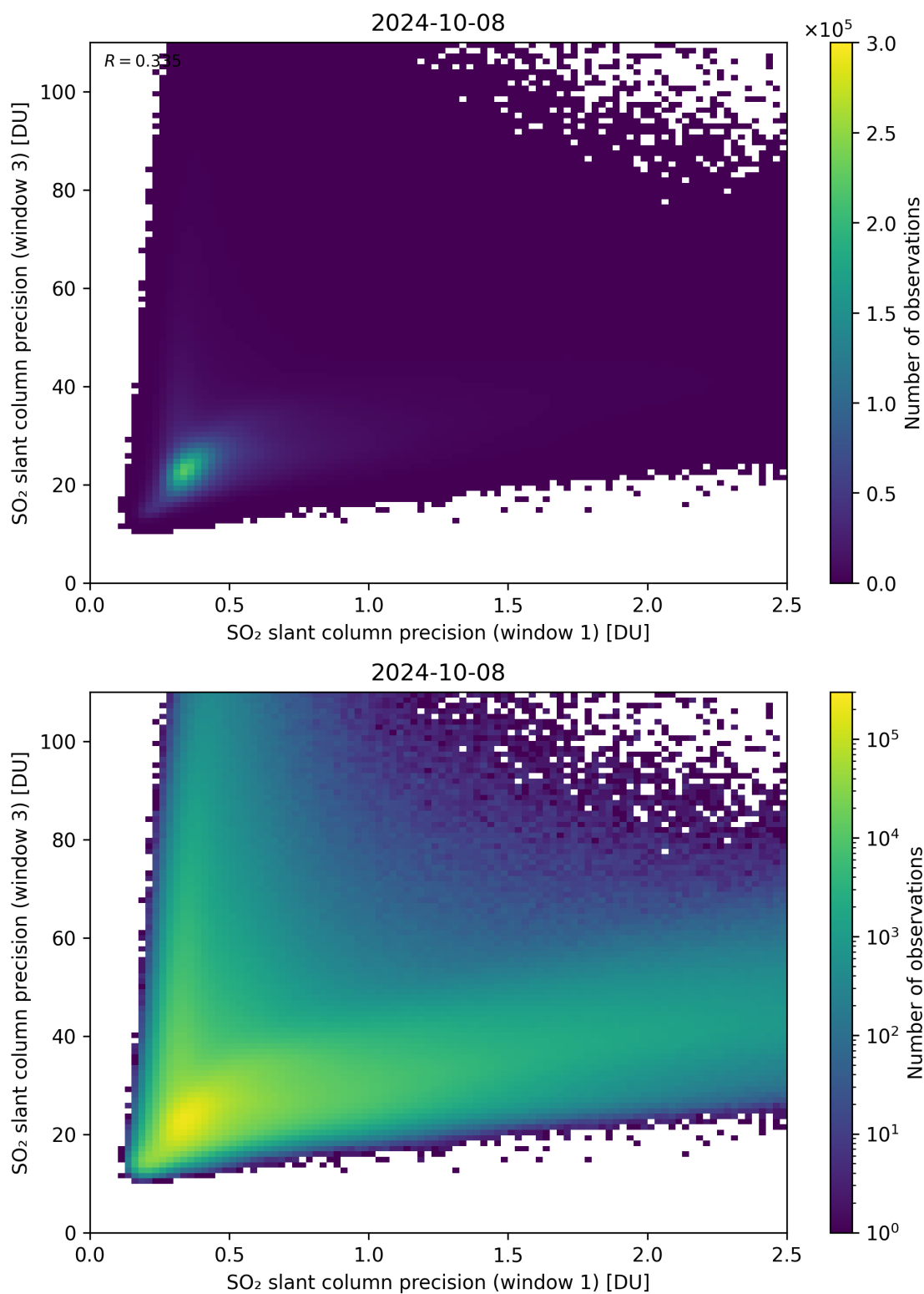
Figure 229: Scatter density plot of “SO 2 slant column precision (window 1)” against “SO 2 slant column precision (window 3)” for 2024-10-08 to 2024-10-09.
