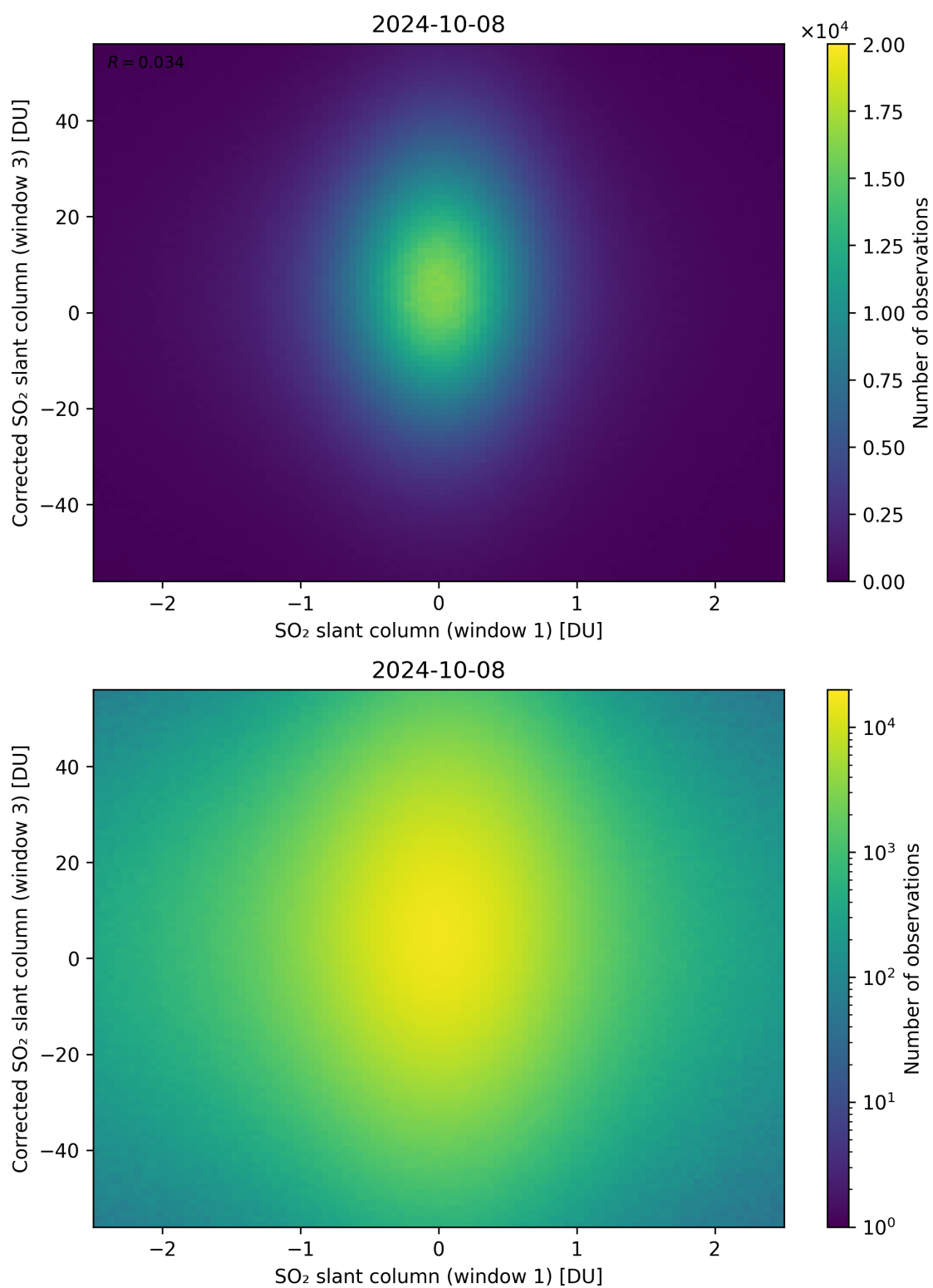
Figure 234: Scatter density plot of “SO 2 slant column (window 1)” against “Corrected SO 2 slant column (window 3)” for 2024-10-08 to 2024-10-09.
