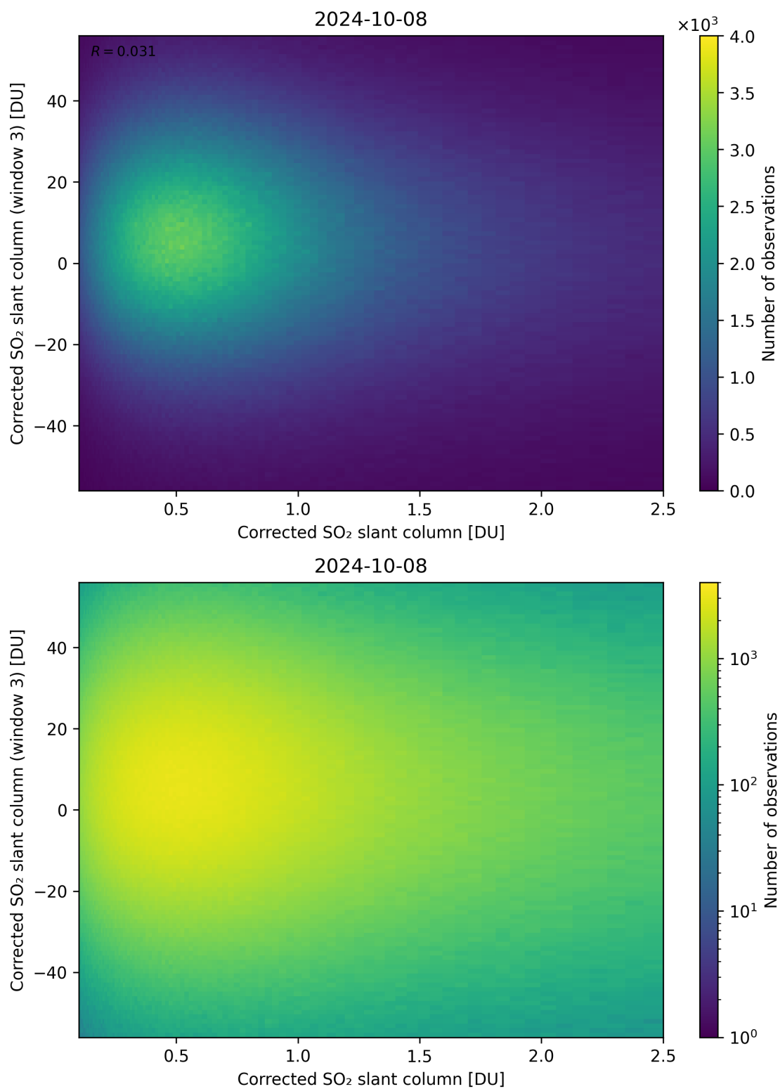
Figure 186: Scatter density plot of “Corrected SO 2 slant column” against “Corrected SO 2 slant column (window 3)” for 2024-10-08 to 2024-10-09.
