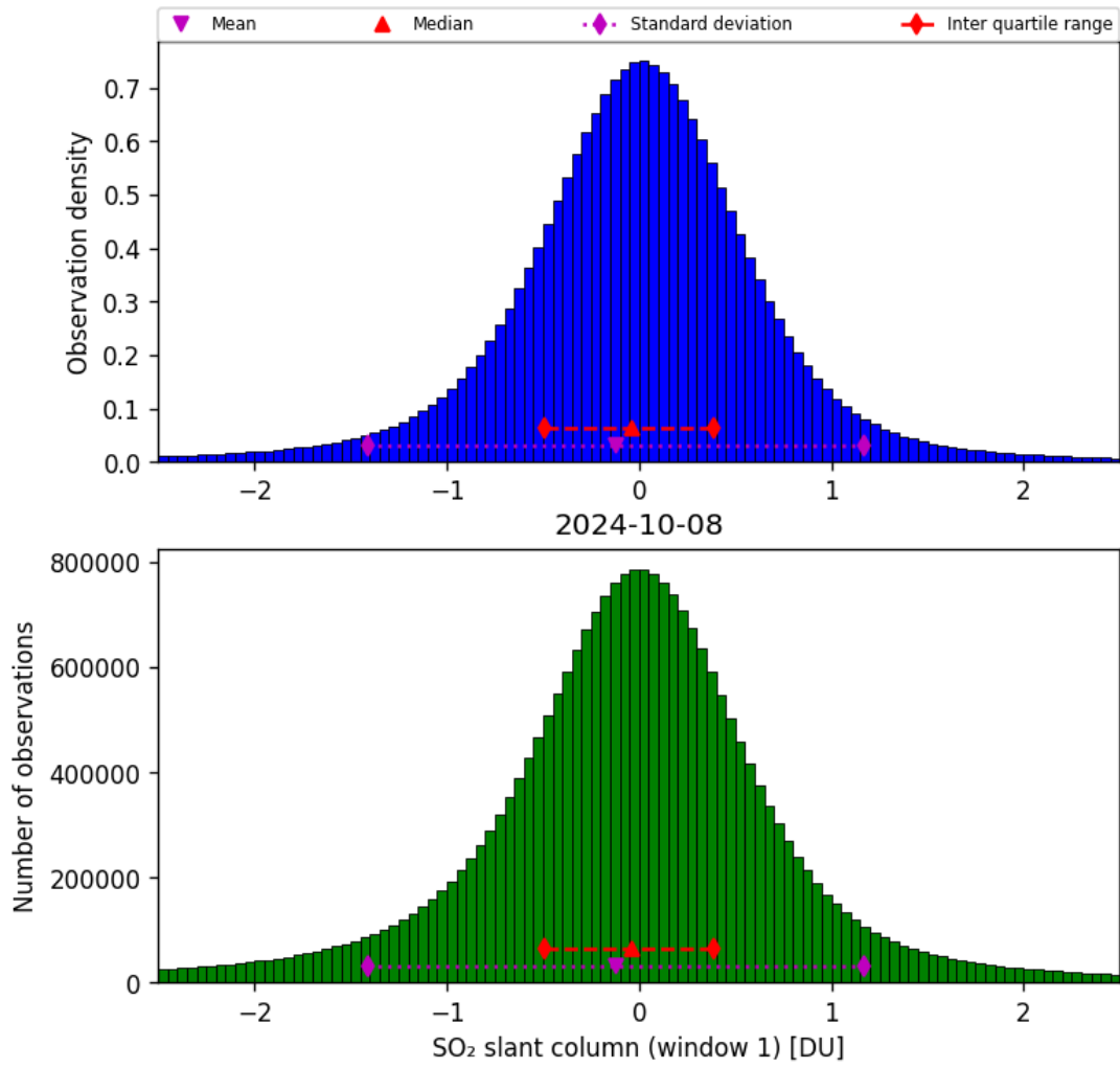
Figure 56: Histogram of “SO 2 slant column (window 1)” for 2024-10-08 to 2024-10-09
