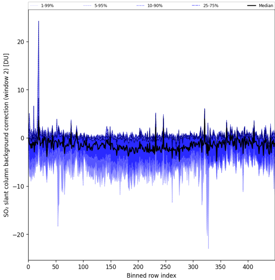
Figure 86: Along track statistics of “SO 2 slant column background correction (window 2)” for 2024-10-08 to 2024-10-09
