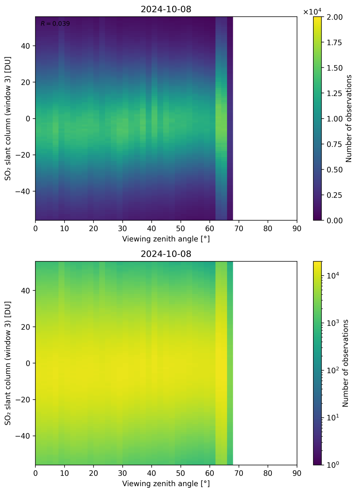
Figure 323: Scatter density plot of “Viewing zenith angle” against “SO 2 slant column (window 3)” for 2024-10-08 to 2024-10-09.
