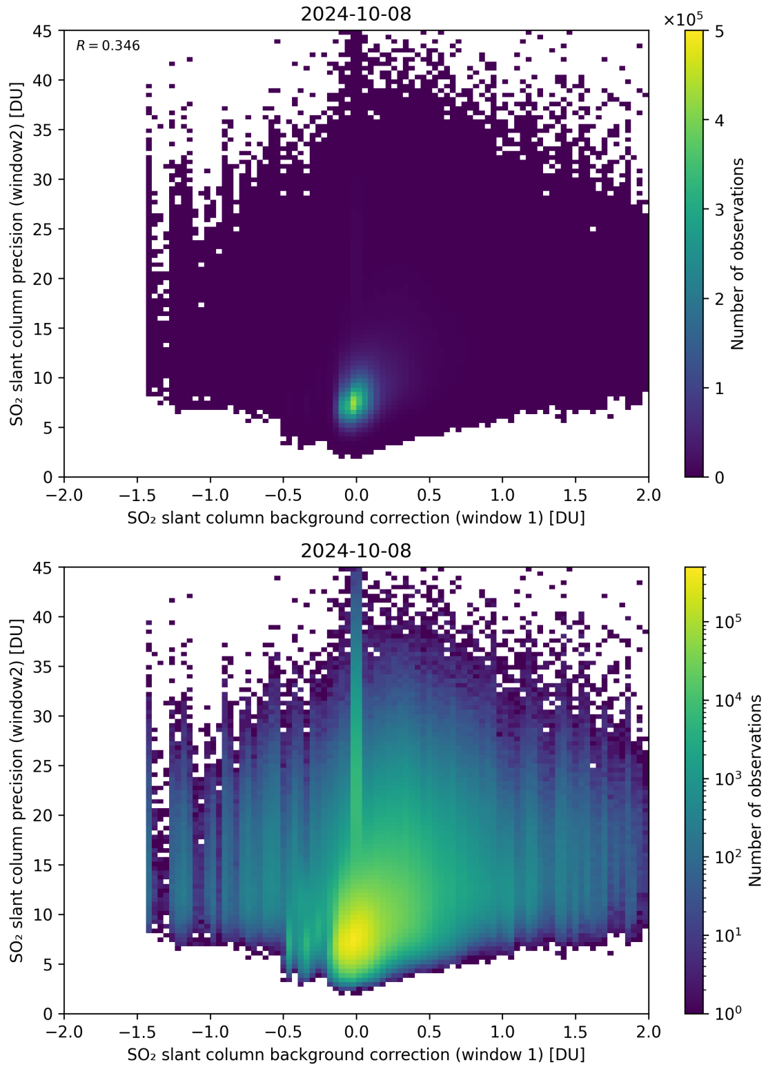
Figure 106: Scatter density plot of “SO 2 slant column background correction (window 1)” against “SO 2 slant column precision (window2)” for 2024-10-08 to 2024-10-09.
