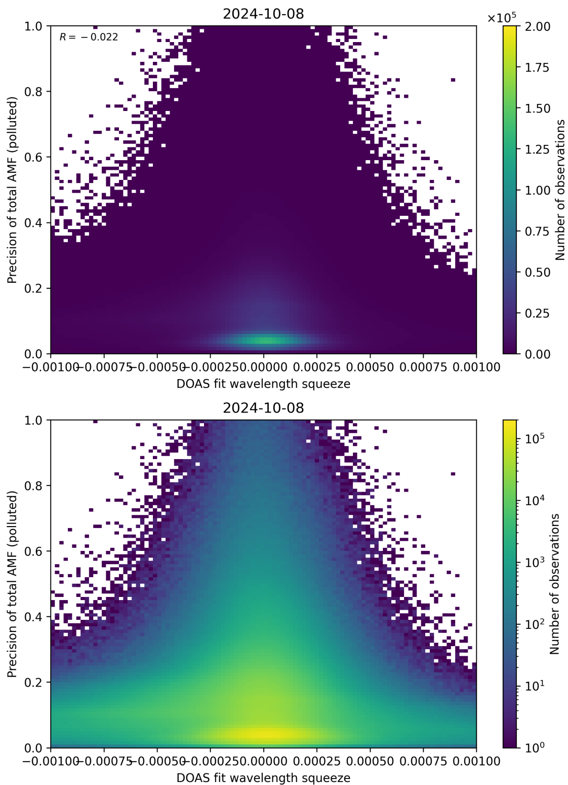
Figure 135: Scatter density plot of “DOAS fit wavelength squeeze” against “Precision of total AMF (polluted)” for 2024-10-08 to 2024-10-09.
