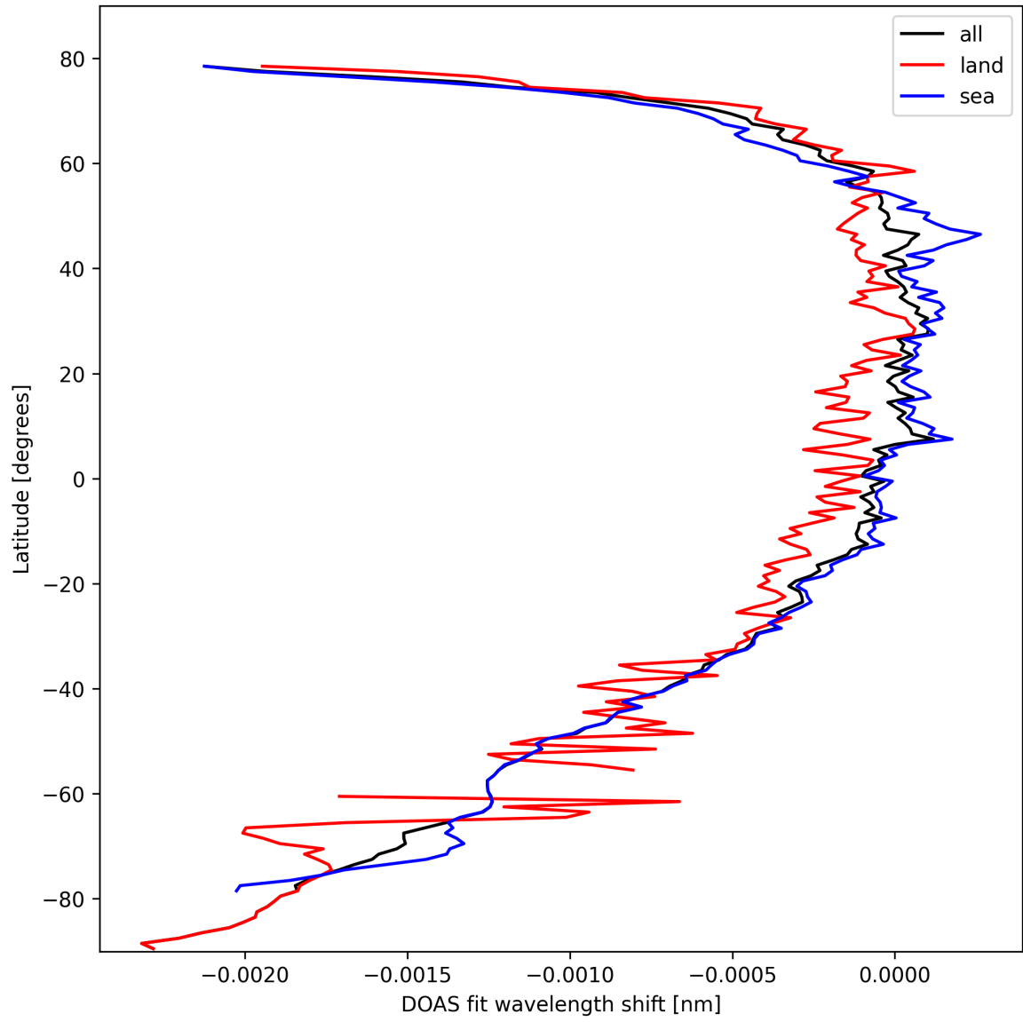
Figure 45: Zonal average of “DOAS fit wavelength shift” for 2024-10-08 to 2024-10-09.
