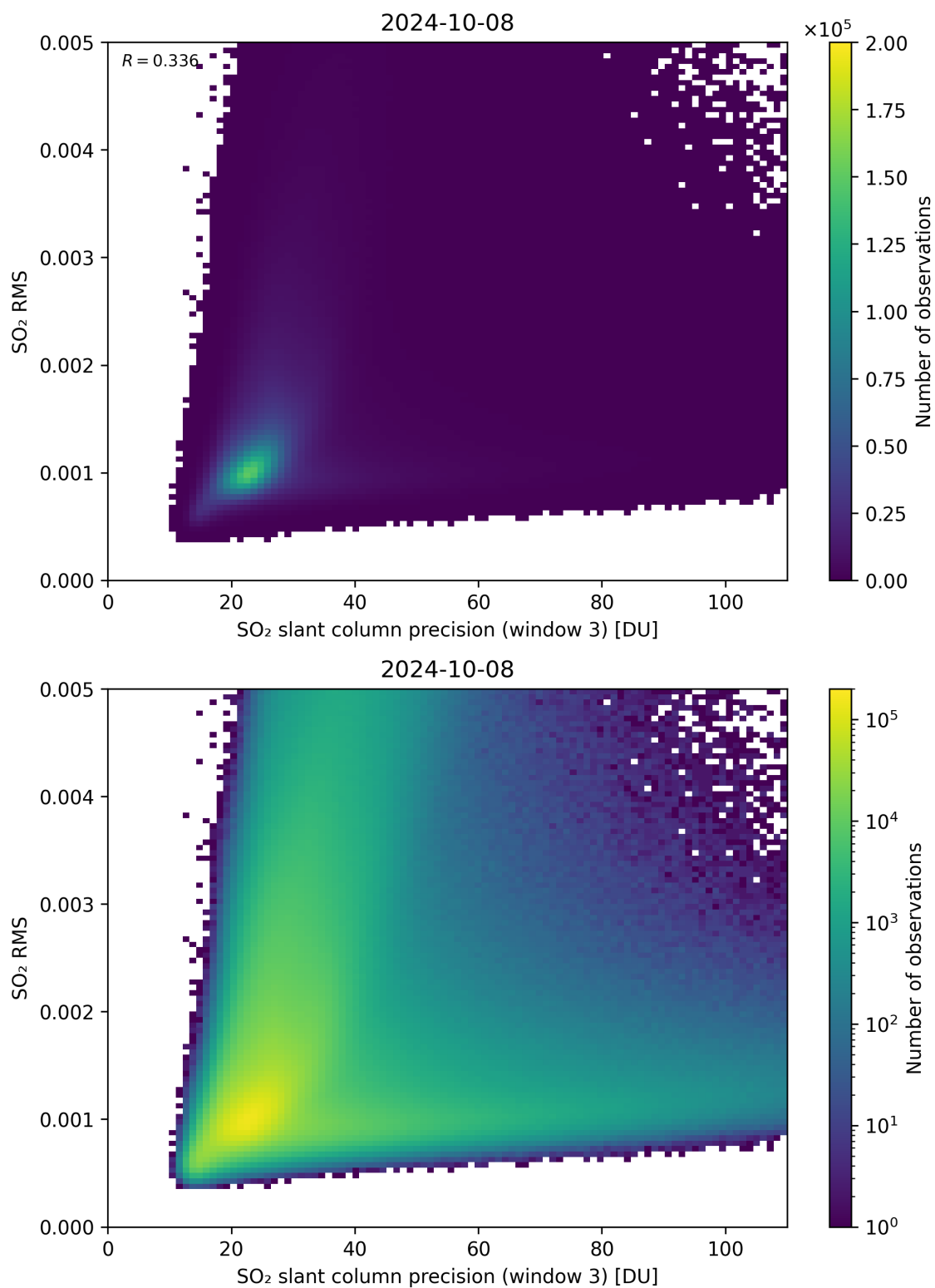
Figure 260: Scatter density plot of “SO 2 slant column precision (window 3)” against “SO 2 RMS” for 2024-10-08 to 2024-10-09.
