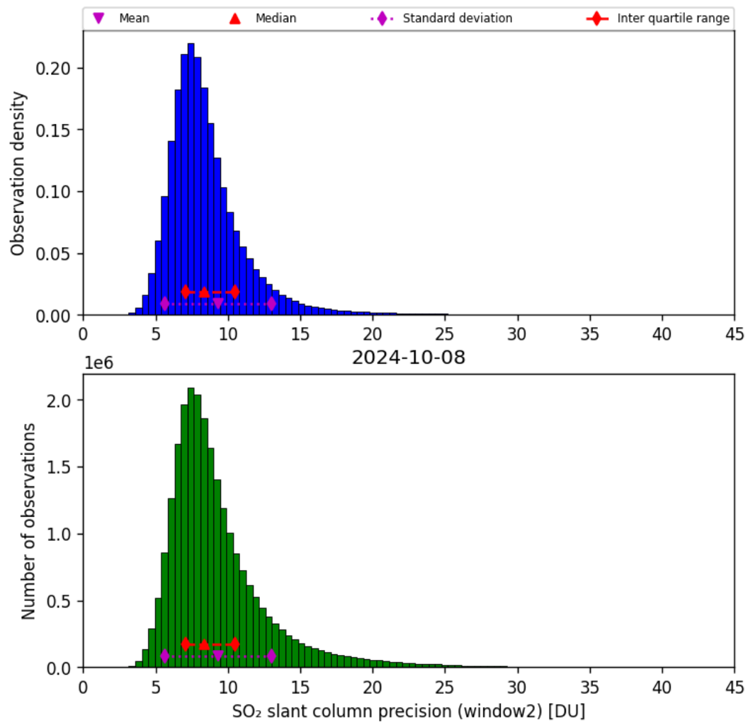
Figure 61: Histogram of “SO 2 slant column precision (window2)” for 2024-10-08 to 2024-10-09
