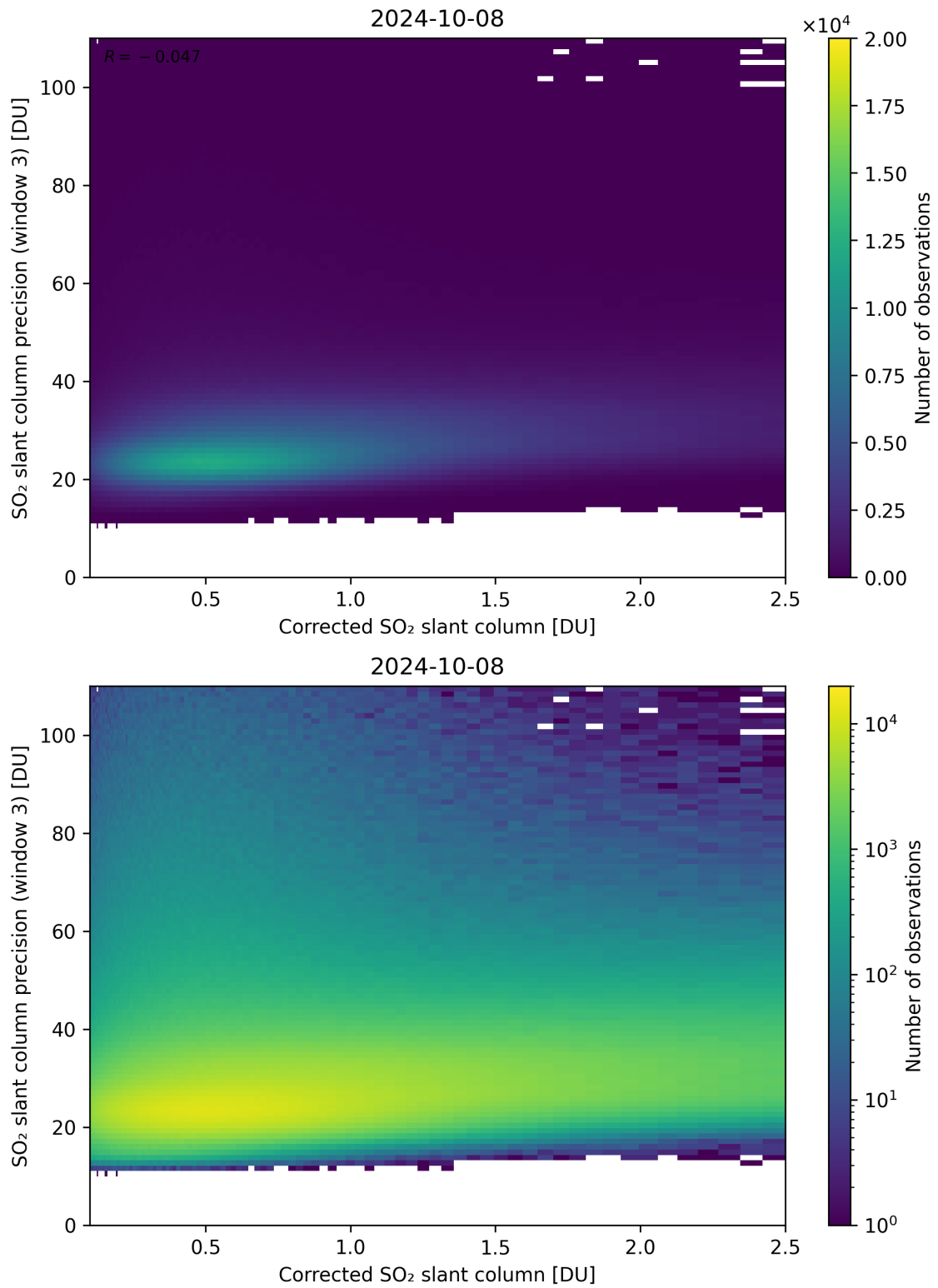
Figure 191: Scatter density plot of “Corrected SO 2 slant column” against “SO 2 slant column precision (window 3)” for 2024-10-08 to 2024-10-09.
