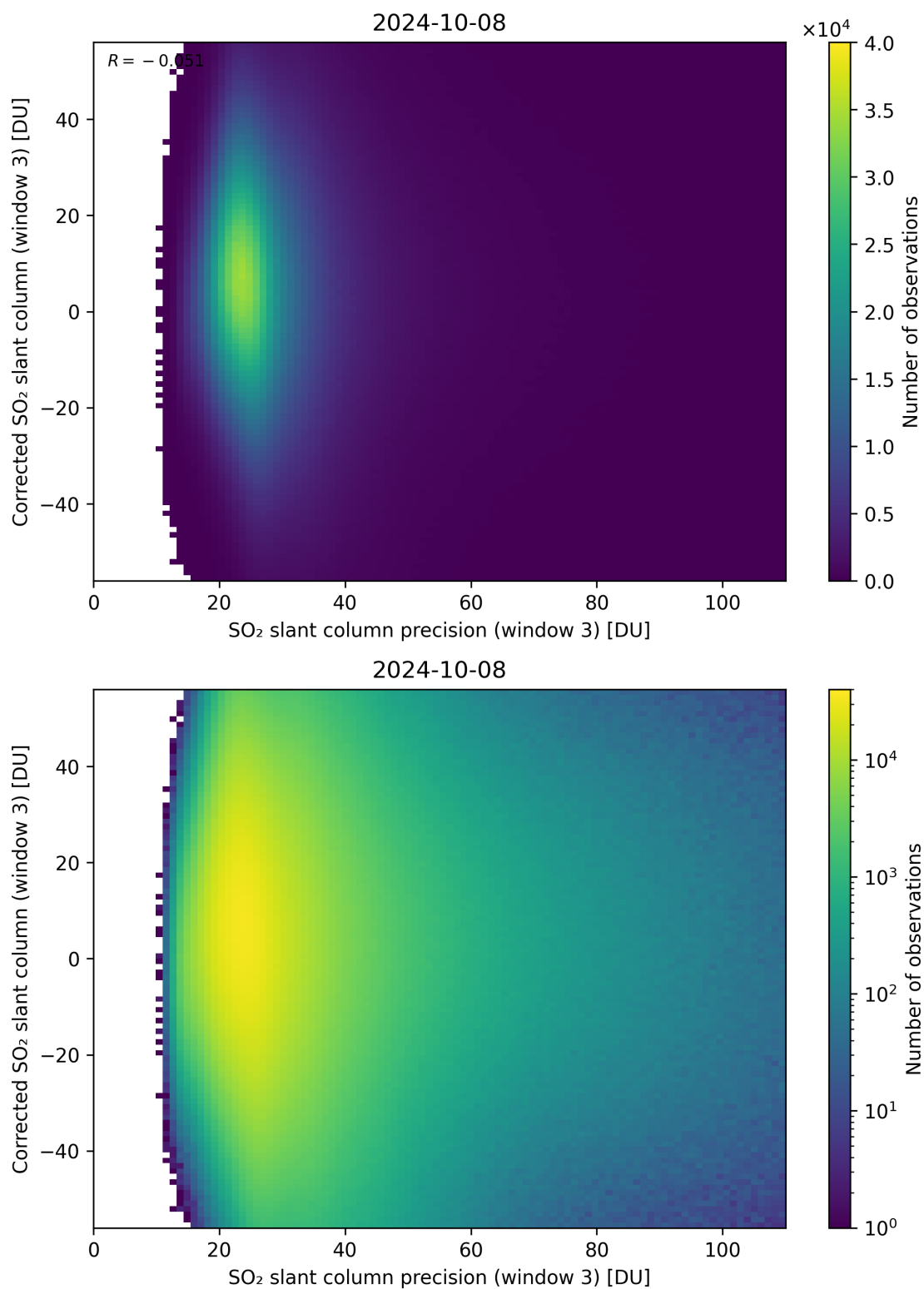
Figure 262: Scatter density plot of “SO 2 slant column precision (window 3)” against “Corrected SO 2 slant column (window 3)” for 2024-10-08 to 2024-10-09.
