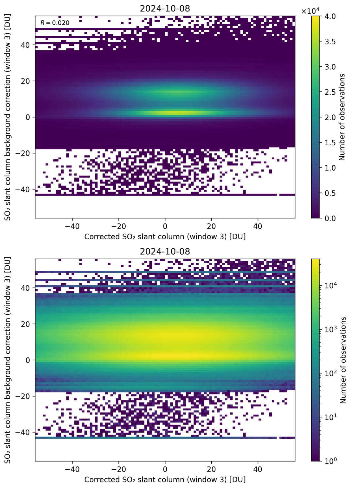
Figure 205: Scatter density plot of “Corrected SO 2 slant column (window 3)” against “SO 2 slant column background correction (window 3)” for 2024-10-08 to 2024-10-09.
