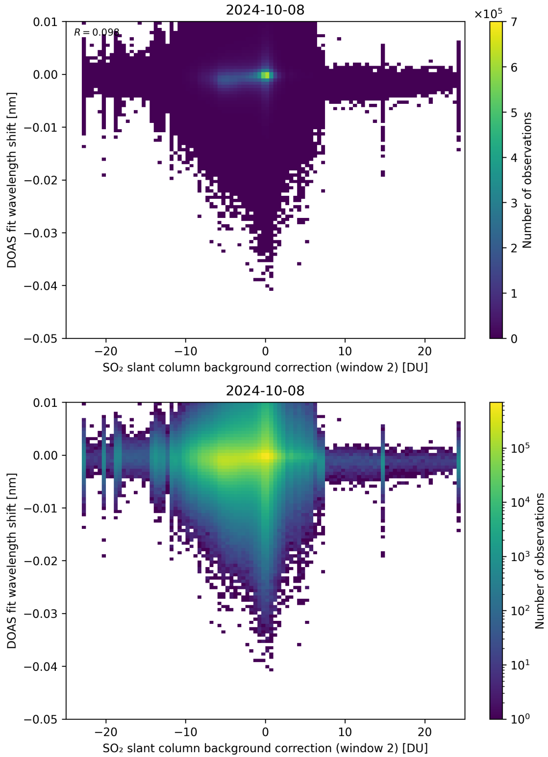
Figure 112: Scatter density plot of “SO 2 slant column background correction (window 2)” against “DOAS fit wavelength shift” for 2024-10-08 to 2024-10-09.
