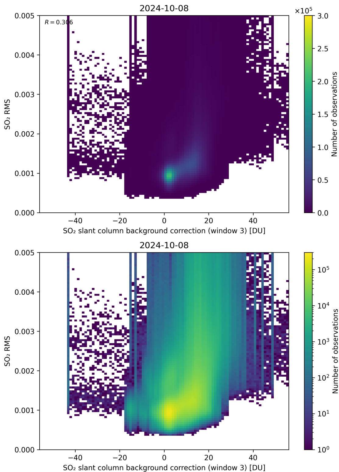
Figure 123: Scatter density plot of “SO 2 slant column background correction (window 3)” against “SO 2 RMS” for 2024-10-08 to 2024-10-09.
