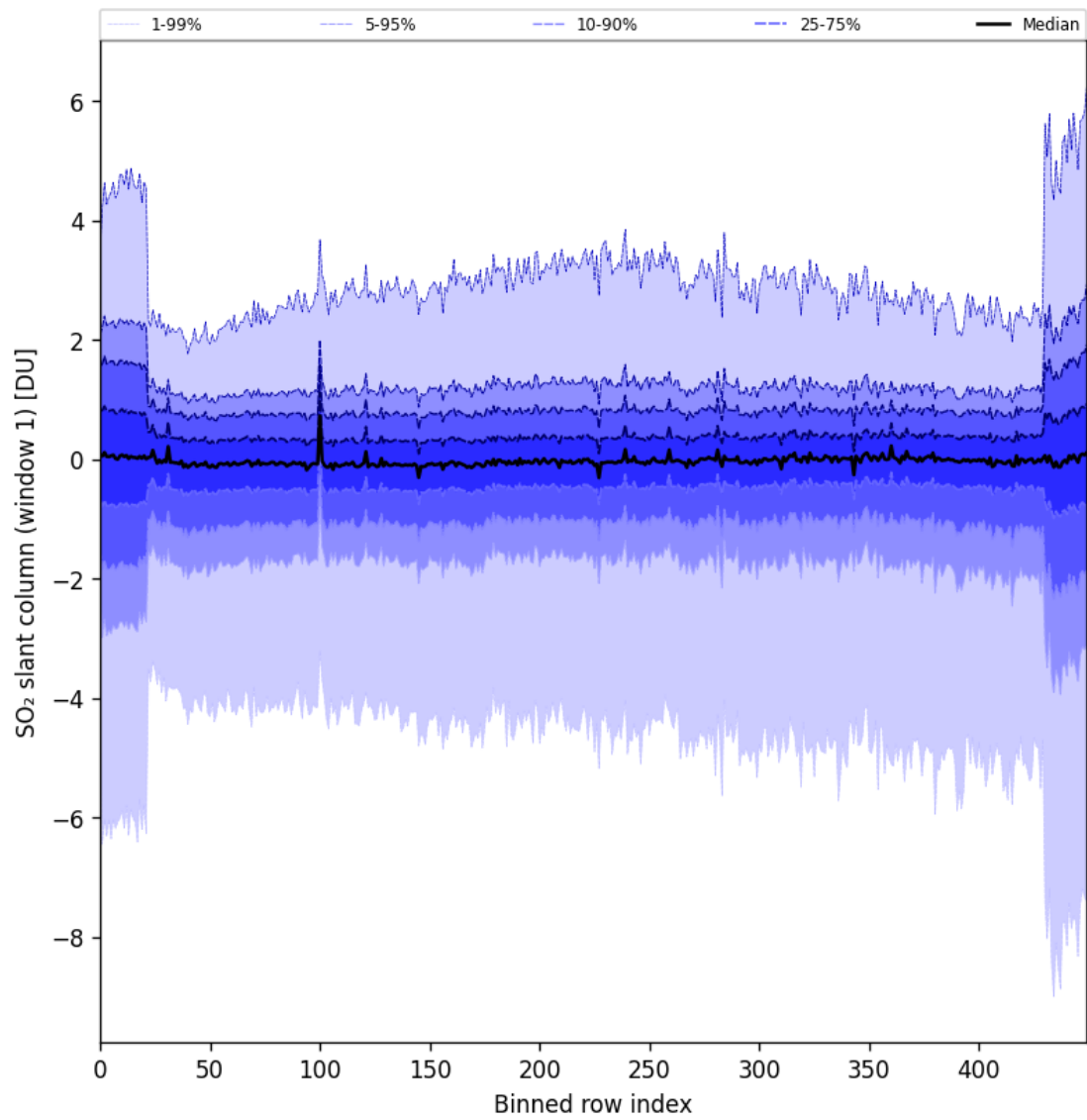
Figure 79: Along track statistics of “SO 2 slant column (window 1)” for 2024-10-08 to 2024-10-09
