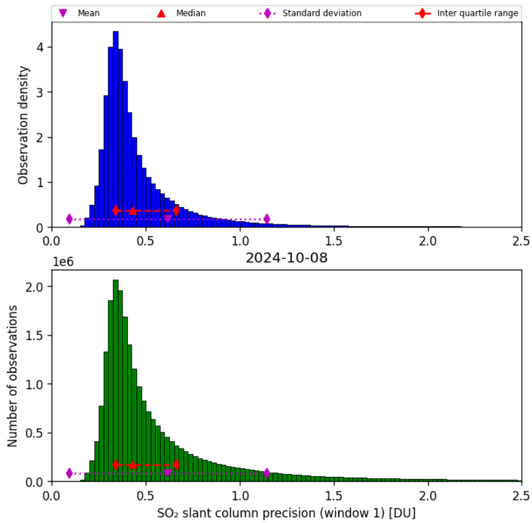
Figure 57: Histogram of “SO 2 slant column precision (window 1)” for 2024-10-08 to 2024-10-09
