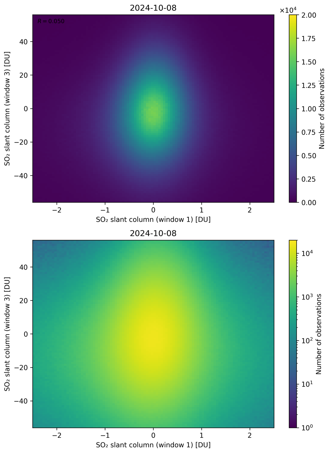
Figure 237: Scatter density plot of “SO 2 slant column (window 1)” against “SO 2 slant column (window 3)” for 2024-10-08 to 2024-10-09.
