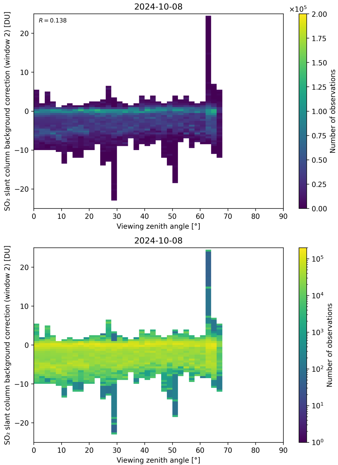
Figure 309: Scatter density plot of “Viewing zenith angle” against “SO 2 slant column background correction (window 2)” for 2024-10-08 to 2024-10-09.
