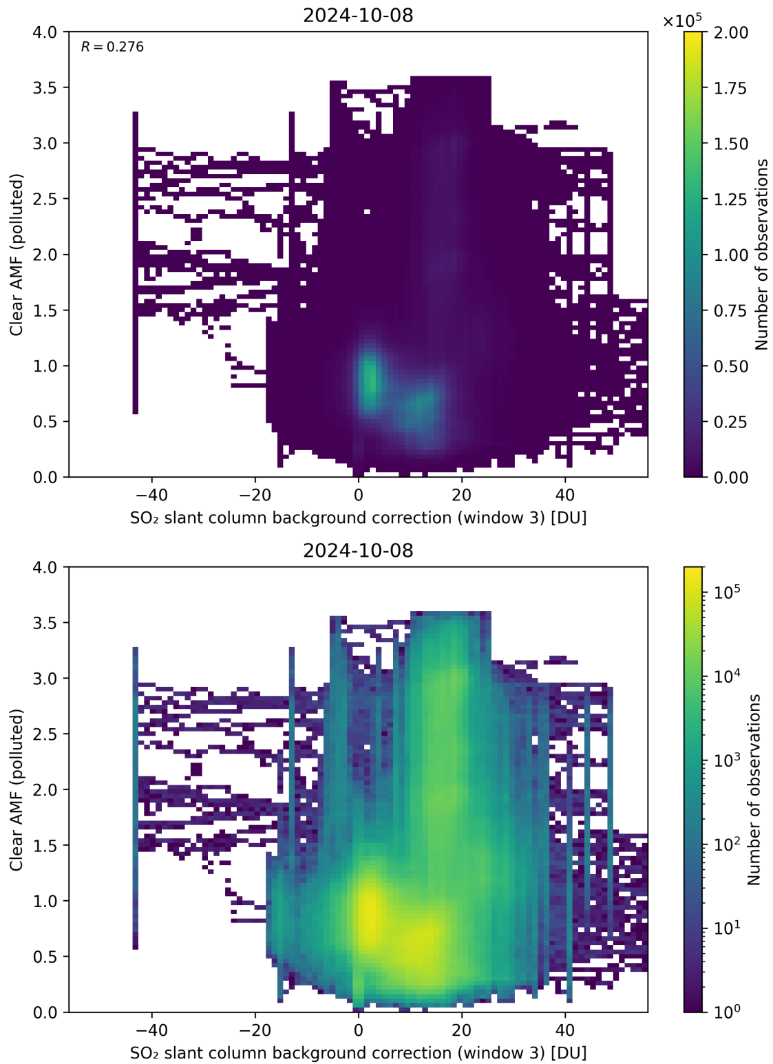
Figure 124: Scatter density plot of “SO 2 slant column background correction (window 3)” against “Clear AMF (polluted)” for 2024-10-08 to 2024-10-09.
