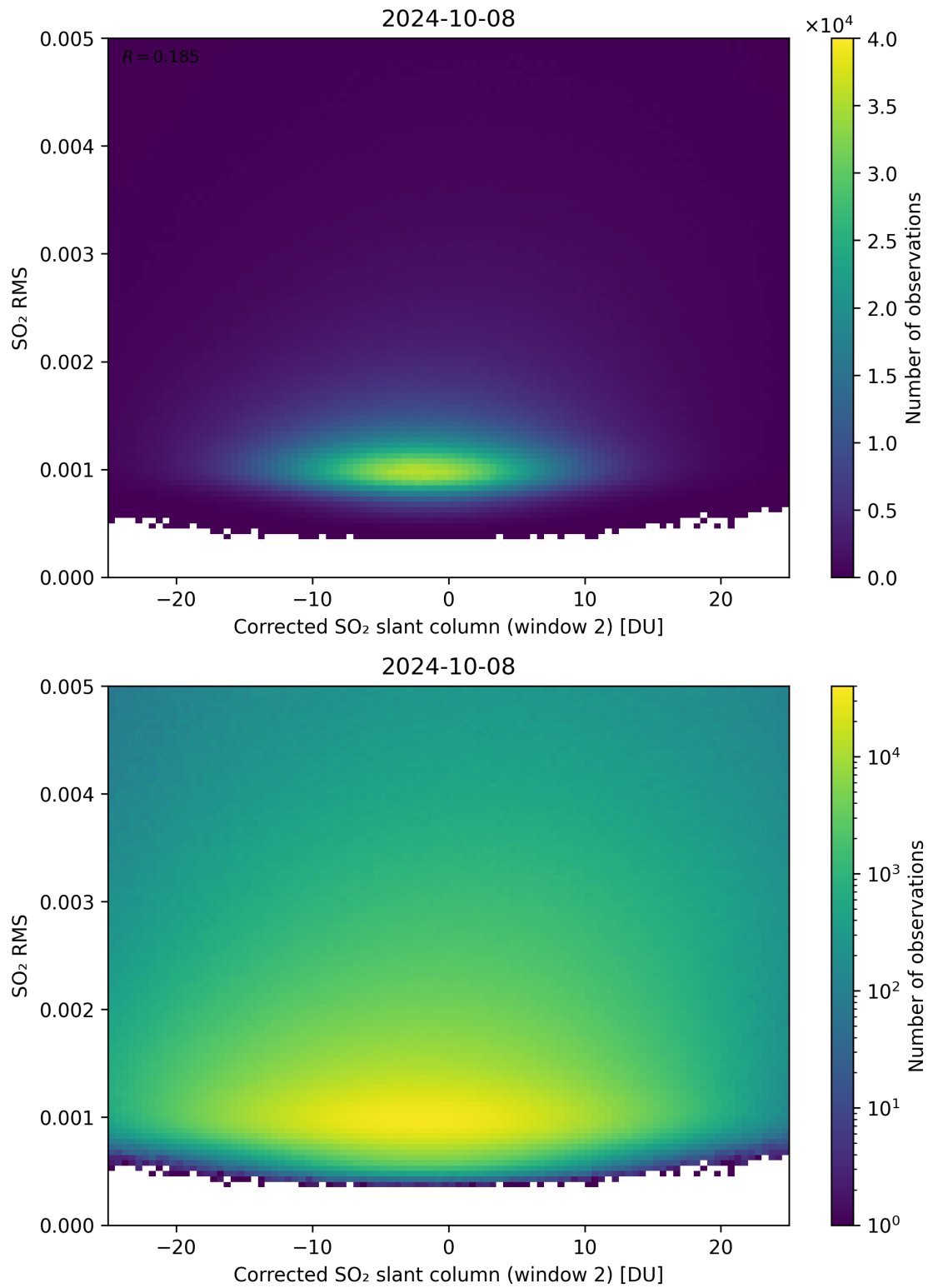
Figure 198: Scatter density plot of “Corrected SO 2 slant column (window 2)” against “SO 2 RMS” for 2024-10-08 to 2024-10-09.
