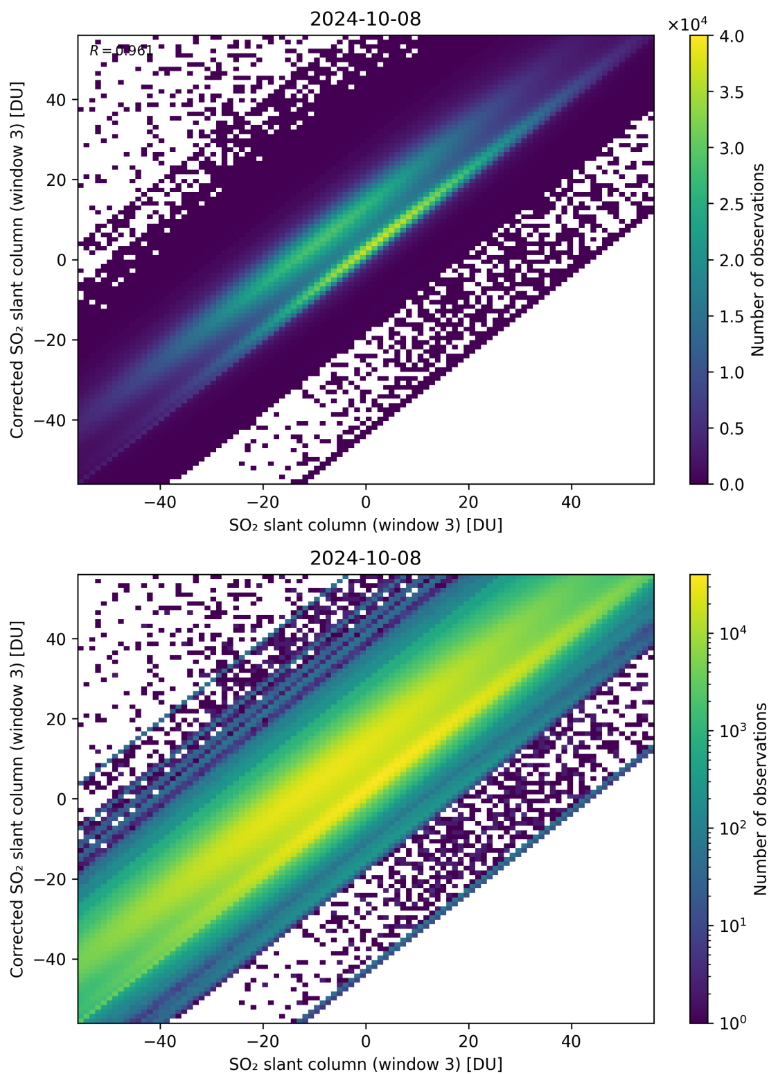
Figure 266: Scatter density plot of “SO 2 slant column (window 3)” against “Corrected SO 2 slant column (window 3)” for 2024-10-08 to 2024-10-09.
