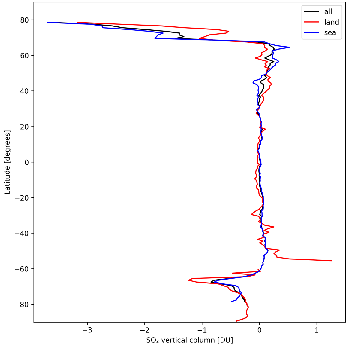
Figure 30: Zonal average of “SO 2 vertical column” for 2024-10-08 to 2024-10-09.
