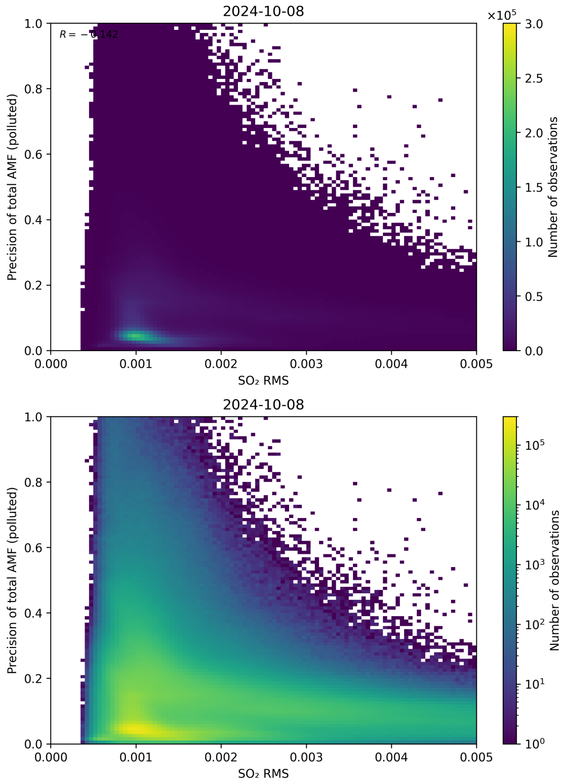
Figure 138: Scatter density plot of “SO 2 RMS” against “Precision of total AMF (polluted)” for 2024-10-08 to 2024-10-09.
