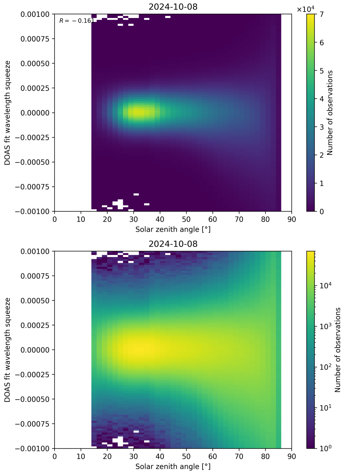
Figure 162: Scatter density plot of “Solar zenith angle” against “DOAS fit wavelength squeeze” for 2024-10-08 to 2024-10-09.
