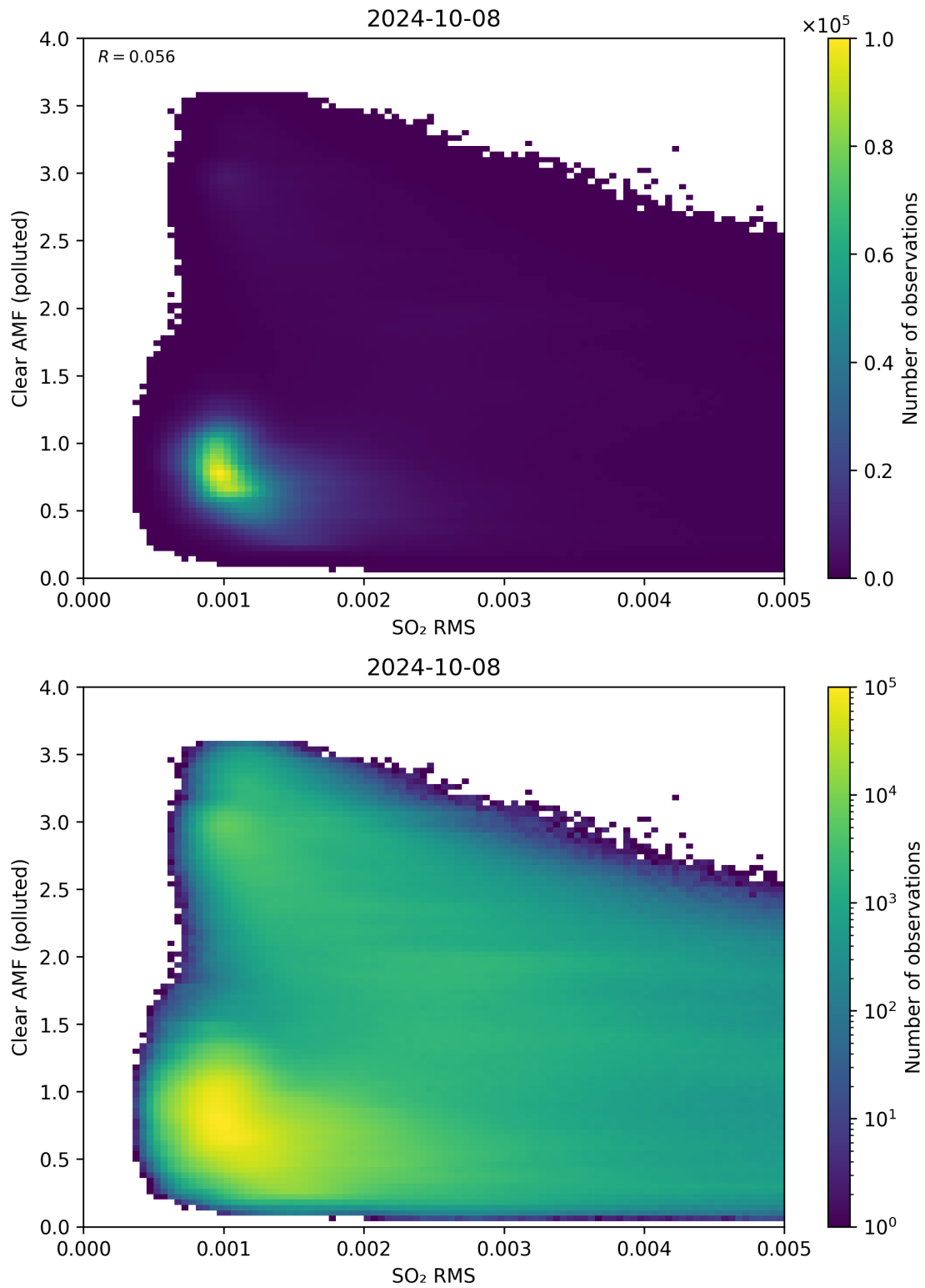
Figure 136: Scatter density plot of “SO 2 RMS” against “Clear AMF (polluted)” for 2024-10-08 to 2024-10-09.
