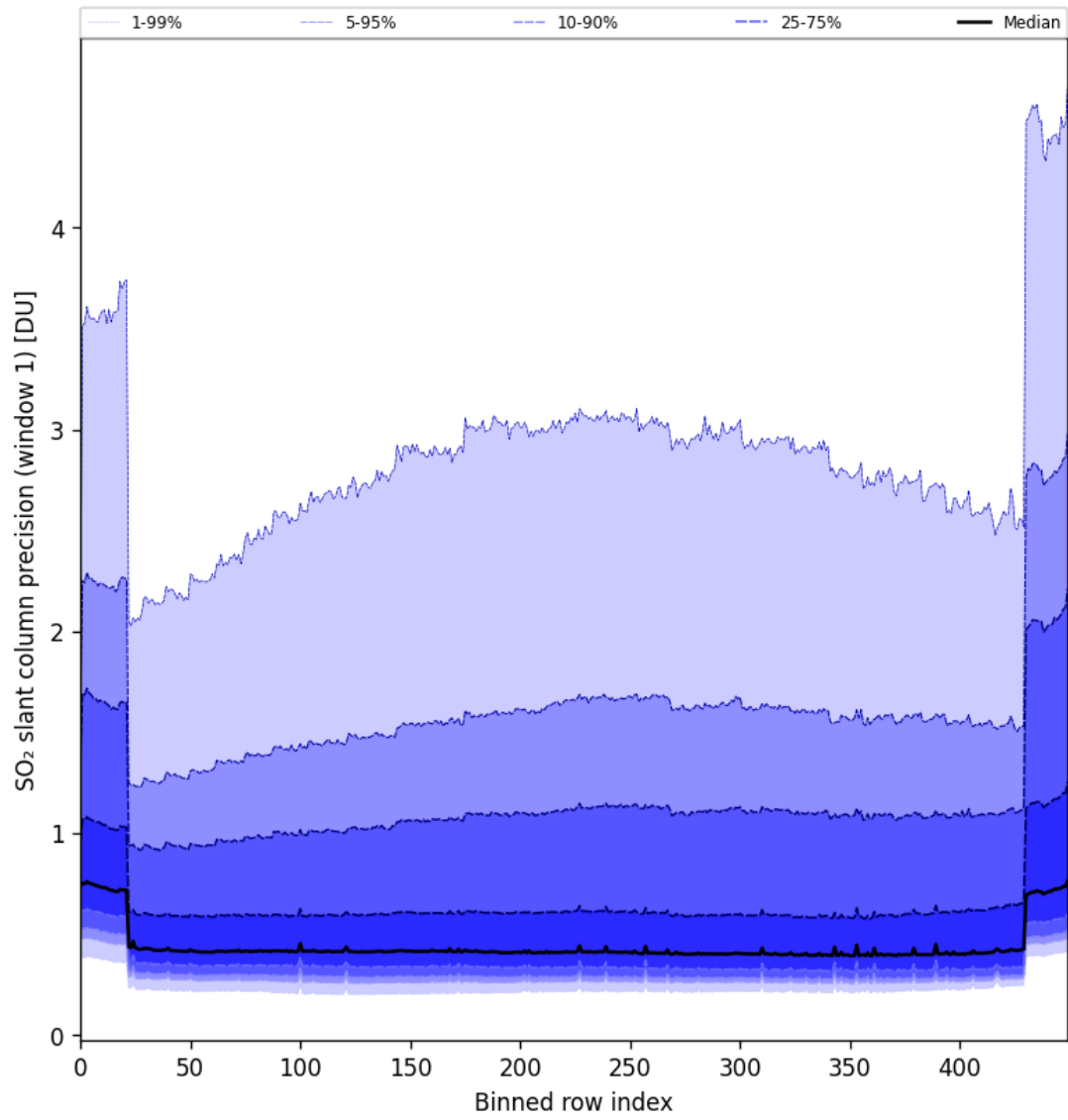
Figure 80: Along track statistics of “SO 2 slant column precision (window 1)” for 2024-10-08 to 2024-10-09
