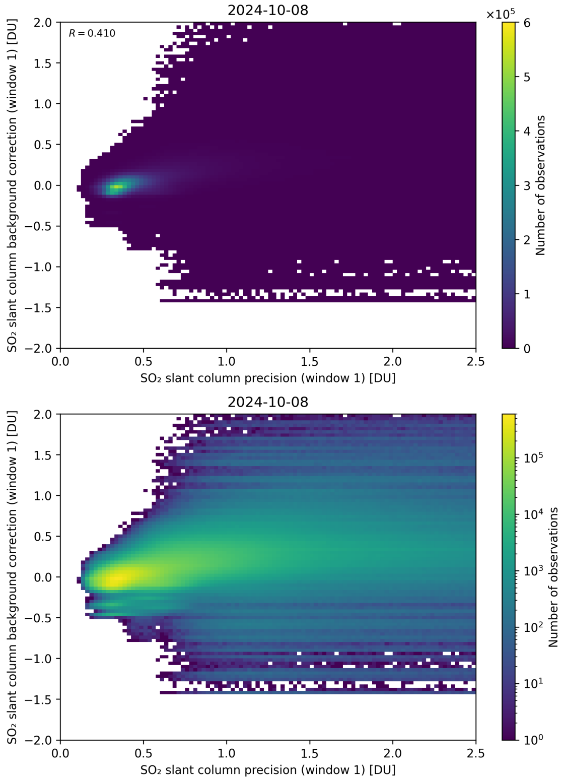
Figure 218: Scatter density plot of “SO 2 slant column precision (window 1)” against “SO 2 slant column background correction (window 1)” for 2024-10-08 to 2024-10-09.
