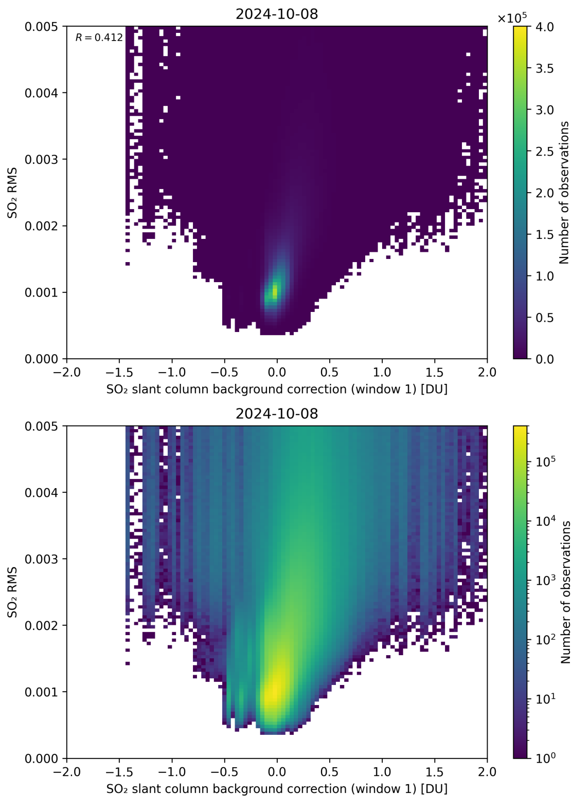
Figure 102: Scatter density plot of “SO 2 slant column background correction (window 1)” against “SO 2 RMS” for 2024-10-08 to 2024-10-09.
