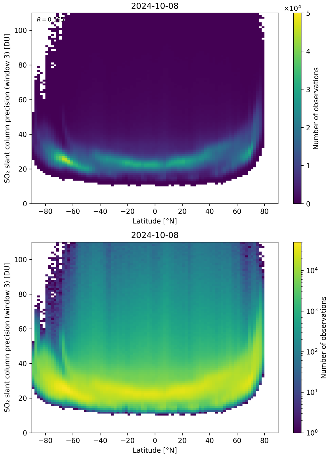
Figure 153: Scatter density plot of “Latitude” against “SO 2 slant column precision (window 3)” for 2024-10-08 to 2024-10-09.
