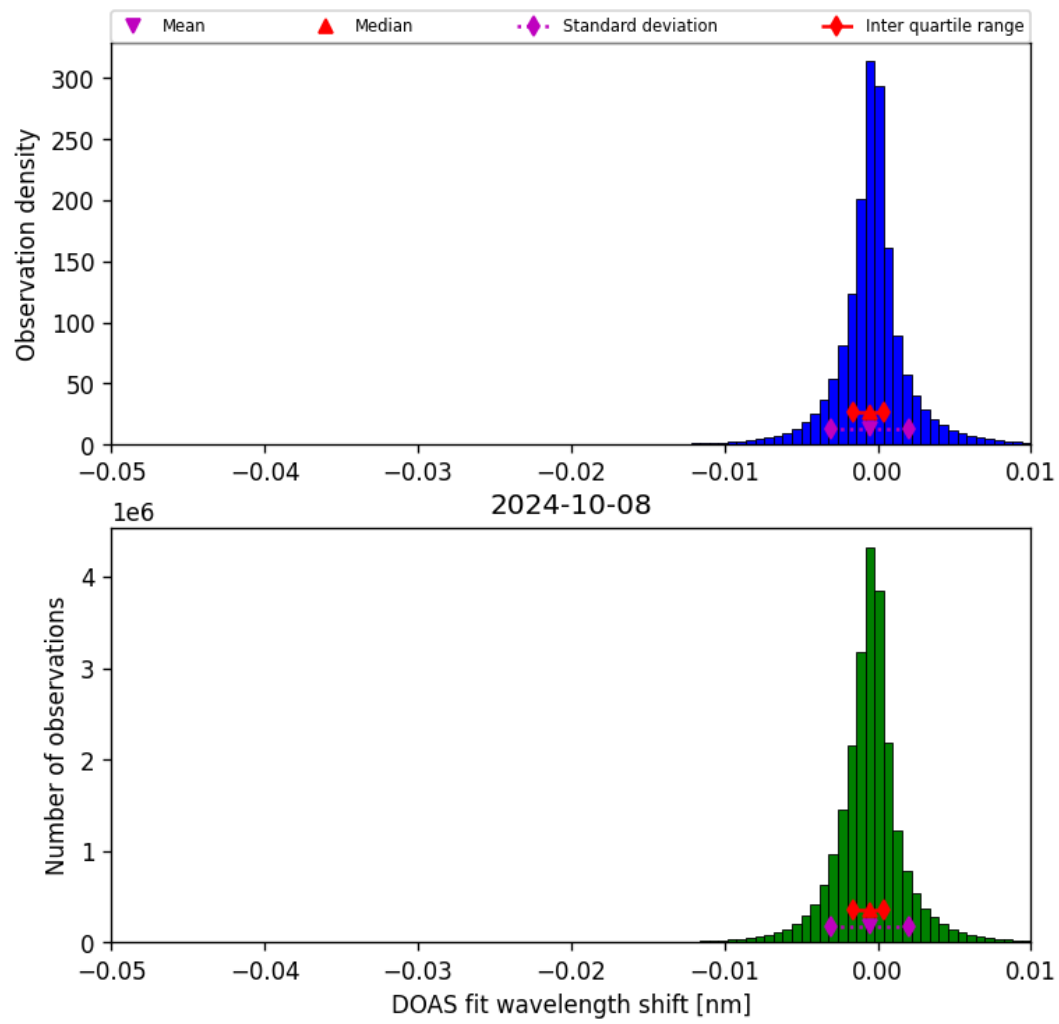
Figure 68: Histogram of “DOAS fit wavelength shift” for 2024-10-08 to 2024-10-09
