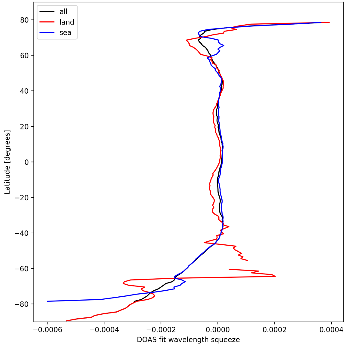
Figure 46: Zonal average of “DOAS fit wavelength squeeze” for 2024-10-08 to 2024-10-09.
