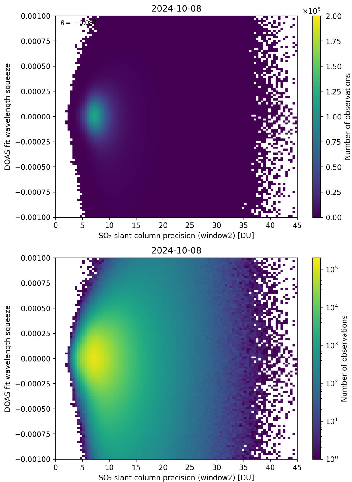
Figure 244: Scatter density plot of “SO 2 slant column precision (window2)” against “DOAS fit wavelength squeeze” for 2024-10-08 to 2024-10-09.
