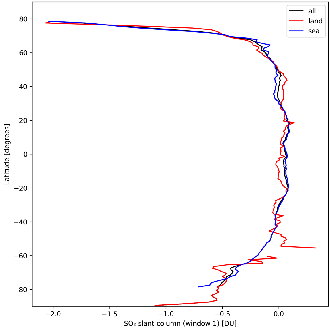
Figure 33: Zonal average of “SO 2 slant column (window 1)” for 2024-10-08 to 2024-10-09.
