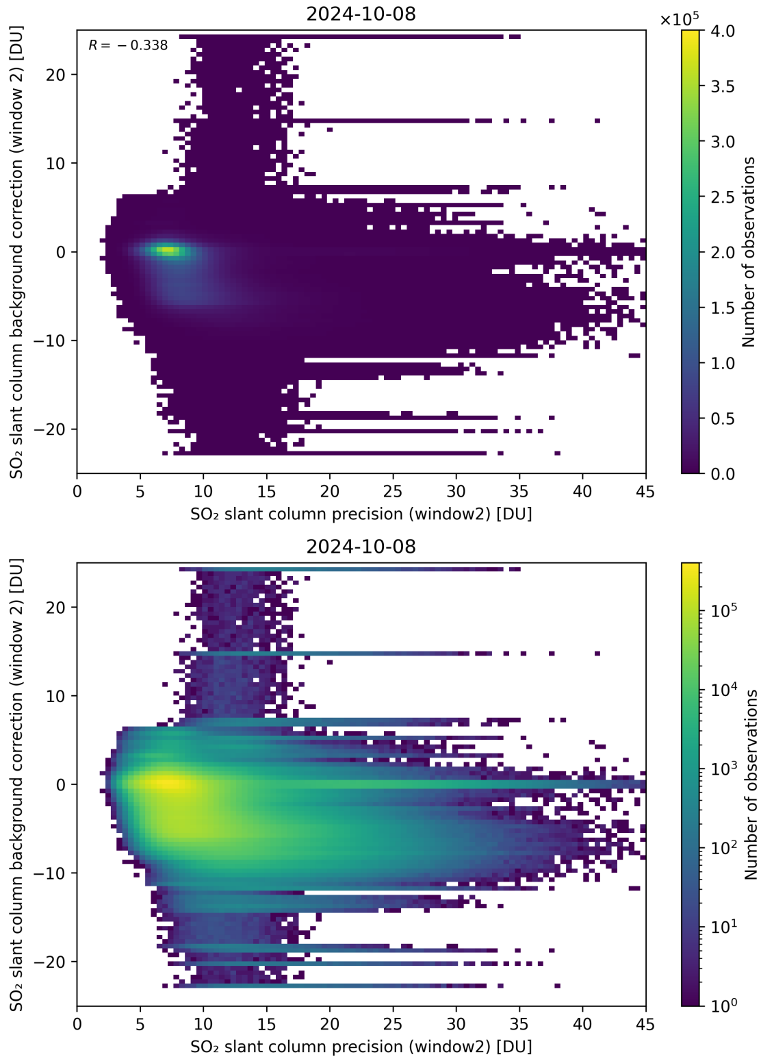
Figure 241: Scatter density plot of “SO 2 slant column precision (window2)” against “SO 2 slant column background correction (window 2)” for 2024-10-08 to 2024-10-09.
