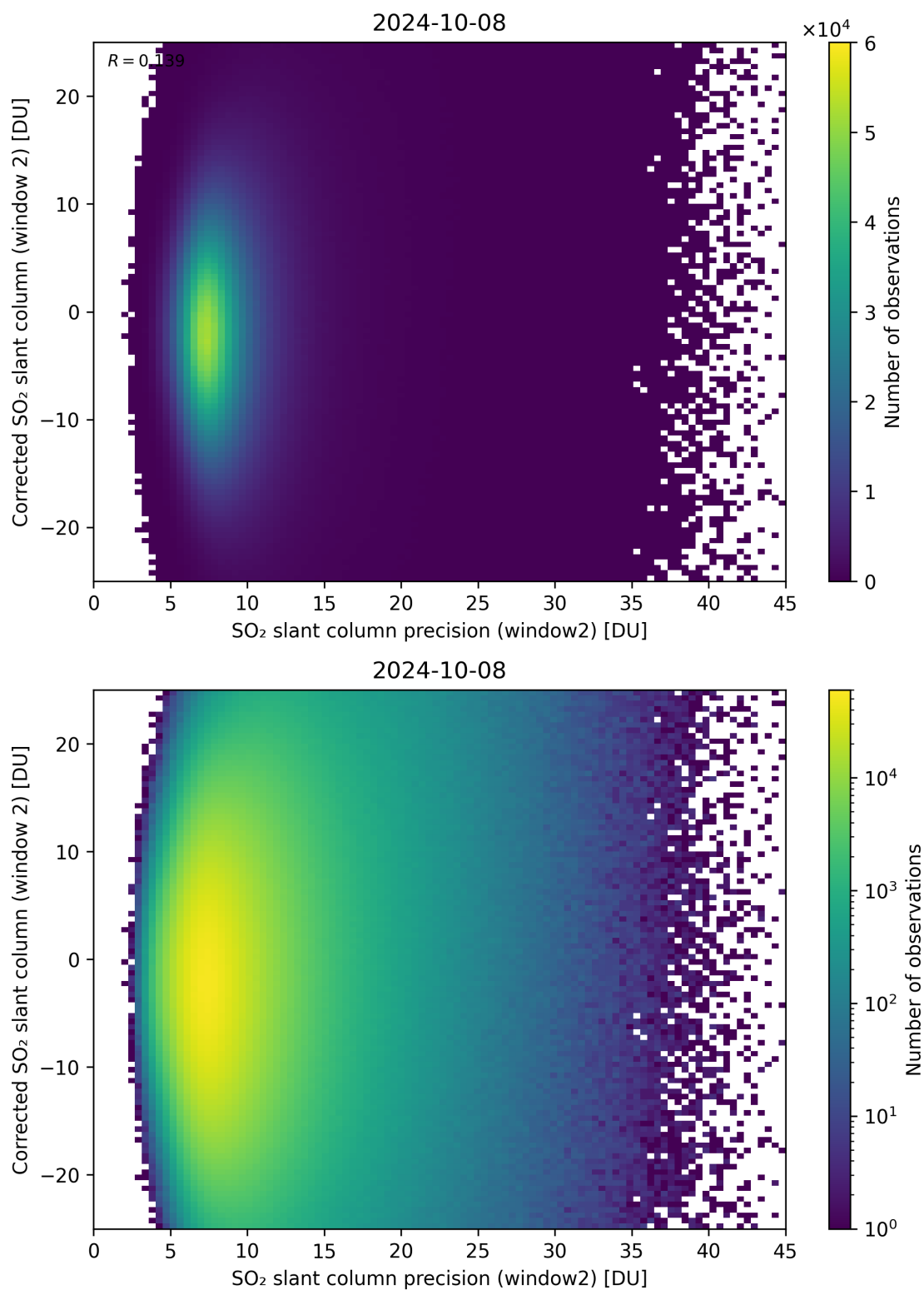
Figure 247: Scatter density plot of “SO 2 slant column precision (window2)” against “Corrected SO 2 slant column (window 2)” for 2024-10-08 to 2024-10-09.
