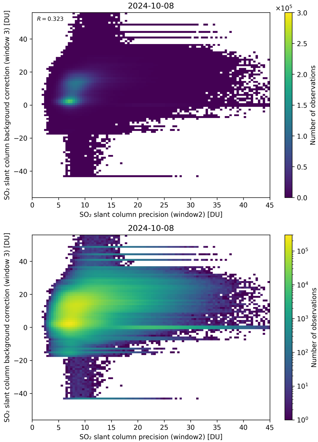
Figure 242: Scatter density plot of “SO 2 slant column precision (window2)” against “SO 2 slant column background correction (window 3)” for 2024-10-08 to 2024-10-09.
