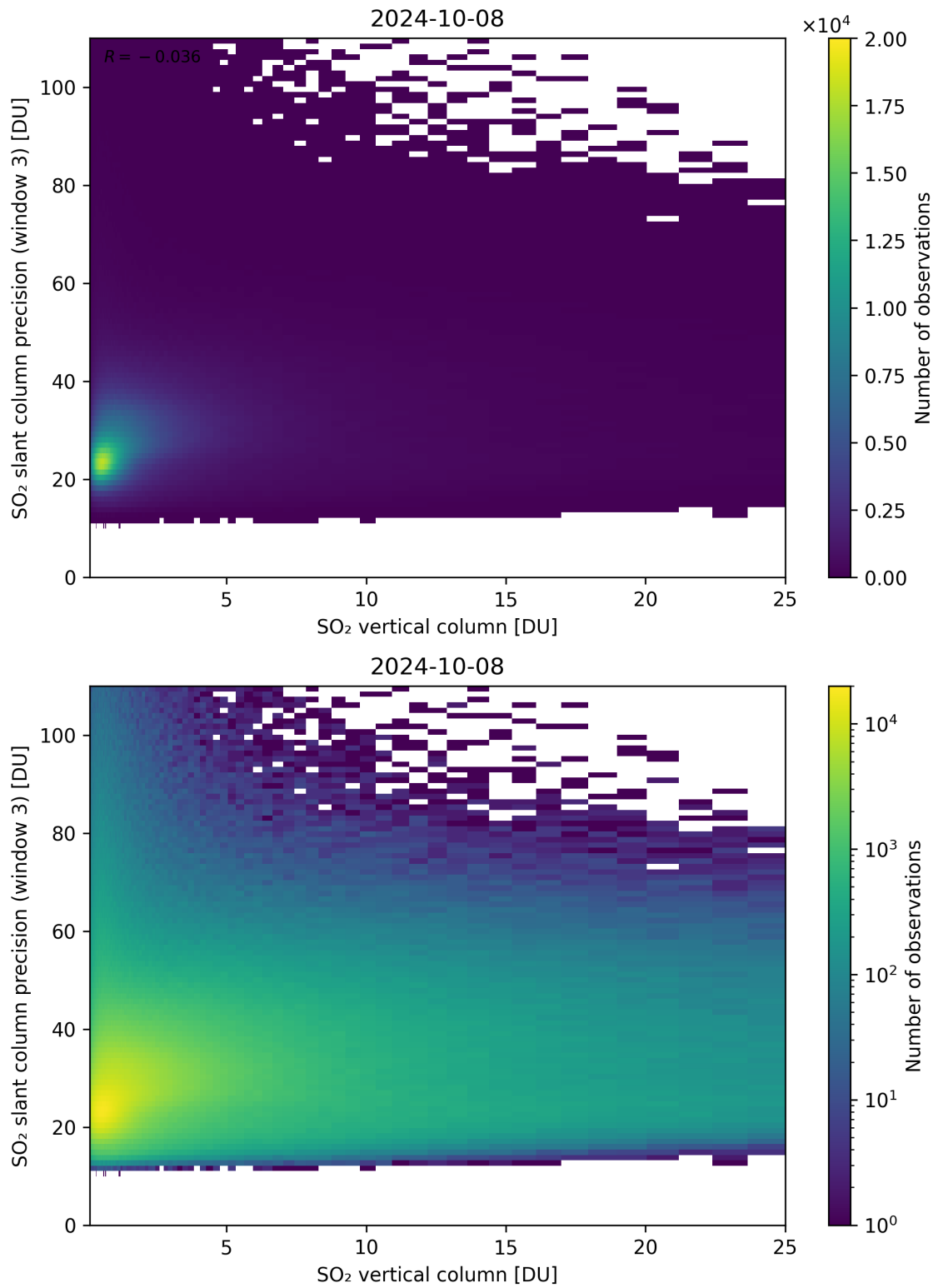
Figure 304: Scatter density plot of “SO 2 vertical column” against “SO 2 slant column precision (window 3)” for 2024-10-08 to 2024-10-09.
