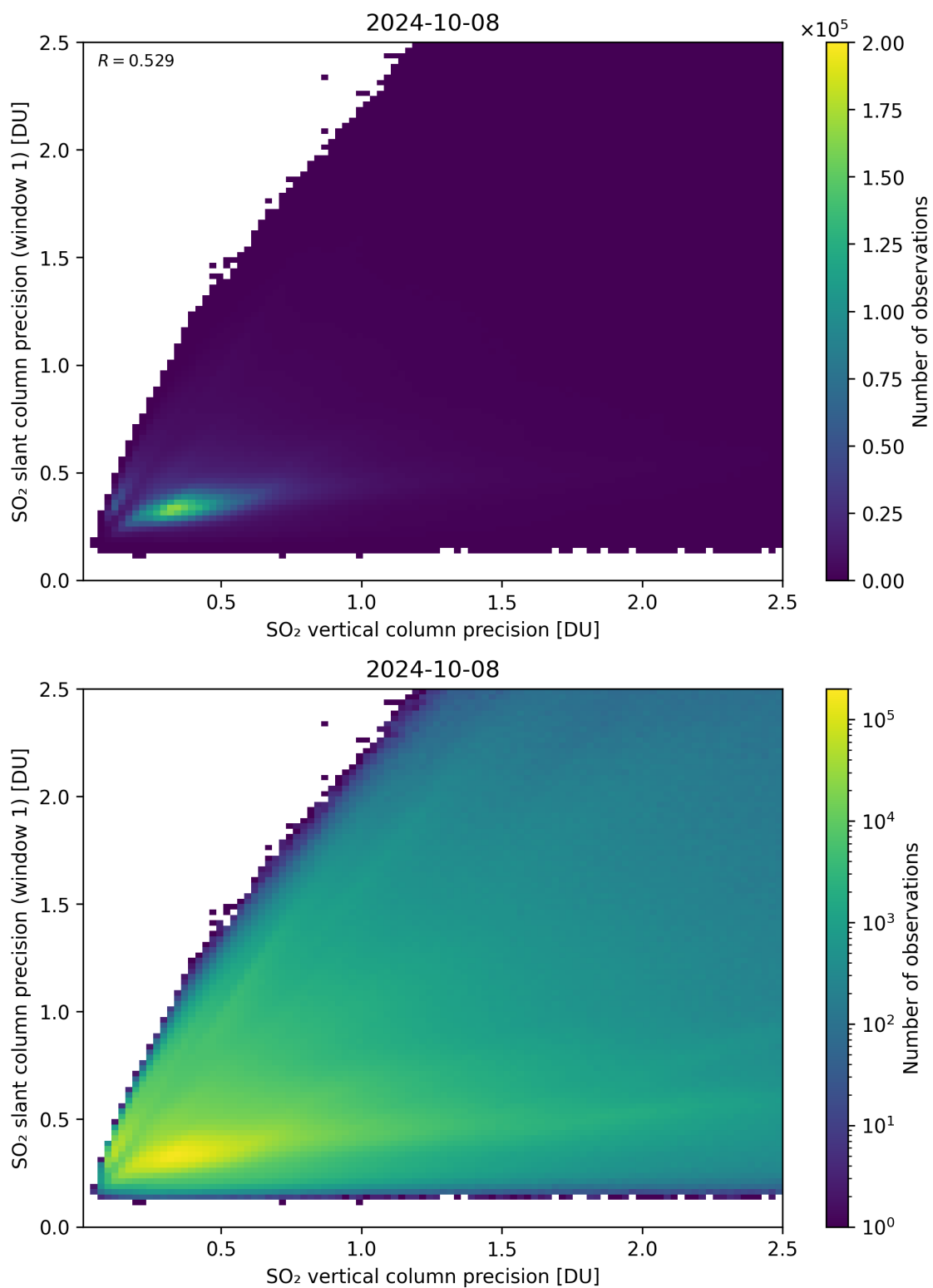
Figure 290: Scatter density plot of “SO 2 vertical column precision” against “SO 2 slant column precision (window 1)” for 2024-10-08 to 2024-10-09.
