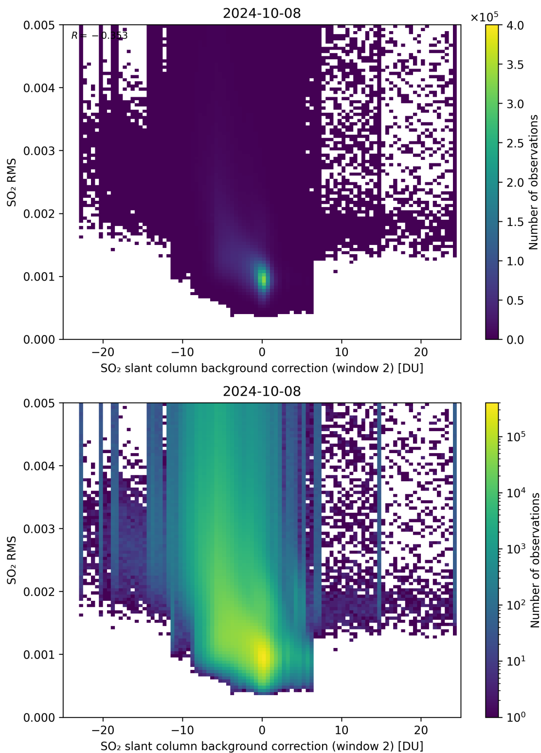
Figure 114: Scatter density plot of “SO 2 slant column background correction (window 2)” against “SO 2 RMS” for 2024-10-08 to 2024-10-09.
