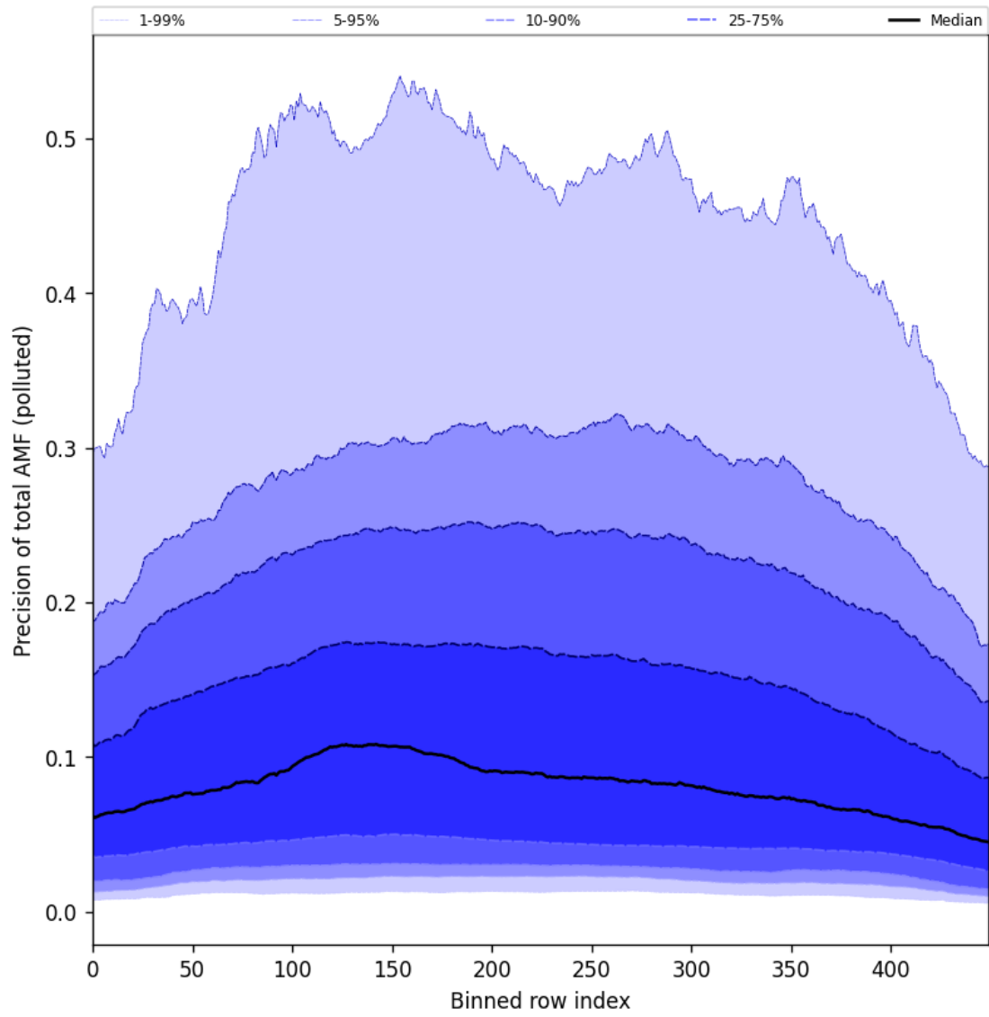
Figure 95: Along track statistics of “Precision of total AMF (polluted)” for 2024-10-08 to 2024-10-09
