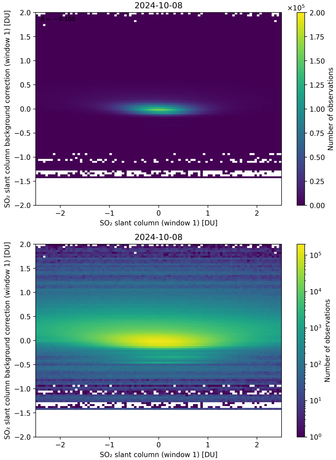
Figure 212: Scatter density plot of "SO 2 slant column (window 1)" against "SO 2 slant column background correction (window 1)" for 2024-10-08 to 2024-10-09.
