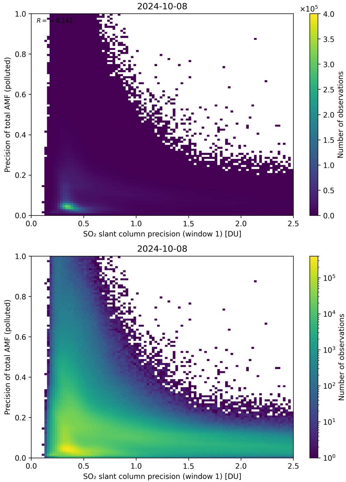
Figure 231: Scatter density plot of “SO 2 slant column precision (window 1)” against “Precision of total AMF (polluted)” for 2024-10-08 to 2024-10-09.
