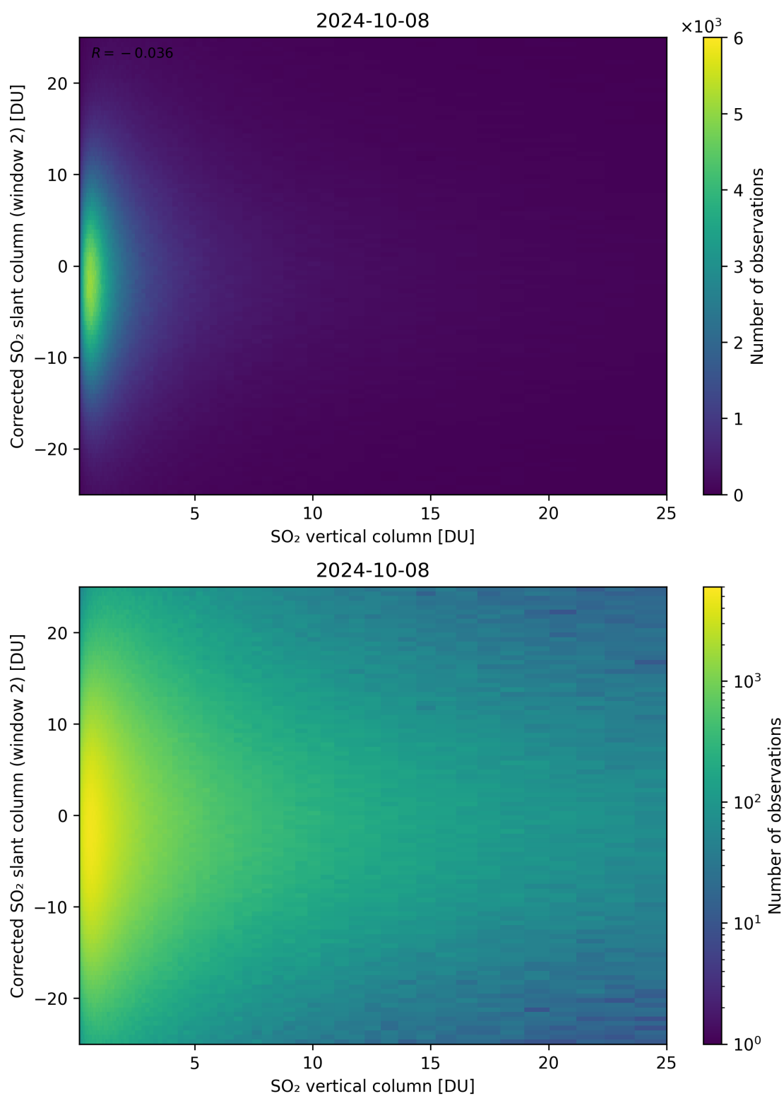
Figure 298: Scatter density plot of “SO 2 vertical column” against “Corrected SO 2 slant column (window 2)” for 2024-10-08 to 2024-10-09.
