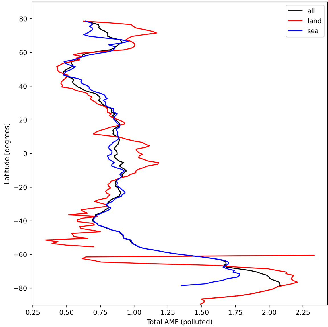
Figure 48: Zonal average of “Total AMF (polluted)” for 2024-10-08 to 2024-10-09.
