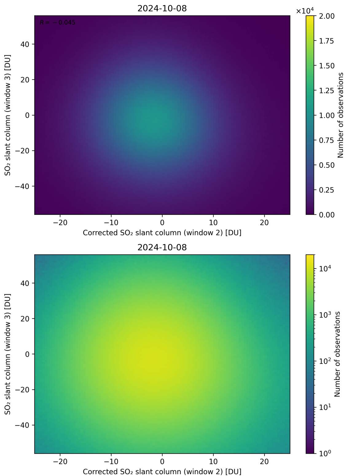
Figure 201: Scatter density plot of “Corrected SO 2 slant column (window 2)” against “SO 2 slant column (window 3)” for 2024-10-08 to 2024-10-09.
