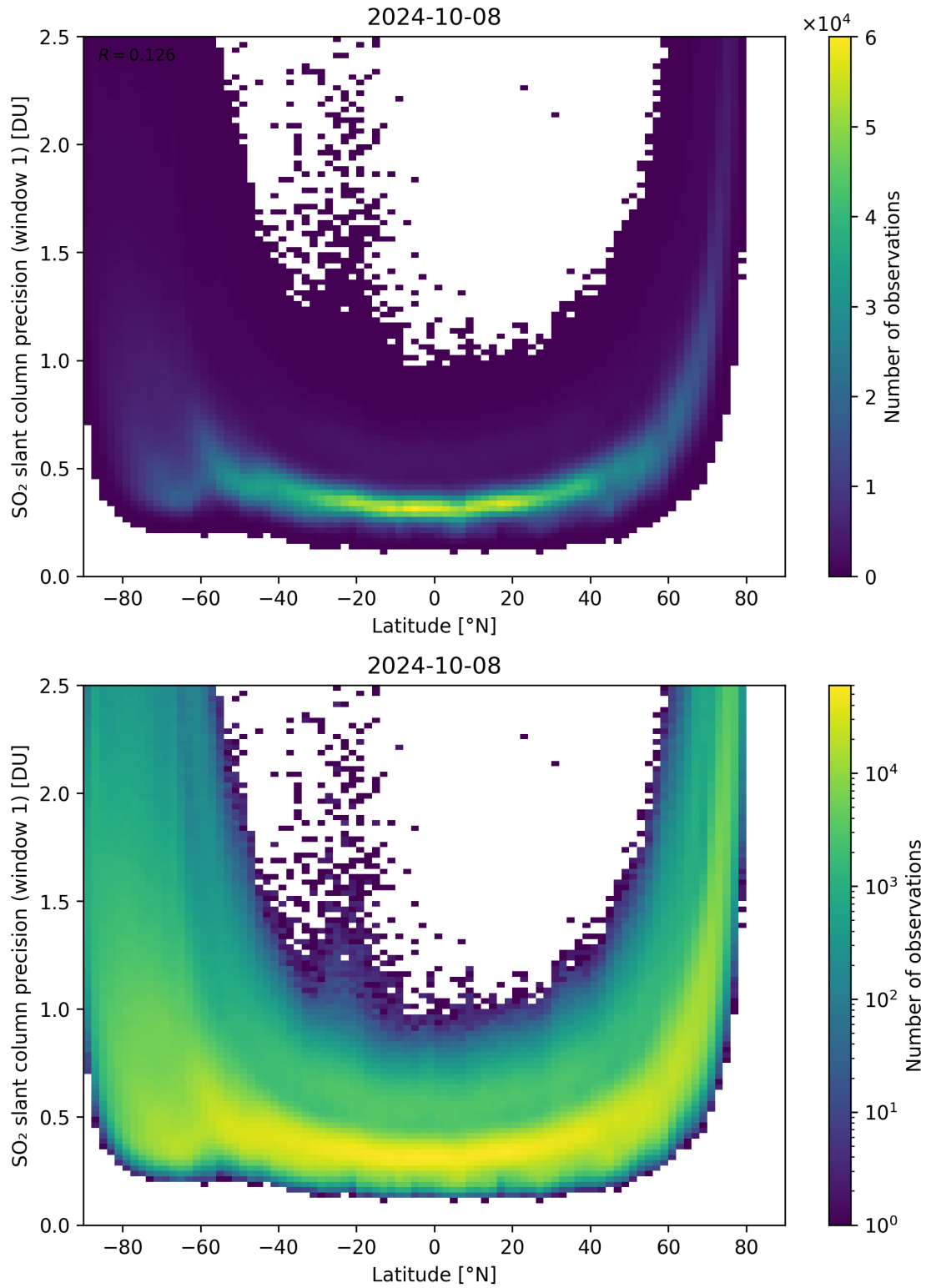
Figure 150: Scatter density plot of “Latitude” against “SO 2 slant column precision (window 1)” for 2024-10-08 to 2024-10-09.
