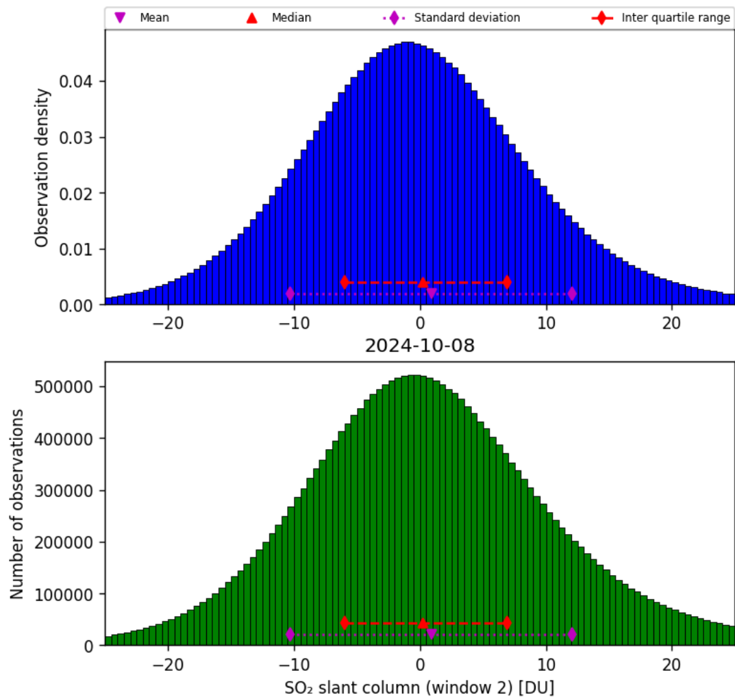
Figure 60: Histogram of “SO 2 slant column (window 2)” for 2024-10-08 to 2024-10-09
