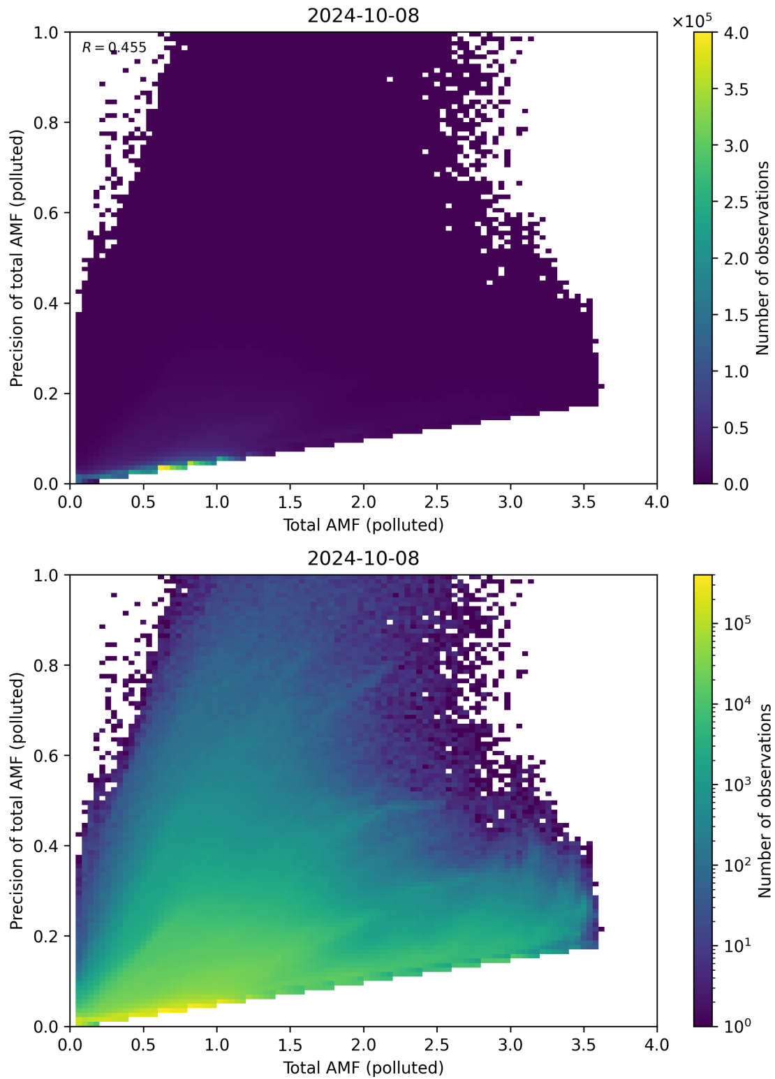
Figure 272: Scatter density plot of “Total AMF (polluted)” against “Precision of total AMF (polluted)” for 2024-10-08 to 2024-10-09.
