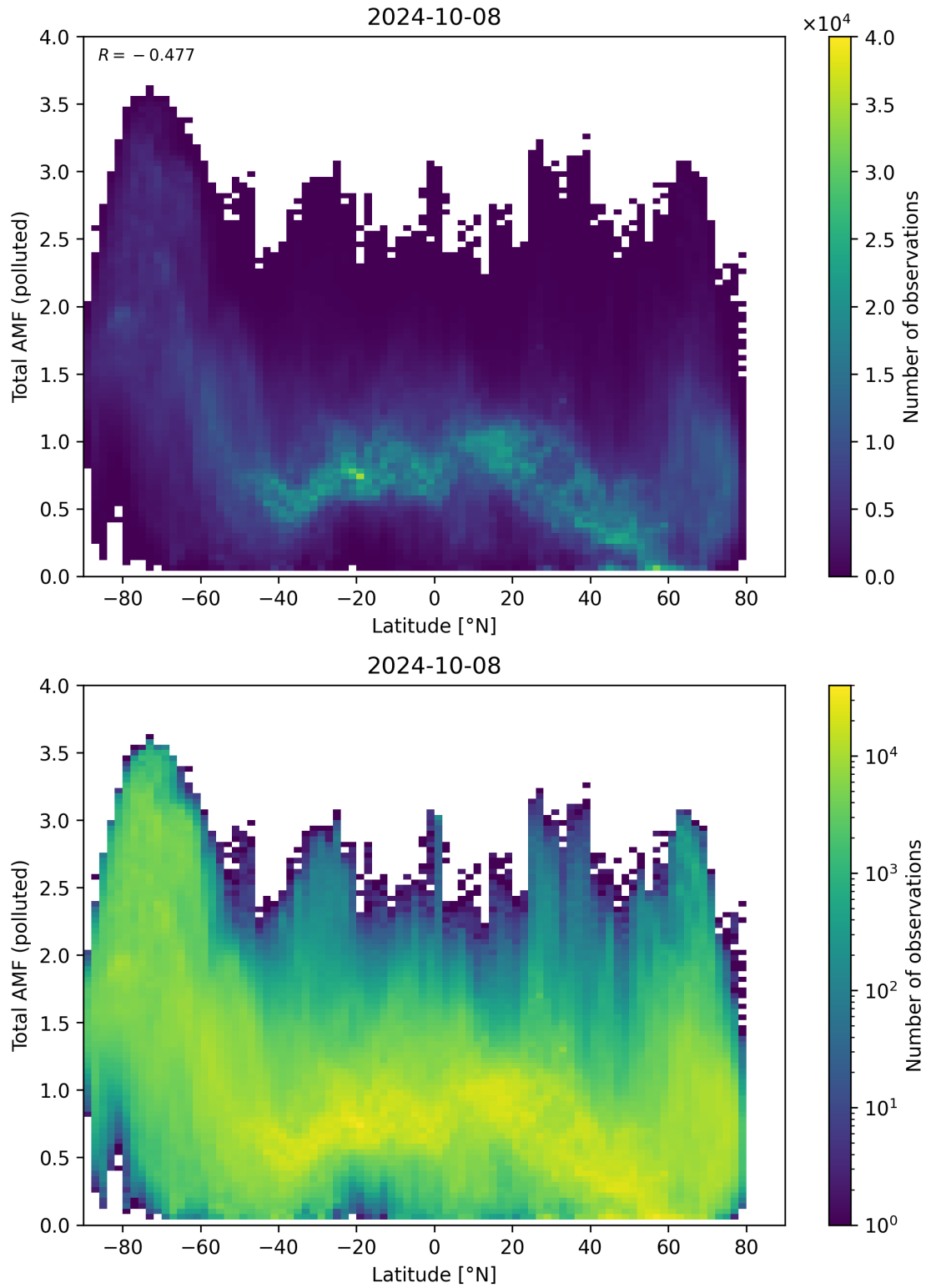
Figure 154: Scatter density plot of “Latitude” against “Total AMF (polluted)” for 2024-10-08 to 2024-10-09.
