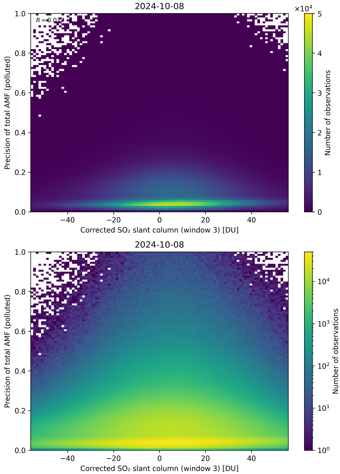
Figure 211: Scatter density plot of “Corrected SO 2 slant column (window 3)” against “Precision of total AMF (polluted)” for 2024-10-08 to 2024-10-09.
