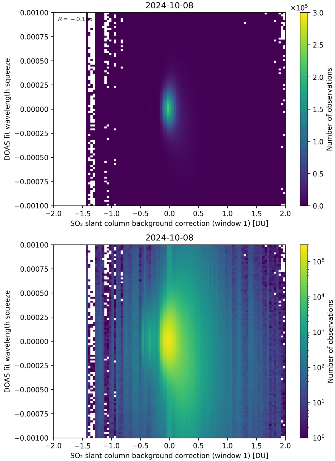
Figure 101: Scatter density plot of “SO 2 slant column background correction (window 1)” against “DOAS fit wavelength squeeze” for 2024-10-08 to 2024-10-09.
