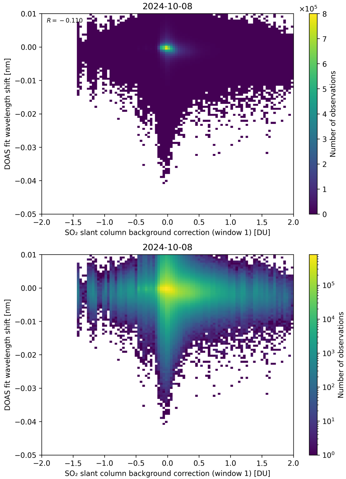
Figure 100: Scatter density plot of “SO 2 slant column background correction (window 1)” against “DOAS fit wavelength shift” for 2024-10-08 to 2024-10-09.
