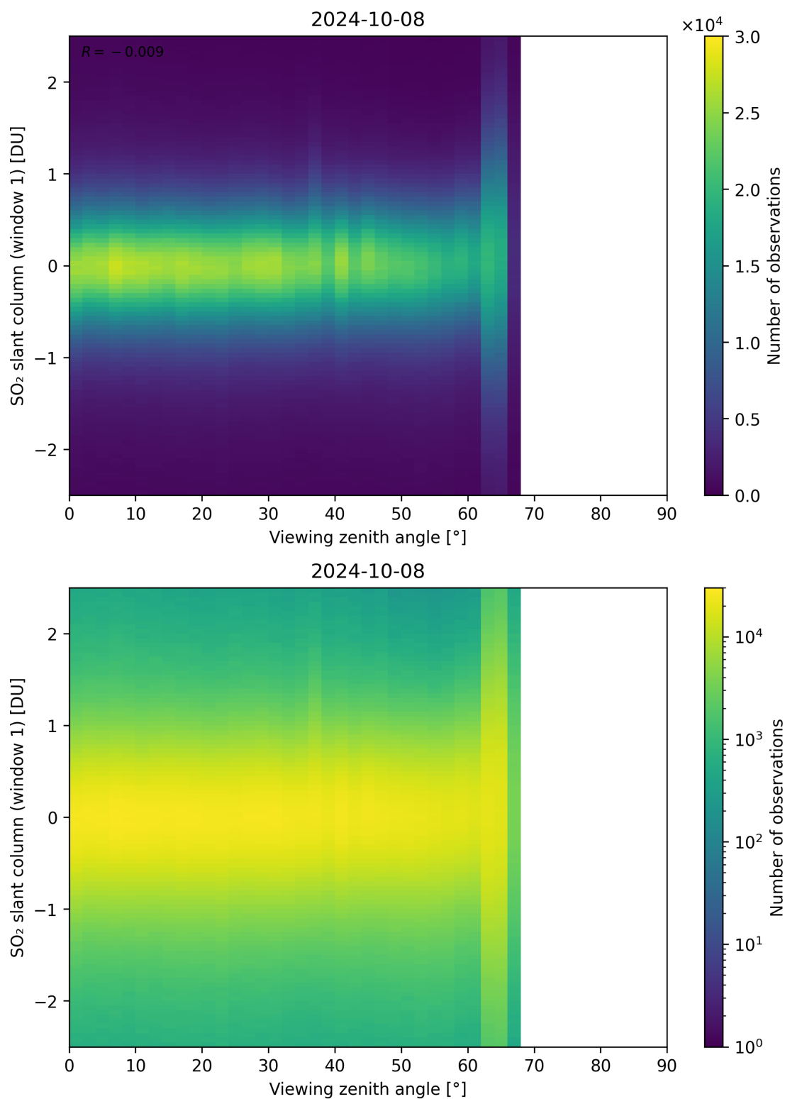
Figure 320: Scatter density plot of “Viewing zenith angle” against “SO 2 slant column (window 1)” for 2024-10-08 to 2024-10-09.
