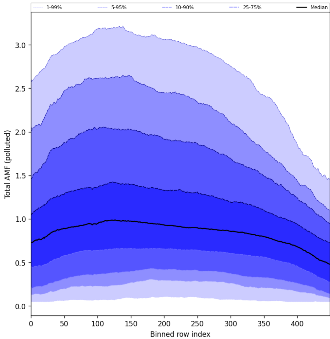
Figure 94: Along track statistics of “Total AMF (polluted)” for 2024-10-08 to 2024-10-09
