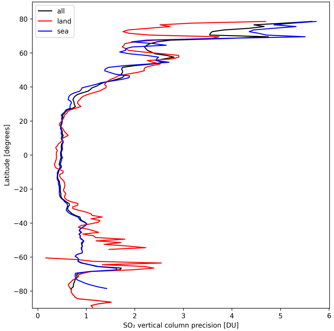
Figure 31: Zonal average of “SO 2 vertical column precision” for 2024-10-08 to 2024-10-09.
