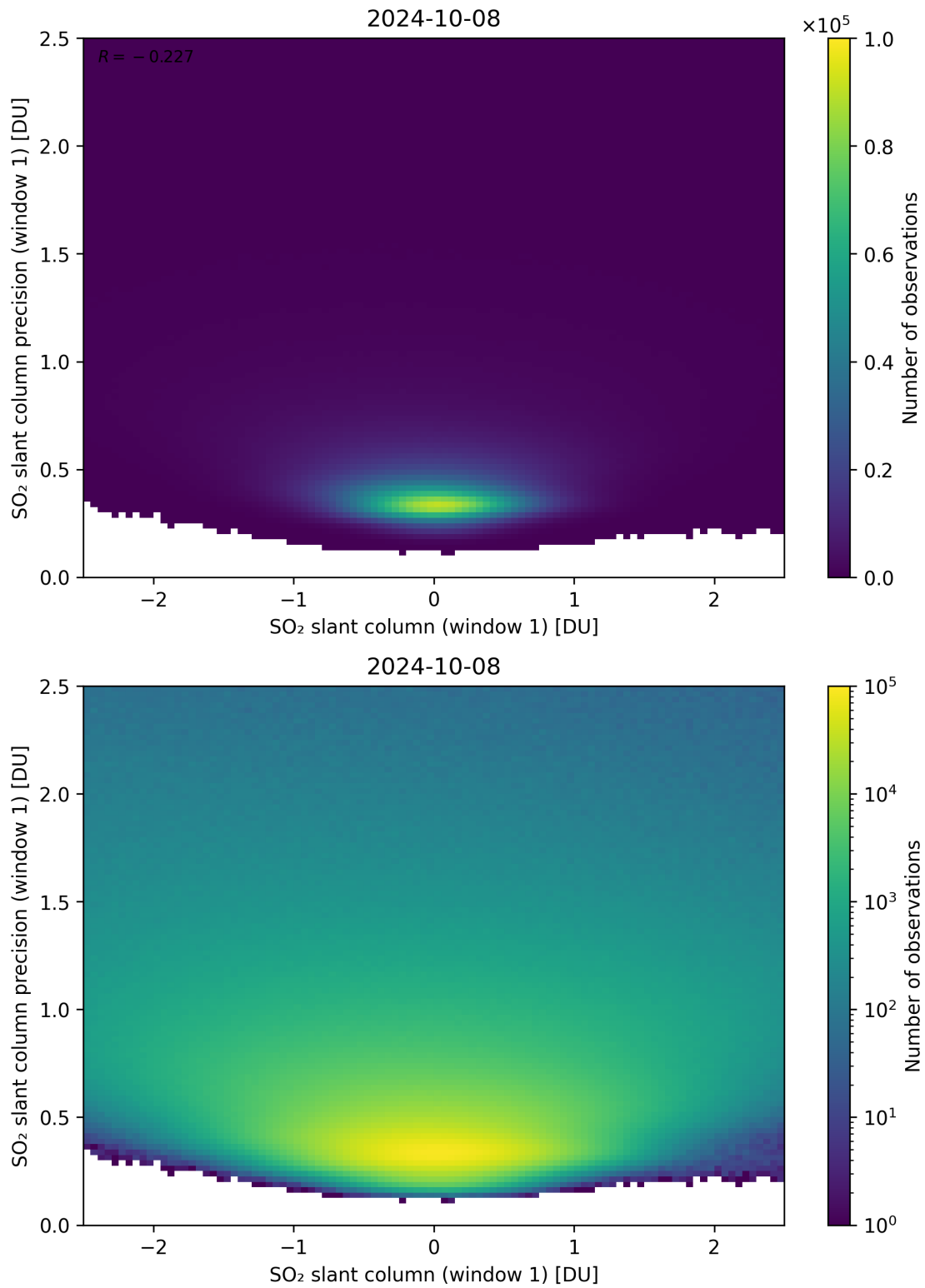
Figure 235: Scatter density plot of “SO 2 slant column (window 1)” against “SO 2 slant column precision (window 1)” for 2024-10-08 to 2024-10-09.
