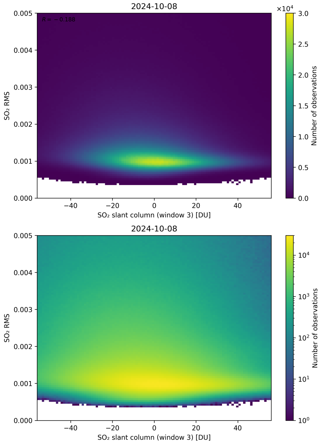
Figure 256: Scatter density plot of “SO 2 slant column (window 3)” against “SO 2 RMS” for 2024-10-08 to 2024-10-09.
