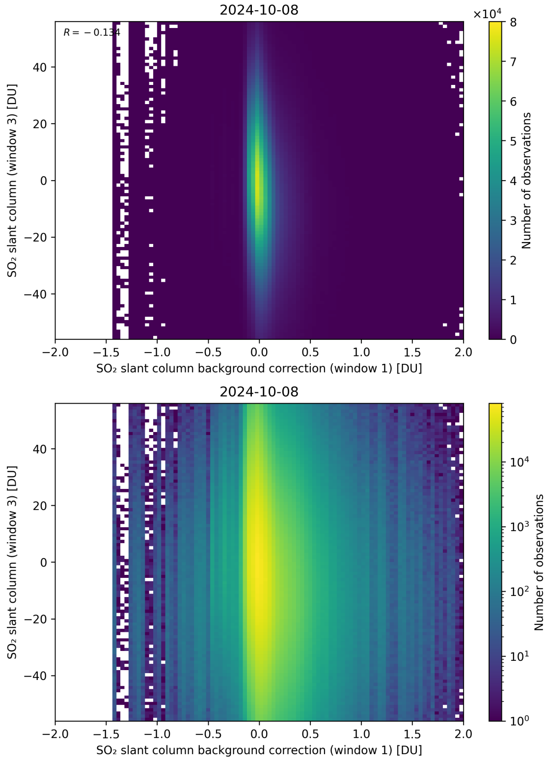
Figure 107: Scatter density plot of “SO 2 slant column background correction (window 1)” against “SO 2 slant column (window 3)” for 2024-10-08 to 2024-10-09.
