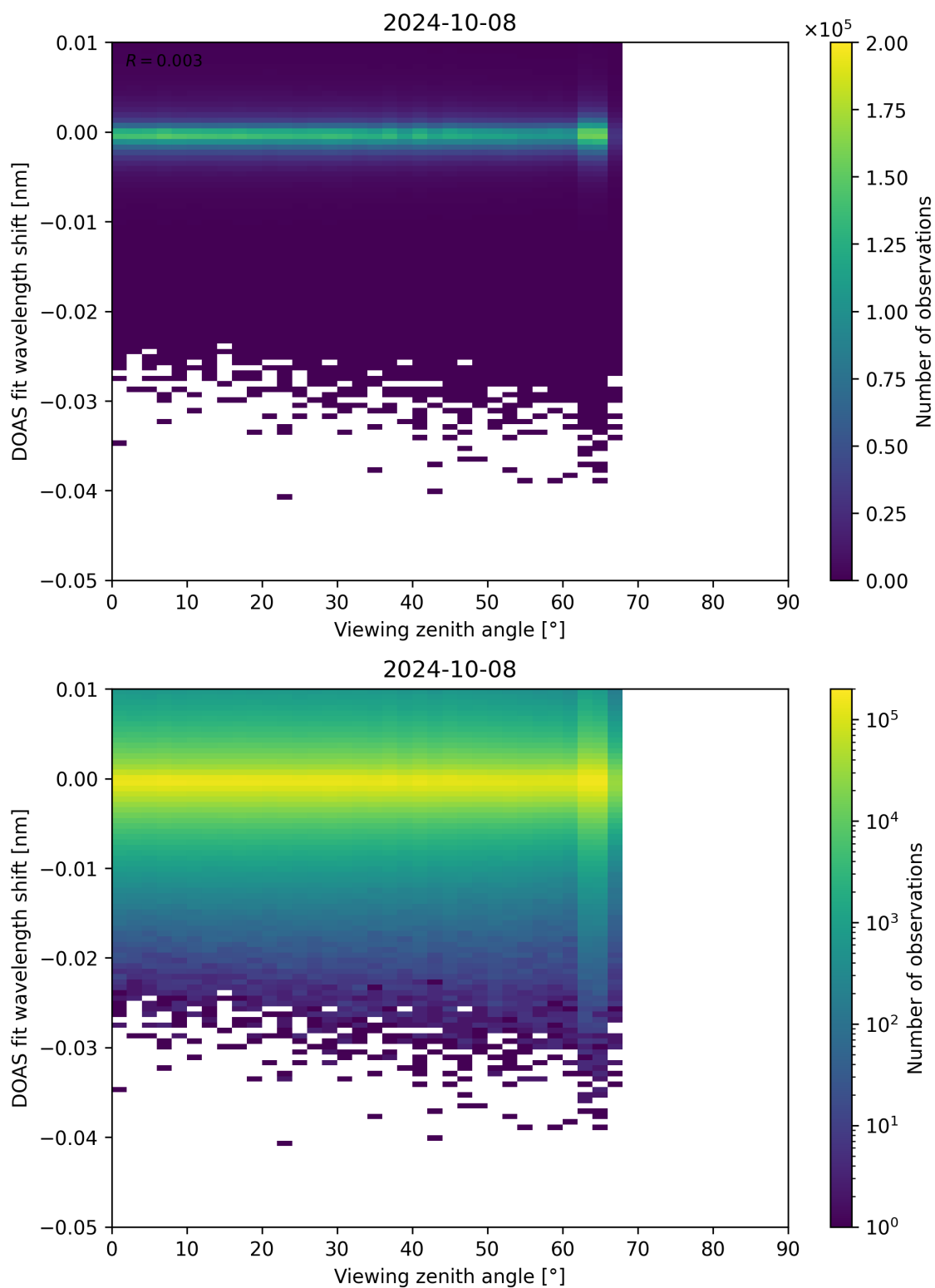
Figure 311: Scatter density plot of “Viewing zenith angle” against “DOAS fit wavelength shift” for 2024-10-08 to 2024-10-09.
