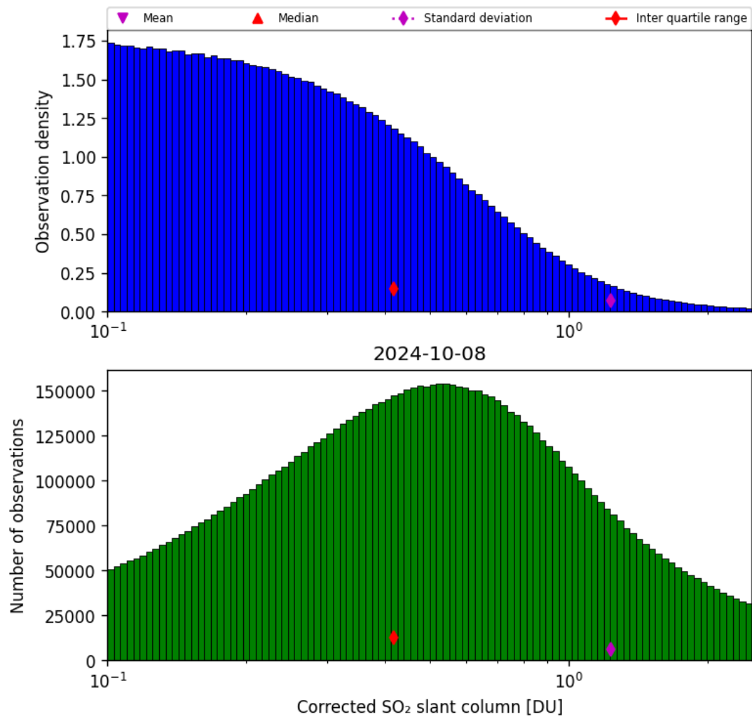
Figure 55: Histogram of “Corrected SO 2 slant column” for 2024-10-08 to 2024-10-09
