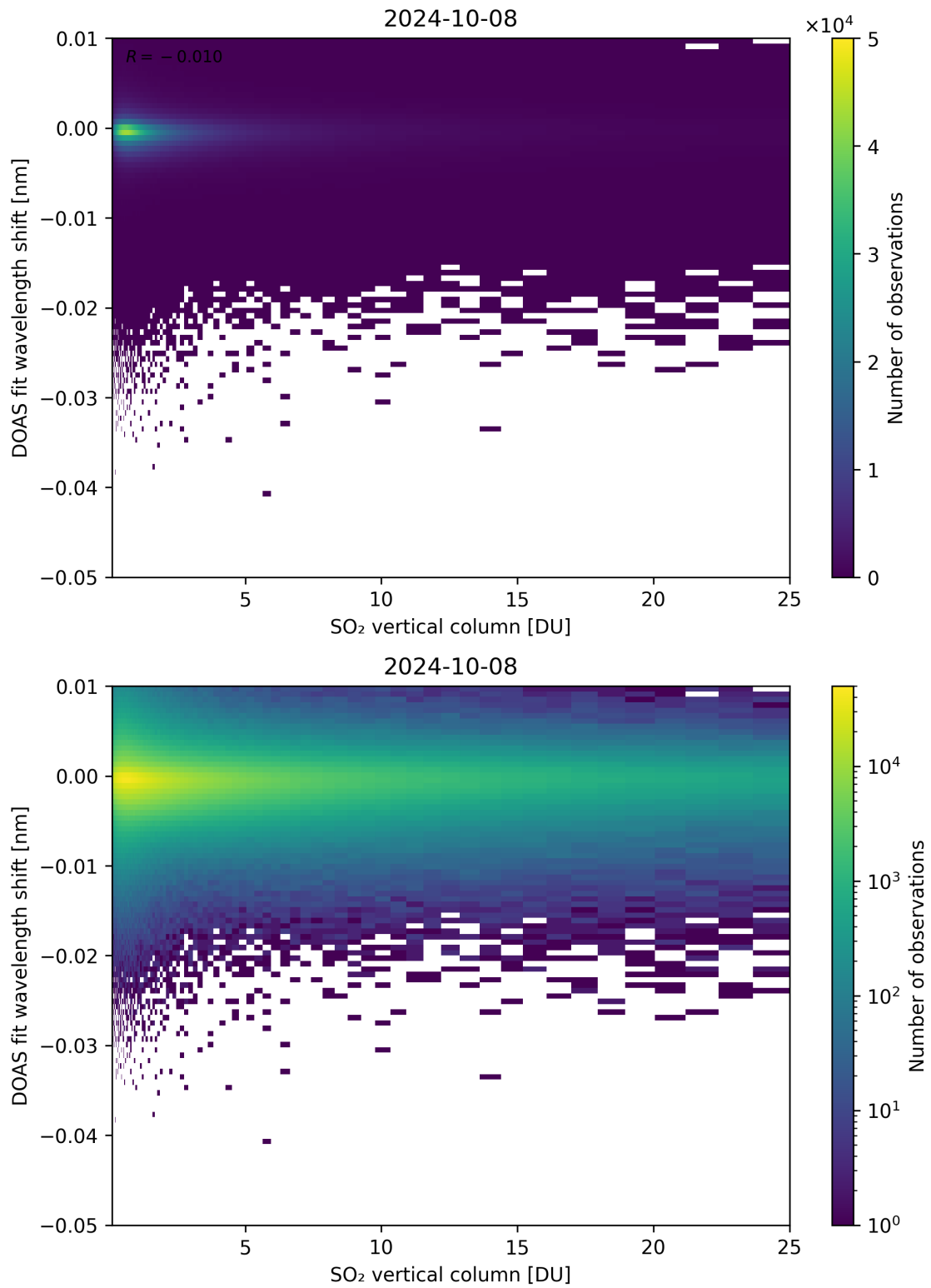
Figure 276: Scatter density plot of “SO 2 vertical column” against “DOAS fit wavelength shift” for 2024-10-08 to 2024-10-09.
