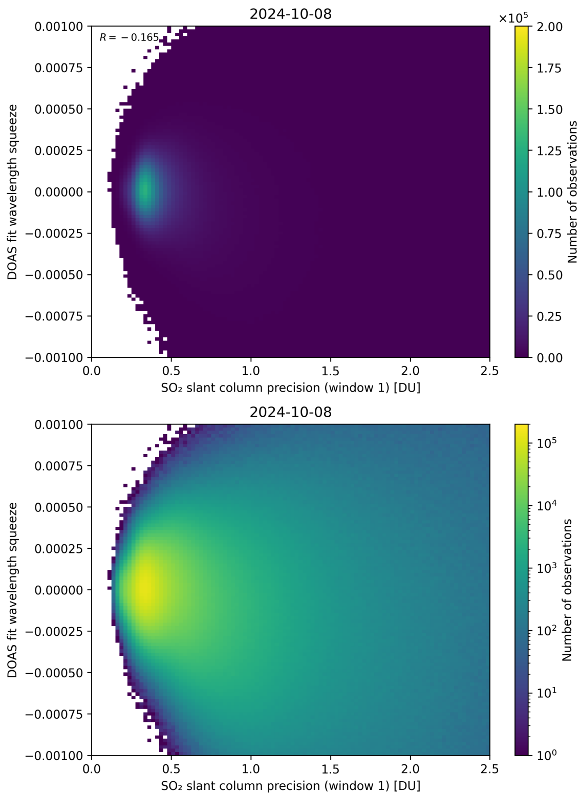
Figure 222: Scatter density plot of “SO 2 slant column precision (window 1)” against “DOAS fit wavelength squeeze” for 2024-10-08 to 2024-10-09.
