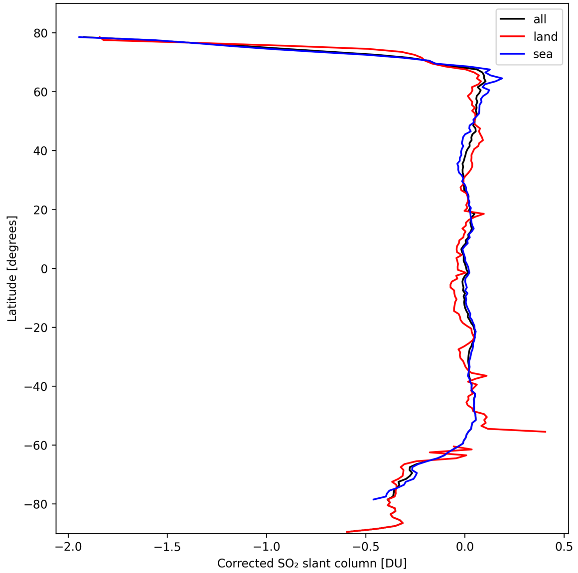
Figure 32: Zonal average of “Corrected SO 2 slant column” for 2024-10-08 to 2024-10-09.
