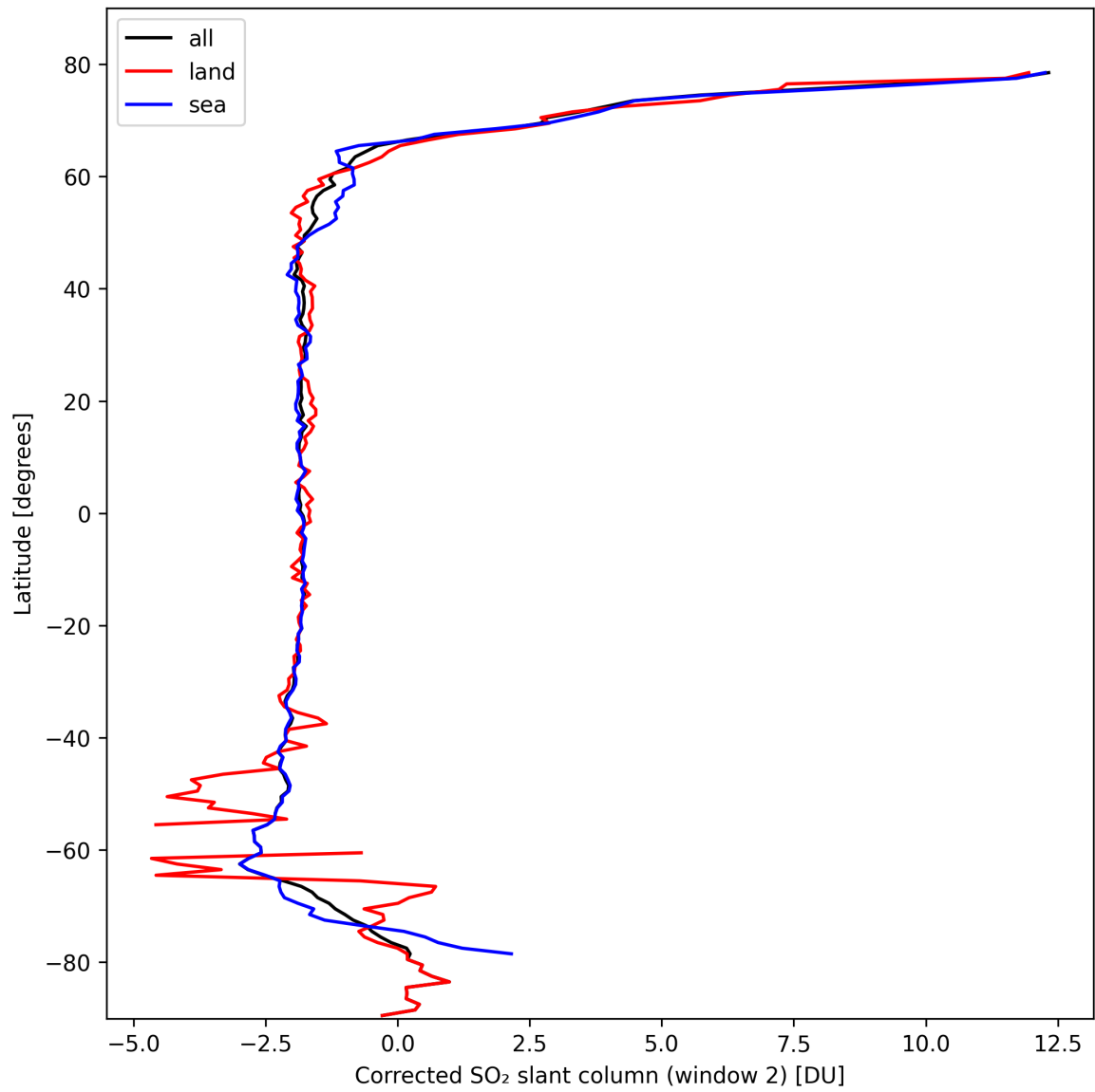
Figure 39: Zonal average of “Corrected SO 2 slant column (window 2)” for 2024-10-08 to 2024-10-09.
