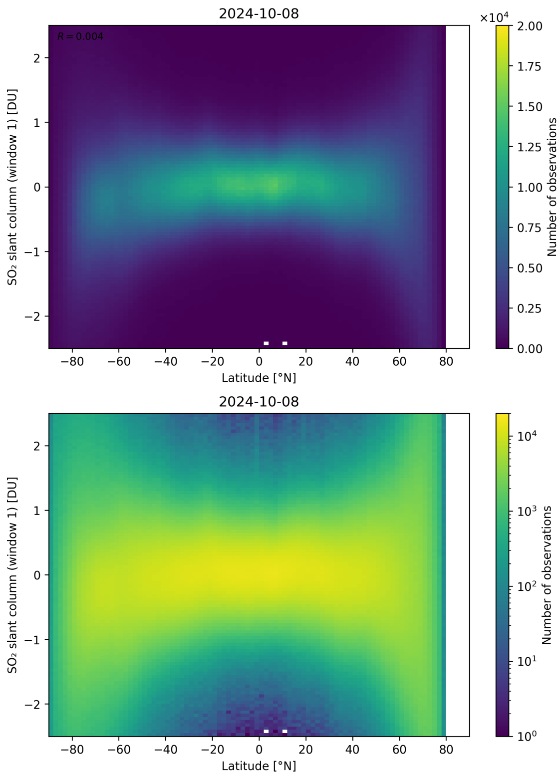
Figure 149: Scatter density plot of “Latitude” against “SO 2 slant column (window 1)” for 2024-10-08 to 2024-10-09.
