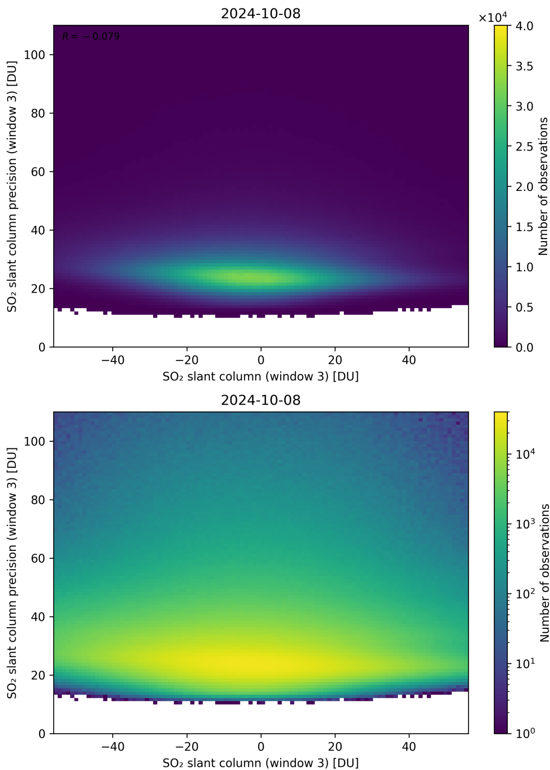
Figure 267: Scatter density plot of “SO 2 slant column (window 3)” against “SO 2 slant column precision (window 3)” for 2024-10-08 to 2024-10-09.
