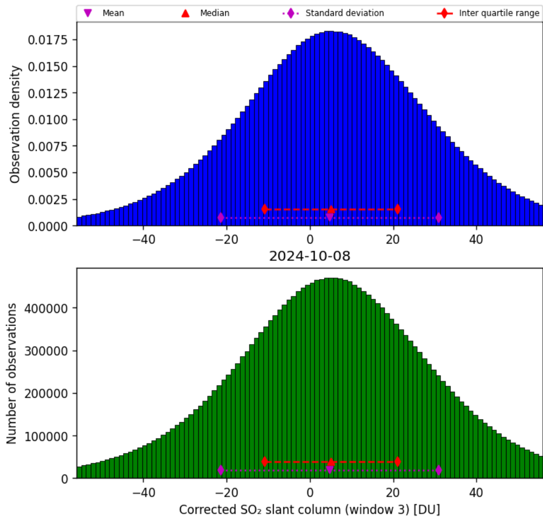
Figure 66: Histogram of “Corrected SO 2 slant column (window 3)” for 2024-10-08 to 2024-10-09
