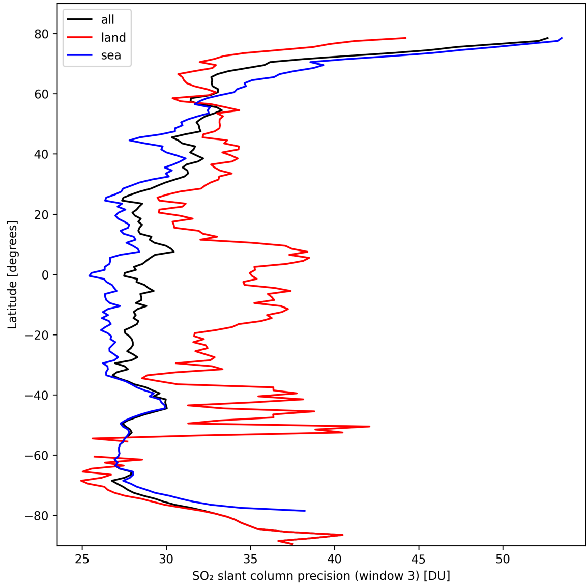
Figure 42: Zonal average of “SO 2 slant column precision (window 3)” for 2024-10-08 to 2024-10-09.
