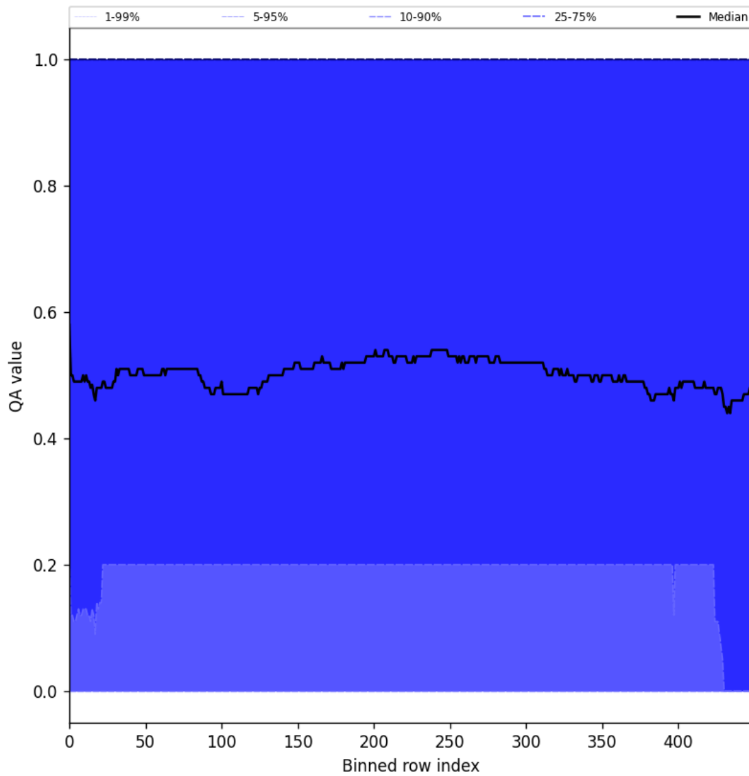
Figure 75: Along track statistics of “QA value” for 2024-10-08 to 2024-10-09
