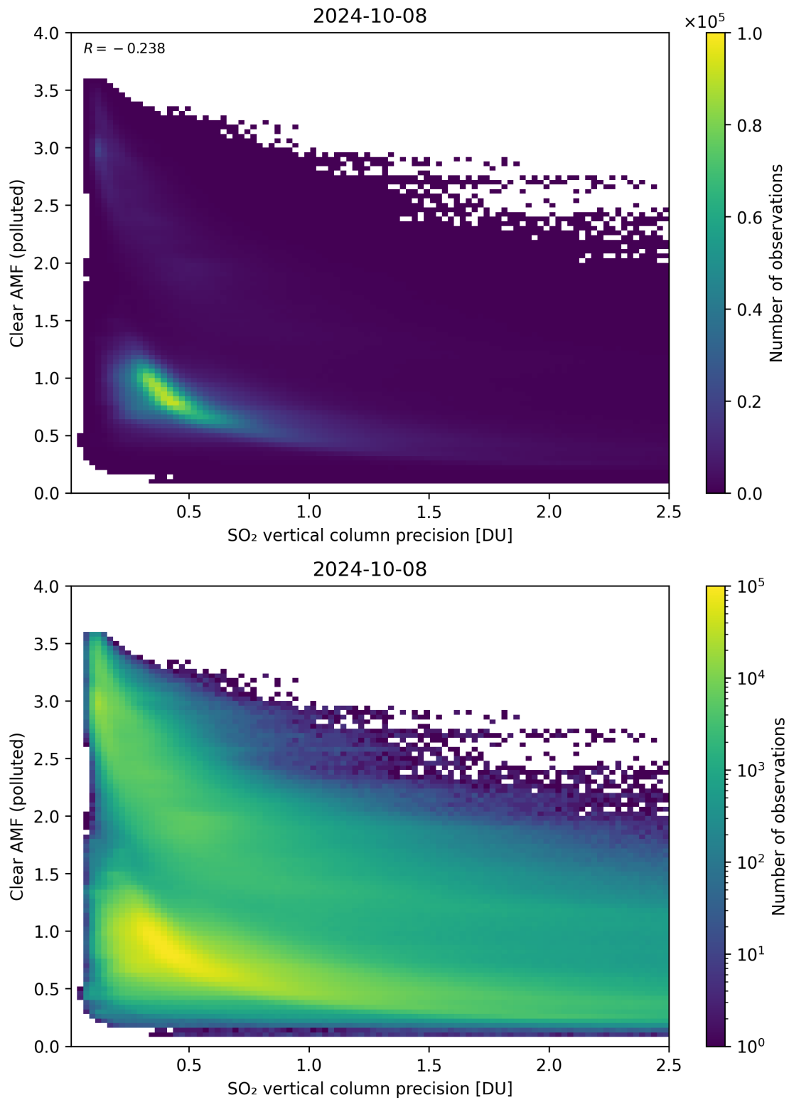
Figure 285: Scatter density plot of “SO 2 vertical column precision” against “Clear AMF (polluted)” for 2024-10-08 to 2024-10-09.
