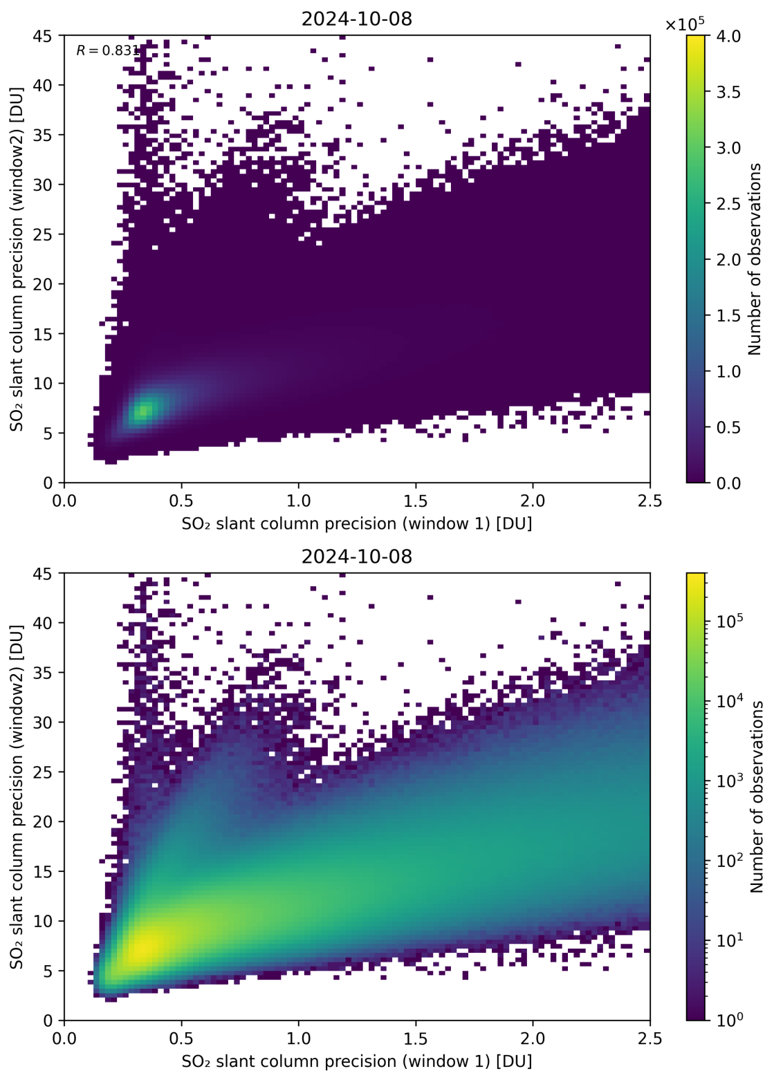
Figure 227: Scatter density plot of “SO 2 slant column precision (window 1)” against “SO 2 slant column precision (window2)” for 2024-10-08 to 2024-10-09.
