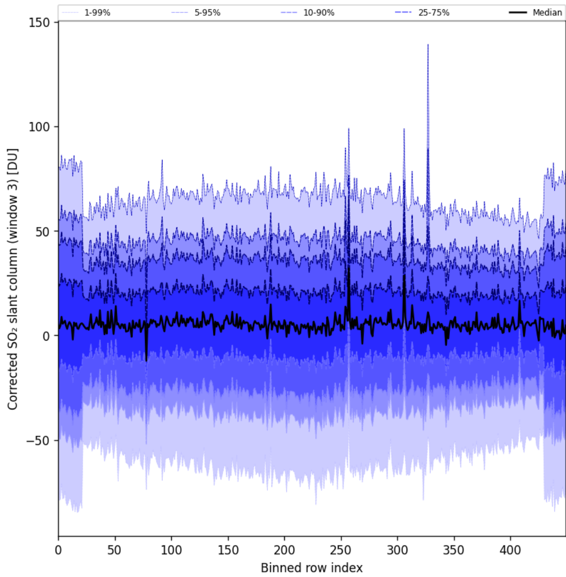
Figure 89: Along track statistics of “Corrected SO 2 slant column (window 3)” for 2024-10-08 to 2024-10-09
