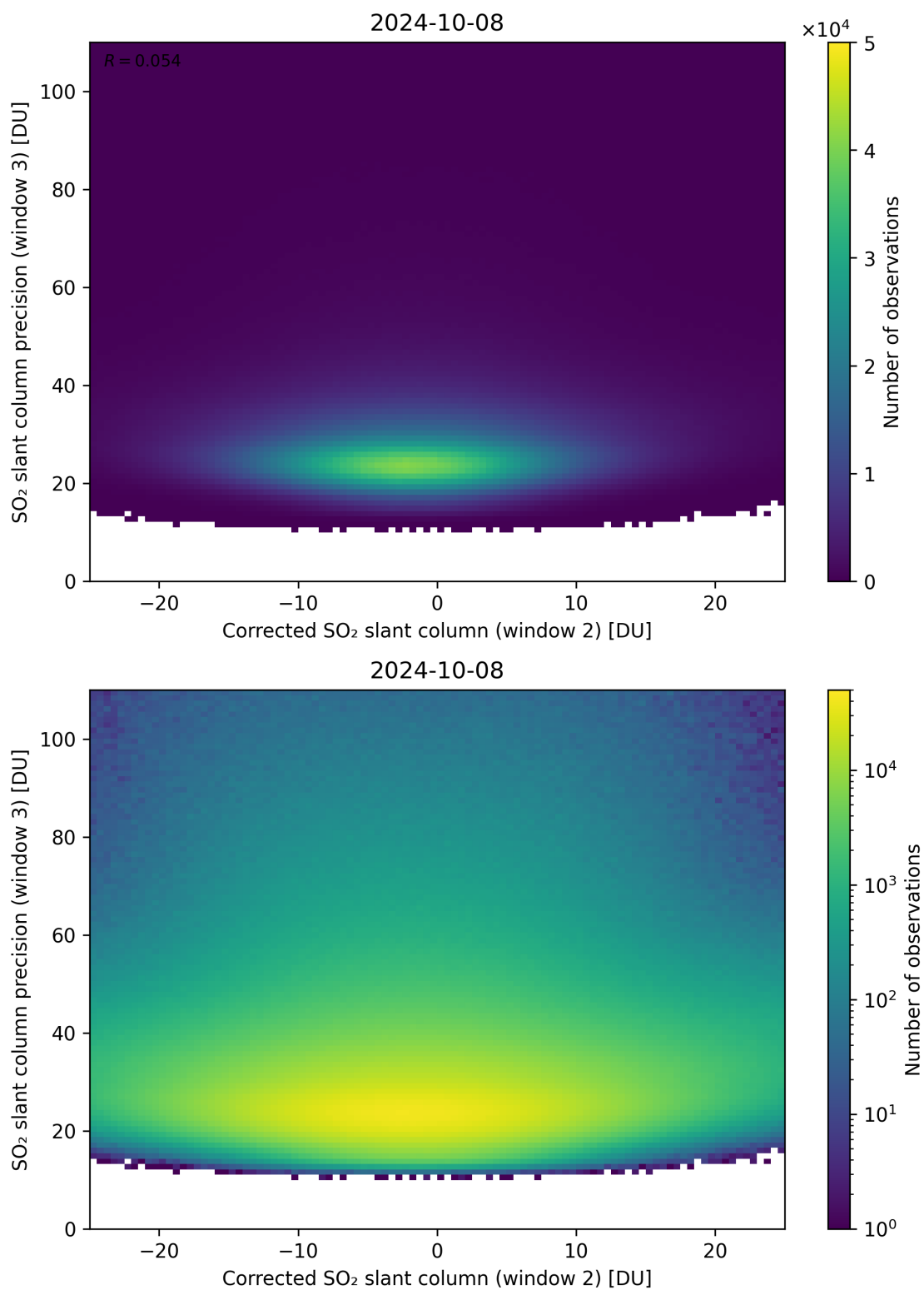
Figure 202: Scatter density plot of “Corrected SO 2 slant column (window 2)” against “SO 2 slant column precision (window 3)” for 2024-10-08 to 2024-10-09.
