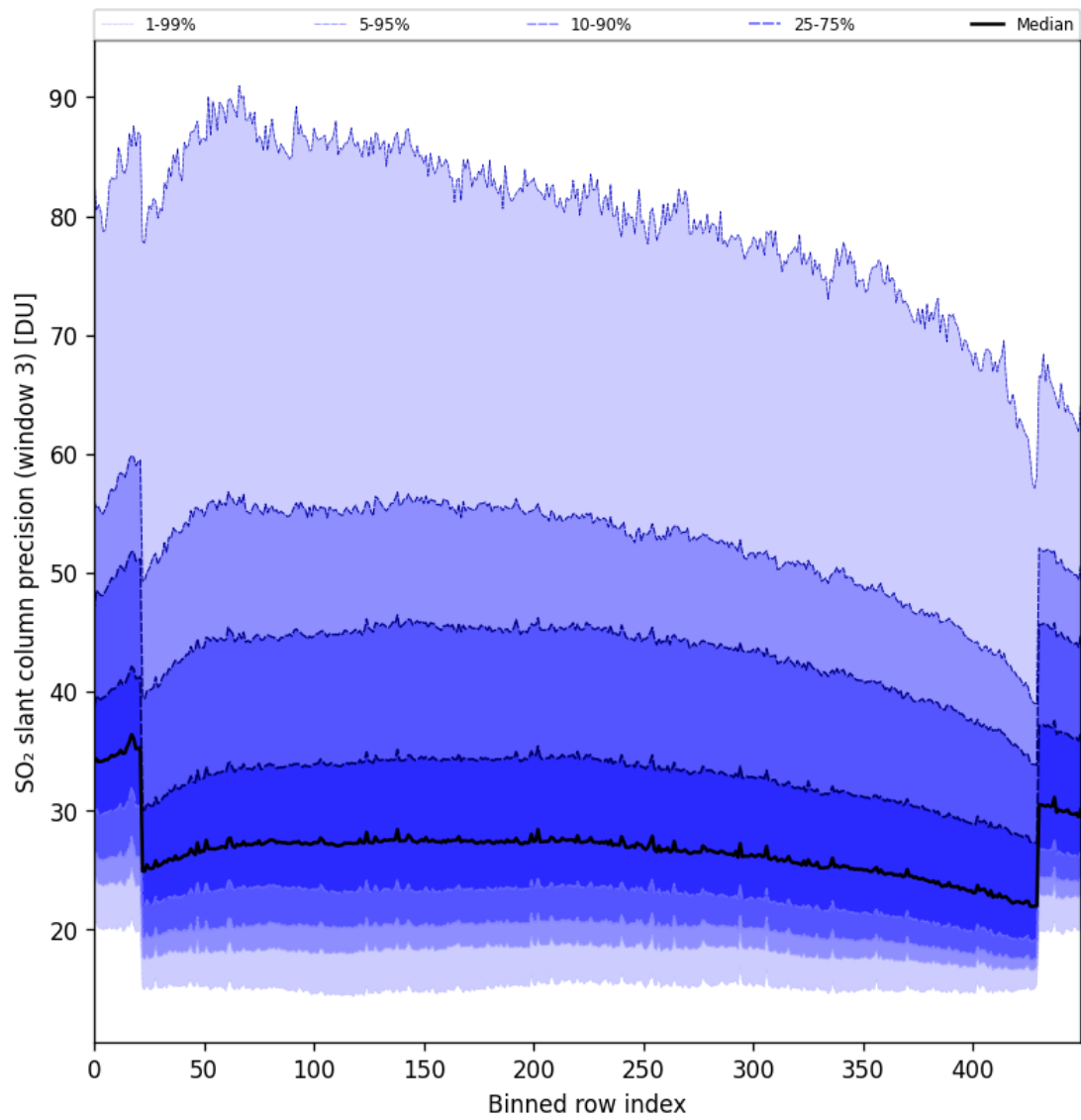
Figure 88: Along track statistics of “SO 2 slant column precision (window 3)” for 2024-10-08 to 2024-10-09
