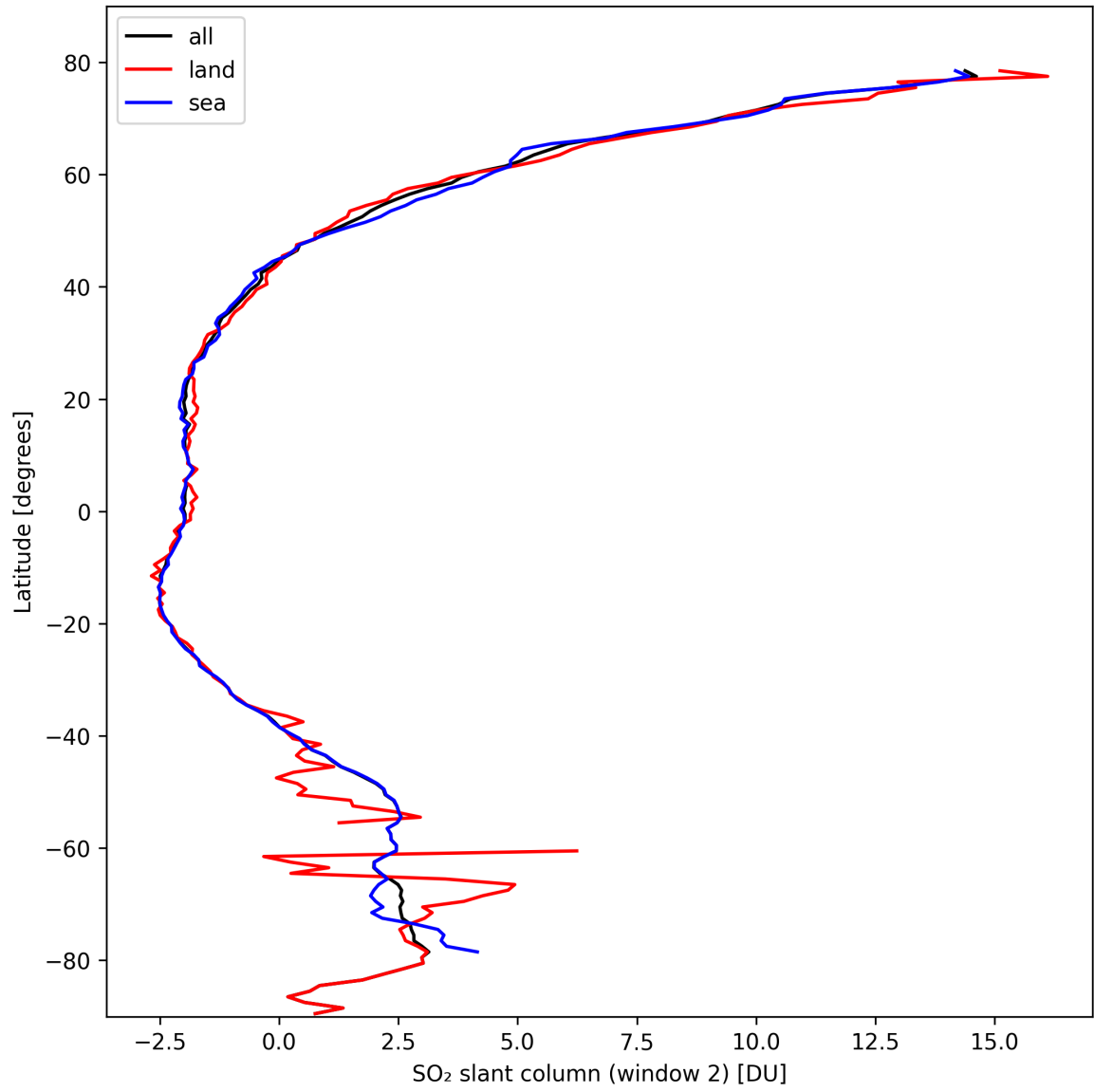
Figure 37: Zonal average of “SO 2 slant column (window 2)” for 2024-10-08 to 2024-10-09.
