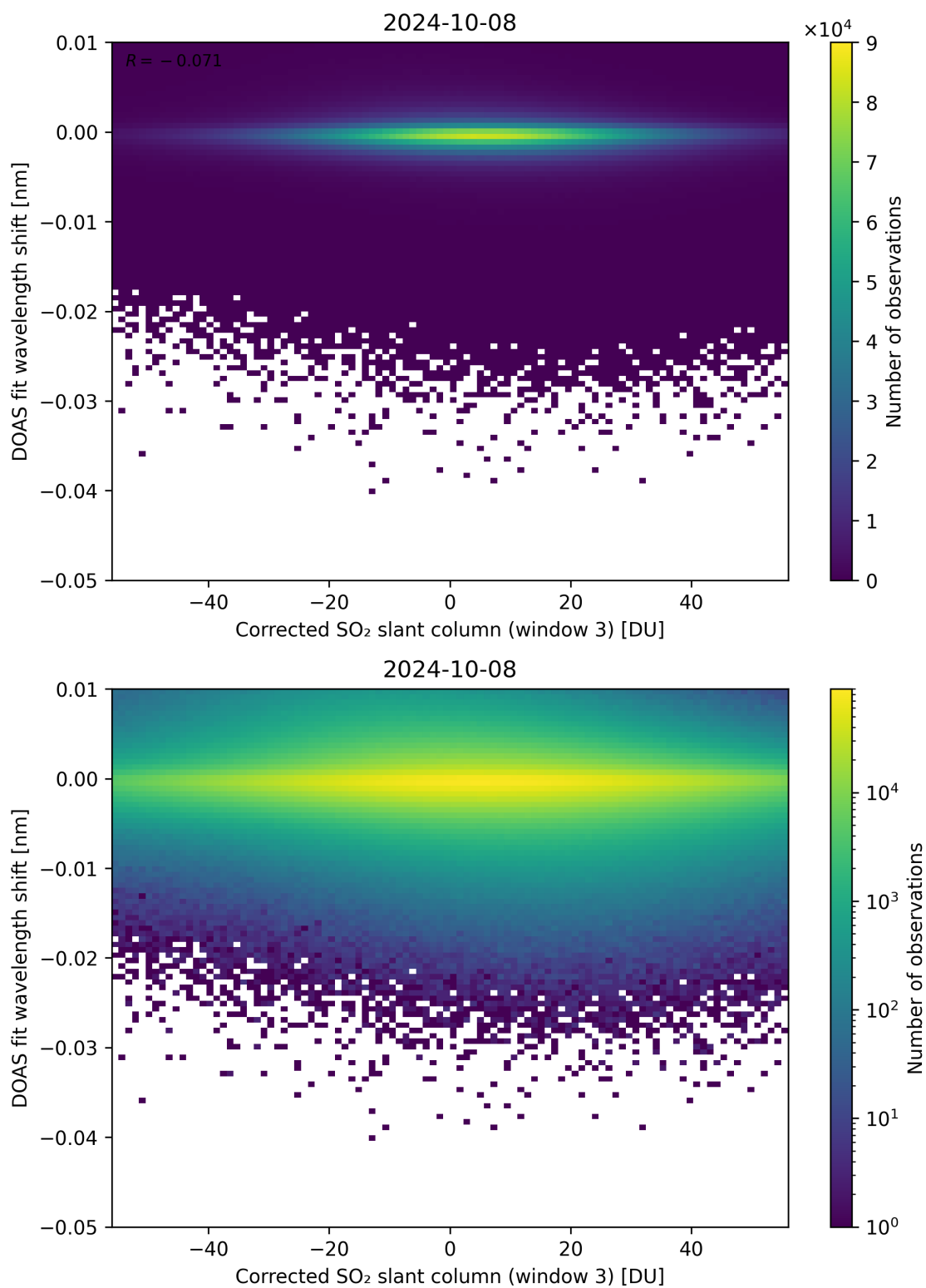
Figure 206: Scatter density plot of “Corrected SO 2 slant column (window 3)” against “DOAS fit wavelength shift” for 2024-10-08 to 2024-10-09.
