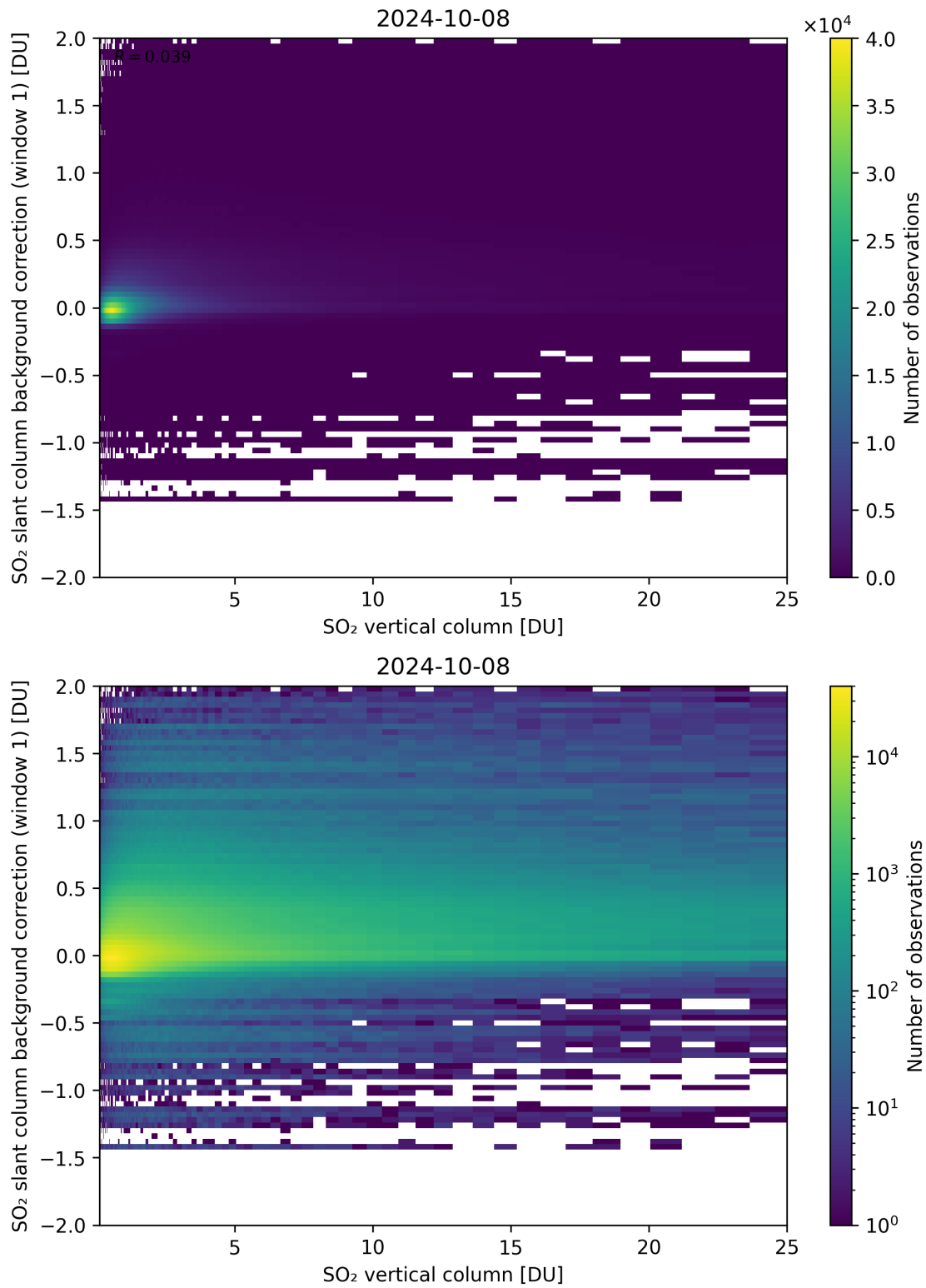
Figure 273: Scatter density plot of “SO 2 vertical column” against “SO 2 slant column background correction (window 1)” for 2024-10-08 to 2024-10-09.
