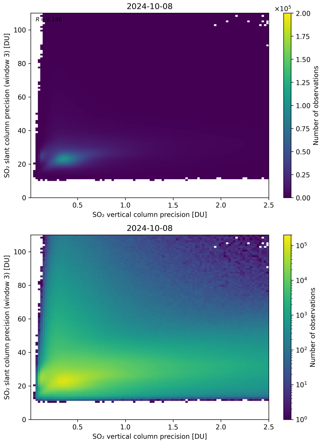
Figure 293: Scatter density plot of “SO 2 vertical column precision” against “SO 2 slant column precision (window 3)” for 2024-10-08 to 2024-10-09.
