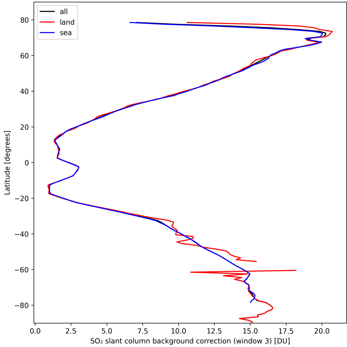
Figure 44: Zonal average of “SO 2 slant column background correction (window 3)” for 2024-10-08 to 2024-10-09.
