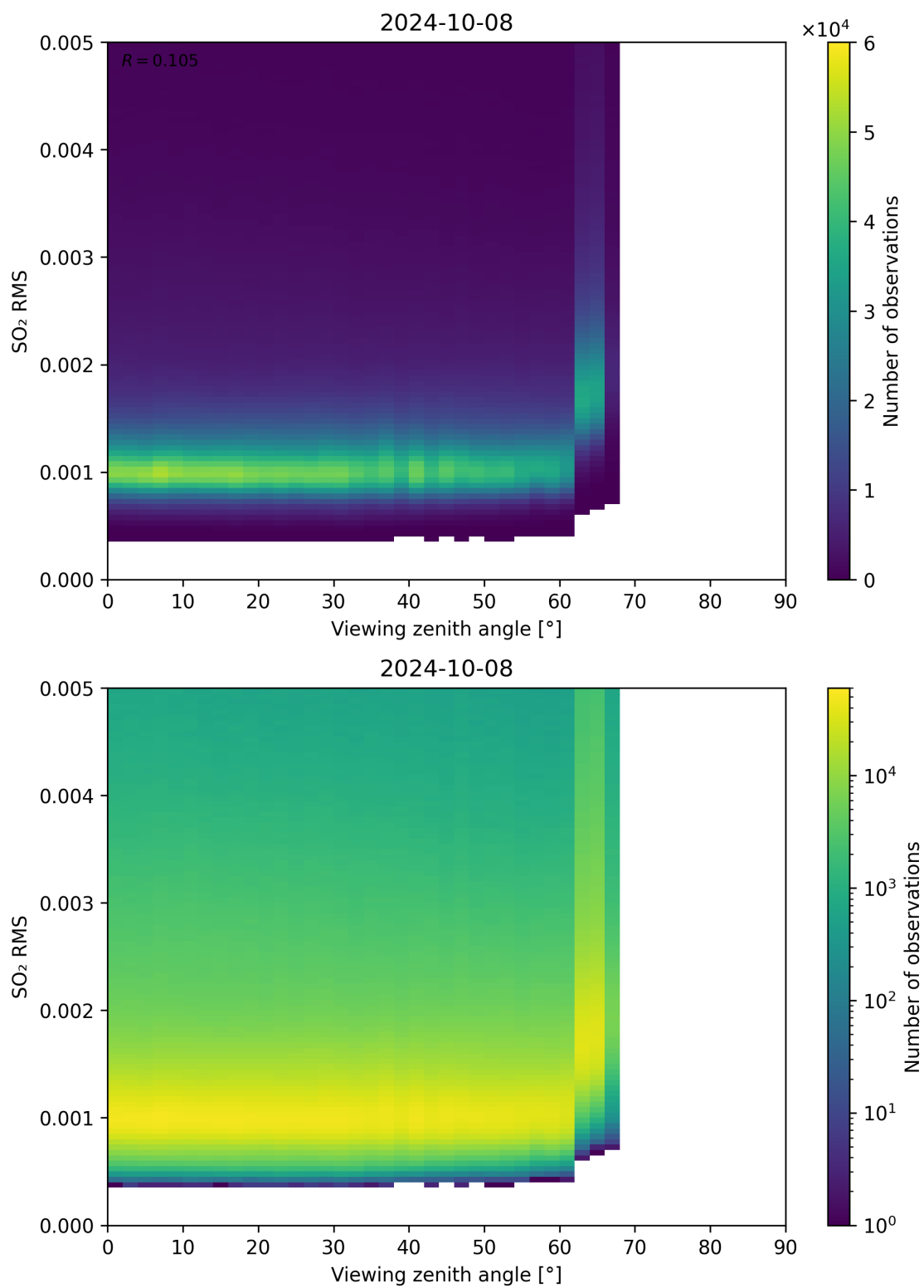
Figure 313: Scatter density plot of “Viewing zenith angle” against “SO 2 RMS” for 2024-10-08 to 2024-10-09.
