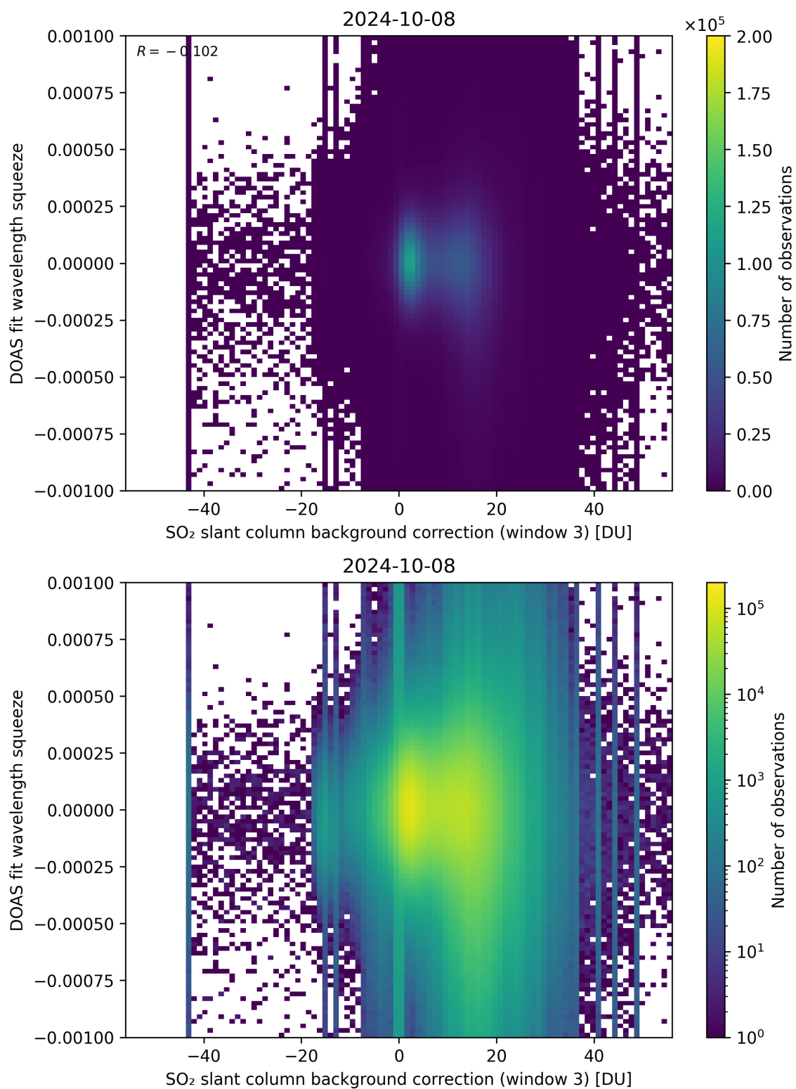
Figure 122: Scatter density plot of “SO 2 slant column background correction (window 3)” against “DOAS fit wavelength squeeze” for 2024-10-08 to 2024-10-09.
