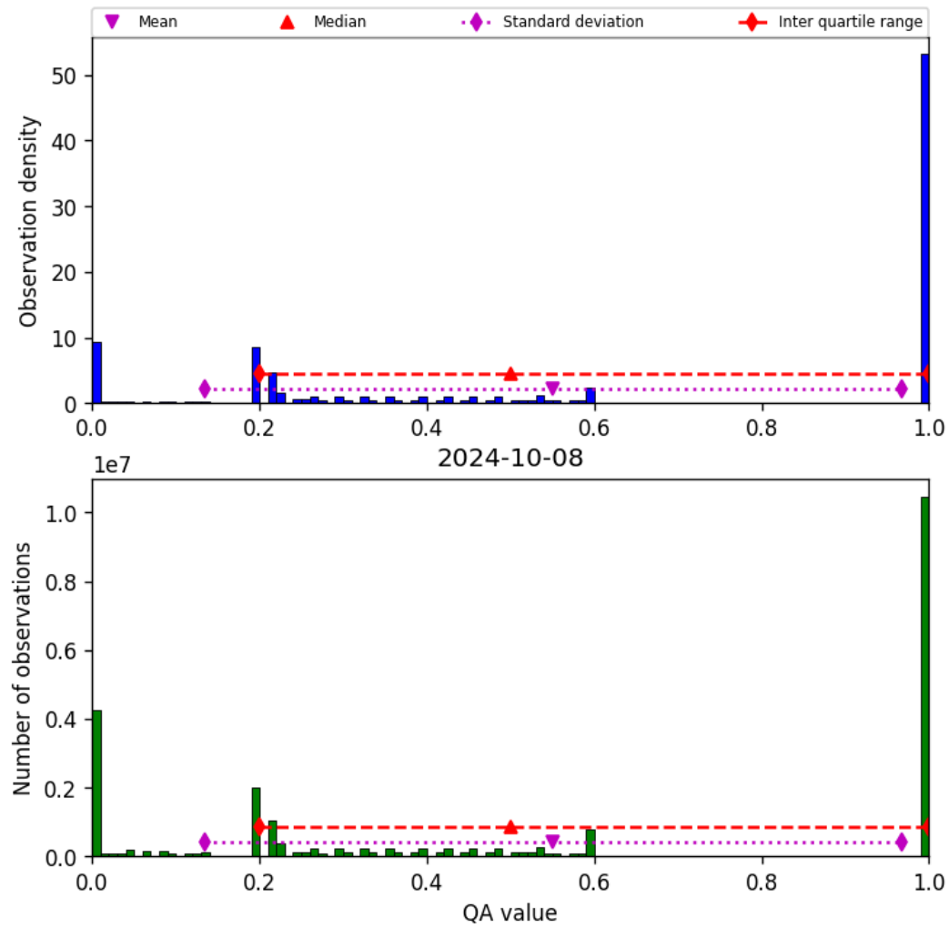
Figure 52: Histogram of “QA value” for 2024-10-08 to 2024-10-09
