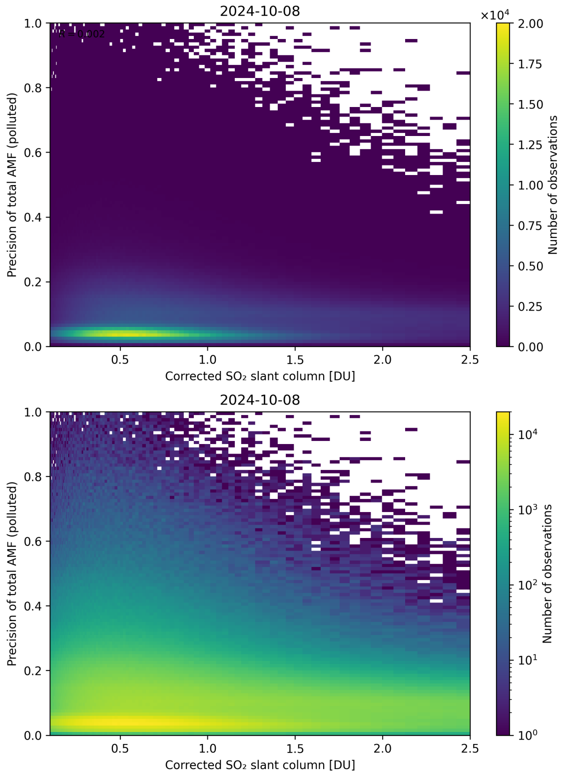
Figure 193: Scatter density plot of “Corrected SO 2 slant column” against “Precision of total AMF (polluted)” for 2024-10-08 to 2024-10-09.
