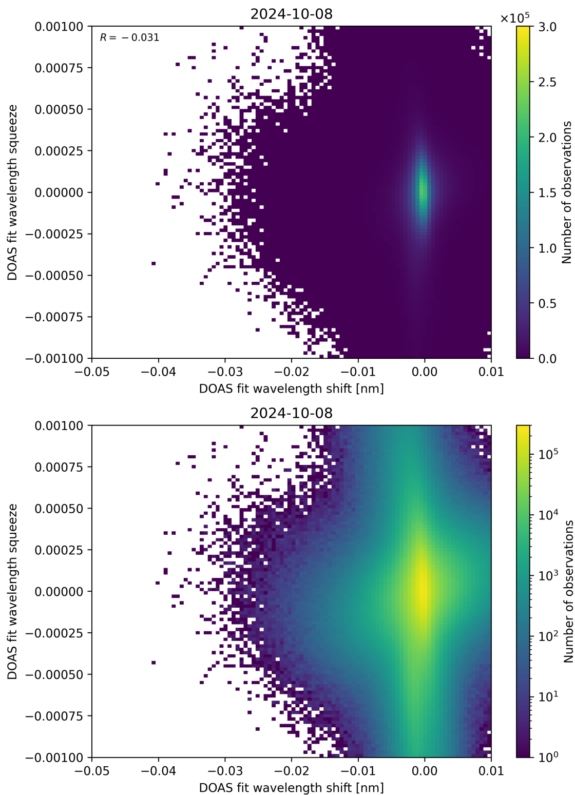
Figure 127: Scatter density plot of “DOAS fit wavelength shift” against “DOAS fit wavelength squeeze” for 2024-10-08 to 2024-10-09.
