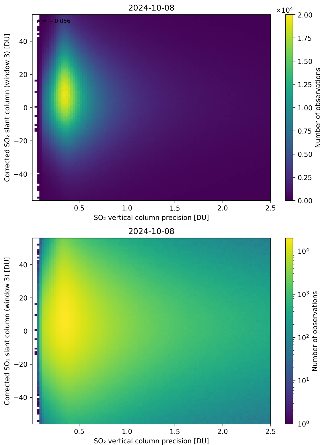
Figure 288: Scatter density plot of “SO 2 vertical column precision” against “Corrected SO 2 slant column (window 3)” for 2024-10-08 to 2024-10-09.
