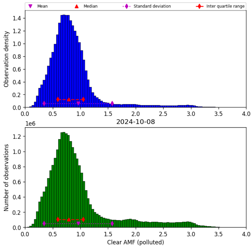
Figure 73: Histogram of “Clear AMF (polluted)” for 2024-10-08 to 2024-10-09
