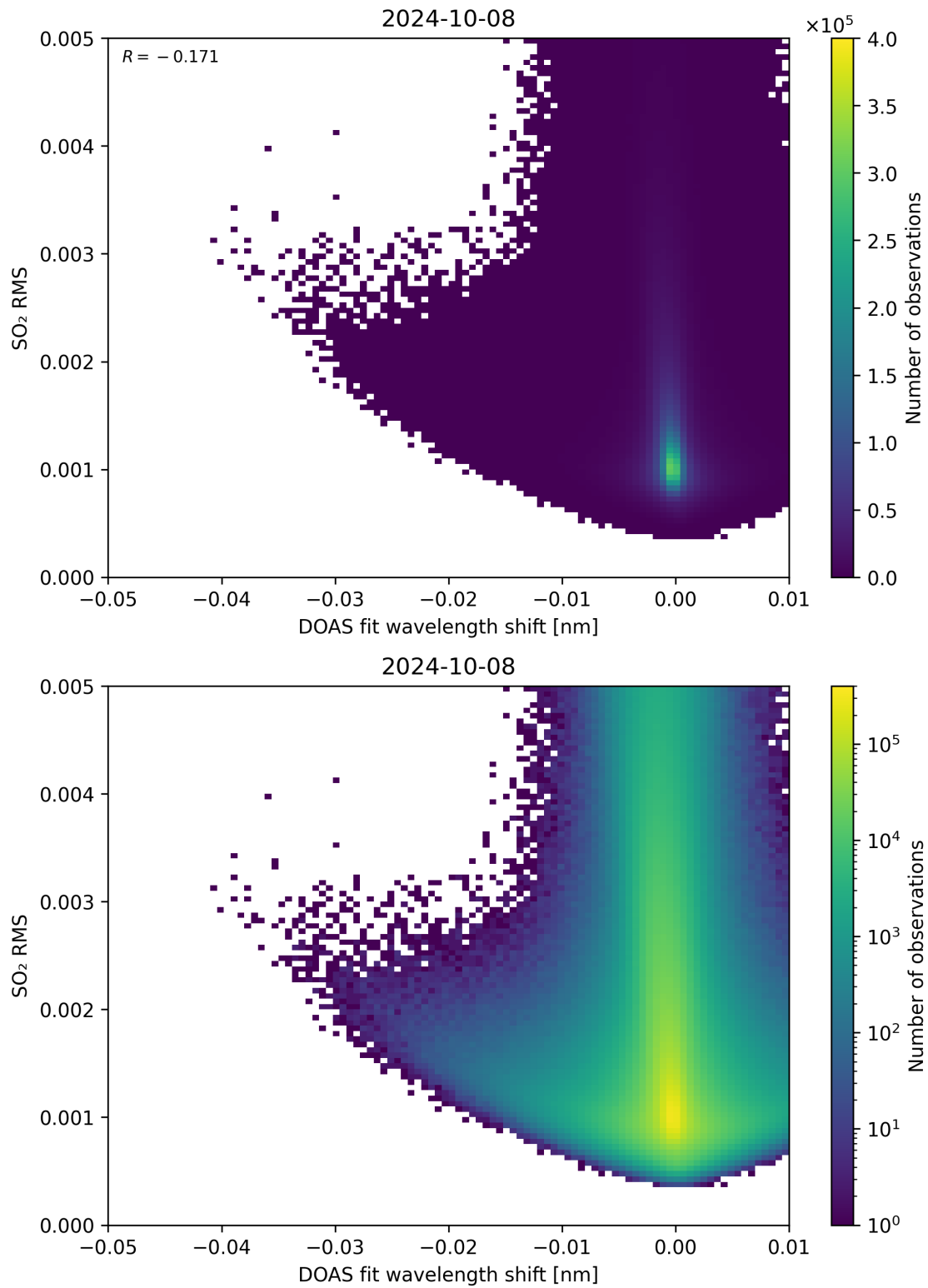
Figure 128: Scatter density plot of “DOAS fit wavelength shift” against “SO 2 RMS” for 2024-10-08 to 2024-10-09.
