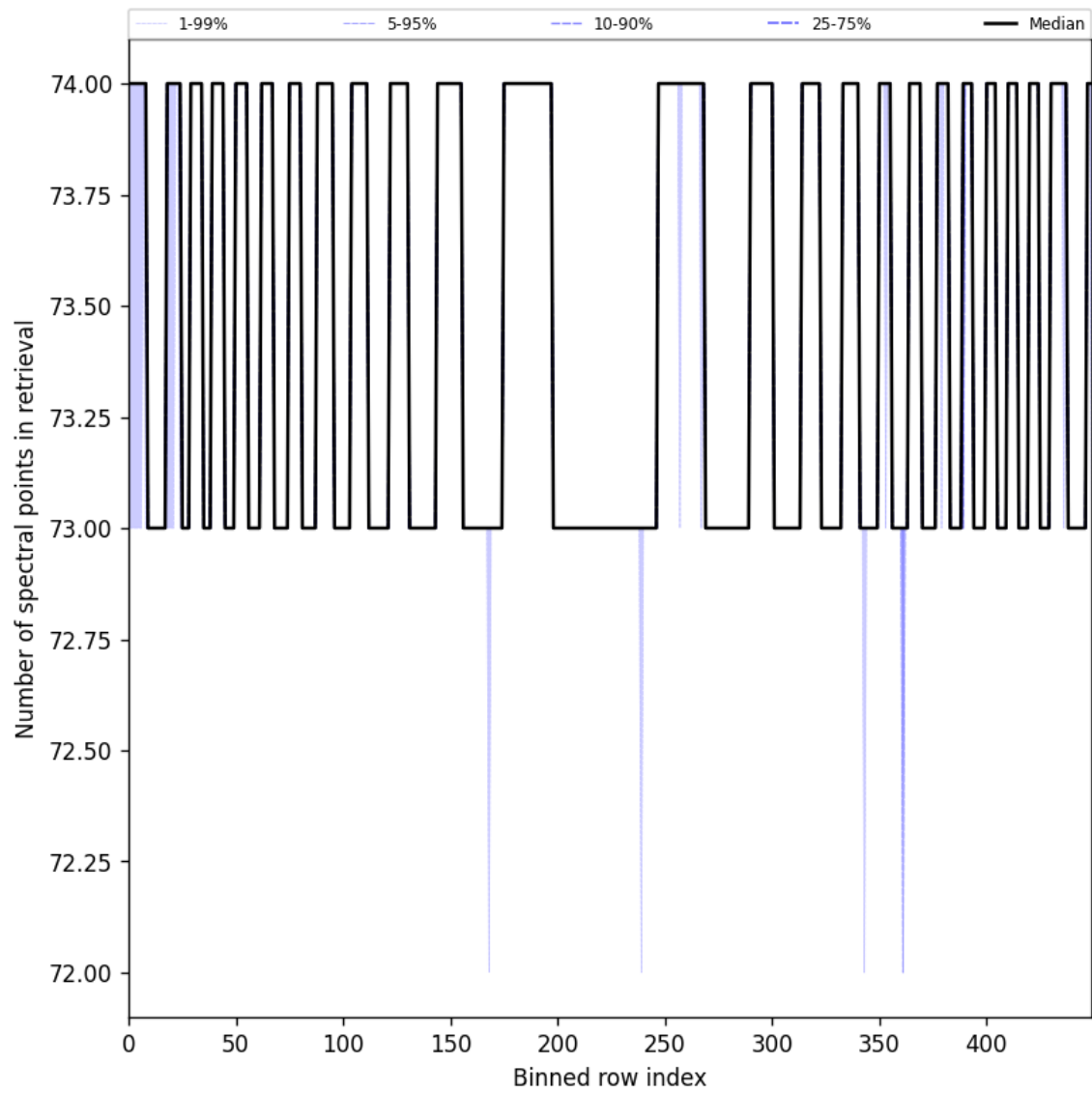
Figure 97: Along track statistics of “Number of spectral points in retrieval” for 2024-10-08 to 2024-10-09
