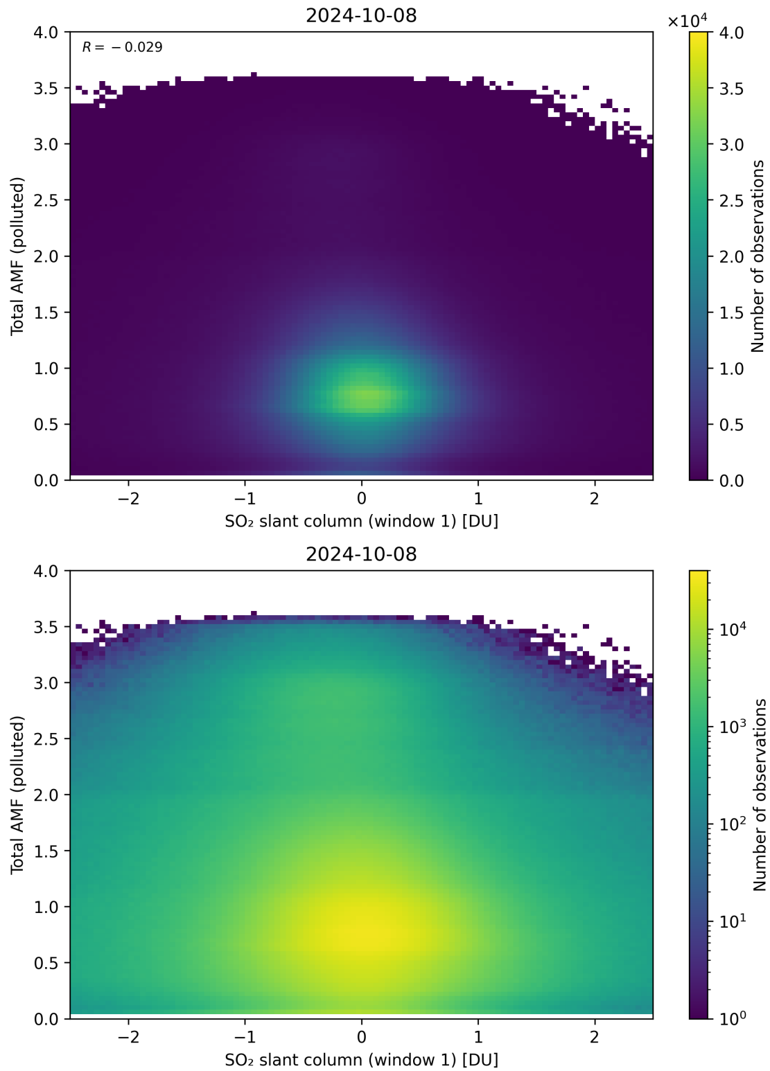
Figure 239: Scatter density plot of “SO 2 slant column (window 1)” against “Total AMF (polluted)” for 2024-10-08 to 2024-10-09.
