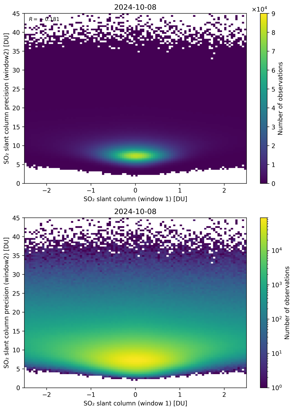
Figure 236: Scatter density plot of “SO 2 slant column (window 1)” against “SO 2 slant column precision (window2)” for 2024-10-08 to 2024-10-09.
