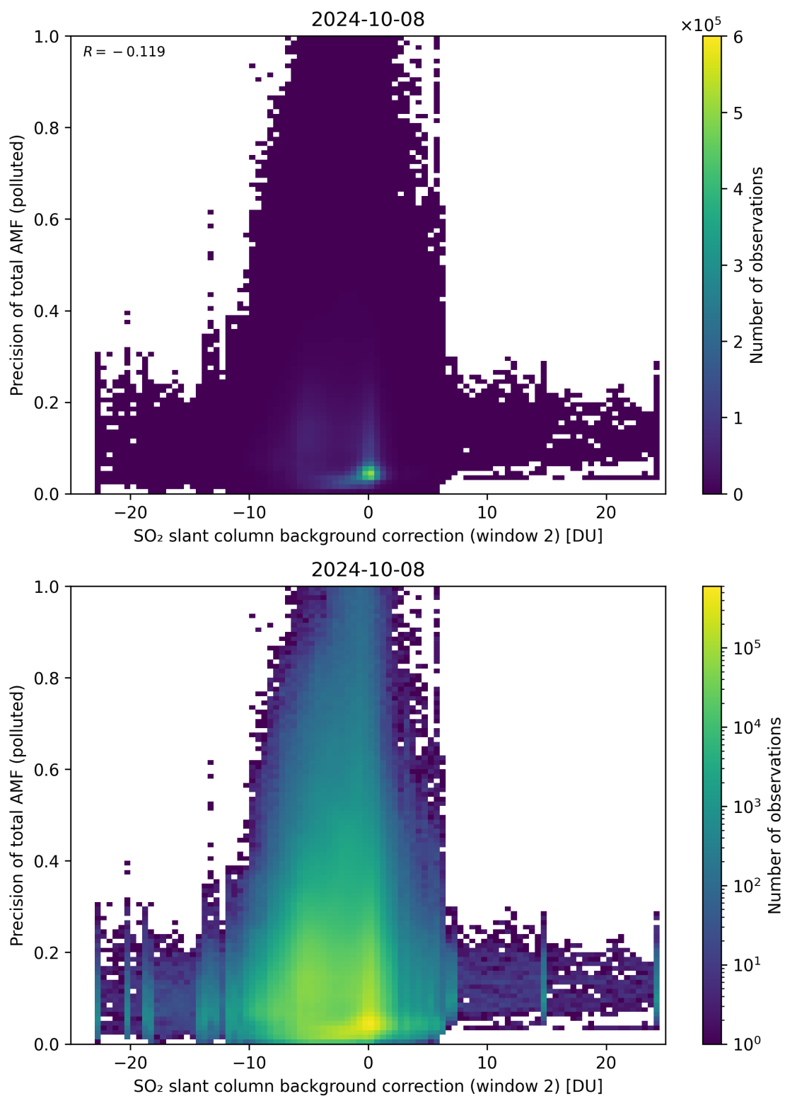
Figure 120: Scatter density plot of “SO 2 slant column background correction (window 2)” against “Precision of total AMF (polluted)” for 2024-10-08 to 2024-10-09.
