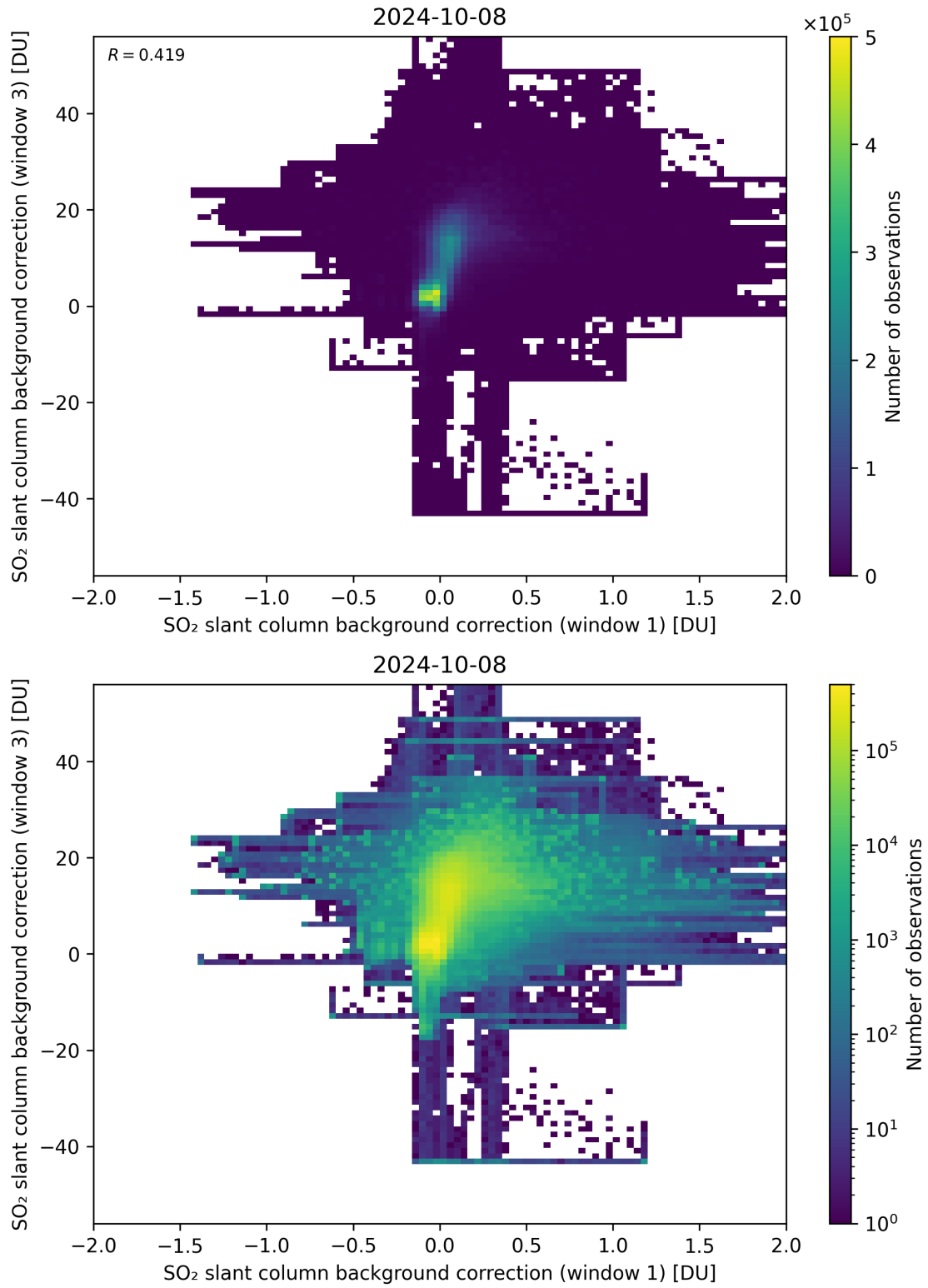
Figure 99: Scatter density plot of “SO 2 slant column background correction (window 1)” against “SO 2 slant column background correction (window 3)” for 2024-10-08 to 2024-10-09.
