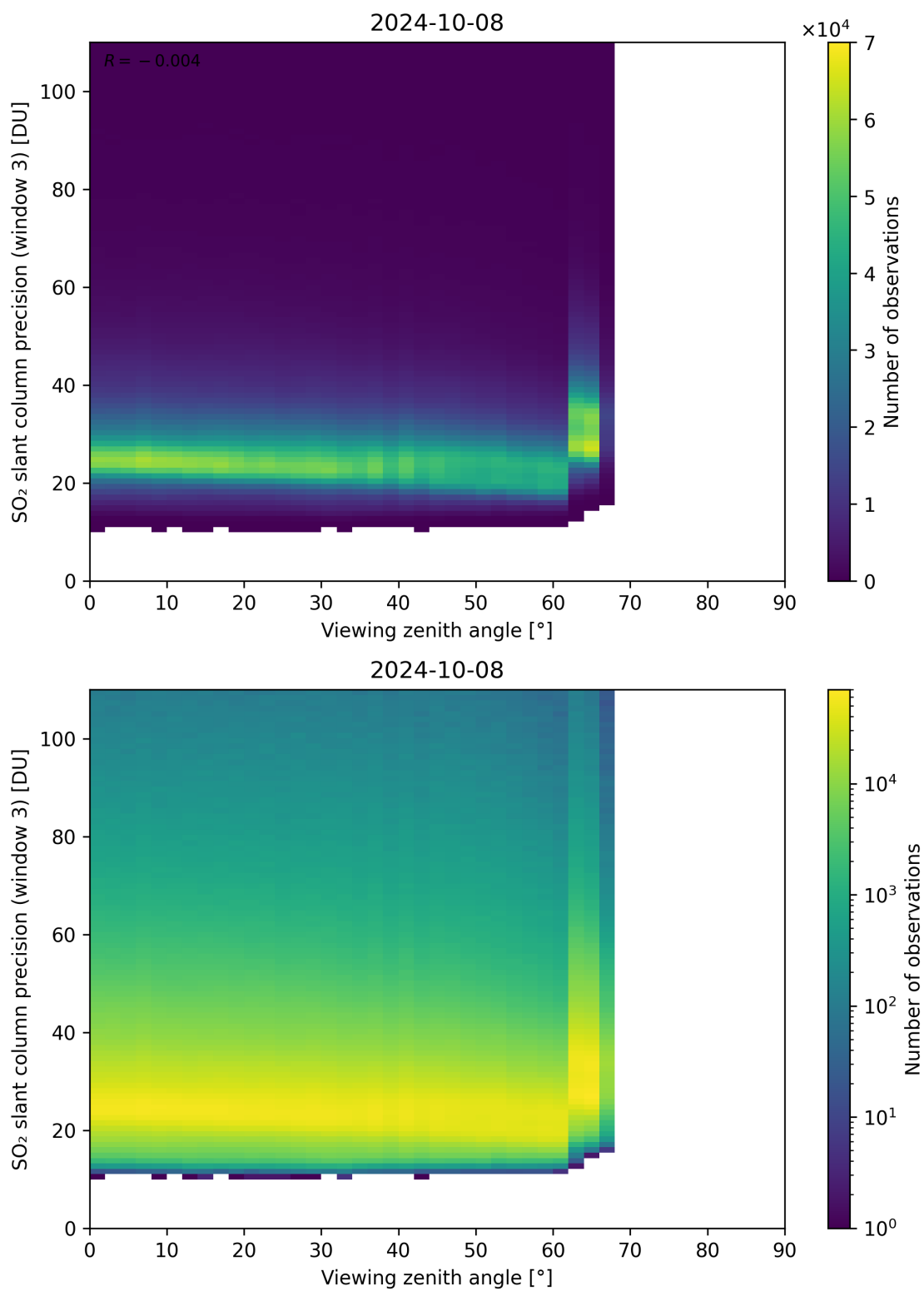
Figure 324: Scatter density plot of “Viewing zenith angle” against “SO 2 slant column precision (window 3)” for 2024-10-08 to 2024-10-09.
