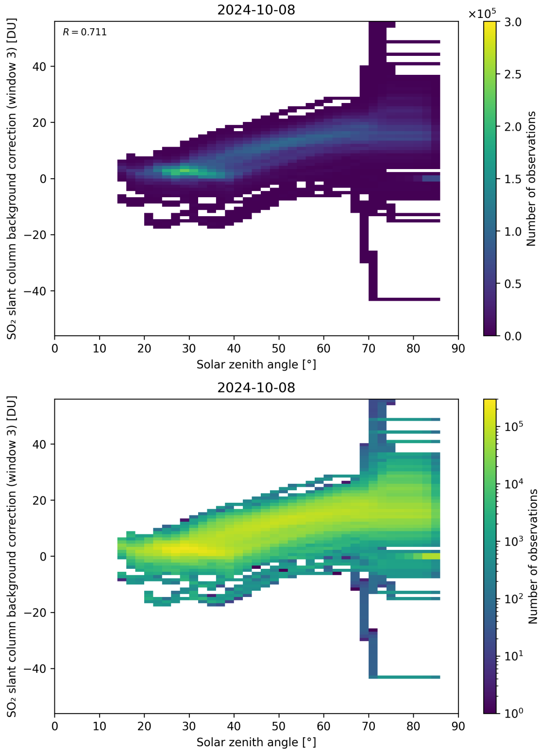
Figure 160: Scatter density plot of “Solar zenith angle” against “SO 2 slant column background correction (window 3)” for 2024-10-08 to 2024-10-09.
