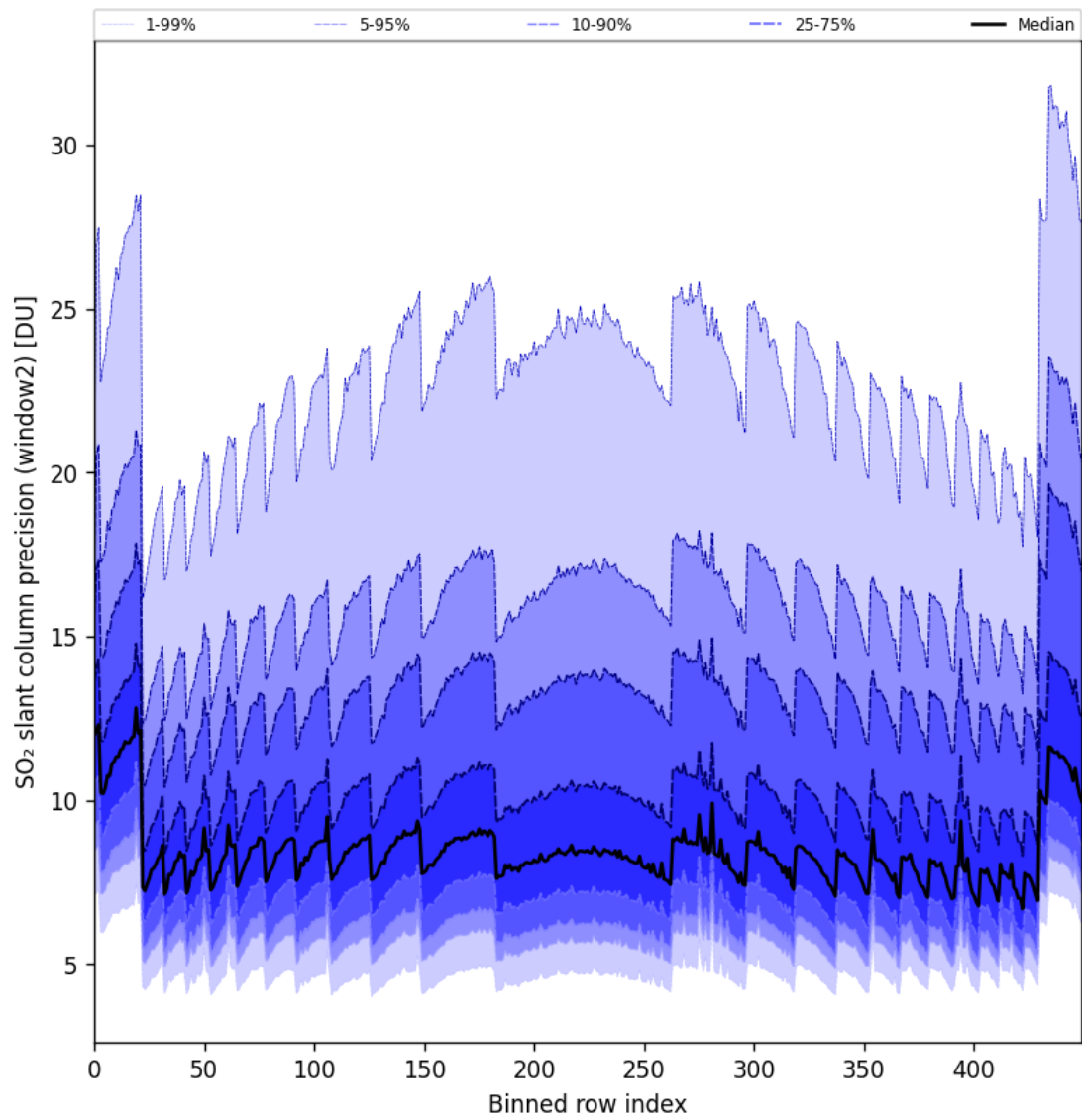
Figure 84: Along track statistics of “SO 2 slant column precision (window2)” for 2024-10-08 to 2024-10-09
