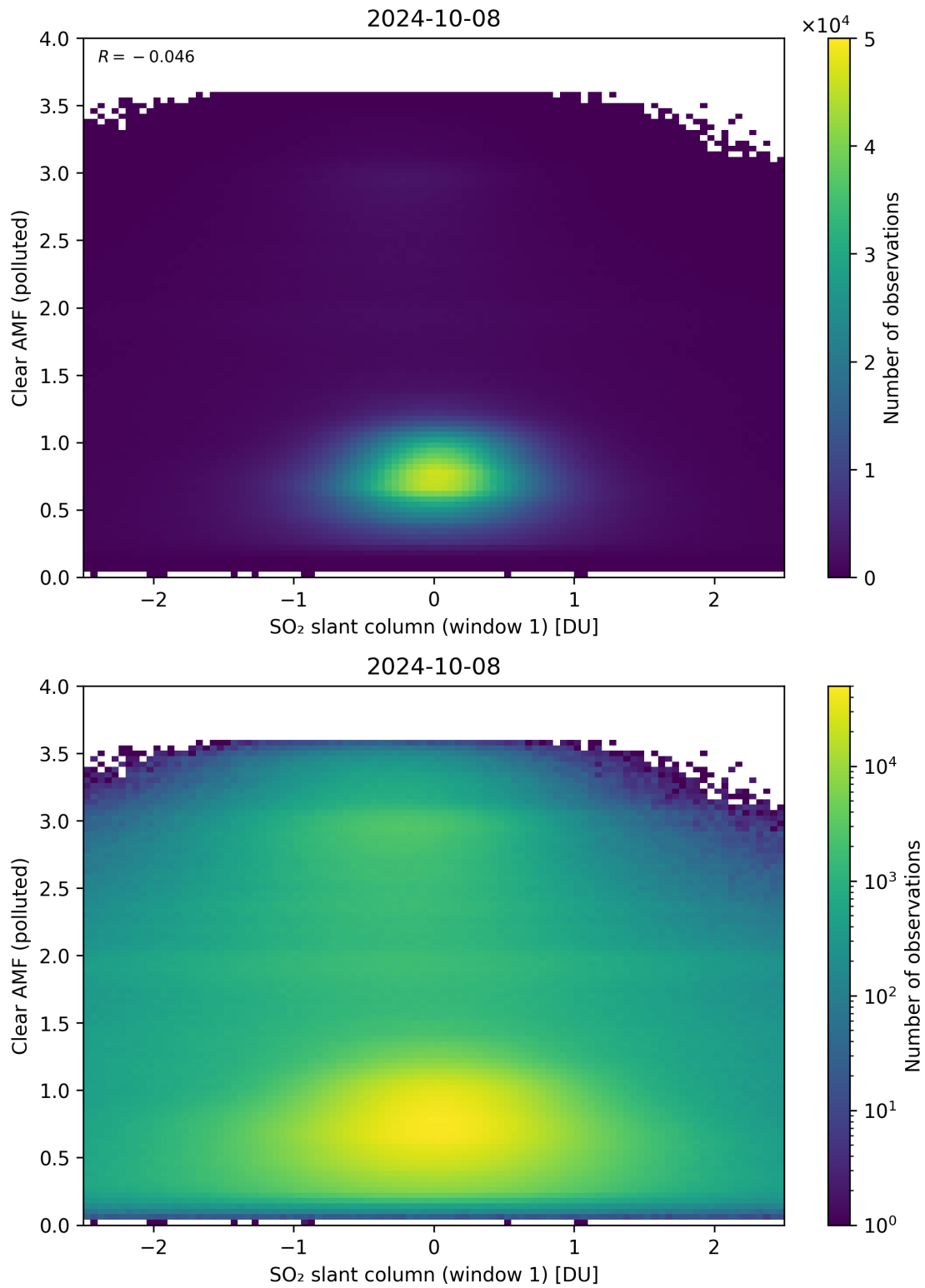
Figure 232: Scatter density plot of “SO 2 slant column (window 1)” against “Clear AMF (polluted)” for 2024-10-08 to 2024-10-09.
