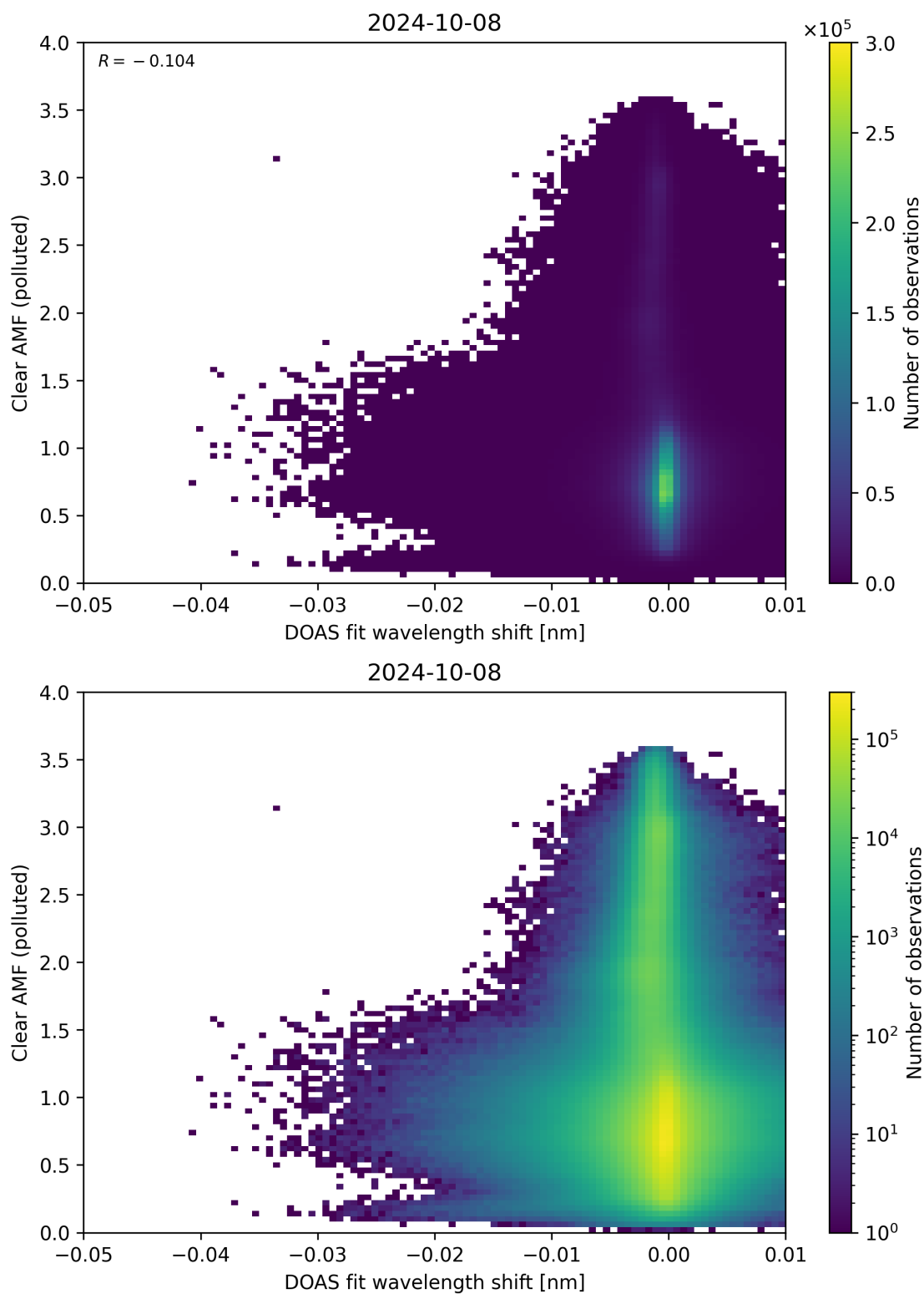
Figure 129: Scatter density plot of “DOAS fit wavelength shift” against “Clear AMF (polluted)” for 2024-10-08 to 2024-10-09.
