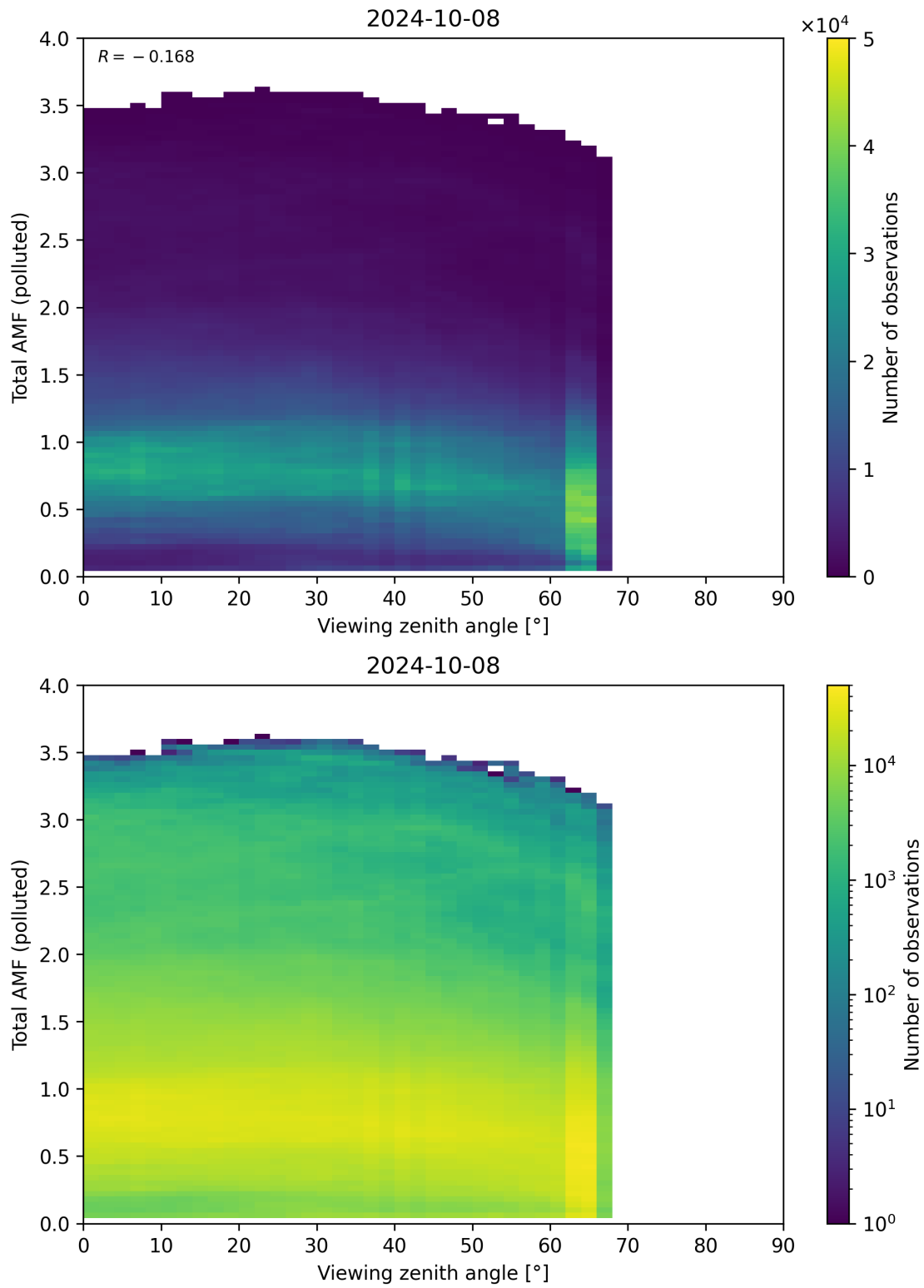
Figure 325: Scatter density plot of “Viewing zenith angle” against “Total AMF (polluted)” for 2024-10-08 to 2024-10-09.
