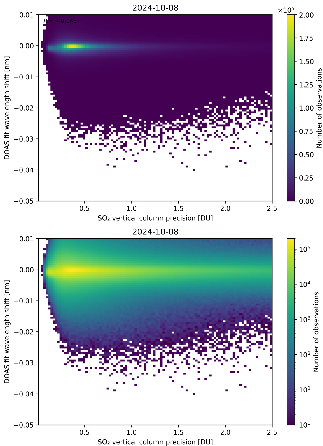
Figure 282: Scatter density plot of “SO 2 vertical column precision” against “DOAS fit wavelength shift” for 2024-10-08 to 2024-10-09.
