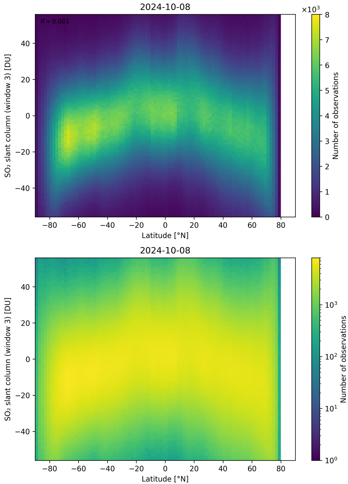
Figure 152: Scatter density plot of “Latitude” against “SO 2 slant column (window 3)” for 2024-10-08 to 2024-10-09.
