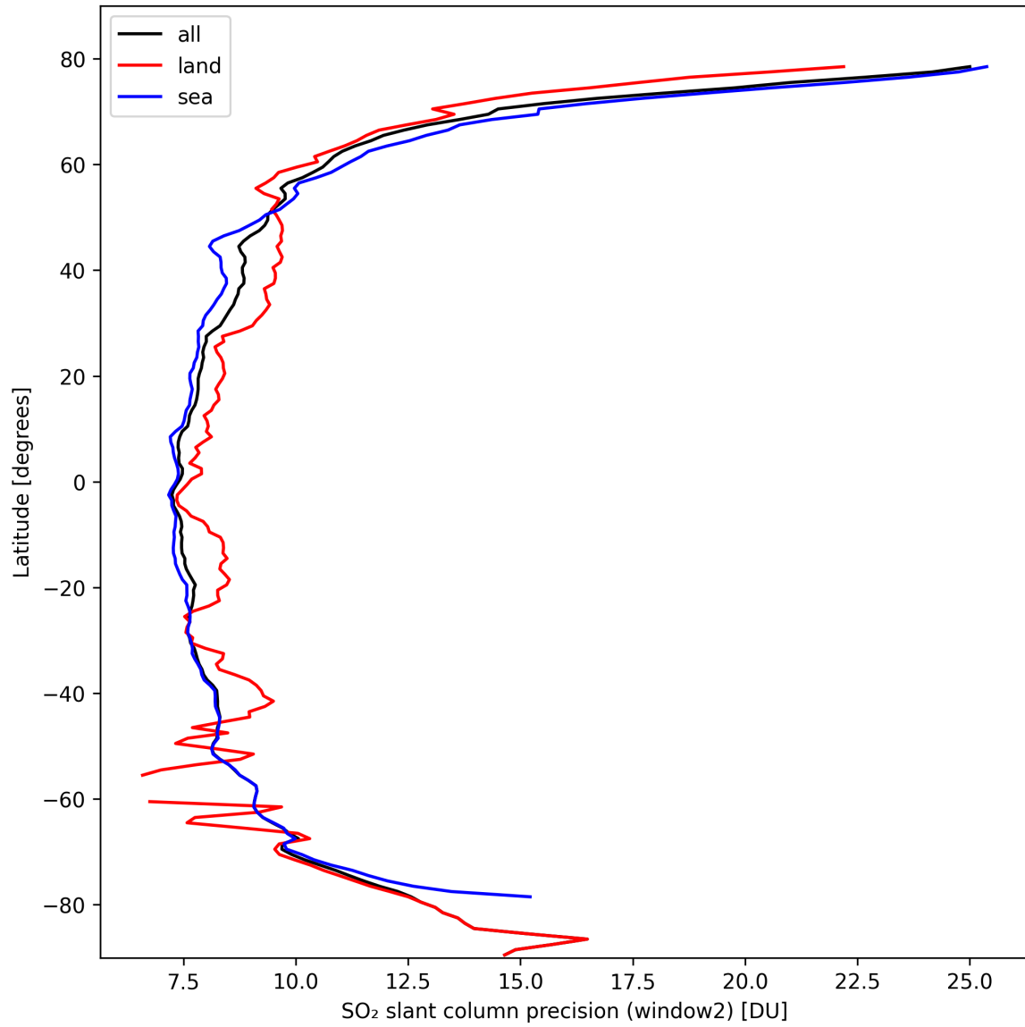
Figure 38: Zonal average of “SO 2 slant column precision (window2)” for 2024-10-08 to 2024-10-10.
