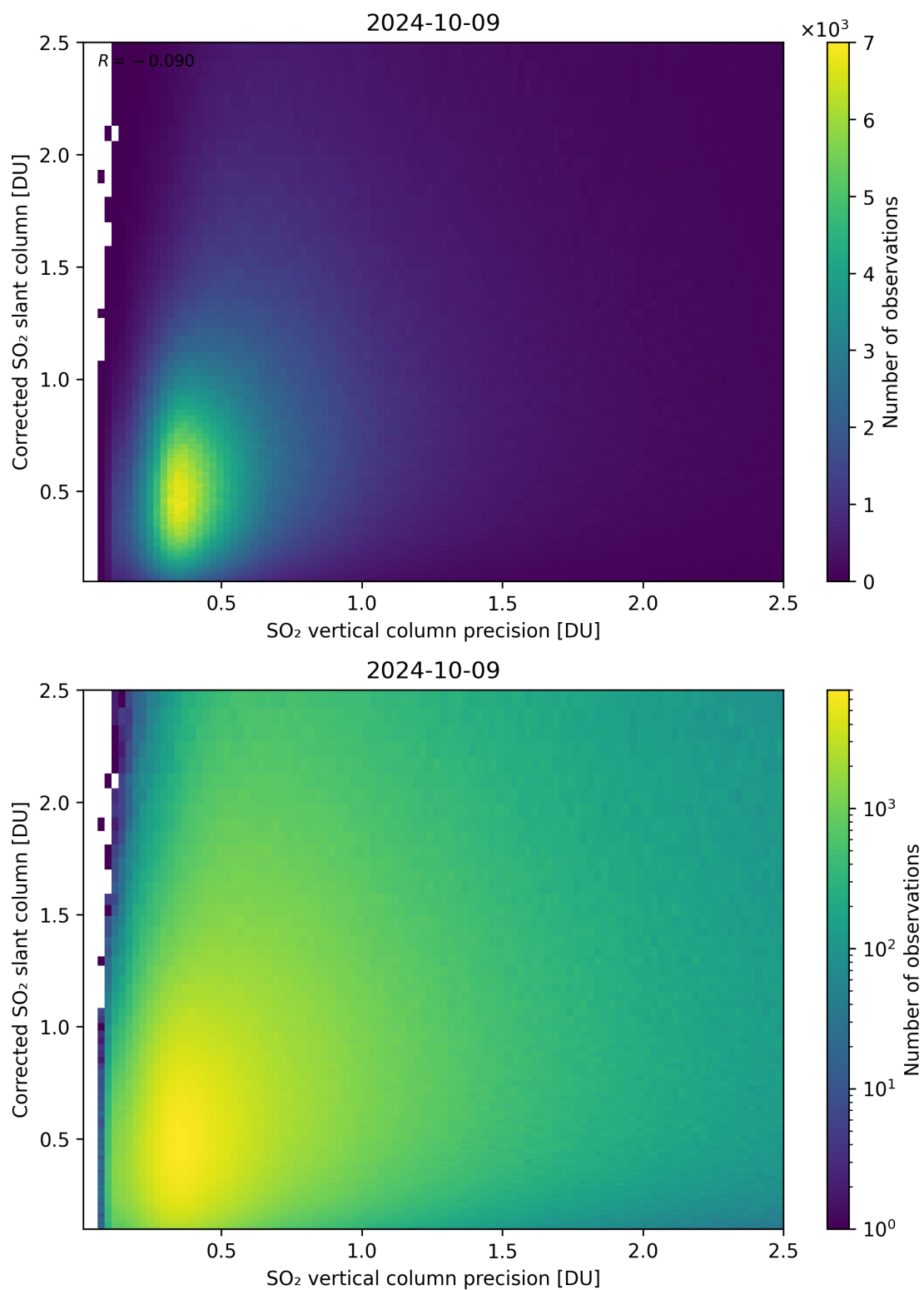
Figure 286: Scatter density plot of “SO 2 vertical column precision” against “Corrected SO 2 slant column” for 2024-10-08 to 2024-10-10.
