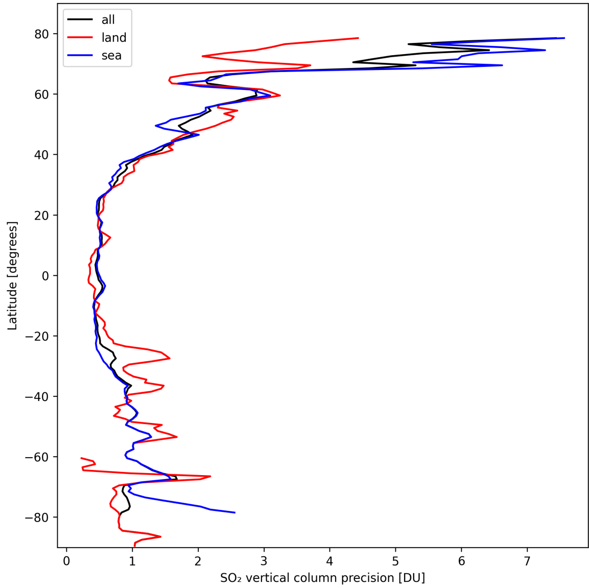
Figure 31: Zonal average of “SO 2 vertical column precision” for 2024-10-08 to 2024-10-10.
