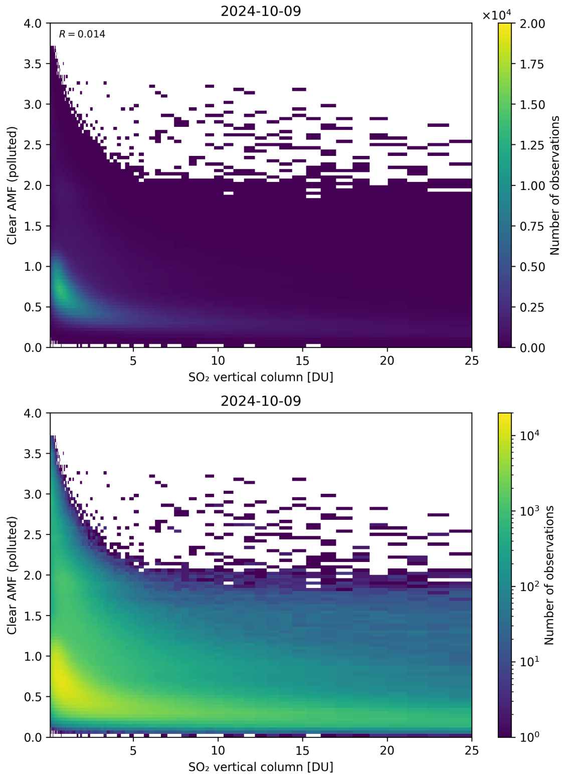
Figure 296: Scatter density plot of “SO 2 vertical column” against “Clear AMF (polluted)” for 2024-10-08 to 2024-10-10.
