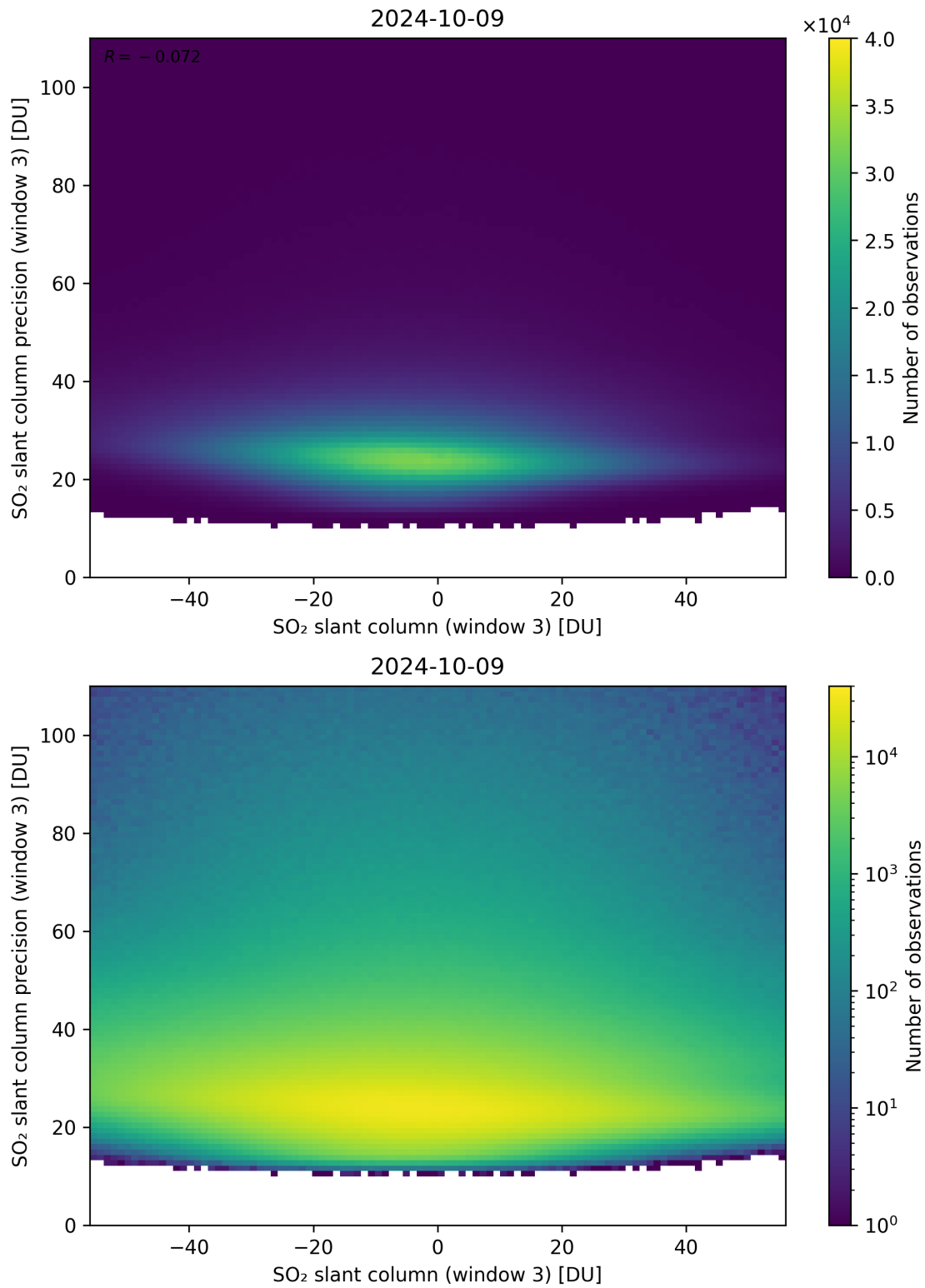
Figure 267: Scatter density plot of “SO 2 slant column (window 3)” against “SO 2 slant column precision (window 3)” for 2024-10-08 to 2024-10-10.
