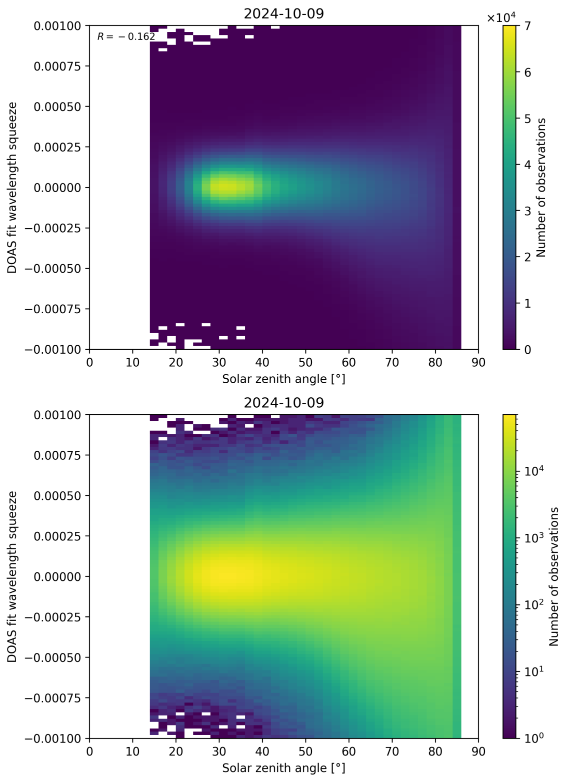
Figure 162: Scatter density plot of “Solar zenith angle” against “DOAS fit wavelength squeeze” for 2024-10-08 to 2024-10-10.
