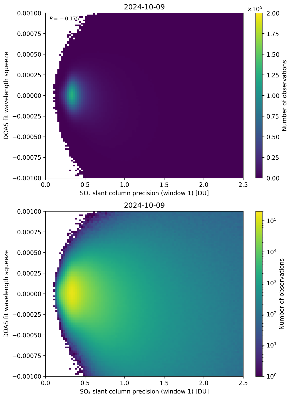
Figure 222: Scatter density plot of “SO 2 slant column precision (window 1)” against “DOAS fit wavelength squeeze” for 2024-10-08 to 2024-10-10.
