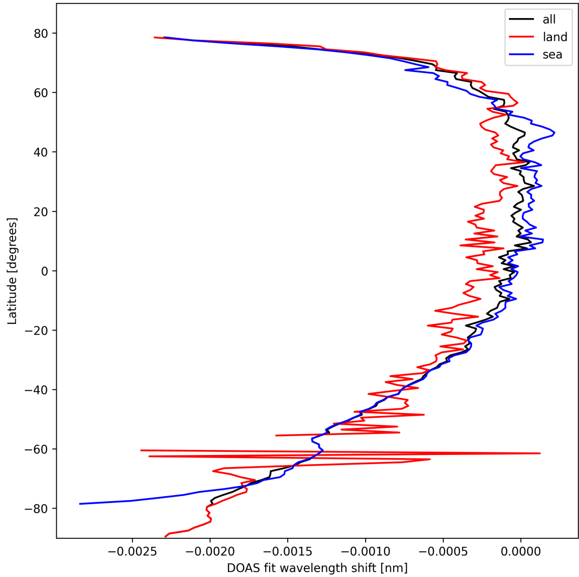
Figure 45: Zonal average of “DOAS fit wavelength shift” for 2024-10-08 to 2024-10-10.
