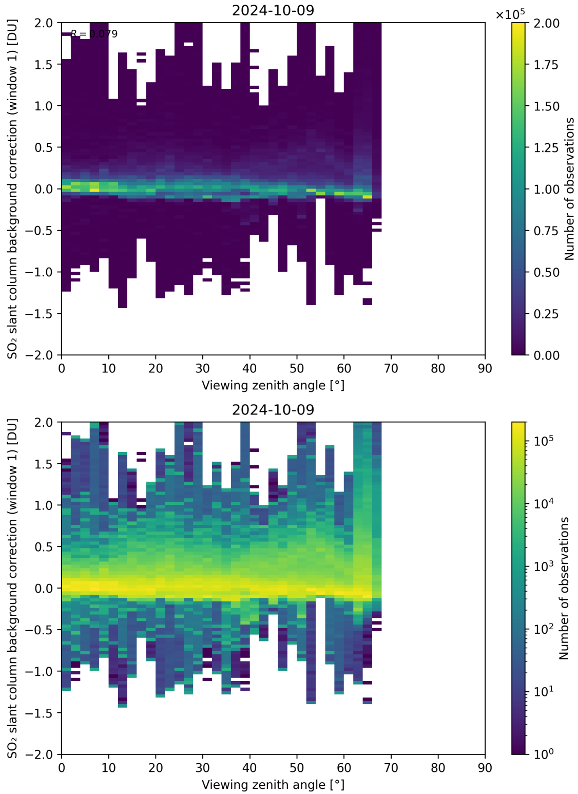
Figure 308: Scatter density plot of “Viewing zenith angle” against “SO 2 slant column background correction (window 1)” for 2024-10-08 to 2024-10-10.
