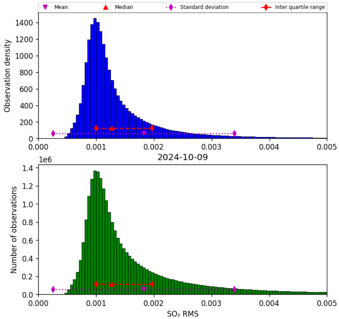
Figure 70: Histogram of “SO 2 RMS” for 2024-10-08 to 2024-10-10
