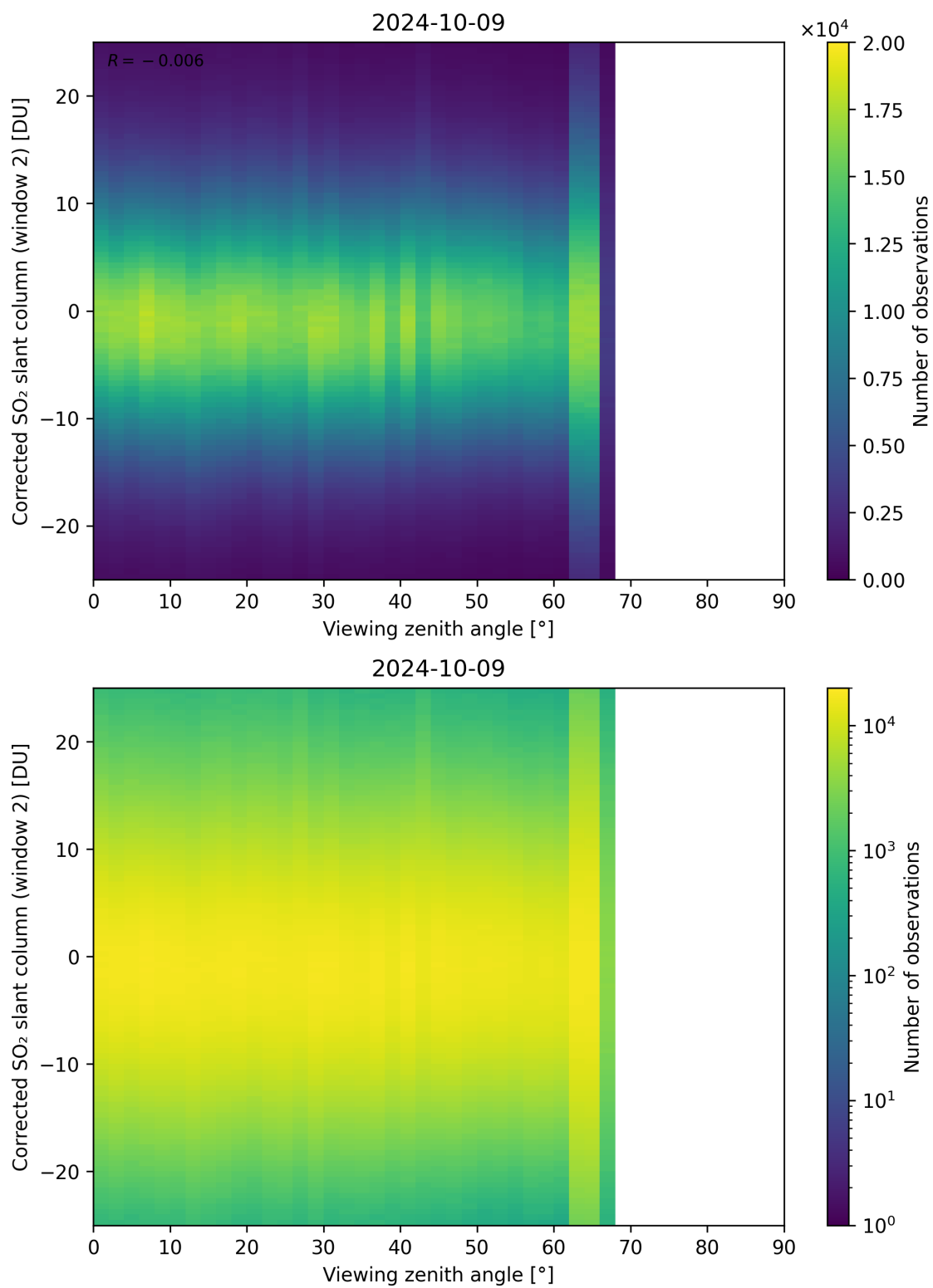
Figure 318: Scatter density plot of “Viewing zenith angle” against “Corrected SO 2 slant column (window 2)” for 2024-10-08 to 2024-10-10.
