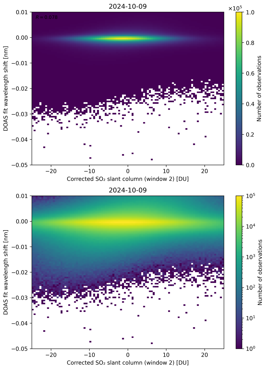
Figure 196: Scatter density plot of “Corrected SO 2 slant column (window 2)” against “DOAS fit wavelength shift” for 2024-10-08 to 2024-10-10.
