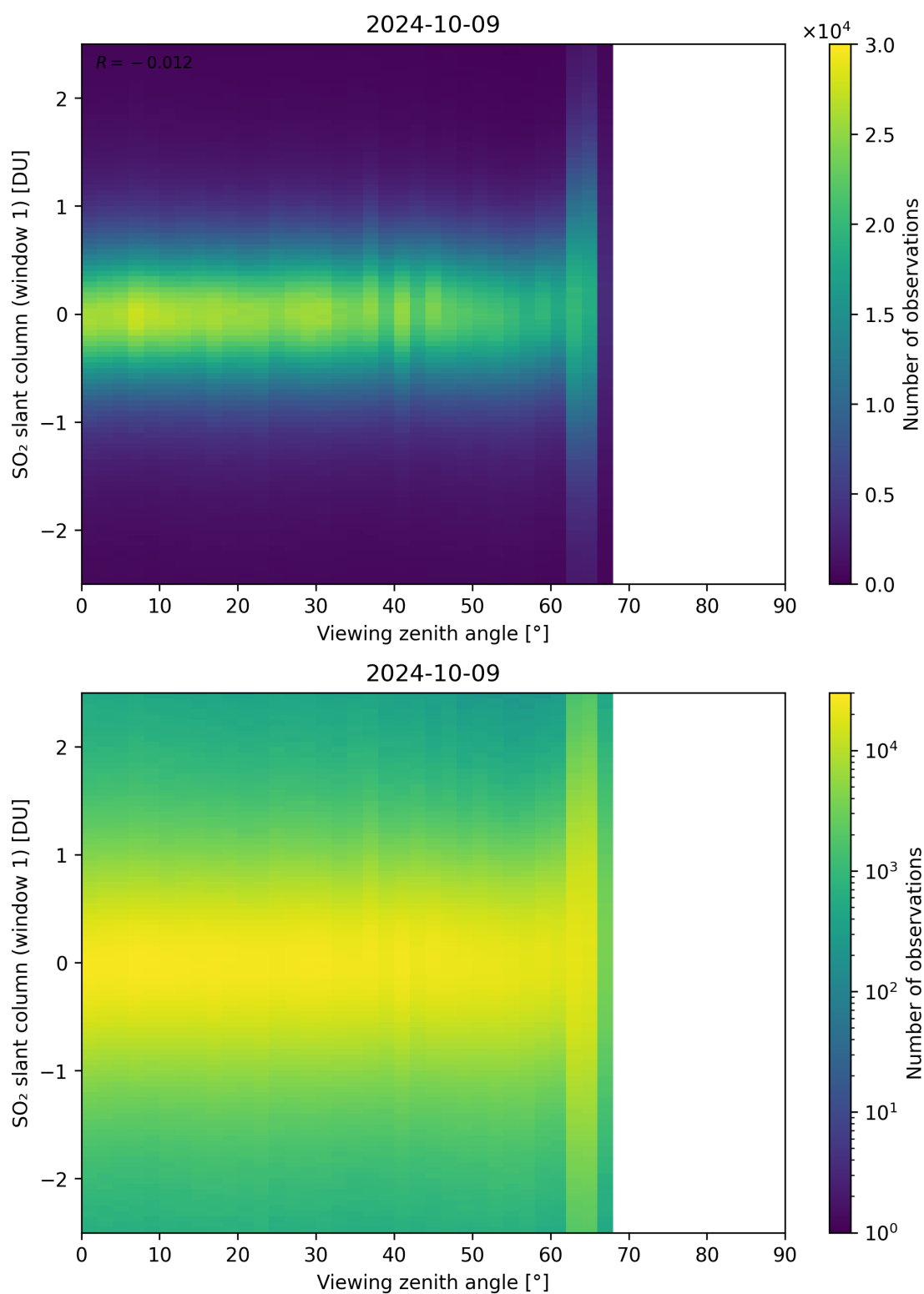
Figure 320: Scatter density plot of “Viewing zenith angle” against “SO 2 slant column (window 1)” for 2024-10-08 to 2024-10-10.
