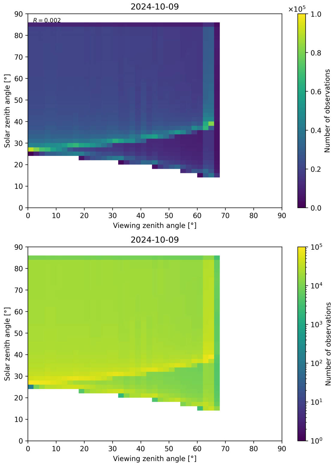
Figure 315: Scatter density plot of “Viewing zenith angle” against “Solar zenith angle” for 2024-10-08 to 2024-10-10.
