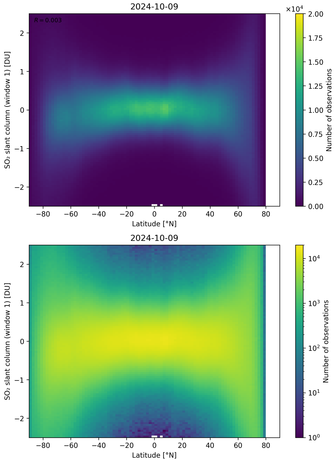
Figure 149: Scatter density plot of “Latitude” against “SO 2 slant column (window 1)” for 2024-10-08 to 2024-10-10.
