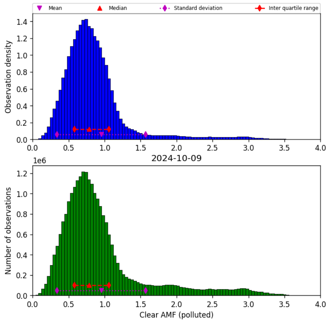
Figure 73: Histogram of “Clear AMF (polluted)” for 2024-10-08 to 2024-10-10
