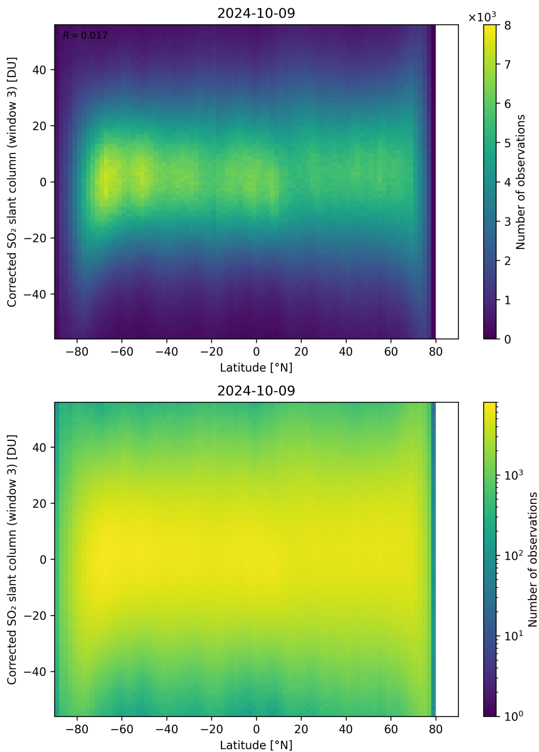
Figure 148: Scatter density plot of “Latitude” against “Corrected SO 2 slant column (window 3)” for 2024-10-08 to 2024-10-10.
