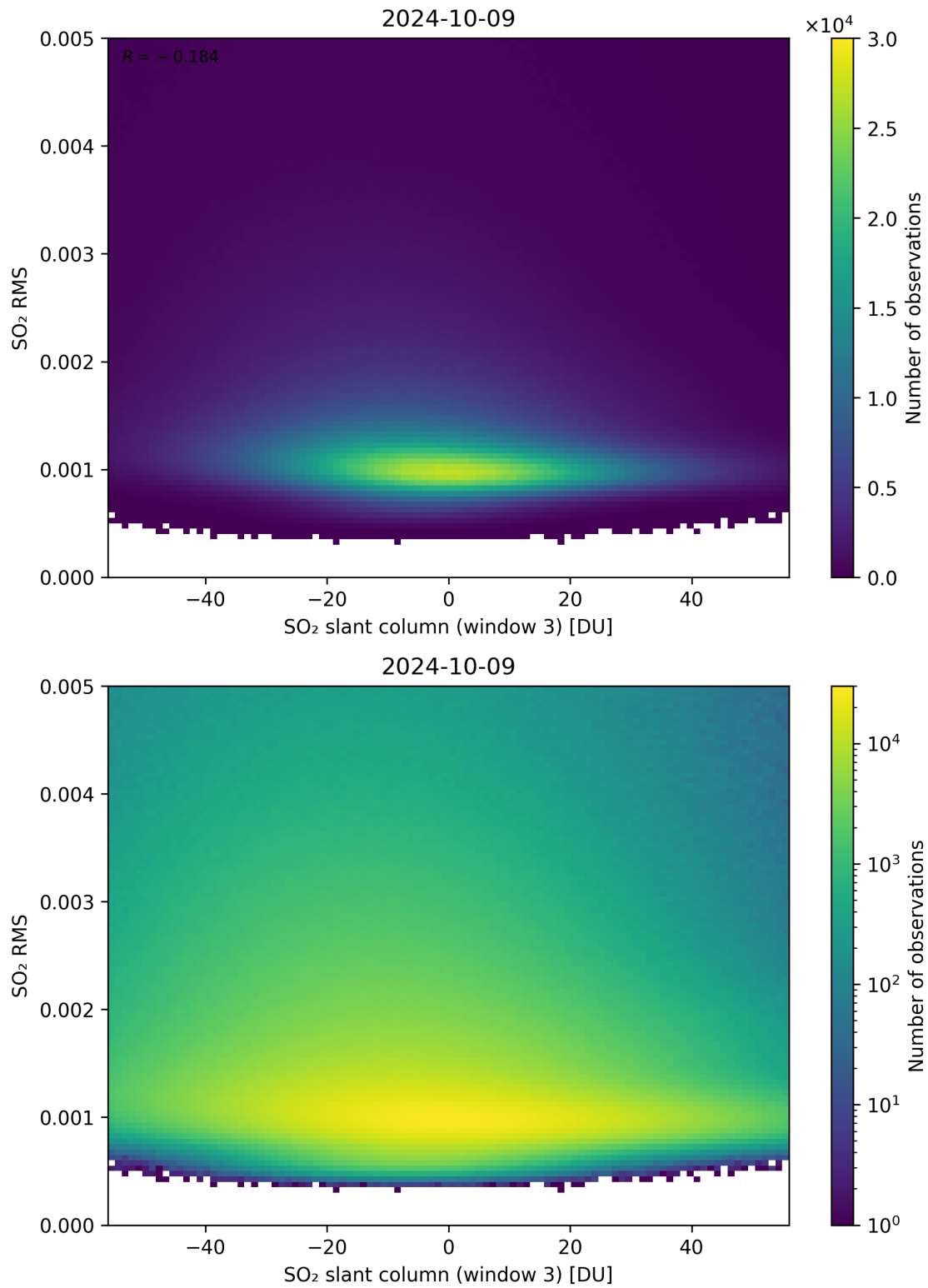
Figure 256: Scatter density plot of “SO 2 slant column (window 3)” against “SO 2 RMS” for 2024-10-08 to 2024-10-10.
