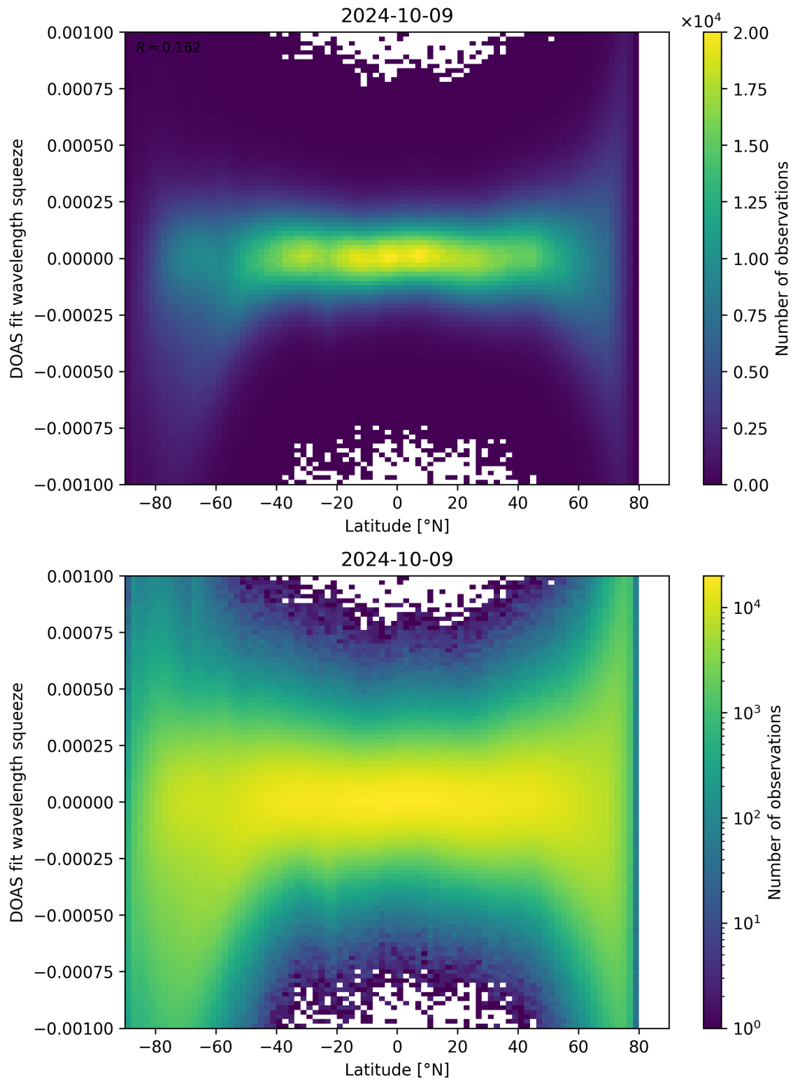
Figure 143: Scatter density plot of “Latitude” against “DOAS fit wavelength squeeze” for 2024-10-08 to 2024-10-10.
