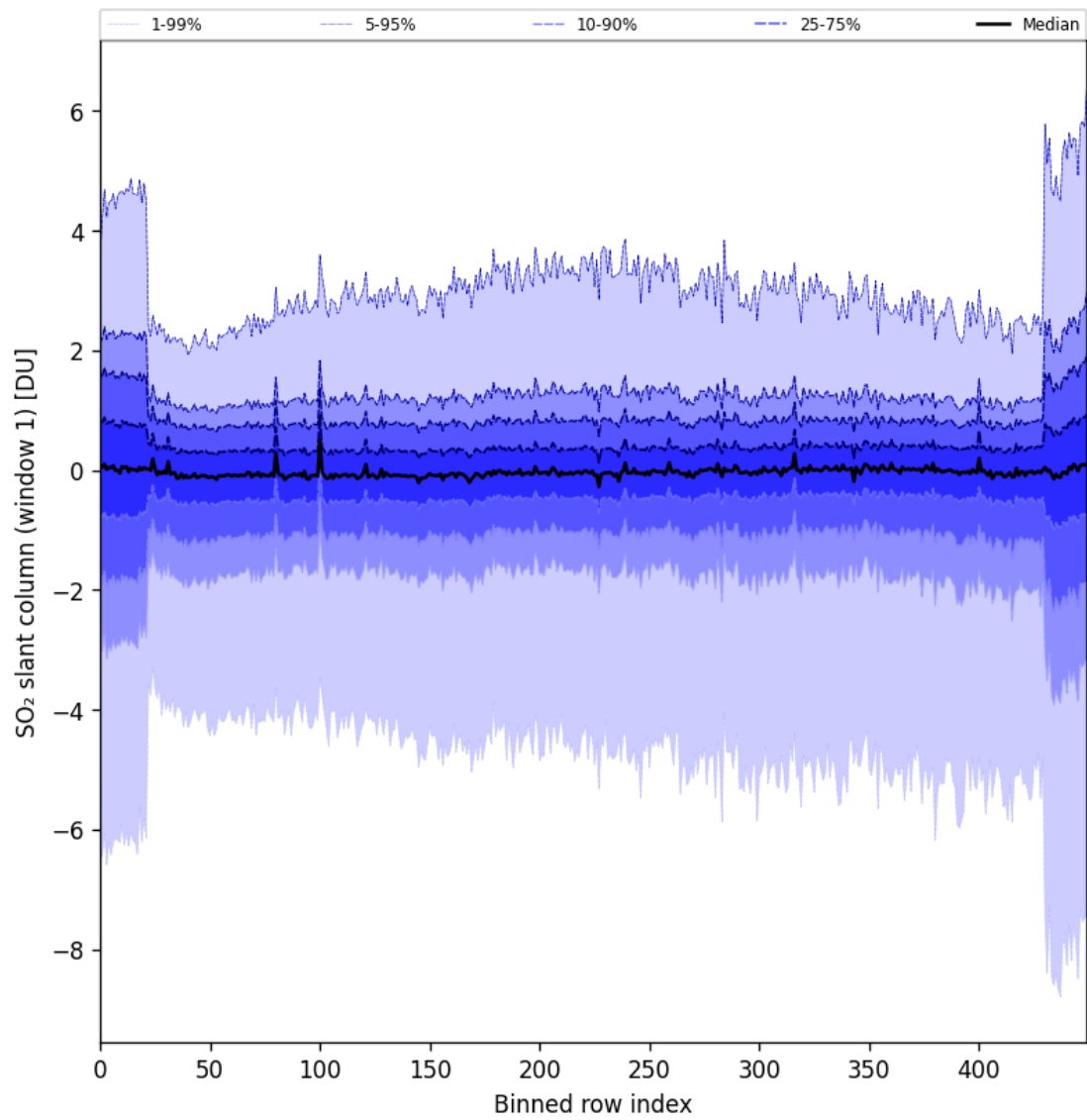
Figure 79: Along track statistics of “SO 2 slant column (window 1)” for 2024-10-08 to 2024-10-10
