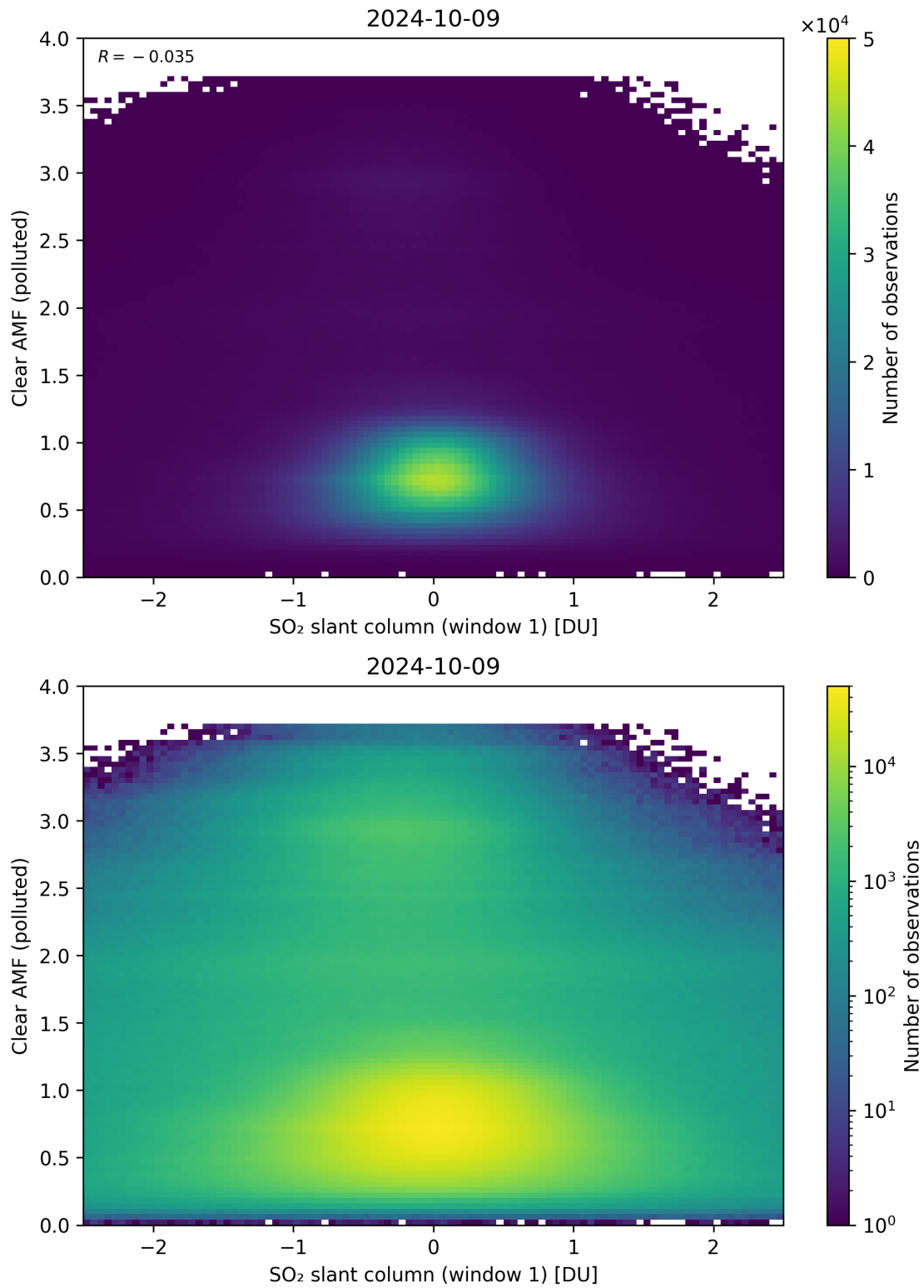
Figure 232: Scatter density plot of “SO 2 slant column (window 1)” against “Clear AMF (polluted)” for 2024-10-08 to 2024-10-10.
