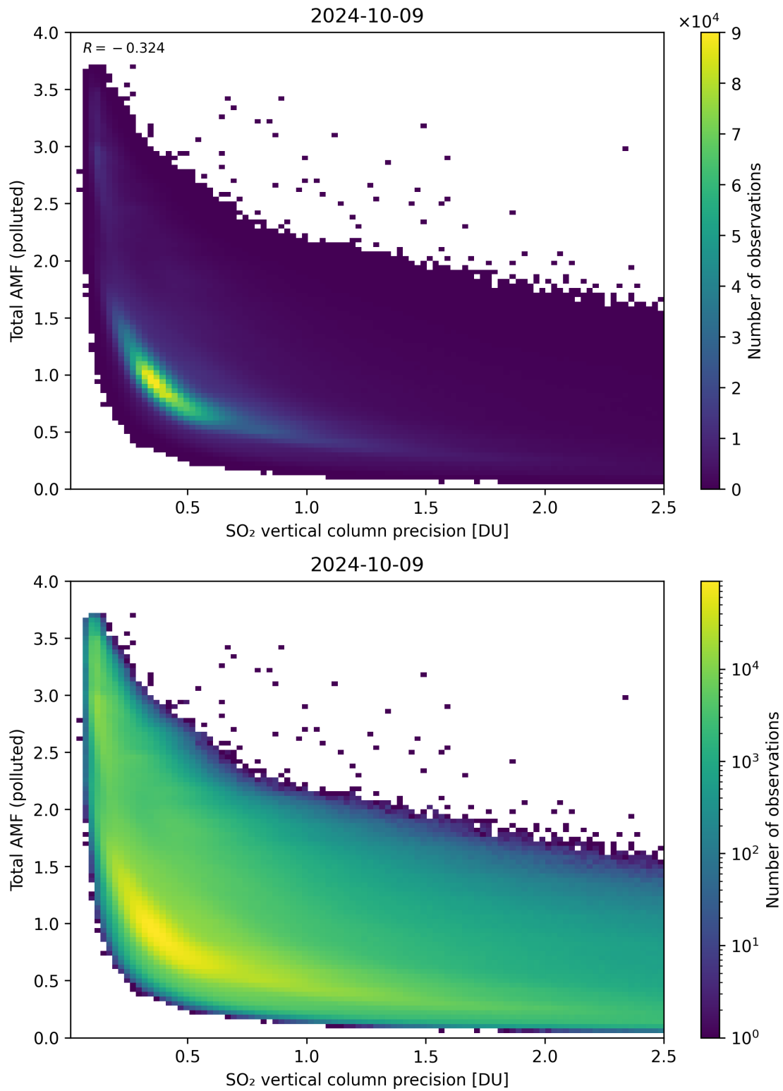
Figure 294: Scatter density plot of “SO 2 vertical column precision” against “Total AMF (polluted)” for 2024-10-08 to 2024-10-10.
