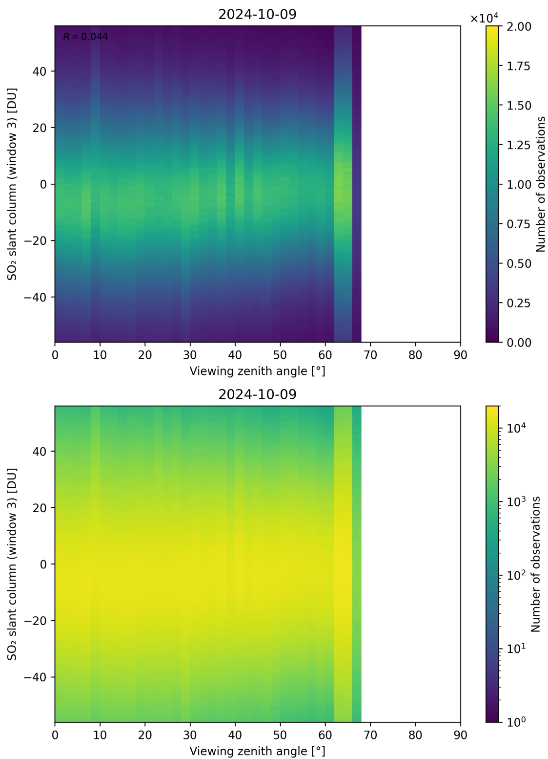
Figure 323: Scatter density plot of “Viewing zenith angle” against “SO 2 slant column (window 3)” for 2024-10-08 to 2024-10-10.
