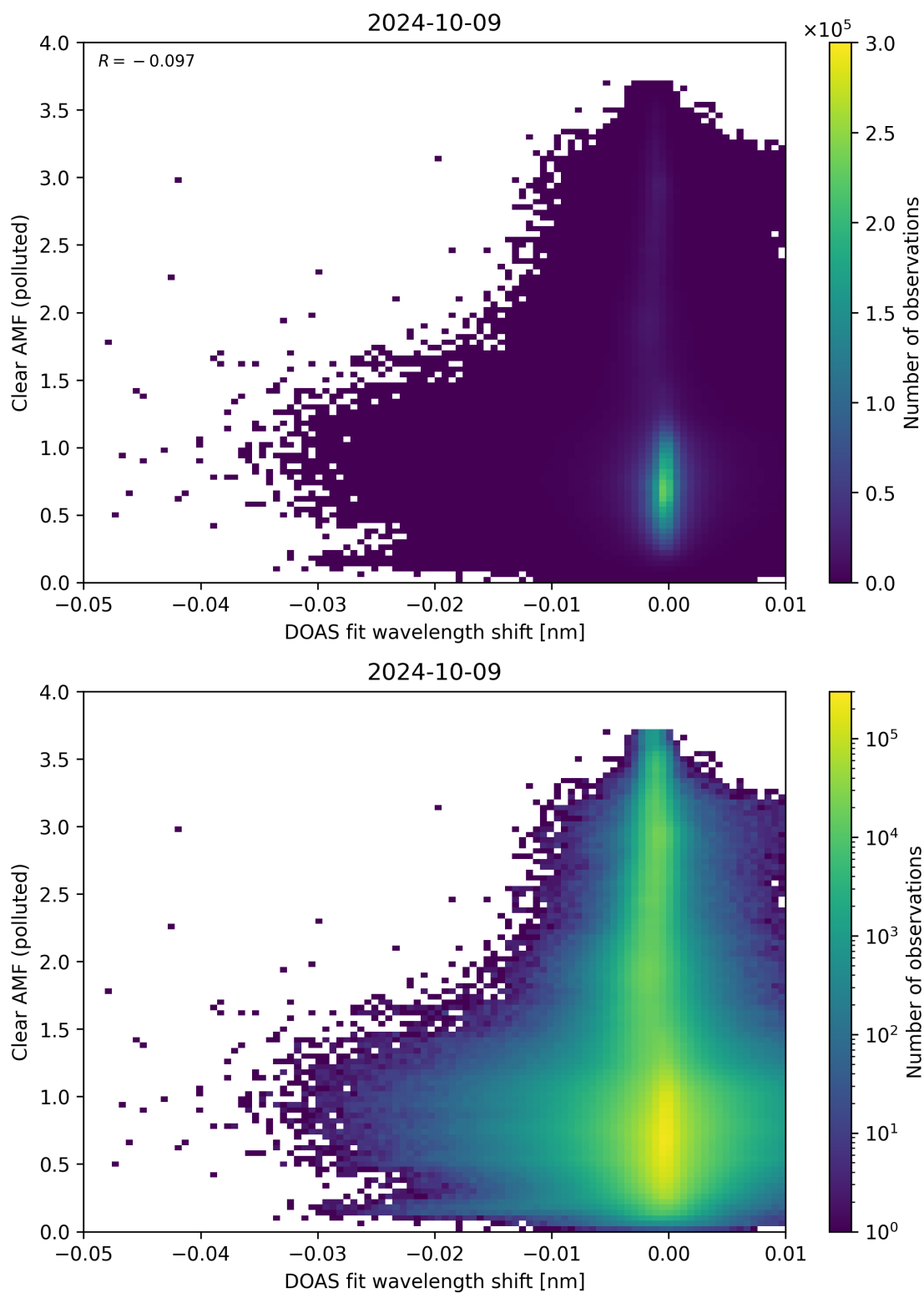
Figure 129: Scatter density plot of “DOAS fit wavelength shift” against “Clear AMF (polluted)” for 2024-10-08 to 2024-10-10.
