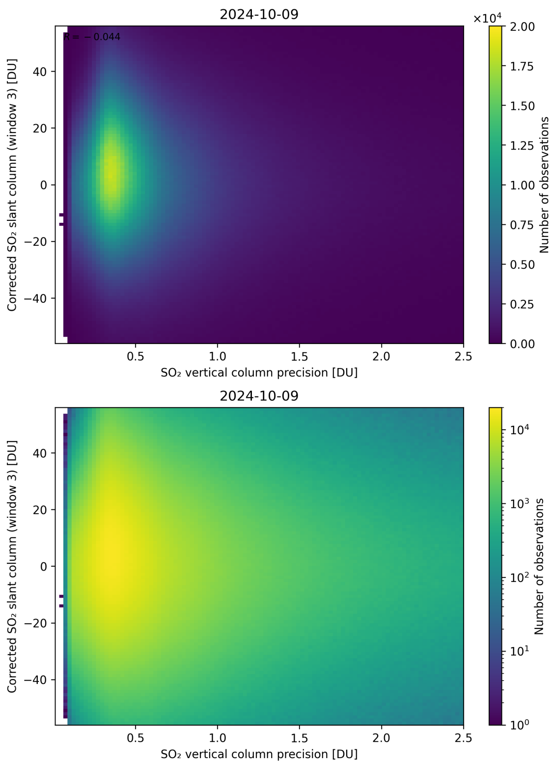
Figure 288: Scatter density plot of “SO 2 vertical column precision” against “Corrected SO 2 slant column (window 3)” for 2024-10-08 to 2024-10-10.
