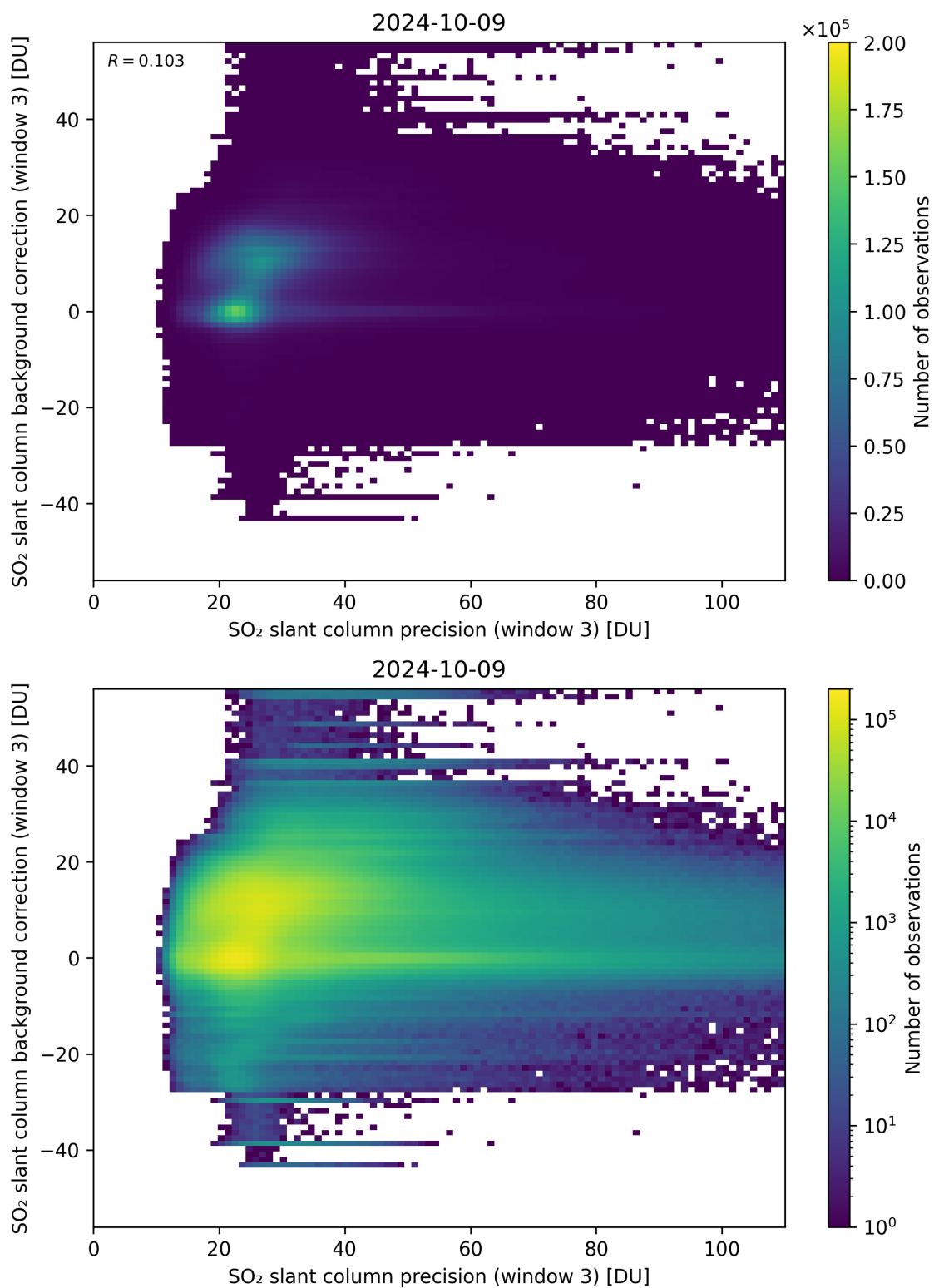
Figure 257: Scatter density plot of “SO 2 slant column precision (window 3)” against “SO 2 slant column background correction (window 3)” for 2024-10-08 to 2024-10-10.
