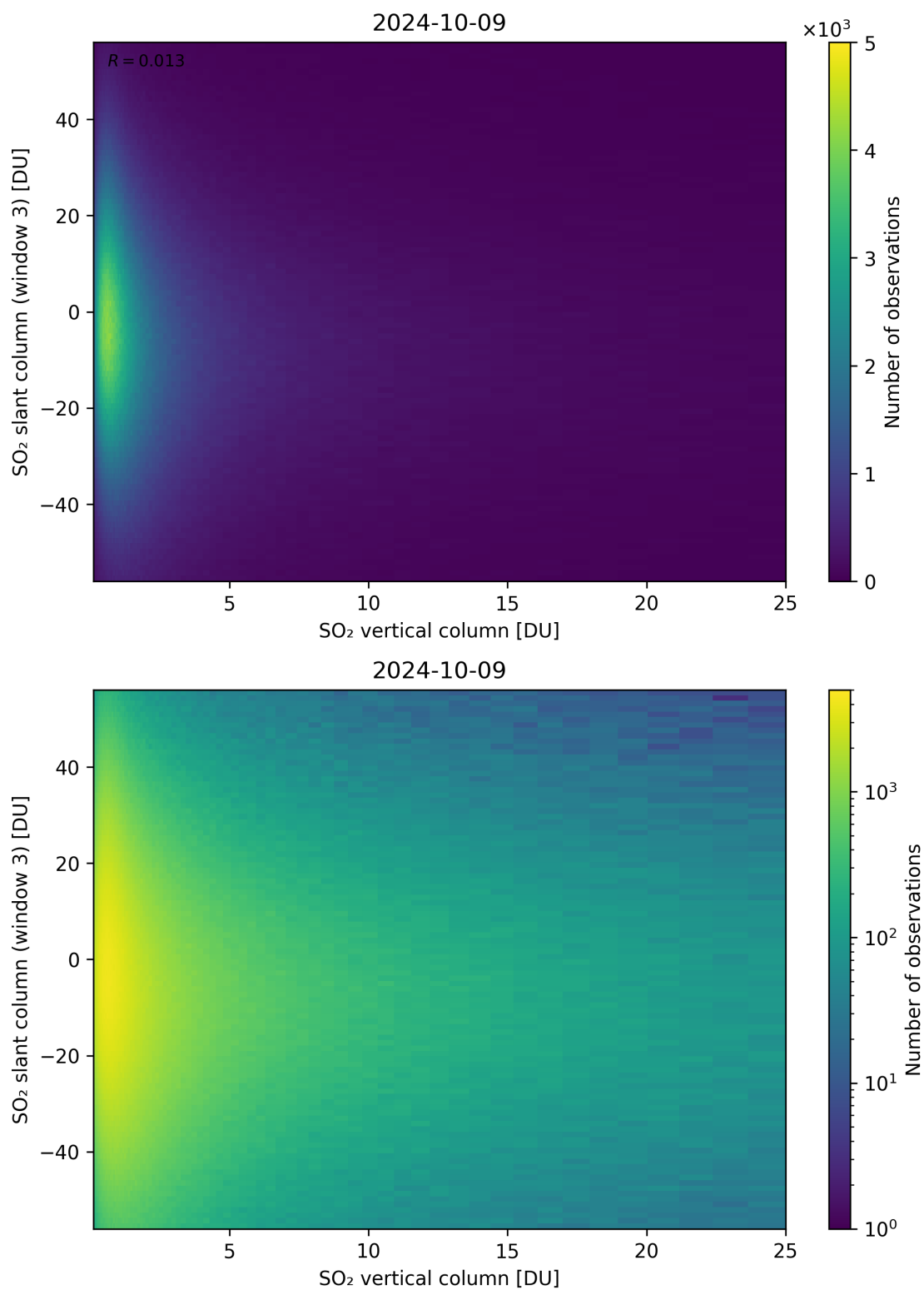
Figure 303: Scatter density plot of “SO 2 vertical column” against “SO 2 slant column (window 3)” for 2024-10-08 to 2024-10-10.
