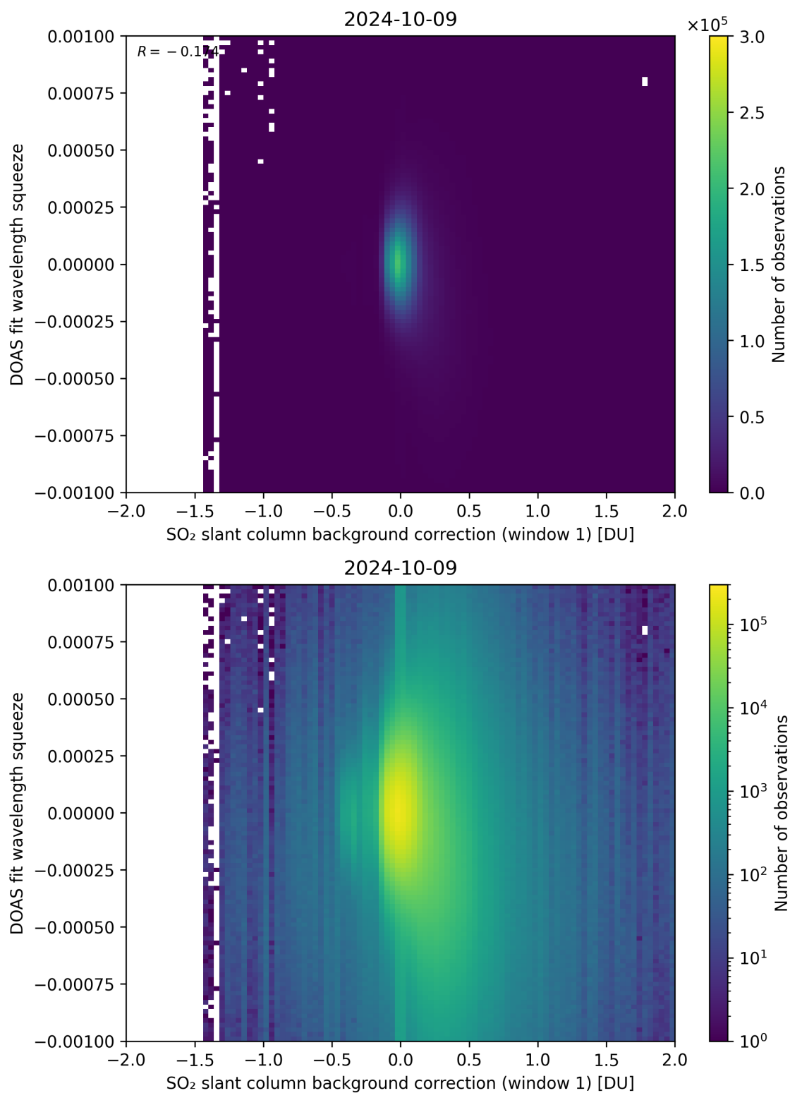
Figure 101: Scatter density plot of “SO 2 slant column background correction (window 1)” against “DOAS fit wavelength squeeze” for 2024-10-08 to 2024-10-10.
