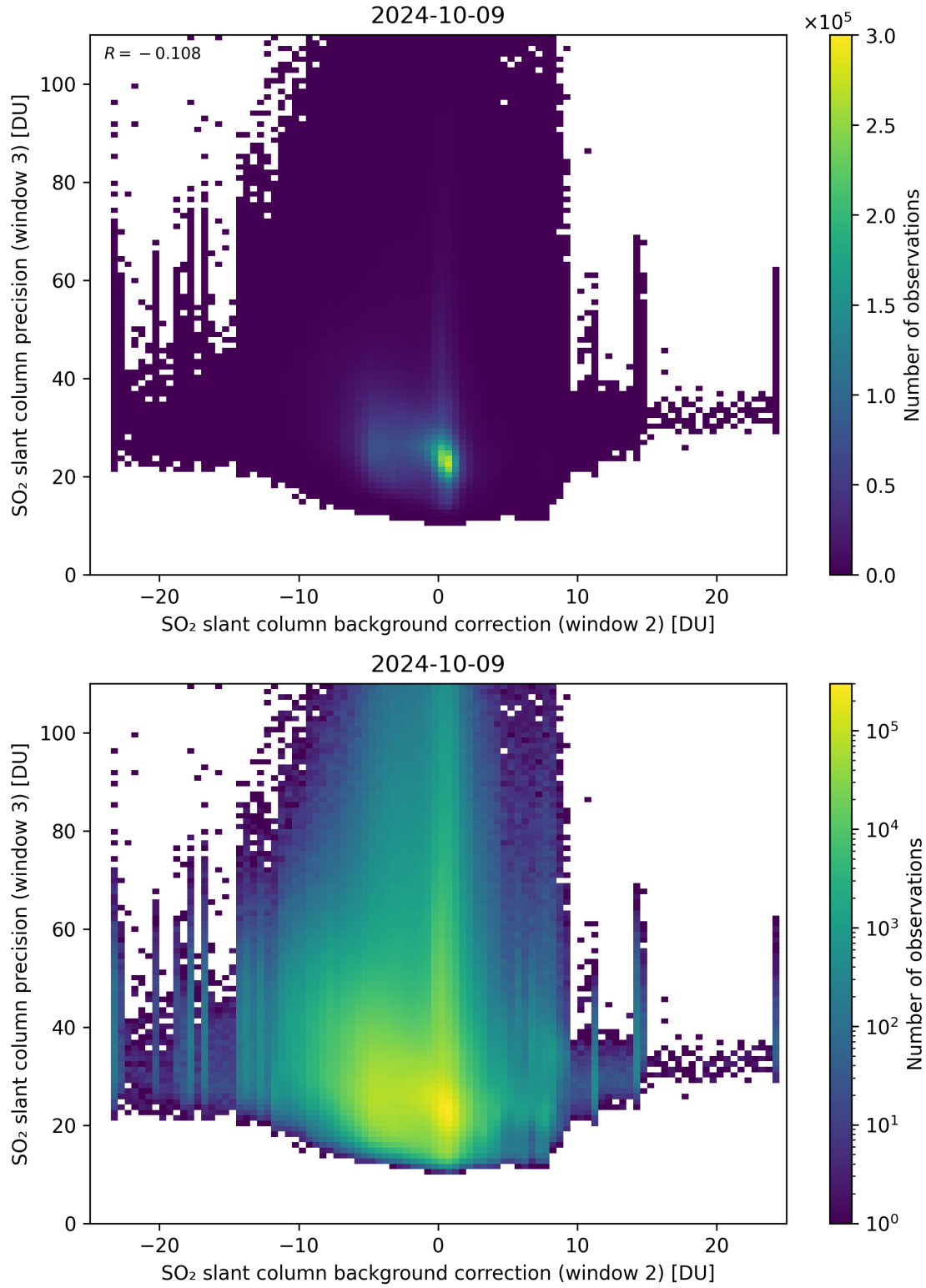
Figure 118: Scatter density plot of “SO 2 slant column background correction (window 2)” against “SO 2 slant column precision (window 3)” for 2024-10-08 to 2024-10-10.
