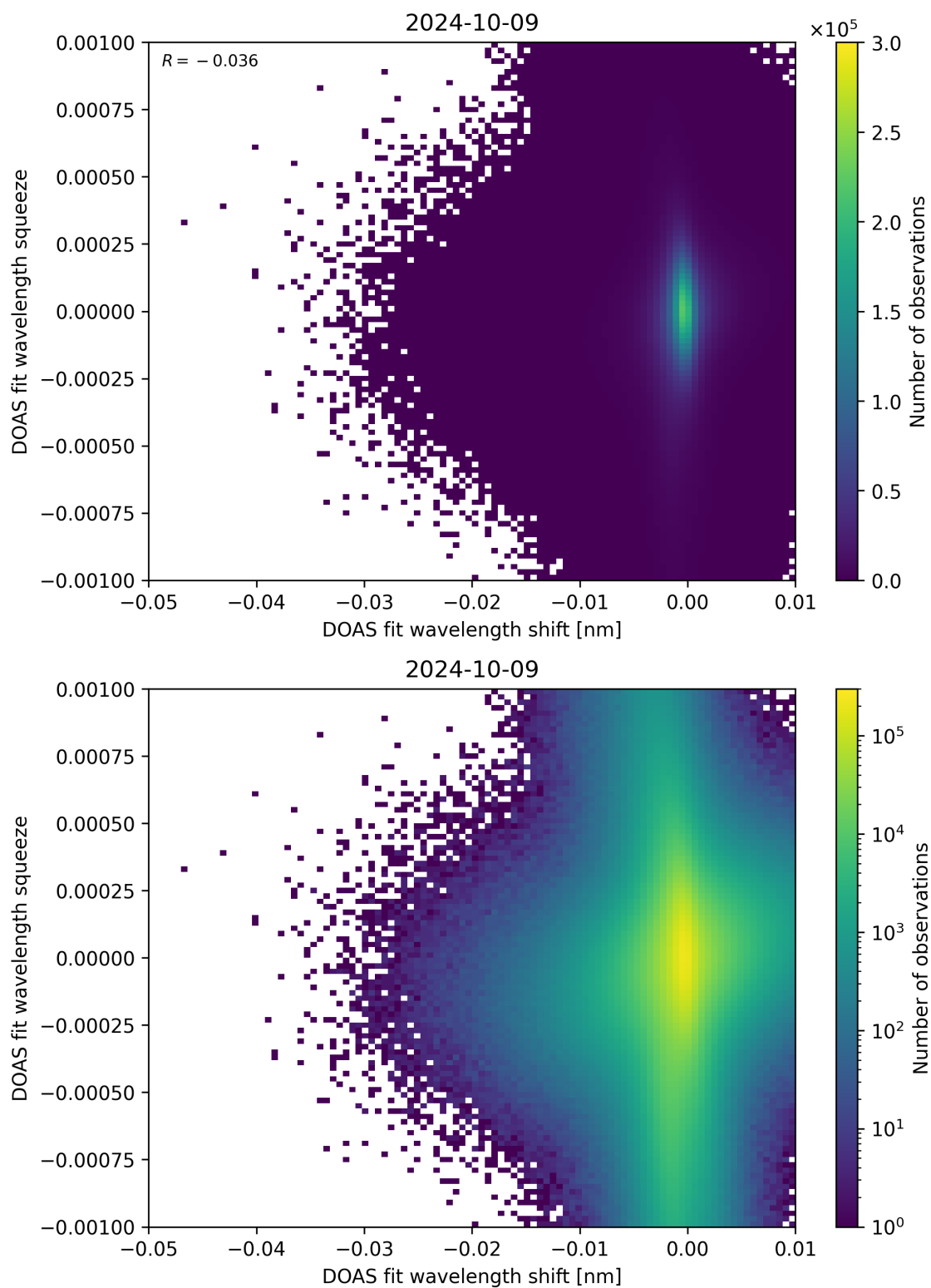
Figure 127: Scatter density plot of “DOAS fit wavelength shift” against “DOAS fit wavelength squeeze” for 2024-10-08 to 2024-10-10.
