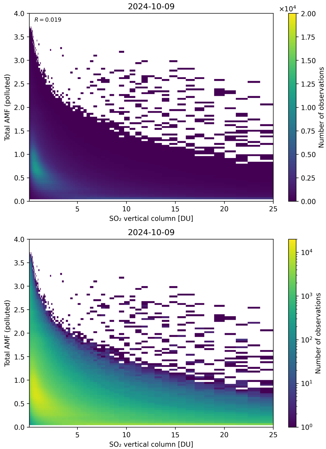
Figure 305: Scatter density plot of “SO 2 vertical column” against “Total AMF (polluted)” for 2024-10-08 to 2024-10-10.
