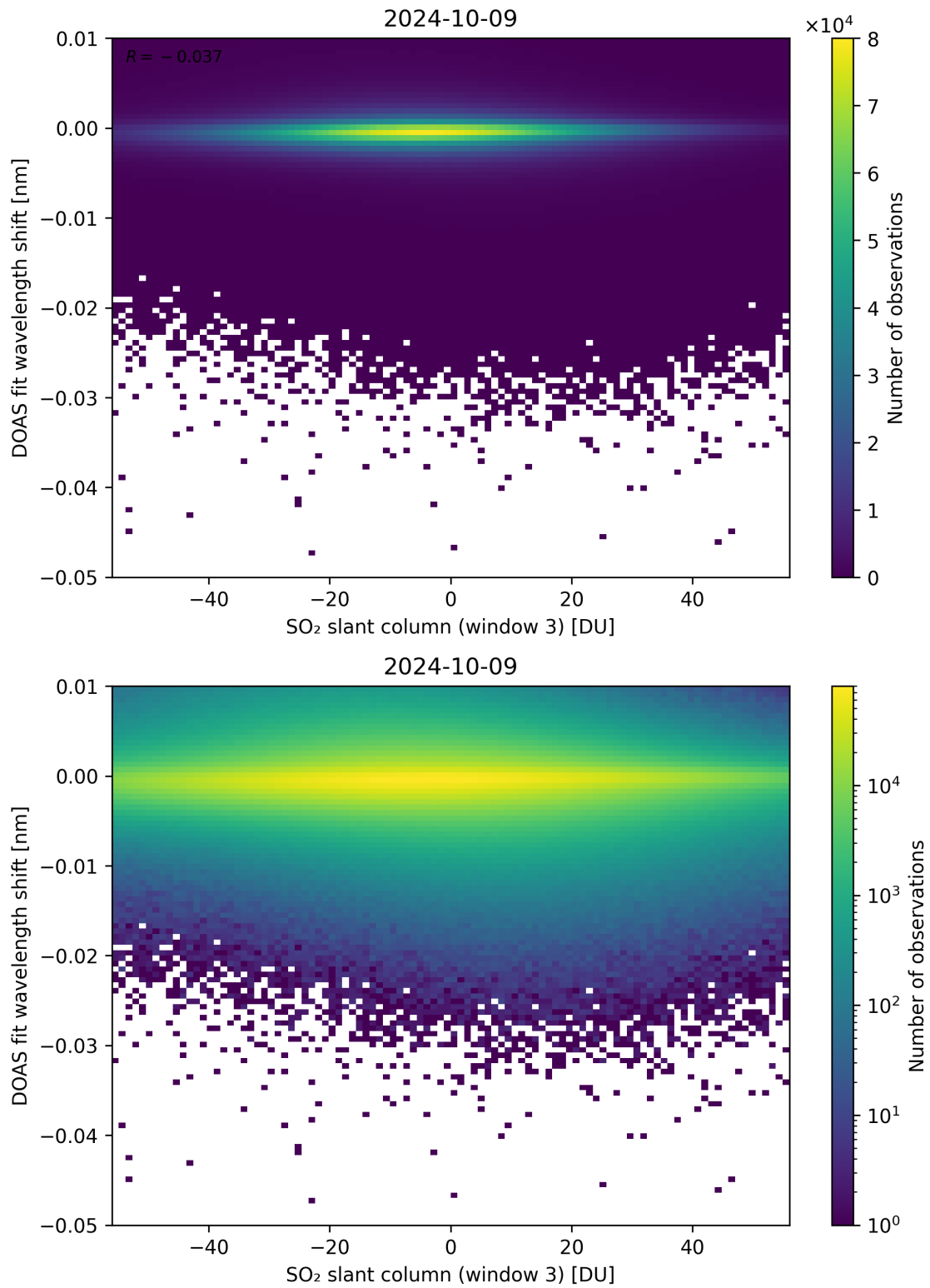
Figure 254: Scatter density plot of “SO 2 slant column (window 3)” against “DOAS fit wavelength shift” for 2024-10-08 to 2024-10-10.
