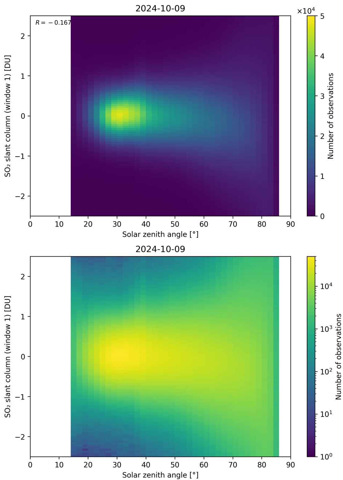
Figure 169: Scatter density plot of “Solar zenith angle” against “SO 2 slant column (window 1)” for 2024-10-08 to 2024-10-10.
