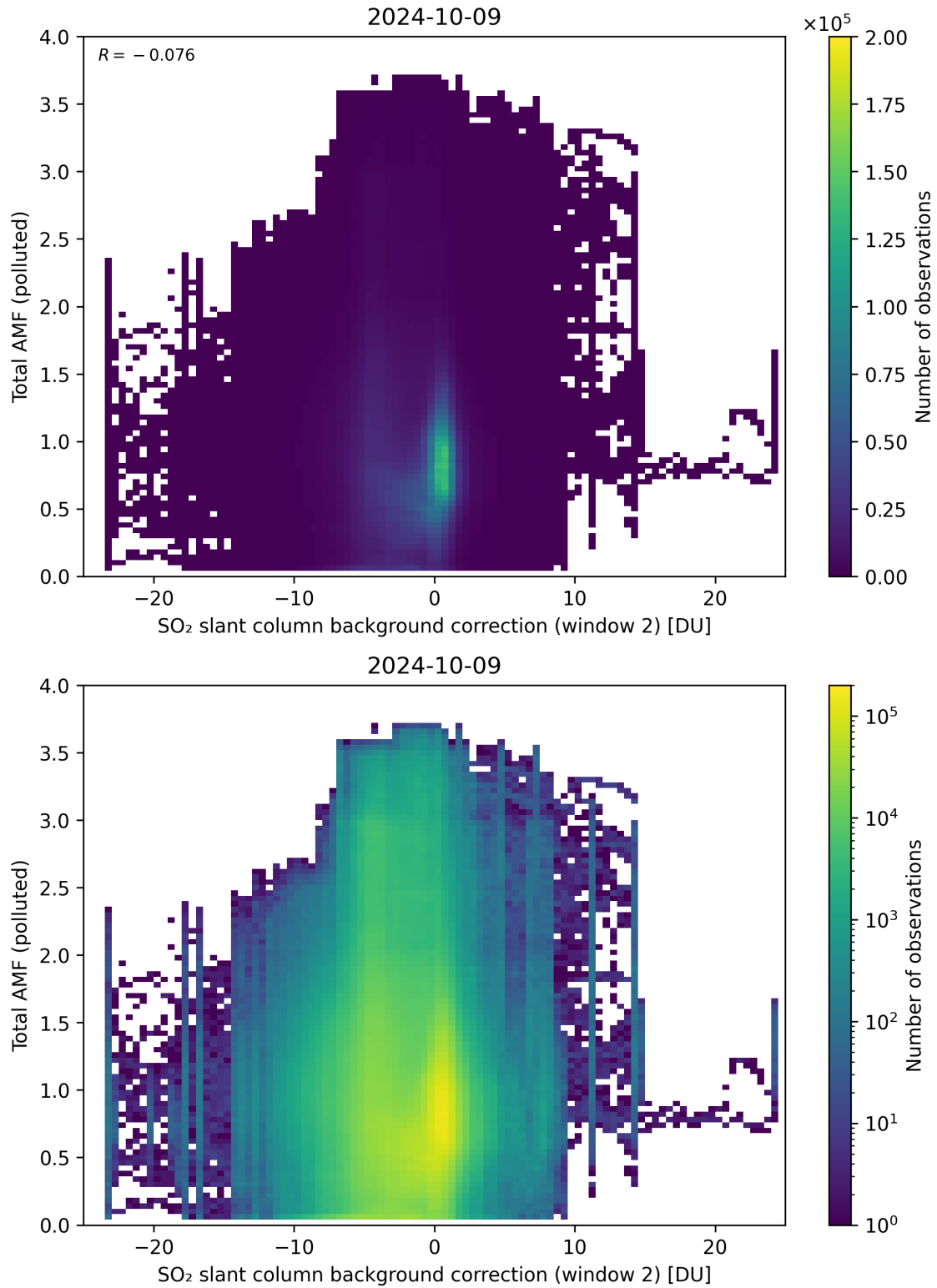
Figure 119: Scatter density plot of “SO 2 slant column background correction (window 2)” against “Total AMF (polluted)” for 2024-10-08 to 2024-10-10.
