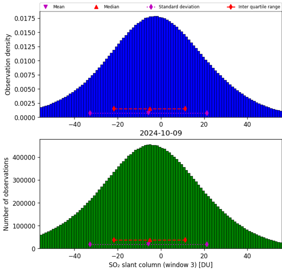
Figure 64: Histogram of “SO 2 slant column (window 3)” for 2024-10-08 to 2024-10-10
