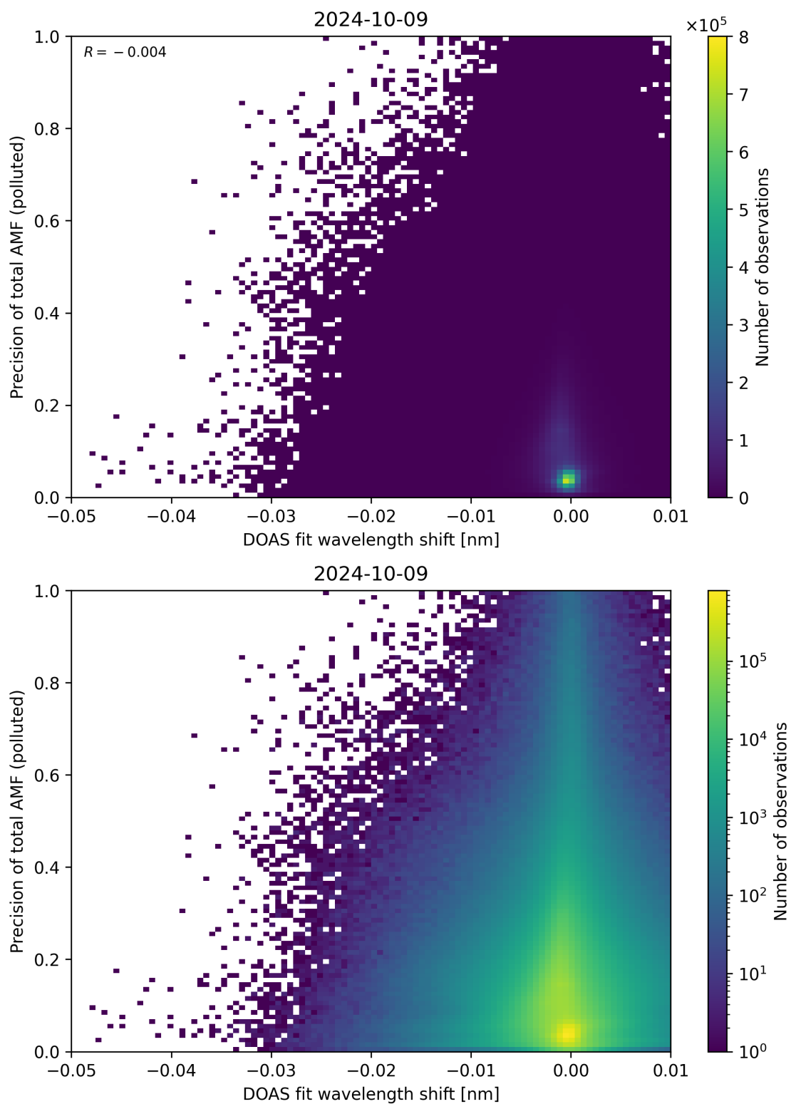
Figure 131: Scatter density plot of “DOAS fit wavelength shift” against “Precision of total AMF (polluted)” for 2024-10-08 to 2024-10-10.
