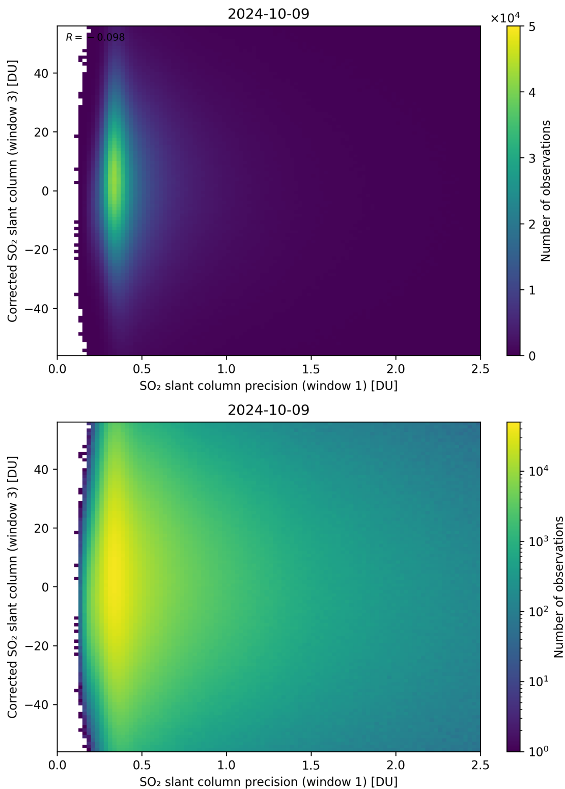
Figure 226: Scatter density plot of “SO 2 slant column precision (window 1)” against “Corrected SO 2 slant column (window 3)” for 2024-10-08 to 2024-10-10.
