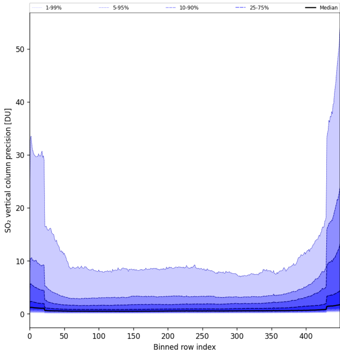
Figure 77: Along track statistics of “SO 2 vertical column precision” for 2024-10-08 to 2024-10-10
