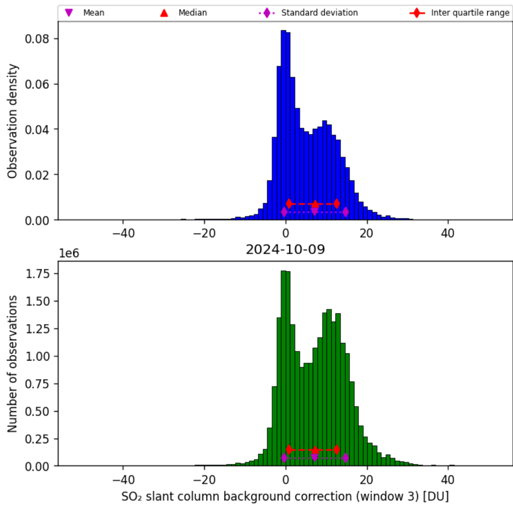
Figure 67: Histogram of “SO 2 slant column background correction (window 3)” for 2024-10-08 to 2024-10-10
