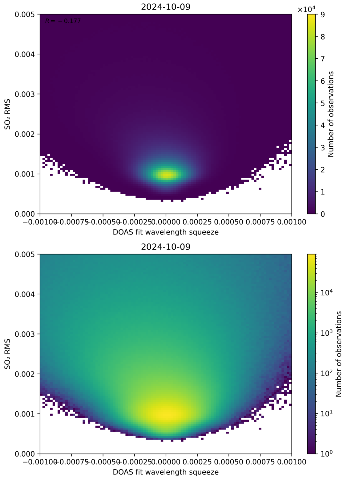
Figure 132: Scatter density plot of “DOAS fit wavelength squeeze” against “SO 2 RMS” for 2024-10-08 to 2024-10-10.
