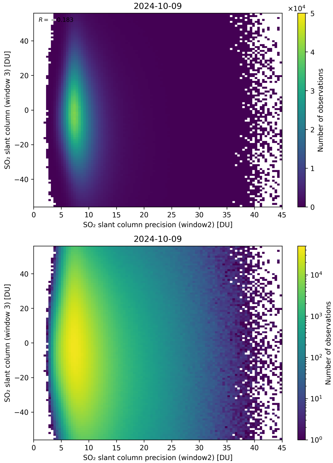
Figure 249: Scatter density plot of “SO 2 slant column precision (window2)” against “SO 2 slant column (window 3)” for 2024-10-08 to 2024-10-10.
