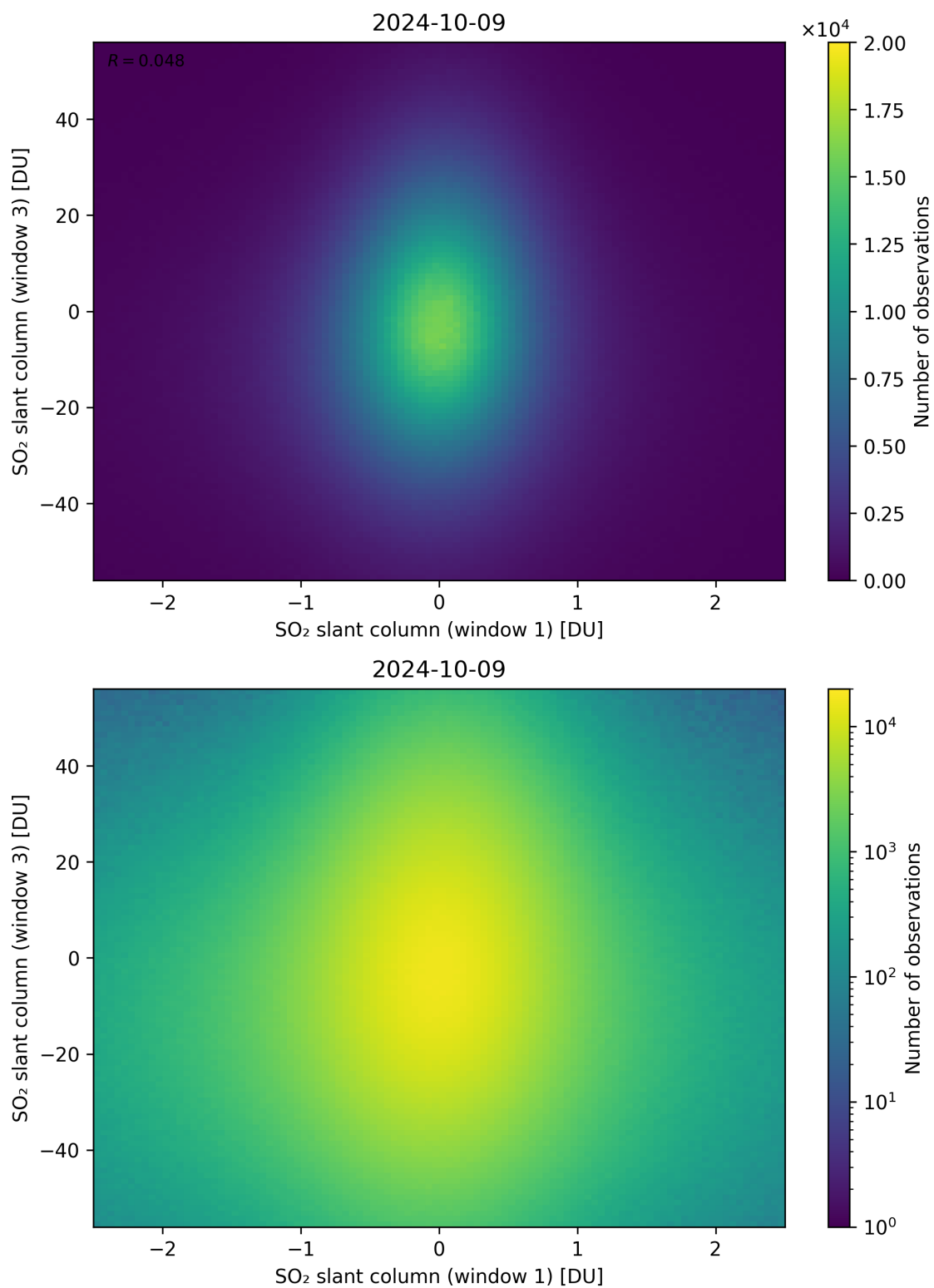
Figure 237: Scatter density plot of “SO 2 slant column (window 1)” against “SO 2 slant column (window 3)” for 2024-10-08 to 2024-10-10.
