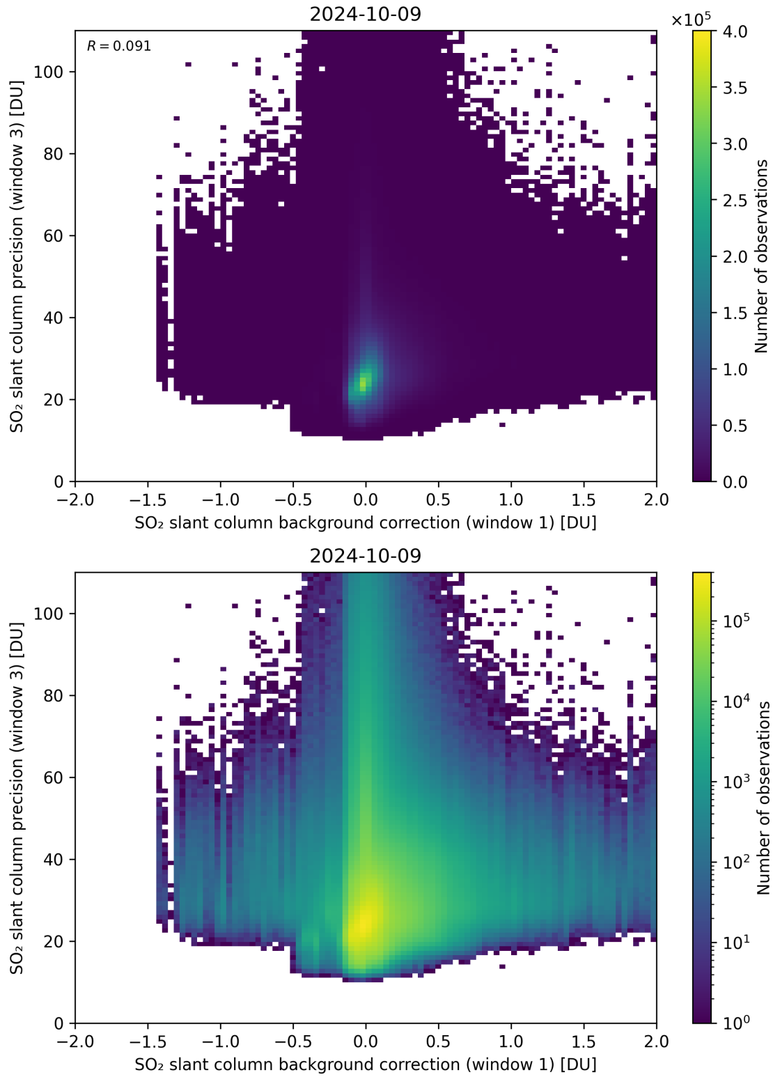
Figure 108: Scatter density plot of “SO 2 slant column background correction (window 1)” against “SO 2 slant column precision (window 3)” for 2024-10-08 to 2024-10-10.
