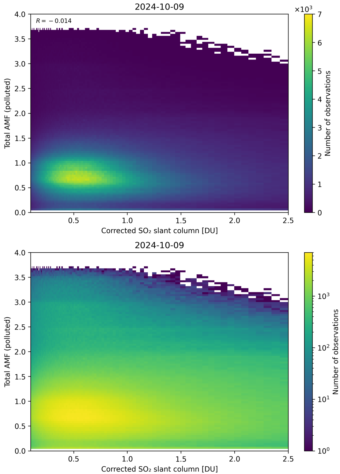
Figure 192: Scatter density plot of “Corrected SO 2 slant column” against “Total AMF (polluted)” for 2024-10-08 to 2024-10-10.
