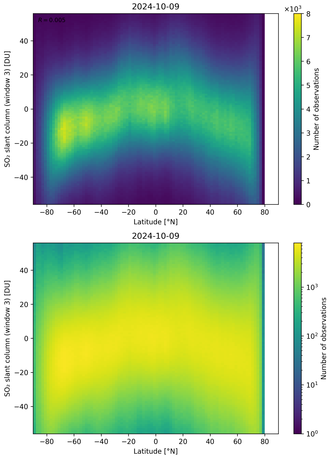
Figure 152: Scatter density plot of “Latitude” against “SO 2 slant column (window 3)” for 2024-10-08 to 2024-10-10.
