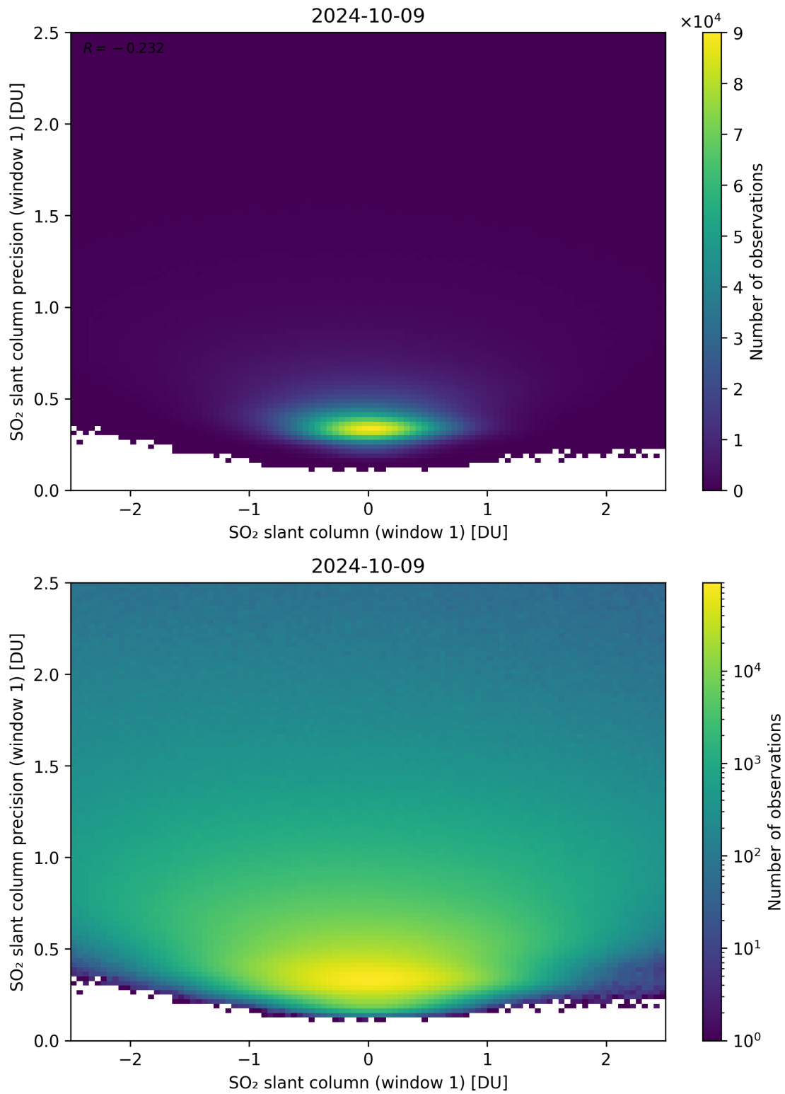
Figure 235: Scatter density plot of “SO 2 slant column (window 1)” against “SO 2 slant column precision (window 1)” for 2024-10-08 to 2024-10-10.
