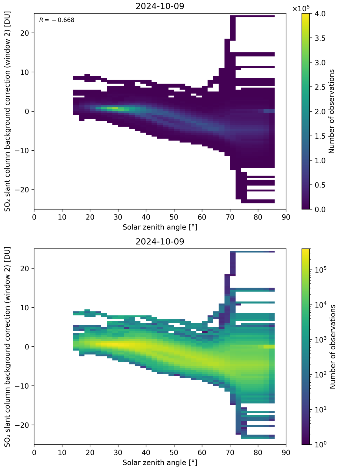
Figure 159: Scatter density plot of “Solar zenith angle” against “SO 2 slant column background correction (window 2)” for 2024-10-08 to 2024-10-10.
