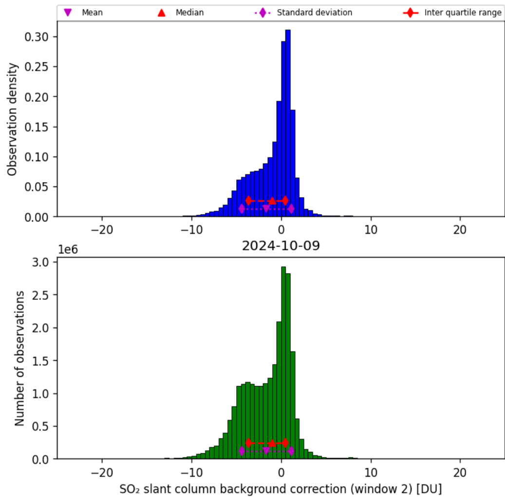
Figure 63: Histogram of “SO 2 slant column background correction (window 2)” for 2024-10-08 to 2024-10-10
