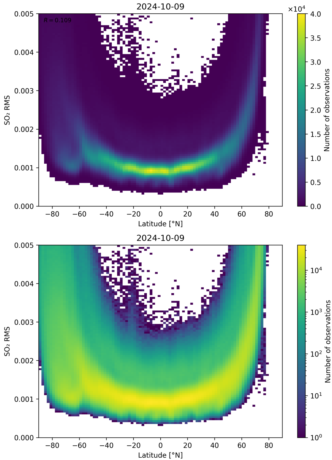
Figure 144: Scatter density plot of “Latitude” against “SO 2 RMS” for 2024-10-08 to 2024-10-10.
