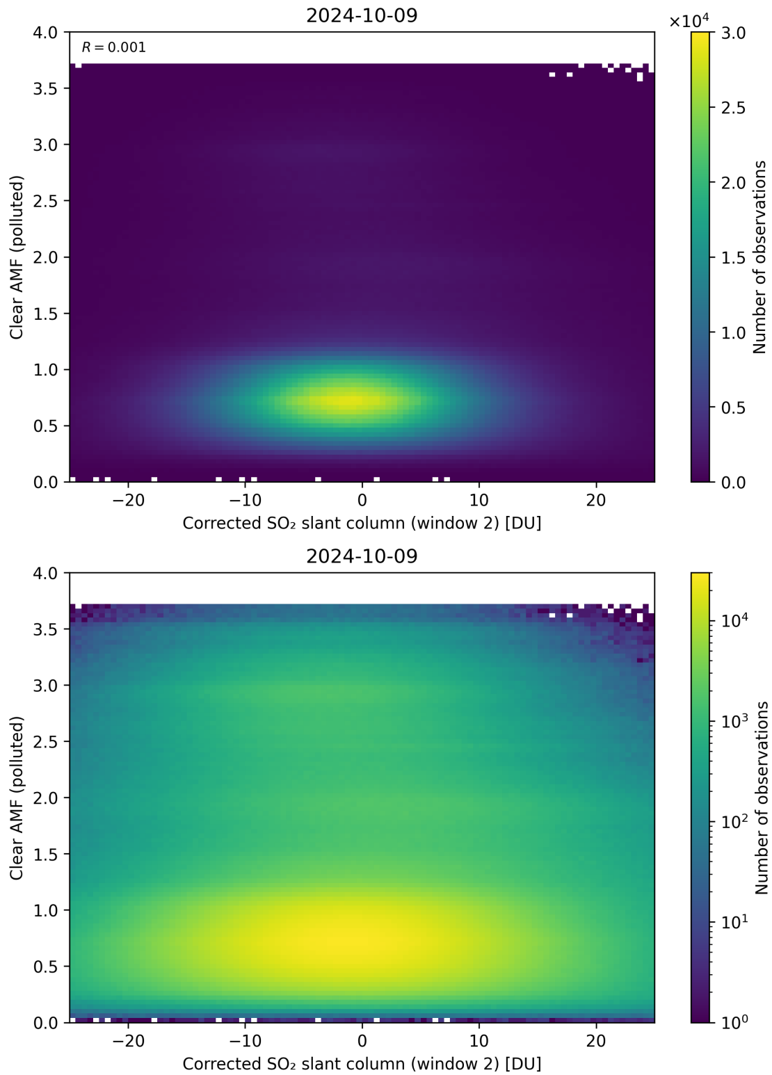
Figure 199: Scatter density plot of “Corrected SO 2 slant column (window 2)” against “Clear AMF (polluted)” for 2024-10-08 to 2024-10-10.
