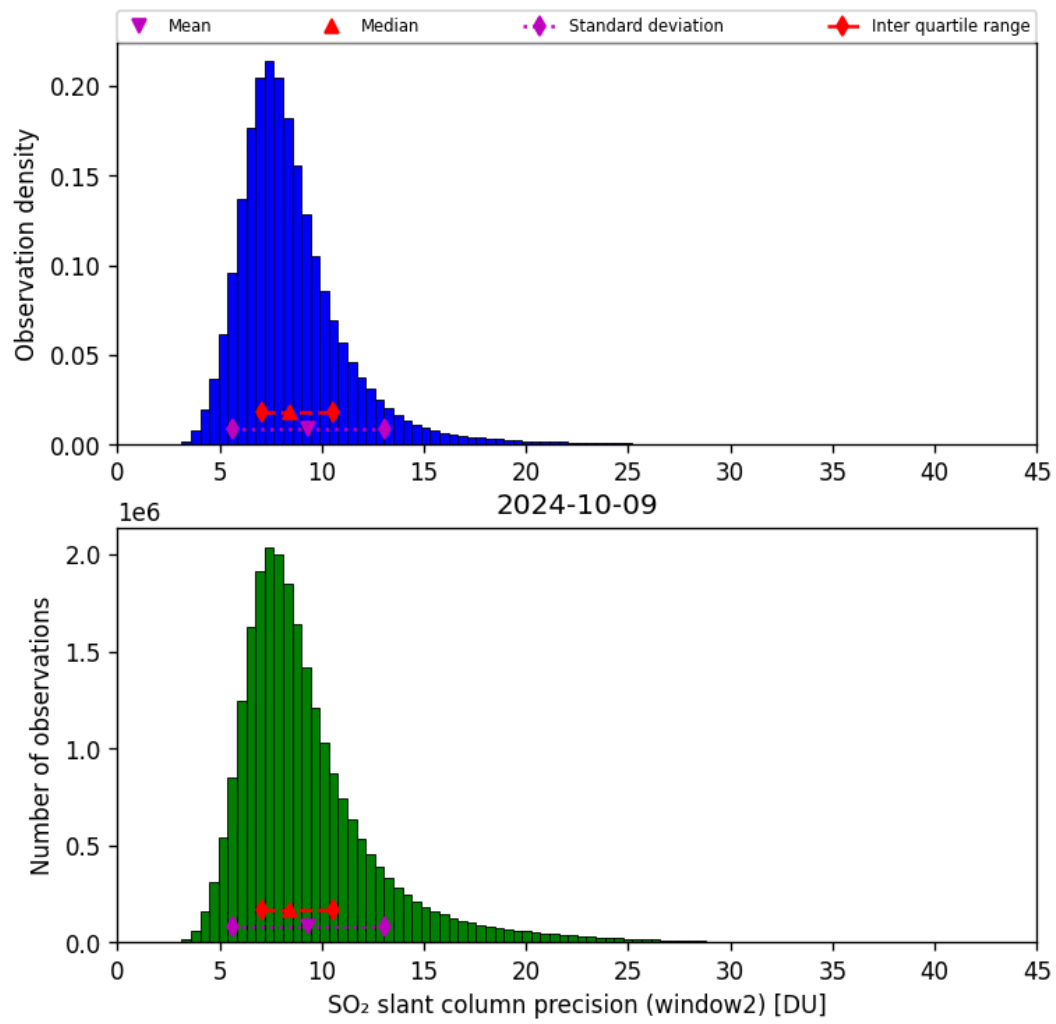
Figure 61: Histogram of “SO 2 slant column precision (window2)” for 2024-10-08 to 2024-10-10
