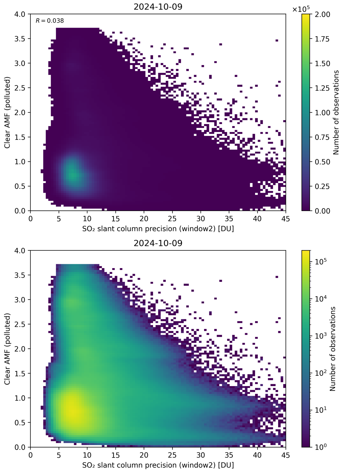
Figure 246: Scatter density plot of “SO 2 slant column precision (window2)” against “Clear AMF (polluted)” for 2024-10-08 to 2024-10-10.
