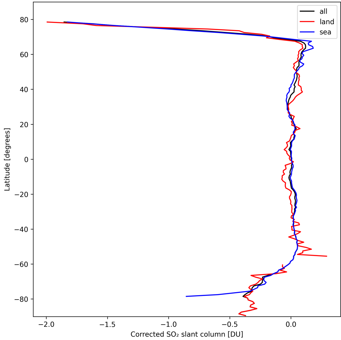
Figure 32: Zonal average of “Corrected SO 2 slant column” for 2024-10-08 to 2024-10-10.
