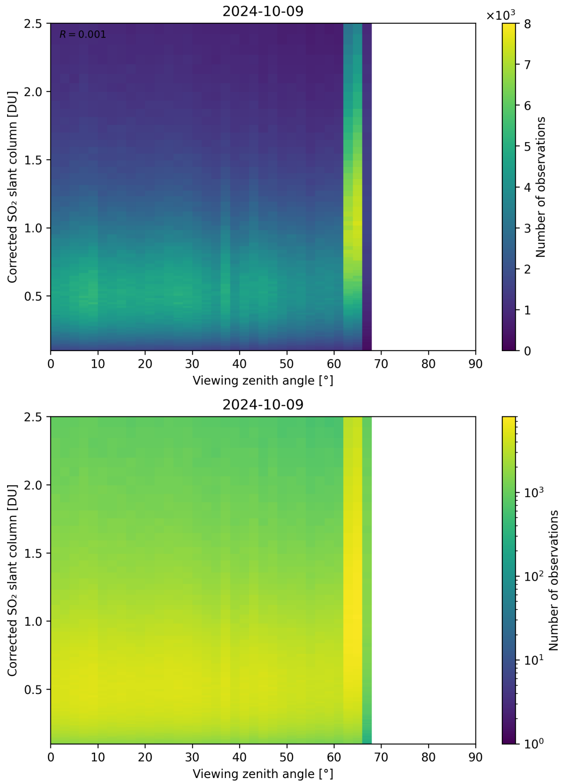
Figure 317: Scatter density plot of “Viewing zenith angle” against “Corrected SO 2 slant column” for 2024-10-08 to 2024-10-10.
