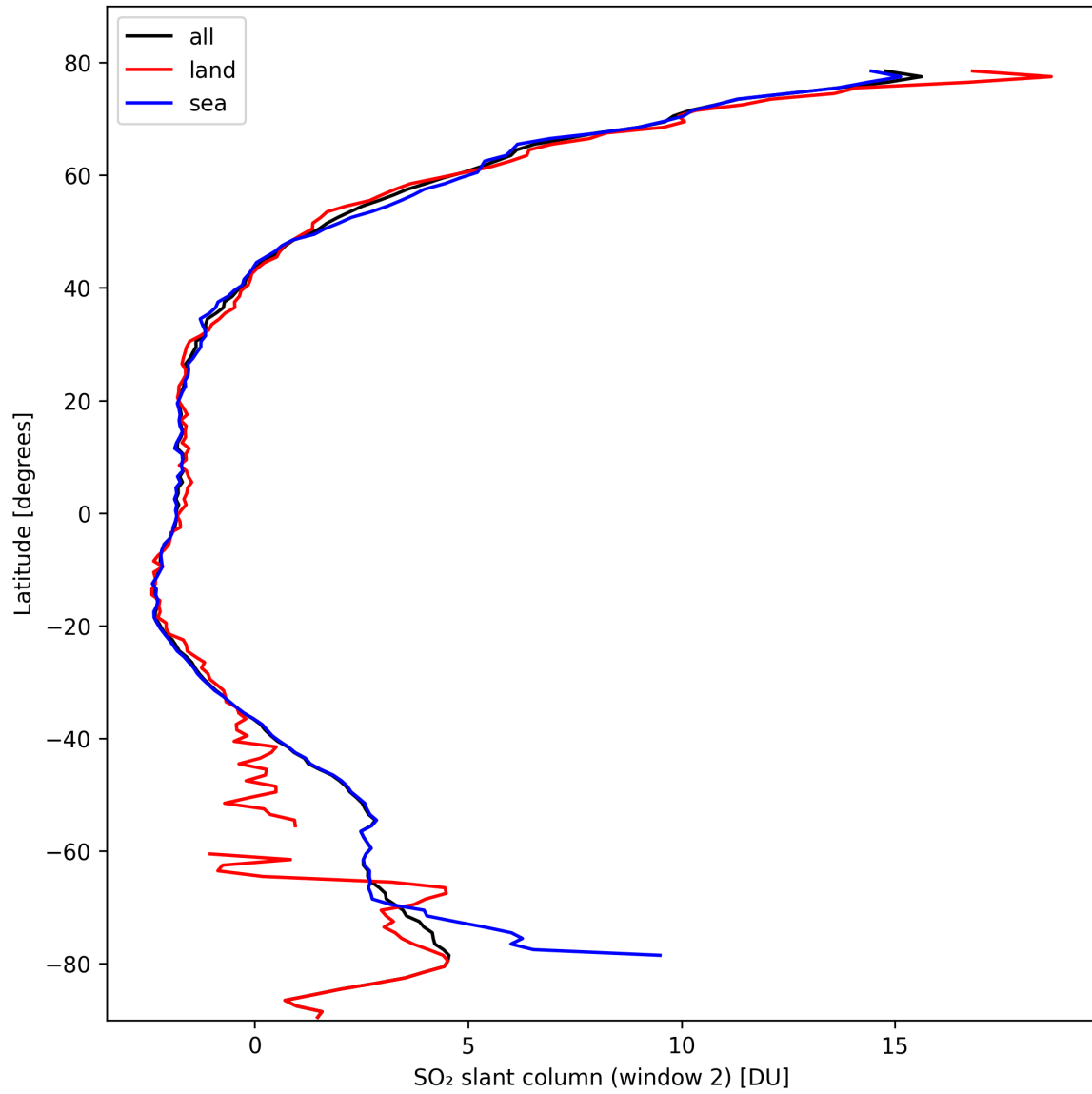
Figure 37: Zonal average of “SO 2 slant column (window 2)” for 2024-10-08 to 2024-10-10.
