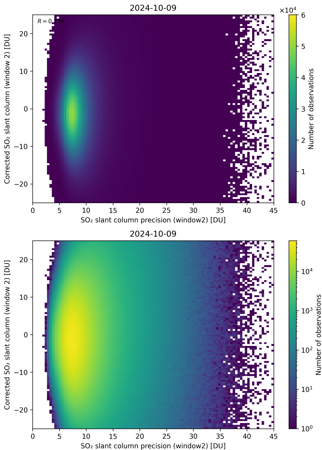
Figure 247: Scatter density plot of “SO 2 slant column precision (window2)” against “Corrected SO 2 slant column (window 2)” for 2024-10-08 to 2024-10-10.
