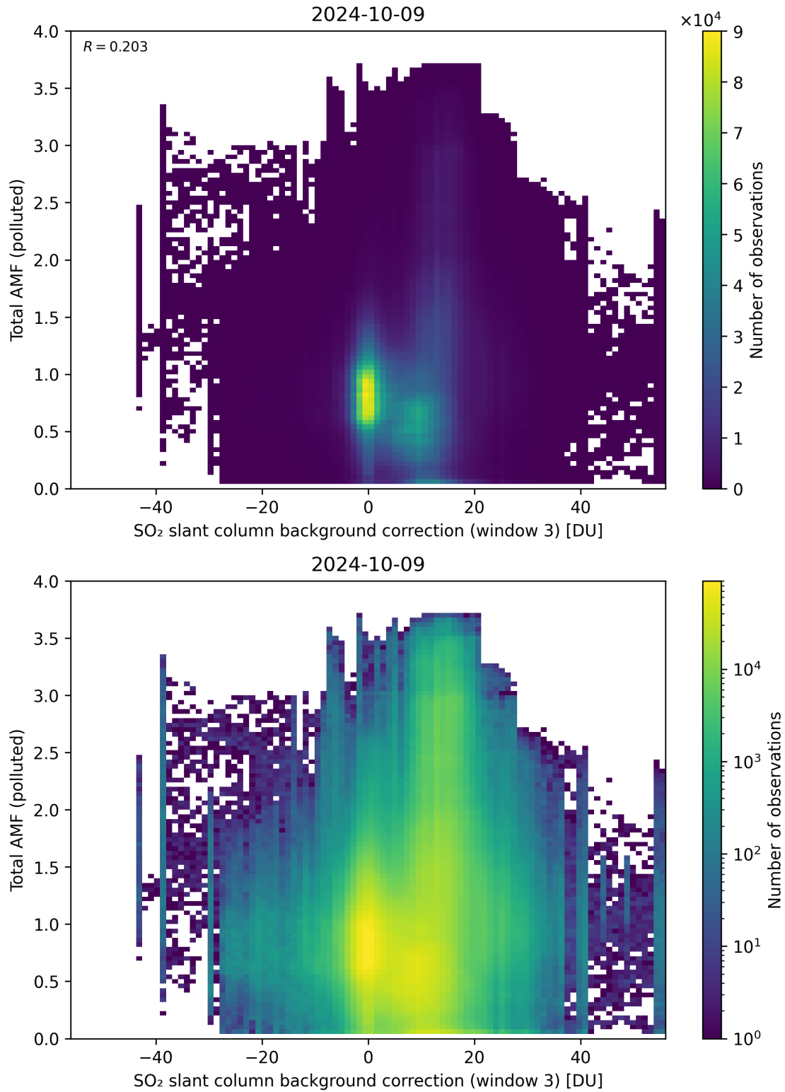
Figure 125: Scatter density plot of “SO 2 slant column background correction (window 3)” against “Total AMF (polluted)” for 2024-10-08 to 2024-10-10.
