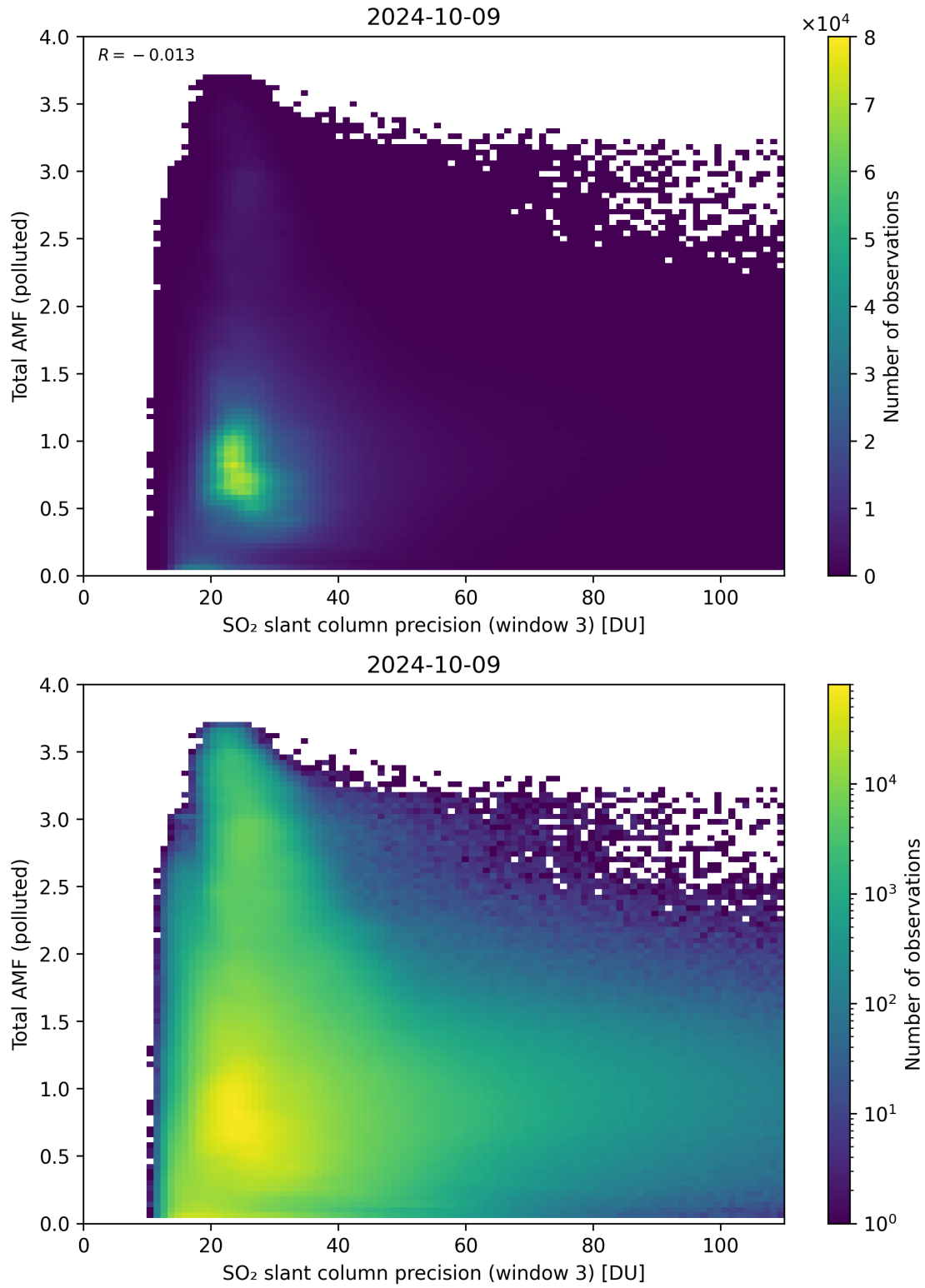
Figure 263: Scatter density plot of “SO 2 slant column precision (window 3)” against “Total AMF (polluted)” for 2024-10-08 to 2024-10-10.
