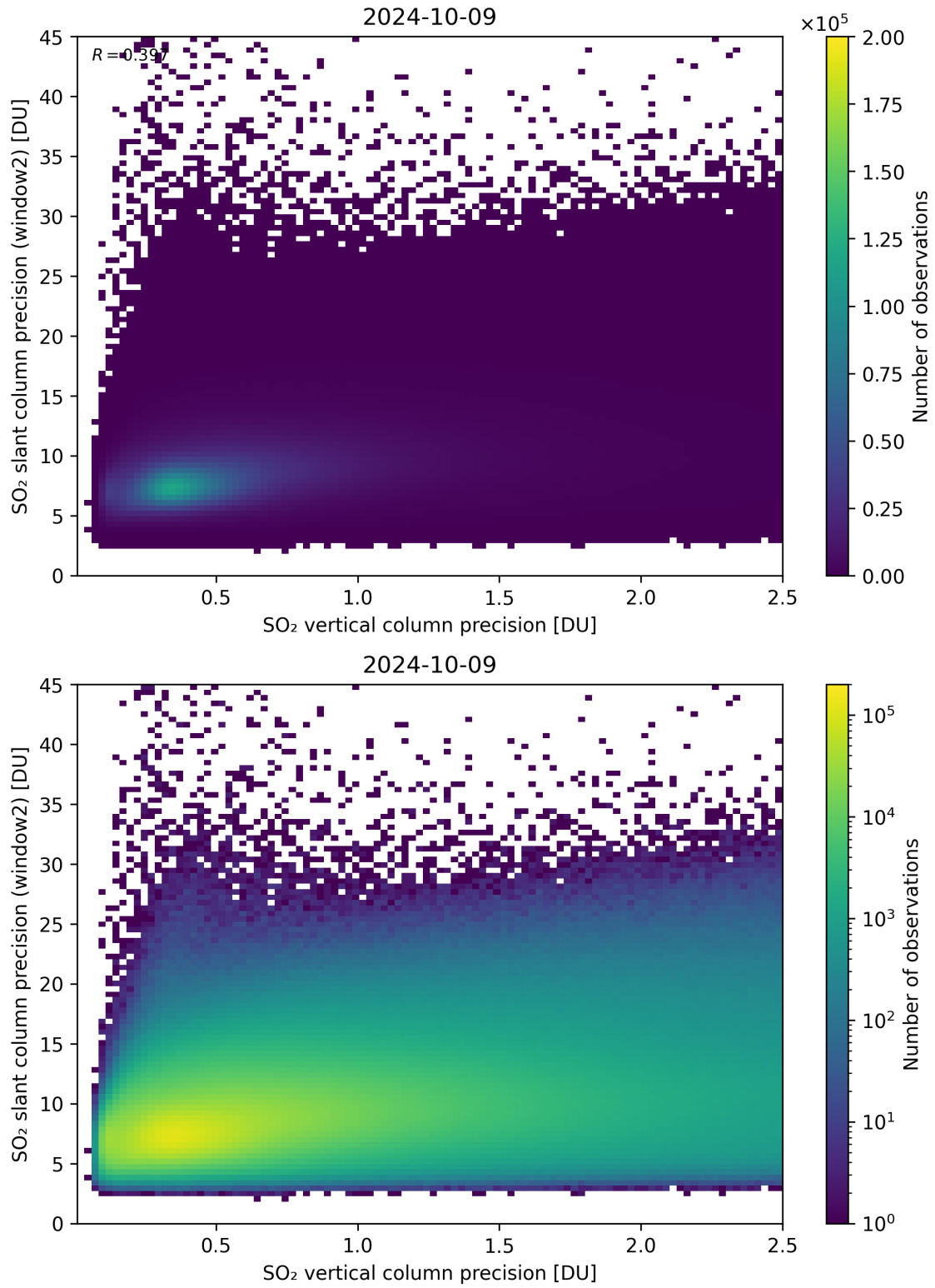
Figure 291: Scatter density plot of “SO 2 vertical column precision” against “SO 2 slant column precision (window2)” for 2024-10-08 to 2024-10-10.
