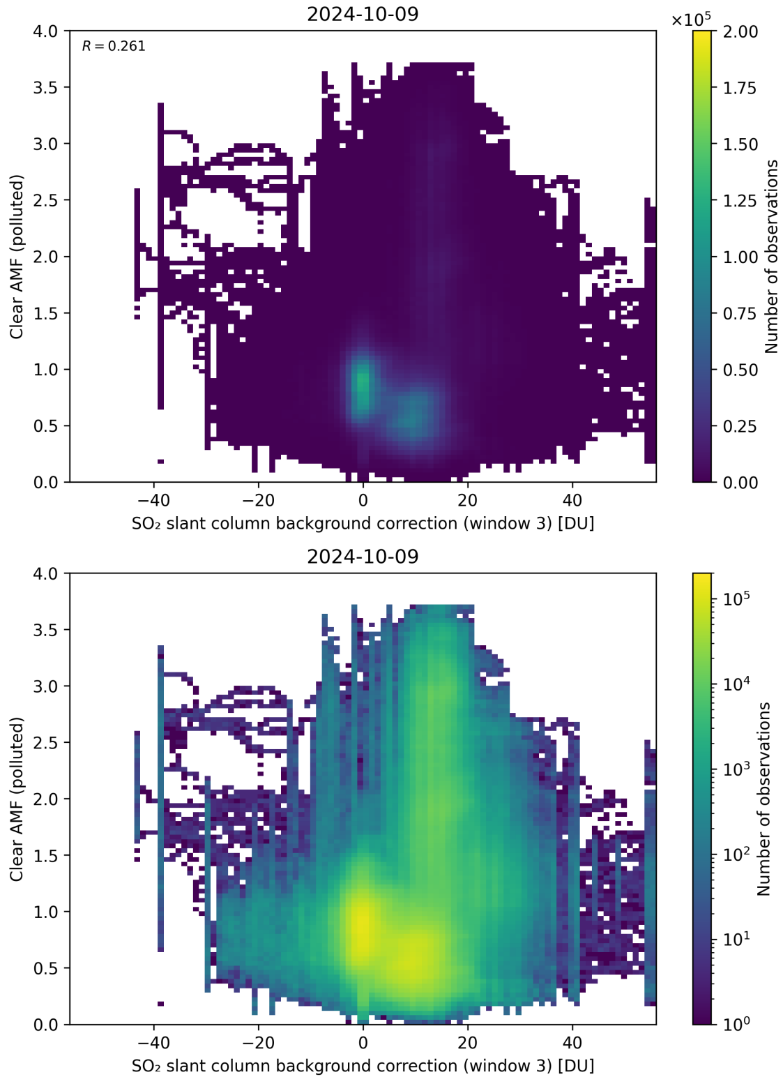
Figure 124: Scatter density plot of “SO 2 slant column background correction (window 3)” against “Clear AMF (polluted)” for 2024-10-08 to 2024-10-10.
