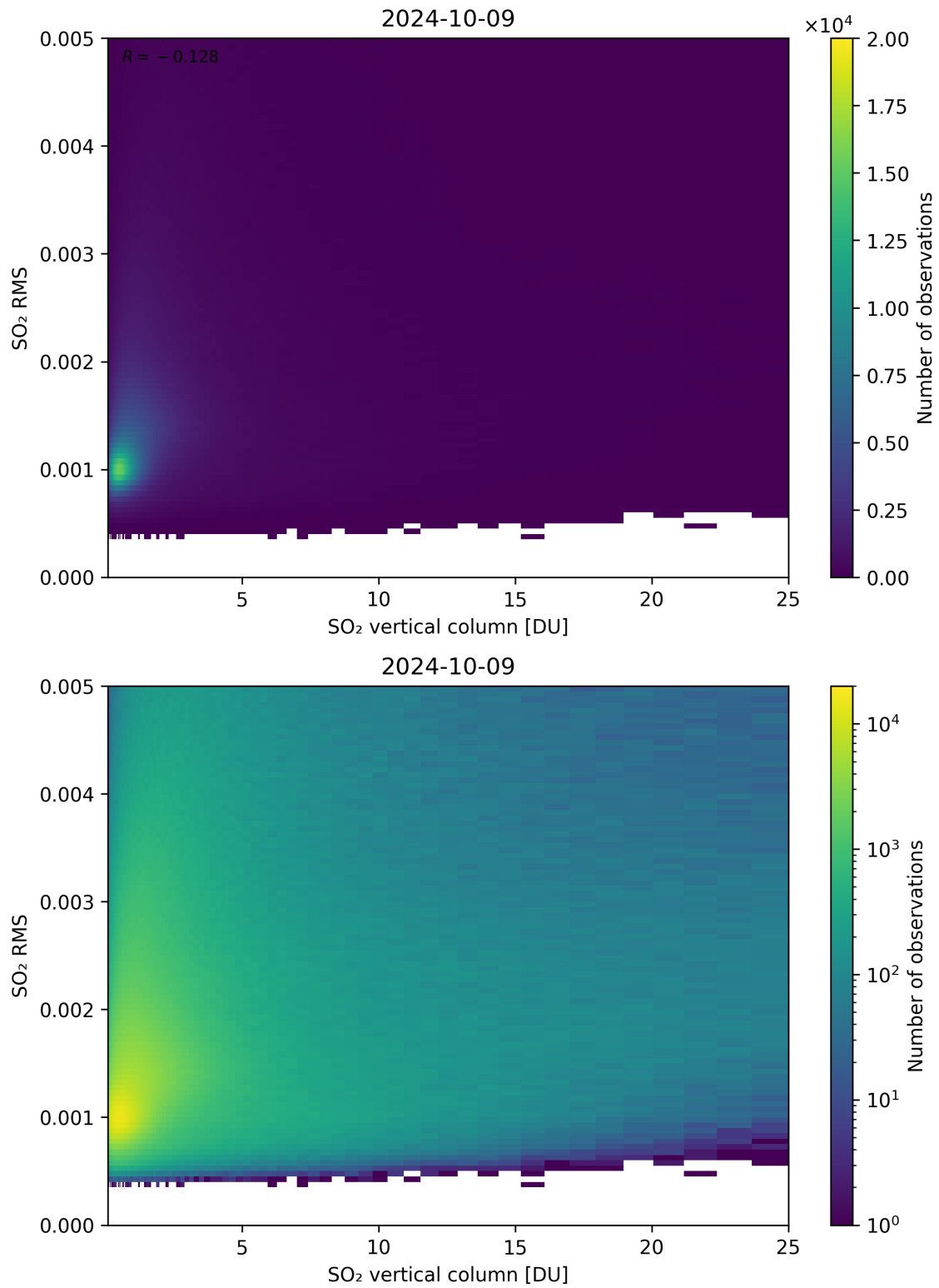
Figure 278: Scatter density plot of “SO 2 vertical column” against “SO 2 RMS” for 2024-10-08 to 2024-10-10.
