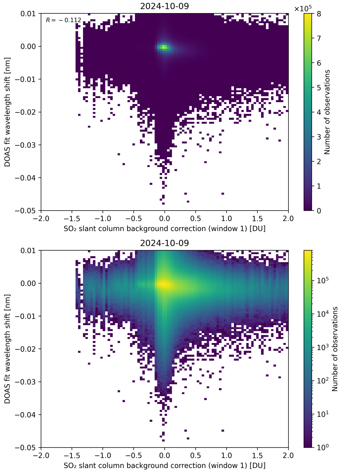
Figure 100: Scatter density plot of “SO 2 slant column background correction (window 1)” against “DOAS fit wavelength shift” for 2024-10-08 to 2024-10-10.
