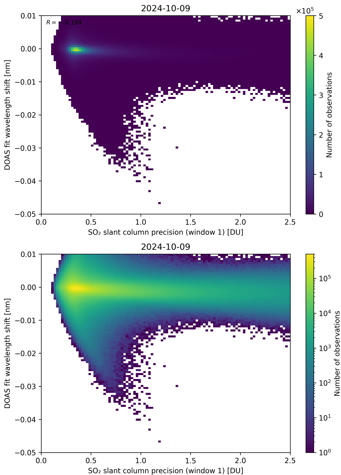
Figure 221: Scatter density plot of “SO 2 slant column precision (window 1)” against “DOAS fit wavelength shift” for 2024-10-08 to 2024-10-10.
