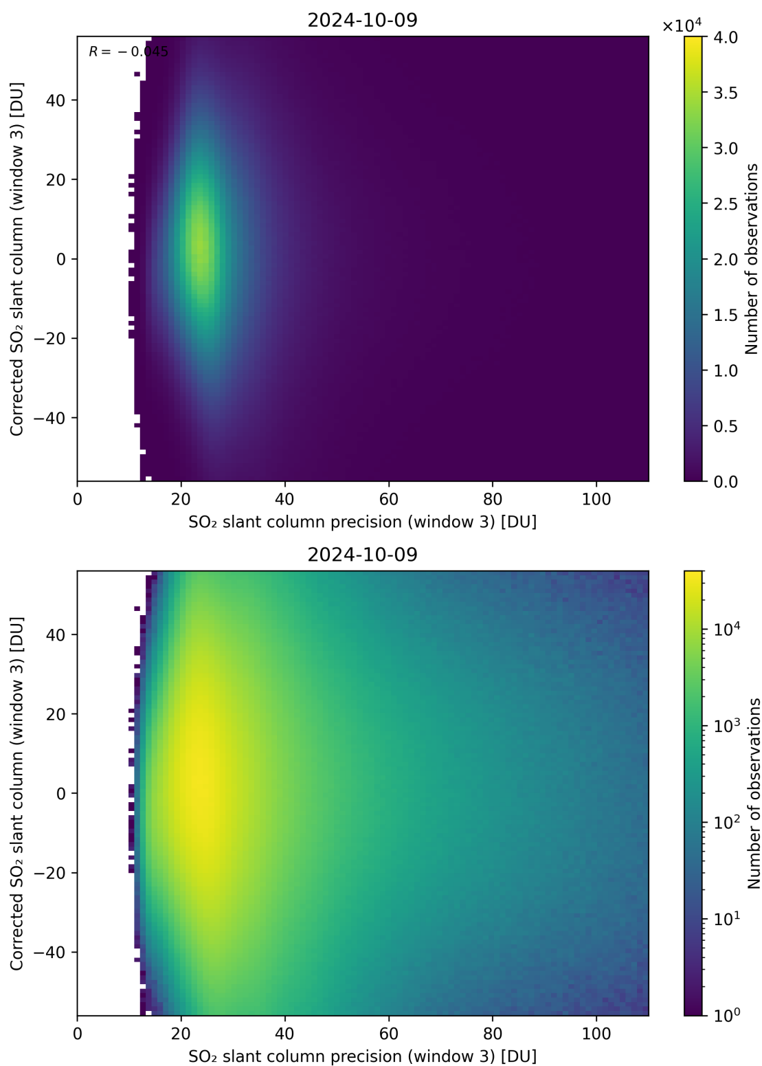
Figure 262: Scatter density plot of “SO 2 slant column precision (window 3)” against “Corrected SO 2 slant column (window 3)” for 2024-10-08 to 2024-10-10.
