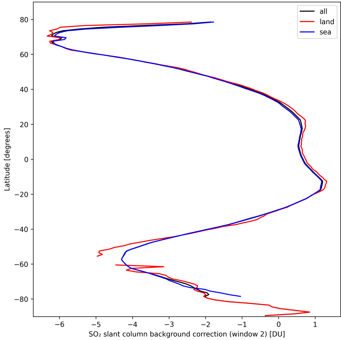
Figure 40: Zonal average of "SO 2 slant column background correction (window 2)" for 2024-10-08 to 2024-10-10.
