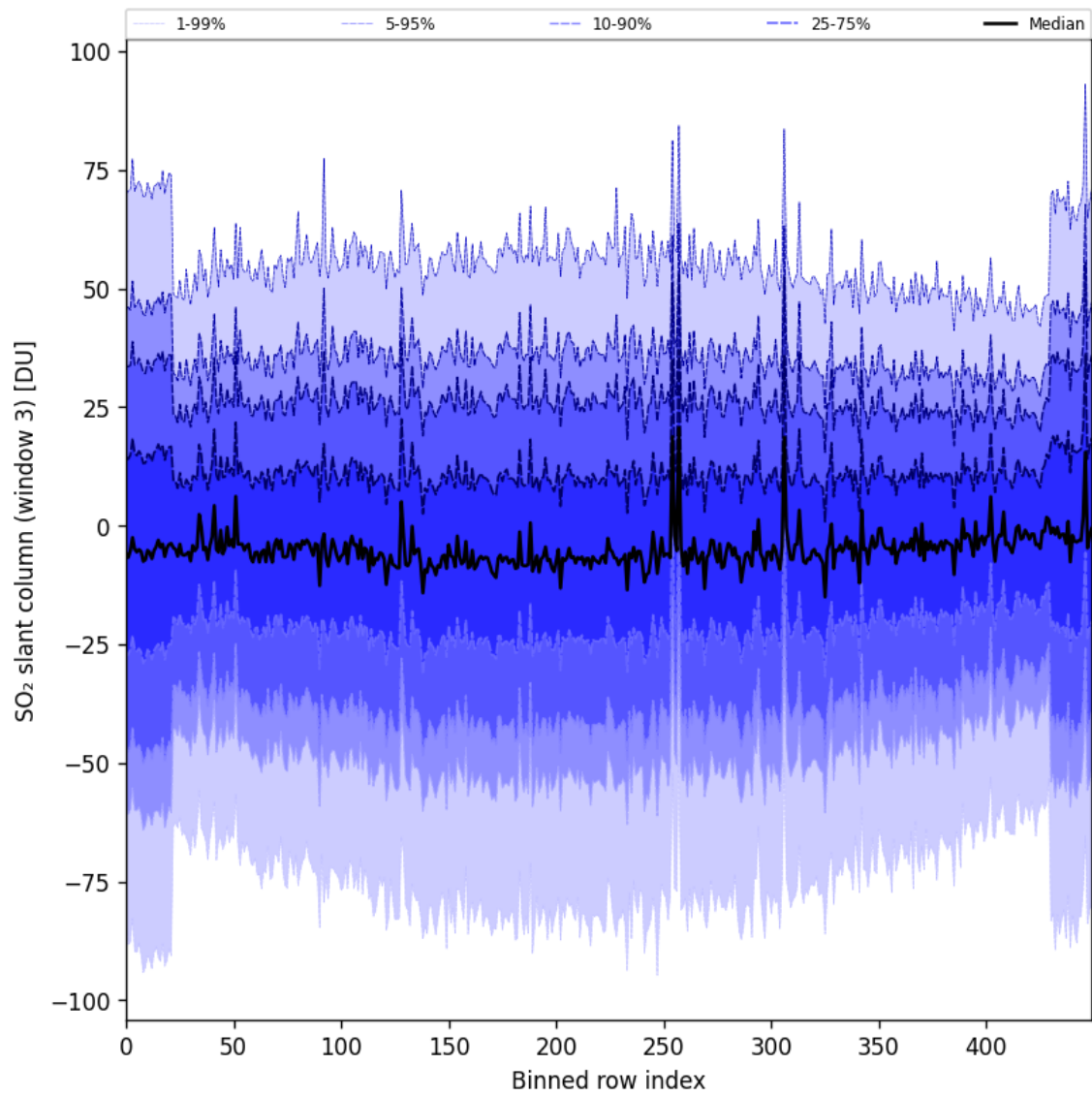
Figure 87: Along track statistics of “SO 2 slant column (window 3)” for 2024-10-08 to 2024-10-10
