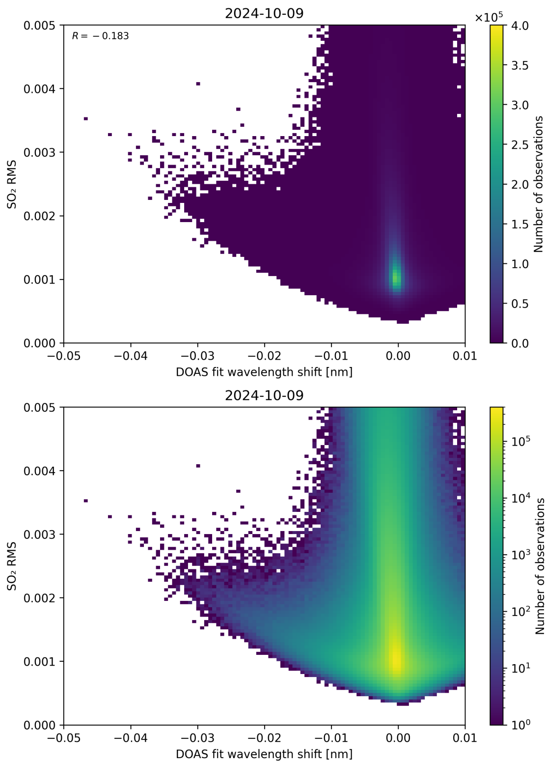
Figure 128: Scatter density plot of “DOAS fit wavelength shift” against “SO 2 RMS” for 2024-10-08 to 2024-10-10.
