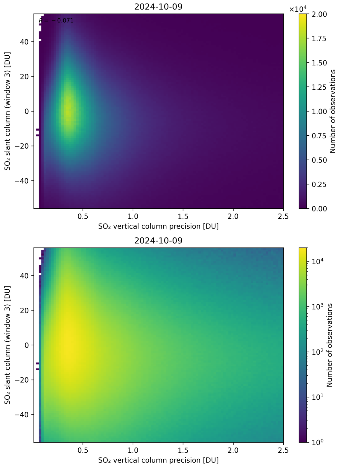
Figure 292: Scatter density plot of “SO 2 vertical column precision” against “SO 2 slant column (window 3)” for 2024-10-08 to 2024-10-10.
