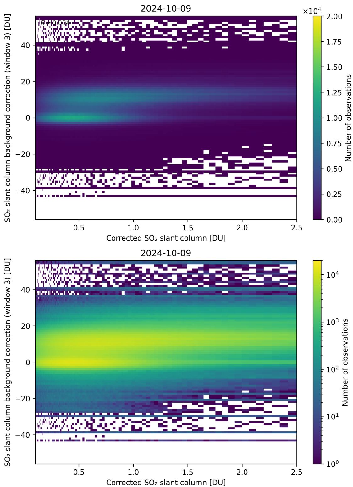
Figure 180: Scatter density plot of “Corrected SO 2 slant column” against “SO 2 slant column background correction (window 3)” for 2024-10-08 to 2024-10-10.
