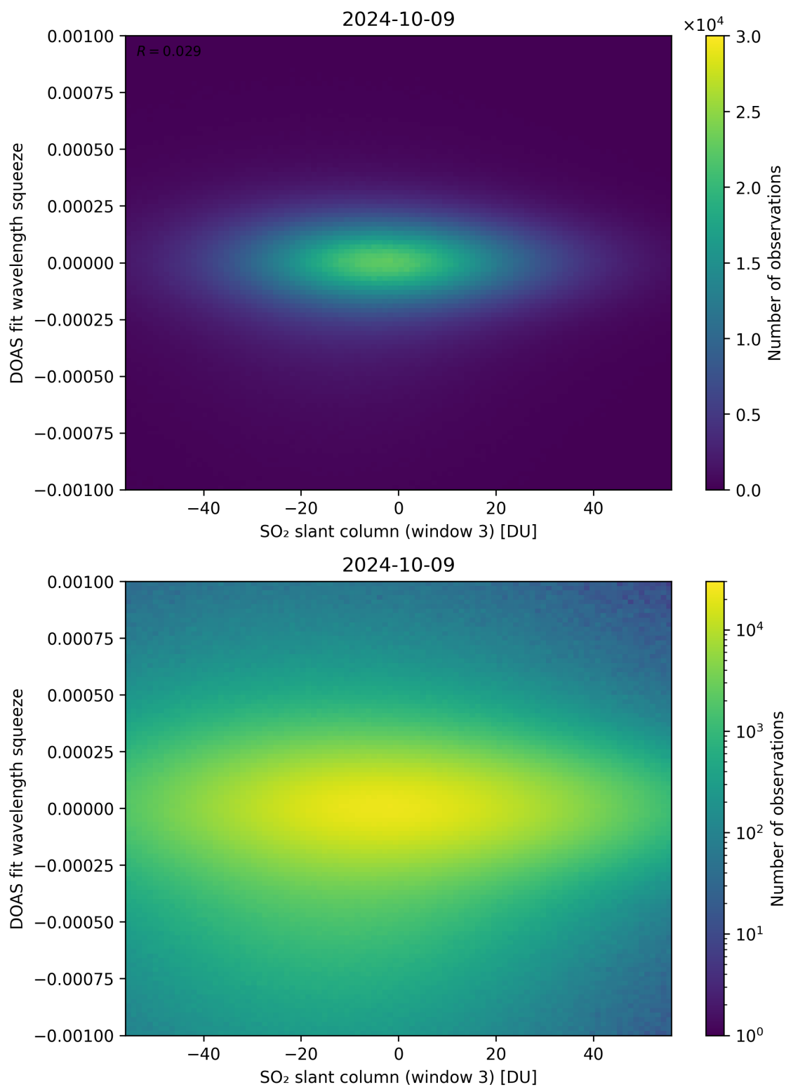
Figure 255: Scatter density plot of “SO 2 slant column (window 3)” against “DOAS fit wavelength squeeze” for 2024-10-08 to 2024-10-10.
