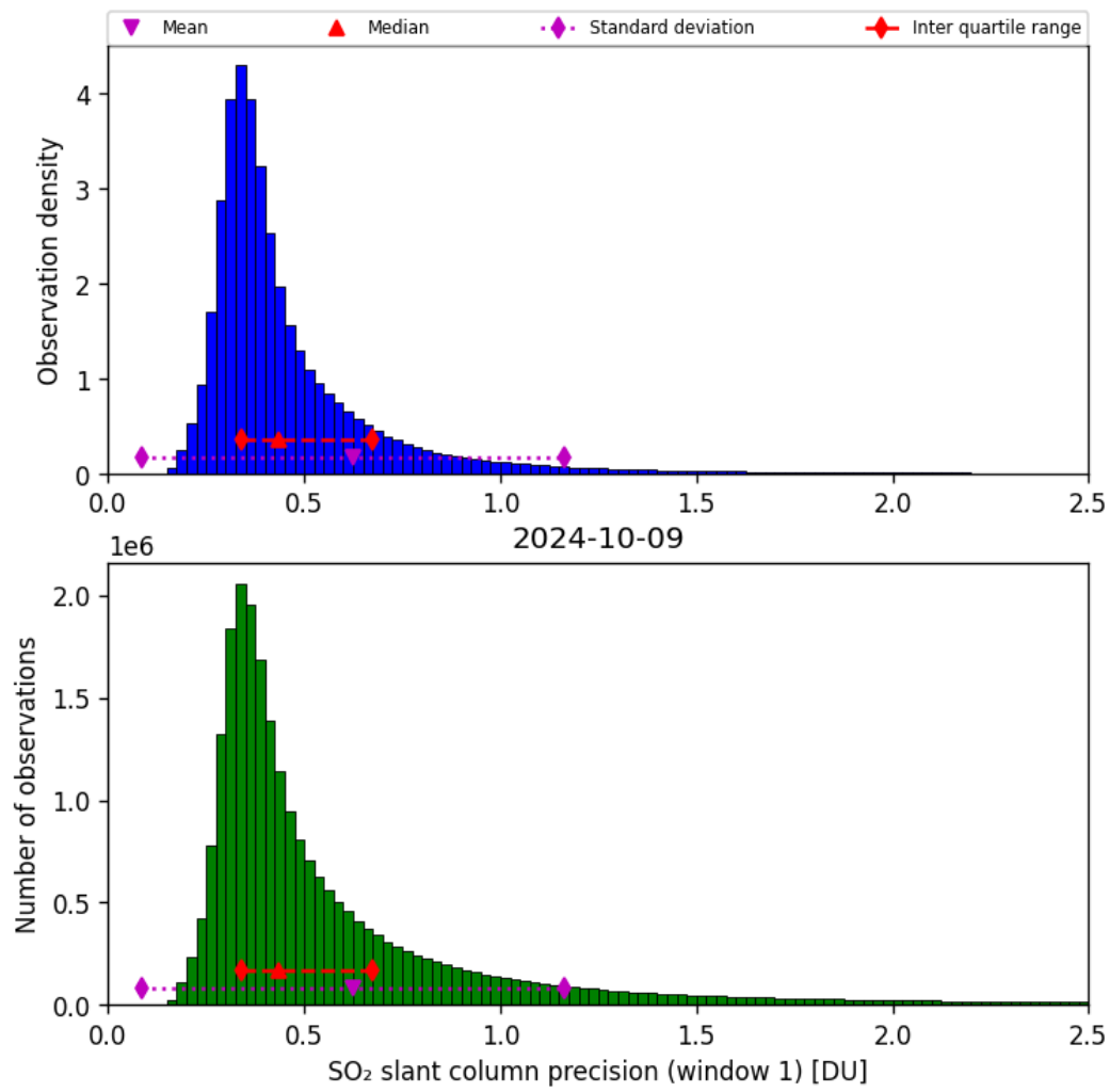
Figure 57: Histogram of “SO 2 slant column precision (window 1)” for 2024-10-08 to 2024-10-10
