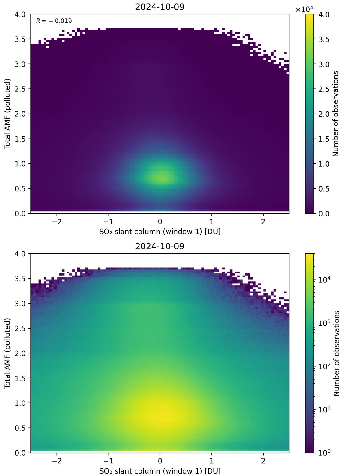
Figure 239: Scatter density plot of “SO 2 slant column (window 1)” against “Total AMF (polluted)” for 2024-10-08 to 2024-10-10.
