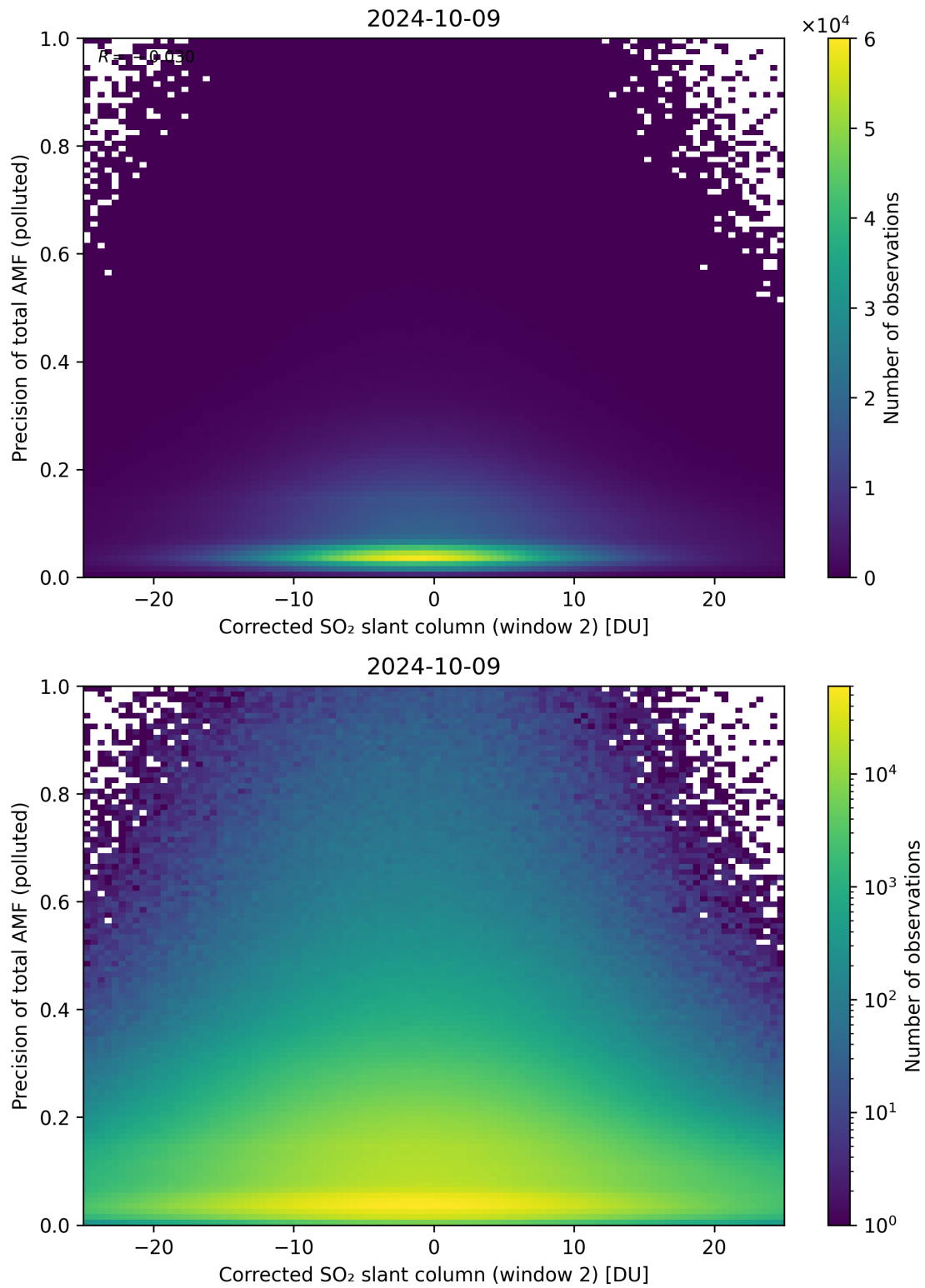
Figure 204: Scatter density plot of “Corrected SO 2 slant column (window 2)” against “Precision of total AMF (polluted)” for 2024-10-08 to 2024-10-10.
