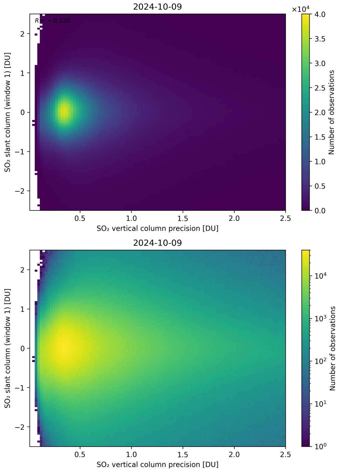
Figure 289: Scatter density plot of “SO 2 vertical column precision” against “SO 2 slant column (window 1)” for 2024-10-08 to 2024-10-10.
