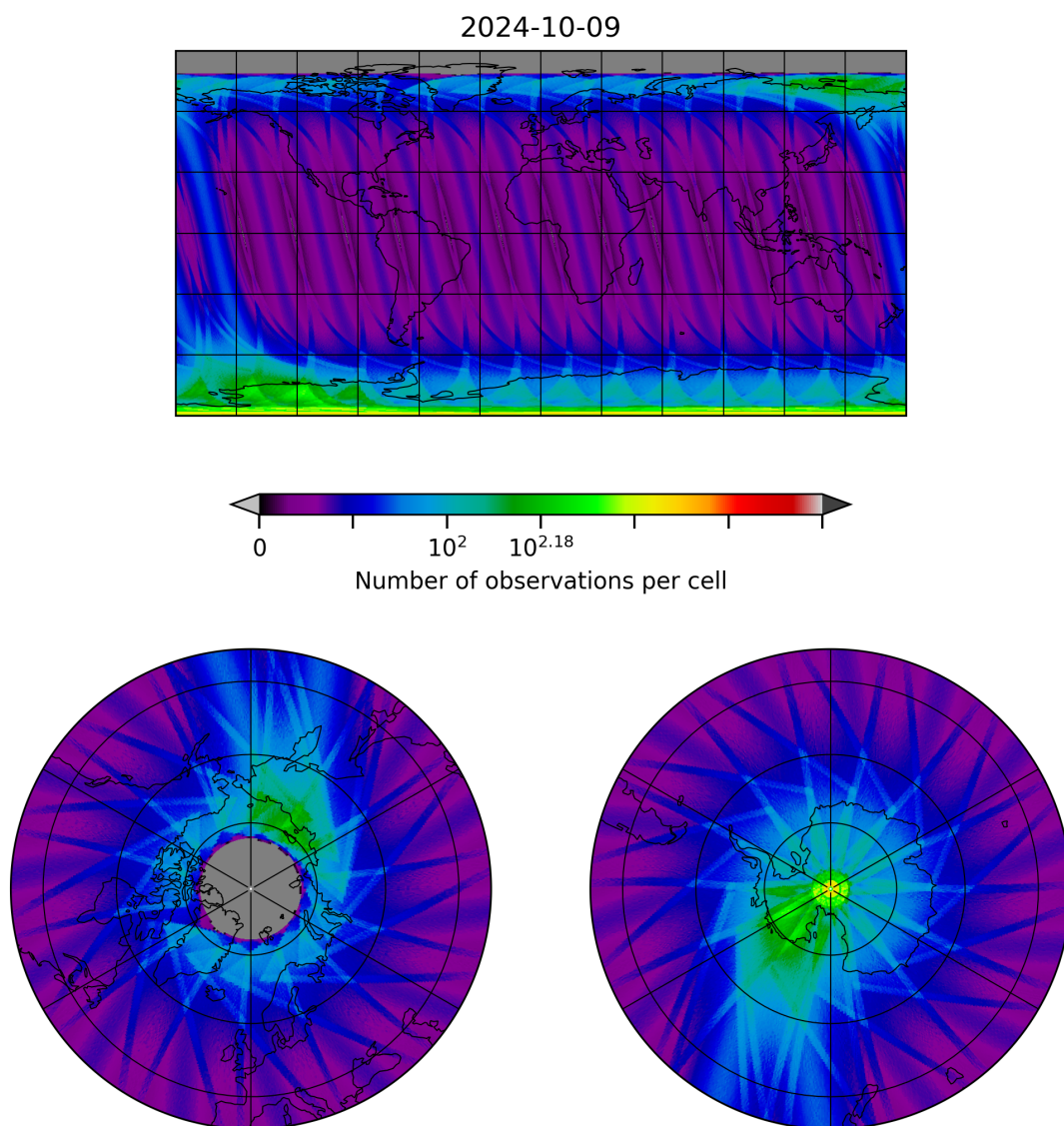
Figure 28: Map of the number of observations for 2024-10-08 to 2024-10-10
