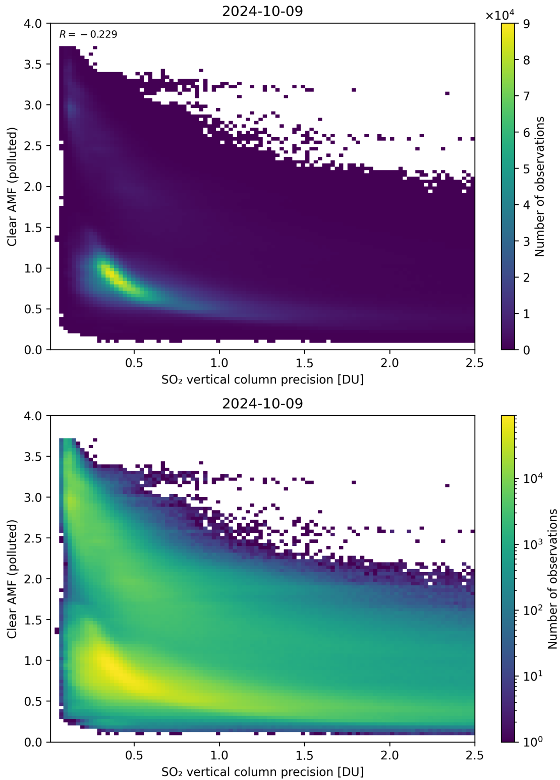
Figure 285: Scatter density plot of “SO 2 vertical column precision” against “Clear AMF (polluted)” for 2024-10-08 to 2024-10-10.
