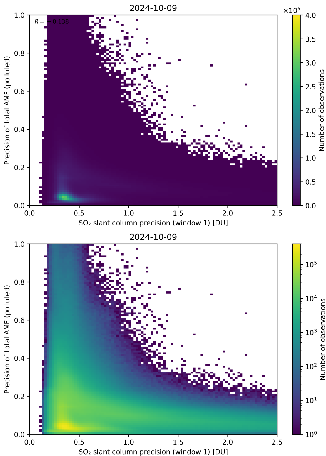
Figure 231: Scatter density plot of “SO 2 slant column precision (window 1)” against “Precision of total AMF (polluted)” for 2024-10-08 to 2024-10-10.
