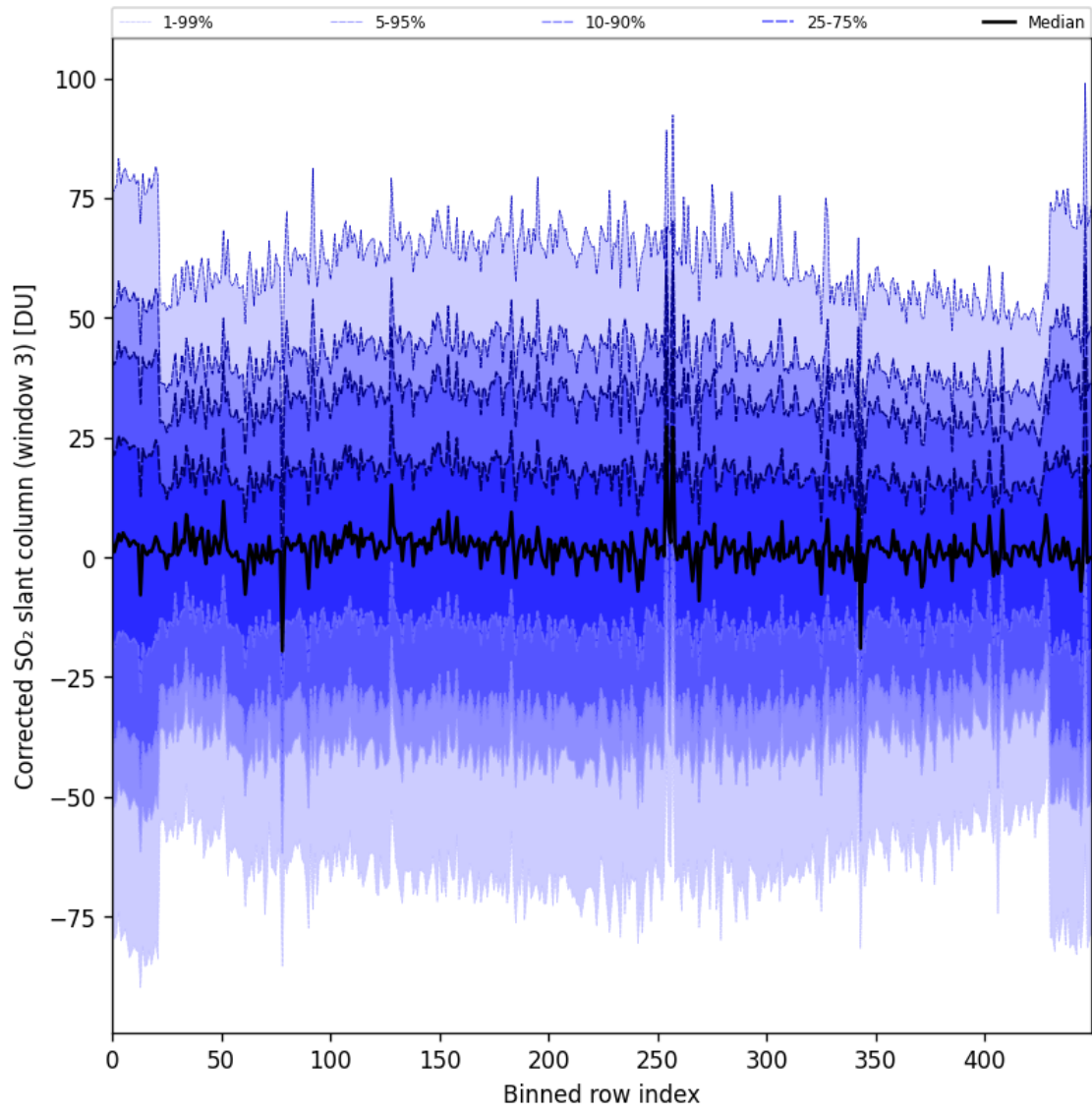
Figure 89: Along track statistics of “Corrected SO 2 slant column (window 3)” for 2024-10-08 to 2024-10-10
