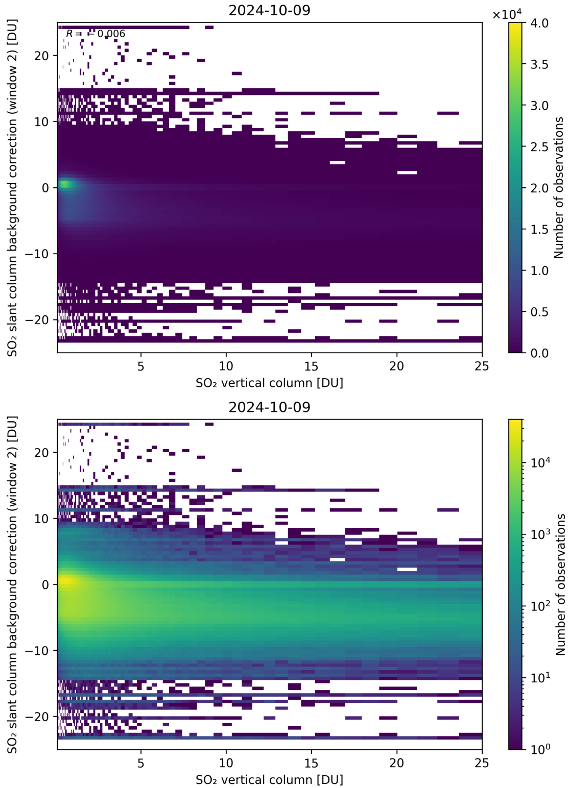
Figure 274: Scatter density plot of “SO 2 vertical column” against “SO 2 slant column background correction (window 2)” for 2024-10-08 to 2024-10-10.
