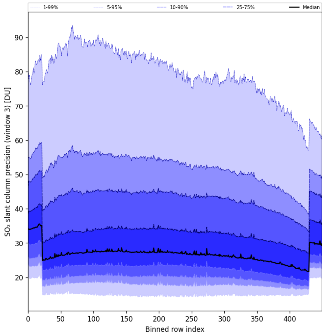
Figure 88: Along track statistics of “SO 2 slant column precision (window 3)” for 2024-10-08 to 2024-10-10
