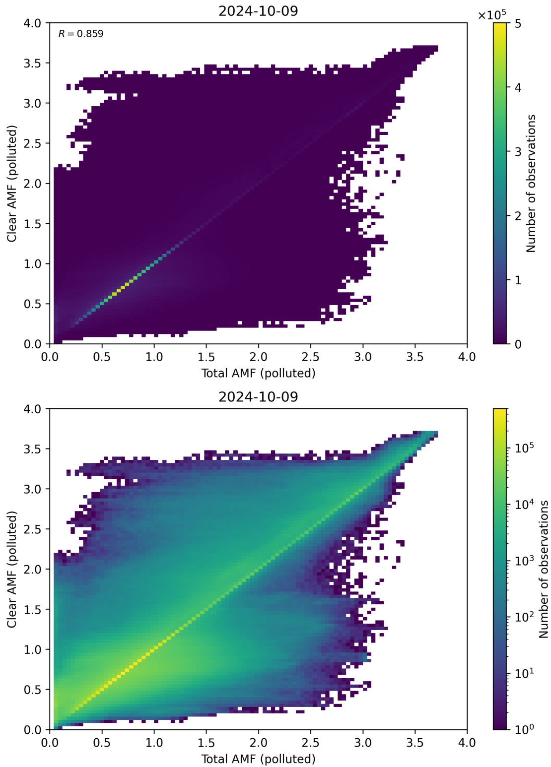
Figure 271: Scatter density plot of “Total AMF (polluted)” against “Clear AMF (polluted)” for 2024-10-08 to 2024-10-10.
