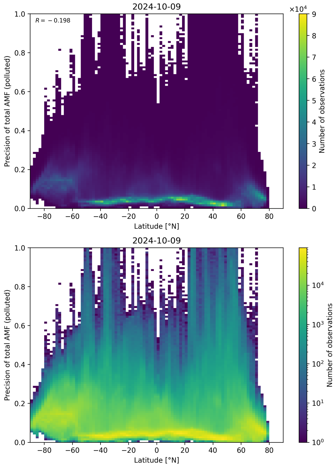
Figure 155: Scatter density plot of “Latitude” against “Precision of total AMF (polluted)” for 2024-10-08 to 2024-10-10.
