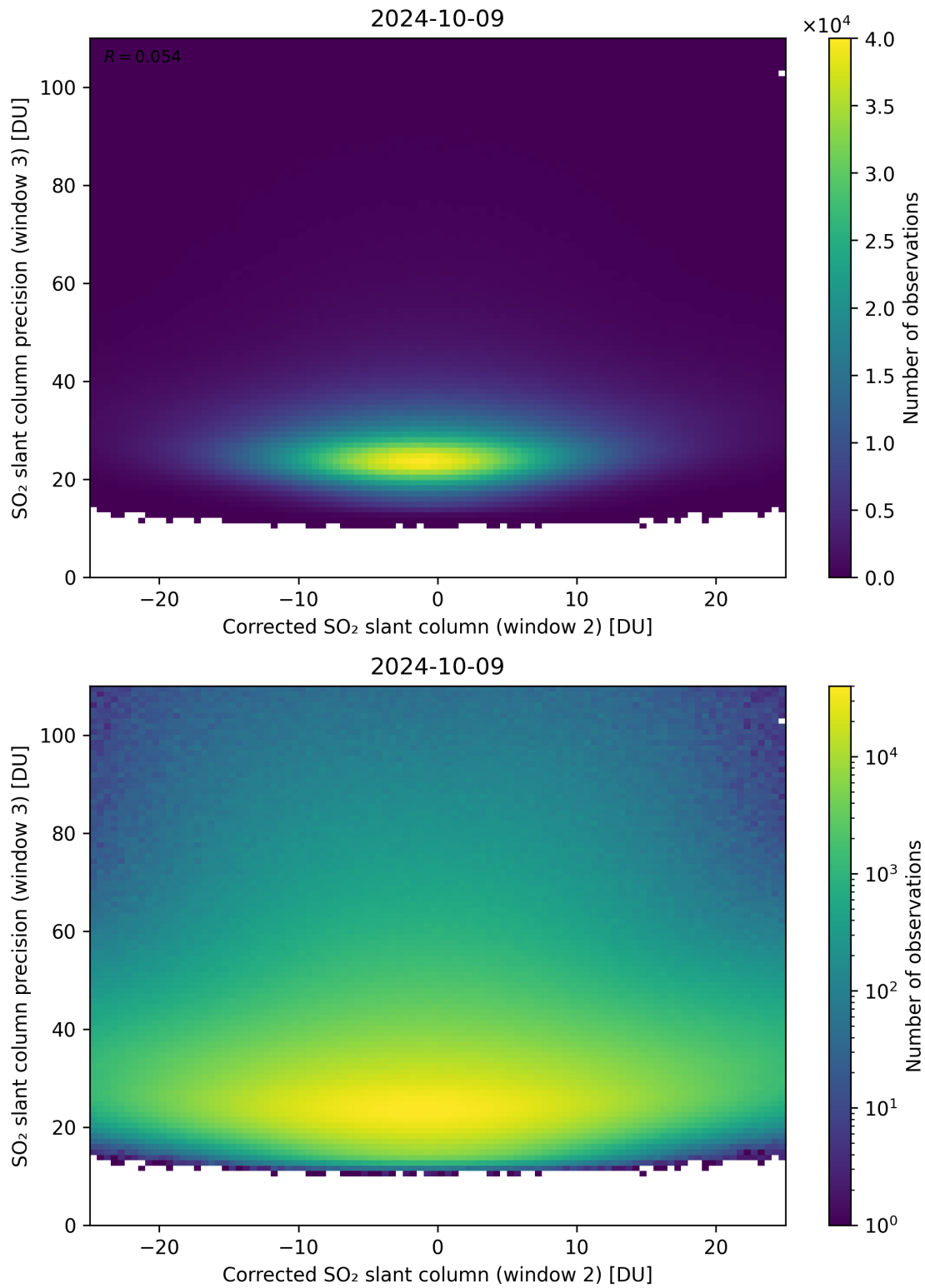
Figure 202: Scatter density plot of “Corrected SO 2 slant column (window 2)” against “SO 2 slant column precision (window 3)” for 2024-10-08 to 2024-10-10.
