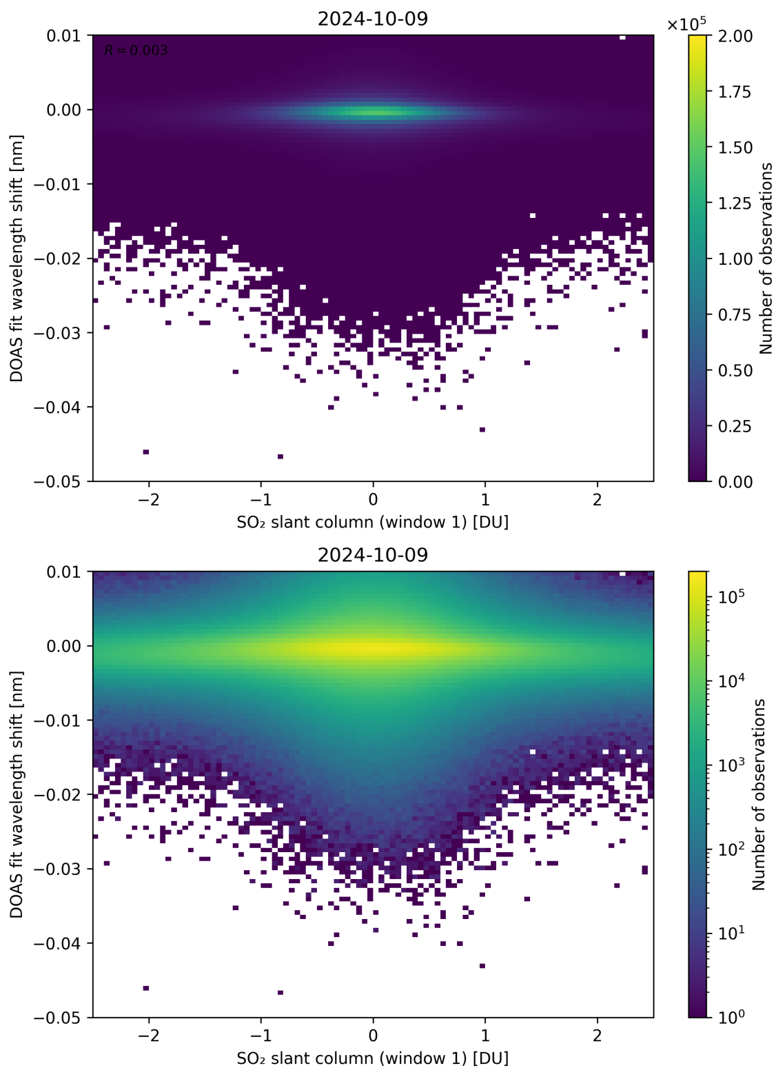
Figure 215: Scatter density plot of “SO 2 slant column (window 1)” against “DOAS fit wavelength shift” for 2024-10-08 to 2024-10-10.
