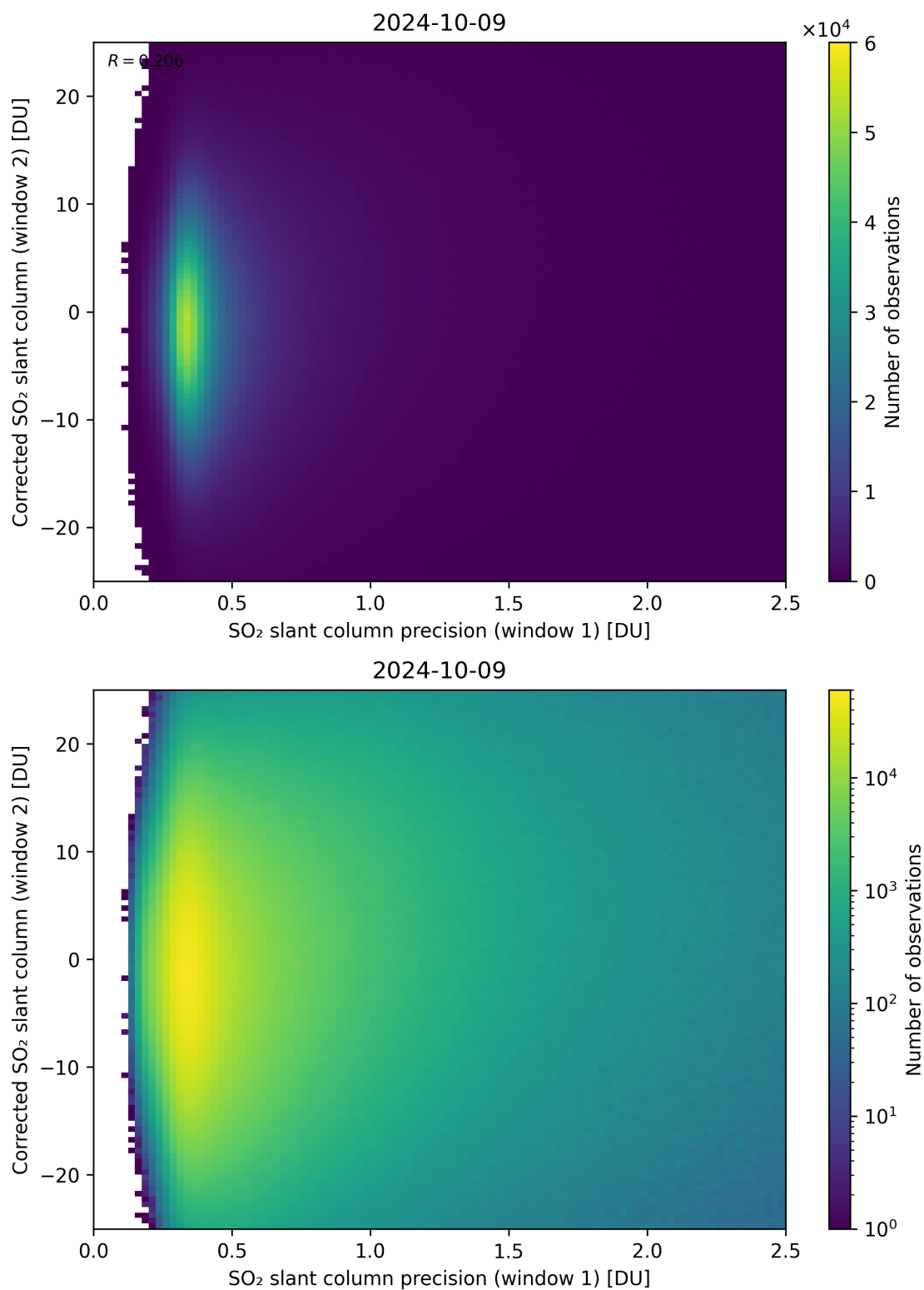
Figure 225: Scatter density plot of “SO 2 slant column precision (window 1)” against “Corrected SO 2 slant column (window 2)” for 2024-10-08 to 2024-10-10.
