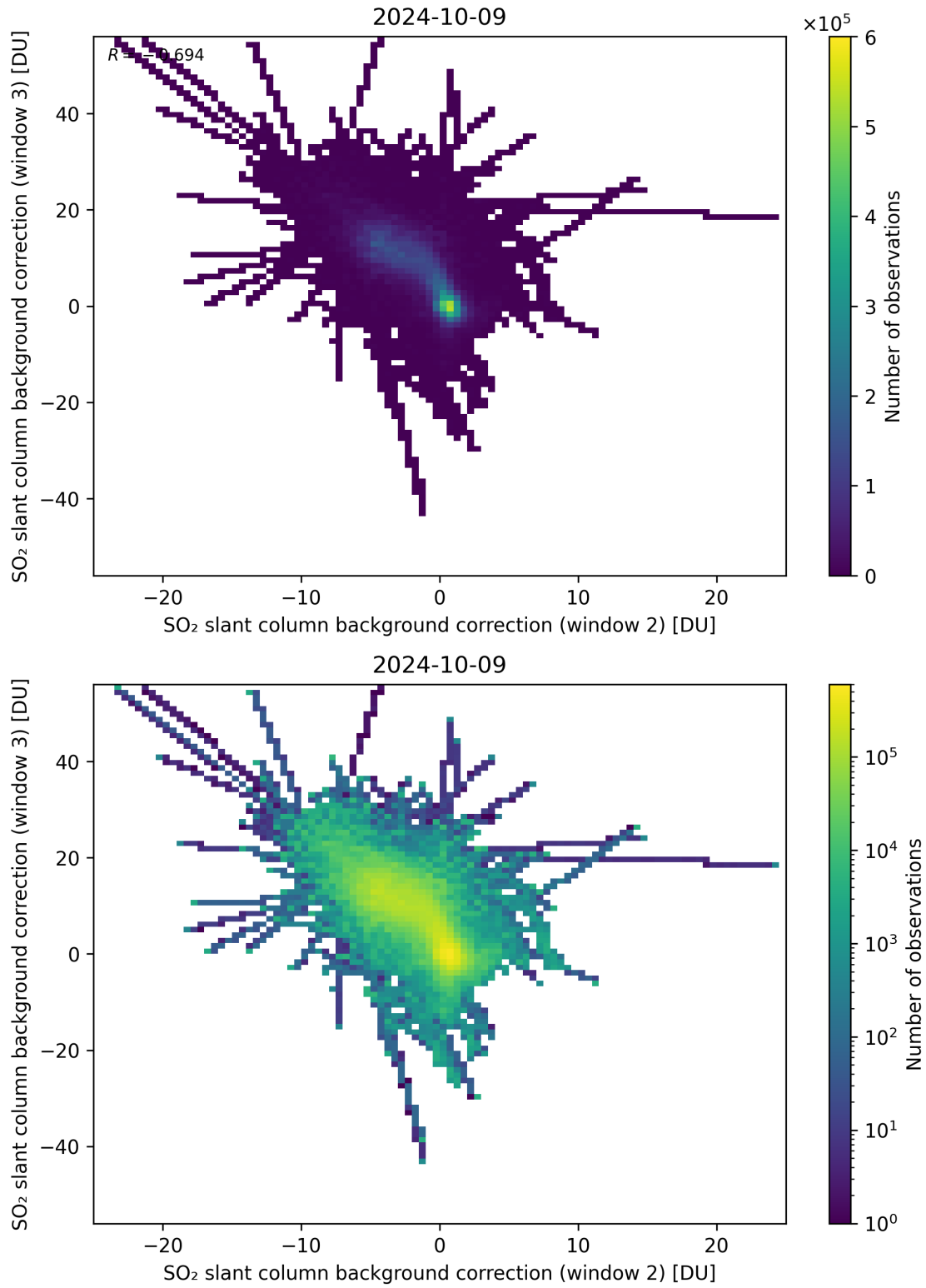
Figure 111: Scatter density plot of “SO 2 slant column background correction (window 2)” against “SO 2 slant column background correction (window 3)” for 2024-10-08 to 2024-10-10.
