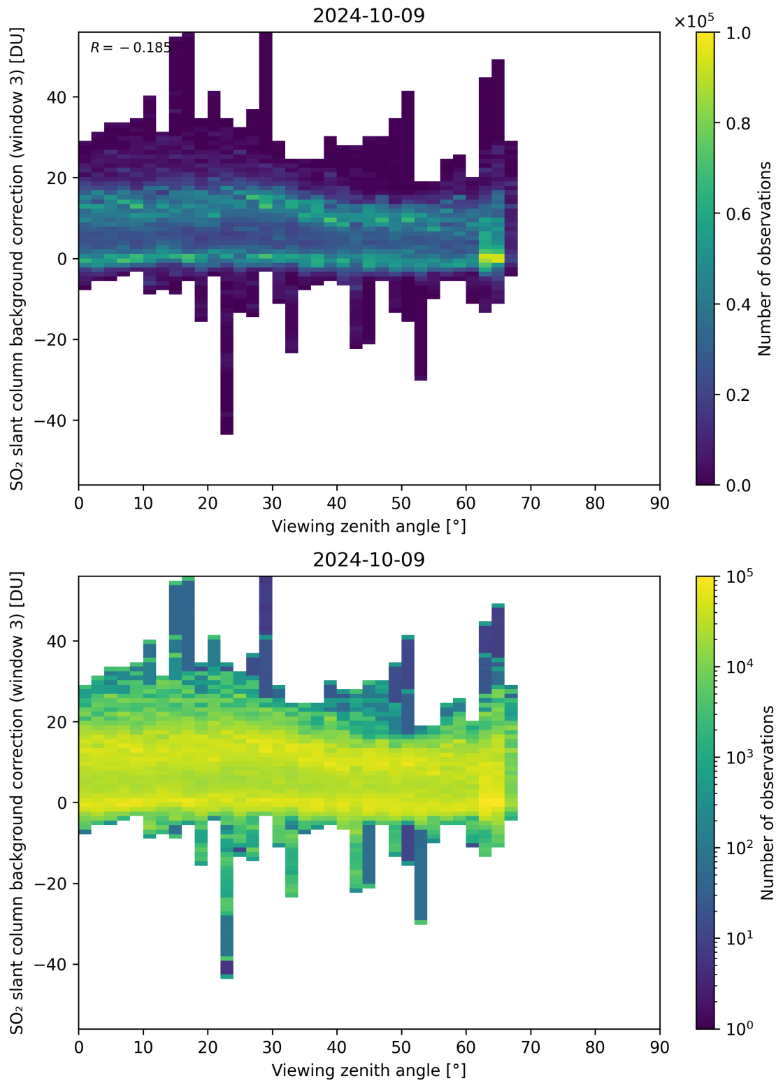
Figure 310: Scatter density plot of “Viewing zenith angle” against “SO 2 slant column background correction (window 3)” for 2024-10-08 to 2024-10-10.
