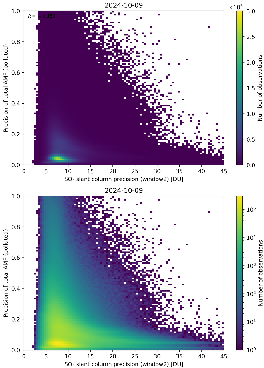
Figure 252: Scatter density plot of “SO 2 slant column precision (window2)” against “Precision of total AMF (polluted)” for 2024-10-08 to 2024-10-10.
