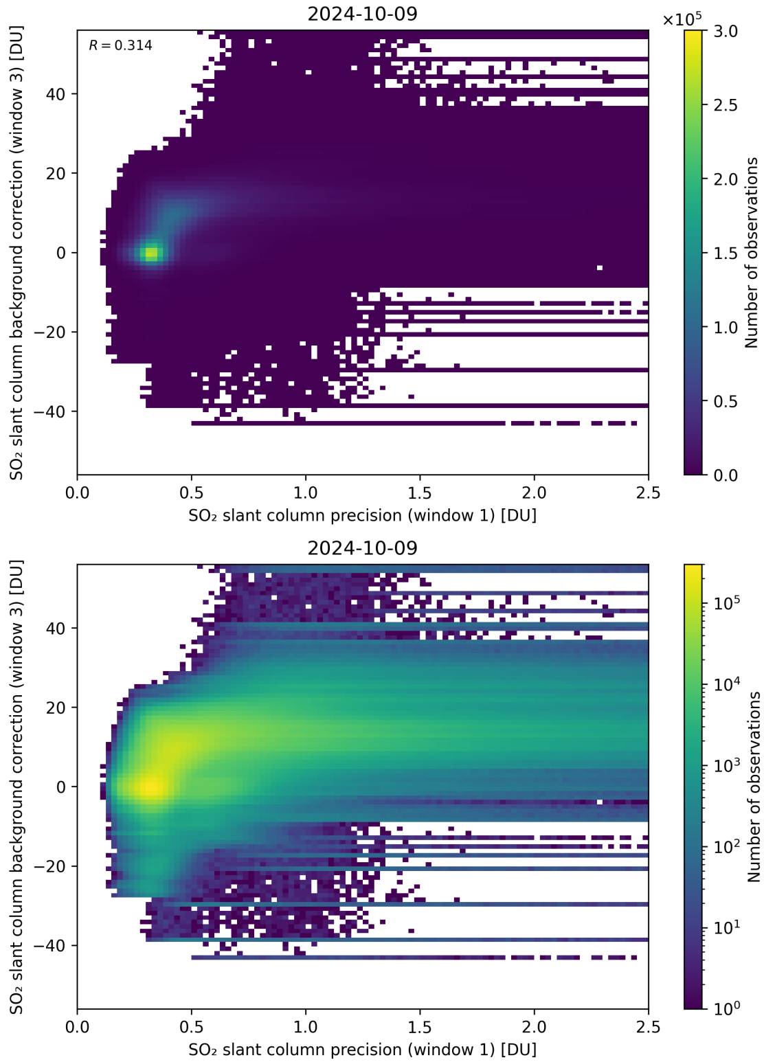
Figure 220: Scatter density plot of “SO 2 slant column precision (window 1)” against “SO 2 slant column background correction (window 3)” for 2024-10-08 to 2024-10-10.
