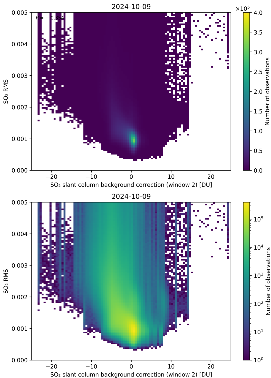
Figure 114: Scatter density plot of “SO 2 slant column background correction (window 2)” against “SO 2 RMS” for 2024-10-08 to 2024-10-10.
