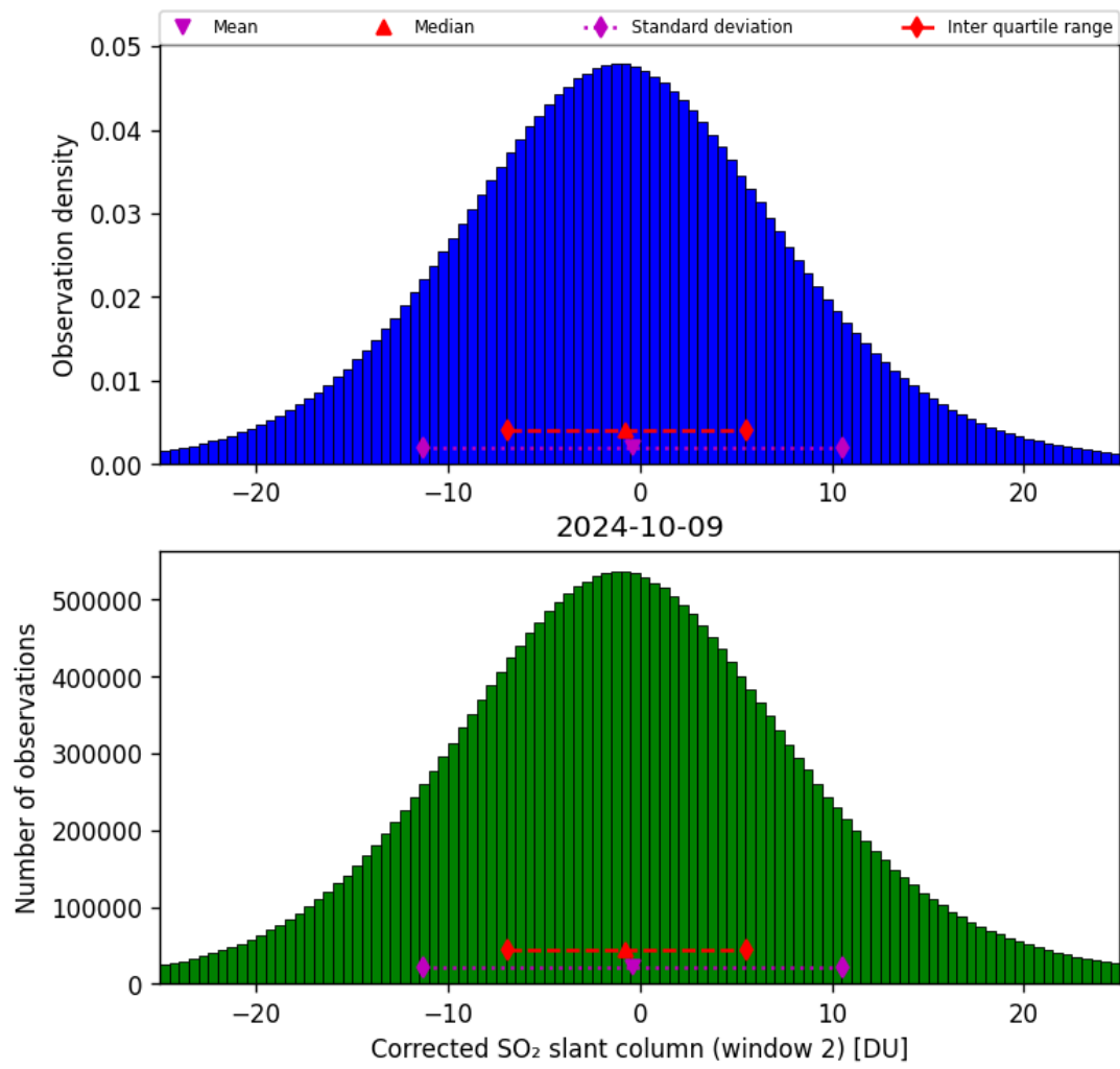
Figure 62: Histogram of “Corrected SO 2 slant column (window 2)” for 2024-10-08 to 2024-10-10
