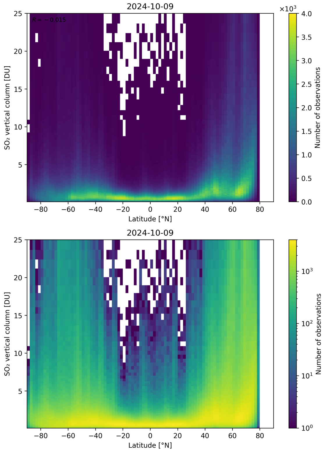
Figure 156: Scatter density plot of “Latitude” against “SO 2 vertical column” for 2024-10-08 to 2024-10-10.
