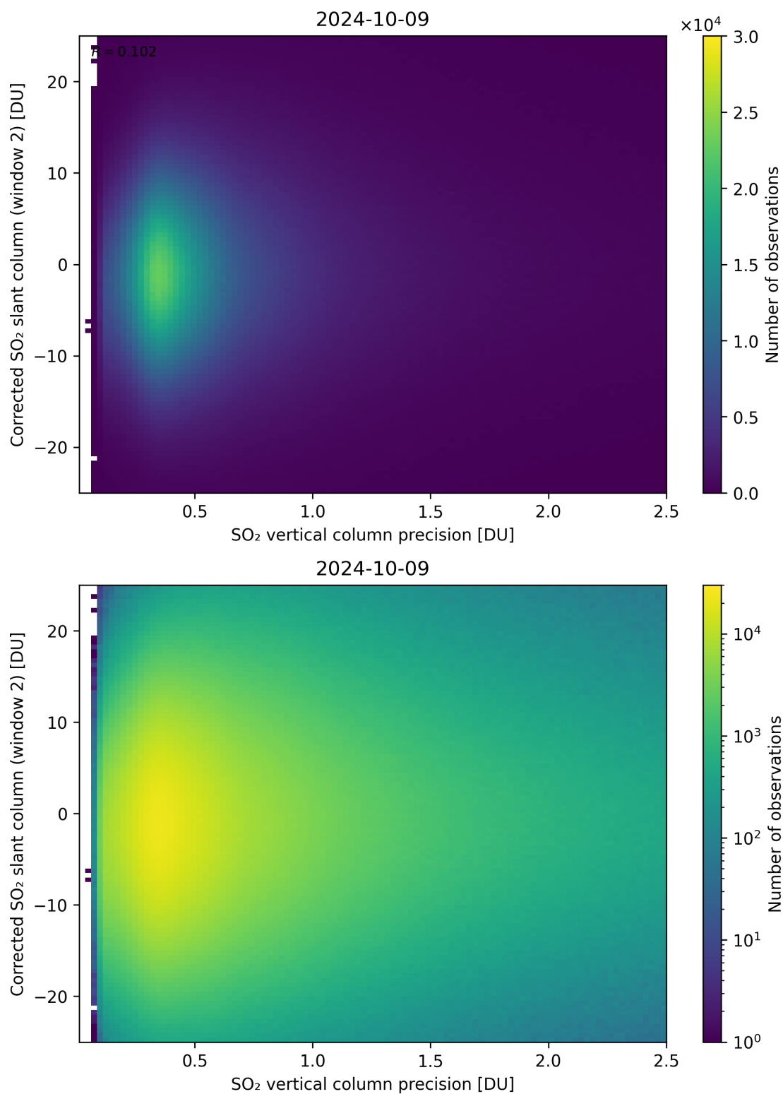
Figure 287: Scatter density plot of “SO 2 vertical column precision” against “Corrected SO 2 slant column (window 2)” for 2024-10-08 to 2024-10-10.
