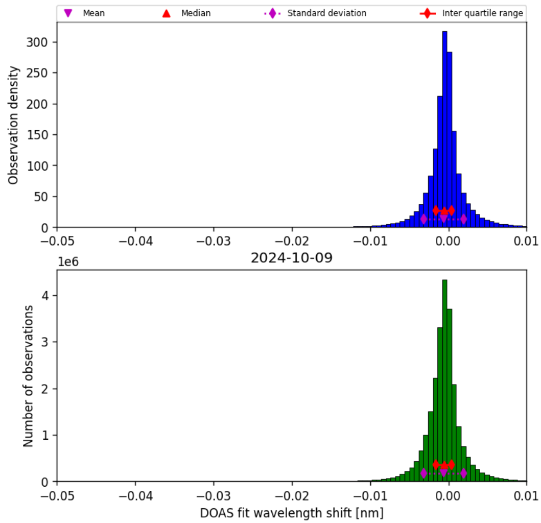
Figure 68: Histogram of “DOAS fit wavelength shift” for 2024-10-08 to 2024-10-10
