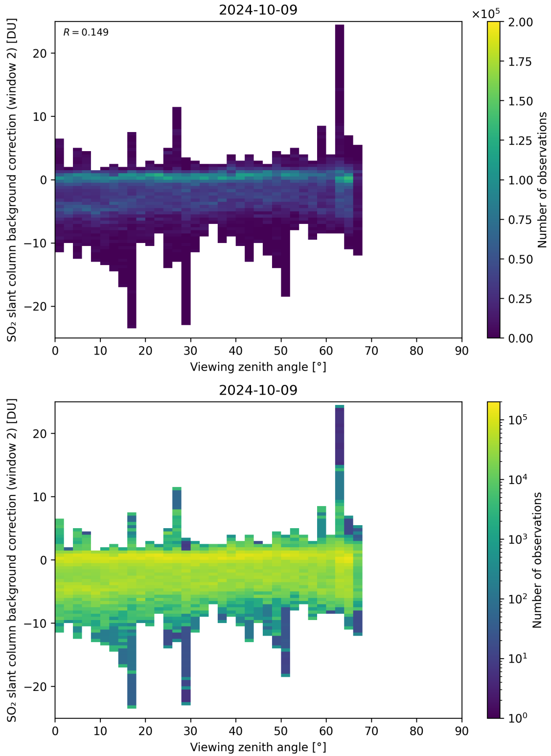
Figure 309: Scatter density plot of “Viewing zenith angle” against “SO 2 slant column background correction (window 2)” for 2024-10-08 to 2024-10-10.
