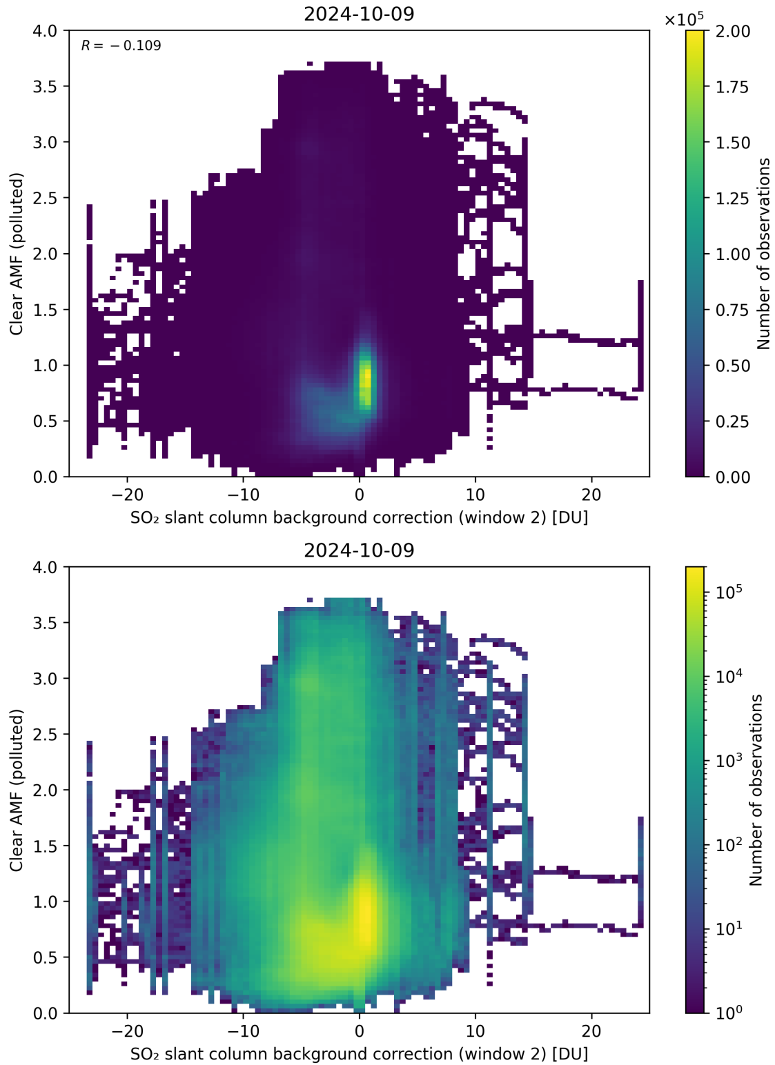
Figure 115: Scatter density plot of “SO 2 slant column background correction (window 2)” against “Clear AMF (polluted)” for 2024-10-08 to 2024-10-10.
