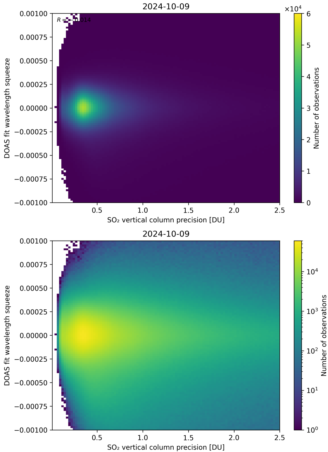
Figure 283: Scatter density plot of “SO 2 vertical column precision” against “DOAS fit wavelength squeeze” for 2024-10-08 to 2024-10-10.
