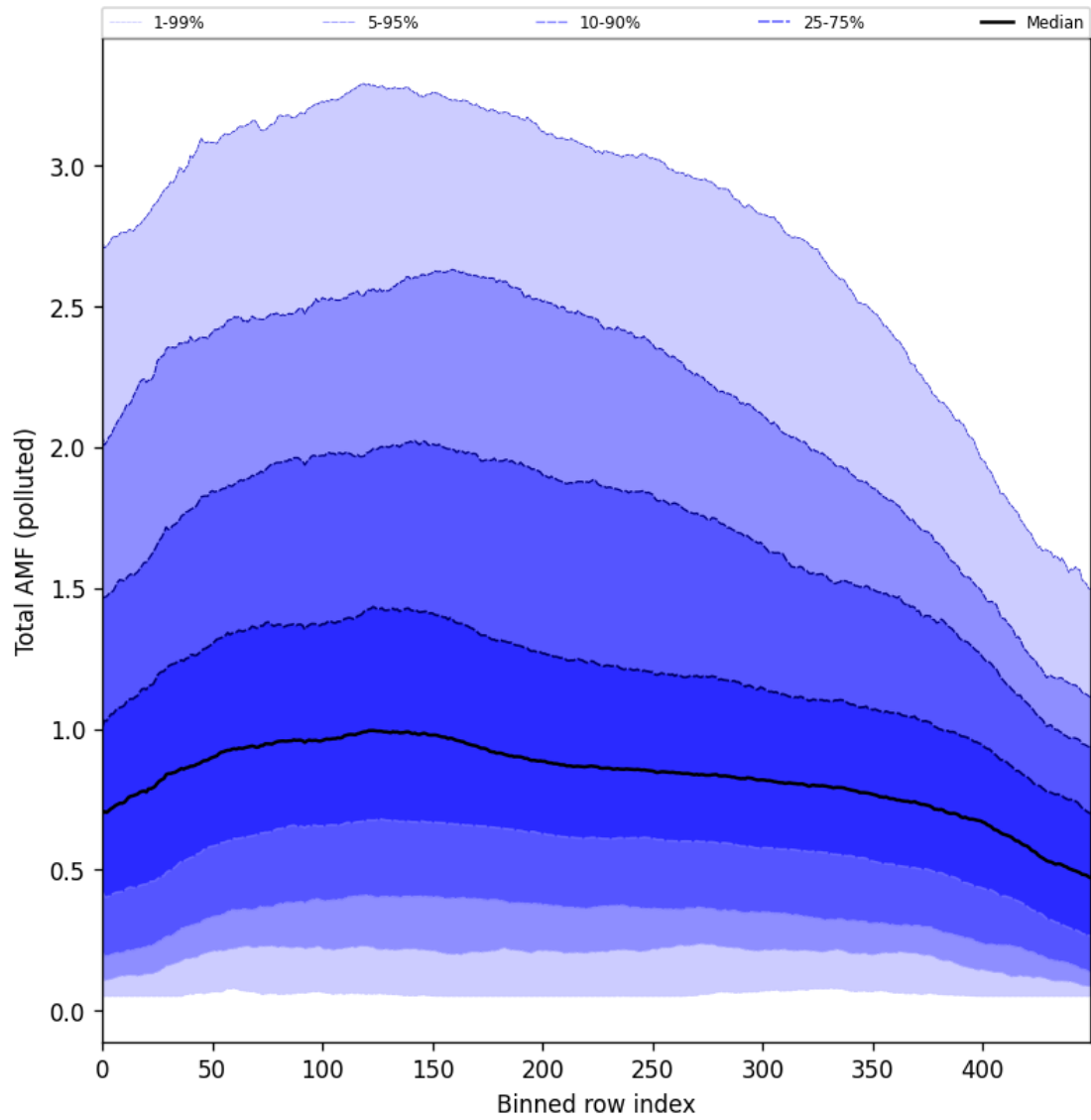
Figure 94: Along track statistics of “Total AMF (polluted)” for 2024-10-08 to 2024-10-10
