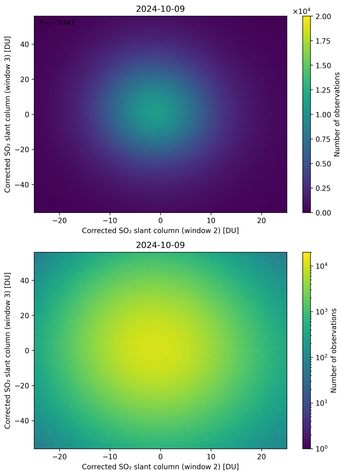
Figure 200: Scatter density plot of “Corrected SO 2 slant column (window 2)” against “Corrected SO 2 slant column (window 3)” for 2024-10-08 to 2024-10-10.
