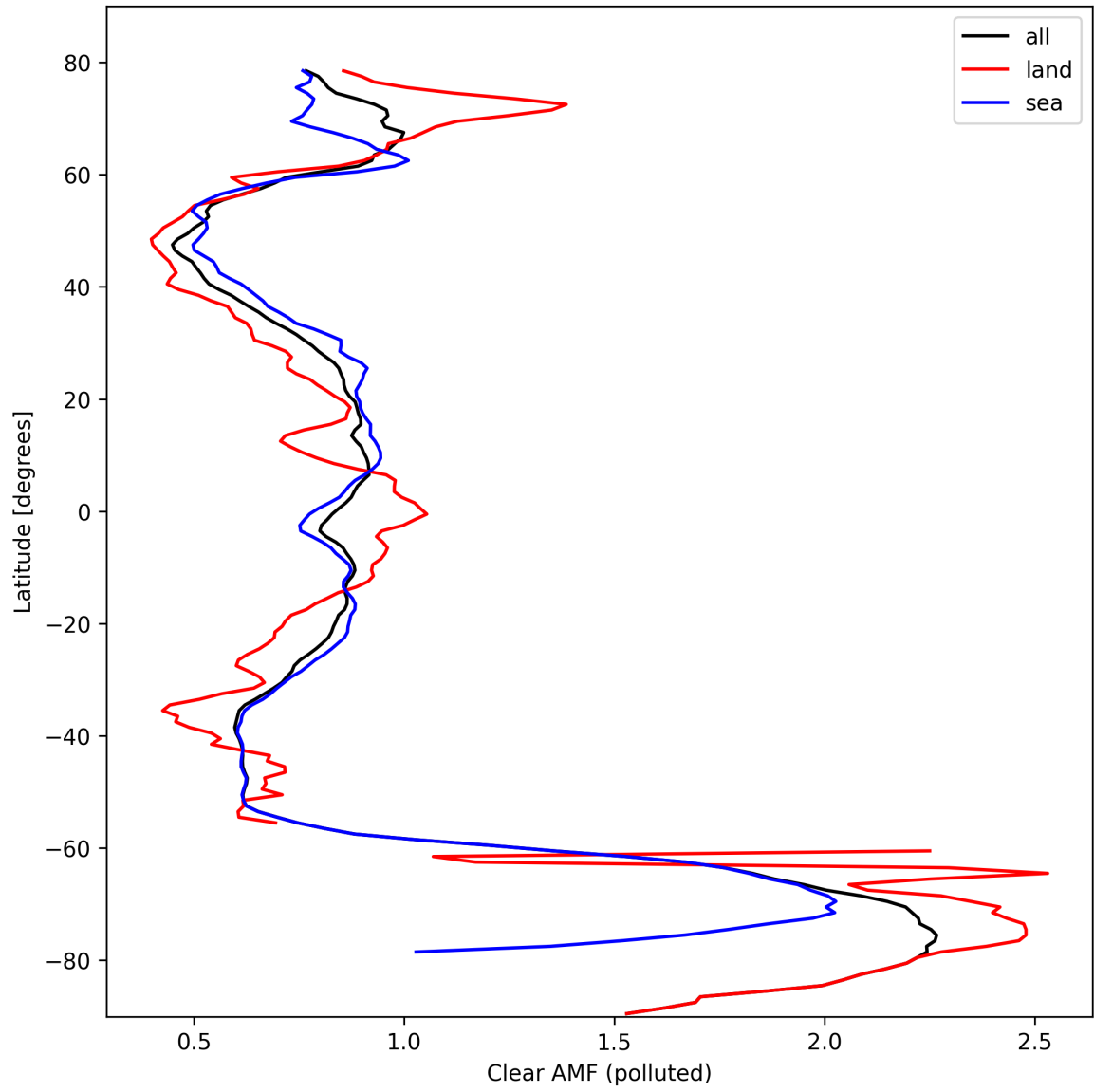
Figure 50: Zonal average of “Clear AMF (polluted)” for 2024-10-08 to 2024-10-10.
