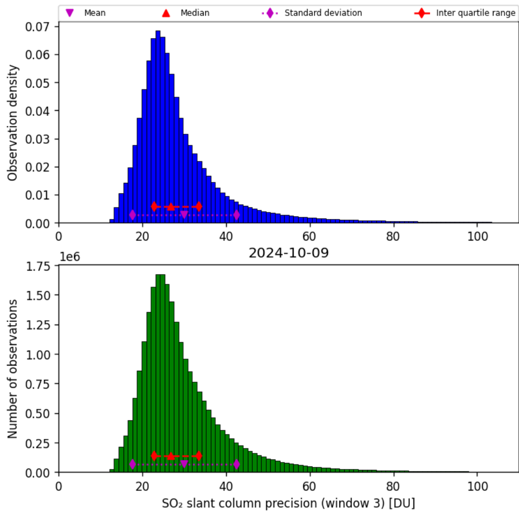
Figure 65: Histogram of “SO 2 slant column precision (window 3)” for 2024-10-08 to 2024-10-10
