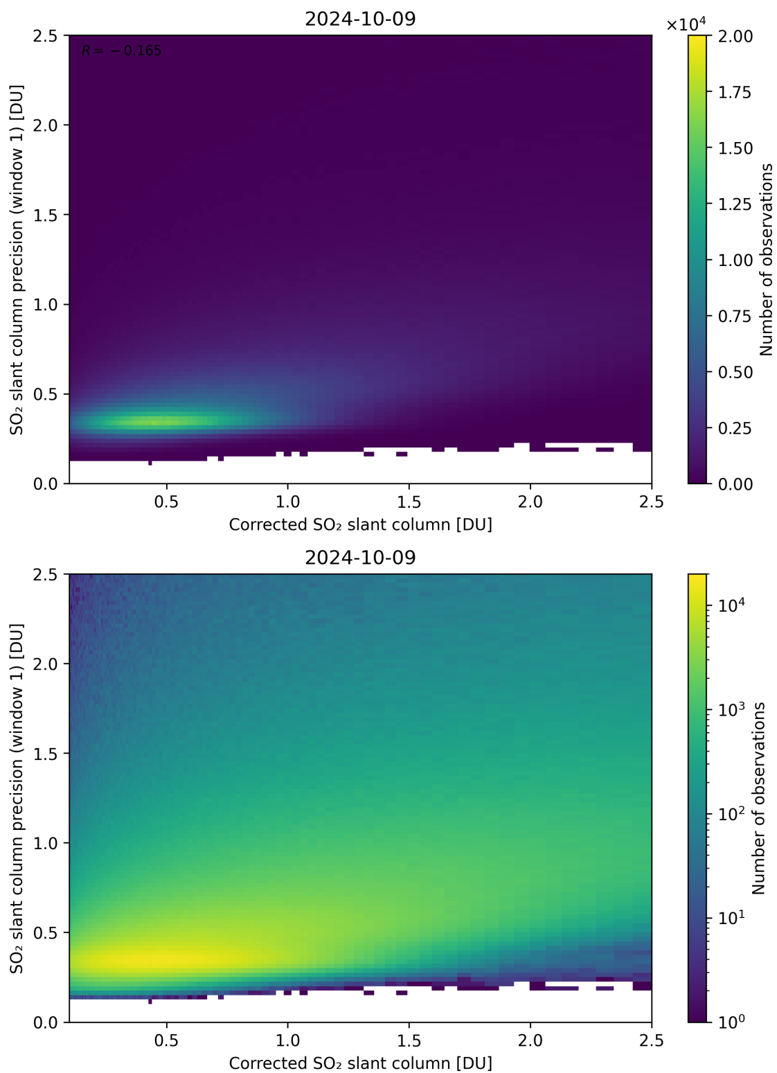
Figure 188: Scatter density plot of “Corrected SO 2 slant column” against “SO 2 slant column precision (window 1)” for 2024-10-08 to 2024-10-10.
