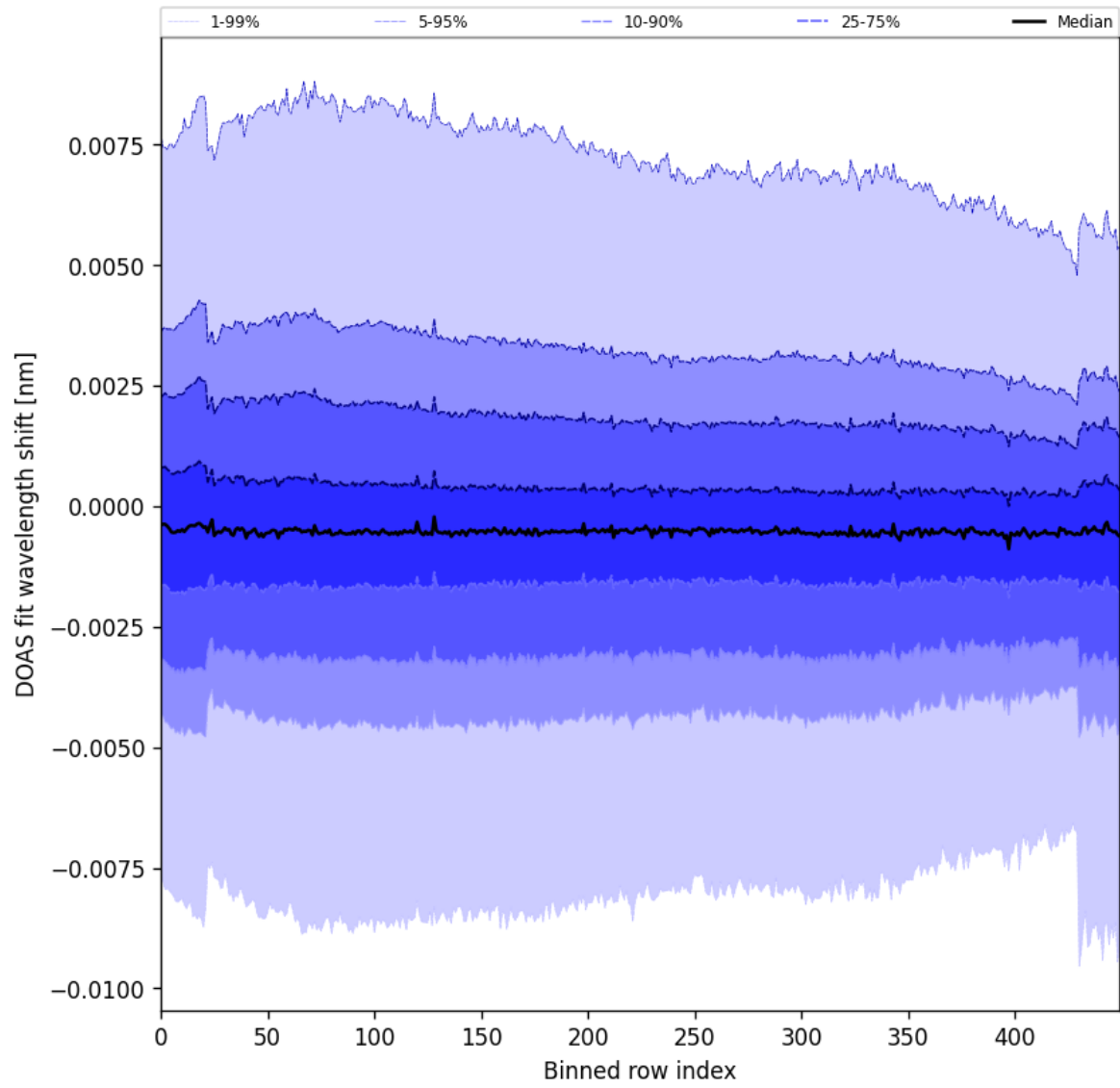
Figure 91: Along track statistics of “DOAS fit wavelength shift” for 2024-10-08 to 2024-10-10
