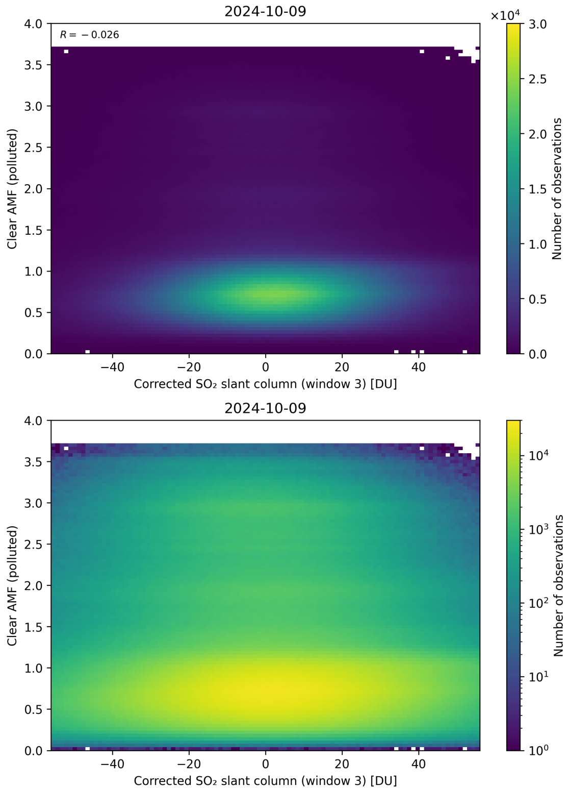
Figure 209: Scatter density plot of “Corrected SO 2 slant column (window 3)” against “Clear AMF (polluted)” for 2024-10-08 to 2024-10-10.
