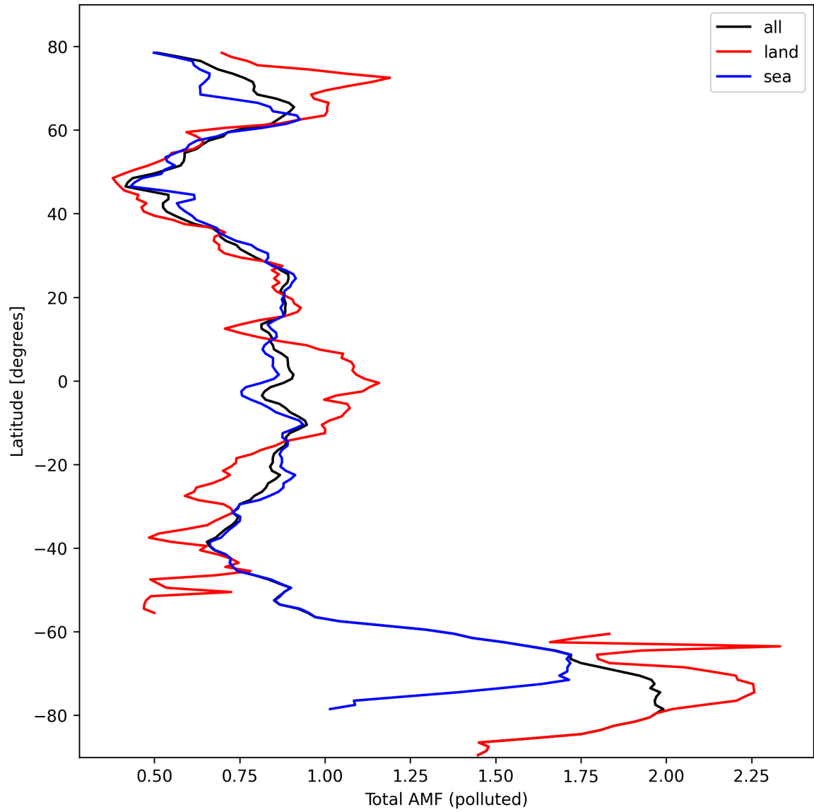
Figure 48: Zonal average of “Total AMF (polluted)” for 2024-10-08 to 2024-10-10.
