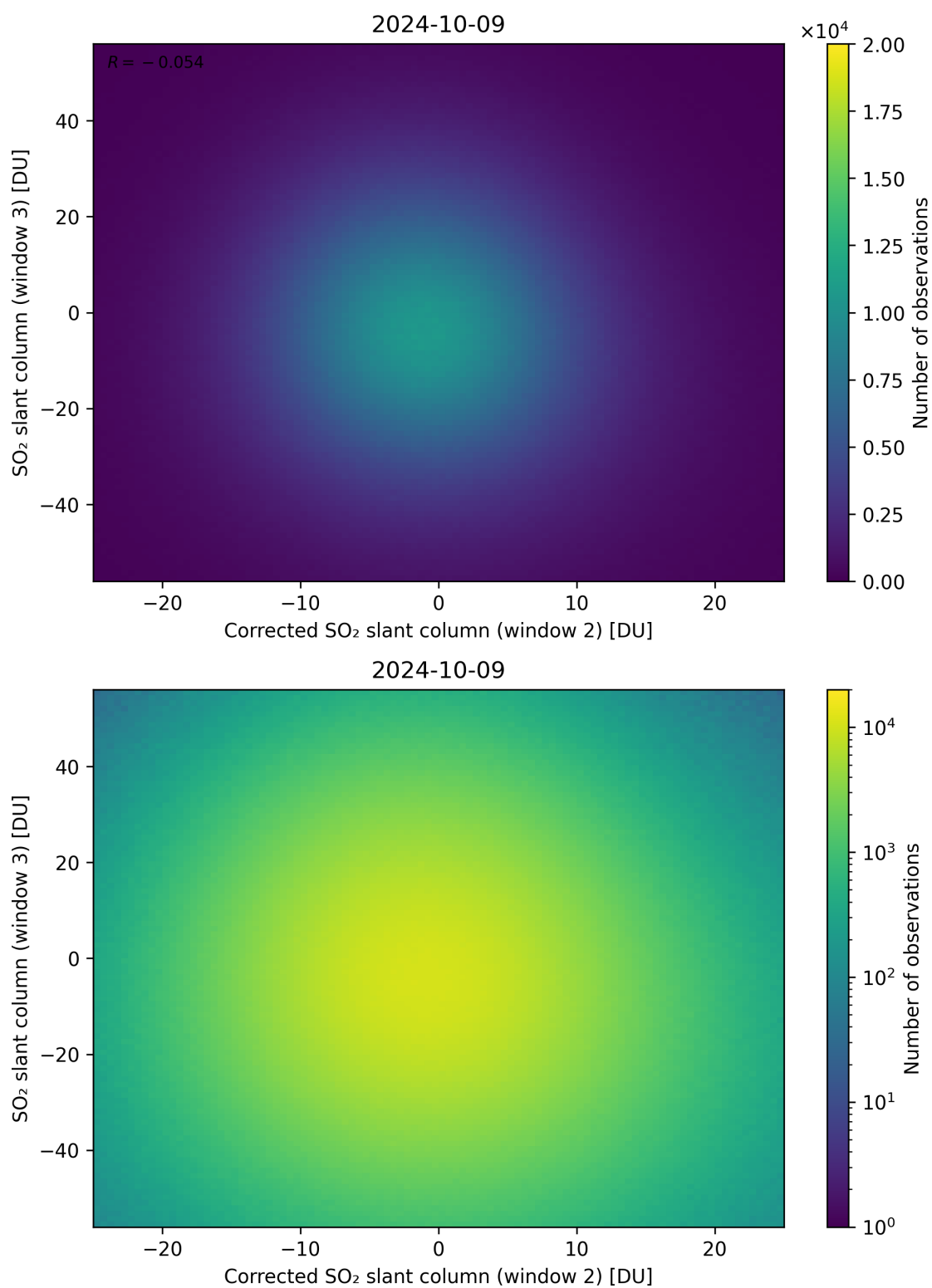
Figure 201: Scatter density plot of “Corrected SO 2 slant column (window 2)” against “SO 2 slant column (window 3)” for 2024-10-08 to 2024-10-10.
