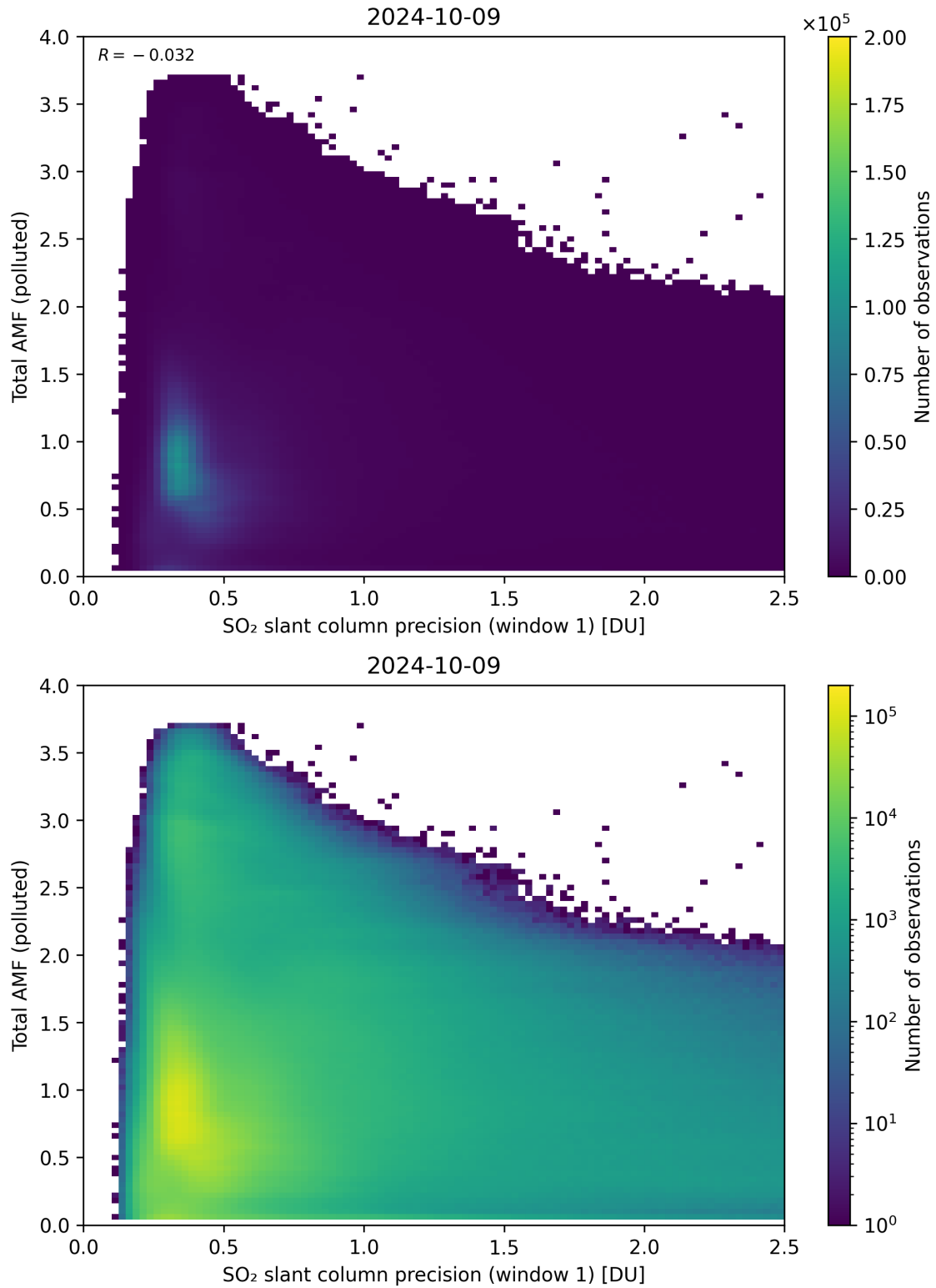
Figure 230: Scatter density plot of “SO 2 slant column precision (window 1)” against “Total AMF (polluted)” for 2024-10-08 to 2024-10-10.
