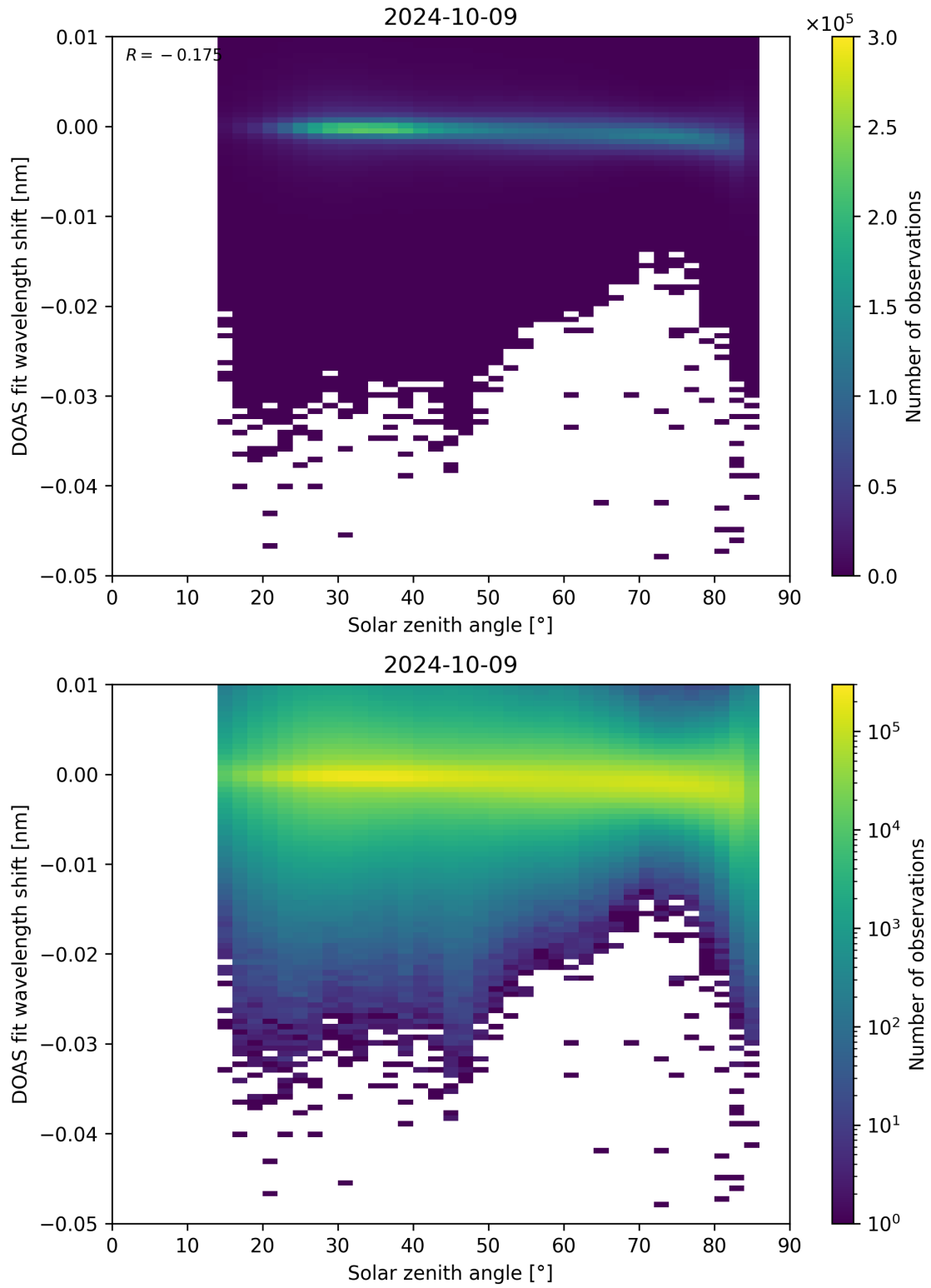
Figure 161: Scatter density plot of “Solar zenith angle” against “DOAS fit wavelength shift” for 2024-10-08 to 2024-10-10.
