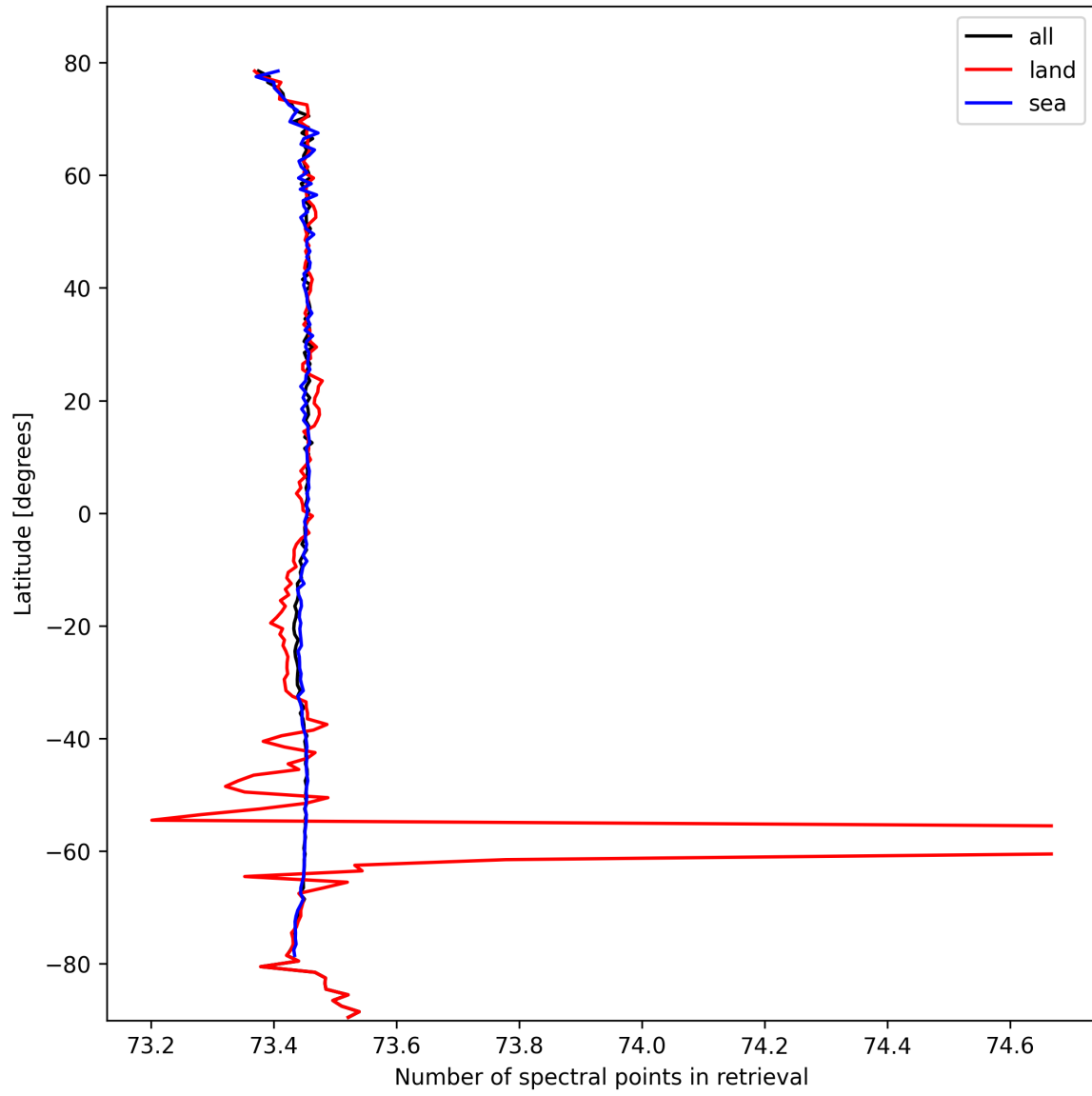
Figure 51: Zonal average of “Number of spectral points in retrieval” for 2024-10-08 to 2024-10-10.
