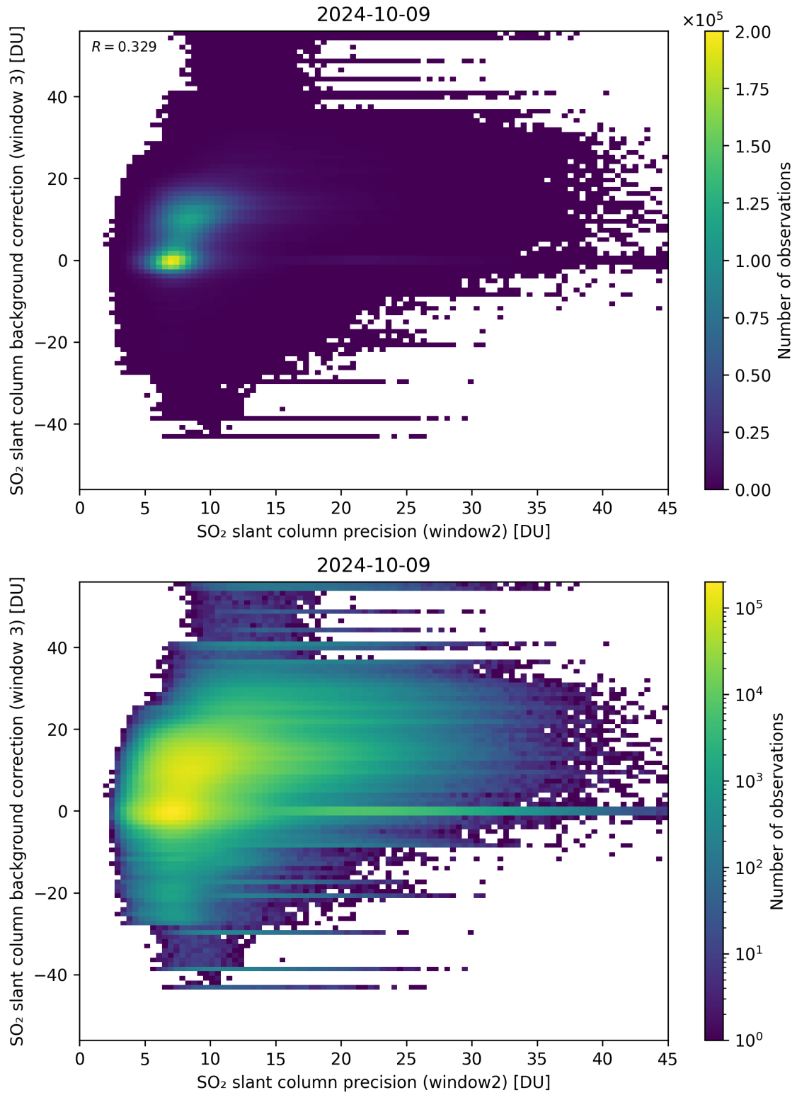
Figure 242: Scatter density plot of “SO 2 slant column precision (window2)” against “SO 2 slant column background correction (window 3)” for 2024-10-08 to 2024-10-10.
