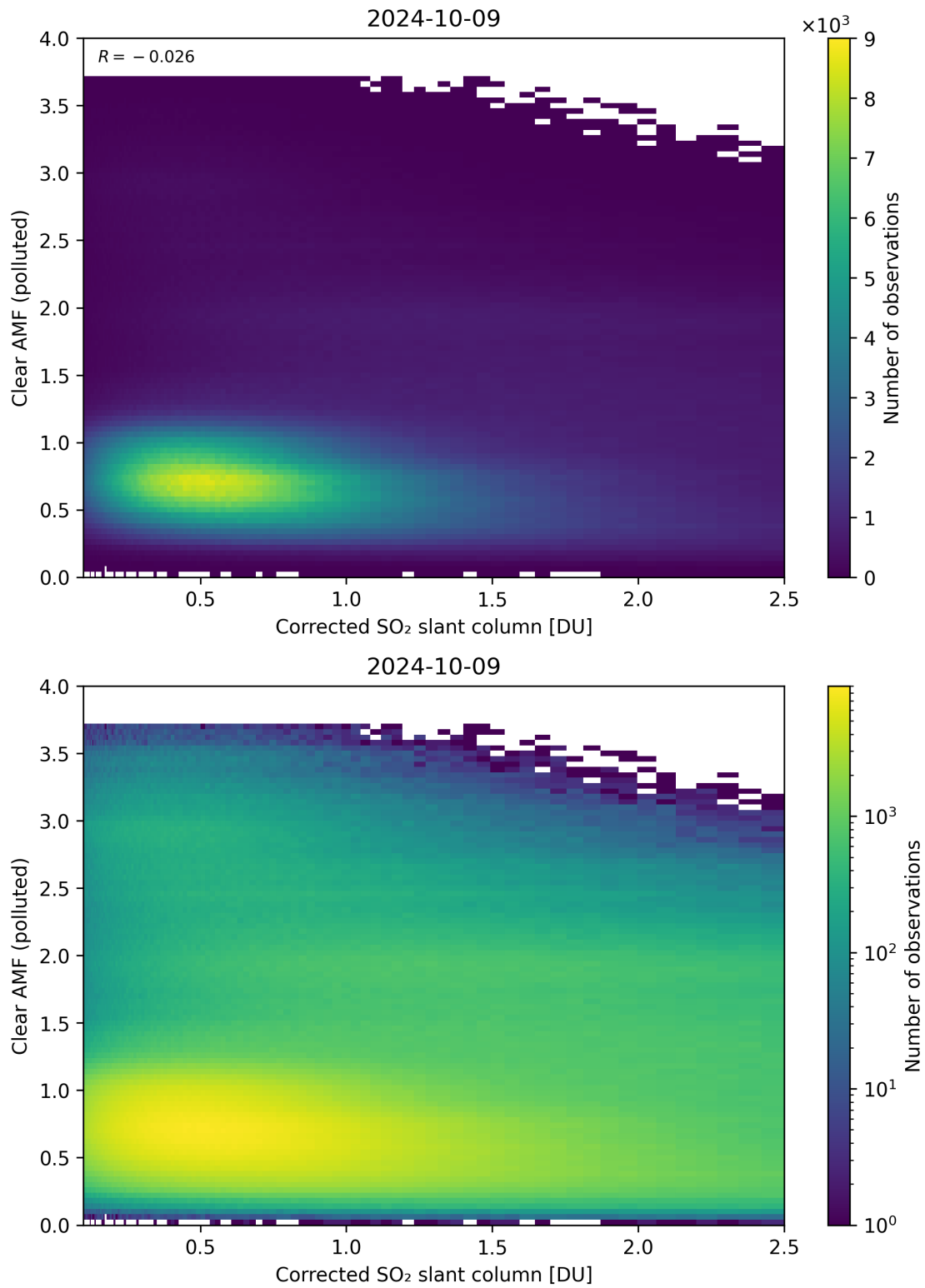
Figure 184: Scatter density plot of “Corrected SO 2 slant column” against “Clear AMF (polluted)” for 2024-10-08 to 2024-10-10.
