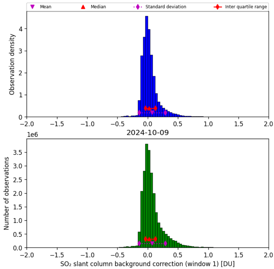
Figure 59: Histogram of “SO 2 slant column background correction (window 1)” for 2024-10-08 to 2024-10-10
