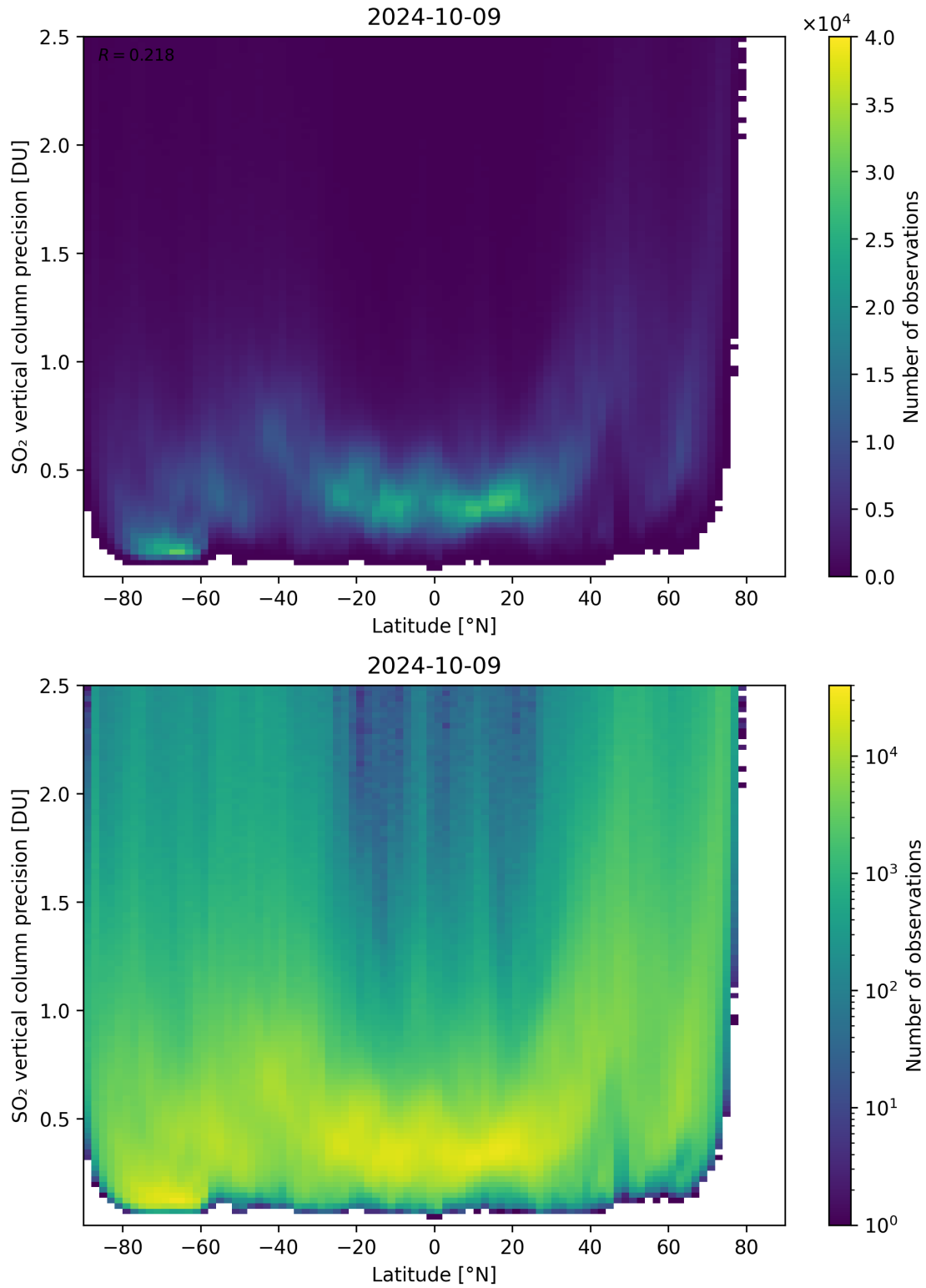
Figure 157: Scatter density plot of “Latitude” against “SO 2 vertical column precision” for 2024-10-08 to 2024-10-10.
