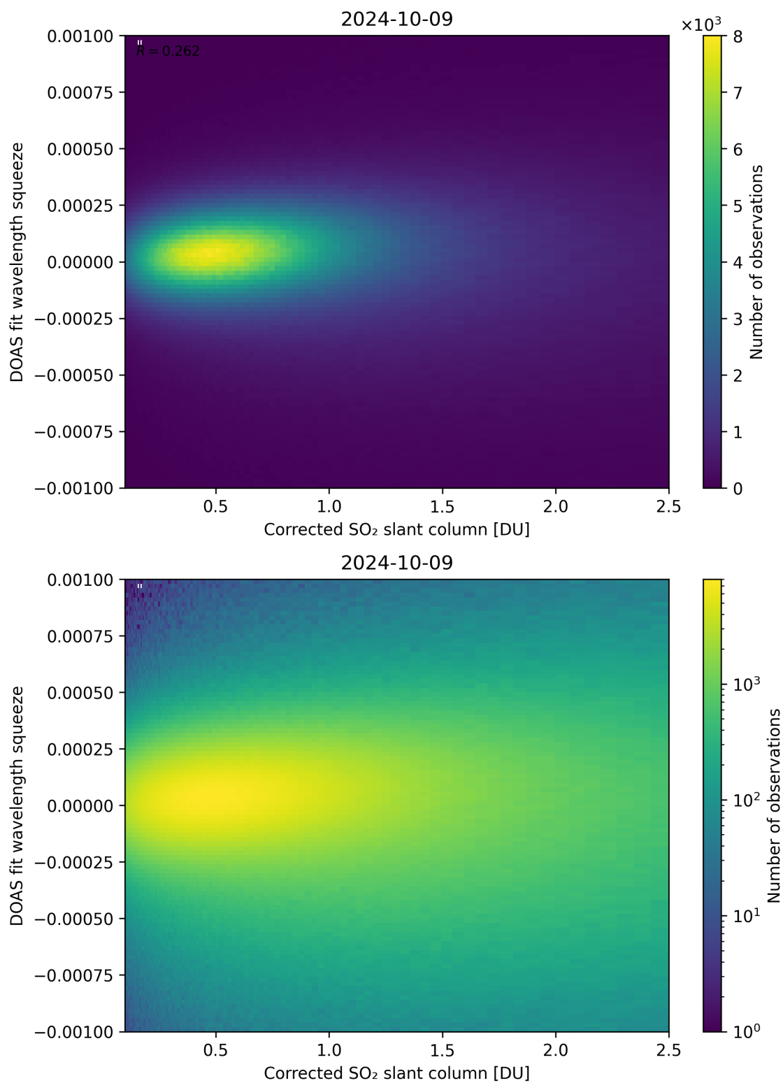
Figure 182: Scatter density plot of “Corrected SO 2 slant column” against “DOAS fit wavelength squeeze” for 2024-10-08 to 2024-10-10.
