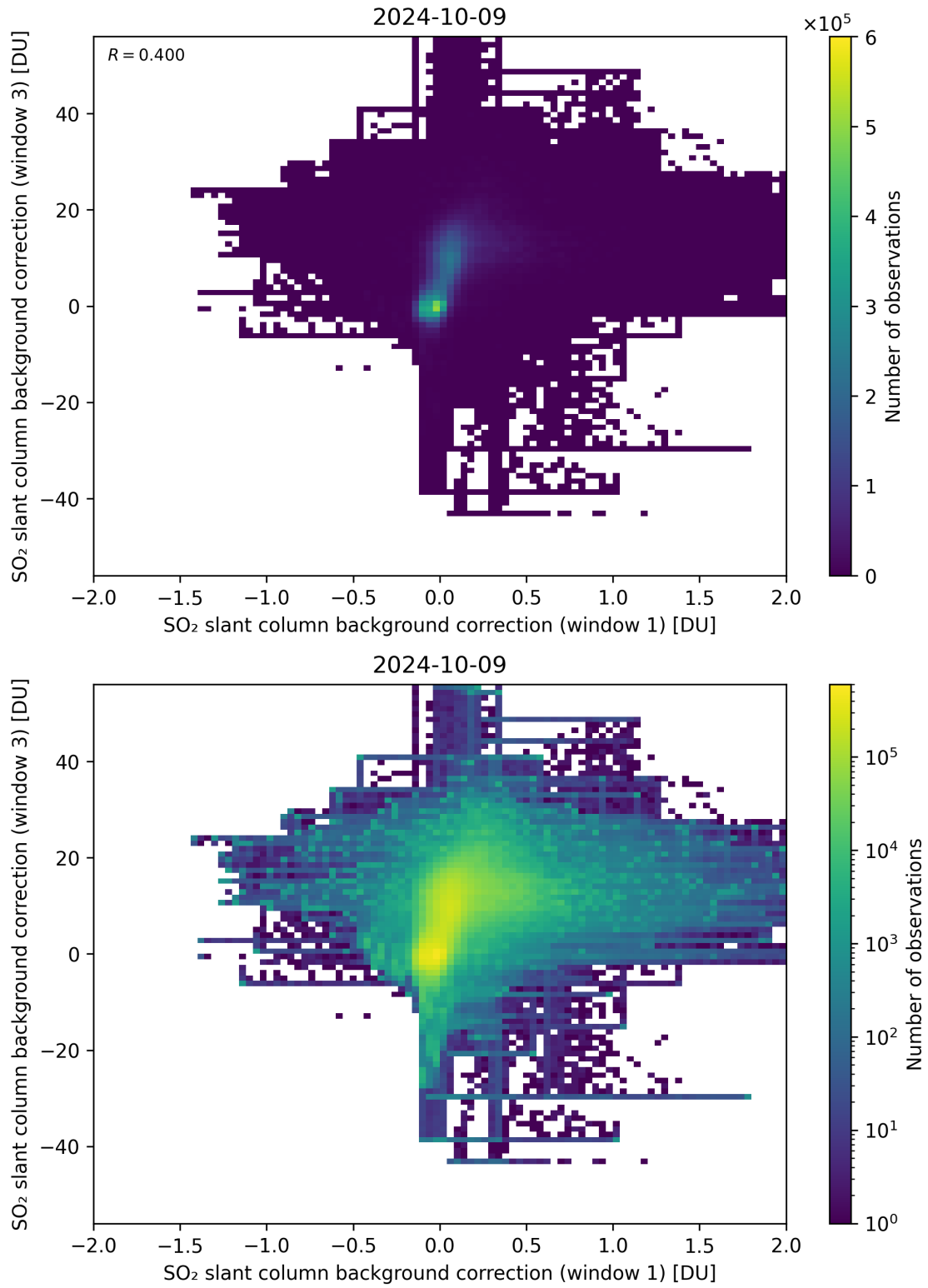
Figure 99: Scatter density plot of “SO 2 slant column background correction (window 1)” against “SO 2 slant column background correction (window 3)” for 2024-10-08 to 2024-10-10.
