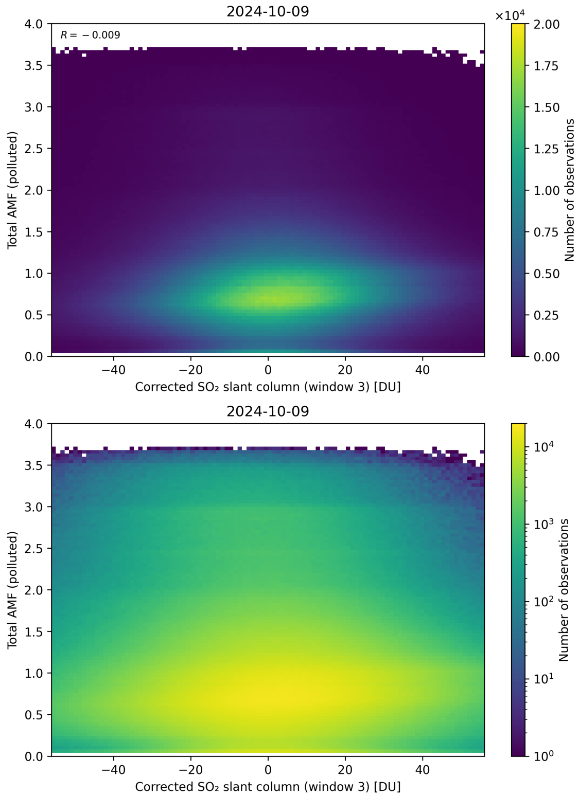
Figure 210: Scatter density plot of “Corrected SO 2 slant column (window 3)” against “Total AMF (polluted)” for 2024-10-08 to 2024-10-10.
