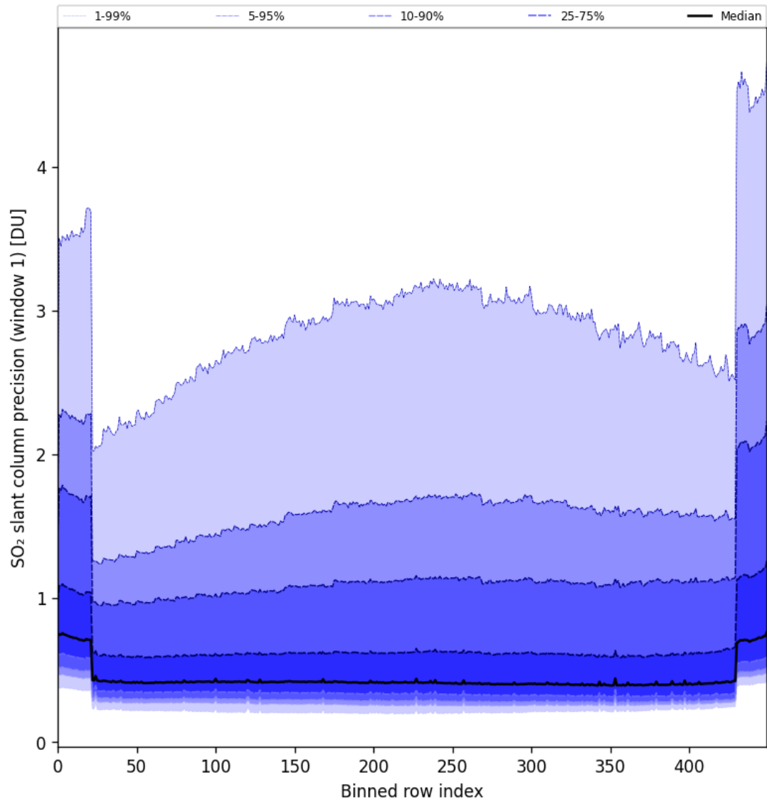
Figure 80: Along track statistics of "SO 2 slant column precision (window 1)" for 2024-10-08 to 2024-10-10
