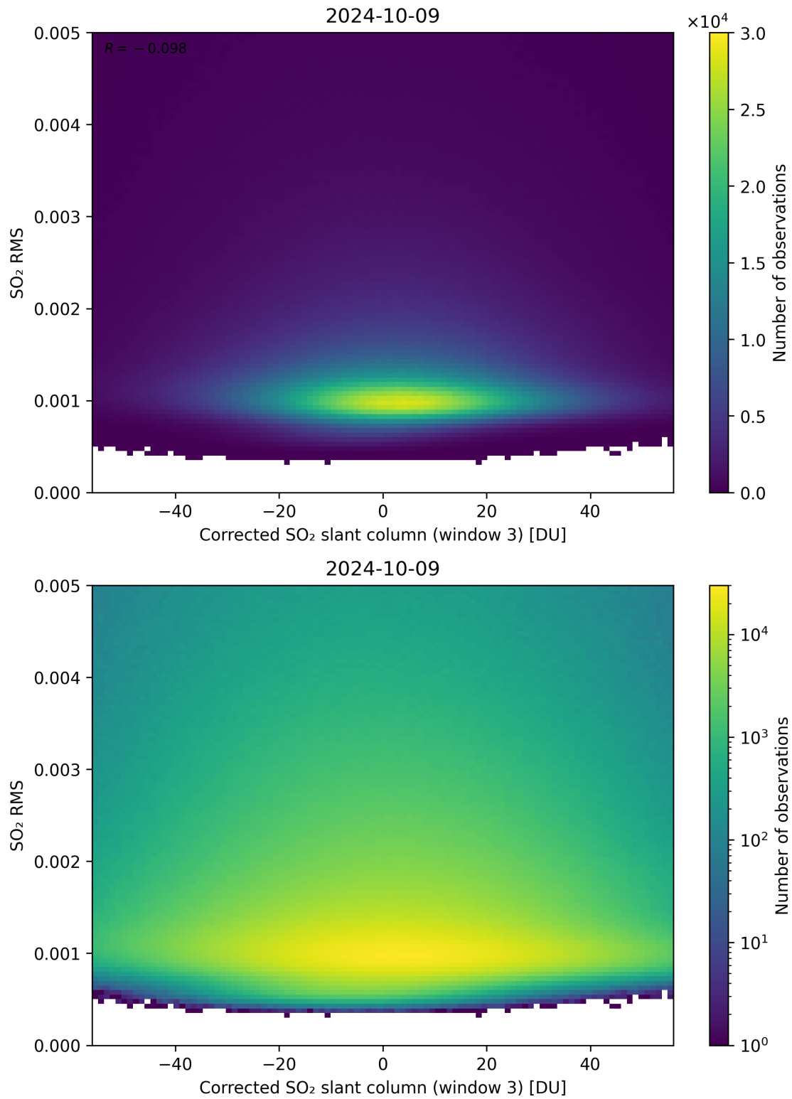
Figure 208: Scatter density plot of “Corrected SO 2 slant column (window 3)” against “SO 2 RMS” for 2024-10-08 to 2024-10-10.
