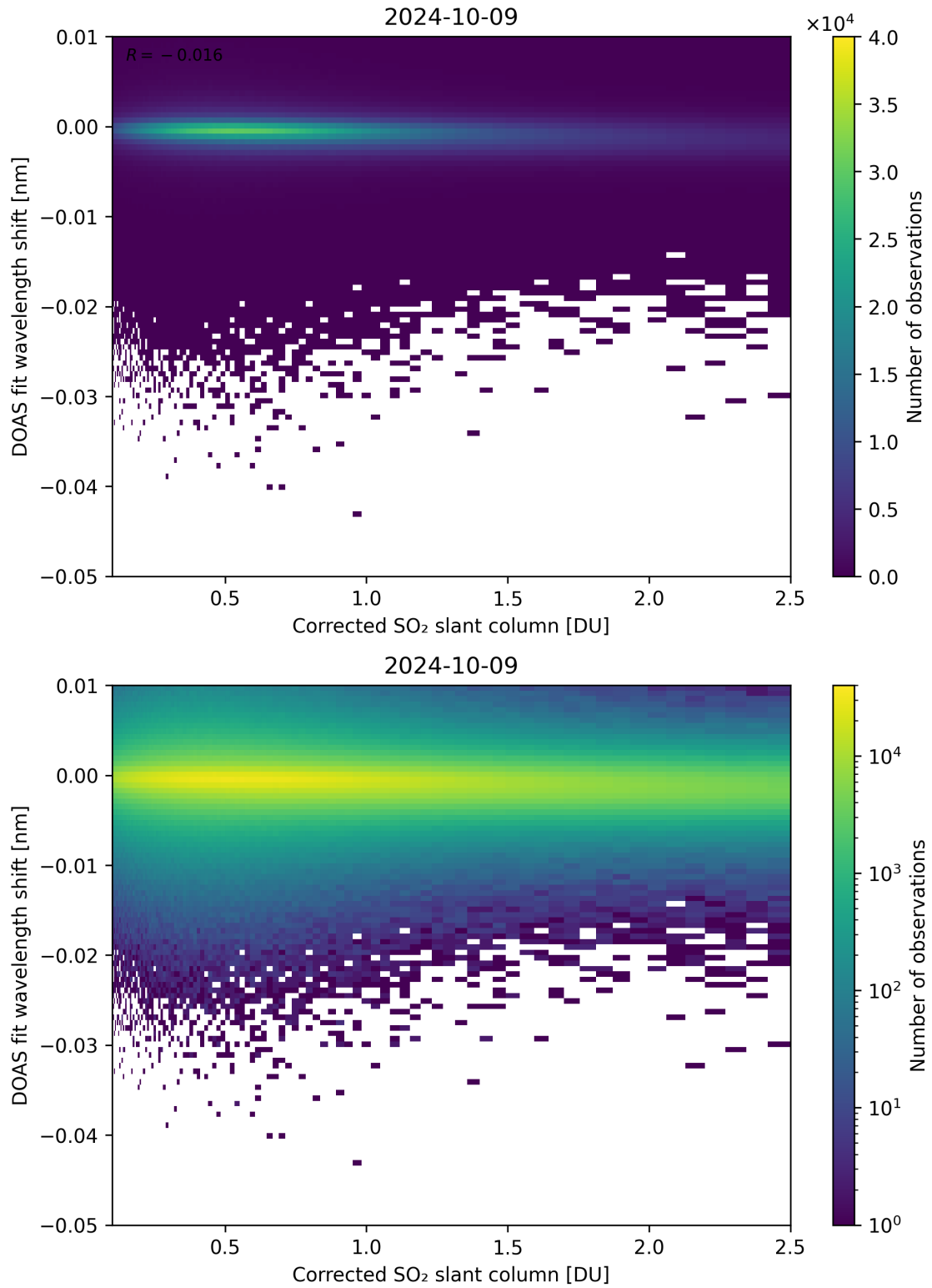
Figure 181: Scatter density plot of “Corrected SO 2 slant column” against “DOAS fit wavelength shift” for 2024-10-08 to 2024-10-10.
