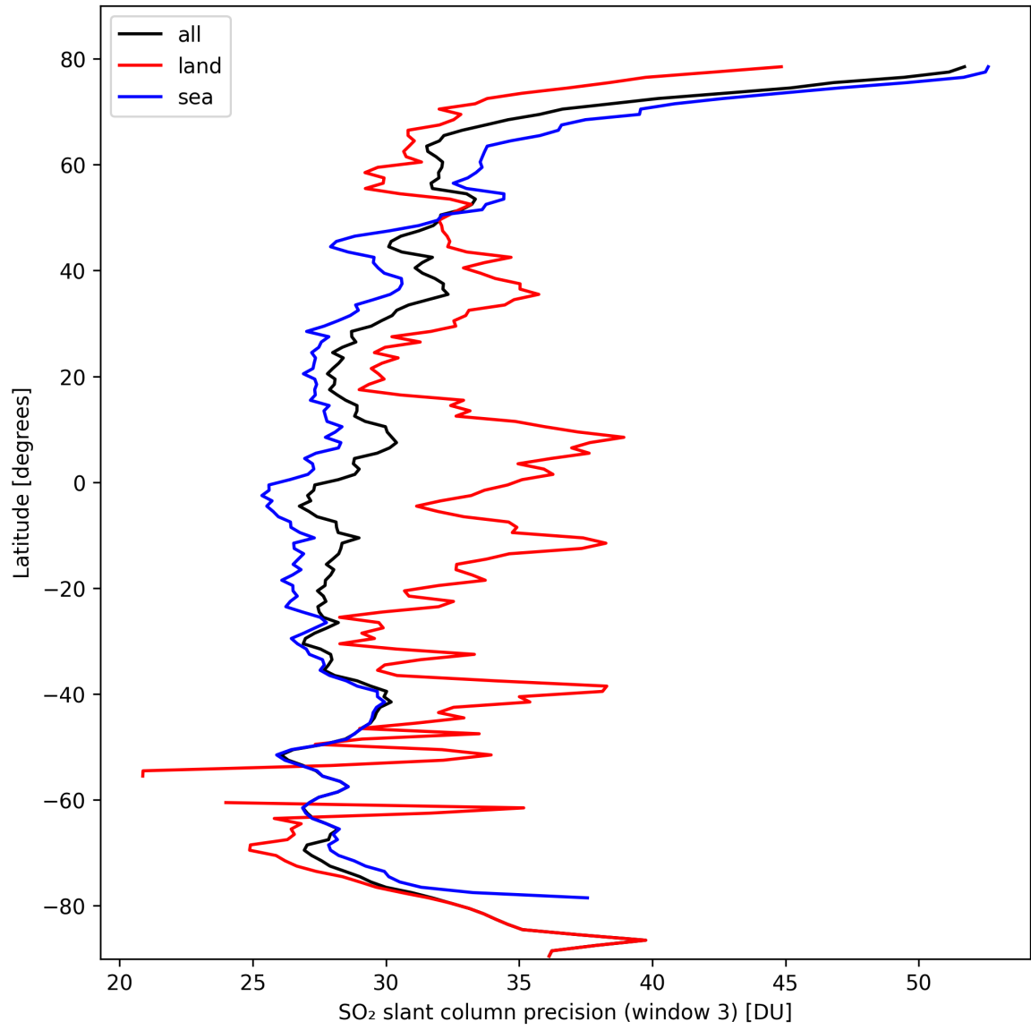
Figure 42: Zonal average of “SO 2 slant column precision (window 3)” for 2024-10-08 to 2024-10-10.
