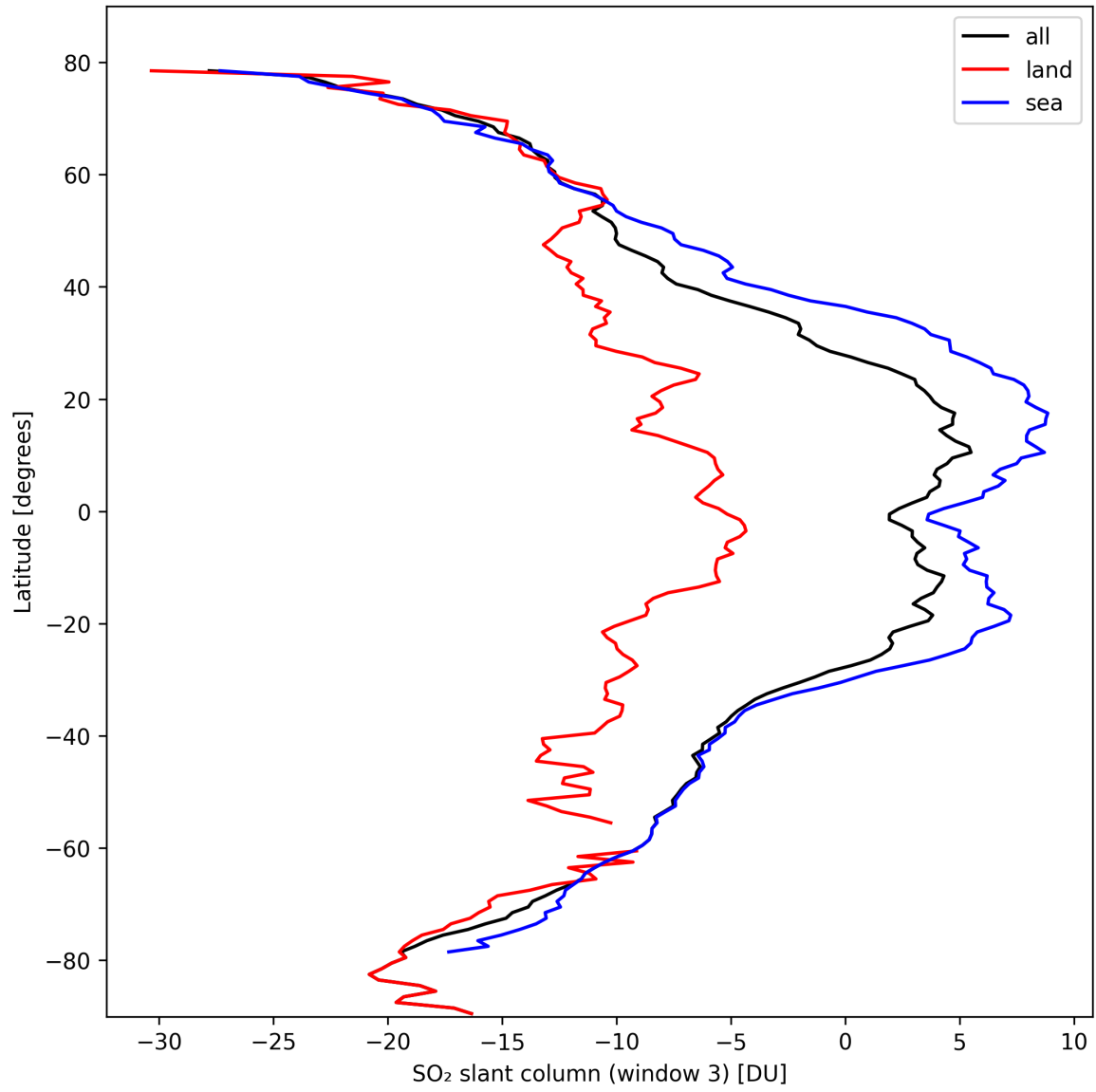
Figure 41: Zonal average of “SO 2 slant column (window 3)” for 2024-10-08 to 2024-10-10.
