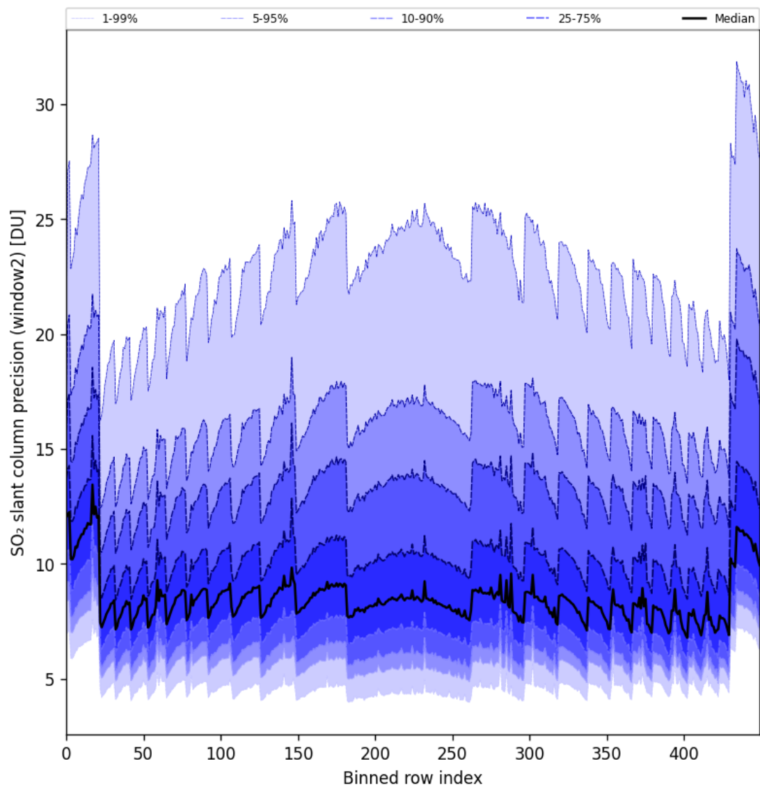
Figure 84: Along track statistics of “SO 2 slant column precision (window2)” for 2024-10-08 to 2024-10-10
