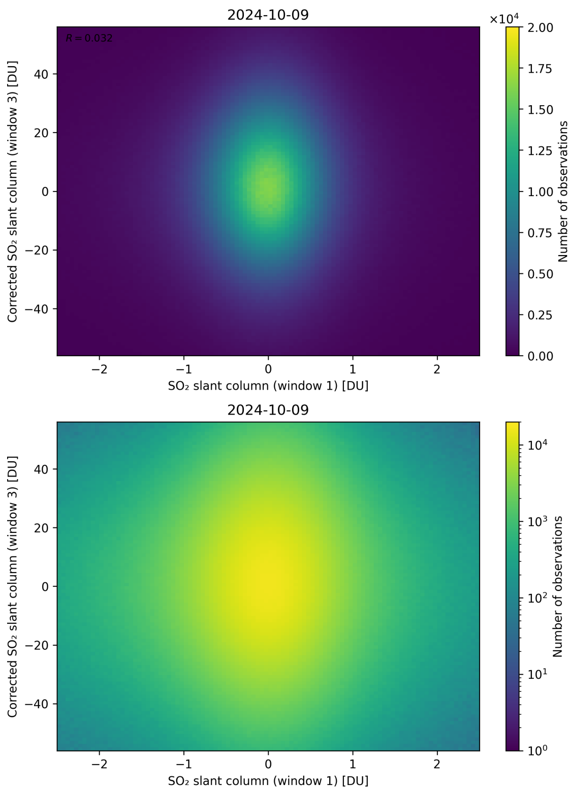
Figure 234: Scatter density plot of “SO 2 slant column (window 1)” against “Corrected SO 2 slant column (window 3)” for 2024-10-08 to 2024-10-10.
