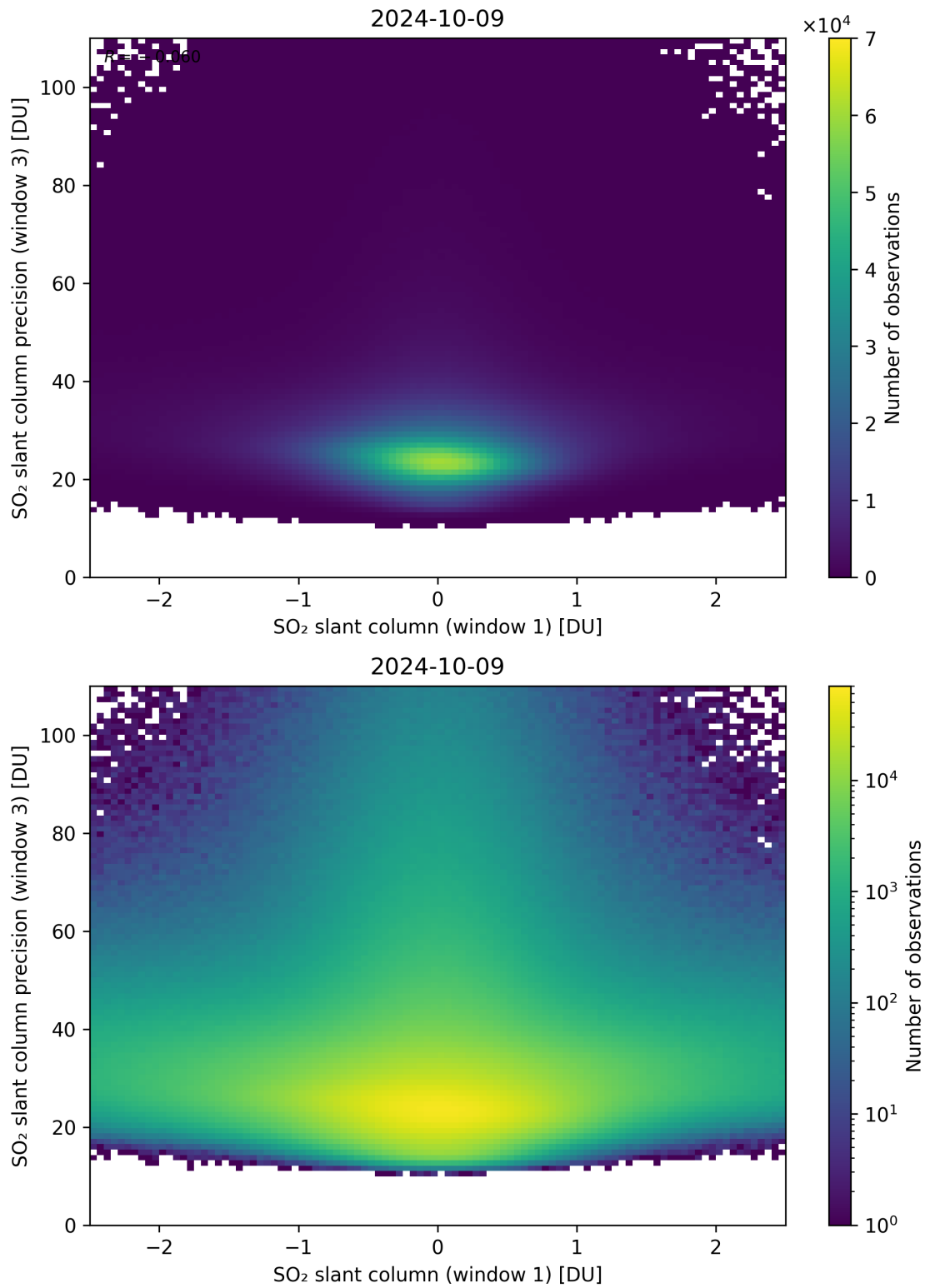
Figure 238: Scatter density plot of “SO 2 slant column (window 1)” against “SO 2 slant column precision (window 3)” for 2024-10-08 to 2024-10-10.
