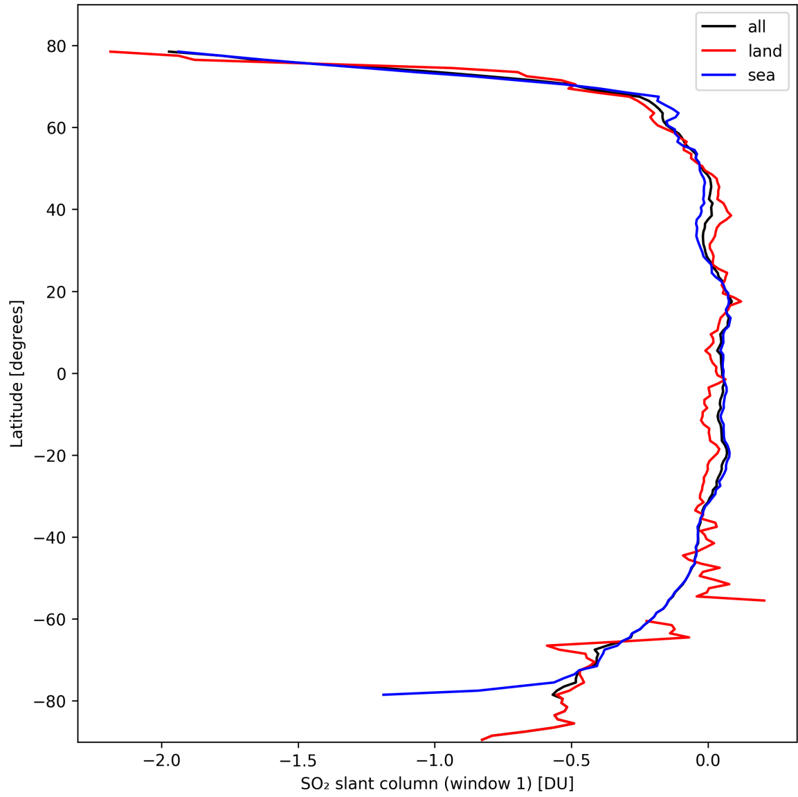
Figure 33: Zonal average of “SO 2 slant column (window 1)” for 2024-10-08 to 2024-10-10.
