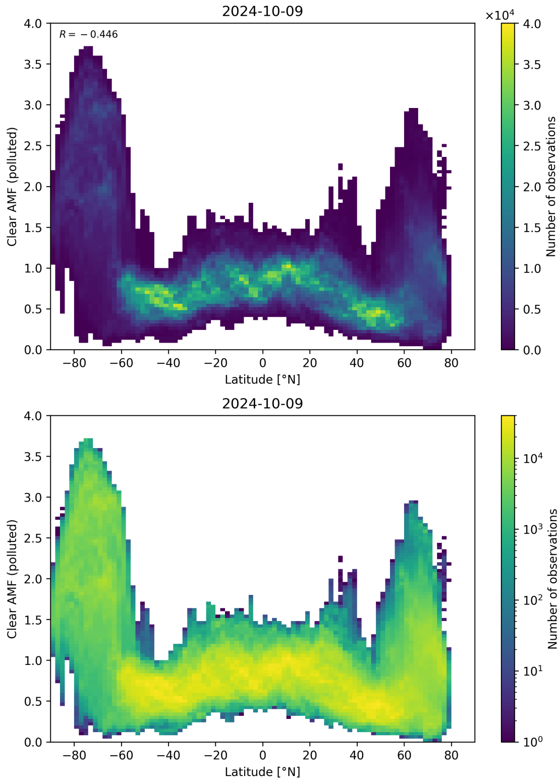
Figure 145: Scatter density plot of “Latitude” against “Clear AMF (polluted)” for 2024-10-08 to 2024-10-10.
