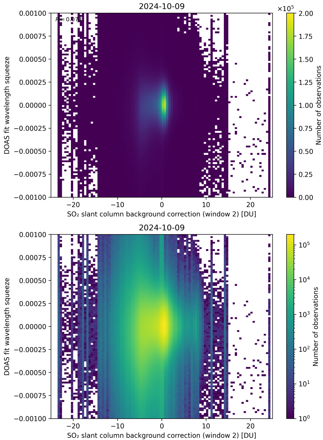
Figure 113: Scatter density plot of “SO 2 slant column background correction (window 2)” against “DOAS fit wavelength squeeze” for 2024-10-08 to 2024-10-10.
