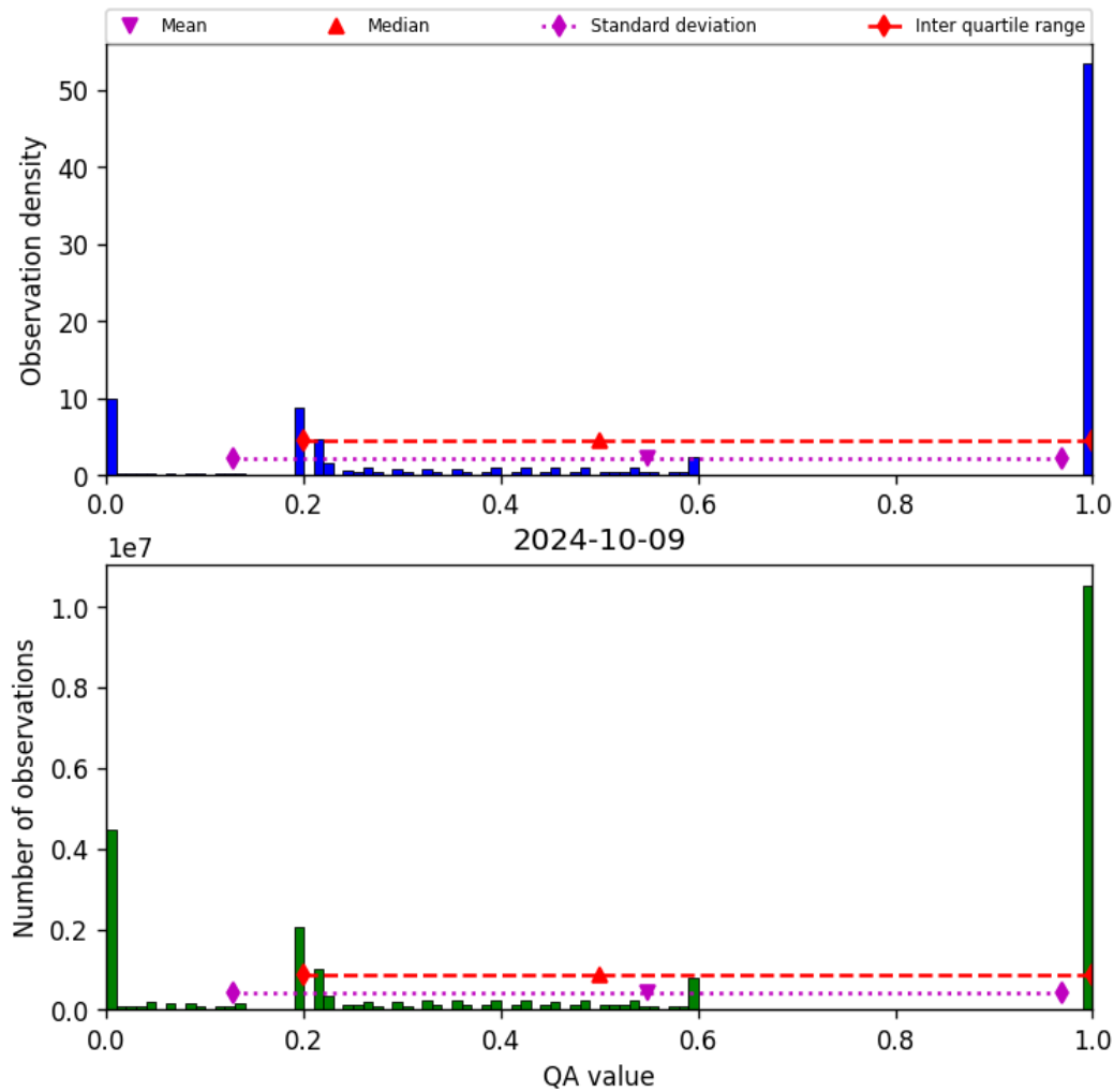
Figure 52: Histogram of “QA value” for 2024-10-08 to 2024-10-10
