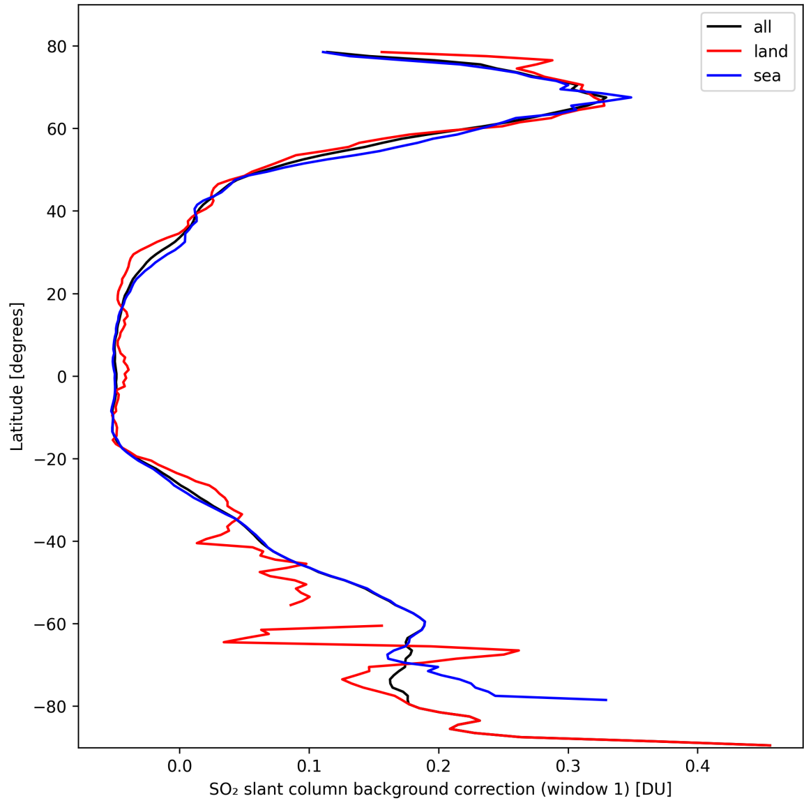
Figure 36: Zonal average of “SO 2 slant column background correction (window 1)” for 2024-10-08 to 2024-10-10.
