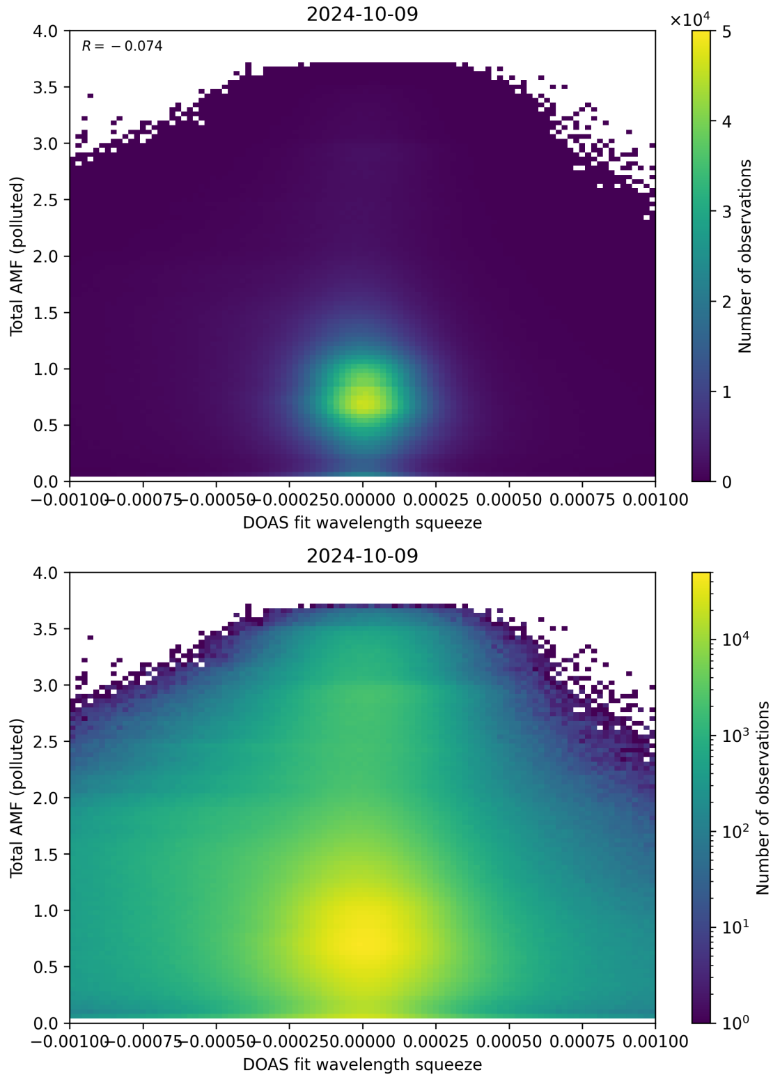
Figure 134: Scatter density plot of “DOAS fit wavelength squeeze” against “Total AMF (polluted)” for 2024-10-08 to 2024-10-10.
