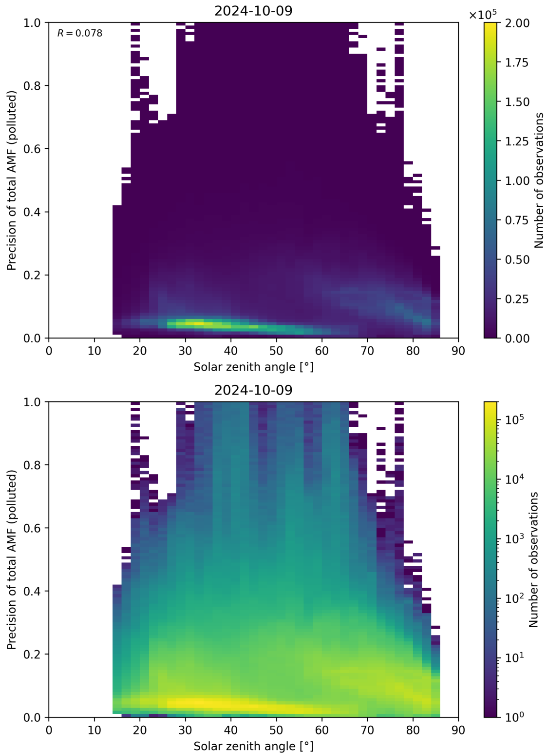
Figure 175: Scatter density plot of “Solar zenith angle” against “Precision of total AMF (polluted)” for 2024-10-08 to 2024-10-10.
