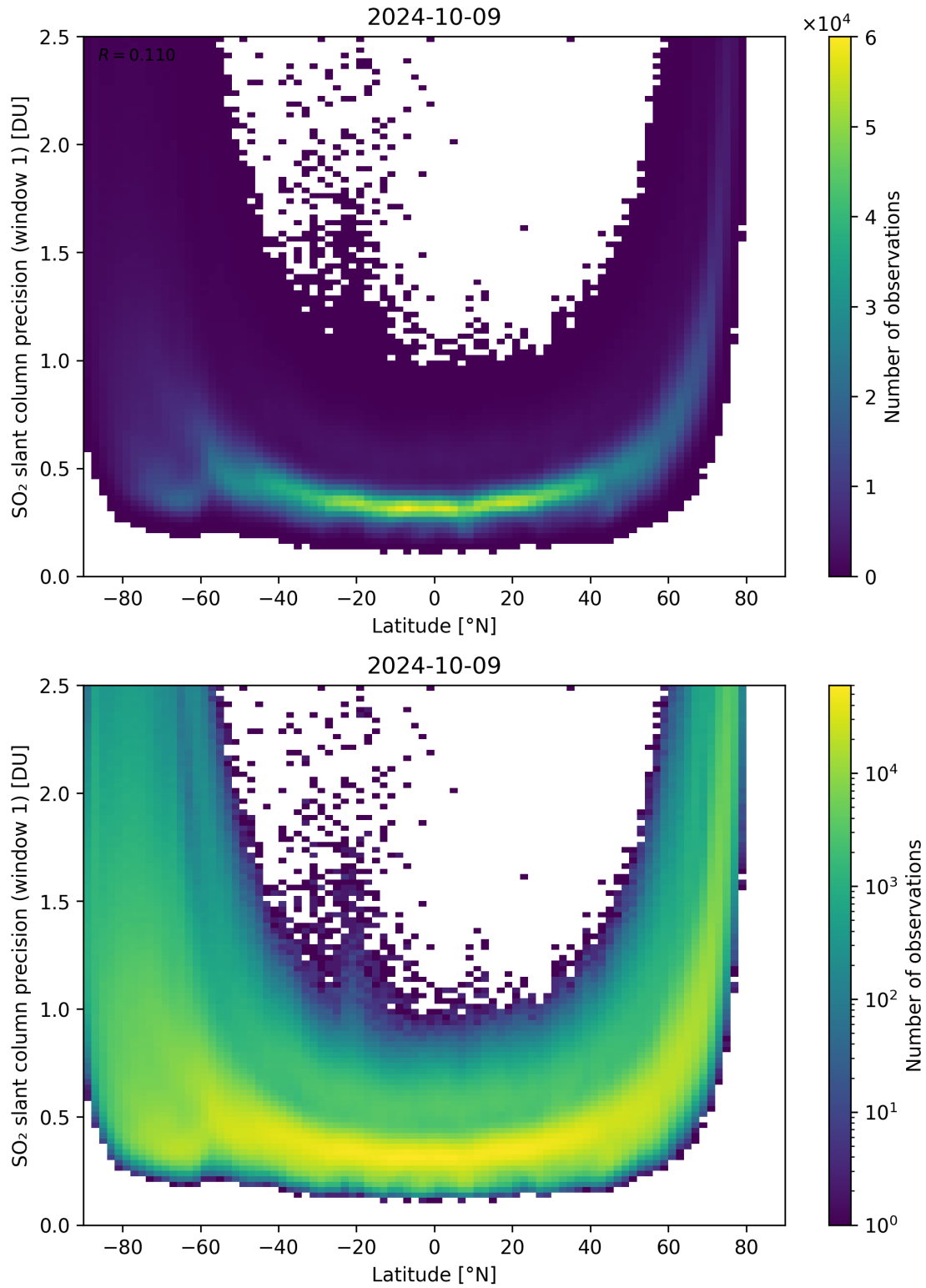
Figure 150: Scatter density plot of “Latitude” against “SO 2 slant column precision (window 1)” for 2024-10-08 to 2024-10-10.
