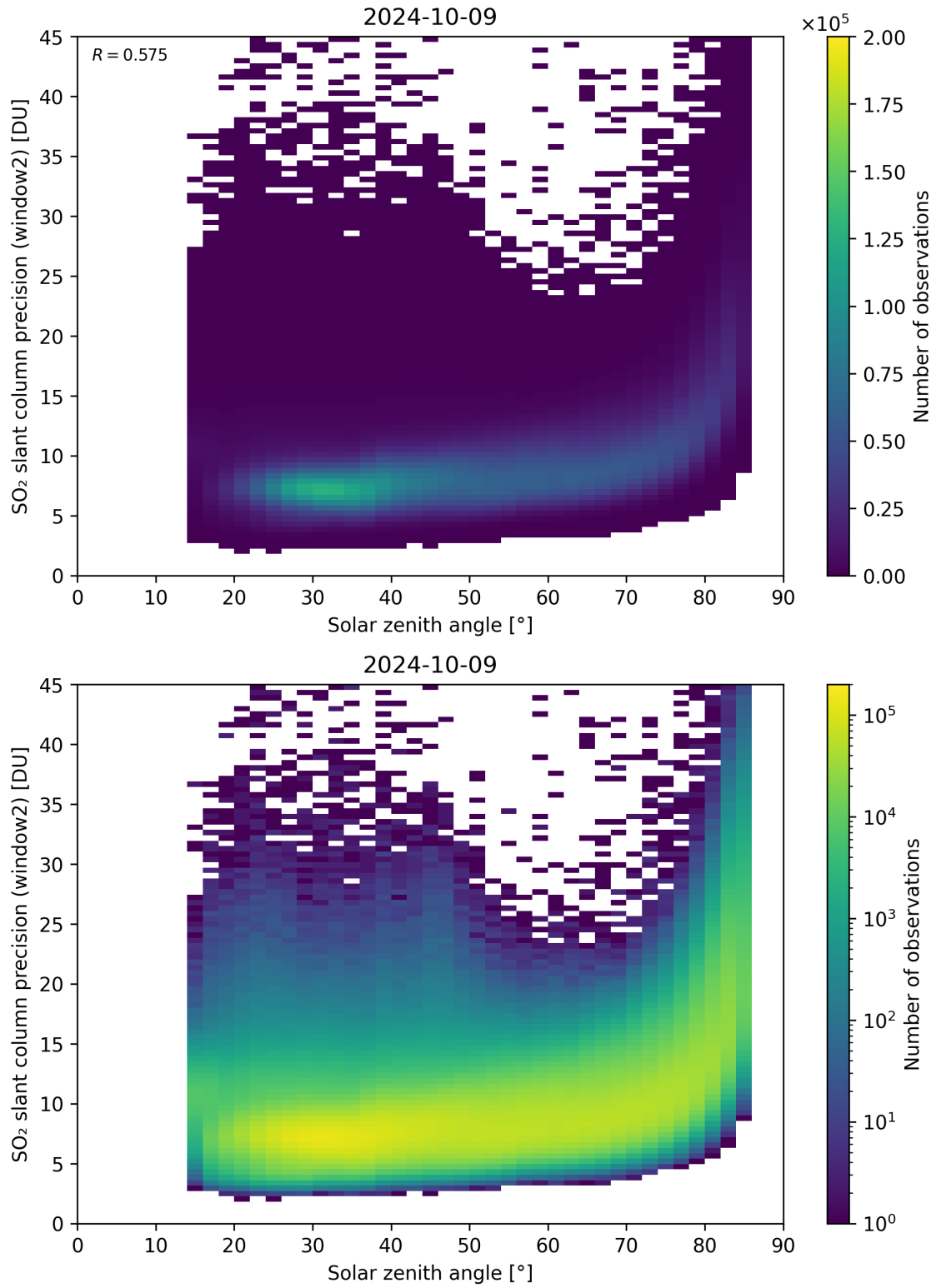
Figure 171: Scatter density plot of “Solar zenith angle” against “SO 2 slant column precision (window2)” for 2024-10-08 to 2024-10-10.
