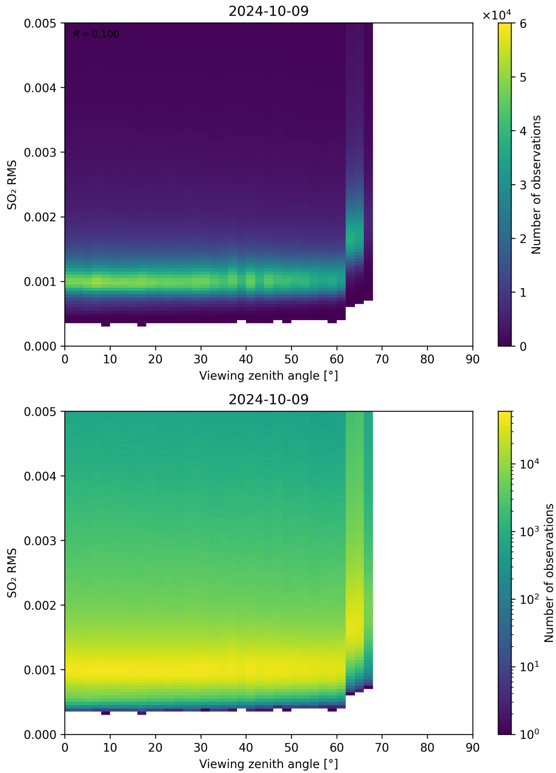
Figure 313: Scatter density plot of “Viewing zenith angle” against “SO 2 RMS” for 2024-10-08 to 2024-10-10.
