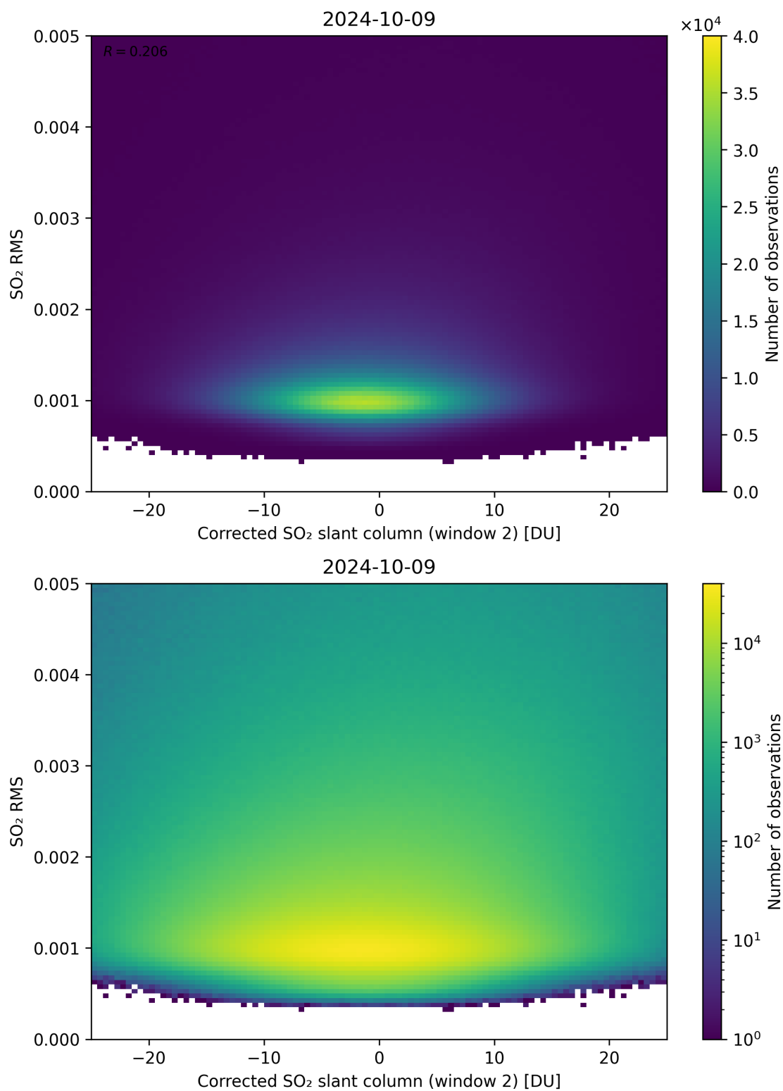
Figure 198: Scatter density plot of “Corrected SO 2 slant column (window 2)” against “SO 2 RMS” for 2024-10-08 to 2024-10-10.
