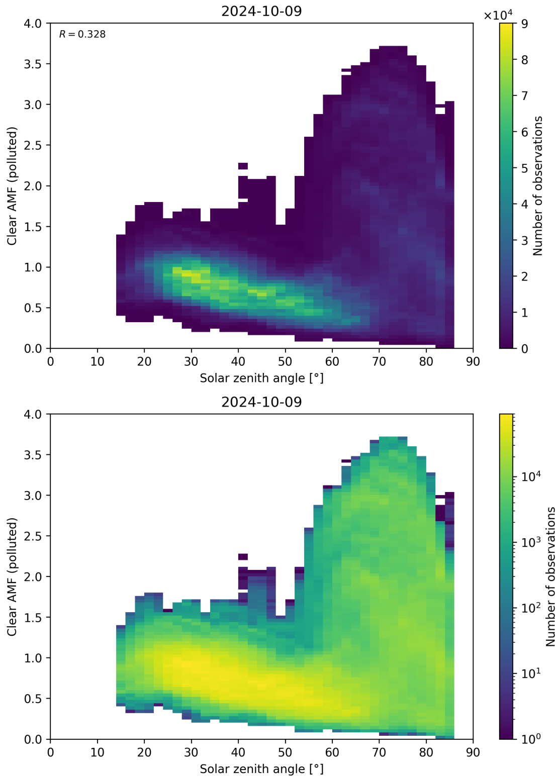
Figure 165: Scatter density plot of “Solar zenith angle” against “Clear AMF (polluted)” for 2024-10-08 to 2024-10-10.
