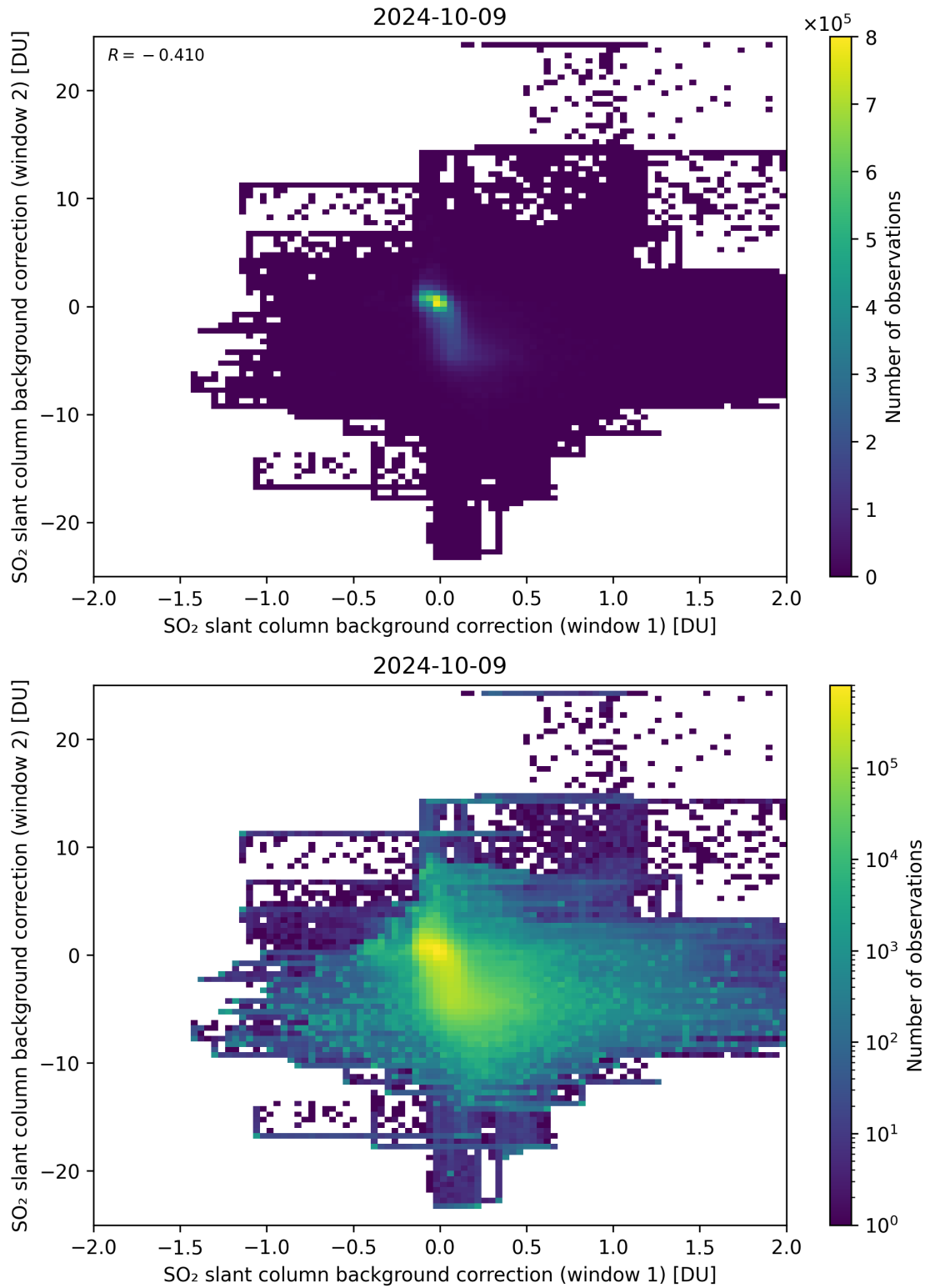
Figure 98: Scatter density plot of “SO 2 slant column background correction (window 1)” against “SO 2 slant column background correction (window 2)” for 2024-10-08 to 2024-10-10.
