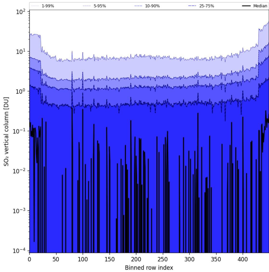
Figure 76: Along track statistics of “SO 2 vertical column” for 2024-10-08 to 2024-10-10
