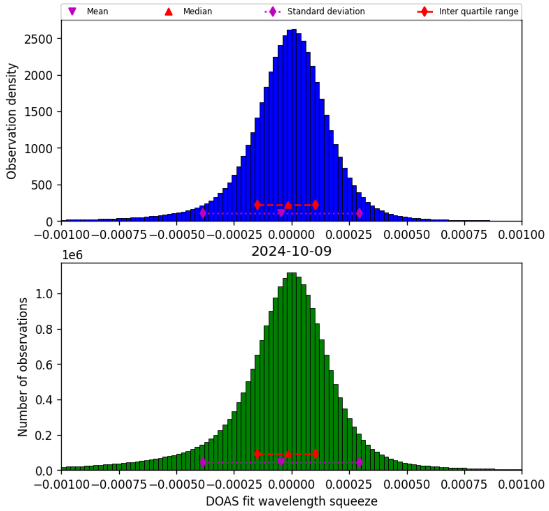
Figure 69: Histogram of “DOAS fit wavelength squeeze” for 2024-10-08 to 2024-10-10
