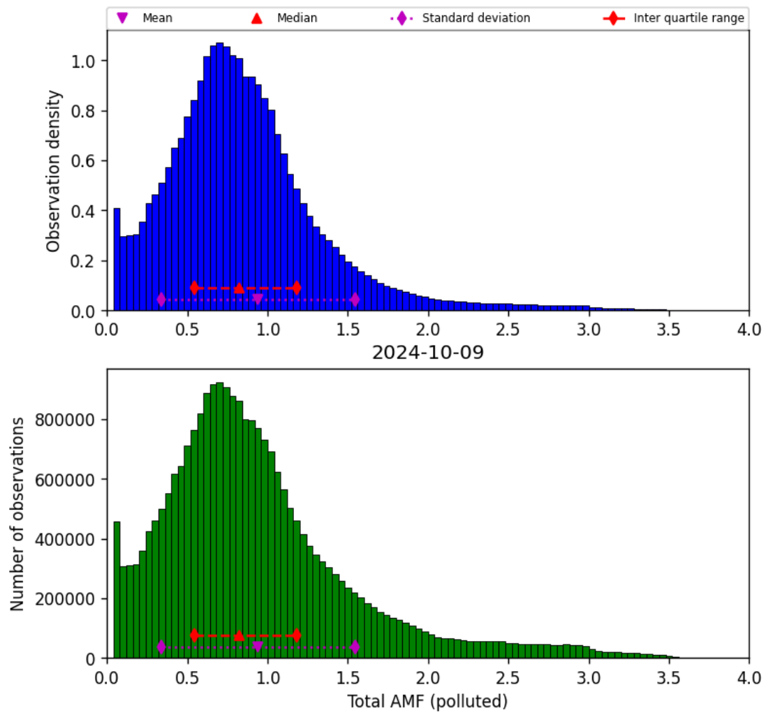
Figure 71: Histogram of “Total AMF (polluted)” for 2024-10-08 to 2024-10-10
