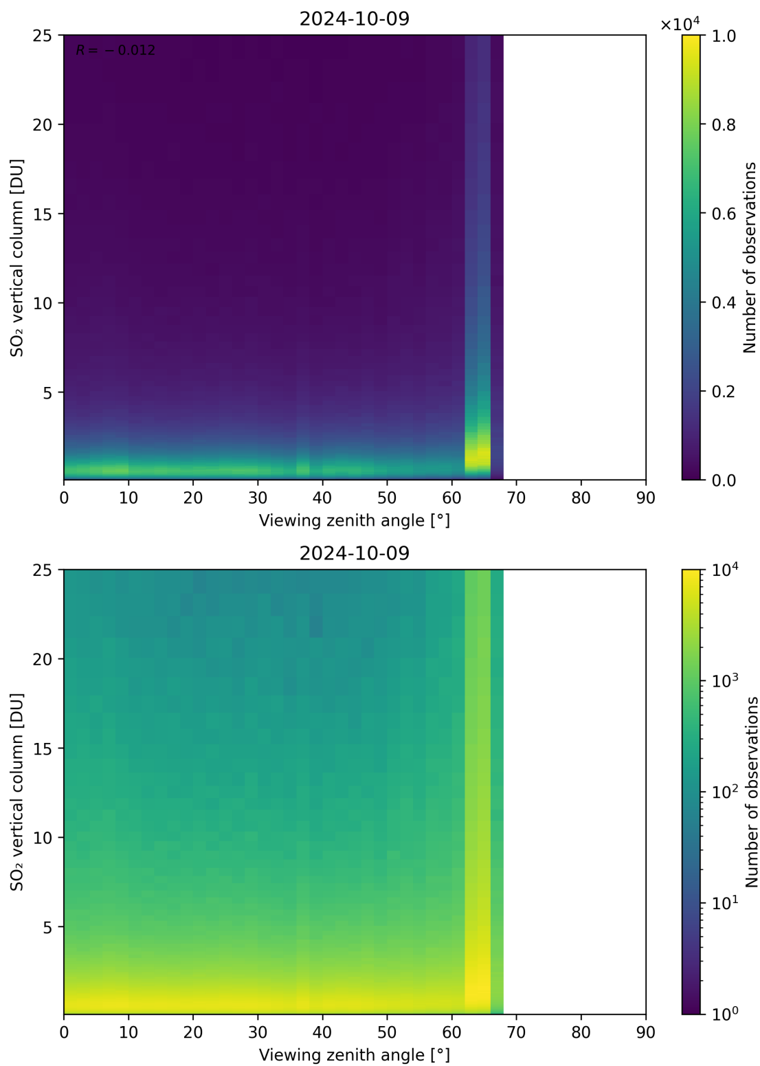
Figure 327: Scatter density plot of “Viewing zenith angle” against “SO 2 vertical column” for 2024-10-08 to 2024-10-10.
