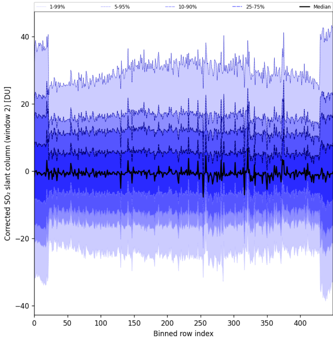
Figure 85: Along track statistics of “Corrected SO 2 slant column (window 2)” for 2024-10-08 to 2024-10-10
