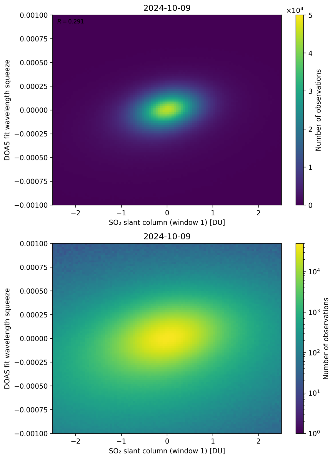
Figure 216: Scatter density plot of “SO 2 slant column (window 1)” against “DOAS fit wavelength squeeze” for 2024-10-08 to 2024-10-10.
