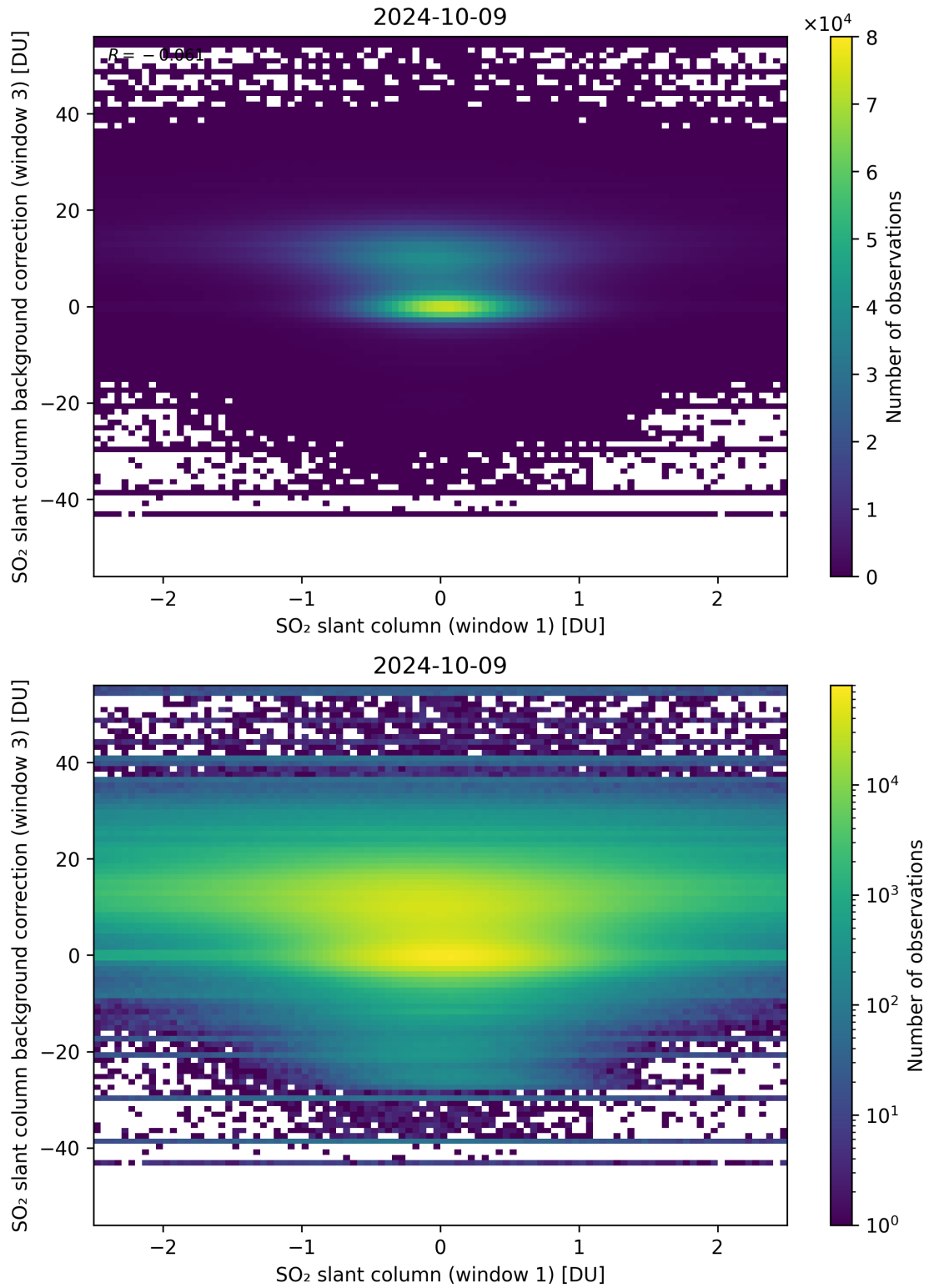
Figure 214: Scatter density plot of “SO 2 slant column (window 1)” against “SO 2 slant column background correction (window 3)” for 2024-10-08 to 2024-10-10.
