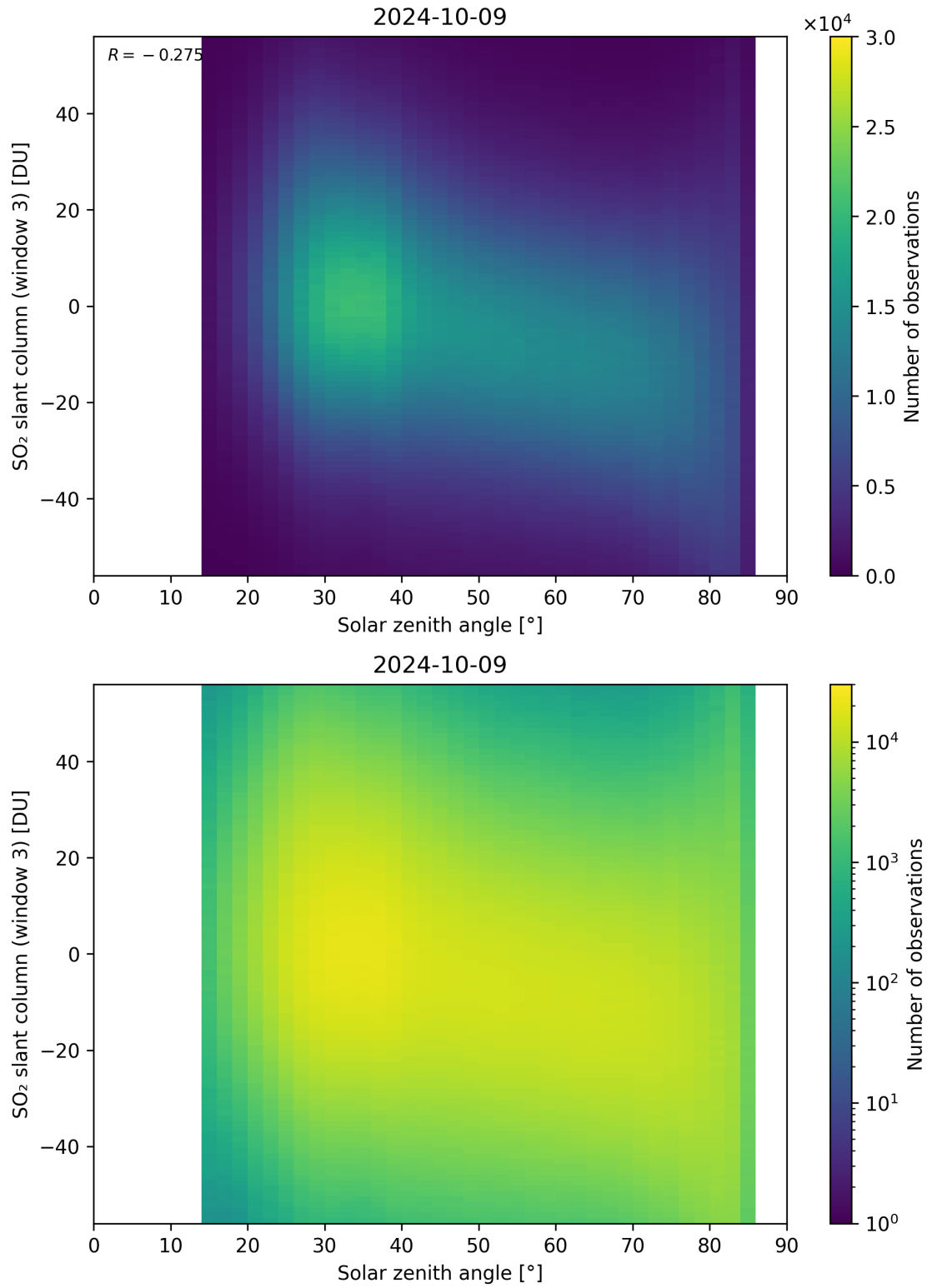
Figure 172: Scatter density plot of “Solar zenith angle” against “SO 2 slant column (window 3)” for 2024-10-08 to 2024-10-10.
