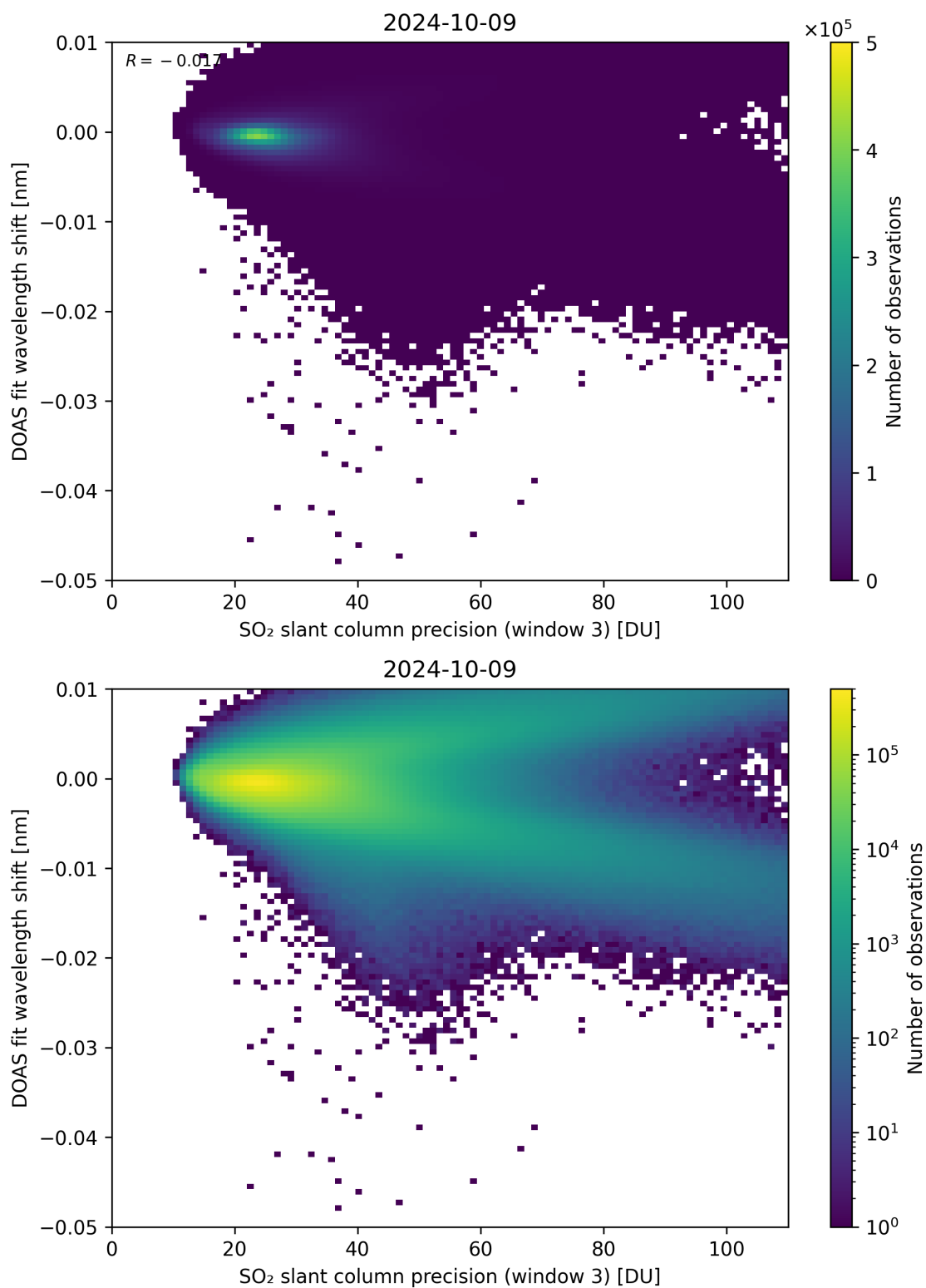
Figure 258: Scatter density plot of “SO 2 slant column precision (window 3)” against “DOAS fit wavelength shift” for 2024-10-08 to 2024-10-10.
