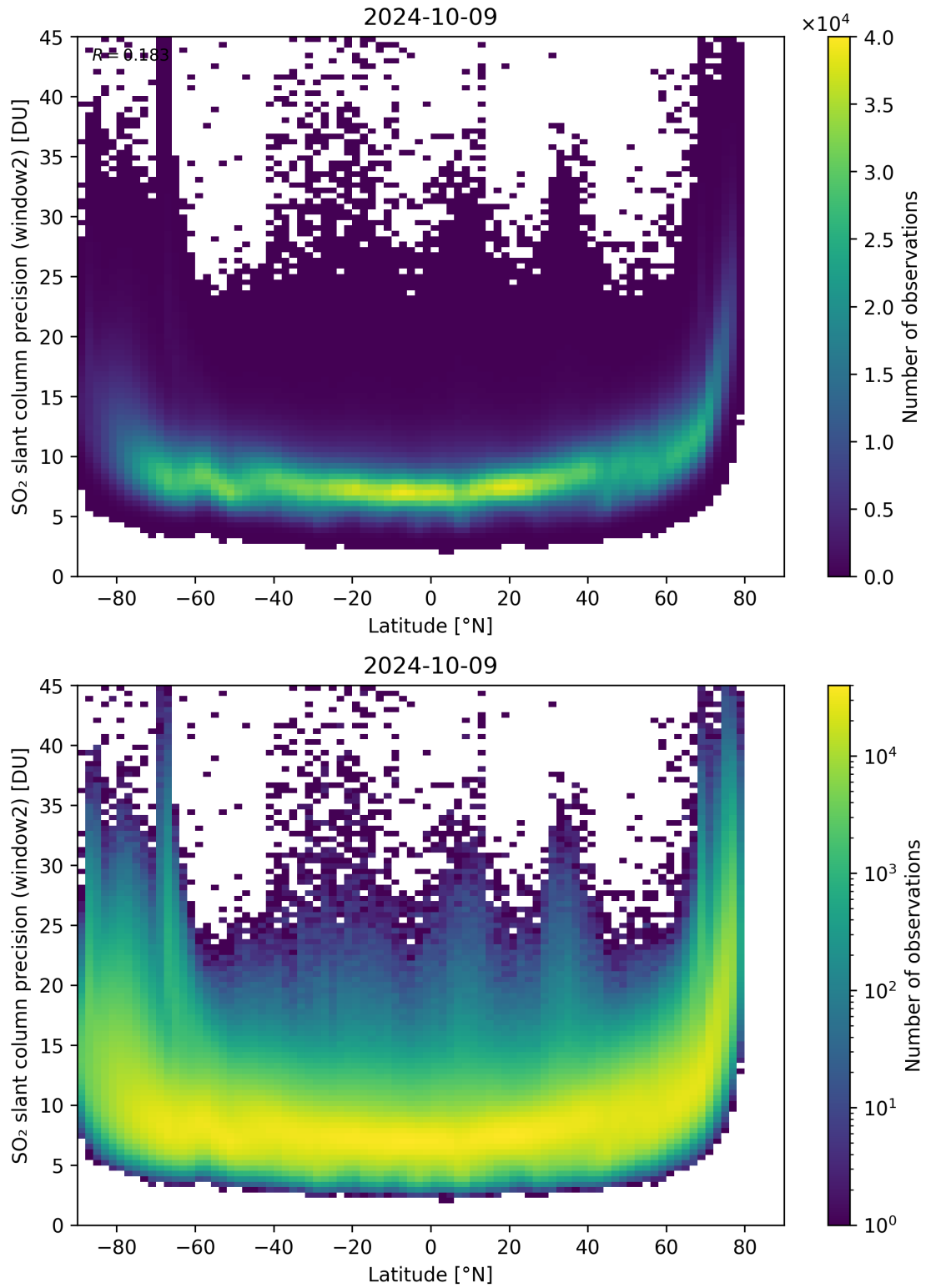
Figure 151: Scatter density plot of “Latitude” against “SO 2 slant column precision (window2)” for 2024-10-08 to 2024-10-10.
