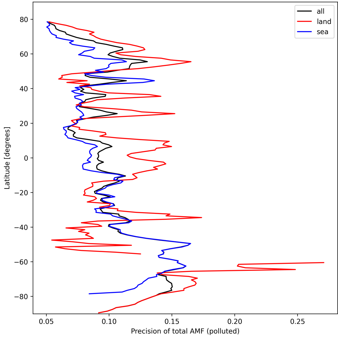
Figure 49: Zonal average of “Precision of total AMF (polluted)” for 2024-10-08 to 2024-10-10.
