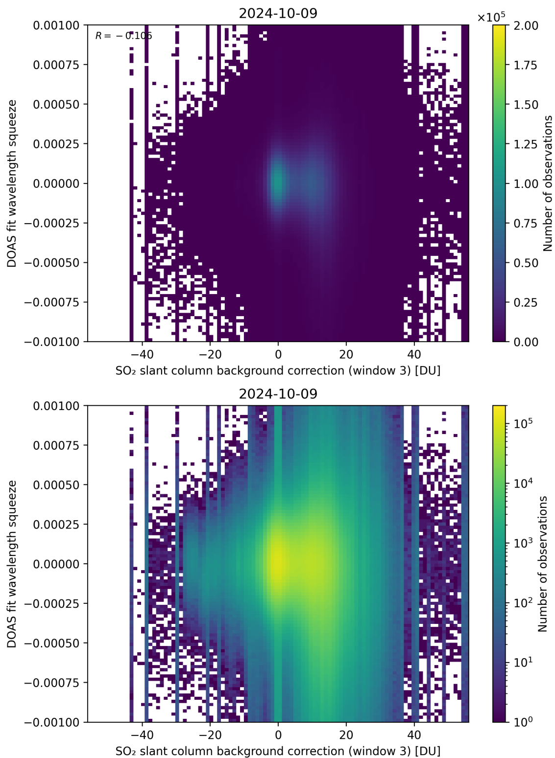
Figure 122: Scatter density plot of “SO 2 slant column background correction (window 3)” against “DOAS fit wavelength squeeze” for 2024-10-08 to 2024-10-10.
