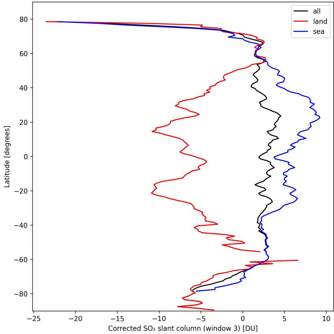
Figure 43: Zonal average of “Corrected SO 2 slant column (window 3)” for 2024-10-08 to 2024-10-10.
