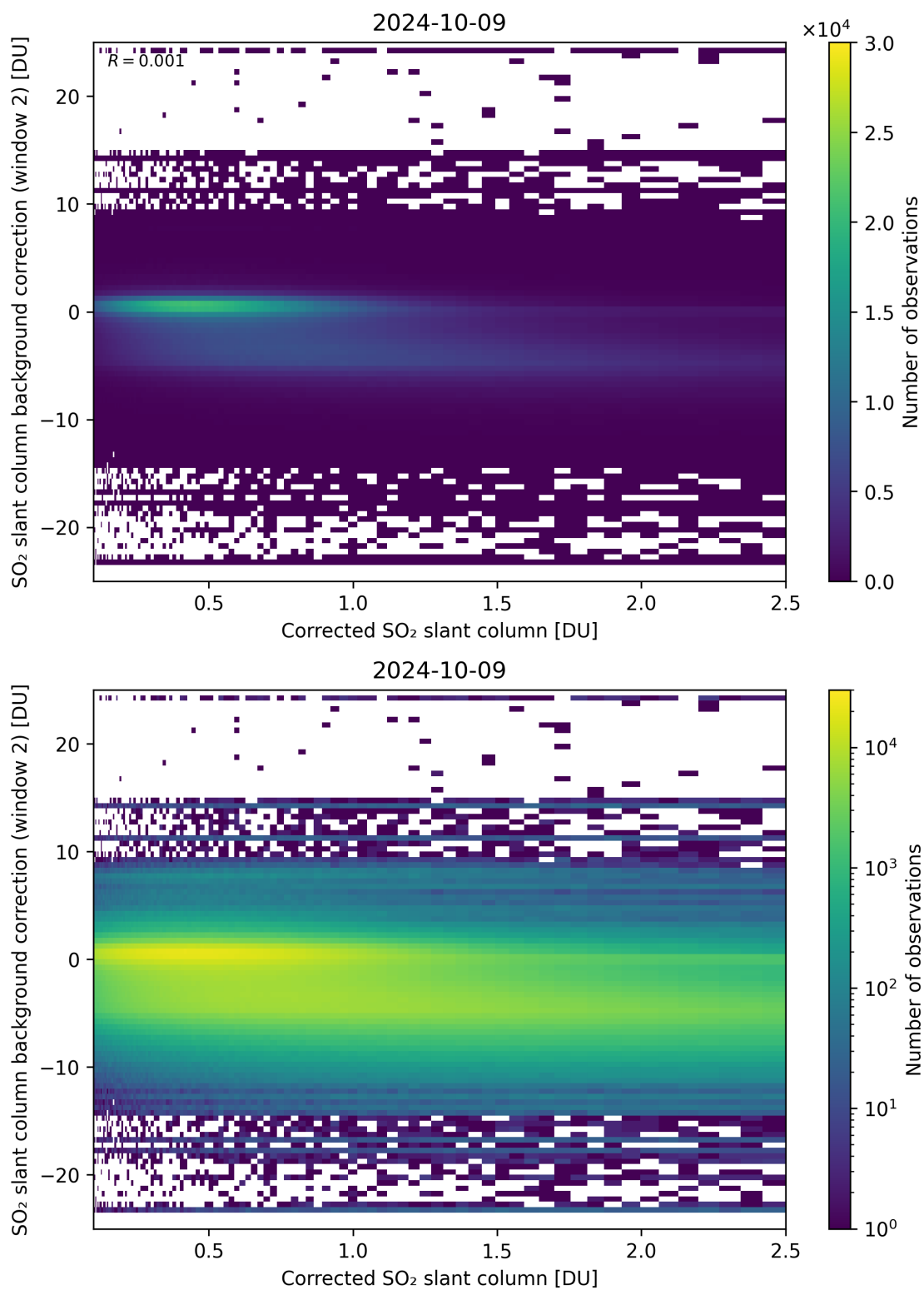
Figure 179: Scatter density plot of “Corrected SO 2 slant column” against “SO 2 slant column background correction (window 2)” for 2024-10-08 to 2024-10-10.
