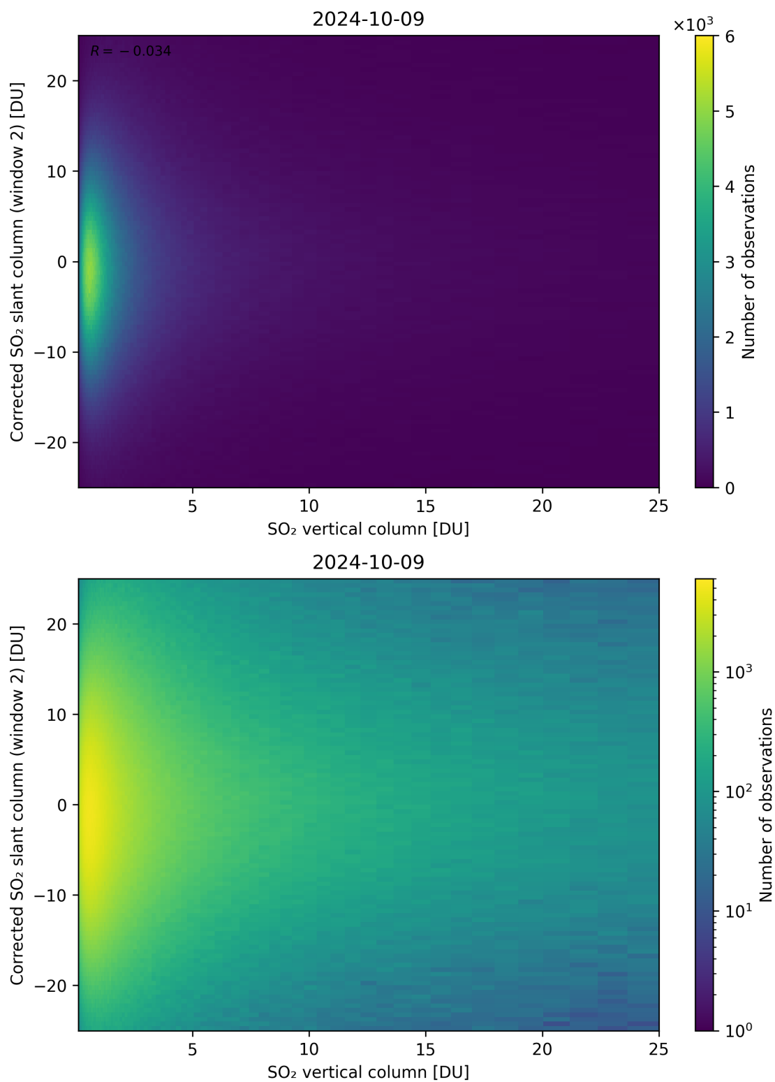
Figure 298: Scatter density plot of “SO 2 vertical column” against “Corrected SO 2 slant column (window 2)” for 2024-10-08 to 2024-10-10.
