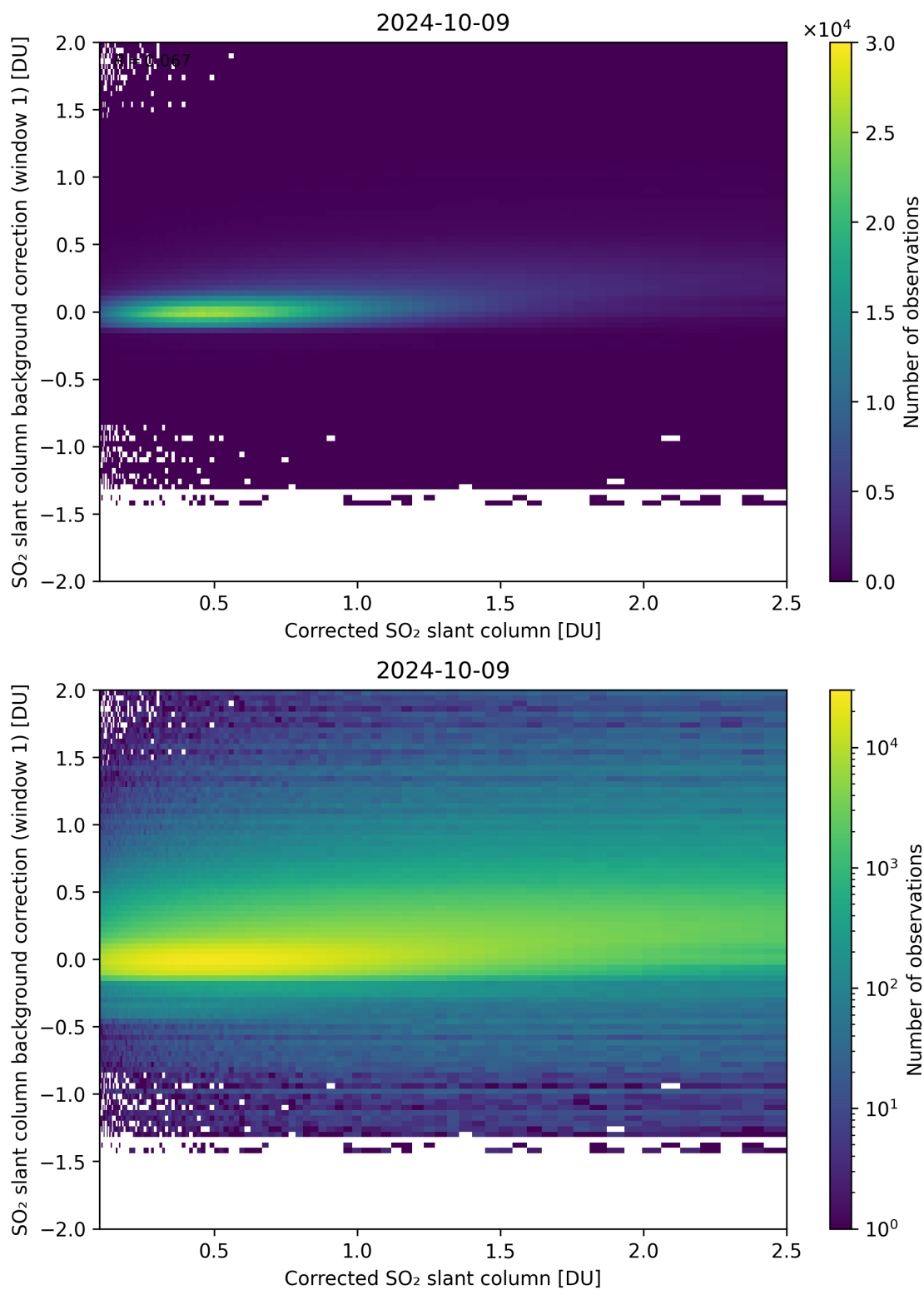
Figure 178: Scatter density plot of “Corrected SO 2 slant column” against “SO 2 slant column background correction (window 1)” for 2024-10-08 to 2024-10-10.
