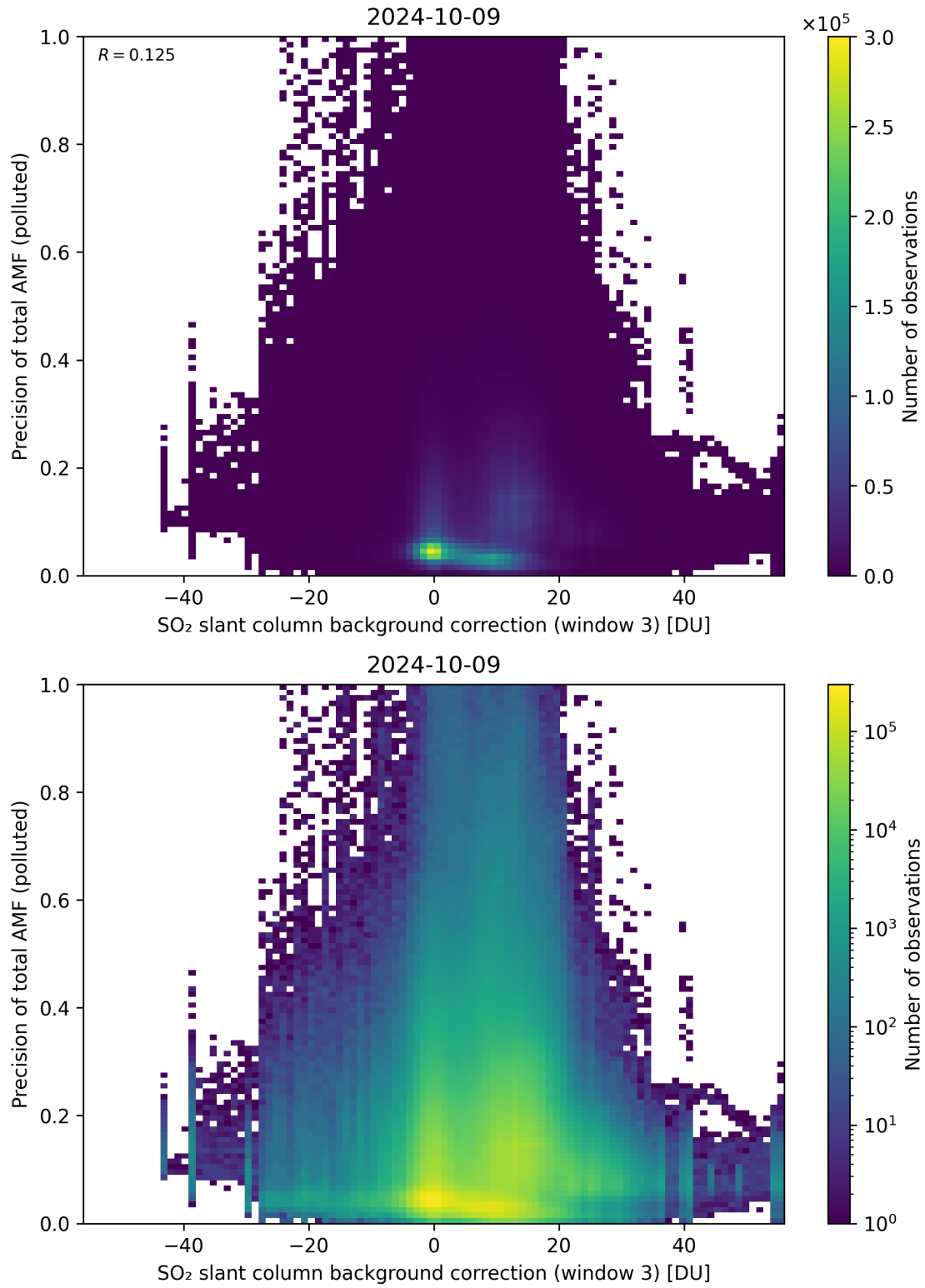
Figure 126: Scatter density plot of “SO 2 slant column background correction (window 3)” against “Precision of total AMF (polluted)” for 2024-10-08 to 2024-10-10.
