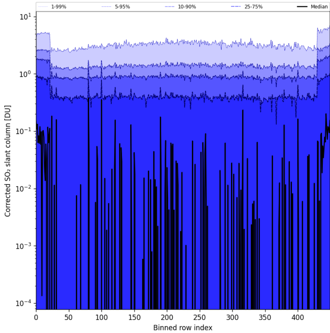
Figure 78: Along track statistics of “Corrected SO 2 slant column” for 2024-10-08 to 2024-10-10
