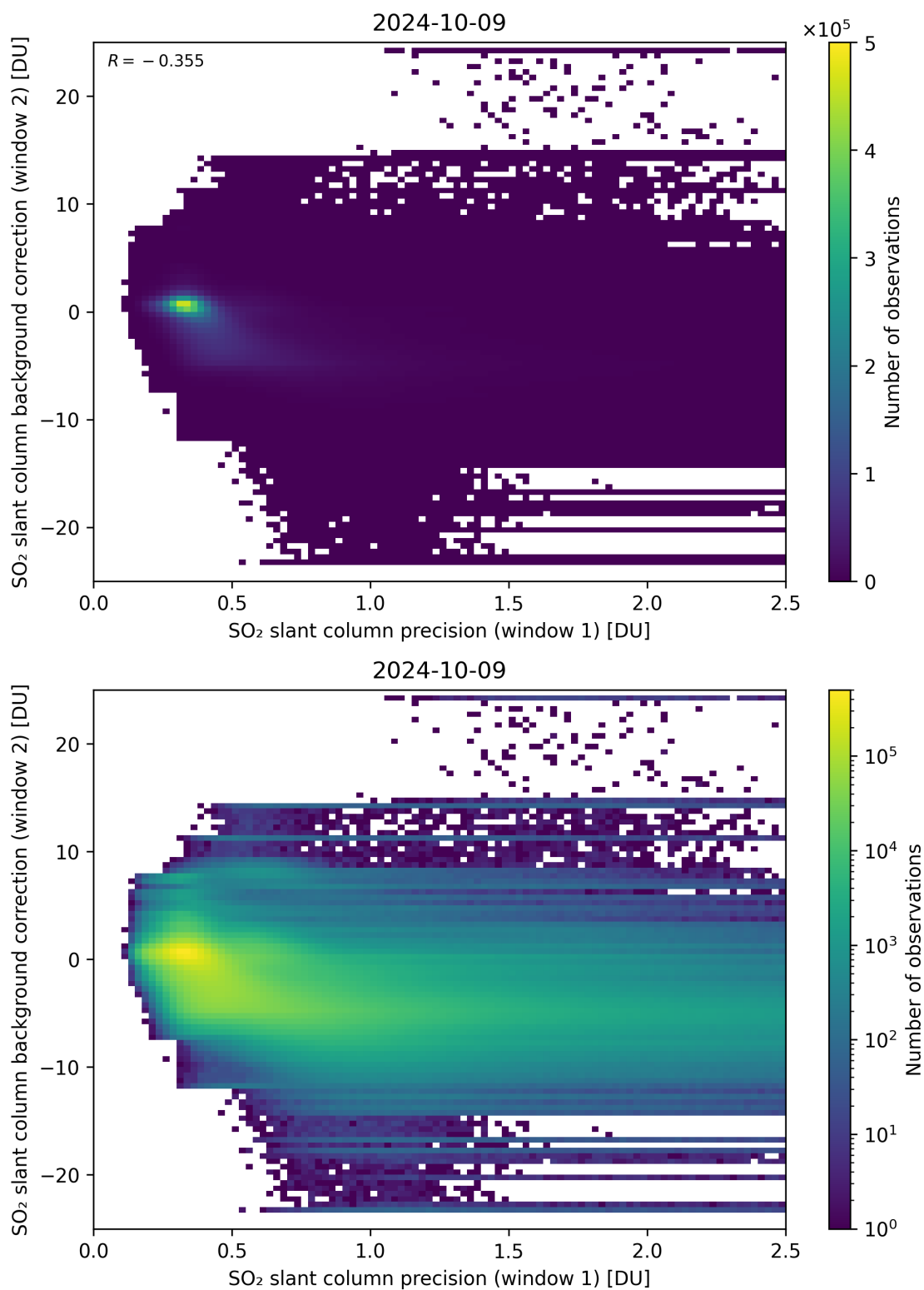
Figure 219: Scatter density plot of “SO 2 slant column precision (window 1)” against “SO 2 slant column background correction (window 2)” for 2024-10-08 to 2024-10-10.
