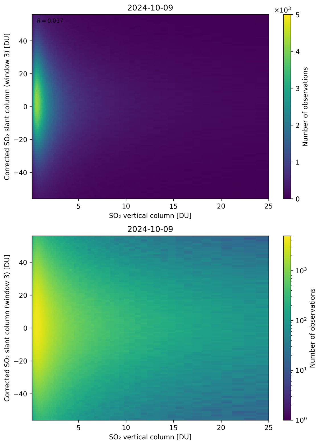
Figure 299: Scatter density plot of “SO 2 vertical column” against “Corrected SO 2 slant column (window 3)” for 2024-10-08 to 2024-10-10.
