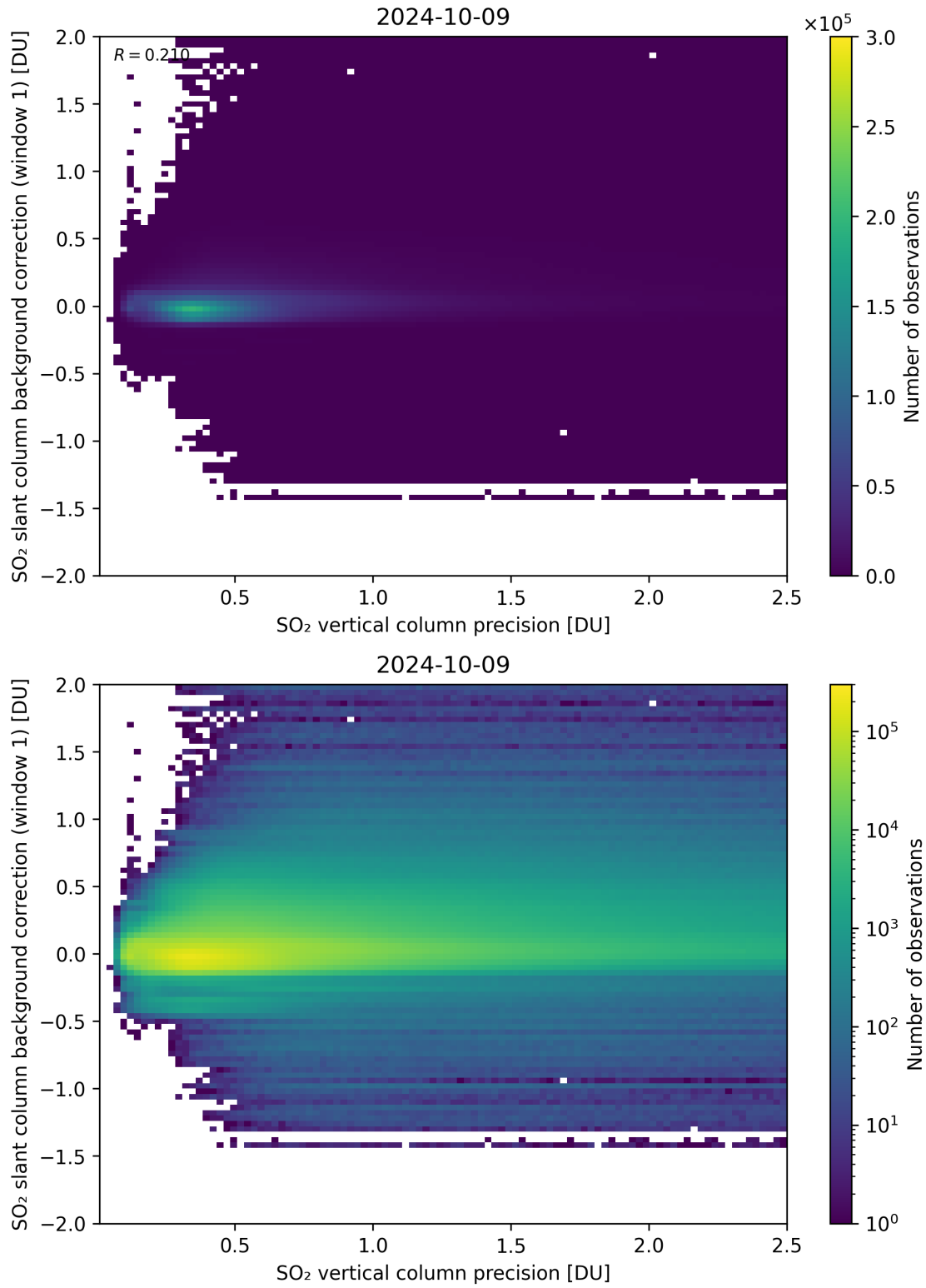
Figure 279: Scatter density plot of “SO 2 vertical column precision” against “SO 2 slant column background correction (window 1)” for 2024-10-08 to 2024-10-10.
