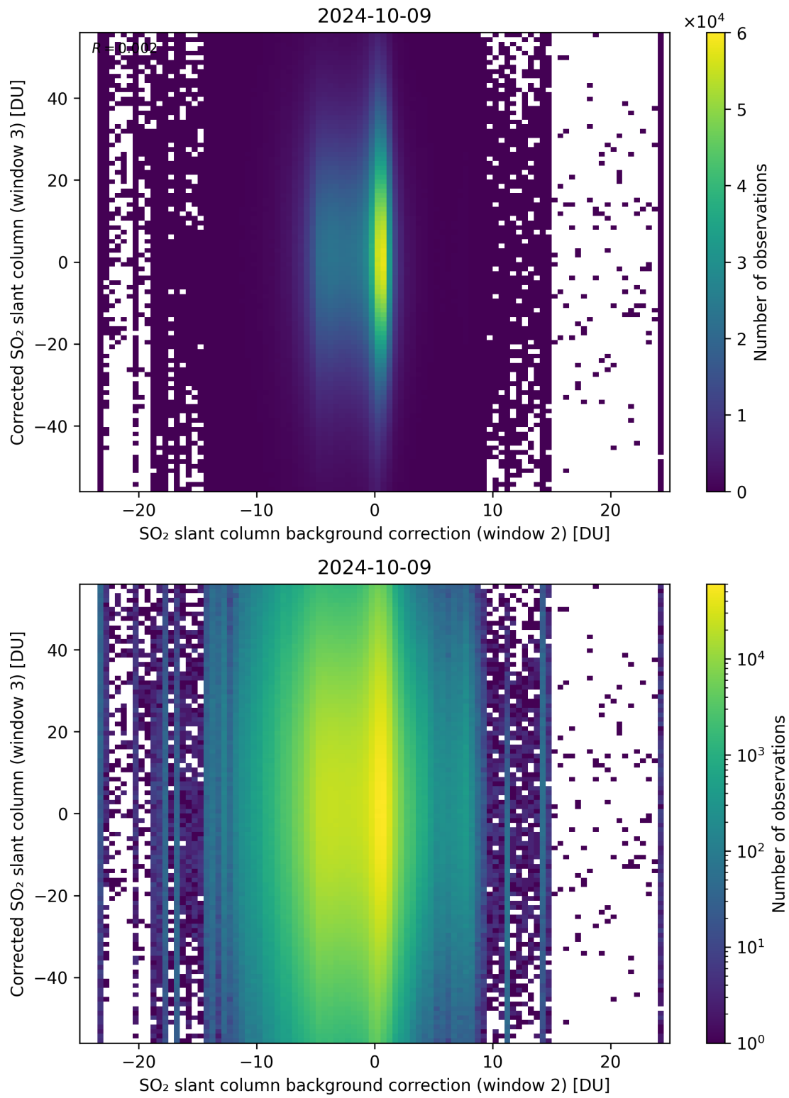
Figure 116: Scatter density plot of “SO 2 slant column background correction (window 2)” against “Corrected SO 2 slant column (window 3)” for 2024-10-08 to 2024-10-10.
