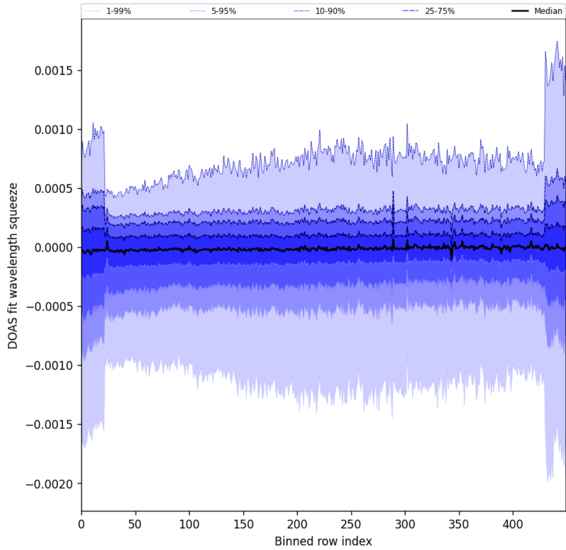
Figure 92: Along track statistics of “DOAS fit wavelength squeeze” for 2024-10-08 to 2024-10-10
