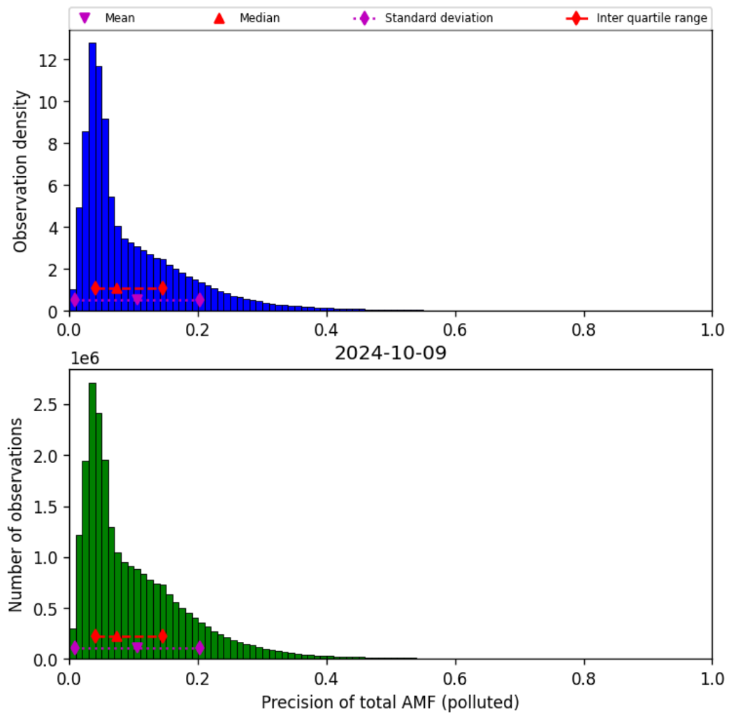
Figure 72: Histogram of “Precision of total AMF (polluted)” for 2024-10-08 to 2024-10-10
