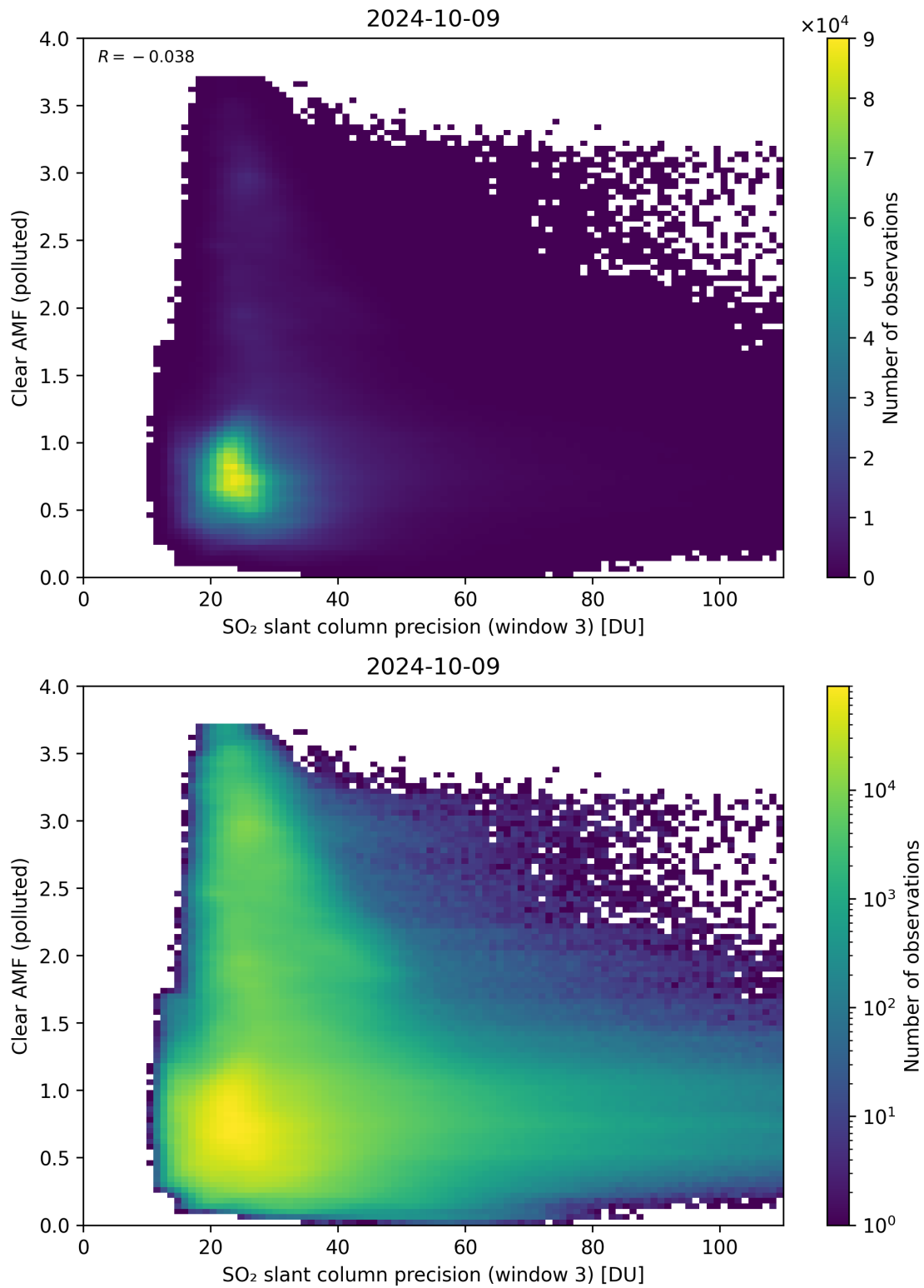
Figure 261: Scatter density plot of “SO 2 slant column precision (window 3)” against “Clear AMF (polluted)” for 2024-10-08 to 2024-10-10.
