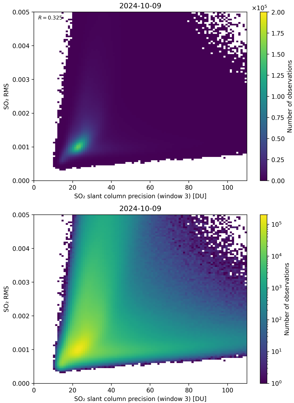
Figure 260: Scatter density plot of “SO 2 slant column precision (window 3)” against “SO 2 RMS” for 2024-10-08 to 2024-10-10.
