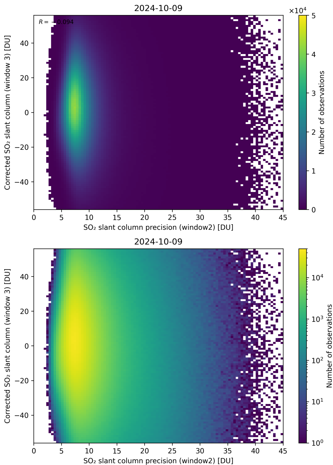
Figure 248: Scatter density plot of “SO 2 slant column precision (window2)” against “Corrected SO 2 slant column (window 3)” for 2024-10-08 to 2024-10-10.
