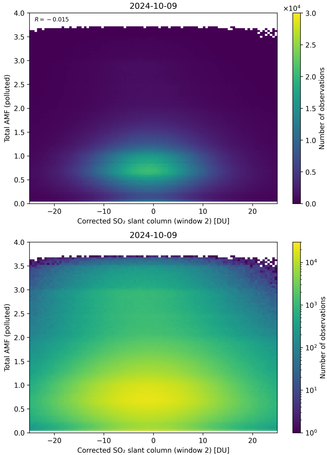
Figure 203: Scatter density plot of “Corrected SO 2 slant column (window 2)” against “Total AMF (polluted)” for 2024-10-08 to 2024-10-10.
