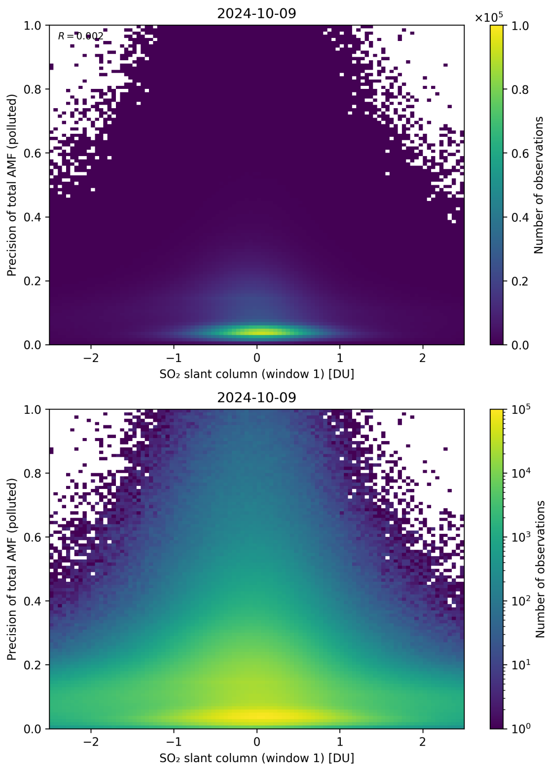
Figure 240: Scatter density plot of “SO 2 slant column (window 1)” against “Precision of total AMF (polluted)” for 2024-10-08 to 2024-10-10.
