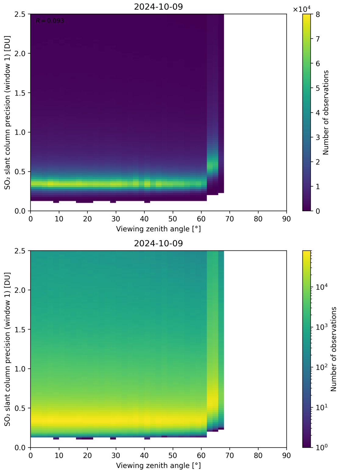
Figure 321: Scatter density plot of “Viewing zenith angle” against “SO 2 slant column precision (window 1)” for 2024-10-08 to 2024-10-10.
