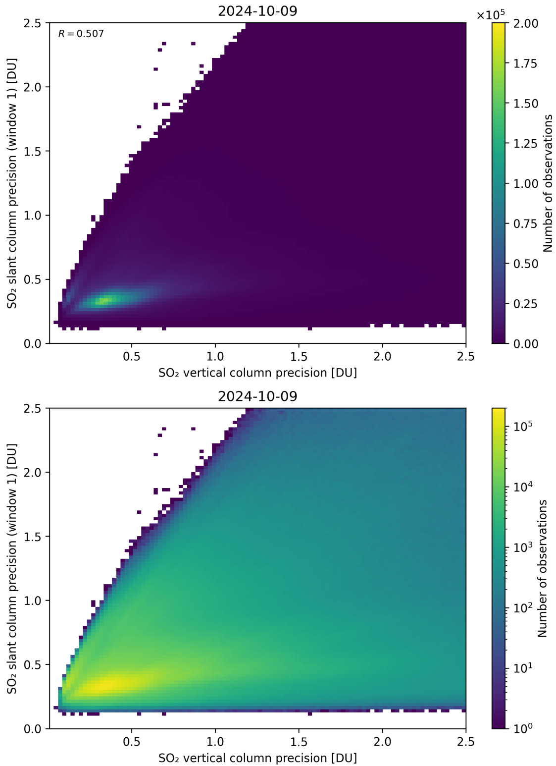
Figure 290: Scatter density plot of “SO 2 vertical column precision” against “SO 2 slant column precision (window 1)” for 2024-10-08 to 2024-10-10.
