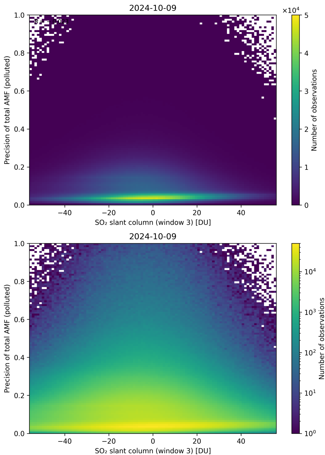
Figure 269: Scatter density plot of “SO 2 slant column (window 3)” against “Precision of total AMF (polluted)” for 2024-10-08 to 2024-10-10.
