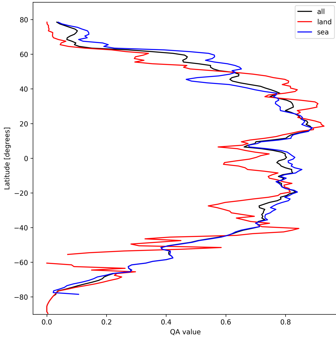
Figure 29: Zonal average of “QA value” for 2024-10-08 to 2024-10-10.
