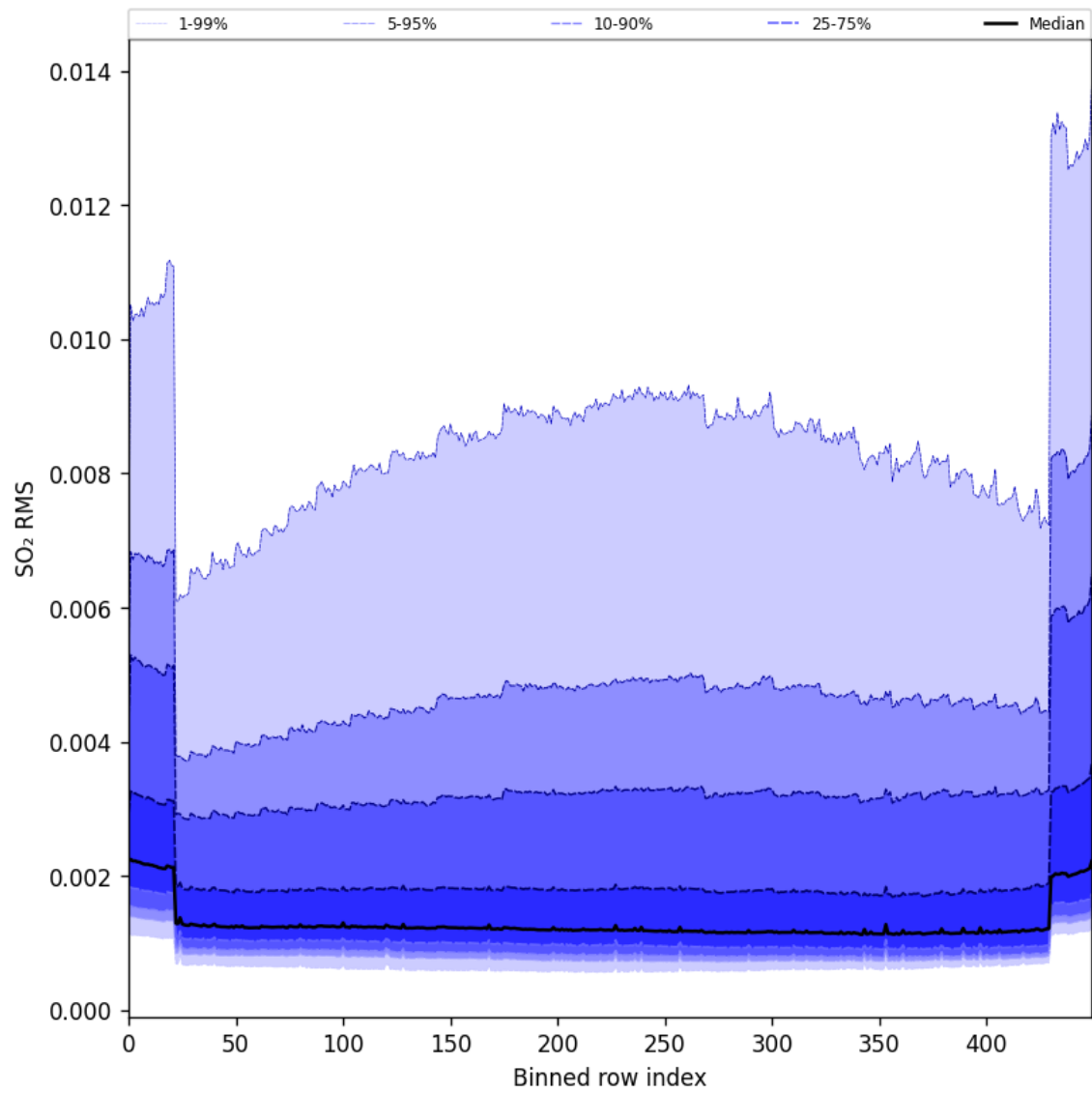
Figure 93: Along track statistics of “SO 2 RMS” for 2024-10-08 to 2024-10-10
