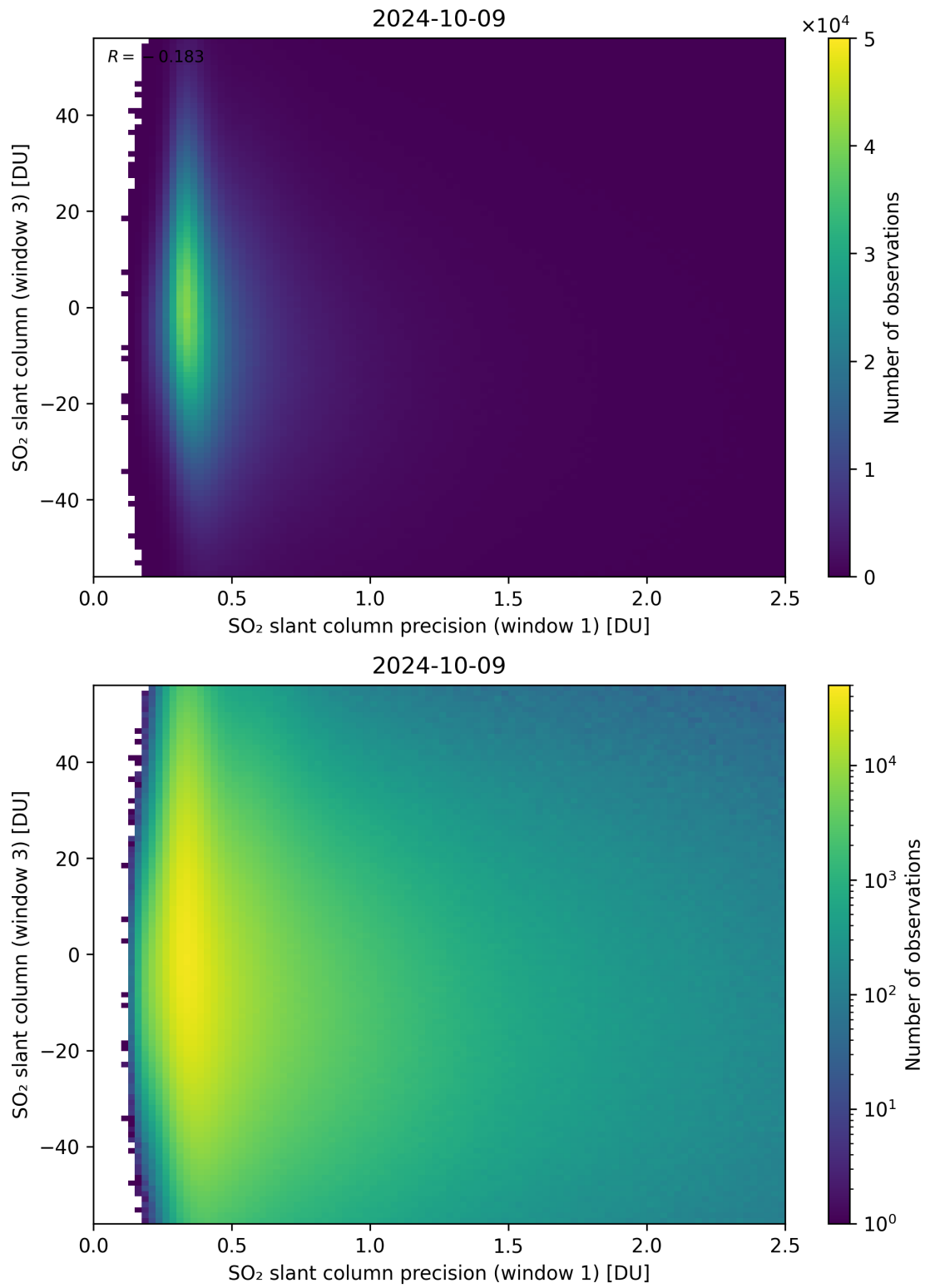
Figure 228: Scatter density plot of “SO 2 slant column precision (window 1)” against “SO 2 slant column (window 3)” for 2024-10-08 to 2024-10-10.
