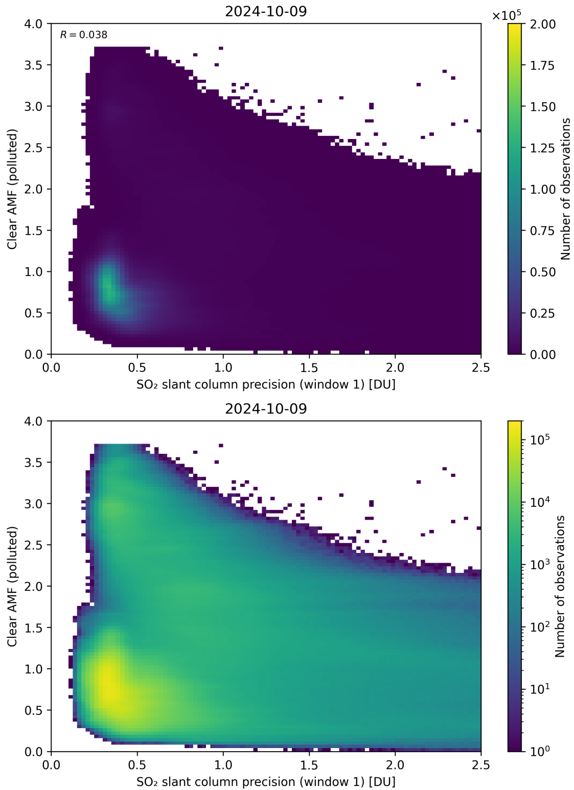
Figure 224: Scatter density plot of “SO 2 slant column precision (window 1)” against “Clear AMF (polluted)” for 2024-10-08 to 2024-10-10.
