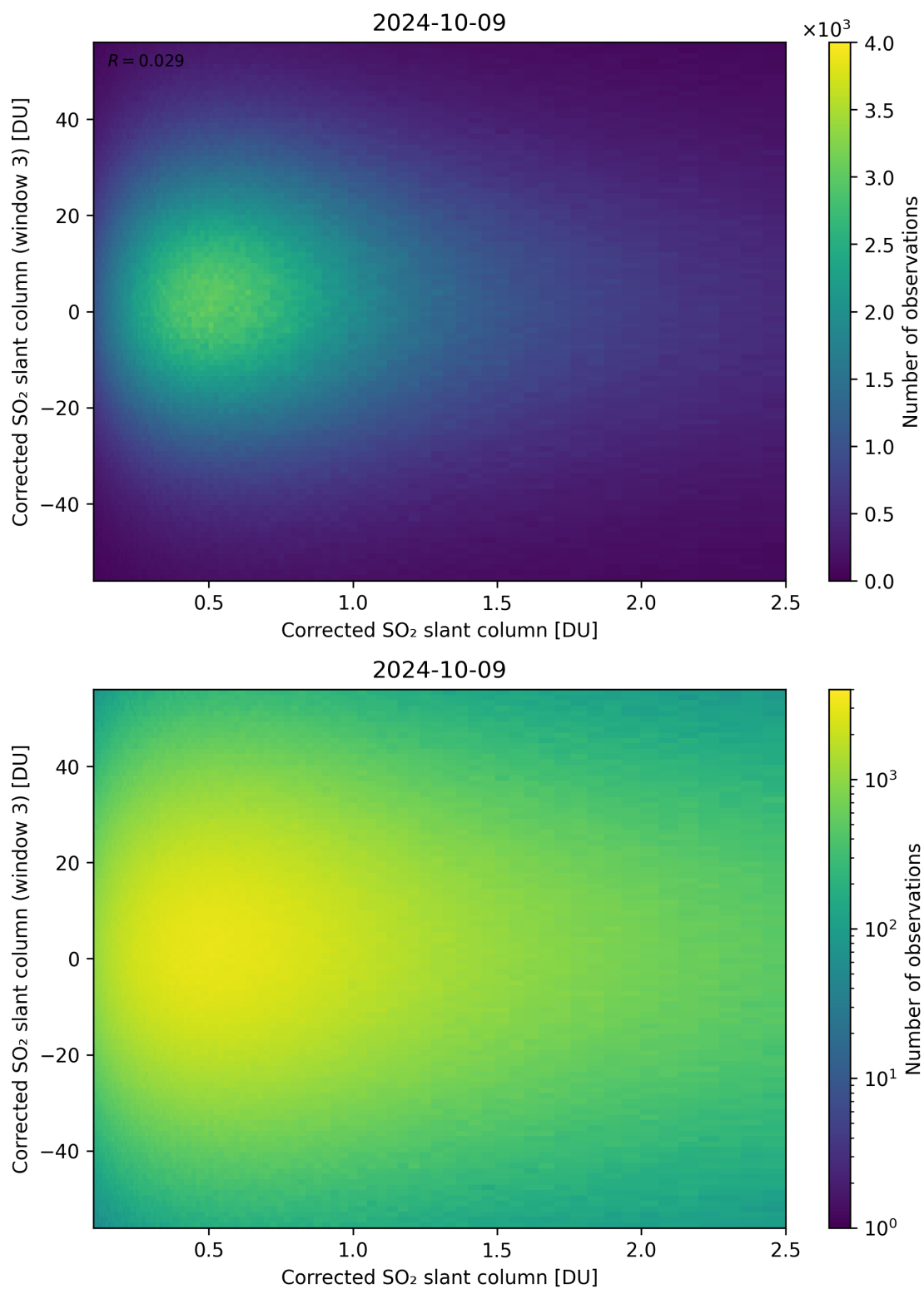
Figure 186: Scatter density plot of “Corrected SO 2 slant column” against “Corrected SO 2 slant column (window 3)” for 2024-10-08 to 2024-10-10.
