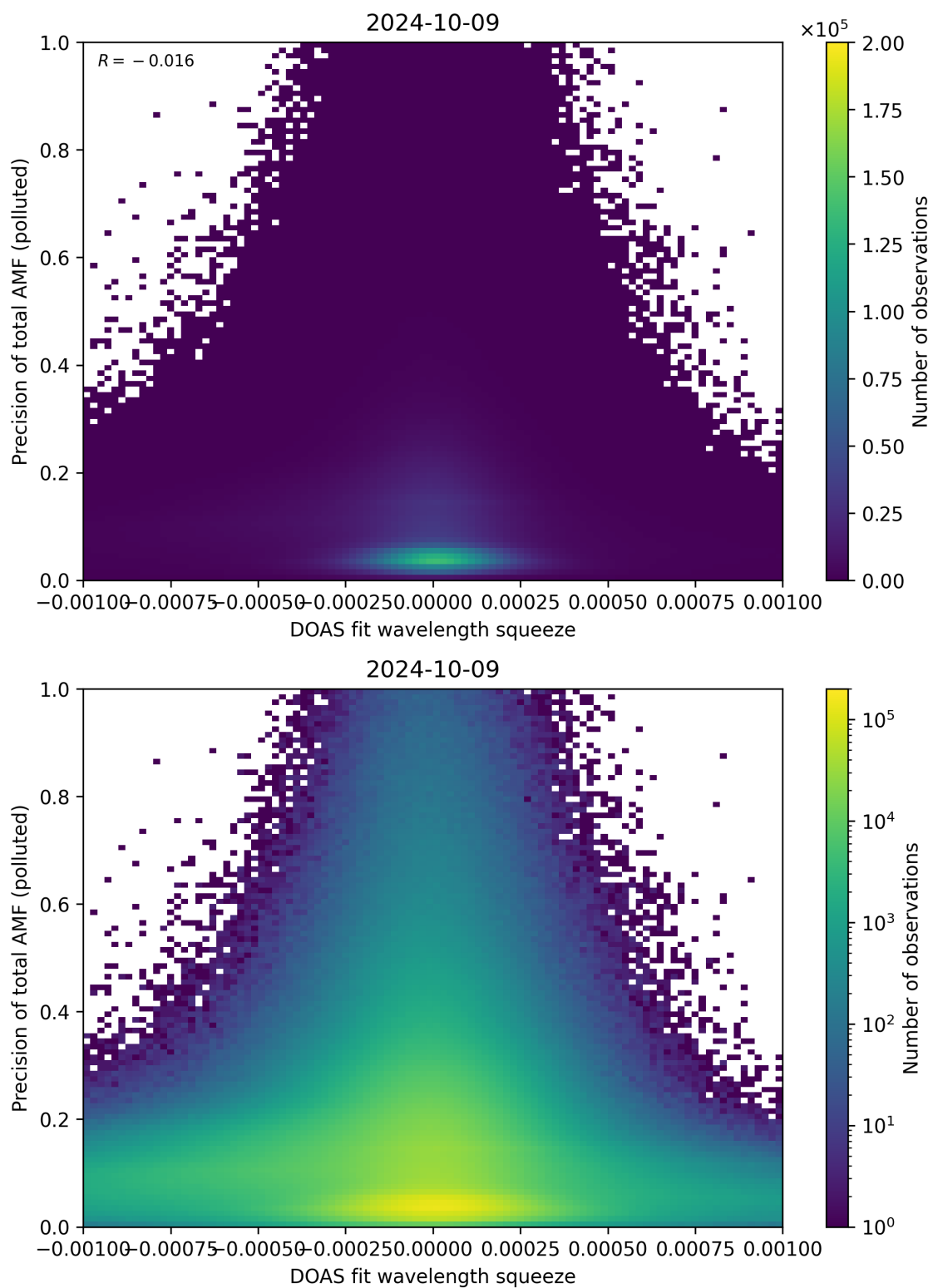
Figure 135: Scatter density plot of “DOAS fit wavelength squeeze” against “Precision of total AMF (polluted)” for 2024-10-08 to 2024-10-10.
