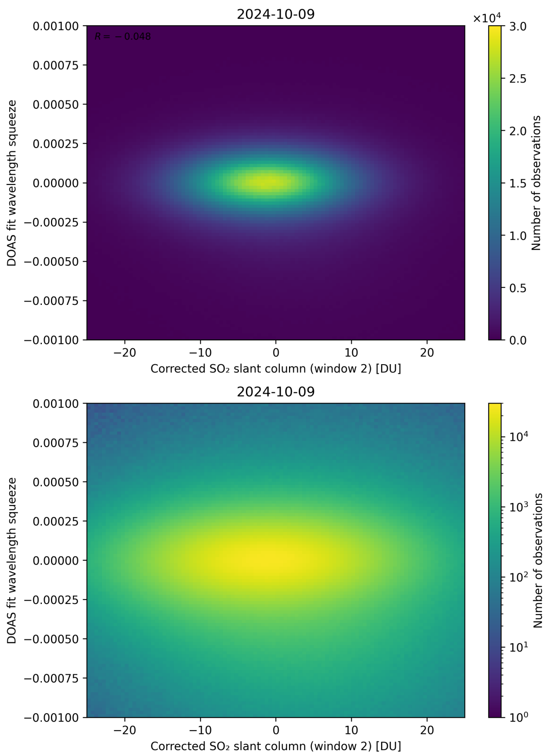
Figure 197: Scatter density plot of “Corrected SO 2 slant column (window 2)” against “DOAS fit wavelength squeeze” for 2024-10-08 to 2024-10-10.
