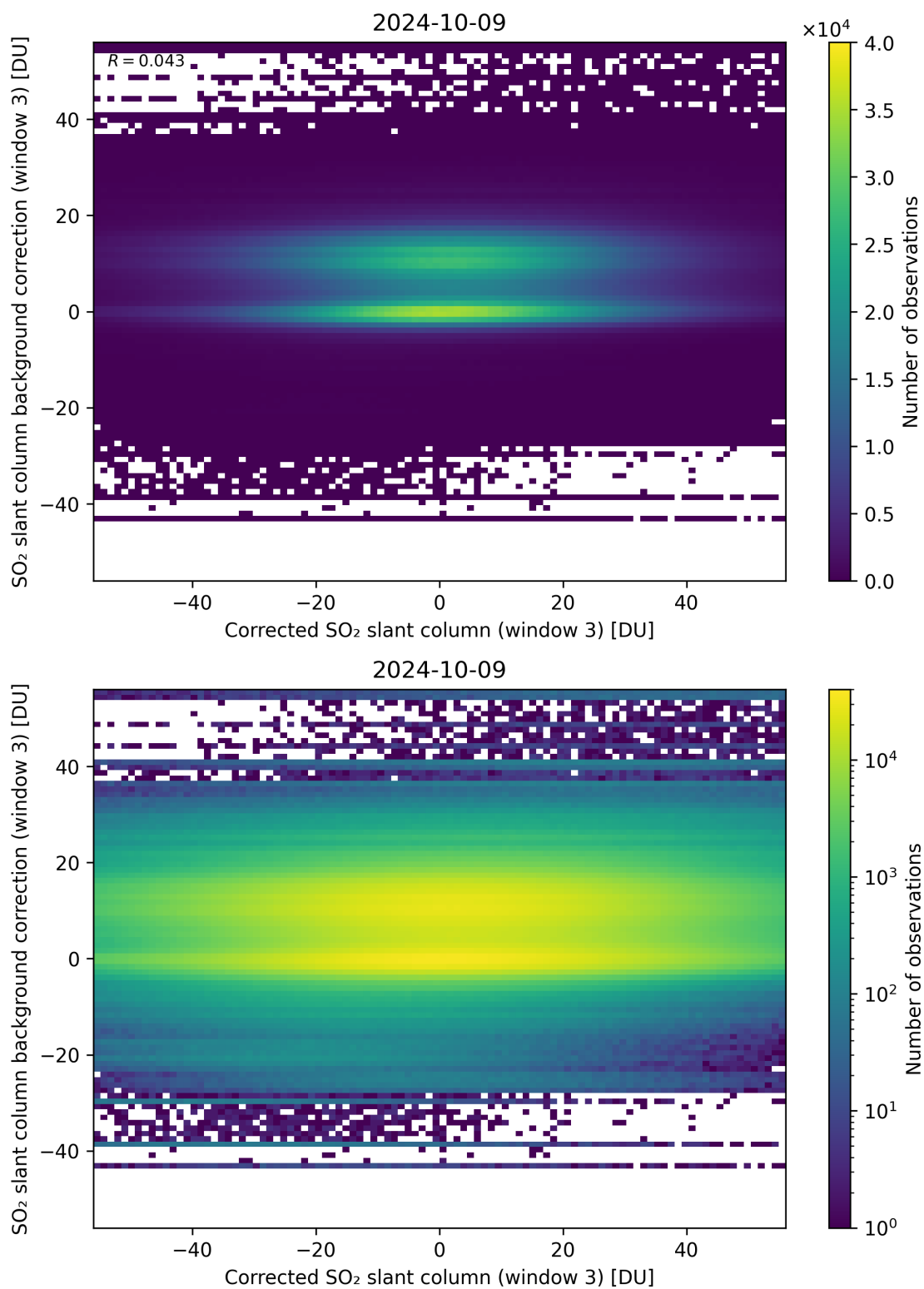
Figure 205: Scatter density plot of “Corrected SO 2 slant column (window 3)” against “SO 2 slant column background correction (window 3)” for 2024-10-08 to 2024-10-10.
