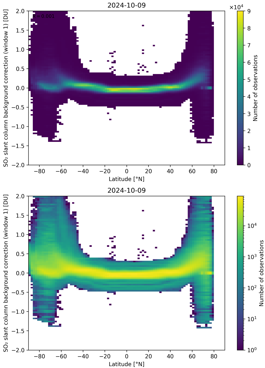
Figure 139: Scatter density plot of “Latitude” against “SO 2 slant column background correction (window 1)” for 2024-10-08 to 2024-10-10.
