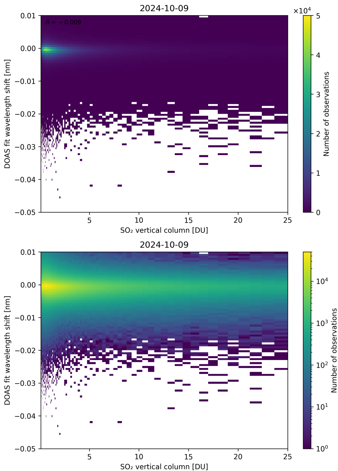
Figure 276: Scatter density plot of “SO 2 vertical column” against “DOAS fit wavelength shift” for 2024-10-08 to 2024-10-10.
