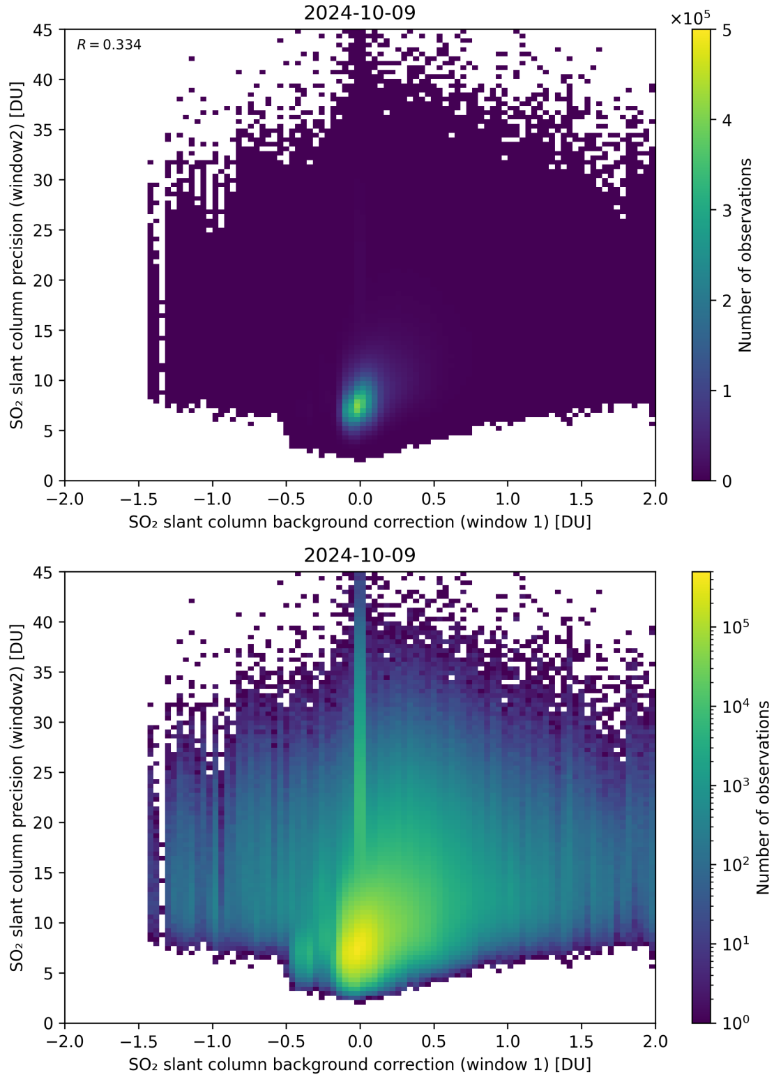
Figure 106: Scatter density plot of “SO 2 slant column background correction (window 1)” against “SO 2 slant column precision (window2)” for 2024-10-08 to 2024-10-10.
