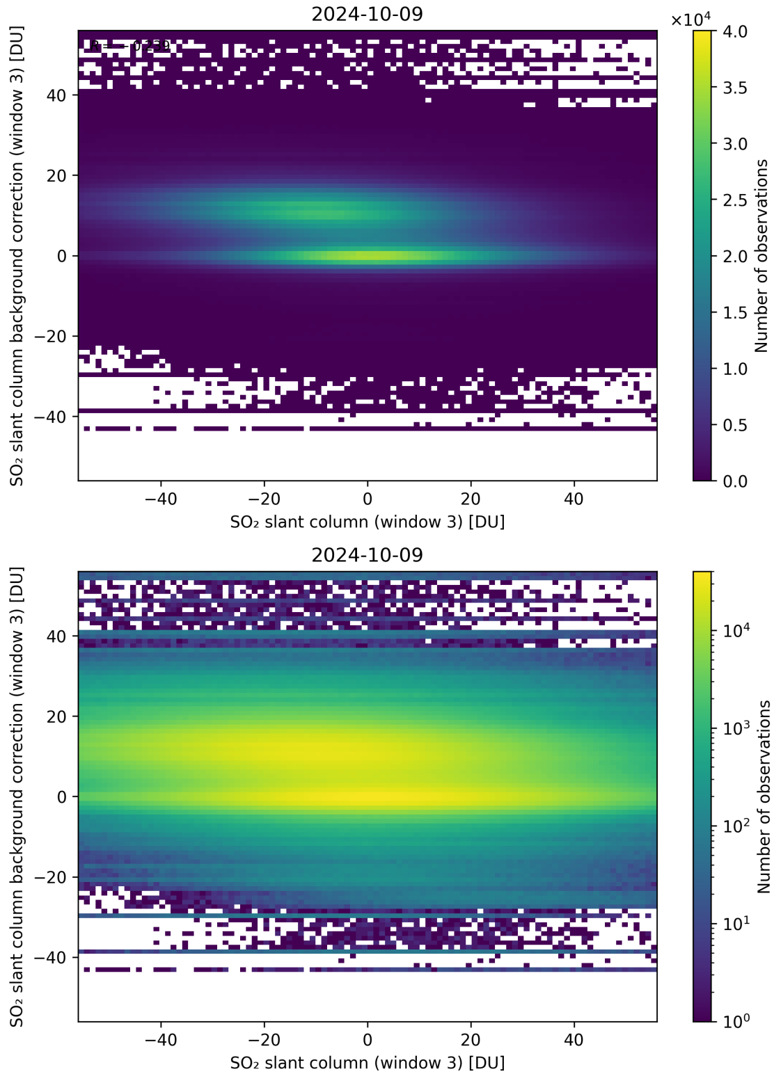
Figure 253: Scatter density plot of “SO 2 slant column (window 3)” against “SO 2 slant column background correction (window 3)” for 2024-10-08 to 2024-10-10.
