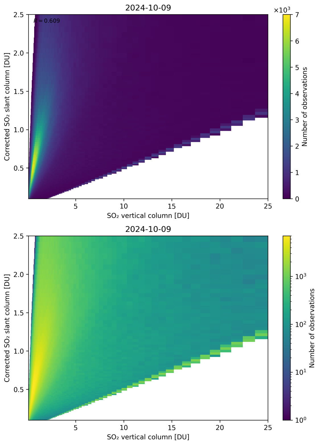
Figure 297: Scatter density plot of “SO 2 vertical column” against “Corrected SO 2 slant column” for 2024-10-08 to 2024-10-10.
