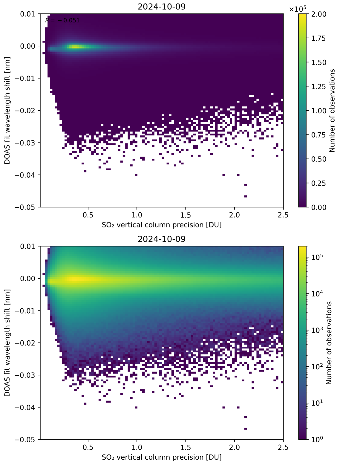
Figure 282: Scatter density plot of “SO 2 vertical column precision” against “DOAS fit wavelength shift” for 2024-10-08 to 2024-10-10.
