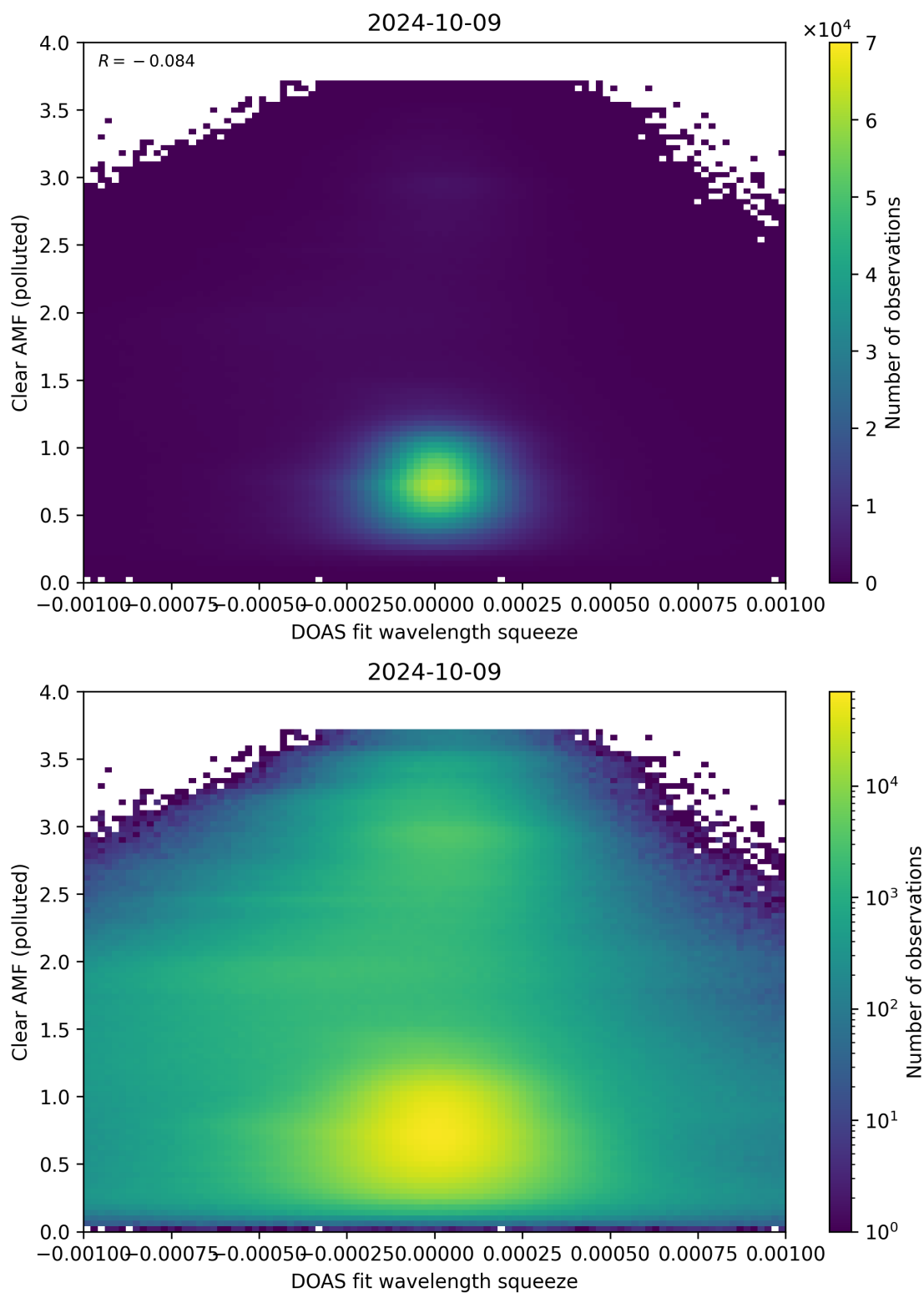
Figure 133: Scatter density plot of “DOAS fit wavelength squeeze” against “Clear AMF (polluted)” for 2024-10-08 to 2024-10-10.
