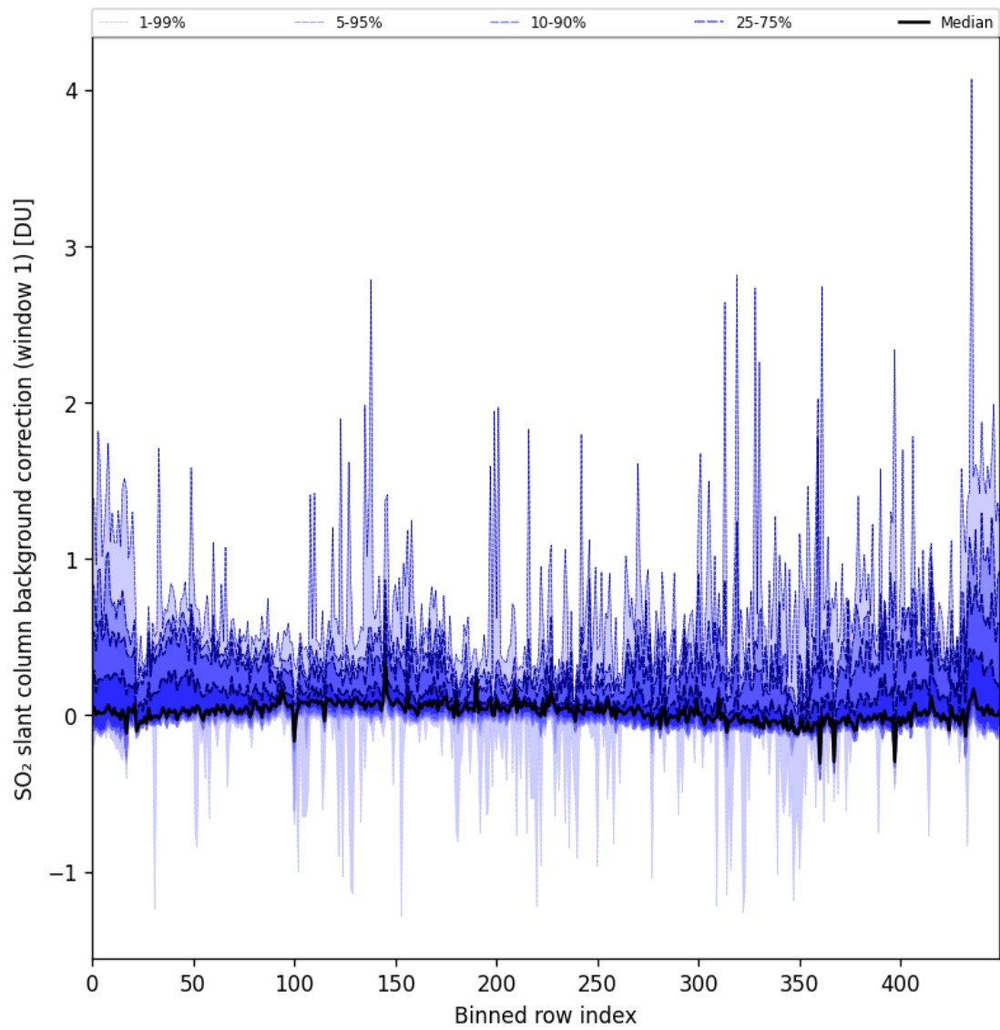
Figure 82: Along track statistics of “SO 2 slant column background correction (window 1)” for 2024-10-08 to 2024-10-10
