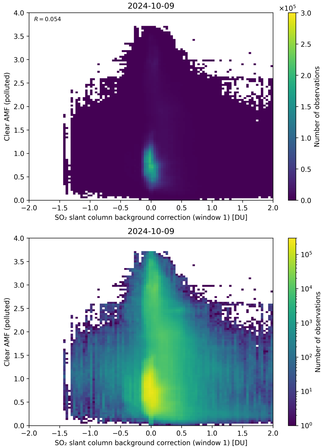
Figure 103: Scatter density plot of “SO 2 slant column background correction (window 1)” against “Clear AMF (polluted)” for 2024-10-08 to 2024-10-10.
