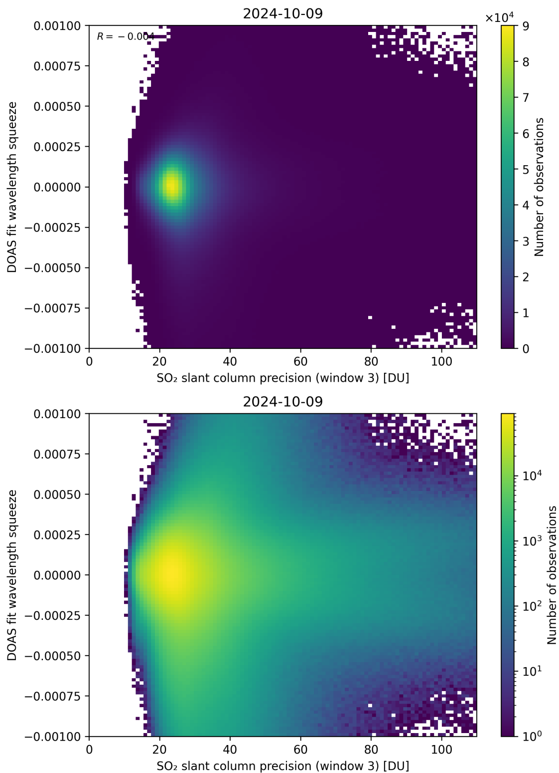
Figure 259: Scatter density plot of “SO 2 slant column precision (window 3)” against “DOAS fit wavelength squeeze” for 2024-10-08 to 2024-10-10.
