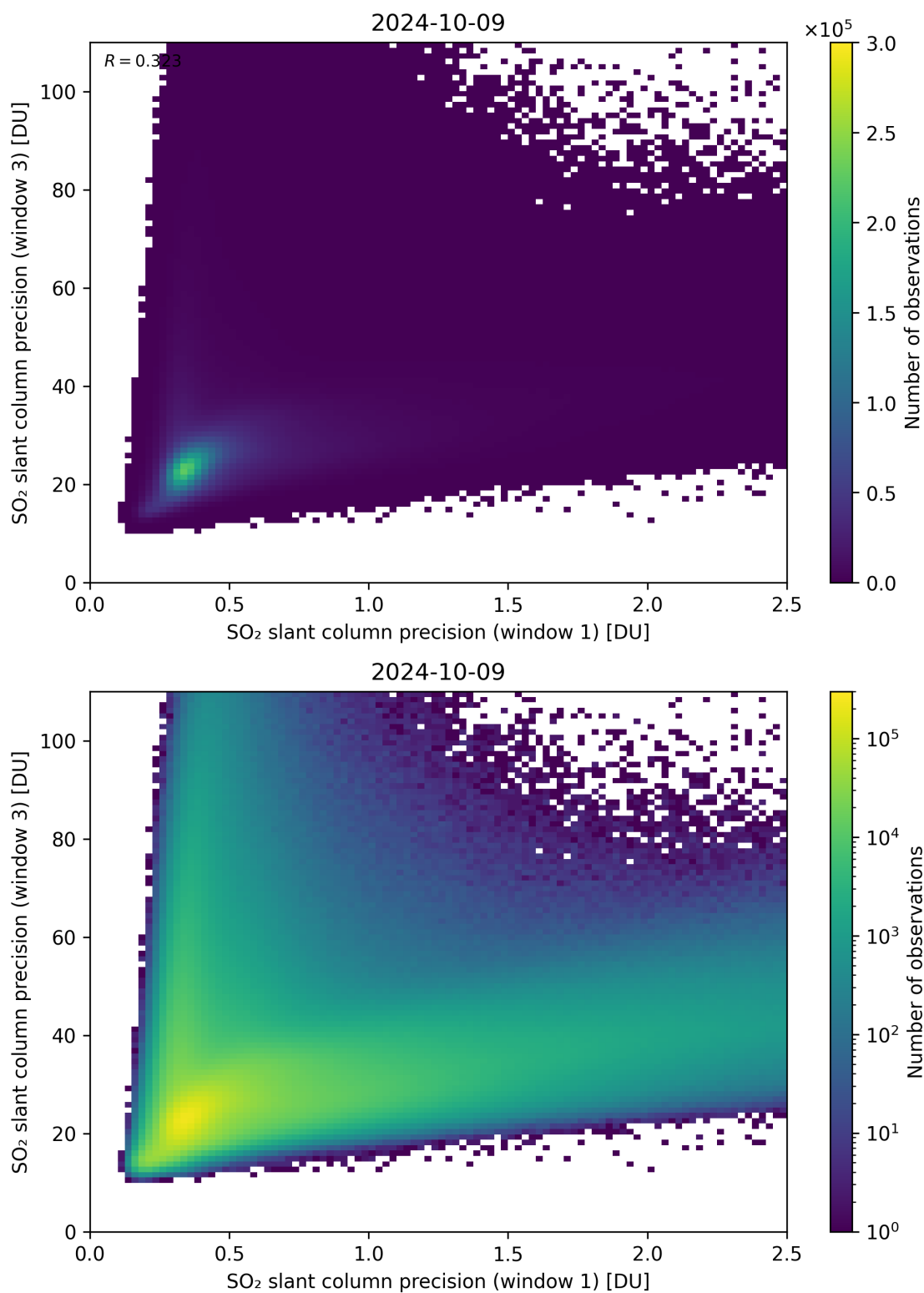
Figure 229: Scatter density plot of “SO 2 slant column precision (window 1)” against “SO 2 slant column precision (window 3)” for 2024-10-08 to 2024-10-10.
