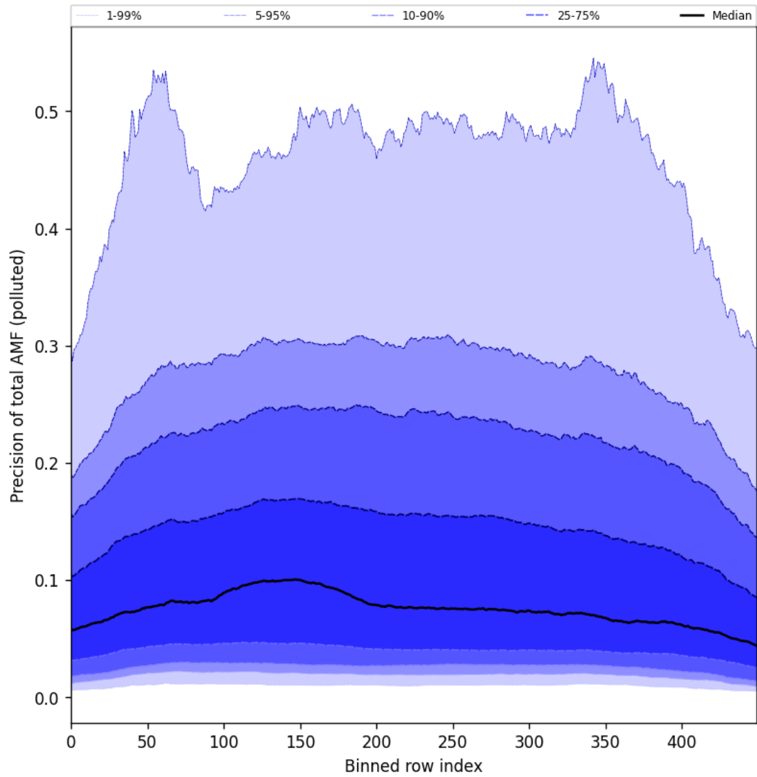
Figure 95: Along track statistics of “Precision of total AMF (polluted)” for 2024-10-08 to 2024-10-10
