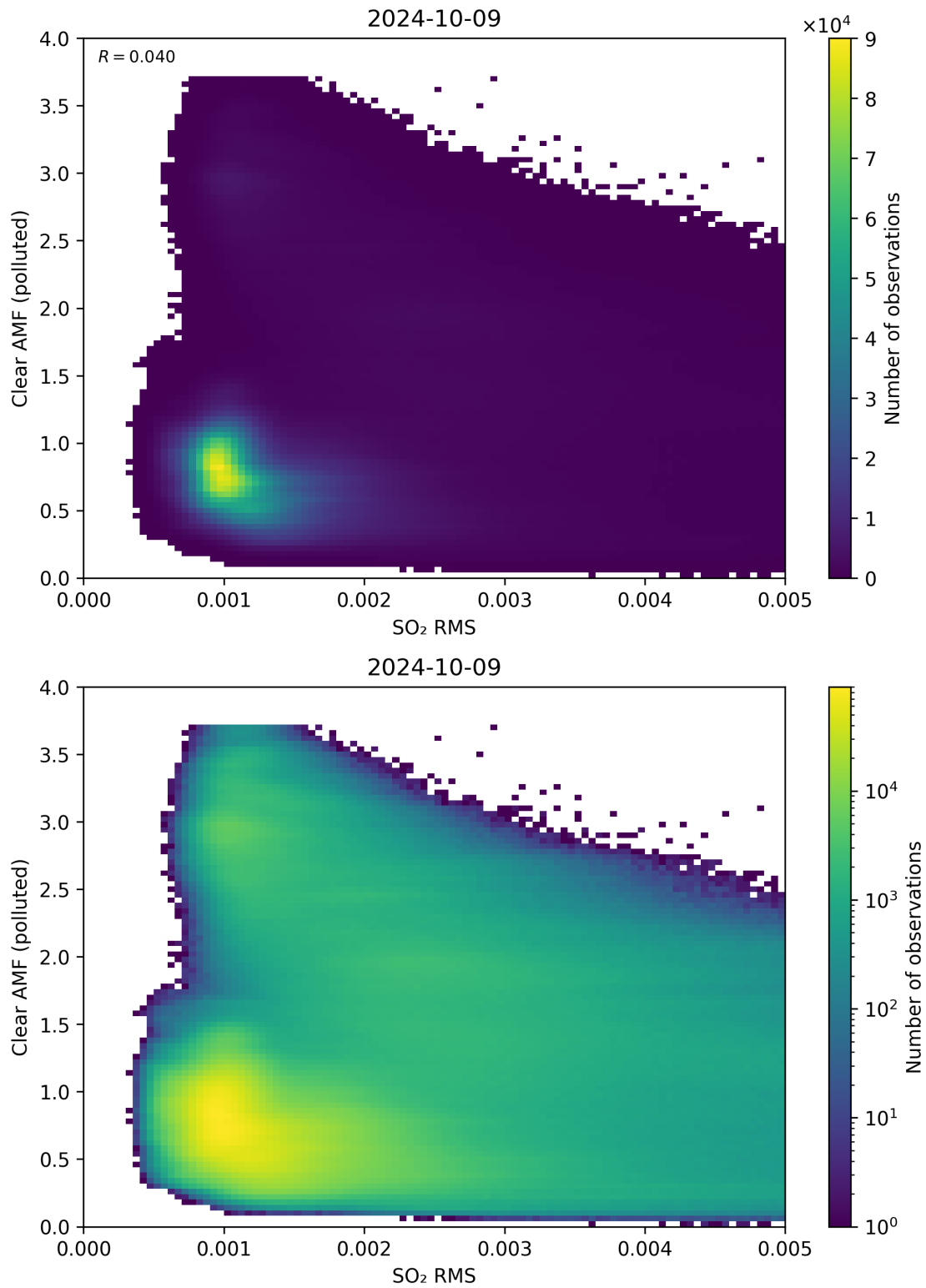
Figure 136: Scatter density plot of “SO 2 RMS” against “Clear AMF (polluted)” for 2024-10-08 to 2024-10-10.
