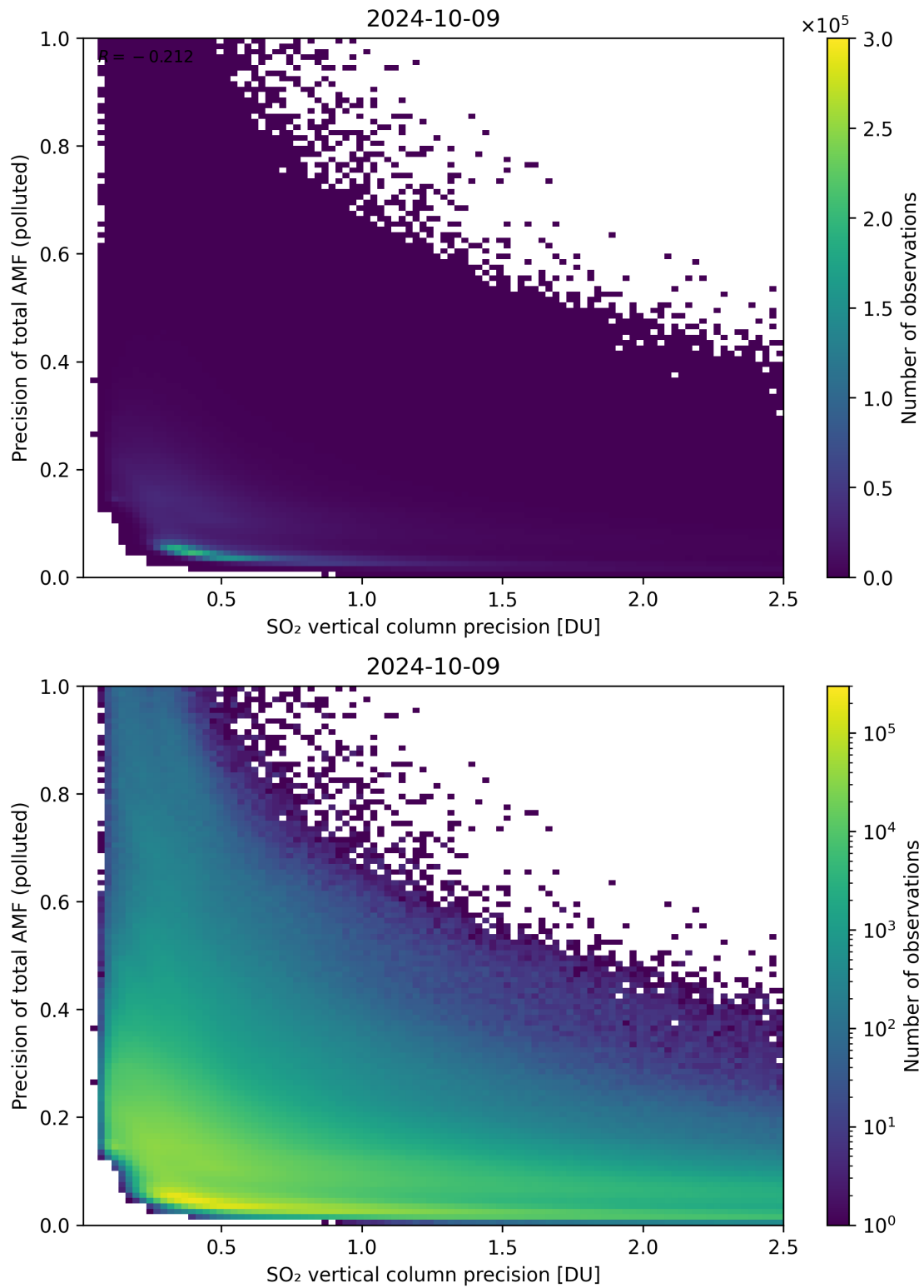
Figure 295: Scatter density plot of “SO 2 vertical column precision” against “Precision of total AMF (polluted)” for 2024-10-08 to 2024-10-10.
