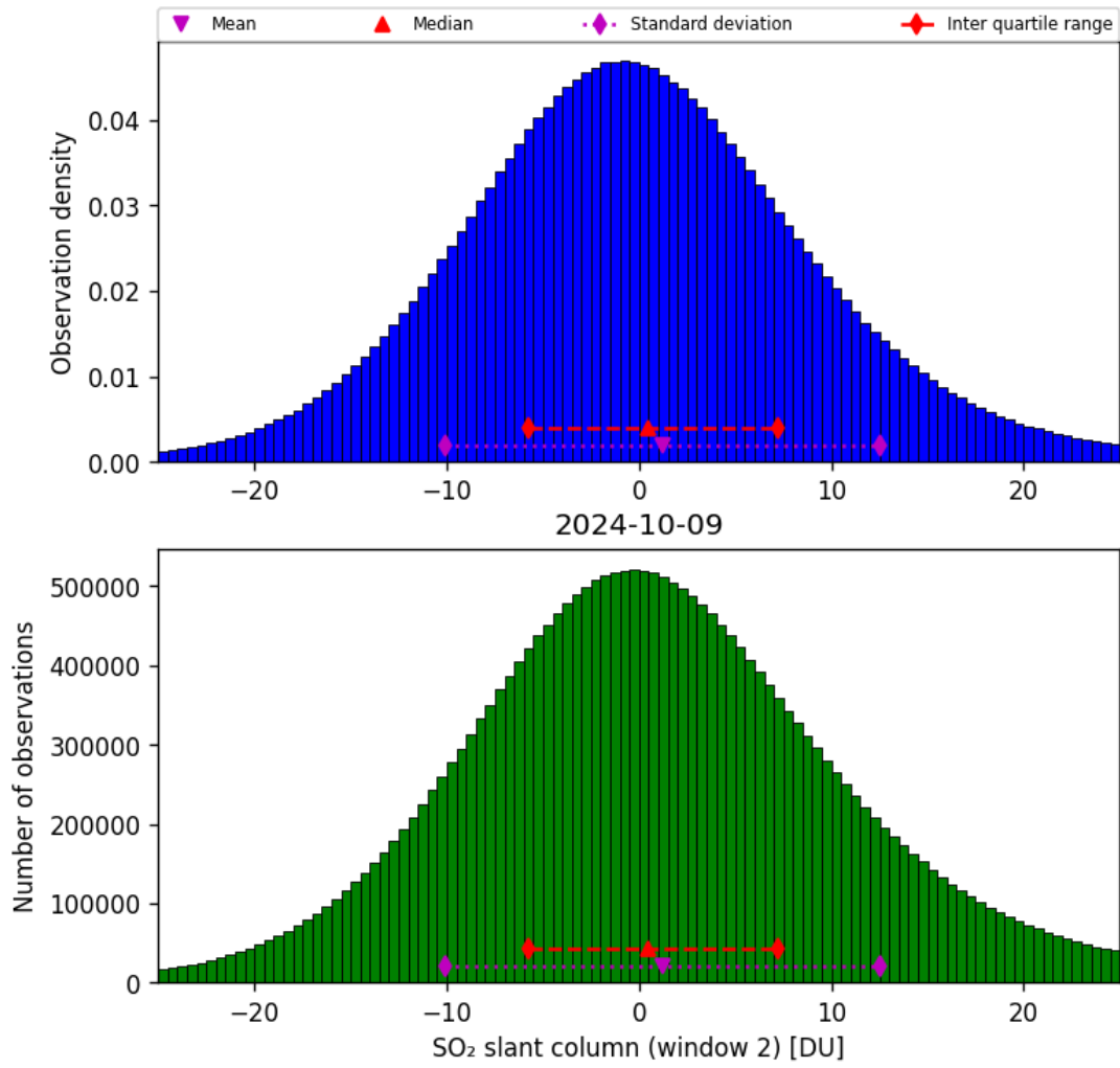
Figure 60: Histogram of “SO 2 slant column (window 2)” for 2024-10-08 to 2024-10-10
