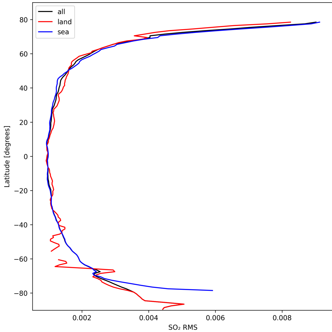
Figure 47: Zonal average of “SO 2 RMS” for 2024-10-08 to 2024-10-10.
