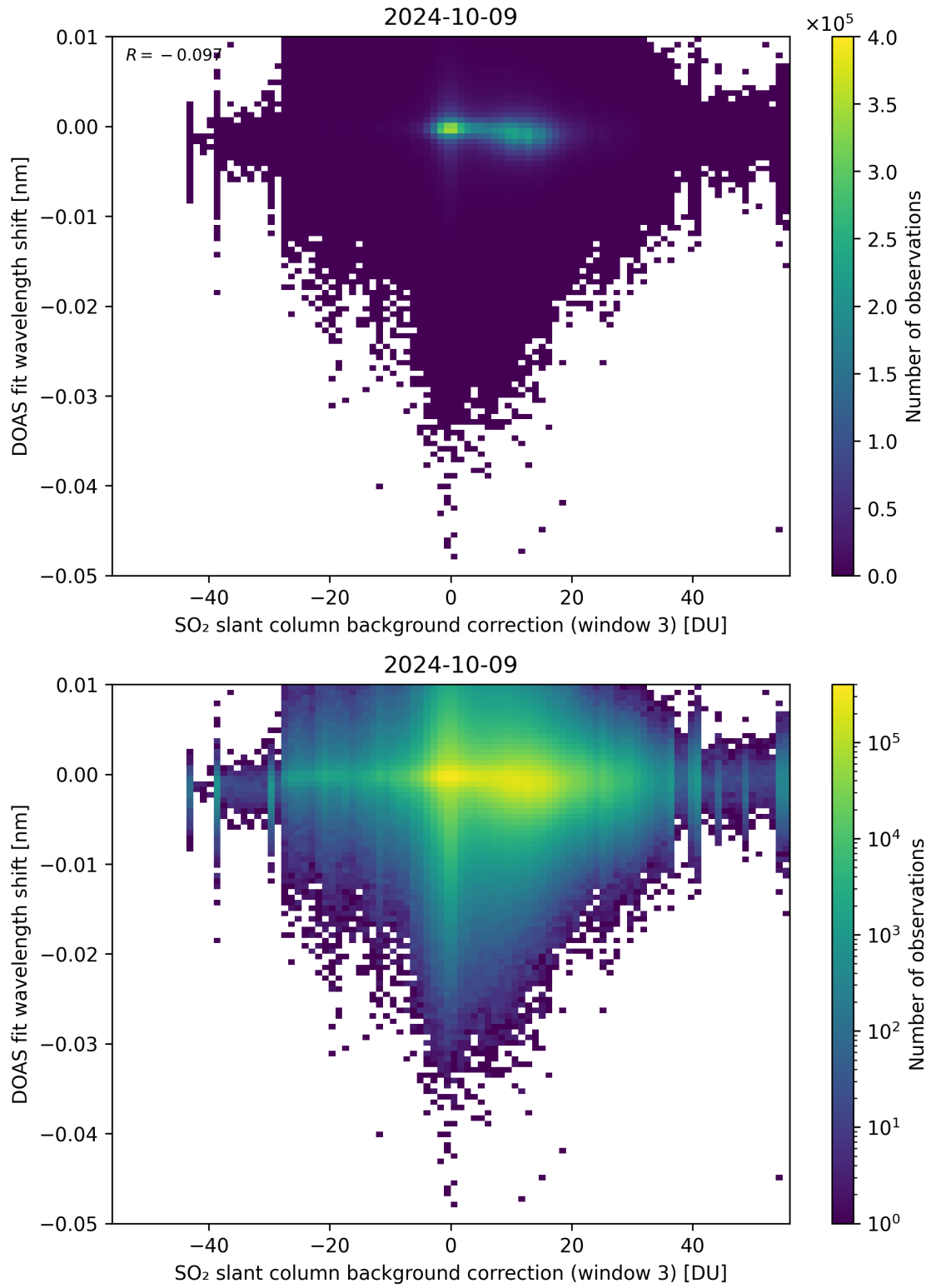
Figure 121: Scatter density plot of “SO 2 slant column background correction (window 3)” against “DOAS fit wavelength shift” for 2024-10-08 to 2024-10-10.
