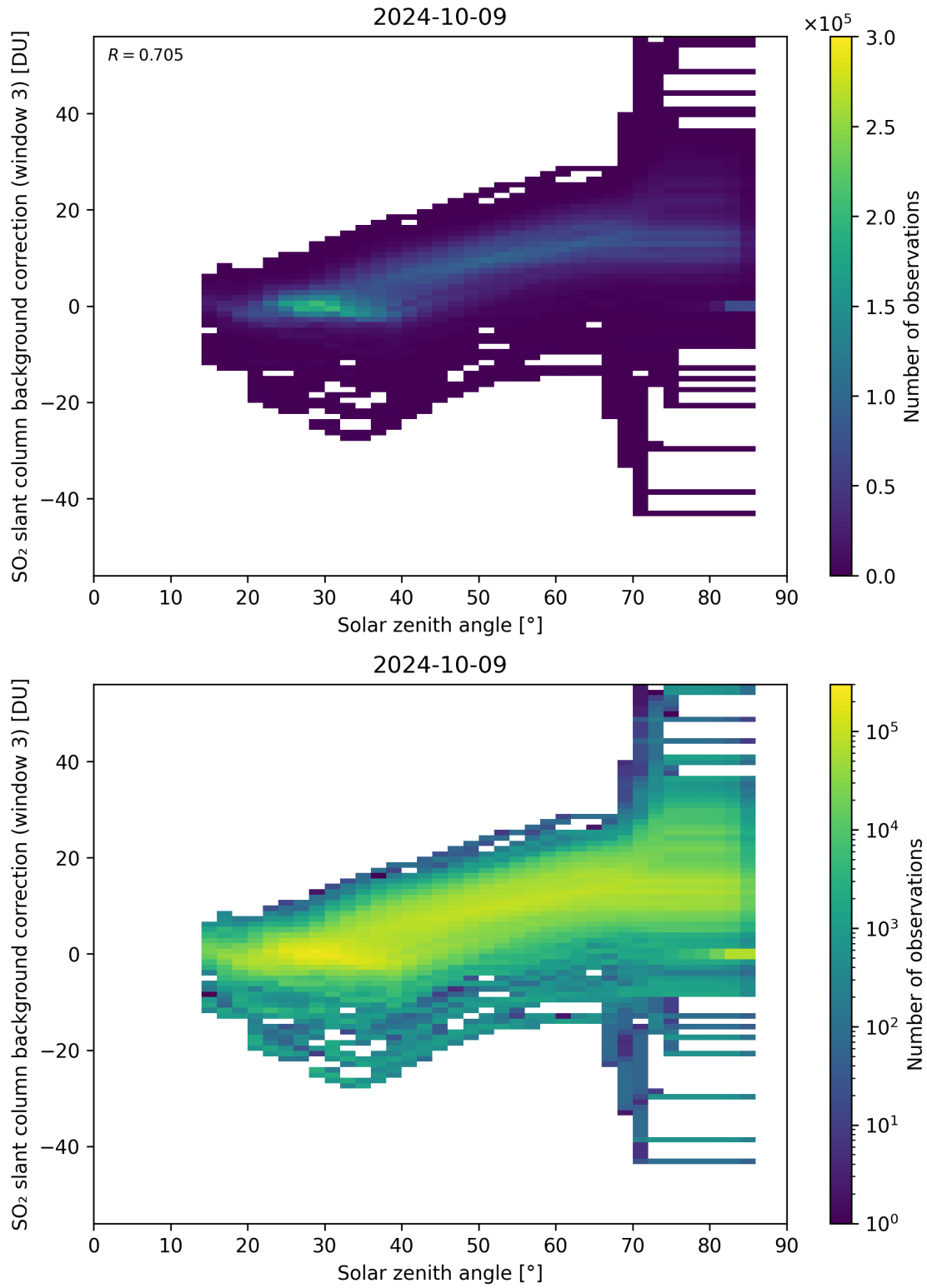
Figure 160: Scatter density plot of “Solar zenith angle” against “SO 2 slant column background correction (window 3)” for 2024-10-08 to 2024-10-10.
