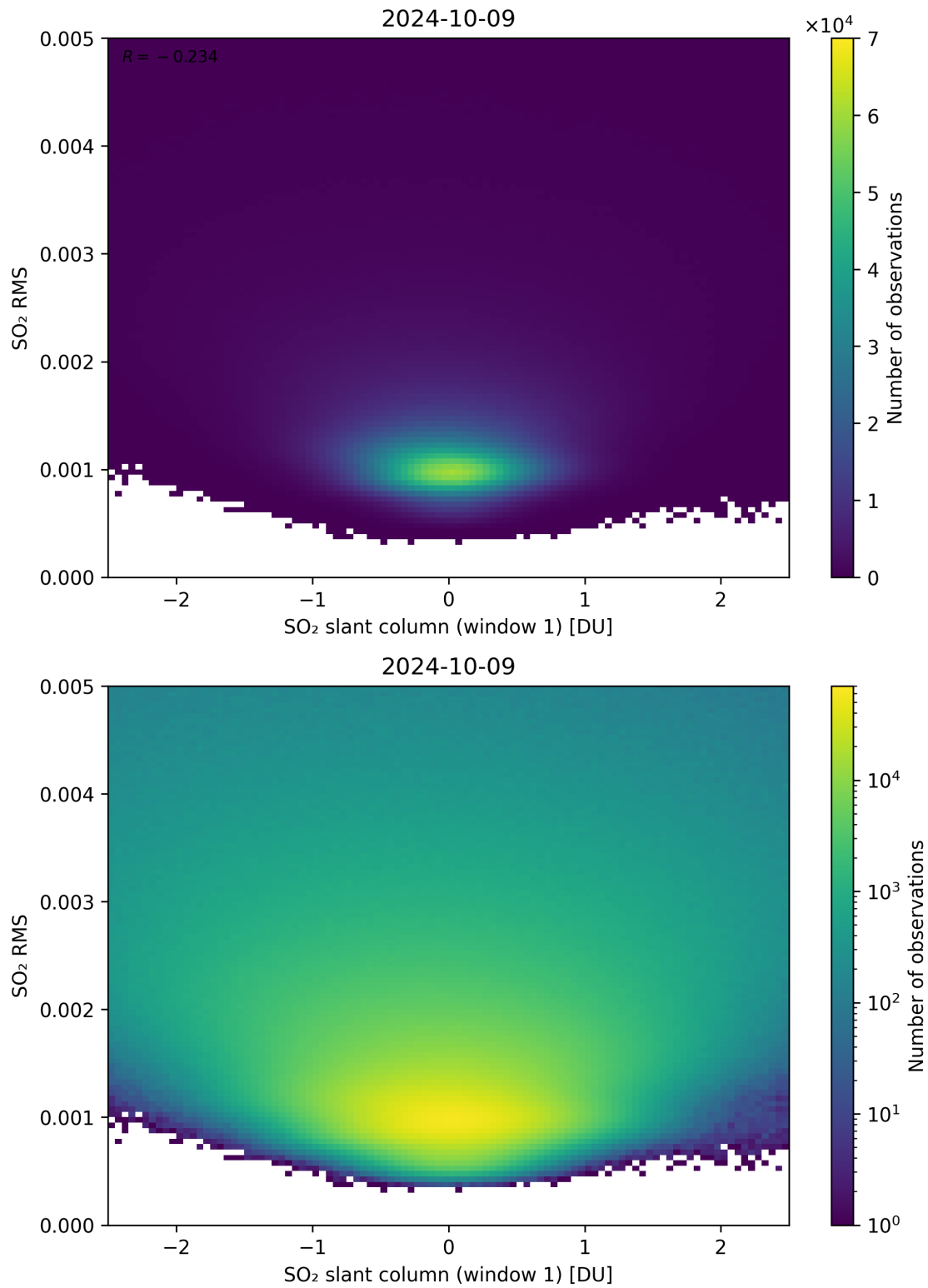
Figure 217: Scatter density plot of “SO 2 slant column (window 1)” against “SO 2 RMS” for 2024-10-08 to 2024-10-10.
