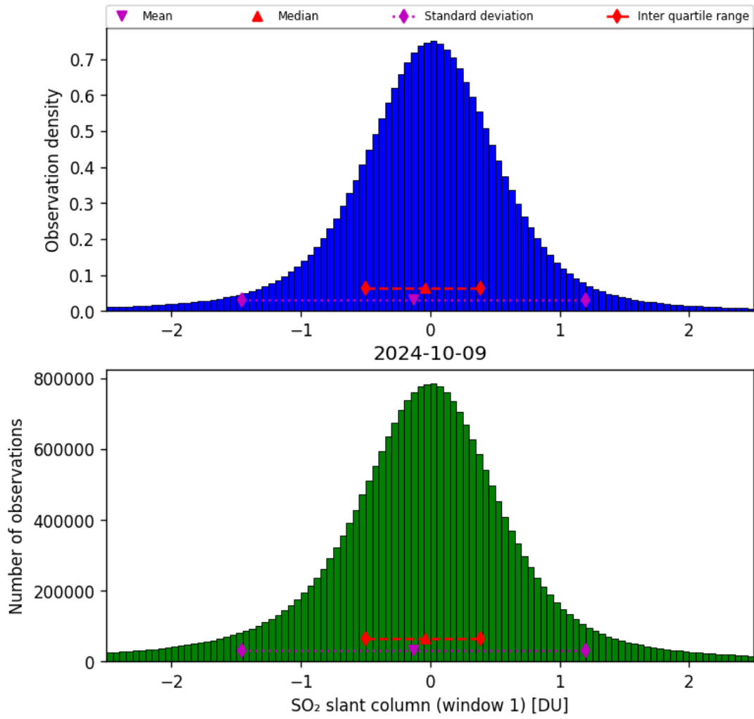
Figure 56: Histogram of “SO 2 slant column (window 1)” for 2024-10-08 to 2024-10-10
