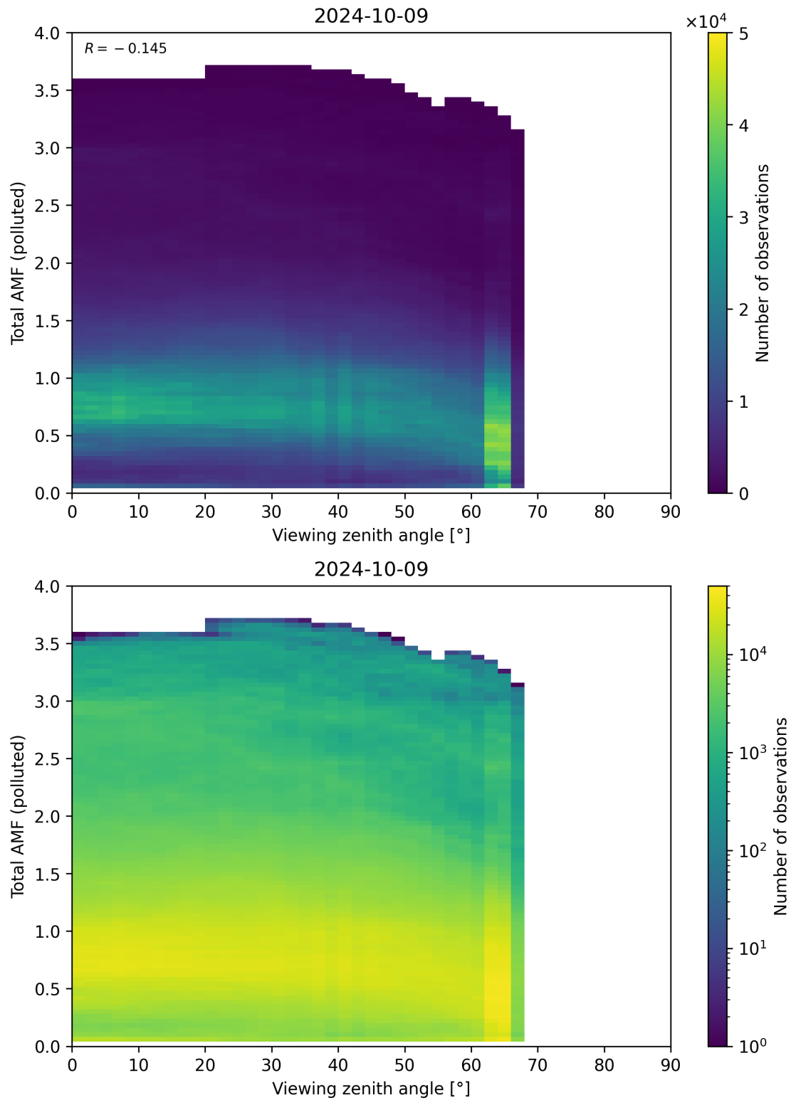
Figure 325: Scatter density plot of “Viewing zenith angle” against “Total AMF (polluted)” for 2024-10-08 to 2024-10-10.
