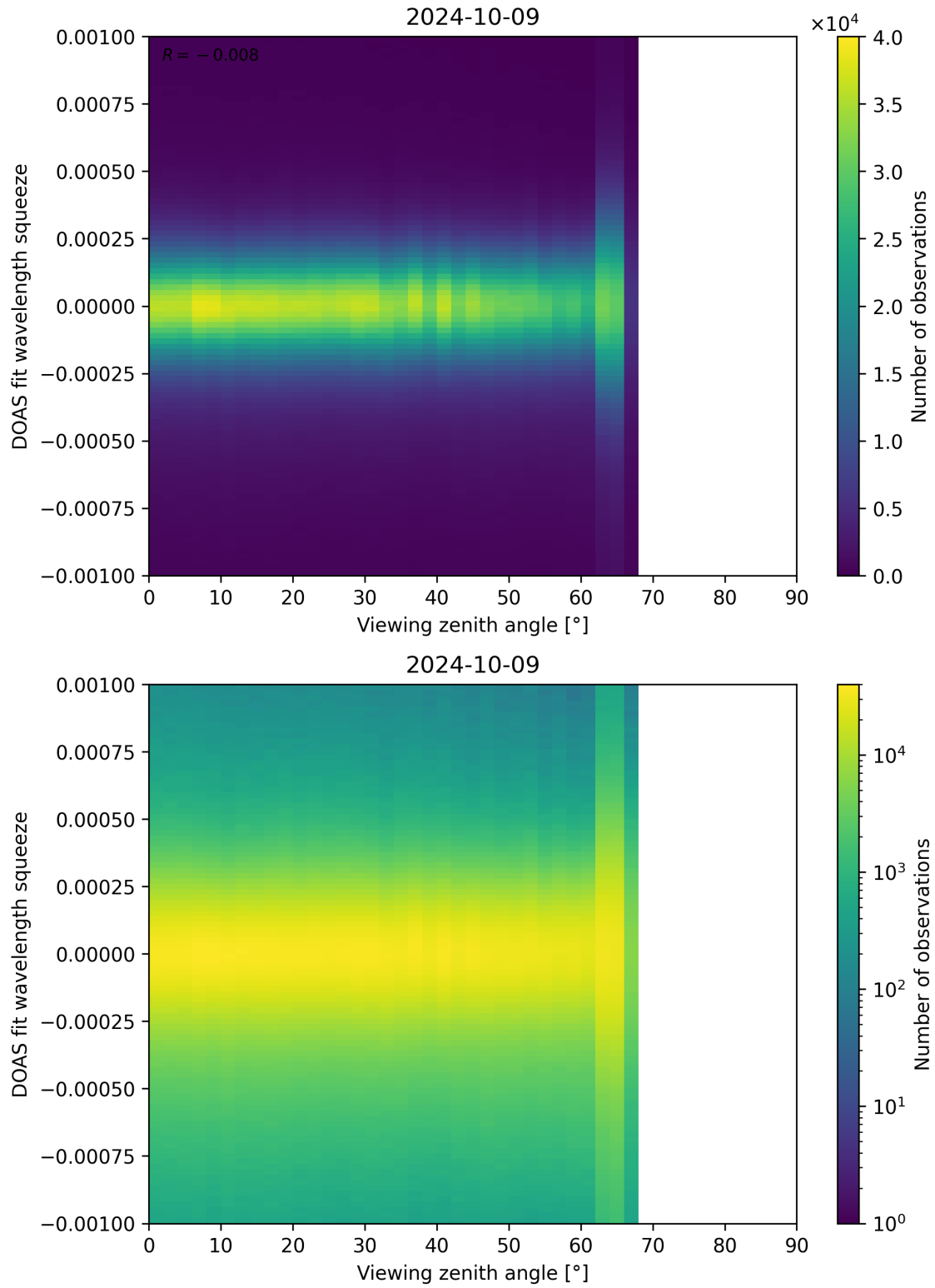
Figure 312: Scatter density plot of “Viewing zenith angle” against “DOAS fit wavelength squeeze” for 2024-10-08 to 2024-10-10.
