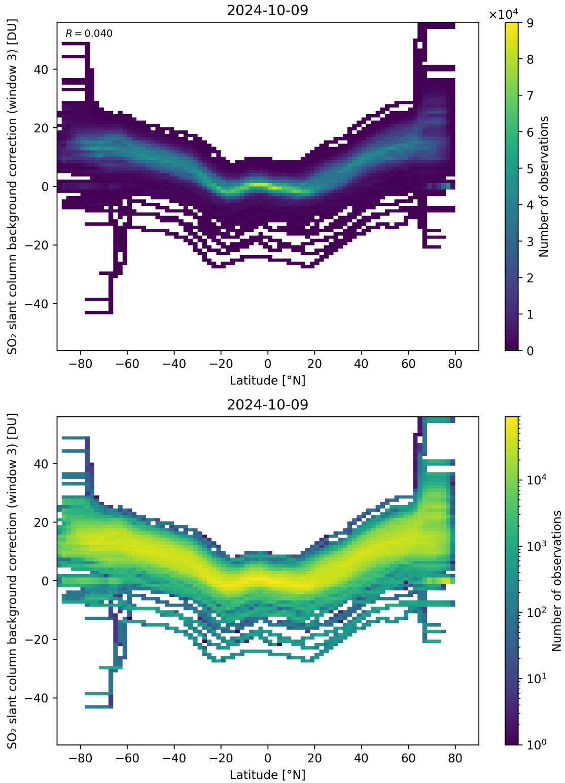
Figure 141: Scatter density plot of “Latitude” against “SO 2 slant column background correction (window 3)” for 2024-10-08 to 2024-10-10.
