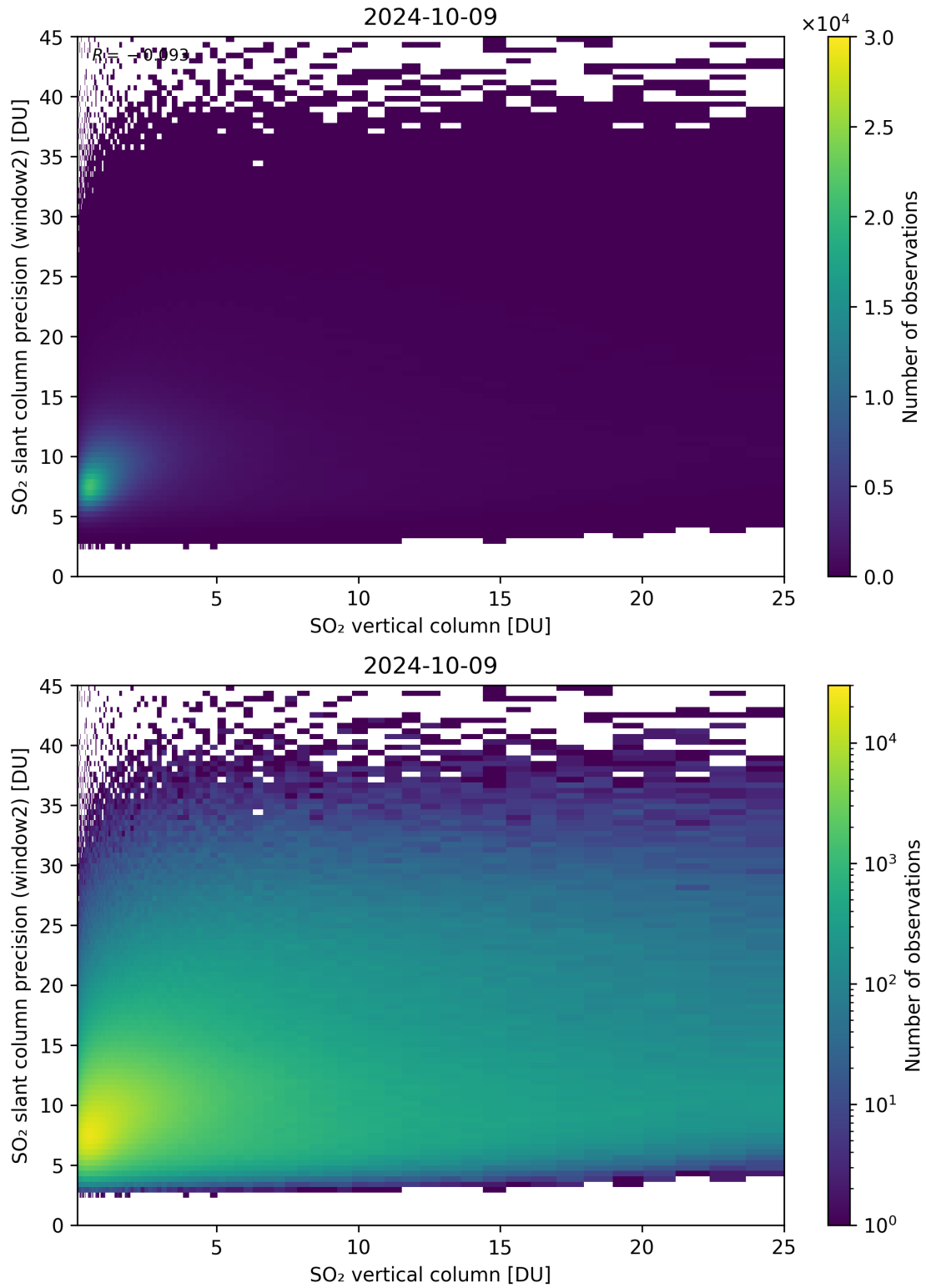
Figure 302: Scatter density plot of “SO 2 vertical column” against “SO 2 slant column precision (window2)” for 2024-10-08 to 2024-10-10.
