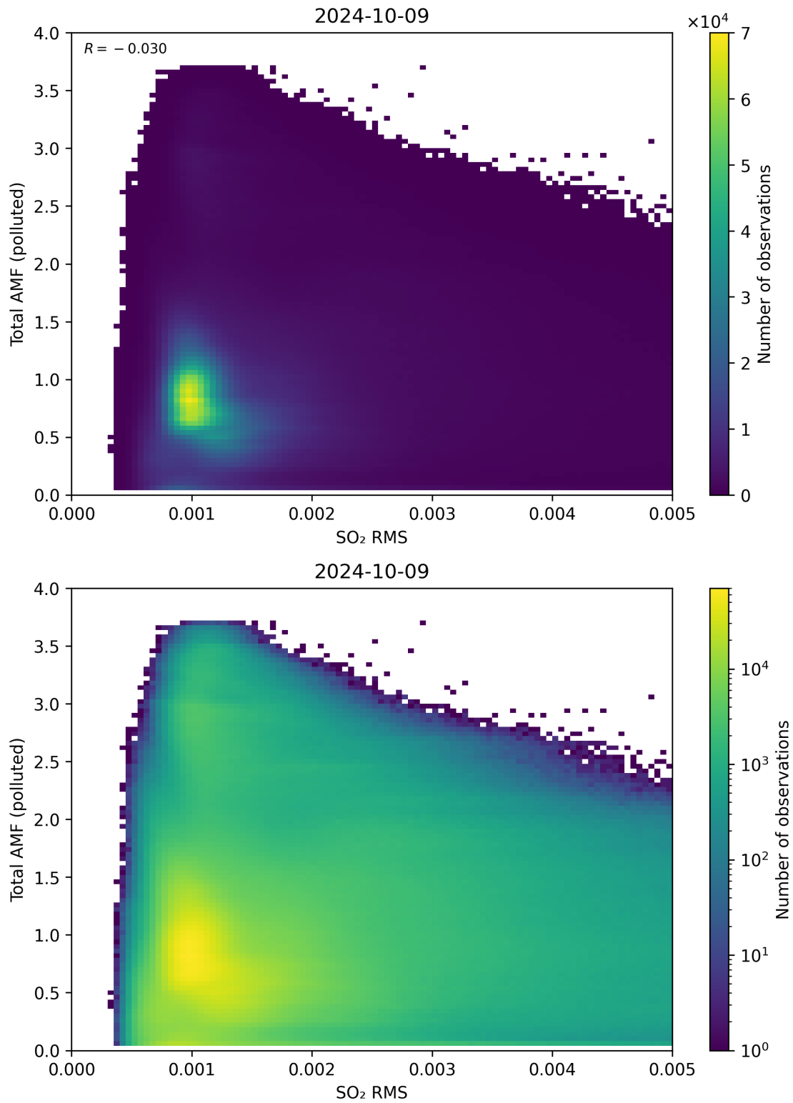
Figure 137: Scatter density plot of “SO 2 RMS” against “Total AMF (polluted)” for 2024-10-08 to 2024-10-10.
