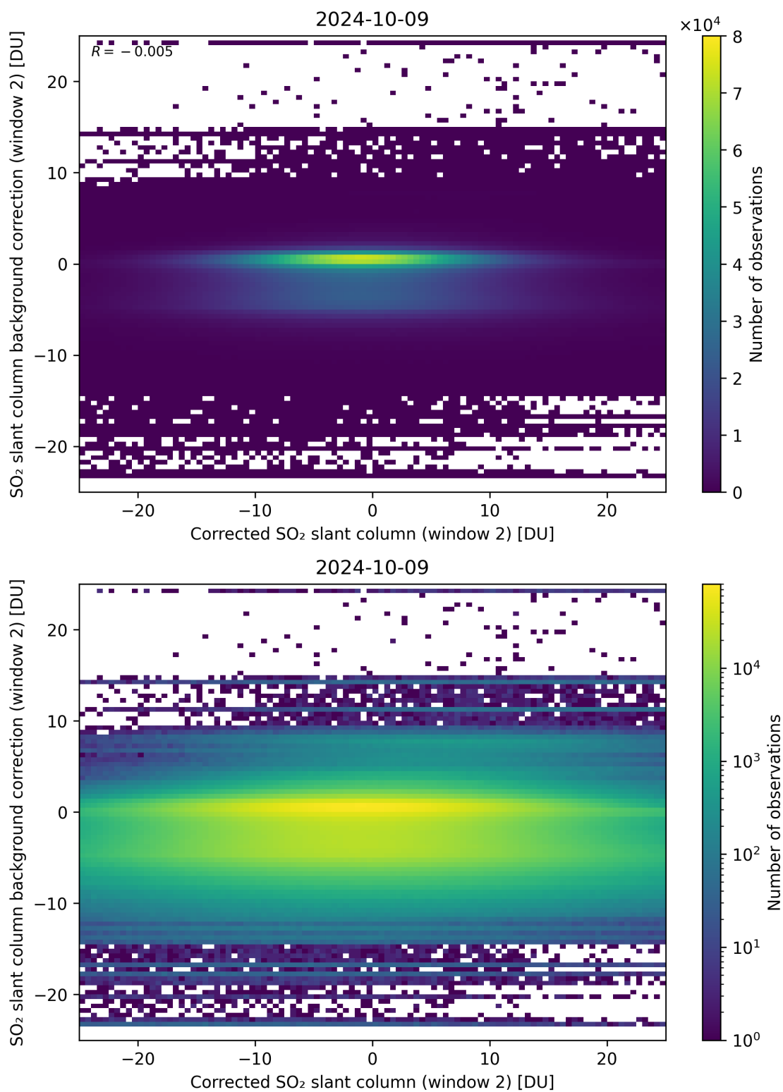
Figure 194: Scatter density plot of “Corrected SO 2 slant column (window 2)” against “SO 2 slant column background correction (window 2)” for 2024-10-08 to 2024-10-10.
