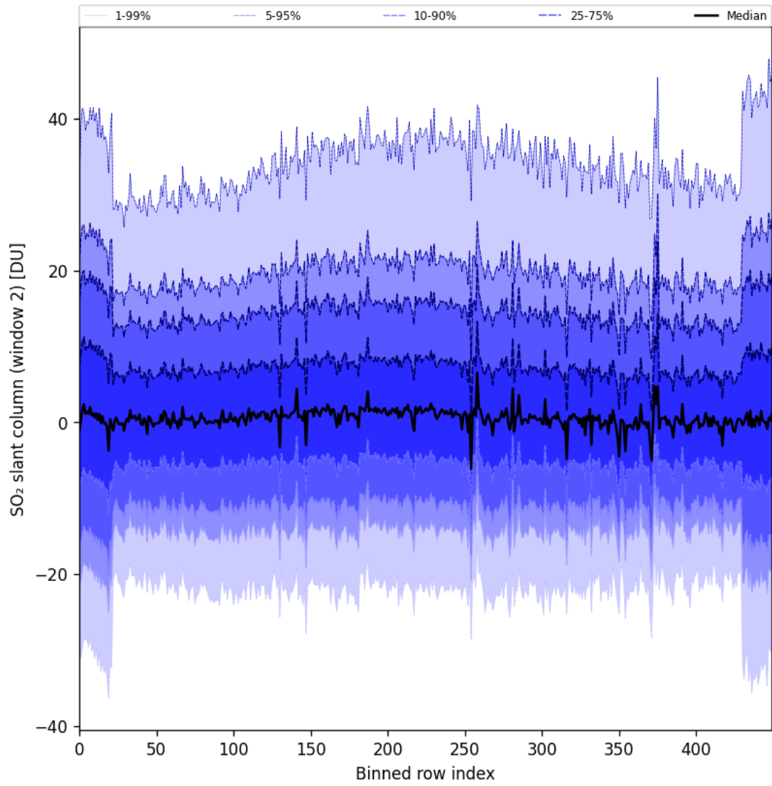
Figure 83: Along track statistics of “SO 2 slant column (window 2)” for 2024-10-08 to 2024-10-10
