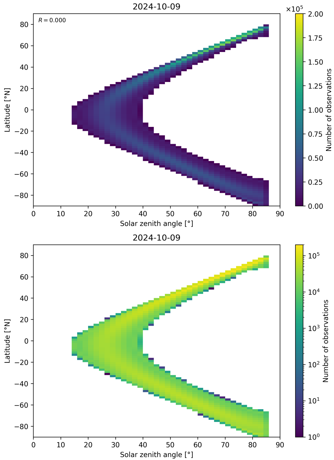
Figure 164: Scatter density plot of “Solar zenith angle” against “Latitude” for 2024-10-08 to 2024-10-10.
