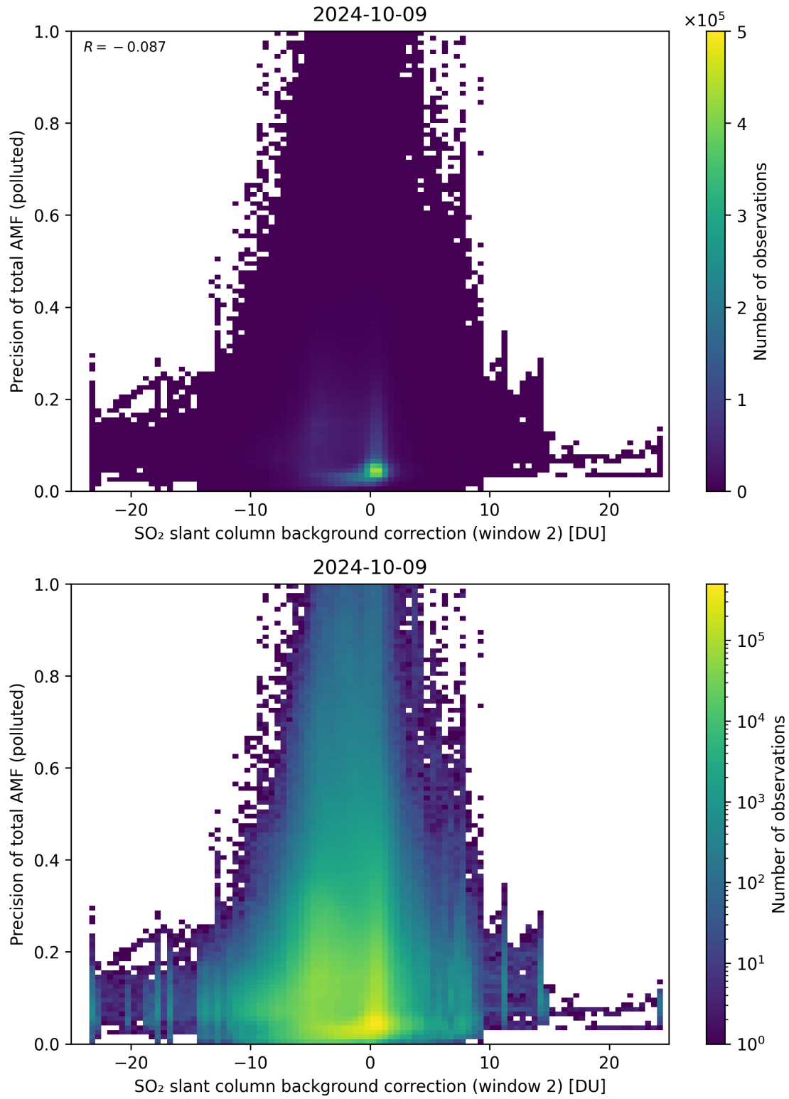
Figure 120: Scatter density plot of “SO 2 slant column background correction (window 2)” against “Precision of total AMF (polluted)” for 2024-10-08 to 2024-10-10.
