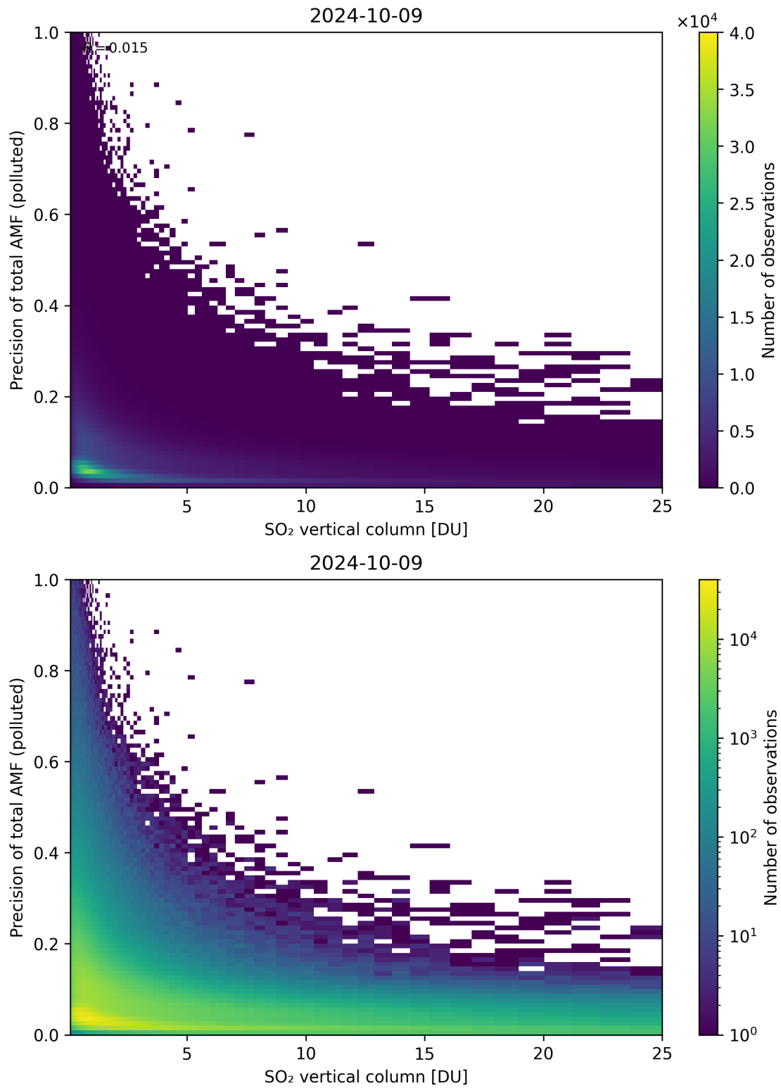
Figure 306: Scatter density plot of “SO 2 vertical column” against “Precision of total AMF (polluted)” for 2024-10-08 to 2024-10-10.
