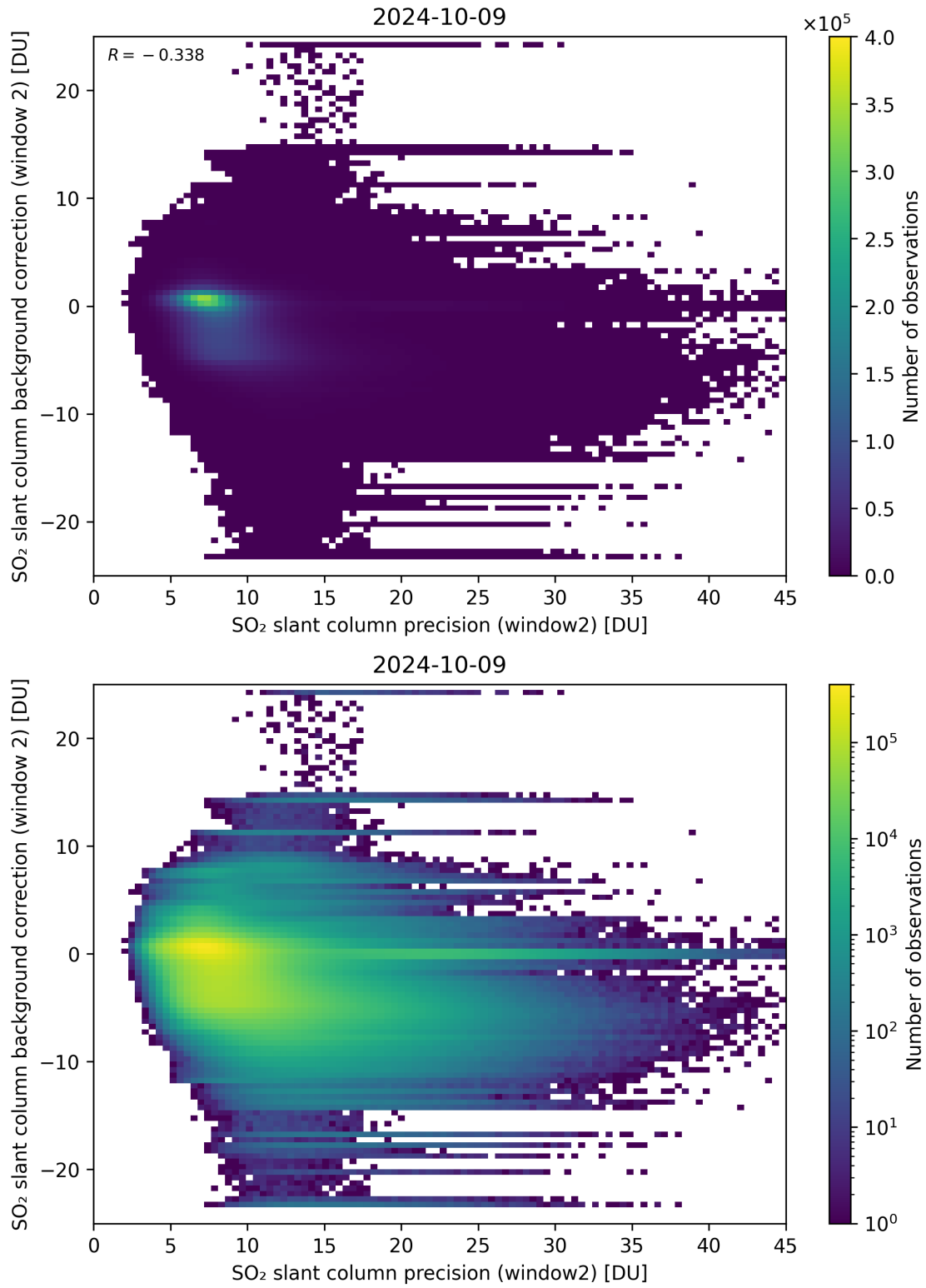
Figure 241: Scatter density plot of “SO 2 slant column precision (window2)” against “SO 2 slant column background correction (window 2)” for 2024-10-08 to 2024-10-10.
