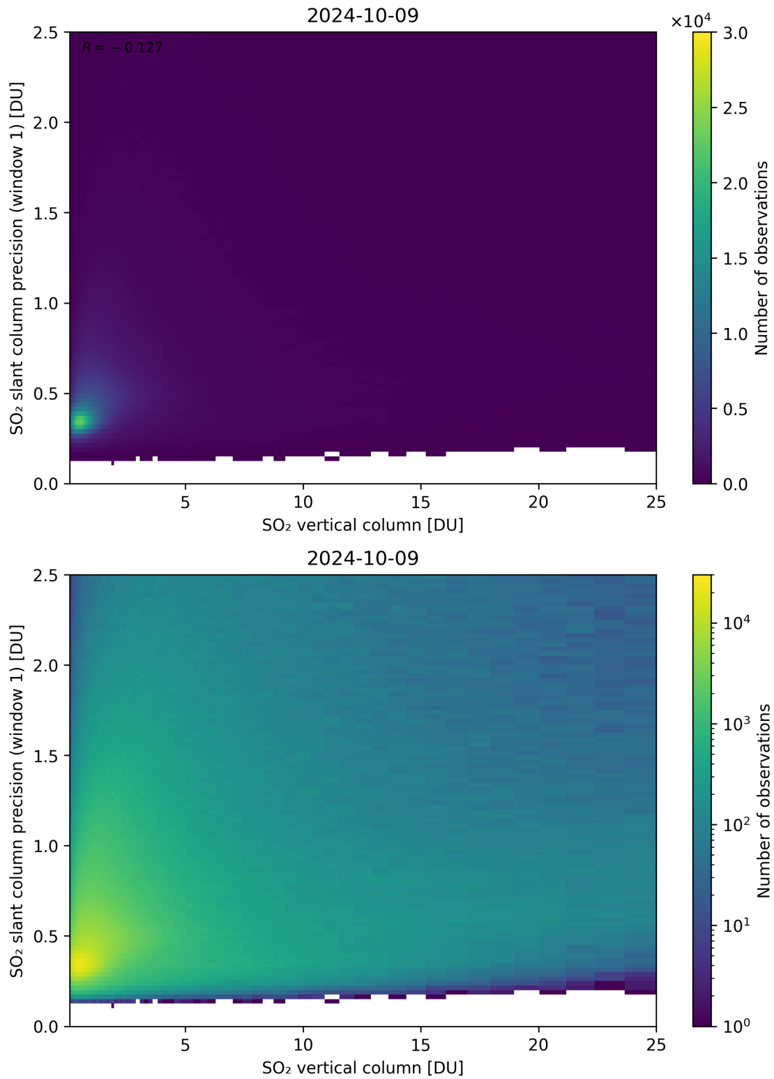
Figure 301: Scatter density plot of “SO 2 vertical column” against “SO 2 slant column precision (window 1)” for 2024-10-08 to 2024-10-10.
