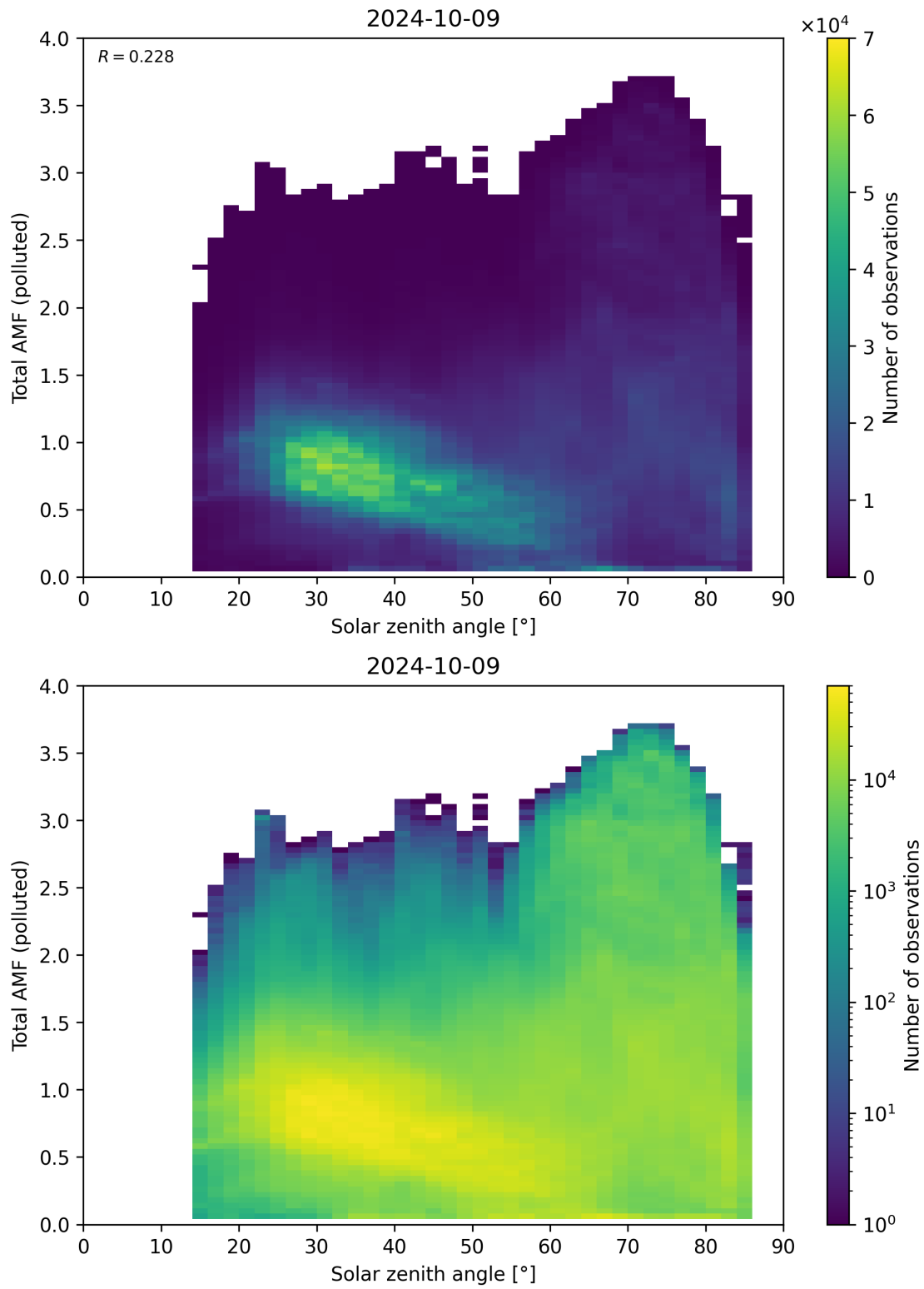
Figure 174: Scatter density plot of “Solar zenith angle” against “Total AMF (polluted)” for 2024-10-08 to 2024-10-10.
