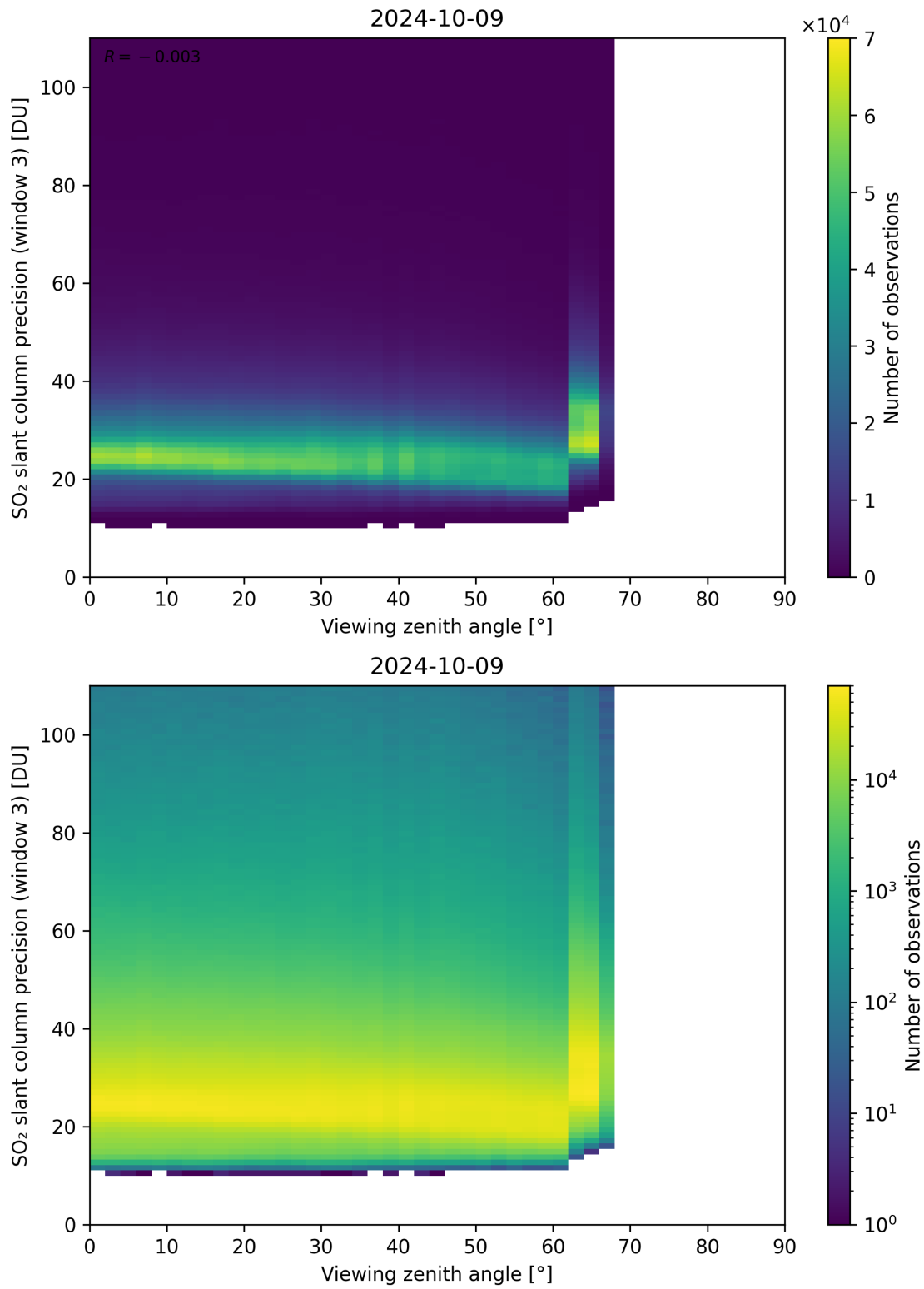
Figure 324: Scatter density plot of “Viewing zenith angle” against “SO 2 slant column precision (window 3)” for 2024-10-08 to 2024-10-10.
