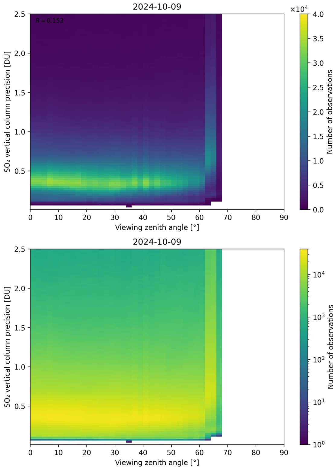
Figure 328: Scatter density plot of “Viewing zenith angle” against “SO 2 vertical column precision” for 2024-10-08 to 2024-10-10.
