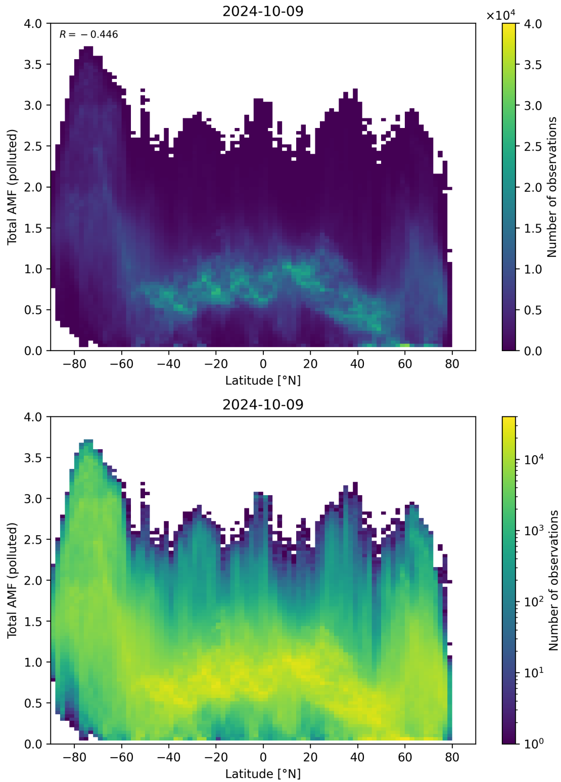
Figure 154: Scatter density plot of “Latitude” against “Total AMF (polluted)” for 2024-10-08 to 2024-10-10.
