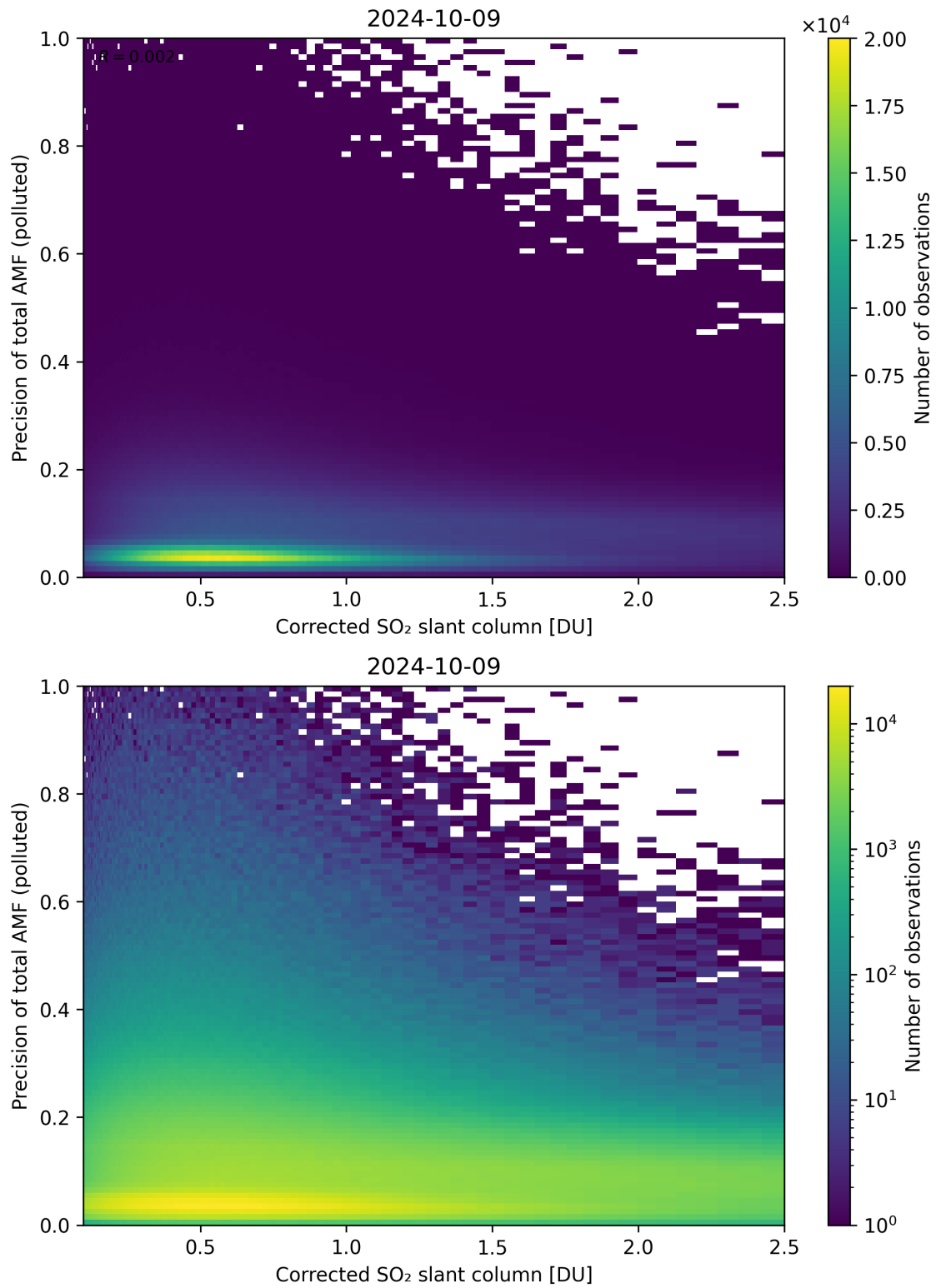
Figure 193: Scatter density plot of “Corrected SO 2 slant column” against “Precision of total AMF (polluted)” for 2024-10-08 to 2024-10-10.
