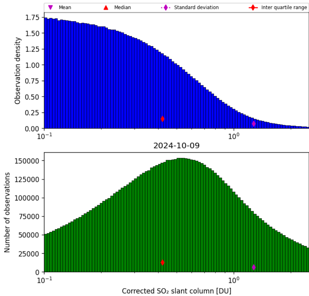
Figure 55: Histogram of “Corrected SO 2 slant column” for 2024-10-08 to 2024-10-10
