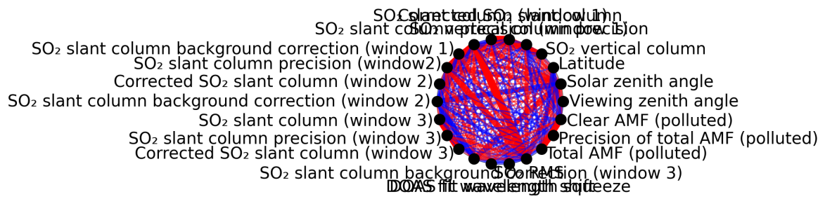
Figure 1: Map of correlation graph for 2024-10-08 to 2024-10-10.
