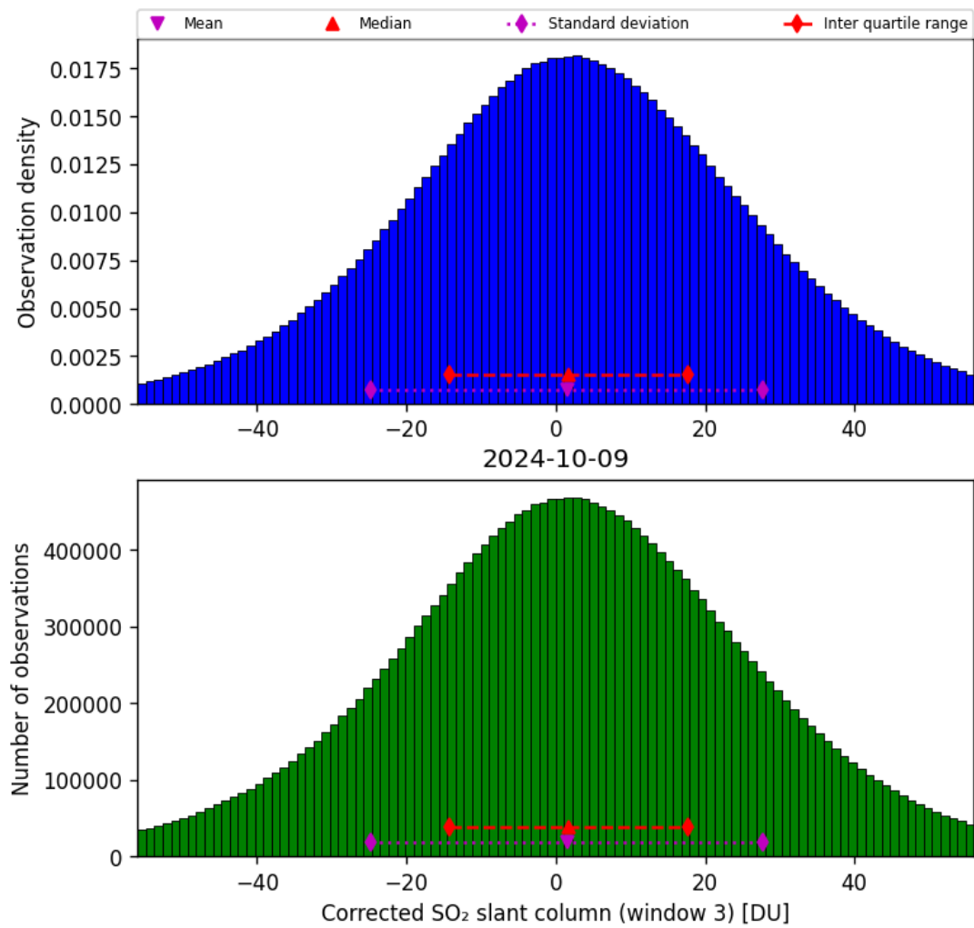
Figure 66: Histogram of “Corrected SO 2 slant column (window 3)” for 2024-10-08 to 2024-10-10
