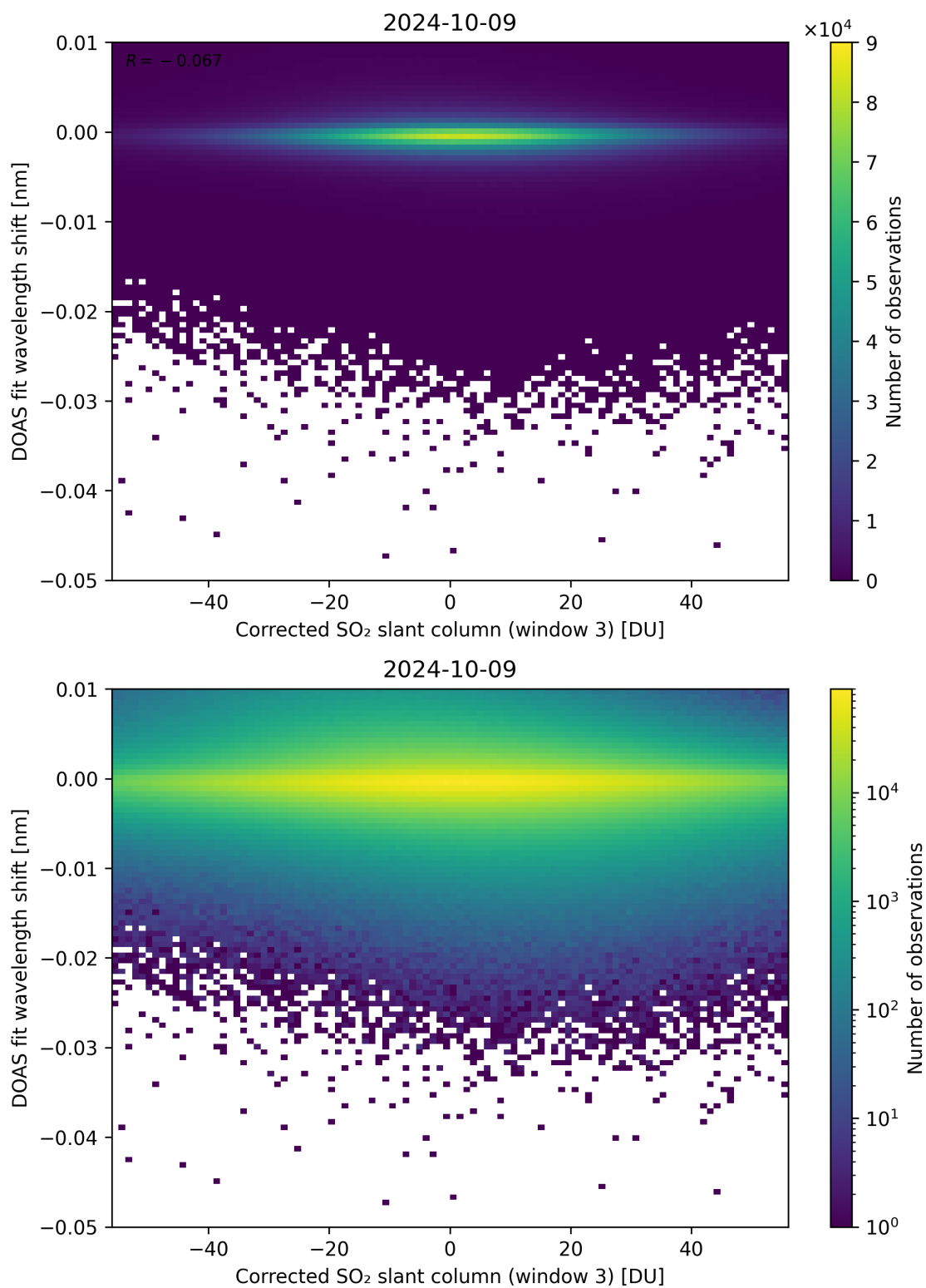
Figure 206: Scatter density plot of “Corrected SO 2 slant column (window 3)” against “DOAS fit wavelength shift” for 2024-10-08 to 2024-10-10.
