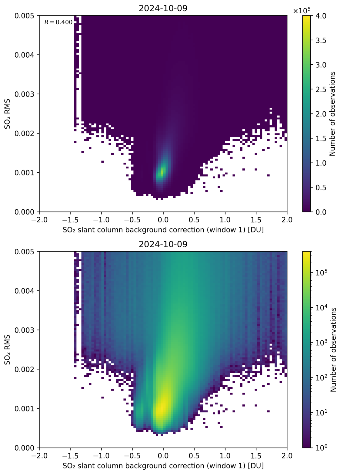
Figure 102: Scatter density plot of “SO 2 slant column background correction (window 1)” against “SO 2 RMS” for 2024-10-08 to 2024-10-10.
