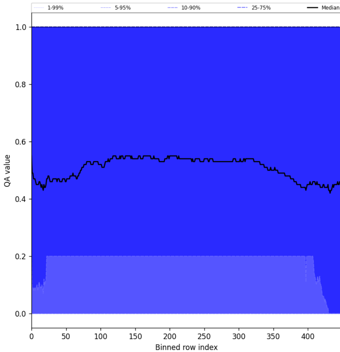
Figure 75: Along track statistics of “QA value” for 2024-10-08 to 2024-10-10
