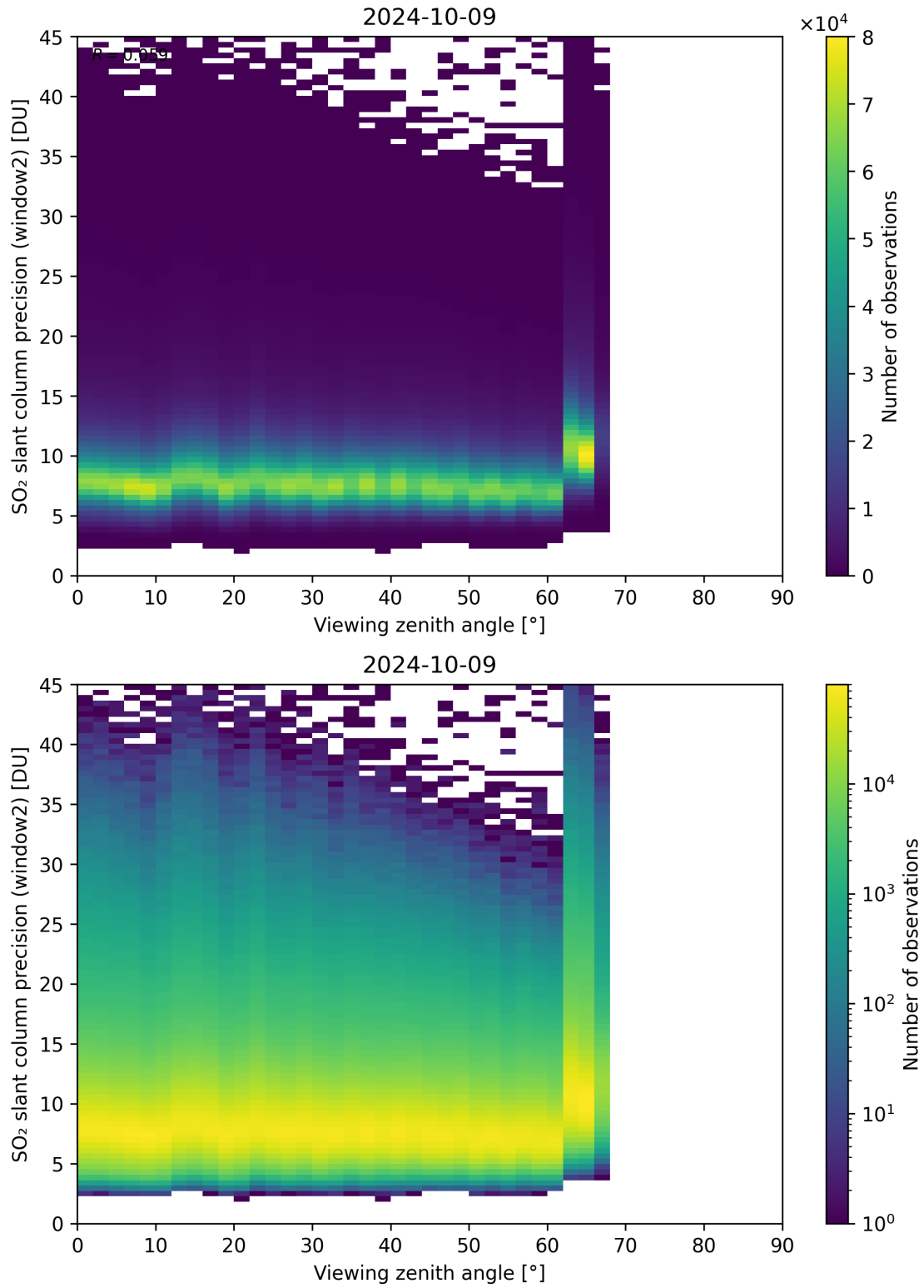
Figure 322: Scatter density plot of “Viewing zenith angle” against “SO 2 slant column precision (window2)” for 2024-10-08 to 2024-10-10.
