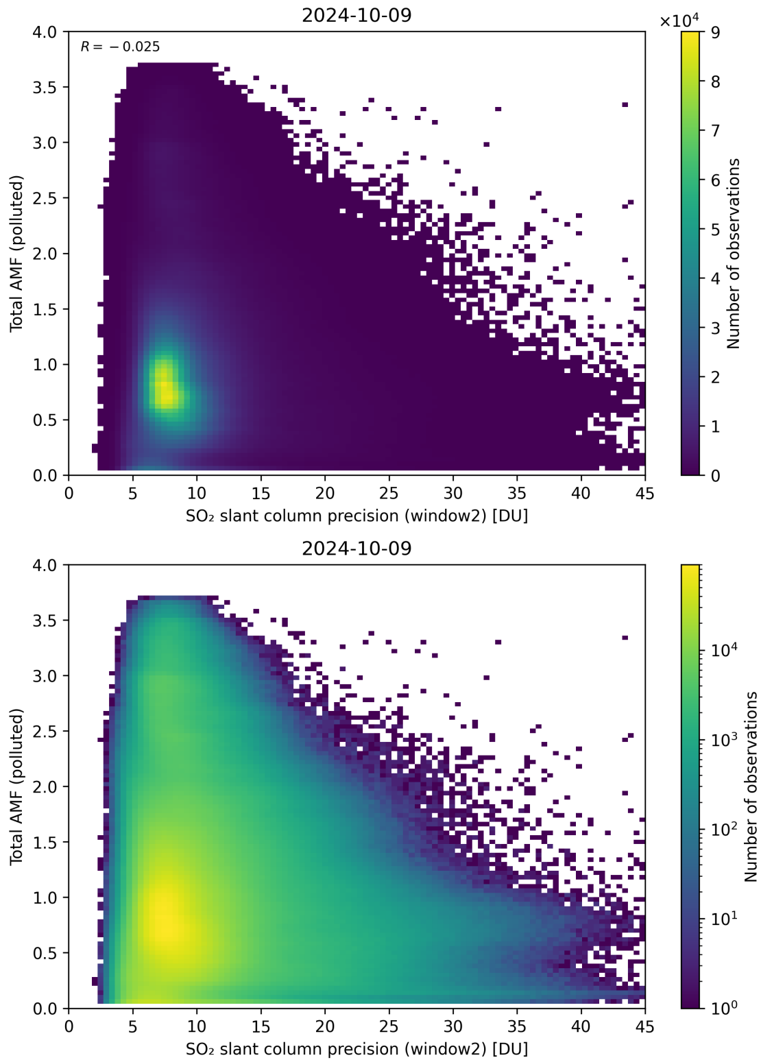
Figure 251: Scatter density plot of “SO 2 slant column precision (window2)” against “Total AMF (polluted)” for 2024-10-08 to 2024-10-10.
