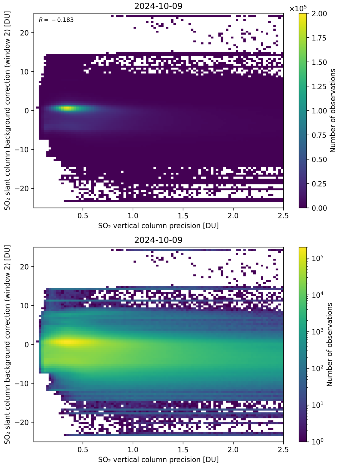
Figure 280: Scatter density plot of “SO 2 vertical column precision” against “SO 2 slant column background correction (window 2)” for 2024-10-08 to 2024-10-10.
