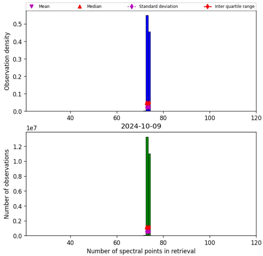
Figure 74: Histogram of “Number of spectral points in retrieval” for 2024-10-08 to 2024-10-10
