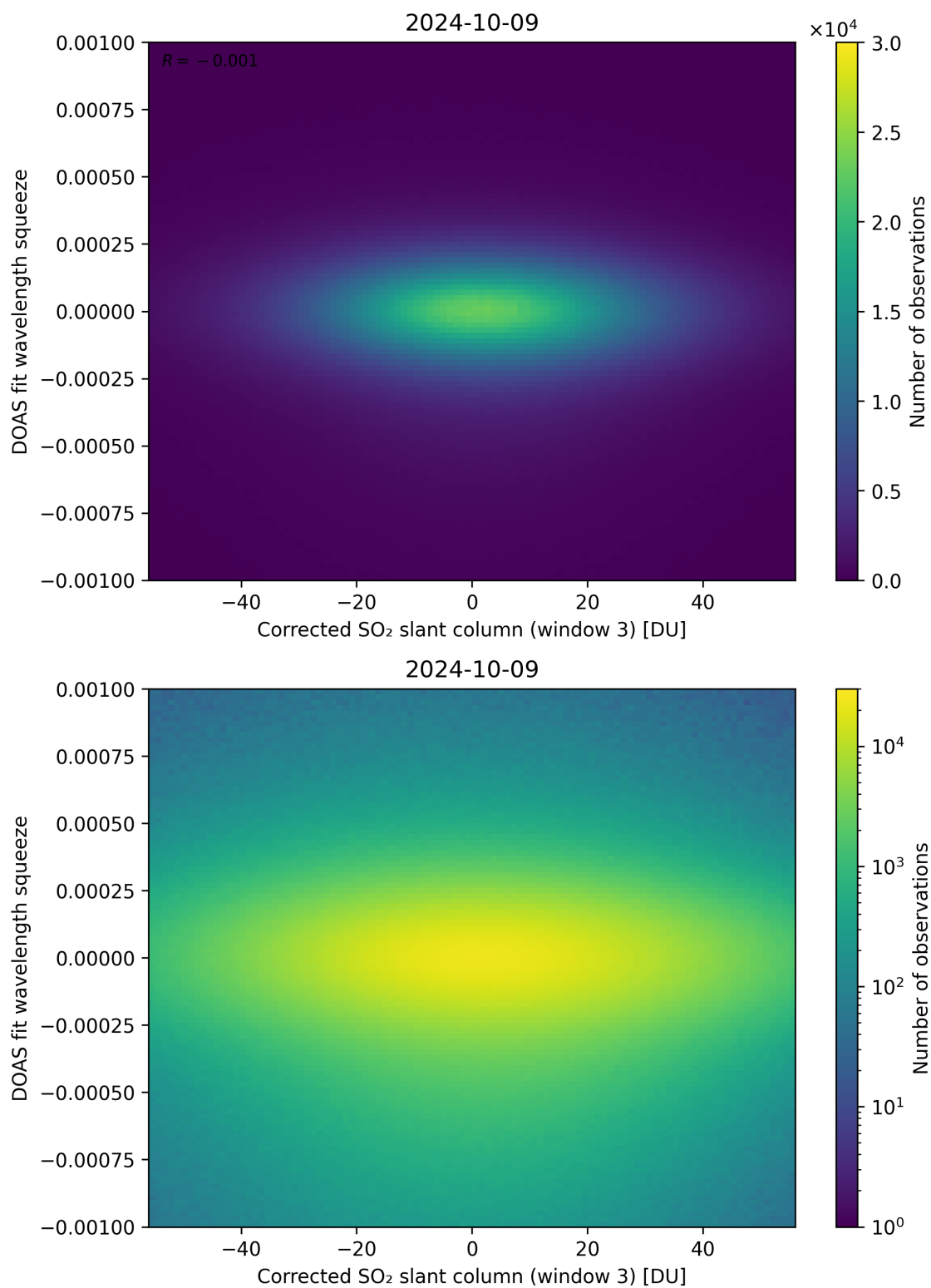
Figure 207: Scatter density plot of “Corrected SO 2 slant column (window 3)” against “DOAS fit wavelength squeeze” for 2024-10-08 to 2024-10-10.
