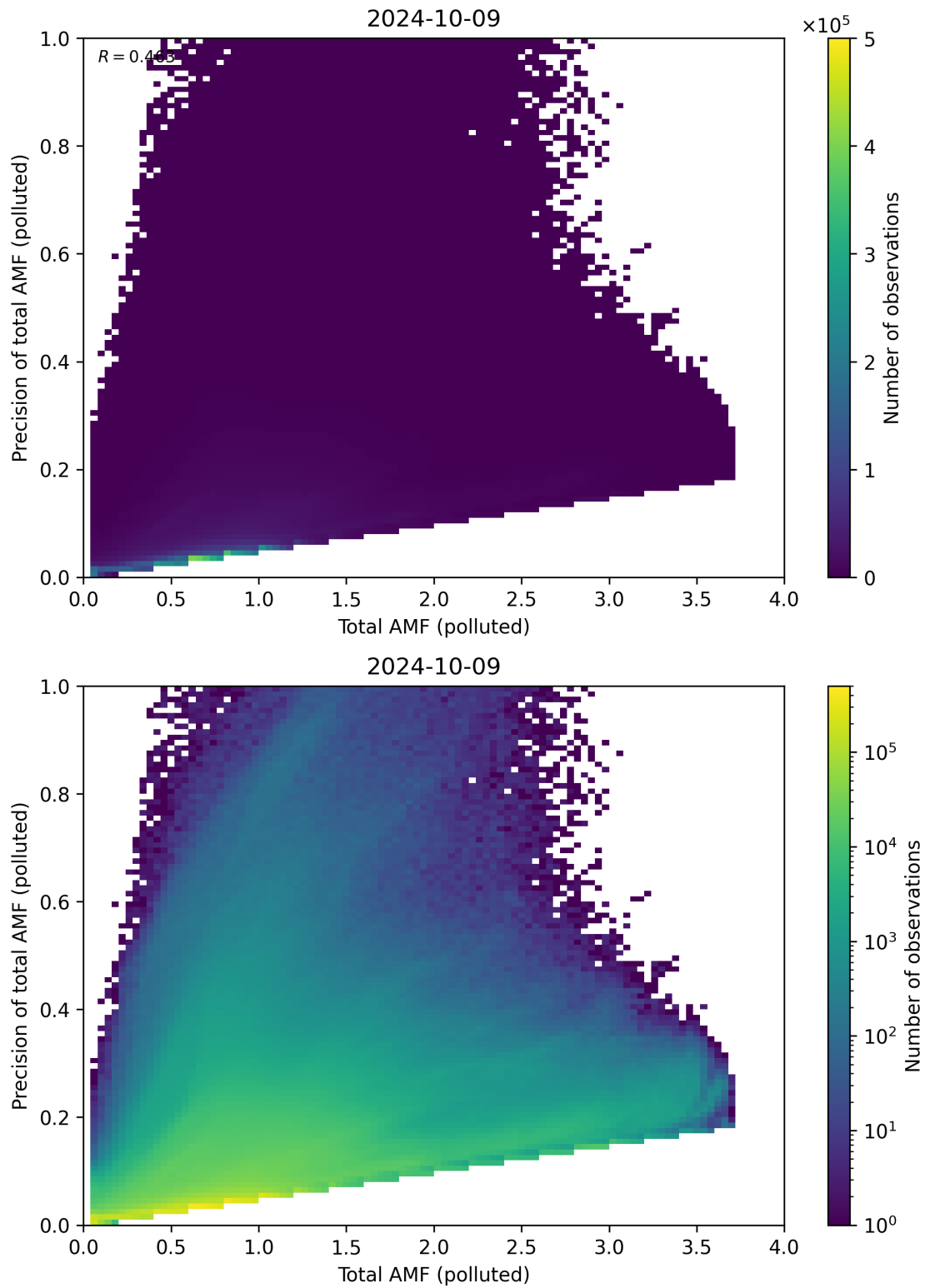
Figure 272: Scatter density plot of “Total AMF (polluted)” against “Precision of total AMF (polluted)” for 2024-10-08 to 2024-10-10.
