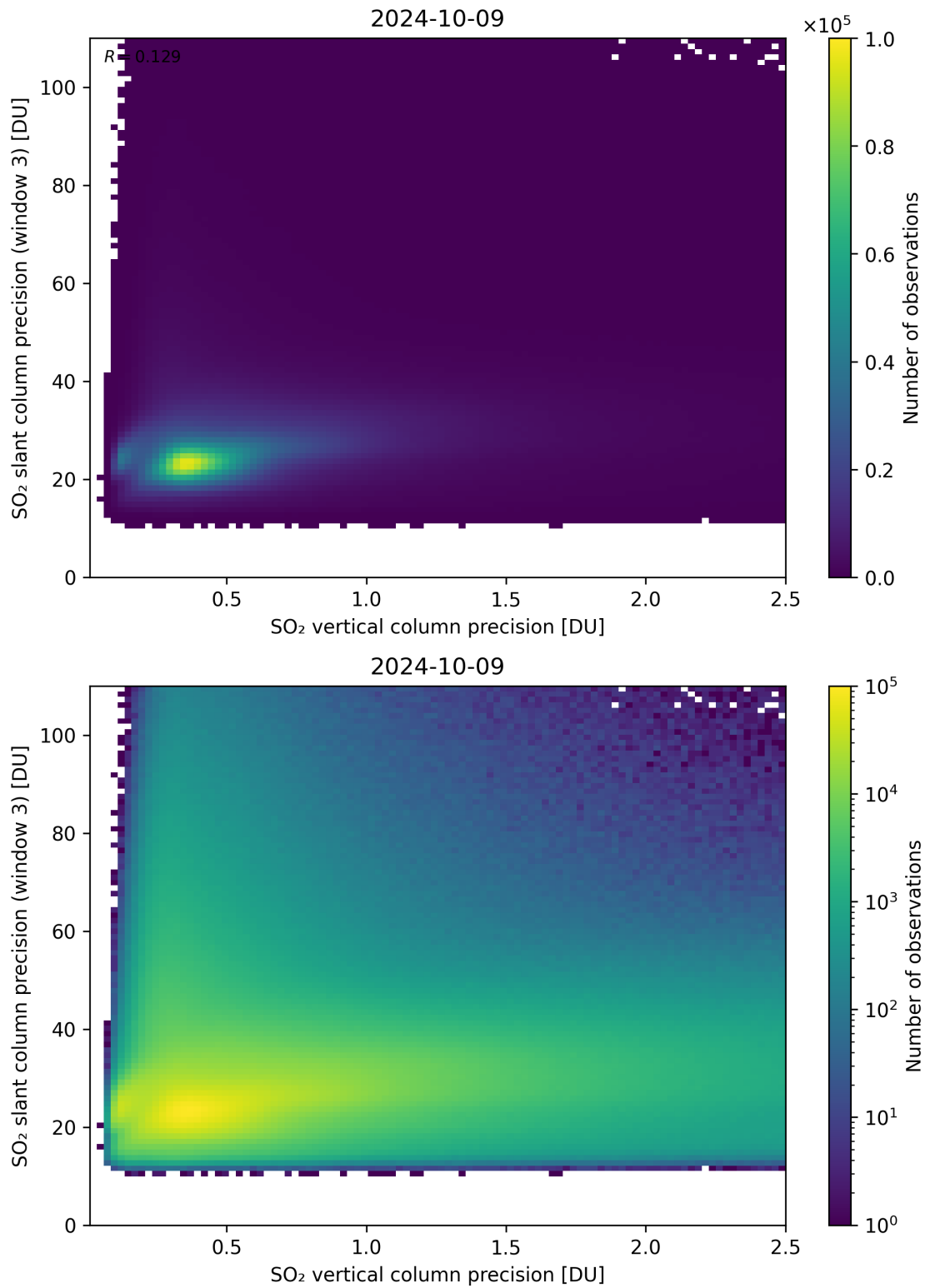
Figure 293: Scatter density plot of “SO 2 vertical column precision” against “SO 2 slant column precision (window 3)” for 2024-10-08 to 2024-10-10.
