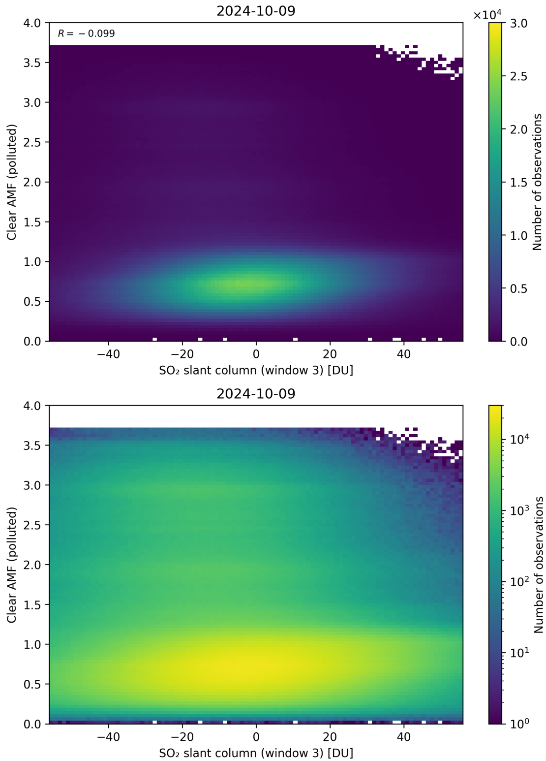
Figure 265: Scatter density plot of “SO 2 slant column (window 3)” against “Clear AMF (polluted)” for 2024-10-08 to 2024-10-10.
