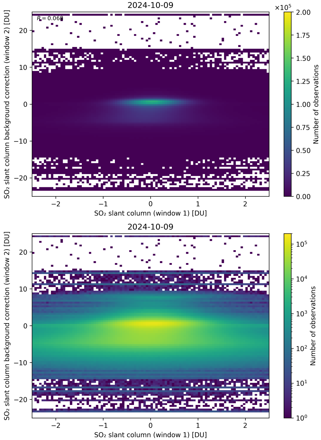
Figure 213: Scatter density plot of “SO 2 slant column (window 1)” against “SO 2 slant column background correction (window 2)” for 2024-10-08 to 2024-10-10.
