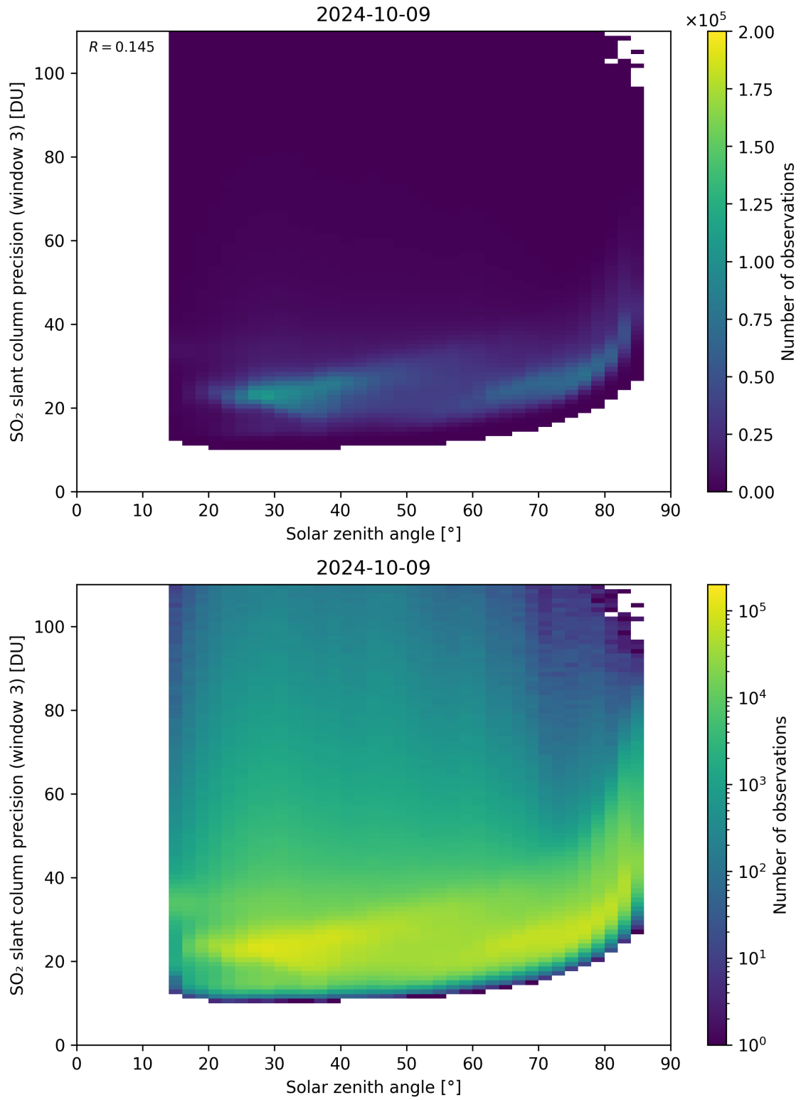
Figure 173: Scatter density plot of “Solar zenith angle” against “SO 2 slant column precision (window 3)” for 2024-10-08 to 2024-10-10.
