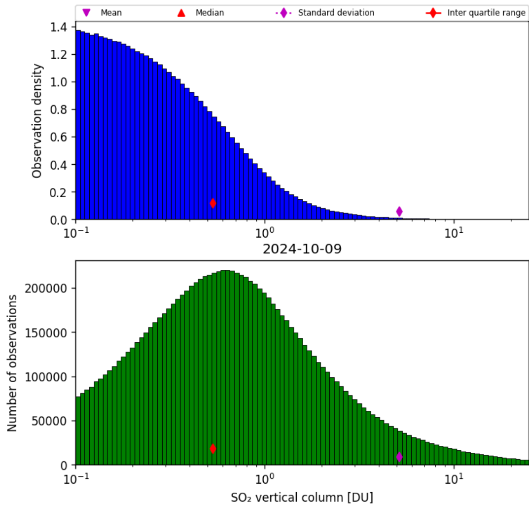
Figure 53: Histogram of “SO 2 vertical column” for 2024-10-08 to 2024-10-10
