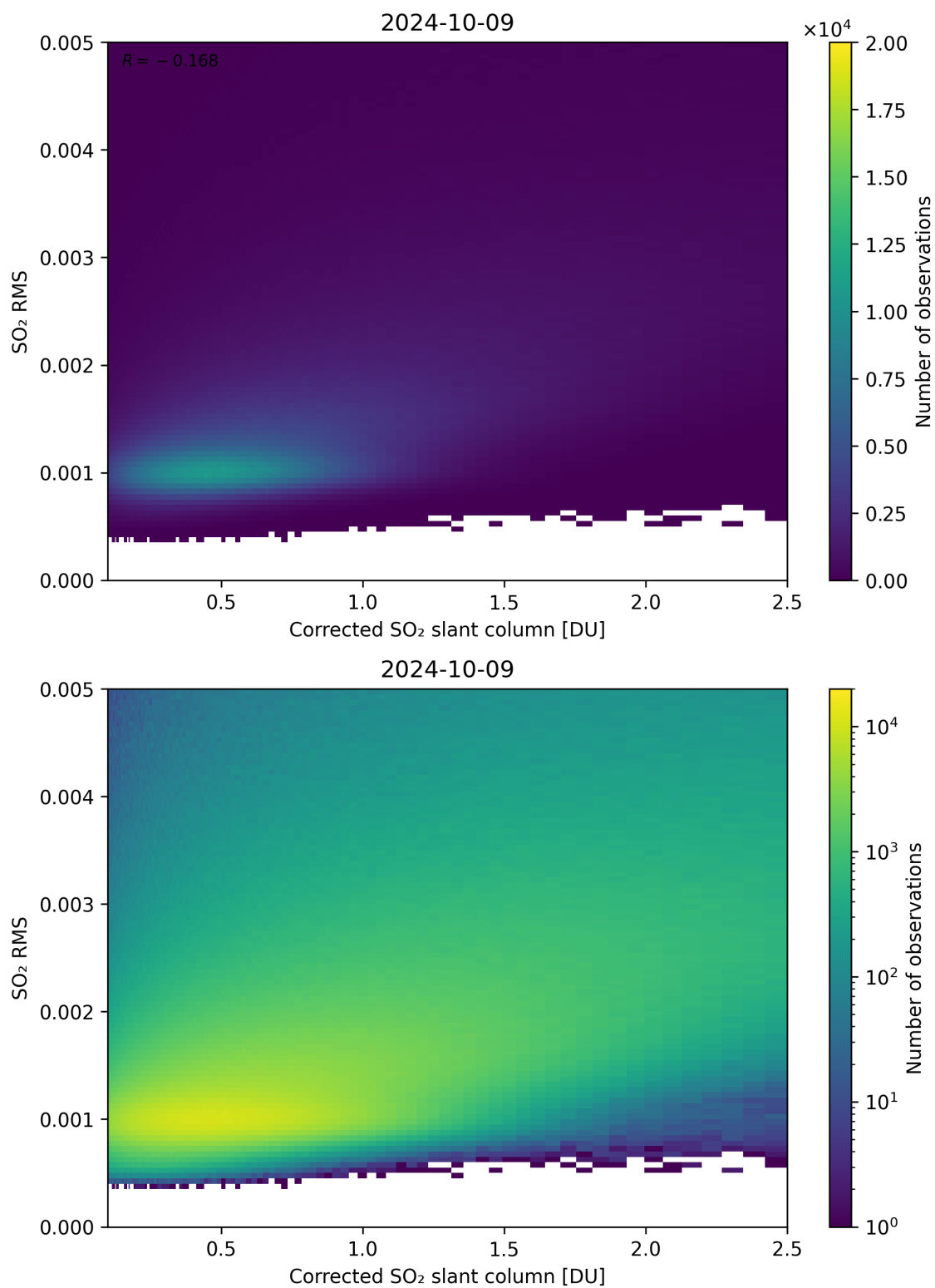
Figure 183: Scatter density plot of “Corrected SO 2 slant column” against “SO 2 RMS” for 2024-10-08 to 2024-10-10.
