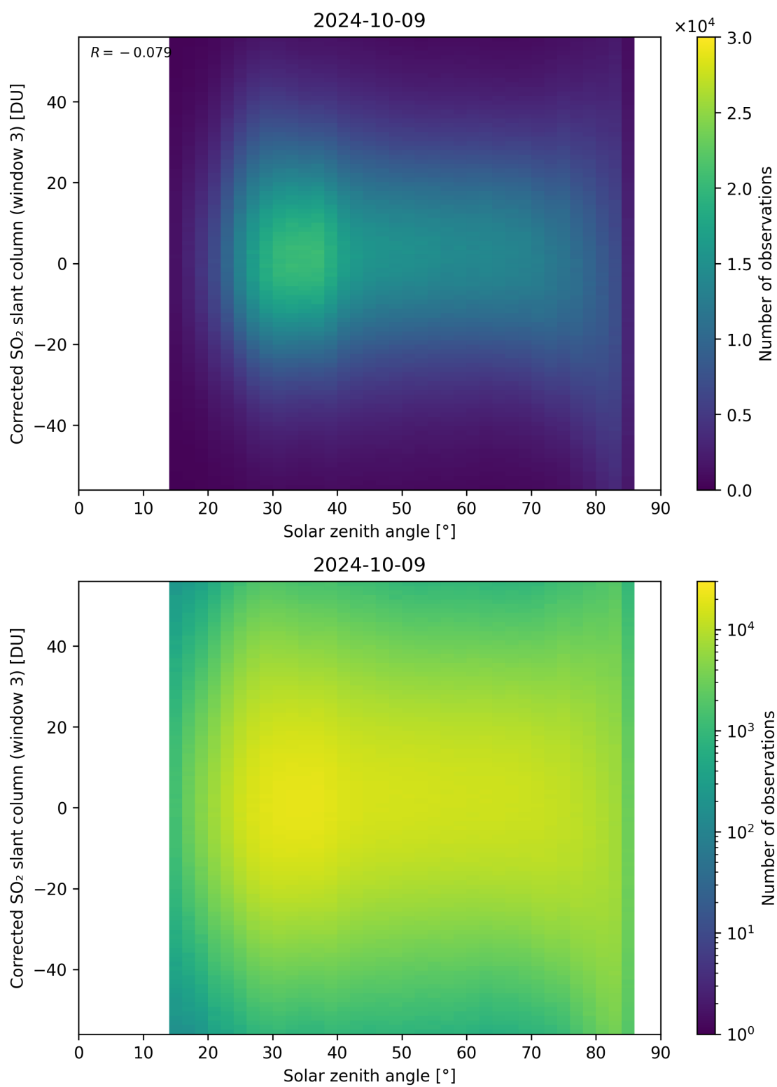
Figure 168: Scatter density plot of “Solar zenith angle” against “Corrected SO 2 slant column (window 3)” for 2024-10-08 to 2024-10-10.
