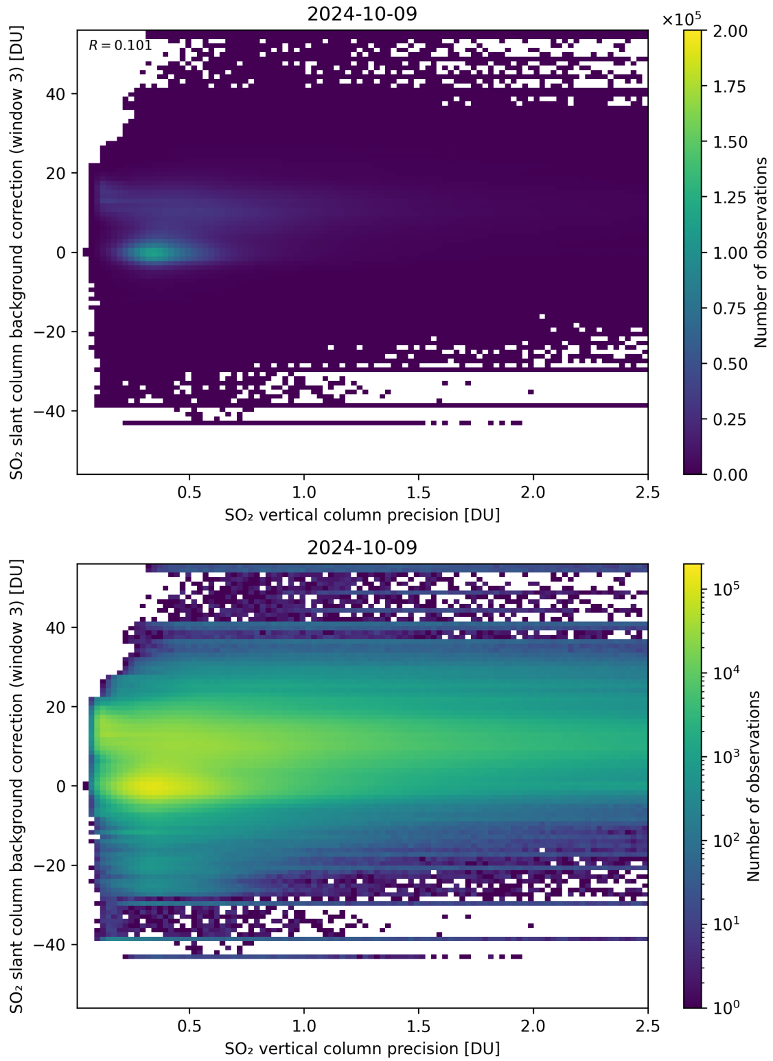
Figure 281: Scatter density plot of “SO 2 vertical column precision” against “SO 2 slant column background correction (window 3)” for 2024-10-08 to 2024-10-10.
