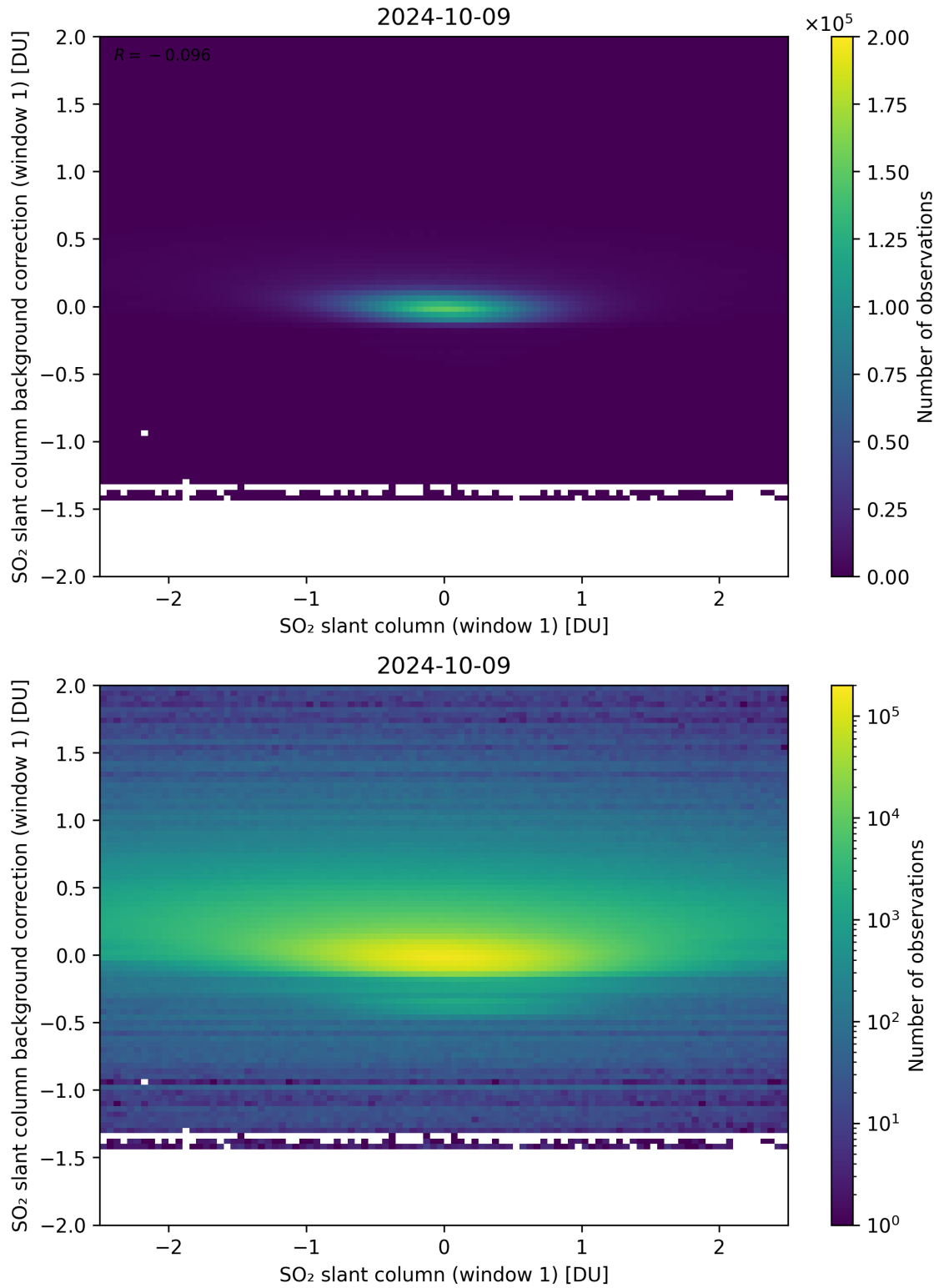
Figure 212: Scatter density plot of “SO 2 slant column (window 1)” against “SO 2 slant column background correction (window 1)” for 2024-10-08 to 2024-10-10.
