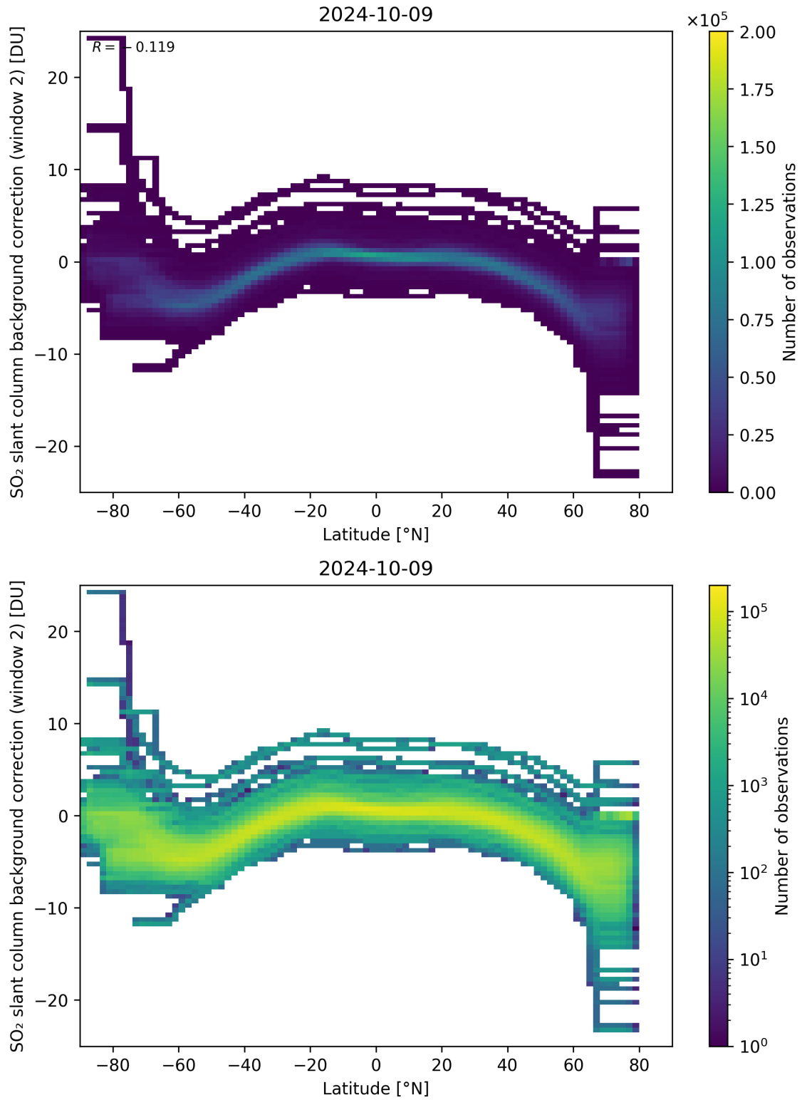
Figure 140: Scatter density plot of “Latitude” against “SO 2 slant column background correction (window 2)” for 2024-10-08 to 2024-10-10.
