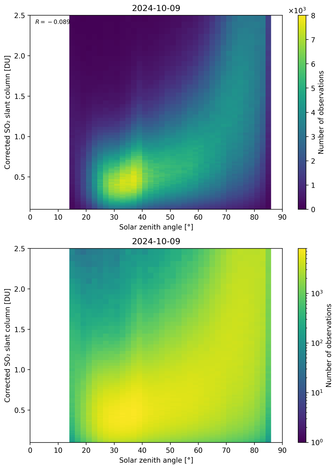
Figure 166: Scatter density plot of “Solar zenith angle” against “Corrected SO 2 slant column” for 2024-10-08 to 2024-10-10.
