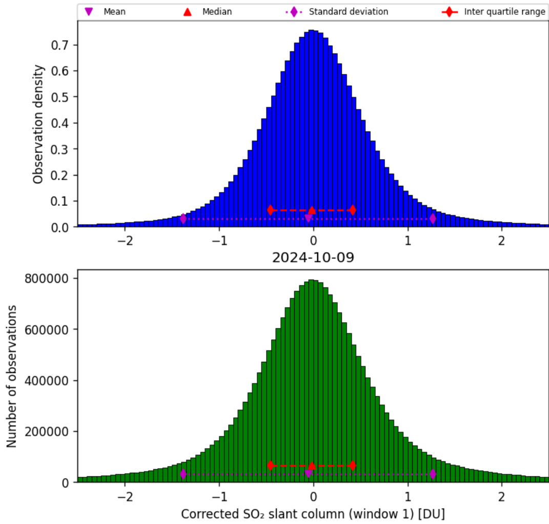
Figure 58: Histogram of “Corrected SO 2 slant column (window 1)” for 2024-10-08 to 2024-10-10
