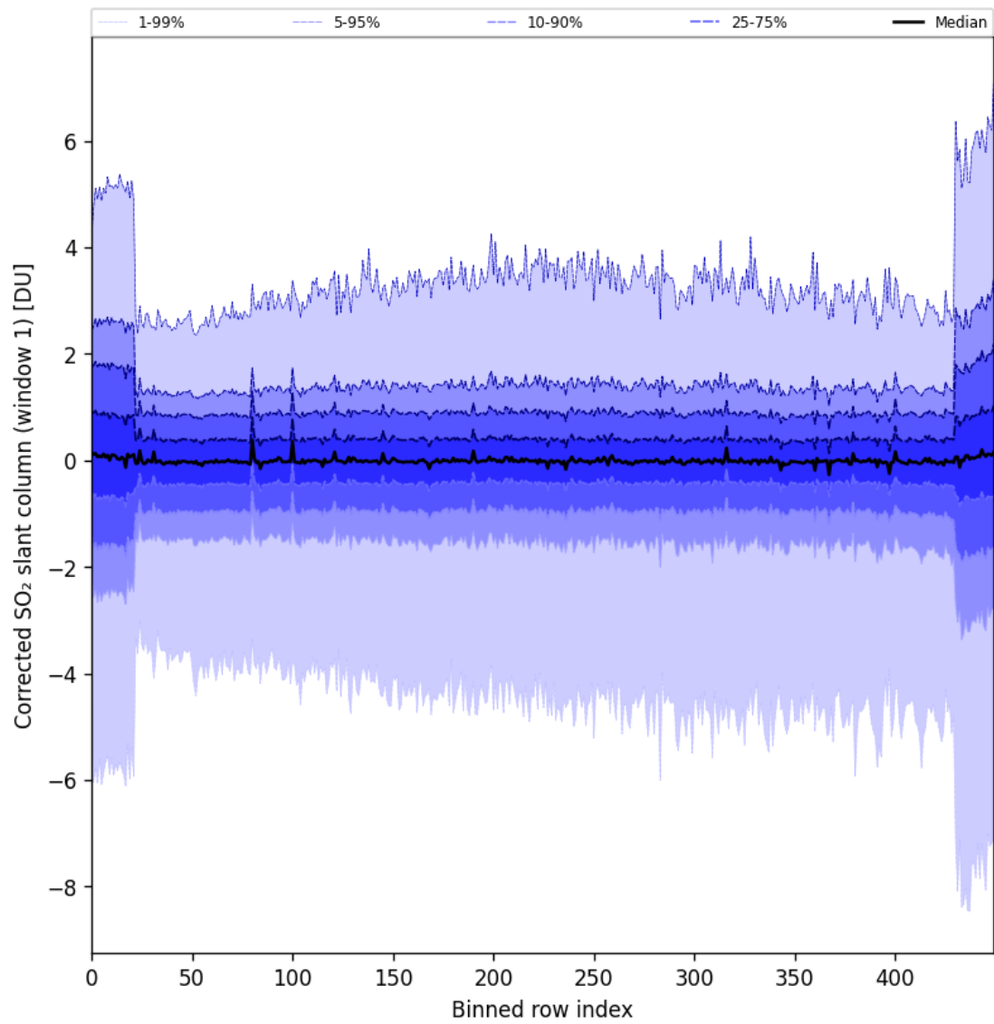
Figure 81: Along track statistics of “Corrected SO 2 slant column (window 1)” for 2024-10-08 to 2024-10-10
