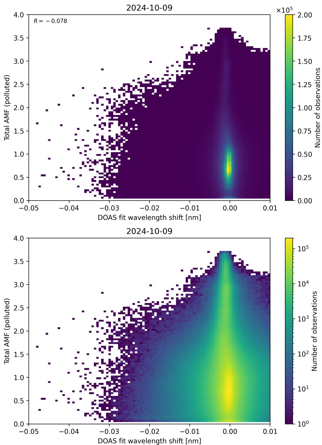
Figure 130: Scatter density plot of “DOAS fit wavelength shift” against “Total AMF (polluted)” for 2024-10-08 to 2024-10-10.
