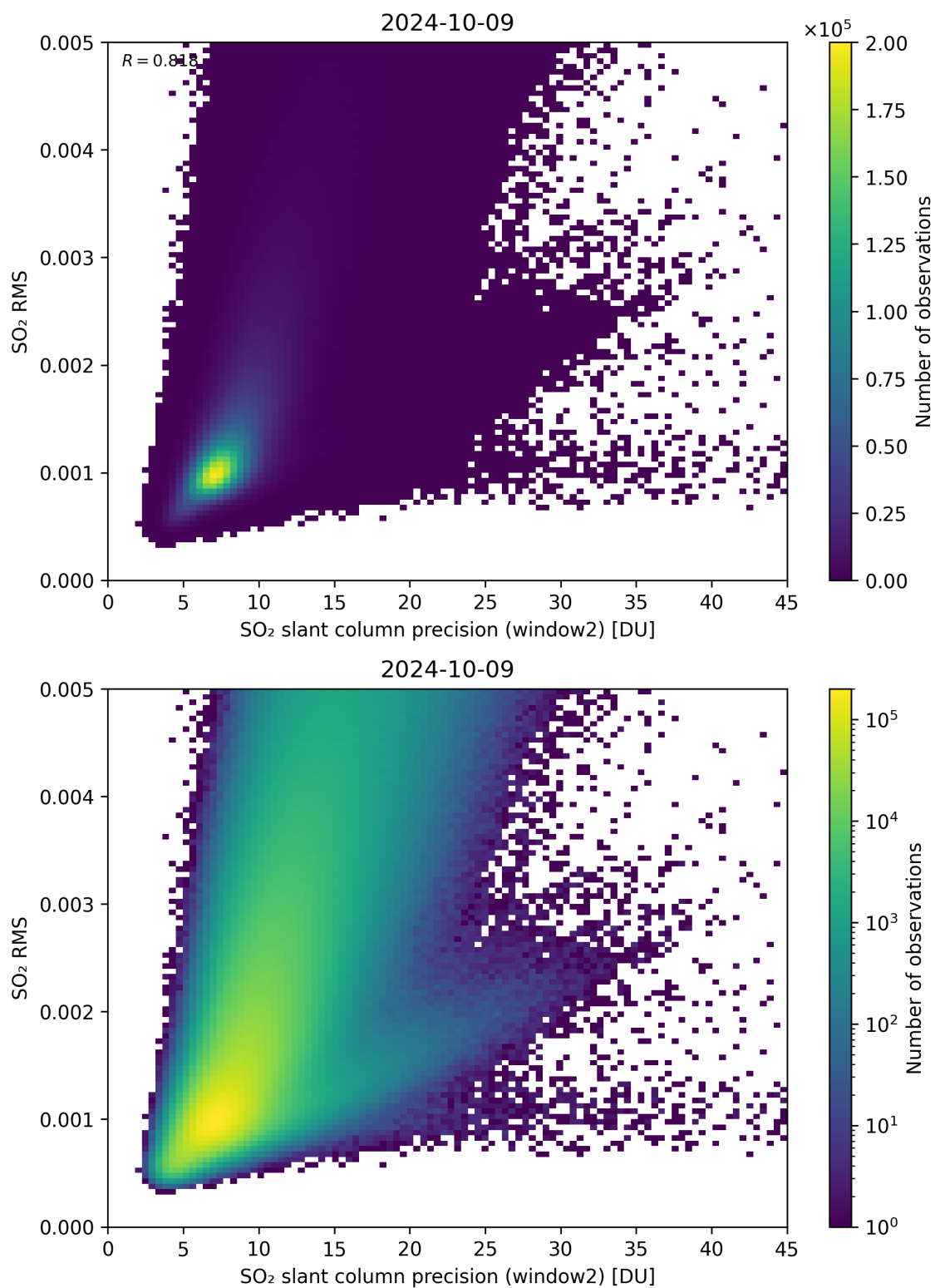
Figure 245: Scatter density plot of “SO 2 slant column precision (window2)” against “SO 2 RMS” for 2024-10-08 to 2024-10-10.
