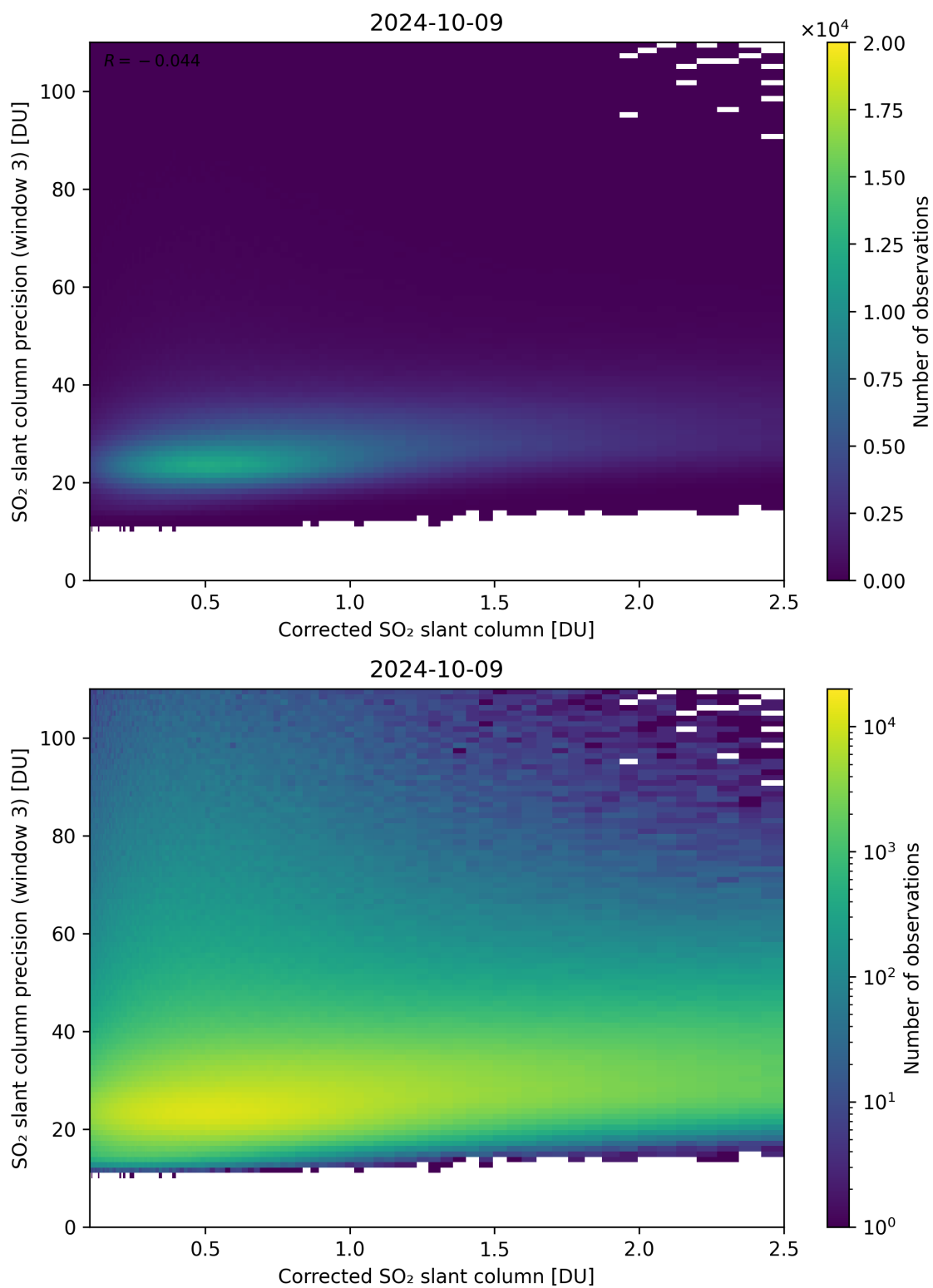
Figure 191: Scatter density plot of “Corrected SO 2 slant column” against “SO 2 slant column precision (window 3)” for 2024-10-08 to 2024-10-10.
