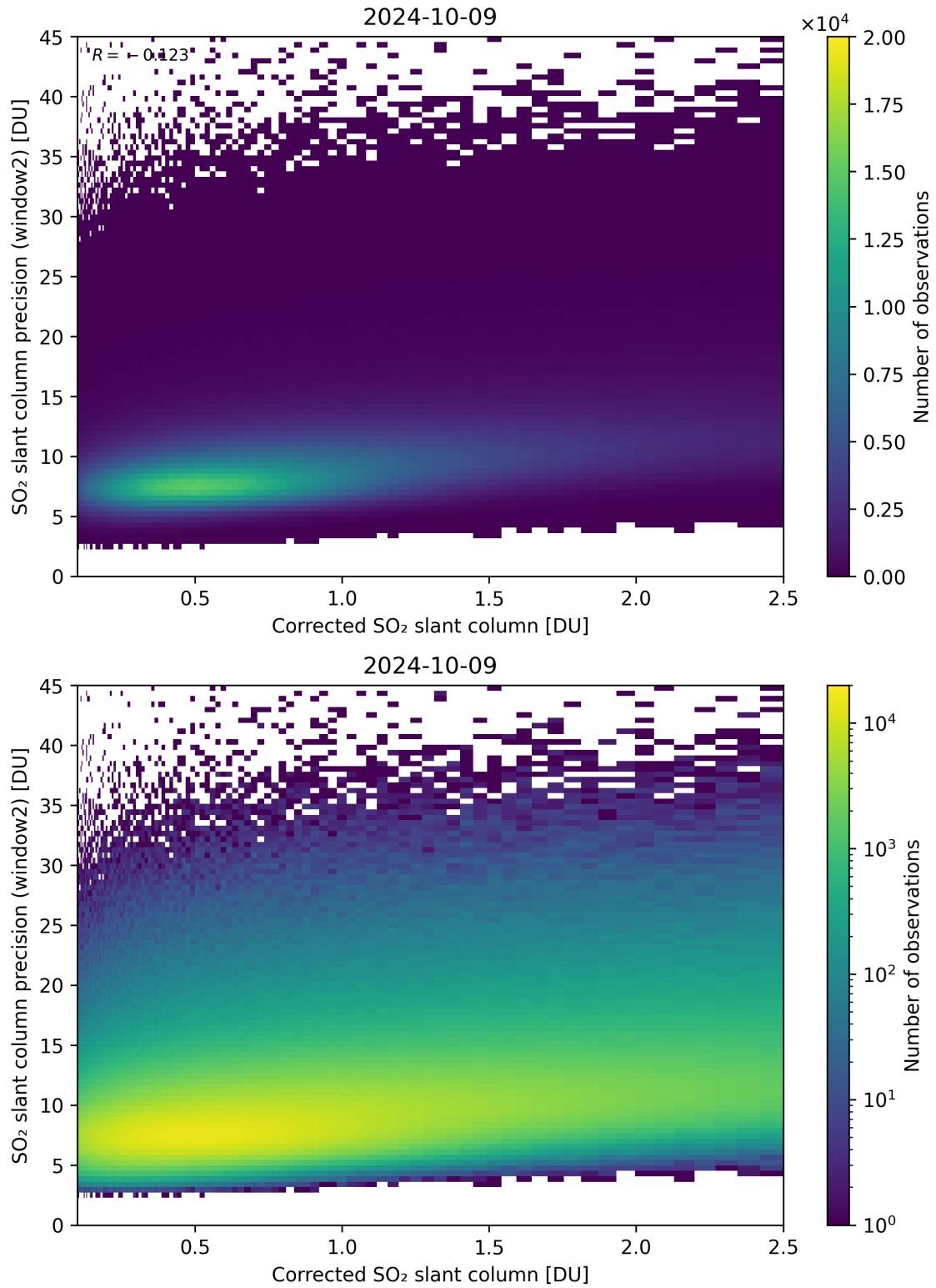
Figure 189: Scatter density plot of “Corrected SO 2 slant column” against “SO 2 slant column precision (window2)” for 2024-10-08 to 2024-10-10.
