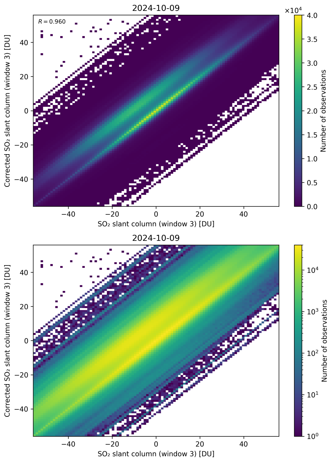
Figure 266: Scatter density plot of “SO 2 slant column (window 3)” against “Corrected SO 2 slant column (window 3)” for 2024-10-08 to 2024-10-10.
