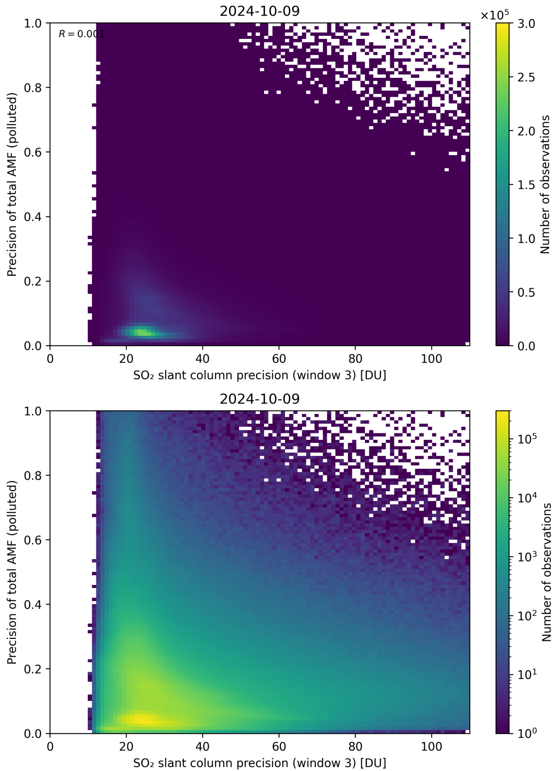
Figure 264: Scatter density plot of “SO 2 slant column precision (window 3)” against “Precision of total AMF (polluted)” for 2024-10-08 to 2024-10-10.
