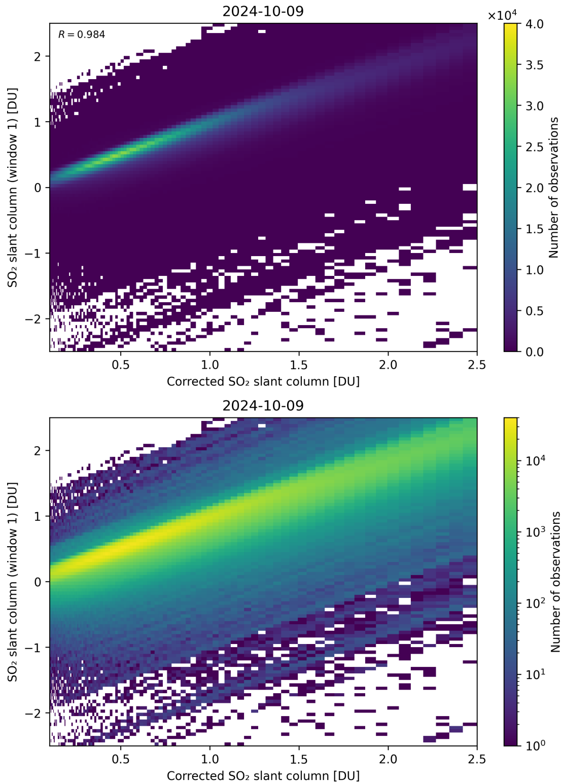
Figure 187: Scatter density plot of “Corrected SO 2 slant column” against “SO 2 slant column (window 1)” for 2024-10-08 to 2024-10-10.
