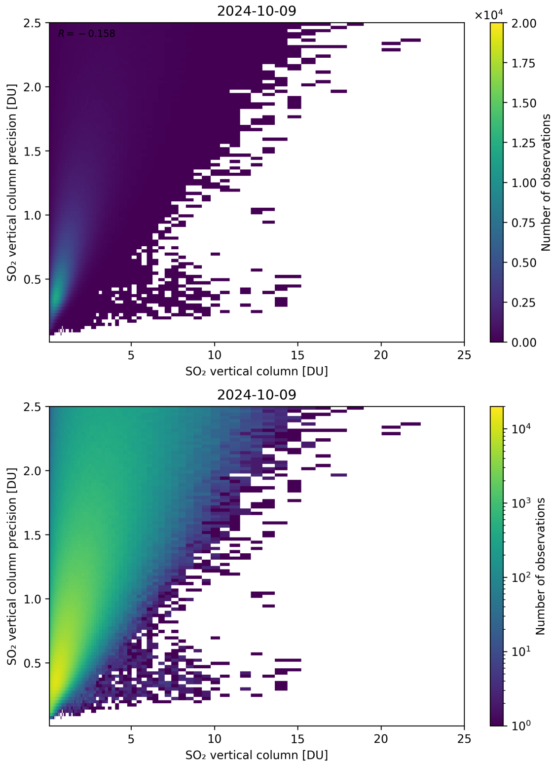
Figure 307: Scatter density plot of “SO 2 vertical column” against “SO 2 vertical column precision” for 2024-10-08 to 2024-10-10.
