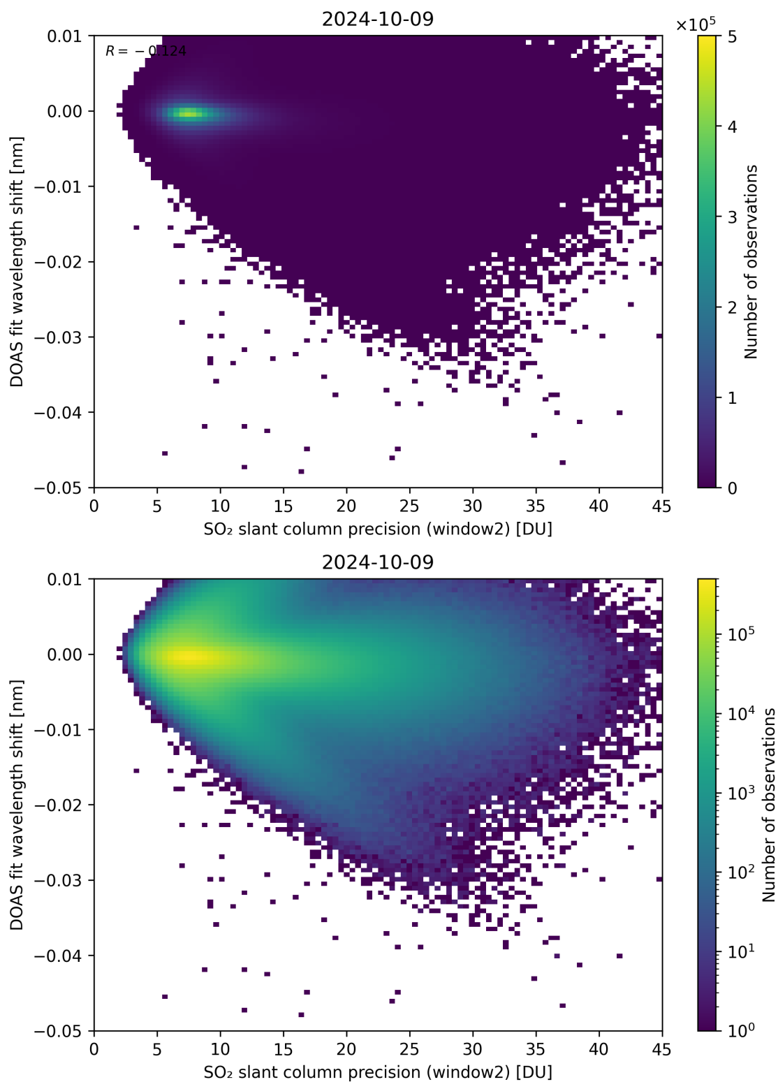
Figure 243: Scatter density plot of “SO 2 slant column precision (window2)” against “DOAS fit wavelength shift” for 2024-10-08 to 2024-10-10.
