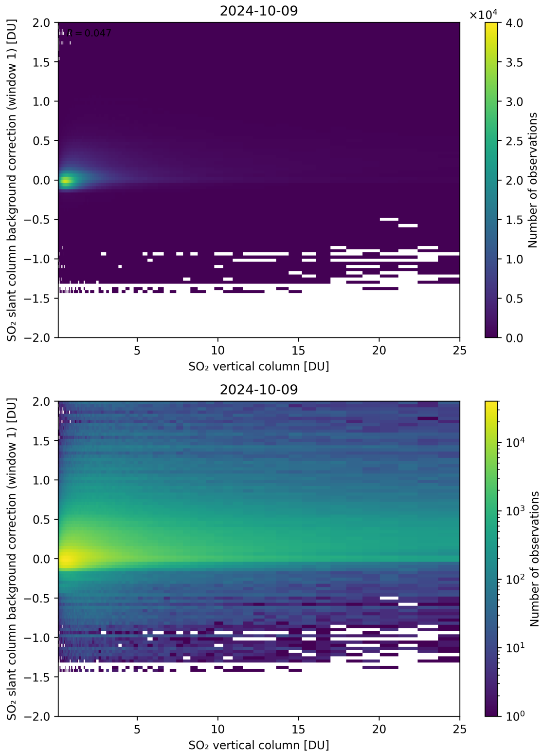
Figure 273: Scatter density plot of “SO 2 vertical column” against “SO 2 slant column background correction (window 1)” for 2024-10-08 to 2024-10-10.
