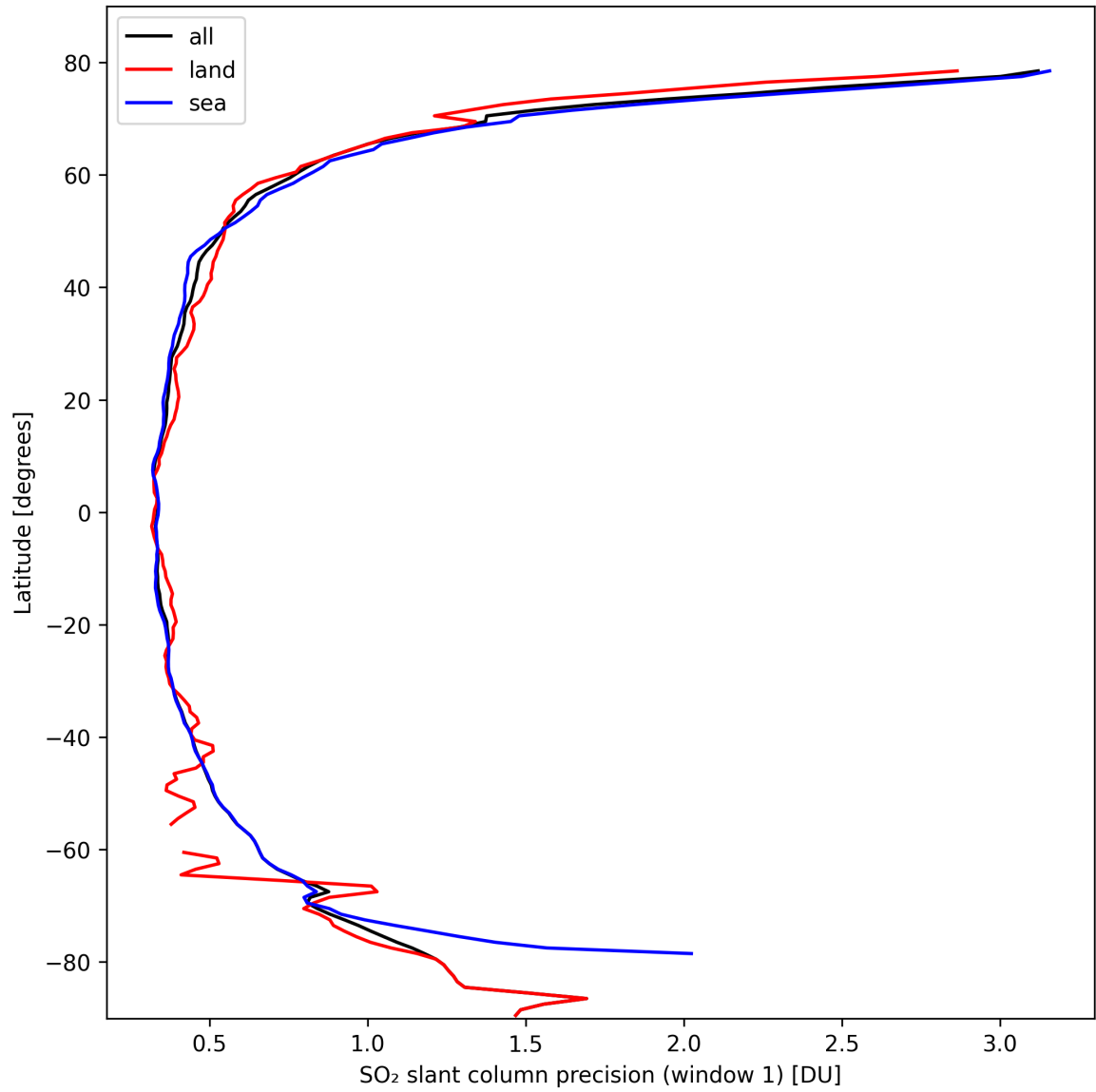
Figure 34: Zonal average of “SO 2 slant column precision (window 1)” for 2024-10-08 to 2024-10-10.
