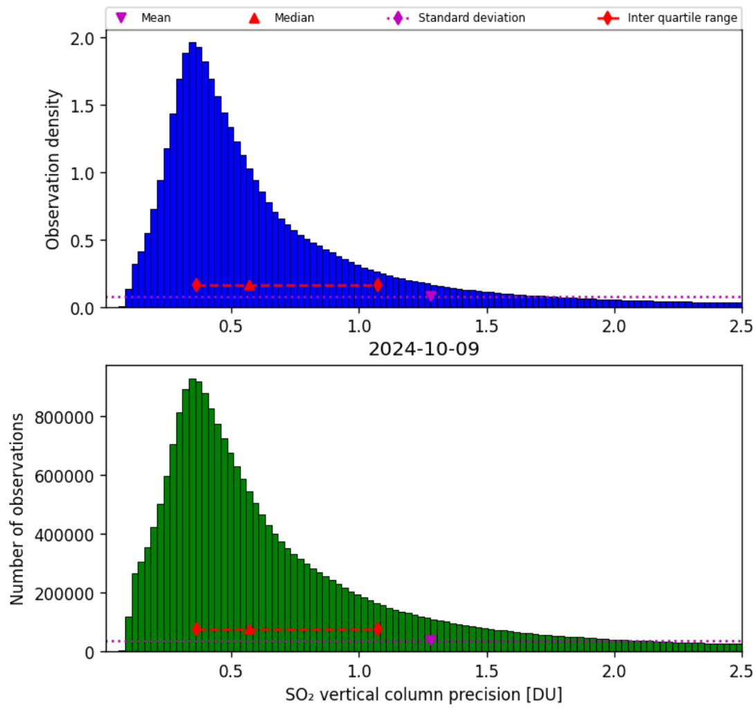
Figure 54: Histogram of “SO 2 vertical column precision” for 2024-10-08 to 2024-10-10
