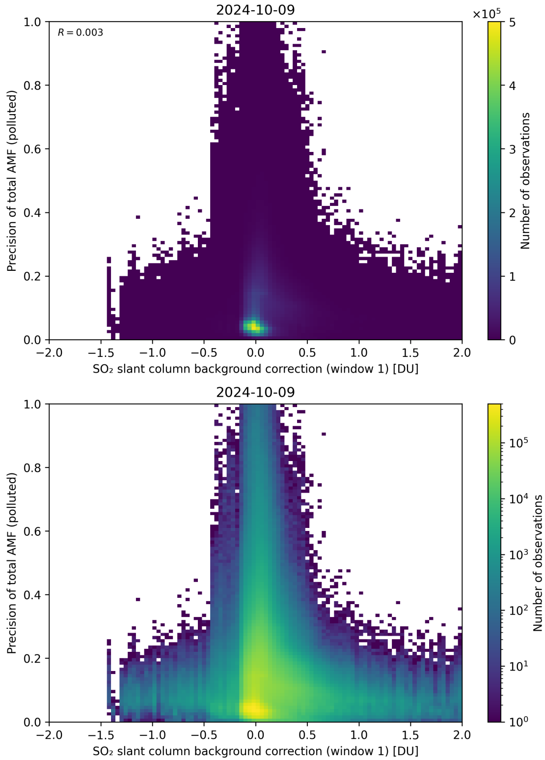
Figure 110: Scatter density plot of “SO 2 slant column background correction (window 1)” against “Precision of total AMF (polluted)” for 2024-10-08 to 2024-10-10.
