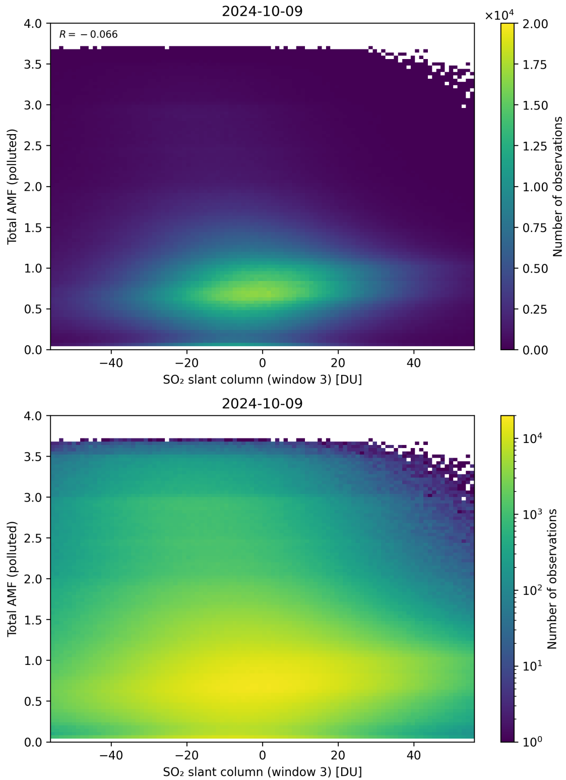
Figure 268: Scatter density plot of “SO 2 slant column (window 3)” against “Total AMF (polluted)” for 2024-10-08 to 2024-10-10.
