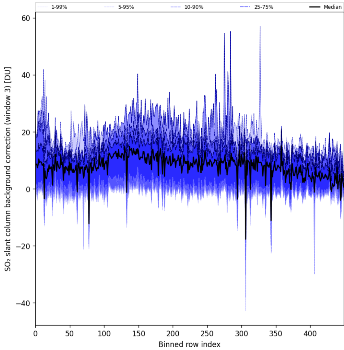
Figure 90: Along track statistics of “SO 2 slant column background correction (window 3)” for 2024-10-08 to 2024-10-10
