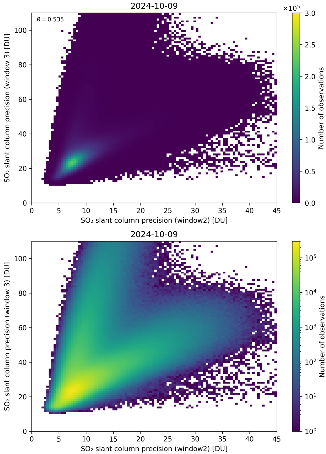
Figure 250: Scatter density plot of “SO 2 slant column precision (window2)” against “SO 2 slant column precision (window 3)” for 2024-10-08 to 2024-10-10.
