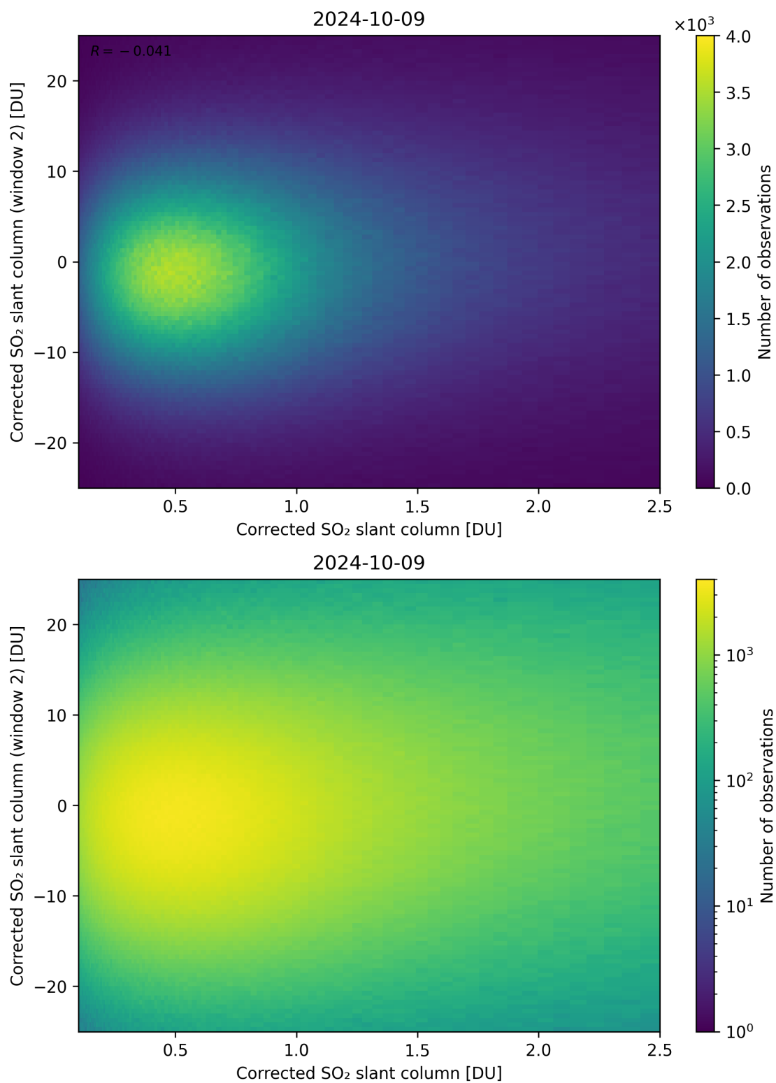
Figure 185: Scatter density plot of “Corrected SO 2 slant column” against “Corrected SO 2 slant column (window 2)” for 2024-10-08 to 2024-10-10.
