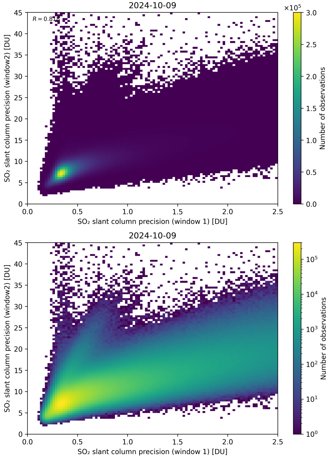
Figure 227: Scatter density plot of “SO 2 slant column precision (window 1)” against “SO 2 slant column precision (window2)” for 2024-10-08 to 2024-10-10.
