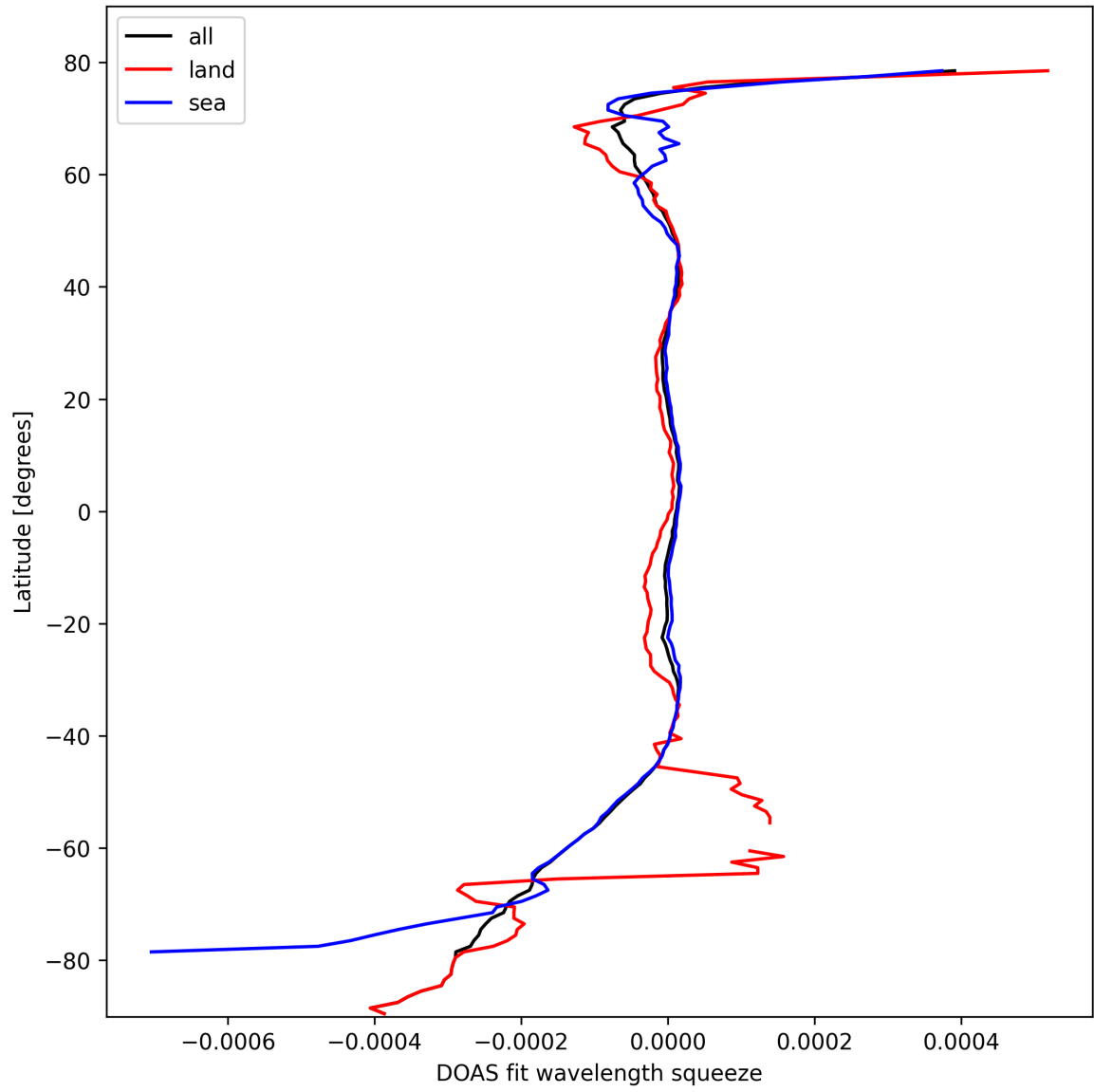
Figure 46: Zonal average of “DOAS fit wavelength squeeze” for 2024-10-08 to 2024-10-10.
