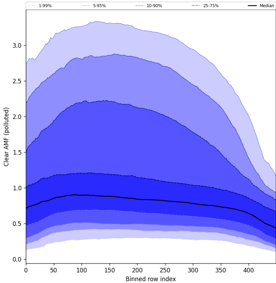
Figure 96: Along track statistics of “Clear AMF (polluted)” for 2024-10-08 to 2024-10-10
