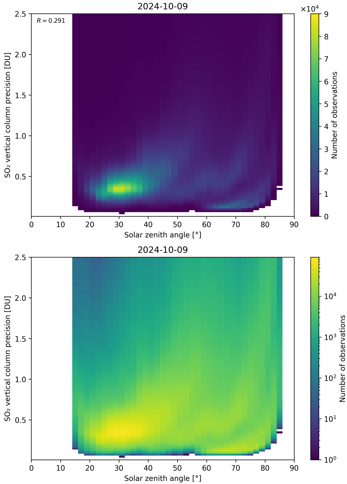
Figure 177: Scatter density plot of “Solar zenith angle” against “SO 2 vertical column precision” for 2024-10-08 to 2024-10-10.
