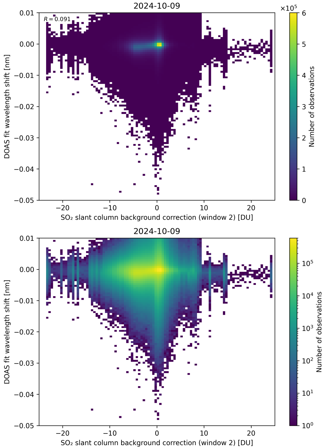
Figure 112: Scatter density plot of “SO 2 slant column background correction (window 2)” against “DOAS fit wavelength shift” for 2024-10-08 to 2024-10-10.
