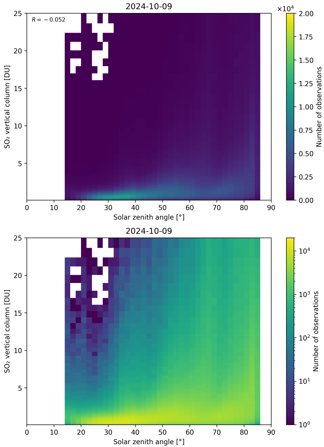
Figure 176: Scatter density plot of “Solar zenith angle” against “SO 2 vertical column” for 2024-10-08 to 2024-10-10.
