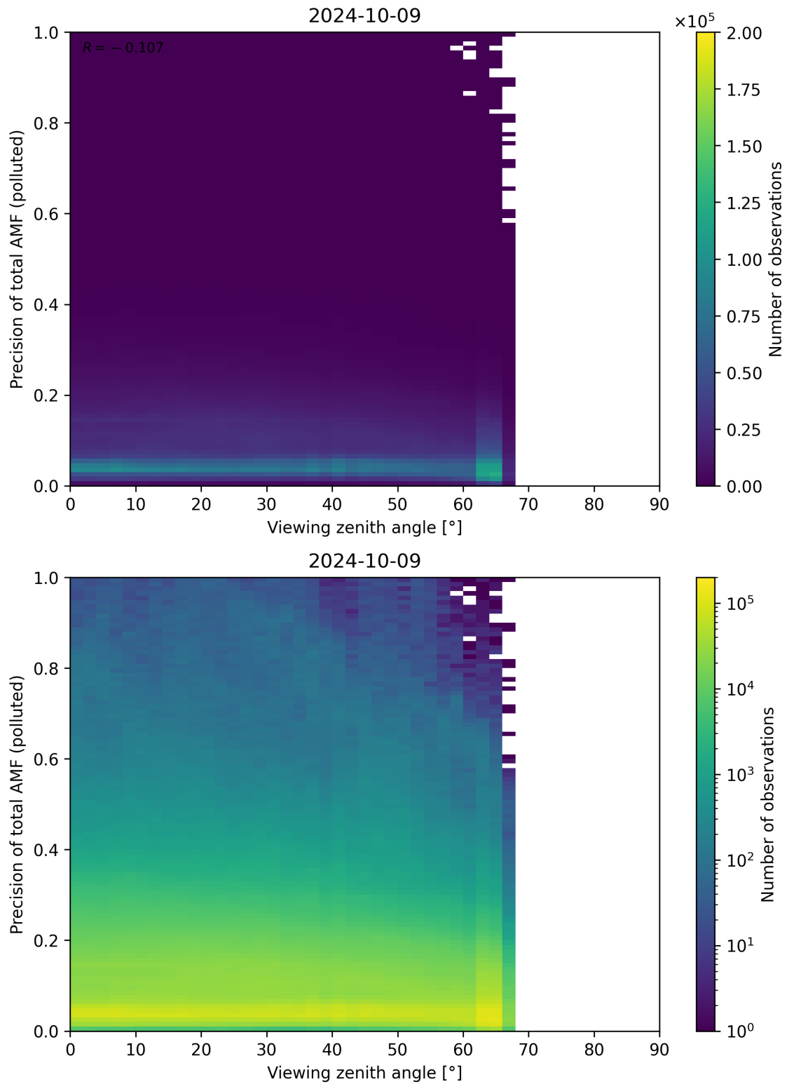
Figure 326: Scatter density plot of “Viewing zenith angle” against “Precision of total AMF (polluted)” for 2024-10-08 to 2024-10-10.
