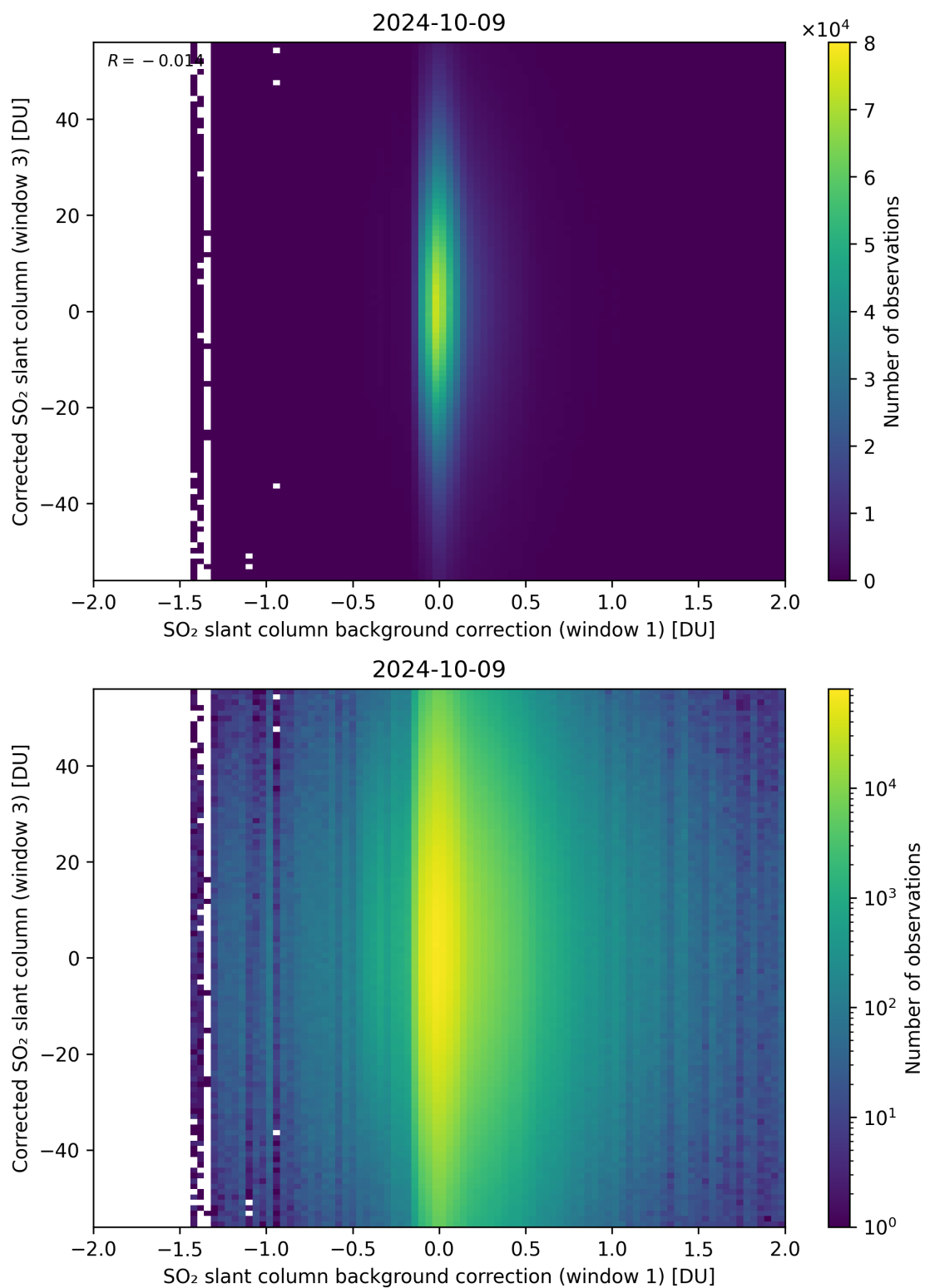
Figure 105: Scatter density plot of “SO 2 slant column background correction (window 1)” against “Corrected SO 2 slant column (window 3)” for 2024-10-08 to 2024-10-10.
