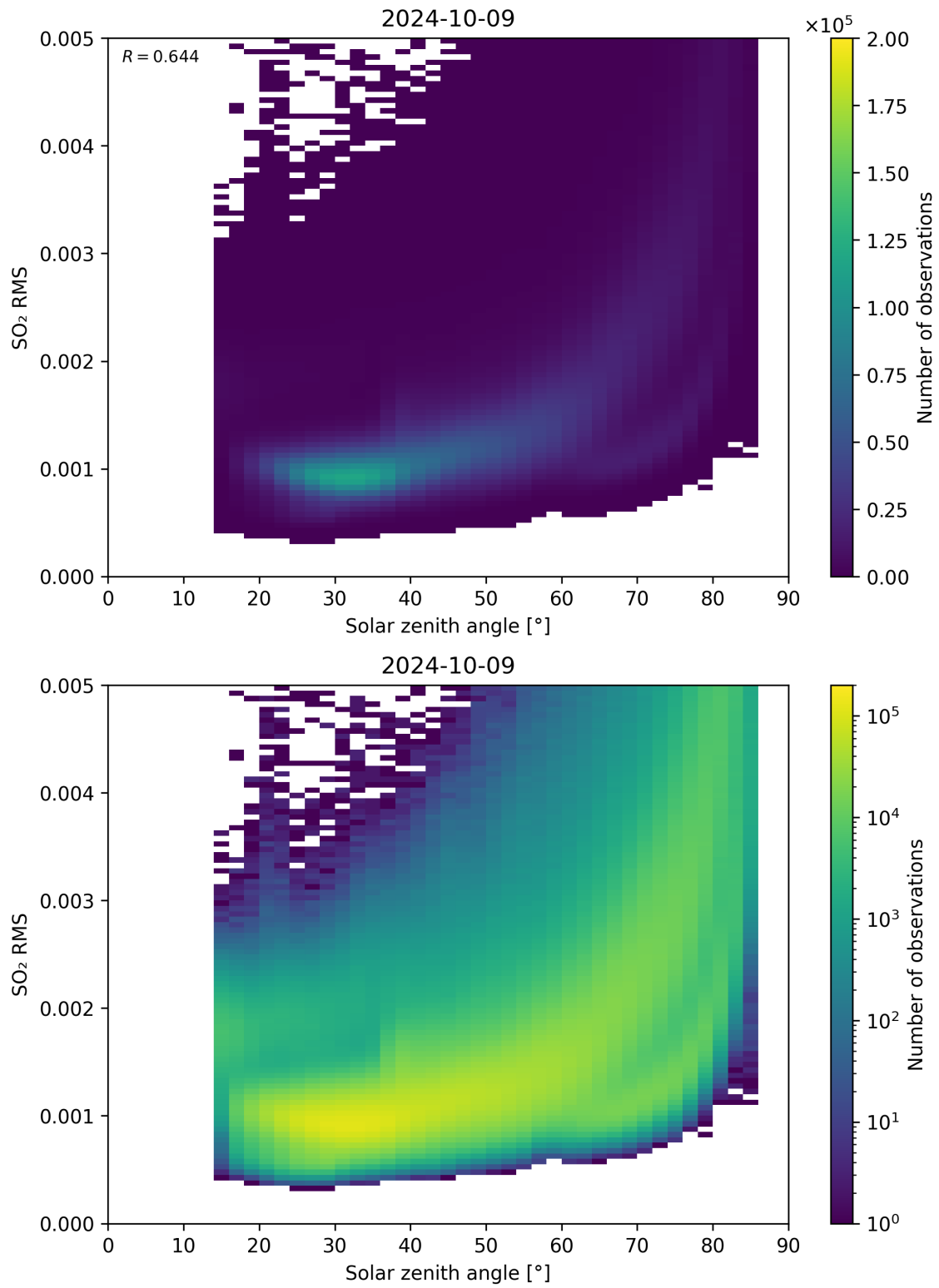
Figure 163: Scatter density plot of “Solar zenith angle” against “SO 2 RMS” for 2024-10-08 to 2024-10-10.
