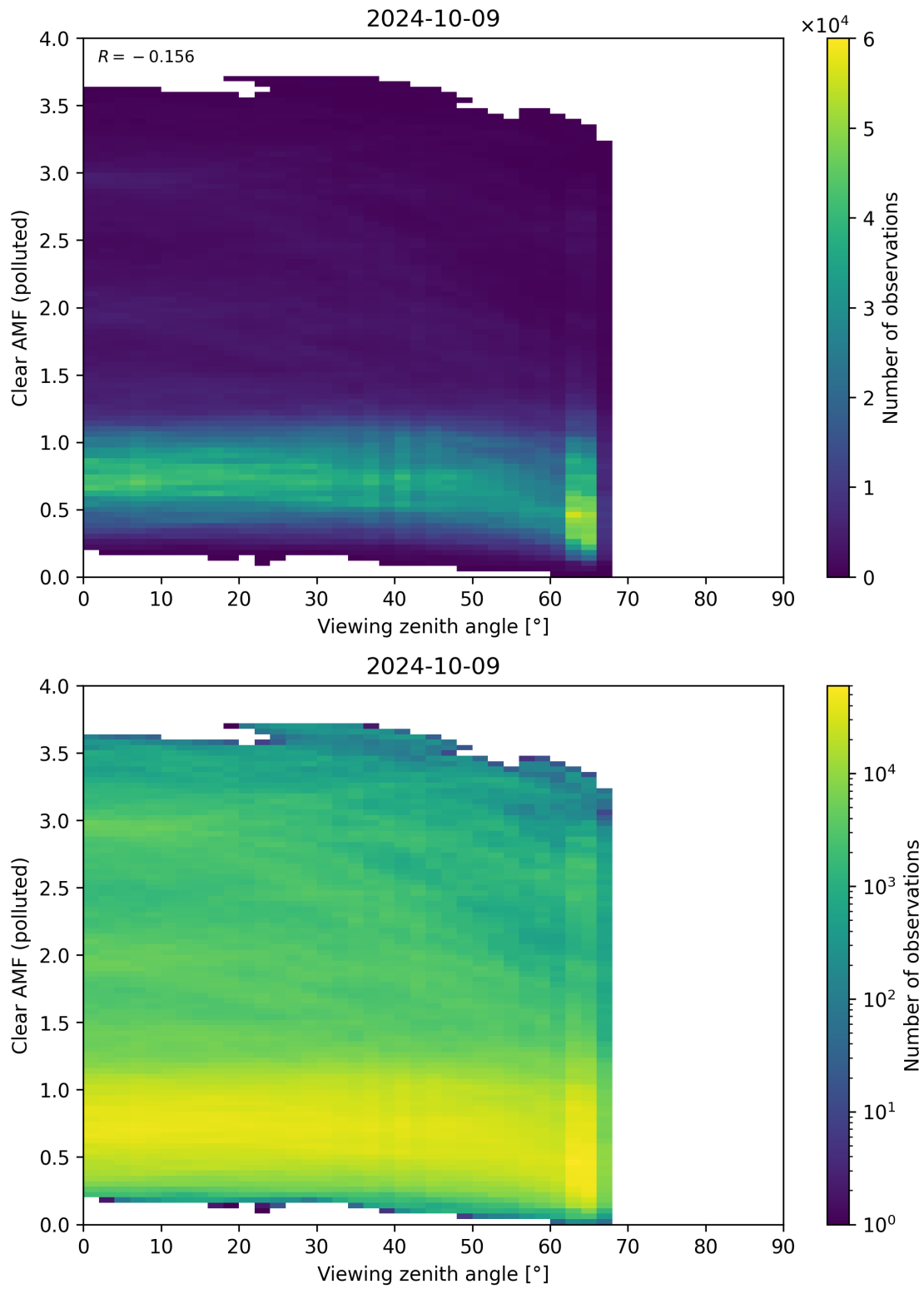
Figure 316: Scatter density plot of “Viewing zenith angle” against “Clear AMF (polluted)” for 2024-10-08 to 2024-10-10.
