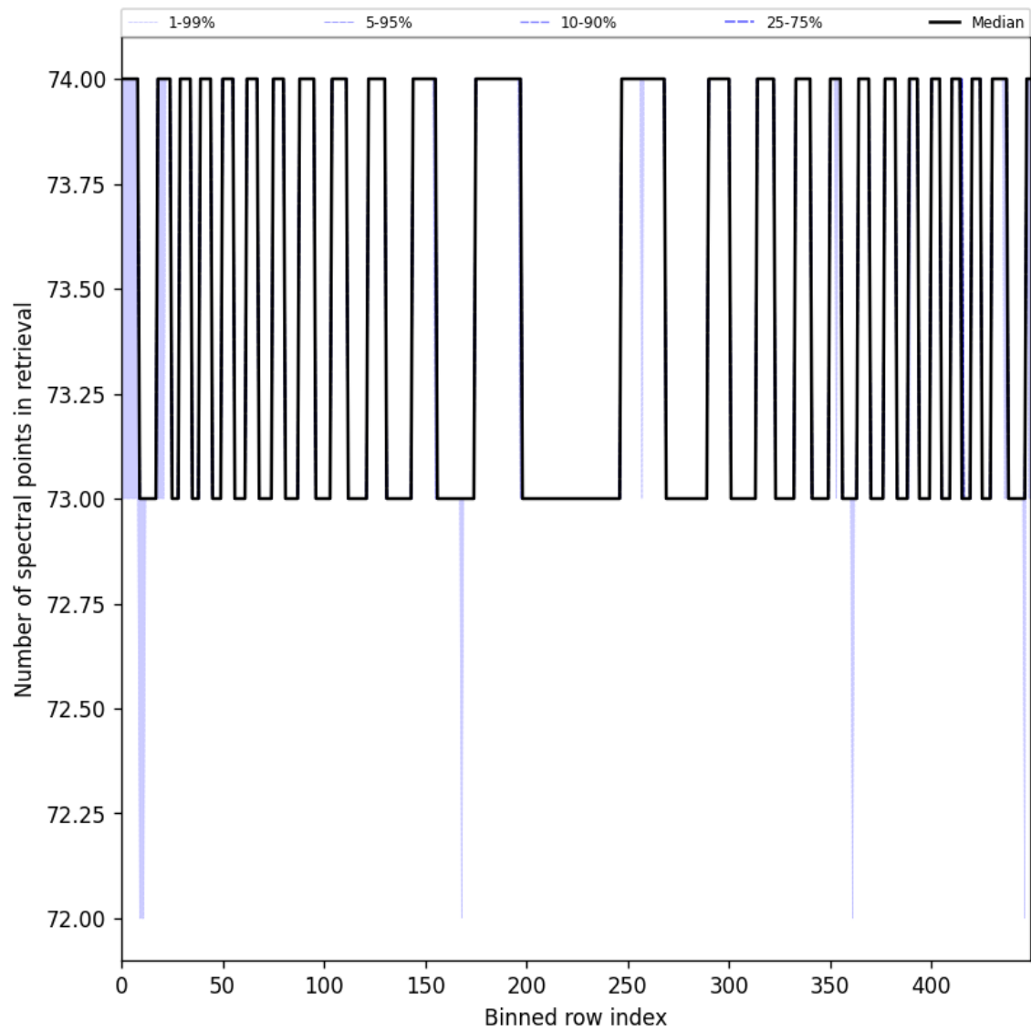
Figure 97: Along track statistics of “Number of spectral points in retrieval” for 2024-10-08 to 2024-10-10
