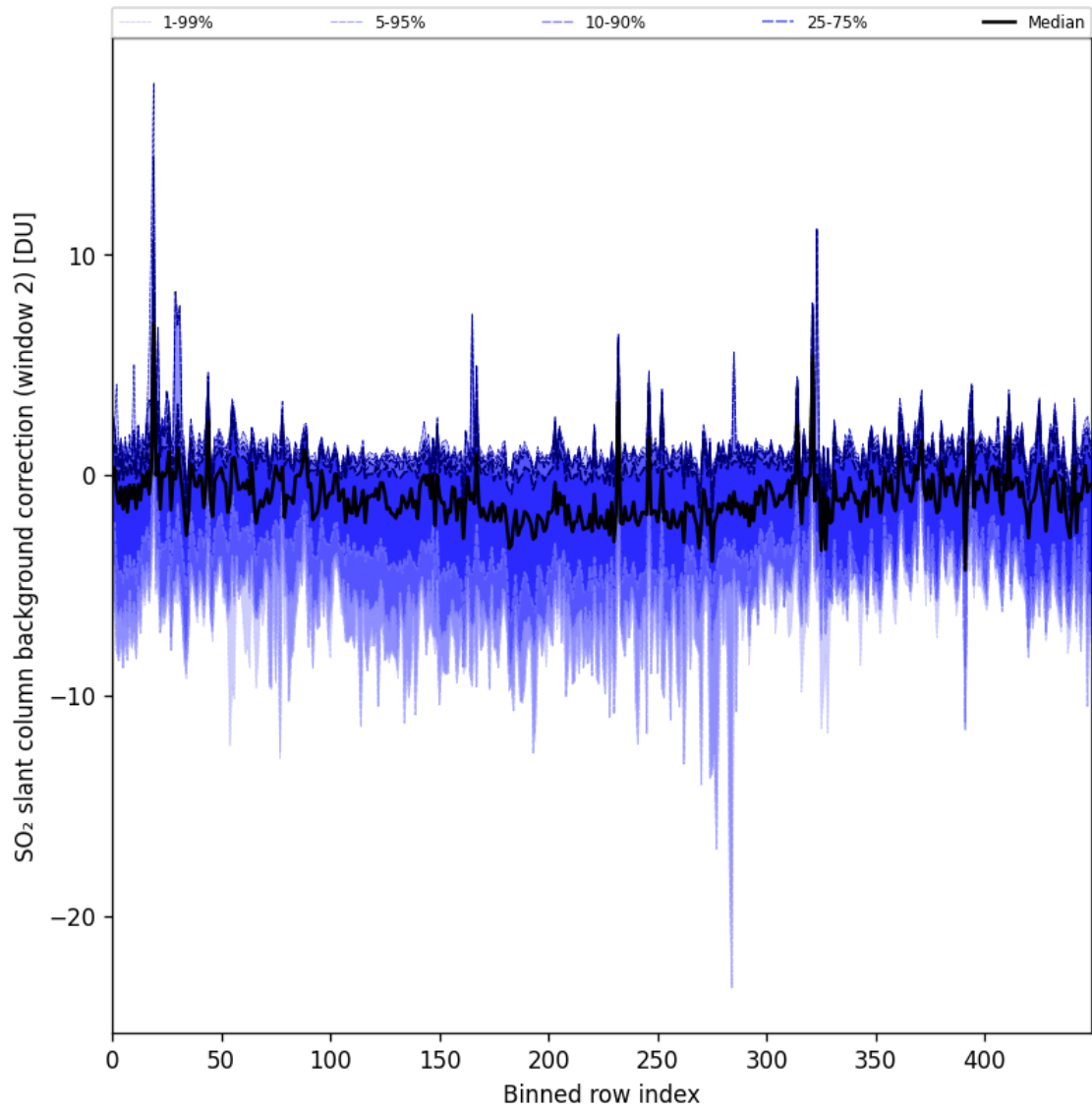
Figure 86: Along track statistics of “SO 2 slant column background correction (window 2)” for 2024-10-08 to 2024-10-10
