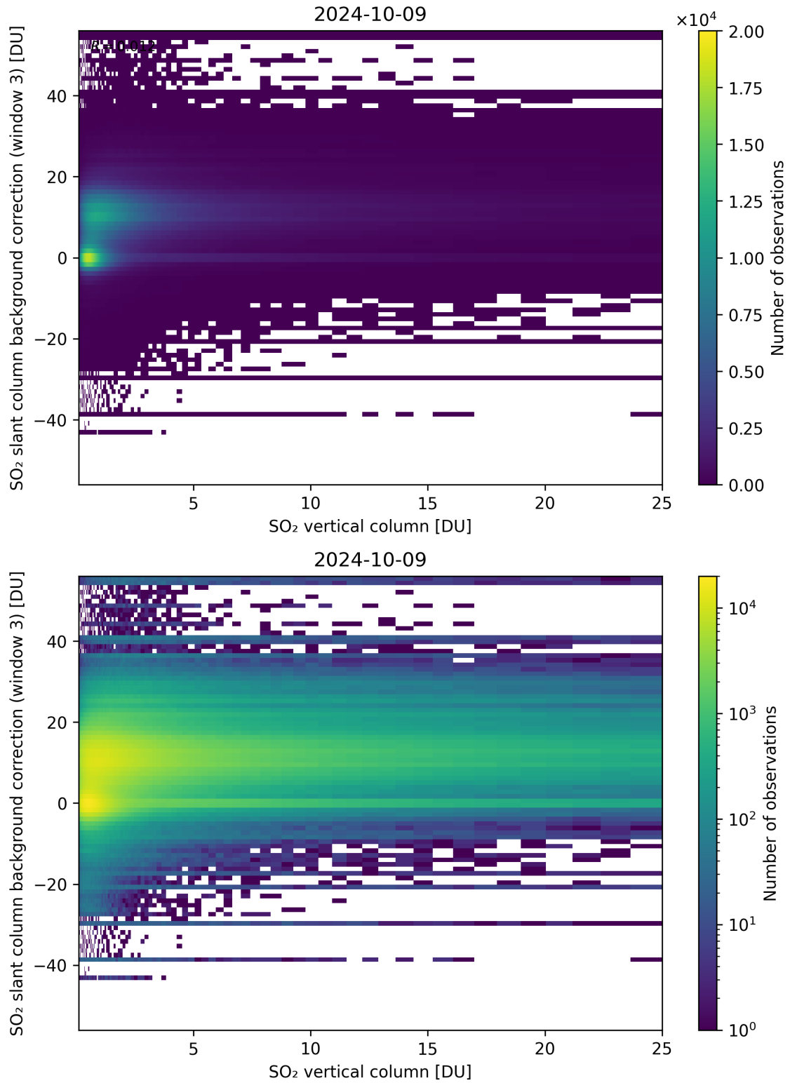
Figure 275: Scatter density plot of “SO 2 vertical column” against “SO 2 slant column background correction (window 3)” for 2024-10-08 to 2024-10-10.
