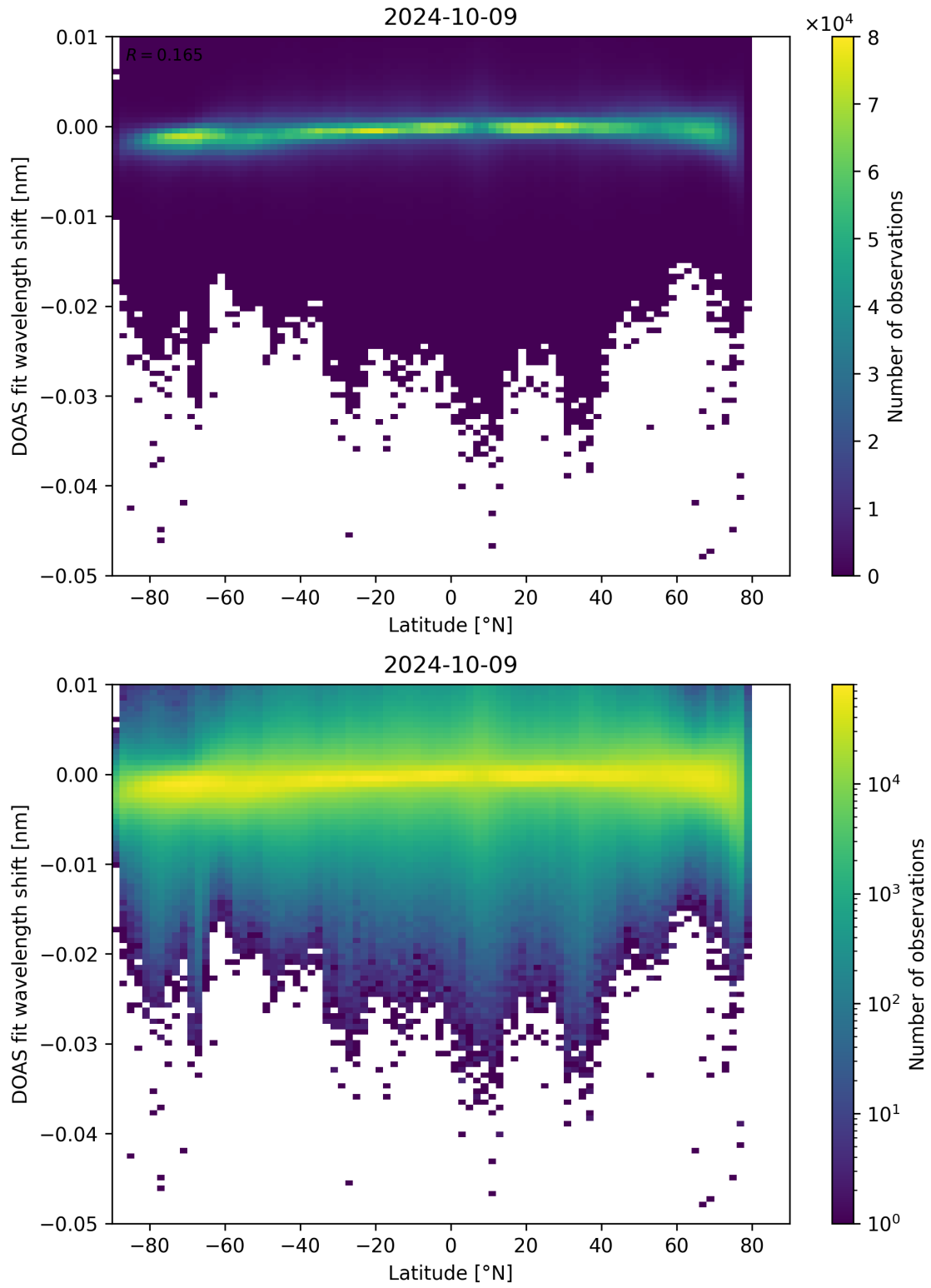
Figure 142: Scatter density plot of “Latitude” against “DOAS fit wavelength shift” for 2024-10-08 to 2024-10-10.
