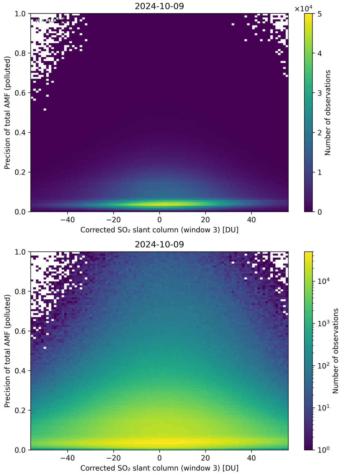
Figure 211: Scatter density plot of “Corrected SO 2 slant column (window 3)” against “Precision of total AMF (polluted)” for 2024-10-08 to 2024-10-10.
