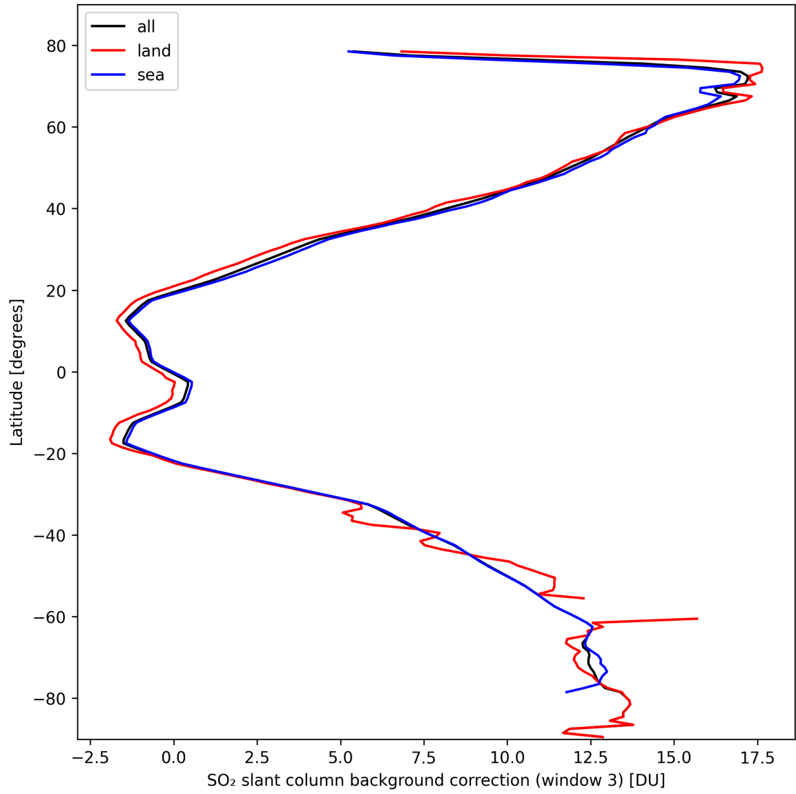
Figure 44: Zonal average of “SO 2 slant column background correction (window 3)” for 2024-10-08 to 2024-10-10.
