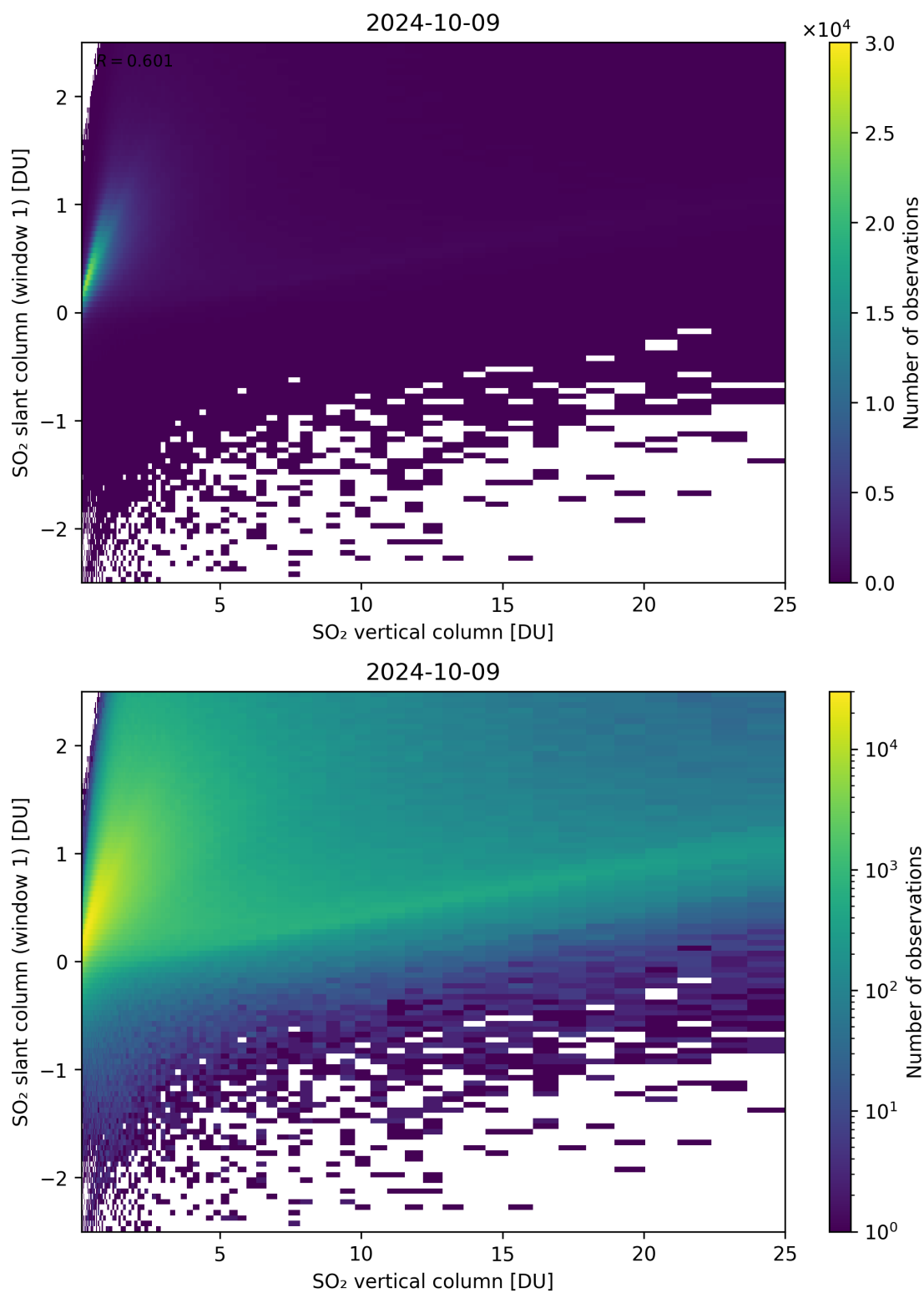
Figure 300: Scatter density plot of “SO 2 vertical column” against “SO 2 slant column (window 1)” for 2024-10-08 to 2024-10-10.
