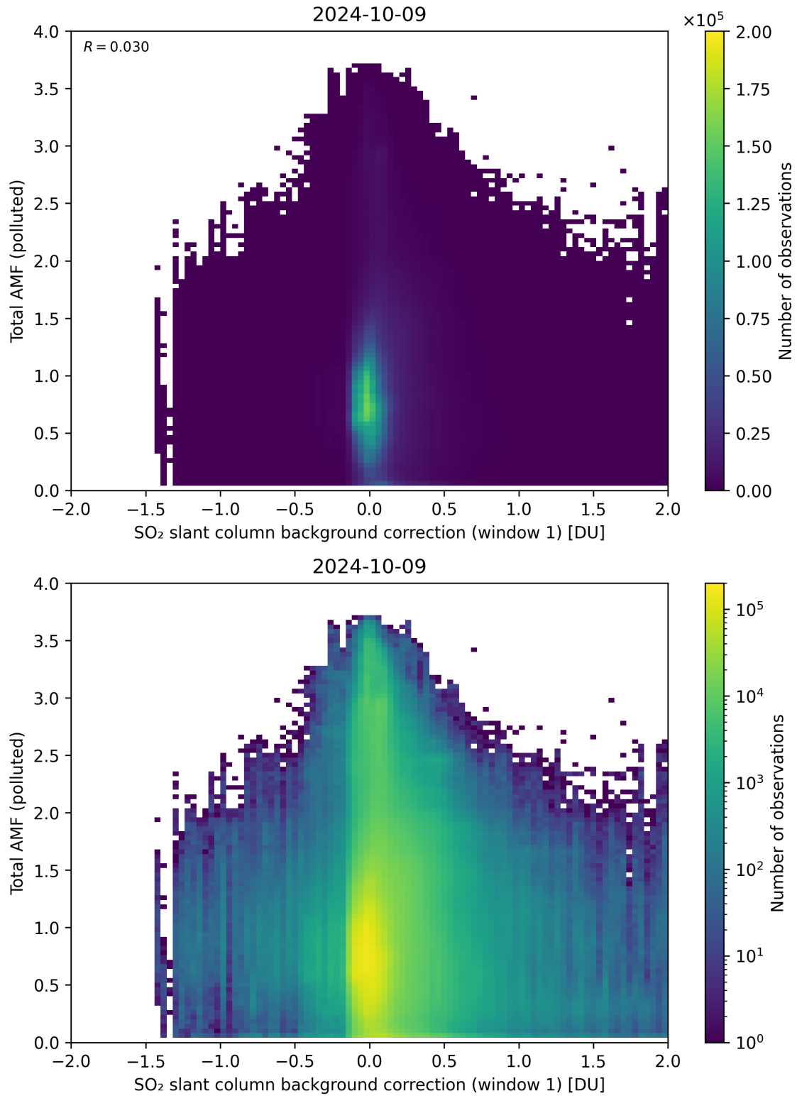
Figure 109: Scatter density plot of “SO 2 slant column background correction (window 1)” against “Total AMF (polluted)” for 2024-10-08 to 2024-10-10.
