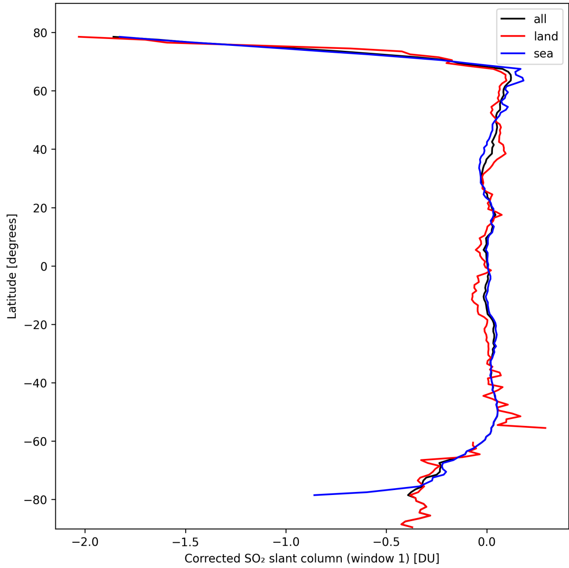
Figure 35: Zonal average of “Corrected SO 2 slant column (window 1)” for 2024-10-08 to 2024-10-10.
