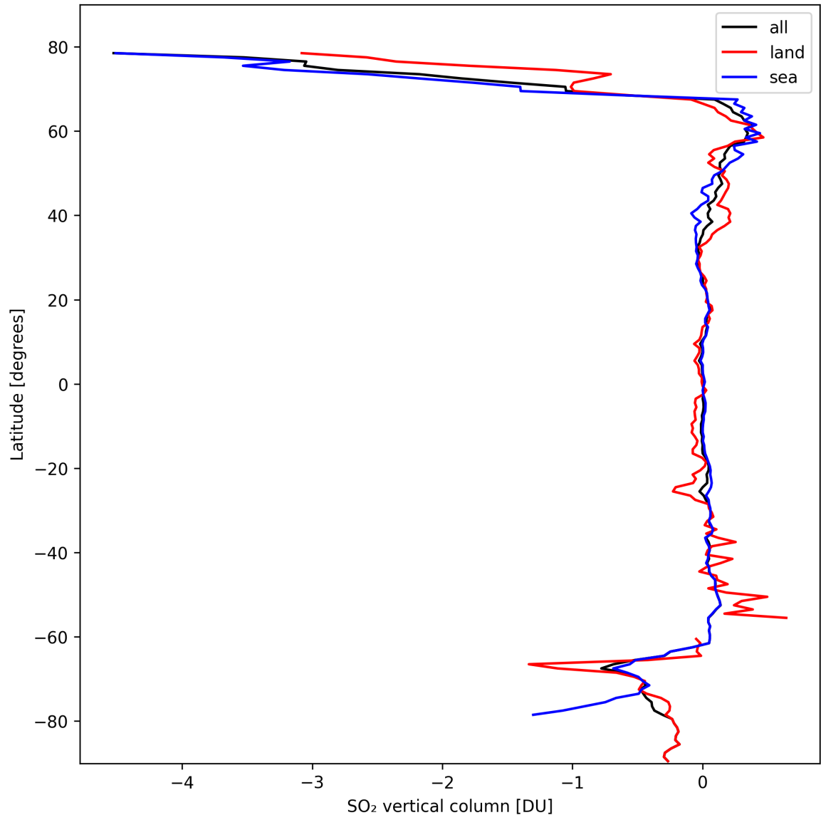
Figure 30: Zonal average of “SO 2 vertical column” for 2024-10-08 to 2024-10-10.
