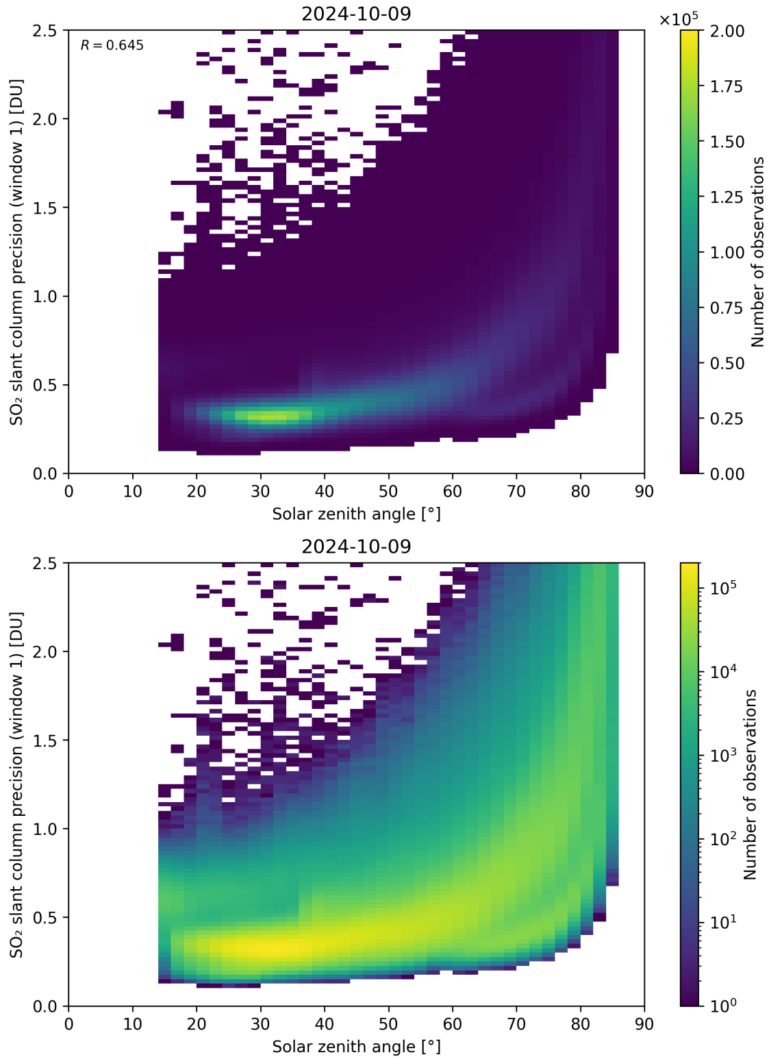
Figure 170: Scatter density plot of “Solar zenith angle” against “SO 2 slant column precision (window 1)” for 2024-10-08 to 2024-10-10.
