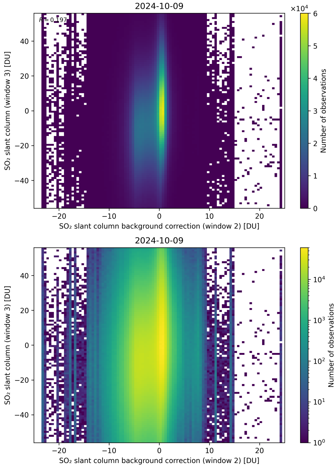
Figure 117: Scatter density plot of “SO 2 slant column background correction (window 2)” against “SO 2 slant column (window 3)” for 2024-10-08 to 2024-10-10.
