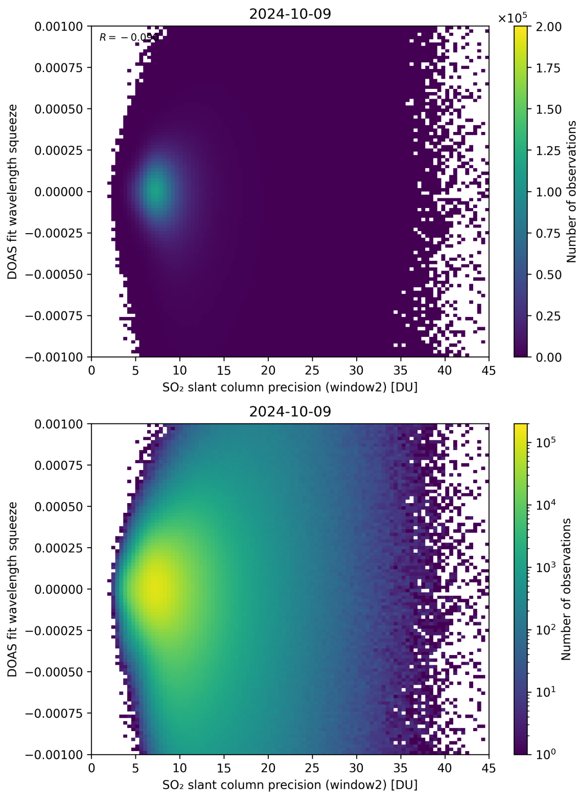
Figure 244: Scatter density plot of “SO 2 slant column precision (window2)” against “DOAS fit wavelength squeeze” for 2024-10-08 to 2024-10-10.
