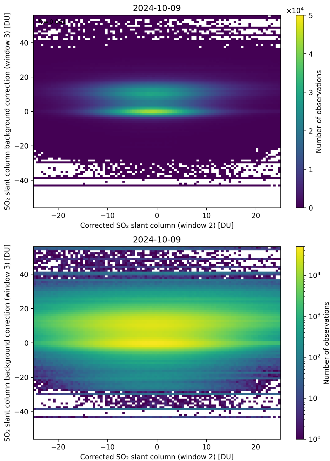
Figure 195: Scatter density plot of “Corrected SO 2 slant column (window 2)” against “SO 2 slant column background correction (window 3)” for 2024-10-08 to 2024-10-10.
