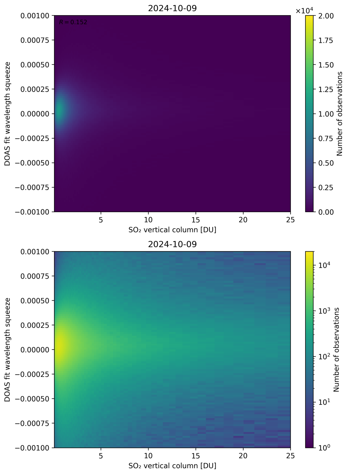
Figure 277: Scatter density plot of “SO 2 vertical column” against “DOAS fit wavelength squeeze” for 2024-10-08 to 2024-10-10.
