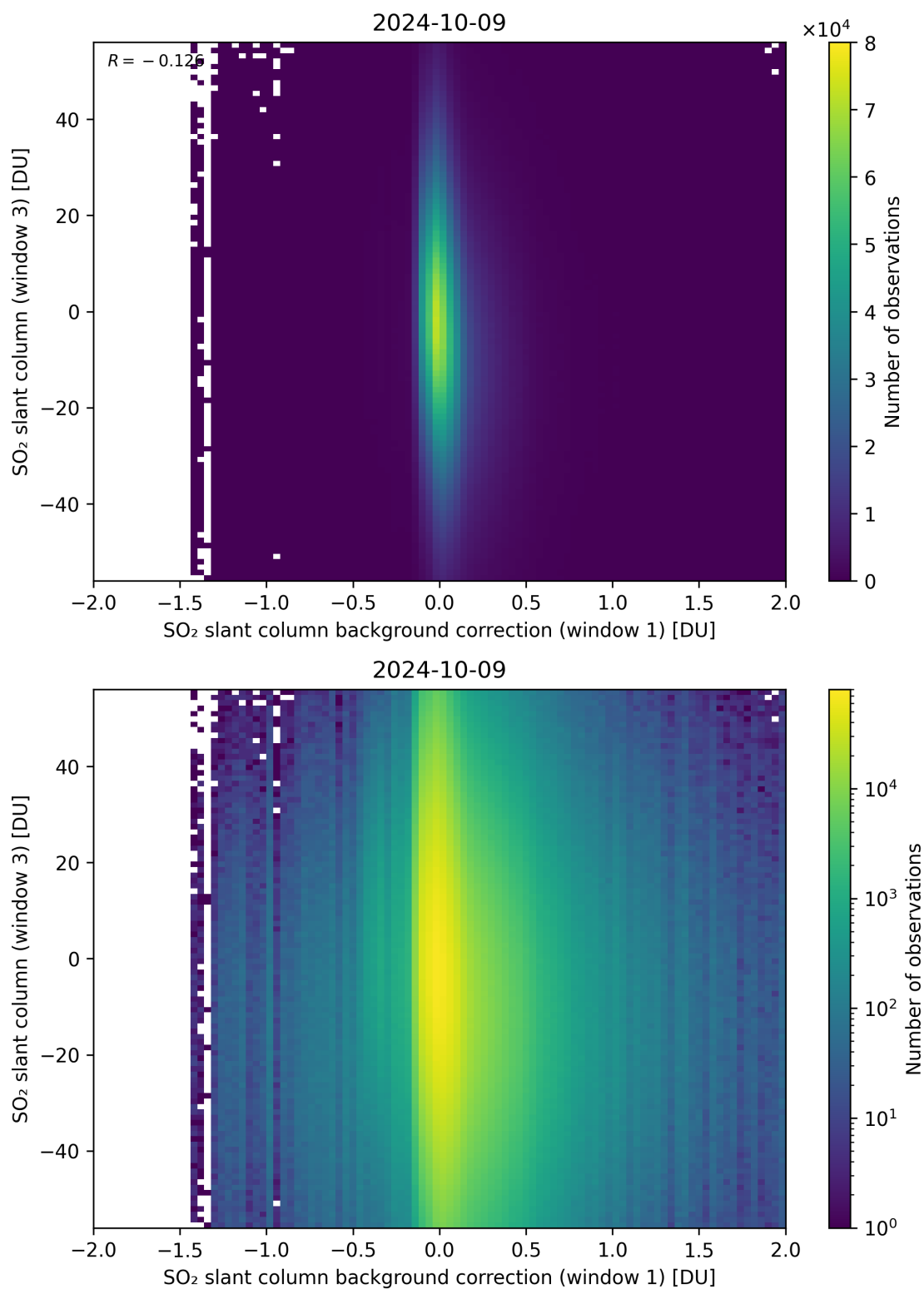
Figure 107: Scatter density plot of “SO 2 slant column background correction (window 1)” against “SO 2 slant column (window 3)” for 2024-10-08 to 2024-10-10.
