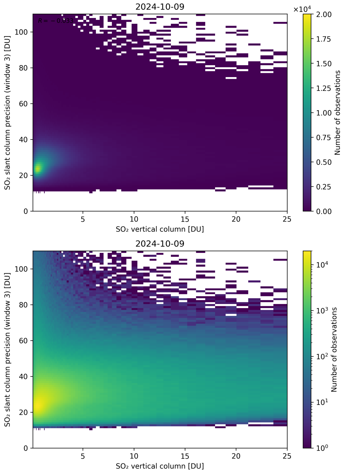
Figure 304: Scatter density plot of “SO 2 vertical column” against “SO 2 slant column precision (window 3)” for 2024-10-08 to 2024-10-10.
