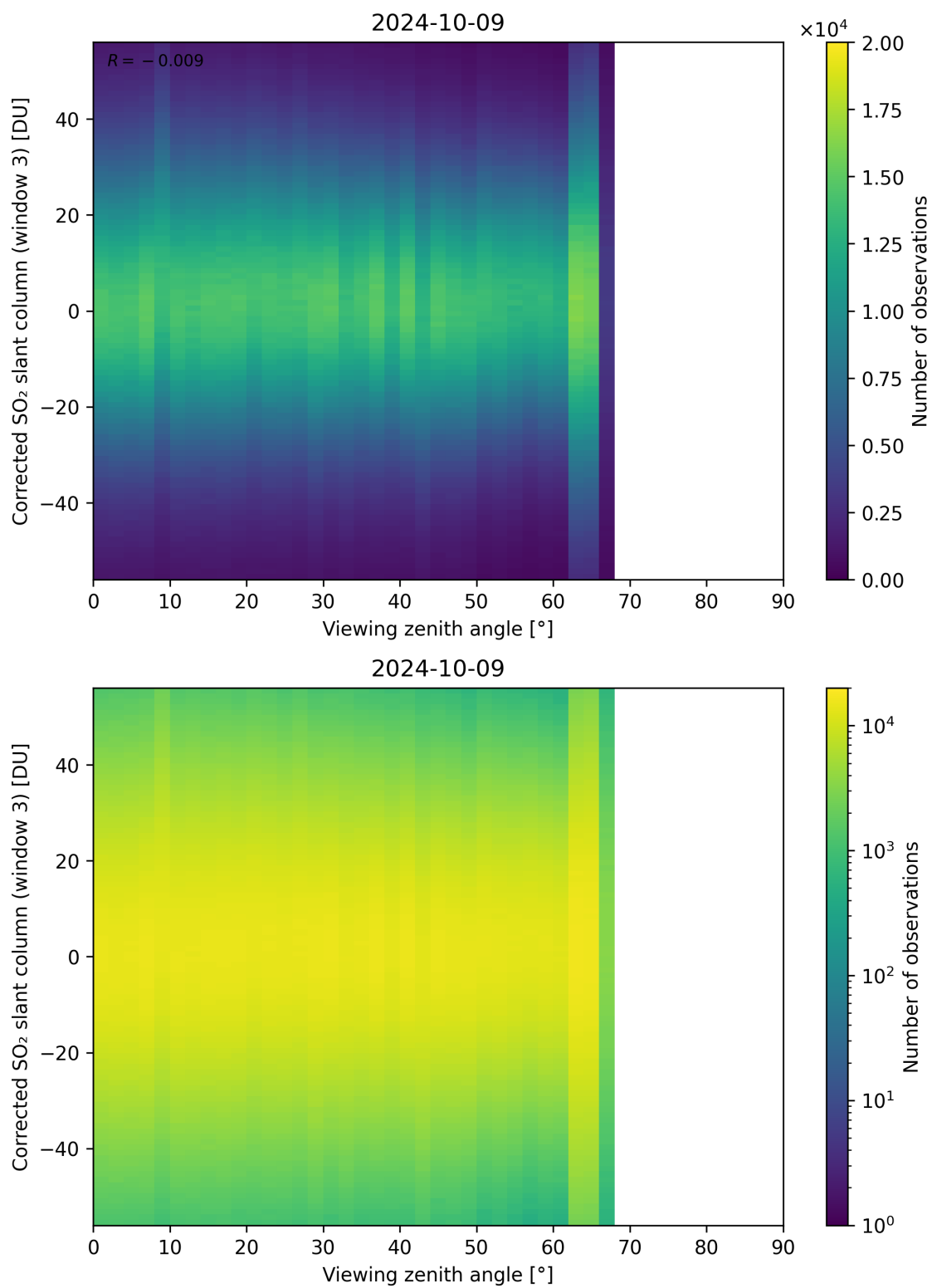
Figure 319: Scatter density plot of “Viewing zenith angle” against “Corrected SO 2 slant column (window 3)” for 2024-10-08 to 2024-10-10.
