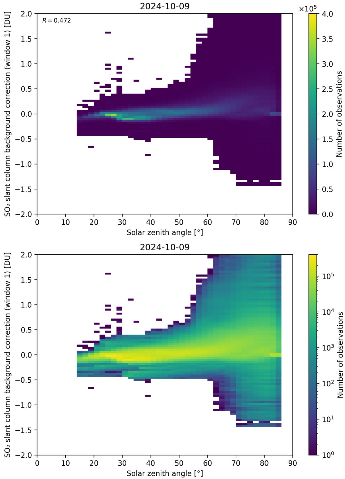
Figure 158: Scatter density plot of “Solar zenith angle” against “SO 2 slant column background correction (window 1)” for 2024-10-08 to 2024-10-10.
