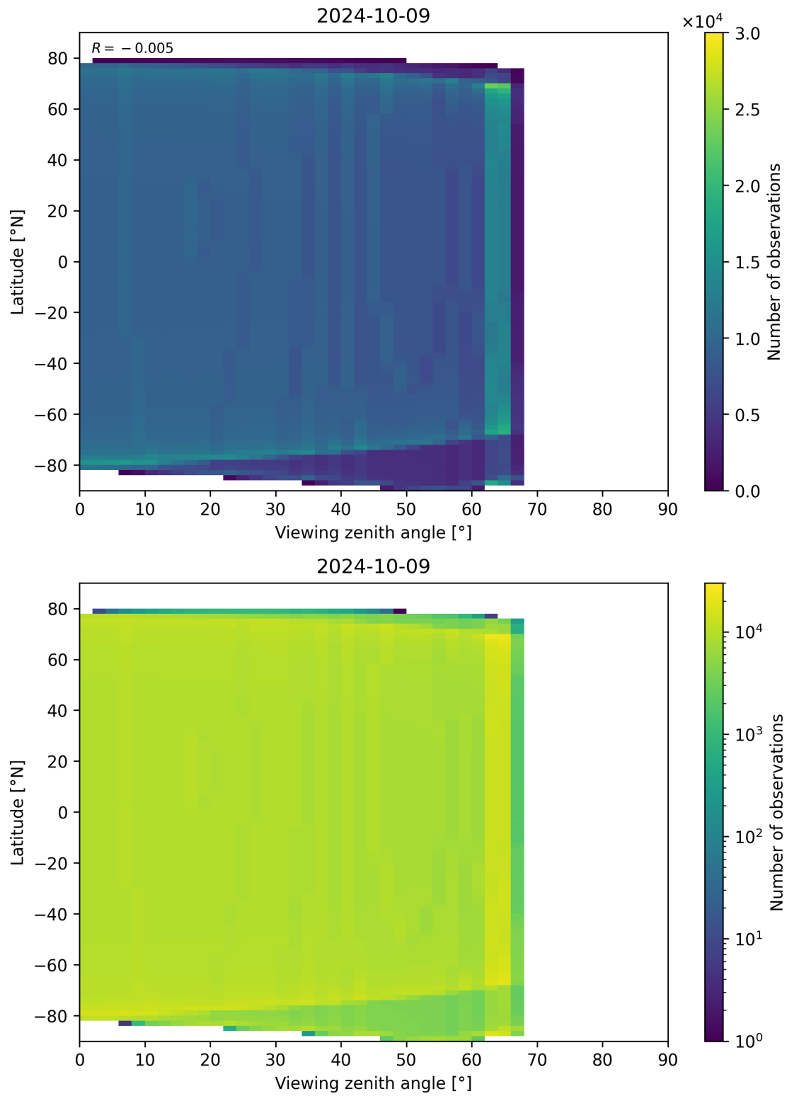
Figure 314: Scatter density plot of “Viewing zenith angle” against “Latitude” for 2024-10-08 to 2024-10-10.
