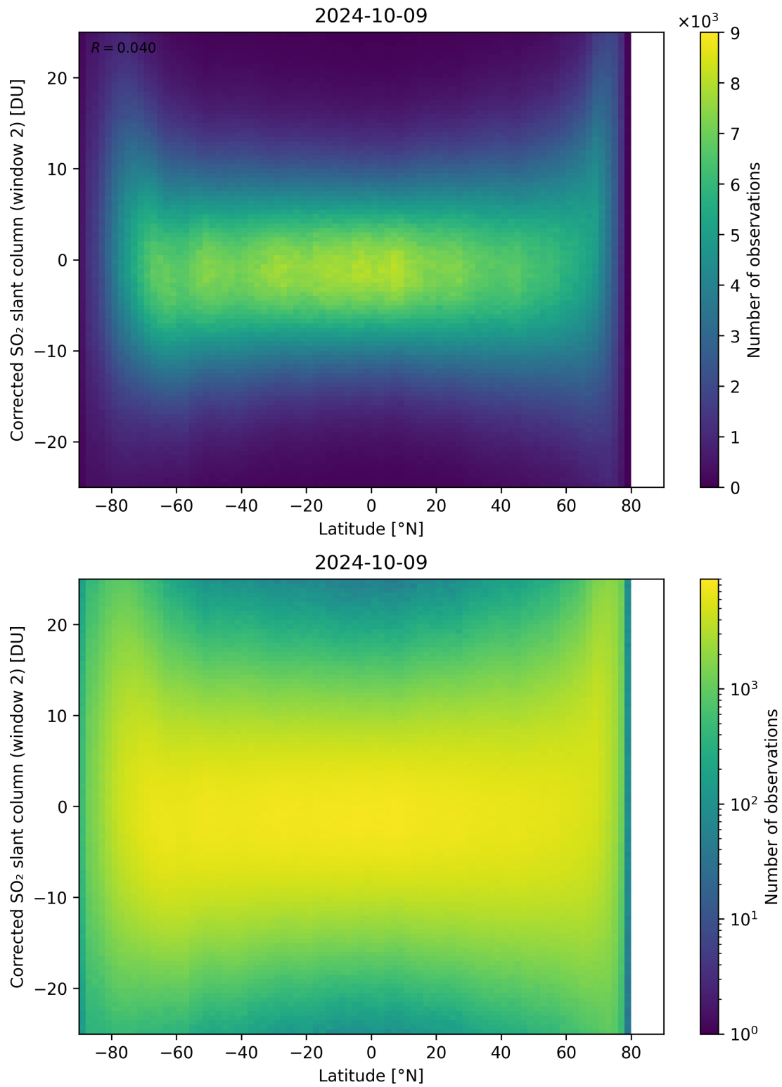
Figure 147: Scatter density plot of “Latitude” against “Corrected SO 2 slant column (window 2)” for 2024-10-08 to 2024-10-10.
