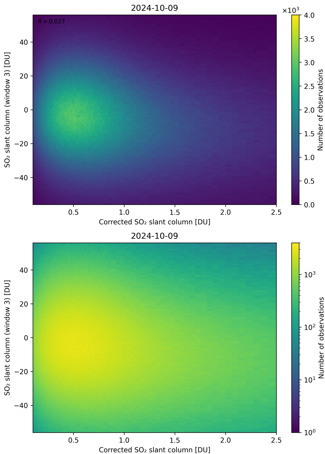
Figure 190: Scatter density plot of “Corrected SO 2 slant column” against “SO 2 slant column (window 3)” for 2024-10-08 to 2024-10-10.
