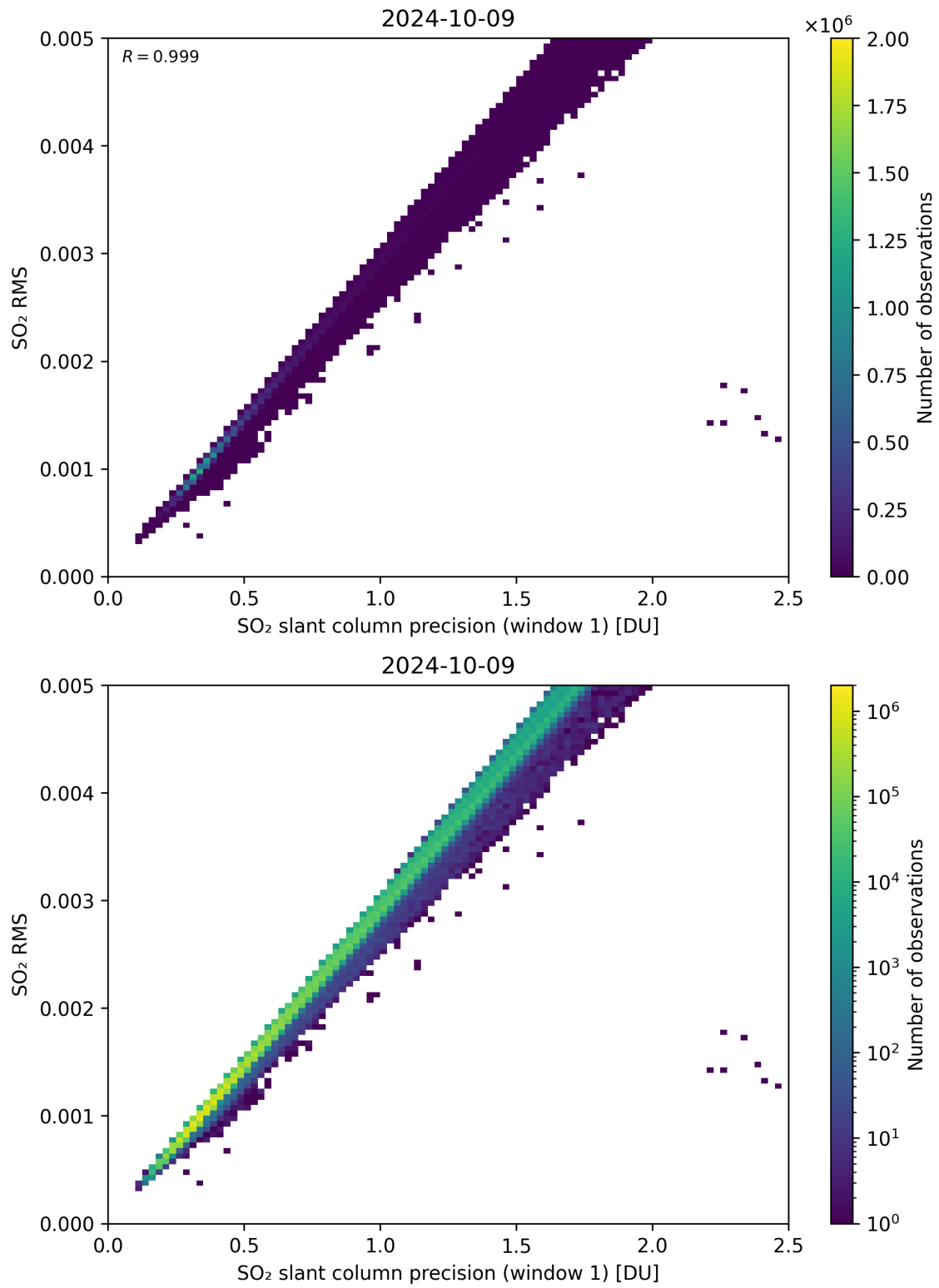
Figure 223: Scatter density plot of “SO 2 slant column precision (window 1)” against “SO 2 RMS” for 2024-10-08 to 2024-10-10.
