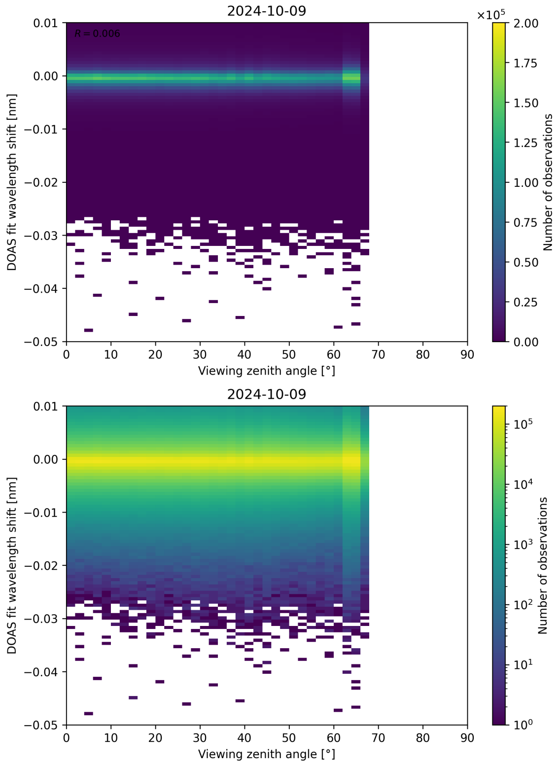
Figure 311: Scatter density plot of “Viewing zenith angle” against “DOAS fit wavelength shift” for 2024-10-08 to 2024-10-10.
