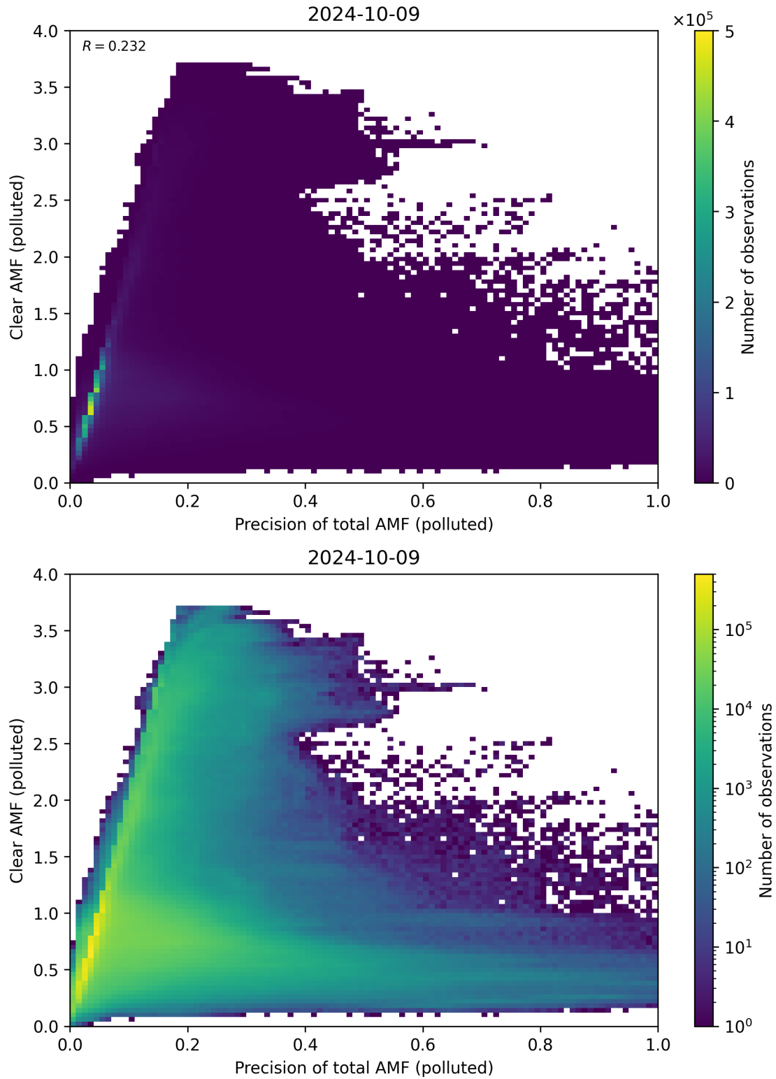
Figure 270: Scatter density plot of “Precision of total AMF (polluted)” against “Clear AMF (polluted)” for 2024-10-08 to 2024-10-10.
