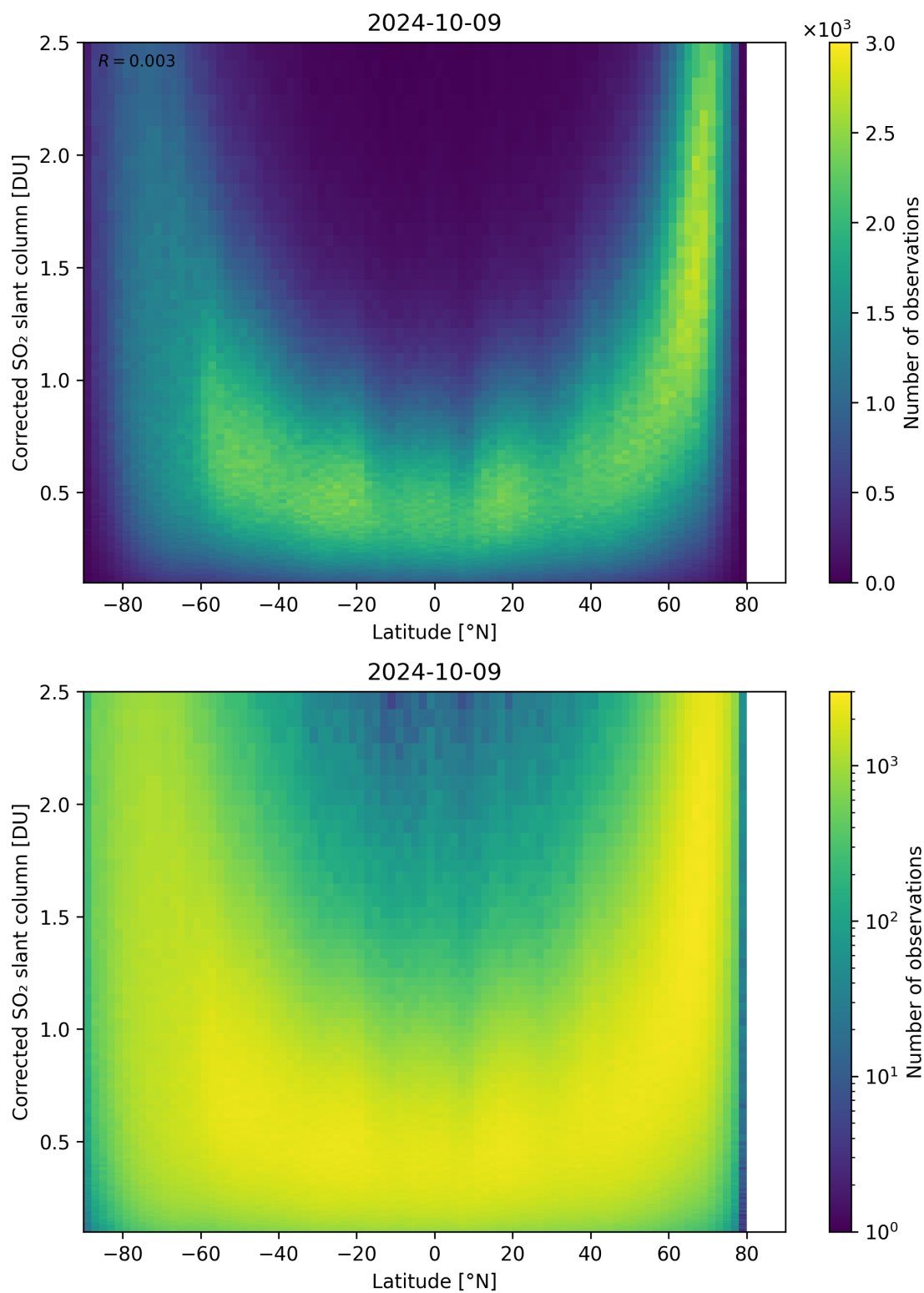
Figure 146: Scatter density plot of “Latitude” against “Corrected SO 2 slant column” for 2024-10-08 to 2024-10-10.
