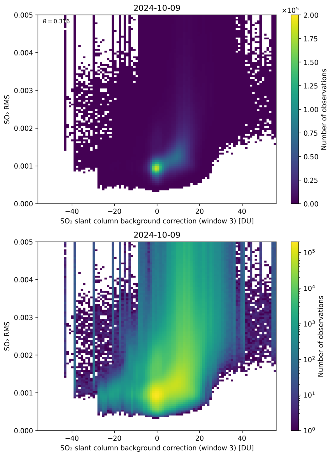
Figure 123: Scatter density plot of “SO 2 slant column background correction (window 3)” against “SO 2 RMS” for 2024-10-08 to 2024-10-10.
