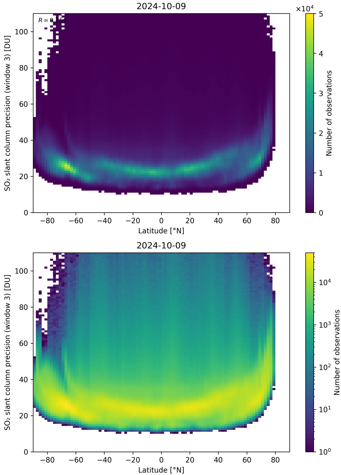
Figure 153: Scatter density plot of “Latitude” against “SO 2 slant column precision (window 3)” for 2024-10-08 to 2024-10-10.
