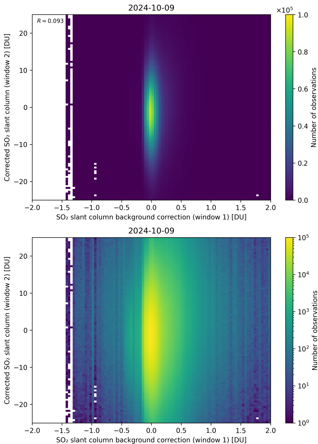
Figure 104: Scatter density plot of “SO 2 slant column background correction (window 1)” against “Corrected SO 2 slant column (window 2)” for 2024-10-08 to 2024-10-10.
