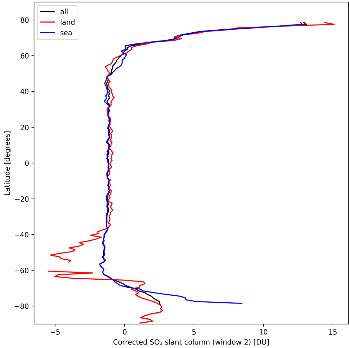
Figure 39: Zonal average of “Corrected SO 2 slant column (window 2)” for 2024-10-08 to 2024-10-10.
