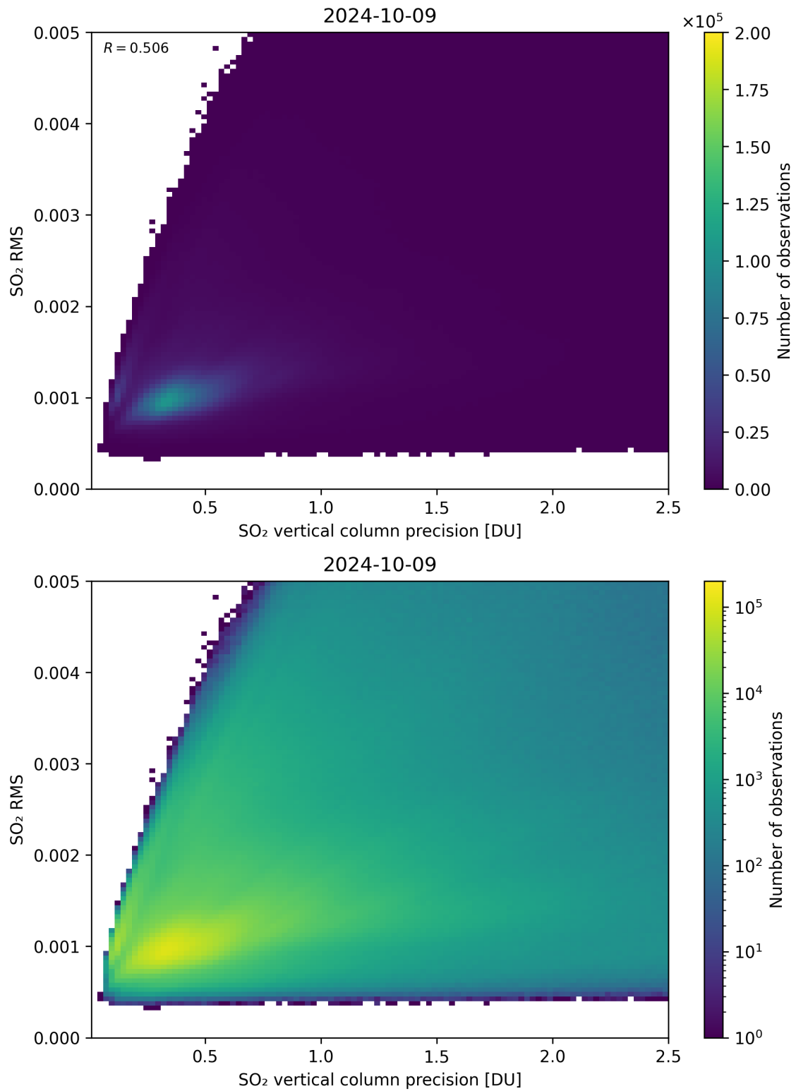
Figure 284: Scatter density plot of “SO 2 vertical column precision” against “SO 2 RMS” for 2024-10-08 to 2024-10-10.
