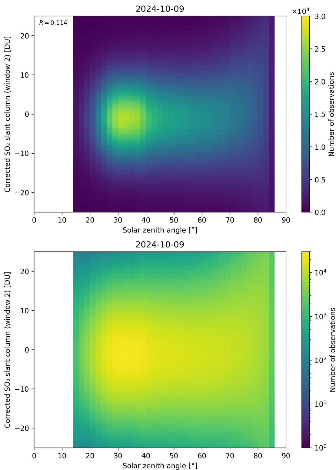
Figure 167: Scatter density plot of “Solar zenith angle” against “Corrected SO 2 slant column (window 2)” for 2024-10-08 to 2024-10-10.
