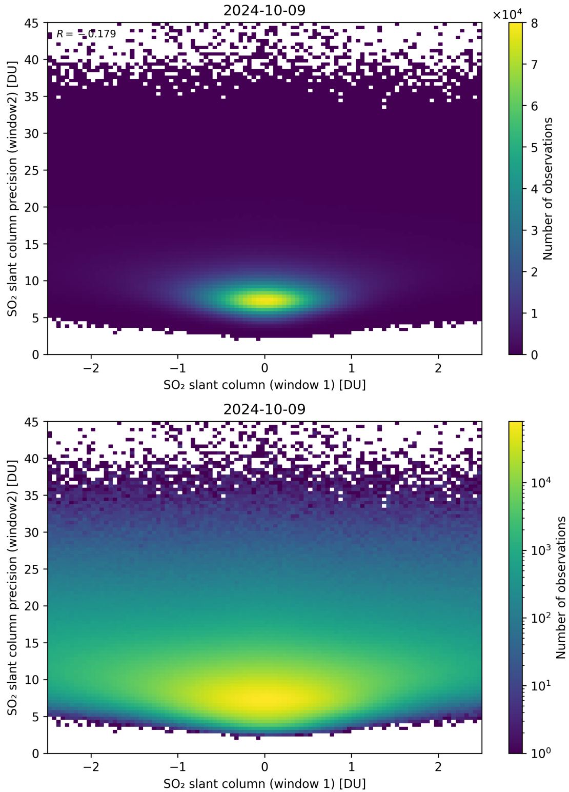
Figure 236: Scatter density plot of “SO 2 slant column (window 1)” against “SO 2 slant column precision (window2)” for 2024-10-08 to 2024-10-10.
