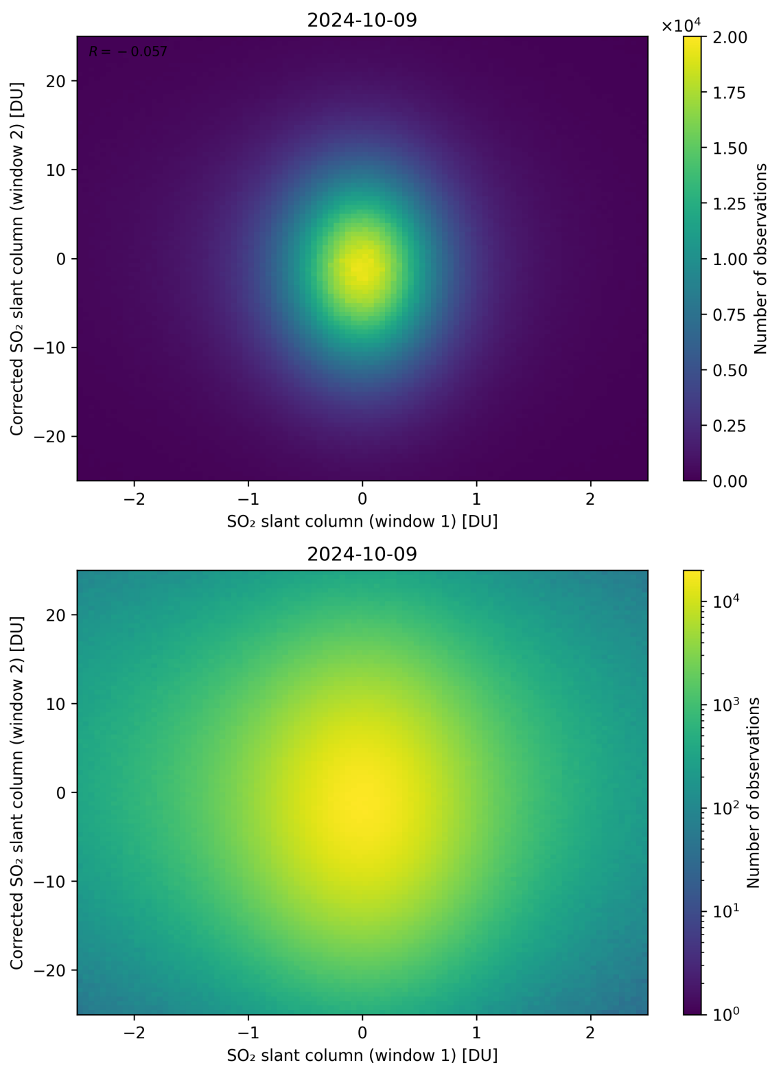
Figure 233: Scatter density plot of “SO 2 slant column (window 1)” against “Corrected SO 2 slant column (window 2)” for 2024-10-08 to 2024-10-10.
