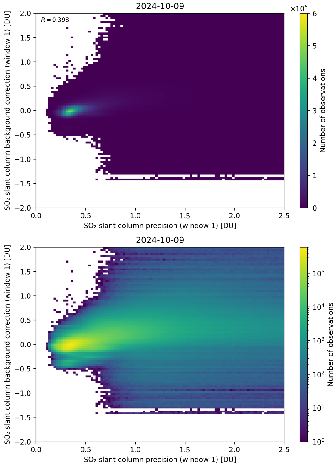
Figure 218: Scatter density plot of “SO 2 slant column precision (window 1)” against “SO 2 slant column background correction (window 1)” for 2024-10-08 to 2024-10-10.
