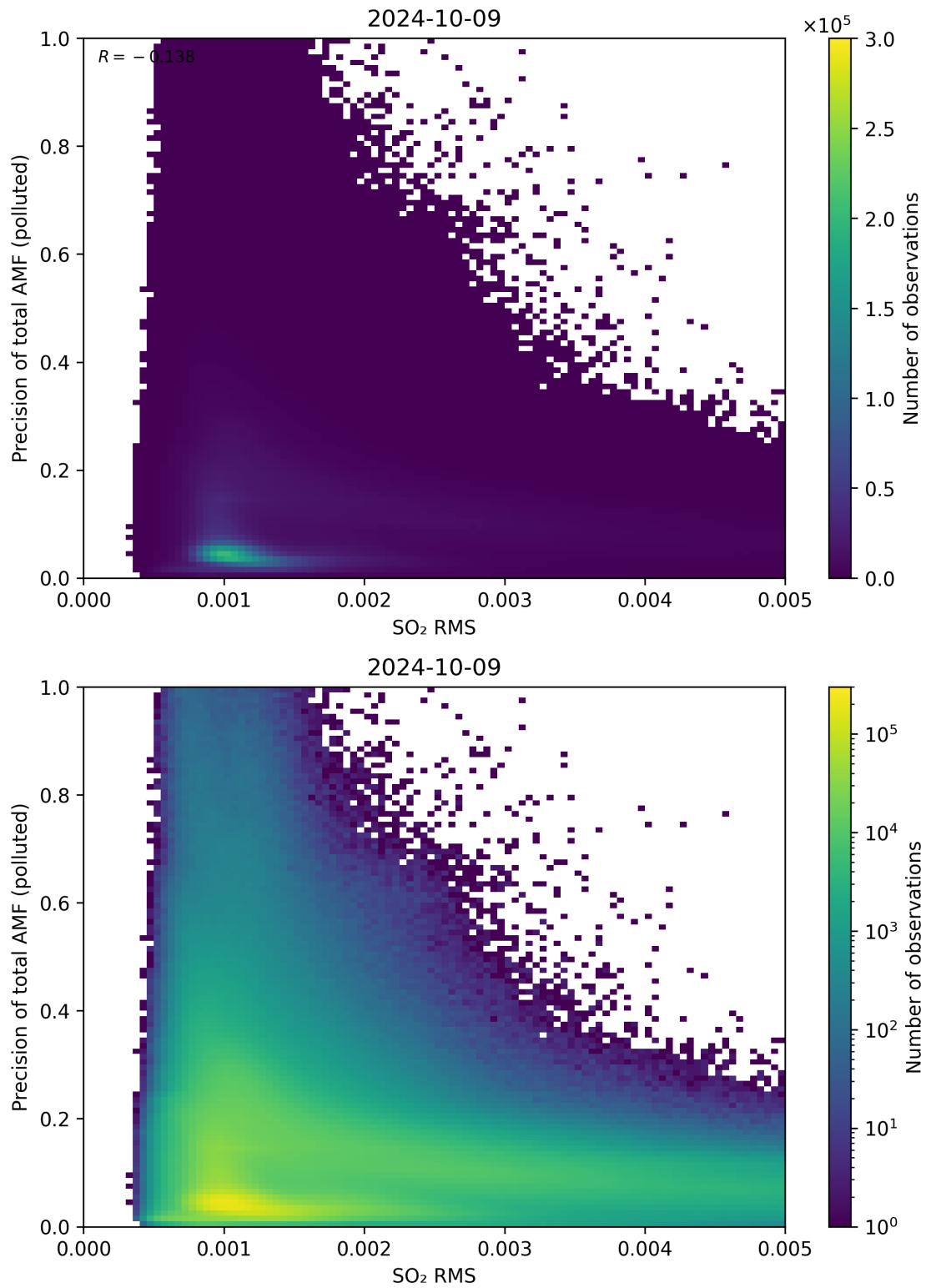
Figure 138: Scatter density plot of “SO 2 RMS” against “Precision of total AMF (polluted)” for 2024-10-08 to 2024-10-10.
