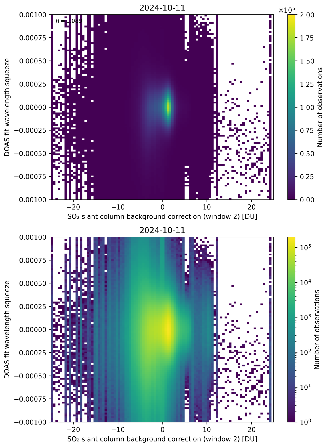
Figure 113: Scatter density plot of “SO 2 slant column background correction (window 2)” against “DOAS fit wavelength squeeze” for 2024-10-10 to 2024-10-12.
