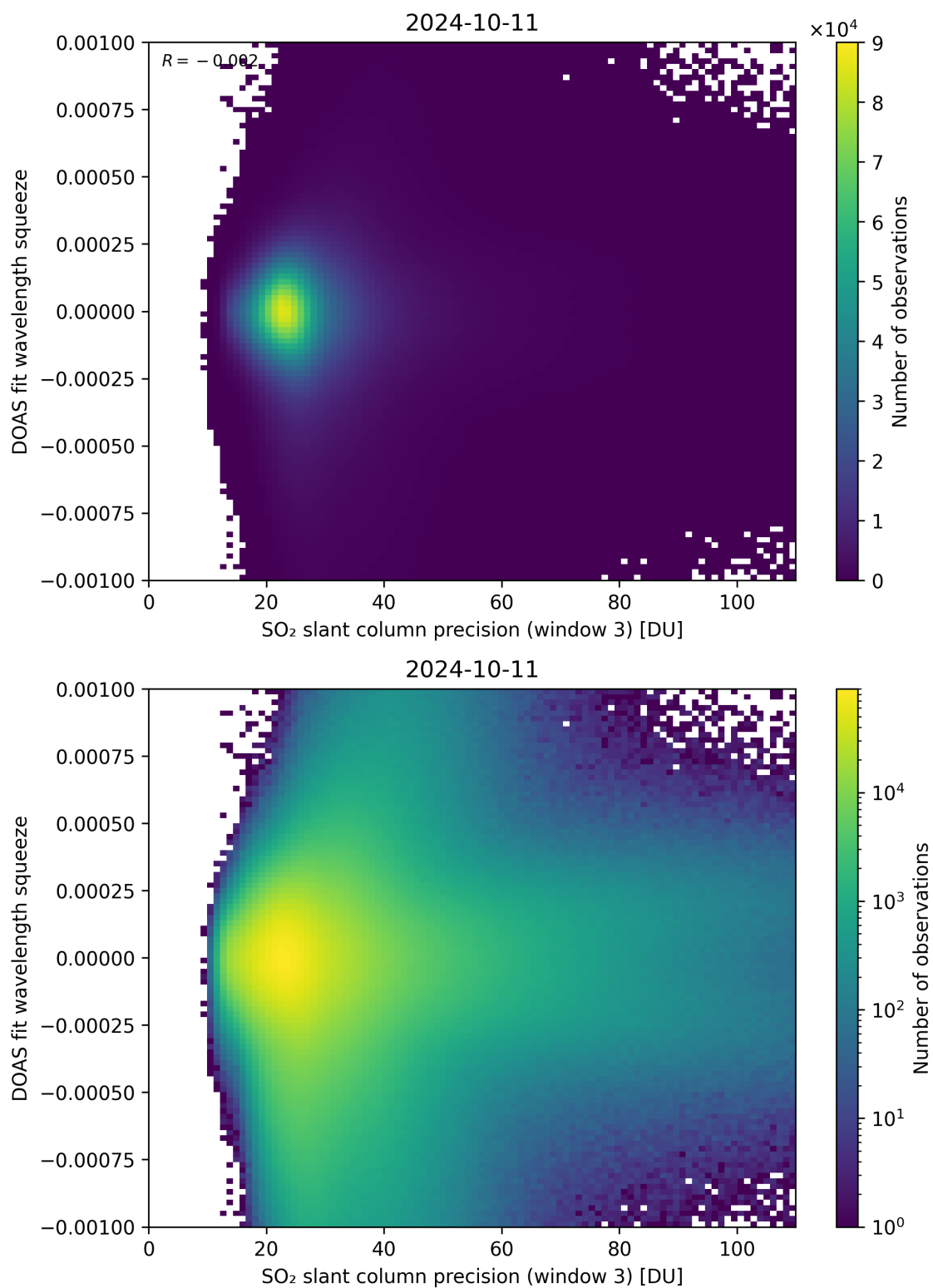
Figure 259: Scatter density plot of “SO 2 slant column precision (window 3)” against “DOAS fit wavelength squeeze” for 2024-10-10 to 2024-10-12.
