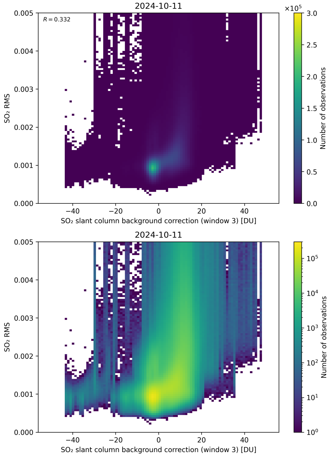
Figure 123: Scatter density plot of “SO 2 slant column background correction (window 3)” against “SO 2 RMS” for 2024-10-10 to 2024-10-12.
