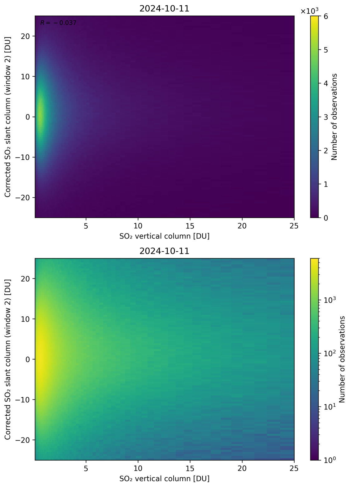
Figure 298: Scatter density plot of “SO 2 vertical column” against “Corrected SO 2 slant column (window 2)” for 2024-10-10 to 2024-10-12.
