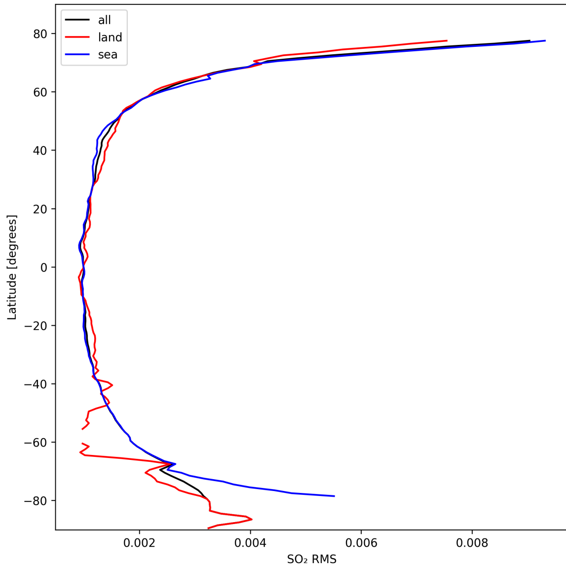
Figure 47: Zonal average of “SO 2 RMS” for 2024-10-10 to 2024-10-12.
