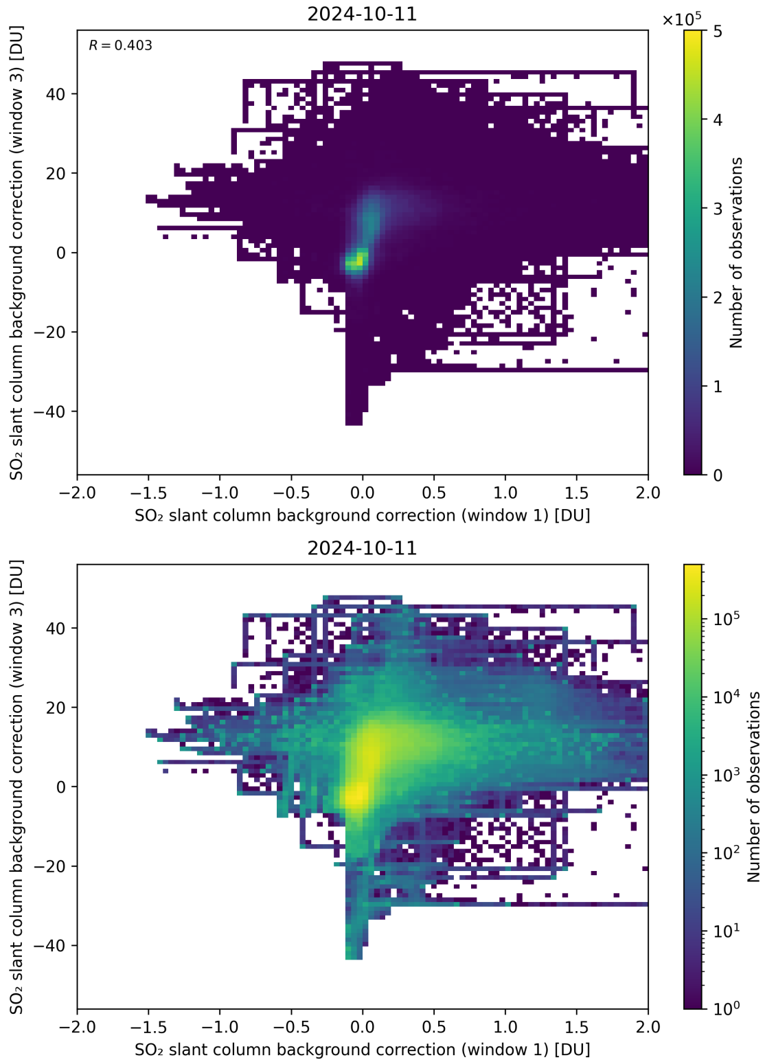
Figure 99: Scatter density plot of “SO 2 slant column background correction (window 1)” against “SO 2 slant column background correction (window 3)” for 2024-10-10 to 2024-10-12.
