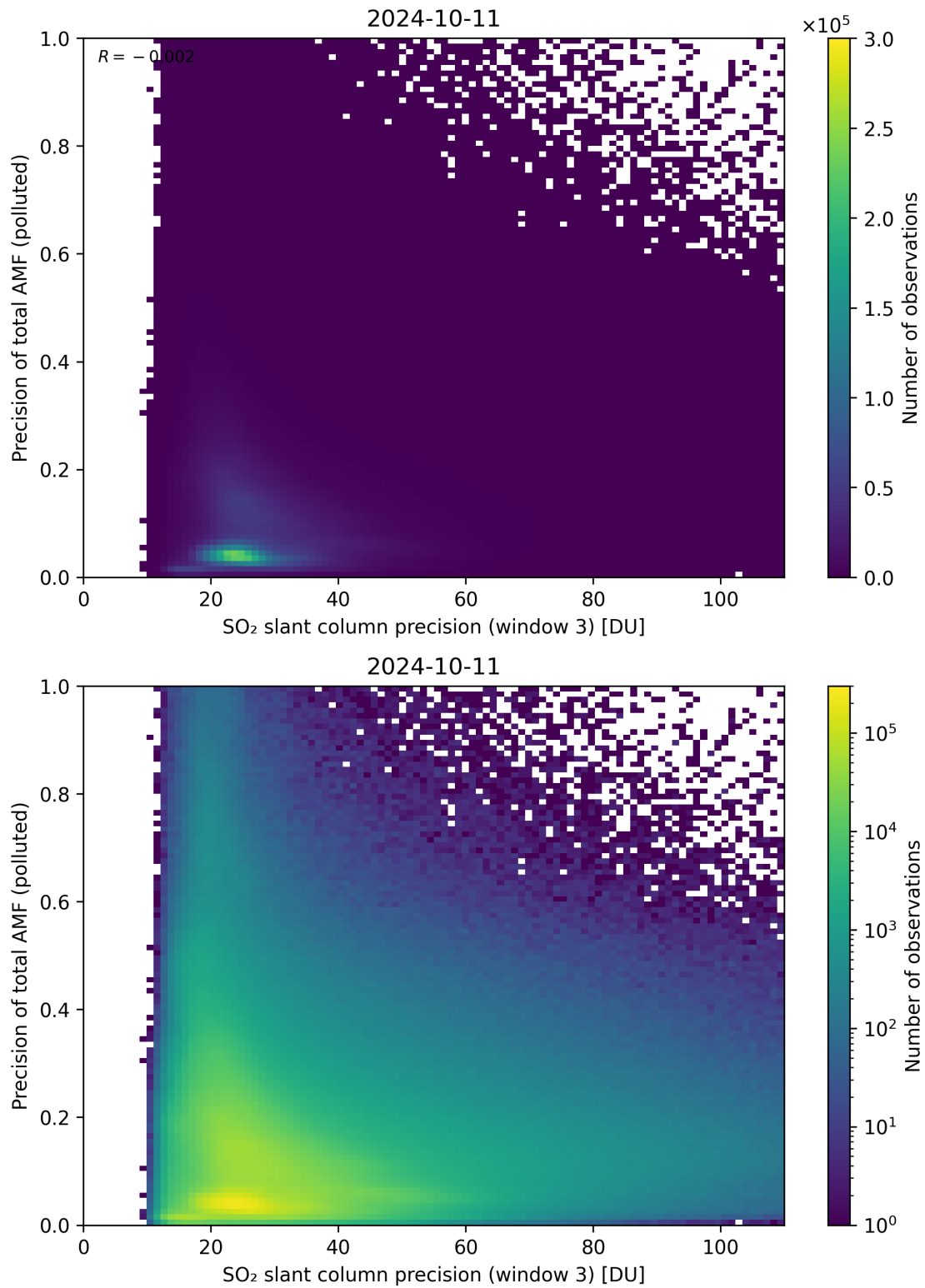
Figure 264: Scatter density plot of “SO 2 slant column precision (window 3)” against “Precision of total AMF (polluted)” for 2024-10-10 to 2024-10-12.
