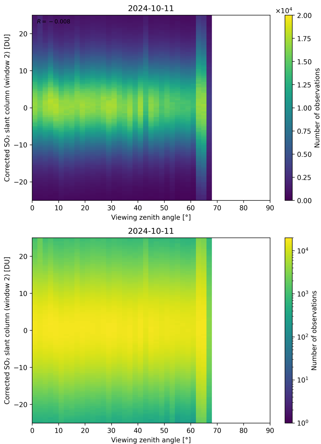
Figure 318: Scatter density plot of “Viewing zenith angle” against “Corrected SO 2 slant column (window 2)” for 2024-10-10 to 2024-10-12.
