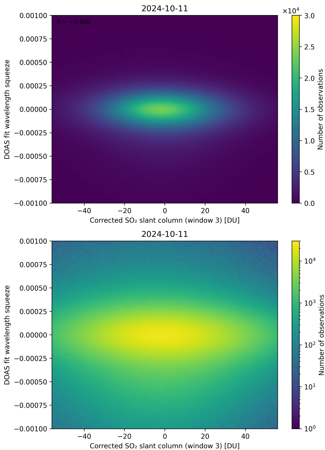
Figure 207: Scatter density plot of “Corrected SO 2 slant column (window 3)” against “DOAS fit wavelength squeeze” for 2024-10-10 to 2024-10-12.
