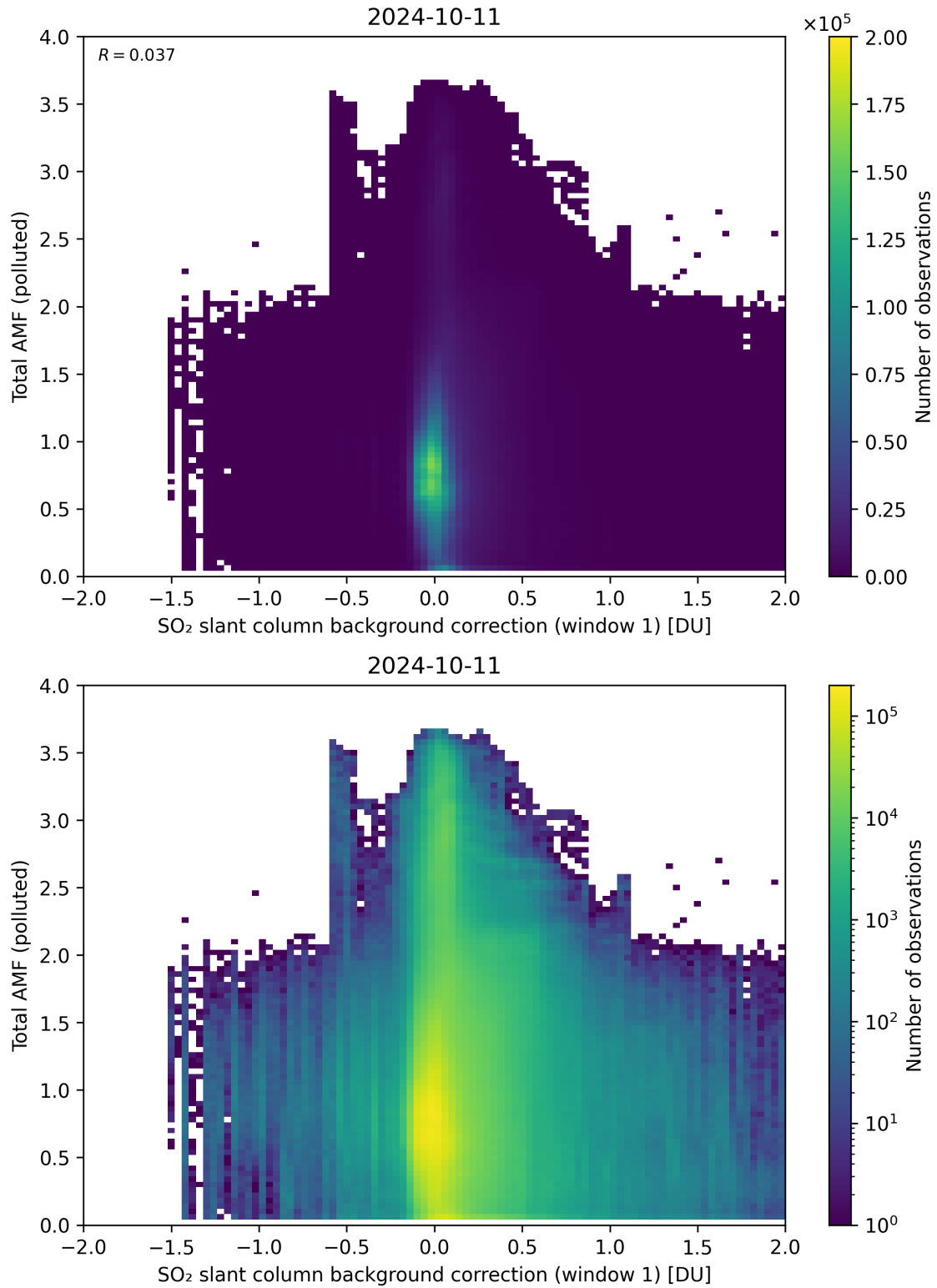
Figure 109: Scatter density plot of “SO 2 slant column background correction (window 1)” against “Total AMF (polluted)” for 2024-10-10 to 2024-10-12.
