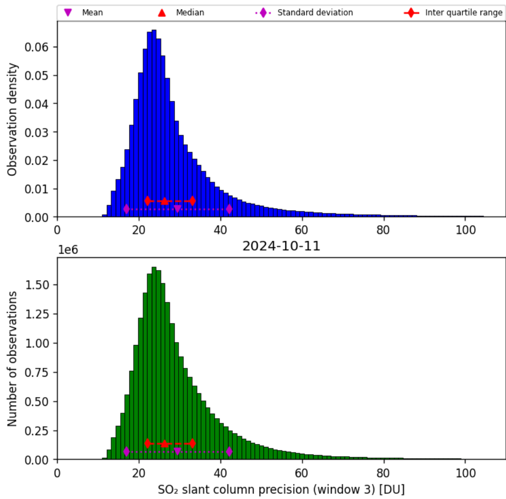
Figure 65: Histogram of “SO 2 slant column precision (window 3)” for 2024-10-10 to 2024-10-12
