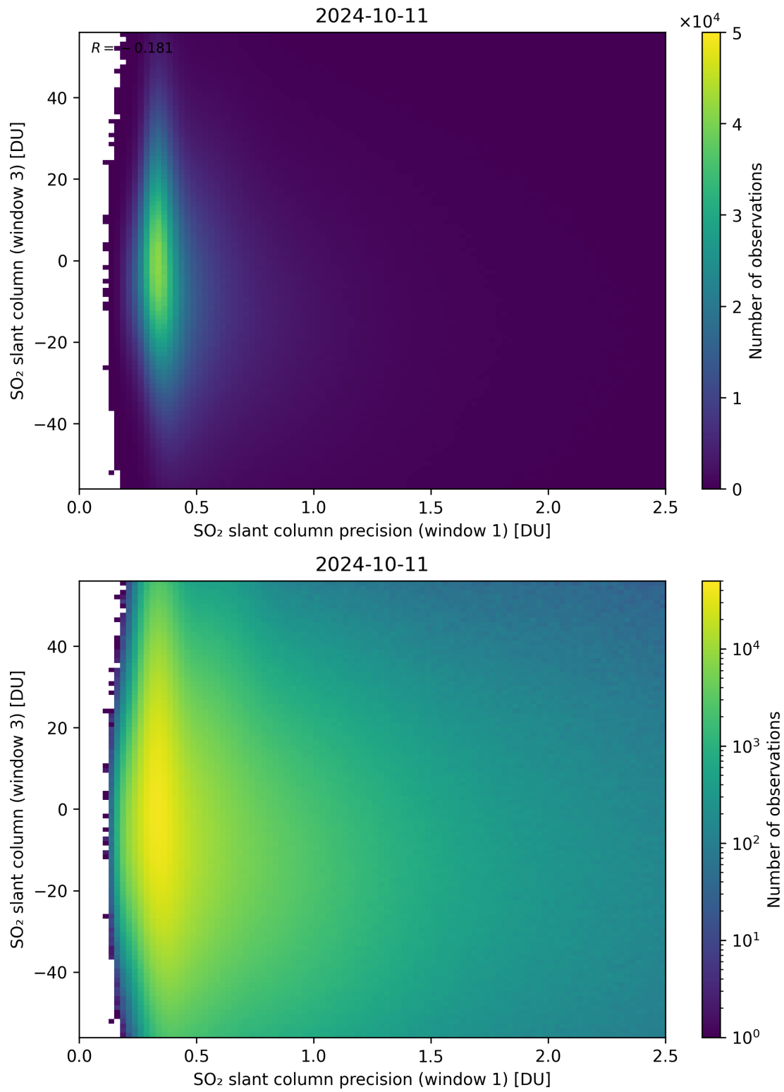
Figure 228: Scatter density plot of “SO 2 slant column precision (window 1)” against “SO 2 slant column (window 3)” for 2024-10-10 to 2024-10-12.
