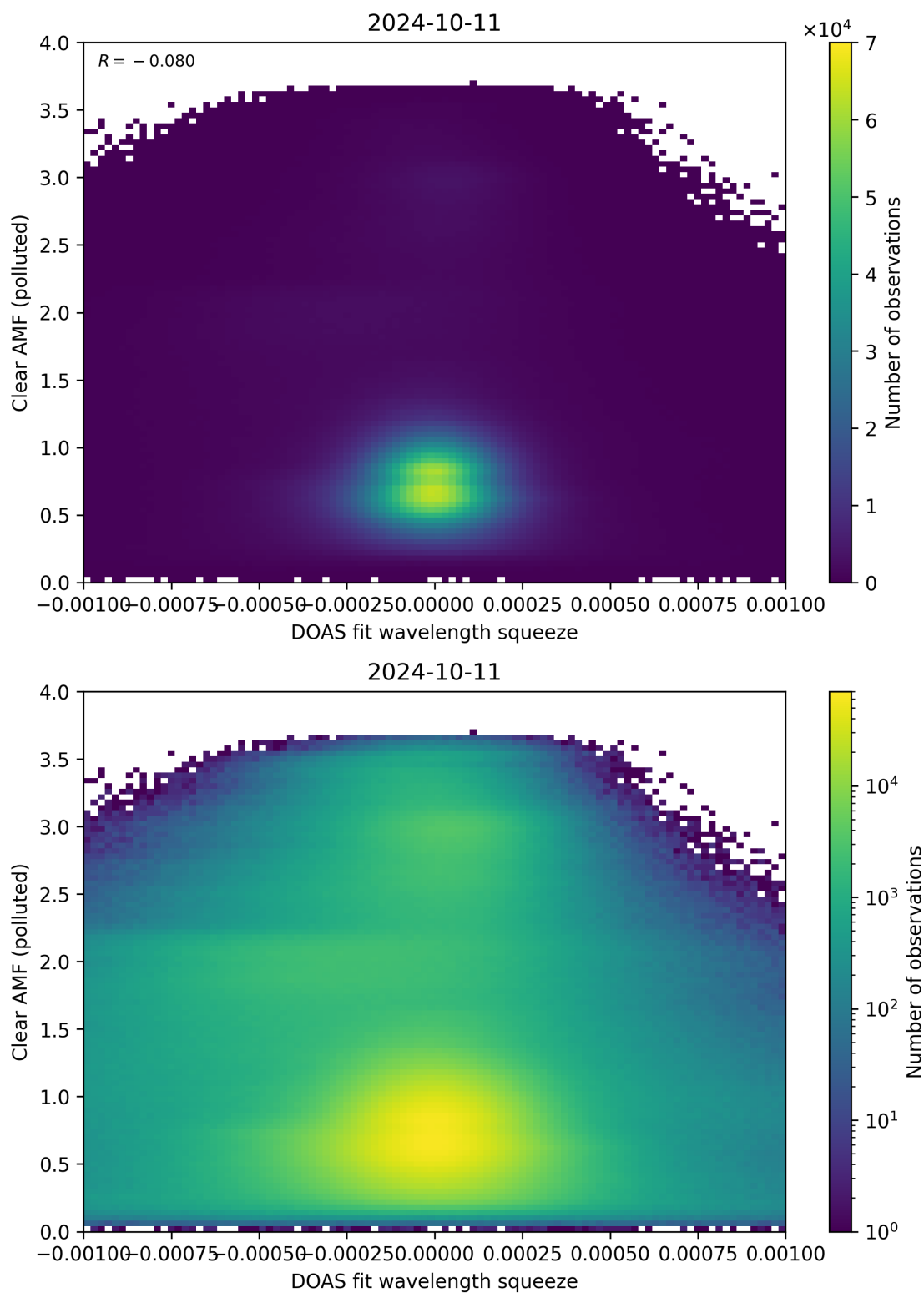
Figure 133: Scatter density plot of “DOAS fit wavelength squeeze” against “Clear AMF (polluted)” for 2024-10-10 to 2024-10-12.
