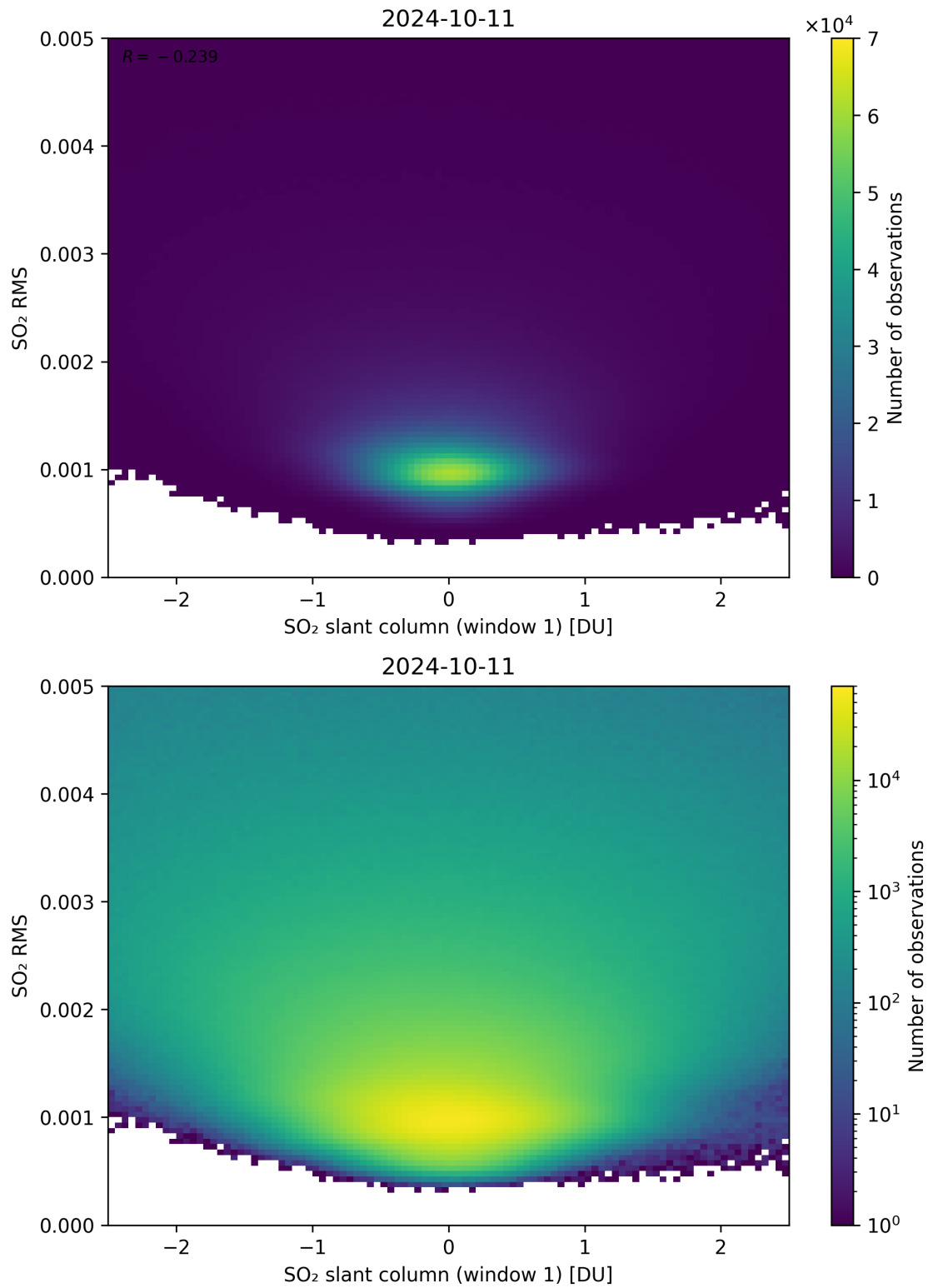
Figure 217: Scatter density plot of “SO 2 slant column (window 1)” against “SO 2 RMS” for 2024-10-10 to 2024-10-12.
