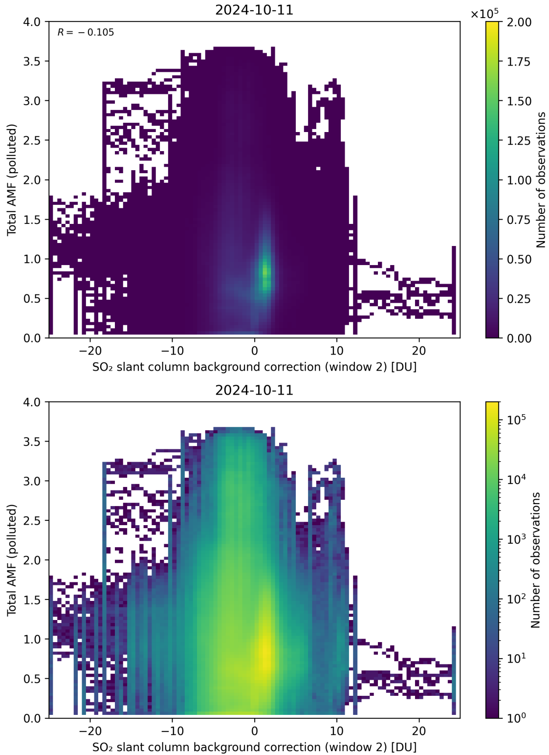
Figure 119: Scatter density plot of “SO 2 slant column background correction (window 2)” against “Total AMF (polluted)” for 2024-10-10 to 2024-10-12.
