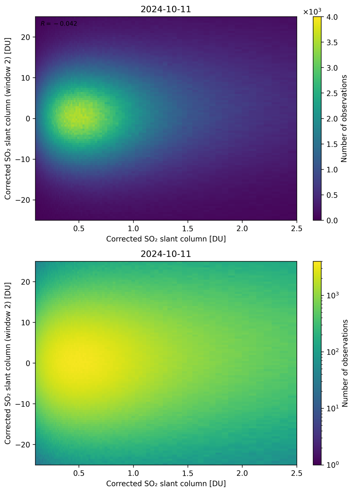
Figure 185: Scatter density plot of “Corrected SO 2 slant column” against “Corrected SO 2 slant column (window 2)” for 2024-10-10 to 2024-10-12.
