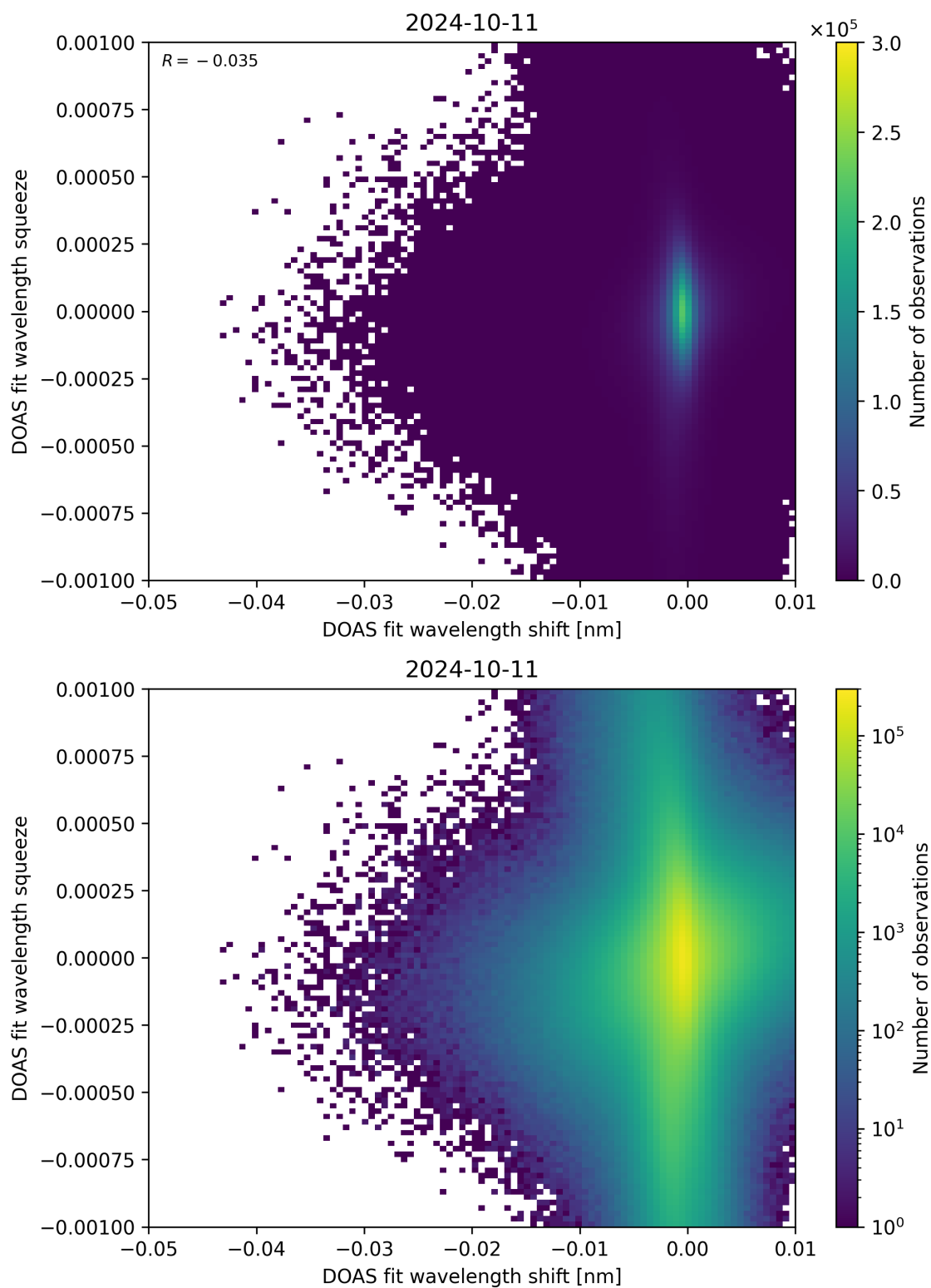
Figure 127: Scatter density plot of “DOAS fit wavelength shift” against “DOAS fit wavelength squeeze” for 2024-10-10 to 2024-10-12.
