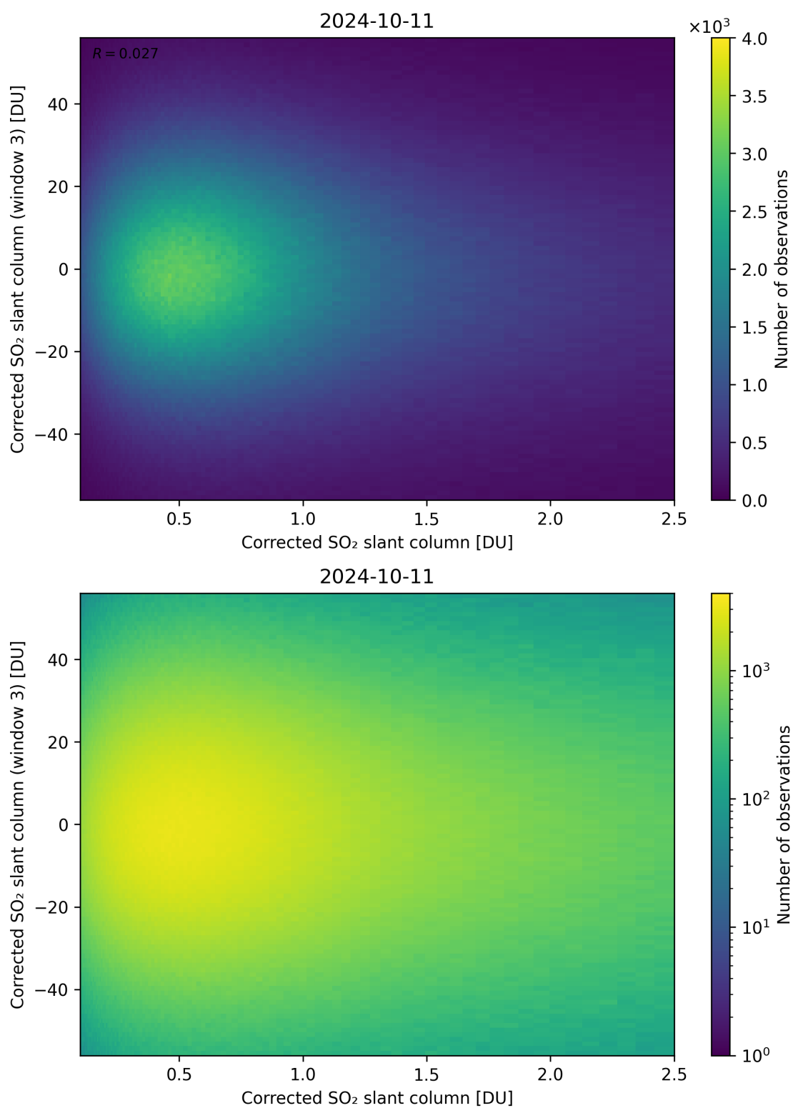
Figure 186: Scatter density plot of “Corrected SO 2 slant column” against “Corrected SO 2 slant column (window 3)” for 2024-10-10 to 2024-10-12.
