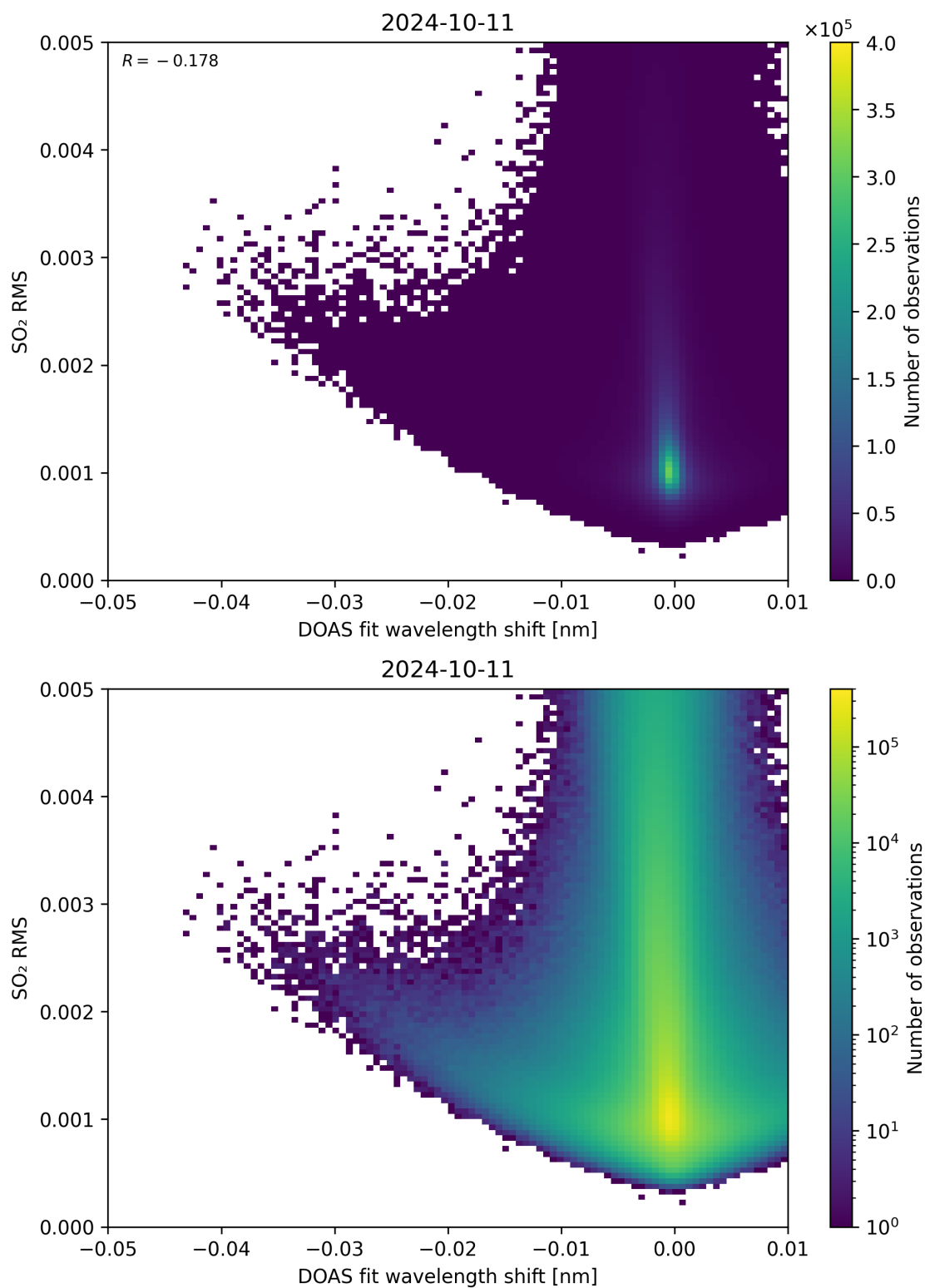
Figure 128: Scatter density plot of “DOAS fit wavelength shift” against “SO 2 RMS” for 2024-10-10 to 2024-10-12.
