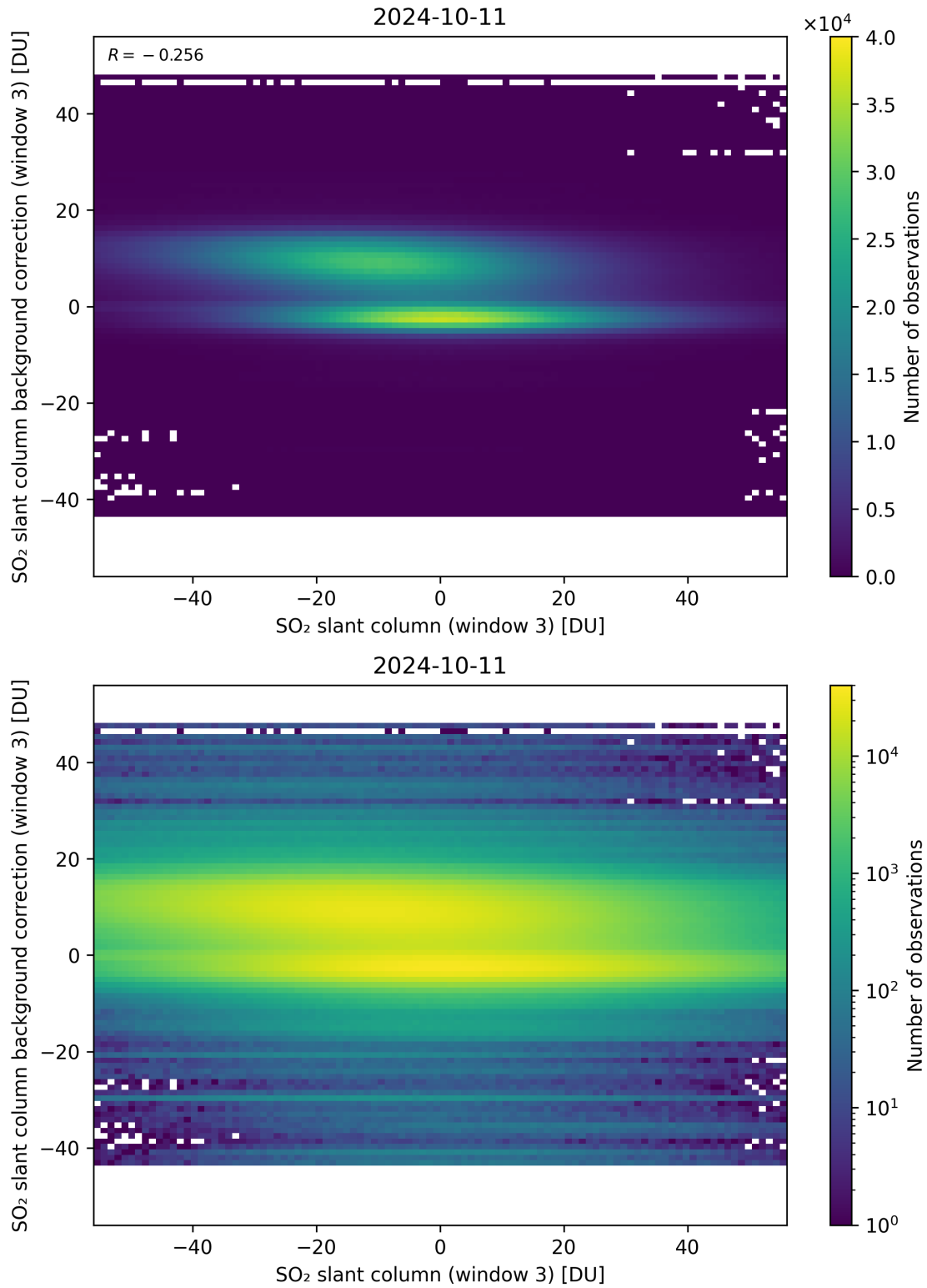
Figure 253: Scatter density plot of “SO 2 slant column (window 3)” against “SO 2 slant column background correction (window 3)” for 2024-10-10 to 2024-10-12.
