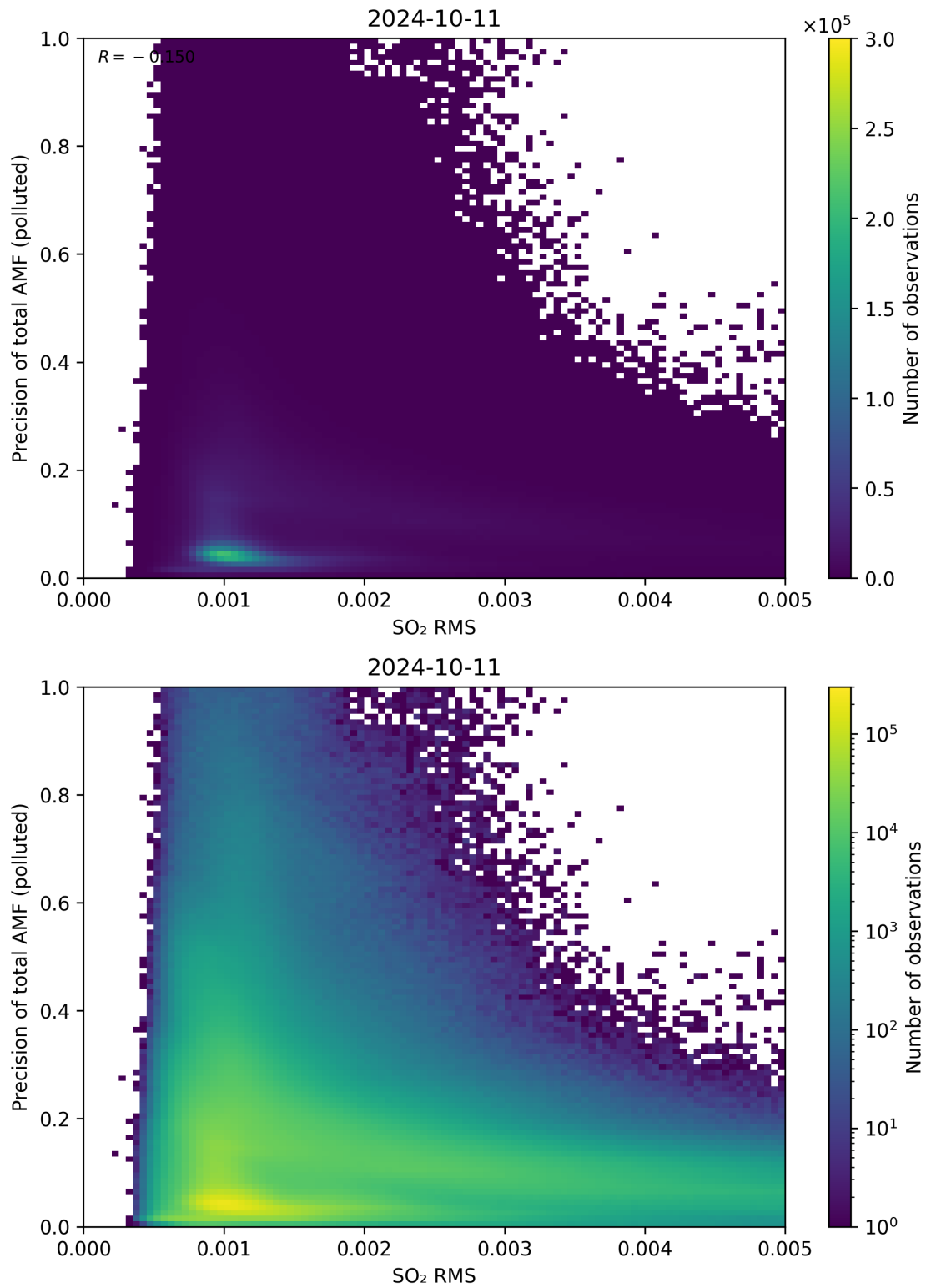
Figure 138: Scatter density plot of “SO 2 RMS” against “Precision of total AMF (polluted)” for 2024-10-10 to 2024-10-12.
