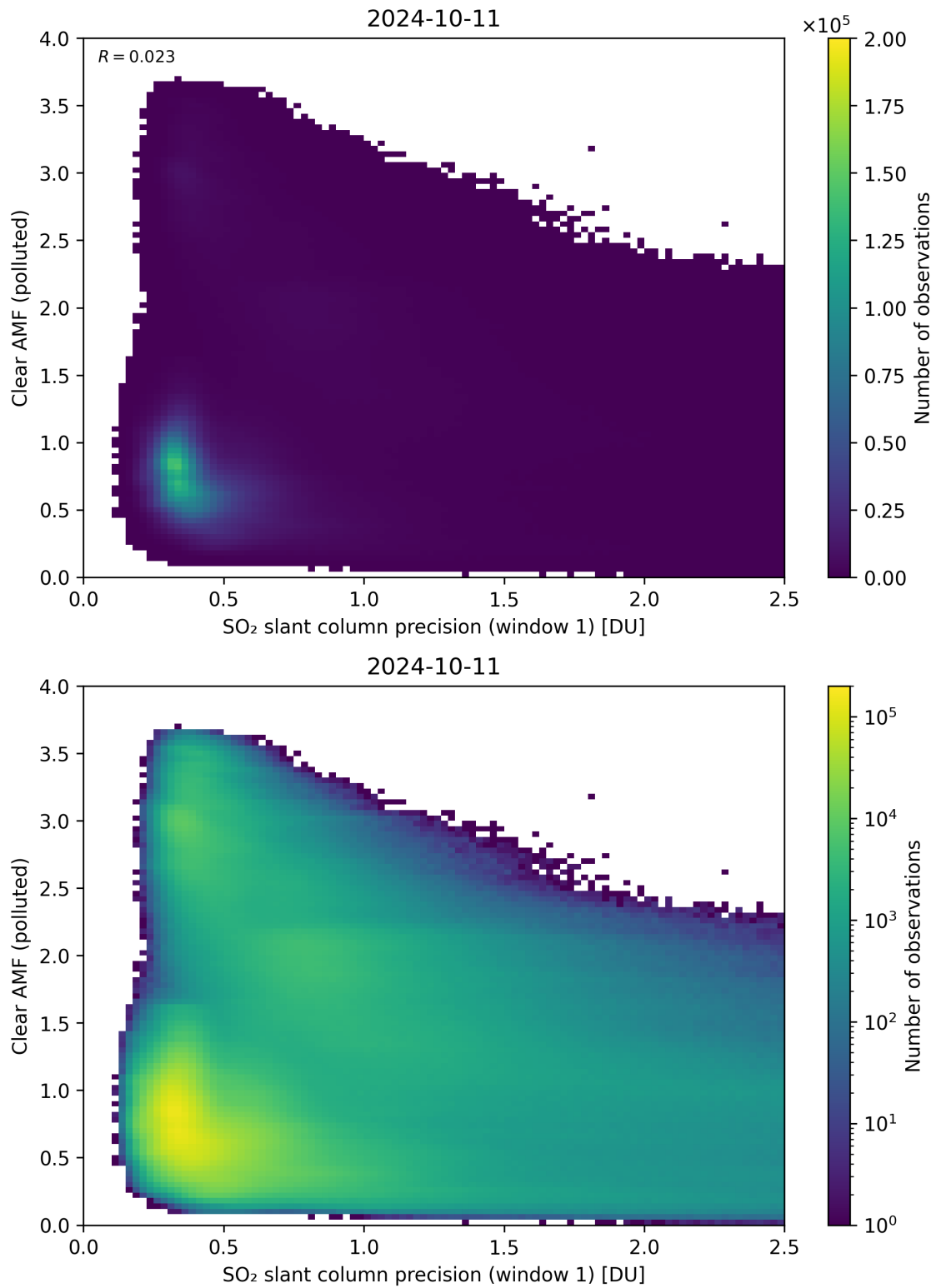
Figure 224: Scatter density plot of “SO 2 slant column precision (window 1)” against “Clear AMF (polluted)” for 2024-10-10 to 2024-10-12.
