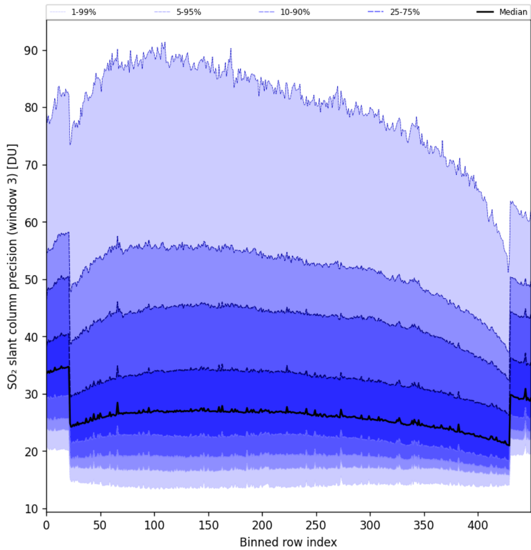
Figure 88: Along track statistics of “SO 2 slant column precision (window 3)” for 2024-10-10 to 2024-10-12
