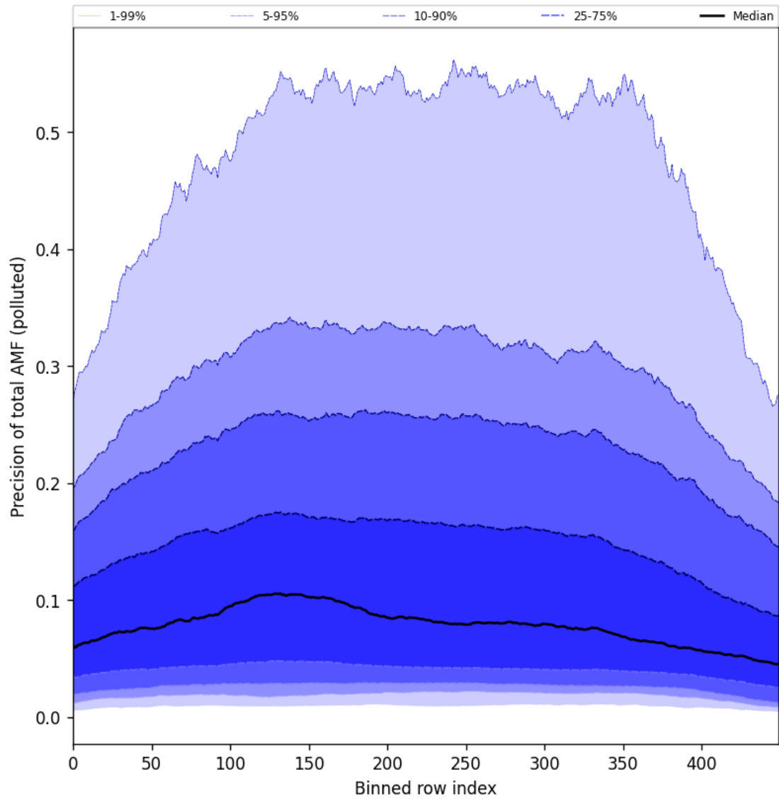
Figure 95: Along track statistics of “Precision of total AMF (polluted)” for 2024-10-10 to 2024-10-12
