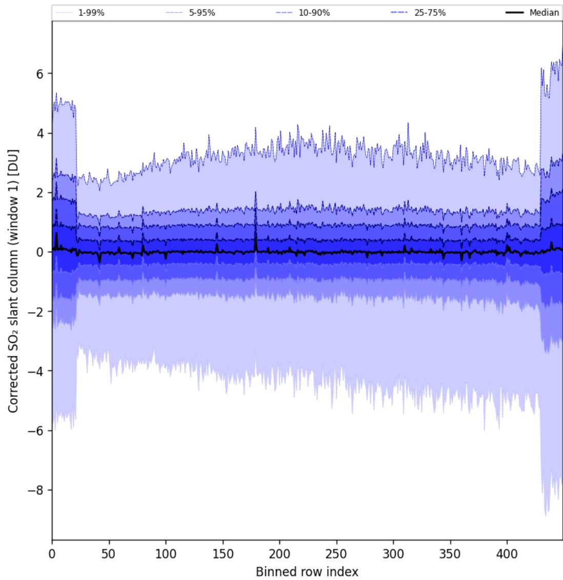
Figure 81: Along track statistics of “Corrected SO 2 slant column (window 1)” for 2024-10-10 to 2024-10-12
