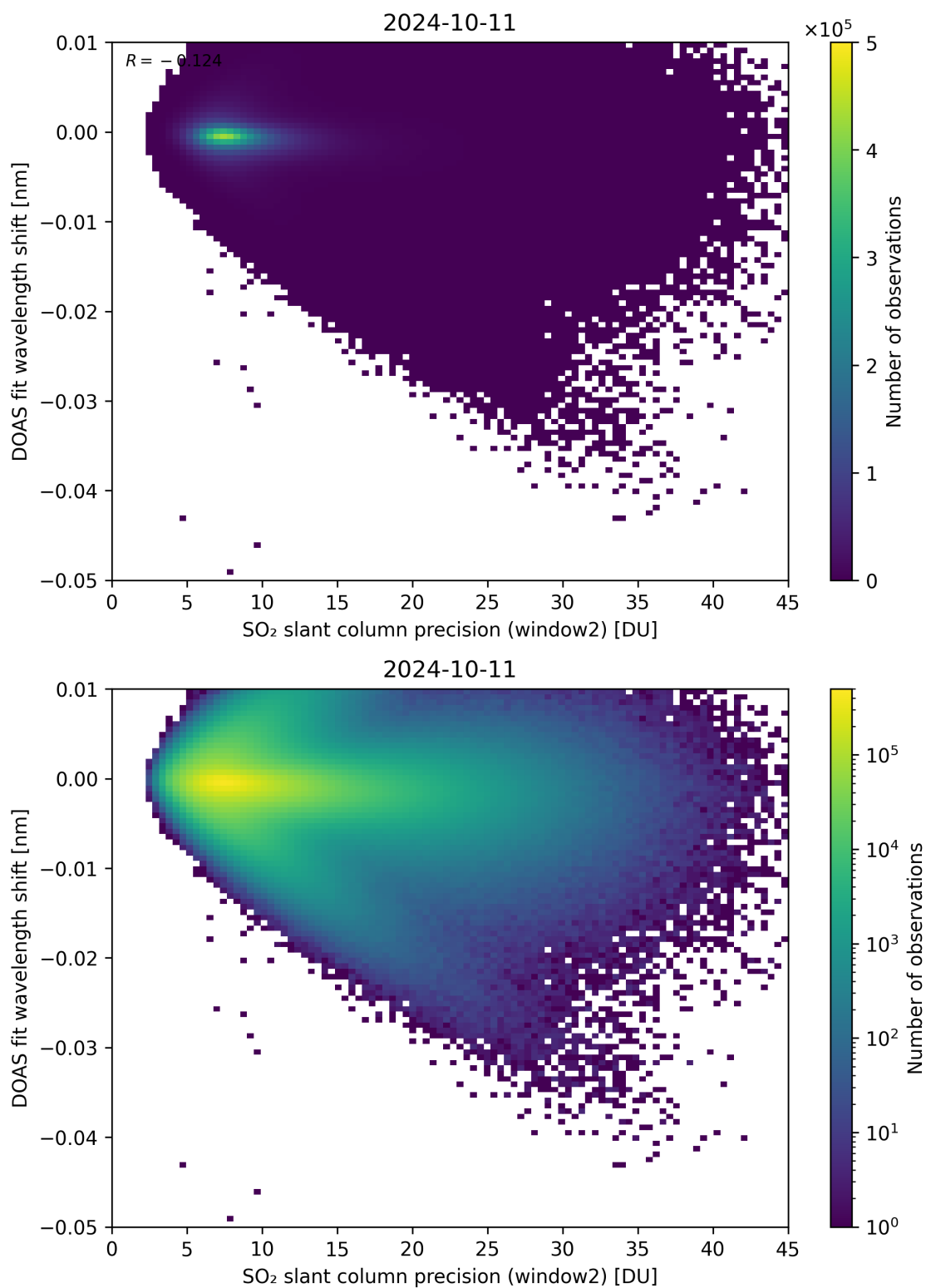
Figure 243: Scatter density plot of “SO 2 slant column precision (window2)” against “DOAS fit wavelength shift” for 2024-10-10 to 2024-10-12.
