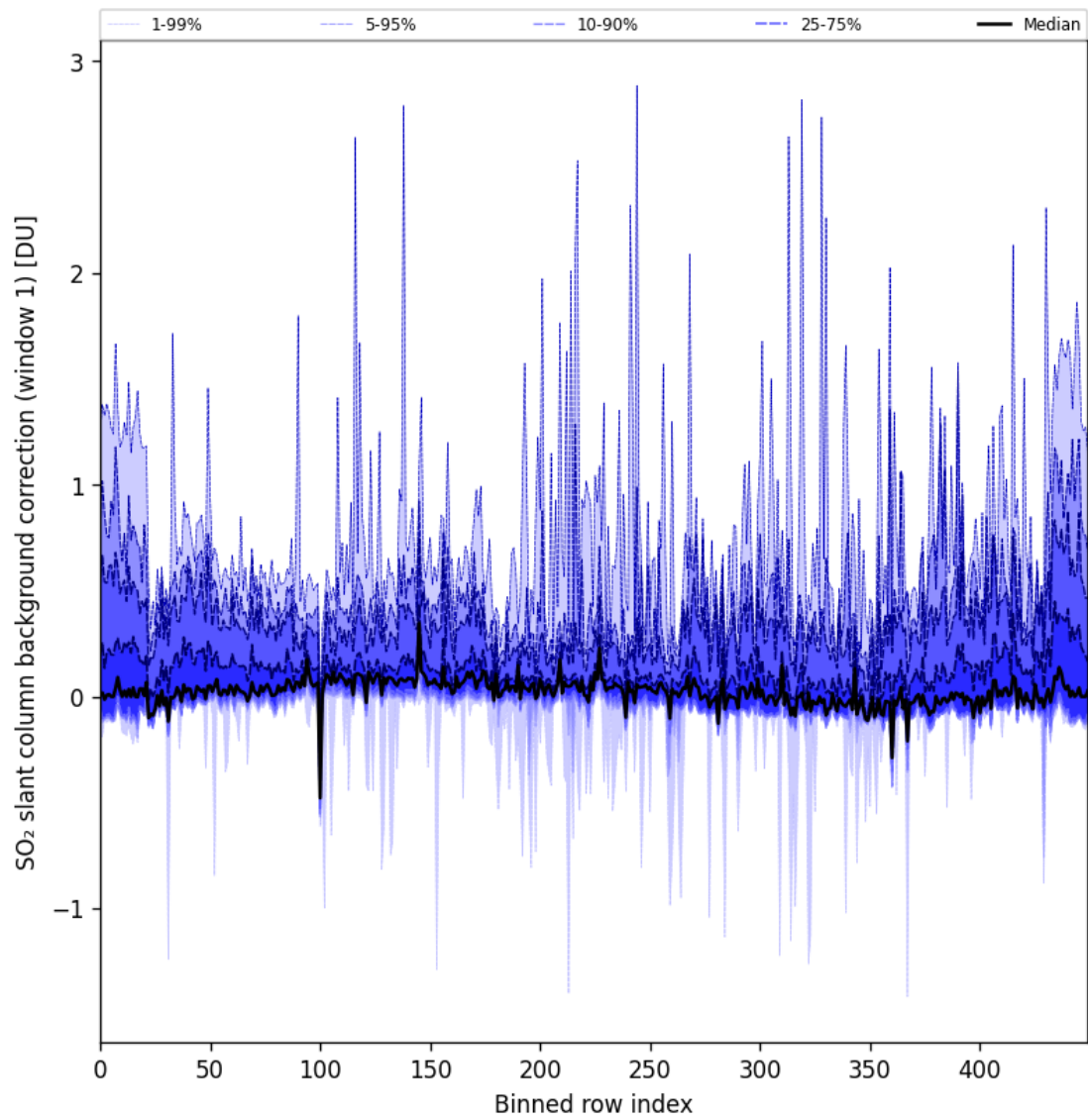
Figure 82: Along track statistics of “SO 2 slant column background correction (window 1)” for 2024-10-10 to 2024-10-12
