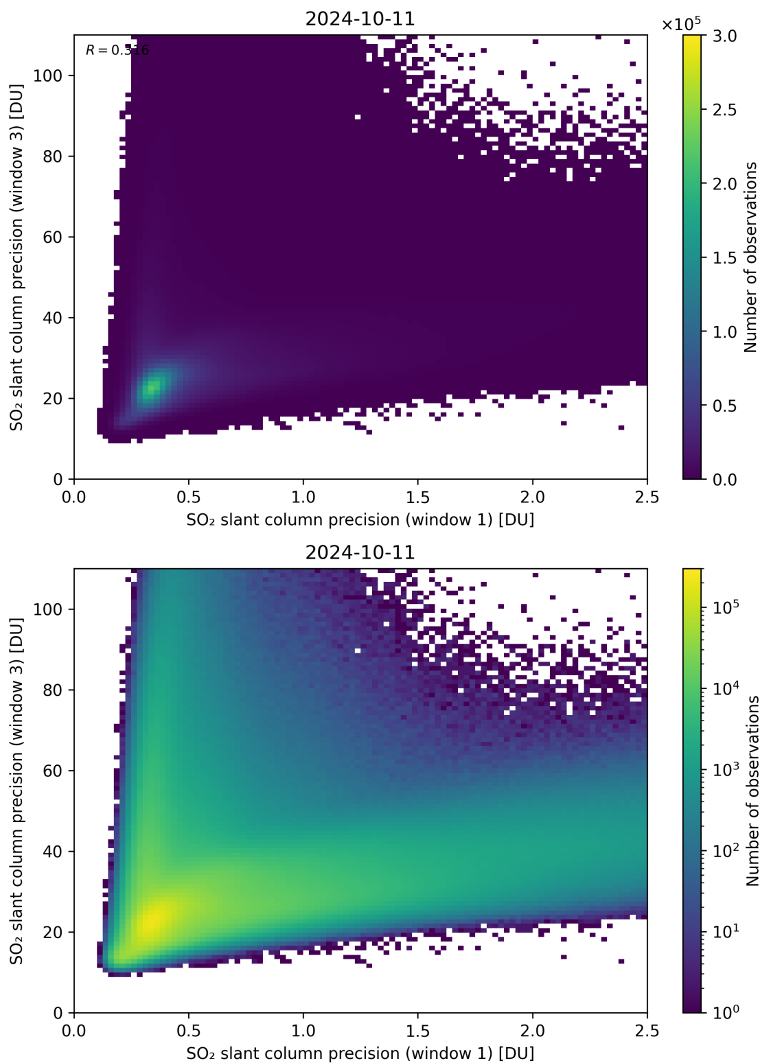
Figure 229: Scatter density plot of “SO 2 slant column precision (window 1)” against “SO 2 slant column precision (window 3)” for 2024-10-10 to 2024-10-12.
