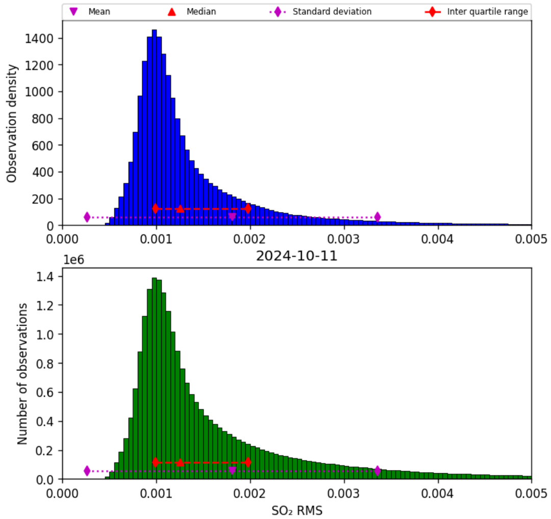
Figure 70: Histogram of “SO 2 RMS” for 2024-10-10 to 2024-10-12
