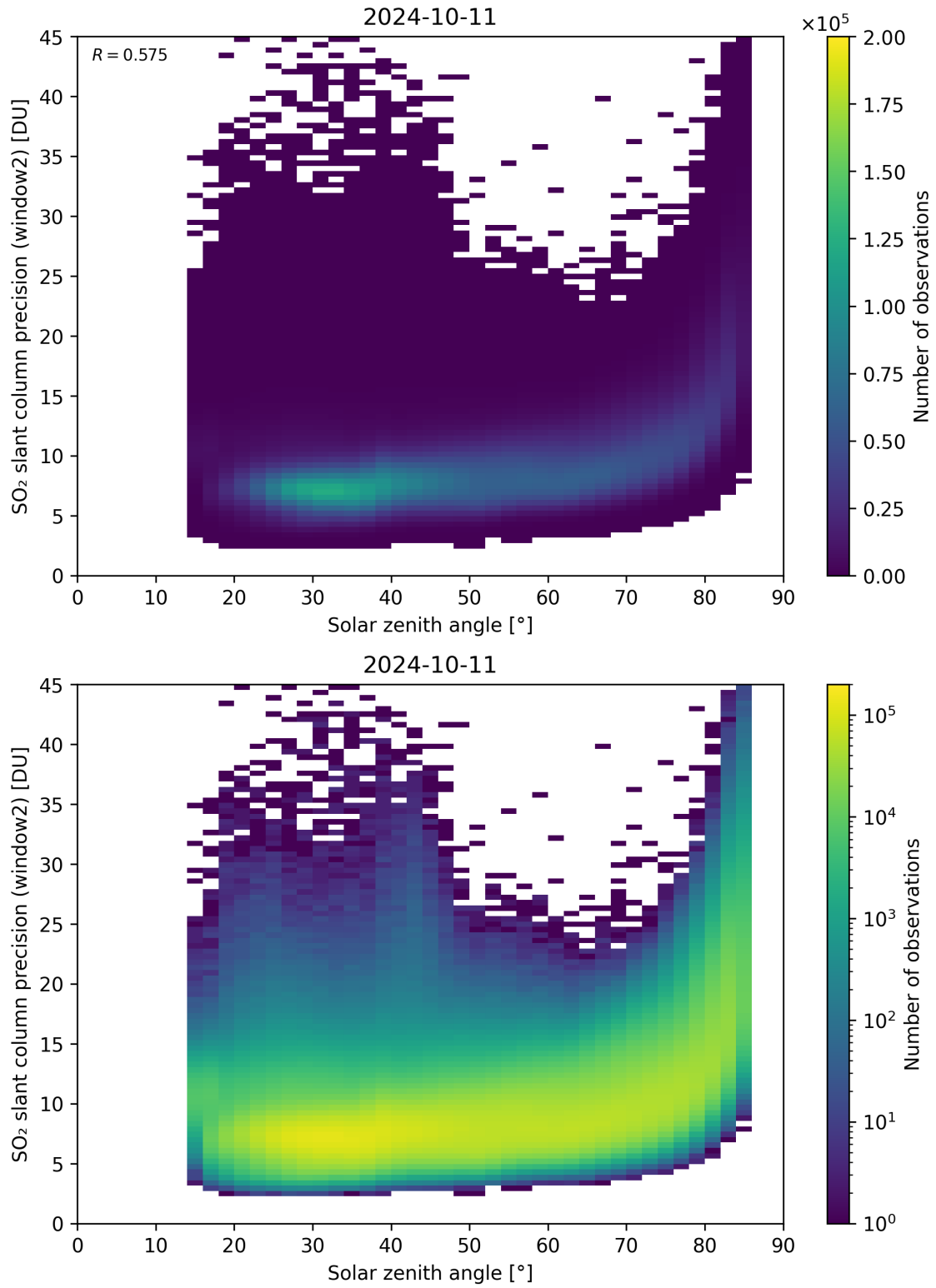
Figure 171: Scatter density plot of “Solar zenith angle” against “SO 2 slant column precision (window2)” for 2024-10-10 to 2024-10-12.
