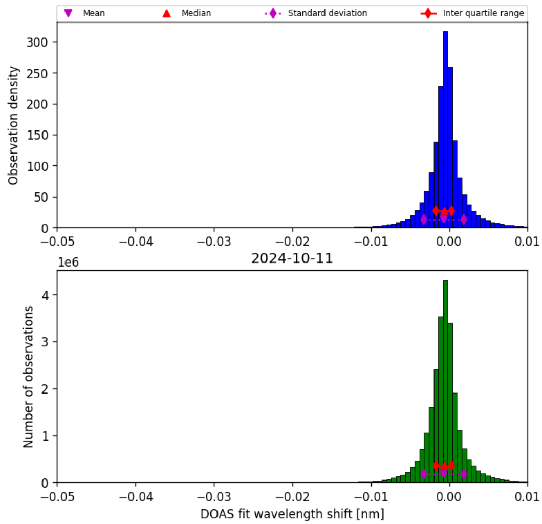
Figure 68: Histogram of “DOAS fit wavelength shift” for 2024-10-10 to 2024-10-12
