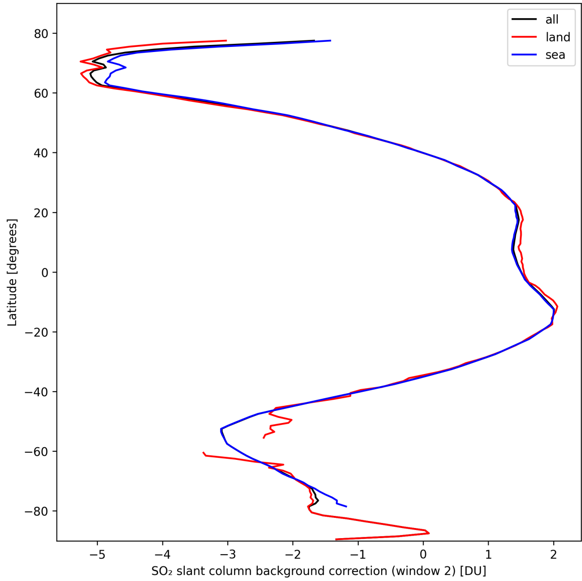
Figure 40: Zonal average of "SO 2 slant column background correction (window 2)" for 2024-10-10 to 2024-10-12.
