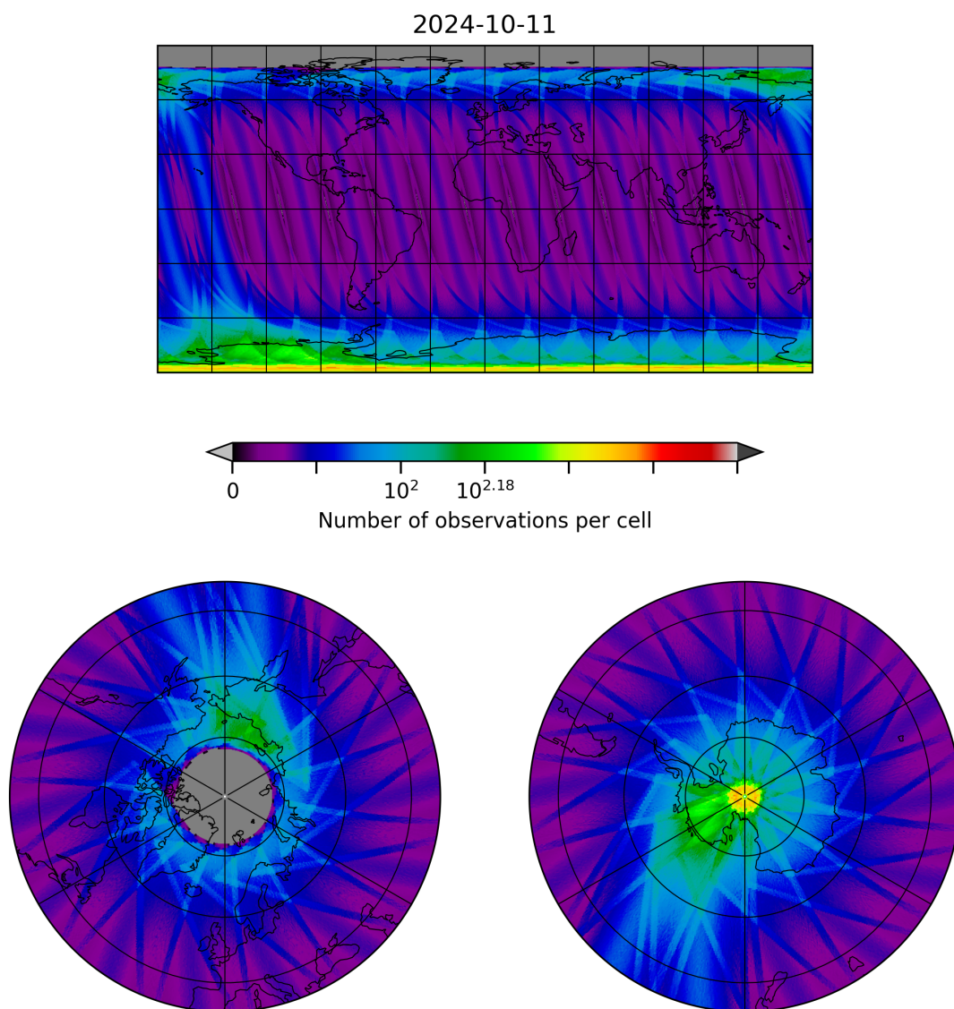
Figure 28: Map of the number of observations for 2024-10-10 to 2024-10-12
