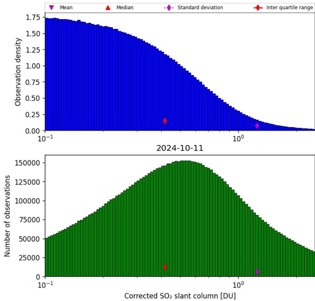
Figure 55: Histogram of "Corrected SO 2 slant column" for 2024-10-10 to 2024-10-12
