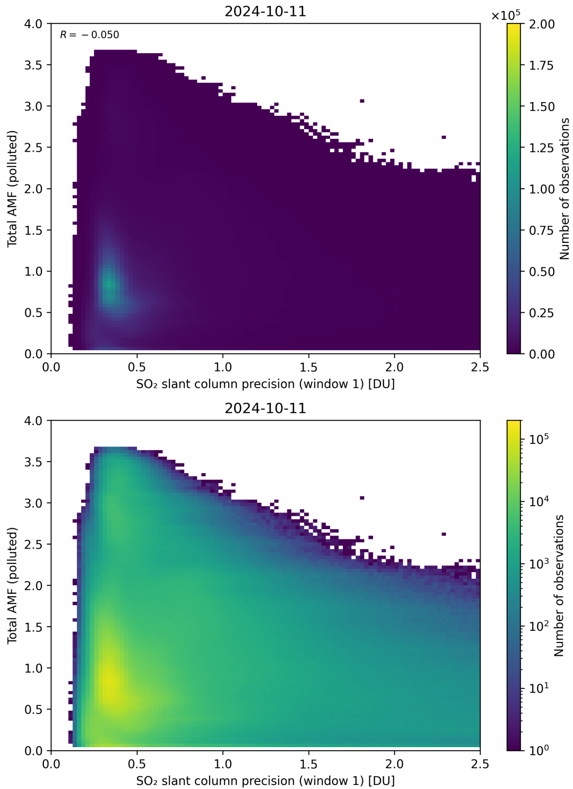
Figure 230: Scatter density plot of “SO 2 slant column precision (window 1)” against “Total AMF (polluted)” for 2024-10-10 to 2024-10-12.
