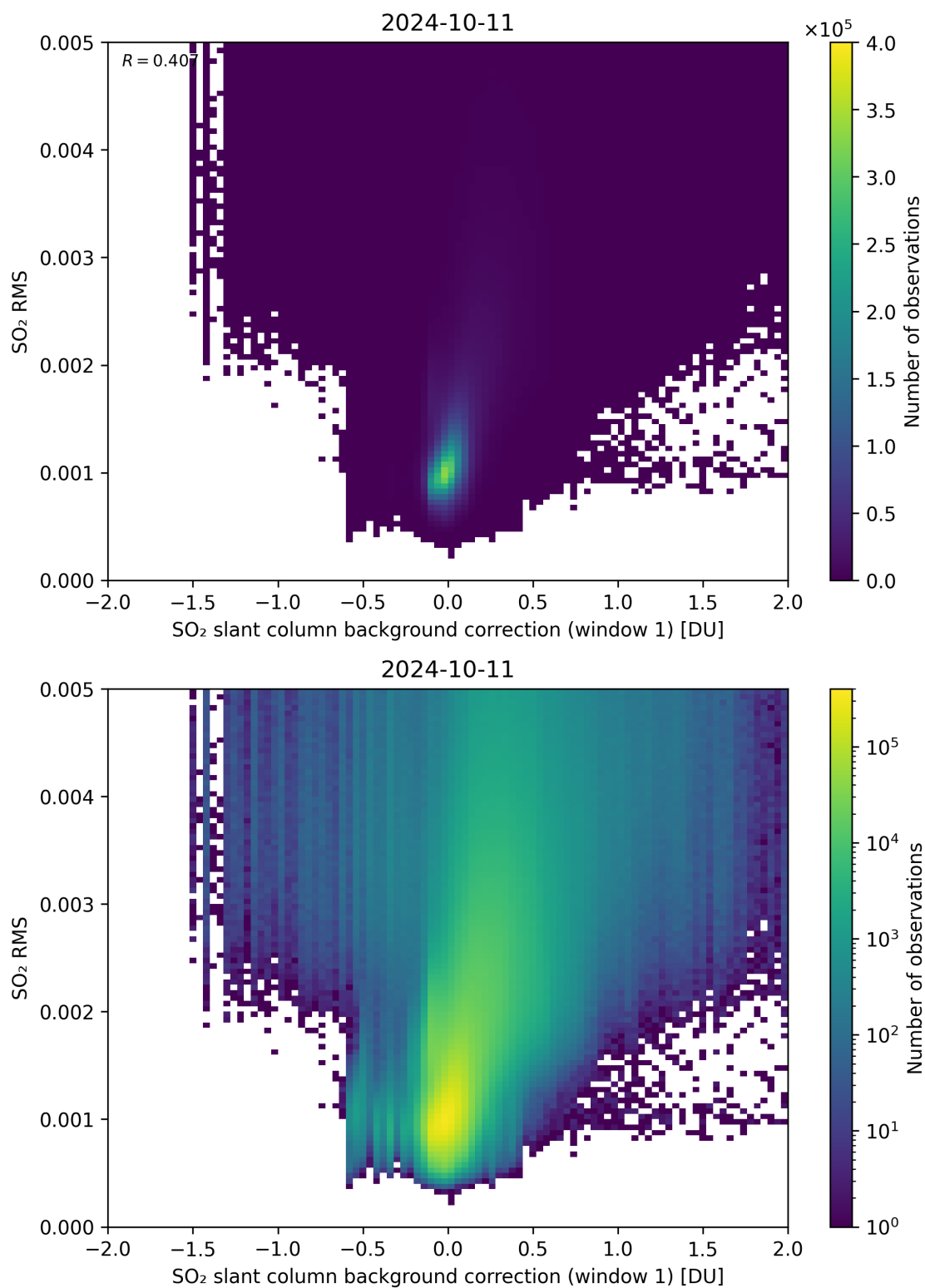
Figure 102: Scatter density plot of “SO 2 slant column background correction (window 1)” against “SO 2 RMS” for 2024-10-10 to 2024-10-12.
