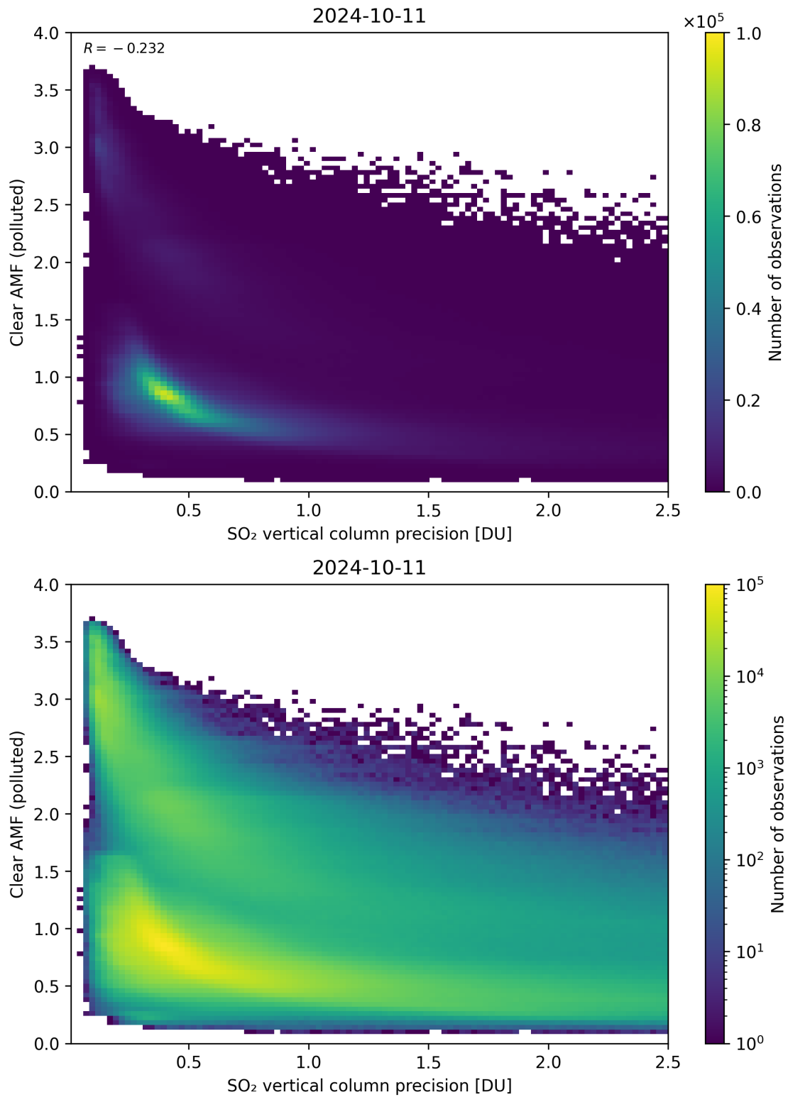
Figure 285: Scatter density plot of “SO 2 vertical column precision” against “Clear AMF (polluted)” for 2024-10-10 to 2024-10-12.
