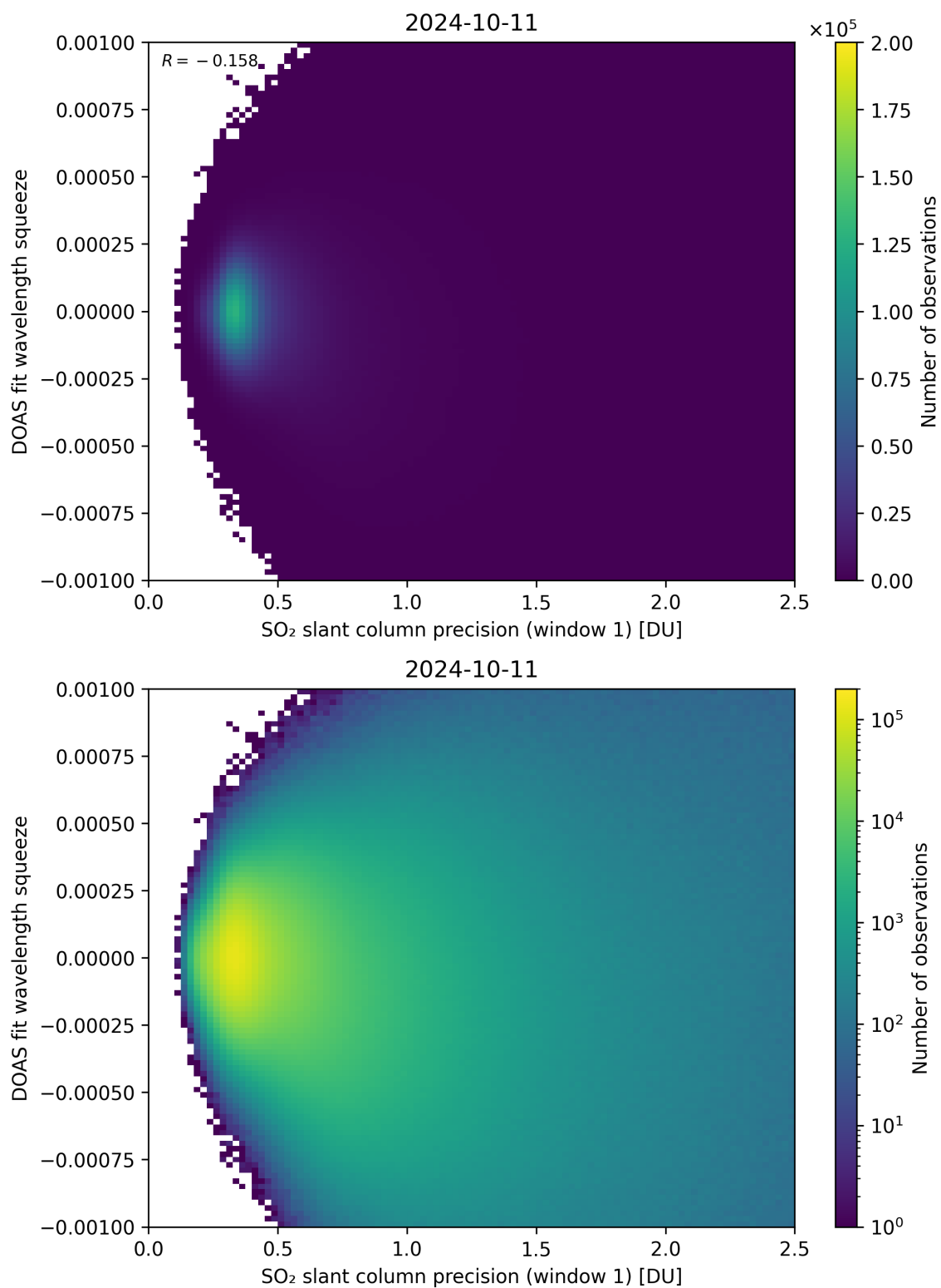
Figure 222: Scatter density plot of “SO 2 slant column precision (window 1)” against “DOAS fit wavelength squeeze” for 2024-10-10 to 2024-10-12.
