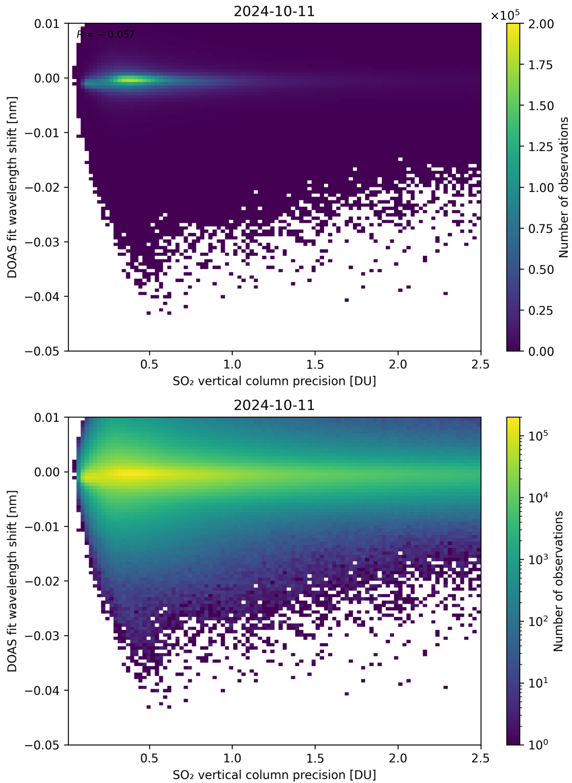
Figure 282: Scatter density plot of “SO 2 vertical column precision” against “DOAS fit wavelength shift” for 2024-10-10 to 2024-10-12.
