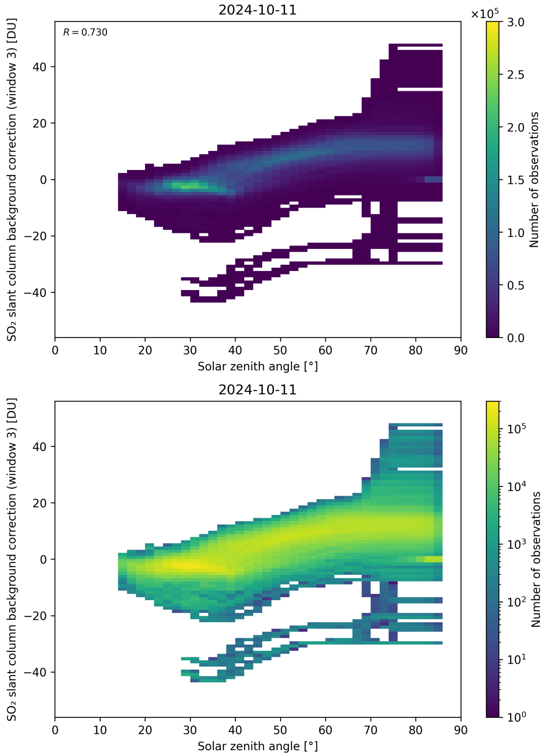
Figure 160: Scatter density plot of “Solar zenith angle” against “SO 2 slant column background correction (window 3)” for 2024-10-10 to 2024-10-12.
