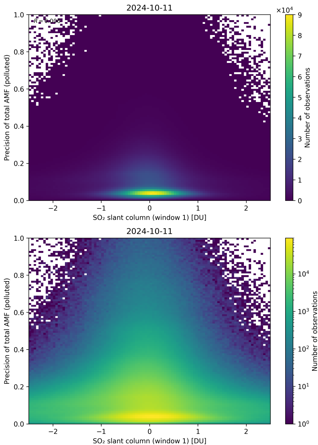
Figure 240: Scatter density plot of “SO 2 slant column (window 1)” against “Precision of total AMF (polluted)” for 2024-10-10 to 2024-10-12.
