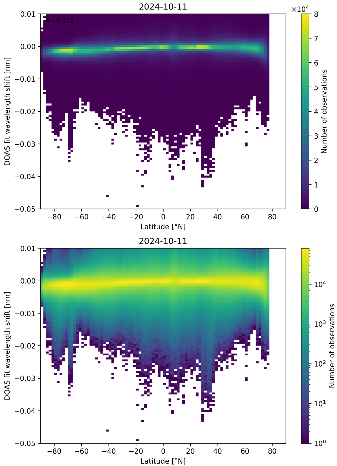
Figure 142: Scatter density plot of “Latitude” against “DOAS fit wavelength shift” for 2024-10-10 to 2024-10-12.
