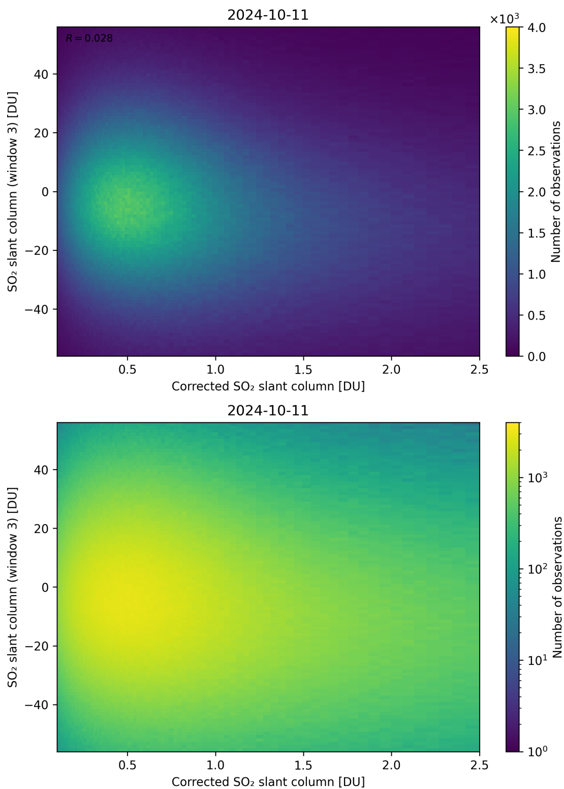
Figure 190: Scatter density plot of “Corrected SO 2 slant column” against “SO 2 slant column (window 3)” for 2024-10-10 to 2024-10-12.
