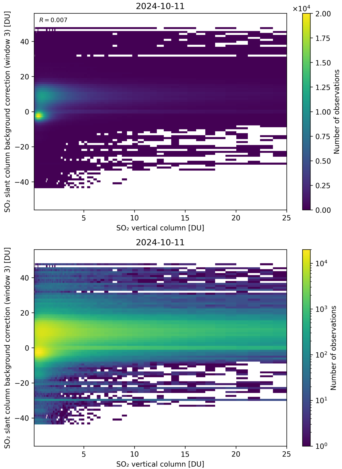
Figure 275: Scatter density plot of “SO 2 vertical column” against “SO 2 slant column background correction (window 3)” for 2024-10-10 to 2024-10-12.
