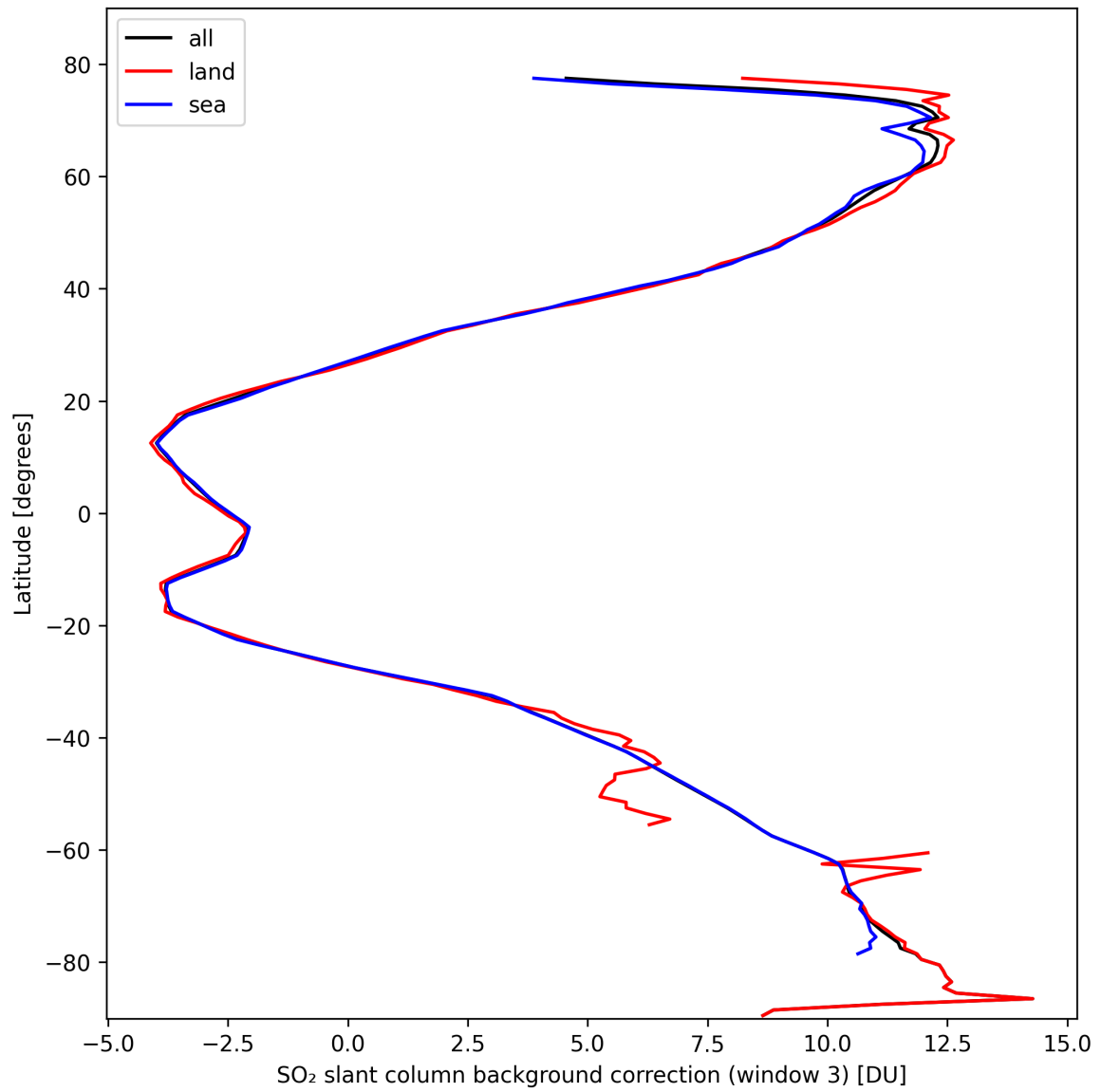
Figure 44: Zonal average of “SO 2 slant column background correction (window 3)” for 2024-10-10 to 2024-10-12.
