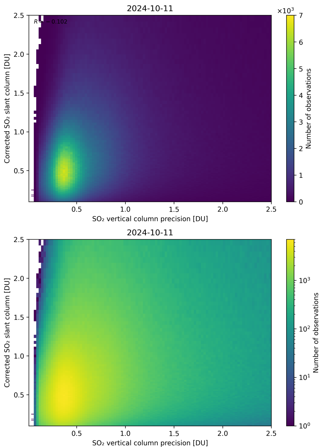
Figure 286: Scatter density plot of “SO 2 vertical column precision” against “Corrected SO 2 slant column” for 2024-10-10 to 2024-10-12.
