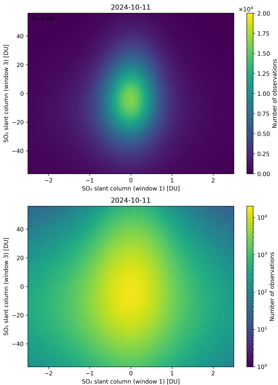
Figure 237: Scatter density plot of “SO 2 slant column (window 1)” against “SO 2 slant column (window 3)” for 2024-10-10 to 2024-10-12.
