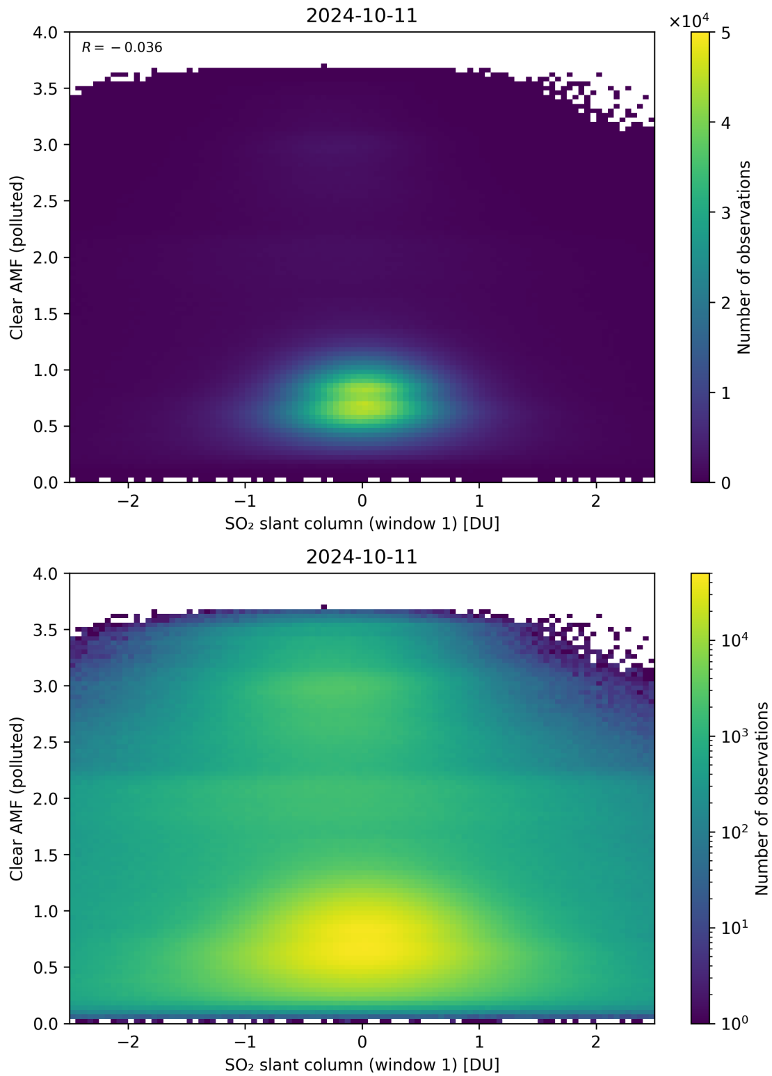
Figure 232: Scatter density plot of “SO 2 slant column (window 1)” against “Clear AMF (polluted)” for 2024-10-10 to 2024-10-12.
