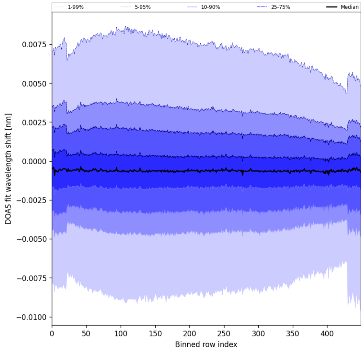
Figure 91: Along track statistics of “DOAS fit wavelength shift” for 2024-10-10 to 2024-10-12
