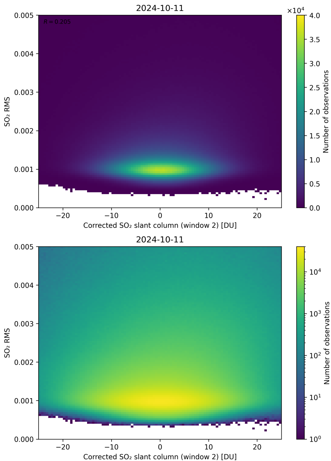
Figure 198: Scatter density plot of “Corrected SO 2 slant column (window 2)” against “SO 2 RMS” for 2024-10-10 to 2024-10-12.
