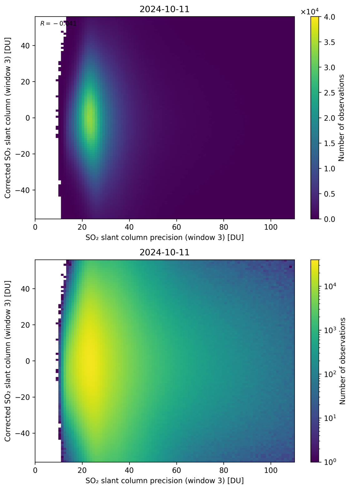
Figure 262: Scatter density plot of “SO 2 slant column precision (window 3)” against “Corrected SO 2 slant column (window 3)” for 2024-10-10 to 2024-10-12.
