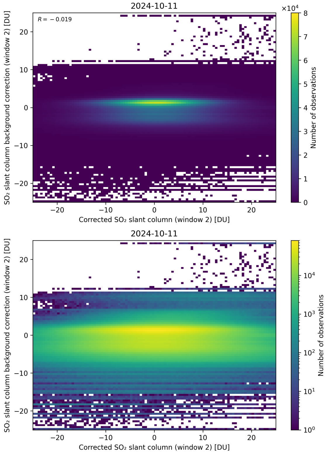
Figure 194: Scatter density plot of “Corrected SO 2 slant column (window 2)” against “SO 2 slant column background correction (window 2)” for 2024-10-10 to 2024-10-12.
