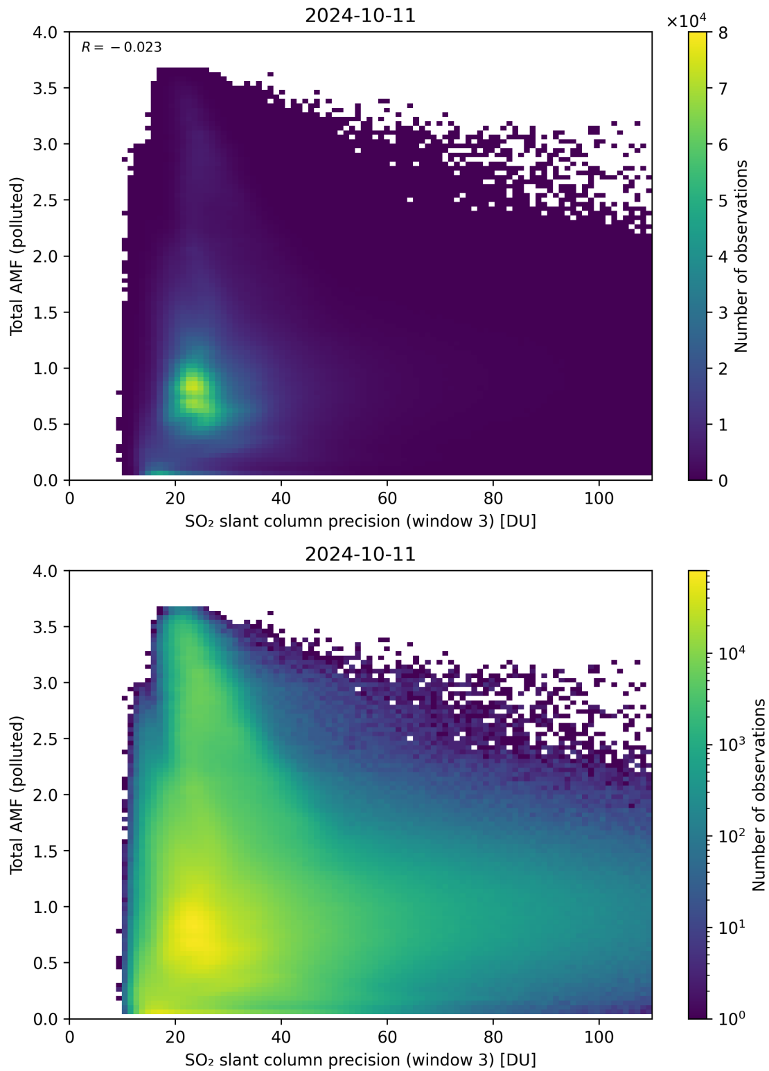
Figure 263: Scatter density plot of “SO 2 slant column precision (window 3)” against “Total AMF (polluted)” for 2024-10-10 to 2024-10-12.
