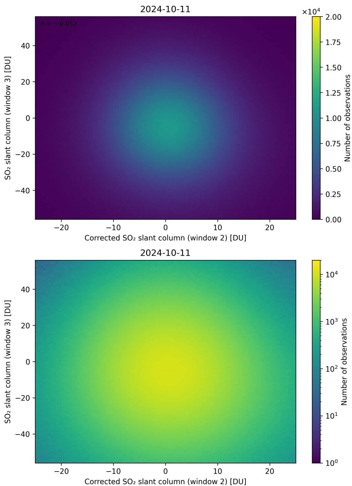
Figure 201: Scatter density plot of “Corrected SO 2 slant column (window 2)” against “SO 2 slant column (window 3)” for 2024-10-10 to 2024-10-12.
