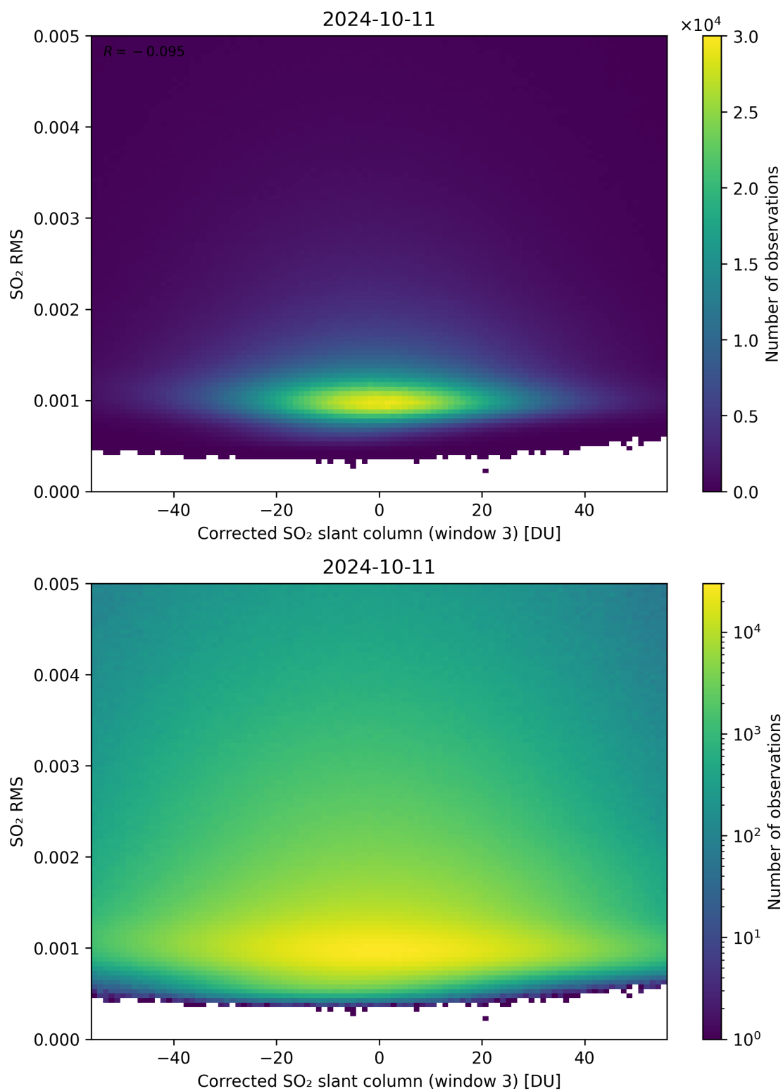
Figure 208: Scatter density plot of “Corrected SO 2 slant column (window 3)” against “SO 2 RMS” for 2024-10-10 to 2024-10-12.
