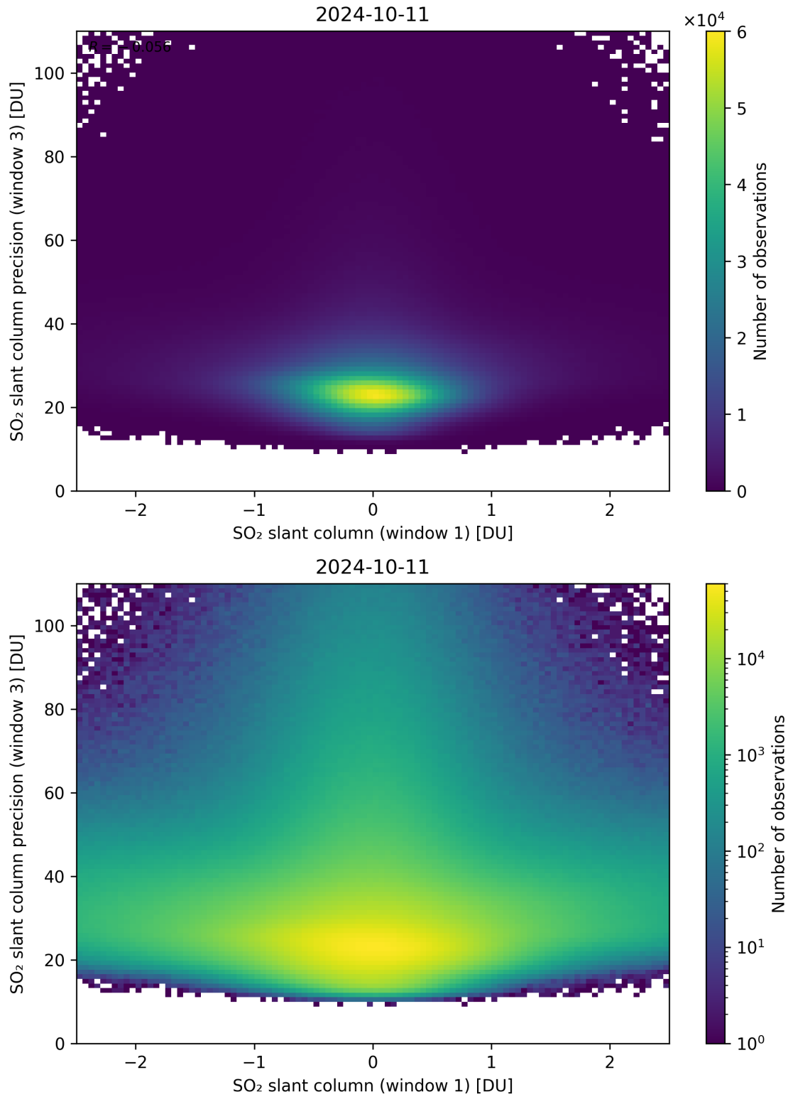
Figure 238: Scatter density plot of “SO 2 slant column (window 1)” against “SO 2 slant column precision (window 3)” for 2024-10-10 to 2024-10-12.
