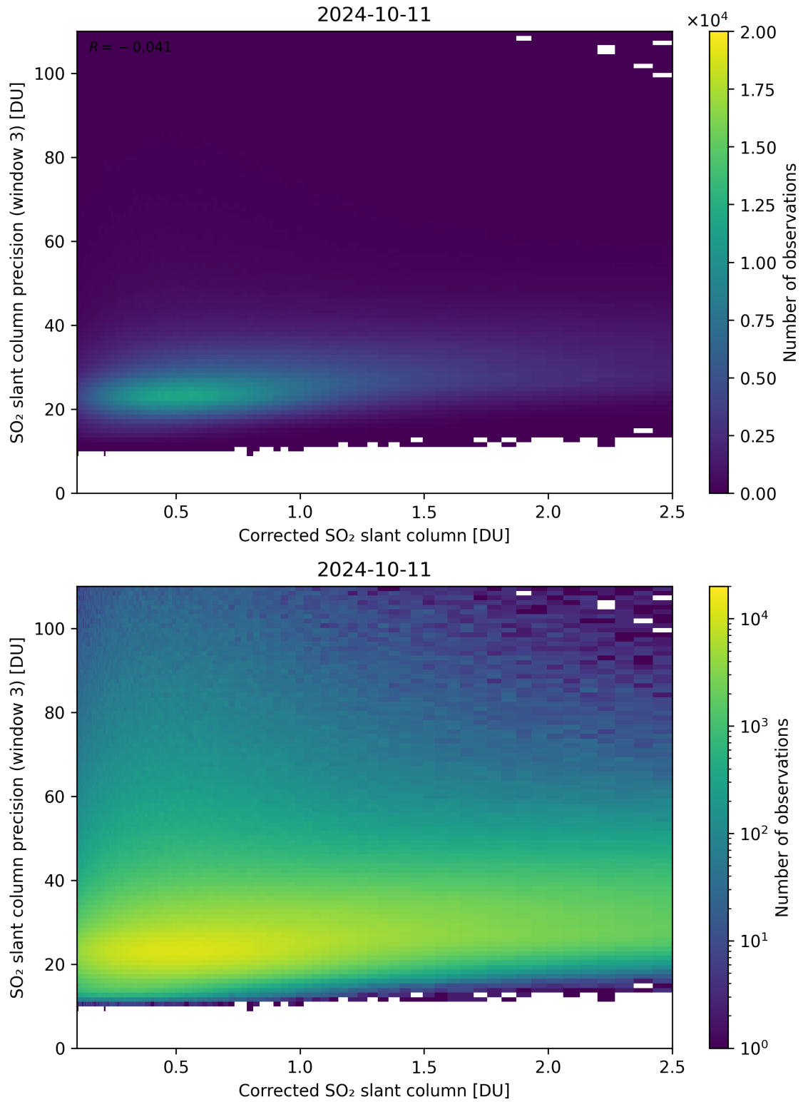
Figure 191: Scatter density plot of “Corrected SO 2 slant column” against “SO 2 slant column precision (window 3)” for 2024-10-10 to 2024-10-12.
