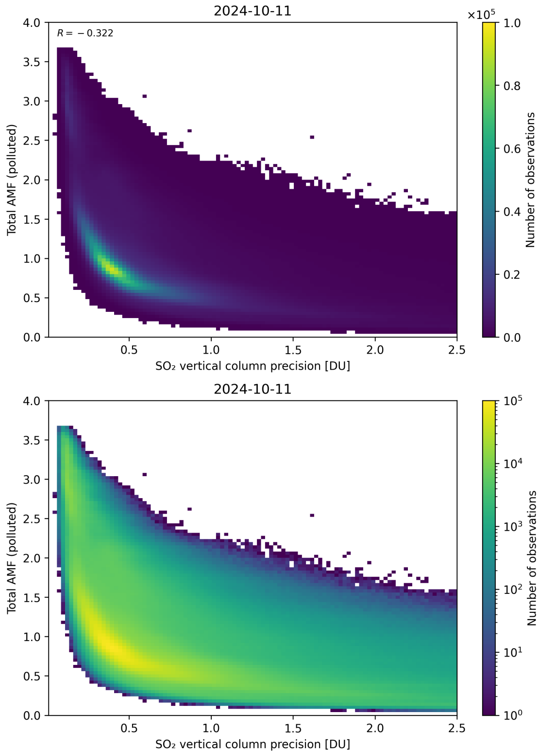
Figure 294: Scatter density plot of “SO 2 vertical column precision” against “Total AMF (polluted)” for 2024-10-10 to 2024-10-12.
