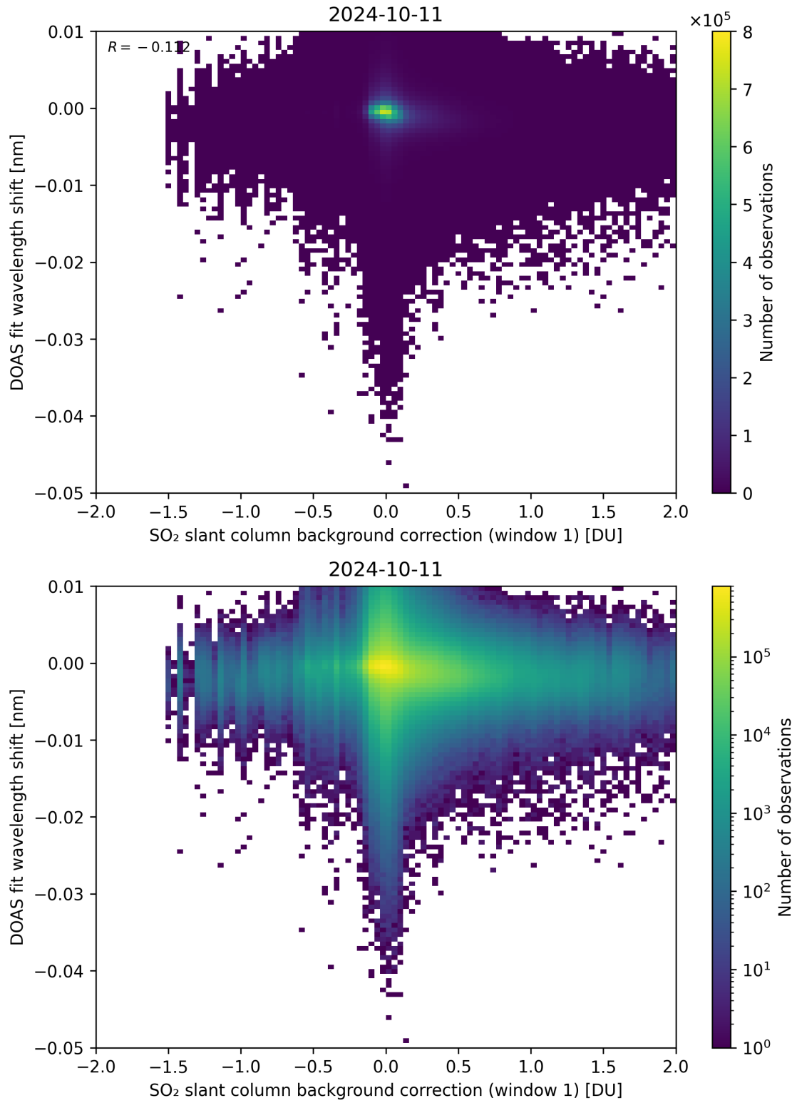
Figure 100: Scatter density plot of “SO 2 slant column background correction (window 1)” against “DOAS fit wavelength shift” for 2024-10-10 to 2024-10-12.
