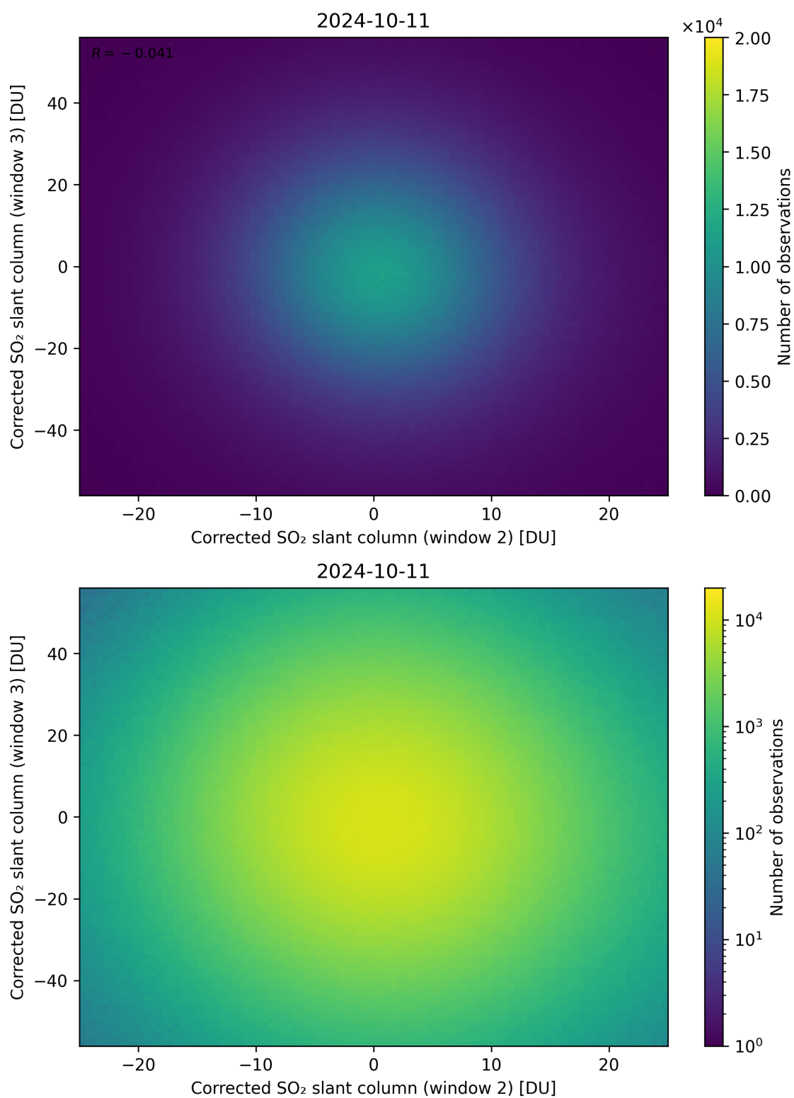
Figure 200: Scatter density plot of “Corrected SO 2 slant column (window 2)” against “Corrected SO 2 slant column (window 3)” for 2024-10-10 to 2024-10-12.
