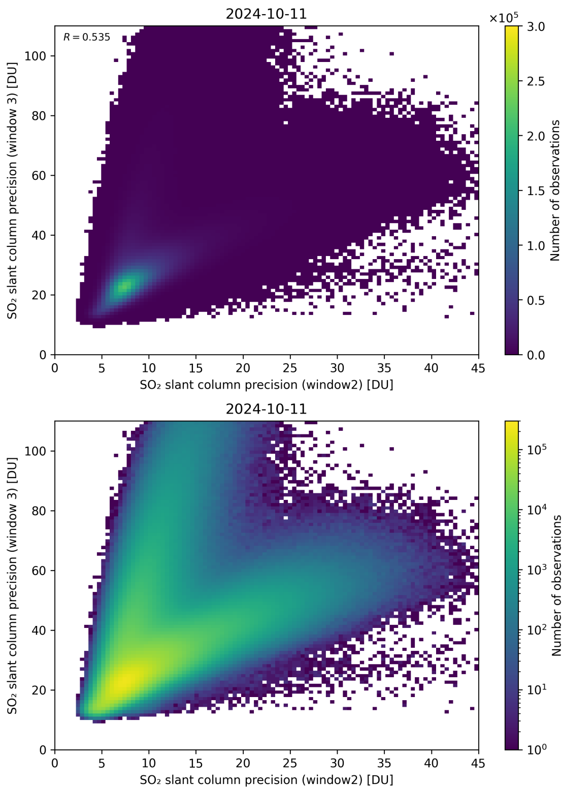
Figure 250: Scatter density plot of “SO 2 slant column precision (window2)” against “SO 2 slant column precision (window 3)” for 2024-10-10 to 2024-10-12.
