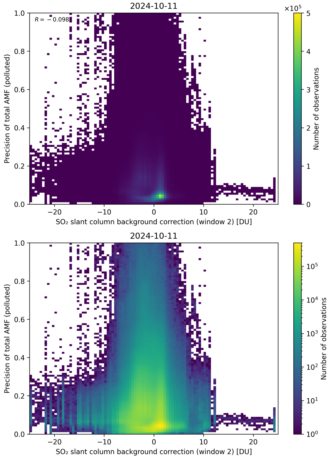
Figure 120: Scatter density plot of “SO 2 slant column background correction (window 2)” against “Precision of total AMF (polluted)” for 2024-10-10 to 2024-10-12.
