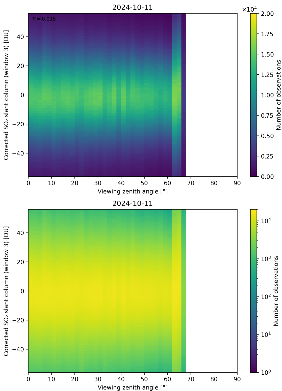
Figure 319: Scatter density plot of “Viewing zenith angle” against “Corrected SO 2 slant column (window 3)” for 2024-10-10 to 2024-10-12.
