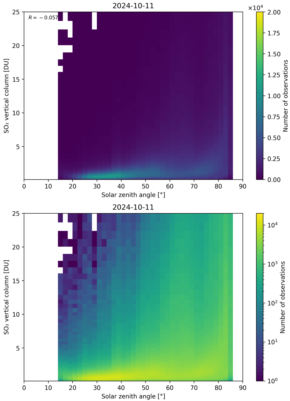
Figure 176: Scatter density plot of “Solar zenith angle” against “SO 2 vertical column” for 2024-10-10 to 2024-10-12.
