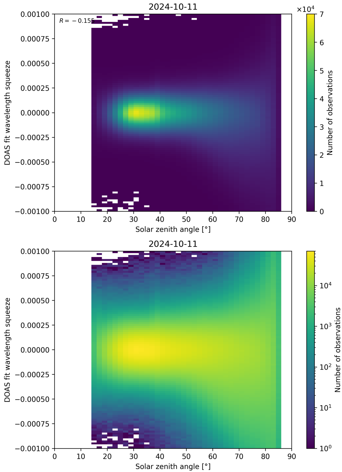
Figure 162: Scatter density plot of “Solar zenith angle” against “DOAS fit wavelength squeeze” for 2024-10-10 to 2024-10-12.
