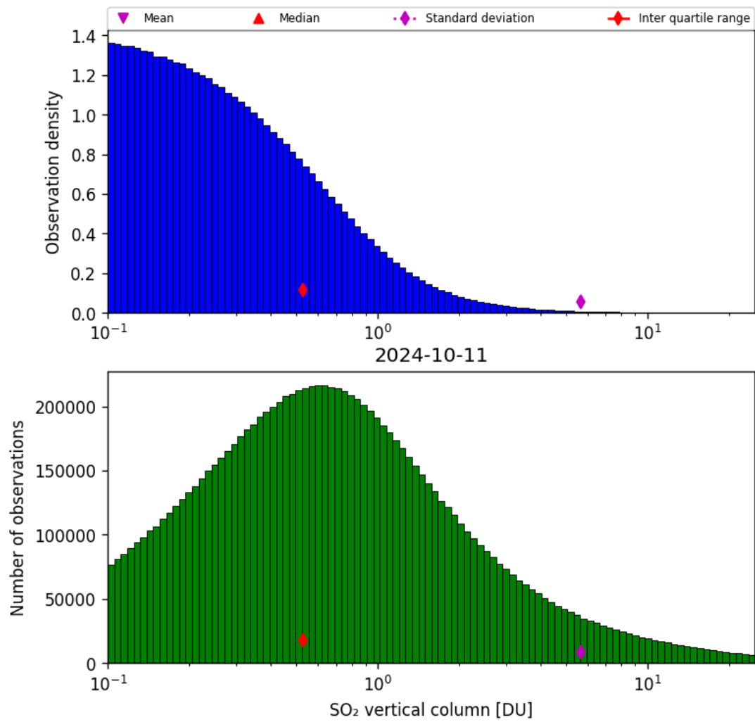
Figure 53: Histogram of “SO 2 vertical column” for 2024-10-10 to 2024-10-12
