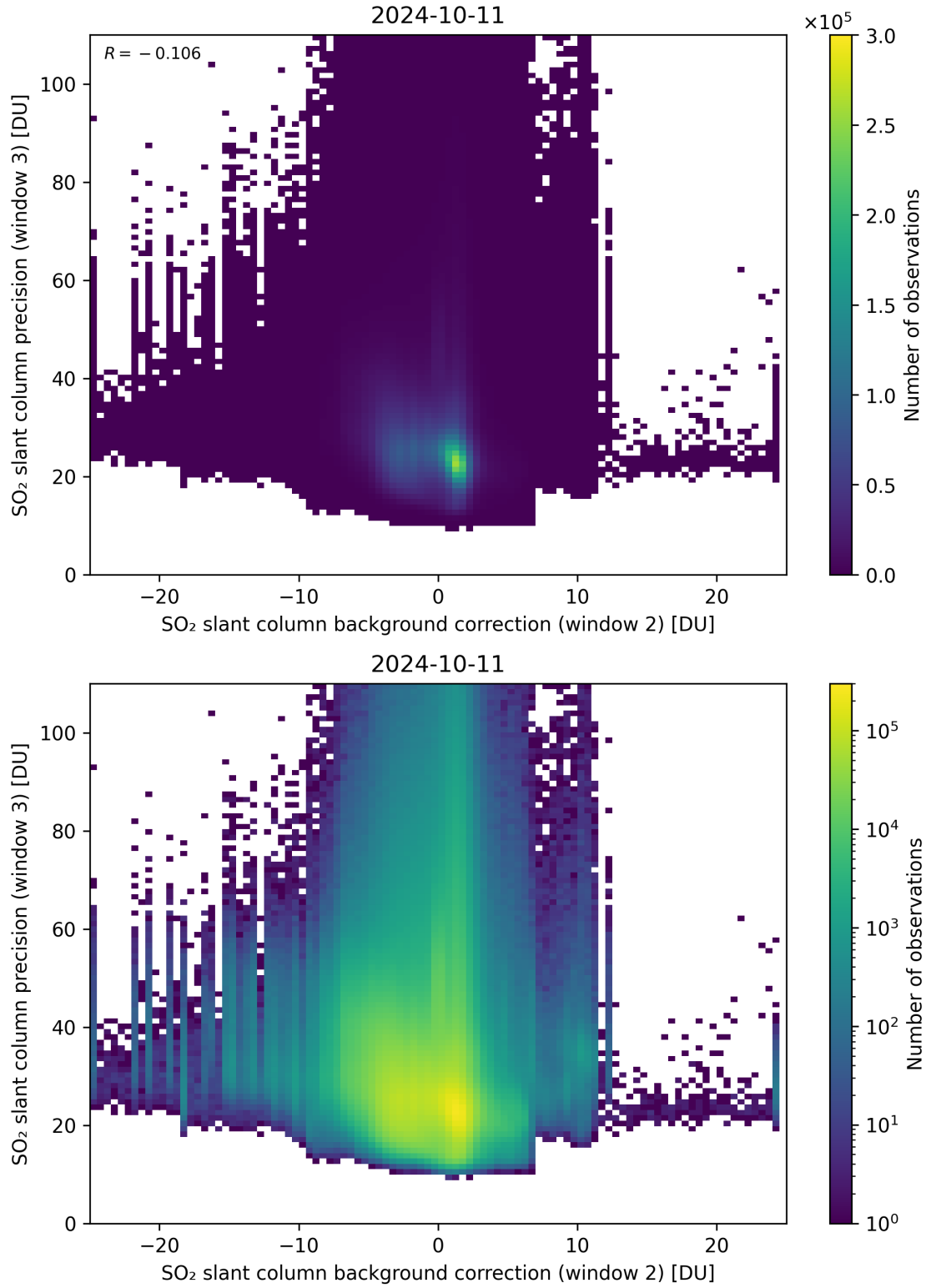
Figure 118: Scatter density plot of “SO 2 slant column background correction (window 2)” against “SO 2 slant column precision (window 3)” for 2024-10-10 to 2024-10-12.
