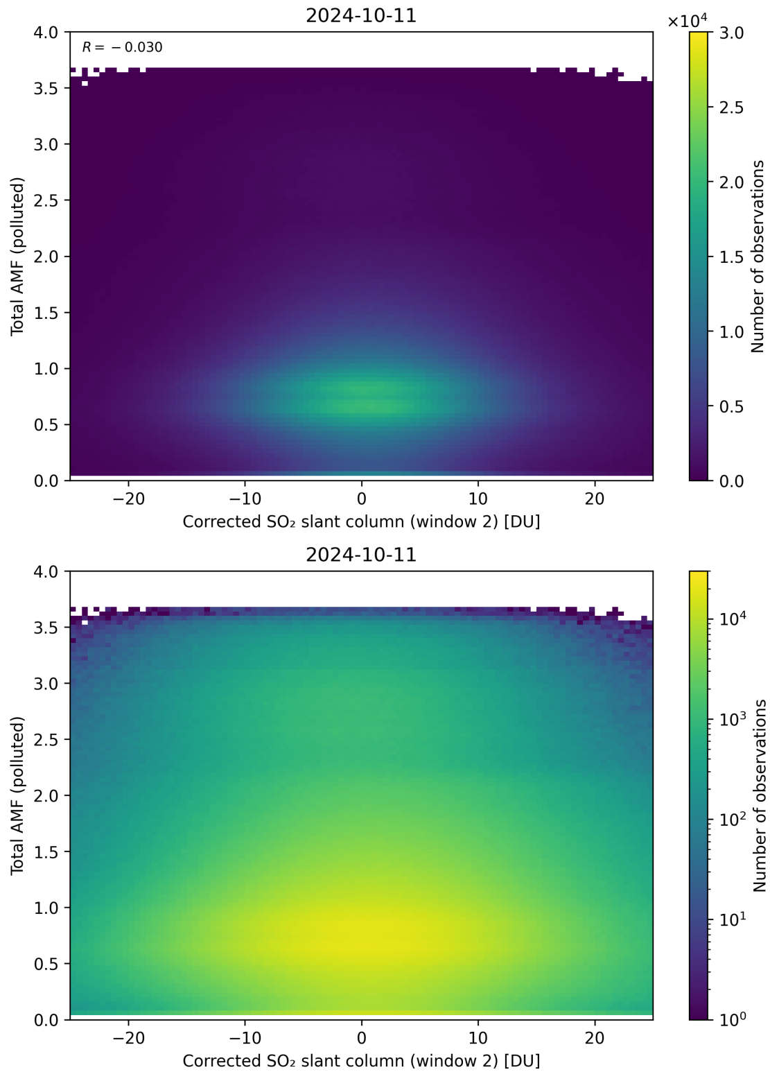
Figure 203: Scatter density plot of “Corrected SO 2 slant column (window 2)” against “Total AMF (polluted)” for 2024-10-10 to 2024-10-12.
