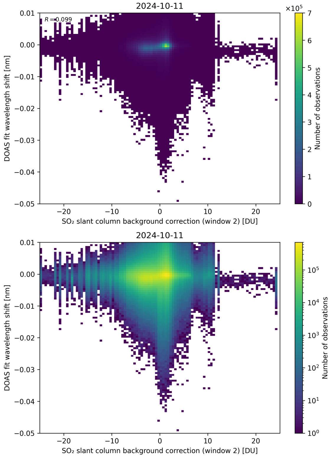
Figure 112: Scatter density plot of “SO 2 slant column background correction (window 2)” against “DOAS fit wavelength shift” for 2024-10-10 to 2024-10-12.
