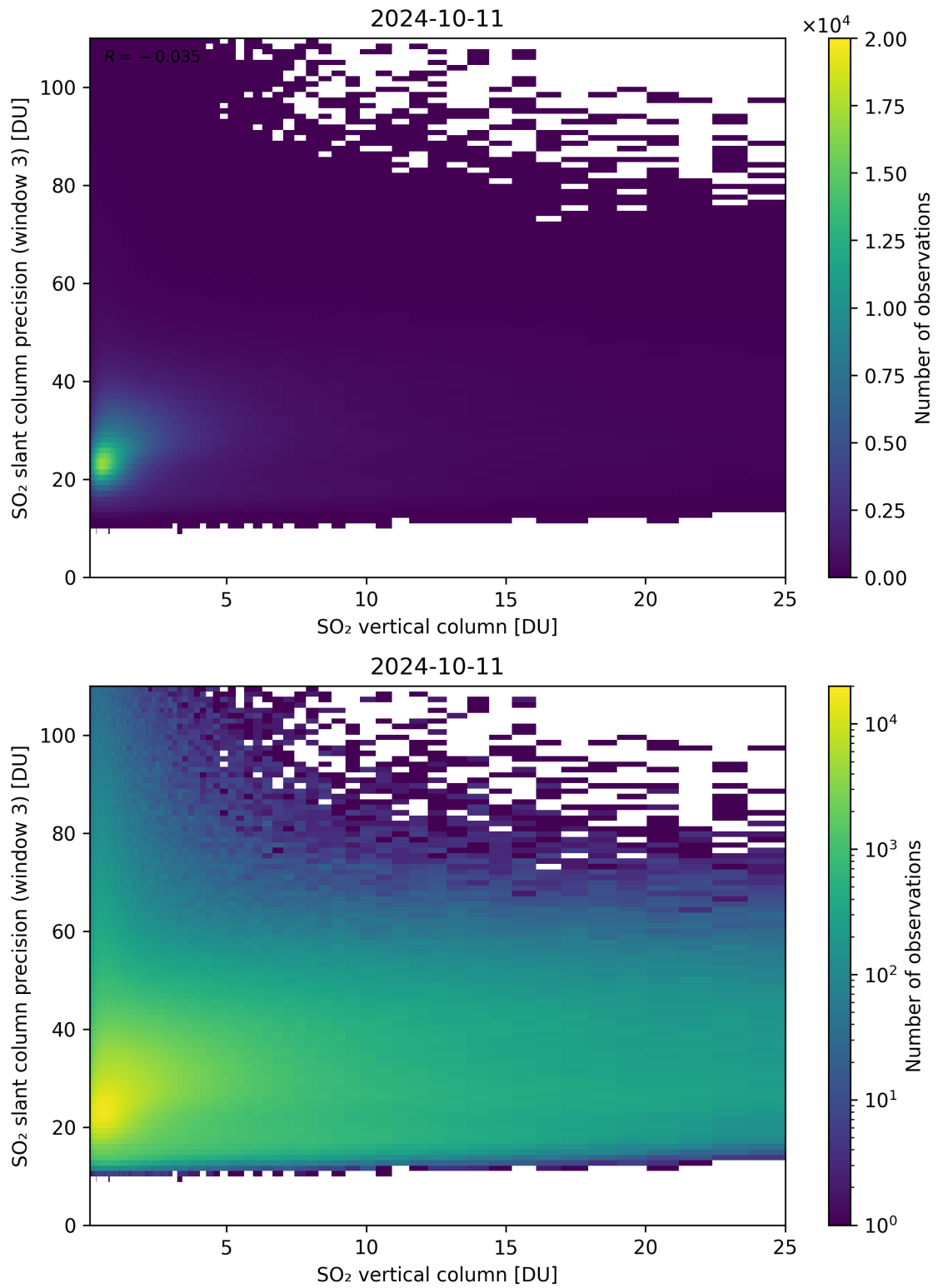
Figure 304: Scatter density plot of “SO 2 vertical column” against “SO 2 slant column precision (window 3)” for 2024-10-10 to 2024-10-12.
