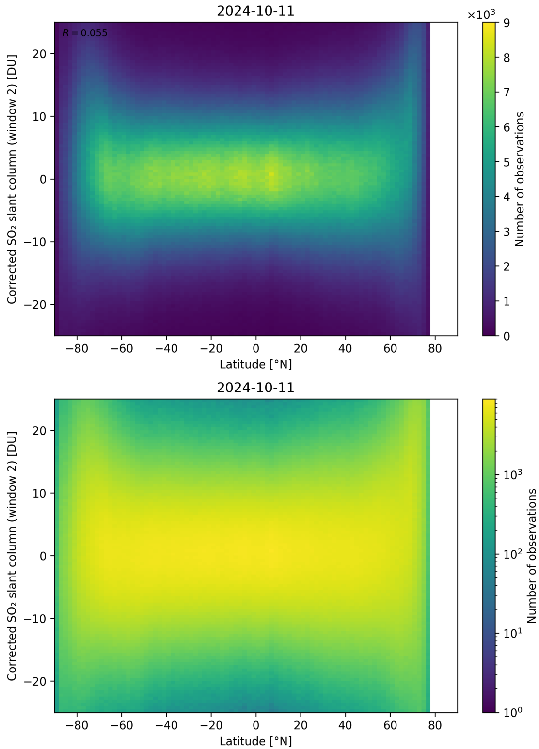
Figure 147: Scatter density plot of “Latitude” against “Corrected SO 2 slant column (window 2)” for 2024-10-10 to 2024-10-12.
