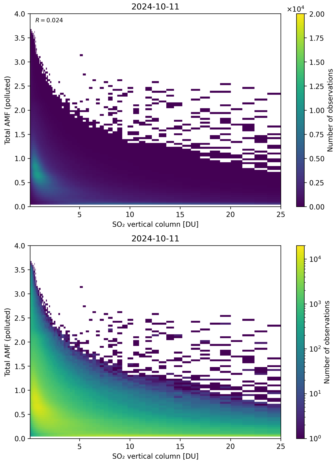
Figure 305: Scatter density plot of “SO 2 vertical column” against “Total AMF (polluted)” for 2024-10-10 to 2024-10-12.
