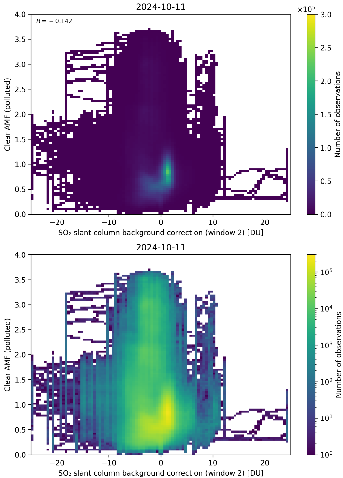
Figure 115: Scatter density plot of “SO 2 slant column background correction (window 2)” against “Clear AMF (polluted)” for 2024-10-10 to 2024-10-12.
