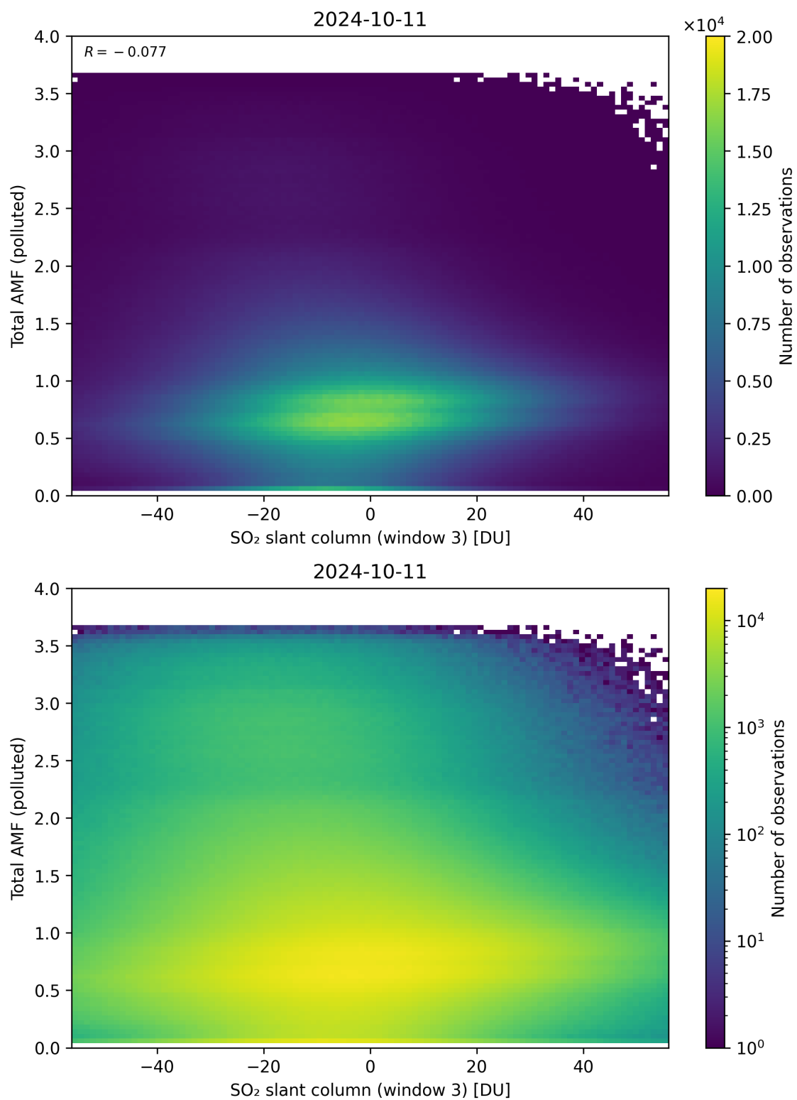
Figure 268: Scatter density plot of “SO 2 slant column (window 3)” against “Total AMF (polluted)” for 2024-10-10 to 2024-10-12.
