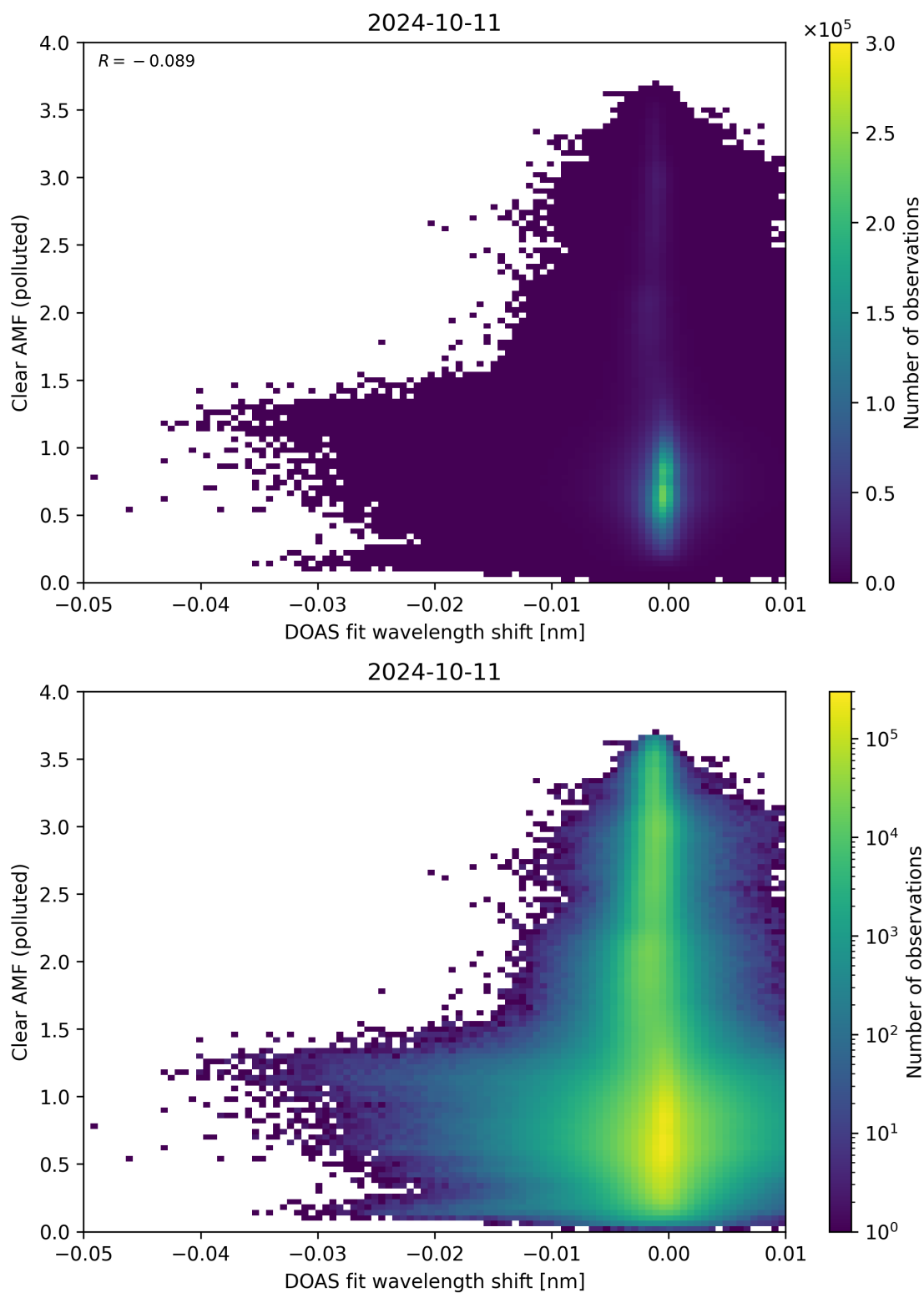
Figure 129: Scatter density plot of “DOAS fit wavelength shift” against “Clear AMF (polluted)” for 2024-10-10 to 2024-10-12.
