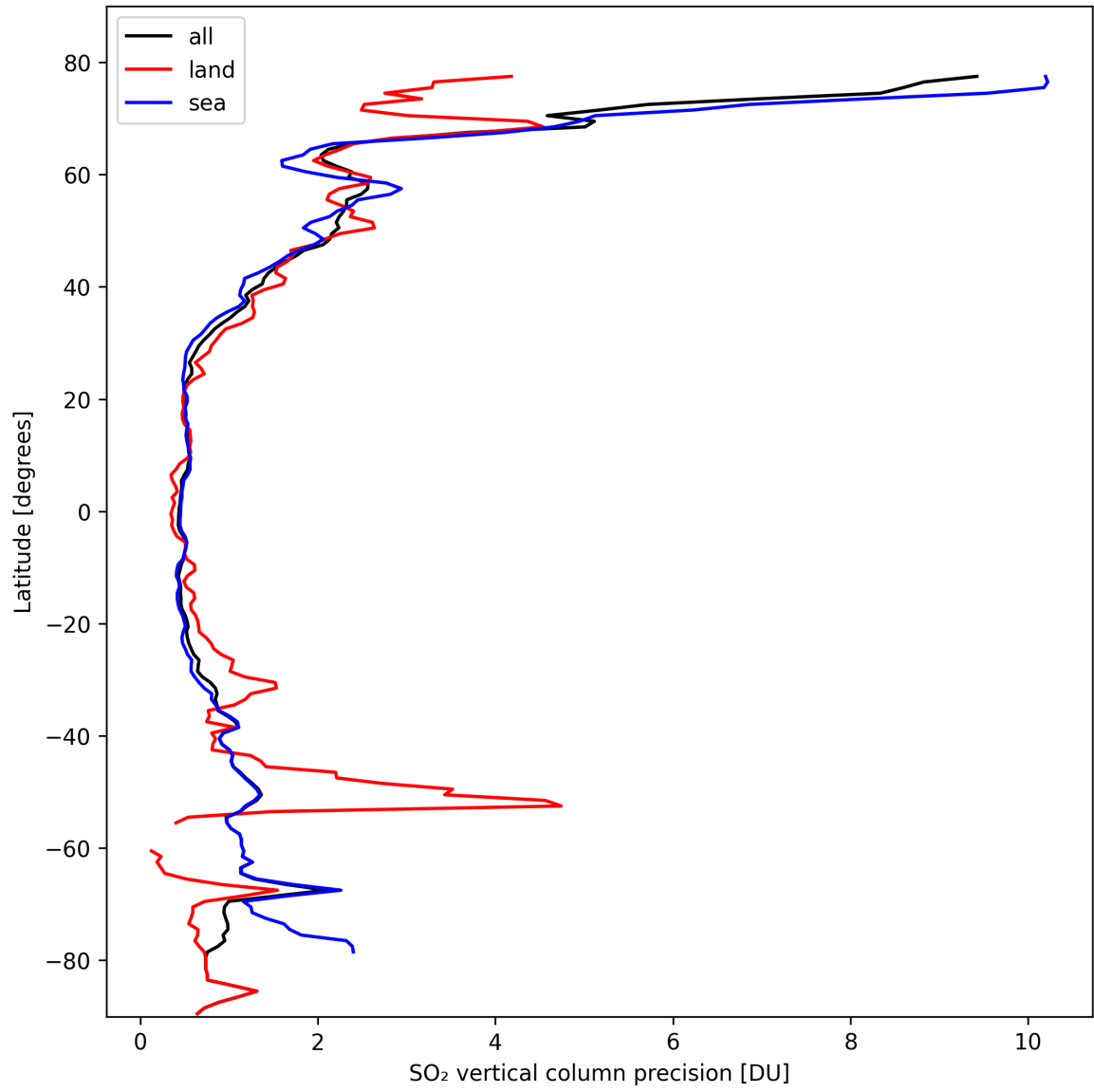
Figure 31: Zonal average of “SO 2 vertical column precision” for 2024-10-10 to 2024-10-12.
