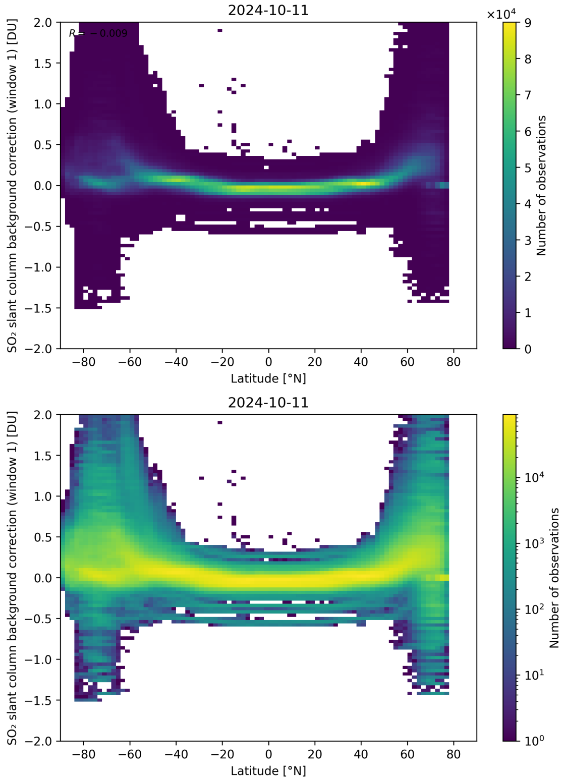
Figure 139: Scatter density plot of “Latitude” against “SO 2 slant column background correction (window 1)” for 2024-10-10 to 2024-10-12.
