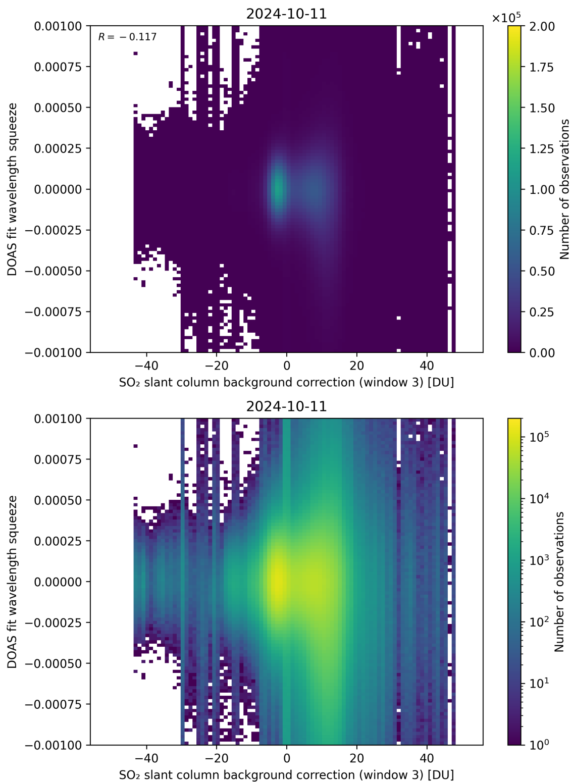
Figure 122: Scatter density plot of “SO 2 slant column background correction (window 3)” against “DOAS fit wavelength squeeze” for 2024-10-10 to 2024-10-12.
