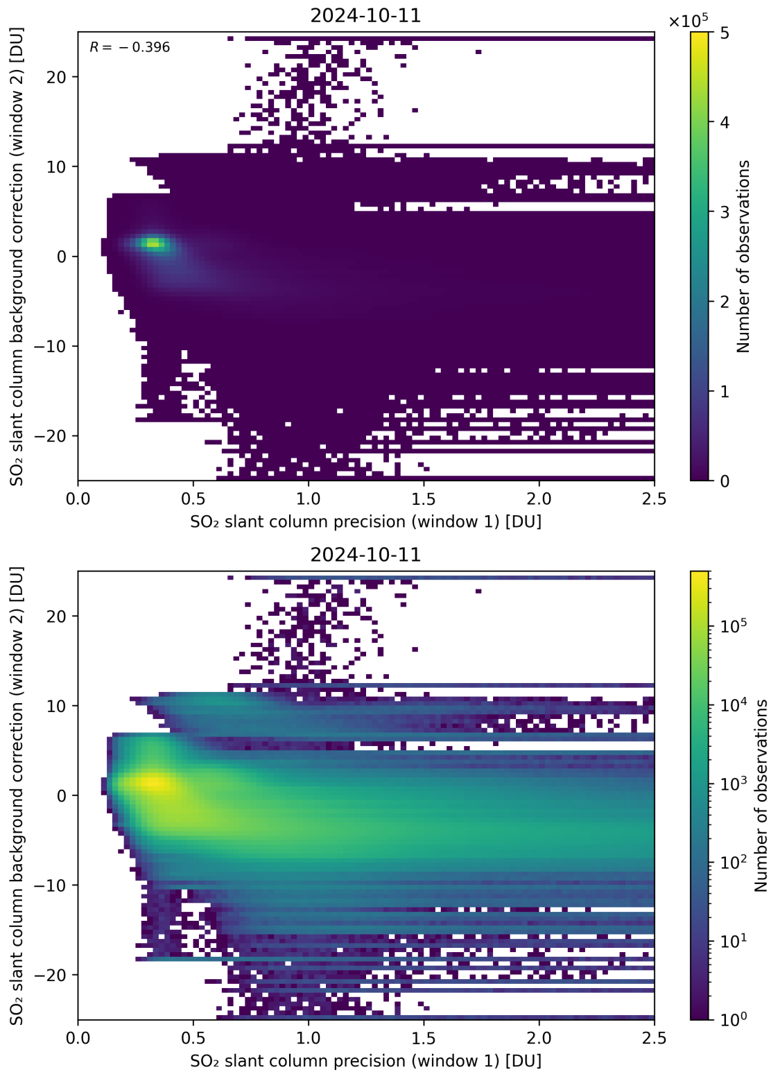
Figure 219: Scatter density plot of “SO 2 slant column precision (window 1)” against “SO 2 slant column background correction (window 2)” for 2024-10-10 to 2024-10-12.
