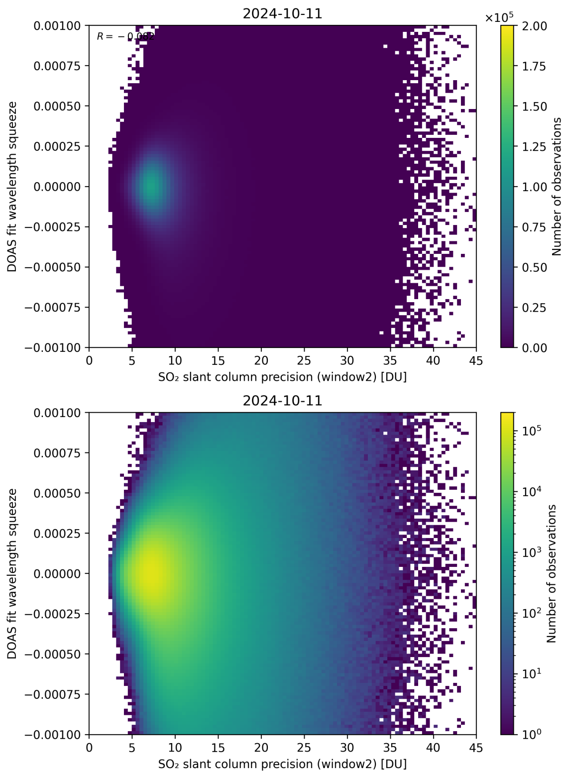
Figure 244: Scatter density plot of “SO 2 slant column precision (window2)” against “DOAS fit wavelength squeeze” for 2024-10-10 to 2024-10-12.
