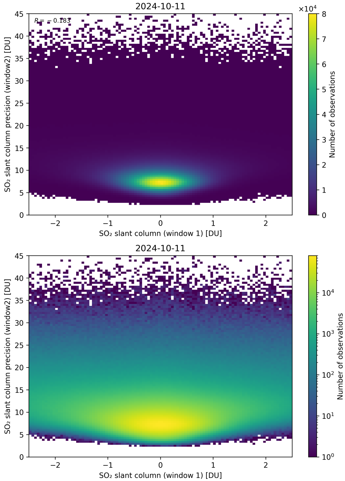
Figure 236: Scatter density plot of “SO 2 slant column (window 1)” against “SO 2 slant column precision (window2)” for 2024-10-10 to 2024-10-12.
