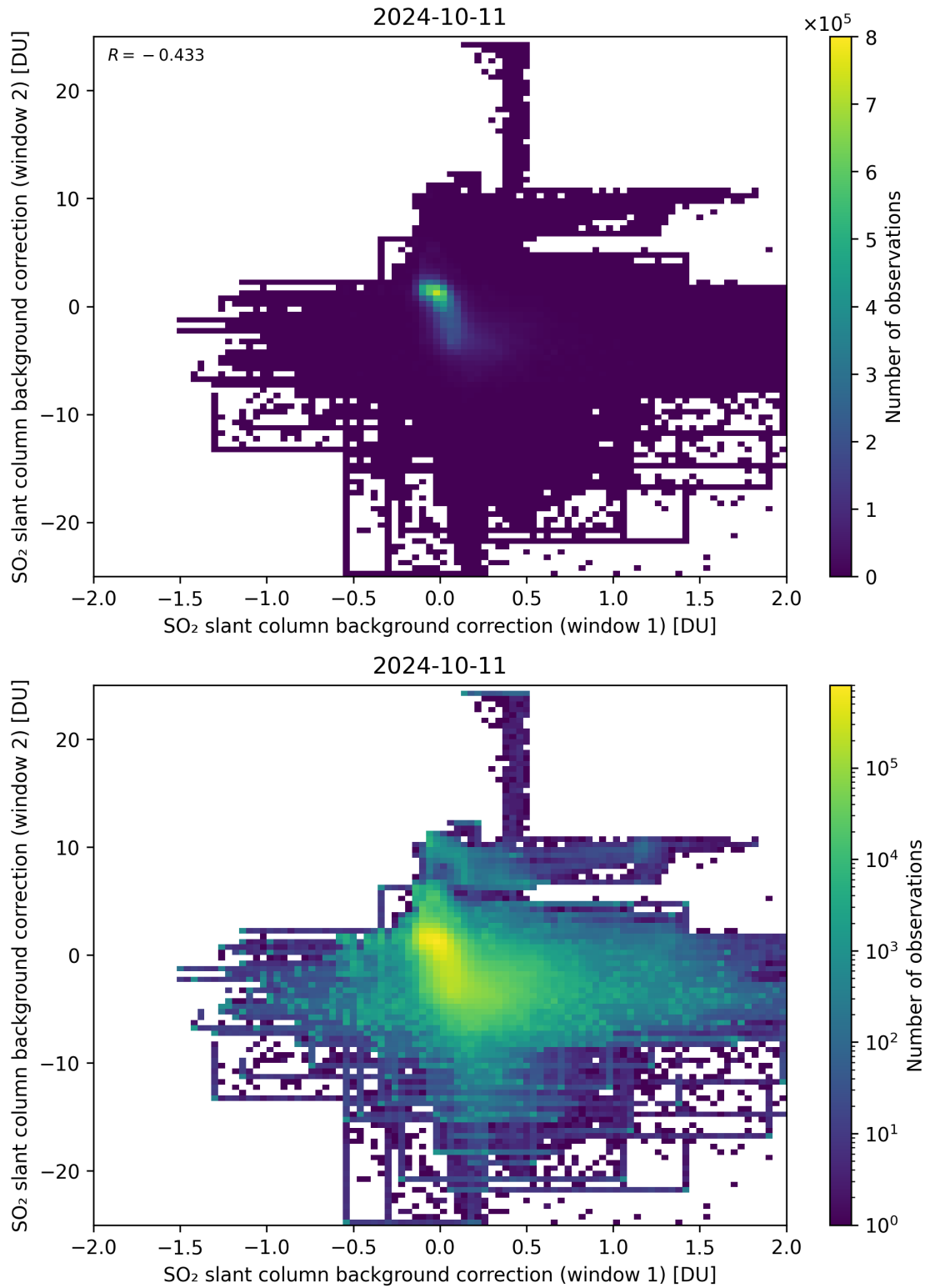
Figure 98: Scatter density plot of “SO 2 slant column background correction (window 1)” against “SO 2 slant column background correction (window 2)” for 2024-10-10 to 2024-10-12.
