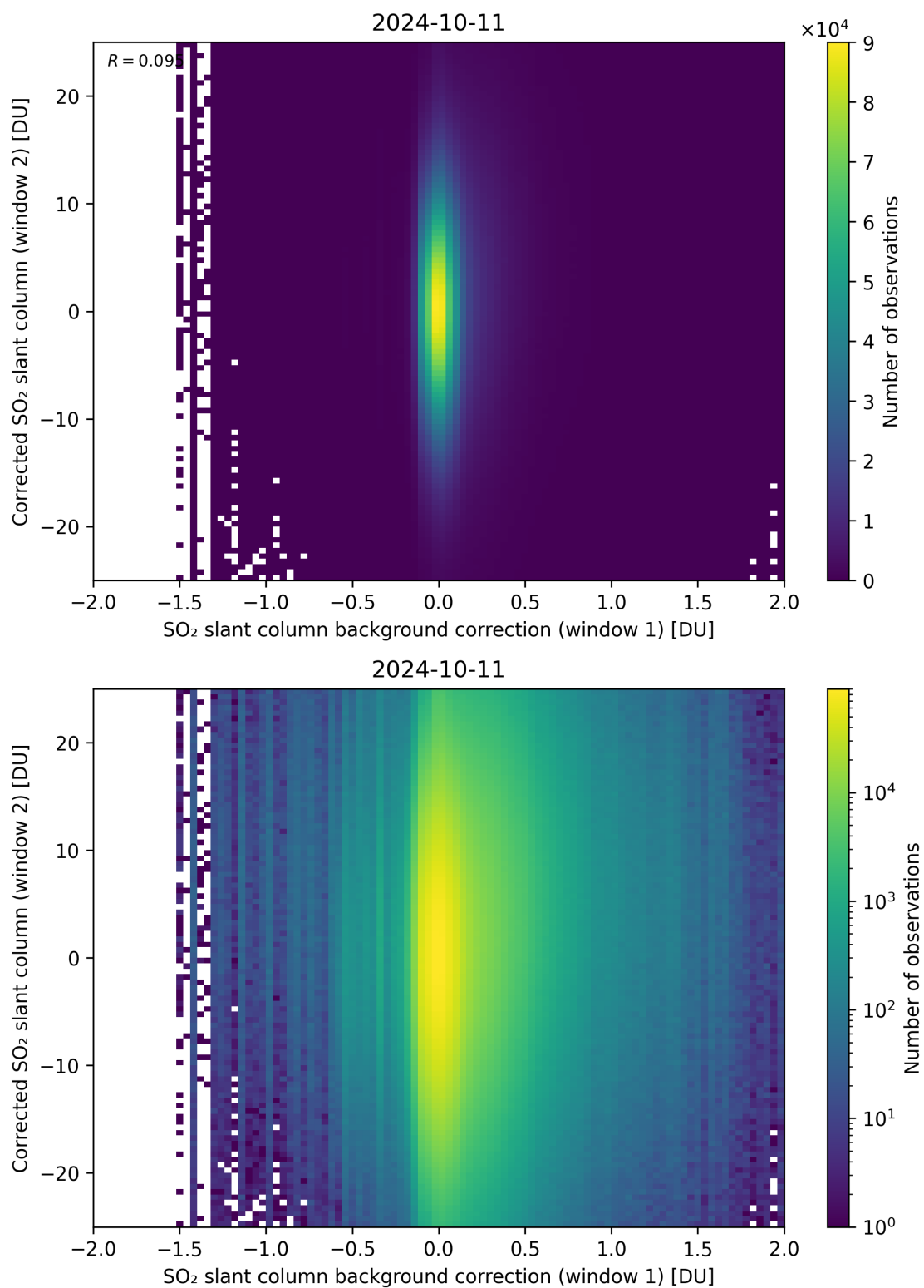
Figure 104: Scatter density plot of “SO 2 slant column background correction (window 1)” against “Corrected SO 2 slant column (window 2)” for 2024-10-10 to 2024-10-12.
