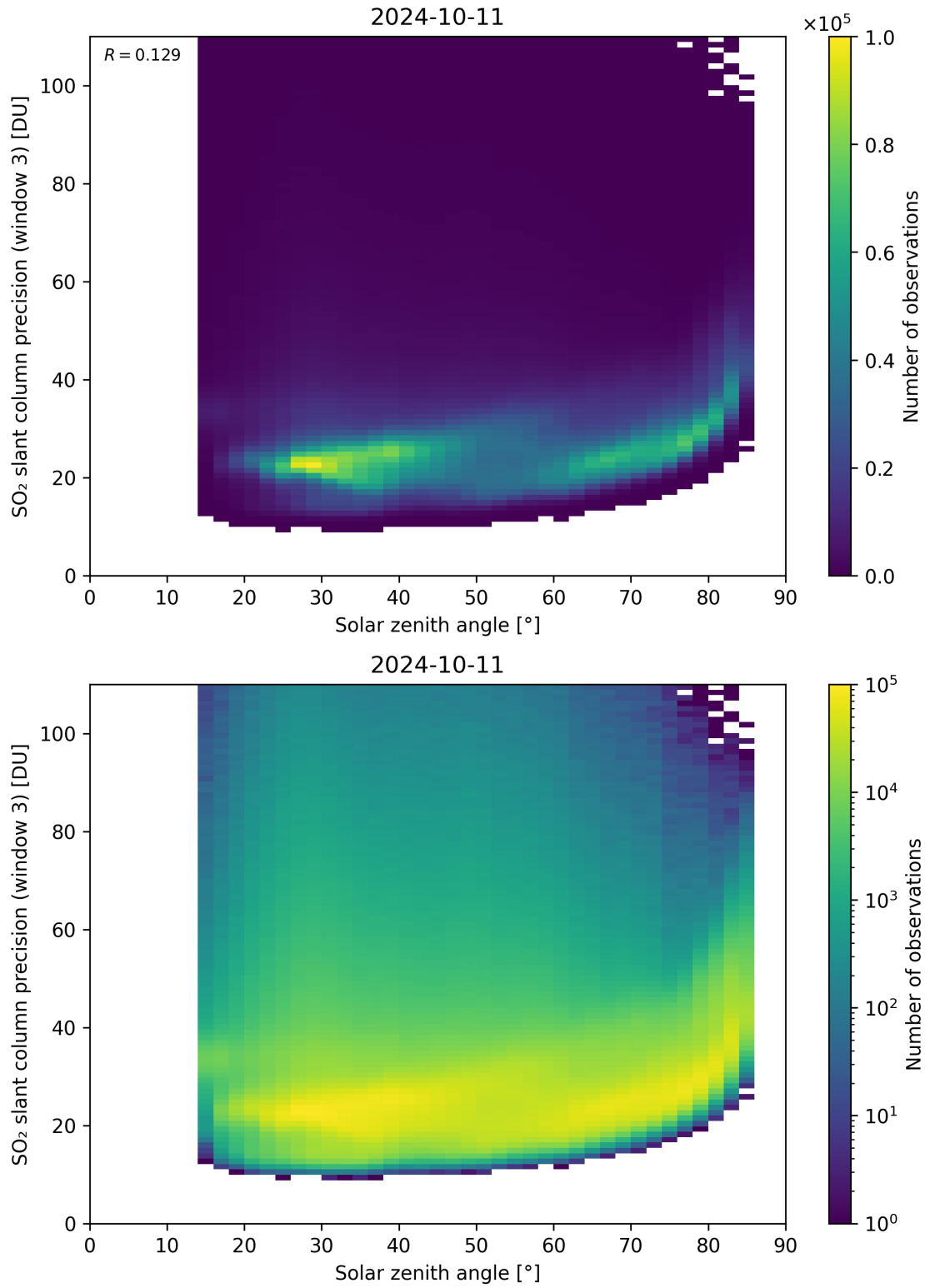
Figure 173: Scatter density plot of “Solar zenith angle” against “SO 2 slant column precision (window 3)” for 2024-10-10 to 2024-10-12.
