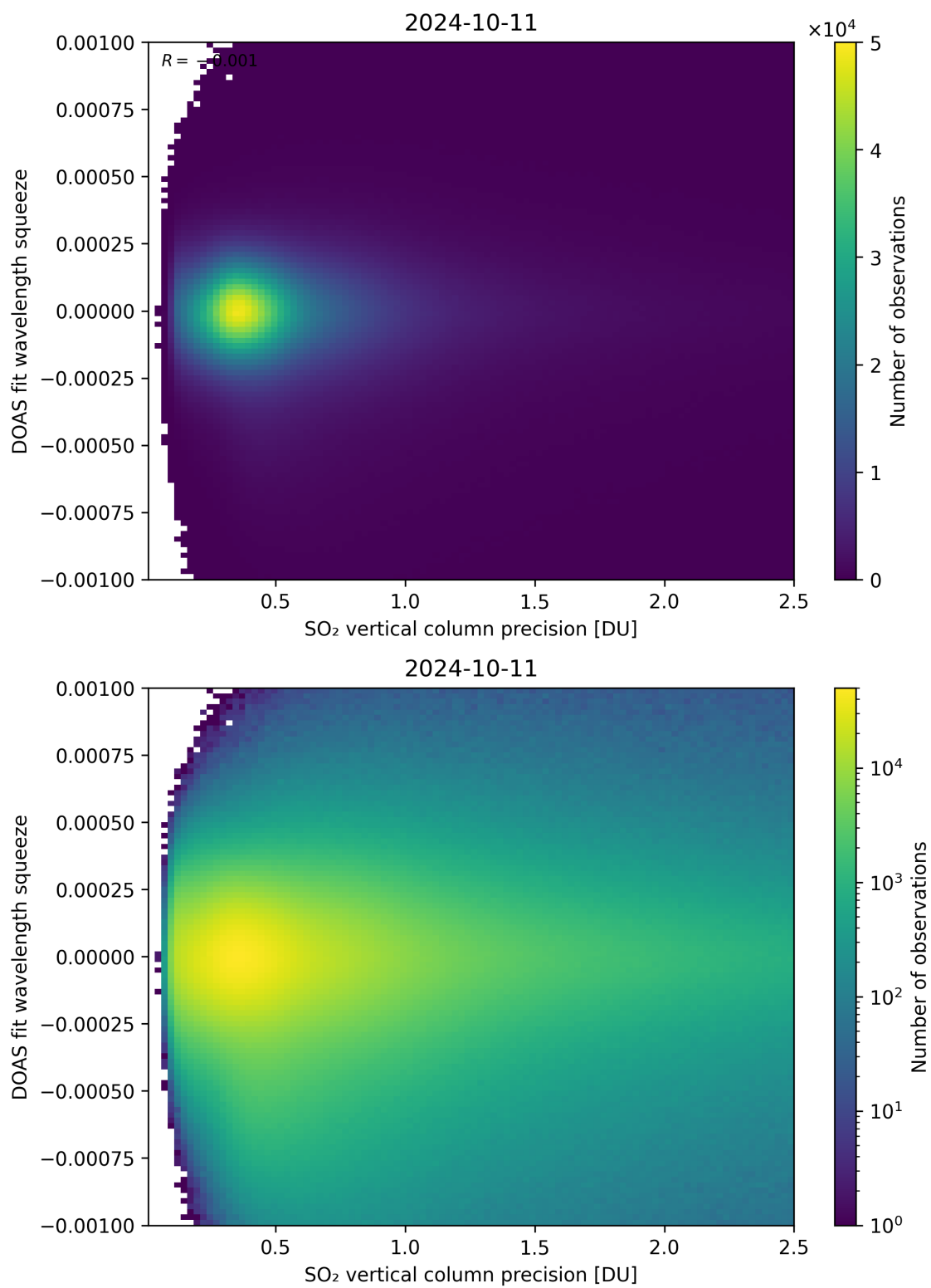
Figure 283: Scatter density plot of “SO 2 vertical column precision” against “DOAS fit wavelength squeeze” for 2024-10-10 to 2024-10-12.
