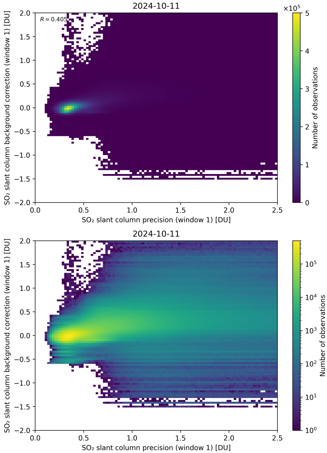
Figure 218: Scatter density plot of “SO 2 slant column precision (window 1)” against “SO 2 slant column background correction (window 1)” for 2024-10-10 to 2024-10-12.
