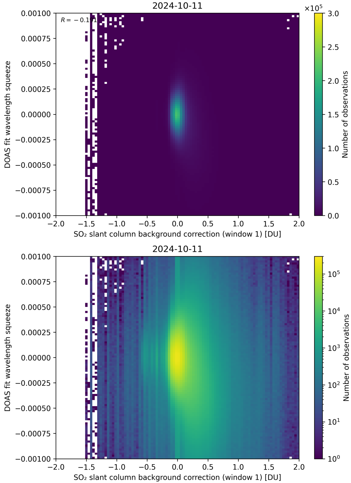
Figure 101: Scatter density plot of “SO 2 slant column background correction (window 1)” against “DOAS fit wavelength squeeze” for 2024-10-10 to 2024-10-12.
