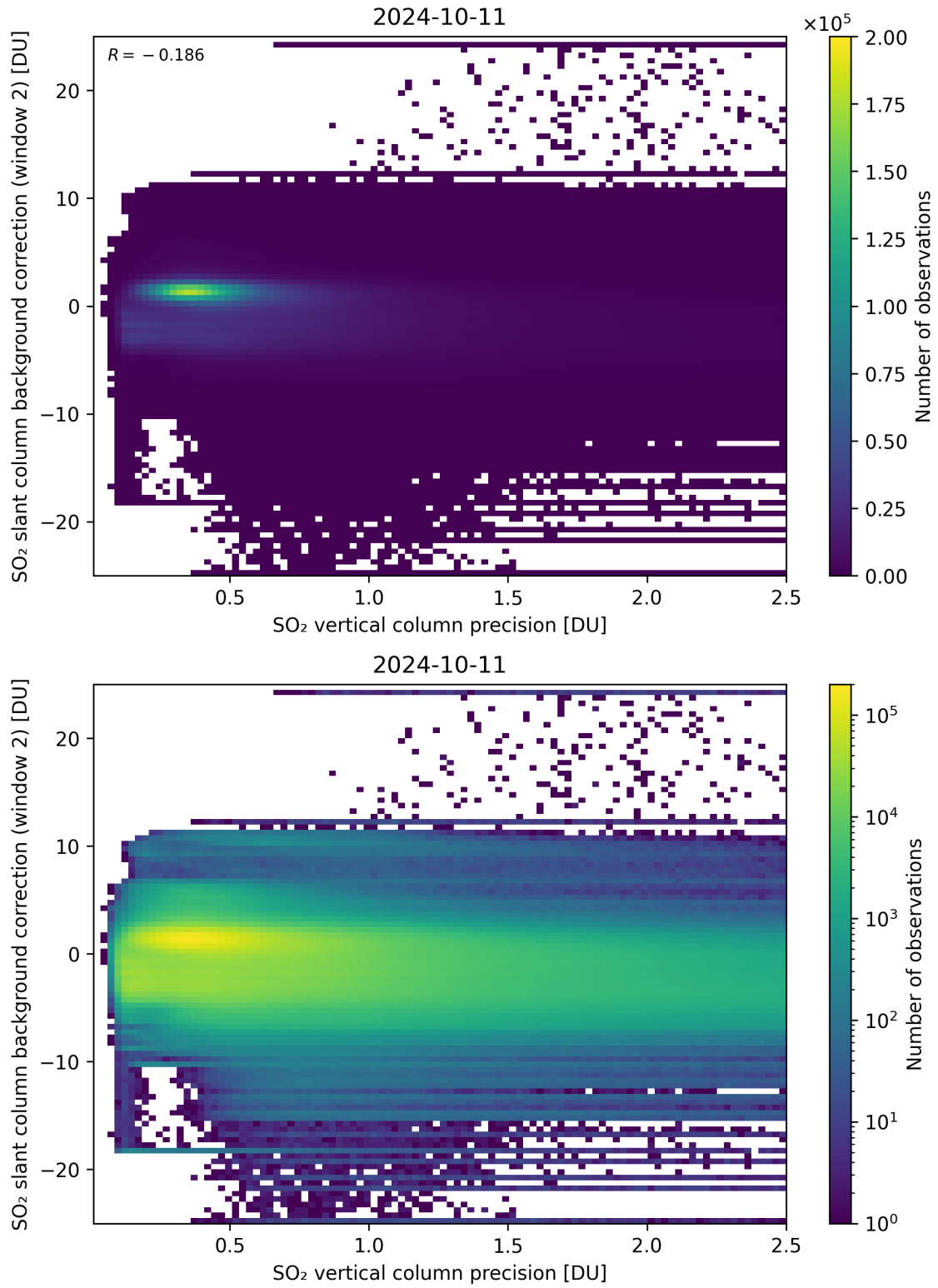
Figure 280: Scatter density plot of “SO 2 vertical column precision” against “SO 2 slant column background correction (window 2)” for 2024-10-10 to 2024-10-12.
