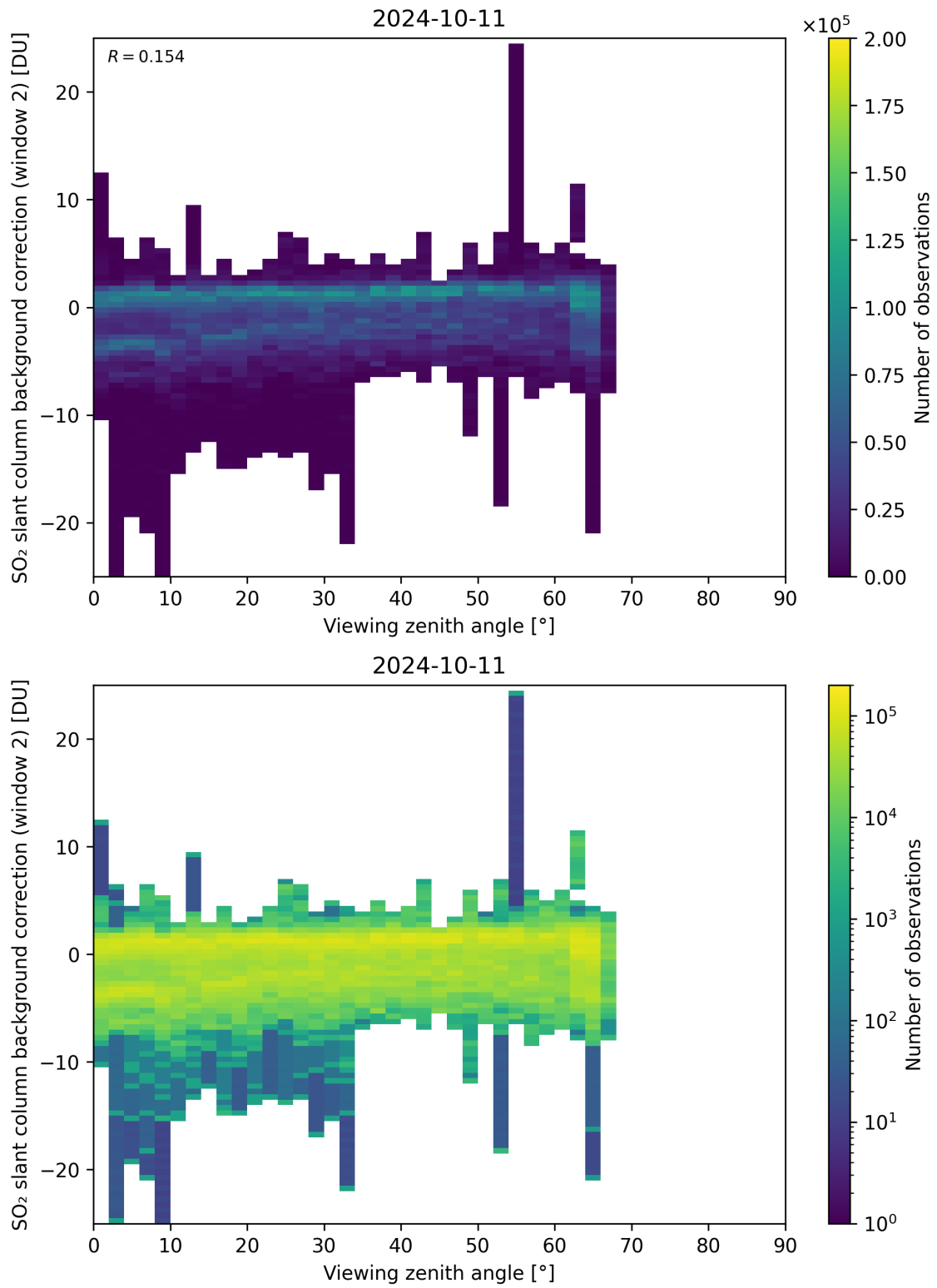
Figure 309: Scatter density plot of “Viewing zenith angle” against “SO 2 slant column background correction (window 2)” for 2024-10-10 to 2024-10-12.
