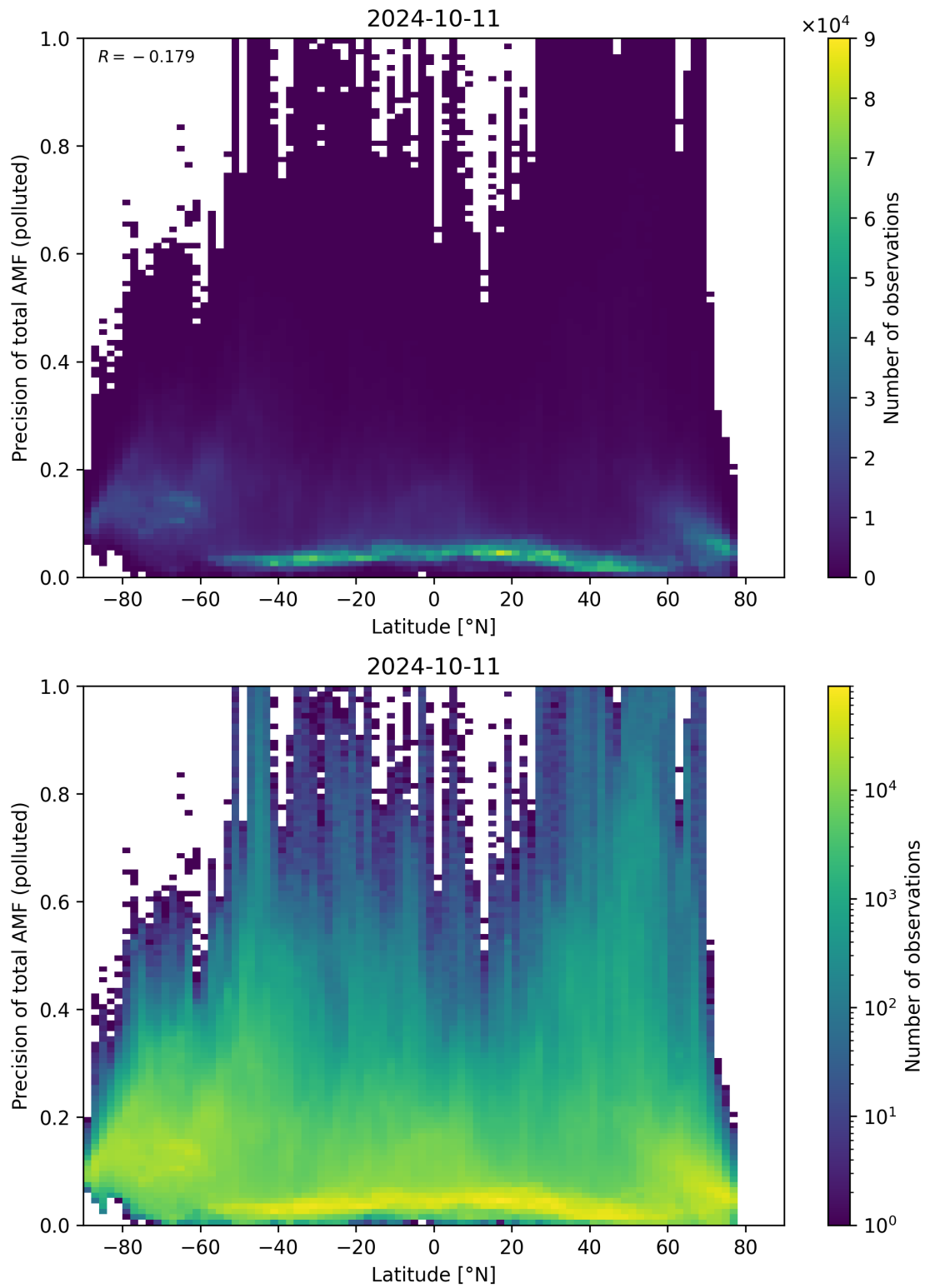
Figure 155: Scatter density plot of “Latitude” against “Precision of total AMF (polluted)” for 2024-10-10 to 2024-10-12.
