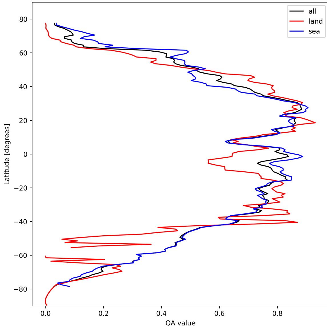
Figure 29: Zonal average of “QA value” for 2024-10-10 to 2024-10-12.
