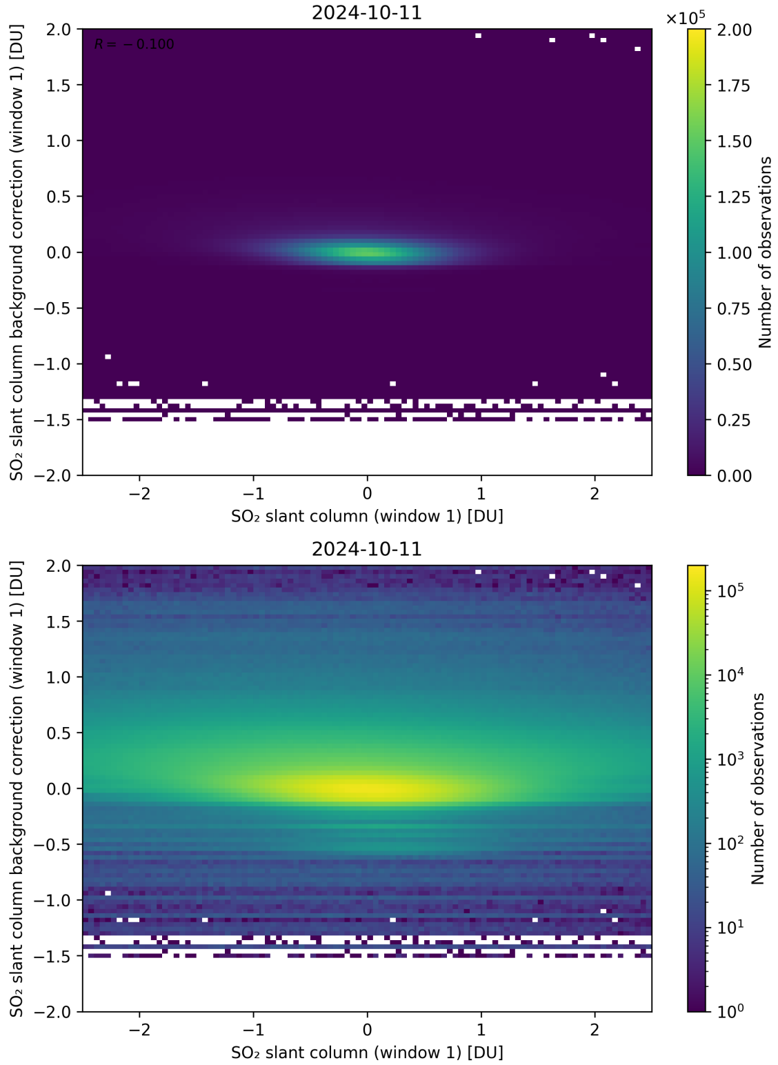
Figure 212: Scatter density plot of “SO 2 slant column (window 1)” against “SO 2 slant column background correction (window 1)” for 2024-10-10 to 2024-10-12.
