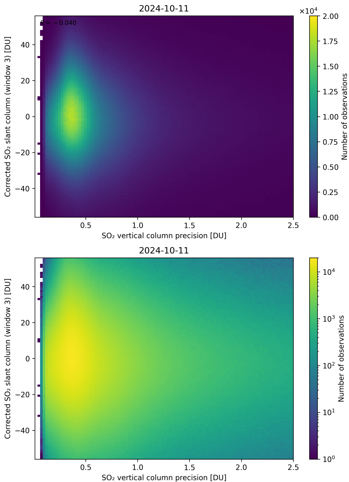
Figure 288: Scatter density plot of “SO 2 vertical column precision” against “Corrected SO 2 slant column (window 3)” for 2024-10-10 to 2024-10-12.
