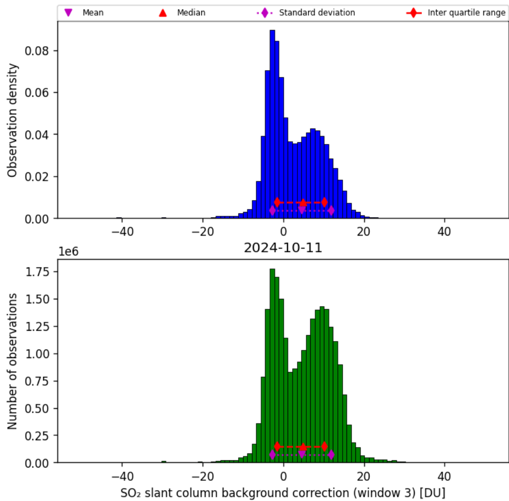
Figure 67: Histogram of “SO 2 slant column background correction (window 3)” for 2024-10-10 to 2024-10-12
