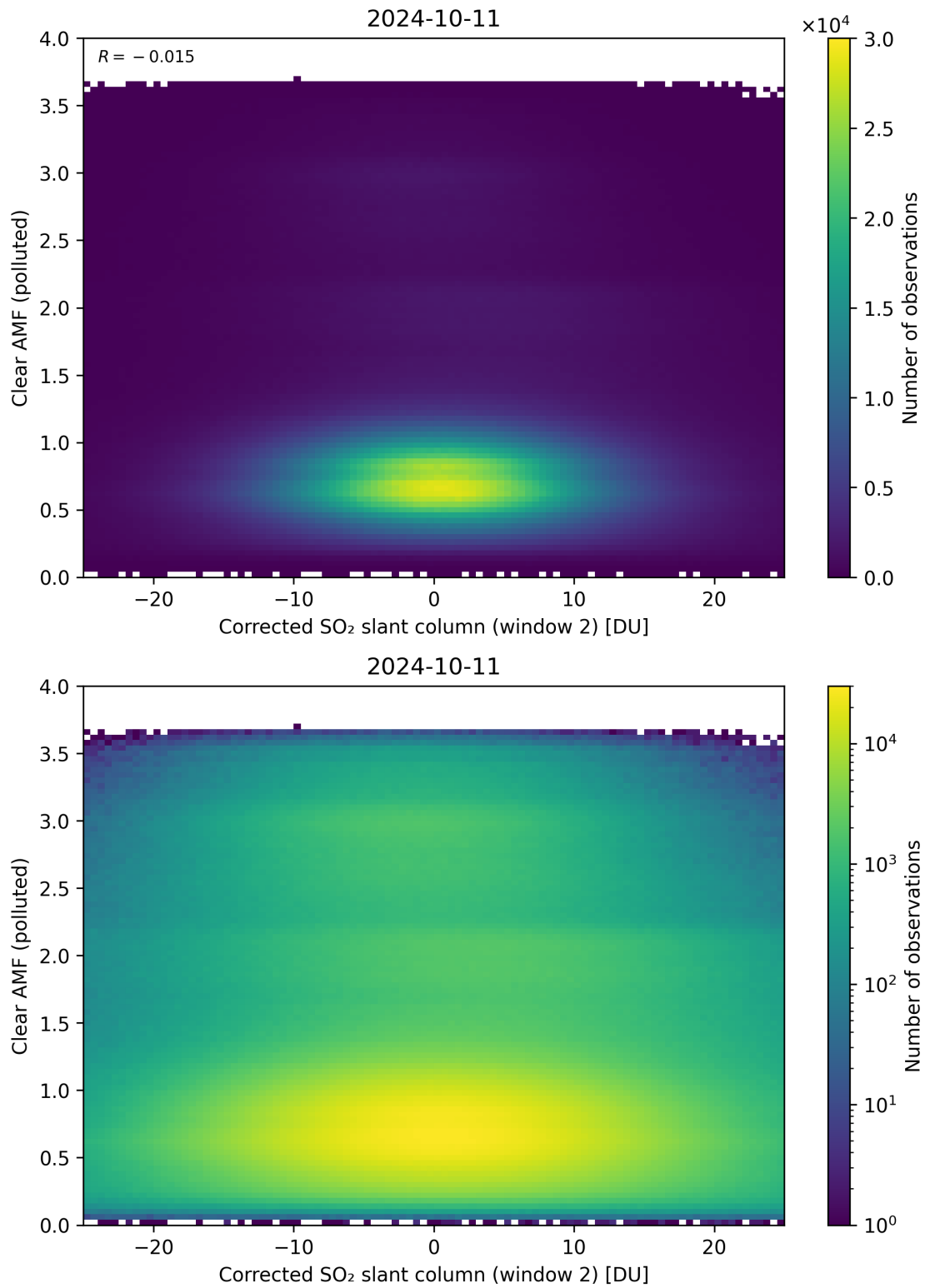
Figure 199: Scatter density plot of “Corrected SO 2 slant column (window 2)” against “Clear AMF (polluted)” for 2024-10-10 to 2024-10-12.
