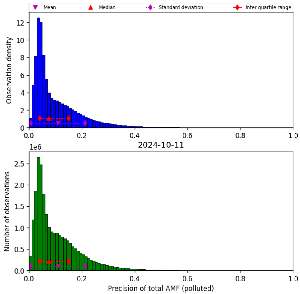
Figure 72: Histogram of “Precision of total AMF (polluted)” for 2024-10-10 to 2024-10-12
