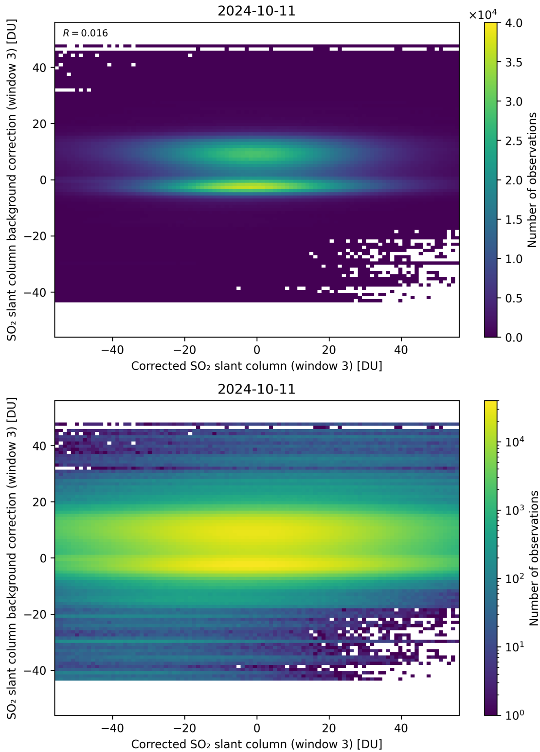
Figure 205: Scatter density plot of “Corrected SO 2 slant column (window 3)” against “SO 2 slant column background correction (window 3)” for 2024-10-10 to 2024-10-12.
