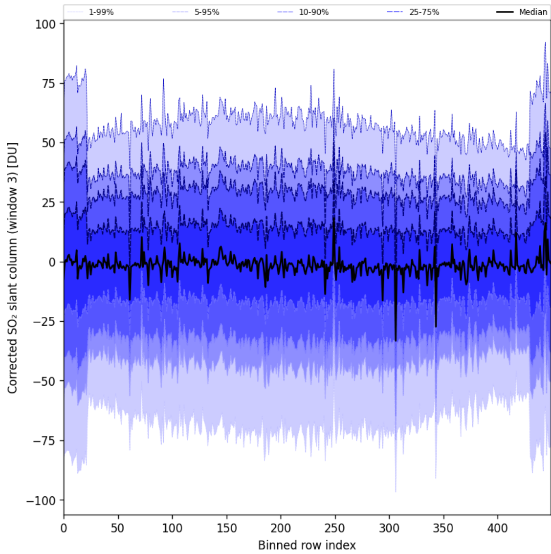
Figure 89: Along track statistics of “Corrected SO 2 slant column (window 3)” for 2024-10-10 to 2024-10-12
