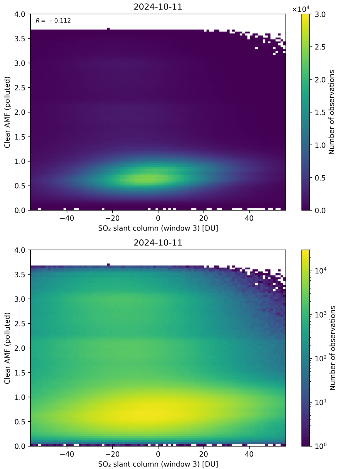
Figure 265: Scatter density plot of “SO 2 slant column (window 3)” against “Clear AMF (polluted)” for 2024-10-10 to 2024-10-12.
