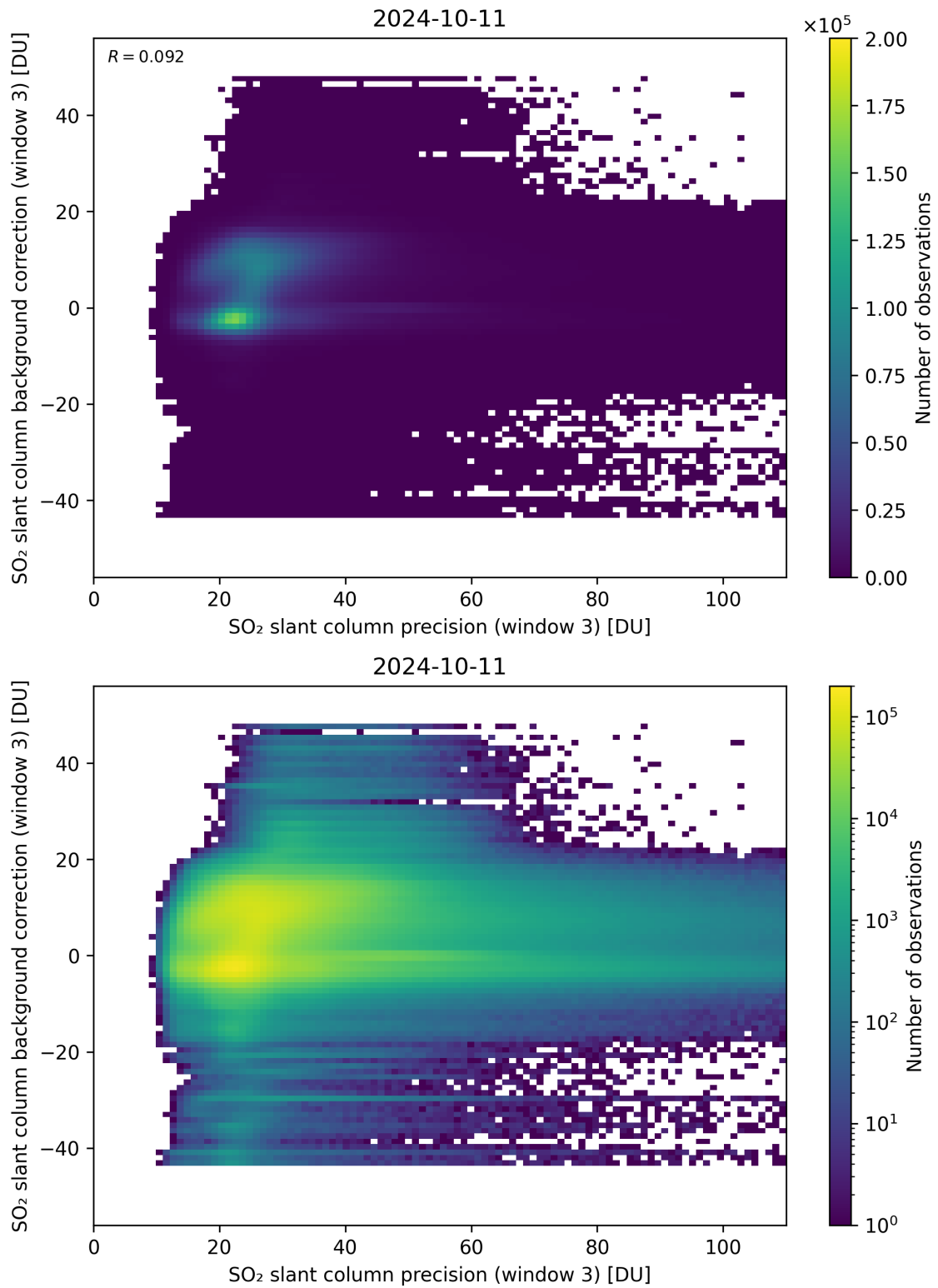
Figure 257: Scatter density plot of “SO 2 slant column precision (window 3)” against “SO 2 slant column background correction (window 3)” for 2024-10-10 to 2024-10-12.
