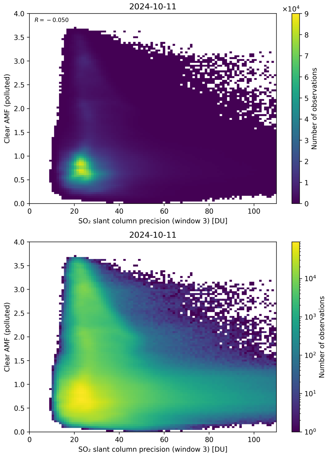
Figure 261: Scatter density plot of “SO 2 slant column precision (window 3)” against “Clear AMF (polluted)” for 2024-10-10 to 2024-10-12.
