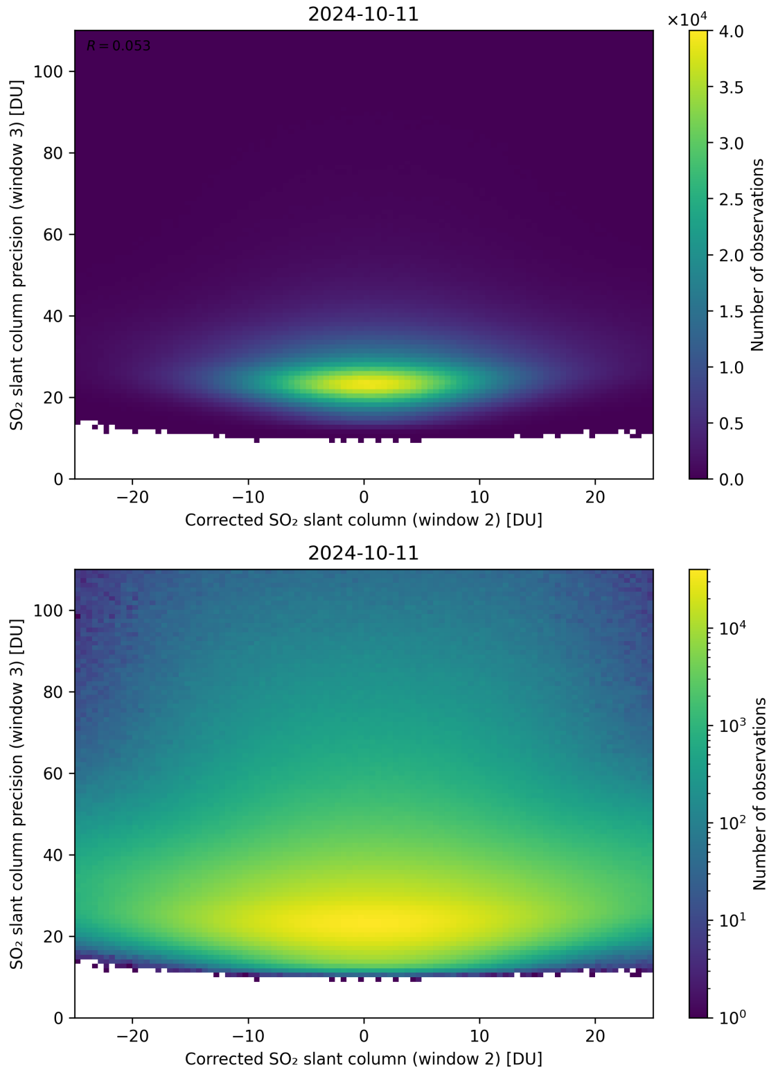
Figure 202: Scatter density plot of “Corrected SO 2 slant column (window 2)” against “SO 2 slant column precision (window 3)” for 2024-10-10 to 2024-10-12.
