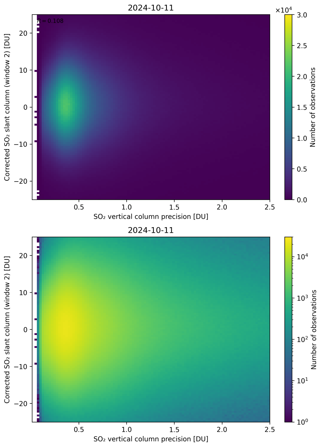
Figure 287: Scatter density plot of “SO 2 vertical column precision” against “Corrected SO 2 slant column (window 2)” for 2024-10-10 to 2024-10-12.
