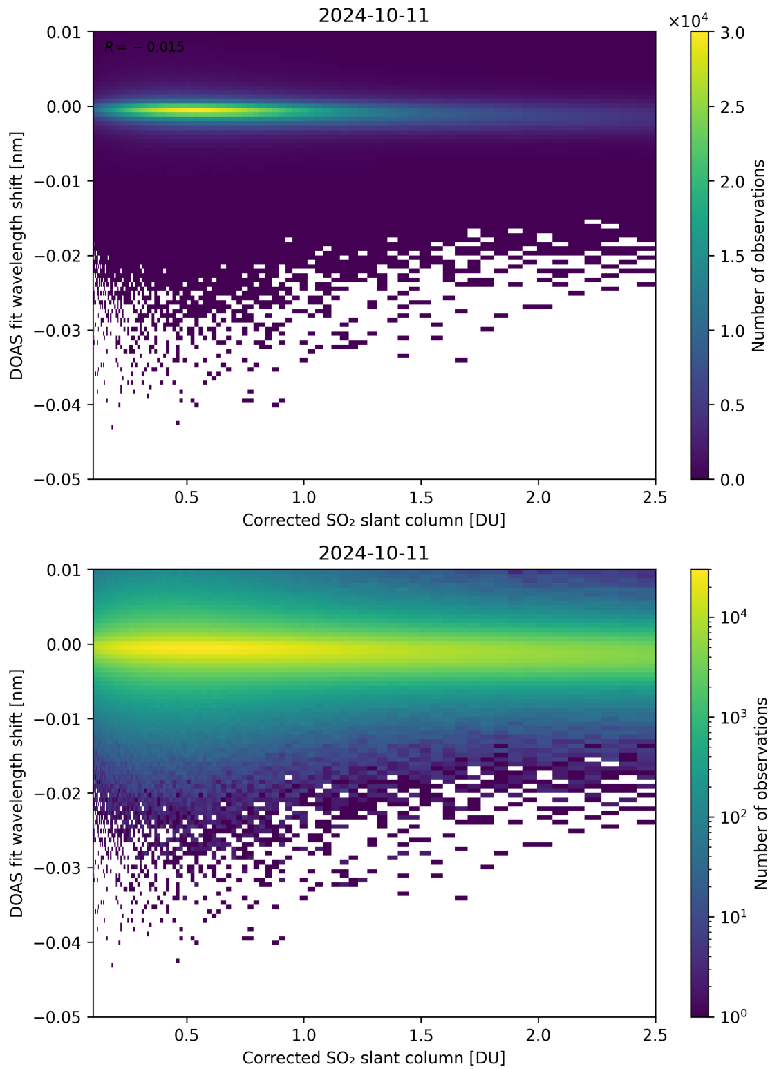
Figure 181: Scatter density plot of “Corrected SO 2 slant column” against “DOAS fit wavelength shift” for 2024-10-10 to 2024-10-12.
