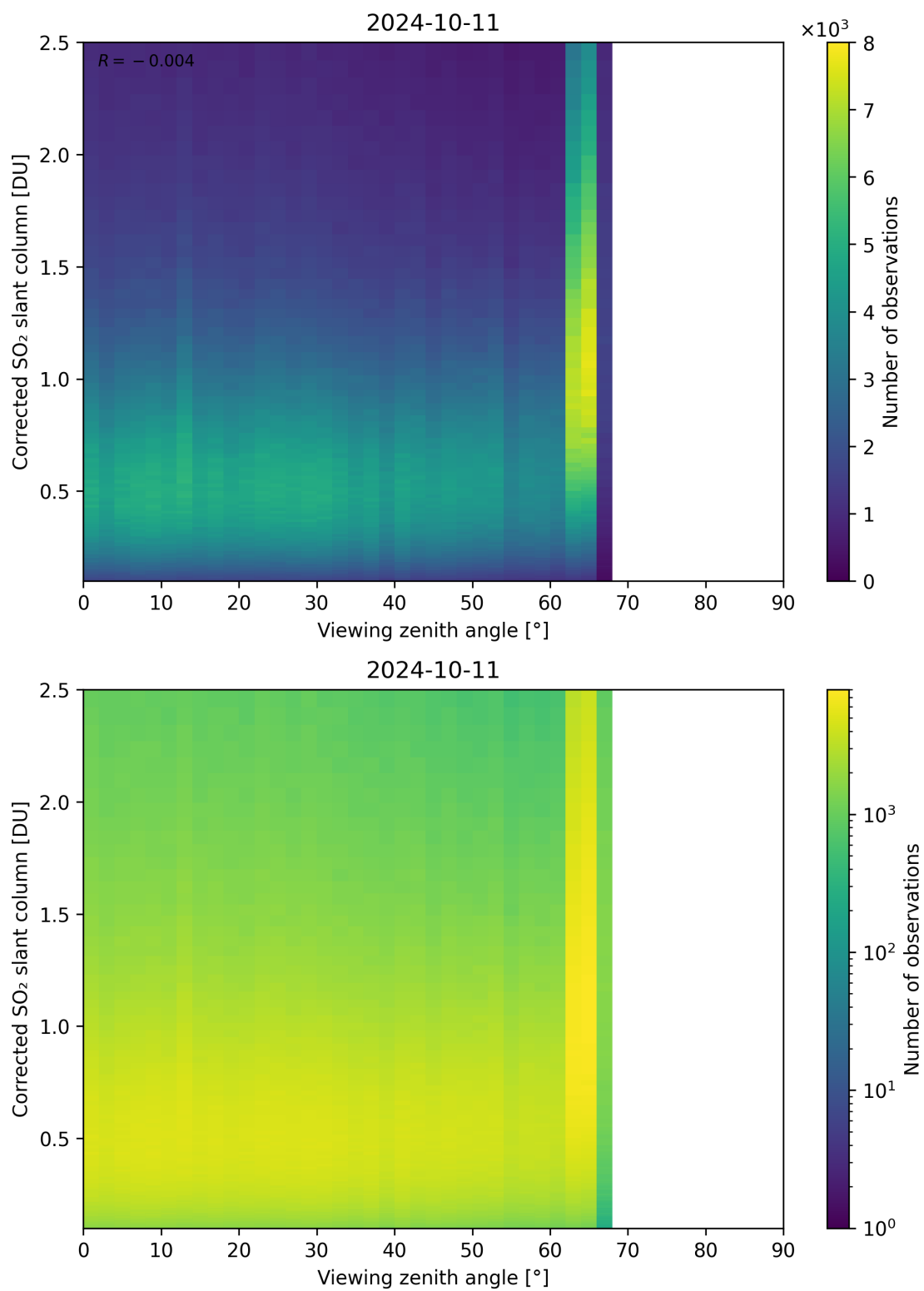
Figure 317: Scatter density plot of “Viewing zenith angle” against “Corrected SO 2 slant column” for 2024-10-10 to 2024-10-12.
