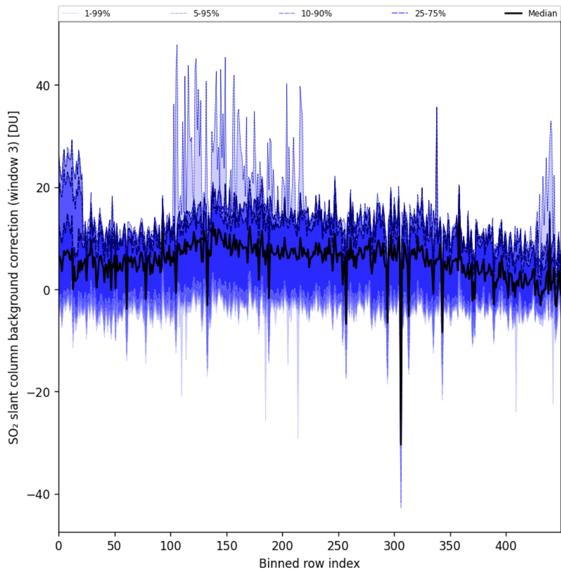
Figure 90: Along track statistics of “SO 2 slant column background correction (window 3)” for 2024-10-10 to 2024-10-12
