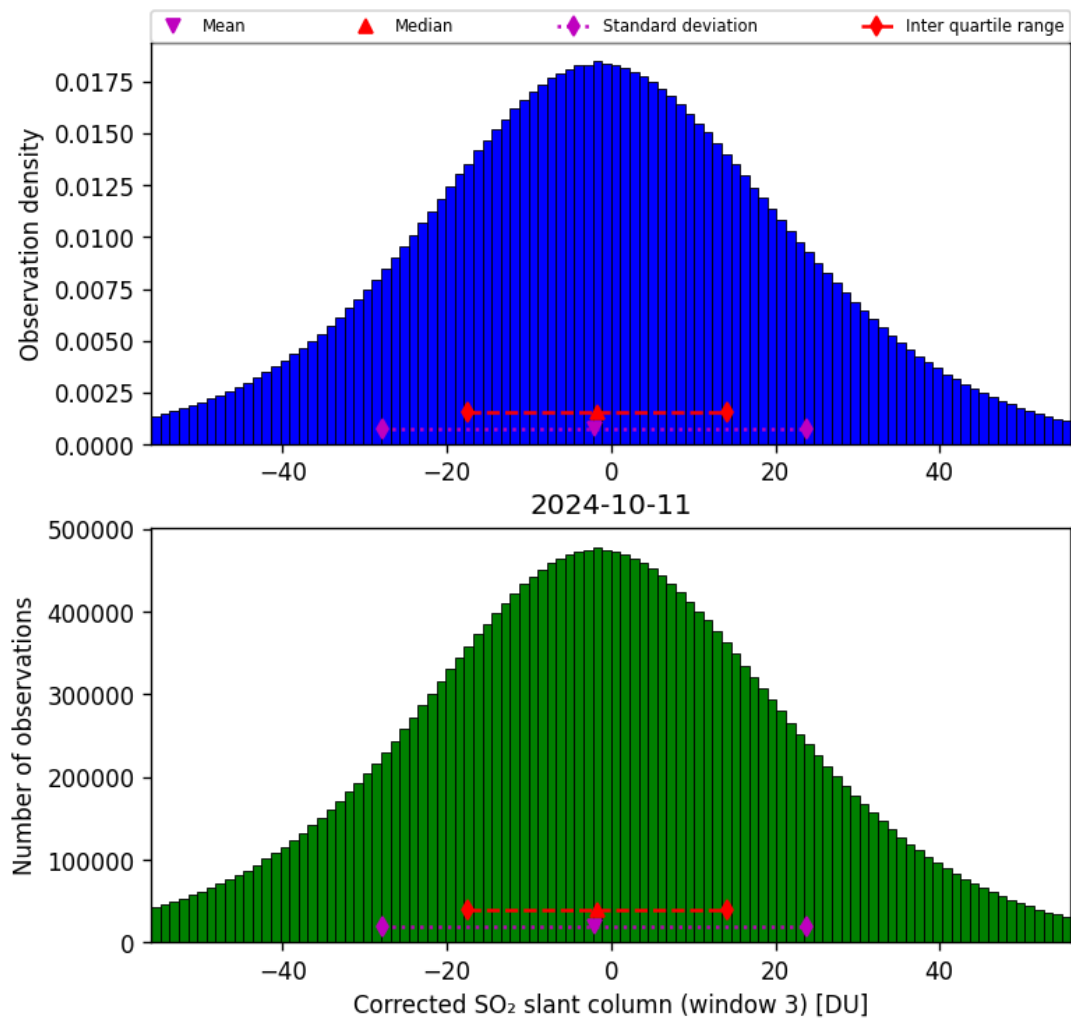
Figure 66: Histogram of “Corrected SO 2 slant column (window 3)” for 2024-10-10 to 2024-10-12
