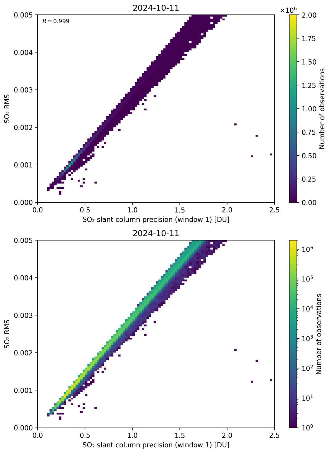
Figure 223: Scatter density plot of “SO 2 slant column precision (window 1)” against “SO 2 RMS” for 2024-10-10 to 2024-10-12.
