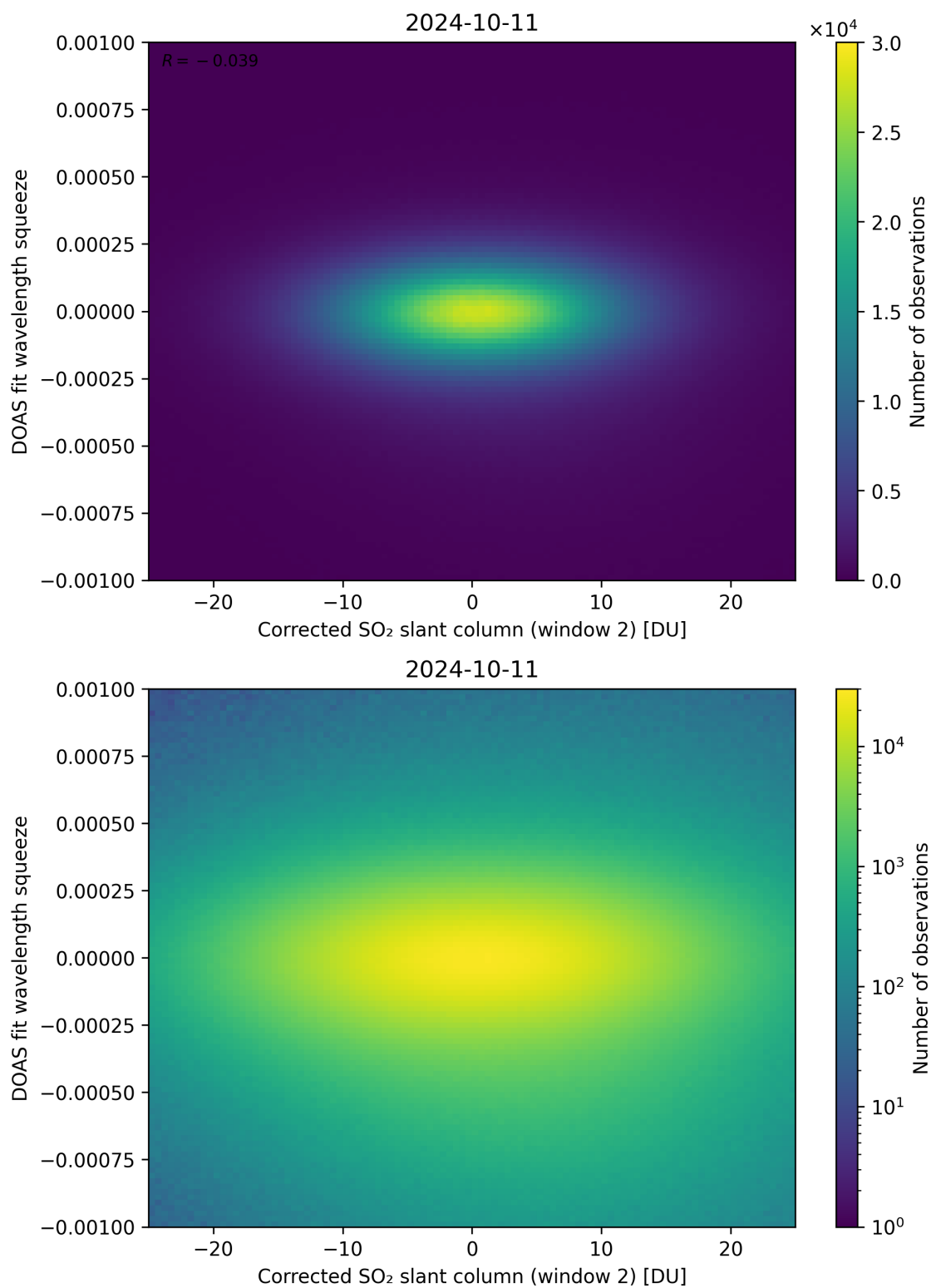
Figure 197: Scatter density plot of “Corrected SO 2 slant column (window 2)” against “DOAS fit wavelength squeeze” for 2024-10-10 to 2024-10-12.
