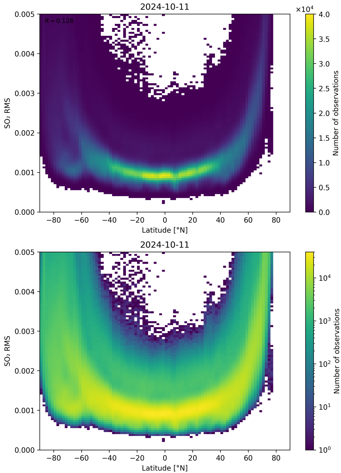
Figure 144: Scatter density plot of “Latitude” against “SO 2 RMS” for 2024-10-10 to 2024-10-12.
