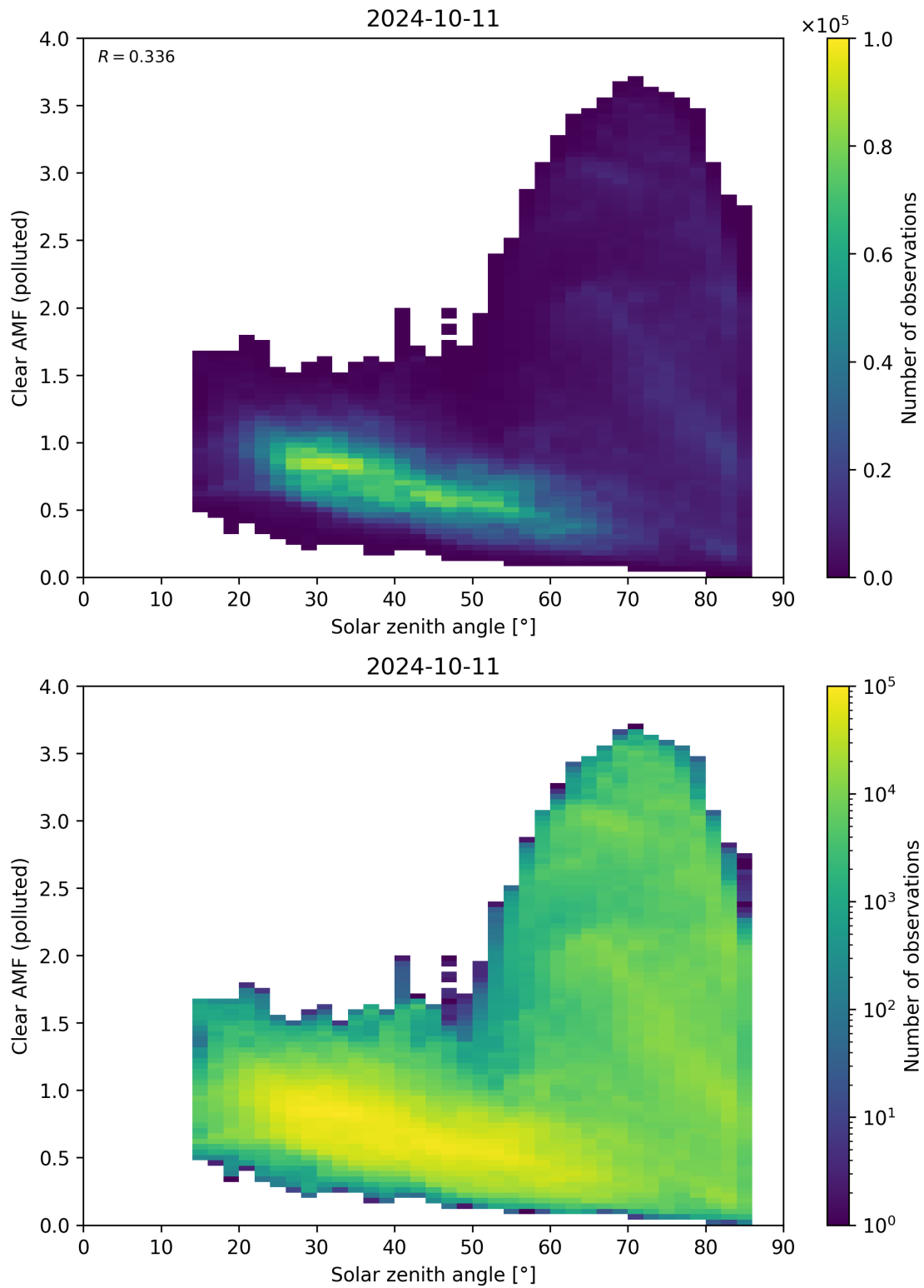
Figure 165: Scatter density plot of “Solar zenith angle” against “Clear AMF (polluted)” for 2024-10-10 to 2024-10-12.
