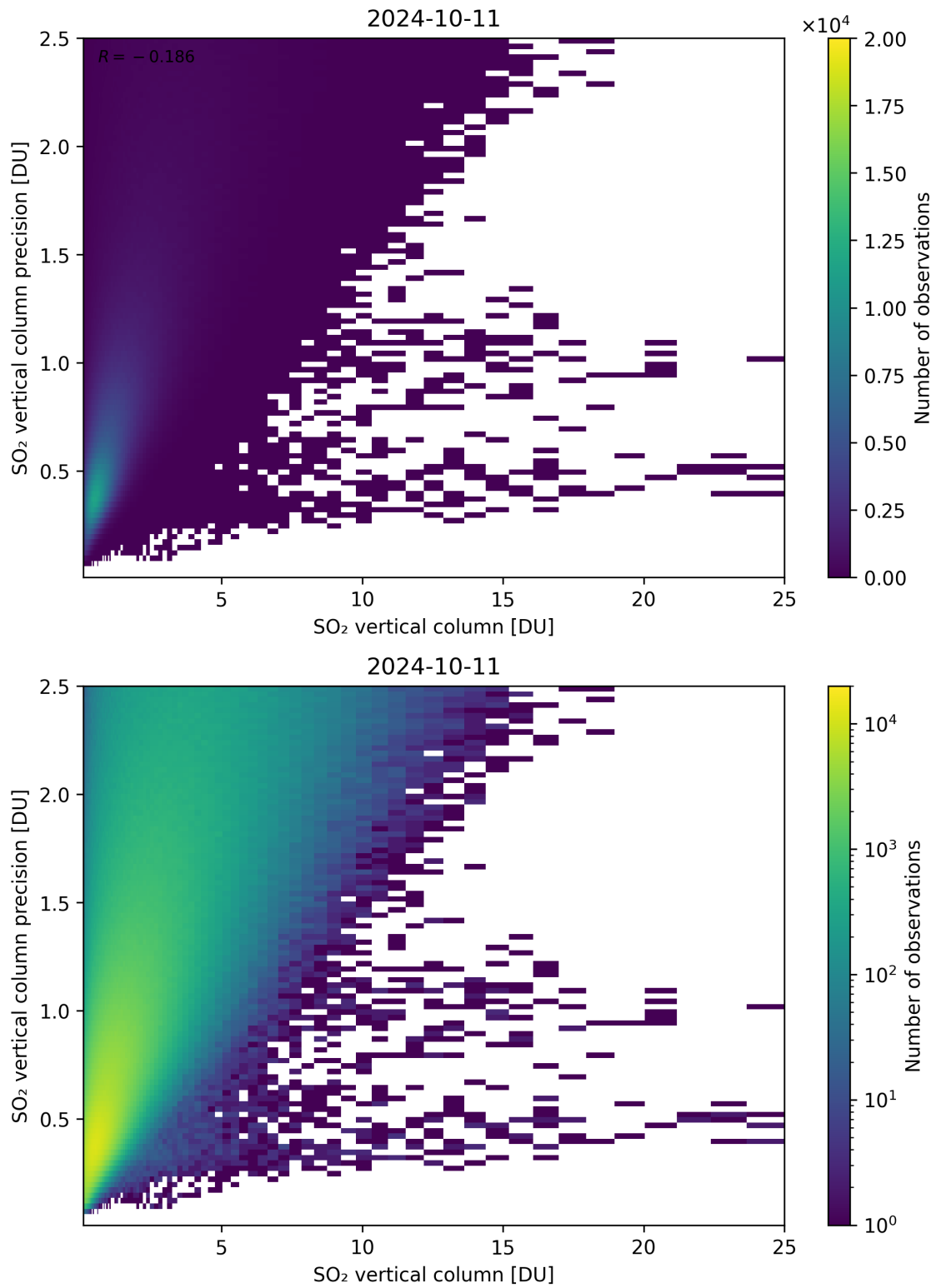
Figure 307: Scatter density plot of “SO 2 vertical column” against “SO 2 vertical column precision” for 2024-10-10 to 2024-10-12.
