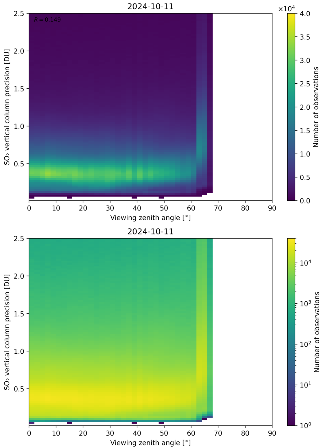
Figure 328: Scatter density plot of “Viewing zenith angle” against “SO 2 vertical column precision” for 2024-10-10 to 2024-10-12.
