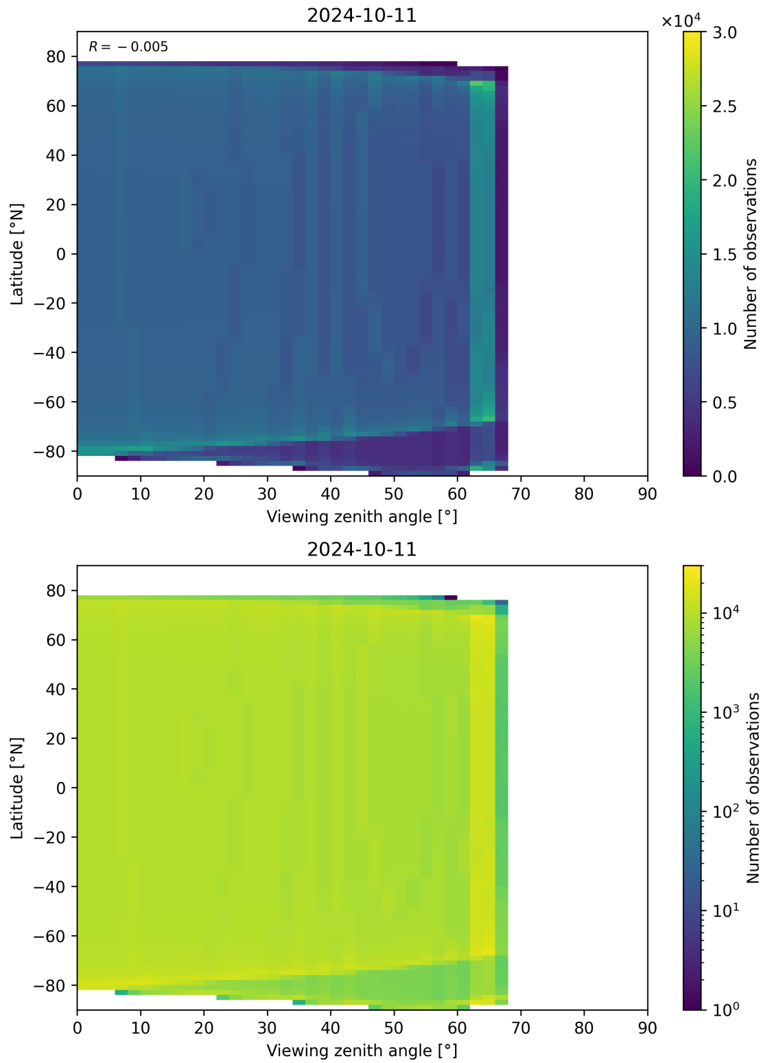
Figure 314: Scatter density plot of “Viewing zenith angle” against “Latitude” for 2024-10-10 to 2024-10-12.
