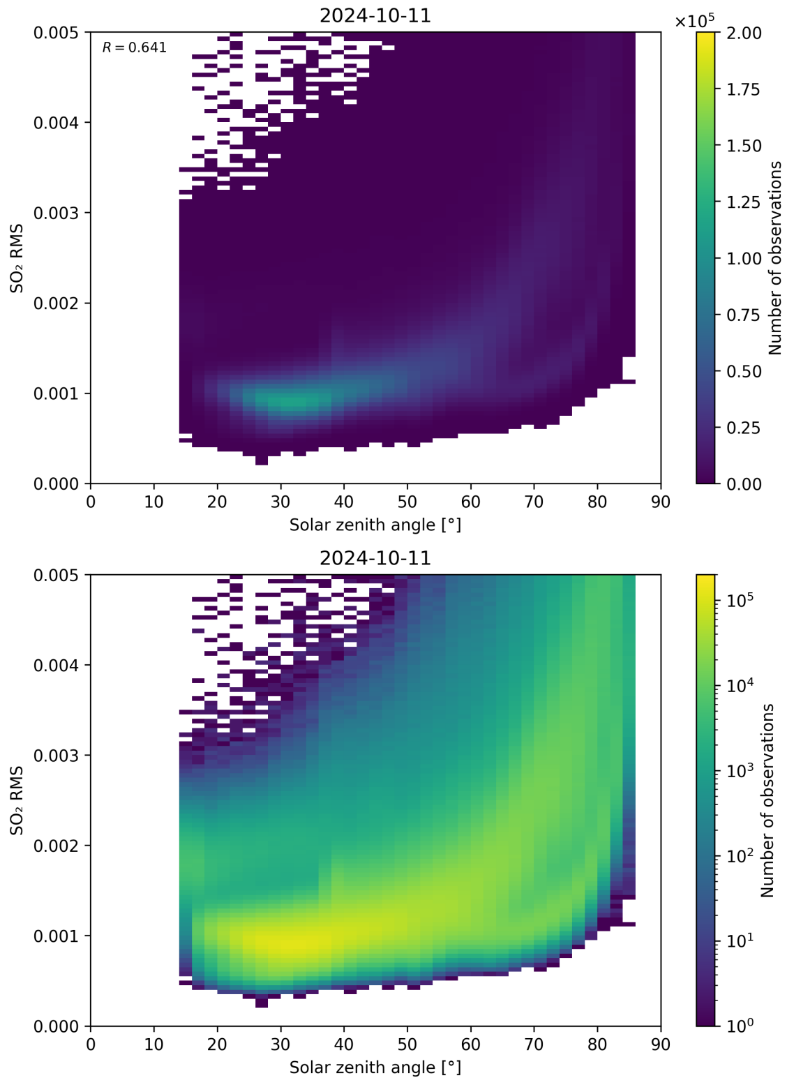
Figure 163: Scatter density plot of “Solar zenith angle” against “SO 2 RMS” for 2024-10-10 to 2024-10-12.
