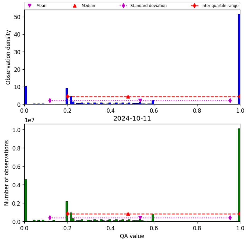
Figure 52: Histogram of “QA value” for 2024-10-10 to 2024-10-12
