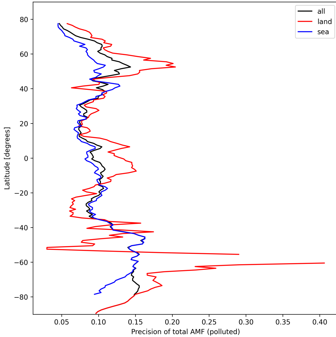
Figure 49: Zonal average of “Precision of total AMF (polluted)” for 2024-10-10 to 2024-10-12.
