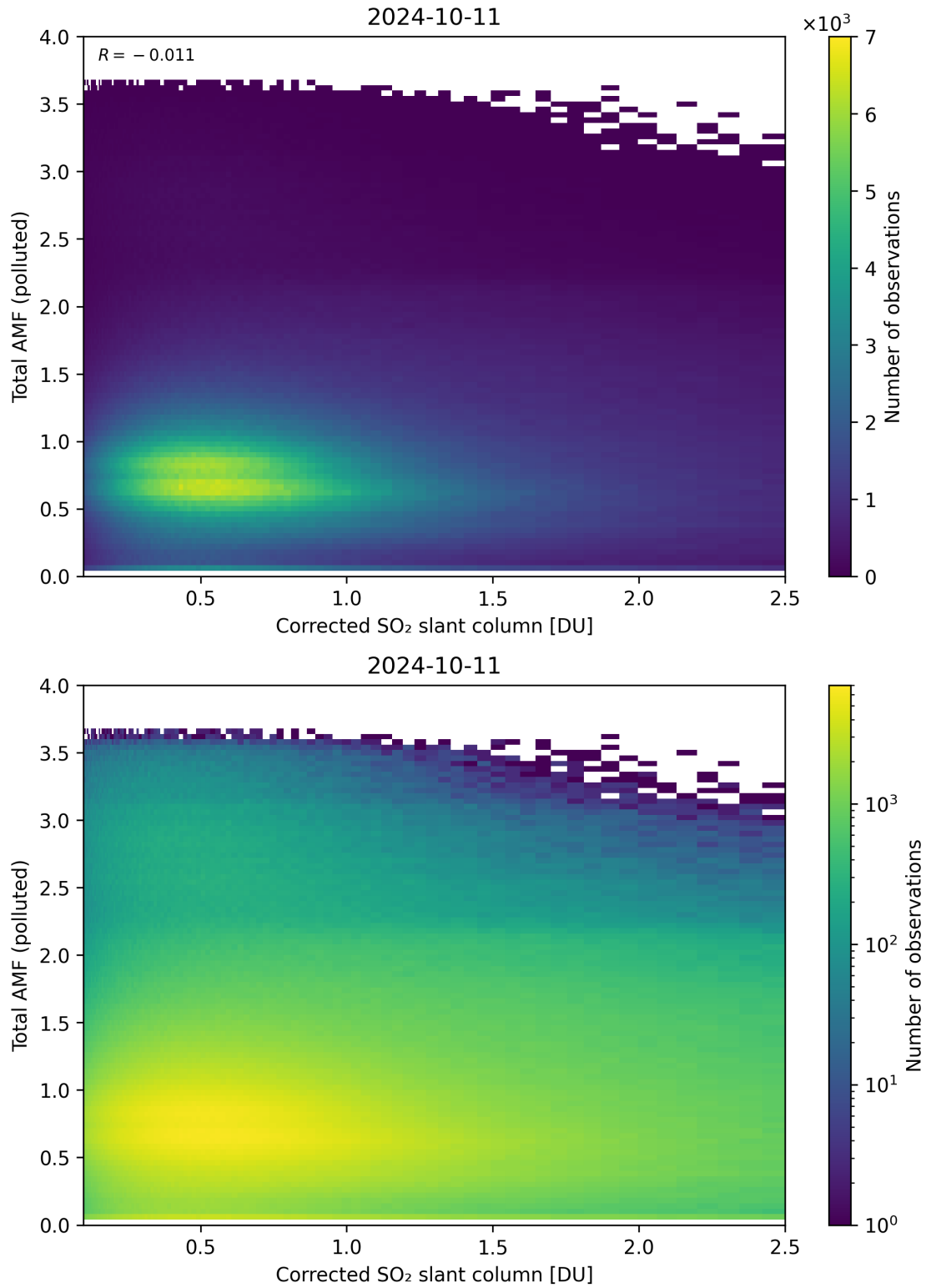
Figure 192: Scatter density plot of “Corrected SO 2 slant column” against “Total AMF (polluted)” for 2024-10-10 to 2024-10-12.
