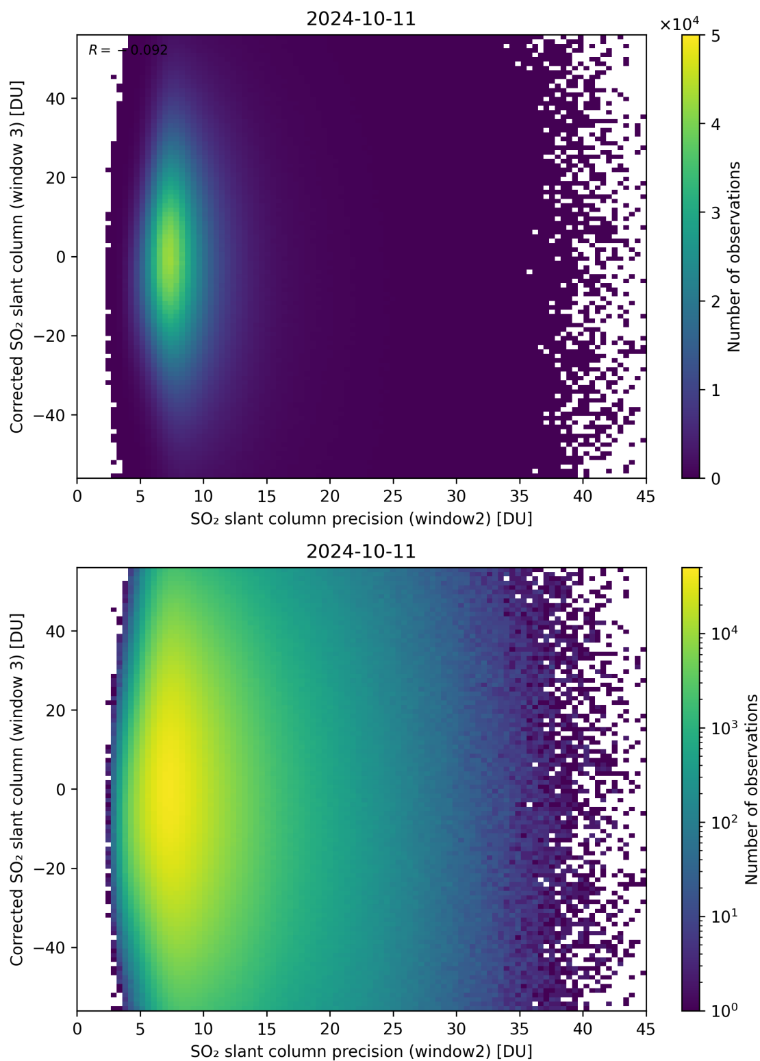
Figure 248: Scatter density plot of “SO 2 slant column precision (window2)” against “Corrected SO 2 slant column (window 3)” for 2024-10-10 to 2024-10-12.
