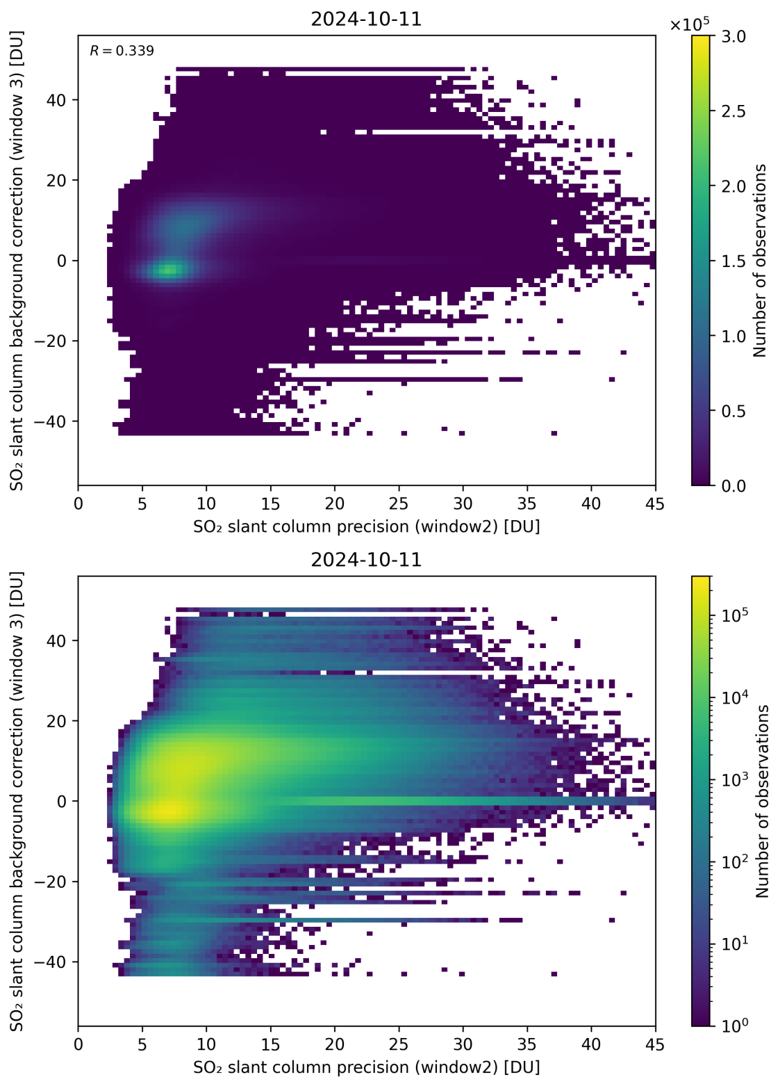
Figure 242: Scatter density plot of “SO 2 slant column precision (window2)” against “SO 2 slant column background correction (window 3)” for 2024-10-10 to 2024-10-12.
