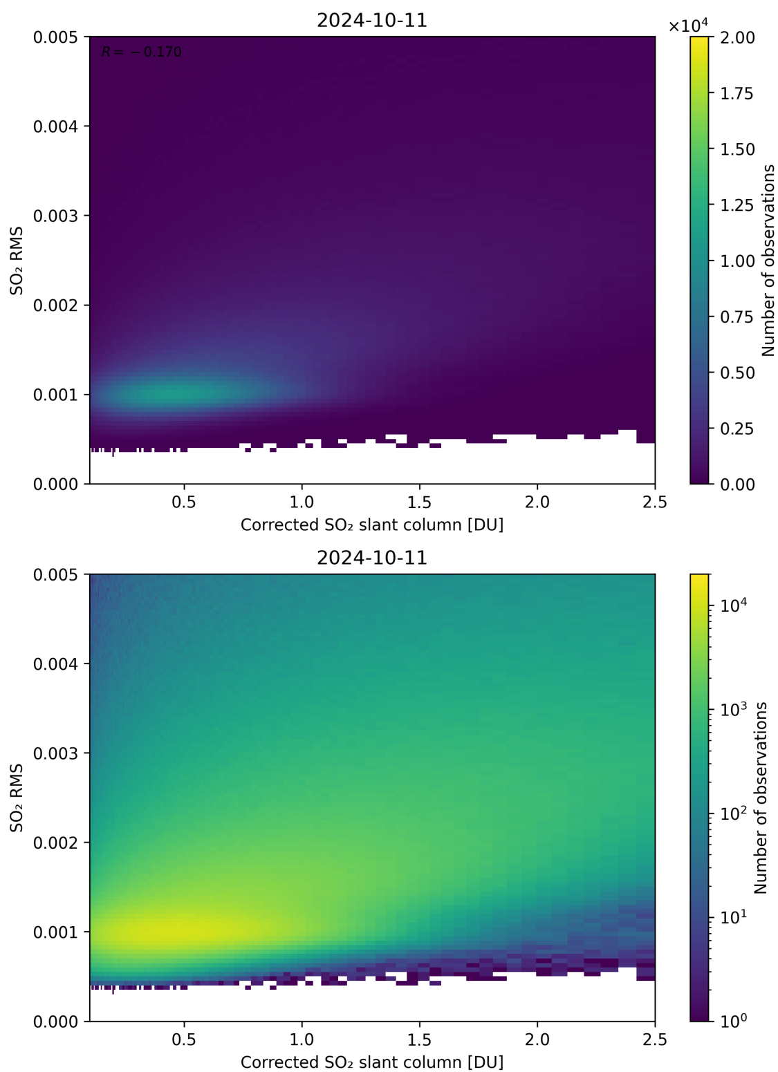
Figure 183: Scatter density plot of “Corrected SO 2 slant column” against “SO 2 RMS” for 2024-10-10 to 2024-10-12.
