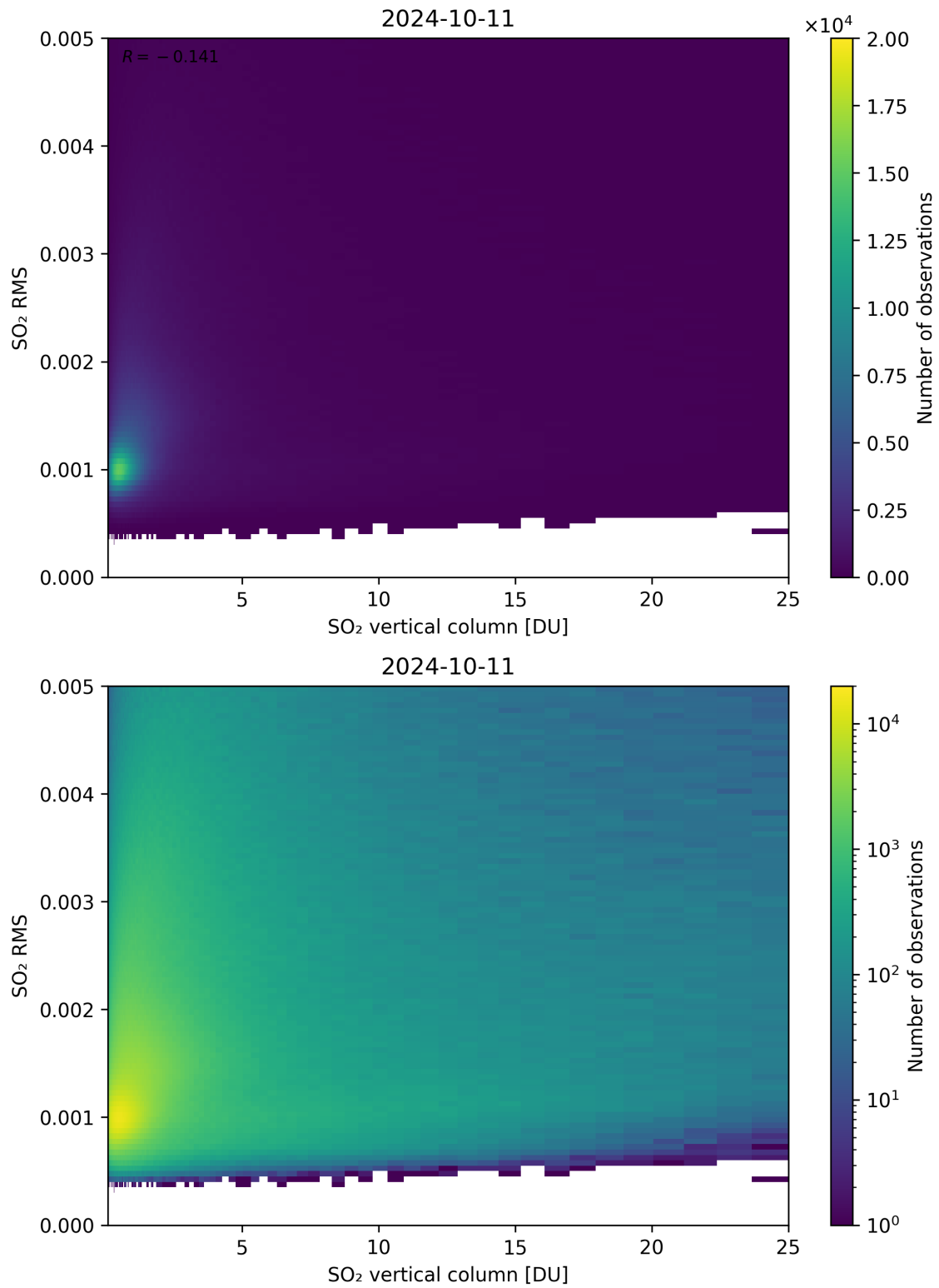
Figure 278: Scatter density plot of “SO 2 vertical column” against “SO 2 RMS” for 2024-10-10 to 2024-10-12.
