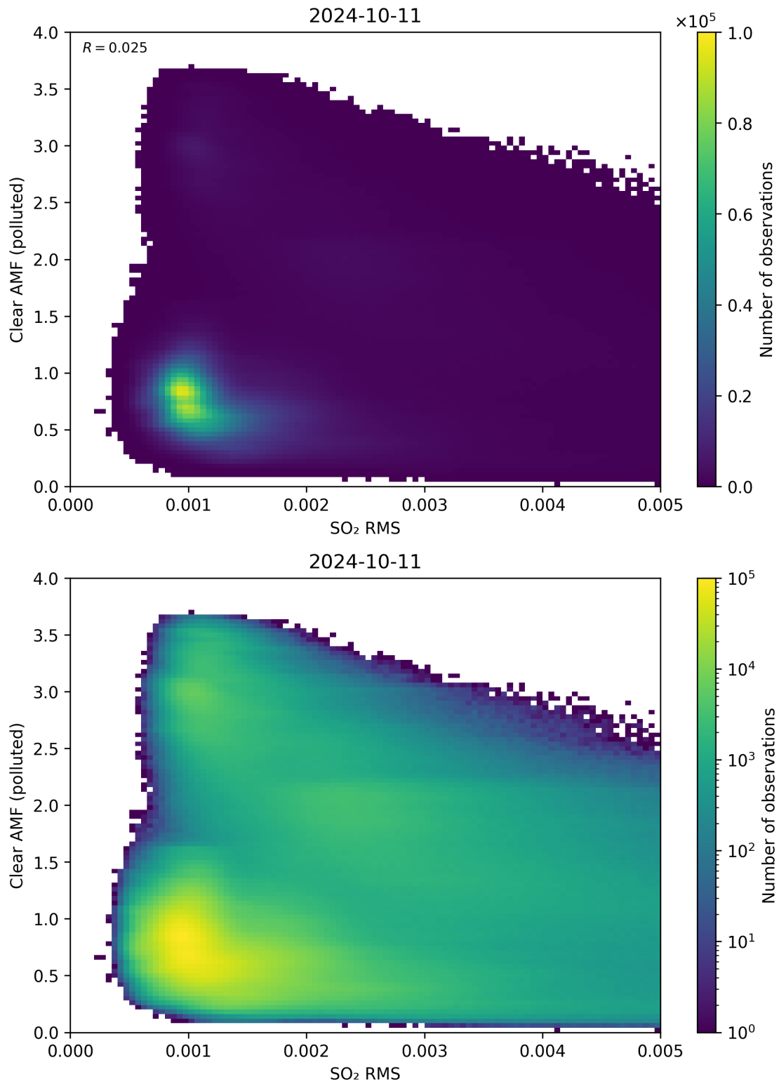
Figure 136: Scatter density plot of “SO 2 RMS” against “Clear AMF (polluted)” for 2024-10-10 to 2024-10-12.
