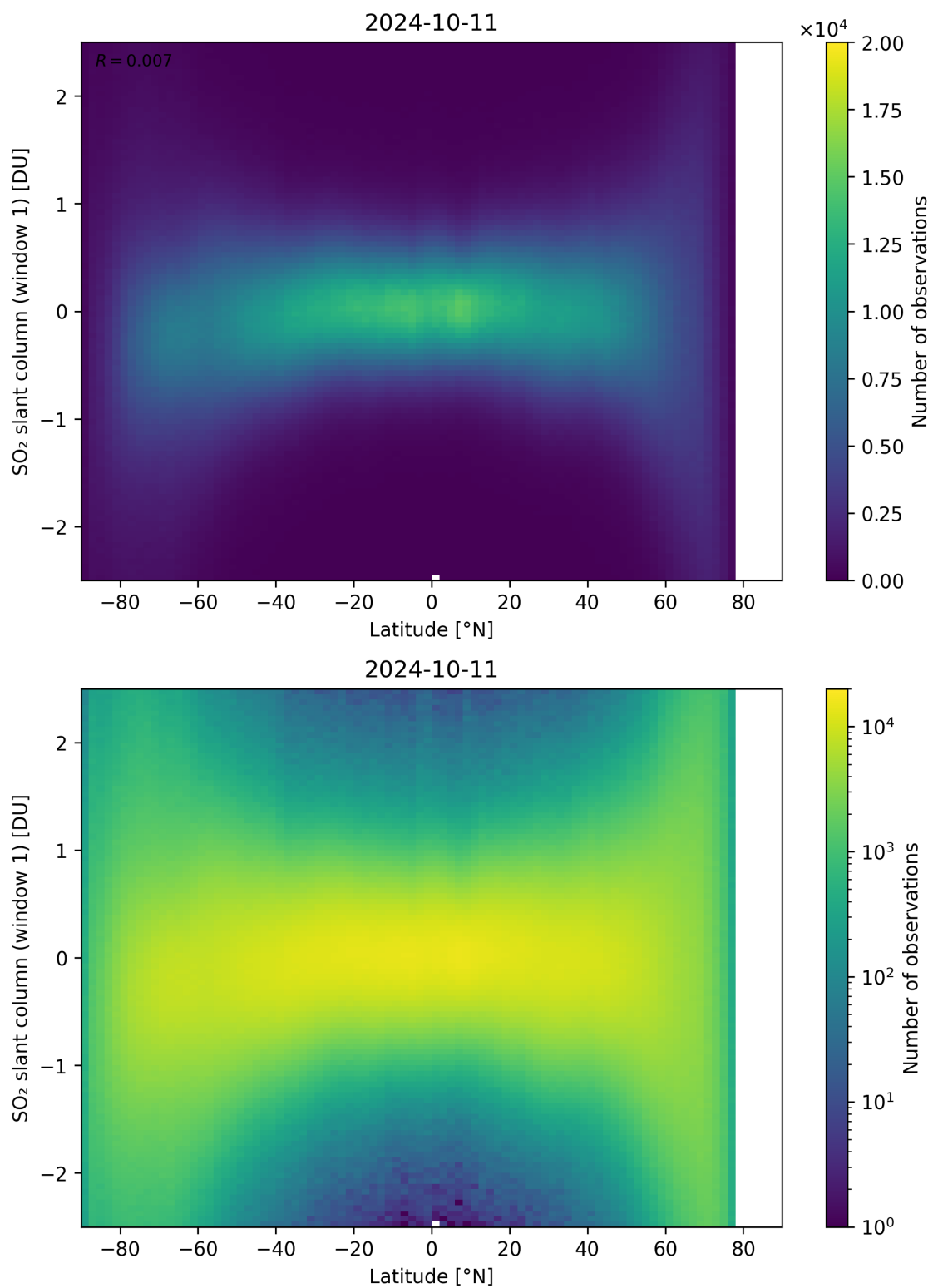
Figure 149: Scatter density plot of “Latitude” against “SO 2 slant column (window 1)” for 2024-10-10 to 2024-10-12.
