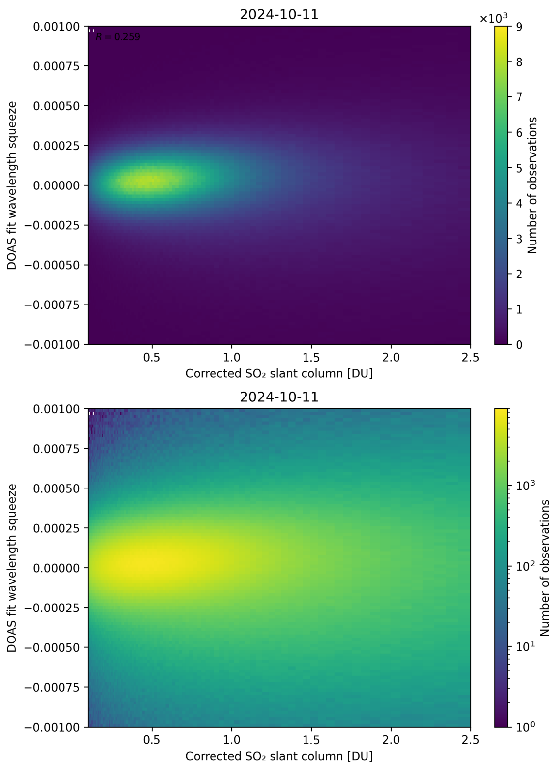
Figure 182: Scatter density plot of “Corrected SO 2 slant column” against “DOAS fit wavelength squeeze” for 2024-10-10 to 2024-10-12.
