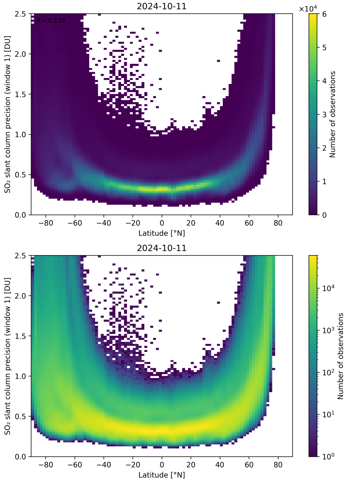
Figure 150: Scatter density plot of “Latitude” against “SO 2 slant column precision (window 1)” for 2024-10-10 to 2024-10-12.
