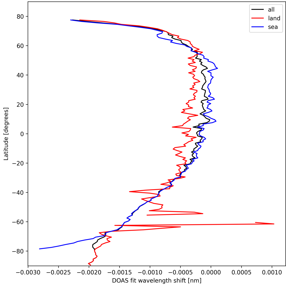
Figure 45: Zonal average of “DOAS fit wavelength shift” for 2024-10-10 to 2024-10-12.
