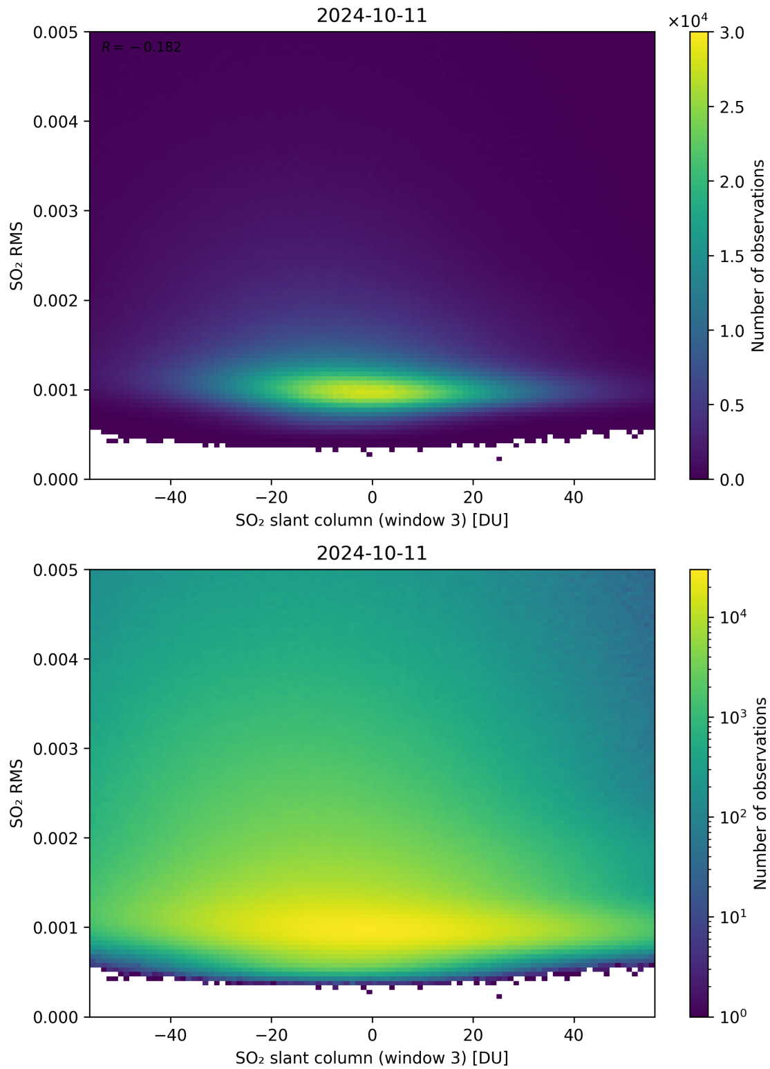
Figure 256: Scatter density plot of “SO 2 slant column (window 3)” against “SO 2 RMS” for 2024-10-10 to 2024-10-12.
