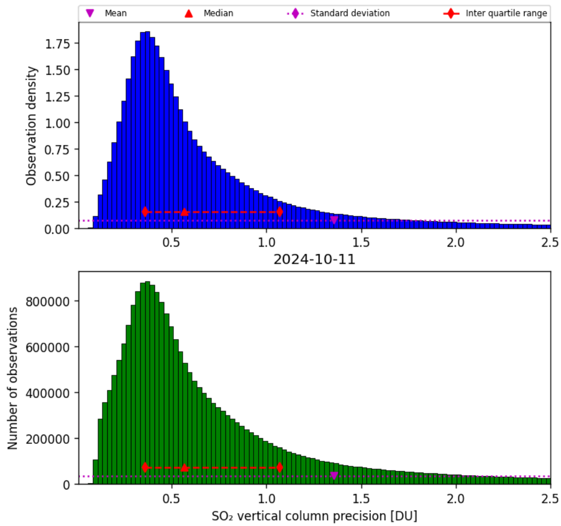
Figure 54: Histogram of “SO 2 vertical column precision” for 2024-10-10 to 2024-10-12
