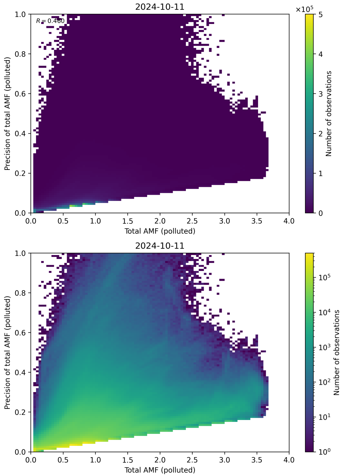
Figure 272: Scatter density plot of “Total AMF (polluted)” against “Precision of total AMF (polluted)” for 2024-10-10 to 2024-10-12.
