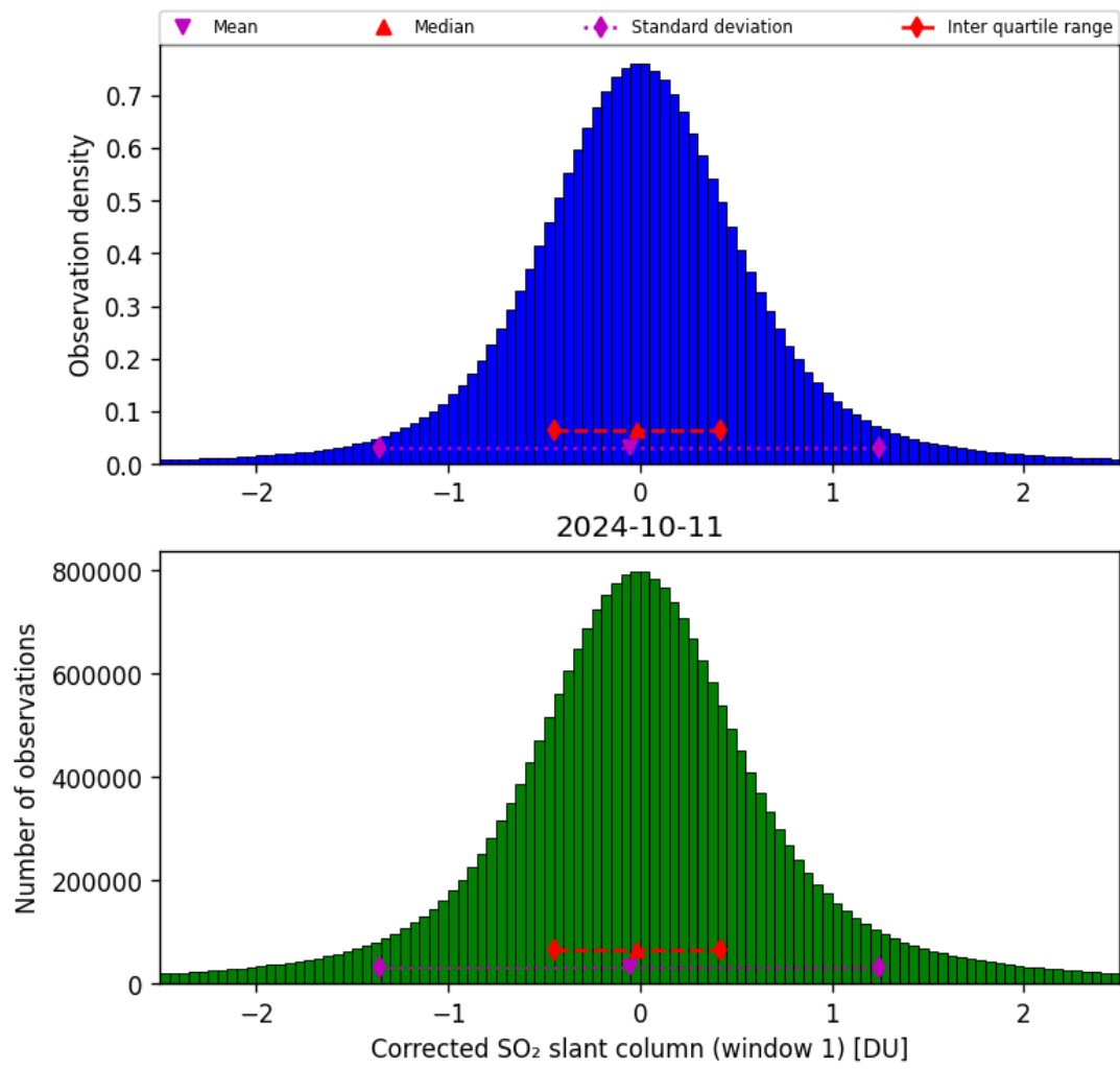
Figure 58: Histogram of “Corrected SO 2 slant column (window 1)” for 2024-10-10 to 2024-10-12
