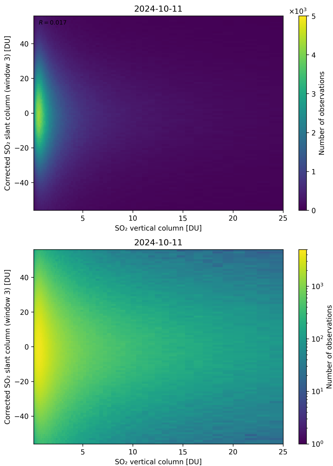
Figure 299: Scatter density plot of “SO 2 vertical column” against “Corrected SO 2 slant column (window 3)” for 2024-10-10 to 2024-10-12.
