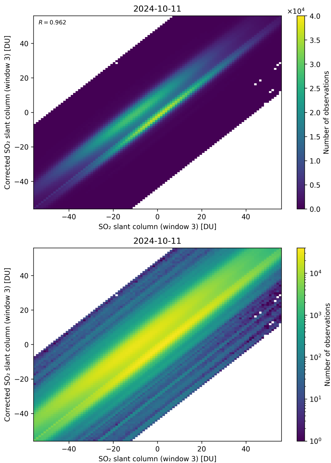
Figure 266: Scatter density plot of “SO 2 slant column (window 3)” against “Corrected SO 2 slant column (window 3)” for 2024-10-10 to 2024-10-12.
