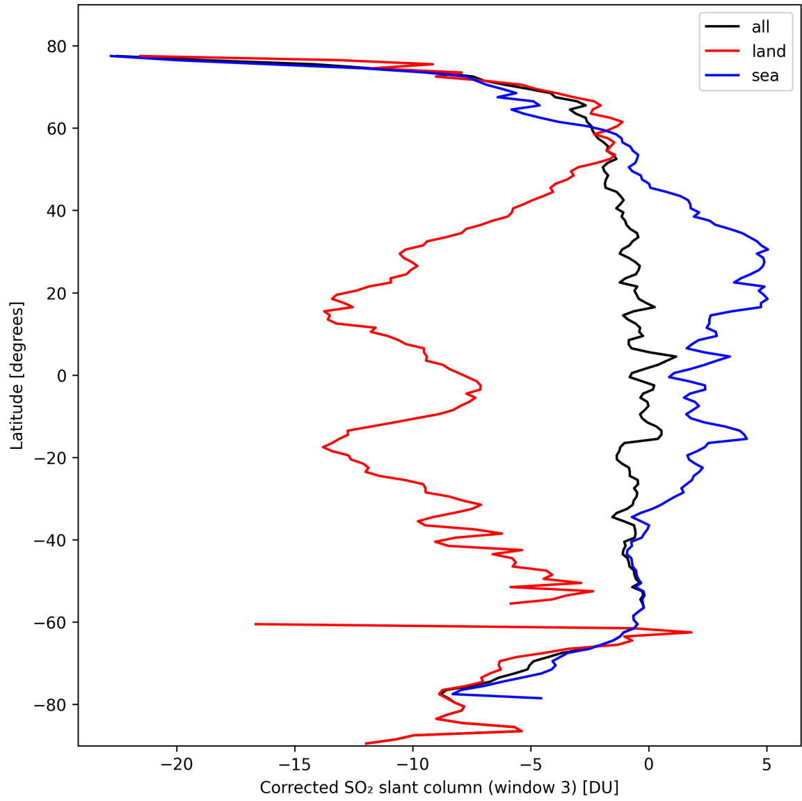
Figure 43: Zonal average of “Corrected SO 2 slant column (window 3)” for 2024-10-10 to 2024-10-12.
