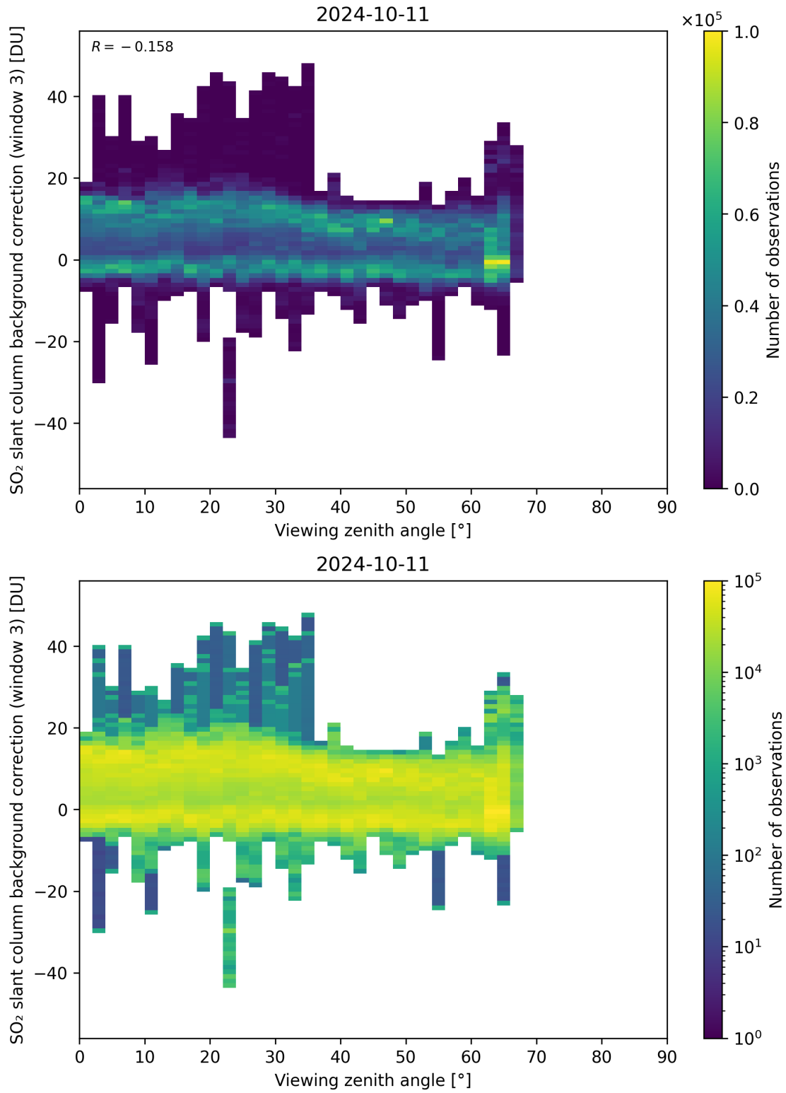
Figure 310: Scatter density plot of “Viewing zenith angle” against “SO 2 slant column background correction (window 3)” for 2024-10-10 to 2024-10-12.
