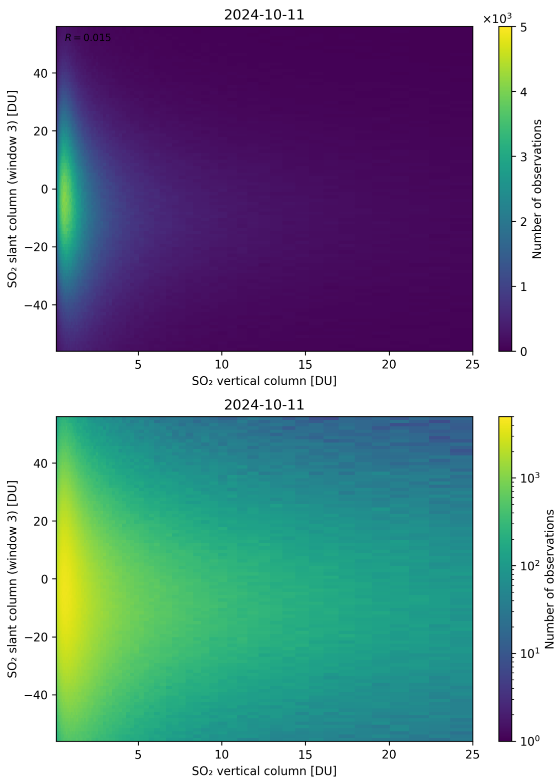
Figure 303: Scatter density plot of “SO 2 vertical column” against “SO 2 slant column (window 3)” for 2024-10-10 to 2024-10-12.
