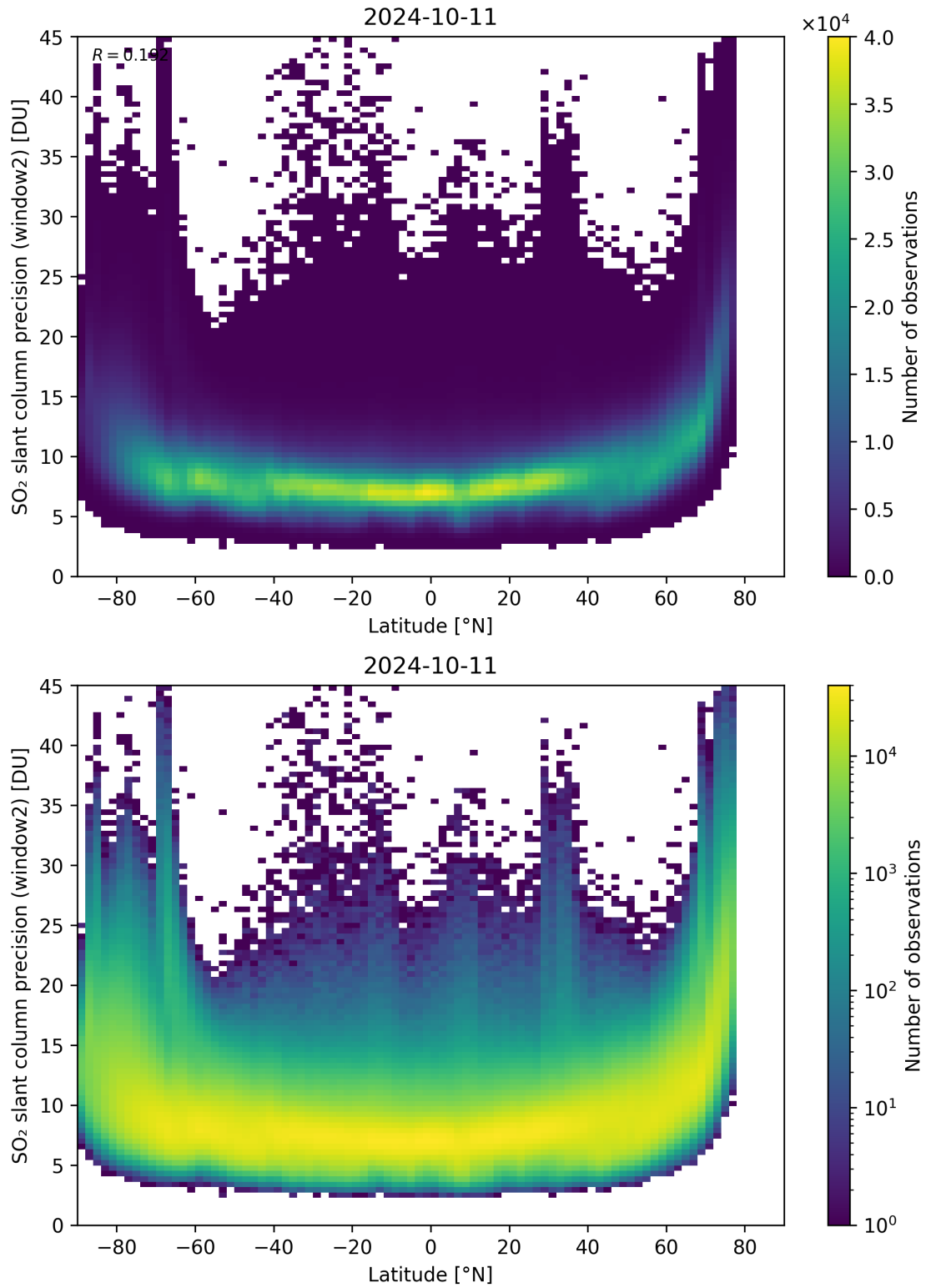
Figure 151: Scatter density plot of “Latitude” against “SO 2 slant column precision (window2)” for 2024-10-10 to 2024-10-12.
