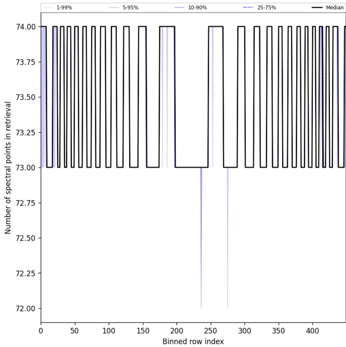
Figure 97: Along track statistics of “Number of spectral points in retrieval” for 2024-10-10 to 2024-10-12
