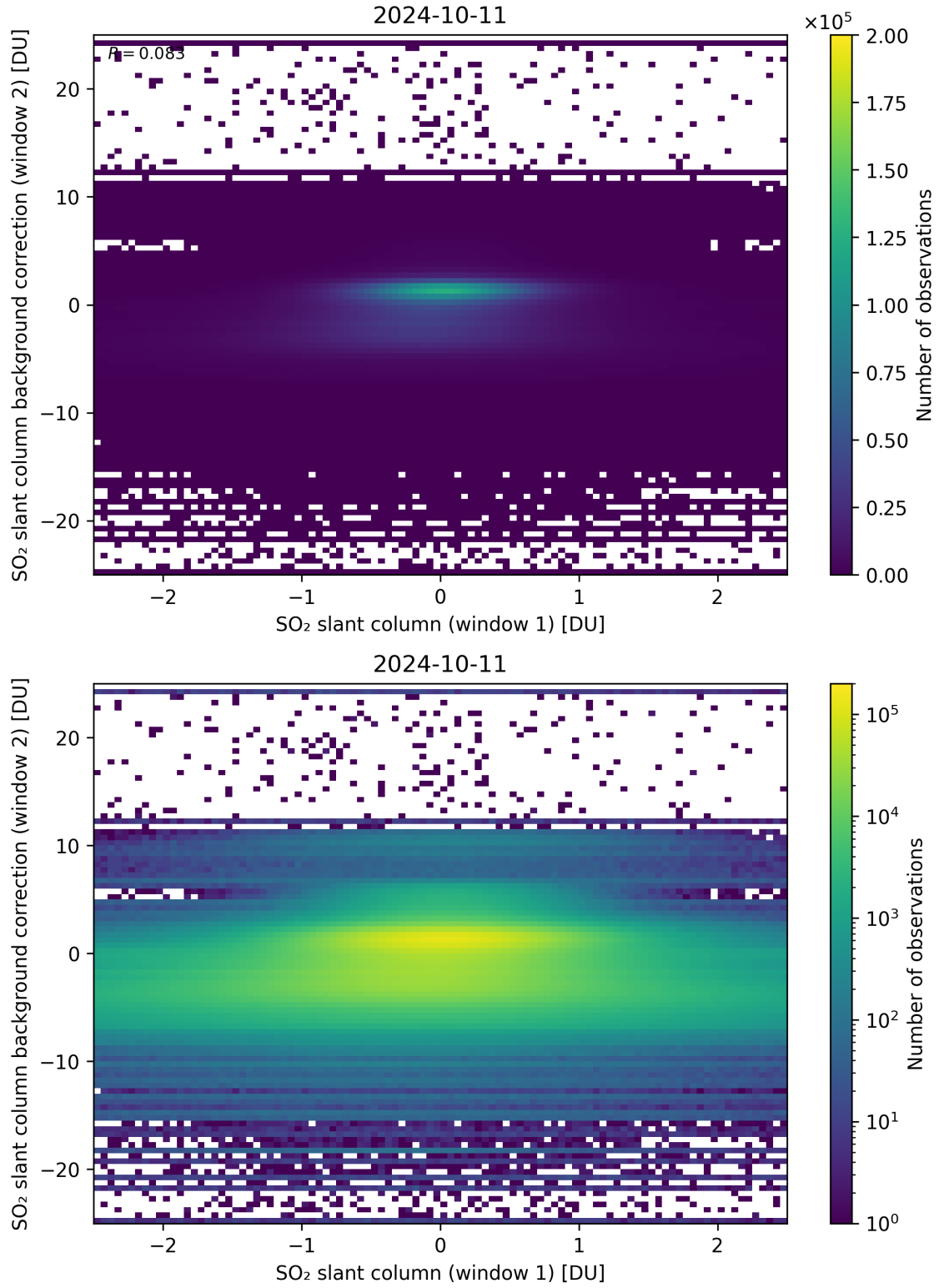
Figure 213: Scatter density plot of “SO 2 slant column (window 1)” against “SO 2 slant column background correction (window 2)” for 2024-10-10 to 2024-10-12.
