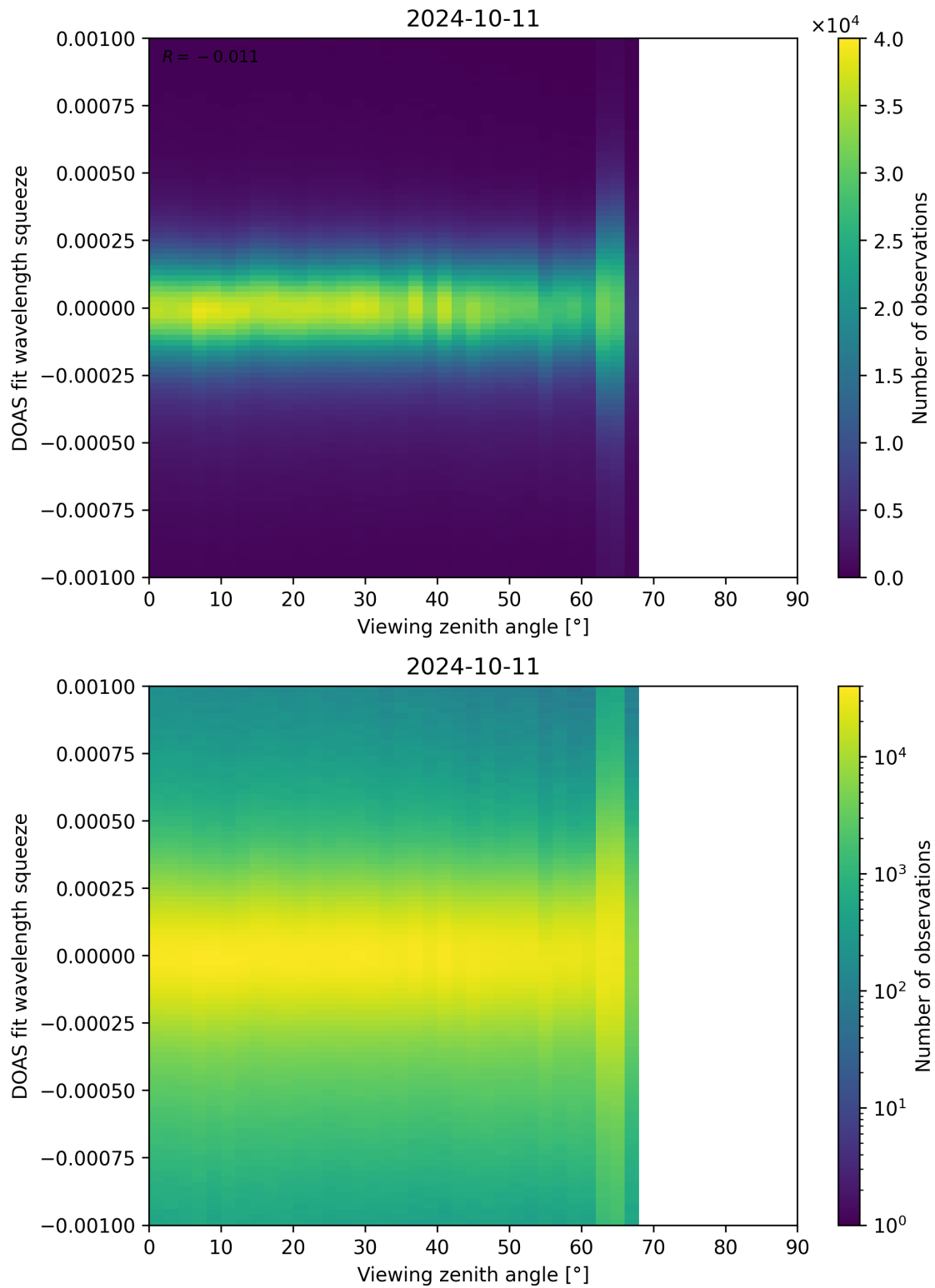
Figure 312: Scatter density plot of “Viewing zenith angle” against “DOAS fit wavelength squeeze” for 2024-10-10 to 2024-10-12.
