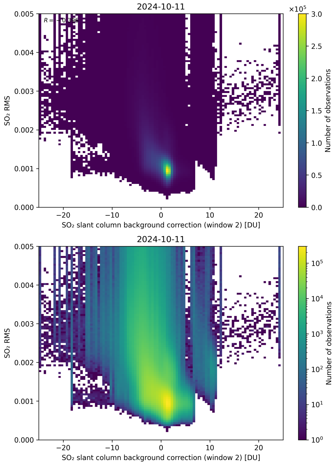
Figure 114: Scatter density plot of “SO 2 slant column background correction (window 2)” against “SO 2 RMS” for 2024-10-10 to 2024-10-12.
