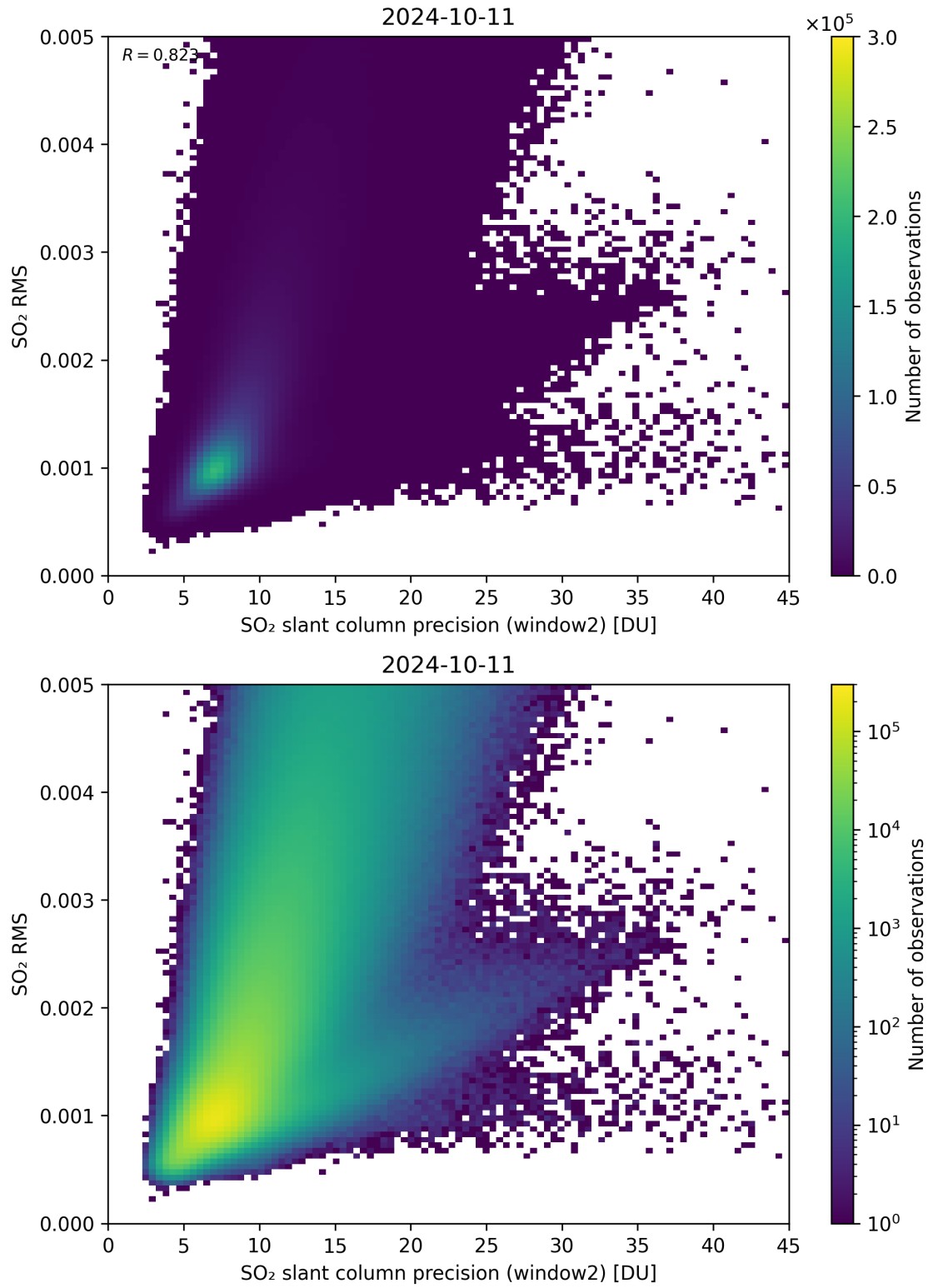
Figure 245: Scatter density plot of “SO 2 slant column precision (window2)” against “SO 2 RMS” for 2024-10-10 to 2024-10-12.
