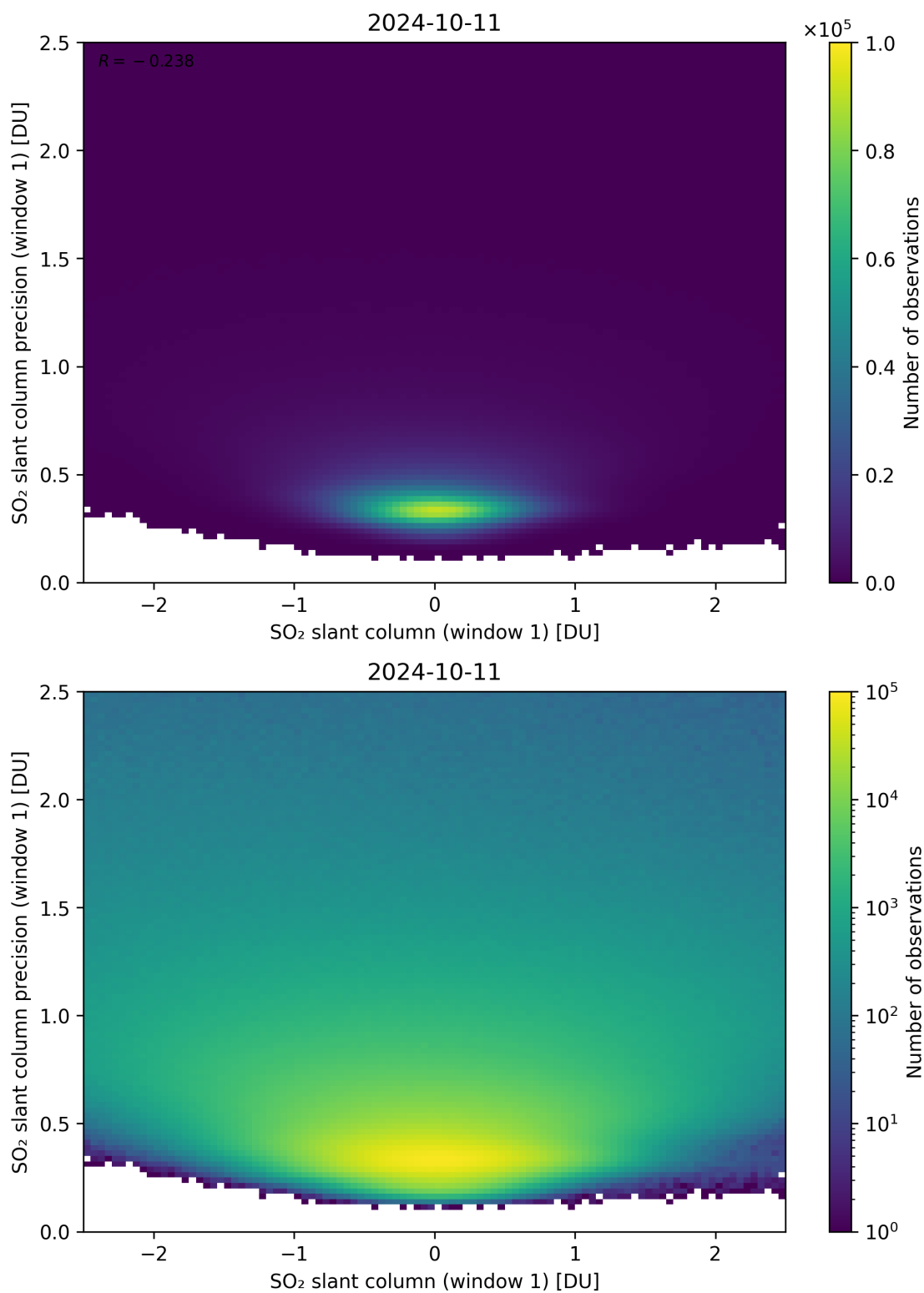
Figure 235: Scatter density plot of “SO 2 slant column (window 1)” against “SO 2 slant column precision (window 1)” for 2024-10-10 to 2024-10-12.
