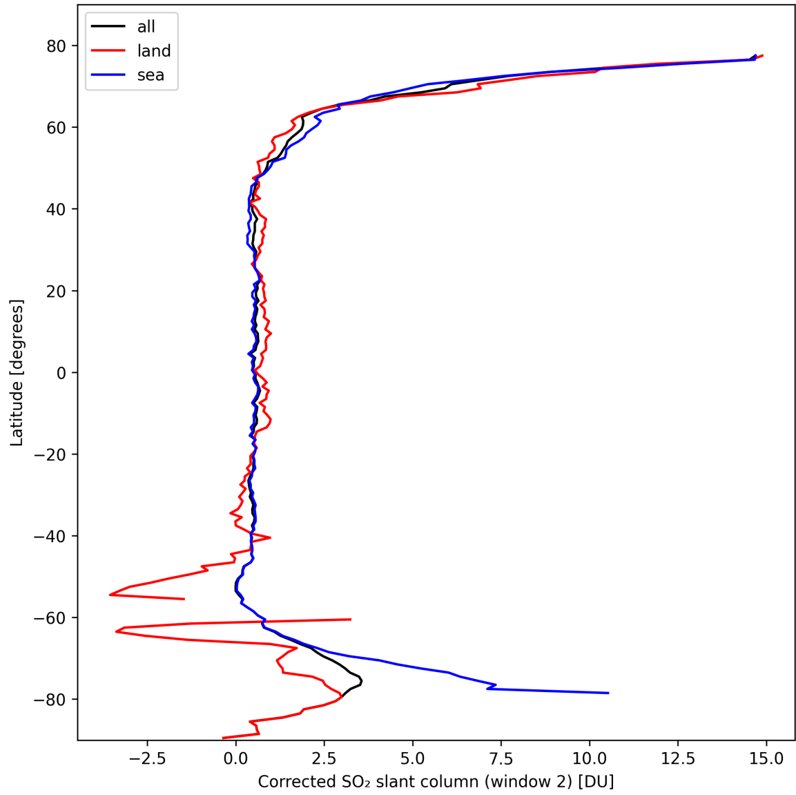
Figure 39: Zonal average of “Corrected SO 2 slant column (window 2)” for 2024-10-10 to 2024-10-12.
