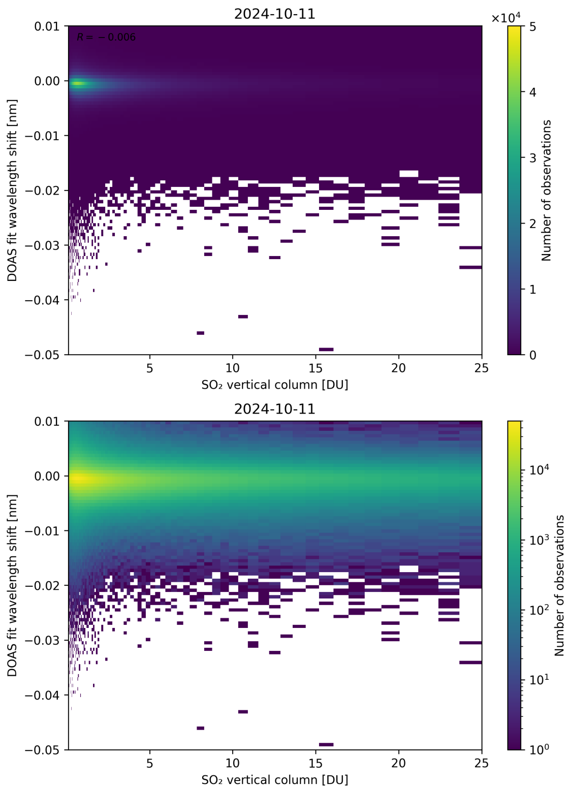
Figure 276: Scatter density plot of “SO 2 vertical column” against “DOAS fit wavelength shift” for 2024-10-10 to 2024-10-12.
