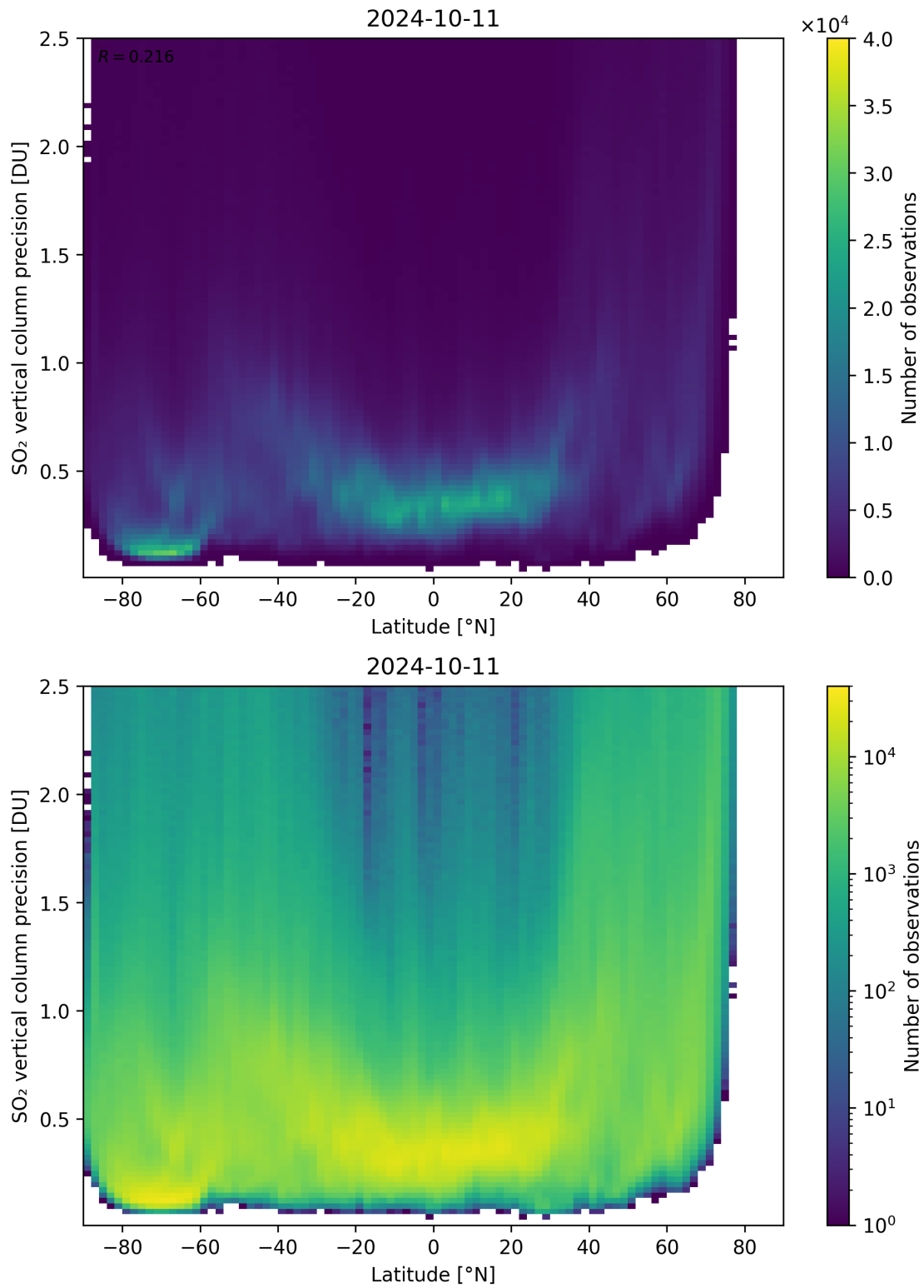
Figure 157: Scatter density plot of “Latitude” against “SO 2 vertical column precision” for 2024-10-10 to 2024-10-12.
