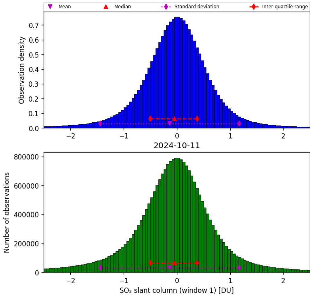
Figure 56: Histogram of “SO 2 slant column (window 1)” for 2024-10-10 to 2024-10-12
