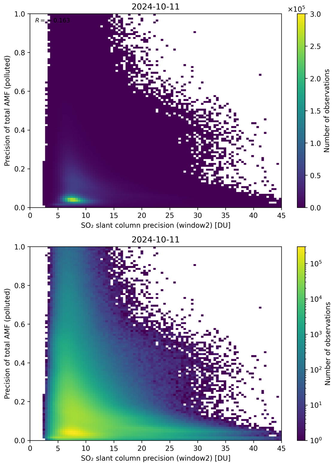
Figure 252: Scatter density plot of “SO 2 slant column precision (window2)” against “Precision of total AMF (polluted)” for 2024-10-10 to 2024-10-12.
