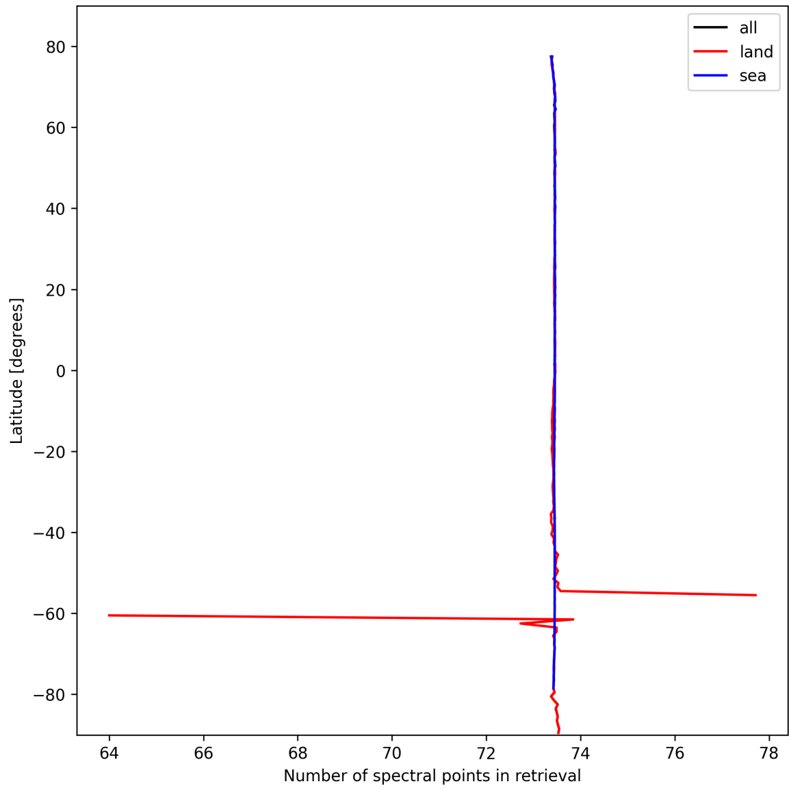
Figure 51: Zonal average of “Number of spectral points in retrieval” for 2024-10-10 to 2024-10-12.
