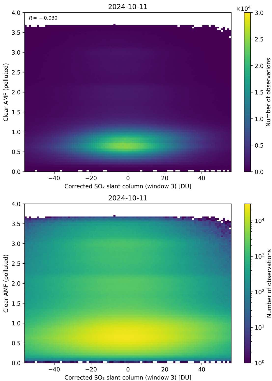
Figure 209: Scatter density plot of “Corrected SO 2 slant column (window 3)” against “Clear AMF (polluted)” for 2024-10-10 to 2024-10-12.
