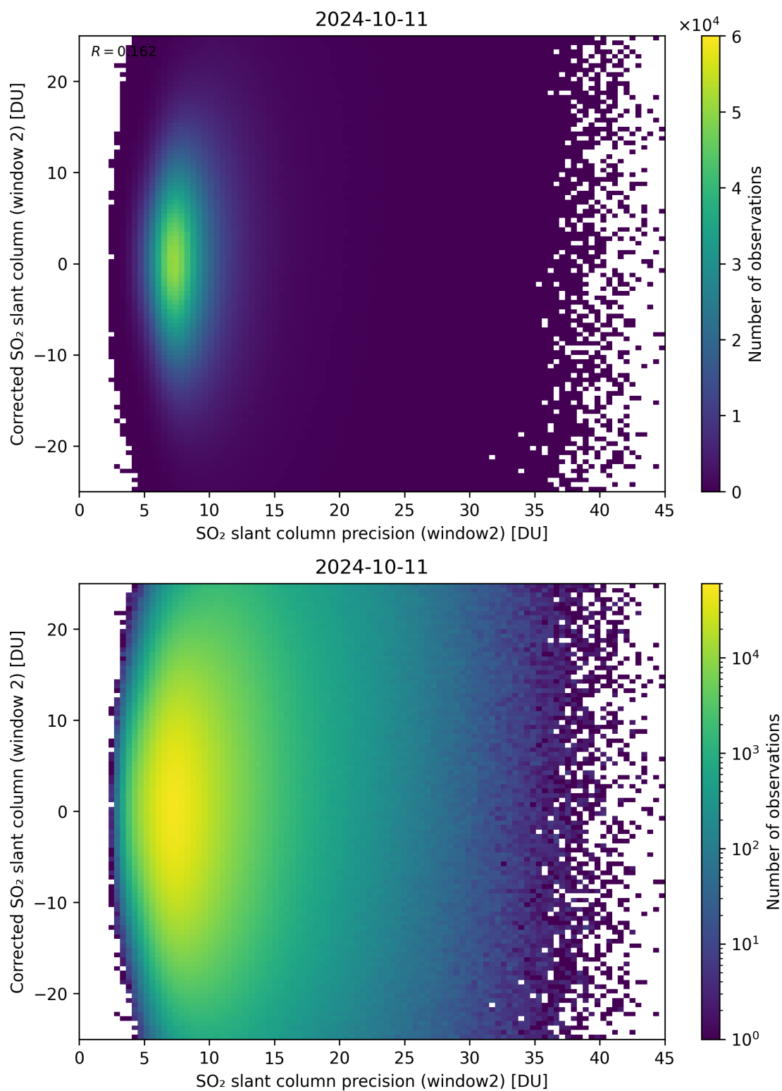
Figure 247: Scatter density plot of “SO 2 slant column precision (window2)” against “Corrected SO 2 slant column (window 2)” for 2024-10-10 to 2024-10-12.
