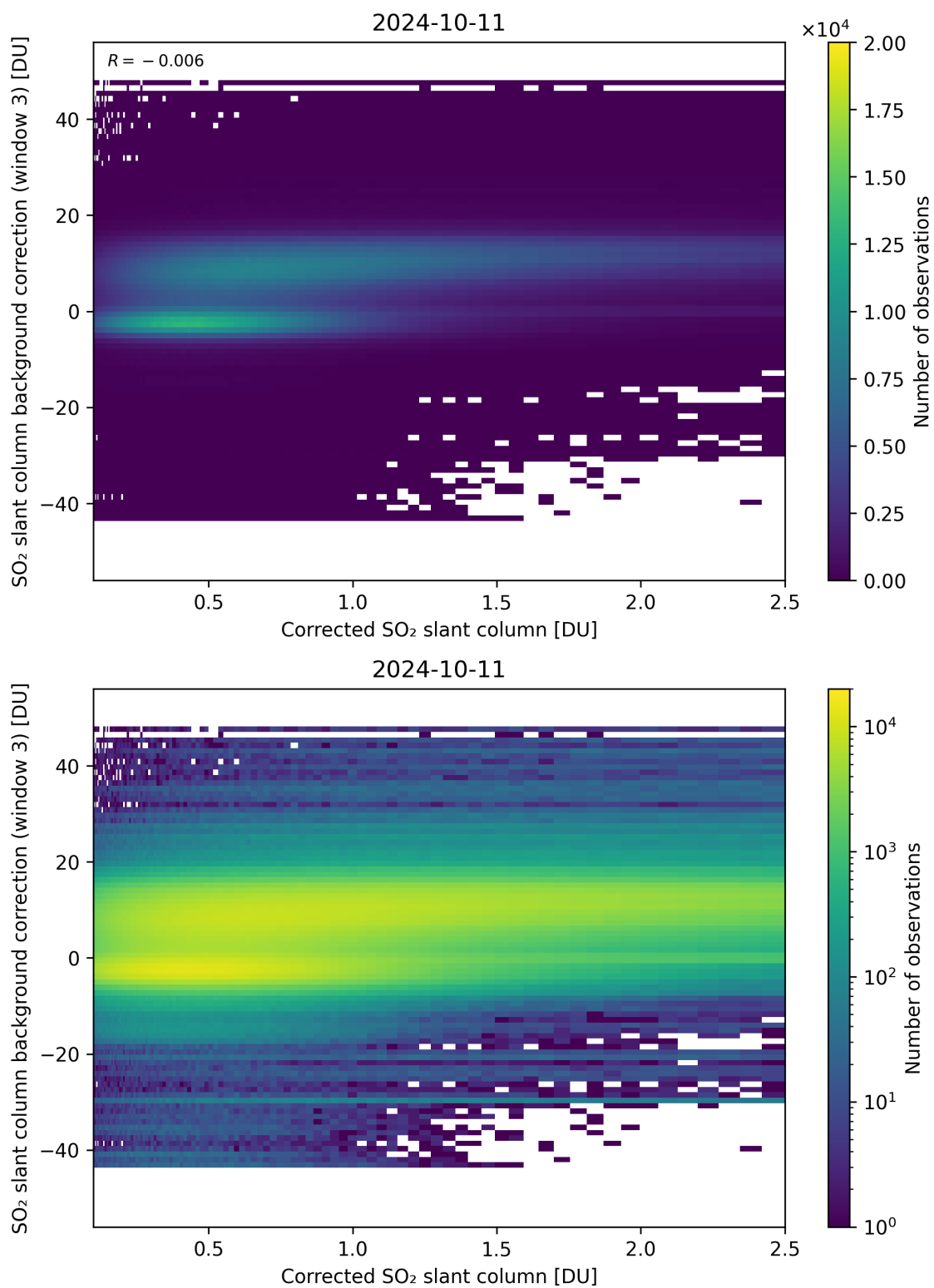
Figure 180: Scatter density plot of “Corrected SO 2 slant column” against “SO 2 slant column background correction (window 3)” for 2024-10-10 to 2024-10-12.
