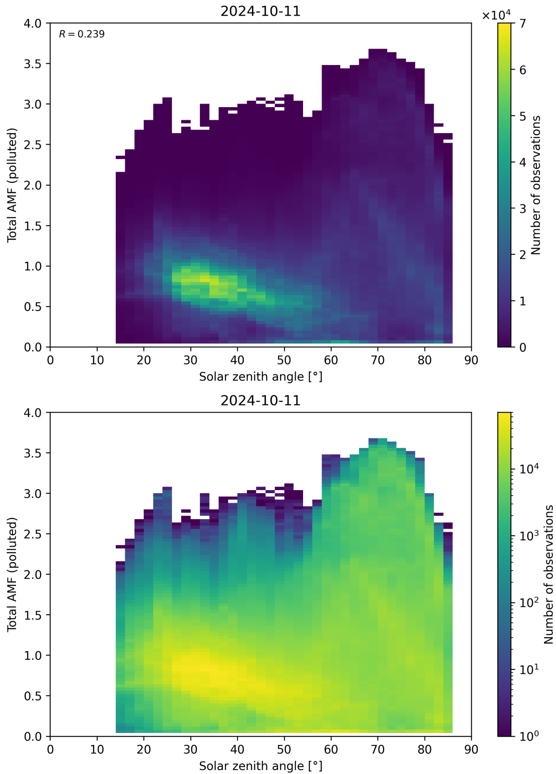
Figure 174: Scatter density plot of “Solar zenith angle” against “Total AMF (polluted)” for 2024-10-10 to 2024-10-12.
