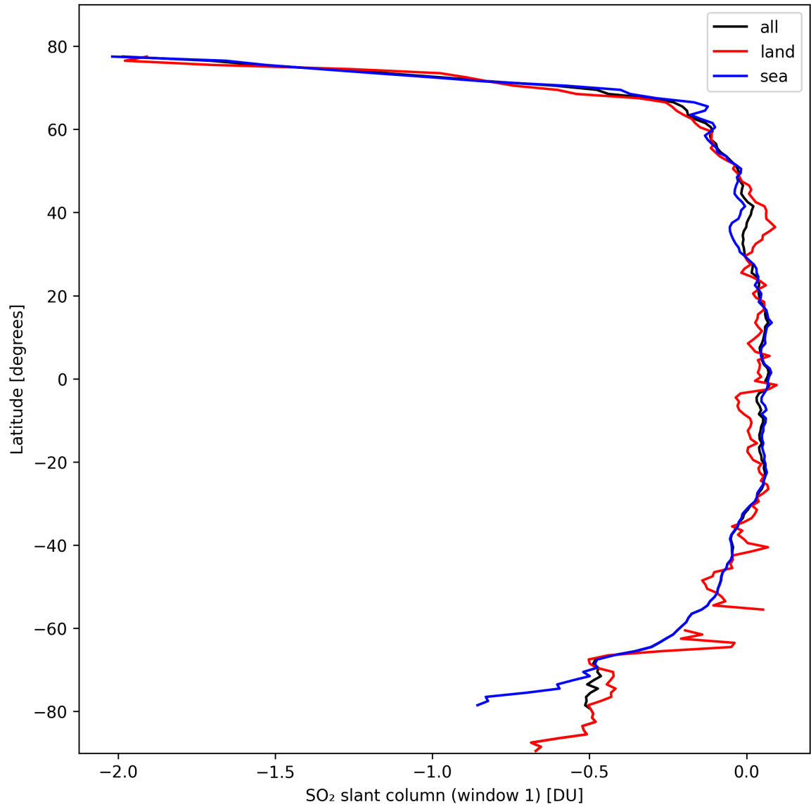
Figure 33: Zonal average of “SO 2 slant column (window 1)” for 2024-10-10 to 2024-10-12.
