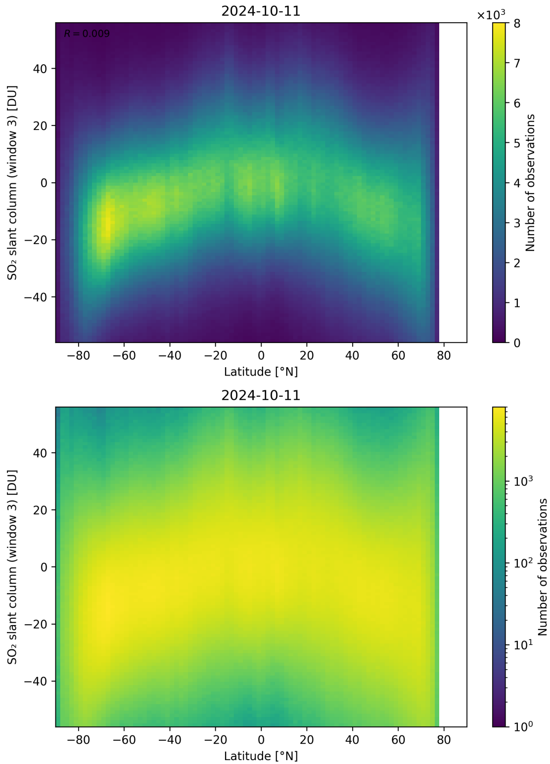
Figure 152: Scatter density plot of “Latitude” against “SO 2 slant column (window 3)” for 2024-10-10 to 2024-10-12.
