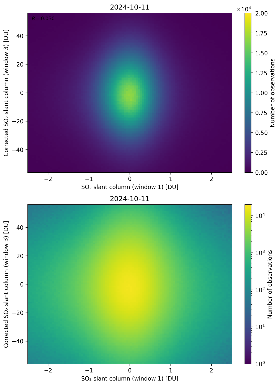
Figure 234: Scatter density plot of “SO 2 slant column (window 1)” against “Corrected SO 2 slant column (window 3)” for 2024-10-10 to 2024-10-12.
