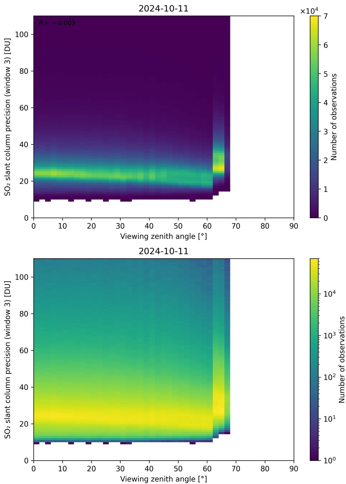
Figure 324: Scatter density plot of “Viewing zenith angle” against “SO 2 slant column precision (window 3)” for 2024-10-10 to 2024-10-12.
