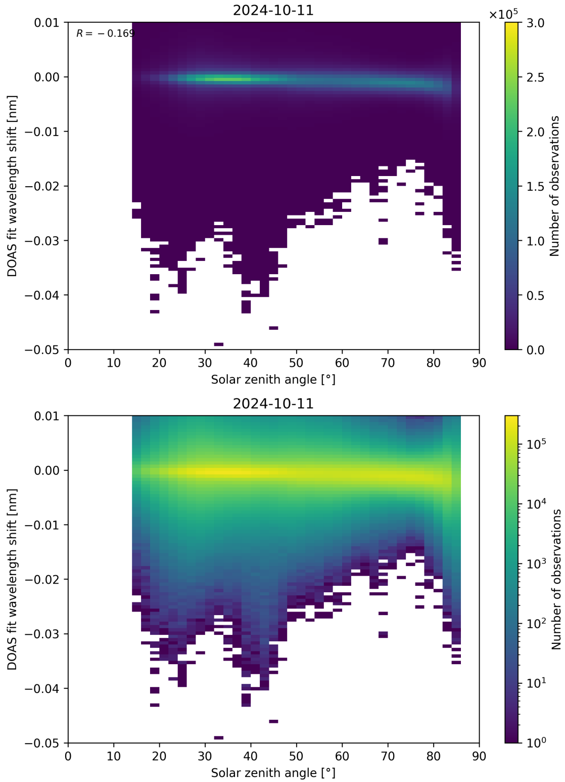
Figure 161: Scatter density plot of “Solar zenith angle” against “DOAS fit wavelength shift” for 2024-10-10 to 2024-10-12.
