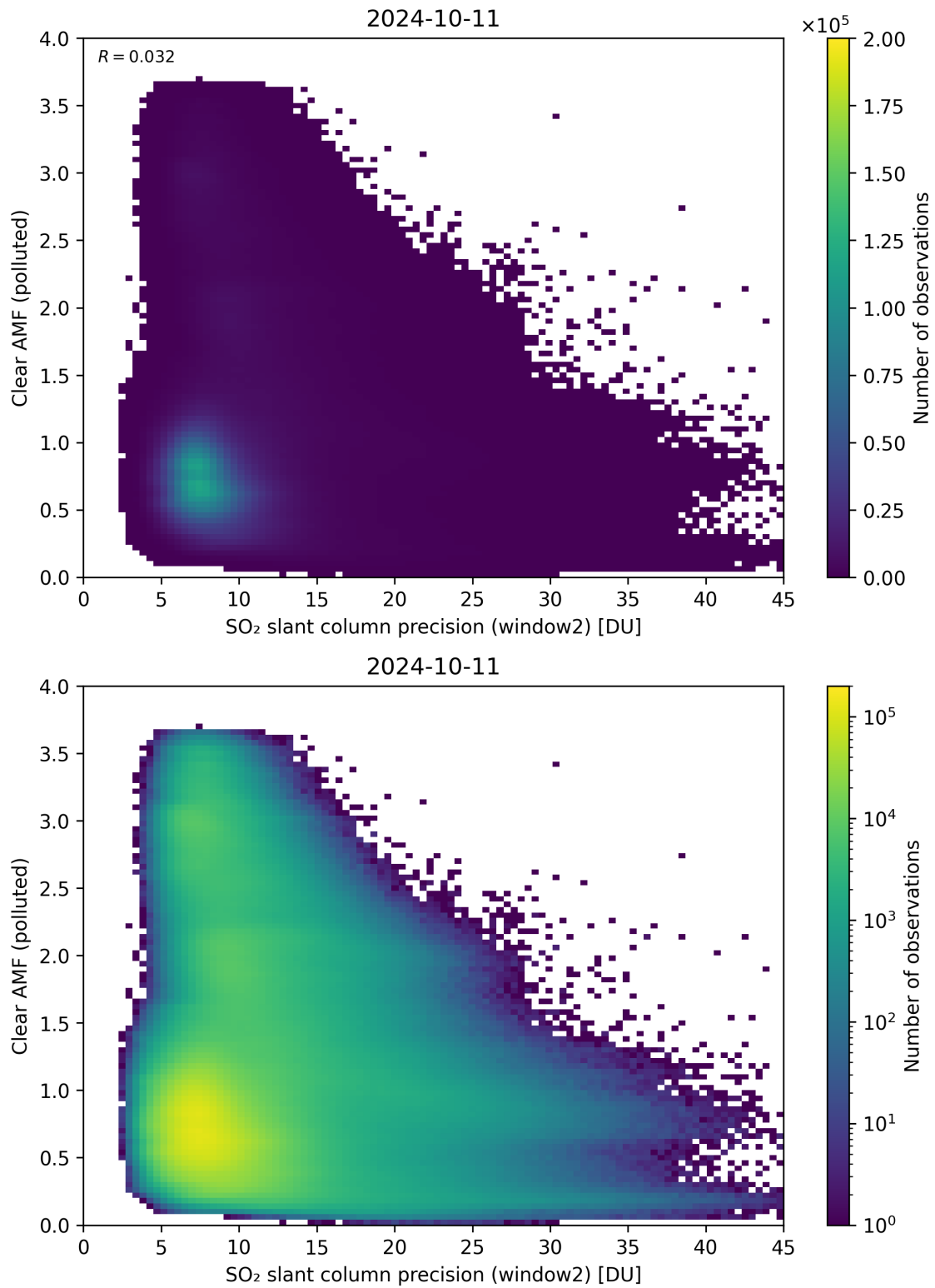
Figure 246: Scatter density plot of “SO 2 slant column precision (window2)” against “Clear AMF (polluted)” for 2024-10-10 to 2024-10-12.
