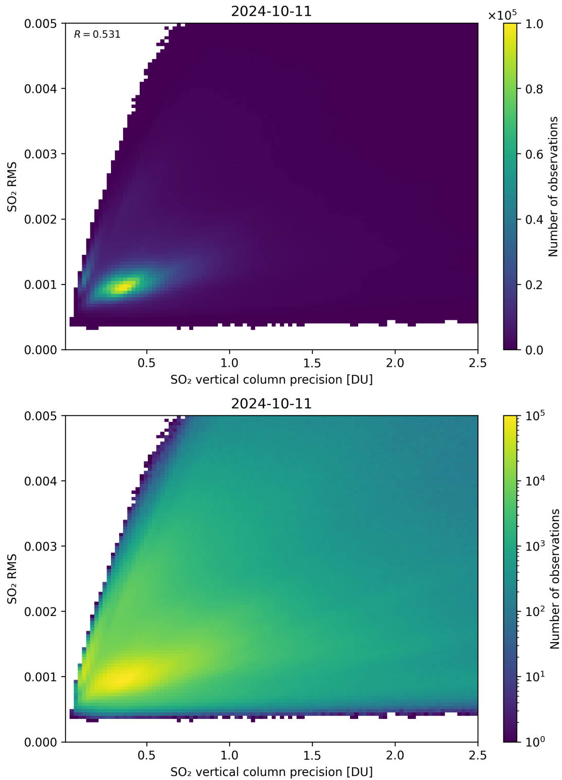
Figure 284: Scatter density plot of “SO 2 vertical column precision” against “SO 2 RMS” for 2024-10-10 to 2024-10-12.
