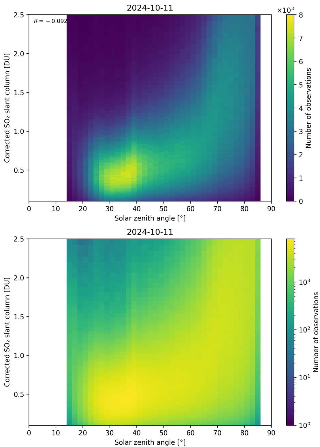
Figure 166: Scatter density plot of “Solar zenith angle” against “Corrected SO 2 slant column” for 2024-10-10 to 2024-10-12.
