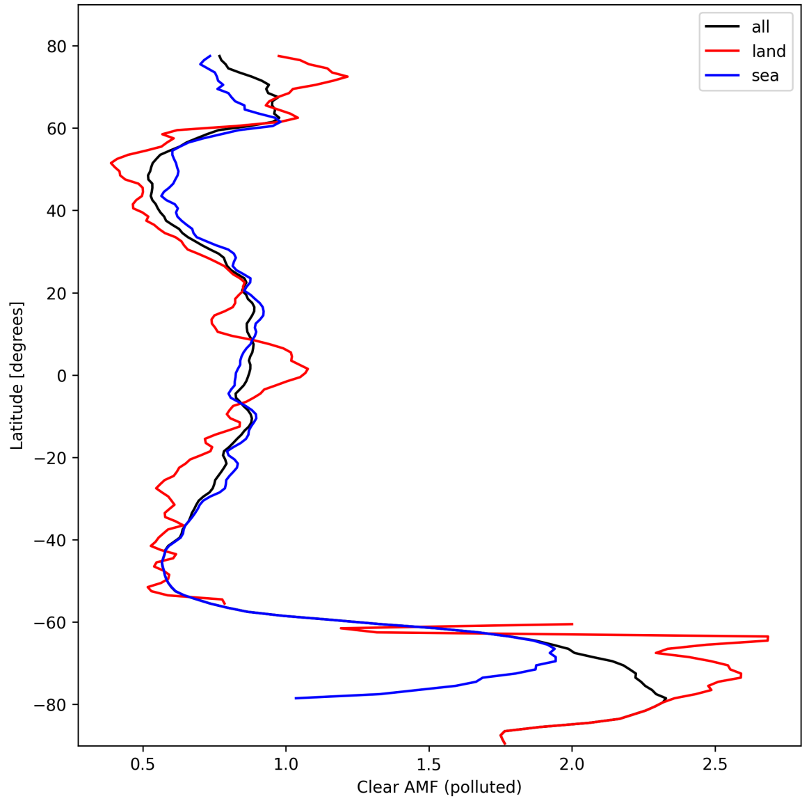
Figure 50: Zonal average of “Clear AMF (polluted)” for 2024-10-10 to 2024-10-12.
