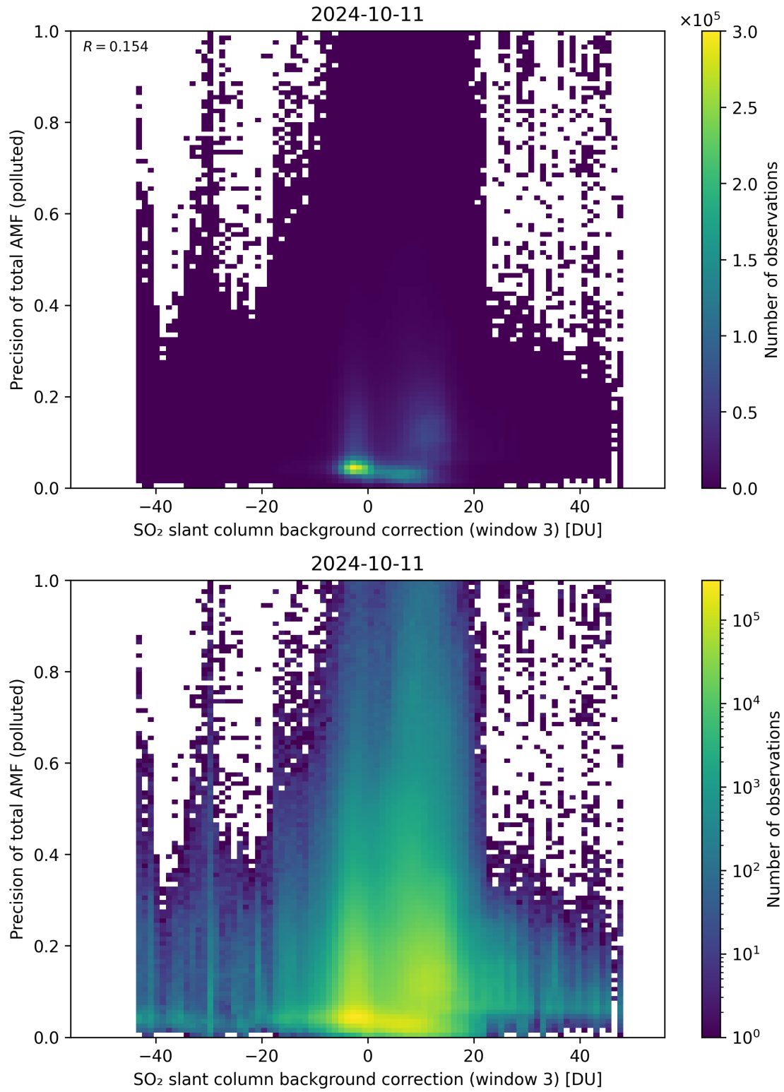
Figure 126: Scatter density plot of “SO 2 slant column background correction (window 3)” against “Precision of total AMF (polluted)” for 2024-10-10 to 2024-10-12.
