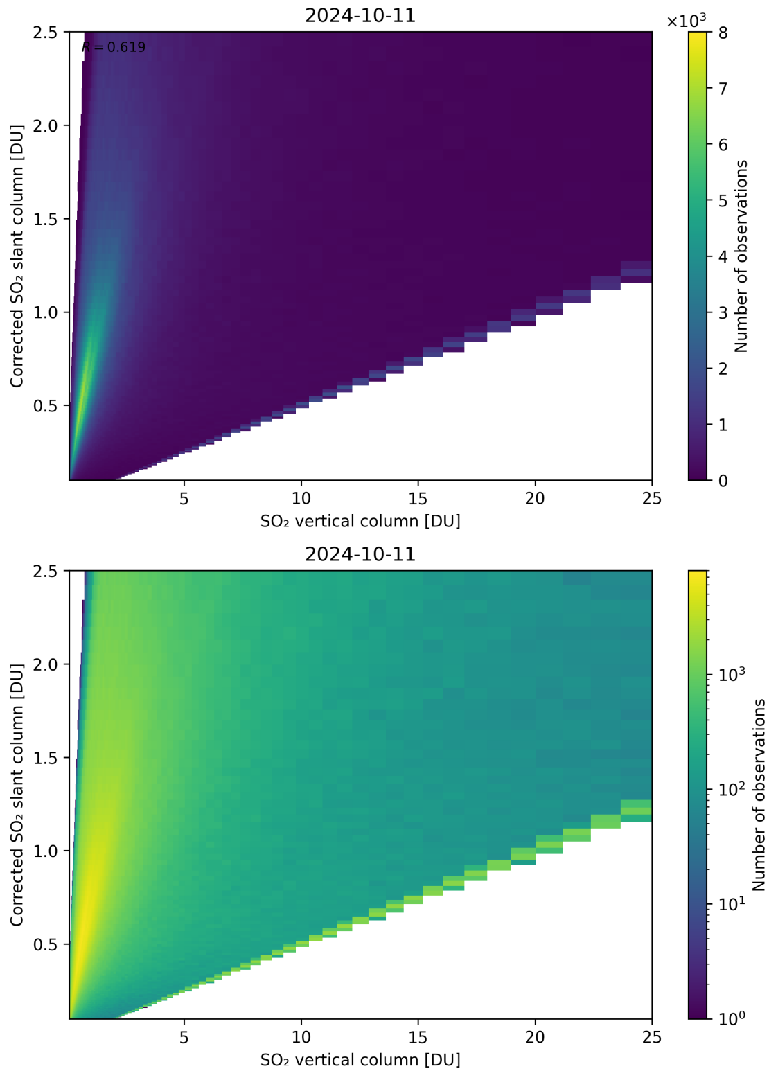
Figure 297: Scatter density plot of “SO 2 vertical column” against “Corrected SO 2 slant column” for 2024-10-10 to 2024-10-12.
