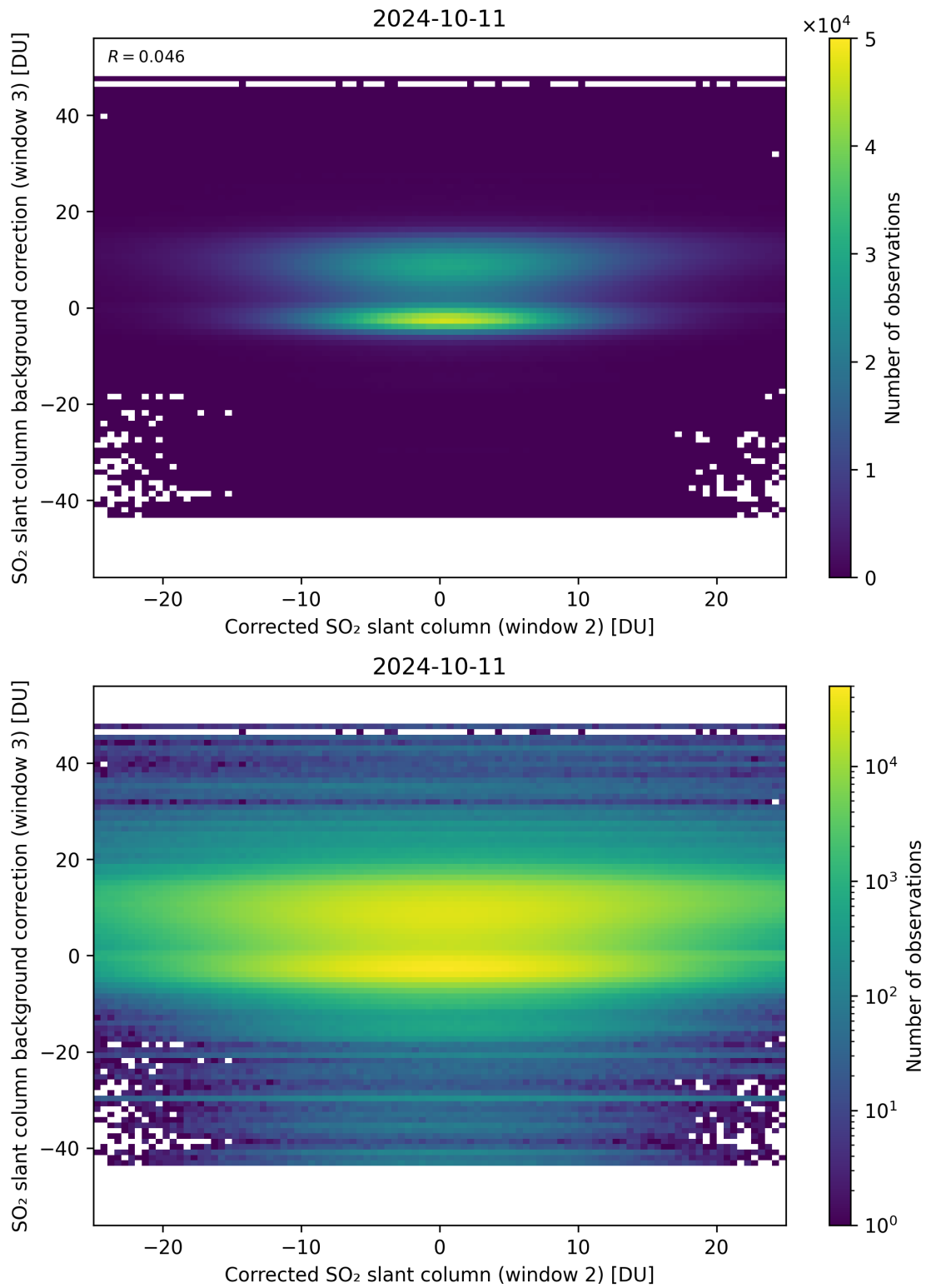
Figure 195: Scatter density plot of “Corrected SO 2 slant column (window 2)” against “SO 2 slant column background correction (window 3)” for 2024-10-10 to 2024-10-12.
