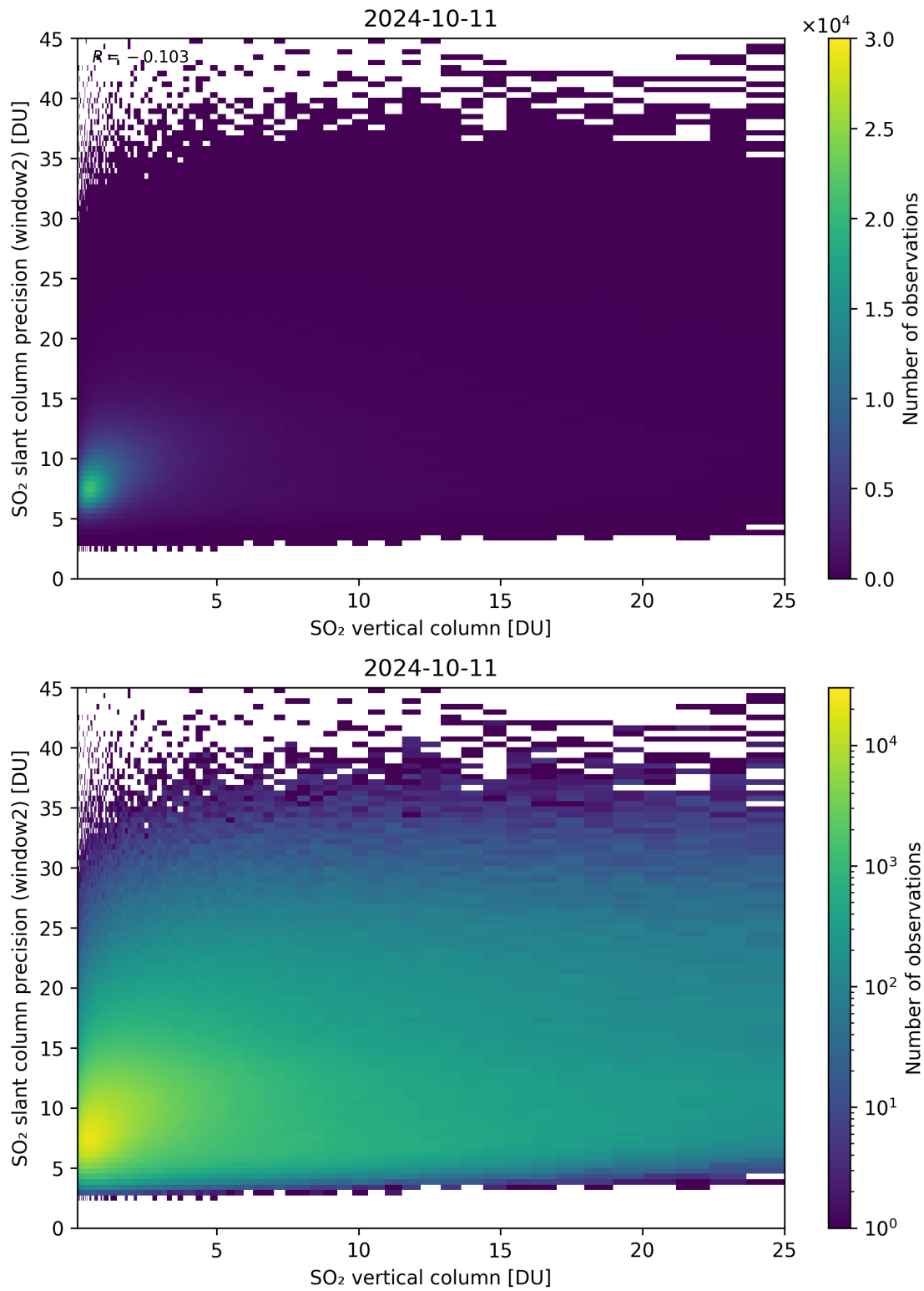
Figure 302: Scatter density plot of “SO 2 vertical column” against “SO 2 slant column precision (window2)” for 2024-10-10 to 2024-10-12.
