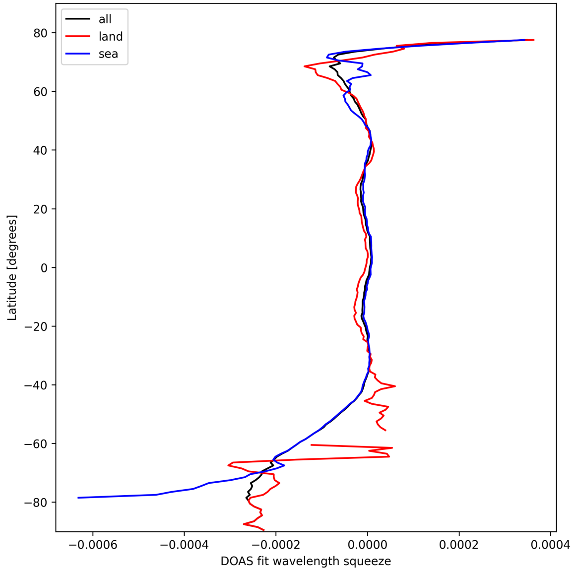
Figure 46: Zonal average of “DOAS fit wavelength squeeze” for 2024-10-10 to 2024-10-12.
