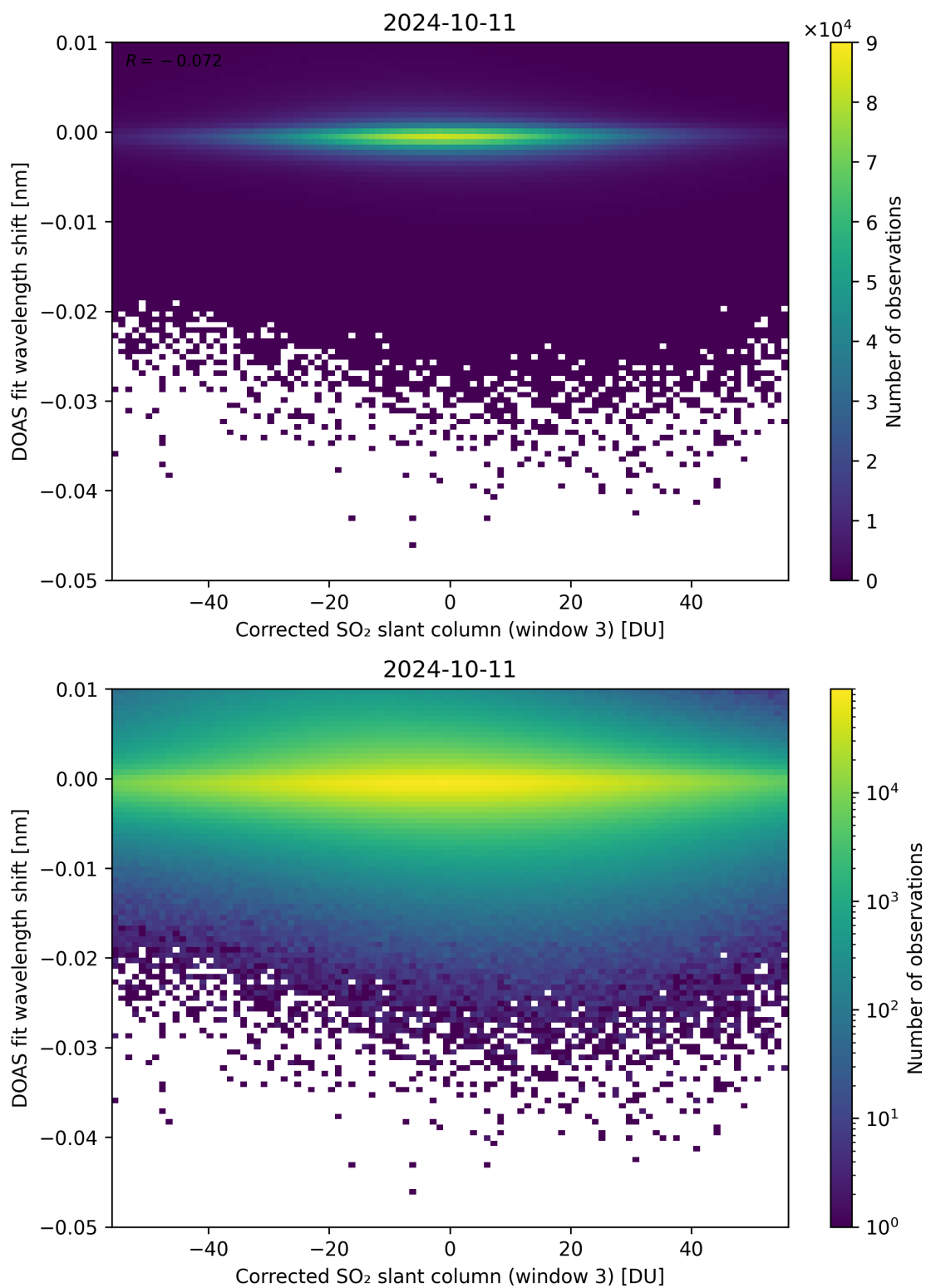
Figure 206: Scatter density plot of “Corrected SO 2 slant column (window 3)” against “DOAS fit wavelength shift” for 2024-10-10 to 2024-10-12.
