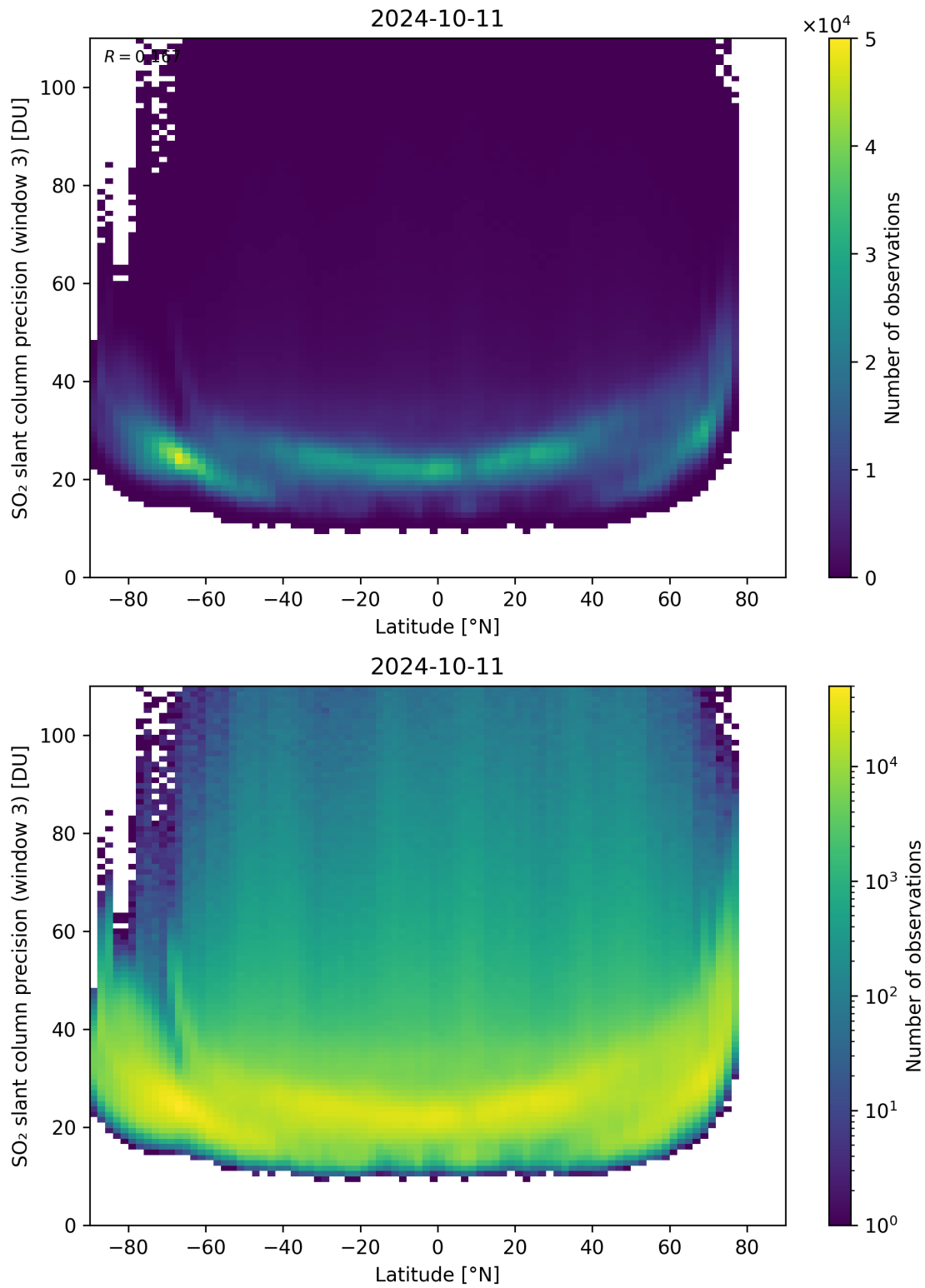
Figure 153: Scatter density plot of “Latitude” against “SO 2 slant column precision (window 3)” for 2024-10-10 to 2024-10-12.
