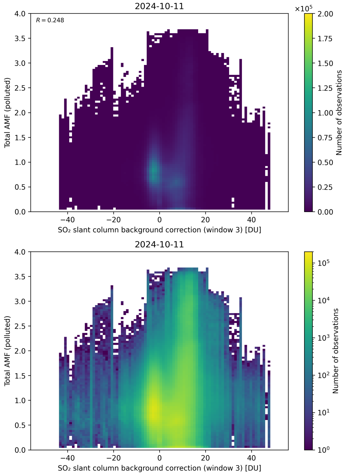
Figure 125: Scatter density plot of “SO 2 slant column background correction (window 3)” against “Total AMF (polluted)” for 2024-10-10 to 2024-10-12.
