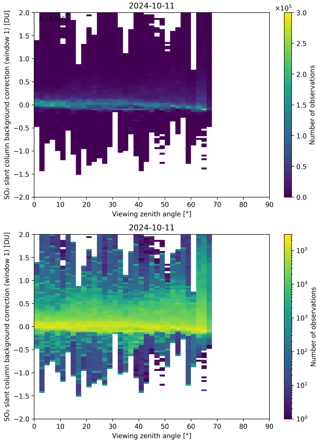
Figure 308: Scatter density plot of “Viewing zenith angle” against “SO 2 slant column background correction (window 1)” for 2024-10-10 to 2024-10-12.
