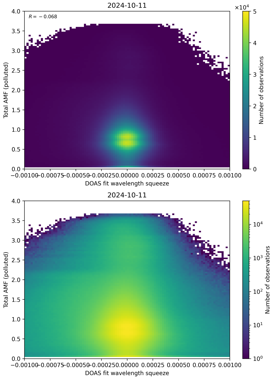
Figure 134: Scatter density plot of “DOAS fit wavelength squeeze” against “Total AMF (polluted)” for 2024-10-10 to 2024-10-12.
