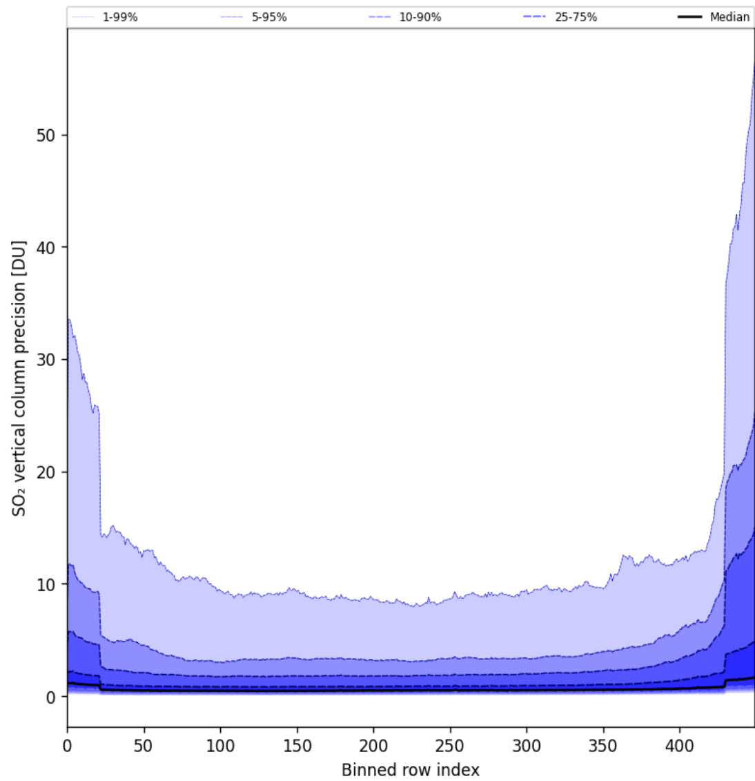
Figure 77: Along track statistics of “SO 2 vertical column precision” for 2024-10-10 to 2024-10-12
