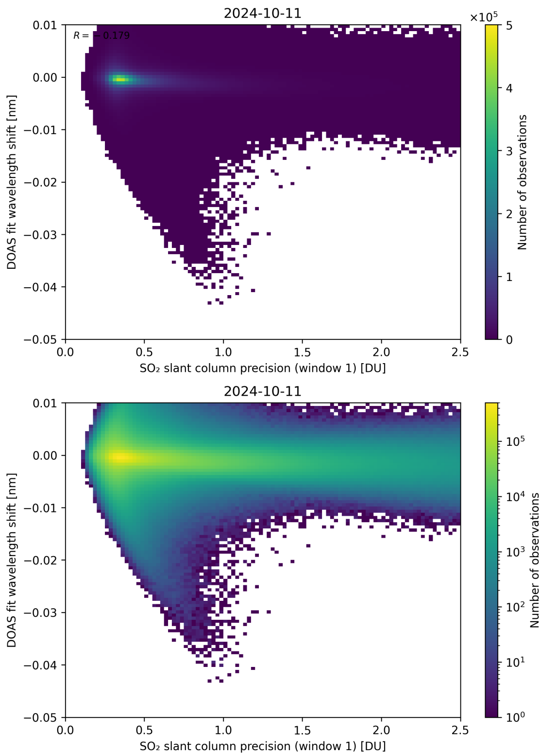
Figure 221: Scatter density plot of “SO 2 slant column precision (window 1)” against “DOAS fit wavelength shift” for 2024-10-10 to 2024-10-12.
