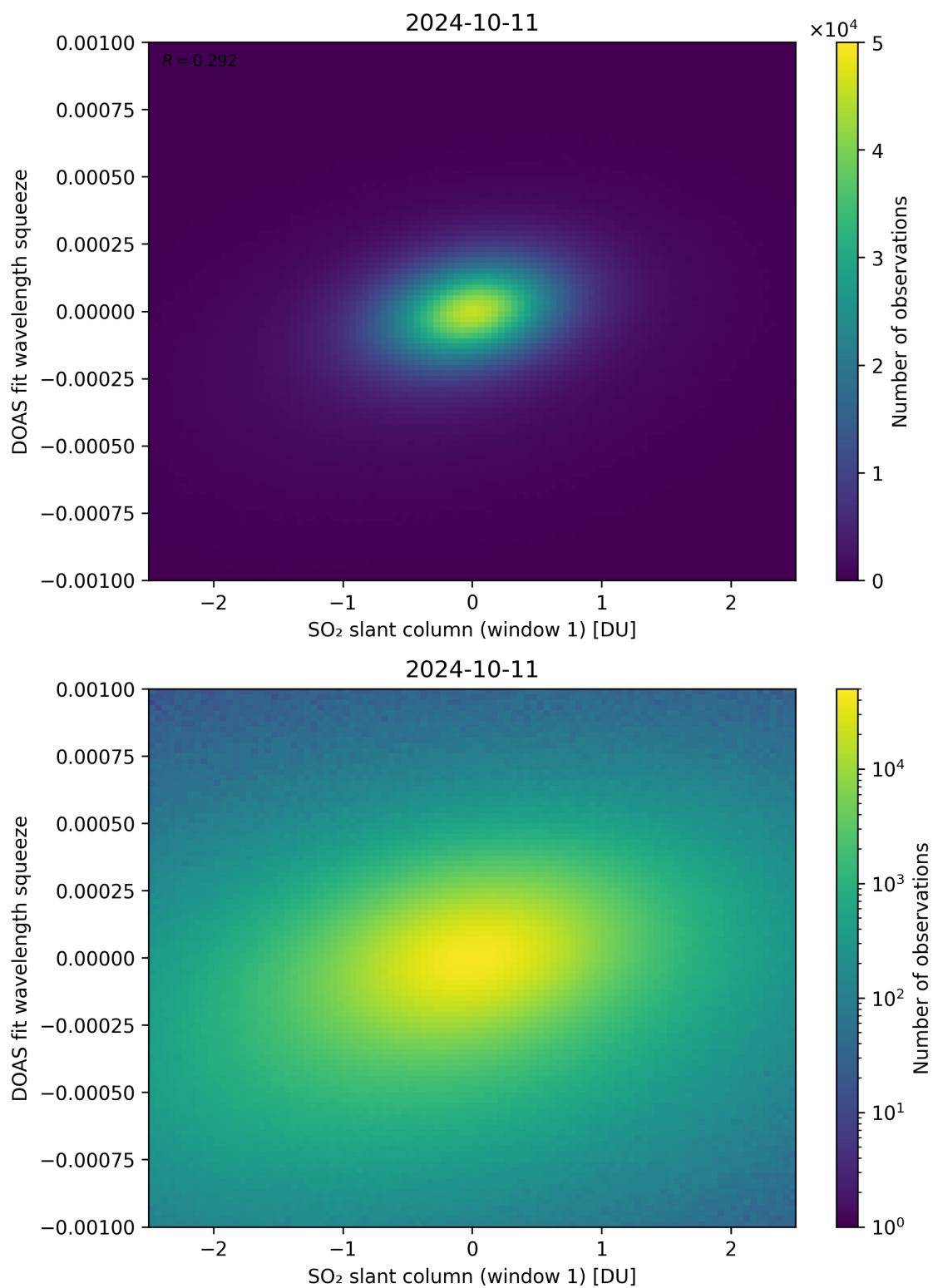
Figure 216: Scatter density plot of “SO 2 slant column (window 1)” against “DOAS fit wavelength squeeze” for 2024-10-10 to 2024-10-12.
