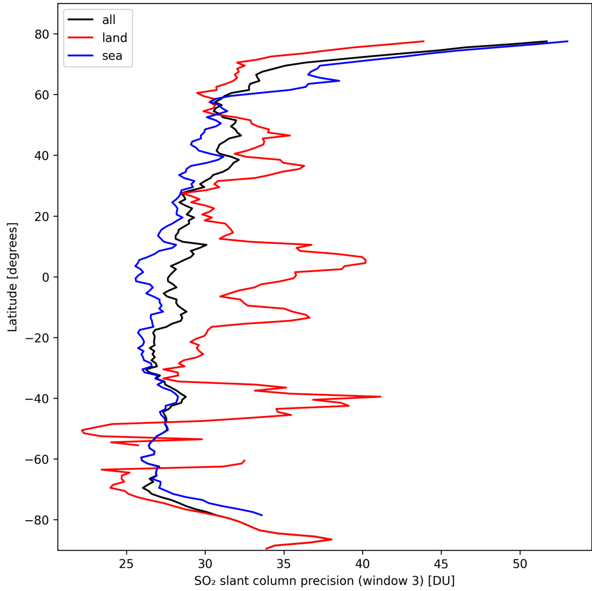
Figure 42: Zonal average of “SO 2 slant column precision (window 3)” for 2024-10-10 to 2024-10-12.
