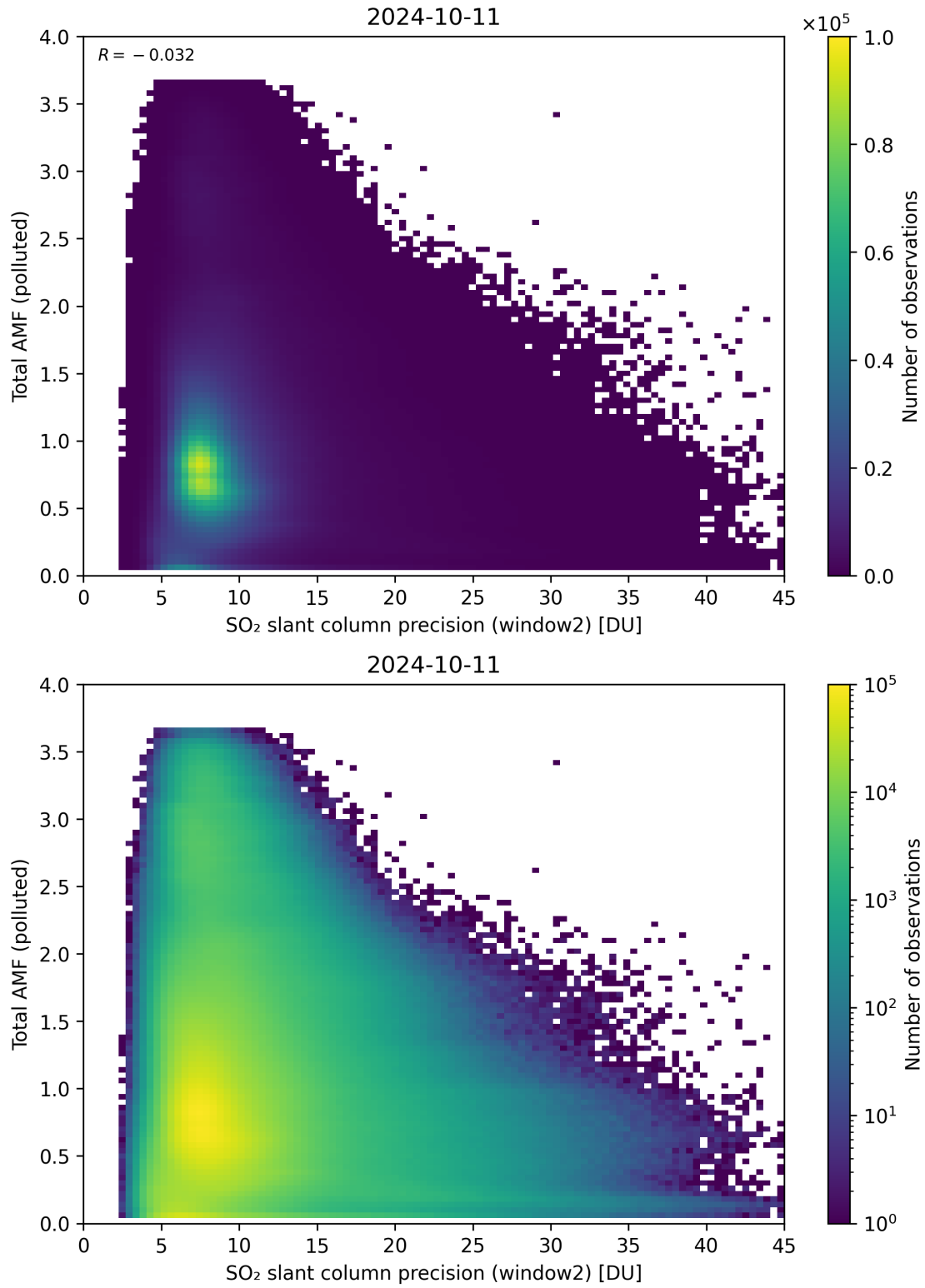
Figure 251: Scatter density plot of “SO 2 slant column precision (window2)” against “Total AMF (polluted)” for 2024-10-10 to 2024-10-12.
