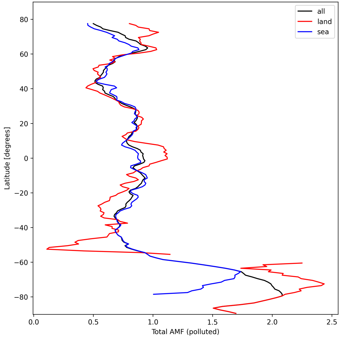
Figure 48: Zonal average of “Total AMF (polluted)” for 2024-10-10 to 2024-10-12.
