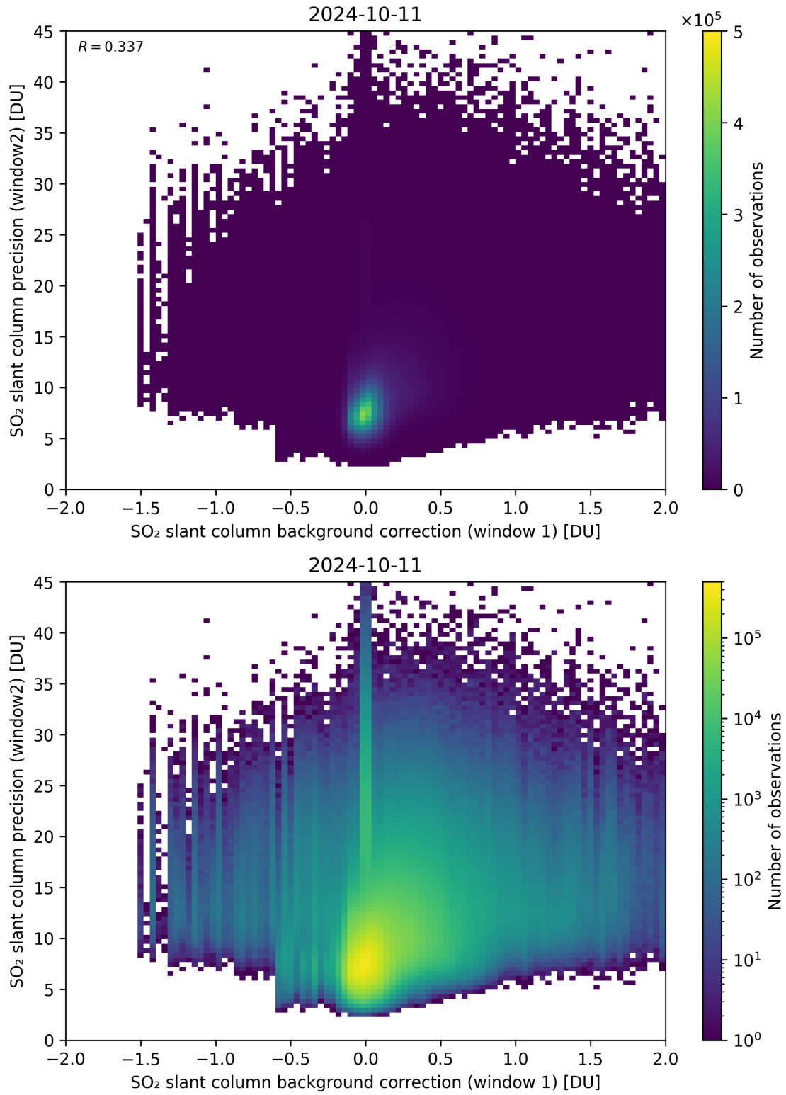
Figure 106: Scatter density plot of “SO 2 slant column background correction (window 1)” against “SO 2 slant column precision (window2)” for 2024-10-10 to 2024-10-12.
