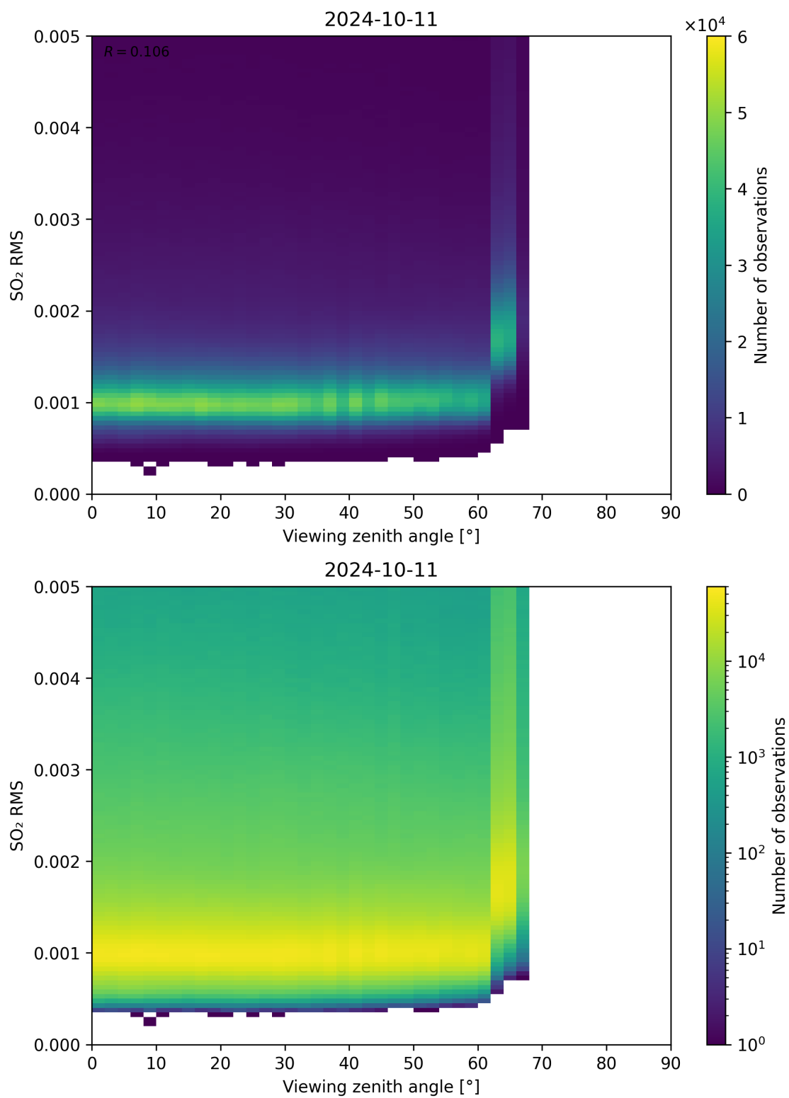
Figure 313: Scatter density plot of “Viewing zenith angle” against “SO 2 RMS” for 2024-10-10 to 2024-10-12.
