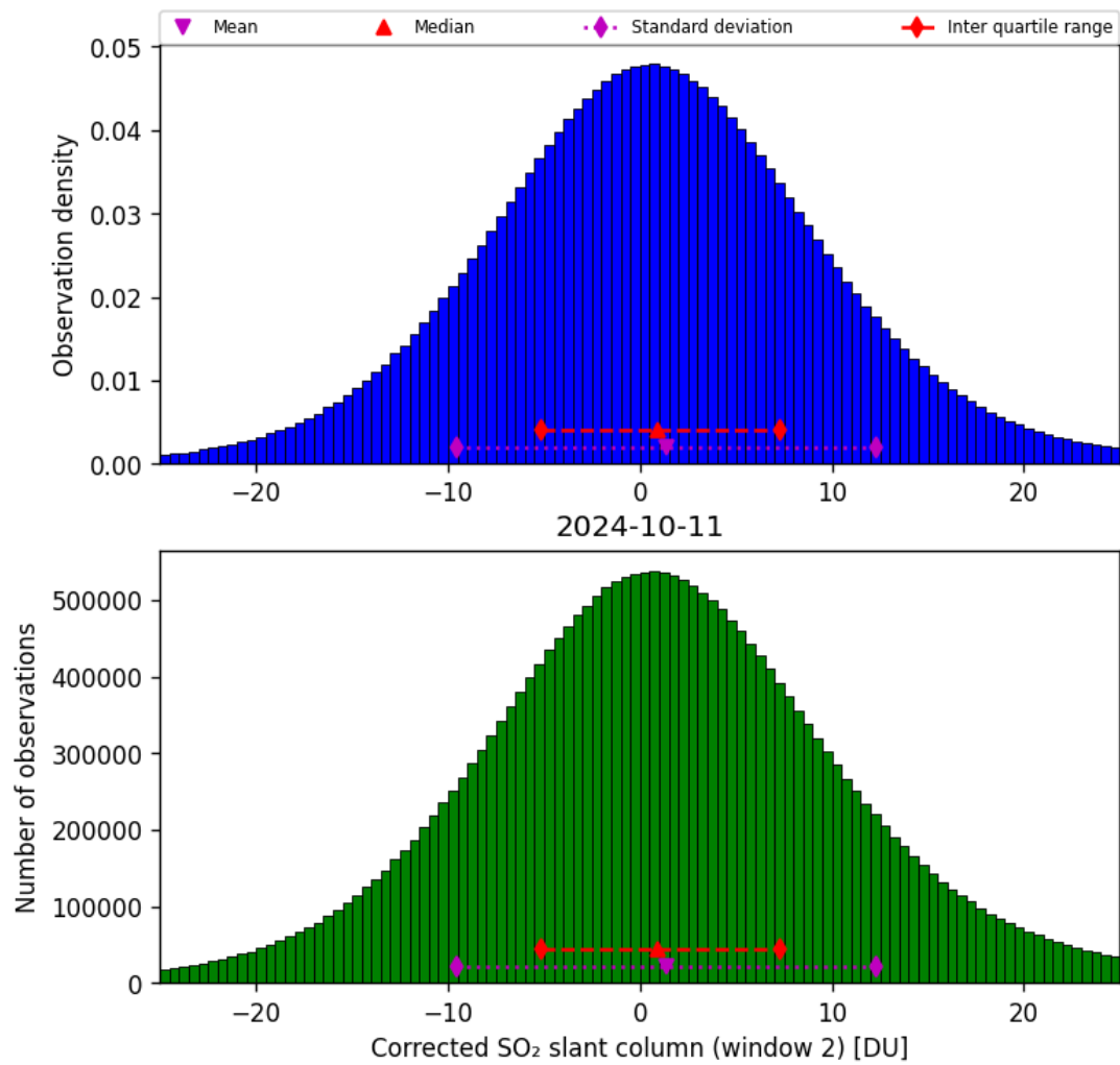
Figure 62: Histogram of “Corrected SO 2 slant column (window 2)” for 2024-10-10 to 2024-10-12
