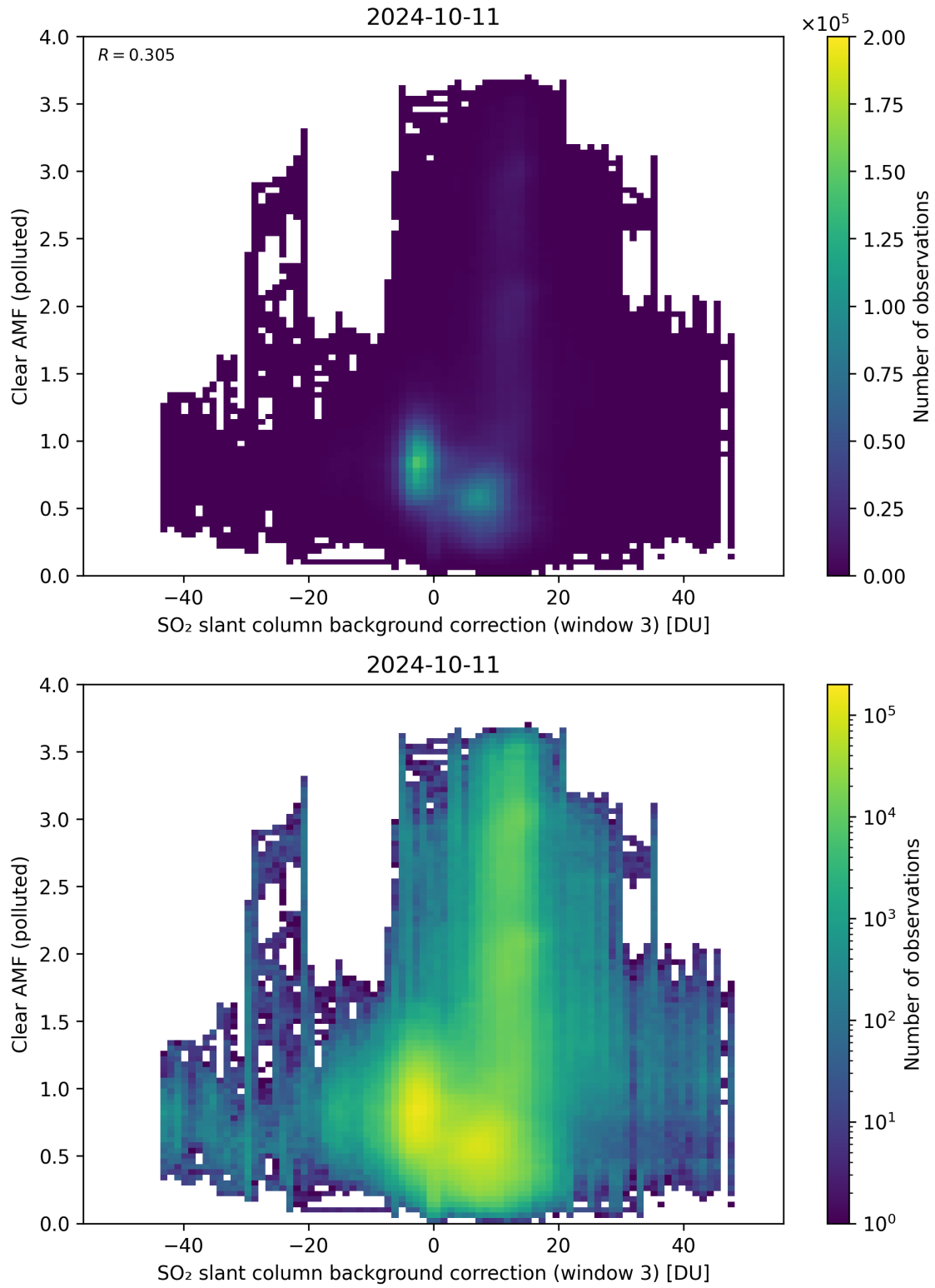
Figure 124: Scatter density plot of “SO 2 slant column background correction (window 3)” against “Clear AMF (polluted)” for 2024-10-10 to 2024-10-12.
