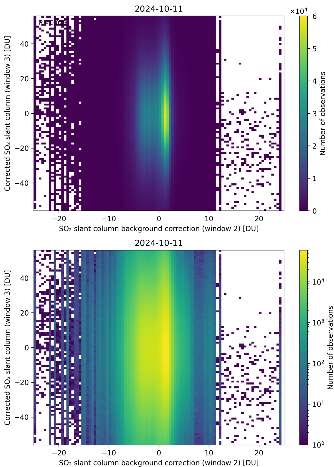
Figure 116: Scatter density plot of “SO 2 slant column background correction (window 2)” against “Corrected SO 2 slant column (window 3)” for 2024-10-10 to 2024-10-12.
