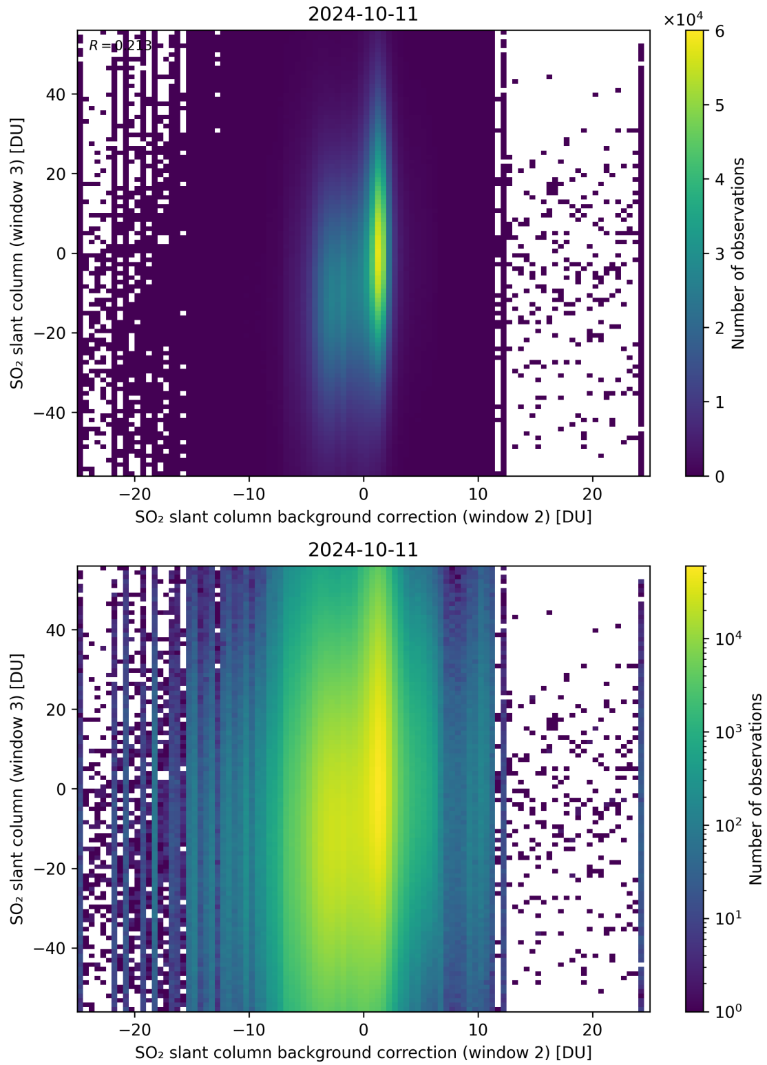
Figure 117: Scatter density plot of “SO 2 slant column background correction (window 2)” against “SO 2 slant column (window 3)” for 2024-10-10 to 2024-10-12.
