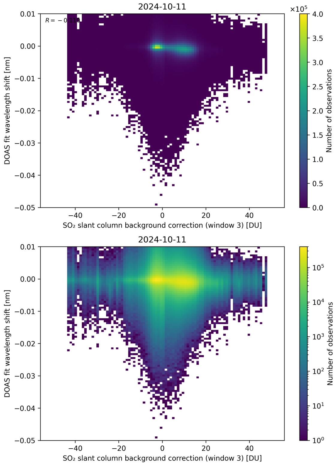
Figure 121: Scatter density plot of “SO 2 slant column background correction (window 3)” against “DOAS fit wavelength shift” for 2024-10-10 to 2024-10-12.
