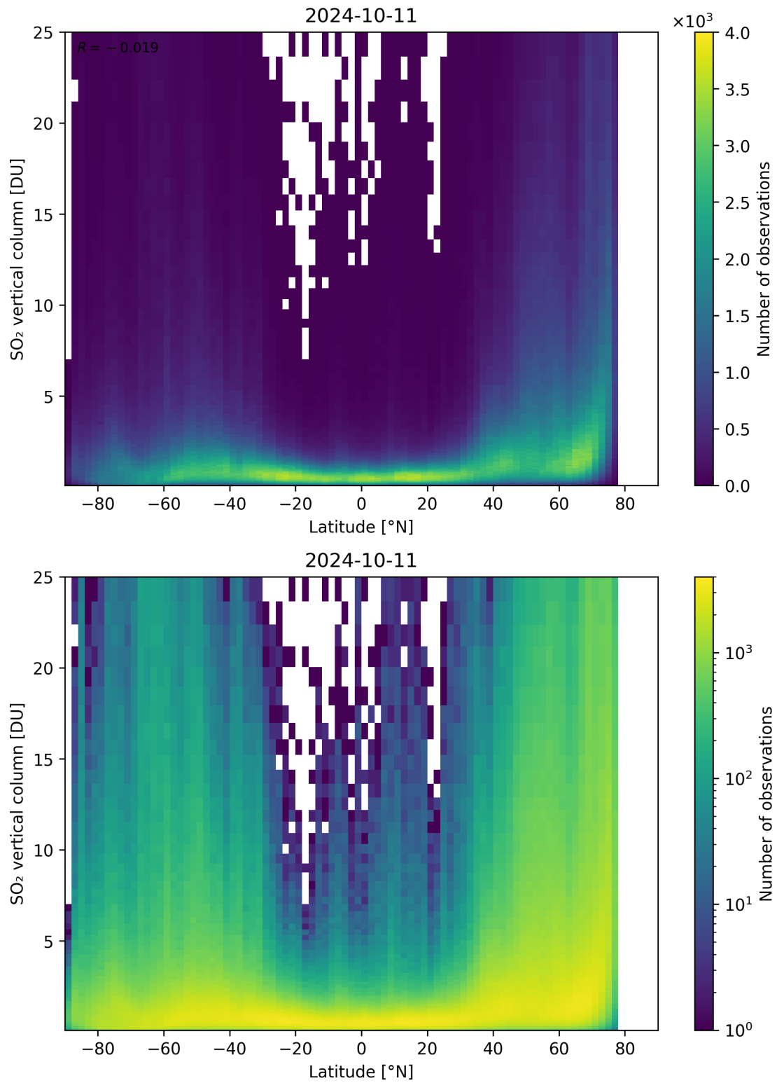
Figure 156: Scatter density plot of “Latitude” against “SO 2 vertical column” for 2024-10-10 to 2024-10-12.
