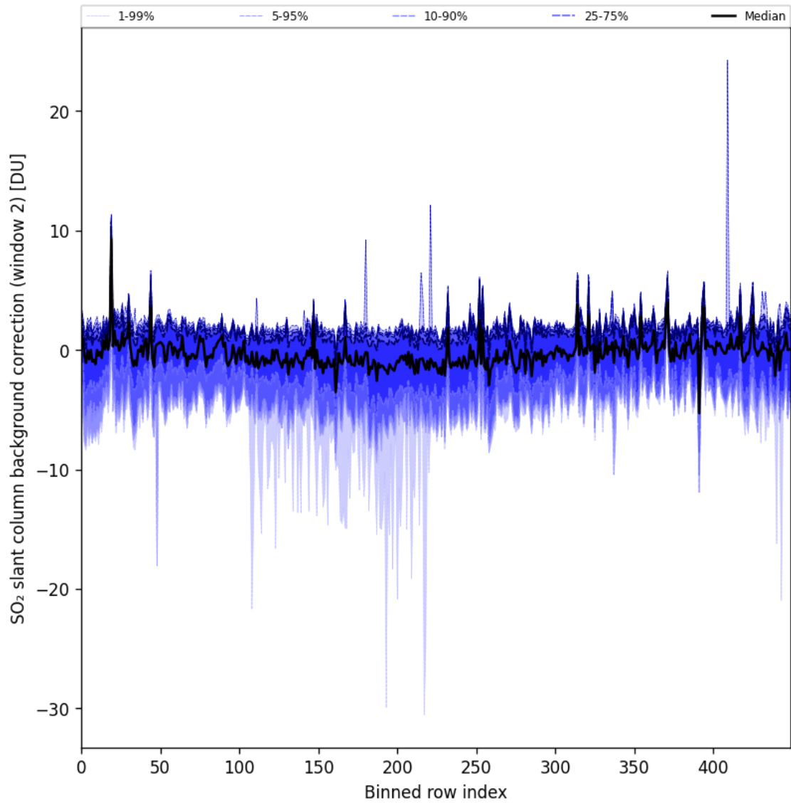
Figure 86: Along track statistics of “SO 2 slant column background correction (window 2)” for 2024-10-10 to 2024-10-12
