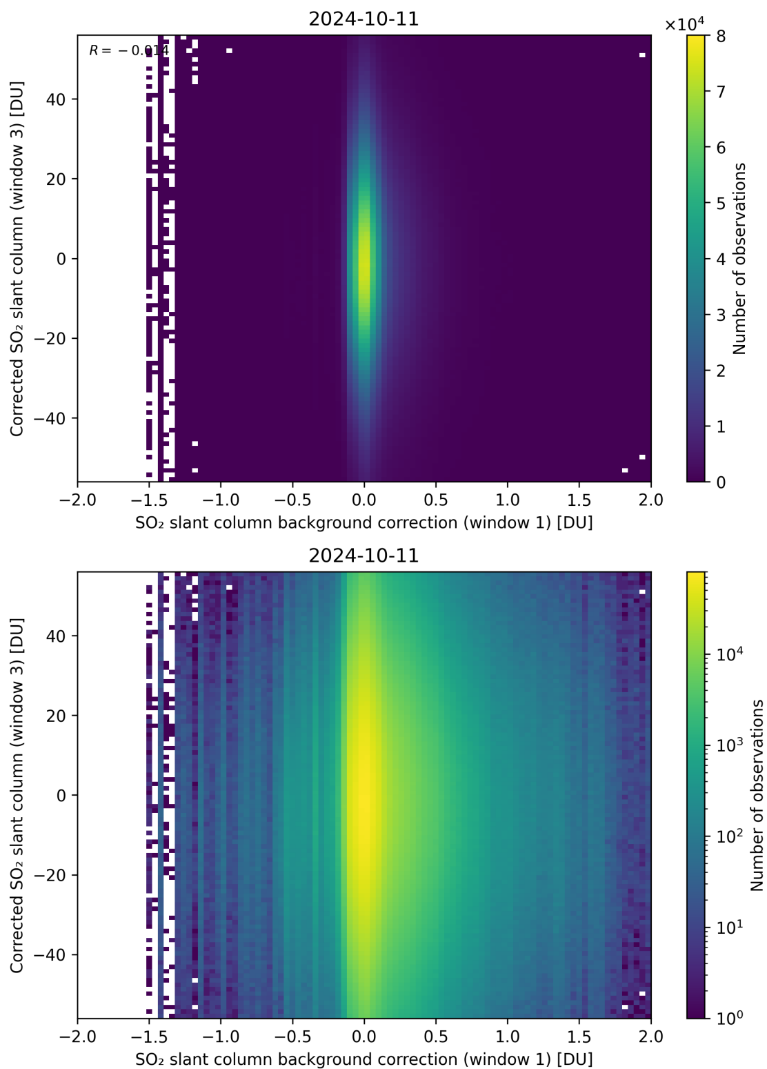
Figure 105: Scatter density plot of “SO 2 slant column background correction (window 1)” against “Corrected SO 2 slant column (window 3)” for 2024-10-10 to 2024-10-12.
