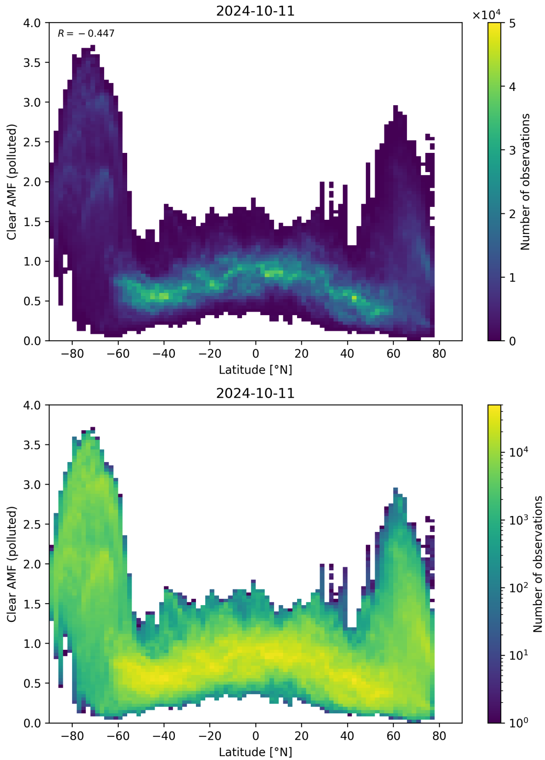
Figure 145: Scatter density plot of “Latitude” against “Clear AMF (polluted)” for 2024-10-10 to 2024-10-12.
