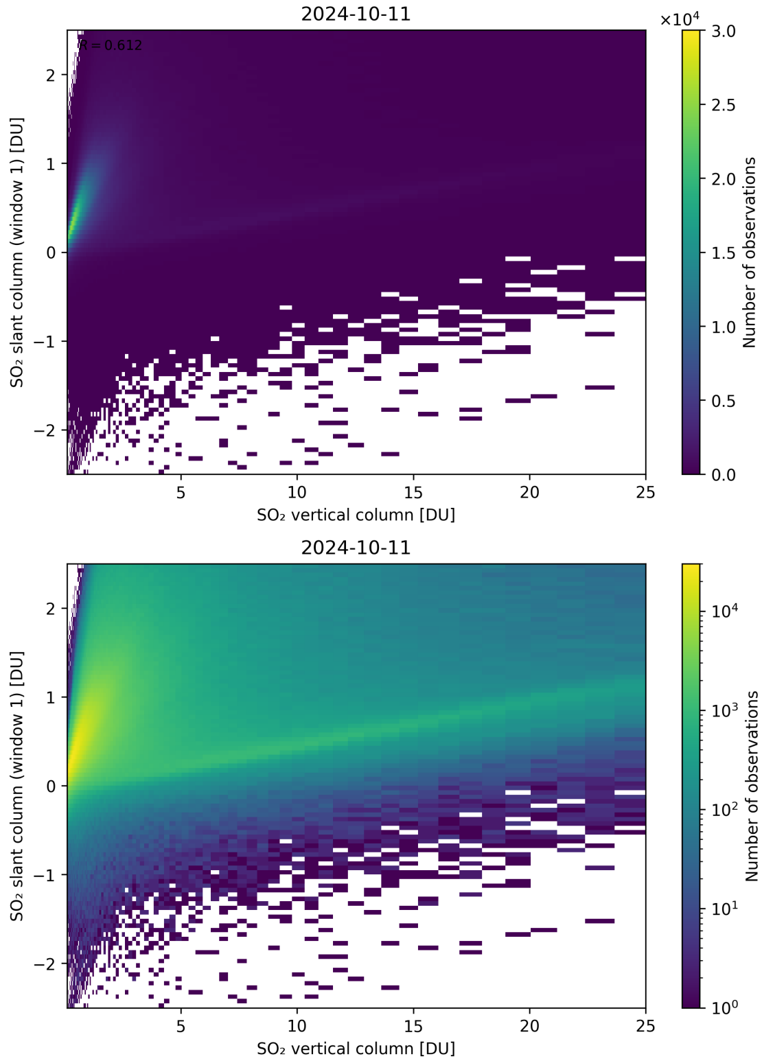
Figure 300: Scatter density plot of “SO 2 vertical column” against “SO 2 slant column (window 1)” for 2024-10-10 to 2024-10-12.
