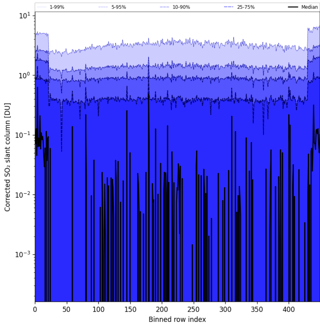
Figure 78: Along track statistics of “Corrected SO 2 slant column” for 2024-10-10 to 2024-10-12
