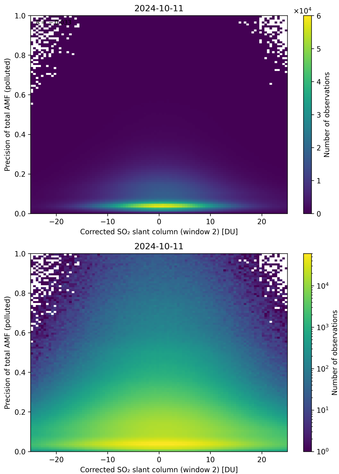
Figure 204: Scatter density plot of “Corrected SO 2 slant column (window 2)” against “Precision of total AMF (polluted)” for 2024-10-10 to 2024-10-12.
