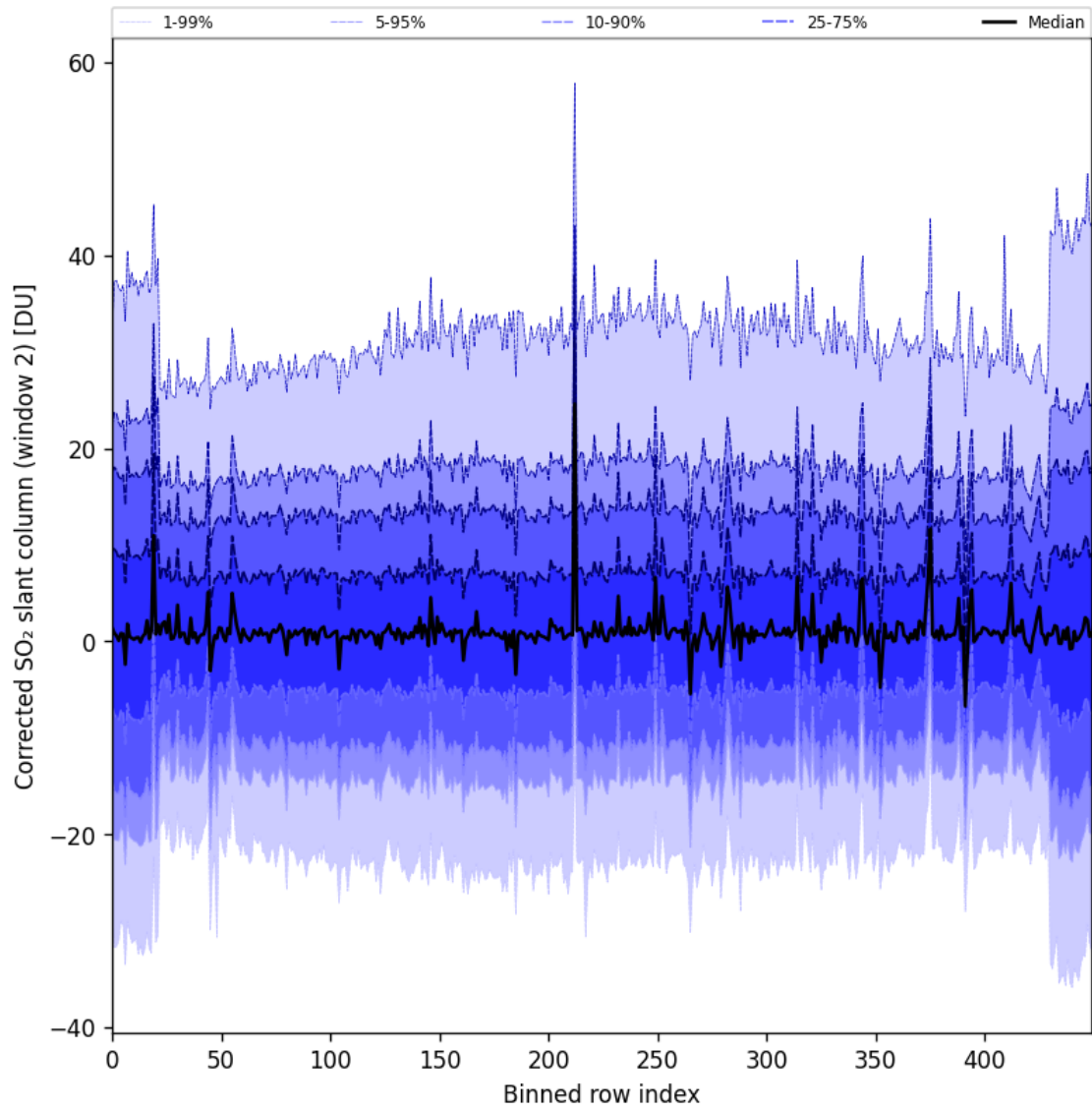
Figure 85: Along track statistics of “Corrected SO 2 slant column (window 2)” for 2024-10-10 to 2024-10-12
