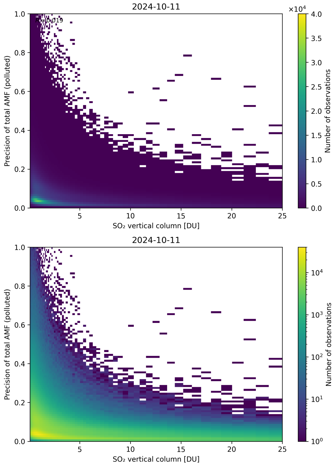
Figure 306: Scatter density plot of “SO 2 vertical column” against “Precision of total AMF (polluted)” for 2024-10-10 to 2024-10-12.
