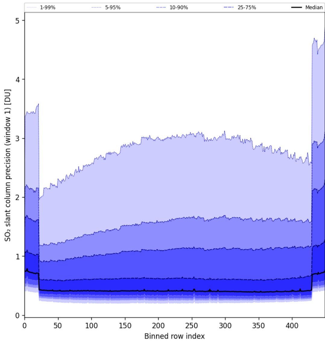
Figure 80: Along track statistics of “SO 2 slant column precision (window 1)” for 2024-10-10 to 2024-10-12
