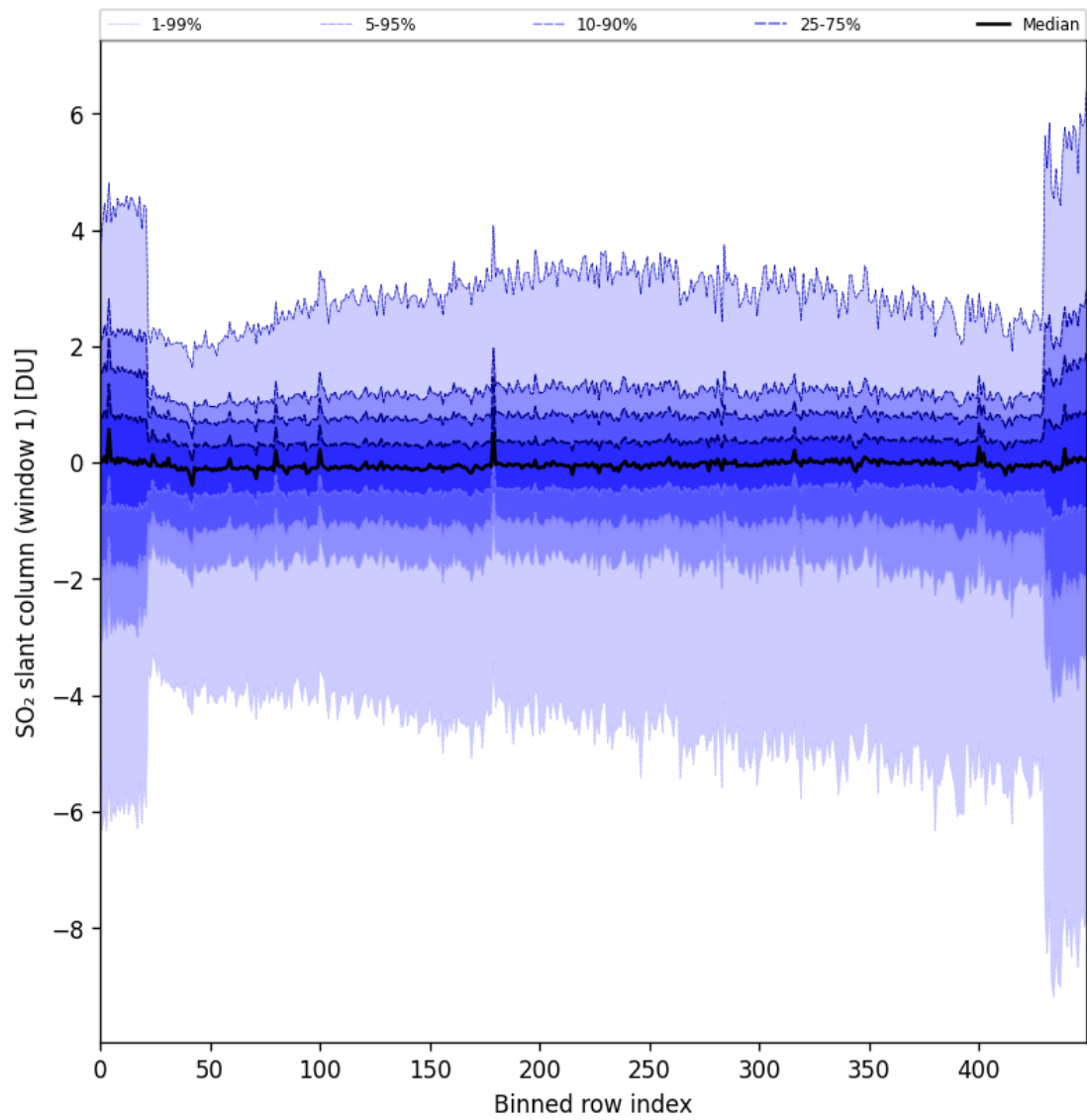
Figure 79: Along track statistics of “SO 2 slant column (window 1)” for 2024-10-10 to 2024-10-12
