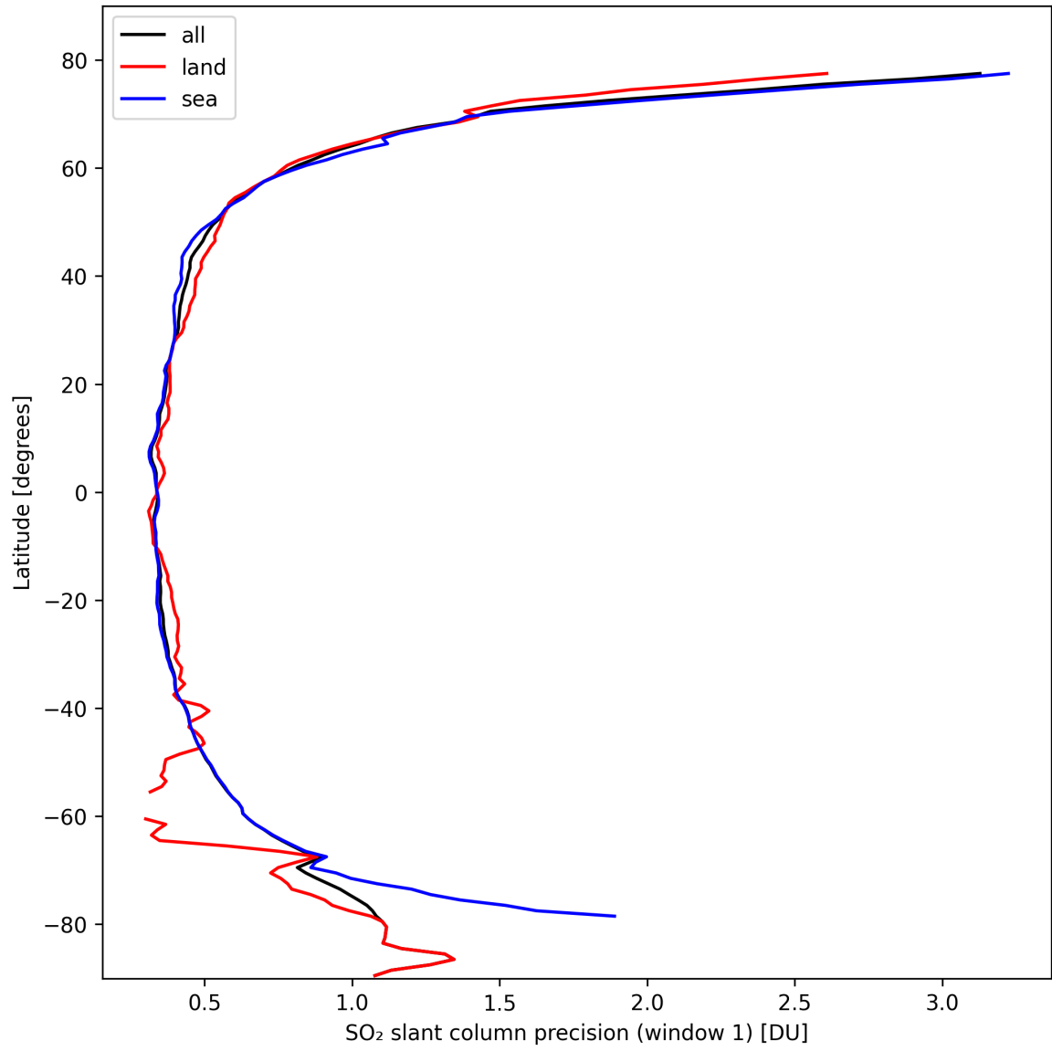
Figure 34: Zonal average of “SO 2 slant column precision (window 1)” for 2024-10-10 to 2024-10-12.
