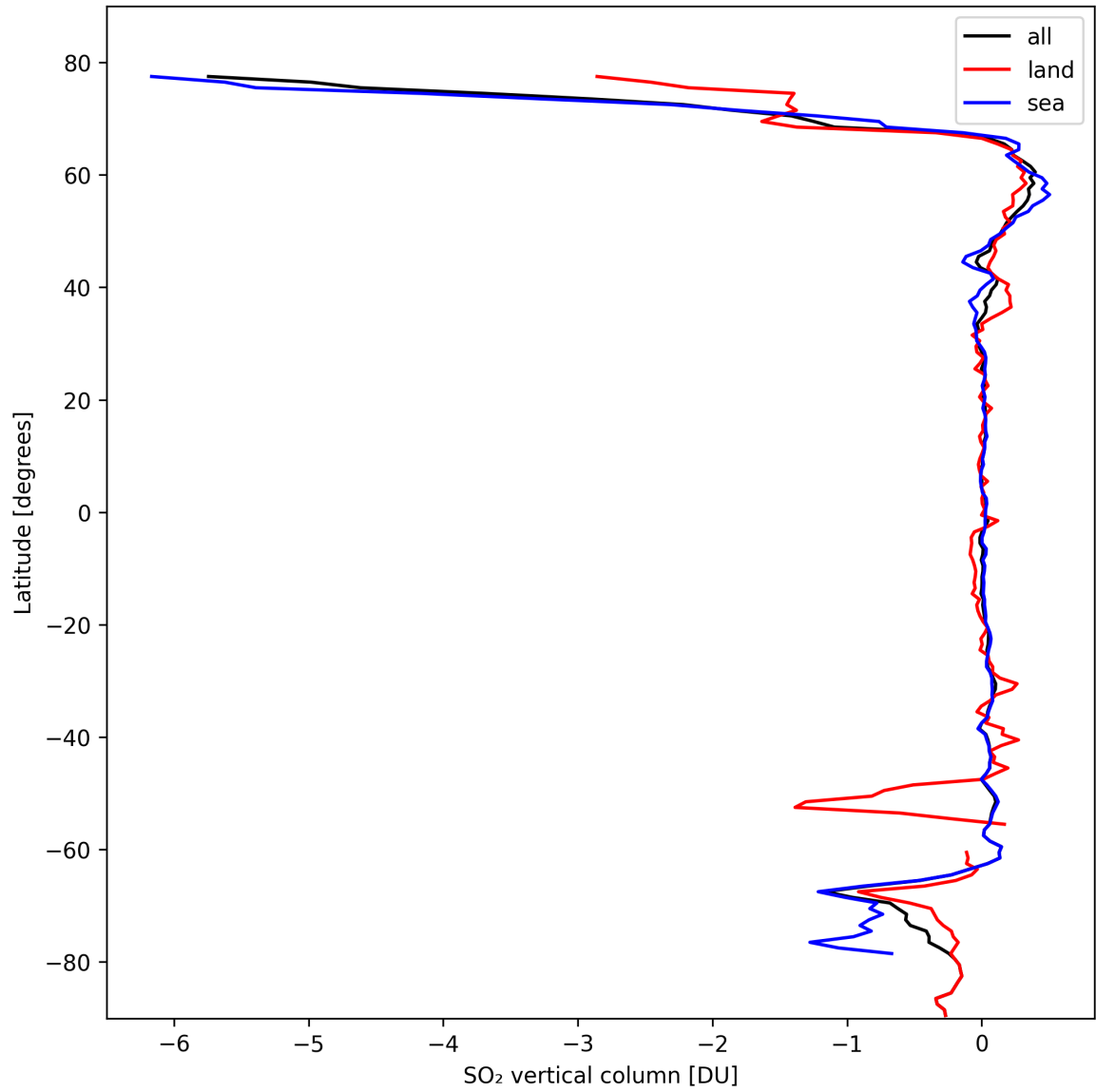
Figure 30: Zonal average of “SO 2 vertical column” for 2024-10-10 to 2024-10-12.
