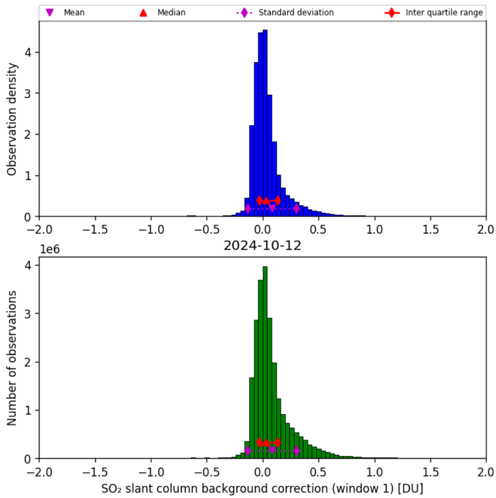
Figure 59: Histogram of “SO 2 slant column background correction (window 1)” for 2024-10-11 to 2024-10-13
