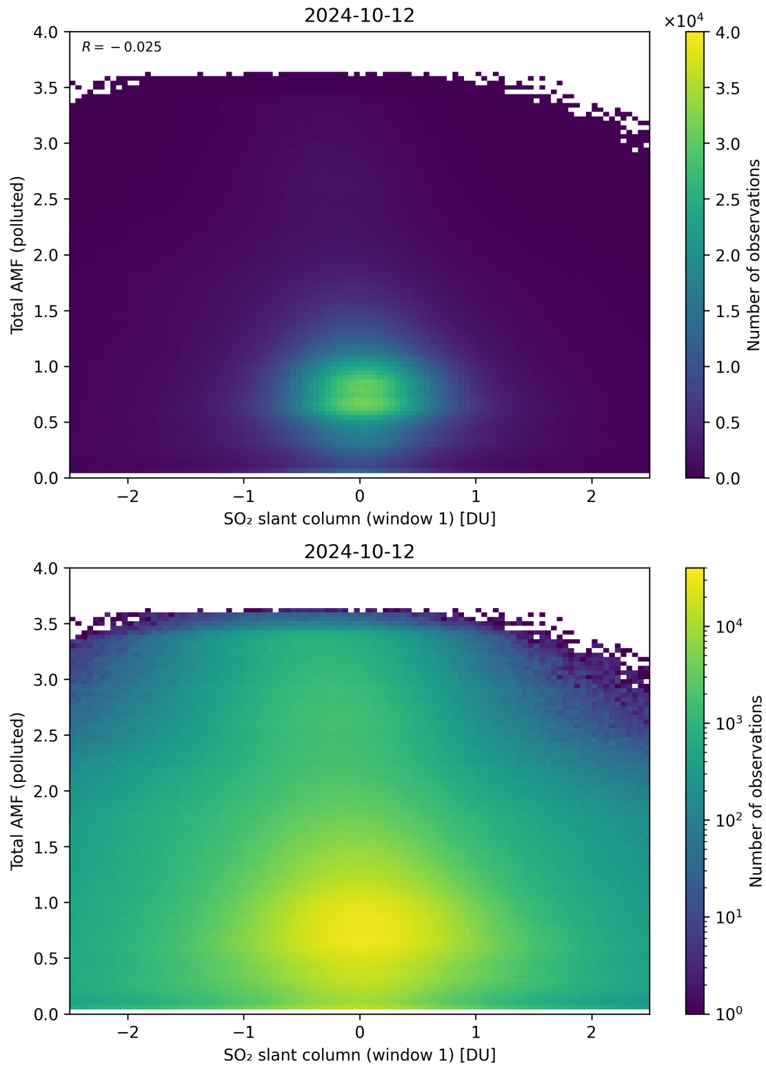
Figure 239: Scatter density plot of “SO 2 slant column (window 1)” against “Total AMF (polluted)” for 2024-10-11 to 2024-10-13.
