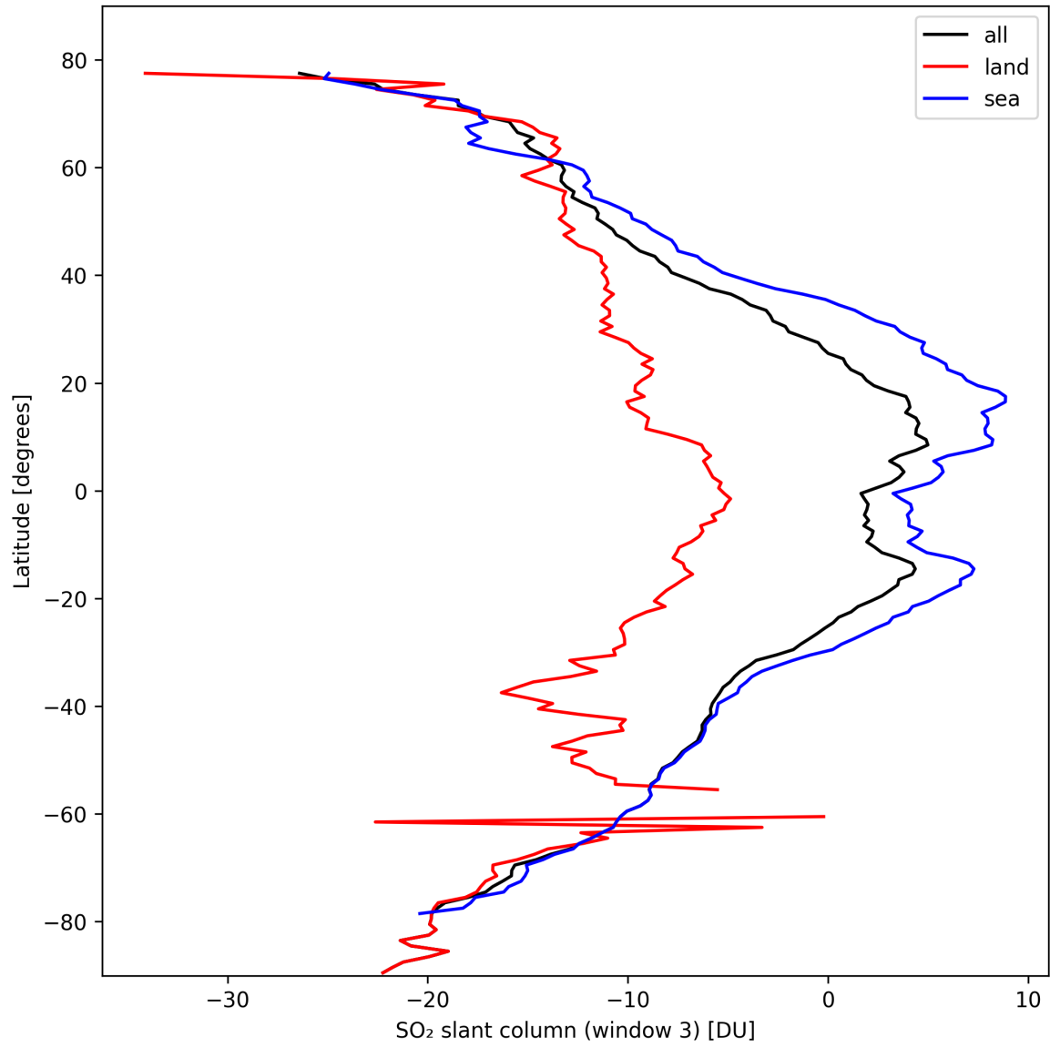
Figure 41: Zonal average of “SO 2 slant column (window 3)” for 2024-10-11 to 2024-10-13.
