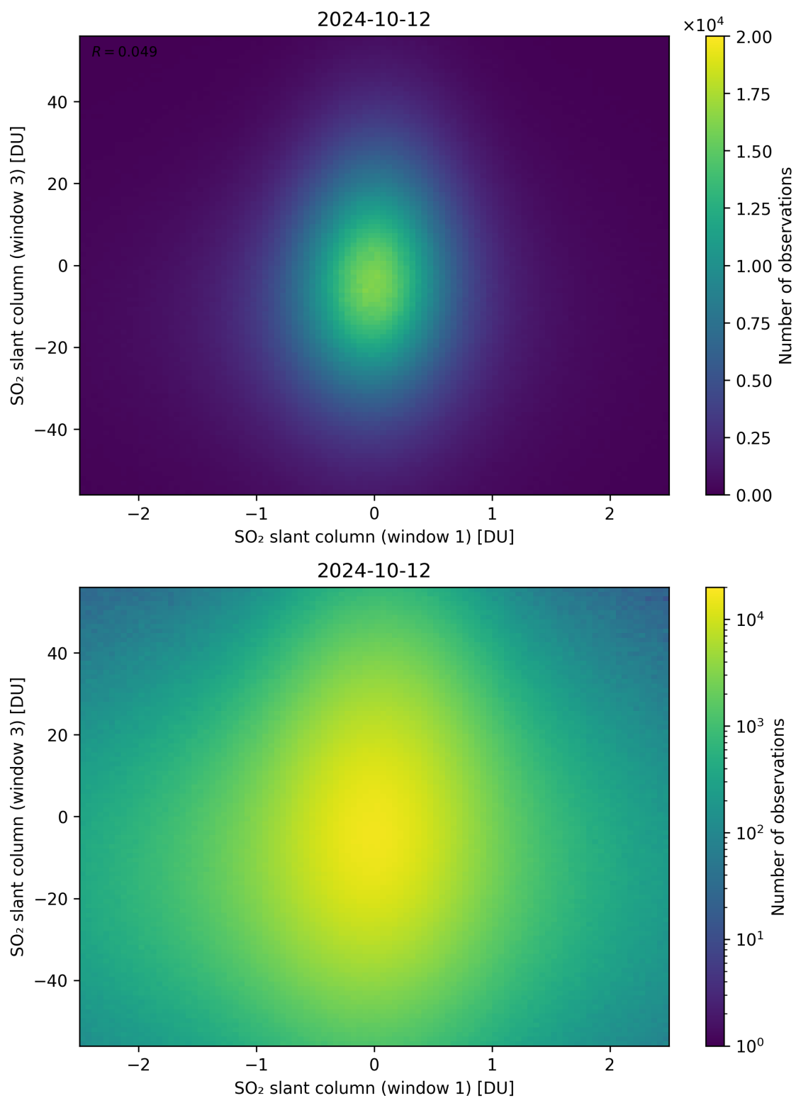
Figure 237: Scatter density plot of “SO 2 slant column (window 1)” against “SO 2 slant column (window 3)” for 2024-10-11 to 2024-10-13.
