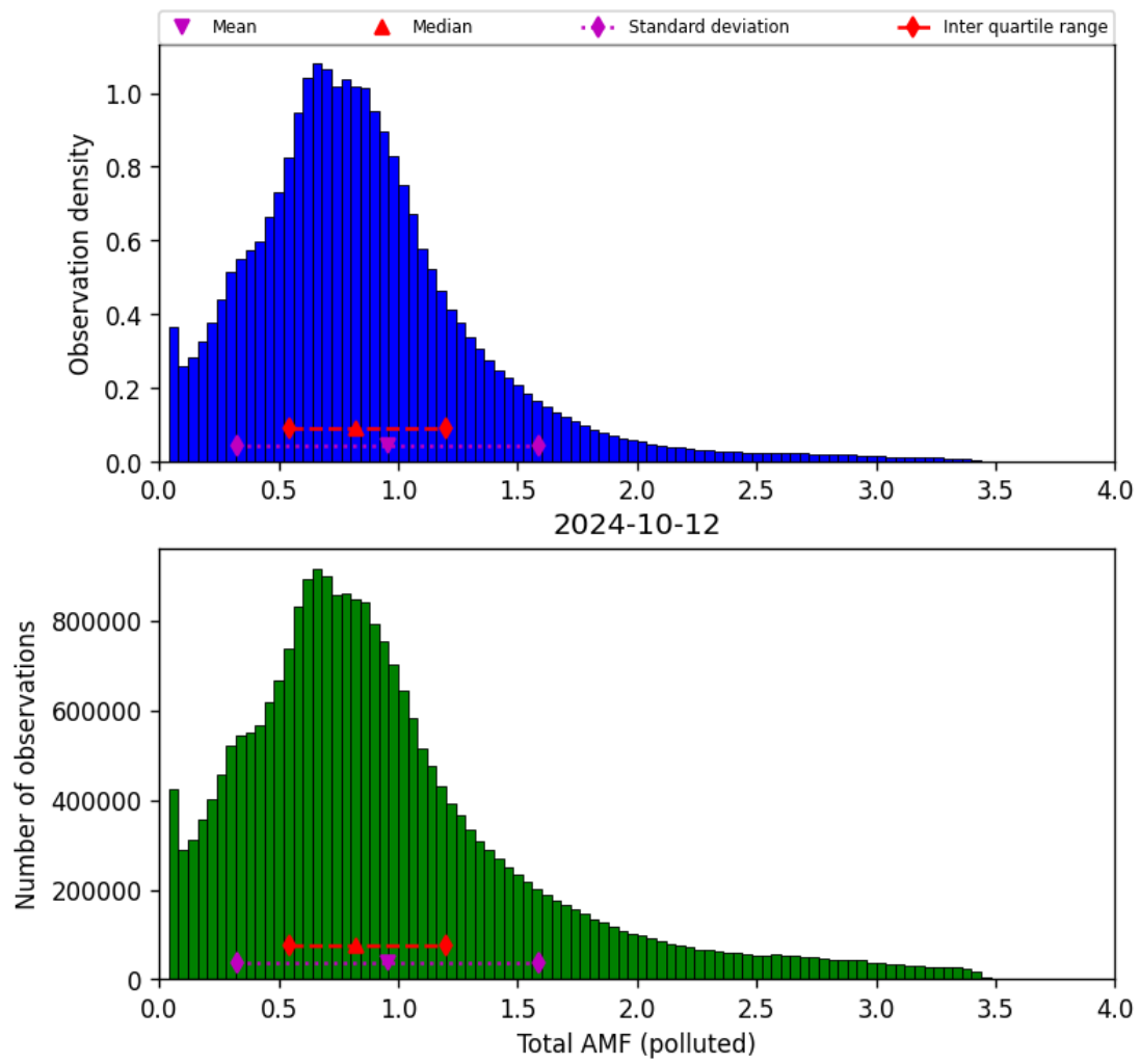
Figure 71: Histogram of “Total AMF (polluted)” for 2024-10-11 to 2024-10-13
