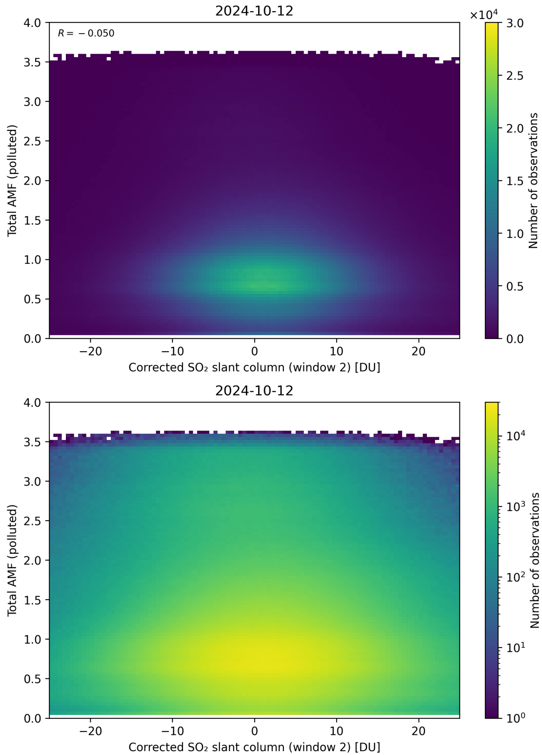
Figure 203: Scatter density plot of “Corrected SO 2 slant column (window 2)” against “Total AMF (polluted)” for 2024-10-11 to 2024-10-13.
