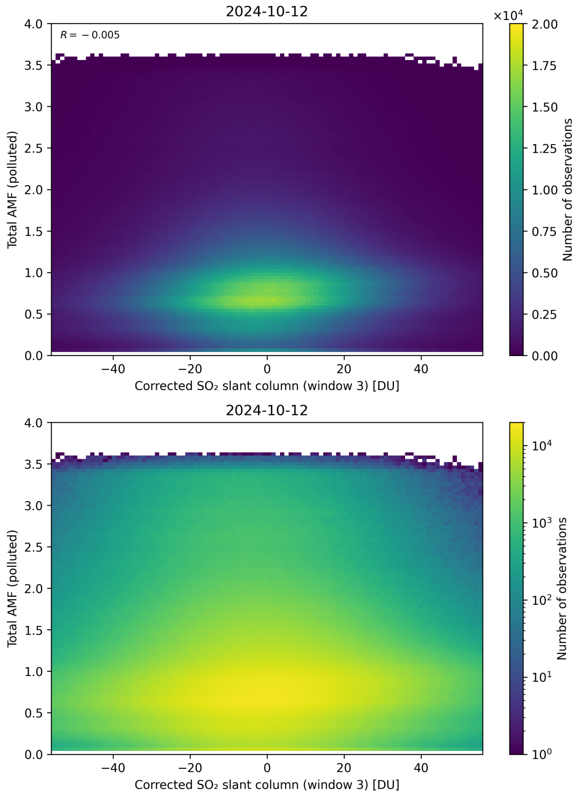
Figure 210: Scatter density plot of “Corrected SO 2 slant column (window 3)” against “Total AMF (polluted)” for 2024-10-11 to 2024-10-13.
