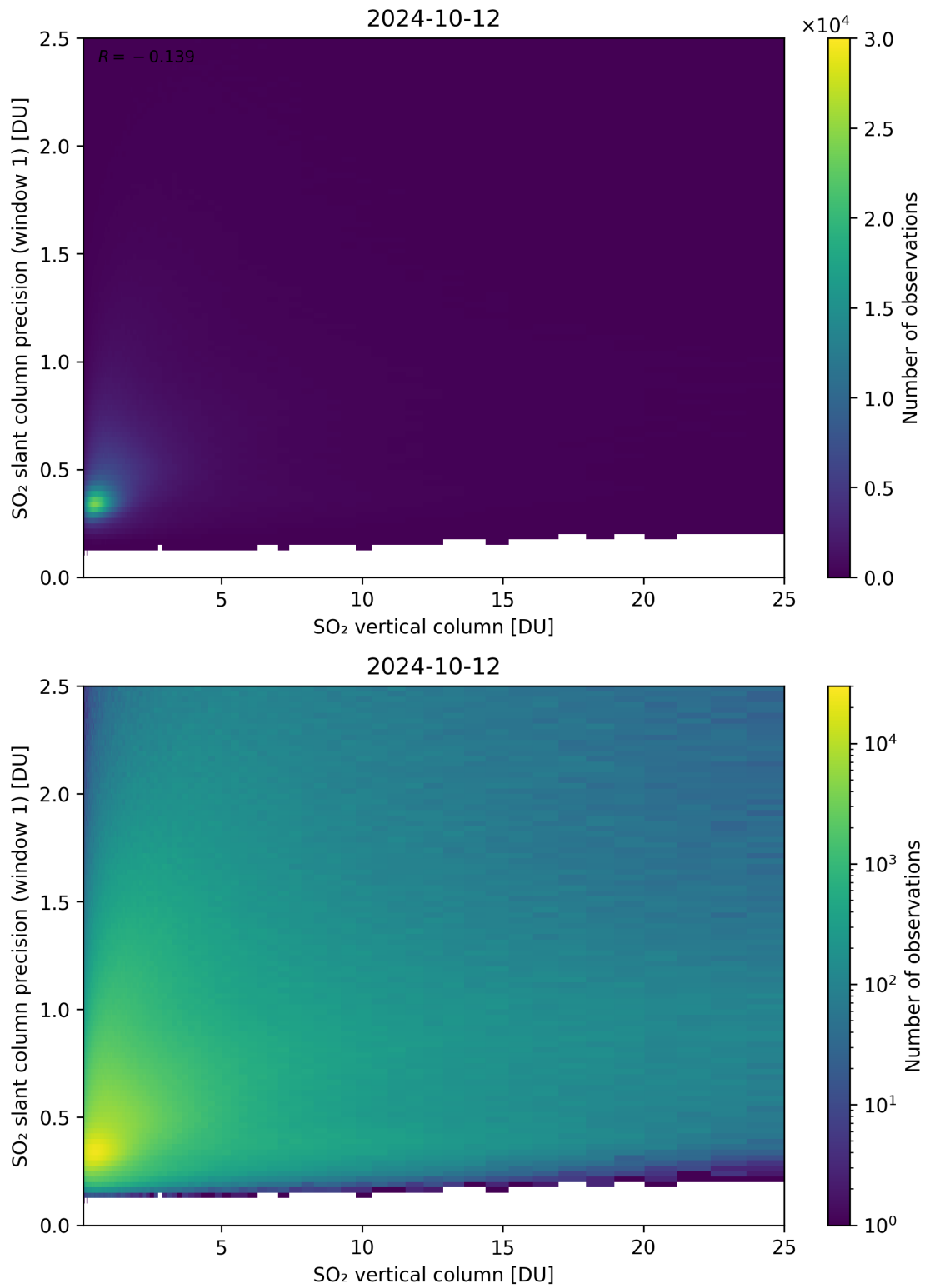
Figure 301: Scatter density plot of “SO 2 vertical column” against “SO 2 slant column precision (window 1)” for 2024-10-11 to 2024-10-13.
