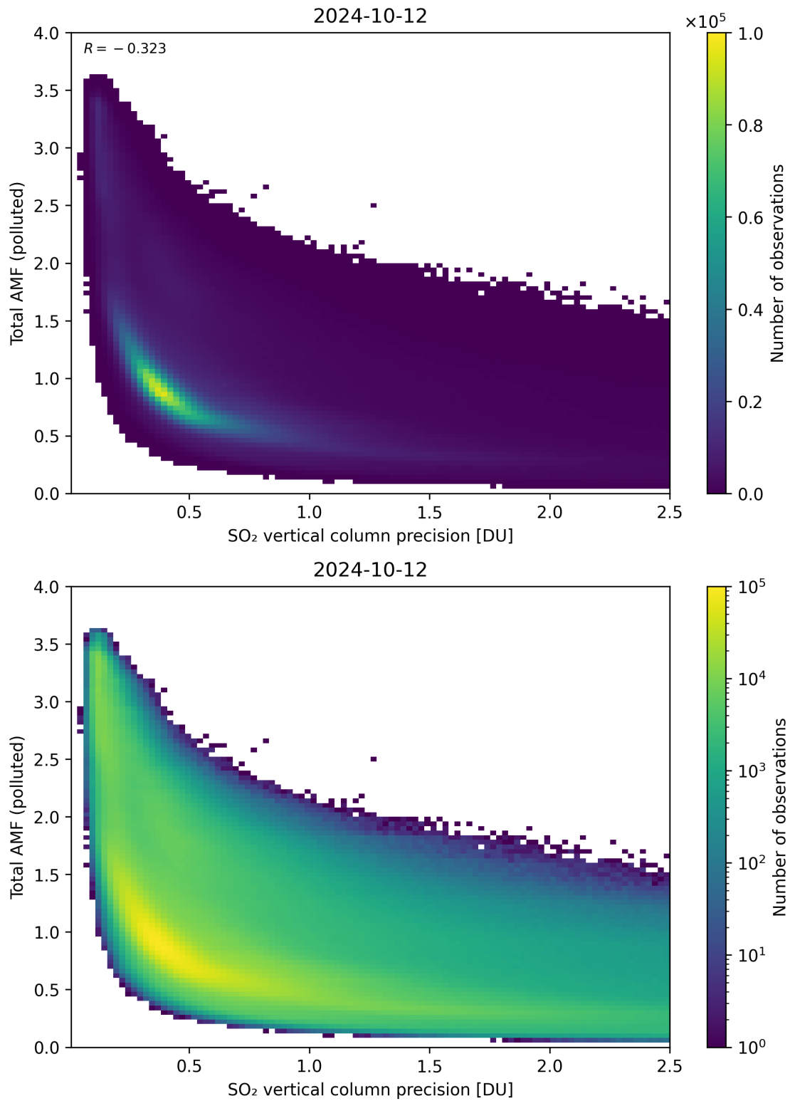
Figure 294: Scatter density plot of “SO 2 vertical column precision” against “Total AMF (polluted)” for 2024-10-11 to 2024-10-13.
