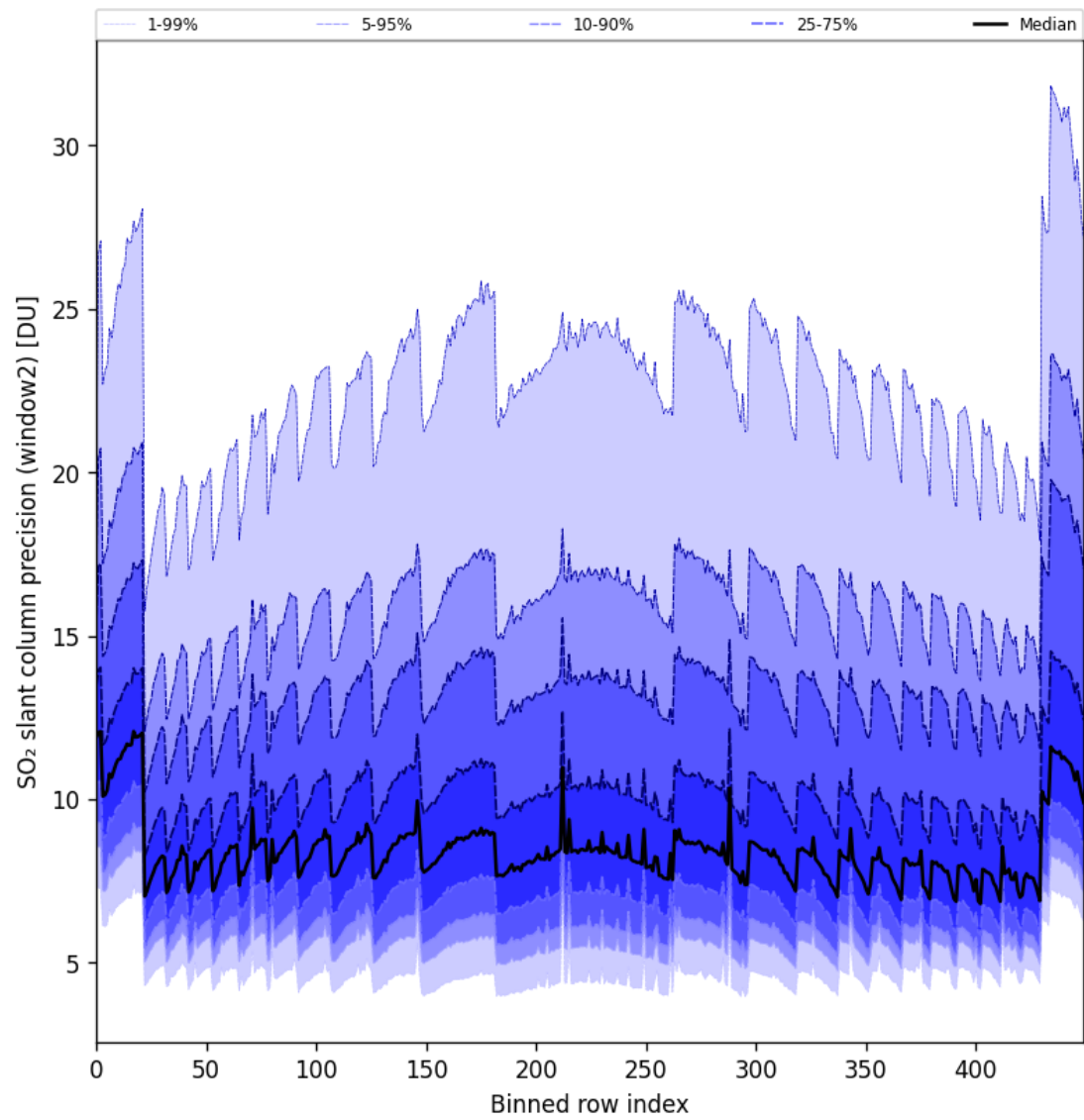
Figure 84: Along track statistics of “SO 2 slant column precision (window2)” for 2024-10-11 to 2024-10-13
