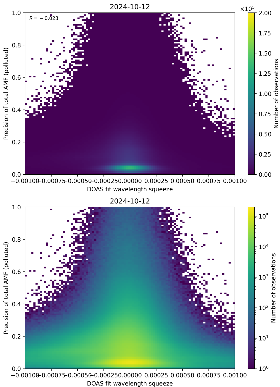
Figure 135: Scatter density plot of “DOAS fit wavelength squeeze” against “Precision of total AMF (polluted)” for 2024-10-11 to 2024-10-13.
