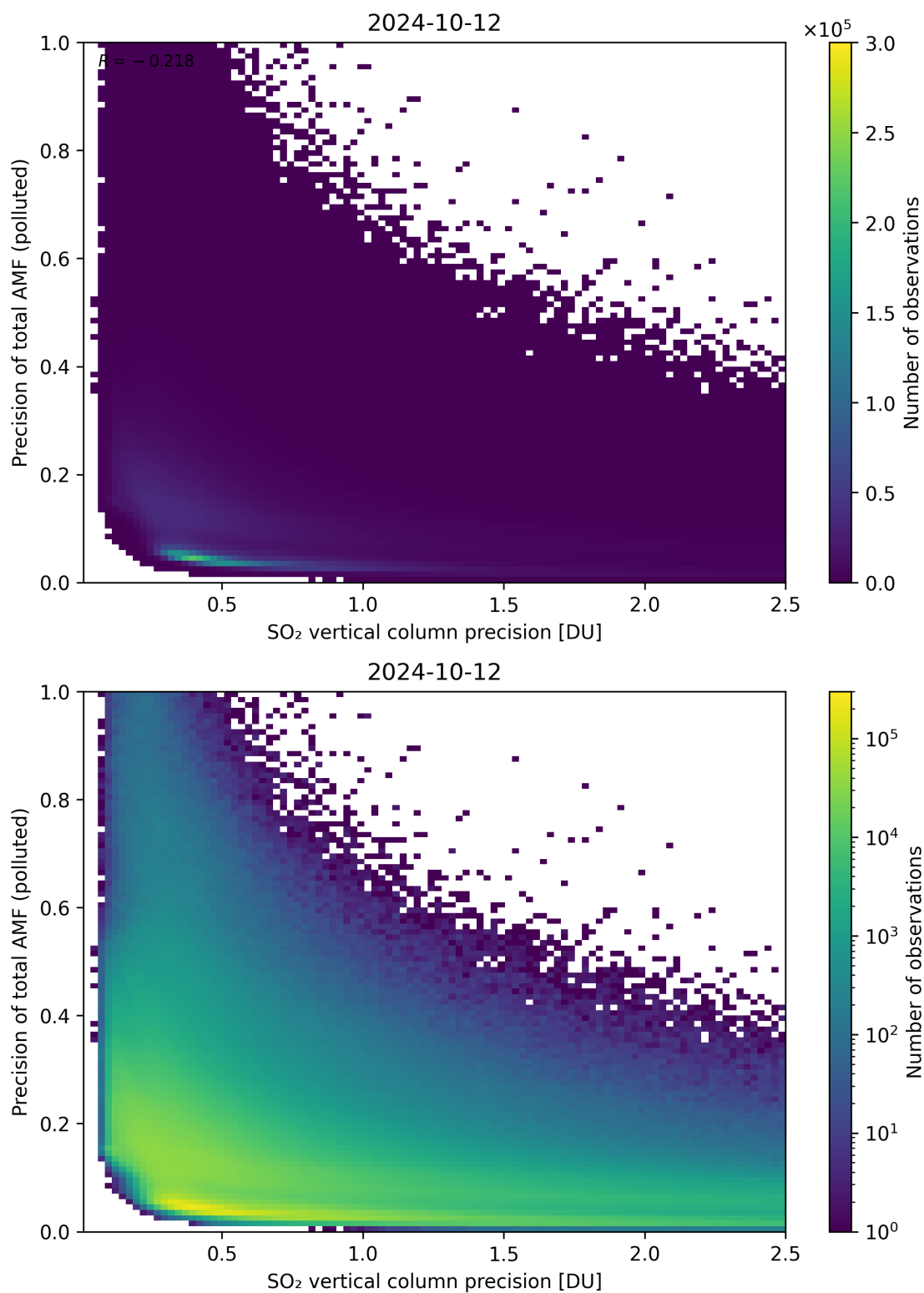
Figure 295: Scatter density plot of “SO 2 vertical column precision” against “Precision of total AMF (polluted)” for 2024-10-11 to 2024-10-13.
