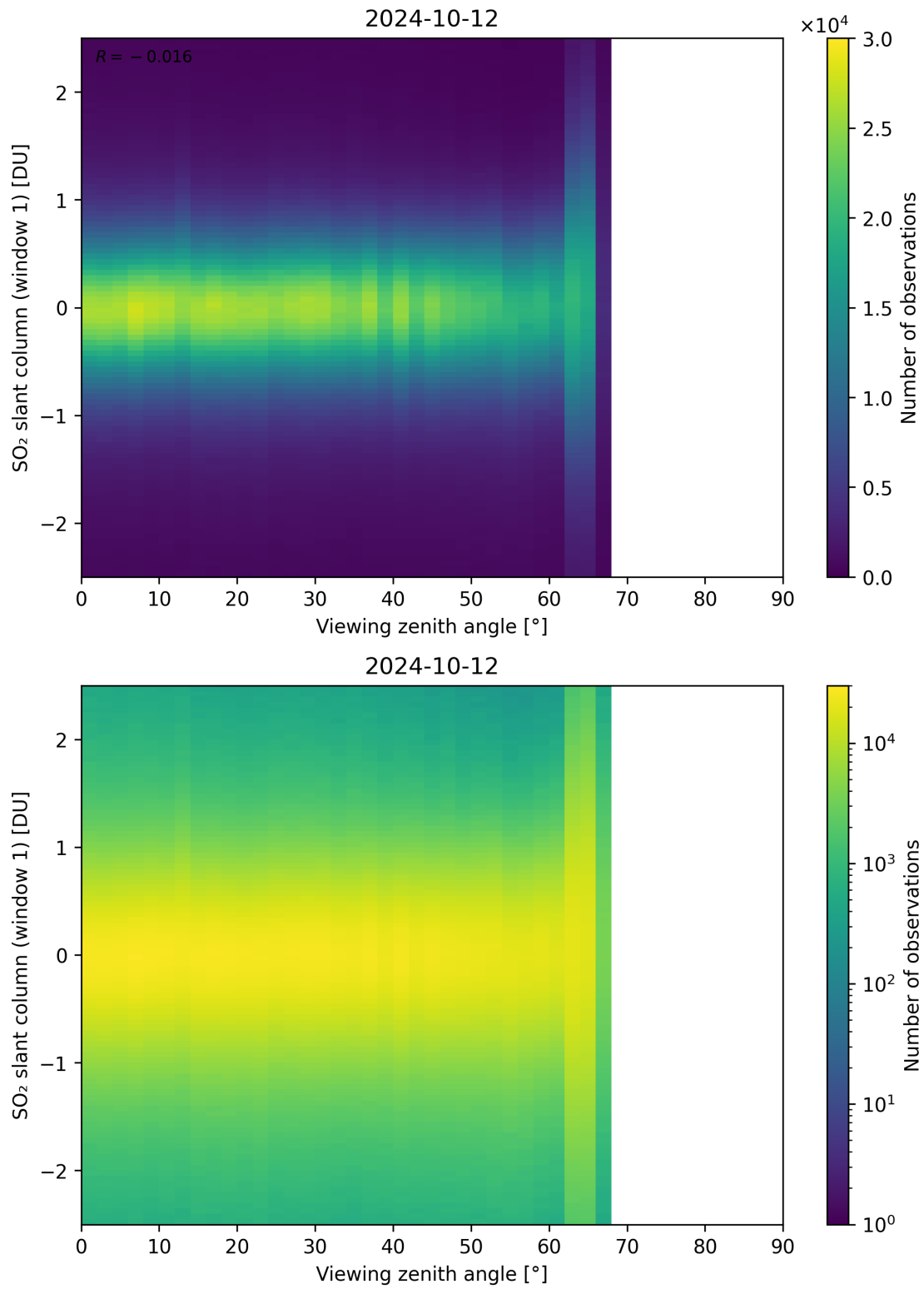
Figure 320: Scatter density plot of “Viewing zenith angle” against “SO 2 slant column (window 1)” for 2024-10-11 to 2024-10-13.
