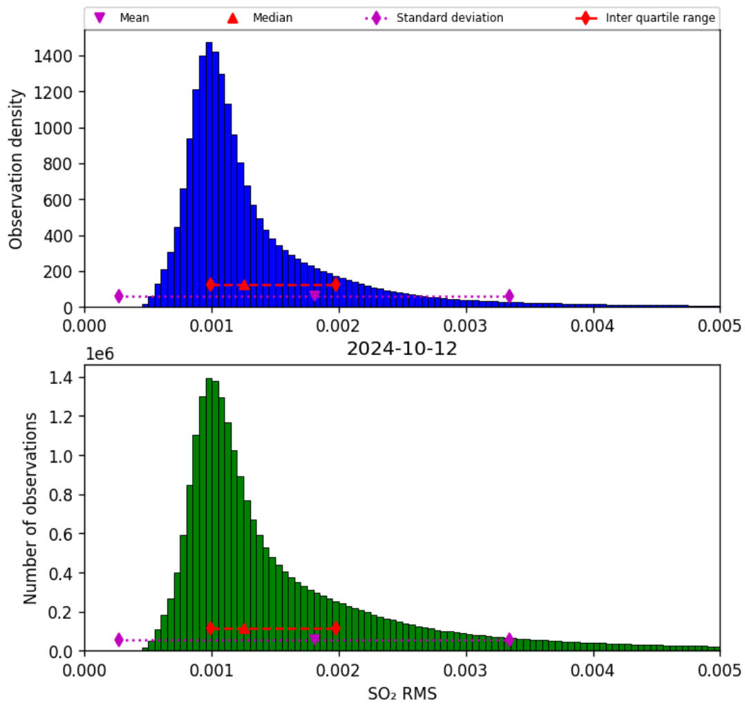
Figure 70: Histogram of “SO 2 RMS” for 2024-10-11 to 2024-10-13
