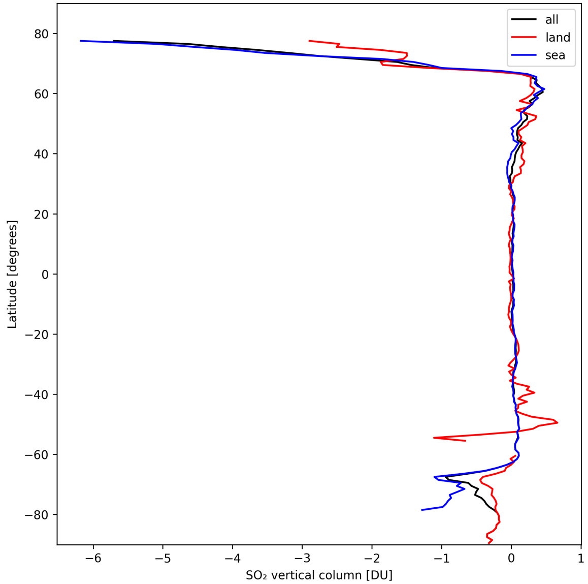
Figure 30: Zonal average of “SO 2 vertical column” for 2024-10-11 to 2024-10-13.
