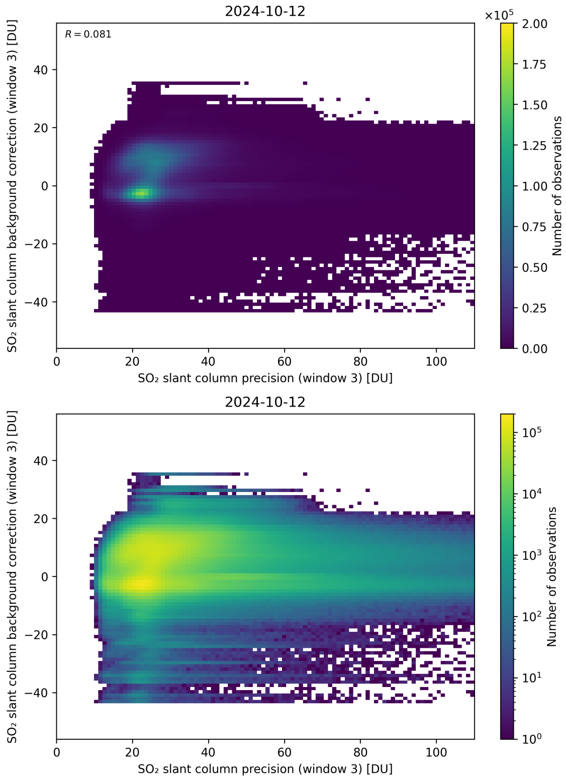
Figure 257: Scatter density plot of “SO 2 slant column precision (window 3)” against “SO 2 slant column background correction (window 3)” for 2024-10-11 to 2024-10-13.
