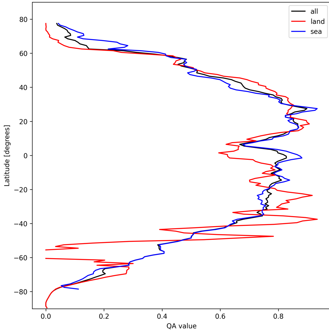
Figure 29: Zonal average of “QA value” for 2024-10-11 to 2024-10-13.
