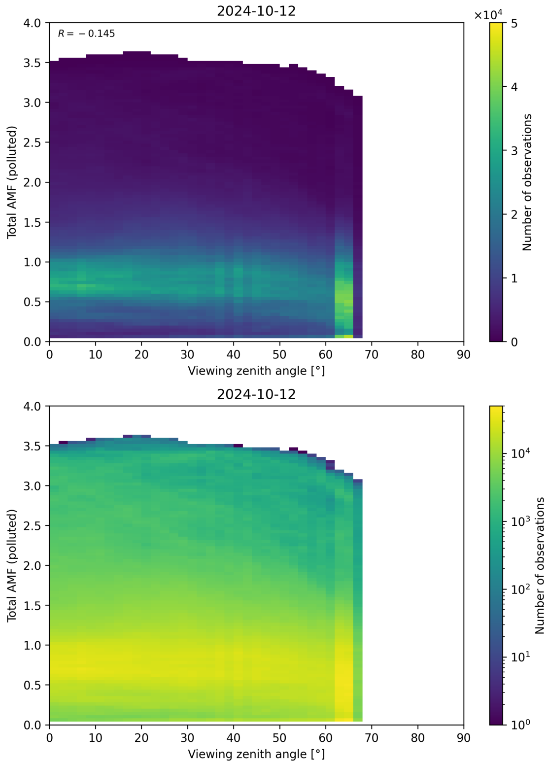
Figure 325: Scatter density plot of “Viewing zenith angle” against “Total AMF (polluted)” for 2024-10-11 to 2024-10-13.
