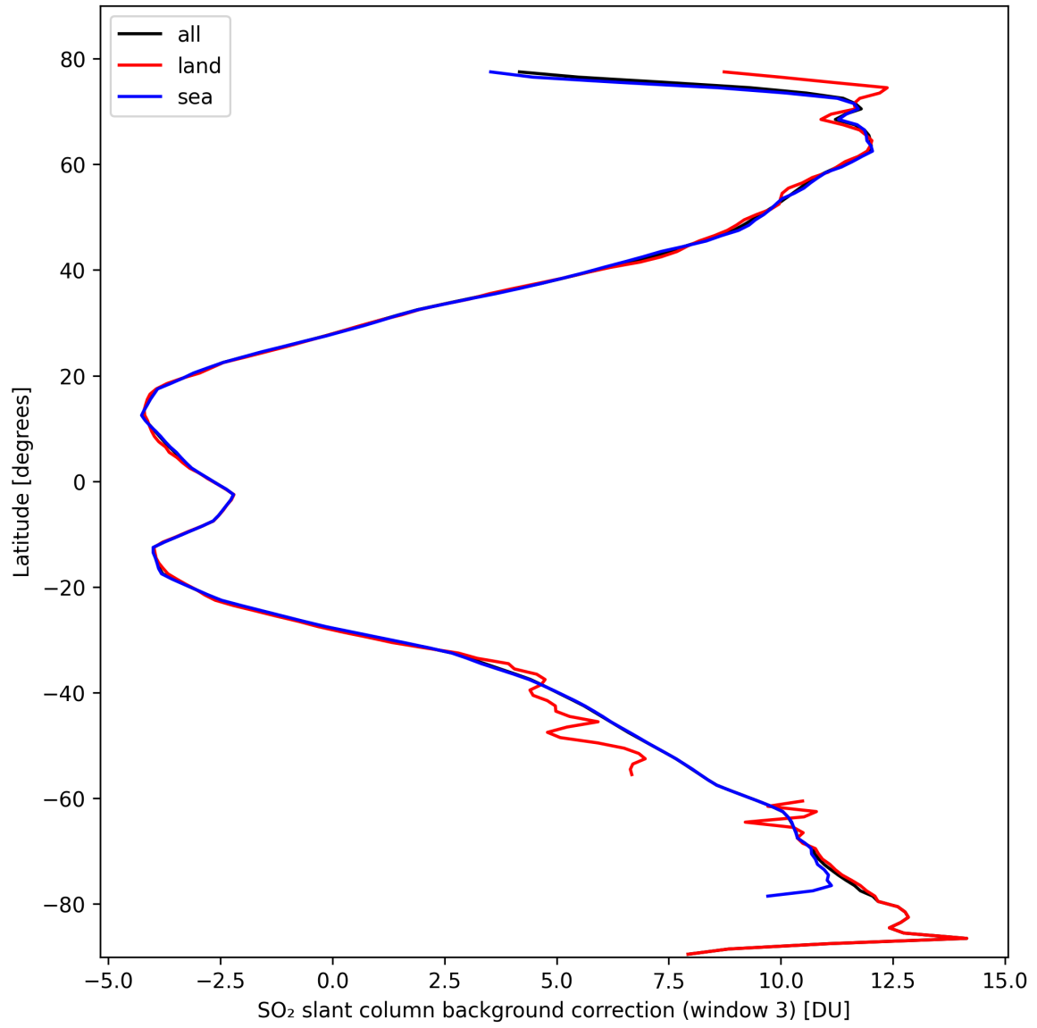
Figure 44: Zonal average of “SO 2 slant column background correction (window 3)” for 2024-10-11 to 2024-10-13.
