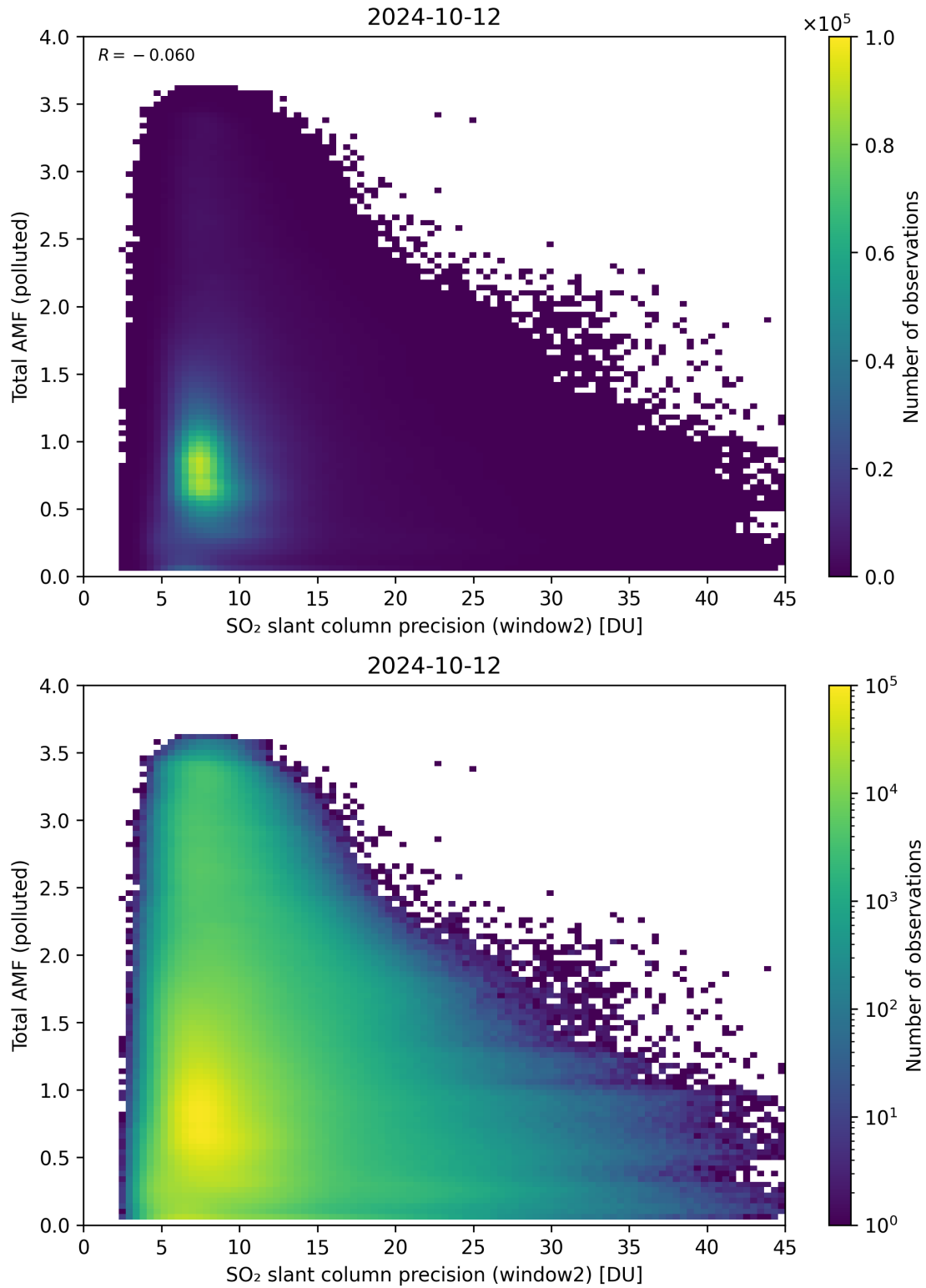
Figure 251: Scatter density plot of “SO 2 slant column precision (window2)” against “Total AMF (polluted)” for 2024-10-11 to 2024-10-13.
