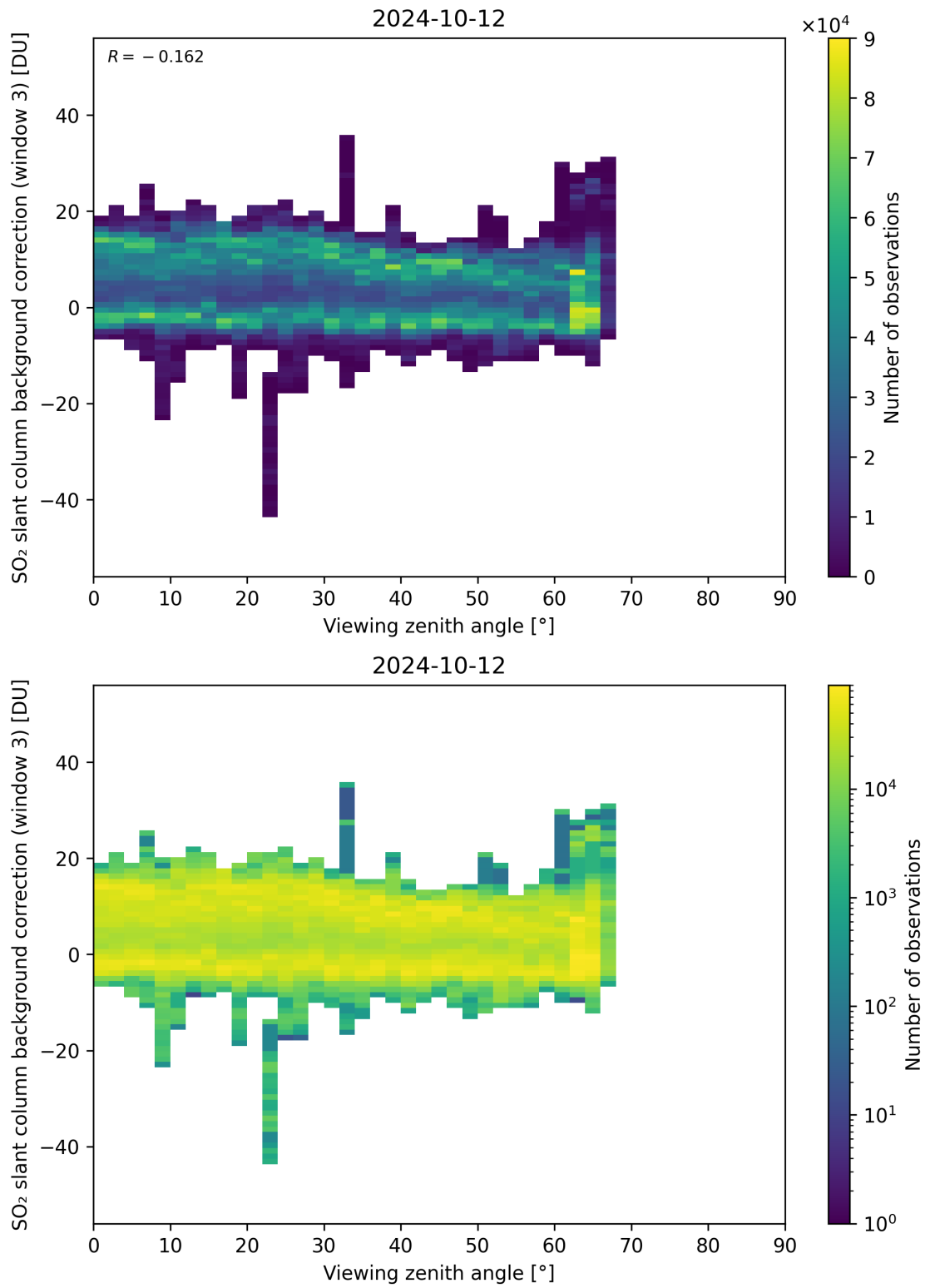
Figure 310: Scatter density plot of “Viewing zenith angle” against “SO 2 slant column background correction (window 3)” for 2024-10-11 to 2024-10-13.
