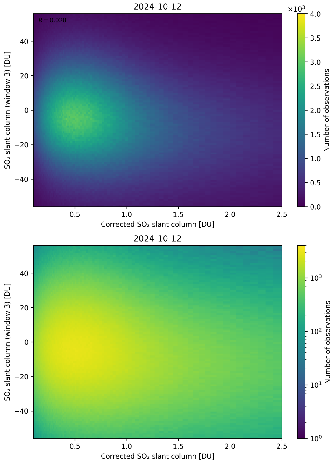
Figure 190: Scatter density plot of “Corrected SO 2 slant column” against “SO 2 slant column (window 3)” for 2024-10-11 to 2024-10-13.
