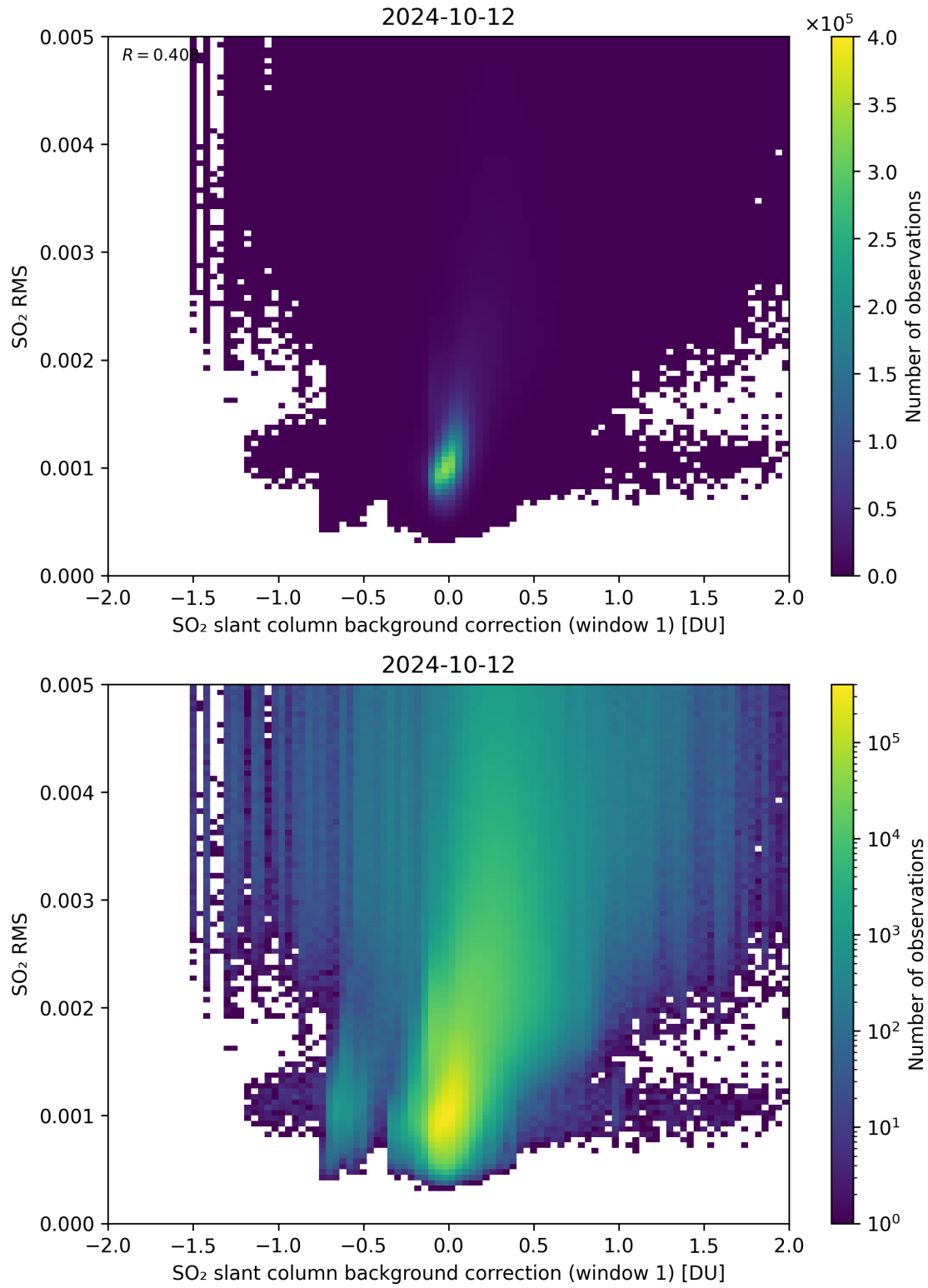
Figure 102: Scatter density plot of “SO 2 slant column background correction (window 1)” against “SO 2 RMS” for 2024-10-11 to 2024-10-13.
