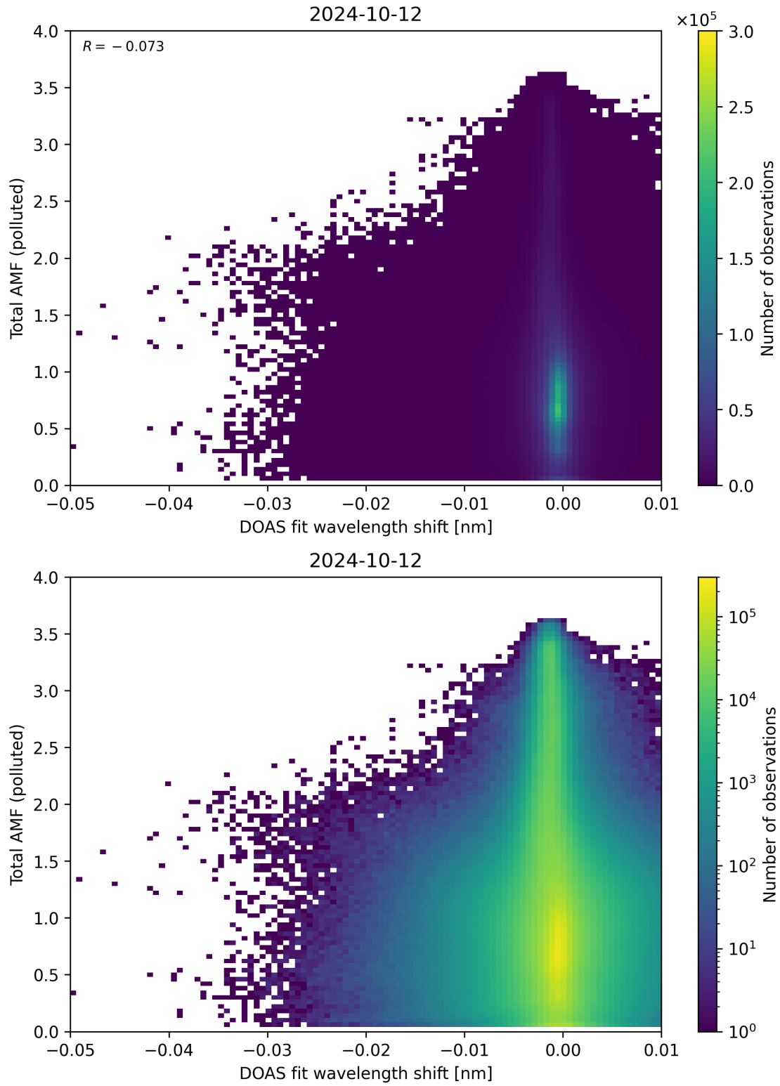
Figure 130: Scatter density plot of “DOAS fit wavelength shift” against “Total AMF (polluted)” for 2024-10-11 to 2024-10-13.
