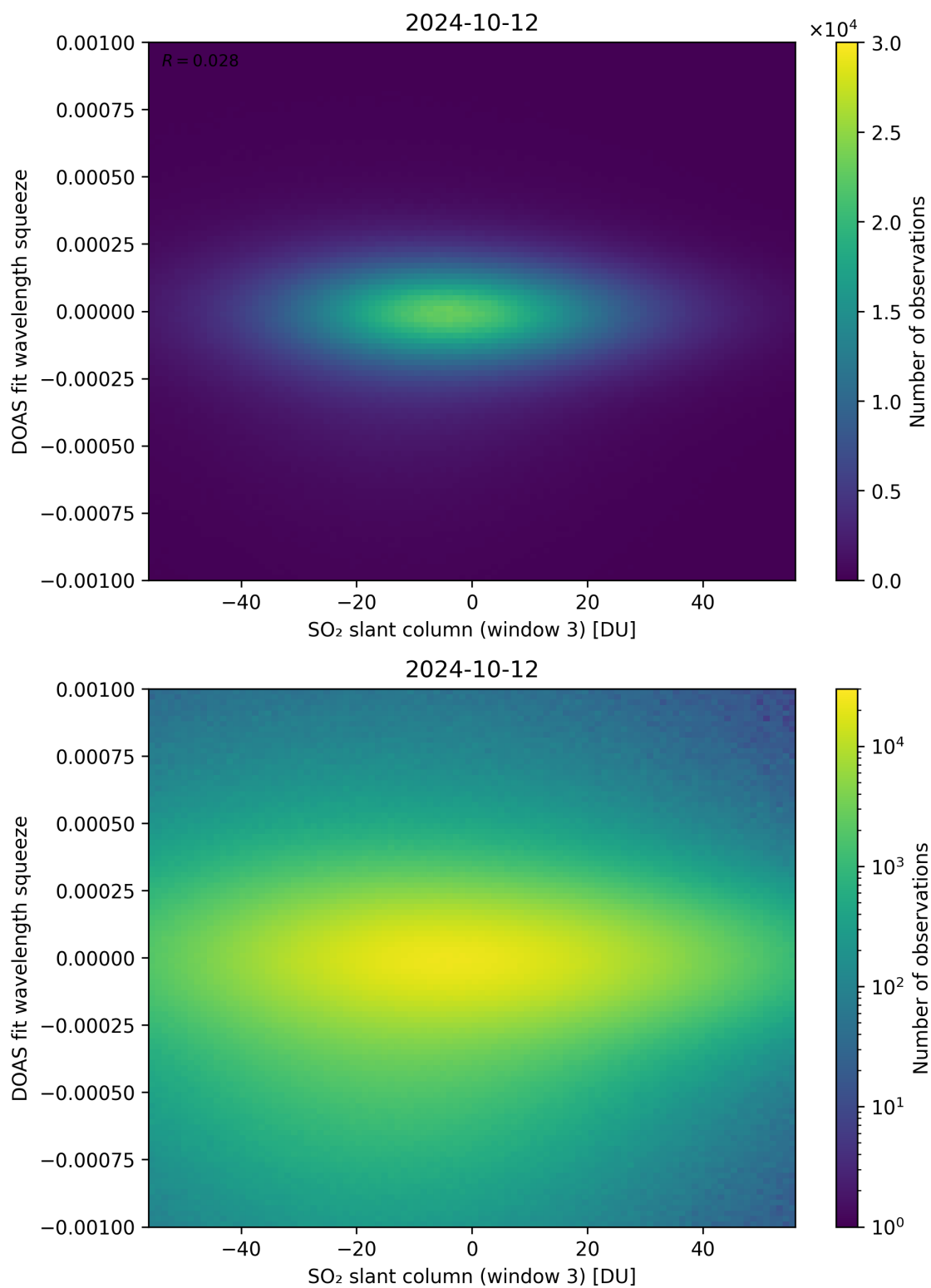
Figure 255: Scatter density plot of “SO 2 slant column (window 3)” against “DOAS fit wavelength squeeze” for 2024-10-11 to 2024-10-13.
