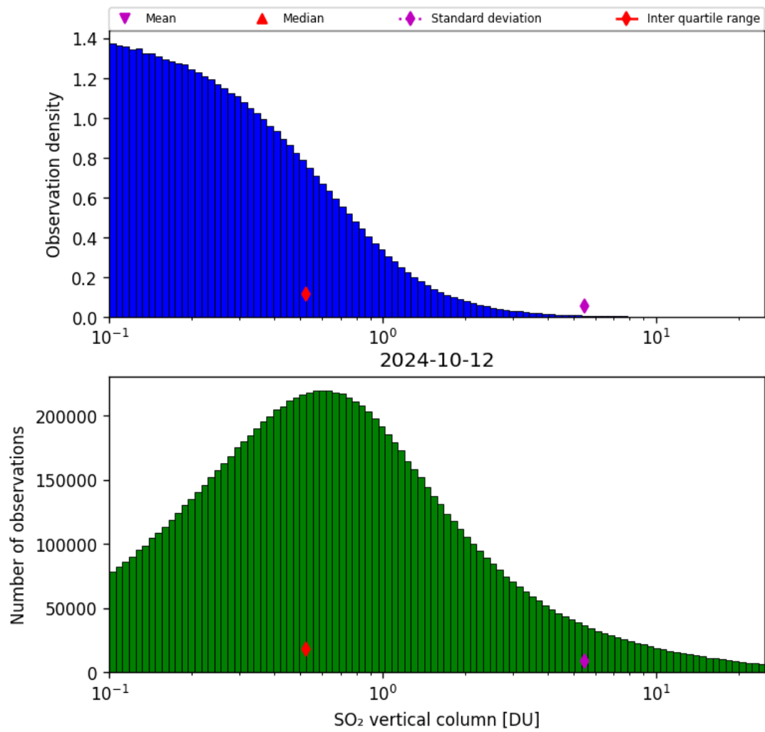
Figure 53: Histogram of “SO 2 vertical column” for 2024-10-11 to 2024-10-13
