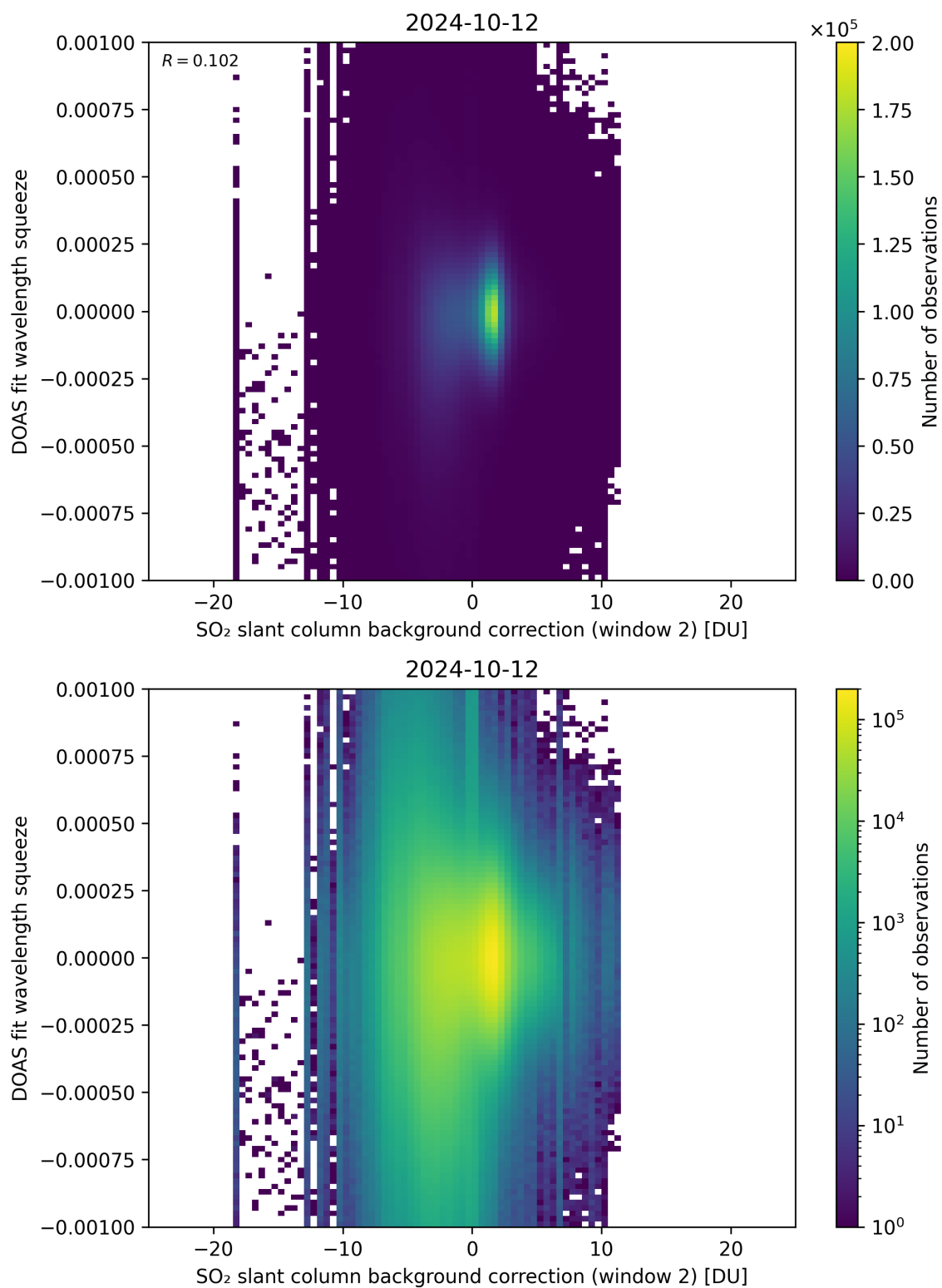
Figure 113: Scatter density plot of “SO 2 slant column background correction (window 2)” against “DOAS fit wavelength squeeze” for 2024-10-11 to 2024-10-13.
