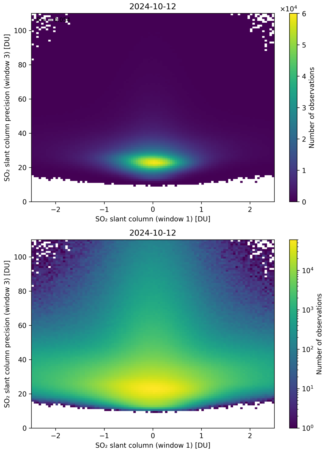
Figure 238: Scatter density plot of “SO 2 slant column (window 1)” against “SO 2 slant column precision (window 3)” for 2024-10-11 to 2024-10-13.
