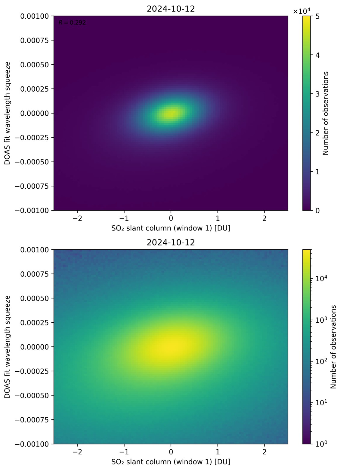
Figure 216: Scatter density plot of “SO 2 slant column (window 1)” against “DOAS fit wavelength squeeze” for 2024-10-11 to 2024-10-13.
