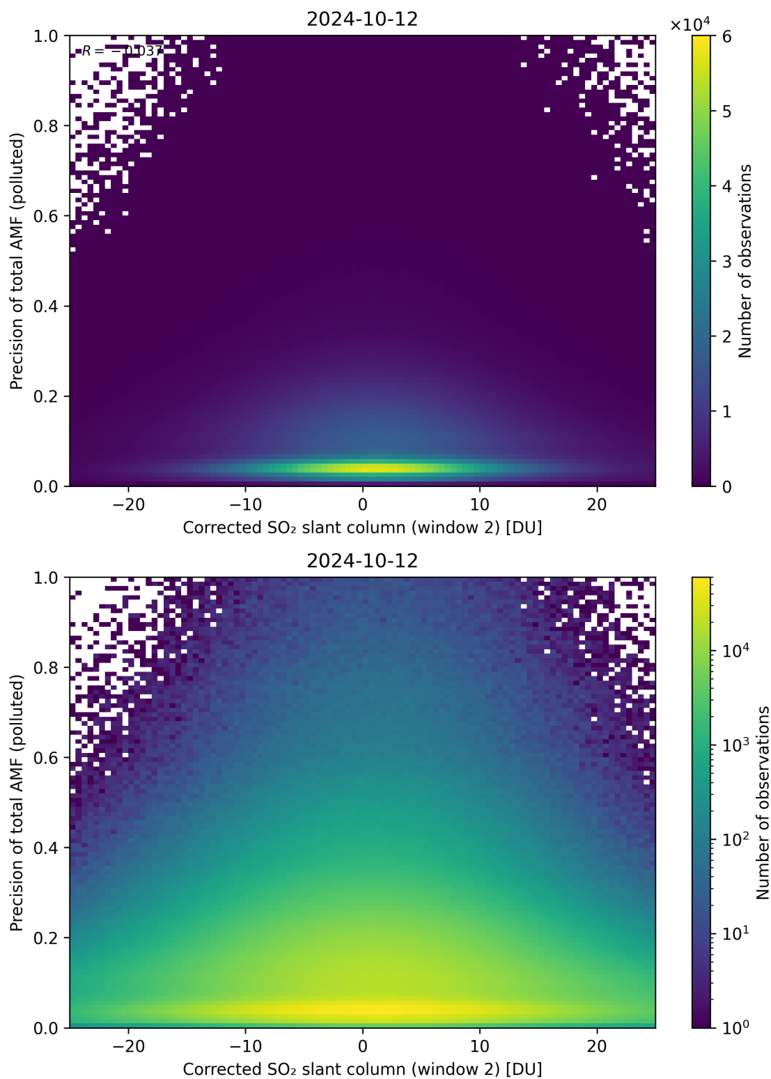
Figure 204: Scatter density plot of “Corrected SO 2 slant column (window 2)” against “Precision of total AMF (polluted)” for 2024-10-11 to 2024-10-13.
