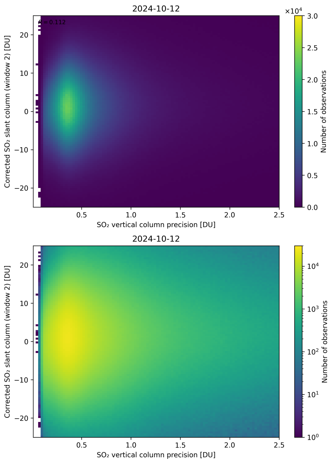
Figure 287: Scatter density plot of “SO 2 vertical column precision” against “Corrected SO 2 slant column (window 2)” for 2024-10-11 to 2024-10-13.
