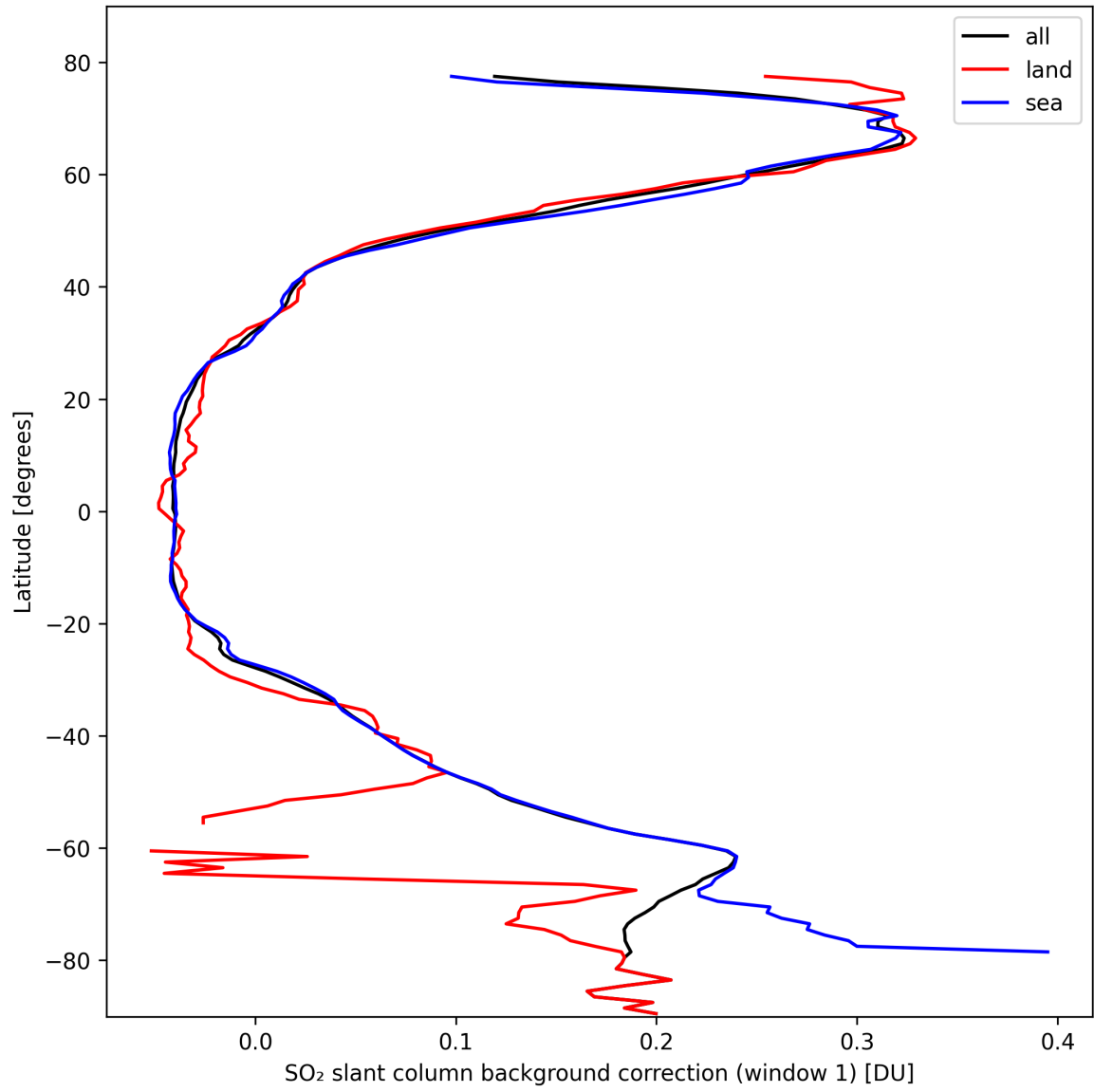
Figure 36: Zonal average of “SO 2 slant column background correction (window 1)” for 2024-10-11 to 2024-10-13.
