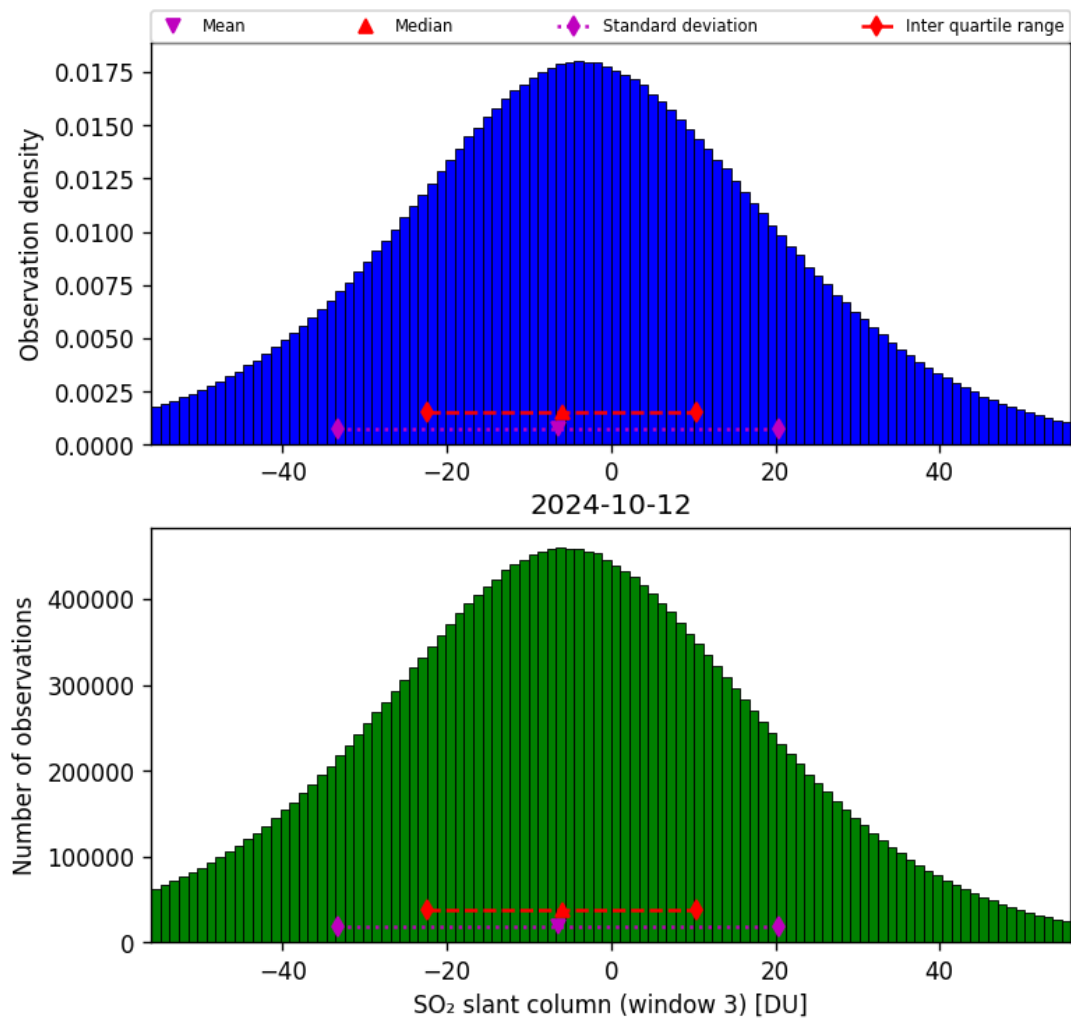
Figure 64: Histogram of “SO 2 slant column (window 3)” for 2024-10-11 to 2024-10-13
