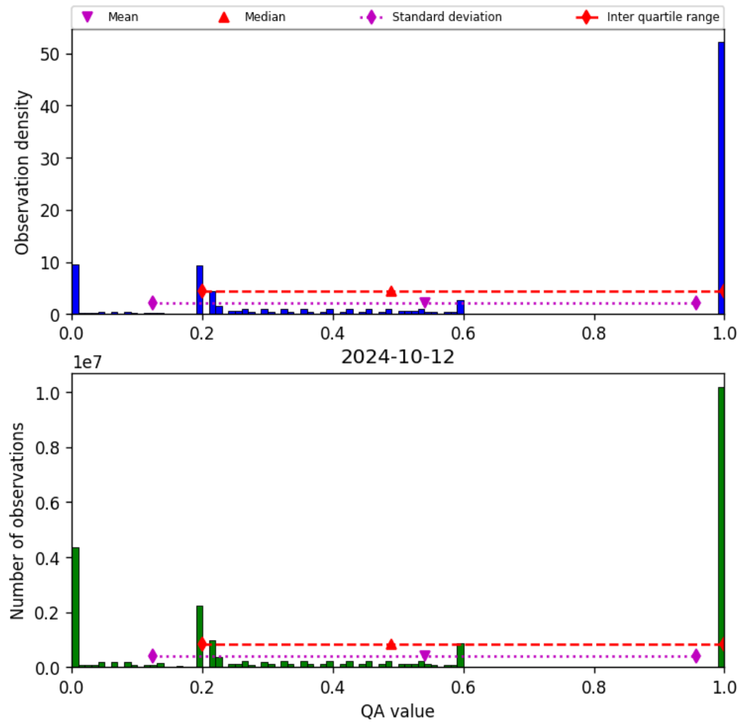
Figure 52: Histogram of “QA value” for 2024-10-11 to 2024-10-13
