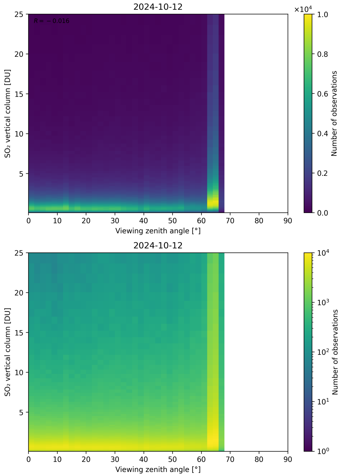
Figure 327: Scatter density plot of “Viewing zenith angle” against “SO 2 vertical column” for 2024-10-11 to 2024-10-13.
