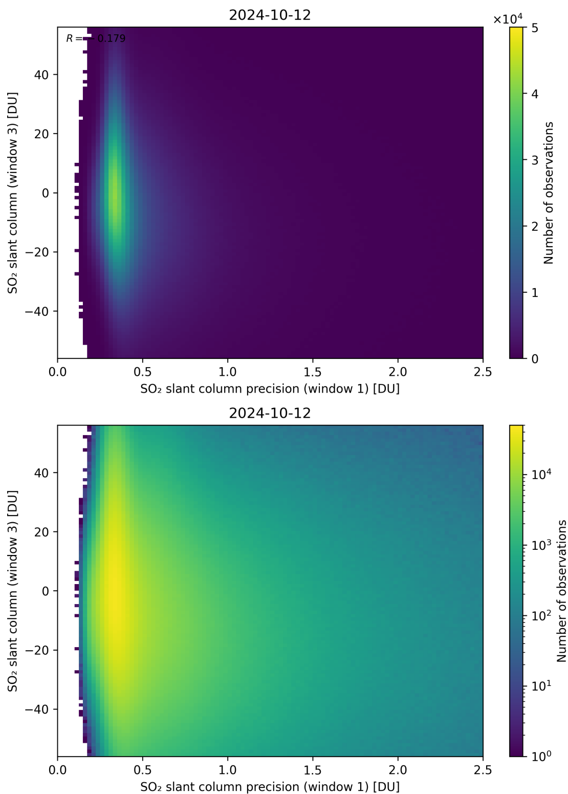
Figure 228: Scatter density plot of “SO 2 slant column precision (window 1)” against “SO 2 slant column (window 3)” for 2024-10-11 to 2024-10-13.
