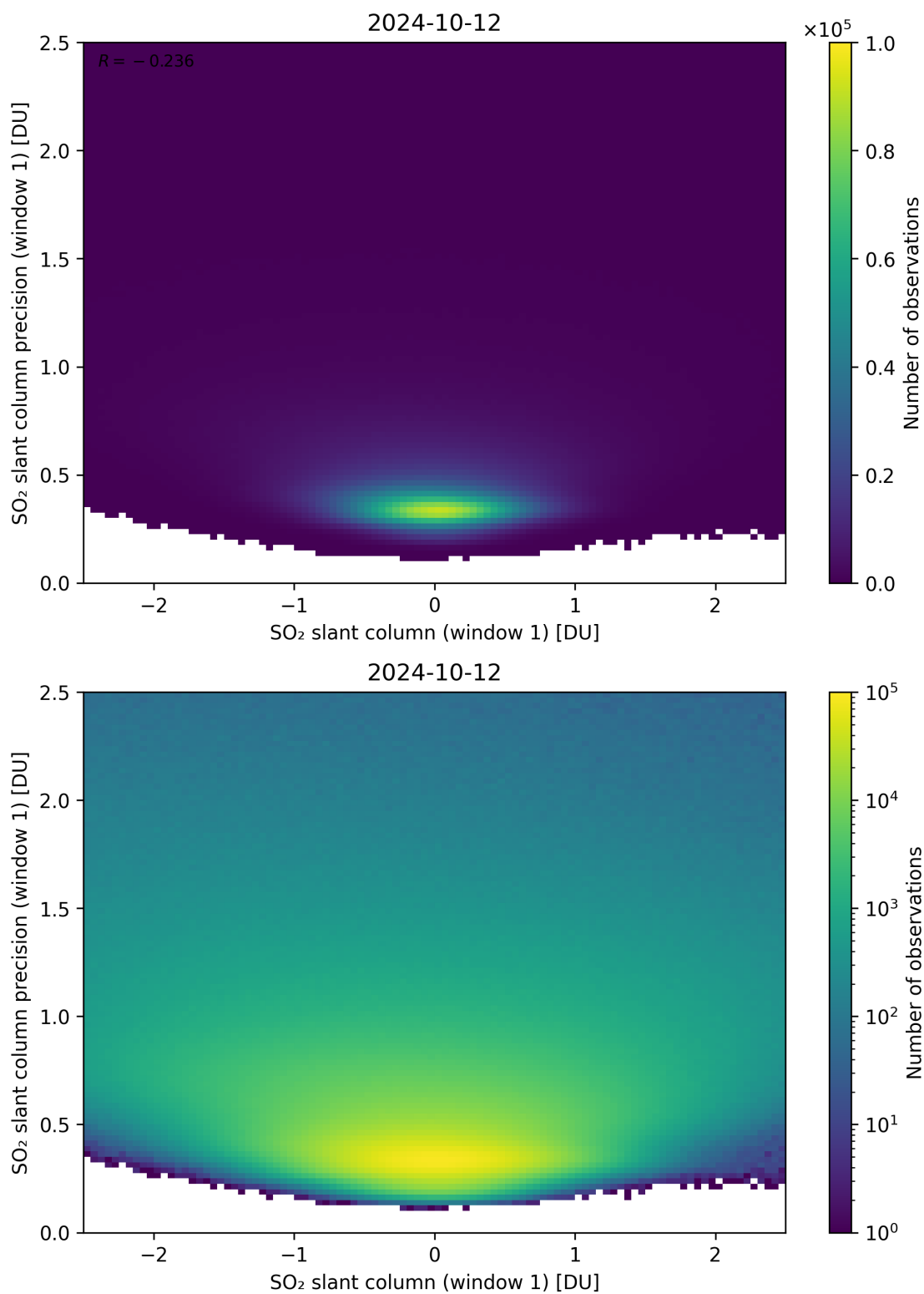
Figure 235: Scatter density plot of “SO 2 slant column (window 1)” against “SO 2 slant column precision (window 1)” for 2024-10-11 to 2024-10-13.
