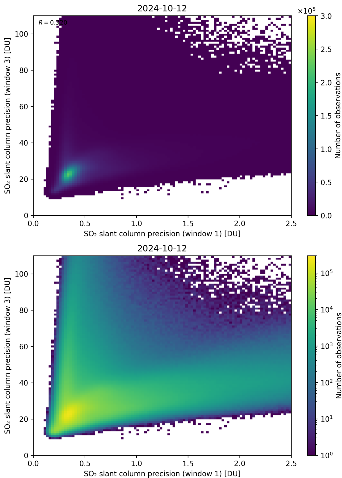
Figure 229: Scatter density plot of “SO 2 slant column precision (window 1)” against “SO 2 slant column precision (window 3)” for 2024-10-11 to 2024-10-13.
