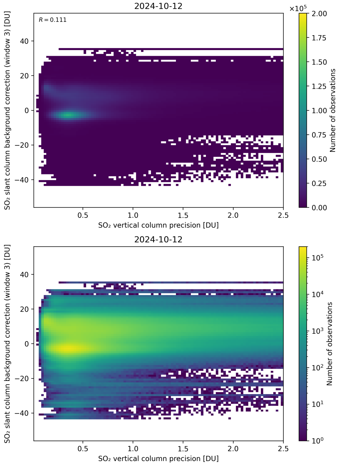
Figure 281: Scatter density plot of “SO 2 vertical column precision” against “SO 2 slant column background correction (window 3)” for 2024-10-11 to 2024-10-13.
