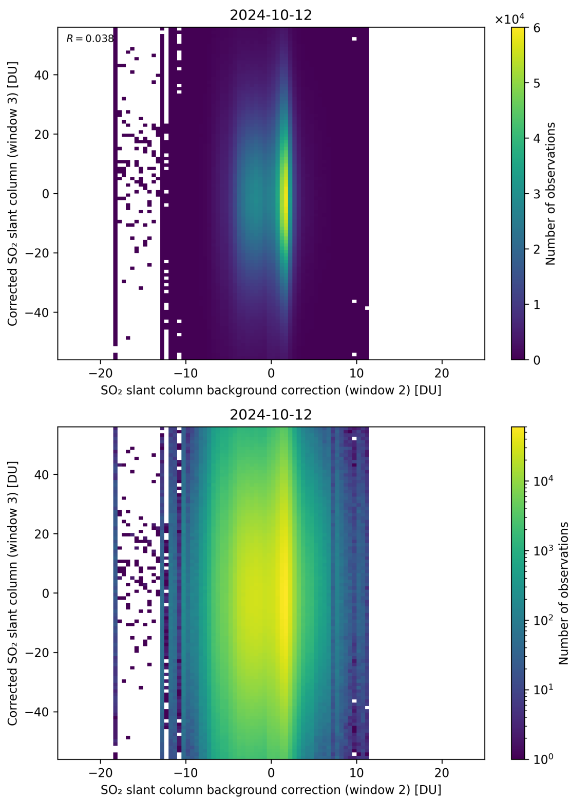
Figure 116: Scatter density plot of “SO 2 slant column background correction (window 2)” against “Corrected SO 2 slant column (window 3)” for 2024-10-11 to 2024-10-13.
