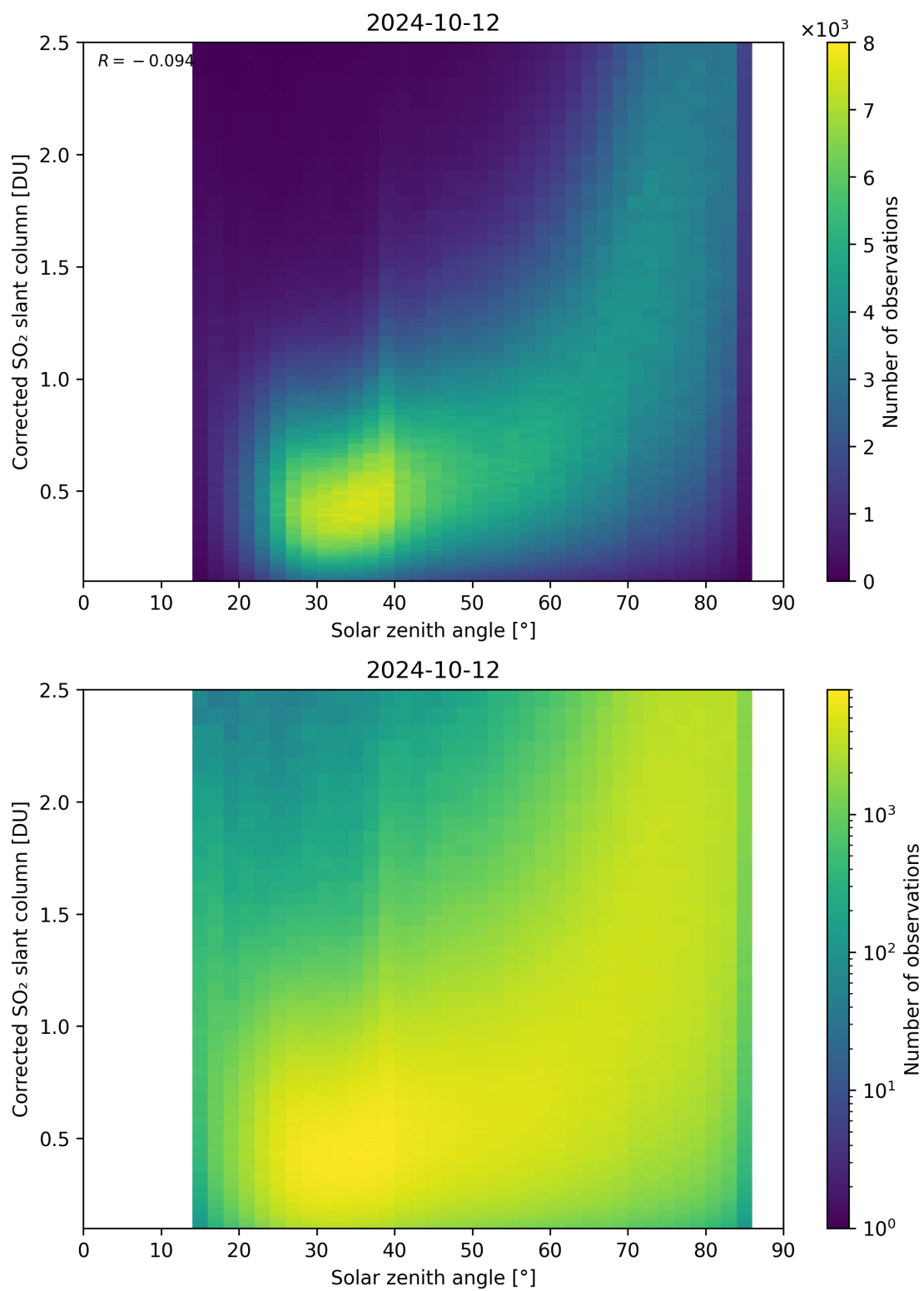
Figure 166: Scatter density plot of “Solar zenith angle” against “Corrected SO 2 slant column” for 2024-10-11 to 2024-10-13.
