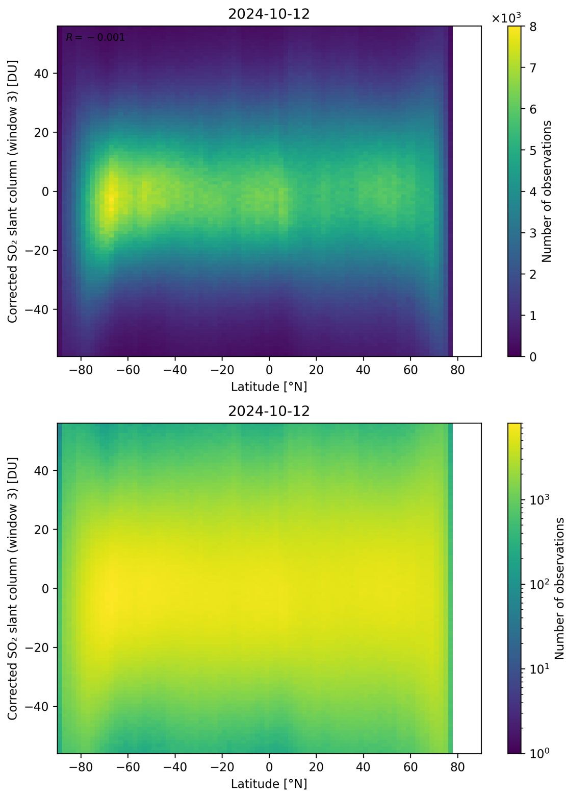
Figure 148: Scatter density plot of “Latitude” against “Corrected SO 2 slant column (window 3)” for 2024-10-11 to 2024-10-13.
