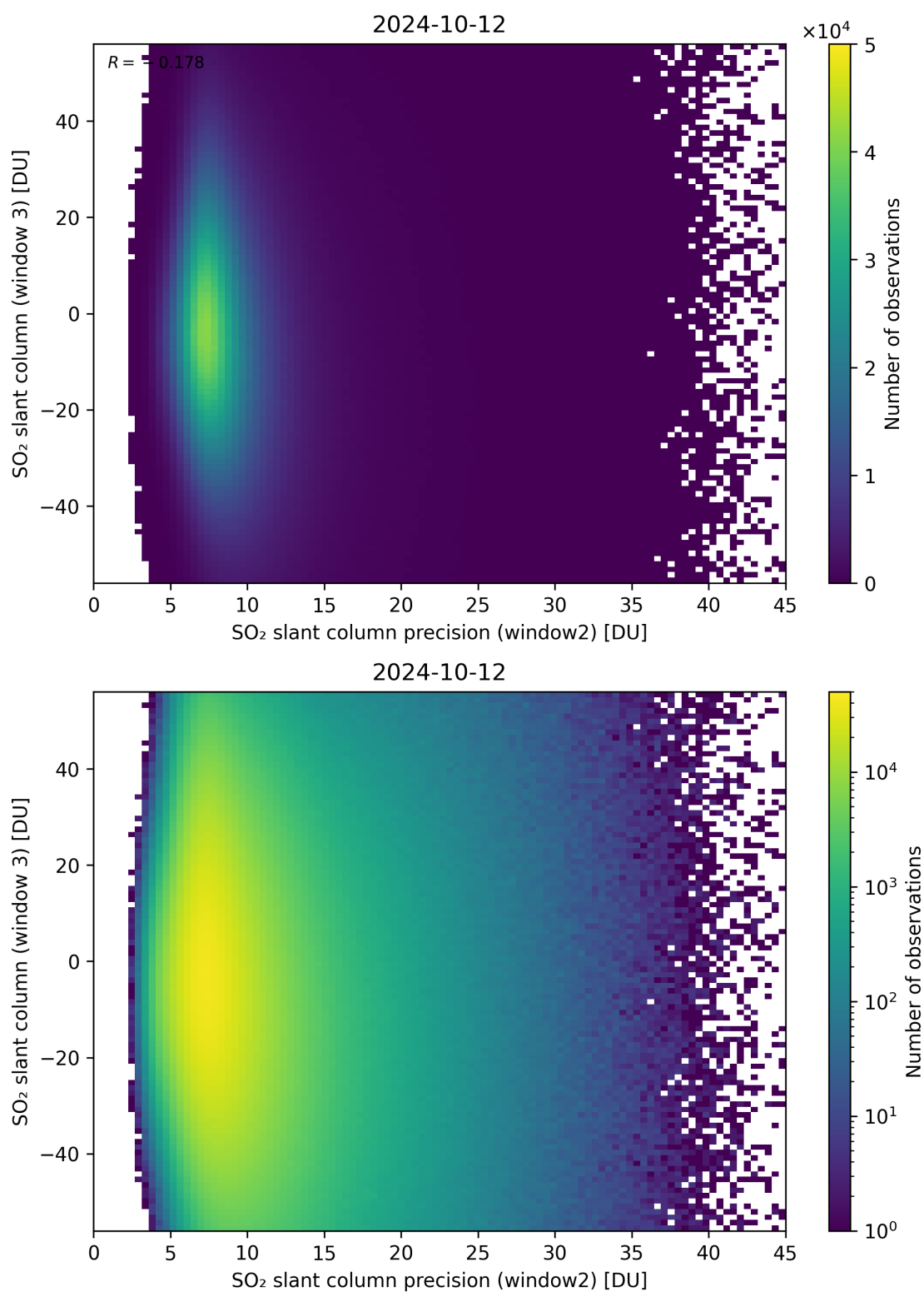
Figure 249: Scatter density plot of “SO 2 slant column precision (window2)” against “SO 2 slant column (window 3)” for 2024-10-11 to 2024-10-13.
