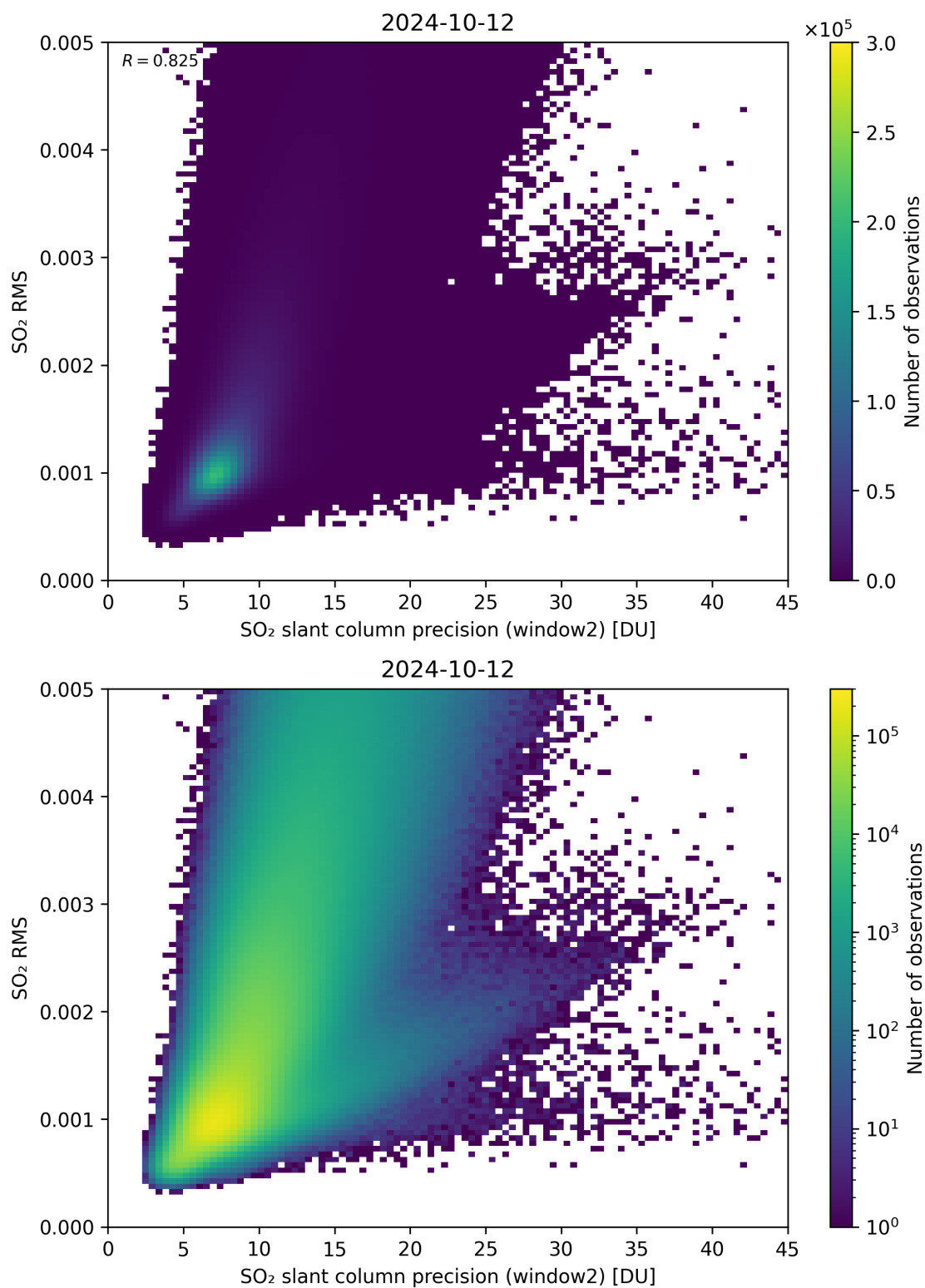
Figure 245: Scatter density plot of “SO 2 slant column precision (window2)” against “SO 2 RMS” for 2024-10-11 to 2024-10-13.
