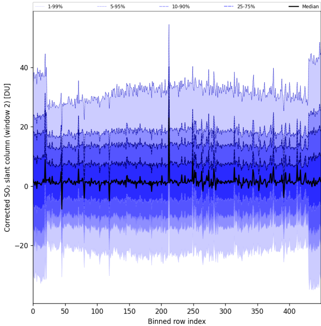
Figure 85: Along track statistics of “Corrected SO 2 slant column (window 2)” for 2024-10-11 to 2024-10-13
