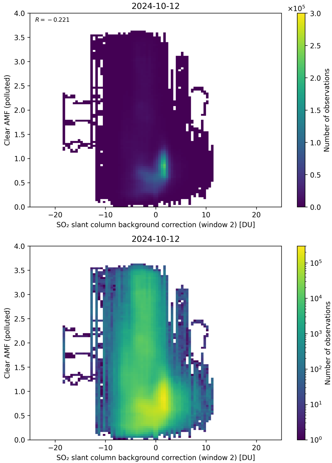
Figure 115: Scatter density plot of “SO 2 slant column background correction (window 2)” against “Clear AMF (polluted)” for 2024-10-11 to 2024-10-13.
