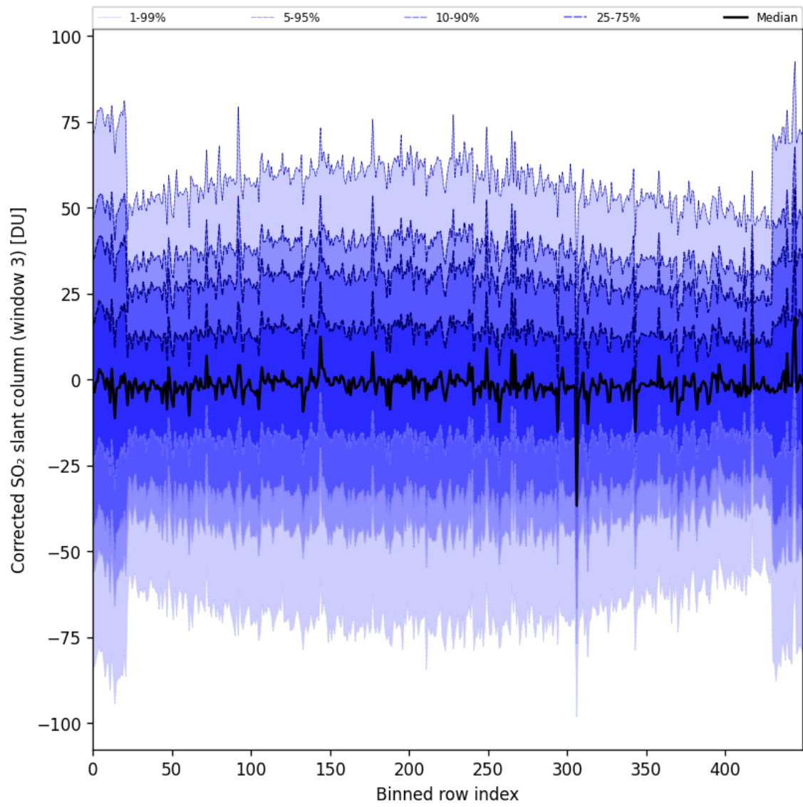
Figure 89: Along track statistics of “Corrected SO 2 slant column (window 3)” for 2024-10-11 to 2024-10-13
