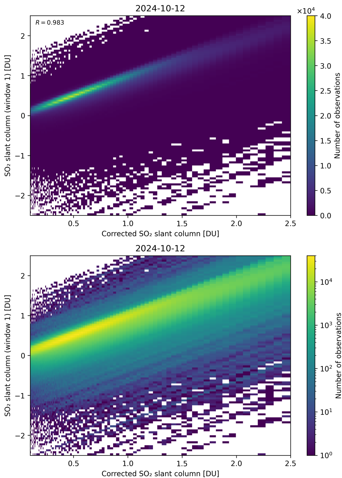
Figure 187: Scatter density plot of “Corrected SO 2 slant column” against “SO 2 slant column (window 1)” for 2024-10-11 to 2024-10-13.
