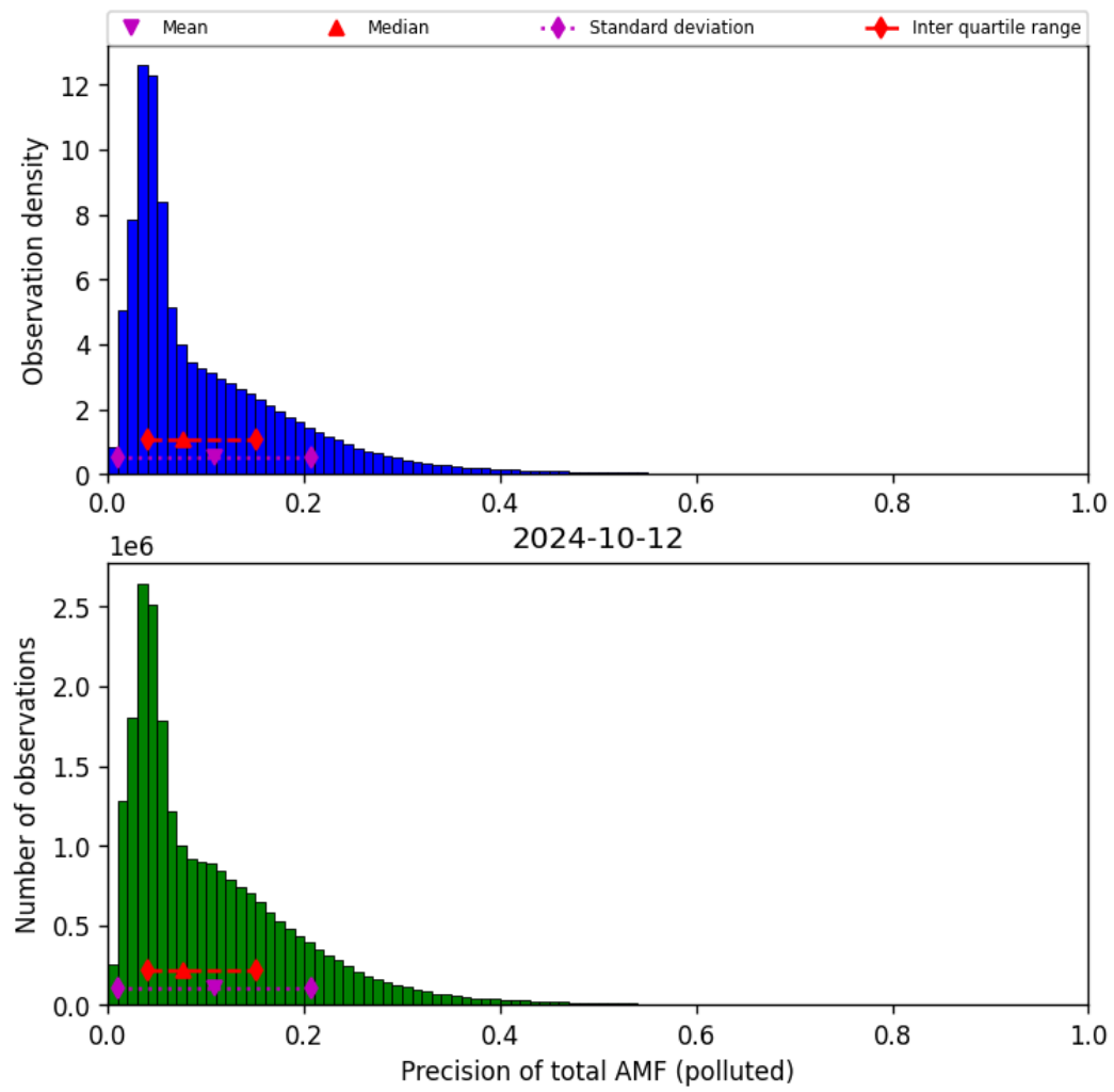
Figure 72: Histogram of “Precision of total AMF (polluted)” for 2024-10-11 to 2024-10-13
