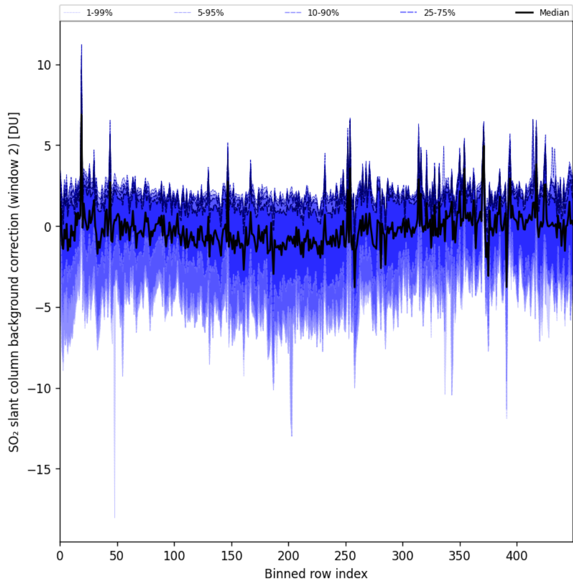
Figure 86: Along track statistics of “SO 2 slant column background correction (window 2)” for 2024-10-11 to 2024-10-13
