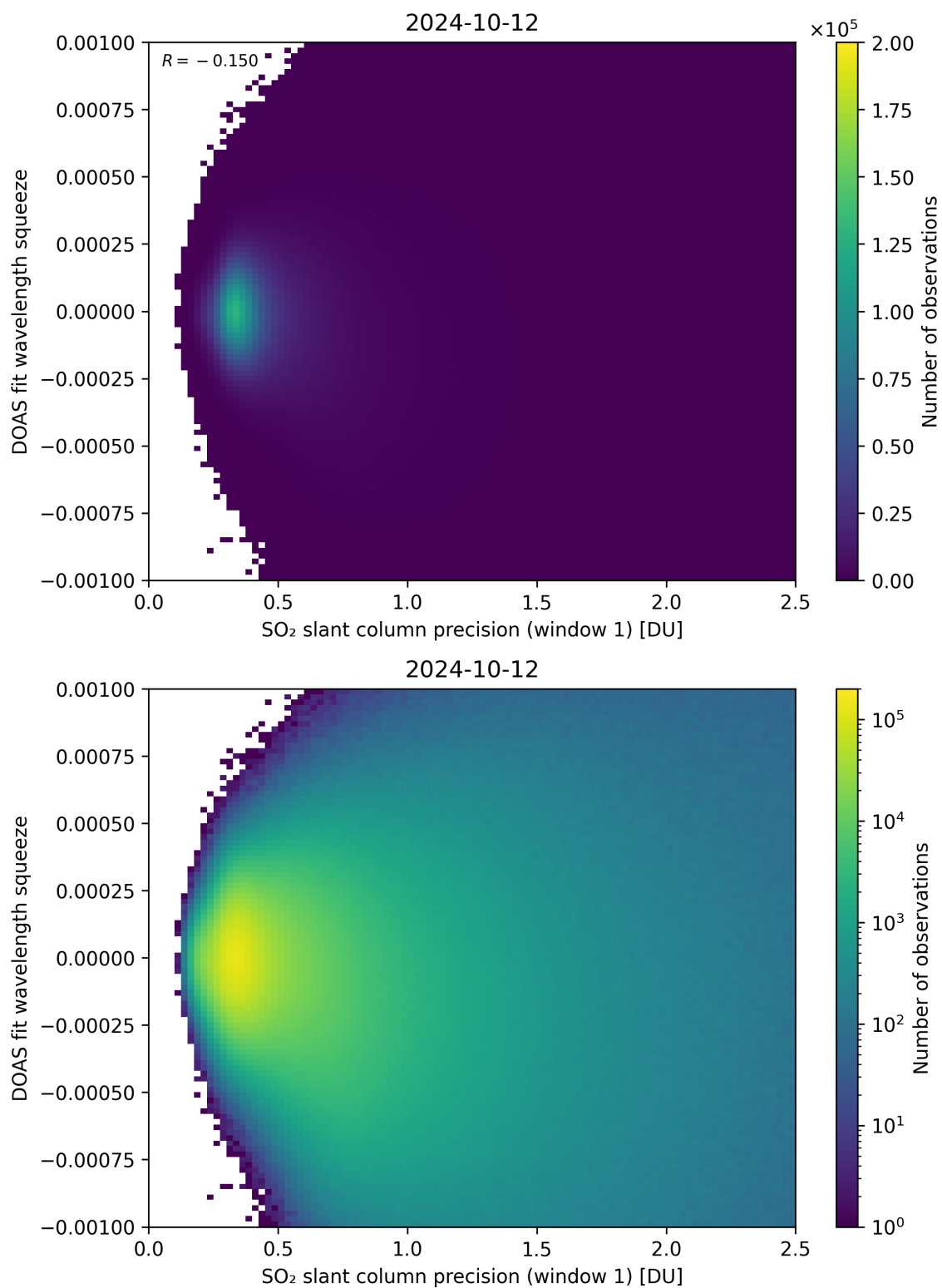
Figure 222: Scatter density plot of “SO 2 slant column precision (window 1)” against “DOAS fit wavelength squeeze” for 2024-10-11 to 2024-10-13.
