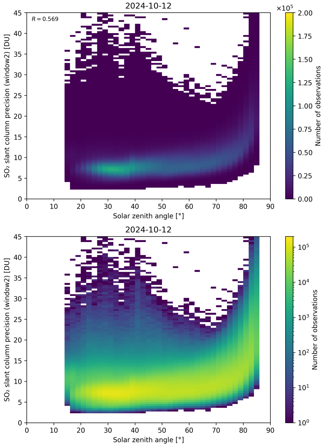
Figure 171: Scatter density plot of “Solar zenith angle” against “SO 2 slant column precision (window2)” for 2024-10-11 to 2024-10-13.
