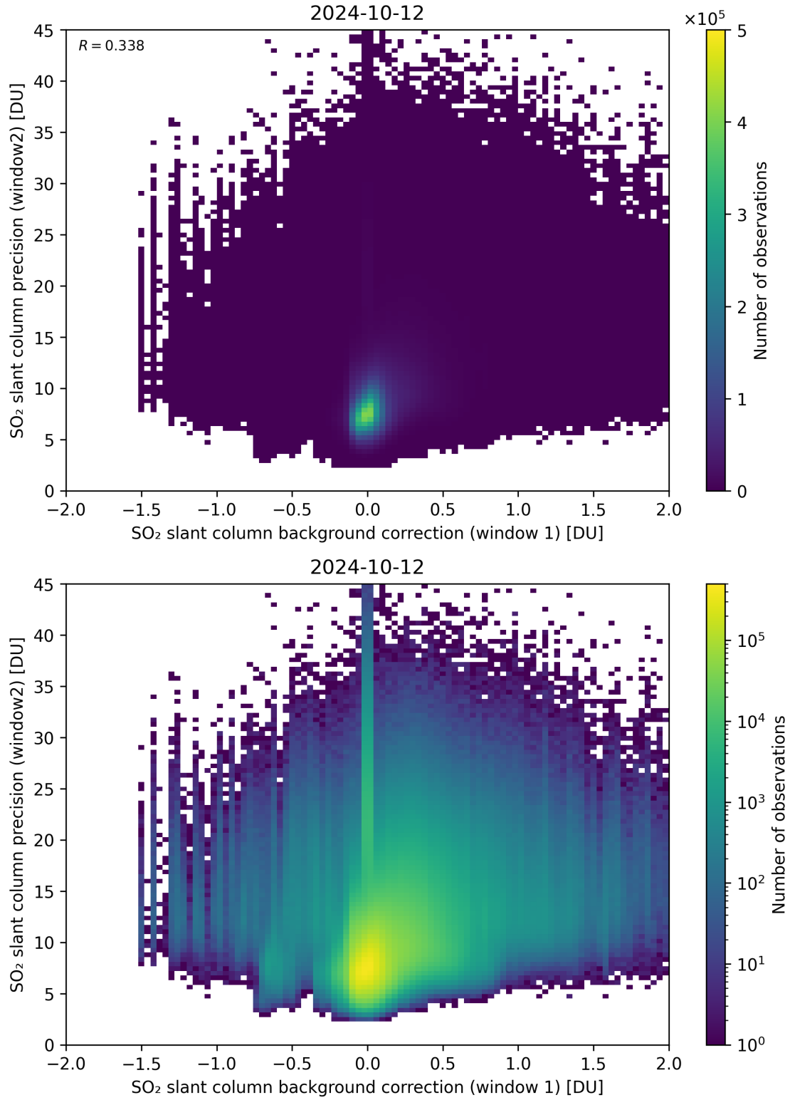
Figure 106: Scatter density plot of “SO 2 slant column background correction (window 1)” against “SO 2 slant column precision (window2)” for 2024-10-11 to 2024-10-13.
