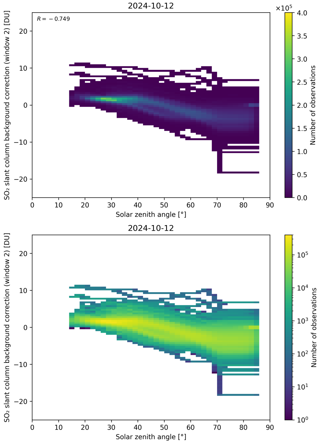
Figure 159: Scatter density plot of “Solar zenith angle” against “SO 2 slant column background correction (window 2)” for 2024-10-11 to 2024-10-13.
