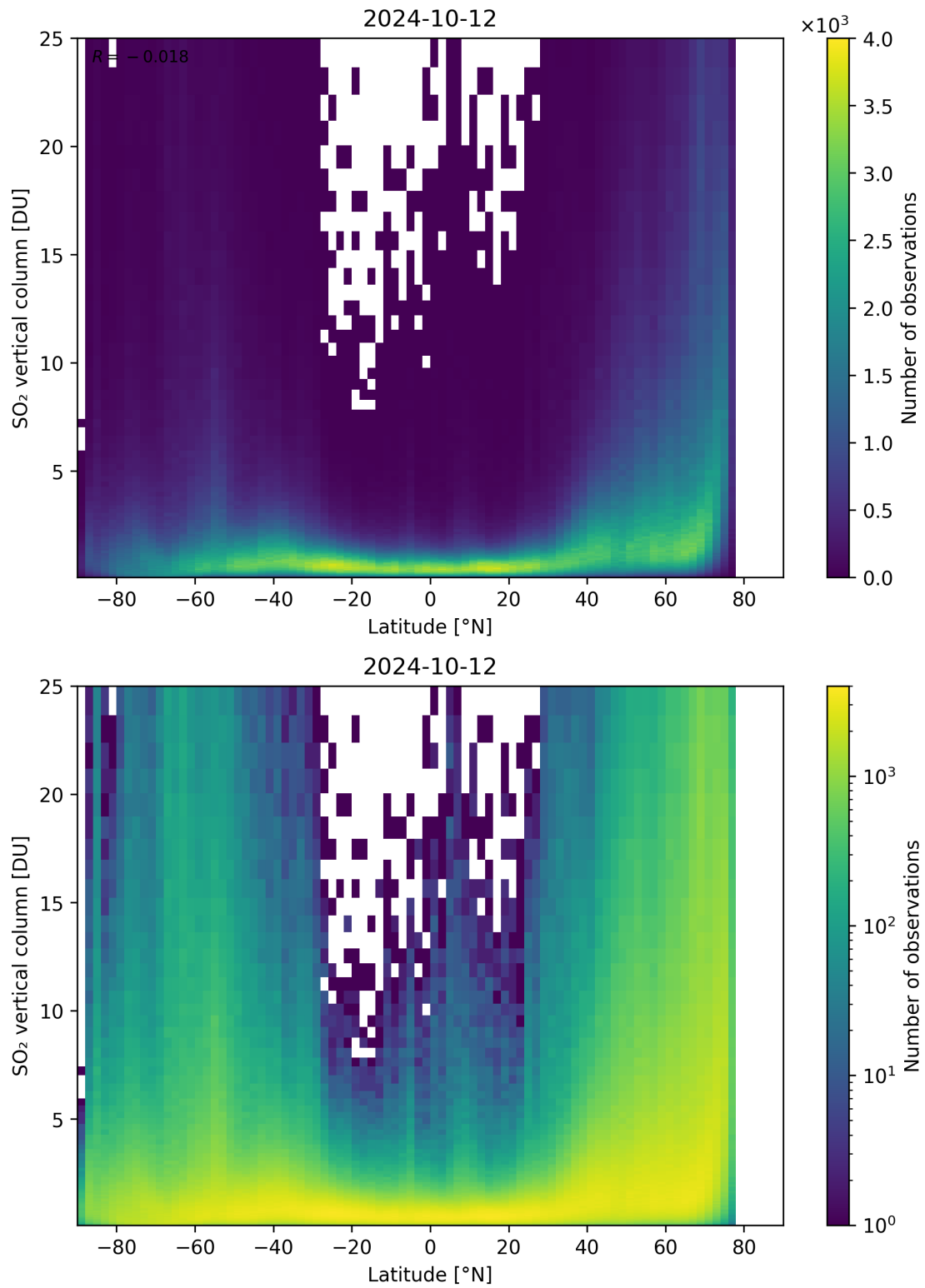
Figure 156: Scatter density plot of “Latitude” against “SO 2 vertical column” for 2024-10-11 to 2024-10-13.
