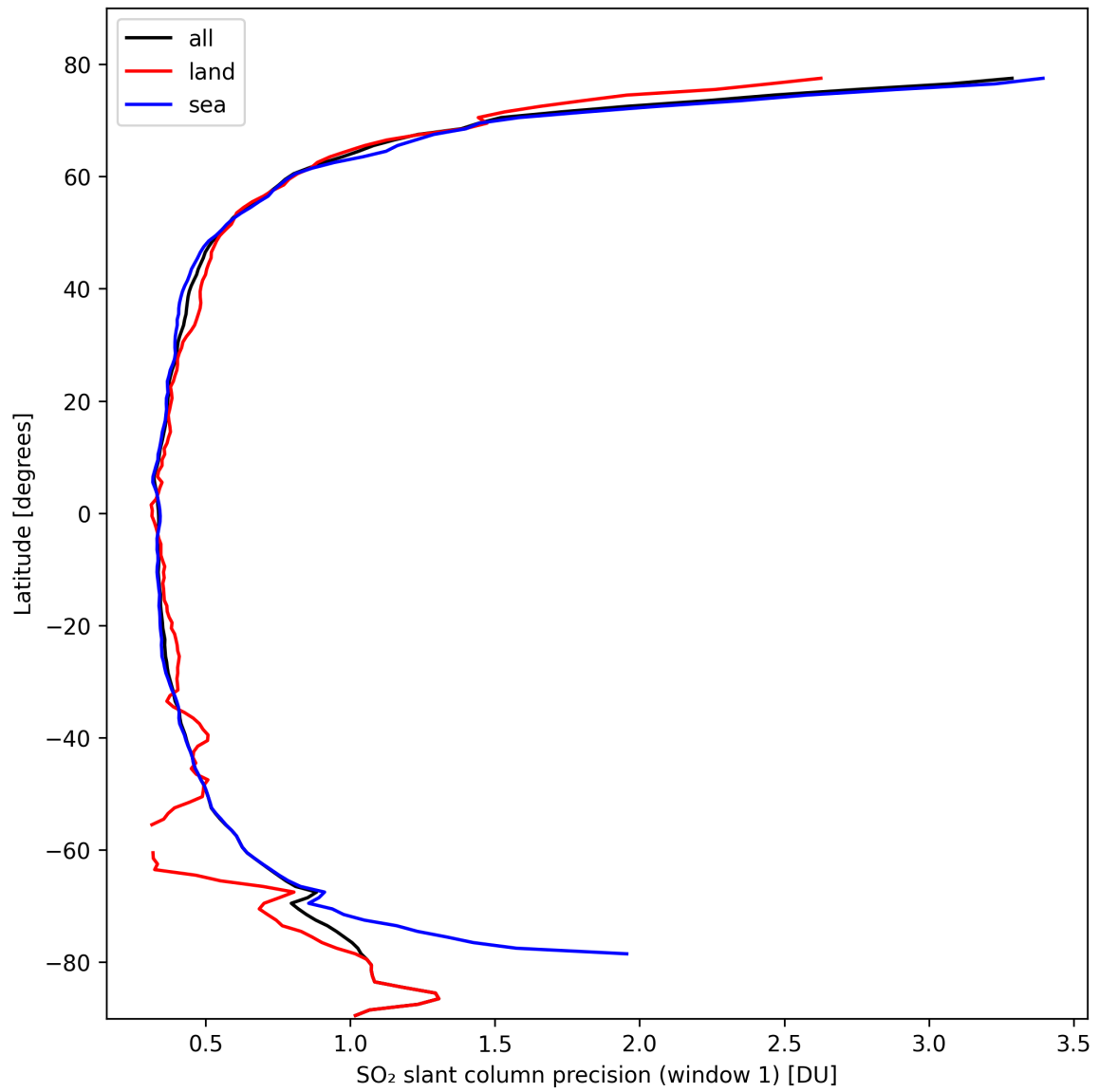
Figure 34: Zonal average of “SO 2 slant column precision (window 1)” for 2024-10-11 to 2024-10-13.
