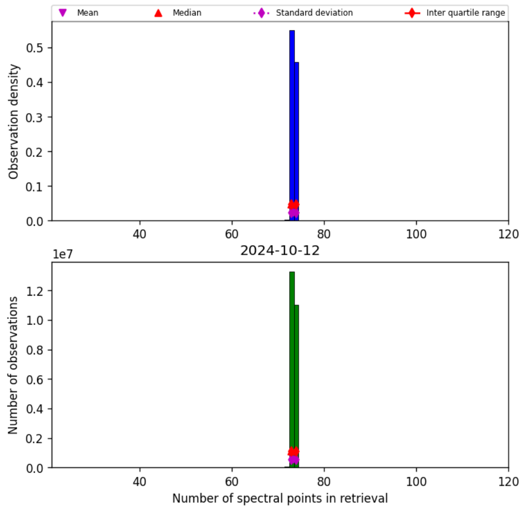
Figure 74: Histogram of “Number of spectral points in retrieval” for 2024-10-11 to 2024-10-13
