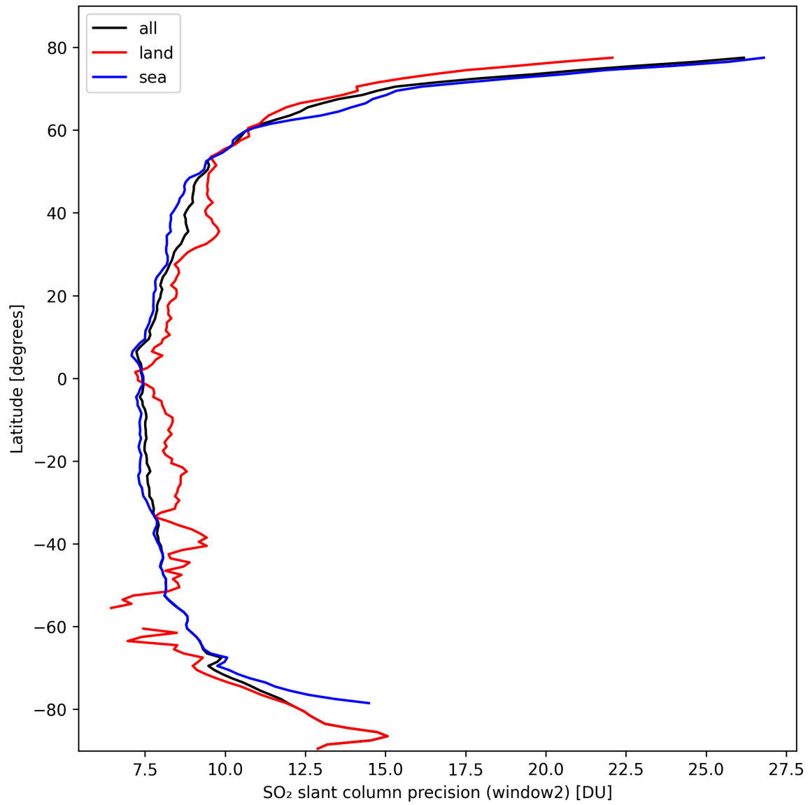
Figure 38: Zonal average of “SO 2 slant column precision (window2)” for 2024-10-11 to 2024-10-13.
