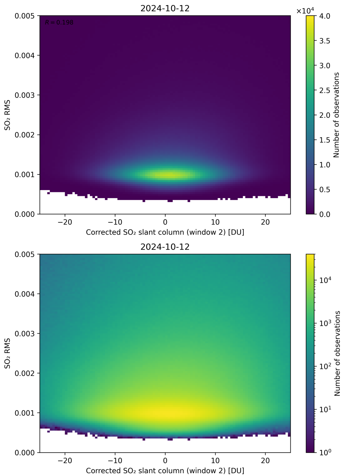
Figure 198: Scatter density plot of “Corrected SO 2 slant column (window 2)” against “SO 2 RMS” for 2024-10-11 to 2024-10-13.
