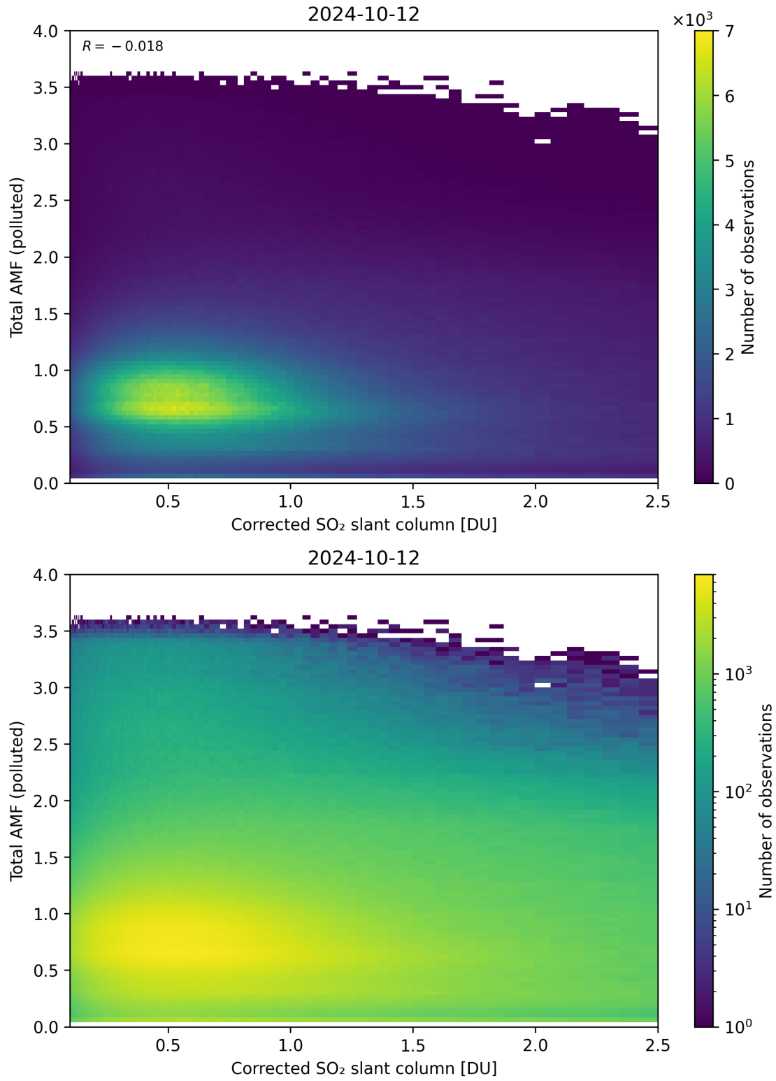
Figure 192: Scatter density plot of “Corrected SO 2 slant column” against “Total AMF (polluted)” for 2024-10-11 to 2024-10-13.
