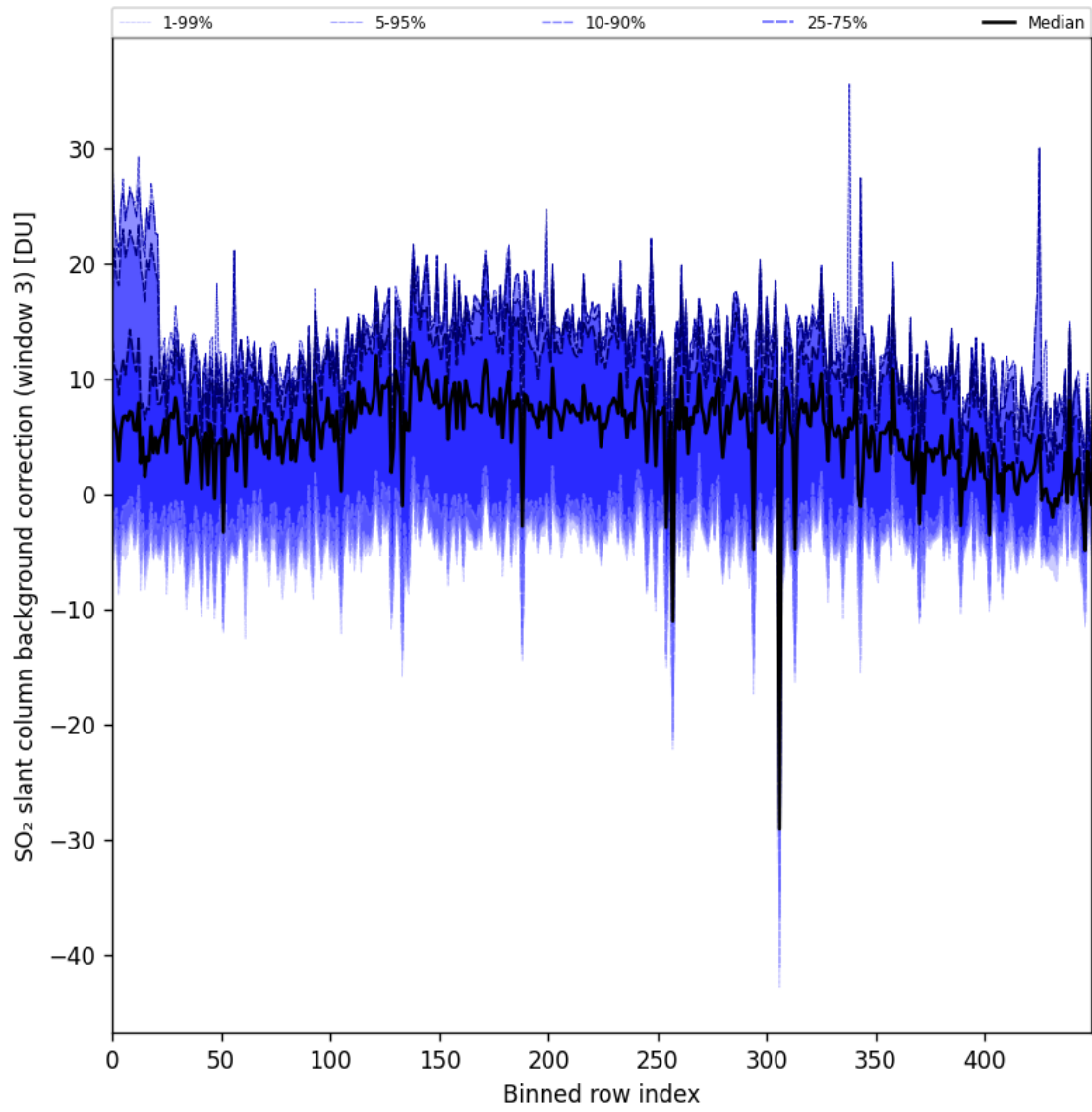
Figure 90: Along track statistics of “SO 2 slant column background correction (window 3)” for 2024-10-11 to 2024-10-13
