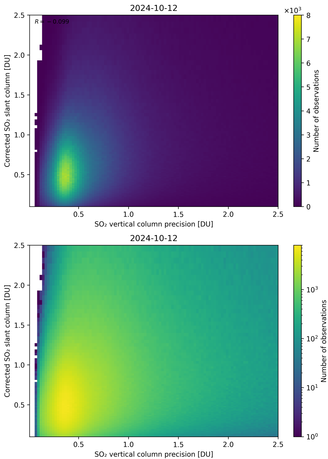
Figure 286: Scatter density plot of “SO 2 vertical column precision” against “Corrected SO 2 slant column” for 2024-10-11 to 2024-10-13.
