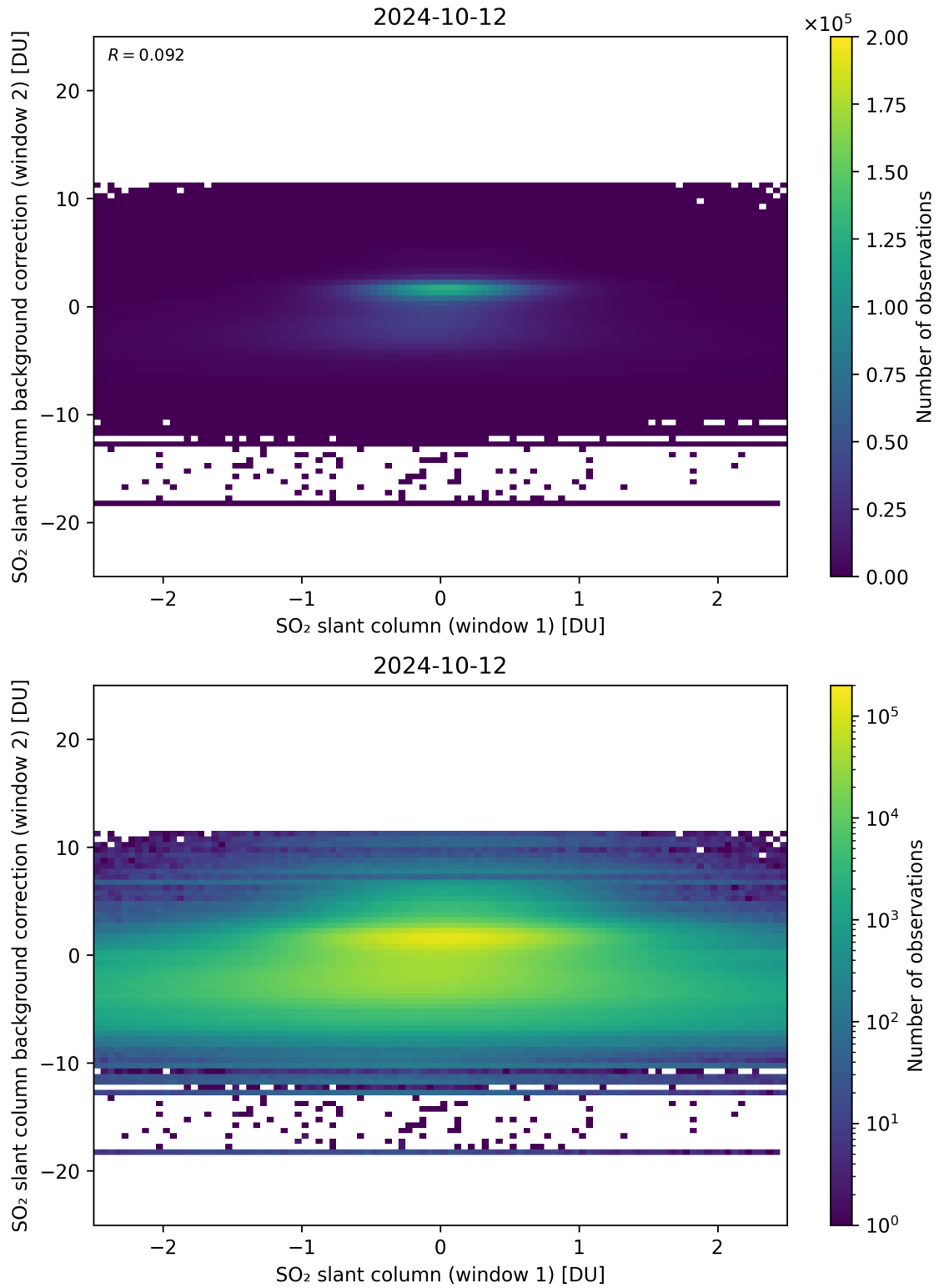
Figure 213: Scatter density plot of “SO 2 slant column (window 1)” against “SO 2 slant column background correction (window 2)” for 2024-10-11 to 2024-10-13.
