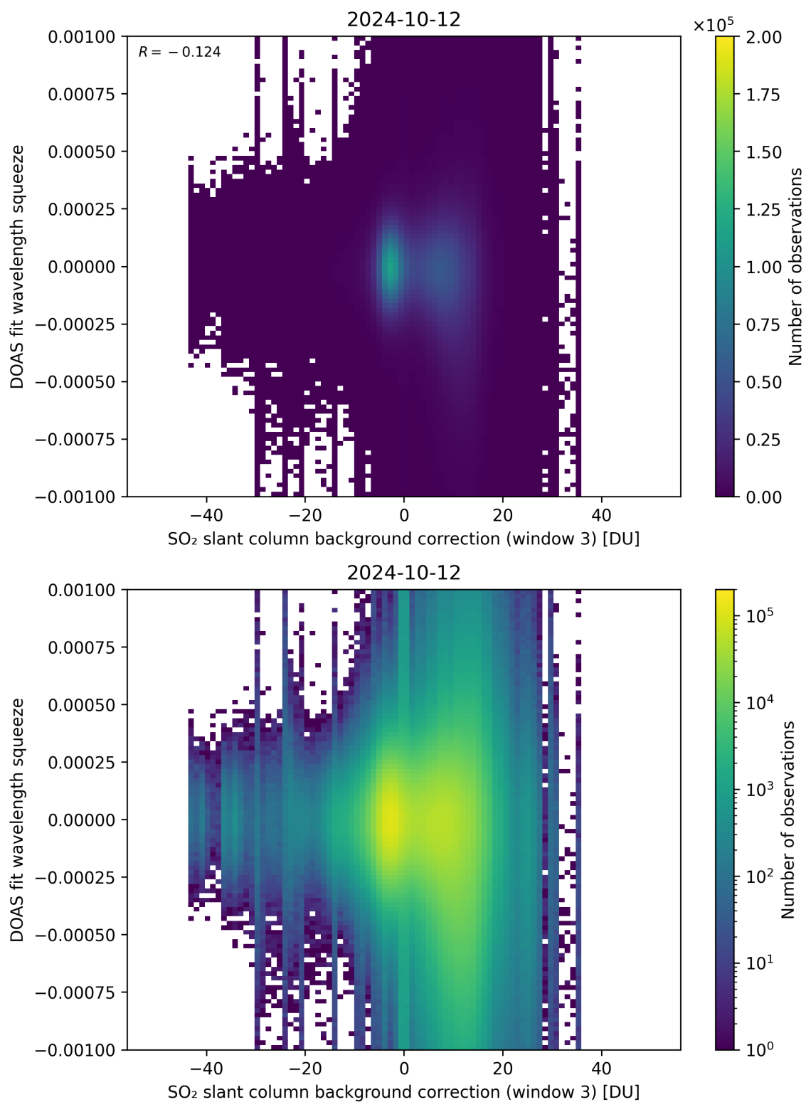
Figure 122: Scatter density plot of “SO 2 slant column background correction (window 3)” against “DOAS fit wavelength squeeze” for 2024-10-11 to 2024-10-13.
