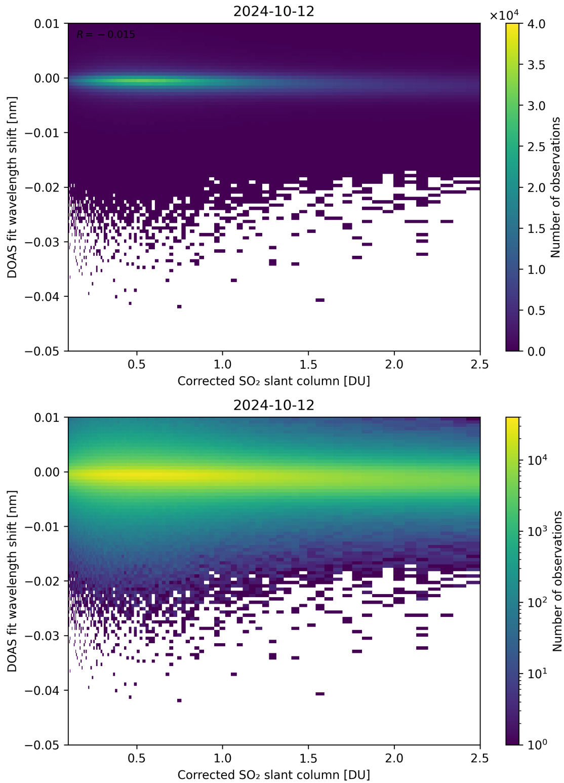
Figure 181: Scatter density plot of “Corrected SO 2 slant column” against “DOAS fit wavelength shift” for 2024-10-11 to 2024-10-13.
