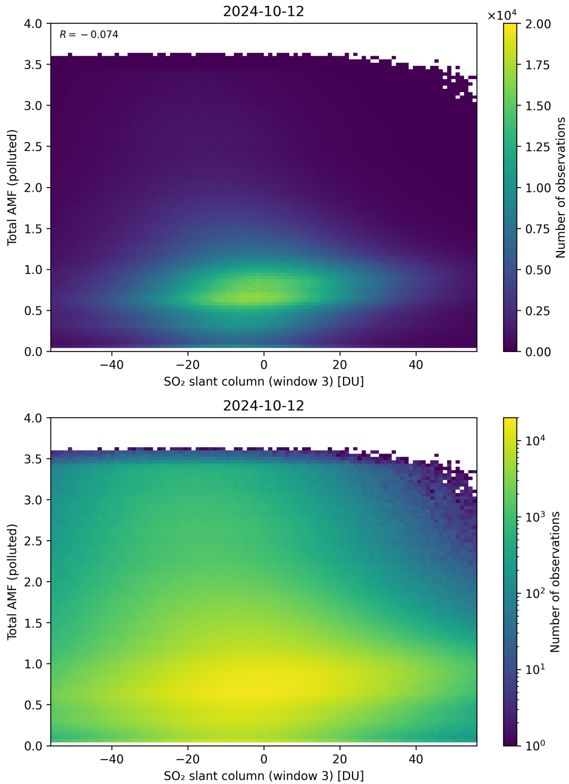
Figure 268: Scatter density plot of “SO 2 slant column (window 3)” against “Total AMF (polluted)” for 2024-10-11 to 2024-10-13.
