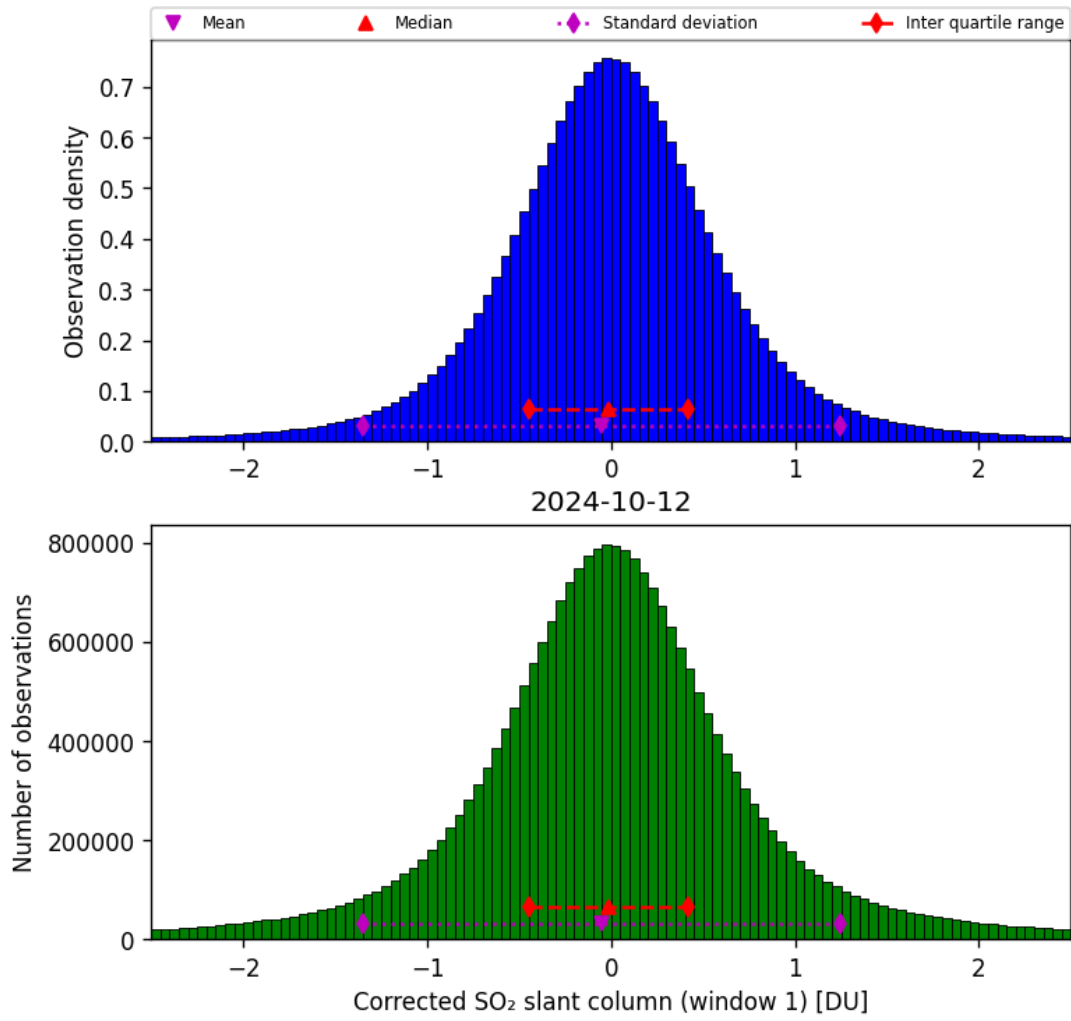
Figure 58: Histogram of “Corrected SO 2 slant column (window 1)” for 2024-10-11 to 2024-10-13
