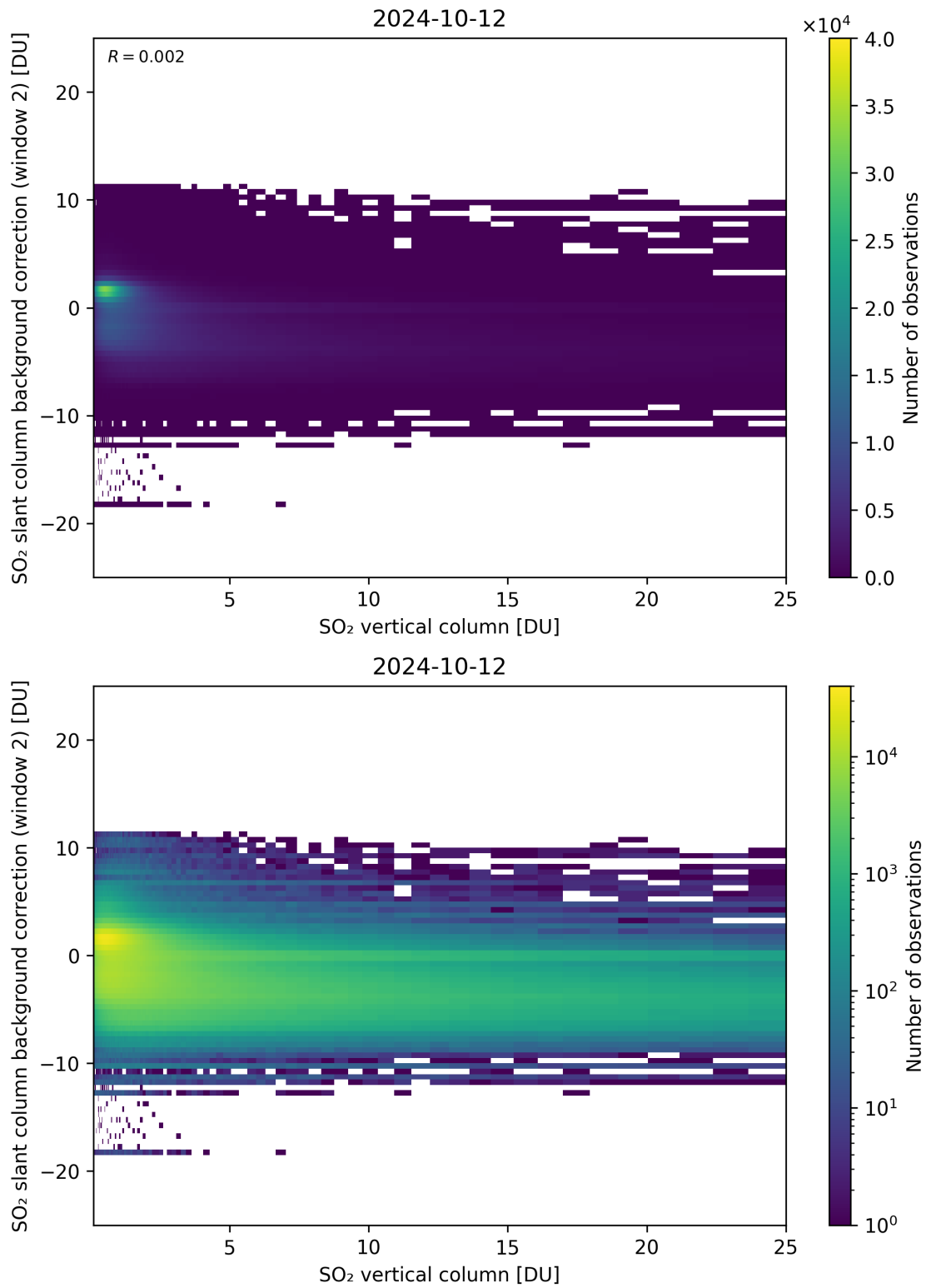
Figure 274: Scatter density plot of “SO 2 vertical column” against “SO 2 slant column background correction (window 2)” for 2024-10-11 to 2024-10-13.
