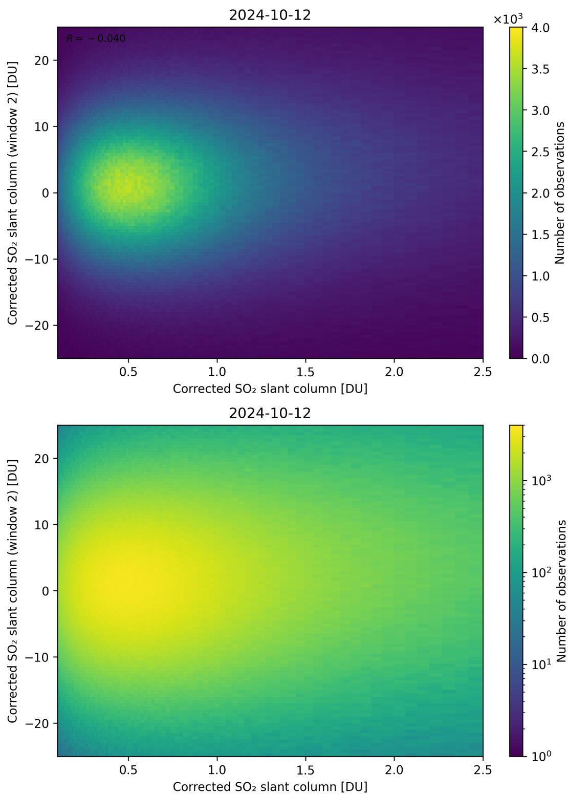
Figure 185: Scatter density plot of “Corrected SO 2 slant column” against “Corrected SO 2 slant column (window 2)” for 2024-10-11 to 2024-10-13.
