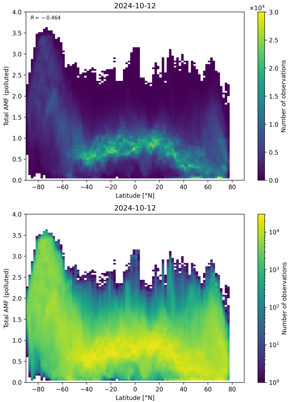
Figure 154: Scatter density plot of “Latitude” against “Total AMF (polluted)” for 2024-10-11 to 2024-10-13.
