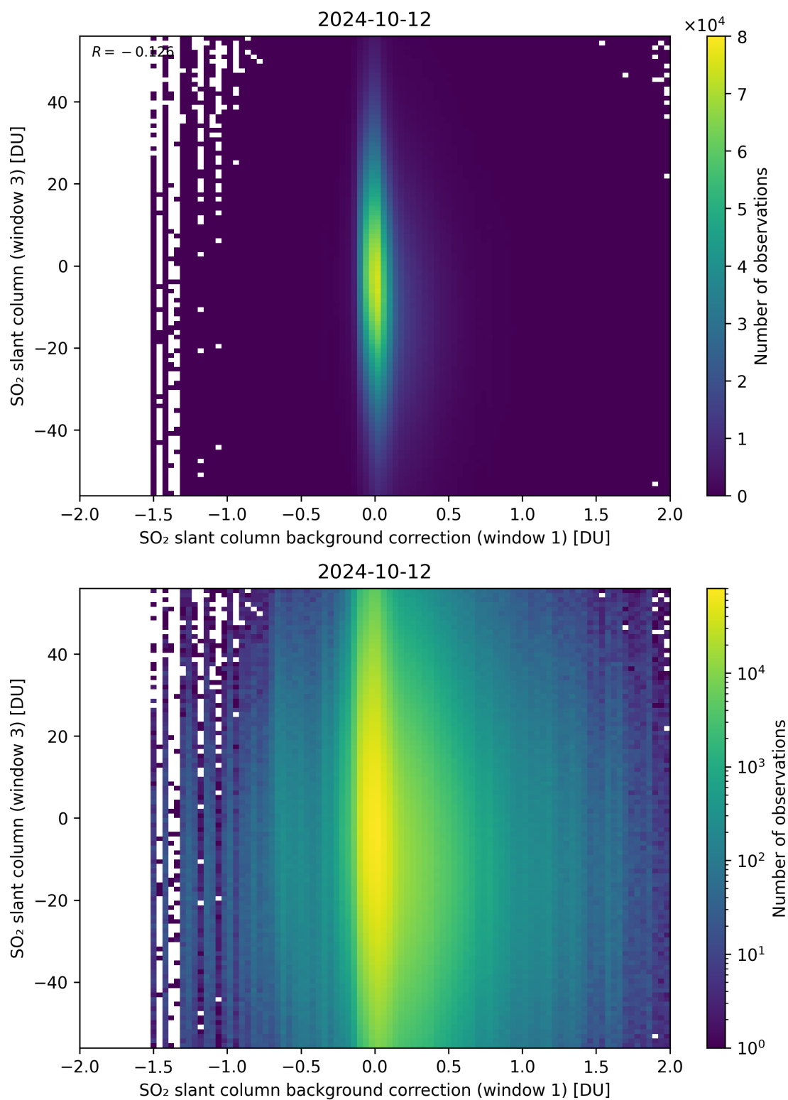
Figure 107: Scatter density plot of “SO 2 slant column background correction (window 1)” against “SO 2 slant column (window 3)” for 2024-10-11 to 2024-10-13.
