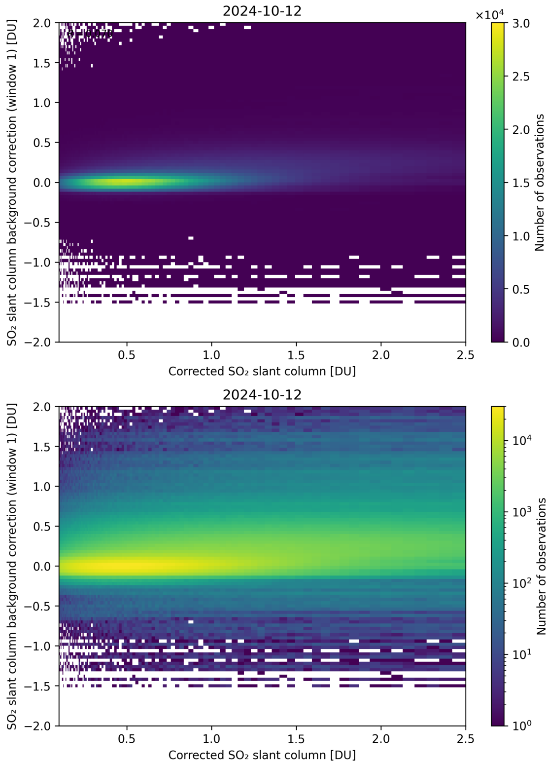
Figure 178: Scatter density plot of “Corrected SO 2 slant column” against “SO 2 slant column background correction (window 1)” for 2024-10-11 to 2024-10-13.
