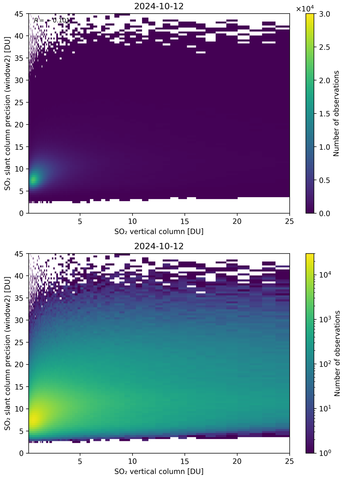
Figure 302: Scatter density plot of “SO 2 vertical column” against “SO 2 slant column precision (window2)” for 2024-10-11 to 2024-10-13.
