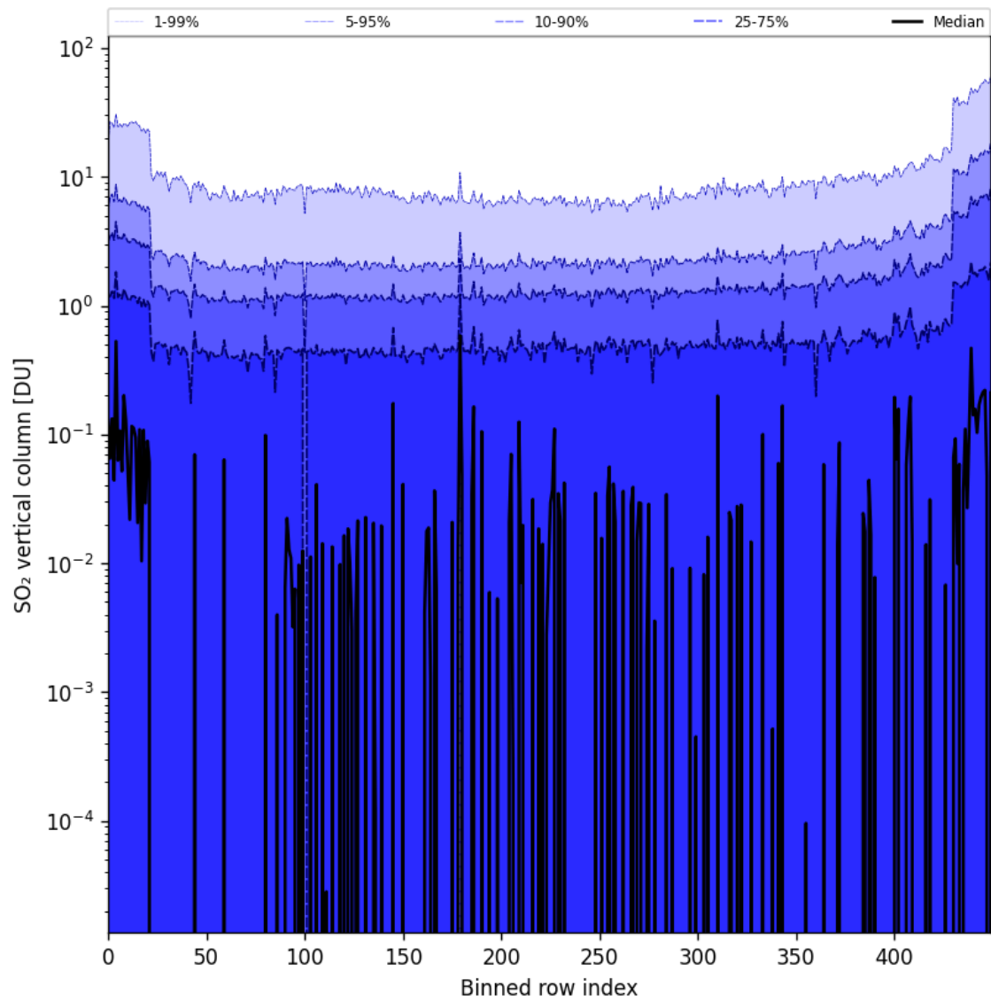
Figure 76: Along track statistics of “SO 2 vertical column” for 2024-10-11 to 2024-10-13
