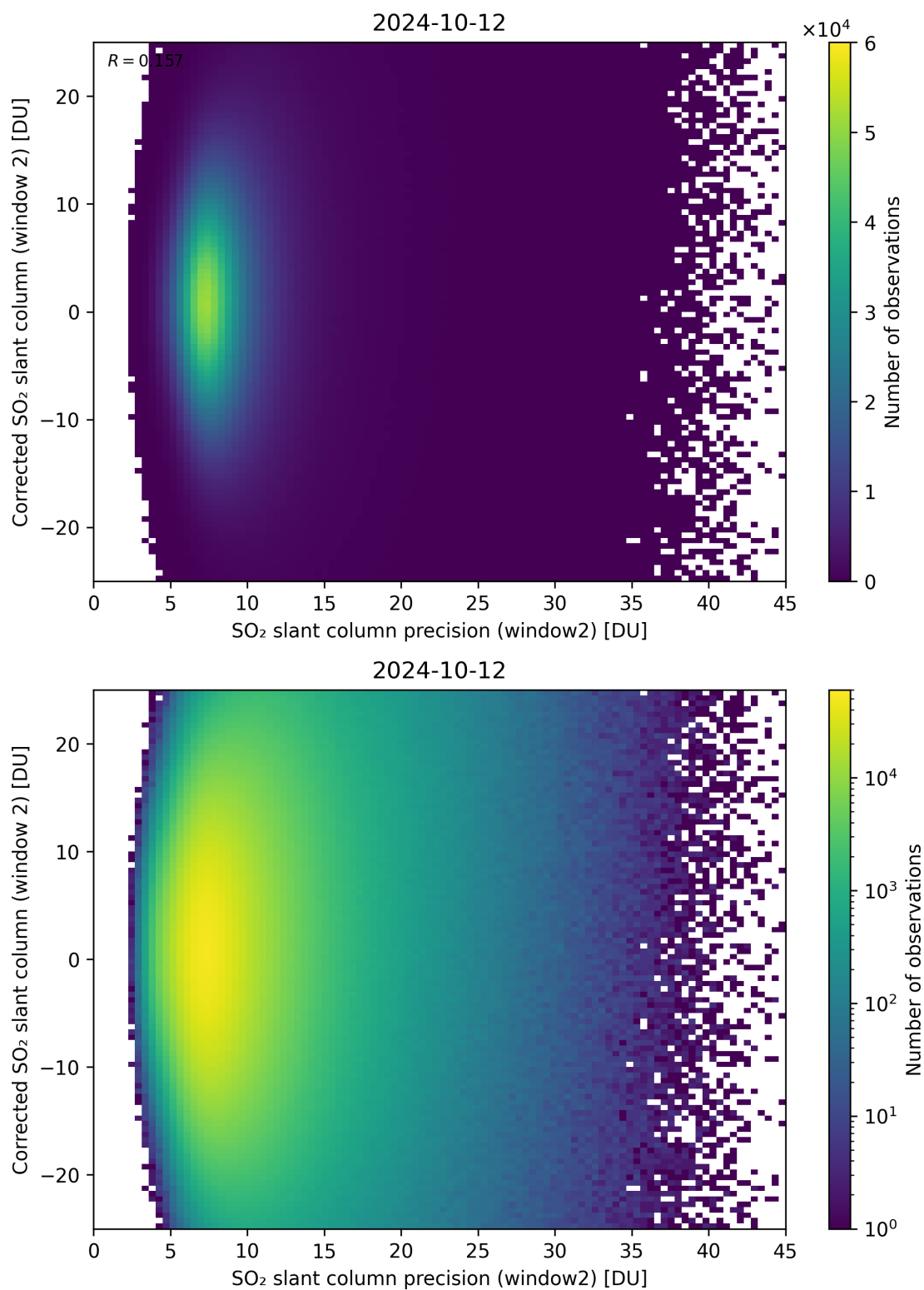
Figure 247: Scatter density plot of “SO 2 slant column precision (window2)” against “Corrected SO 2 slant column (window 2)” for 2024-10-11 to 2024-10-13.
