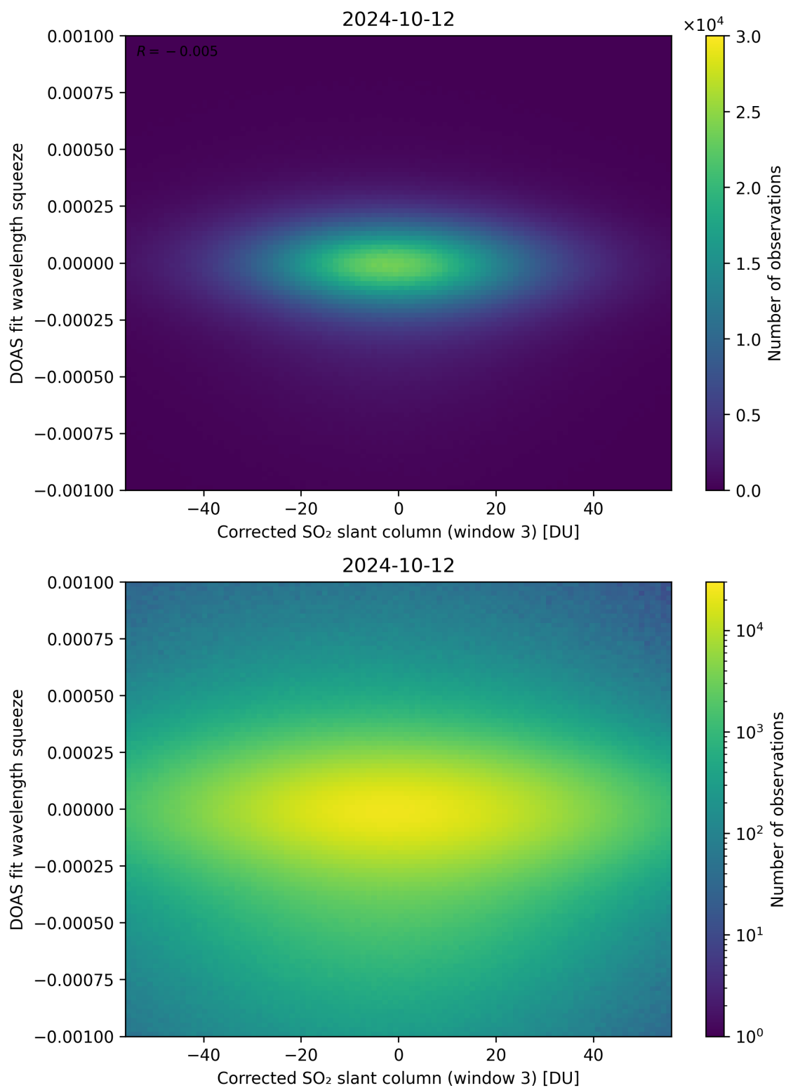
Figure 207: Scatter density plot of “Corrected SO 2 slant column (window 3)” against “DOAS fit wavelength squeeze” for 2024-10-11 to 2024-10-13.
