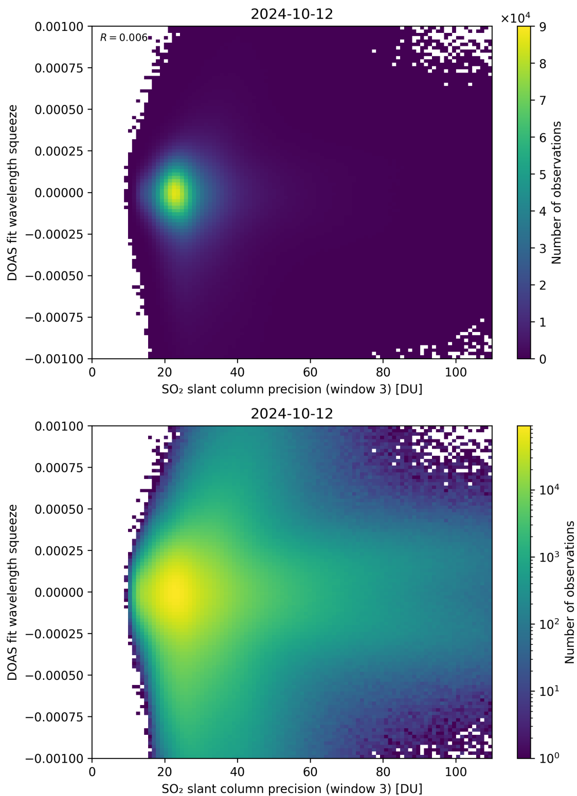
Figure 259: Scatter density plot of “SO 2 slant column precision (window 3)” against “DOAS fit wavelength squeeze” for 2024-10-11 to 2024-10-13.
