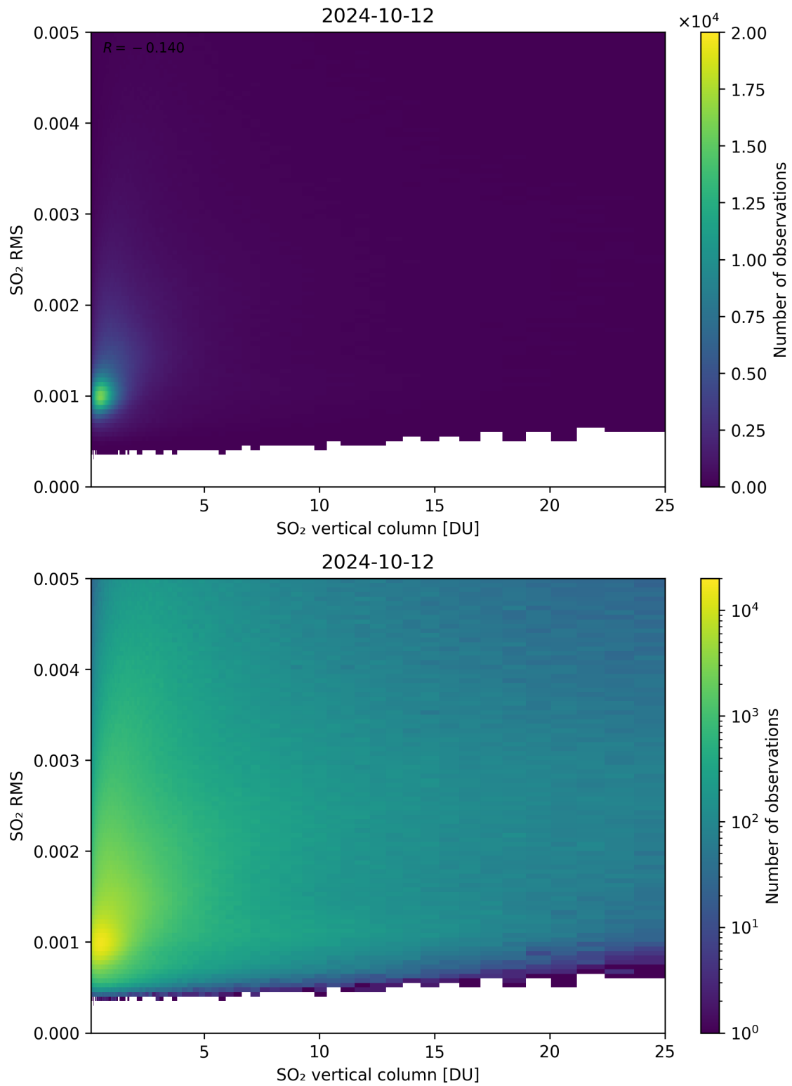
Figure 278: Scatter density plot of “SO 2 vertical column” against “SO 2 RMS” for 2024-10-11 to 2024-10-13.
