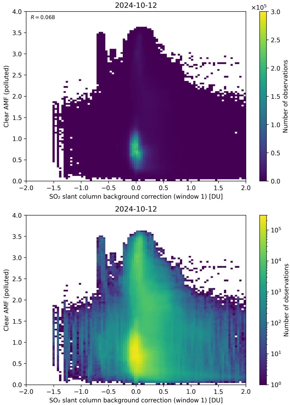
Figure 103: Scatter density plot of “SO 2 slant column background correction (window 1)” against “Clear AMF (polluted)” for 2024-10-11 to 2024-10-13.
