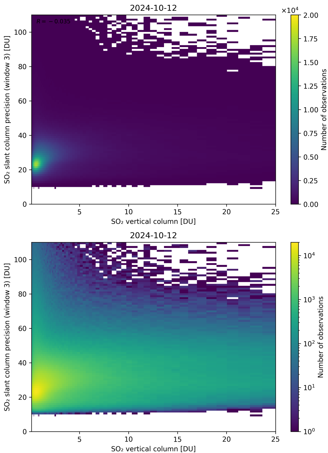
Figure 304: Scatter density plot of “SO 2 vertical column” against “SO 2 slant column precision (window 3)” for 2024-10-11 to 2024-10-13.
