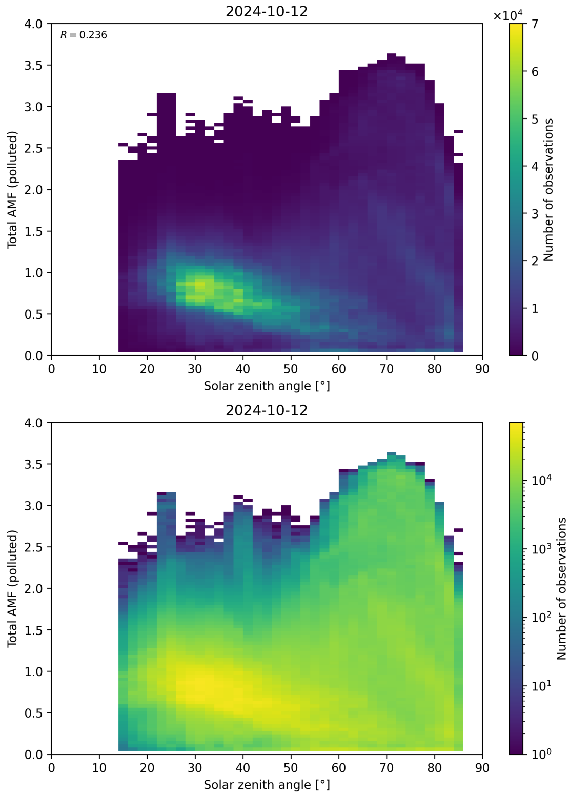
Figure 174: Scatter density plot of “Solar zenith angle” against “Total AMF (polluted)” for 2024-10-11 to 2024-10-13.
