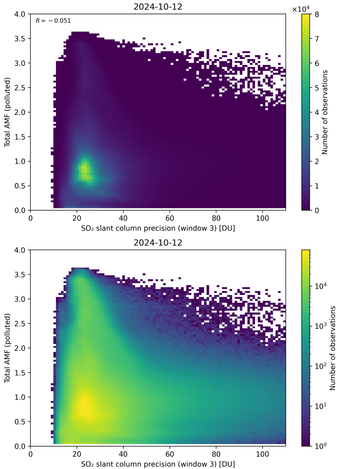
Figure 263: Scatter density plot of “SO 2 slant column precision (window 3)” against “Total AMF (polluted)” for 2024-10-11 to 2024-10-13.
