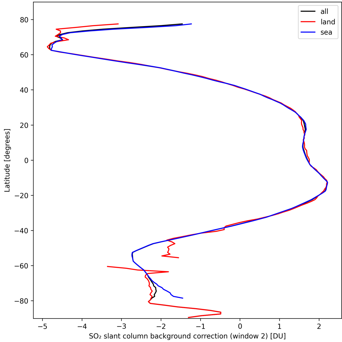
Figure 40: Zonal average of “SO 2 slant column background correction (window 2)” for 2024-10-11 to 2024-10-13.
