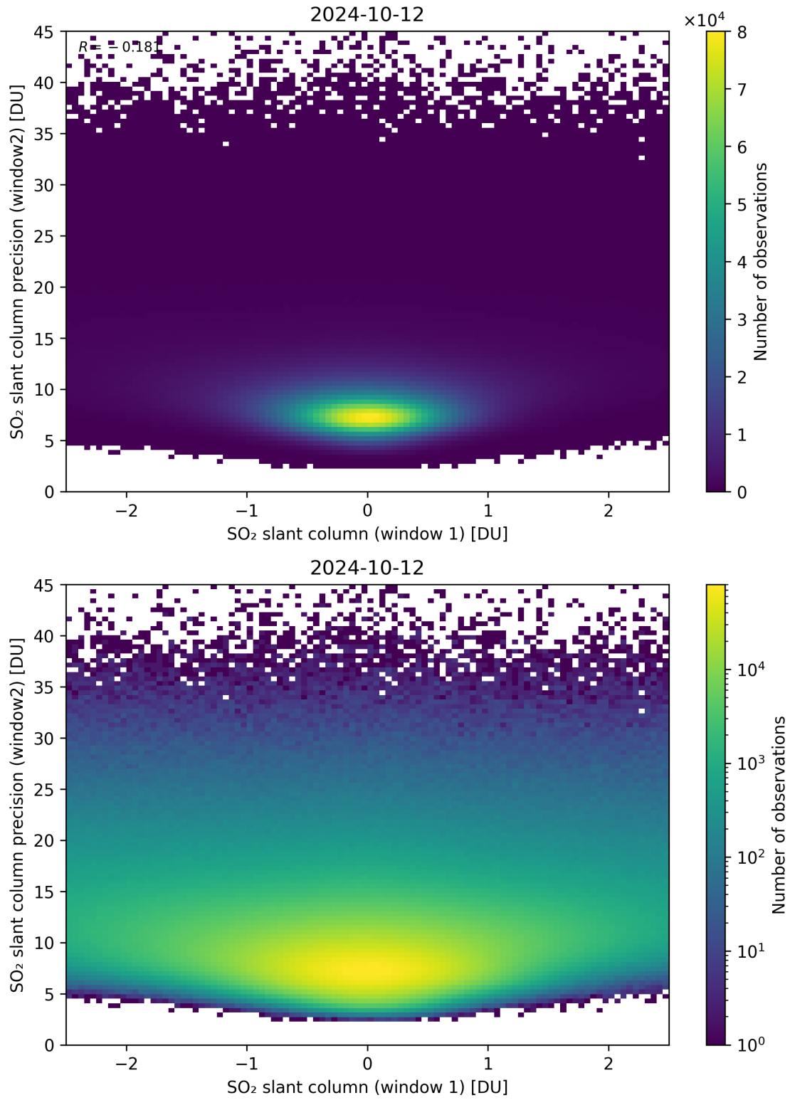
Figure 236: Scatter density plot of “SO 2 slant column (window 1)” against “SO 2 slant column precision (window2)” for 2024-10-11 to 2024-10-13.
