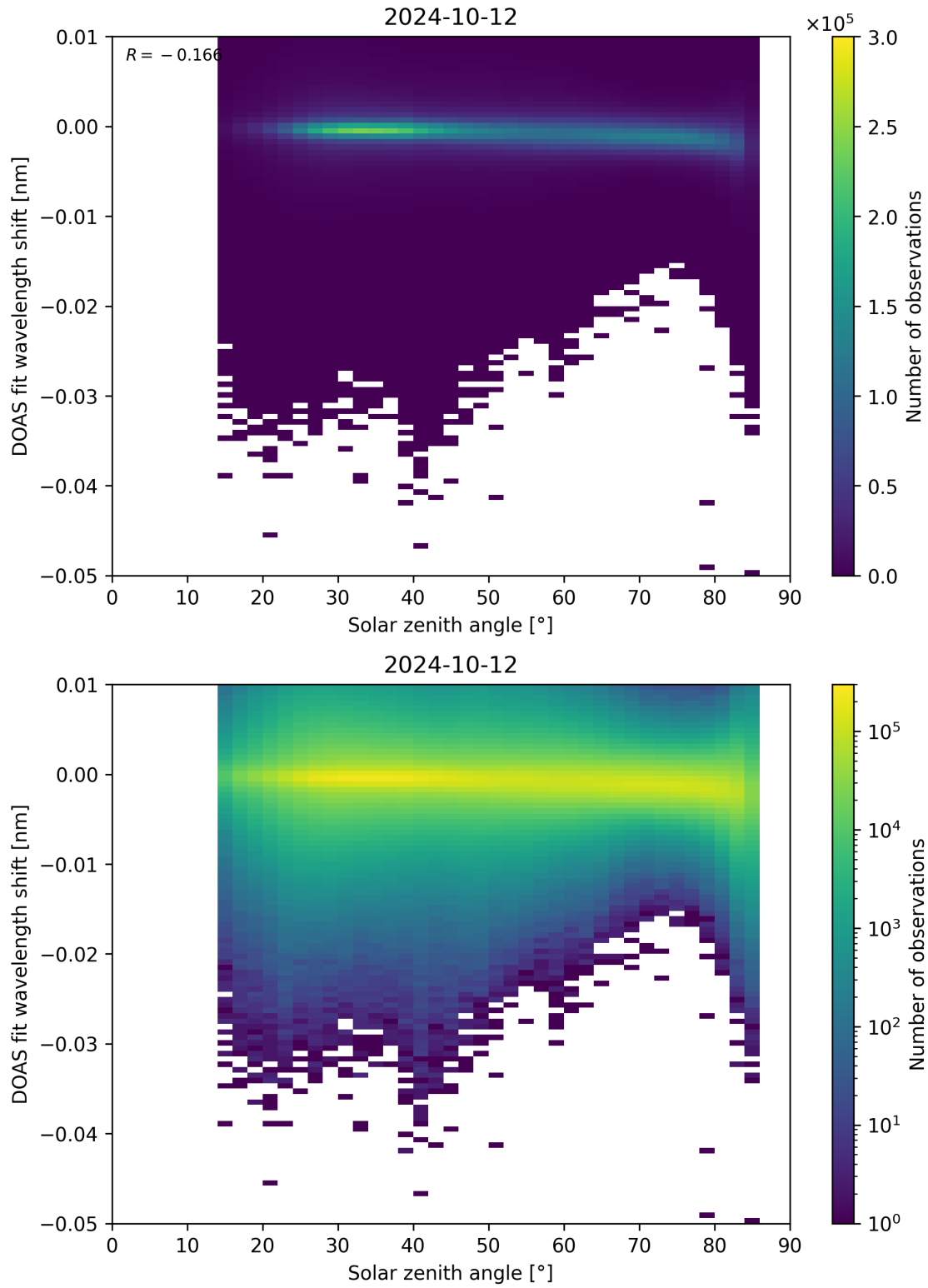
Figure 161: Scatter density plot of “Solar zenith angle” against “DOAS fit wavelength shift” for 2024-10-11 to 2024-10-13.
