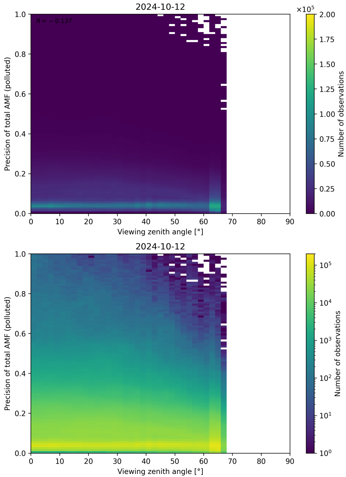
Figure 326: Scatter density plot of “Viewing zenith angle” against “Precision of total AMF (polluted)” for 2024-10-11 to 2024-10-13.
