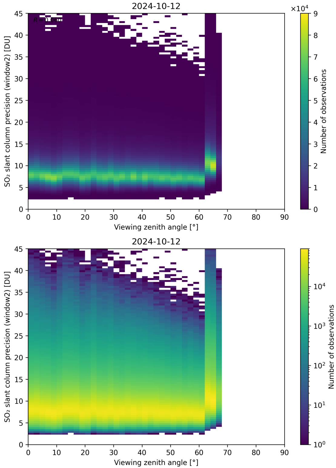
Figure 322: Scatter density plot of “Viewing zenith angle” against “SO 2 slant column precision (window2)” for 2024-10-11 to 2024-10-13.
