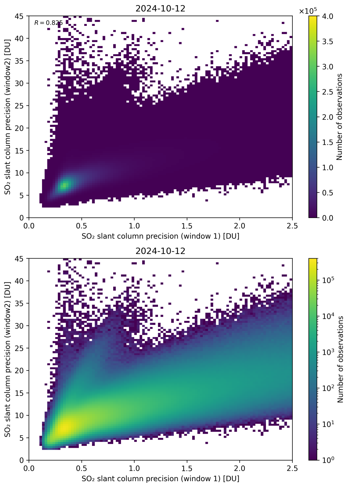
Figure 227: Scatter density plot of “SO 2 slant column precision (window 1)” against “SO 2 slant column precision (window2)” for 2024-10-11 to 2024-10-13.
