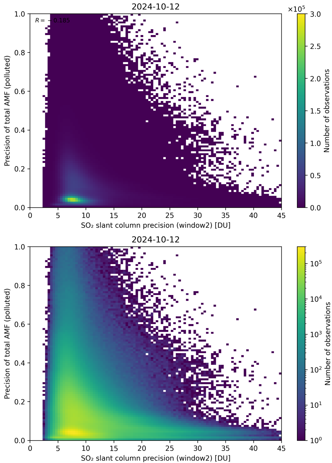
Figure 252: Scatter density plot of “SO 2 slant column precision (window2)” against “Precision of total AMF (polluted)” for 2024-10-11 to 2024-10-13.
