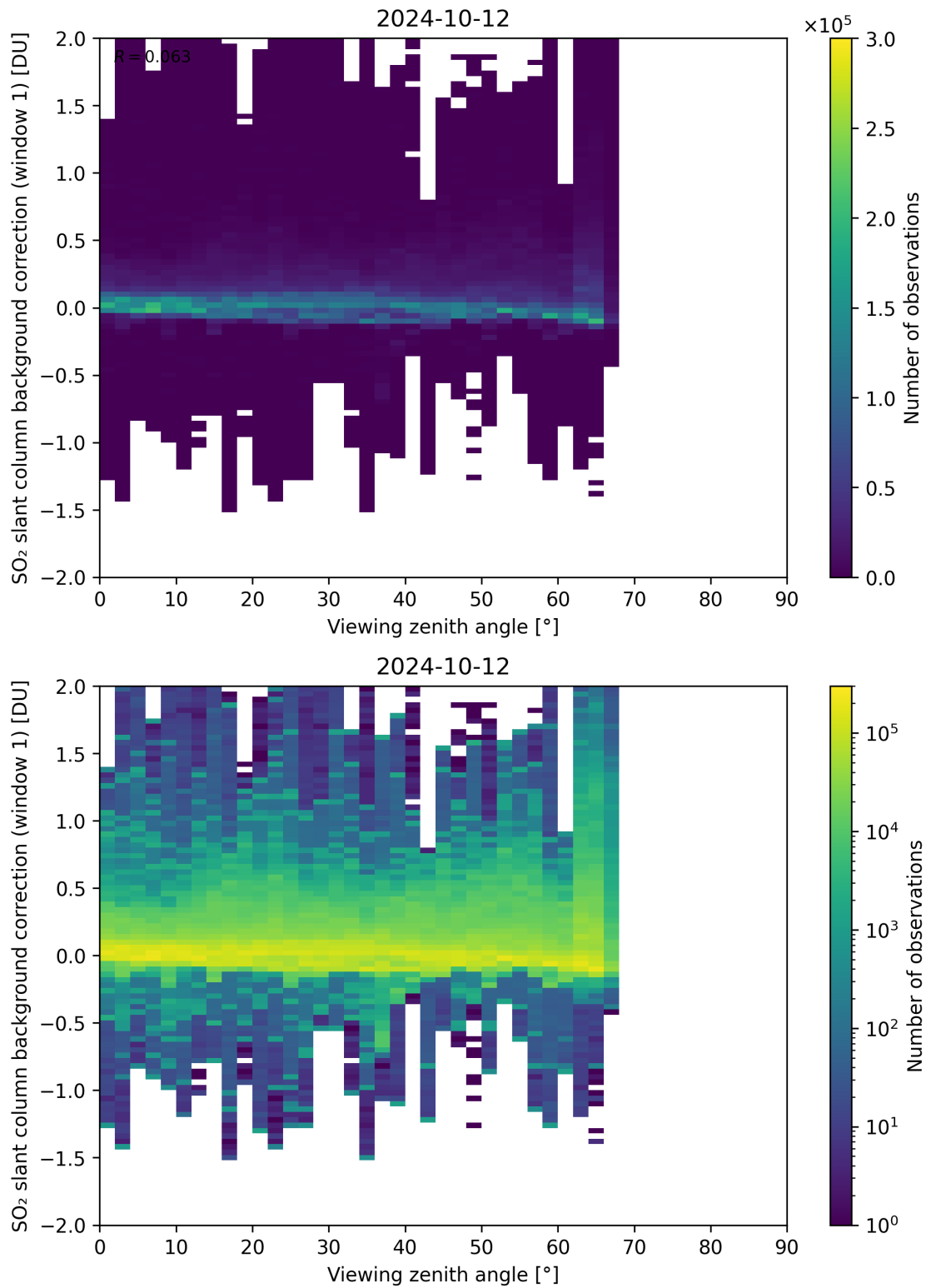
Figure 308: Scatter density plot of “Viewing zenith angle” against “SO 2 slant column background correction (window 1)” for 2024-10-11 to 2024-10-13.
