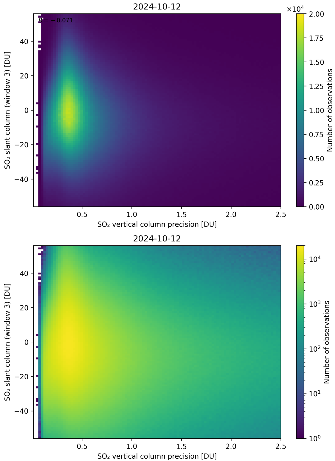
Figure 292: Scatter density plot of “SO 2 vertical column precision” against “SO 2 slant column (window 3)” for 2024-10-11 to 2024-10-13.
