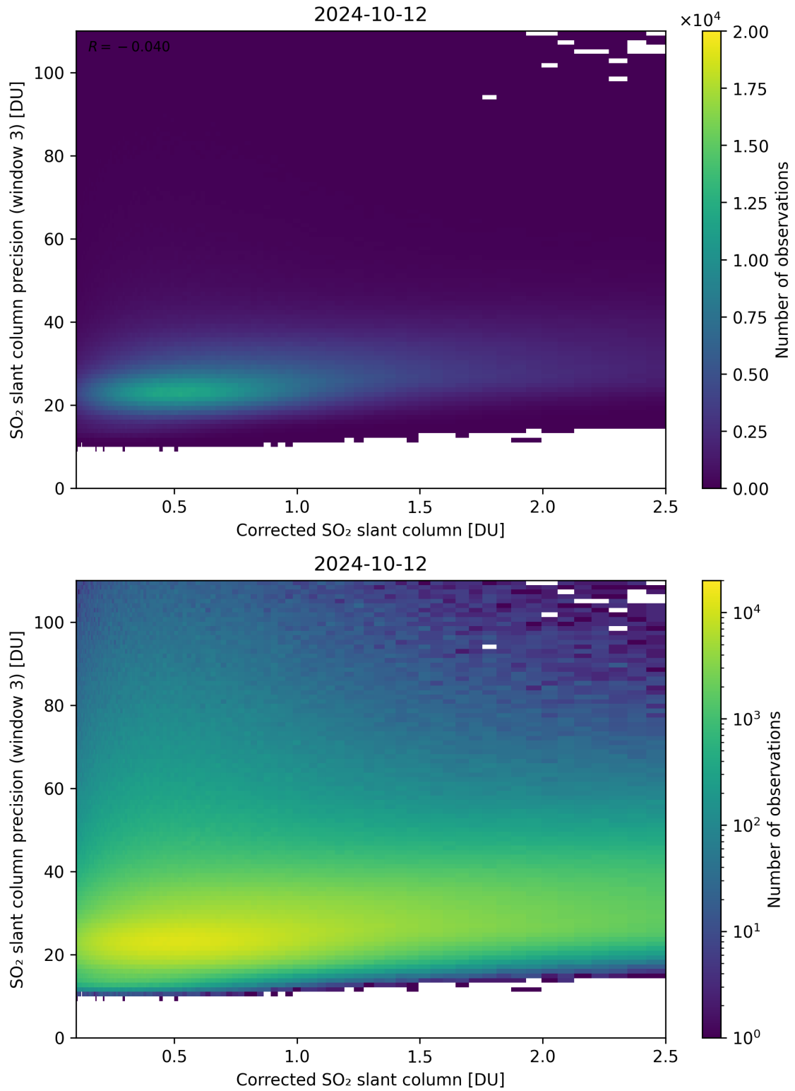
Figure 191: Scatter density plot of “Corrected SO 2 slant column” against “SO 2 slant column precision (window 3)” for 2024-10-11 to 2024-10-13.
