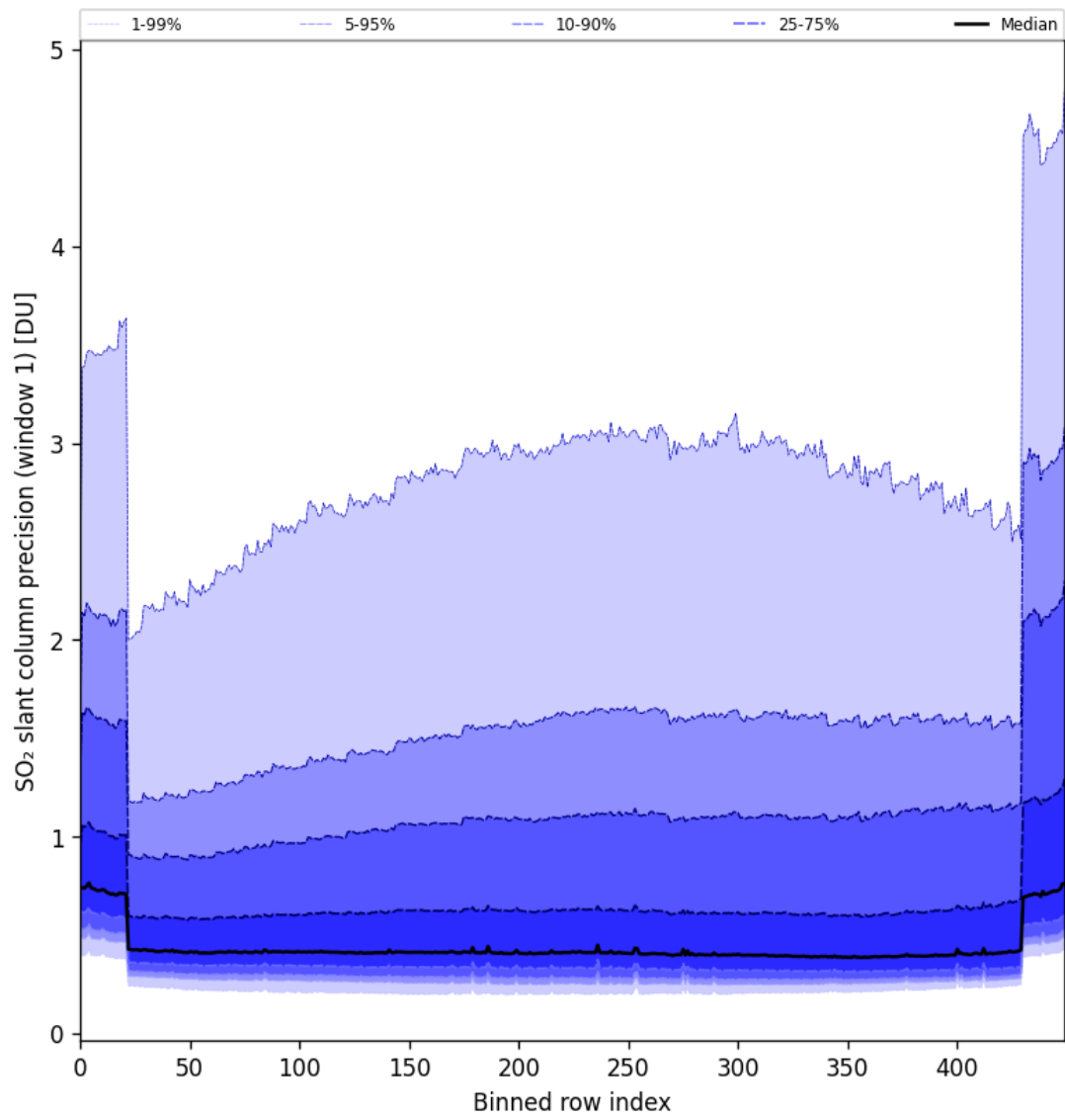
Figure 80: Along track statistics of “SO 2 slant column precision (window 1)” for 2024-10-11 to 2024-10-13
