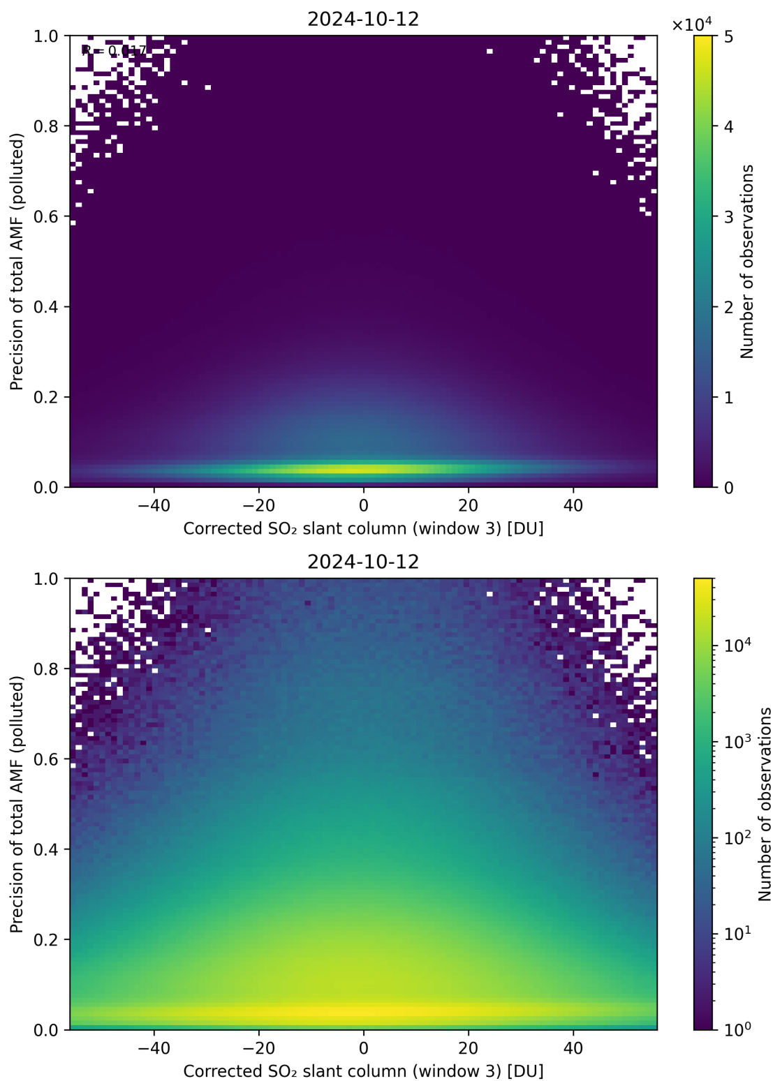
Figure 211: Scatter density plot of “Corrected SO 2 slant column (window 3)” against “Precision of total AMF (polluted)” for 2024-10-11 to 2024-10-13.
