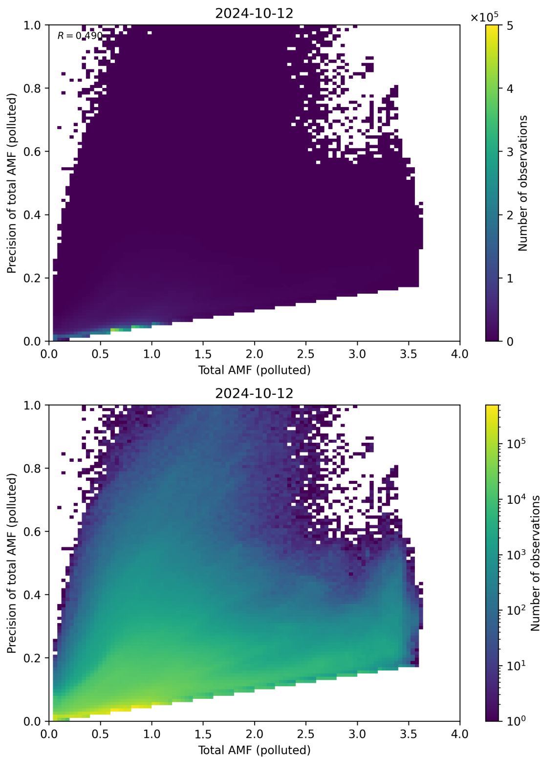
Figure 272: Scatter density plot of “Total AMF (polluted)” against “Precision of total AMF (polluted)” for 2024-10-11 to 2024-10-13.
