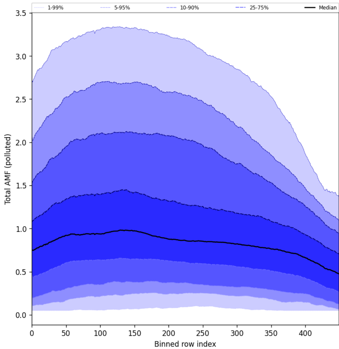
Figure 94: Along track statistics of “Total AMF (polluted)” for 2024-10-11 to 2024-10-13
