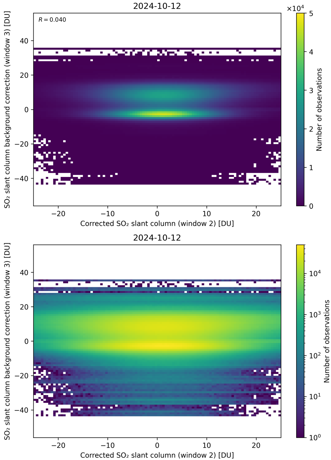
Figure 195: Scatter density plot of “Corrected SO 2 slant column (window 2)” against “SO 2 slant column background correction (window 3)” for 2024-10-11 to 2024-10-13.
