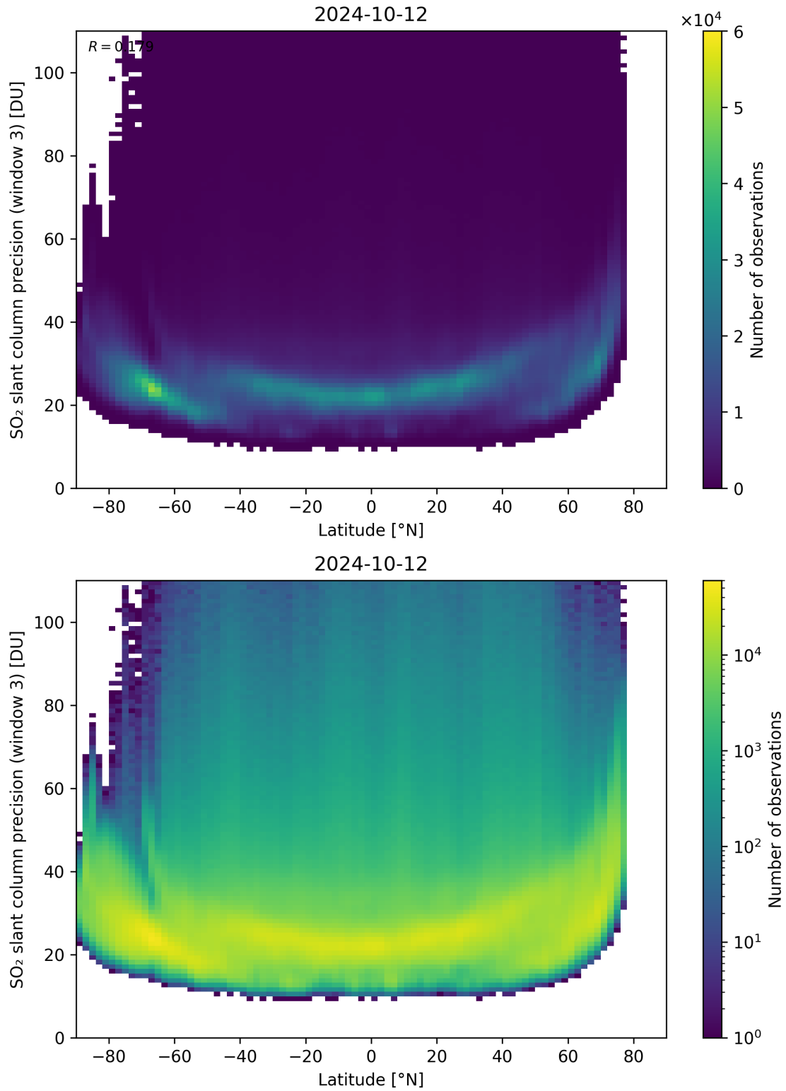
Figure 153: Scatter density plot of “Latitude” against “SO 2 slant column precision (window 3)” for 2024-10-11 to 2024-10-13.
