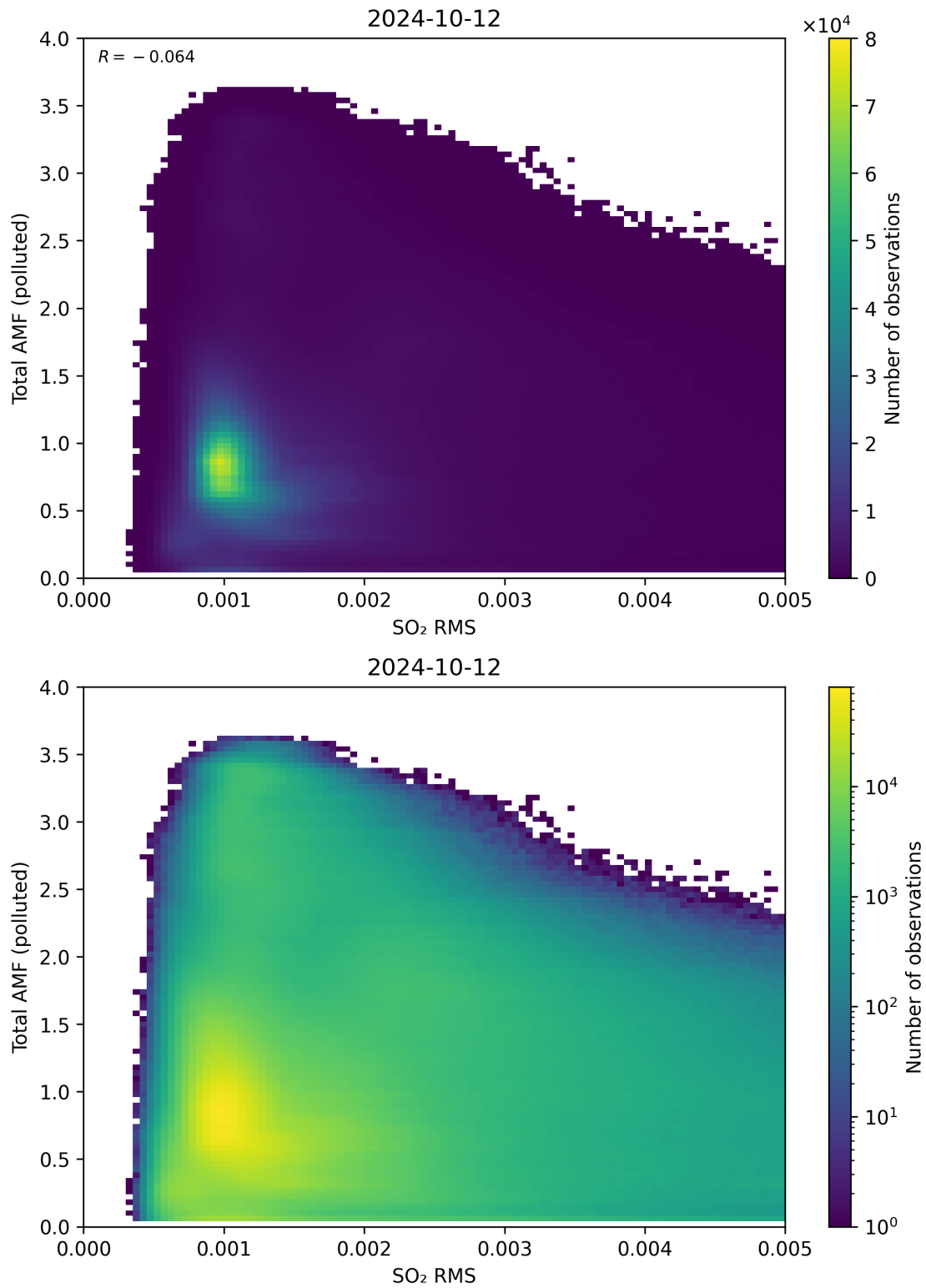
Figure 137: Scatter density plot of “SO 2 RMS” against “Total AMF (polluted)” for 2024-10-11 to 2024-10-13.
