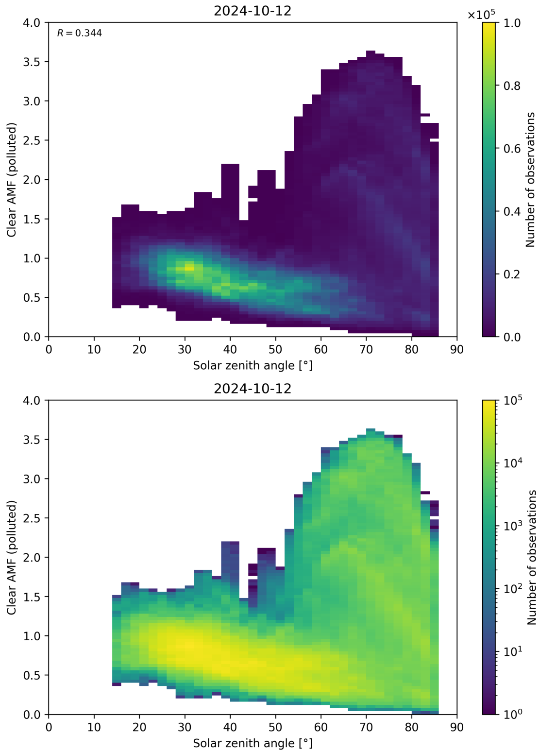
Figure 165: Scatter density plot of “Solar zenith angle” against “Clear AMF (polluted)” for 2024-10-11 to 2024-10-13.
