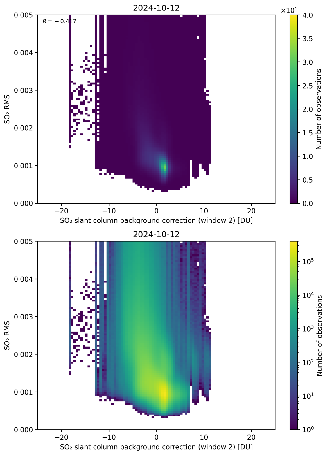
Figure 114: Scatter density plot of “SO 2 slant column background correction (window 2)” against “SO 2 RMS” for 2024-10-11 to 2024-10-13.
