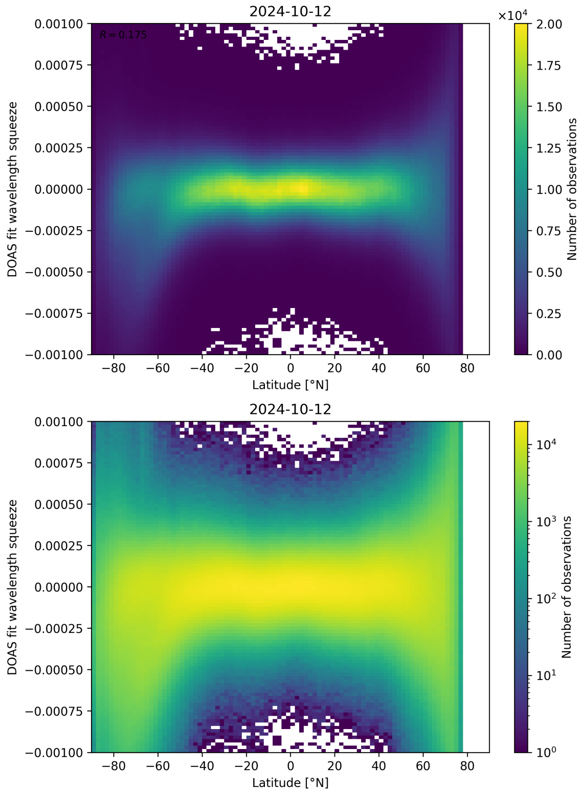
Figure 143: Scatter density plot of “Latitude” against “DOAS fit wavelength squeeze” for 2024-10-11 to 2024-10-13.
