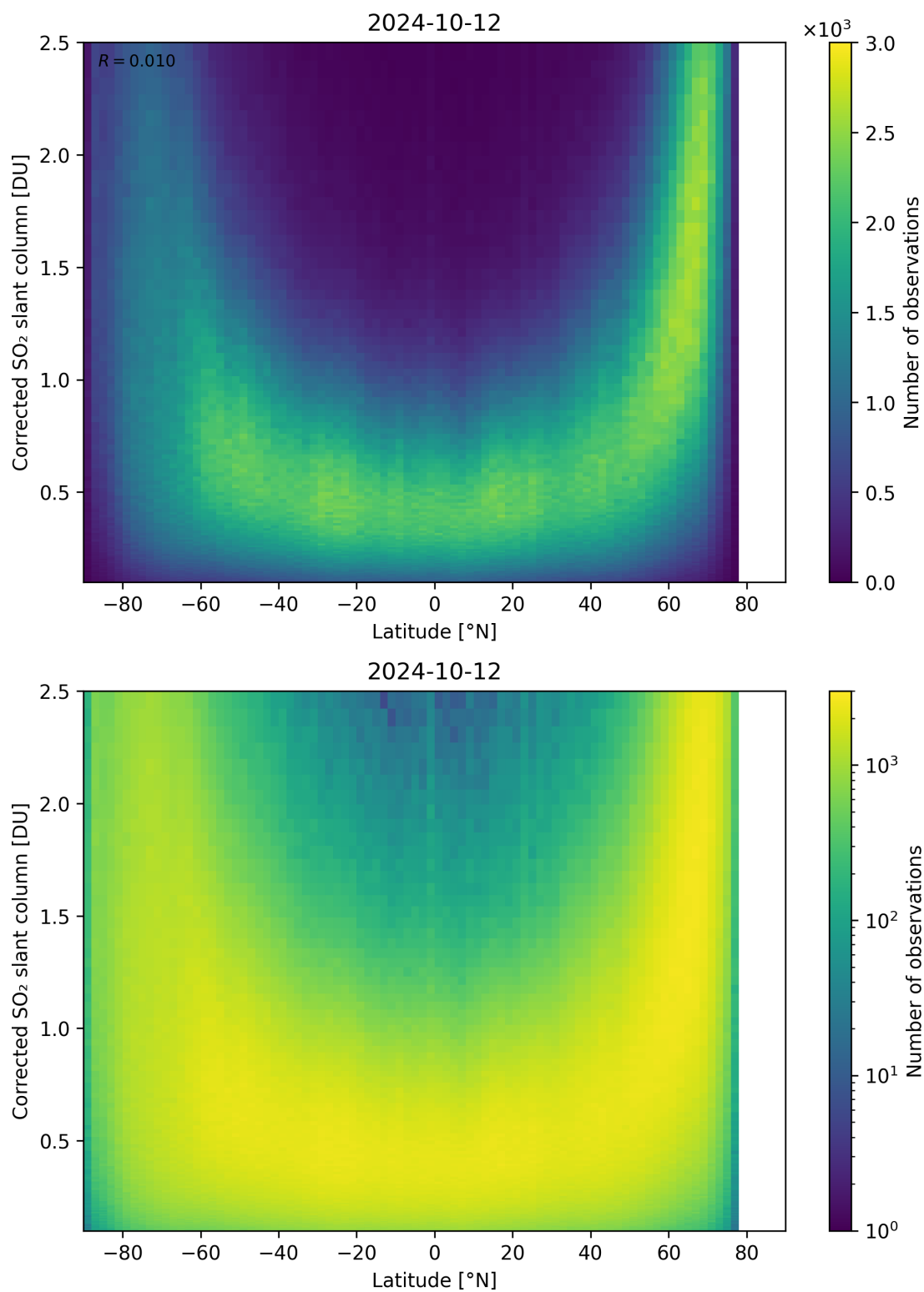
Figure 146: Scatter density plot of “Latitude” against “Corrected SO 2 slant column” for 2024-10-11 to 2024-10-13.
