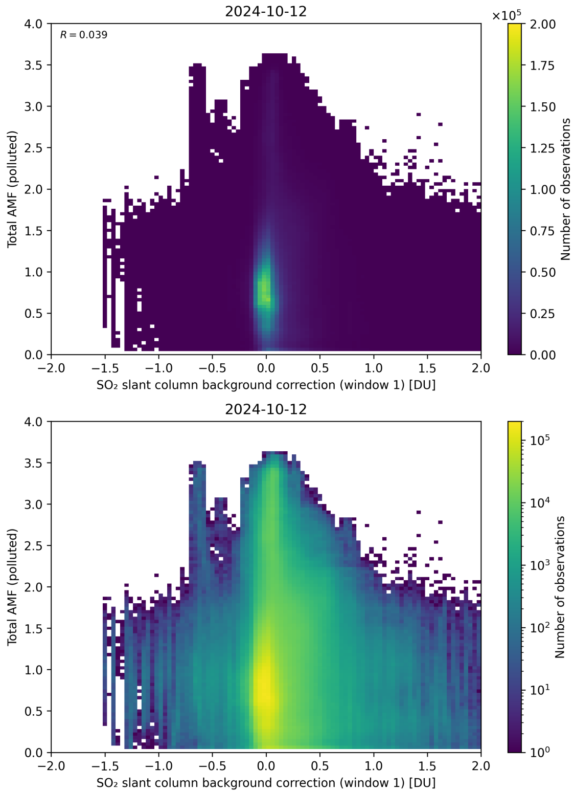
Figure 109: Scatter density plot of “SO 2 slant column background correction (window 1)” against “Total AMF (polluted)” for 2024-10-11 to 2024-10-13.
