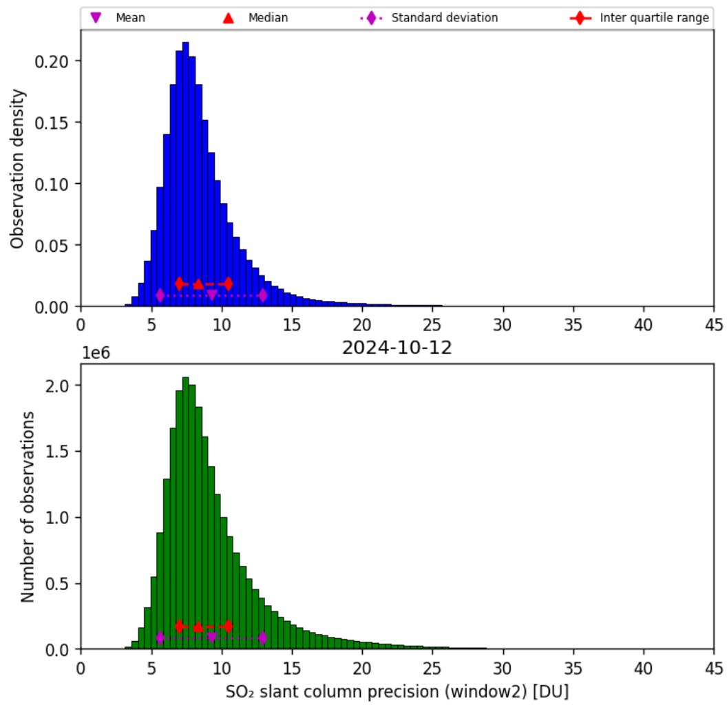
Figure 61: Histogram of “SO 2 slant column precision (window2)” for 2024-10-11 to 2024-10-13
