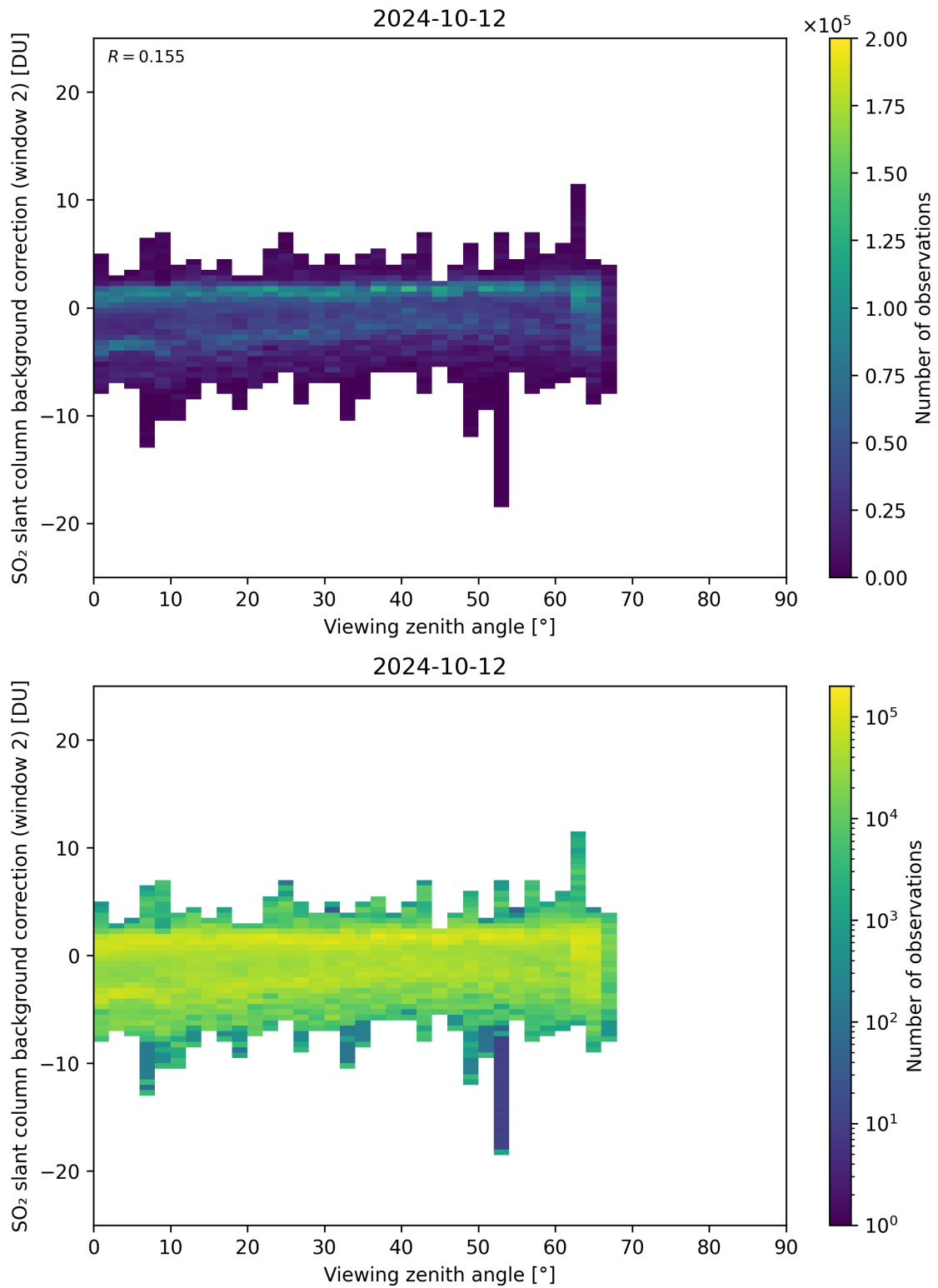
Figure 309: Scatter density plot of “Viewing zenith angle” against “SO 2 slant column background correction (window 2)” for 2024-10-11 to 2024-10-13.
