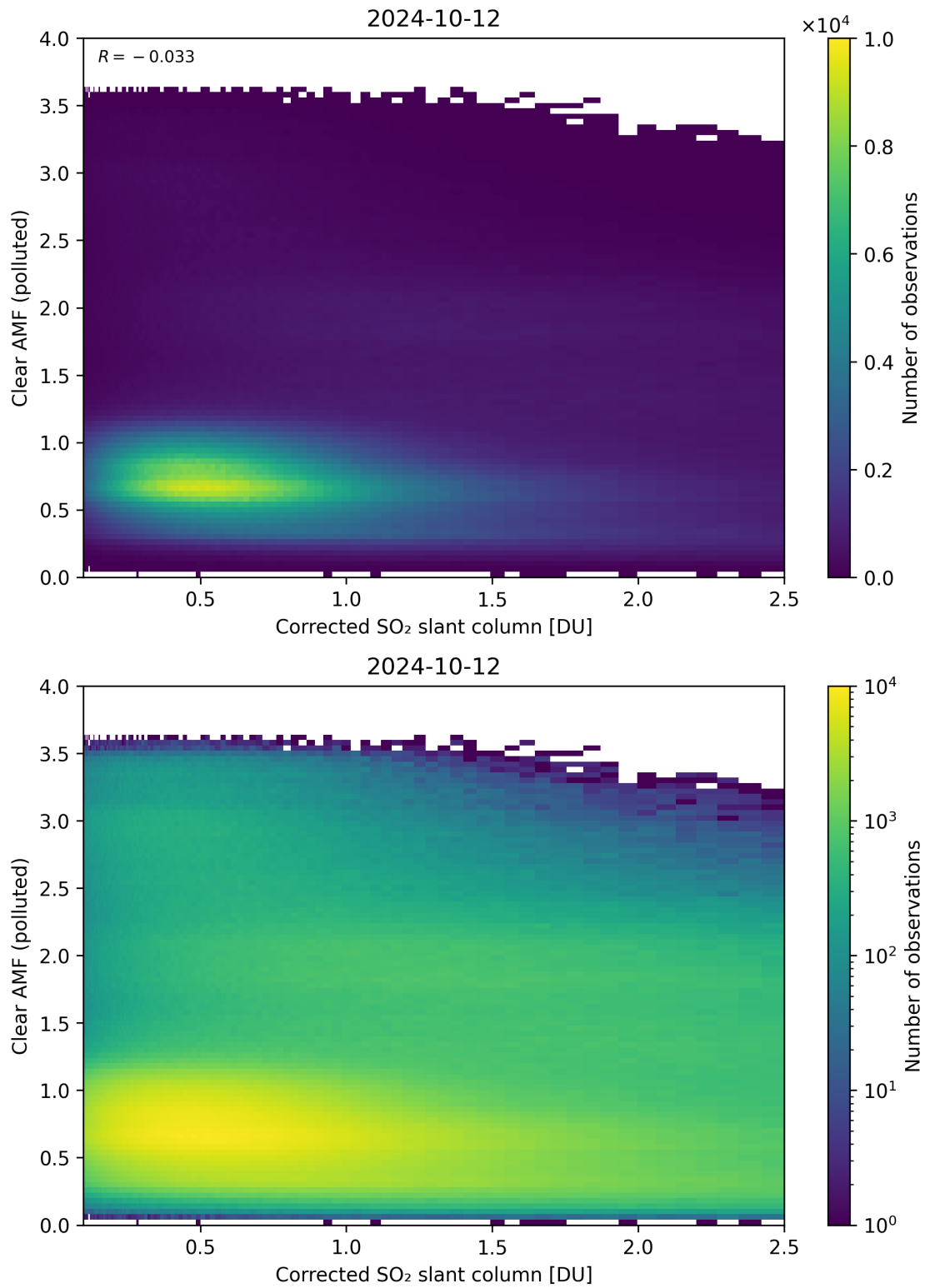
Figure 184: Scatter density plot of “Corrected SO 2 slant column” against “Clear AMF (polluted)” for 2024-10-11 to 2024-10-13.
