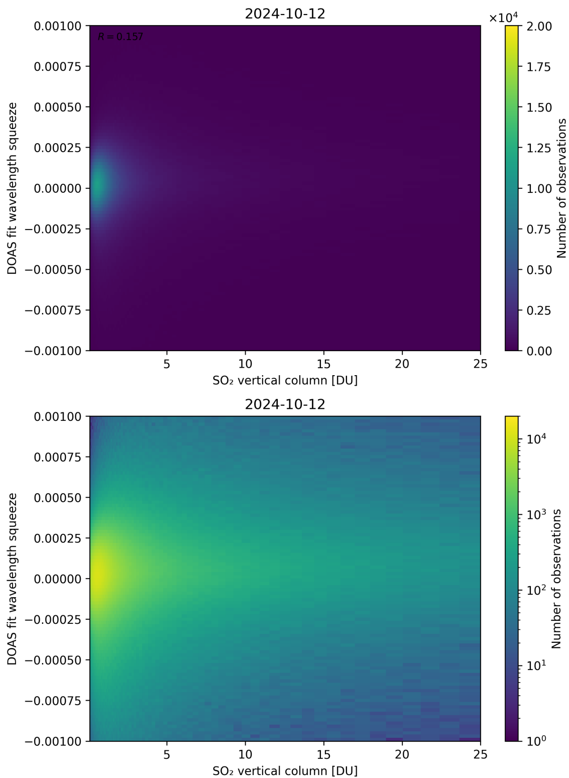
Figure 277: Scatter density plot of “SO 2 vertical column” against “DOAS fit wavelength squeeze” for 2024-10-11 to 2024-10-13.
