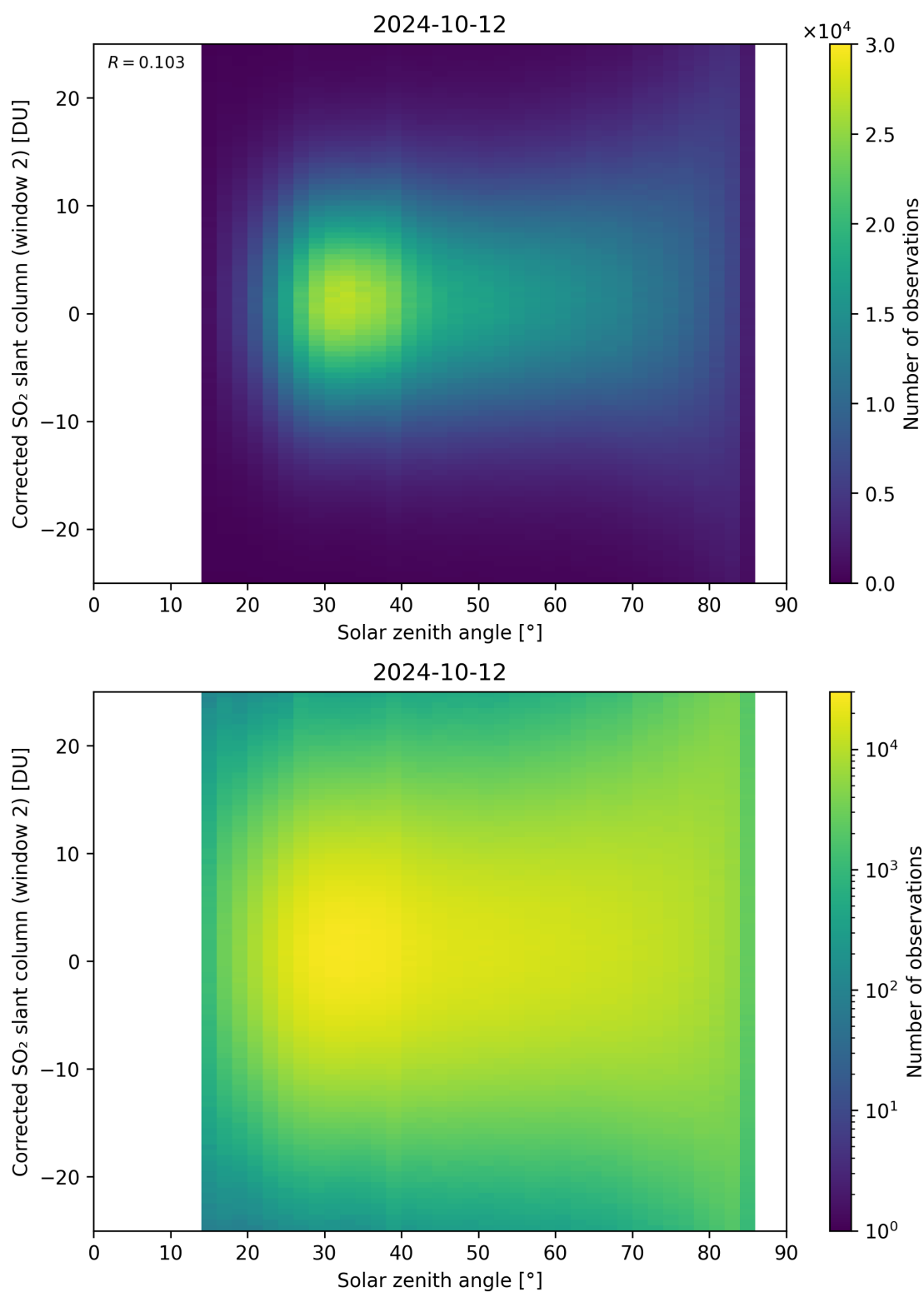
Figure 167: Scatter density plot of “Solar zenith angle” against “Corrected SO 2 slant column (window 2)” for 2024-10-11 to 2024-10-13.
