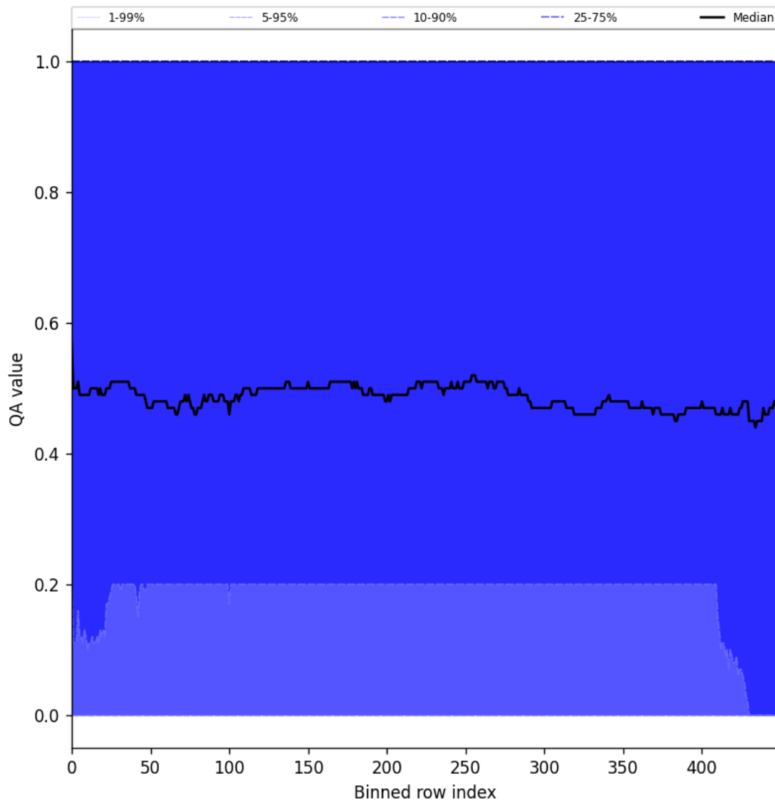
Figure 75: Along track statistics of “QA value” for 2024-10-11 to 2024-10-13
