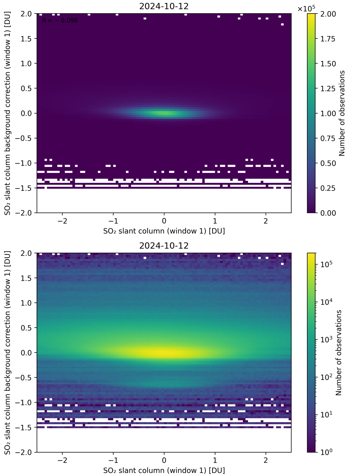
Figure 212: Scatter density plot of “SO 2 slant column (window 1)” against “SO 2 slant column background correction (window 1)” for 2024-10-11 to 2024-10-13.
