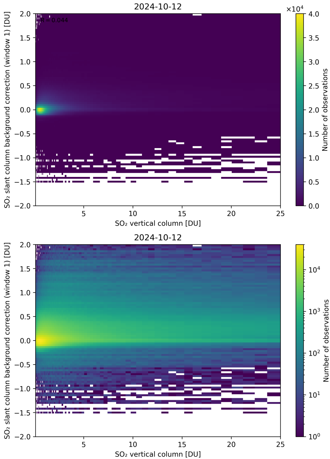
Figure 273: Scatter density plot of “SO 2 vertical column” against “SO 2 slant column background correction (window 1)” for 2024-10-11 to 2024-10-13.
