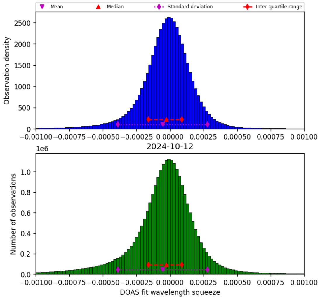
Figure 69: Histogram of “DOAS fit wavelength squeeze” for 2024-10-11 to 2024-10-13
