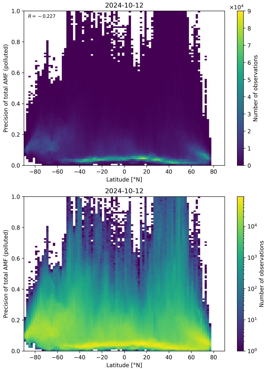
Figure 155: Scatter density plot of “Latitude” against “Precision of total AMF (polluted)” for 2024-10-11 to 2024-10-13.
