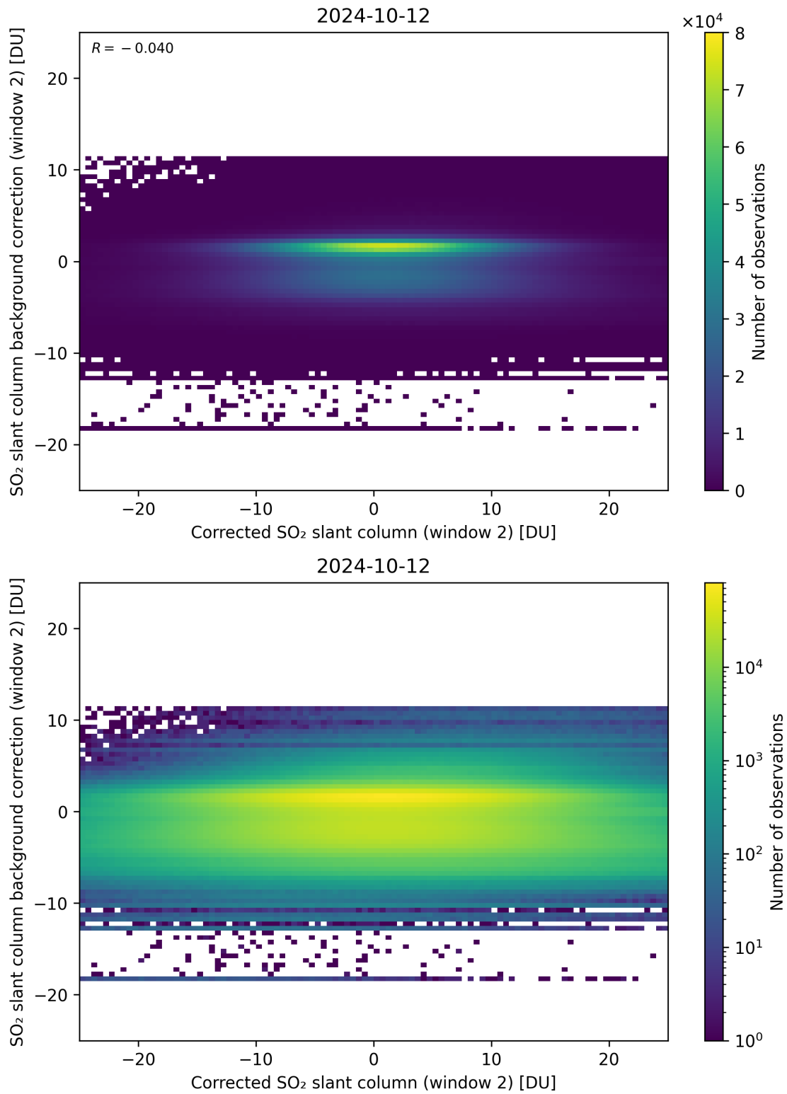
Figure 194: Scatter density plot of “Corrected SO 2 slant column (window 2)” against “SO 2 slant column background correction (window 2)” for 2024-10-11 to 2024-10-13.
