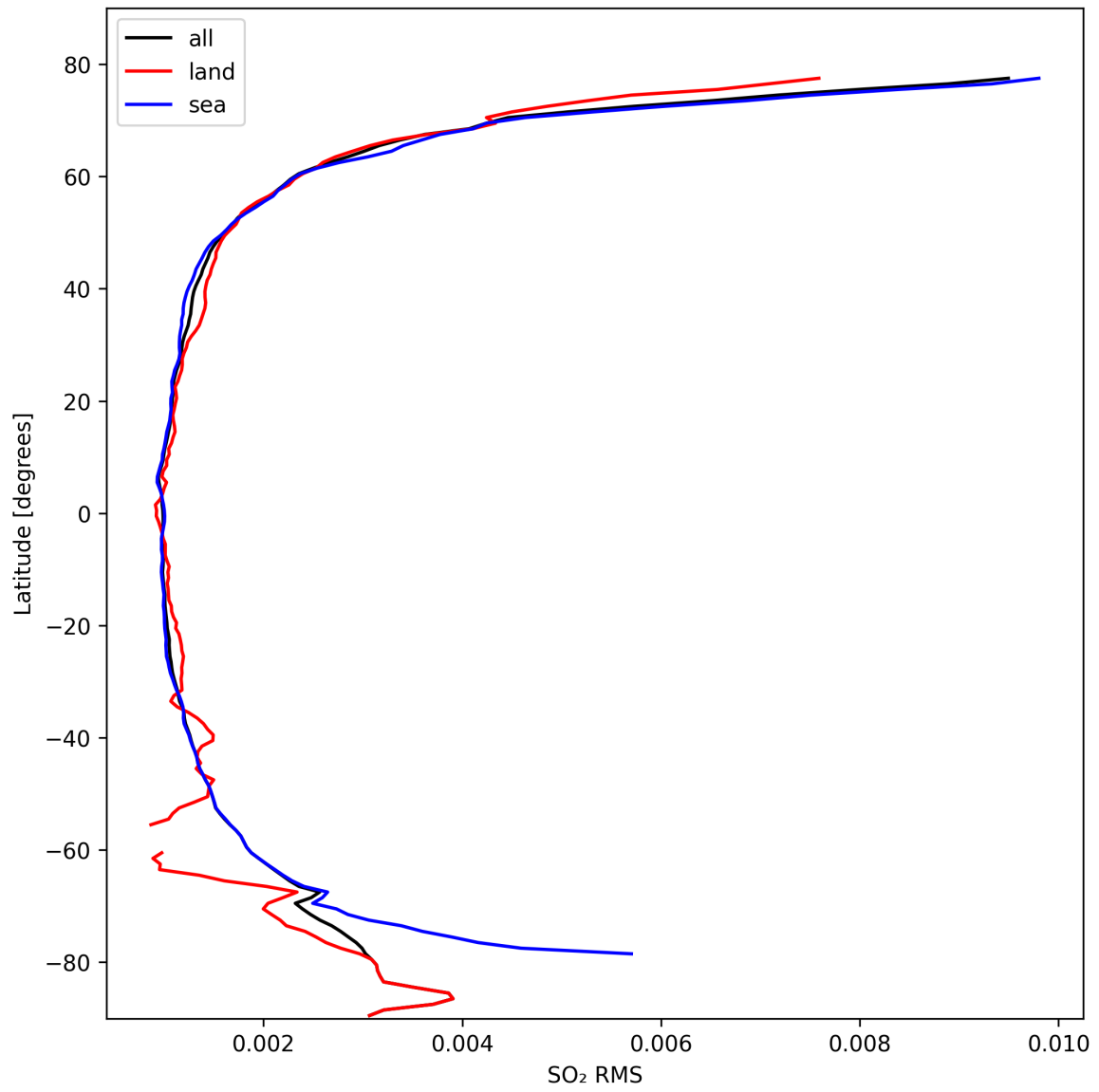
Figure 47: Zonal average of “SO 2 RMS” for 2024-10-11 to 2024-10-13.
