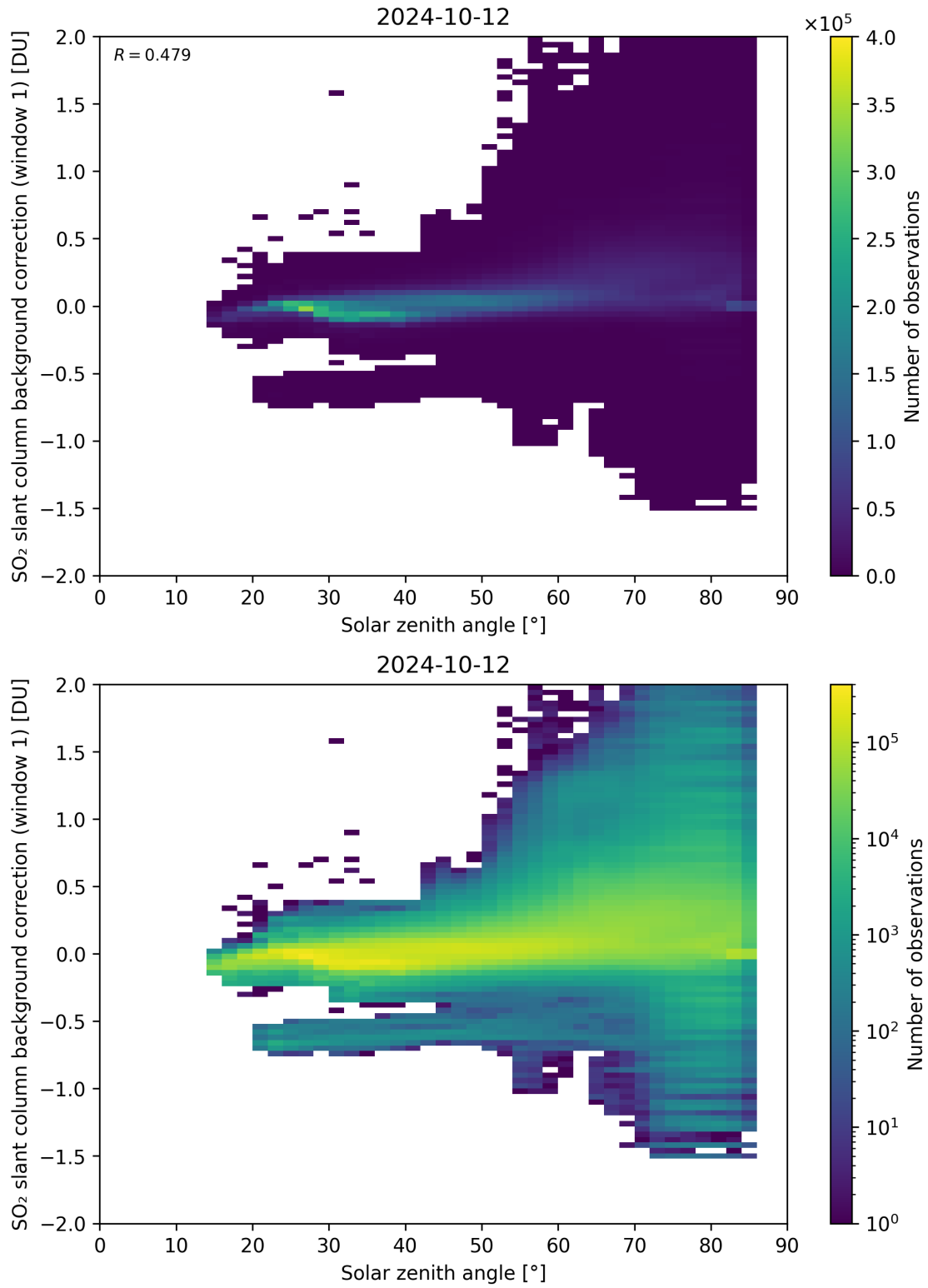
Figure 158: Scatter density plot of “Solar zenith angle” against “SO 2 slant column background correction (window 1)” for 2024-10-11 to 2024-10-13.
