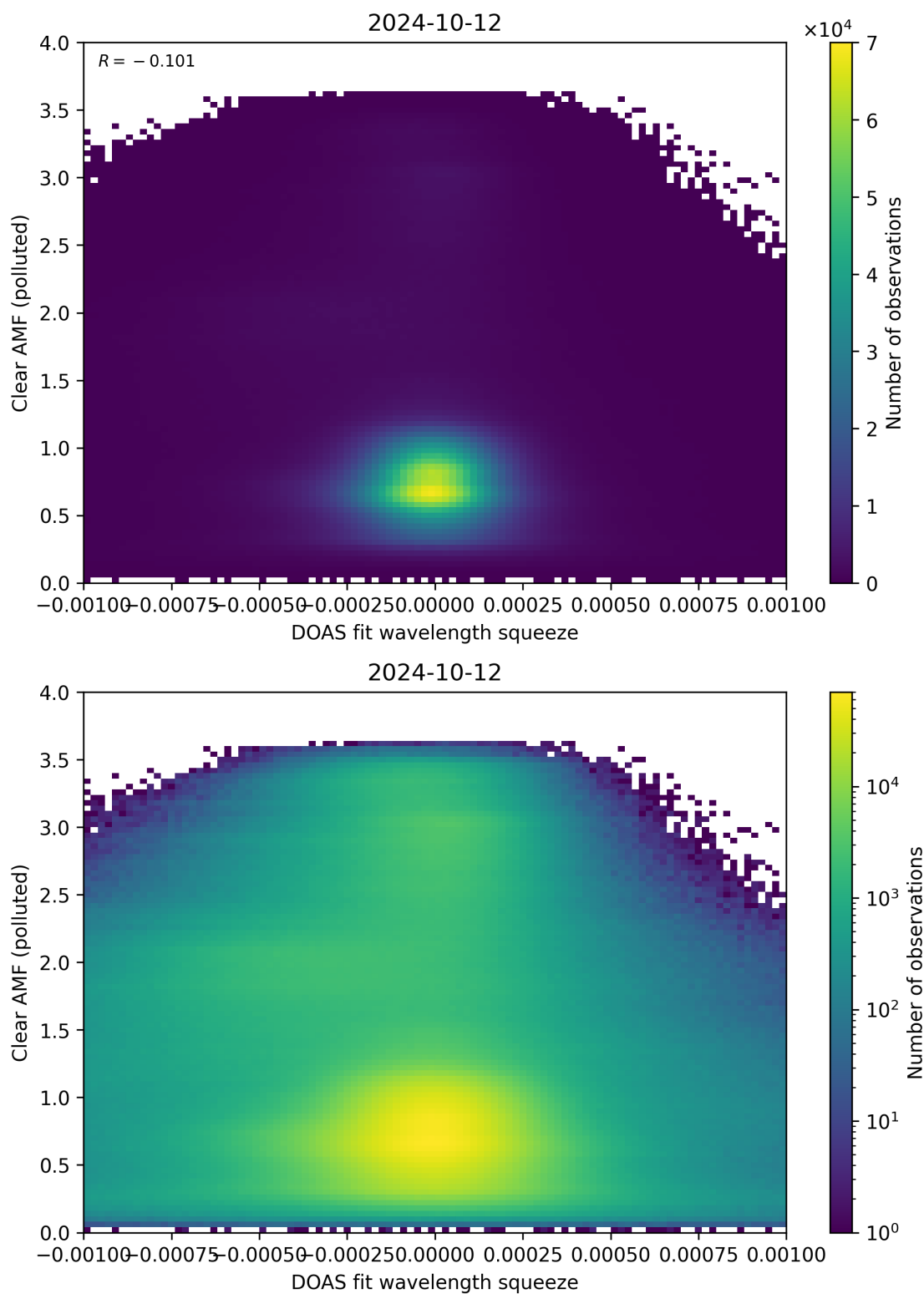
Figure 133: Scatter density plot of “DOAS fit wavelength squeeze” against “Clear AMF (polluted)” for 2024-10-11 to 2024-10-13.
