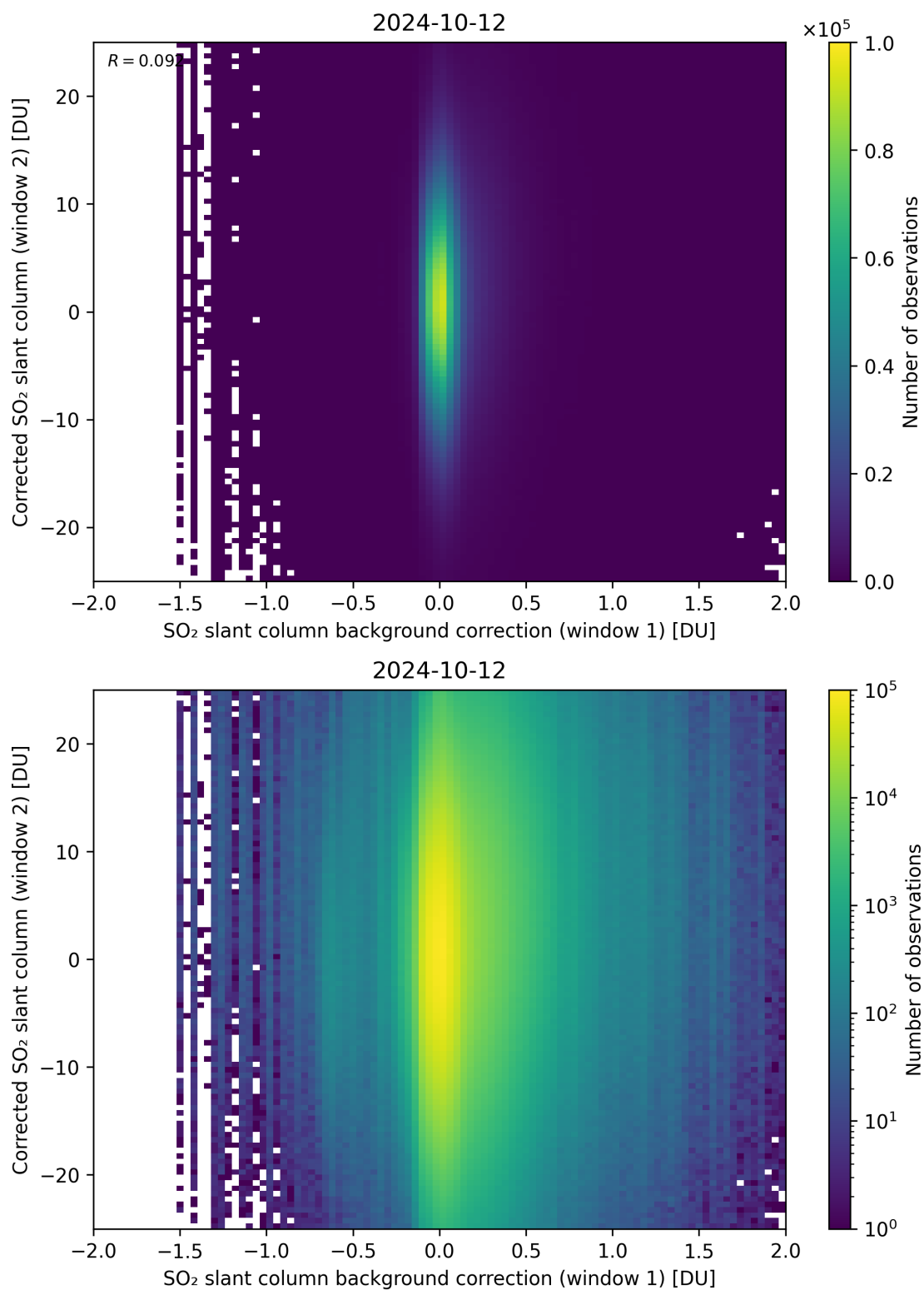
Figure 104: Scatter density plot of “SO 2 slant column background correction (window 1)” against “Corrected SO 2 slant column (window 2)” for 2024-10-11 to 2024-10-13.
