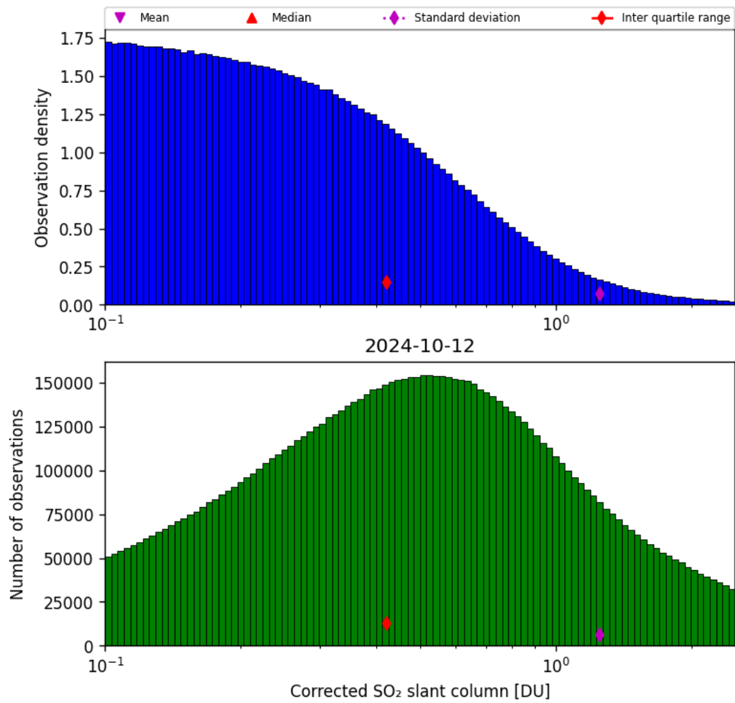
Figure 55: Histogram of “Corrected SO 2 slant column” for 2024-10-11 to 2024-10-13
