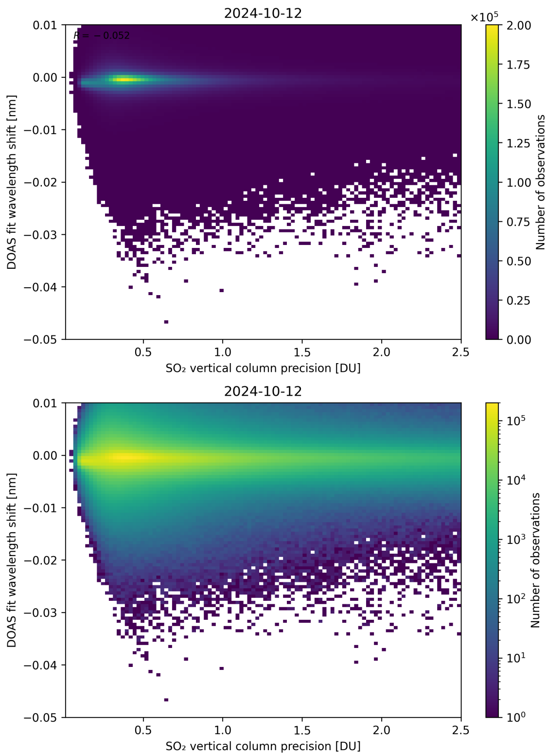
Figure 282: Scatter density plot of “SO 2 vertical column precision” against “DOAS fit wavelength shift” for 2024-10-11 to 2024-10-13.
