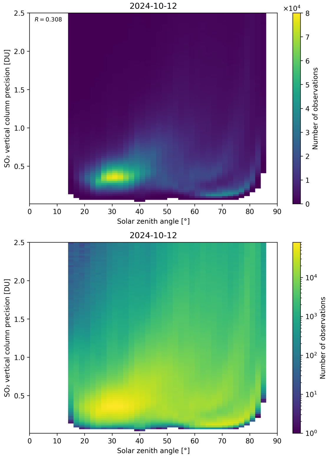
Figure 177: Scatter density plot of “Solar zenith angle” against “SO 2 vertical column precision” for 2024-10-11 to 2024-10-13.
