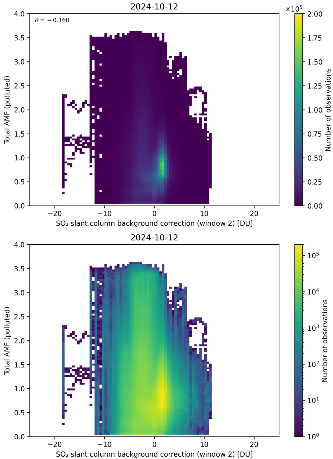
Figure 119: Scatter density plot of “SO 2 slant column background correction (window 2)” against “Total AMF (polluted)” for 2024-10-11 to 2024-10-13.
