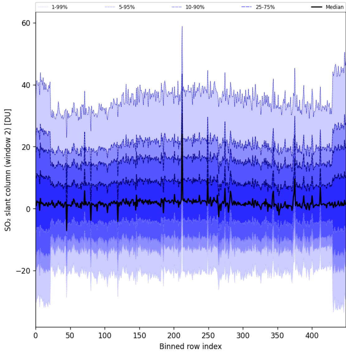
Figure 83: Along track statistics of “SO 2 slant column (window 2)” for 2024-10-11 to 2024-10-13
