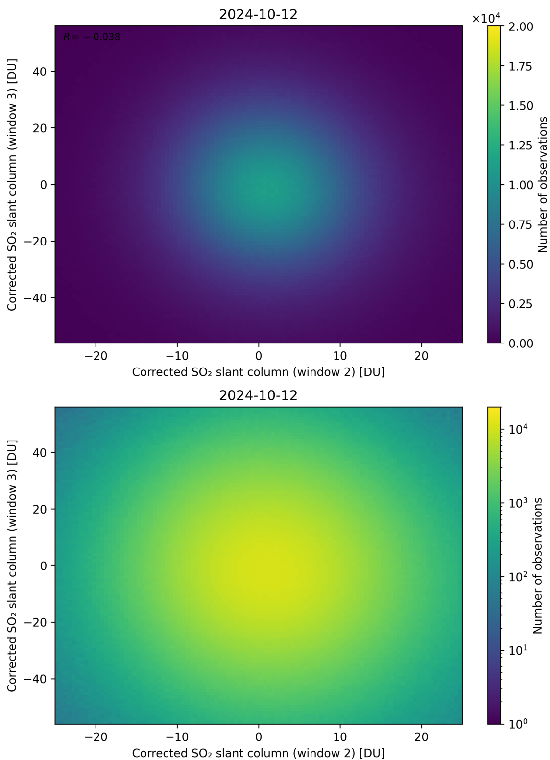
Figure 200: Scatter density plot of “Corrected SO 2 slant column (window 2)” against “Corrected SO 2 slant column (window 3)” for 2024-10-11 to 2024-10-13.
