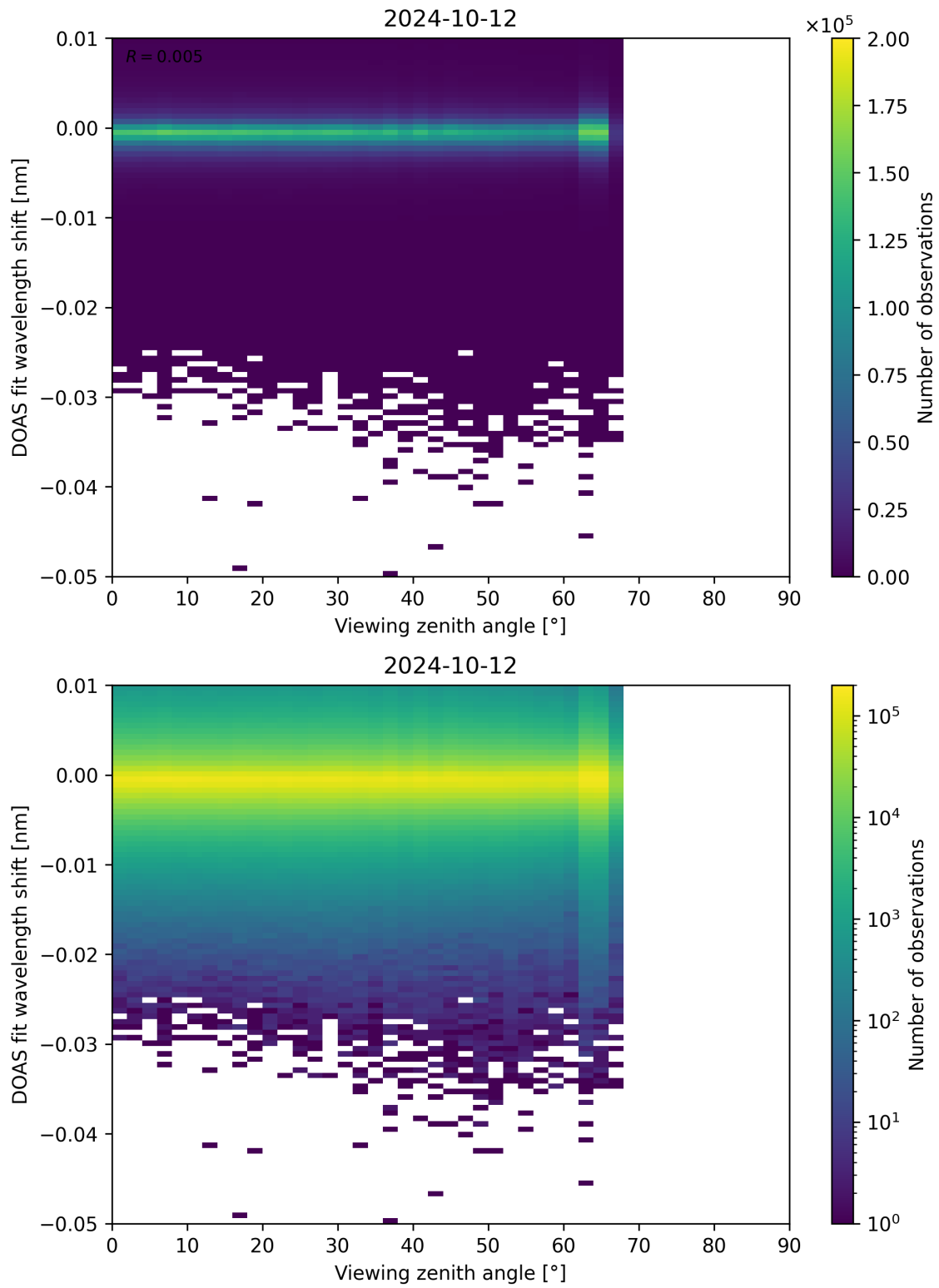
Figure 311: Scatter density plot of “Viewing zenith angle” against “DOAS fit wavelength shift” for 2024-10-11 to 2024-10-13.
