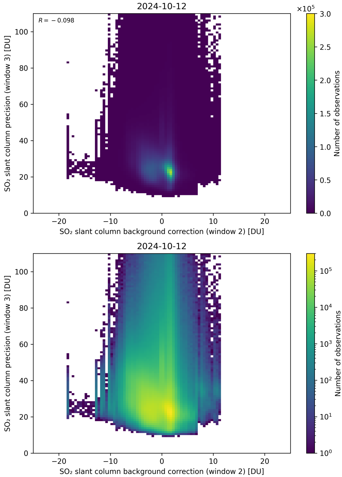
Figure 118: Scatter density plot of “SO 2 slant column background correction (window 2)” against “SO 2 slant column precision (window 3)” for 2024-10-11 to 2024-10-13.
