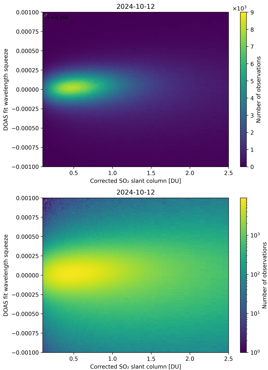
Figure 182: Scatter density plot of “Corrected SO 2 slant column” against “DOAS fit wavelength squeeze” for 2024-10-11 to 2024-10-13.
