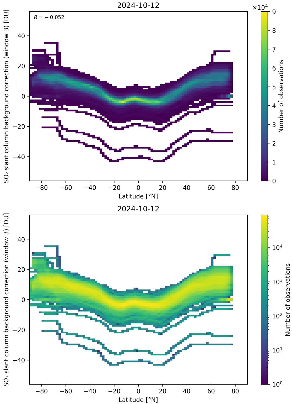
Figure 141: Scatter density plot of “Latitude” against “SO 2 slant column background correction (window 3)” for 2024-10-11 to 2024-10-13.
