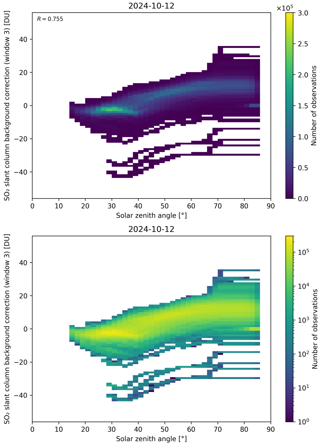
Figure 160: Scatter density plot of “Solar zenith angle” against “SO 2 slant column background correction (window 3)” for 2024-10-11 to 2024-10-13.
