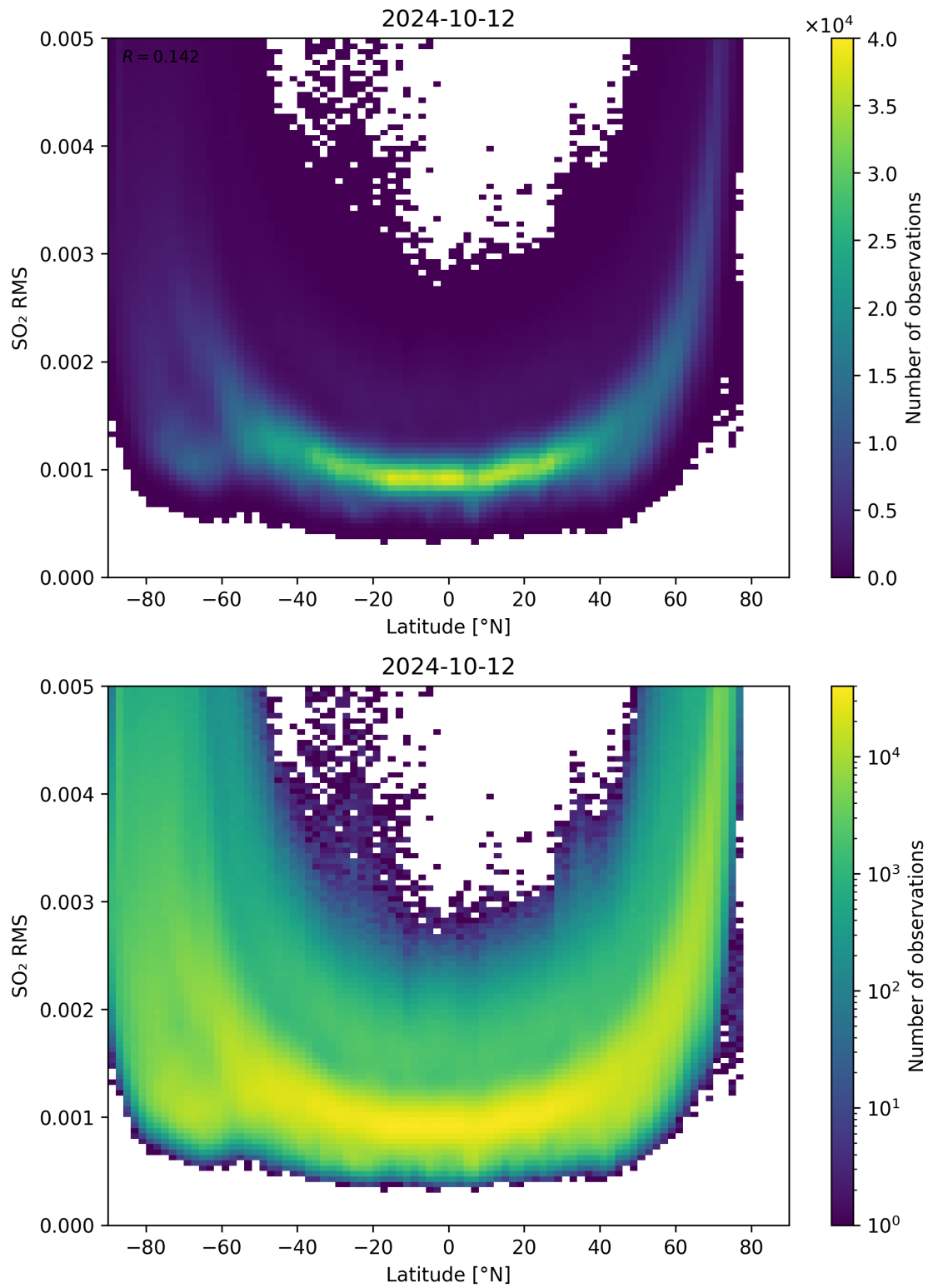
Figure 144: Scatter density plot of “Latitude” against “SO 2 RMS” for 2024-10-11 to 2024-10-13.
