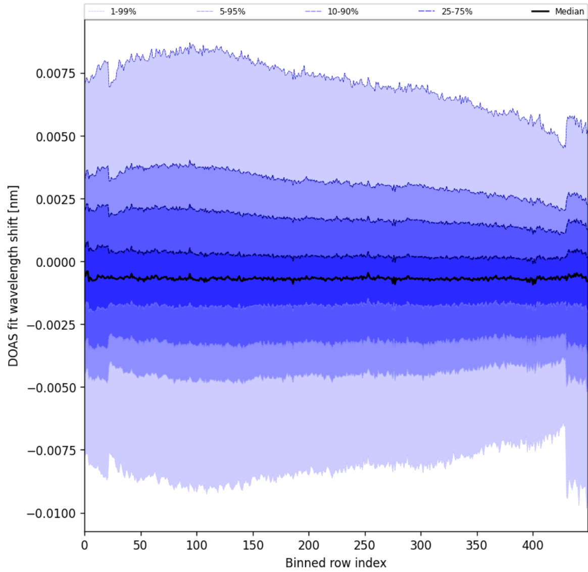
Figure 91: Along track statistics of “DOAS fit wavelength shift” for 2024-10-11 to 2024-10-13
