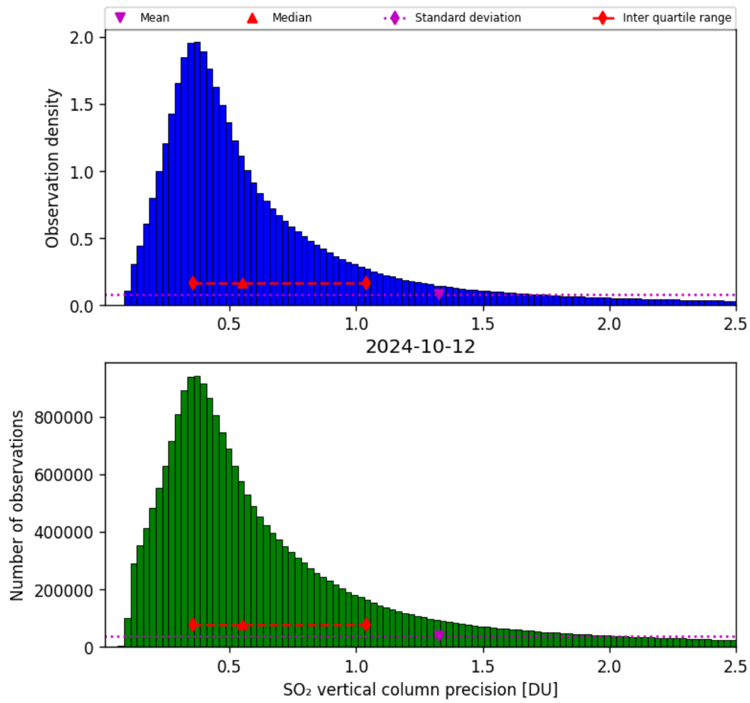
Figure 54: Histogram of “SO 2 vertical column precision” for 2024-10-11 to 2024-10-13
