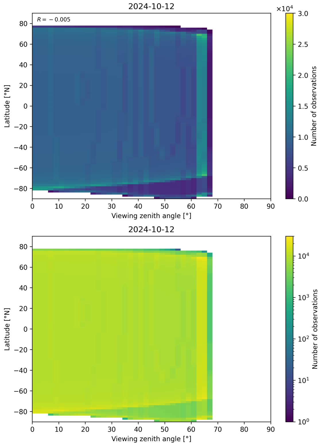
Figure 314: Scatter density plot of “Viewing zenith angle” against “Latitude” for 2024-10-11 to 2024-10-13.
