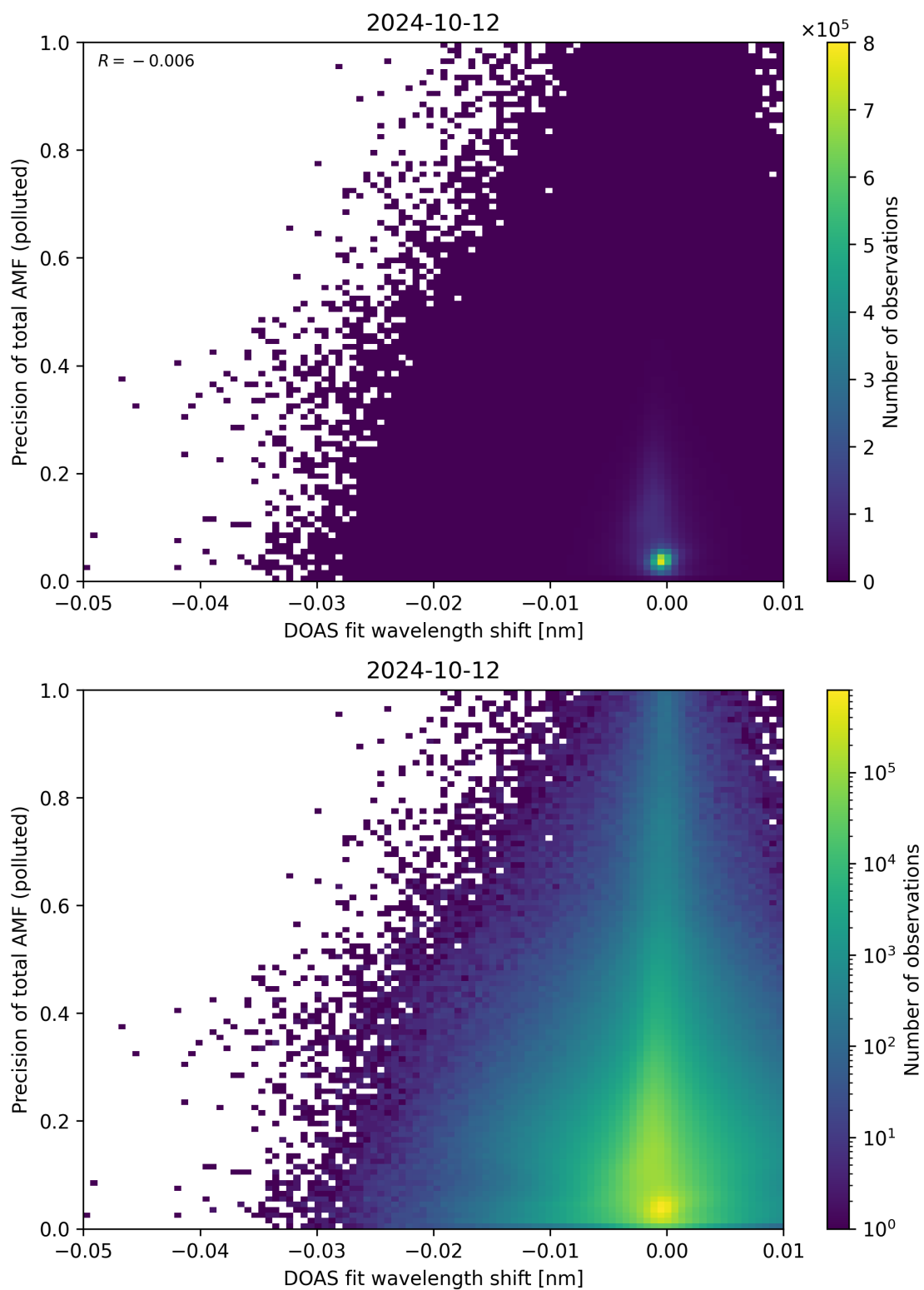
Figure 131: Scatter density plot of “DOAS fit wavelength shift” against “Precision of total AMF (polluted)” for 2024-10-11 to 2024-10-13.
