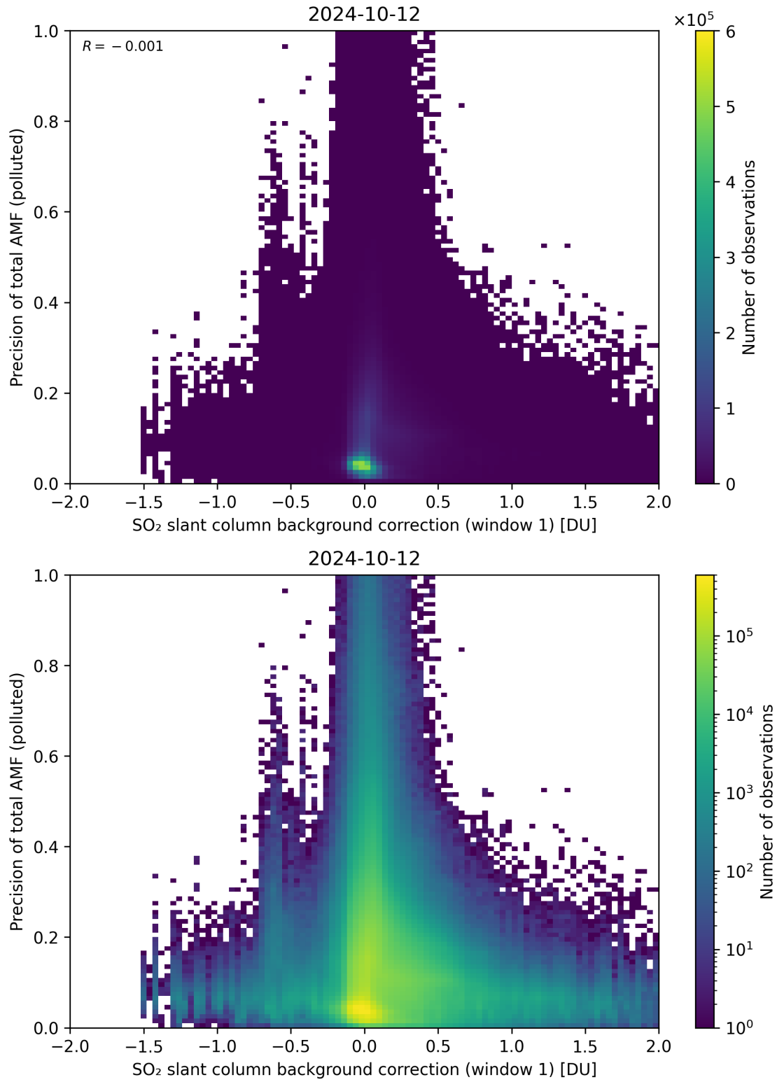
Figure 110: Scatter density plot of “SO 2 slant column background correction (window 1)” against “Precision of total AMF (polluted)” for 2024-10-11 to 2024-10-13.
