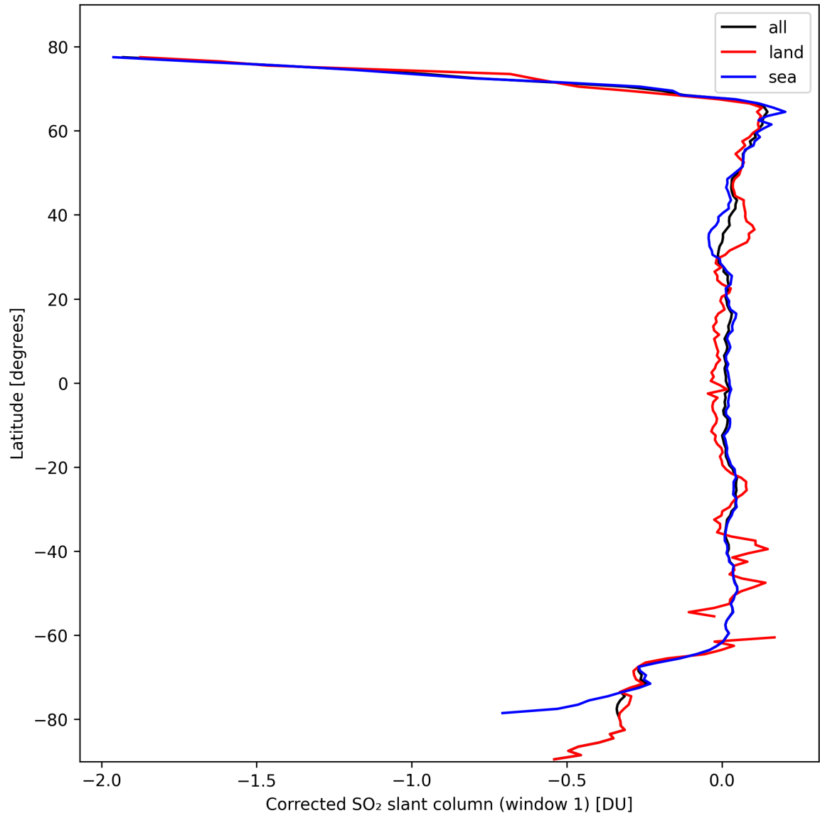
Figure 35: Zonal average of “Corrected SO 2 slant column (window 1)” for 2024-10-11 to 2024-10-13.
