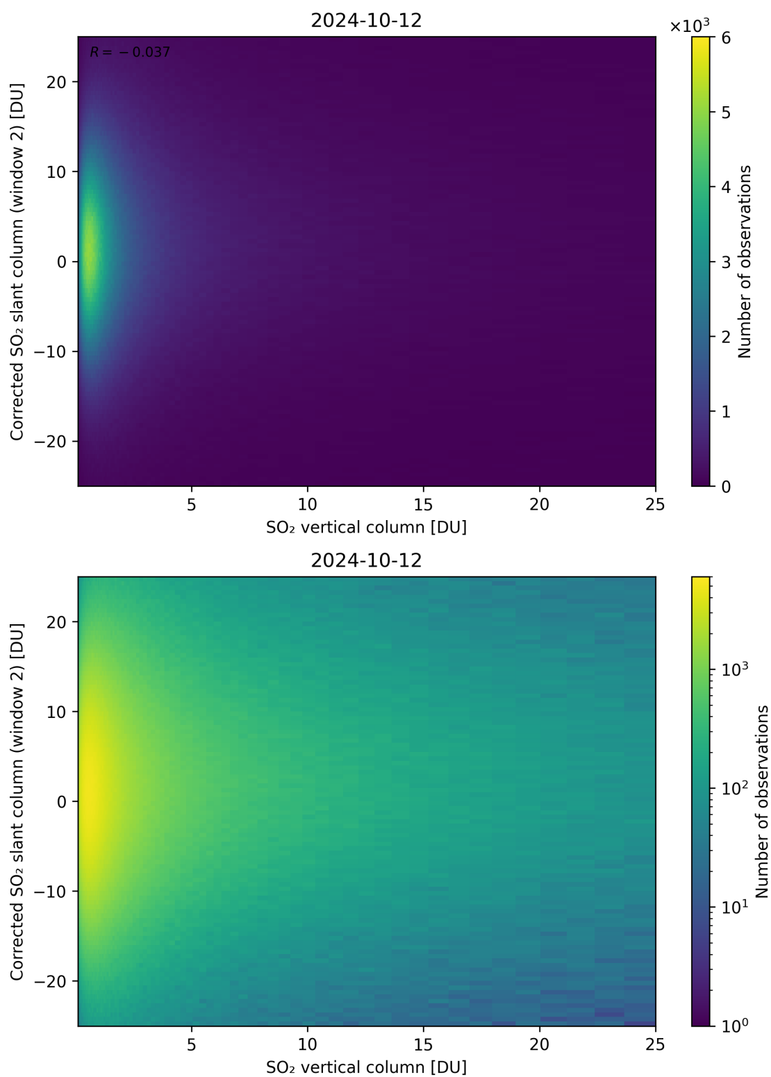
Figure 298: Scatter density plot of “SO 2 vertical column” against “Corrected SO 2 slant column (window 2)” for 2024-10-11 to 2024-10-13.
