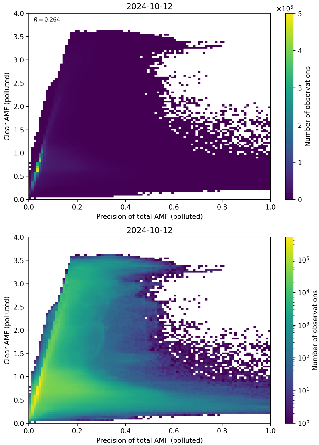
Figure 270: Scatter density plot of “Precision of total AMF (polluted)” against “Clear AMF (polluted)” for 2024-10-11 to 2024-10-13.
