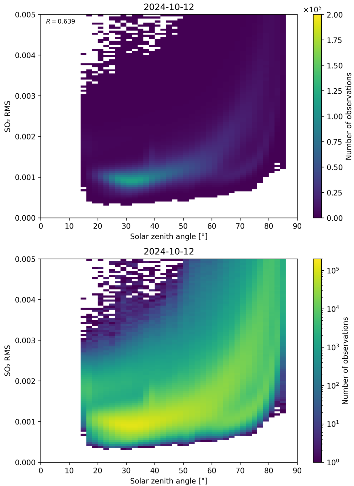
Figure 163: Scatter density plot of “Solar zenith angle” against “SO 2 RMS” for 2024-10-11 to 2024-10-13.
