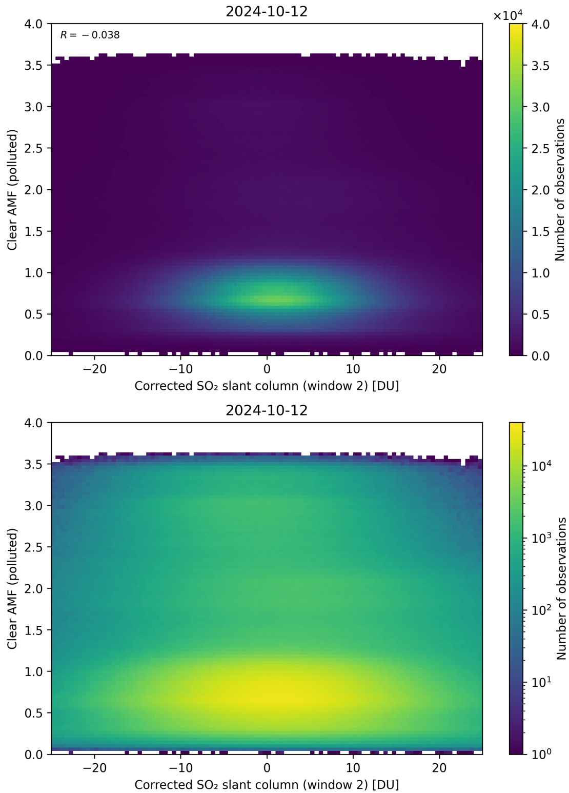
Figure 199: Scatter density plot of “Corrected SO 2 slant column (window 2)” against “Clear AMF (polluted)” for 2024-10-11 to 2024-10-13.
