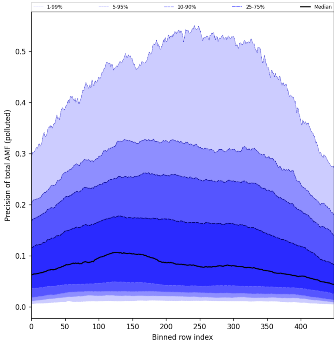
Figure 95: Along track statistics of “Precision of total AMF (polluted)” for 2024-10-11 to 2024-10-13
