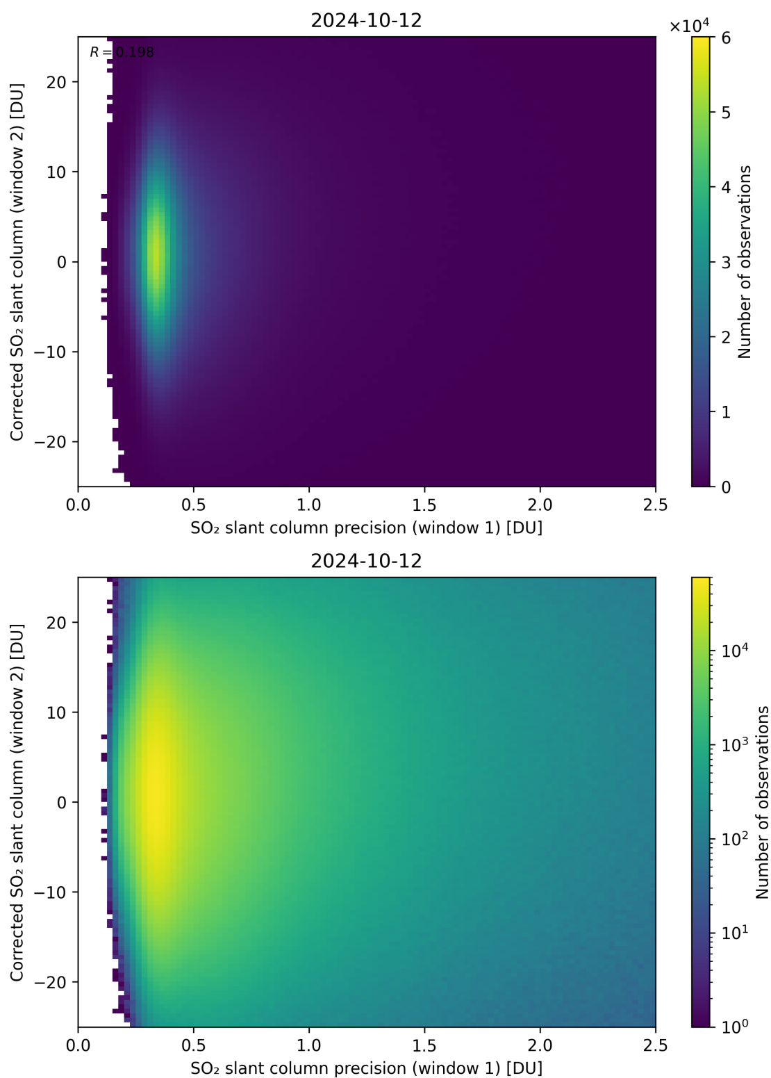
Figure 225: Scatter density plot of “SO 2 slant column precision (window 1)” against “Corrected SO 2 slant column (window 2)” for 2024-10-11 to 2024-10-13.
