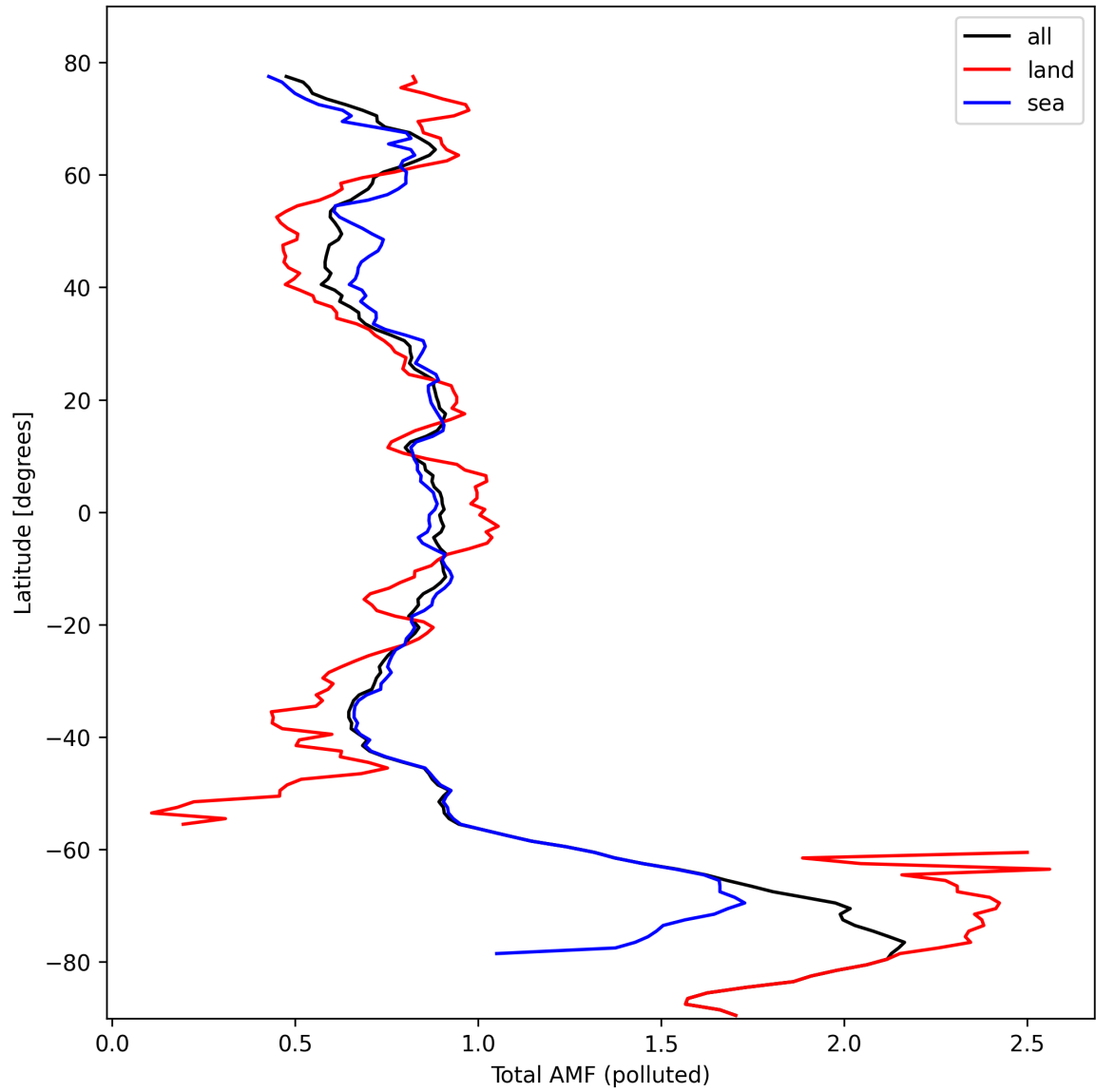
Figure 48: Zonal average of “Total AMF (polluted)” for 2024-10-11 to 2024-10-13.
