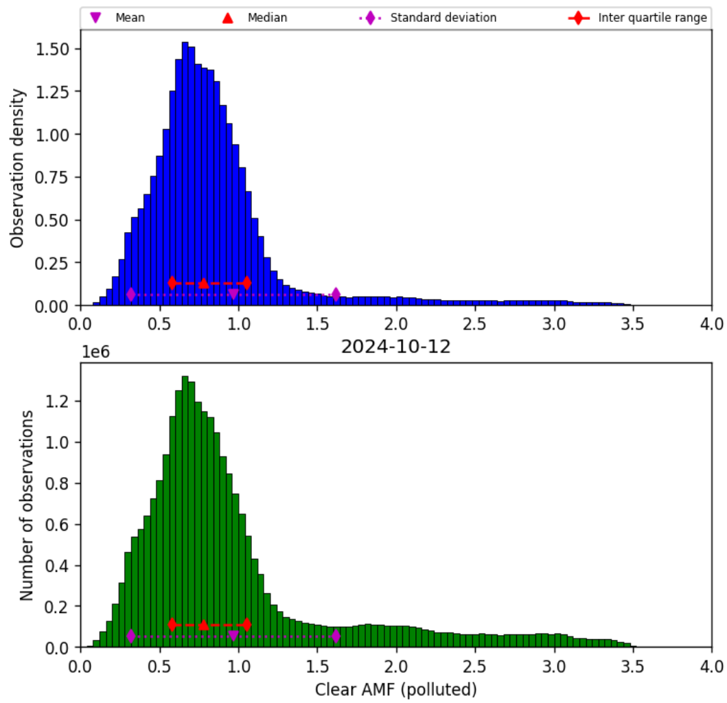
Figure 73: Histogram of “Clear AMF (polluted)” for 2024-10-11 to 2024-10-13
