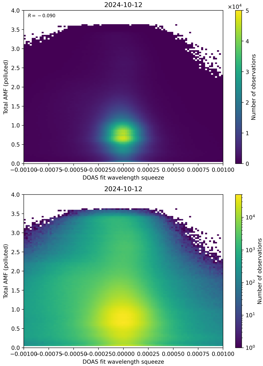
Figure 134: Scatter density plot of “DOAS fit wavelength squeeze” against “Total AMF (polluted)” for 2024-10-11 to 2024-10-13.
