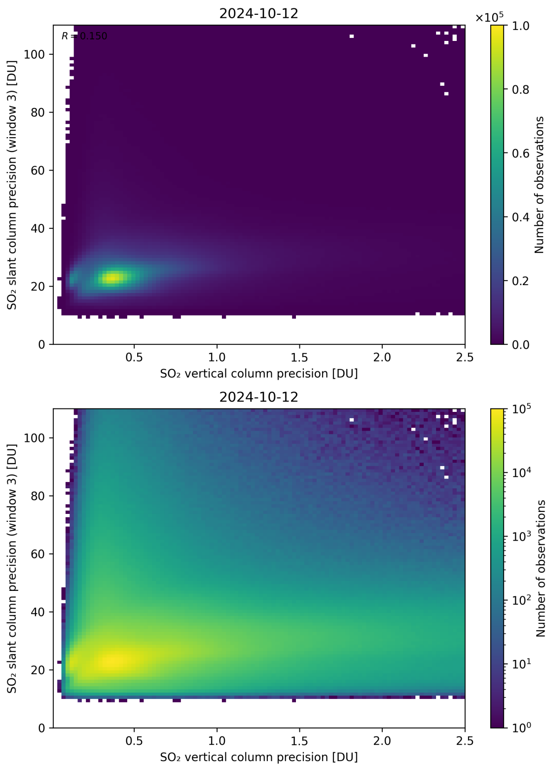
Figure 293: Scatter density plot of “SO 2 vertical column precision” against “SO 2 slant column precision (window 3)” for 2024-10-11 to 2024-10-13.
