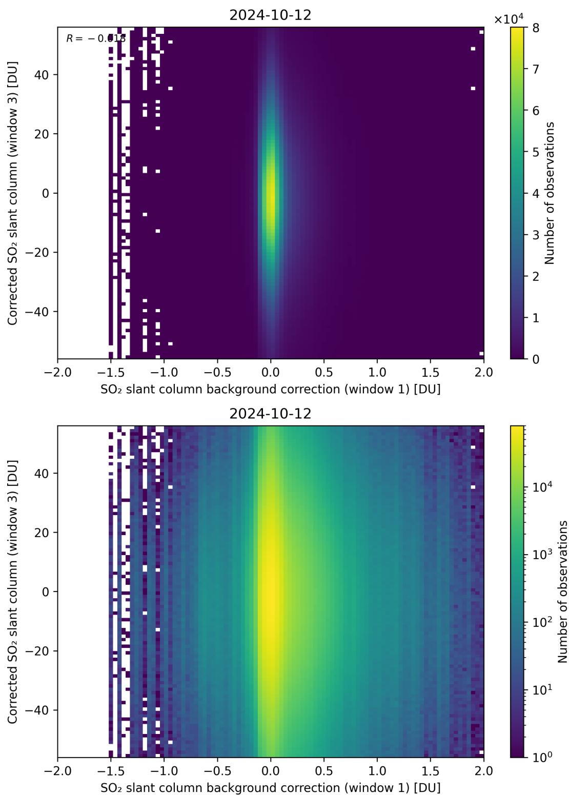
Figure 105: Scatter density plot of “SO 2 slant column background correction (window 1)” against “Corrected SO 2 slant column (window 3)” for 2024-10-11 to 2024-10-13.
