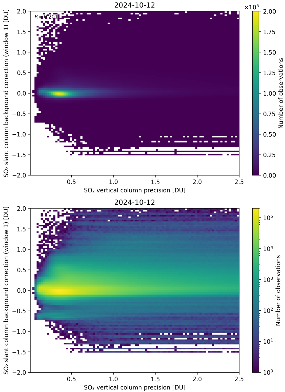
Figure 279: Scatter density plot of “SO 2 vertical column precision” against “SO 2 slant column background correction (window 1)” for 2024-10-11 to 2024-10-13.
