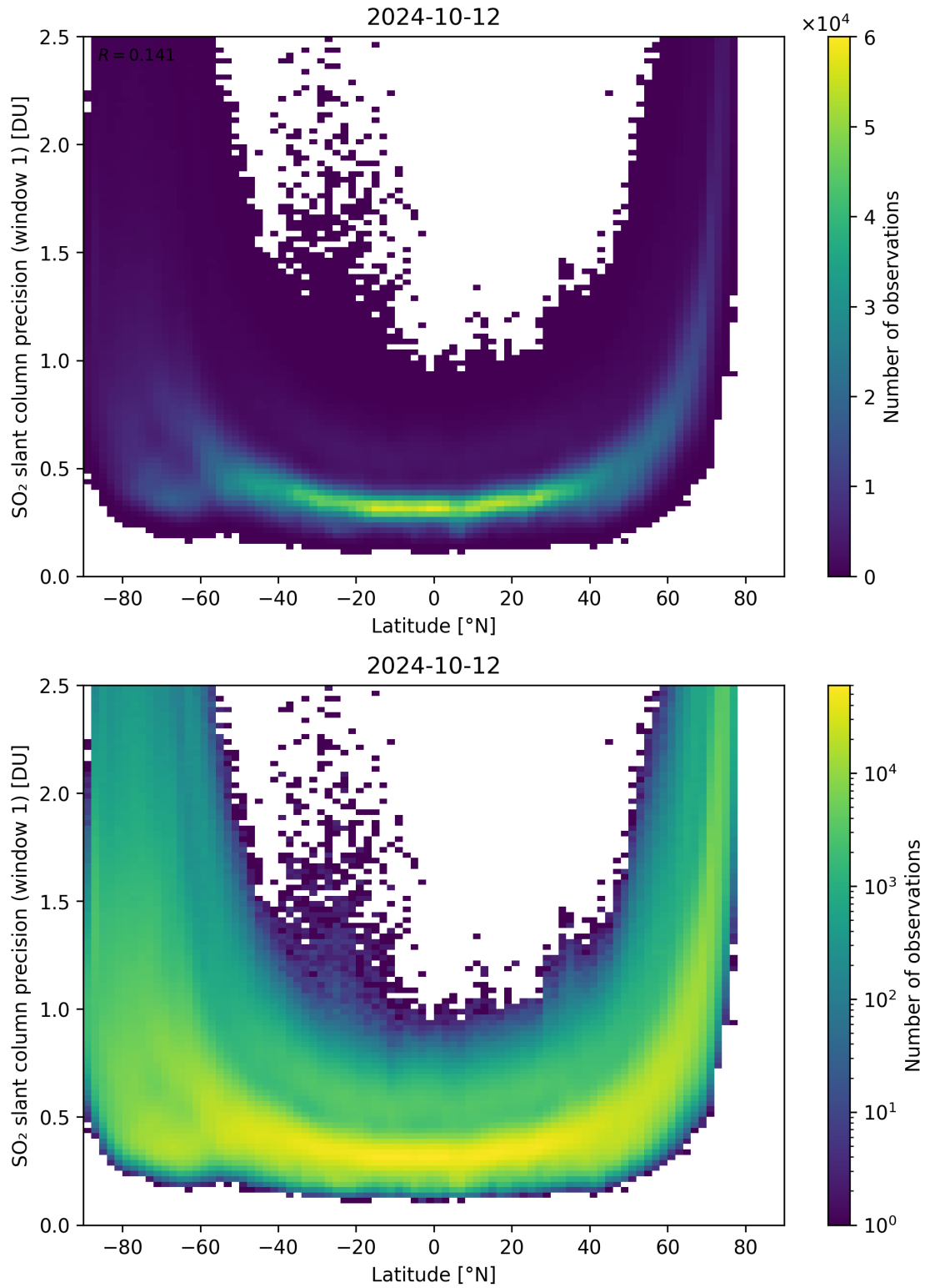
Figure 150: Scatter density plot of “Latitude” against “SO 2 slant column precision (window 1)” for 2024-10-11 to 2024-10-13.
