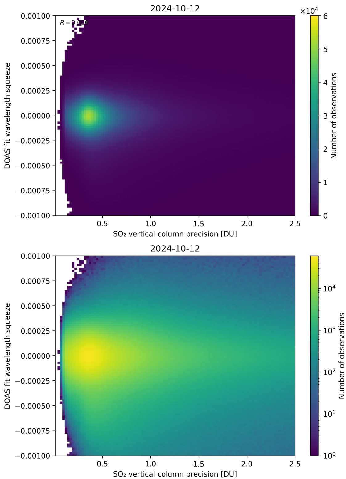
Figure 283: Scatter density plot of “SO 2 vertical column precision” against “DOAS fit wavelength squeeze” for 2024-10-11 to 2024-10-13.
