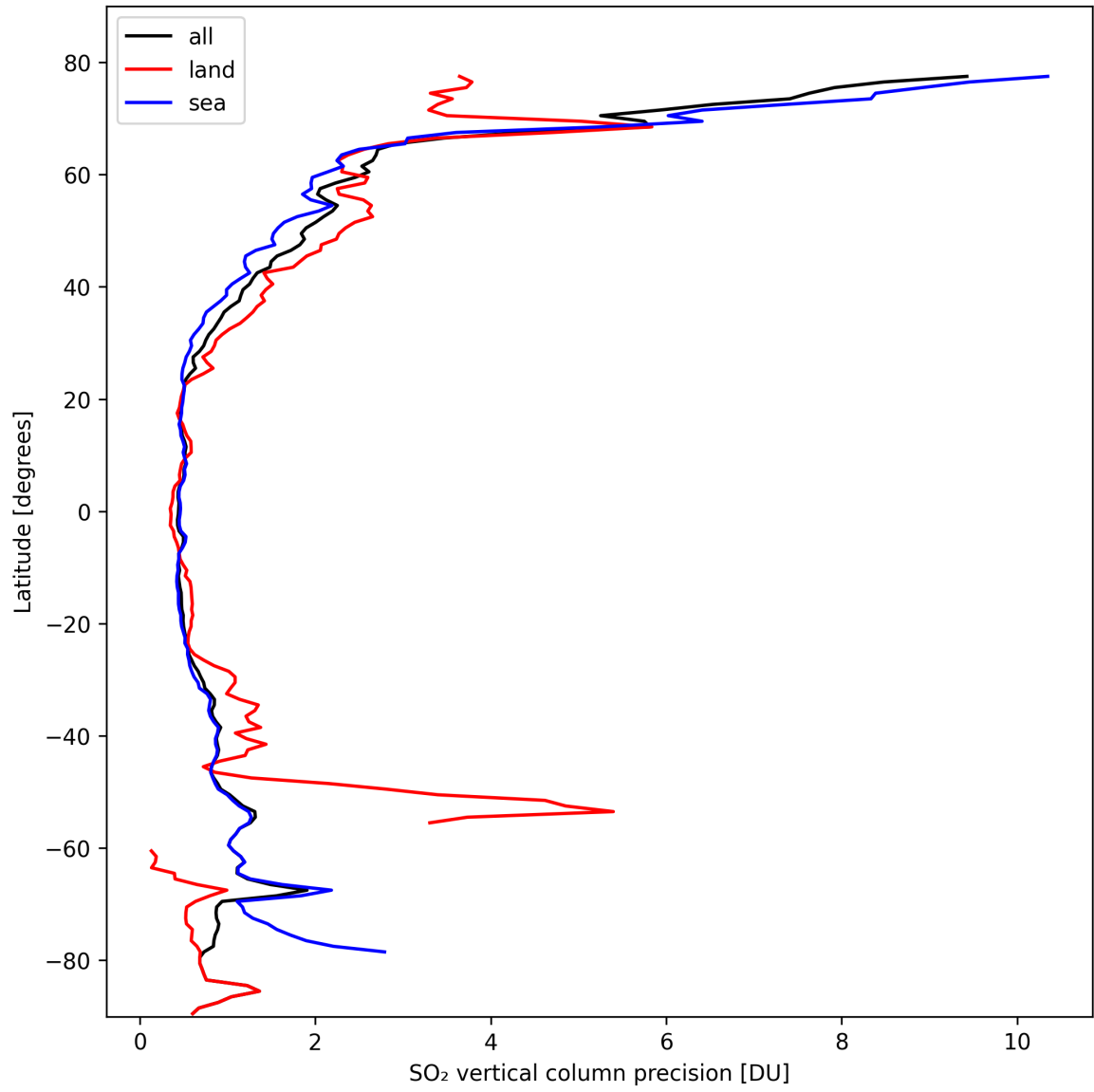
Figure 31: Zonal average of “SO 2 vertical column precision” for 2024-10-11 to 2024-10-13.
