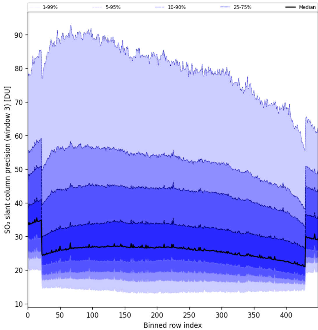
Figure 88: Along track statistics of “SO 2 slant column precision (window 3)” for 2024-10-11 to 2024-10-13
