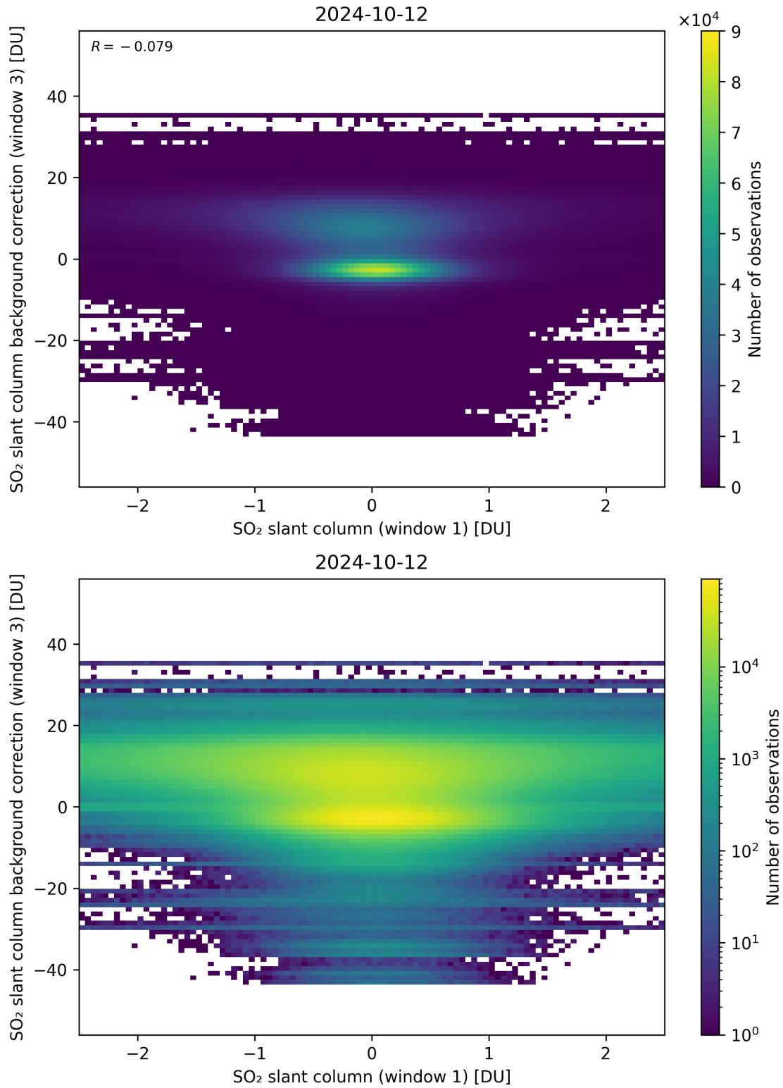
Figure 214: Scatter density plot of “SO 2 slant column (window 1)” against “SO 2 slant column background correction (window 3)” for 2024-10-11 to 2024-10-13.
