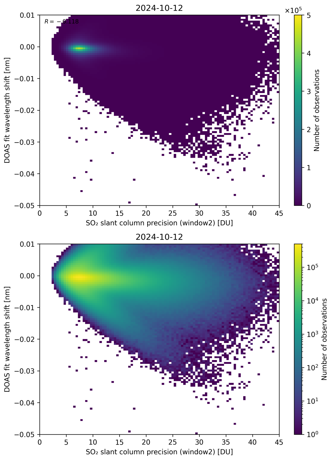
Figure 243: Scatter density plot of “SO 2 slant column precision (window2)” against “DOAS fit wavelength shift” for 2024-10-11 to 2024-10-13.
