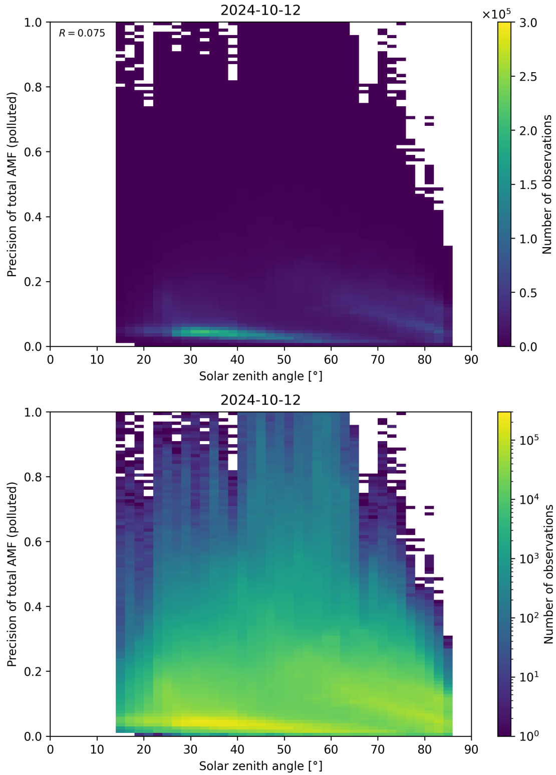
Figure 175: Scatter density plot of “Solar zenith angle” against “Precision of total AMF (polluted)” for 2024-10-11 to 2024-10-13.
