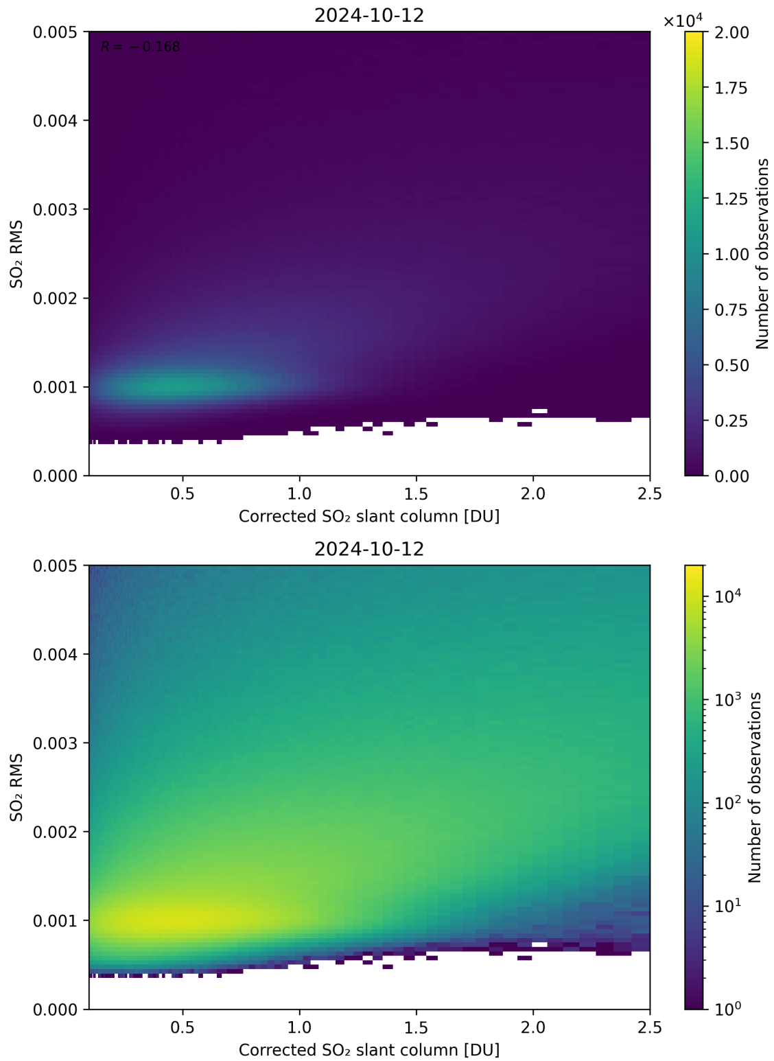
Figure 183: Scatter density plot of “Corrected SO 2 slant column” against “SO 2 RMS” for 2024-10-11 to 2024-10-13.
