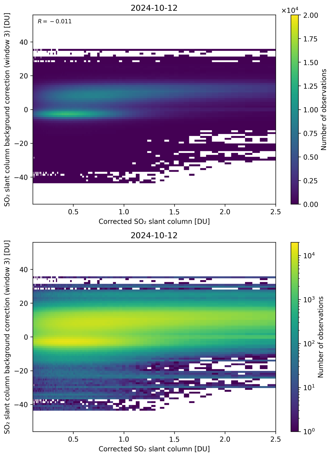
Figure 180: Scatter density plot of “Corrected SO 2 slant column” against “SO 2 slant column background correction (window 3)” for 2024-10-11 to 2024-10-13.
