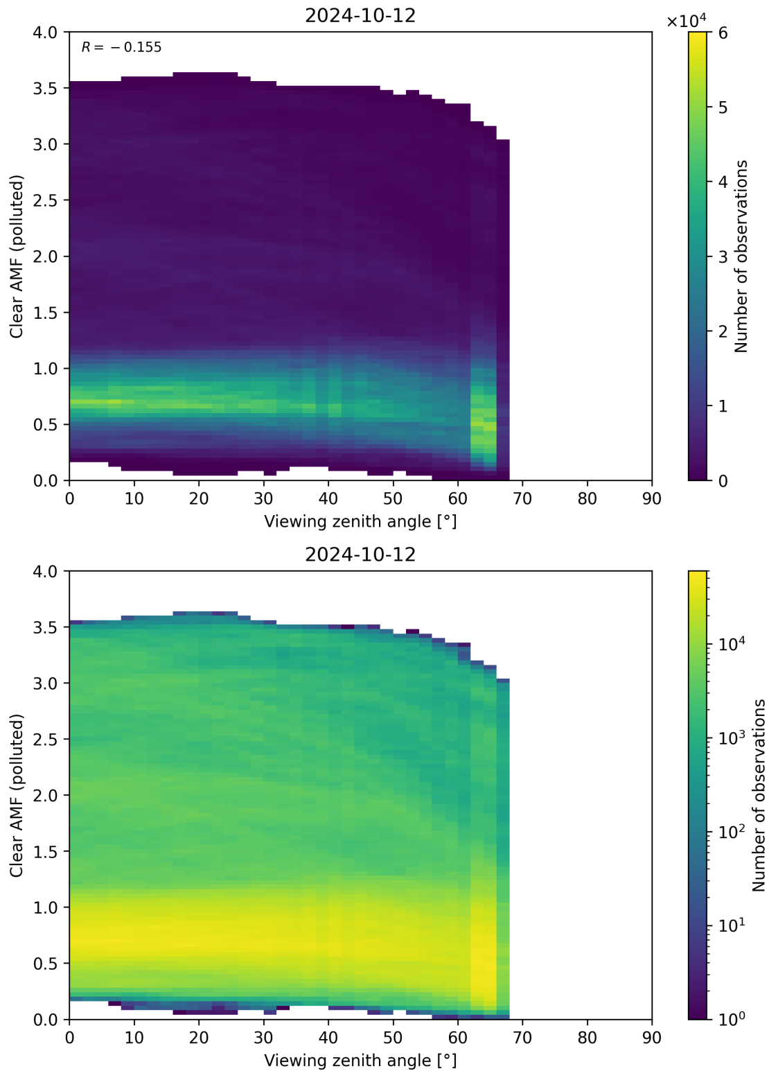
Figure 316: Scatter density plot of “Viewing zenith angle” against “Clear AMF (polluted)” for 2024-10-11 to 2024-10-13.
