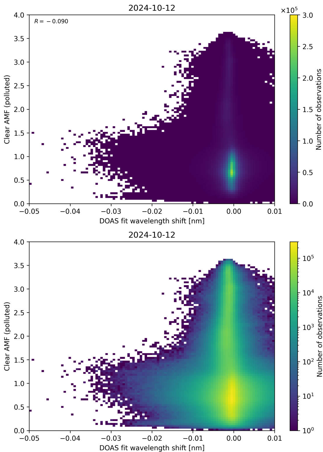
Figure 129: Scatter density plot of “DOAS fit wavelength shift” against “Clear AMF (polluted)” for 2024-10-11 to 2024-10-13.
