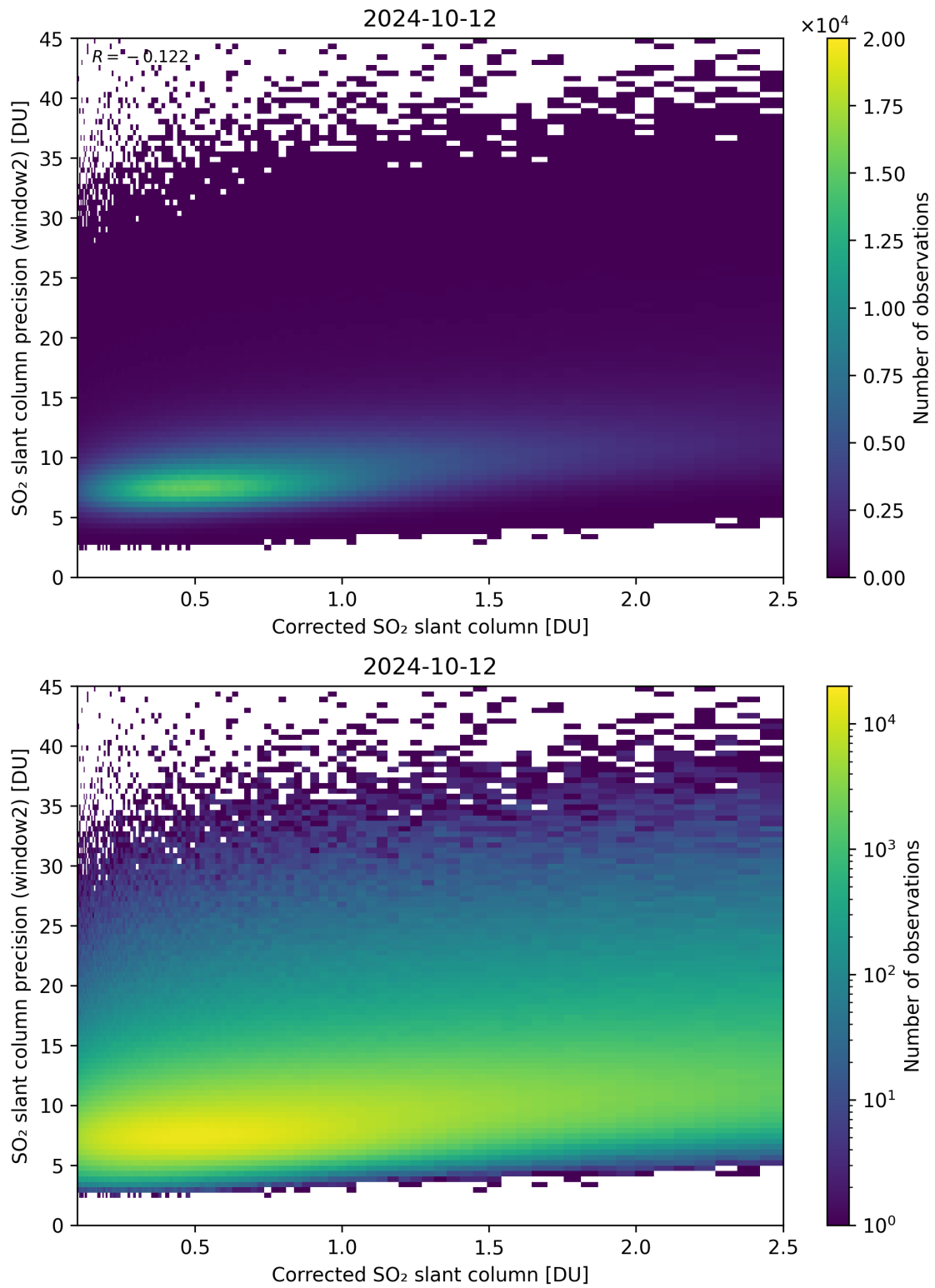
Figure 189: Scatter density plot of “Corrected SO 2 slant column” against “SO 2 slant column precision (window2)” for 2024-10-11 to 2024-10-13.
