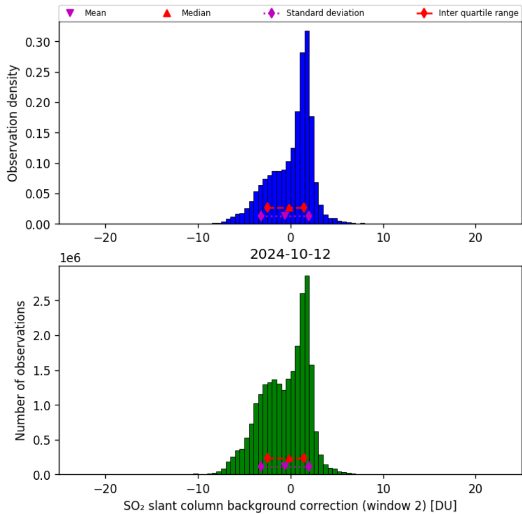
Figure 63: Histogram of “SO 2 slant column background correction (window 2)” for 2024-10-11 to 2024-10-13
