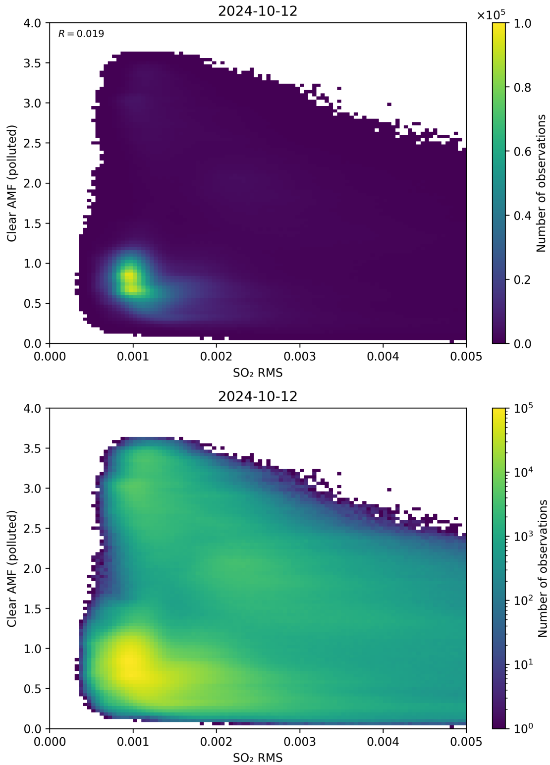
Figure 136: Scatter density plot of “SO 2 RMS” against “Clear AMF (polluted)” for 2024-10-11 to 2024-10-13.
