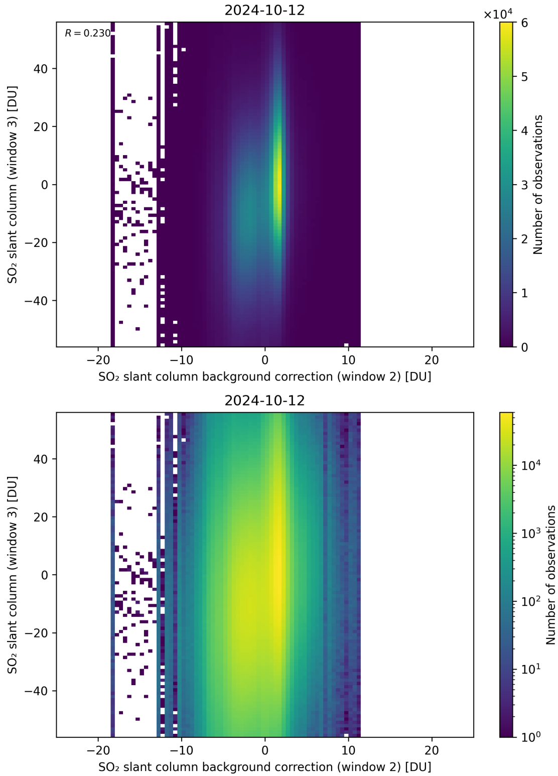
Figure 117: Scatter density plot of “SO 2 slant column background correction (window 2)” against “SO 2 slant column (window 3)” for 2024-10-11 to 2024-10-13.
