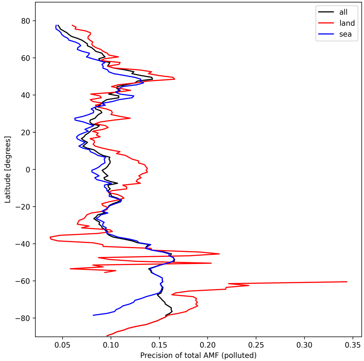
Figure 49: Zonal average of “Precision of total AMF (polluted)” for 2024-10-11 to 2024-10-13.
