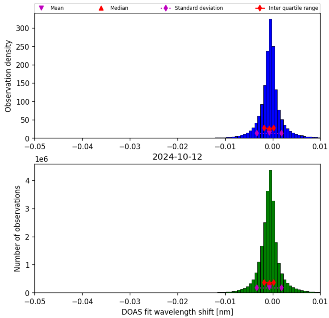
Figure 68: Histogram of “DOAS fit wavelength shift” for 2024-10-11 to 2024-10-13
