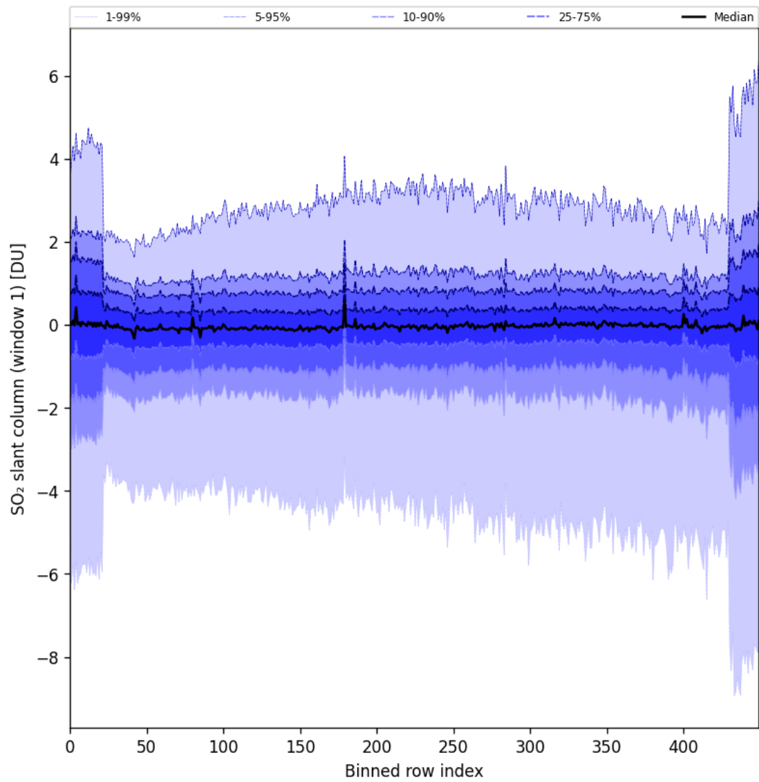
Figure 79: Along track statistics of “SO 2 slant column (window 1)” for 2024-10-11 to 2024-10-13
