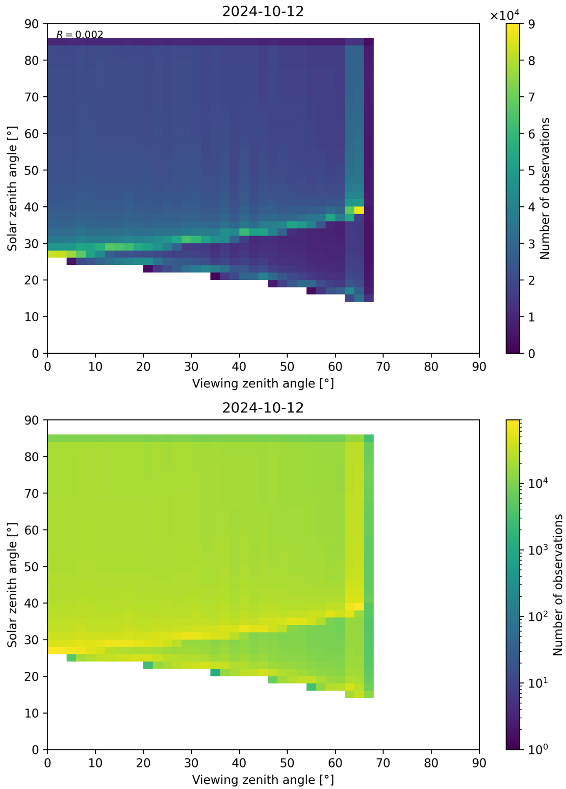
Figure 315: Scatter density plot of “Viewing zenith angle” against “Solar zenith angle” for 2024-10-11 to 2024-10-13.
