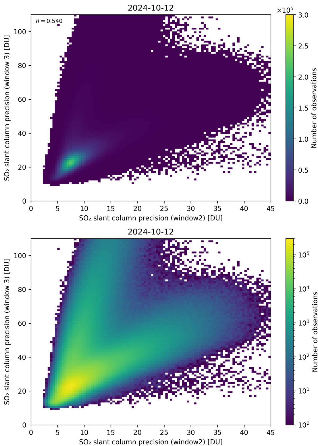
Figure 250: Scatter density plot of “SO 2 slant column precision (window2)” against “SO 2 slant column precision (window 3)” for 2024-10-11 to 2024-10-13.
