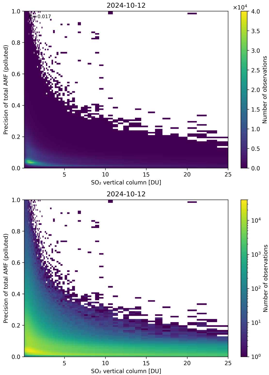
Figure 306: Scatter density plot of “SO 2 vertical column” against “Precision of total AMF (polluted)” for 2024-10-11 to 2024-10-13.
