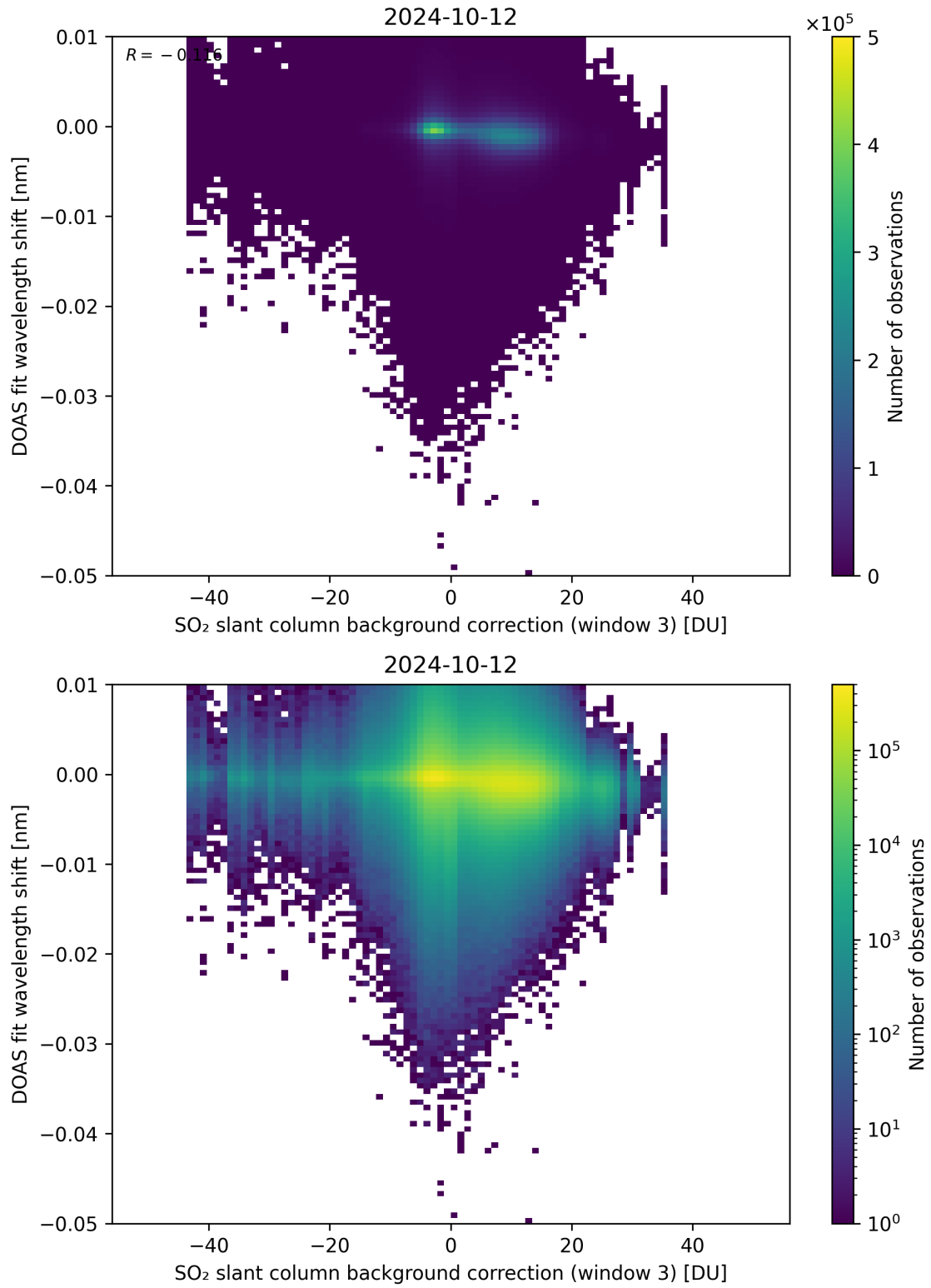
Figure 121: Scatter density plot of “SO 2 slant column background correction (window 3)” against “DOAS fit wavelength shift” for 2024-10-11 to 2024-10-13.
