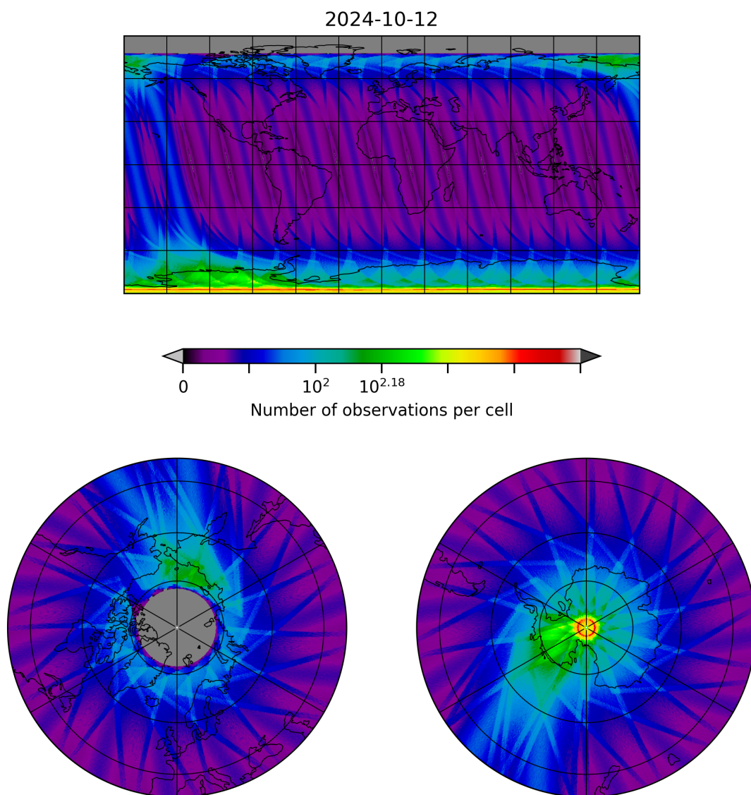
Figure 28: Map of the number of observations for 2024-10-11 to 2024-10-13
