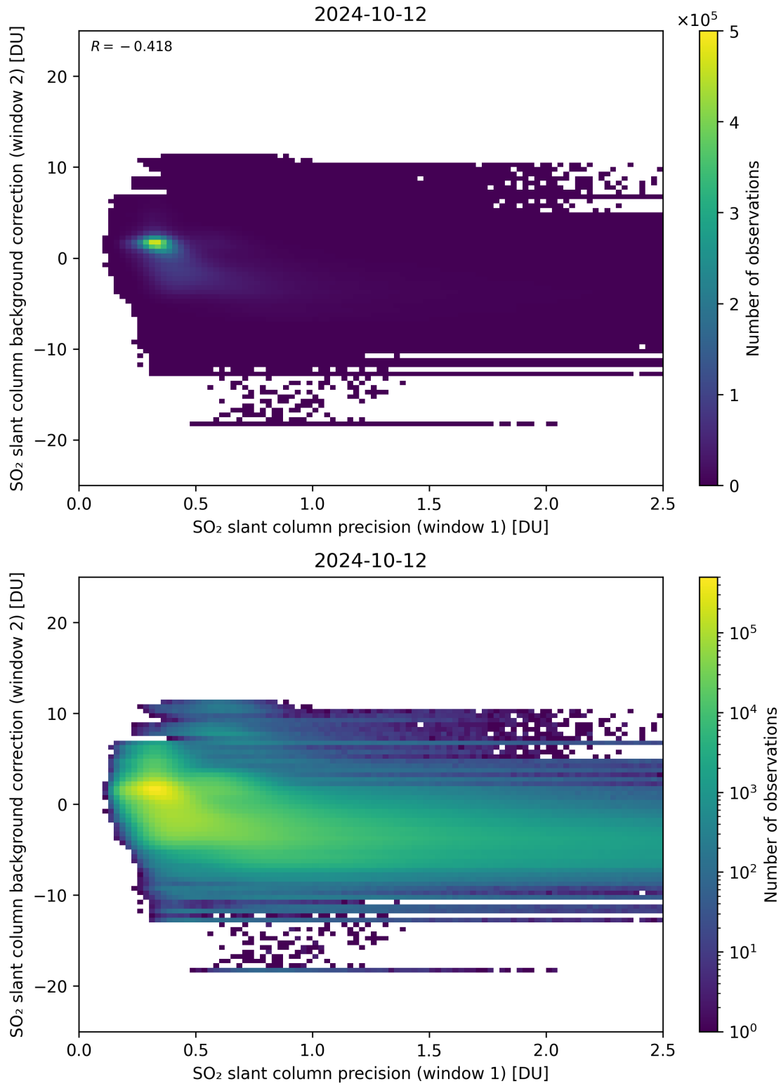
Figure 219: Scatter density plot of “SO 2 slant column precision (window 1)” against “SO 2 slant column background correction (window 2)” for 2024-10-11 to 2024-10-13.
