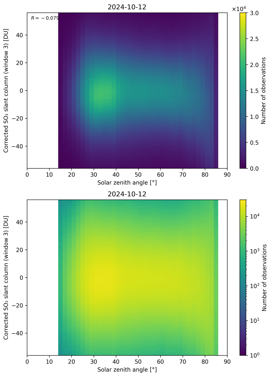
Figure 168: Scatter density plot of “Solar zenith angle” against “Corrected SO 2 slant column (window 3)” for 2024-10-11 to 2024-10-13.
