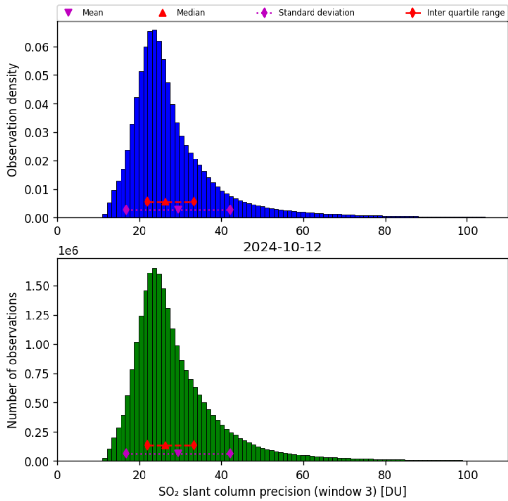
Figure 65: Histogram of “SO 2 slant column precision (window 3)” for 2024-10-11 to 2024-10-13
