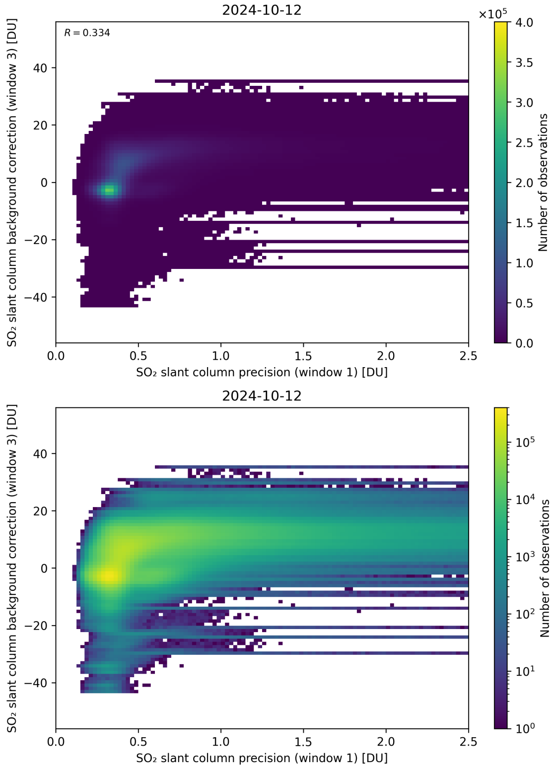
Figure 220: Scatter density plot of “SO 2 slant column precision (window 1)” against “SO 2 slant column background correction (window 3)” for 2024-10-11 to 2024-10-13.
