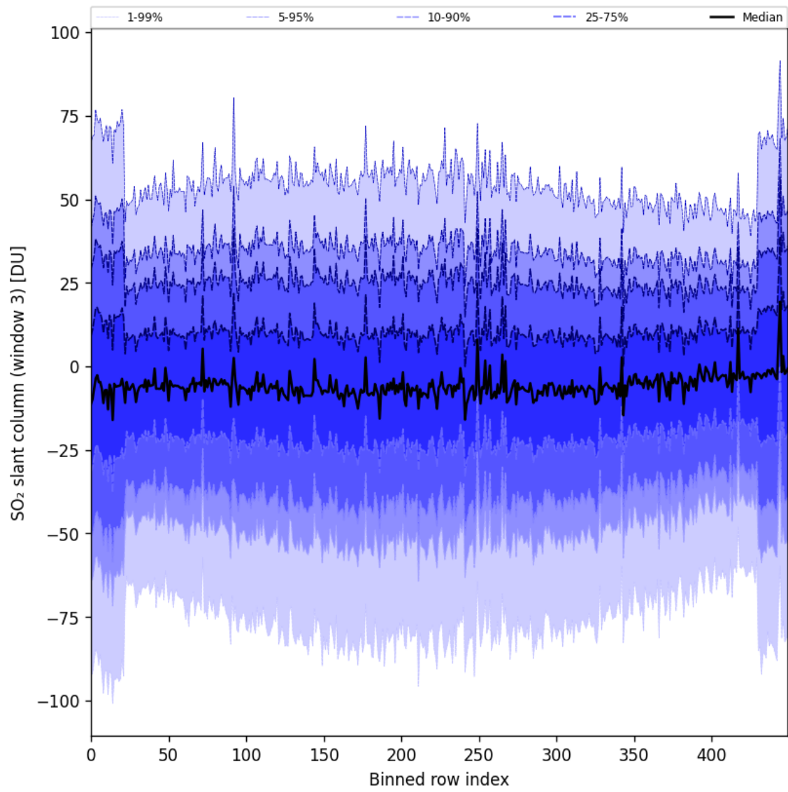
Figure 87: Along track statistics of “SO 2 slant column (window 3)” for 2024-10-11 to 2024-10-13
