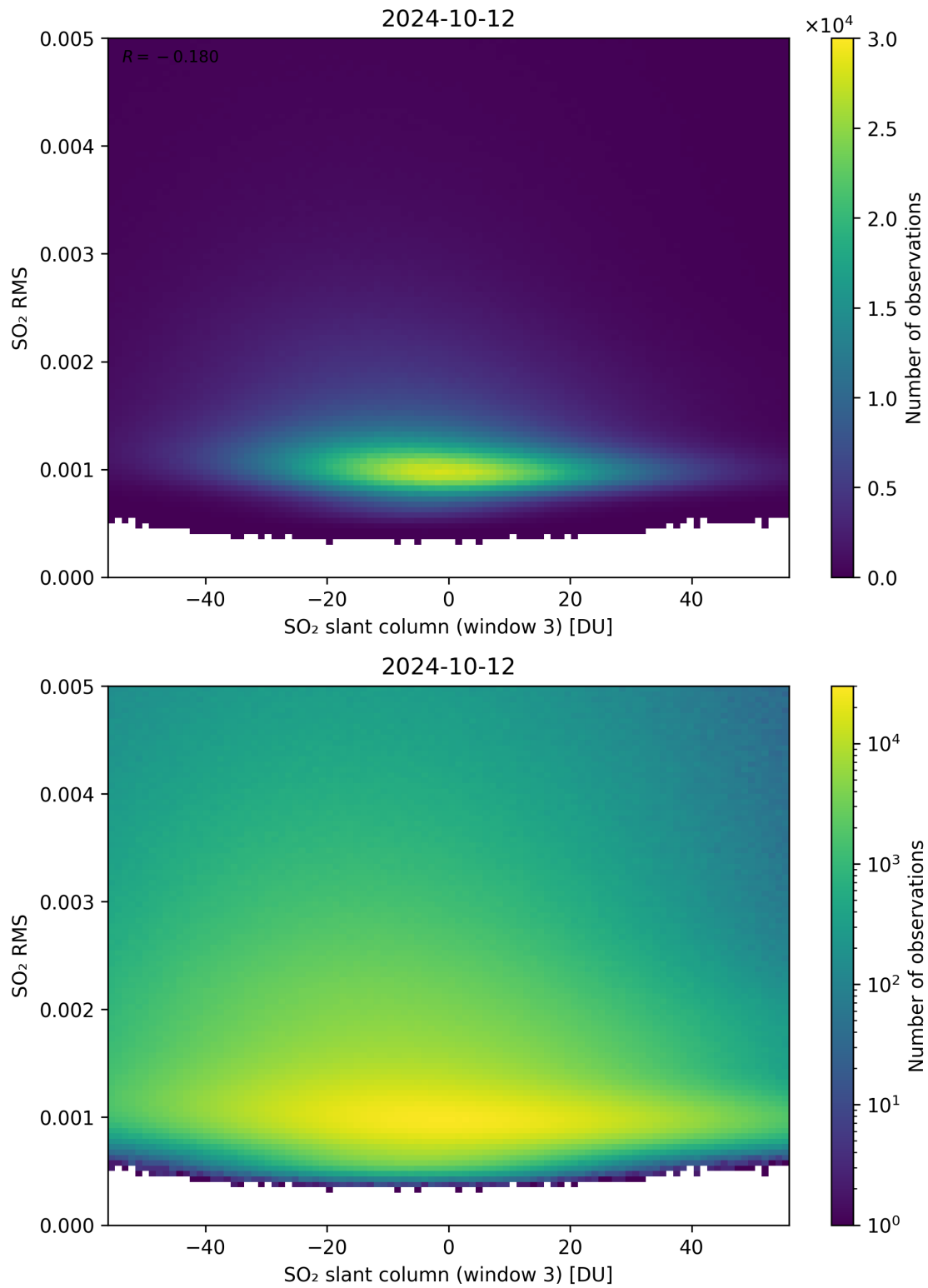
Figure 256: Scatter density plot of “SO 2 slant column (window 3)” against “SO 2 RMS” for 2024-10-11 to 2024-10-13.
