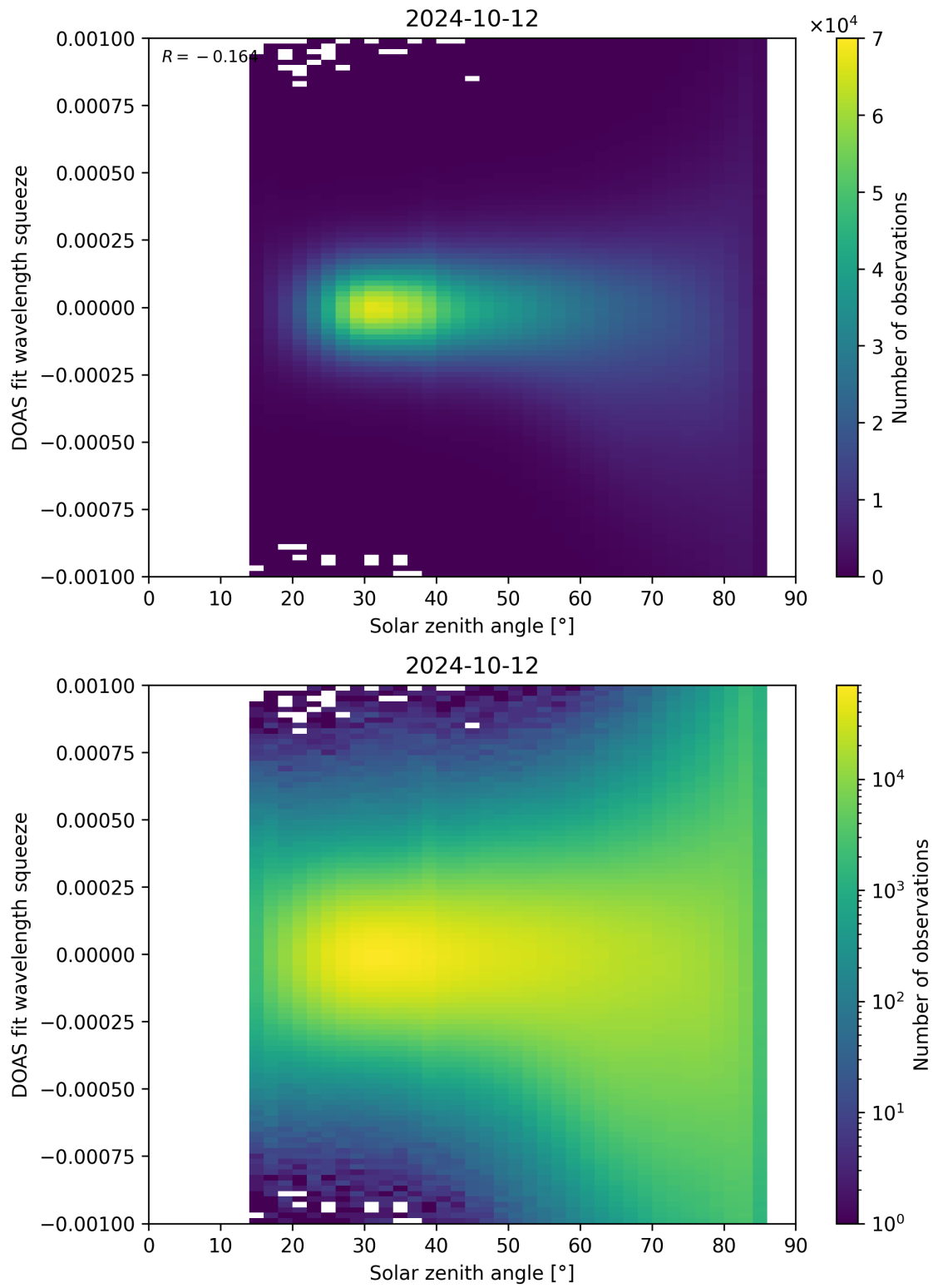
Figure 162: Scatter density plot of “Solar zenith angle” against “DOAS fit wavelength squeeze” for 2024-10-11 to 2024-10-13.
