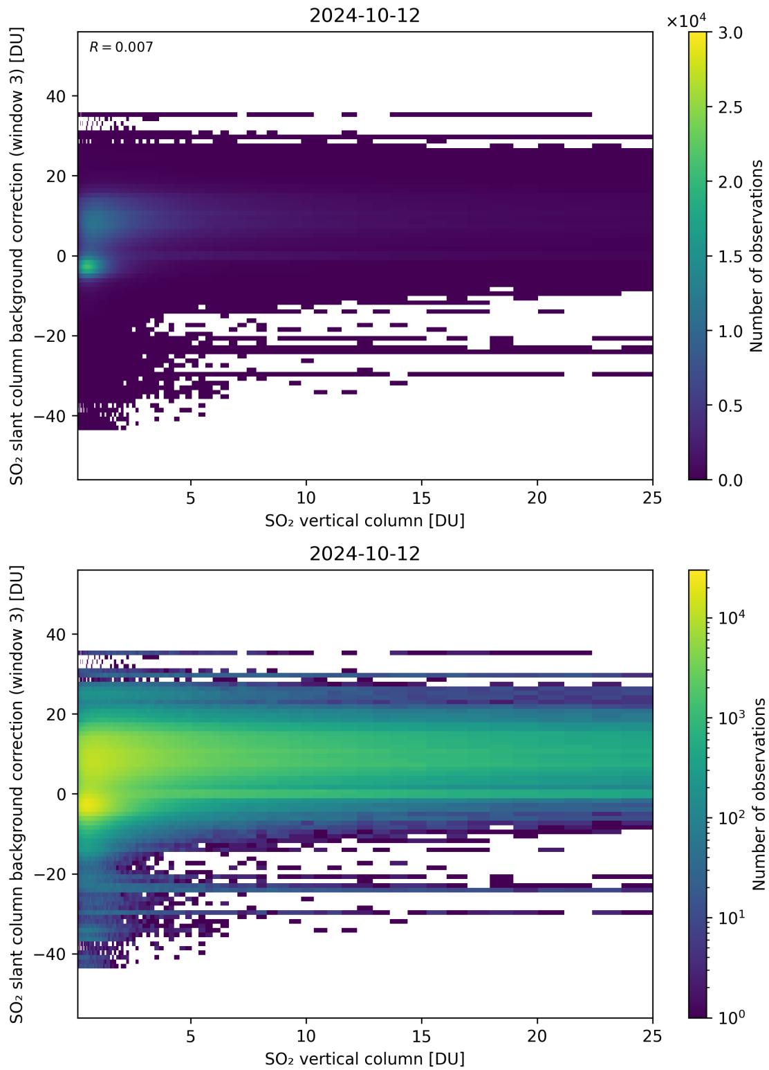
Figure 275: Scatter density plot of “SO 2 vertical column” against “SO 2 slant column background correction (window 3)” for 2024-10-11 to 2024-10-13.
