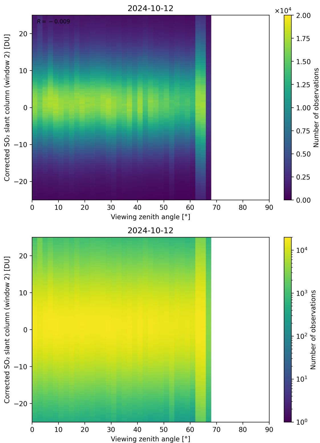
Figure 318: Scatter density plot of “Viewing zenith angle” against “Corrected SO 2 slant column (window 2)” for 2024-10-11 to 2024-10-13.
