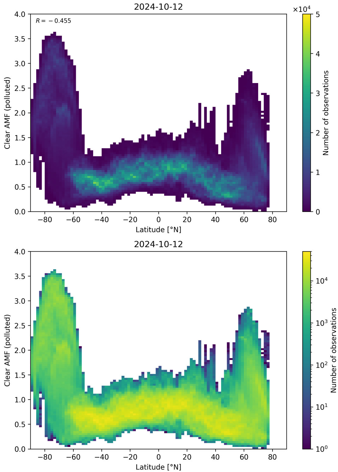
Figure 145: Scatter density plot of “Latitude” against “Clear AMF (polluted)” for 2024-10-11 to 2024-10-13.
