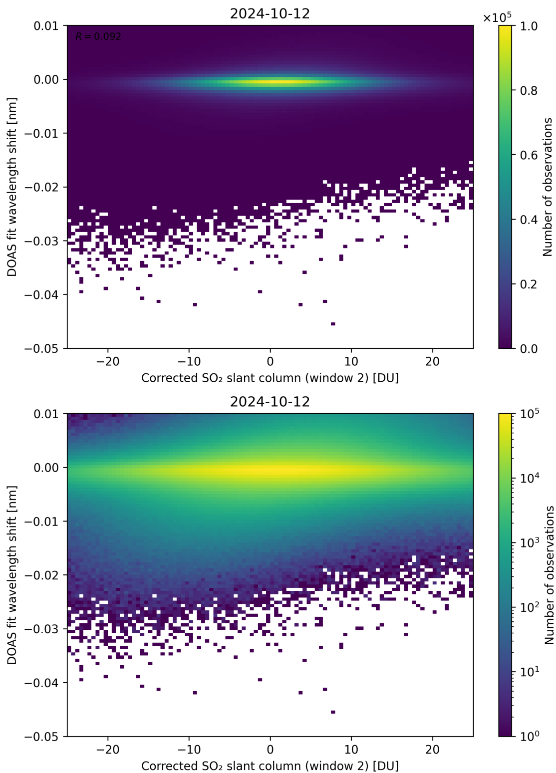
Figure 196: Scatter density plot of “Corrected SO 2 slant column (window 2)” against “DOAS fit wavelength shift” for 2024-10-11 to 2024-10-13.
