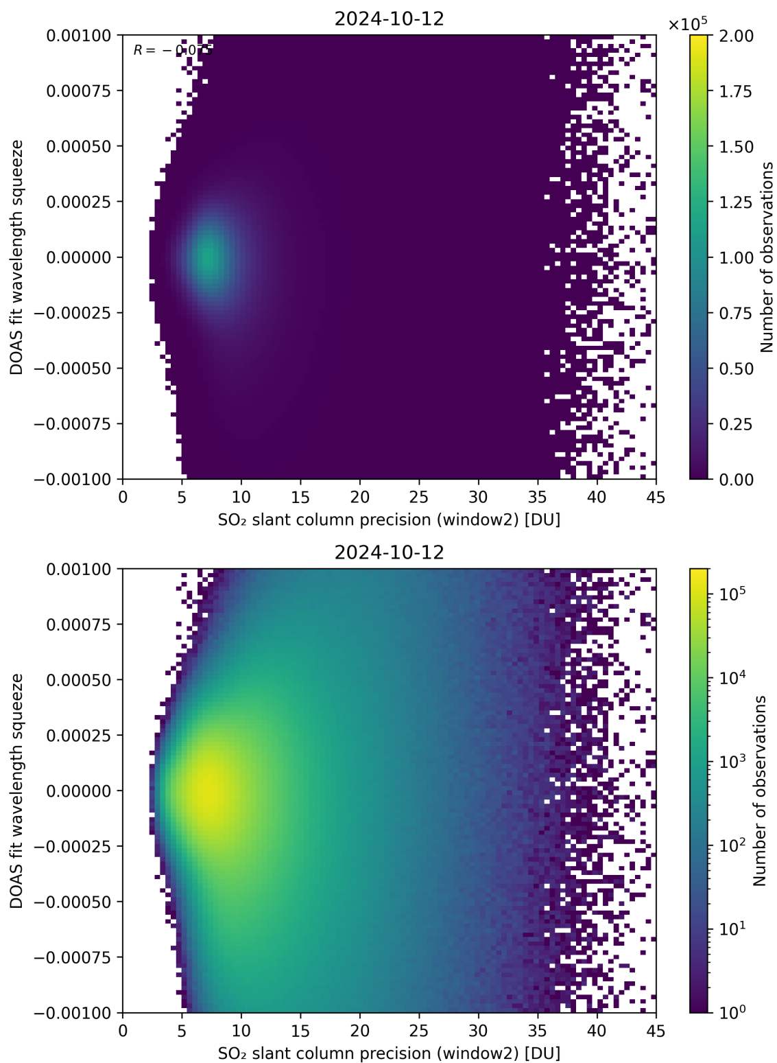
Figure 244: Scatter density plot of “SO 2 slant column precision (window2)” against “DOAS fit wavelength squeeze” for 2024-10-11 to 2024-10-13.
