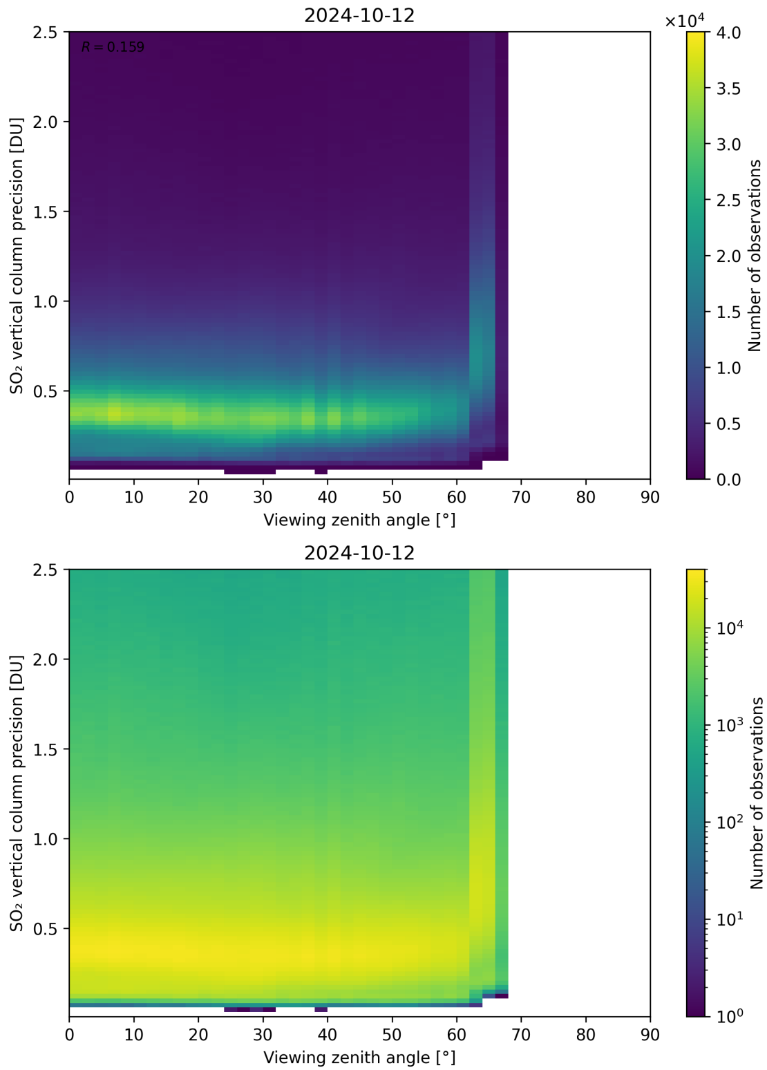
Figure 328: Scatter density plot of “Viewing zenith angle” against “SO 2 vertical column precision” for 2024-10-11 to 2024-10-13.
