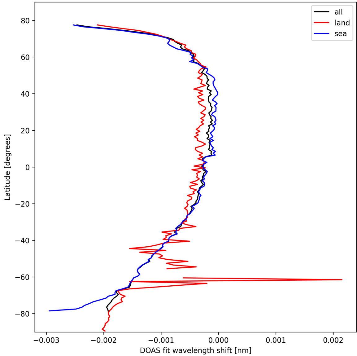
Figure 45: Zonal average of “DOAS fit wavelength shift” for 2024-10-11 to 2024-10-13.
