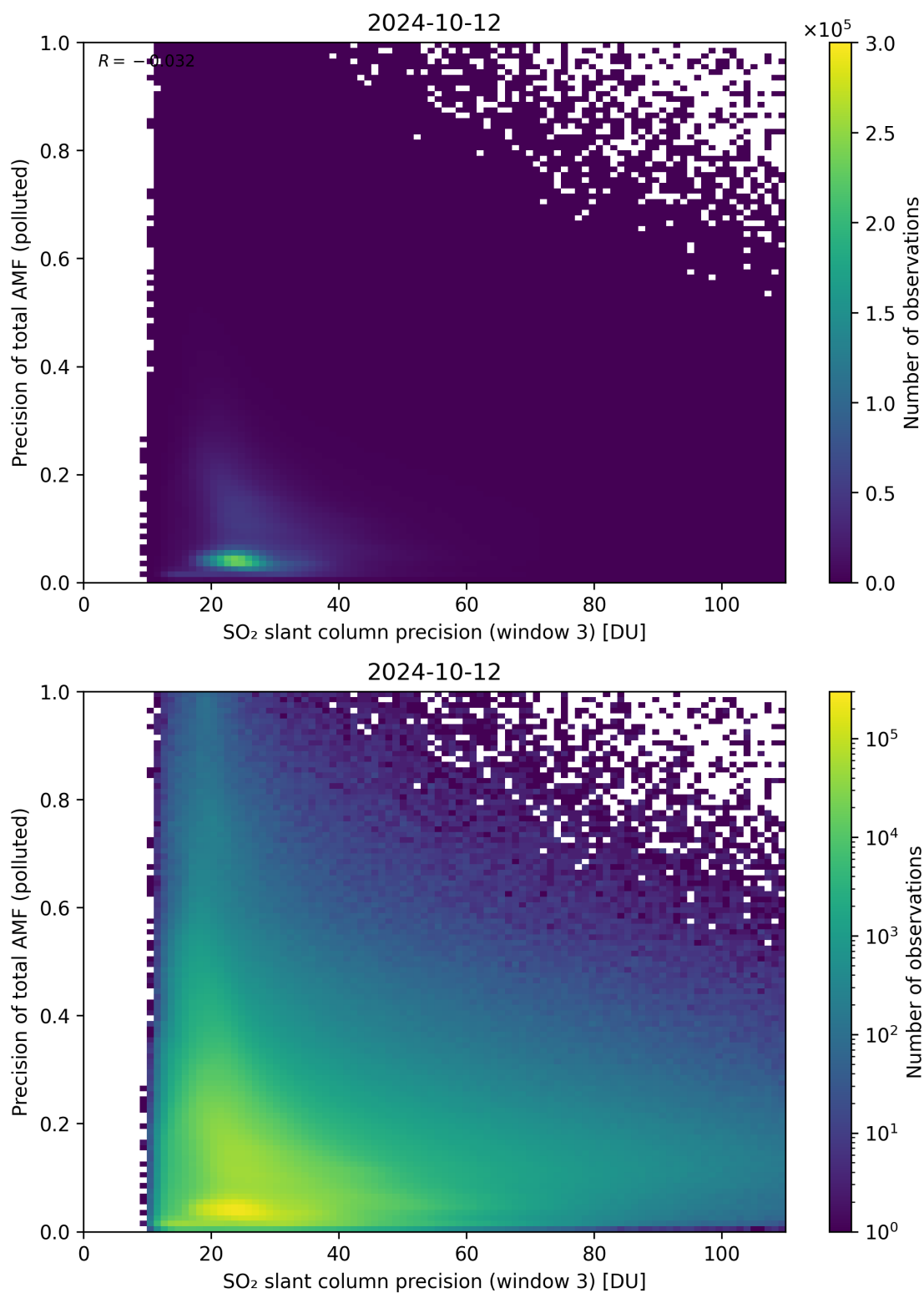
Figure 264: Scatter density plot of “SO 2 slant column precision (window 3)” against “Precision of total AMF (polluted)” for 2024-10-11 to 2024-10-13.
