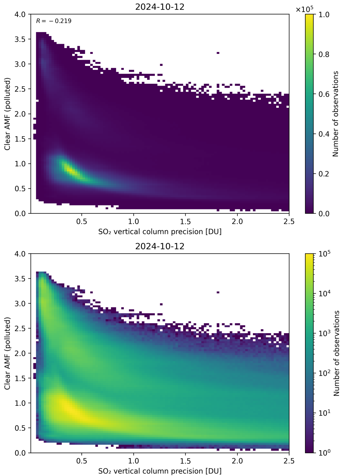
Figure 285: Scatter density plot of “SO 2 vertical column precision” against “Clear AMF (polluted)” for 2024-10-11 to 2024-10-13.
