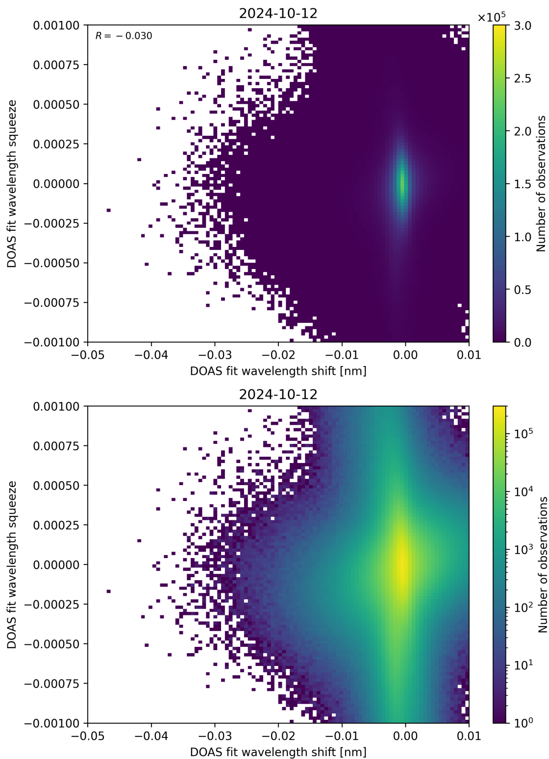
Figure 127: Scatter density plot of “DOAS fit wavelength shift” against “DOAS fit wavelength squeeze” for 2024-10-11 to 2024-10-13.
