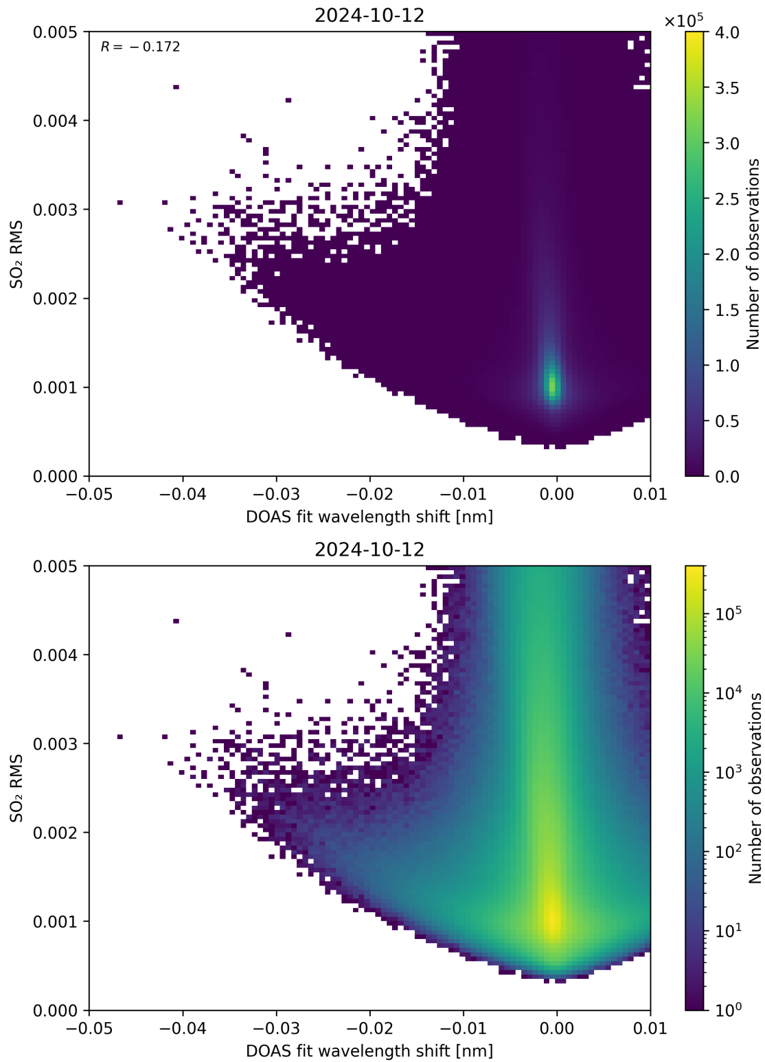
Figure 128: Scatter density plot of “DOAS fit wavelength shift” against “SO 2 RMS” for 2024-10-11 to 2024-10-13.
