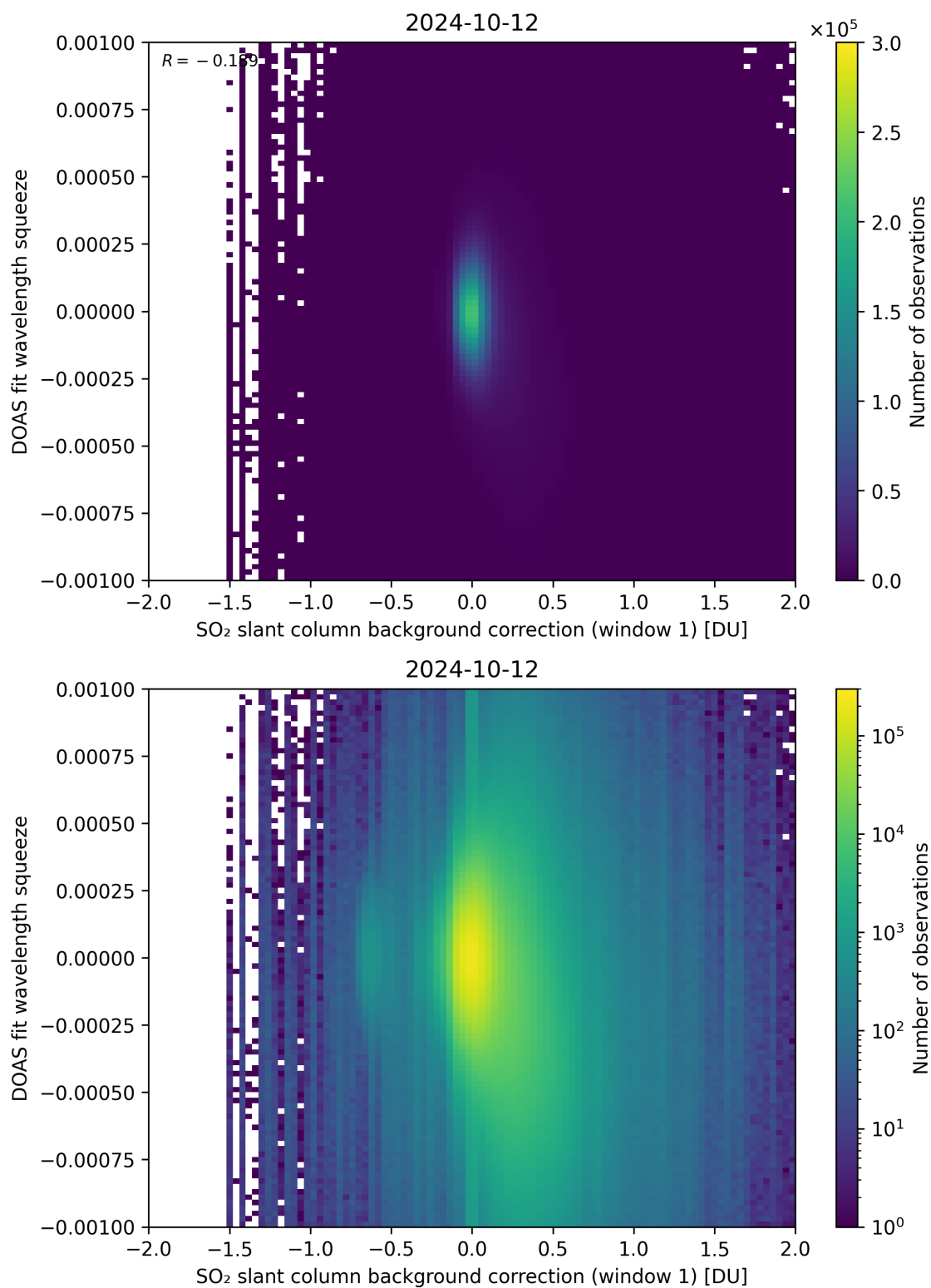
Figure 101: Scatter density plot of “SO 2 slant column background correction (window 1)” against “DOAS fit wavelength squeeze” for 2024-10-11 to 2024-10-13.
