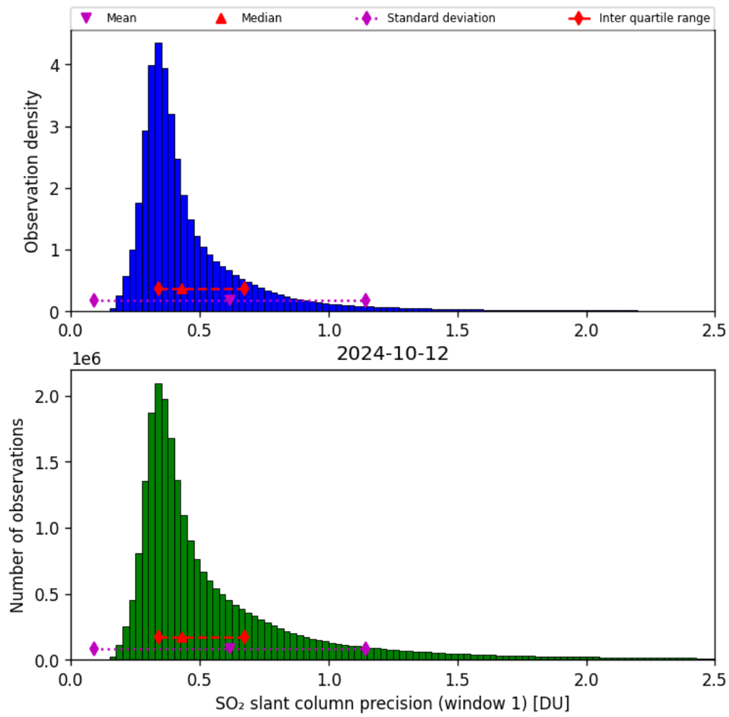
Figure 57: Histogram of “SO 2 slant column precision (window 1)” for 2024-10-11 to 2024-10-13
