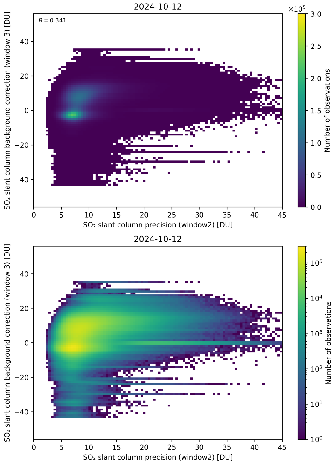
Figure 242: Scatter density plot of “SO 2 slant column precision (window2)” against “SO 2 slant column background correction (window 3)” for 2024-10-11 to 2024-10-13.
