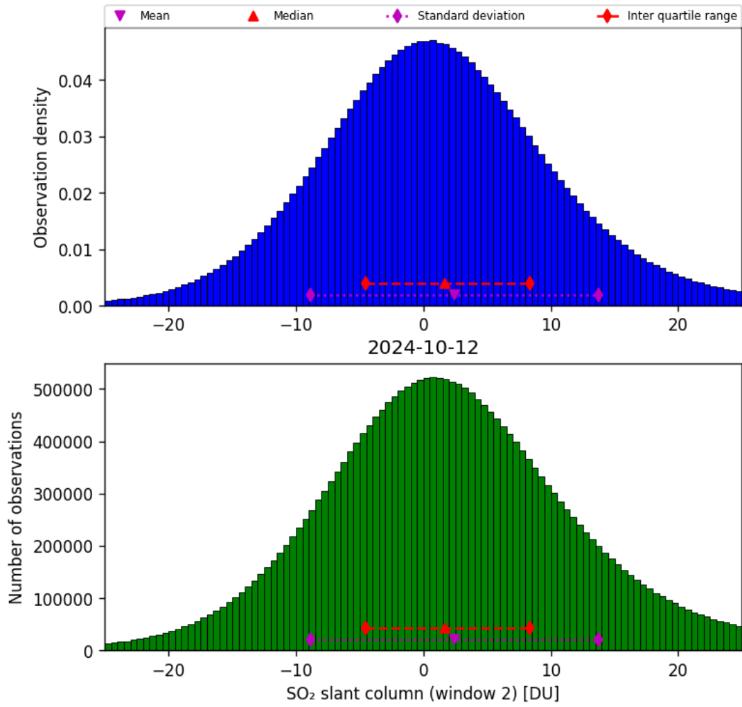
Figure 60: Histogram of “SO 2 slant column (window 2)” for 2024-10-11 to 2024-10-13
