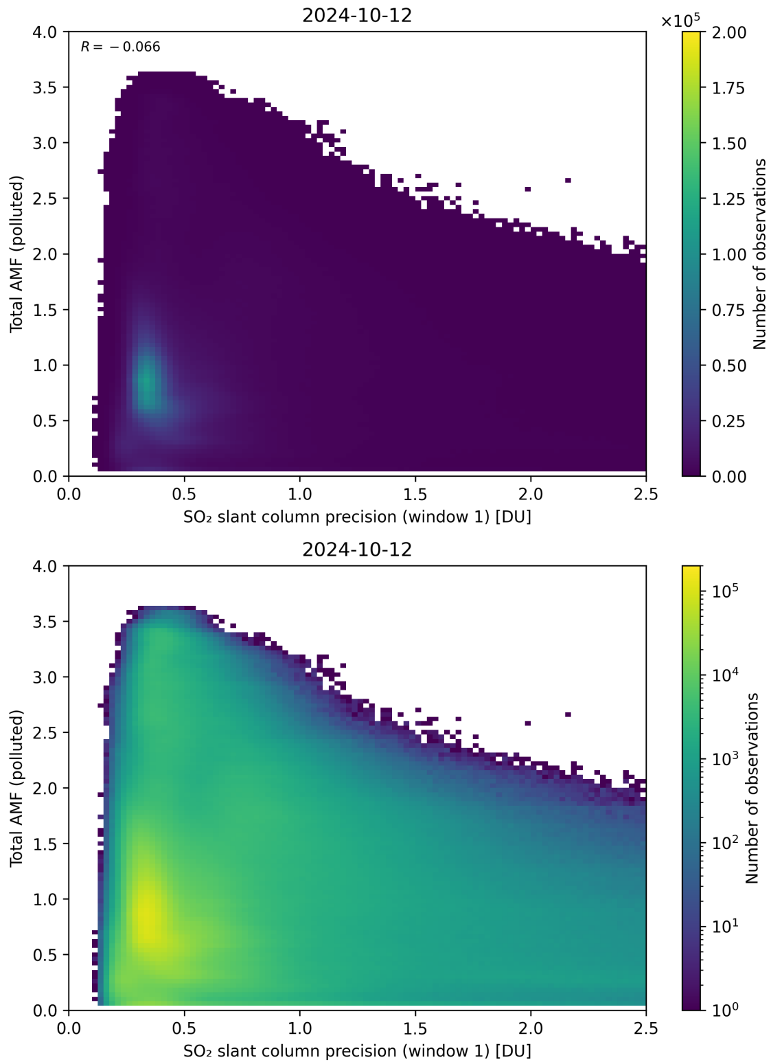
Figure 230: Scatter density plot of “SO 2 slant column precision (window 1)” against “Total AMF (polluted)” for 2024-10-11 to 2024-10-13.
