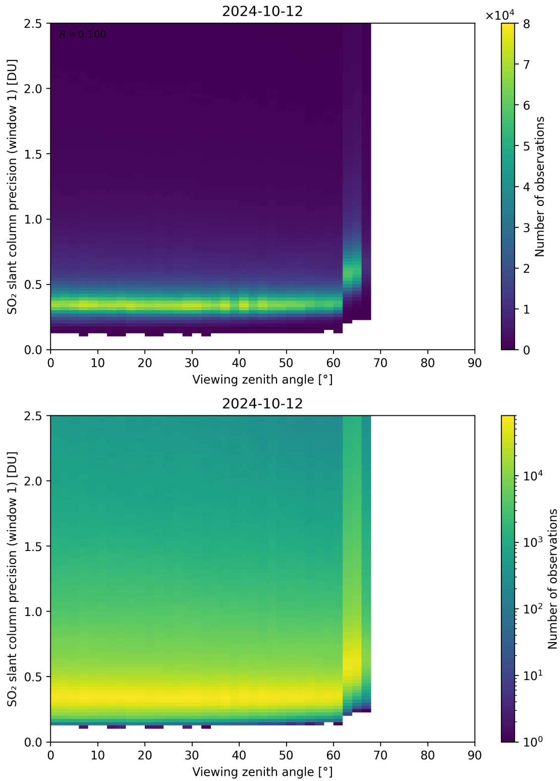
Figure 321: Scatter density plot of “Viewing zenith angle” against “SO 2 slant column precision (window 1)” for 2024-10-11 to 2024-10-13.
