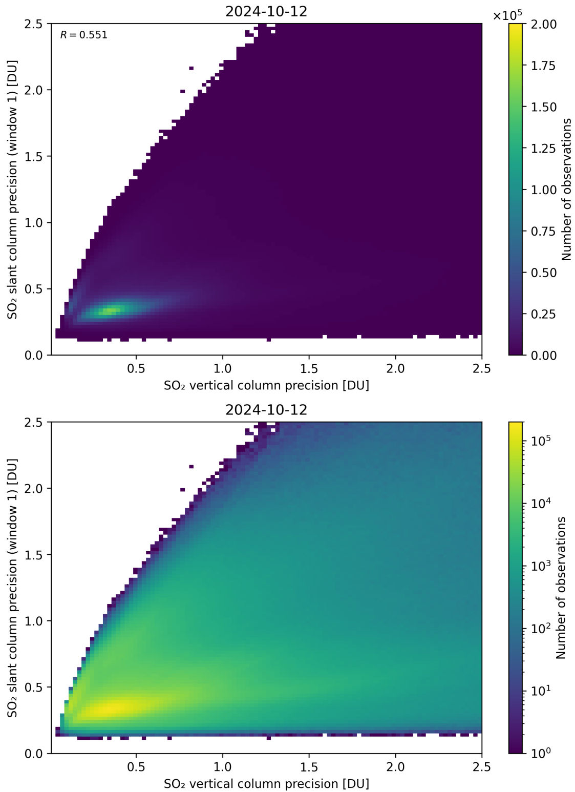
Figure 290: Scatter density plot of “SO 2 vertical column precision” against “SO 2 slant column precision (window 1)” for 2024-10-11 to 2024-10-13.
