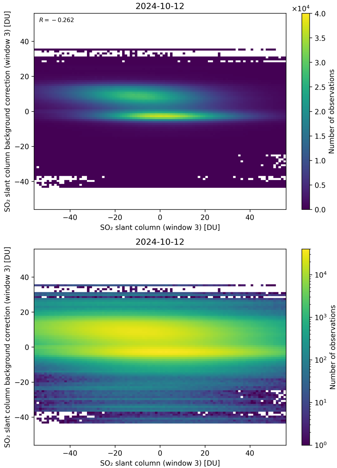
Figure 253: Scatter density plot of “SO 2 slant column (window 3)” against “SO 2 slant column background correction (window 3)” for 2024-10-11 to 2024-10-13.
