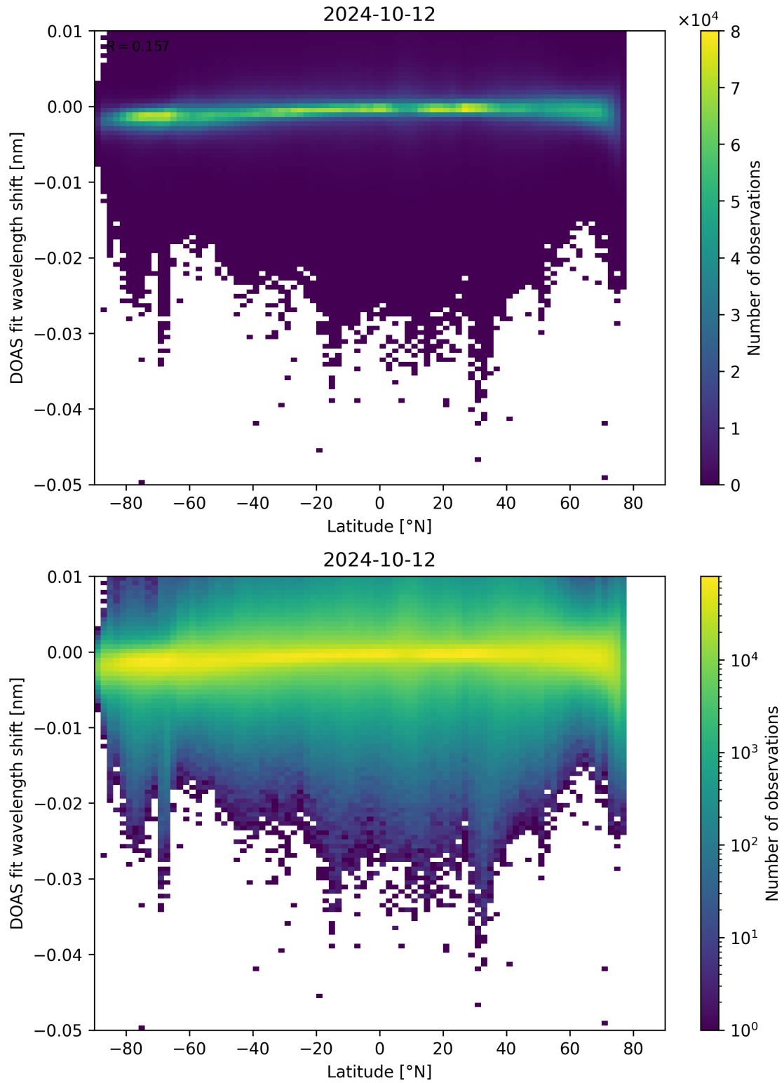
Figure 142: Scatter density plot of “Latitude” against “DOAS fit wavelength shift” for 2024-10-11 to 2024-10-13.
