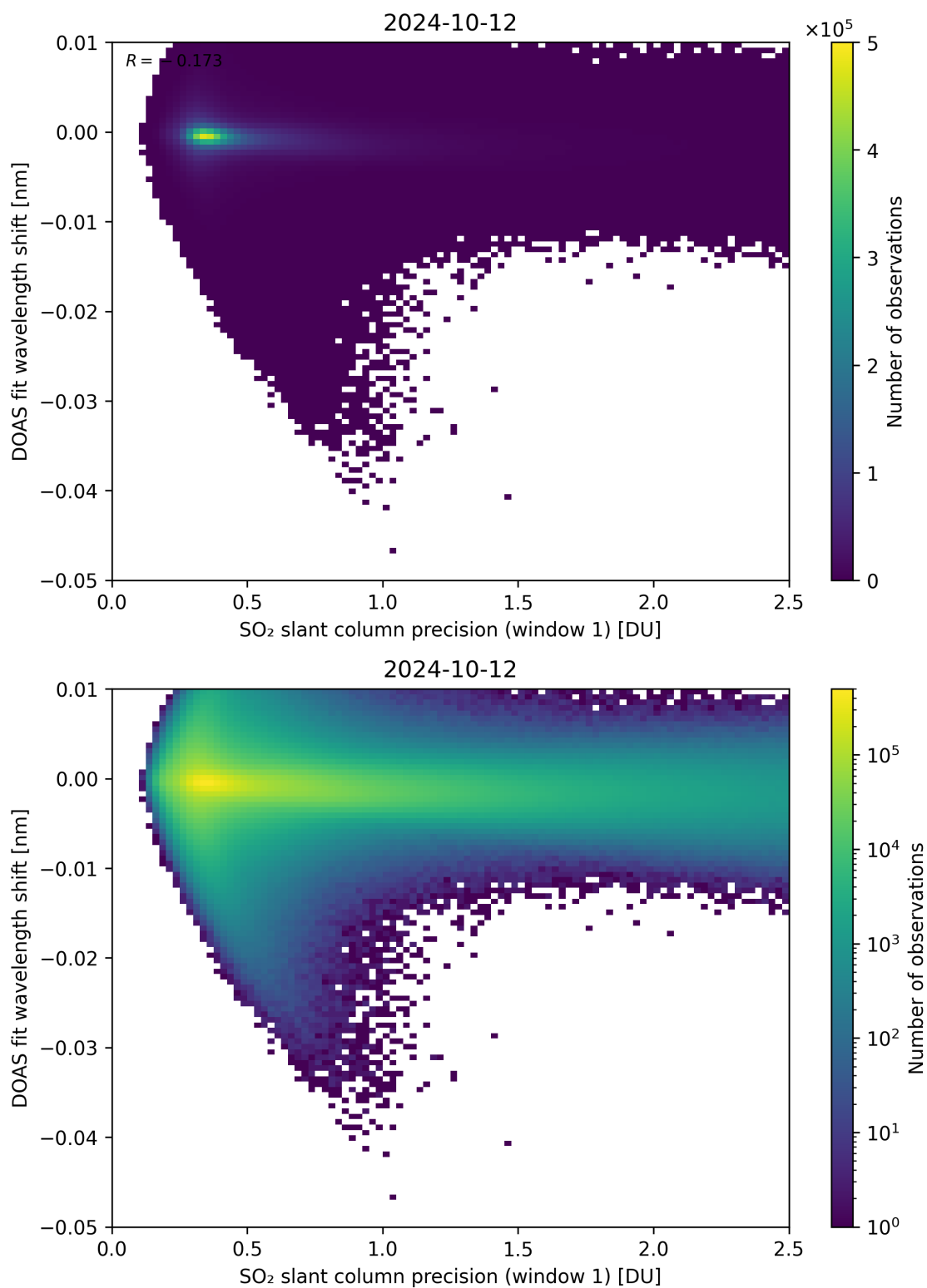
Figure 221: Scatter density plot of “SO 2 slant column precision (window 1)” against “DOAS fit wavelength shift” for 2024-10-11 to 2024-10-13.
