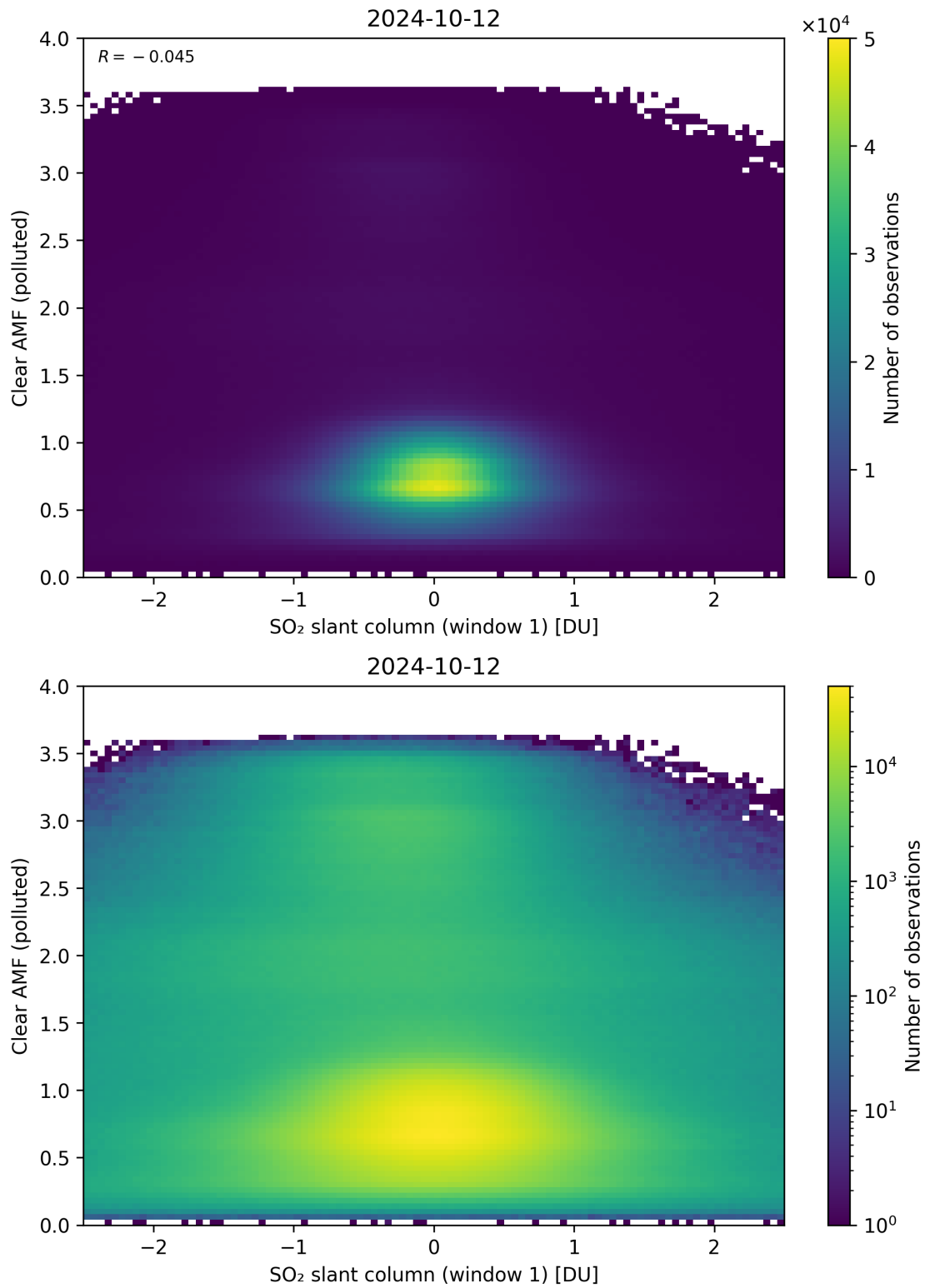
Figure 232: Scatter density plot of “SO 2 slant column (window 1)” against “Clear AMF (polluted)” for 2024-10-11 to 2024-10-13.
