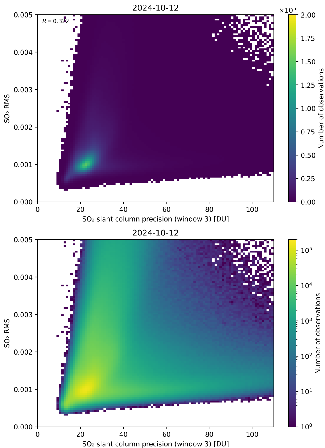
Figure 260: Scatter density plot of “SO 2 slant column precision (window 3)” against “SO 2 RMS” for 2024-10-11 to 2024-10-13.
