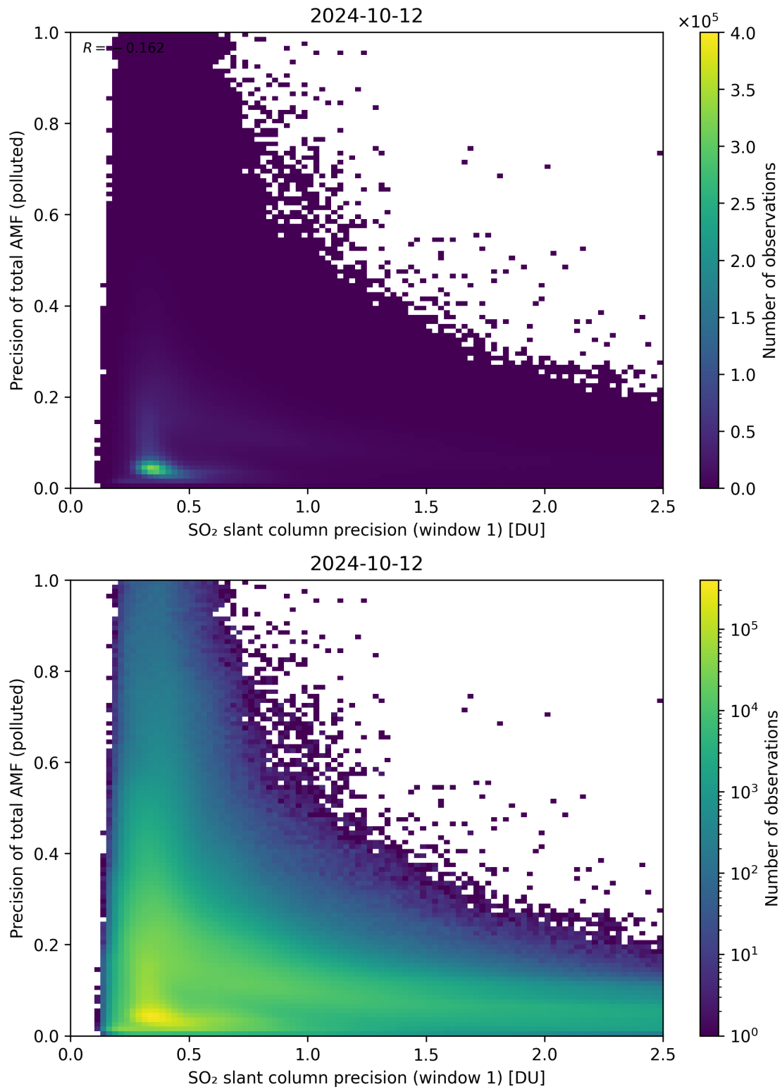
Figure 231: Scatter density plot of “SO 2 slant column precision (window 1)” against “Precision of total AMF (polluted)” for 2024-10-11 to 2024-10-13.
