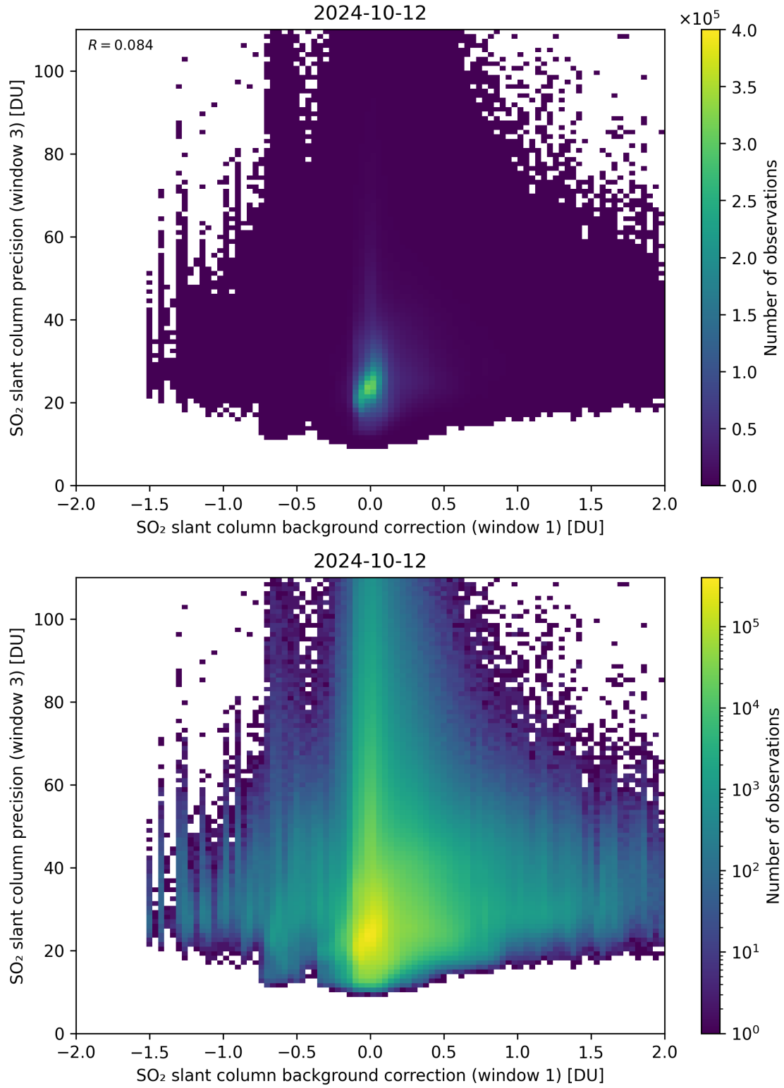
Figure 108: Scatter density plot of “SO 2 slant column background correction (window 1)” against “SO 2 slant column precision (window 3)” for 2024-10-11 to 2024-10-13.
