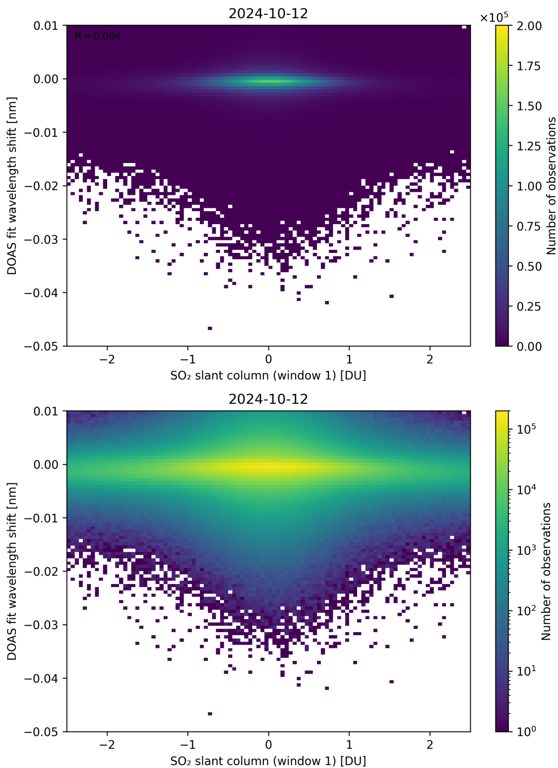
Figure 215: Scatter density plot of “SO 2 slant column (window 1)” against “DOAS fit wavelength shift” for 2024-10-11 to 2024-10-13.
