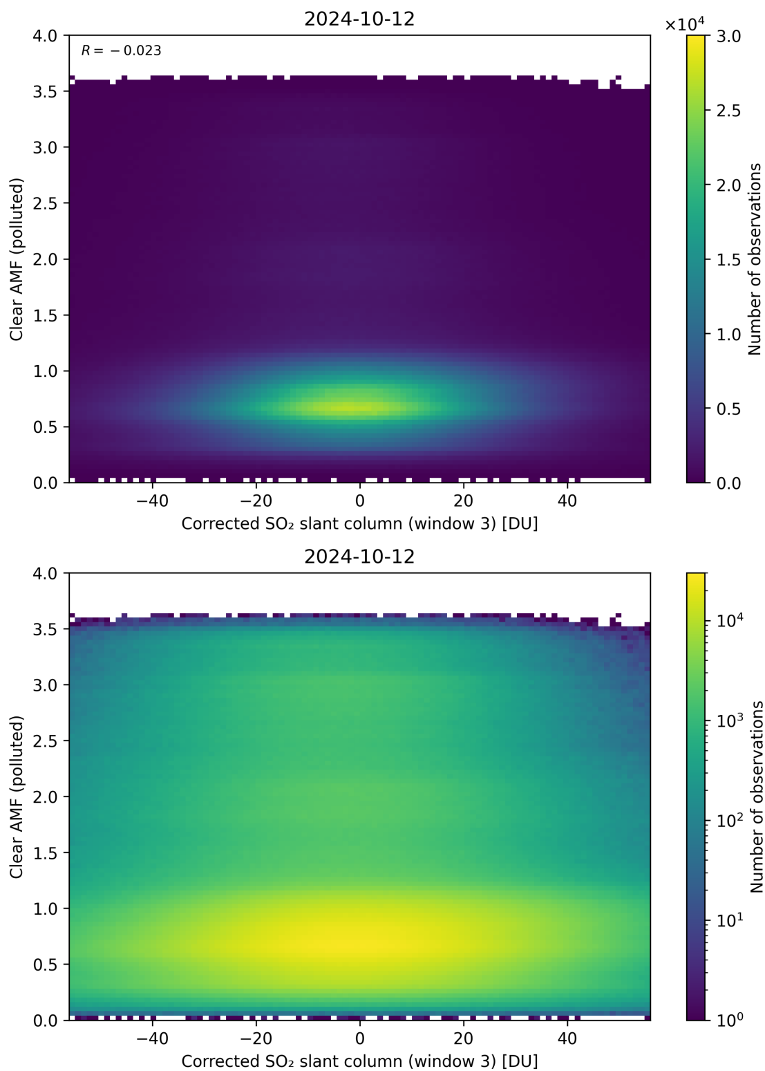
Figure 209: Scatter density plot of “Corrected SO 2 slant column (window 3)” against “Clear AMF (polluted)” for 2024-10-11 to 2024-10-13.
