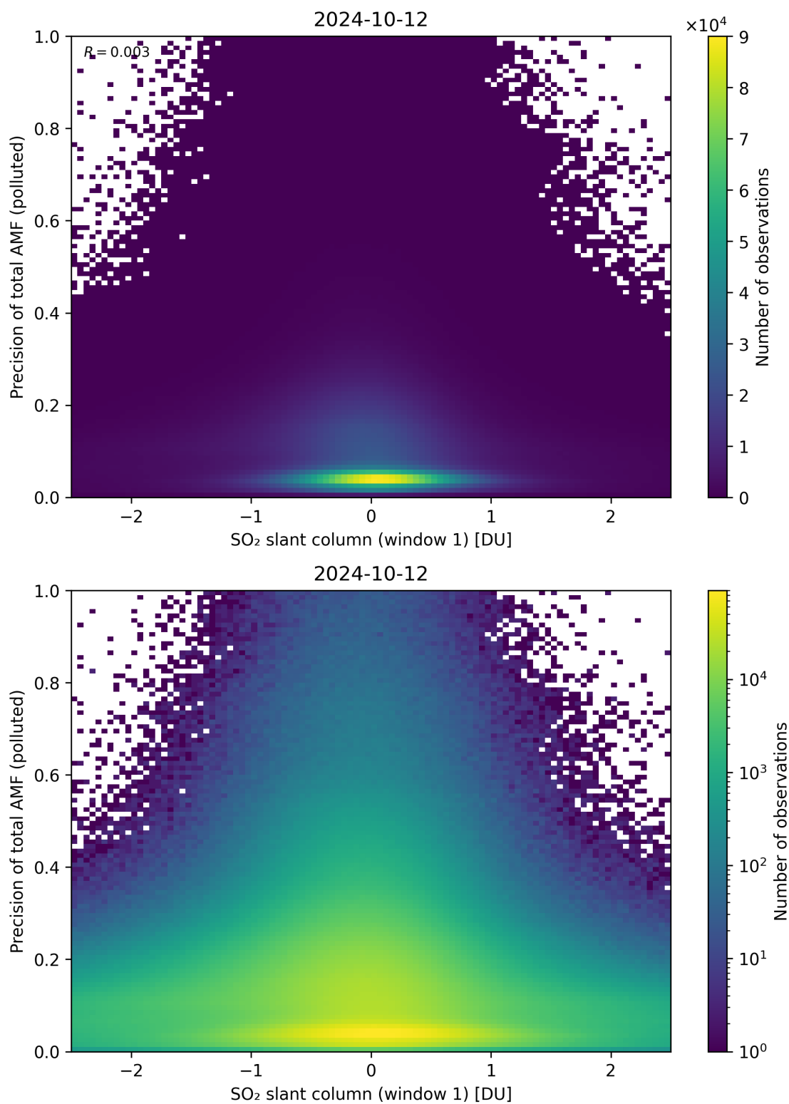
Figure 240: Scatter density plot of “SO 2 slant column (window 1)” against “Precision of total AMF (polluted)” for 2024-10-11 to 2024-10-13.
