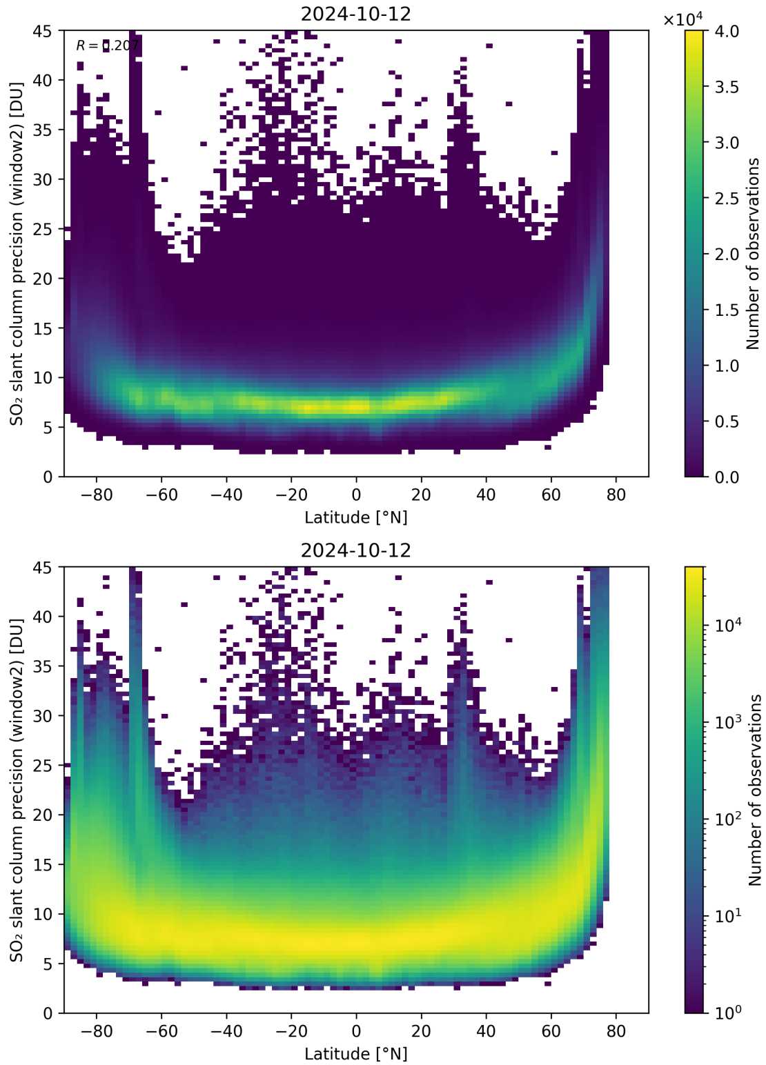
Figure 151: Scatter density plot of “Latitude” against “SO 2 slant column precision (window2)” for 2024-10-11 to 2024-10-13.
