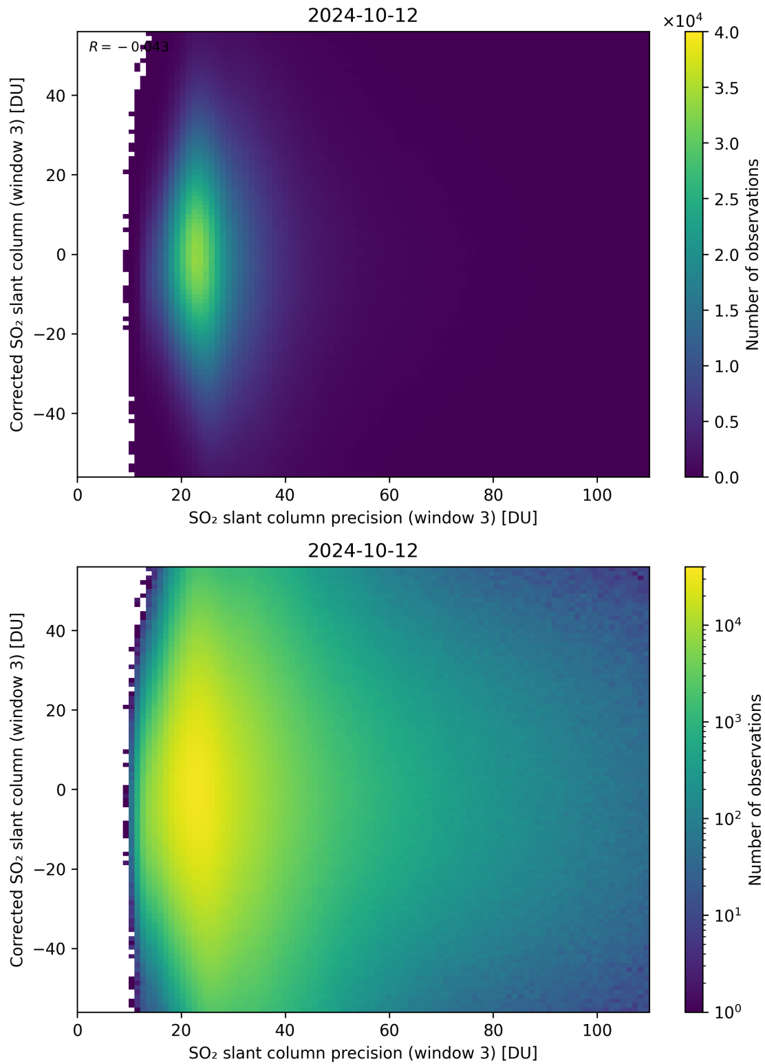
Figure 262: Scatter density plot of “SO 2 slant column precision (window 3)” against “Corrected SO 2 slant column (window 3)” for 2024-10-11 to 2024-10-13.
