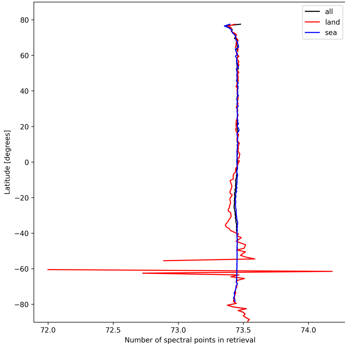
Figure 51: Zonal average of “Number of spectral points in retrieval” for 2024-10-11 to 2024-10-13.
