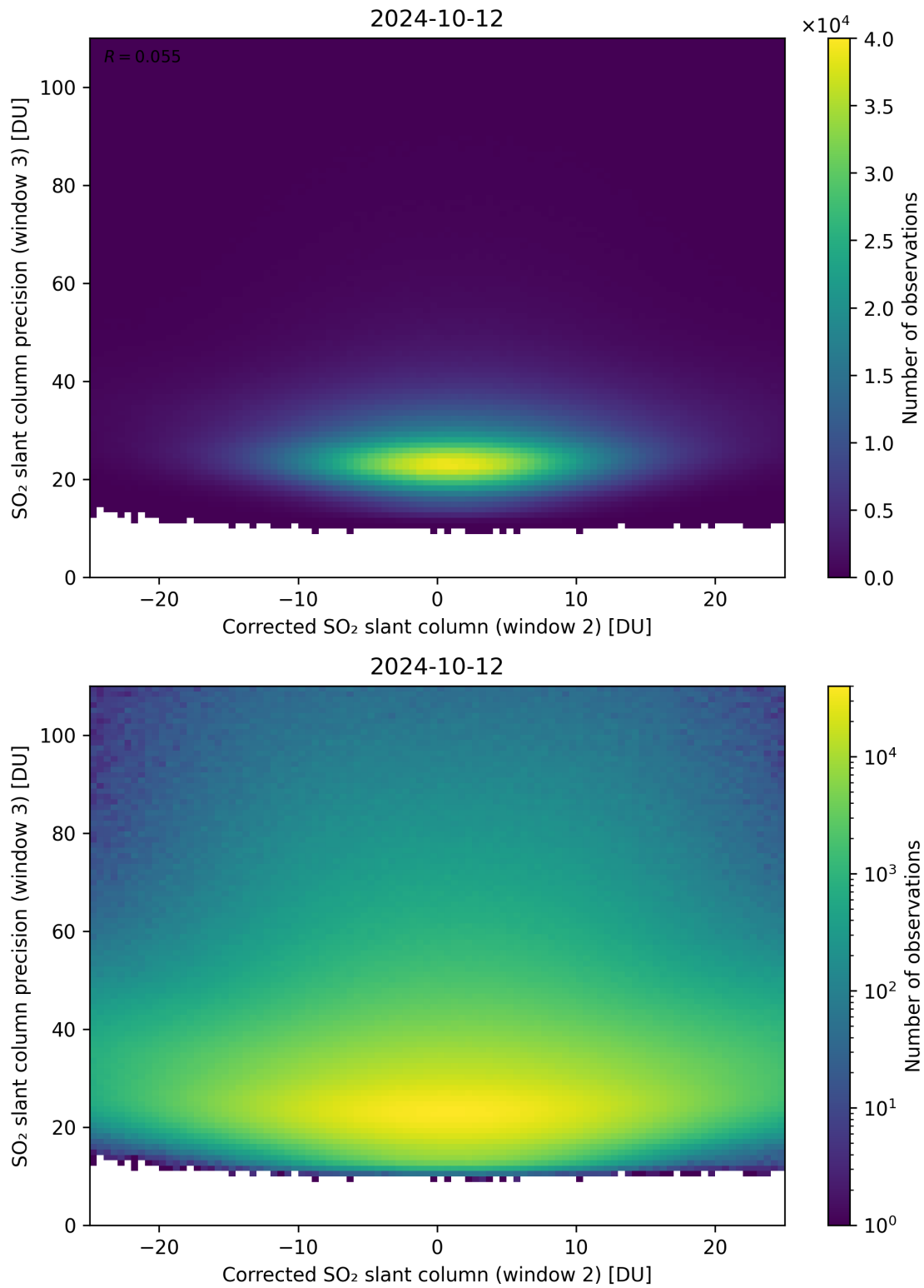
Figure 202: Scatter density plot of “Corrected SO 2 slant column (window 2)” against “SO 2 slant column precision (window 3)” for 2024-10-11 to 2024-10-13.
