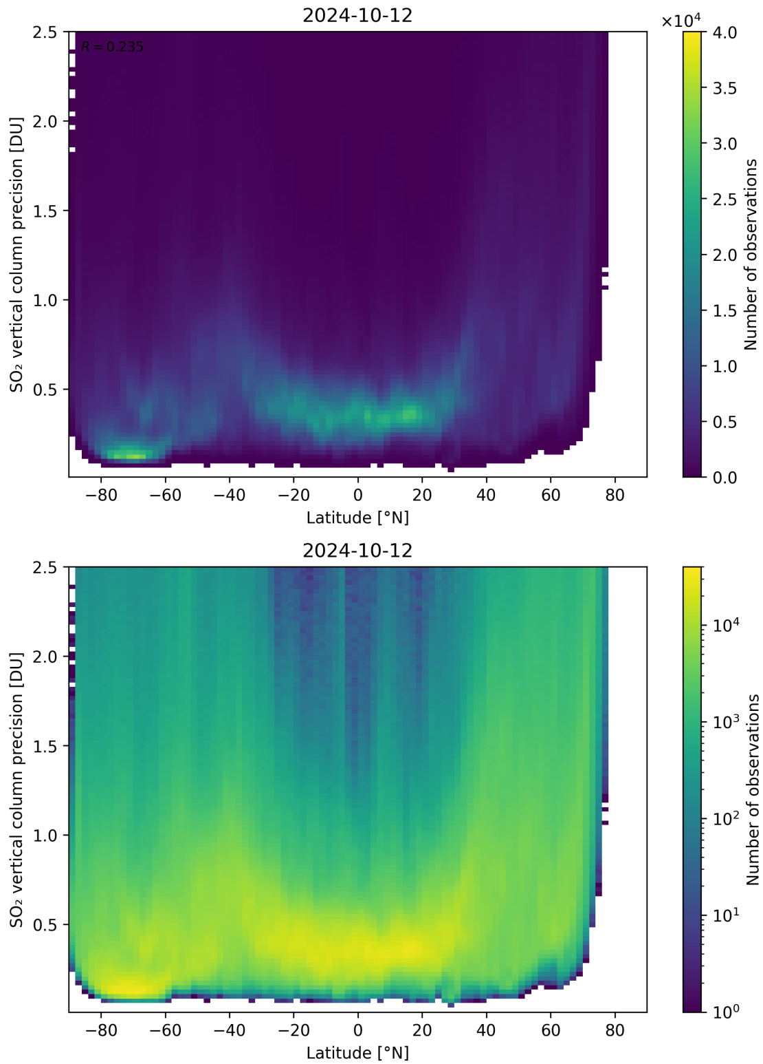
Figure 157: Scatter density plot of “Latitude” against “SO 2 vertical column precision” for 2024-10-11 to 2024-10-13.
