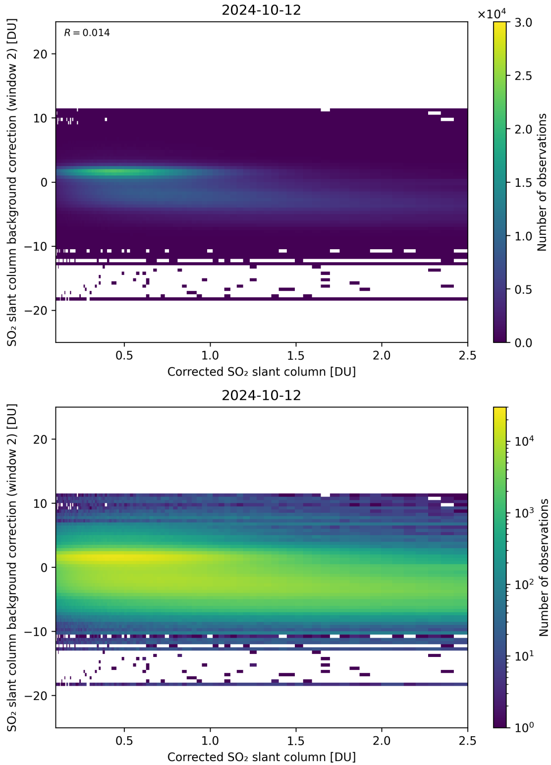
Figure 179: Scatter density plot of “Corrected SO 2 slant column” against “SO 2 slant column background correction (window 2)” for 2024-10-11 to 2024-10-13.
