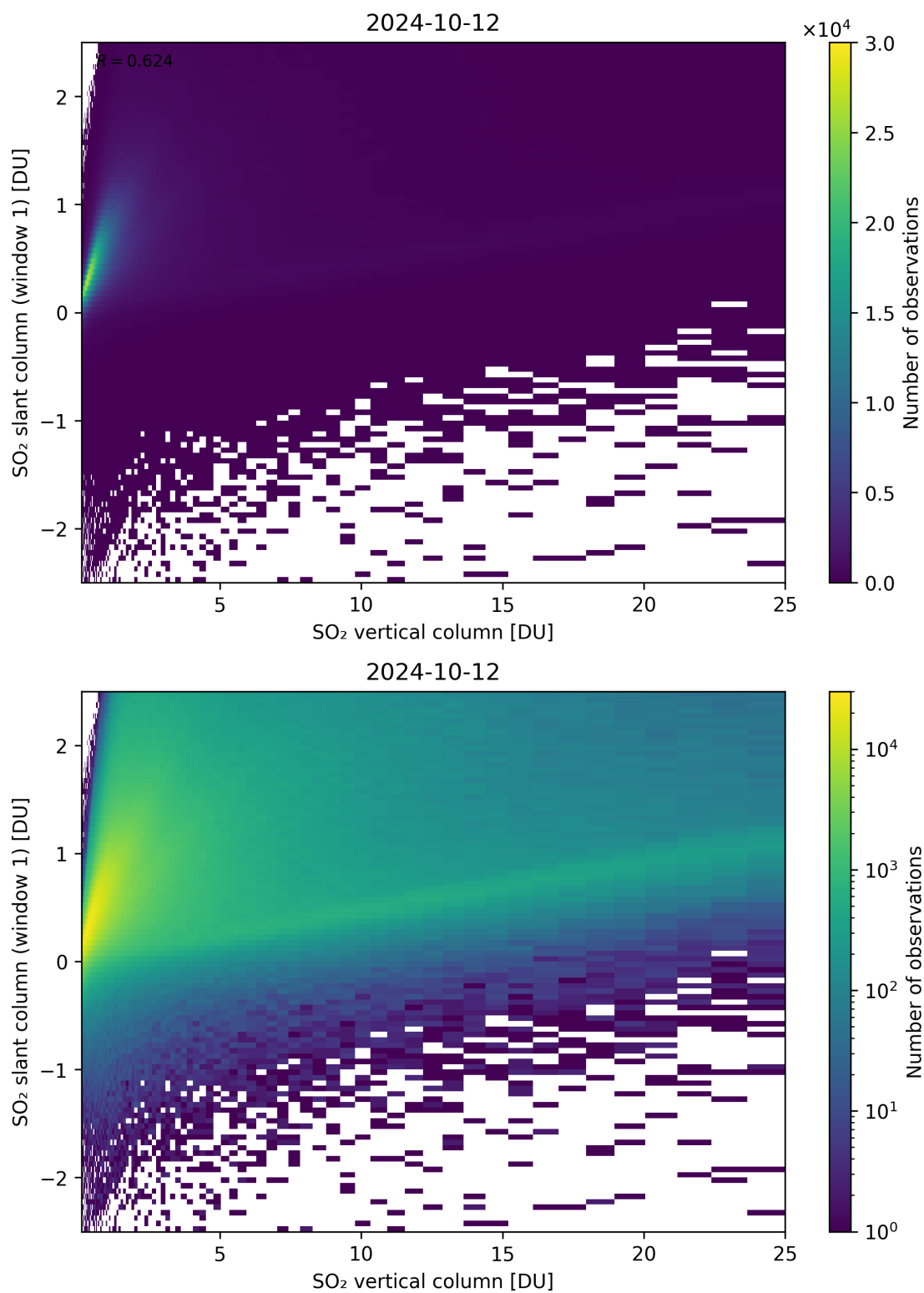
Figure 300: Scatter density plot of “SO 2 vertical column” against “SO 2 slant column (window 1)” for 2024-10-11 to 2024-10-13.
