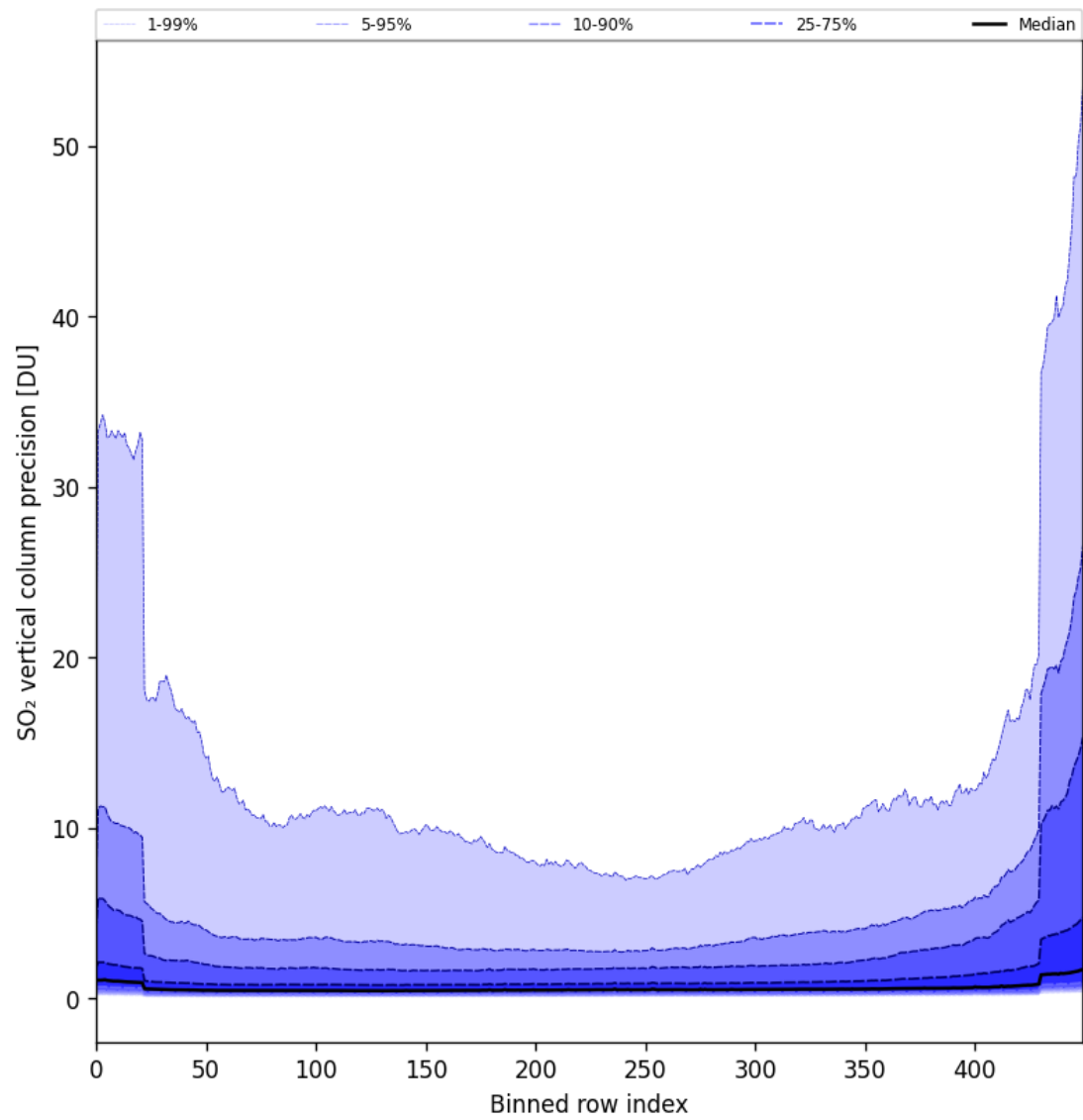
Figure 77: Along track statistics of “SO 2 vertical column precision” for 2024-10-11 to 2024-10-13
