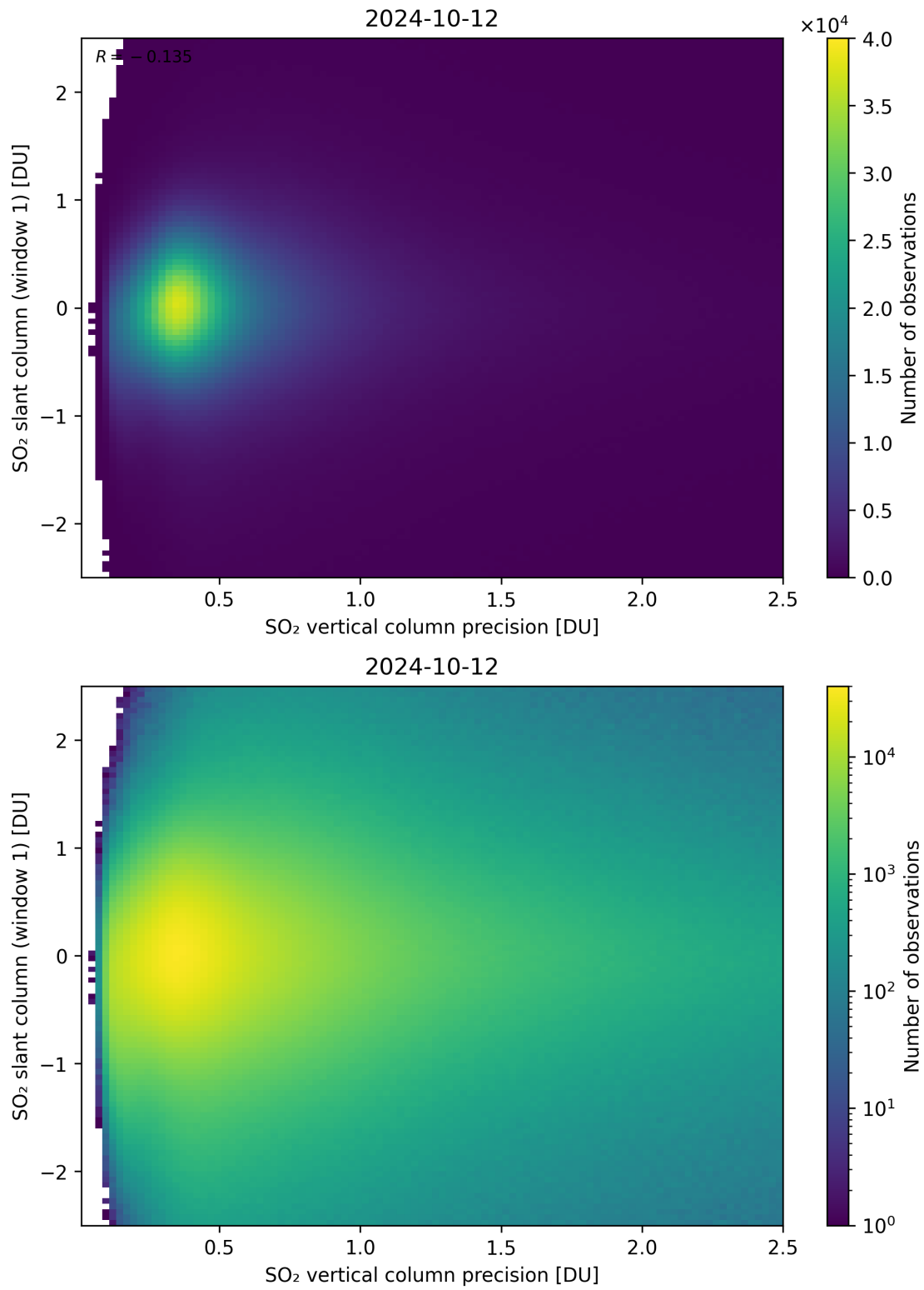
Figure 289: Scatter density plot of “SO 2 vertical column precision” against “SO 2 slant column (window 1)” for 2024-10-11 to 2024-10-13.
