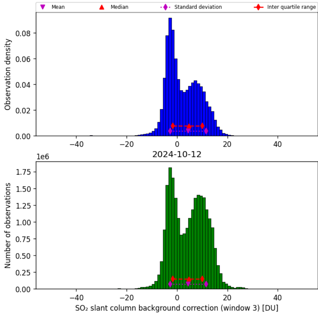
Figure 67: Histogram of “SO 2 slant column background correction (window 3)” for 2024-10-11 to 2024-10-13
