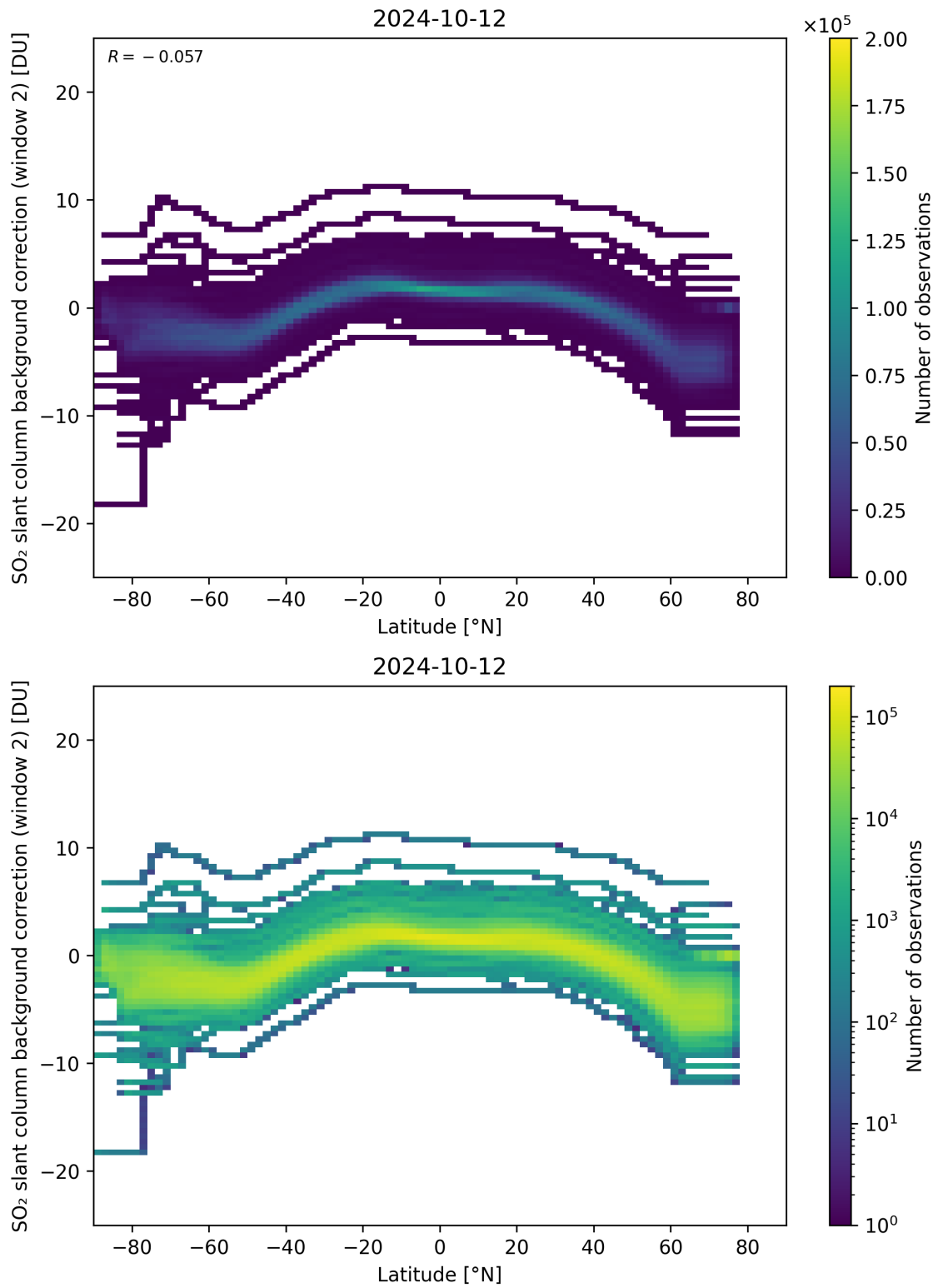
Figure 140: Scatter density plot of “Latitude” against “SO 2 slant column background correction (window 2)” for 2024-10-11 to 2024-10-13.
