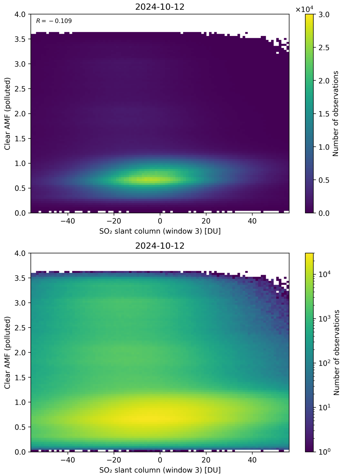
Figure 265: Scatter density plot of “SO 2 slant column (window 3)” against “Clear AMF (polluted)” for 2024-10-11 to 2024-10-13.
