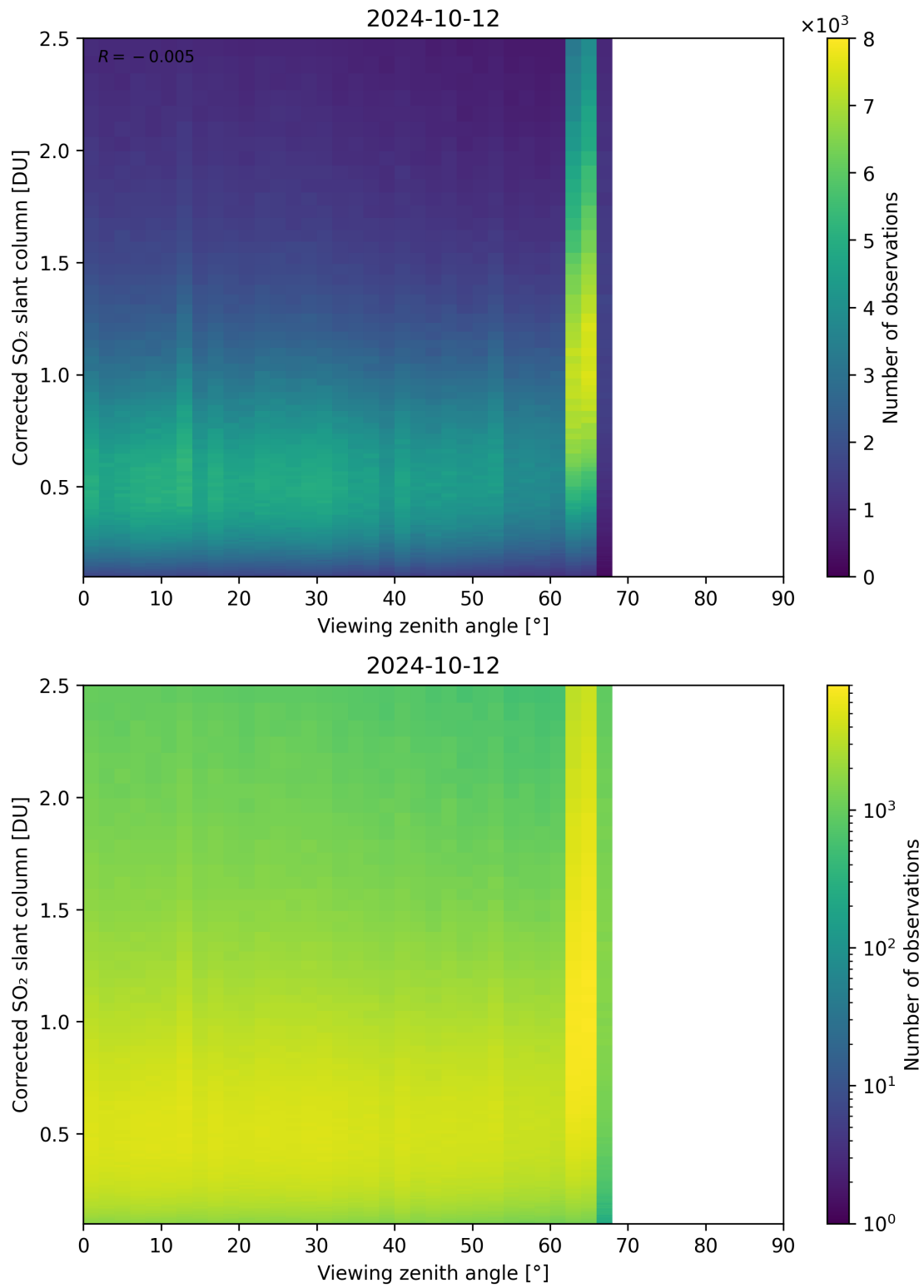
Figure 317: Scatter density plot of “Viewing zenith angle” against “Corrected SO 2 slant column” for 2024-10-11 to 2024-10-13.
