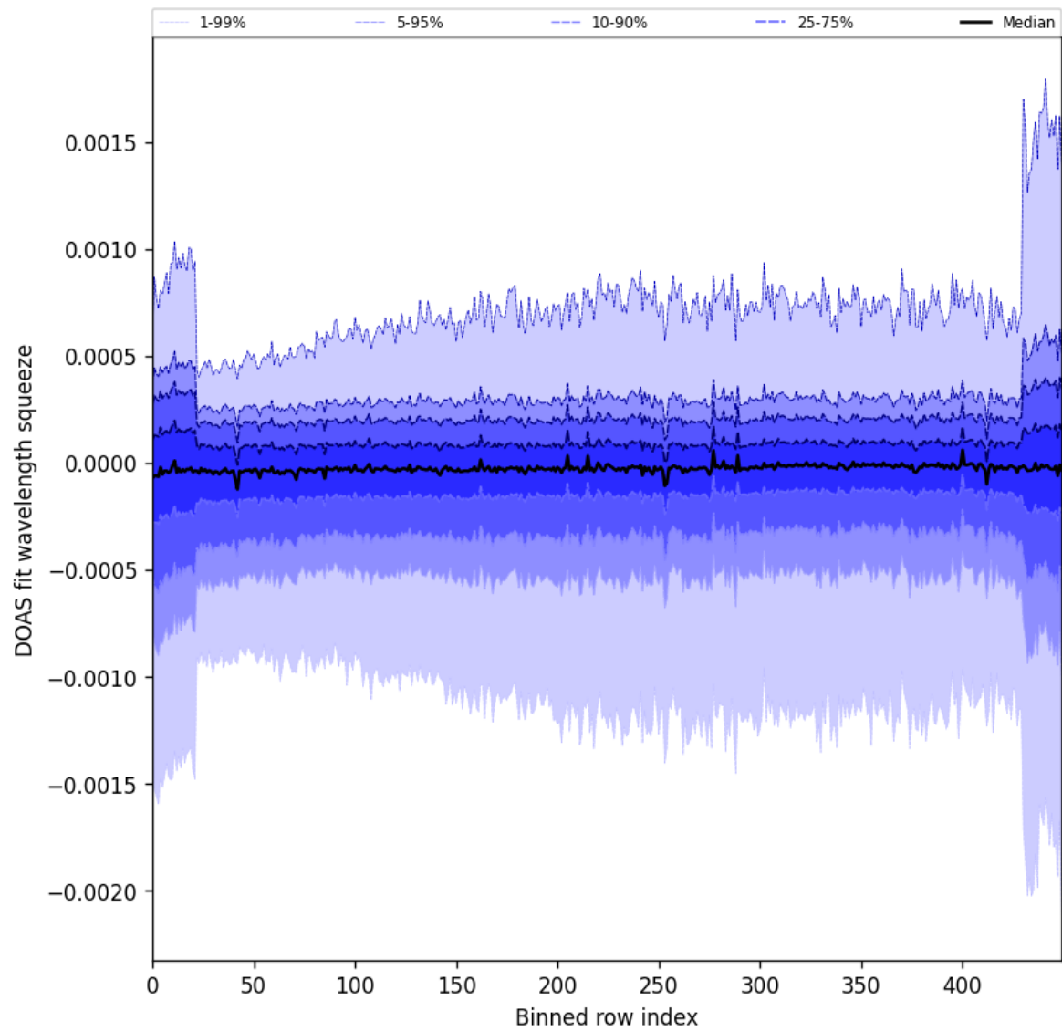
Figure 92: Along track statistics of “DOAS fit wavelength squeeze” for 2024-10-11 to 2024-10-13
