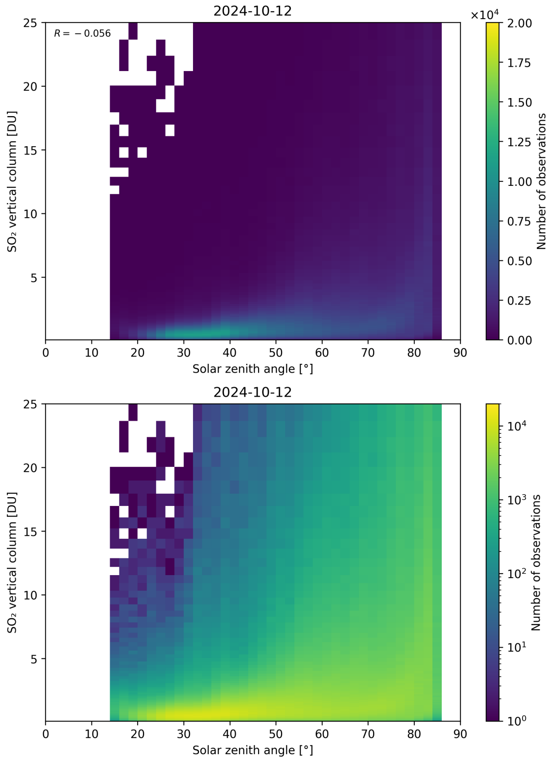
Figure 176: Scatter density plot of “Solar zenith angle” against “SO 2 vertical column” for 2024-10-11 to 2024-10-13.
