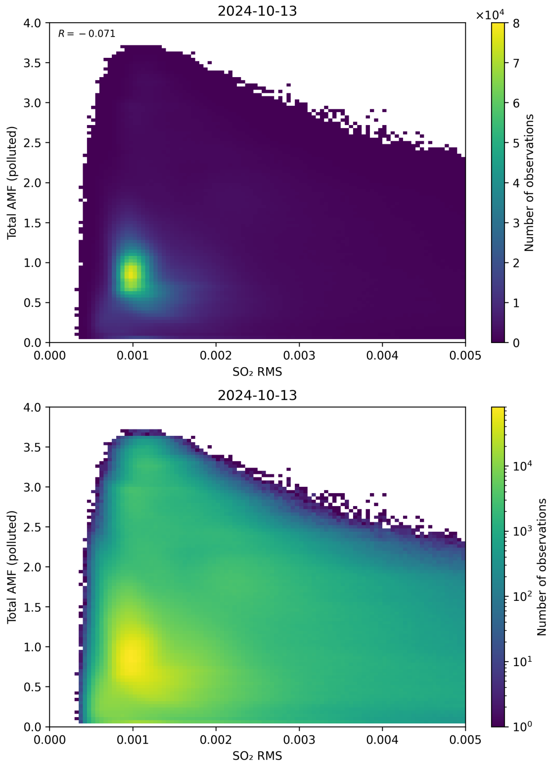
Figure 137: Scatter density plot of “SO 2 RMS” against “Total AMF (polluted)” for 2024-10-12 to 2024-10-14.
