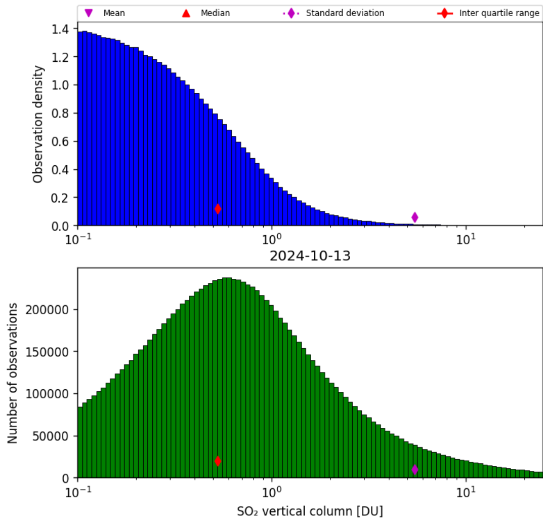
Figure 53: Histogram of “SO 2 vertical column” for 2024-10-12 to 2024-10-14
