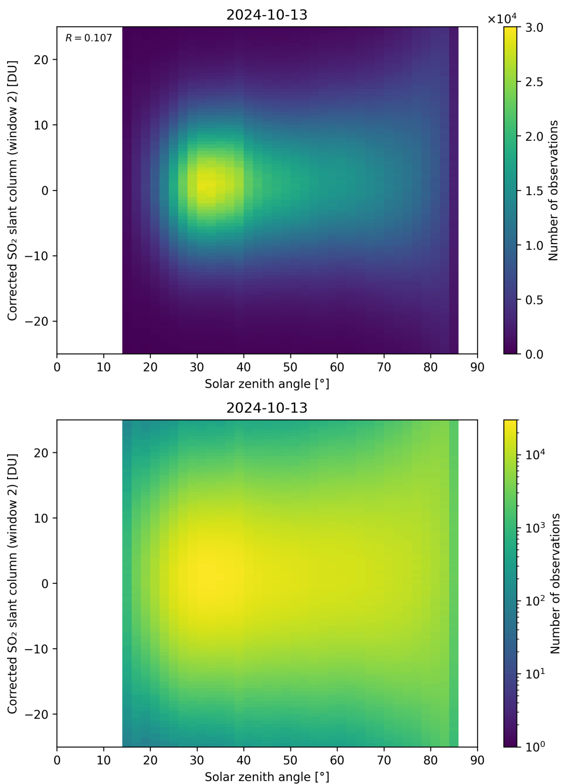
Figure 167: Scatter density plot of “Solar zenith angle” against “Corrected SO 2 slant column (window 2)” for 2024-10-12 to 2024-10-14.
