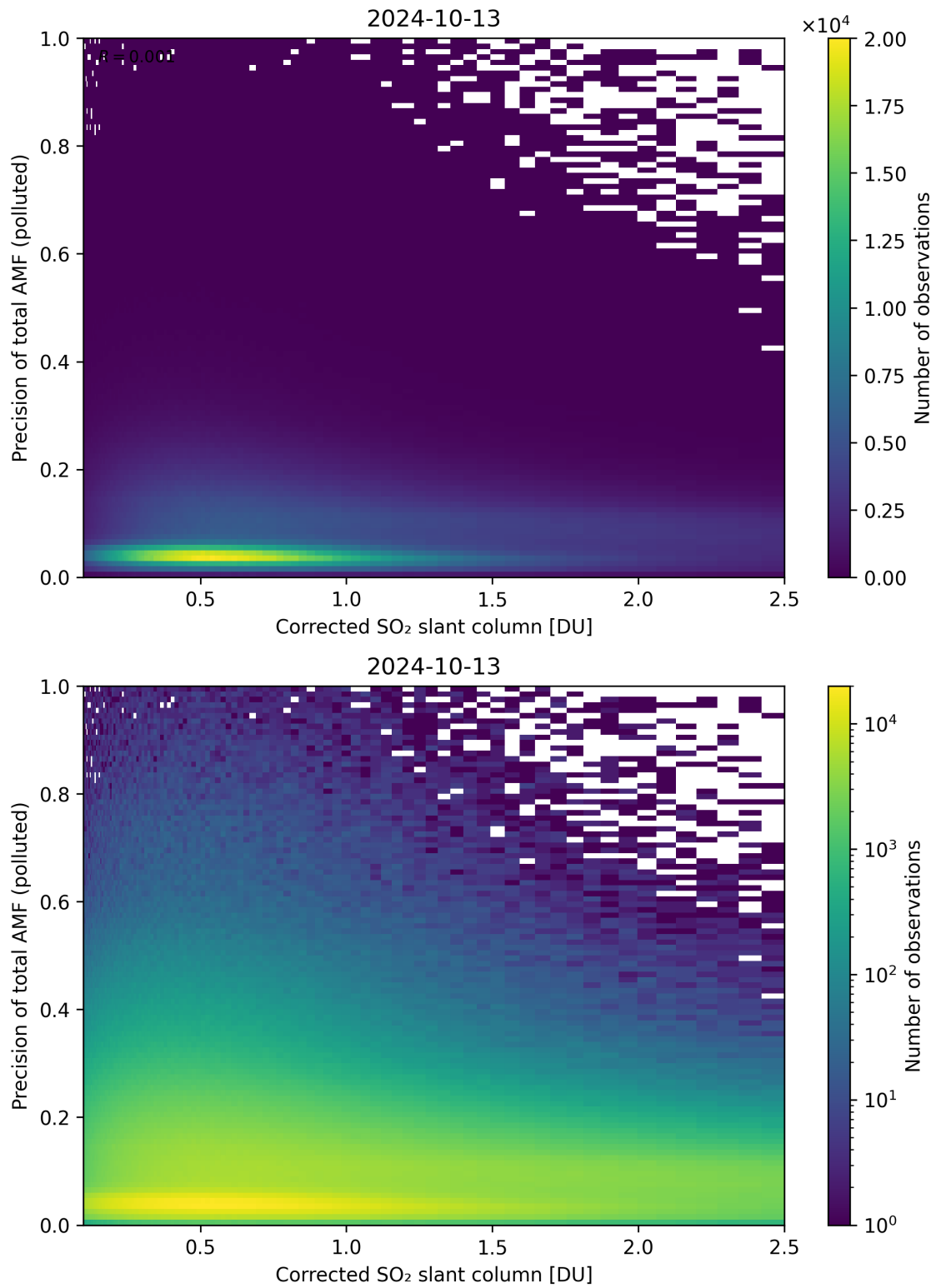
Figure 193: Scatter density plot of “Corrected SO 2 slant column” against “Precision of total AMF (polluted)” for 2024-10-12 to 2024-10-14.
