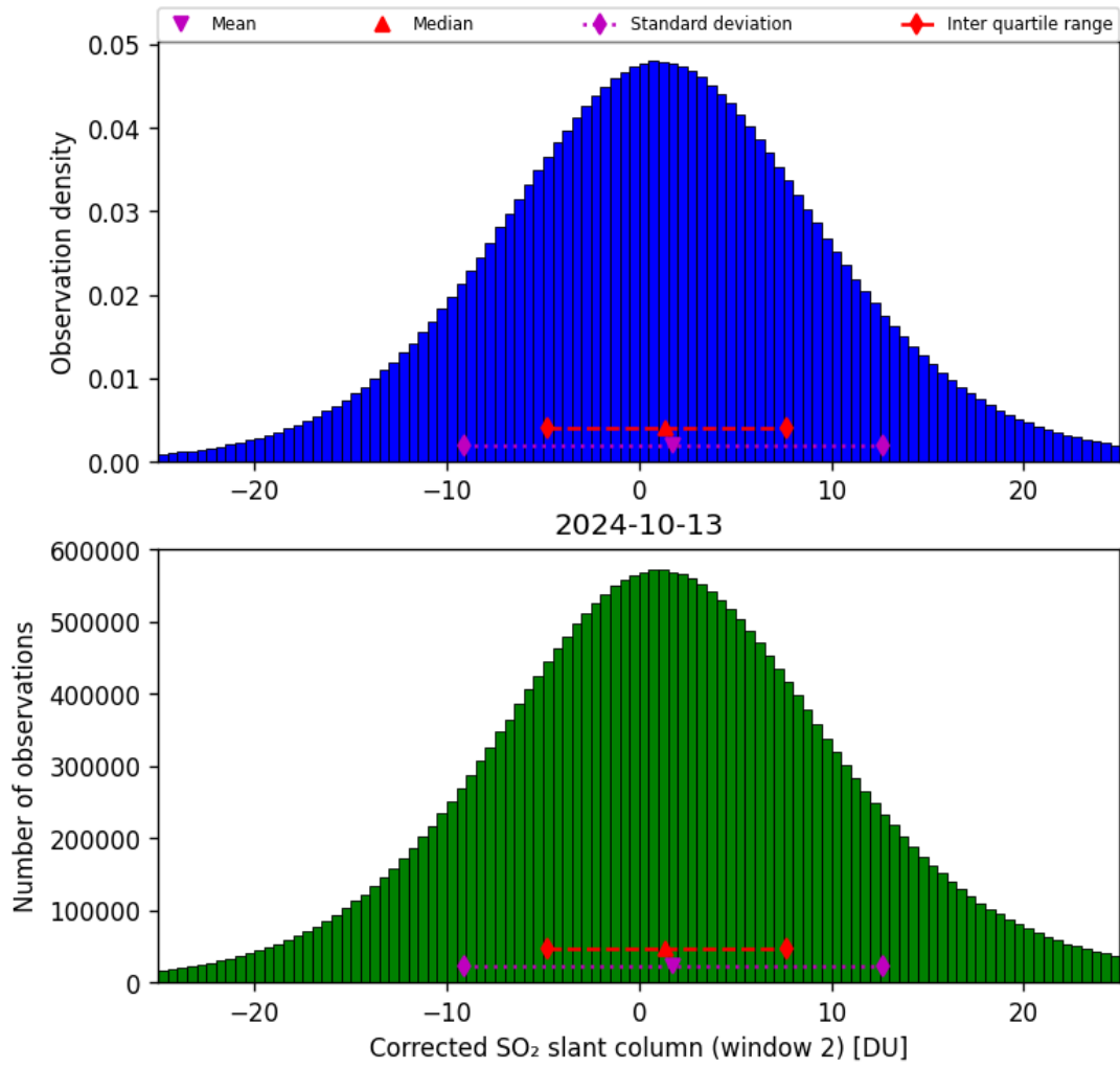
Figure 62: Histogram of “Corrected SO 2 slant column (window 2)” for 2024-10-12 to 2024-10-14
