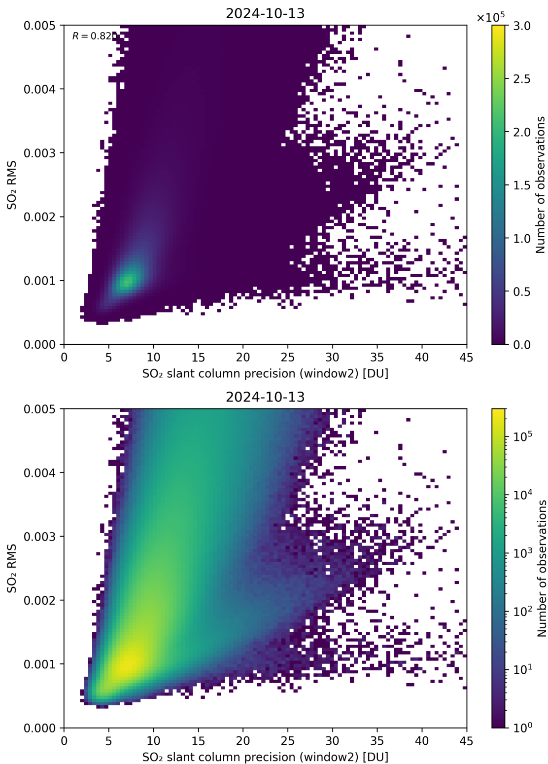
Figure 245: Scatter density plot of “SO 2 slant column precision (window2)” against “SO 2 RMS” for 2024-10-12 to 2024-10-14.
