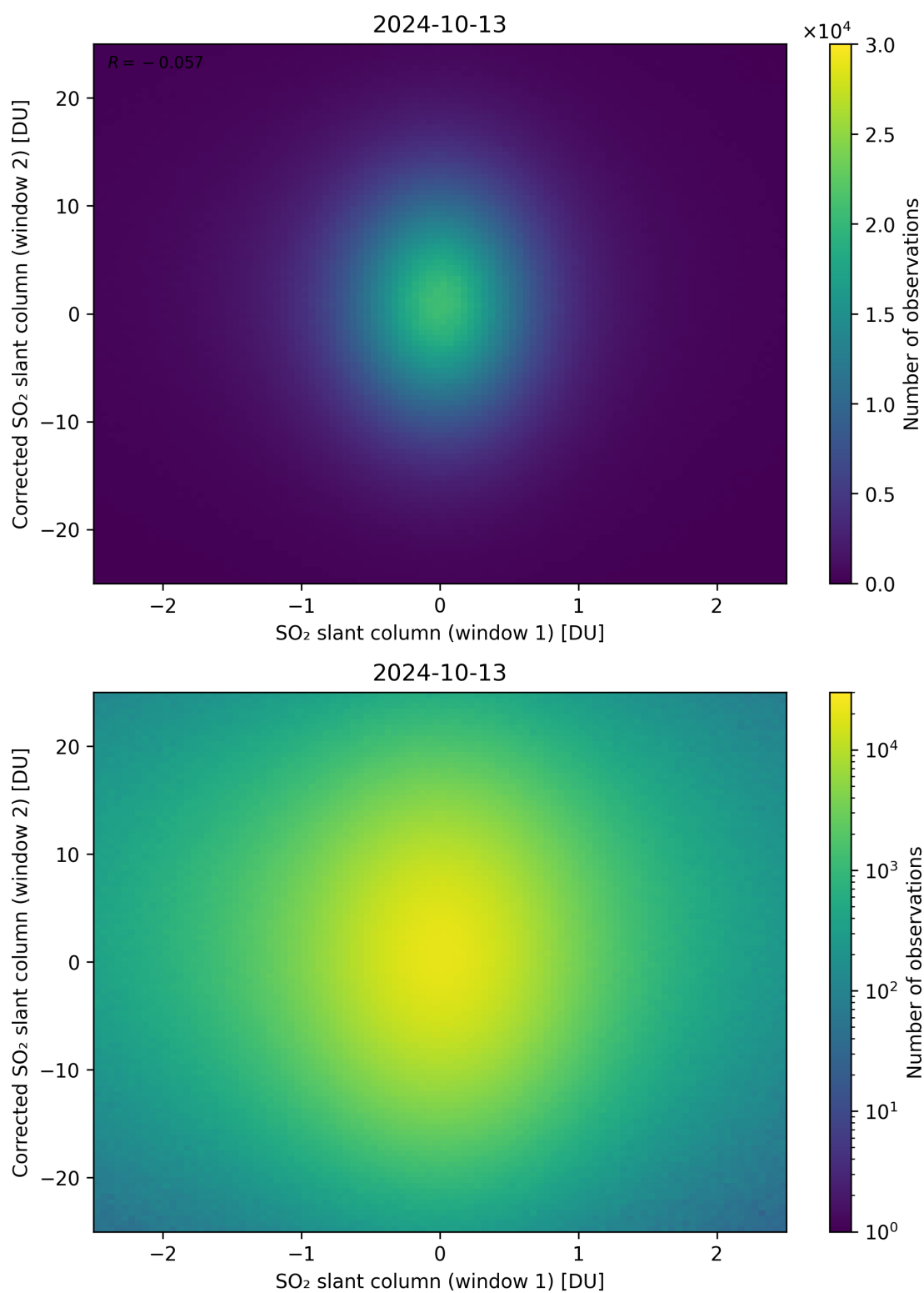
Figure 233: Scatter density plot of “SO 2 slant column (window 1)” against “Corrected SO 2 slant column (window 2)” for 2024-10-12 to 2024-10-14.
