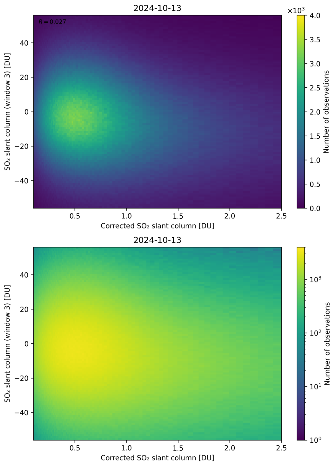
Figure 190: Scatter density plot of “Corrected SO 2 slant column” against “SO 2 slant column (window 3)” for 2024-10-12 to 2024-10-14.
