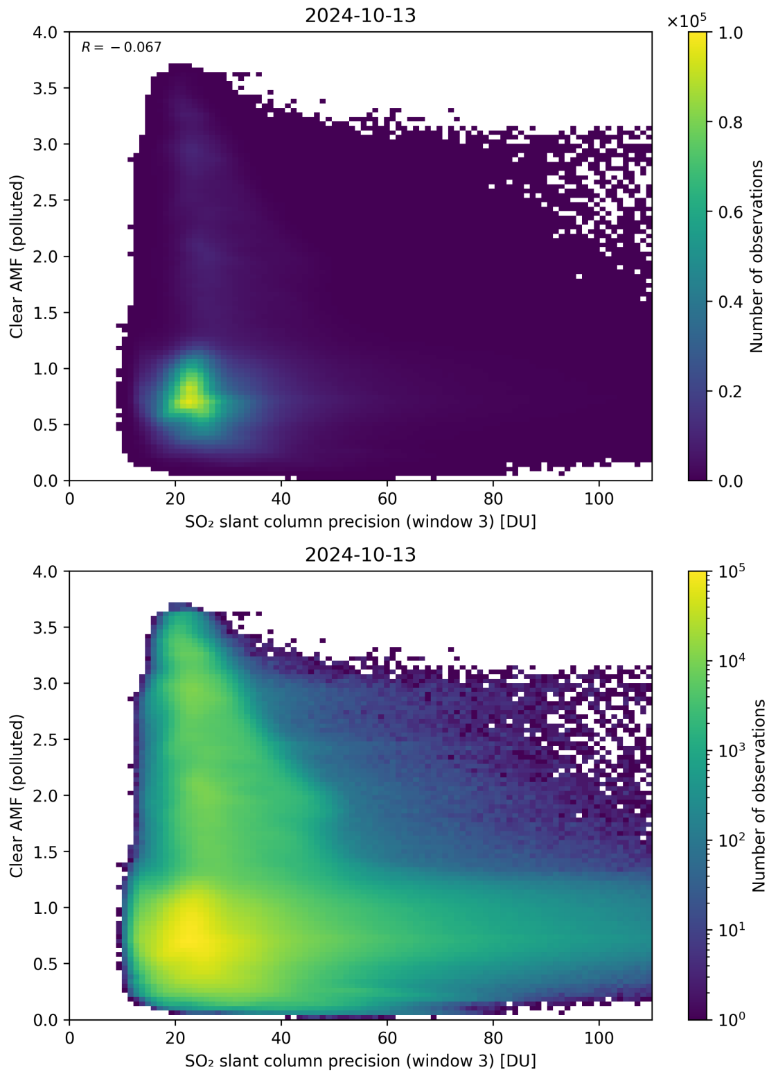
Figure 261: Scatter density plot of “SO 2 slant column precision (window 3)” against “Clear AMF (polluted)” for 2024-10-12 to 2024-10-14.
