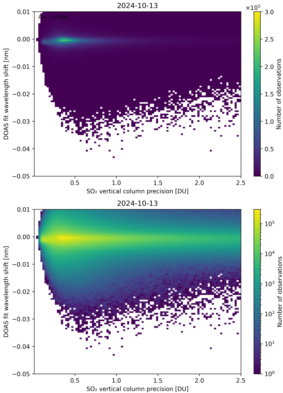
Figure 282: Scatter density plot of “SO 2 vertical column precision” against “DOAS fit wavelength shift” for 2024-10-12 to 2024-10-14.
