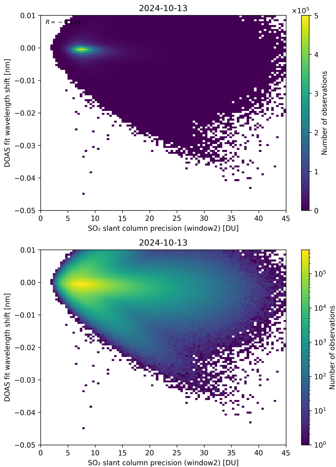
Figure 243: Scatter density plot of “SO 2 slant column precision (window2)” against “DOAS fit wavelength shift” for 2024-10-12 to 2024-10-14.
