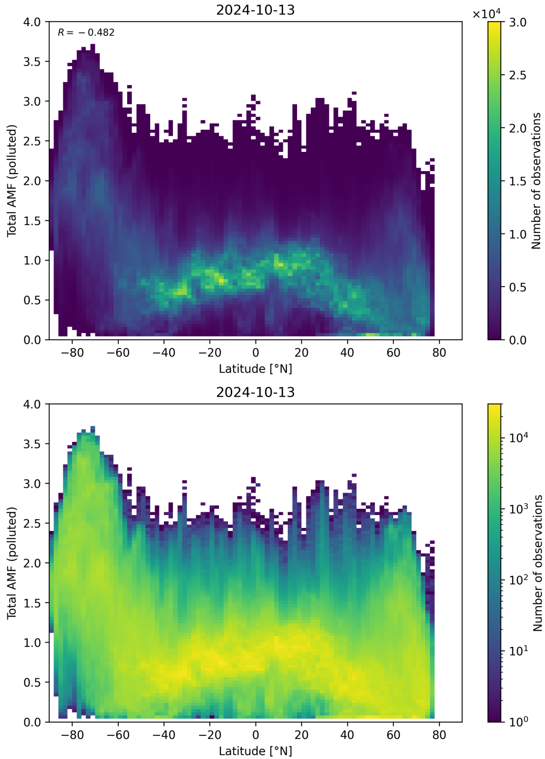
Figure 154: Scatter density plot of “Latitude” against “Total AMF (polluted)” for 2024-10-12 to 2024-10-14.
