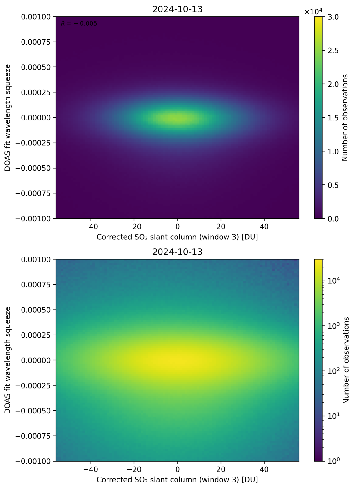
Figure 207: Scatter density plot of “Corrected SO 2 slant column (window 3)” against “DOAS fit wavelength squeeze” for 2024-10-12 to 2024-10-14.
