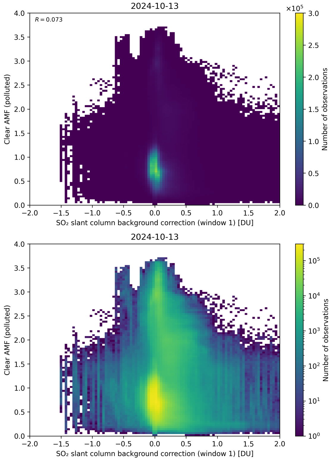
Figure 103: Scatter density plot of “SO 2 slant column background correction (window 1)” against “Clear AMF (polluted)” for 2024-10-12 to 2024-10-14.
