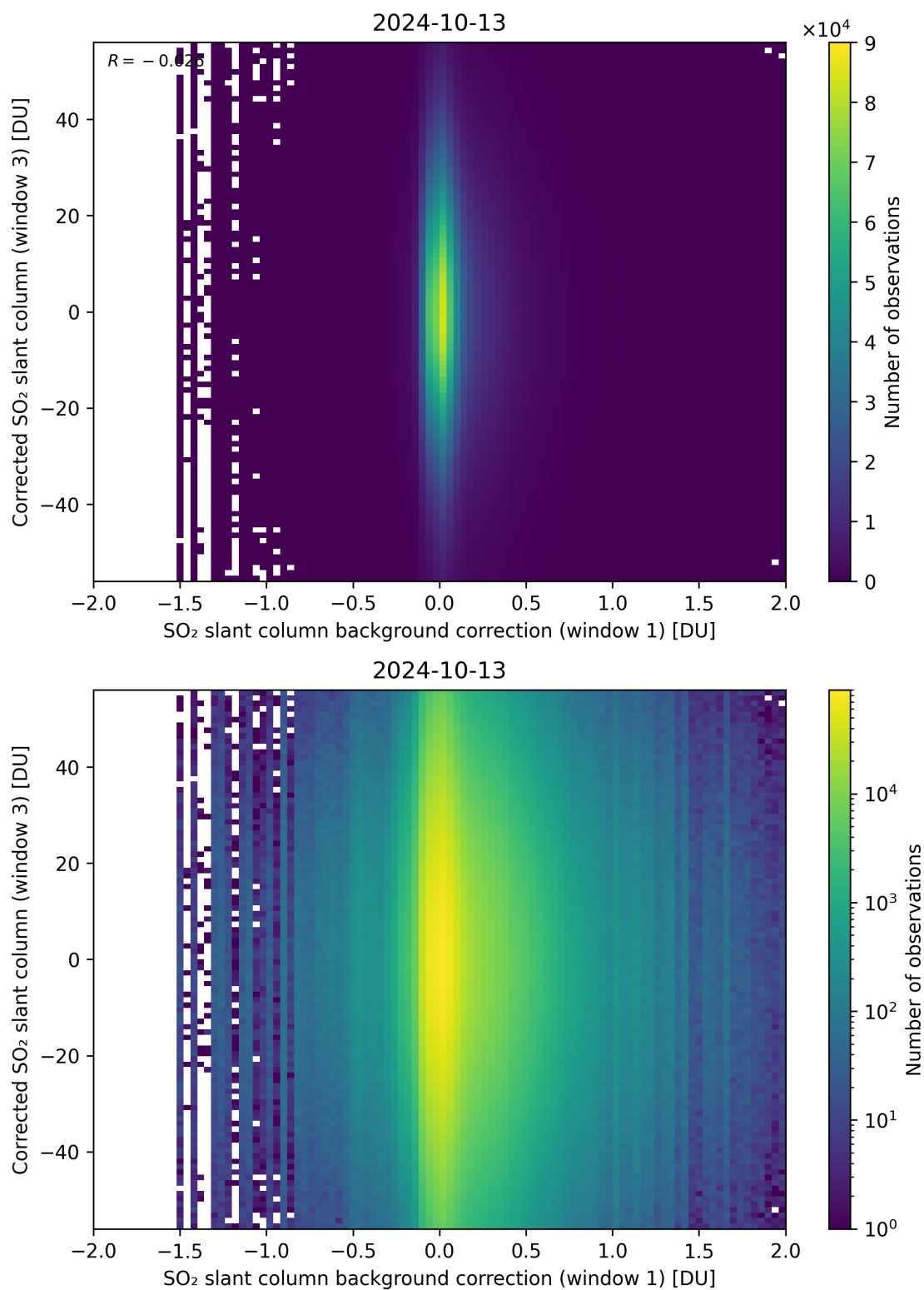
Figure 105: Scatter density plot of “SO 2 slant column background correction (window 1)” against “Corrected SO 2 slant column (window 3)” for 2024-10-12 to 2024-10-14.
