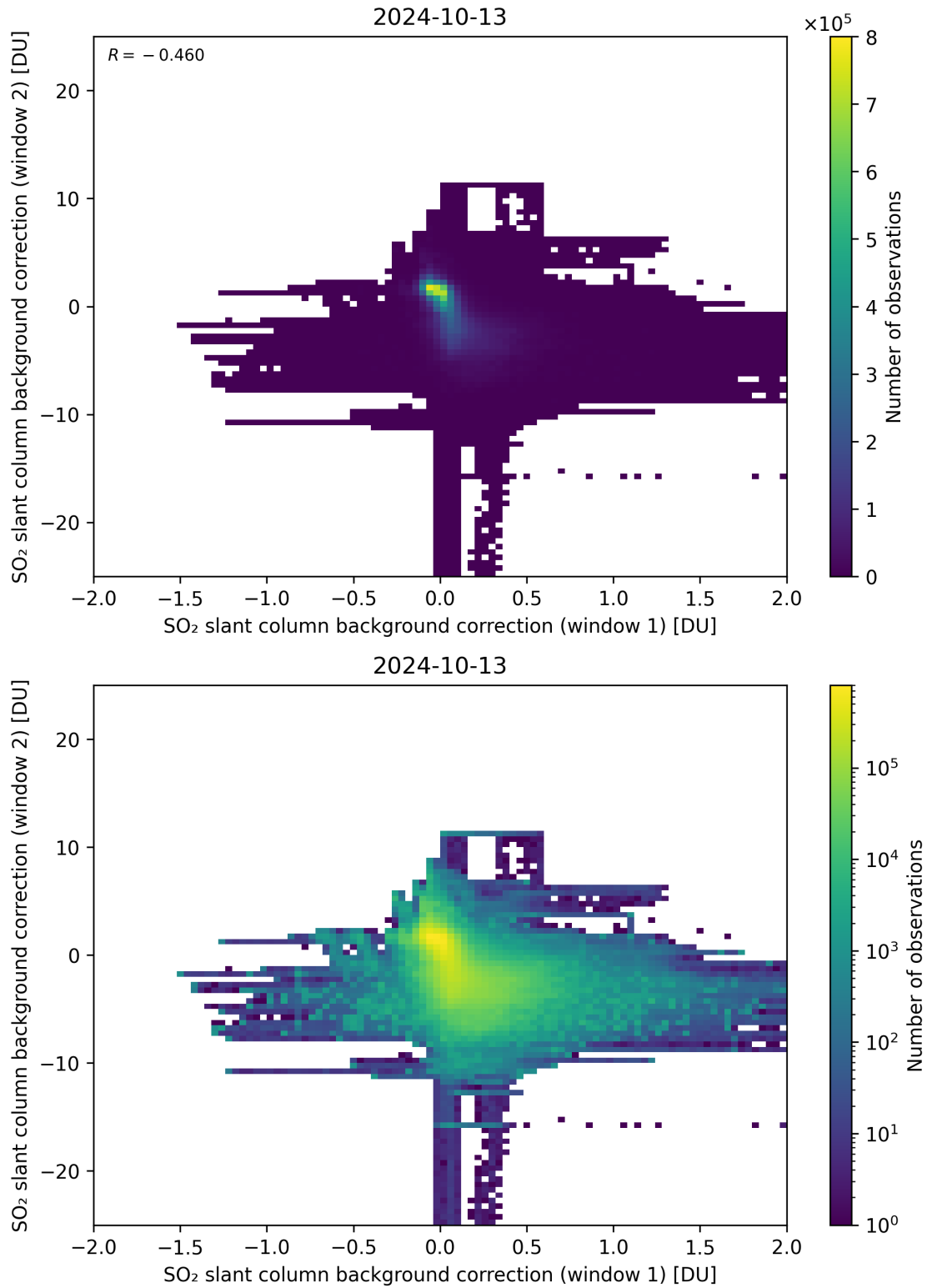
Figure 98: Scatter density plot of “SO 2 slant column background correction (window 1)” against “SO 2 slant column background correction (window 2)” for 2024-10-12 to 2024-10-14.
