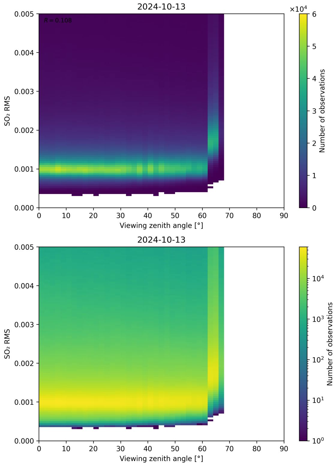
Figure 313: Scatter density plot of “Viewing zenith angle” against “SO 2 RMS” for 2024-10-12 to 2024-10-14.
