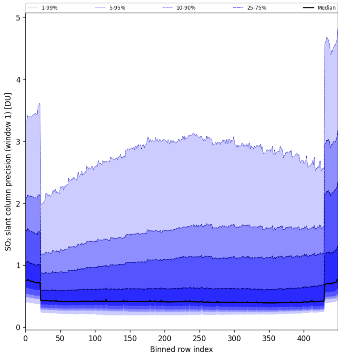
Figure 80: Along track statistics of “SO 2 slant column precision (window 1)” for 2024-10-12 to 2024-10-14
