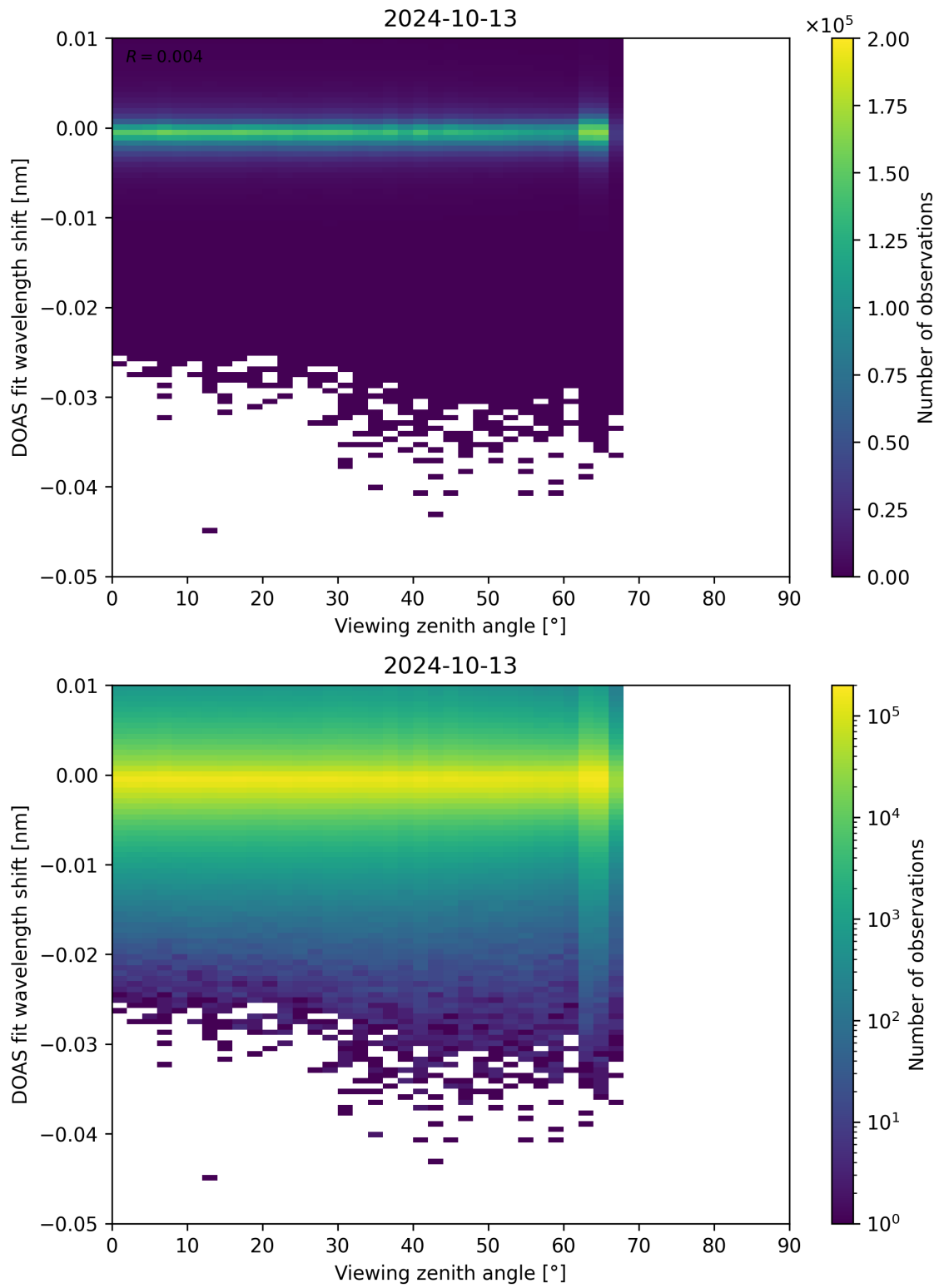
Figure 311: Scatter density plot of “Viewing zenith angle” against “DOAS fit wavelength shift” for 2024-10-12 to 2024-10-14.
