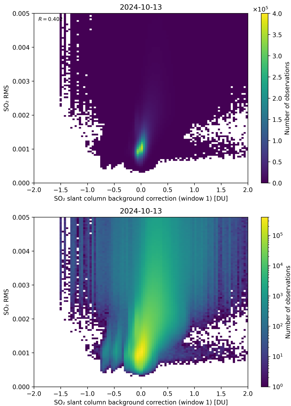
Figure 102: Scatter density plot of “SO 2 slant column background correction (window 1)” against “SO 2 RMS” for 2024-10-12 to 2024-10-14.
