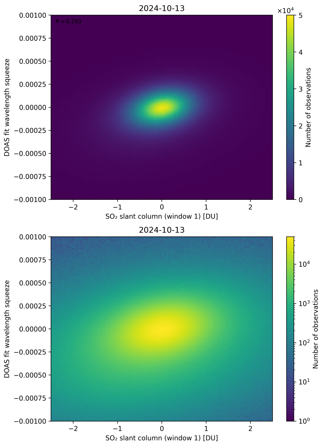
Figure 216: Scatter density plot of “SO 2 slant column (window 1)” against “DOAS fit wavelength squeeze” for 2024-10-12 to 2024-10-14.
