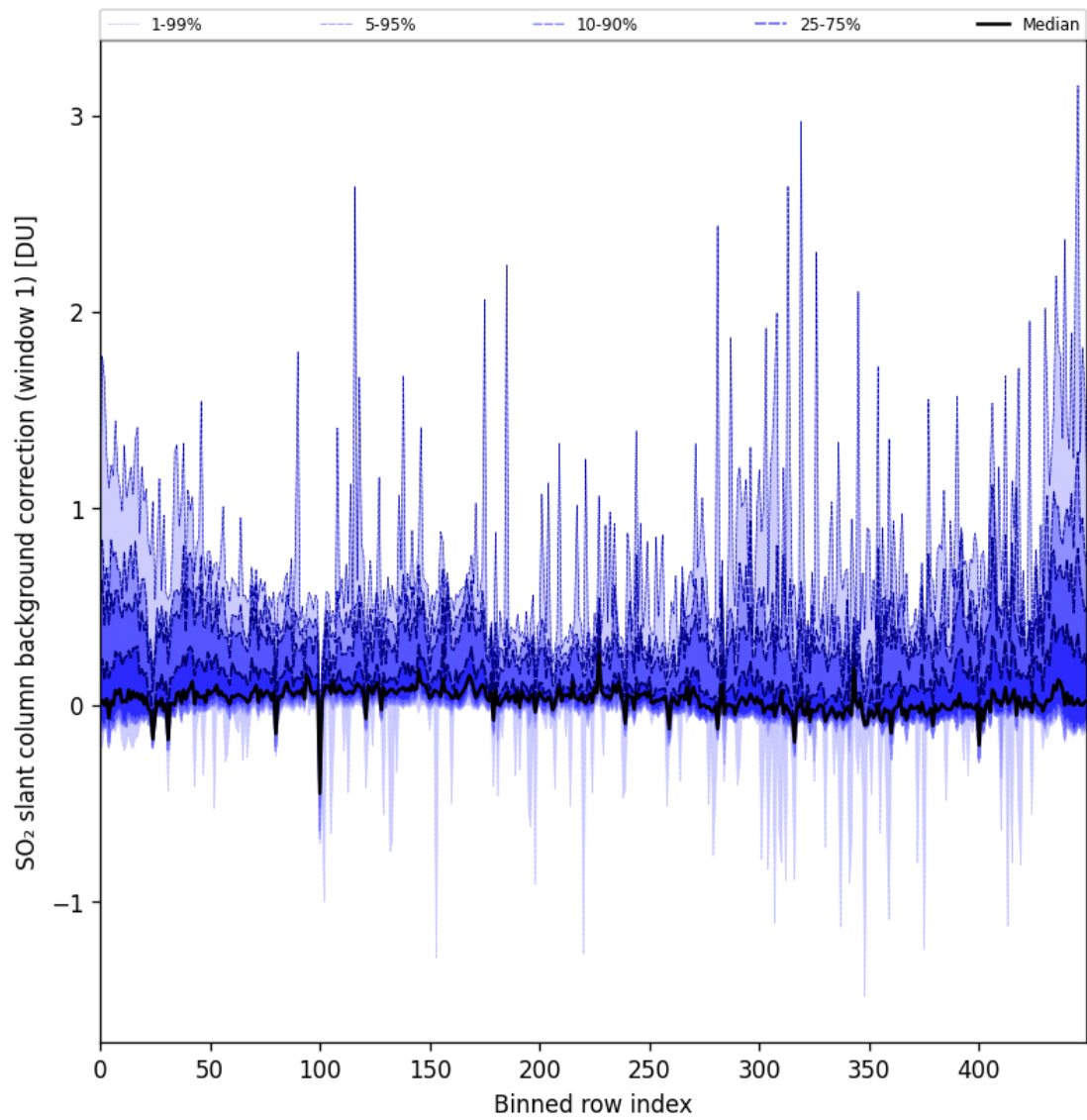
Figure 82: Along track statistics of “SO 2 slant column background correction (window 1)” for 2024-10-12 to 2024-10-14
