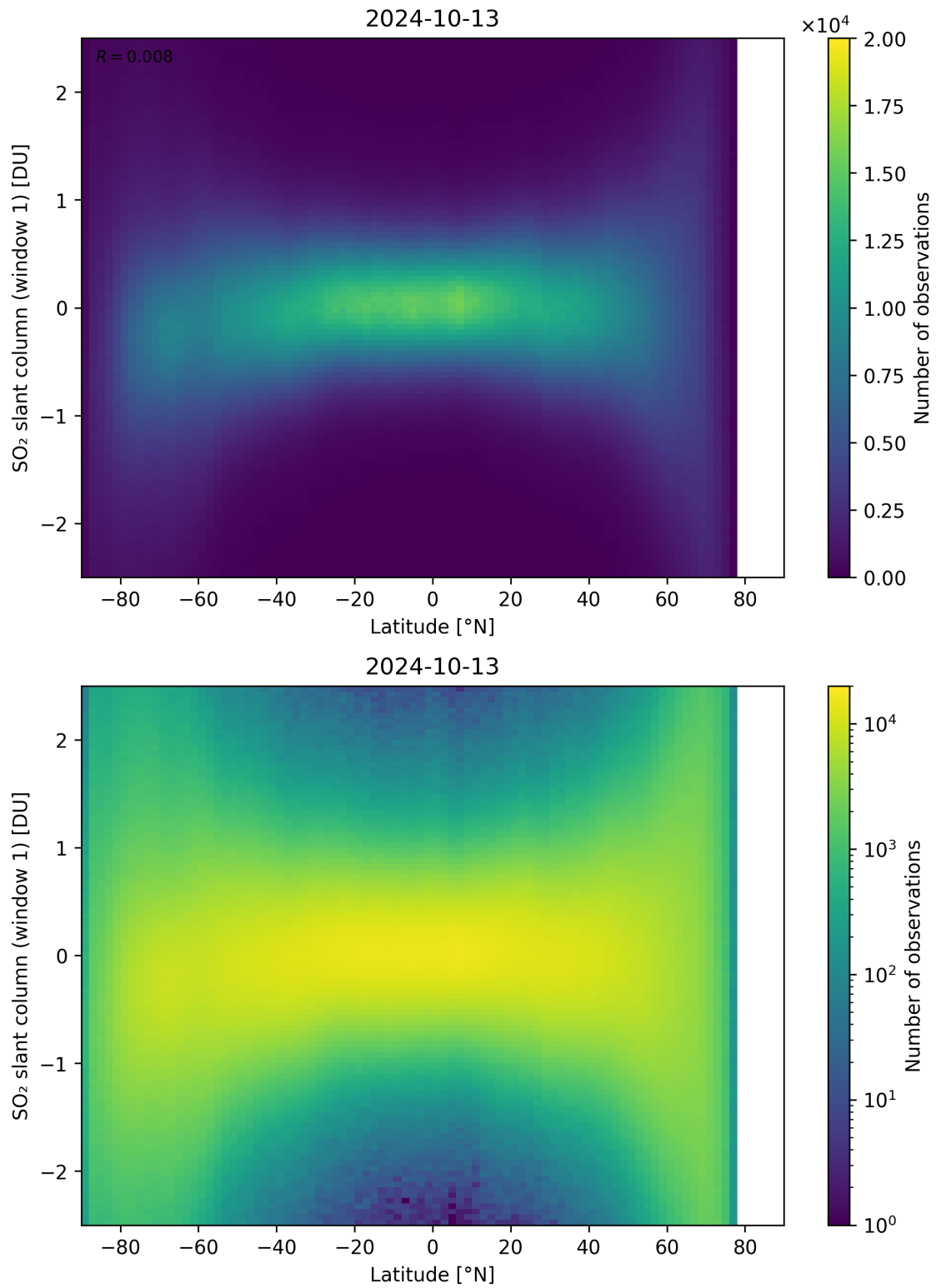
Figure 149: Scatter density plot of “Latitude” against “SO 2 slant column (window 1)” for 2024-10-12 to 2024-10-14.
