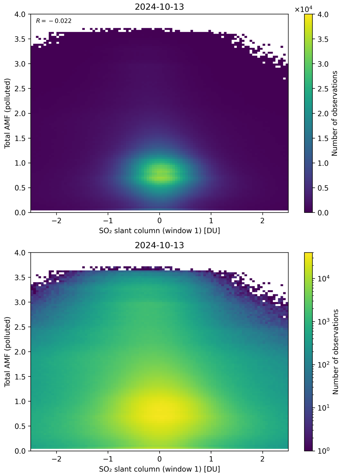
Figure 239: Scatter density plot of “SO 2 slant column (window 1)” against “Total AMF (polluted)” for 2024-10-12 to 2024-10-14.
