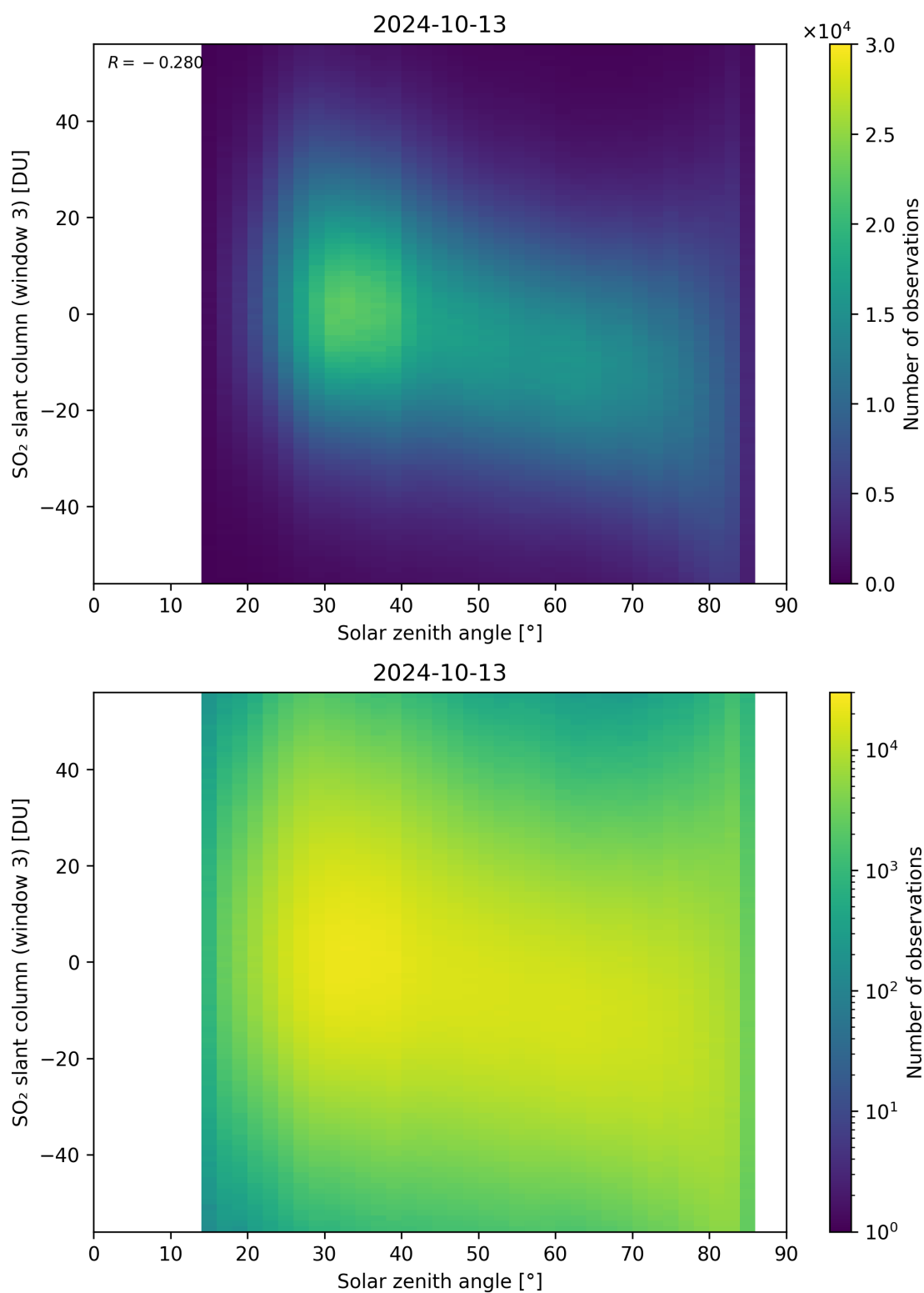
Figure 172: Scatter density plot of “Solar zenith angle” against “SO 2 slant column (window 3)” for 2024-10-12 to 2024-10-14.
