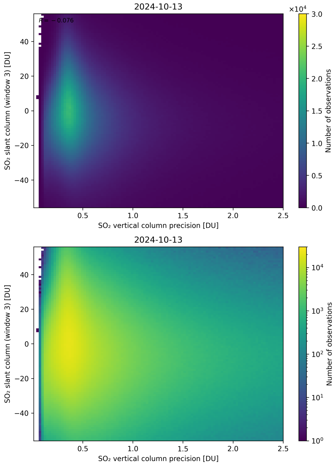
Figure 292: Scatter density plot of “SO 2 vertical column precision” against “SO 2 slant column (window 3)” for 2024-10-12 to 2024-10-14.
