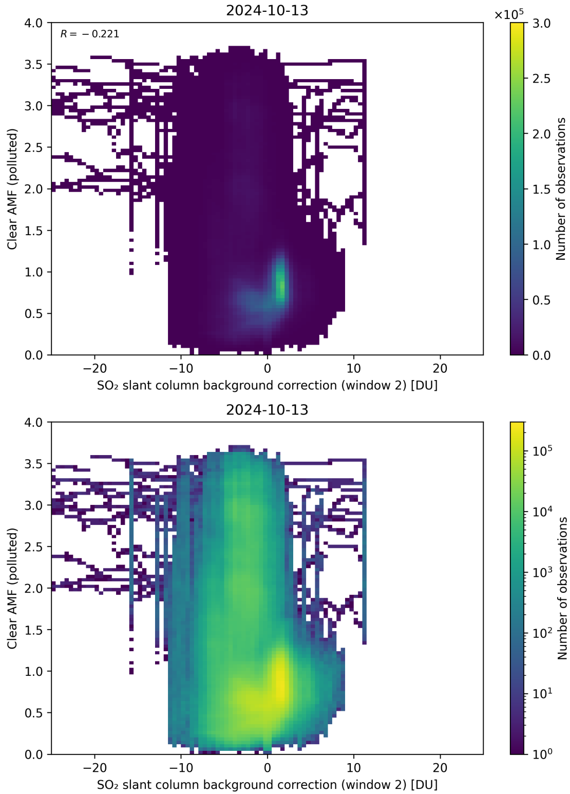
Figure 115: Scatter density plot of “SO 2 slant column background correction (window 2)” against “Clear AMF (polluted)” for 2024-10-12 to 2024-10-14.
