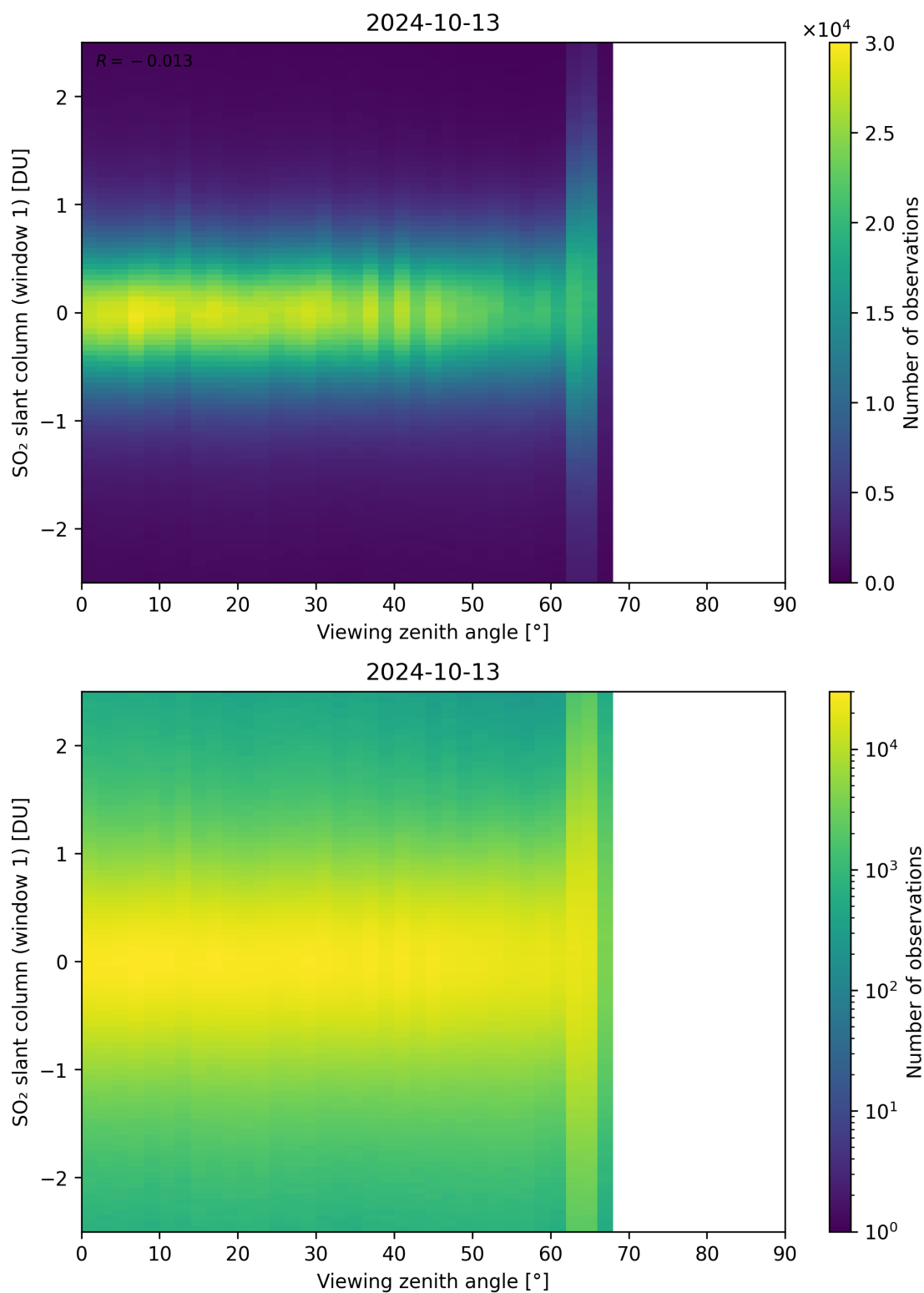
Figure 320: Scatter density plot of “Viewing zenith angle” against “SO 2 slant column (window 1)” for 2024-10-12 to 2024-10-14.
