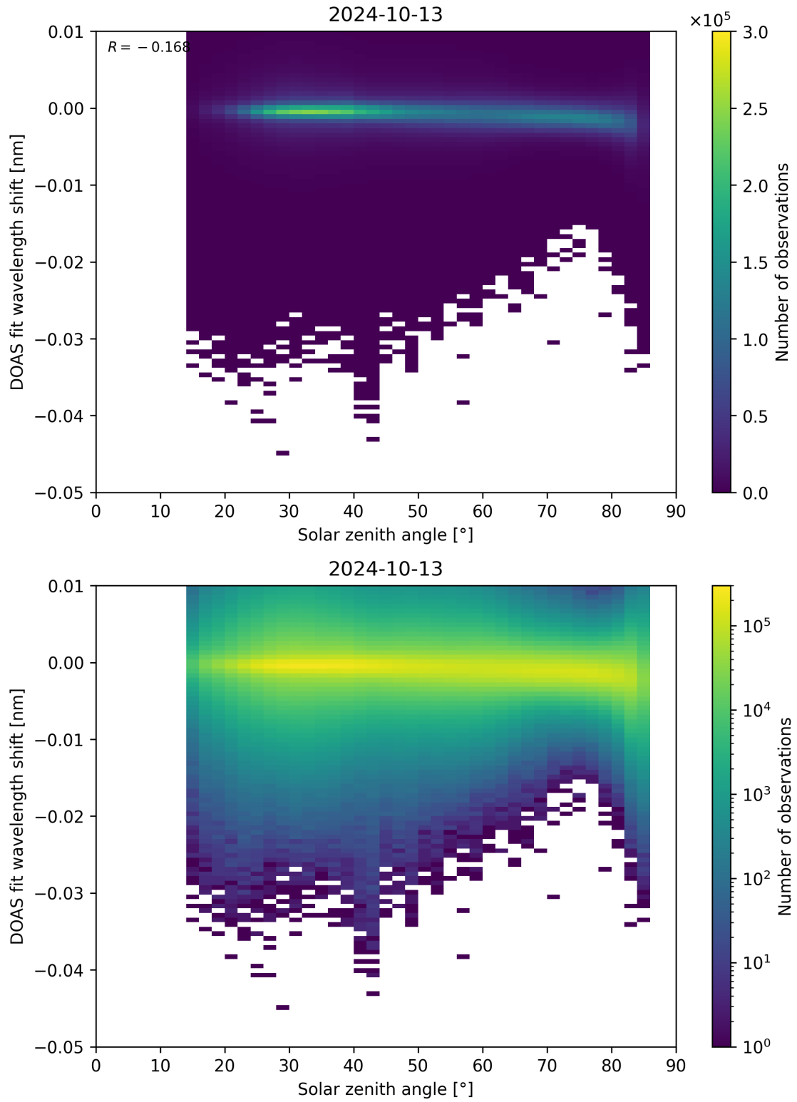
Figure 161: Scatter density plot of “Solar zenith angle” against “DOAS fit wavelength shift” for 2024-10-12 to 2024-10-14.
