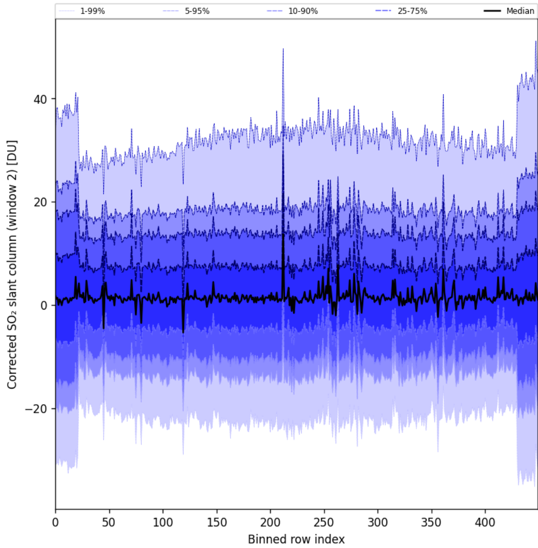
Figure 85: Along track statistics of “Corrected SO 2 slant column (window 2)” for 2024-10-12 to 2024-10-14
