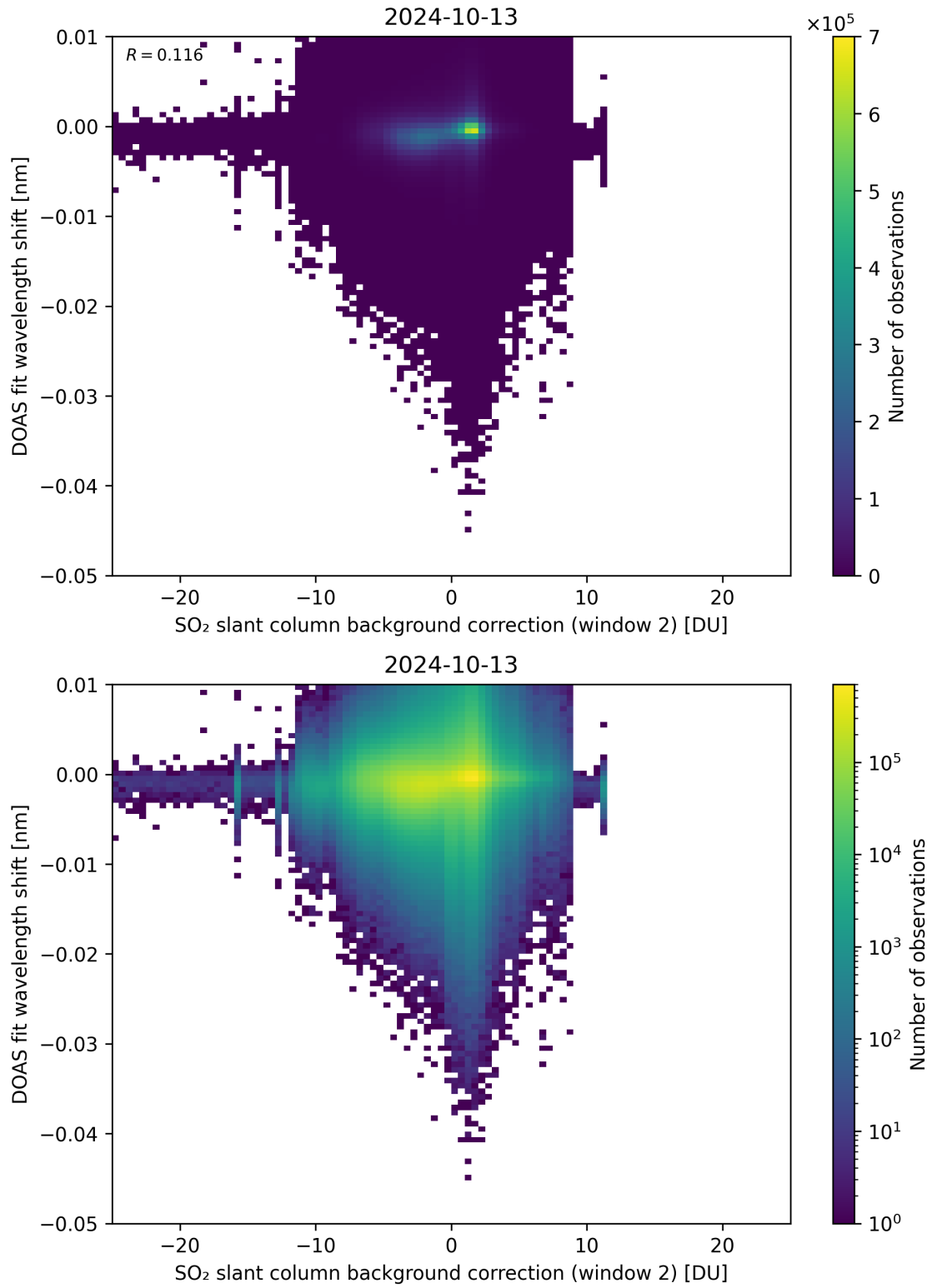
Figure 112: Scatter density plot of “SO 2 slant column background correction (window 2)” against “DOAS fit wavelength shift” for 2024-10-12 to 2024-10-14.
