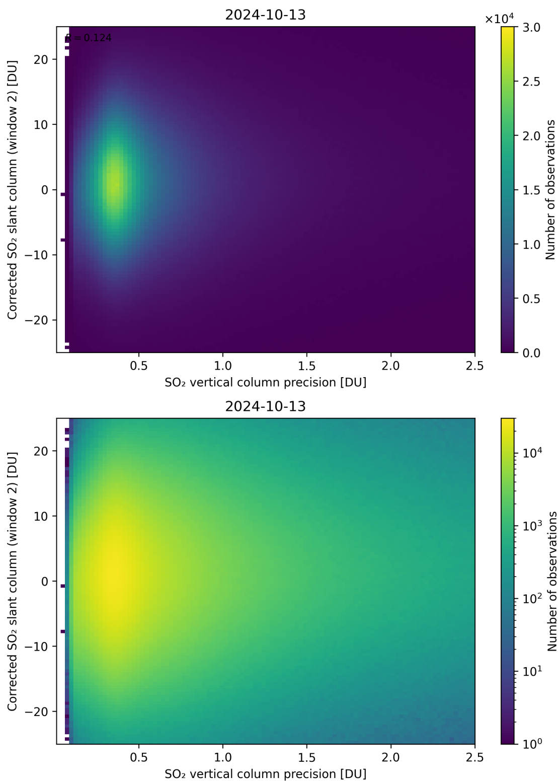
Figure 287: Scatter density plot of “SO 2 vertical column precision” against “Corrected SO 2 slant column (window 2)” for 2024-10-12 to 2024-10-14.
