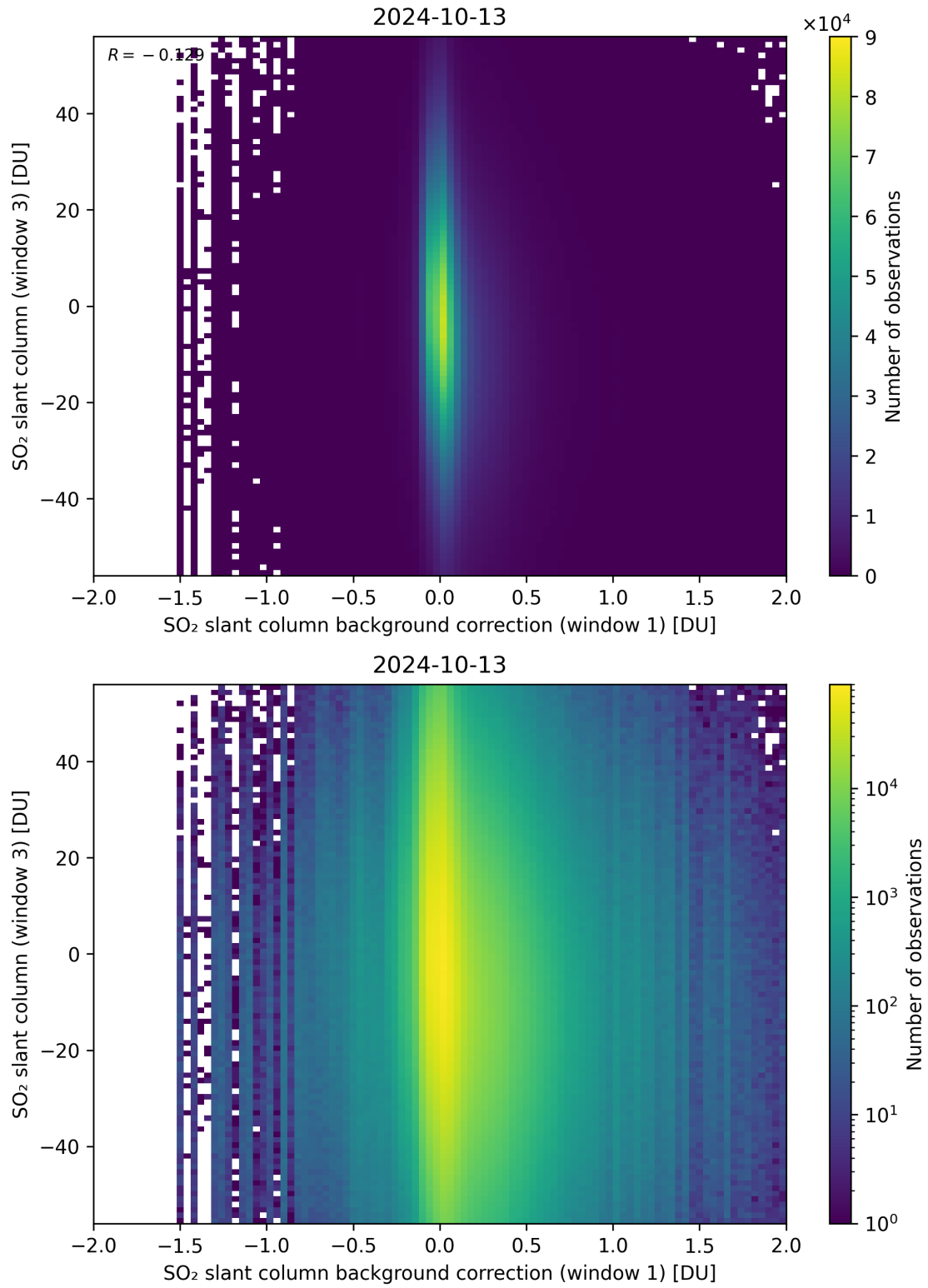
Figure 107: Scatter density plot of “SO 2 slant column background correction (window 1)” against “SO 2 slant column (window 3)” for 2024-10-12 to 2024-10-14.
