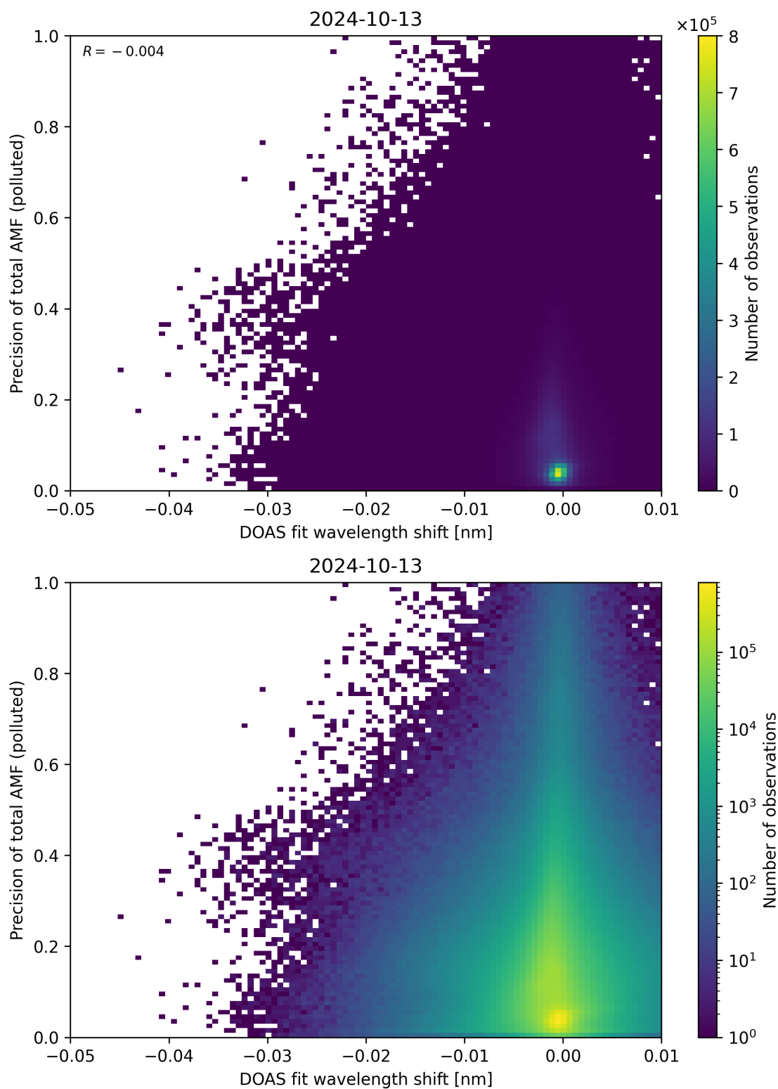
Figure 131: Scatter density plot of “DOAS fit wavelength shift” against “Precision of total AMF (polluted)” for 2024-10-12 to 2024-10-14.
