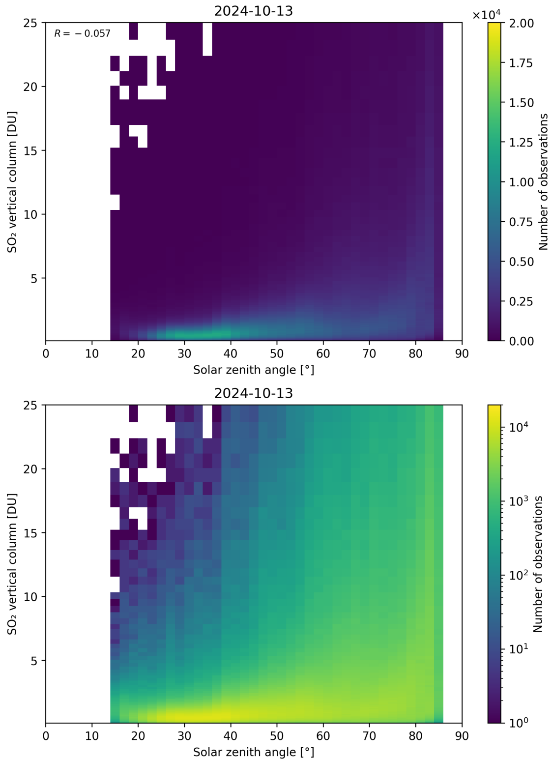
Figure 176: Scatter density plot of “Solar zenith angle” against “SO 2 vertical column” for 2024-10-12 to 2024-10-14.
