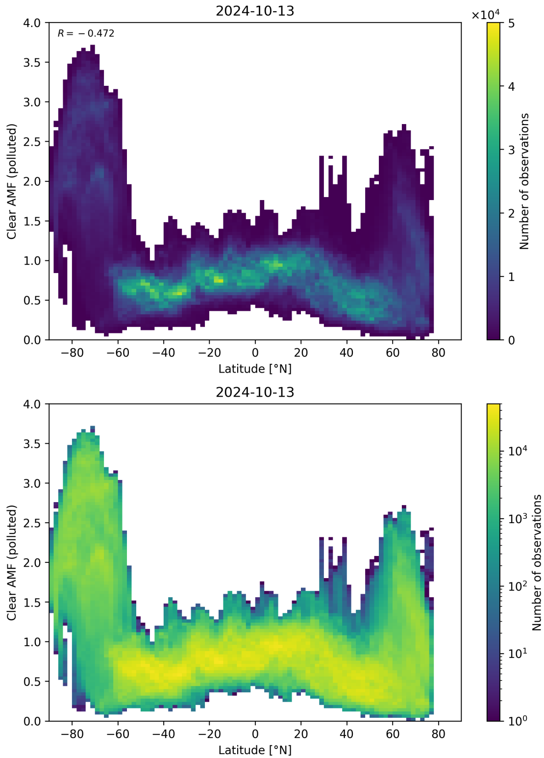
Figure 145: Scatter density plot of “Latitude” against “Clear AMF (polluted)” for 2024-10-12 to 2024-10-14.
