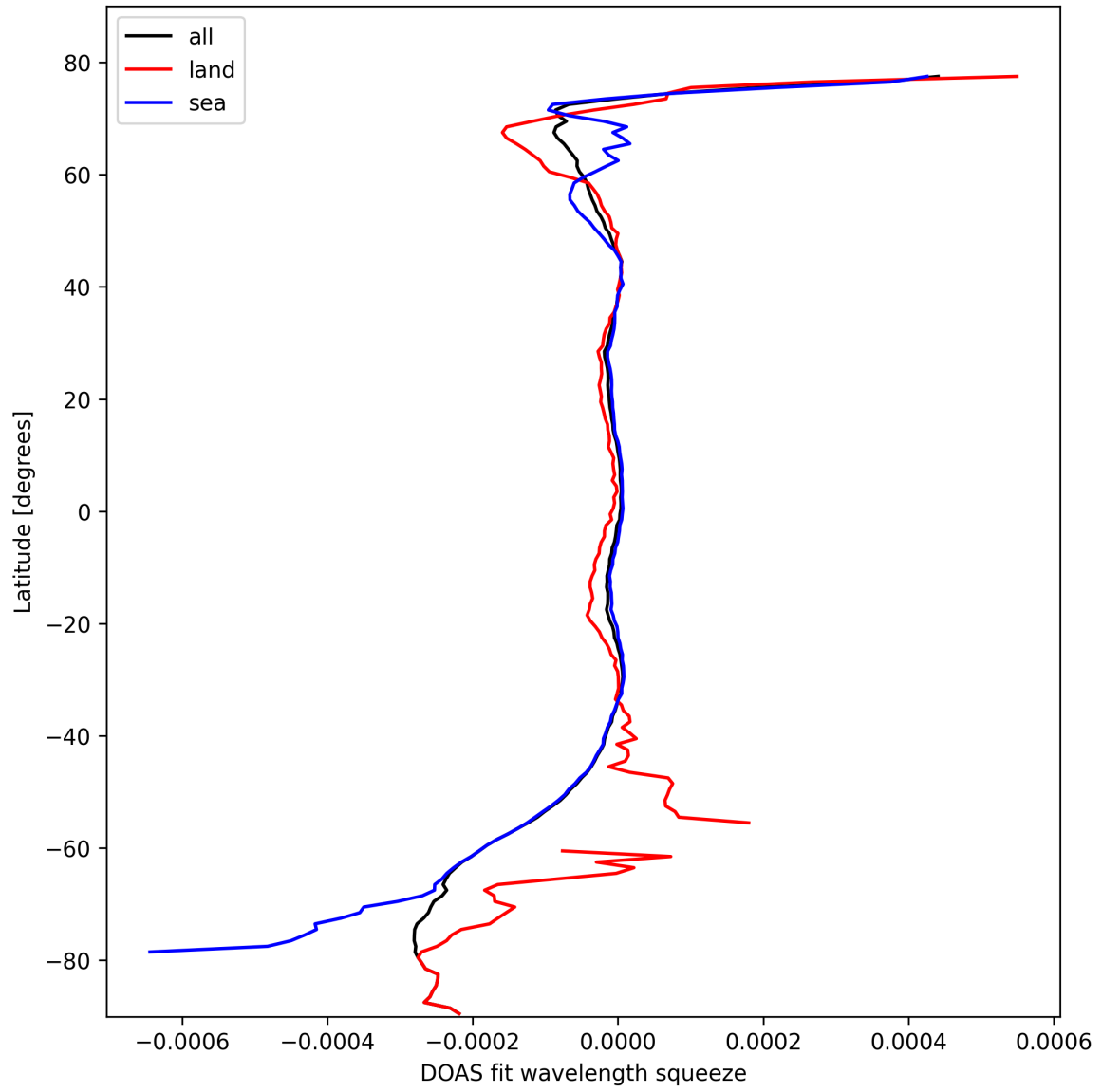
Figure 46: Zonal average of “DOAS fit wavelength squeeze” for 2024-10-12 to 2024-10-14.
