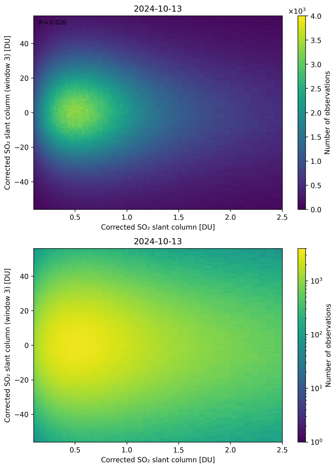
Figure 186: Scatter density plot of “Corrected SO 2 slant column” against “Corrected SO 2 slant column (window 3)” for 2024-10-12 to 2024-10-14.
