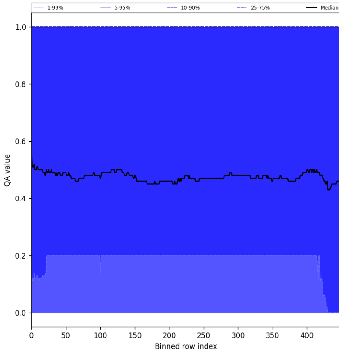
Figure 75: Along track statistics of “QA value” for 2024-10-12 to 2024-10-14
