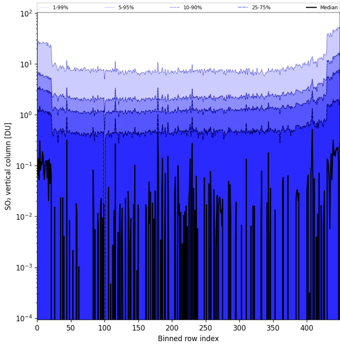
Figure 76: Along track statistics of “SO 2 vertical column” for 2024-10-12 to 2024-10-14
