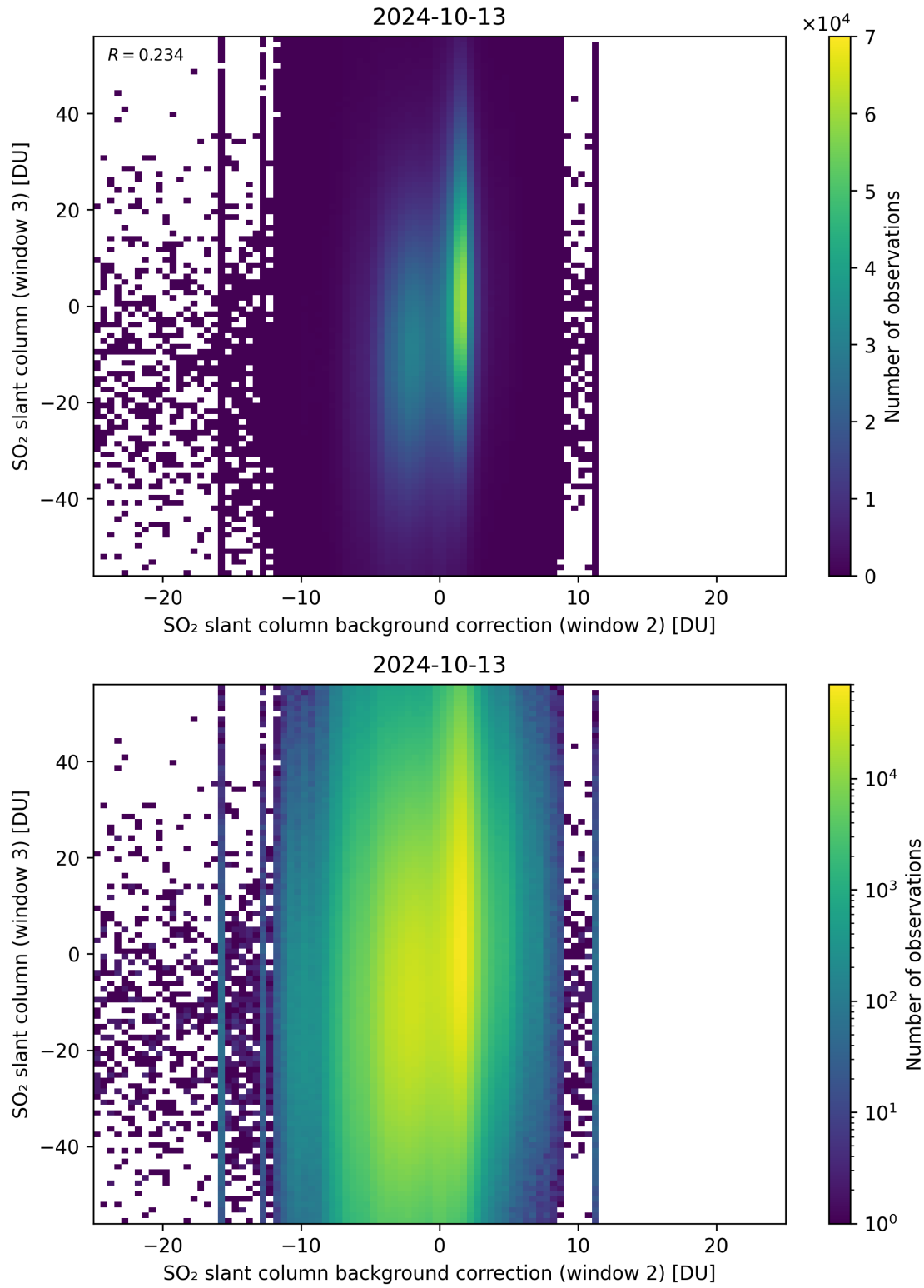
Figure 117: Scatter density plot of “SO 2 slant column background correction (window 2)” against “SO 2 slant column (window 3)” for 2024-10-12 to 2024-10-14.
