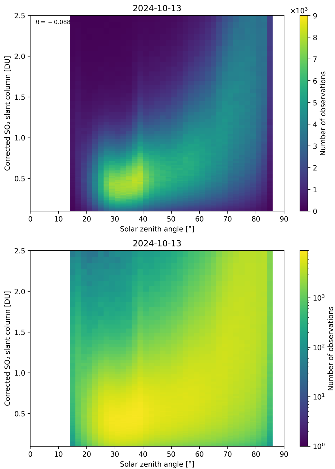
Figure 166: Scatter density plot of “Solar zenith angle” against “Corrected SO 2 slant column” for 2024-10-12 to 2024-10-14.
