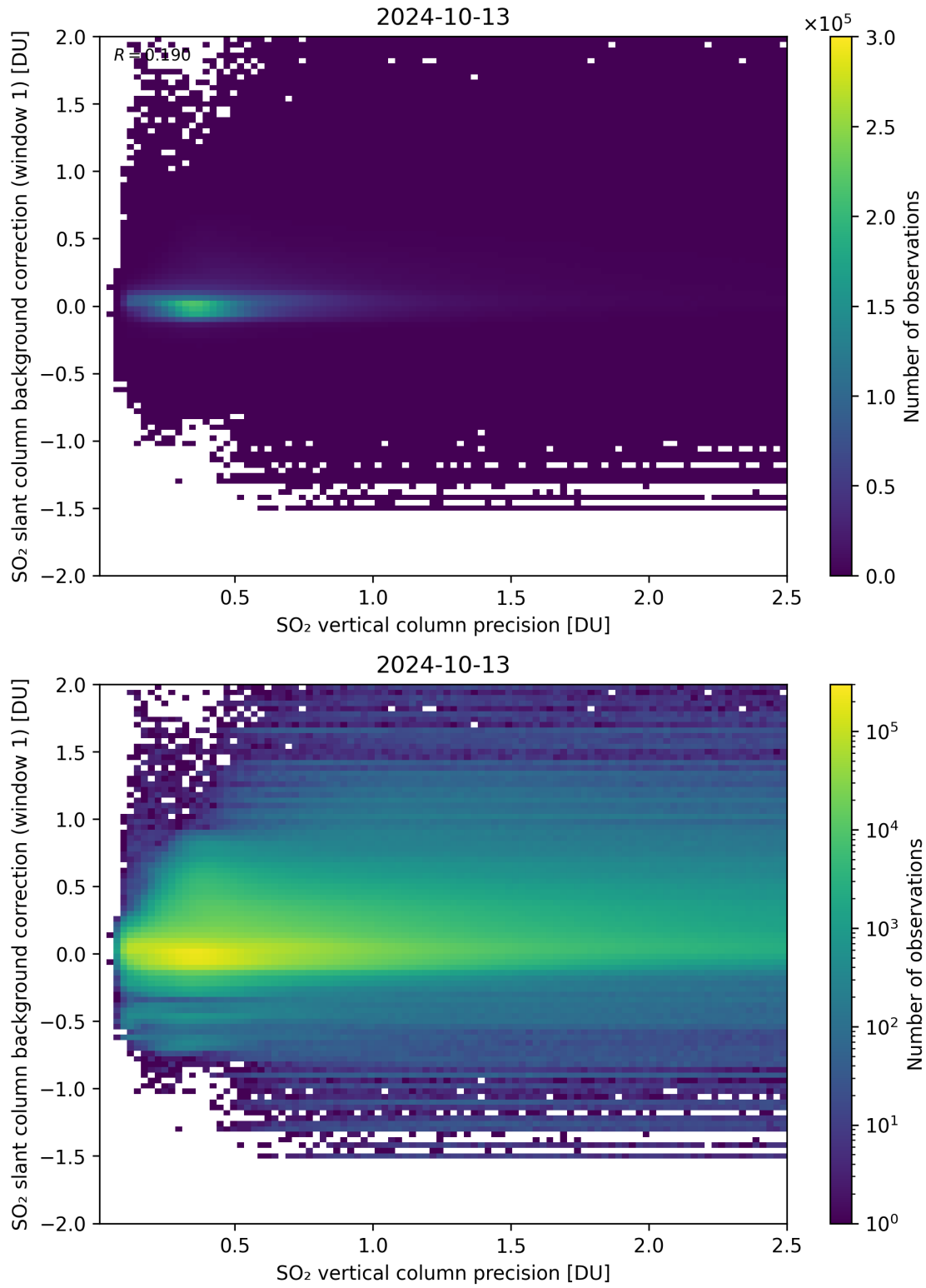
Figure 279: Scatter density plot of “SO 2 vertical column precision” against “SO 2 slant column background correction (window 1)” for 2024-10-12 to 2024-10-14.
