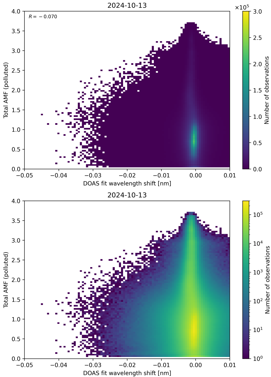
Figure 130: Scatter density plot of “DOAS fit wavelength shift” against “Total AMF (polluted)” for 2024-10-12 to 2024-10-14.
