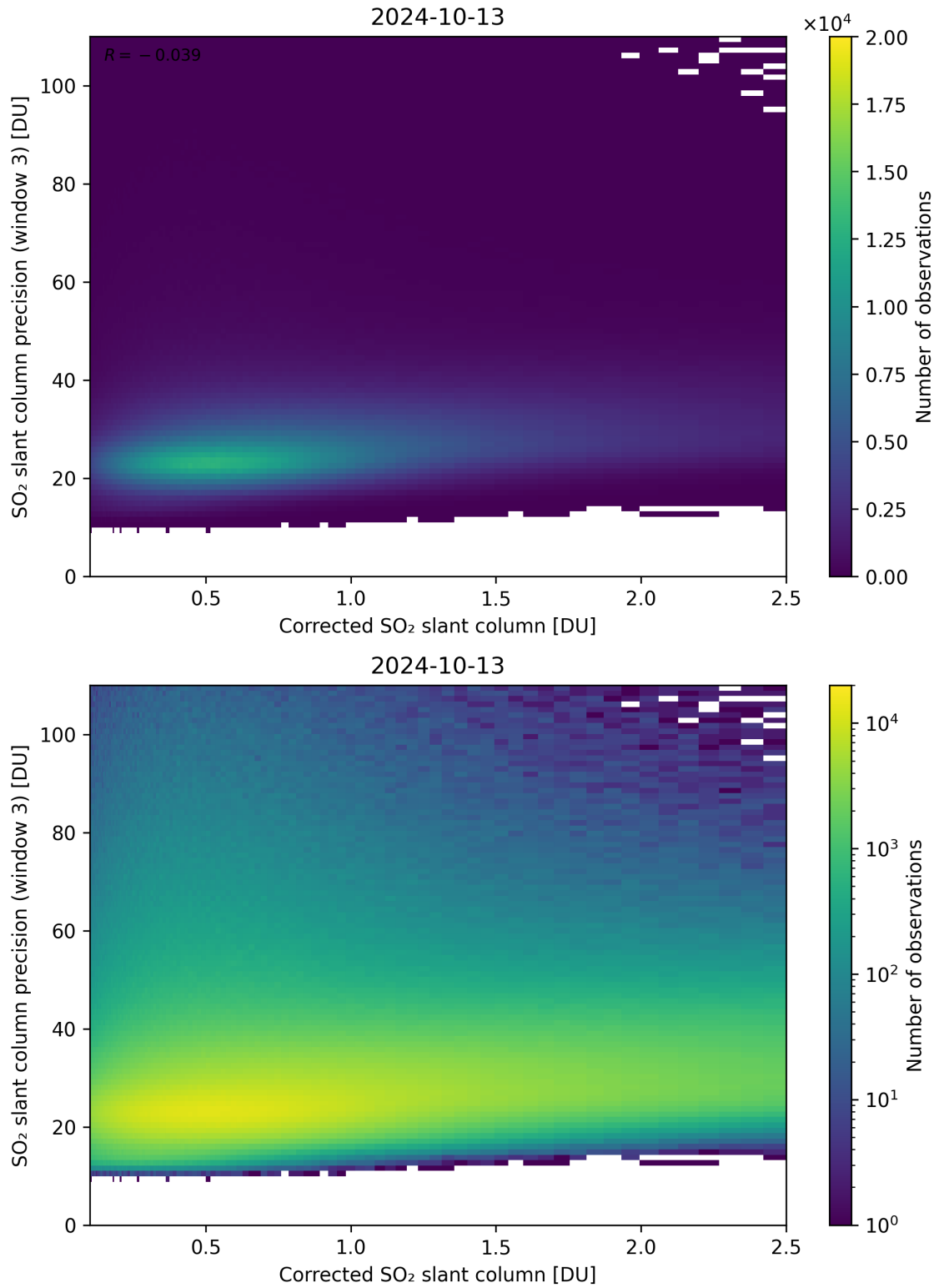
Figure 191: Scatter density plot of “Corrected SO 2 slant column” against “SO 2 slant column precision (window 3)” for 2024-10-12 to 2024-10-14.
