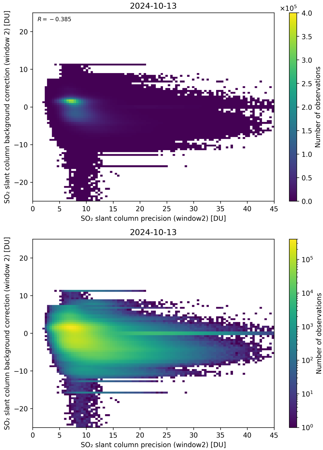
Figure 241: Scatter density plot of “SO 2 slant column precision (window2)” against “SO 2 slant column background correction (window 2)” for 2024-10-12 to 2024-10-14.
