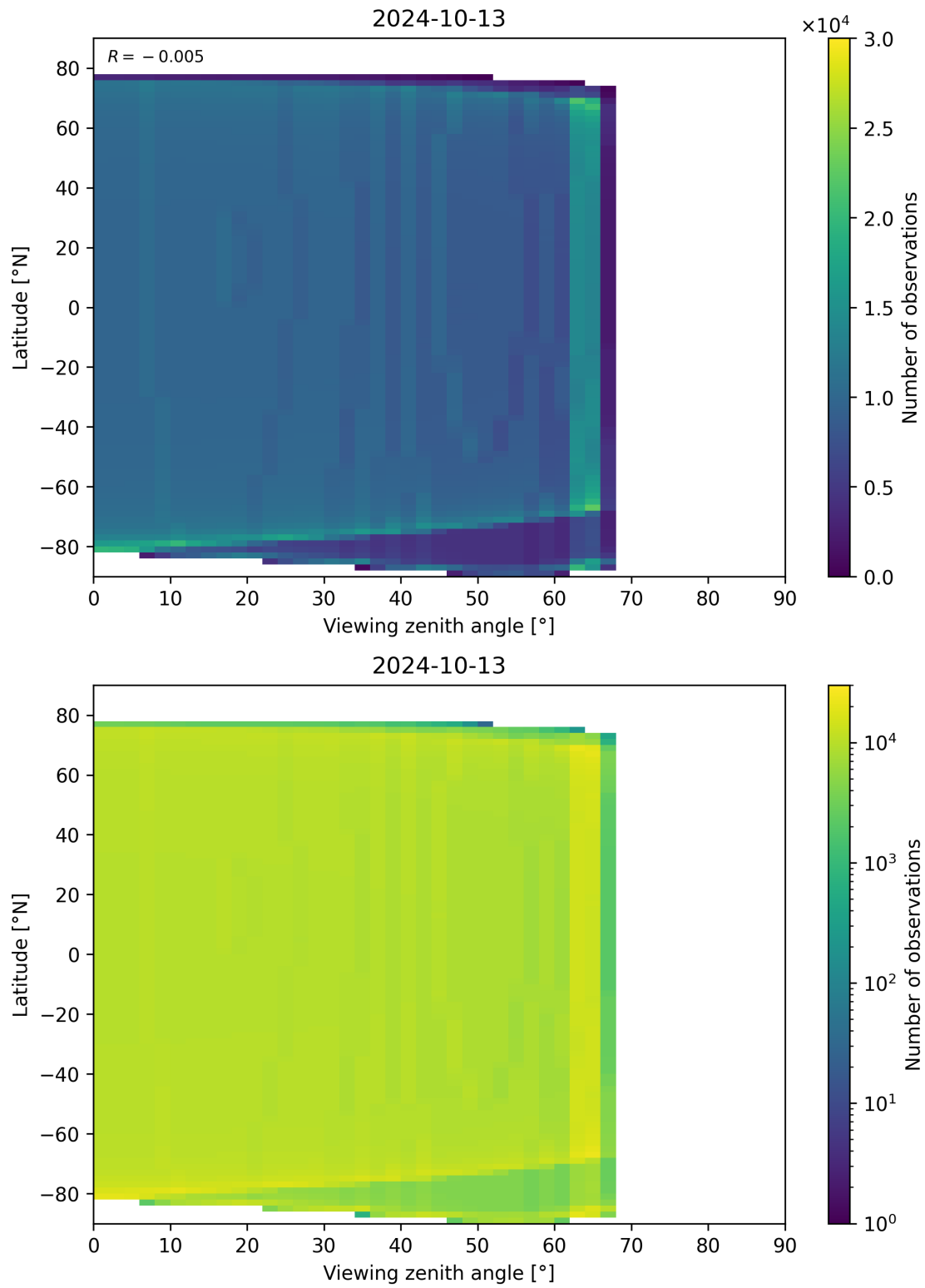
Figure 314: Scatter density plot of “Viewing zenith angle” against “Latitude” for 2024-10-12 to 2024-10-14.
