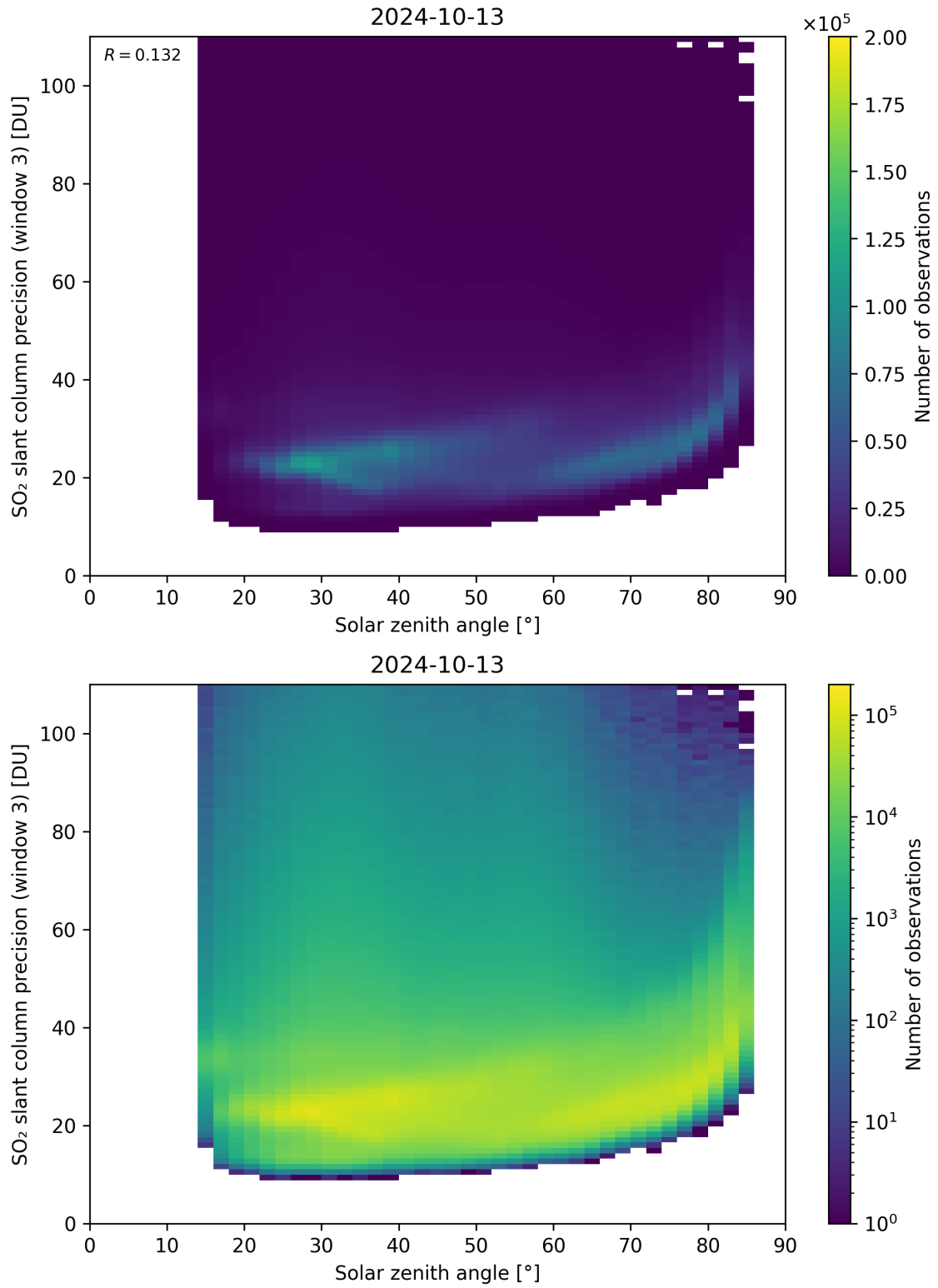
Figure 173: Scatter density plot of “Solar zenith angle” against “SO 2 slant column precision (window 3)” for 2024-10-12 to 2024-10-14.
