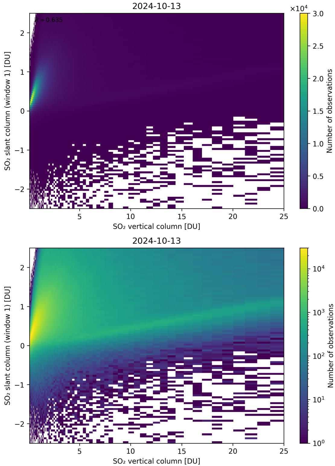
Figure 300: Scatter density plot of “SO 2 vertical column” against “SO 2 slant column (window 1)” for 2024-10-12 to 2024-10-14.
