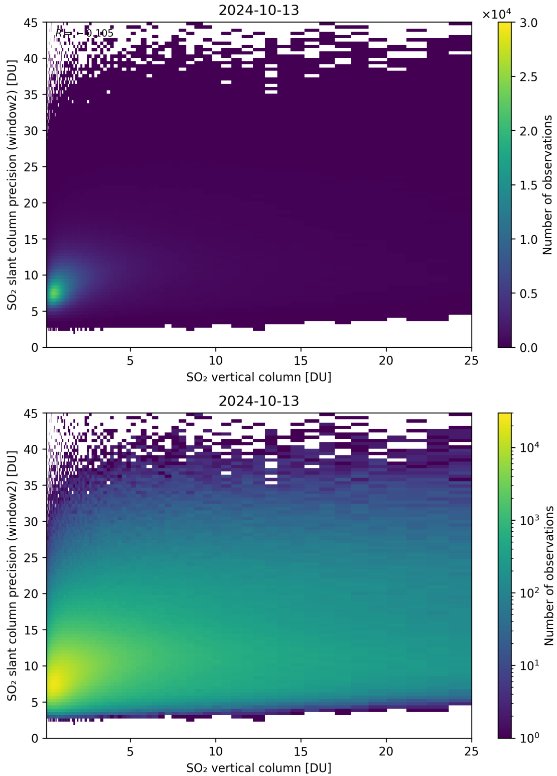
Figure 302: Scatter density plot of “SO 2 vertical column” against “SO 2 slant column precision (window2)” for 2024-10-12 to 2024-10-14.
