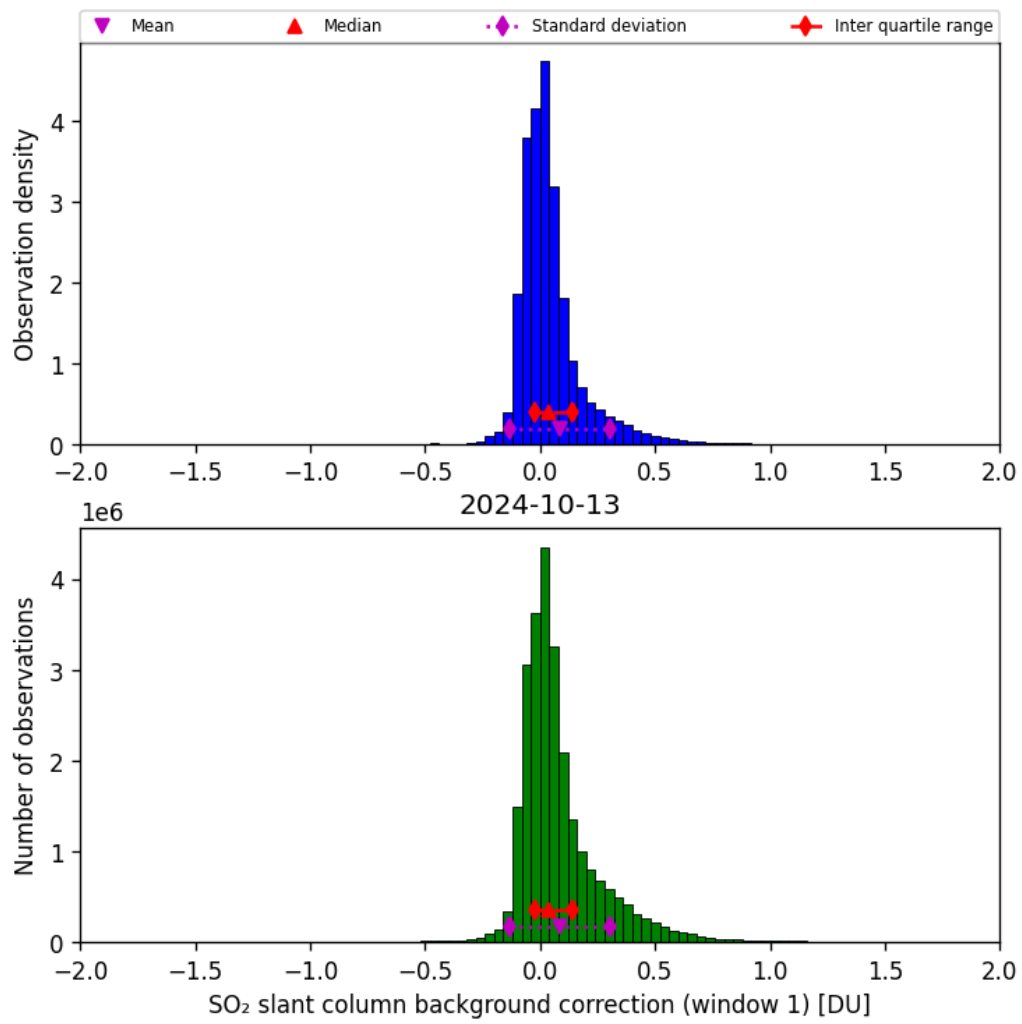
Figure 59: Histogram of “SO 2 slant column background correction (window 1)” for 2024-10-12 to 2024-10-14
