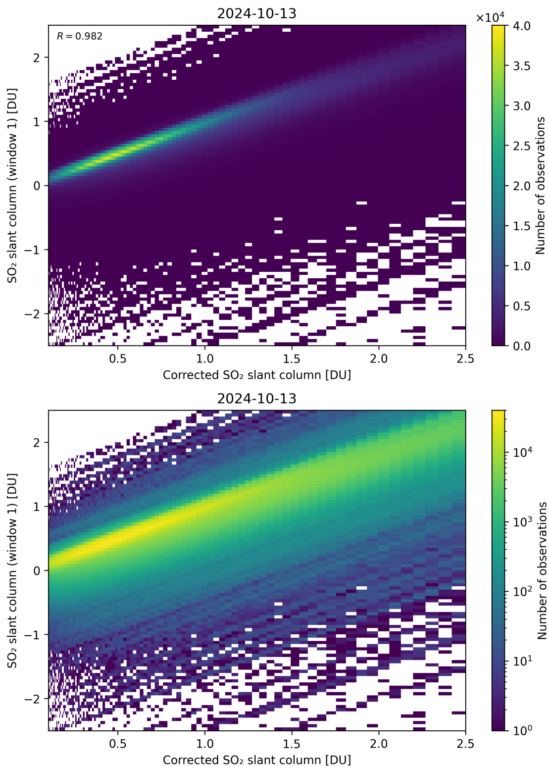
Figure 187: Scatter density plot of “Corrected SO 2 slant column” against “SO 2 slant column (window 1)” for 2024-10-12 to 2024-10-14.
