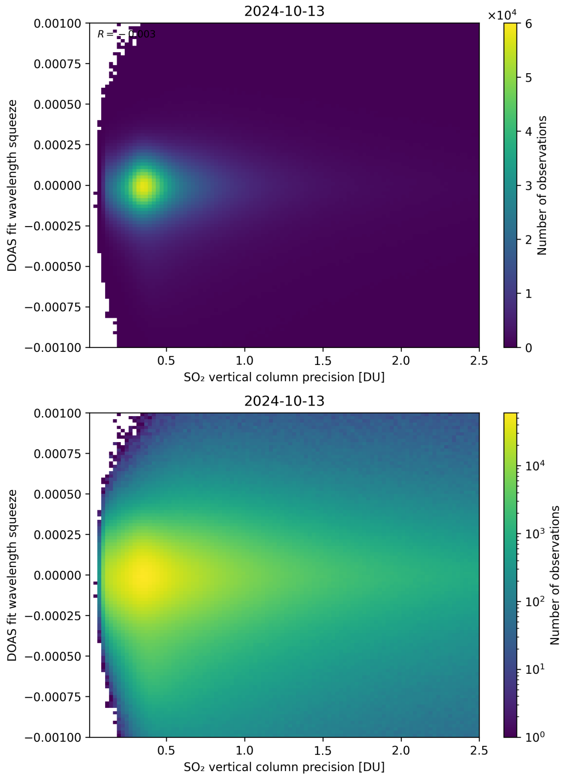
Figure 283: Scatter density plot of “SO 2 vertical column precision” against “DOAS fit wavelength squeeze” for 2024-10-12 to 2024-10-14.
