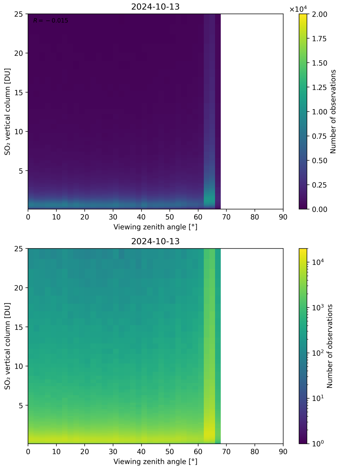
Figure 327: Scatter density plot of “Viewing zenith angle” against “SO 2 vertical column” for 2024-10-12 to 2024-10-14.
