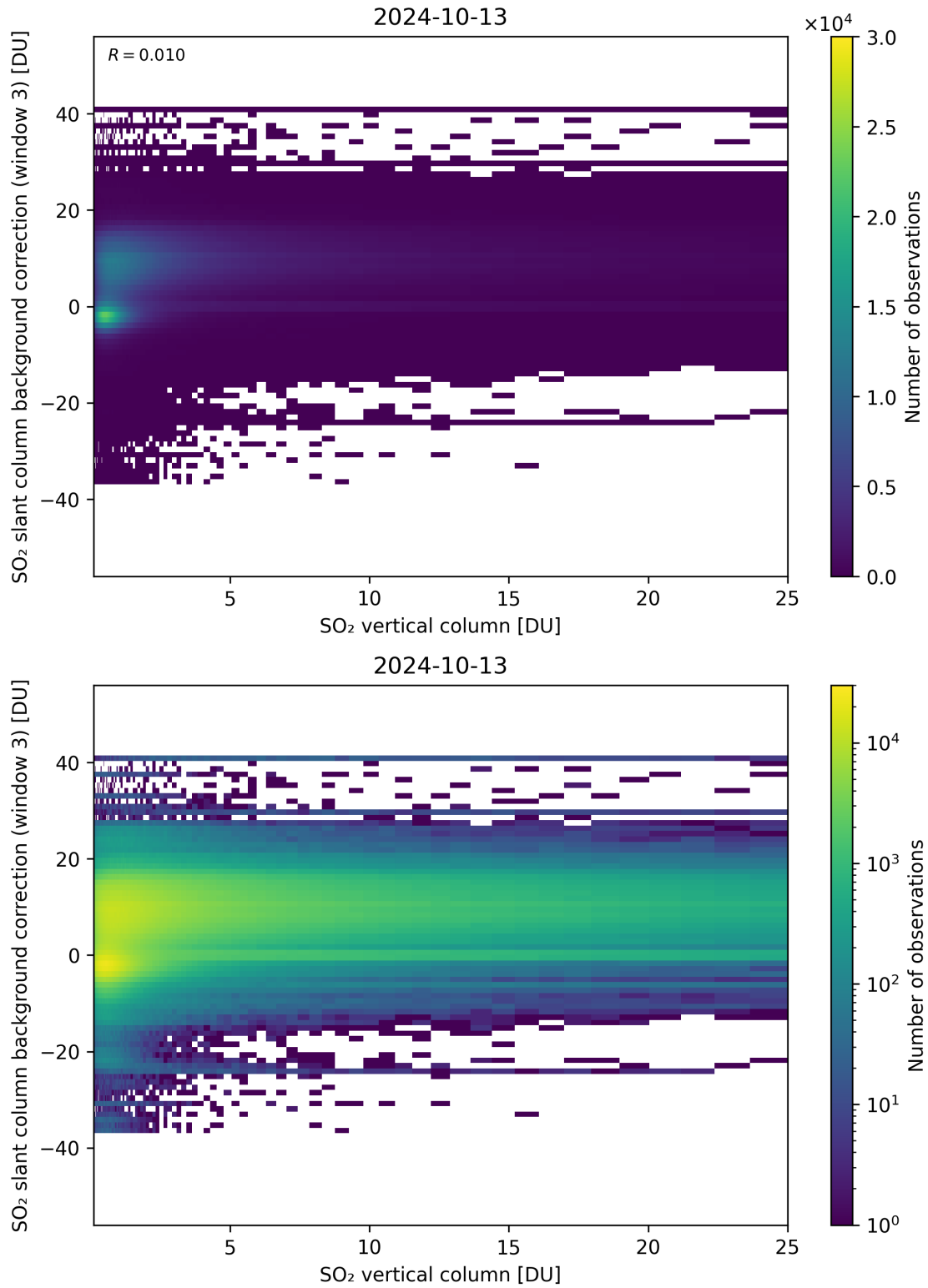
Figure 275: Scatter density plot of “SO 2 vertical column” against “SO 2 slant column background correction (window 3)” for 2024-10-12 to 2024-10-14.
