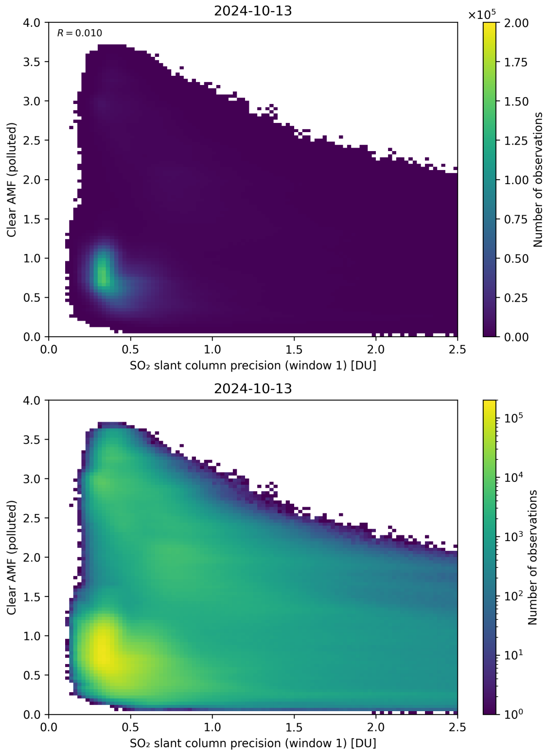
Figure 224: Scatter density plot of “SO 2 slant column precision (window 1)” against “Clear AMF (polluted)” for 2024-10-12 to 2024-10-14.
