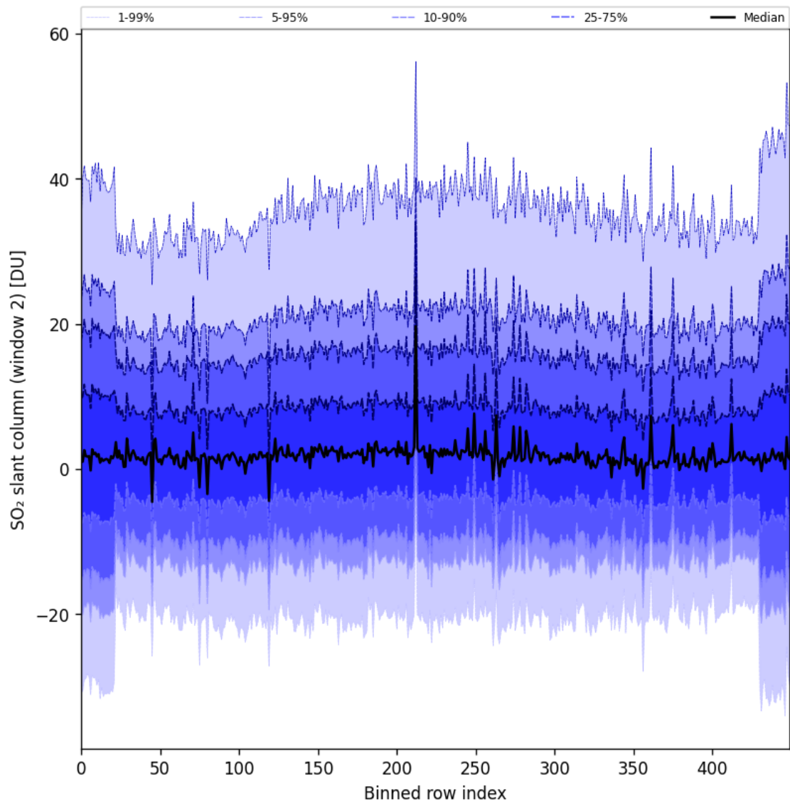
Figure 83: Along track statistics of “SO 2 slant column (window 2)” for 2024-10-12 to 2024-10-14
