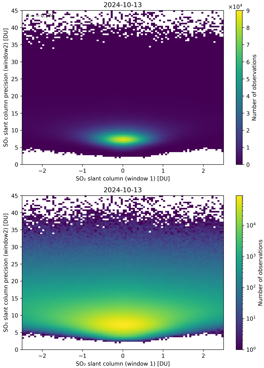
Figure 236: Scatter density plot of “SO 2 slant column (window 1)” against “SO 2 slant column precision (window2)” for 2024-10-12 to 2024-10-14.
