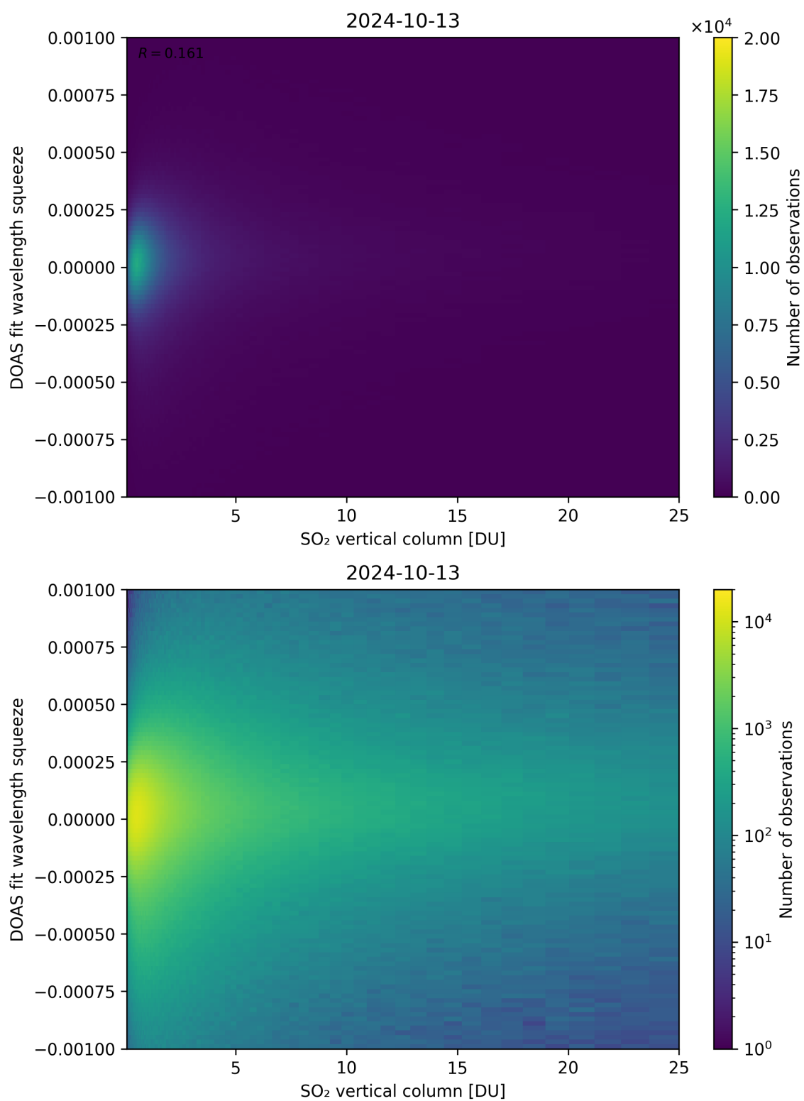
Figure 277: Scatter density plot of “SO 2 vertical column” against “DOAS fit wavelength squeeze” for 2024-10-12 to 2024-10-14.
