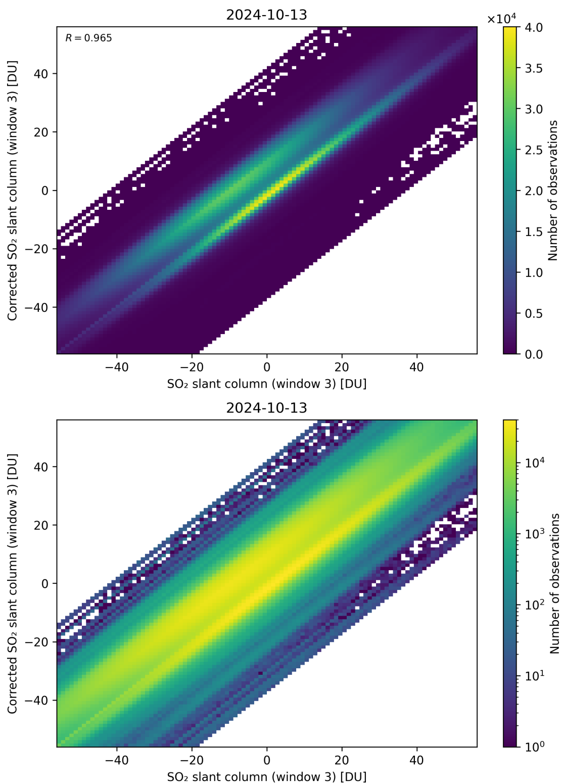
Figure 266: Scatter density plot of “SO 2 slant column (window 3)” against “Corrected SO 2 slant column (window 3)” for 2024-10-12 to 2024-10-14.
