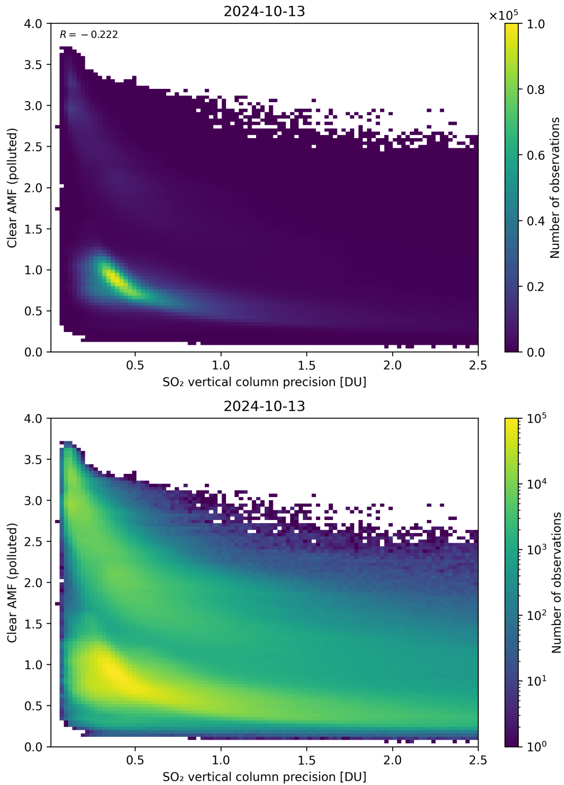
Figure 285: Scatter density plot of “SO 2 vertical column precision” against “Clear AMF (polluted)” for 2024-10-12 to 2024-10-14.
