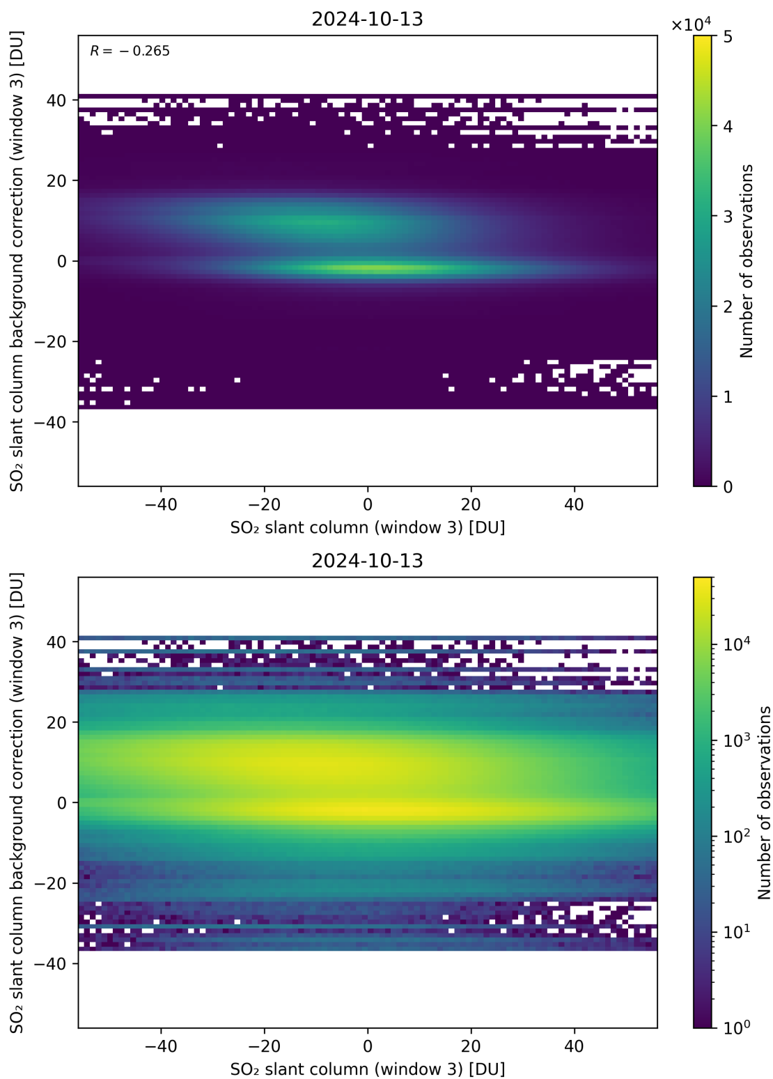
Figure 253: Scatter density plot of “SO 2 slant column (window 3)” against “SO 2 slant column background correction (window 3)” for 2024-10-12 to 2024-10-14.
