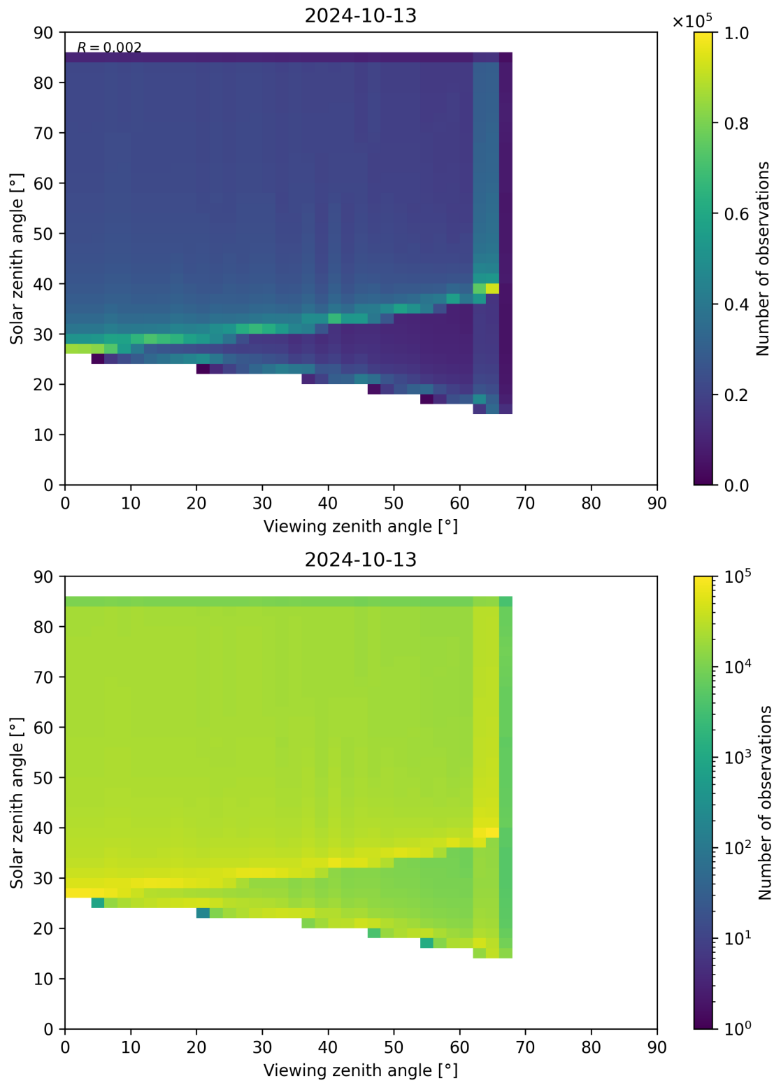
Figure 315: Scatter density plot of “Viewing zenith angle” against “Solar zenith angle” for 2024-10-12 to 2024-10-14.
