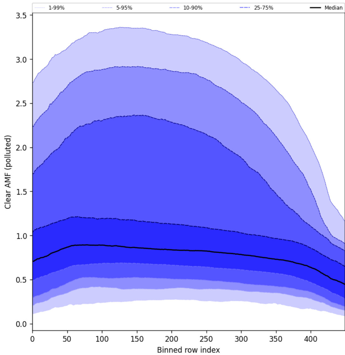
Figure 96: Along track statistics of “Clear AMF (polluted)” for 2024-10-12 to 2024-10-14
