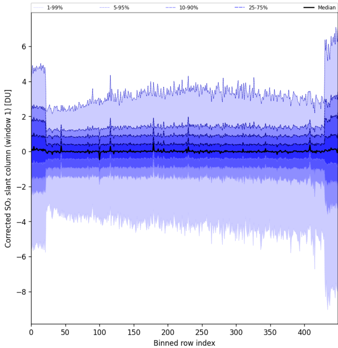
Figure 81: Along track statistics of “Corrected SO 2 slant column (window 1)” for 2024-10-12 to 2024-10-14
