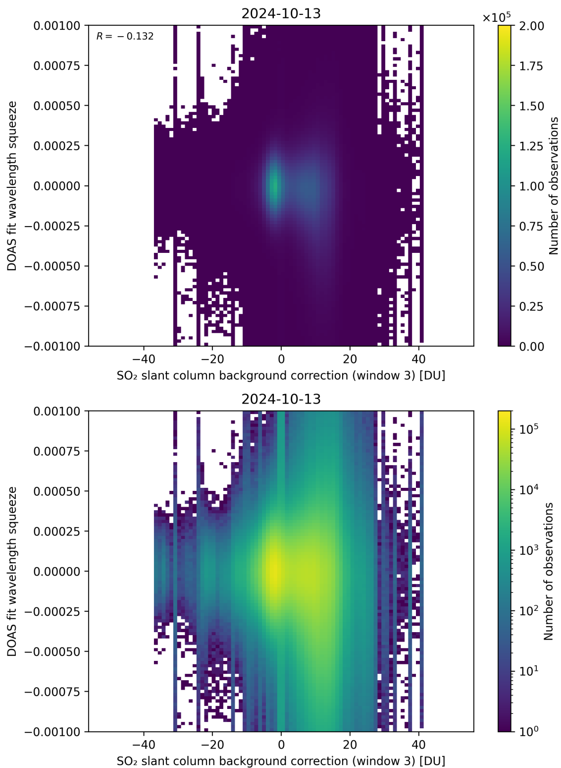
Figure 122: Scatter density plot of “SO 2 slant column background correction (window 3)” against “DOAS fit wavelength squeeze” for 2024-10-12 to 2024-10-14.
