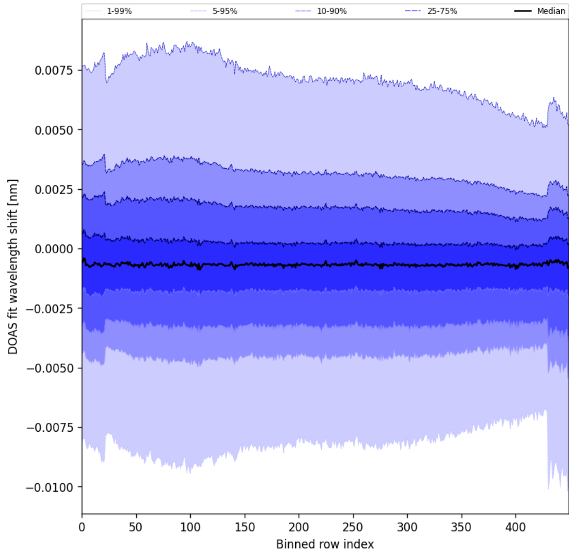
Figure 91: Along track statistics of “DOAS fit wavelength shift” for 2024-10-12 to 2024-10-14
