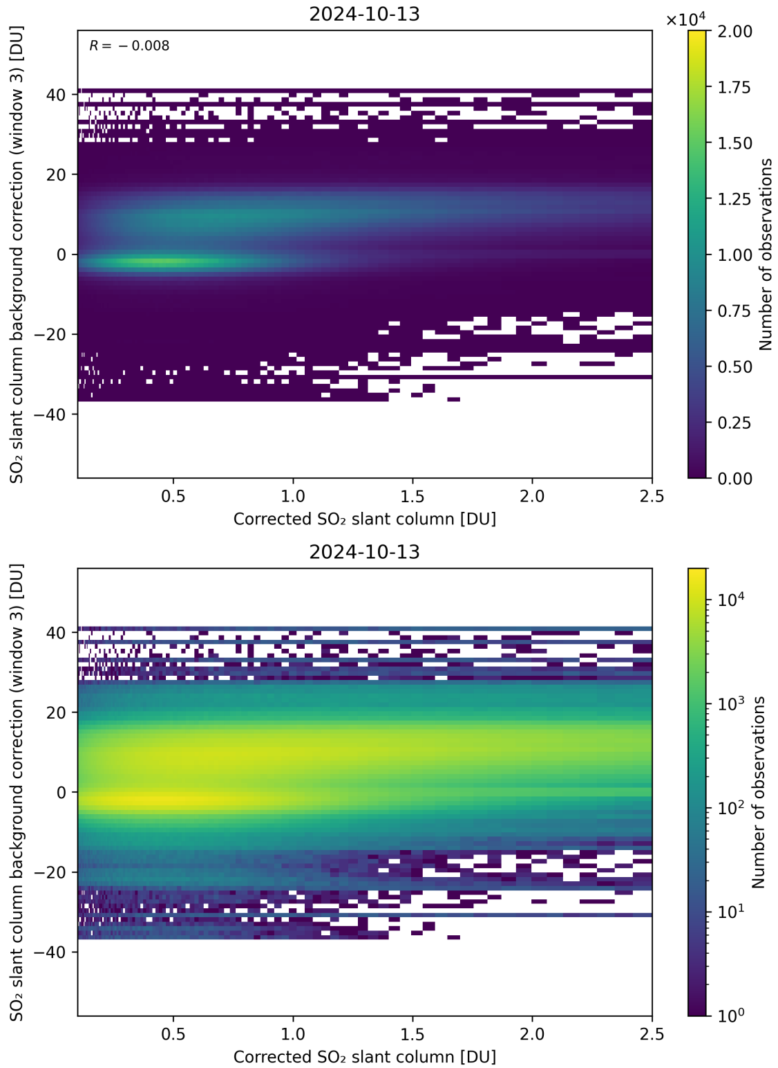
Figure 180: Scatter density plot of “Corrected SO 2 slant column” against “SO 2 slant column background correction (window 3)” for 2024-10-12 to 2024-10-14.
