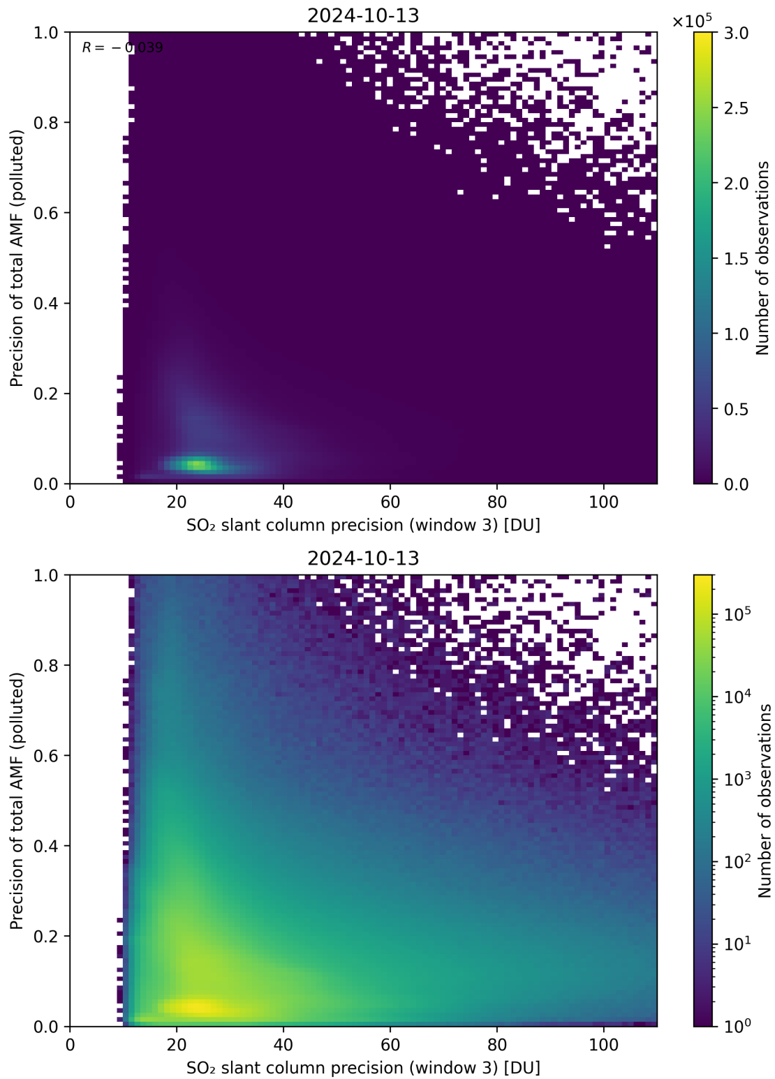
Figure 264: Scatter density plot of “SO 2 slant column precision (window 3)” against “Precision of total AMF (polluted)” for 2024-10-12 to 2024-10-14.
