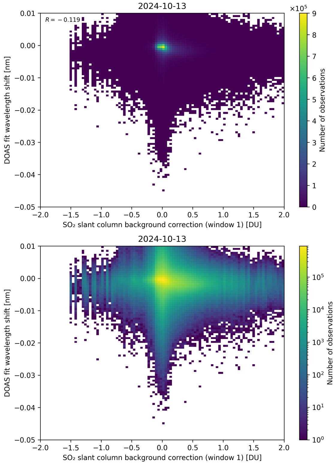
Figure 100: Scatter density plot of “SO 2 slant column background correction (window 1)” against “DOAS fit wavelength shift” for 2024-10-12 to 2024-10-14.
