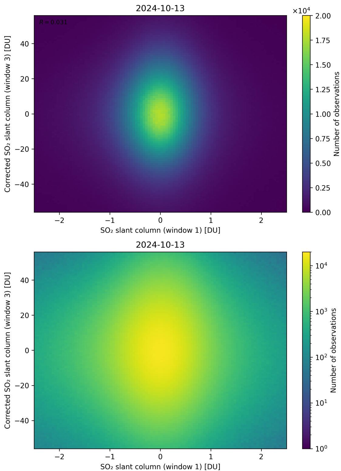
Figure 234: Scatter density plot of “SO 2 slant column (window 1)” against “Corrected SO 2 slant column (window 3)” for 2024-10-12 to 2024-10-14.
