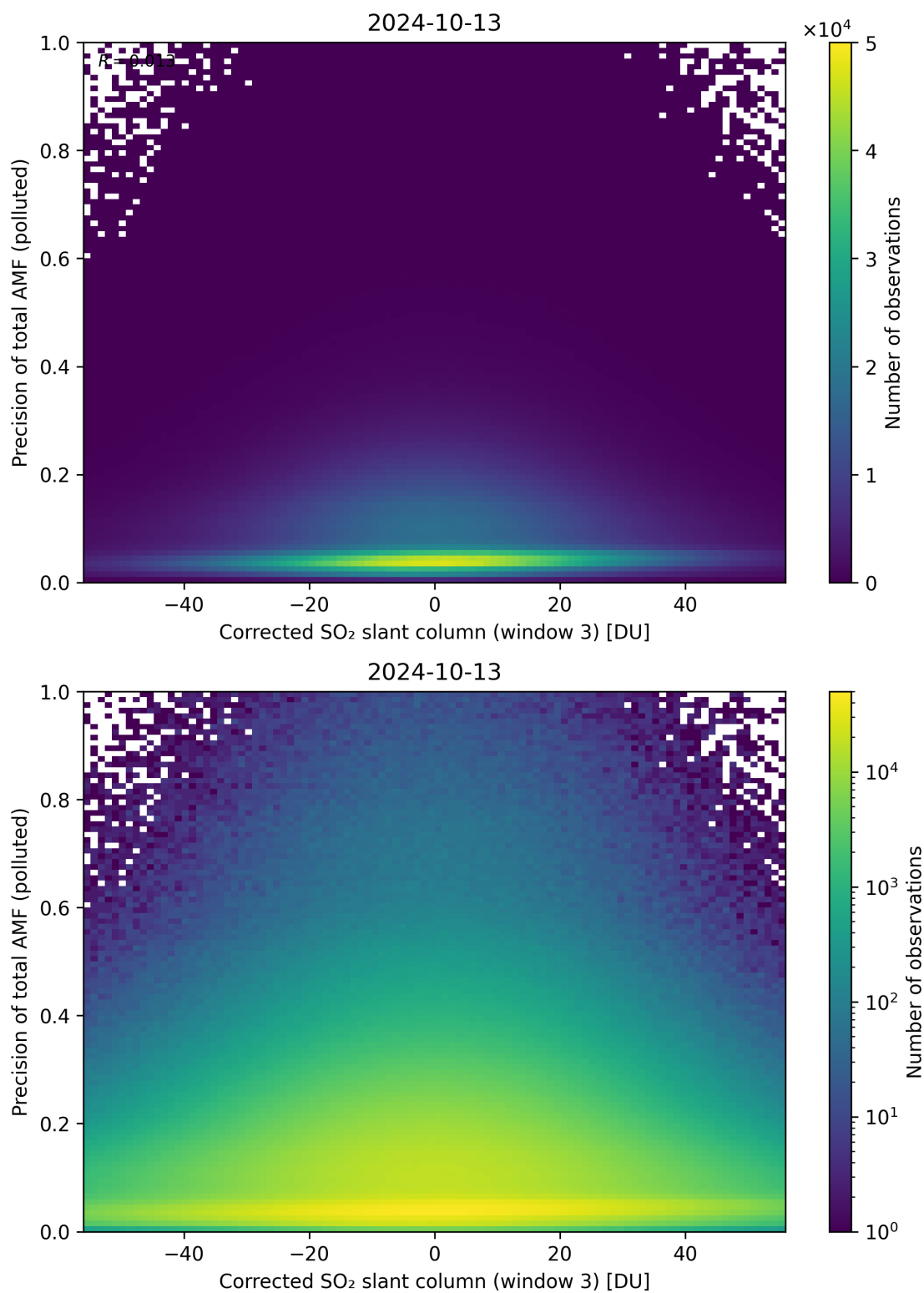
Figure 211: Scatter density plot of “Corrected SO 2 slant column (window 3)” against “Precision of total AMF (polluted)” for 2024-10-12 to 2024-10-14.
