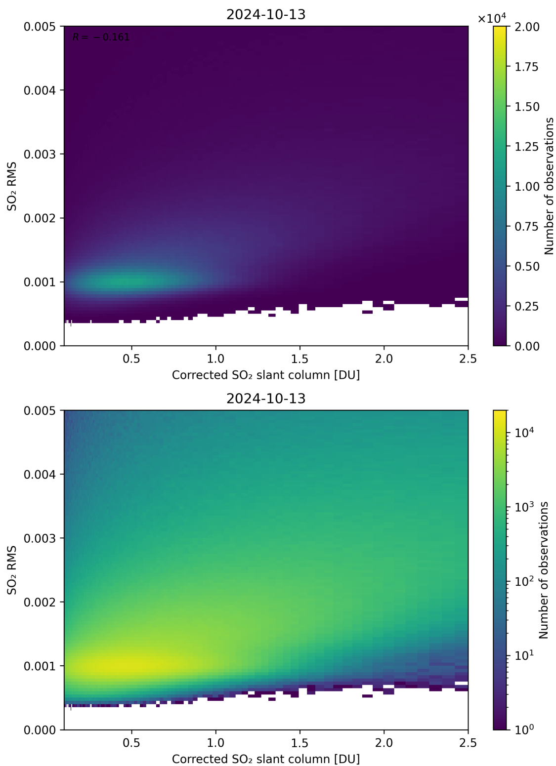
Figure 183: Scatter density plot of “Corrected SO 2 slant column” against “SO 2 RMS” for 2024-10-12 to 2024-10-14.
