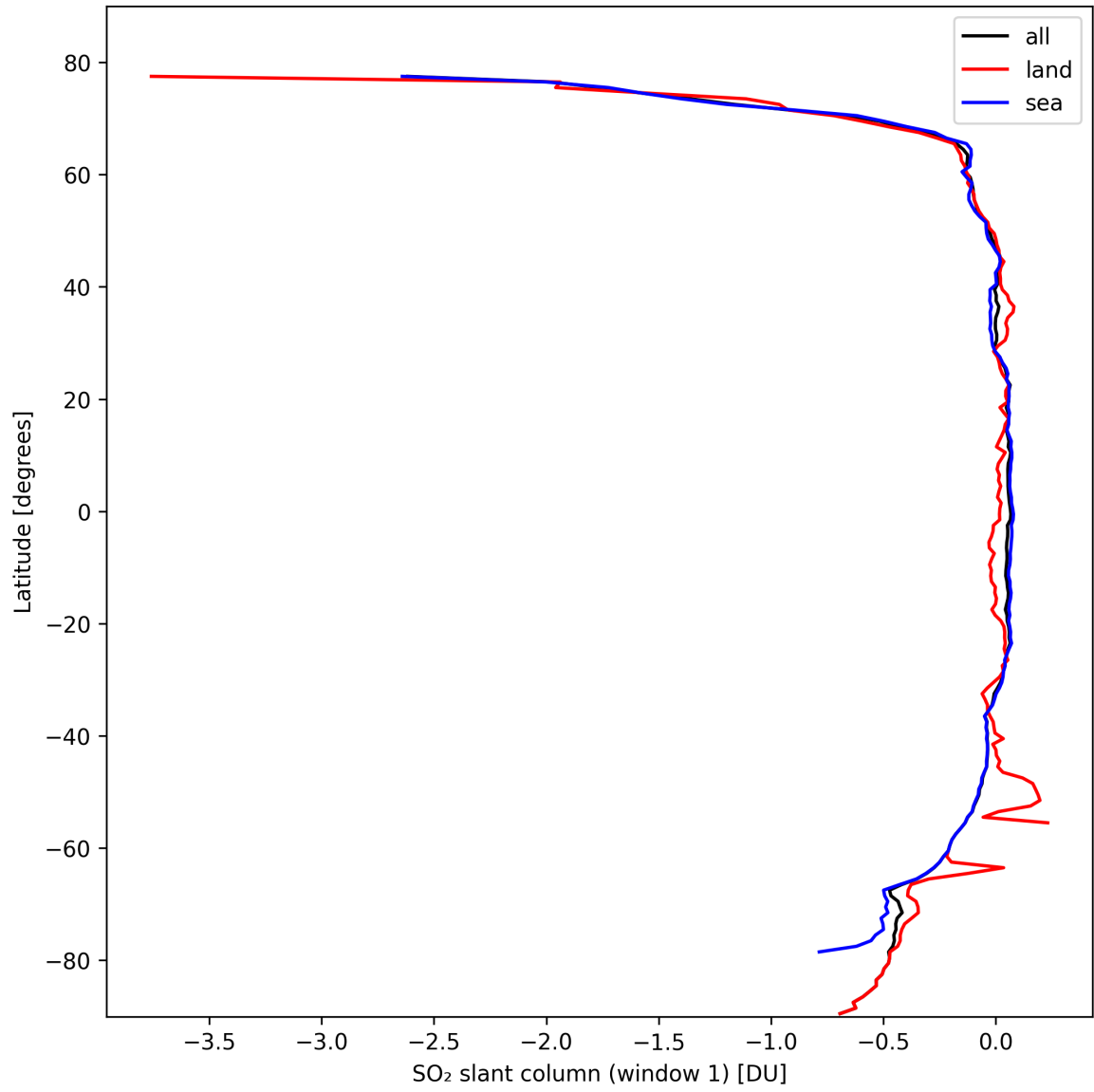
Figure 33: Zonal average of “SO 2 slant column (window 1)” for 2024-10-12 to 2024-10-14.
