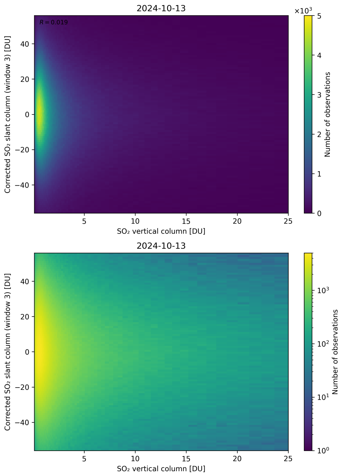
Figure 299: Scatter density plot of “SO 2 vertical column” against “Corrected SO 2 slant column (window 3)” for 2024-10-12 to 2024-10-14.
