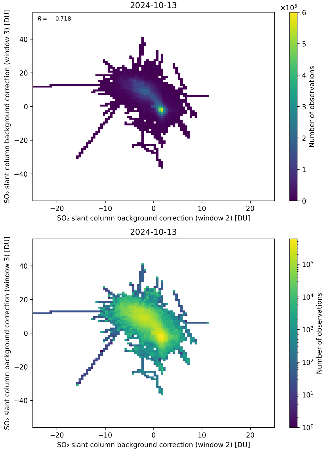
Figure 111: Scatter density plot of “SO 2 slant column background correction (window 2)” against “SO 2 slant column background correction (window 3)” for 2024-10-12 to 2024-10-14.
