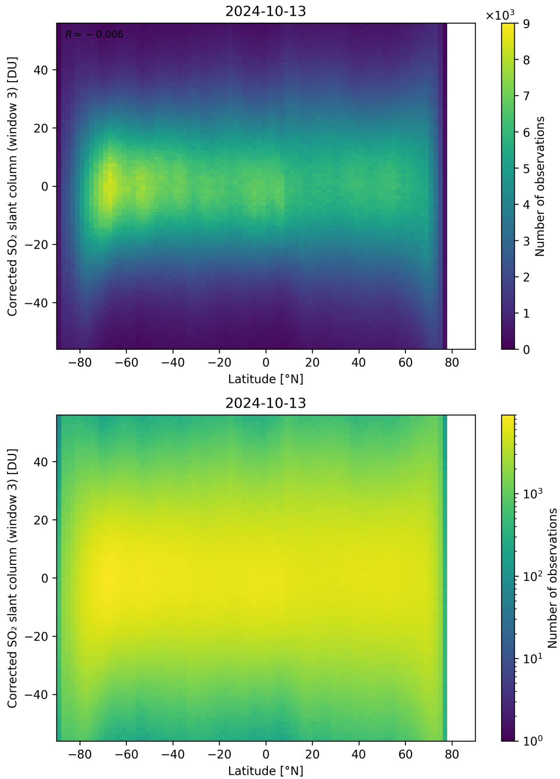
Figure 148: Scatter density plot of “Latitude” against “Corrected SO 2 slant column (window 3)” for 2024-10-12 to 2024-10-14.
