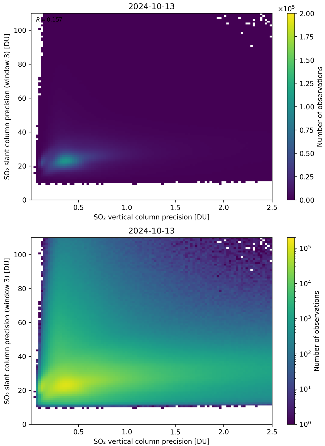
Figure 293: Scatter density plot of “SO 2 vertical column precision” against “SO 2 slant column precision (window 3)” for 2024-10-12 to 2024-10-14.
