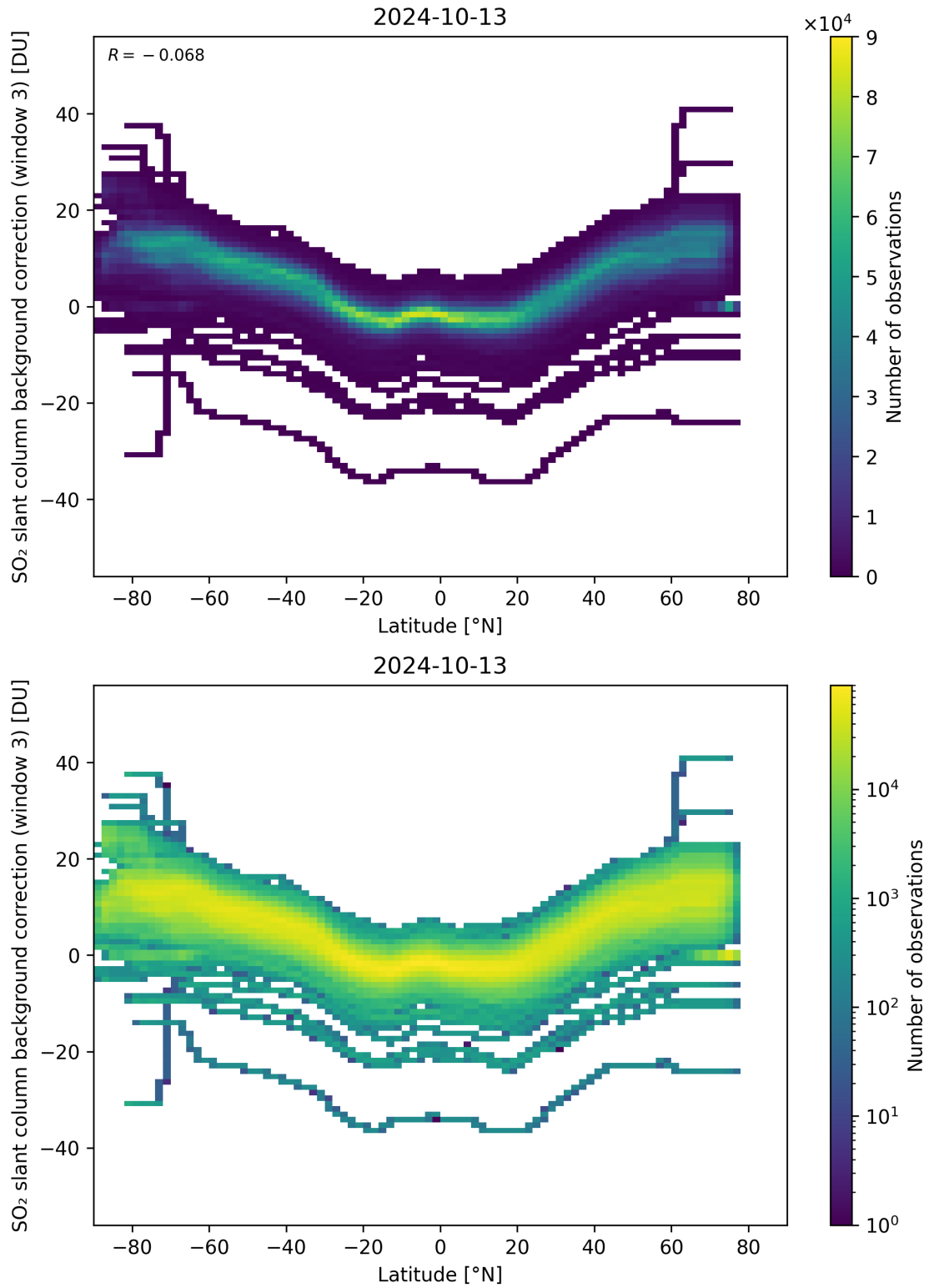
Figure 141: Scatter density plot of “Latitude” against “SO 2 slant column background correction (window 3)” for 2024-10-12 to 2024-10-14.
