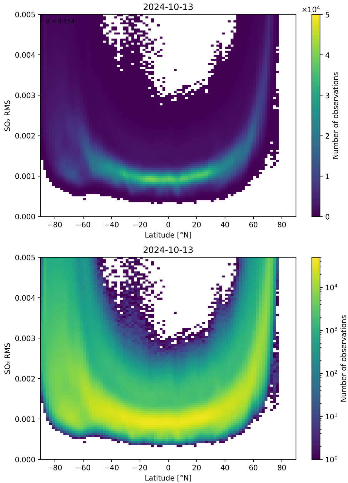
Figure 144: Scatter density plot of “Latitude” against “SO 2 RMS” for 2024-10-12 to 2024-10-14.
