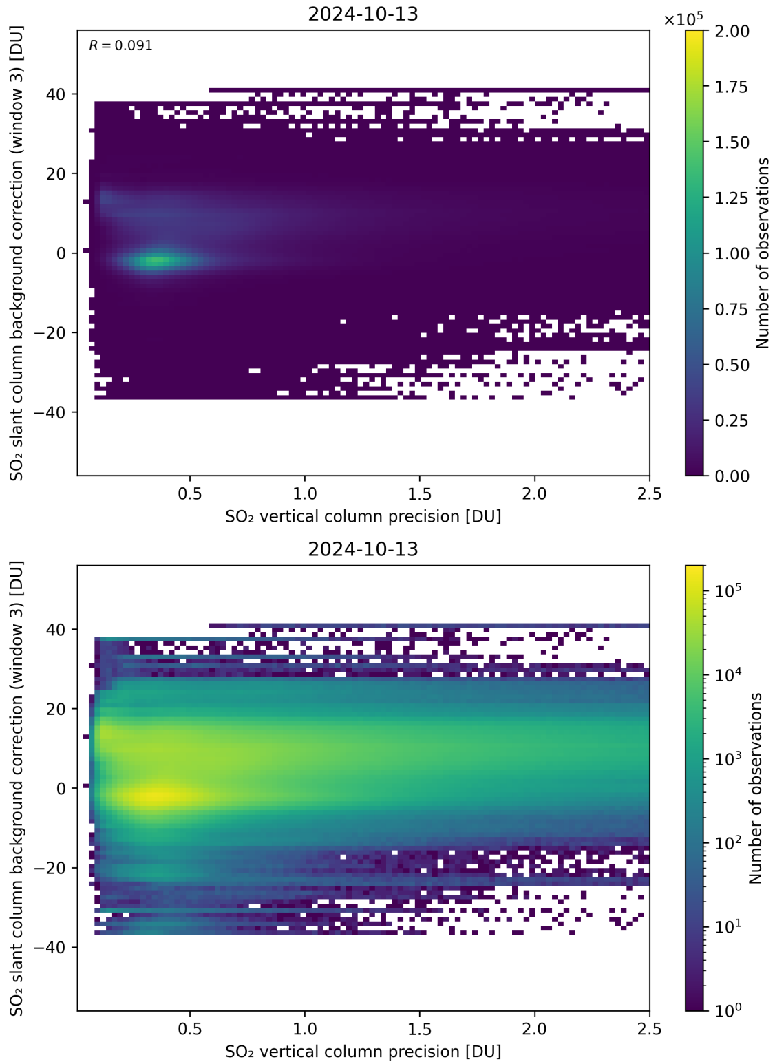
Figure 281: Scatter density plot of “SO 2 vertical column precision” against “SO 2 slant column background correction (window 3)” for 2024-10-12 to 2024-10-14.
