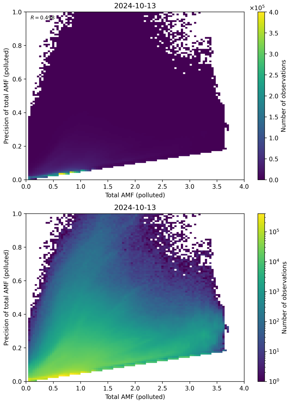
Figure 272: Scatter density plot of “Total AMF (polluted)” against “Precision of total AMF (polluted)” for 2024-10-12 to 2024-10-14.
