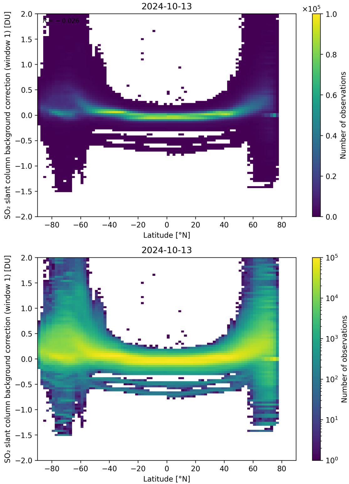
Figure 139: Scatter density plot of “Latitude” against “SO 2 slant column background correction (window 1)” for 2024-10-12 to 2024-10-14.
