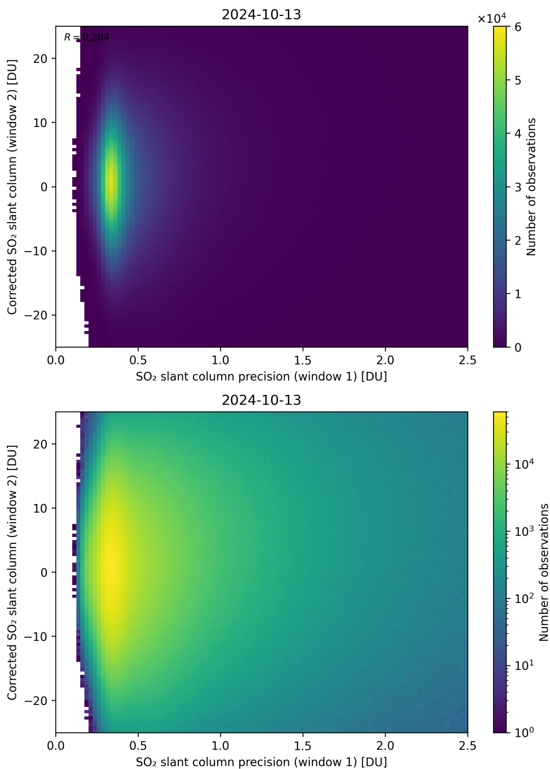
Figure 225: Scatter density plot of “SO 2 slant column precision (window 1)” against “Corrected SO 2 slant column (window 2)” for 2024-10-12 to 2024-10-14.
