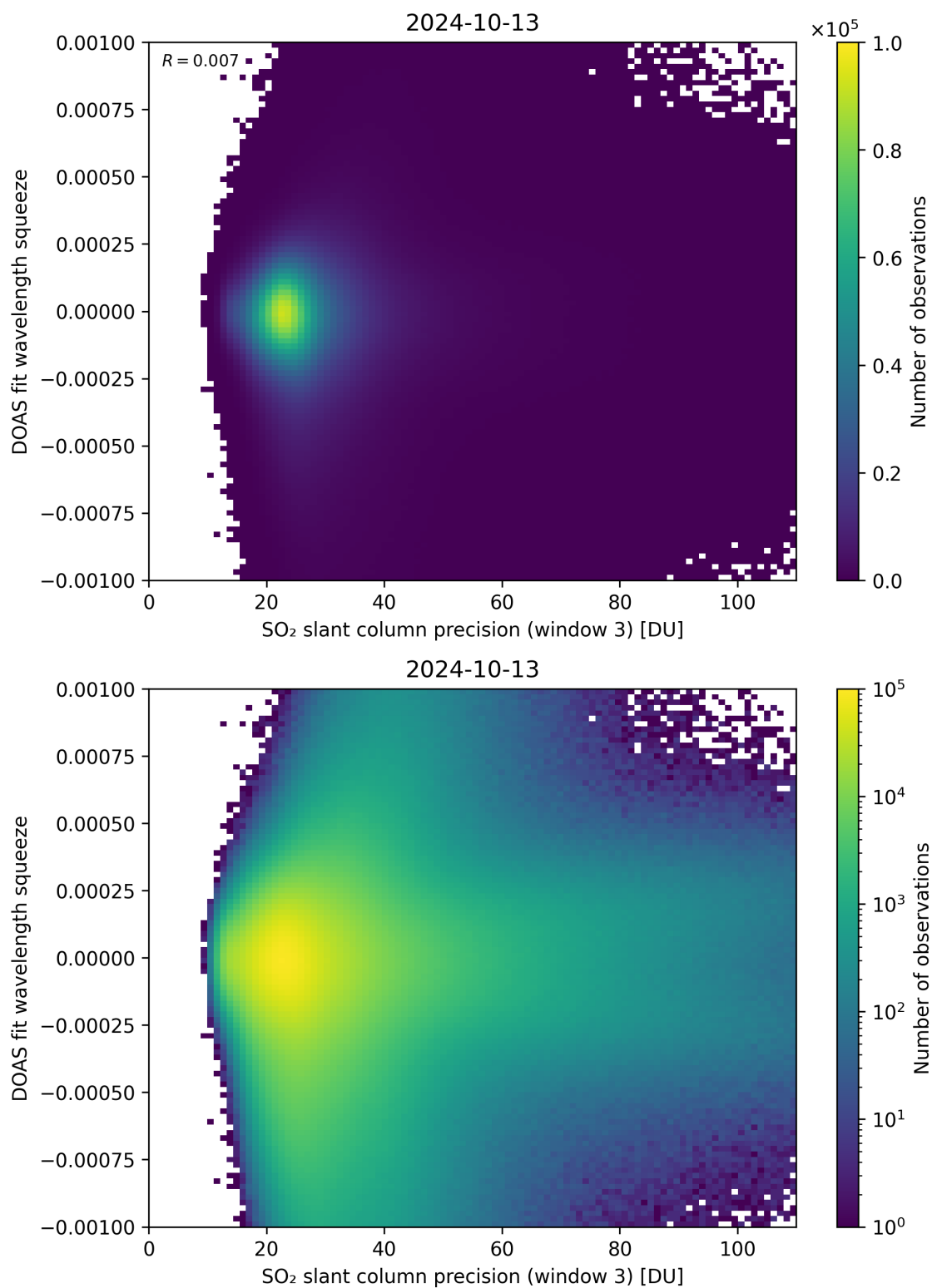
Figure 259: Scatter density plot of “SO 2 slant column precision (window 3)” against “DOAS fit wavelength squeeze” for 2024-10-12 to 2024-10-14.
