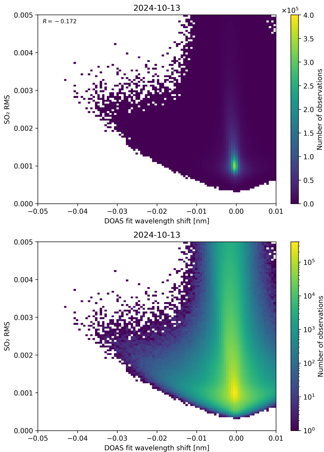
Figure 128: Scatter density plot of “DOAS fit wavelength shift” against “SO 2 RMS” for 2024-10-12 to 2024-10-14.
