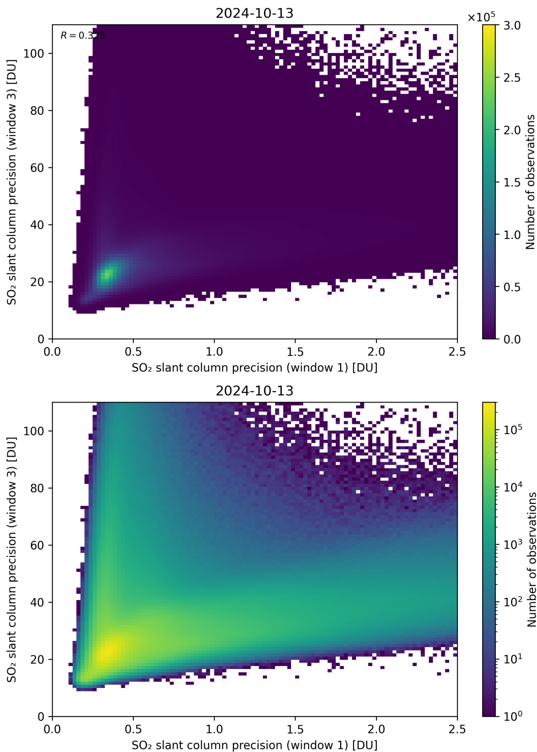
Figure 229: Scatter density plot of “SO 2 slant column precision (window 1)” against “SO 2 slant column precision (window 3)” for 2024-10-12 to 2024-10-14.
