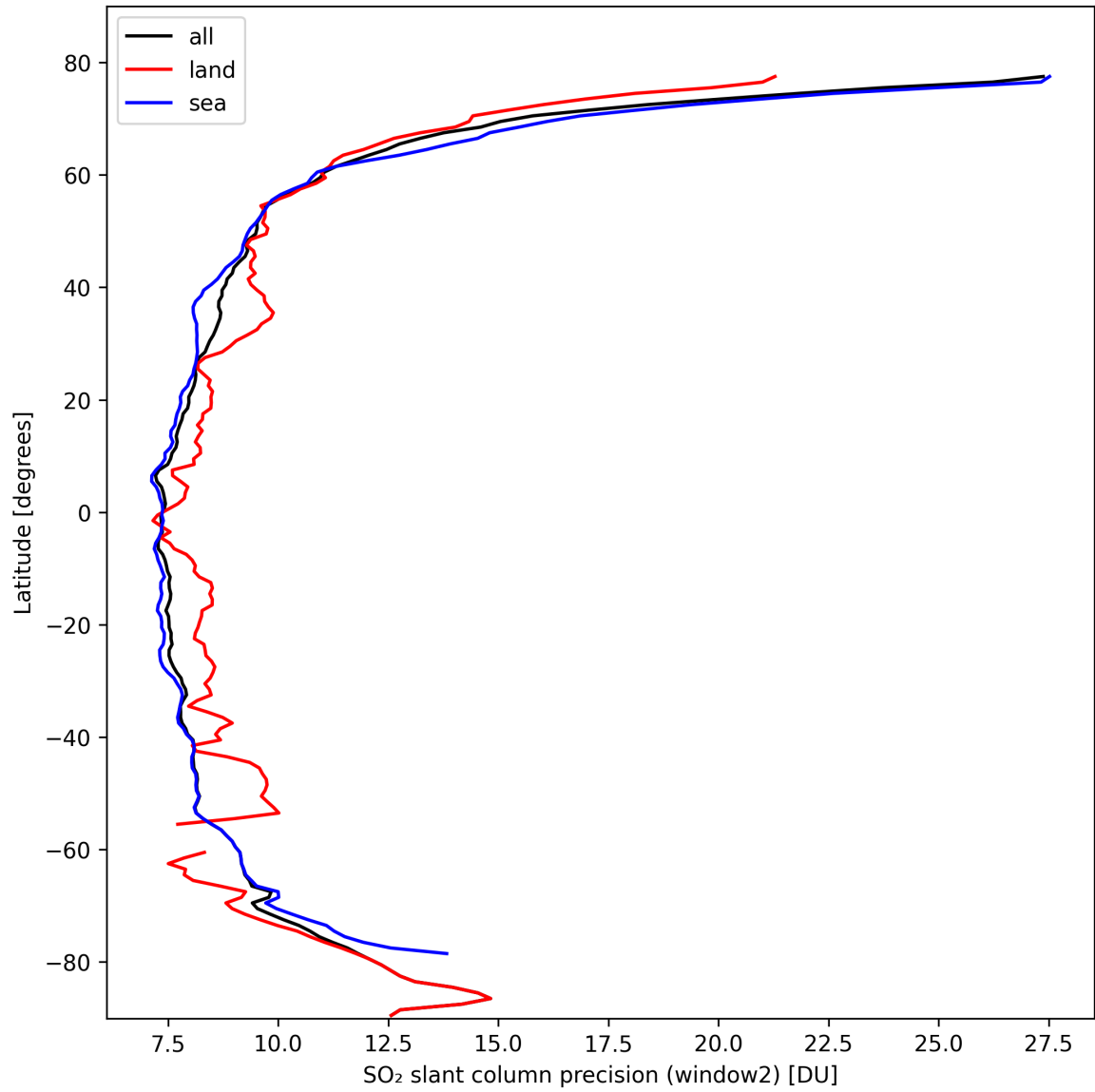
Figure 38: Zonal average of “SO 2 slant column precision (window2)” for 2024-10-12 to 2024-10-14.
