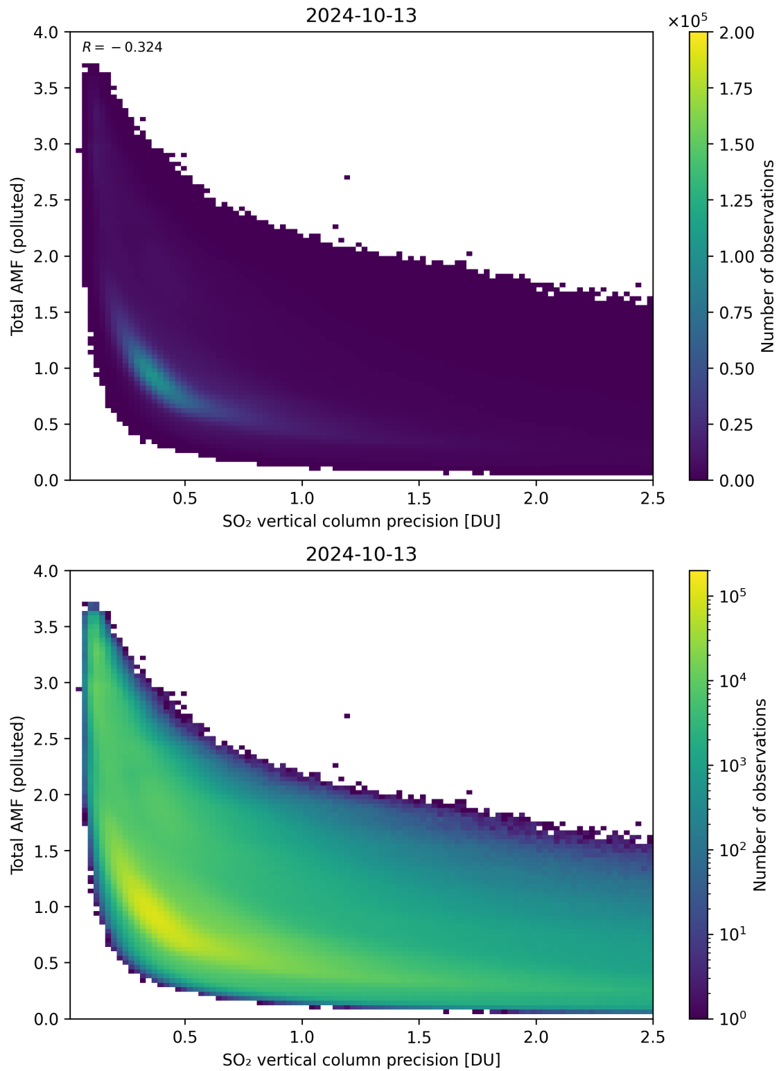
Figure 294: Scatter density plot of “SO 2 vertical column precision” against “Total AMF (polluted)” for 2024-10-12 to 2024-10-14.
