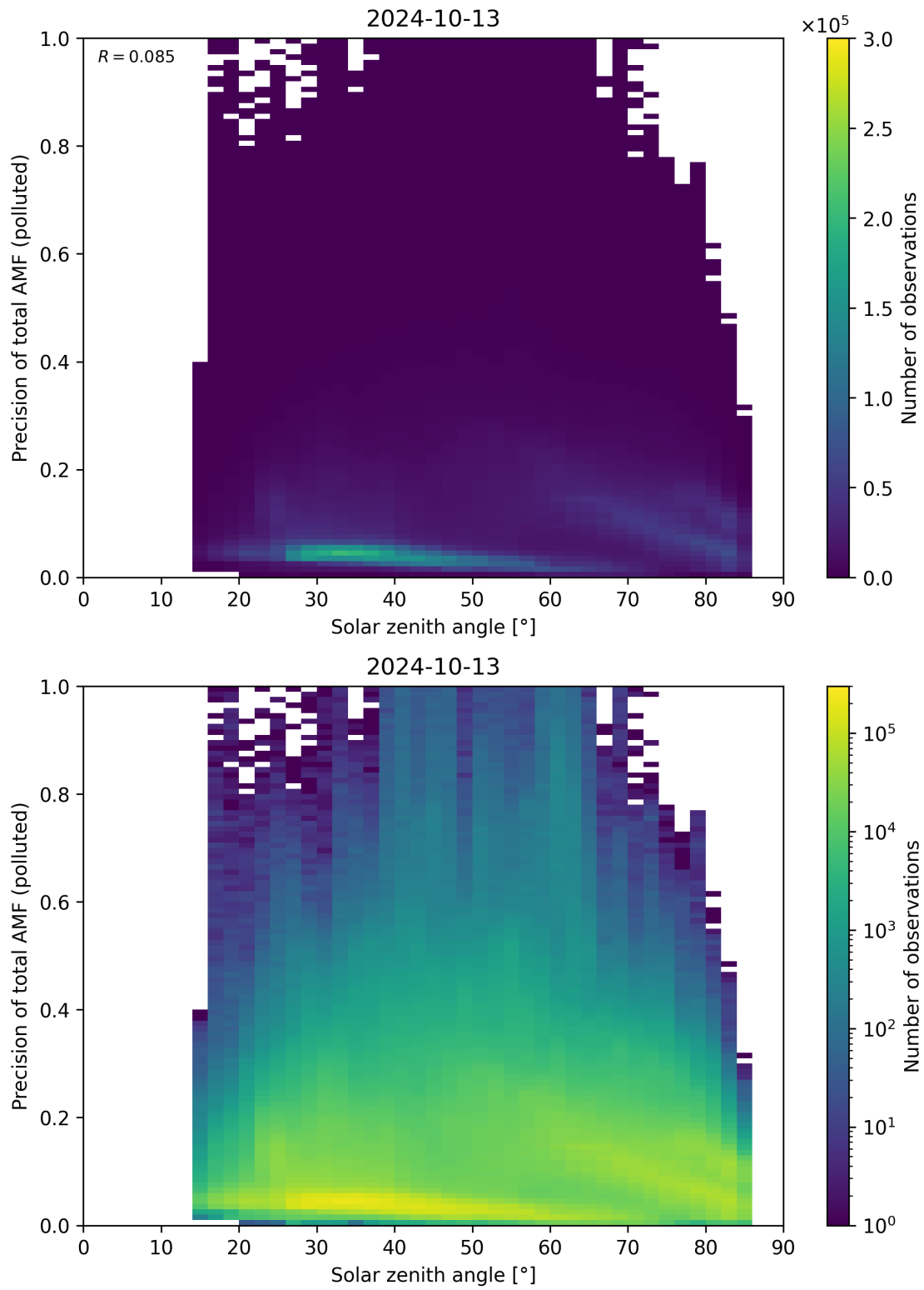
Figure 175: Scatter density plot of “Solar zenith angle” against “Precision of total AMF (polluted)” for 2024-10-12 to 2024-10-14.
