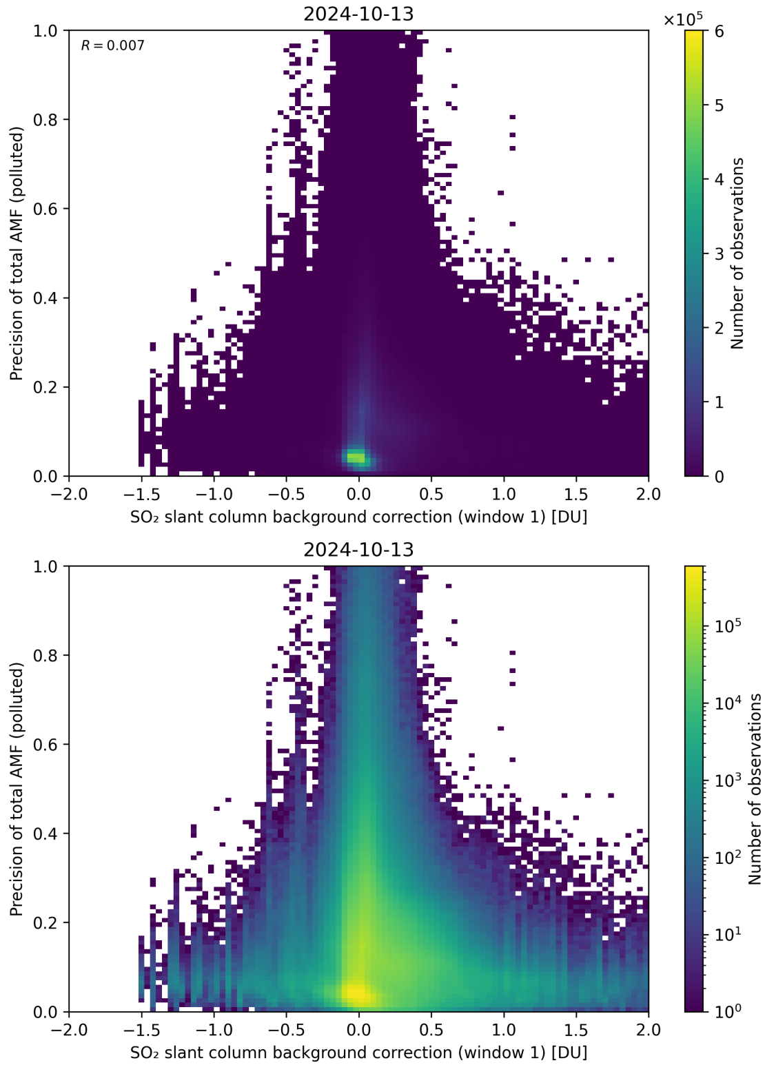
Figure 110: Scatter density plot of “SO 2 slant column background correction (window 1)” against “Precision of total AMF (polluted)” for 2024-10-12 to 2024-10-14.
