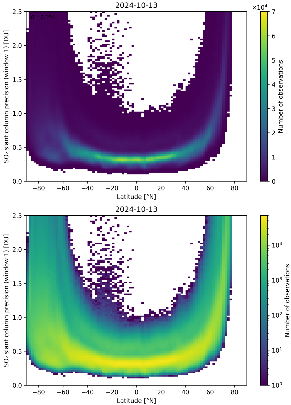
Figure 150: Scatter density plot of “Latitude” against “SO 2 slant column precision (window 1)” for 2024-10-12 to 2024-10-14.
