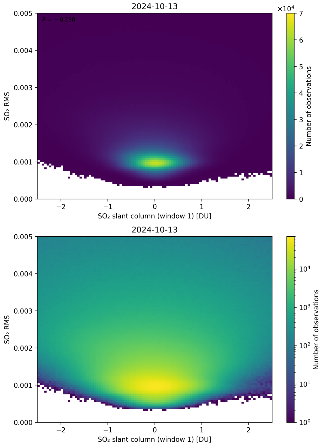
Figure 217: Scatter density plot of “SO 2 slant column (window 1)” against “SO 2 RMS” for 2024-10-12 to 2024-10-14.
