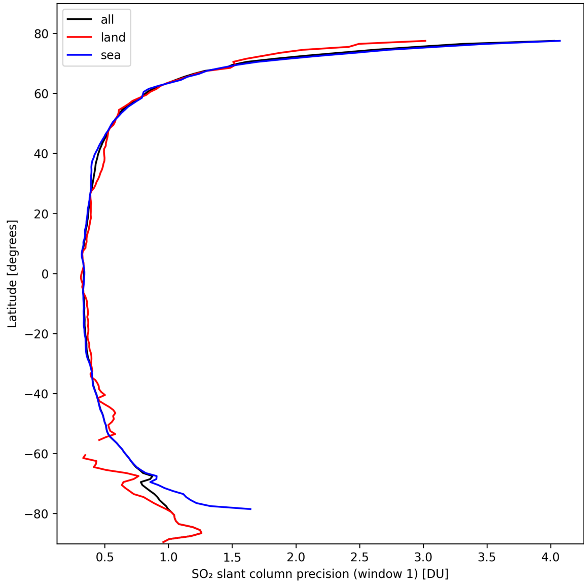
Figure 34: Zonal average of “SO 2 slant column precision (window 1)” for 2024-10-12 to 2024-10-14.
