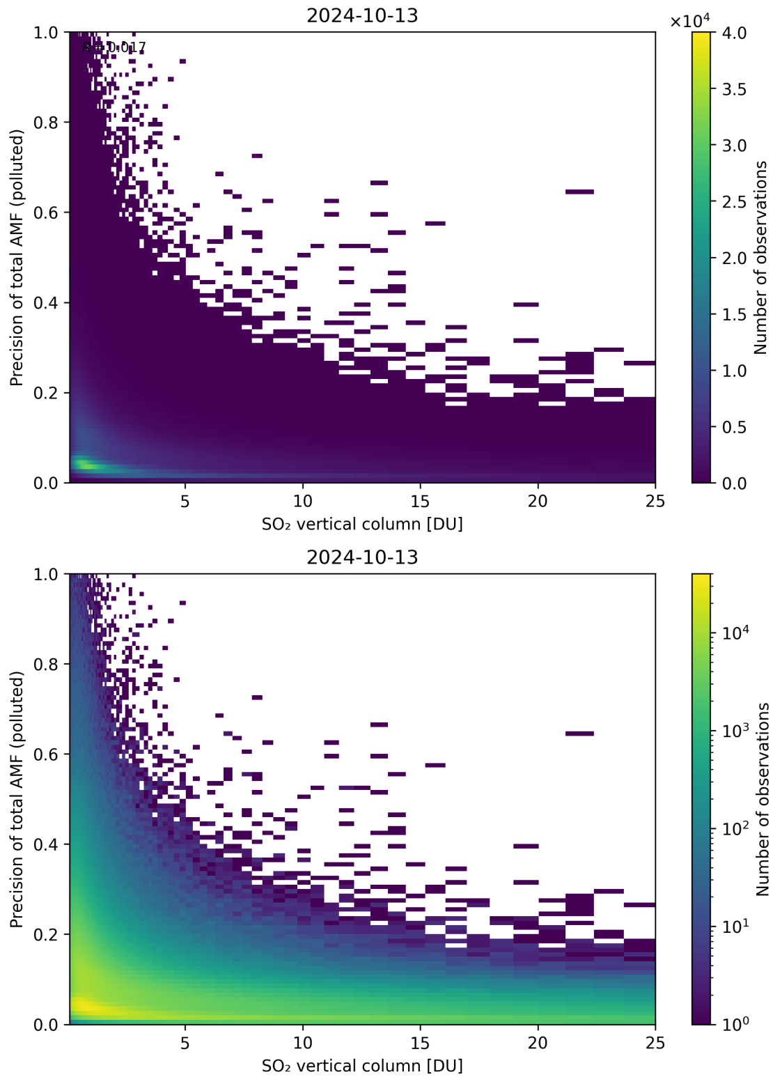
Figure 306: Scatter density plot of “SO 2 vertical column” against “Precision of total AMF (polluted)” for 2024-10-12 to 2024-10-14.
