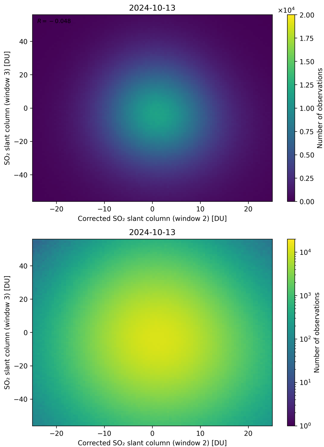
Figure 201: Scatter density plot of “Corrected SO 2 slant column (window 2)” against “SO 2 slant column (window 3)” for 2024-10-12 to 2024-10-14.
