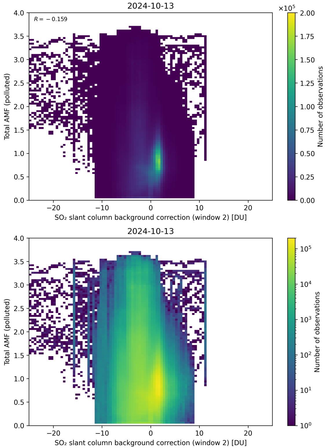
Figure 119: Scatter density plot of “SO 2 slant column background correction (window 2)” against “Total AMF (polluted)” for 2024-10-12 to 2024-10-14.
