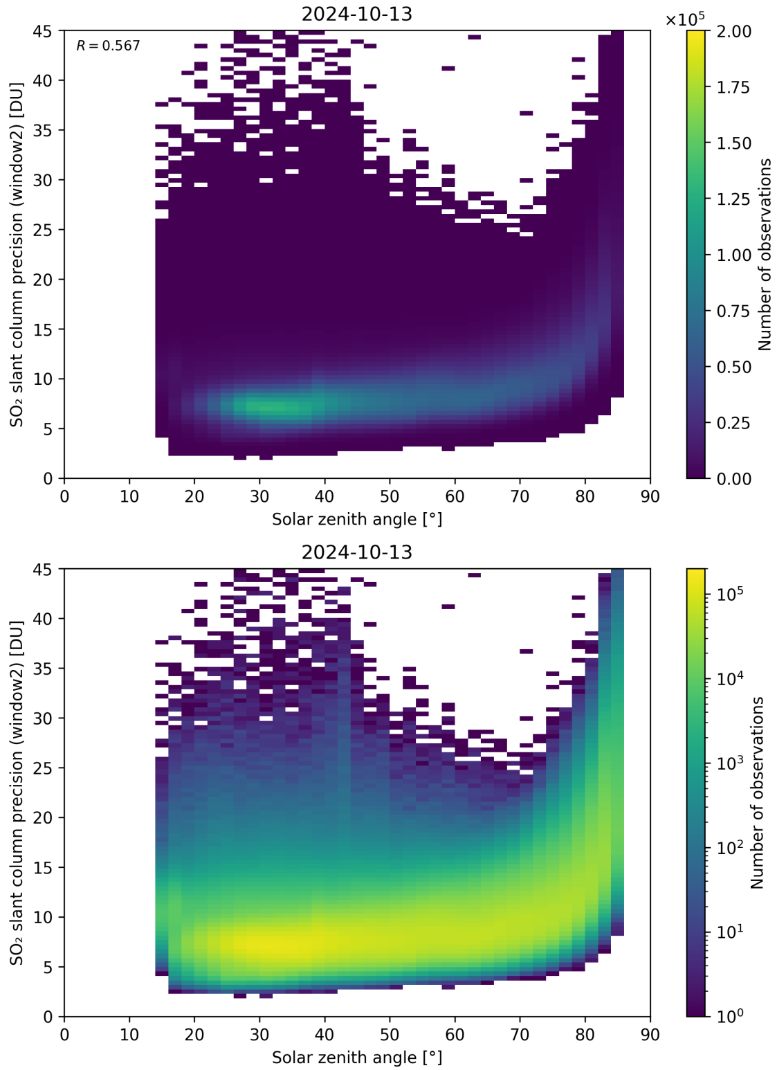
Figure 171: Scatter density plot of “Solar zenith angle” against “SO 2 slant column precision (window2)” for 2024-10-12 to 2024-10-14.
