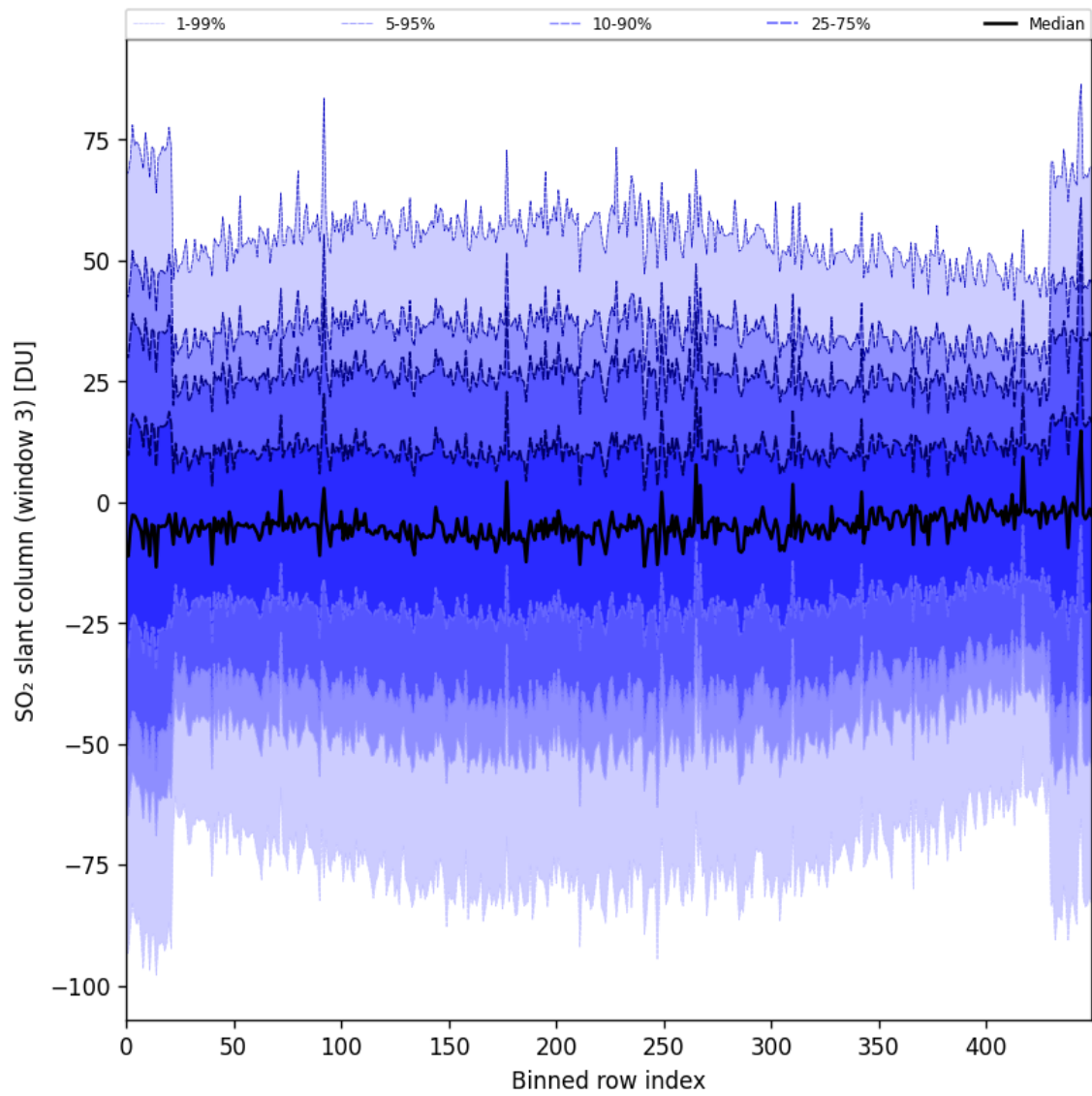
Figure 87: Along track statistics of “SO 2 slant column (window 3)” for 2024-10-12 to 2024-10-14
