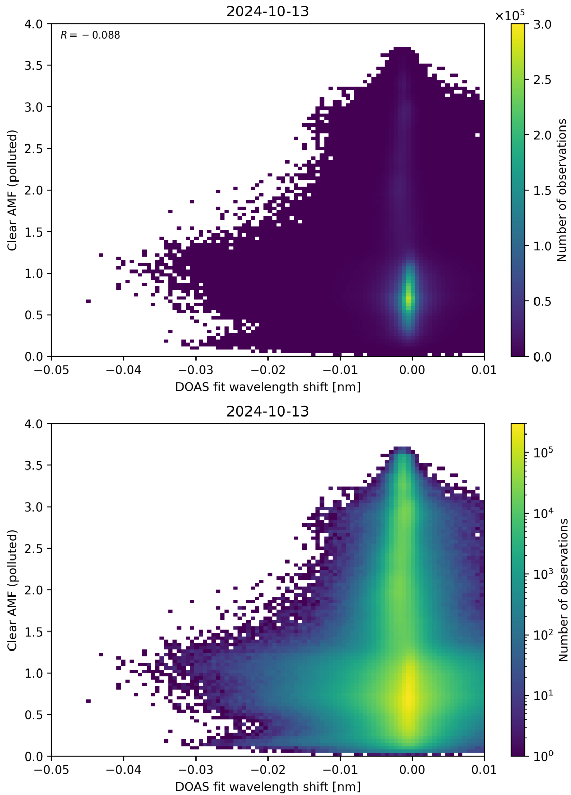
Figure 129: Scatter density plot of “DOAS fit wavelength shift” against “Clear AMF (polluted)” for 2024-10-12 to 2024-10-14.
