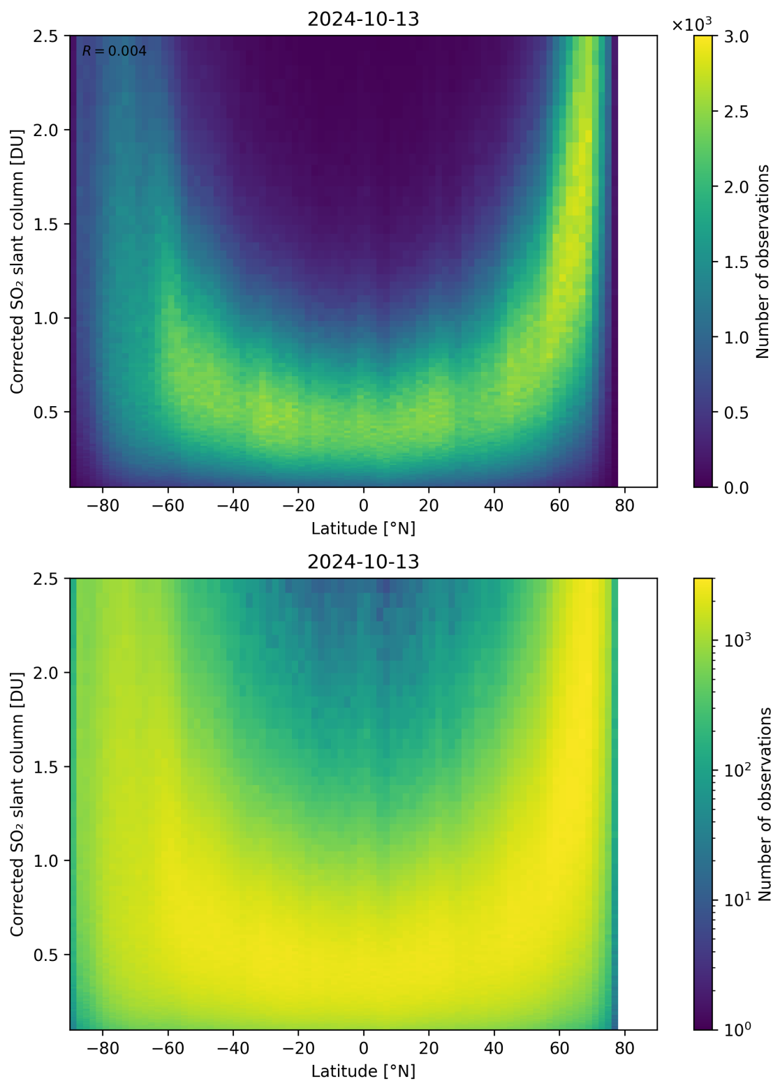
Figure 146: Scatter density plot of “Latitude” against “Corrected SO 2 slant column” for 2024-10-12 to 2024-10-14.
