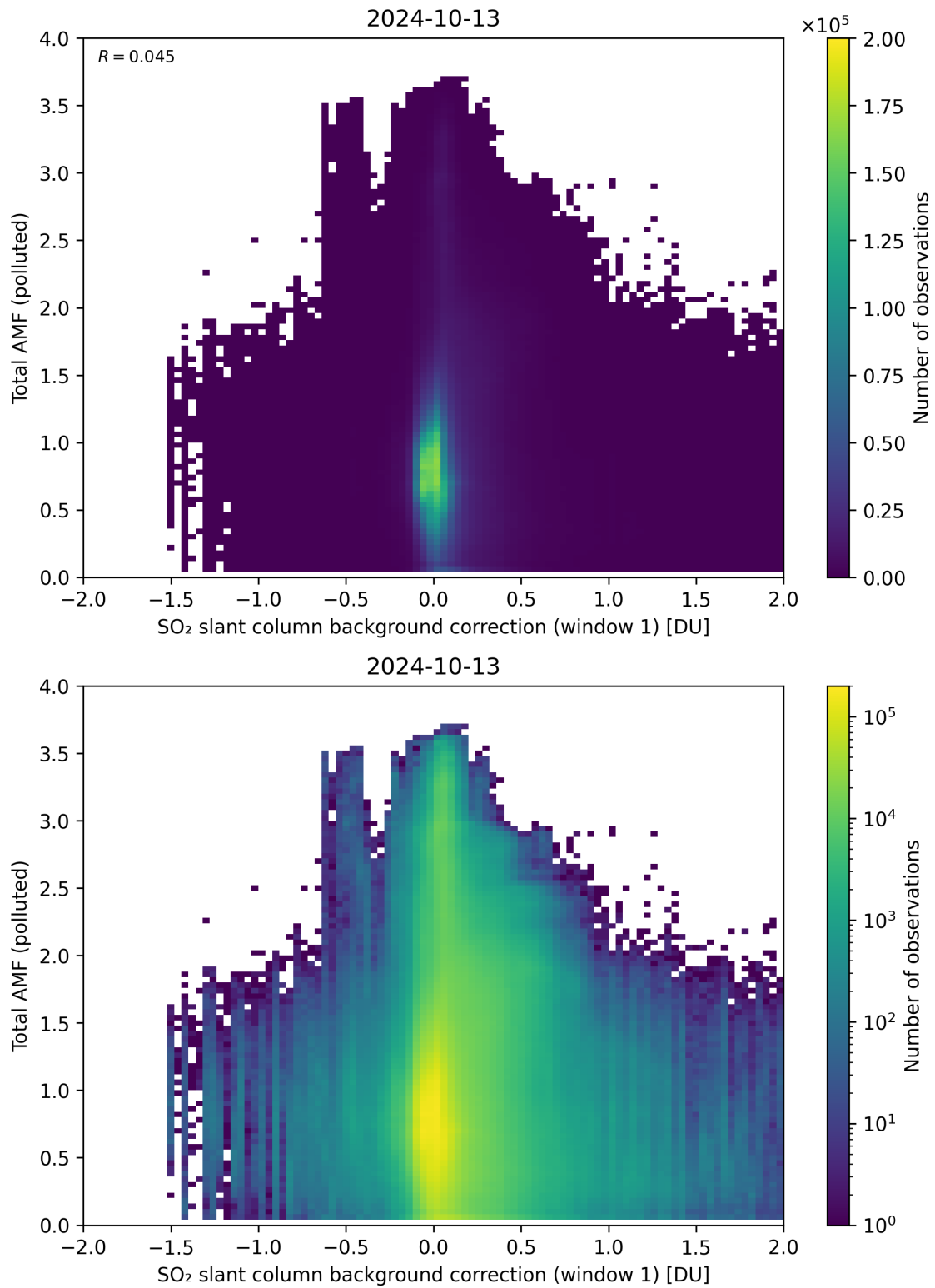
Figure 109: Scatter density plot of “SO 2 slant column background correction (window 1)” against “Total AMF (polluted)” for 2024-10-12 to 2024-10-14.
