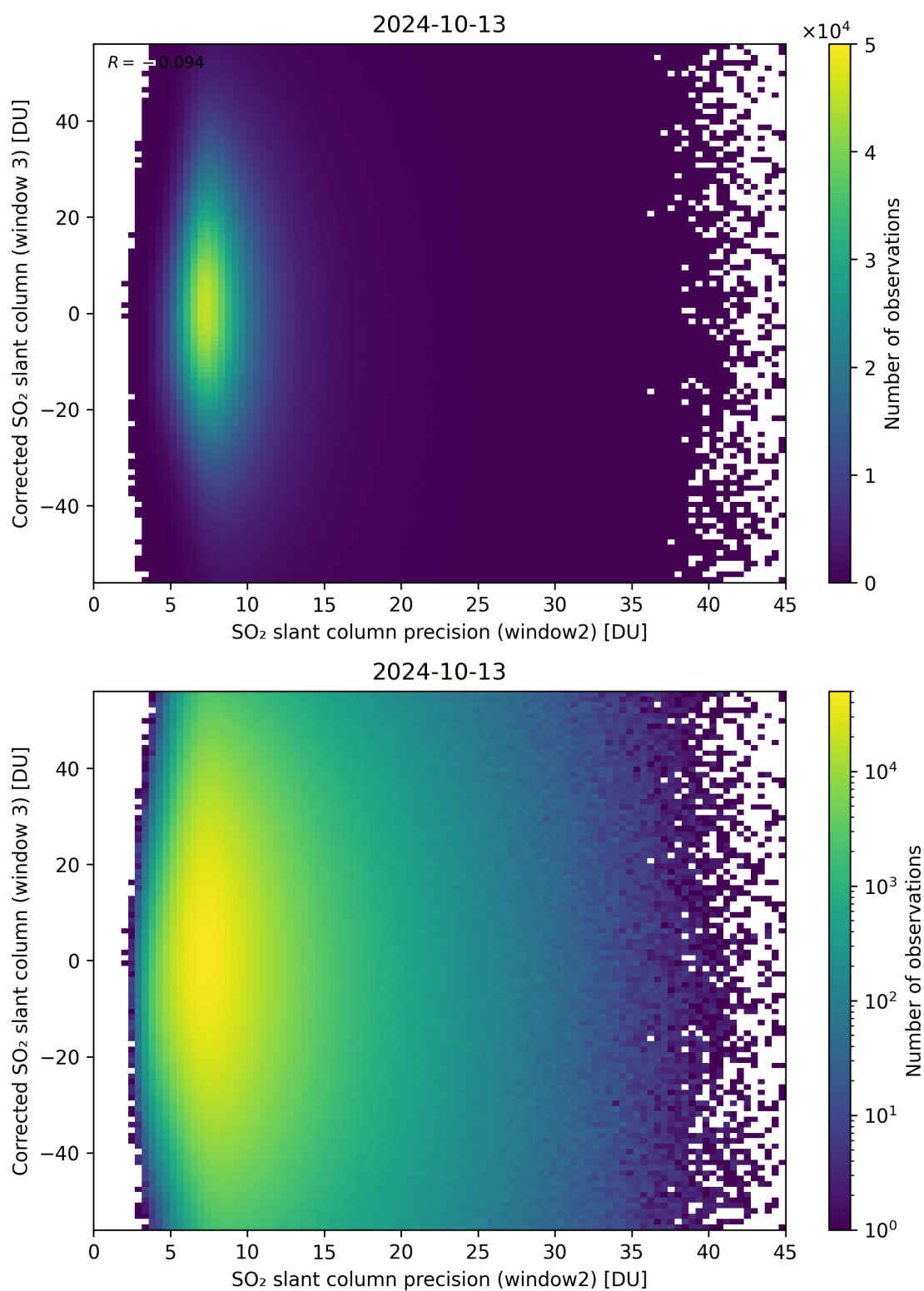
Figure 248: Scatter density plot of “SO 2 slant column precision (window2)” against “Corrected SO 2 slant column (window 3)” for 2024-10-12 to 2024-10-14.
