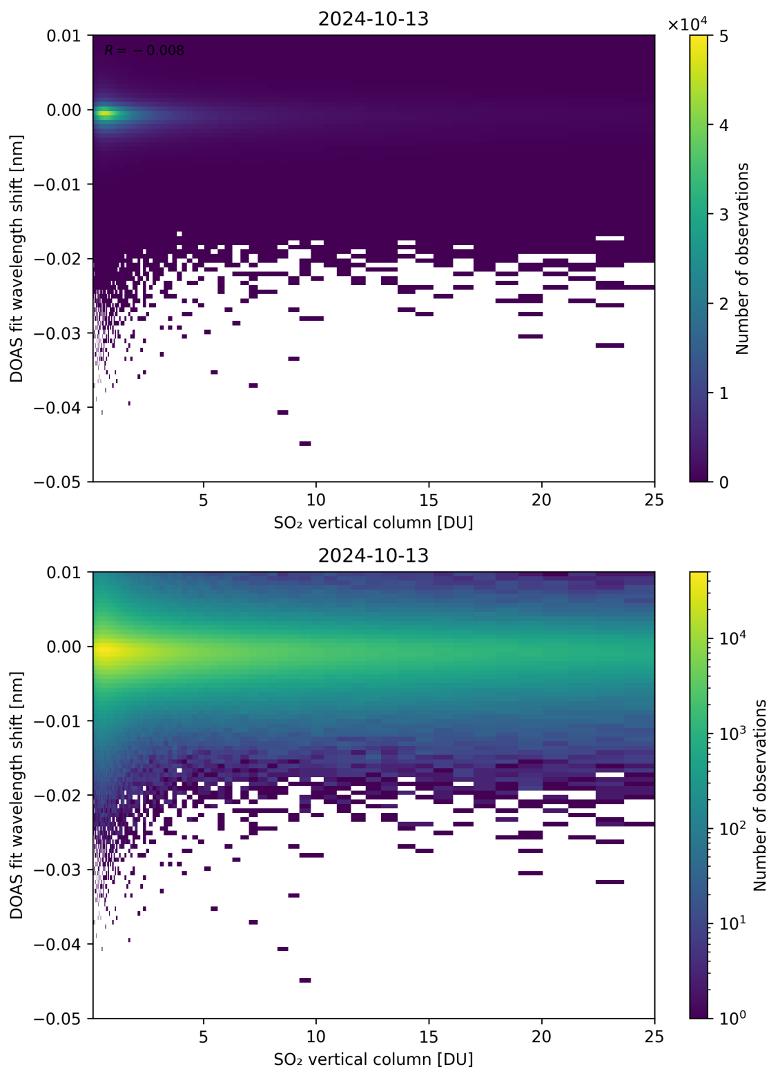
Figure 276: Scatter density plot of “SO 2 vertical column” against “DOAS fit wavelength shift” for 2024-10-12 to 2024-10-14.
