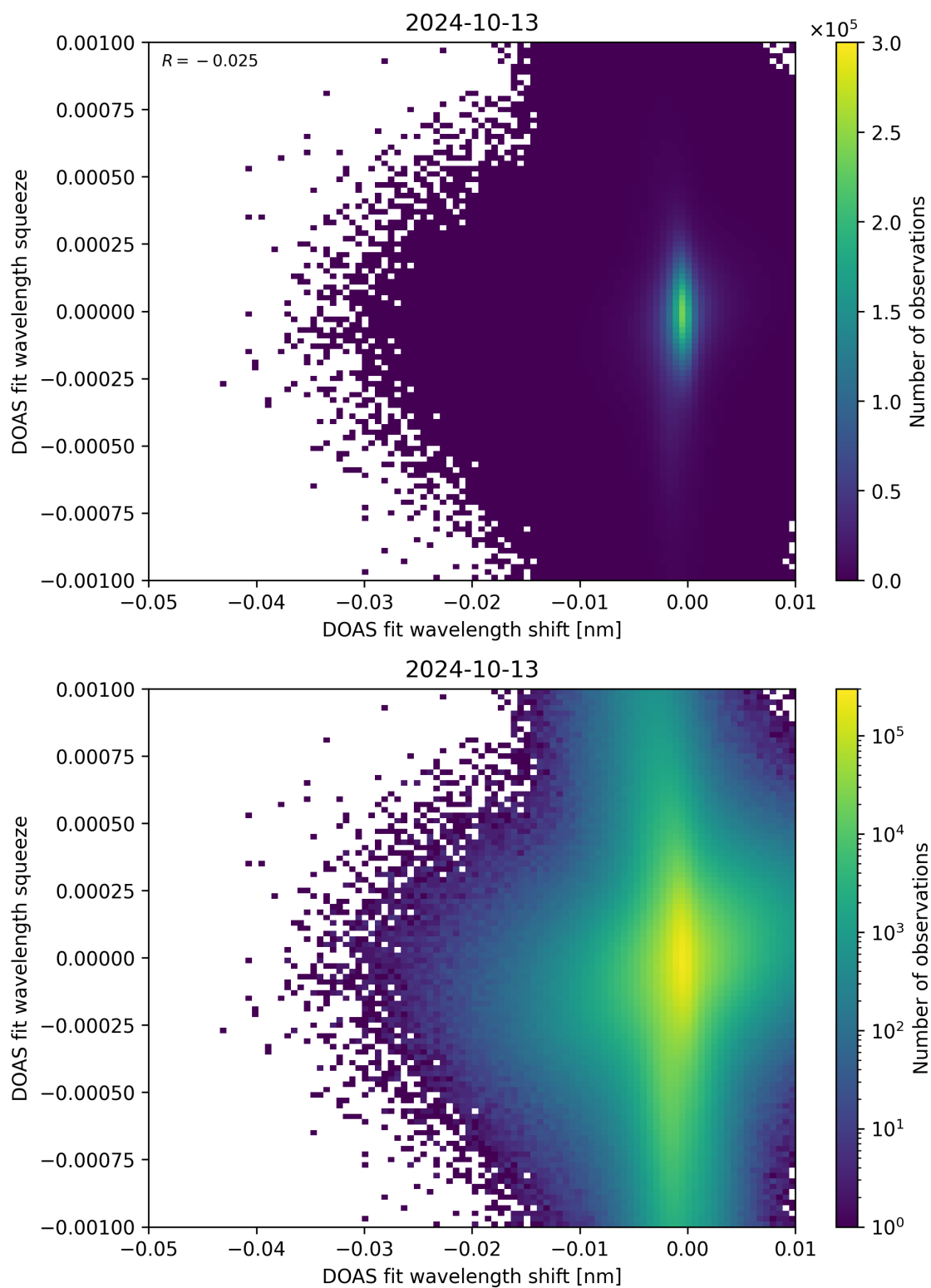
Figure 127: Scatter density plot of “DOAS fit wavelength shift” against “DOAS fit wavelength squeeze” for 2024-10-12 to 2024-10-14.
