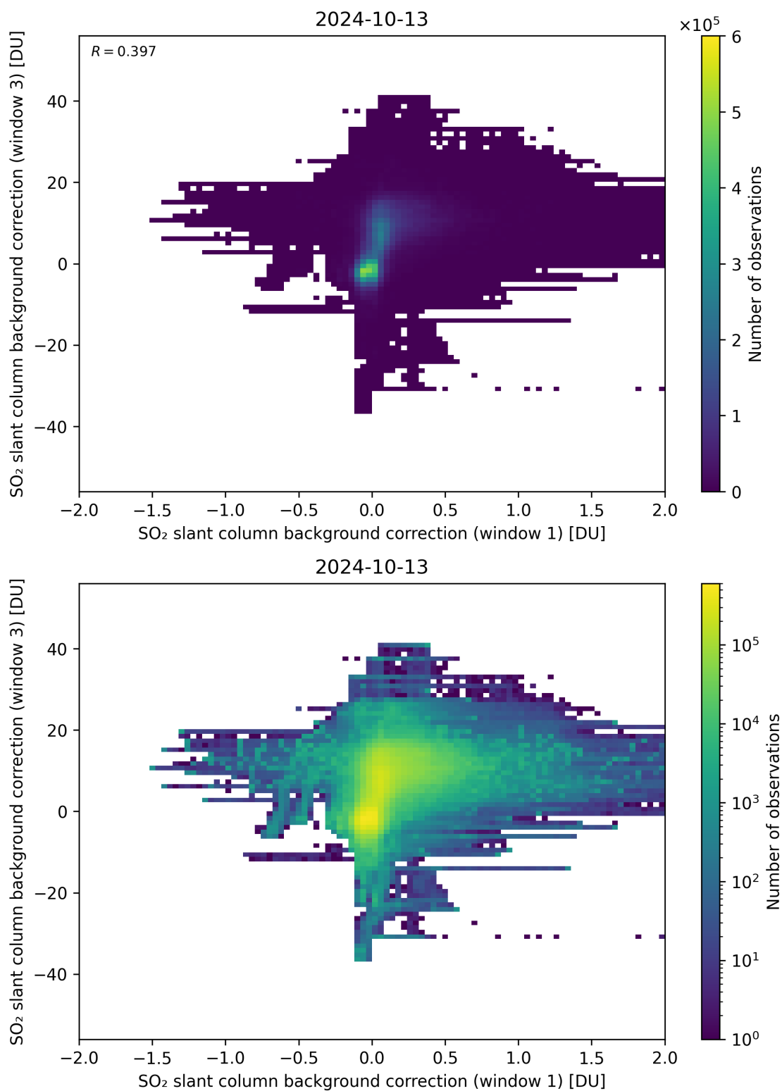
Figure 99: Scatter density plot of “SO 2 slant column background correction (window 1)” against “SO 2 slant column background correction (window 3)” for 2024-10-12 to 2024-10-14.
