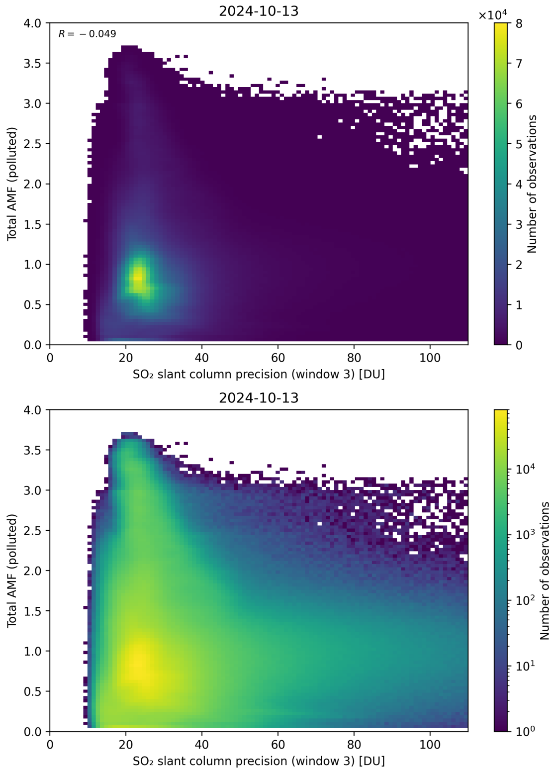
Figure 263: Scatter density plot of “SO 2 slant column precision (window 3)” against “Total AMF (polluted)” for 2024-10-12 to 2024-10-14.
