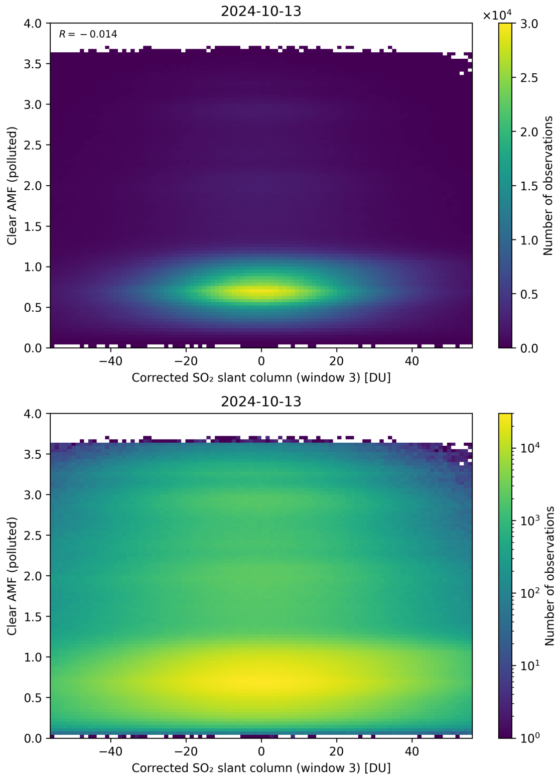
Figure 209: Scatter density plot of “Corrected SO 2 slant column (window 3)” against “Clear AMF (polluted)” for 2024-10-12 to 2024-10-14.
