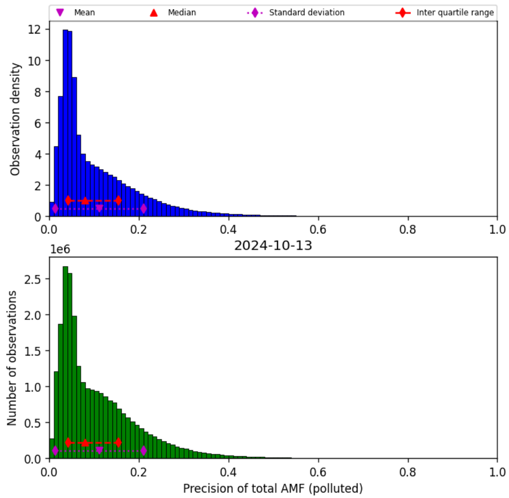
Figure 72: Histogram of “Precision of total AMF (polluted)” for 2024-10-12 to 2024-10-14
