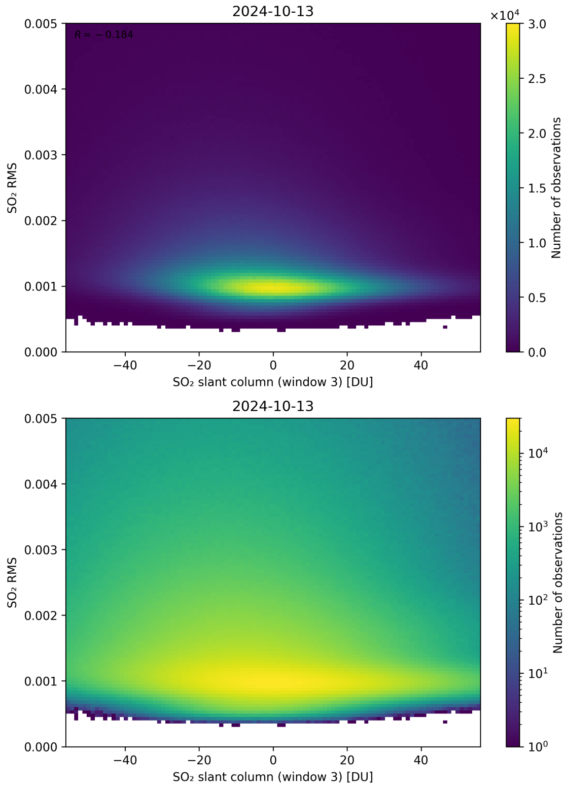
Figure 256: Scatter density plot of “SO 2 slant column (window 3)” against “SO 2 RMS” for 2024-10-12 to 2024-10-14.
