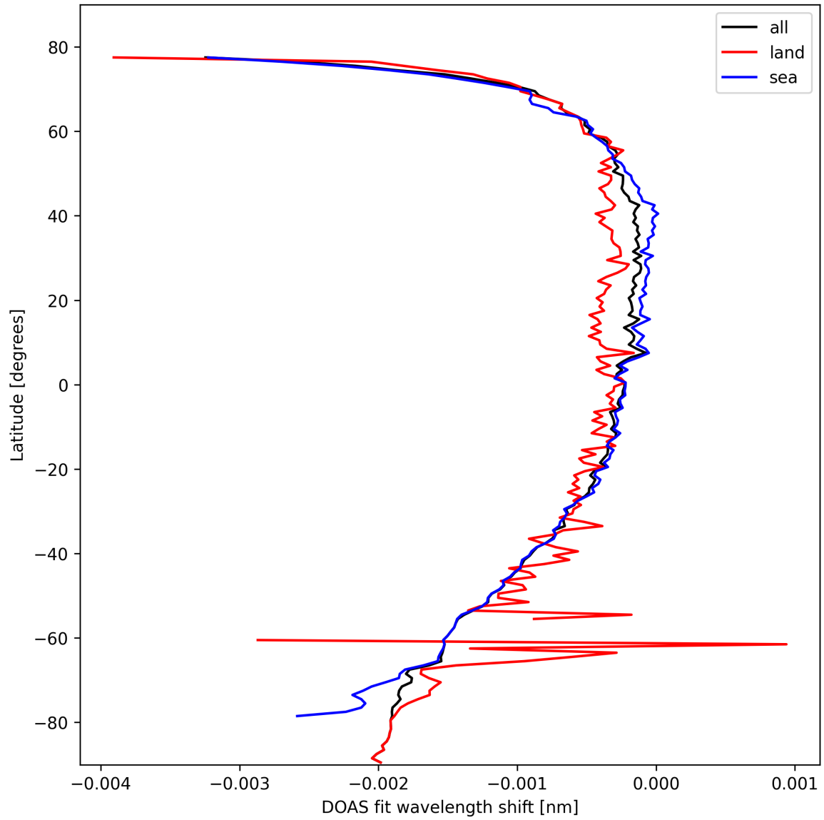
Figure 45: Zonal average of “DOAS fit wavelength shift” for 2024-10-12 to 2024-10-14.
