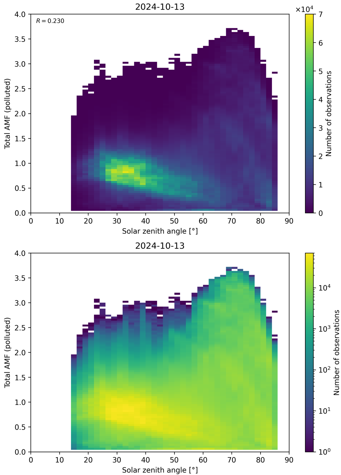
Figure 174: Scatter density plot of “Solar zenith angle” against “Total AMF (polluted)” for 2024-10-12 to 2024-10-14.
