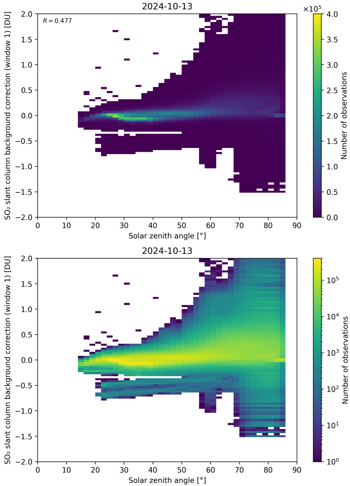
Figure 158: Scatter density plot of “Solar zenith angle” against “SO 2 slant column background correction (window 1)” for 2024-10-12 to 2024-10-14.
