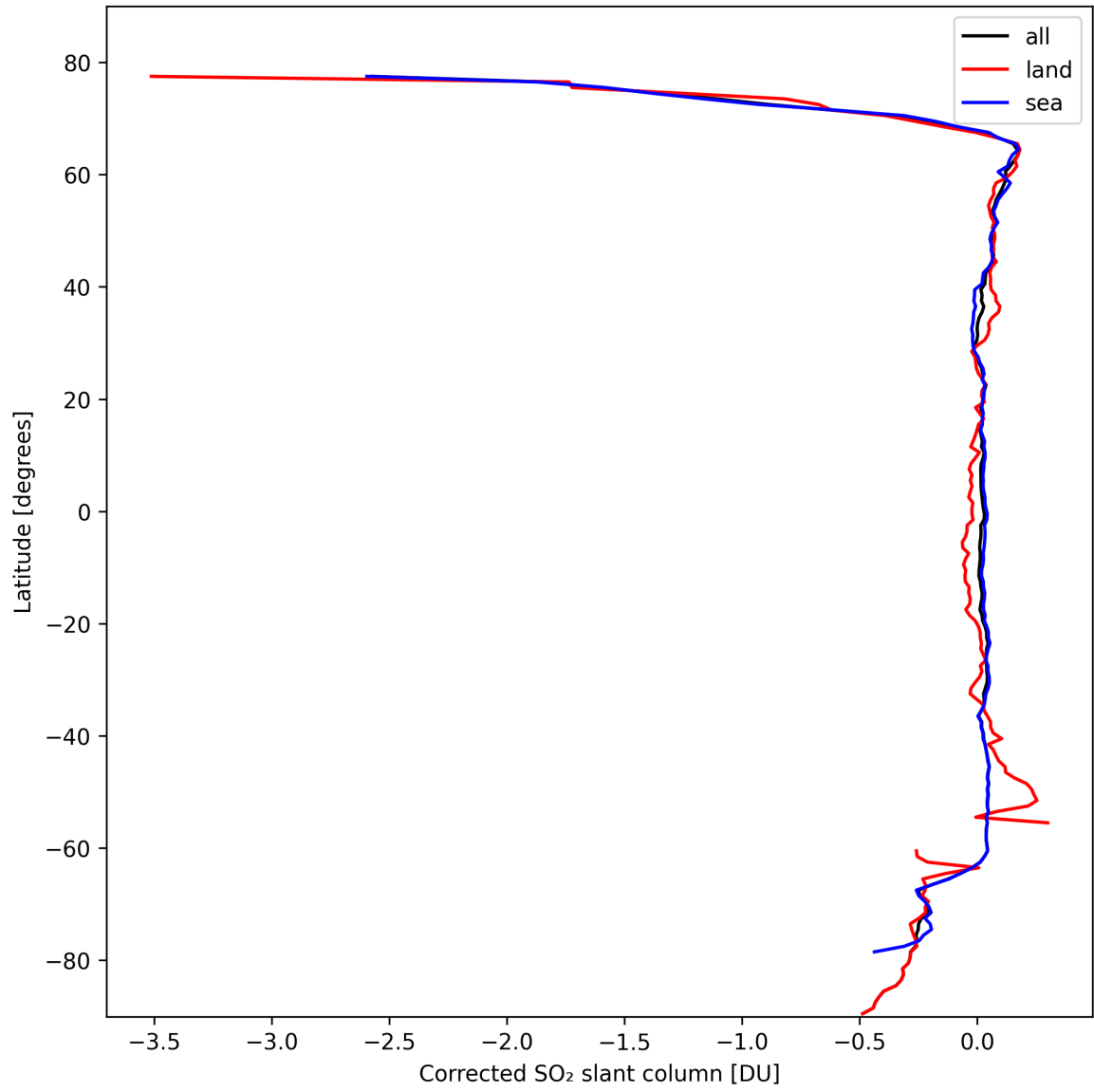
Figure 32: Zonal average of “Corrected SO 2 slant column” for 2024-10-12 to 2024-10-14.
