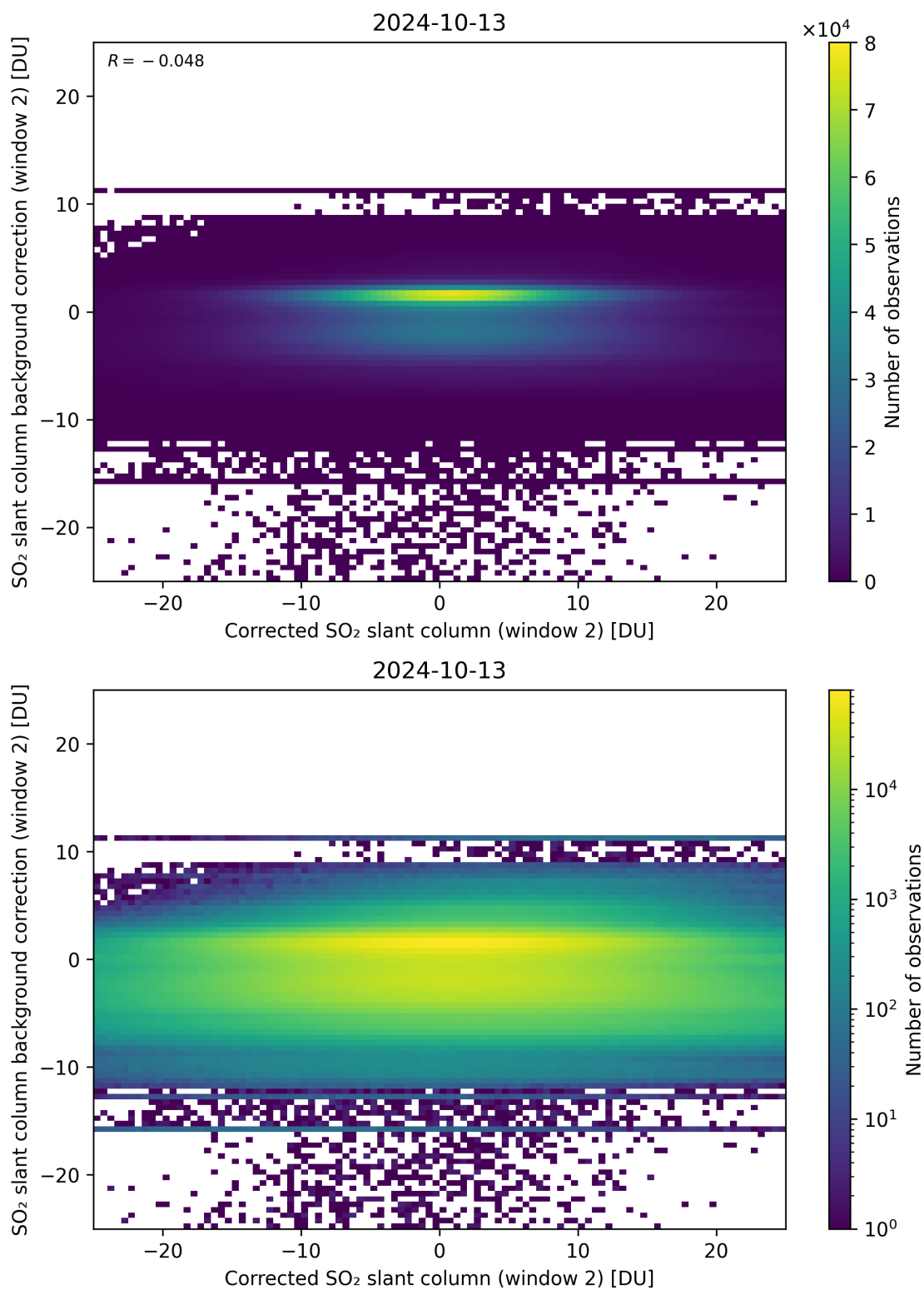
Figure 194: Scatter density plot of “Corrected SO 2 slant column (window 2)” against “SO 2 slant column background correction (window 2)” for 2024-10-12 to 2024-10-14.
