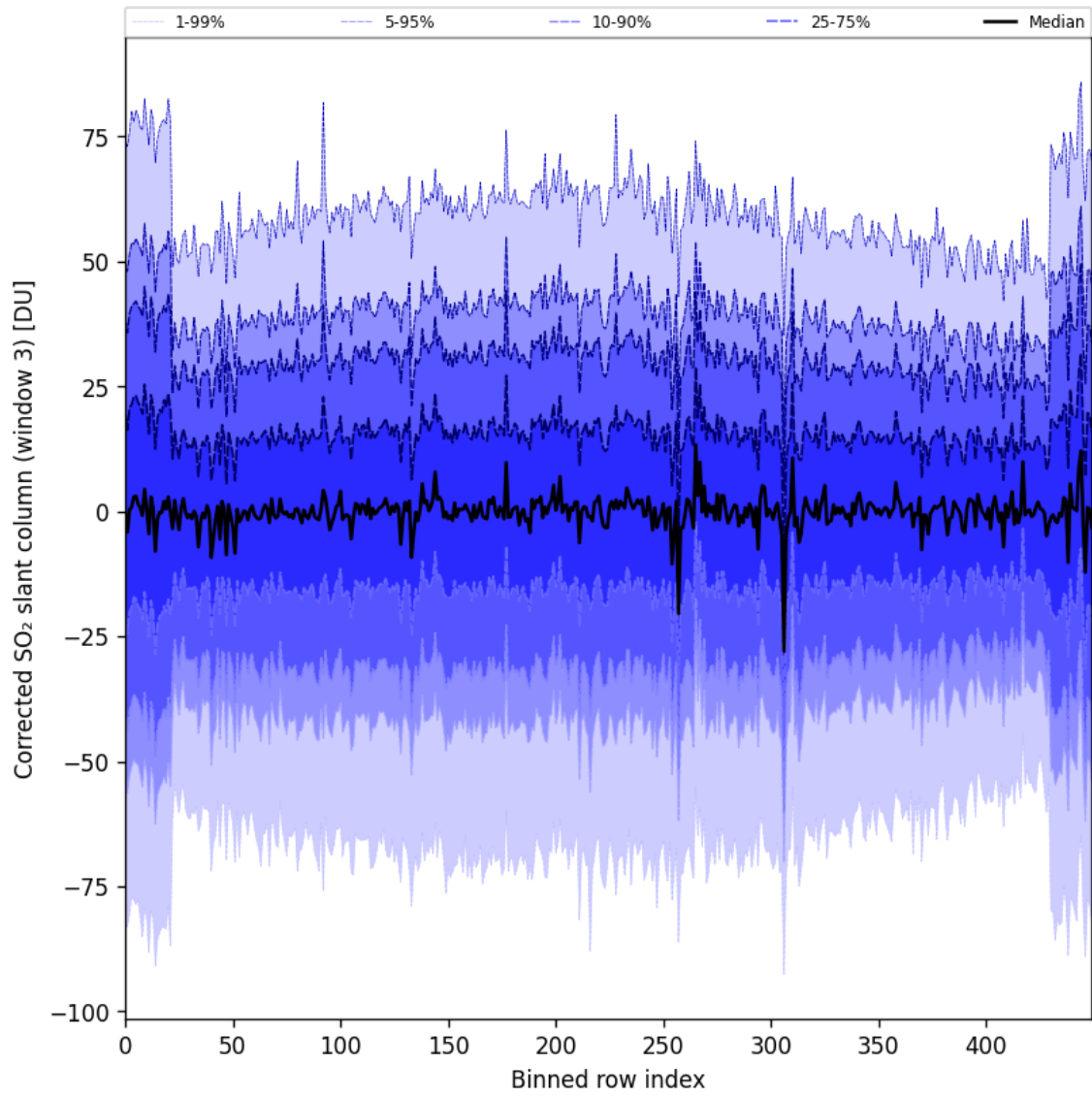
Figure 89: Along track statistics of “Corrected SO 2 slant column (window 3)” for 2024-10-12 to 2024-10-14
