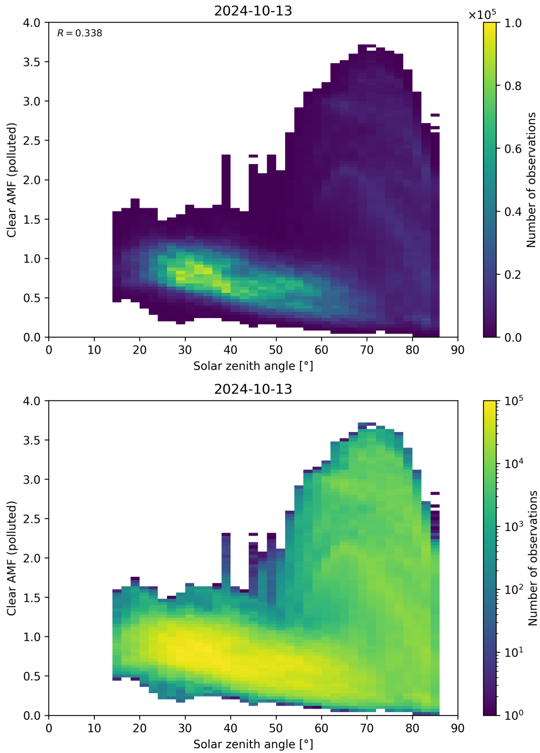
Figure 165: Scatter density plot of “Solar zenith angle” against “Clear AMF (polluted)” for 2024-10-12 to 2024-10-14.
