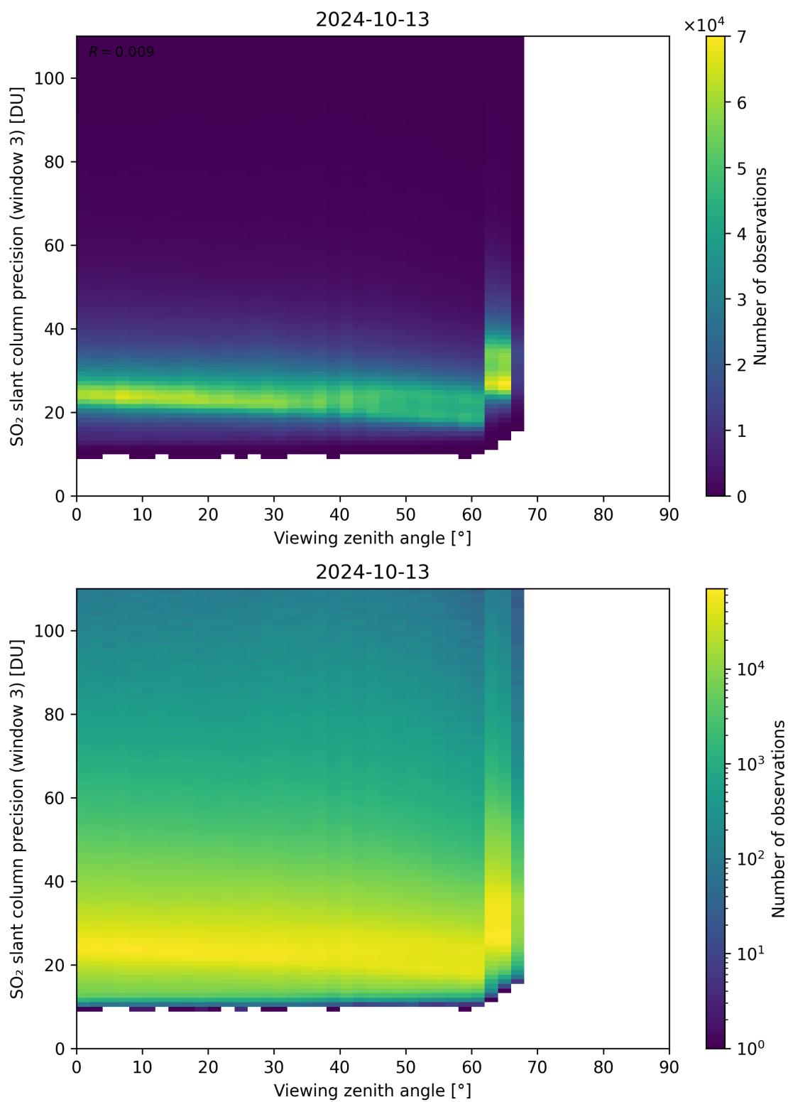
Figure 324: Scatter density plot of “Viewing zenith angle” against “SO 2 slant column precision (window 3)” for 2024-10-12 to 2024-10-14.
