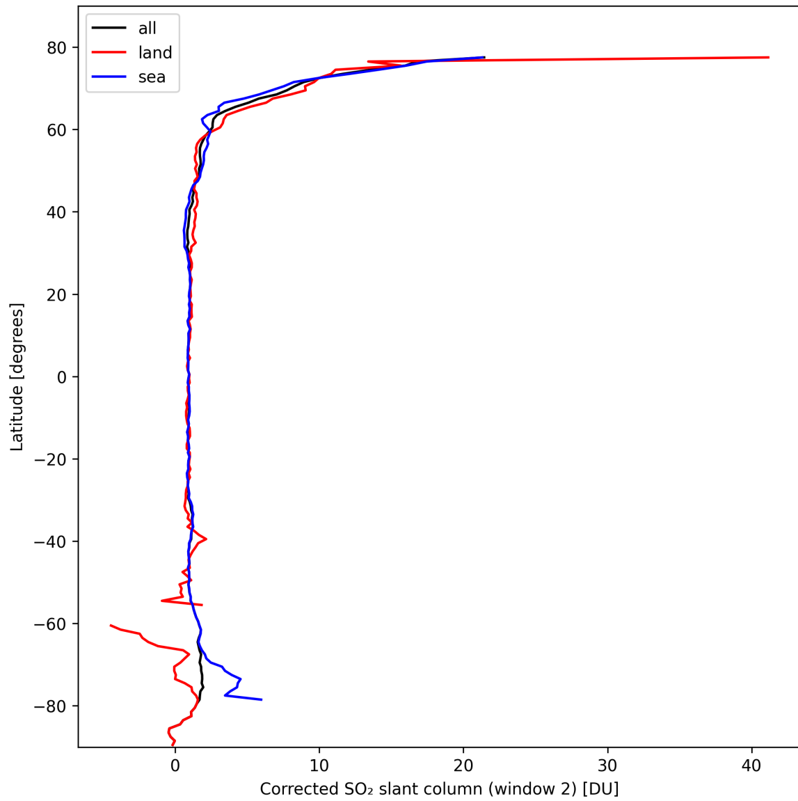
Figure 39: Zonal average of “Corrected SO 2 slant column (window 2)” for 2024-10-12 to 2024-10-14.
