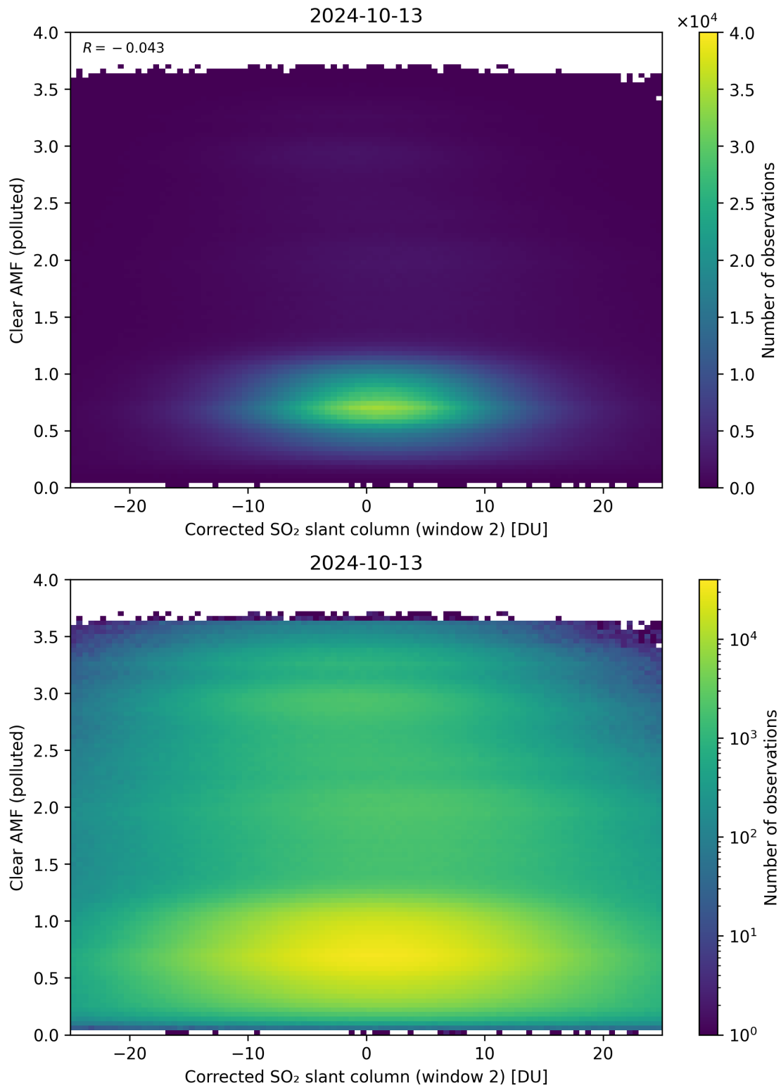
Figure 199: Scatter density plot of “Corrected SO 2 slant column (window 2)” against “Clear AMF (polluted)” for 2024-10-12 to 2024-10-14.
