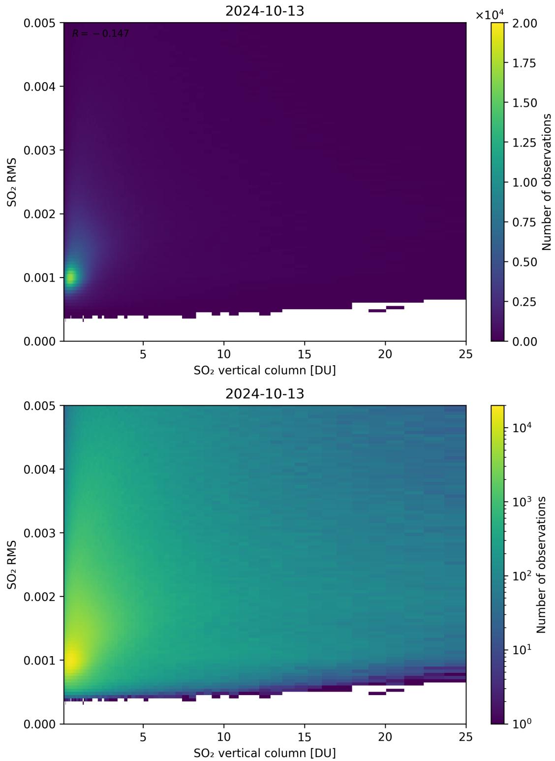
Figure 278: Scatter density plot of “SO 2 vertical column” against “SO 2 RMS” for 2024-10-12 to 2024-10-14.
