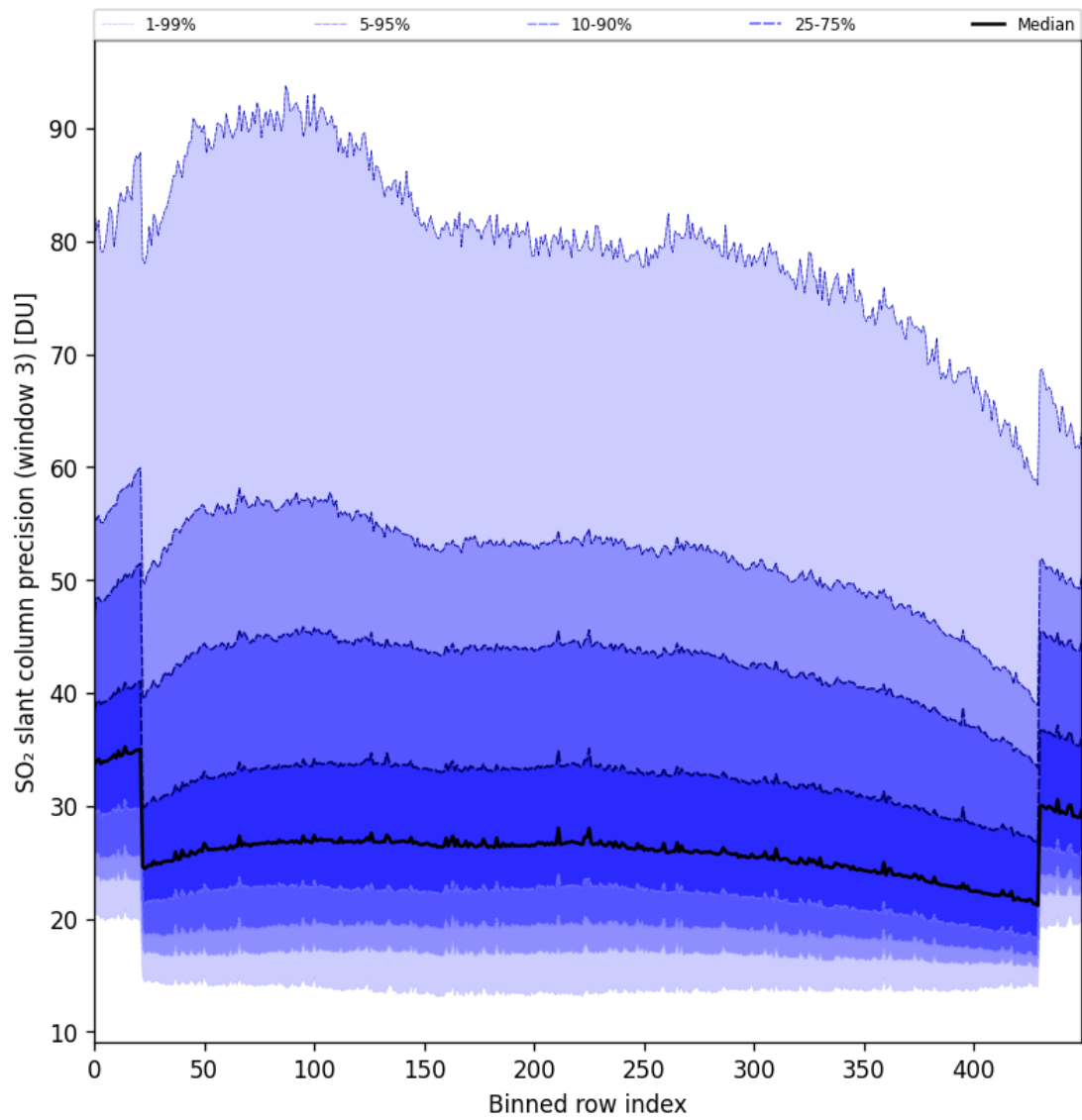
Figure 88: Along track statistics of “SO 2 slant column precision (window 3)” for 2024-10-12 to 2024-10-14
