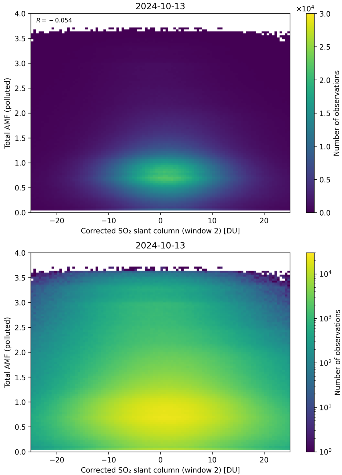
Figure 203: Scatter density plot of “Corrected SO 2 slant column (window 2)” against “Total AMF (polluted)” for 2024-10-12 to 2024-10-14.
