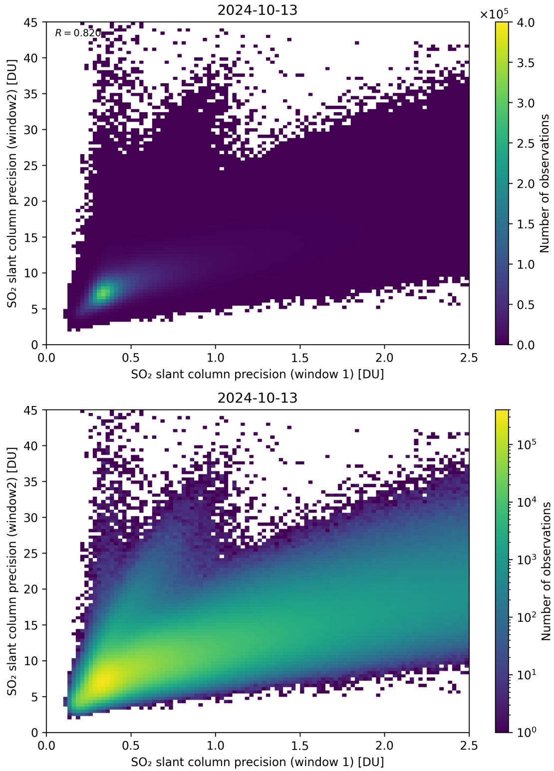
Figure 227: Scatter density plot of “SO 2 slant column precision (window 1)” against “SO 2 slant column precision (window2)” for 2024-10-12 to 2024-10-14.
