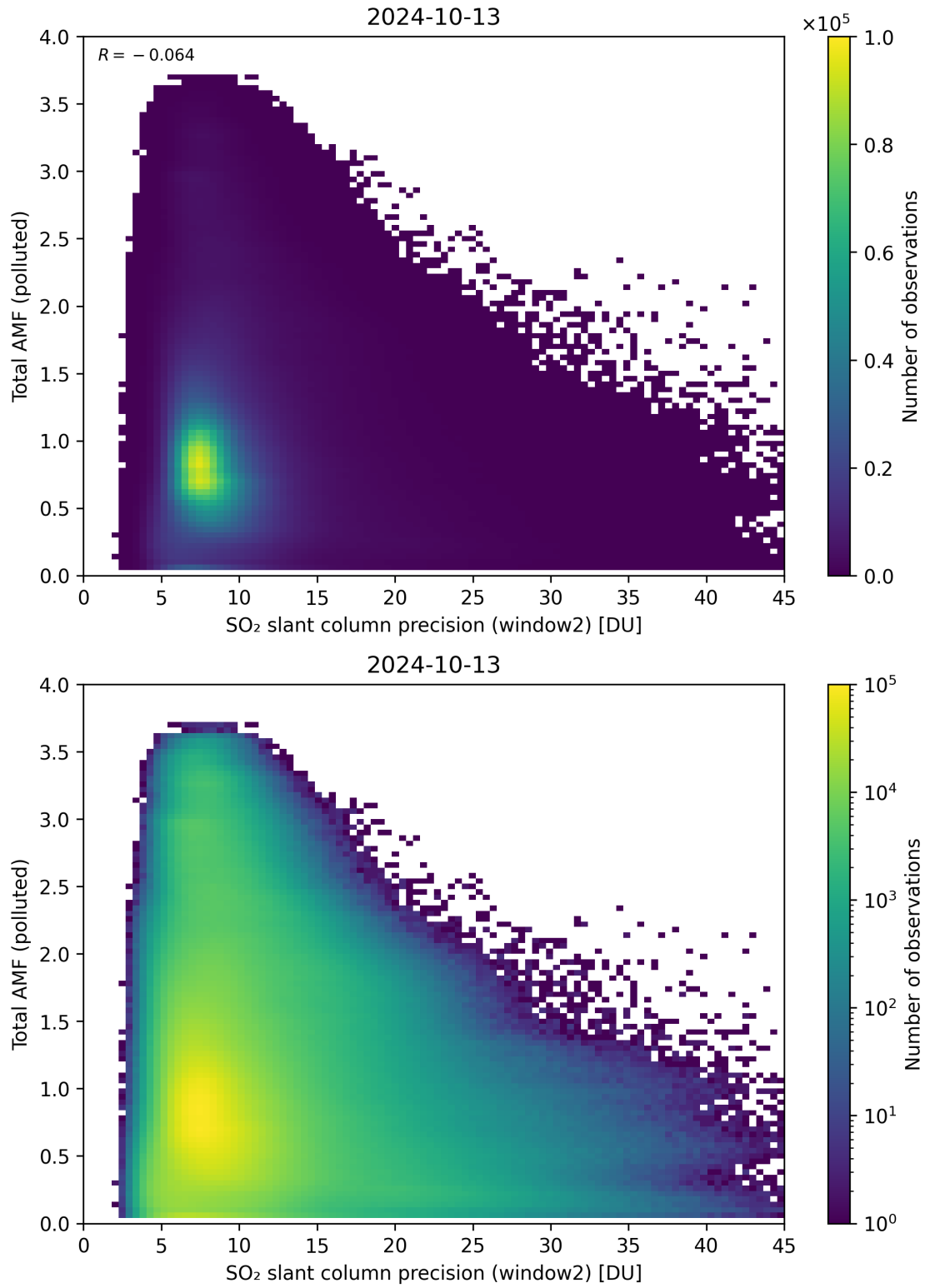
Figure 251: Scatter density plot of “SO 2 slant column precision (window2)” against “Total AMF (polluted)” for 2024-10-12 to 2024-10-14.
