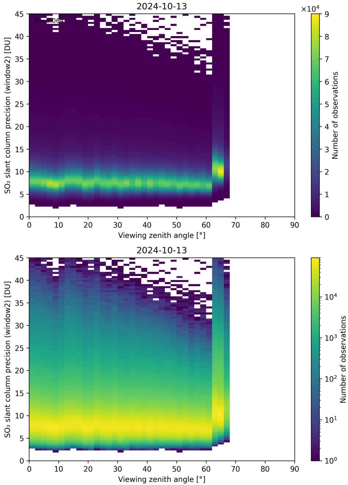
Figure 322: Scatter density plot of “Viewing zenith angle” against “SO 2 slant column precision (window2)” for 2024-10-12 to 2024-10-14.
