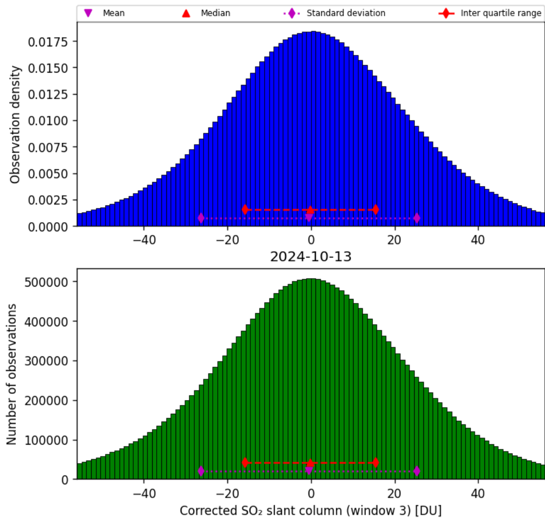
Figure 66: Histogram of “Corrected SO 2 slant column (window 3)” for 2024-10-12 to 2024-10-14
