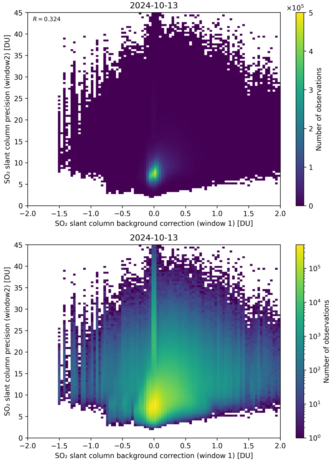
Figure 106: Scatter density plot of “SO 2 slant column background correction (window 1)” against “SO 2 slant column precision (window2)” for 2024-10-12 to 2024-10-14.
