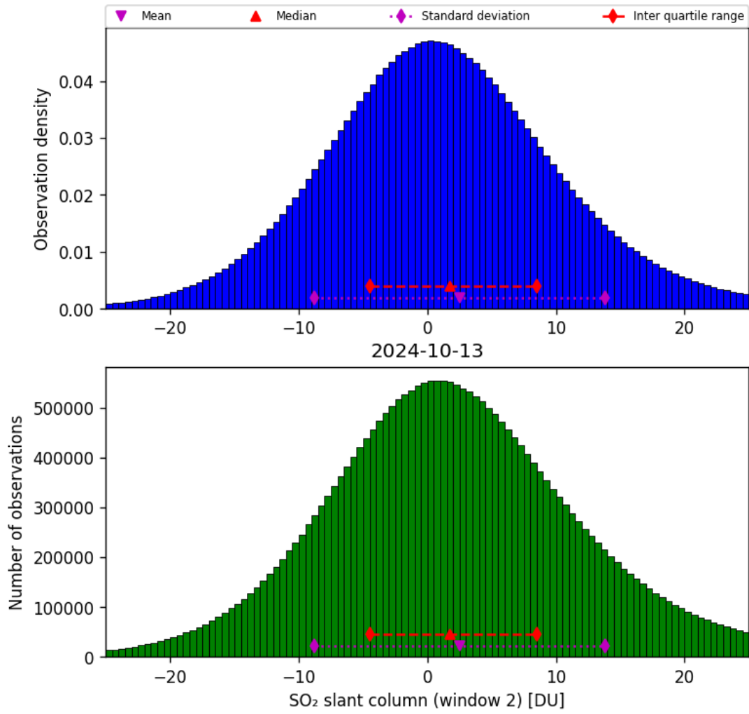
Figure 60: Histogram of “SO 2 slant column (window 2)” for 2024-10-12 to 2024-10-14
