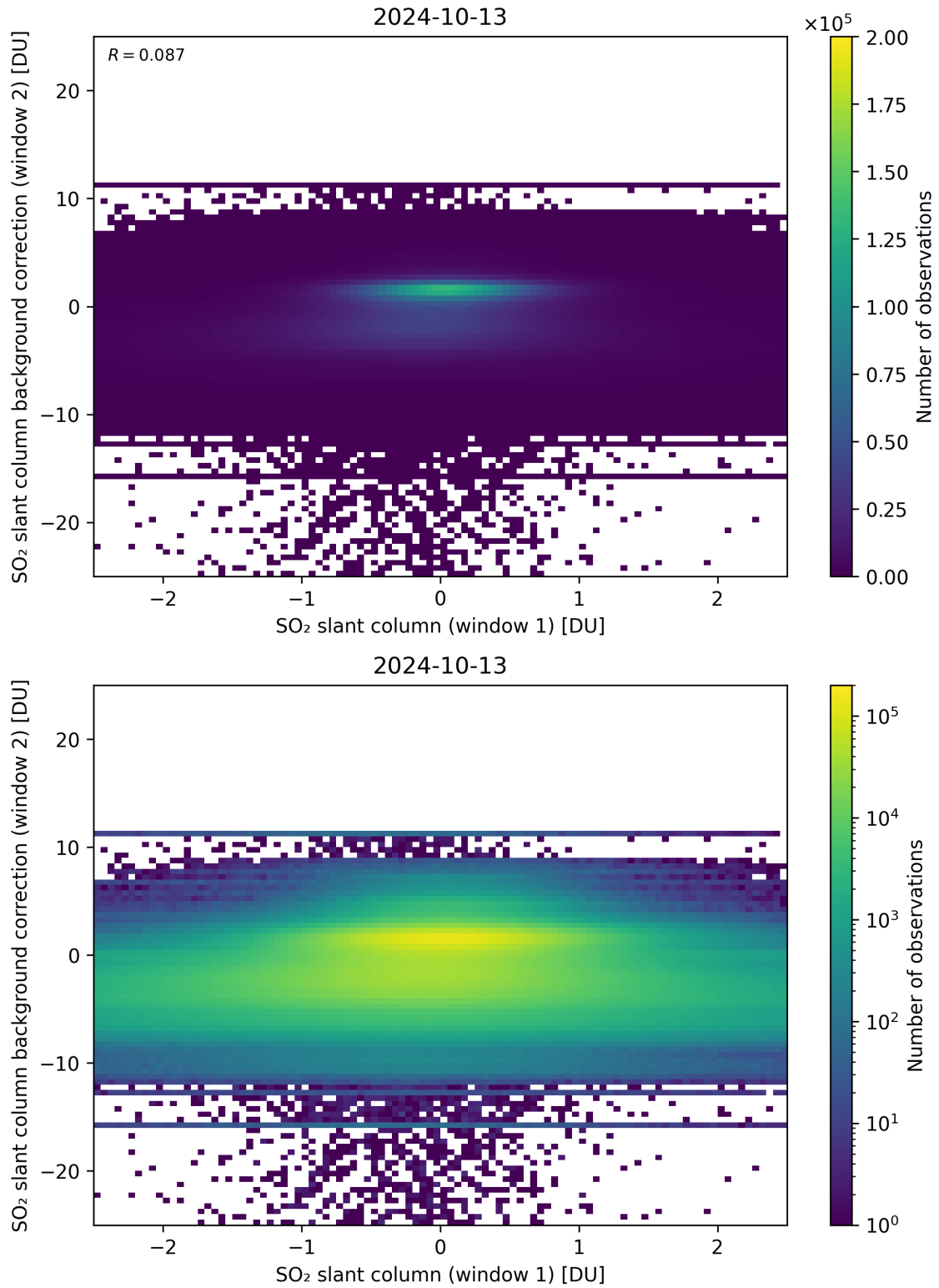
Figure 213: Scatter density plot of “SO 2 slant column (window 1)” against “SO 2 slant column background correction (window 2)” for 2024-10-12 to 2024-10-14.
