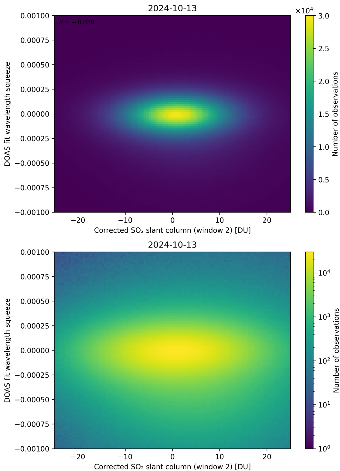
Figure 197: Scatter density plot of “Corrected SO 2 slant column (window 2)” against “DOAS fit wavelength squeeze” for 2024-10-12 to 2024-10-14.
