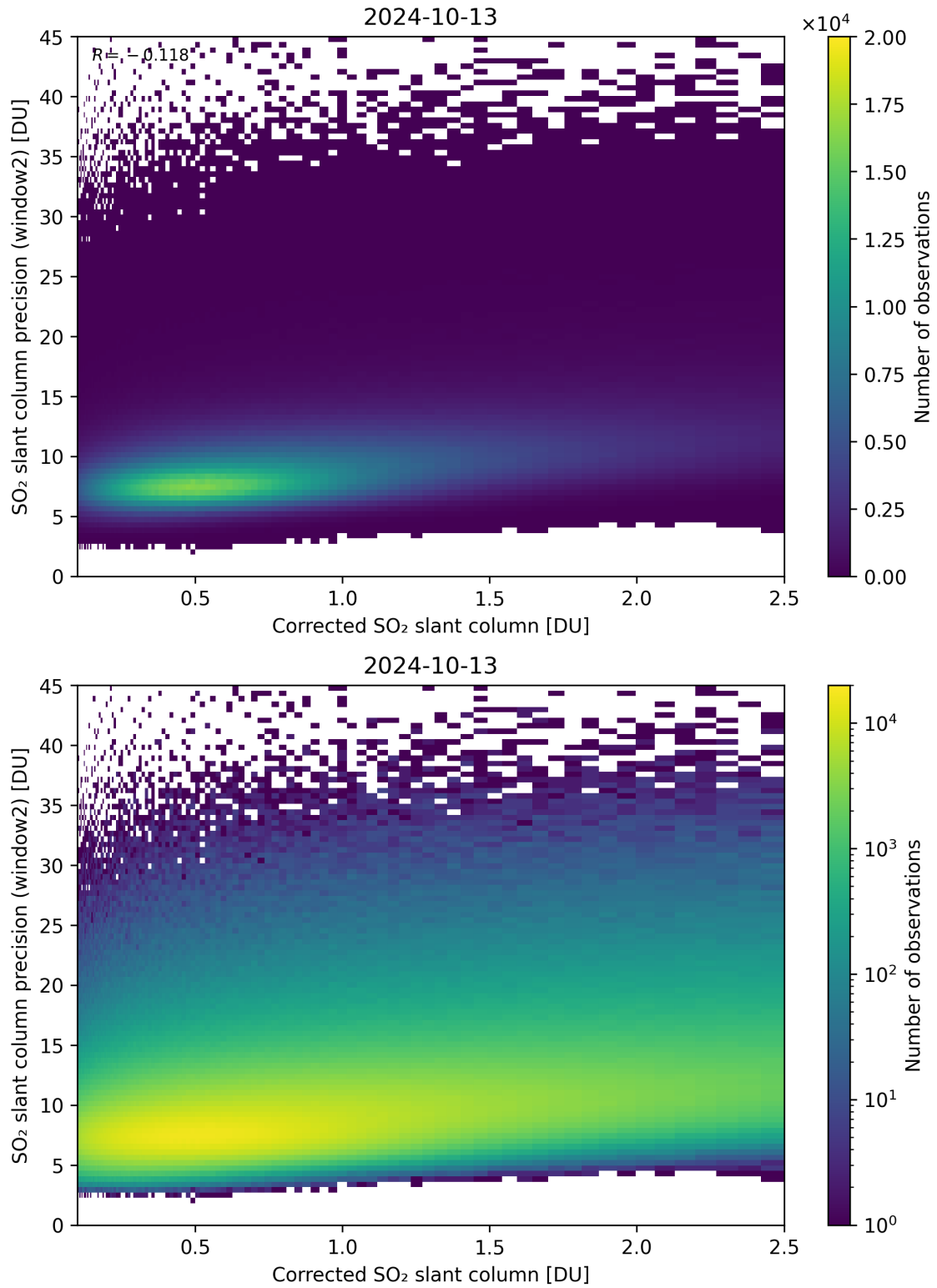
Figure 189: Scatter density plot of “Corrected SO 2 slant column” against “SO 2 slant column precision (window2)” for 2024-10-12 to 2024-10-14.
