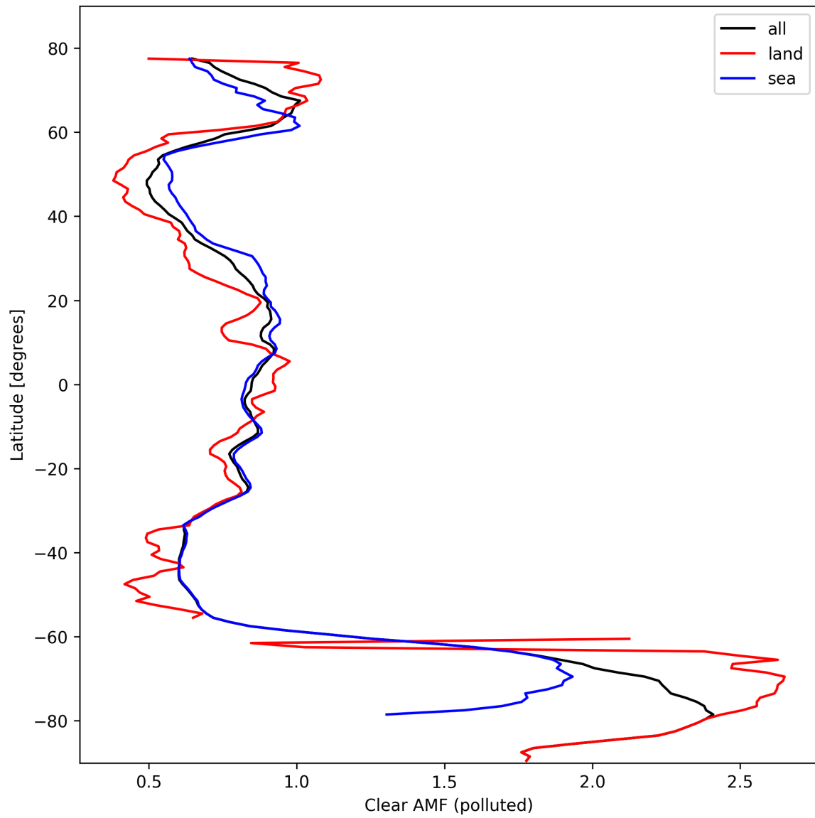
Figure 50: Zonal average of “Clear AMF (polluted)” for 2024-10-12 to 2024-10-14.
