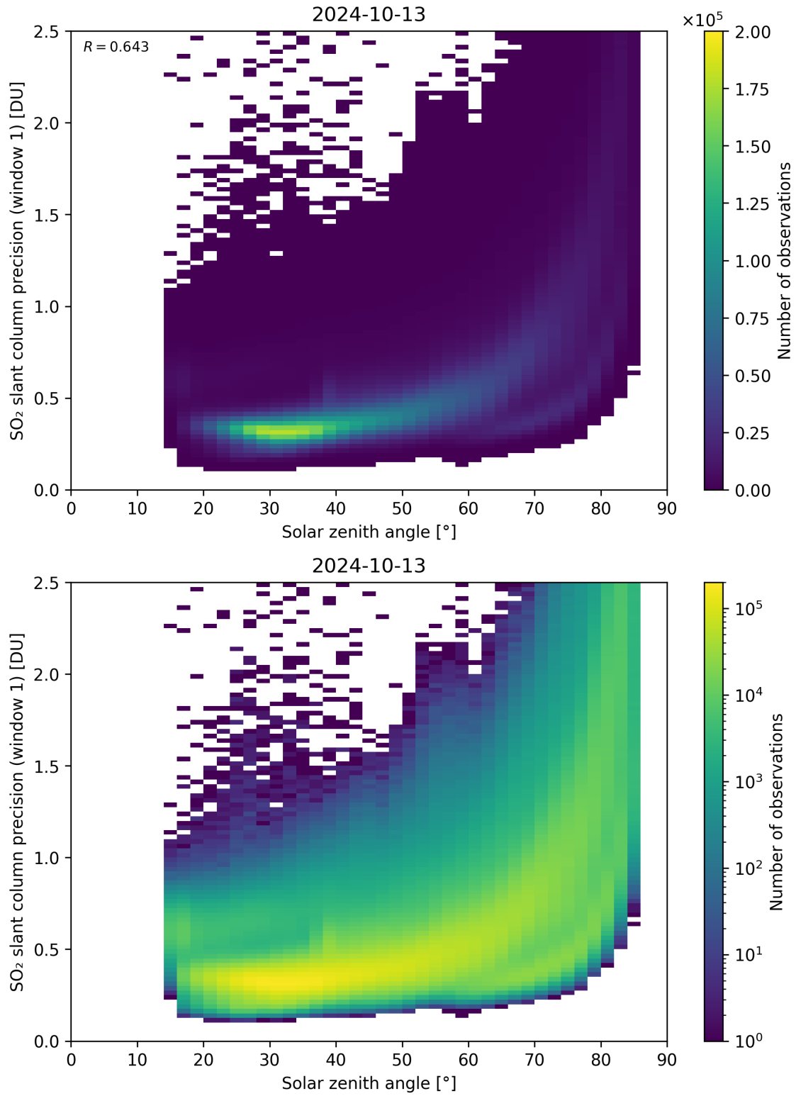
Figure 170: Scatter density plot of “Solar zenith angle” against “SO 2 slant column precision (window 1)” for 2024-10-12 to 2024-10-14.
