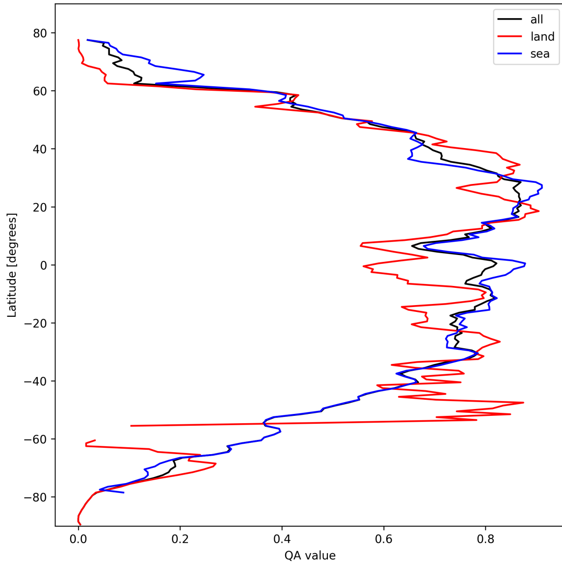
Figure 29: Zonal average of “QA value” for 2024-10-12 to 2024-10-14.
