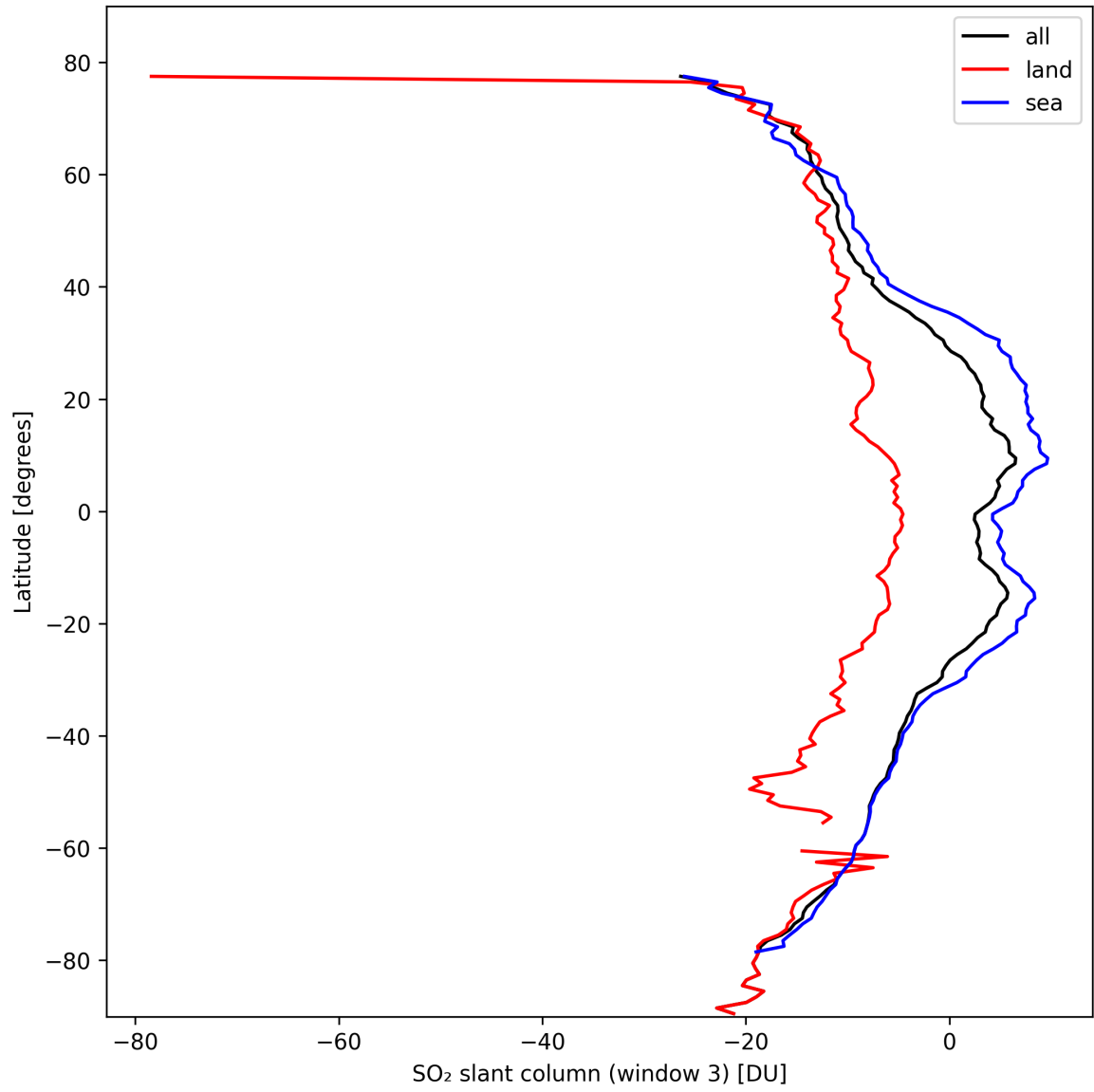
Figure 41: Zonal average of “SO 2 slant column (window 3)” for 2024-10-12 to 2024-10-14.
