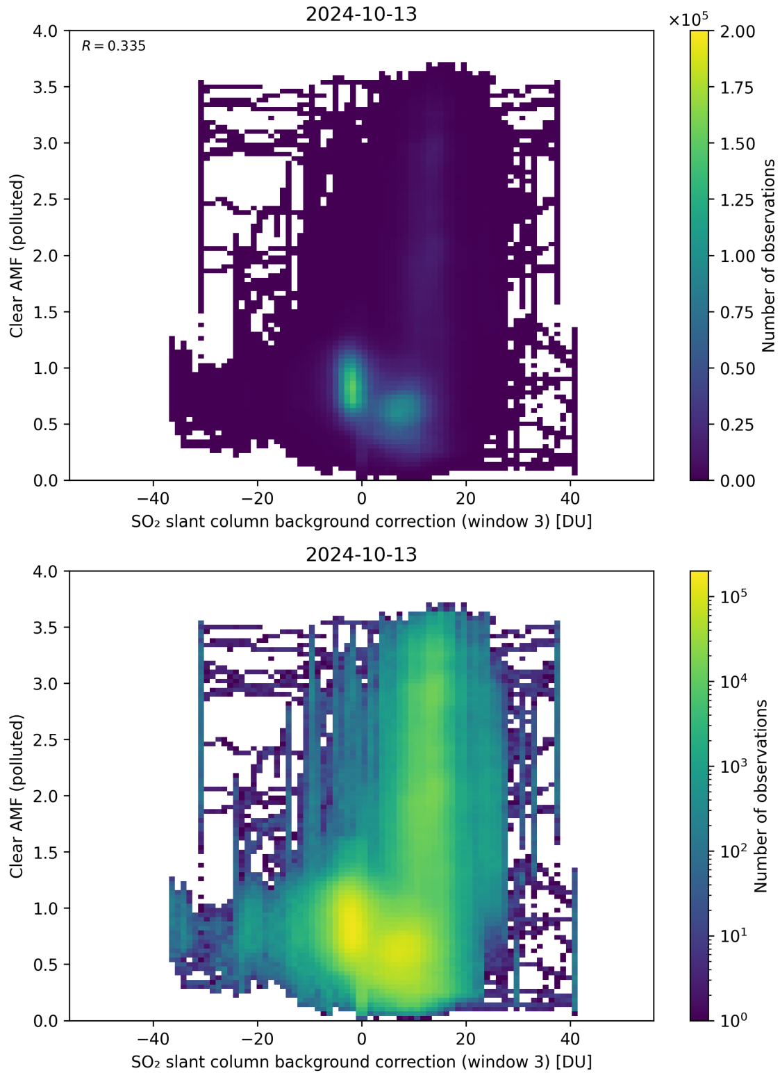
Figure 124: Scatter density plot of “SO 2 slant column background correction (window 3)” against “Clear AMF (polluted)” for 2024-10-12 to 2024-10-14.
