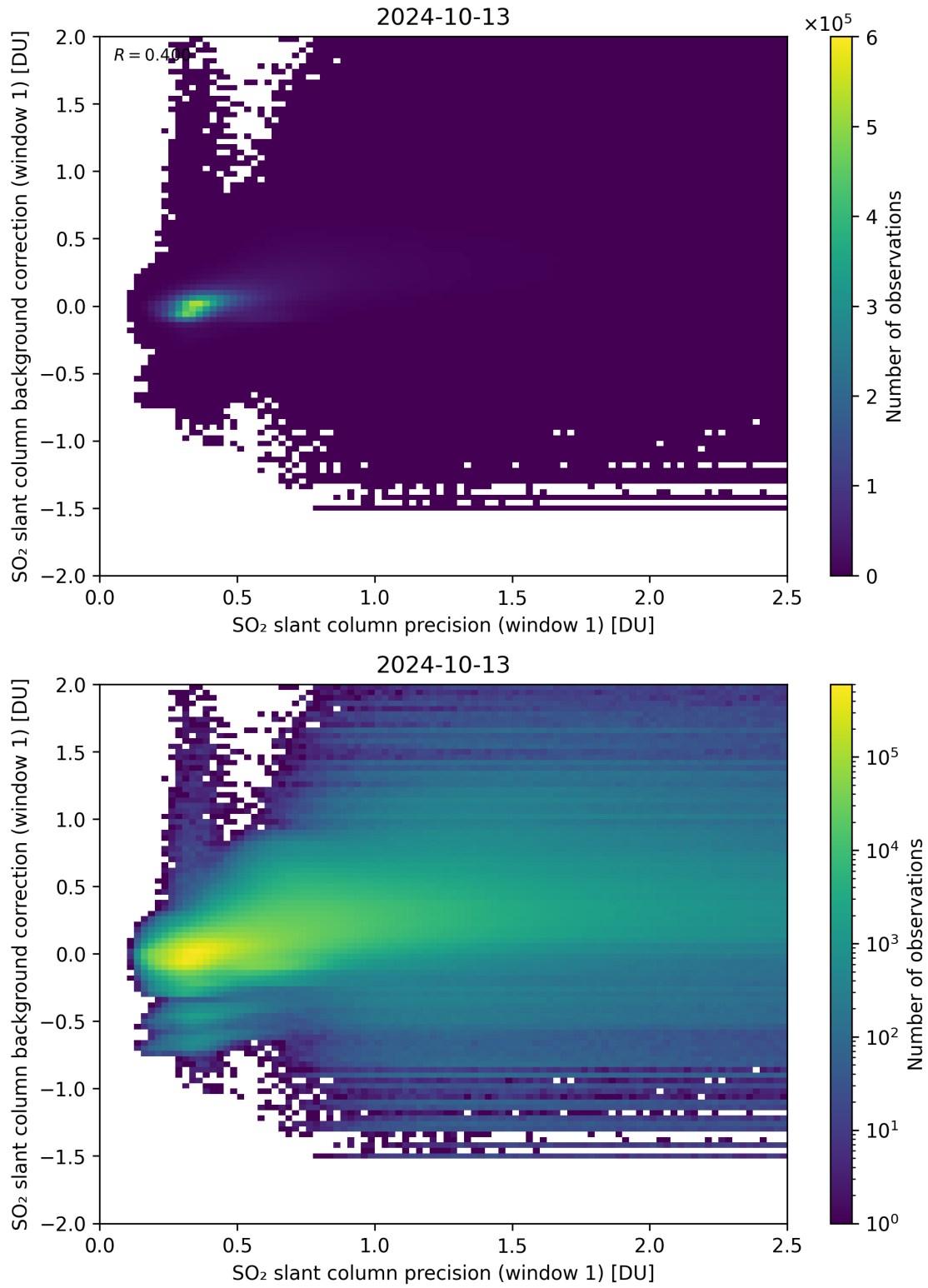
Figure 218: Scatter density plot of “SO 2 slant column precision (window 1)” against “SO 2 slant column background correction (window 1)” for 2024-10-12 to 2024-10-14.
