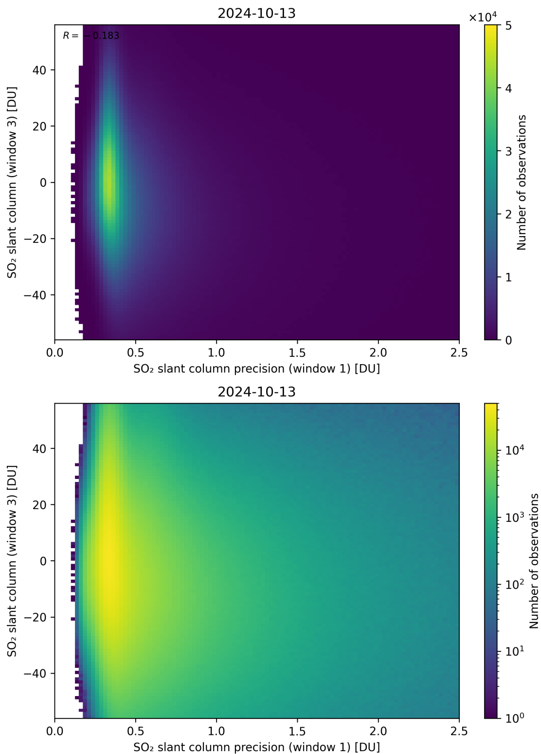
Figure 228: Scatter density plot of “SO 2 slant column precision (window 1)” against “SO 2 slant column (window 3)” for 2024-10-12 to 2024-10-14.
