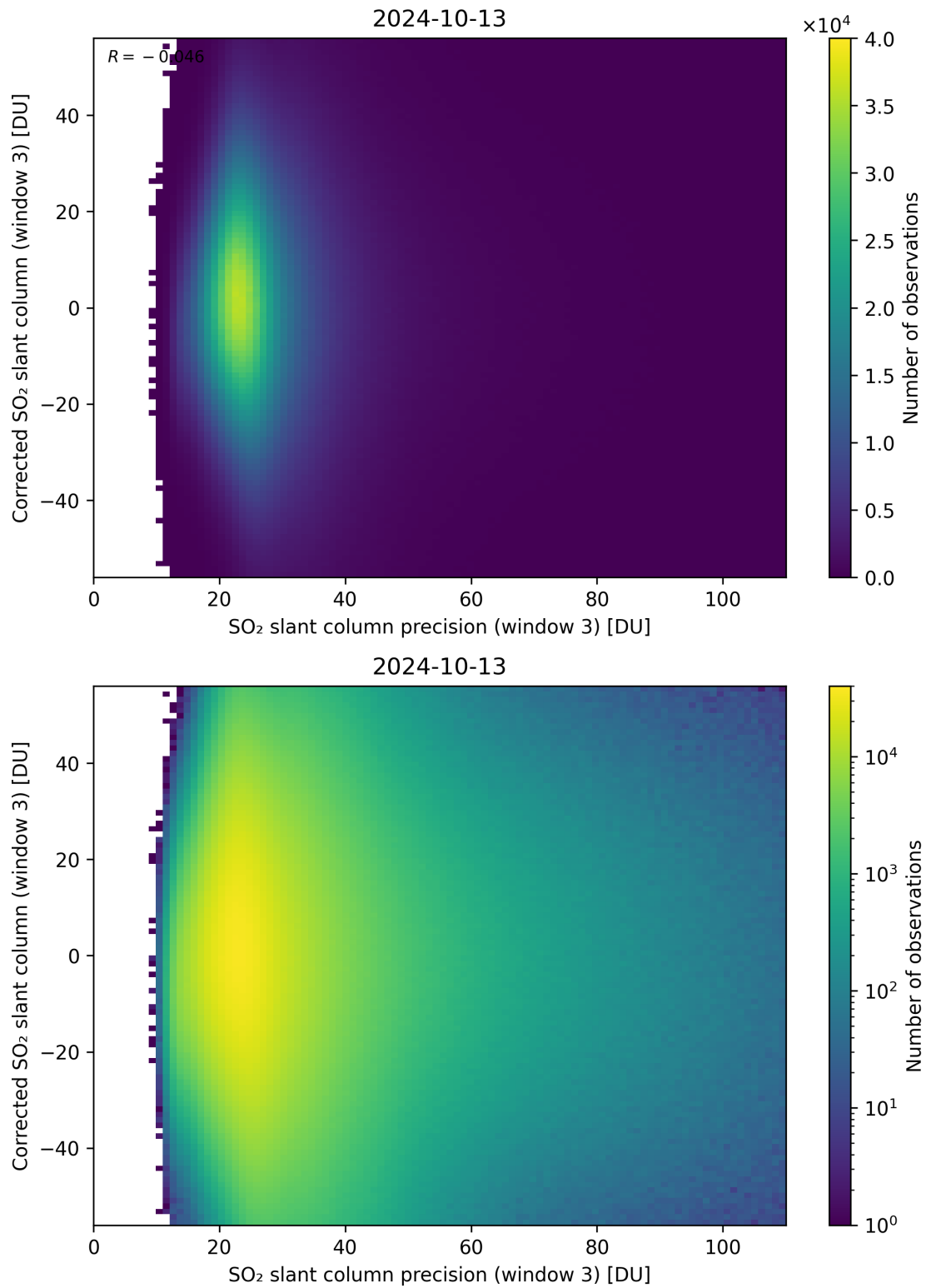
Figure 262: Scatter density plot of “SO 2 slant column precision (window 3)” against “Corrected SO 2 slant column (window 3)” for 2024-10-12 to 2024-10-14.
