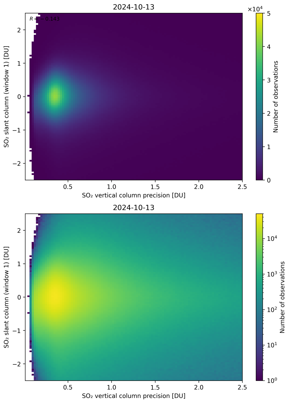
Figure 289: Scatter density plot of “SO 2 vertical column precision” against “SO 2 slant column (window 1)” for 2024-10-12 to 2024-10-14.
