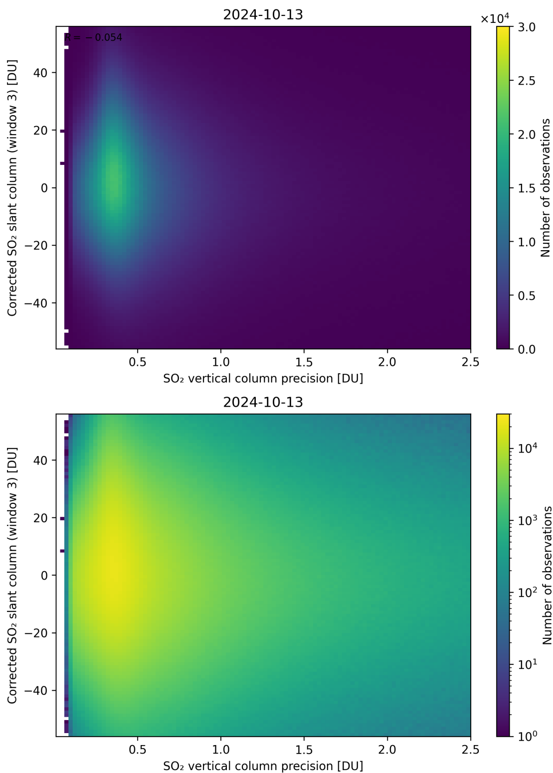
Figure 288: Scatter density plot of “SO 2 vertical column precision” against “Corrected SO 2 slant column (window 3)” for 2024-10-12 to 2024-10-14.
