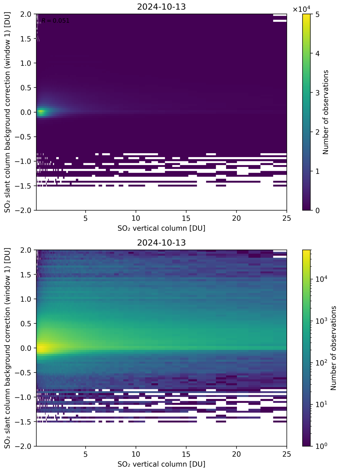
Figure 273: Scatter density plot of “SO 2 vertical column” against “SO 2 slant column background correction (window 1)” for 2024-10-12 to 2024-10-14.
