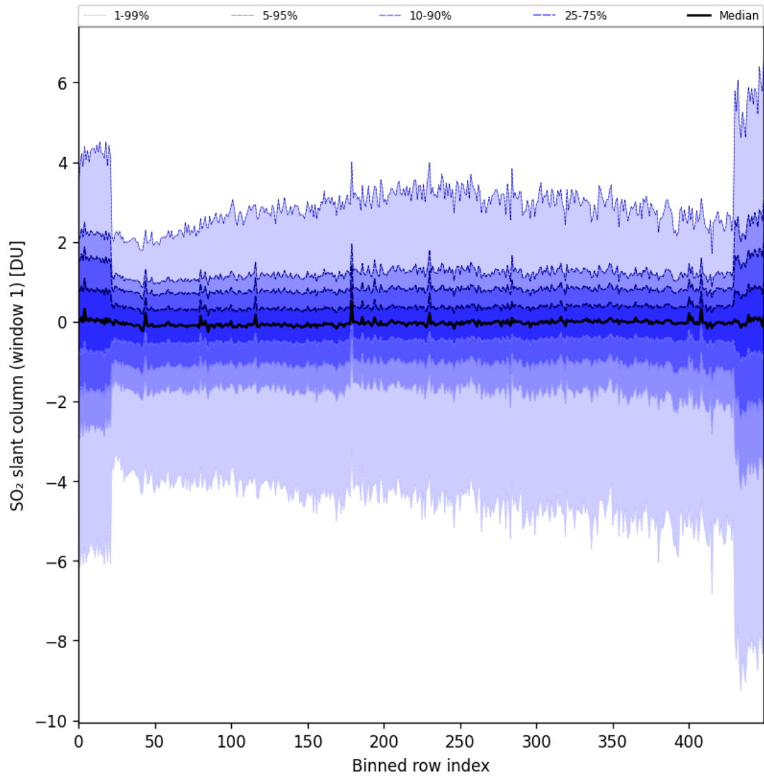
Figure 79: Along track statistics of “SO 2 slant column (window 1)” for 2024-10-12 to 2024-10-14
