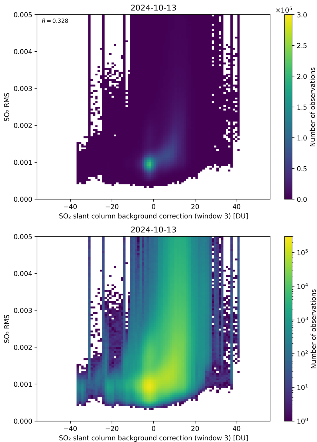
Figure 123: Scatter density plot of “SO 2 slant column background correction (window 3)” against “SO 2 RMS” for 2024-10-12 to 2024-10-14.
