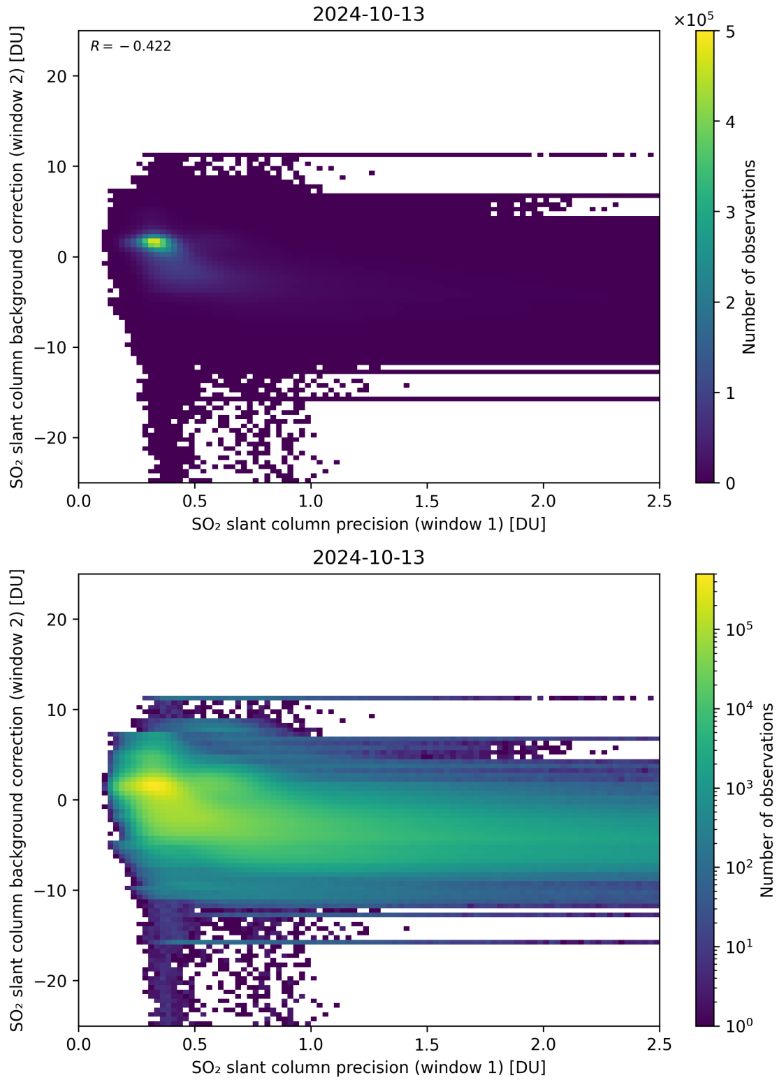
Figure 219: Scatter density plot of “SO 2 slant column precision (window 1)” against “SO 2 slant column background correction (window 2)” for 2024-10-12 to 2024-10-14.
