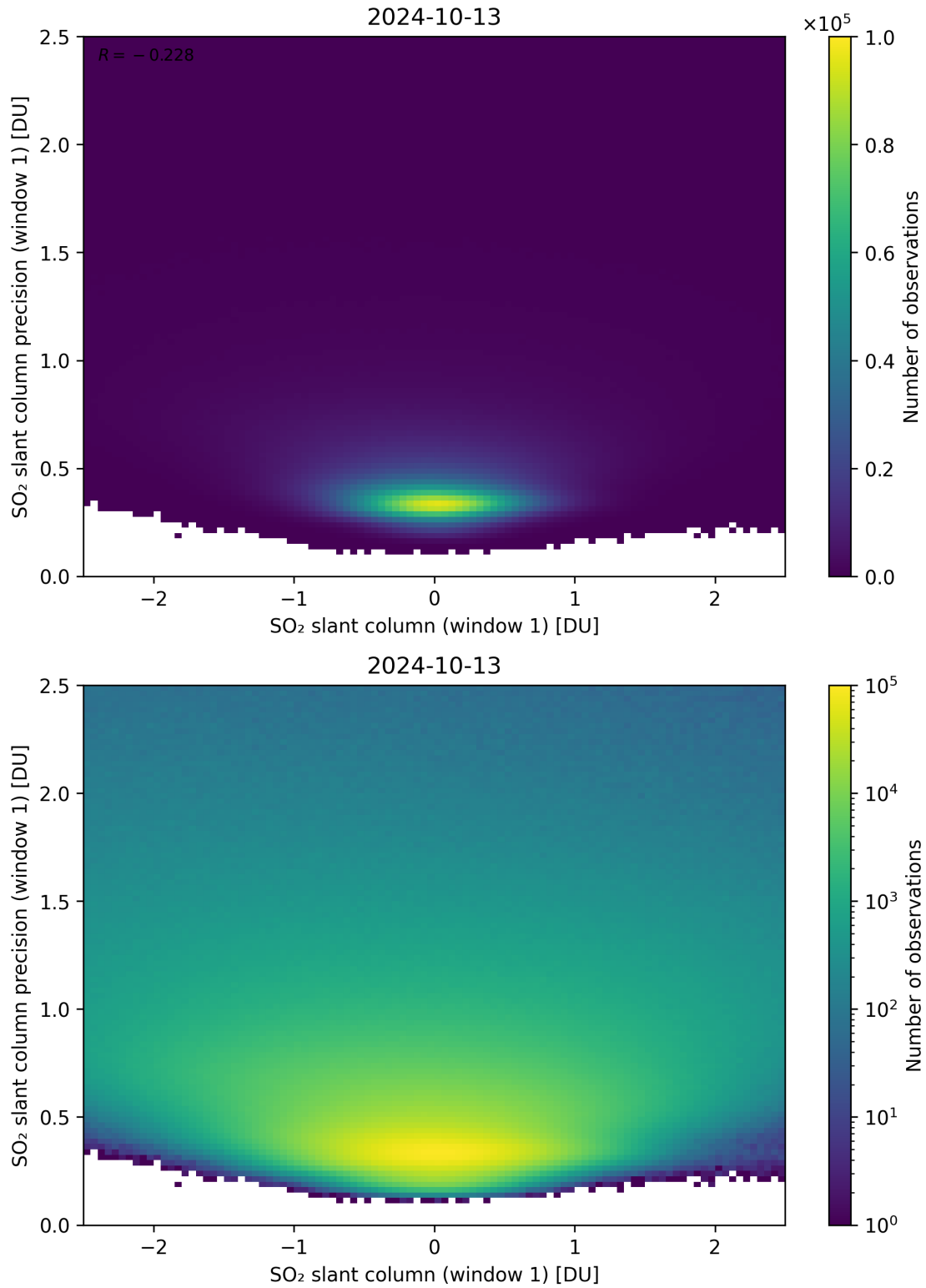
Figure 235: Scatter density plot of “SO 2 slant column (window 1)” against “SO 2 slant column precision (window 1)” for 2024-10-12 to 2024-10-14.
