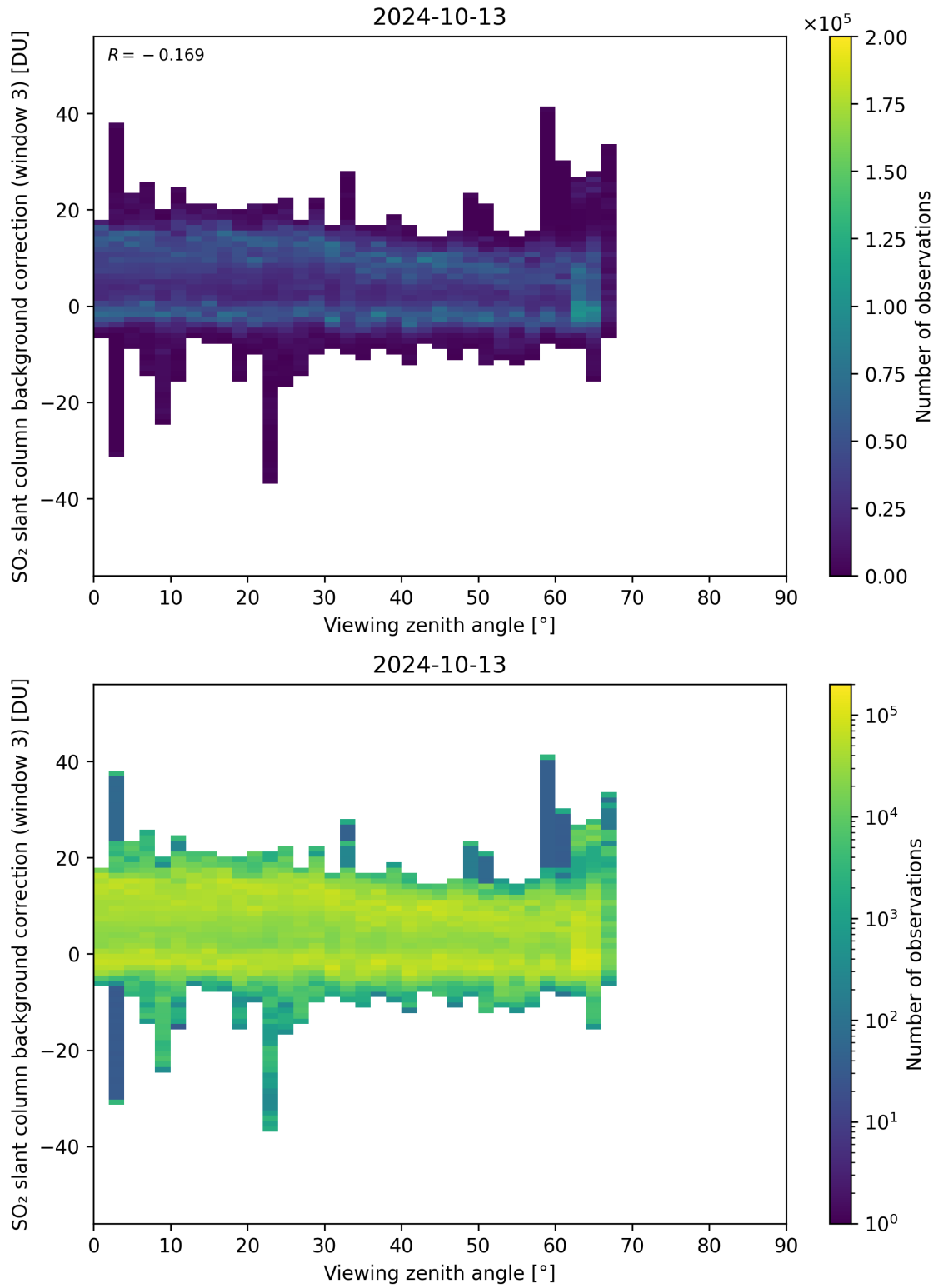
Figure 310: Scatter density plot of “Viewing zenith angle” against “SO 2 slant column background correction (window 3)” for 2024-10-12 to 2024-10-14.
