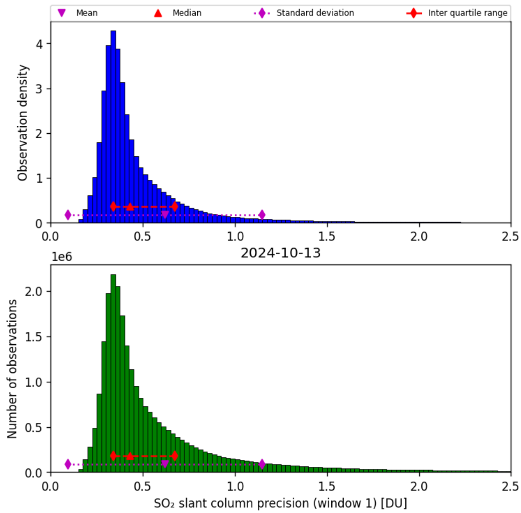
Figure 57: Histogram of “SO 2 slant column precision (window 1)” for 2024-10-12 to 2024-10-14
