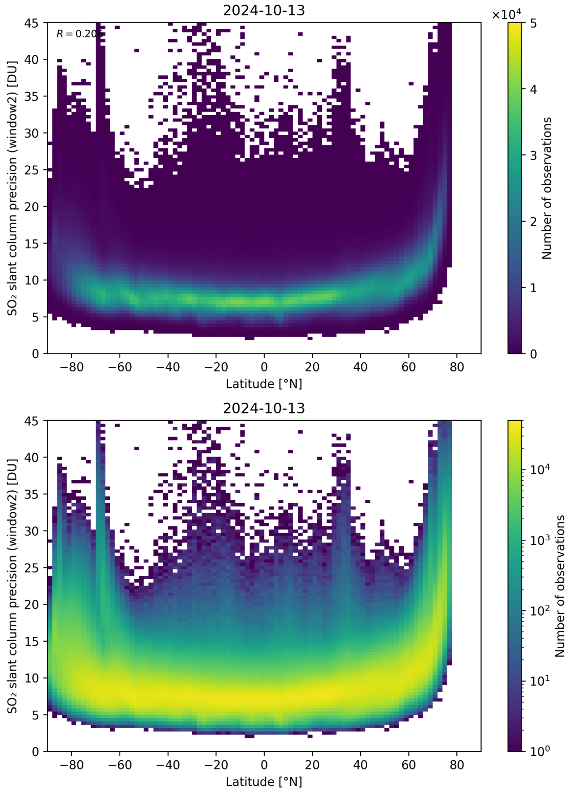
Figure 151: Scatter density plot of “Latitude” against “SO 2 slant column precision (window2)” for 2024-10-12 to 2024-10-14.
