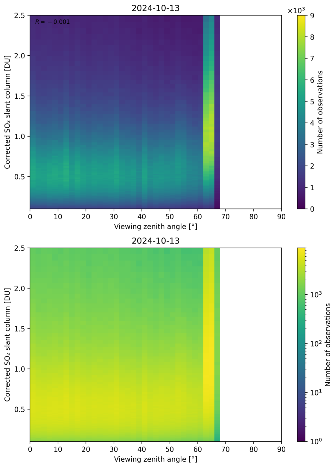
Figure 317: Scatter density plot of “Viewing zenith angle” against “Corrected SO 2 slant column” for 2024-10-12 to 2024-10-14.
