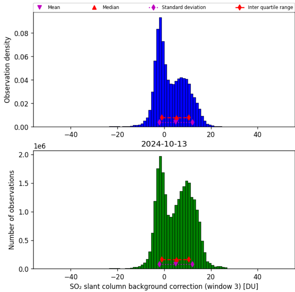
Figure 67: Histogram of “SO 2 slant column background correction (window 3)” for 2024-10-12 to 2024-10-14
