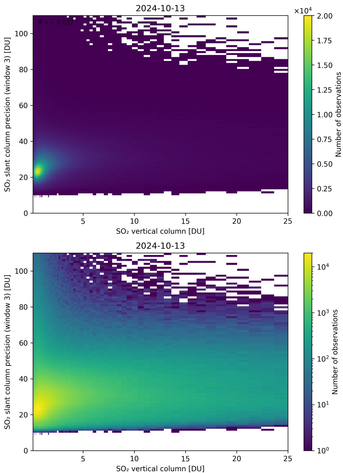
Figure 304: Scatter density plot of “SO 2 vertical column” against “SO 2 slant column precision (window 3)” for 2024-10-12 to 2024-10-14.
