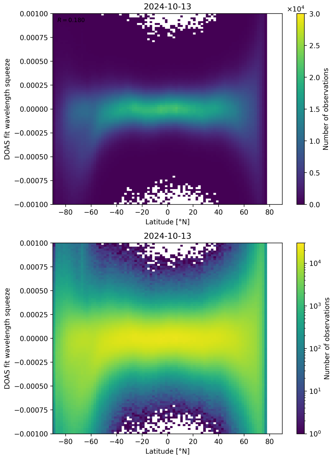
Figure 143: Scatter density plot of “Latitude” against “DOAS fit wavelength squeeze” for 2024-10-12 to 2024-10-14.
