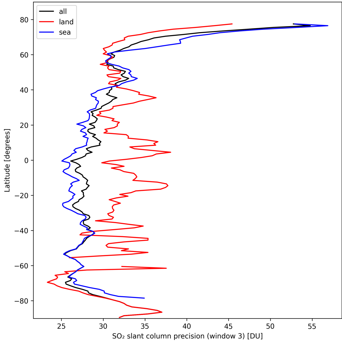
Figure 42: Zonal average of “SO 2 slant column precision (window 3)” for 2024-10-12 to 2024-10-14.
