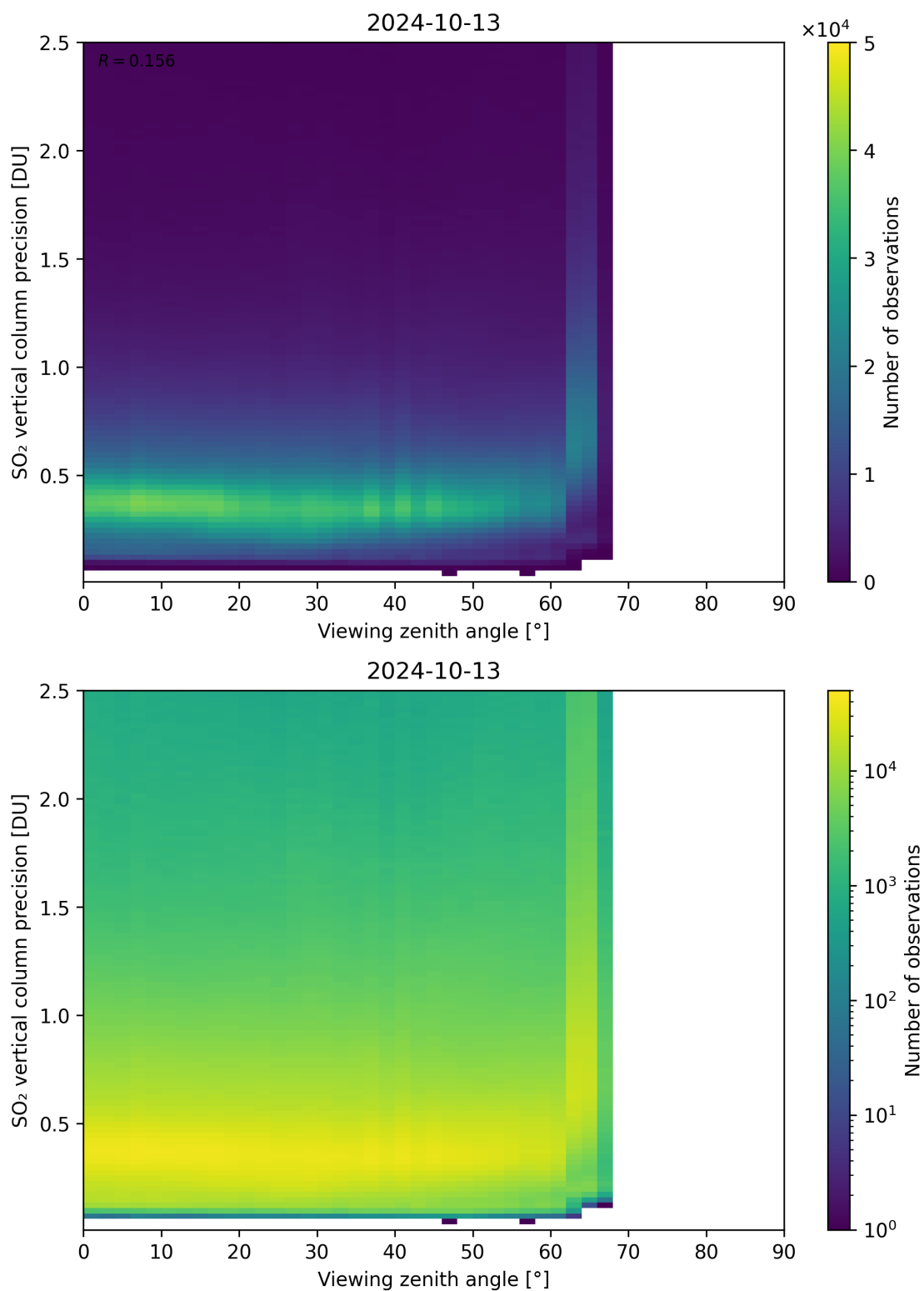
Figure 328: Scatter density plot of “Viewing zenith angle” against “SO 2 vertical column precision” for 2024-10-12 to 2024-10-14.
