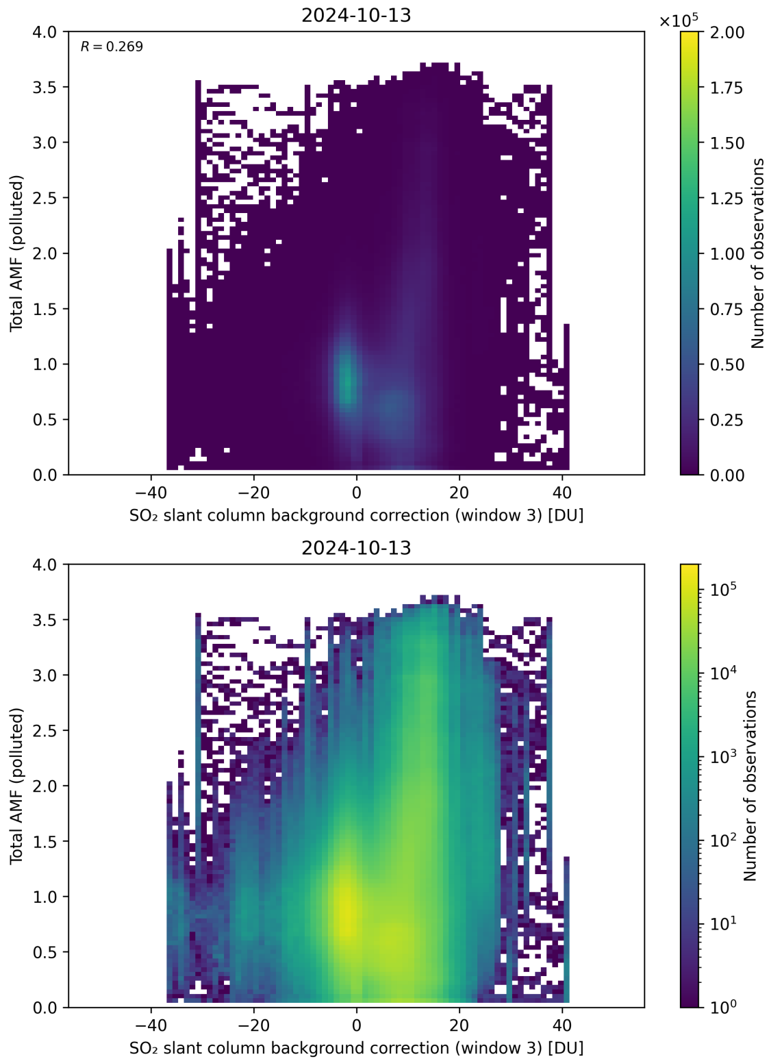
Figure 125: Scatter density plot of “SO 2 slant column background correction (window 3)” against “Total AMF (polluted)” for 2024-10-12 to 2024-10-14.
