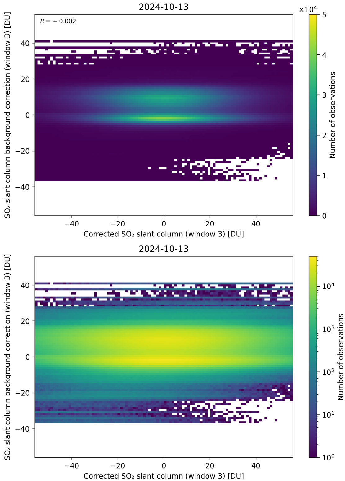
Figure 205: Scatter density plot of “Corrected SO 2 slant column (window 3)” against “SO 2 slant column background correction (window 3)” for 2024-10-12 to 2024-10-14.
