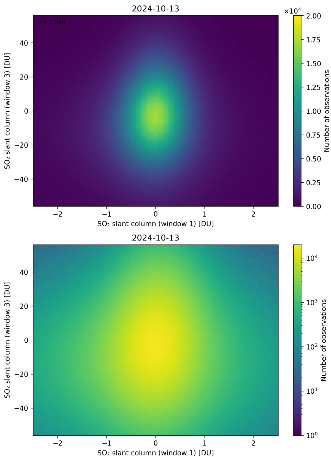
Figure 237: Scatter density plot of “SO 2 slant column (window 1)” against “SO 2 slant column (window 3)” for 2024-10-12 to 2024-10-14.
