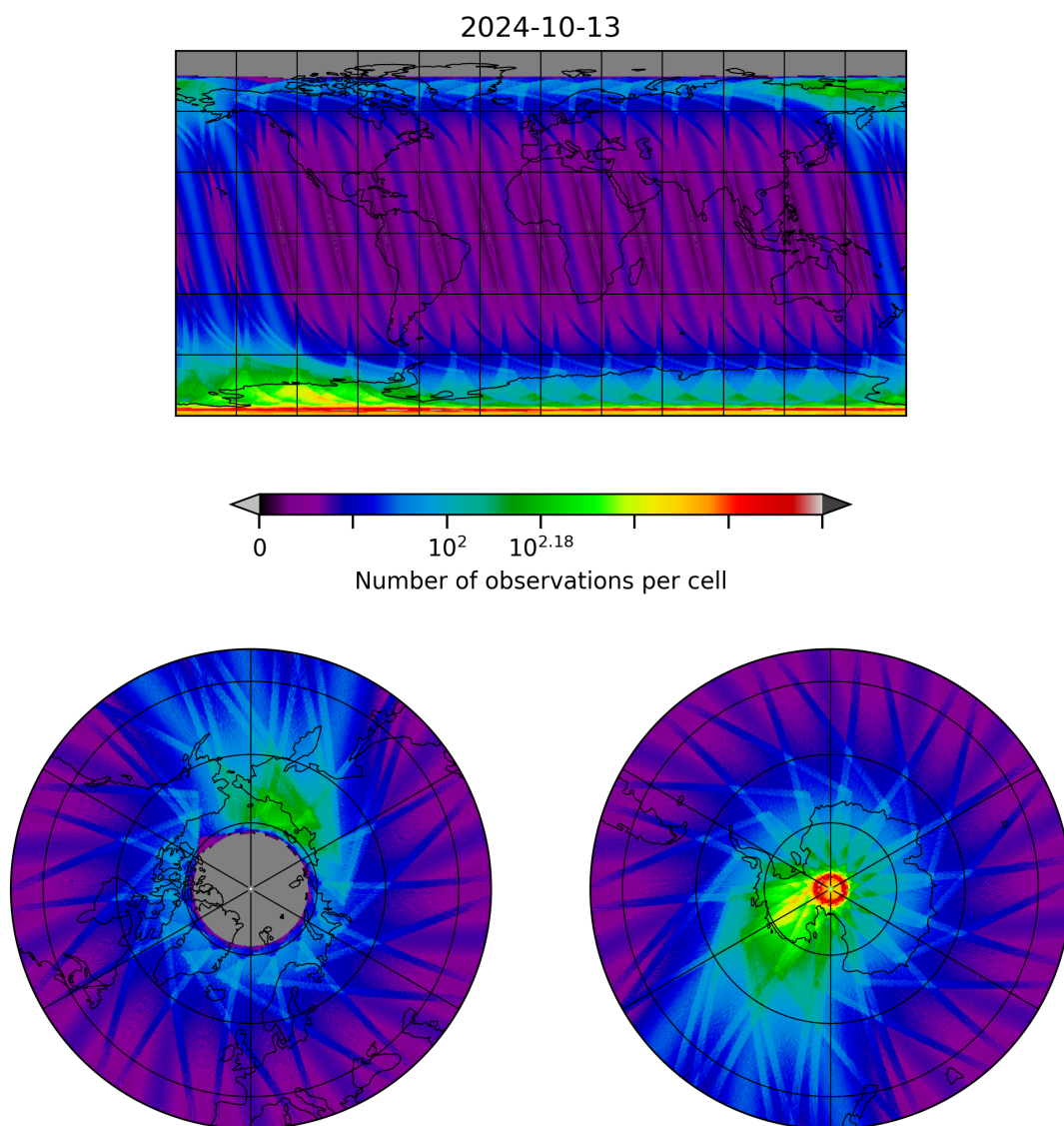
Figure 28: Map of the number of observations for 2024-10-12 to 2024-10-14
