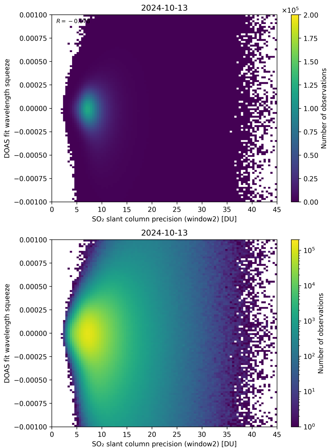
Figure 244: Scatter density plot of “SO 2 slant column precision (window2)” against “DOAS fit wavelength squeeze” for 2024-10-12 to 2024-10-14.
