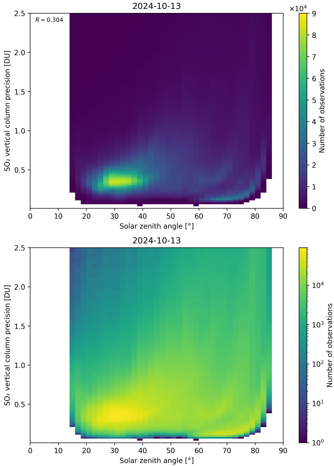
Figure 177: Scatter density plot of “Solar zenith angle” against “SO 2 vertical column precision” for 2024-10-12 to 2024-10-14.
