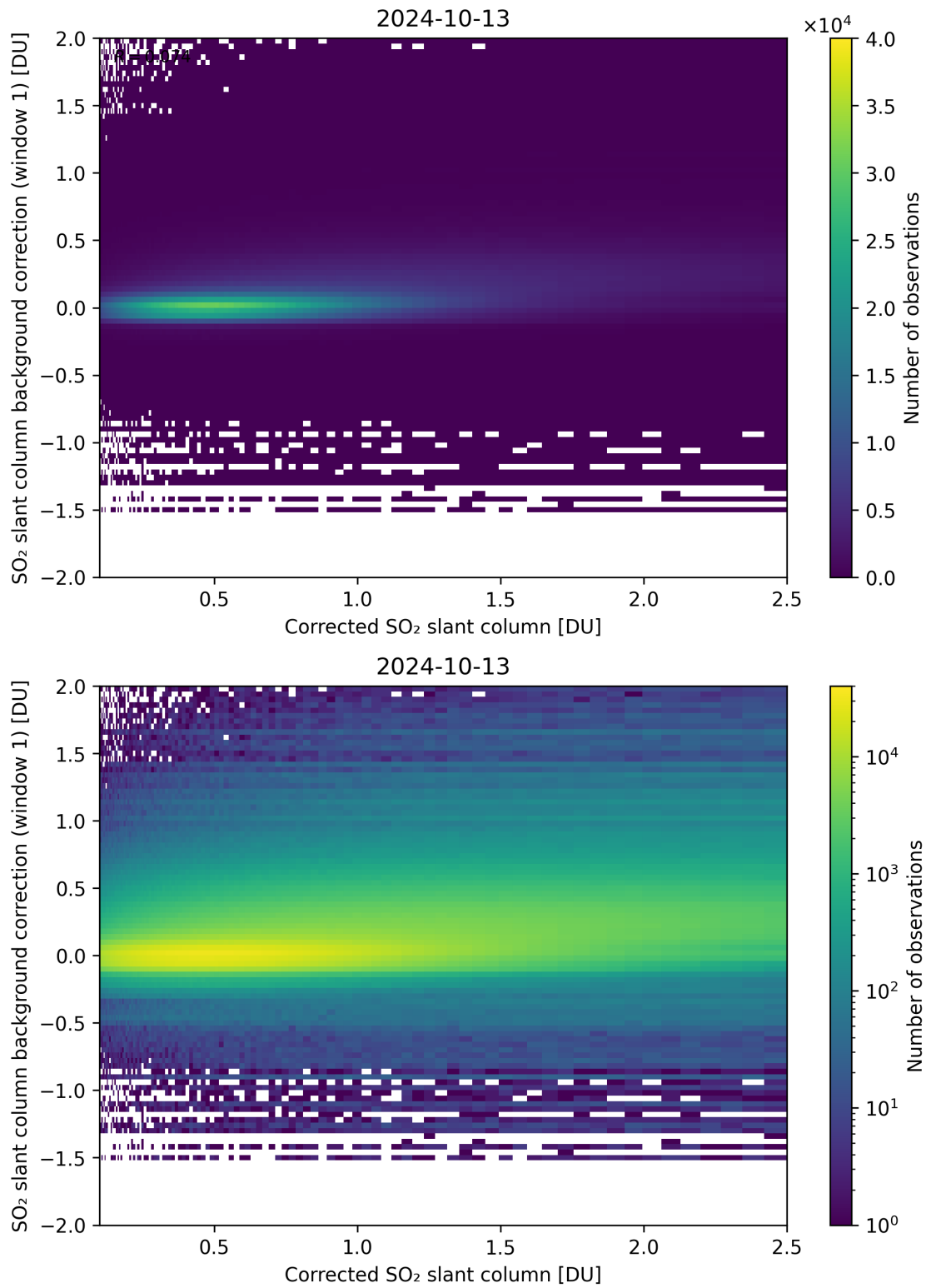
Figure 178: Scatter density plot of “Corrected SO 2 slant column” against “SO 2 slant column background correction (window 1)” for 2024-10-12 to 2024-10-14.
