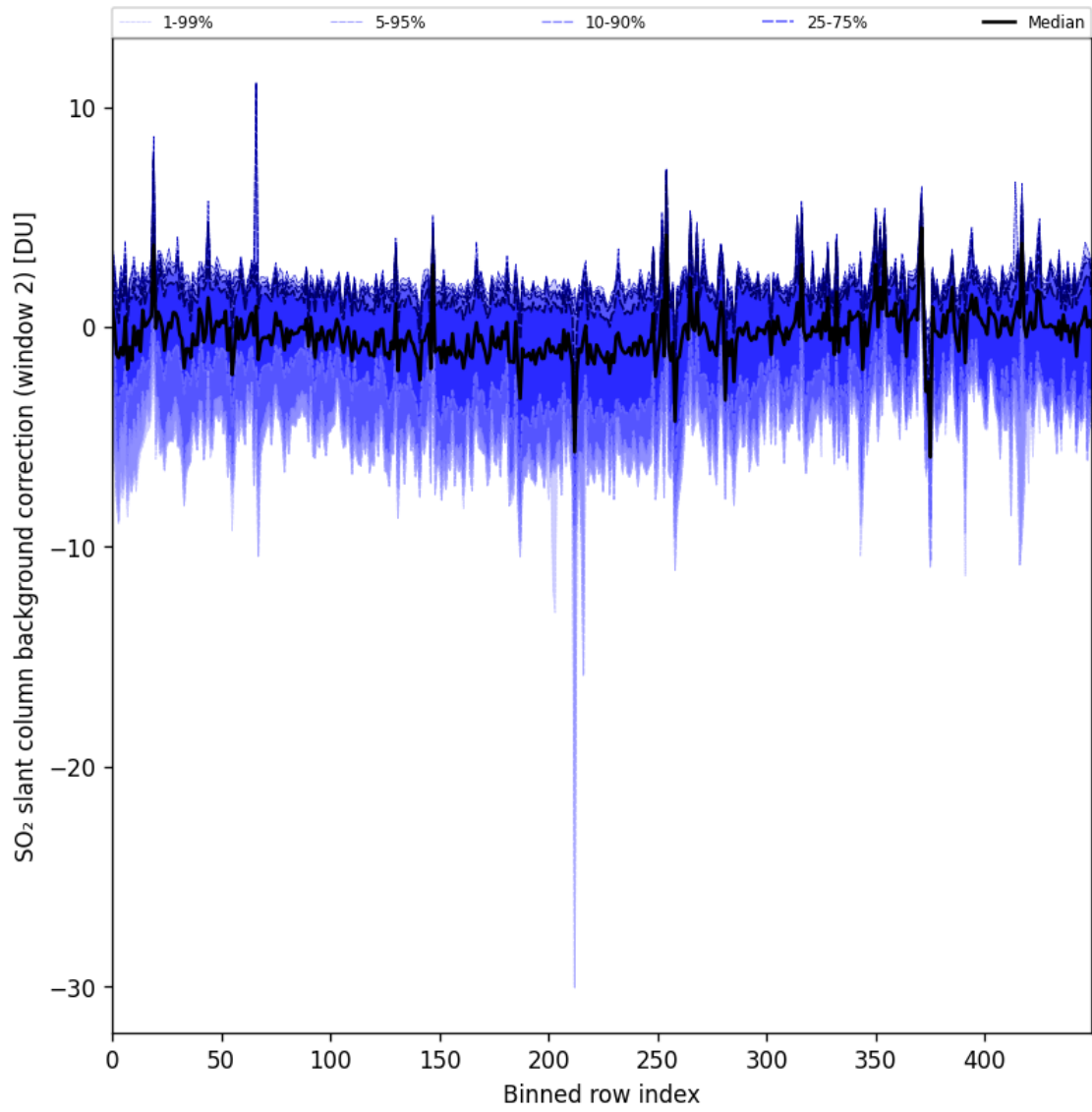
Figure 86: Along track statistics of “SO 2 slant column background correction (window 2)” for 2024-10-12 to 2024-10-14
