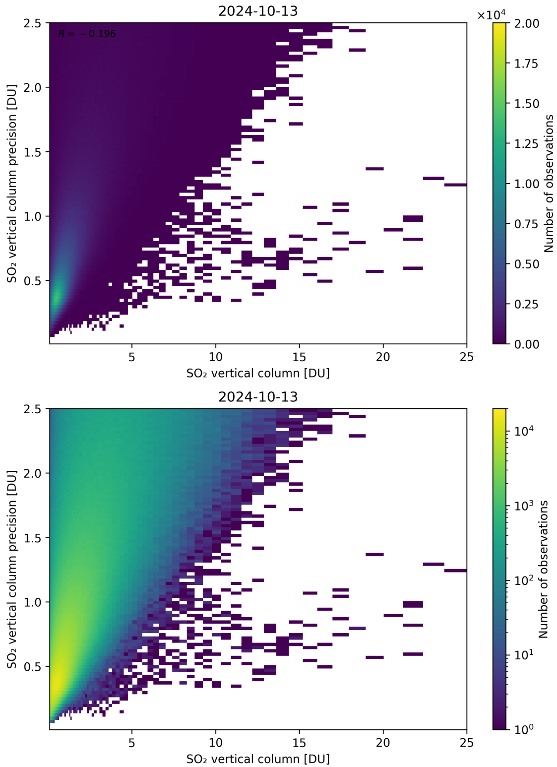
Figure 307: Scatter density plot of “SO 2 vertical column” against “SO 2 vertical column precision” for 2024-10-12 to 2024-10-14.
