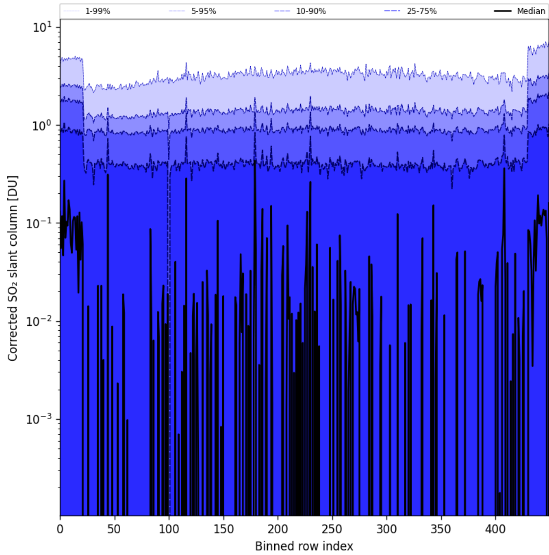
Figure 78: Along track statistics of “Corrected SO 2 slant column” for 2024-10-12 to 2024-10-14
