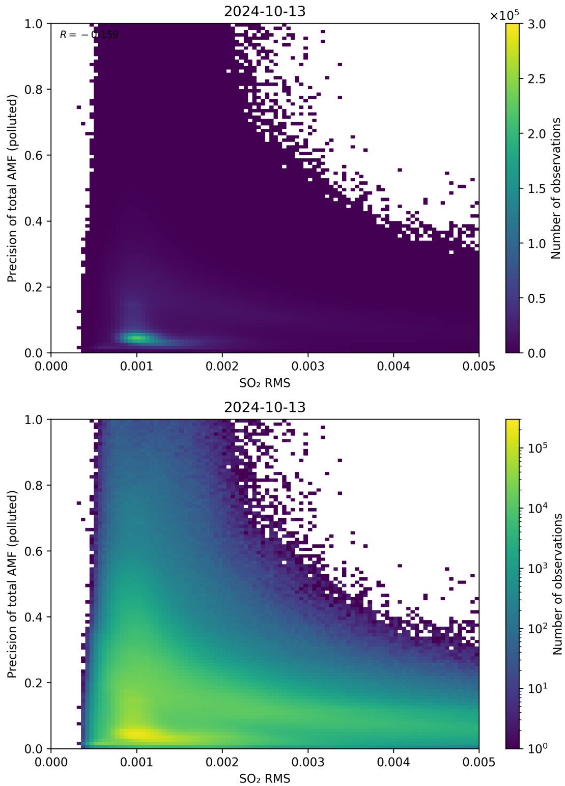
Figure 138: Scatter density plot of “SO 2 RMS” against “Precision of total AMF (polluted)” for 2024-10-12 to 2024-10-14.
