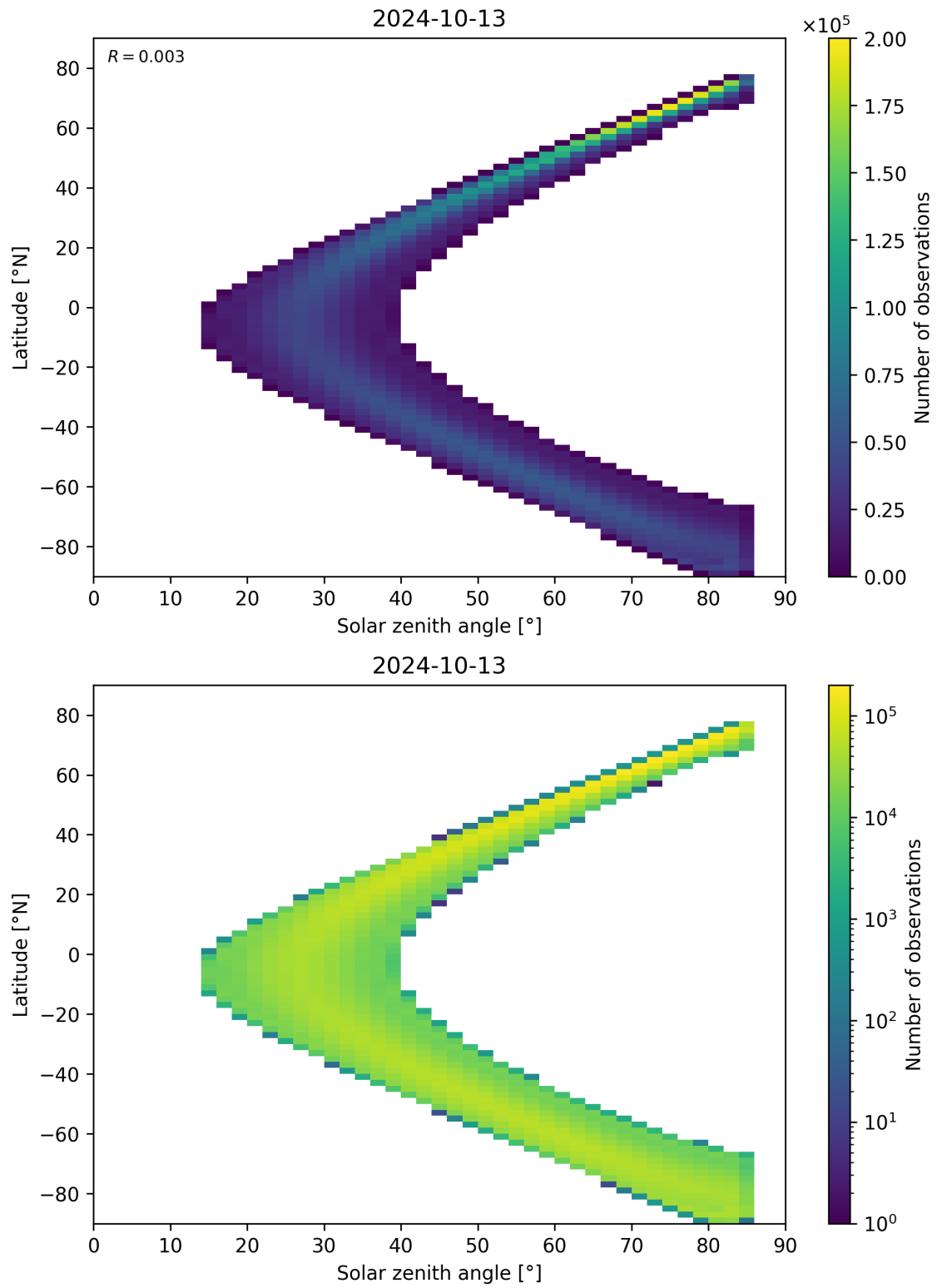
Figure 164: Scatter density plot of “Solar zenith angle” against “Latitude” for 2024-10-12 to 2024-10-14.
