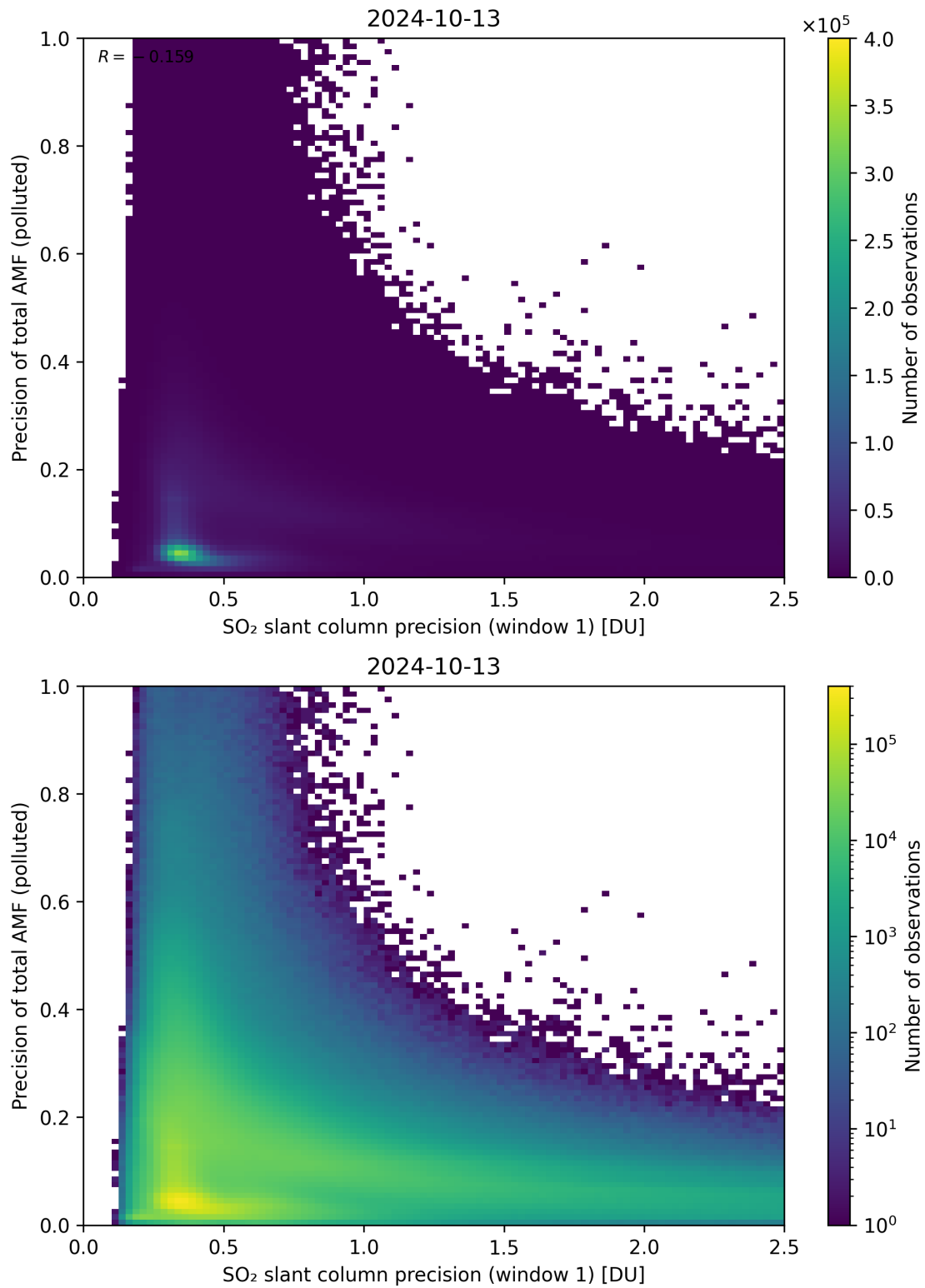
Figure 231: Scatter density plot of “SO 2 slant column precision (window 1)” against “Precision of total AMF (polluted)” for 2024-10-12 to 2024-10-14.
