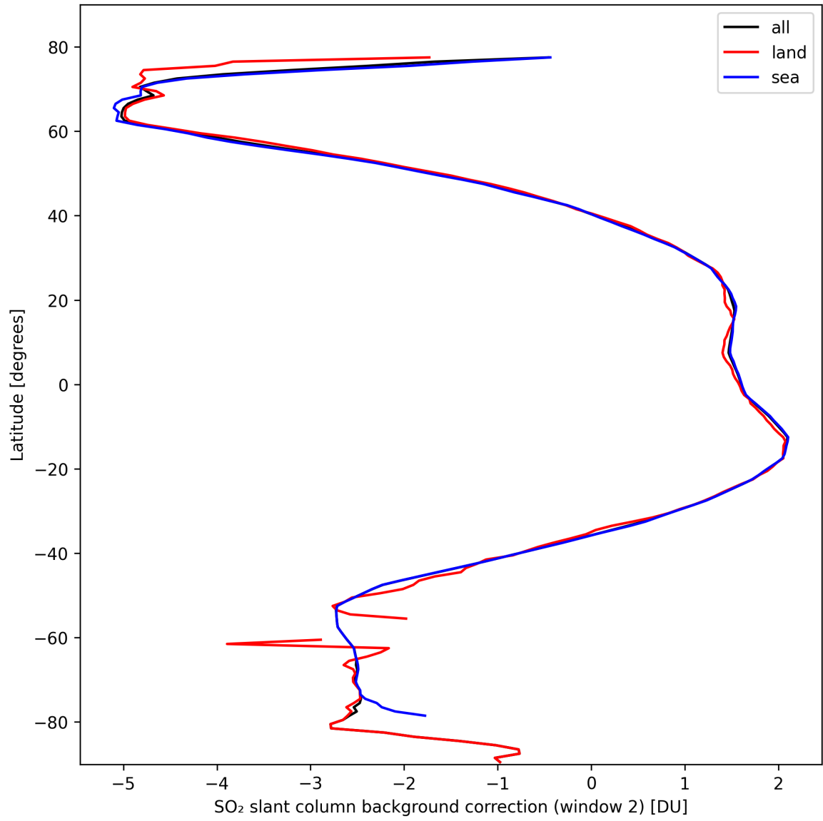
Figure 40: Zonal average of “SO 2 slant column background correction (window 2)” for 2024-10-12 to 2024-10-14.
