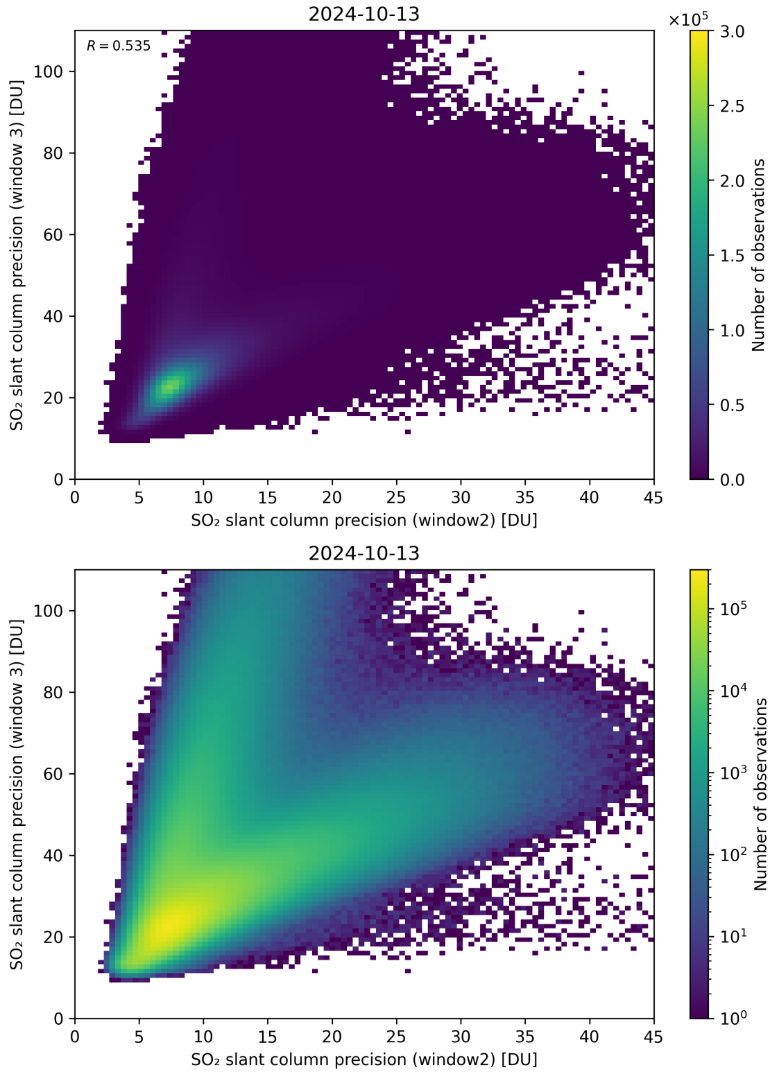
Figure 250: Scatter density plot of “SO 2 slant column precision (window2)” against “SO 2 slant column precision (window 3)” for 2024-10-12 to 2024-10-14.
