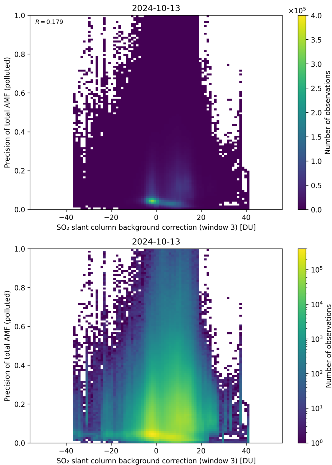
Figure 126: Scatter density plot of “SO 2 slant column background correction (window 3)” against “Precision of total AMF (polluted)” for 2024-10-12 to 2024-10-14.
