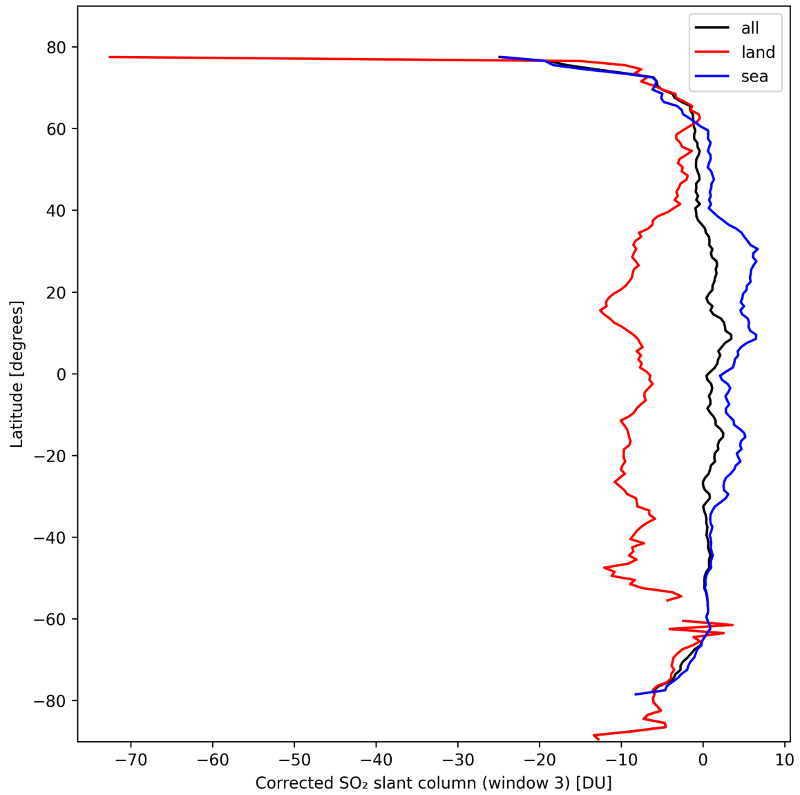
Figure 43: Zonal average of “Corrected SO 2 slant column (window 3)” for 2024-10-12 to 2024-10-14.
