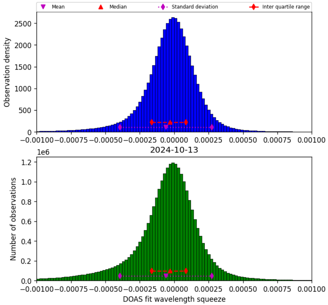
Figure 69: Histogram of “DOAS fit wavelength squeeze” for 2024-10-12 to 2024-10-14
