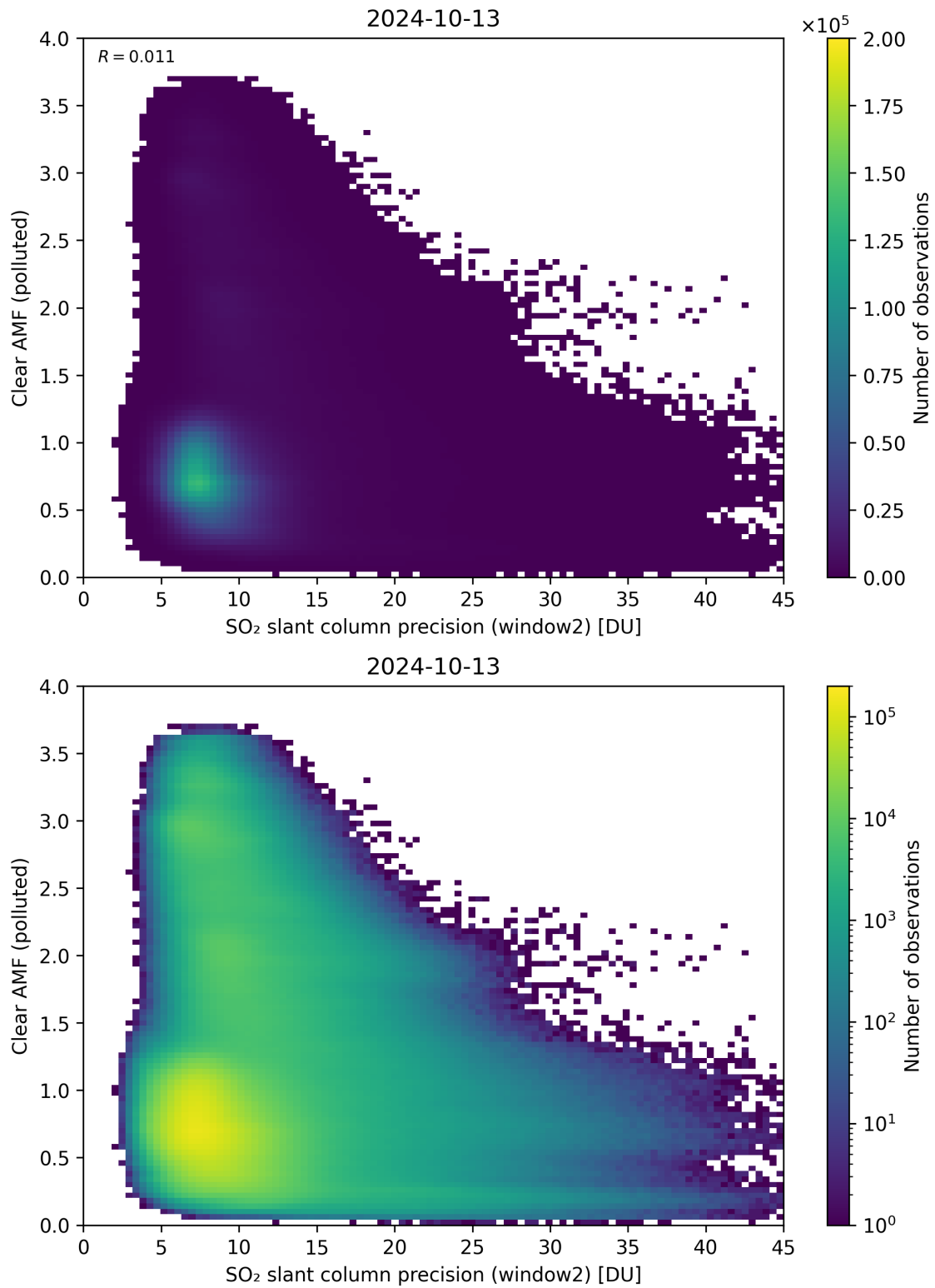
Figure 246: Scatter density plot of “SO 2 slant column precision (window2)” against “Clear AMF (polluted)” for 2024-10-12 to 2024-10-14.
