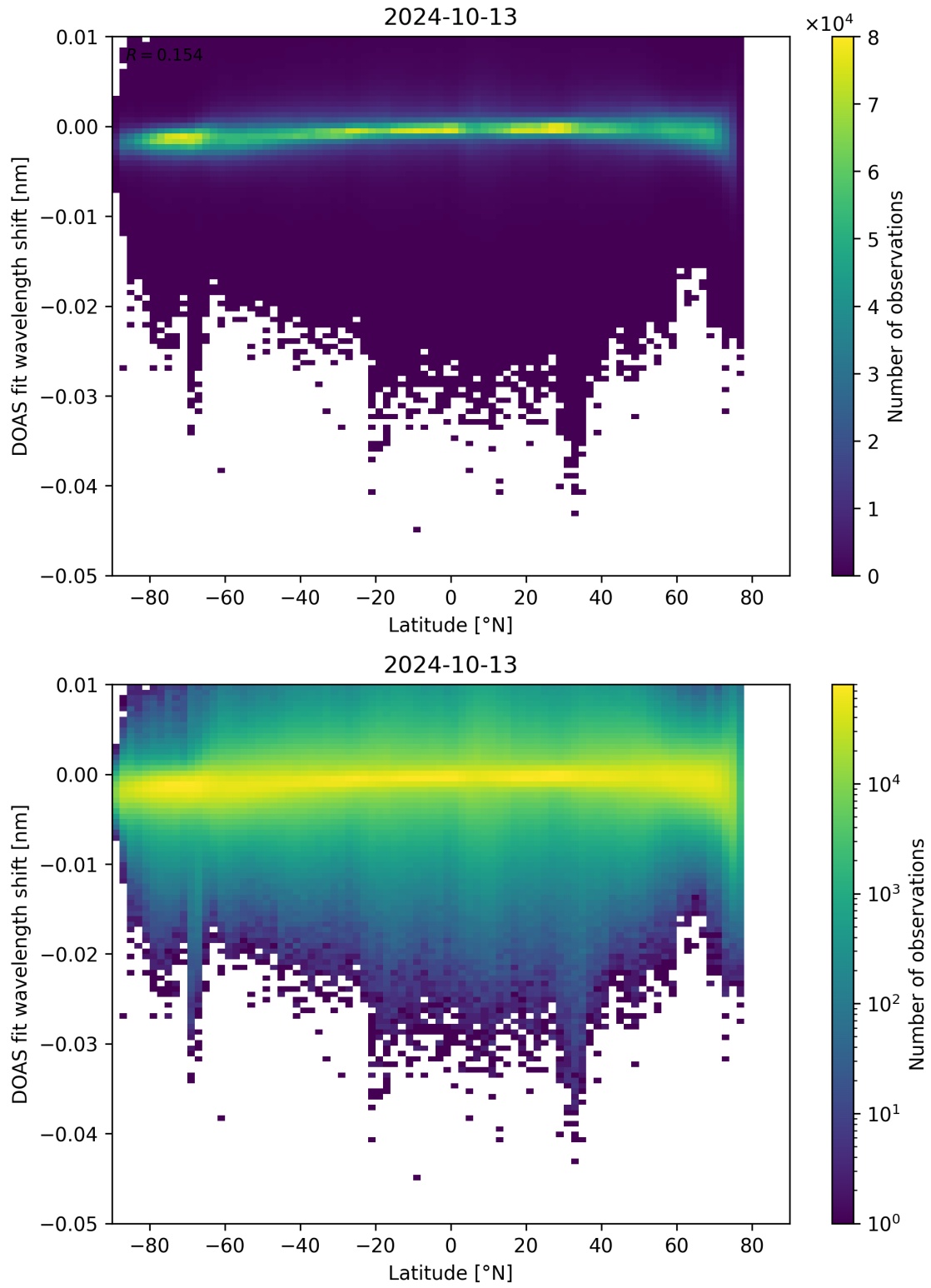
Figure 142: Scatter density plot of “Latitude” against “DOAS fit wavelength shift” for 2024-10-12 to 2024-10-14.
