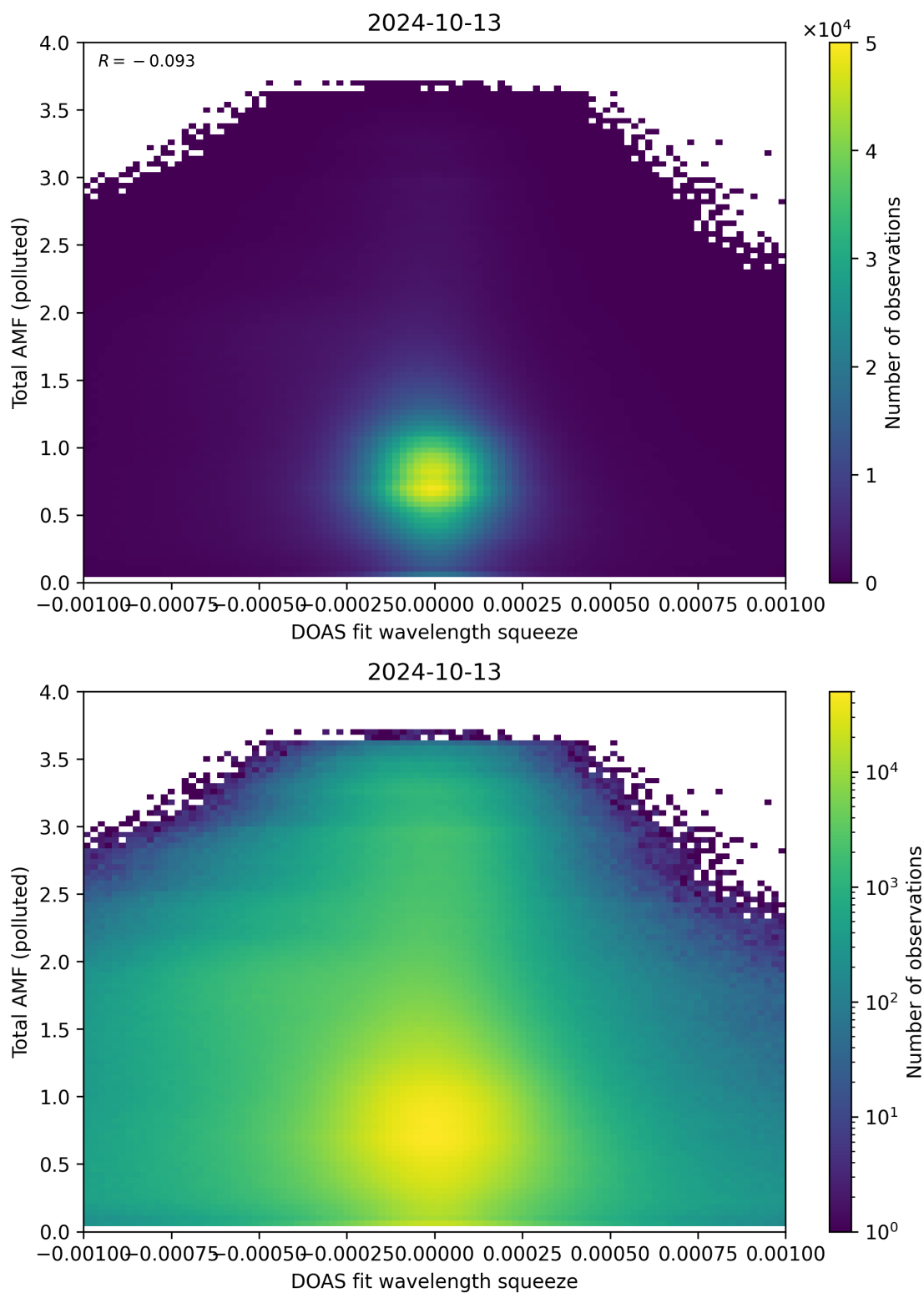
Figure 134: Scatter density plot of “DOAS fit wavelength squeeze” against “Total AMF (polluted)” for 2024-10-12 to 2024-10-14.
