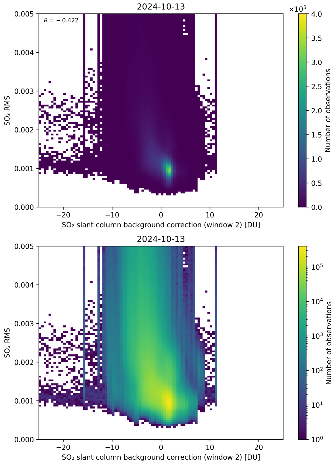
Figure 114: Scatter density plot of “SO 2 slant column background correction (window 2)” against “SO 2 RMS” for 2024-10-12 to 2024-10-14.
