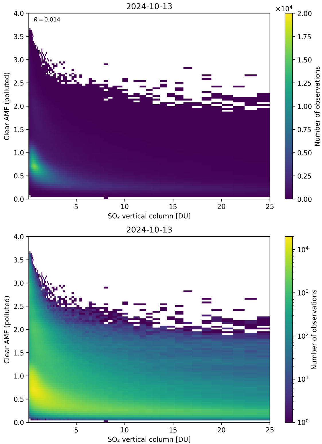
Figure 296: Scatter density plot of “SO 2 vertical column” against “Clear AMF (polluted)” for 2024-10-12 to 2024-10-14.
