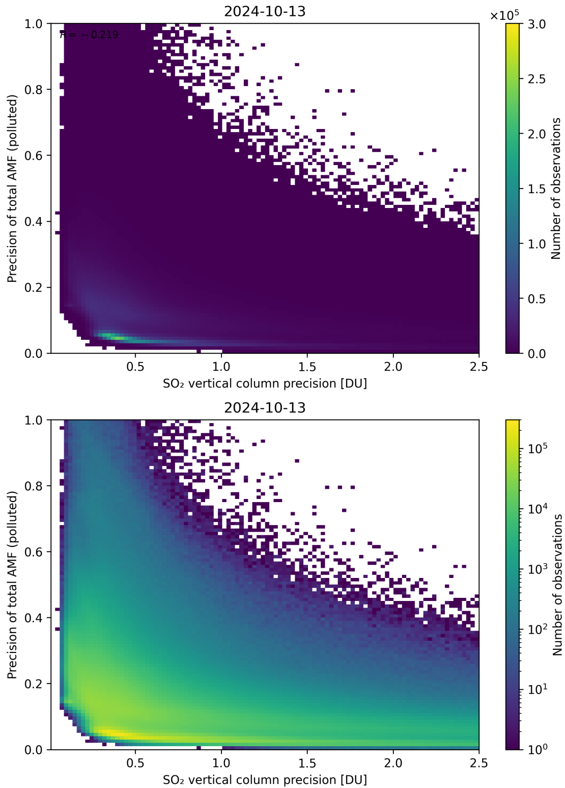
Figure 295: Scatter density plot of “SO 2 vertical column precision” against “Precision of total AMF (polluted)” for 2024-10-12 to 2024-10-14.
