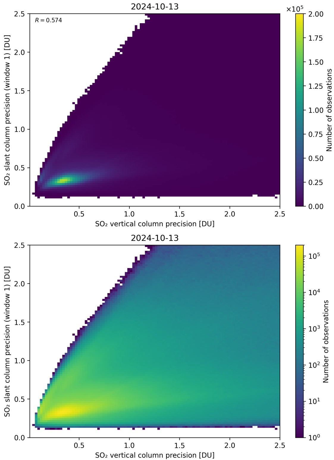
Figure 290: Scatter density plot of “SO 2 vertical column precision” against “SO 2 slant column precision (window 1)” for 2024-10-12 to 2024-10-14.
