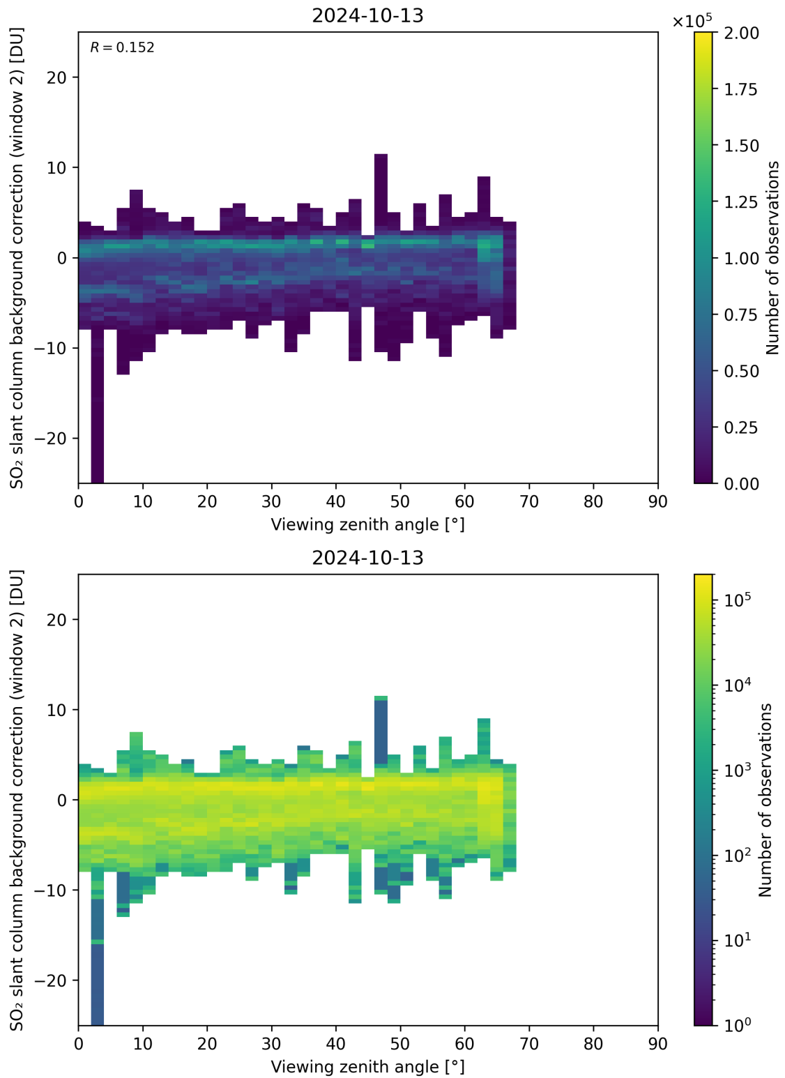
Figure 309: Scatter density plot of “Viewing zenith angle” against “SO 2 slant column background correction (window 2)” for 2024-10-12 to 2024-10-14.
