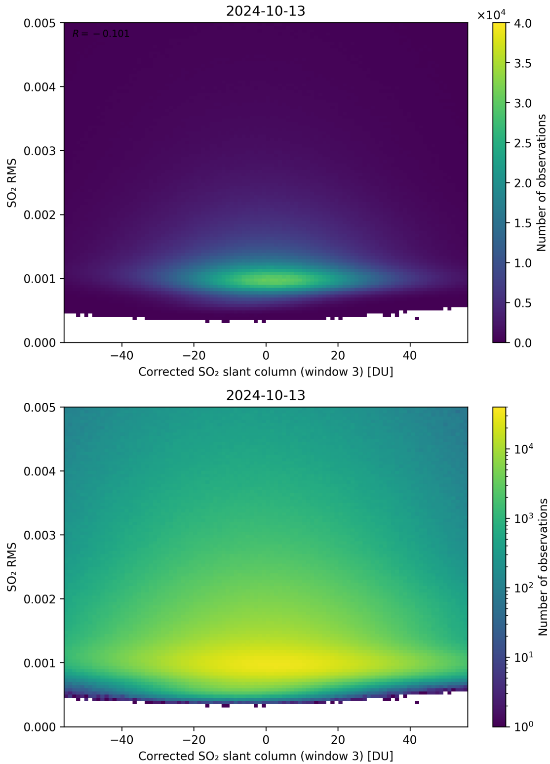
Figure 208: Scatter density plot of “Corrected SO 2 slant column (window 3)” against “SO 2 RMS” for 2024-10-12 to 2024-10-14.
