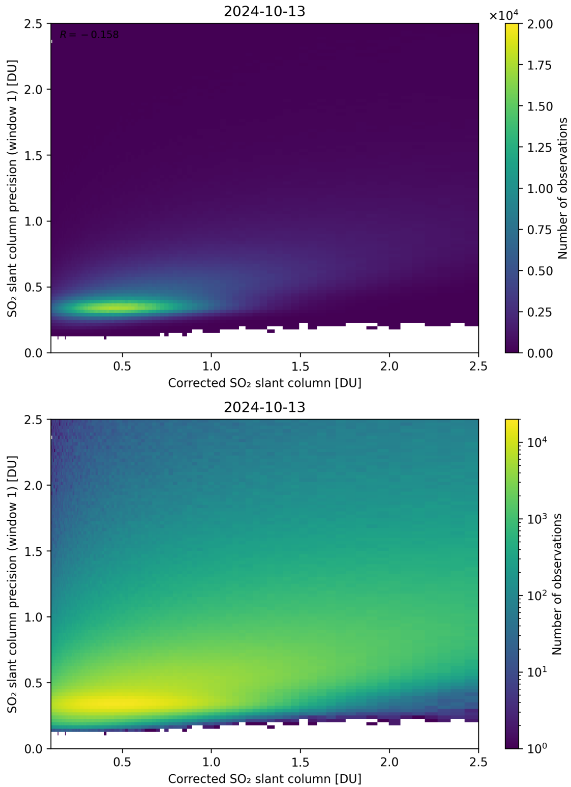
Figure 188: Scatter density plot of “Corrected SO 2 slant column” against “SO 2 slant column precision (window 1)” for 2024-10-12 to 2024-10-14.
