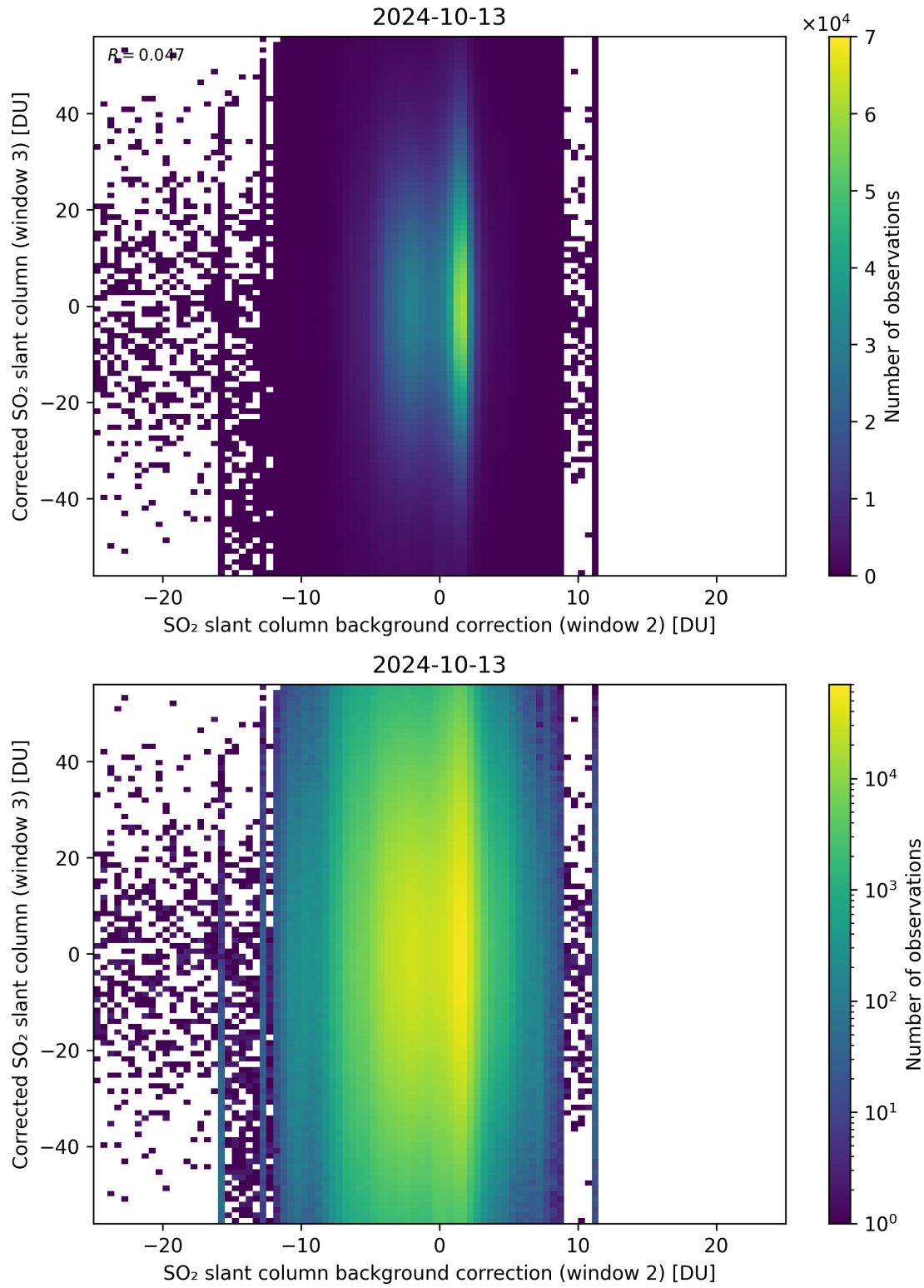
Figure 116: Scatter density plot of “SO 2 slant column background correction (window 2)” against “Corrected SO 2 slant column (window 3)” for 2024-10-12 to 2024-10-14.
