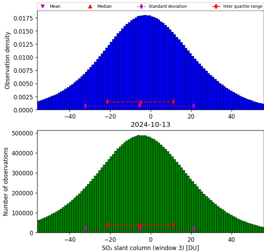
Figure 64: Histogram of “SO 2 slant column (window 3)” for 2024-10-12 to 2024-10-14
