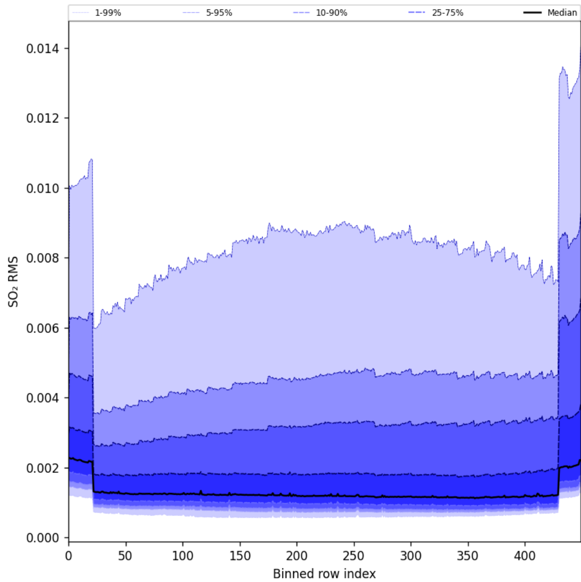
Figure 93: Along track statistics of “SO 2 RMS” for 2024-10-12 to 2024-10-14
