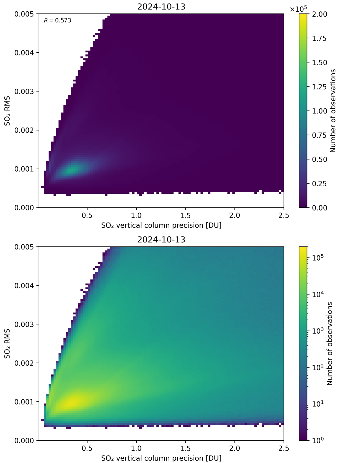
Figure 284: Scatter density plot of “SO 2 vertical column precision” against “SO 2 RMS” for 2024-10-12 to 2024-10-14.
