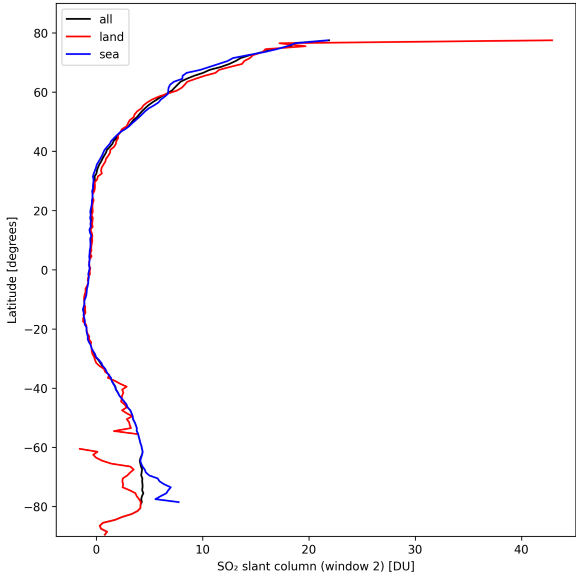
Figure 37: Zonal average of “SO 2 slant column (window 2)” for 2024-10-12 to 2024-10-14.
