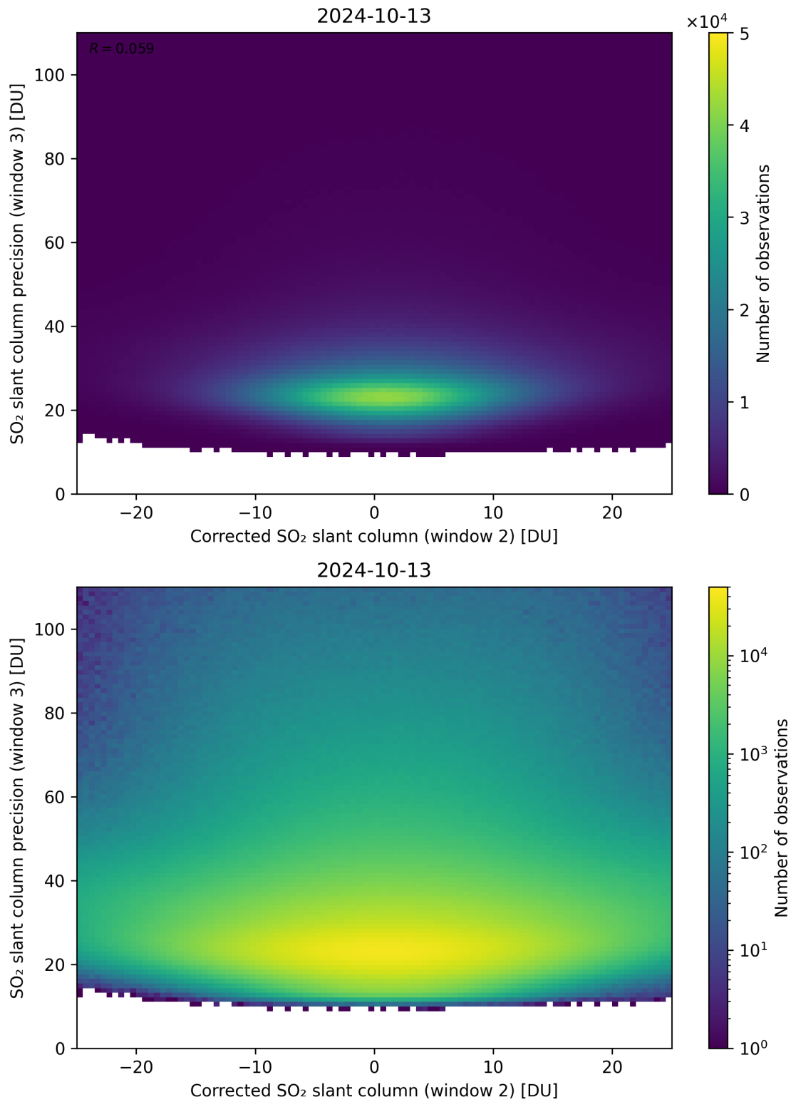
Figure 202: Scatter density plot of “Corrected SO 2 slant column (window 2)” against “SO 2 slant column precision (window 3)” for 2024-10-12 to 2024-10-14.
