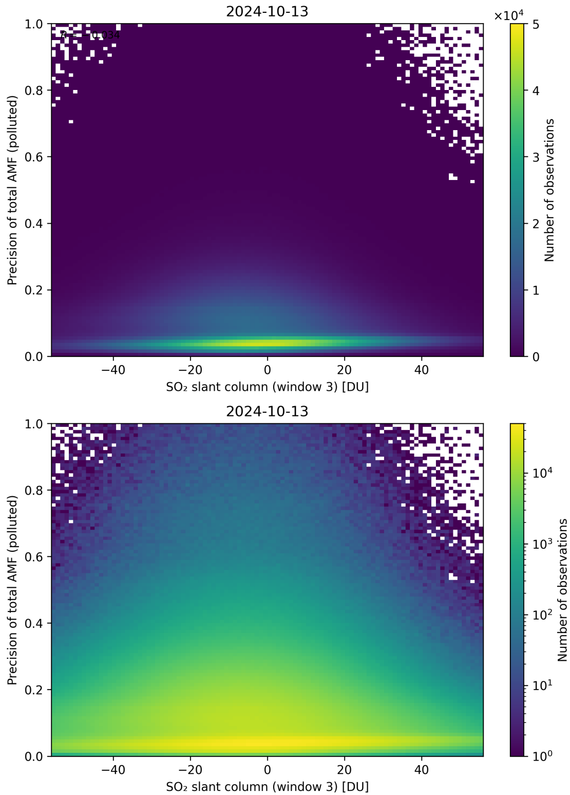
Figure 269: Scatter density plot of “SO 2 slant column (window 3)” against “Precision of total AMF (polluted)” for 2024-10-12 to 2024-10-14.
