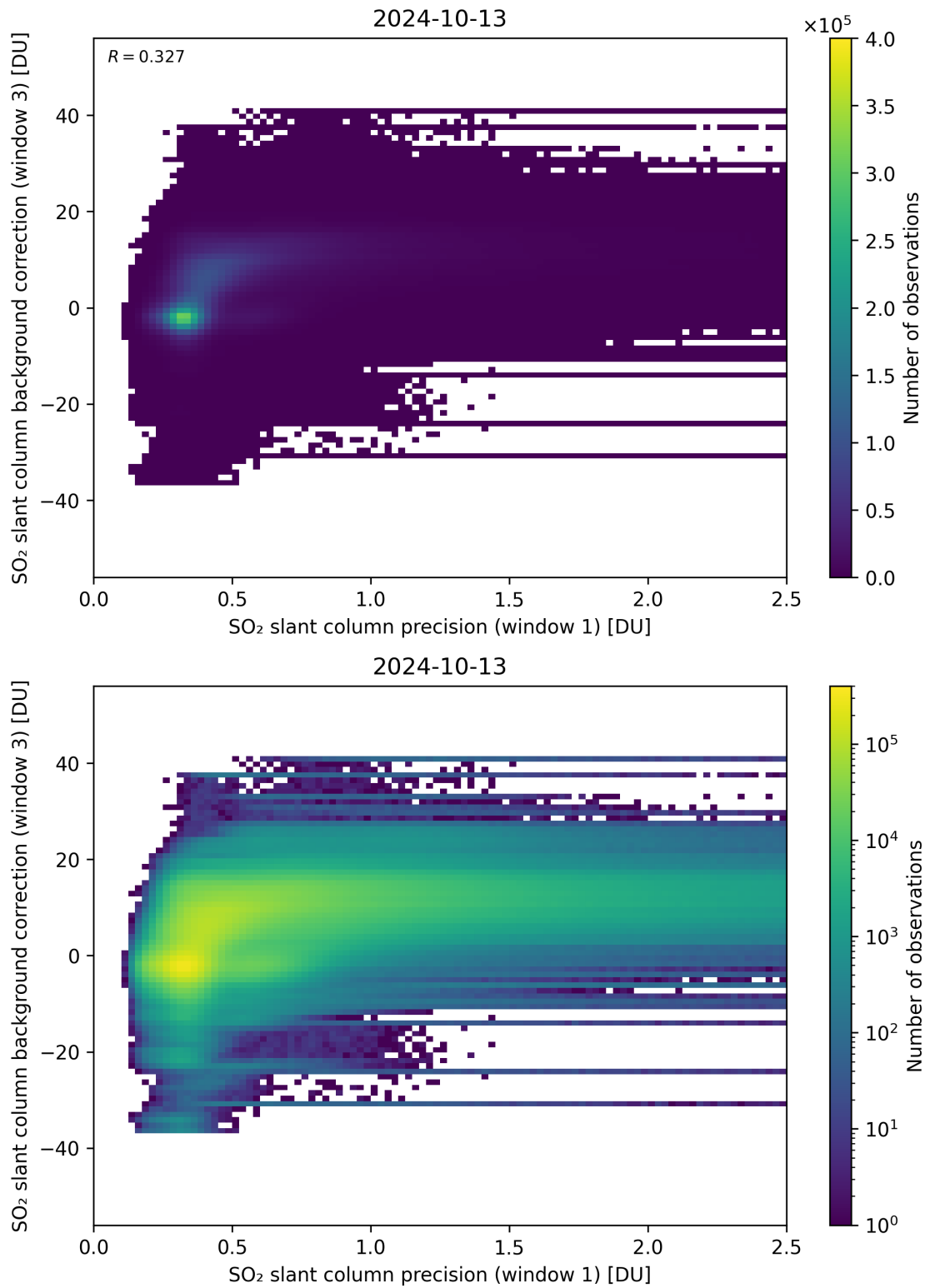
Figure 220: Scatter density plot of “SO 2 slant column precision (window 1)” against “SO 2 slant column background correction (window 3)” for 2024-10-12 to 2024-10-14.
