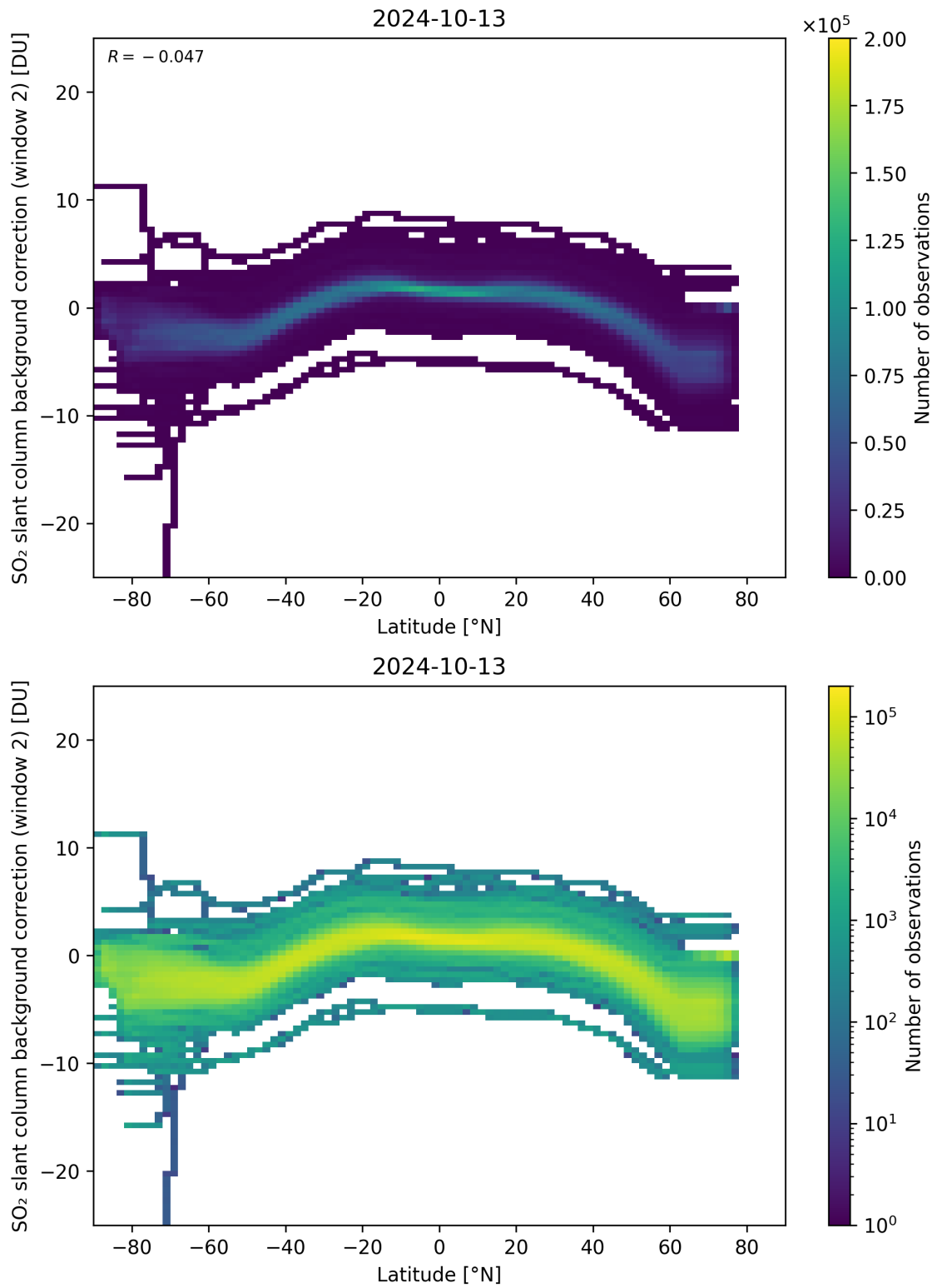
Figure 140: Scatter density plot of “Latitude” against “SO 2 slant column background correction (window 2)” for 2024-10-12 to 2024-10-14.
