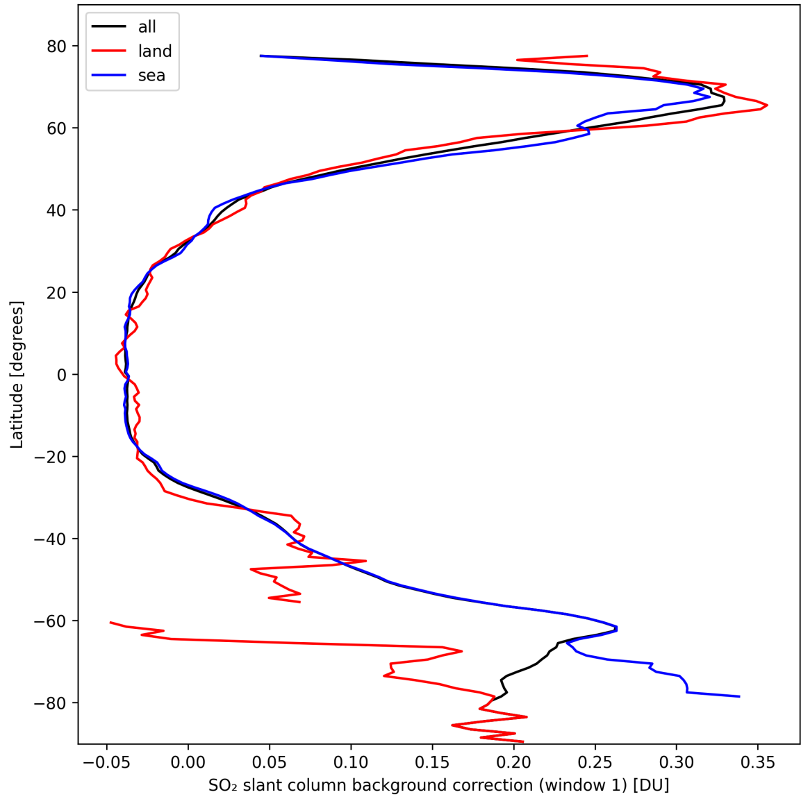
Figure 36: Zonal average of “SO 2 slant column background correction (window 1)” for 2024-10-12 to 2024-10-14.
