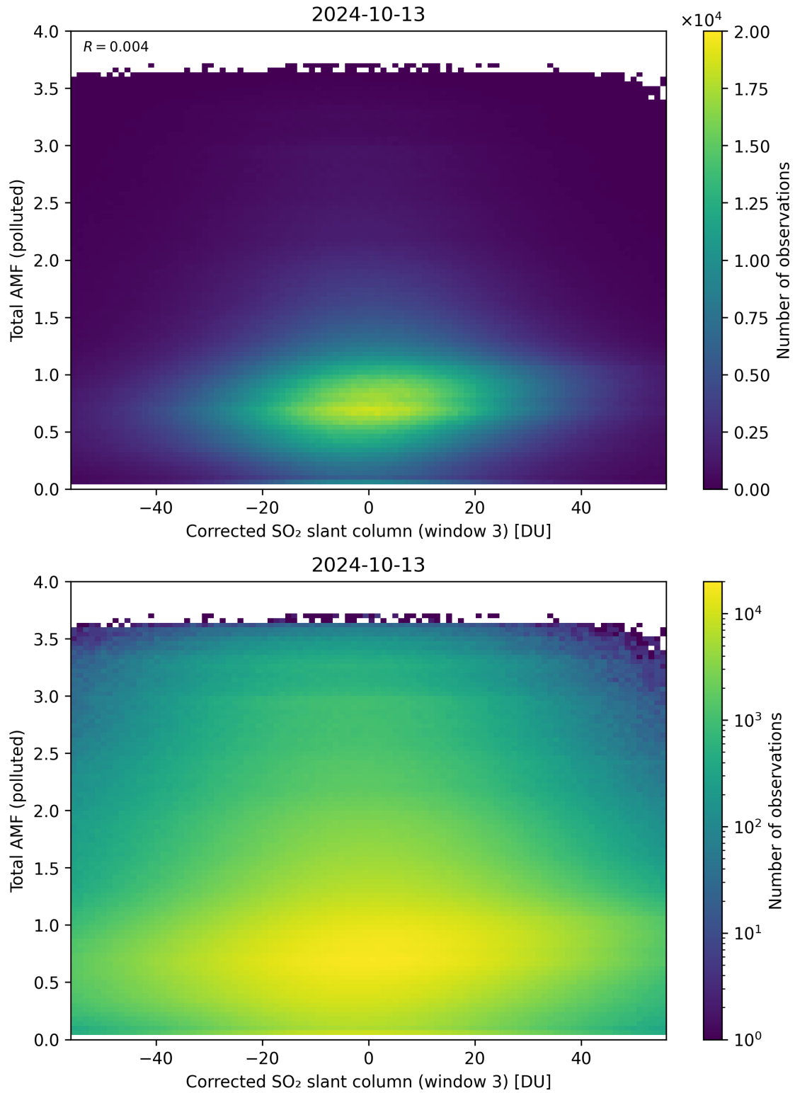
Figure 210: Scatter density plot of “Corrected SO 2 slant column (window 3)” against “Total AMF (polluted)” for 2024-10-12 to 2024-10-14.
