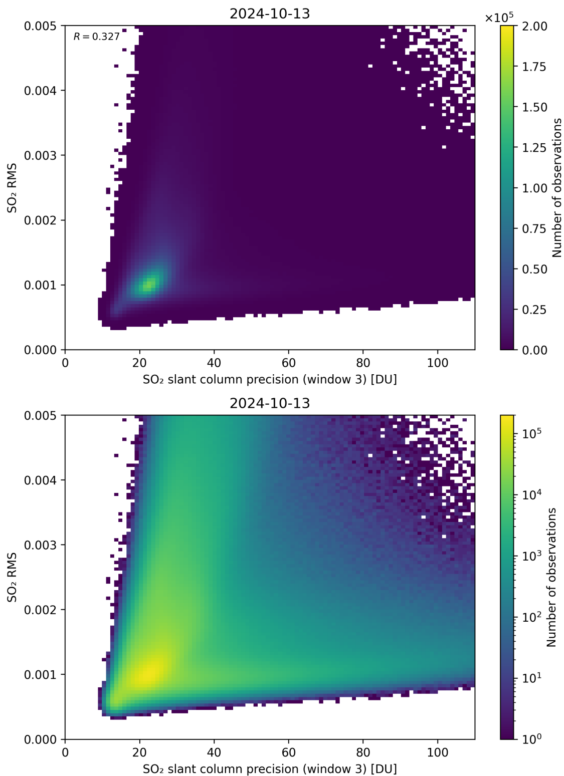
Figure 260: Scatter density plot of “SO 2 slant column precision (window 3)” against “SO 2 RMS” for 2024-10-12 to 2024-10-14.
