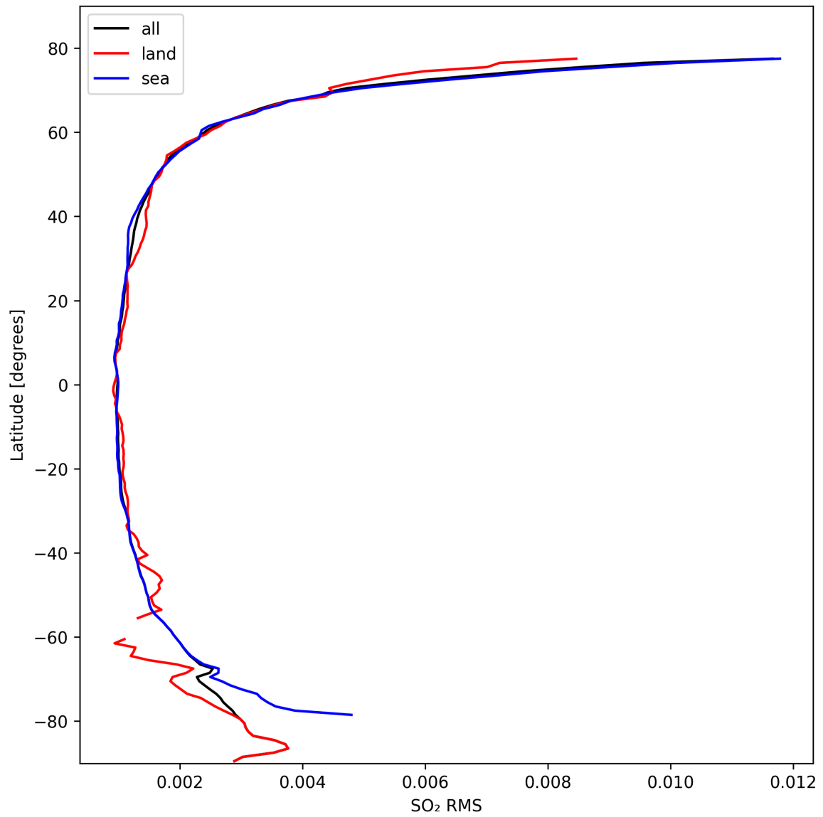
Figure 47: Zonal average of “SO 2 RMS” for 2024-10-12 to 2024-10-14.
