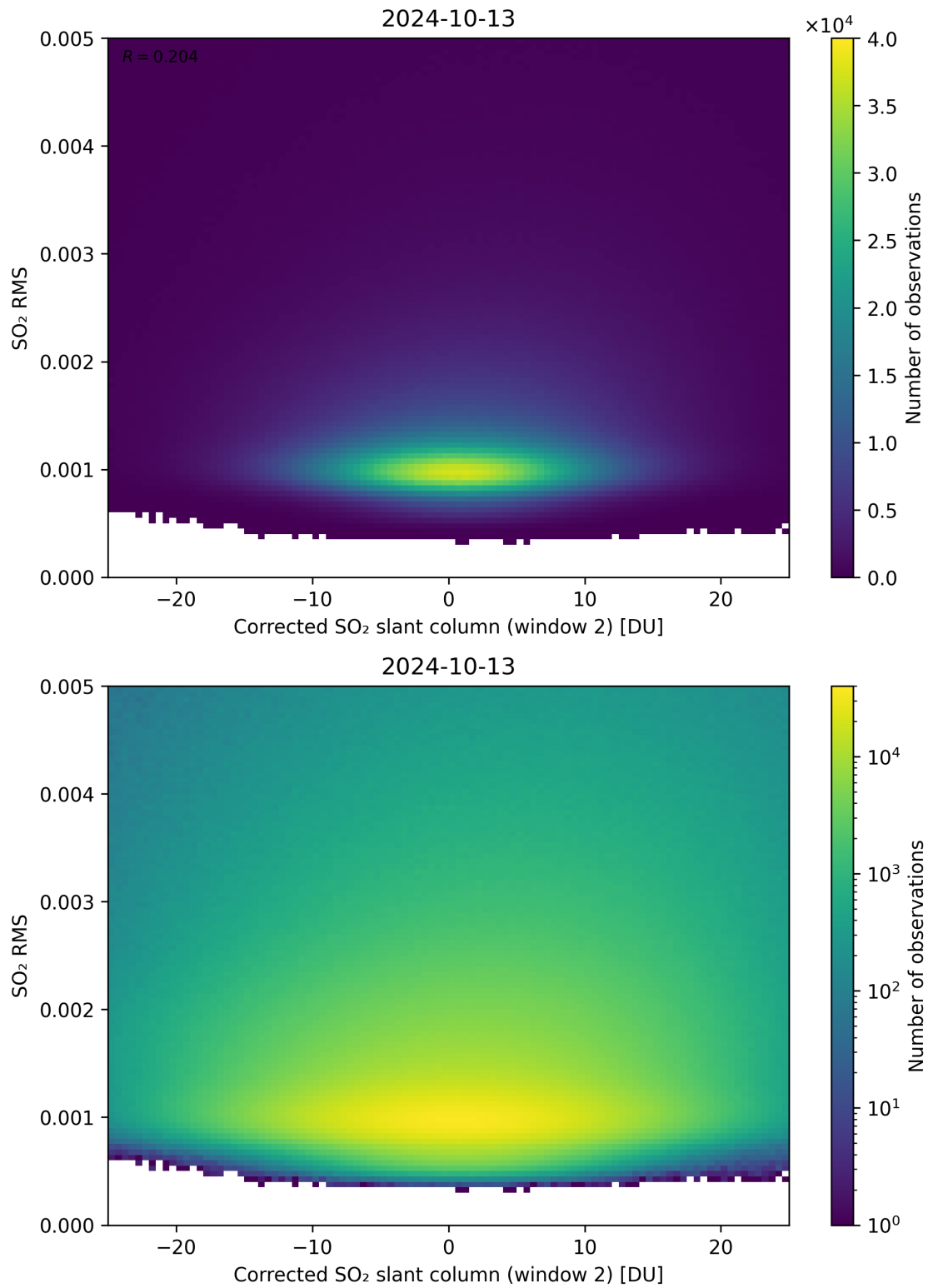
Figure 198: Scatter density plot of “Corrected SO 2 slant column (window 2)” against “SO 2 RMS” for 2024-10-12 to 2024-10-14.
