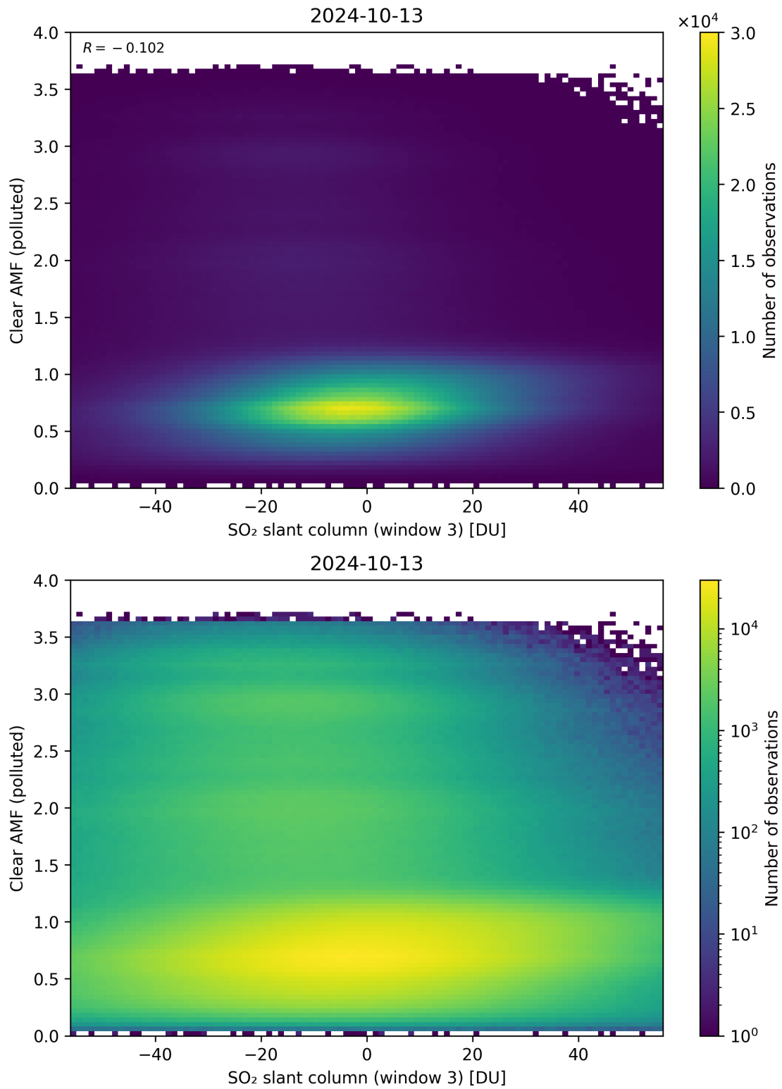
Figure 265: Scatter density plot of “SO 2 slant column (window 3)” against “Clear AMF (polluted)” for 2024-10-12 to 2024-10-14.
