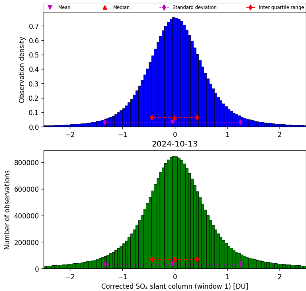
Figure 58: Histogram of “Corrected SO 2 slant column (window 1)” for 2024-10-12 to 2024-10-14
