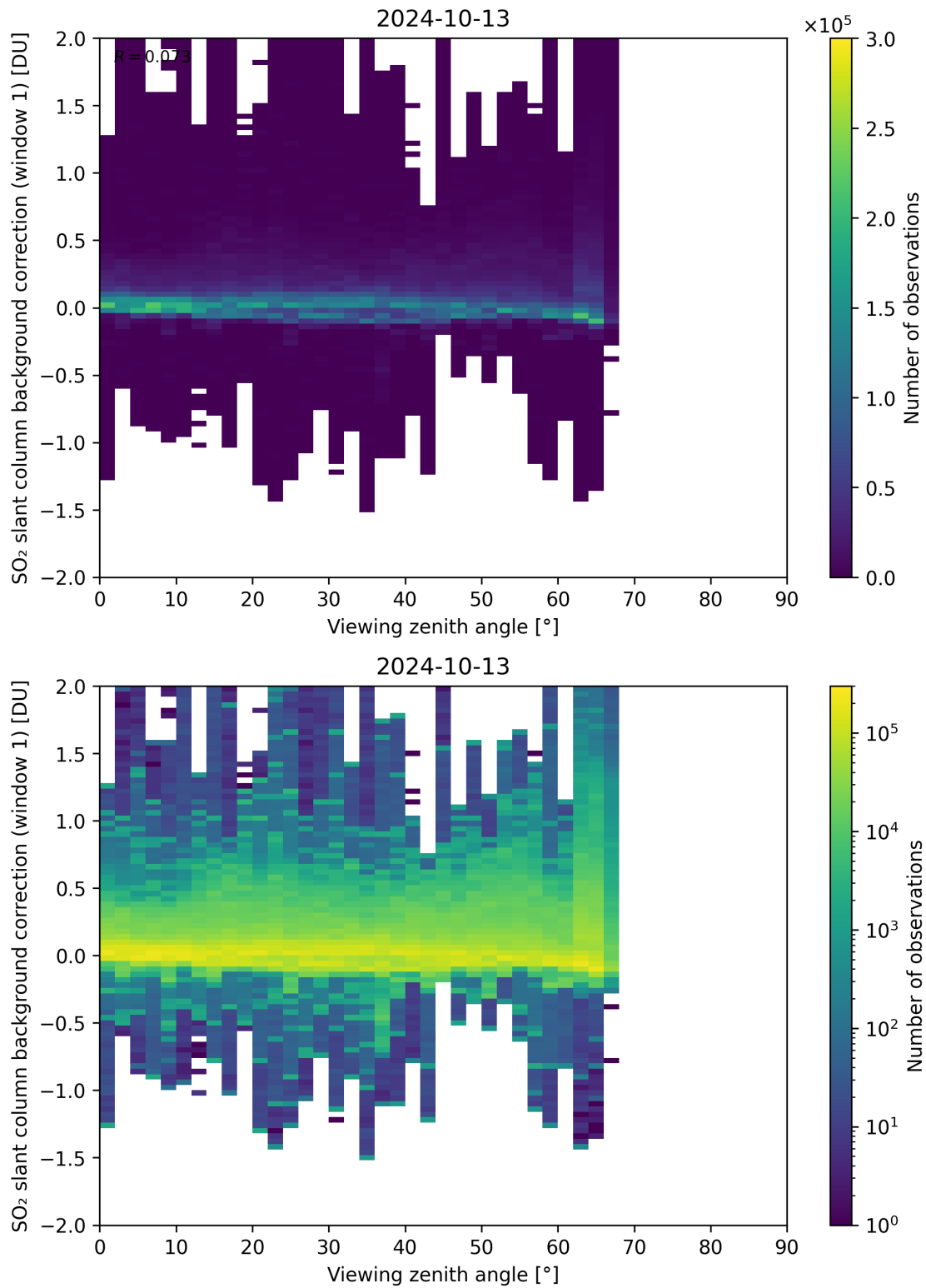
Figure 308: Scatter density plot of “Viewing zenith angle” against “SO 2 slant column background correction (window 1)” for 2024-10-12 to 2024-10-14.
