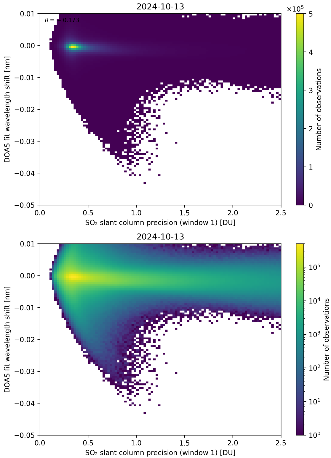
Figure 221: Scatter density plot of “SO 2 slant column precision (window 1)” against “DOAS fit wavelength shift” for 2024-10-12 to 2024-10-14.
