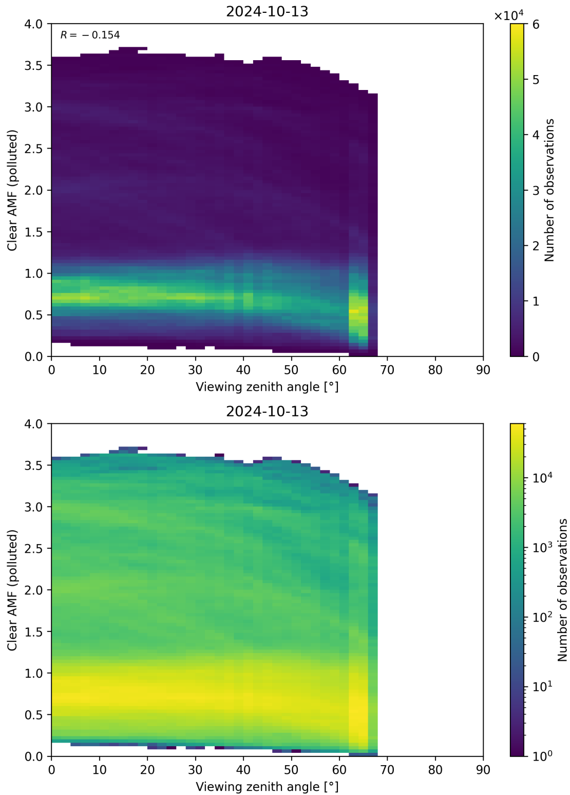
Figure 316: Scatter density plot of “Viewing zenith angle” against “Clear AMF (polluted)” for 2024-10-12 to 2024-10-14.
