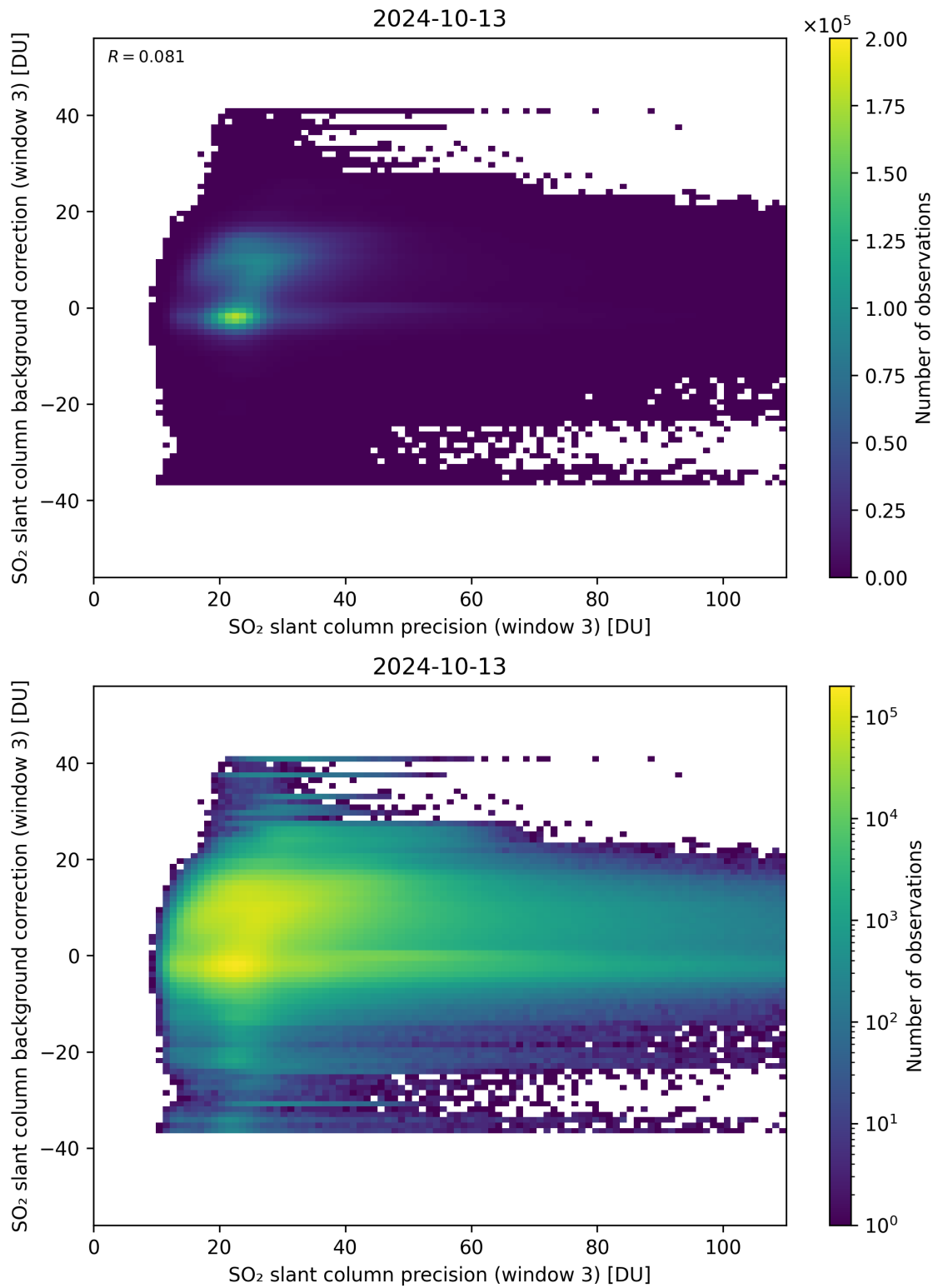
Figure 257: Scatter density plot of “SO 2 slant column precision (window 3)” against “SO 2 slant column background correction (window 3)” for 2024-10-12 to 2024-10-14.
