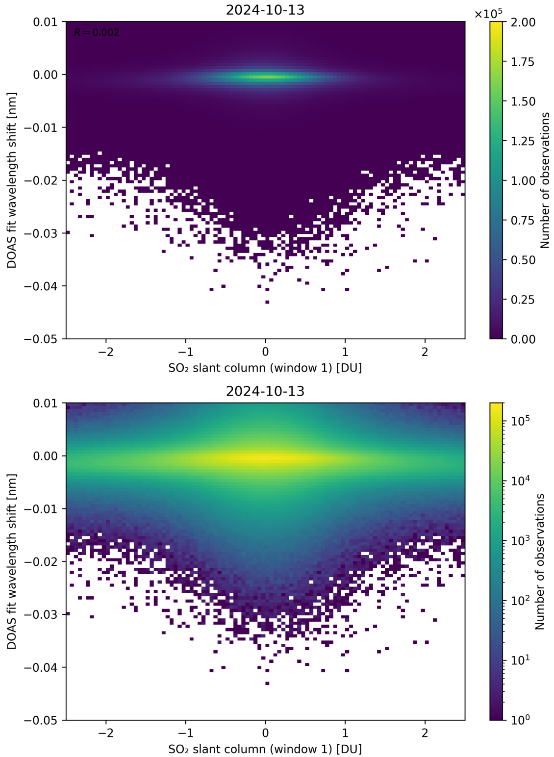
Figure 215: Scatter density plot of “SO 2 slant column (window 1)” against “DOAS fit wavelength shift” for 2024-10-12 to 2024-10-14.
