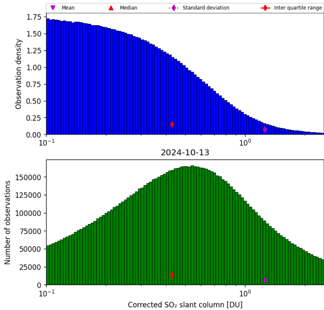
Figure 55: Histogram of “Corrected SO 2 slant column” for 2024-10-12 to 2024-10-14
