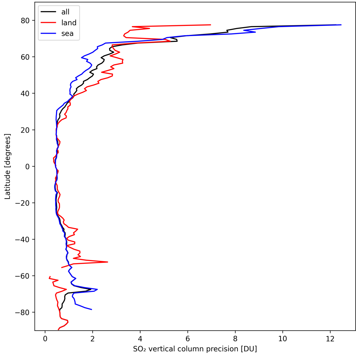
Figure 31: Zonal average of “SO 2 vertical column precision” for 2024-10-12 to 2024-10-14.
