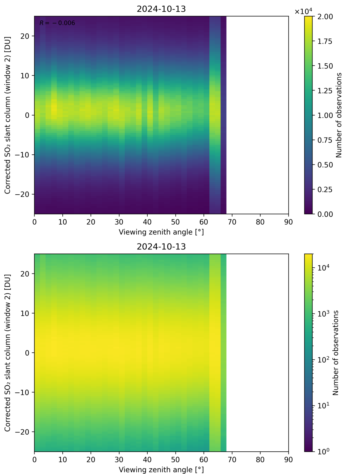
Figure 318: Scatter density plot of “Viewing zenith angle” against “Corrected SO 2 slant column (window 2)” for 2024-10-12 to 2024-10-14.
