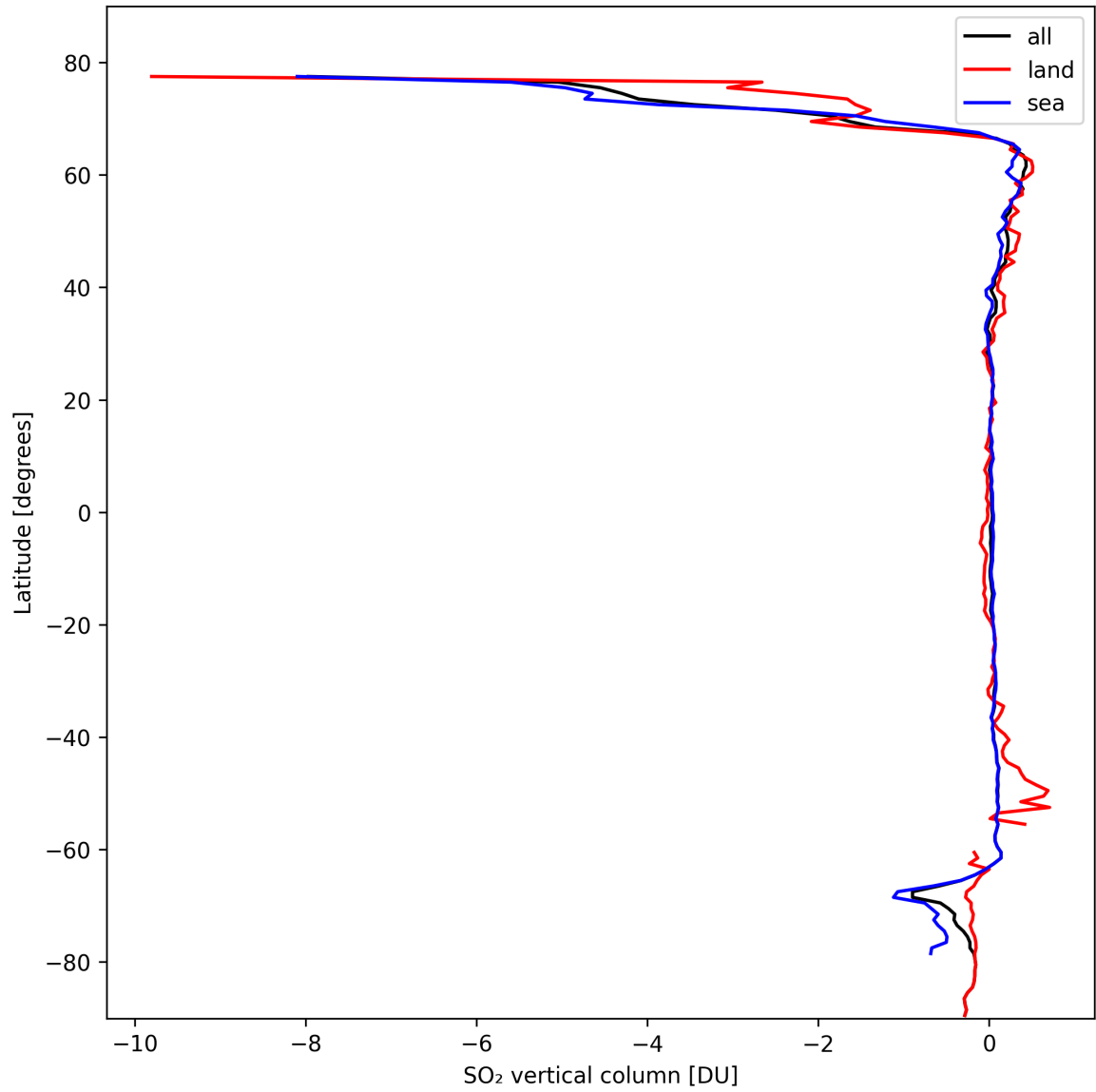
Figure 30: Zonal average of “SO 2 vertical column” for 2024-10-12 to 2024-10-14.
