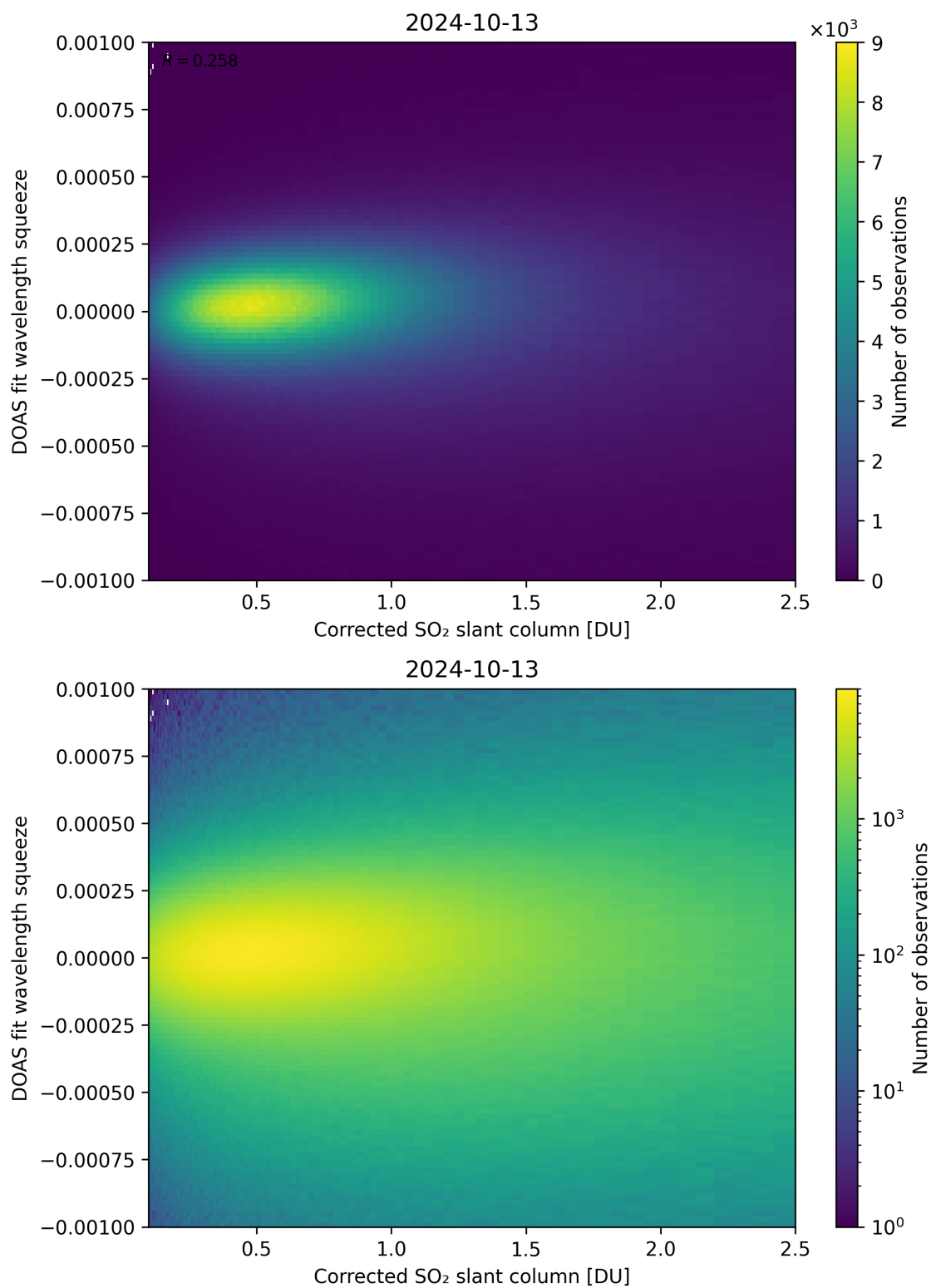
Figure 182: Scatter density plot of “Corrected SO 2 slant column” against “DOAS fit wavelength squeeze” for 2024-10-12 to 2024-10-14.
