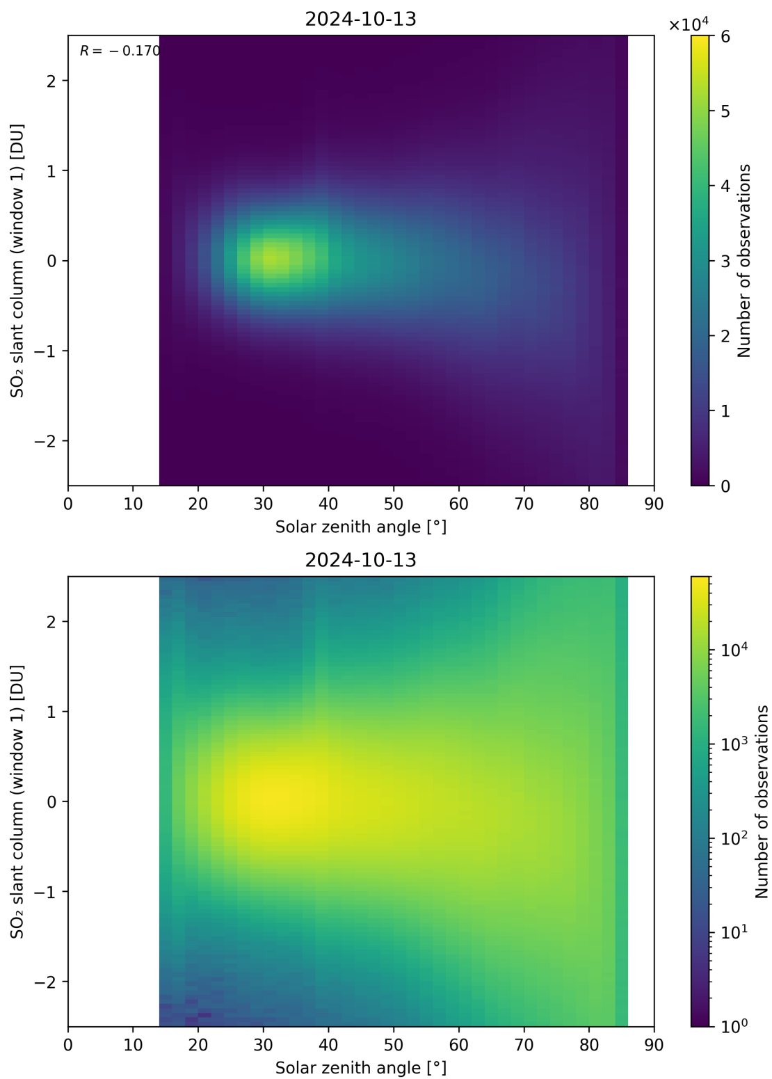
Figure 169: Scatter density plot of “Solar zenith angle” against “SO 2 slant column (window 1)” for 2024-10-12 to 2024-10-14.
