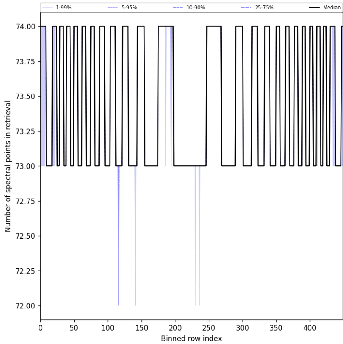
Figure 97: Along track statistics of “Number of spectral points in retrieval” for 2024-10-12 to 2024-10-14
