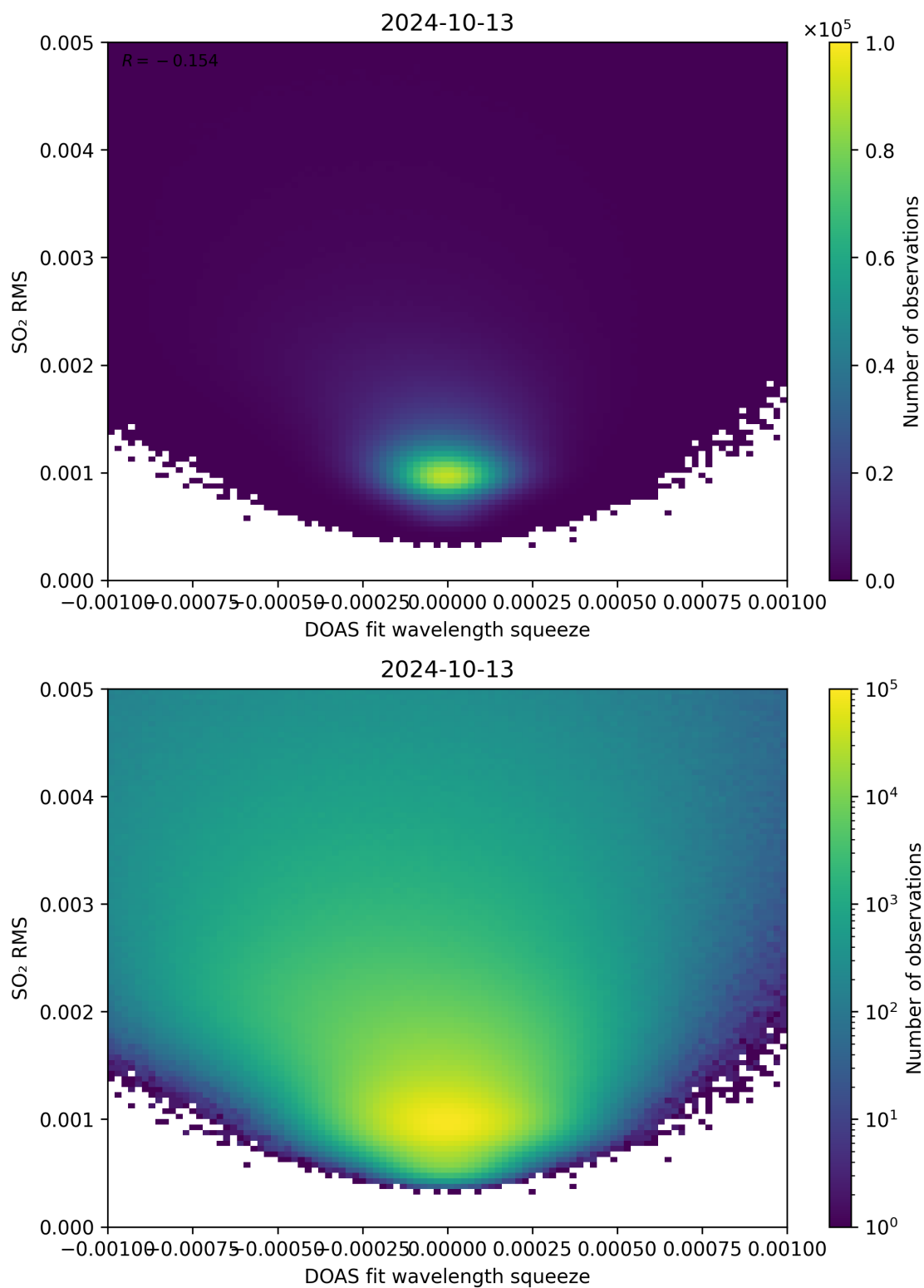
Figure 132: Scatter density plot of “DOAS fit wavelength squeeze” against “SO 2 RMS” for 2024-10-12 to 2024-10-14.
