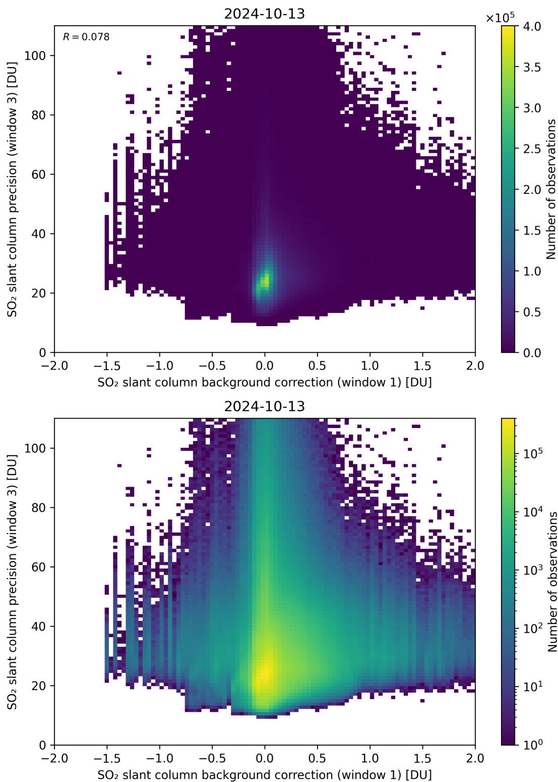
Figure 108: Scatter density plot of “SO 2 slant column background correction (window 1)” against “SO 2 slant column precision (window 3)” for 2024-10-12 to 2024-10-14.
