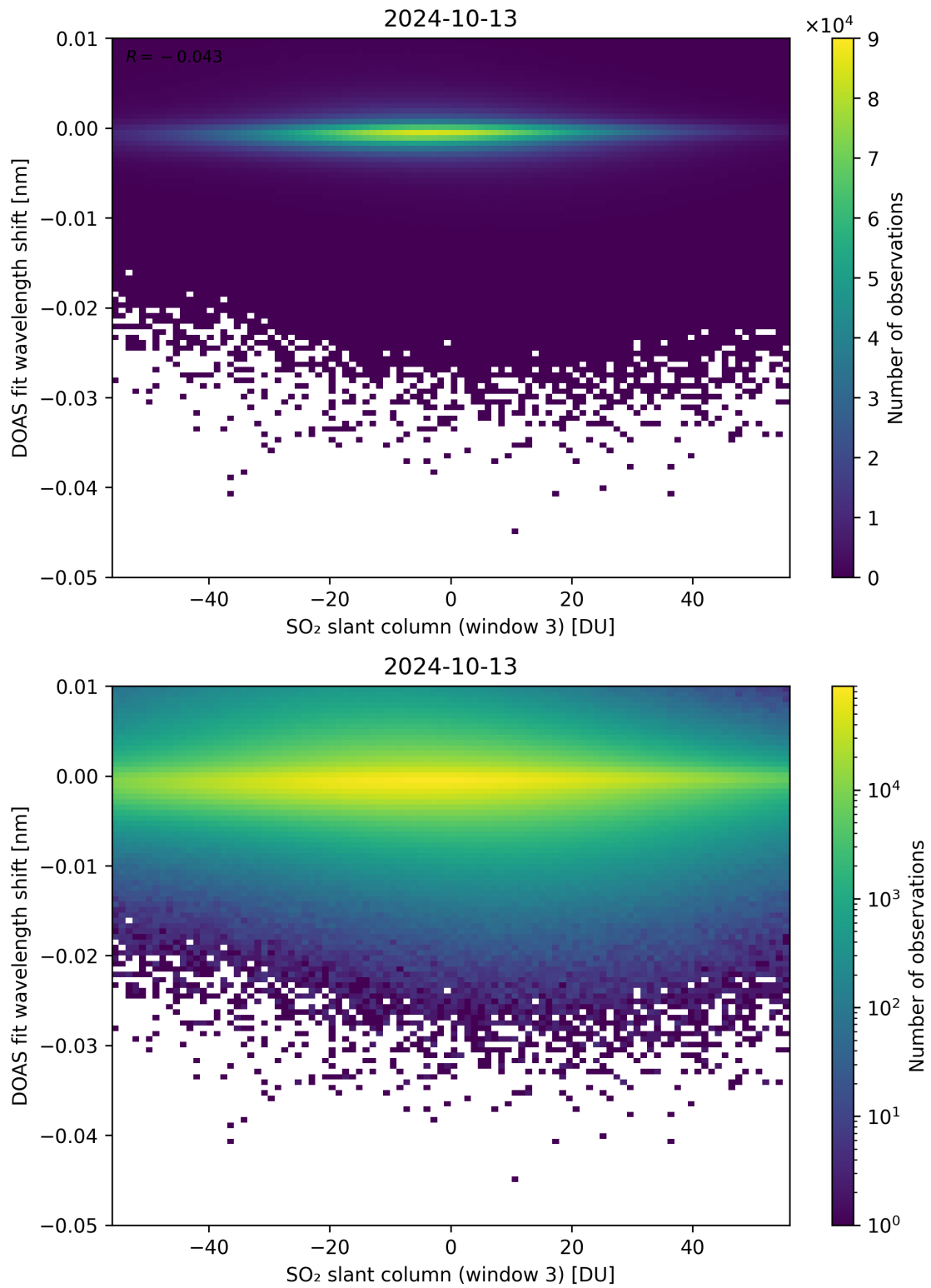
Figure 254: Scatter density plot of “SO 2 slant column (window 3)” against “DOAS fit wavelength shift” for 2024-10-12 to 2024-10-14.
