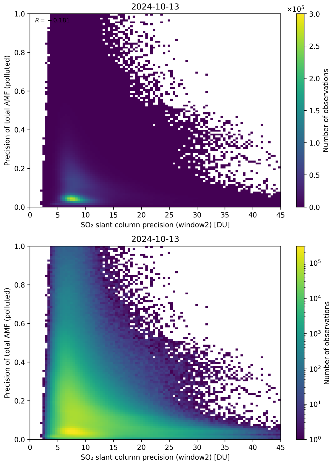
Figure 252: Scatter density plot of “SO 2 slant column precision (window2)” against “Precision of total AMF (polluted)” for 2024-10-12 to 2024-10-14.
