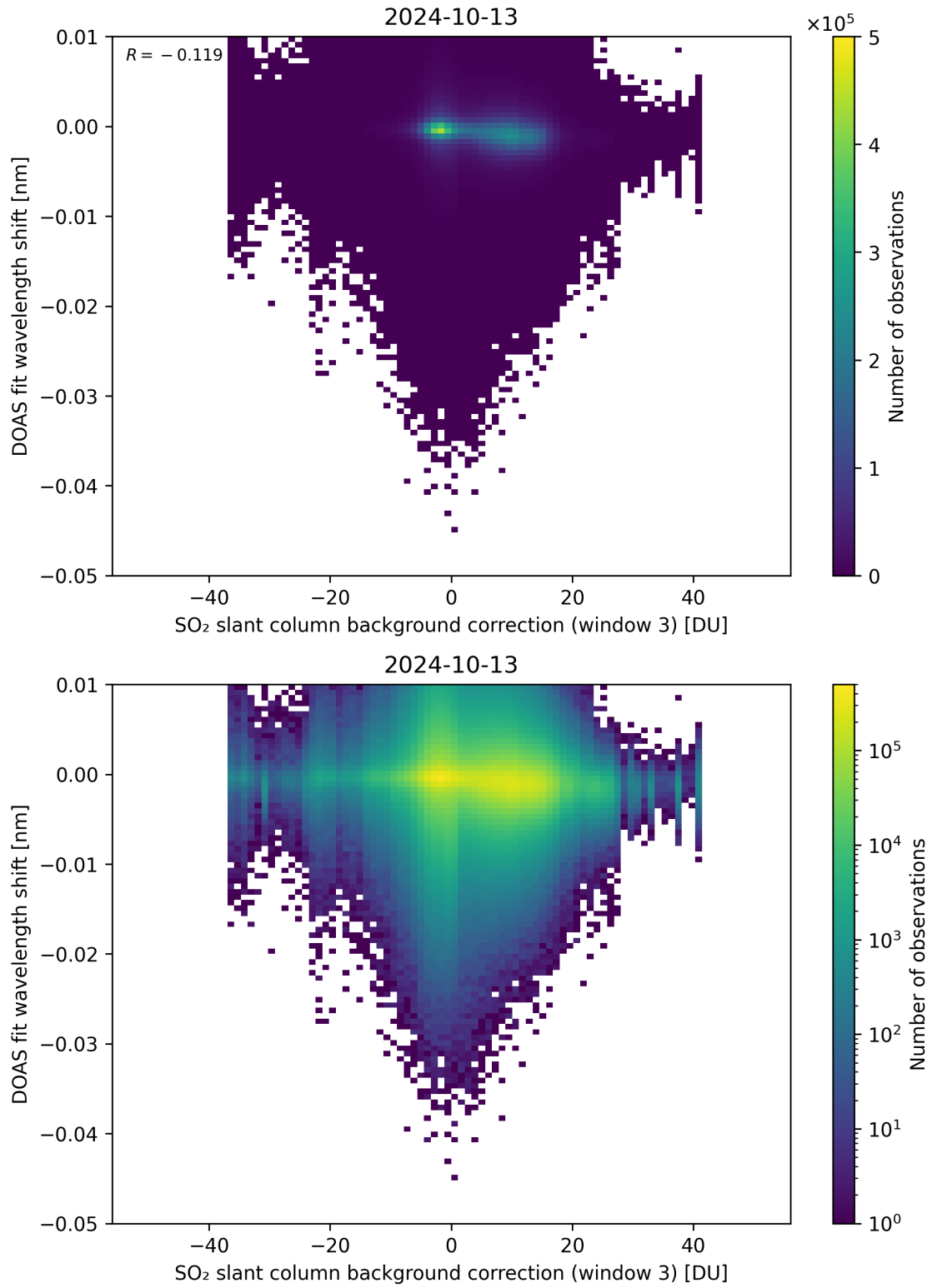
Figure 121: Scatter density plot of “SO 2 slant column background correction (window 3)” against “DOAS fit wavelength shift” for 2024-10-12 to 2024-10-14.
