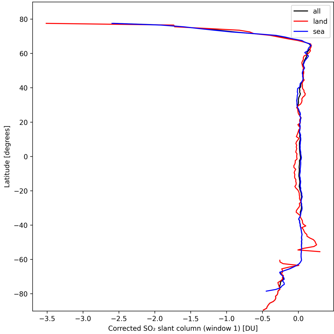
Figure 35: Zonal average of “Corrected SO 2 slant column (window 1)” for 2024-10-12 to 2024-10-14.
