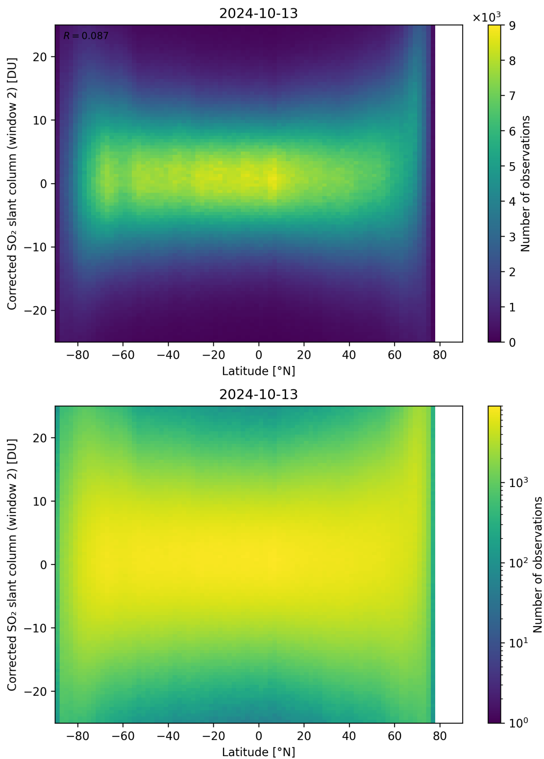
Figure 147: Scatter density plot of “Latitude” against “Corrected SO 2 slant column (window 2)” for 2024-10-12 to 2024-10-14.
