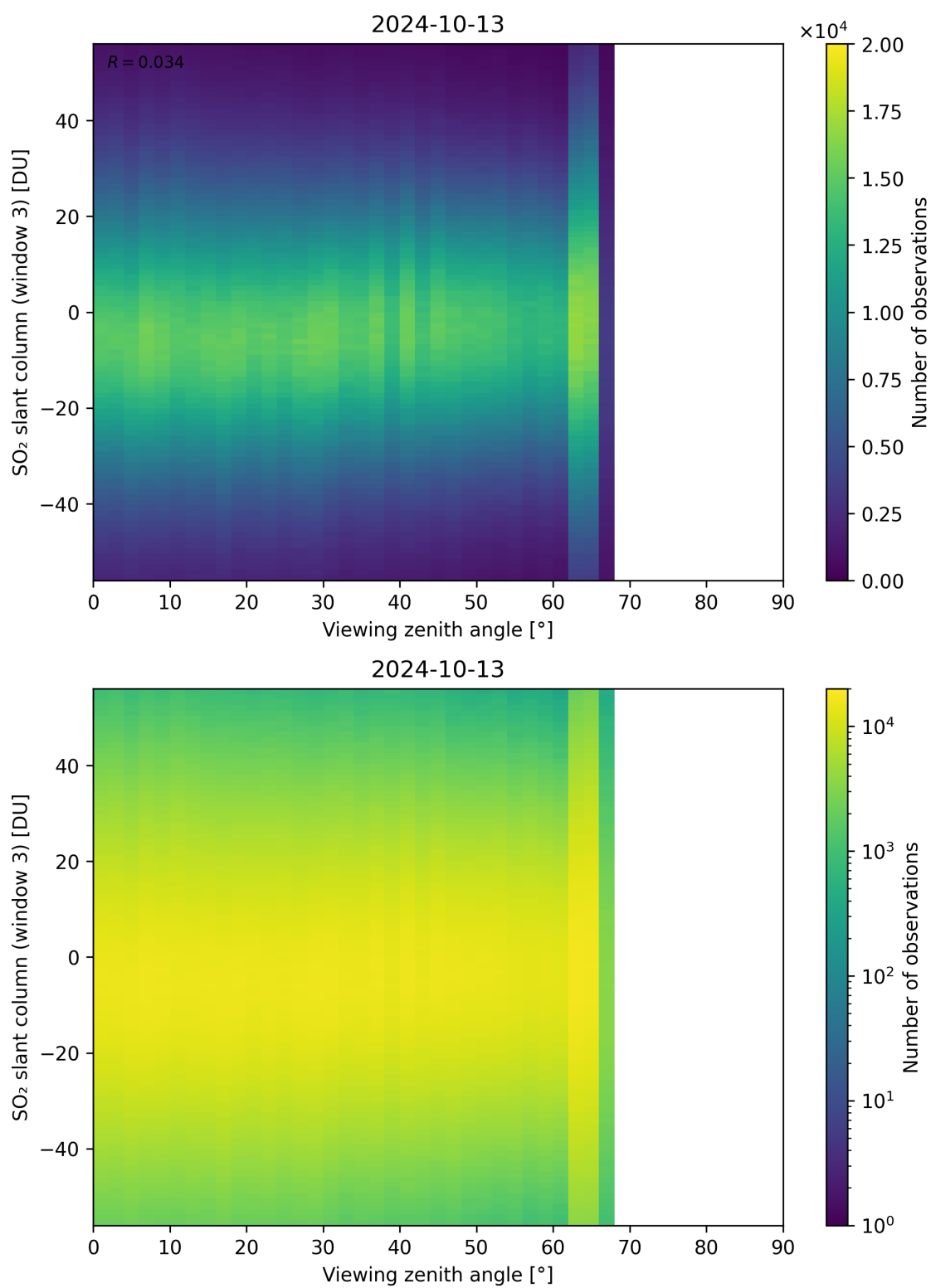
Figure 323: Scatter density plot of “Viewing zenith angle” against “SO 2 slant column (window 3)” for 2024-10-12 to 2024-10-14.
