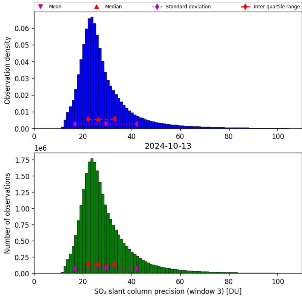
Figure 65: Histogram of “SO 2 slant column precision (window 3)” for 2024-10-12 to 2024-10-14
