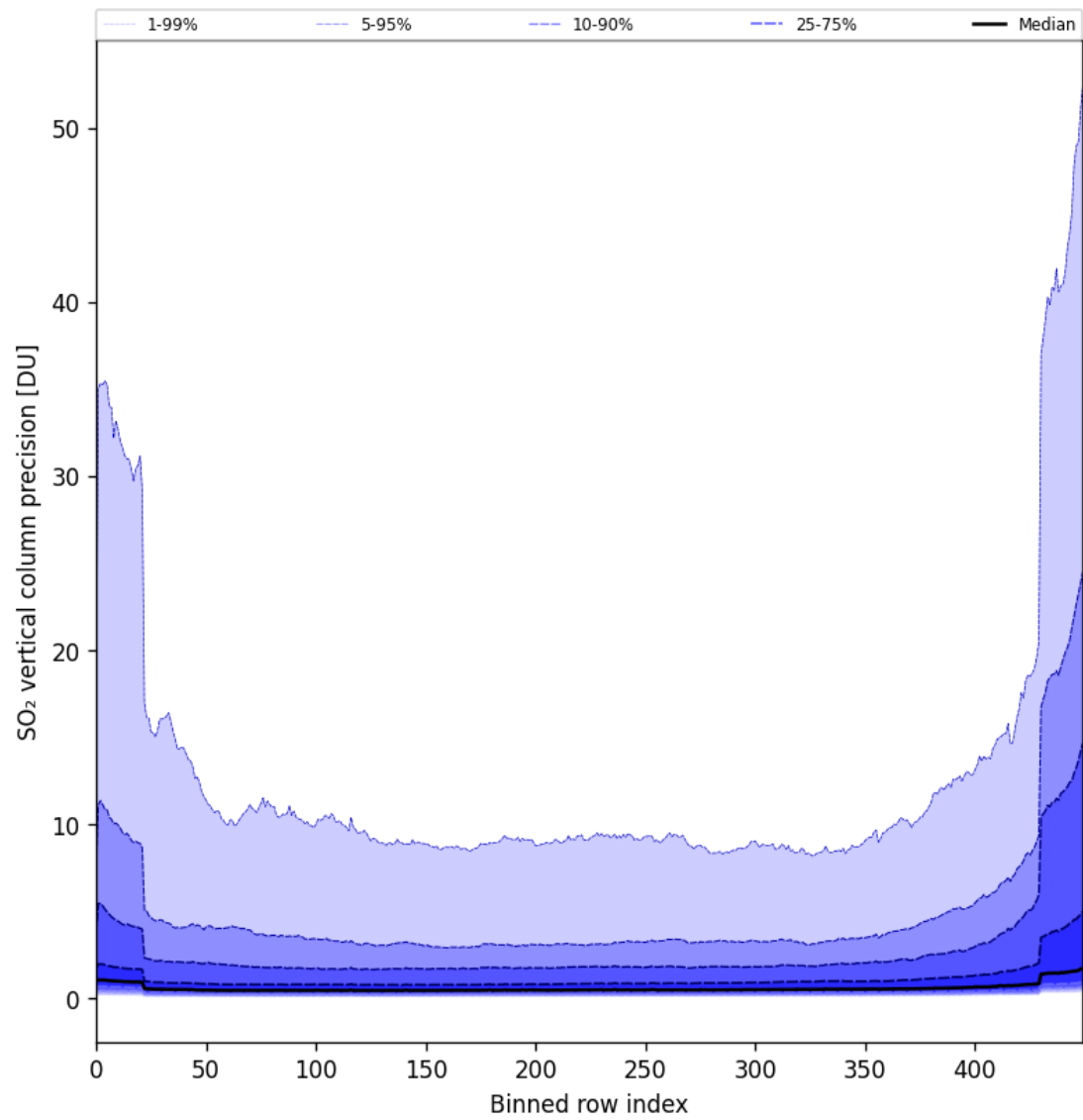
Figure 77: Along track statistics of “SO 2 vertical column precision” for 2024-10-12 to 2024-10-14
