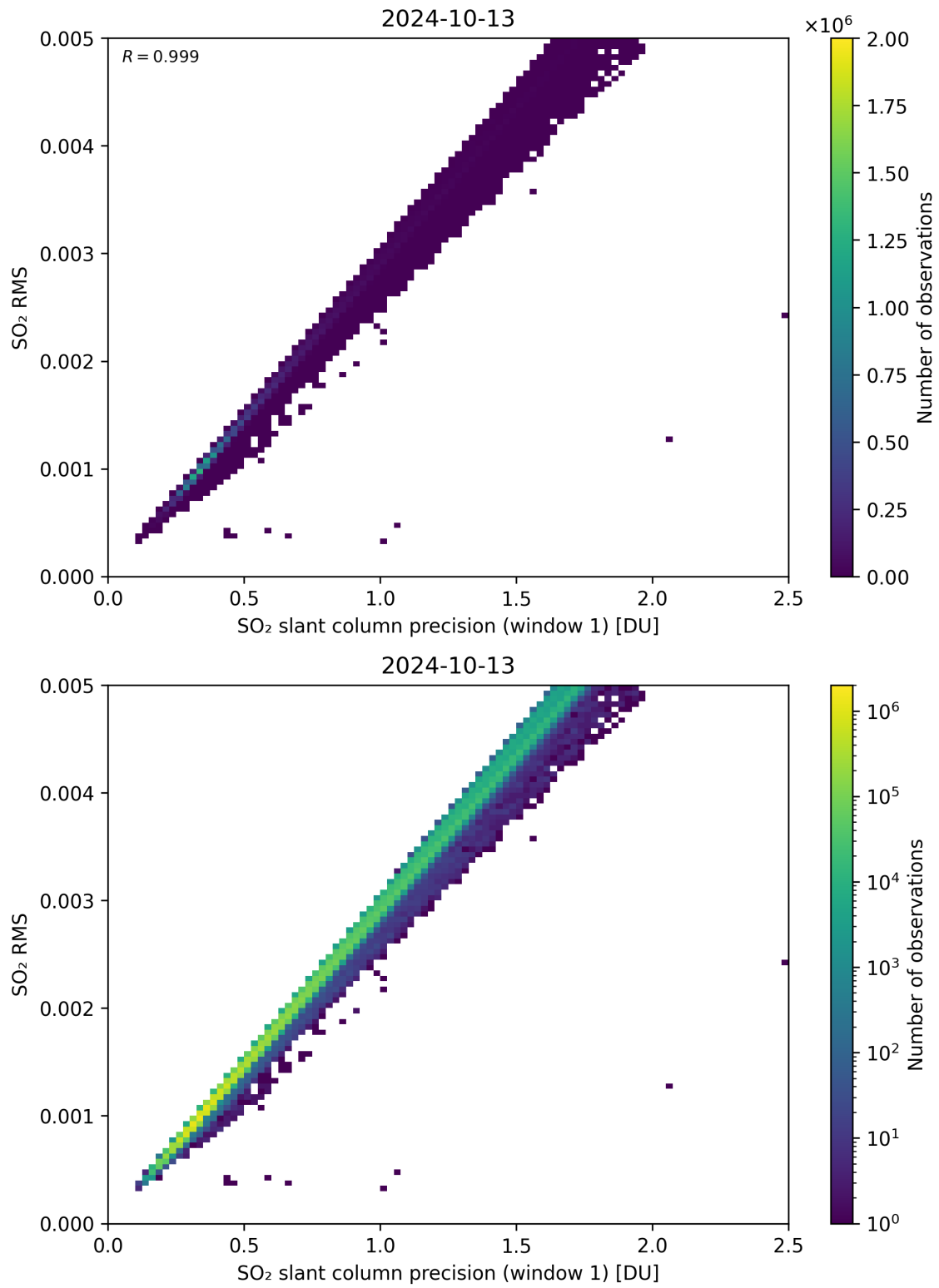
Figure 223: Scatter density plot of “SO 2 slant column precision (window 1)” against “SO 2 RMS” for 2024-10-12 to 2024-10-14.
