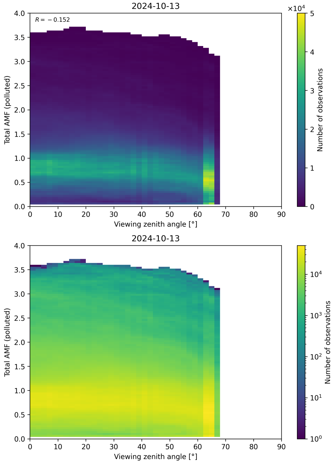
Figure 325: Scatter density plot of “Viewing zenith angle” against “Total AMF (polluted)” for 2024-10-12 to 2024-10-14.
