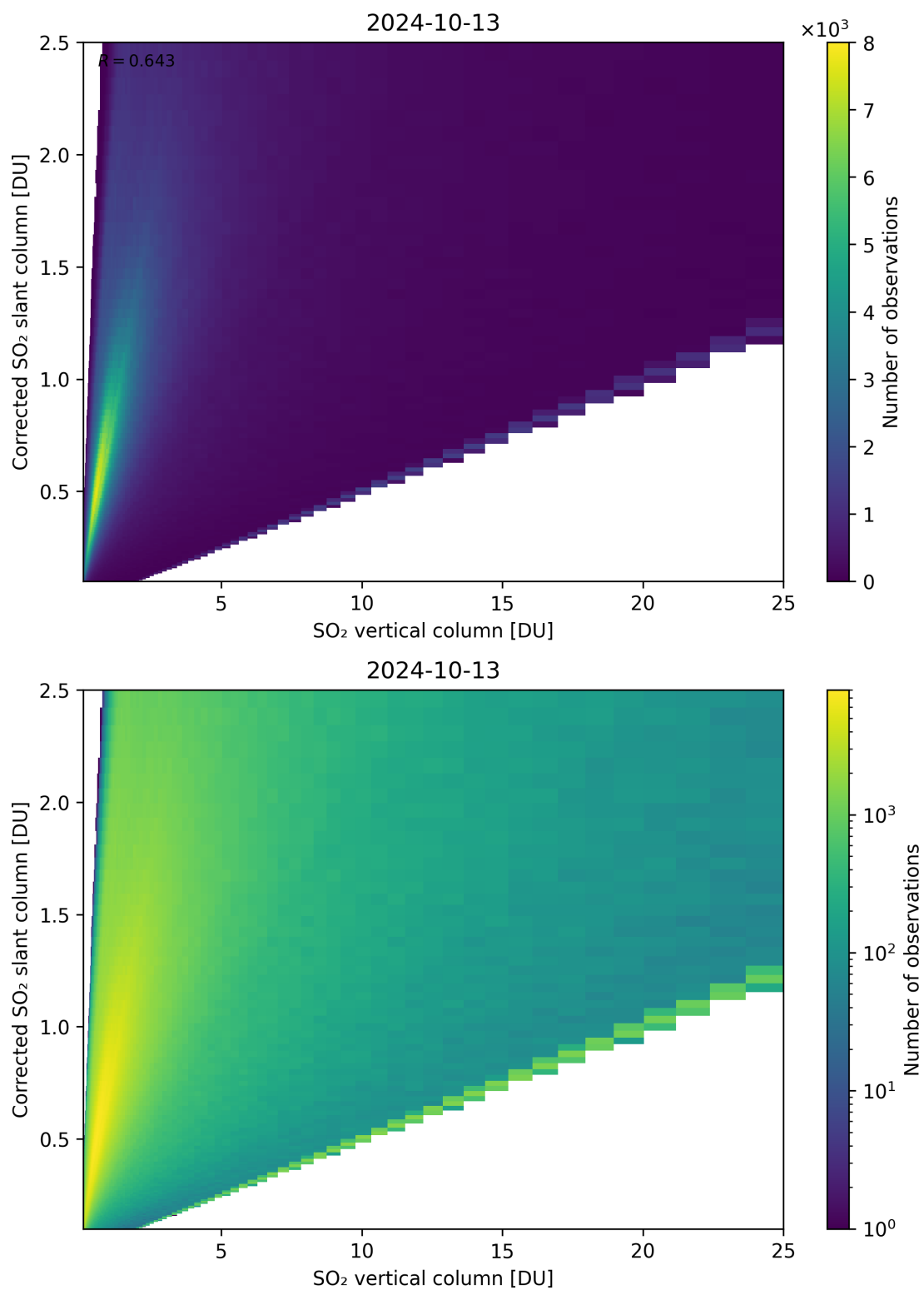
Figure 297: Scatter density plot of “SO 2 vertical column” against “Corrected SO 2 slant column” for 2024-10-12 to 2024-10-14.
