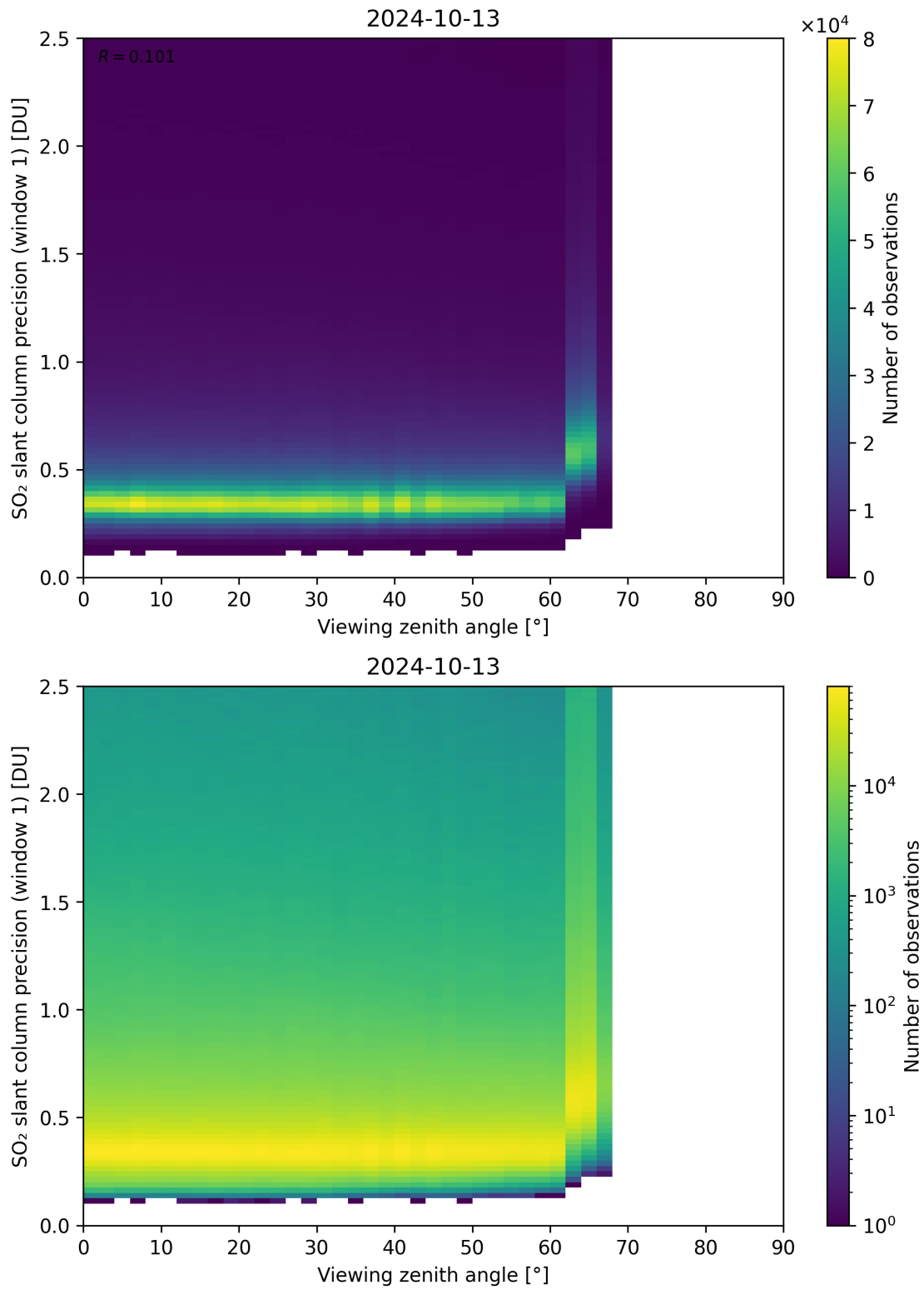
Figure 321: Scatter density plot of “Viewing zenith angle” against “SO 2 slant column precision (window 1)” for 2024-10-12 to 2024-10-14.
