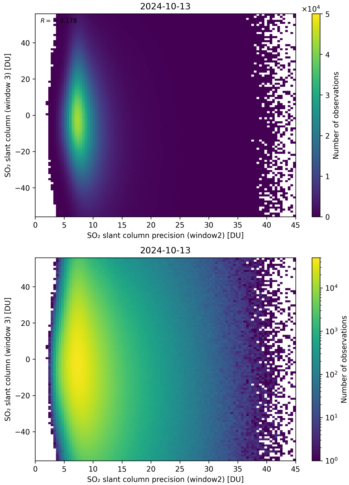
Figure 249: Scatter density plot of “SO 2 slant column precision (window2)” against “SO 2 slant column (window 3)” for 2024-10-12 to 2024-10-14.
