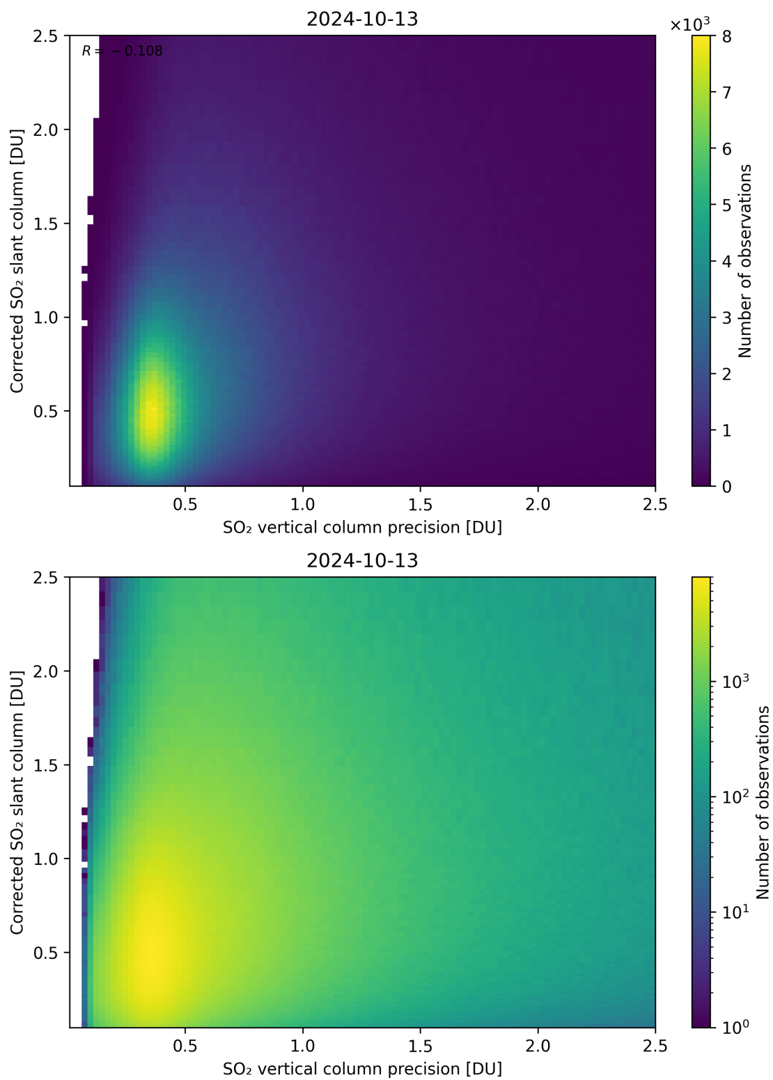
Figure 286: Scatter density plot of “SO 2 vertical column precision” against “Corrected SO 2 slant column” for 2024-10-12 to 2024-10-14.
