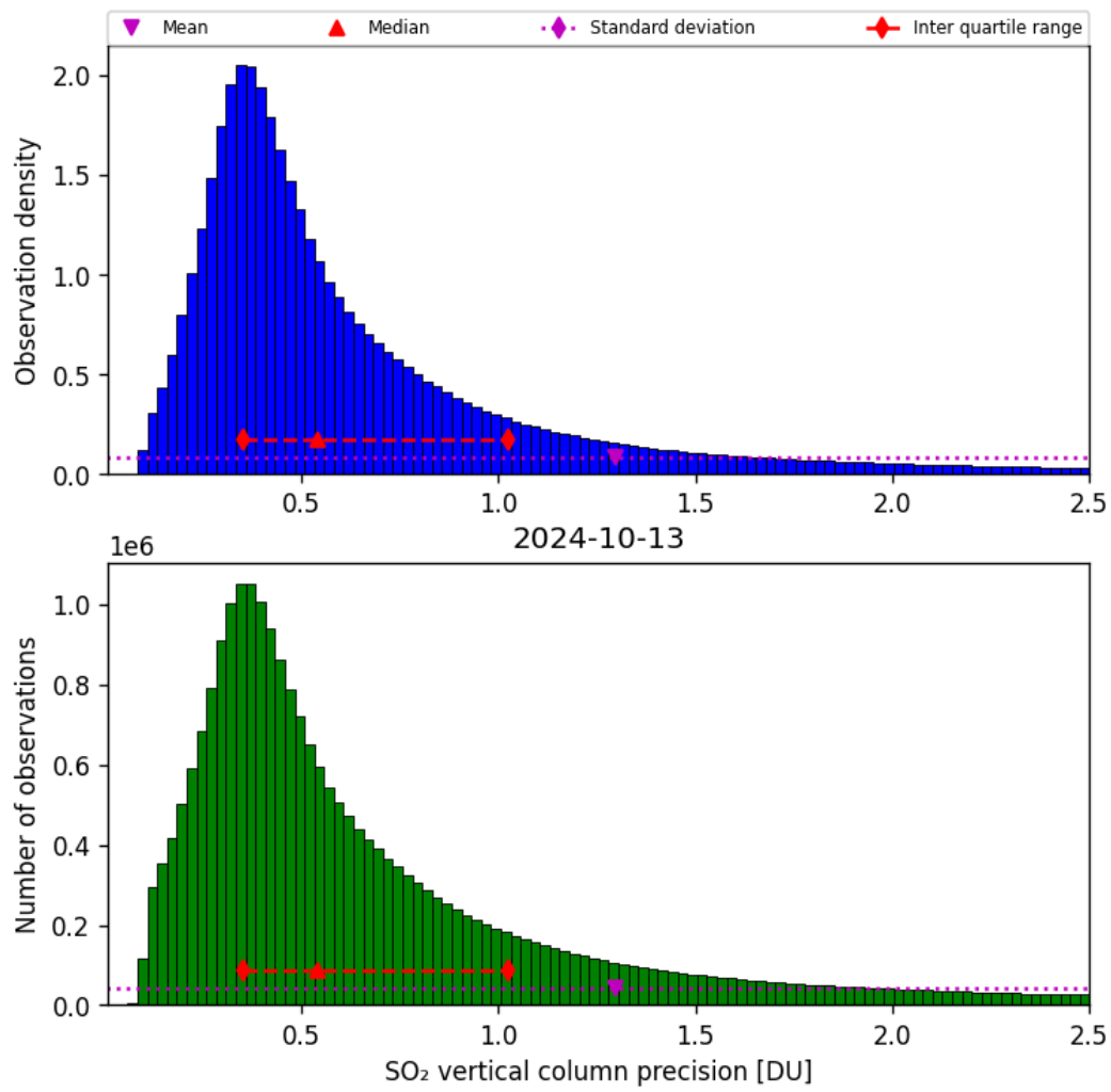
Figure 54: Histogram of “SO 2 vertical column precision” for 2024-10-12 to 2024-10-14
