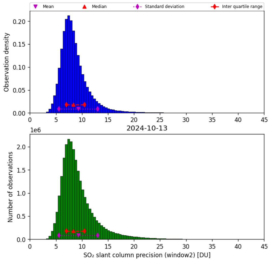
Figure 61: Histogram of “SO 2 slant column precision (window2)” for 2024-10-12 to 2024-10-14
