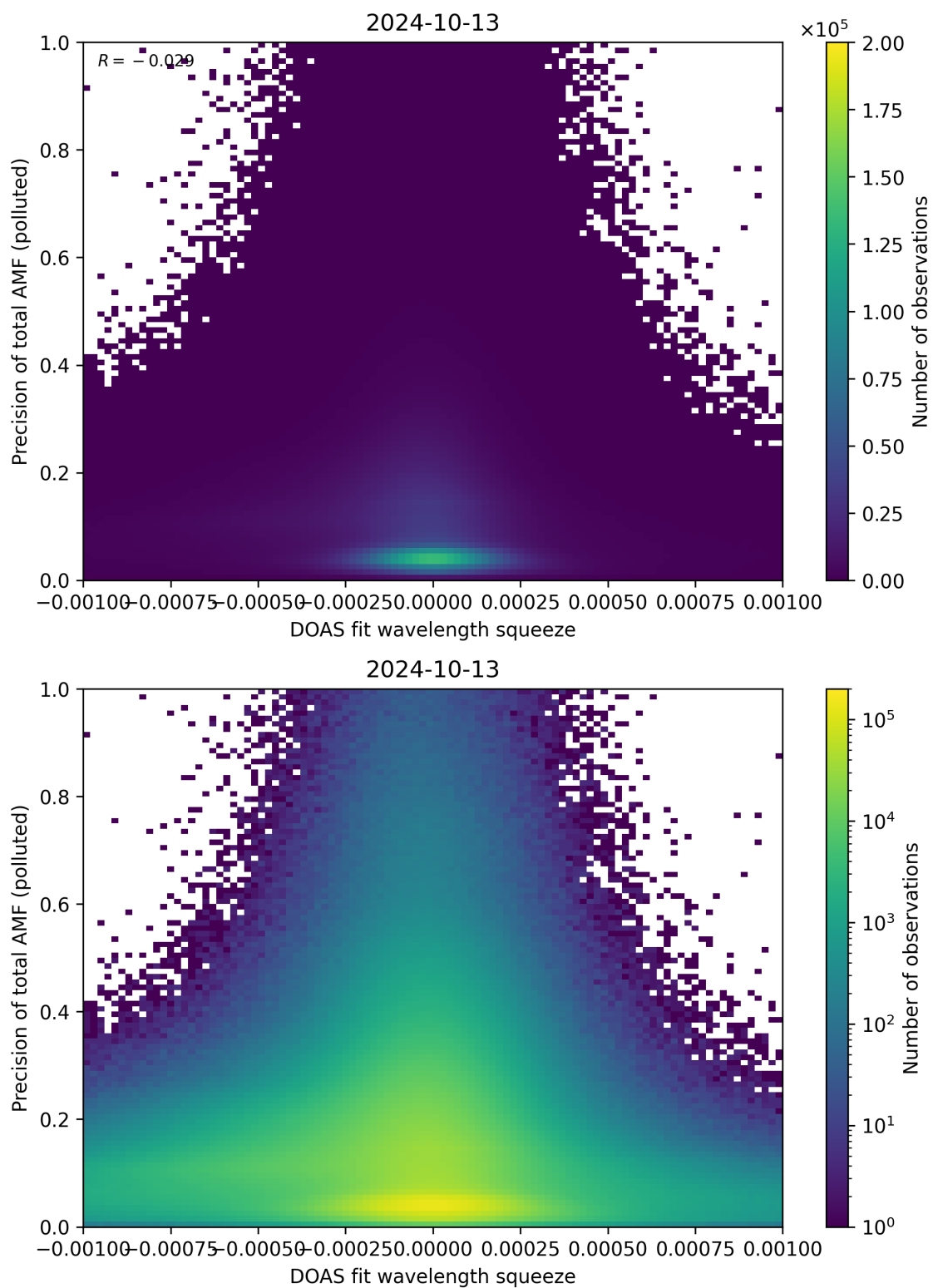
Figure 135: Scatter density plot of “DOAS fit wavelength squeeze” against “Precision of total AMF (polluted)” for 2024-10-12 to 2024-10-14.
