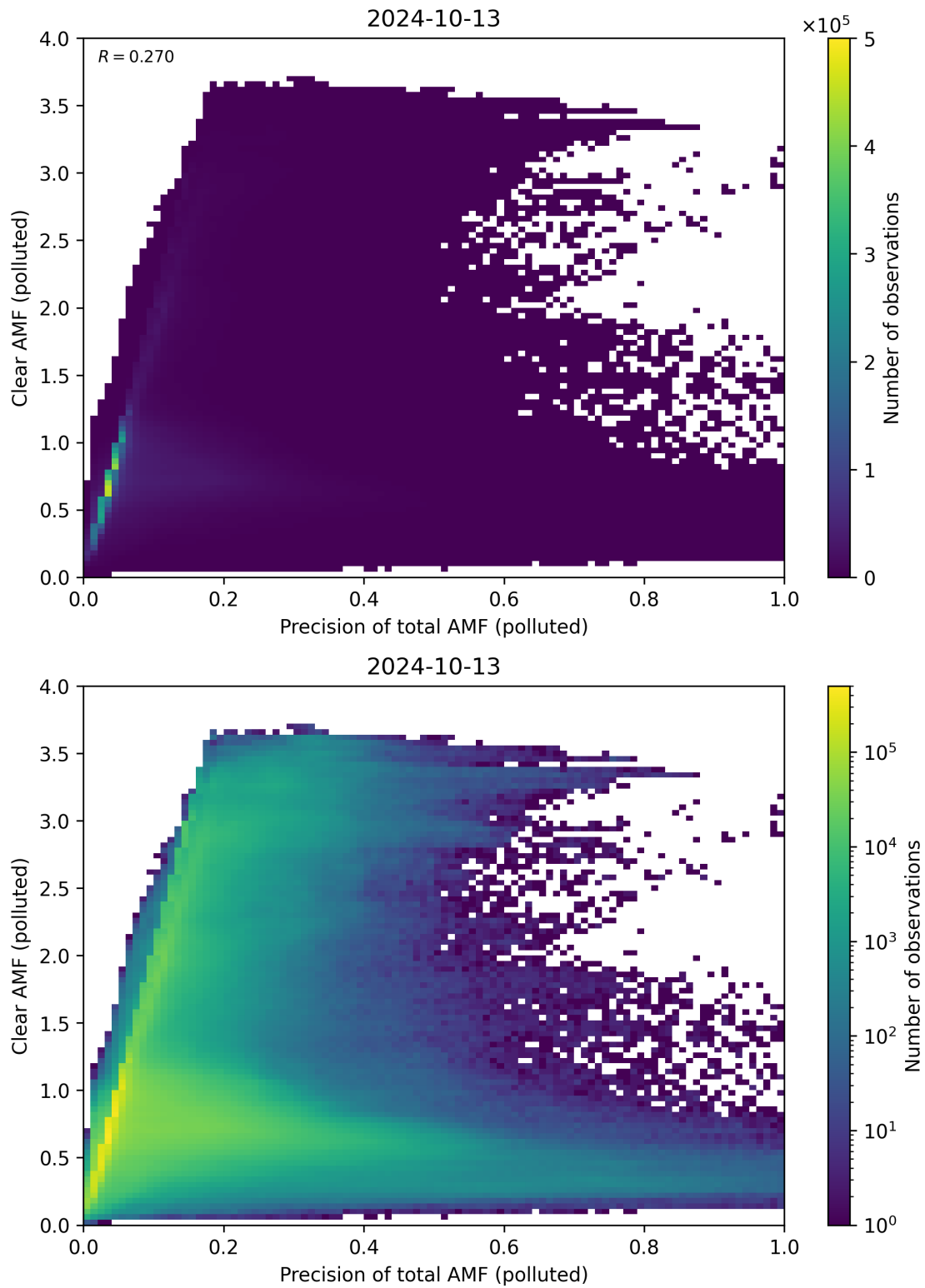
Figure 270: Scatter density plot of “Precision of total AMF (polluted)” against “Clear AMF (polluted)” for 2024-10-12 to 2024-10-14.
