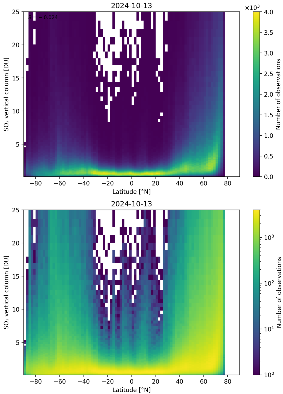
Figure 156: Scatter density plot of “Latitude” against “SO 2 vertical column” for 2024-10-12 to 2024-10-14.
