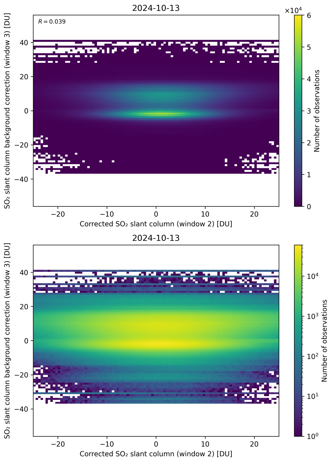
Figure 195: Scatter density plot of “Corrected SO 2 slant column (window 2)” against “SO 2 slant column background correction (window 3)” for 2024-10-12 to 2024-10-14.
