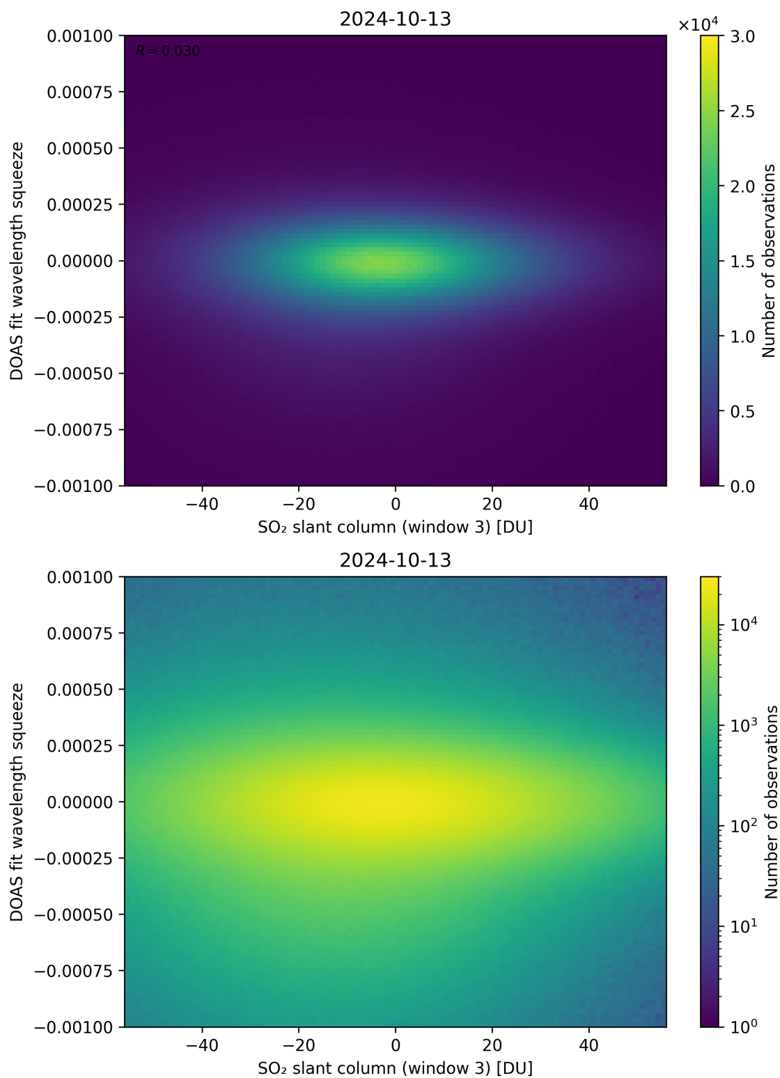
Figure 255: Scatter density plot of “SO 2 slant column (window 3)” against “DOAS fit wavelength squeeze” for 2024-10-12 to 2024-10-14.
