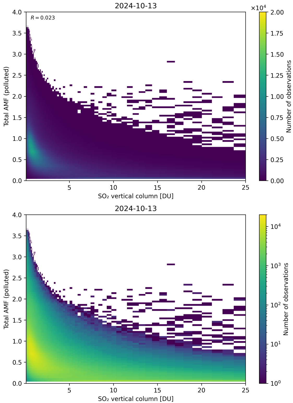
Figure 305: Scatter density plot of “SO 2 vertical column” against “Total AMF (polluted)” for 2024-10-12 to 2024-10-14.
