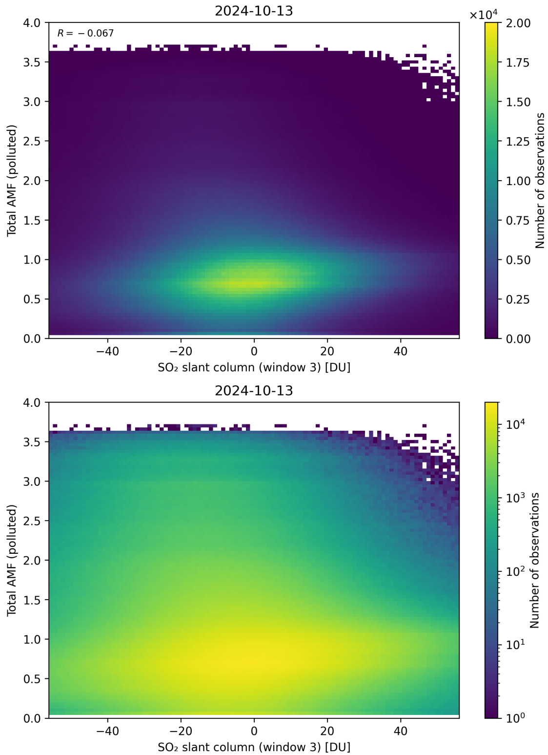
Figure 268: Scatter density plot of “SO 2 slant column (window 3)” against “Total AMF (polluted)” for 2024-10-12 to 2024-10-14.
