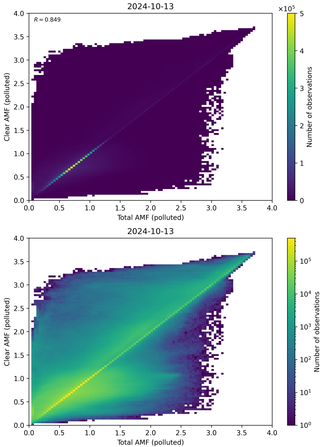
Figure 271: Scatter density plot of “Total AMF (polluted)” against “Clear AMF (polluted)” for 2024-10-12 to 2024-10-14.
