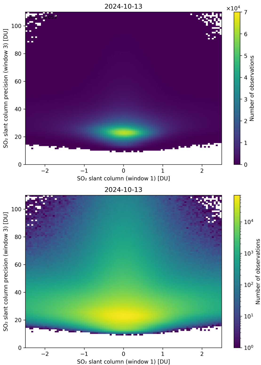
Figure 238: Scatter density plot of “SO 2 slant column (window 1)” against “SO 2 slant column precision (window 3)” for 2024-10-12 to 2024-10-14.
