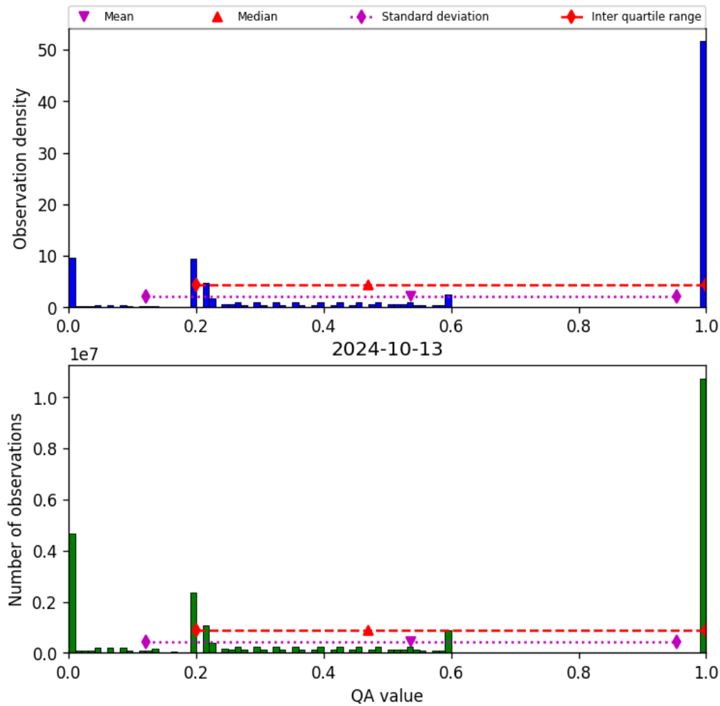
Figure 52: Histogram of “QA value” for 2024-10-12 to 2024-10-14
