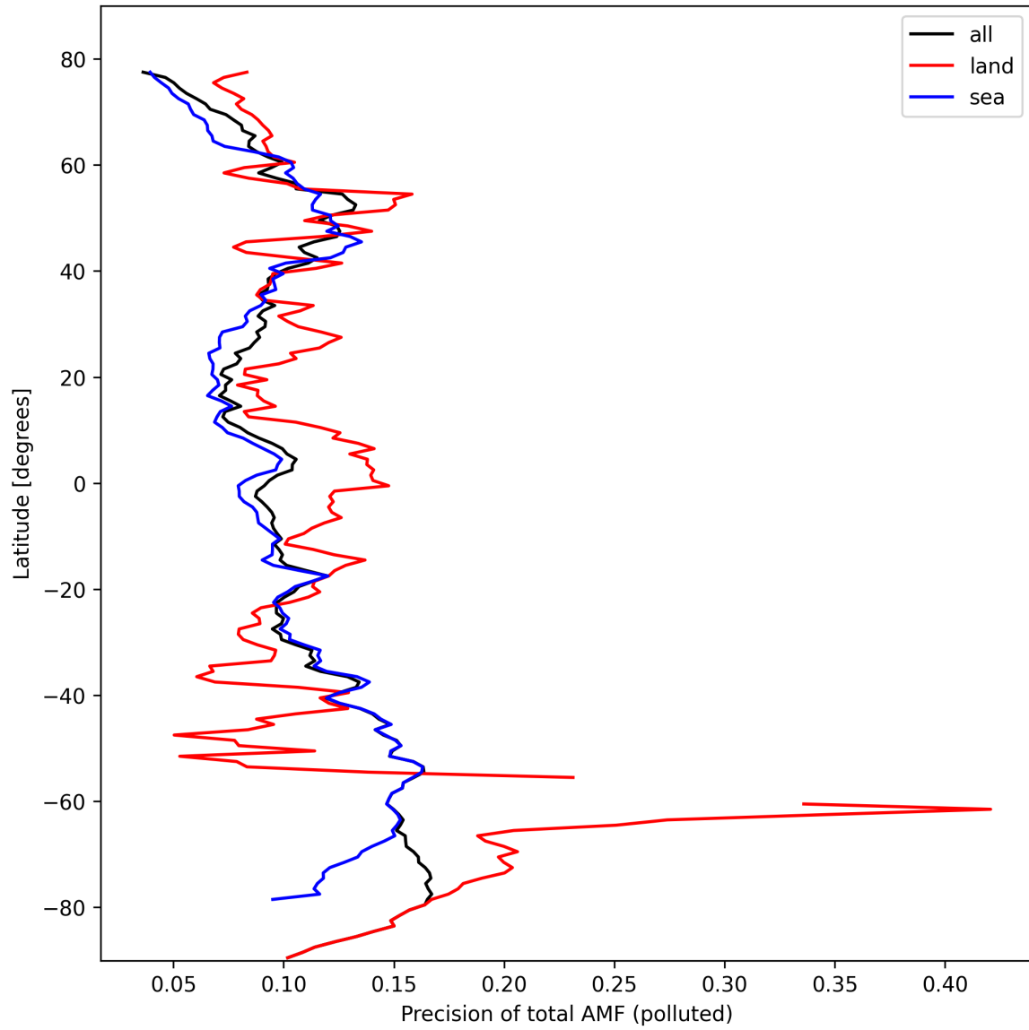
Figure 49: Zonal average of “Precision of total AMF (polluted)” for 2024-10-12 to 2024-10-14.
