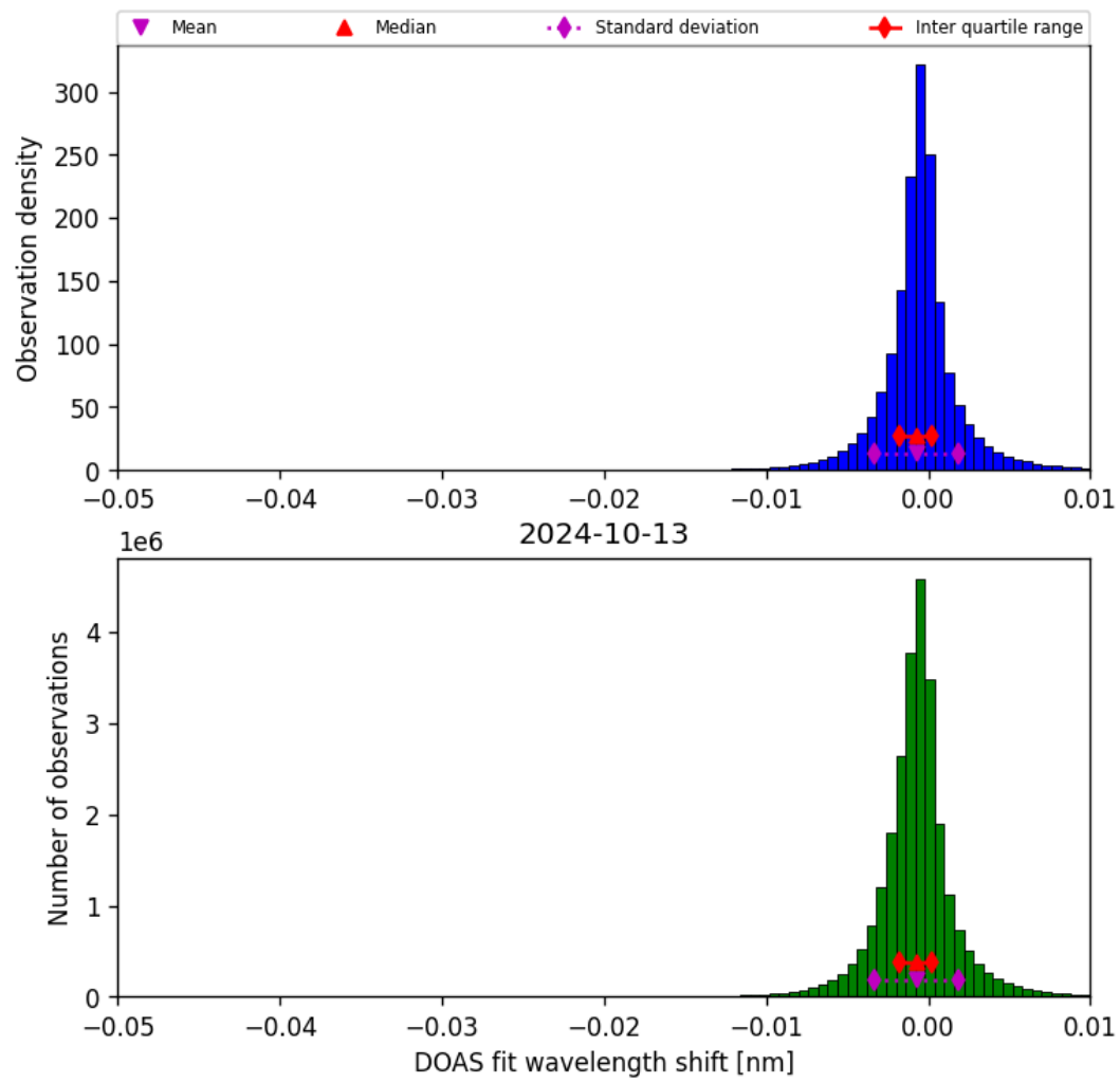
Figure 68: Histogram of “DOAS fit wavelength shift” for 2024-10-12 to 2024-10-14
