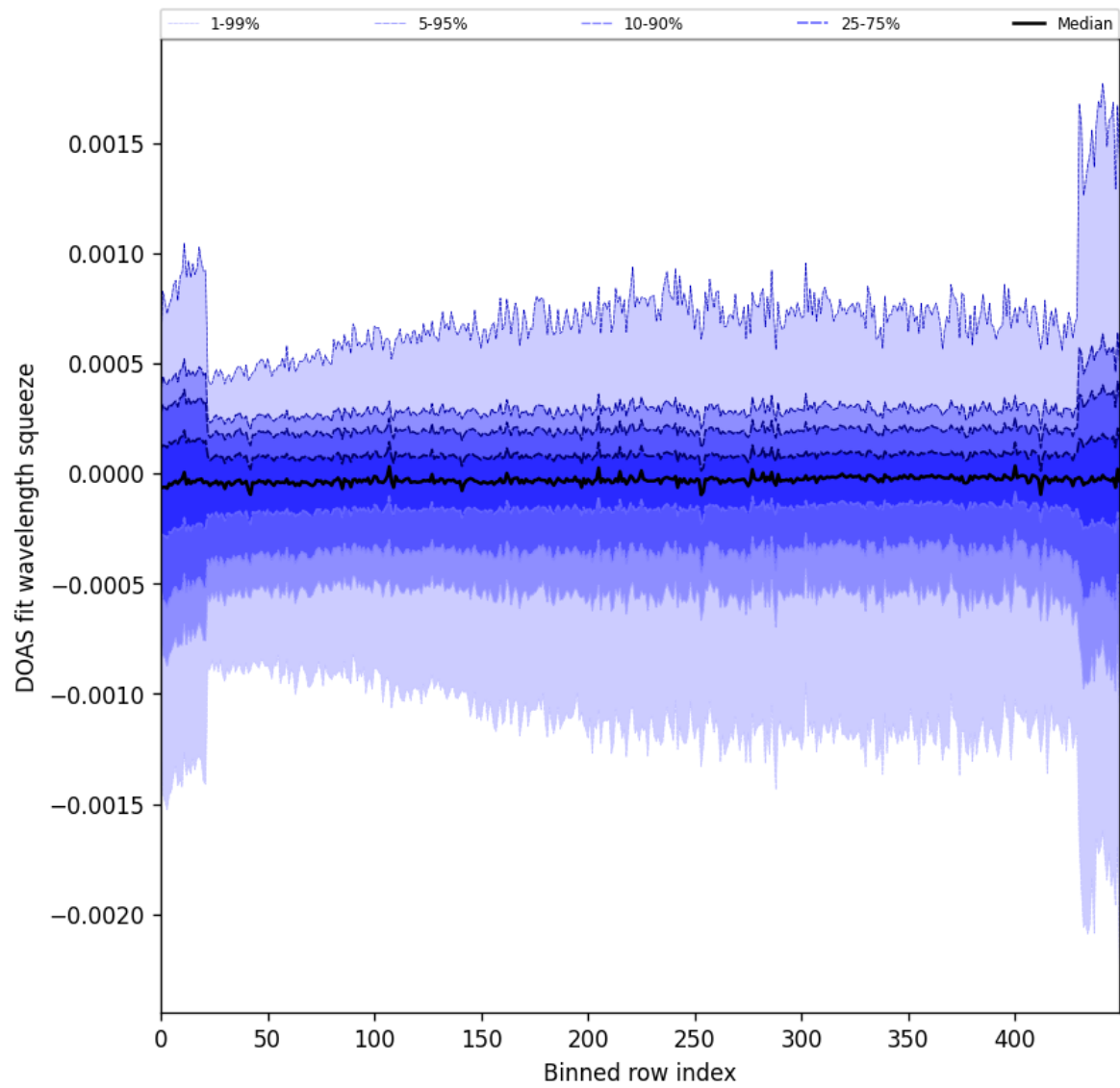
Figure 92: Along track statistics of “DOAS fit wavelength squeeze” for 2024-10-12 to 2024-10-14
