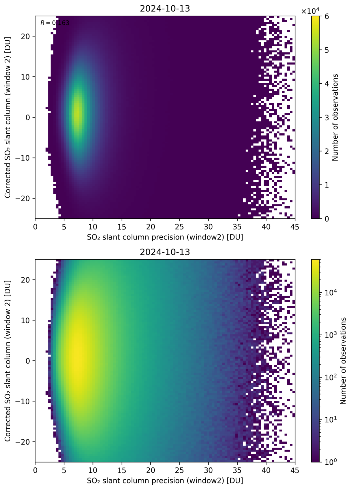
Figure 247: Scatter density plot of “SO 2 slant column precision (window2)” against “Corrected SO 2 slant column (window 2)” for 2024-10-12 to 2024-10-14.
