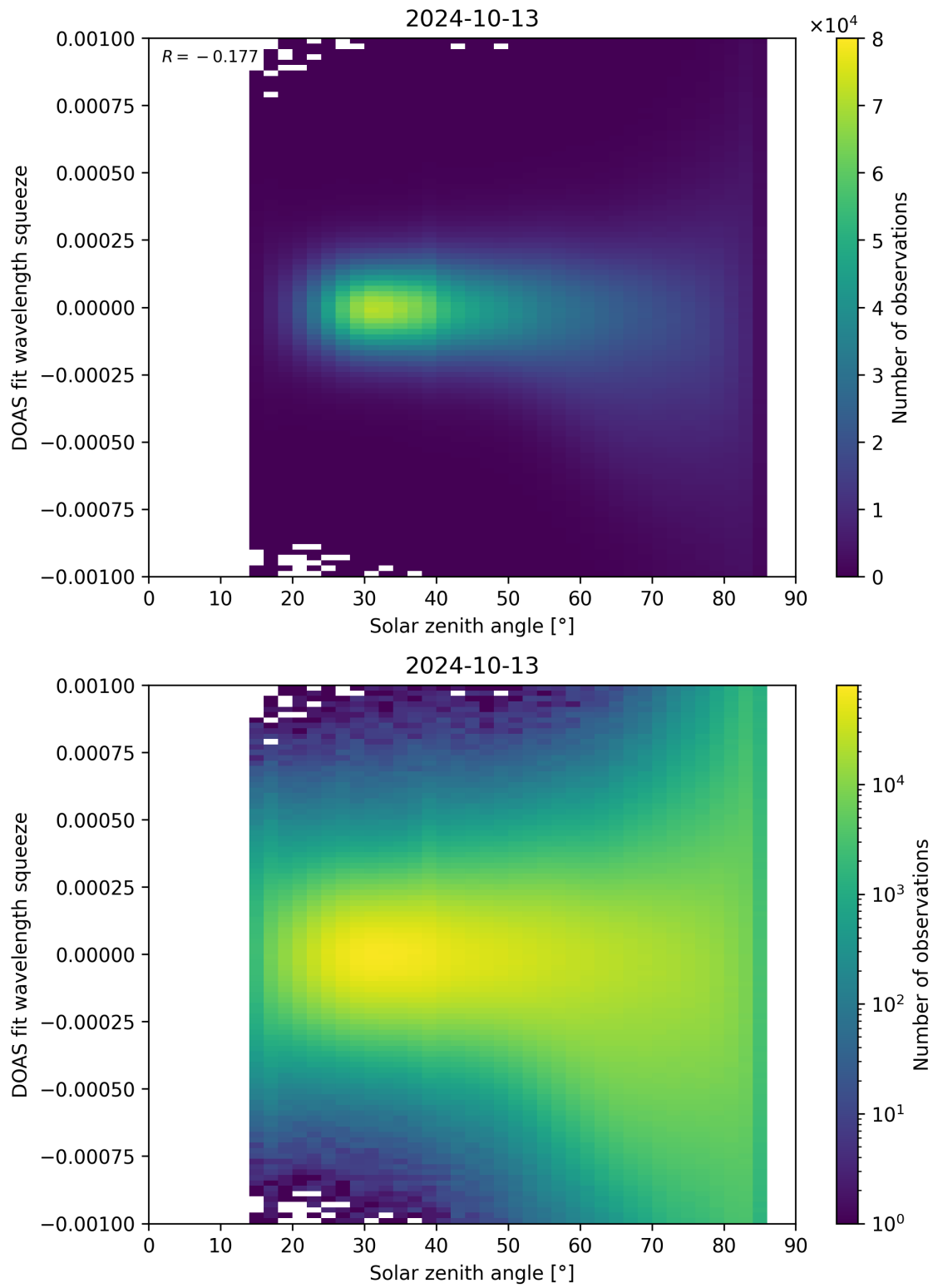
Figure 162: Scatter density plot of “Solar zenith angle” against “DOAS fit wavelength squeeze” for 2024-10-12 to 2024-10-14.
