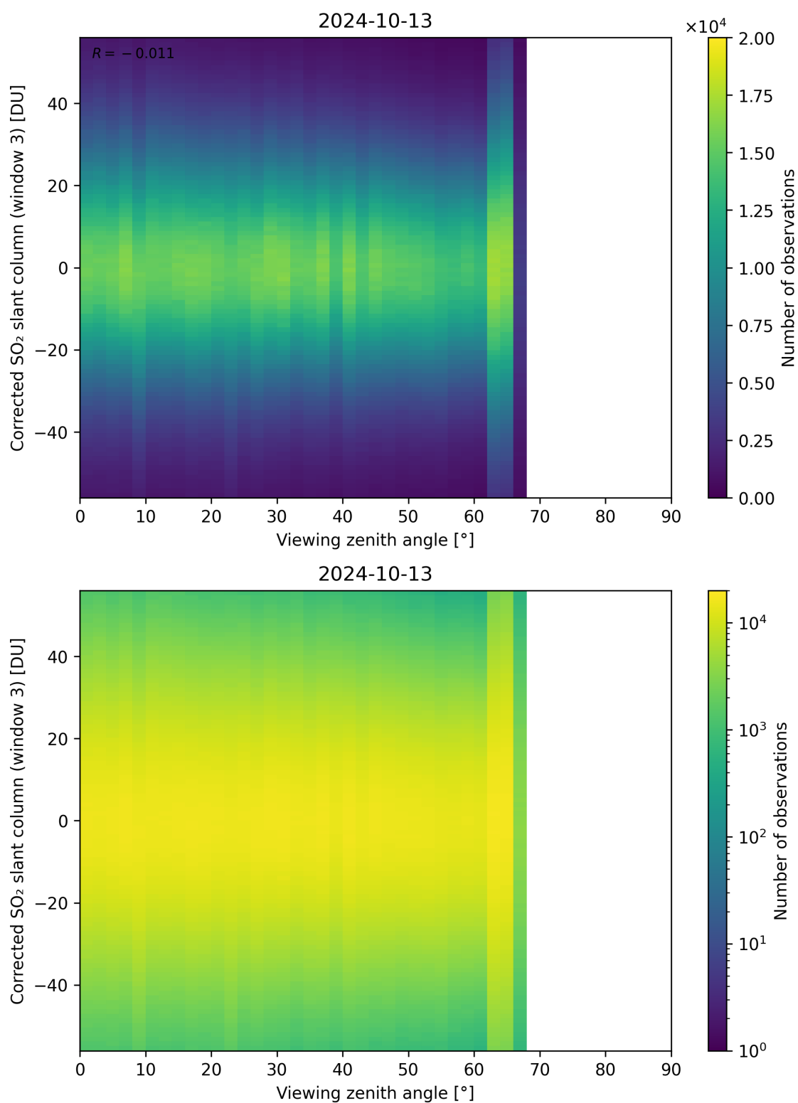
Figure 319: Scatter density plot of “Viewing zenith angle” against “Corrected SO 2 slant column (window 3)” for 2024-10-12 to 2024-10-14.
