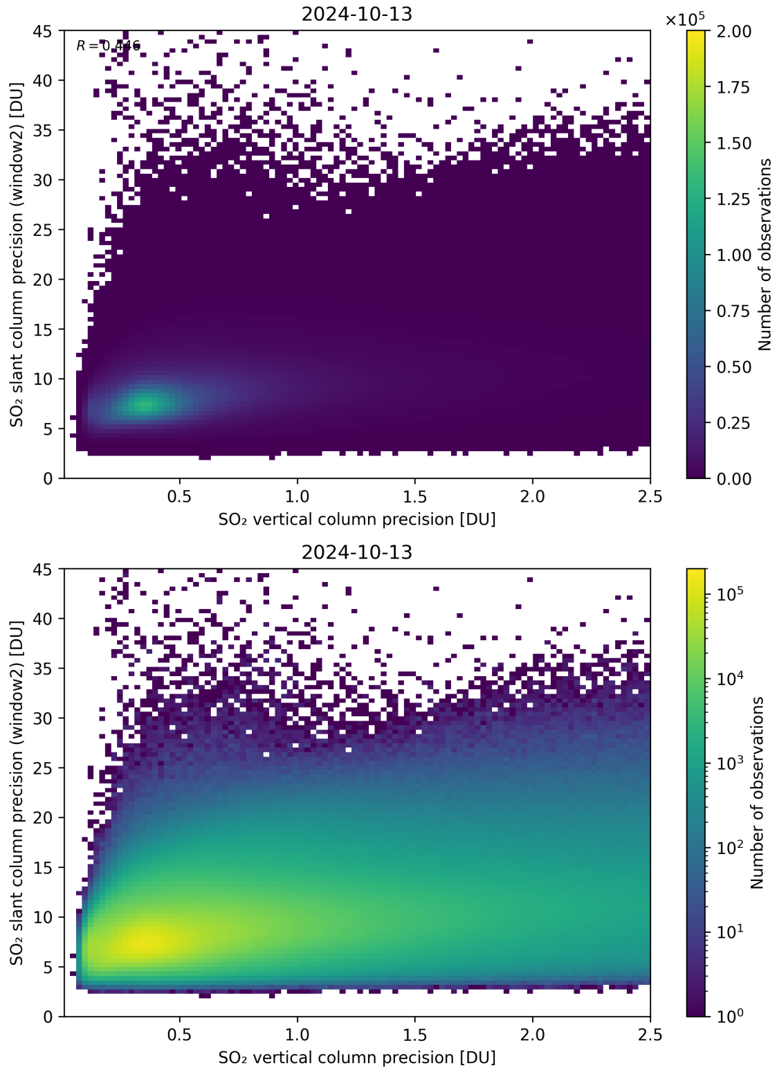
Figure 291: Scatter density plot of “SO 2 vertical column precision” against “SO 2 slant column precision (window2)” for 2024-10-12 to 2024-10-14.
