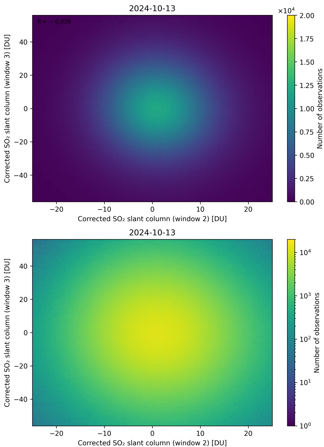
Figure 200: Scatter density plot of “Corrected SO 2 slant column (window 2)” against “Corrected SO 2 slant column (window 3)” for 2024-10-12 to 2024-10-14.
