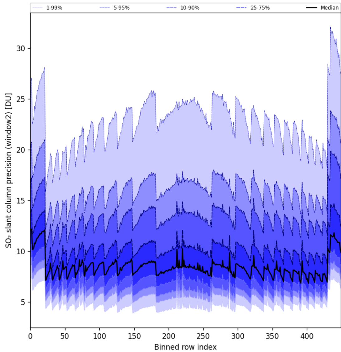
Figure 84: Along track statistics of “SO 2 slant column precision (window2)” for 2024-10-12 to 2024-10-14
