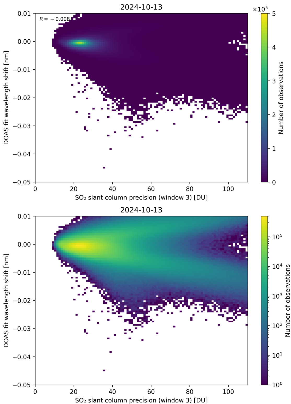
Figure 258: Scatter density plot of “SO 2 slant column precision (window 3)” against “DOAS fit wavelength shift” for 2024-10-12 to 2024-10-14.
