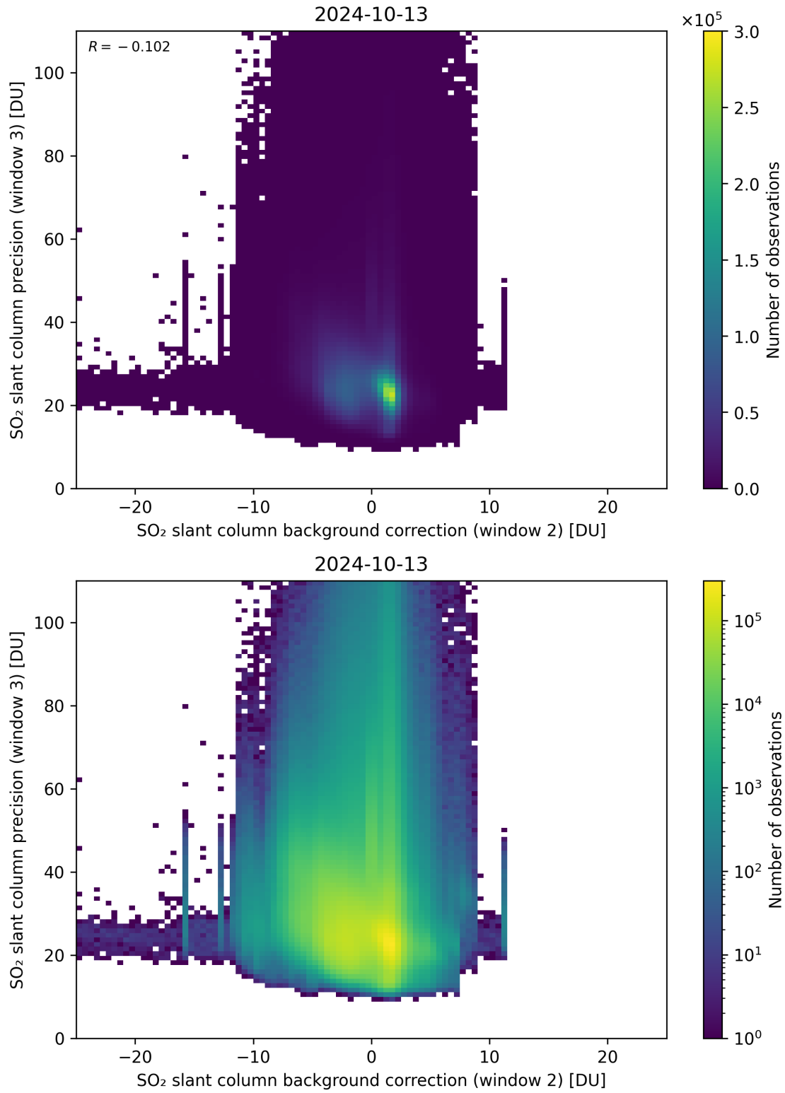
Figure 118: Scatter density plot of “SO 2 slant column background correction (window 2)” against “SO 2 slant column precision (window 3)” for 2024-10-12 to 2024-10-14.
