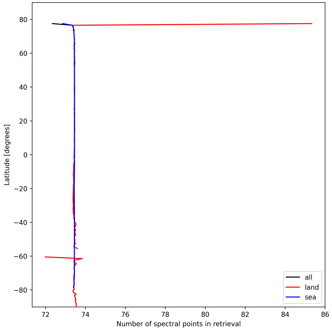
Figure 51: Zonal average of “Number of spectral points in retrieval” for 2024-10-12 to 2024-10-14.
