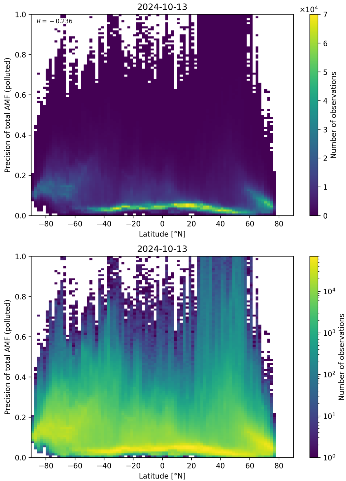
Figure 155: Scatter density plot of “Latitude” against “Precision of total AMF (polluted)” for 2024-10-12 to 2024-10-14.
