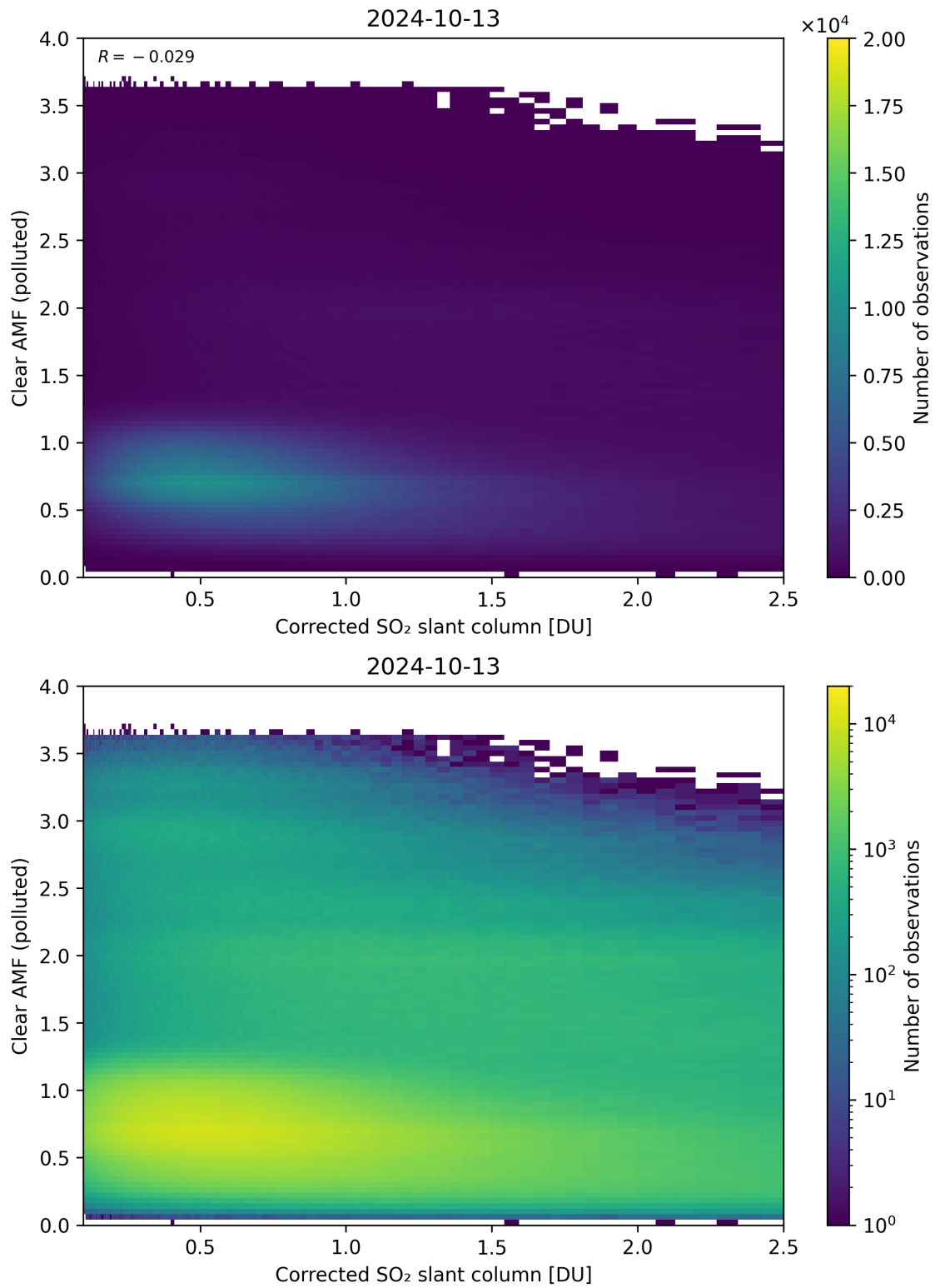
Figure 184: Scatter density plot of “Corrected SO 2 slant column” against “Clear AMF (polluted)” for 2024-10-12 to 2024-10-14.
