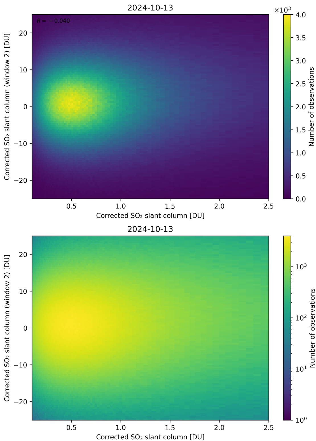
Figure 185: Scatter density plot of “Corrected SO 2 slant column” against “Corrected SO 2 slant column (window 2)” for 2024-10-12 to 2024-10-14.
