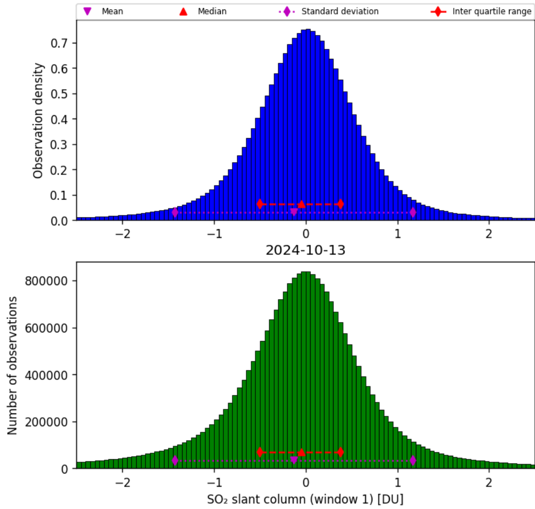
Figure 56: Histogram of “SO 2 slant column (window 1)” for 2024-10-12 to 2024-10-14
