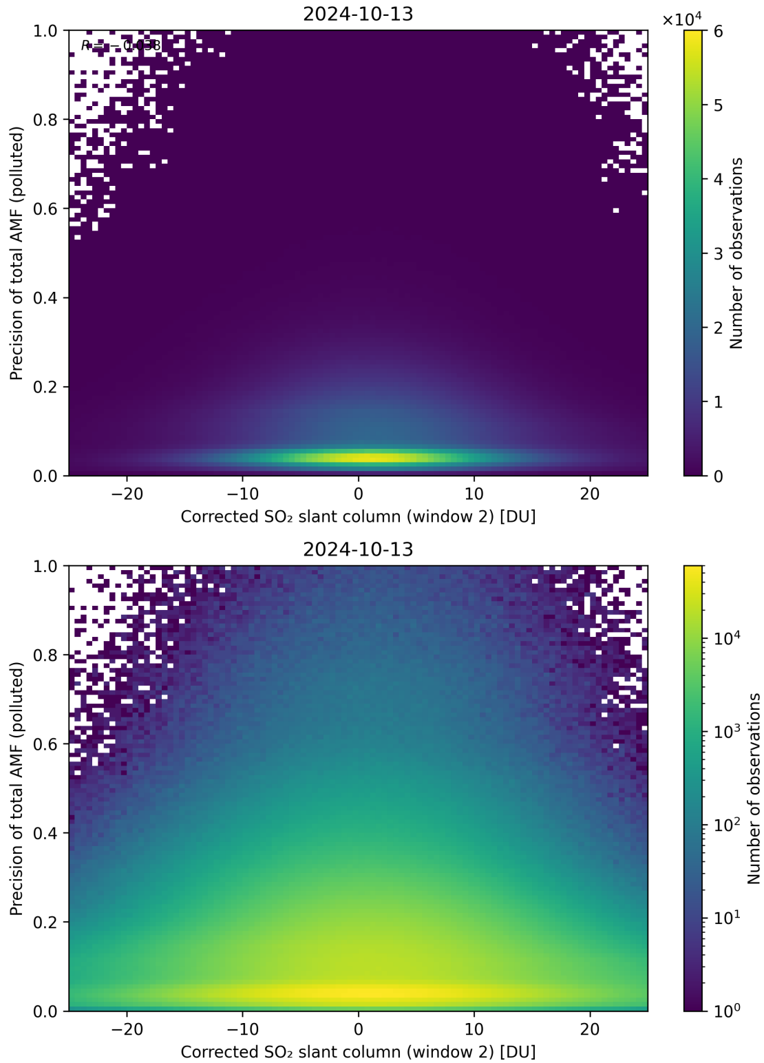
Figure 204: Scatter density plot of “Corrected SO 2 slant column (window 2)” against “Precision of total AMF (polluted)” for 2024-10-12 to 2024-10-14.
