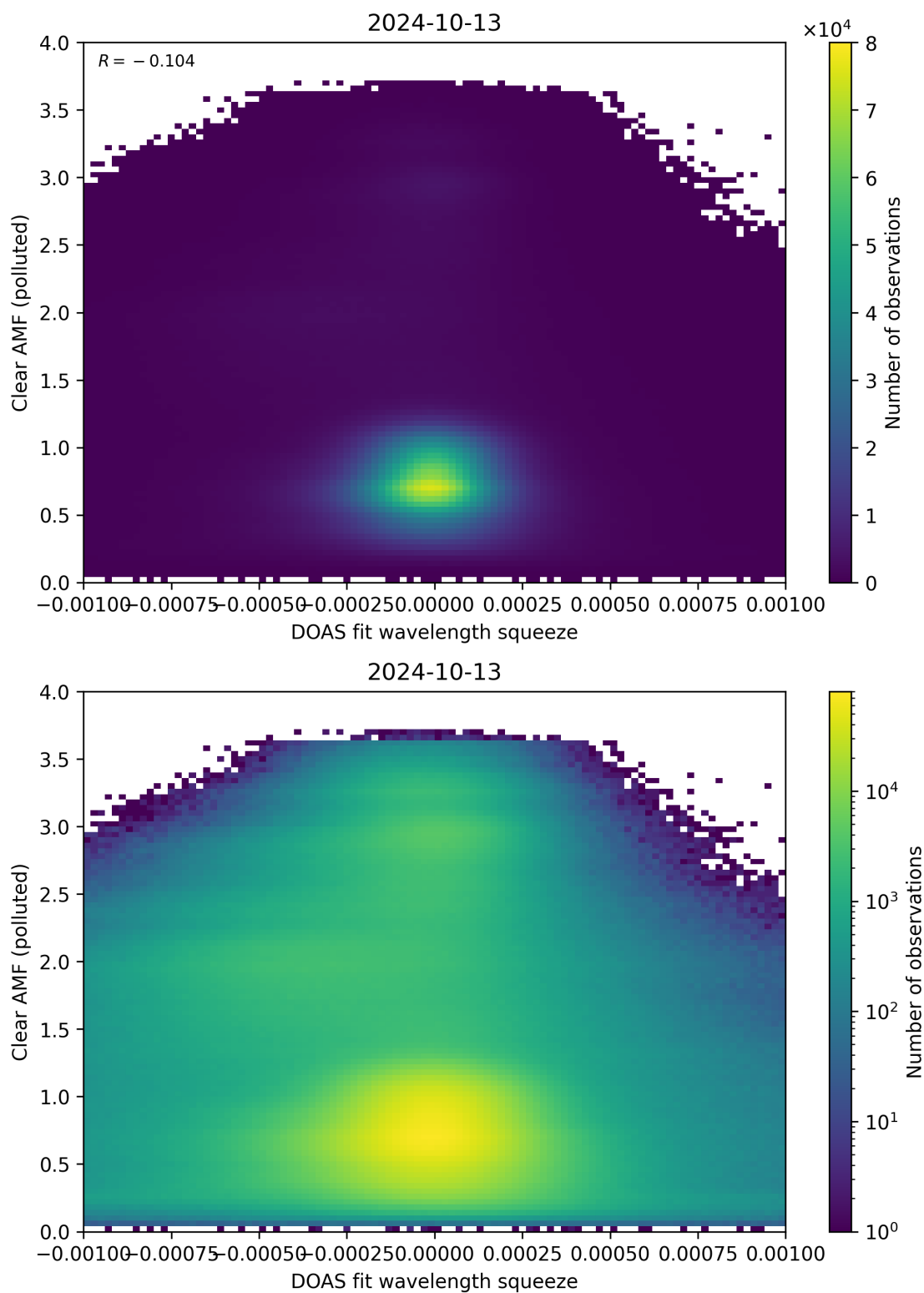
Figure 133: Scatter density plot of “DOAS fit wavelength squeeze” against “Clear AMF (polluted)” for 2024-10-12 to 2024-10-14.
