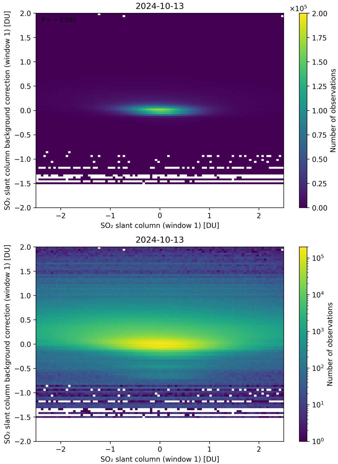
Figure 212: Scatter density plot of “SO 2 slant column (window 1)” against “SO 2 slant column background correction (window 1)” for 2024-10-12 to 2024-10-14.
