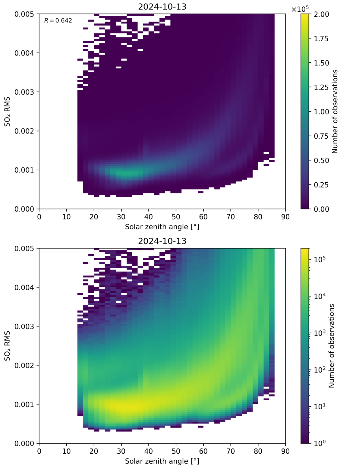
Figure 163: Scatter density plot of “Solar zenith angle” against “SO 2 RMS” for 2024-10-12 to 2024-10-14.
