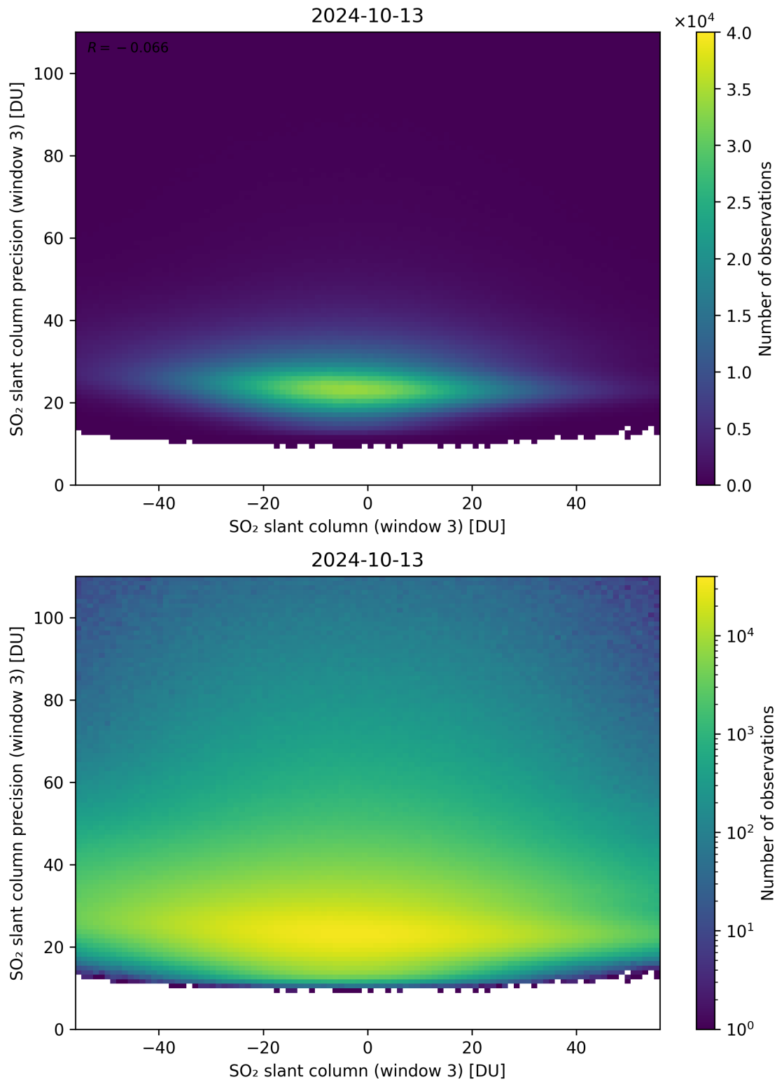
Figure 267: Scatter density plot of “SO 2 slant column (window 3)” against “SO 2 slant column precision (window 3)” for 2024-10-12 to 2024-10-14.
