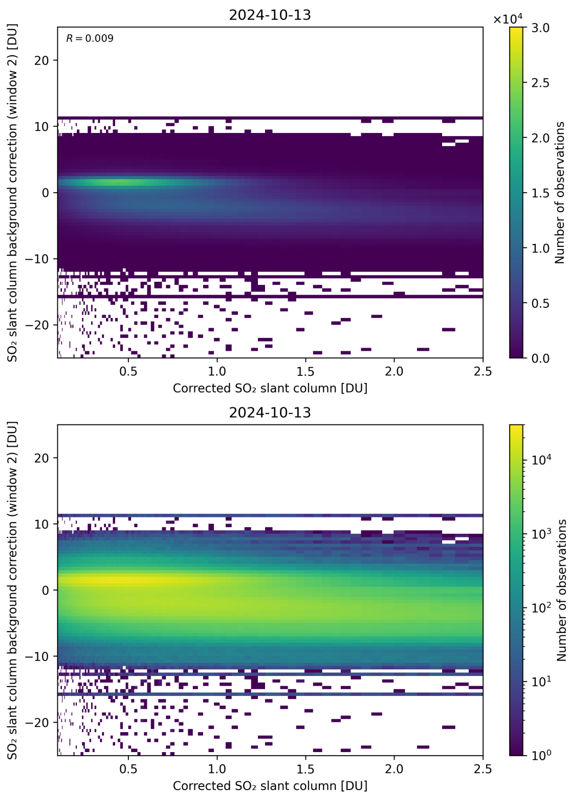
Figure 179: Scatter density plot of “Corrected SO 2 slant column” against “SO 2 slant column background correction (window 2)” for 2024-10-12 to 2024-10-14.
