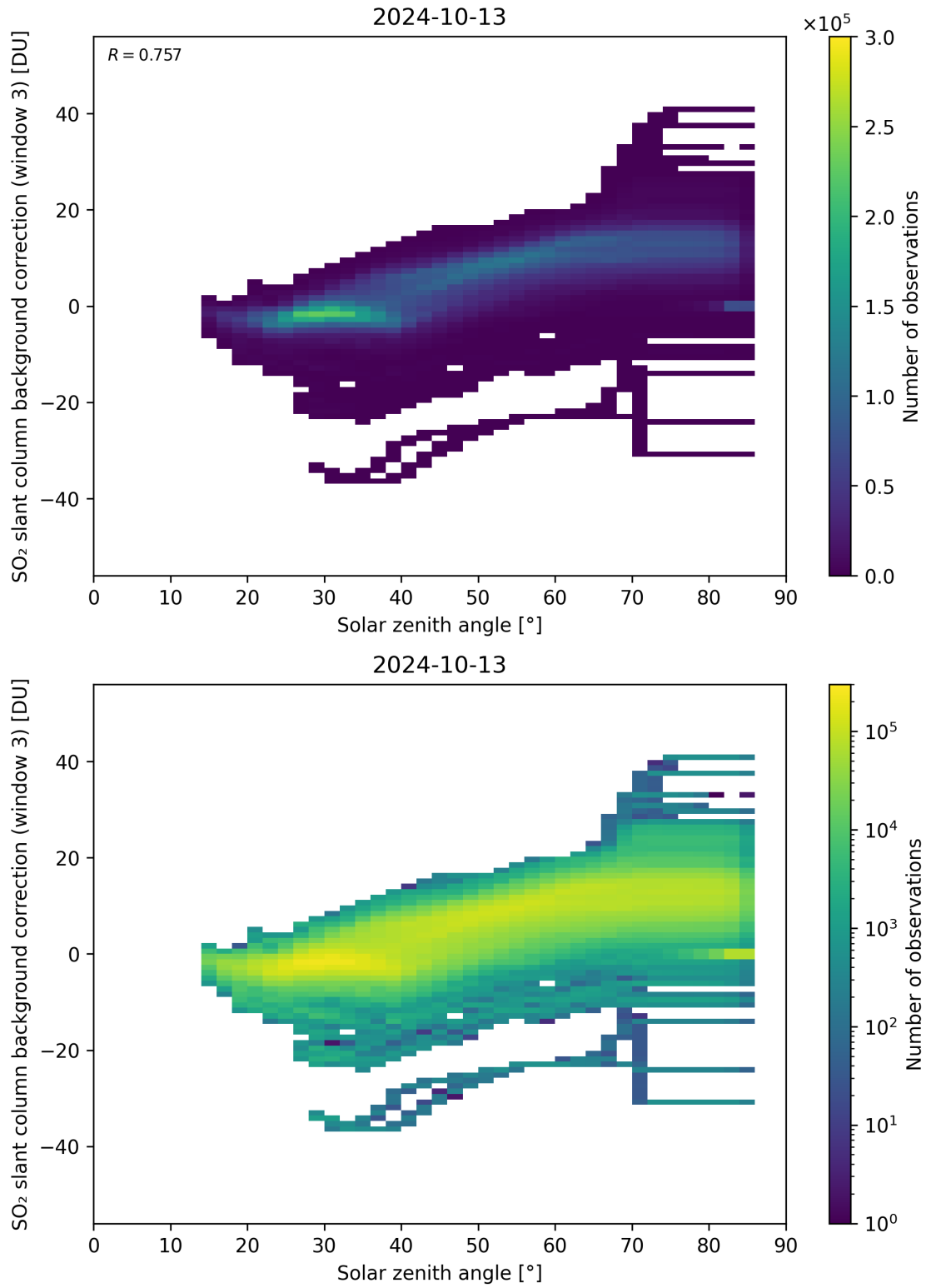
Figure 160: Scatter density plot of “Solar zenith angle” against “SO 2 slant column background correction (window 3)” for 2024-10-12 to 2024-10-14.
