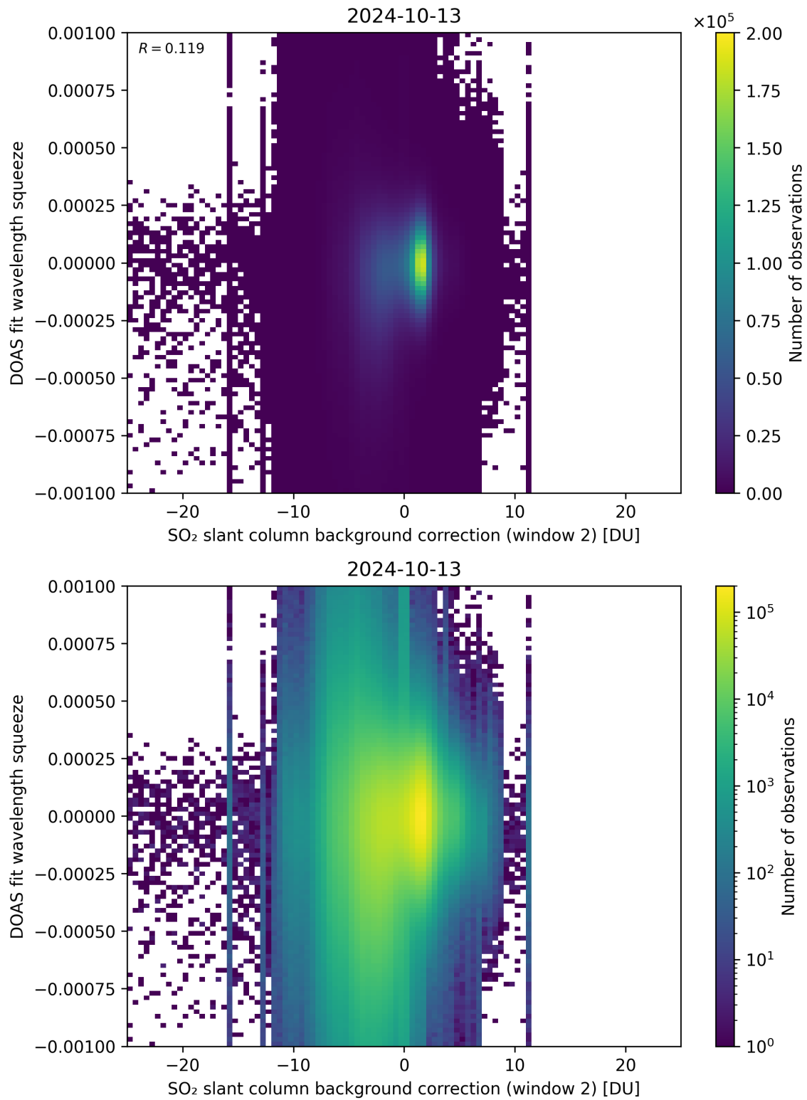
Figure 113: Scatter density plot of “SO 2 slant column background correction (window 2)” against “DOAS fit wavelength squeeze” for 2024-10-12 to 2024-10-14.
