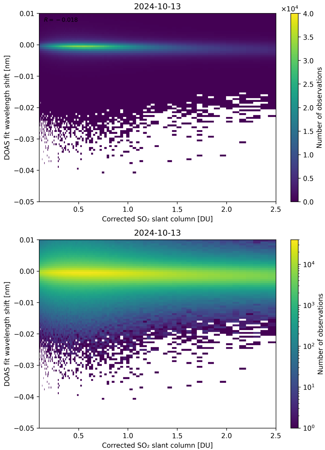
Figure 181: Scatter density plot of “Corrected SO 2 slant column” against “DOAS fit wavelength shift” for 2024-10-12 to 2024-10-14.
