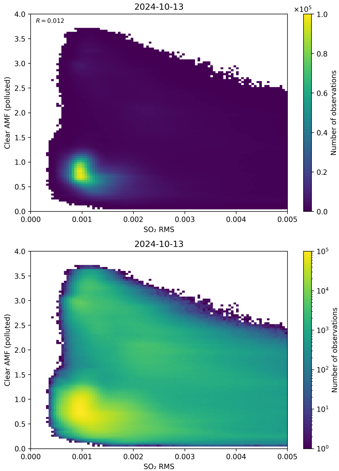
Figure 136: Scatter density plot of “SO 2 RMS” against “Clear AMF (polluted)” for 2024-10-12 to 2024-10-14.
