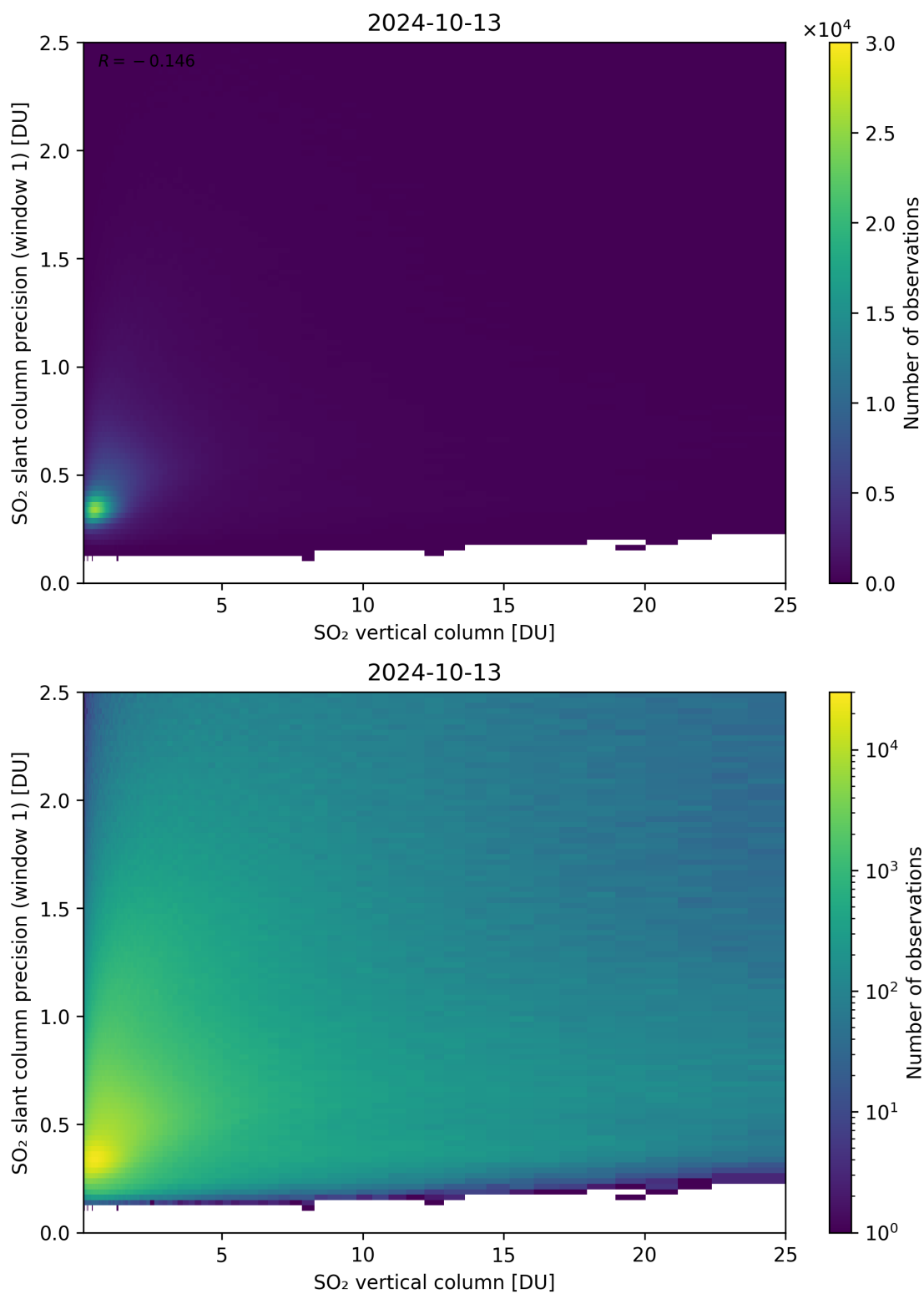
Figure 301: Scatter density plot of “SO 2 vertical column” against “SO 2 slant column precision (window 1)” for 2024-10-12 to 2024-10-14.
