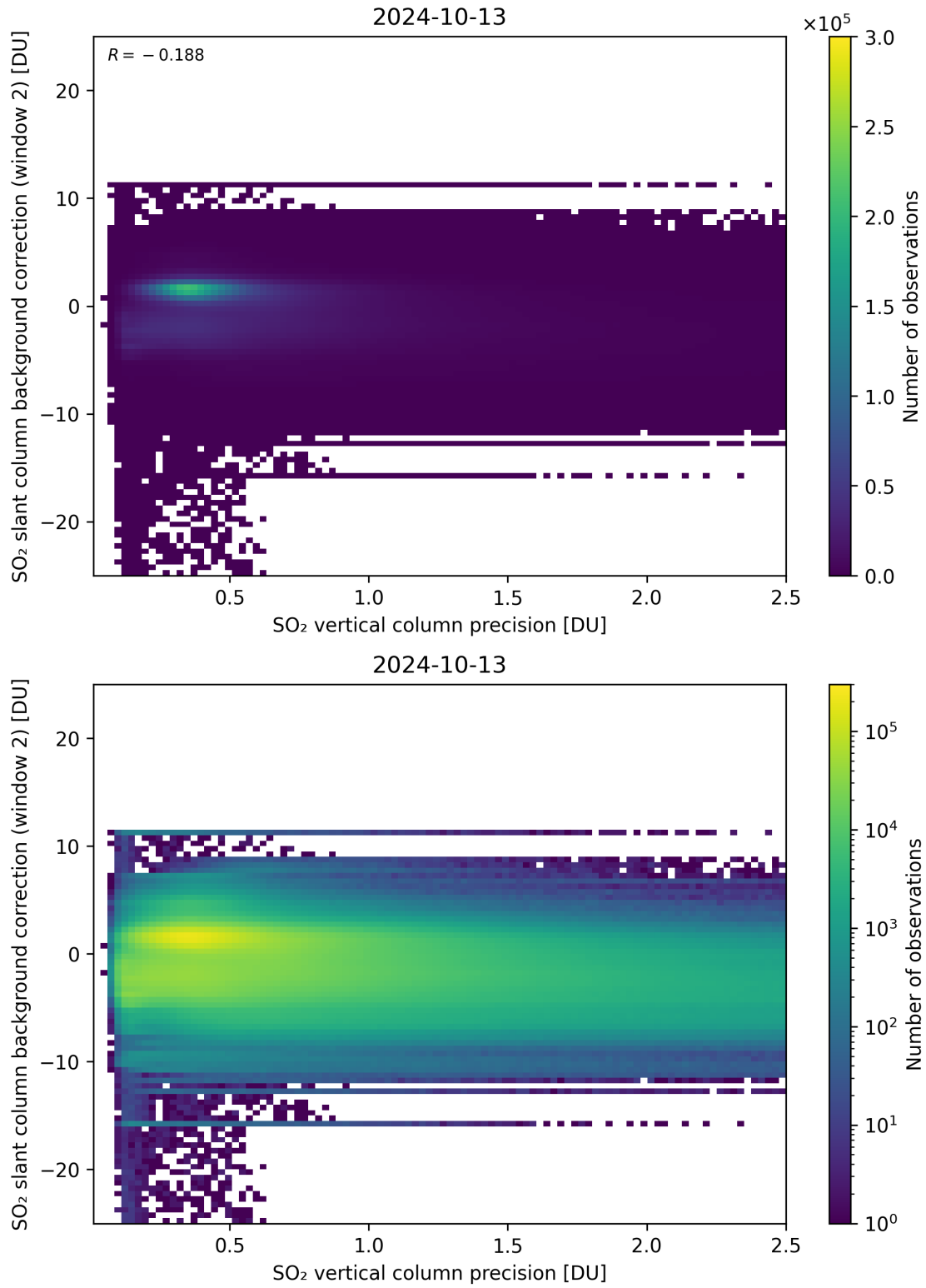
Figure 280: Scatter density plot of “SO 2 vertical column precision” against “SO 2 slant column background correction (window 2)” for 2024-10-12 to 2024-10-14.
