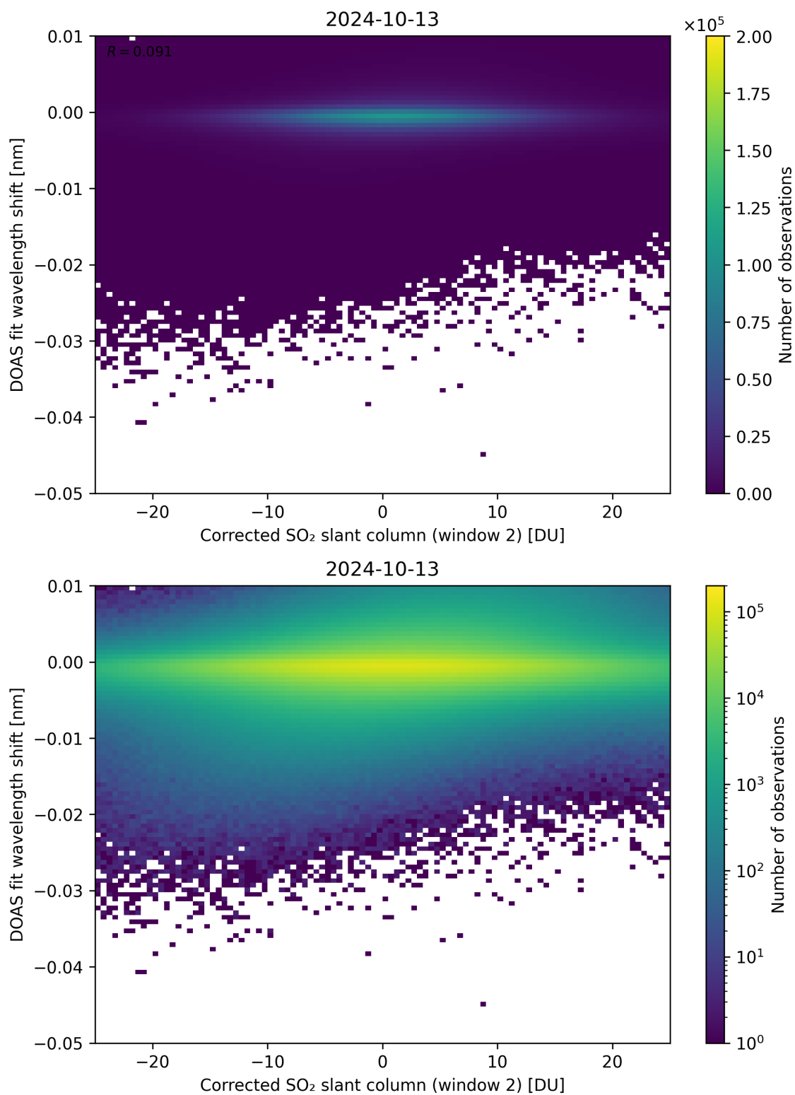
Figure 196: Scatter density plot of “Corrected SO 2 slant column (window 2)” against “DOAS fit wavelength shift” for 2024-10-12 to 2024-10-14.
