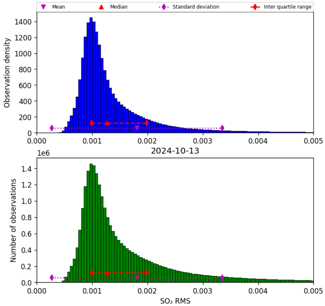
Figure 70: Histogram of “SO 2 RMS” for 2024-10-12 to 2024-10-14
