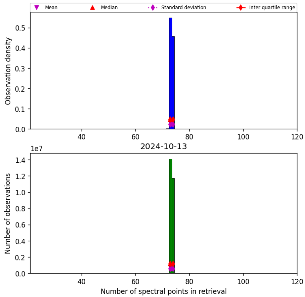
Figure 74: Histogram of “Number of spectral points in retrieval” for 2024-10-12 to 2024-10-14
