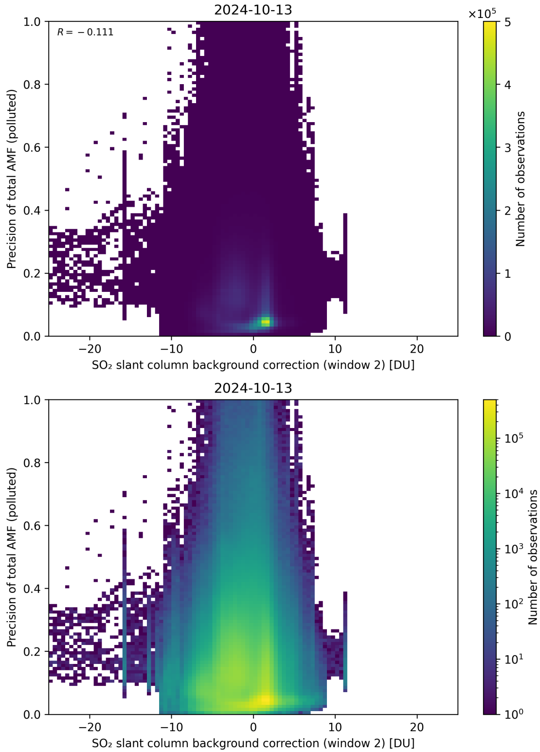
Figure 120: Scatter density plot of “SO 2 slant column background correction (window 2)” against “Precision of total AMF (polluted)” for 2024-10-12 to 2024-10-14.
