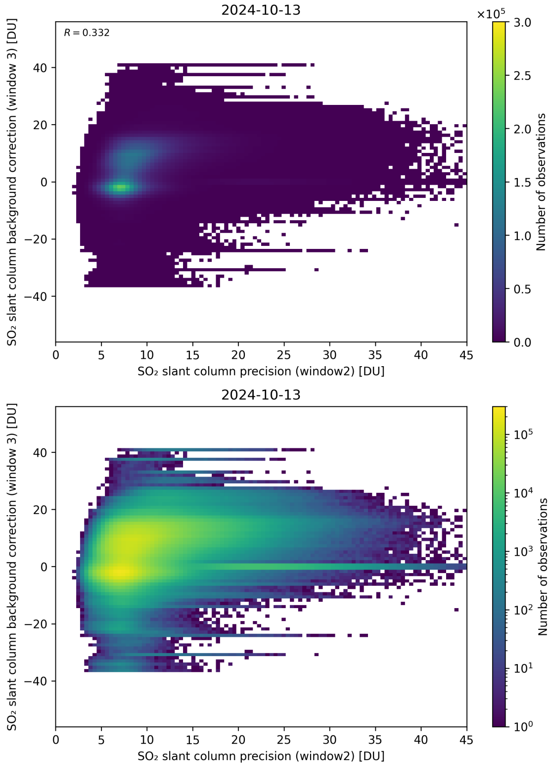
Figure 242: Scatter density plot of “SO 2 slant column precision (window2)” against “SO 2 slant column background correction (window 3)” for 2024-10-12 to 2024-10-14.
