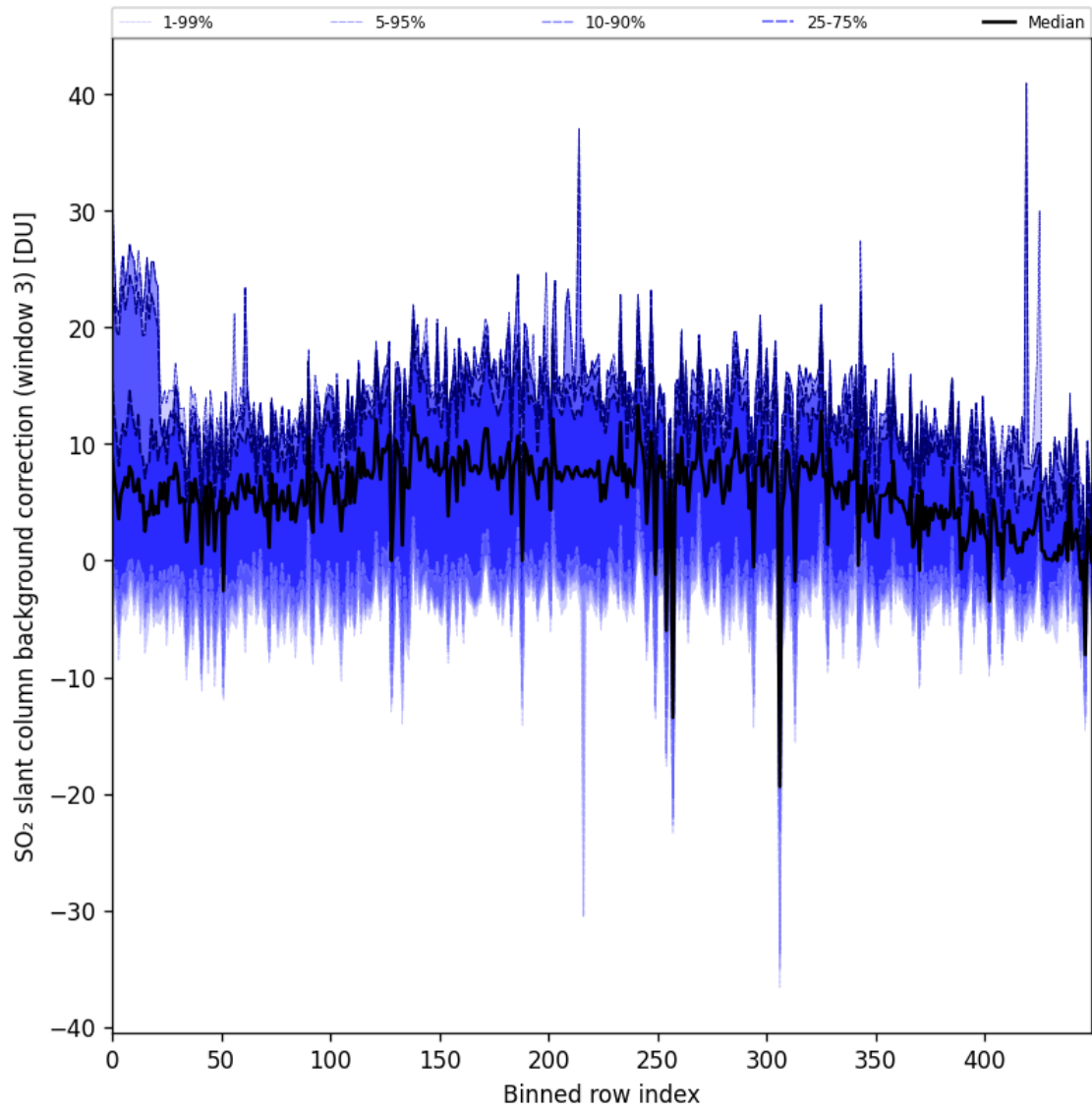
Figure 90: Along track statistics of “SO 2 slant column background correction (window 3)” for 2024-10-12 to 2024-10-14
