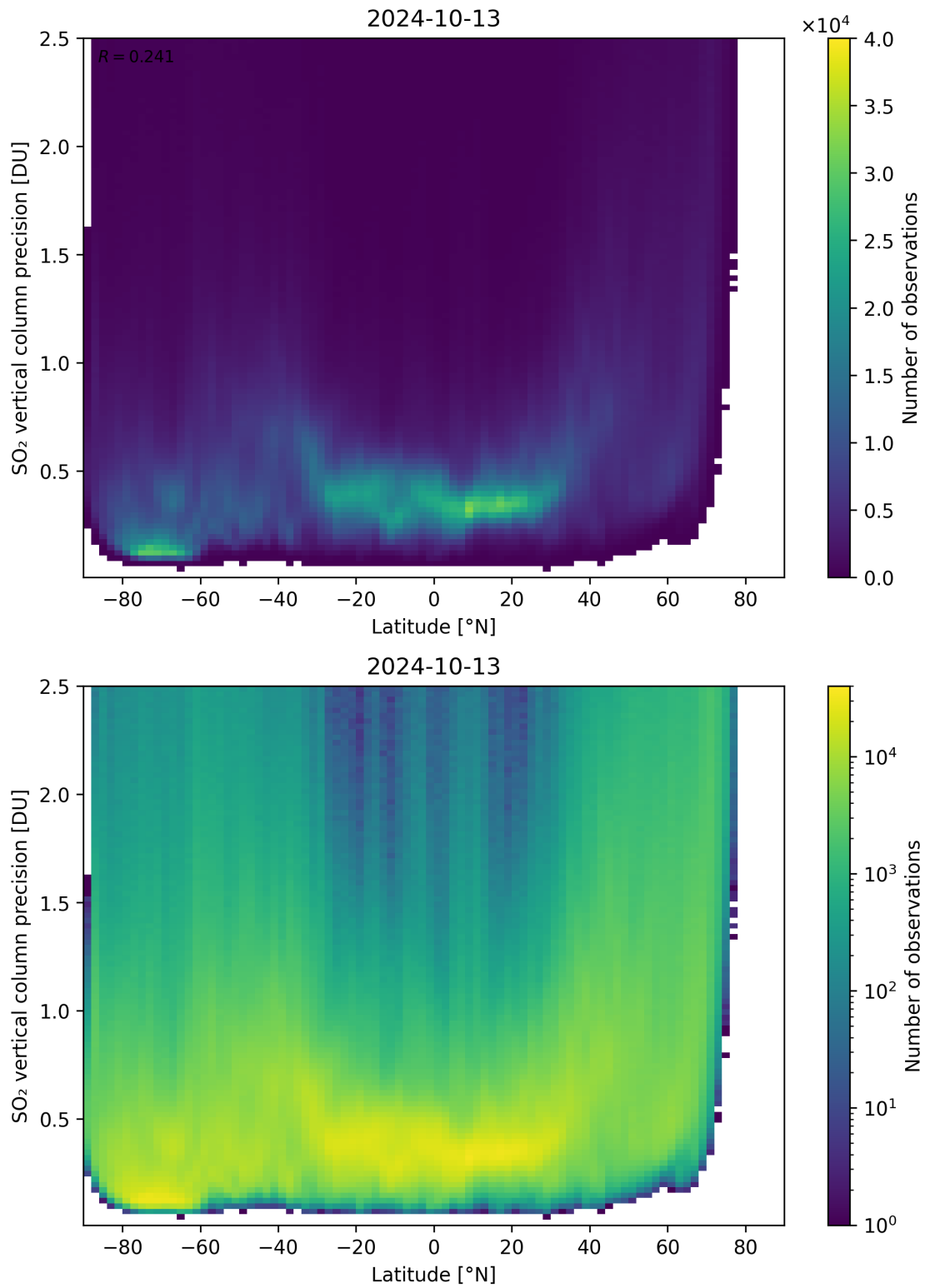
Figure 157: Scatter density plot of “Latitude” against “SO 2 vertical column precision” for 2024-10-12 to 2024-10-14.
