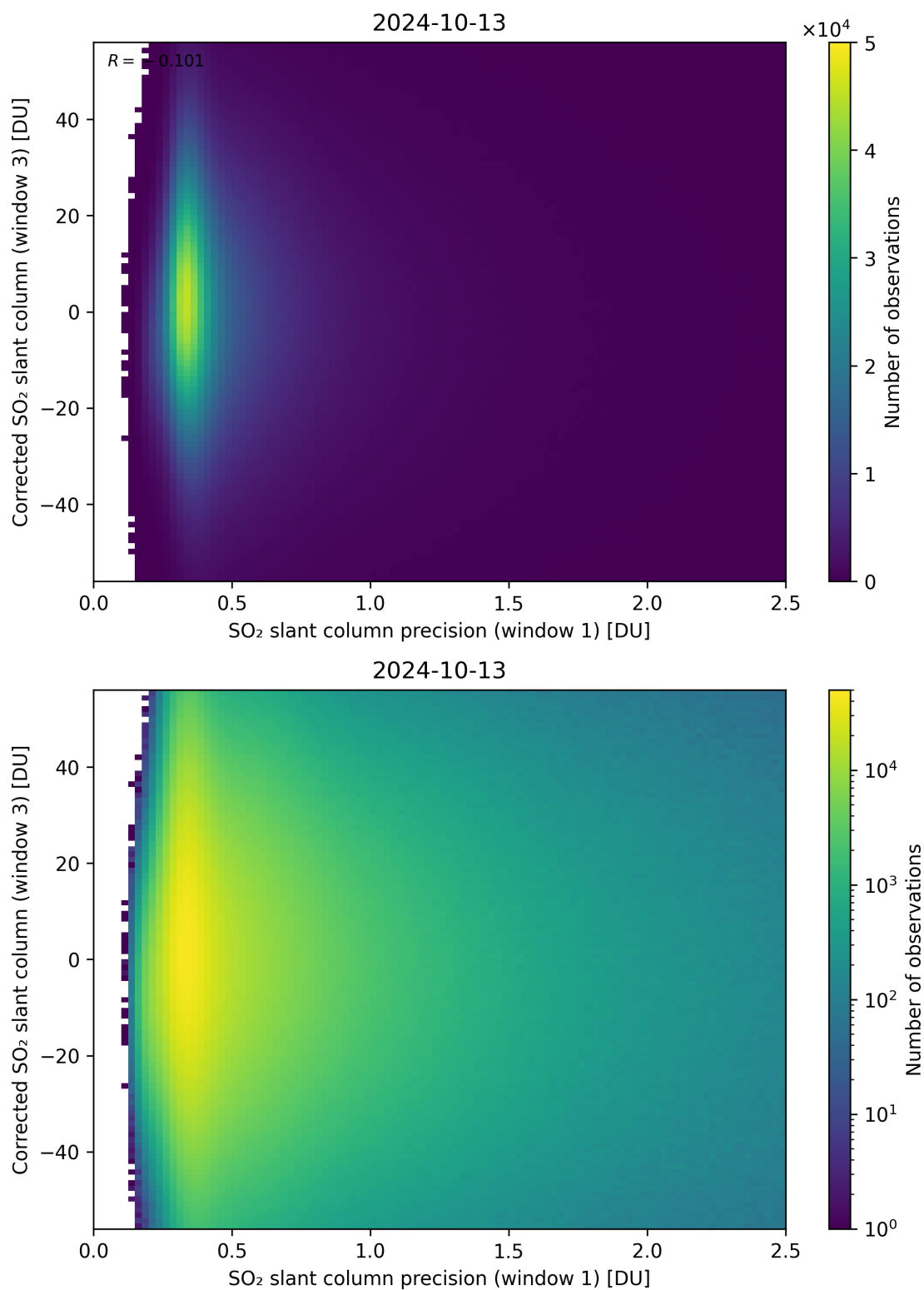
Figure 226: Scatter density plot of “SO 2 slant column precision (window 1)” against “Corrected SO 2 slant column (window 3)” for 2024-10-12 to 2024-10-14.
