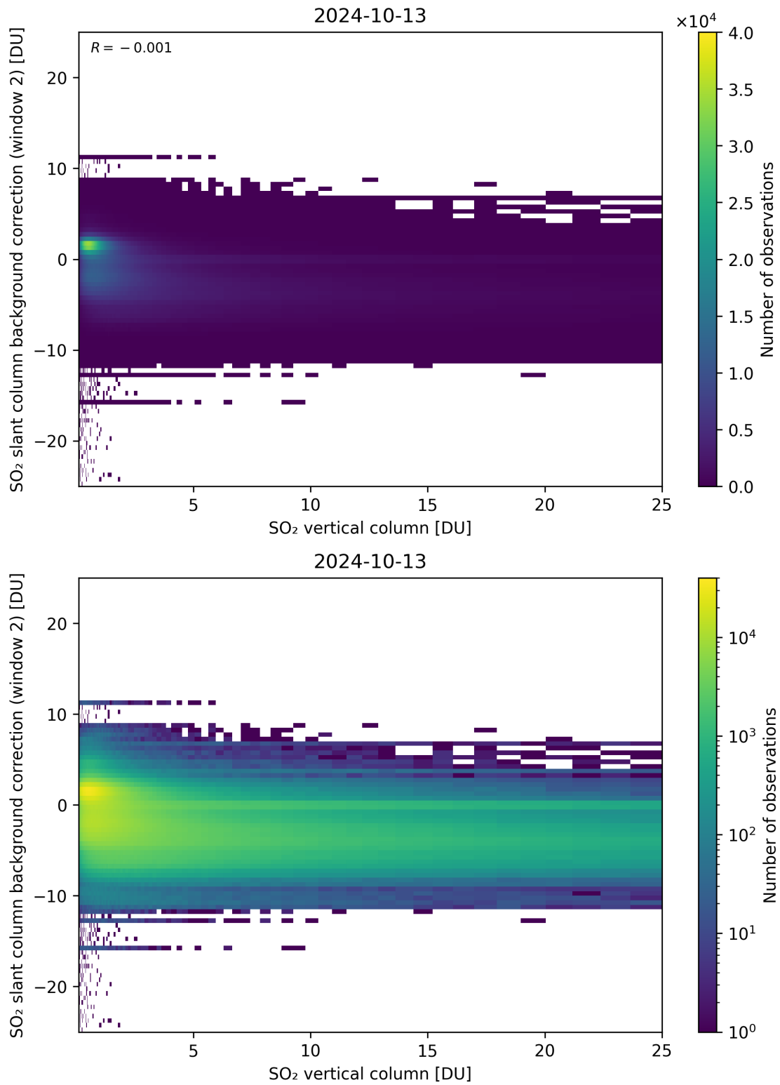
Figure 274: Scatter density plot of “SO 2 vertical column” against “SO 2 slant column background correction (window 2)” for 2024-10-12 to 2024-10-14.
