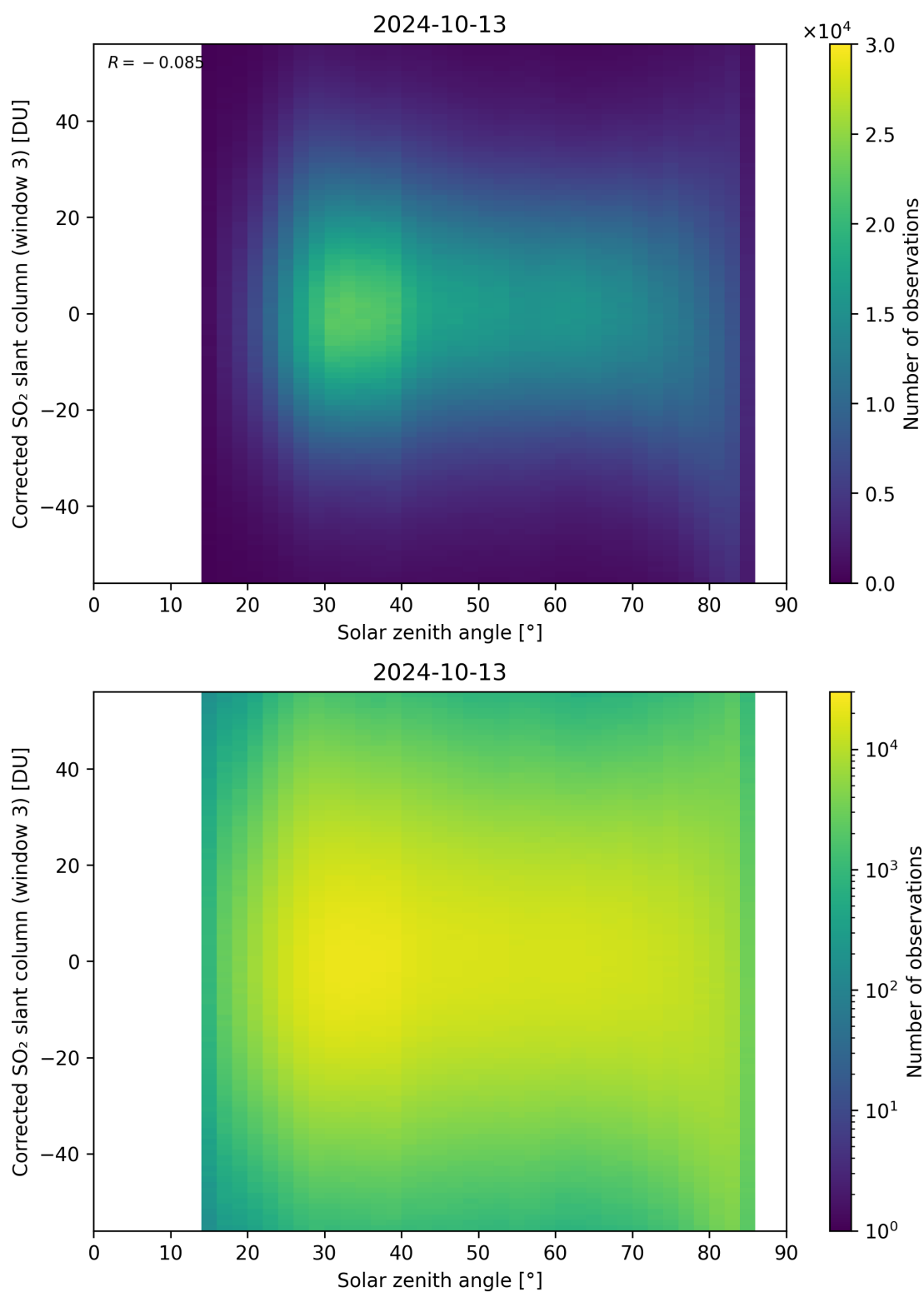
Figure 168: Scatter density plot of “Solar zenith angle” against “Corrected SO 2 slant column (window 3)” for 2024-10-12 to 2024-10-14.
