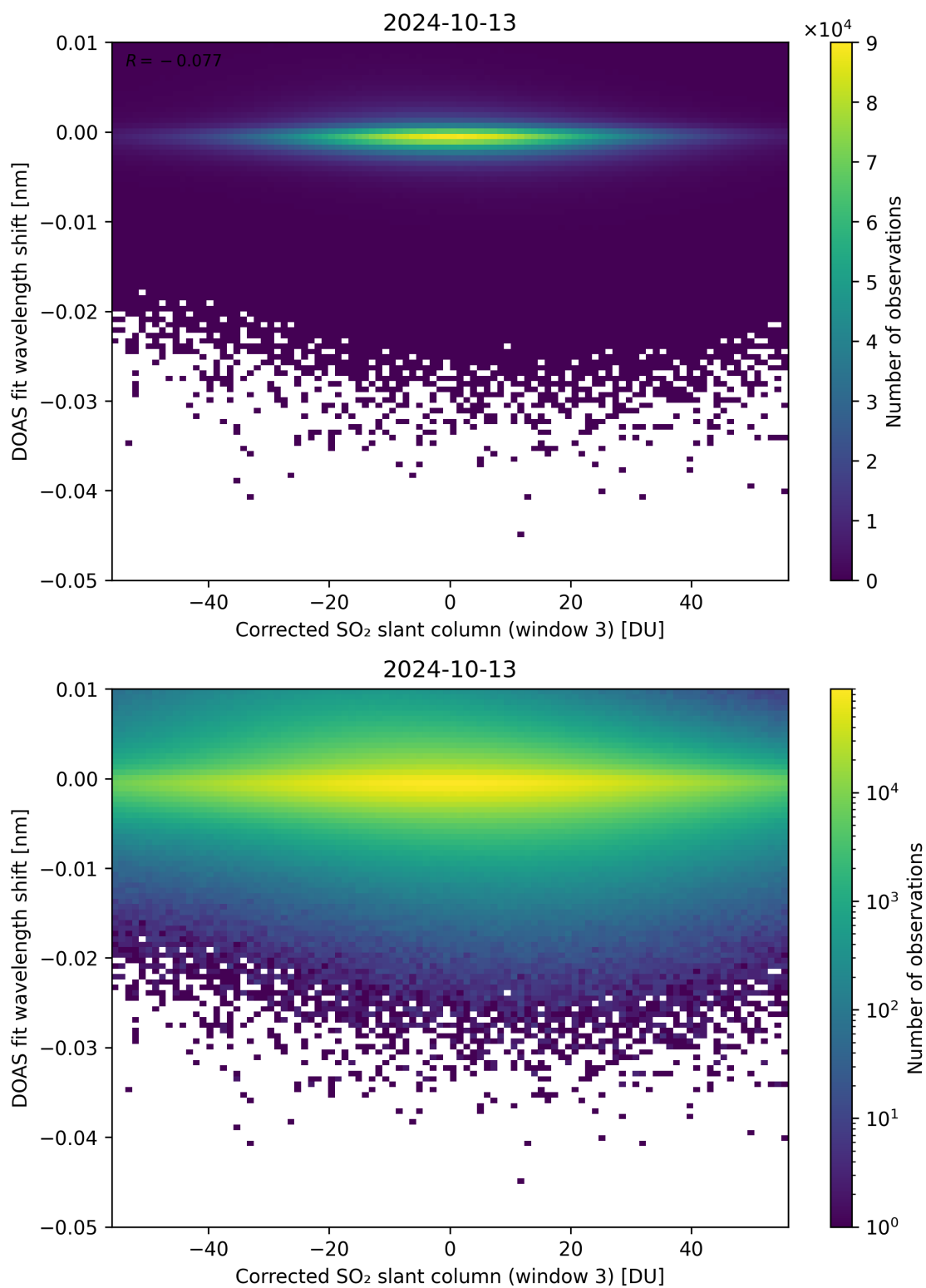
Figure 206: Scatter density plot of “Corrected SO 2 slant column (window 3)” against “DOAS fit wavelength shift” for 2024-10-12 to 2024-10-14.
