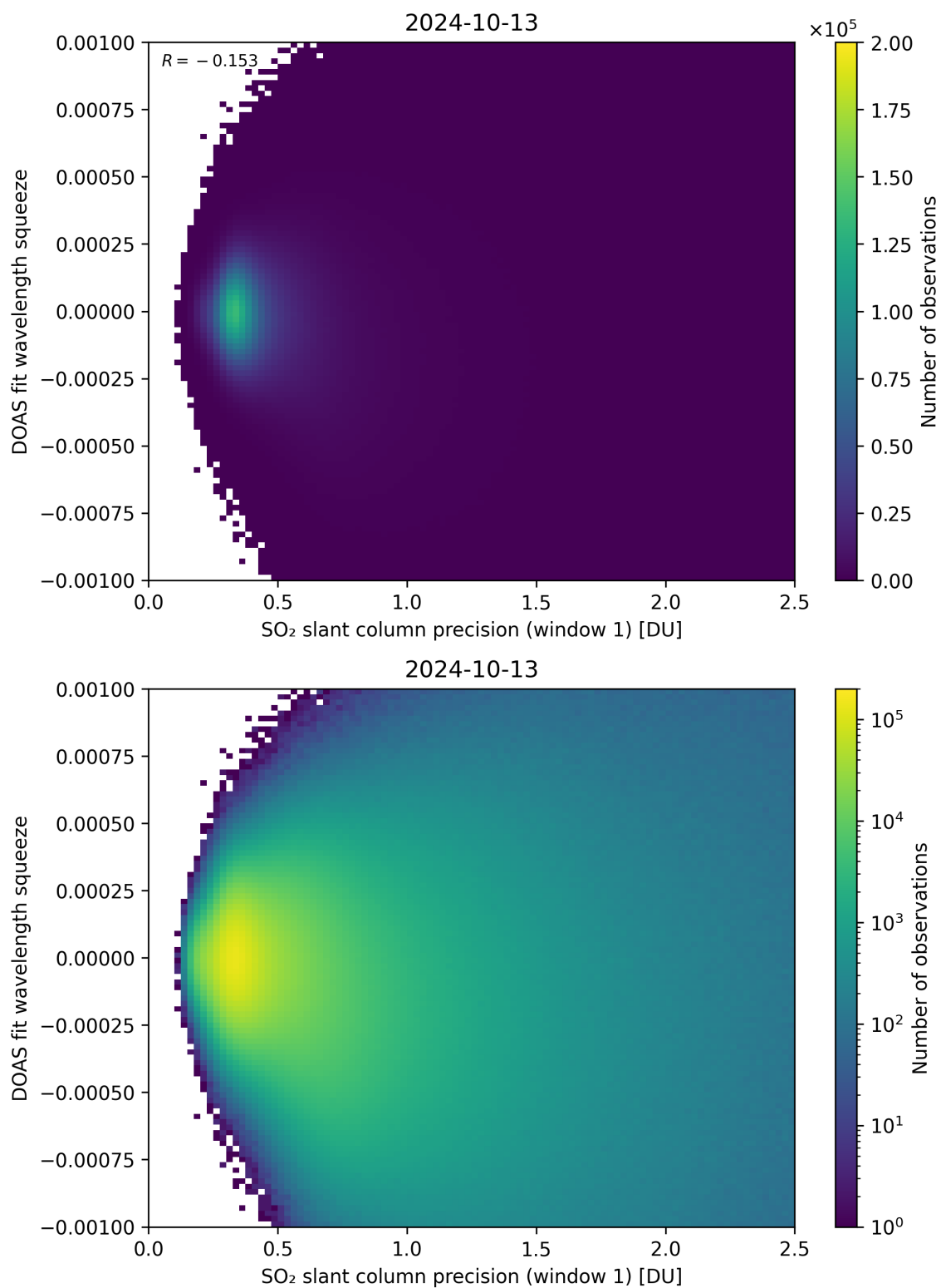
Figure 222: Scatter density plot of “SO 2 slant column precision (window 1)” against “DOAS fit wavelength squeeze” for 2024-10-12 to 2024-10-14.
