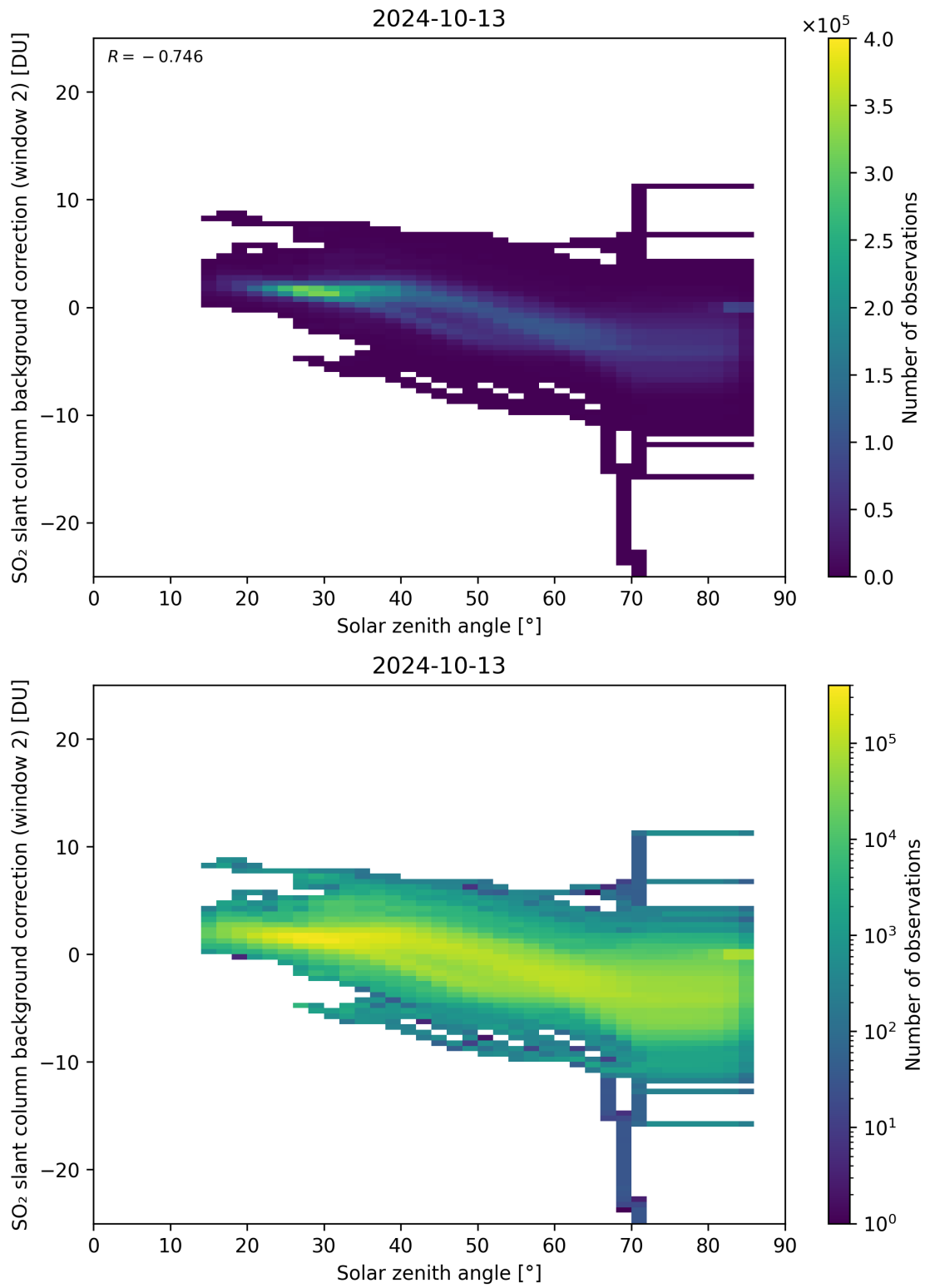
Figure 159: Scatter density plot of “Solar zenith angle” against “SO 2 slant column background correction (window 2)” for 2024-10-12 to 2024-10-14.
