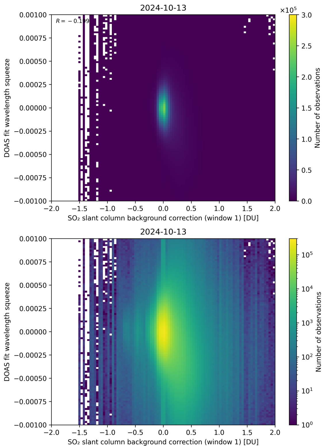
Figure 101: Scatter density plot of “SO 2 slant column background correction (window 1)” against “DOAS fit wavelength squeeze” for 2024-10-12 to 2024-10-14.
