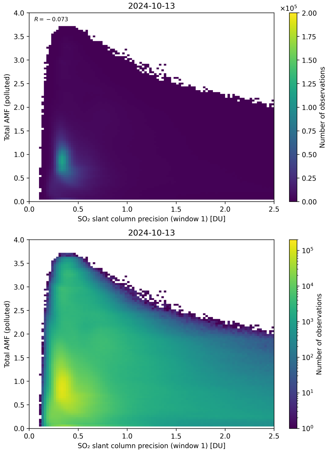
Figure 230: Scatter density plot of “SO 2 slant column precision (window 1)” against “Total AMF (polluted)” for 2024-10-12 to 2024-10-14.
