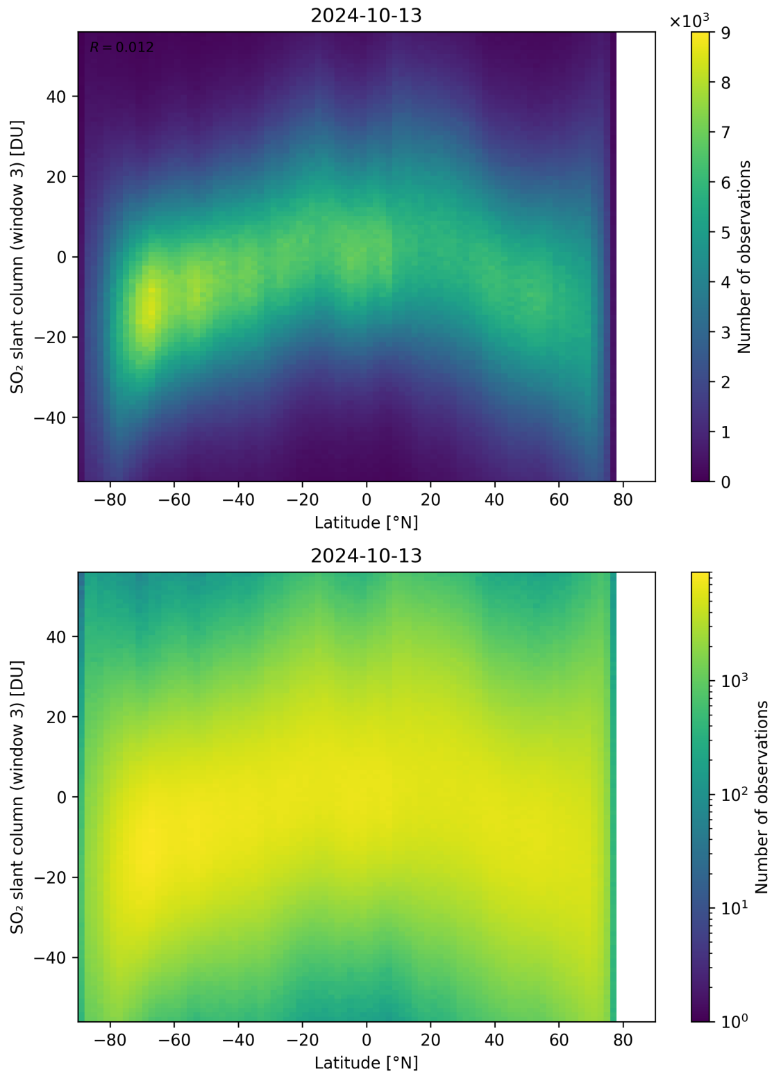
Figure 152: Scatter density plot of “Latitude” against “SO 2 slant column (window 3)” for 2024-10-12 to 2024-10-14.
