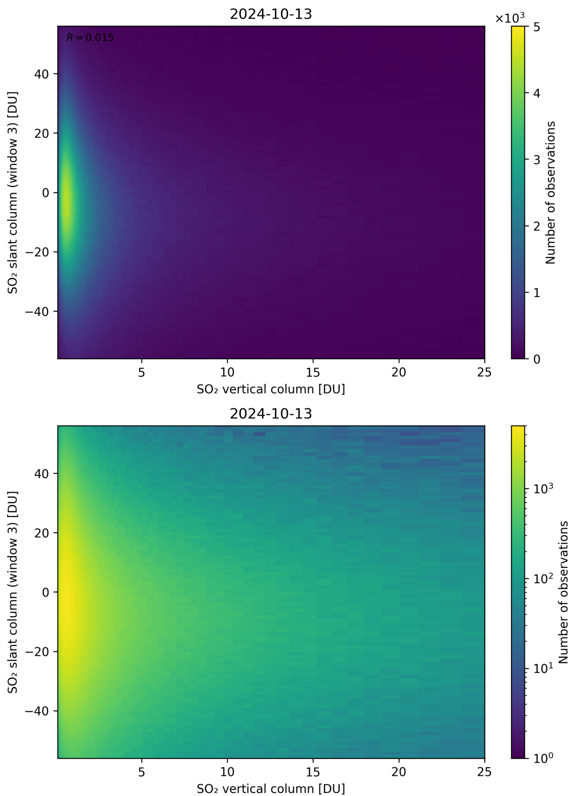
Figure 303: Scatter density plot of “SO 2 vertical column” against “SO 2 slant column (window 3)” for 2024-10-12 to 2024-10-14.
