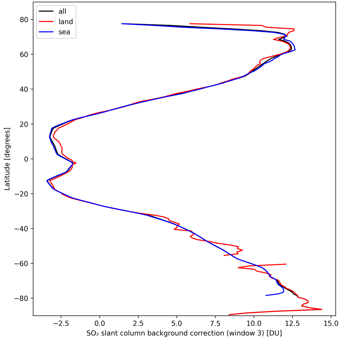
Figure 44: Zonal average of “SO 2 slant column background correction (window 3)” for 2024-10-12 to 2024-10-14.
