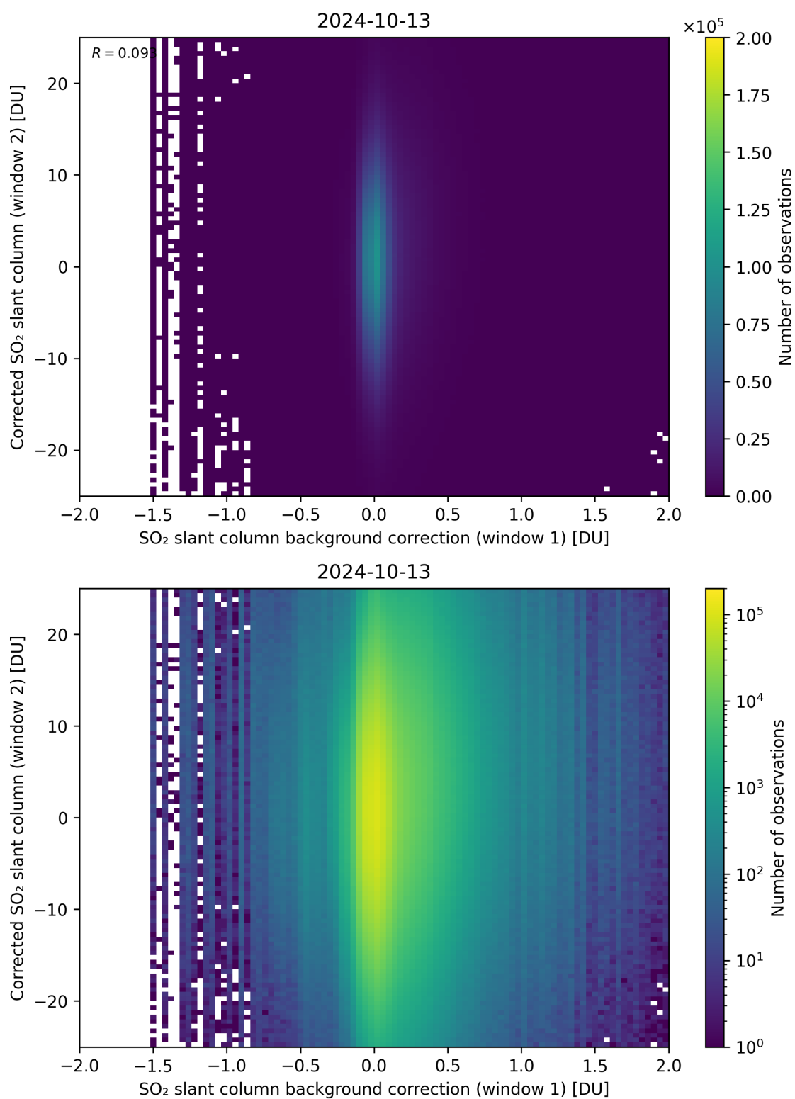
Figure 104: Scatter density plot of “SO 2 slant column background correction (window 1)” against “Corrected SO 2 slant column (window 2)” for 2024-10-12 to 2024-10-14.
