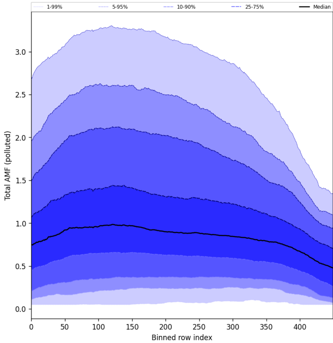
Figure 94: Along track statistics of “Total AMF (polluted)” for 2024-10-12 to 2024-10-14
