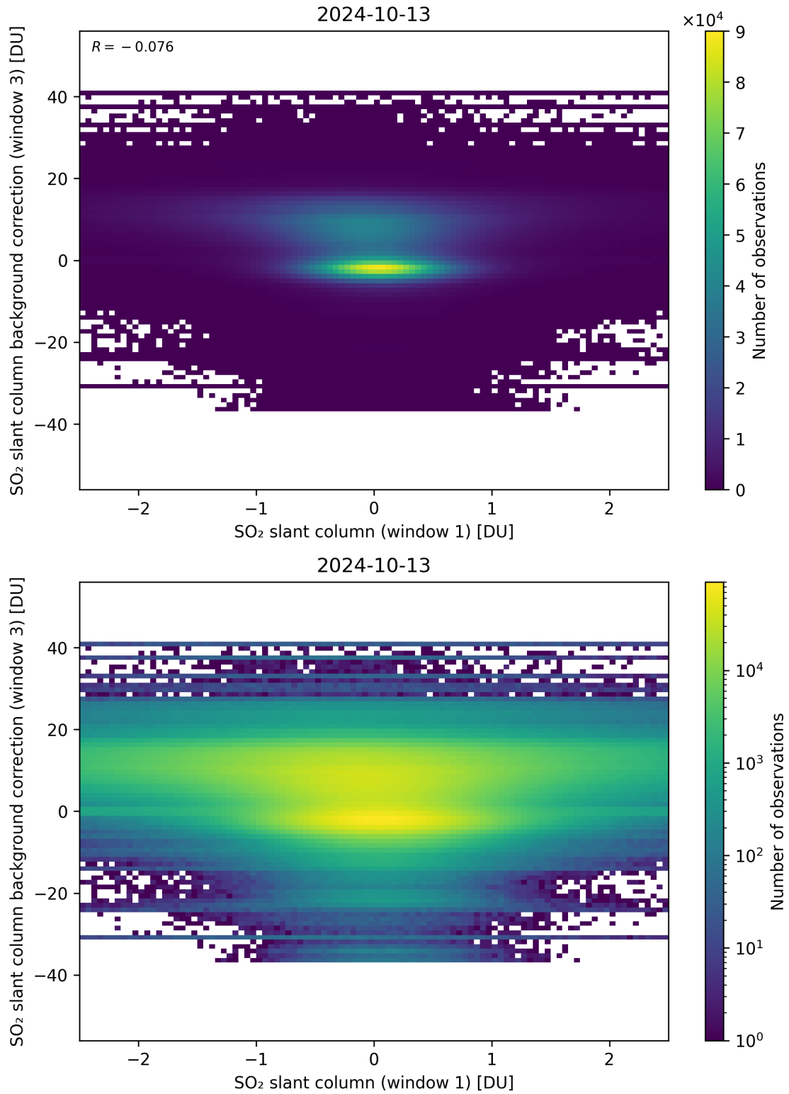
Figure 214: Scatter density plot of “SO 2 slant column (window 1)” against “SO 2 slant column background correction (window 3)” for 2024-10-12 to 2024-10-14.
