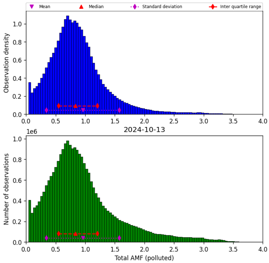
Figure 71: Histogram of “Total AMF (polluted)” for 2024-10-12 to 2024-10-14
