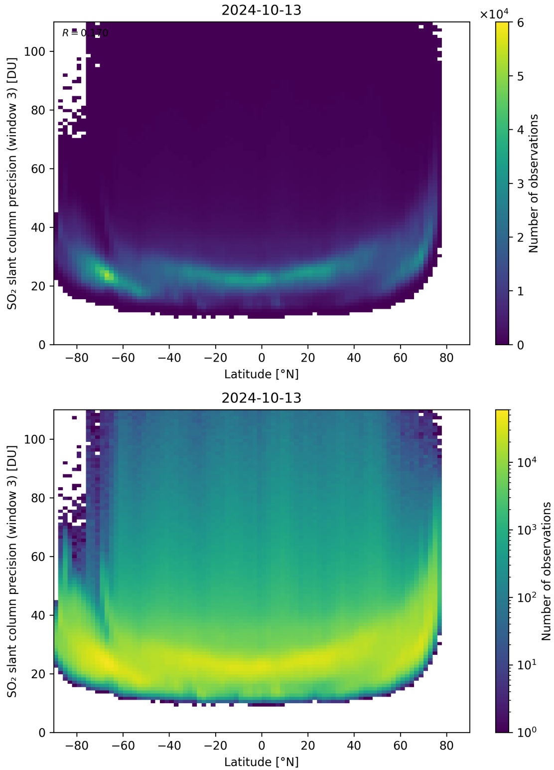
Figure 153: Scatter density plot of “Latitude” against “SO 2 slant column precision (window 3)” for 2024-10-12 to 2024-10-14.
