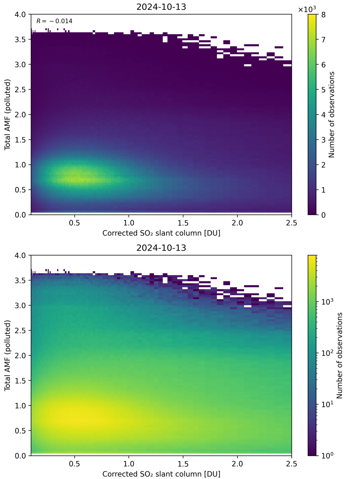
Figure 192: Scatter density plot of “Corrected SO 2 slant column” against “Total AMF (polluted)” for 2024-10-12 to 2024-10-14.
