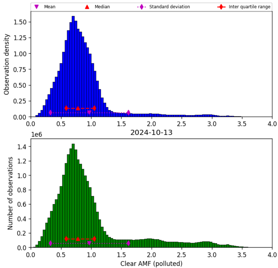
Figure 73: Histogram of “Clear AMF (polluted)” for 2024-10-12 to 2024-10-14
