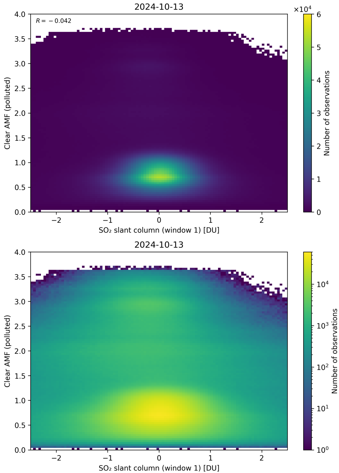
Figure 232: Scatter density plot of “SO 2 slant column (window 1)” against “Clear AMF (polluted)” for 2024-10-12 to 2024-10-14.
