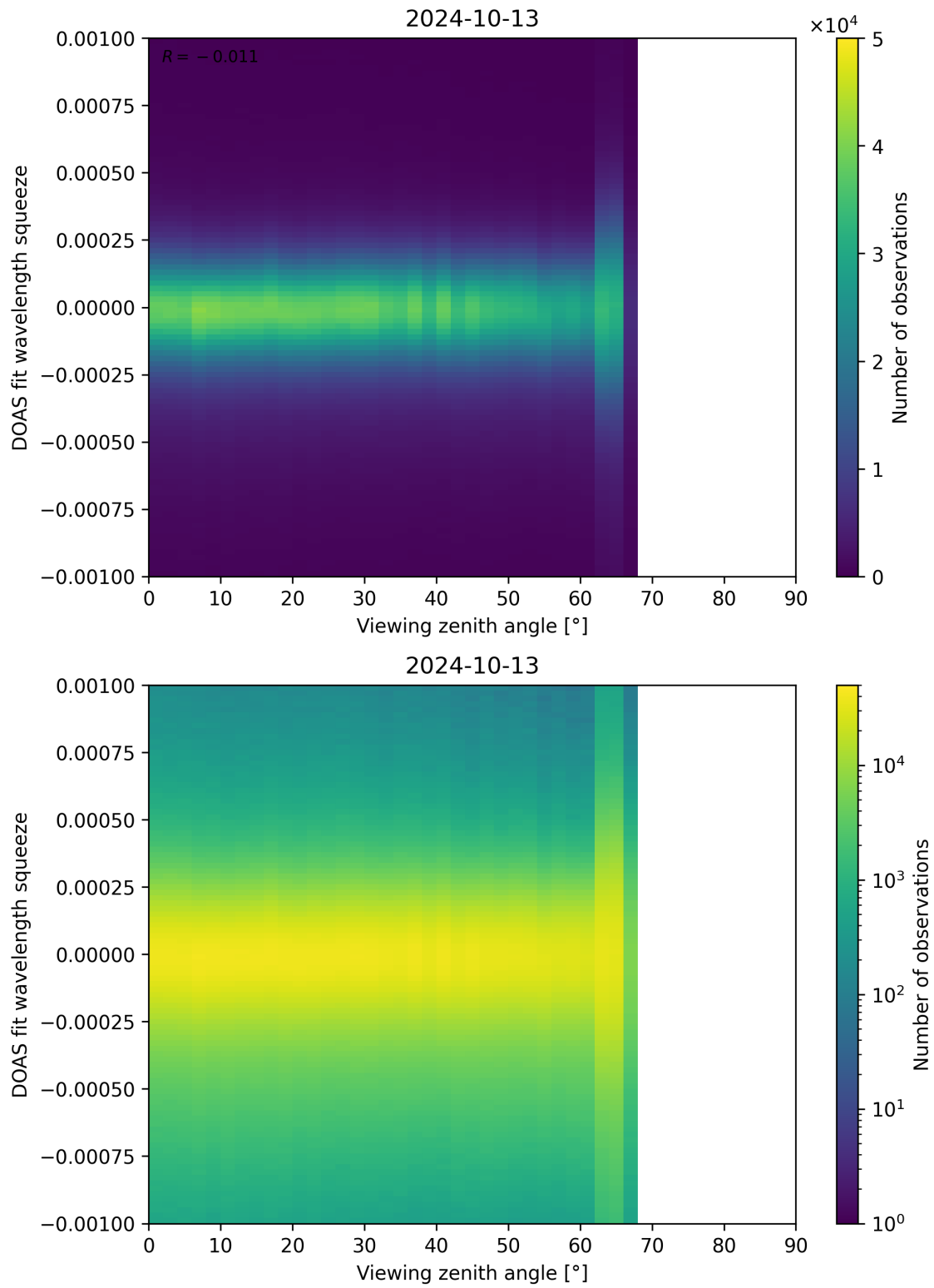
Figure 312: Scatter density plot of “Viewing zenith angle” against “DOAS fit wavelength squeeze” for 2024-10-12 to 2024-10-14.
