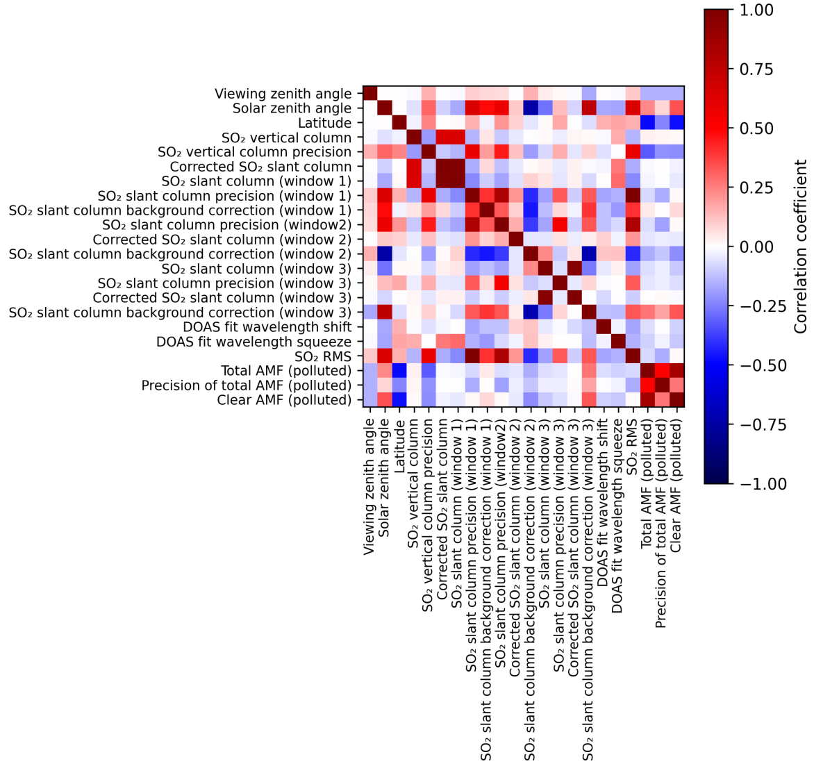
Figure 2: Map of correlation matrix for 2024-10-12 to 2024-10-14.
