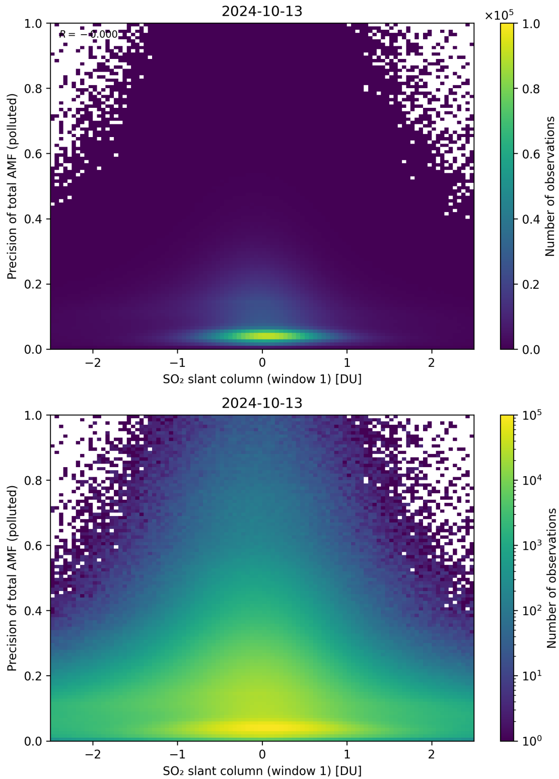
Figure 240: Scatter density plot of “SO 2 slant column (window 1)” against “Precision of total AMF (polluted)” for 2024-10-12 to 2024-10-14.
