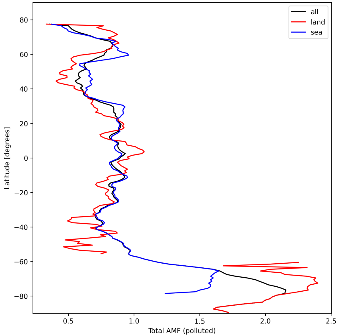
Figure 48: Zonal average of “Total AMF (polluted)” for 2024-10-12 to 2024-10-14.
