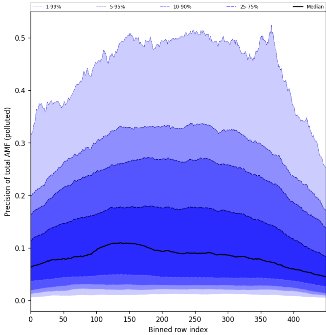
Figure 95: Along track statistics of “Precision of total AMF (polluted)” for 2024-10-12 to 2024-10-14
