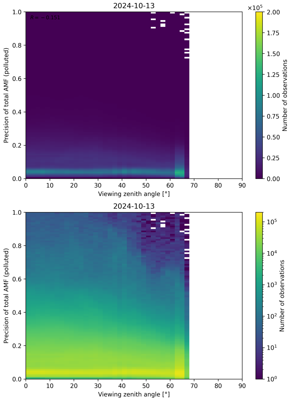
Figure 326: Scatter density plot of “Viewing zenith angle” against “Precision of total AMF (polluted)” for 2024-10-12 to 2024-10-14.
