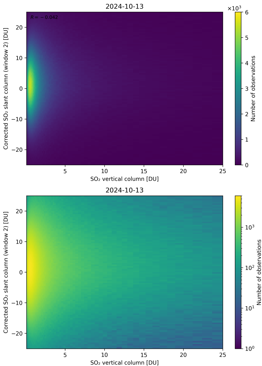
Figure 298: Scatter density plot of “SO 2 vertical column” against “Corrected SO 2 slant column (window 2)” for 2024-10-12 to 2024-10-14.
