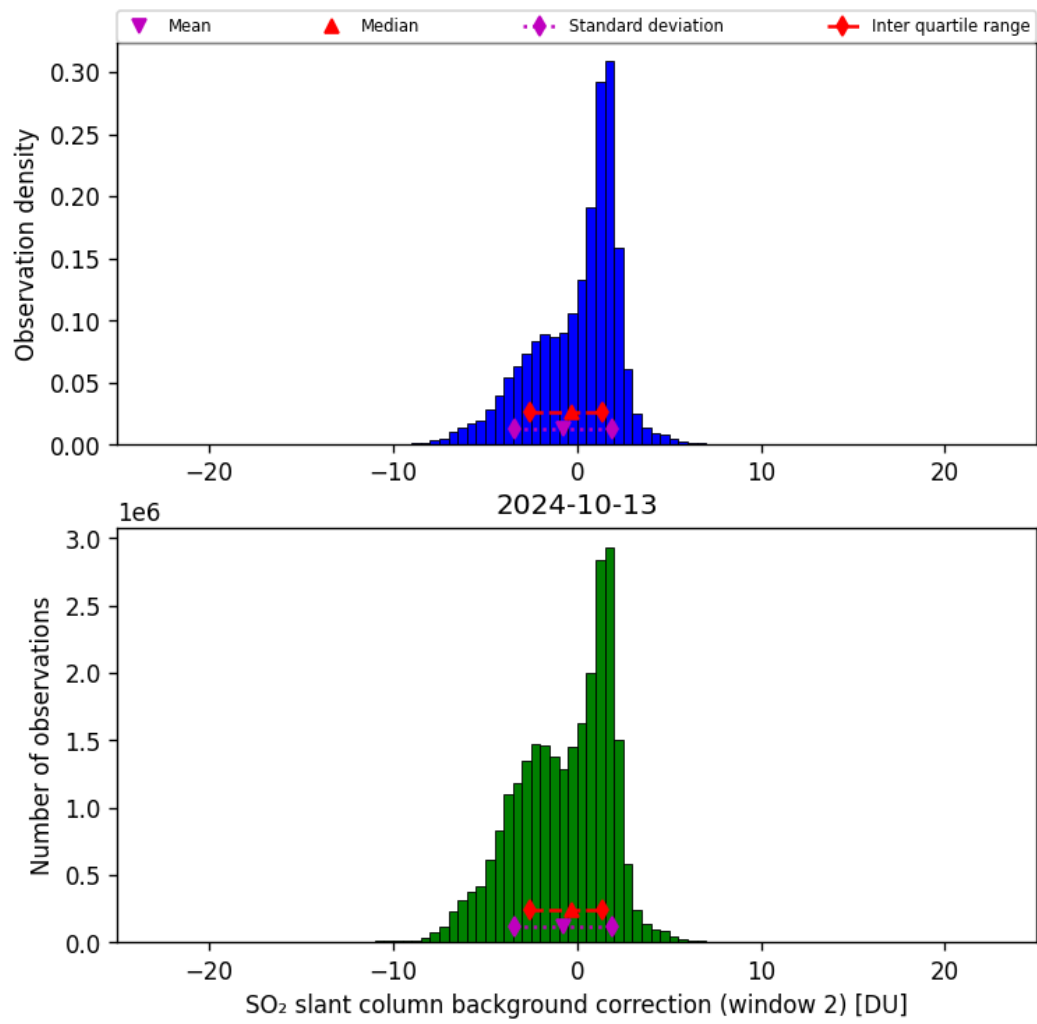
Figure 63: Histogram of “SO 2 slant column background correction (window 2)” for 2024-10-12 to 2024-10-14
