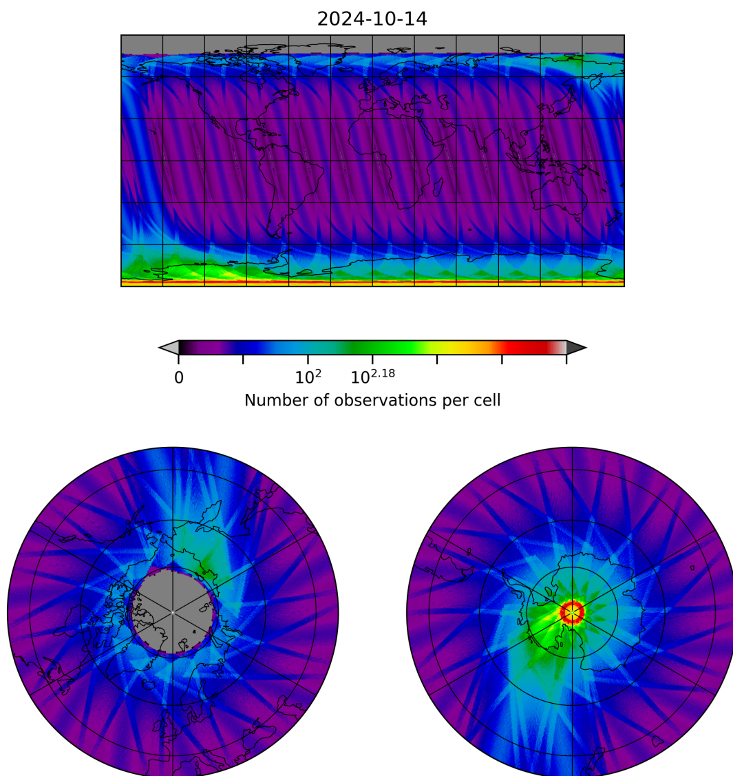
Figure 28: Map of the number of observations for 2024-10-14 to 2024-10-15
