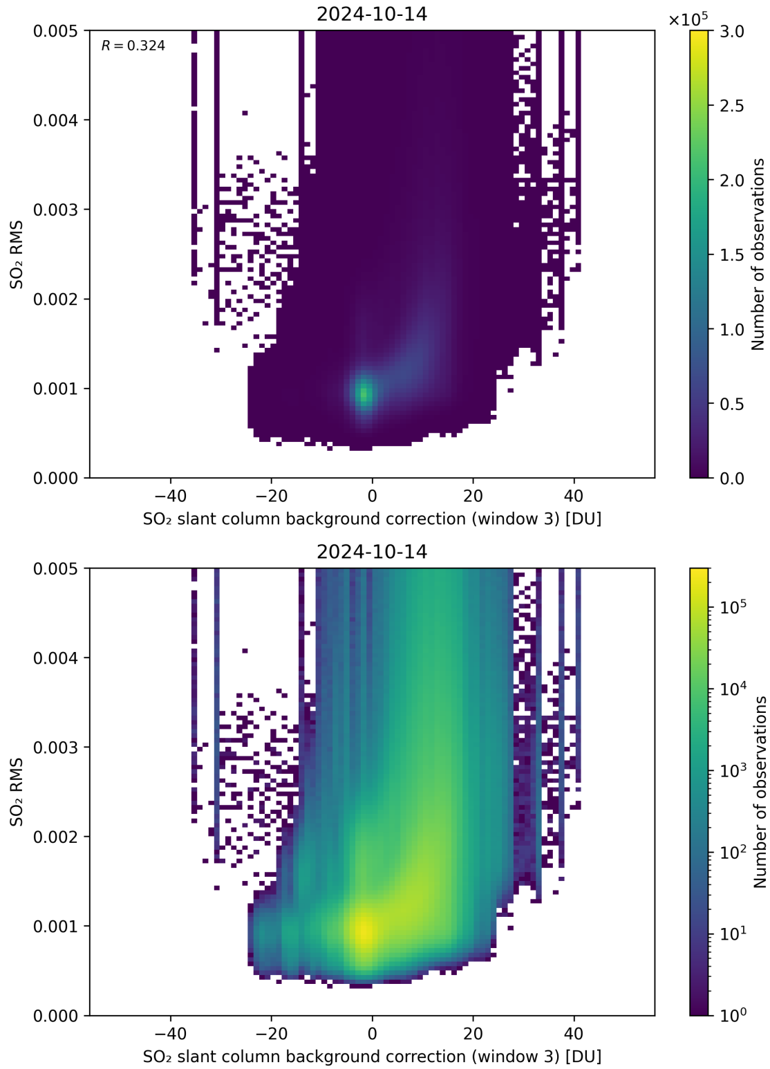
Figure 123: Scatter density plot of “SO 2 slant column background correction (window 3)” against “SO 2 RMS” for 2024-10-14 to 2024-10-15.
