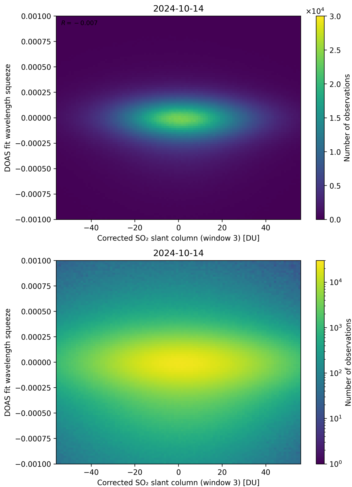
Figure 207: Scatter density plot of “Corrected SO 2 slant column (window 3)” against “DOAS fit wavelength squeeze” for 2024-10-14 to 2024-10-15.
