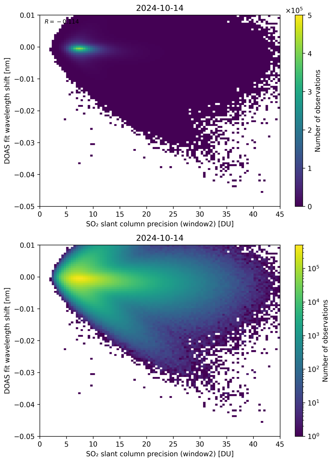
Figure 243: Scatter density plot of “SO 2 slant column precision (window2)” against “DOAS fit wavelength shift” for 2024-10-14 to 2024-10-15.
