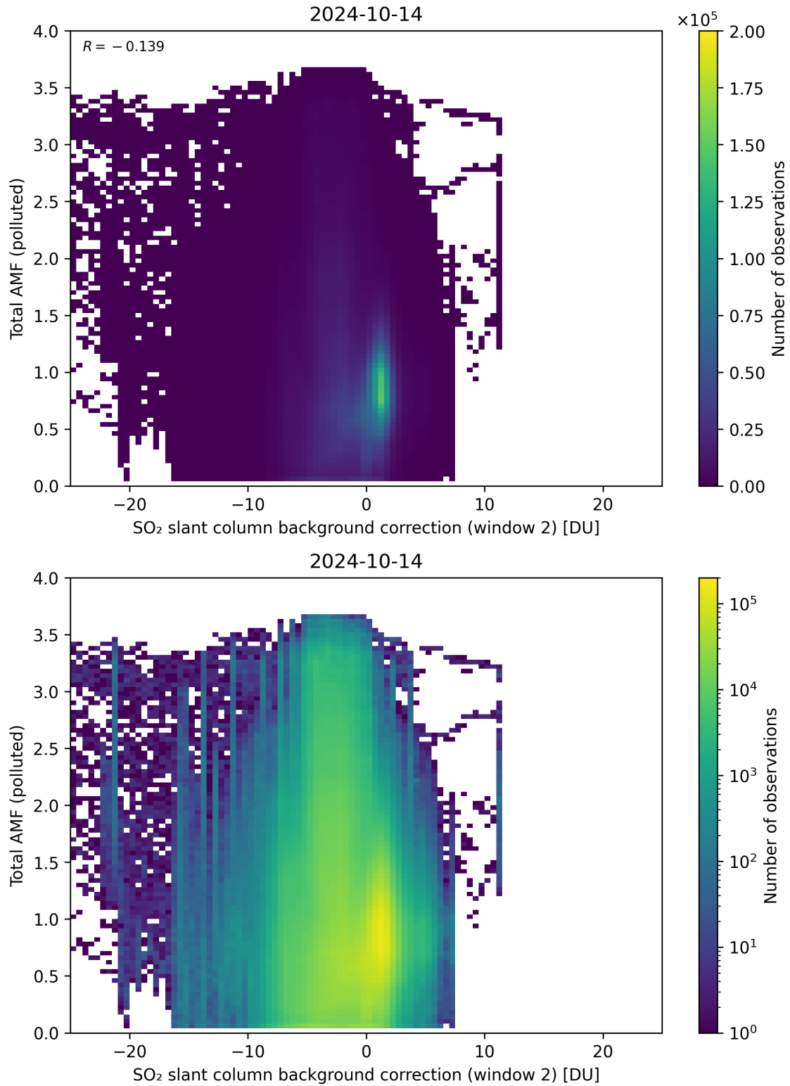
Figure 119: Scatter density plot of “SO 2 slant column background correction (window 2)” against “Total AMF (polluted)” for 2024-10-14 to 2024-10-15.
