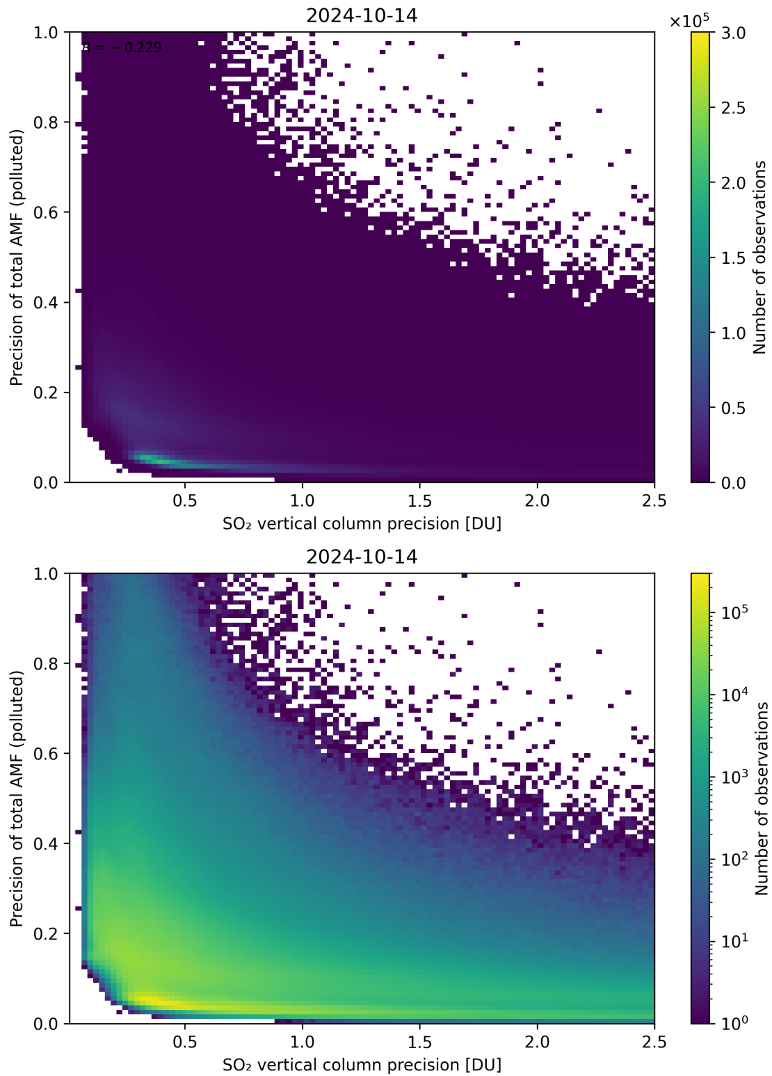
Figure 295: Scatter density plot of “SO 2 vertical column precision” against “Precision of total AMF (polluted)” for 2024-10-14 to 2024-10-15.
