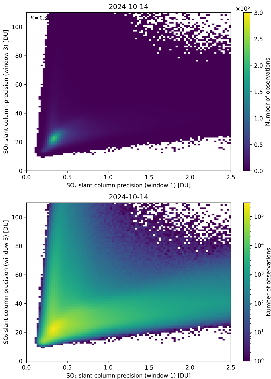
Figure 229: Scatter density plot of “SO 2 slant column precision (window 1)” against “SO 2 slant column precision (window 3)” for 2024-10-14 to 2024-10-15.
