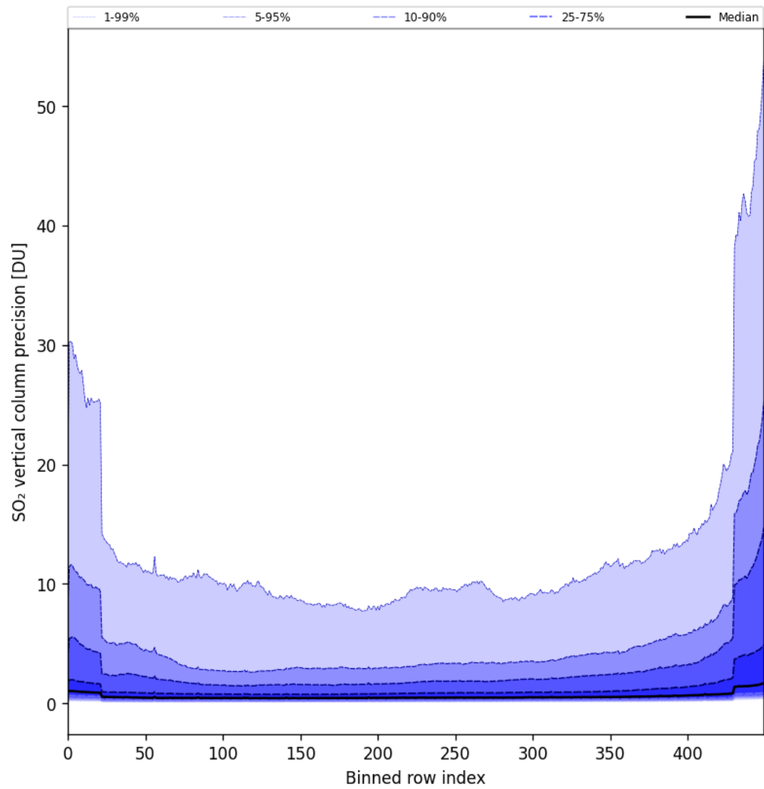
Figure 77: Along track statistics of “SO 2 vertical column precision” for 2024-10-14 to 2024-10-15
