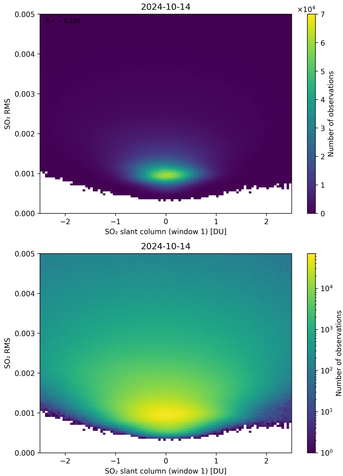
Figure 217: Scatter density plot of “SO 2 slant column (window 1)” against “SO 2 RMS” for 2024-10-14 to 2024-10-15.
