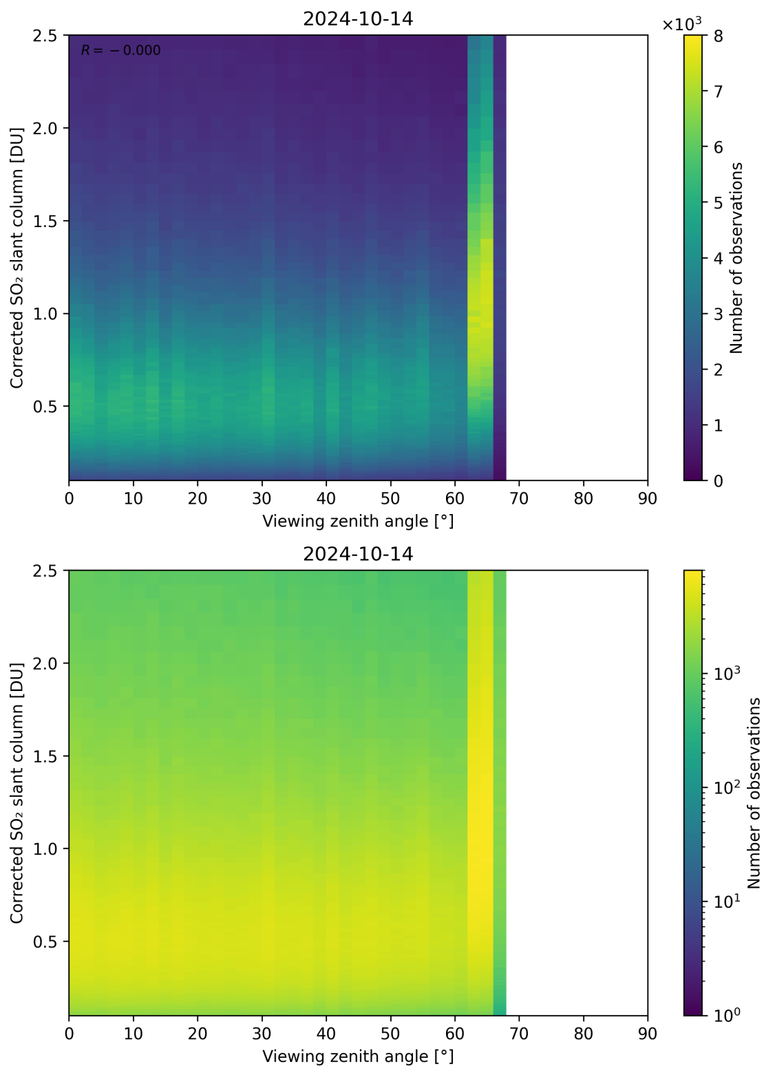
Figure 317: Scatter density plot of “Viewing zenith angle” against “Corrected SO 2 slant column” for 2024-10-14 to 2024-10-15.
