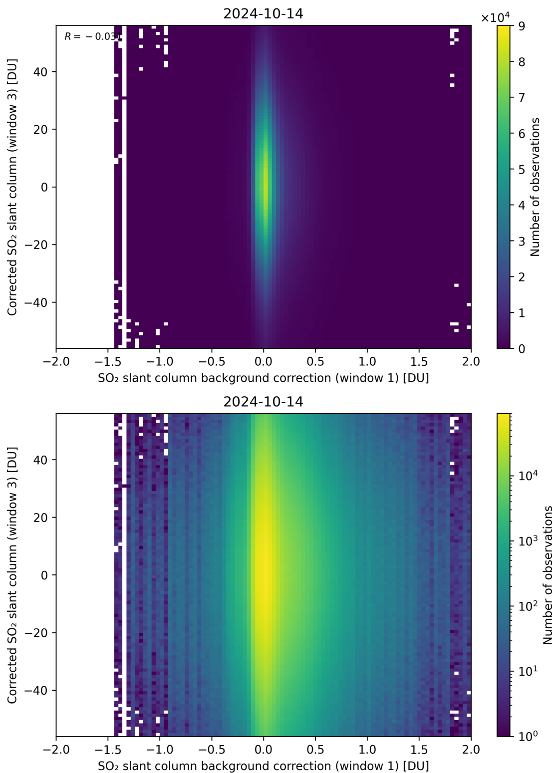
Figure 105: Scatter density plot of “SO 2 slant column background correction (window 1)” against “Corrected SO 2 slant column (window 3)” for 2024-10-14 to 2024-10-15.
