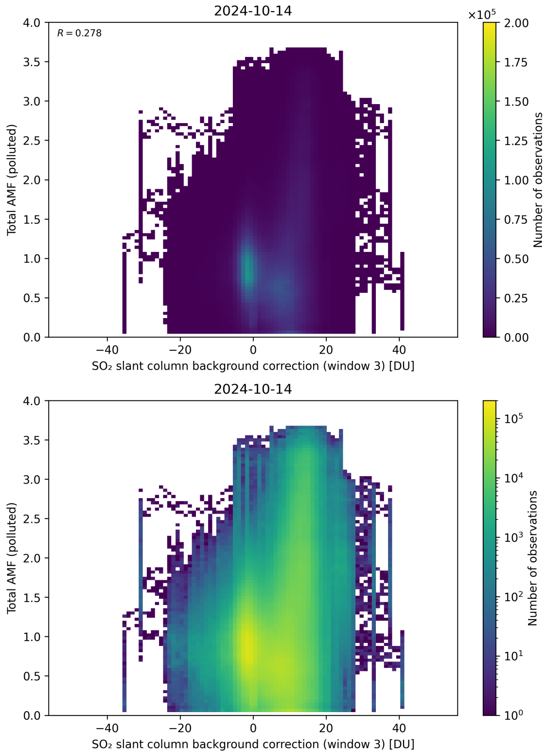
Figure 125: Scatter density plot of “SO 2 slant column background correction (window 3)” against “Total AMF (polluted)” for 2024-10-14 to 2024-10-15.
