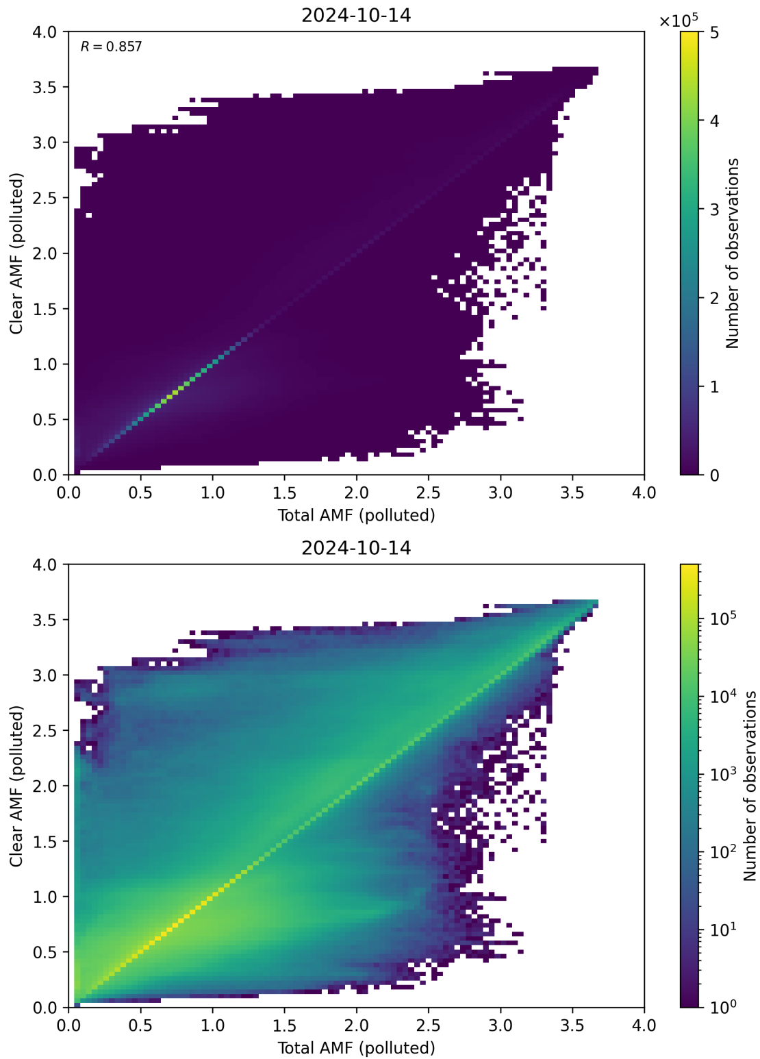
Figure 271: Scatter density plot of “Total AMF (polluted)” against “Clear AMF (polluted)” for 2024-10-14 to 2024-10-15.
