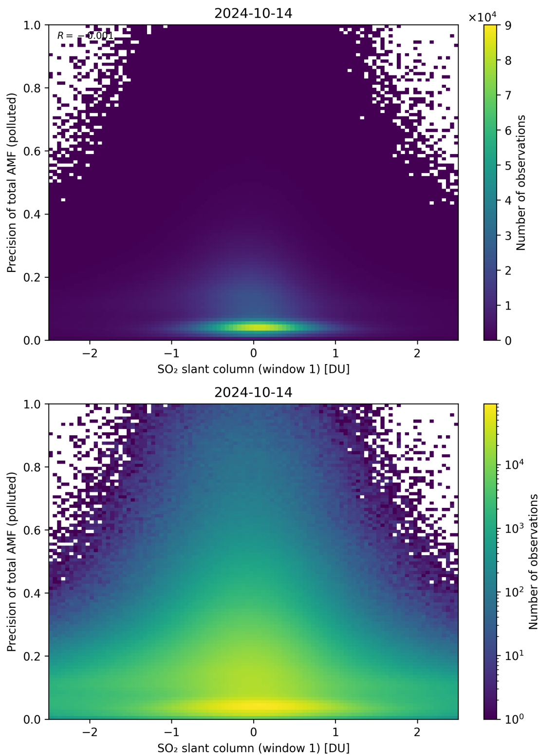
Figure 240: Scatter density plot of “SO 2 slant column (window 1)” against “Precision of total AMF (polluted)” for 2024-10-14 to 2024-10-15.
