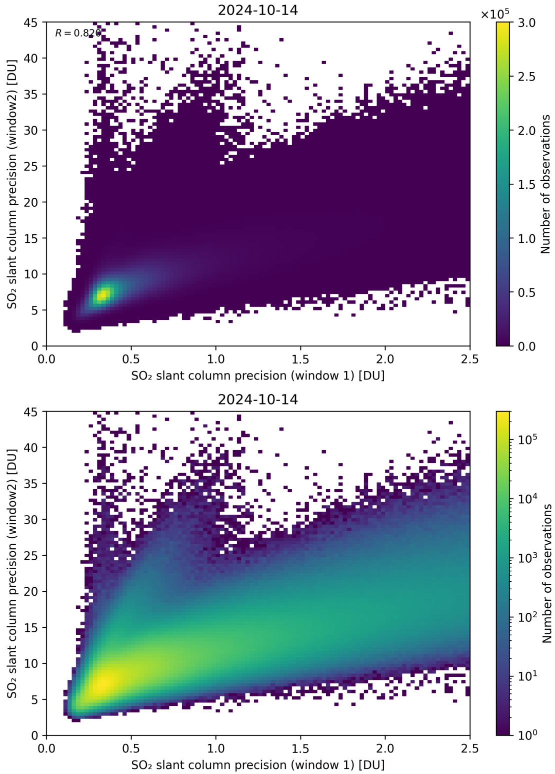
Figure 227: Scatter density plot of “SO 2 slant column precision (window 1)” against “SO 2 slant column precision (window2)” for 2024-10-14 to 2024-10-15.
