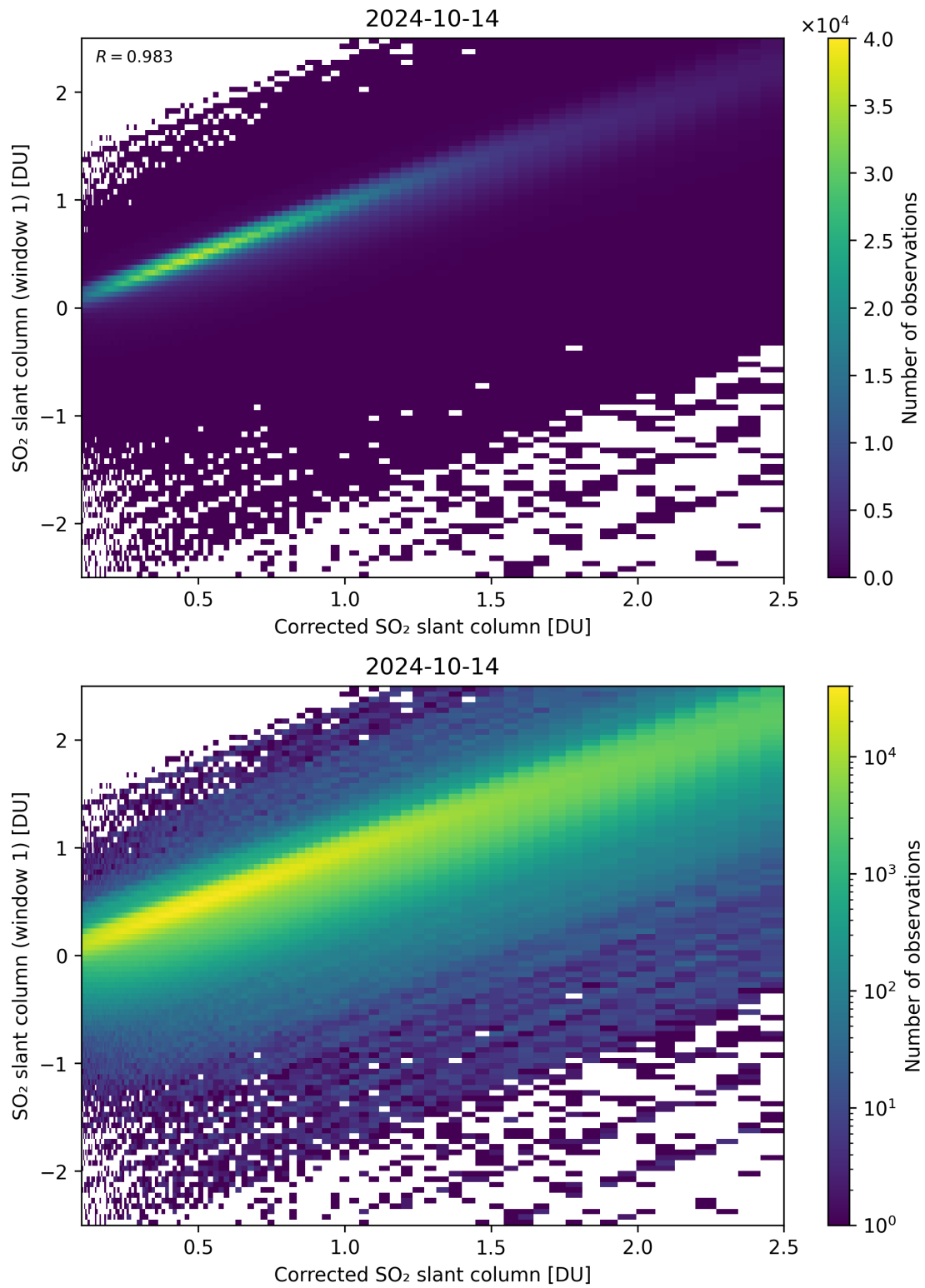
Figure 187: Scatter density plot of “Corrected SO 2 slant column” against “SO 2 slant column (window 1)” for 2024-10-14 to 2024-10-15.
