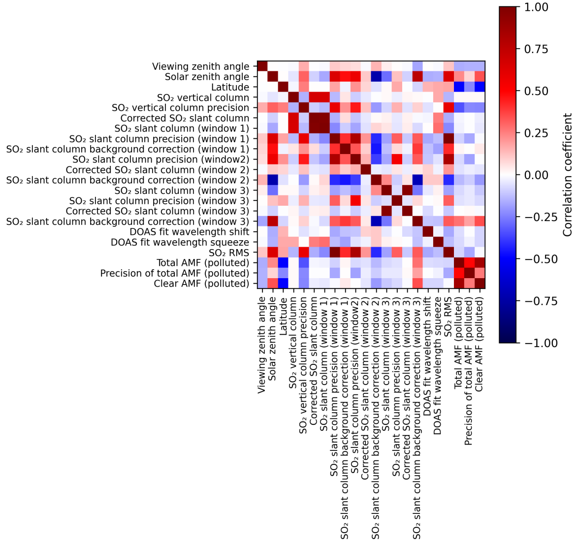
Figure 2: Map of correlation matrix for 2024-10-14 to 2024-10-15.
