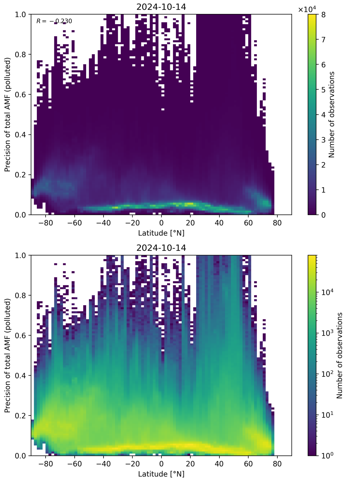
Figure 155: Scatter density plot of “Latitude” against “Precision of total AMF (polluted)” for 2024-10-14 to 2024-10-15.
