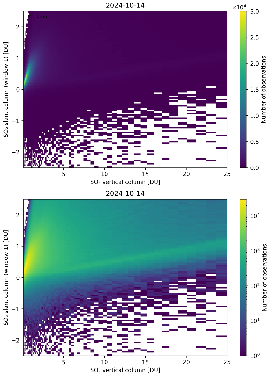
Figure 300: Scatter density plot of “SO 2 vertical column” against “SO 2 slant column (window 1)” for 2024-10-14 to 2024-10-15.
