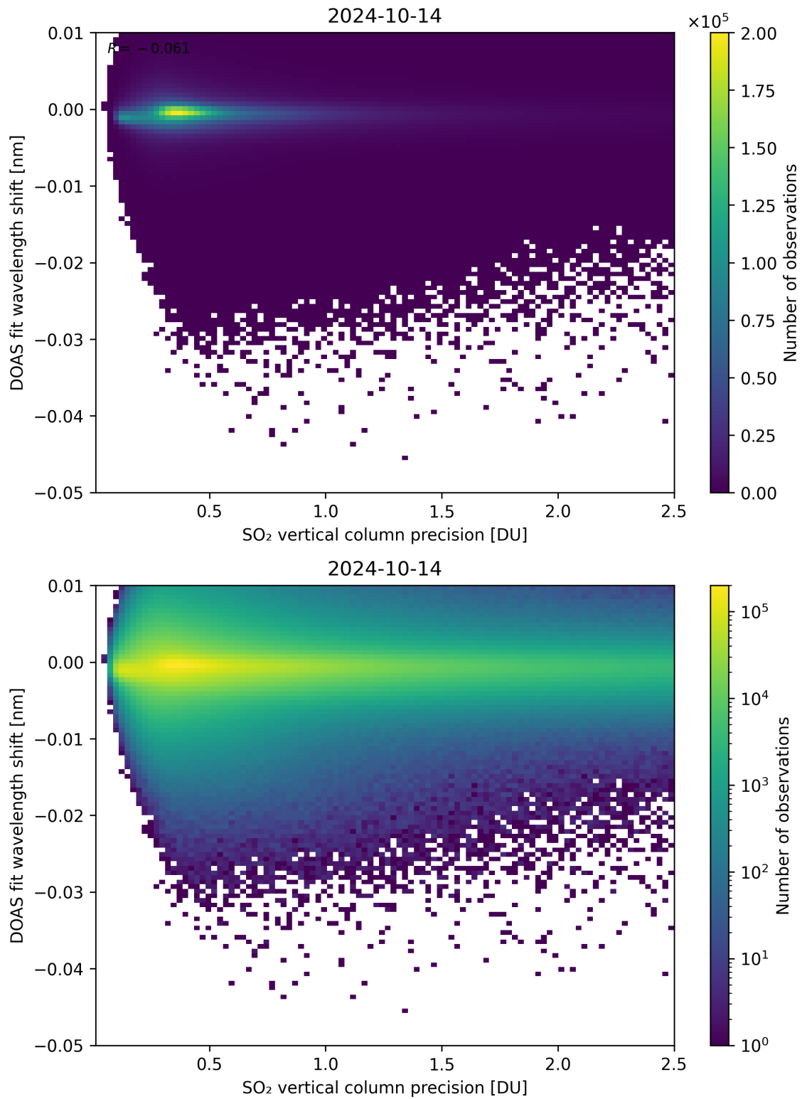
Figure 282: Scatter density plot of “SO 2 vertical column precision” against “DOAS fit wavelength shift” for 2024-10-14 to 2024-10-15.
