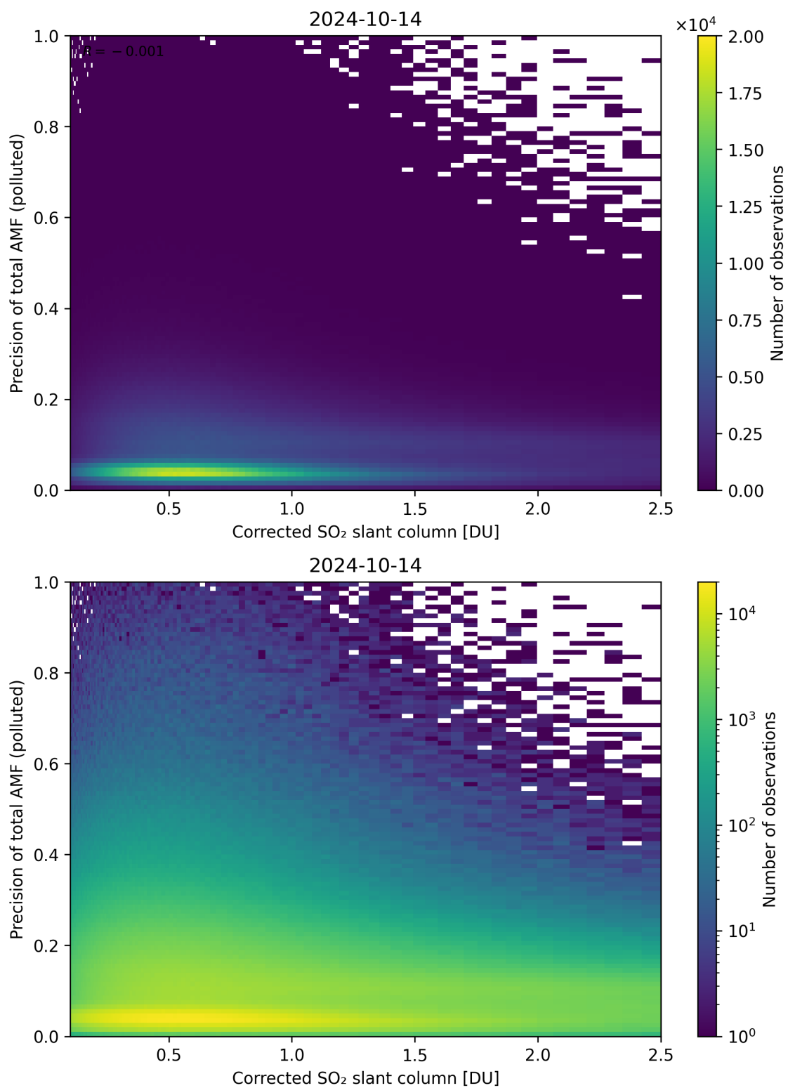
Figure 193: Scatter density plot of “Corrected SO 2 slant column” against “Precision of total AMF (polluted)” for 2024-10-14 to 2024-10-15.
