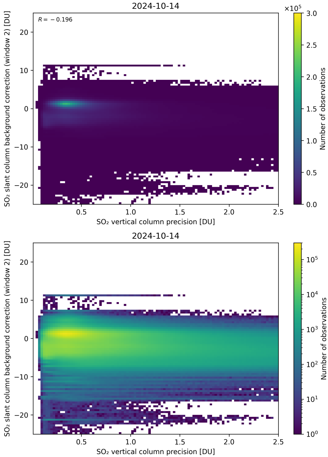
Figure 280: Scatter density plot of “SO 2 vertical column precision” against “SO 2 slant column background correction (window 2)” for 2024-10-14 to 2024-10-15.
