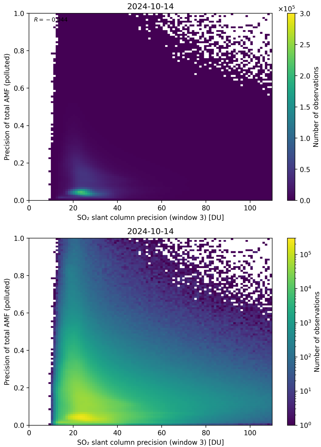
Figure 264: Scatter density plot of “SO 2 slant column precision (window 3)” against “Precision of total AMF (polluted)” for 2024-10-14 to 2024-10-15.
