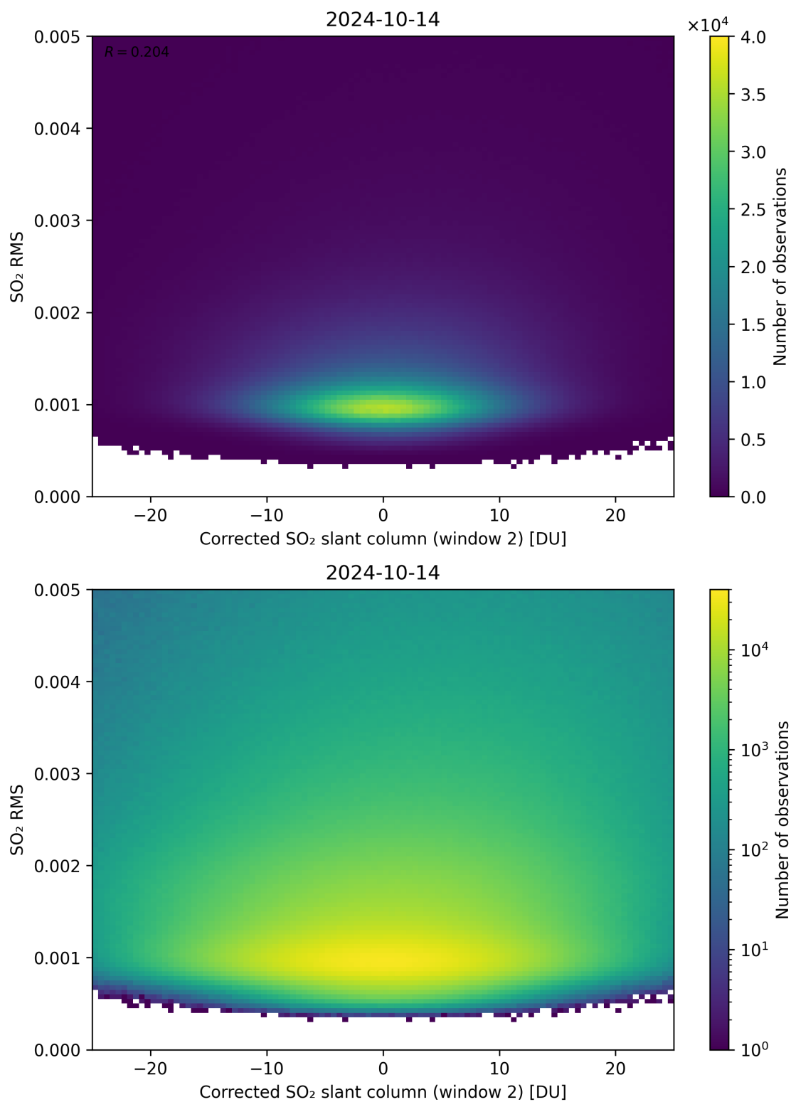
Figure 198: Scatter density plot of “Corrected SO 2 slant column (window 2)” against “SO 2 RMS” for 2024-10-14 to 2024-10-15.
