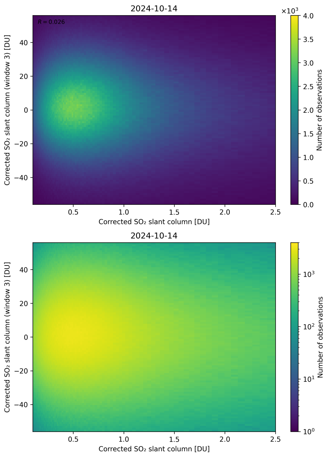
Figure 186: Scatter density plot of “Corrected SO 2 slant column” against “Corrected SO 2 slant column (window 3)” for 2024-10-14 to 2024-10-15.
