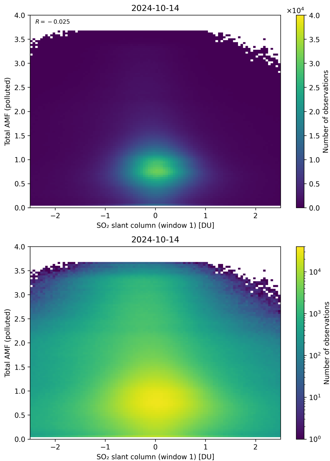
Figure 239: Scatter density plot of “SO 2 slant column (window 1)” against “Total AMF (polluted)” for 2024-10-14 to 2024-10-15.
