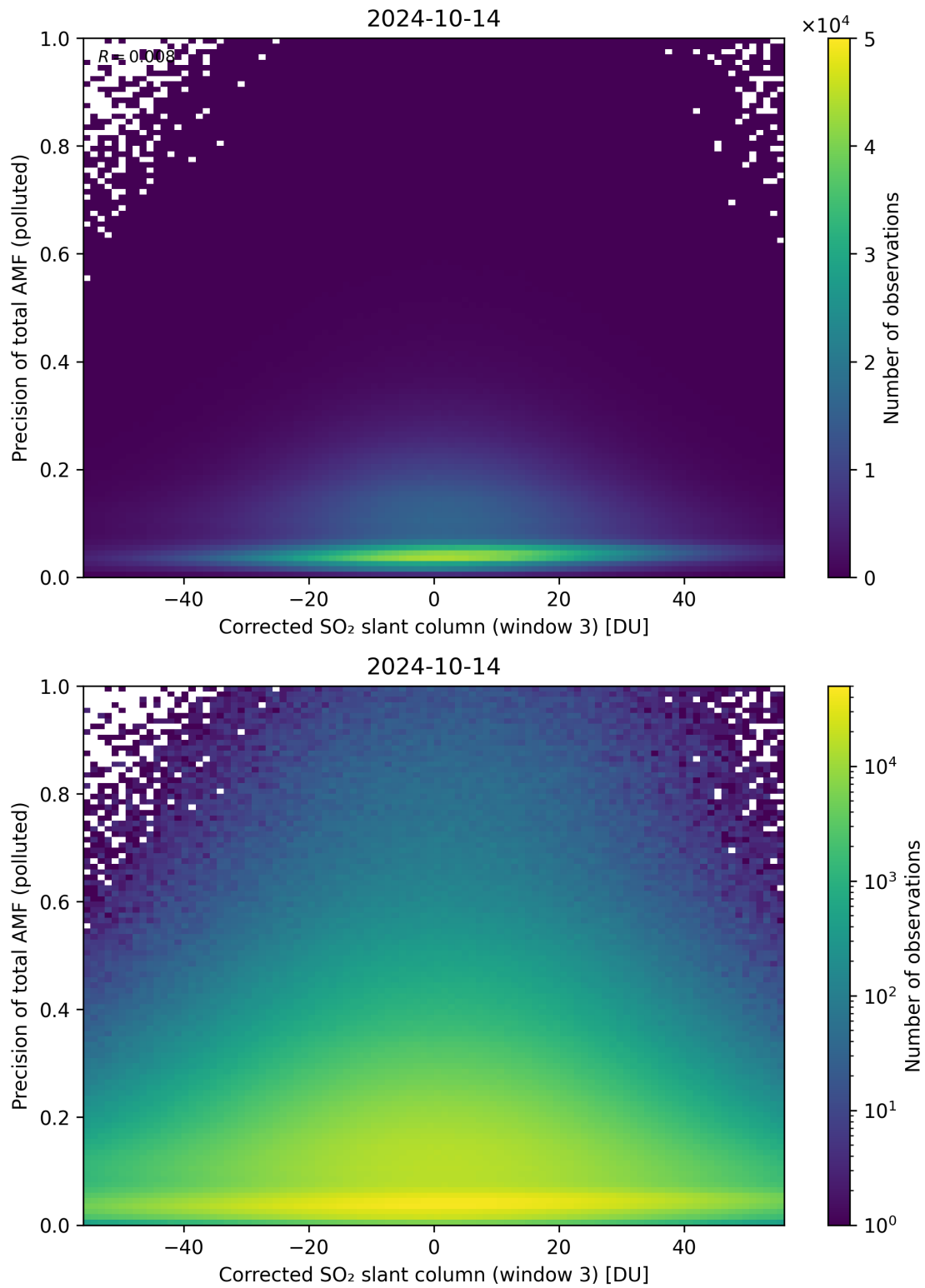
Figure 211: Scatter density plot of “Corrected SO 2 slant column (window 3)” against “Precision of total AMF (polluted)” for 2024-10-14 to 2024-10-15.
