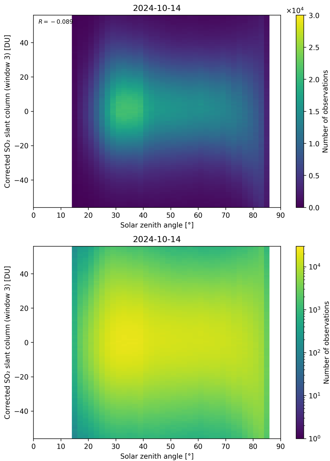
Figure 168: Scatter density plot of “Solar zenith angle” against “Corrected SO 2 slant column (window 3)” for 2024-10-14 to 2024-10-15.
