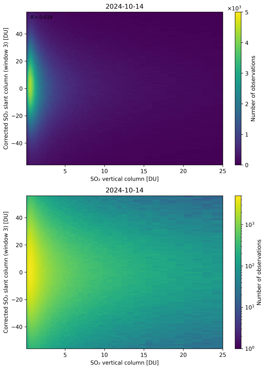
Figure 299: Scatter density plot of “SO 2 vertical column” against “Corrected SO 2 slant column (window 3)” for 2024-10-14 to 2024-10-15.
