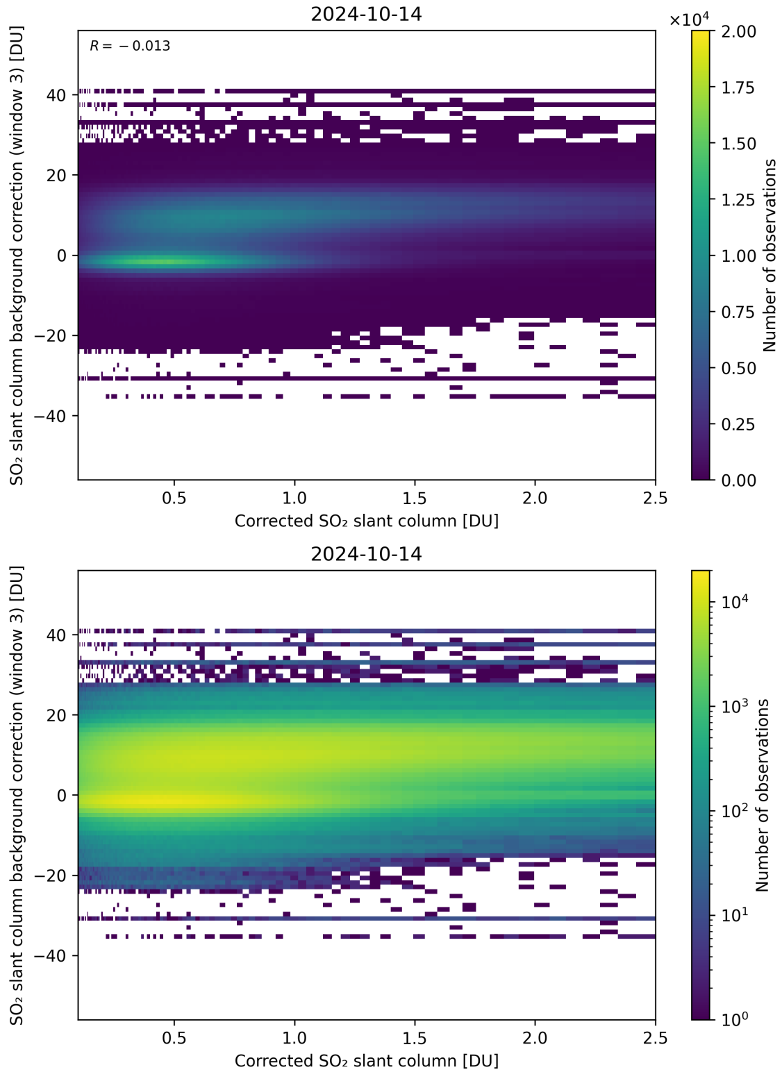
Figure 180: Scatter density plot of “Corrected SO 2 slant column” against “SO 2 slant column background correction (window 3)” for 2024-10-14 to 2024-10-15.
