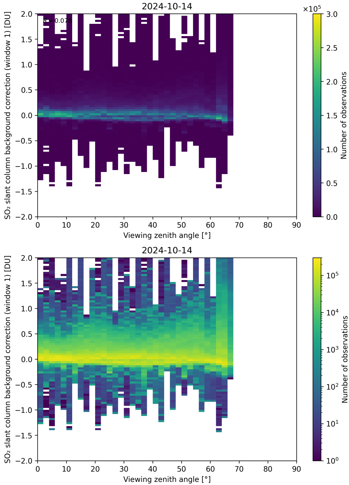
Figure 308: Scatter density plot of “Viewing zenith angle” against “SO 2 slant column background correction (window 1)” for 2024-10-14 to 2024-10-15.
