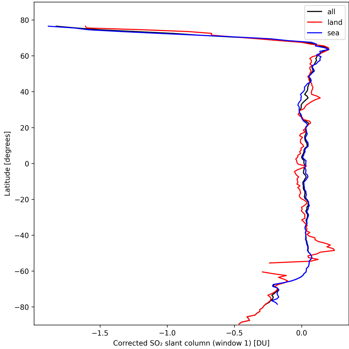
Figure 35: Zonal average of “Corrected SO 2 slant column (window 1)” for 2024-10-14 to 2024-10-15.
