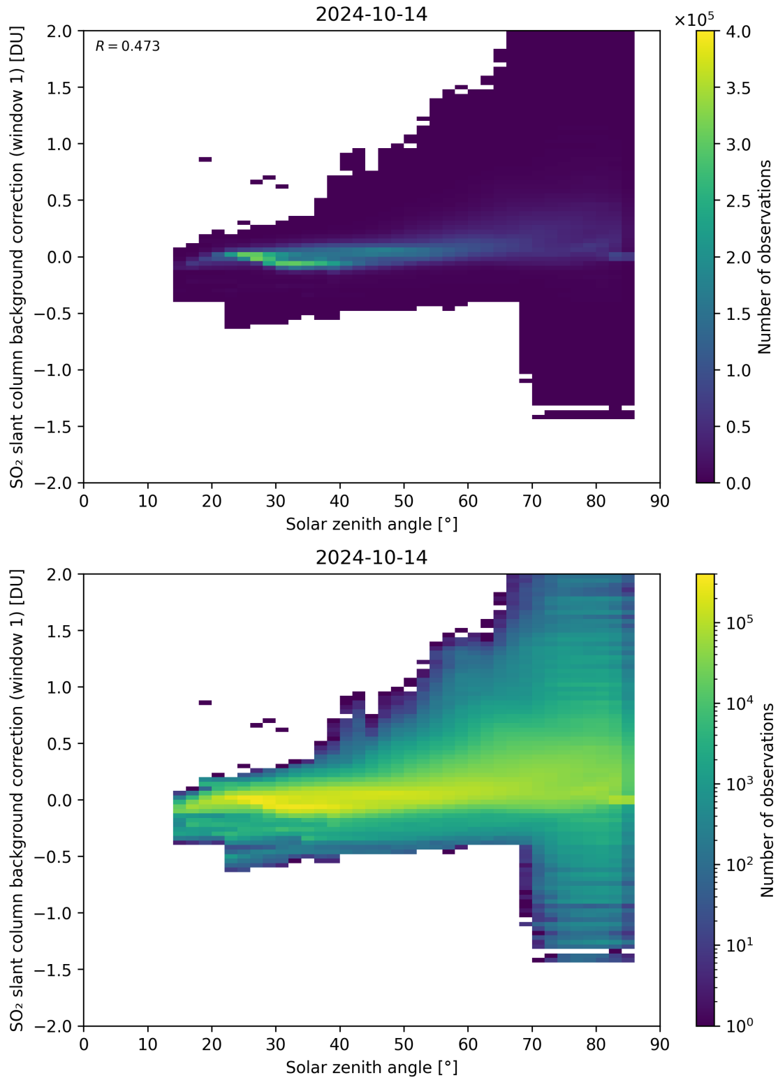
Figure 158: Scatter density plot of “Solar zenith angle” against “SO 2 slant column background correction (window 1)” for 2024-10-14 to 2024-10-15.
