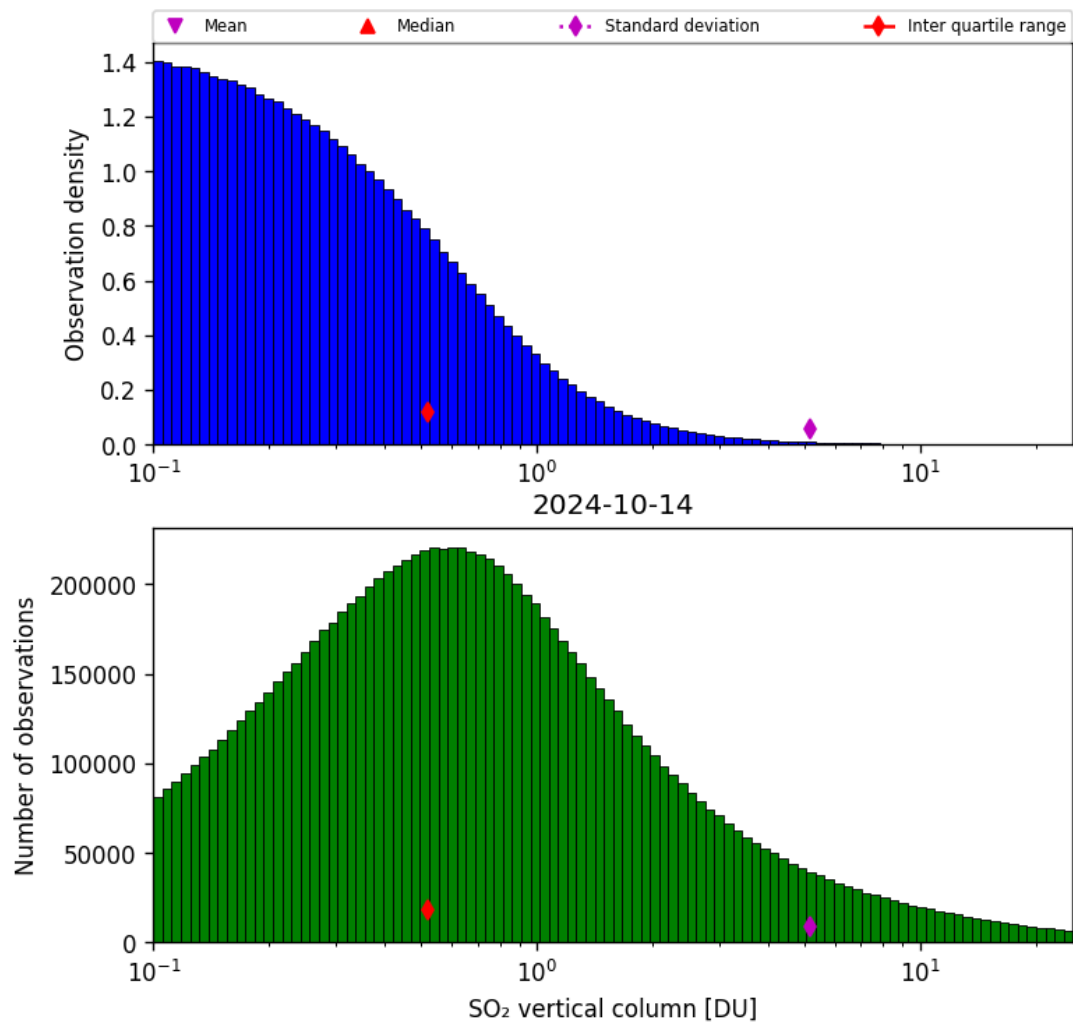
Figure 53: Histogram of “SO 2 vertical column” for 2024-10-14 to 2024-10-15
