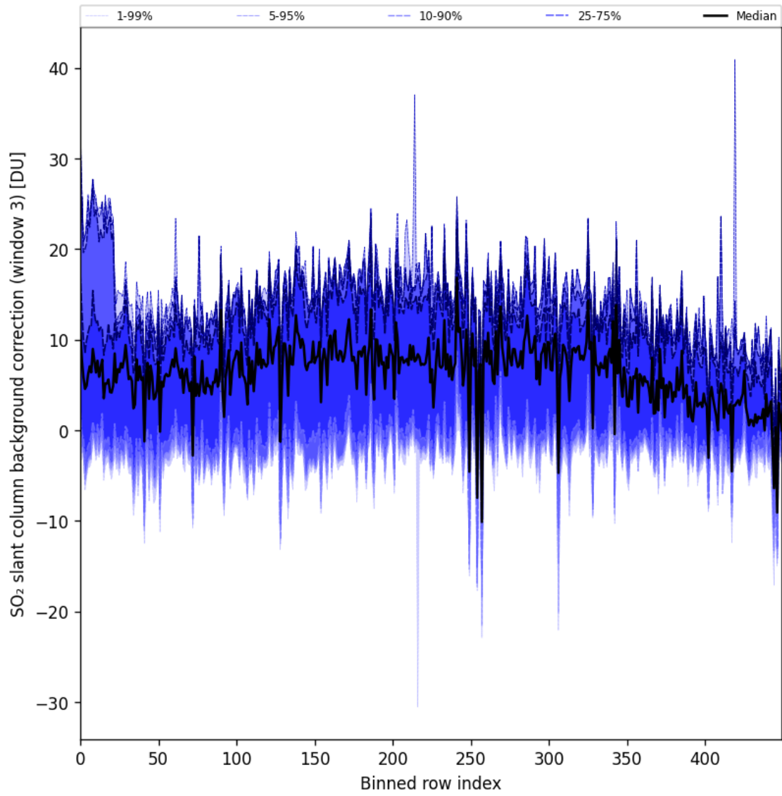
Figure 90: Along track statistics of “SO 2 slant column background correction (window 3)” for 2024-10-14 to 2024-10-15
