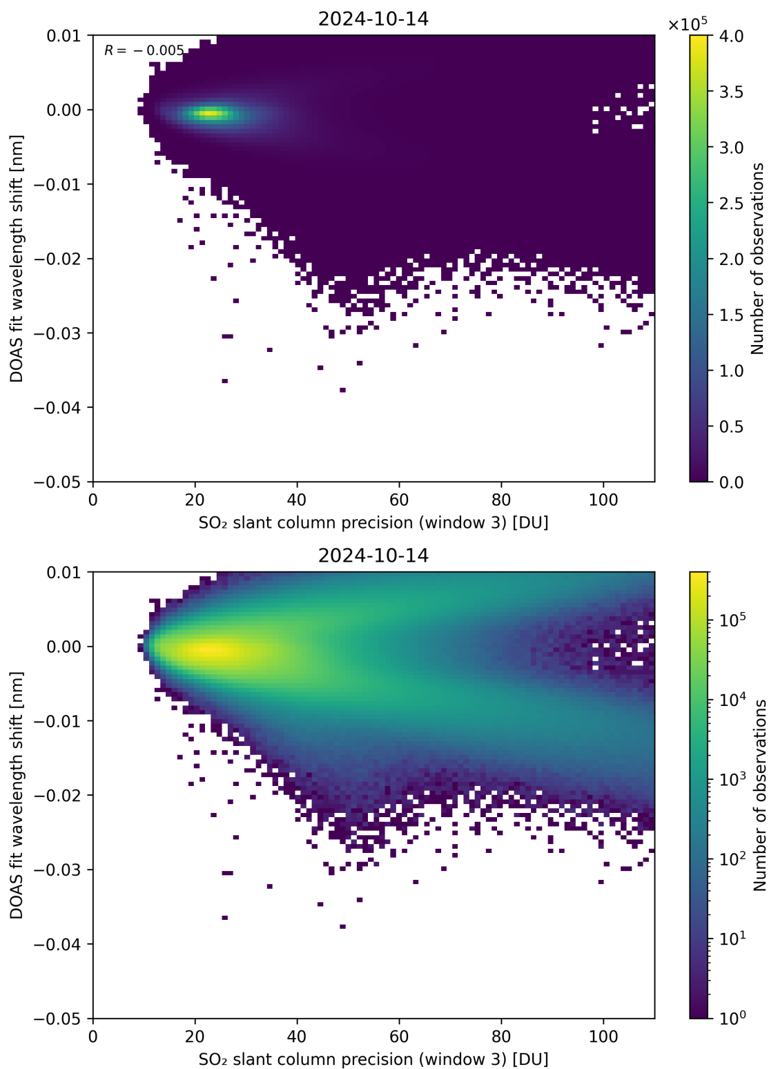
Figure 258: Scatter density plot of “SO 2 slant column precision (window 3)” against “DOAS fit wavelength shift” for 2024-10-14 to 2024-10-15.
