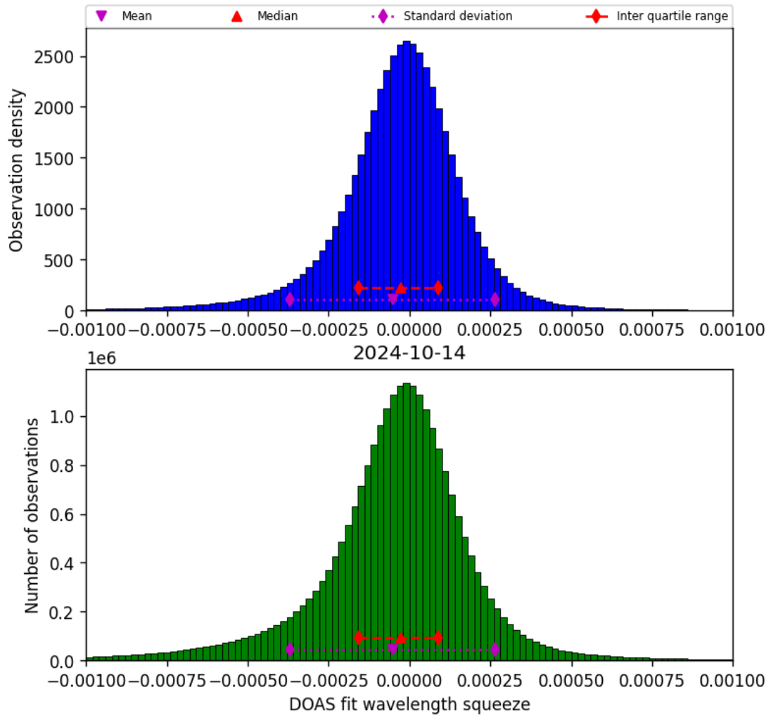
Figure 69: Histogram of “DOAS fit wavelength squeeze” for 2024-10-14 to 2024-10-15
