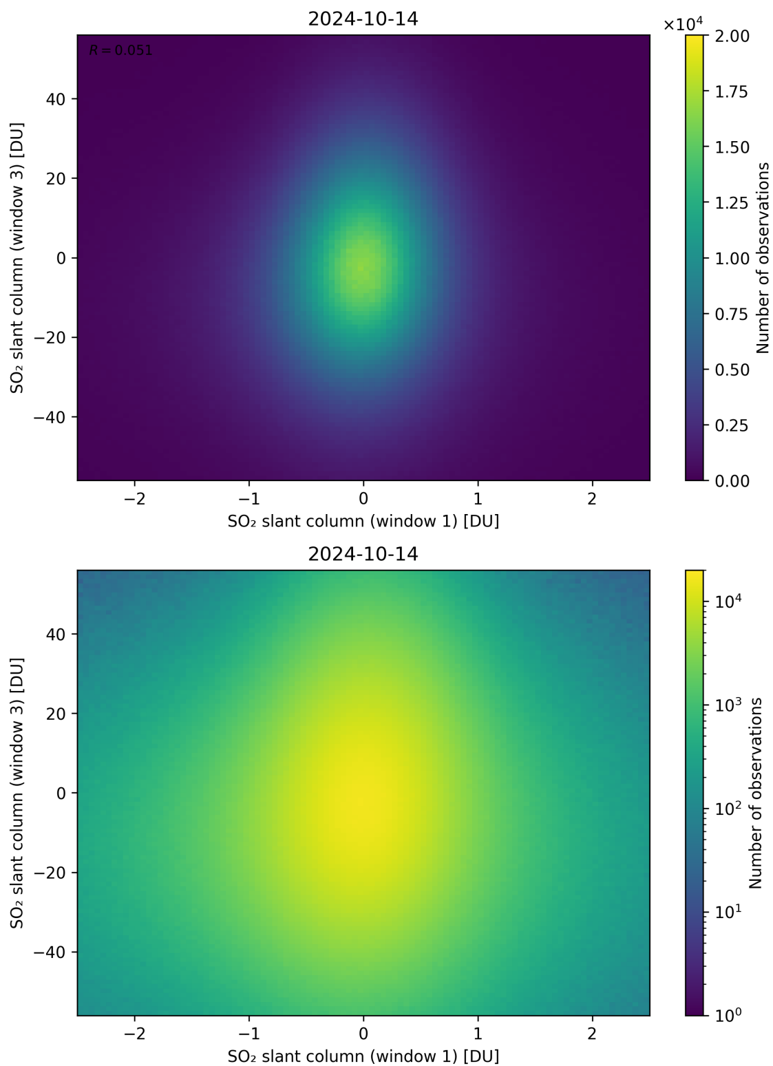
Figure 237: Scatter density plot of “SO 2 slant column (window 1)” against “SO 2 slant column (window 3)” for 2024-10-14 to 2024-10-15.
