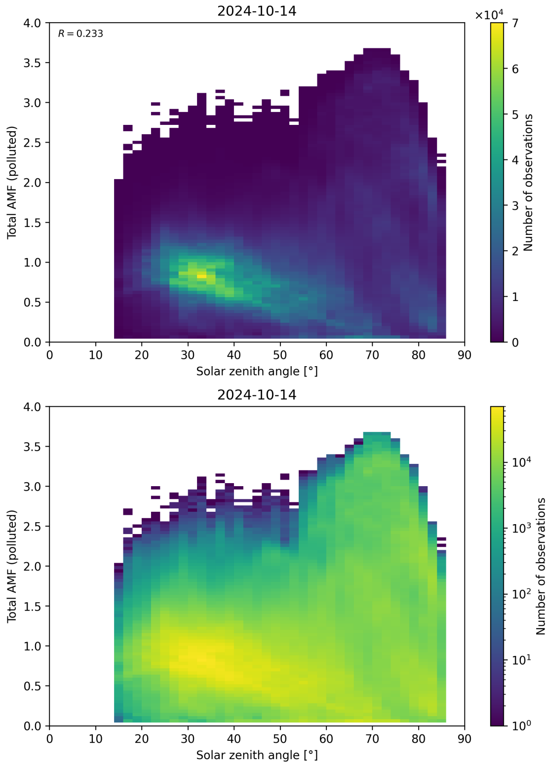
Figure 174: Scatter density plot of “Solar zenith angle” against “Total AMF (polluted)” for 2024-10-14 to 2024-10-15.
