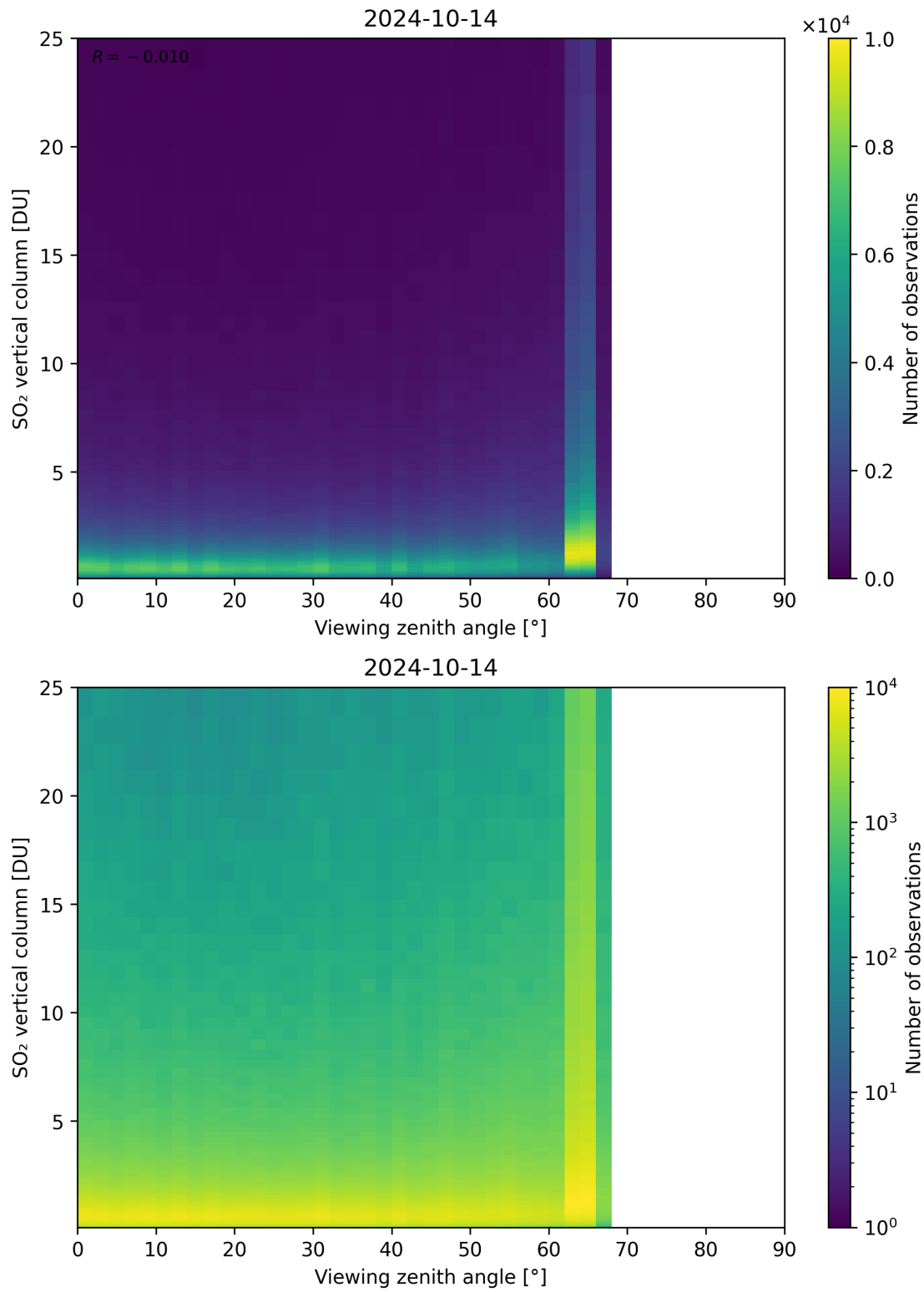
Figure 327: Scatter density plot of “Viewing zenith angle” against “SO 2 vertical column” for 2024-10-14 to 2024-10-15.
