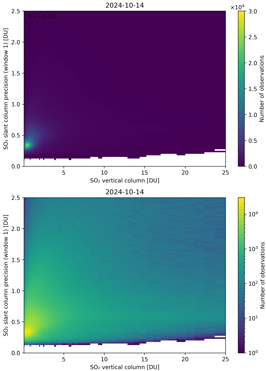
Figure 301: Scatter density plot of “SO 2 vertical column” against “SO 2 slant column precision (window 1)” for 2024-10-14 to 2024-10-15.
