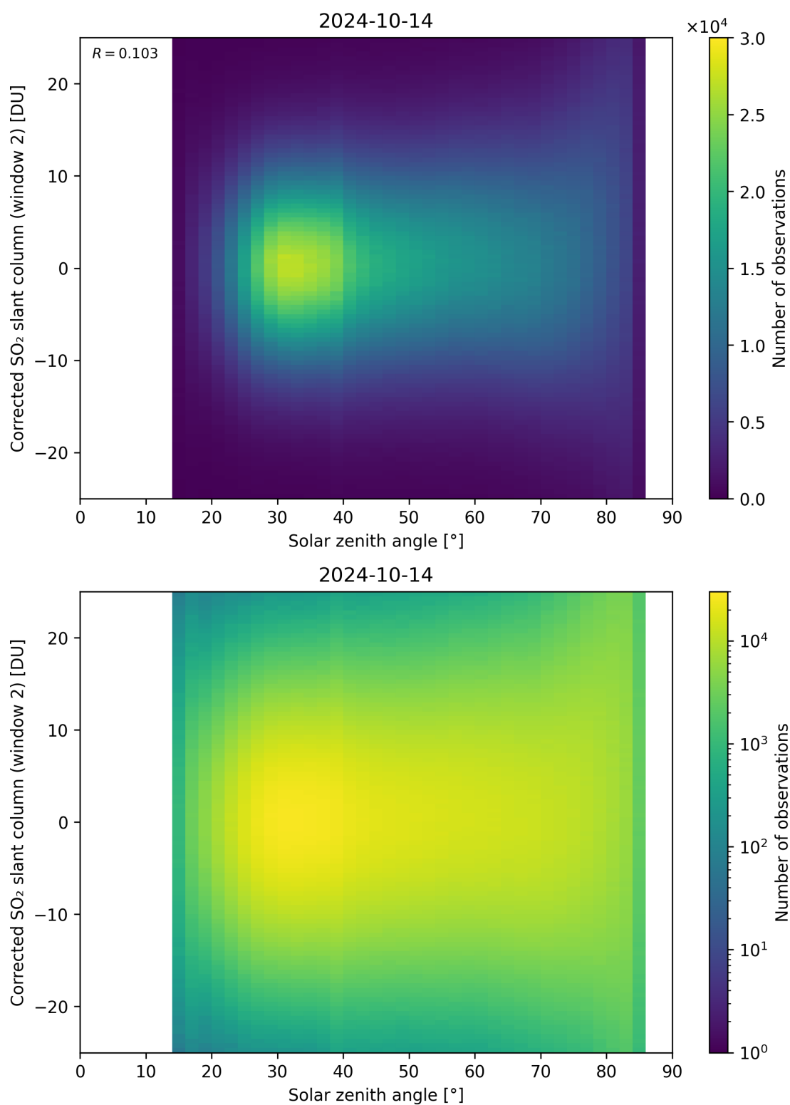
Figure 167: Scatter density plot of “Solar zenith angle” against “Corrected SO 2 slant column (window 2)” for 2024-10-14 to 2024-10-15.
