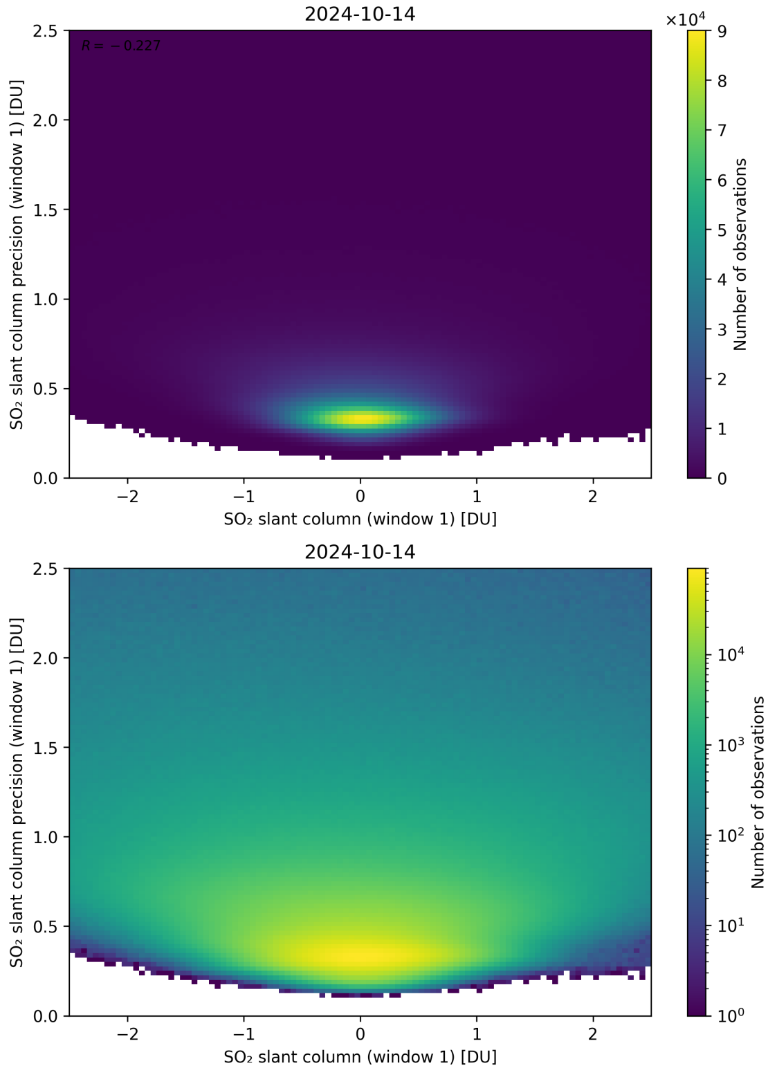
Figure 235: Scatter density plot of “SO 2 slant column (window 1)” against “SO 2 slant column precision (window 1)” for 2024-10-14 to 2024-10-15.
