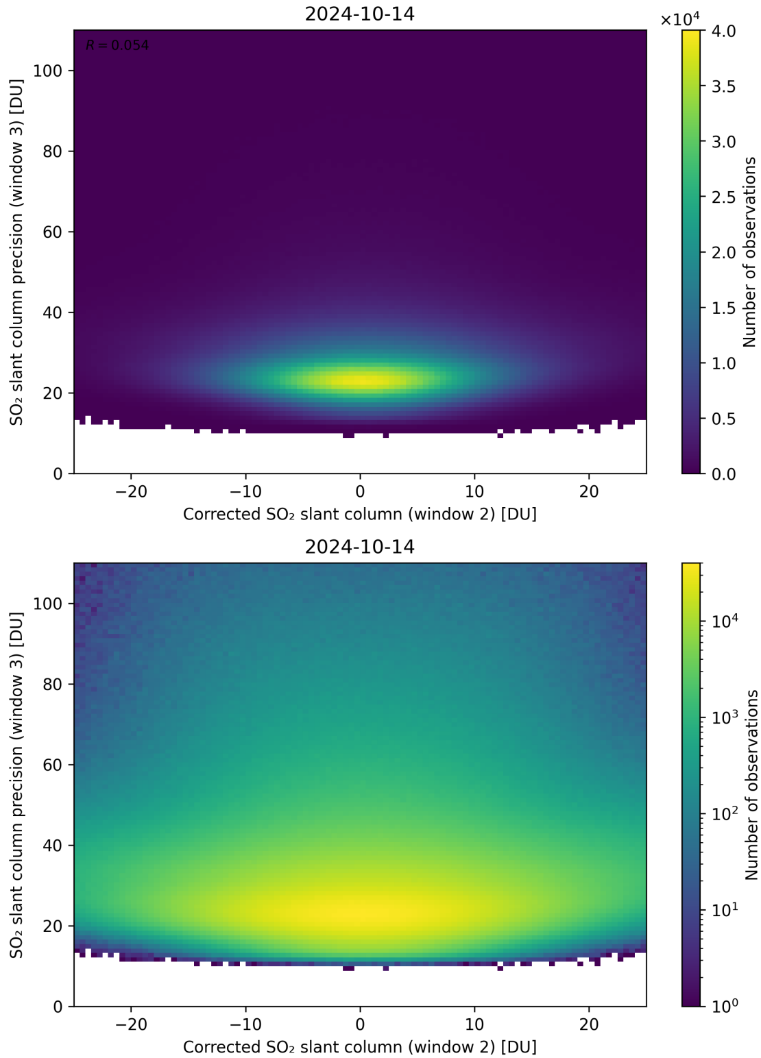
Figure 202: Scatter density plot of “Corrected SO 2 slant column (window 2)” against “SO 2 slant column precision (window 3)” for 2024-10-14 to 2024-10-15.
