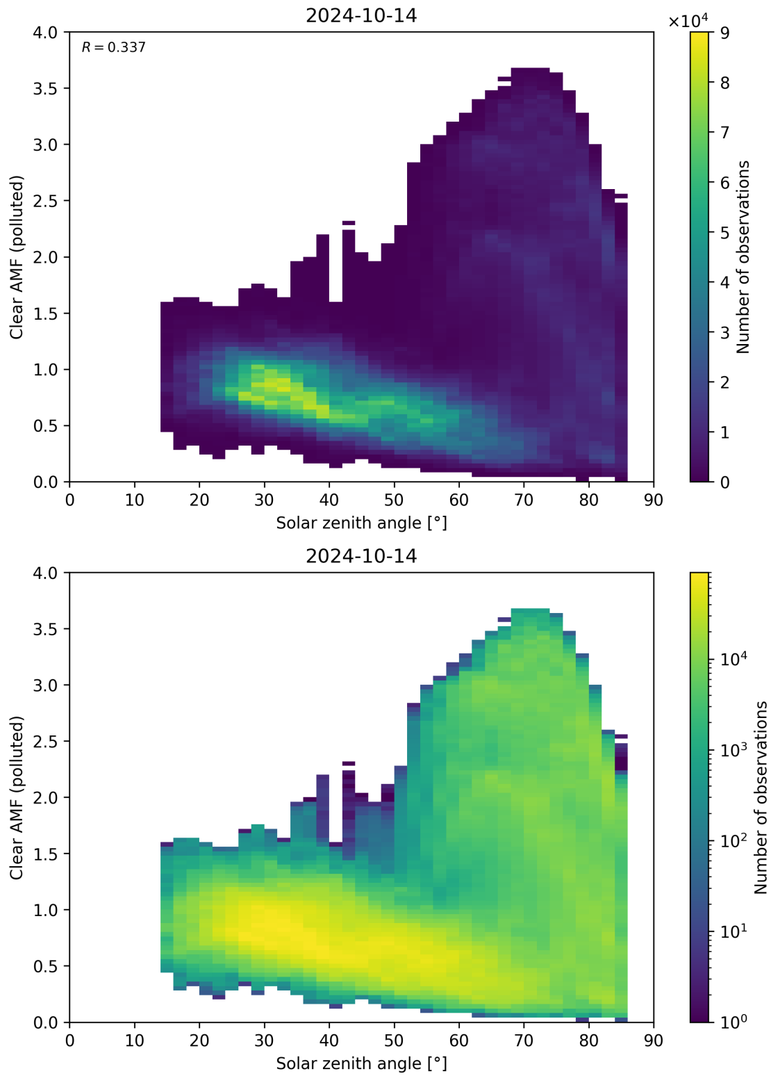
Figure 165: Scatter density plot of “Solar zenith angle” against “Clear AMF (polluted)” for 2024-10-14 to 2024-10-15.
