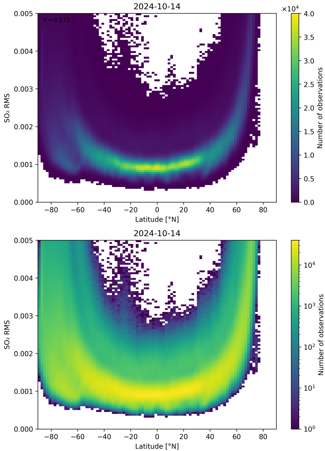
Figure 144: Scatter density plot of “Latitude” against “SO 2 RMS” for 2024-10-14 to 2024-10-15.
