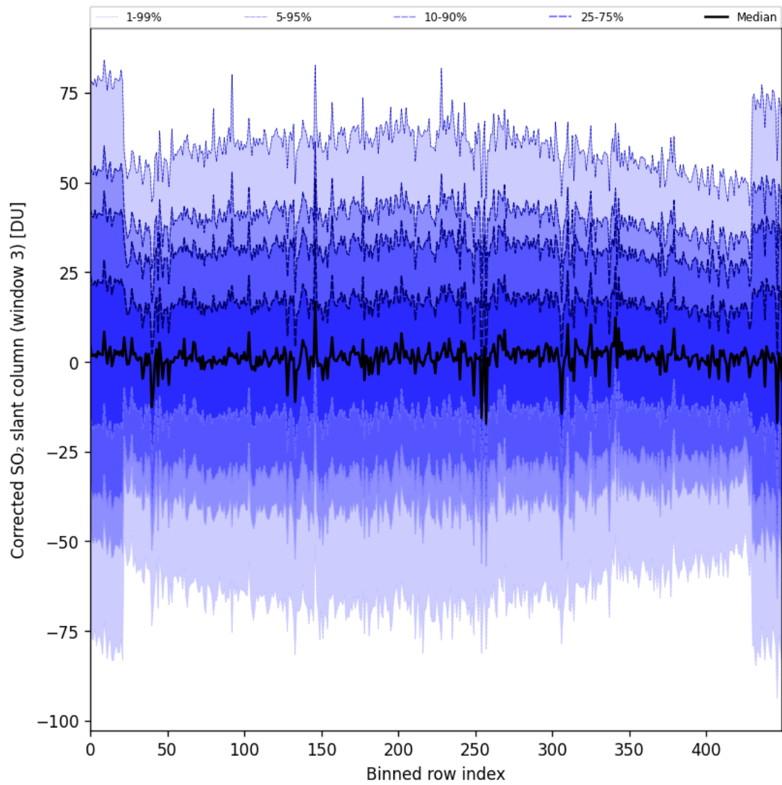
Figure 89: Along track statistics of “Corrected SO 2 slant column (window 3)” for 2024-10-14 to 2024-10-15
