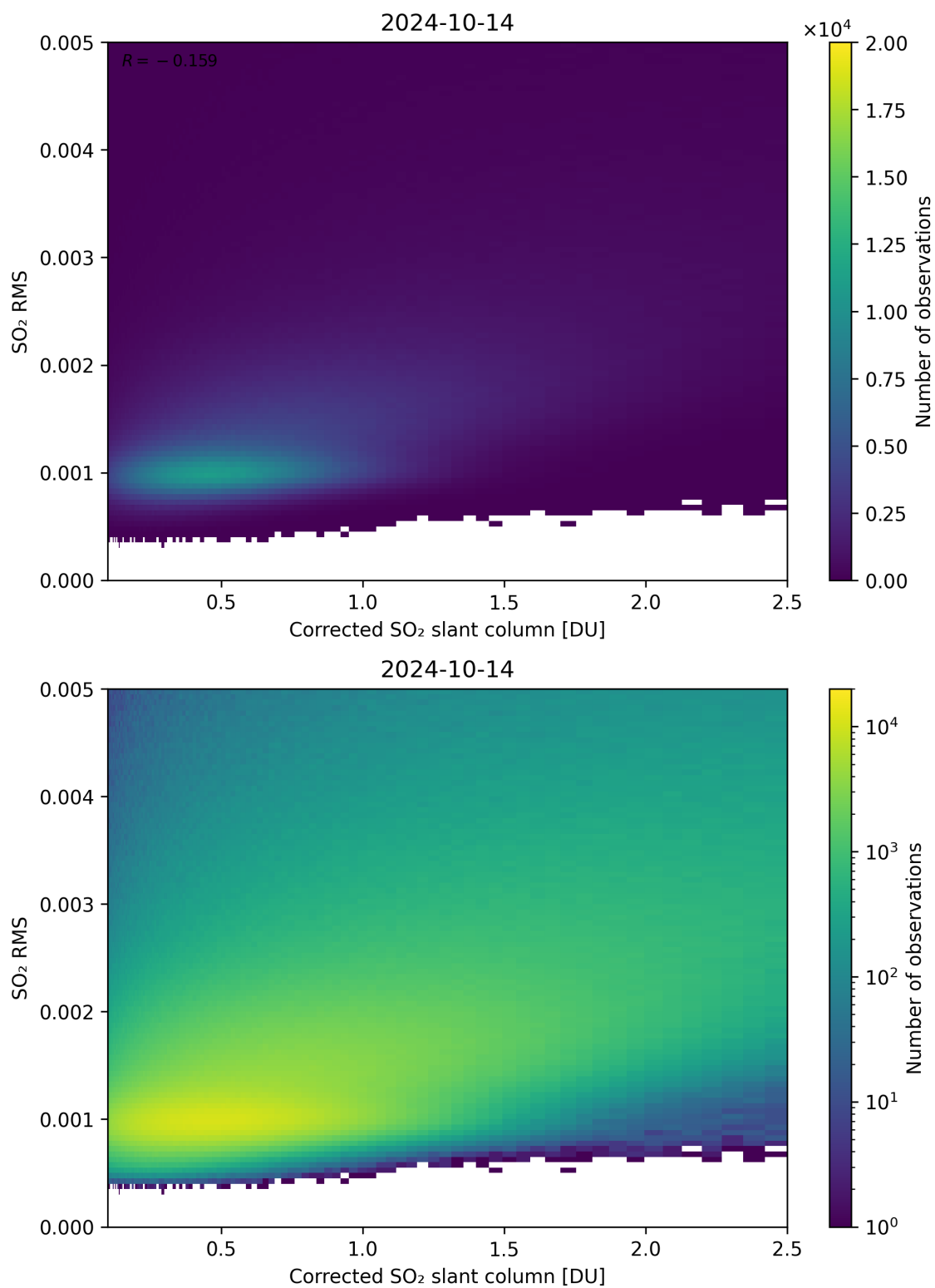
Figure 183: Scatter density plot of “Corrected SO 2 slant column” against “SO 2 RMS” for 2024-10-14 to 2024-10-15.
