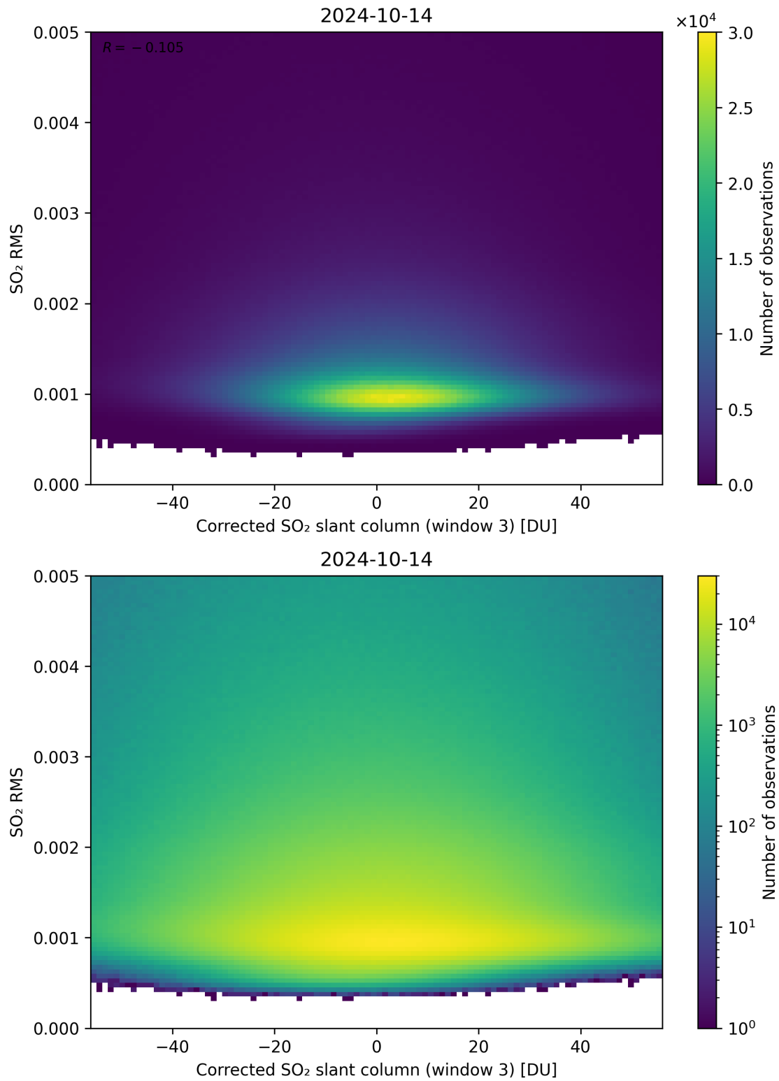
Figure 208: Scatter density plot of “Corrected SO 2 slant column (window 3)” against “SO 2 RMS” for 2024-10-14 to 2024-10-15.
