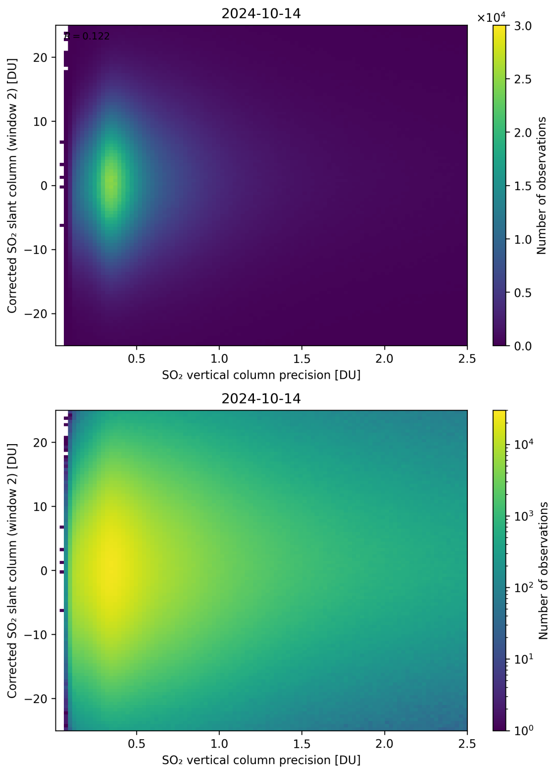
Figure 287: Scatter density plot of “SO 2 vertical column precision” against “Corrected SO 2 slant column (window 2)” for 2024-10-14 to 2024-10-15.
