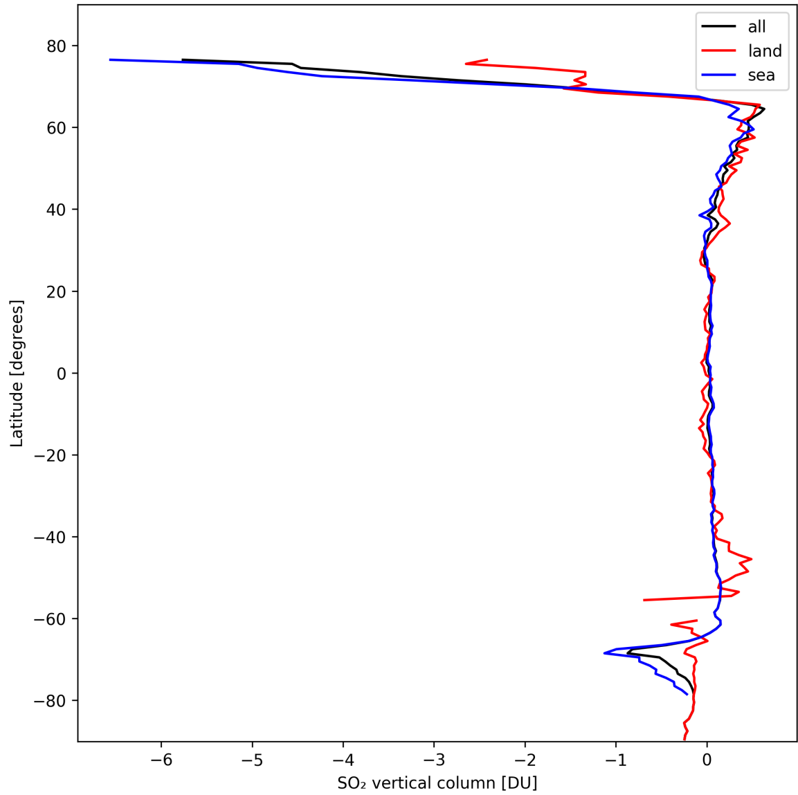
Figure 30: Zonal average of “SO 2 vertical column” for 2024-10-14 to 2024-10-15.
