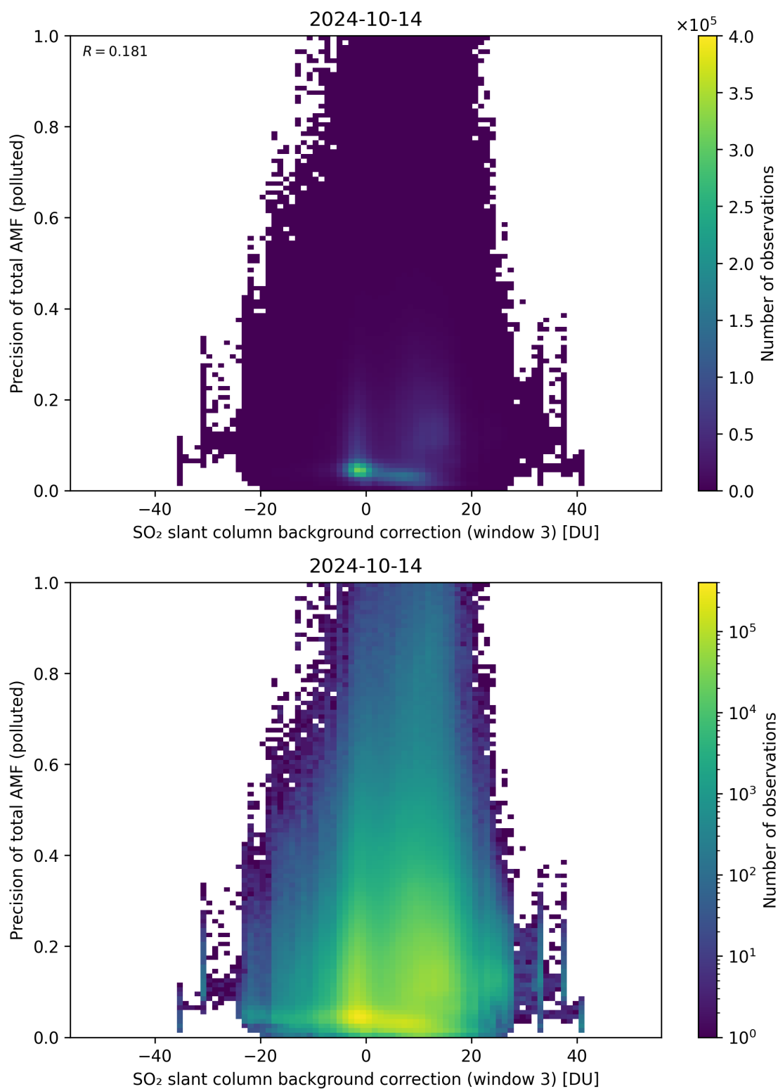
Figure 126: Scatter density plot of “SO 2 slant column background correction (window 3)” against “Precision of total AMF (polluted)” for 2024-10-14 to 2024-10-15.
