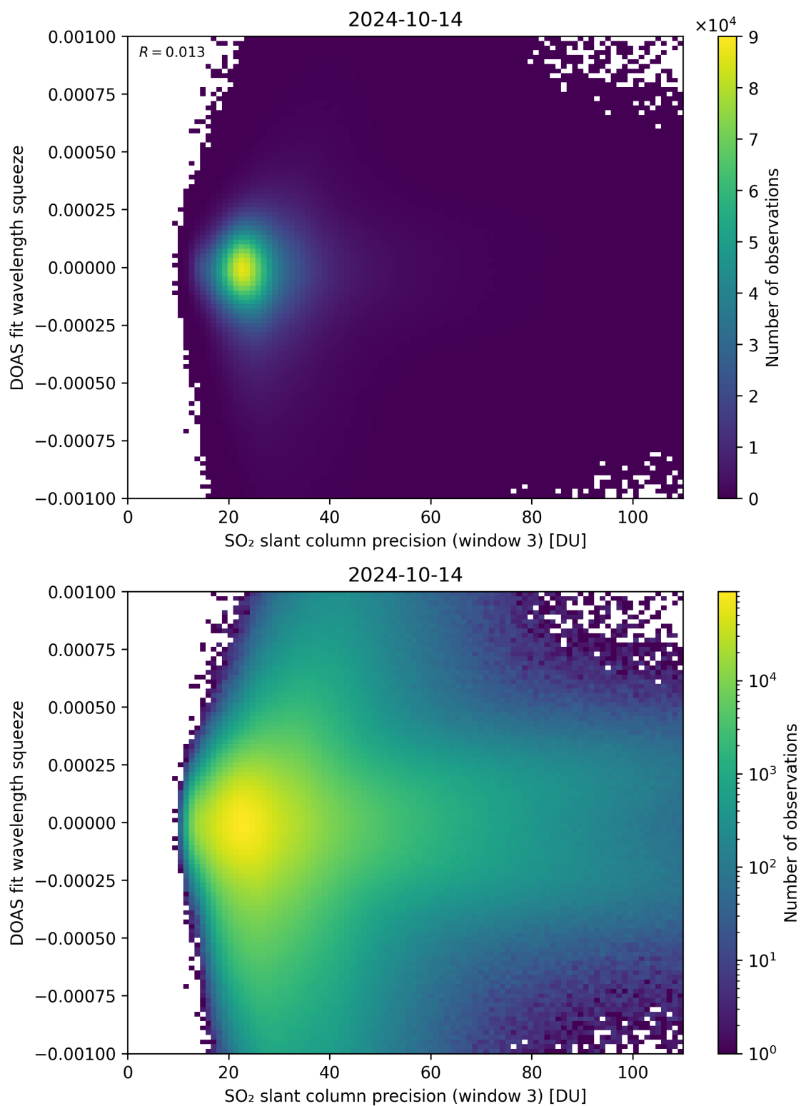
Figure 259: Scatter density plot of “SO 2 slant column precision (window 3)” against “DOAS fit wavelength squeeze” for 2024-10-14 to 2024-10-15.
