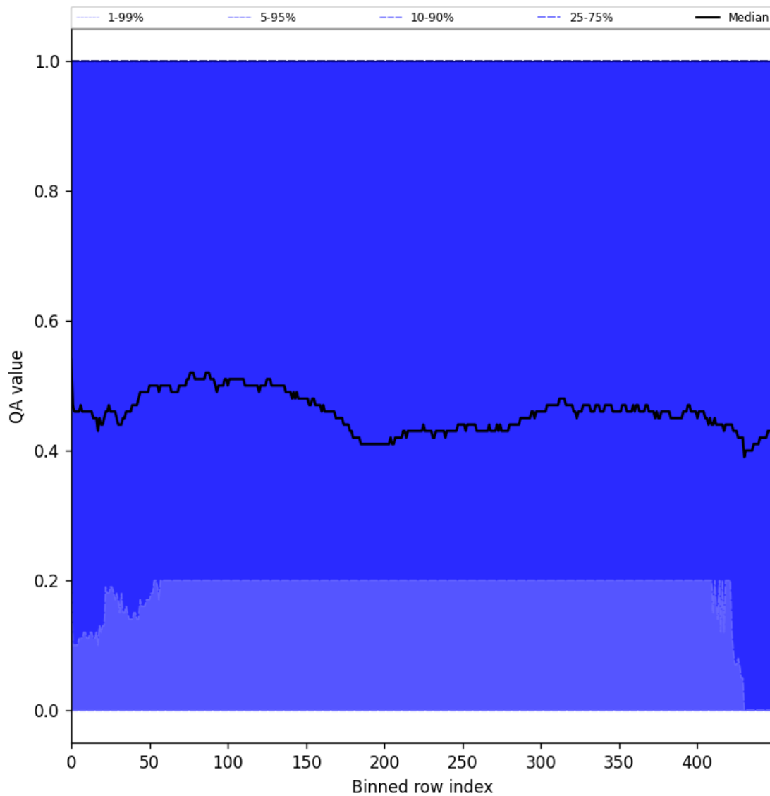
Figure 75: Along track statistics of “QA value” for 2024-10-14 to 2024-10-15
