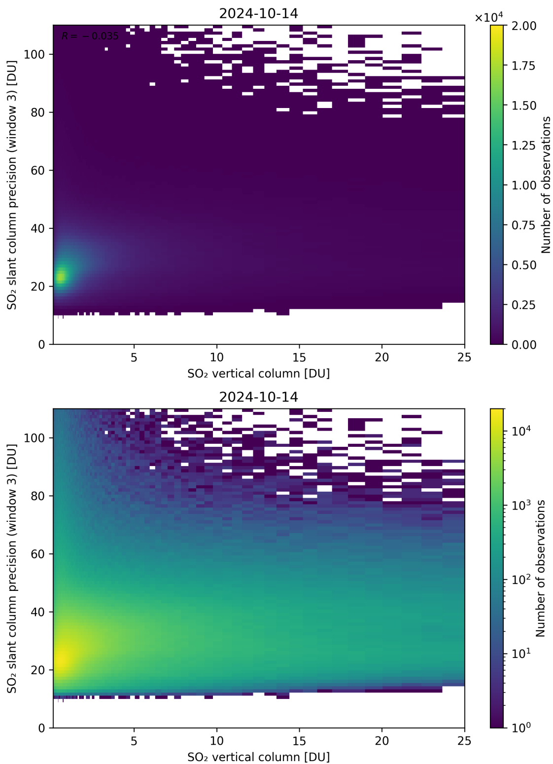
Figure 304: Scatter density plot of “SO 2 vertical column” against “SO 2 slant column precision (window 3)” for 2024-10-14 to 2024-10-15.
