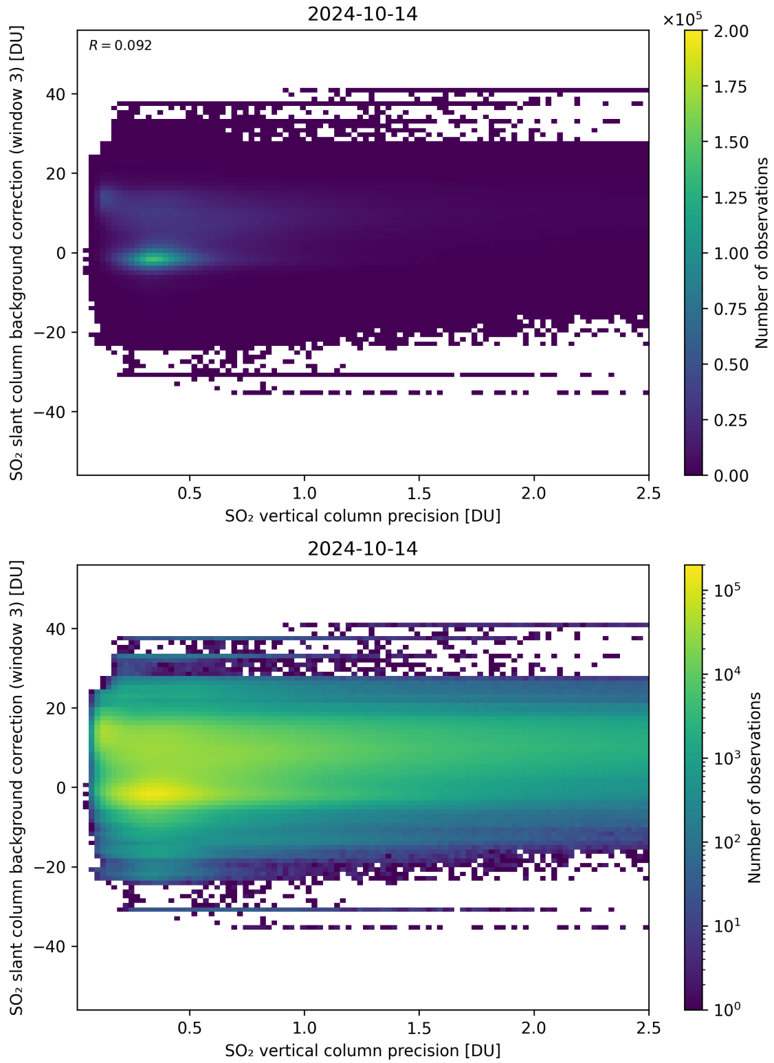
Figure 281: Scatter density plot of “SO 2 vertical column precision” against “SO 2 slant column background correction (window 3)” for 2024-10-14 to 2024-10-15.
