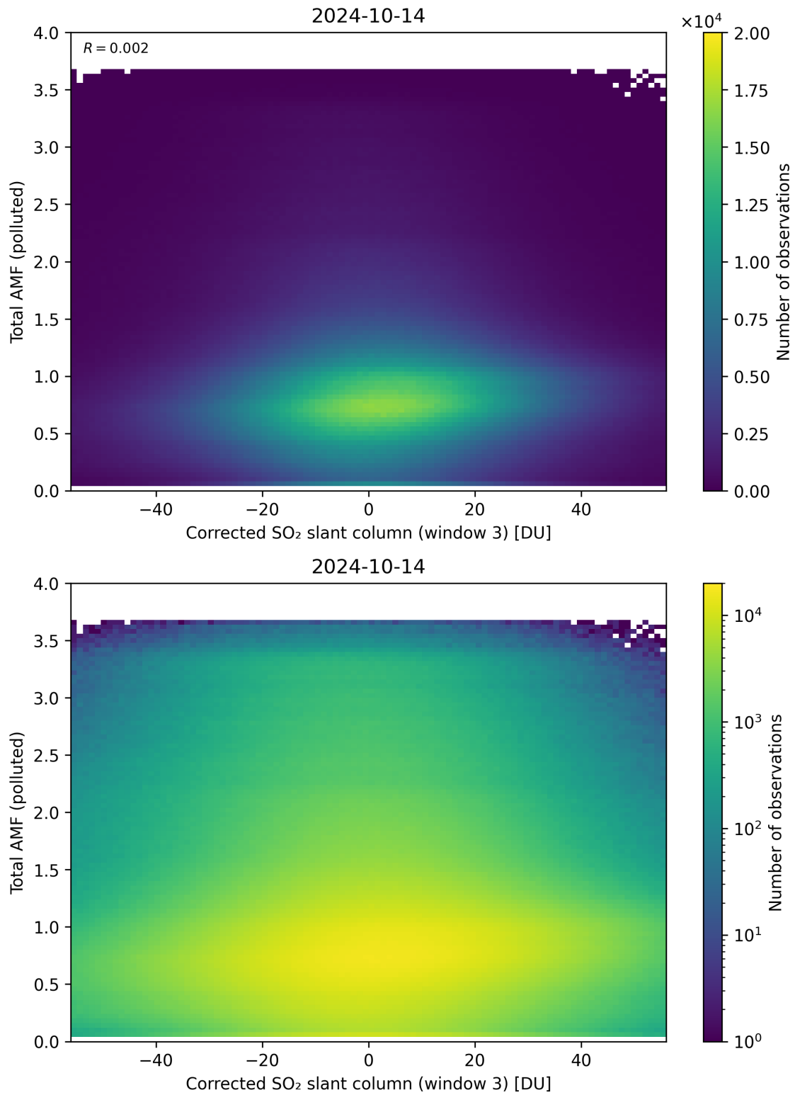
Figure 210: Scatter density plot of “Corrected SO 2 slant column (window 3)” against “Total AMF (polluted)” for 2024-10-14 to 2024-10-15.
