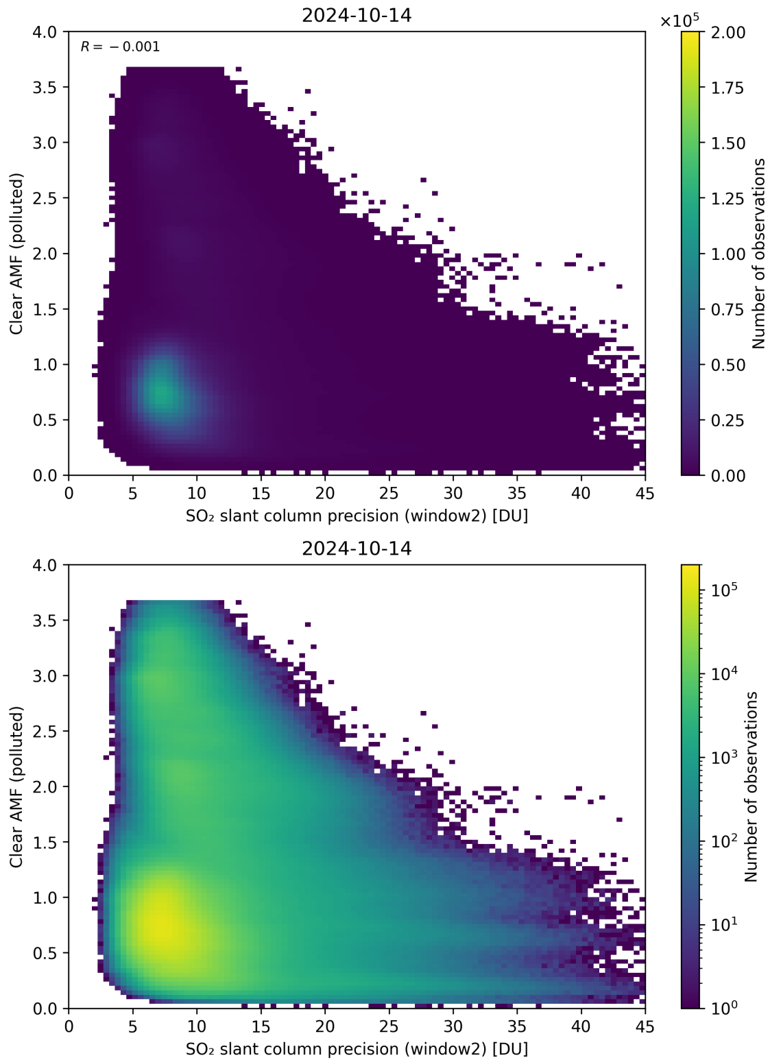
Figure 246: Scatter density plot of “SO 2 slant column precision (window2)” against “Clear AMF (polluted)” for 2024-10-14 to 2024-10-15.
