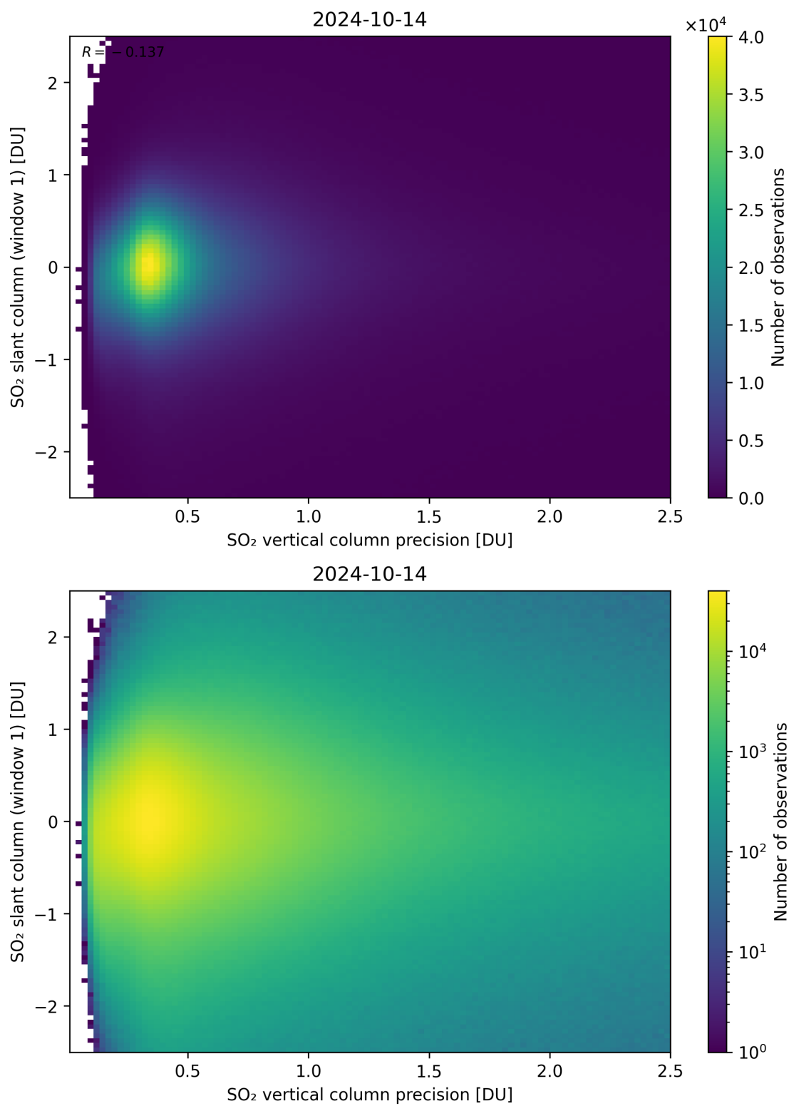
Figure 289: Scatter density plot of “SO 2 vertical column precision” against “SO 2 slant column (window 1)” for 2024-10-14 to 2024-10-15.
