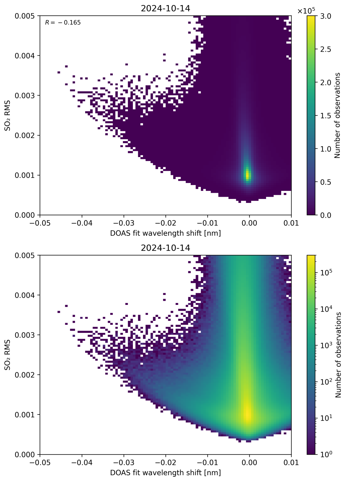
Figure 128: Scatter density plot of “DOAS fit wavelength shift” against “SO 2 RMS” for 2024-10-14 to 2024-10-15.
