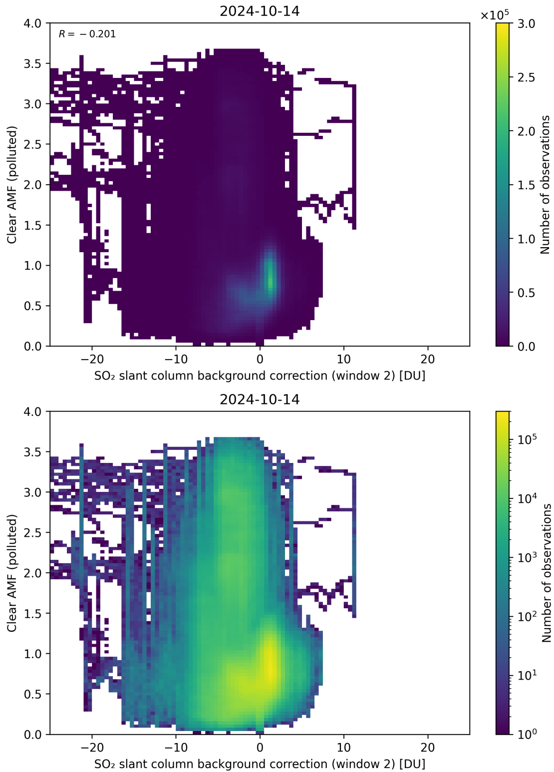
Figure 115: Scatter density plot of “SO 2 slant column background correction (window 2)” against “Clear AMF (polluted)” for 2024-10-14 to 2024-10-15.
