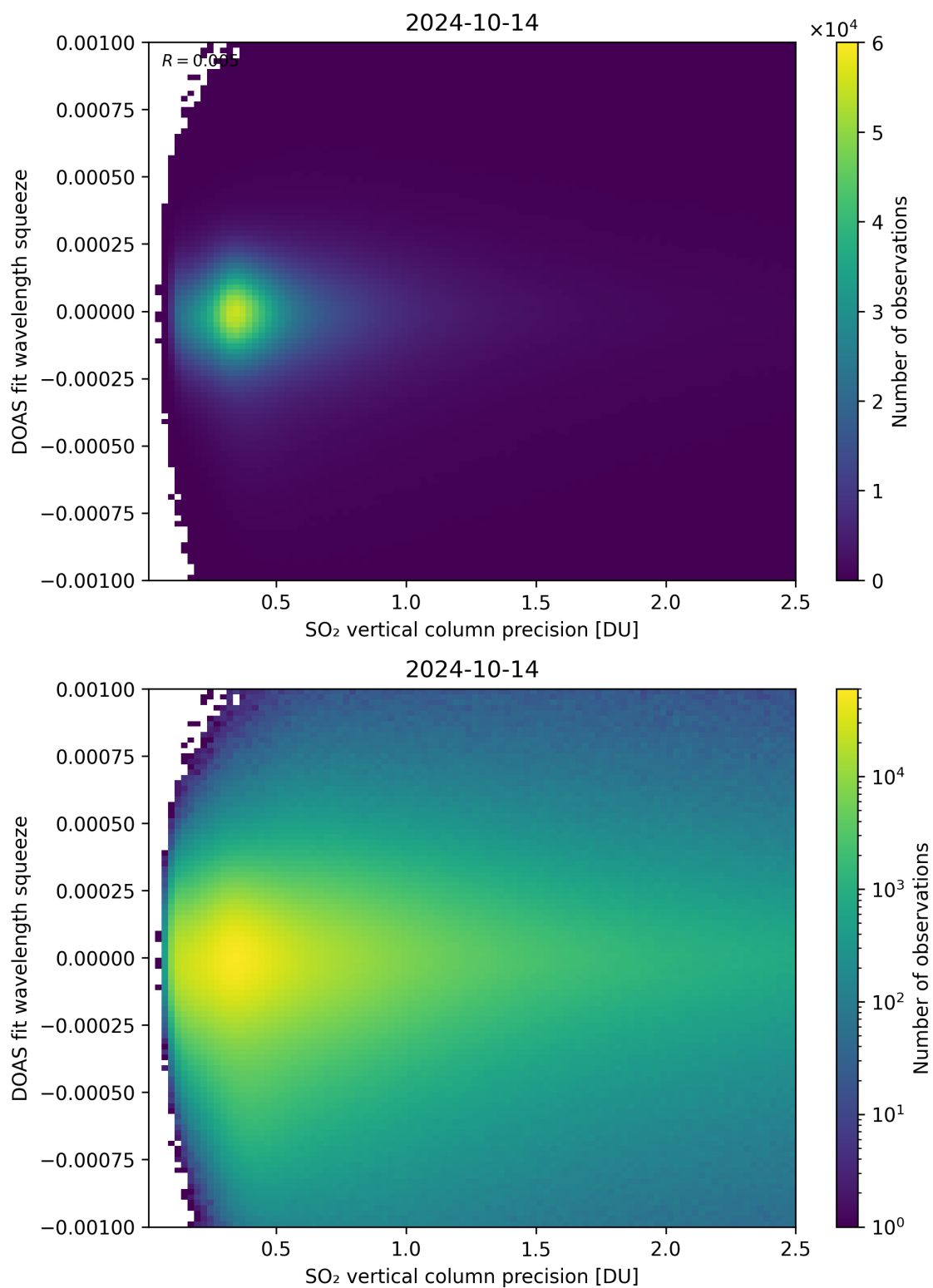
Figure 283: Scatter density plot of “SO 2 vertical column precision” against “DOAS fit wavelength squeeze” for 2024-10-14 to 2024-10-15.
