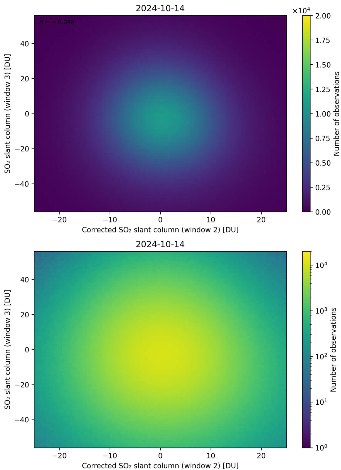
Figure 201: Scatter density plot of “Corrected SO 2 slant column (window 2)” against “SO 2 slant column (window 3)” for 2024-10-14 to 2024-10-15.
