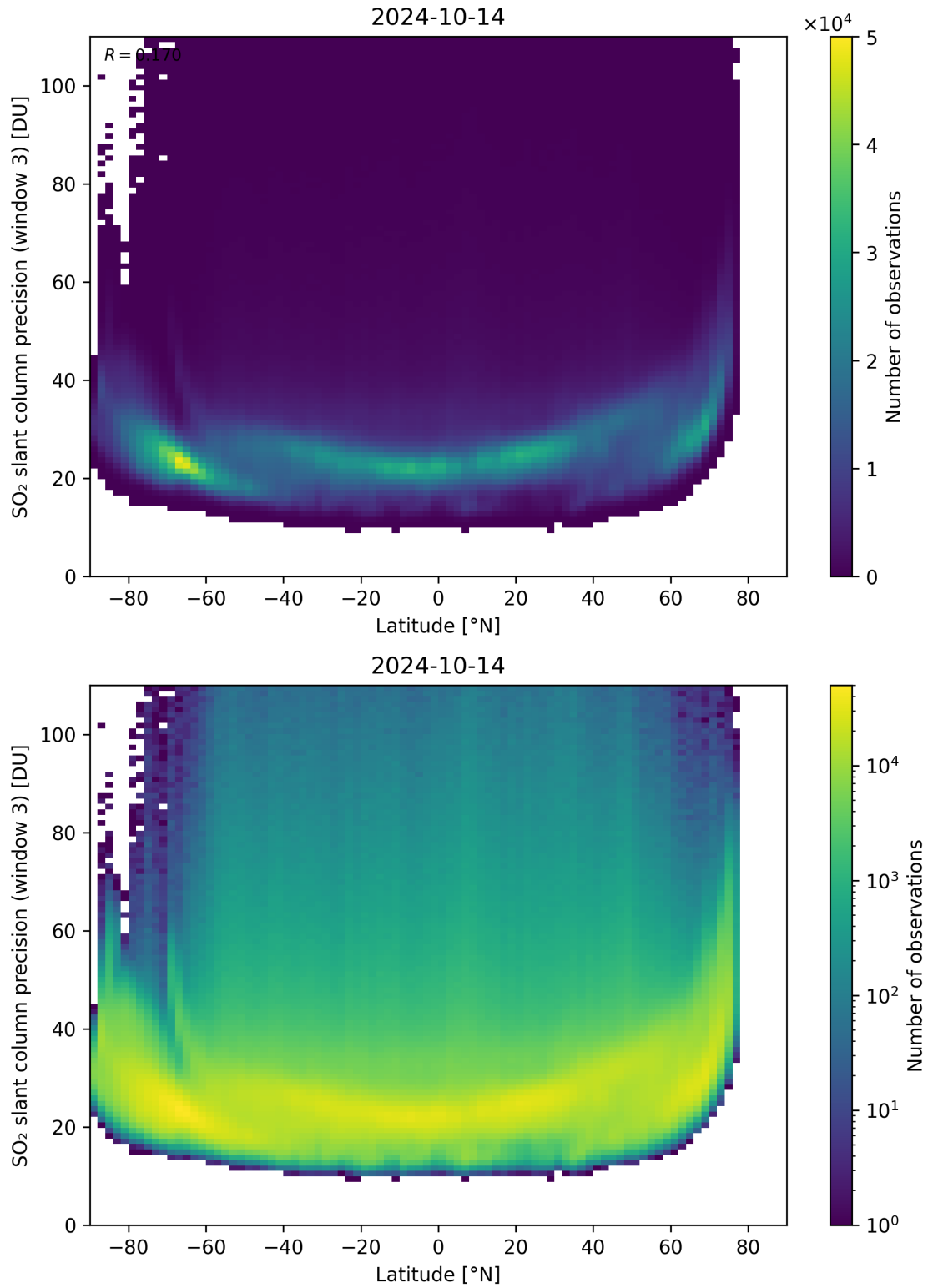
Figure 153: Scatter density plot of “Latitude” against “SO 2 slant column precision (window 3)” for 2024-10-14 to 2024-10-15.
