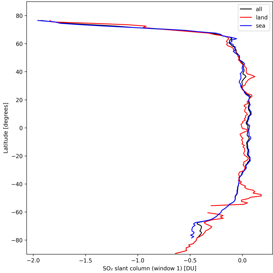
Figure 33: Zonal average of “SO 2 slant column (window 1)” for 2024-10-14 to 2024-10-15.
