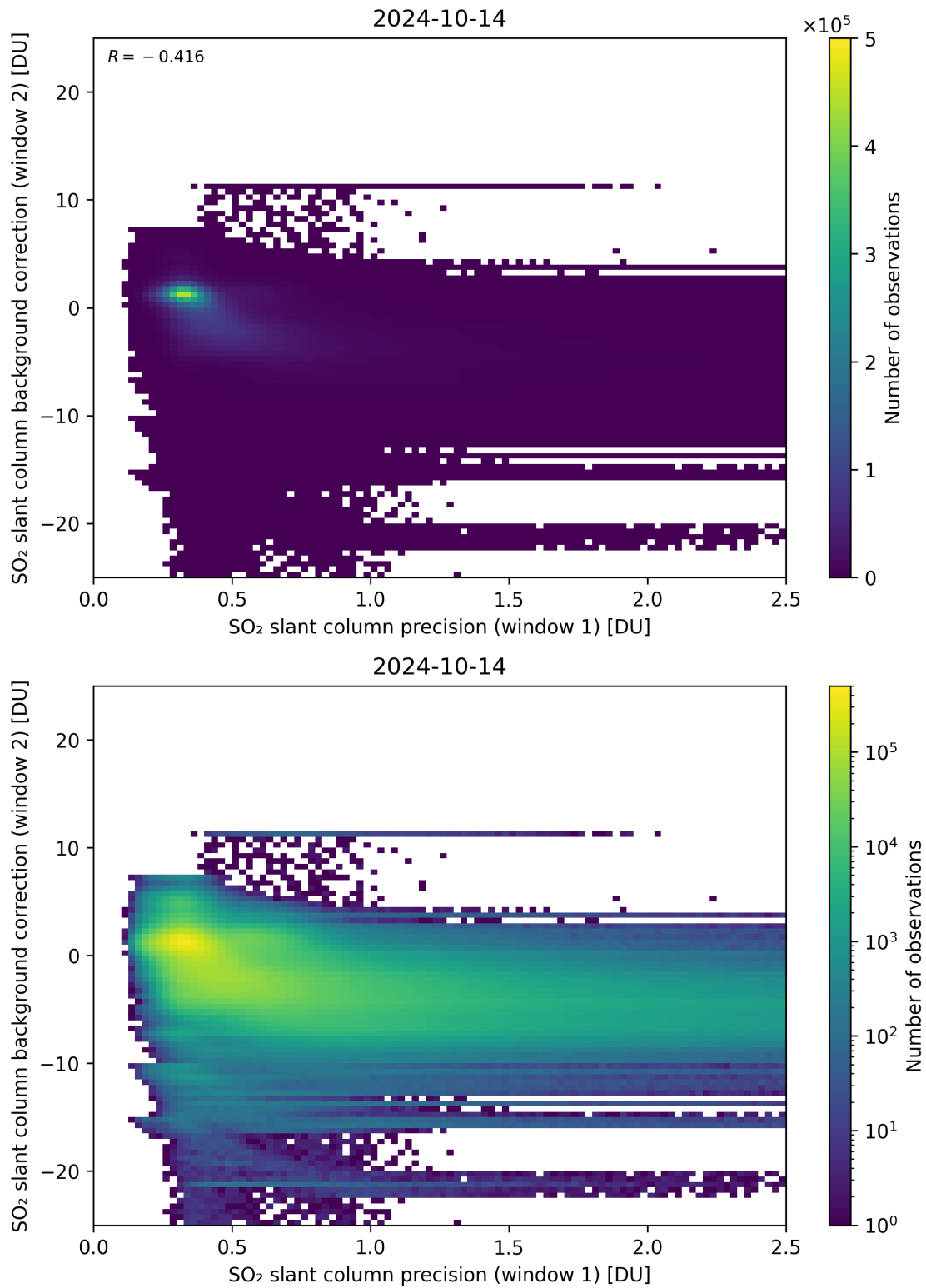
Figure 219: Scatter density plot of “SO 2 slant column precision (window 1)” against “SO 2 slant column background correction (window 2)” for 2024-10-14 to 2024-10-15.
