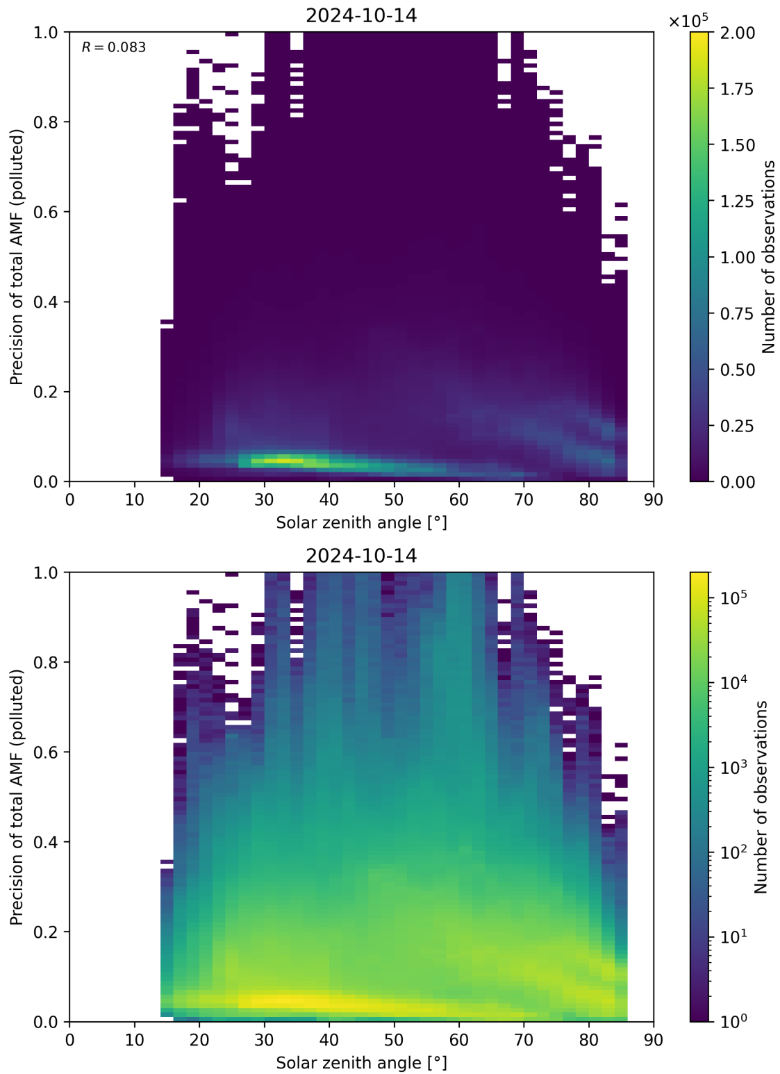
Figure 175: Scatter density plot of “Solar zenith angle” against “Precision of total AMF (polluted)” for 2024-10-14 to 2024-10-15.
