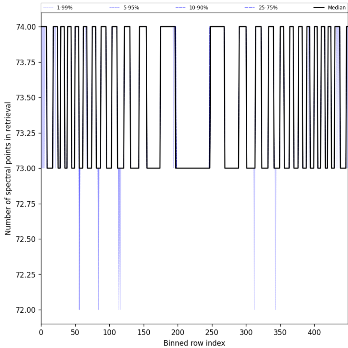
Figure 97: Along track statistics of “Number of spectral points in retrieval” for 2024-10-14 to 2024-10-15
