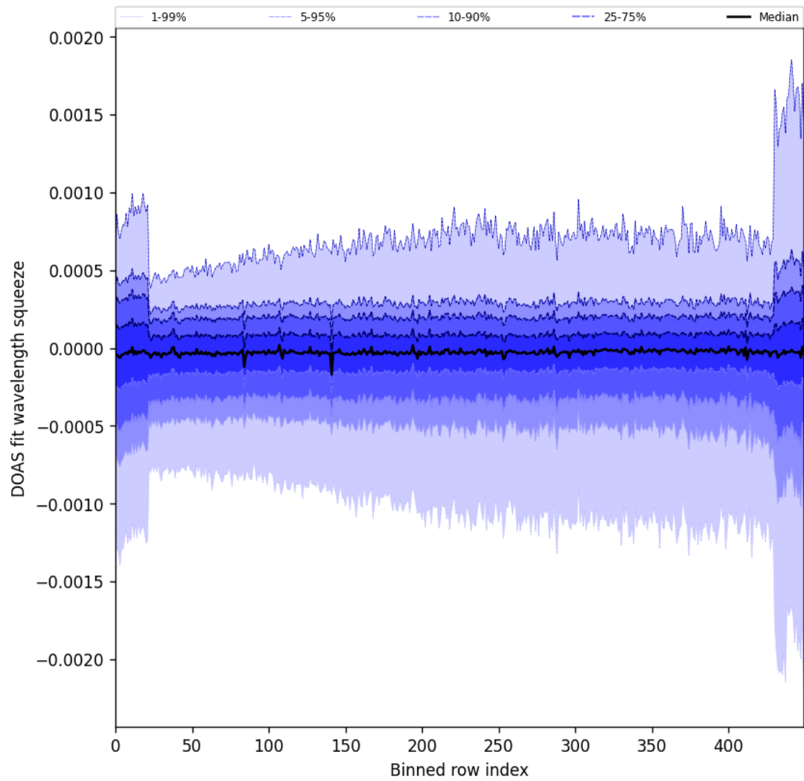
Figure 92: Along track statistics of “DOAS fit wavelength squeeze” for 2024-10-14 to 2024-10-15
