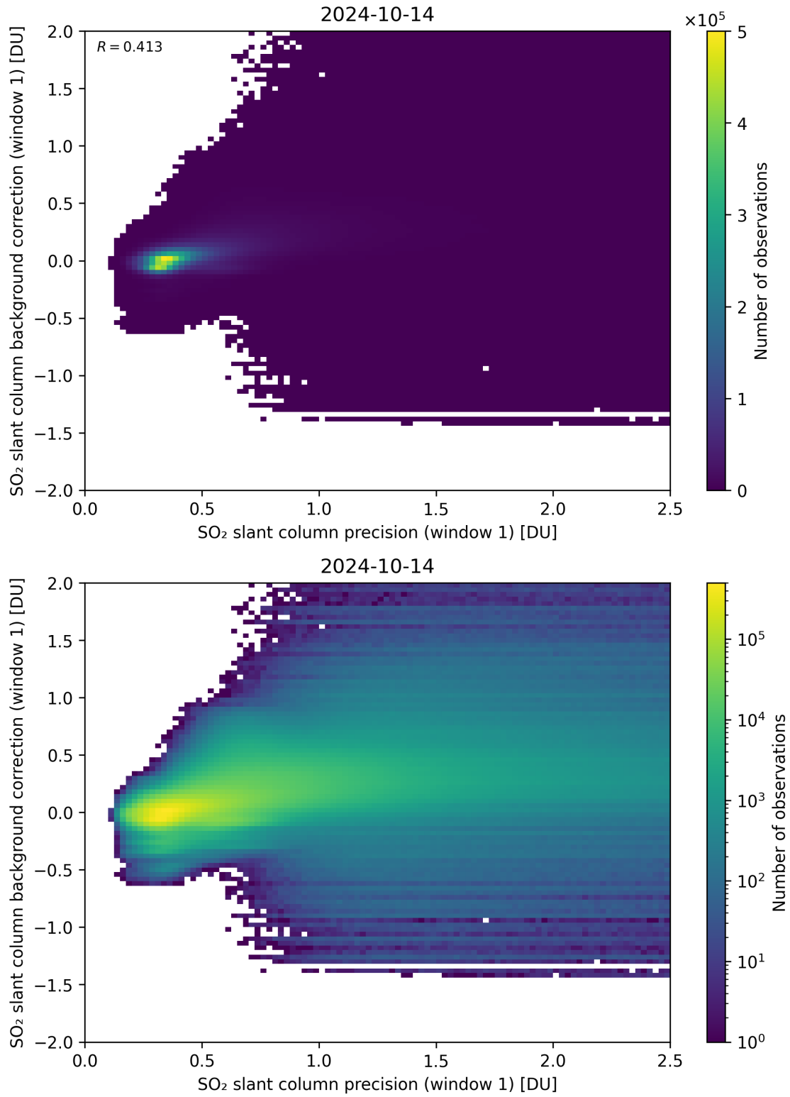
Figure 218: Scatter density plot of “SO 2 slant column precision (window 1)” against “SO 2 slant column background correction (window 1)” for 2024-10-14 to 2024-10-15.
