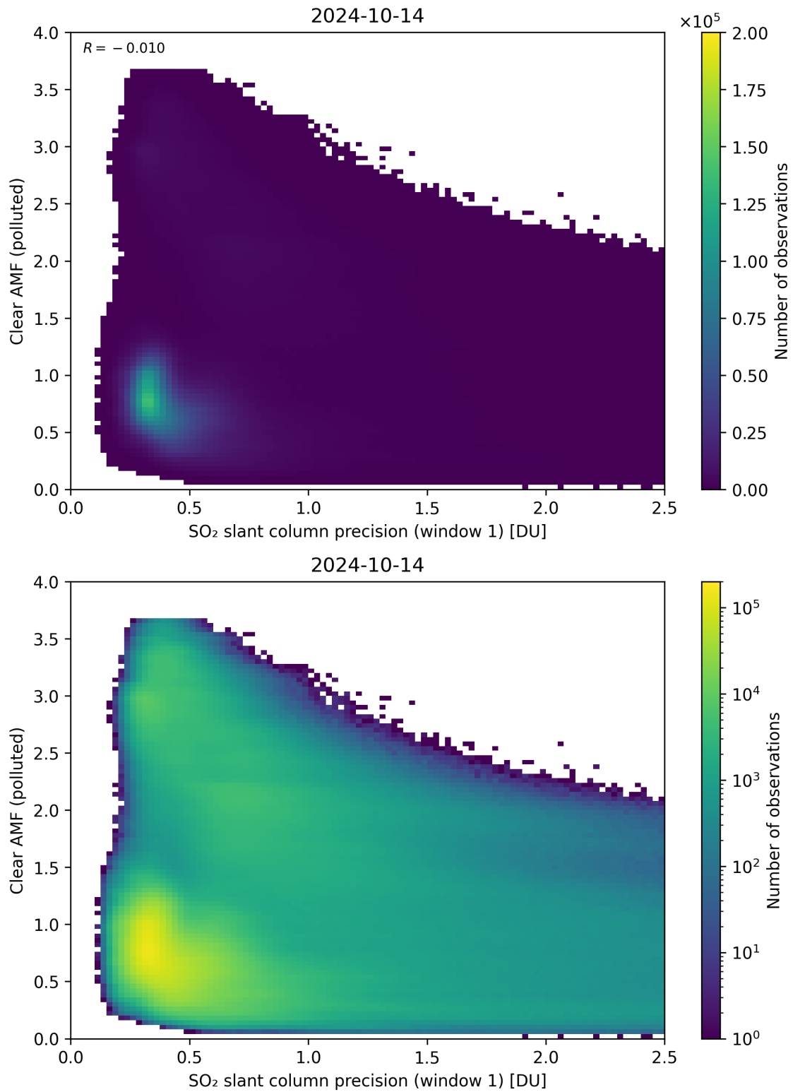
Figure 224: Scatter density plot of “SO 2 slant column precision (window 1)” against “Clear AMF (polluted)” for 2024-10-14 to 2024-10-15.
