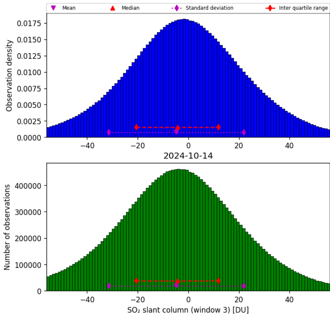
Figure 64: Histogram of “SO 2 slant column (window 3)” for 2024-10-14 to 2024-10-15
