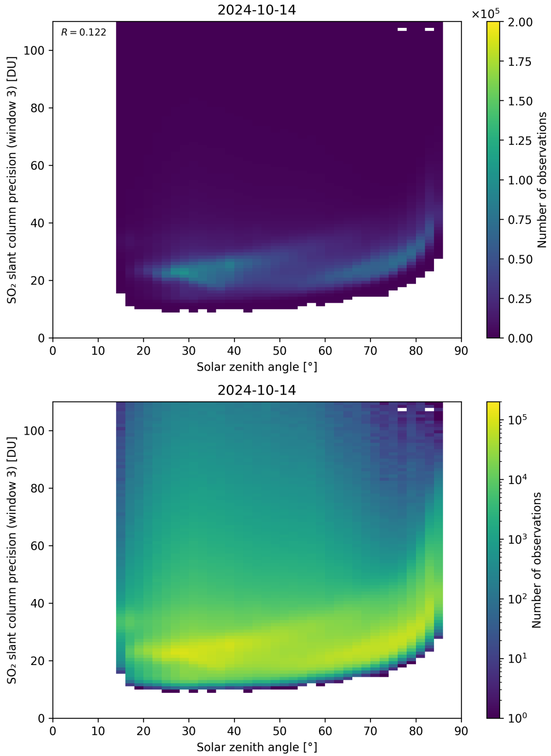
Figure 173: Scatter density plot of “Solar zenith angle” against “SO 2 slant column precision (window 3)” for 2024-10-14 to 2024-10-15.
