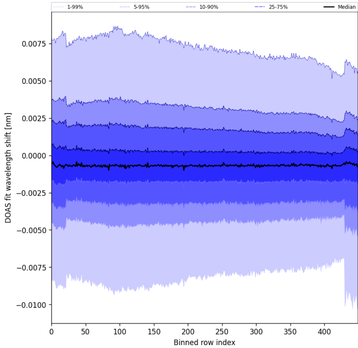
Figure 91: Along track statistics of “DOAS fit wavelength shift” for 2024-10-14 to 2024-10-15
