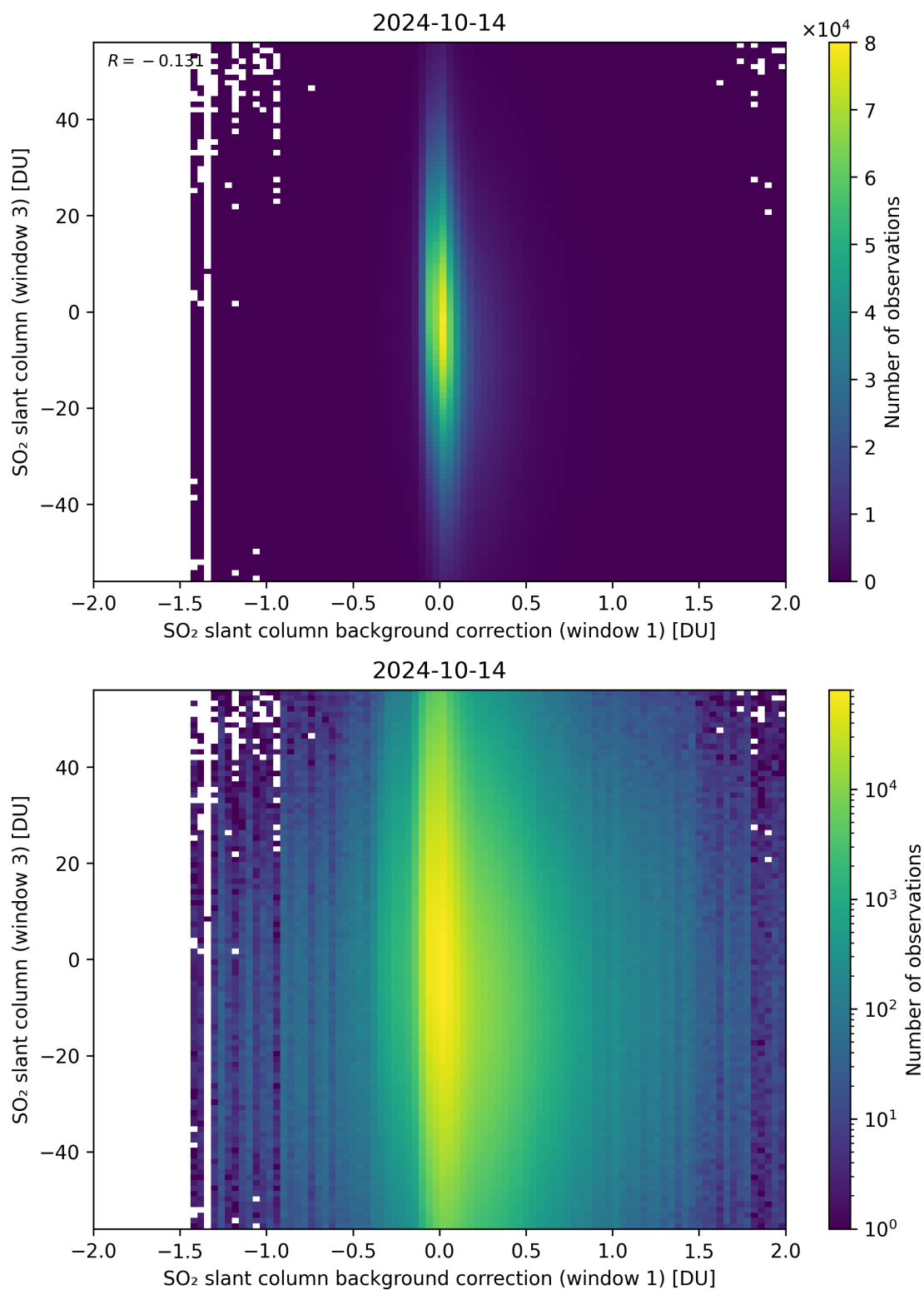
Figure 107: Scatter density plot of “SO 2 slant column background correction (window 1)” against “SO 2 slant column (window 3)” for 2024-10-14 to 2024-10-15.
