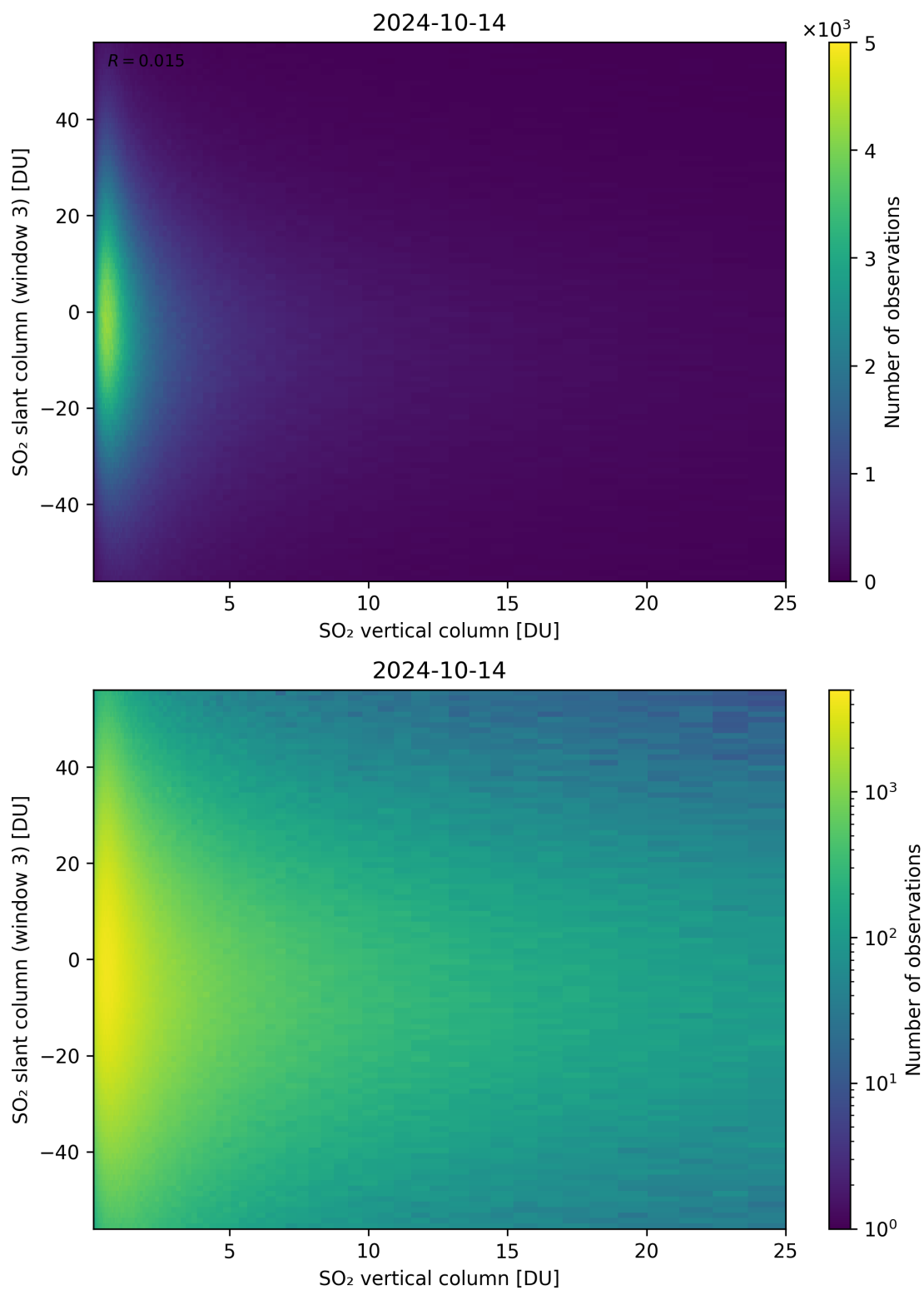
Figure 303: Scatter density plot of “SO 2 vertical column” against “SO 2 slant column (window 3)” for 2024-10-14 to 2024-10-15.
