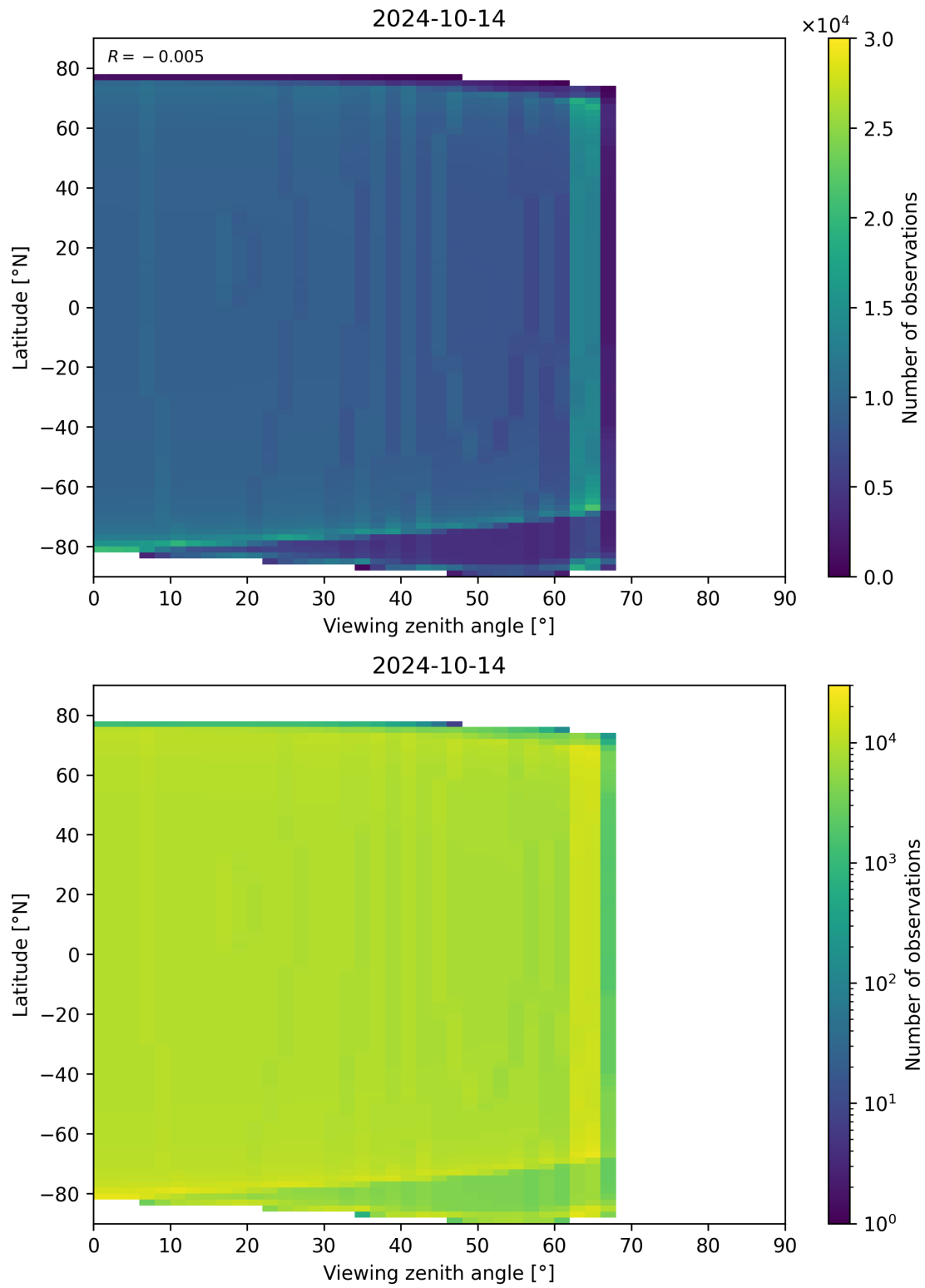
Figure 314: Scatter density plot of “Viewing zenith angle” against “Latitude” for 2024-10-14 to 2024-10-15.
