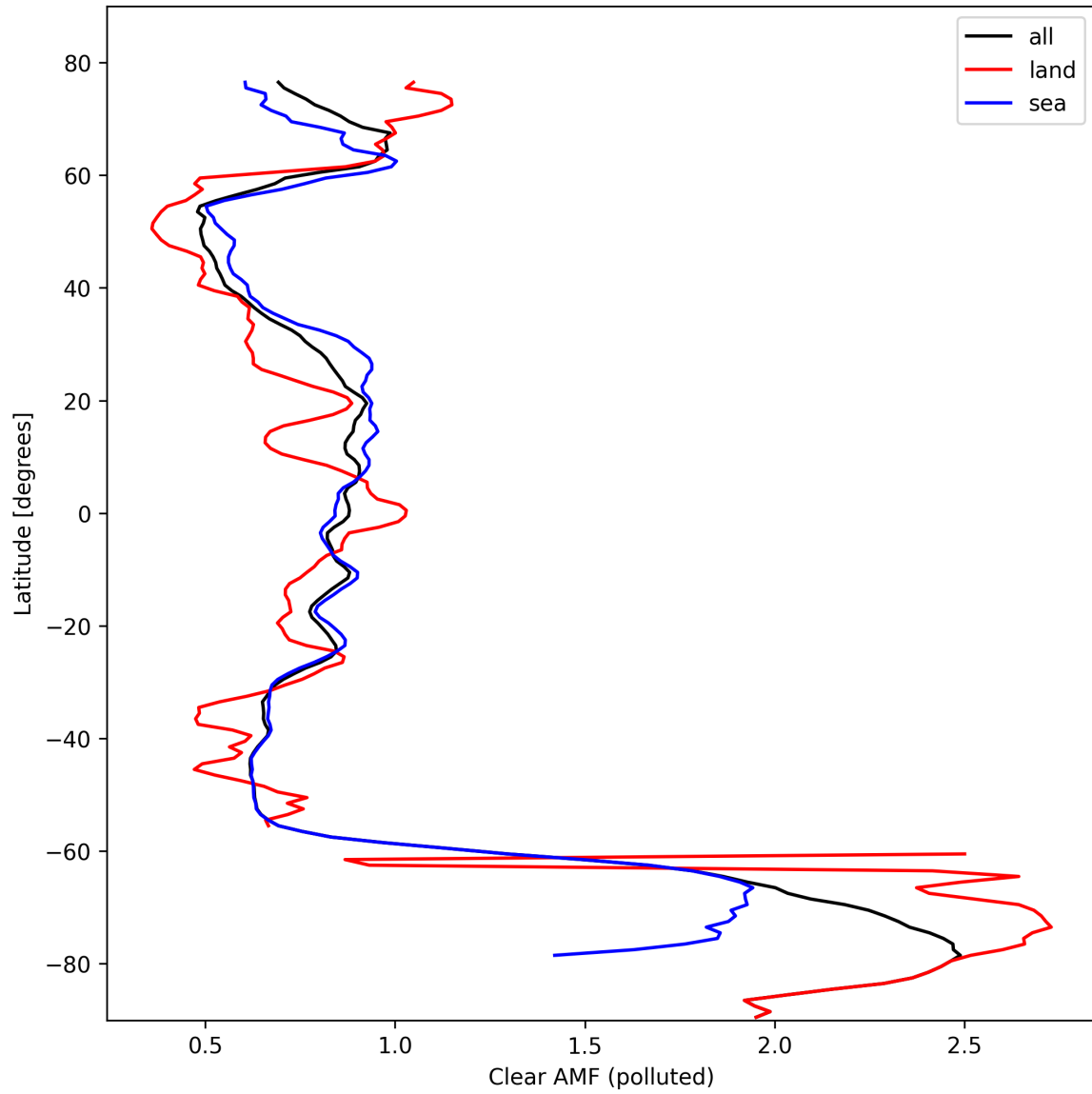
Figure 50: Zonal average of “Clear AMF (polluted)” for 2024-10-14 to 2024-10-15.
