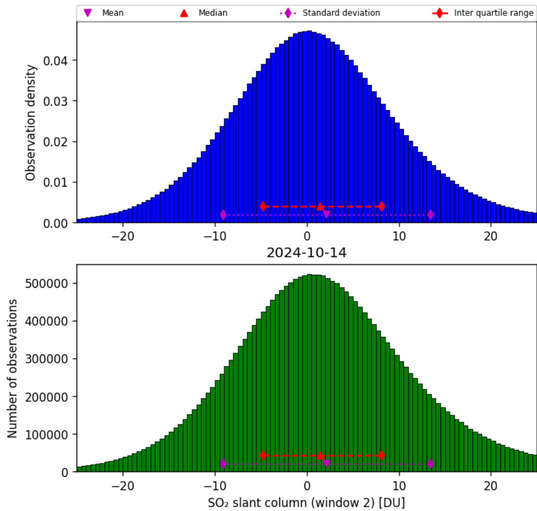
Figure 60: Histogram of “SO 2 slant column (window 2)” for 2024-10-14 to 2024-10-15
