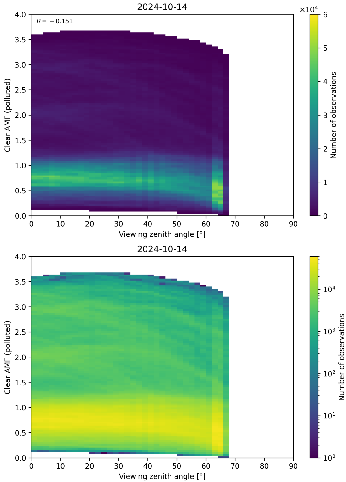
Figure 316: Scatter density plot of “Viewing zenith angle” against “Clear AMF (polluted)” for 2024-10-14 to 2024-10-15.
