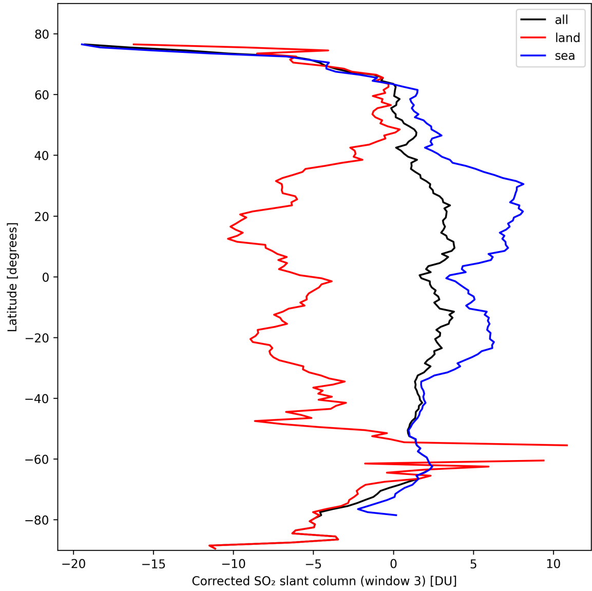
Figure 43: Zonal average of “Corrected SO 2 slant column (window 3)” for 2024-10-14 to 2024-10-15.
