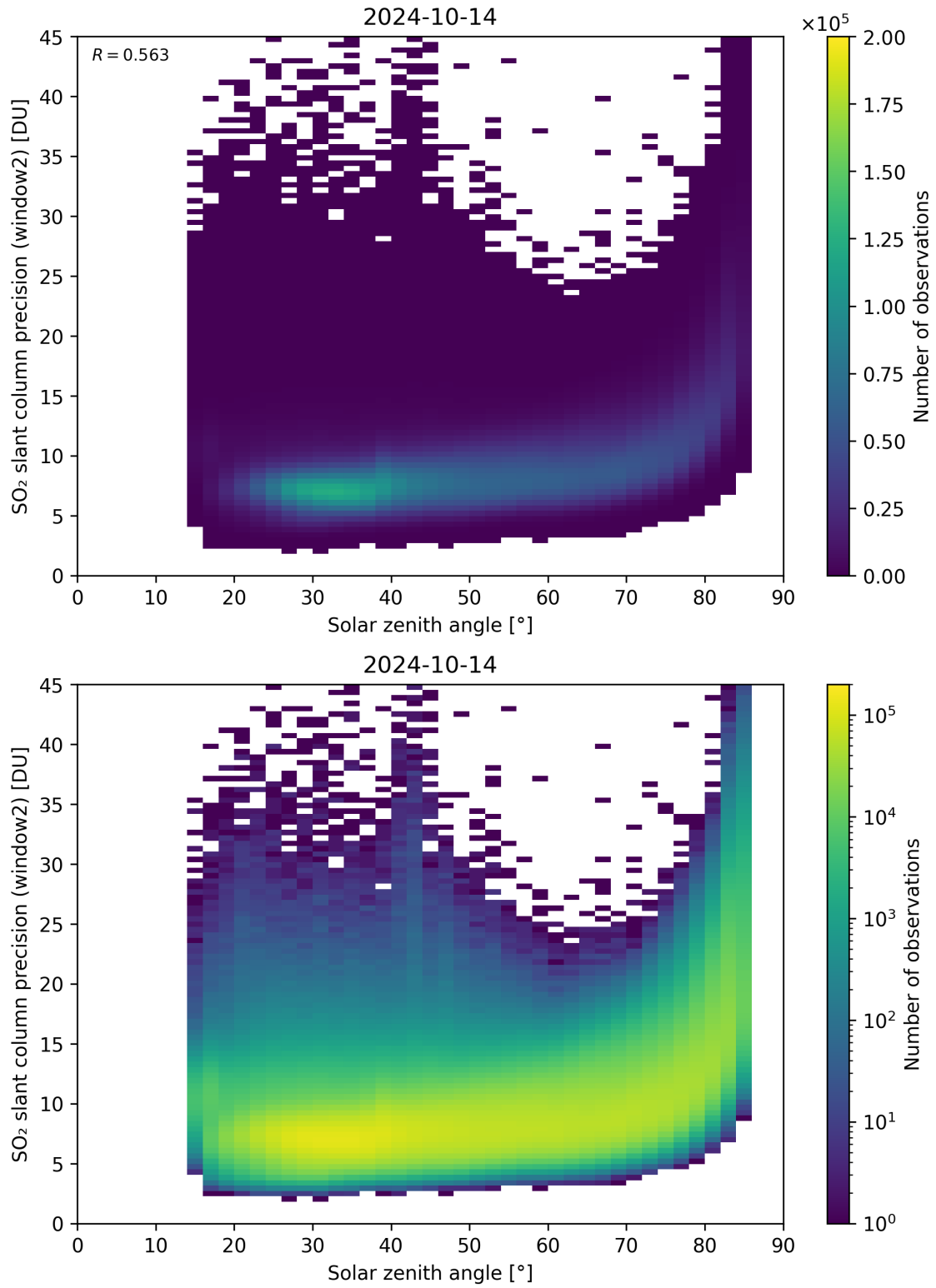
Figure 171: Scatter density plot of “Solar zenith angle” against “SO 2 slant column precision (window2)” for 2024-10-14 to 2024-10-15.
