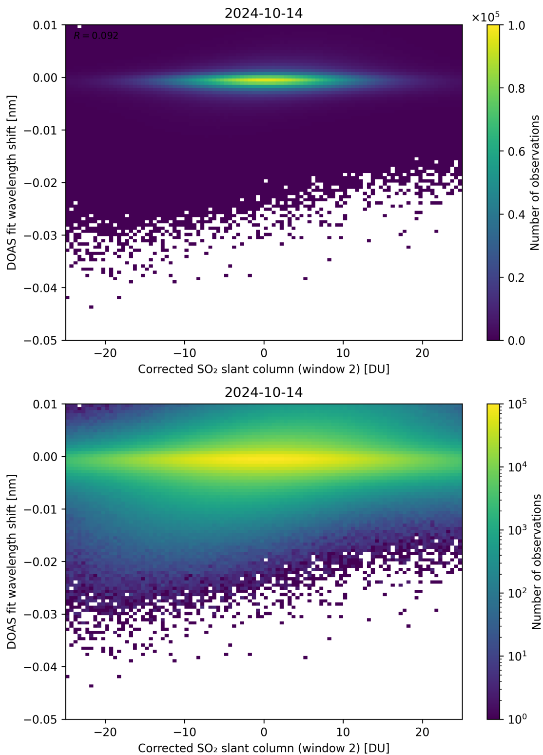
Figure 196: Scatter density plot of “Corrected SO 2 slant column (window 2)” against “DOAS fit wavelength shift” for 2024-10-14 to 2024-10-15.
