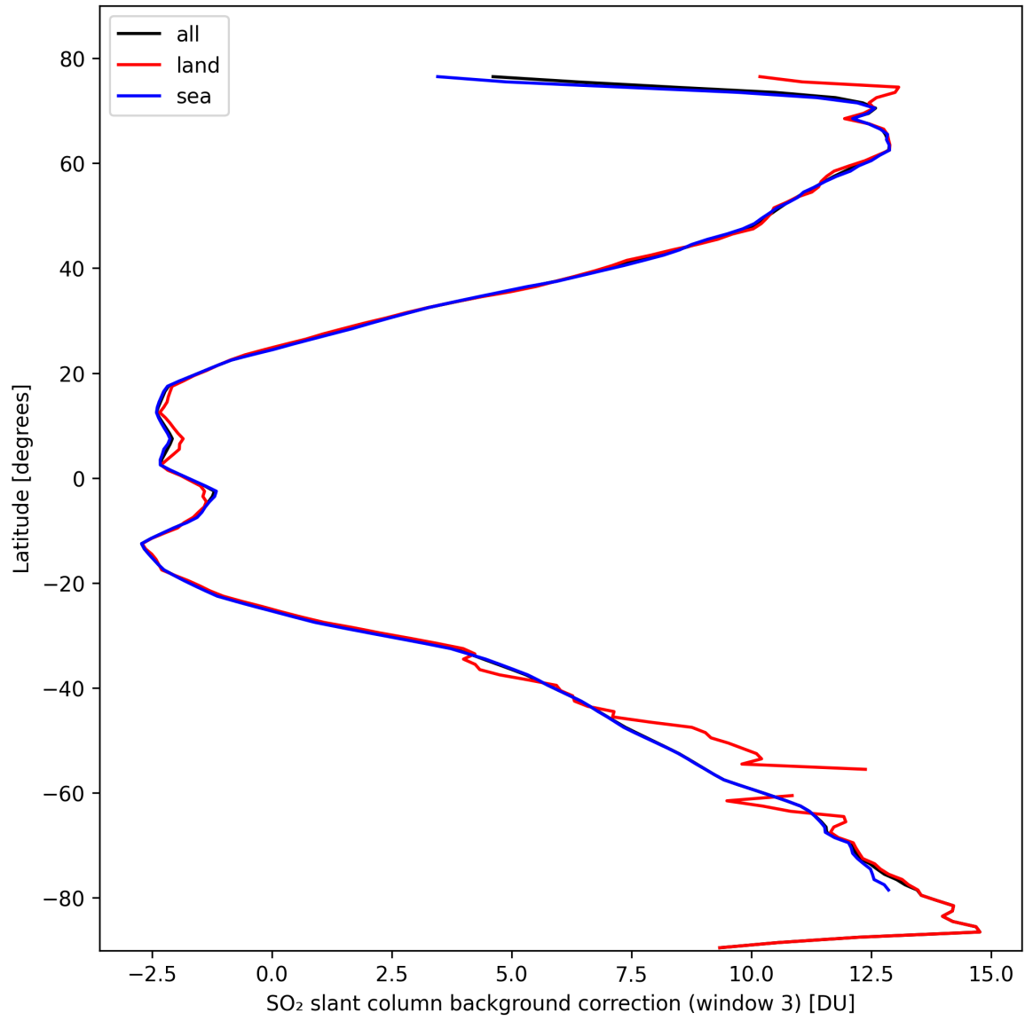
Figure 44: Zonal average of “SO 2 slant column background correction (window 3)” for 2024-10-14 to 2024-10-15.
