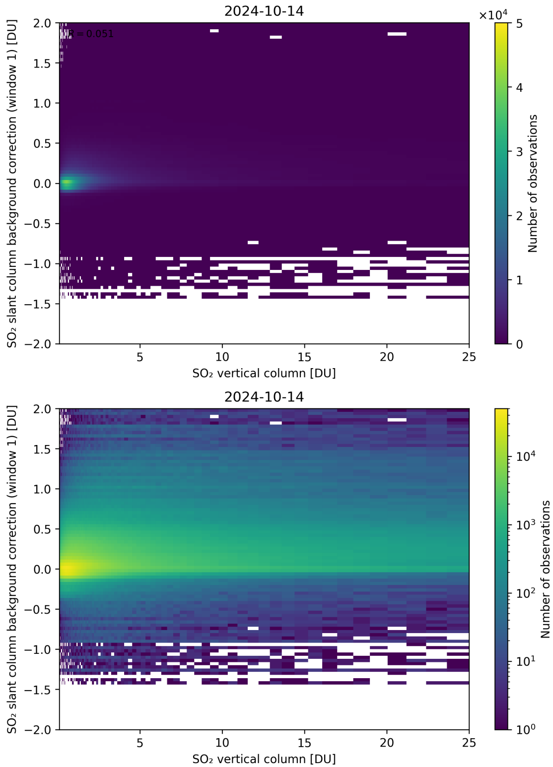
Figure 273: Scatter density plot of “SO 2 vertical column” against “SO 2 slant column background correction (window 1)” for 2024-10-14 to 2024-10-15.
