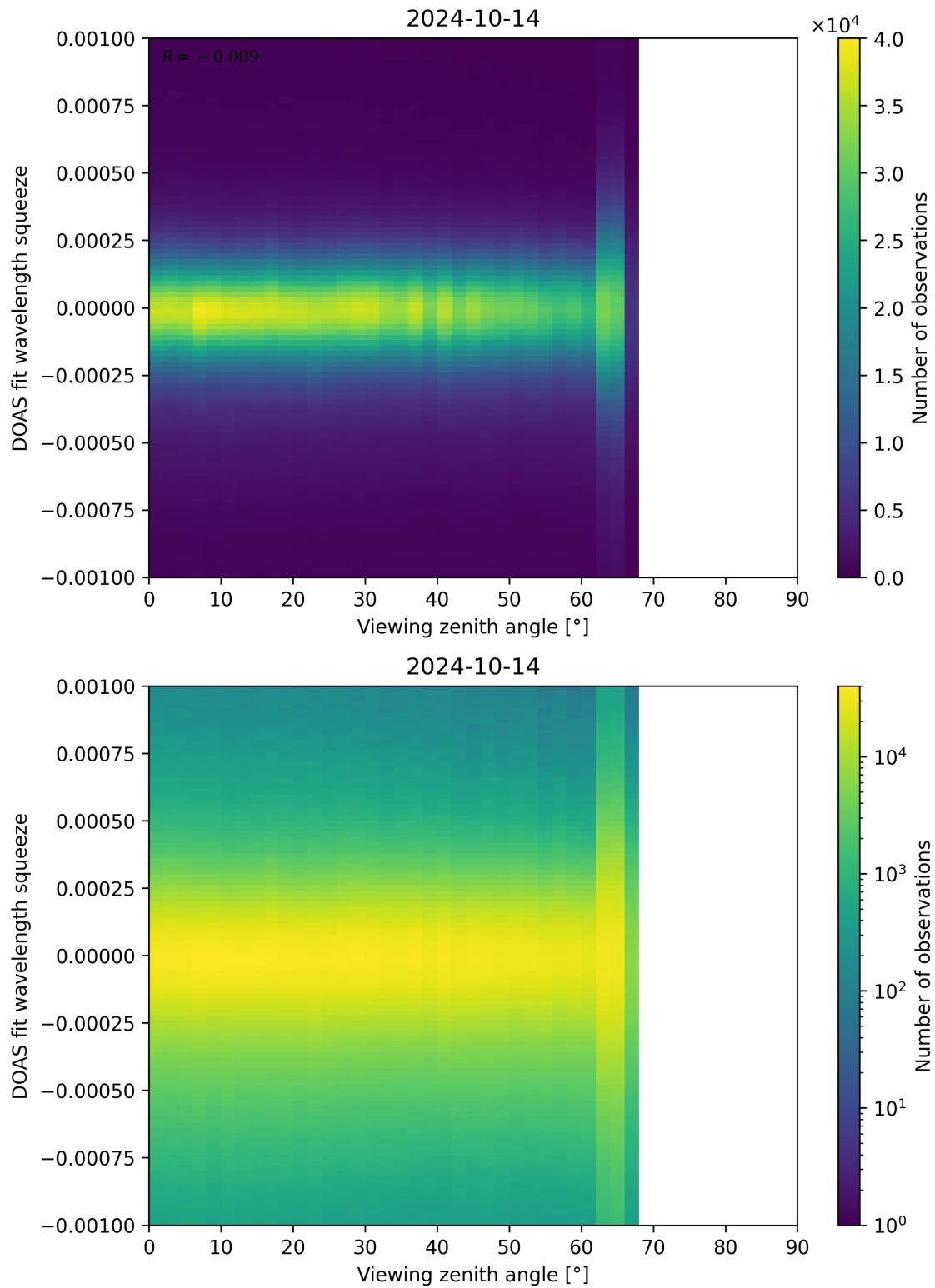
Figure 312: Scatter density plot of “Viewing zenith angle” against “DOAS fit wavelength squeeze” for 2024-10-14 to 2024-10-15.
