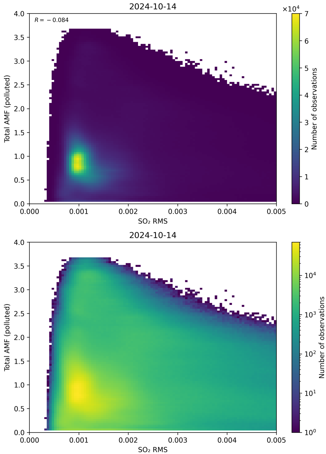
Figure 137: Scatter density plot of “SO 2 RMS” against “Total AMF (polluted)” for 2024-10-14 to 2024-10-15.
