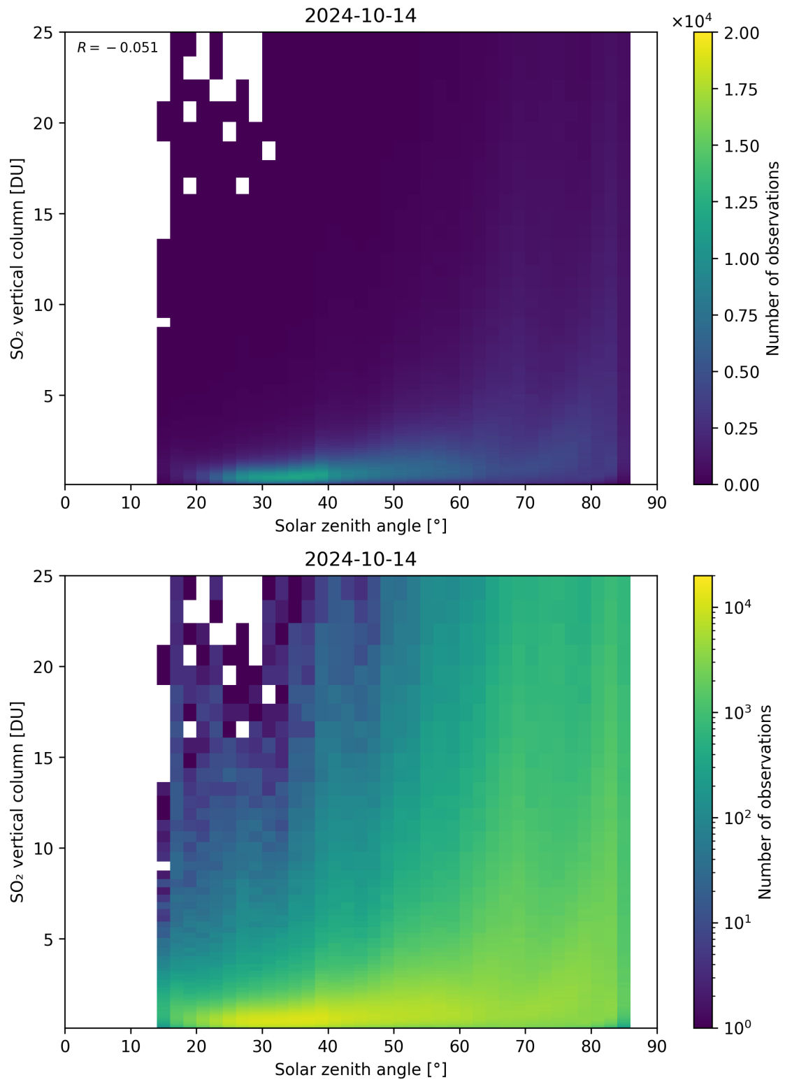
Figure 176: Scatter density plot of “Solar zenith angle” against “SO 2 vertical column” for 2024-10-14 to 2024-10-15.
