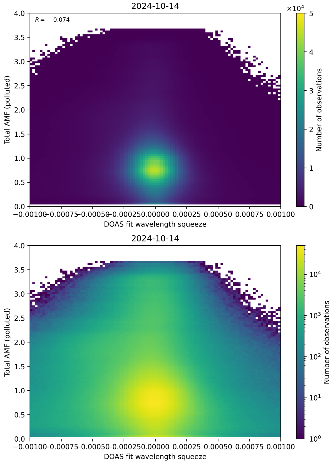
Figure 134: Scatter density plot of “DOAS fit wavelength squeeze” against “Total AMF (polluted)” for 2024-10-14 to 2024-10-15.
