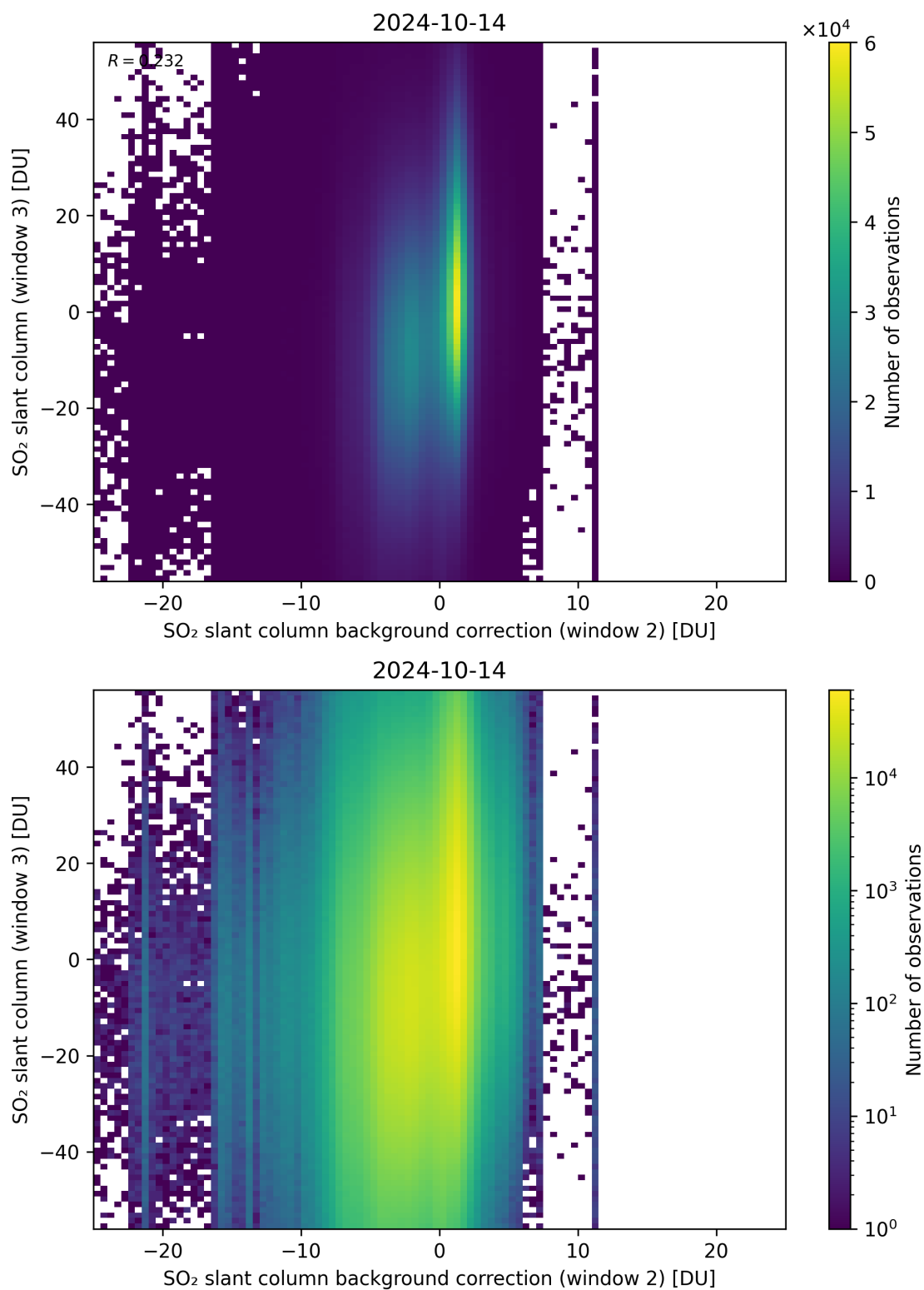
Figure 117: Scatter density plot of “SO 2 slant column background correction (window 2)” against “SO 2 slant column (window 3)” for 2024-10-14 to 2024-10-15.
