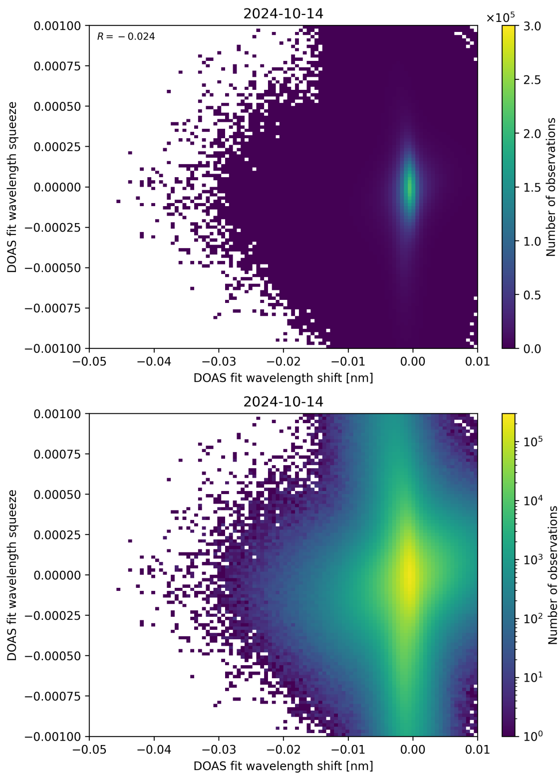
Figure 127: Scatter density plot of “DOAS fit wavelength shift” against “DOAS fit wavelength squeeze” for 2024-10-14 to 2024-10-15.
