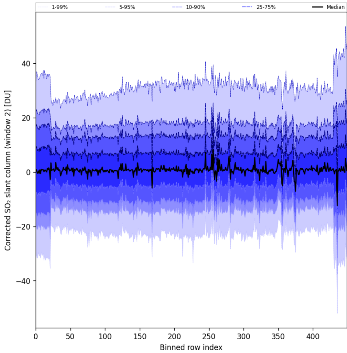
Figure 85: Along track statistics of “Corrected SO 2 slant column (window 2)” for 2024-10-14 to 2024-10-15
