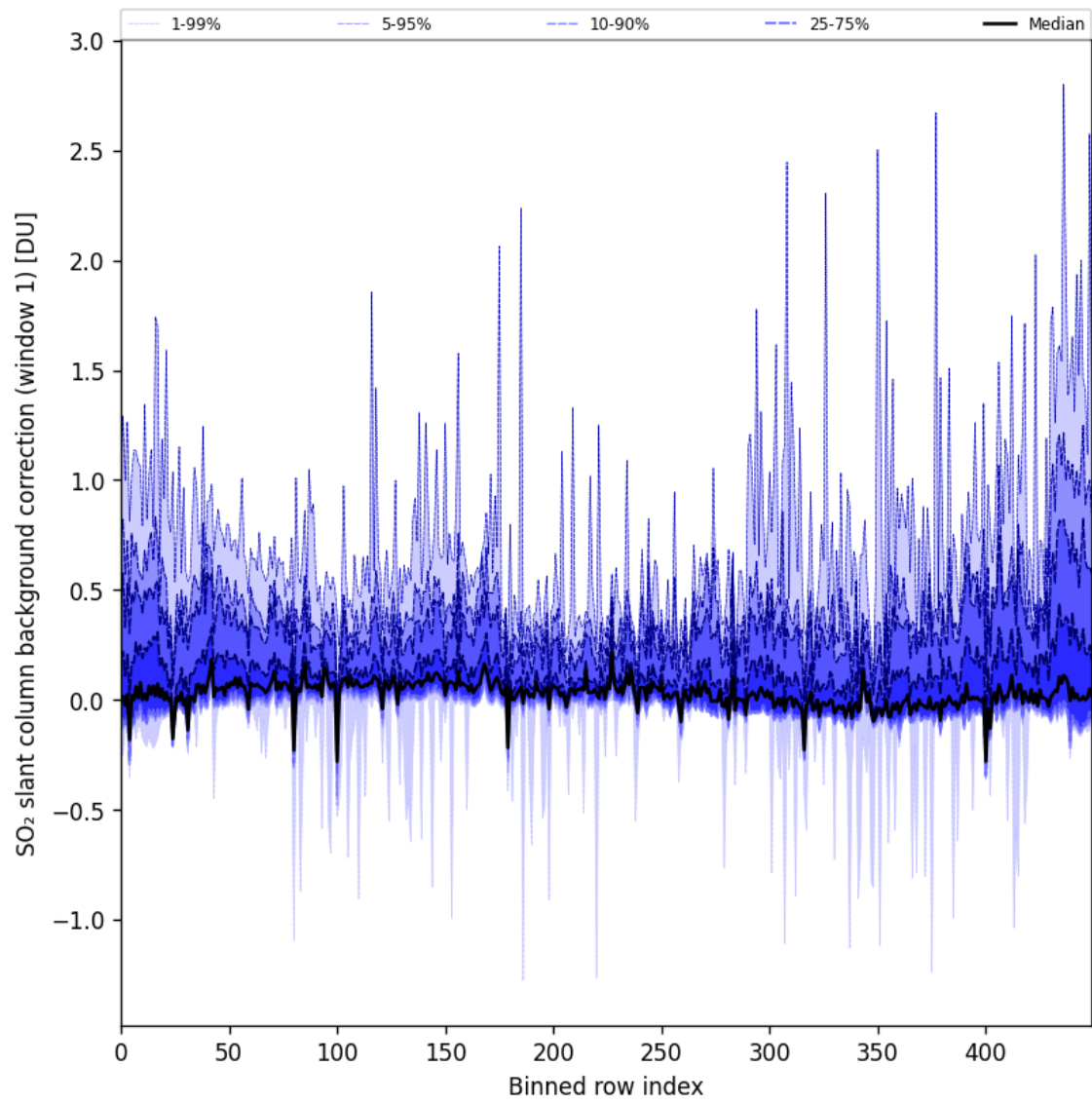
Figure 82: Along track statistics of “SO 2 slant column background correction (window 1)” for 2024-10-14 to 2024-10-15
