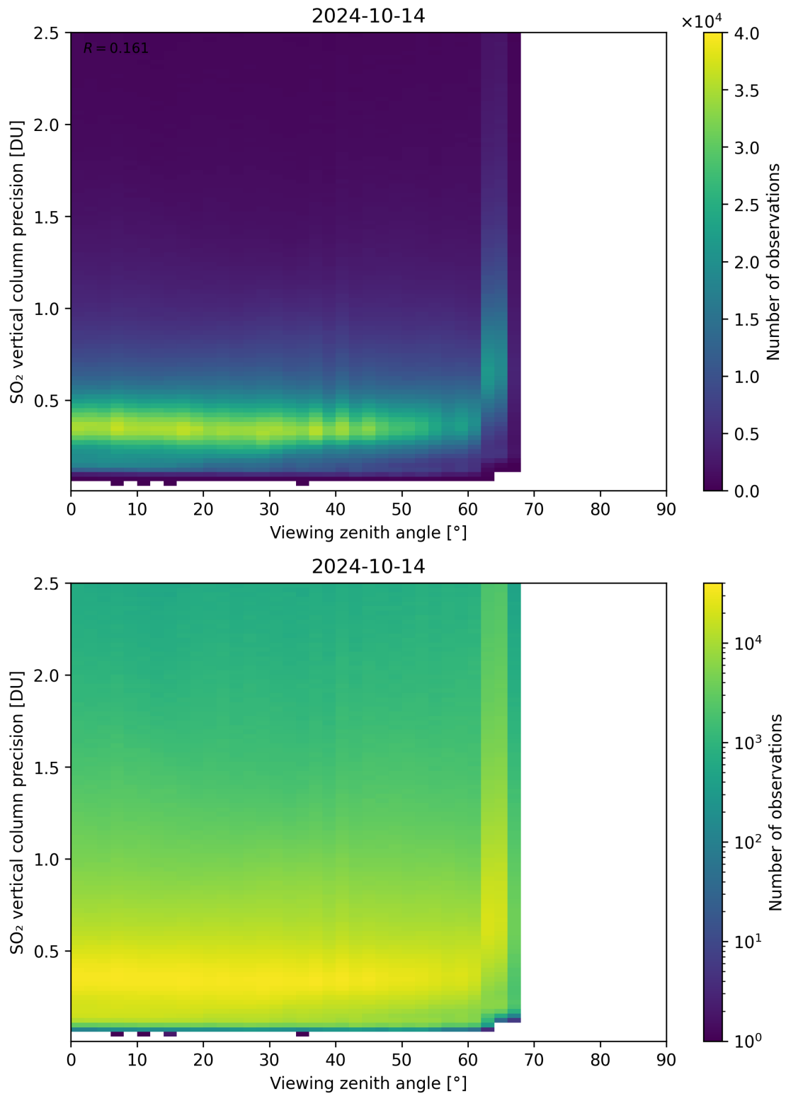
Figure 328: Scatter density plot of “Viewing zenith angle” against “SO 2 vertical column precision” for 2024-10-14 to 2024-10-15.
