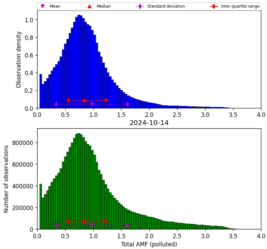
Figure 71: Histogram of “Total AMF (polluted)” for 2024-10-14 to 2024-10-15
