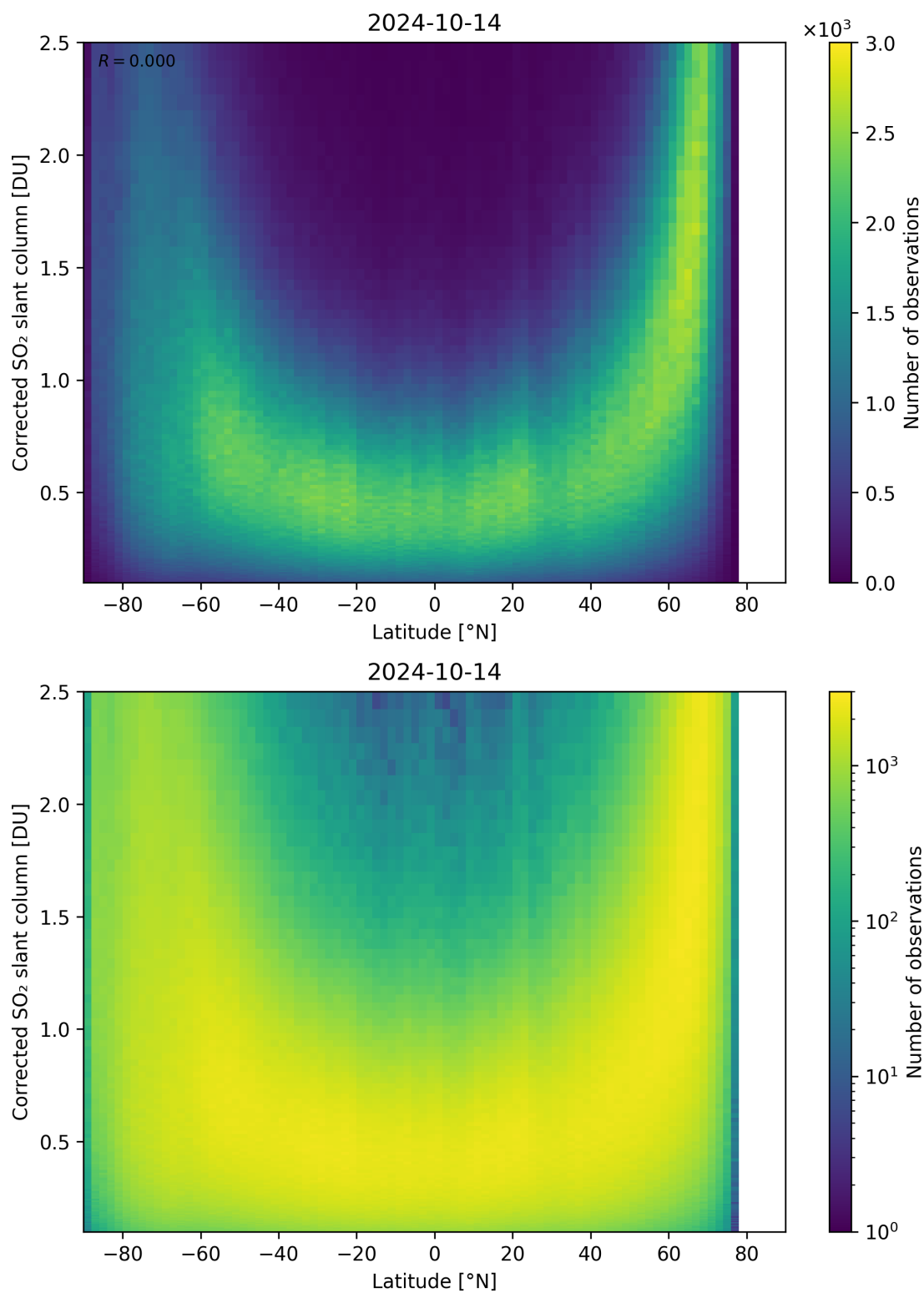
Figure 146: Scatter density plot of “Latitude” against “Corrected SO 2 slant column” for 2024-10-14 to 2024-10-15.
