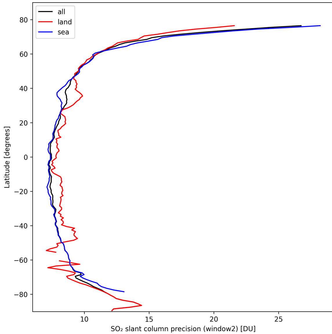
Figure 38: Zonal average of “SO 2 slant column precision (window2)” for 2024-10-14 to 2024-10-15.
