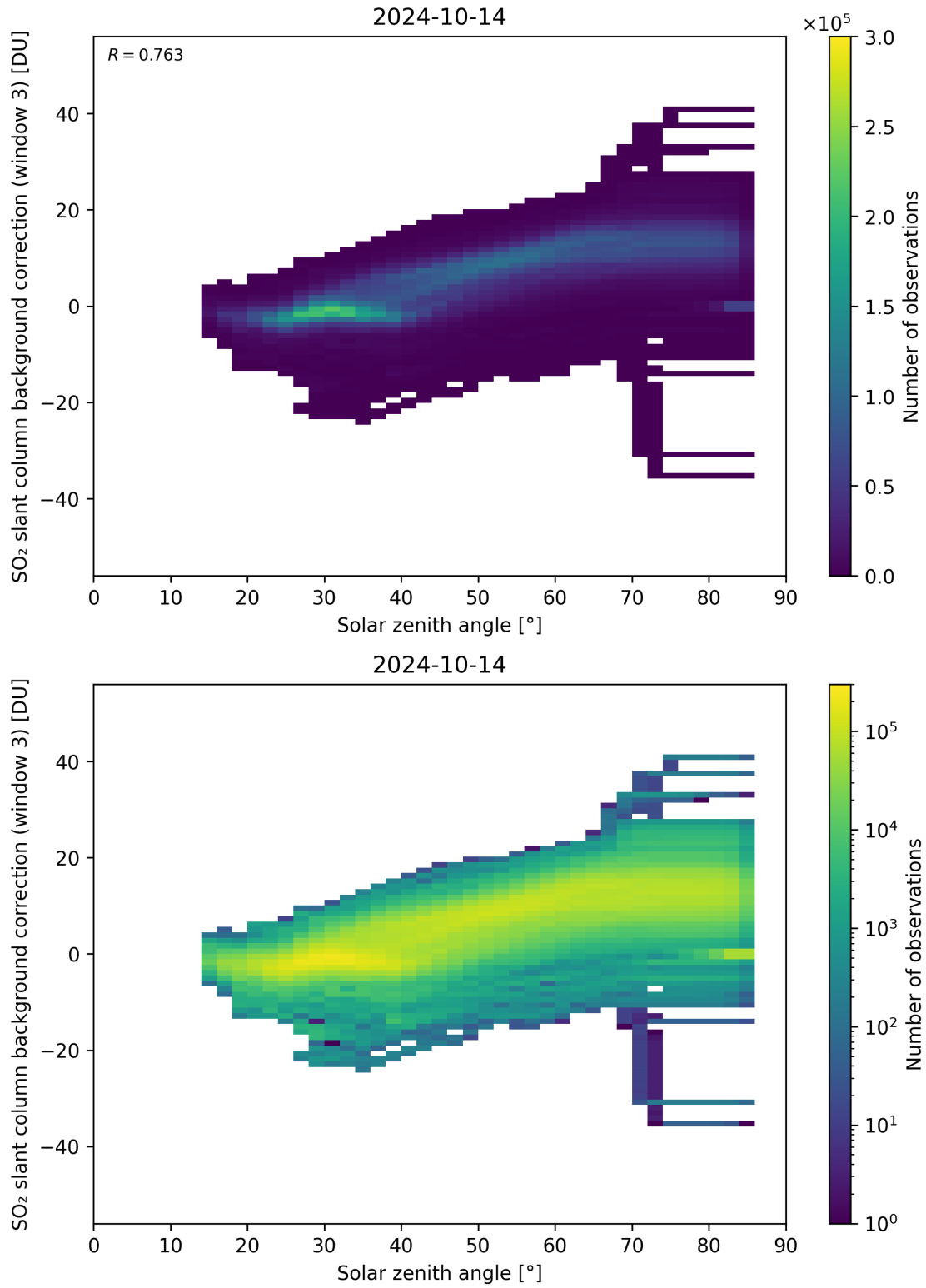
Figure 160: Scatter density plot of “Solar zenith angle” against “SO 2 slant column background correction (window 3)” for 2024-10-14 to 2024-10-15.
