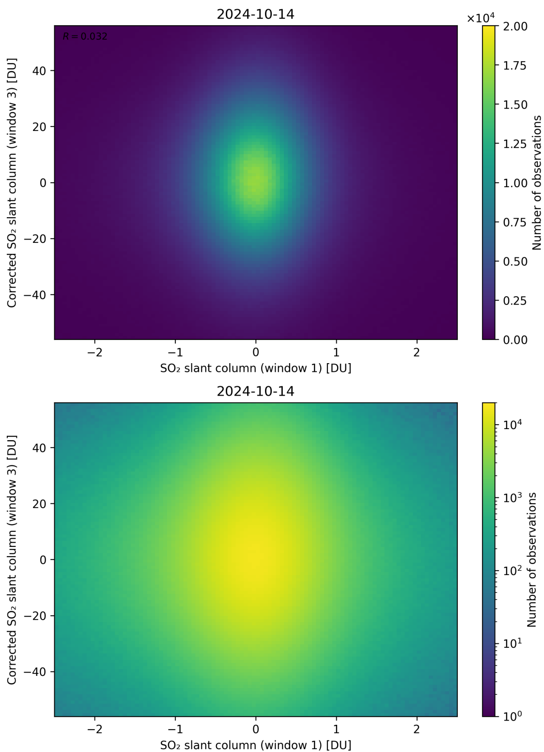
Figure 234: Scatter density plot of “SO 2 slant column (window 1)” against “Corrected SO 2 slant column (window 3)” for 2024-10-14 to 2024-10-15.
