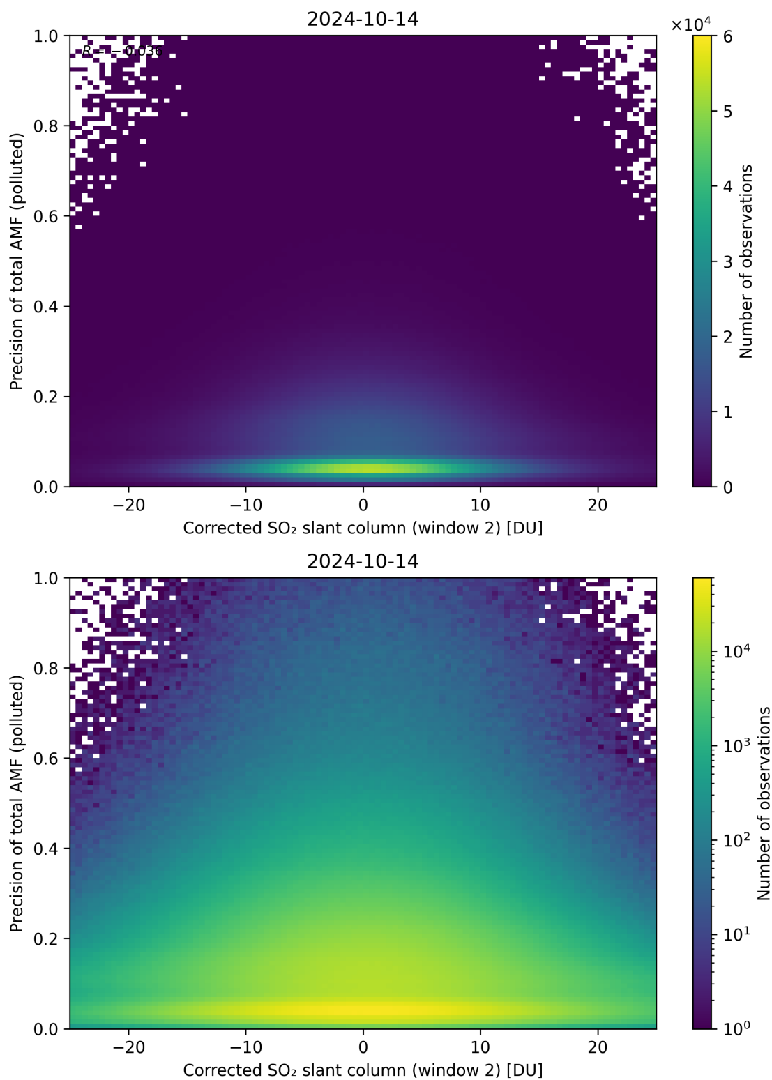
Figure 204: Scatter density plot of “Corrected SO 2 slant column (window 2)” against “Precision of total AMF (polluted)” for 2024-10-14 to 2024-10-15.
