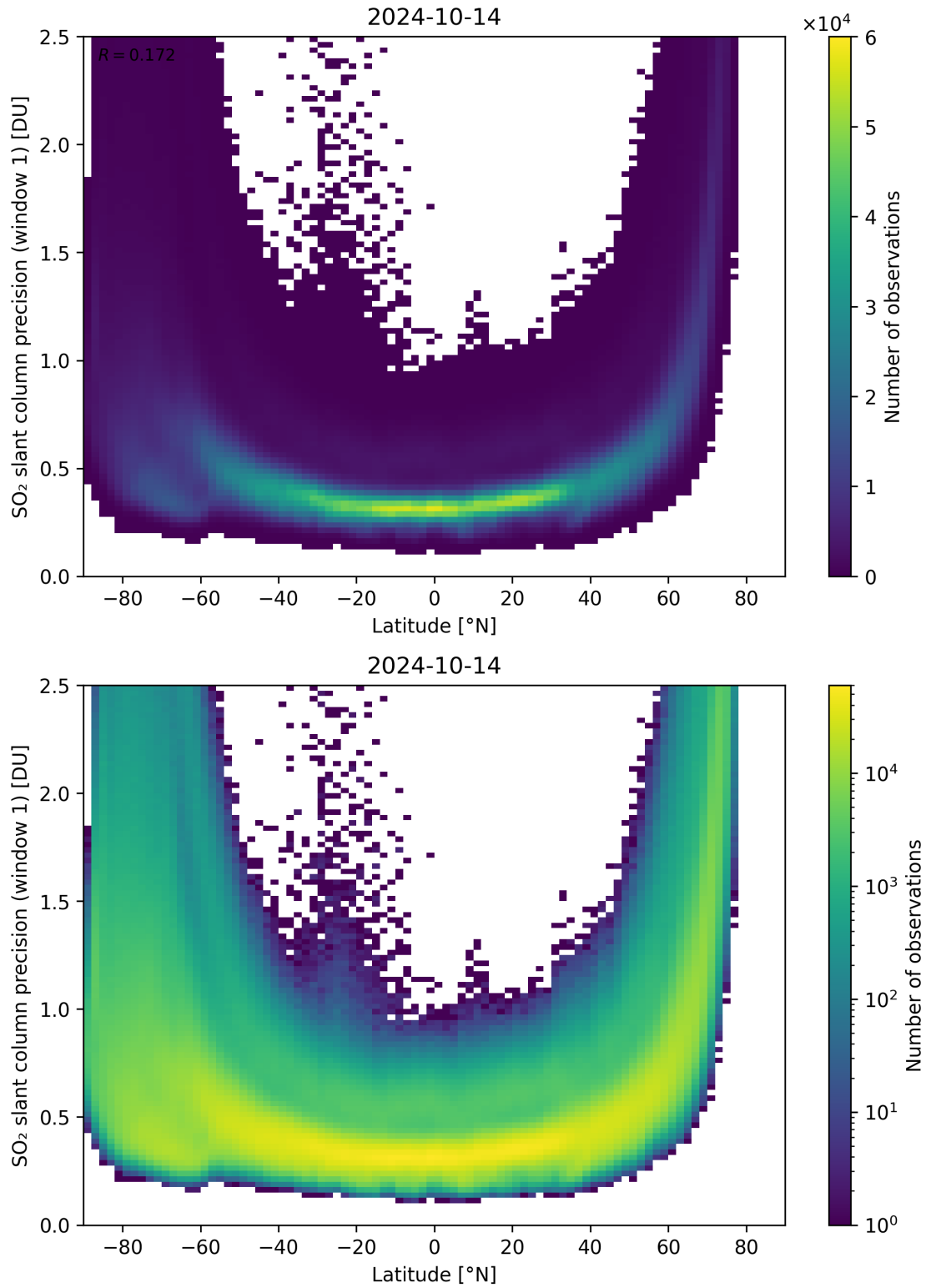
Figure 150: Scatter density plot of “Latitude” against “SO 2 slant column precision (window 1)” for 2024-10-14 to 2024-10-15.
