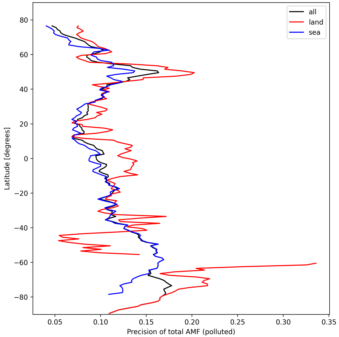
Figure 49: Zonal average of “Precision of total AMF (polluted)” for 2024-10-14 to 2024-10-15.
