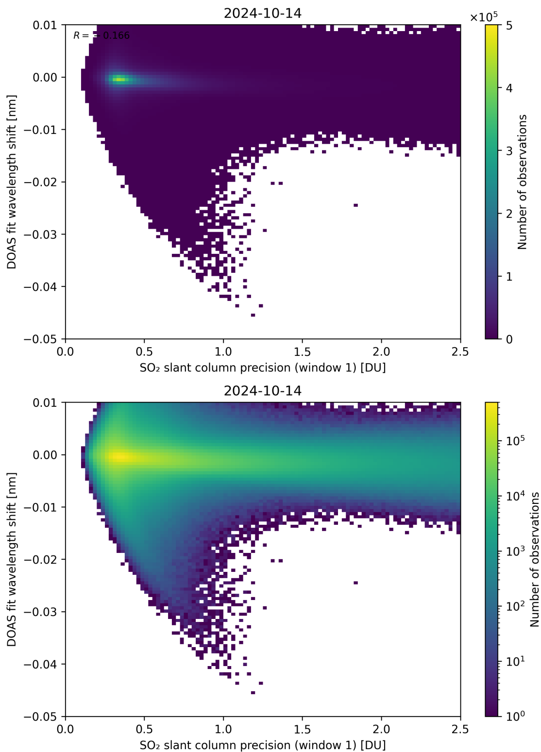
Figure 221: Scatter density plot of “SO 2 slant column precision (window 1)” against “DOAS fit wavelength shift” for 2024-10-14 to 2024-10-15.
