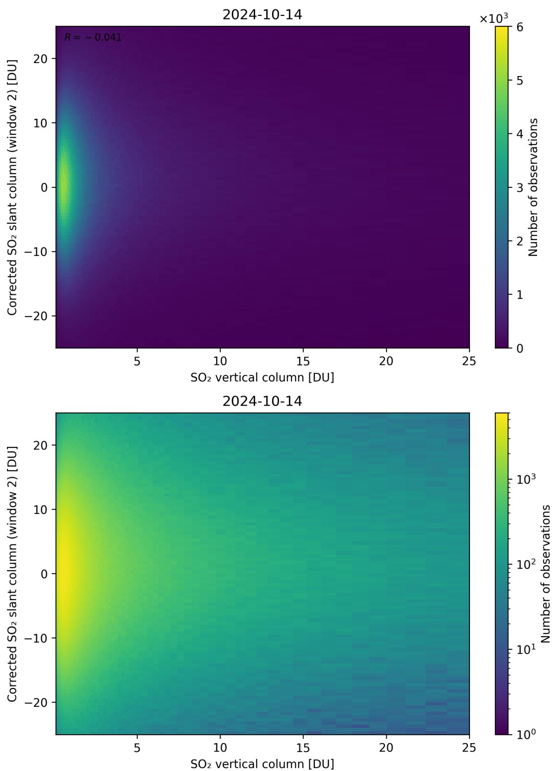
Figure 298: Scatter density plot of “SO 2 vertical column” against “Corrected SO 2 slant column (window 2)” for 2024-10-14 to 2024-10-15.
