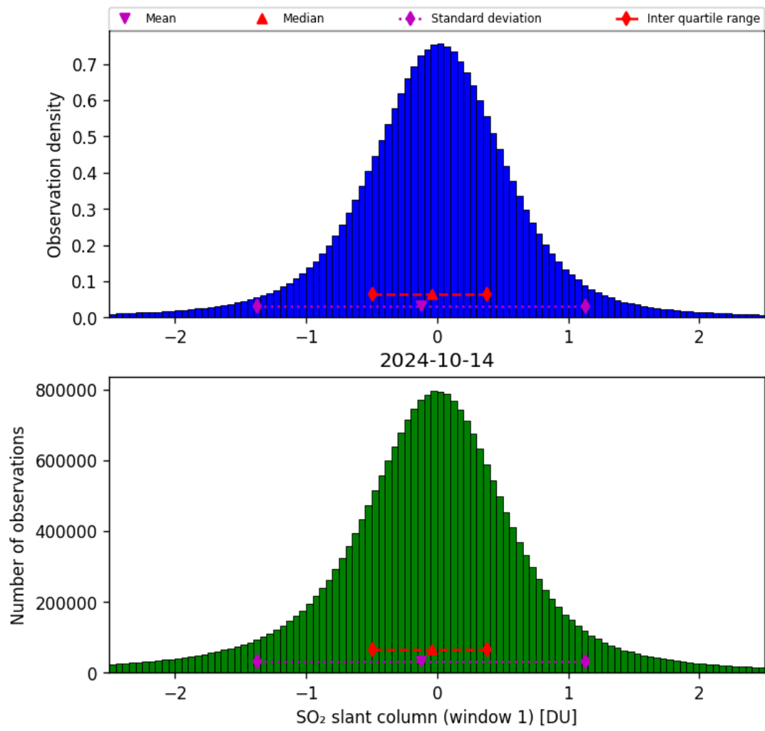
Figure 56: Histogram of “SO 2 slant column (window 1)” for 2024-10-14 to 2024-10-15
