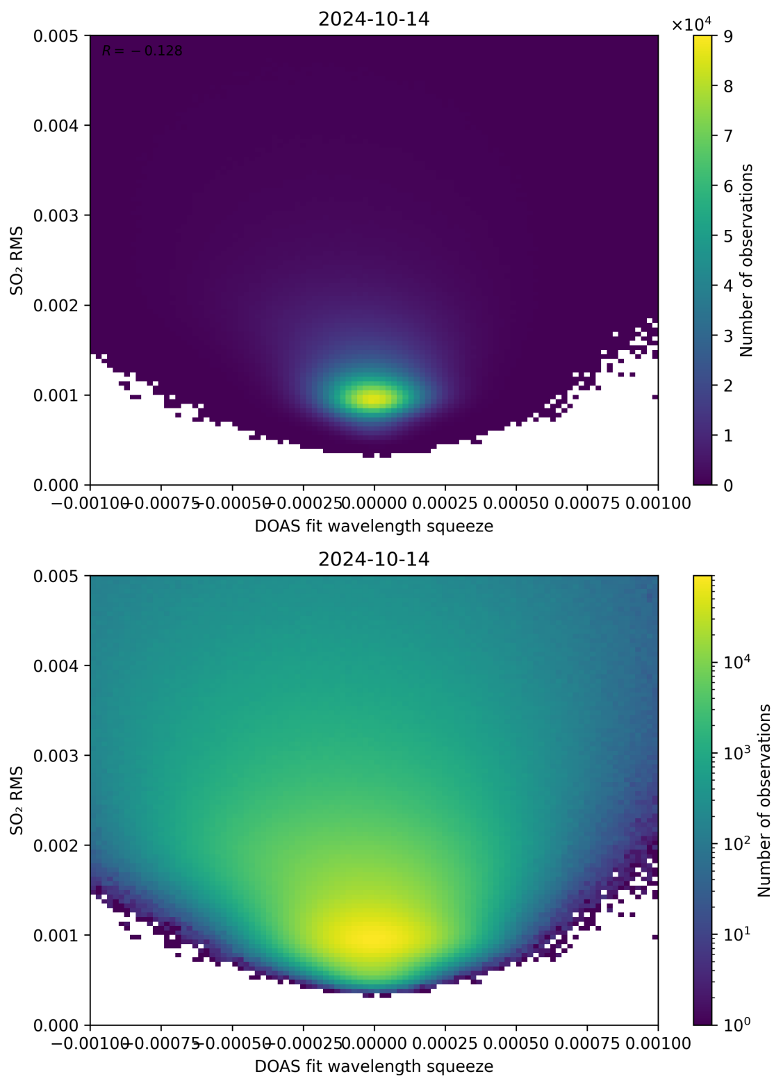
Figure 132: Scatter density plot of “DOAS fit wavelength squeeze” against “SO 2 RMS” for 2024-10-14 to 2024-10-15.
