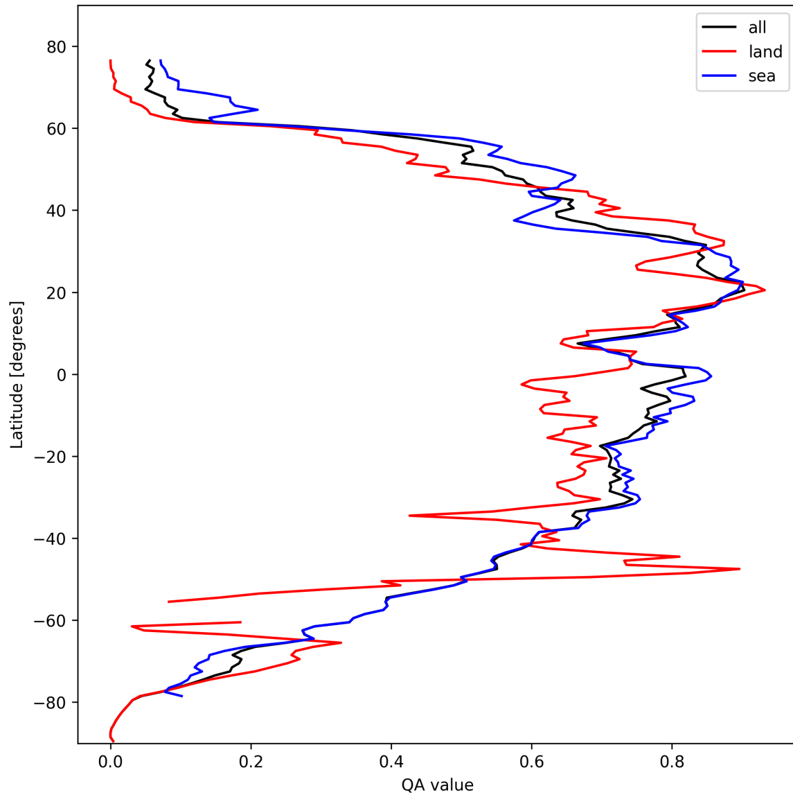
Figure 29: Zonal average of “QA value” for 2024-10-14 to 2024-10-15.
