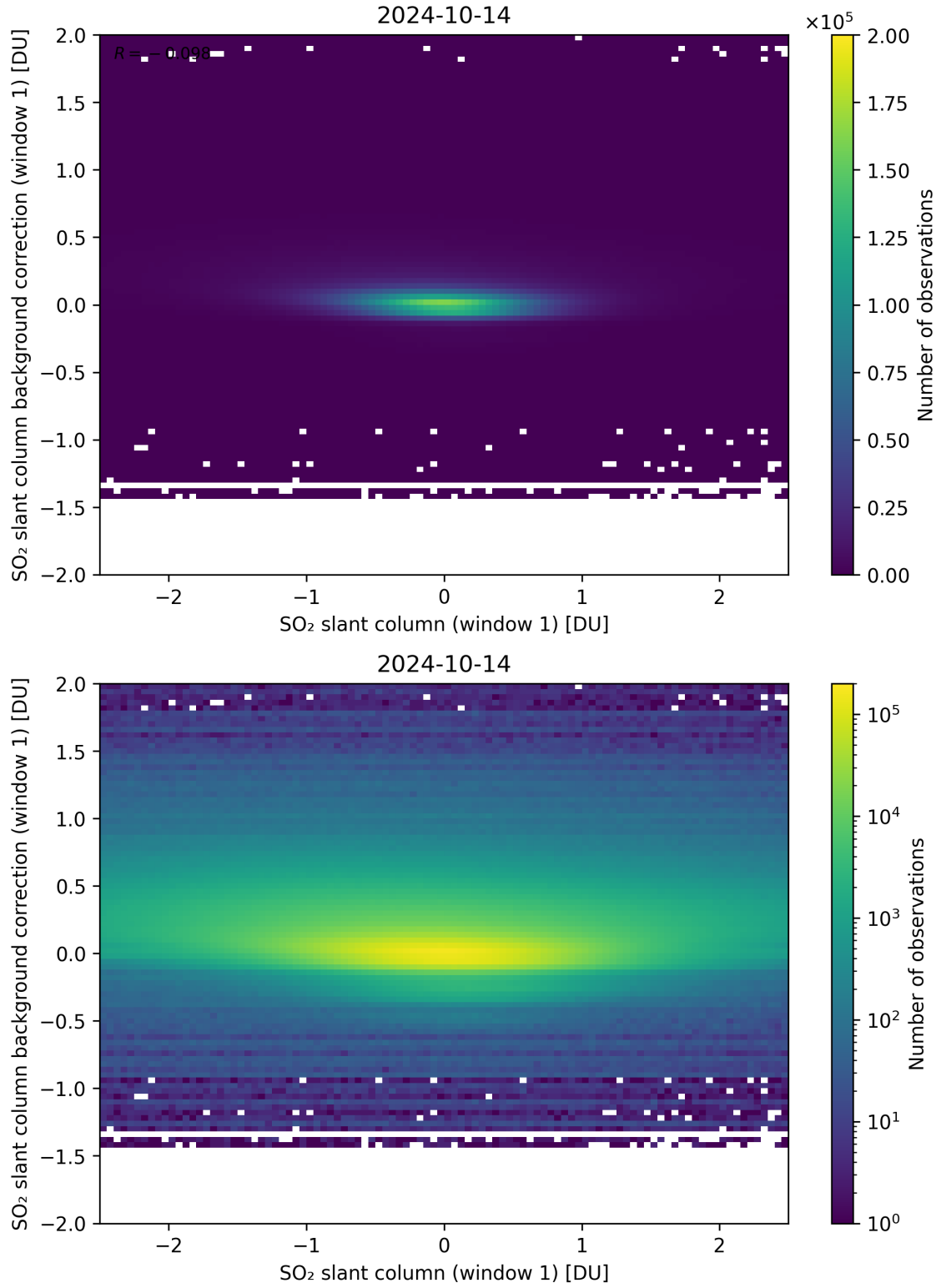
Figure 212: Scatter density plot of “SO 2 slant column (window 1)” against “SO 2 slant column background correction (window 1)” for 2024-10-14 to 2024-10-15.
