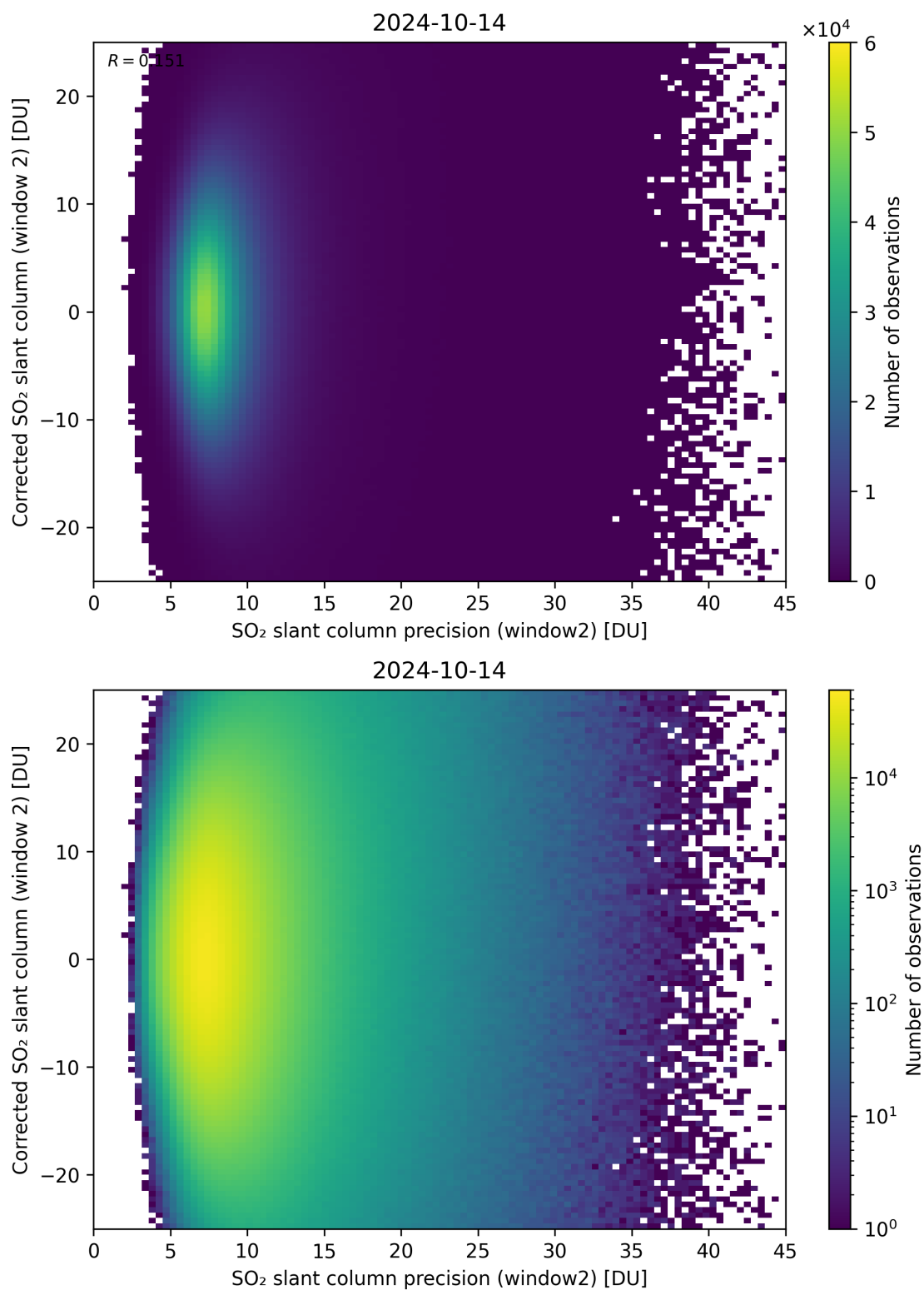
Figure 247: Scatter density plot of “SO 2 slant column precision (window2)” against “Corrected SO 2 slant column (window 2)” for 2024-10-14 to 2024-10-15.
