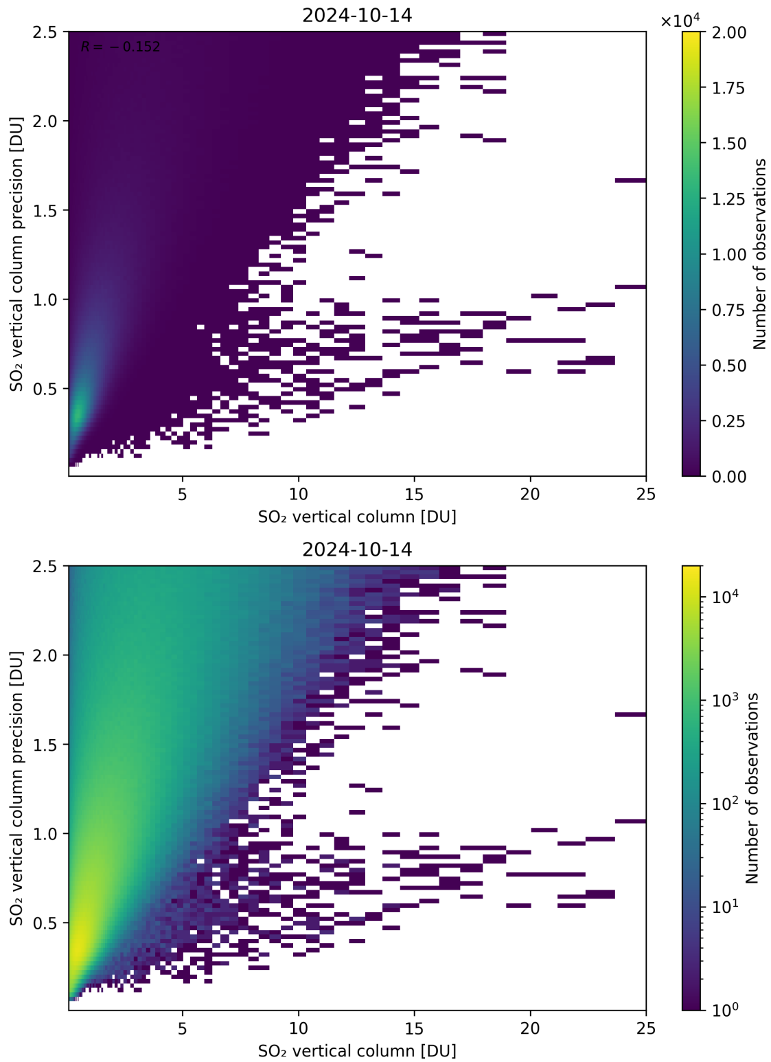
Figure 307: Scatter density plot of “SO 2 vertical column” against “SO 2 vertical column precision” for 2024-10-14 to 2024-10-15.
