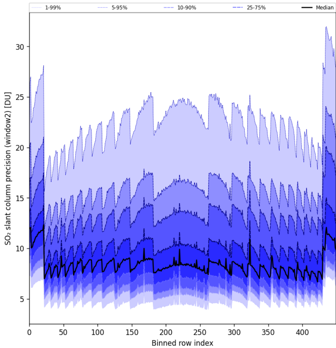
Figure 84: Along track statistics of “SO 2 slant column precision (window2)” for 2024-10-14 to 2024-10-15
