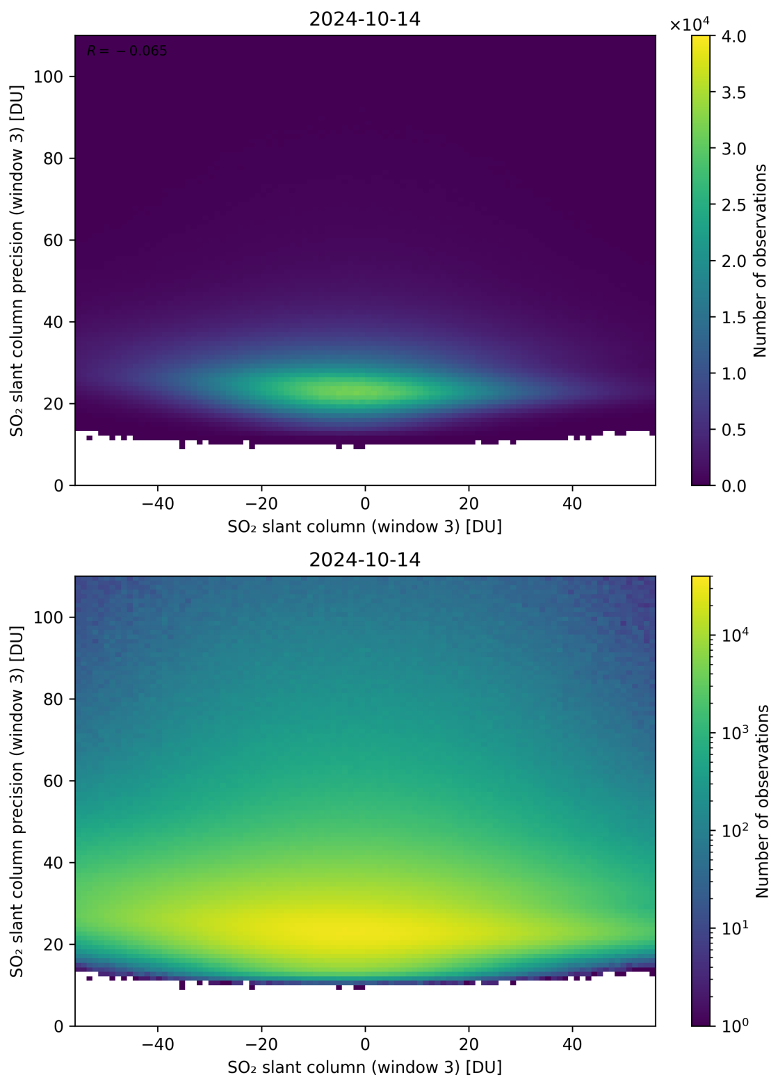
Figure 267: Scatter density plot of “SO 2 slant column (window 3)” against “SO 2 slant column precision (window 3)” for 2024-10-14 to 2024-10-15.
