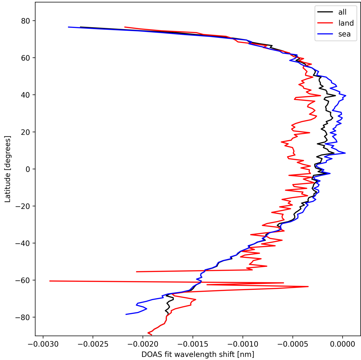
Figure 45: Zonal average of “DOAS fit wavelength shift” for 2024-10-14 to 2024-10-15.
