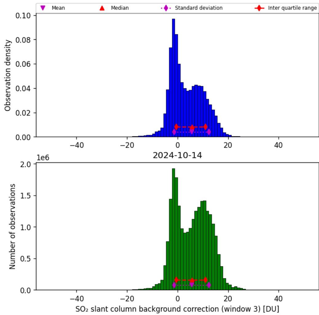
Figure 67: Histogram of “SO 2 slant column background correction (window 3)” for 2024-10-14 to 2024-10-15
