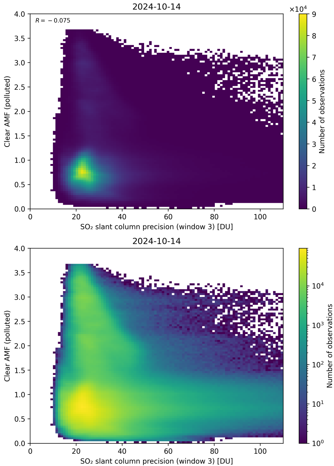
Figure 261: Scatter density plot of “SO 2 slant column precision (window 3)” against “Clear AMF (polluted)” for 2024-10-14 to 2024-10-15.
