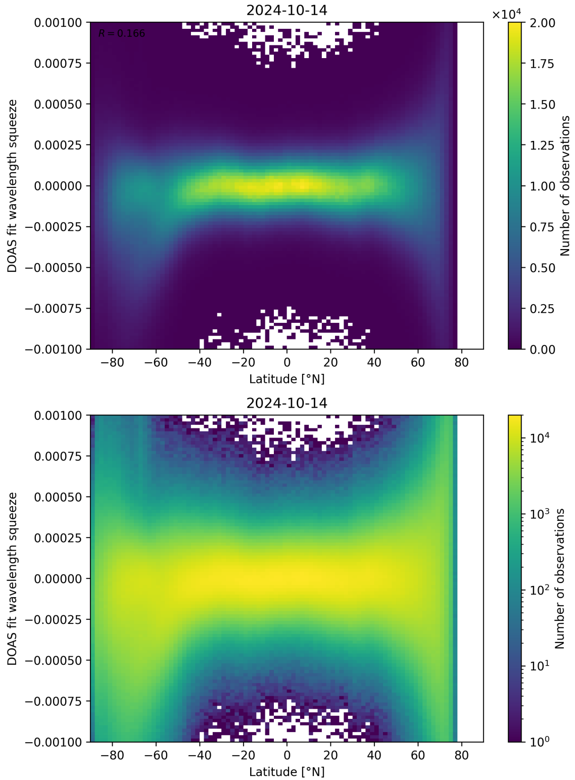
Figure 143: Scatter density plot of “Latitude” against “DOAS fit wavelength squeeze” for 2024-10-14 to 2024-10-15.
