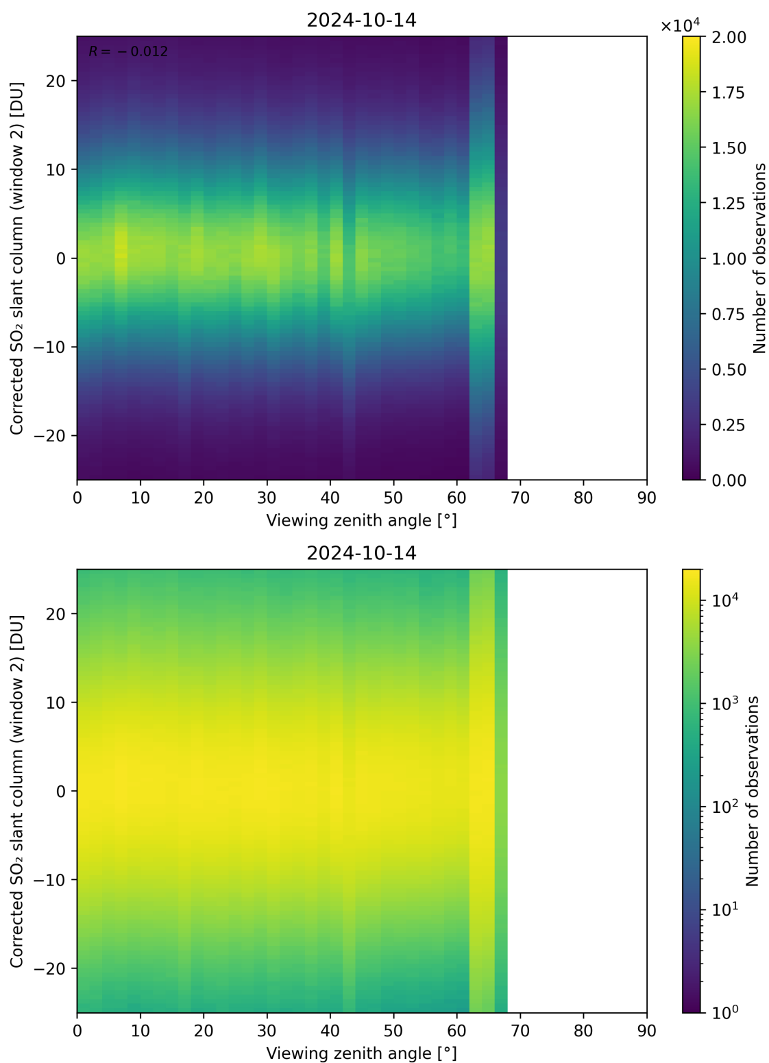
Figure 318: Scatter density plot of “Viewing zenith angle” against “Corrected SO 2 slant column (window 2)” for 2024-10-14 to 2024-10-15.
