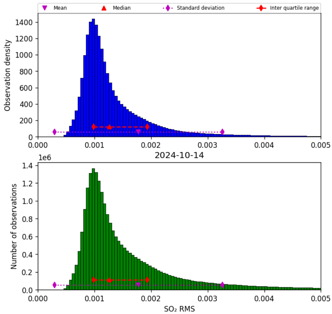
Figure 70: Histogram of "SO 2 RMS" for 2024-10-14 to 2024-10-15
