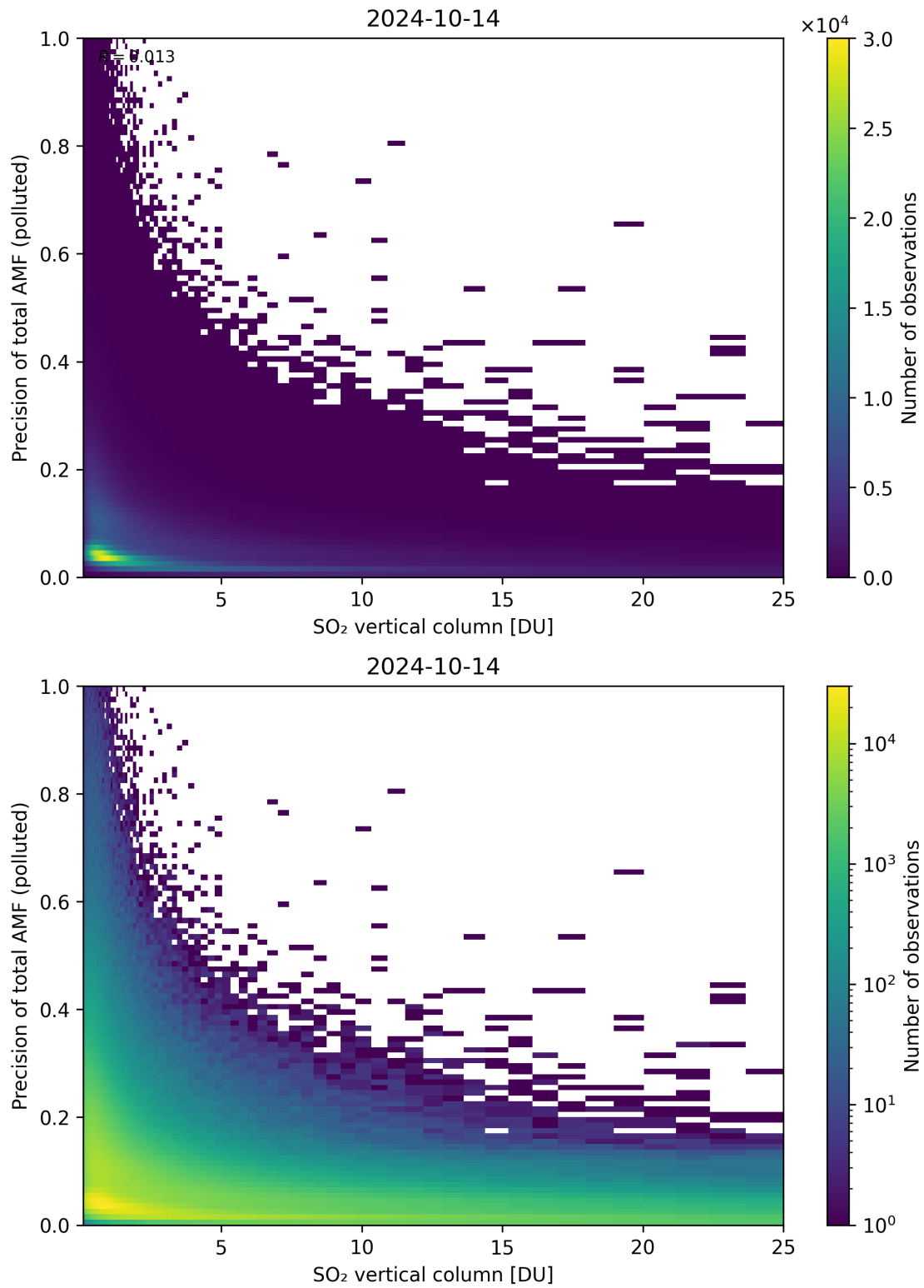
Figure 306: Scatter density plot of “SO 2 vertical column” against “Precision of total AMF (polluted)” for 2024-10-14 to 2024-10-15.
