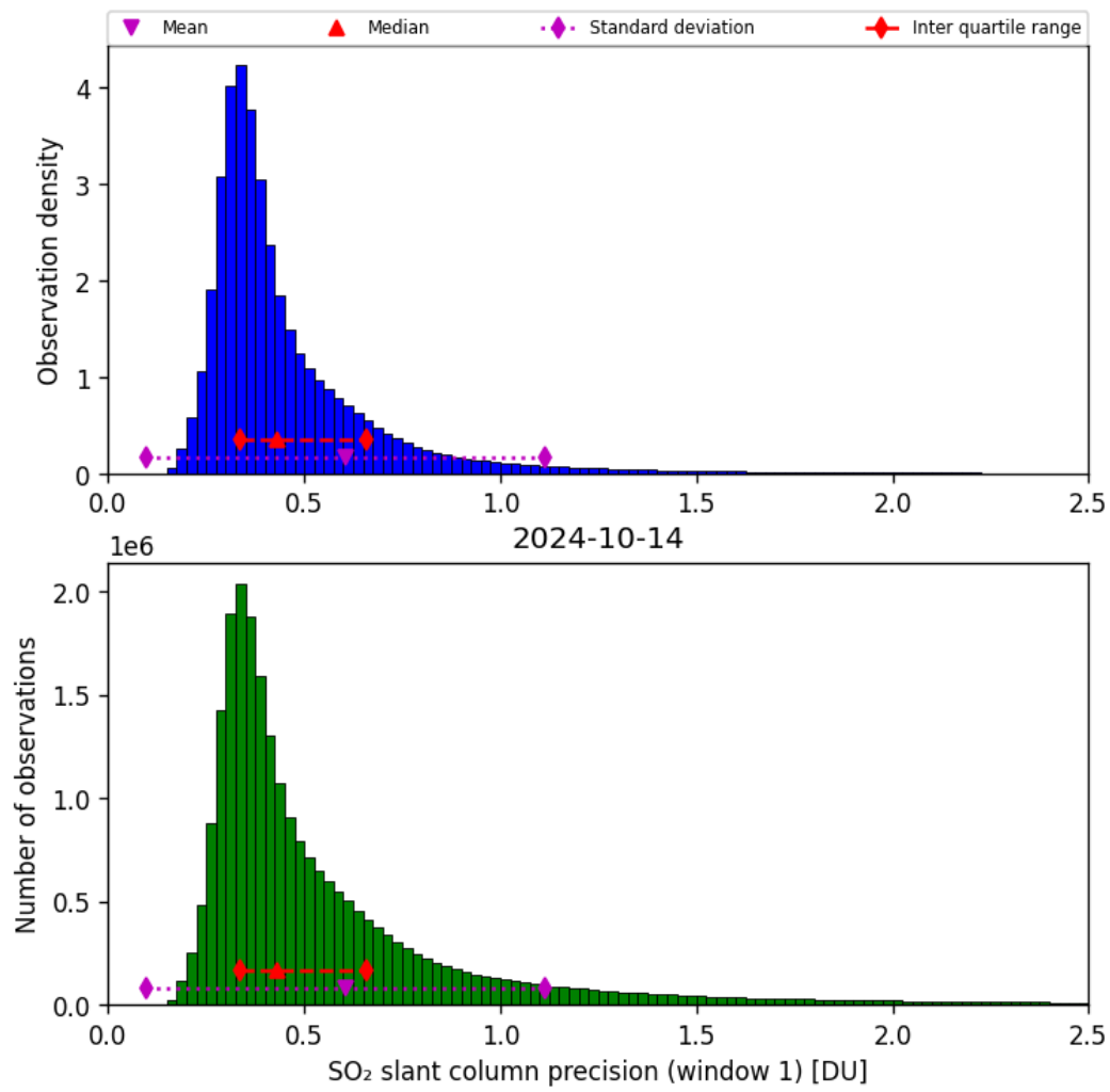
Figure 57: Histogram of “SO 2 slant column precision (window 1)” for 2024-10-14 to 2024-10-15
