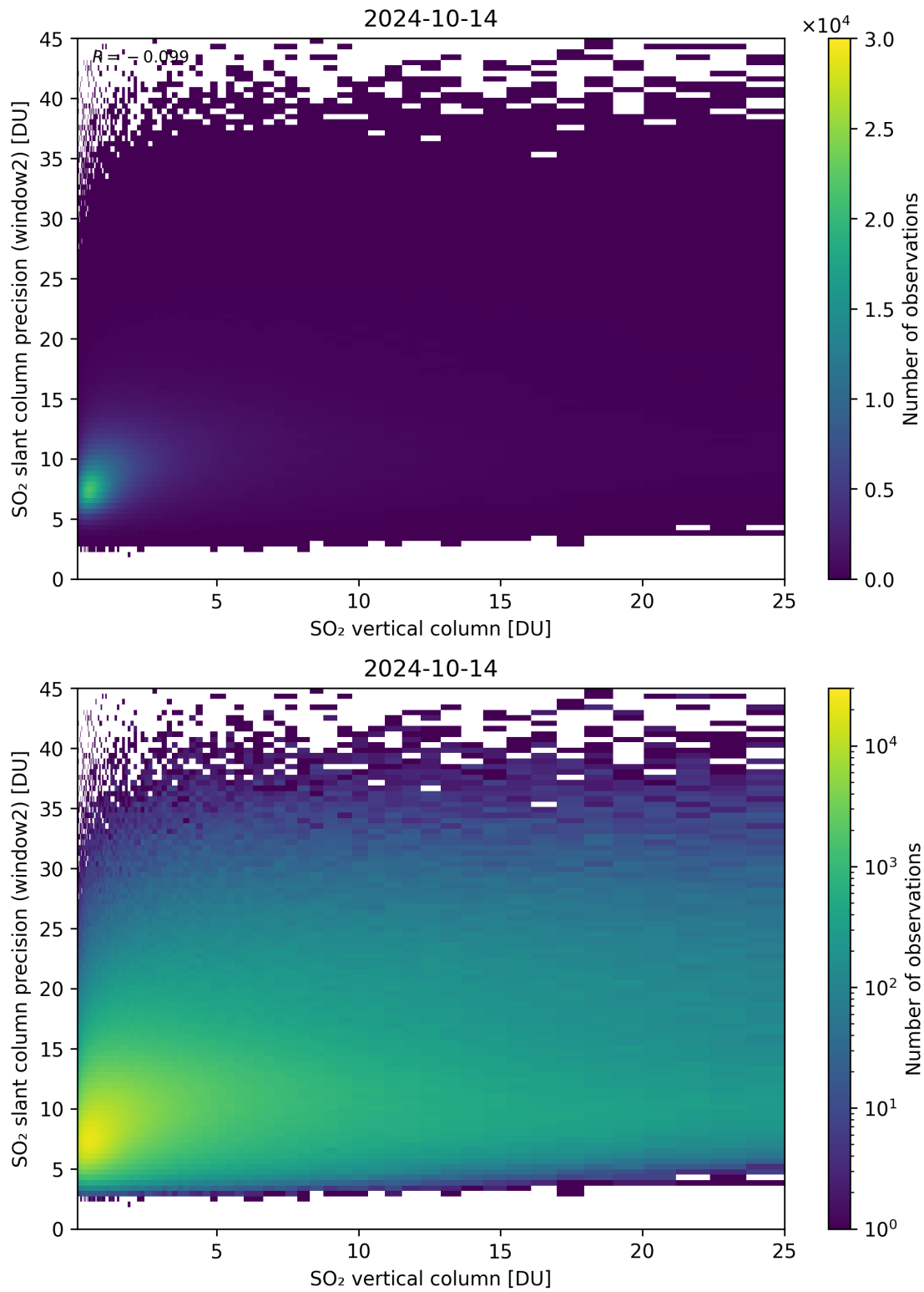
Figure 302: Scatter density plot of “SO 2 vertical column” against “SO 2 slant column precision (window2)” for 2024-10-14 to 2024-10-15.
