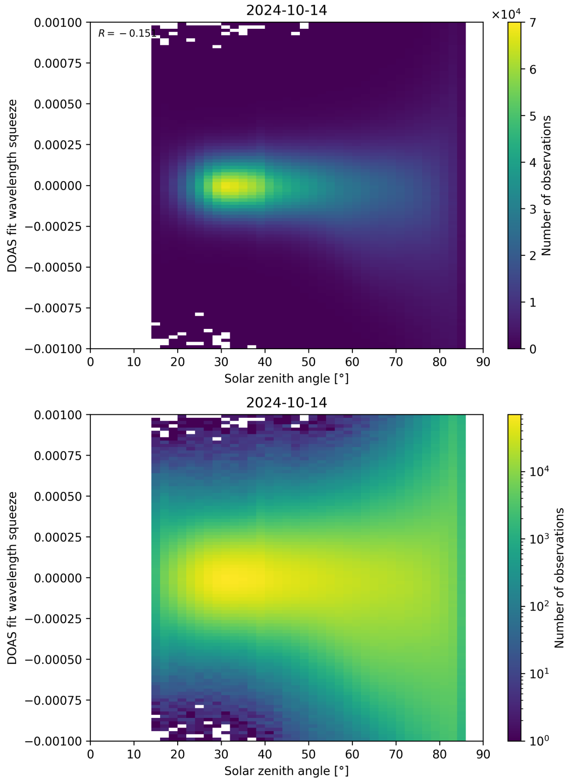
Figure 162: Scatter density plot of “Solar zenith angle” against “DOAS fit wavelength squeeze” for 2024-10-14 to 2024-10-15.
