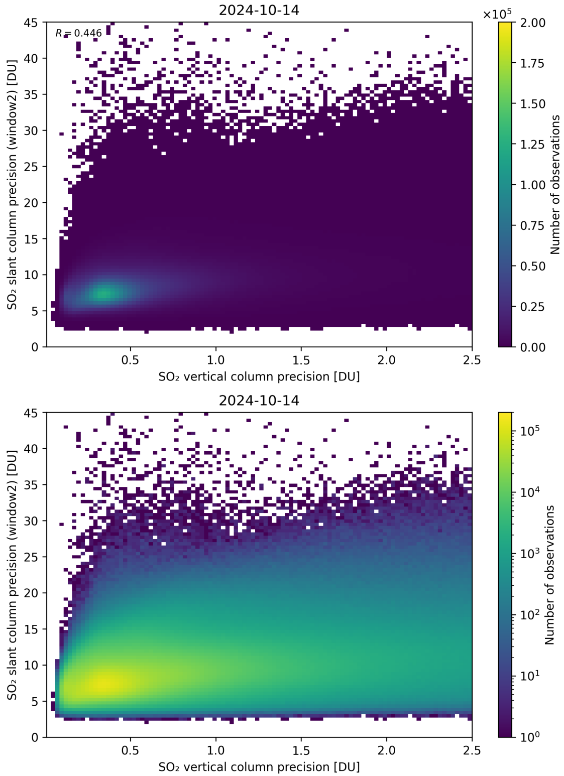
Figure 291: Scatter density plot of “SO 2 vertical column precision” against “SO 2 slant column precision (window2)” for 2024-10-14 to 2024-10-15.
