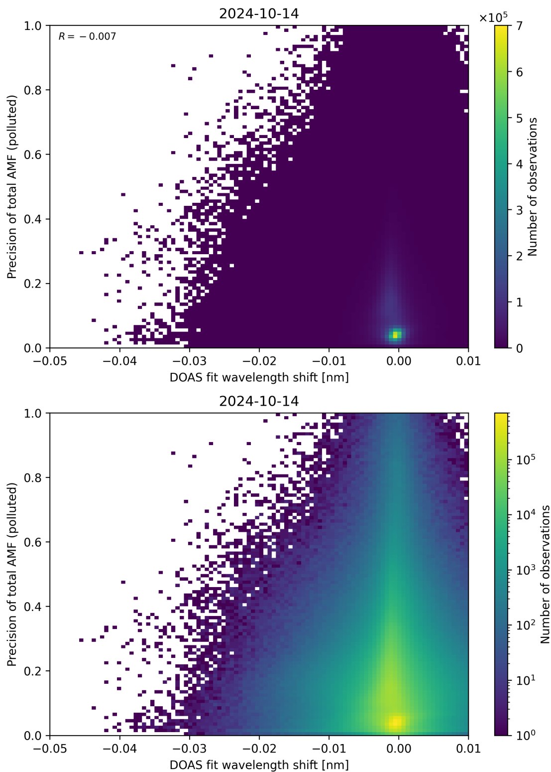
Figure 131: Scatter density plot of “DOAS fit wavelength shift” against “Precision of total AMF (polluted)” for 2024-10-14 to 2024-10-15.
