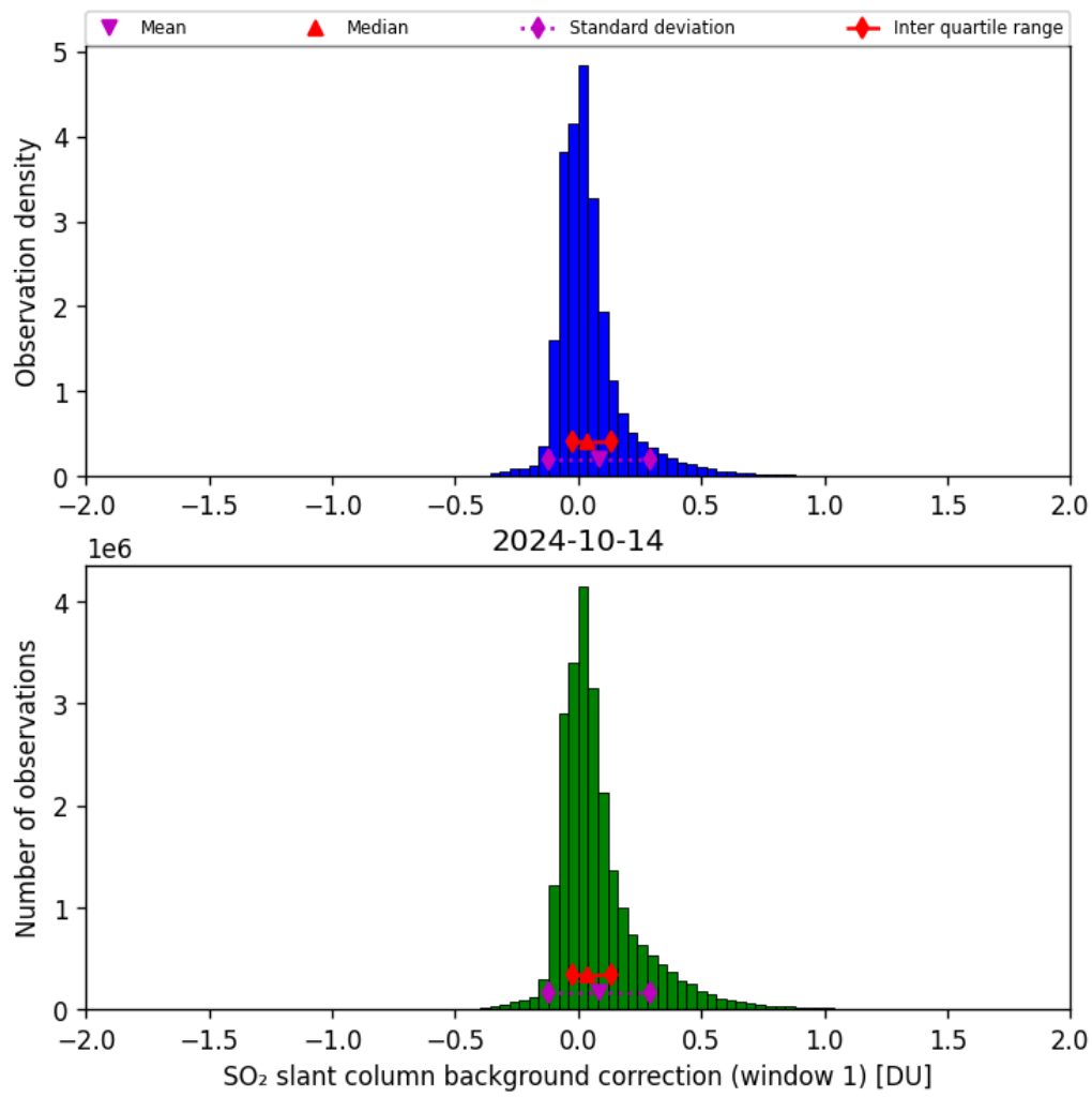
Figure 59: Histogram of “SO 2 slant column background correction (window 1)” for 2024-10-14 to 2024-10-15
