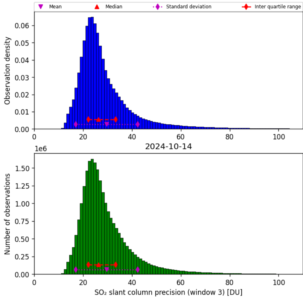
Figure 65: Histogram of “SO 2 slant column precision (window 3)” for 2024-10-14 to 2024-10-15
