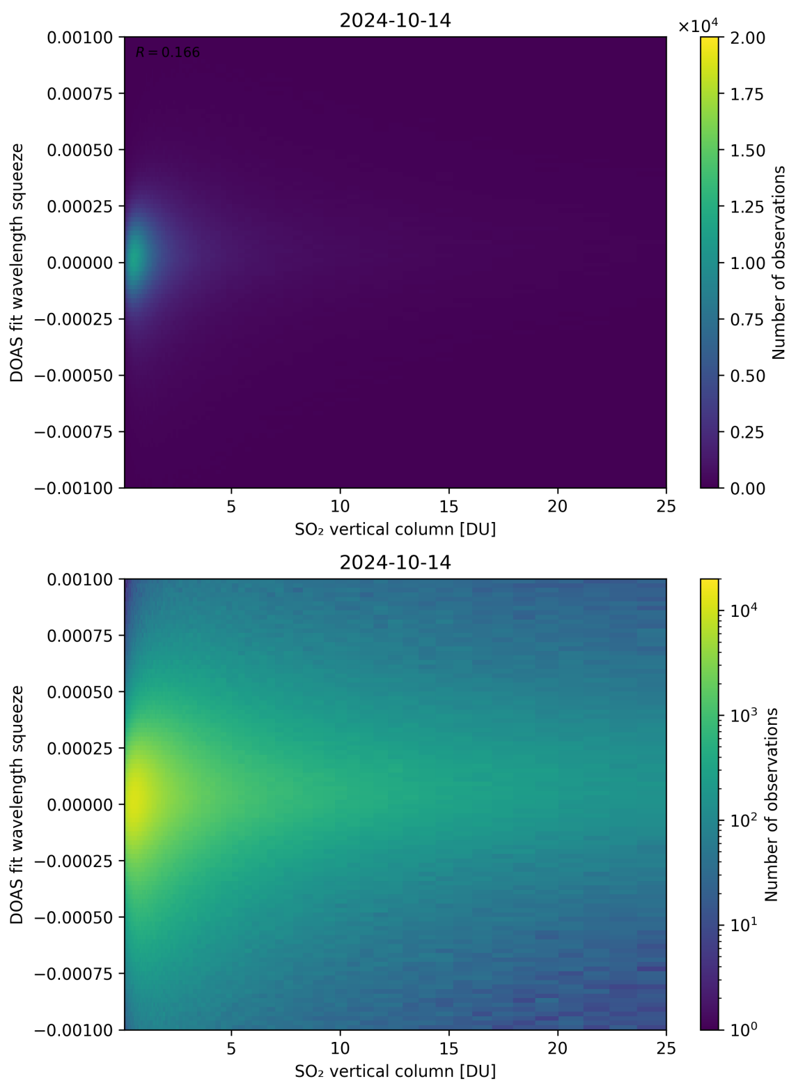
Figure 277: Scatter density plot of “SO 2 vertical column” against “DOAS fit wavelength squeeze” for 2024-10-14 to 2024-10-15.
