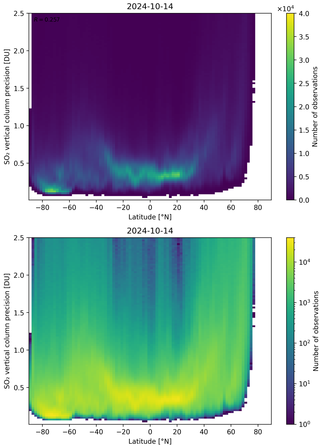
Figure 157: Scatter density plot of “Latitude” against “SO 2 vertical column precision” for 2024-10-14 to 2024-10-15.
