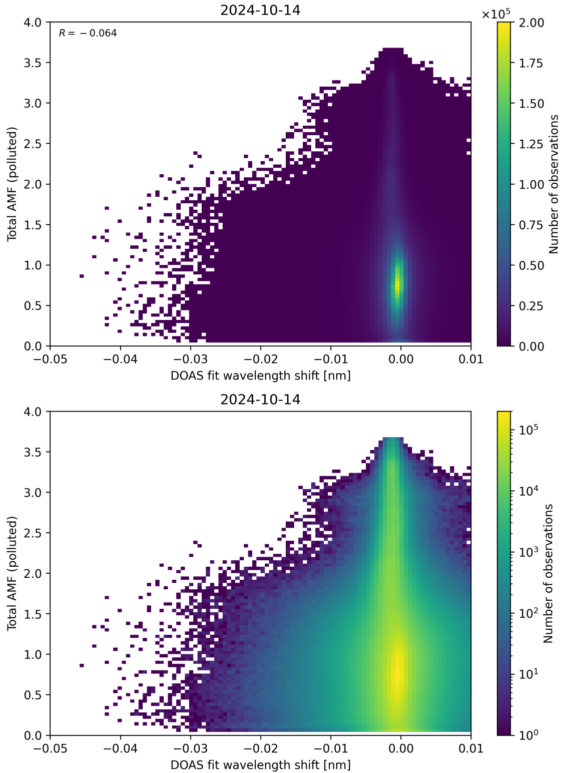
Figure 130: Scatter density plot of “DOAS fit wavelength shift” against “Total AMF (polluted)” for 2024-10-14 to 2024-10-15.
