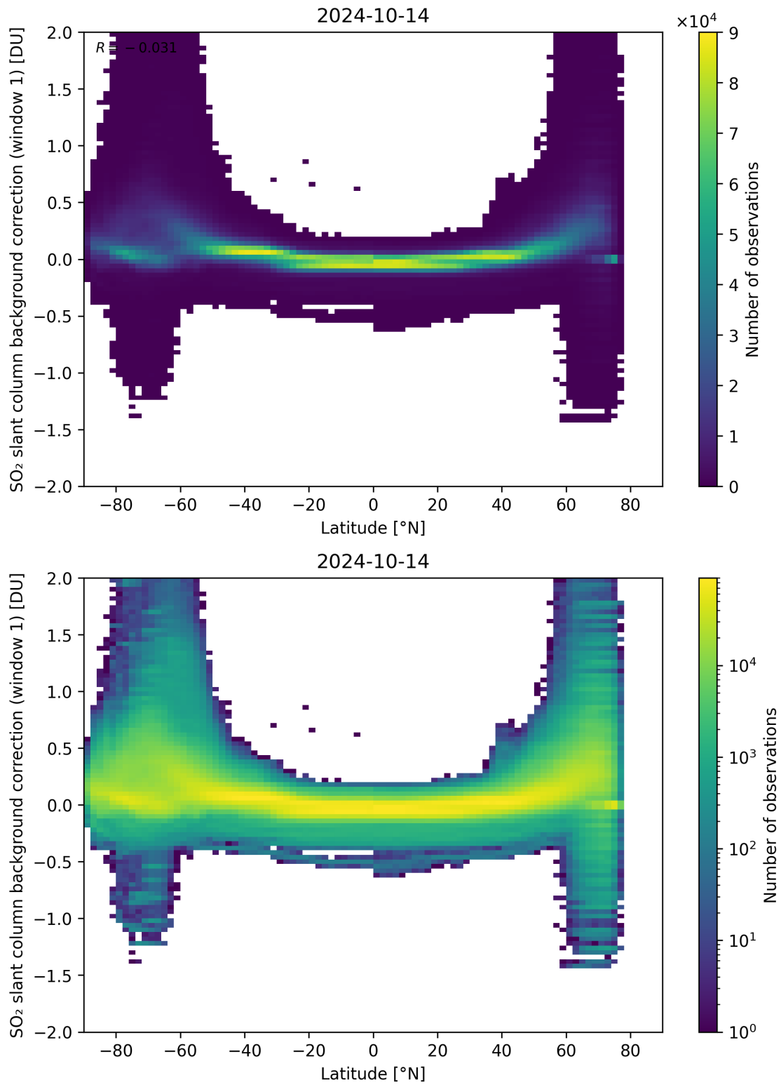
Figure 139: Scatter density plot of “Latitude” against “SO 2 slant column background correction (window 1)” for 2024-10-14 to 2024-10-15.
