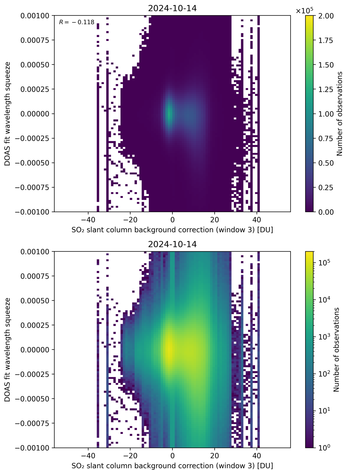
Figure 122: Scatter density plot of “SO 2 slant column background correction (window 3)” against “DOAS fit wavelength squeeze” for 2024-10-14 to 2024-10-15.
