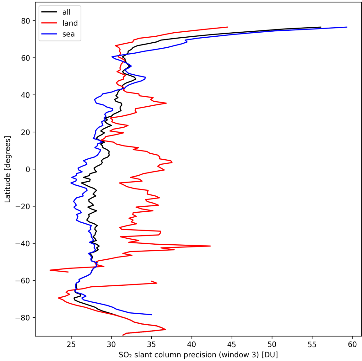
Figure 42: Zonal average of “SO 2 slant column precision (window 3)” for 2024-10-14 to 2024-10-15.
