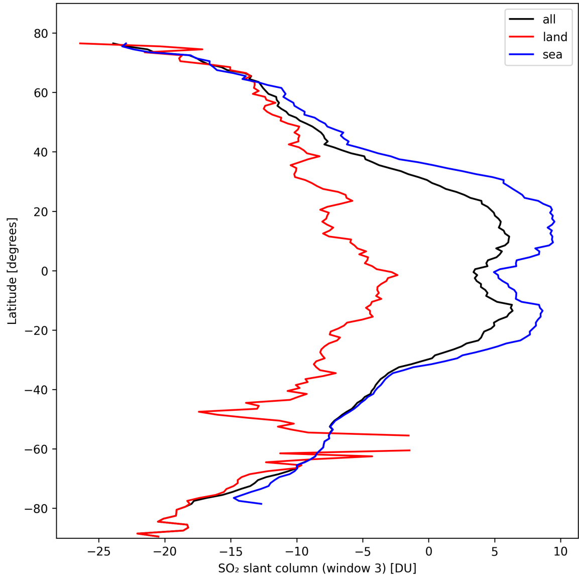
Figure 41: Zonal average of “SO 2 slant column (window 3)” for 2024-10-14 to 2024-10-15.
