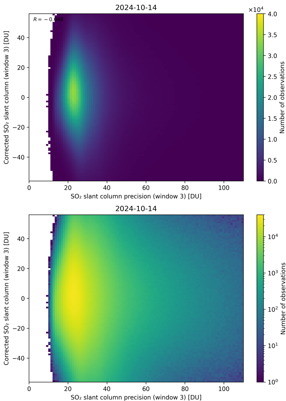
Figure 262: Scatter density plot of “SO 2 slant column precision (window 3)” against “Corrected SO 2 slant column (window 3)” for 2024-10-14 to 2024-10-15.
