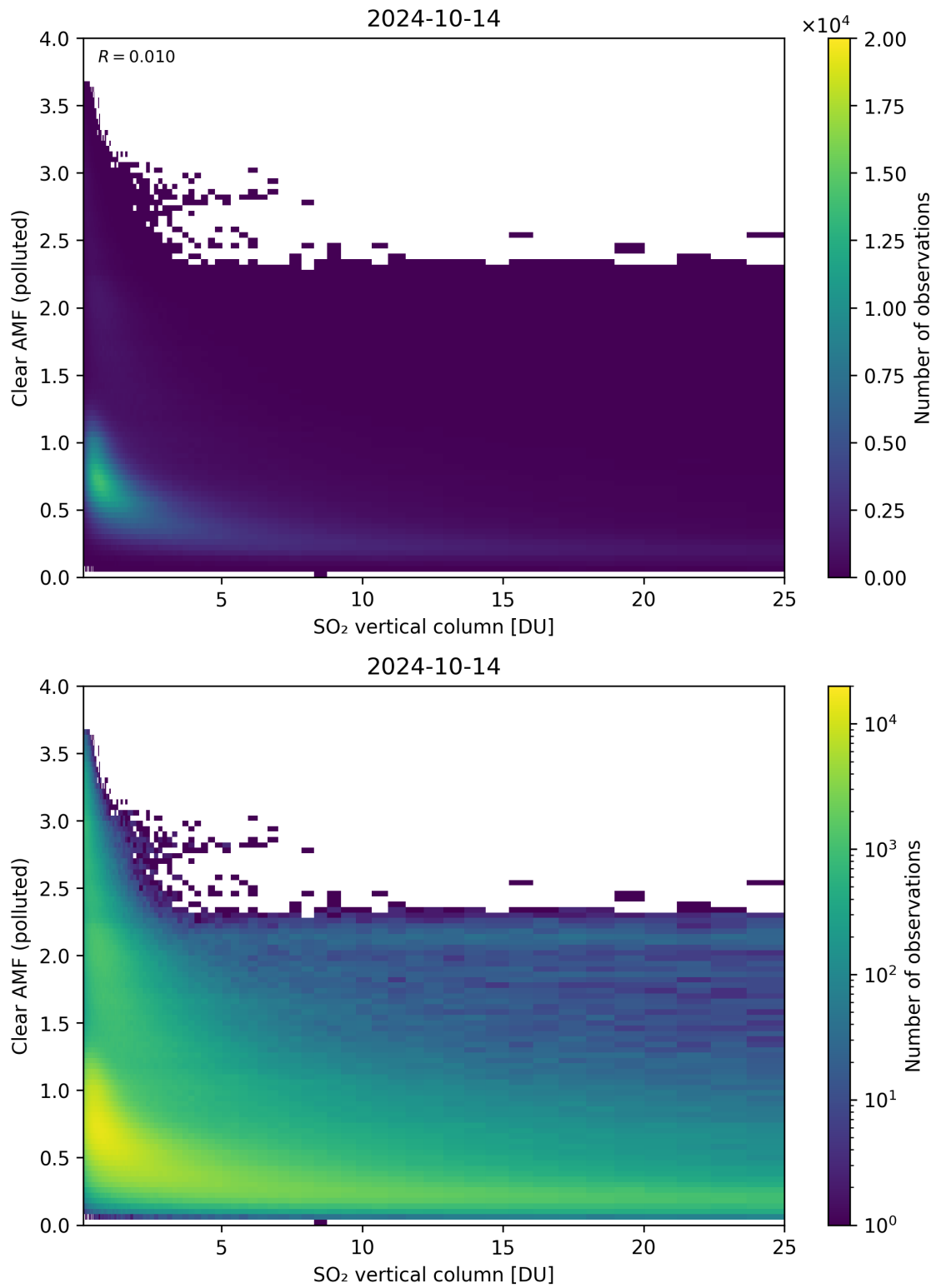
Figure 296: Scatter density plot of “SO 2 vertical column” against “Clear AMF (polluted)” for 2024-10-14 to 2024-10-15.
