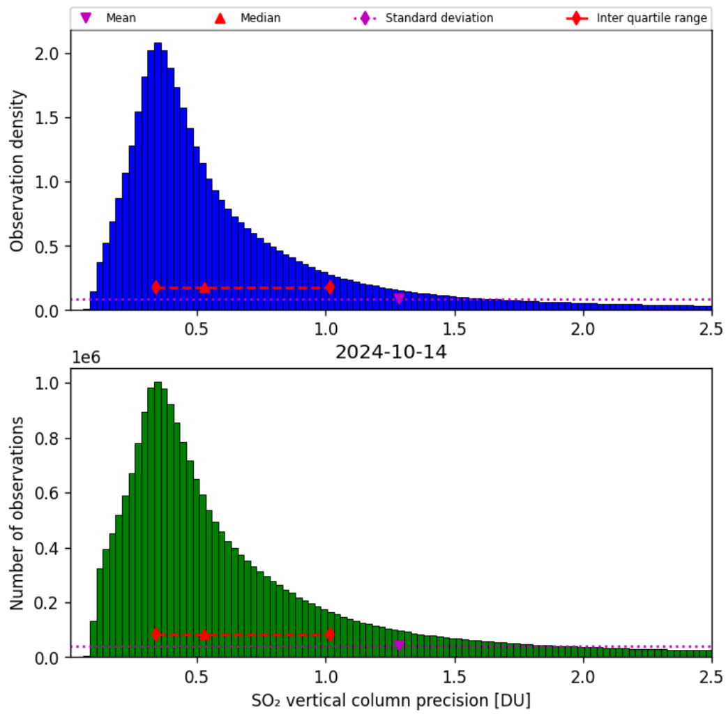
Figure 54: Histogram of “SO 2 vertical column precision” for 2024-10-14 to 2024-10-15
