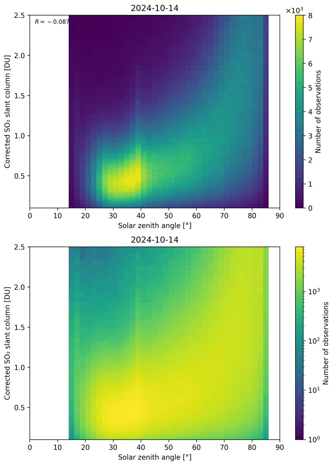
Figure 166: Scatter density plot of “Solar zenith angle” against “Corrected SO 2 slant column” for 2024-10-14 to 2024-10-15.
