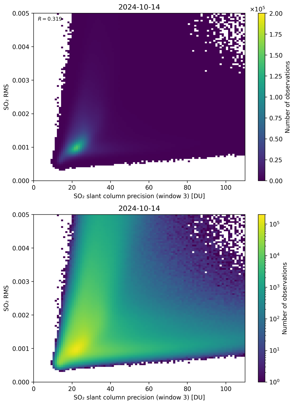
Figure 260: Scatter density plot of “SO 2 slant column precision (window 3)” against “SO 2 RMS” for 2024-10-14 to 2024-10-15.
