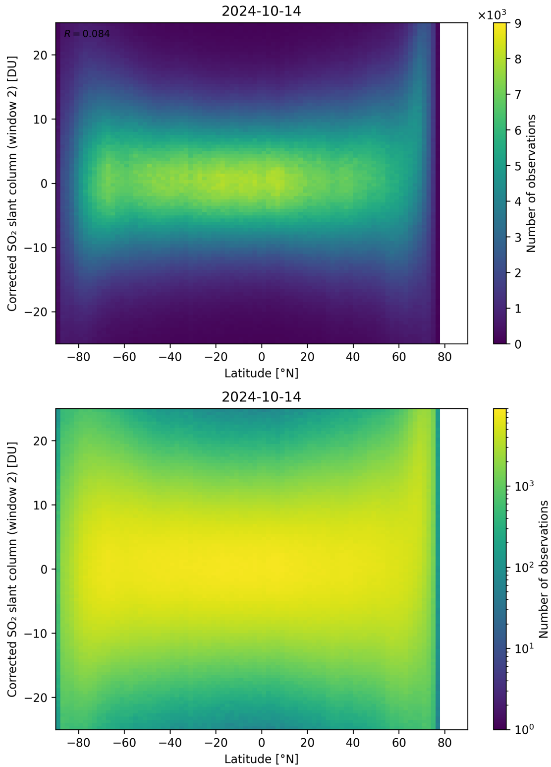
Figure 147: Scatter density plot of “Latitude” against “Corrected SO 2 slant column (window 2)” for 2024-10-14 to 2024-10-15.
