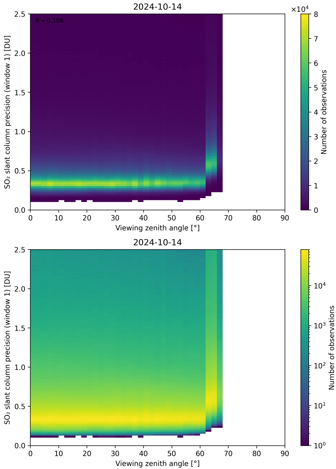
Figure 321: Scatter density plot of “Viewing zenith angle” against “SO 2 slant column precision (window 1)” for 2024-10-14 to 2024-10-15.
