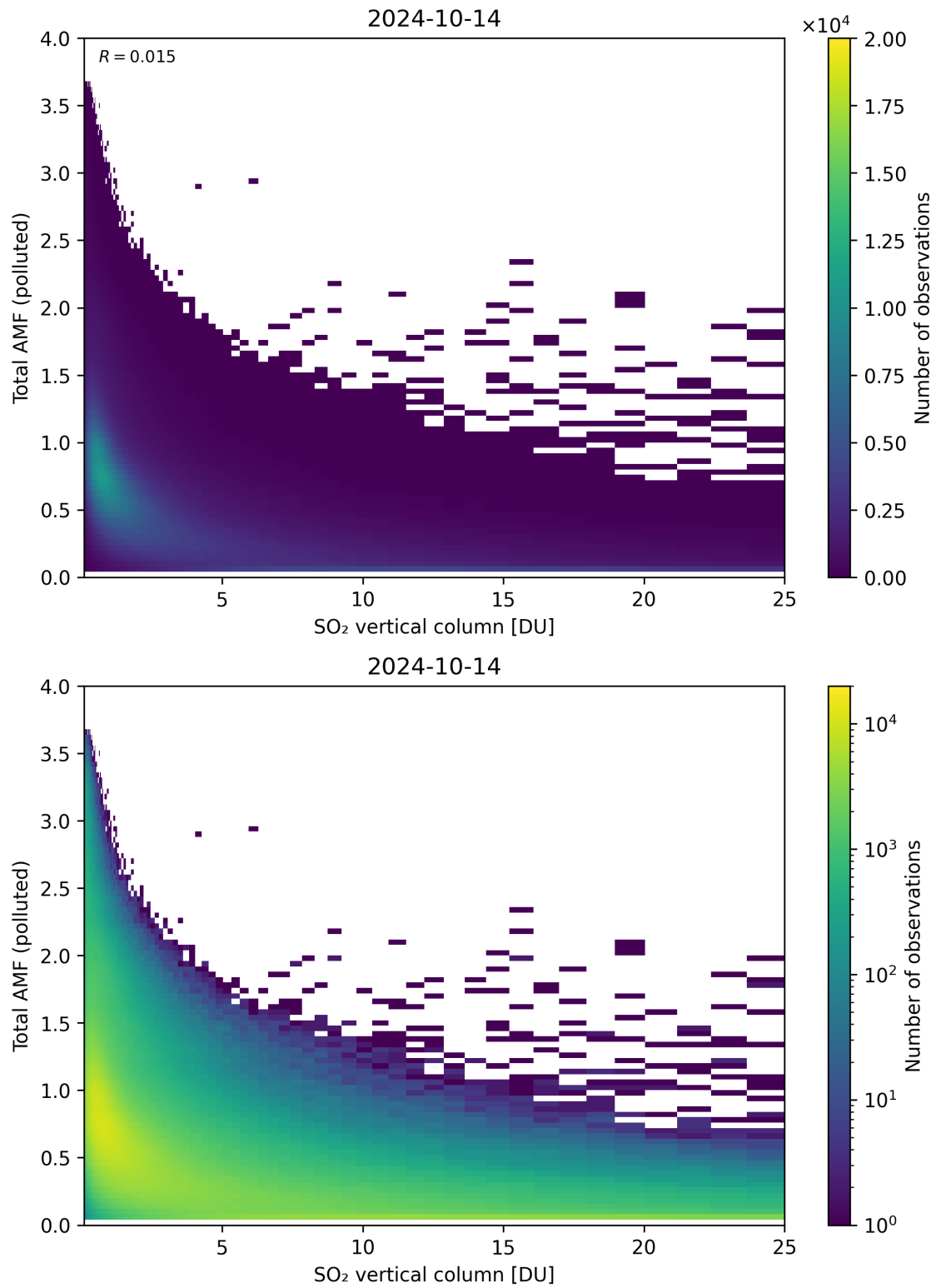
Figure 305: Scatter density plot of “SO 2 vertical column” against “Total AMF (polluted)” for 2024-10-14 to 2024-10-15.
