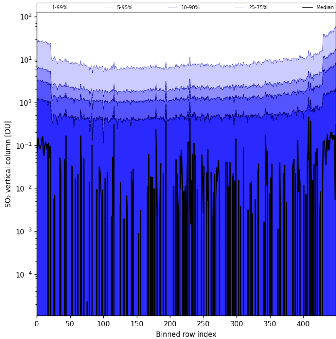
Figure 76: Along track statistics of “SO 2 vertical column” for 2024-10-14 to 2024-10-15
