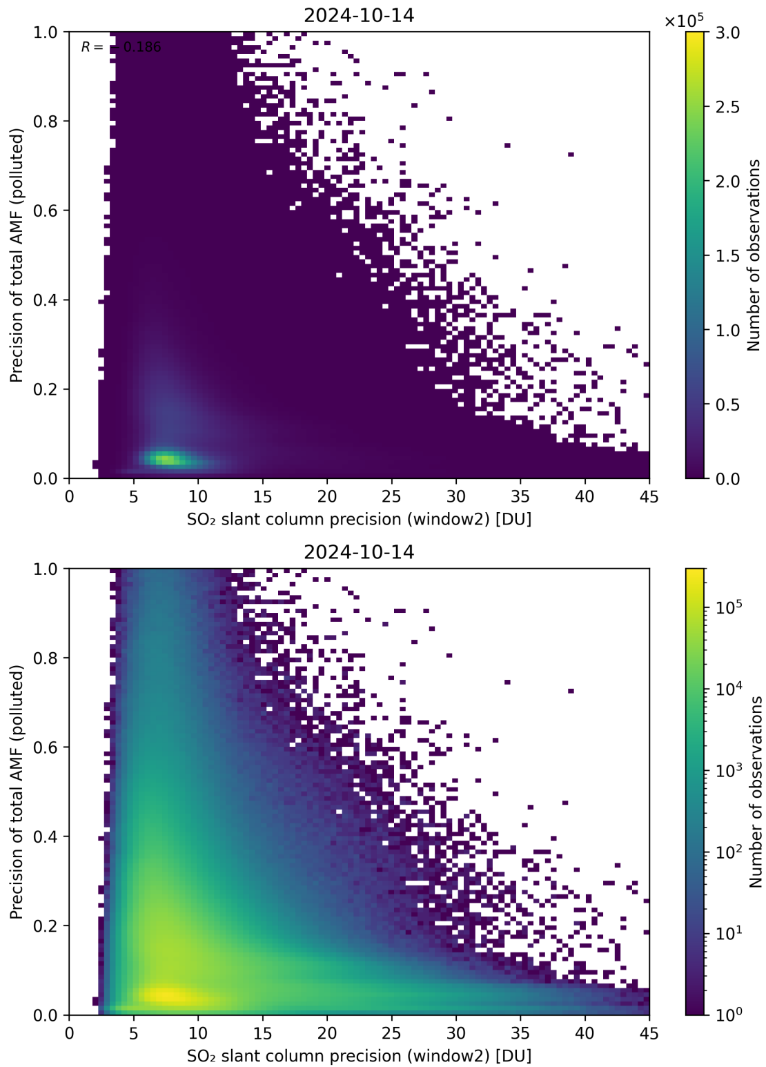
Figure 252: Scatter density plot of “SO 2 slant column precision (window2)” against “Precision of total AMF (polluted)” for 2024-10-14 to 2024-10-15.
