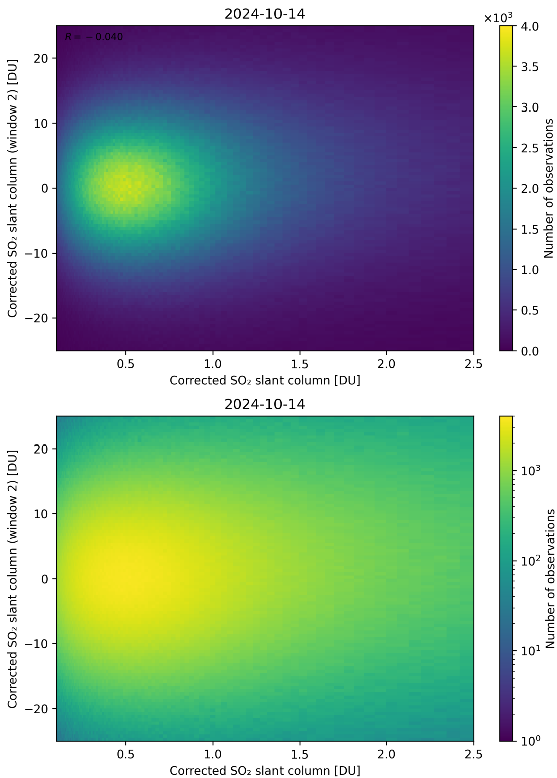
Figure 185: Scatter density plot of “Corrected SO 2 slant column” against “Corrected SO 2 slant column (window 2)” for 2024-10-14 to 2024-10-15.
