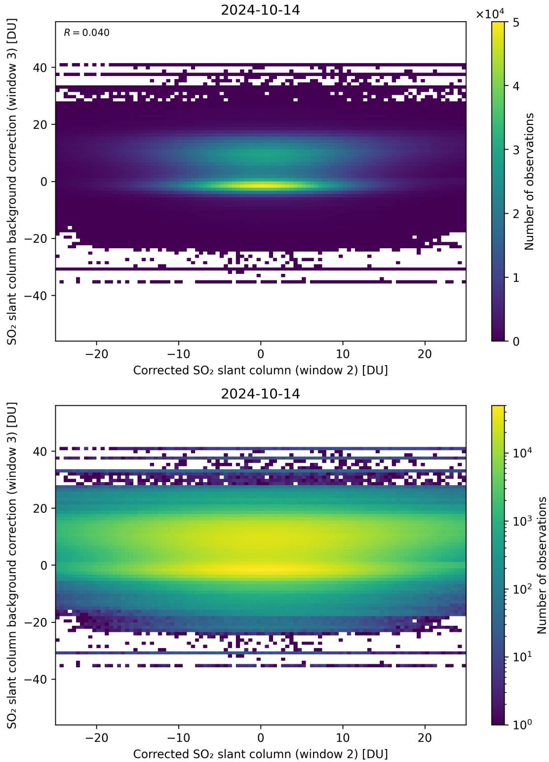
Figure 195: Scatter density plot of “Corrected SO 2 slant column (window 2)” against “SO 2 slant column background correction (window 3)” for 2024-10-14 to 2024-10-15.
