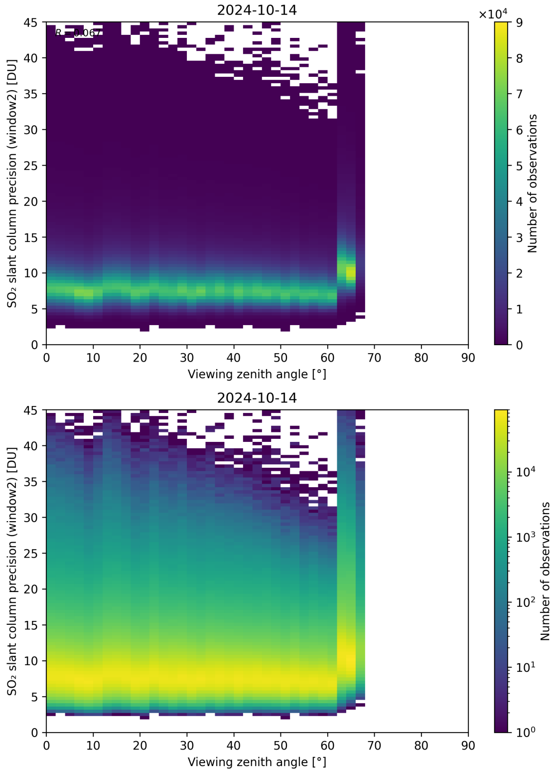
Figure 322: Scatter density plot of “Viewing zenith angle” against “SO 2 slant column precision (window2)” for 2024-10-14 to 2024-10-15.
