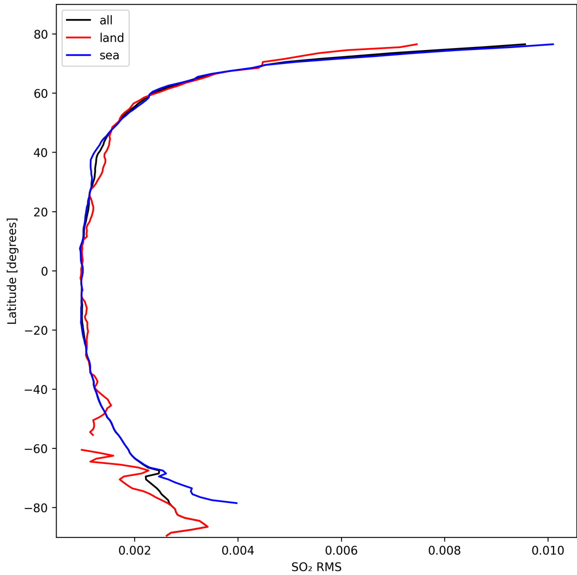
Figure 47: Zonal average of “SO 2 RMS” for 2024-10-14 to 2024-10-15.
