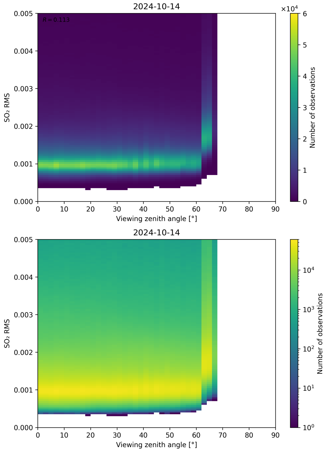
Figure 313: Scatter density plot of “Viewing zenith angle” against “SO 2 RMS” for 2024-10-14 to 2024-10-15.
