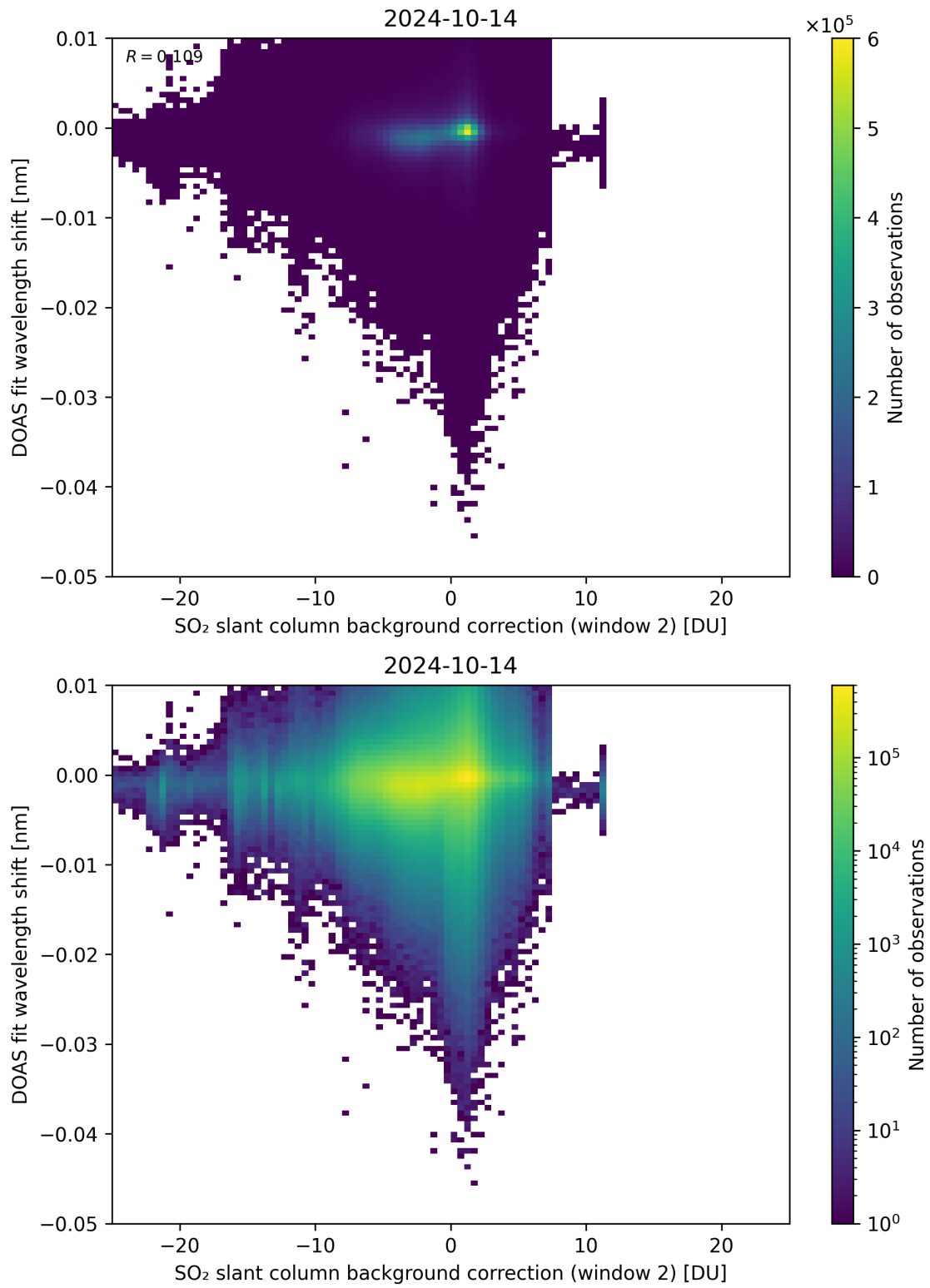
Figure 112: Scatter density plot of “SO 2 slant column background correction (window 2)” against “DOAS fit wavelength shift” for 2024-10-14 to 2024-10-15.
