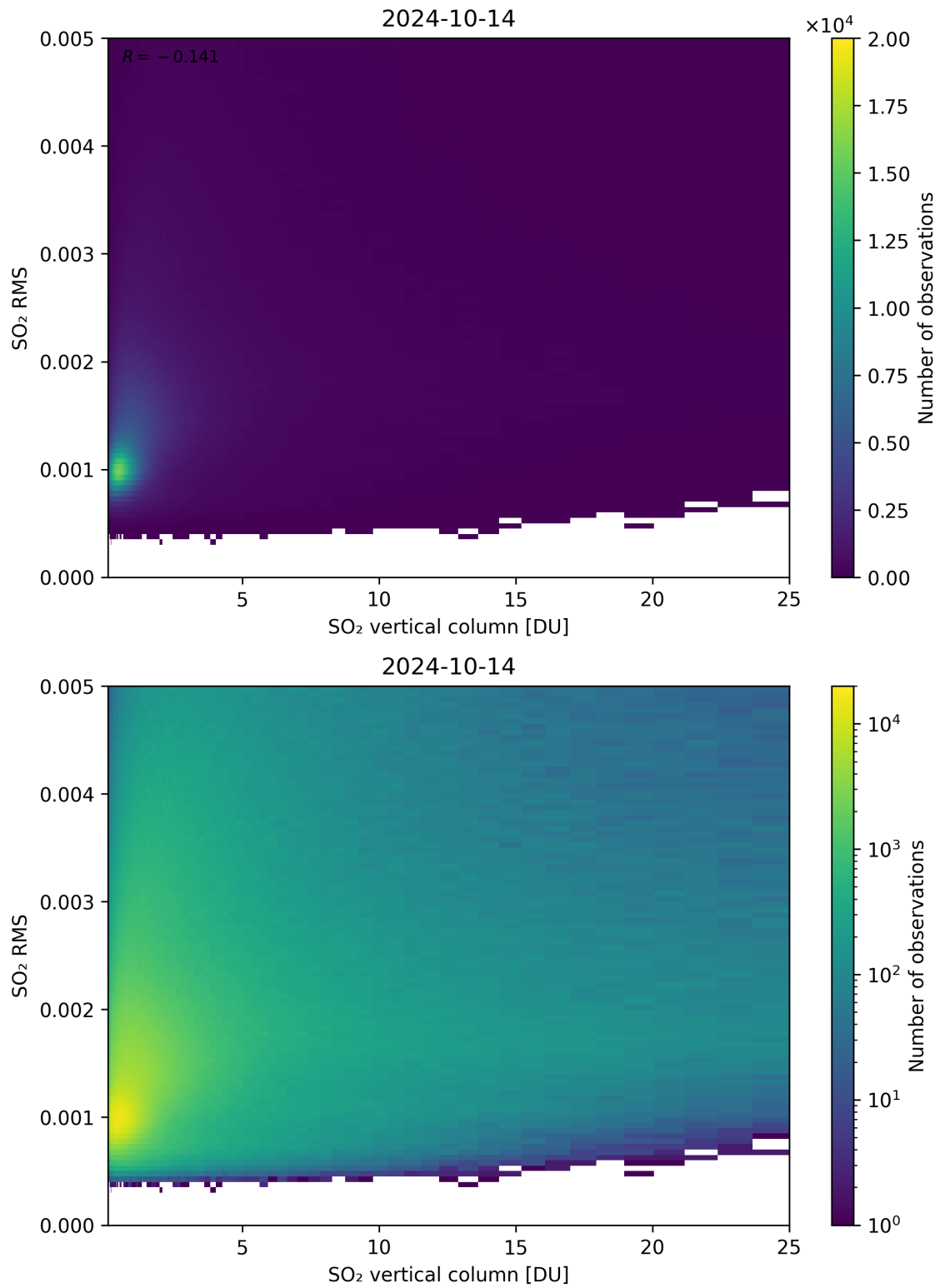
Figure 278: Scatter density plot of “SO 2 vertical column” against “SO 2 RMS” for 2024-10-14 to 2024-10-15.
