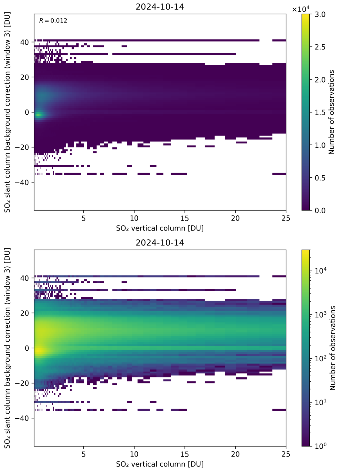
Figure 275: Scatter density plot of “SO 2 vertical column” against “SO 2 slant column background correction (window 3)” for 2024-10-14 to 2024-10-15.
