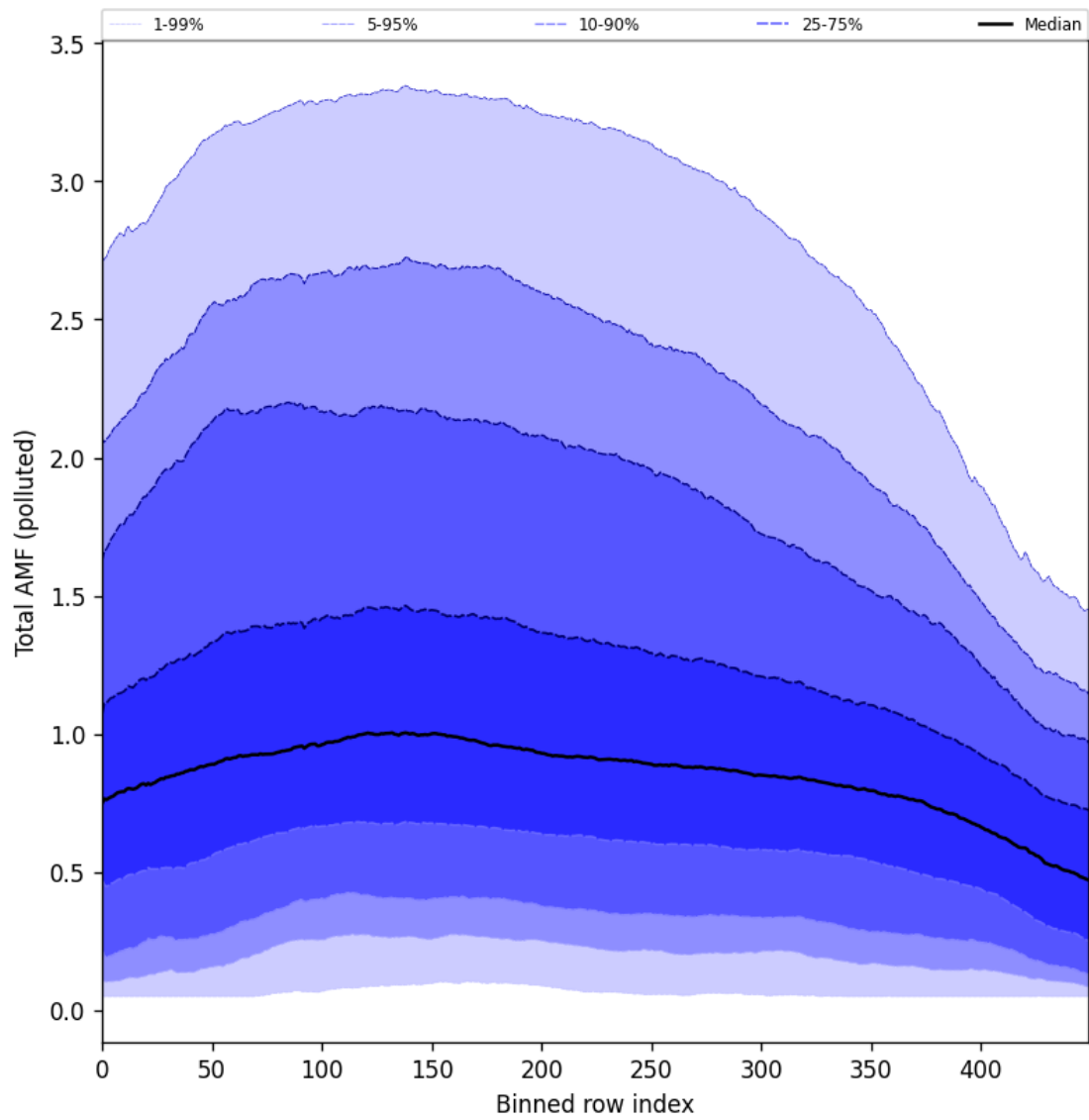
Figure 94: Along track statistics of “Total AMF (polluted)” for 2024-10-14 to 2024-10-15
