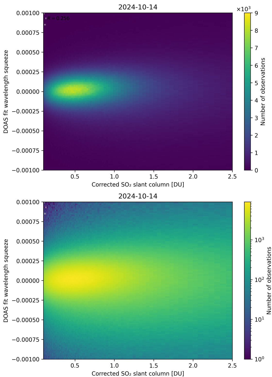
Figure 182: Scatter density plot of “Corrected SO 2 slant column” against “DOAS fit wavelength squeeze” for 2024-10-14 to 2024-10-15.
