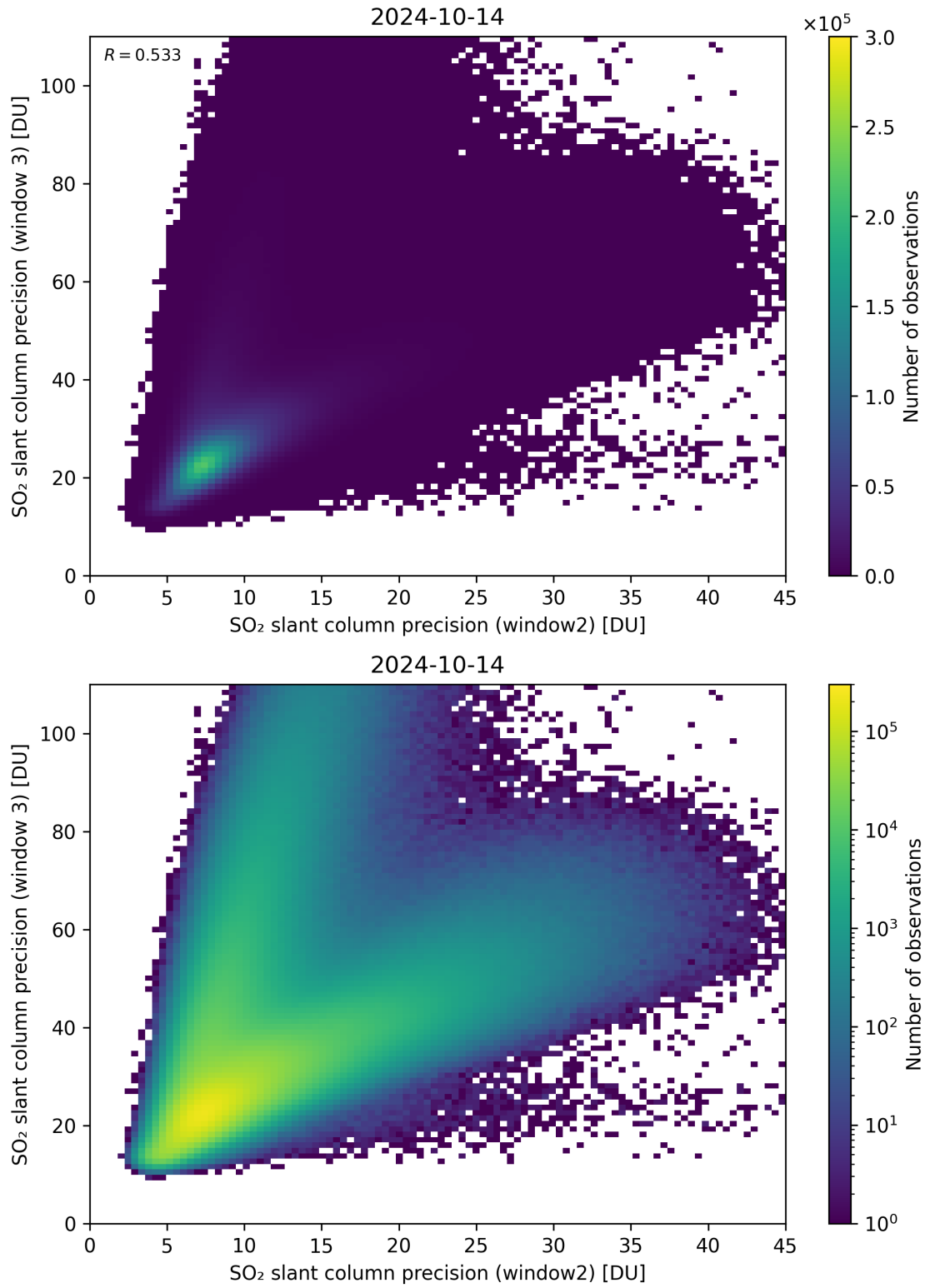
Figure 250: Scatter density plot of “SO 2 slant column precision (window2)” against “SO 2 slant column precision (window 3)” for 2024-10-14 to 2024-10-15.
