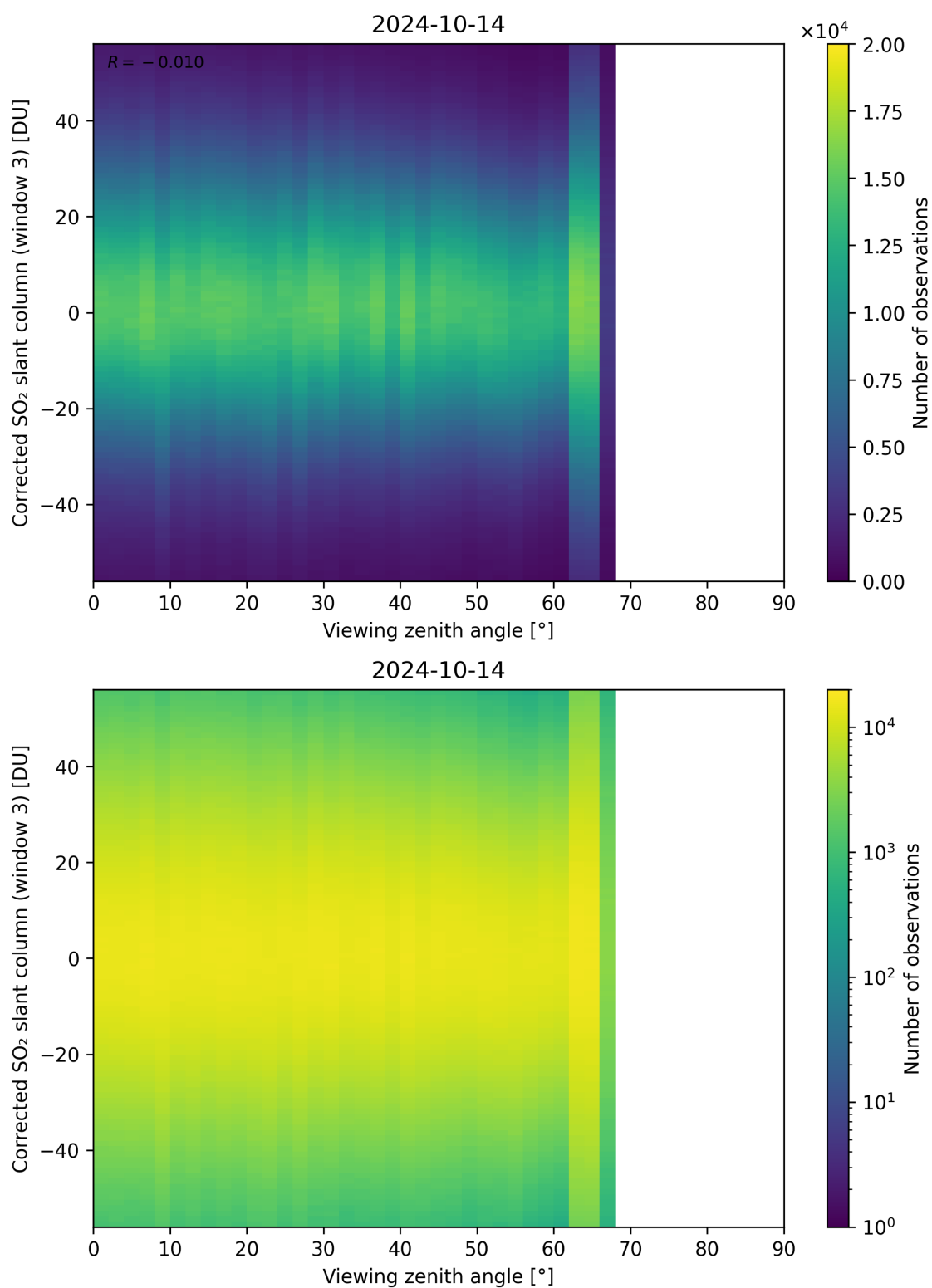
Figure 319: Scatter density plot of “Viewing zenith angle” against “Corrected SO 2 slant column (window 3)” for 2024-10-14 to 2024-10-15.
