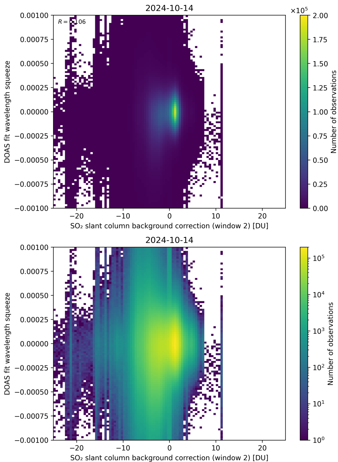
Figure 113: Scatter density plot of “SO 2 slant column background correction (window 2)” against “DOAS fit wavelength squeeze” for 2024-10-14 to 2024-10-15.
