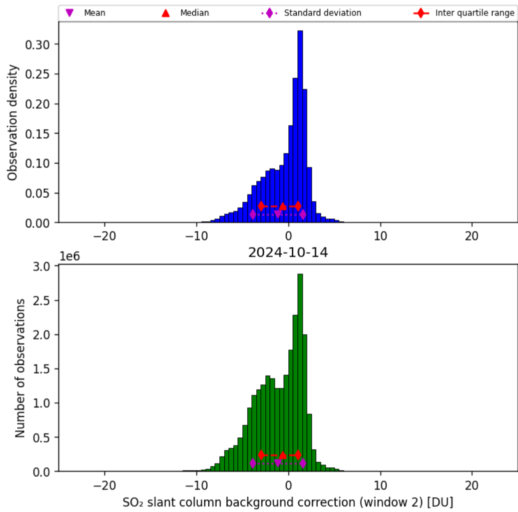
Figure 63: Histogram of “SO 2 slant column background correction (window 2)” for 2024-10-14 to 2024-10-15
