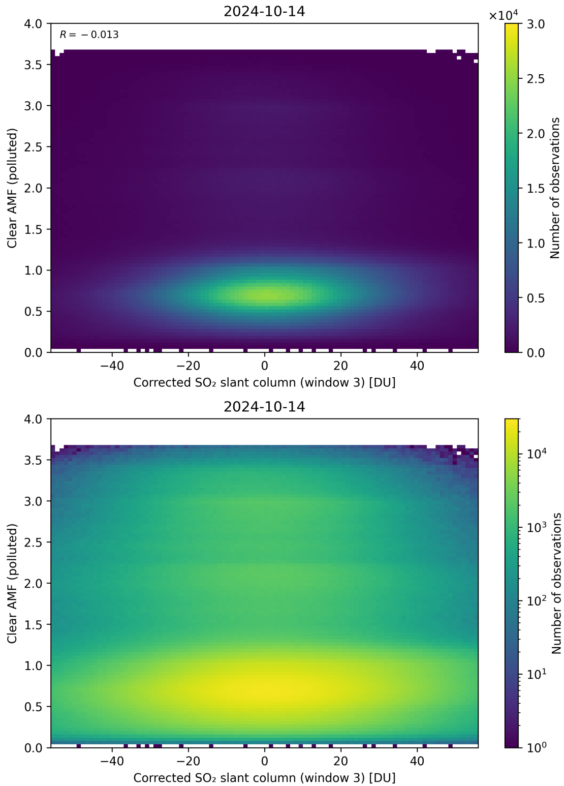
Figure 209: Scatter density plot of “Corrected SO 2 slant column (window 3)” against “Clear AMF (polluted)” for 2024-10-14 to 2024-10-15.
