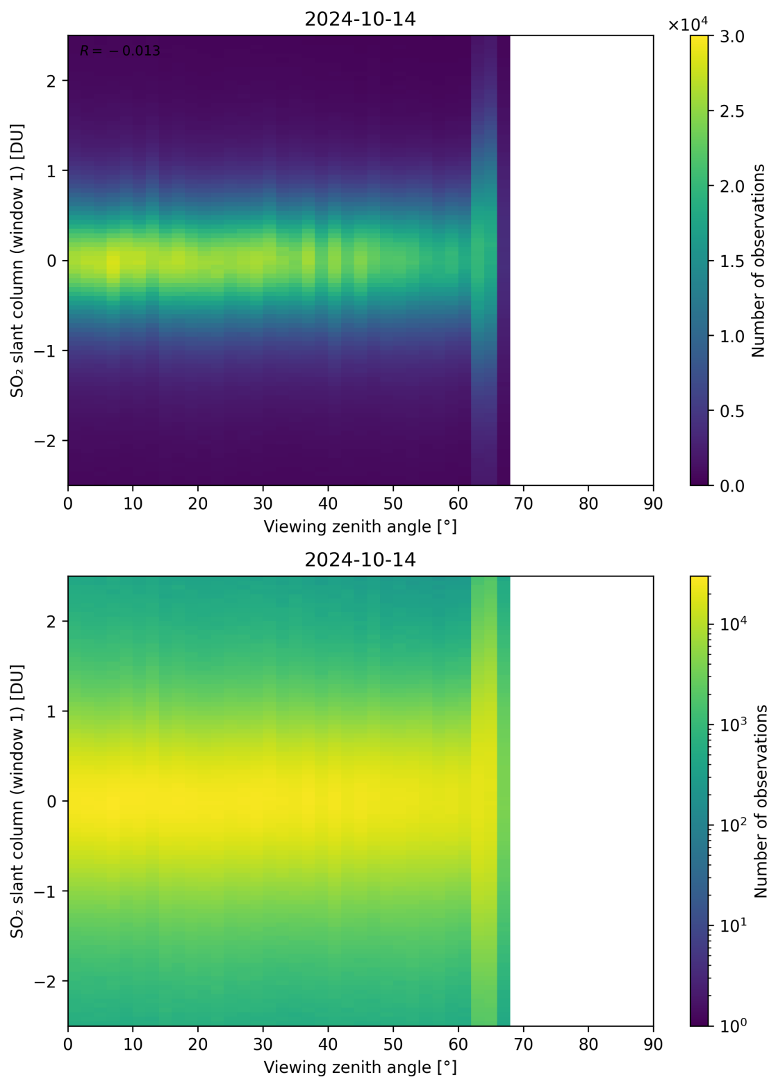
Figure 320: Scatter density plot of “Viewing zenith angle” against “SO 2 slant column (window 1)” for 2024-10-14 to 2024-10-15.
