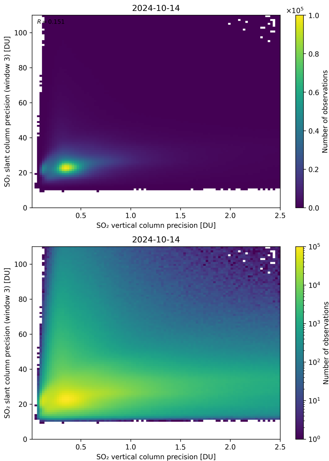
Figure 293: Scatter density plot of “SO 2 vertical column precision” against “SO 2 slant column precision (window 3)” for 2024-10-14 to 2024-10-15.
