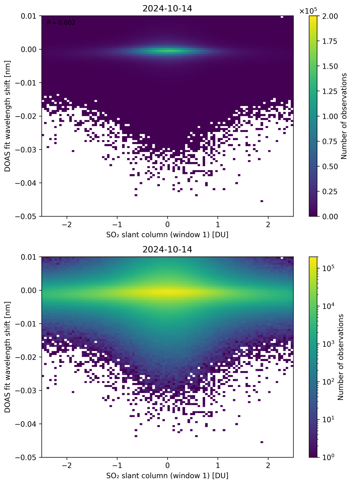
Figure 215: Scatter density plot of “SO 2 slant column (window 1)” against “DOAS fit wavelength shift” for 2024-10-14 to 2024-10-15.
