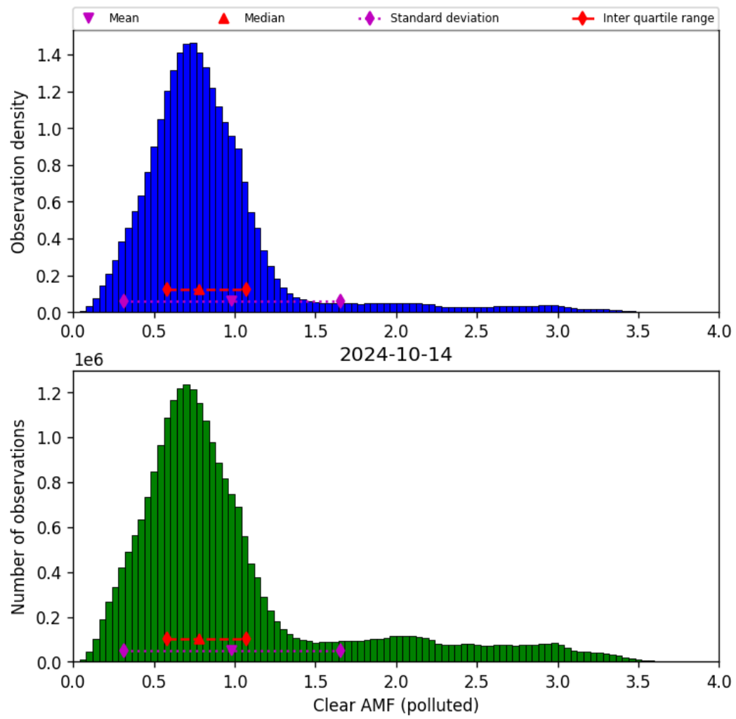
Figure 73: Histogram of “Clear AMF (polluted)” for 2024-10-14 to 2024-10-15
