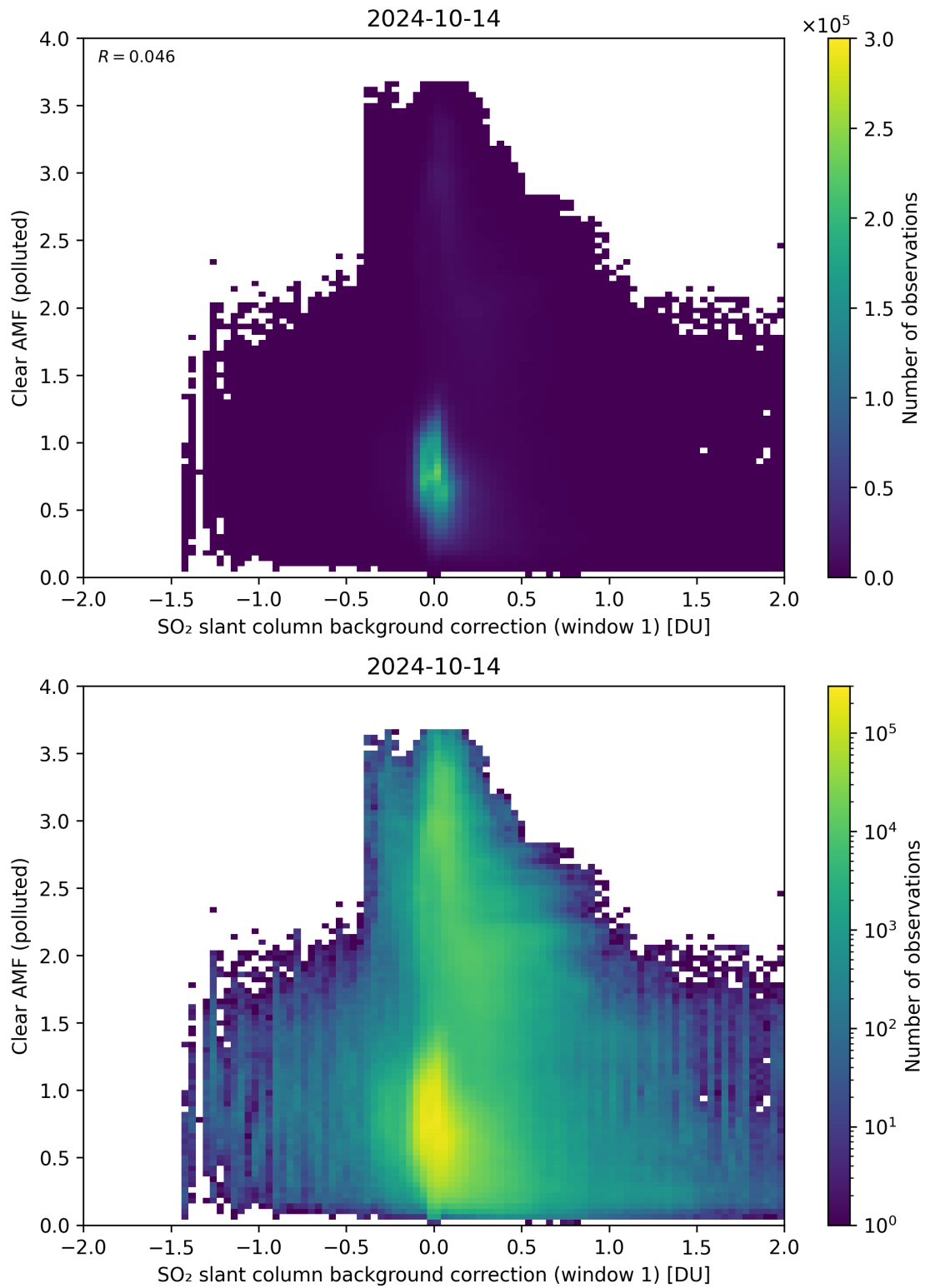
Figure 103: Scatter density plot of “SO 2 slant column background correction (window 1)” against “Clear AMF (polluted)” for 2024-10-14 to 2024-10-15.
