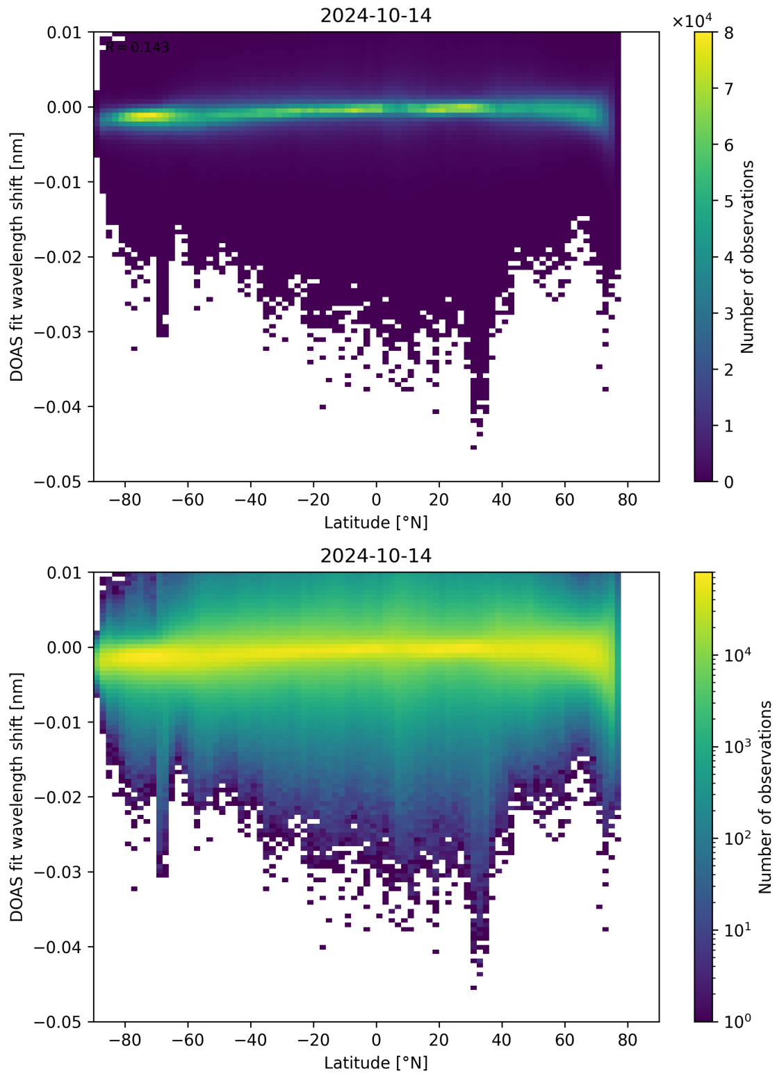
Figure 142: Scatter density plot of “Latitude” against “DOAS fit wavelength shift” for 2024-10-14 to 2024-10-15.
