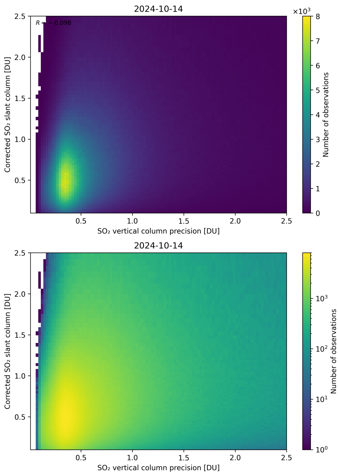
Figure 286: Scatter density plot of “SO 2 vertical column precision” against “Corrected SO 2 slant column” for 2024-10-14 to 2024-10-15.
