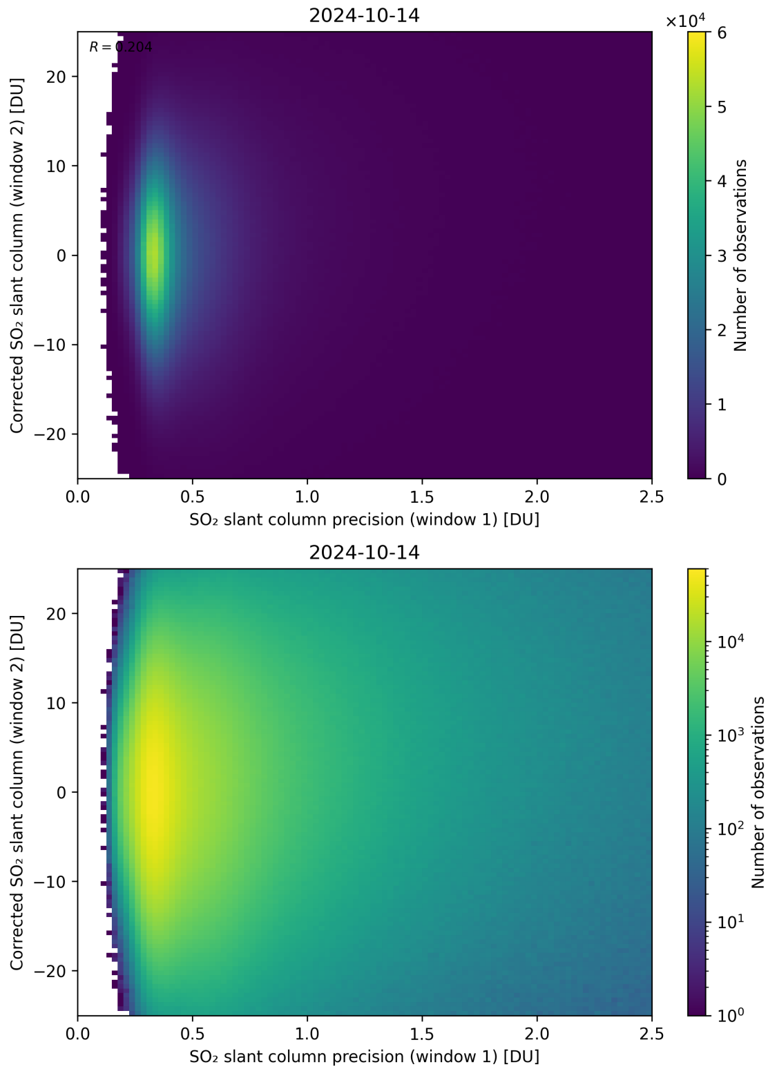
Figure 225: Scatter density plot of “SO 2 slant column precision (window 1)” against “Corrected SO 2 slant column (window 2)” for 2024-10-14 to 2024-10-15.
