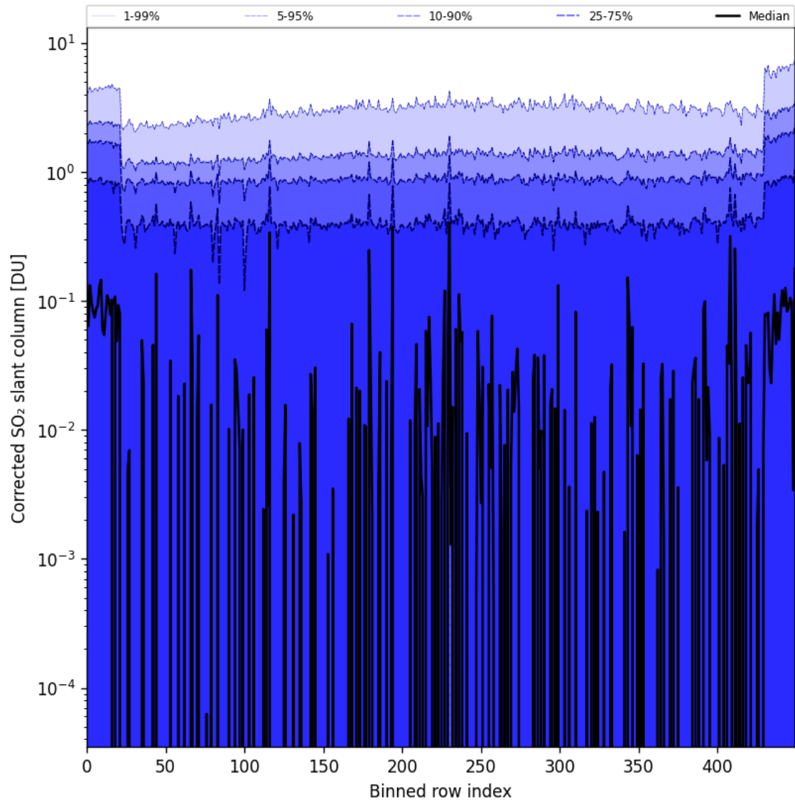
Figure 78: Along track statistics of “Corrected SO 2 slant column” for 2024-10-14 to 2024-10-15
