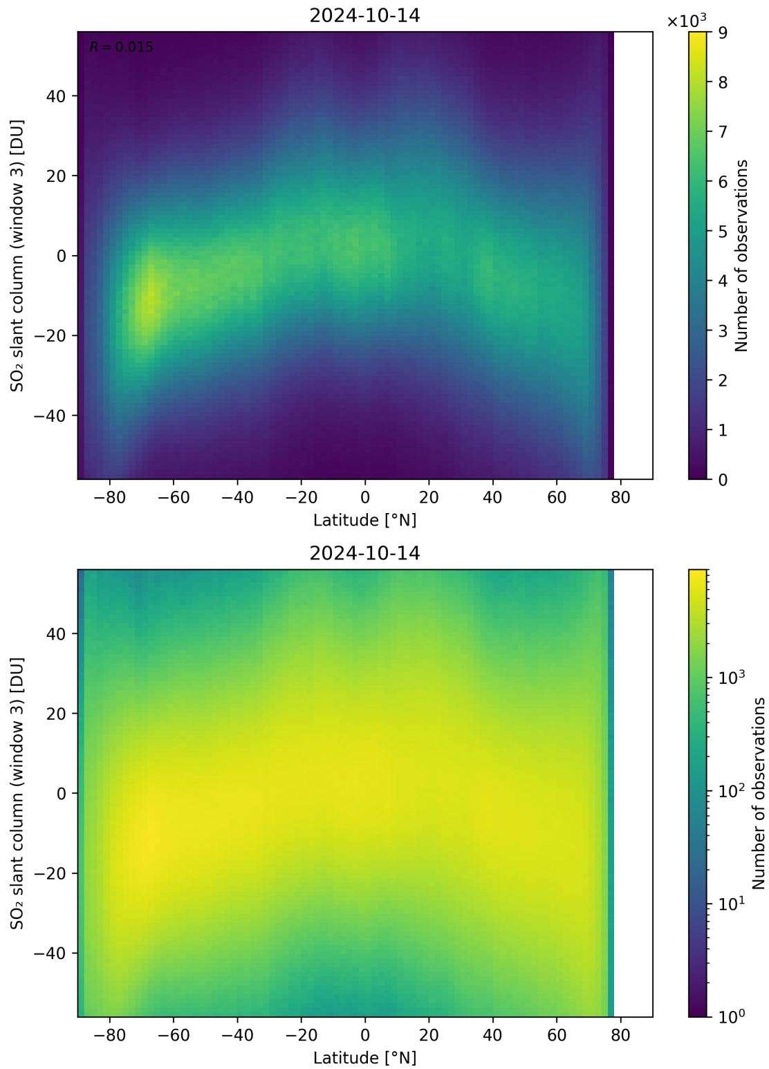
Figure 152: Scatter density plot of “Latitude” against “SO 2 slant column (window 3)” for 2024-10-14 to 2024-10-15.
