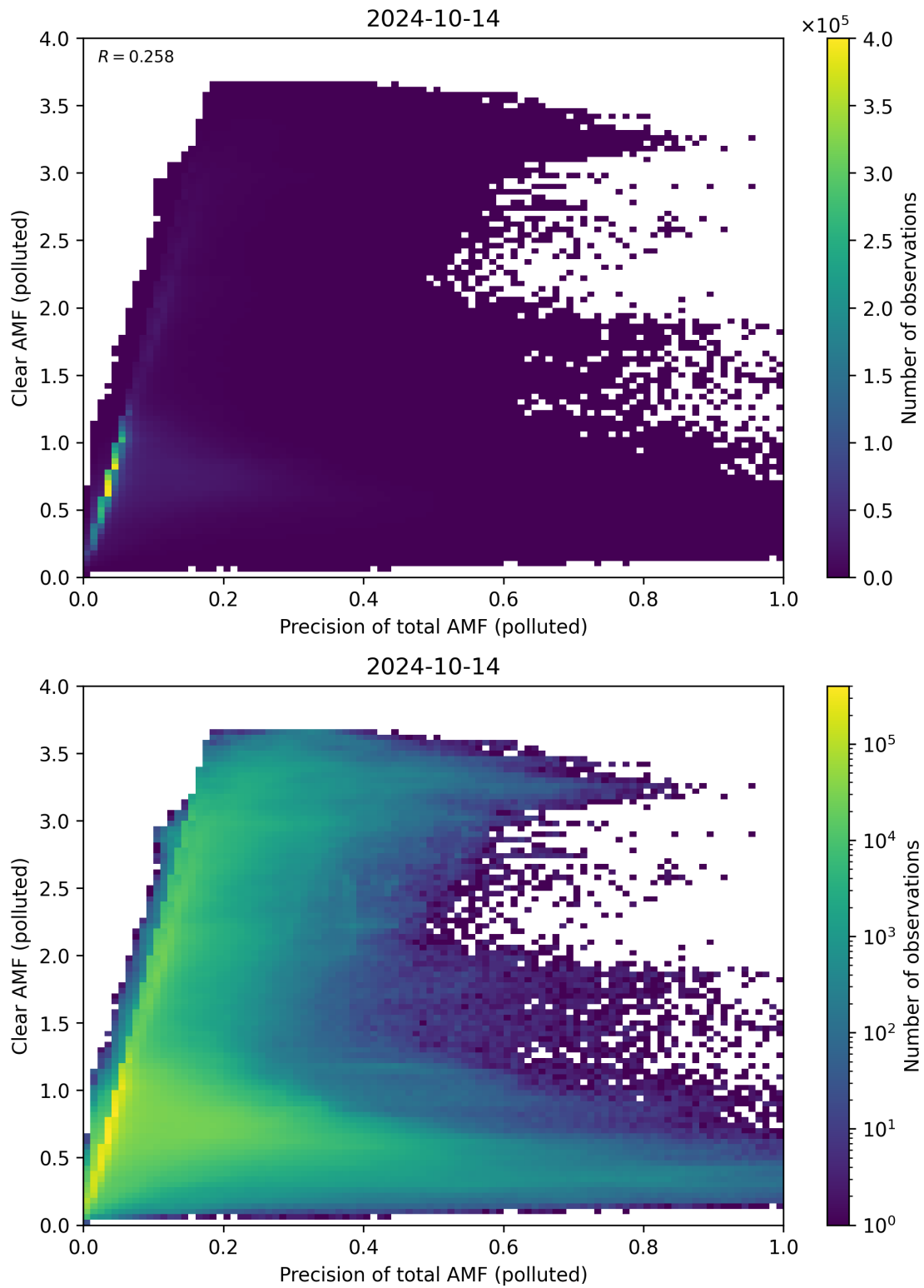
Figure 270: Scatter density plot of “Precision of total AMF (polluted)” against “Clear AMF (polluted)” for 2024-10-14 to 2024-10-15.
