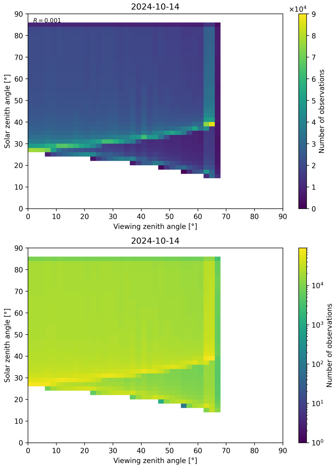
Figure 315: Scatter density plot of “Viewing zenith angle” against “Solar zenith angle” for 2024-10-14 to 2024-10-15.
