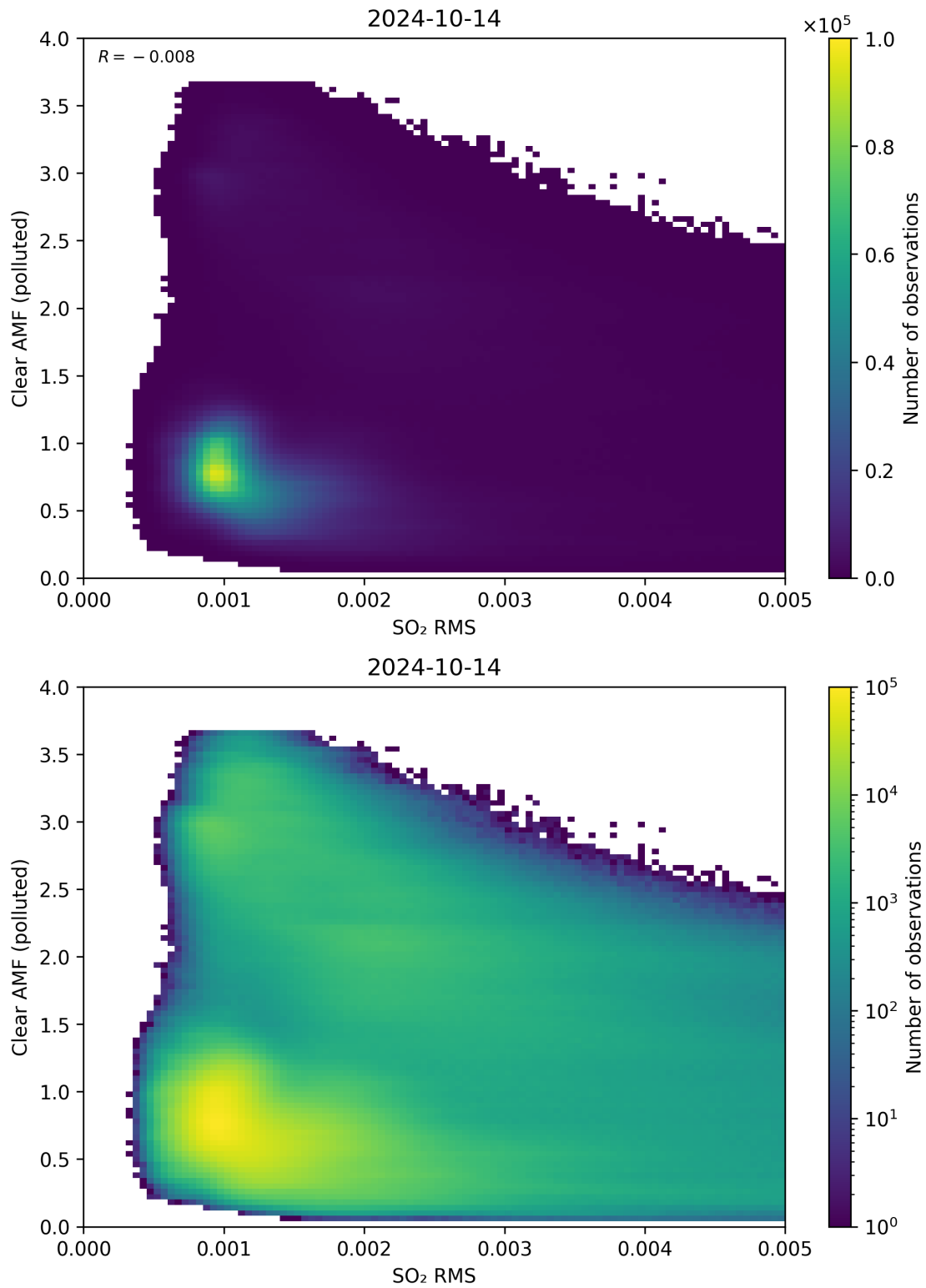
Figure 136: Scatter density plot of “SO 2 RMS” against “Clear AMF (polluted)” for 2024-10-14 to 2024-10-15.
