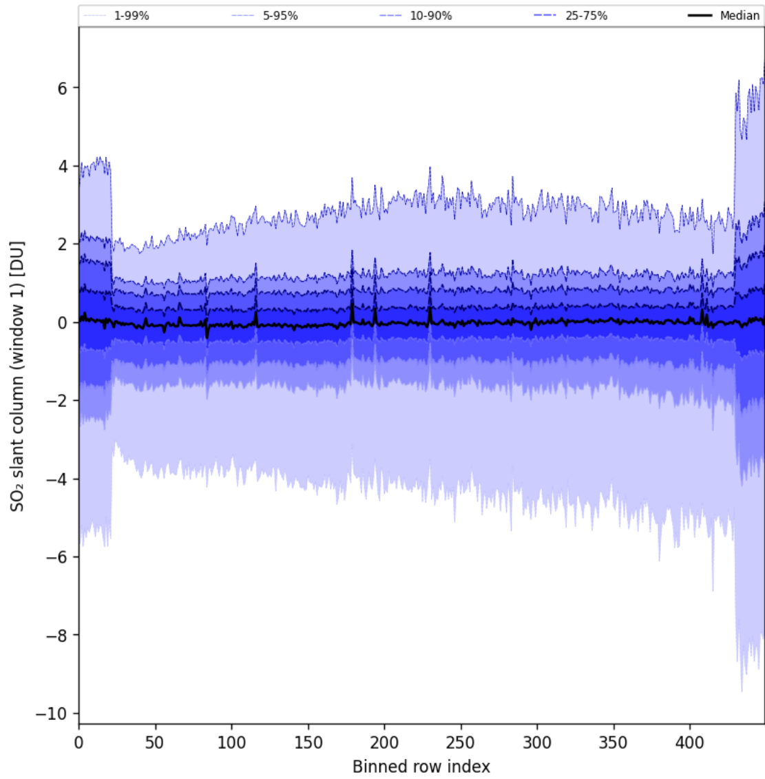
Figure 79: Along track statistics of “SO 2 slant column (window 1)” for 2024-10-14 to 2024-10-15
