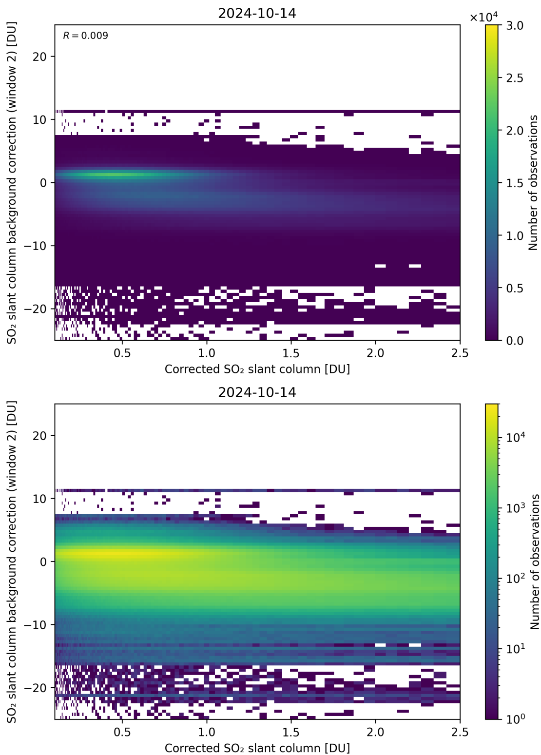
Figure 179: Scatter density plot of “Corrected SO 2 slant column” against “SO 2 slant column background correction (window 2)” for 2024-10-14 to 2024-10-15.
