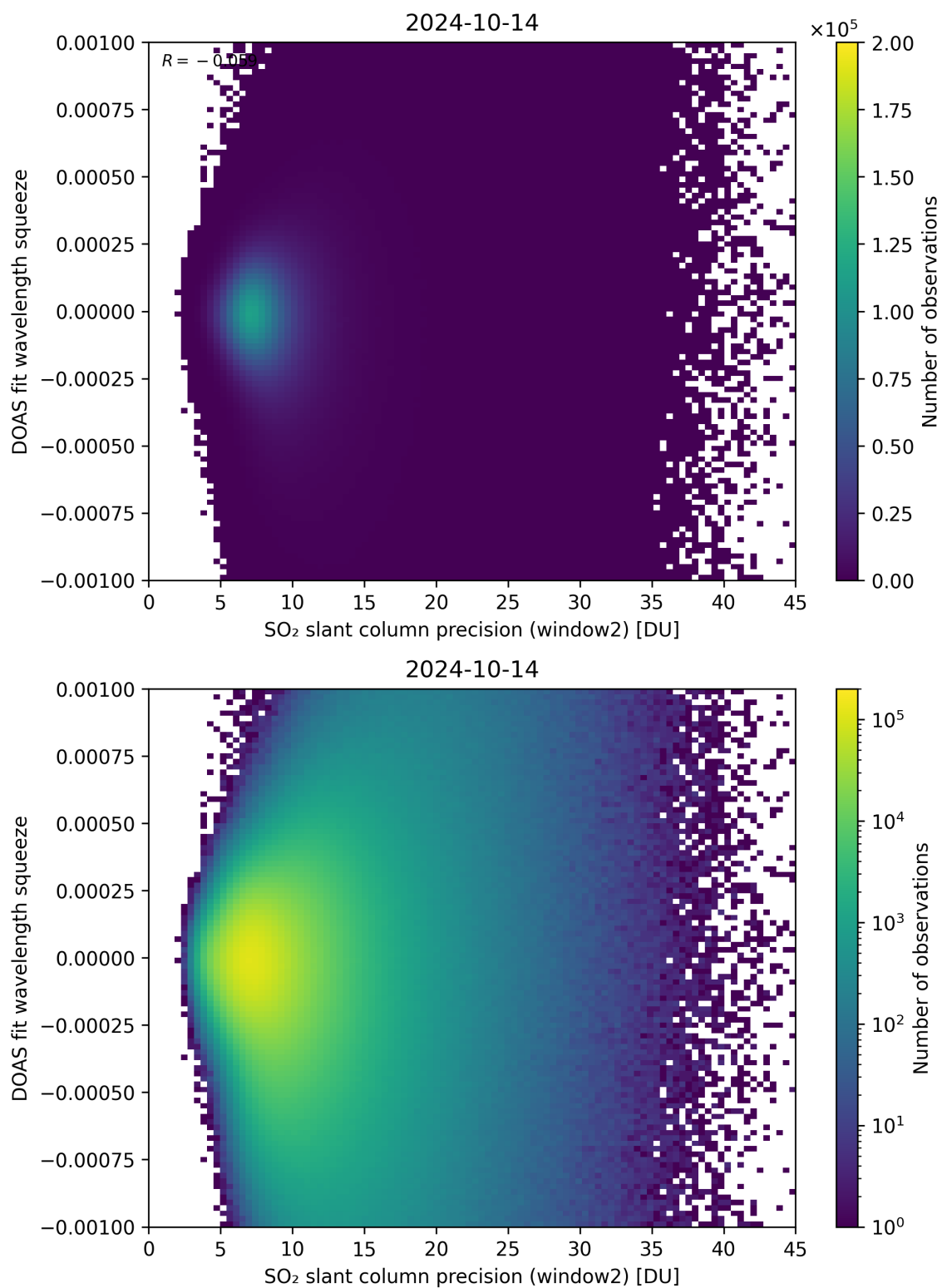
Figure 244: Scatter density plot of “SO 2 slant column precision (window2)” against “DOAS fit wavelength squeeze” for 2024-10-14 to 2024-10-15.
