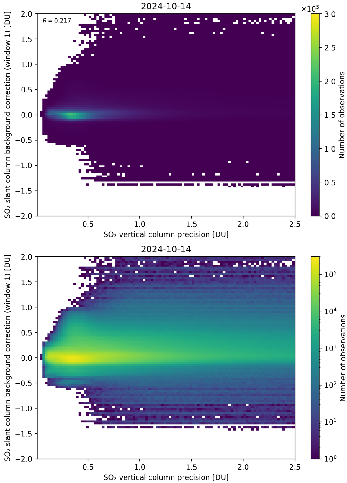
Figure 279: Scatter density plot of “SO 2 vertical column precision” against “SO 2 slant column background correction (window 1)” for 2024-10-14 to 2024-10-15.
