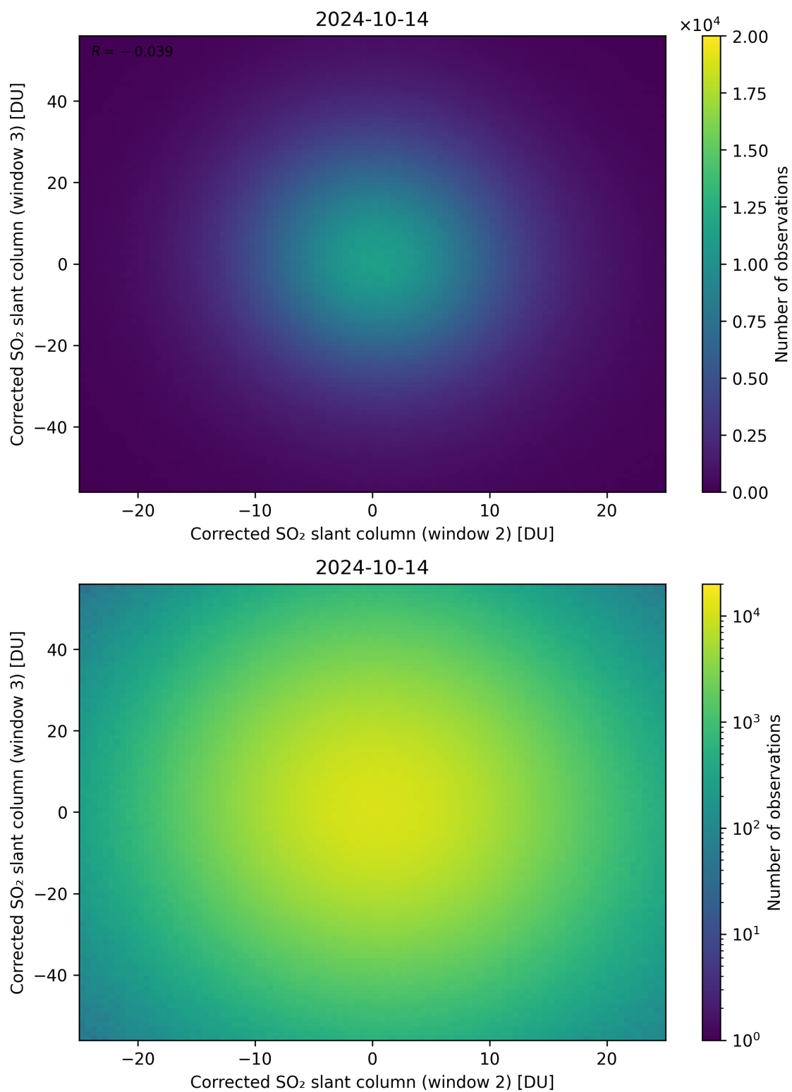
Figure 200: Scatter density plot of “Corrected SO 2 slant column (window 2)” against “Corrected SO 2 slant column (window 3)” for 2024-10-14 to 2024-10-15.
