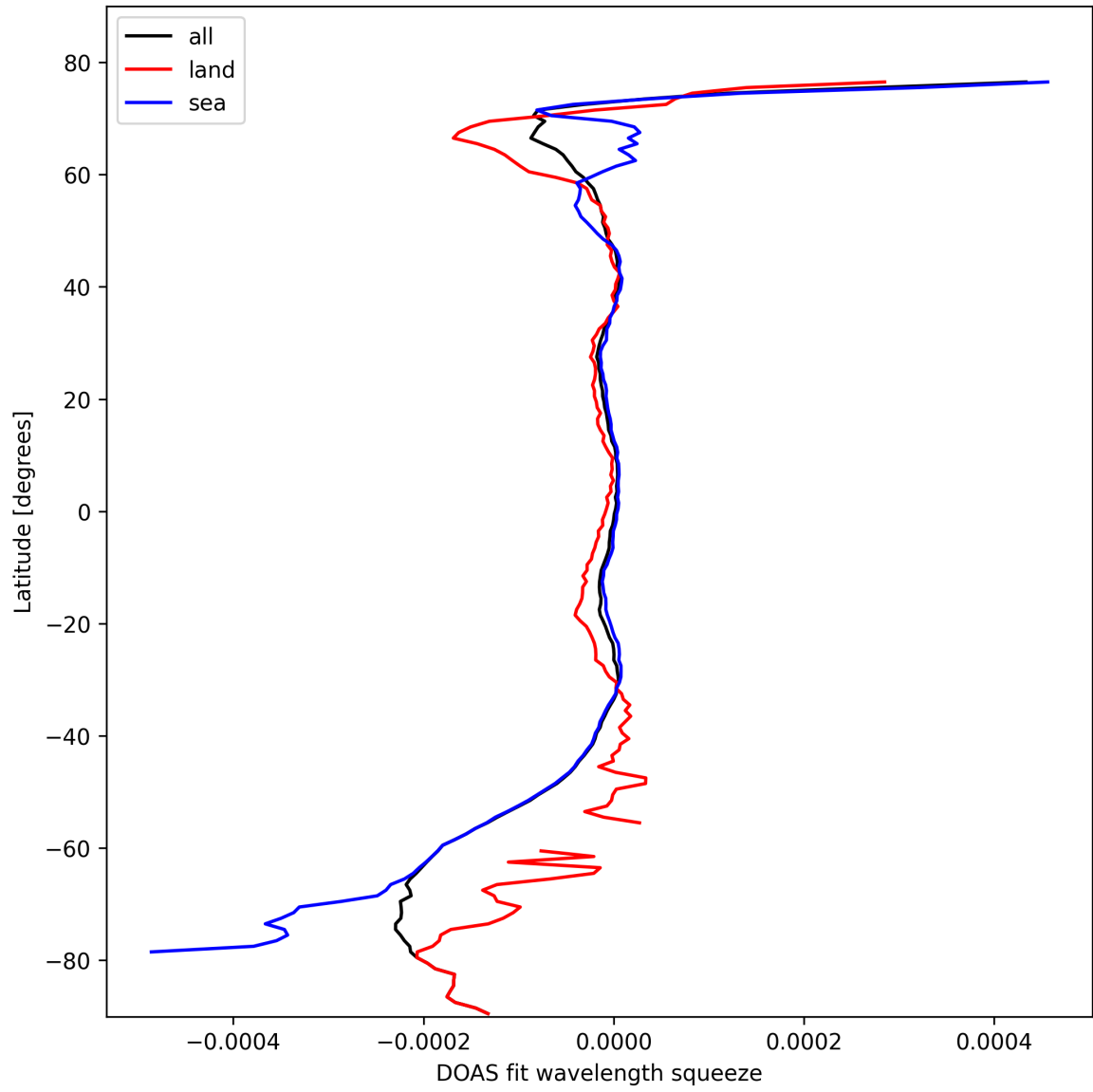
Figure 46: Zonal average of "DOAS fit wavelength squeeze" for 2024-10-14 to 2024-10-15.
