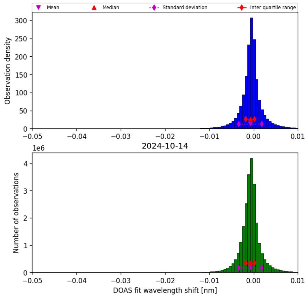
Figure 68: Histogram of “DOAS fit wavelength shift” for 2024-10-14 to 2024-10-15
