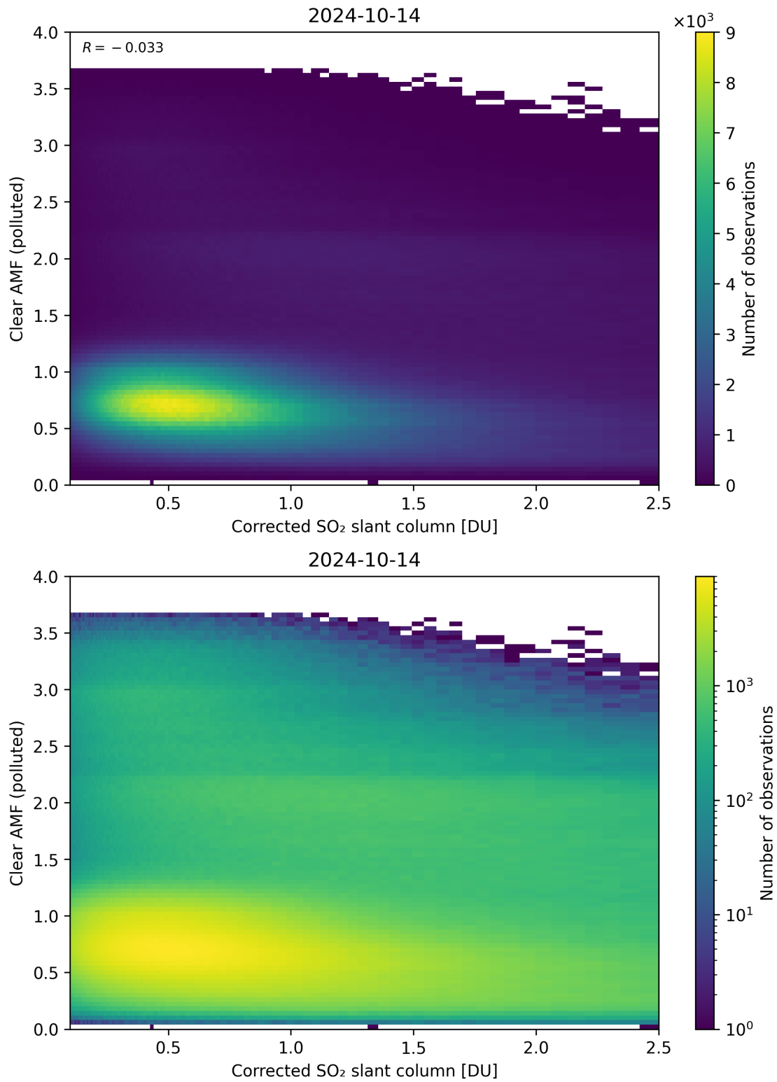
Figure 184: Scatter density plot of “Corrected SO 2 slant column” against “Clear AMF (polluted)” for 2024-10-14 to 2024-10-15.
