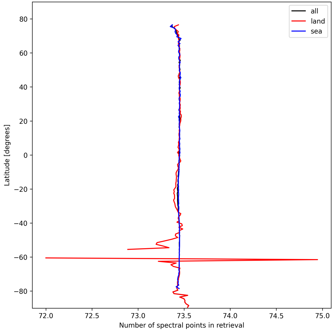
Figure 51: Zonal average of “Number of spectral points in retrieval” for 2024-10-14 to 2024-10-15.
