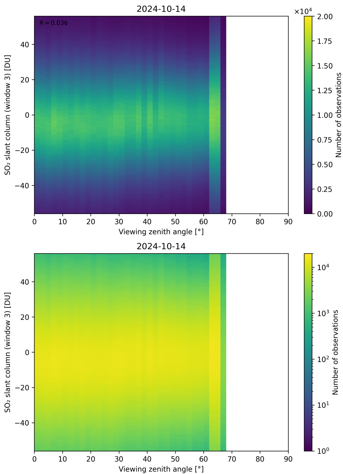
Figure 323: Scatter density plot of “Viewing zenith angle” against “SO 2 slant column (window 3)” for 2024-10-14 to 2024-10-15.
