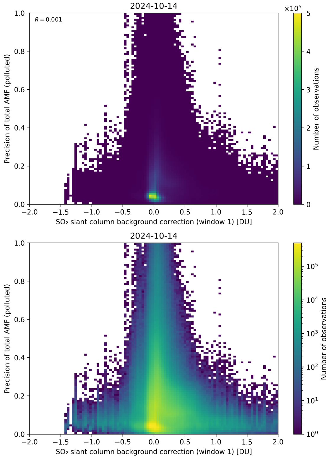
Figure 110: Scatter density plot of “SO 2 slant column background correction (window 1)” against “Precision of total AMF (polluted)” for 2024-10-14 to 2024-10-15.
