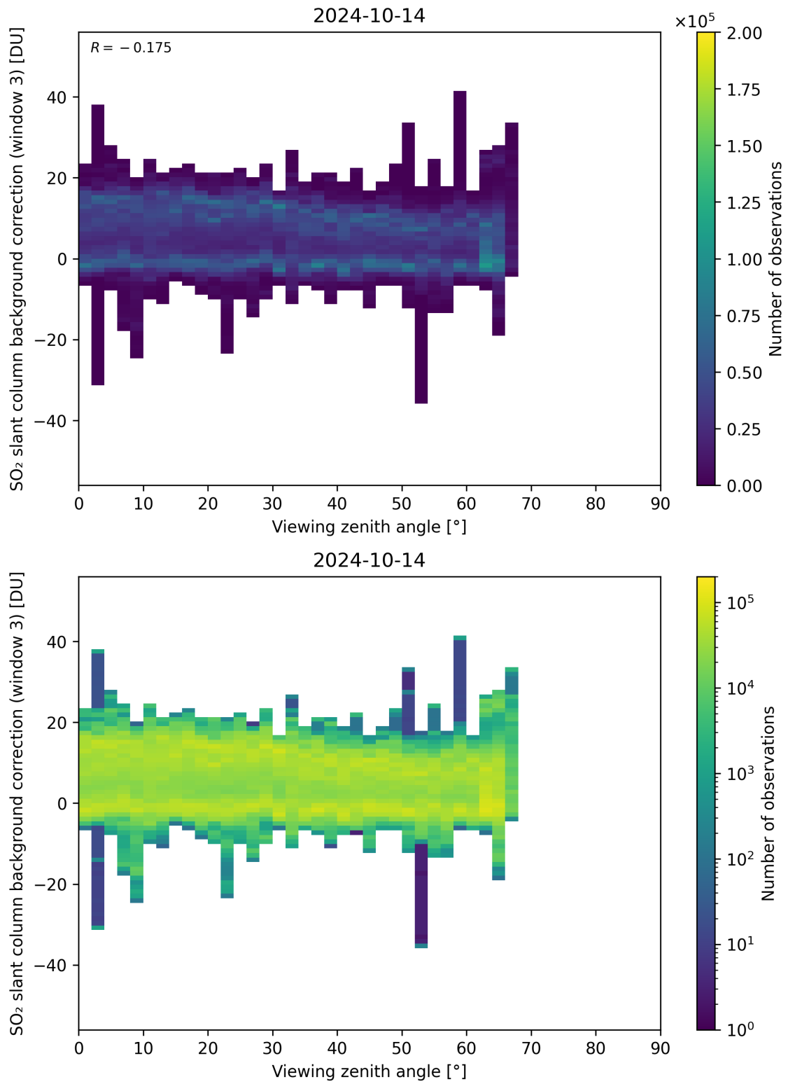
Figure 310: Scatter density plot of “Viewing zenith angle” against “SO 2 slant column background correction (window 3)” for 2024-10-14 to 2024-10-15.
