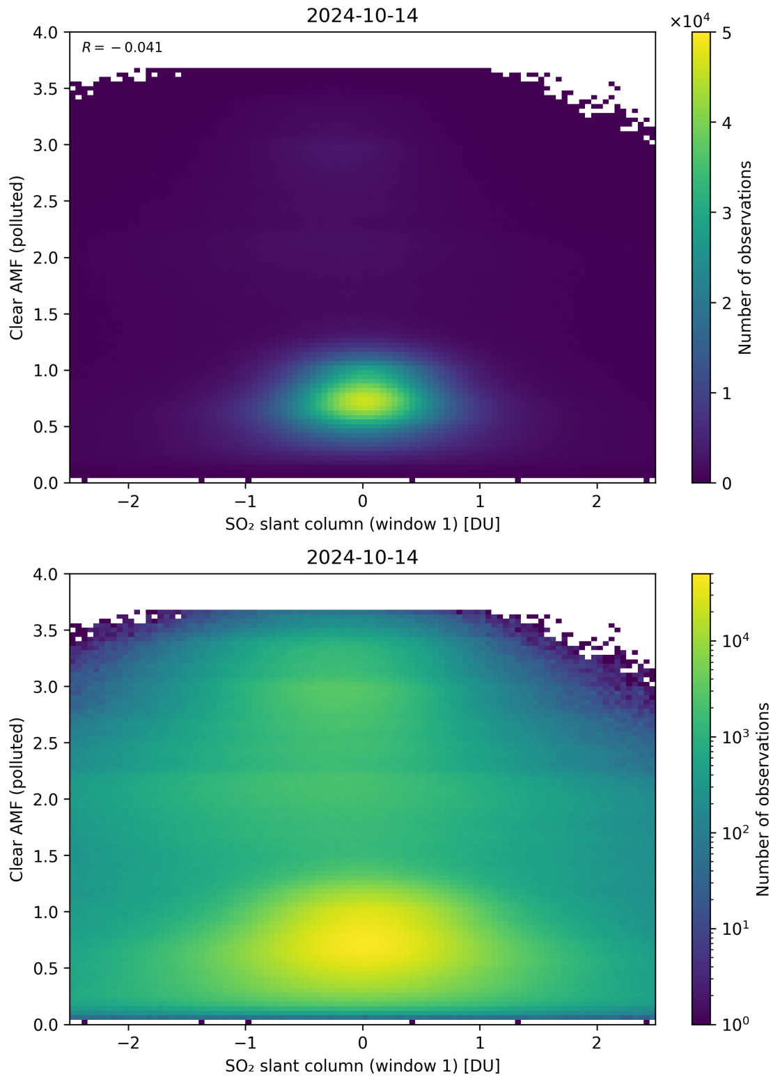
Figure 232: Scatter density plot of “SO 2 slant column (window 1)” against “Clear AMF (polluted)” for 2024-10-14 to 2024-10-15.
