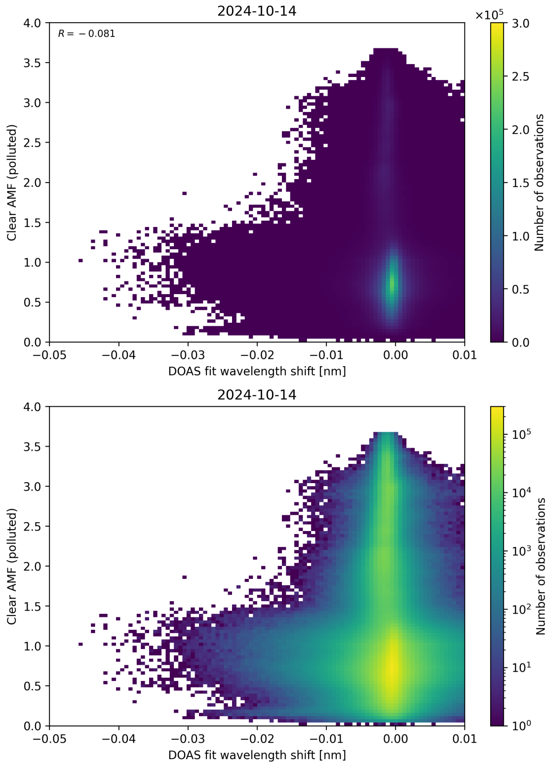
Figure 129: Scatter density plot of “DOAS fit wavelength shift” against “Clear AMF (polluted)” for 2024-10-14 to 2024-10-15.
