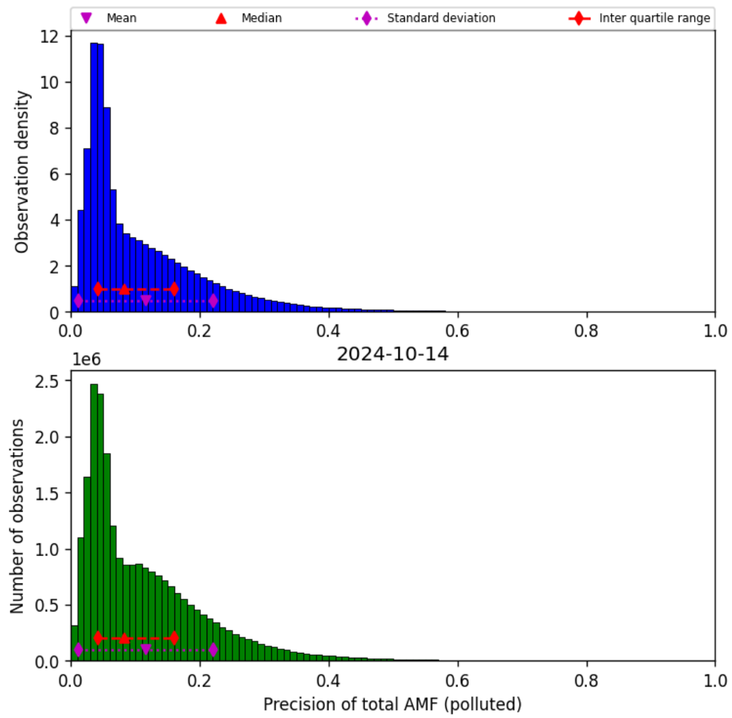
Figure 72: Histogram of “Precision of total AMF (polluted)” for 2024-10-14 to 2024-10-15
