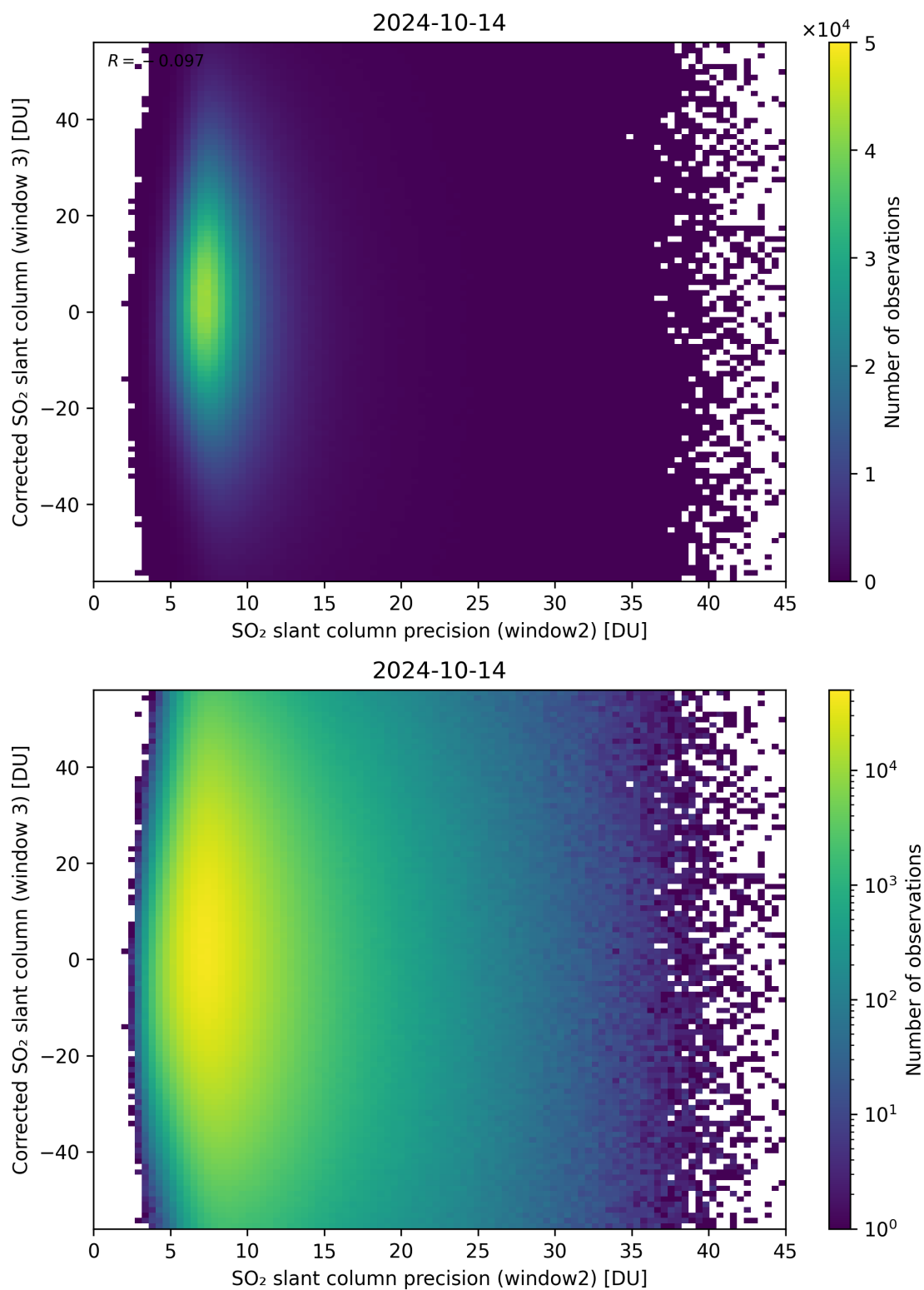
Figure 248: Scatter density plot of “SO 2 slant column precision (window2)” against “Corrected SO 2 slant column (window 3)” for 2024-10-14 to 2024-10-15.
