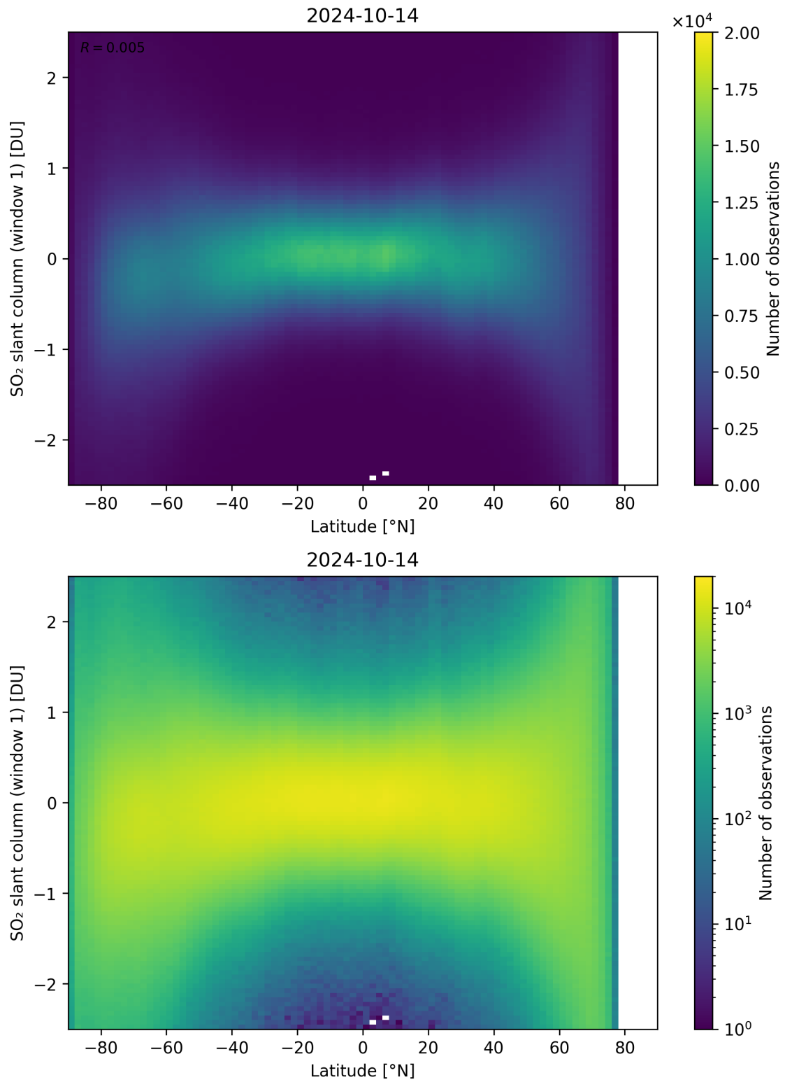
Figure 149: Scatter density plot of “Latitude” against “SO 2 slant column (window 1)” for 2024-10-14 to 2024-10-15.
