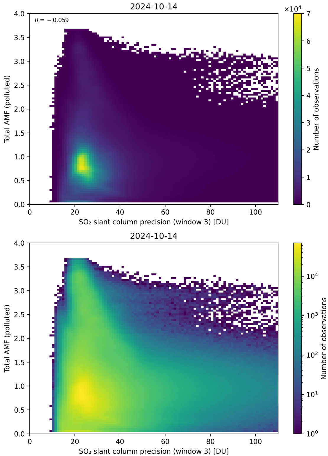
Figure 263: Scatter density plot of “SO 2 slant column precision (window 3)” against “Total AMF (polluted)” for 2024-10-14 to 2024-10-15.
