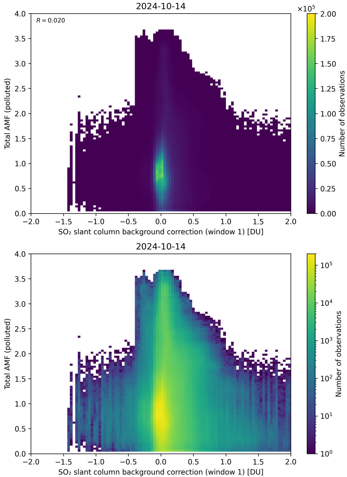
Figure 109: Scatter density plot of “SO 2 slant column background correction (window 1)” against “Total AMF (polluted)” for 2024-10-14 to 2024-10-15.
