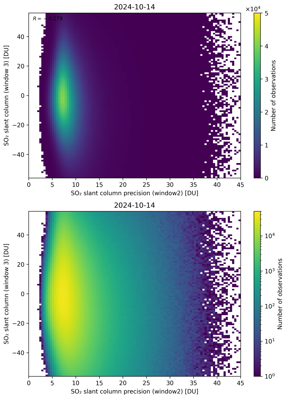
Figure 249: Scatter density plot of “SO 2 slant column precision (window2)” against “SO 2 slant column (window 3)” for 2024-10-14 to 2024-10-15.
