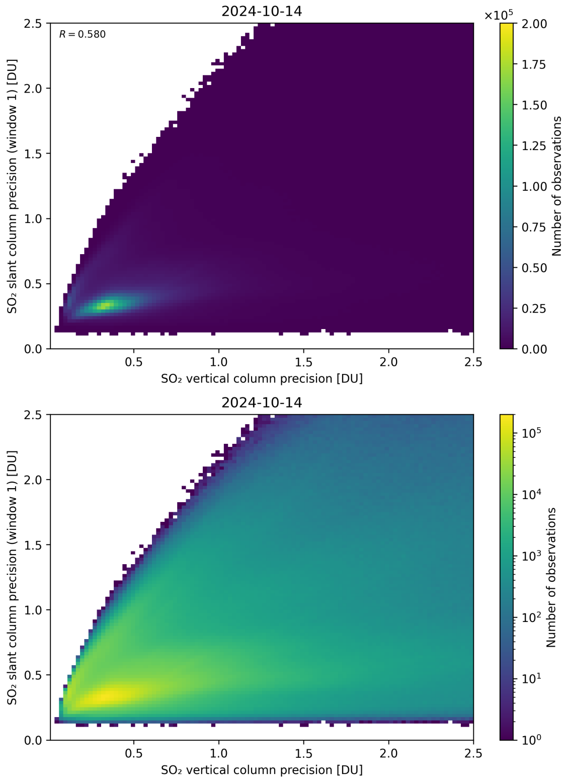
Figure 290: Scatter density plot of “SO 2 vertical column precision” against “SO 2 slant column precision (window 1)” for 2024-10-14 to 2024-10-15.
