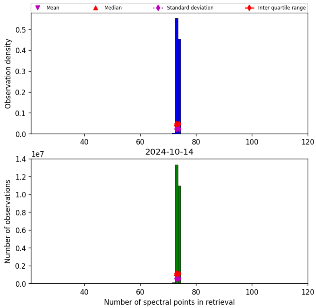
Figure 74: Histogram of “Number of spectral points in retrieval” for 2024-10-14 to 2024-10-15
