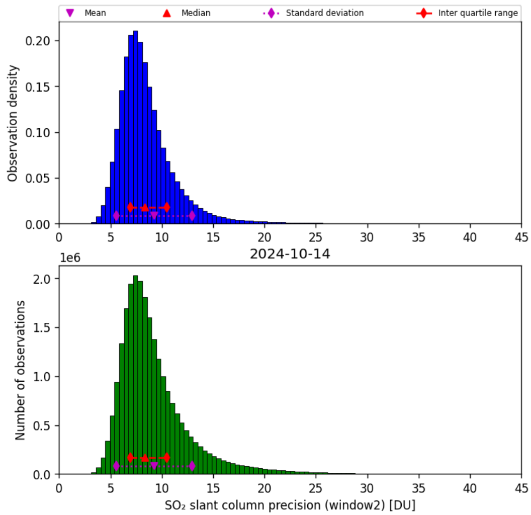
Figure 61: Histogram of “SO 2 slant column precision (window2)” for 2024-10-14 to 2024-10-15
