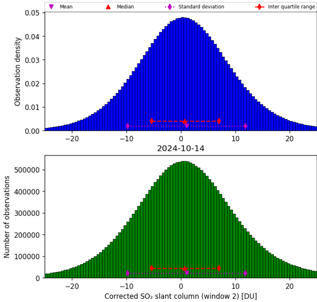
Figure 62: Histogram of “Corrected SO 2 slant column (window 2)” for 2024-10-14 to 2024-10-15
