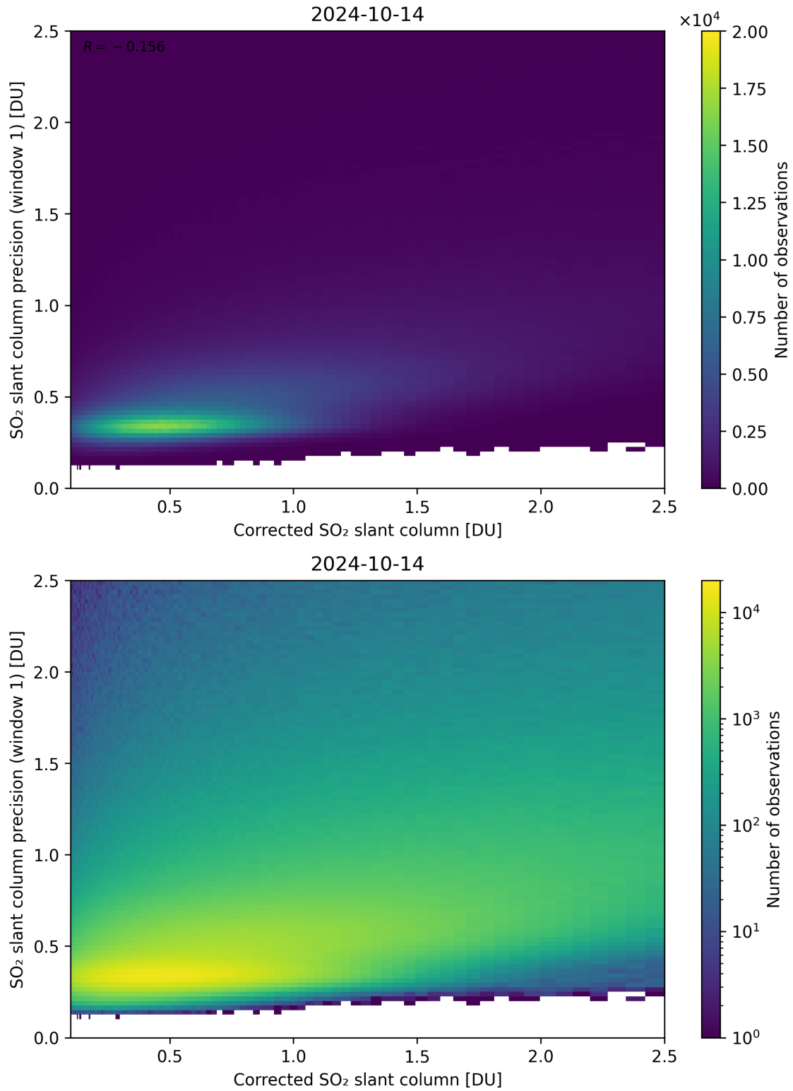
Figure 188: Scatter density plot of “Corrected SO 2 slant column” against “SO 2 slant column precision (window 1)” for 2024-10-14 to 2024-10-15.
