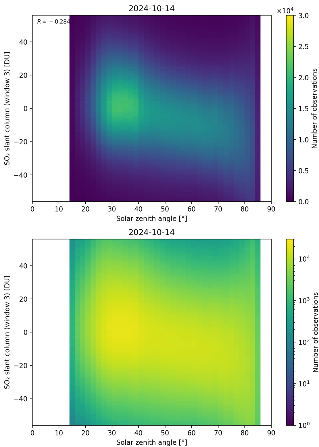
Figure 172: Scatter density plot of “Solar zenith angle” against “SO 2 slant column (window 3)” for 2024-10-14 to 2024-10-15.
