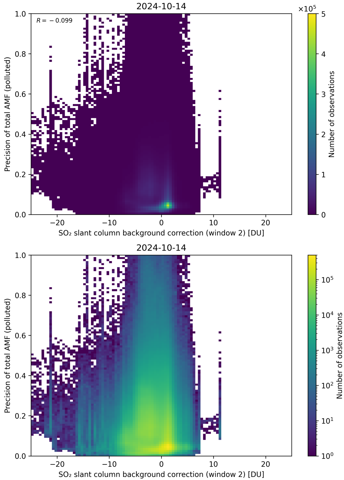
Figure 120: Scatter density plot of “SO 2 slant column background correction (window 2)” against “Precision of total AMF (polluted)” for 2024-10-14 to 2024-10-15.
