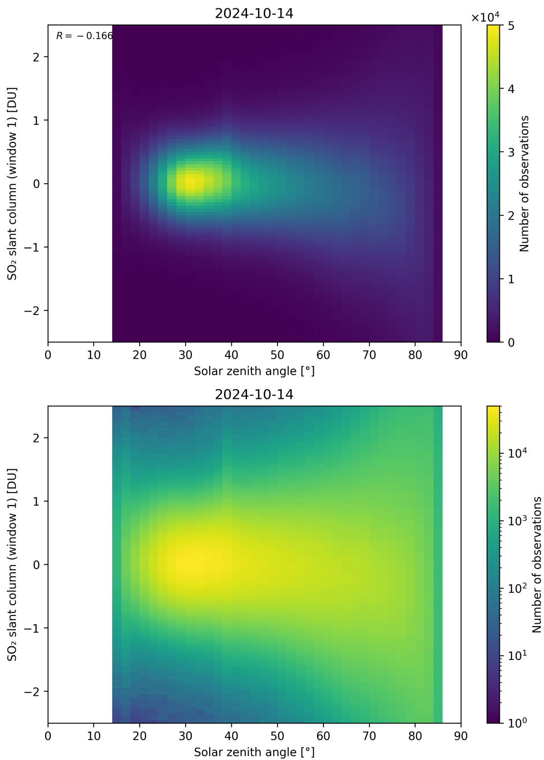
Figure 169: Scatter density plot of “Solar zenith angle” against “SO 2 slant column (window 1)” for 2024-10-14 to 2024-10-15.
