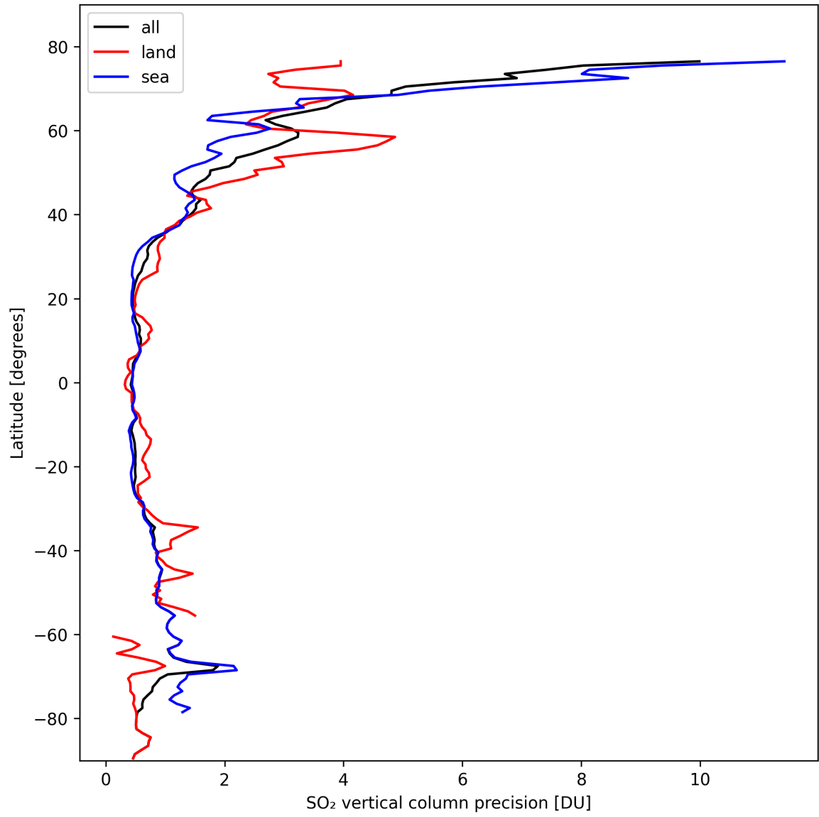
Figure 31: Zonal average of “SO 2 vertical column precision” for 2024-10-14 to 2024-10-15.
