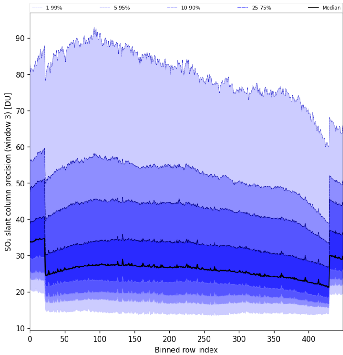
Figure 88: Along track statistics of “SO 2 slant column precision (window 3)” for 2024-10-14 to 2024-10-15
