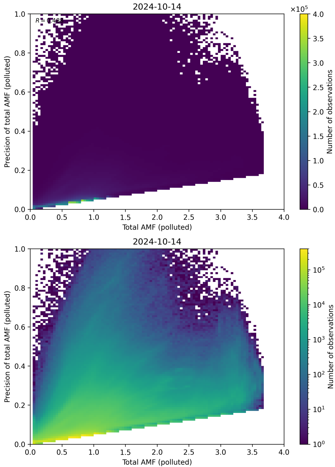
Figure 272: Scatter density plot of “Total AMF (polluted)” against “Precision of total AMF (polluted)” for 2024-10-14 to 2024-10-15.
