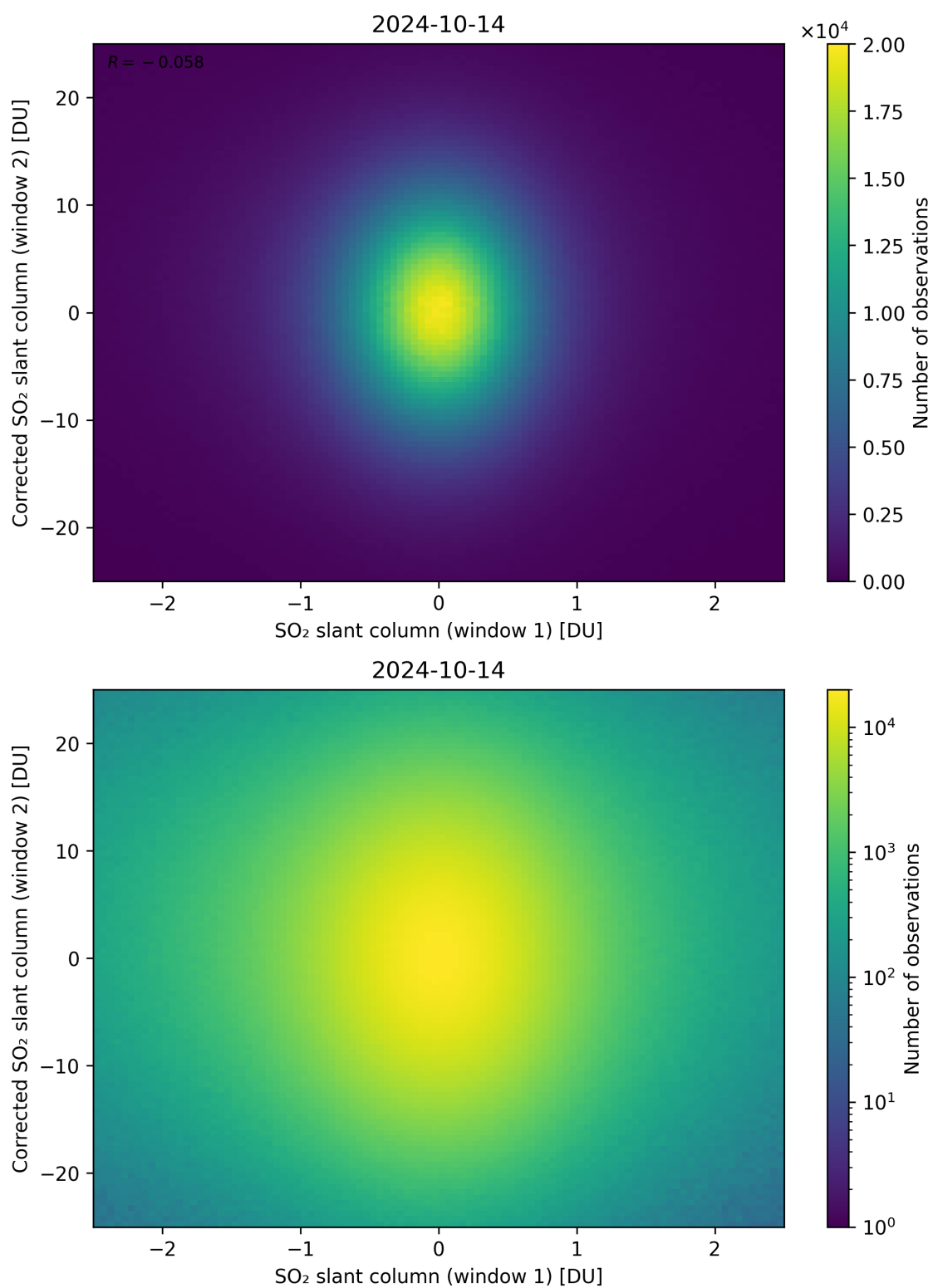
Figure 233: Scatter density plot of “SO 2 slant column (window 1)” against “Corrected SO 2 slant column (window 2)” for 2024-10-14 to 2024-10-15.
