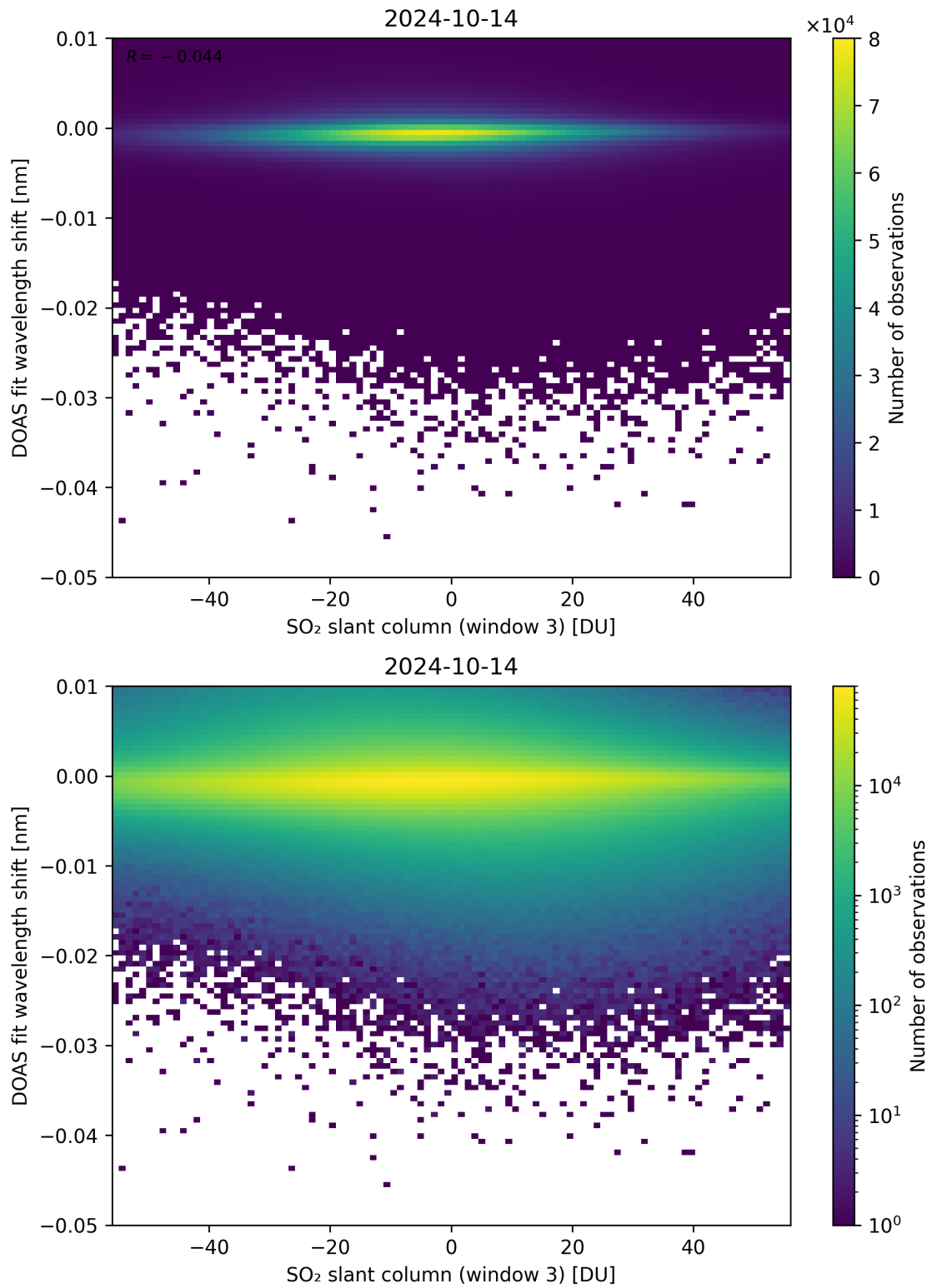
Figure 254: Scatter density plot of “SO 2 slant column (window 3)” against “DOAS fit wavelength shift” for 2024-10-14 to 2024-10-15.
