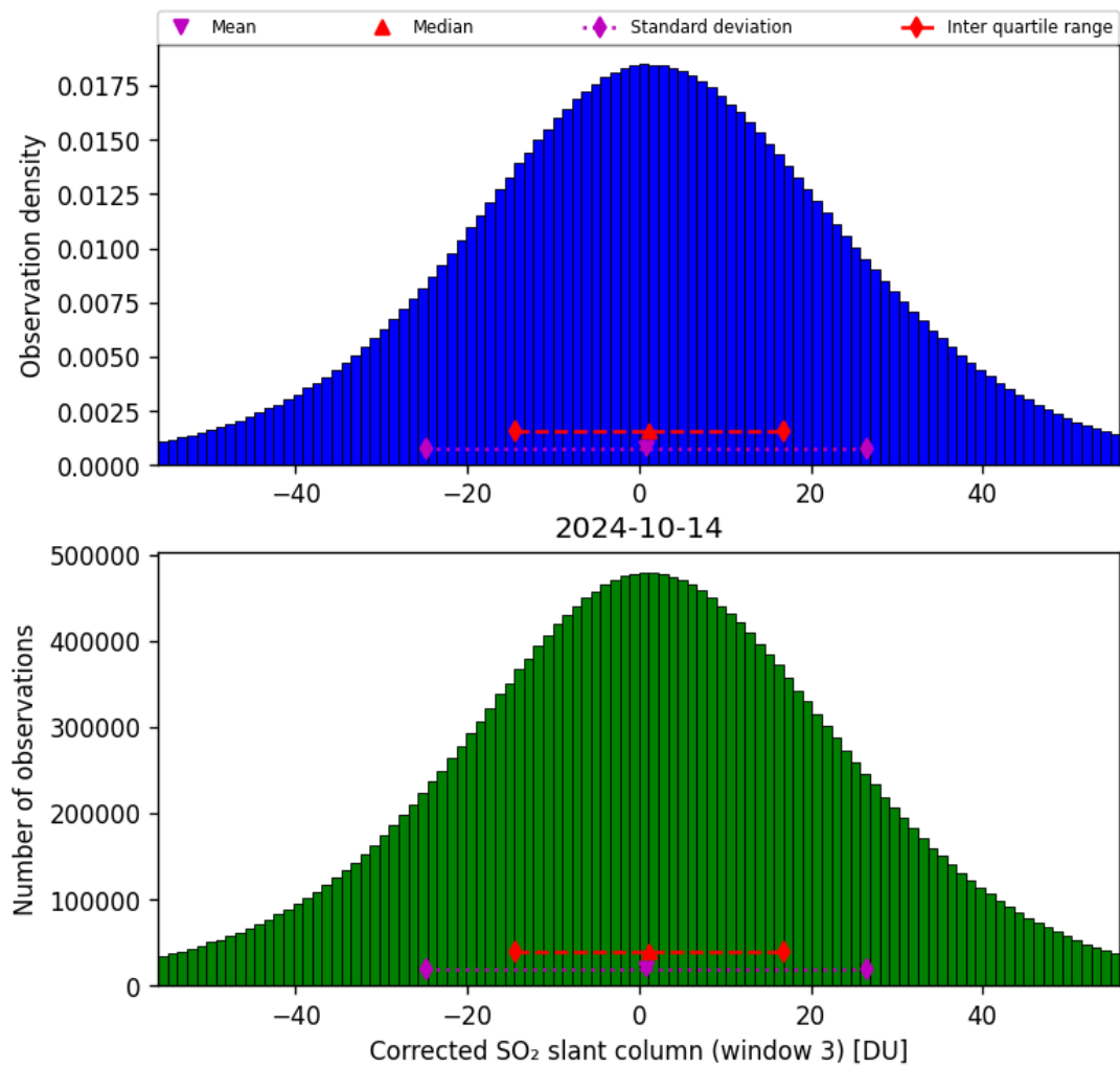
Figure 66: Histogram of “Corrected SO 2 slant column (window 3)” for 2024-10-14 to 2024-10-15
