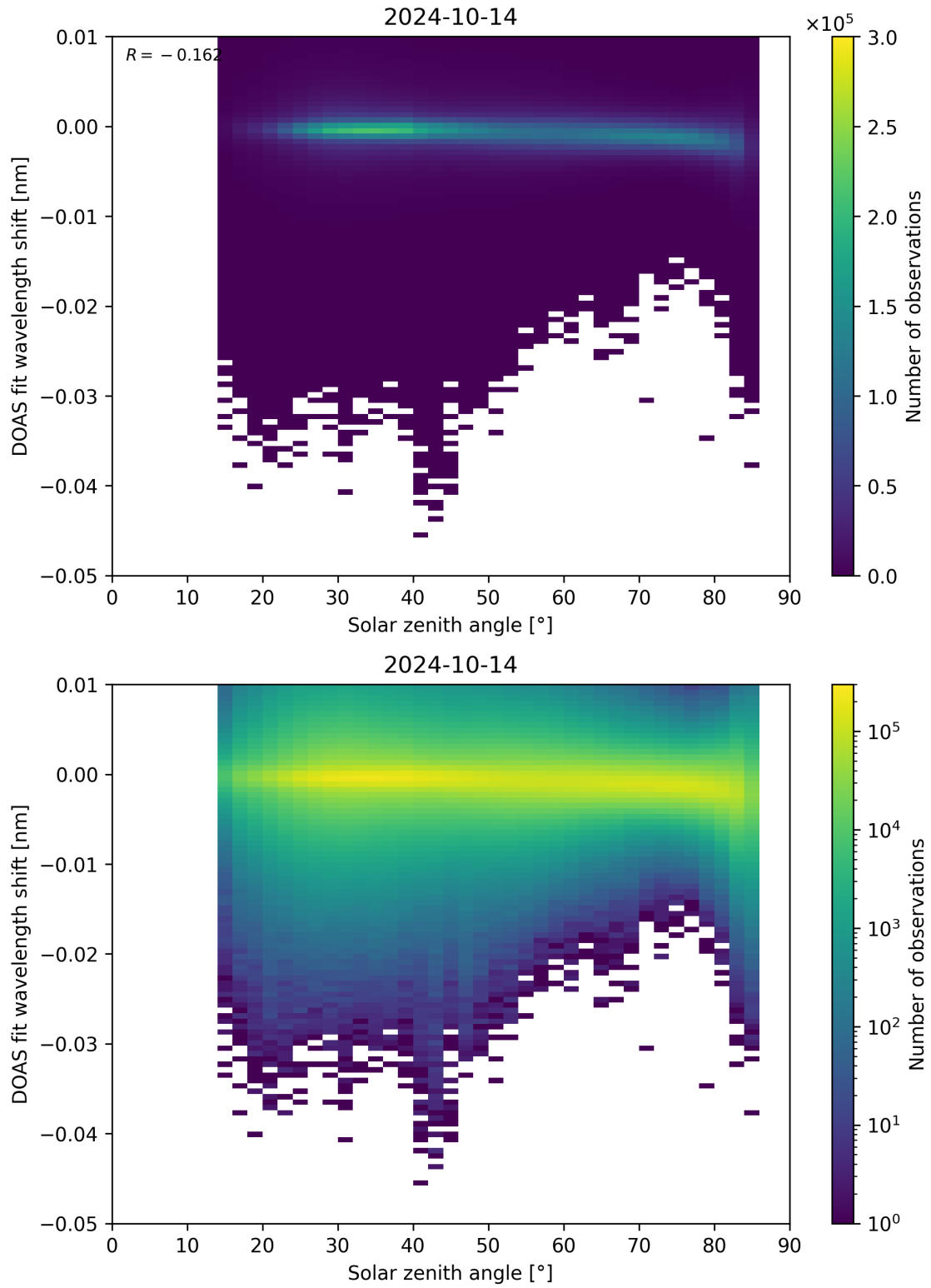
Figure 161: Scatter density plot of “Solar zenith angle” against “DOAS fit wavelength shift” for 2024-10-14 to 2024-10-15.
