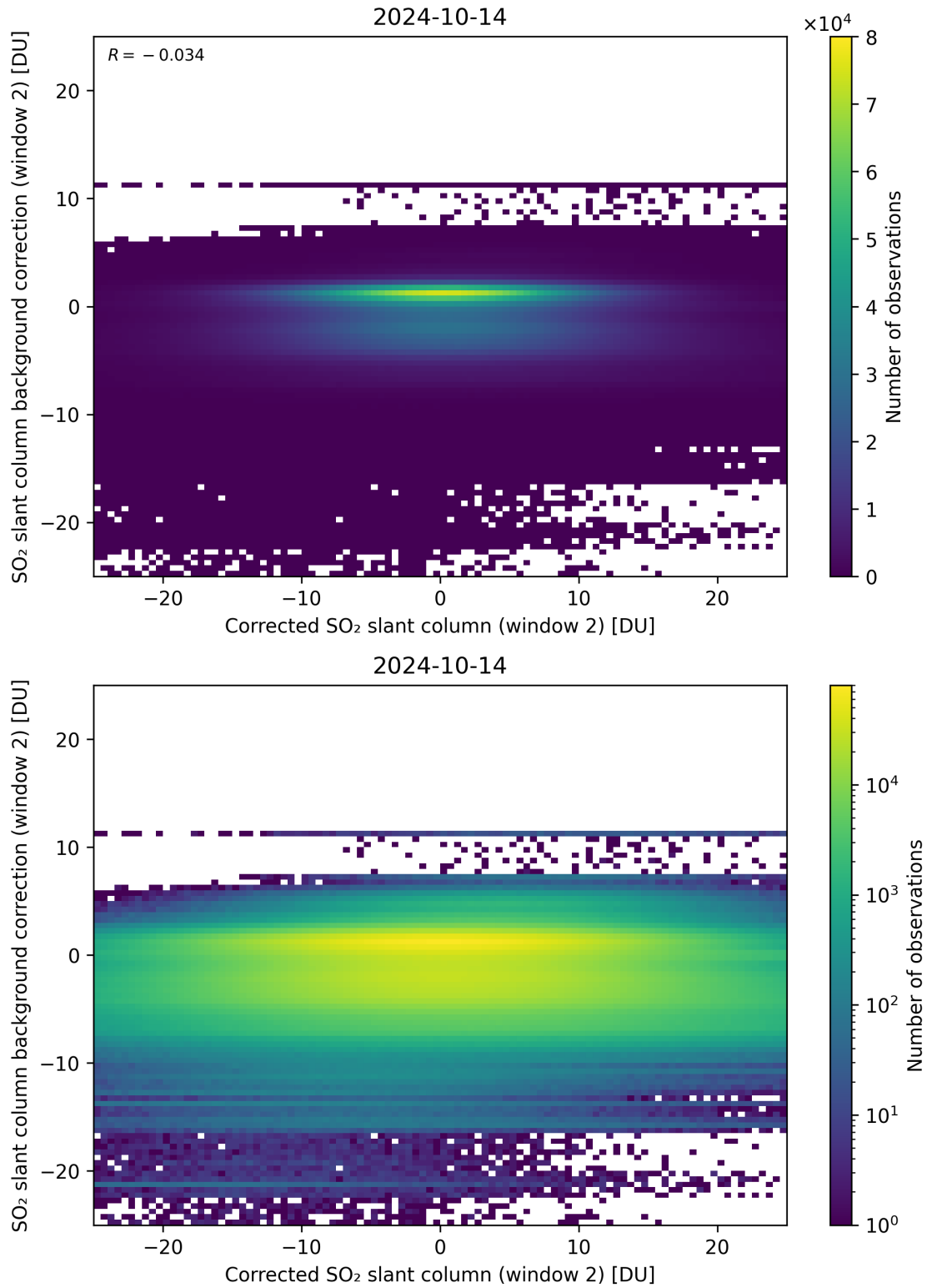
Figure 194: Scatter density plot of “Corrected SO 2 slant column (window 2)” against “SO 2 slant column background correction (window 2)” for 2024-10-14 to 2024-10-15.
