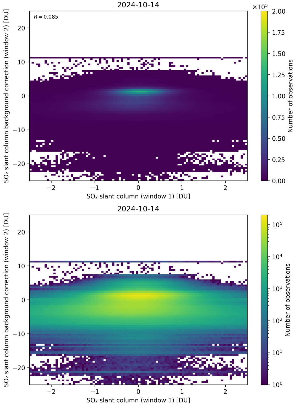
Figure 213: Scatter density plot of “SO 2 slant column (window 1)” against “SO 2 slant column background correction (window 2)” for 2024-10-14 to 2024-10-15.
