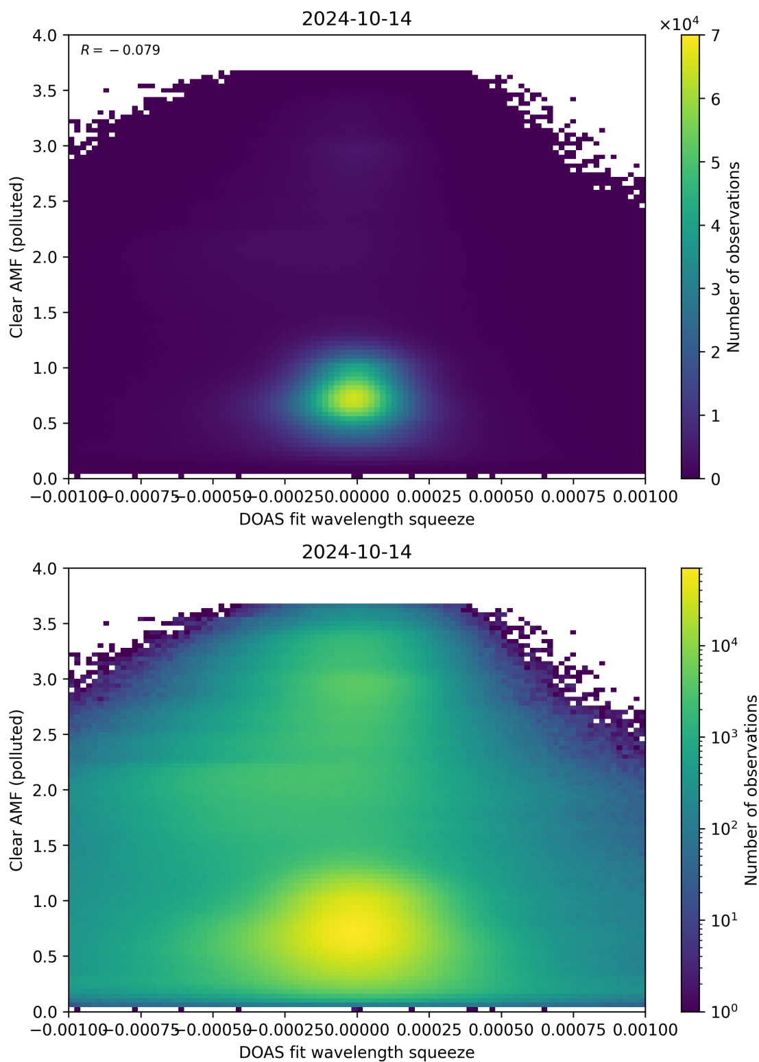
Figure 133: Scatter density plot of “DOAS fit wavelength squeeze” against “Clear AMF (polluted)” for 2024-10-14 to 2024-10-15.
