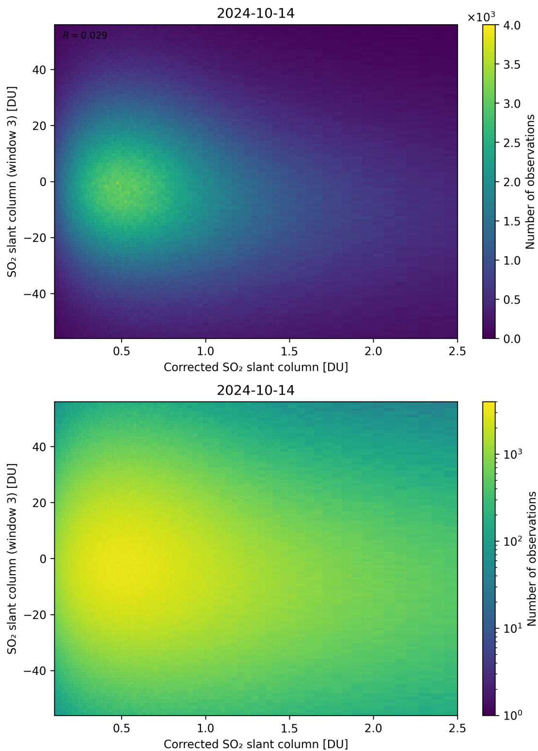
Figure 190: Scatter density plot of “Corrected SO 2 slant column” against “SO 2 slant column (window 3)” for 2024-10-14 to 2024-10-15.
