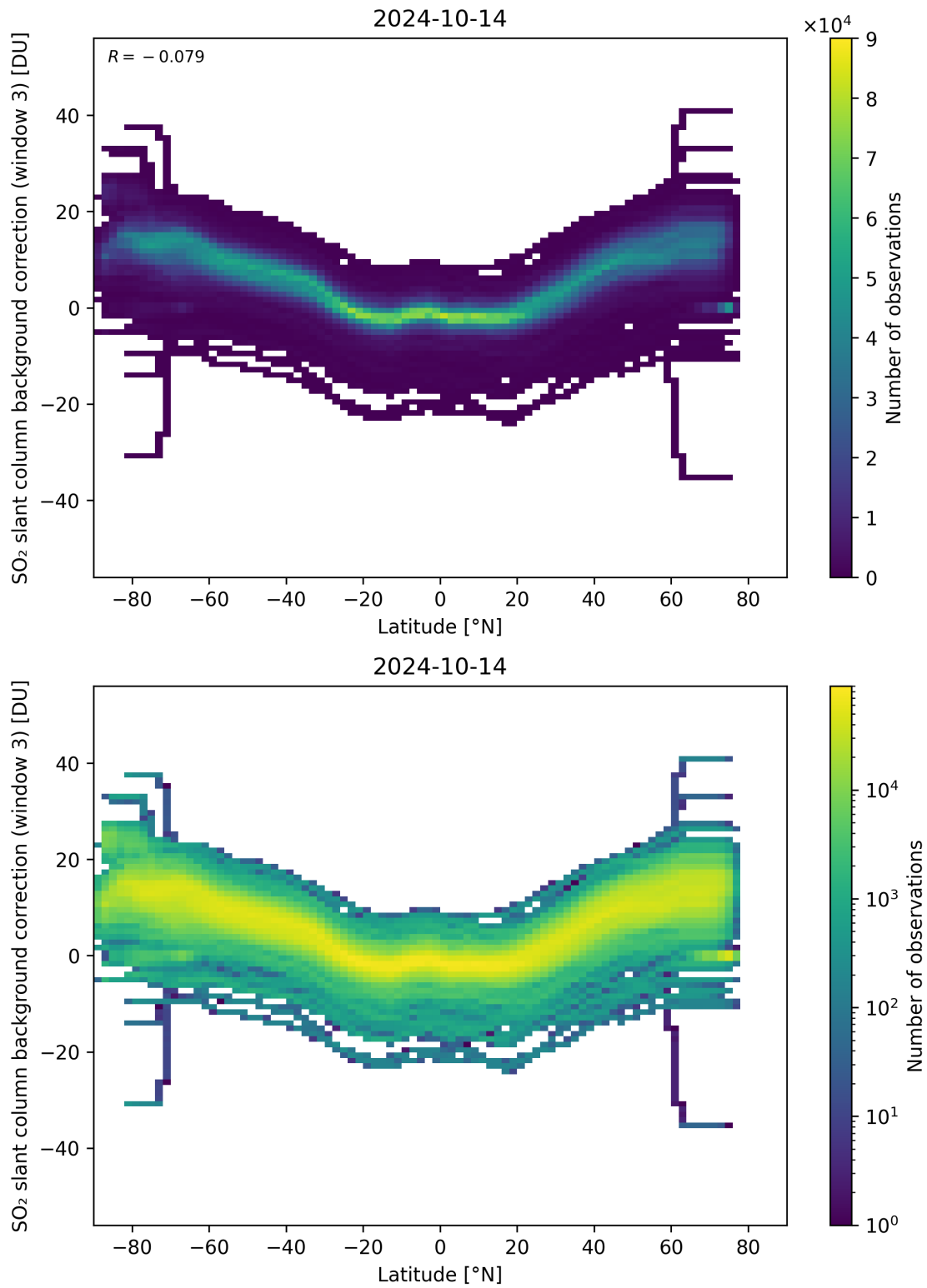
Figure 141: Scatter density plot of “Latitude” against “SO 2 slant column background correction (window 3)” for 2024-10-14 to 2024-10-15.
