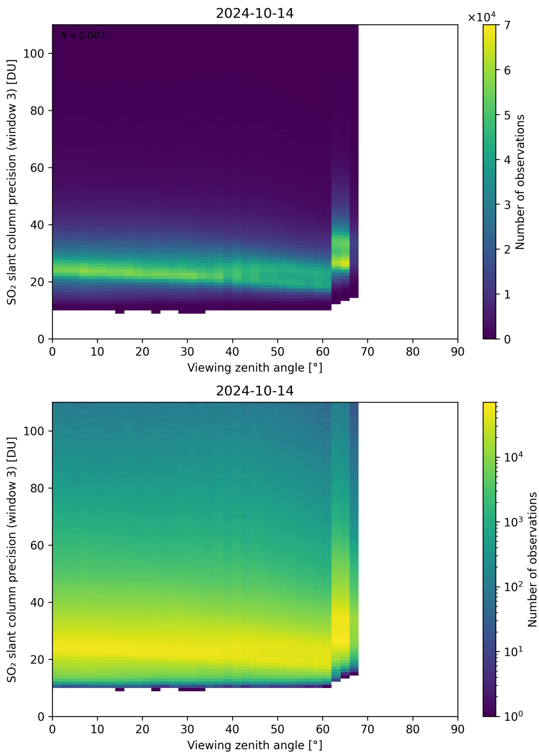
Figure 324: Scatter density plot of “Viewing zenith angle” against “SO 2 slant column precision (window 3)” for 2024-10-14 to 2024-10-15.
