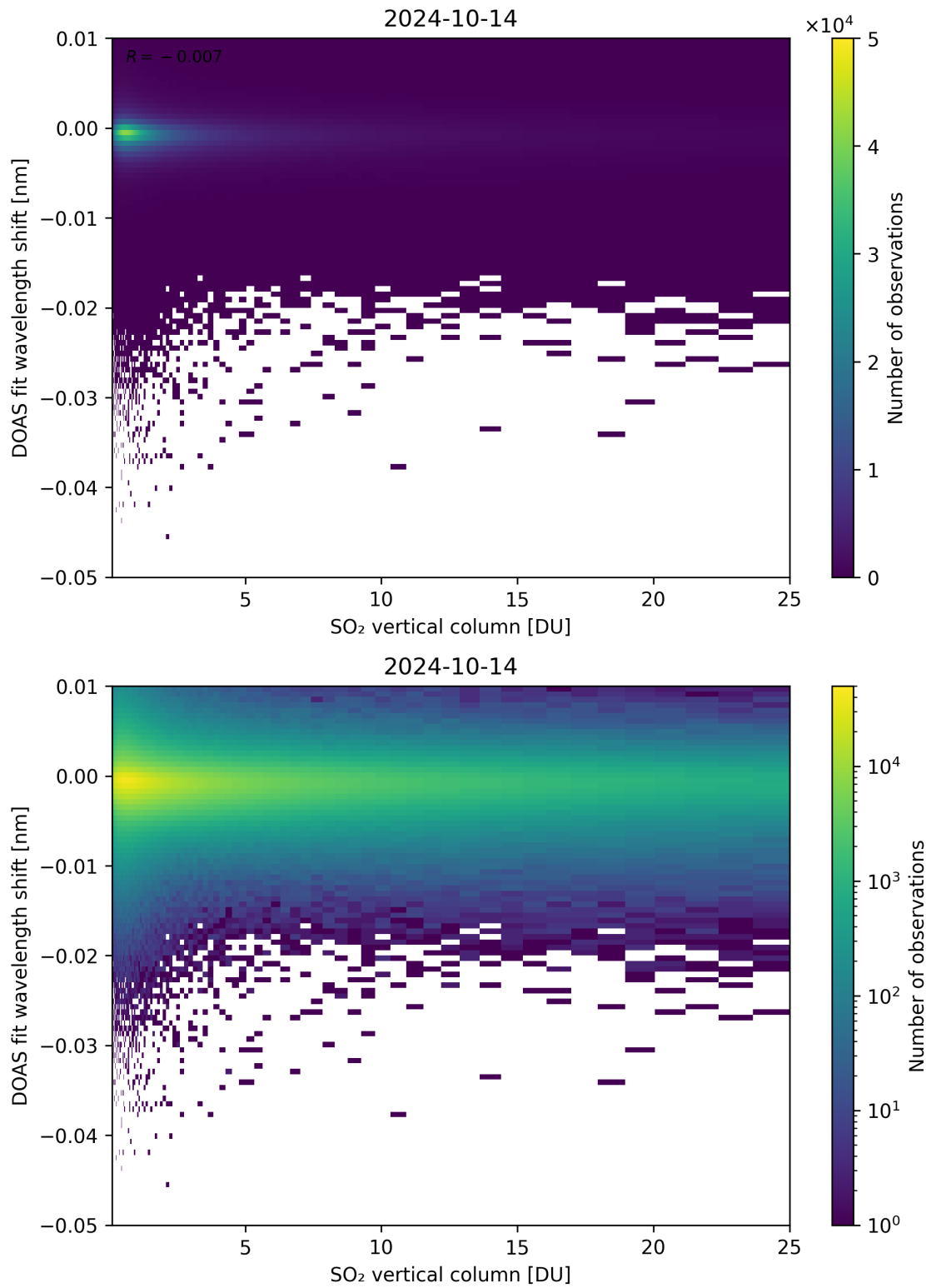
Figure 276: Scatter density plot of “SO 2 vertical column” against “DOAS fit wavelength shift” for 2024-10-14 to 2024-10-15.
