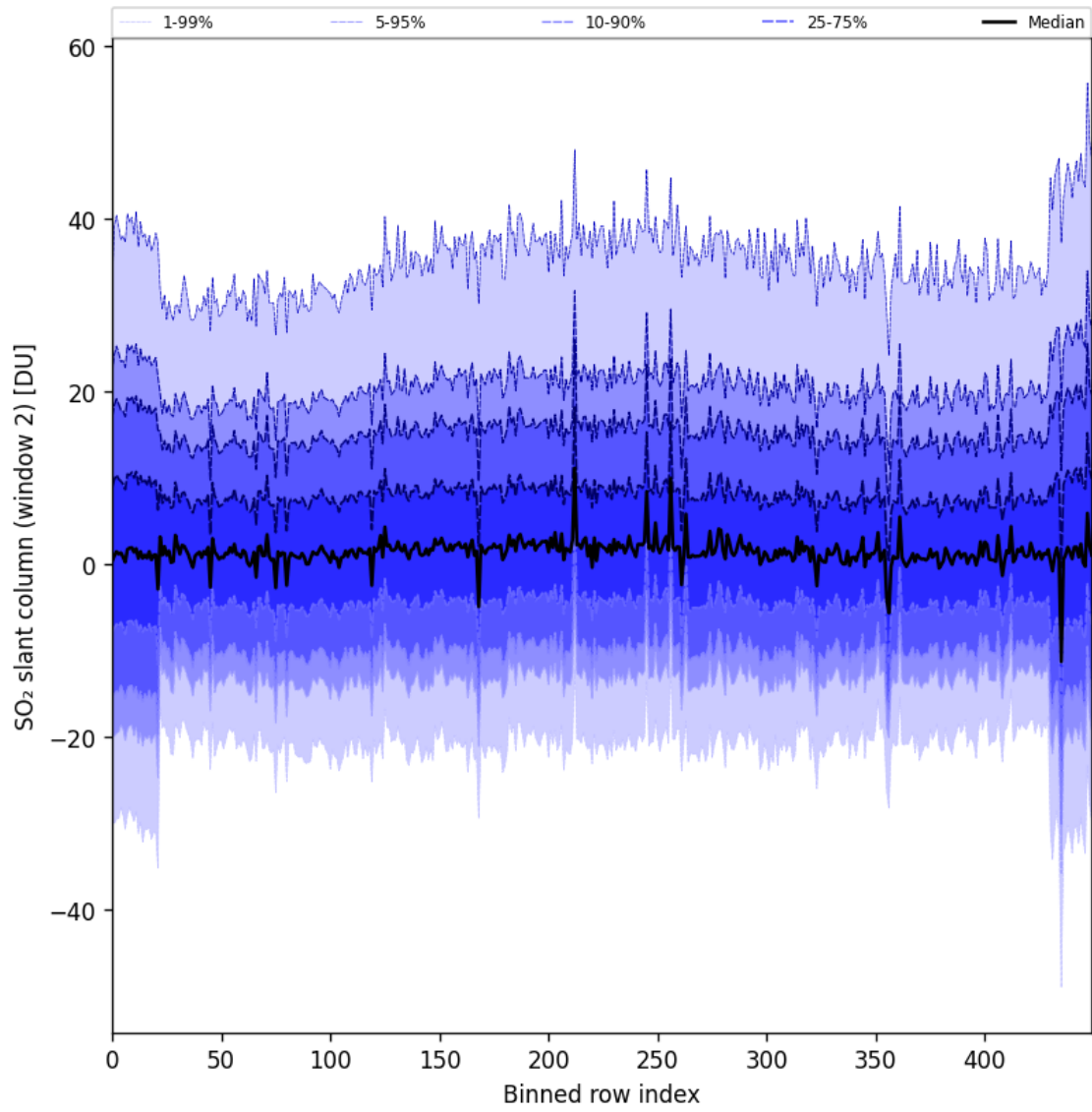
Figure 83: Along track statistics of “SO 2 slant column (window 2)” for 2024-10-14 to 2024-10-15
