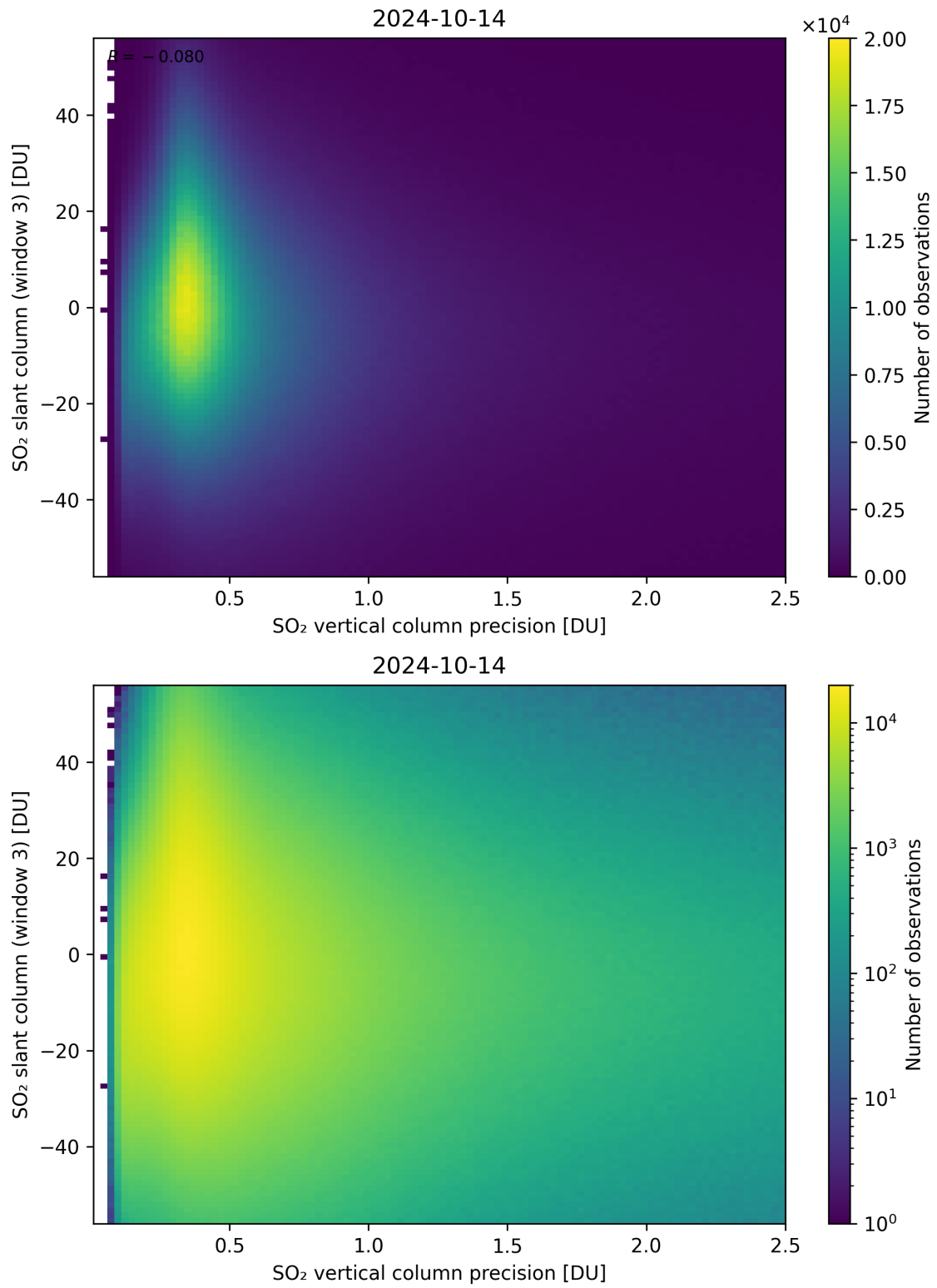
Figure 292: Scatter density plot of “SO 2 vertical column precision” against “SO 2 slant column (window 3)” for 2024-10-14 to 2024-10-15.
