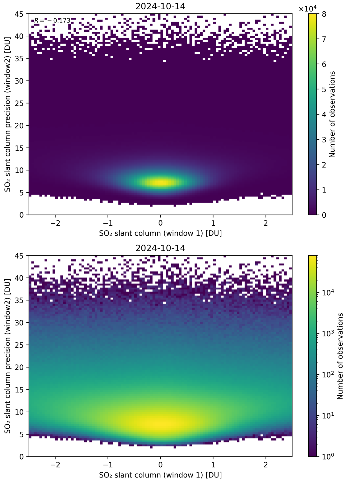
Figure 236: Scatter density plot of “SO 2 slant column (window 1)” against “SO 2 slant column precision (window2)” for 2024-10-14 to 2024-10-15.
