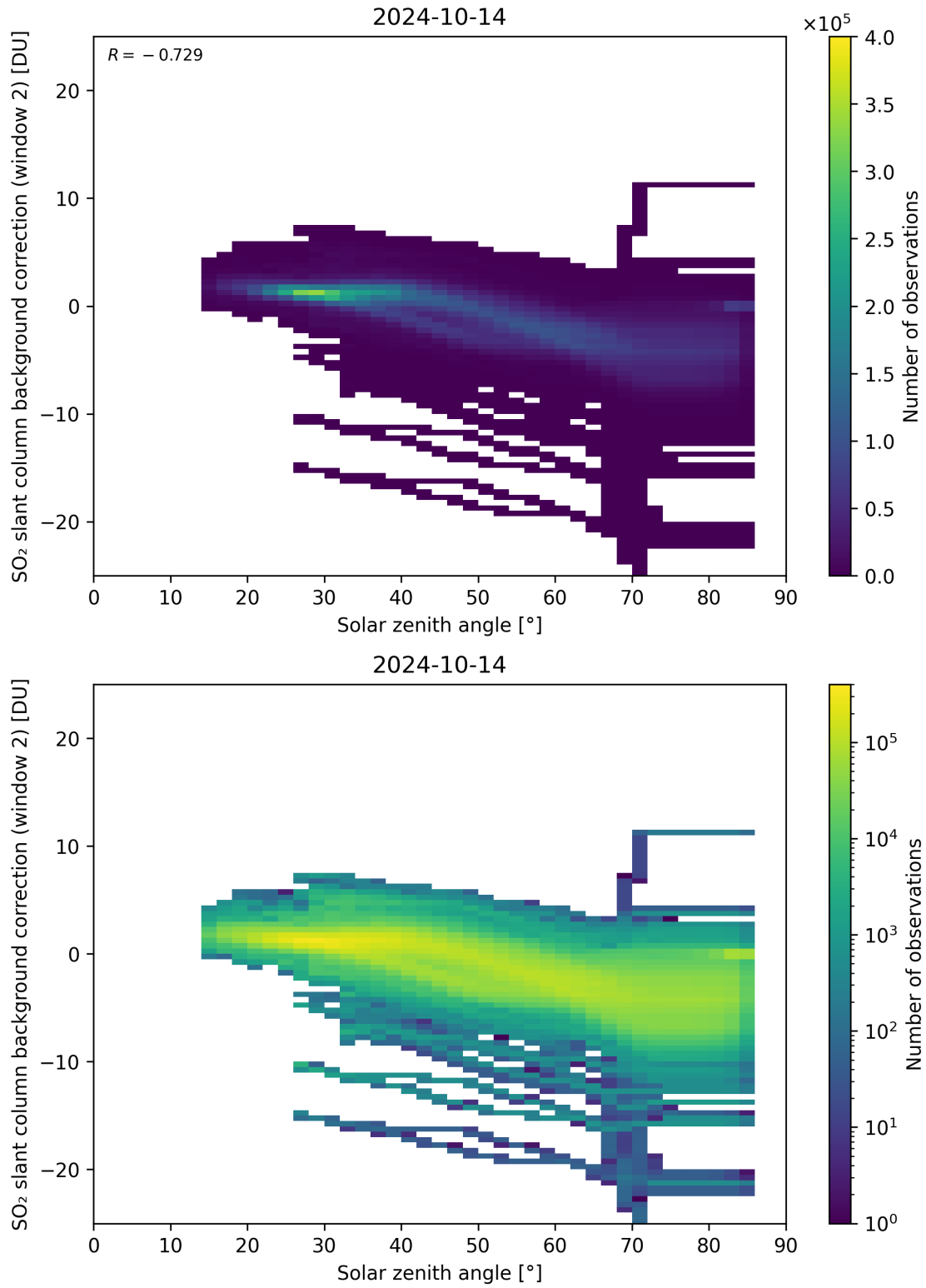
Figure 159: Scatter density plot of “Solar zenith angle” against “SO 2 slant column background correction (window 2)” for 2024-10-14 to 2024-10-15.
