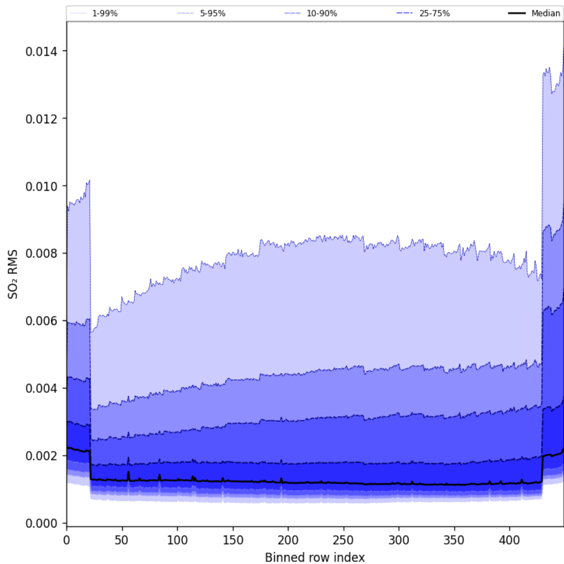
Figure 93: Along track statistics of “SO 2 RMS” for 2024-10-14 to 2024-10-15
