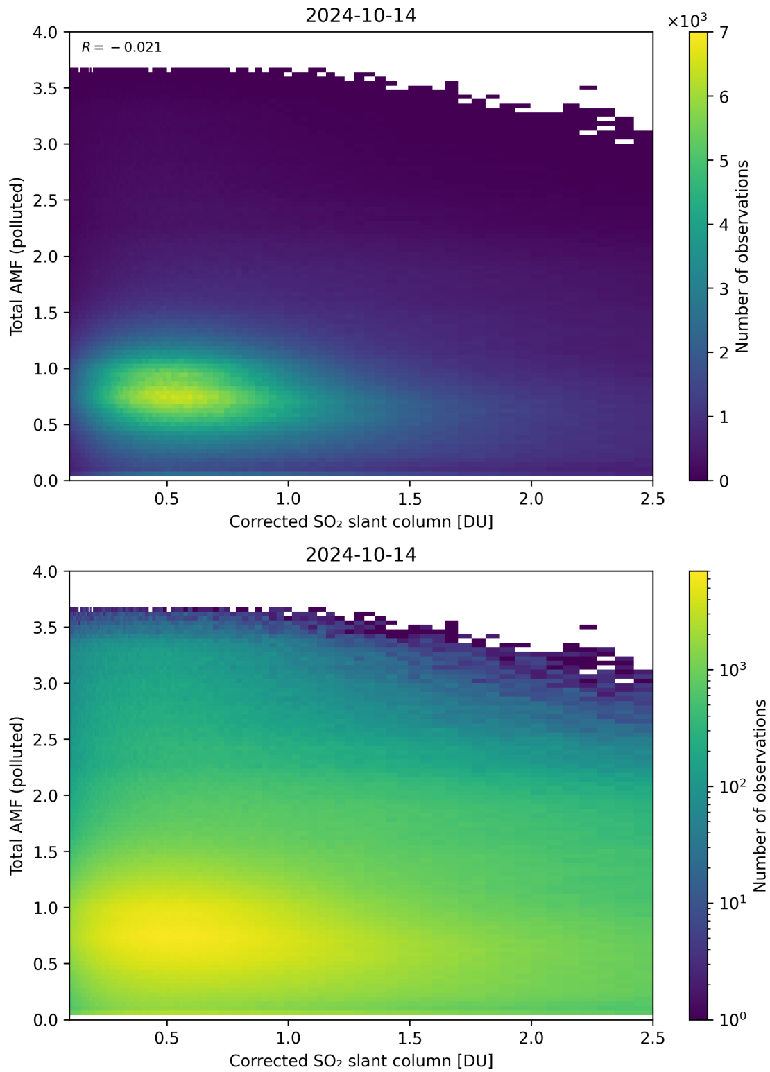
Figure 192: Scatter density plot of “Corrected SO 2 slant column” against “Total AMF (polluted)” for 2024-10-14 to 2024-10-15.
