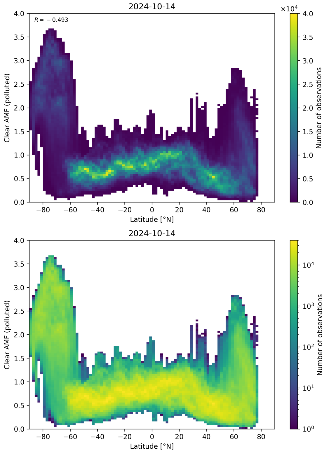
Figure 145: Scatter density plot of “Latitude” against “Clear AMF (polluted)” for 2024-10-14 to 2024-10-15.
