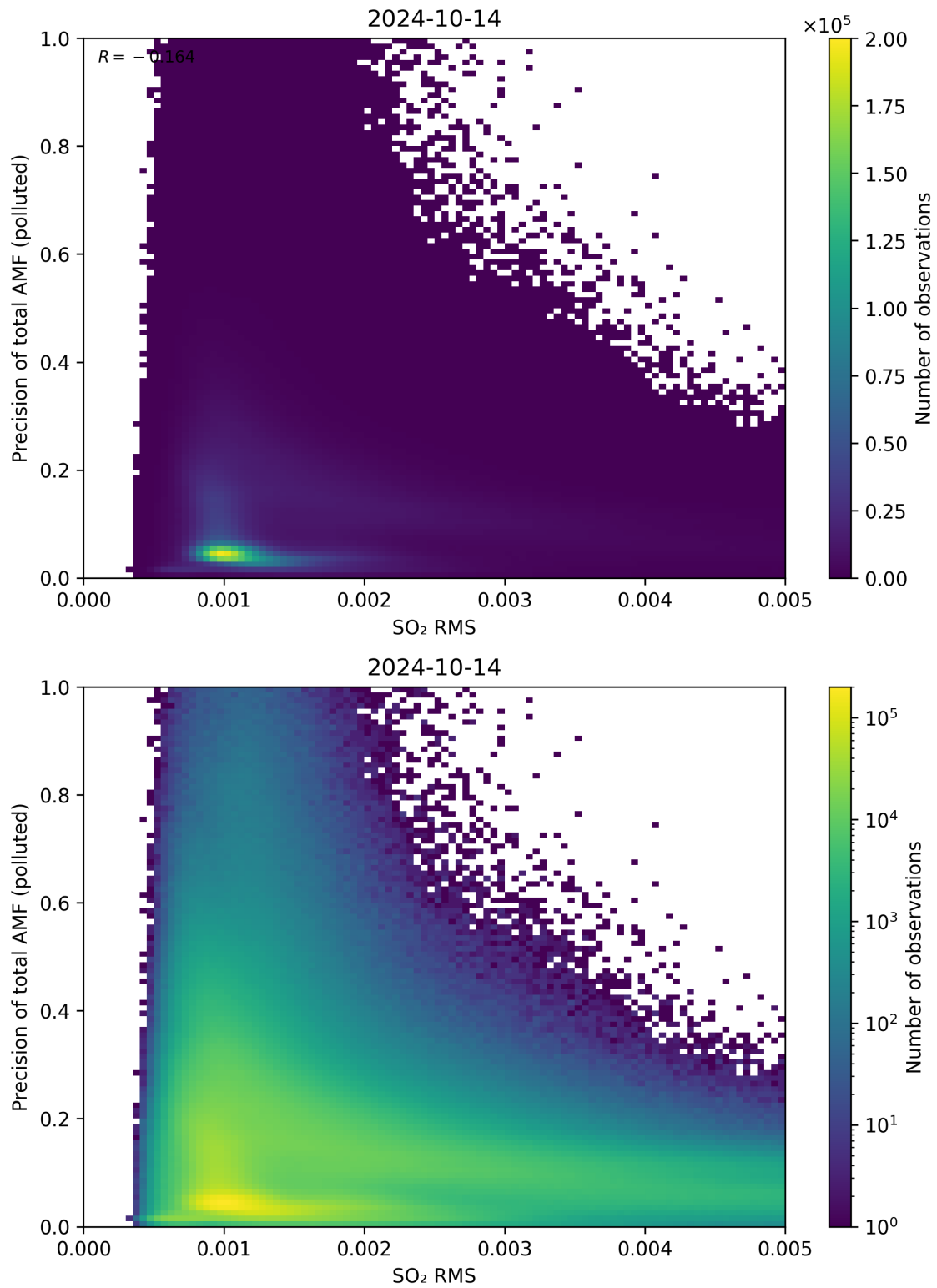
Figure 138: Scatter density plot of “SO 2 RMS” against “Precision of total AMF (polluted)” for 2024-10-14 to 2024-10-15.
