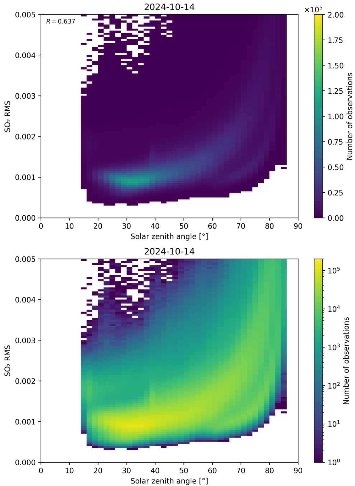
Figure 163: Scatter density plot of “Solar zenith angle” against “SO 2 RMS” for 2024-10-14 to 2024-10-15.
