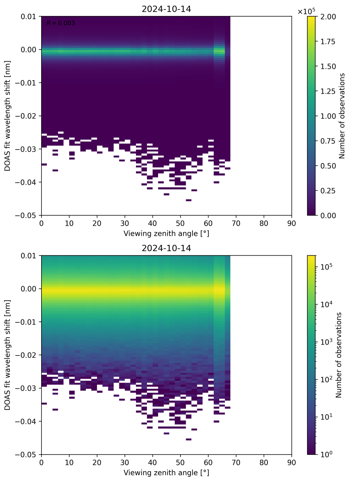
Figure 311: Scatter density plot of “Viewing zenith angle” against “DOAS fit wavelength shift” for 2024-10-14 to 2024-10-15.
