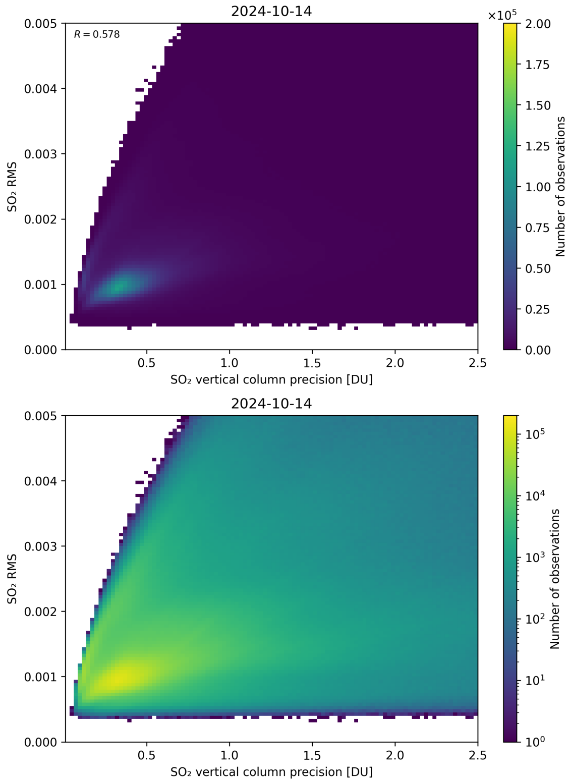
Figure 284: Scatter density plot of “SO 2 vertical column precision” against “SO 2 RMS” for 2024-10-14 to 2024-10-15.
