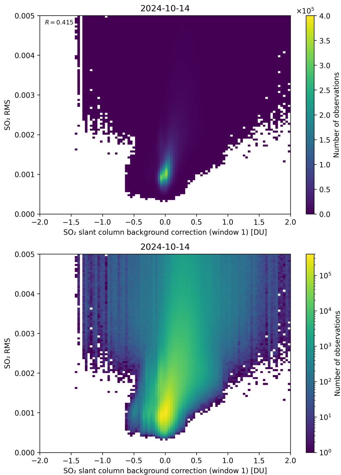
Figure 102: Scatter density plot of “SO 2 slant column background correction (window 1)” against “SO 2 RMS” for 2024-10-14 to 2024-10-15.
