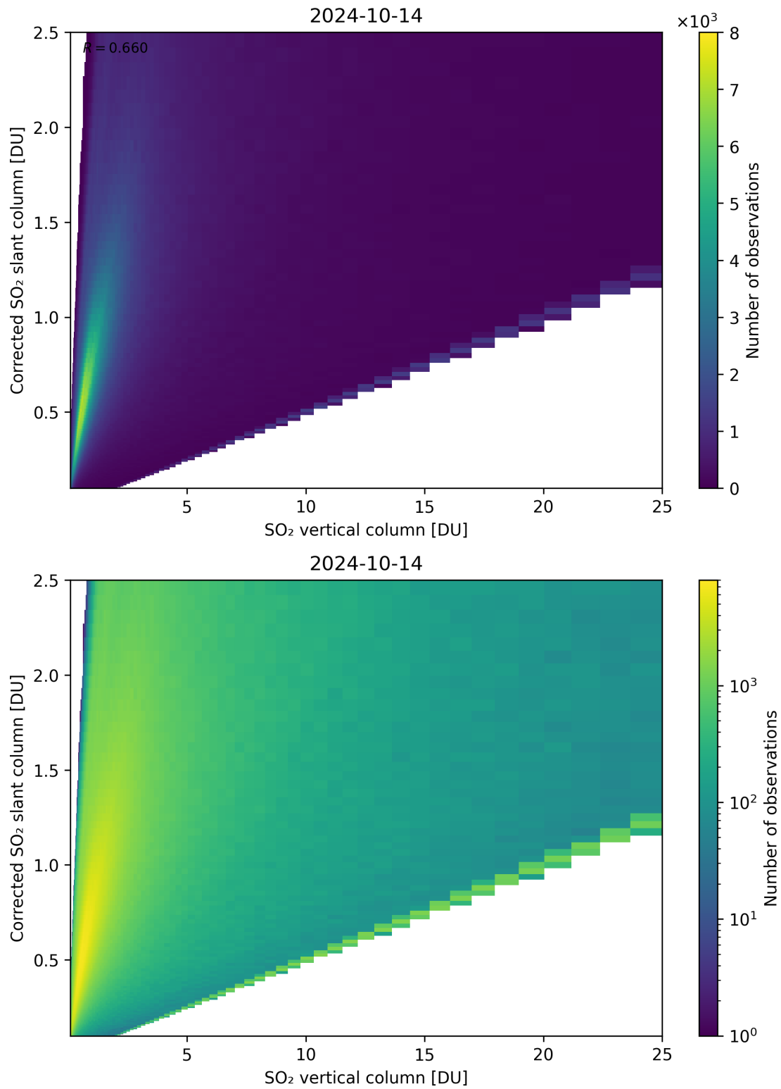
Figure 297: Scatter density plot of “SO 2 vertical column” against “Corrected SO 2 slant column” for 2024-10-14 to 2024-10-15.
