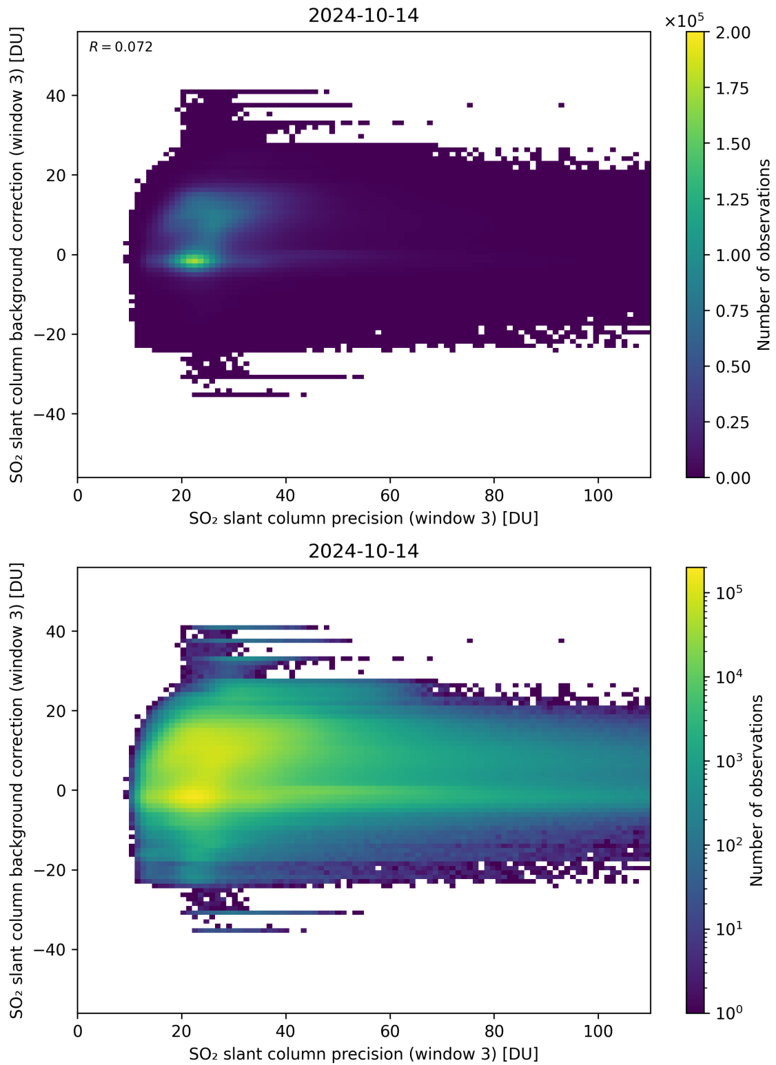
Figure 257: Scatter density plot of “SO 2 slant column precision (window 3)” against “SO 2 slant column background correction (window 3)” for 2024-10-14 to 2024-10-15.
