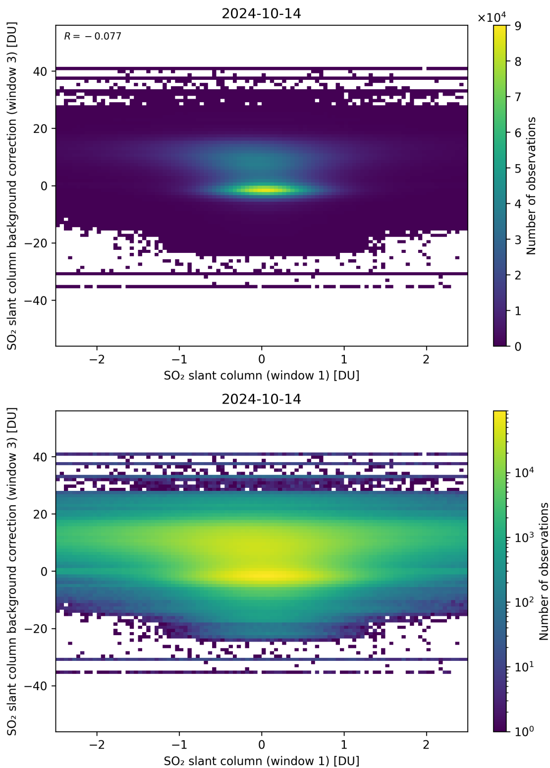
Figure 214: Scatter density plot of “SO 2 slant column (window 1)” against “SO 2 slant column background correction (window 3)” for 2024-10-14 to 2024-10-15.
