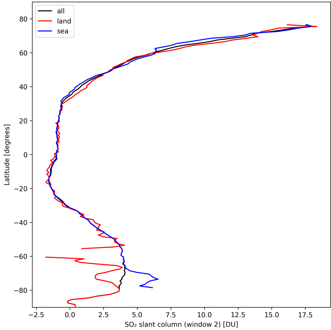
Figure 37: Zonal average of “SO 2 slant column (window 2)” for 2024-10-14 to 2024-10-15.
