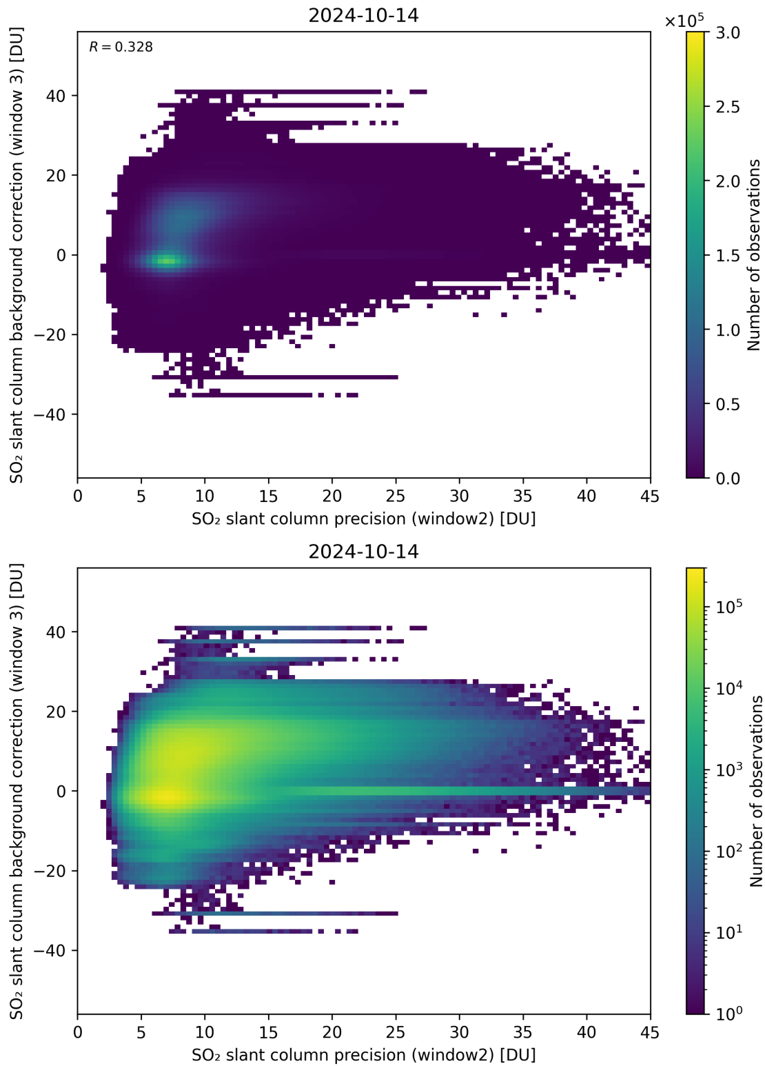
Figure 242: Scatter density plot of “SO 2 slant column precision (window2)” against “SO 2 slant column background correction (window 3)” for 2024-10-14 to 2024-10-15.
