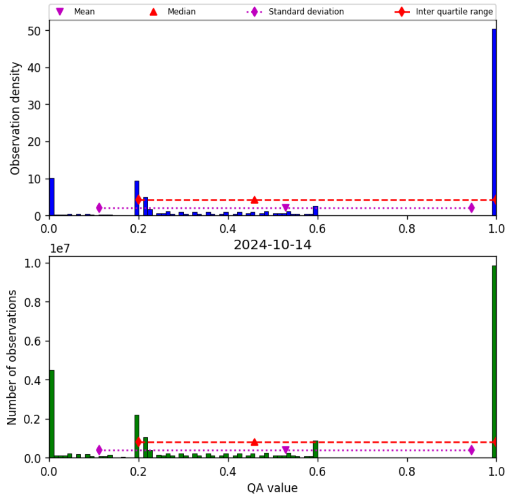
Figure 52: Histogram of “QA value” for 2024-10-14 to 2024-10-15
