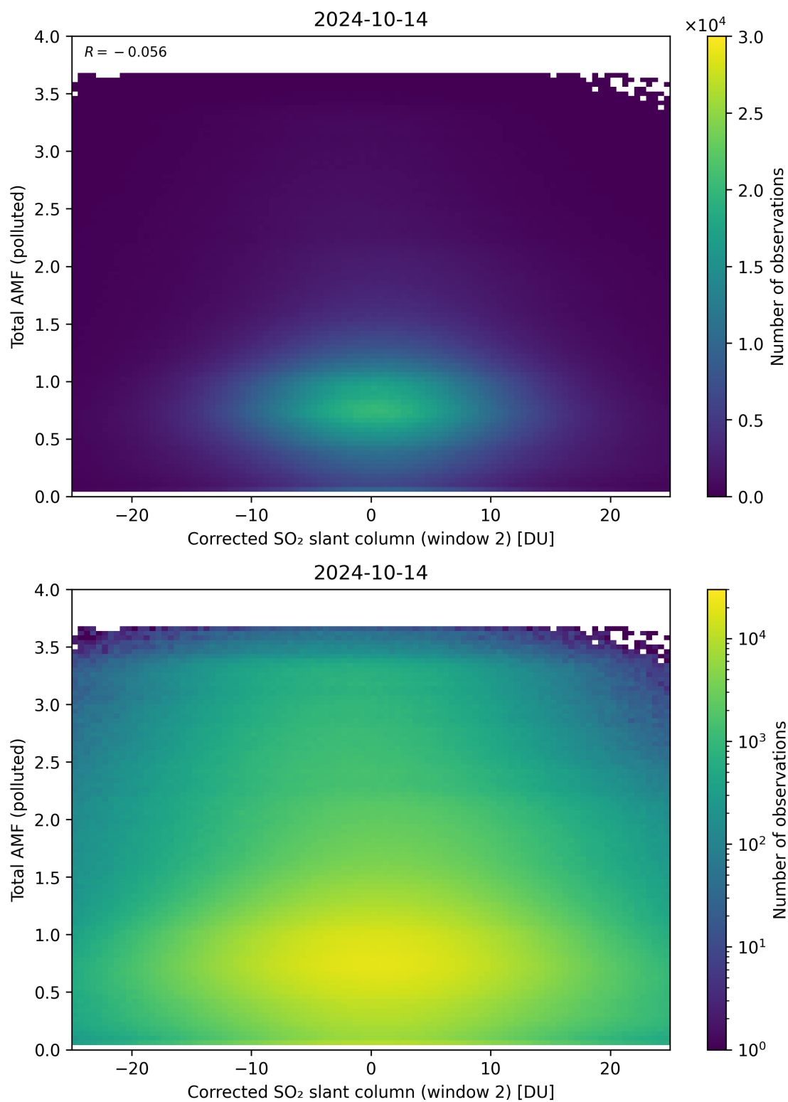
Figure 203: Scatter density plot of “Corrected SO 2 slant column (window 2)” against “Total AMF (polluted)” for 2024-10-14 to 2024-10-15.
