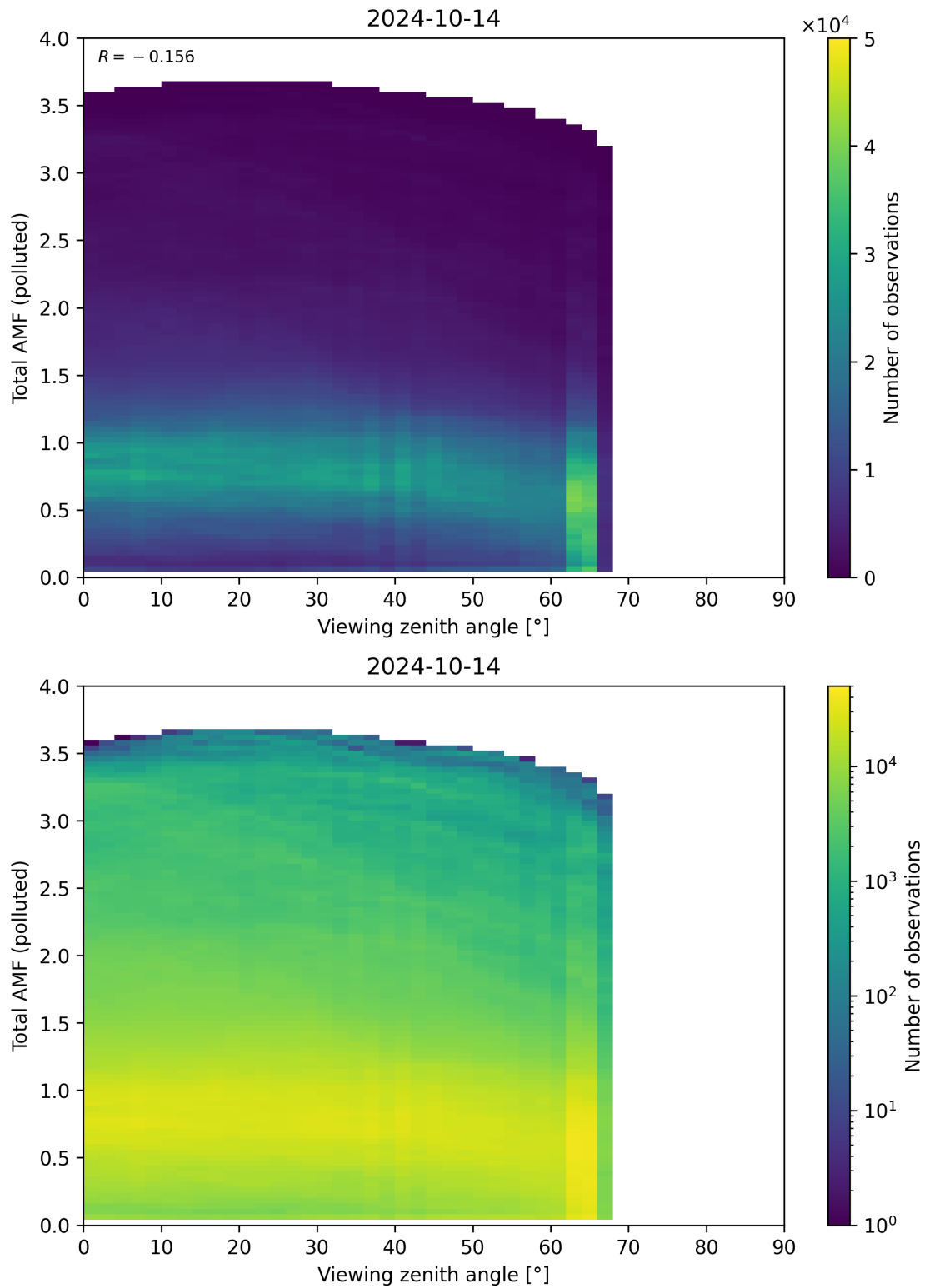
Figure 325: Scatter density plot of “Viewing zenith angle” against “Total AMF (polluted)” for 2024-10-14 to 2024-10-15.
