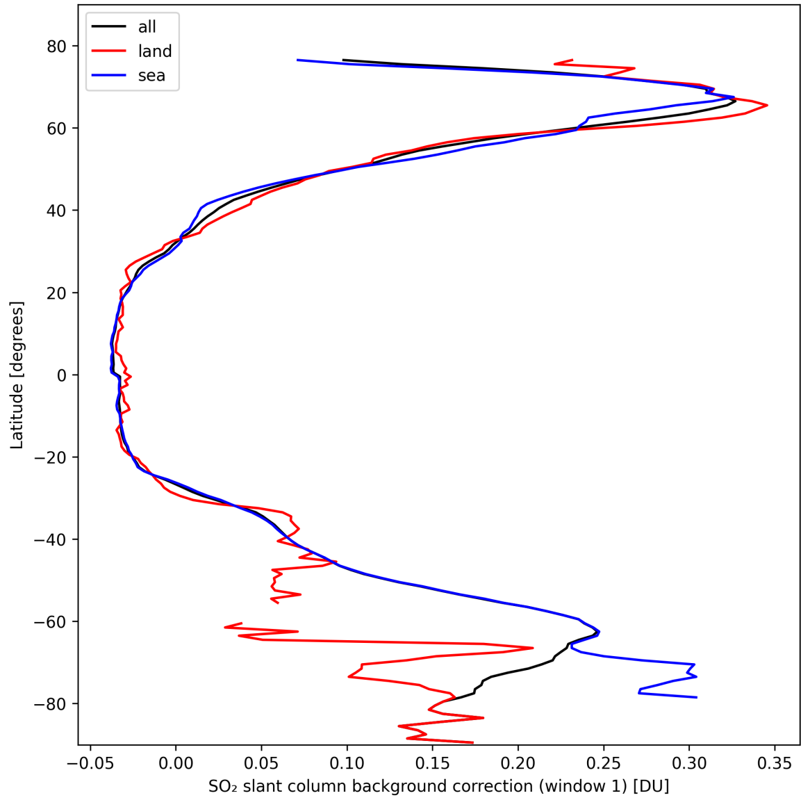
Figure 36: Zonal average of “SO 2 slant column background correction (window 1)” for 2024-10-14 to 2024-10-15.
