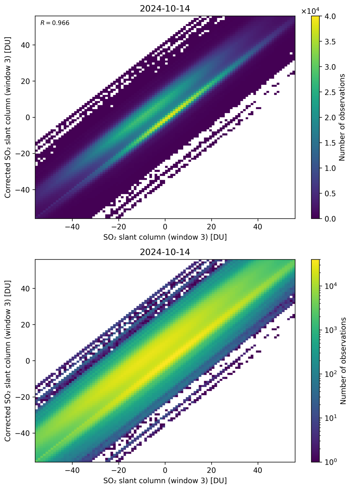
Figure 266: Scatter density plot of “SO 2 slant column (window 3)” against “Corrected SO 2 slant column (window 3)” for 2024-10-14 to 2024-10-15.
