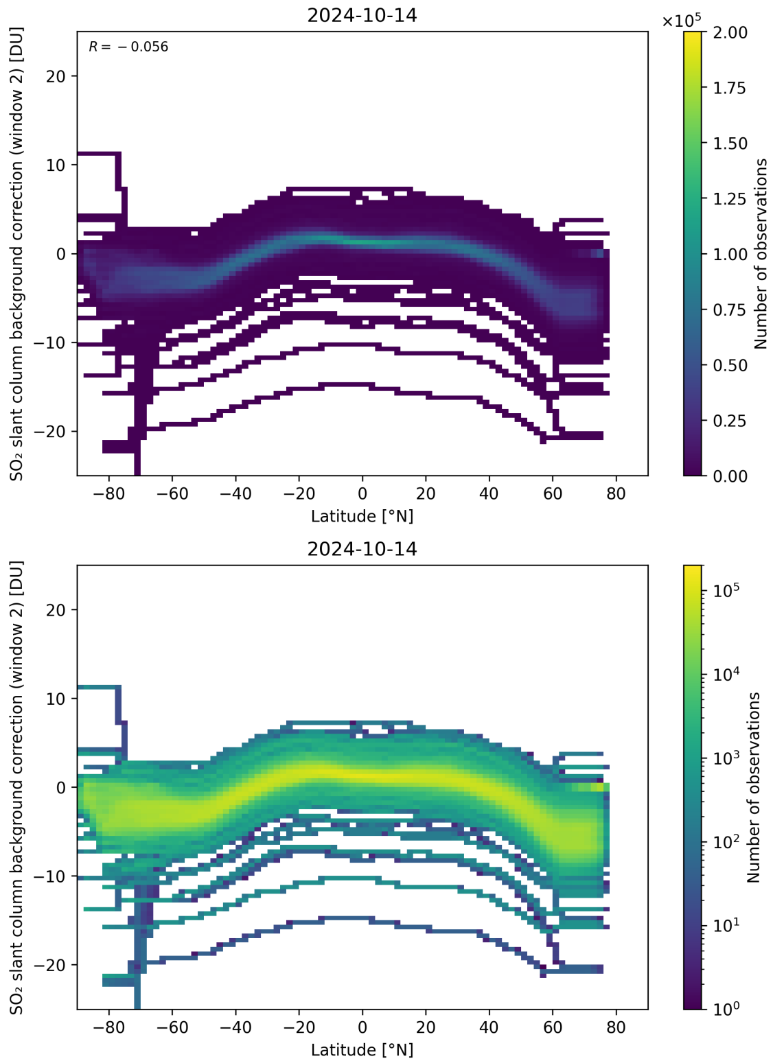
Figure 140: Scatter density plot of “Latitude” against “SO 2 slant column background correction (window 2)” for 2024-10-14 to 2024-10-15.
