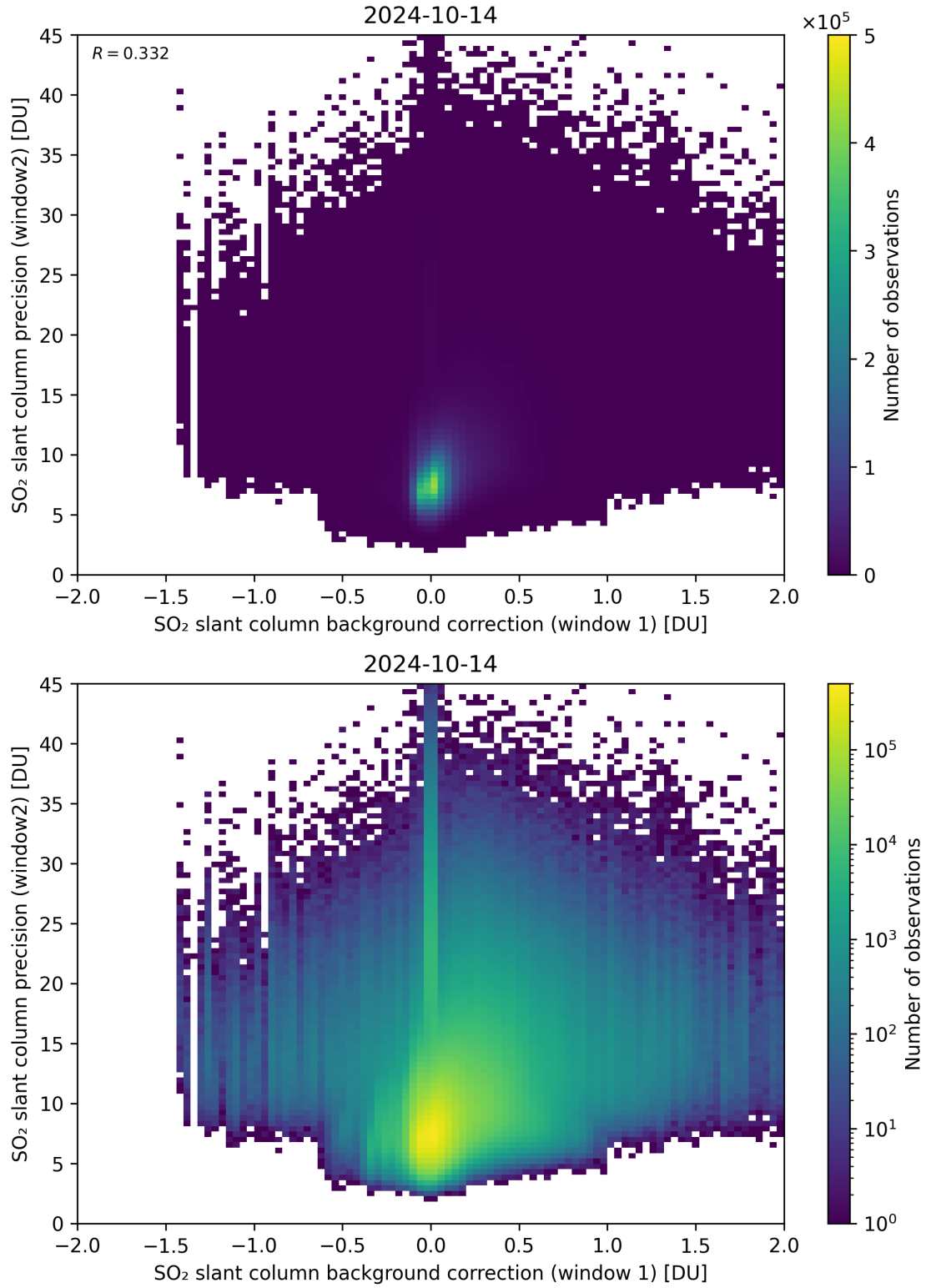
Figure 106: Scatter density plot of “SO 2 slant column background correction (window 1)” against “SO 2 slant column precision (window2)” for 2024-10-14 to 2024-10-15.
