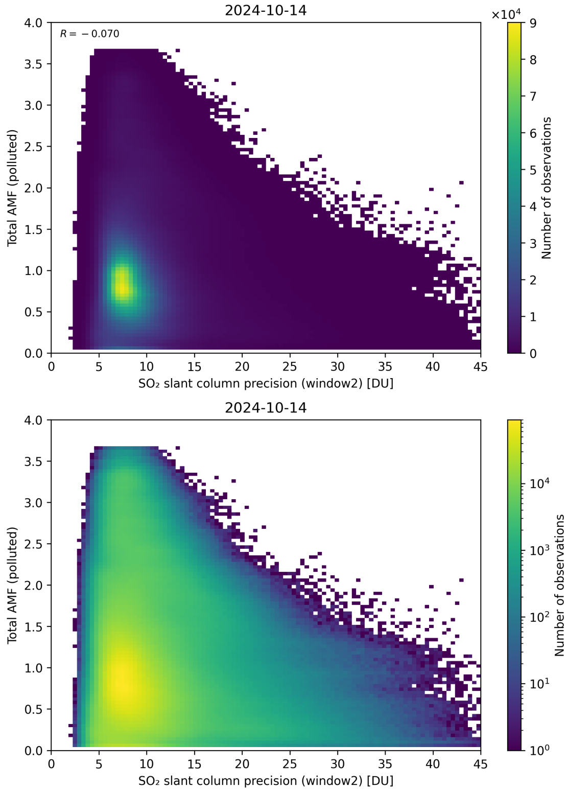
Figure 251: Scatter density plot of “SO 2 slant column precision (window2)” against “Total AMF (polluted)” for 2024-10-14 to 2024-10-15.
