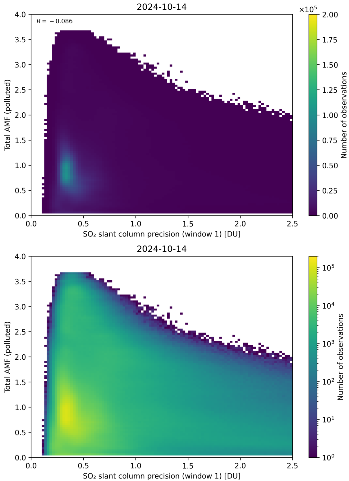
Figure 230: Scatter density plot of “SO 2 slant column precision (window 1)” against “Total AMF (polluted)” for 2024-10-14 to 2024-10-15.
