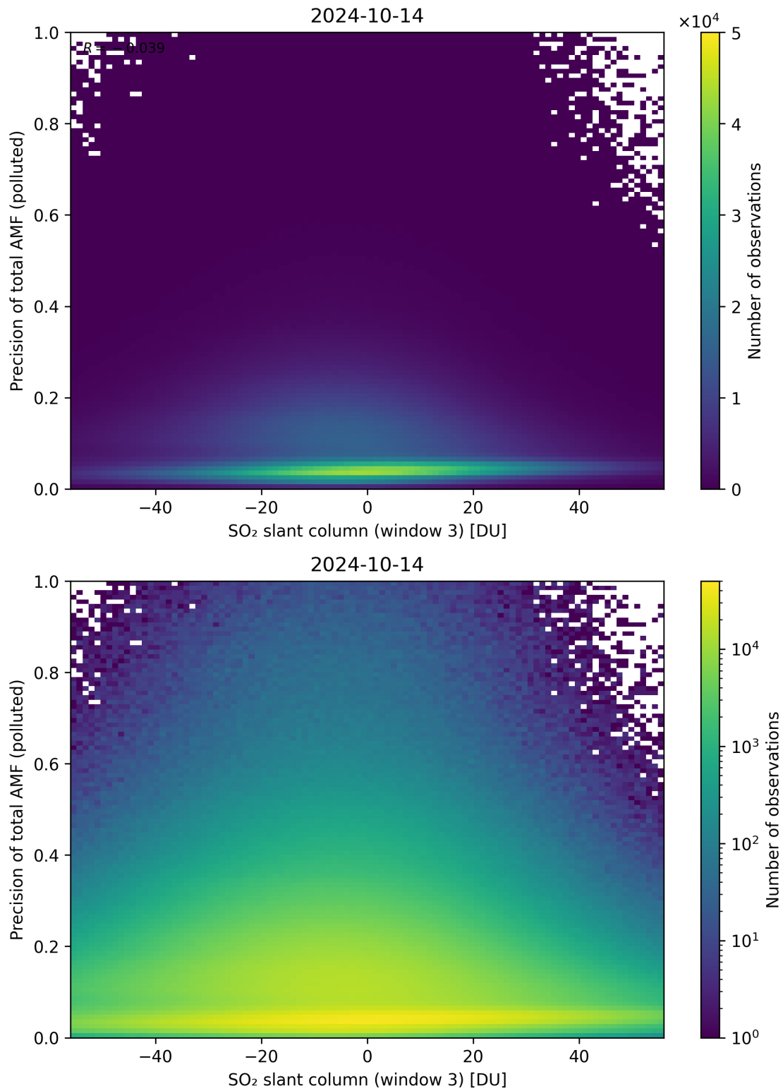
Figure 269: Scatter density plot of “SO 2 slant column (window 3)” against “Precision of total AMF (polluted)” for 2024-10-14 to 2024-10-15.
