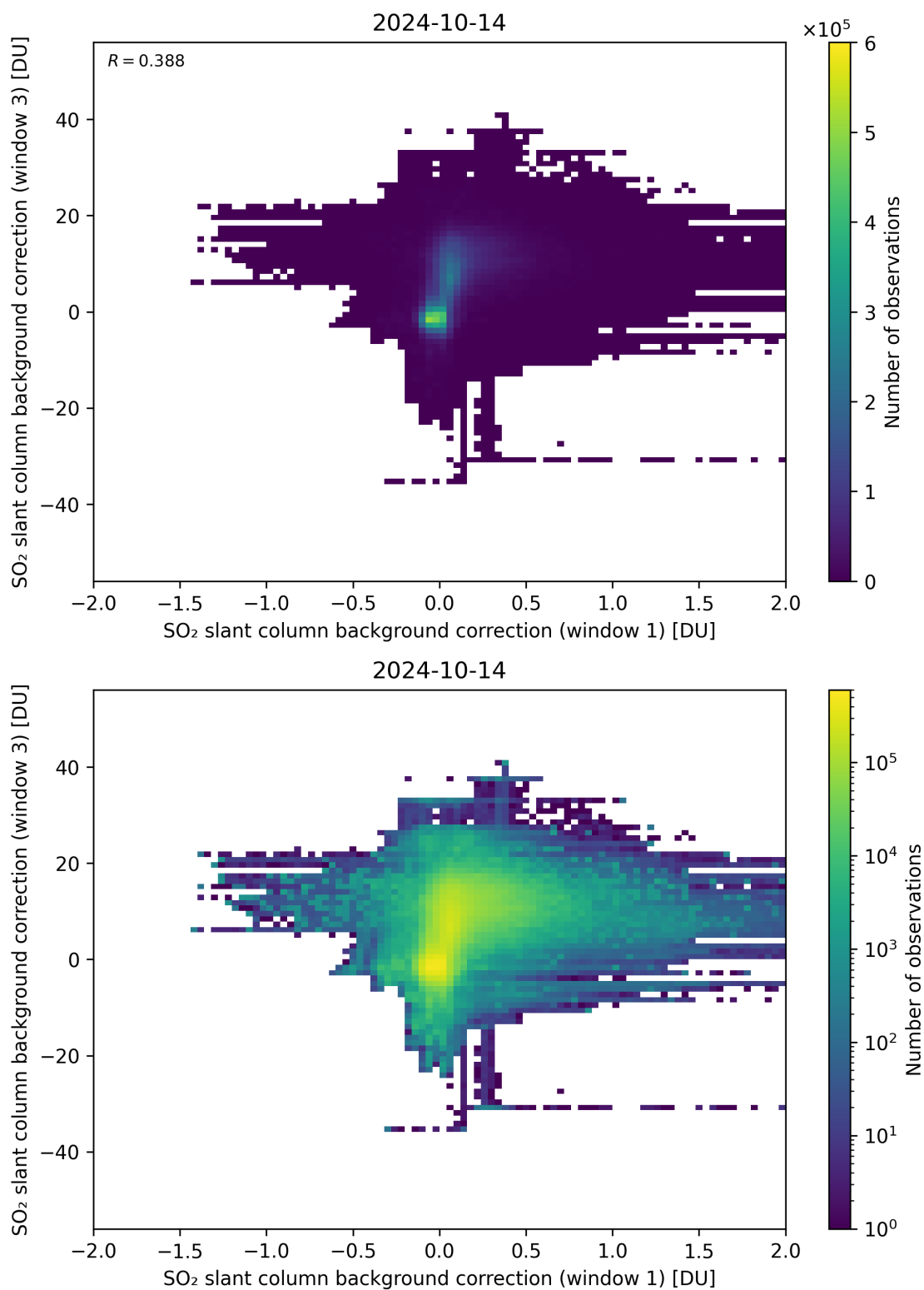
Figure 99: Scatter density plot of “SO 2 slant column background correction (window 1)” against “SO 2 slant column background correction (window 3)” for 2024-10-14 to 2024-10-15.
