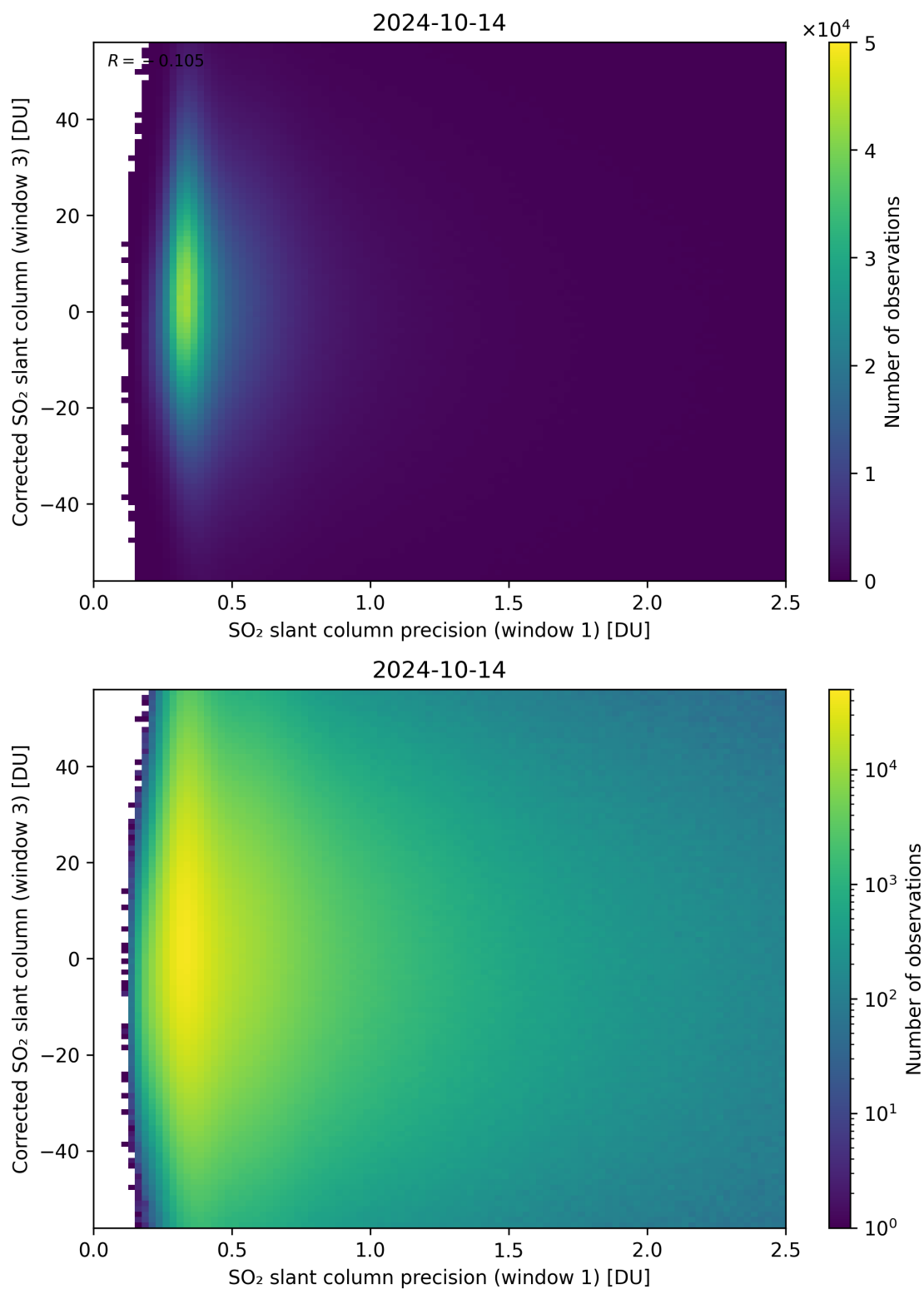
Figure 226: Scatter density plot of “SO 2 slant column precision (window 1)” against “Corrected SO 2 slant column (window 3)” for 2024-10-14 to 2024-10-15.
