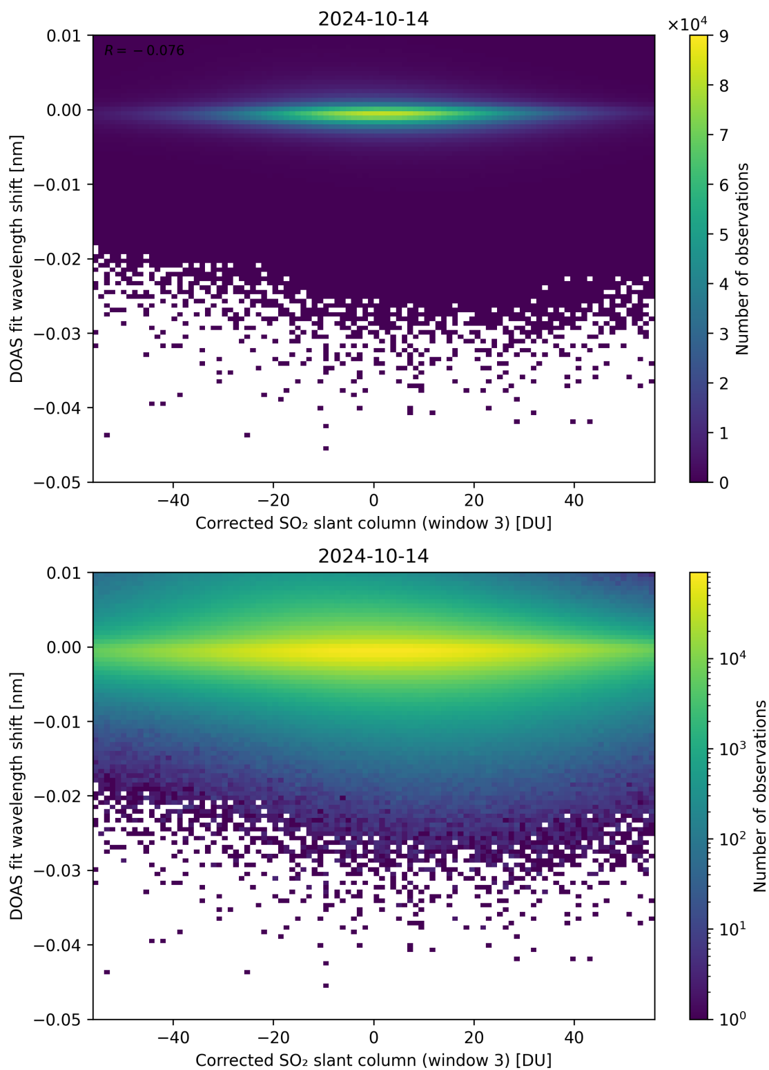
Figure 206: Scatter density plot of “Corrected SO 2 slant column (window 3)” against “DOAS fit wavelength shift” for 2024-10-14 to 2024-10-15.
