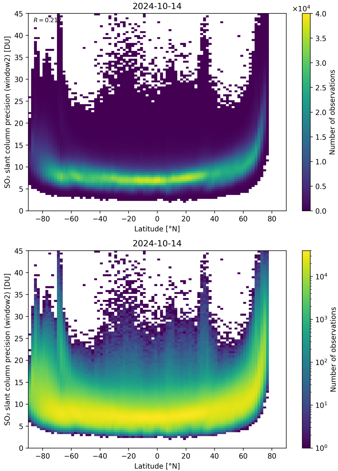
Figure 151: Scatter density plot of “Latitude” against “SO 2 slant column precision (window2)” for 2024-10-14 to 2024-10-15.
