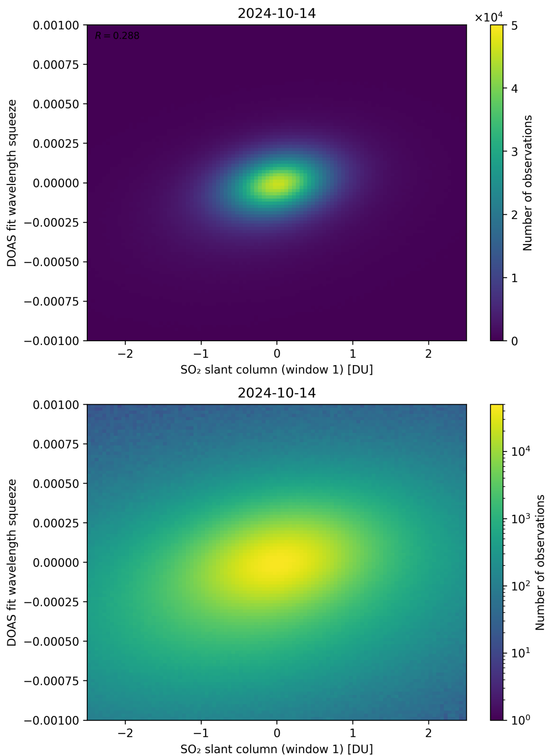
Figure 216: Scatter density plot of “SO 2 slant column (window 1)” against “DOAS fit wavelength squeeze” for 2024-10-14 to 2024-10-15.
