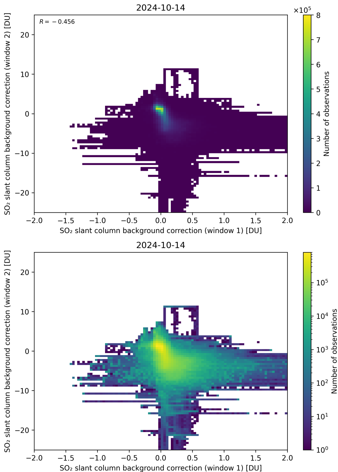
Figure 98: Scatter density plot of “SO 2 slant column background correction (window 1)” against “SO 2 slant column background correction (window 2)” for 2024-10-14 to 2024-10-15.
