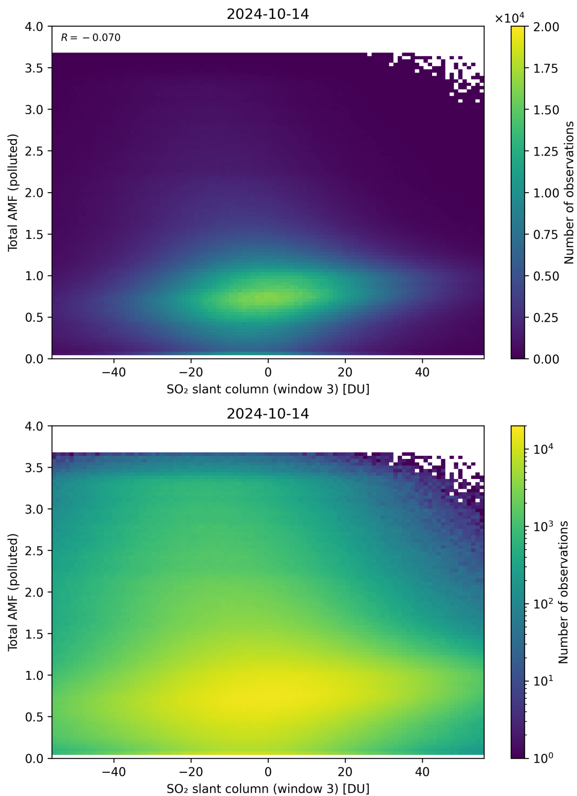
Figure 268: Scatter density plot of “SO 2 slant column (window 3)” against “Total AMF (polluted)” for 2024-10-14 to 2024-10-15.
