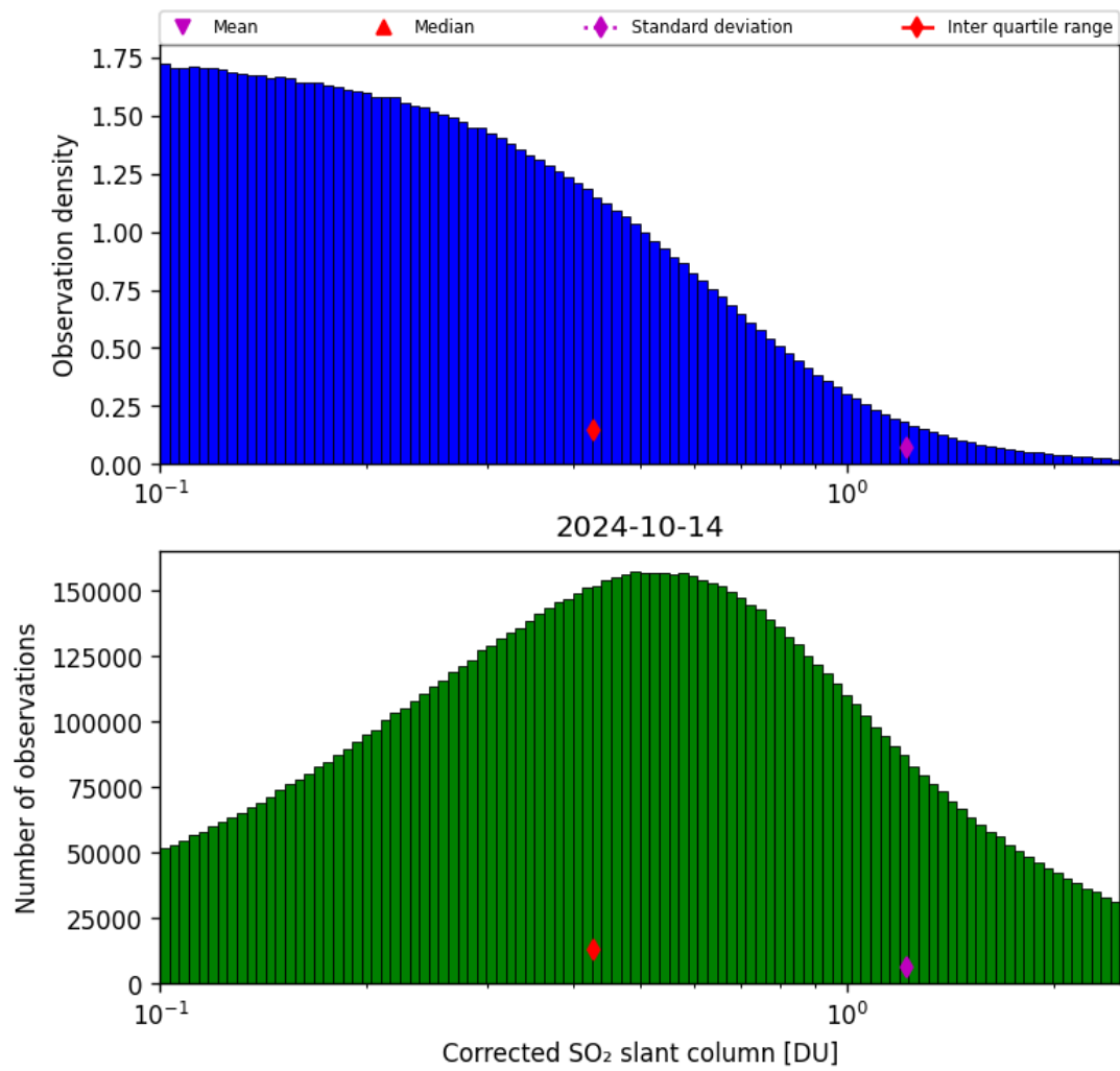
Figure 55: Histogram of “Corrected SO 2 slant column” for 2024-10-14 to 2024-10-15
