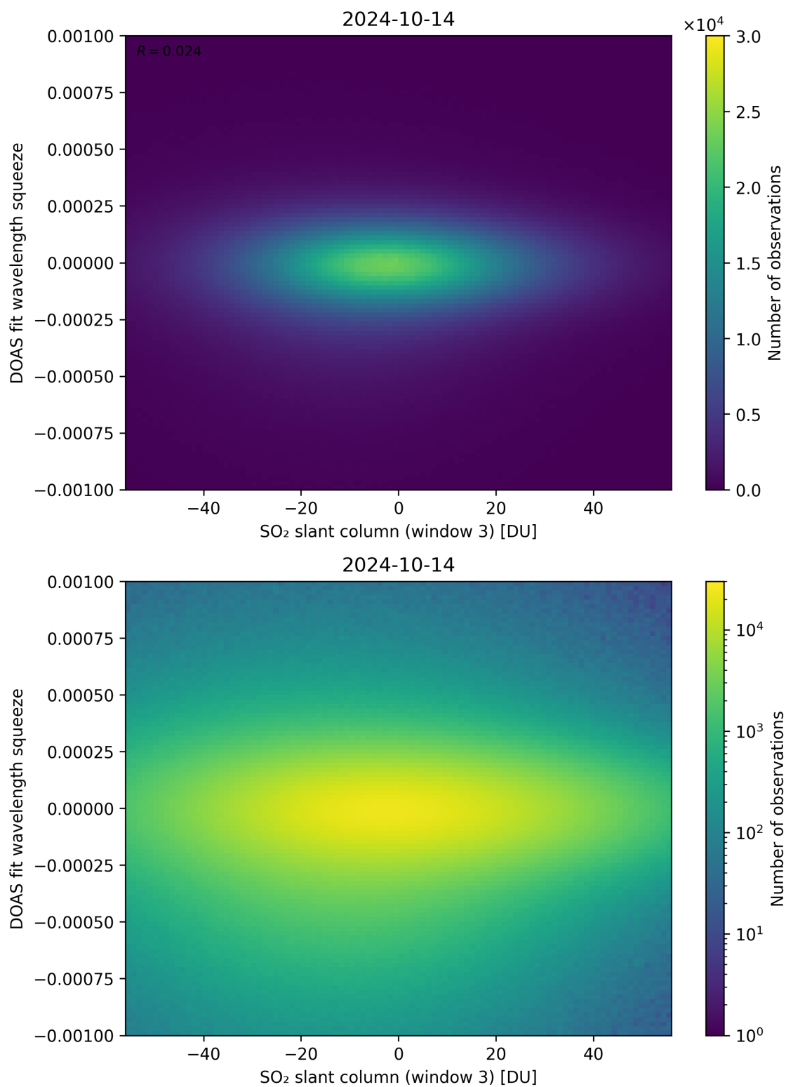
Figure 255: Scatter density plot of “SO 2 slant column (window 3)” against “DOAS fit wavelength squeeze” for 2024-10-14 to 2024-10-15.
