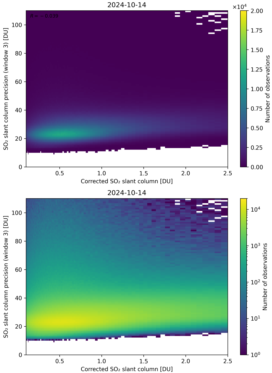
Figure 191: Scatter density plot of “Corrected SO 2 slant column” against “SO 2 slant column precision (window 3)” for 2024-10-14 to 2024-10-15.
