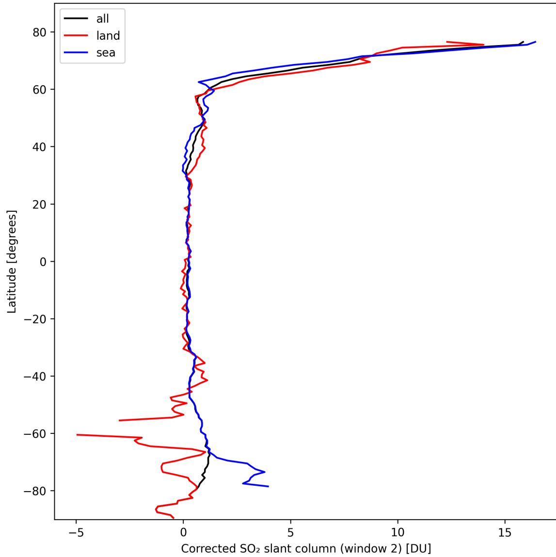
Figure 39: Zonal average of “Corrected SO 2 slant column (window 2)” for 2024-10-14 to 2024-10-15.
