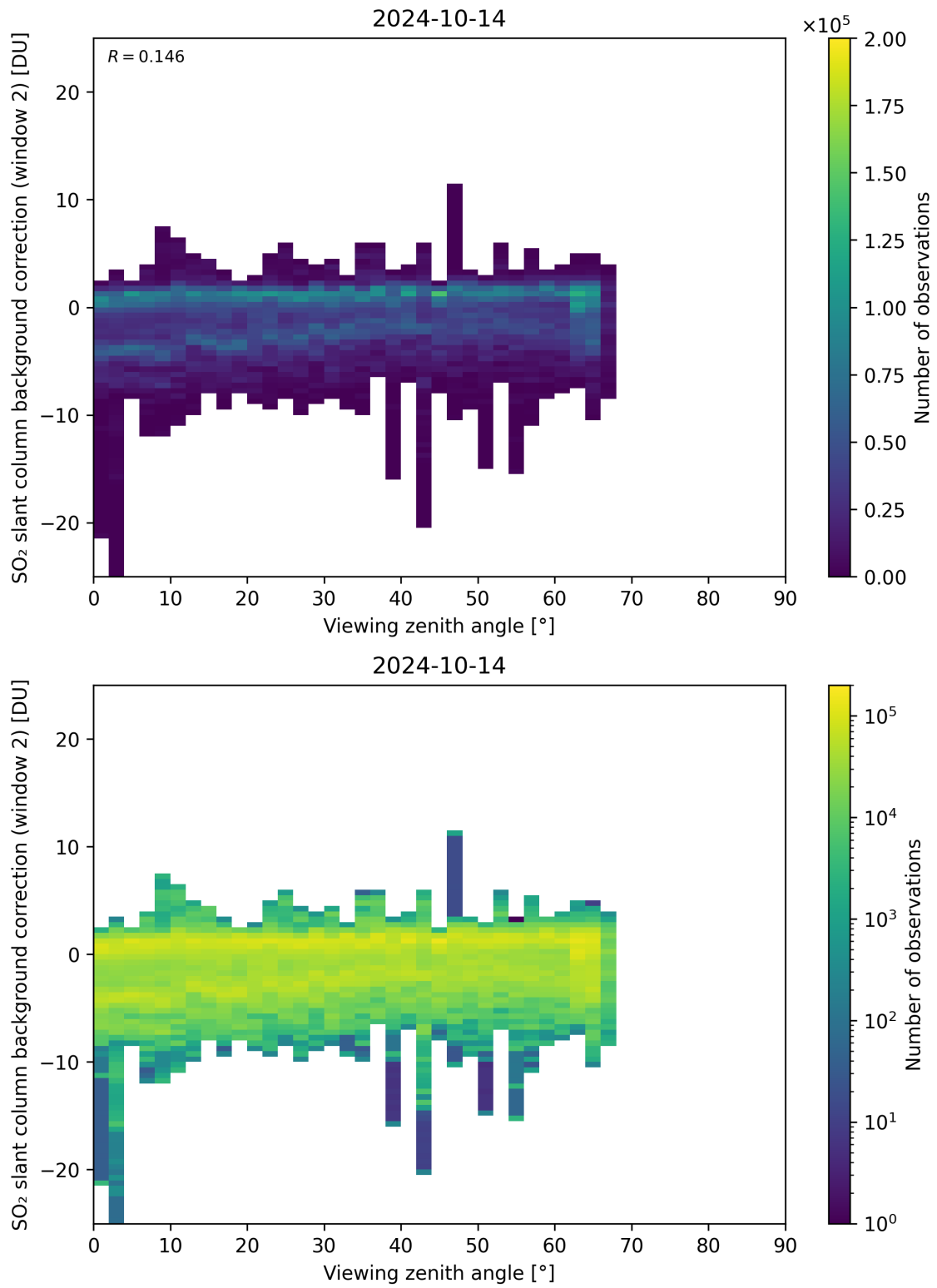
Figure 309: Scatter density plot of “Viewing zenith angle” against “SO 2 slant column background correction (window 2)” for 2024-10-14 to 2024-10-15.
