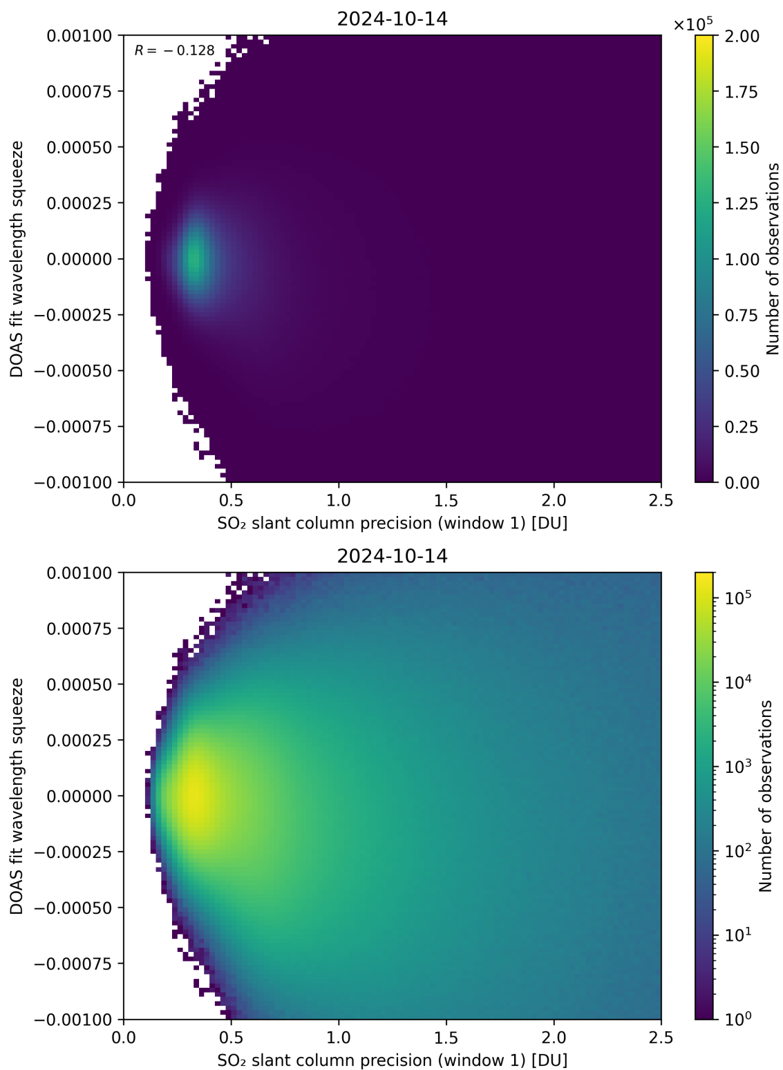
Figure 222: Scatter density plot of “SO 2 slant column precision (window 1)” against “DOAS fit wavelength squeeze” for 2024-10-14 to 2024-10-15.
