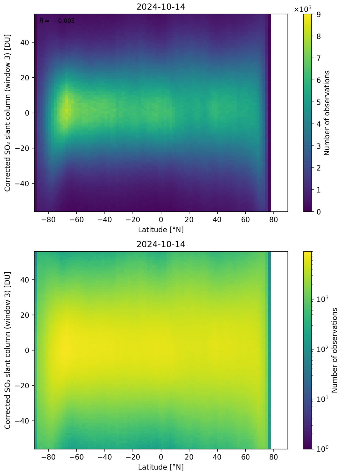
Figure 148: Scatter density plot of “Latitude” against “Corrected SO 2 slant column (window 3)” for 2024-10-14 to 2024-10-15.
