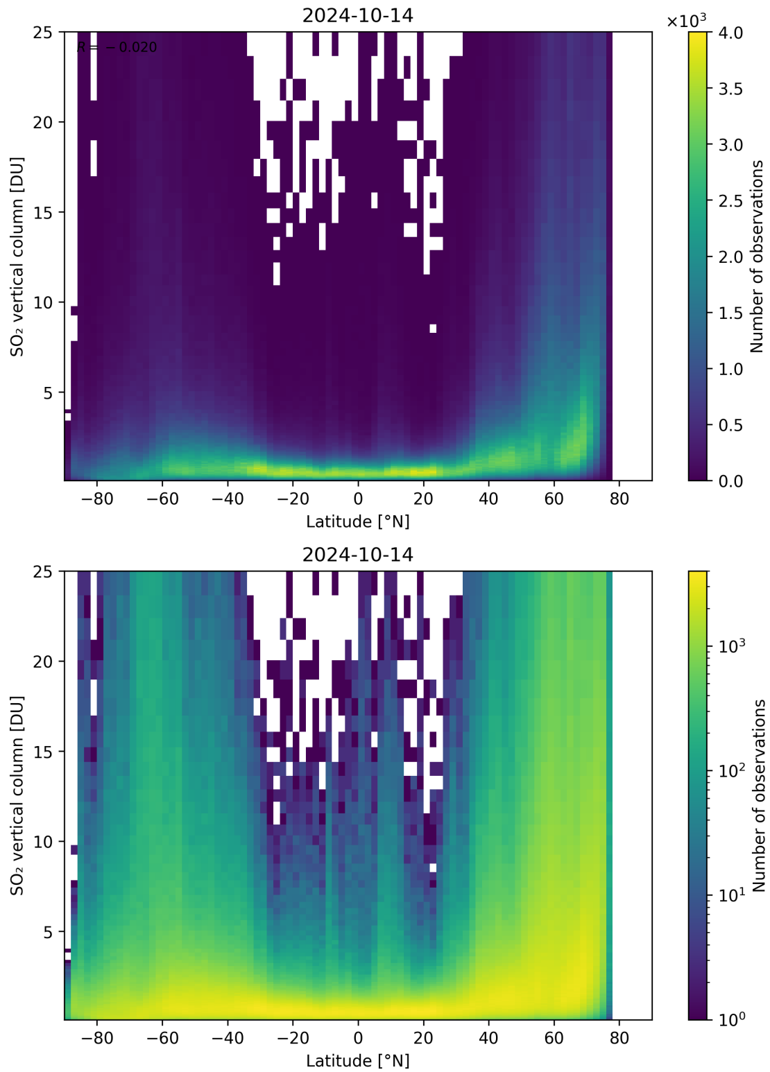
Figure 156: Scatter density plot of “Latitude” against “SO 2 vertical column” for 2024-10-14 to 2024-10-15.
