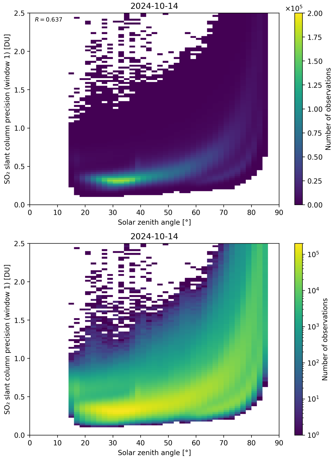
Figure 170: Scatter density plot of “Solar zenith angle” against “SO 2 slant column precision (window 1)” for 2024-10-14 to 2024-10-15.
