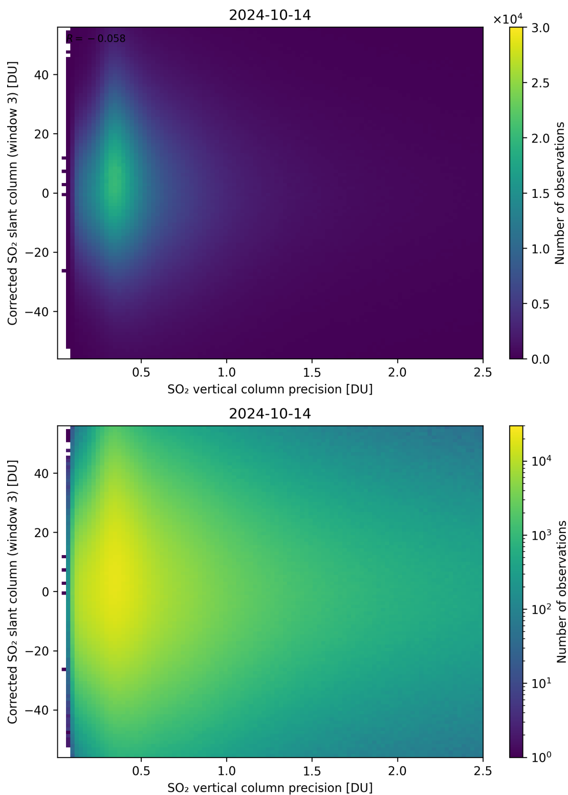
Figure 288: Scatter density plot of “SO 2 vertical column precision” against “Corrected SO 2 slant column (window 3)” for 2024-10-14 to 2024-10-15.
