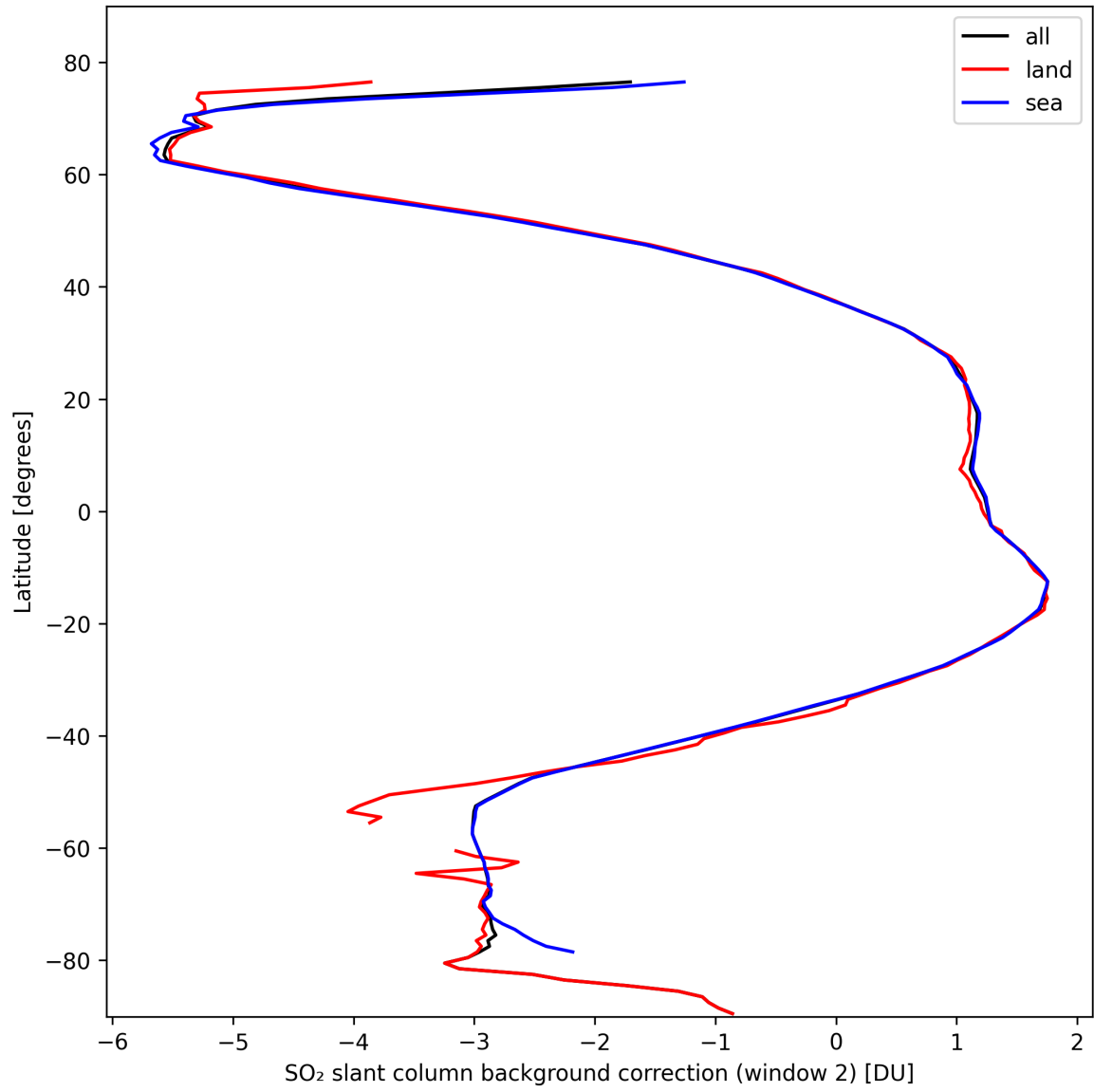
Figure 40: Zonal average of “SO 2 slant column background correction (window 2)” for 2024-10-14 to 2024-10-15.
