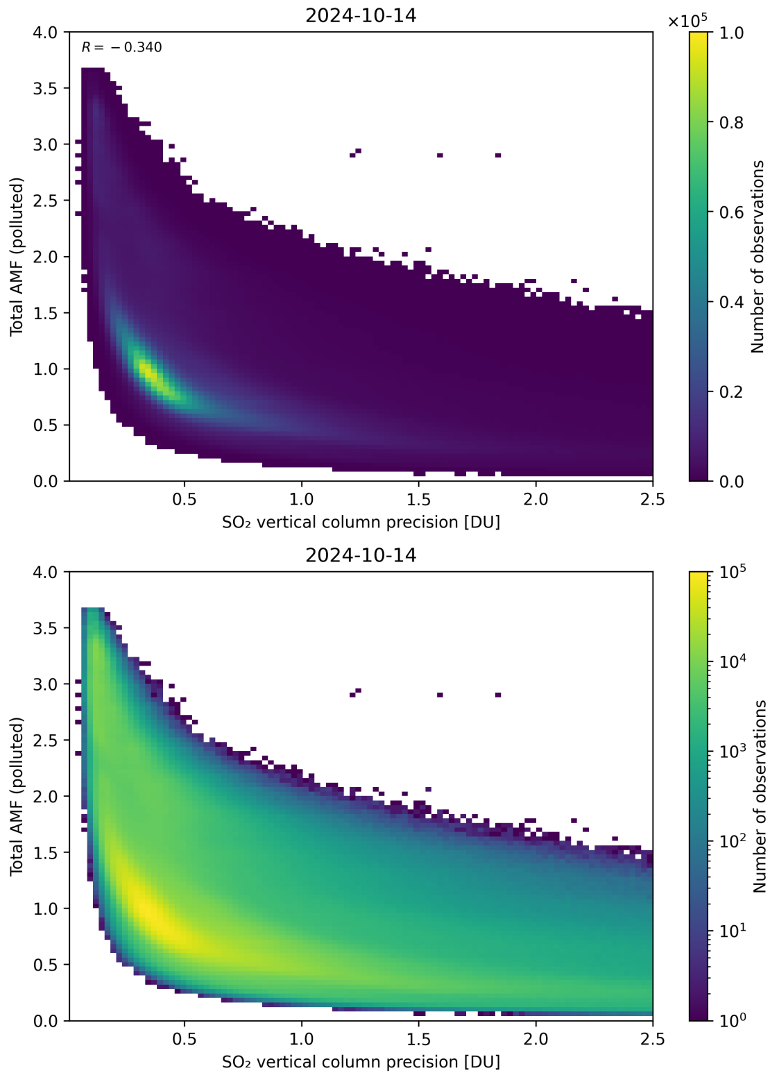
Figure 294: Scatter density plot of “SO 2 vertical column precision” against “Total AMF (polluted)” for 2024-10-14 to 2024-10-15.
