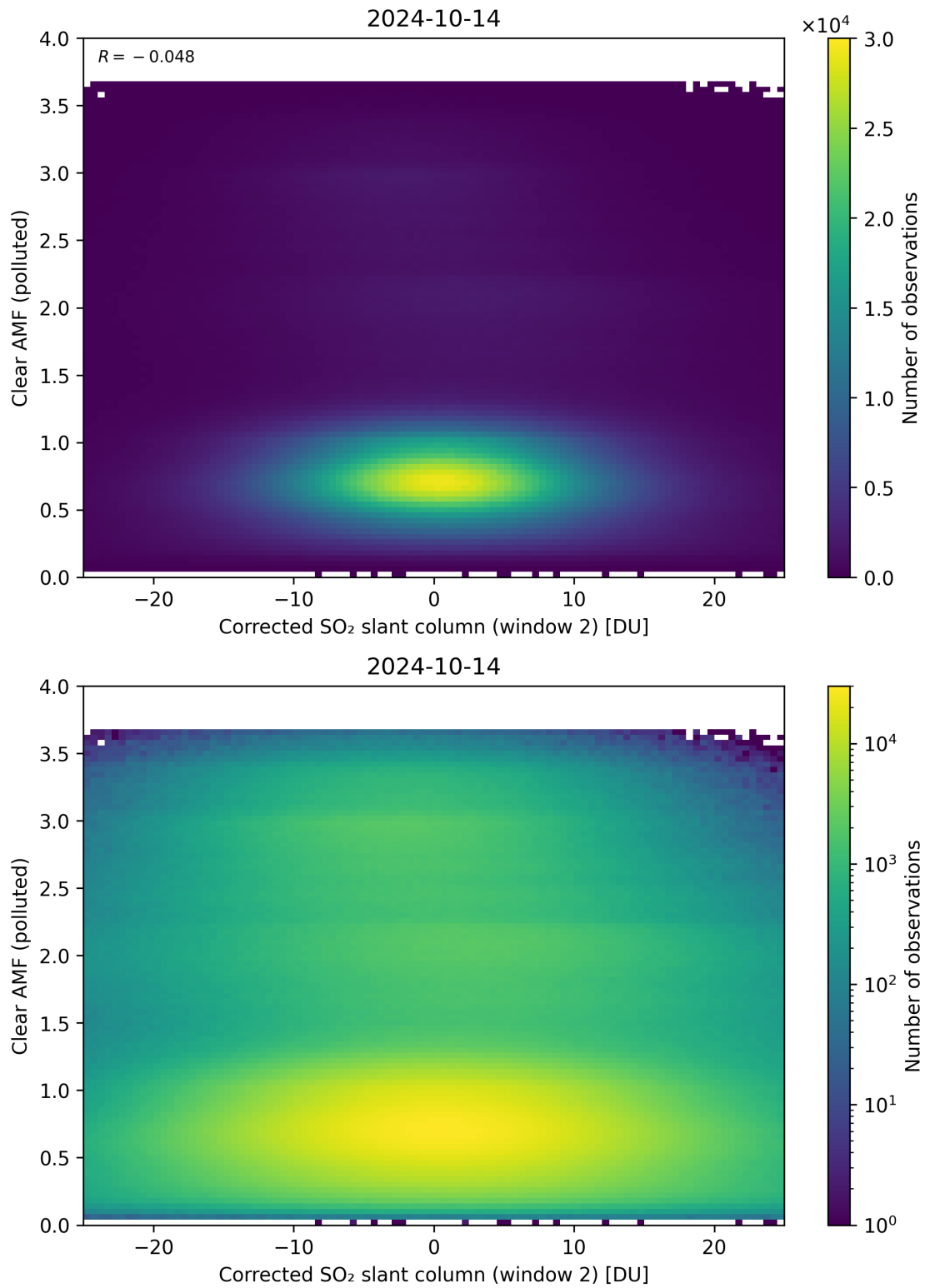
Figure 199: Scatter density plot of “Corrected SO 2 slant column (window 2)” against “Clear AMF (polluted)” for 2024-10-14 to 2024-10-15.
