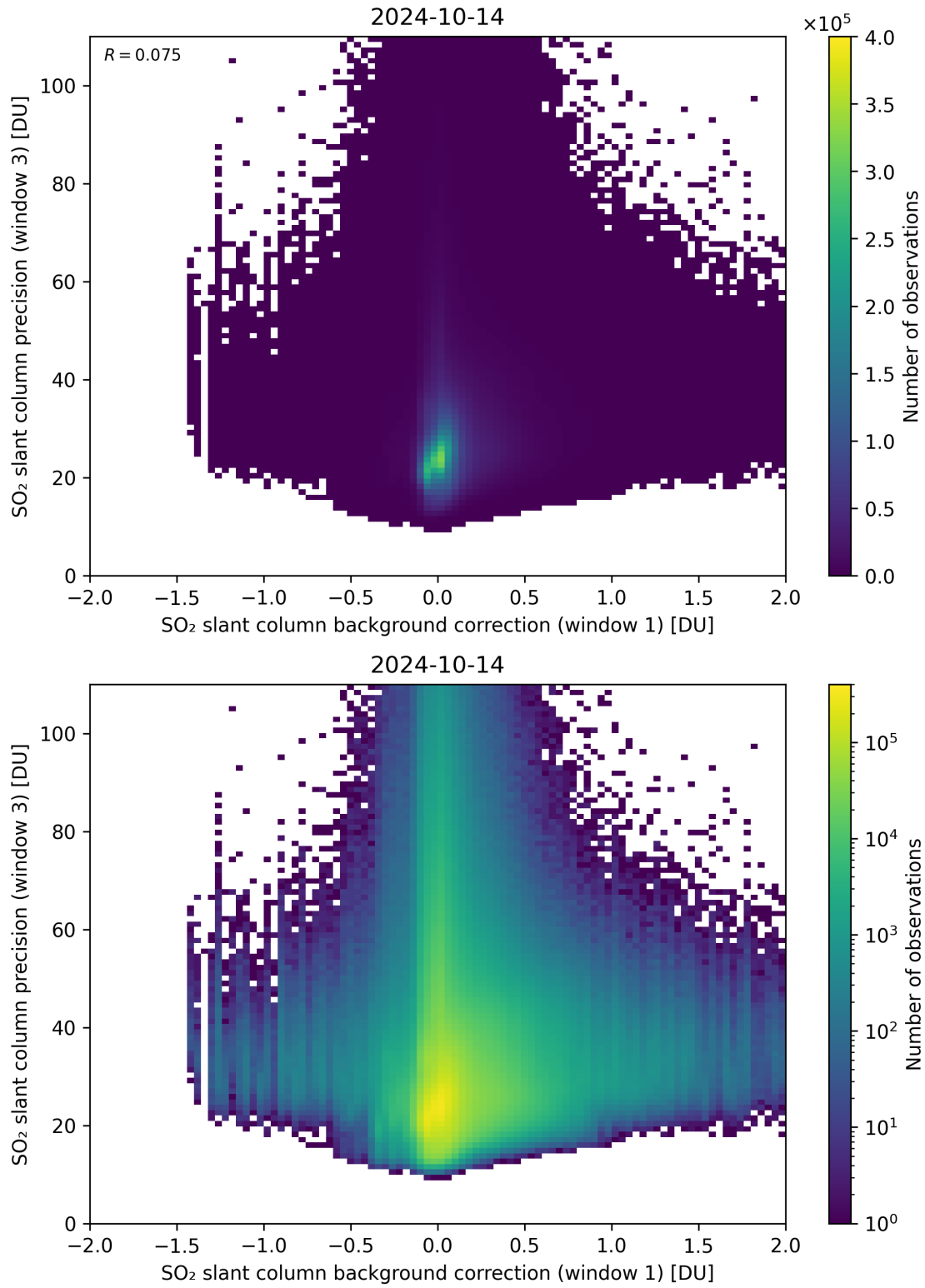
Figure 108: Scatter density plot of “SO 2 slant column background correction (window 1)” against “SO 2 slant column precision (window 3)” for 2024-10-14 to 2024-10-15.
