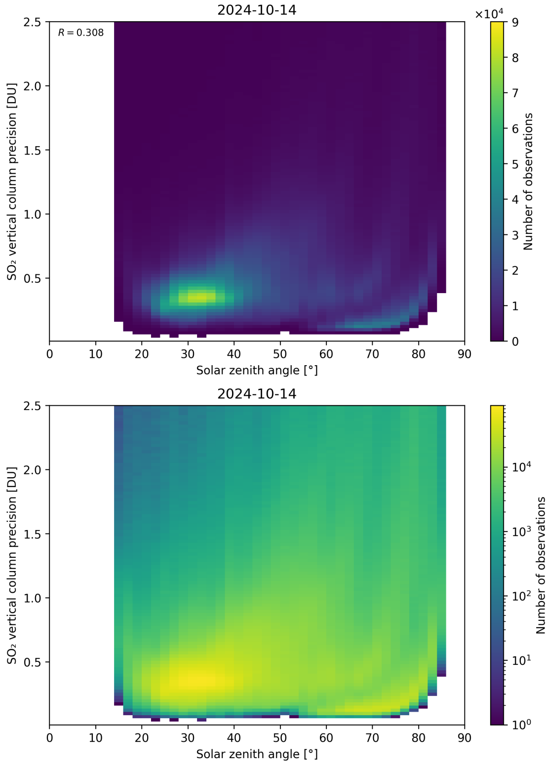
Figure 177: Scatter density plot of “Solar zenith angle” against “SO 2 vertical column precision” for 2024-10-14 to 2024-10-15.
