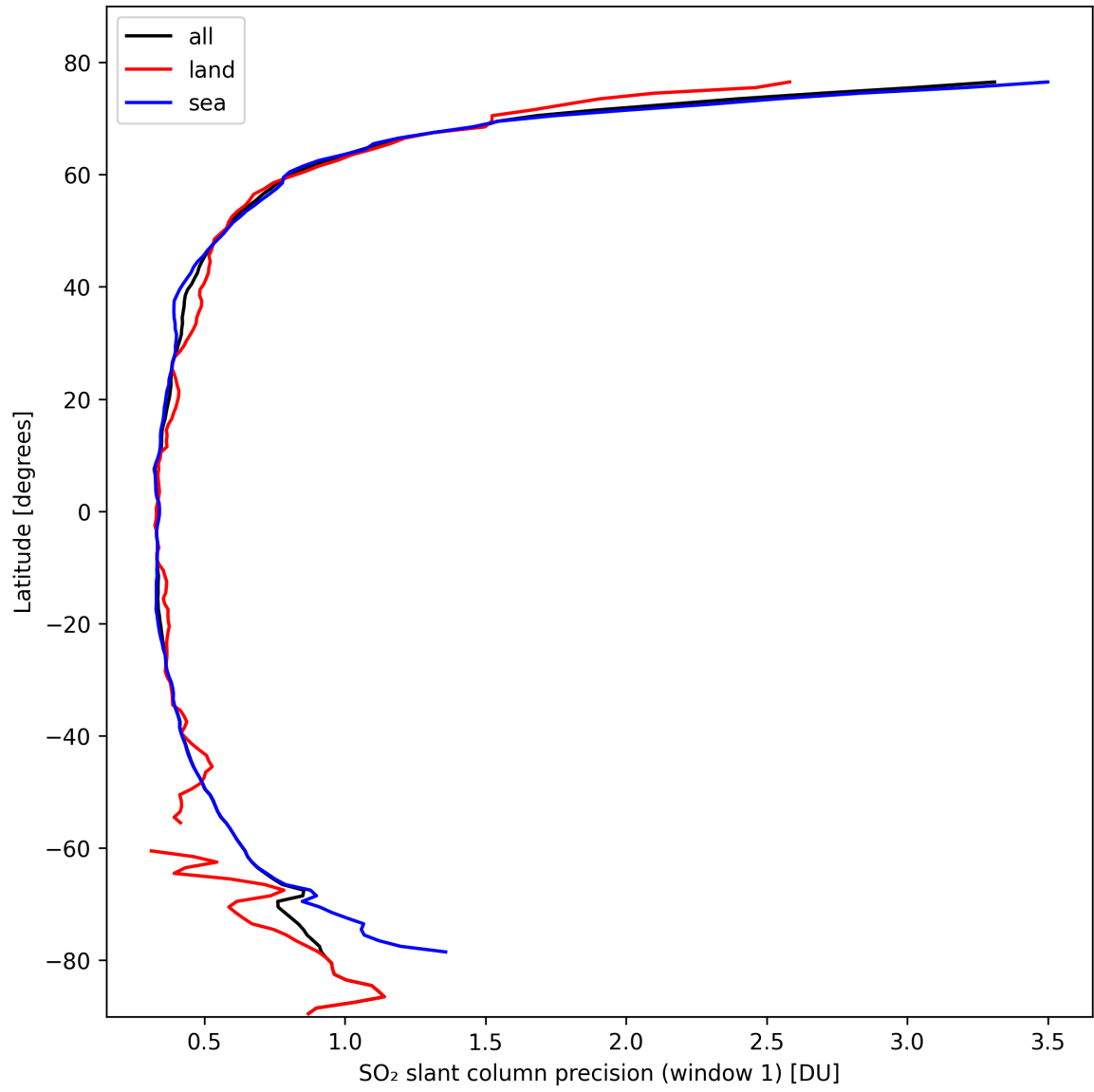
Figure 34: Zonal average of “SO 2 slant column precision (window 1)” for 2024-10-14 to 2024-10-15.
