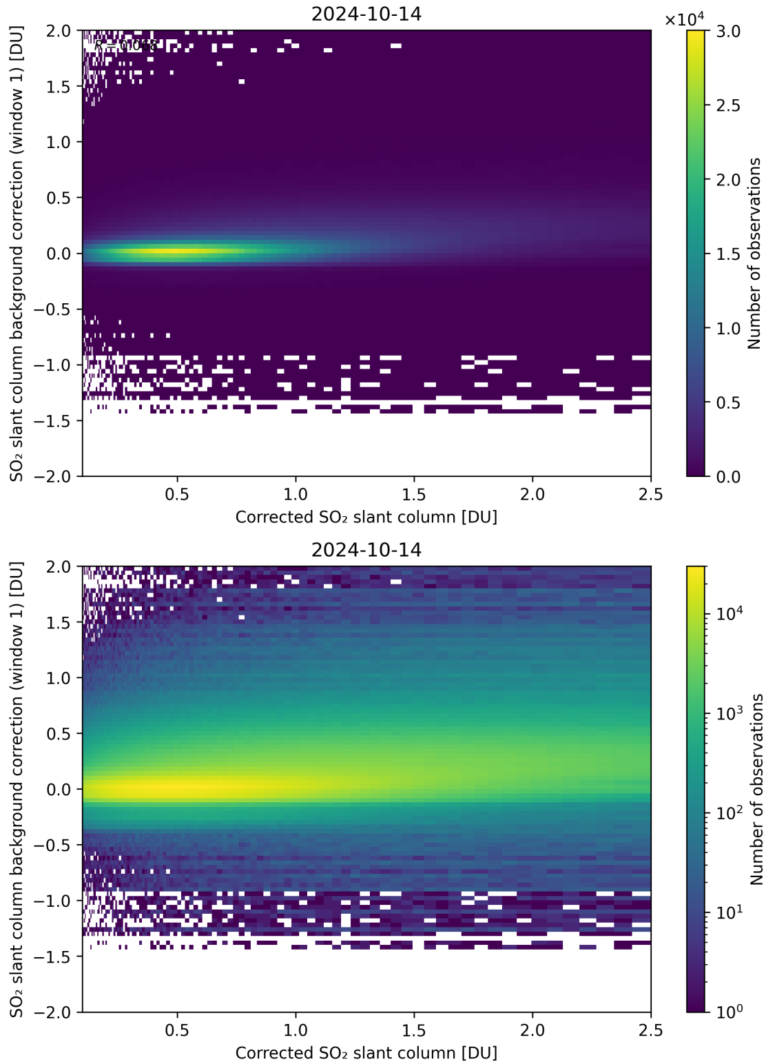
Figure 178: Scatter density plot of “Corrected SO 2 slant column” against “SO 2 slant column background correction (window 1)” for 2024-10-14 to 2024-10-15.
