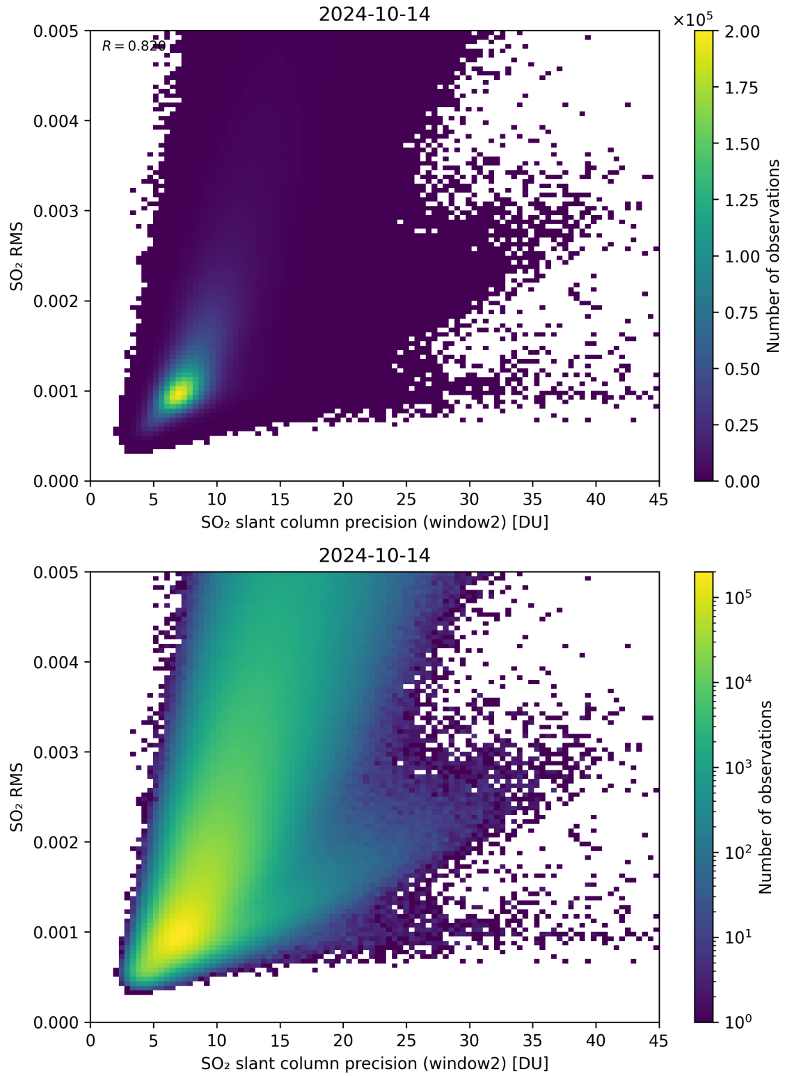
Figure 245: Scatter density plot of “SO 2 slant column precision (window2)” against “SO 2 RMS” for 2024-10-14 to 2024-10-15.
