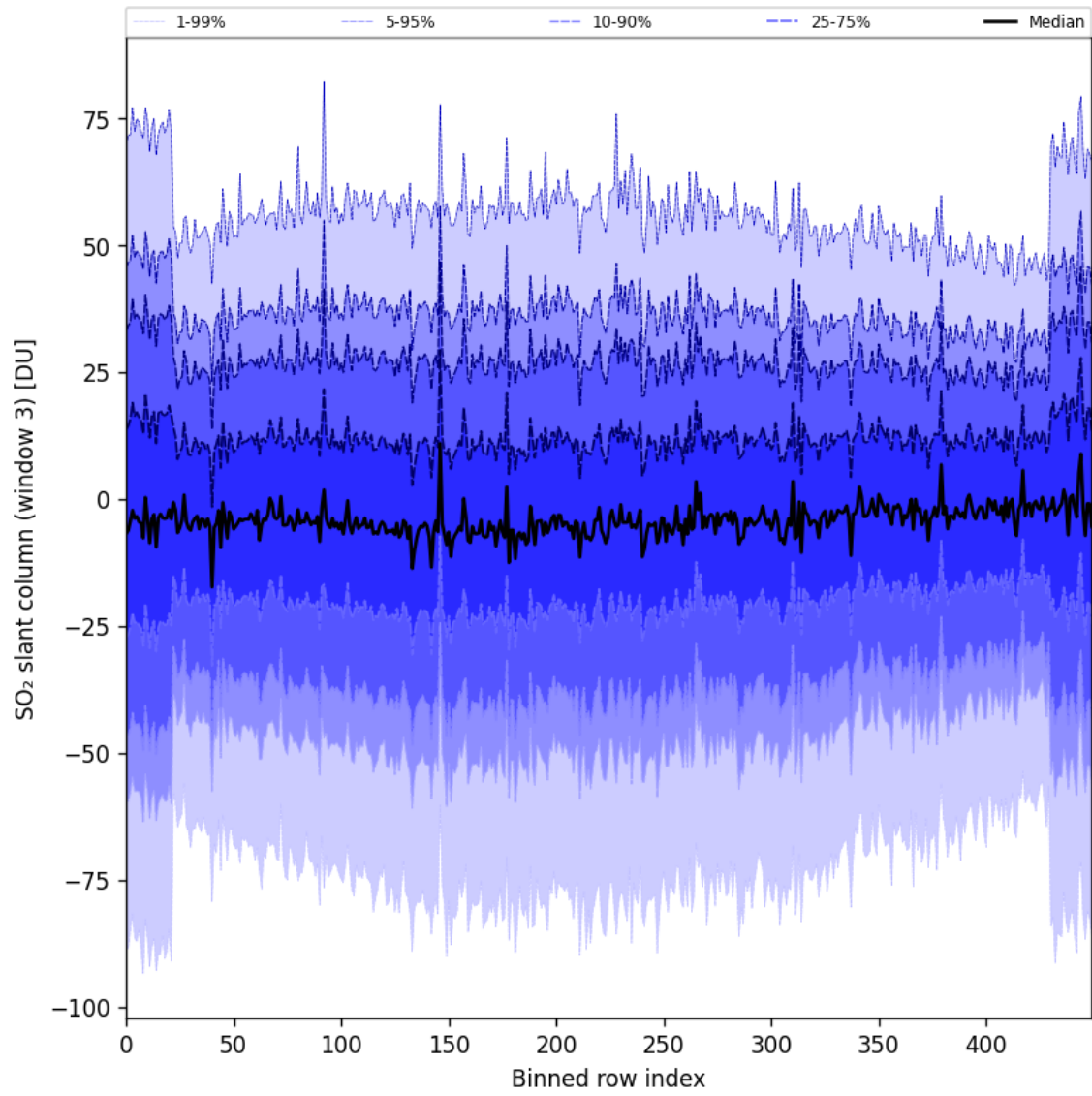
Figure 87: Along track statistics of “SO 2 slant column (window 3)” for 2024-10-14 to 2024-10-15
