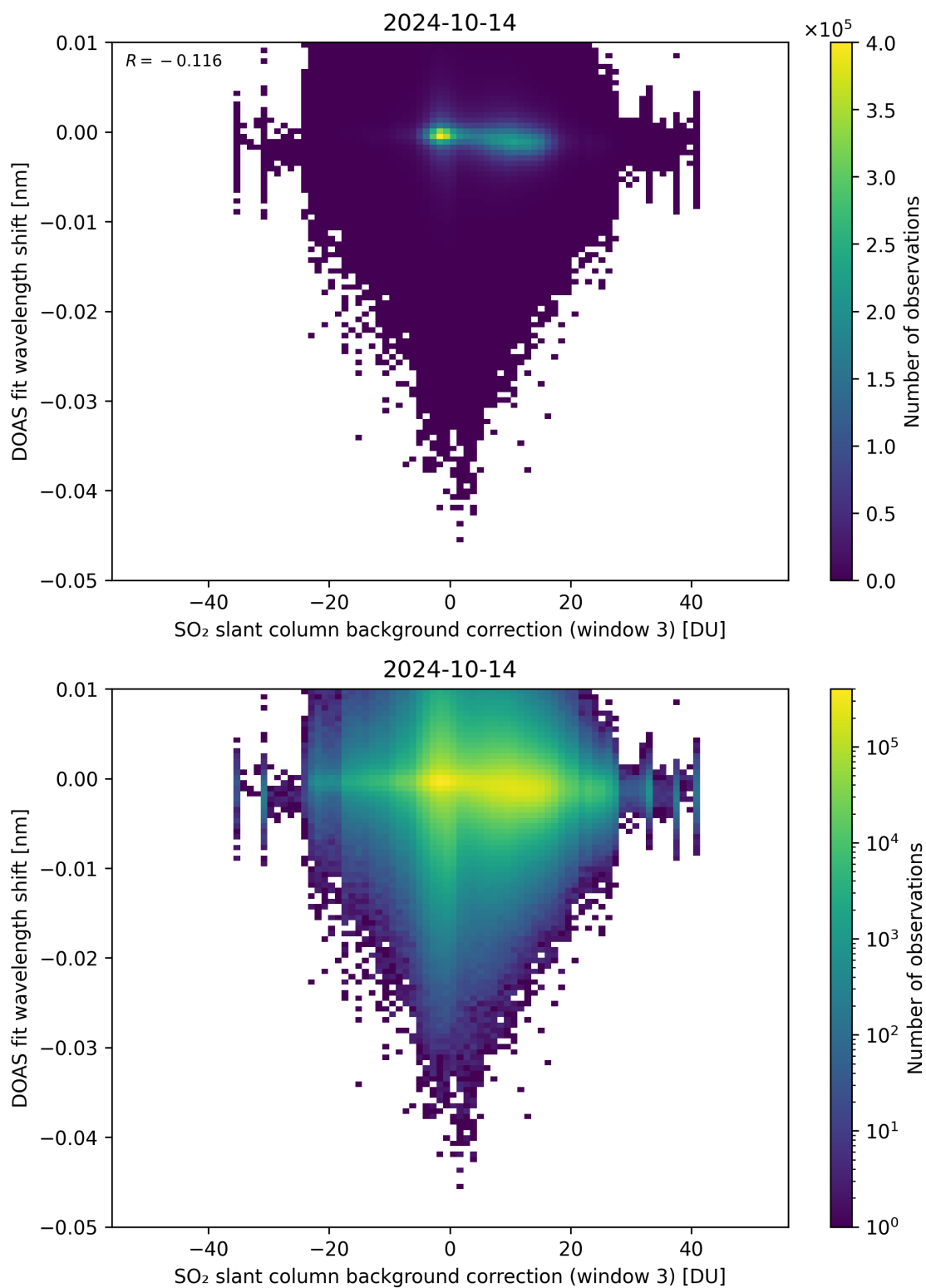
Figure 121: Scatter density plot of “SO 2 slant column background correction (window 3)” against “DOAS fit wavelength shift” for 2024-10-14 to 2024-10-15.
