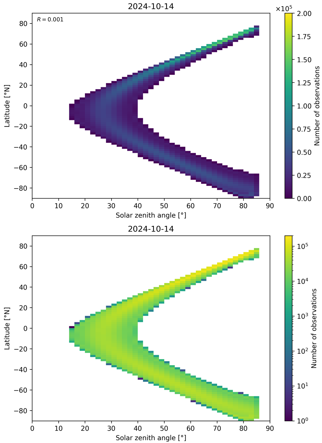
Figure 164: Scatter density plot of “Solar zenith angle” against “Latitude” for 2024-10-14 to 2024-10-15.
