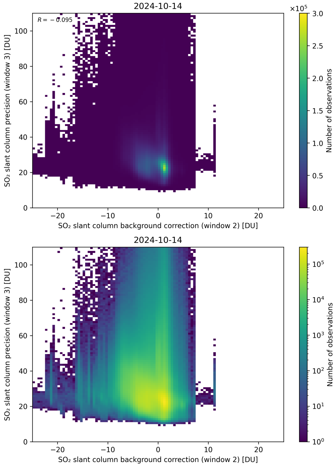
Figure 118: Scatter density plot of “SO 2 slant column background correction (window 2)” against “SO 2 slant column precision (window 3)” for 2024-10-14 to 2024-10-15.
