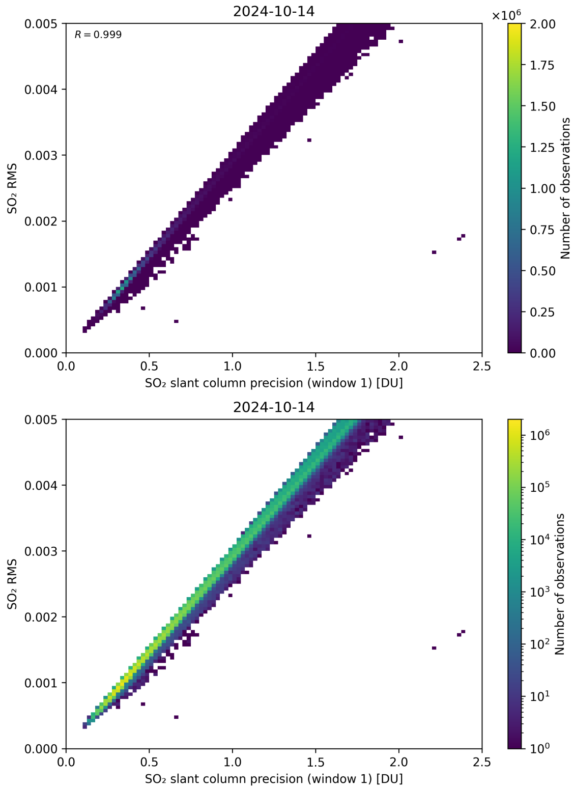
Figure 223: Scatter density plot of “SO 2 slant column precision (window 1)” against “SO 2 RMS” for 2024-10-14 to 2024-10-15.
