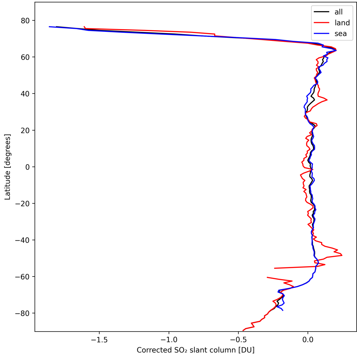
Figure 32: Zonal average of “Corrected SO 2 slant column” for 2024-10-14 to 2024-10-15.
