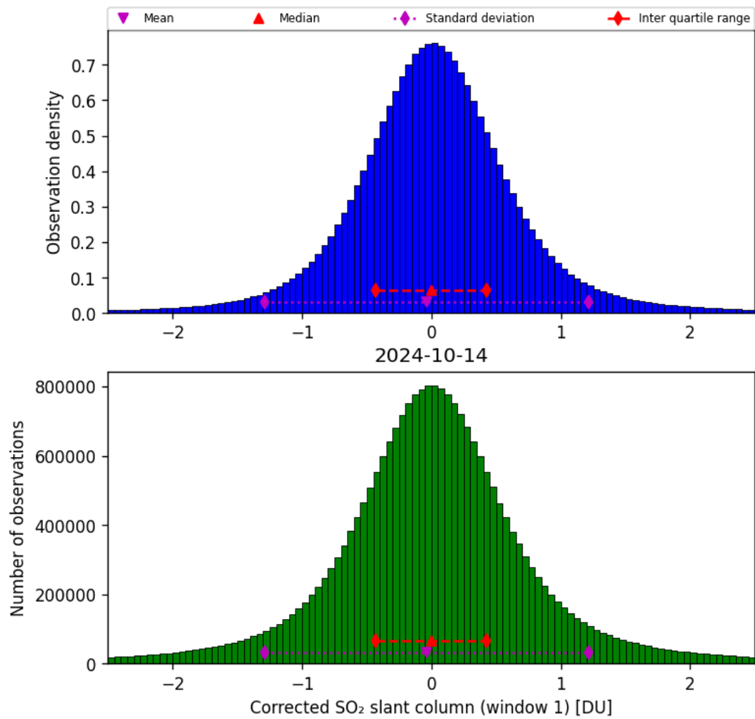
Figure 58: Histogram of “Corrected SO 2 slant column (window 1)” for 2024-10-14 to 2024-10-15
