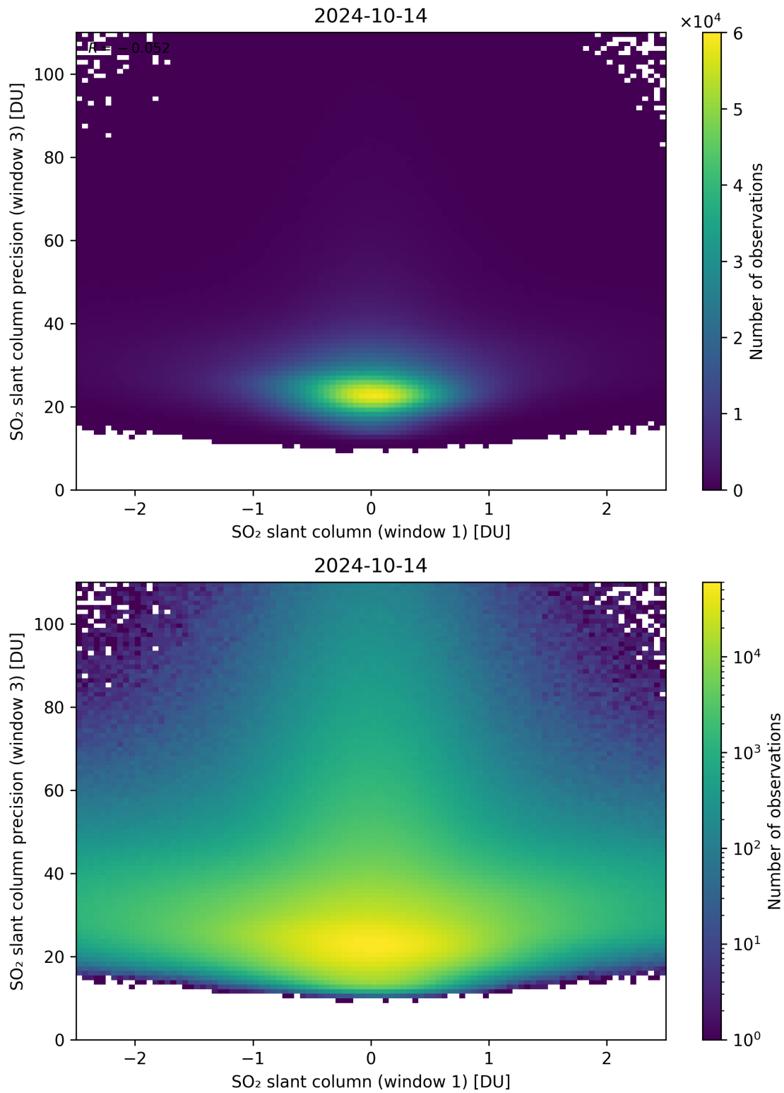
Figure 238: Scatter density plot of “SO 2 slant column (window 1)” against “SO 2 slant column precision (window 3)” for 2024-10-14 to 2024-10-15.
