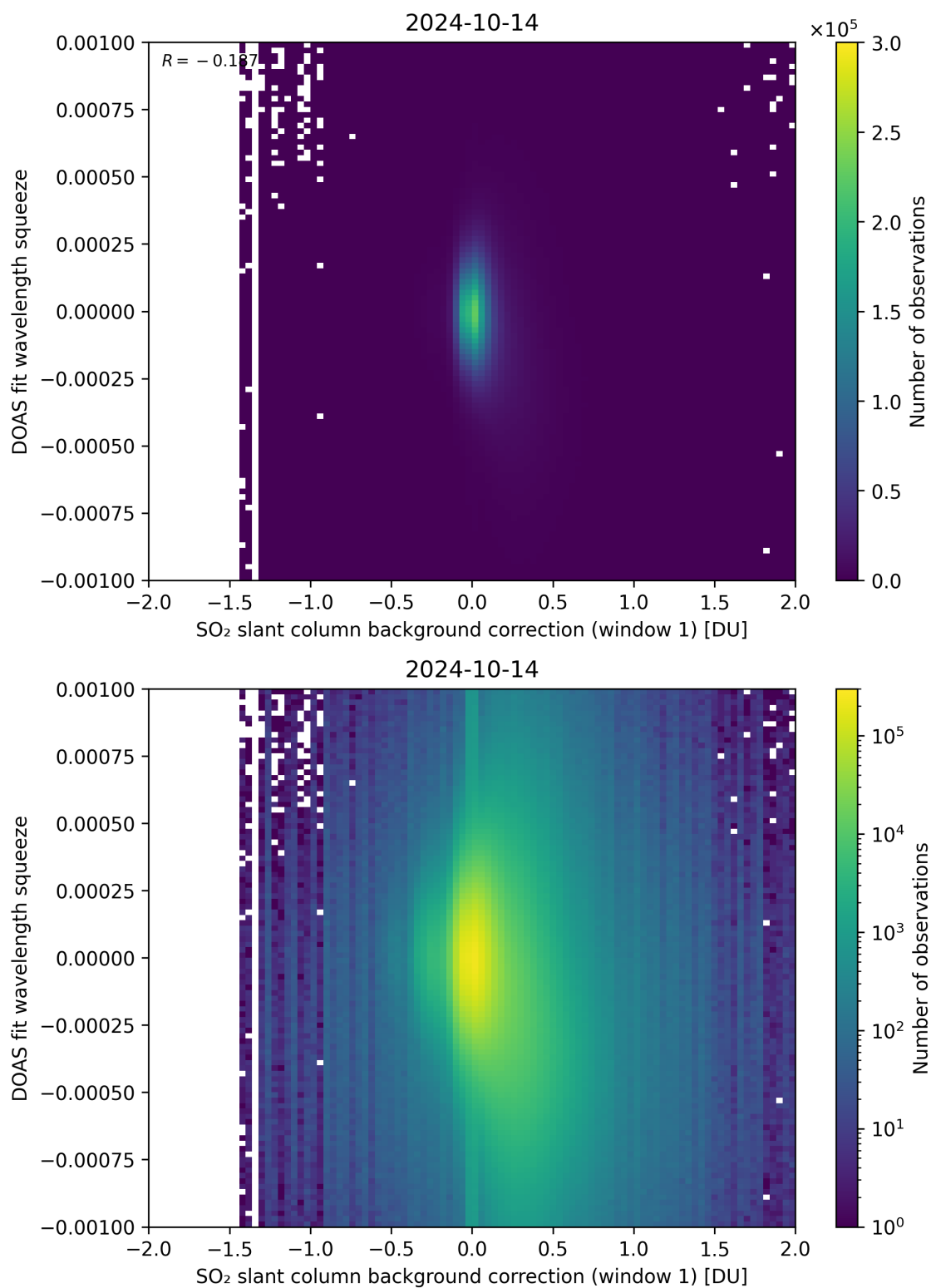
Figure 101: Scatter density plot of “SO 2 slant column background correction (window 1)” against “DOAS fit wavelength squeeze” for 2024-10-14 to 2024-10-15.
