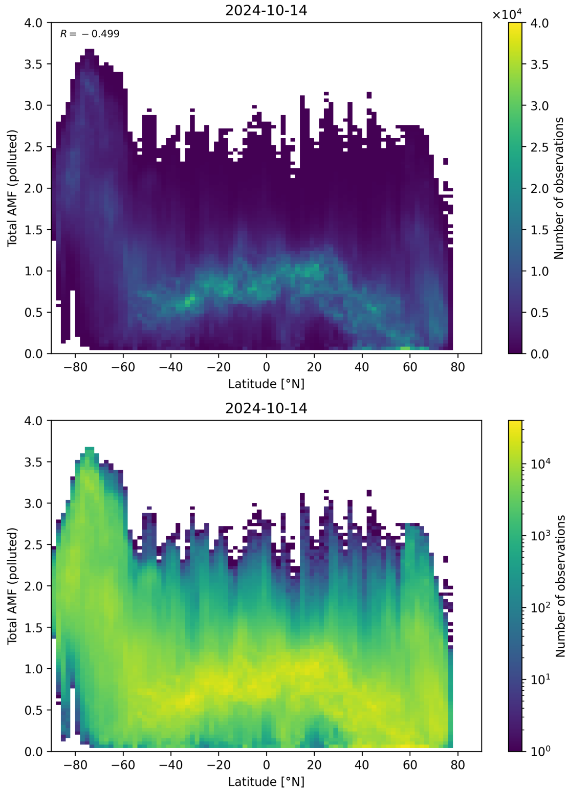
Figure 154: Scatter density plot of “Latitude” against “Total AMF (polluted)” for 2024-10-14 to 2024-10-15.
