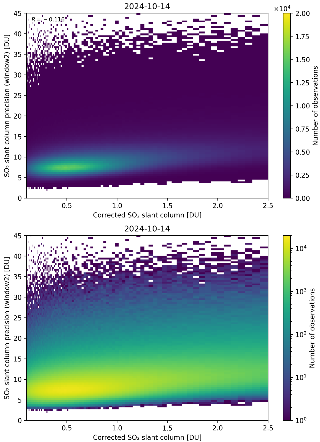
Figure 189: Scatter density plot of “Corrected SO 2 slant column” against “SO 2 slant column precision (window2)” for 2024-10-14 to 2024-10-15.
