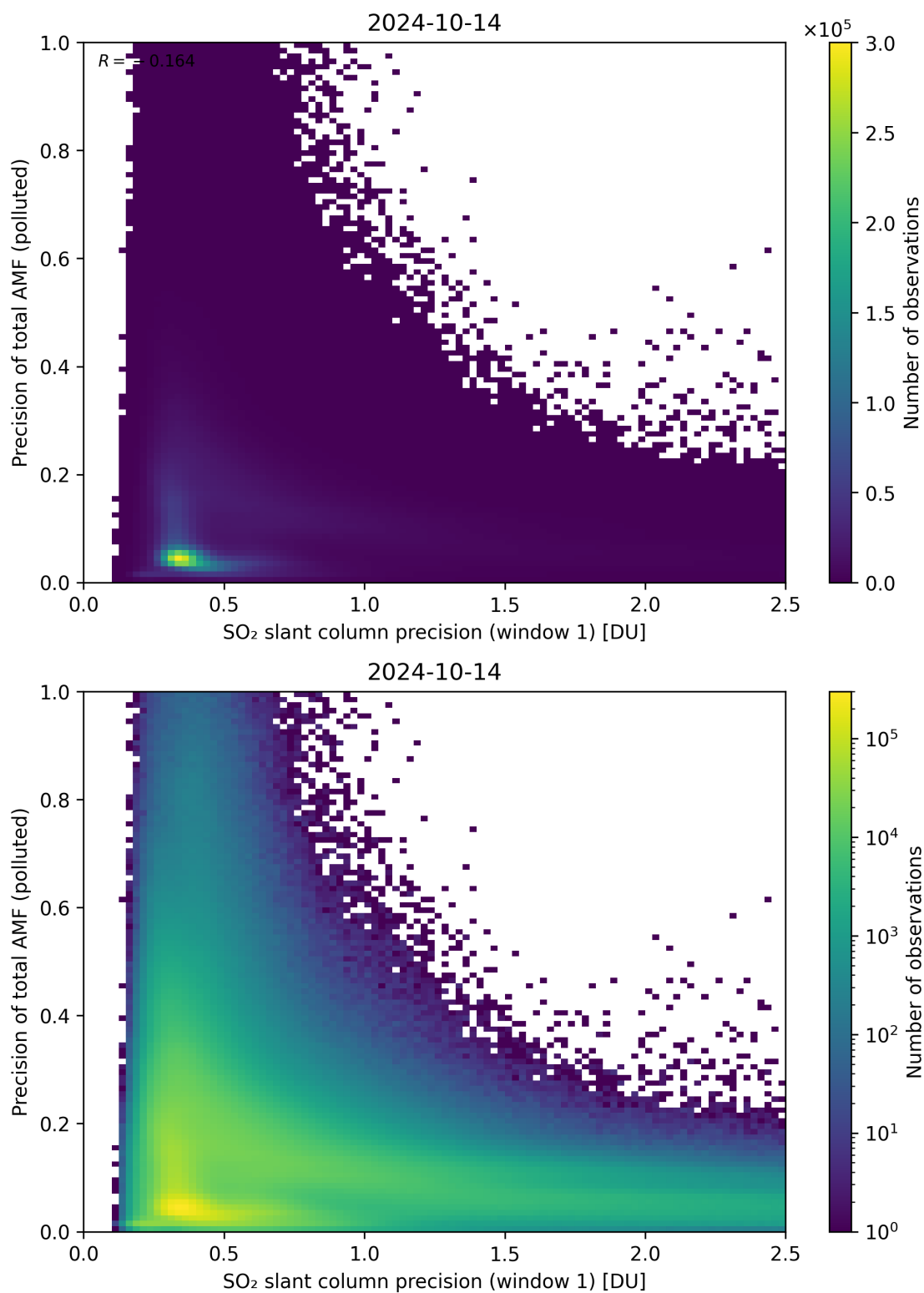
Figure 231: Scatter density plot of “SO 2 slant column precision (window 1)” against “Precision of total AMF (polluted)” for 2024-10-14 to 2024-10-15.
