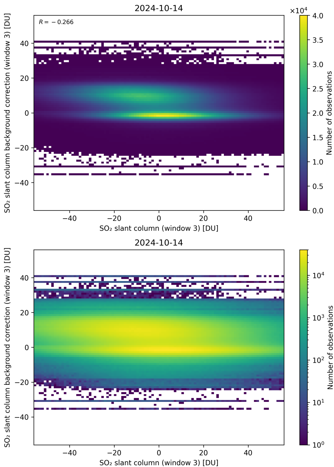
Figure 253: Scatter density plot of “SO 2 slant column (window 3)” against “SO 2 slant column background correction (window 3)” for 2024-10-14 to 2024-10-15.
