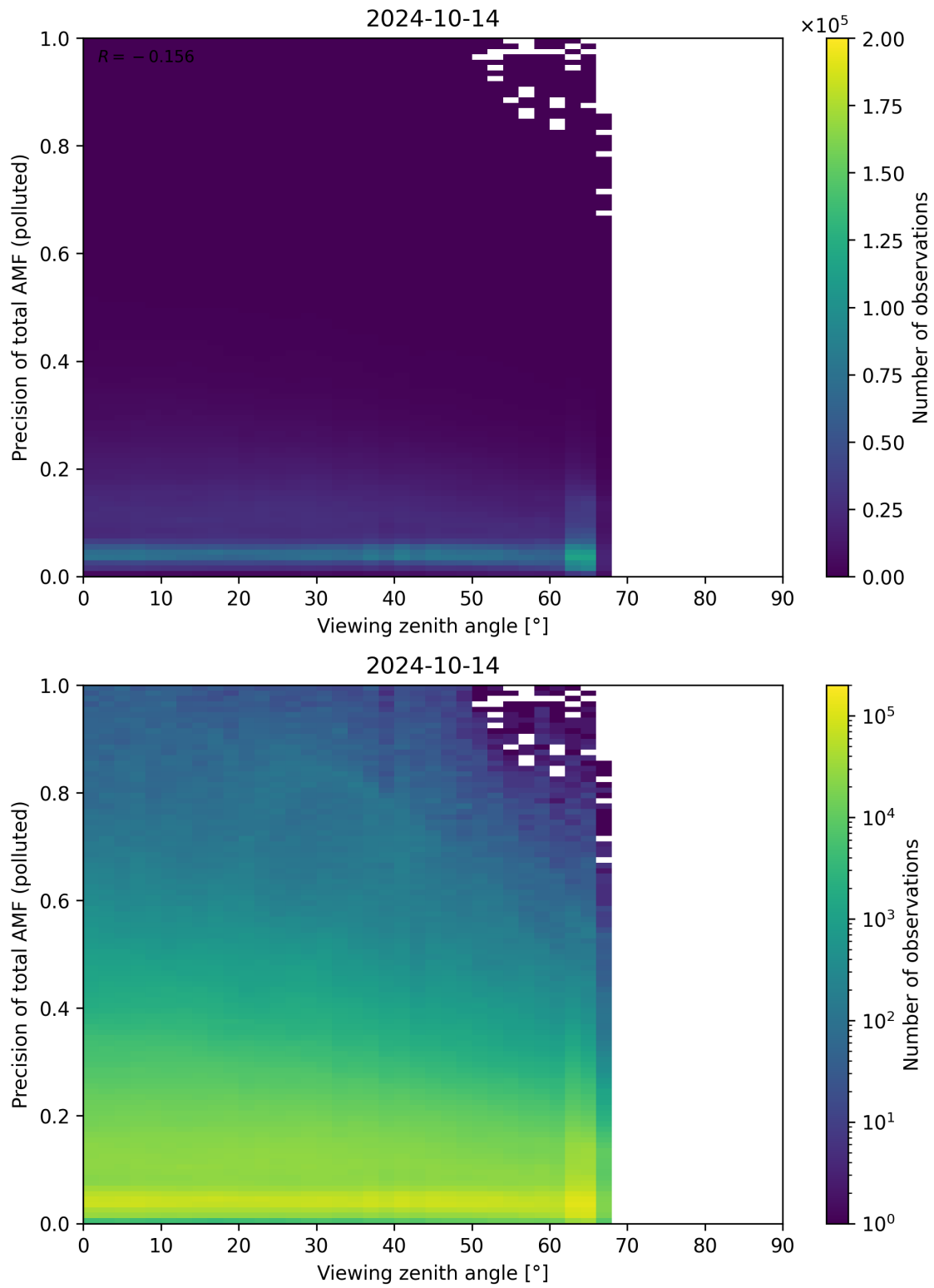
Figure 326: Scatter density plot of “Viewing zenith angle” against “Precision of total AMF (polluted)” for 2024-10-14 to 2024-10-15.
