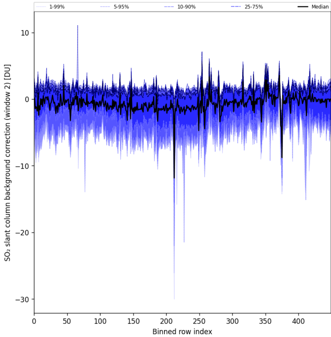
Figure 86: Along track statistics of “SO 2 slant column background correction (window 2)” for 2024-10-14 to 2024-10-15
