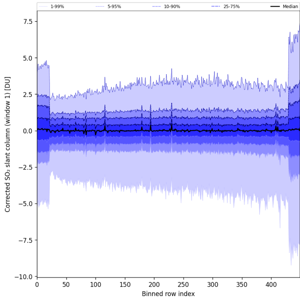
Figure 81: Along track statistics of “Corrected SO 2 slant column (window 1)” for 2024-10-14 to 2024-10-15
