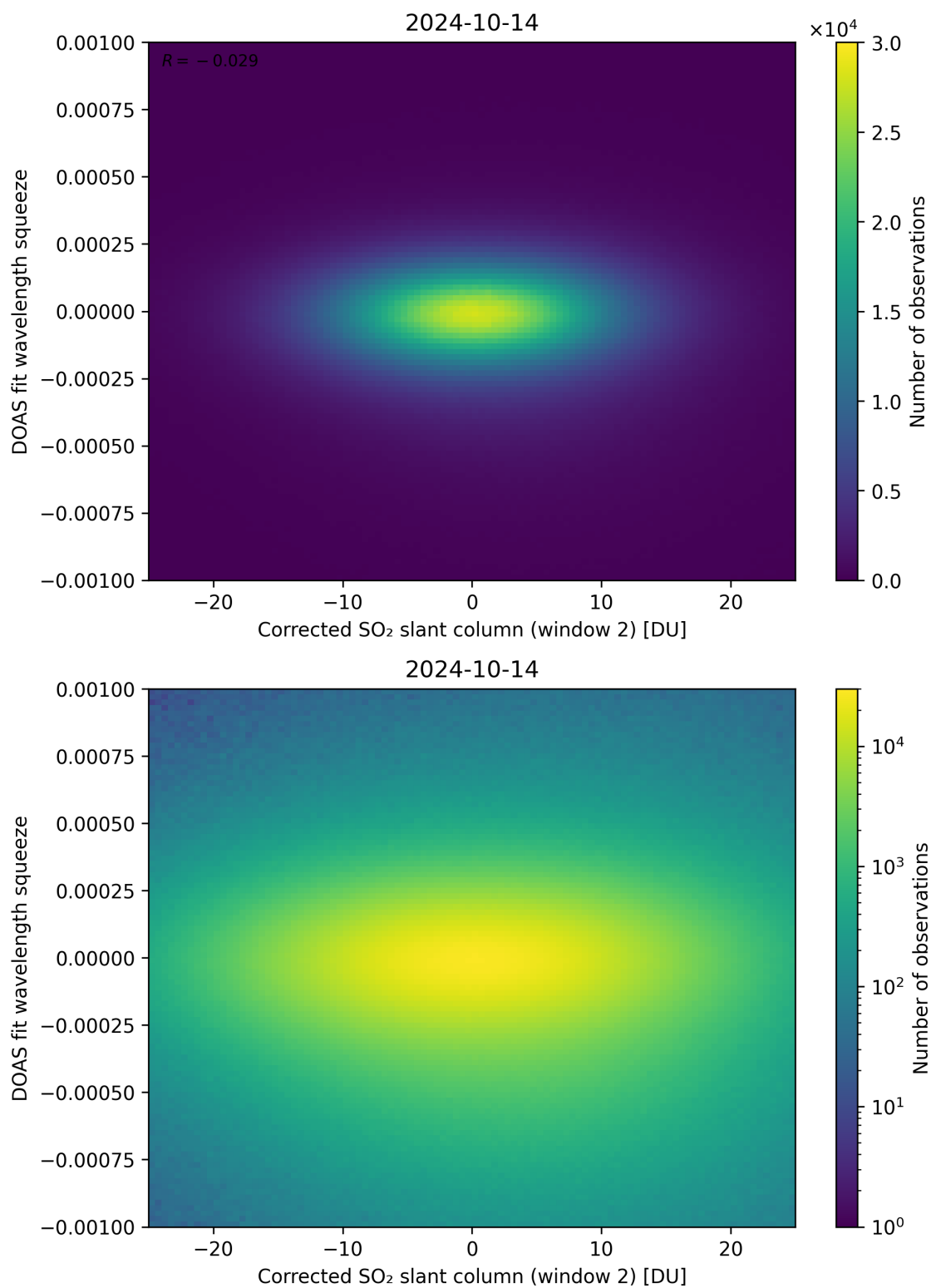
Figure 197: Scatter density plot of “Corrected SO 2 slant column (window 2)” against “DOAS fit wavelength squeeze” for 2024-10-14 to 2024-10-15.
