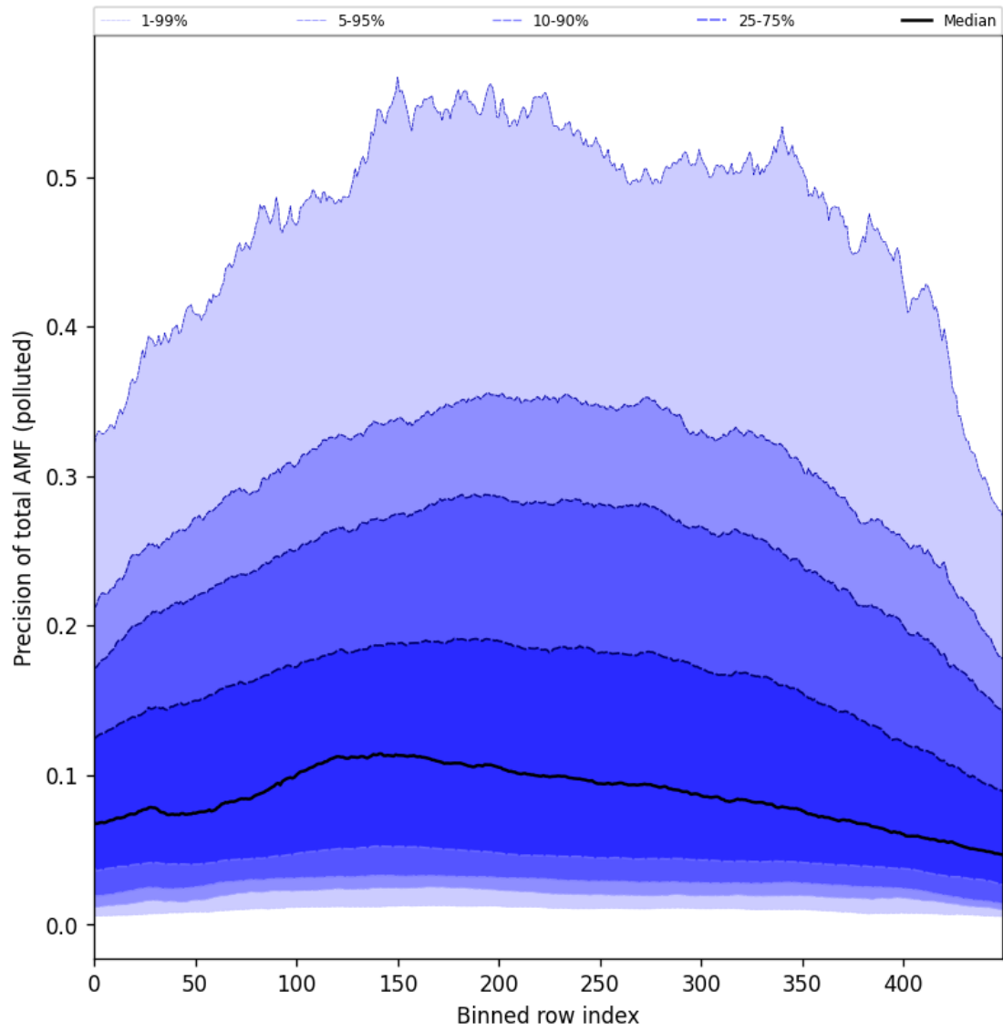
Figure 95: Along track statistics of “Precision of total AMF (polluted)” for 2024-10-14 to 2024-10-15
