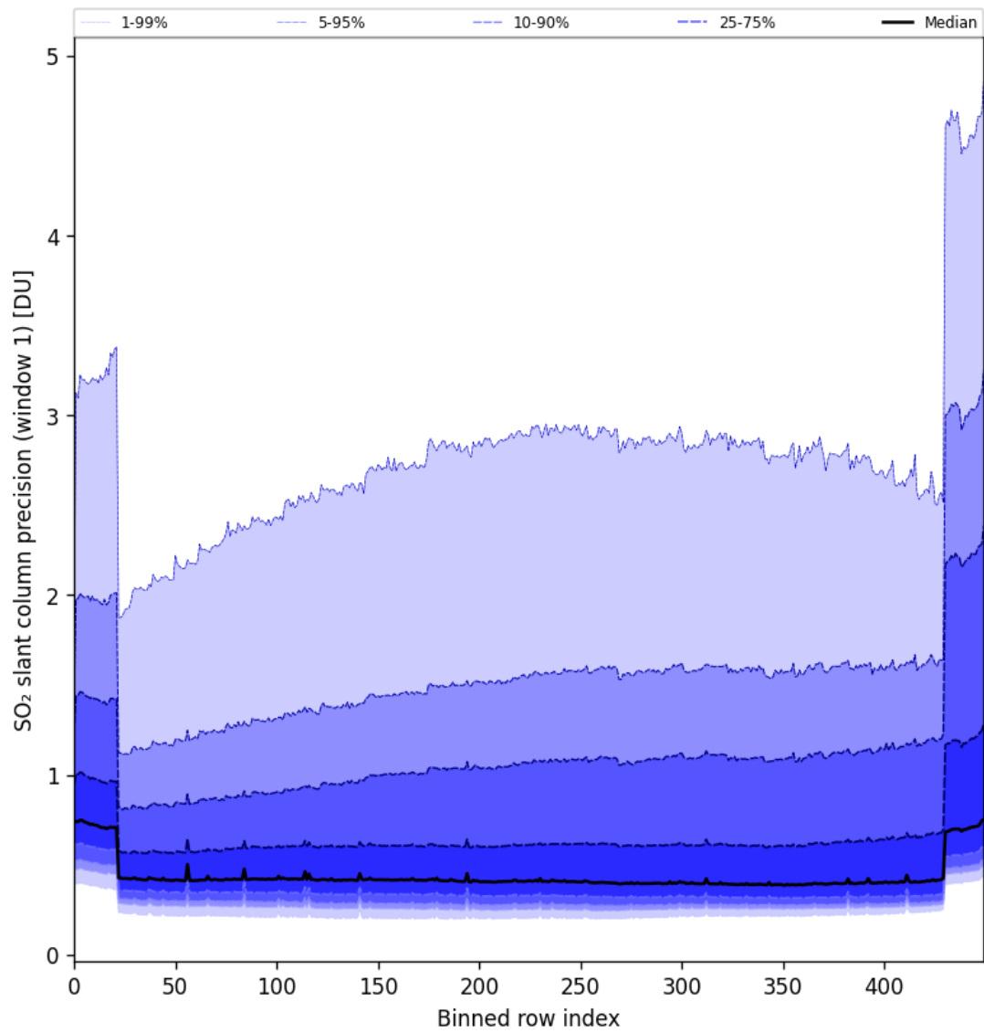
Figure 80: Along track statistics of “SO 2 slant column precision (window 1)” for 2024-10-14 to 2024-10-15
