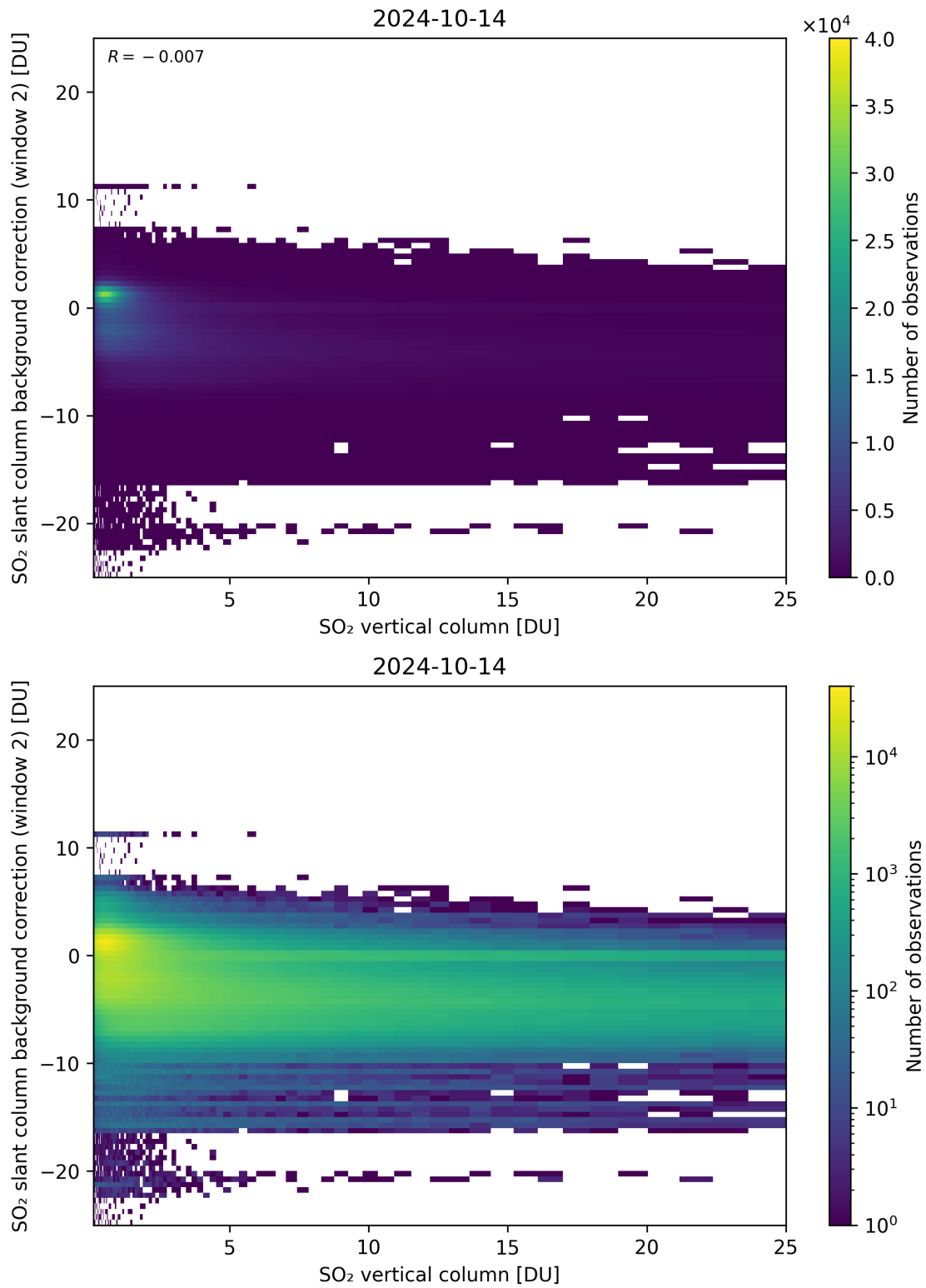
Figure 274: Scatter density plot of “SO 2 vertical column” against “SO 2 slant column background correction (window 2)” for 2024-10-14 to 2024-10-15.
