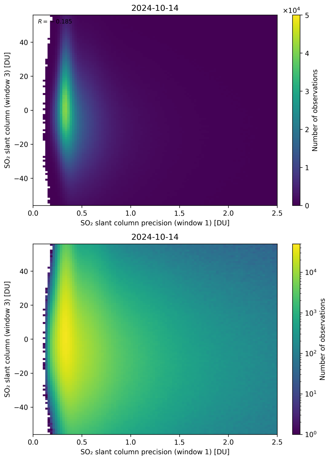
Figure 228: Scatter density plot of “SO 2 slant column precision (window 1)” against “SO 2 slant column (window 3)” for 2024-10-14 to 2024-10-15.
