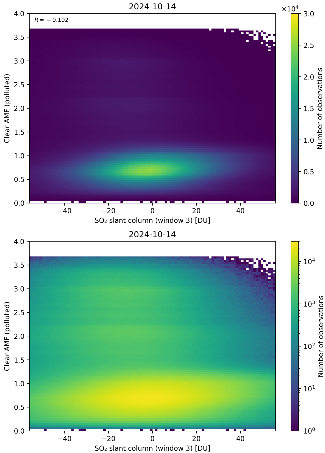
Figure 265: Scatter density plot of “SO 2 slant column (window 3)” against “Clear AMF (polluted)” for 2024-10-14 to 2024-10-15.
