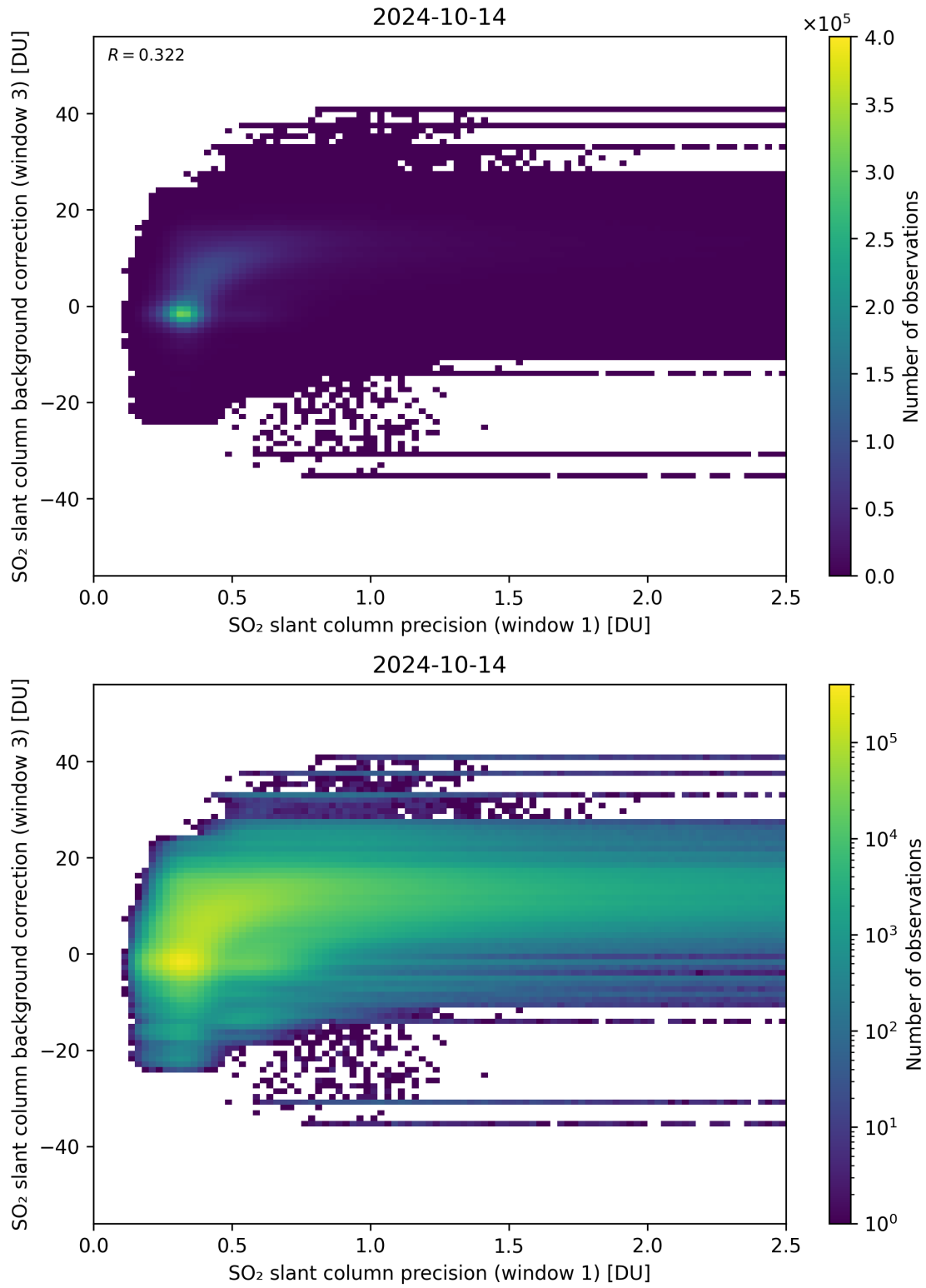
Figure 220: Scatter density plot of “SO 2 slant column precision (window 1)” against “SO 2 slant column background correction (window 3)” for 2024-10-14 to 2024-10-15.
