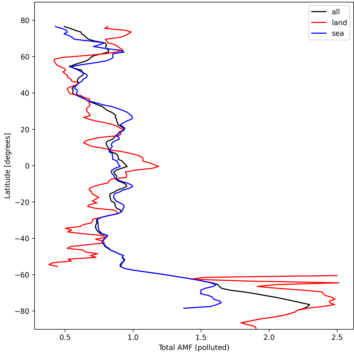
Figure 48: Zonal average of “Total AMF (polluted)” for 2024-10-14 to 2024-10-15.
