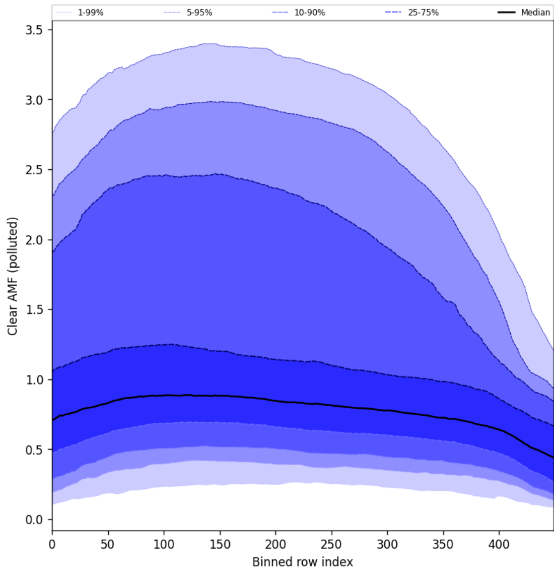
Figure 96: Along track statistics of “Clear AMF (polluted)” for 2024-10-14 to 2024-10-15
