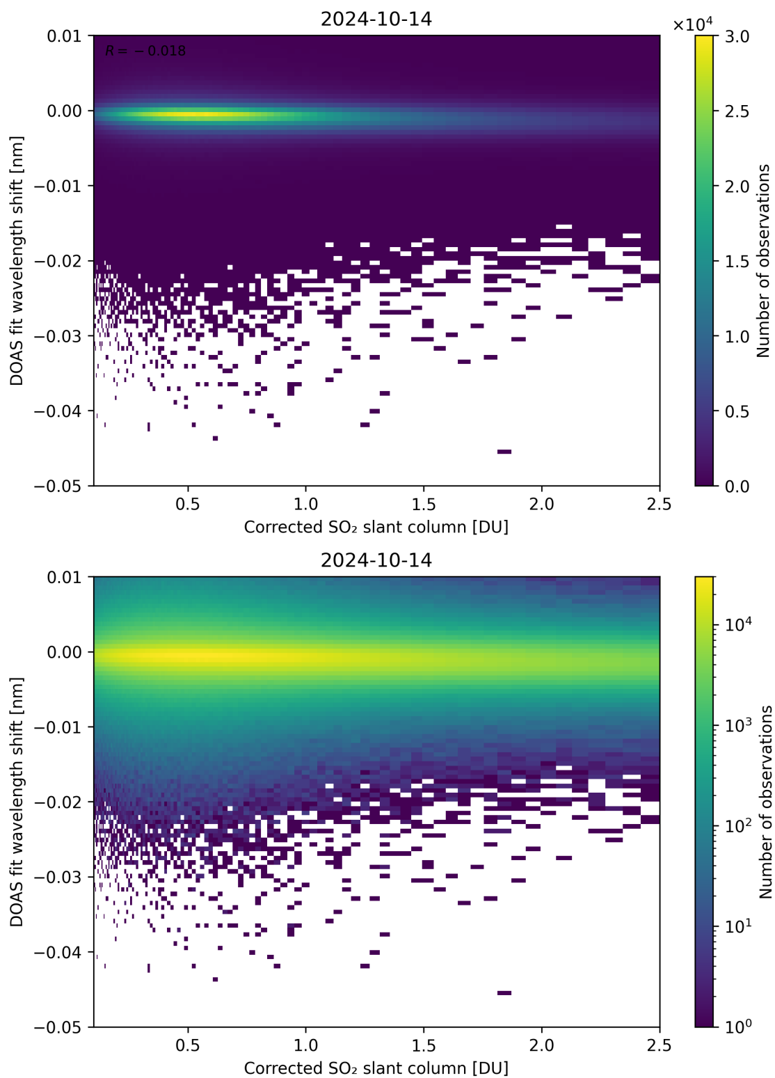
Figure 181: Scatter density plot of “Corrected SO 2 slant column” against “DOAS fit wavelength shift” for 2024-10-14 to 2024-10-15.
