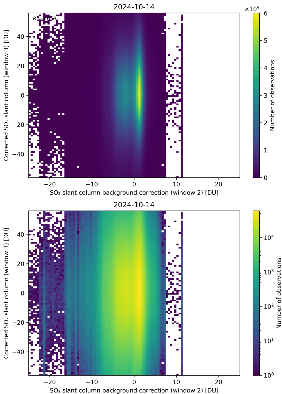
Figure 116: Scatter density plot of “SO 2 slant column background correction (window 2)” against “Corrected SO 2 slant column (window 3)” for 2024-10-14 to 2024-10-15.
