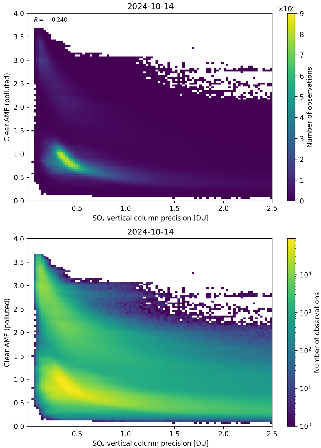
Figure 285: Scatter density plot of “SO 2 vertical column precision” against “Clear AMF (polluted)” for 2024-10-14 to 2024-10-15.
