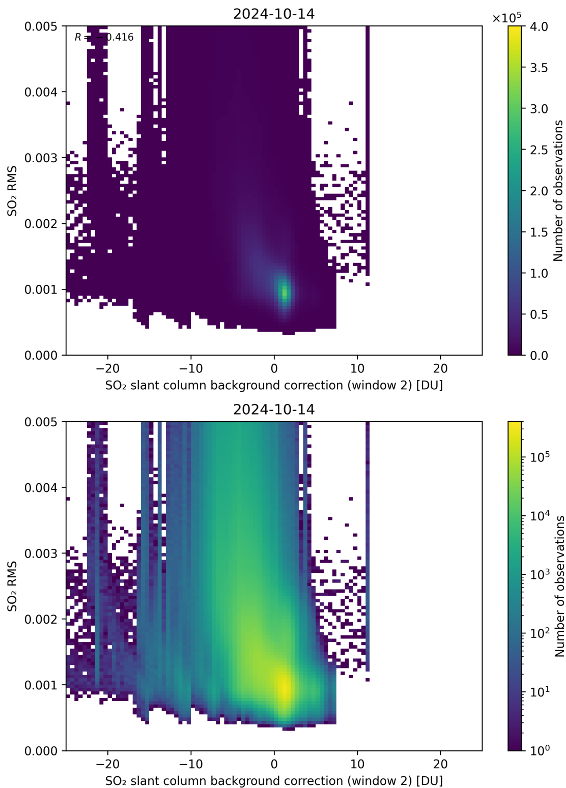
Figure 114: Scatter density plot of “SO 2 slant column background correction (window 2)” against “SO 2 RMS” for 2024-10-14 to 2024-10-15.
