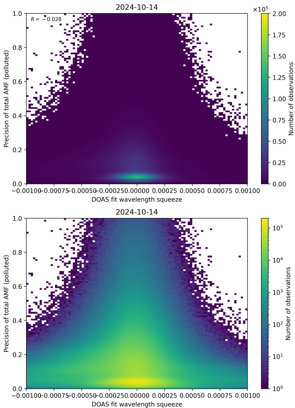
Figure 135: Scatter density plot of “DOAS fit wavelength squeeze” against “Precision of total AMF (polluted)” for 2024-10-14 to 2024-10-15.
