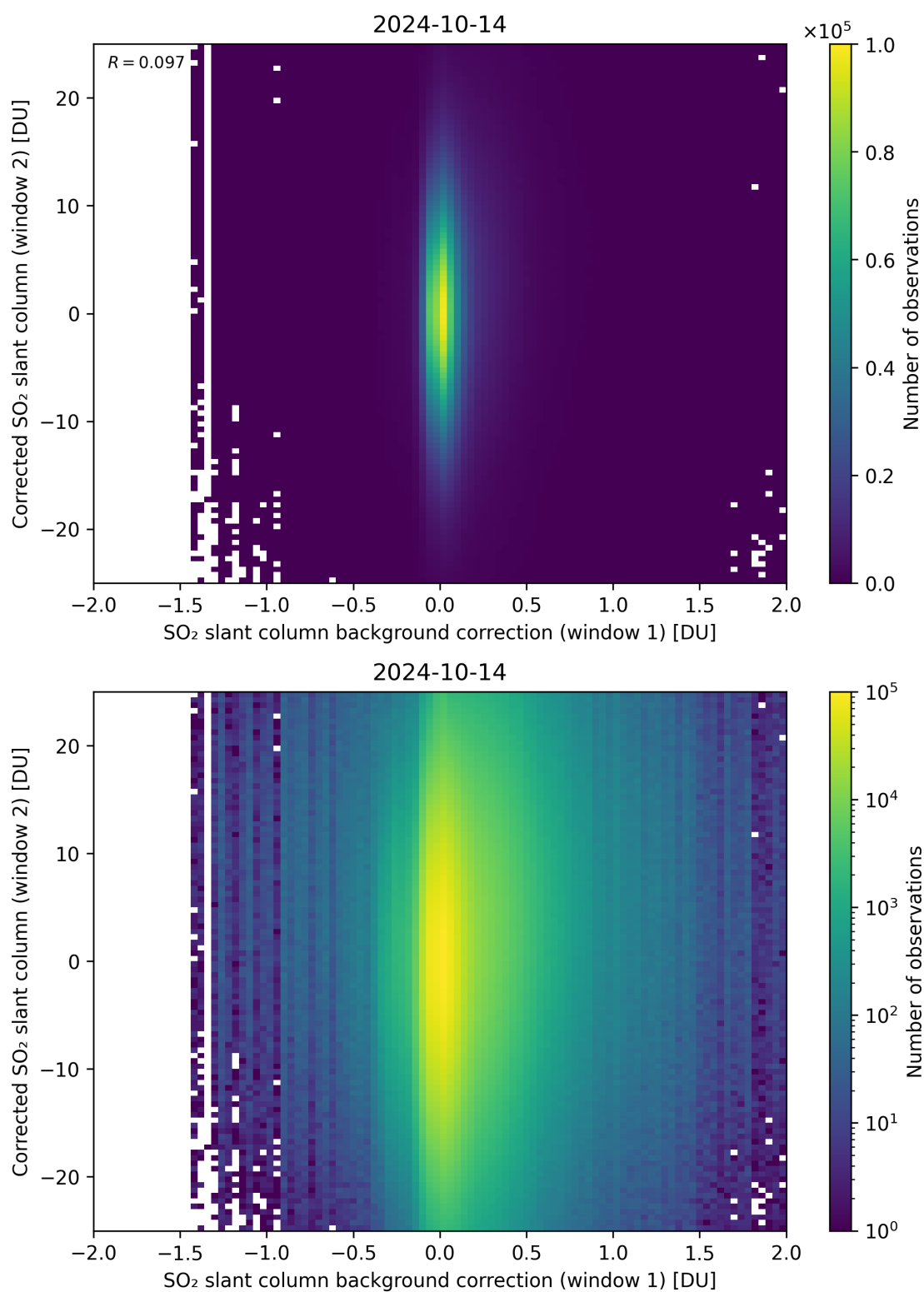
Figure 104: Scatter density plot of “SO 2 slant column background correction (window 1)” against “Corrected SO 2 slant column (window 2)” for 2024-10-14 to 2024-10-15.
