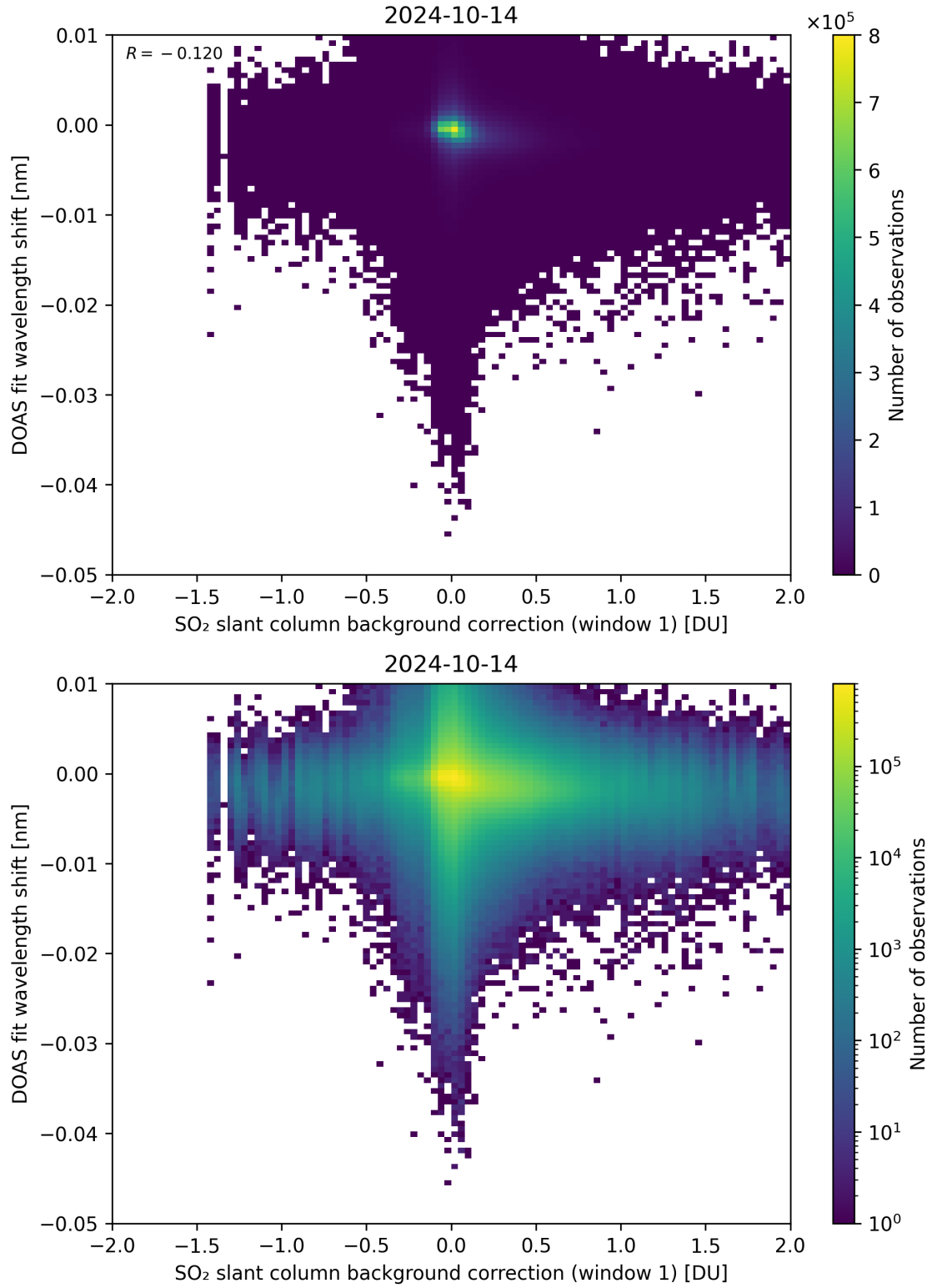
Figure 100: Scatter density plot of “SO 2 slant column background correction (window 1)” against “DOAS fit wavelength shift” for 2024-10-14 to 2024-10-15.
