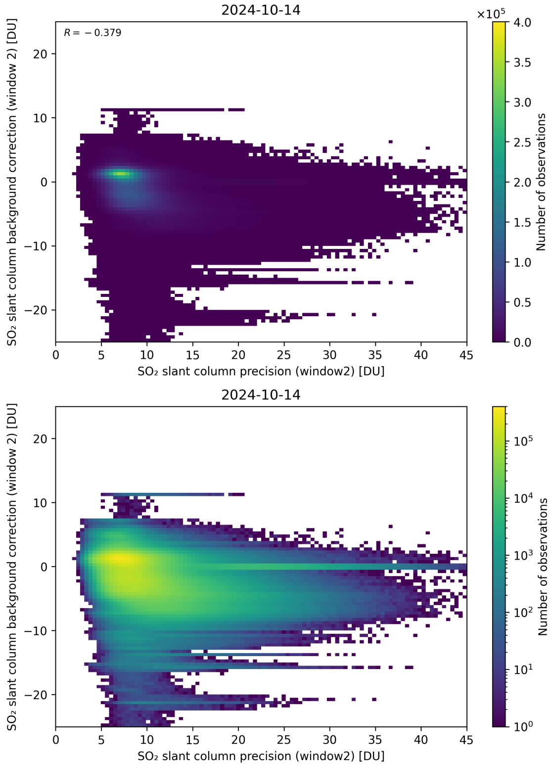
Figure 241: Scatter density plot of “SO 2 slant column precision (window2)” against “SO 2 slant column background correction (window 2)” for 2024-10-14 to 2024-10-15.
