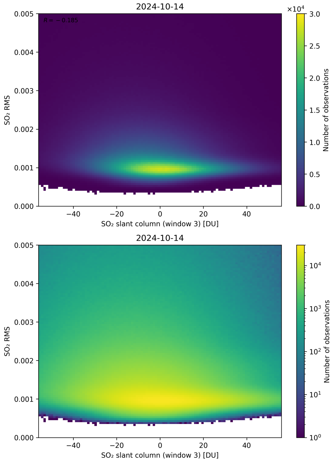
Figure 256: Scatter density plot of “SO 2 slant column (window 3)” against “SO 2 RMS” for 2024-10-14 to 2024-10-15.
