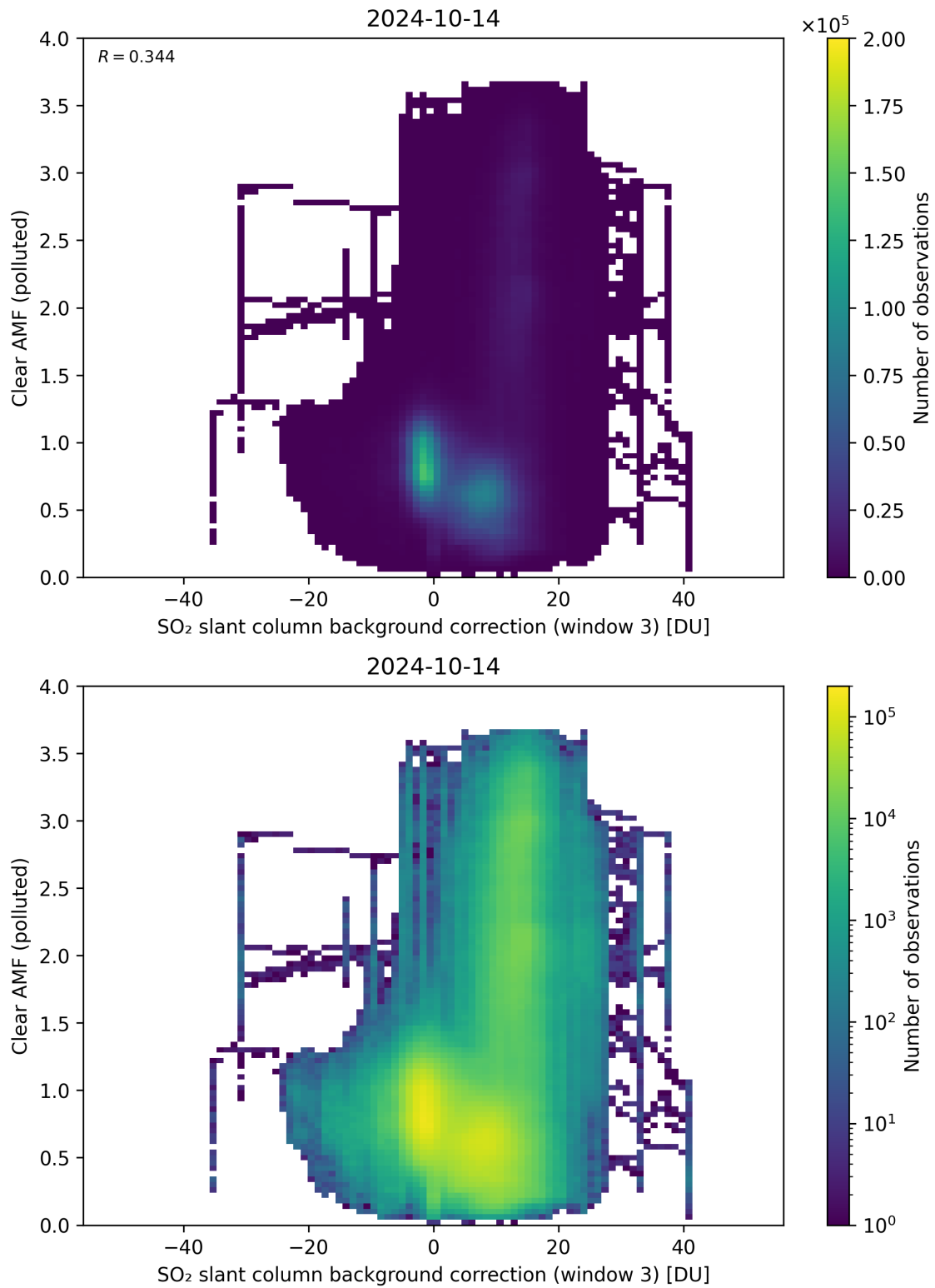
Figure 124: Scatter density plot of “SO 2 slant column background correction (window 3)” against “Clear AMF (polluted)” for 2024-10-14 to 2024-10-15.
