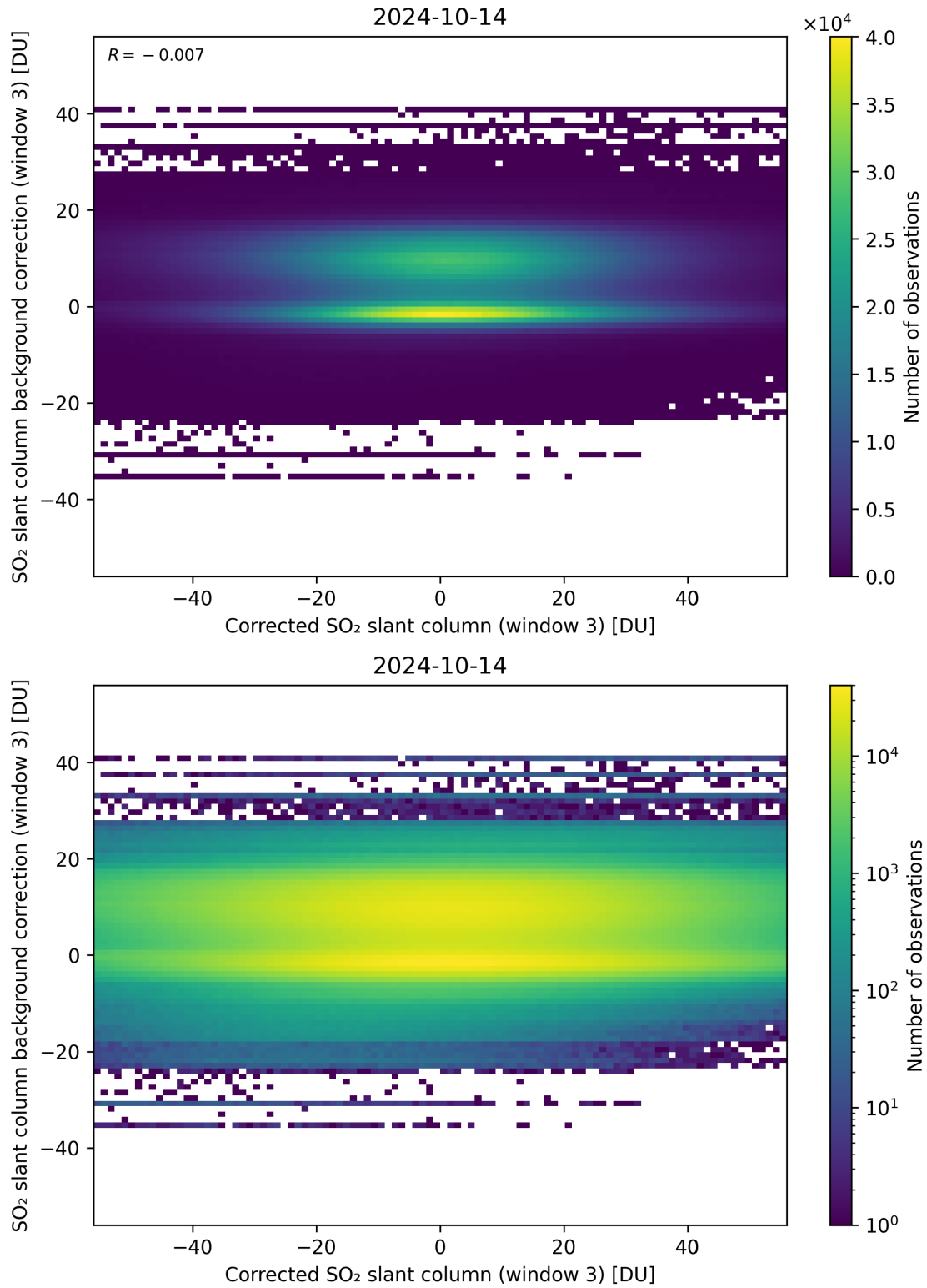
Figure 205: Scatter density plot of “Corrected SO 2 slant column (window 3)” against “SO 2 slant column background correction (window 3)” for 2024-10-14 to 2024-10-15.
