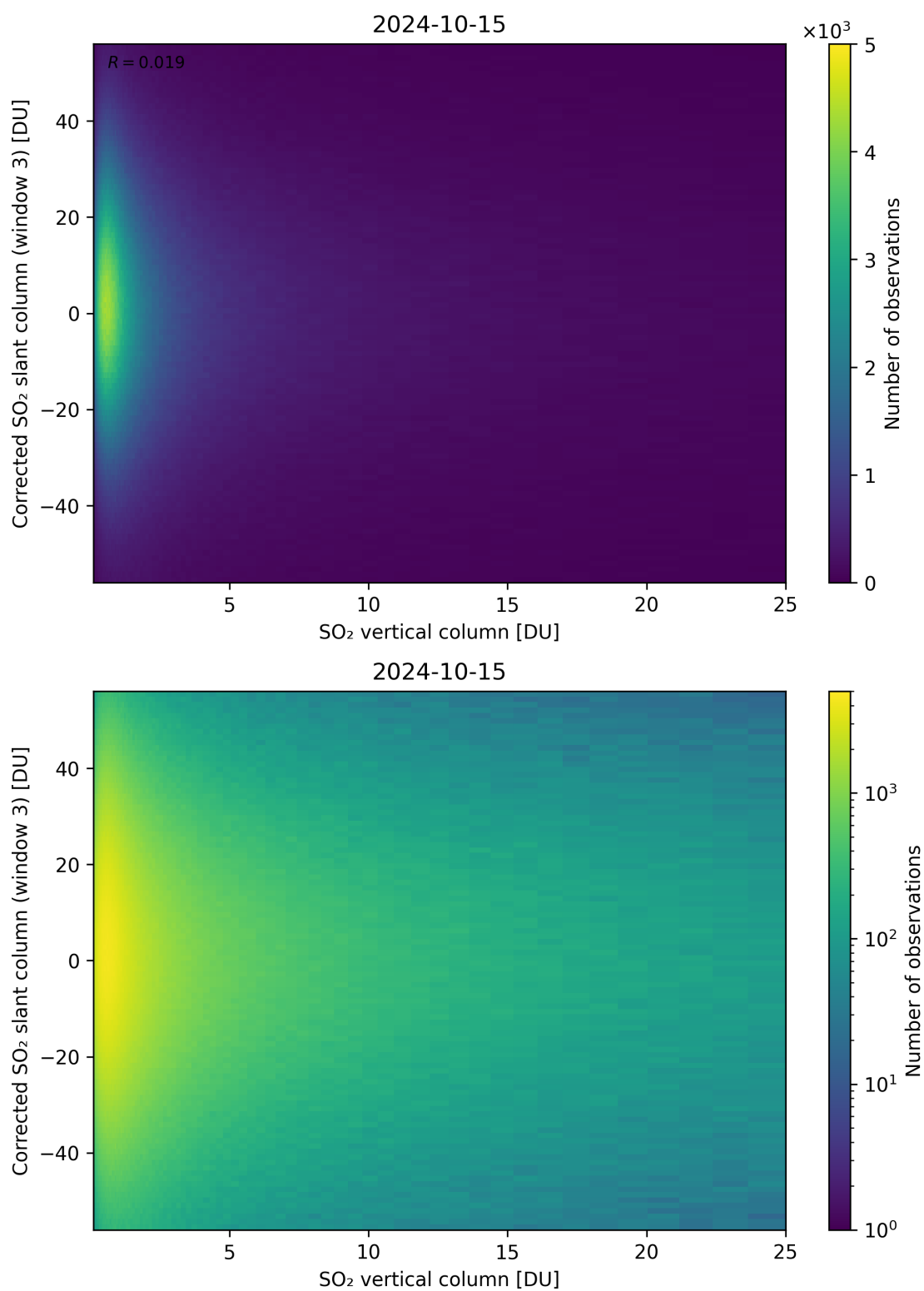
Figure 299: Scatter density plot of “SO 2 vertical column” against “Corrected SO 2 slant column (window 3)” for 2024-10-14 to 2024-10-16.
