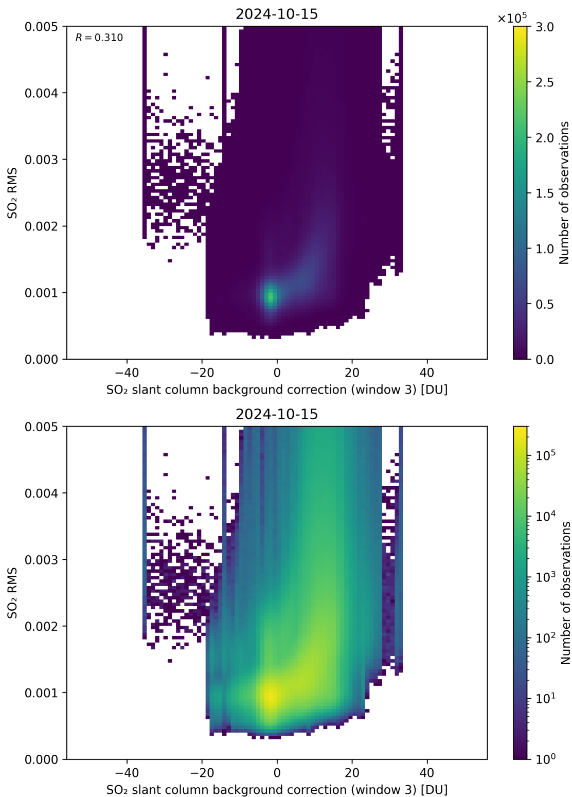
Figure 123: Scatter density plot of “SO 2 slant column background correction (window 3)” against “SO 2 RMS” for 2024-10-14 to 2024-10-16.
