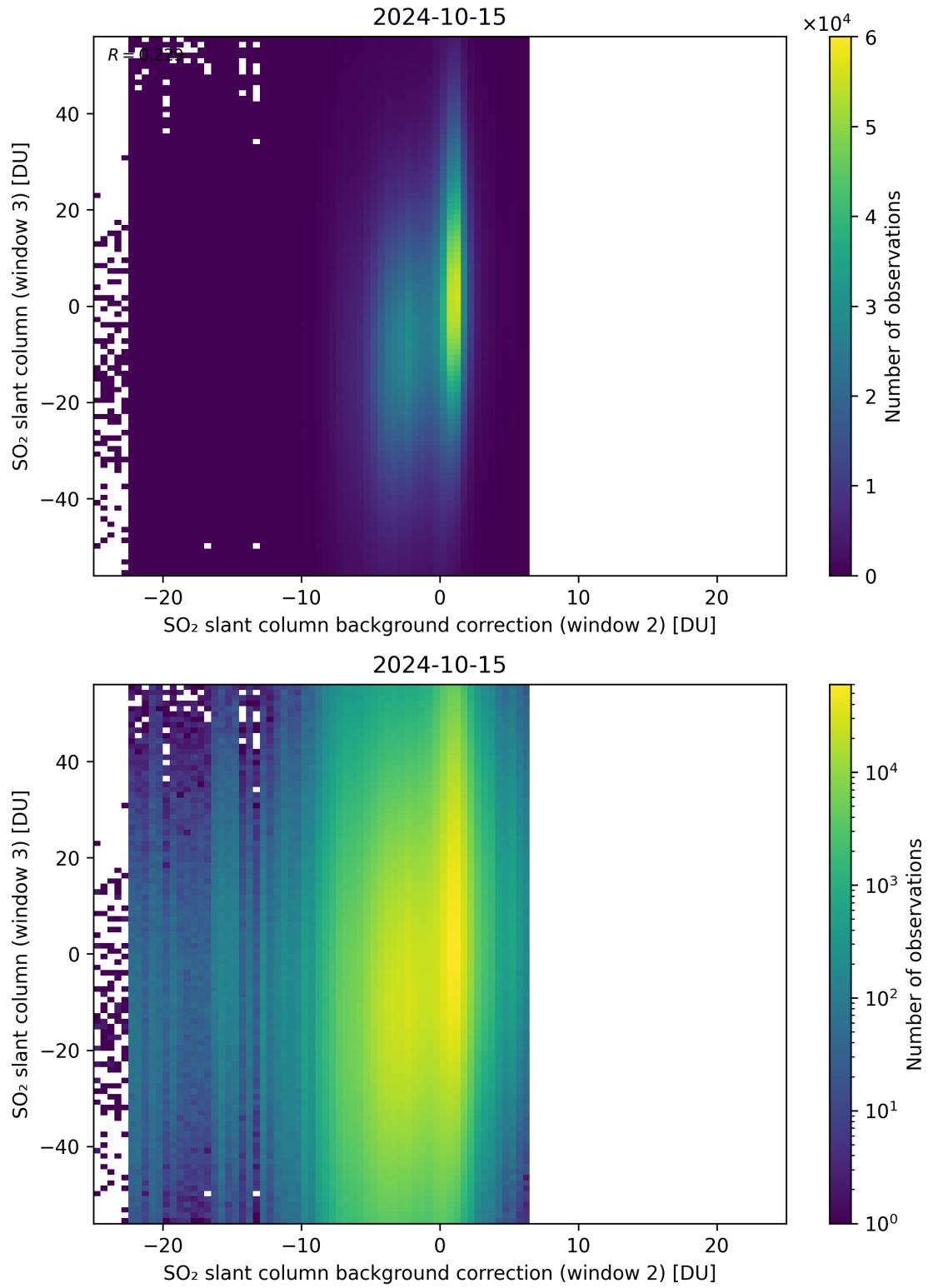
Figure 117: Scatter density plot of “SO 2 slant column background correction (window 2)” against “SO 2 slant column (window 3)” for 2024-10-14 to 2024-10-16.
