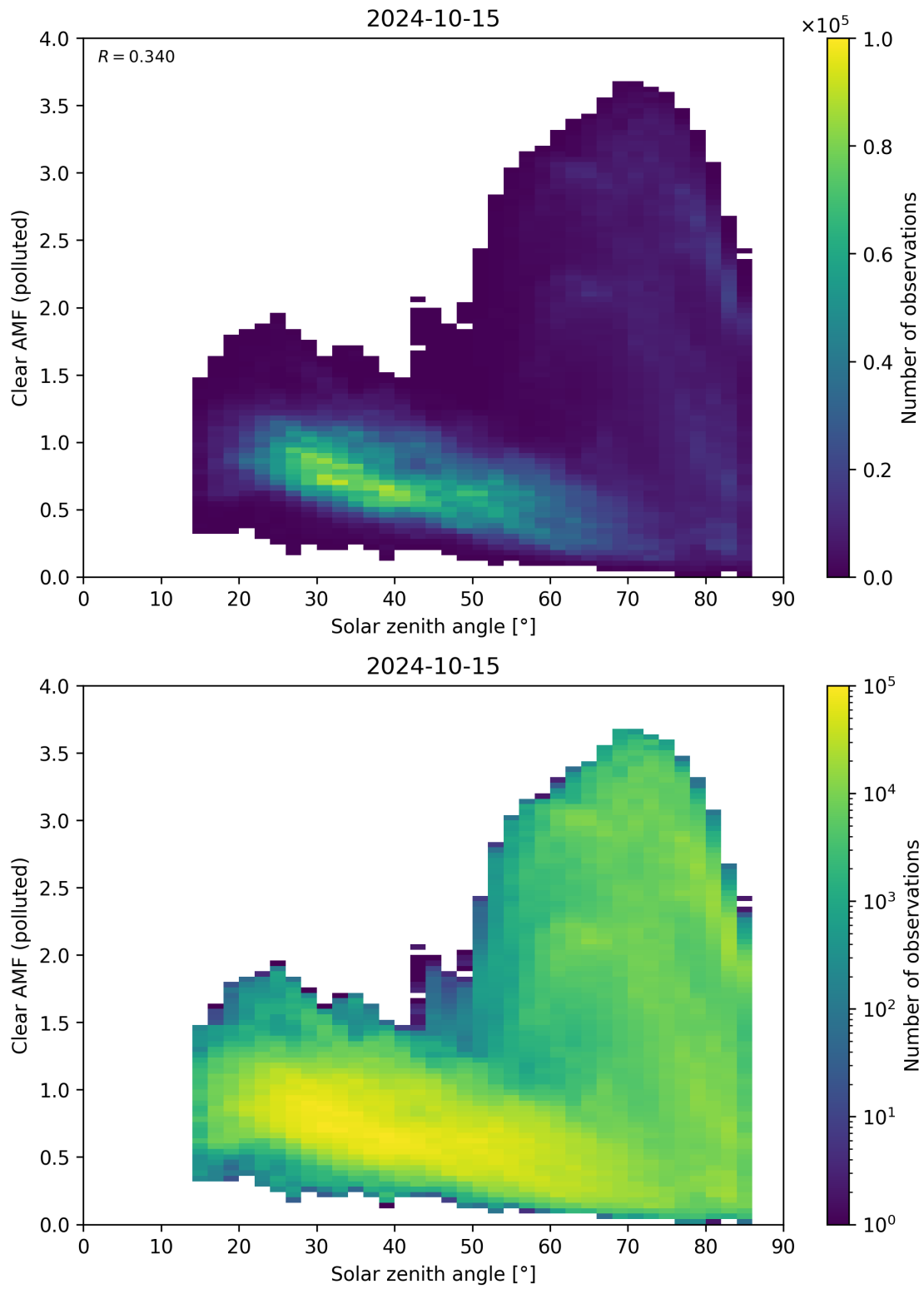
Figure 165: Scatter density plot of “Solar zenith angle” against “Clear AMF (polluted)” for 2024-10-14 to 2024-10-16.
