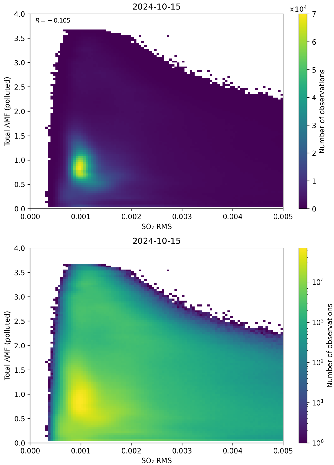
Figure 137: Scatter density plot of “SO 2 RMS” against “Total AMF (polluted)” for 2024-10-14 to 2024-10-16.
