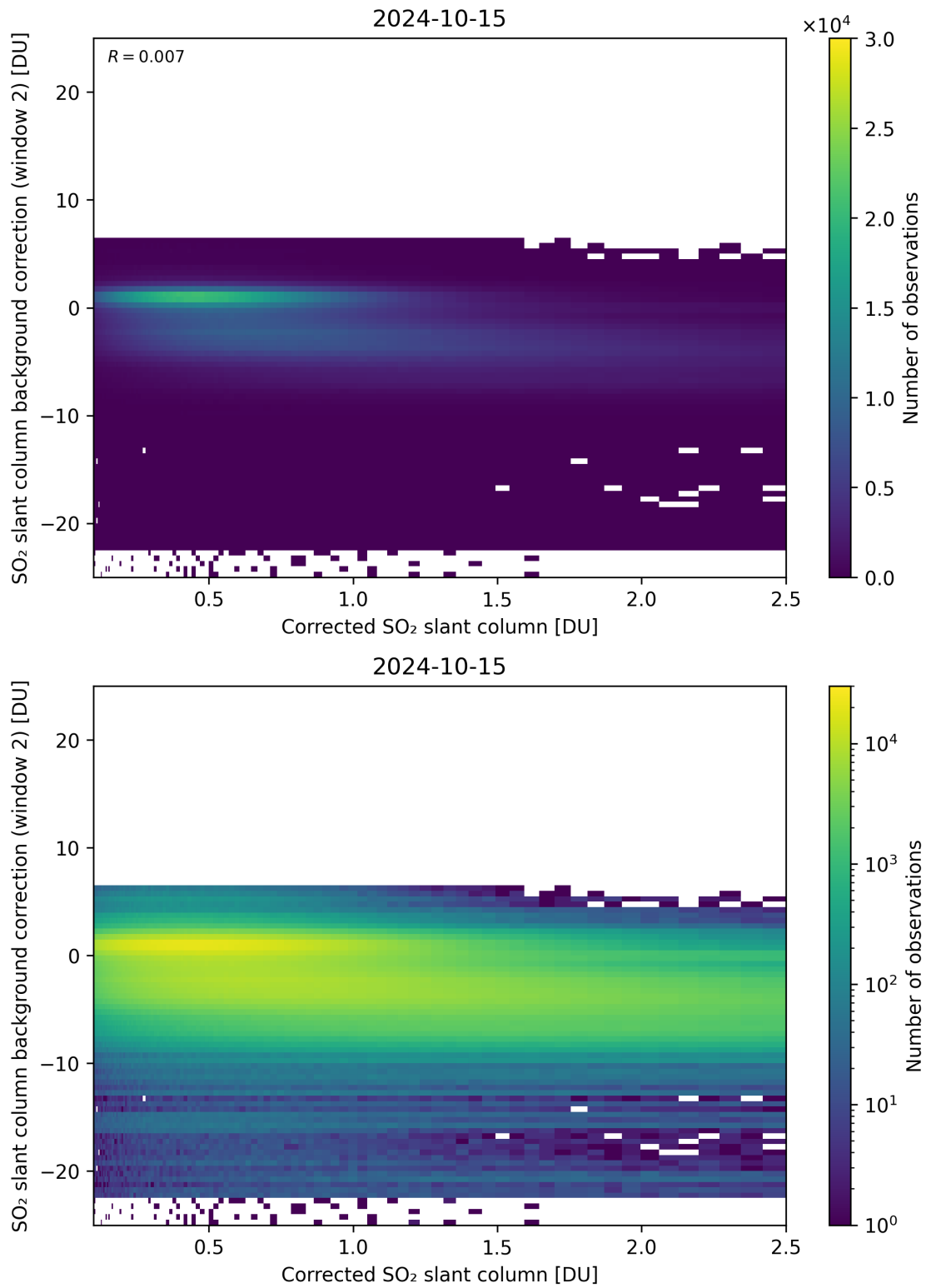
Figure 179: Scatter density plot of “Corrected SO 2 slant column” against “SO 2 slant column background correction (window 2)” for 2024-10-14 to 2024-10-16.
