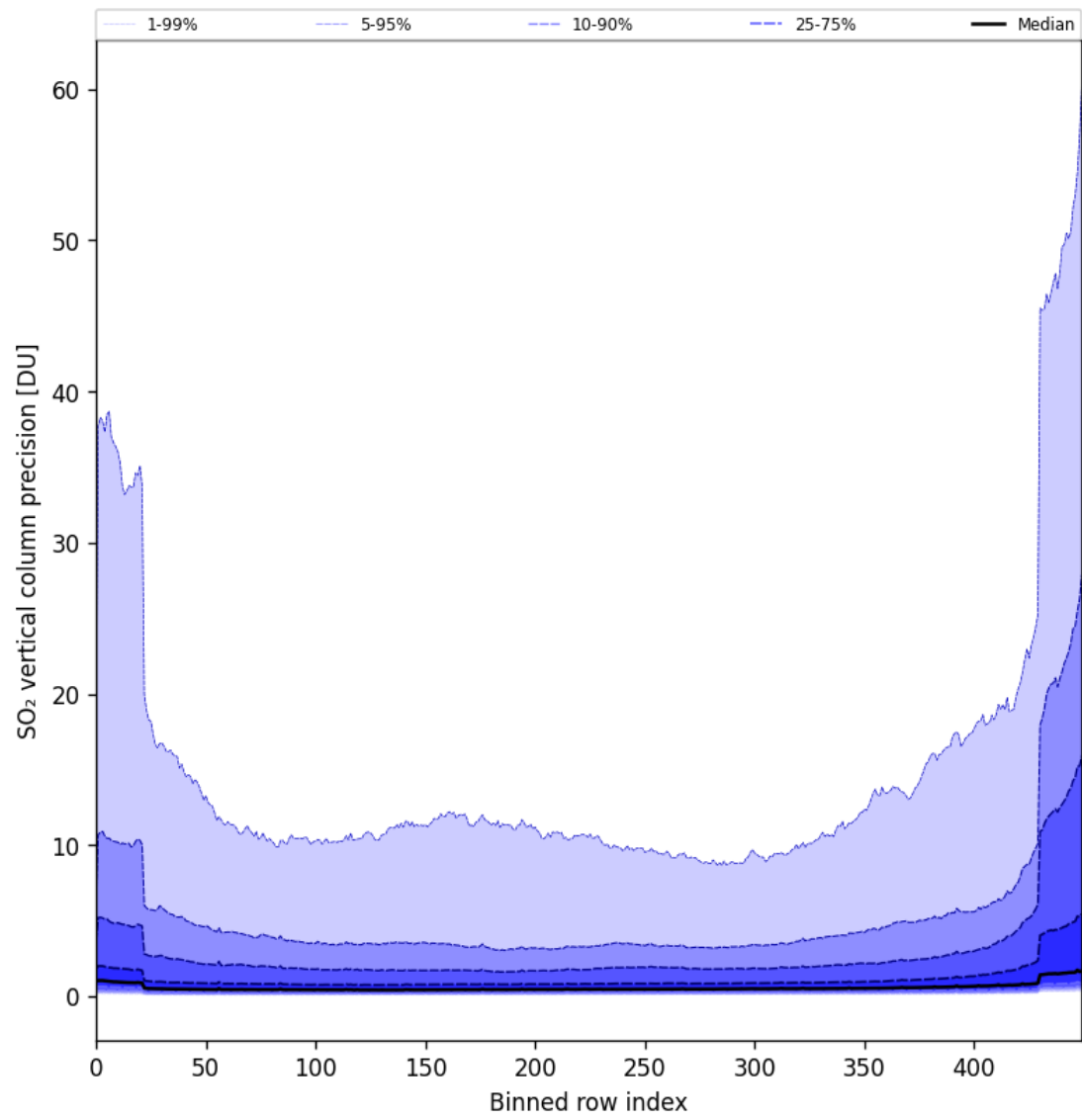
Figure 77: Along track statistics of “SO 2 vertical column precision” for 2024-10-14 to 2024-10-16
