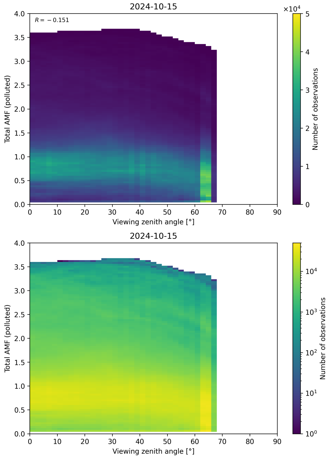
Figure 325: Scatter density plot of “Viewing zenith angle” against “Total AMF (polluted)” for 2024-10-14 to 2024-10-16.
