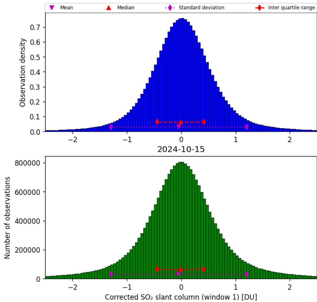
Figure 58: Histogram of “Corrected SO 2 slant column (window 1)” for 2024-10-14 to 2024-10-16
