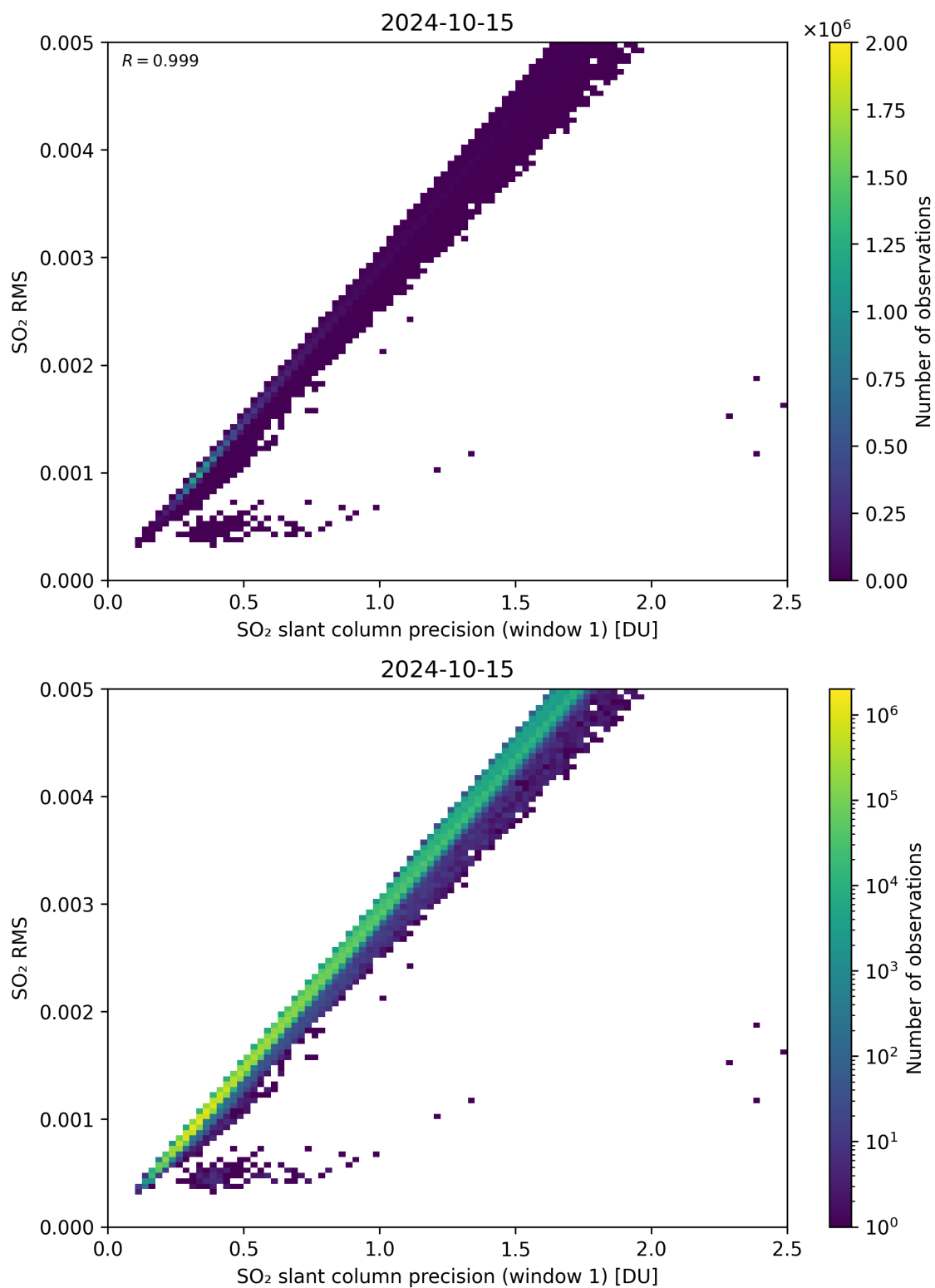
Figure 223: Scatter density plot of “SO 2 slant column precision (window 1)” against “SO 2 RMS” for 2024-10-14 to 2024-10-16.
