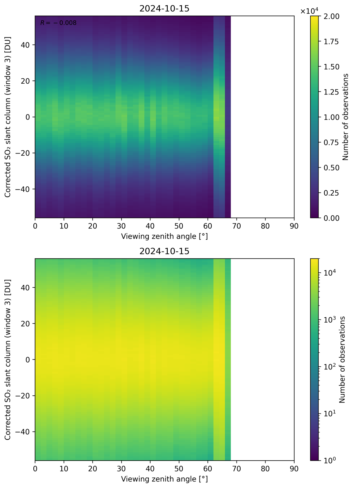
Figure 319: Scatter density plot of “Viewing zenith angle” against “Corrected SO 2 slant column (window 3)” for 2024-10-14 to 2024-10-16.
