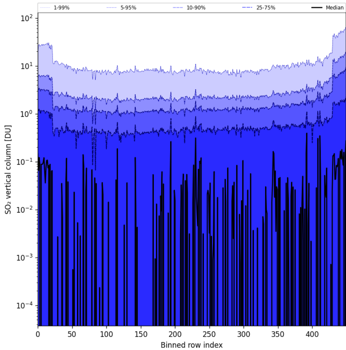
Figure 76: Along track statistics of “SO 2 vertical column” for 2024-10-14 to 2024-10-16
