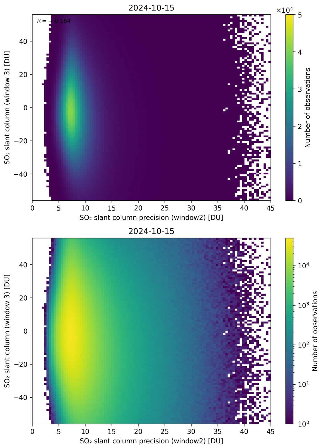
Figure 249: Scatter density plot of “SO 2 slant column precision (window2)” against “SO 2 slant column (window 3)” for 2024-10-14 to 2024-10-16.
