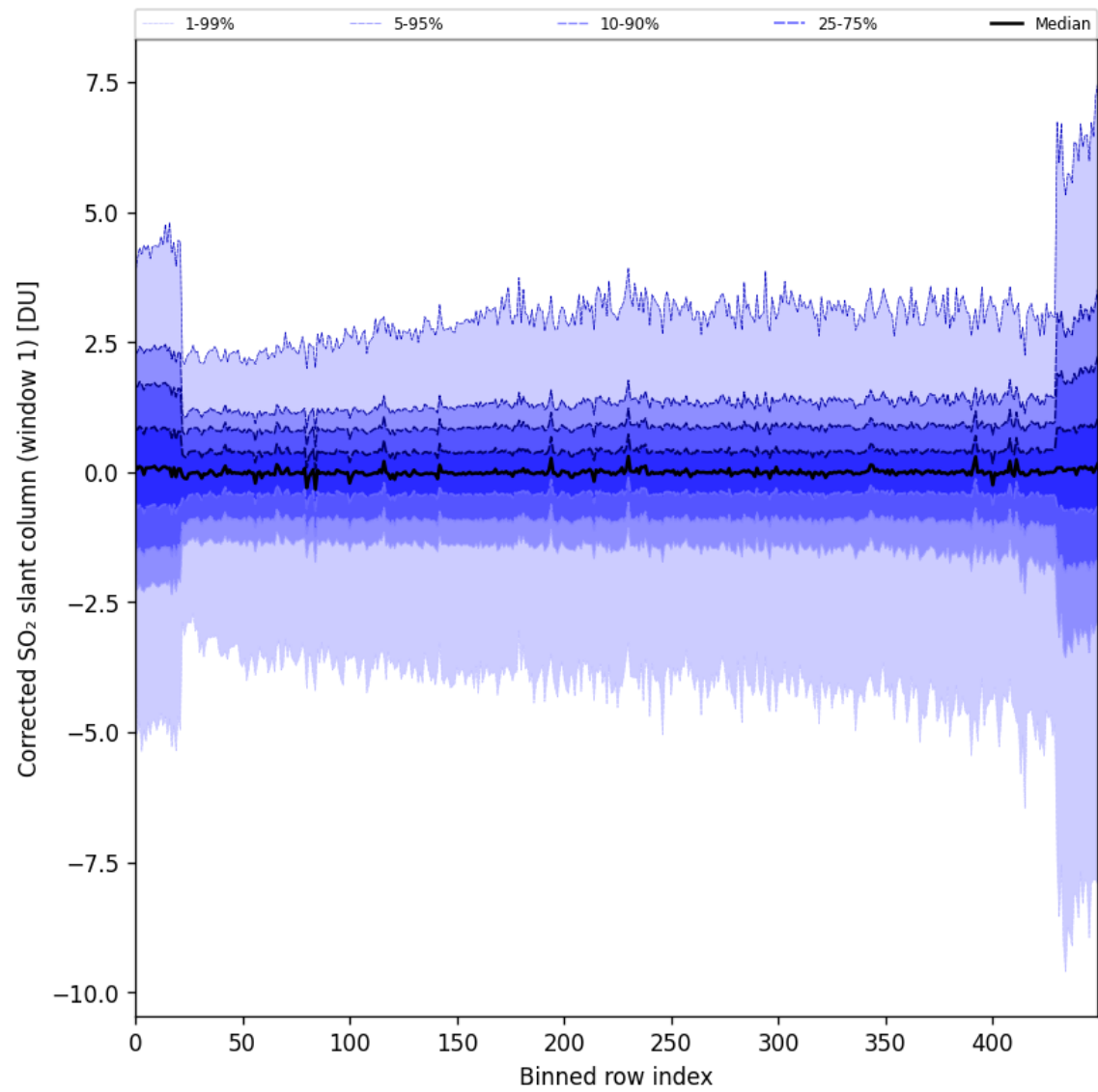
Figure 81: Along track statistics of “Corrected SO 2 slant column (window 1)” for 2024-10-14 to 2024-10-16
