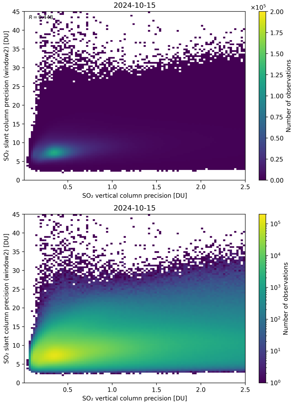
Figure 291: Scatter density plot of “SO 2 vertical column precision” against “SO 2 slant column precision (window2)” for 2024-10-14 to 2024-10-16.
