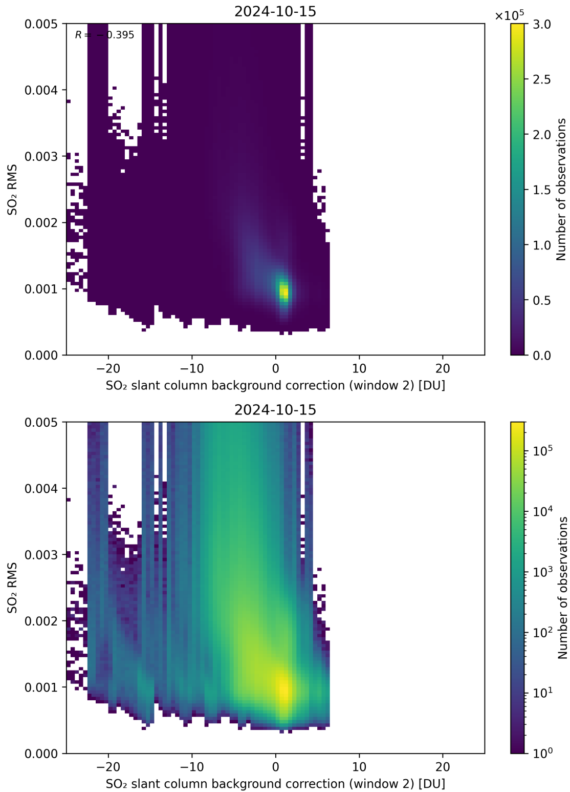
Figure 114: Scatter density plot of “SO 2 slant column background correction (window 2)” against “SO 2 RMS” for 2024-10-14 to 2024-10-16.
