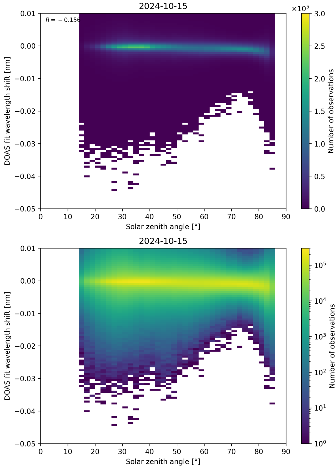
Figure 161: Scatter density plot of “Solar zenith angle” against “DOAS fit wavelength shift” for 2024-10-14 to 2024-10-16.
