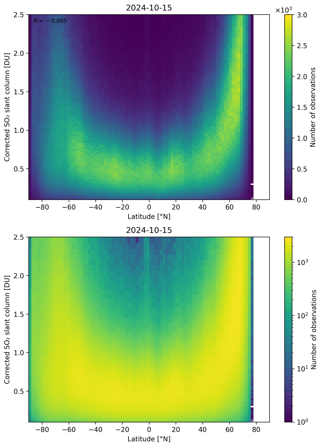
Figure 146: Scatter density plot of “Latitude” against “Corrected SO 2 slant column” for 2024-10-14 to 2024-10-16.
