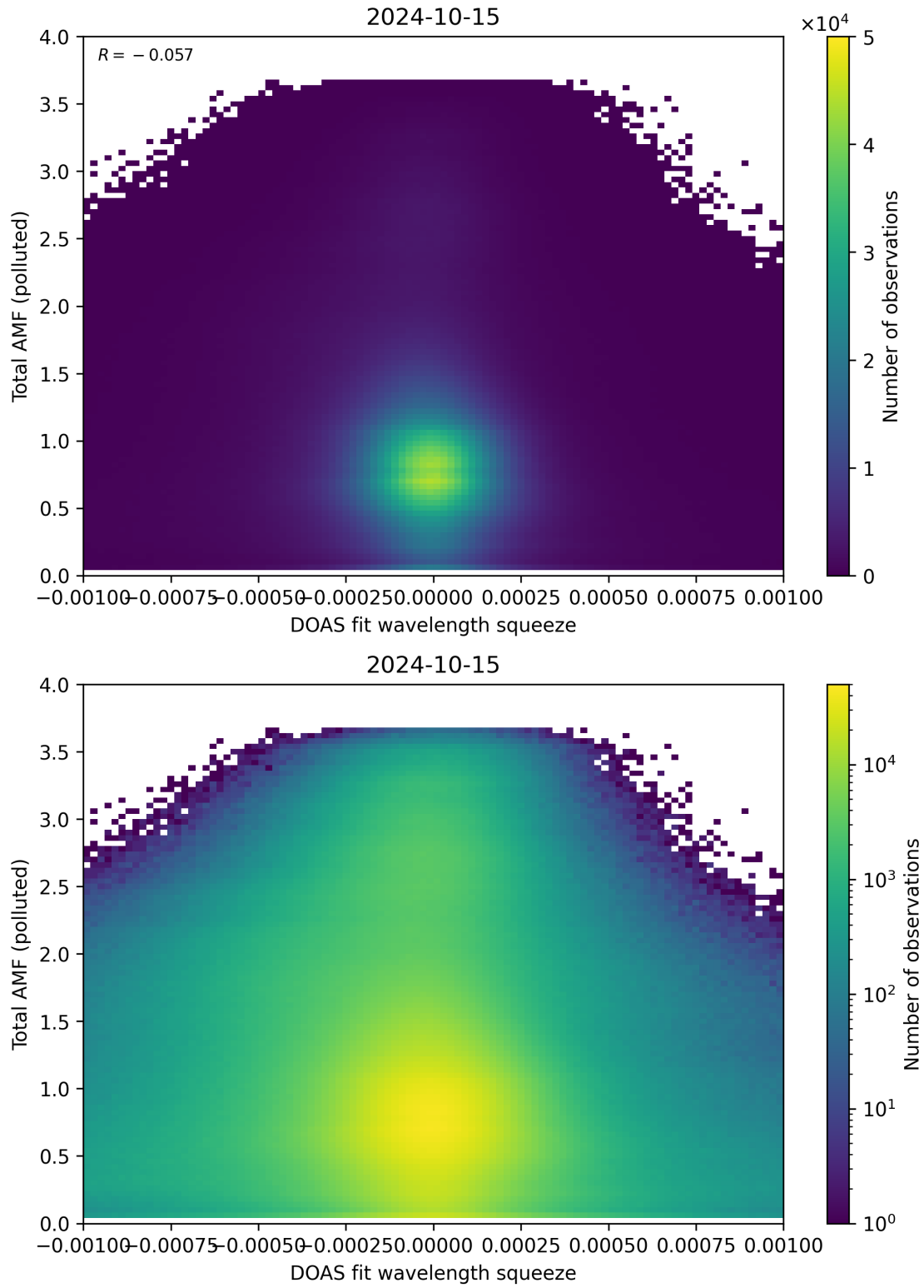
Figure 134: Scatter density plot of “DOAS fit wavelength squeeze” against “Total AMF (polluted)” for 2024-10-14 to 2024-10-16.
