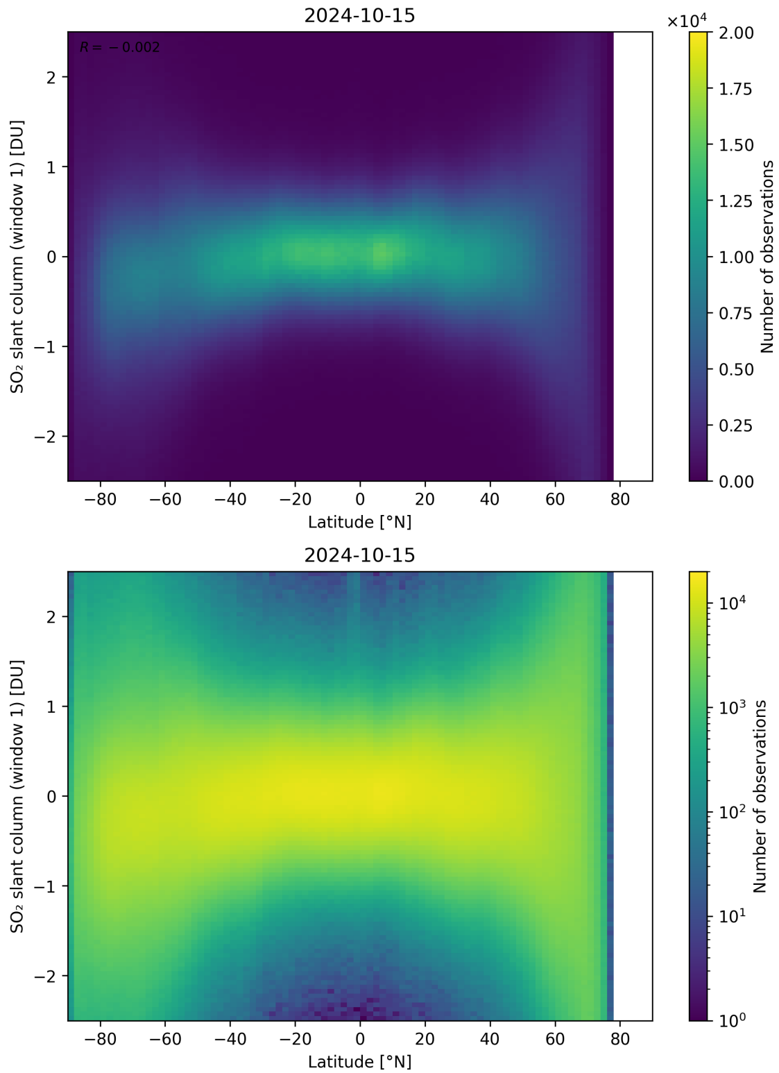
Figure 149: Scatter density plot of “Latitude” against “SO 2 slant column (window 1)” for 2024-10-14 to 2024-10-16.
