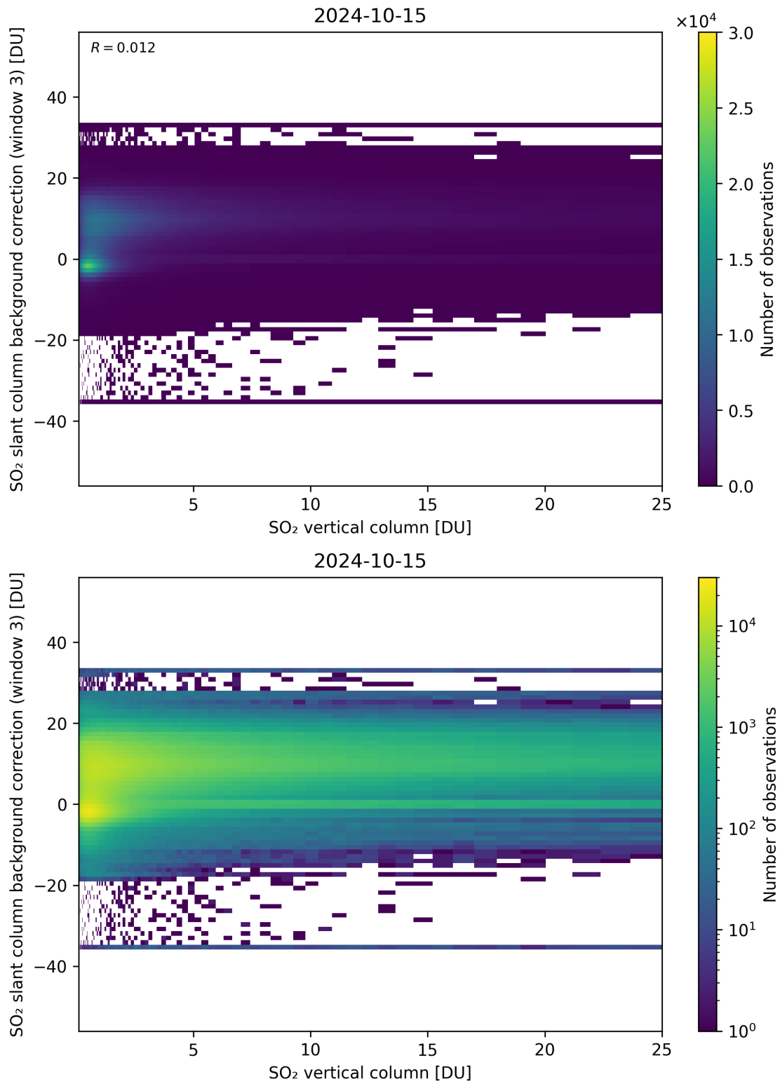
Figure 275: Scatter density plot of “SO 2 vertical column” against “SO 2 slant column background correction (window 3)” for 2024-10-14 to 2024-10-16.
