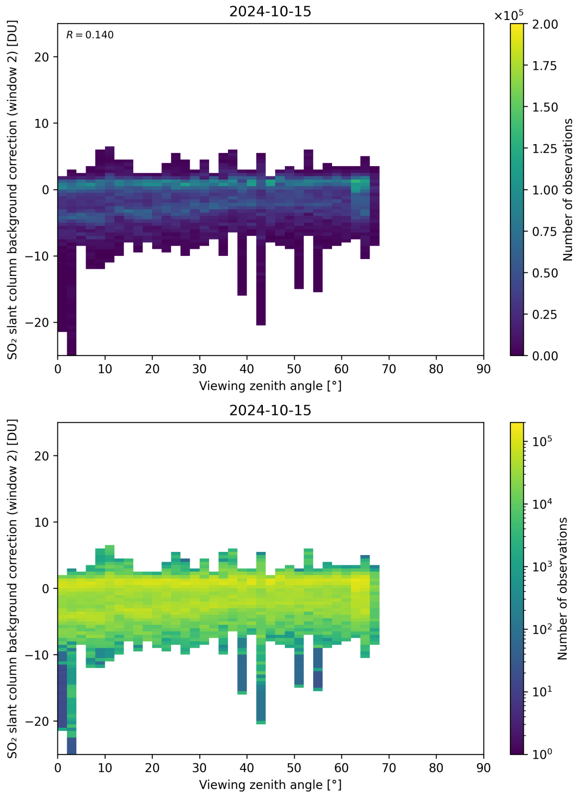
Figure 309: Scatter density plot of “Viewing zenith angle” against “SO 2 slant column background correction (window 2)” for 2024-10-14 to 2024-10-16.
