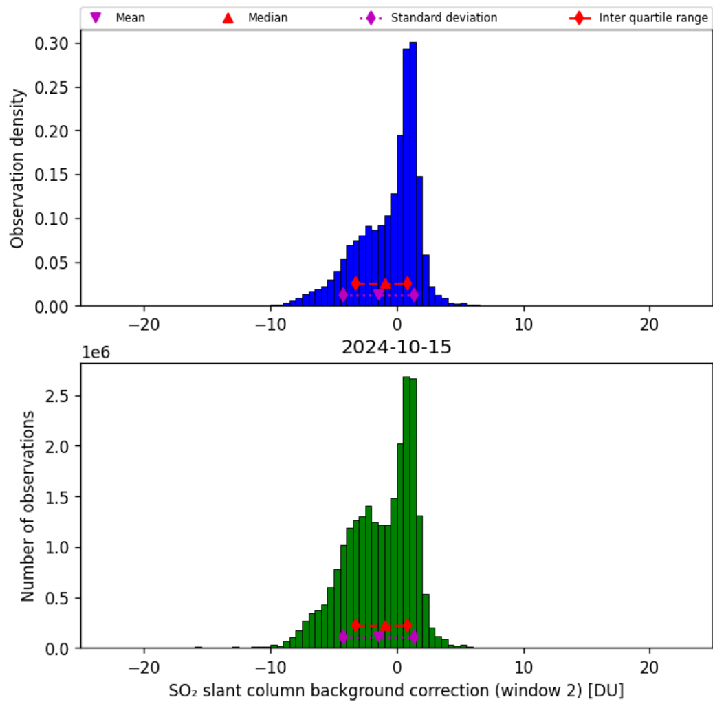
Figure 63: Histogram of “SO 2 slant column background correction (window 2)” for 2024-10-14 to 2024-10-16
