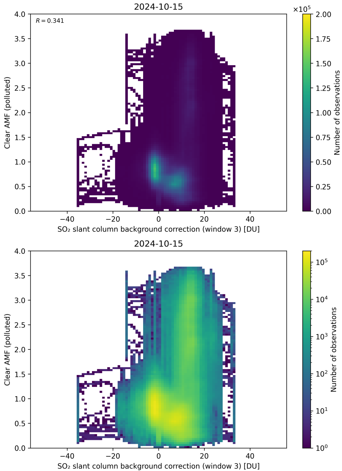
Figure 124: Scatter density plot of “SO 2 slant column background correction (window 3)” against “Clear AMF (polluted)” for 2024-10-14 to 2024-10-16.
