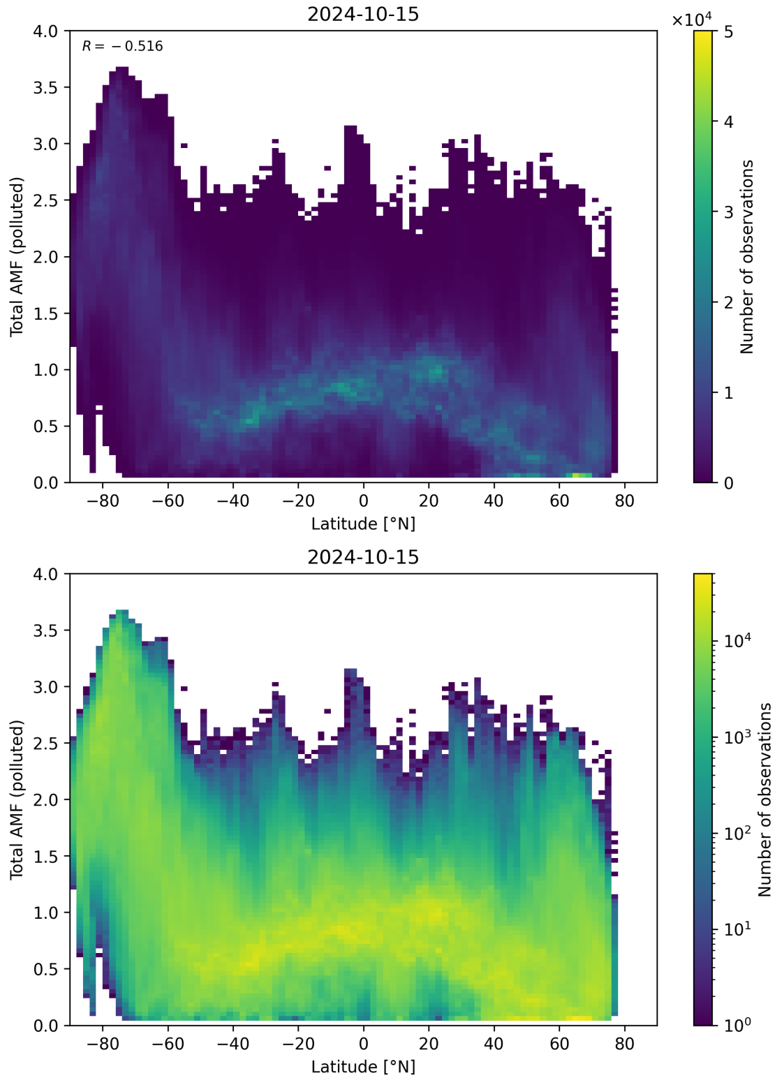
Figure 154: Scatter density plot of “Latitude” against “Total AMF (polluted)” for 2024-10-14 to 2024-10-16.
