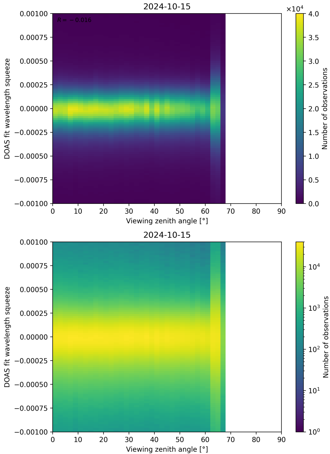
Figure 312: Scatter density plot of “Viewing zenith angle” against “DOAS fit wavelength squeeze” for 2024-10-14 to 2024-10-16.
