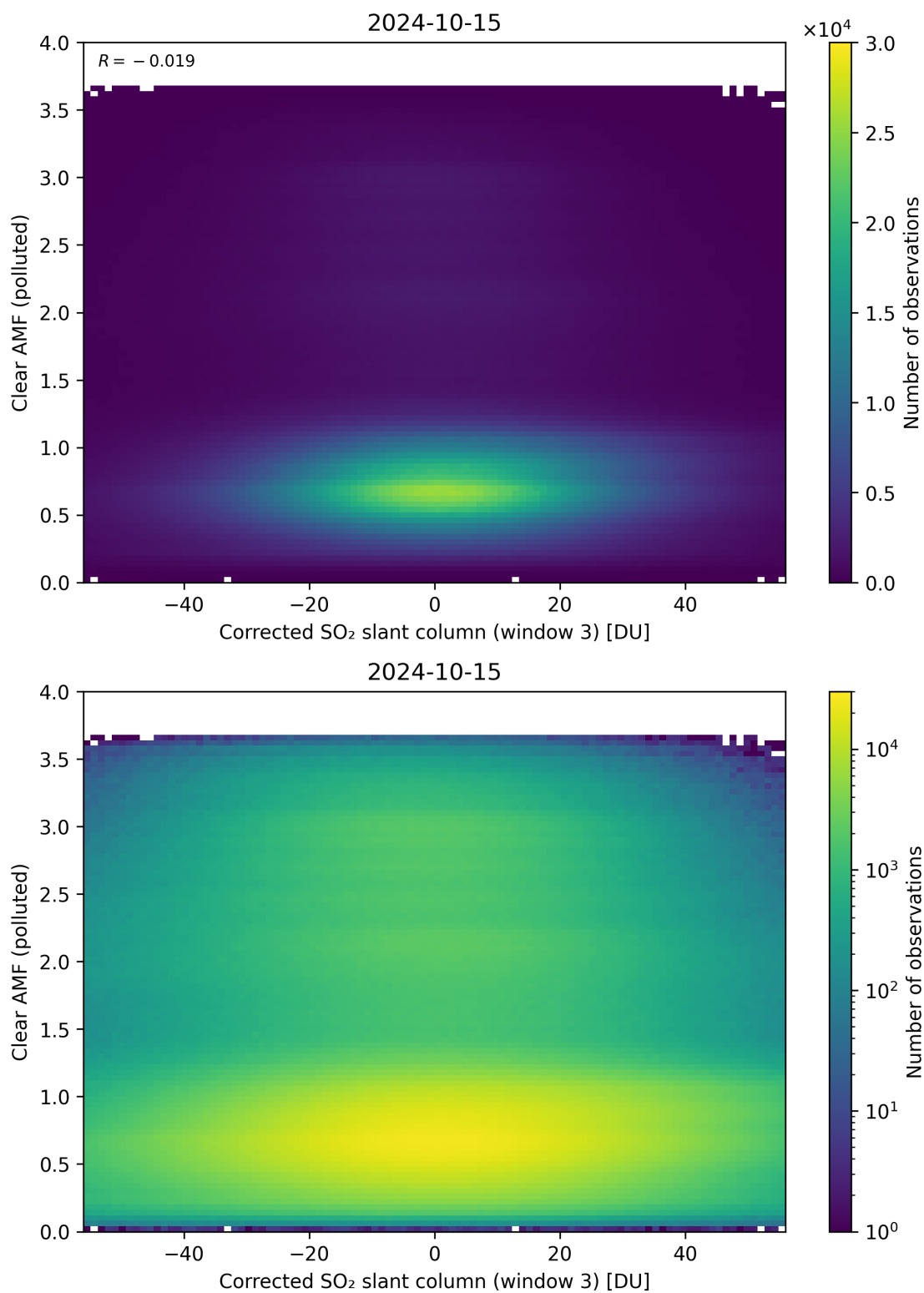
Figure 209: Scatter density plot of “Corrected SO 2 slant column (window 3)” against “Clear AMF (polluted)” for 2024-10-14 to 2024-10-16.
