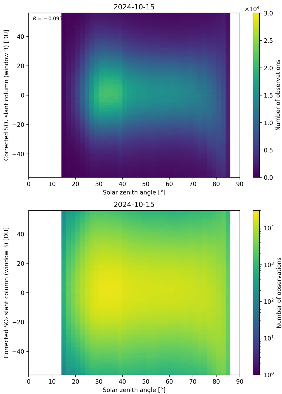
Figure 168: Scatter density plot of “Solar zenith angle” against “Corrected SO 2 slant column (window 3)” for 2024-10-14 to 2024-10-16.
