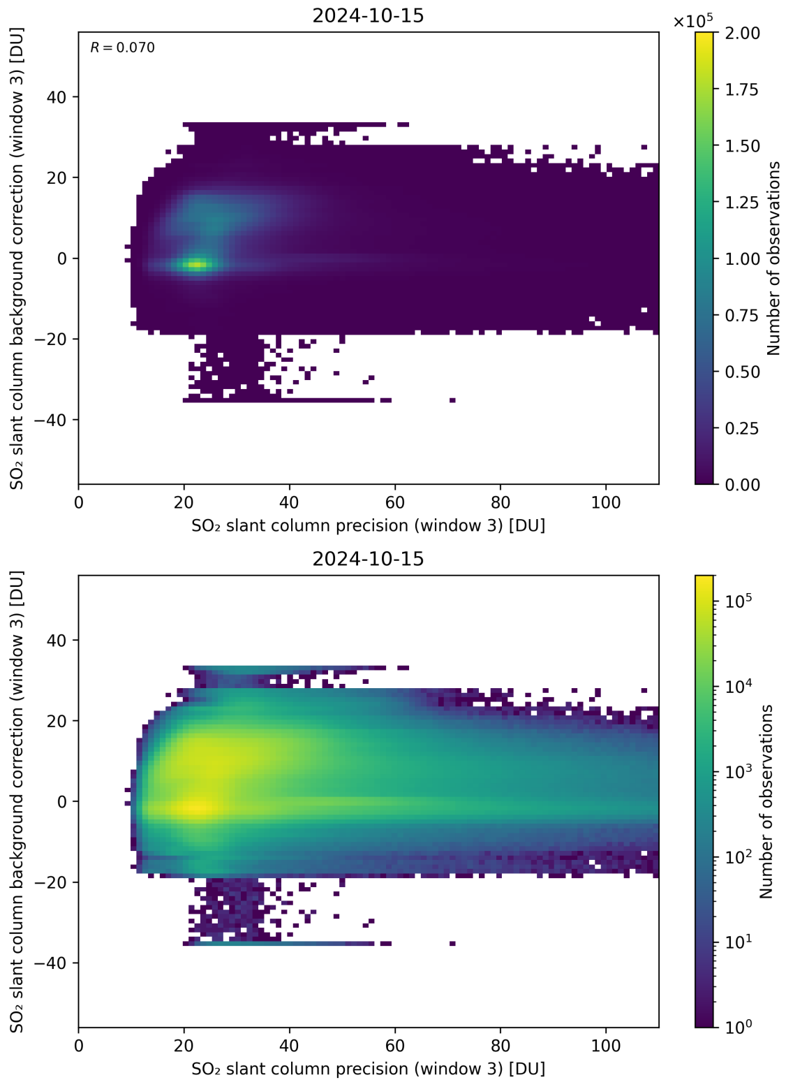
Figure 257: Scatter density plot of “SO 2 slant column precision (window 3)” against “SO 2 slant column background correction (window 3)” for 2024-10-14 to 2024-10-16.
