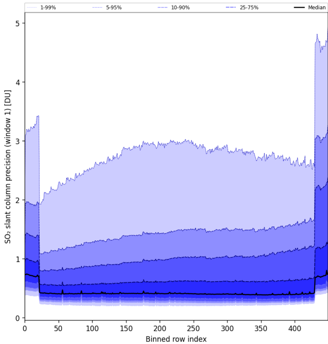
Figure 80: Along track statistics of “SO 2 slant column precision (window 1)” for 2024-10-14 to 2024-10-16
