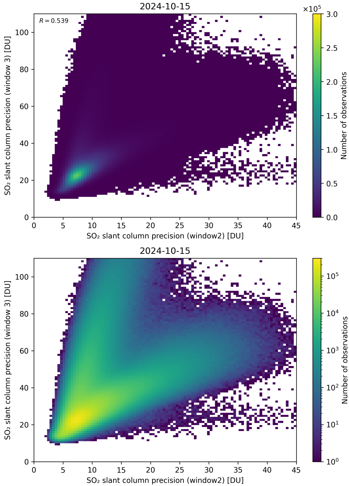
Figure 250: Scatter density plot of “SO 2 slant column precision (window2)” against “SO 2 slant column precision (window 3)” for 2024-10-14 to 2024-10-16.
