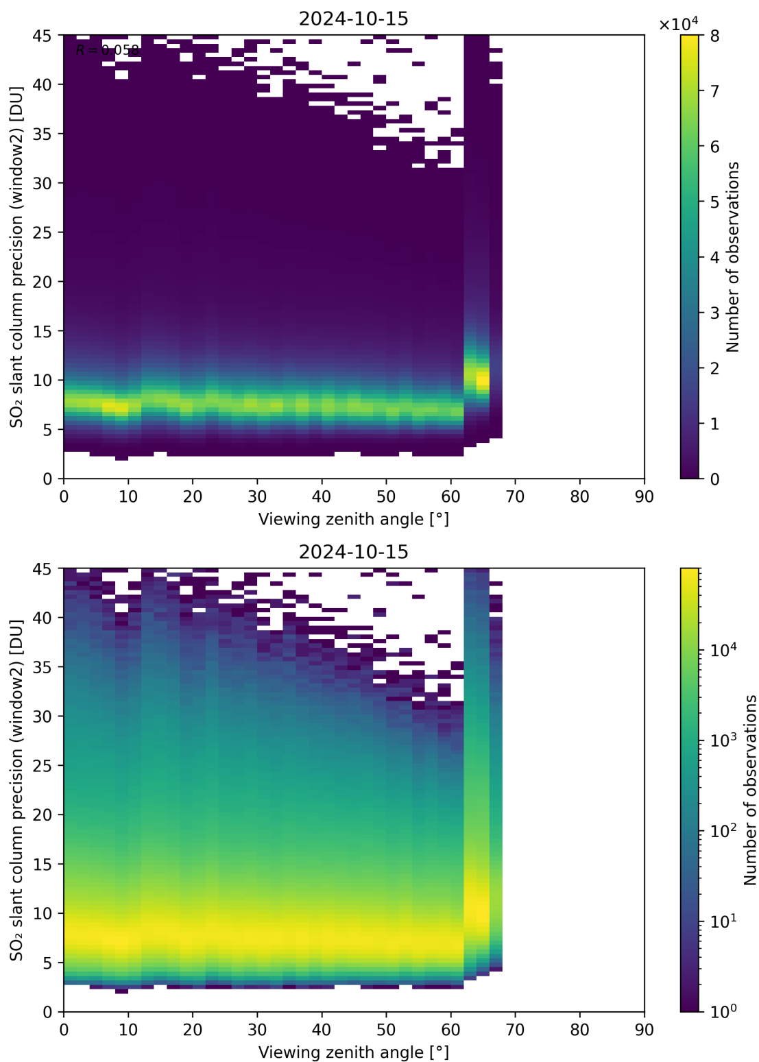
Figure 322: Scatter density plot of “Viewing zenith angle” against “SO 2 slant column precision (window2)” for 2024-10-14 to 2024-10-16.
