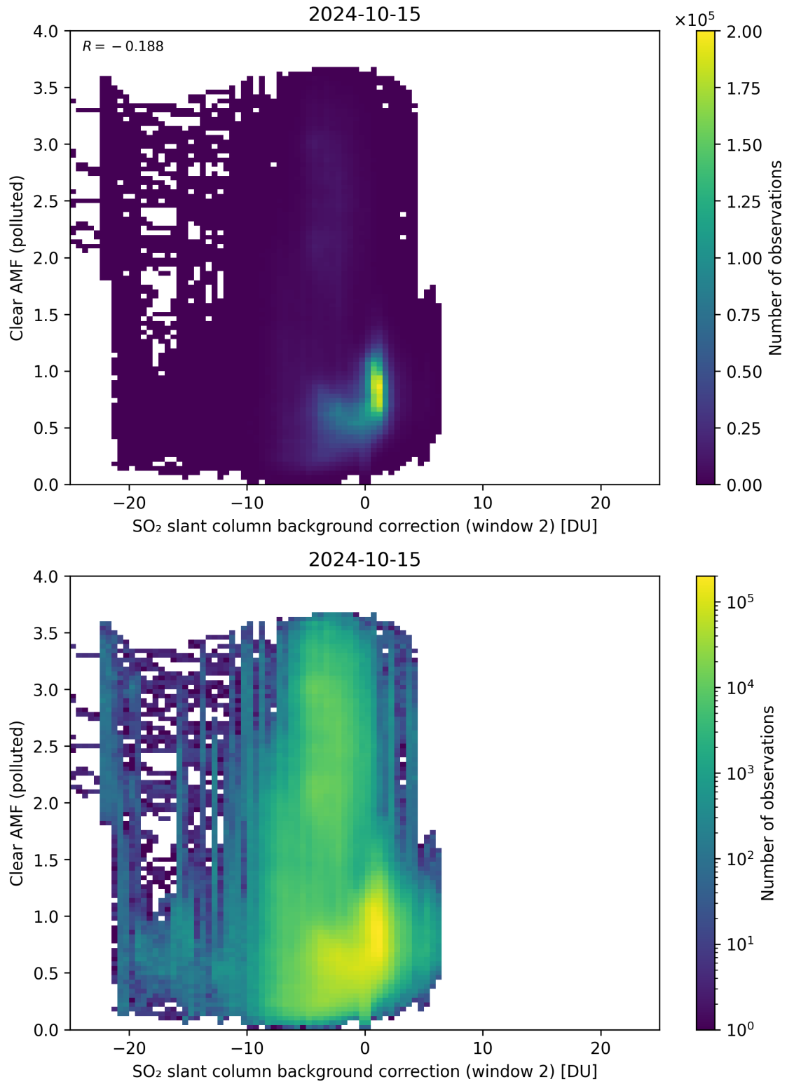
Figure 115: Scatter density plot of “SO 2 slant column background correction (window 2)” against “Clear AMF (polluted)” for 2024-10-14 to 2024-10-16.
