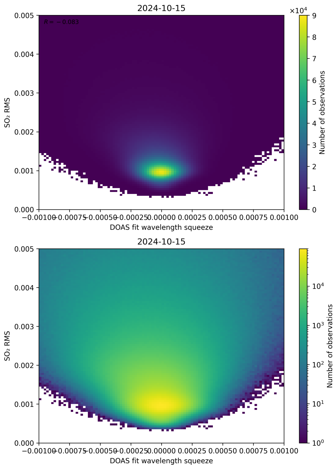
Figure 132: Scatter density plot of “DOAS fit wavelength squeeze” against “SO 2 RMS” for 2024-10-14 to 2024-10-16.
