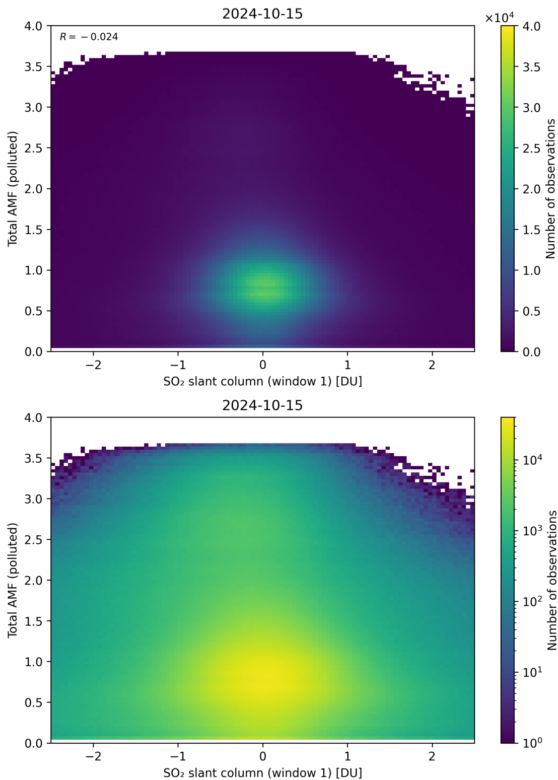
Figure 239: Scatter density plot of “SO 2 slant column (window 1)” against “Total AMF (polluted)” for 2024-10-14 to 2024-10-16.
