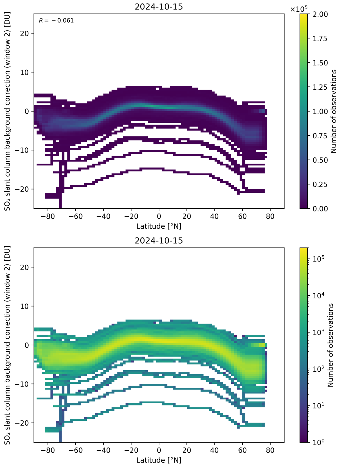
Figure 140: Scatter density plot of “Latitude” against “SO 2 slant column background correction (window 2)” for 2024-10-14 to 2024-10-16.
