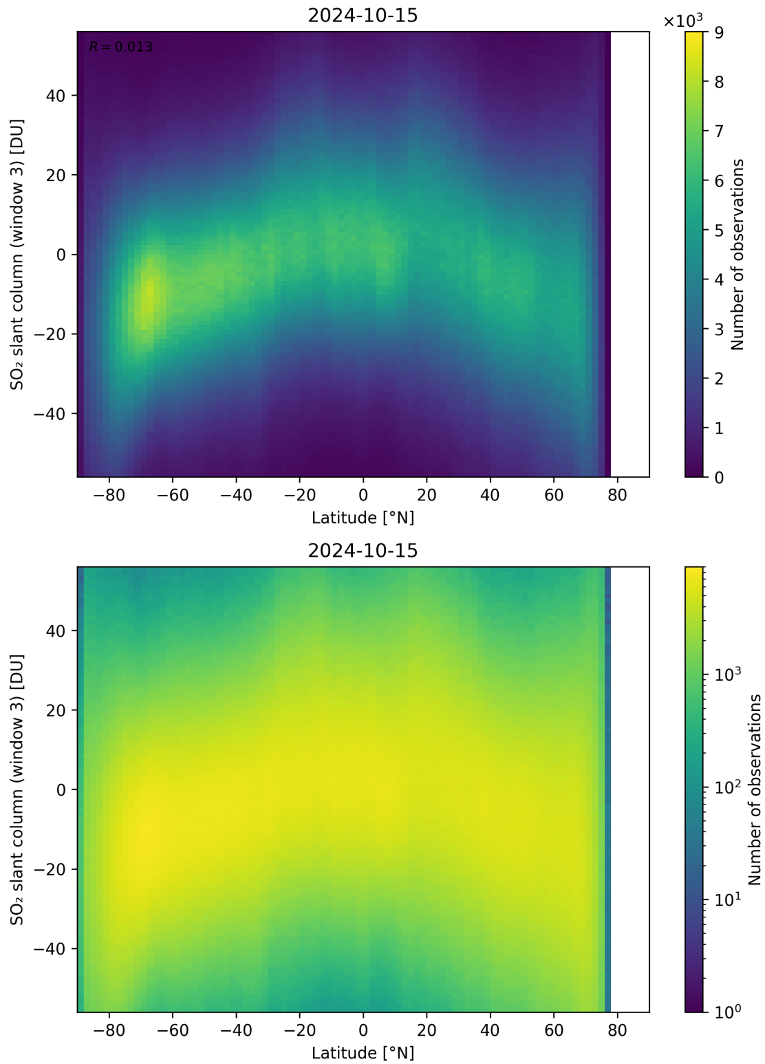
Figure 152: Scatter density plot of “Latitude” against “SO 2 slant column (window 3)” for 2024-10-14 to 2024-10-16.
