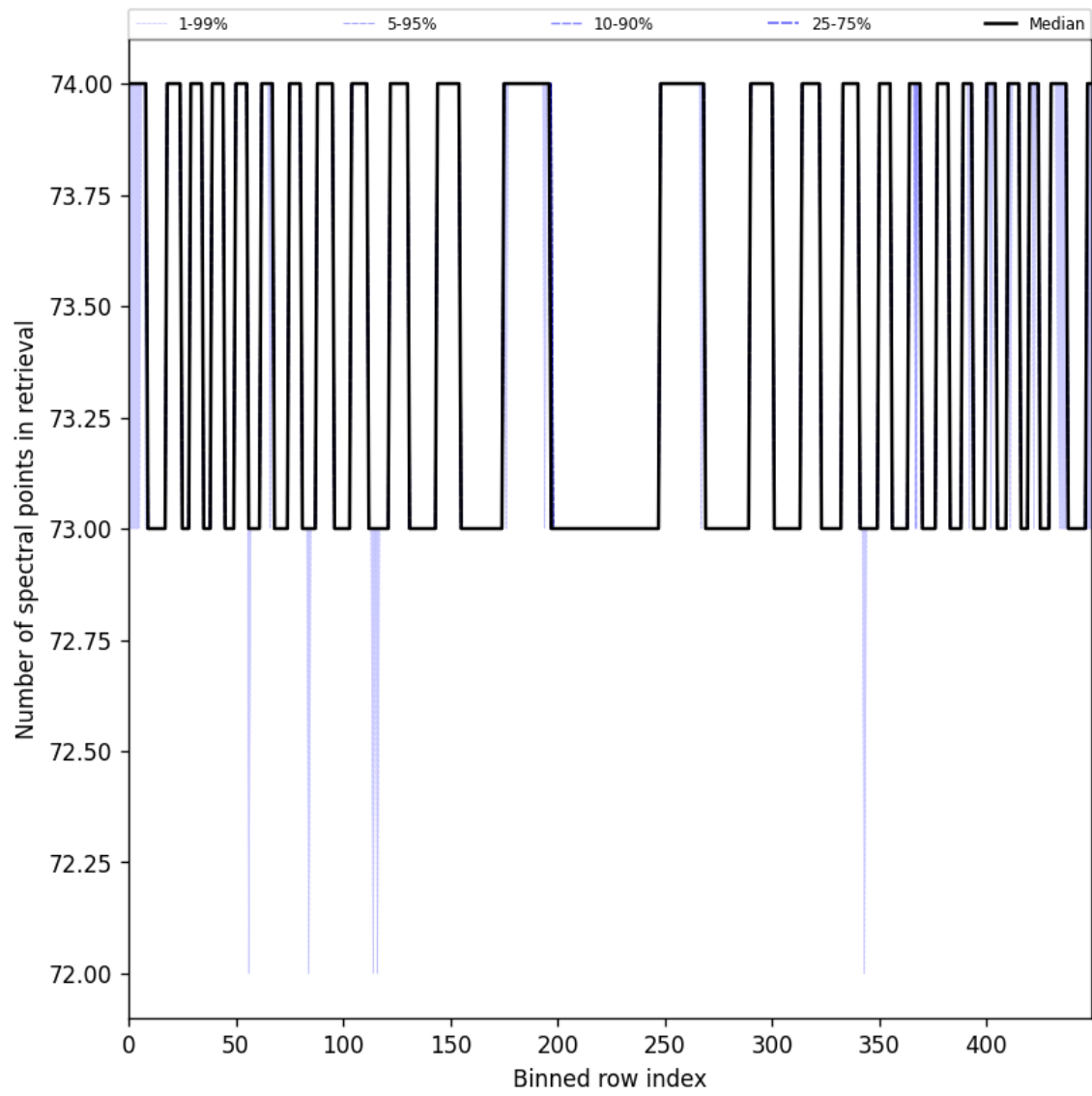
Figure 97: Along track statistics of “Number of spectral points in retrieval” for 2024-10-14 to 2024-10-16
