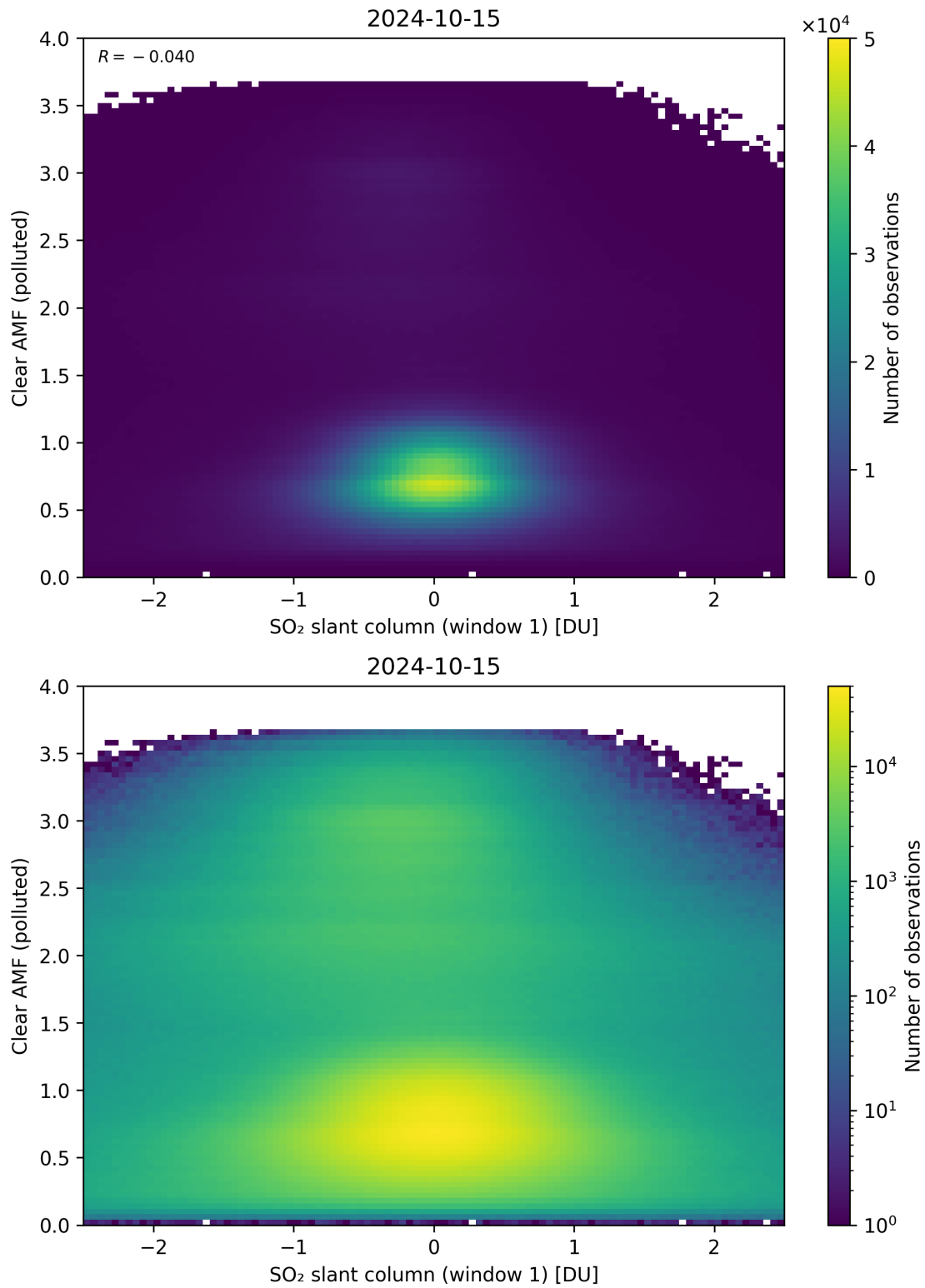
Figure 232: Scatter density plot of “SO 2 slant column (window 1)” against “Clear AMF (polluted)” for 2024-10-14 to 2024-10-16.
