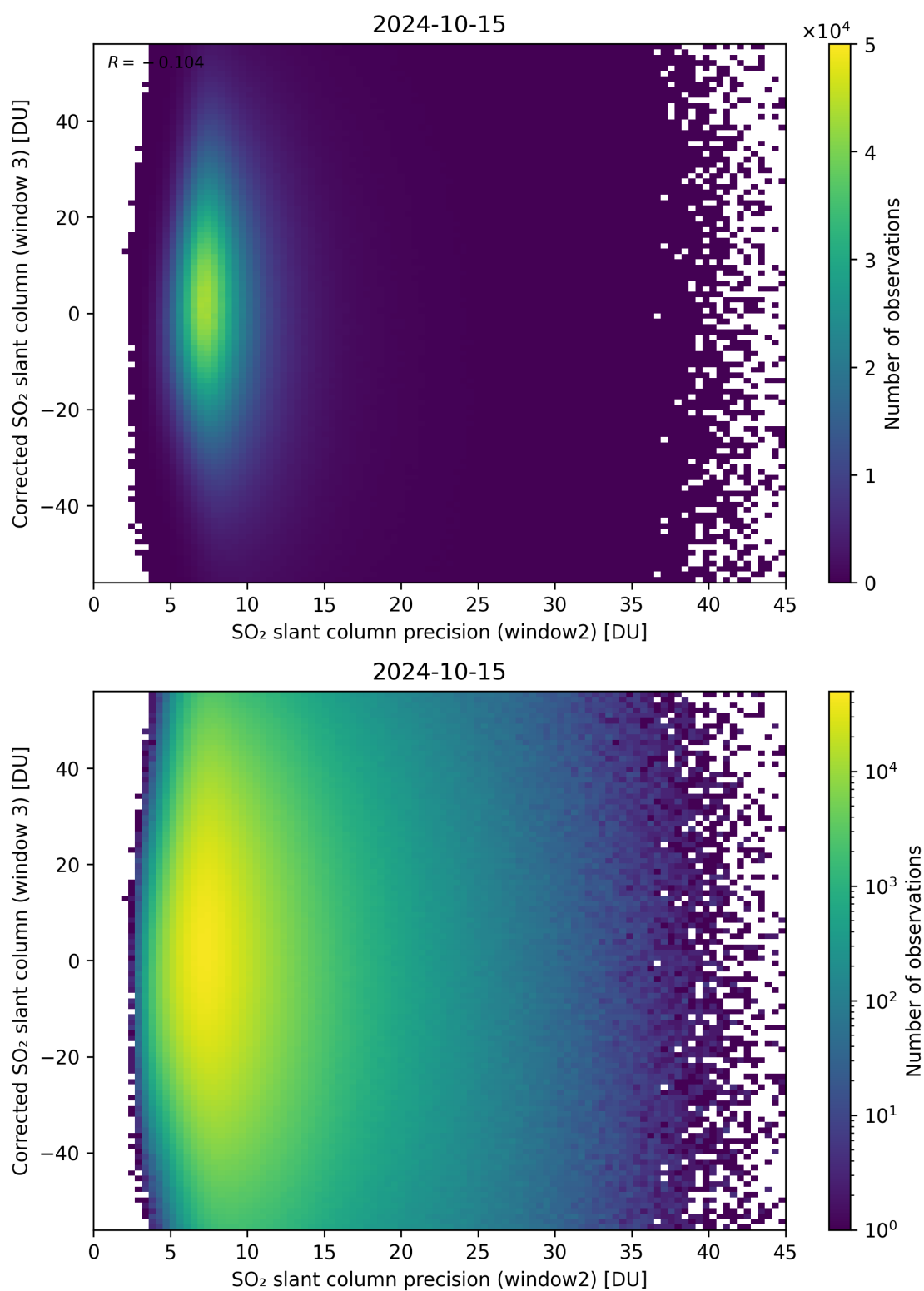
Figure 248: Scatter density plot of “SO 2 slant column precision (window2)” against “Corrected SO 2 slant column (window 3)” for 2024-10-14 to 2024-10-16.
