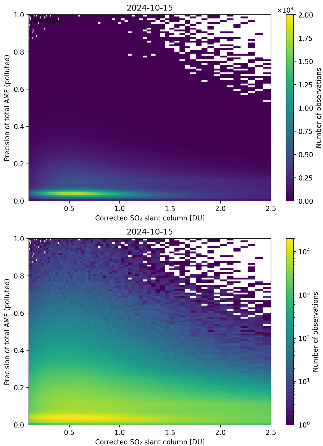
Figure 193: Scatter density plot of “Corrected SO 2 slant column” against “Precision of total AMF (polluted)” for 2024-10-14 to 2024-10-16.
