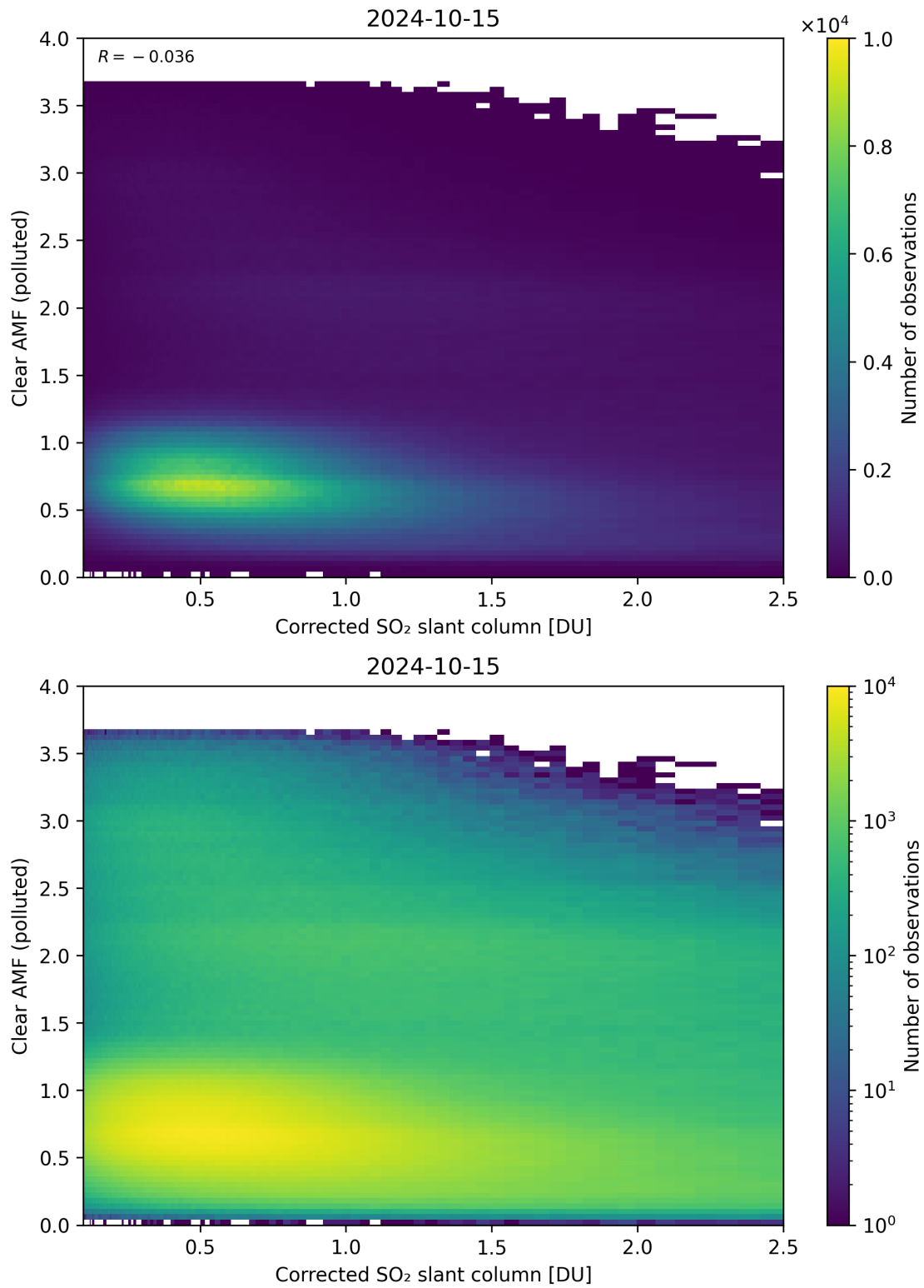
Figure 184: Scatter density plot of “Corrected SO 2 slant column” against “Clear AMF (polluted)” for 2024-10-14 to 2024-10-16.
