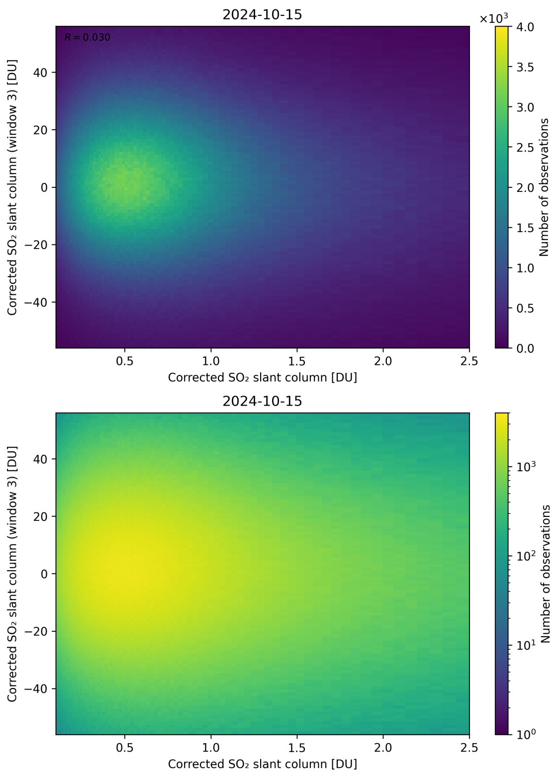
Figure 186: Scatter density plot of “Corrected SO 2 slant column” against “Corrected SO 2 slant column (window 3)” for 2024-10-14 to 2024-10-16.
