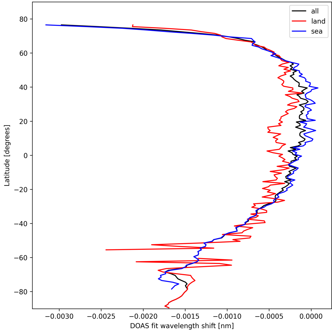
Figure 45: Zonal average of “DOAS fit wavelength shift” for 2024-10-14 to 2024-10-16.
