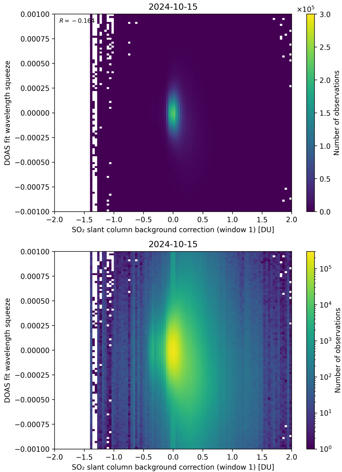
Figure 101: Scatter density plot of “SO 2 slant column background correction (window 1)” against “DOAS fit wavelength squeeze” for 2024-10-14 to 2024-10-16.
