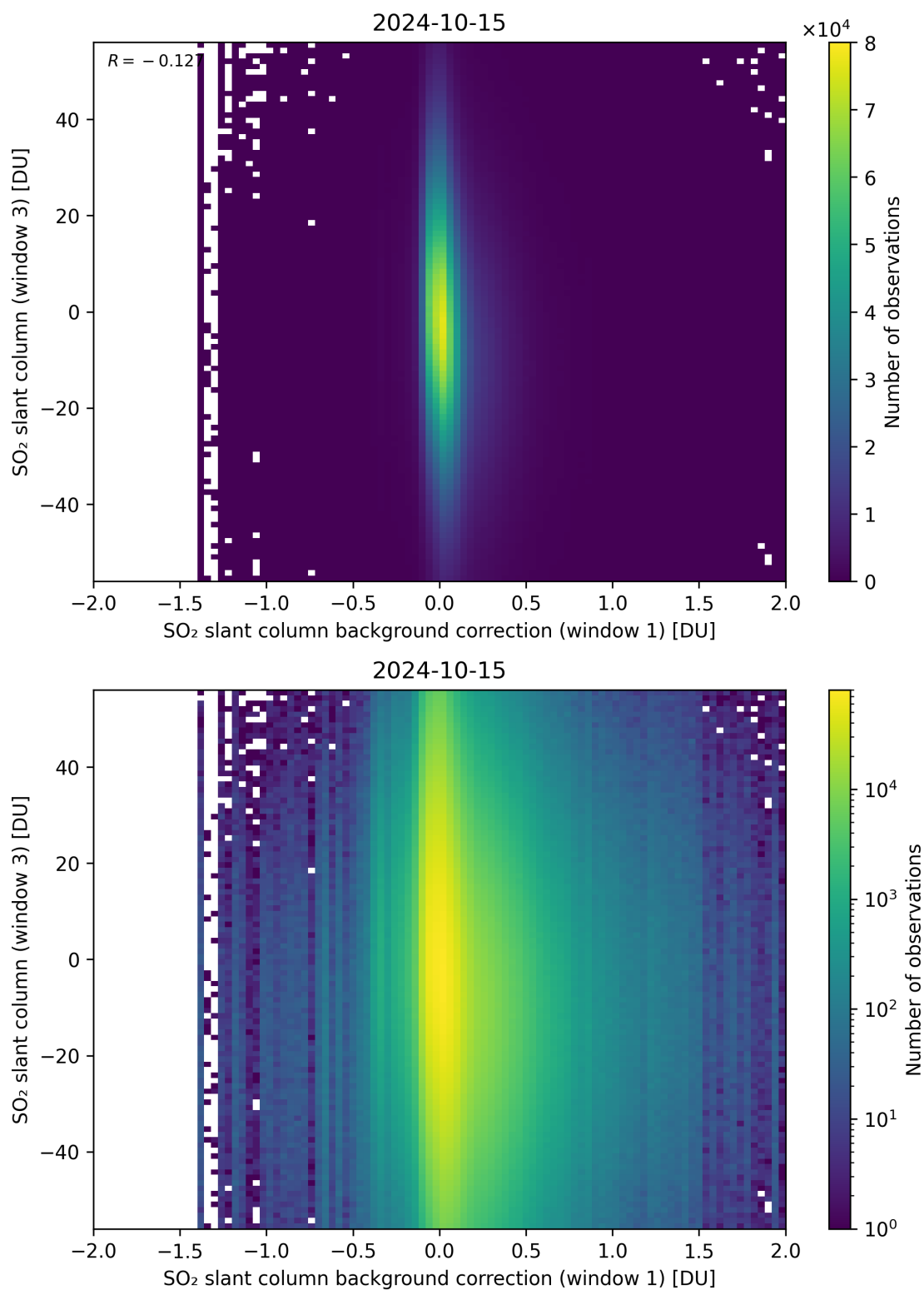
Figure 107: Scatter density plot of “SO 2 slant column background correction (window 1)” against “SO 2 slant column (window 3)” for 2024-10-14 to 2024-10-16.
