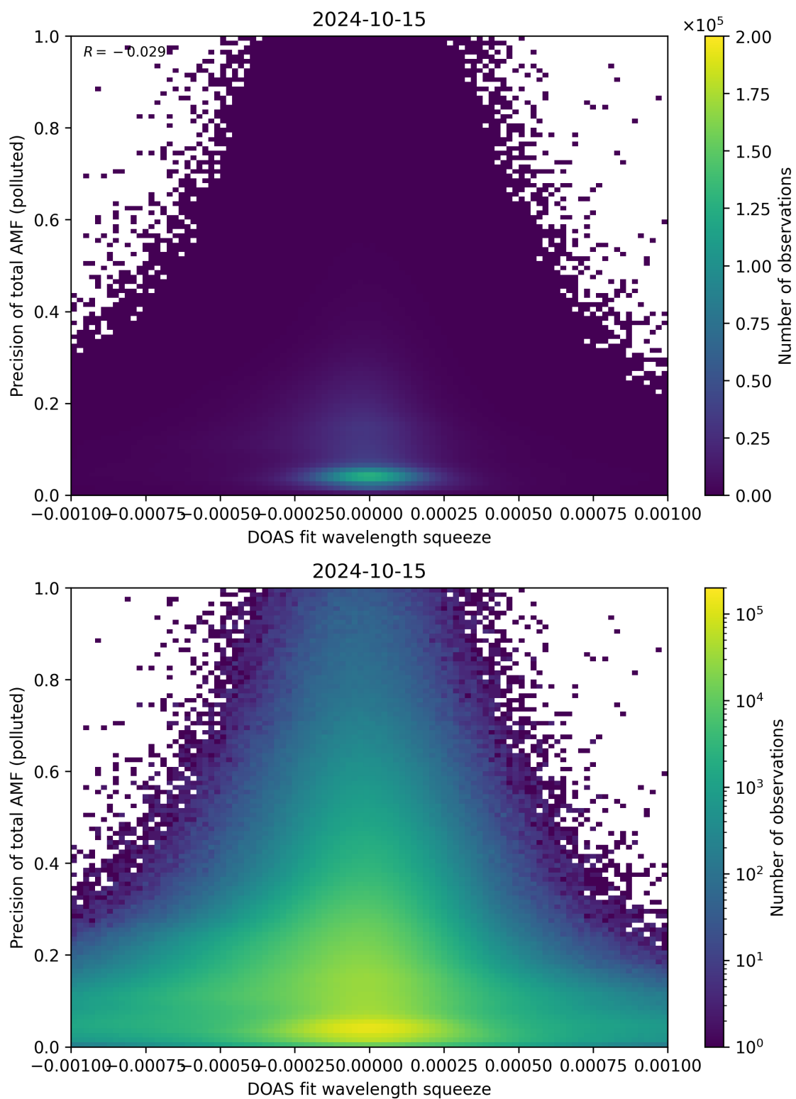
Figure 135: Scatter density plot of “DOAS fit wavelength squeeze” against “Precision of total AMF (polluted)” for 2024-10-14 to 2024-10-16.
