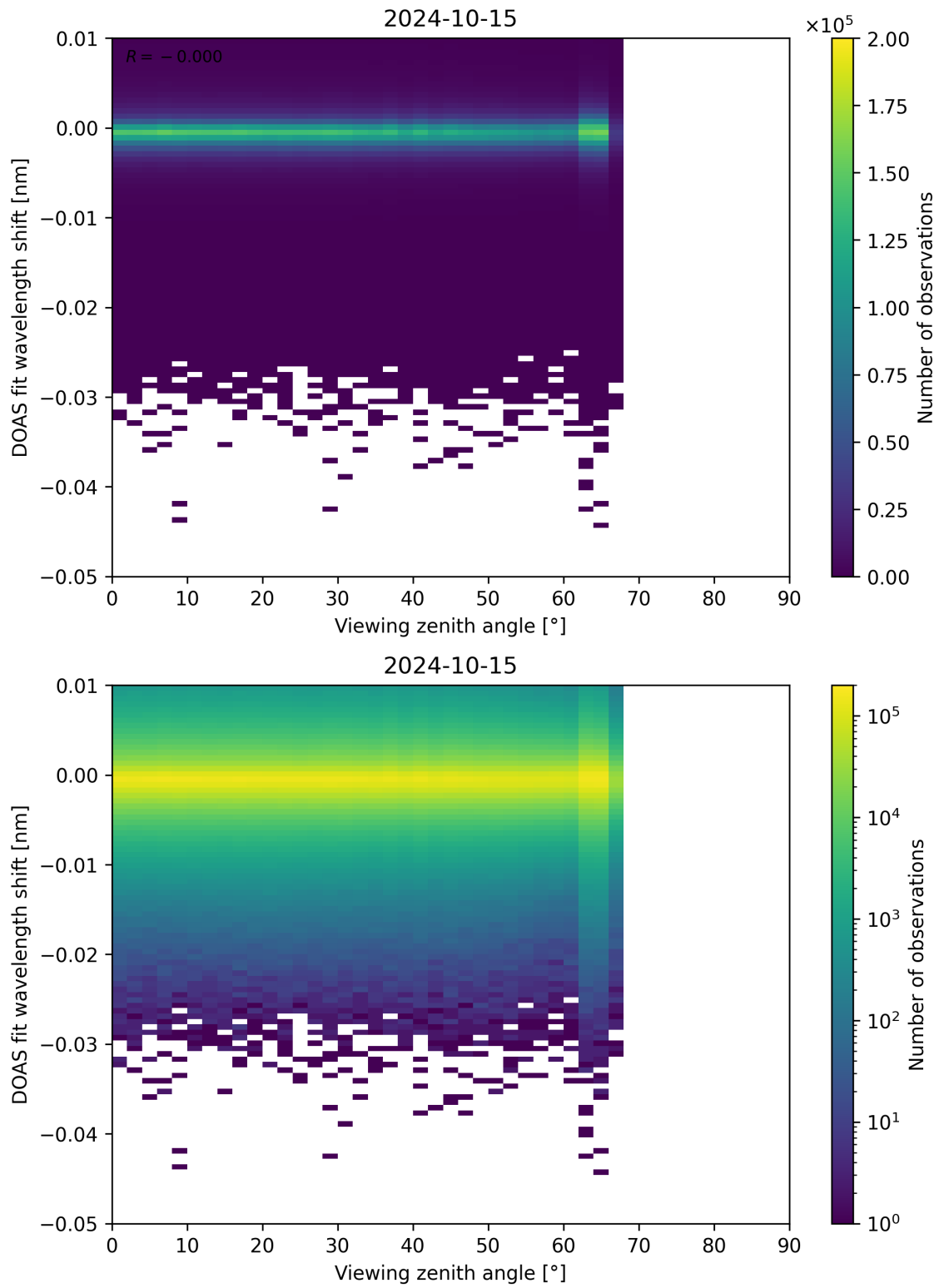
Figure 311: Scatter density plot of “Viewing zenith angle” against “DOAS fit wavelength shift” for 2024-10-14 to 2024-10-16.
