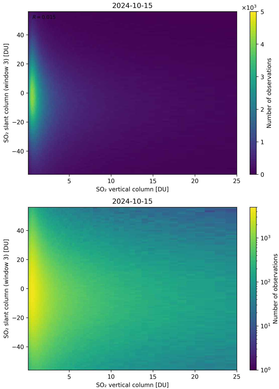
Figure 303: Scatter density plot of “SO 2 vertical column” against “SO 2 slant column (window 3)” for 2024-10-14 to 2024-10-16.
