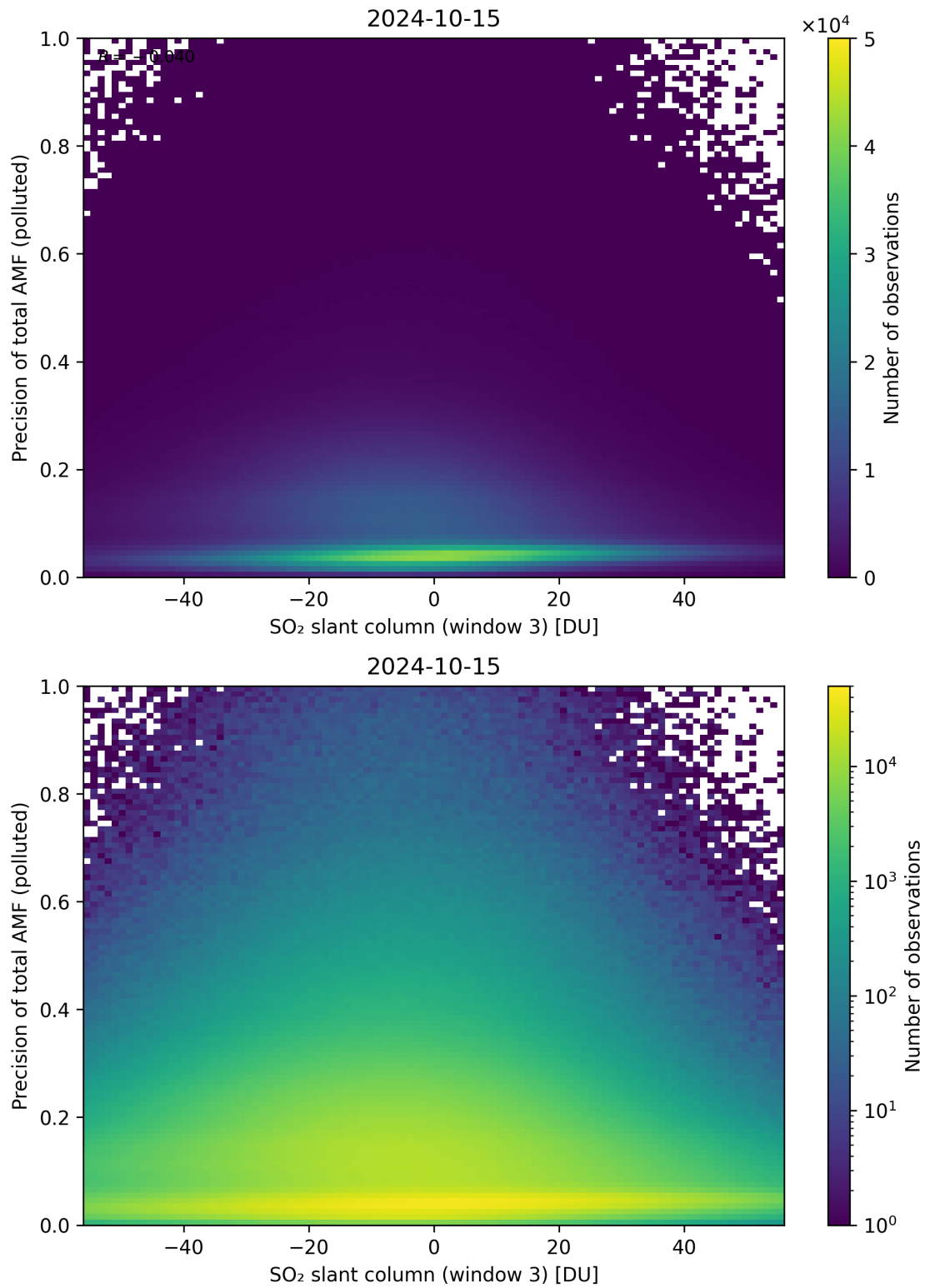
Figure 269: Scatter density plot of “SO 2 slant column (window 3)” against “Precision of total AMF (polluted)” for 2024-10-14 to 2024-10-16.
