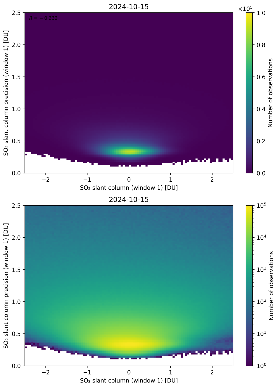
Figure 235: Scatter density plot of “SO 2 slant column (window 1)” against “SO 2 slant column precision (window 1)” for 2024-10-14 to 2024-10-16.
