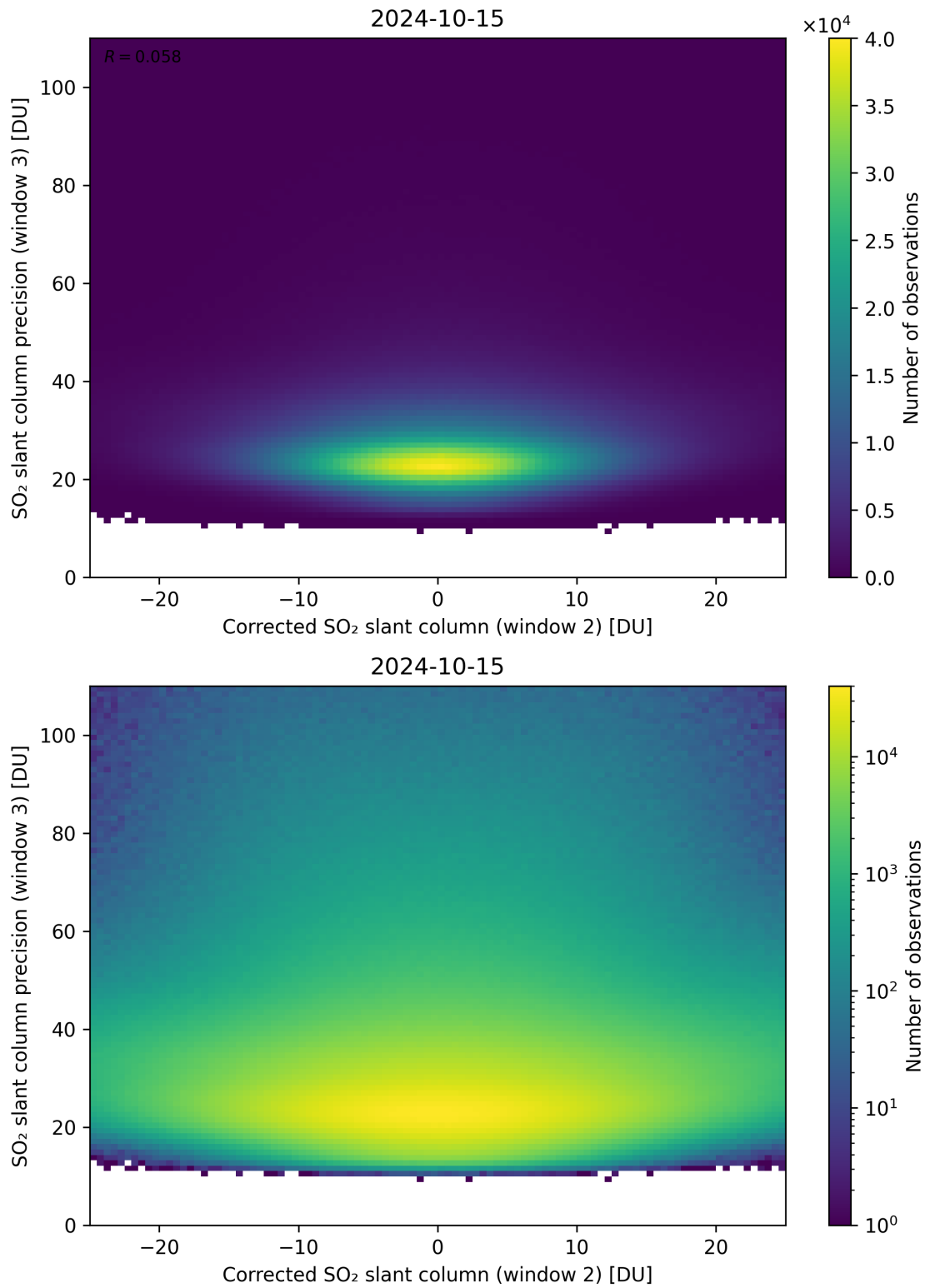
Figure 202: Scatter density plot of “Corrected SO 2 slant column (window 2)” against “SO 2 slant column precision (window 3)” for 2024-10-14 to 2024-10-16.
