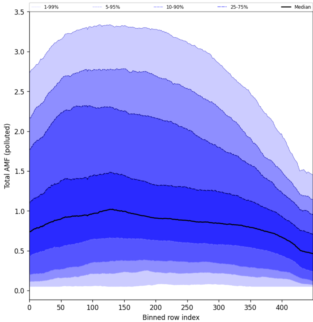
Figure 94: Along track statistics of “Total AMF (polluted)” for 2024-10-14 to 2024-10-16
