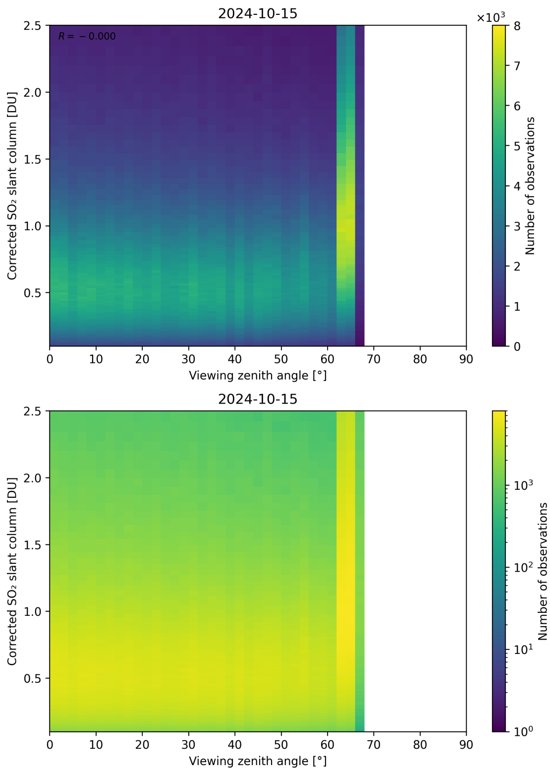
Figure 317: Scatter density plot of “Viewing zenith angle” against “Corrected SO 2 slant column” for 2024-10-14 to 2024-10-16.
