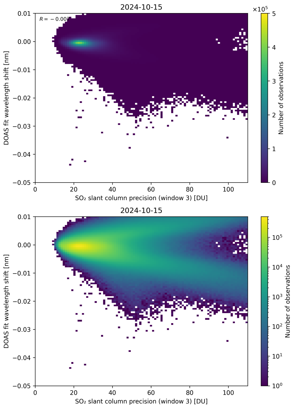
Figure 258: Scatter density plot of “SO 2 slant column precision (window 3)” against “DOAS fit wavelength shift” for 2024-10-14 to 2024-10-16.
