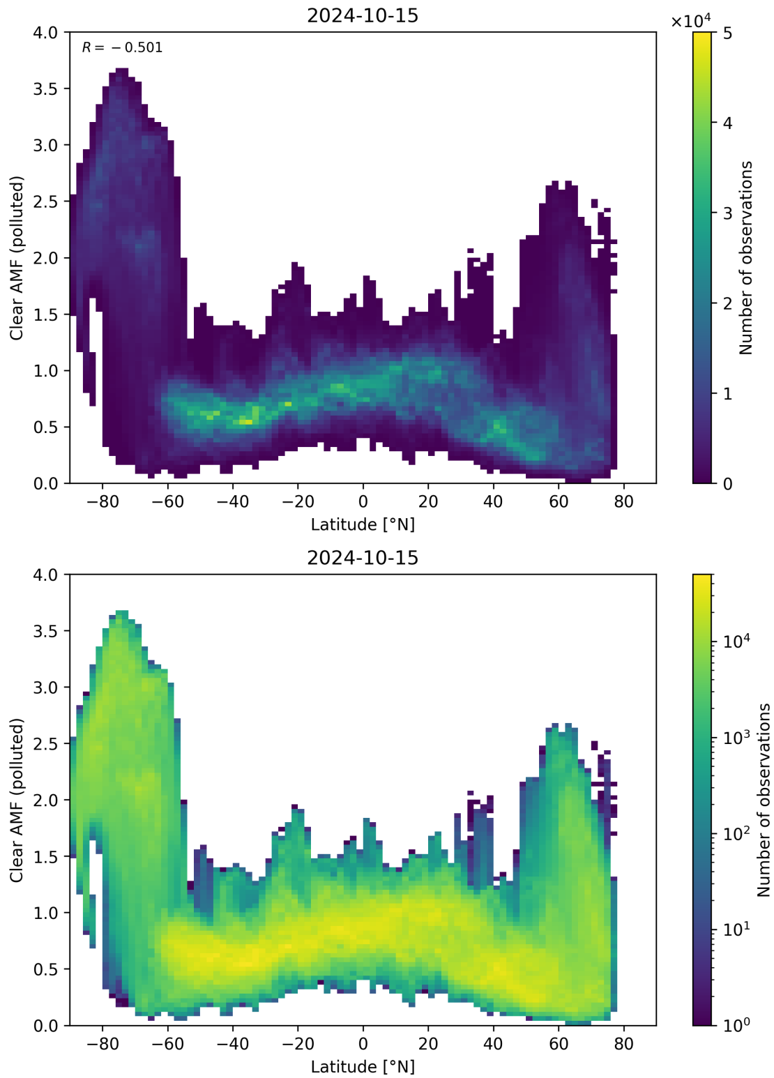
Figure 145: Scatter density plot of “Latitude” against “Clear AMF (polluted)” for 2024-10-14 to 2024-10-16.
