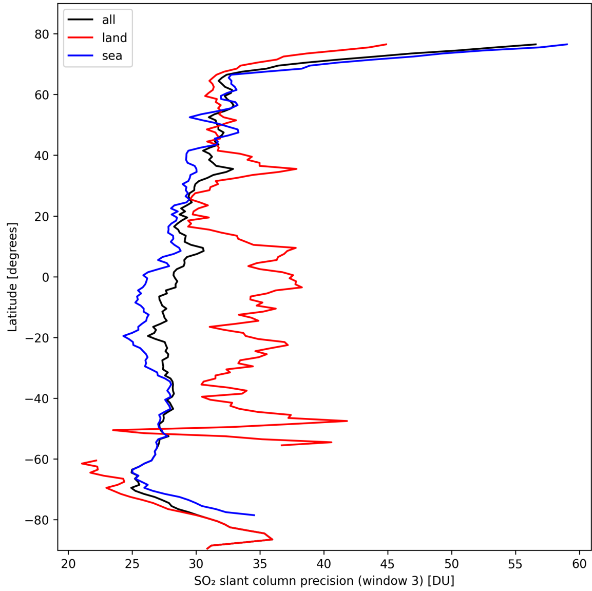
Figure 42: Zonal average of “SO 2 slant column precision (window 3)” for 2024-10-14 to 2024-10-16.
