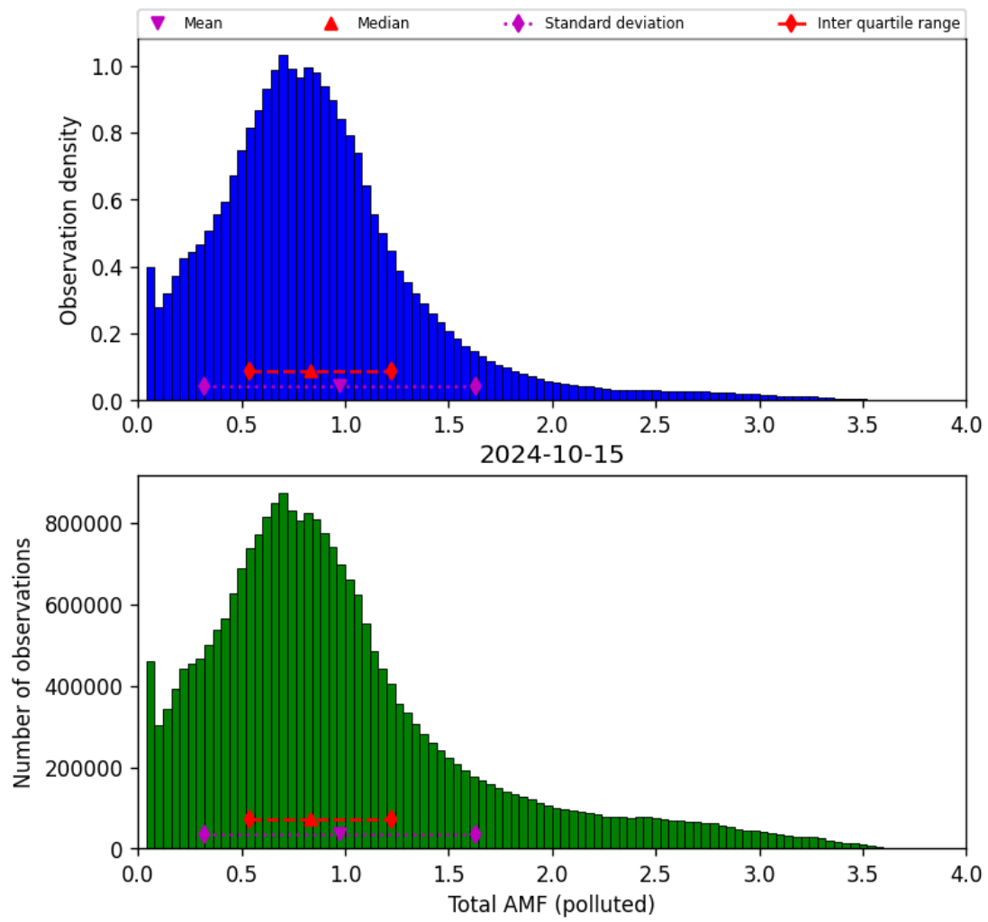
Figure 71: Histogram of “Total AMF (polluted)” for 2024-10-14 to 2024-10-16
