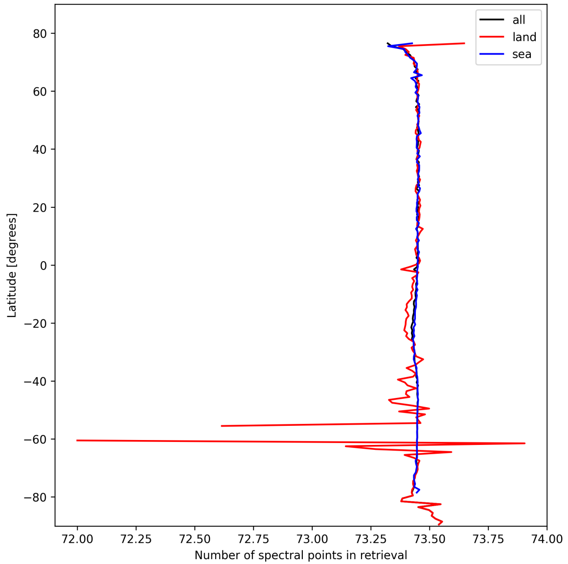
Figure 51: Zonal average of “Number of spectral points in retrieval” for 2024-10-14 to 2024-10-16.
