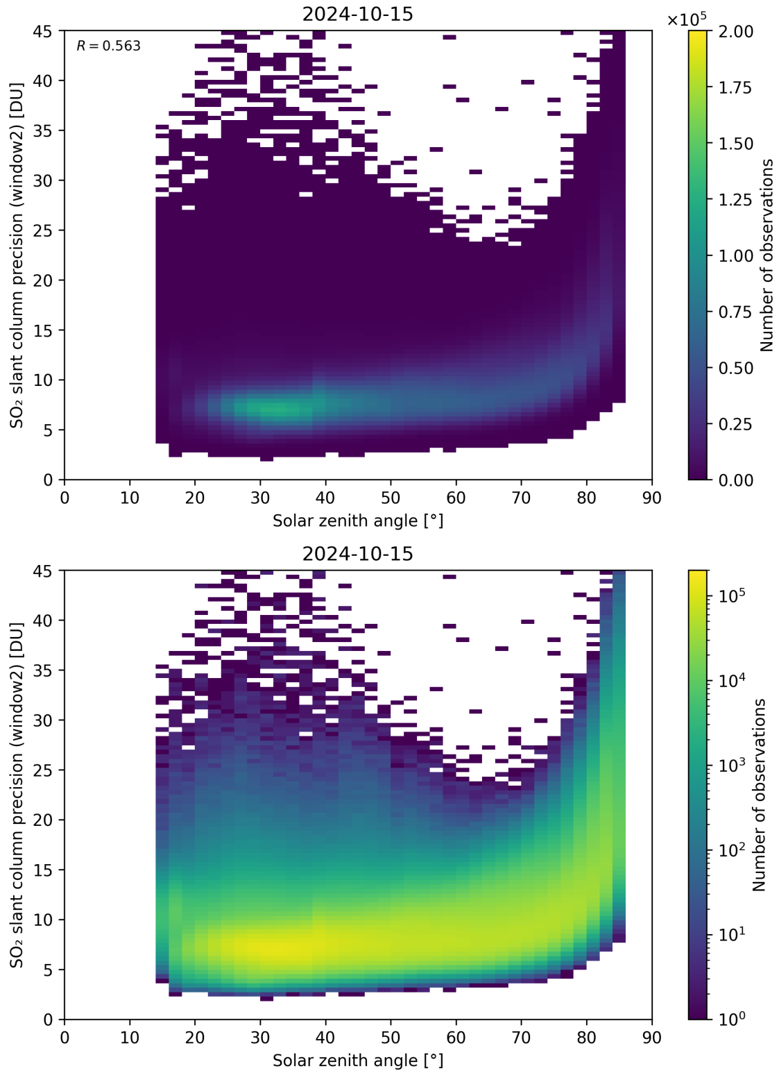
Figure 171: Scatter density plot of “Solar zenith angle” against “SO 2 slant column precision (window2)” for 2024-10-14 to 2024-10-16.
