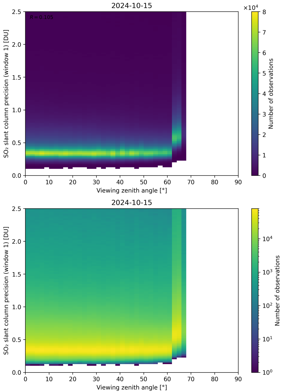
Figure 321: Scatter density plot of “Viewing zenith angle” against “SO 2 slant column precision (window 1)” for 2024-10-14 to 2024-10-16.
