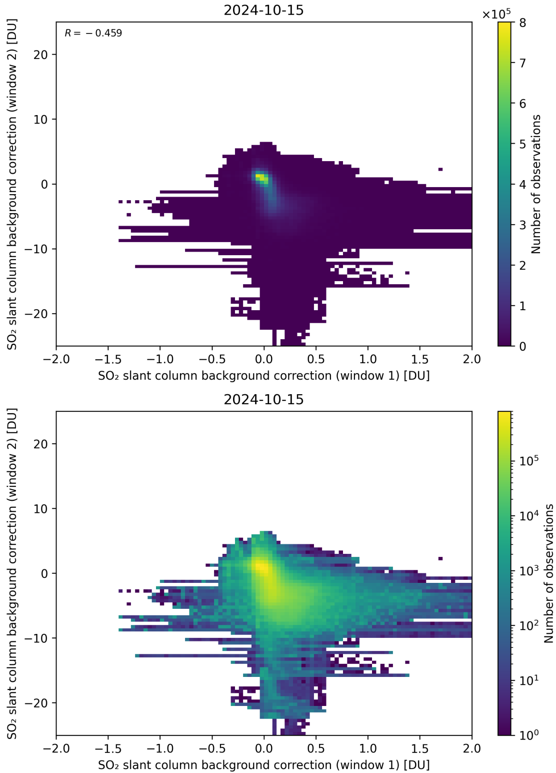
Figure 98: Scatter density plot of “SO 2 slant column background correction (window 1)” against “SO 2 slant column background correction (window 2)” for 2024-10-14 to 2024-10-16.
