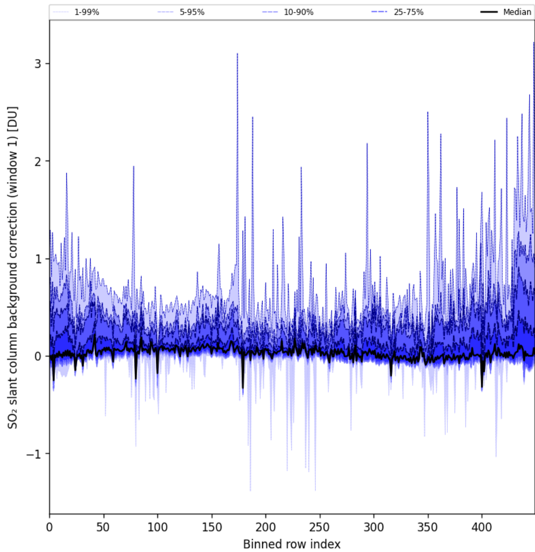
Figure 82: Along track statistics of “SO 2 slant column background correction (window 1)” for 2024-10-14 to 2024-10-16
