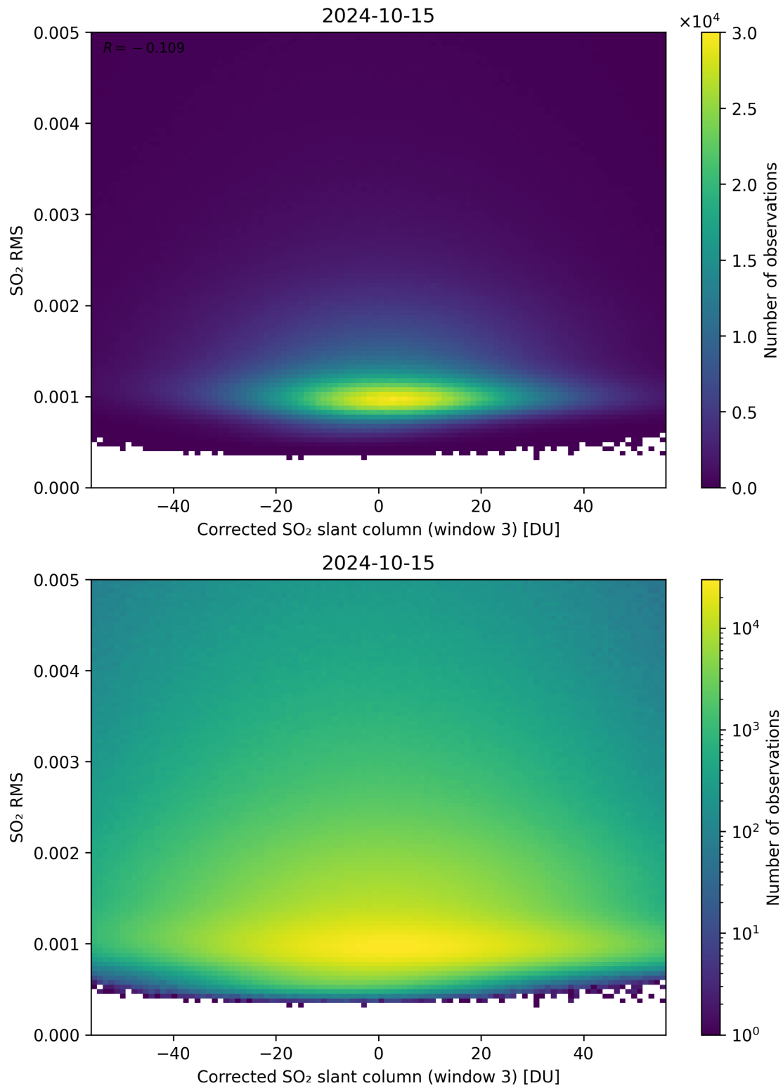
Figure 208: Scatter density plot of “Corrected SO 2 slant column (window 3)” against “SO 2 RMS” for 2024-10-14 to 2024-10-16.
