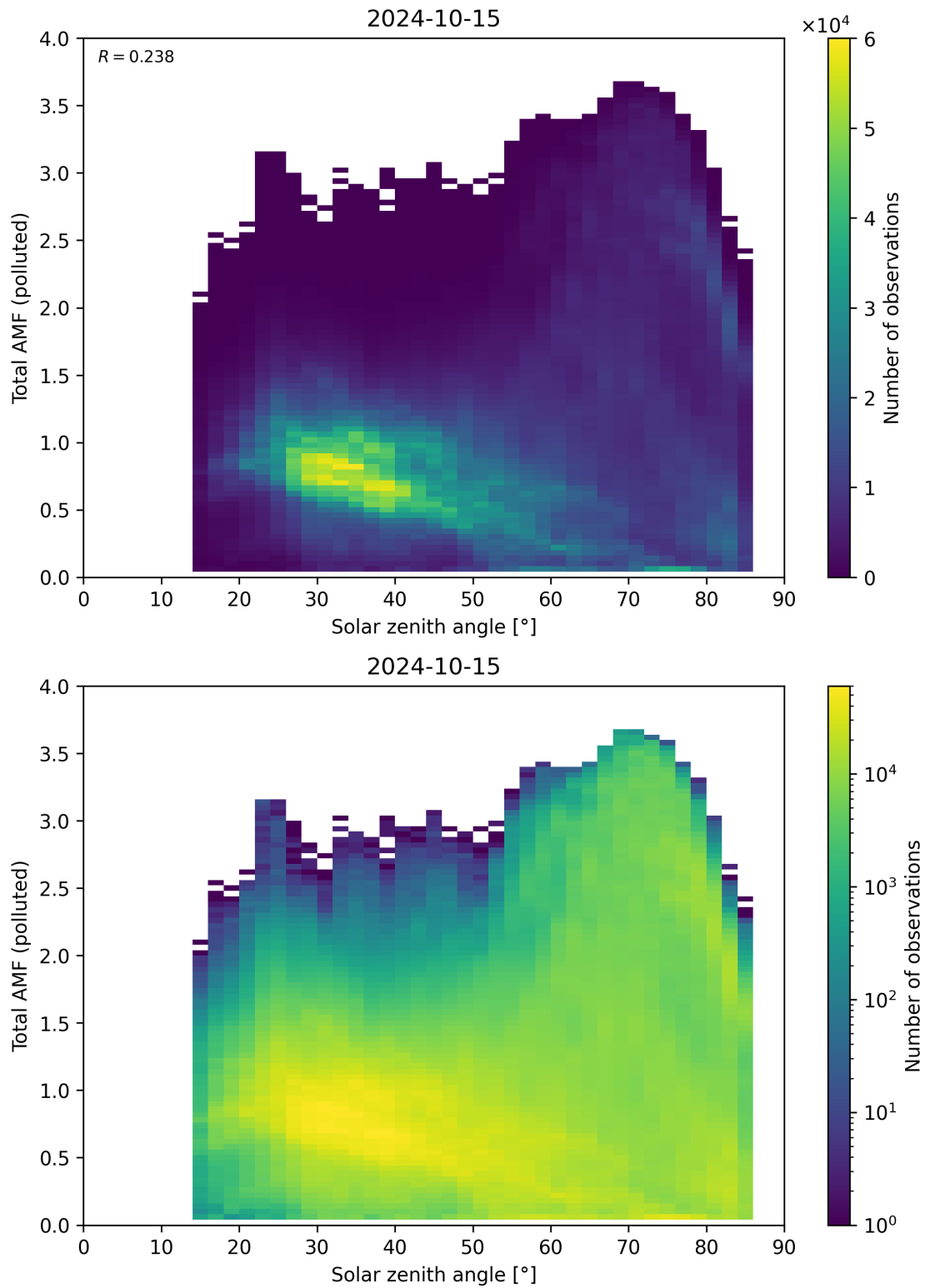
Figure 174: Scatter density plot of “Solar zenith angle” against “Total AMF (polluted)” for 2024-10-14 to 2024-10-16.
