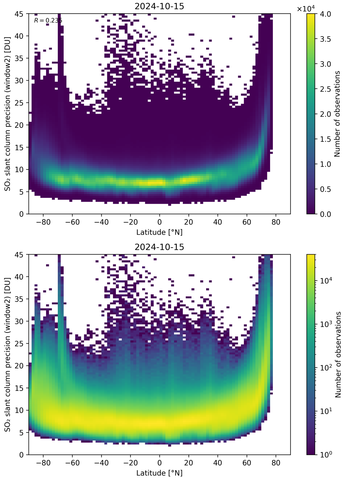
Figure 151: Scatter density plot of “Latitude” against “SO 2 slant column precision (window2)” for 2024-10-14 to 2024-10-16.
