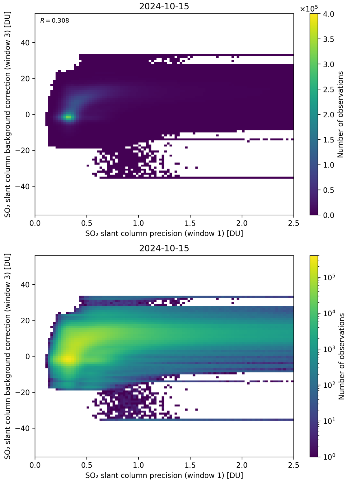
Figure 220: Scatter density plot of “SO 2 slant column precision (window 1)” against “SO 2 slant column background correction (window 3)” for 2024-10-14 to 2024-10-16.
