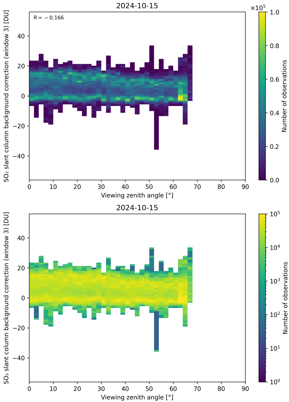
Figure 310: Scatter density plot of “Viewing zenith angle” against “SO 2 slant column background correction (window 3)” for 2024-10-14 to 2024-10-16.
