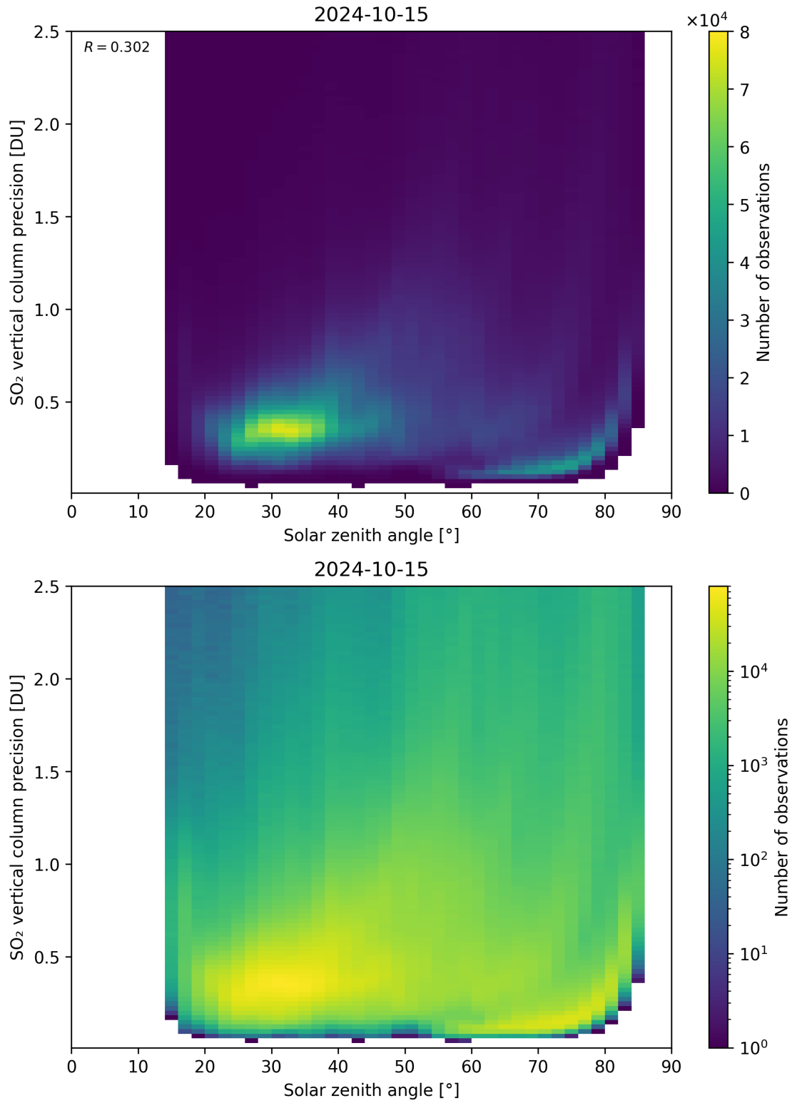
Figure 177: Scatter density plot of “Solar zenith angle” against “SO 2 vertical column precision” for 2024-10-14 to 2024-10-16.
