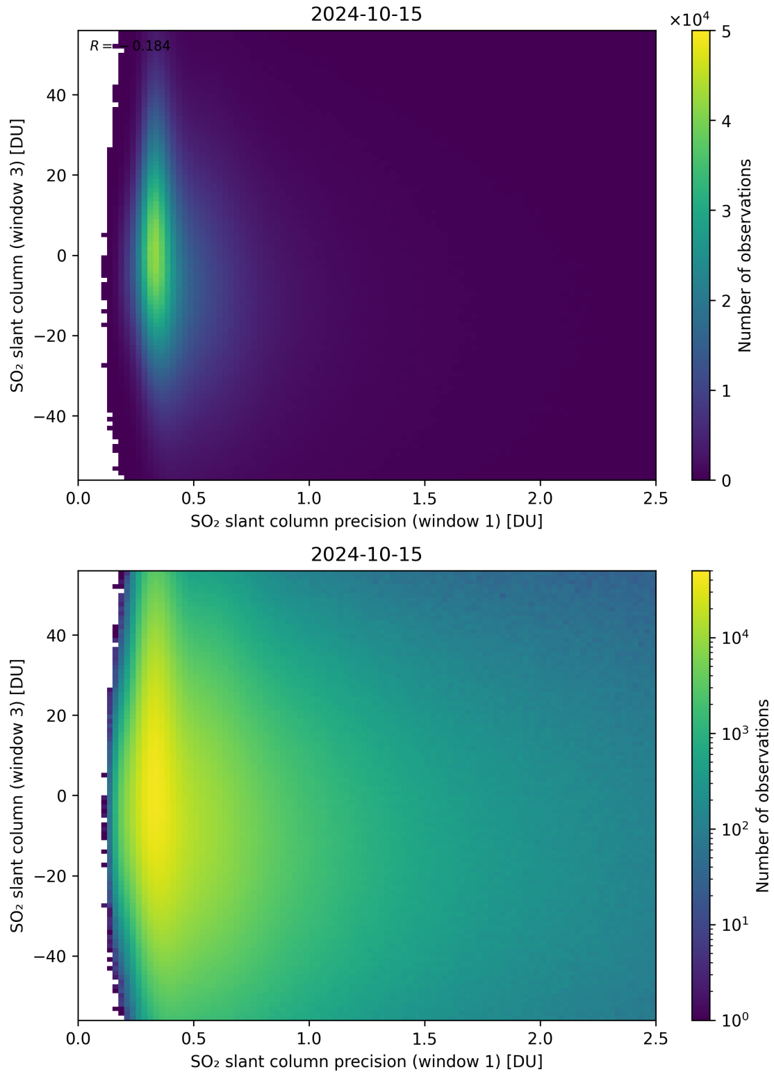
Figure 228: Scatter density plot of “SO 2 slant column precision (window 1)” against “SO 2 slant column (window 3)” for 2024-10-14 to 2024-10-16.
