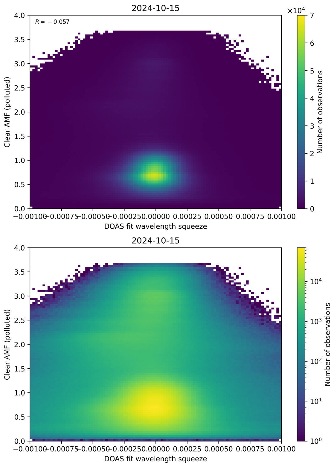
Figure 133: Scatter density plot of “DOAS fit wavelength squeeze” against “Clear AMF (polluted)” for 2024-10-14 to 2024-10-16.
