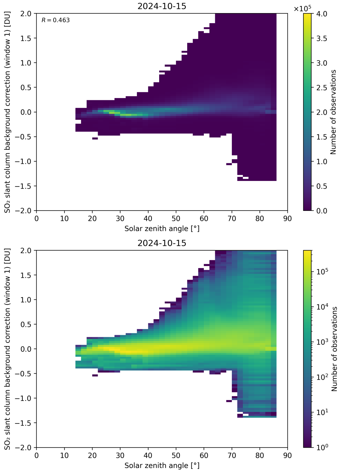
Figure 158: Scatter density plot of “Solar zenith angle” against “SO 2 slant column background correction (window 1)” for 2024-10-14 to 2024-10-16.
