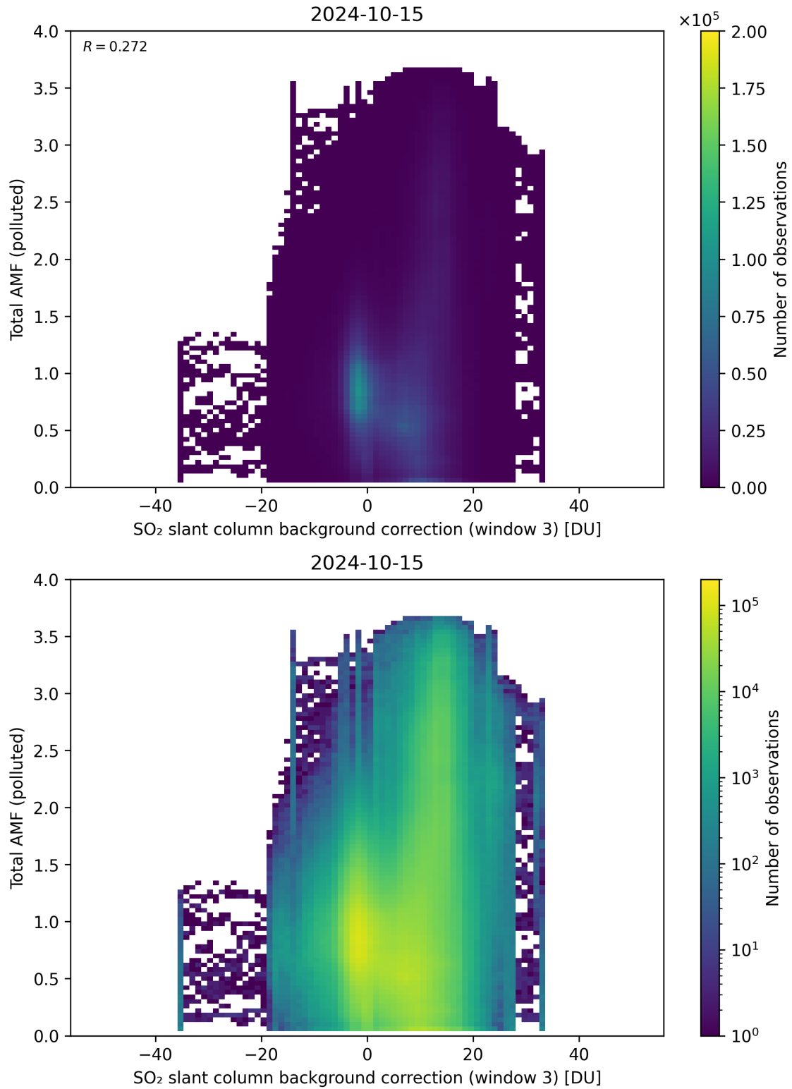
Figure 125: Scatter density plot of “SO 2 slant column background correction (window 3)” against “Total AMF (polluted)” for 2024-10-14 to 2024-10-16.
