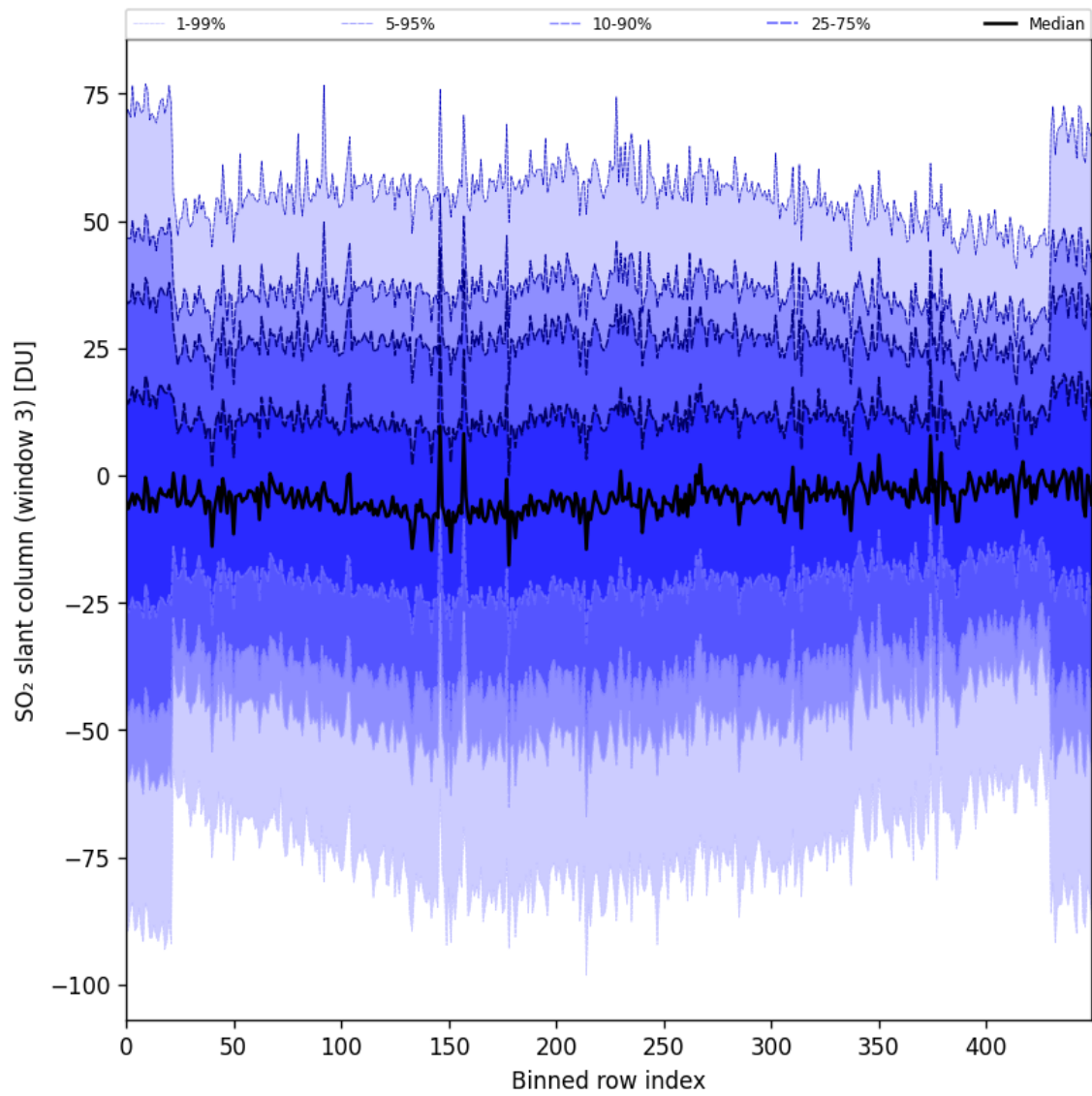
Figure 87: Along track statistics of “SO 2 slant column (window 3)” for 2024-10-14 to 2024-10-16
