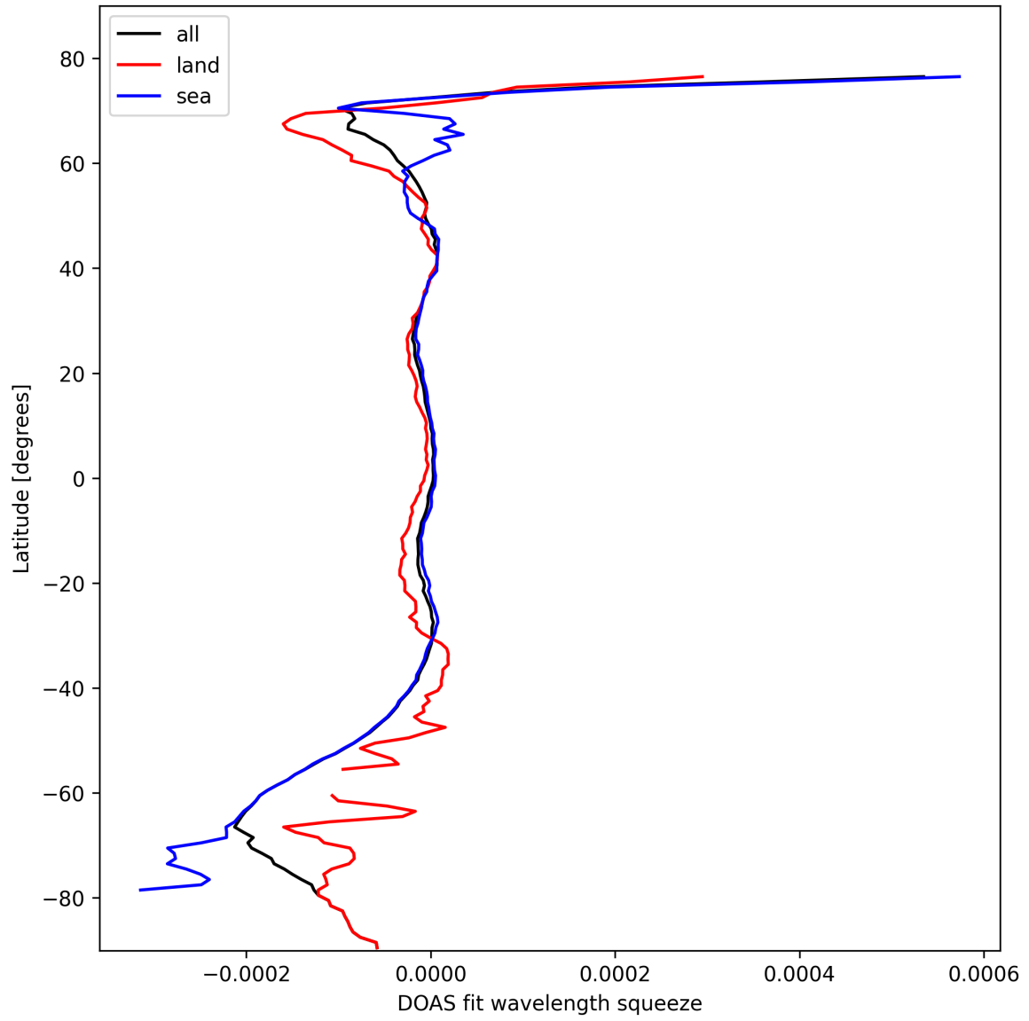
Figure 46: Zonal average of “DOAS fit wavelength squeeze” for 2024-10-14 to 2024-10-16.
