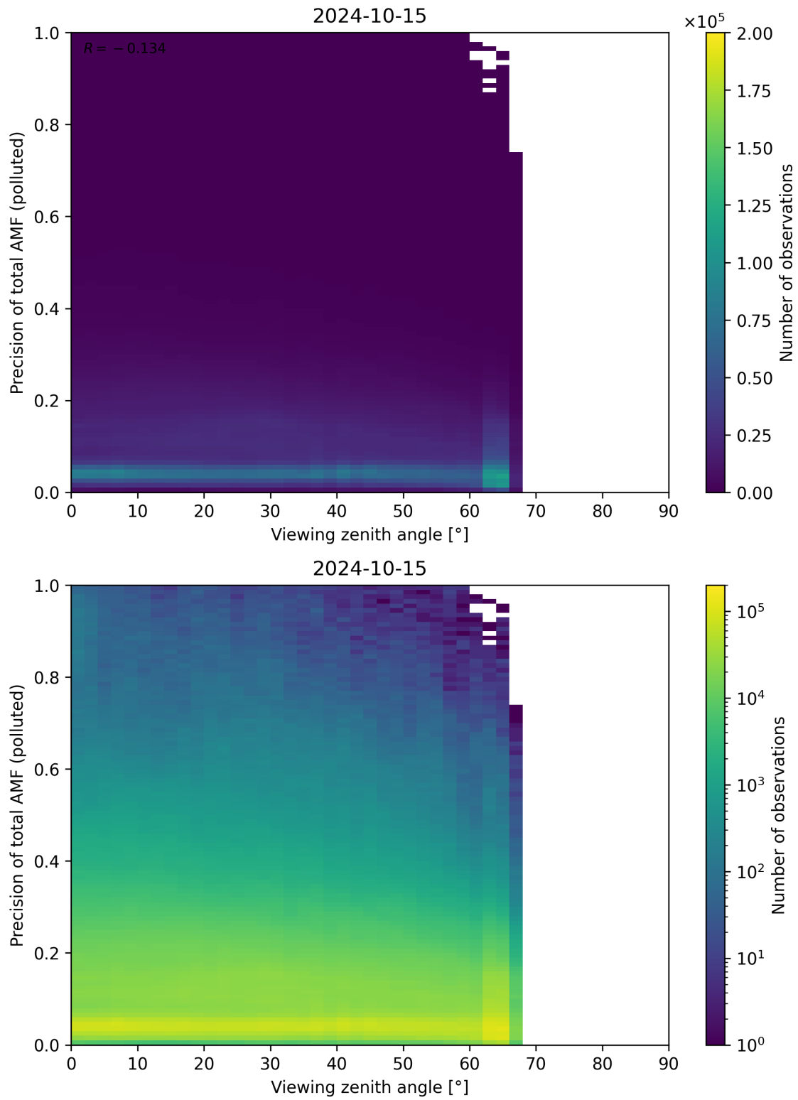
Figure 326: Scatter density plot of “Viewing zenith angle” against “Precision of total AMF (polluted)” for 2024-10-14 to 2024-10-16.
