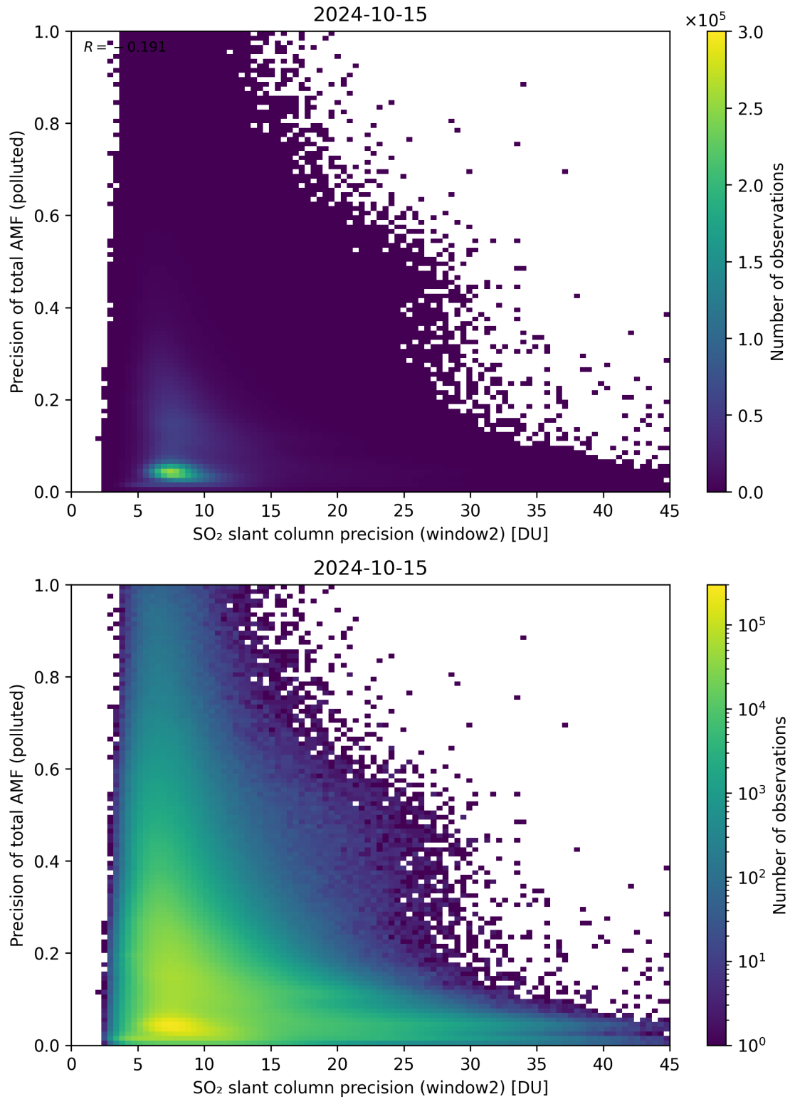
Figure 252: Scatter density plot of “SO 2 slant column precision (window2)” against “Precision of total AMF (polluted)” for 2024-10-14 to 2024-10-16.
