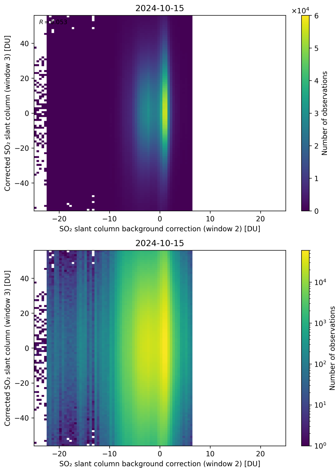
Figure 116: Scatter density plot of “SO 2 slant column background correction (window 2)” against “Corrected SO 2 slant column (window 3)” for 2024-10-14 to 2024-10-16.
