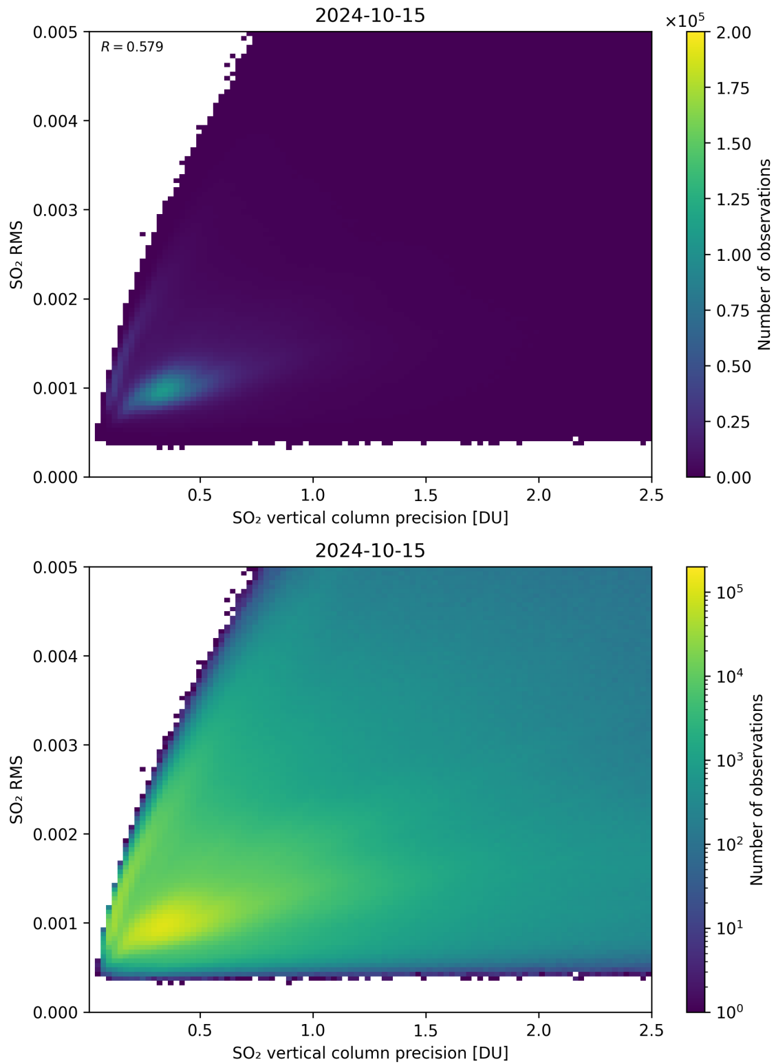
Figure 284: Scatter density plot of “SO 2 vertical column precision” against “SO 2 RMS” for 2024-10-14 to 2024-10-16.
