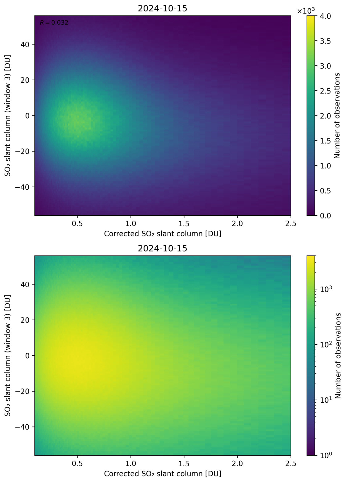
Figure 190: Scatter density plot of “Corrected SO 2 slant column” against “SO 2 slant column (window 3)” for 2024-10-14 to 2024-10-16.
