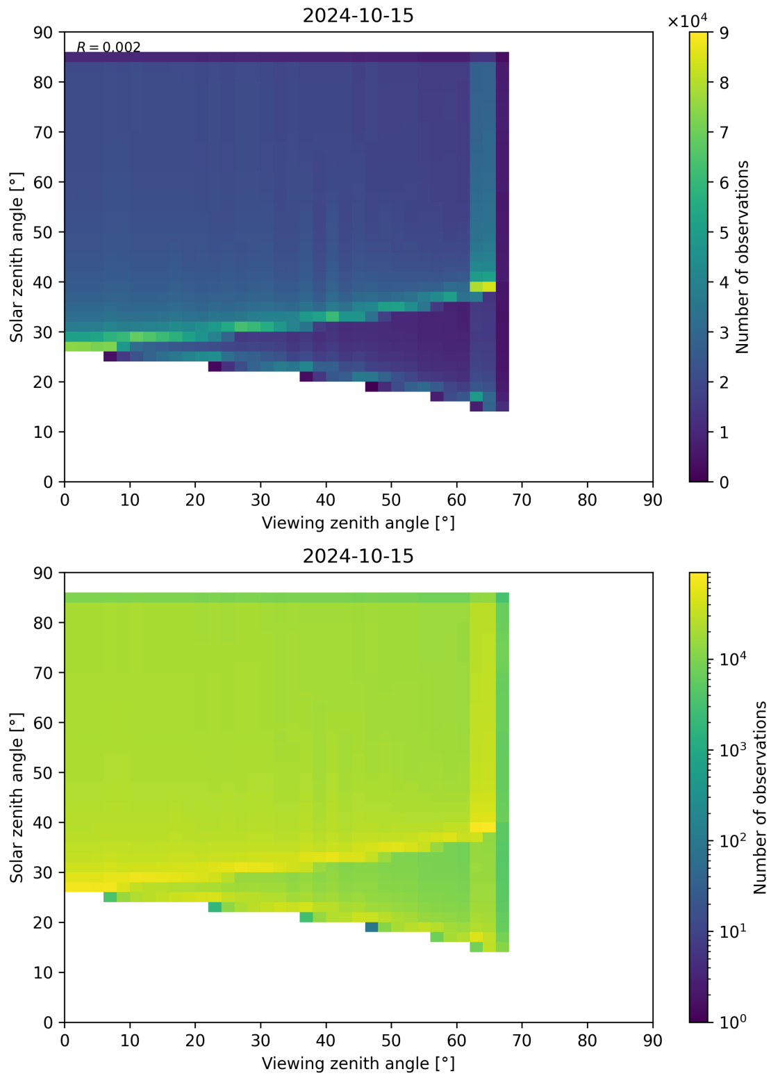
Figure 315: Scatter density plot of “Viewing zenith angle” against “Solar zenith angle” for 2024-10-14 to 2024-10-16.
