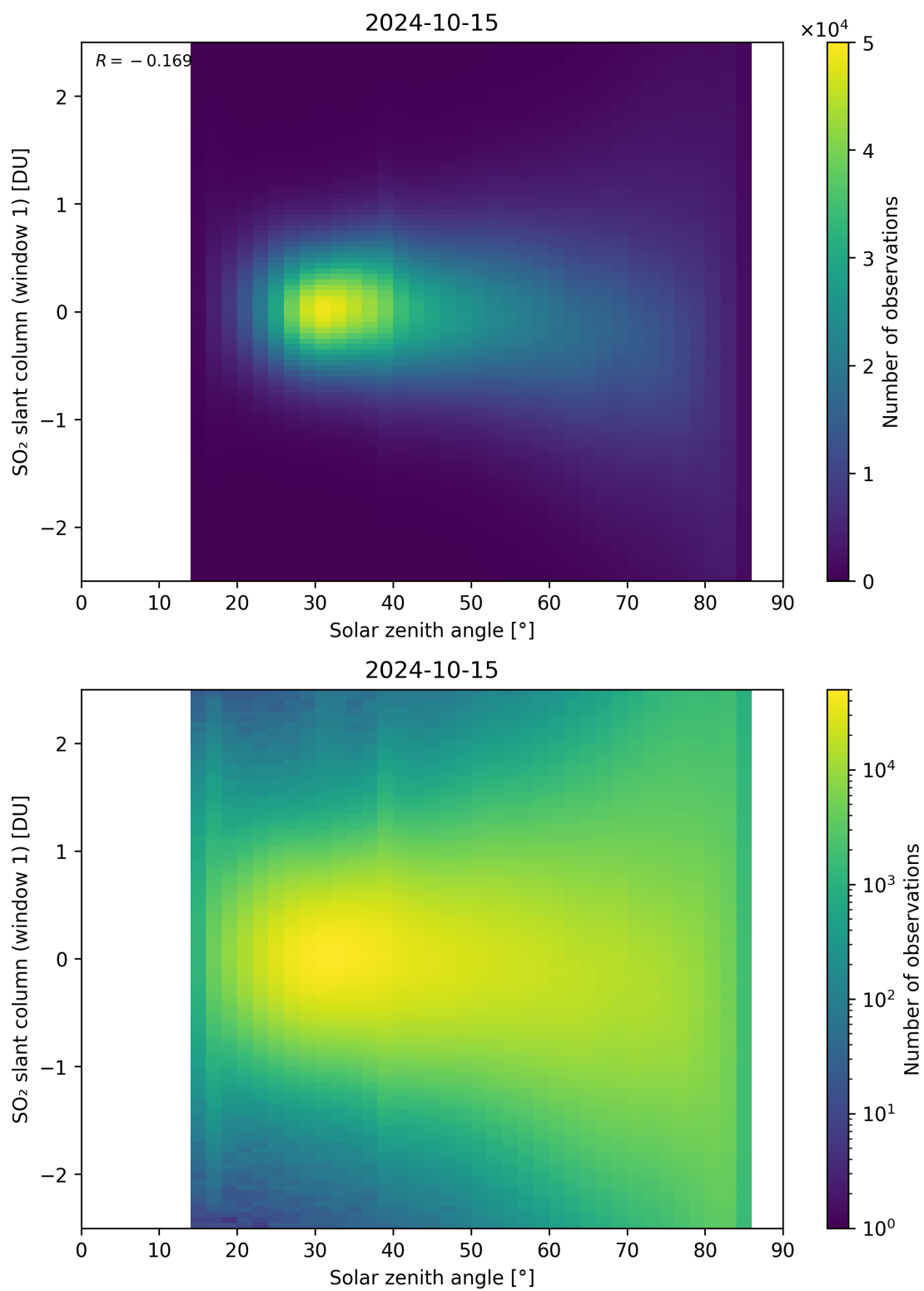
Figure 169: Scatter density plot of “Solar zenith angle” against “SO 2 slant column (window 1)” for 2024-10-14 to 2024-10-16.
