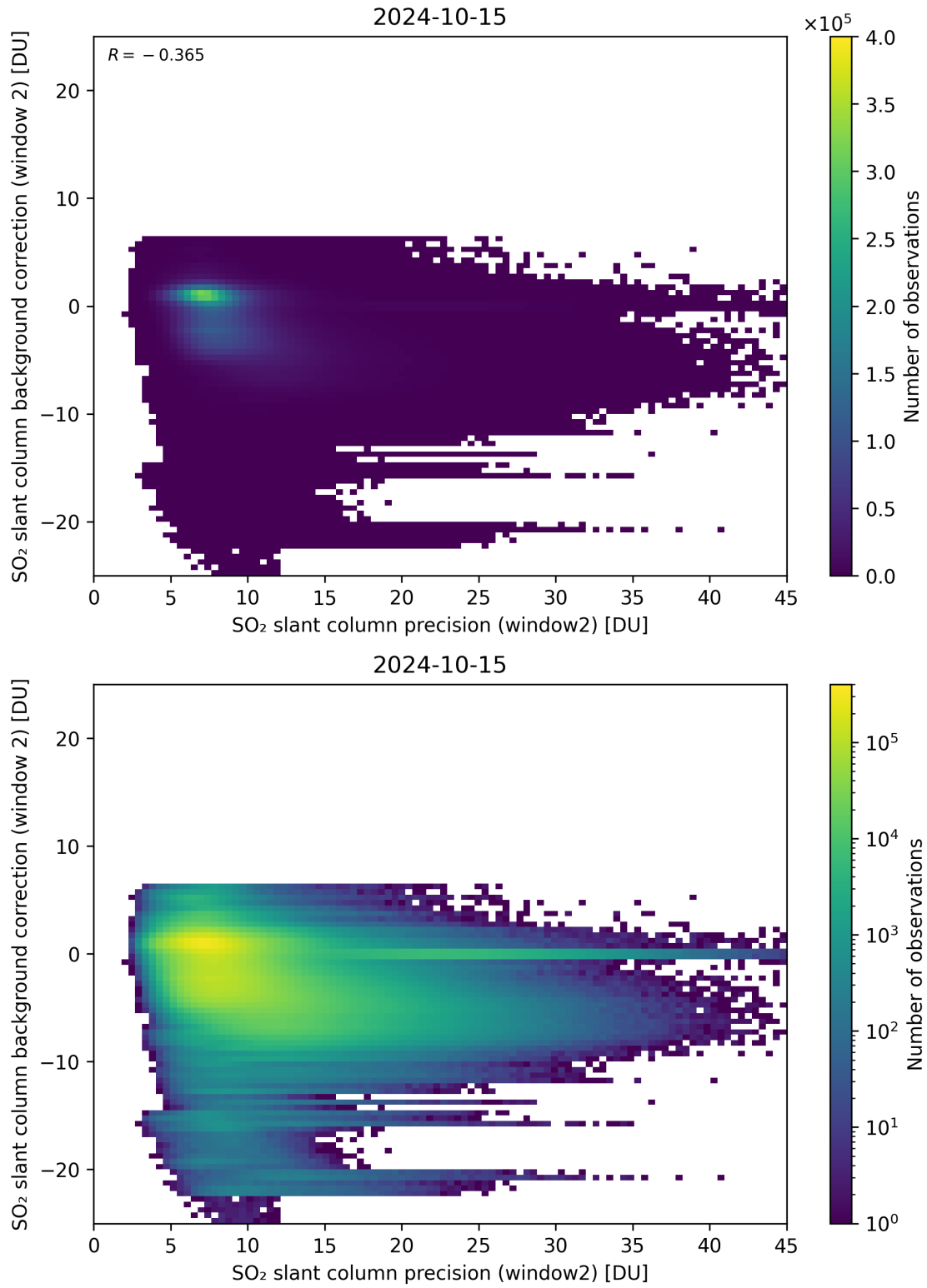
Figure 241: Scatter density plot of “SO 2 slant column precision (window2)” against “SO 2 slant column background correction (window 2)” for 2024-10-14 to 2024-10-16.
