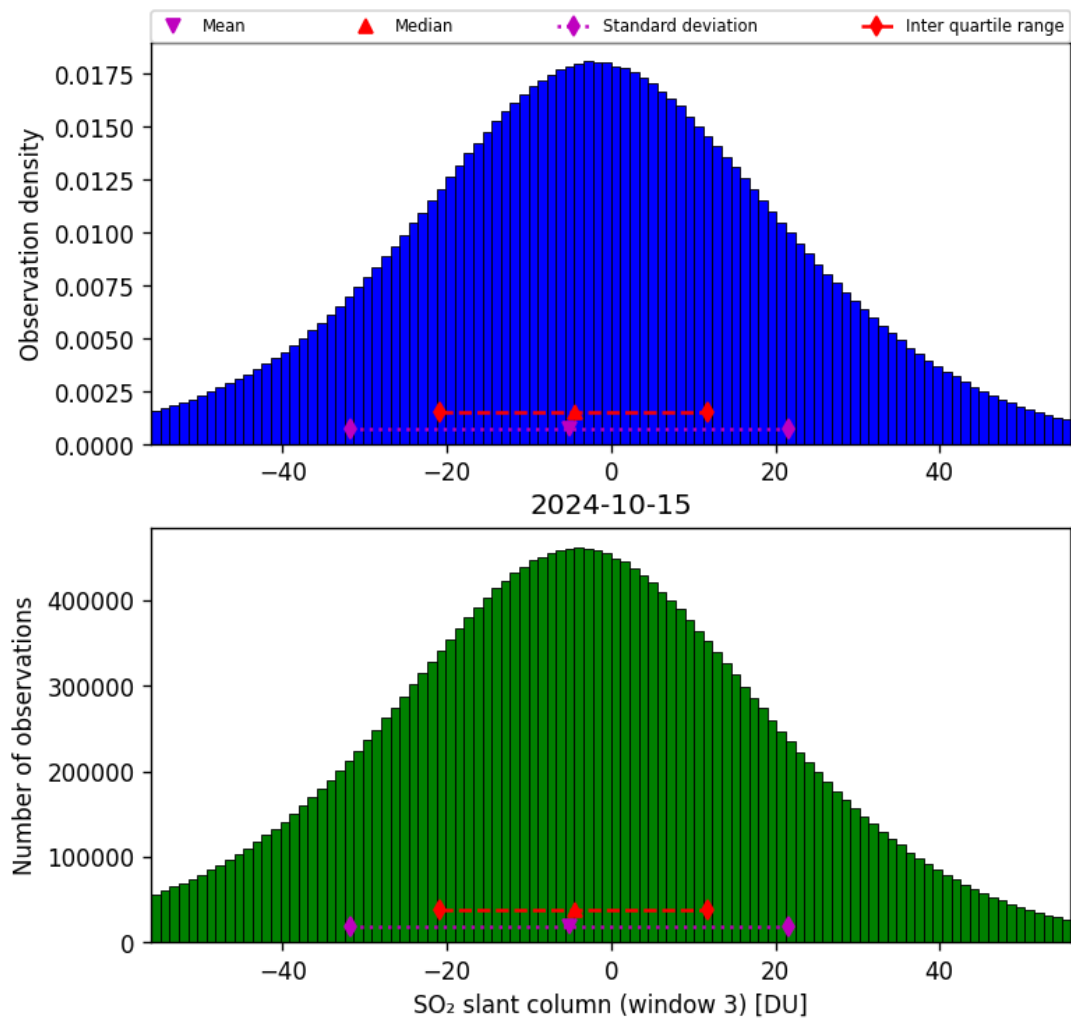
Figure 64: Histogram of “SO 2 slant column (window 3)” for 2024-10-14 to 2024-10-16
