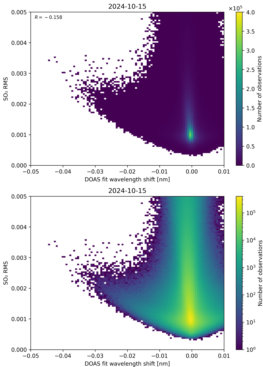
Figure 128: Scatter density plot of “DOAS fit wavelength shift” against “SO 2 RMS” for 2024-10-14 to 2024-10-16.
