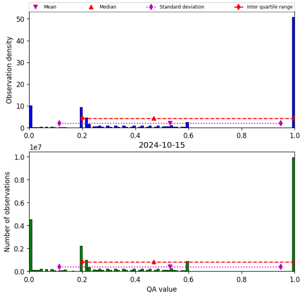
Figure 52: Histogram of “QA value” for 2024-10-14 to 2024-10-16
