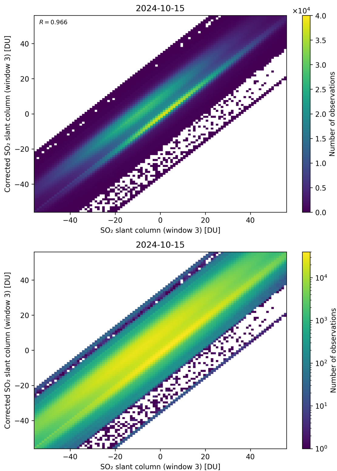
Figure 266: Scatter density plot of “SO 2 slant column (window 3)” against “Corrected SO 2 slant column (window 3)” for 2024-10-14 to 2024-10-16.
