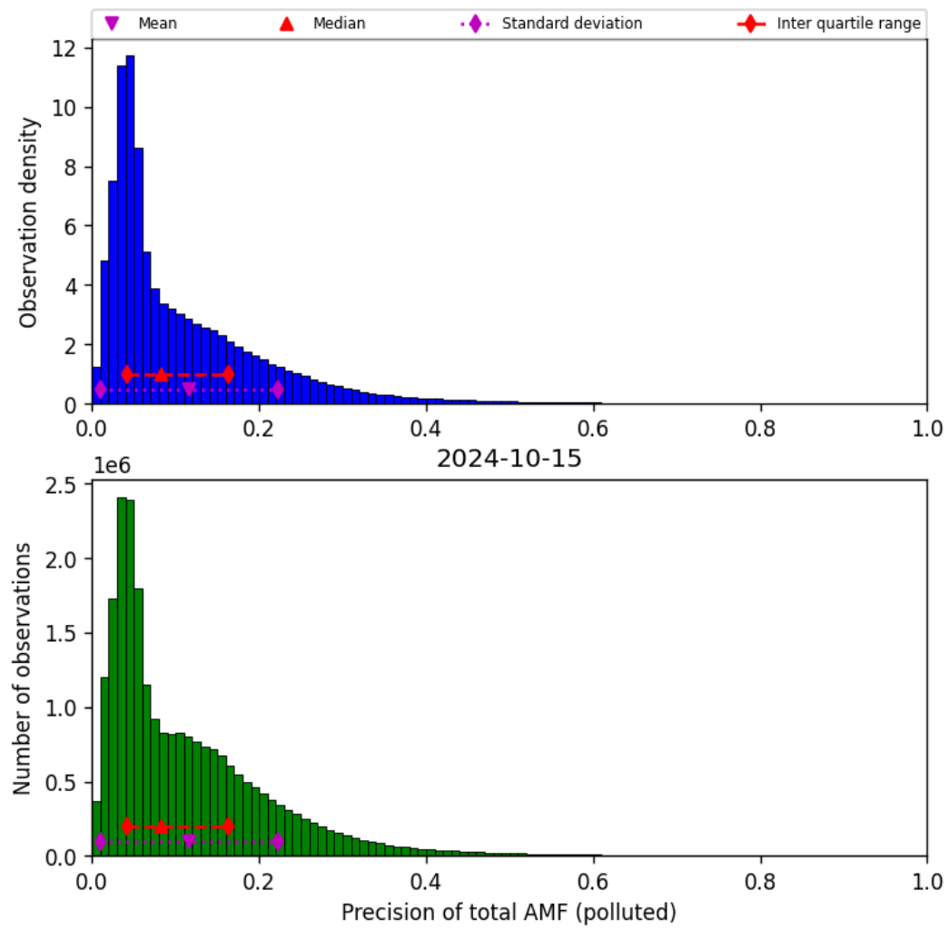
Figure 72: Histogram of “Precision of total AMF (polluted)” for 2024-10-14 to 2024-10-16
