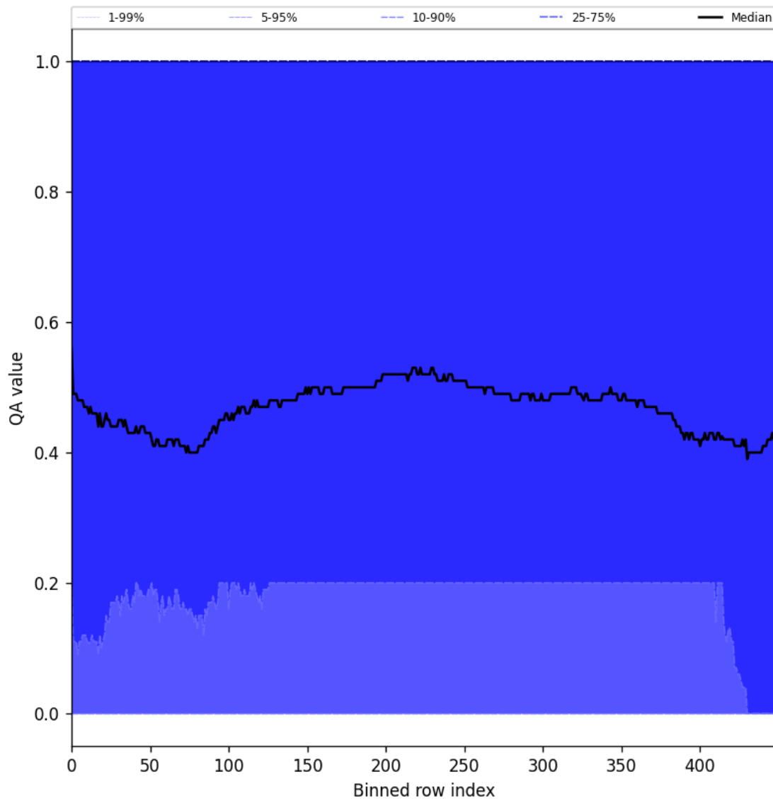
Figure 75: Along track statistics of “QA value” for 2024-10-14 to 2024-10-16
