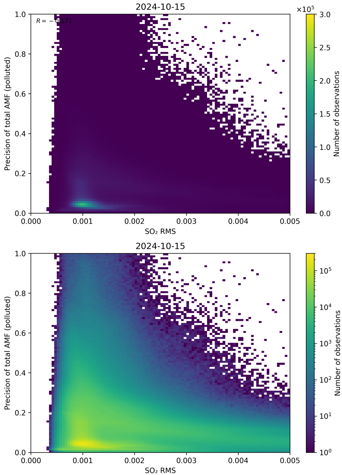
Figure 138: Scatter density plot of “SO 2 RMS” against “Precision of total AMF (polluted)” for 2024-10-14 to 2024-10-16.
