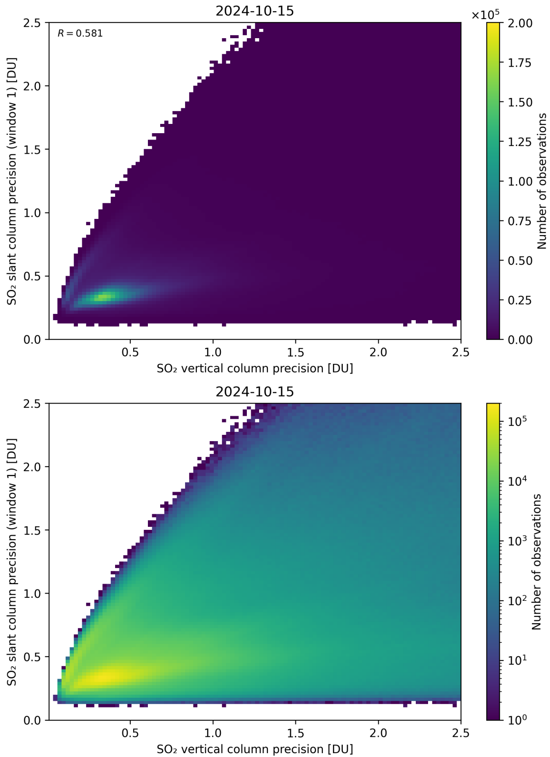
Figure 290: Scatter density plot of “SO 2 vertical column precision” against “SO 2 slant column precision (window 1)” for 2024-10-14 to 2024-10-16.
