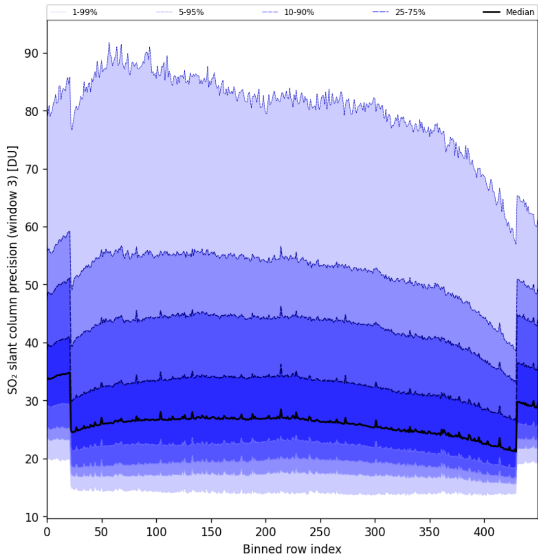
Figure 88: Along track statistics of “SO 2 slant column precision (window 3)” for 2024-10-14 to 2024-10-16
