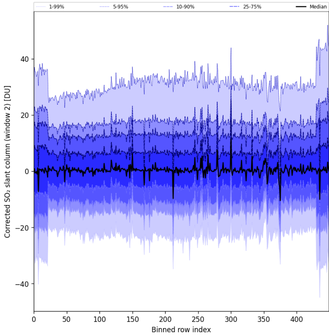
Figure 85: Along track statistics of “Corrected SO 2 slant column (window 2)” for 2024-10-14 to 2024-10-16
