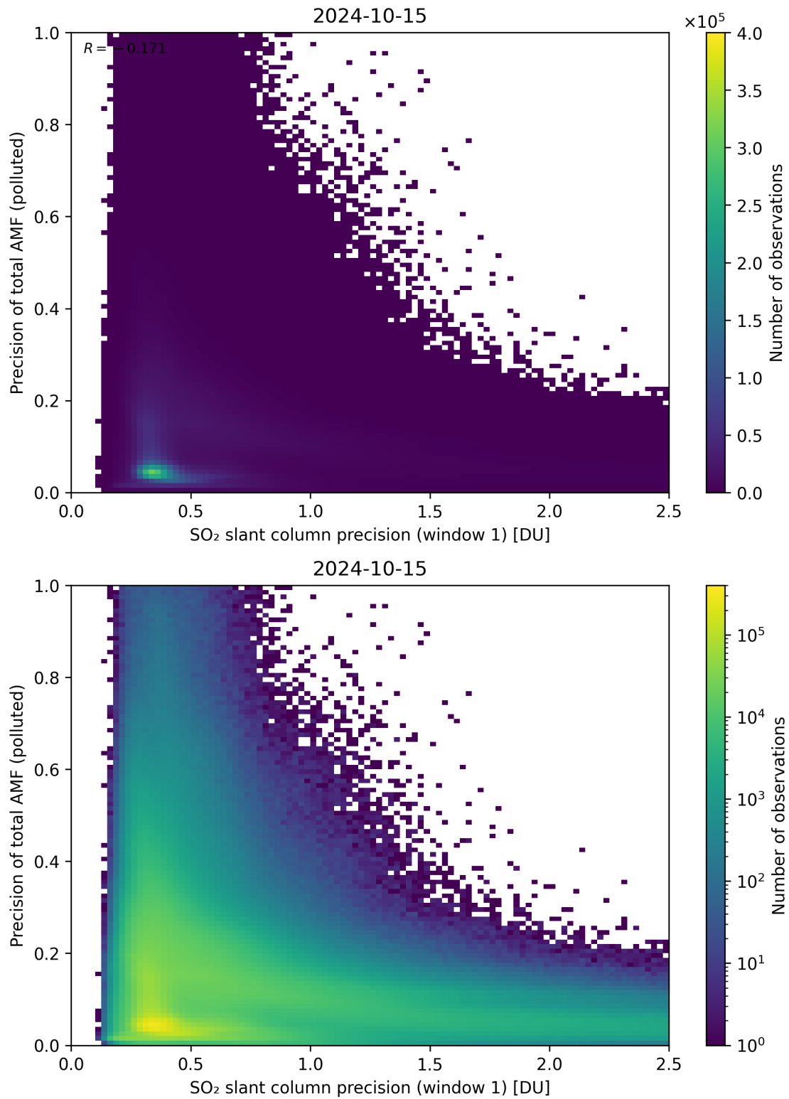
Figure 231: Scatter density plot of “SO 2 slant column precision (window 1)” against “Precision of total AMF (polluted)” for 2024-10-14 to 2024-10-16.
