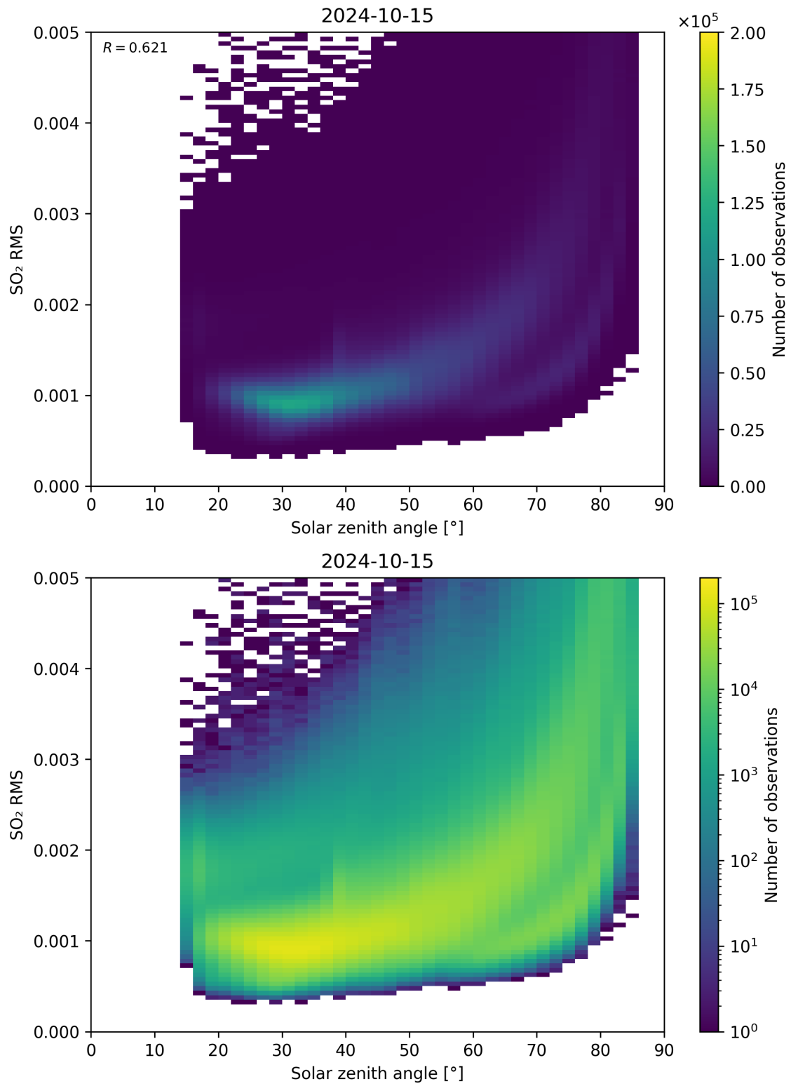
Figure 163: Scatter density plot of “Solar zenith angle” against “SO 2 RMS” for 2024-10-14 to 2024-10-16.
