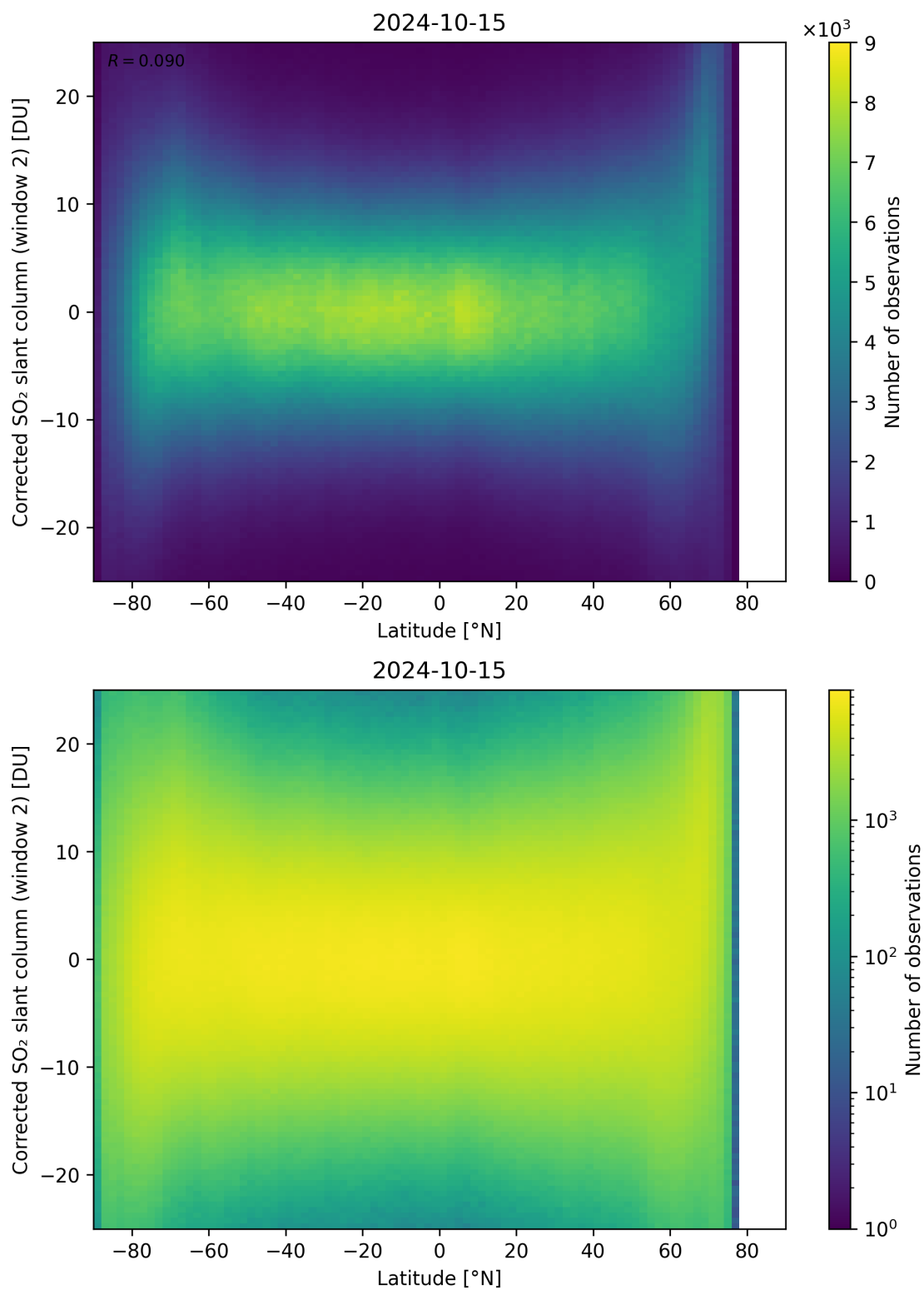
Figure 147: Scatter density plot of “Latitude” against “Corrected SO 2 slant column (window 2)” for 2024-10-14 to 2024-10-16.
