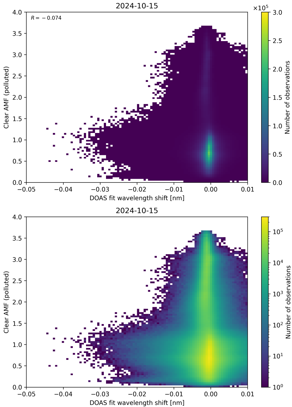
Figure 129: Scatter density plot of “DOAS fit wavelength shift” against “Clear AMF (polluted)” for 2024-10-14 to 2024-10-16.
