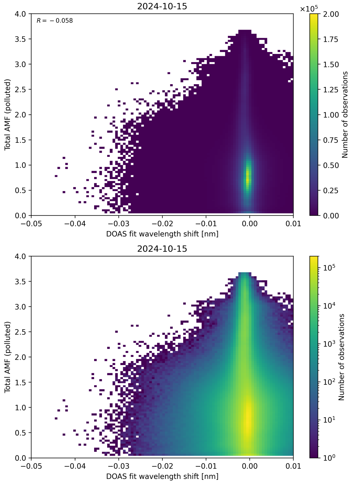
Figure 130: Scatter density plot of “DOAS fit wavelength shift” against “Total AMF (polluted)” for 2024-10-14 to 2024-10-16.
