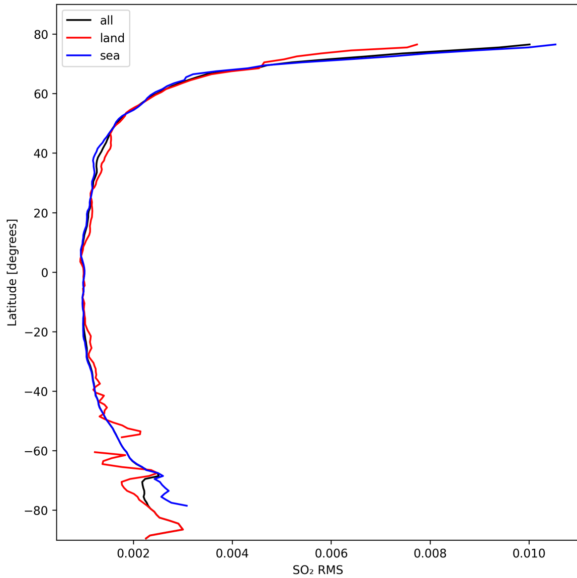
Figure 47: Zonal average of “SO 2 RMS” for 2024-10-14 to 2024-10-16.
