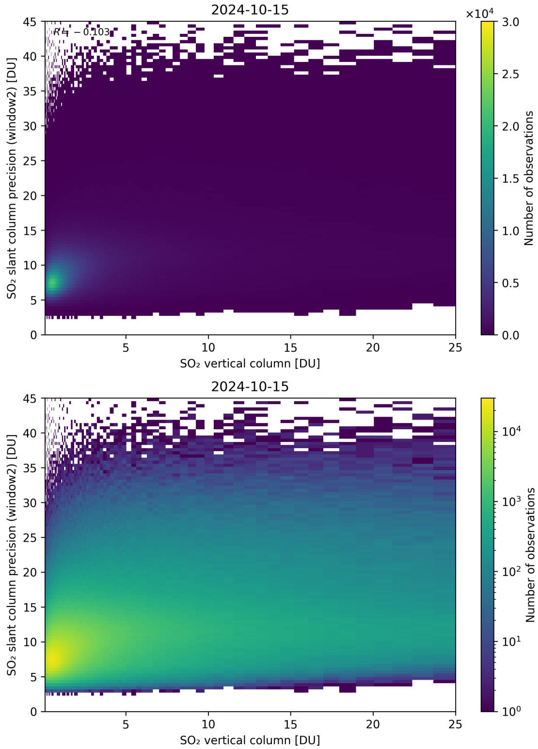
Figure 302: Scatter density plot of “SO 2 vertical column” against “SO 2 slant column precision (window2)” for 2024-10-14 to 2024-10-16.
