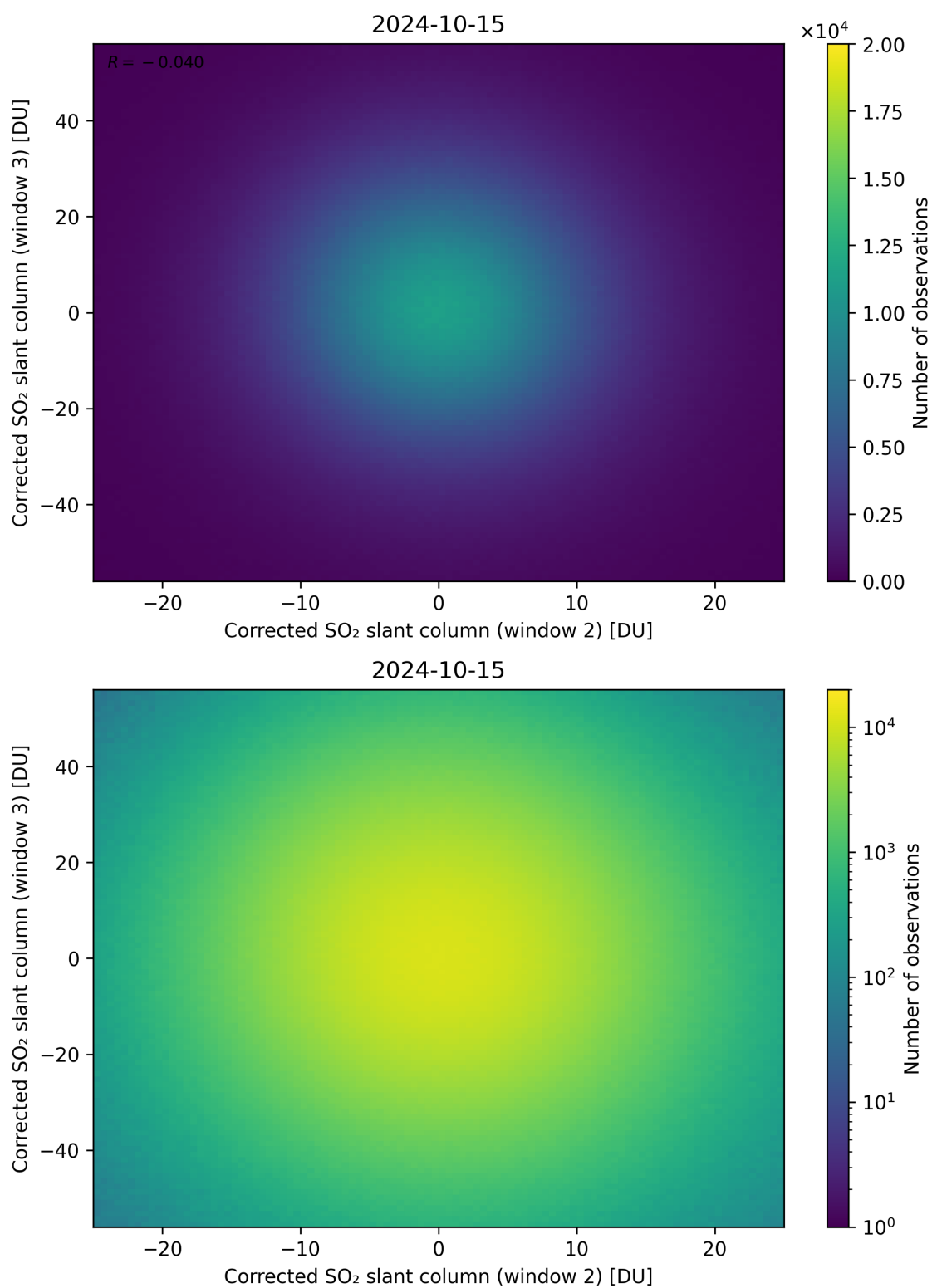
Figure 200: Scatter density plot of “Corrected SO 2 slant column (window 2)” against “Corrected SO 2 slant column (window 3)” for 2024-10-14 to 2024-10-16.
