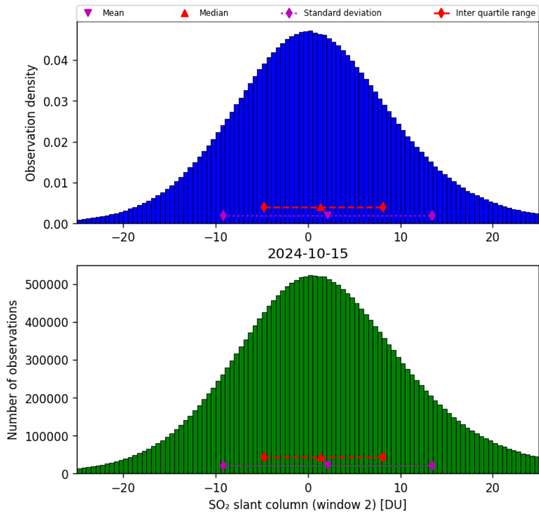
Figure 60: Histogram of “SO 2 slant column (window 2)” for 2024-10-14 to 2024-10-16
