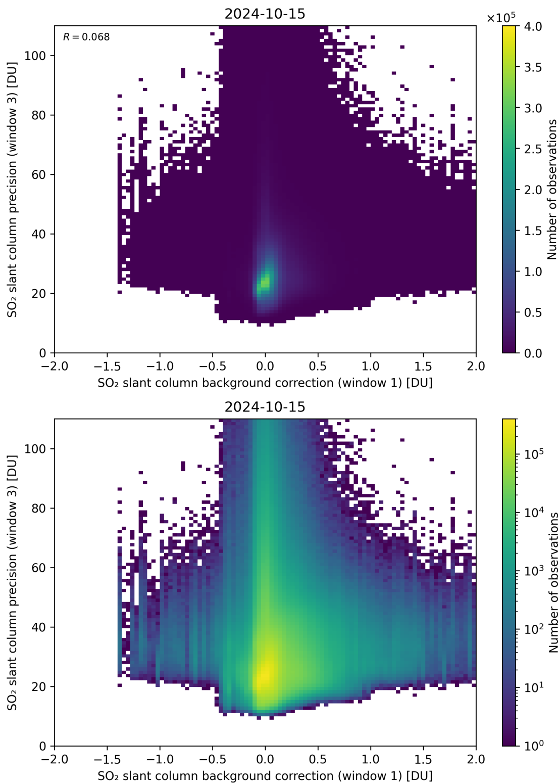
Figure 108: Scatter density plot of “SO 2 slant column background correction (window 1)” against “SO 2 slant column precision (window 3)” for 2024-10-14 to 2024-10-16.
