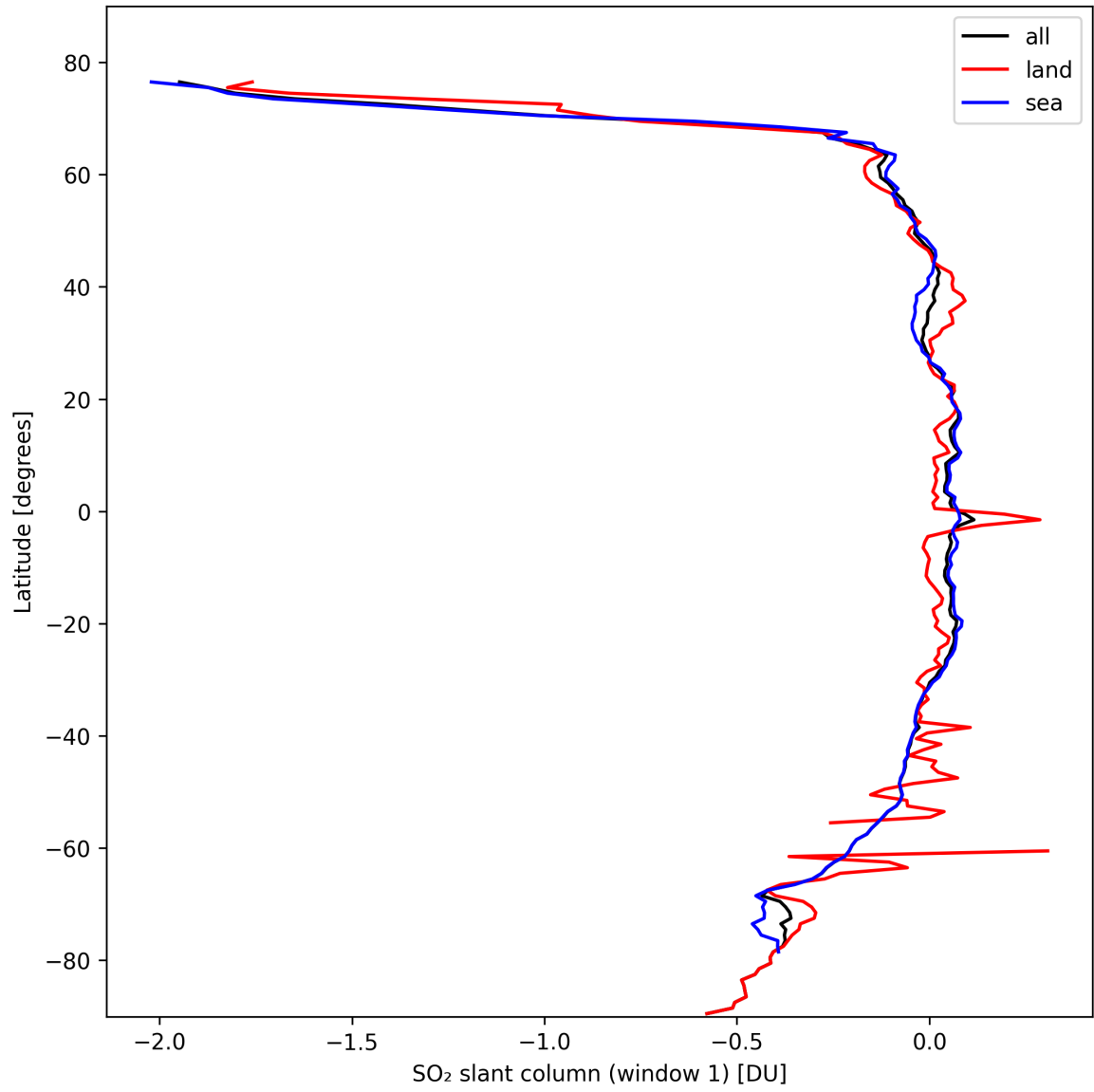
Figure 33: Zonal average of “SO 2 slant column (window 1)” for 2024-10-14 to 2024-10-16.
