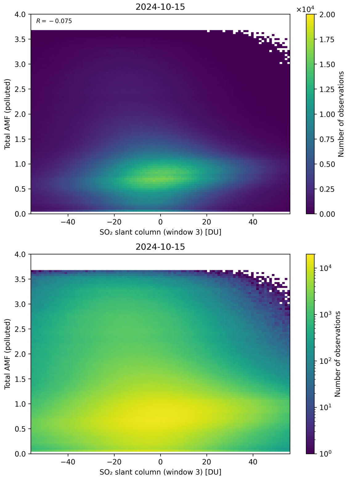
Figure 268: Scatter density plot of “SO 2 slant column (window 3)” against “Total AMF (polluted)” for 2024-10-14 to 2024-10-16.
