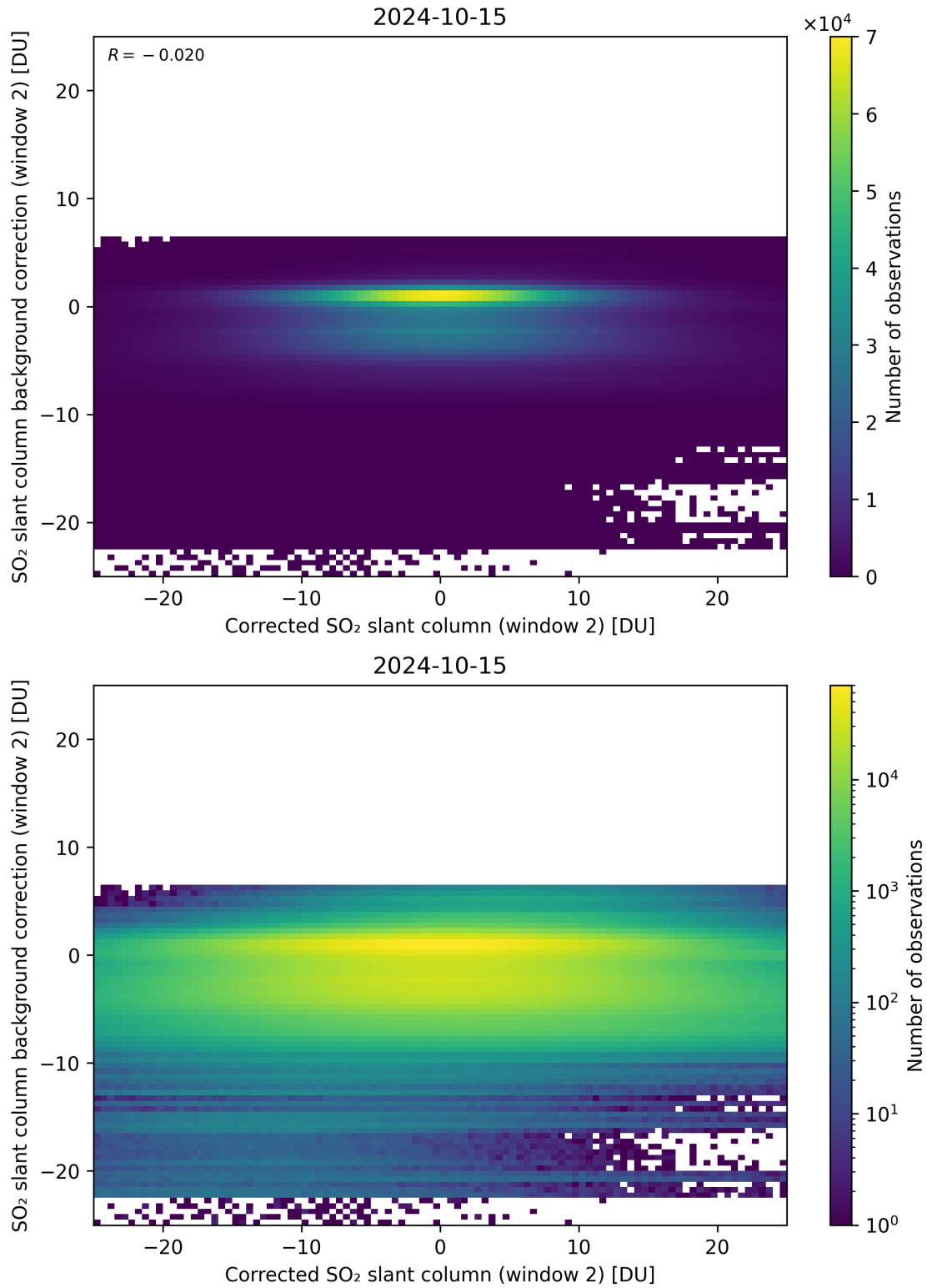
Figure 194: Scatter density plot of “Corrected SO 2 slant column (window 2)” against “SO 2 slant column background correction (window 2)” for 2024-10-14 to 2024-10-16.
