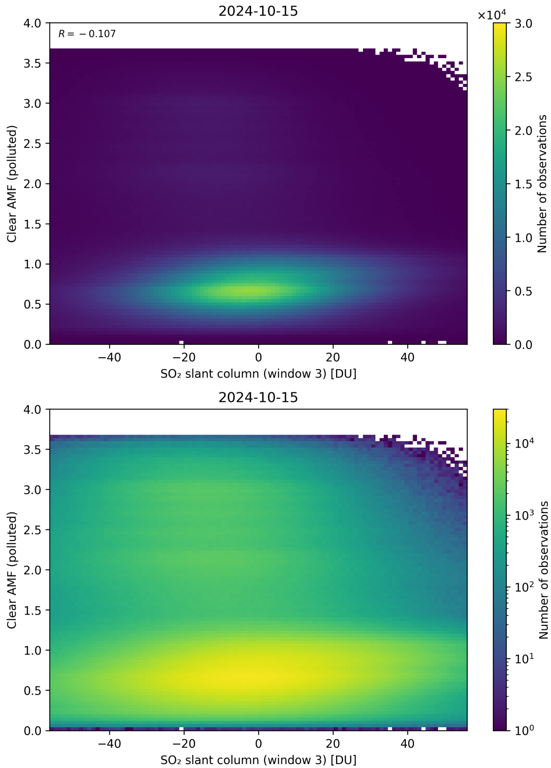
Figure 265: Scatter density plot of “SO 2 slant column (window 3)” against “Clear AMF (polluted)” for 2024-10-14 to 2024-10-16.
