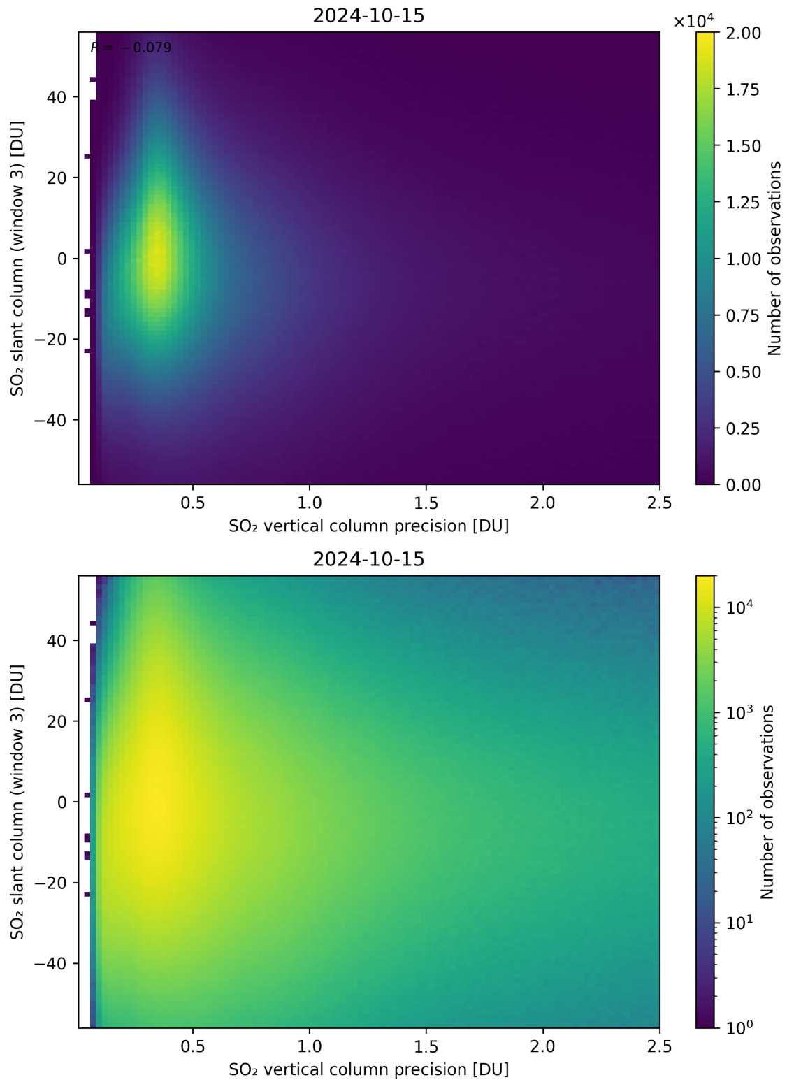
Figure 292: Scatter density plot of “SO 2 vertical column precision” against “SO 2 slant column (window 3)” for 2024-10-14 to 2024-10-16.
