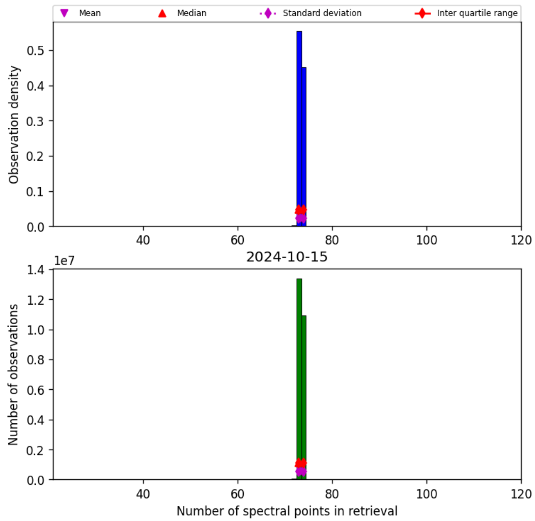
Figure 74: Histogram of “Number of spectral points in retrieval” for 2024-10-14 to 2024-10-16
