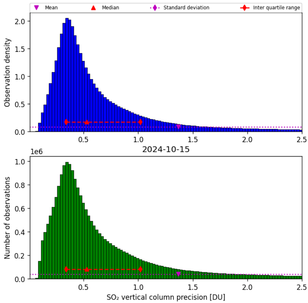
Figure 54: Histogram of “SO 2 vertical column precision” for 2024-10-14 to 2024-10-16
