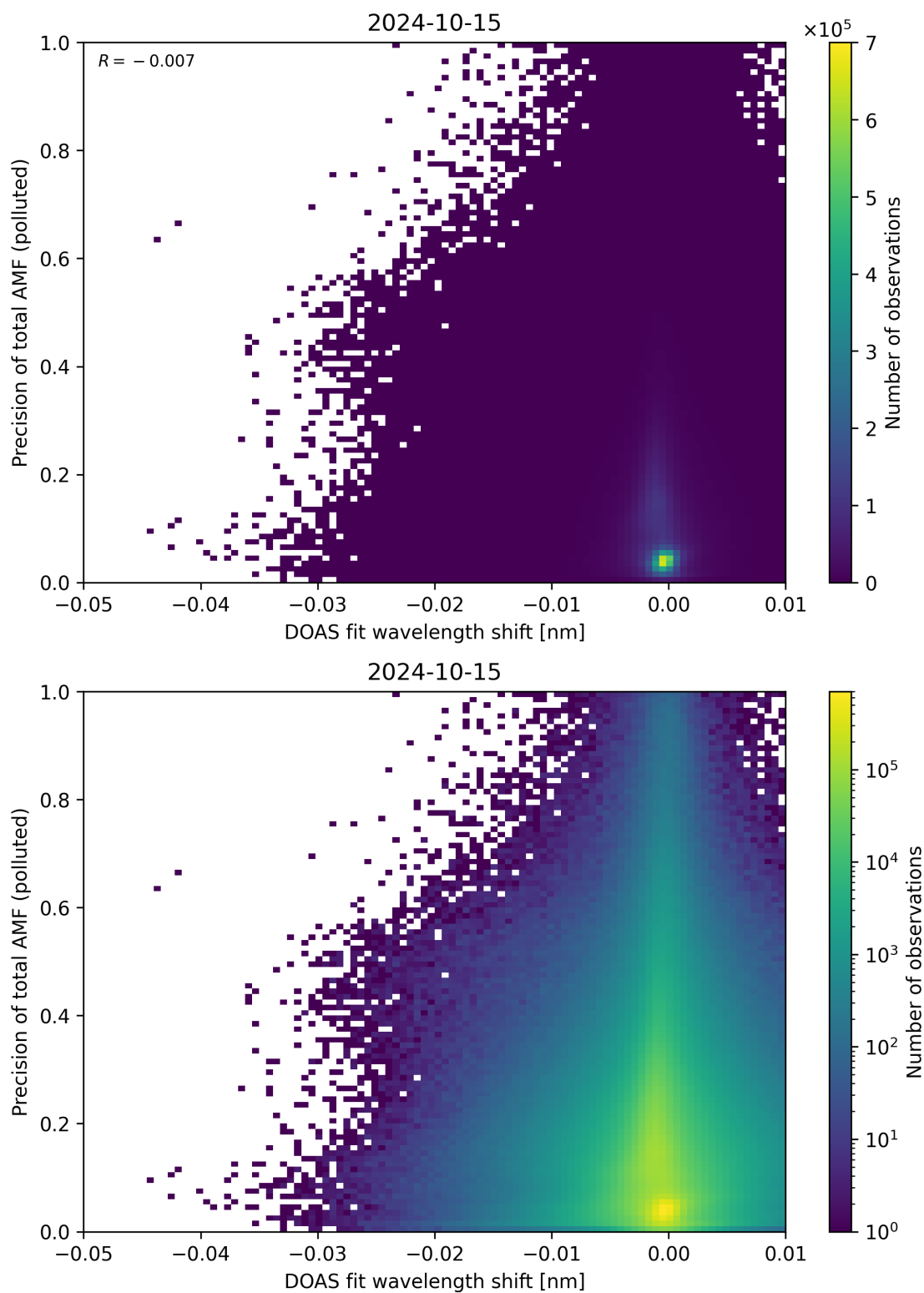
Figure 131: Scatter density plot of “DOAS fit wavelength shift” against “Precision of total AMF (polluted)” for 2024-10-14 to 2024-10-16.
