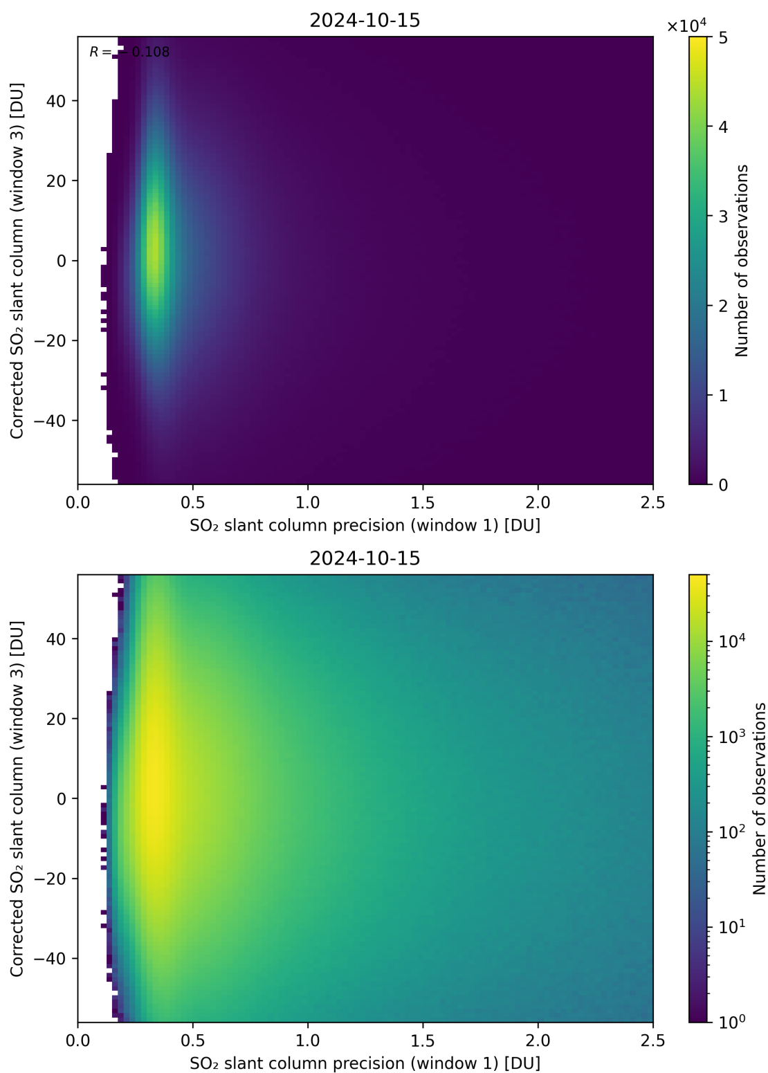
Figure 226: Scatter density plot of “SO 2 slant column precision (window 1)” against “Corrected SO 2 slant column (window 3)” for 2024-10-14 to 2024-10-16.
