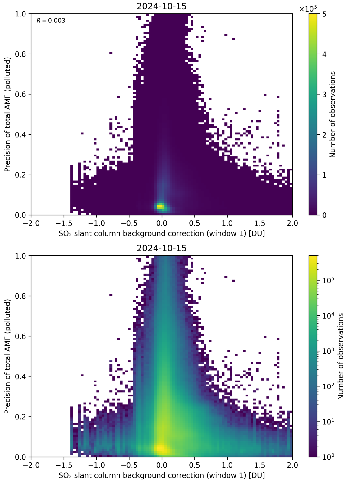
Figure 110: Scatter density plot of “SO 2 slant column background correction (window 1)” against “Precision of total AMF (polluted)” for 2024-10-14 to 2024-10-16.
