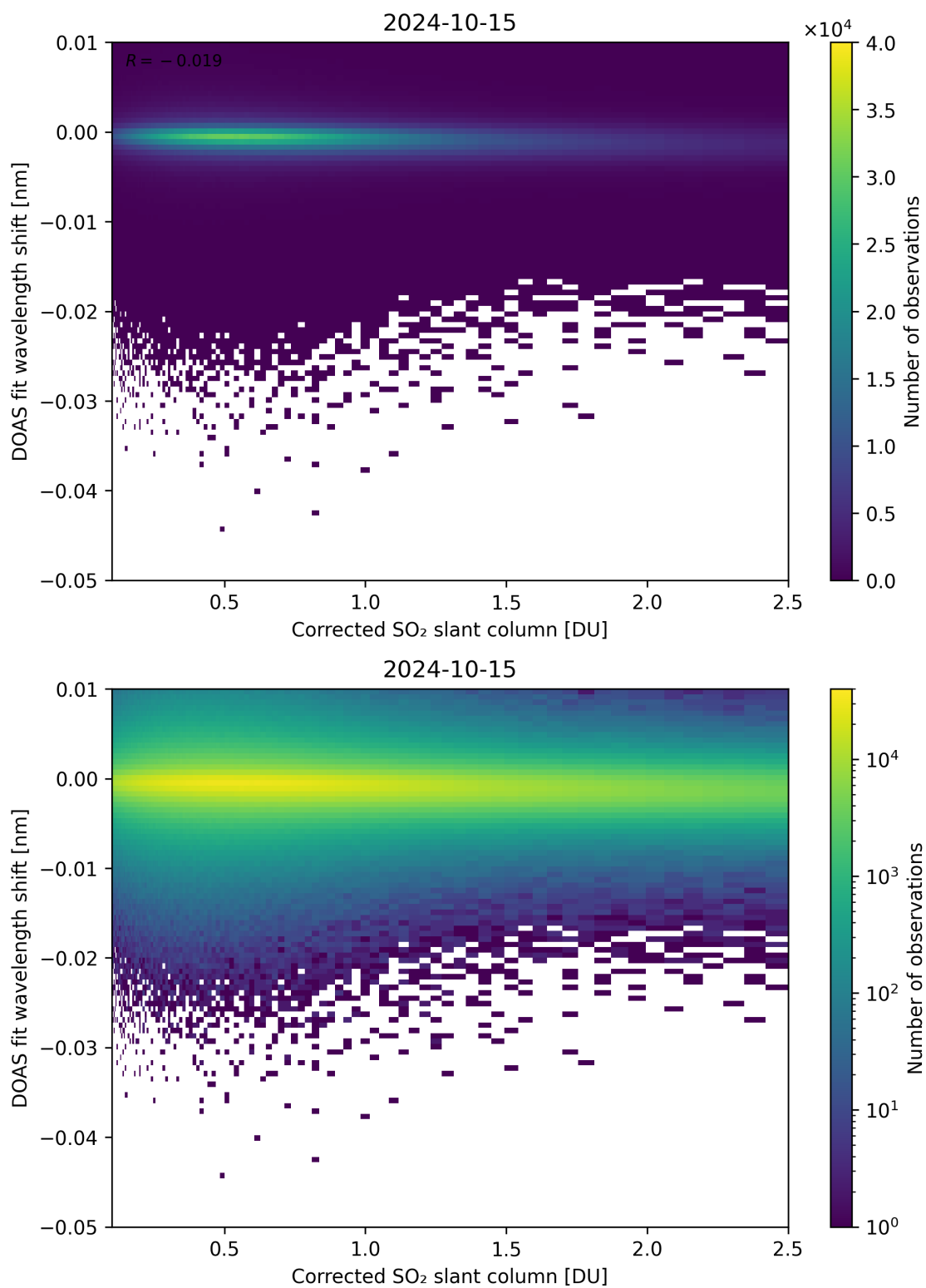
Figure 181: Scatter density plot of “Corrected SO 2 slant column” against “DOAS fit wavelength shift” for 2024-10-14 to 2024-10-16.
