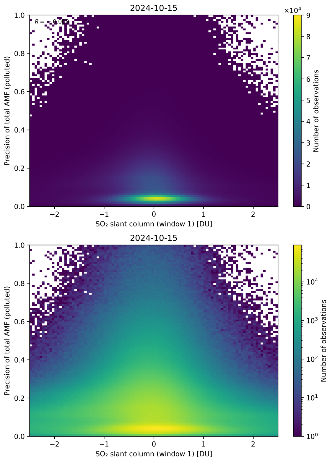
Figure 240: Scatter density plot of “SO 2 slant column (window 1)” against “Precision of total AMF (polluted)” for 2024-10-14 to 2024-10-16.
