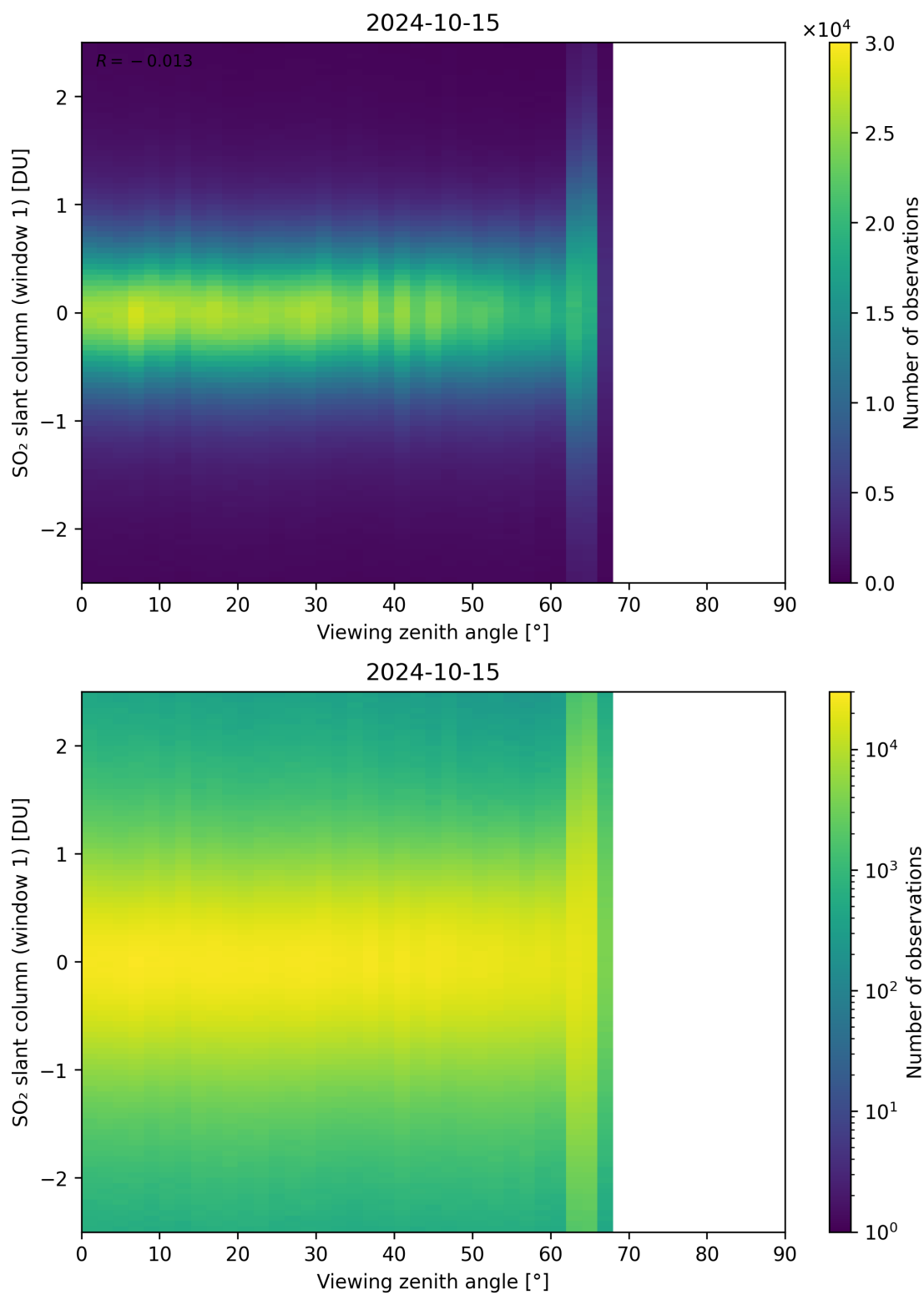
Figure 320: Scatter density plot of “Viewing zenith angle” against “SO 2 slant column (window 1)” for 2024-10-14 to 2024-10-16.
