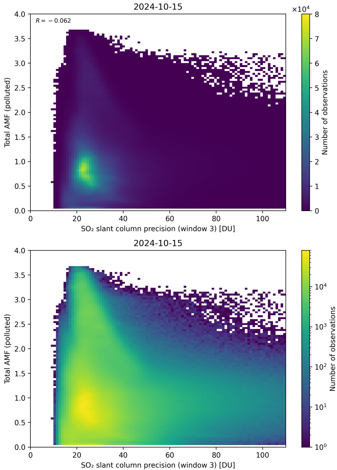
Figure 263: Scatter density plot of “SO 2 slant column precision (window 3)” against “Total AMF (polluted)” for 2024-10-14 to 2024-10-16.
