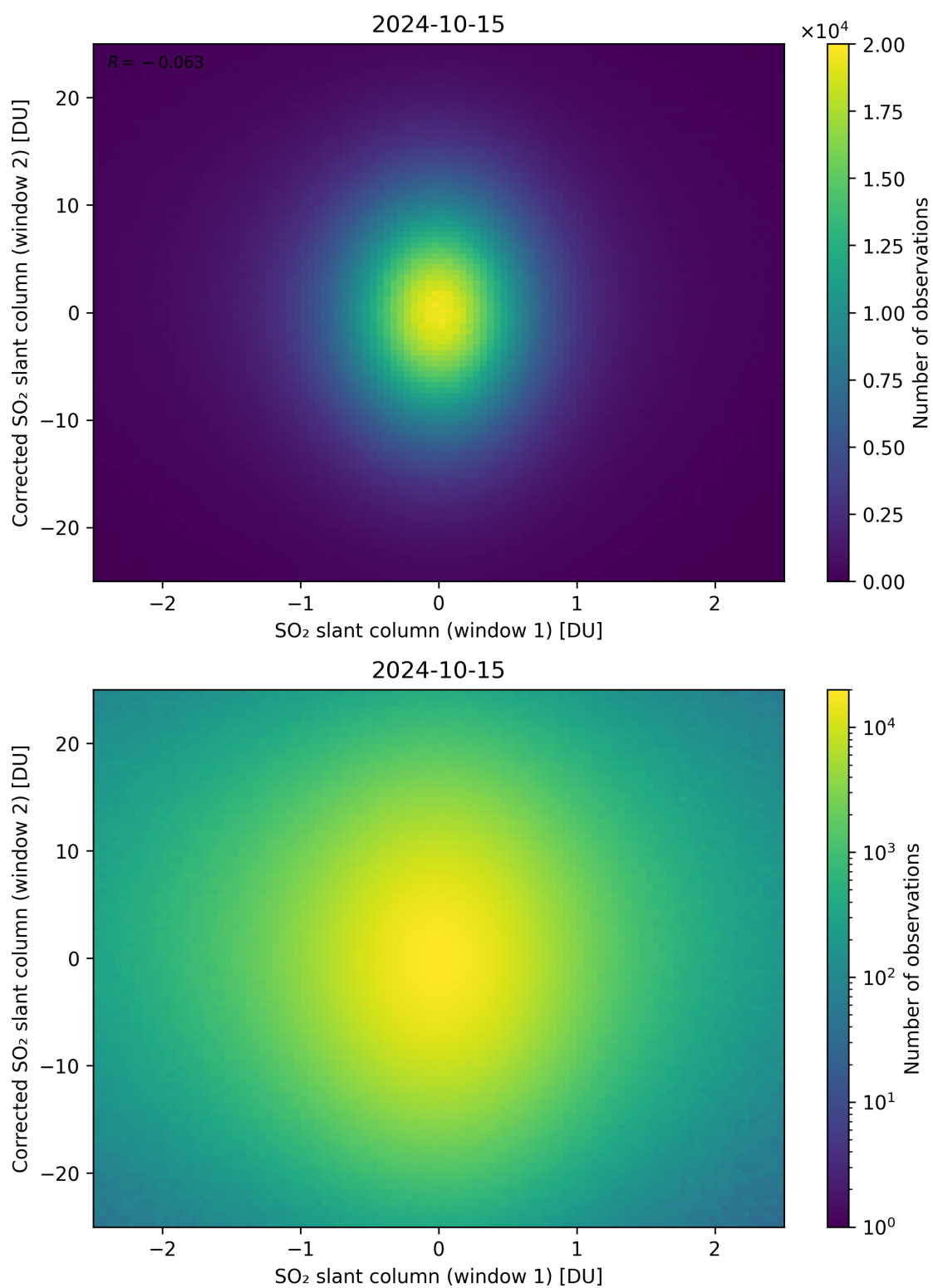
Figure 233: Scatter density plot of “SO 2 slant column (window 1)” against “Corrected SO 2 slant column (window 2)” for 2024-10-14 to 2024-10-16.
