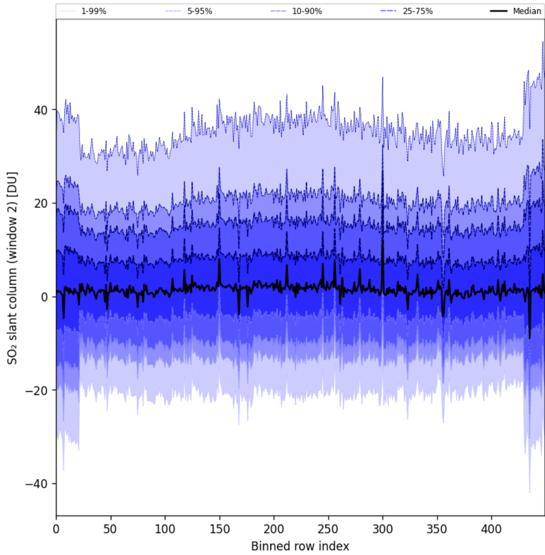
Figure 83: Along track statistics of “SO 2 slant column (window 2)” for 2024-10-14 to 2024-10-16
