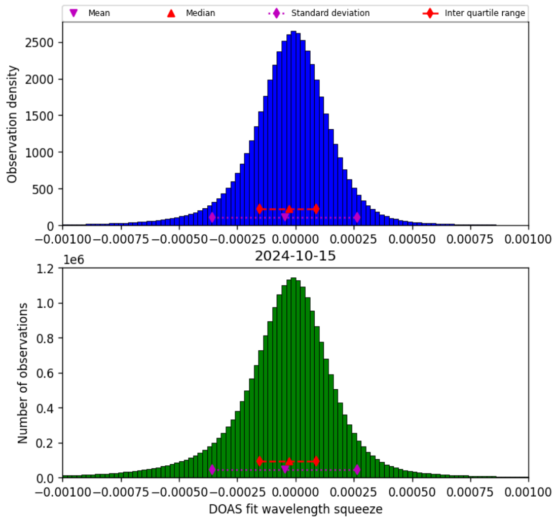
Figure 69: Histogram of “DOAS fit wavelength squeeze” for 2024-10-14 to 2024-10-16
