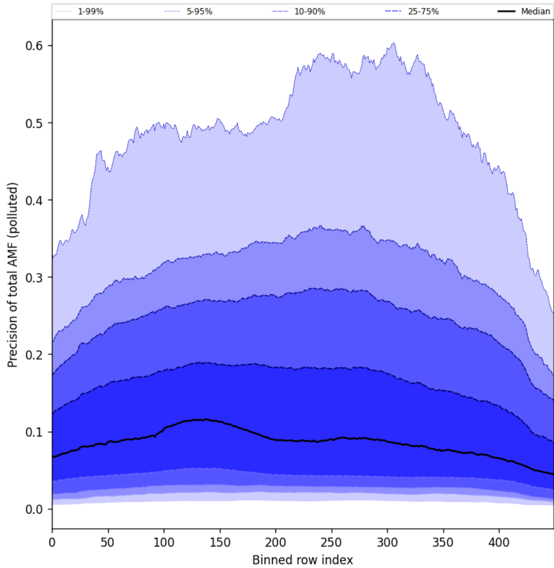
Figure 95: Along track statistics of “Precision of total AMF (polluted)” for 2024-10-14 to 2024-10-16
