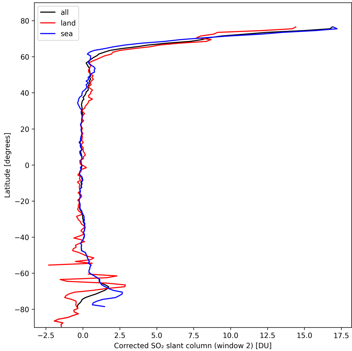
Figure 39: Zonal average of “Corrected SO 2 slant column (window 2)” for 2024-10-14 to 2024-10-16.
