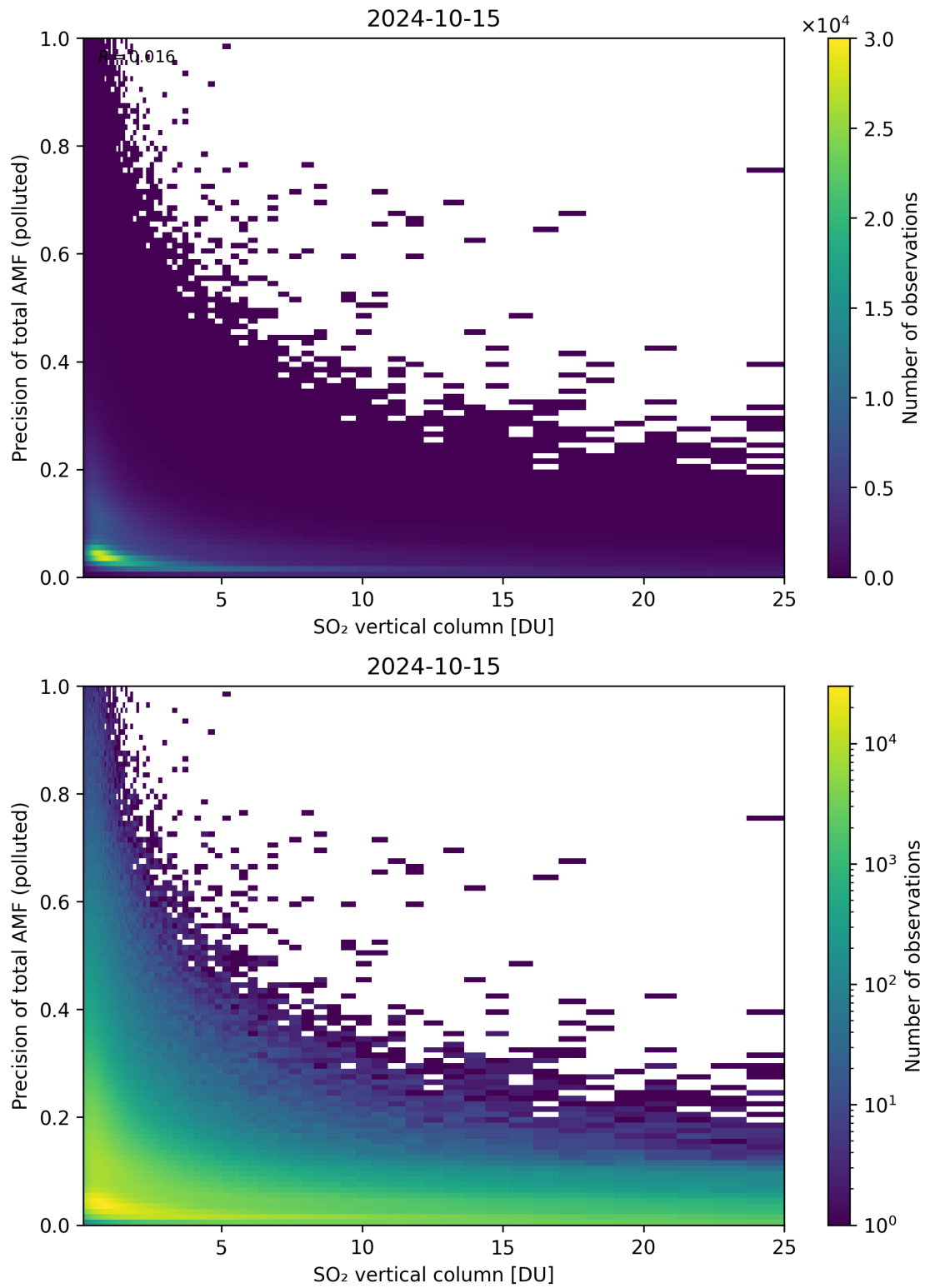
Figure 306: Scatter density plot of “SO 2 vertical column” against “Precision of total AMF (polluted)” for 2024-10-14 to 2024-10-16.
