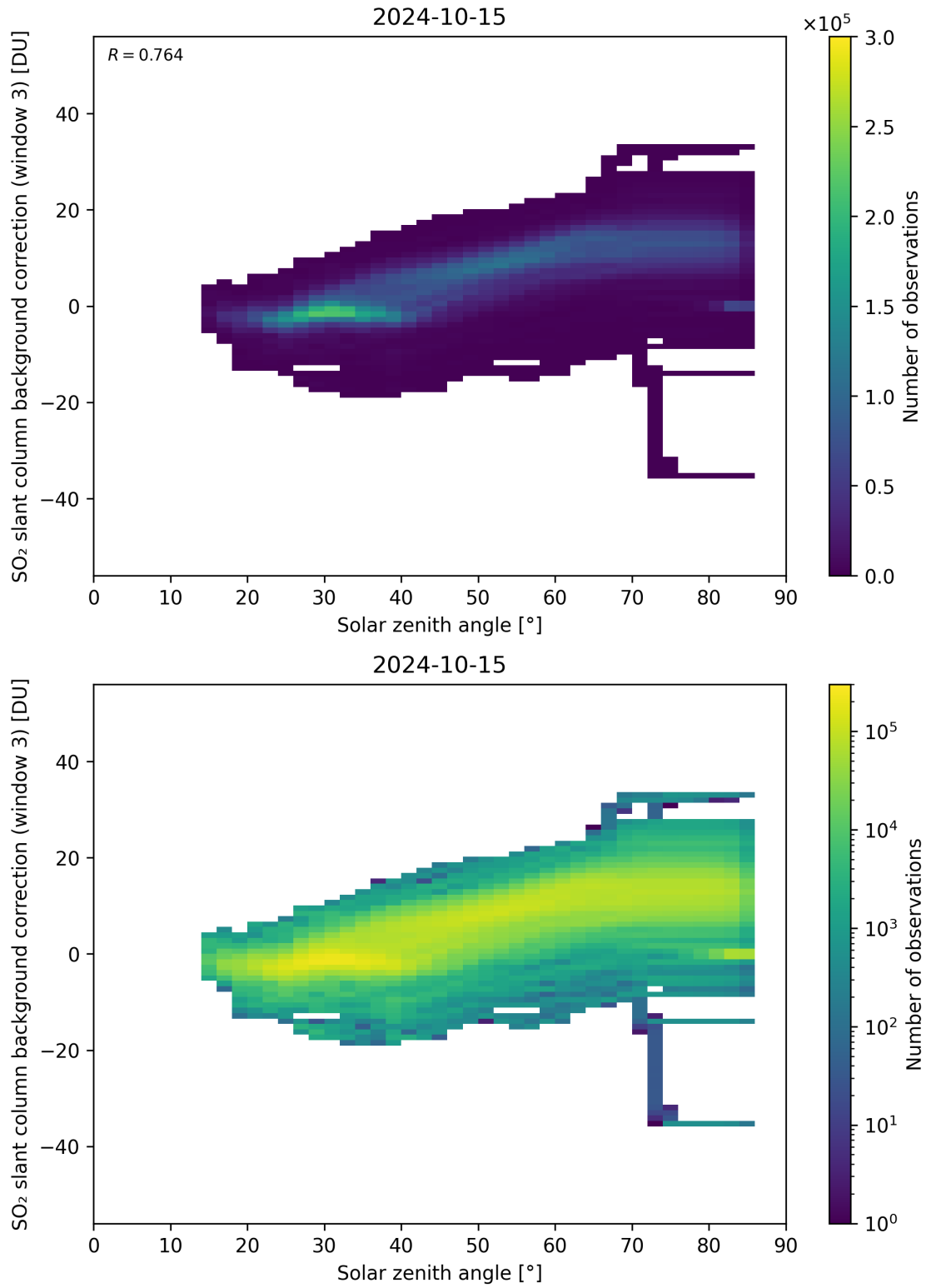
Figure 160: Scatter density plot of “Solar zenith angle” against “SO 2 slant column background correction (window 3)” for 2024-10-14 to 2024-10-16.
