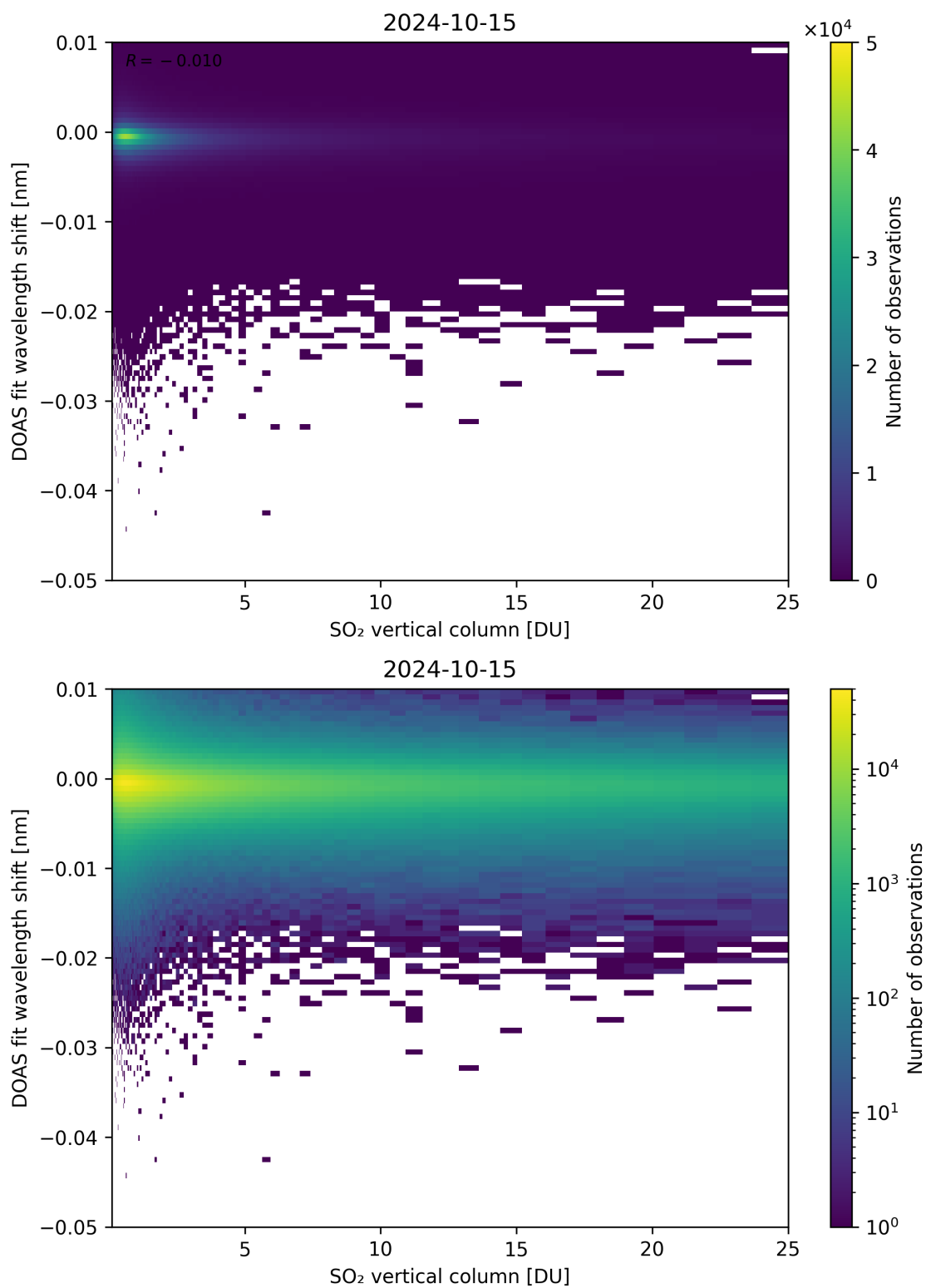
Figure 276: Scatter density plot of “SO 2 vertical column” against “DOAS fit wavelength shift” for 2024-10-14 to 2024-10-16.
