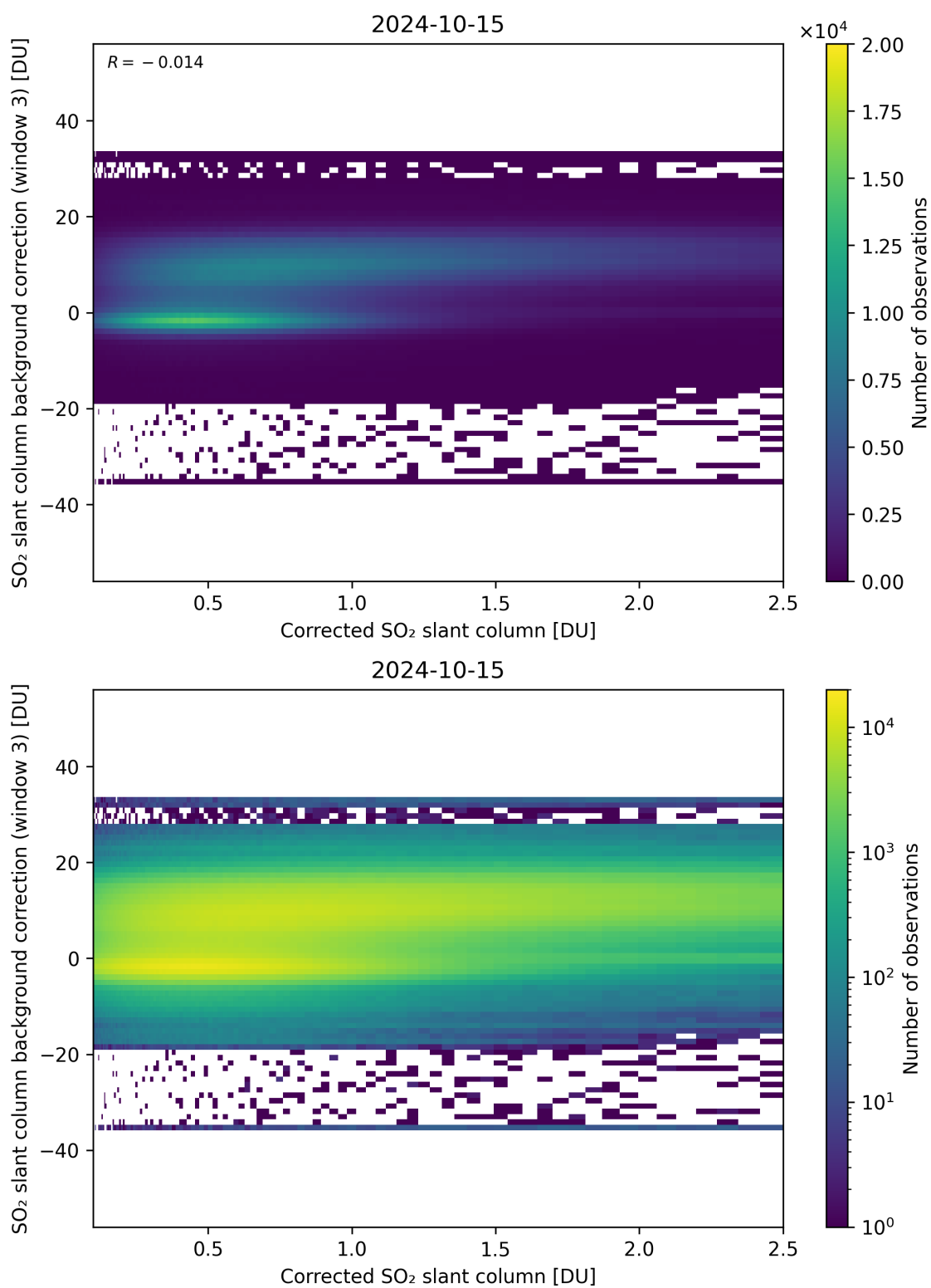
Figure 180: Scatter density plot of “Corrected SO 2 slant column” against “SO 2 slant column background correction (window 3)” for 2024-10-14 to 2024-10-16.
