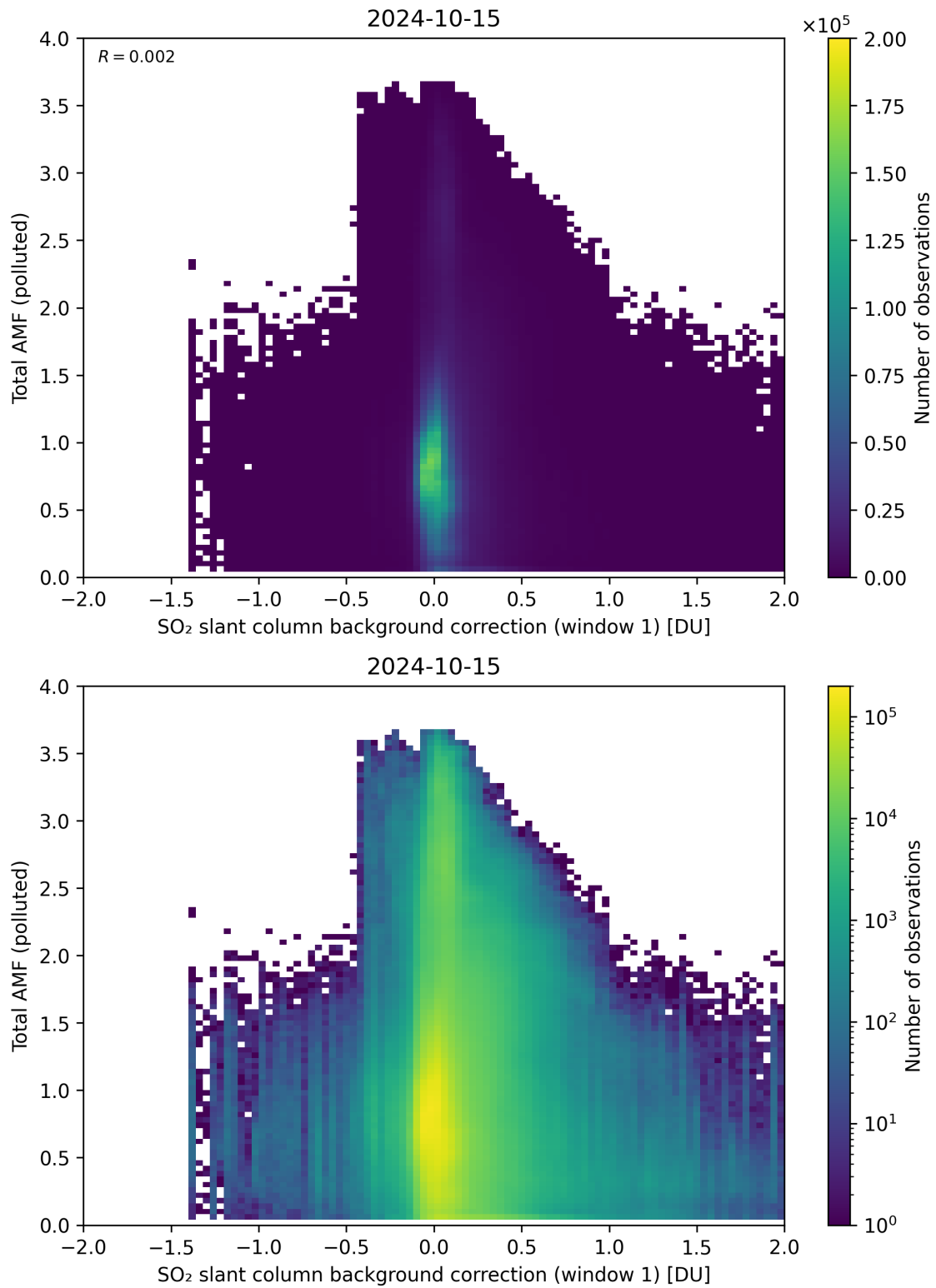
Figure 109: Scatter density plot of “SO 2 slant column background correction (window 1)” against “Total AMF (polluted)” for 2024-10-14 to 2024-10-16.
