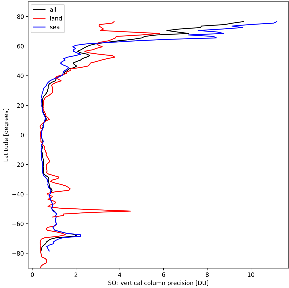
Figure 31: Zonal average of “SO 2 vertical column precision” for 2024-10-14 to 2024-10-16.
