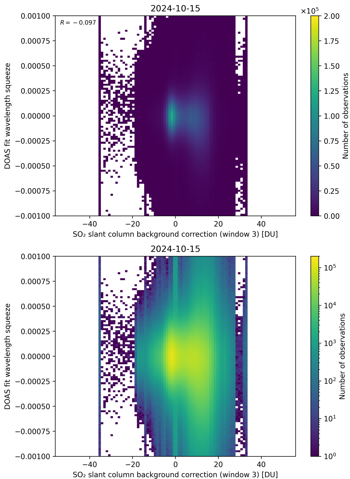
Figure 122: Scatter density plot of “SO 2 slant column background correction (window 3)” against “DOAS fit wavelength squeeze” for 2024-10-14 to 2024-10-16.
