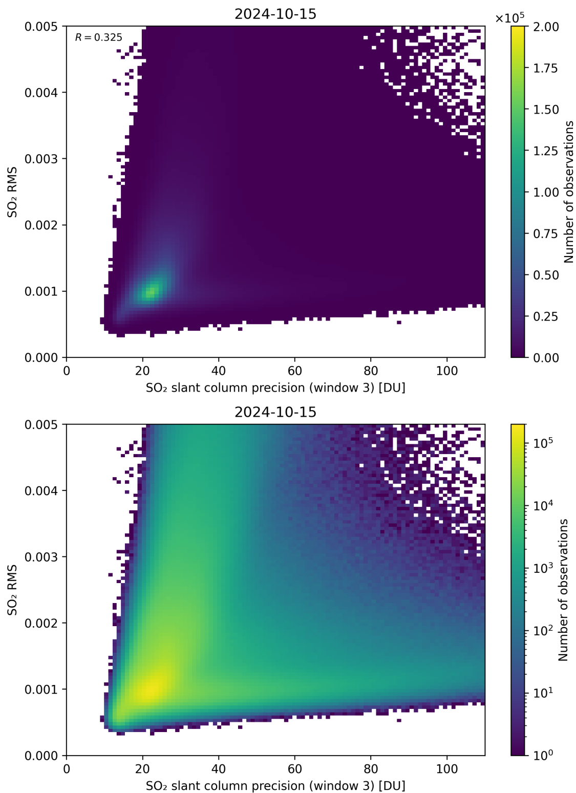
Figure 260: Scatter density plot of “SO 2 slant column precision (window 3)” against “SO 2 RMS” for 2024-10-14 to 2024-10-16.
