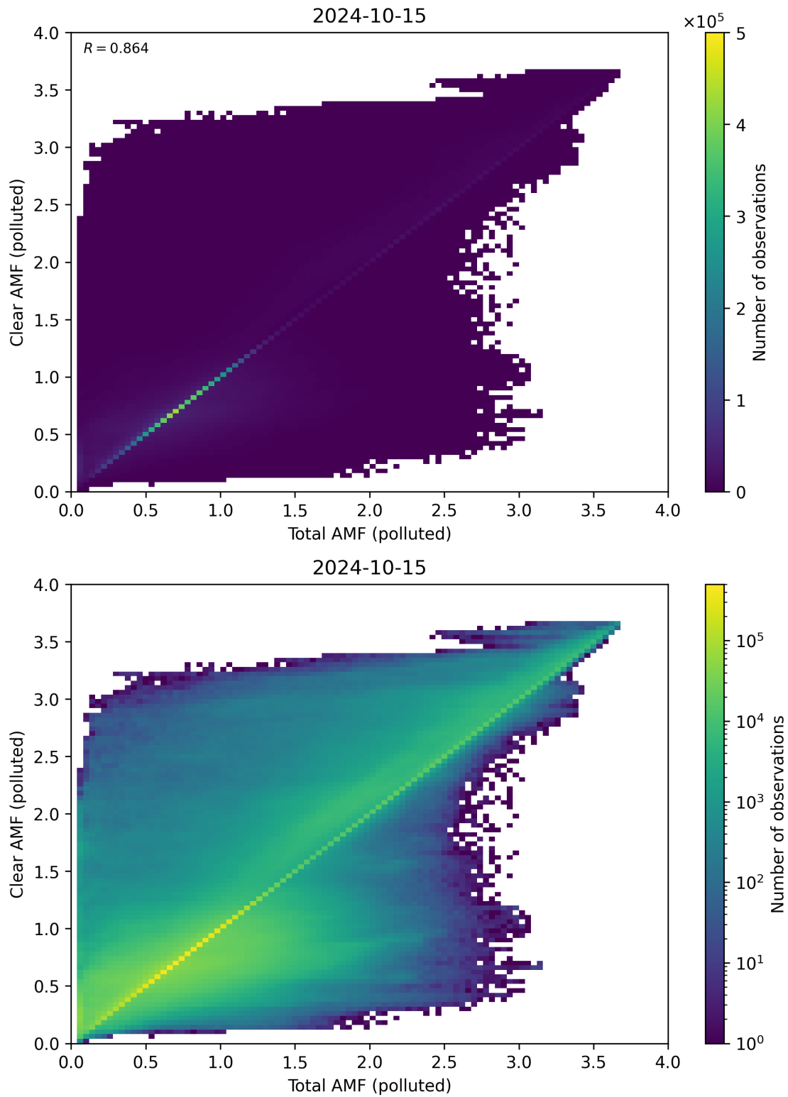
Figure 271: Scatter density plot of “Total AMF (polluted)” against “Clear AMF (polluted)” for 2024-10-14 to 2024-10-16.
