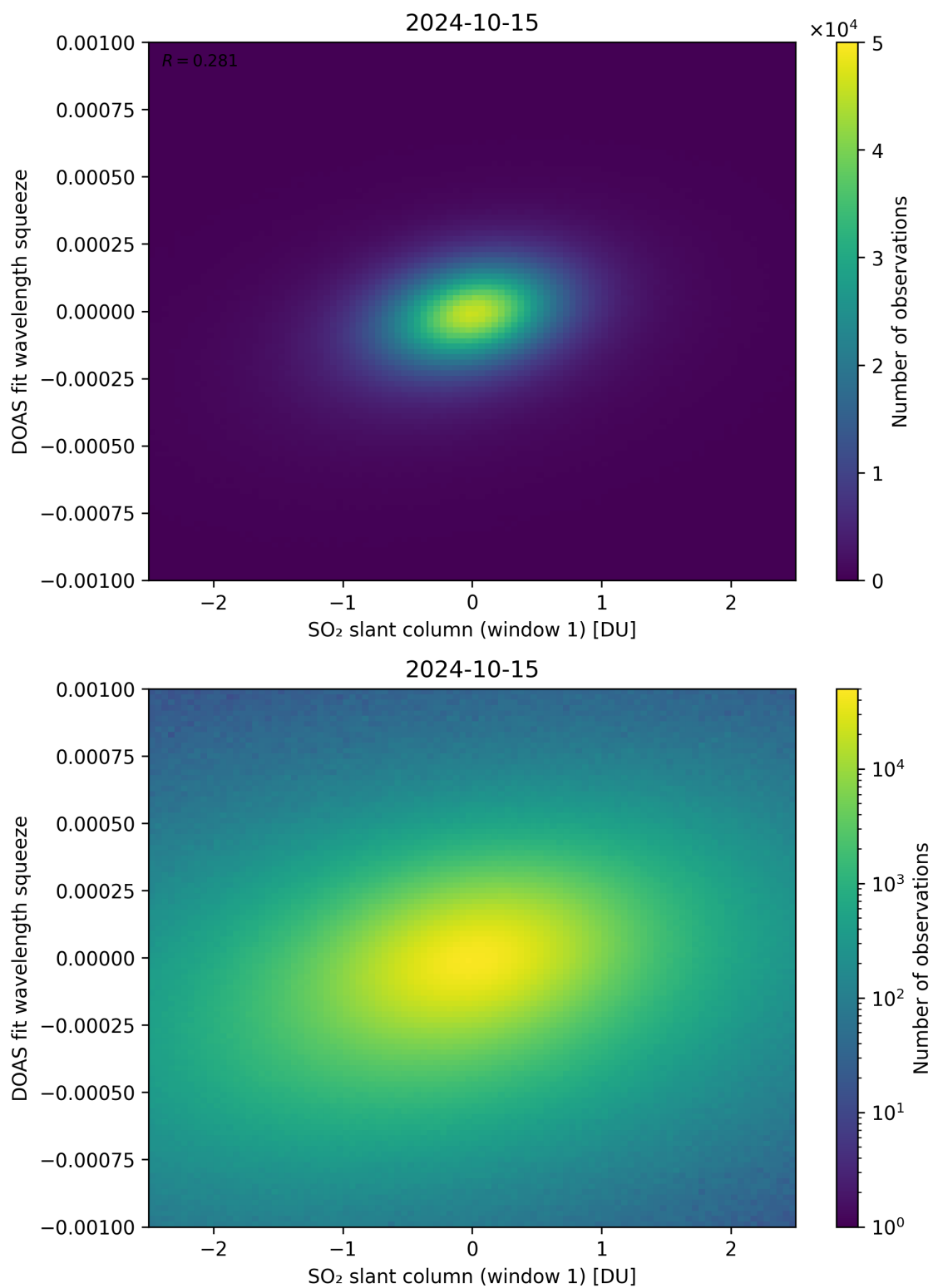
Figure 216: Scatter density plot of “SO 2 slant column (window 1)” against “DOAS fit wavelength squeeze” for 2024-10-14 to 2024-10-16.
