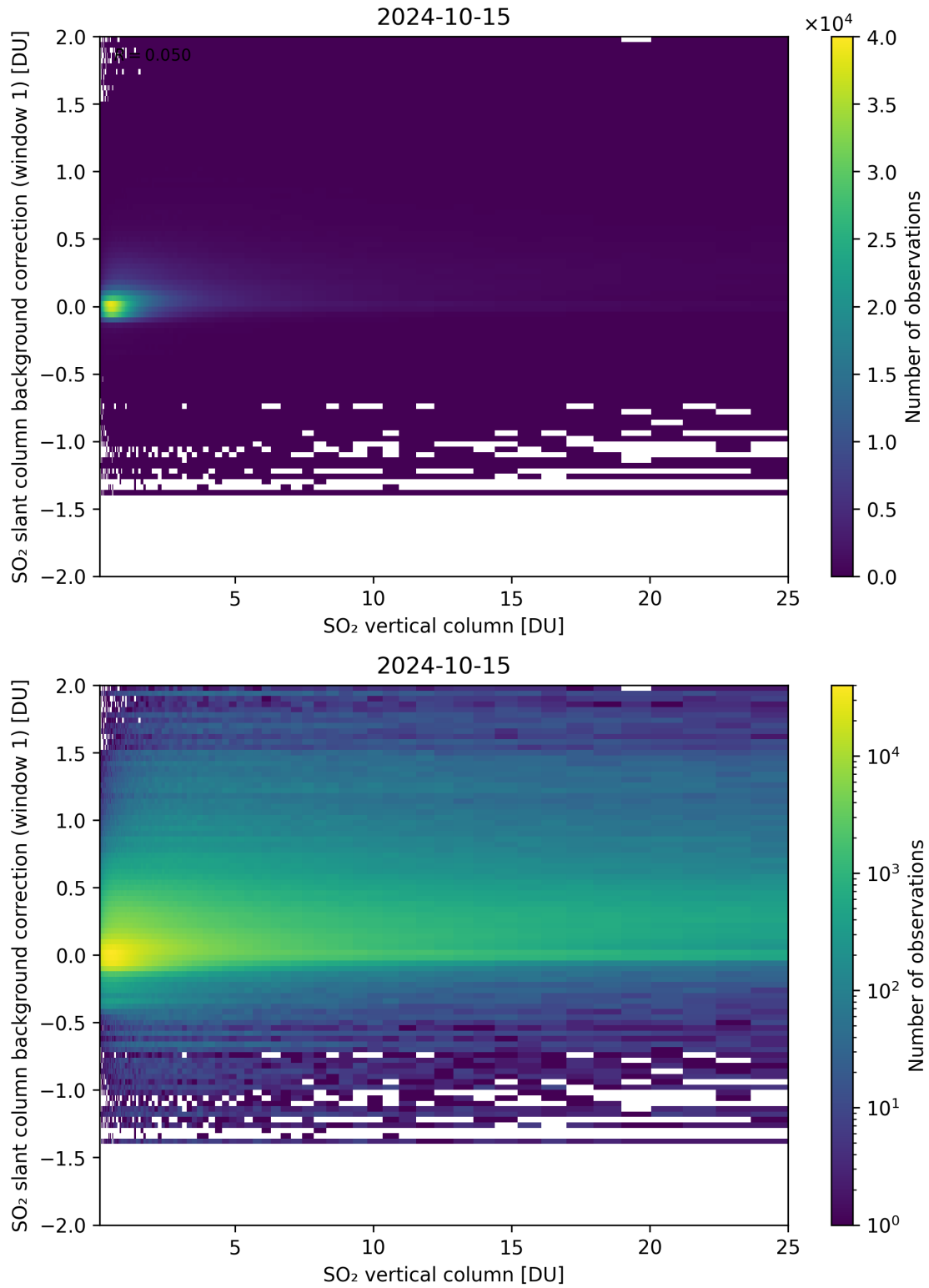
Figure 273: Scatter density plot of “SO 2 vertical column” against “SO 2 slant column background correction (window 1)” for 2024-10-14 to 2024-10-16.
