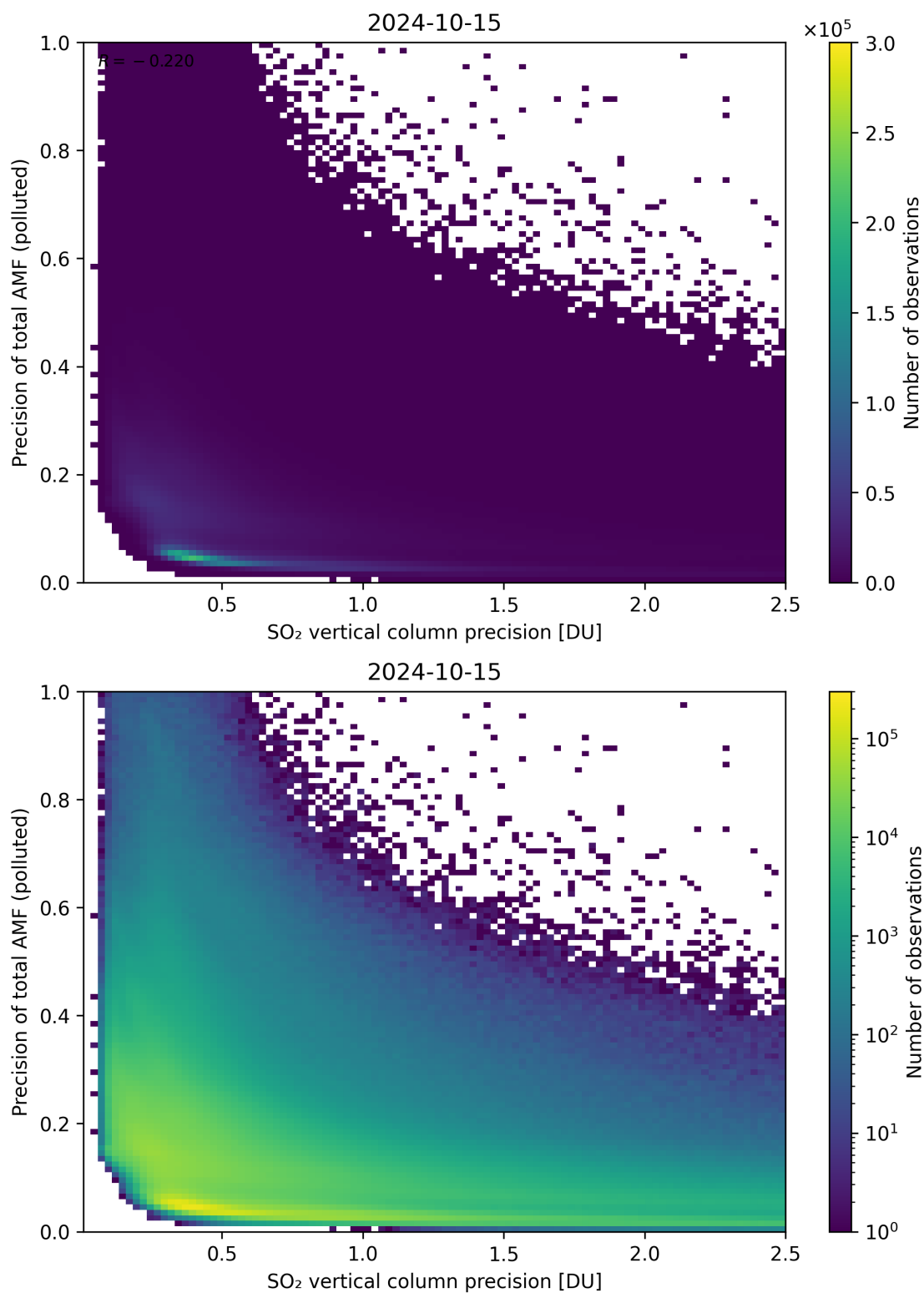
Figure 295: Scatter density plot of “SO 2 vertical column precision” against “Precision of total AMF (polluted)” for 2024-10-14 to 2024-10-16.
