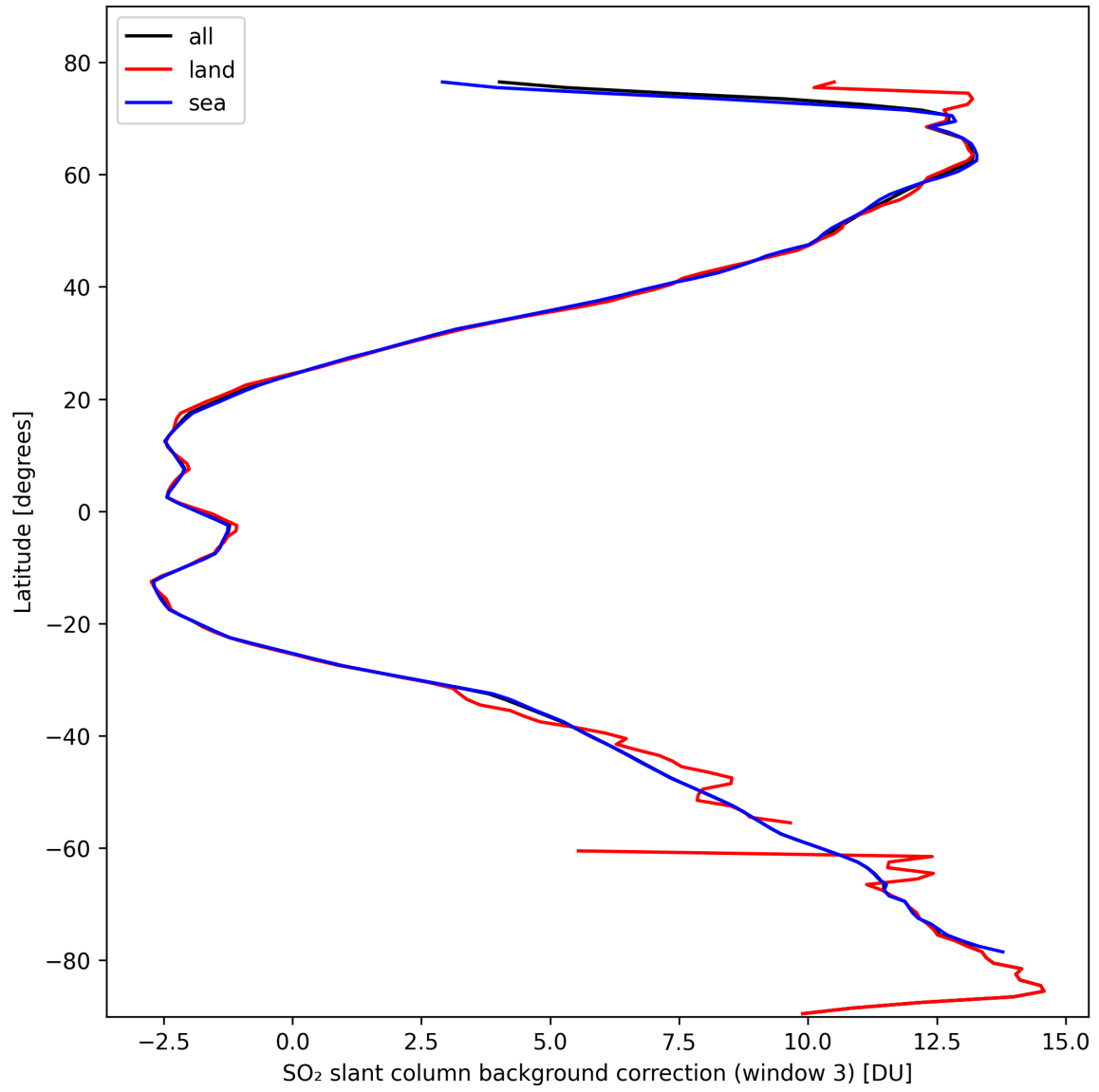
Figure 44: Zonal average of “SO 2 slant column background correction (window 3)” for 2024-10-14 to 2024-10-16.
