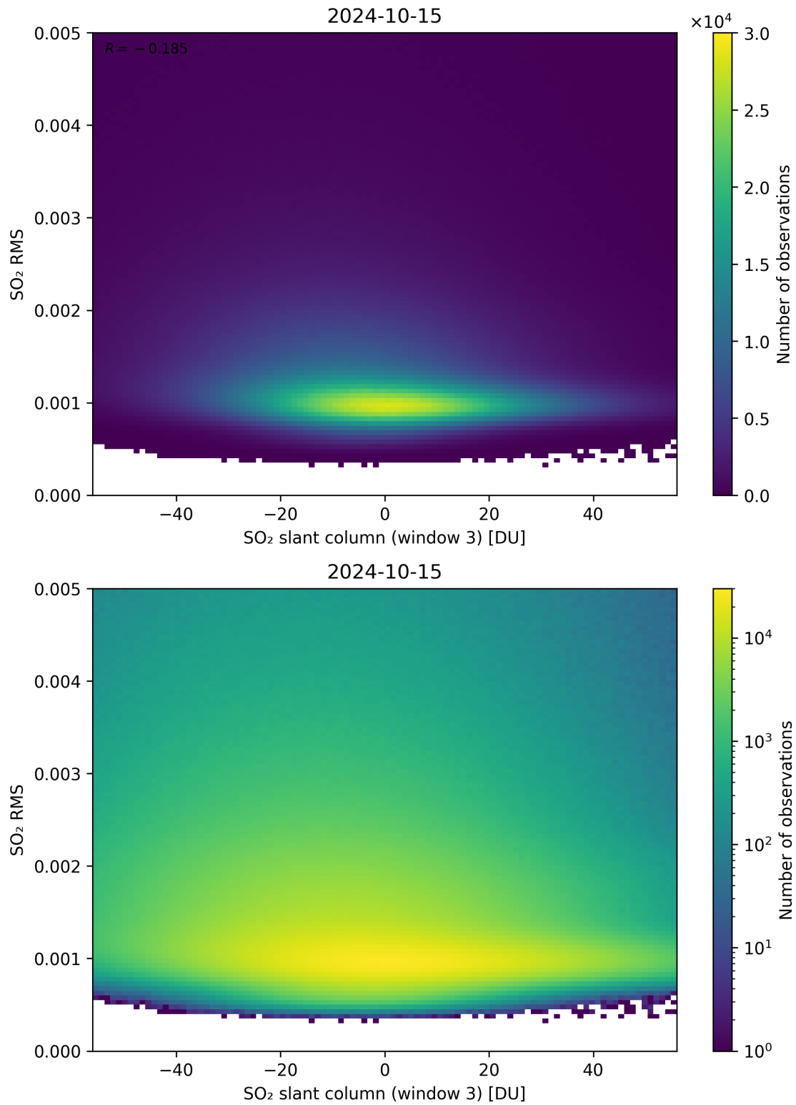
Figure 256: Scatter density plot of “SO 2 slant column (window 3)” against “SO 2 RMS” for 2024-10-14 to 2024-10-16.
