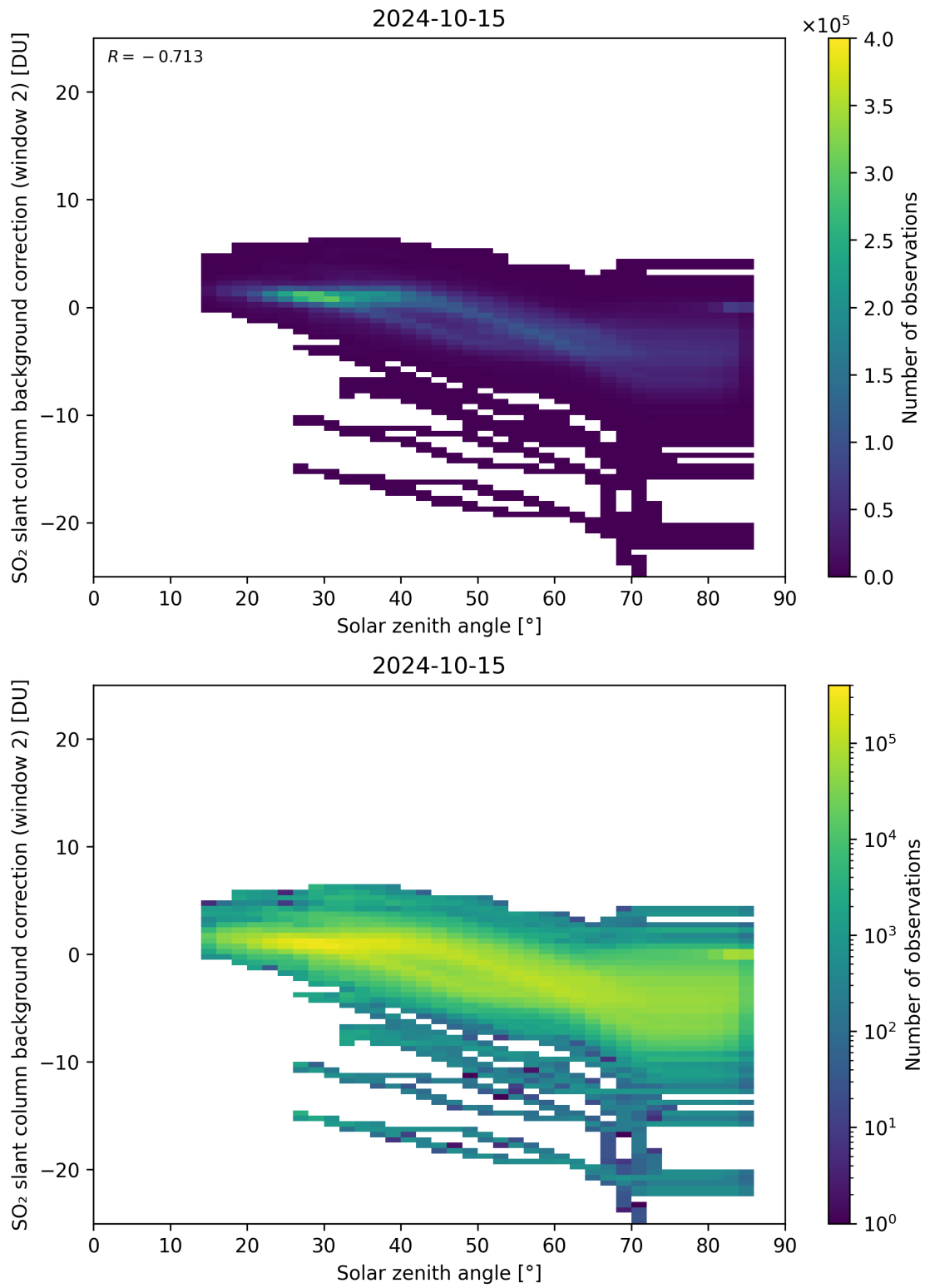
Figure 159: Scatter density plot of “Solar zenith angle” against “SO 2 slant column background correction (window 2)” for 2024-10-14 to 2024-10-16.
