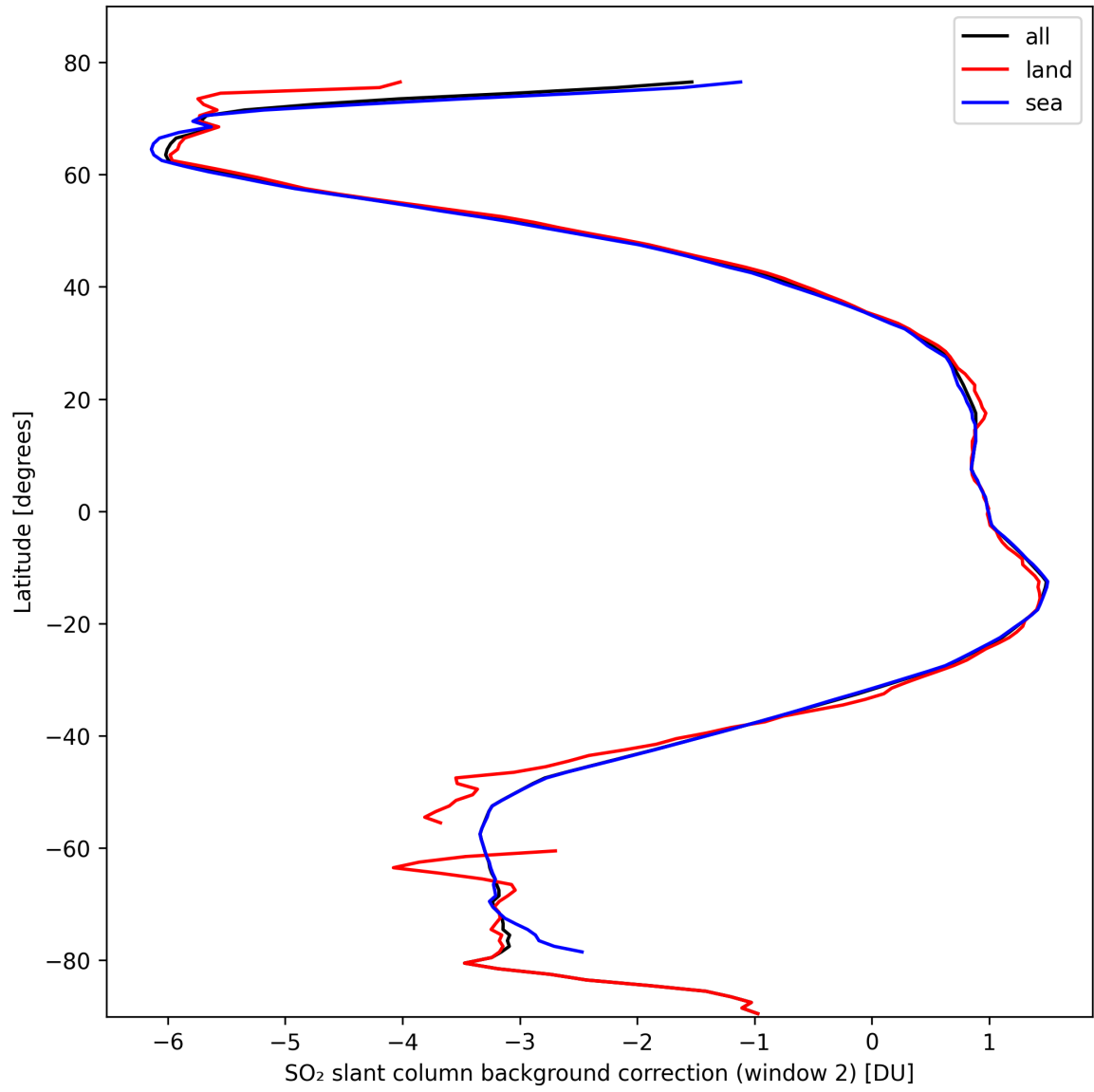
Figure 40: Zonal average of "SO 2 slant column background correction (window 2)" for 2024-10-14 to 2024-10-16.
