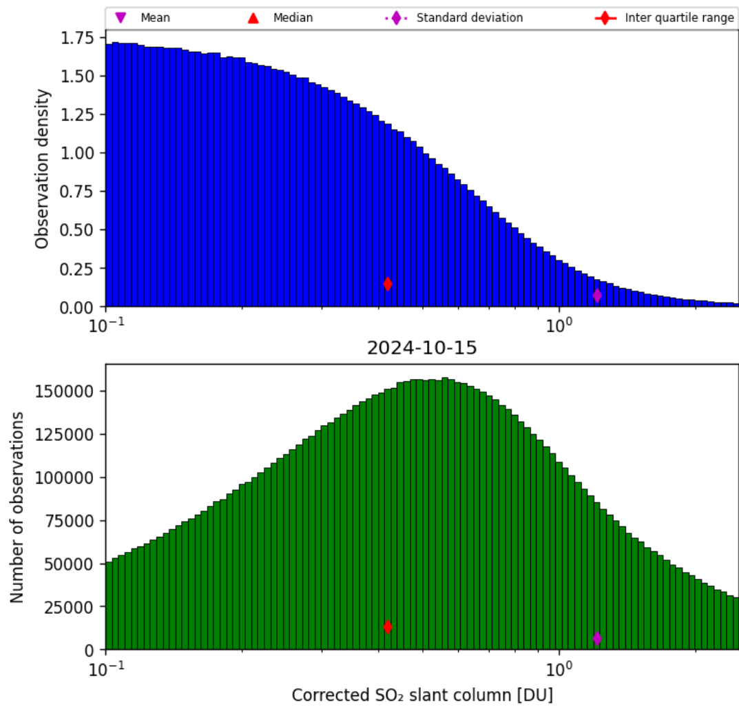
Figure 55: Histogram of “Corrected SO 2 slant column” for 2024-10-14 to 2024-10-16
