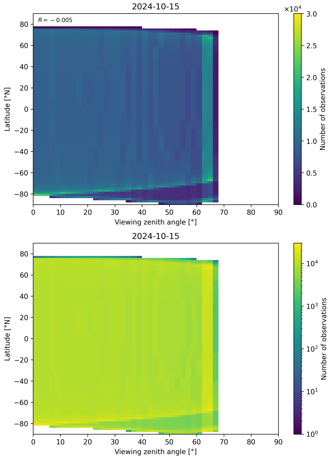
Figure 314: Scatter density plot of “Viewing zenith angle” against “Latitude” for 2024-10-14 to 2024-10-16.
