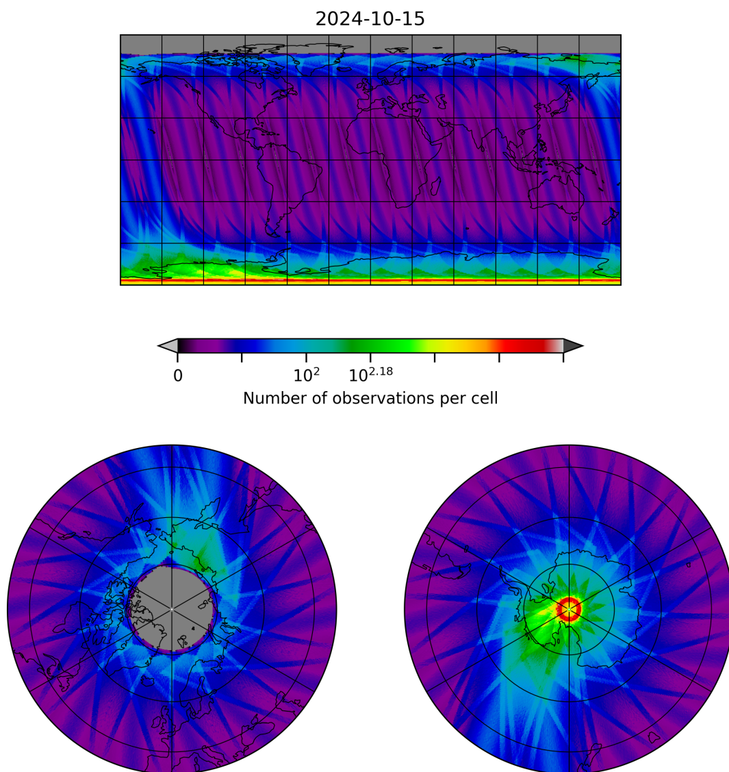
Figure 28: Map of the number of observations for 2024-10-14 to 2024-10-16
