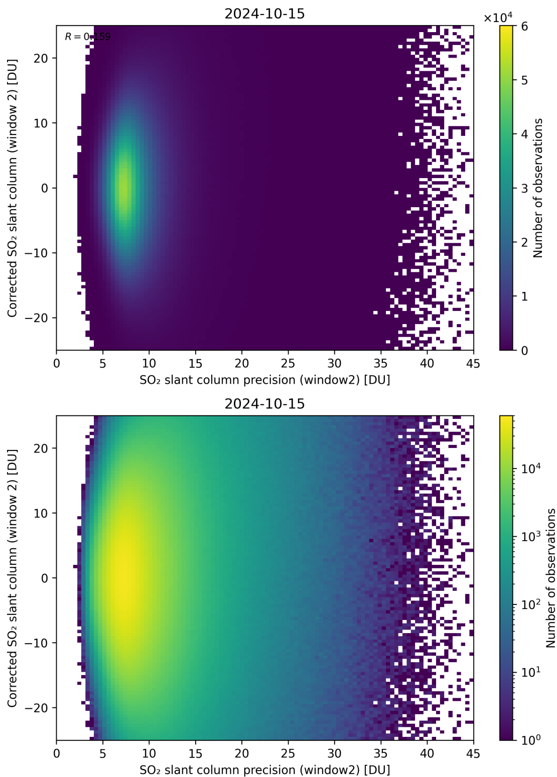
Figure 247: Scatter density plot of “SO 2 slant column precision (window2)” against “Corrected SO 2 slant column (window 2)” for 2024-10-14 to 2024-10-16.
