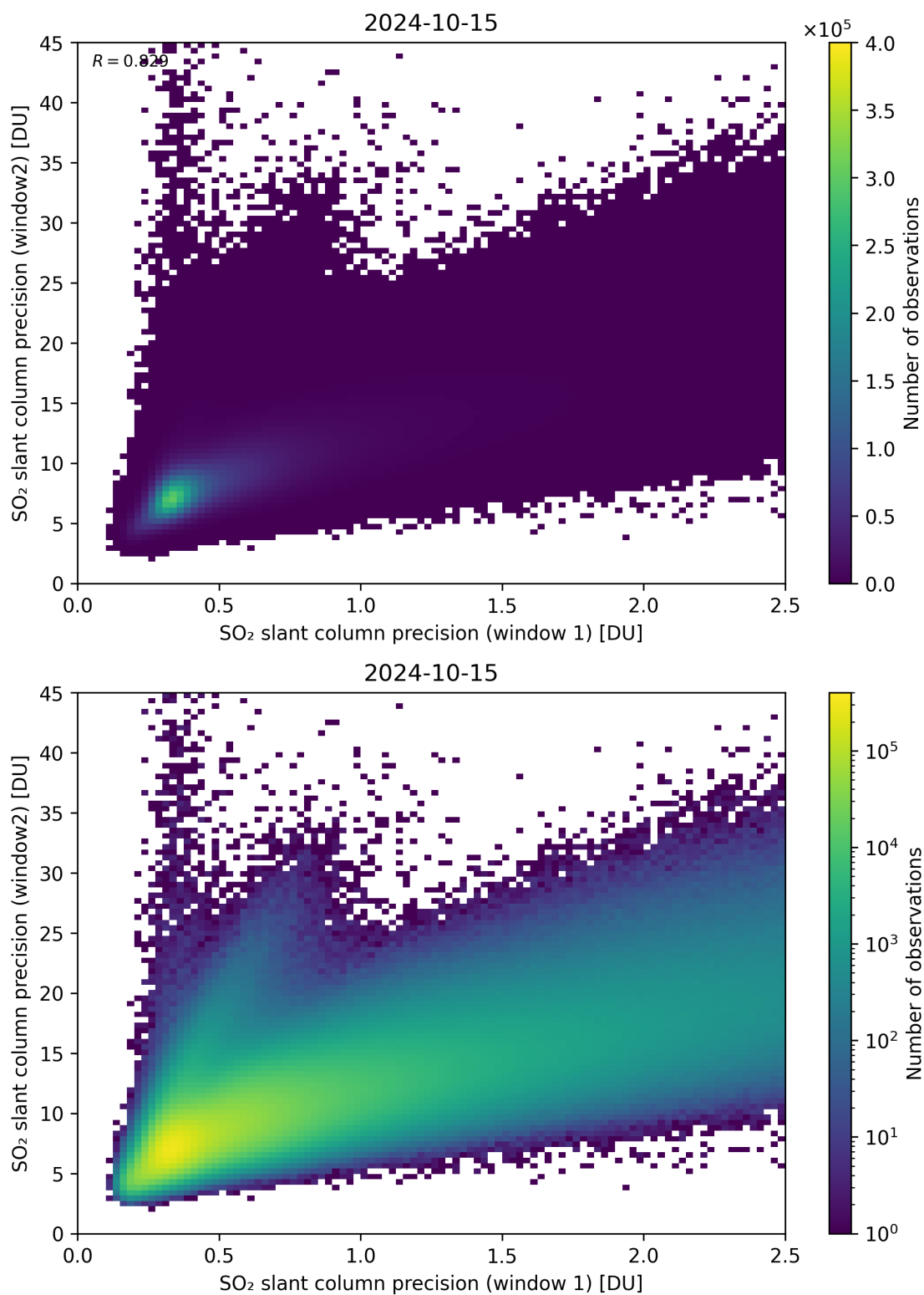
Figure 227: Scatter density plot of “SO 2 slant column precision (window 1)” against “SO 2 slant column precision (window2)” for 2024-10-14 to 2024-10-16.
