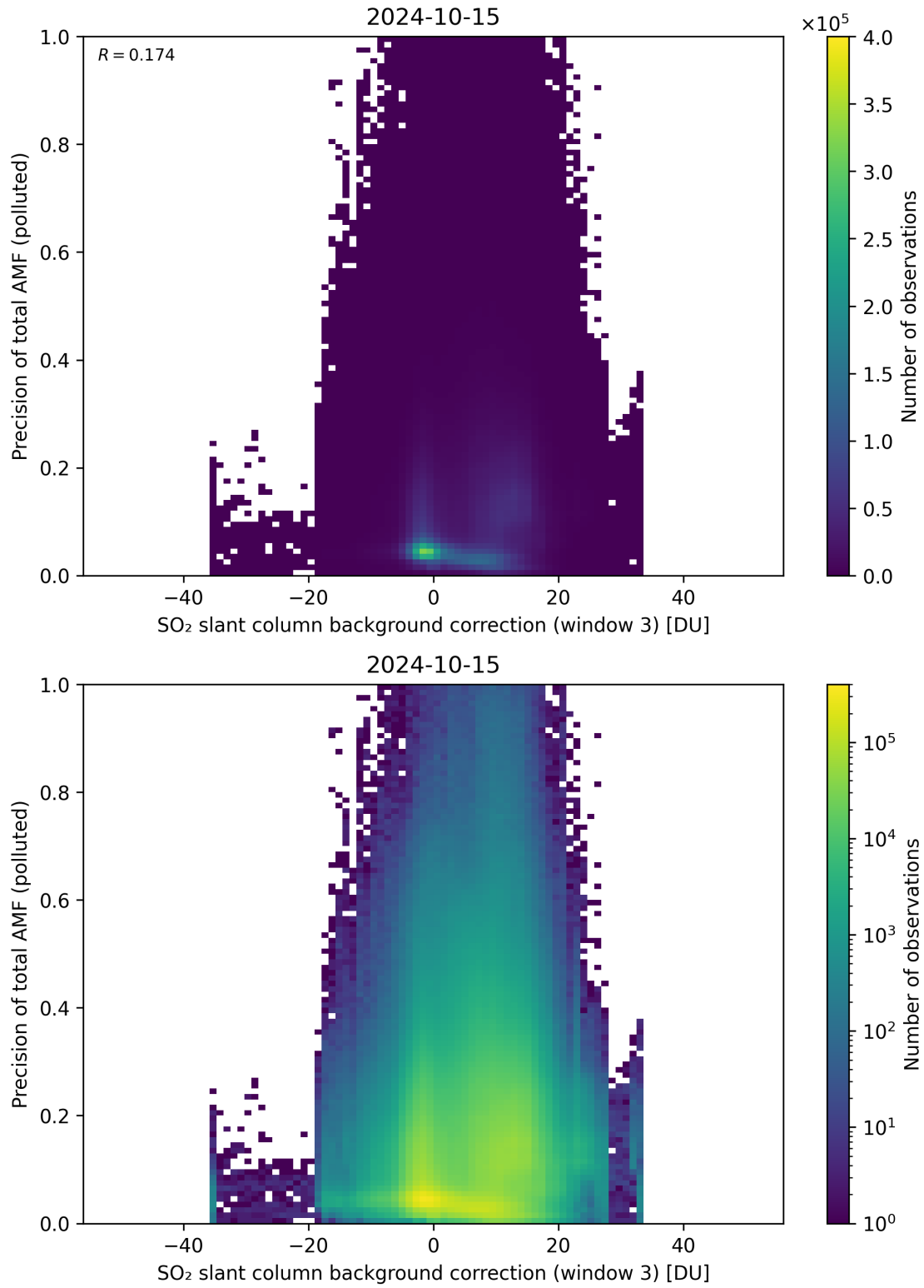
Figure 126: Scatter density plot of “SO 2 slant column background correction (window 3)” against “Precision of total AMF (polluted)” for 2024-10-14 to 2024-10-16.
