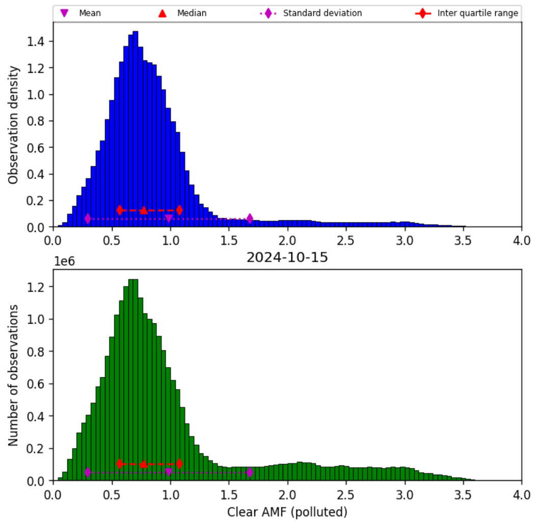
Figure 73: Histogram of “Clear AMF (polluted)” for 2024-10-14 to 2024-10-16
