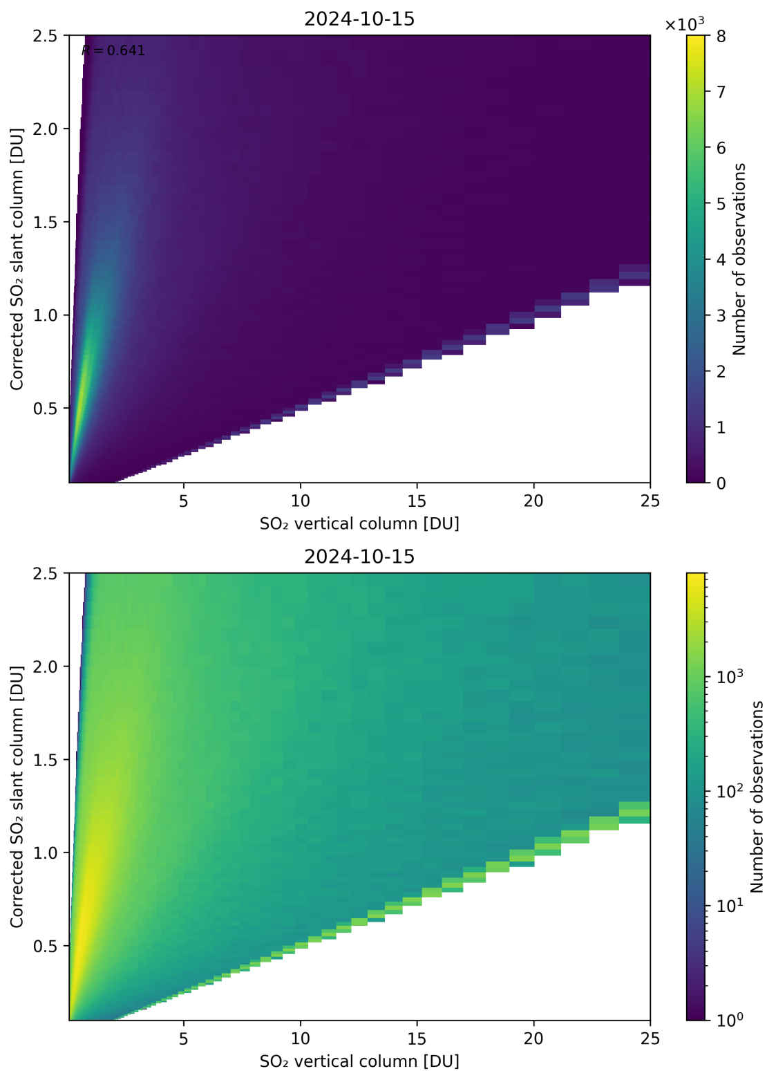
Figure 297: Scatter density plot of “SO 2 vertical column” against “Corrected SO 2 slant column” for 2024-10-14 to 2024-10-16.
