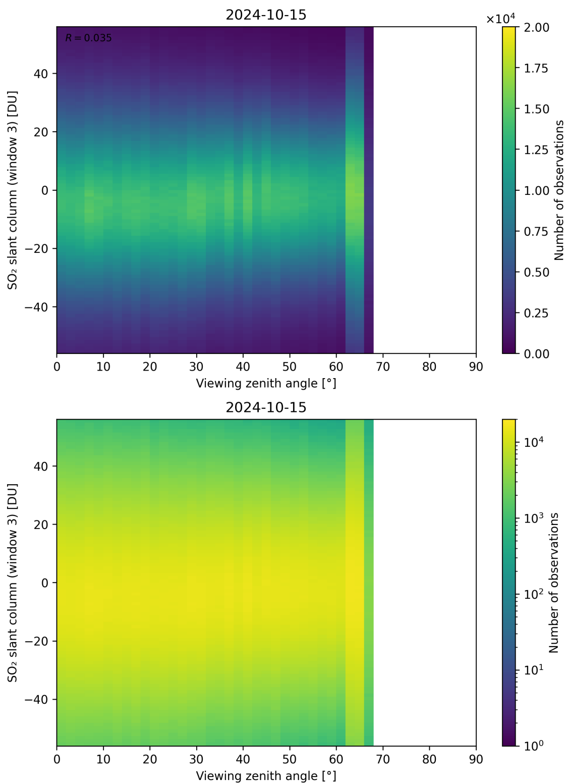
Figure 323: Scatter density plot of “Viewing zenith angle” against “SO 2 slant column (window 3)” for 2024-10-14 to 2024-10-16.
