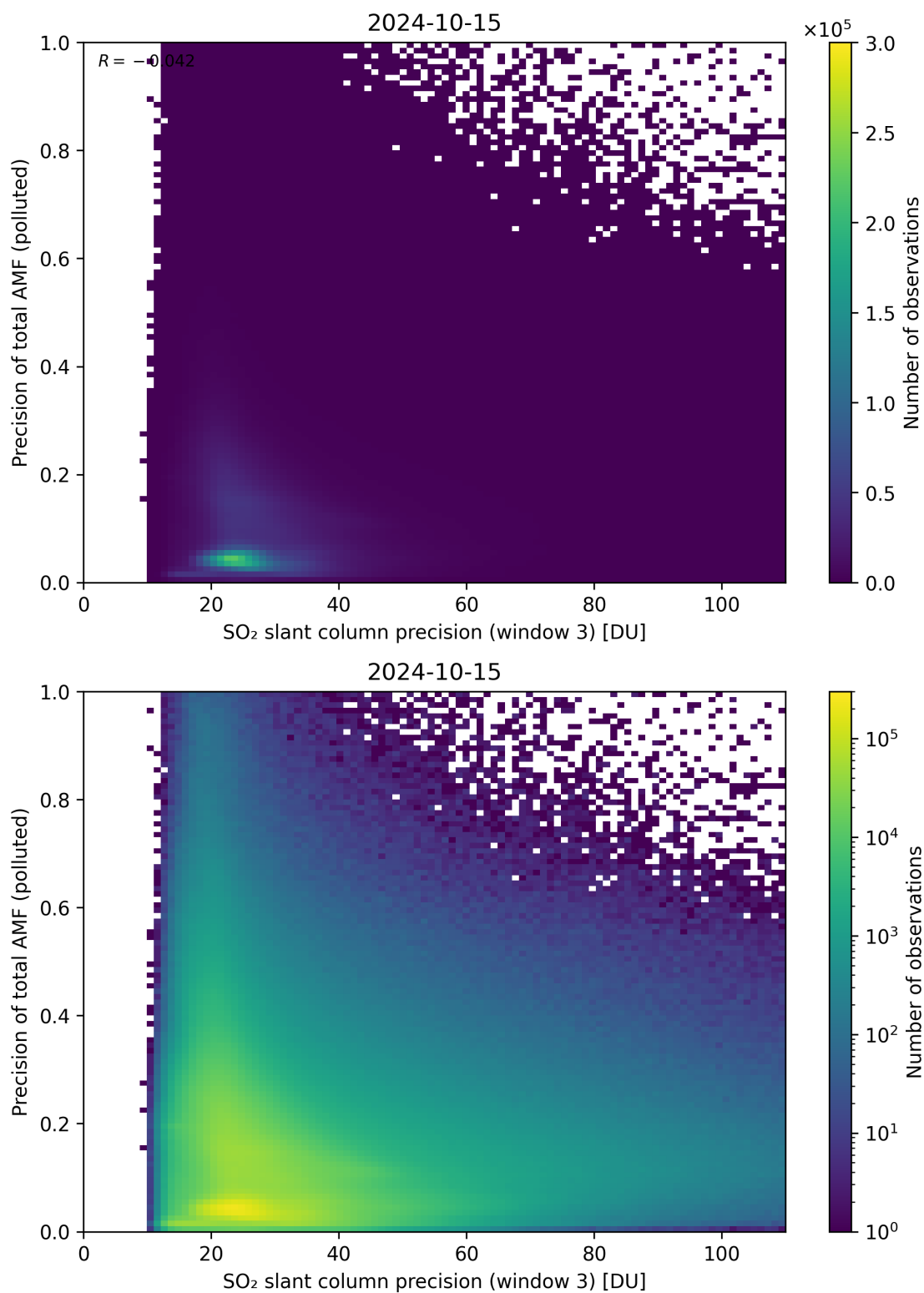
Figure 264: Scatter density plot of “SO 2 slant column precision (window 3)” against “Precision of total AMF (polluted)” for 2024-10-14 to 2024-10-16.
