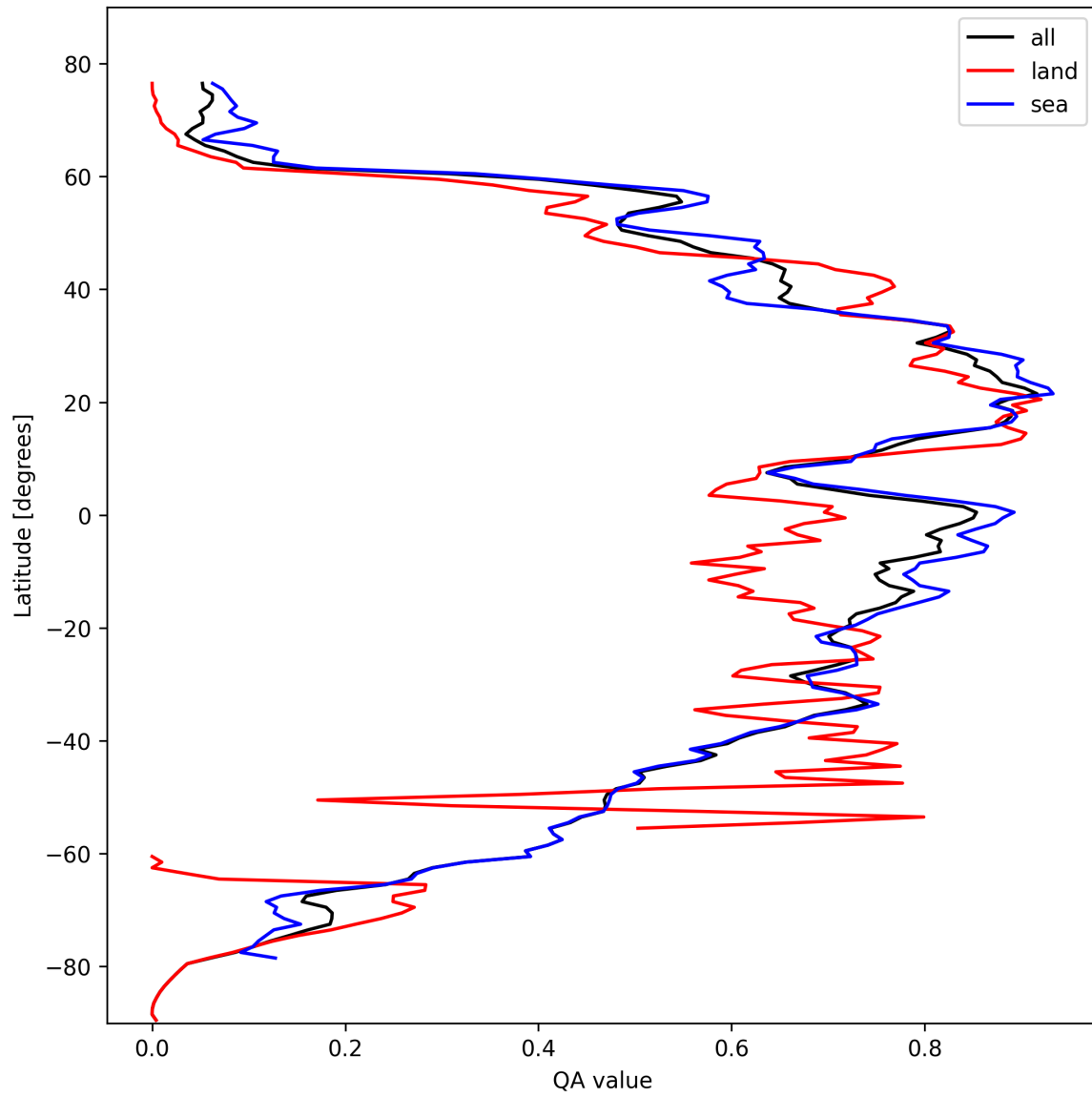
Figure 29: Zonal average of “QA value” for 2024-10-14 to 2024-10-16.
