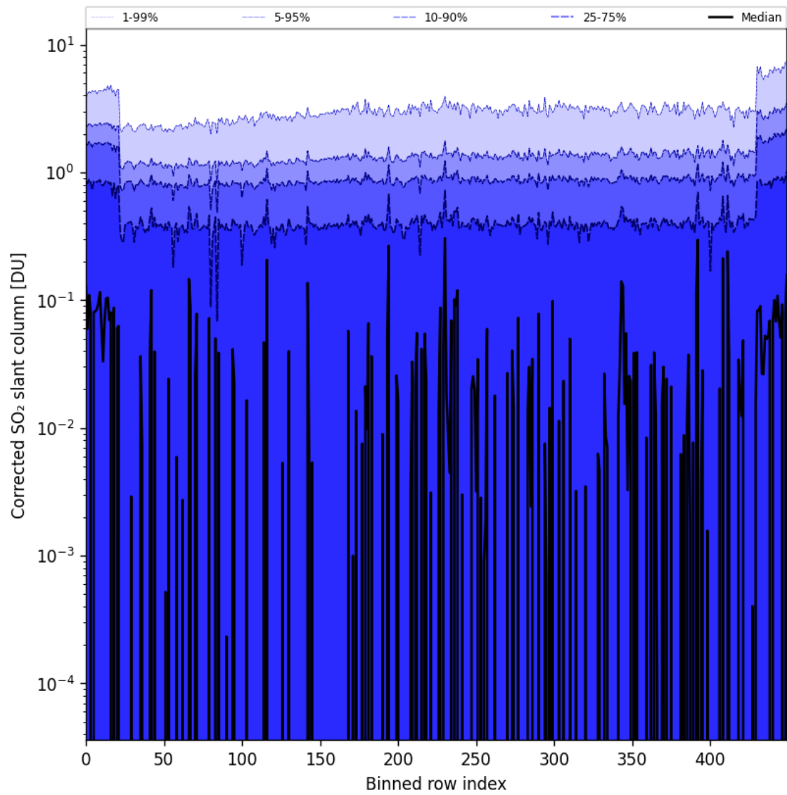
Figure 78: Along track statistics of “Corrected SO 2 slant column” for 2024-10-14 to 2024-10-16
