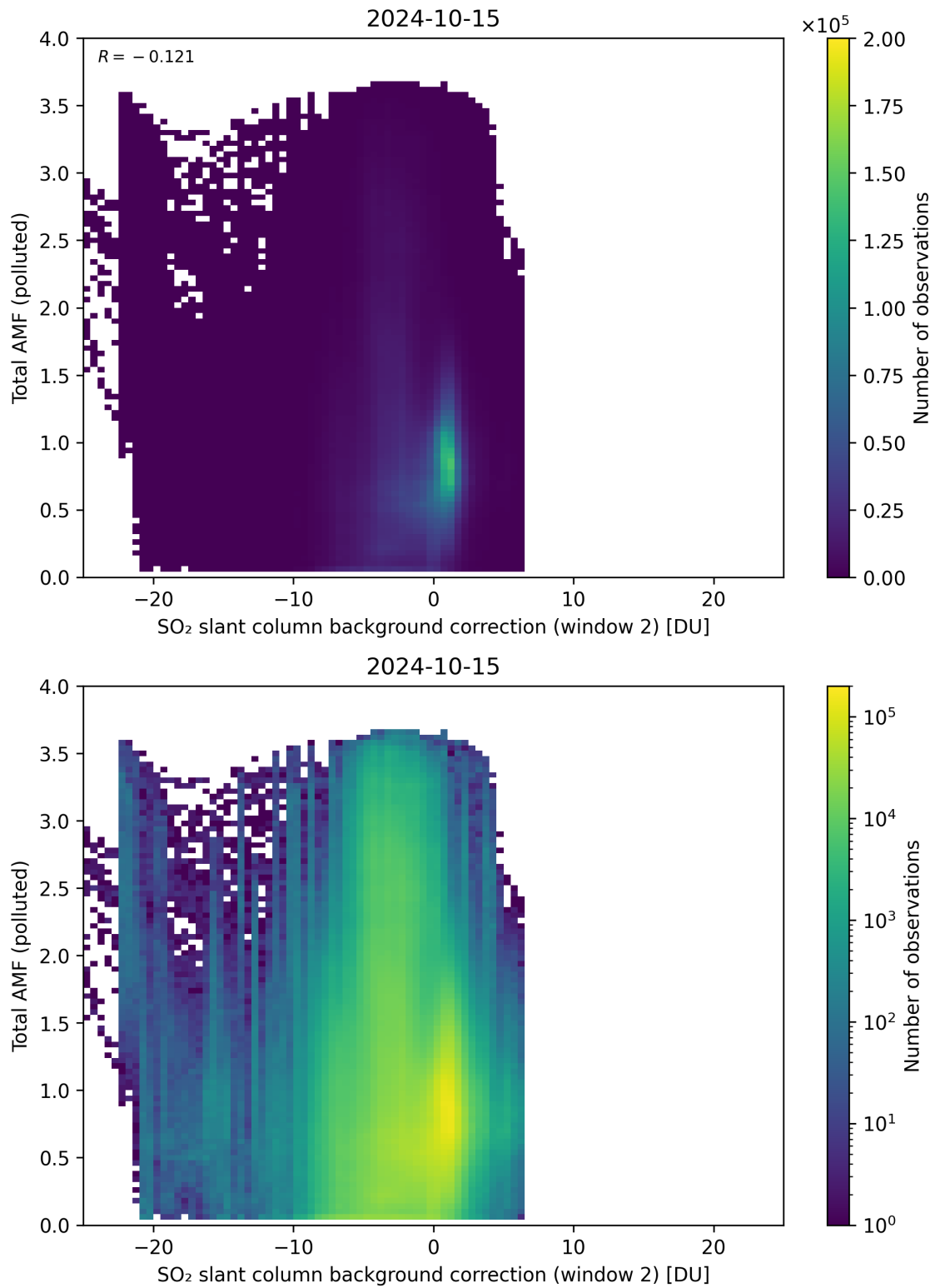
Figure 119: Scatter density plot of “SO 2 slant column background correction (window 2)” against “Total AMF (polluted)” for 2024-10-14 to 2024-10-16.
