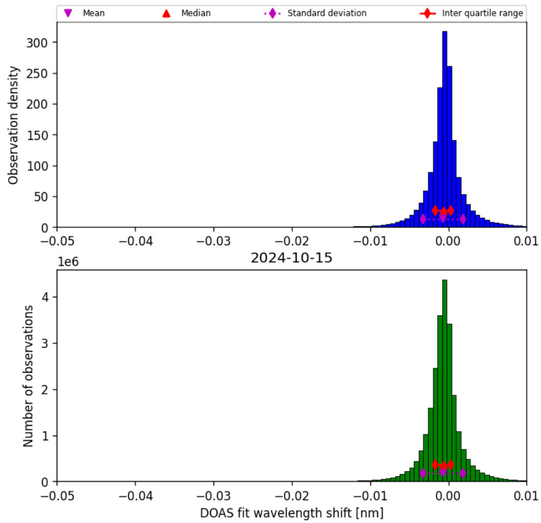
Figure 68: Histogram of “DOAS fit wavelength shift” for 2024-10-14 to 2024-10-16
