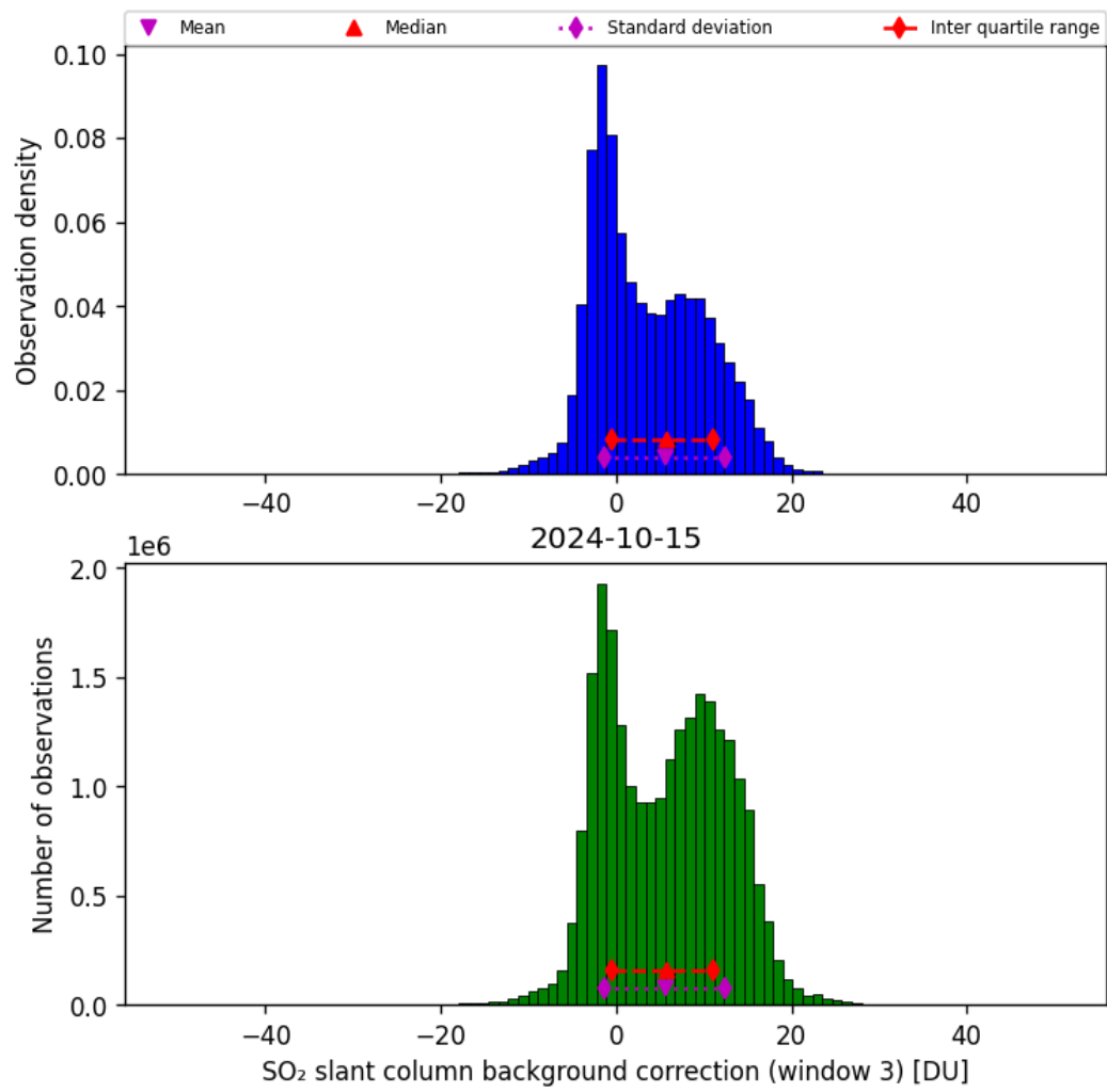
Figure 67: Histogram of “SO 2 slant column background correction (window 3)” for 2024-10-14 to 2024-10-16
