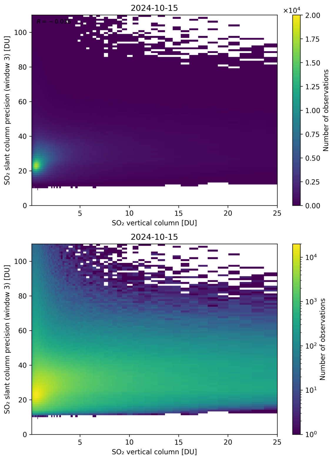
Figure 304: Scatter density plot of “SO 2 vertical column” against “SO 2 slant column precision (window 3)” for 2024-10-14 to 2024-10-16.
