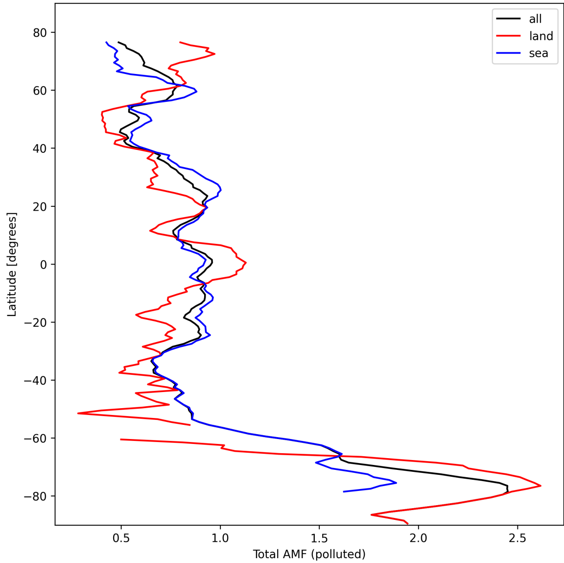
Figure 48: Zonal average of “Total AMF (polluted)” for 2024-10-14 to 2024-10-16.
