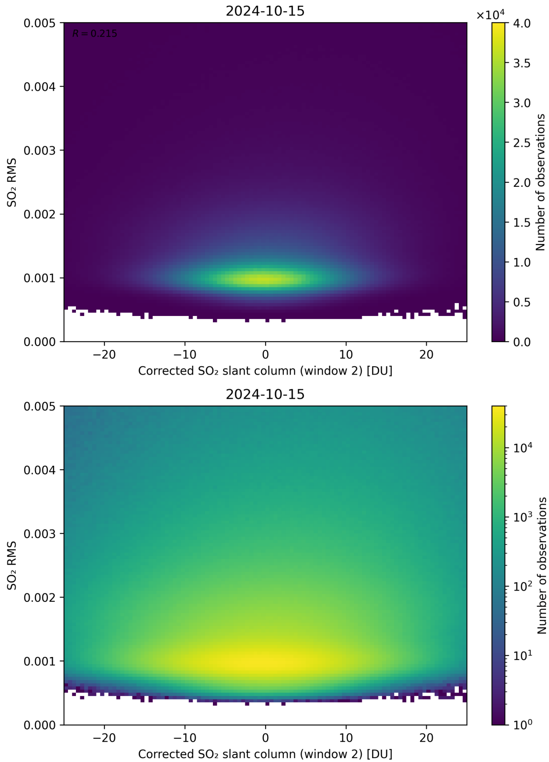
Figure 198: Scatter density plot of “Corrected SO 2 slant column (window 2)” against “SO 2 RMS” for 2024-10-14 to 2024-10-16.
