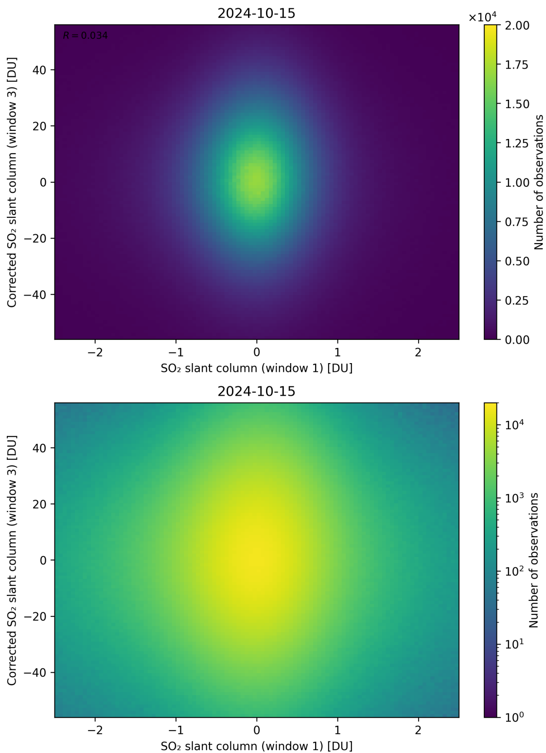
Figure 234: Scatter density plot of “SO 2 slant column (window 1)” against “Corrected SO 2 slant column (window 3)” for 2024-10-14 to 2024-10-16.
