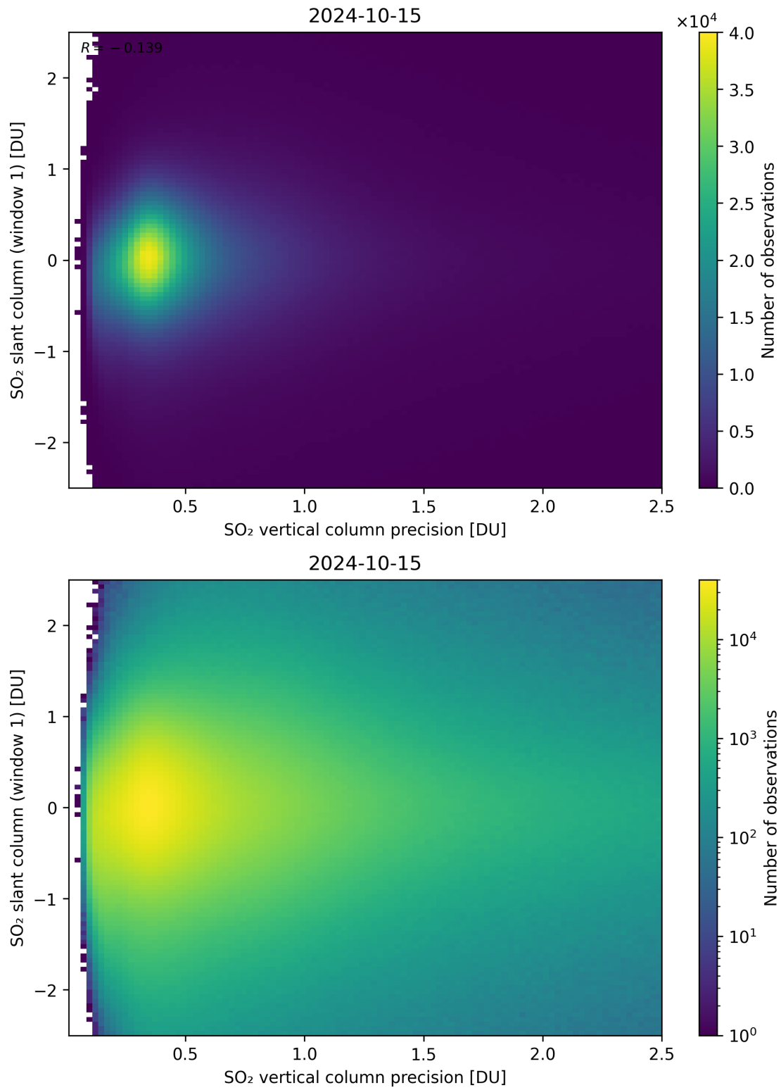
Figure 289: Scatter density plot of “SO 2 vertical column precision” against “SO 2 slant column (window 1)” for 2024-10-14 to 2024-10-16.
