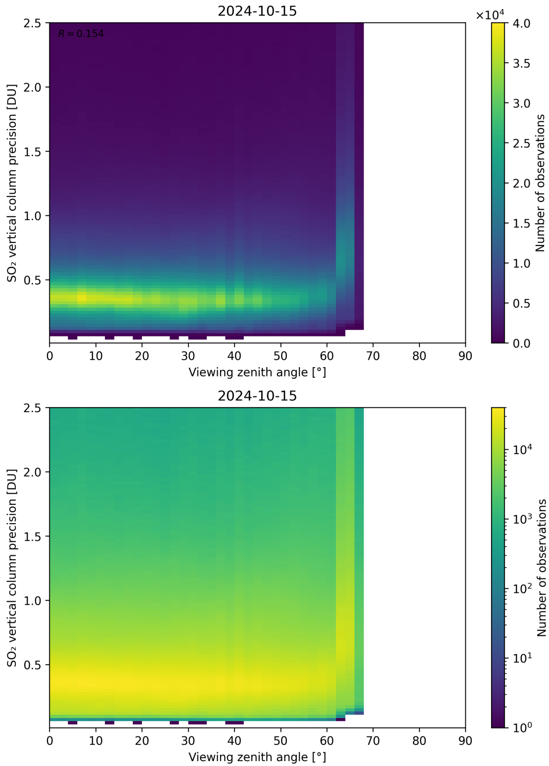
Figure 328: Scatter density plot of “Viewing zenith angle” against “SO 2 vertical column precision” for 2024-10-14 to 2024-10-16.
