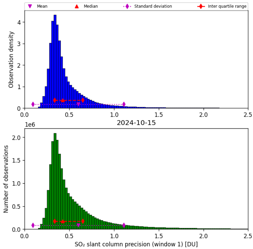
Figure 57: Histogram of “SO 2 slant column precision (window 1)” for 2024-10-14 to 2024-10-16
