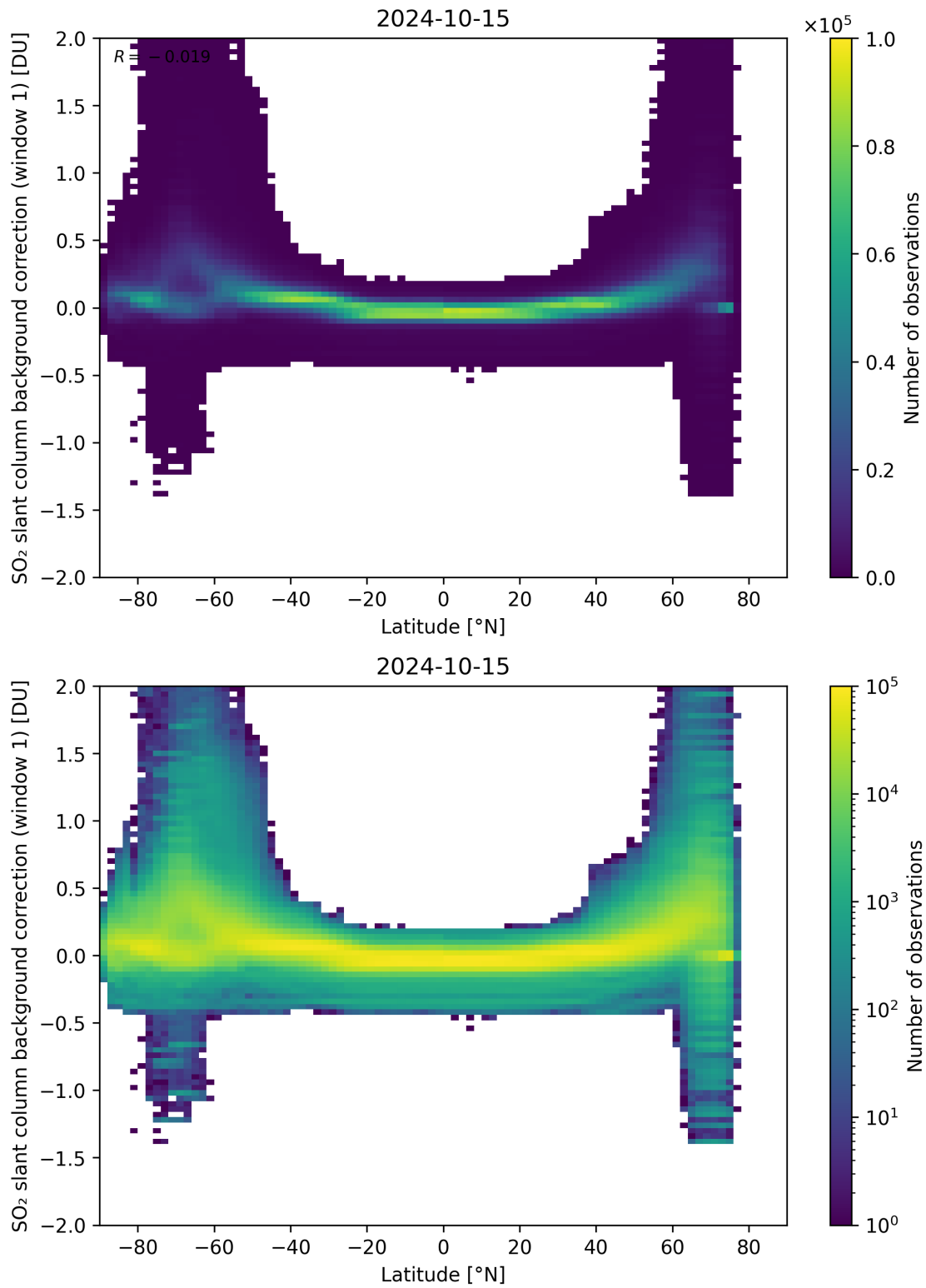
Figure 139: Scatter density plot of “Latitude” against “SO 2 slant column background correction (window 1)” for 2024-10-14 to 2024-10-16.
