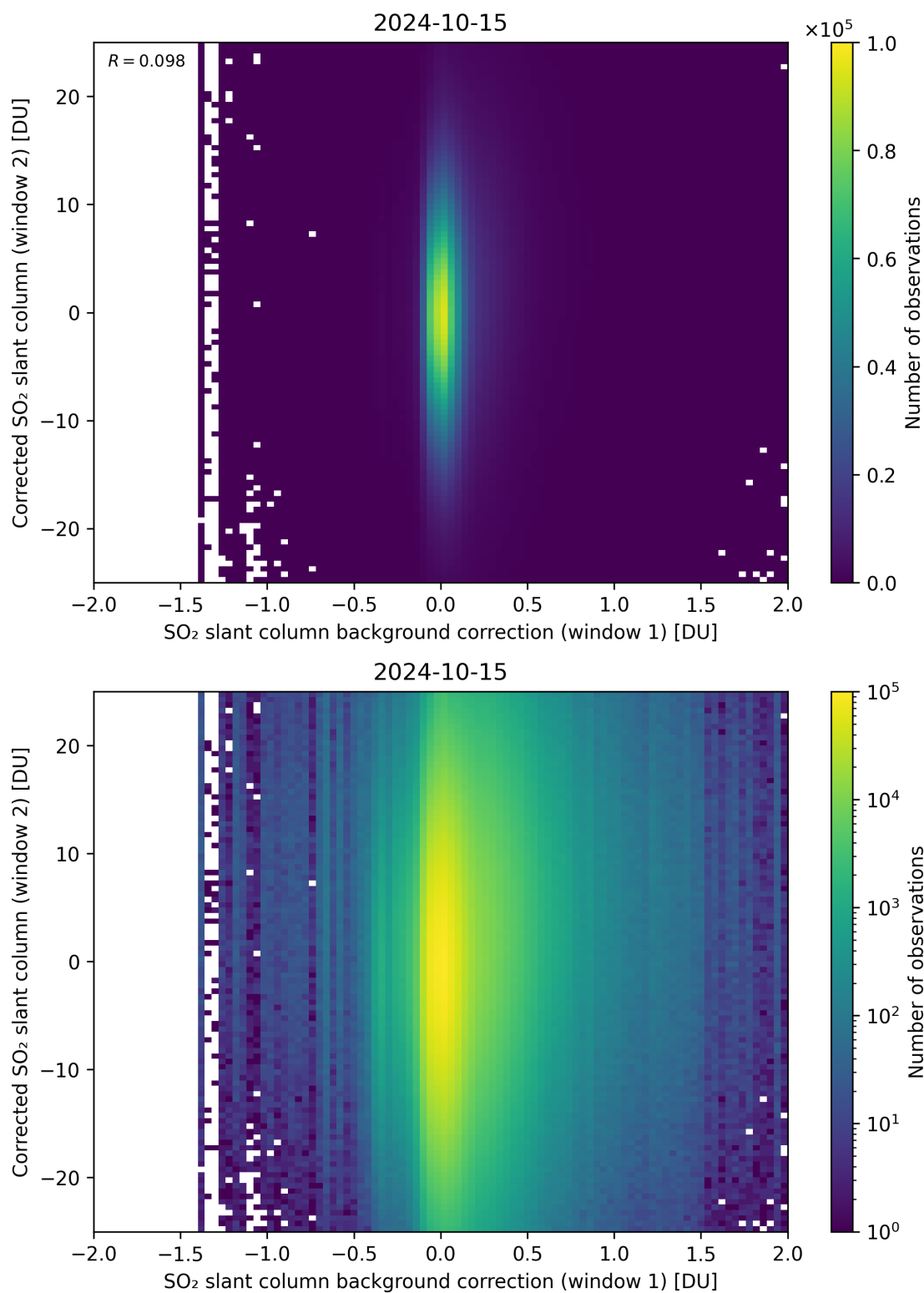
Figure 104: Scatter density plot of “SO 2 slant column background correction (window 1)” against “Corrected SO 2 slant column (window 2)” for 2024-10-14 to 2024-10-16.
