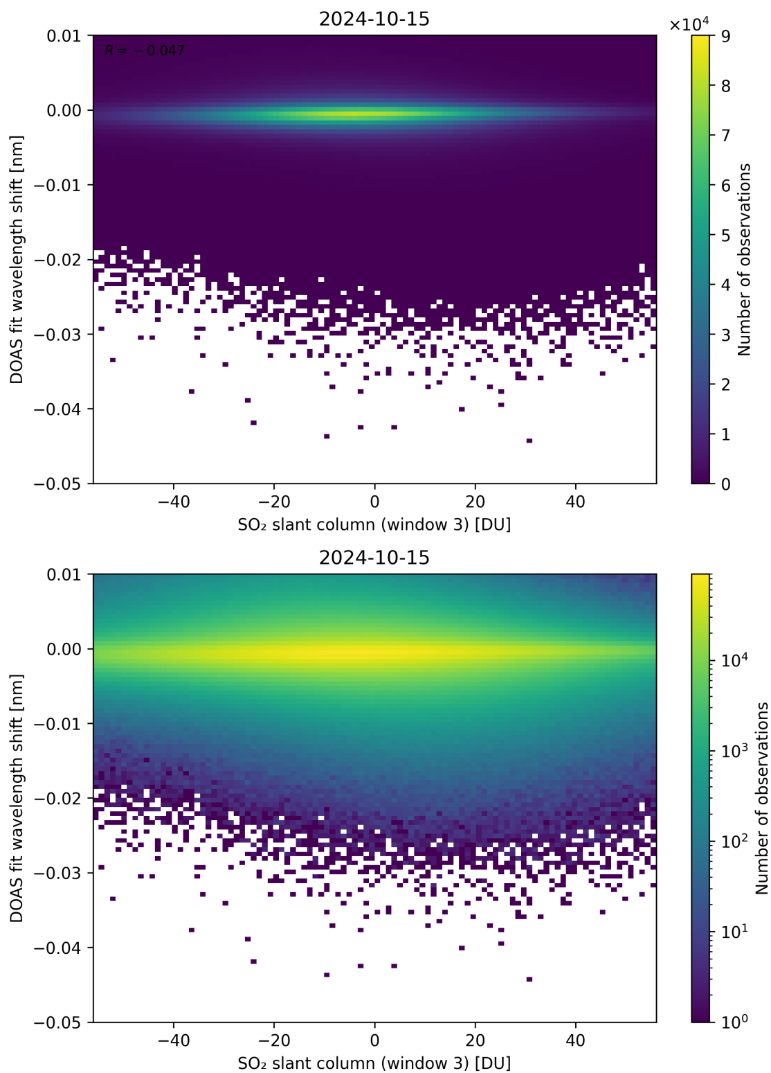
Figure 254: Scatter density plot of “SO 2 slant column (window 3)” against “DOAS fit wavelength shift” for 2024-10-14 to 2024-10-16.
