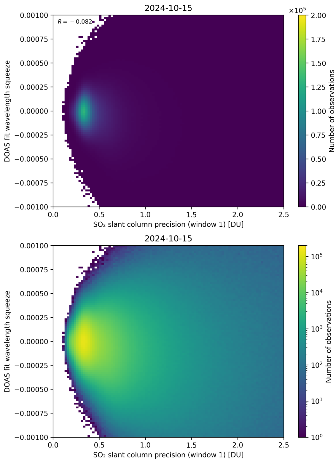
Figure 222: Scatter density plot of “SO 2 slant column precision (window 1)” against “DOAS fit wavelength squeeze” for 2024-10-14 to 2024-10-16.
