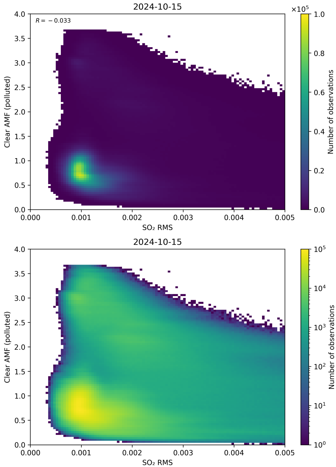
Figure 136: Scatter density plot of “SO 2 RMS” against “Clear AMF (polluted)” for 2024-10-14 to 2024-10-16.
