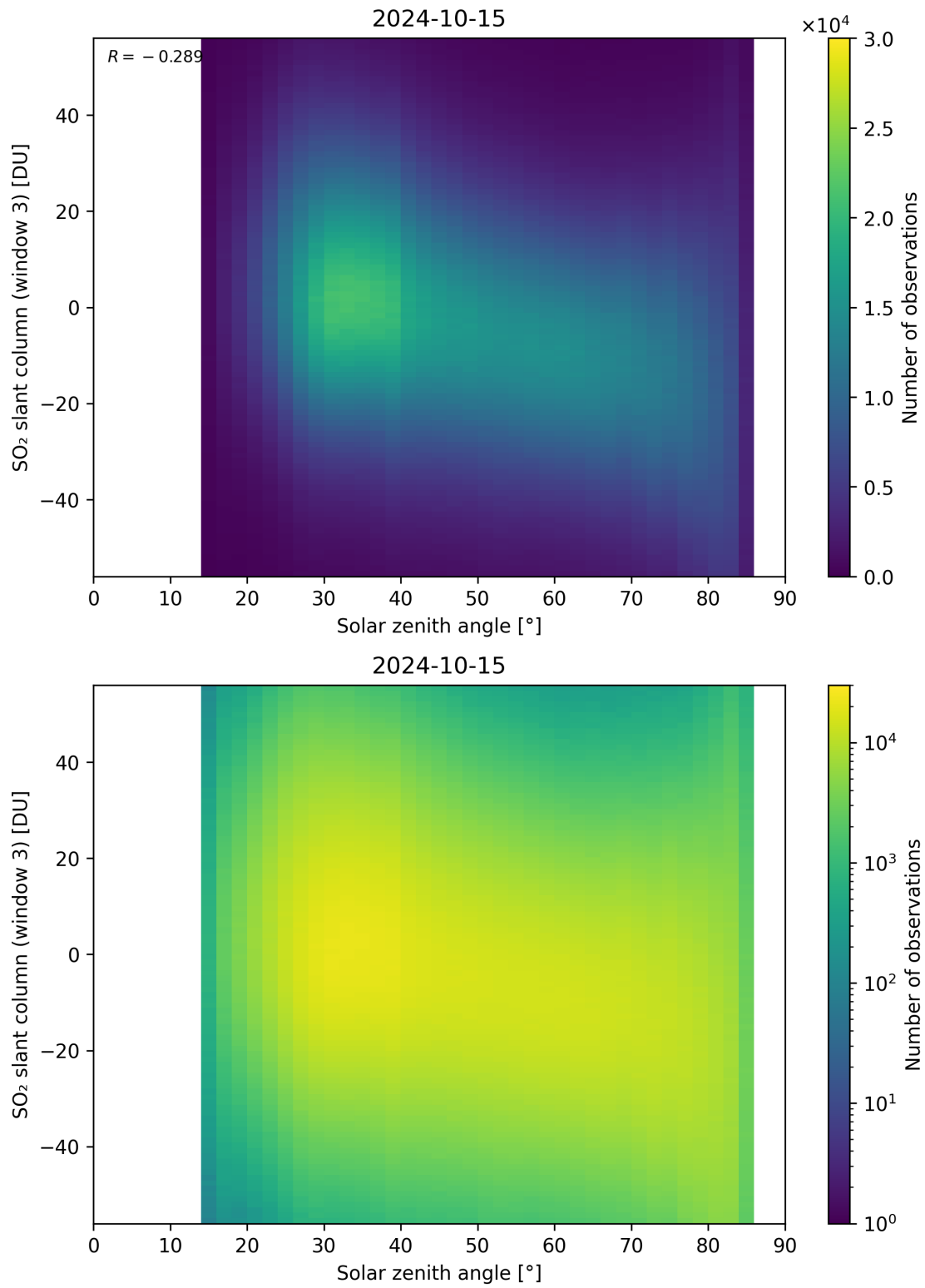
Figure 172: Scatter density plot of “Solar zenith angle” against “SO 2 slant column (window 3)” for 2024-10-14 to 2024-10-16.
