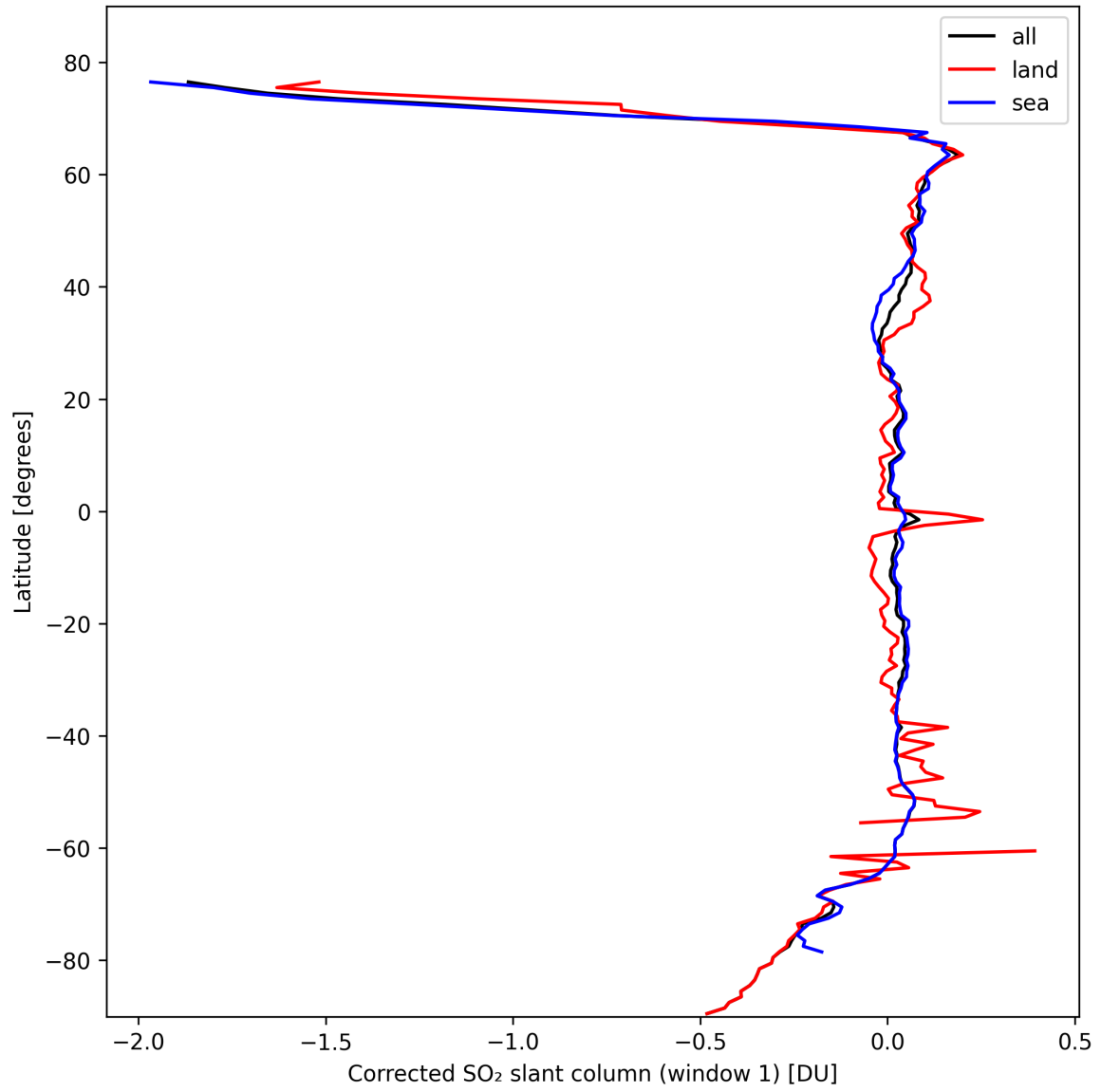
Figure 35: Zonal average of “Corrected SO 2 slant column (window 1)” for 2024-10-14 to 2024-10-16.
