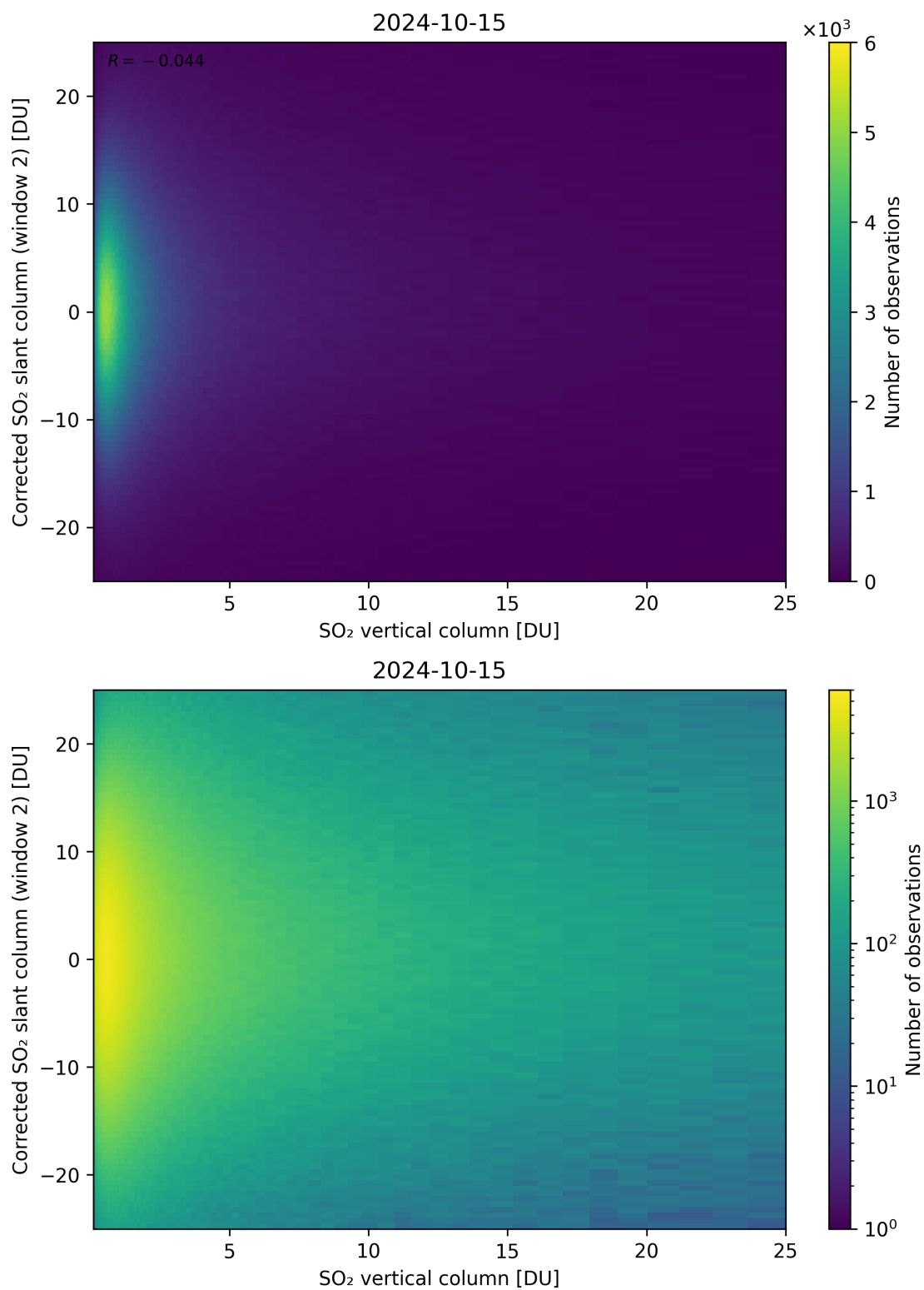
Figure 298: Scatter density plot of “SO 2 vertical column” against “Corrected SO 2 slant column (window 2)” for 2024-10-14 to 2024-10-16.
