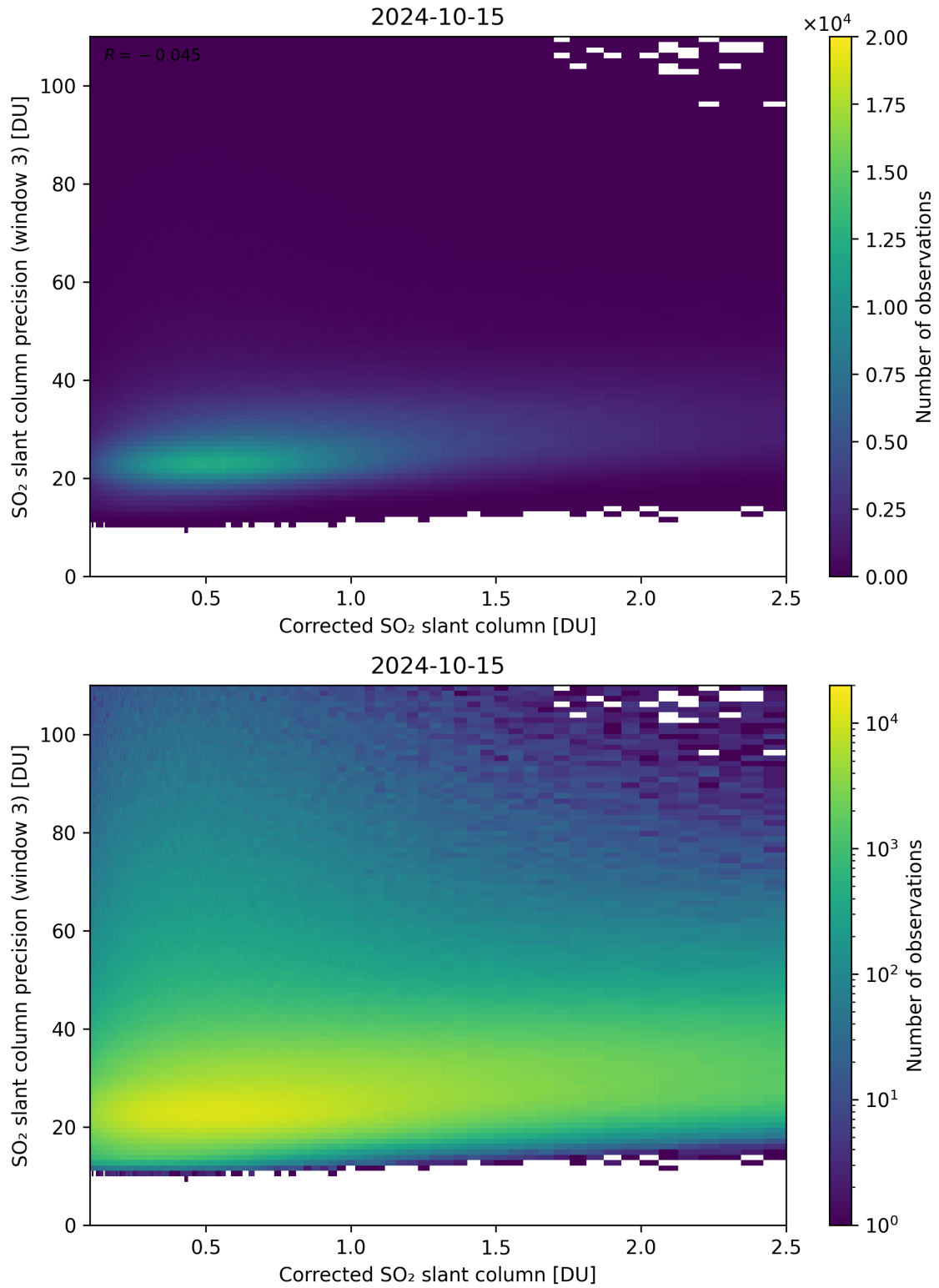
Figure 191: Scatter density plot of “Corrected SO 2 slant column” against “SO 2 slant column precision (window 3)” for 2024-10-14 to 2024-10-16.
