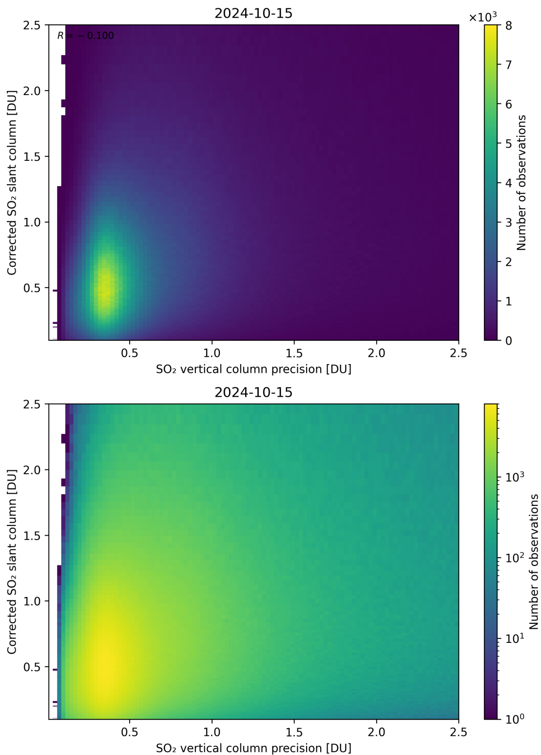
Figure 286: Scatter density plot of “SO 2 vertical column precision” against “Corrected SO 2 slant column” for 2024-10-14 to 2024-10-16.
