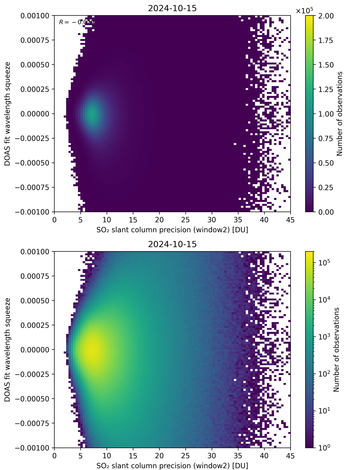
Figure 244: Scatter density plot of “SO 2 slant column precision (window2)” against “DOAS fit wavelength squeeze” for 2024-10-14 to 2024-10-16.
