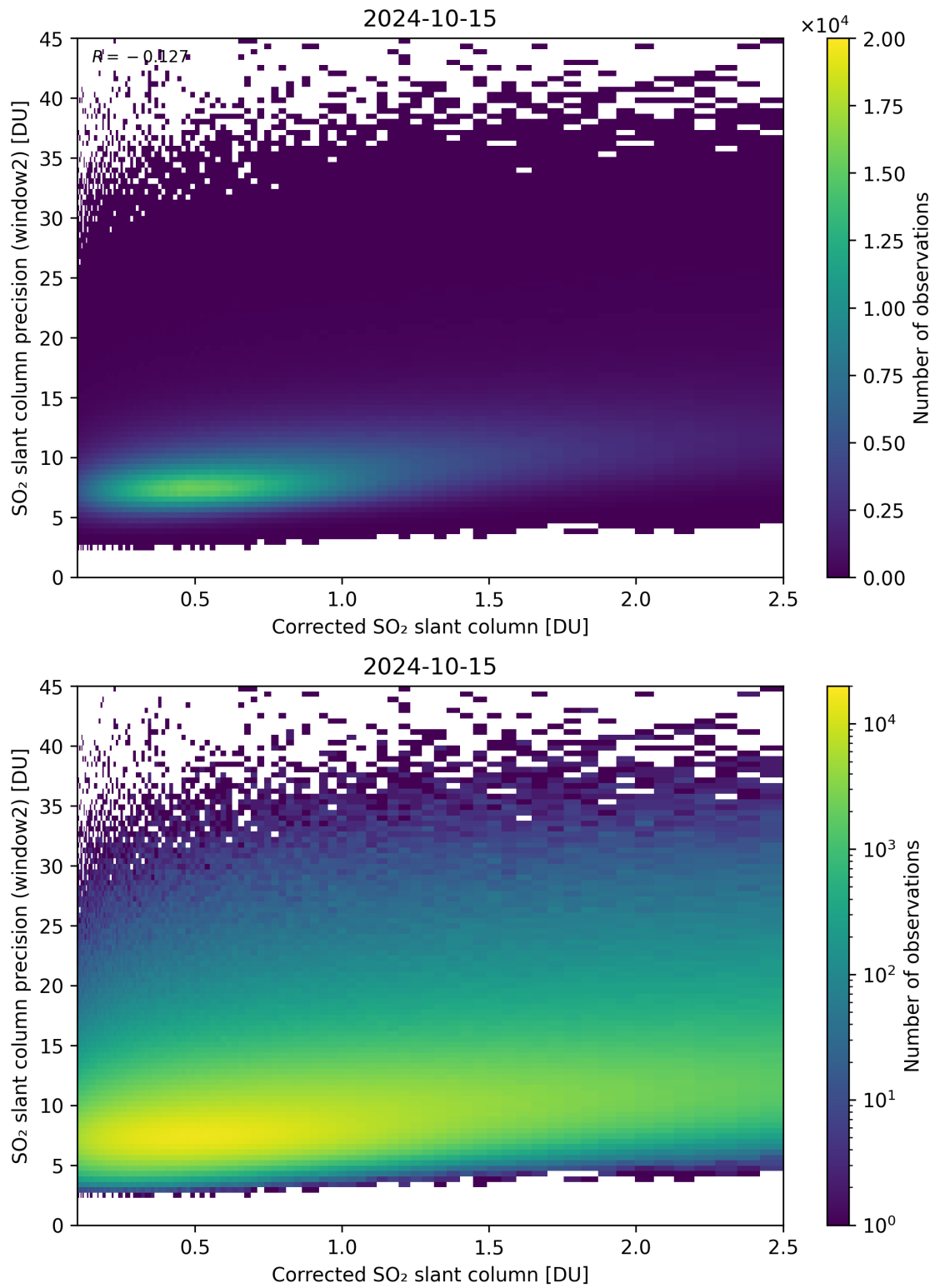
Figure 189: Scatter density plot of “Corrected SO 2 slant column” against “SO 2 slant column precision (window2)” for 2024-10-14 to 2024-10-16.
