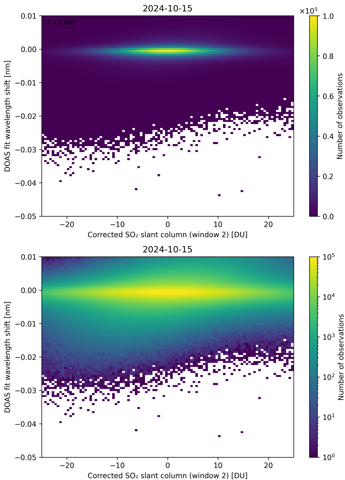
Figure 196: Scatter density plot of “Corrected SO 2 slant column (window 2)” against “DOAS fit wavelength shift” for 2024-10-14 to 2024-10-16.
