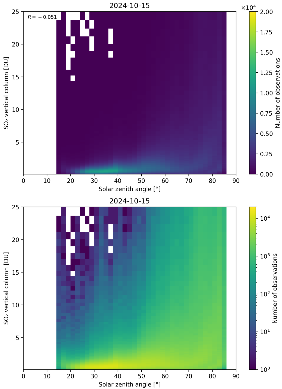
Figure 176: Scatter density plot of “Solar zenith angle” against “SO 2 vertical column” for 2024-10-14 to 2024-10-16.
