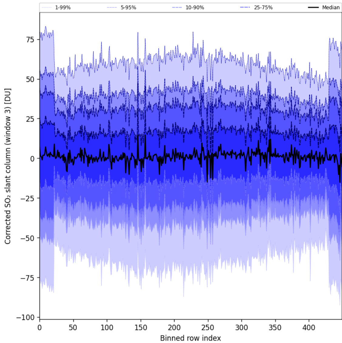
Figure 89: Along track statistics of “Corrected SO 2 slant column (window 3)” for 2024-10-14 to 2024-10-16
