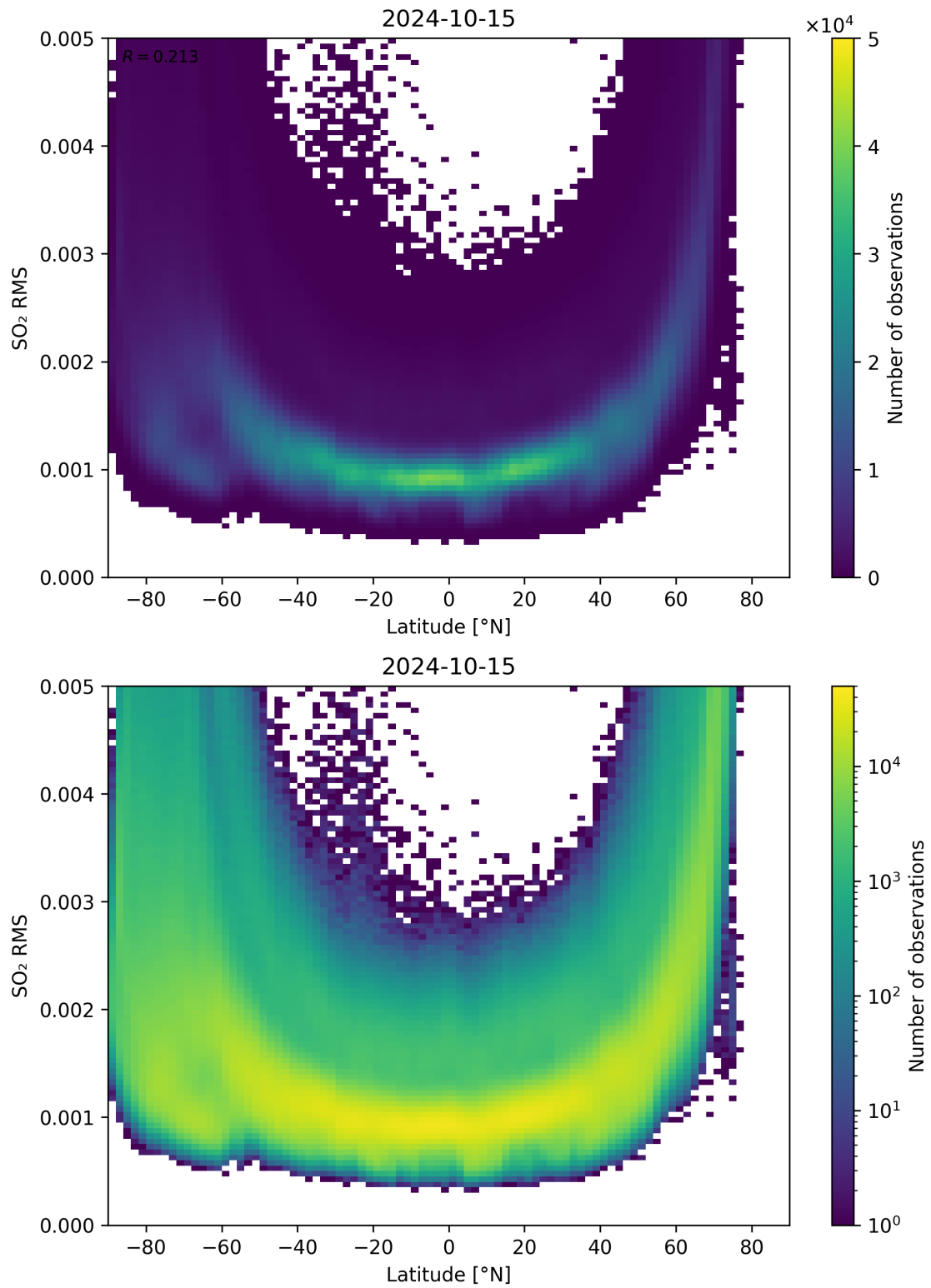
Figure 144: Scatter density plot of “Latitude” against “SO 2 RMS” for 2024-10-14 to 2024-10-16.
