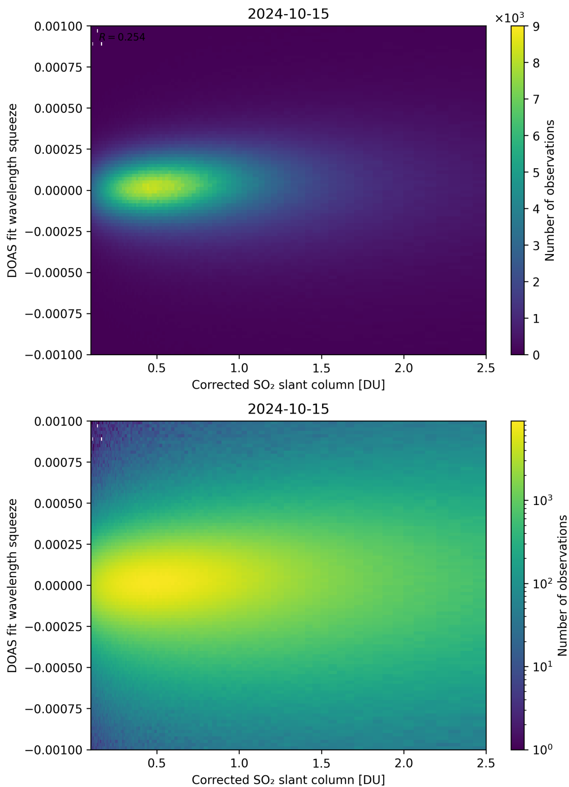
Figure 182: Scatter density plot of “Corrected SO 2 slant column” against “DOAS fit wavelength squeeze” for 2024-10-14 to 2024-10-16.
