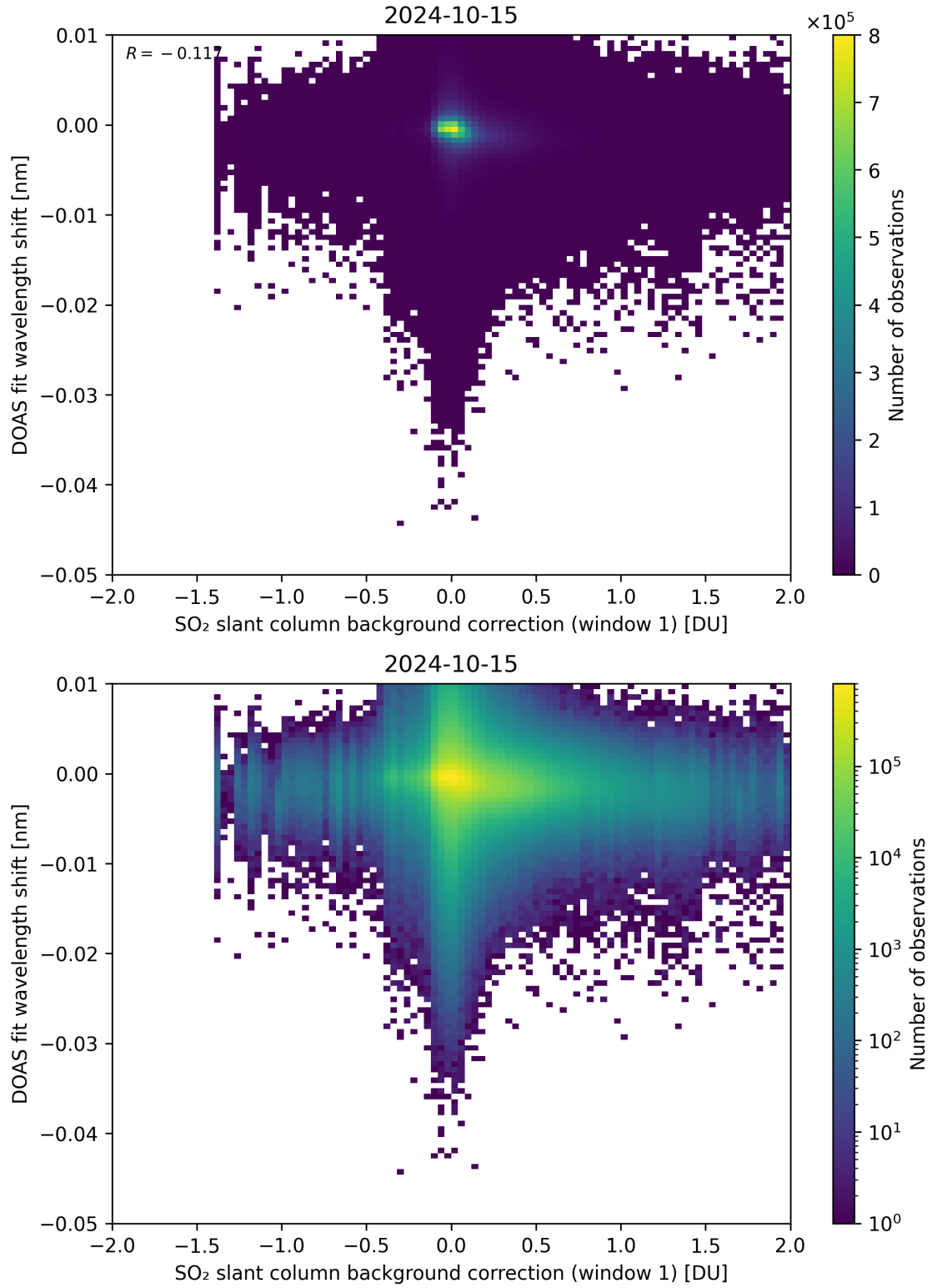
Figure 100: Scatter density plot of “SO 2 slant column background correction (window 1)” against “DOAS fit wavelength shift” for 2024-10-14 to 2024-10-16.
