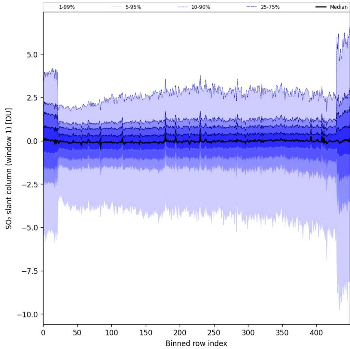
Figure 79: Along track statistics of “SO 2 slant column (window 1)” for 2024-10-14 to 2024-10-16
