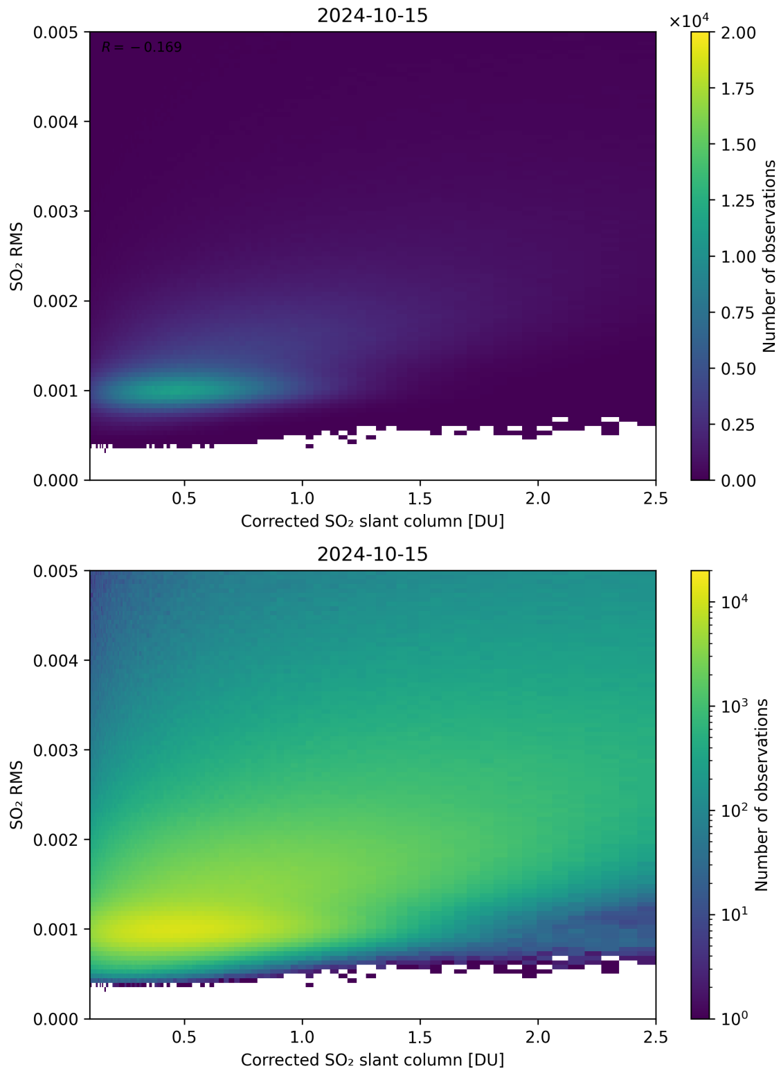
Figure 183: Scatter density plot of “Corrected SO 2 slant column” against “SO 2 RMS” for 2024-10-14 to 2024-10-16.
