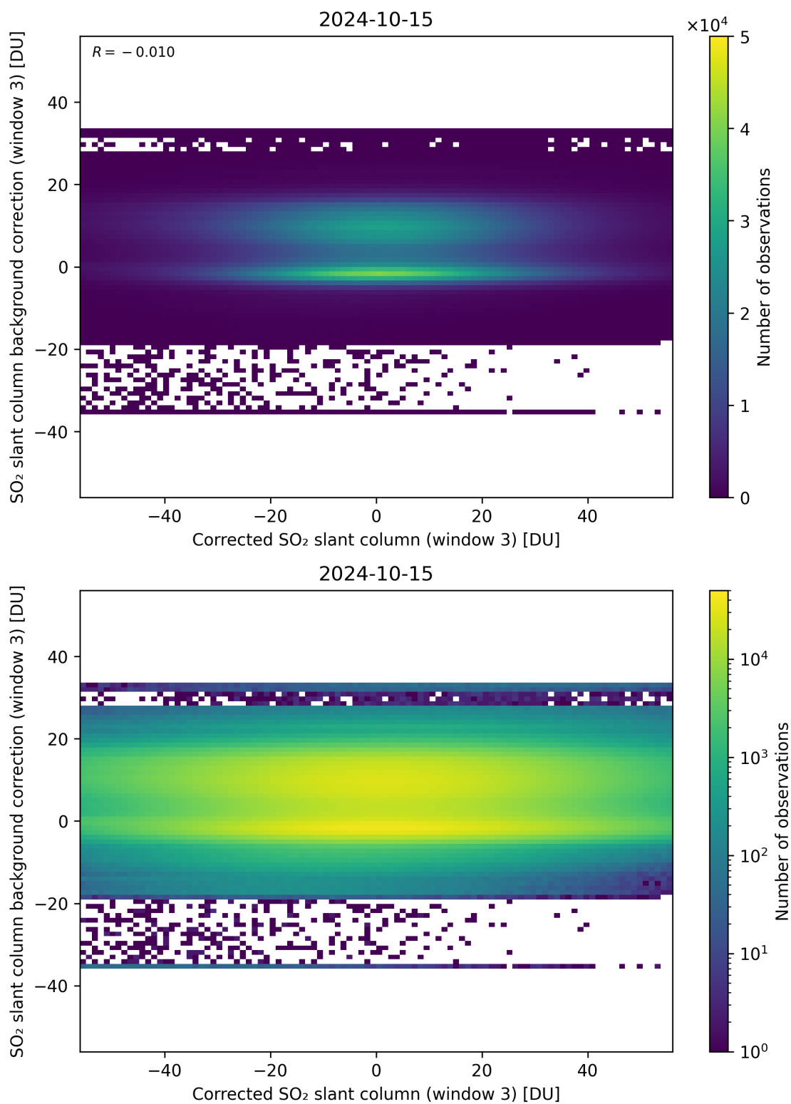
Figure 205: Scatter density plot of “Corrected SO 2 slant column (window 3)” against “SO 2 slant column background correction (window 3)” for 2024-10-14 to 2024-10-16.
