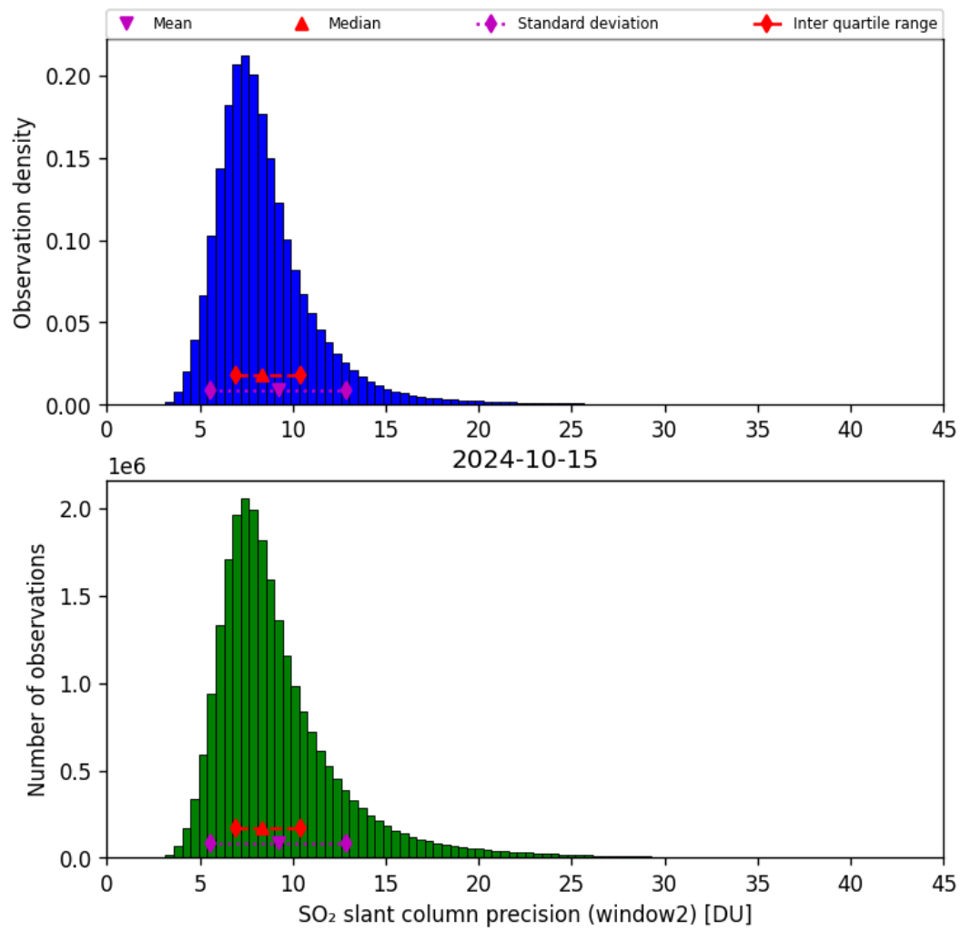
Figure 61: Histogram of “SO 2 slant column precision (window2)” for 2024-10-14 to 2024-10-16
