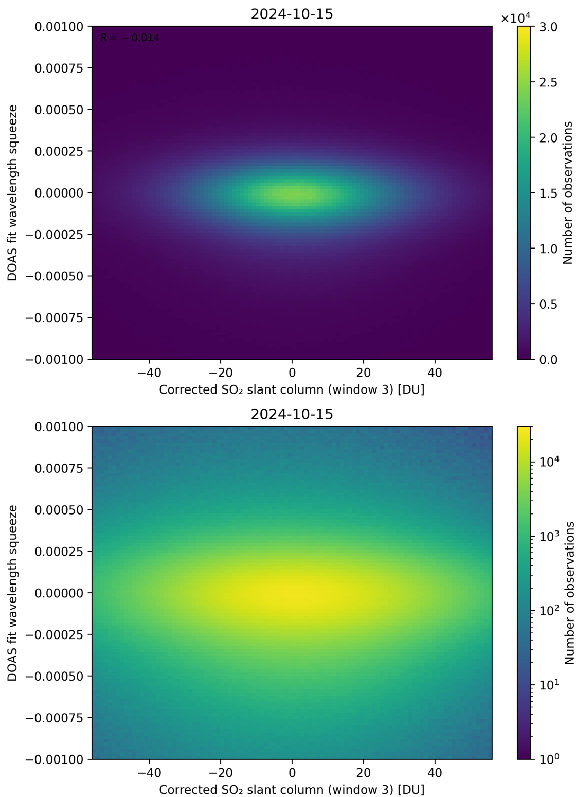
Figure 207: Scatter density plot of “Corrected SO 2 slant column (window 3)” against “DOAS fit wavelength squeeze” for 2024-10-14 to 2024-10-16.
