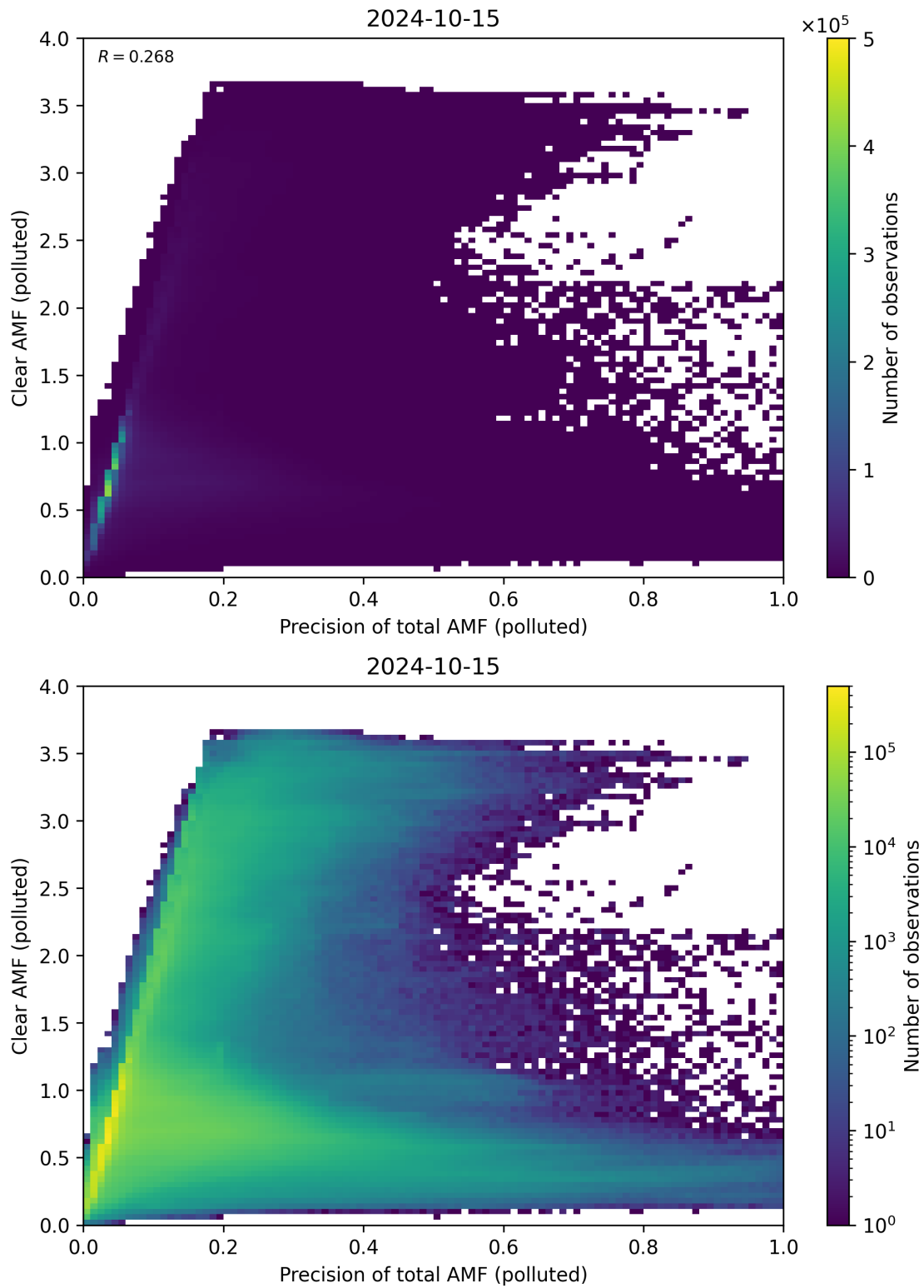
Figure 270: Scatter density plot of “Precision of total AMF (polluted)” against “Clear AMF (polluted)” for 2024-10-14 to 2024-10-16.
