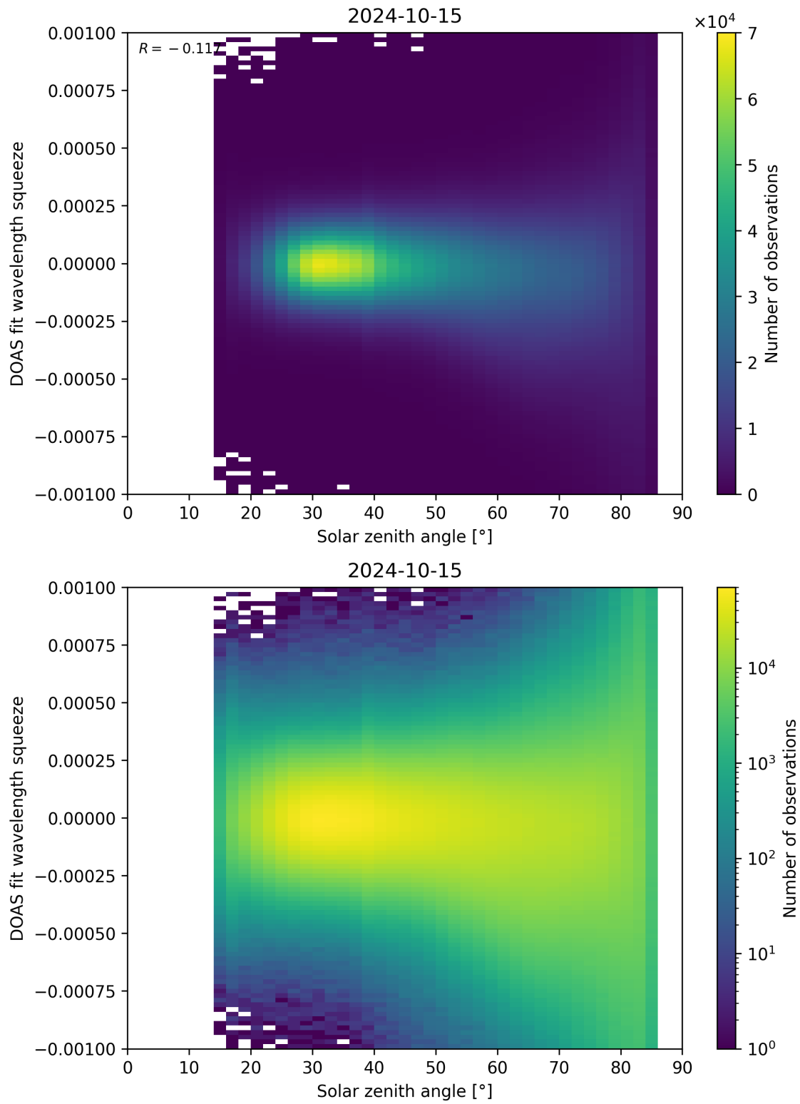
Figure 162: Scatter density plot of “Solar zenith angle” against “DOAS fit wavelength squeeze” for 2024-10-14 to 2024-10-16.
