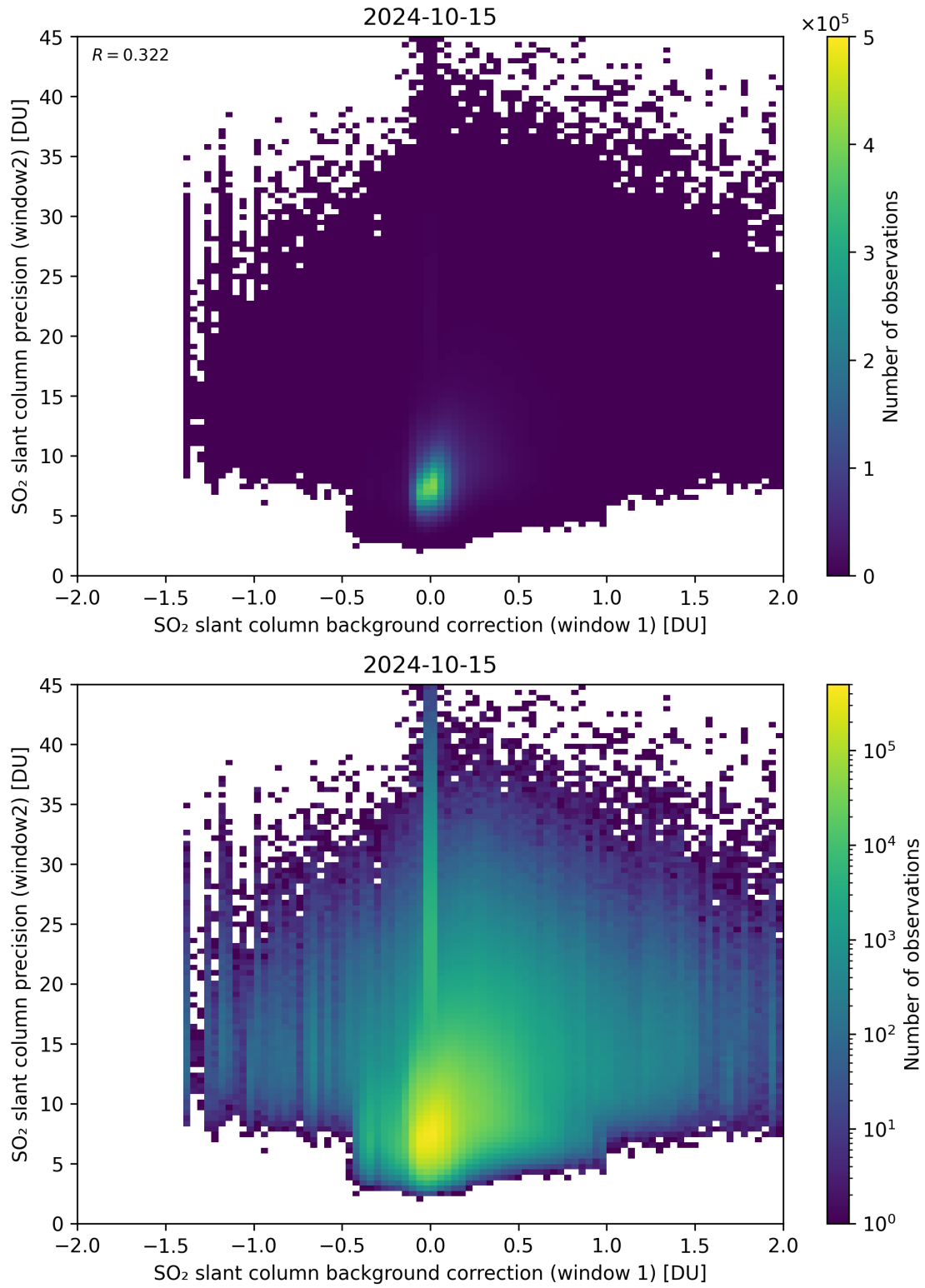
Figure 106: Scatter density plot of “SO 2 slant column background correction (window 1)” against “SO 2 slant column precision (window2)” for 2024-10-14 to 2024-10-16.
