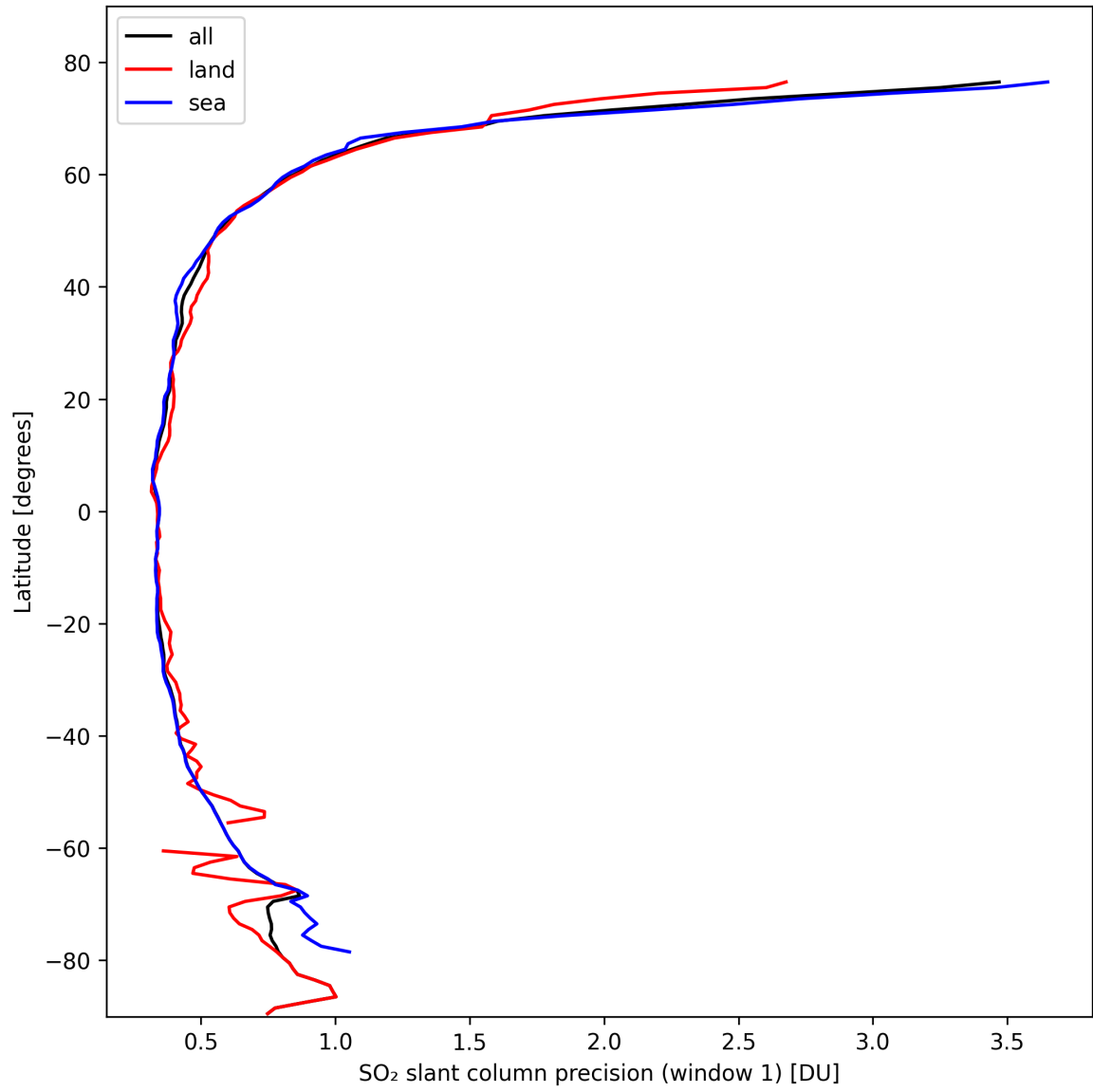
Figure 34: Zonal average of “SO 2 slant column precision (window 1)” for 2024-10-14 to 2024-10-16.
