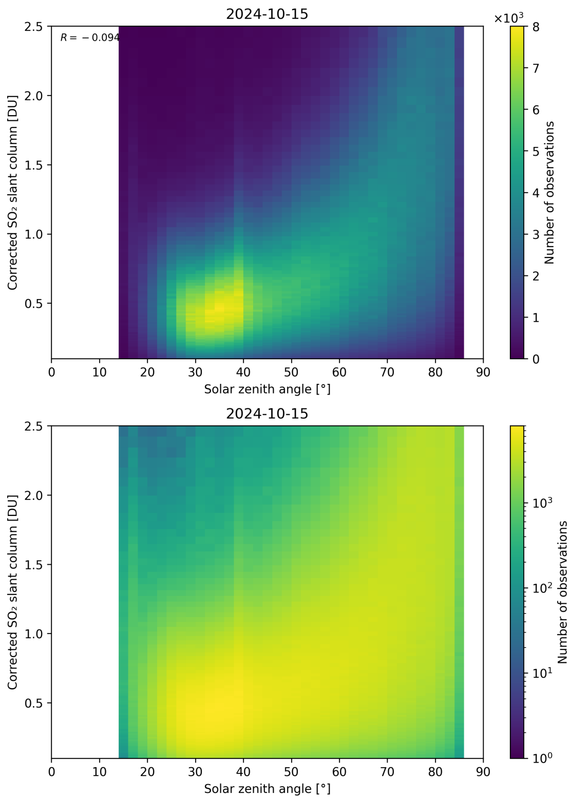
Figure 166: Scatter density plot of “Solar zenith angle” against “Corrected SO 2 slant column” for 2024-10-14 to 2024-10-16.
