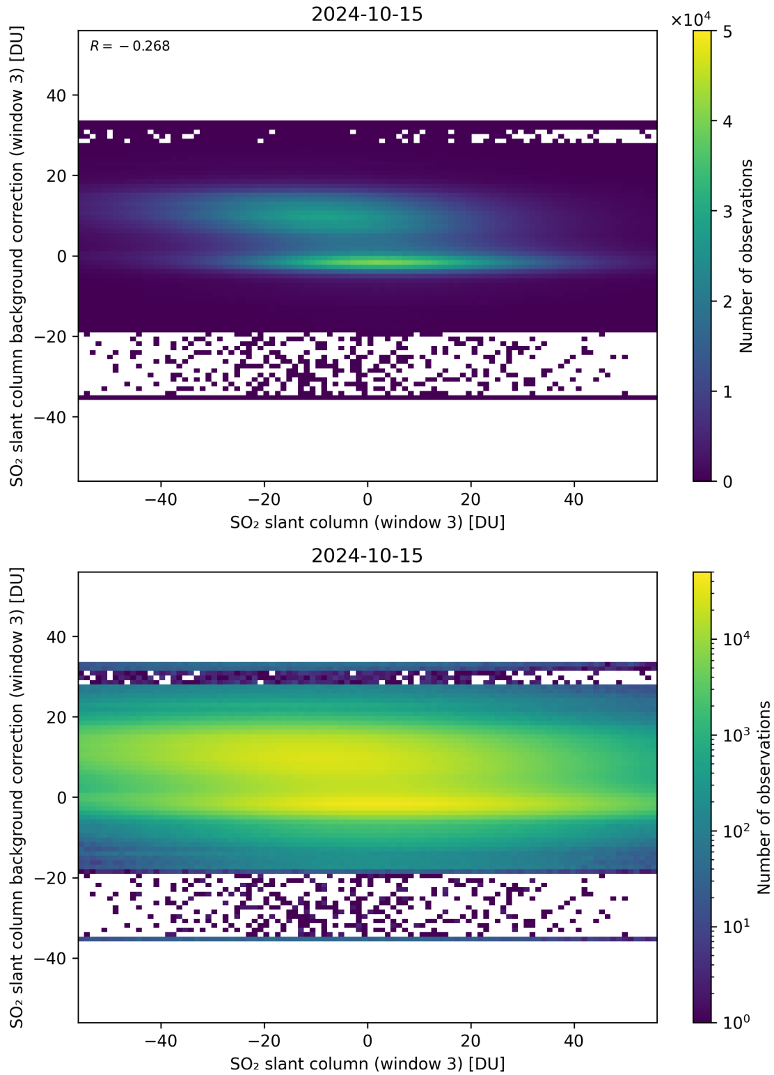
Figure 253: Scatter density plot of “SO 2 slant column (window 3)” against “SO 2 slant column background correction (window 3)” for 2024-10-14 to 2024-10-16.
