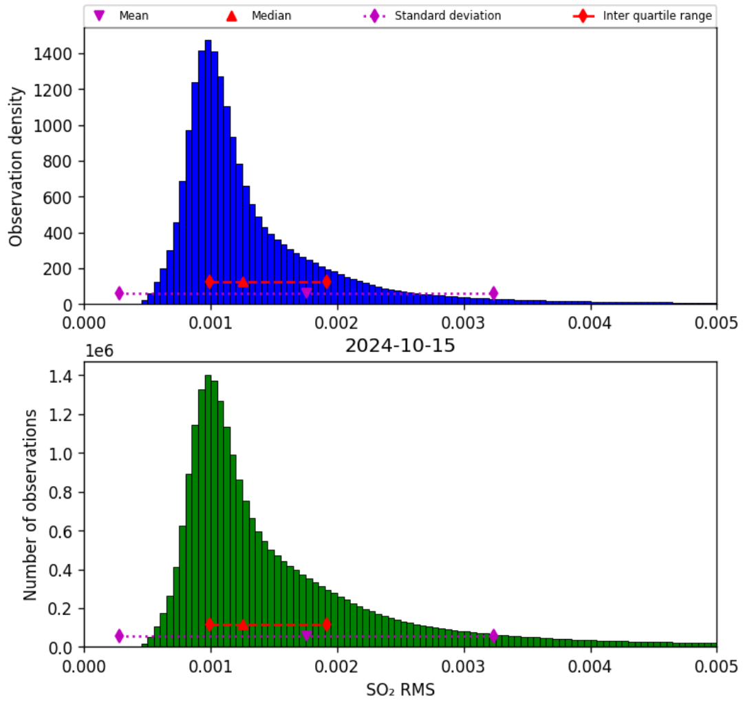
Figure 70: Histogram of “SO 2 RMS” for 2024-10-14 to 2024-10-16
