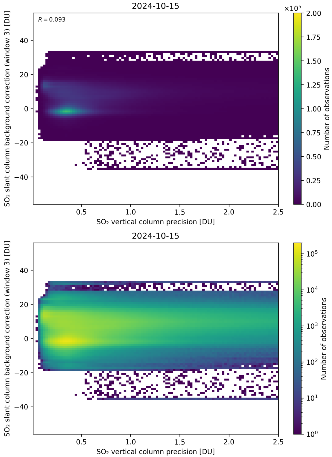
Figure 281: Scatter density plot of “SO 2 vertical column precision” against “SO 2 slant column background correction (window 3)” for 2024-10-14 to 2024-10-16.
