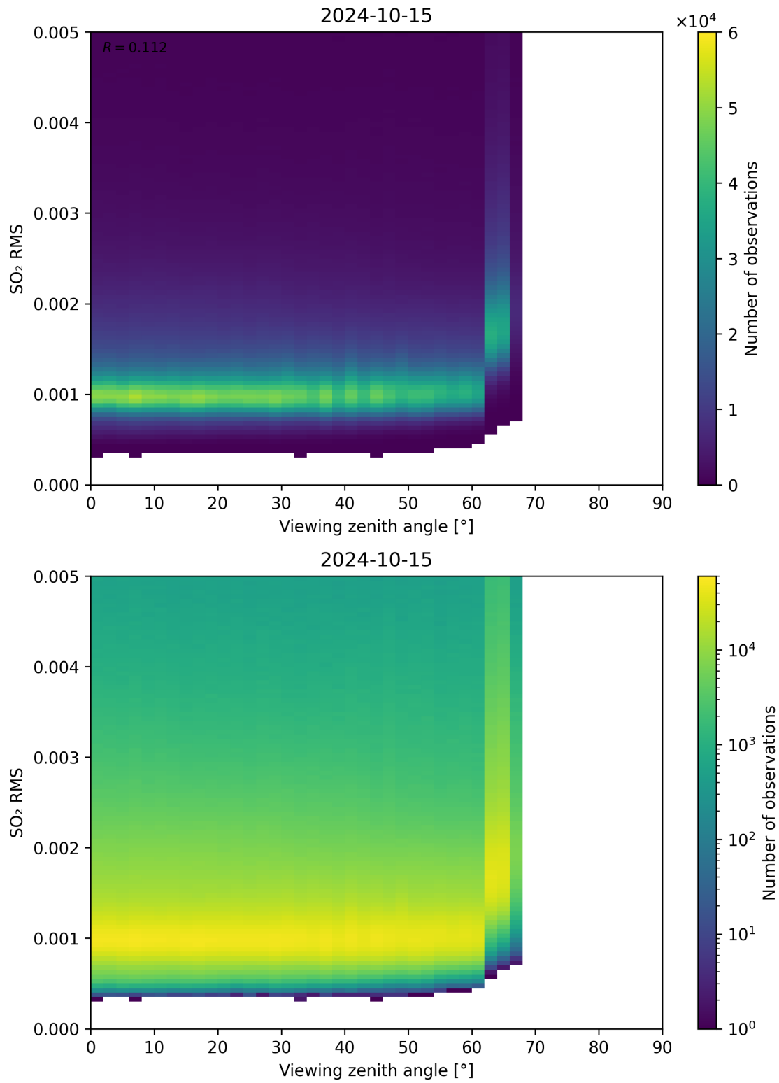
Figure 313: Scatter density plot of “Viewing zenith angle” against “SO 2 RMS” for 2024-10-14 to 2024-10-16.
