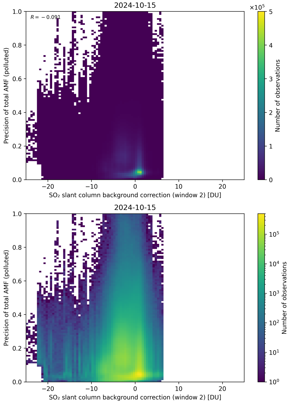
Figure 120: Scatter density plot of “SO 2 slant column background correction (window 2)” against “Precision of total AMF (polluted)” for 2024-10-14 to 2024-10-16.
