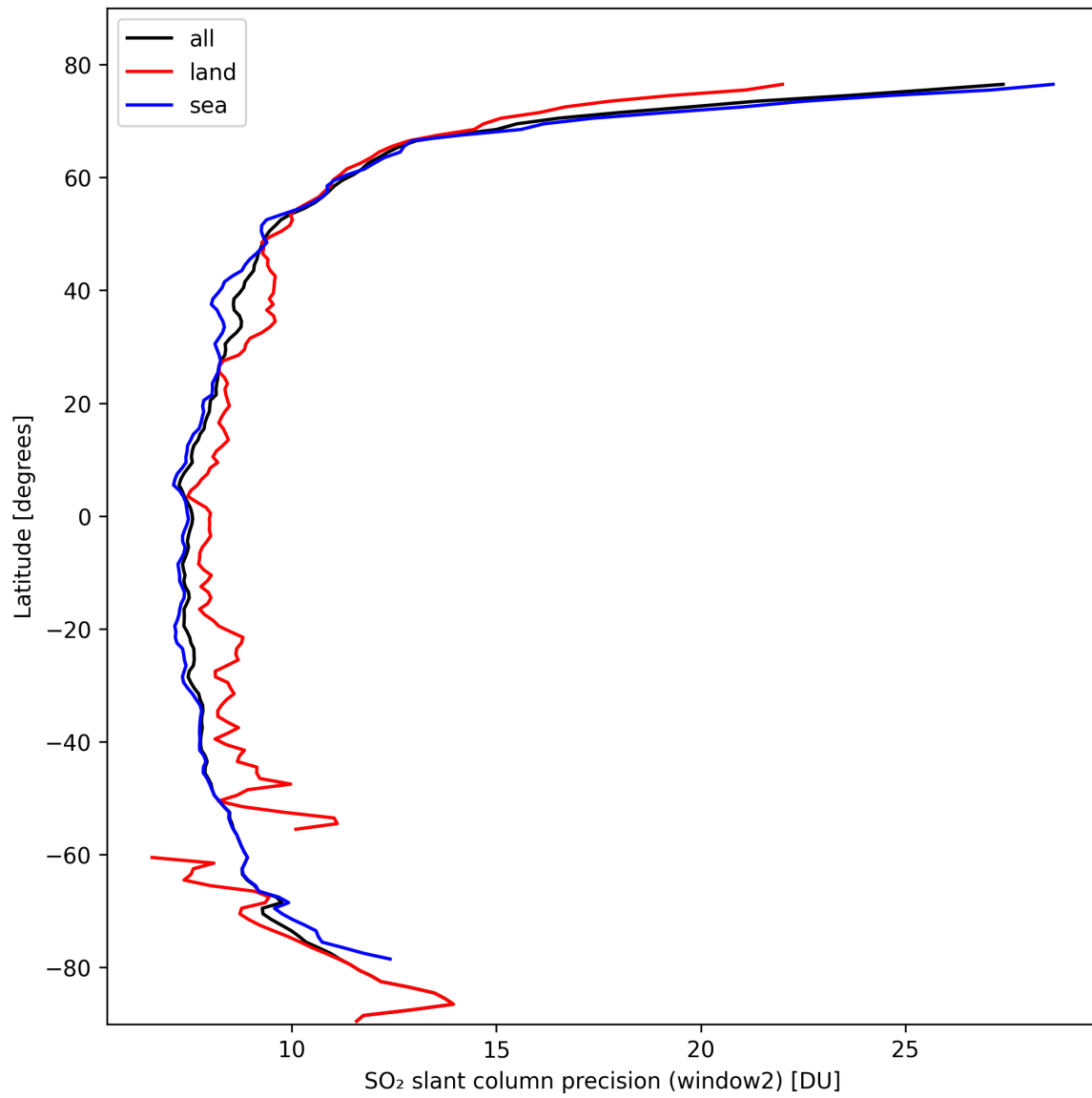
Figure 38: Zonal average of “SO 2 slant column precision (window2)” for 2024-10-14 to 2024-10-16.
