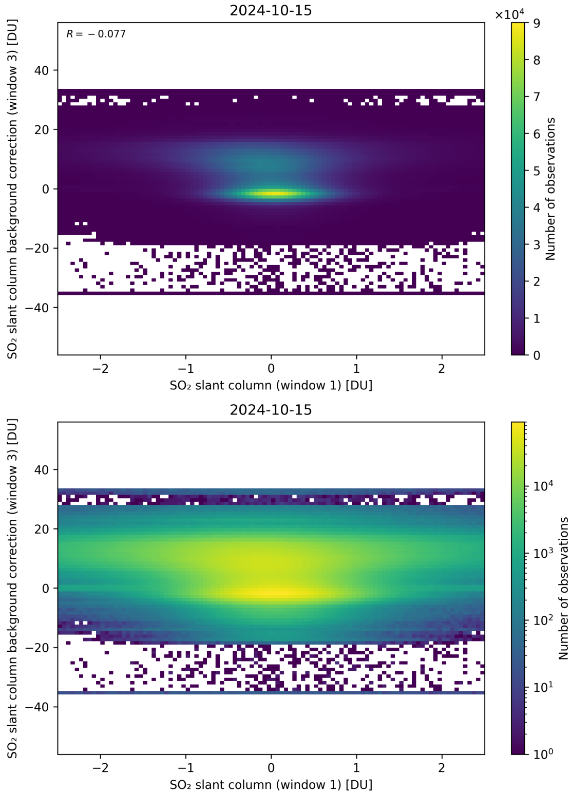
Figure 214: Scatter density plot of “SO 2 slant column (window 1)” against “SO 2 slant column background correction (window 3)” for 2024-10-14 to 2024-10-16.
