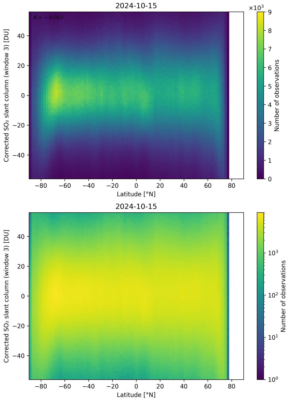
Figure 148: Scatter density plot of “Latitude” against “Corrected SO 2 slant column (window 3)” for 2024-10-14 to 2024-10-16.
