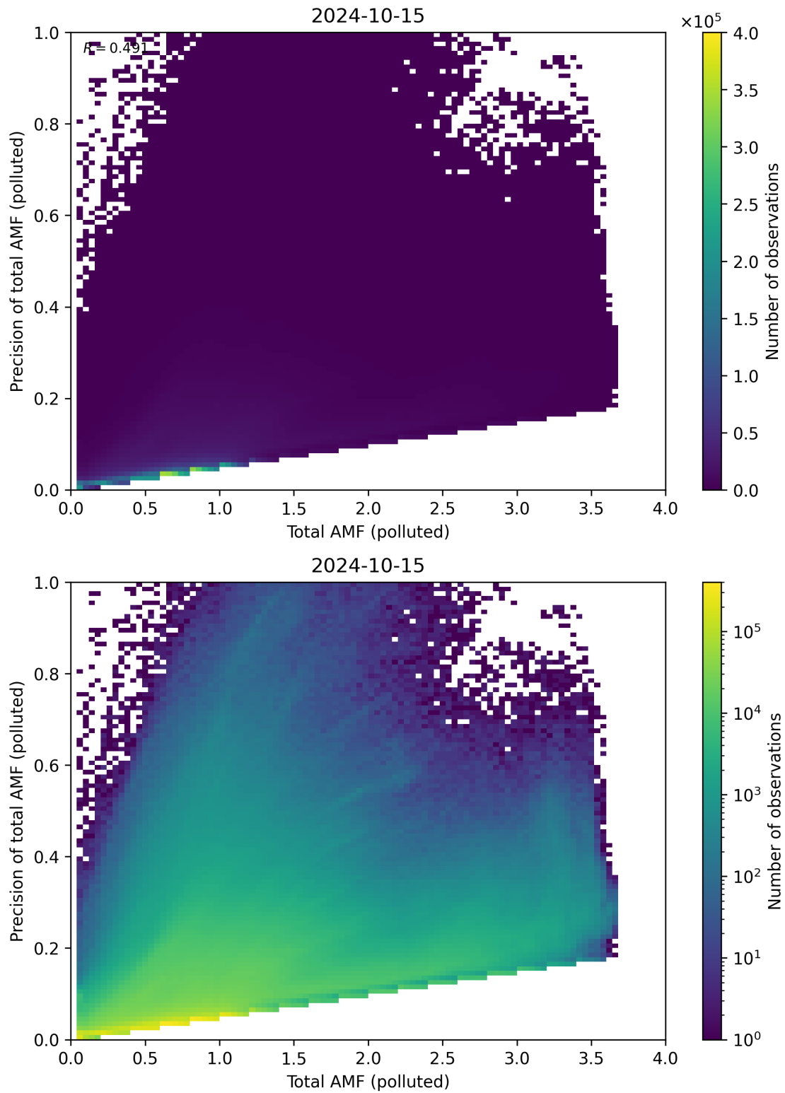
Figure 272: Scatter density plot of “Total AMF (polluted)” against “Precision of total AMF (polluted)” for 2024-10-14 to 2024-10-16.
