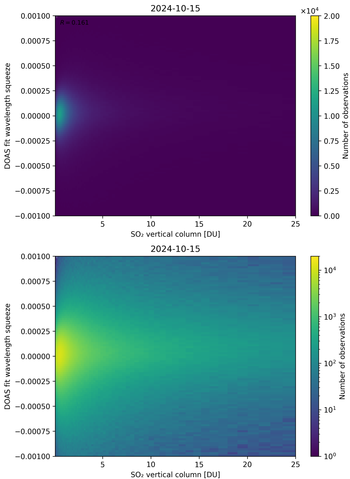
Figure 277: Scatter density plot of “SO 2 vertical column” against “DOAS fit wavelength squeeze” for 2024-10-14 to 2024-10-16.
