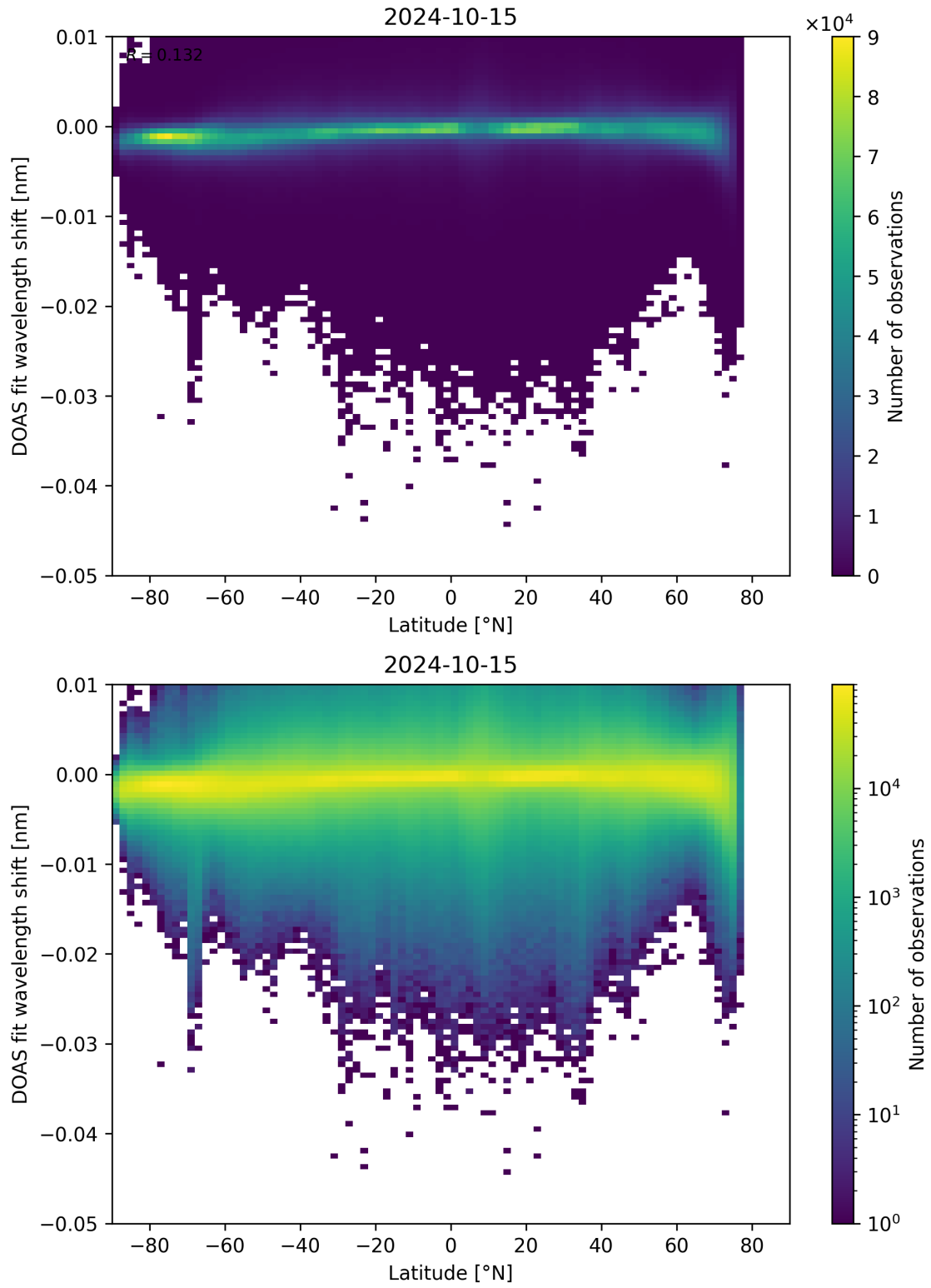
Figure 142: Scatter density plot of “Latitude” against “DOAS fit wavelength shift” for 2024-10-14 to 2024-10-16.
