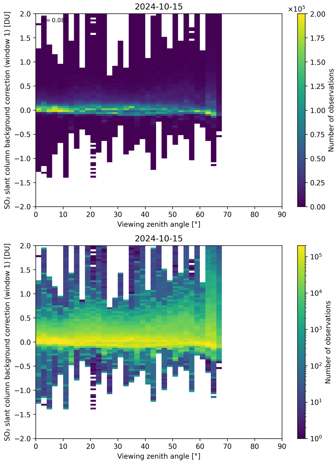
Figure 308: Scatter density plot of “Viewing zenith angle” against “SO 2 slant column background correction (window 1)” for 2024-10-14 to 2024-10-16.
