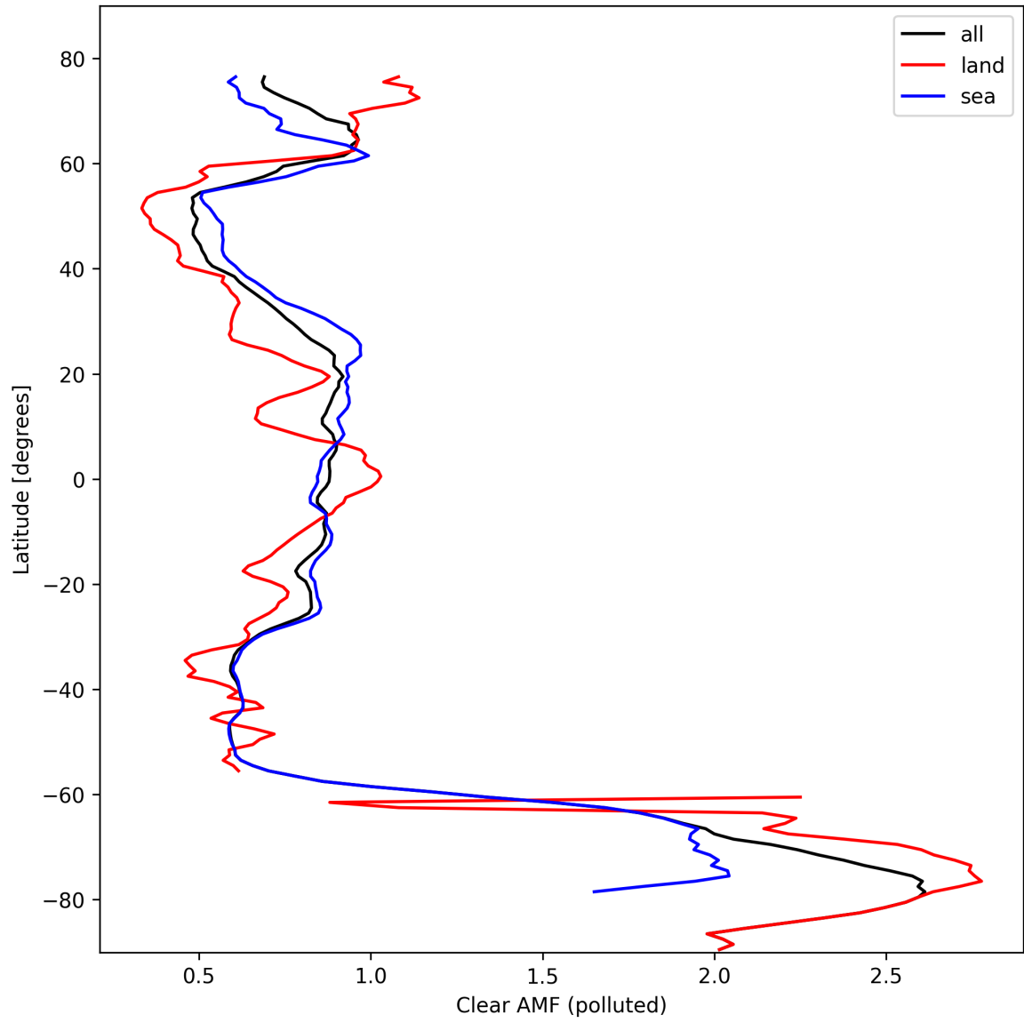
Figure 50: Zonal average of “Clear AMF (polluted)” for 2024-10-14 to 2024-10-16.
