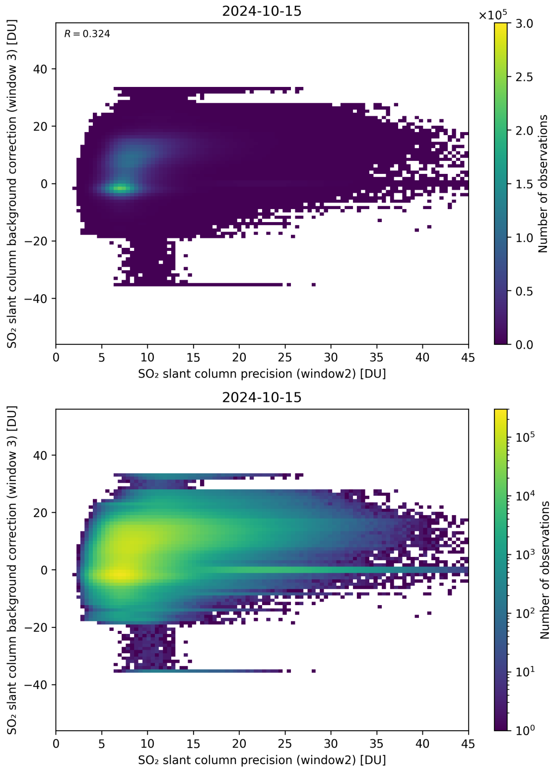
Figure 242: Scatter density plot of “SO 2 slant column precision (window2)” against “SO 2 slant column background correction (window 3)” for 2024-10-14 to 2024-10-16.
