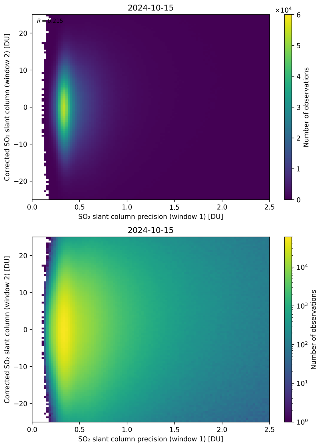
Figure 225: Scatter density plot of “SO 2 slant column precision (window 1)” against “Corrected SO 2 slant column (window 2)” for 2024-10-14 to 2024-10-16.
