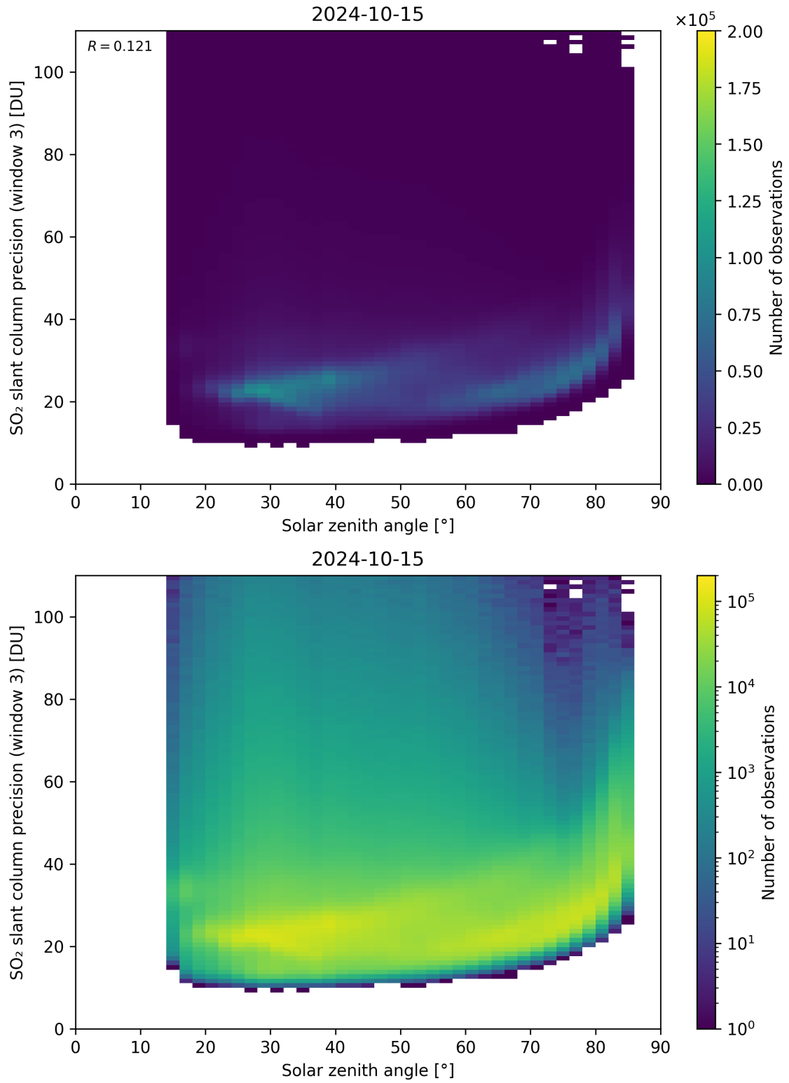
Figure 173: Scatter density plot of “Solar zenith angle” against “SO 2 slant column precision (window 3)” for 2024-10-14 to 2024-10-16.
