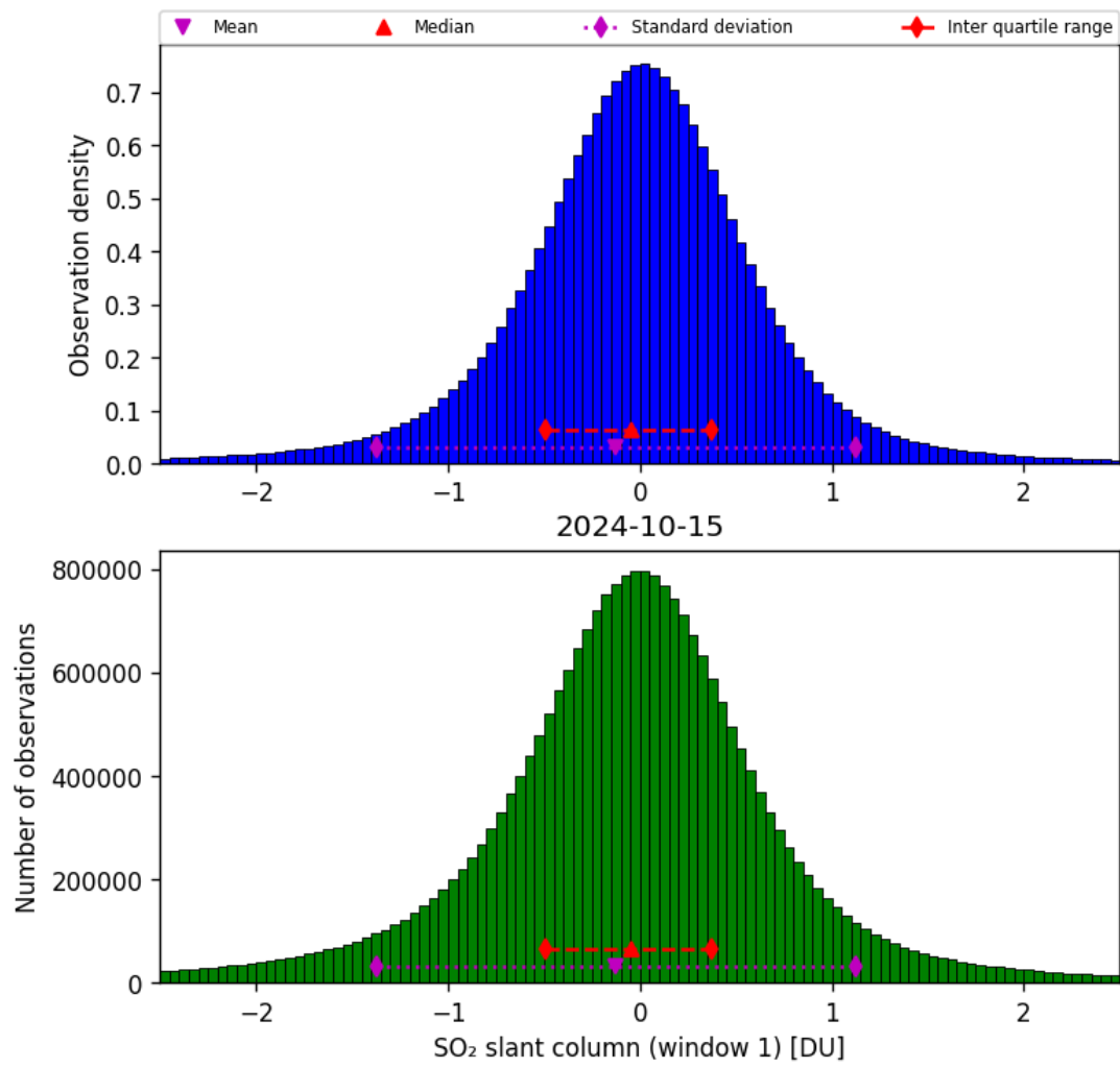
Figure 56: Histogram of “SO 2 slant column (window 1)” for 2024-10-14 to 2024-10-16
