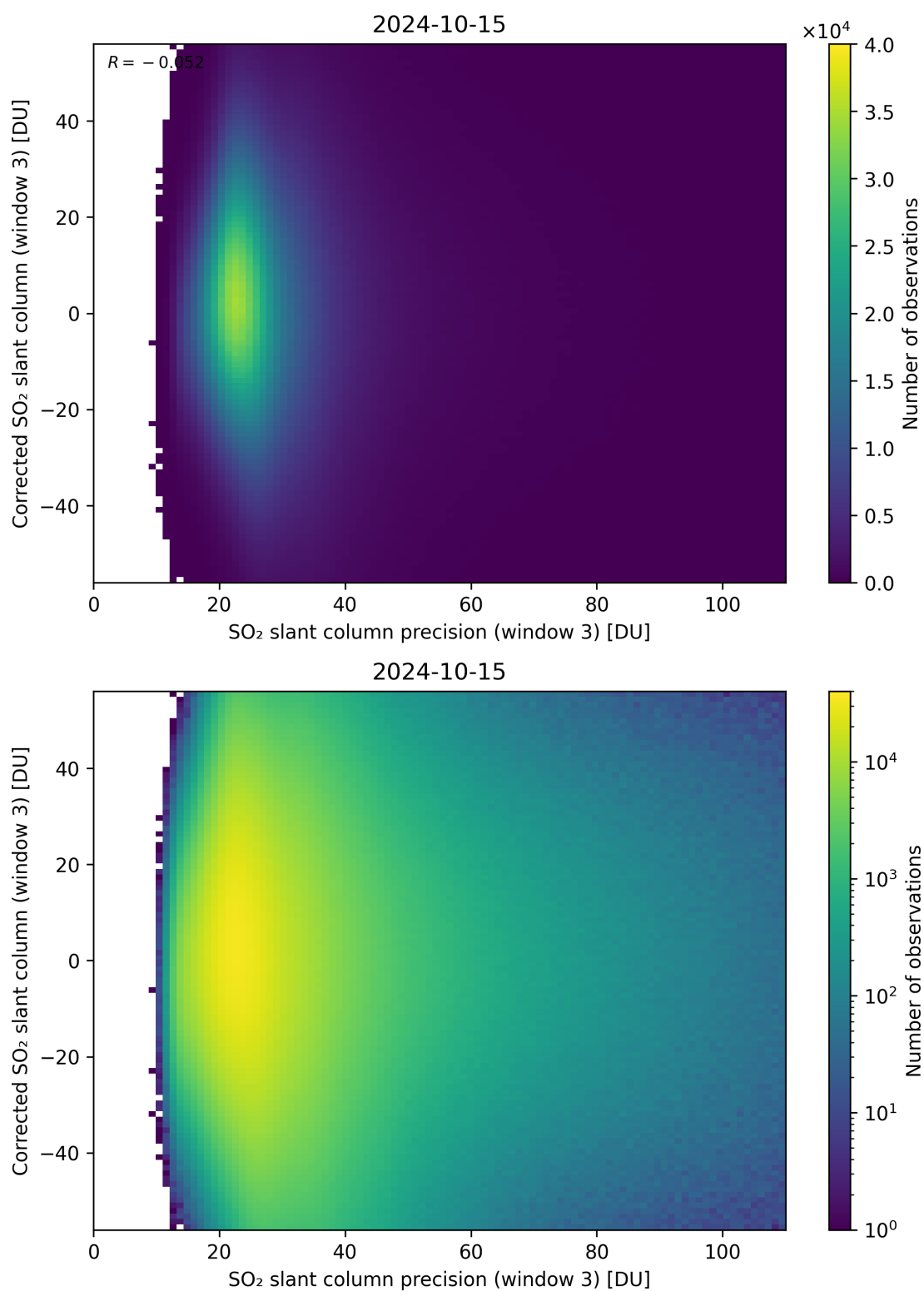
Figure 262: Scatter density plot of “SO 2 slant column precision (window 3)” against “Corrected SO 2 slant column (window 3)” for 2024-10-14 to 2024-10-16.
