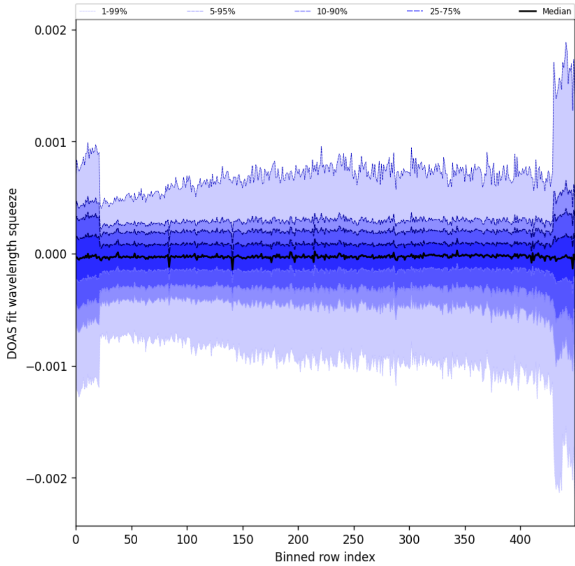
Figure 92: Along track statistics of “DOAS fit wavelength squeeze” for 2024-10-14 to 2024-10-16
