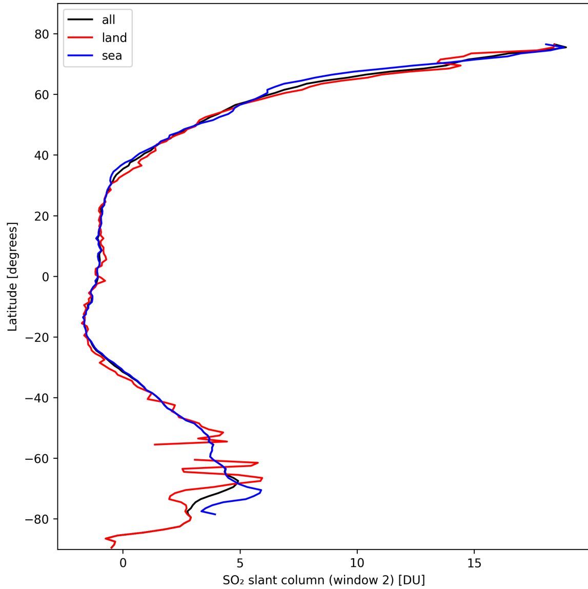
Figure 37: Zonal average of “SO 2 slant column (window 2)” for 2024-10-14 to 2024-10-16.
