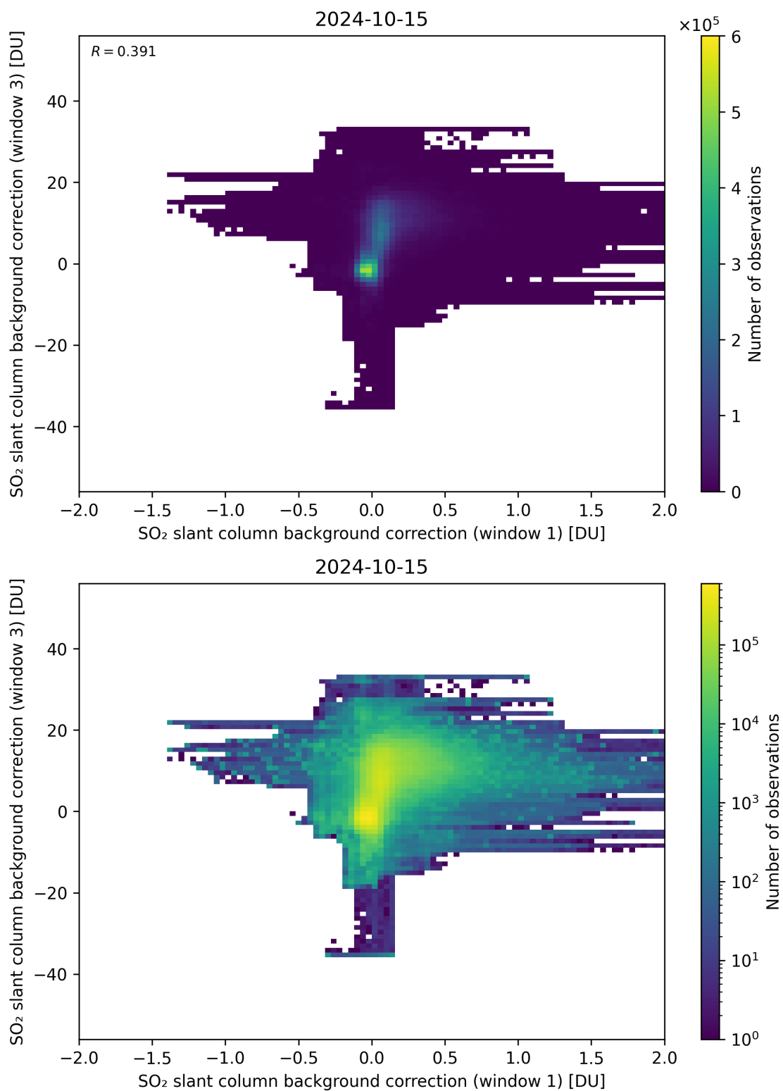
Figure 99: Scatter density plot of “SO 2 slant column background correction (window 1)” against “SO 2 slant column background correction (window 3)” for 2024-10-14 to 2024-10-16.
