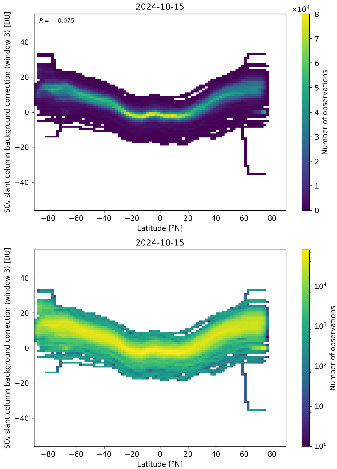
Figure 141: Scatter density plot of “Latitude” against “SO 2 slant column background correction (window 3)” for 2024-10-14 to 2024-10-16.
