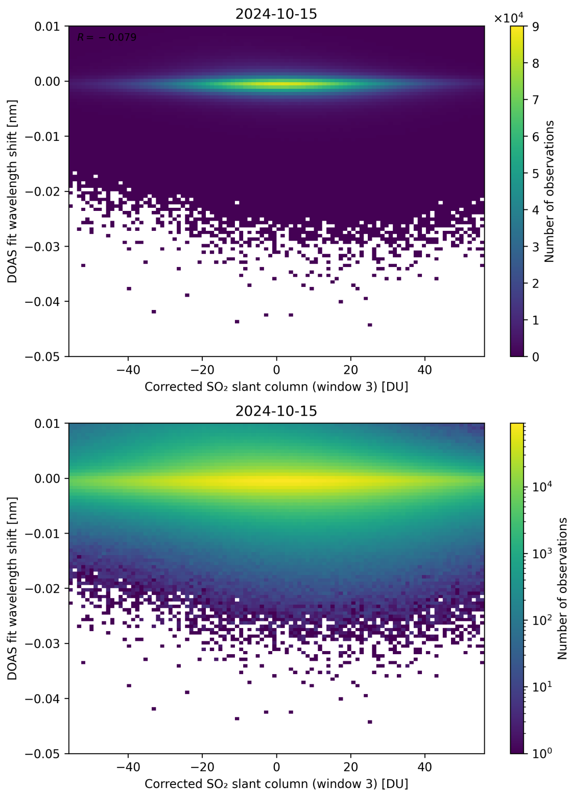
Figure 206: Scatter density plot of “Corrected SO 2 slant column (window 3)” against “DOAS fit wavelength shift” for 2024-10-14 to 2024-10-16.
