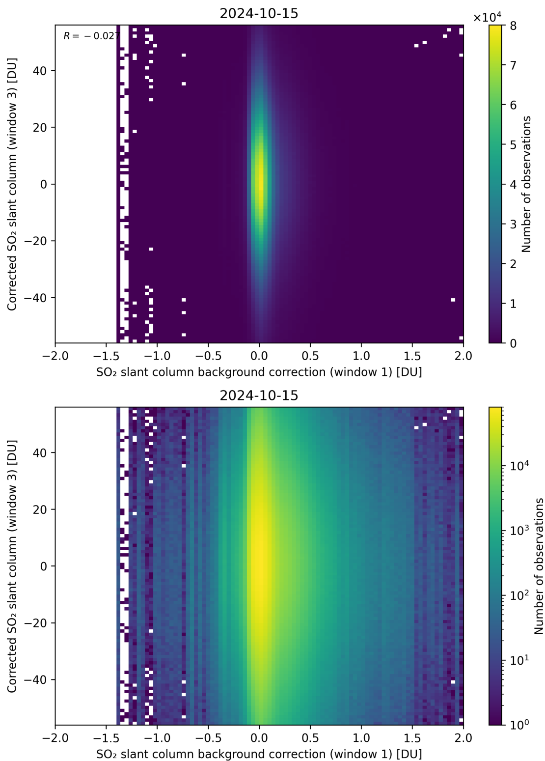
Figure 105: Scatter density plot of “SO 2 slant column background correction (window 1)” against “Corrected SO 2 slant column (window 3)” for 2024-10-14 to 2024-10-16.
