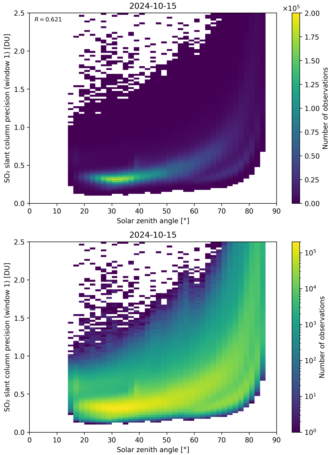
Figure 170: Scatter density plot of “Solar zenith angle” against “SO 2 slant column precision (window 1)” for 2024-10-14 to 2024-10-16.
