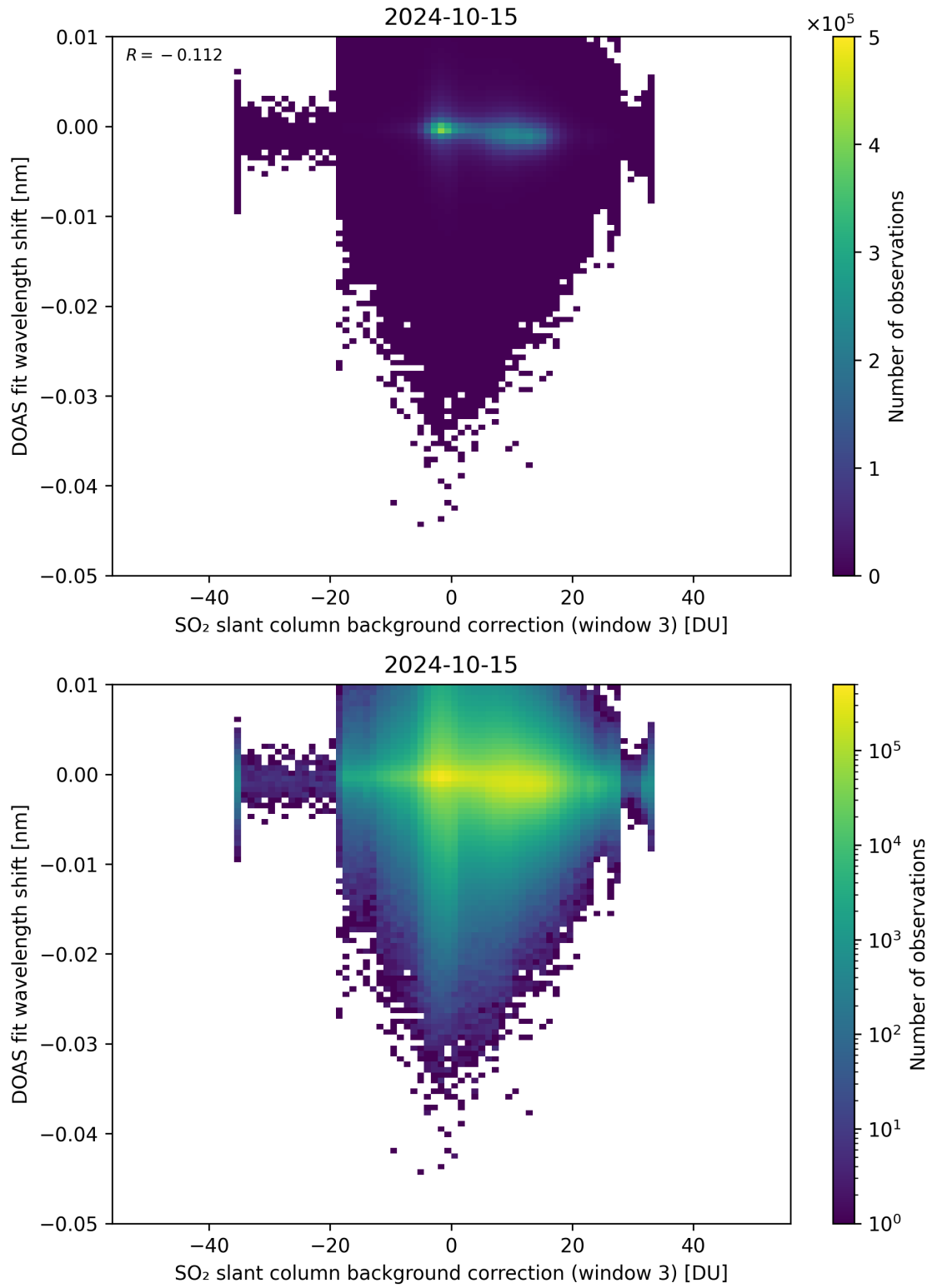
Figure 121: Scatter density plot of “SO 2 slant column background correction (window 3)” against “DOAS fit wavelength shift” for 2024-10-14 to 2024-10-16.
