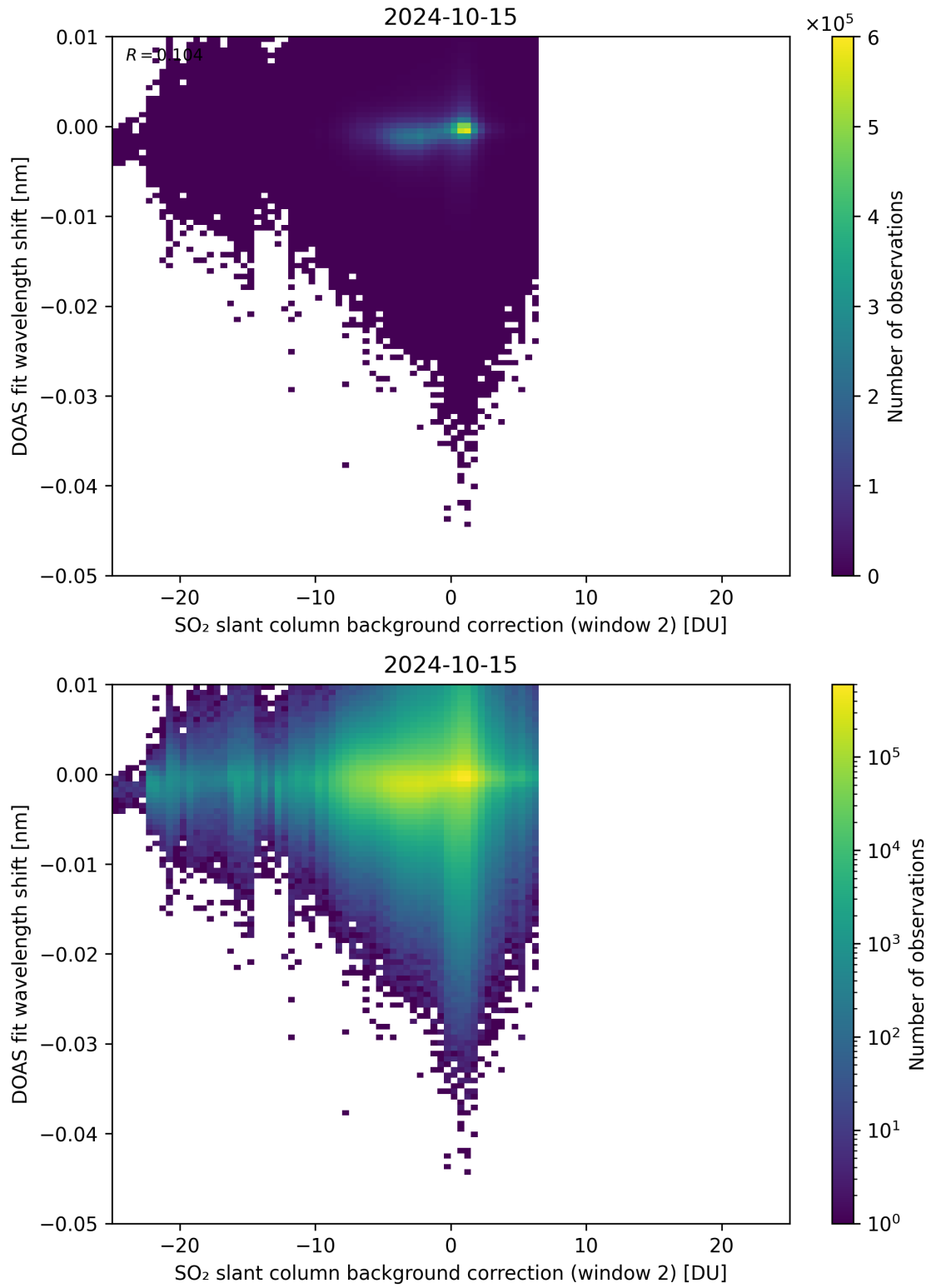
Figure 112: Scatter density plot of “SO 2 slant column background correction (window 2)” against “DOAS fit wavelength shift” for 2024-10-14 to 2024-10-16.
