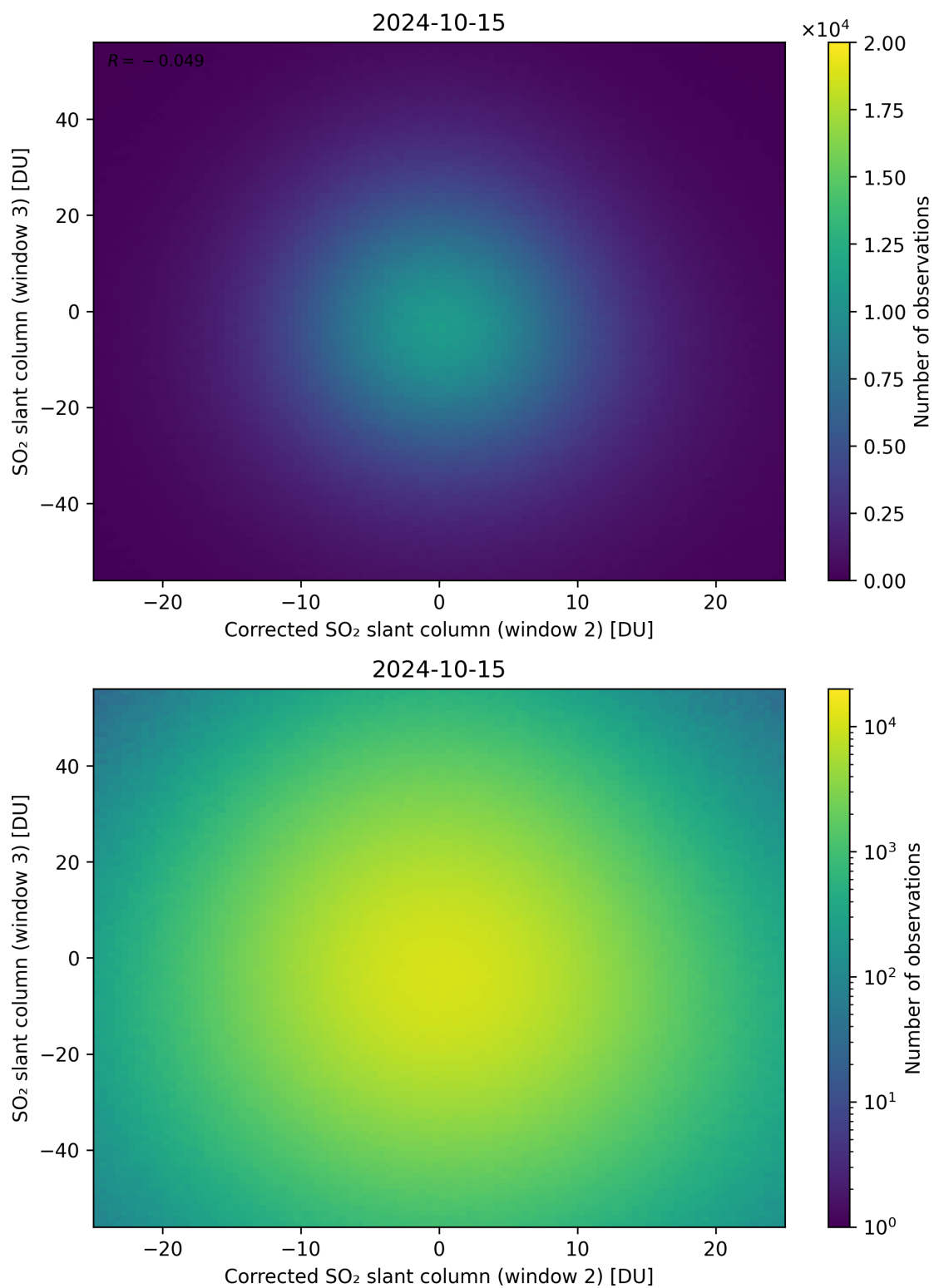
Figure 201: Scatter density plot of “Corrected SO 2 slant column (window 2)” against “SO 2 slant column (window 3)” for 2024-10-14 to 2024-10-16.
