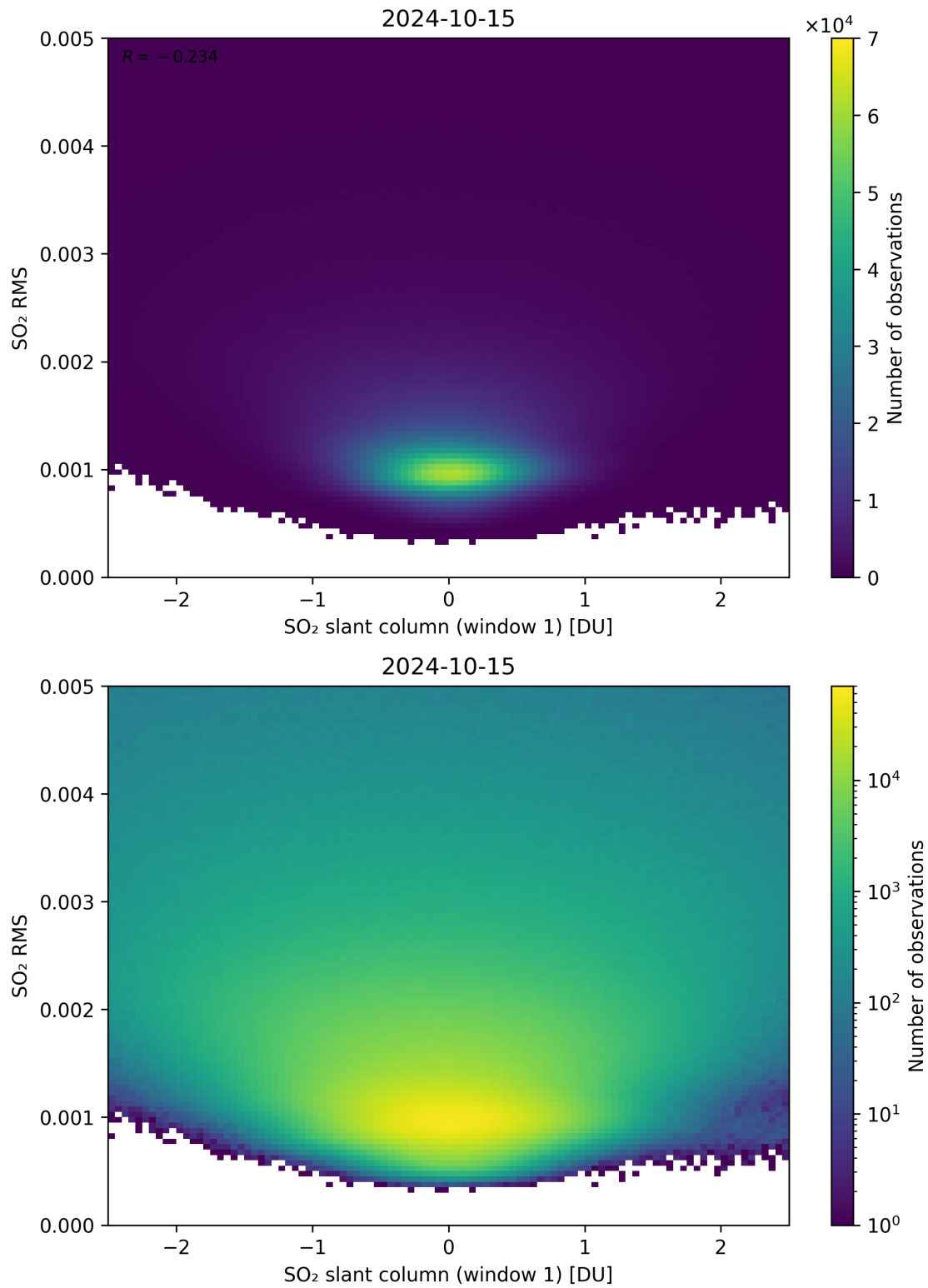
Figure 217: Scatter density plot of “SO 2 slant column (window 1)” against “SO 2 RMS” for 2024-10-14 to 2024-10-16.
