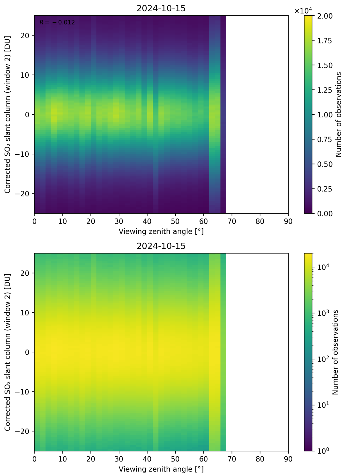
Figure 318: Scatter density plot of “Viewing zenith angle” against “Corrected SO 2 slant column (window 2)” for 2024-10-14 to 2024-10-16.
