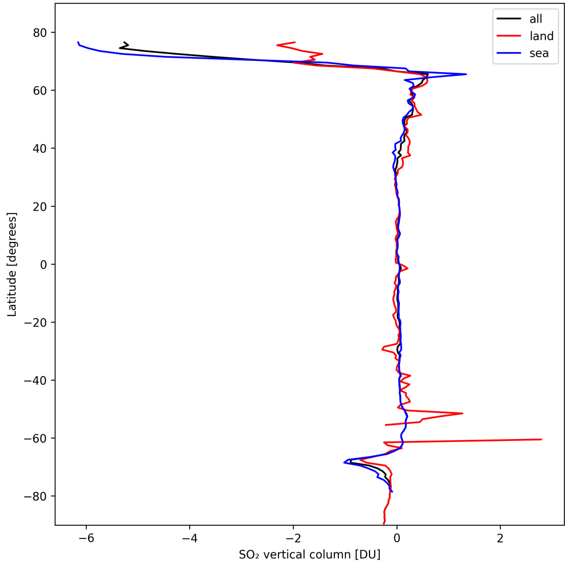
Figure 30: Zonal average of “SO 2 vertical column” for 2024-10-14 to 2024-10-16.
