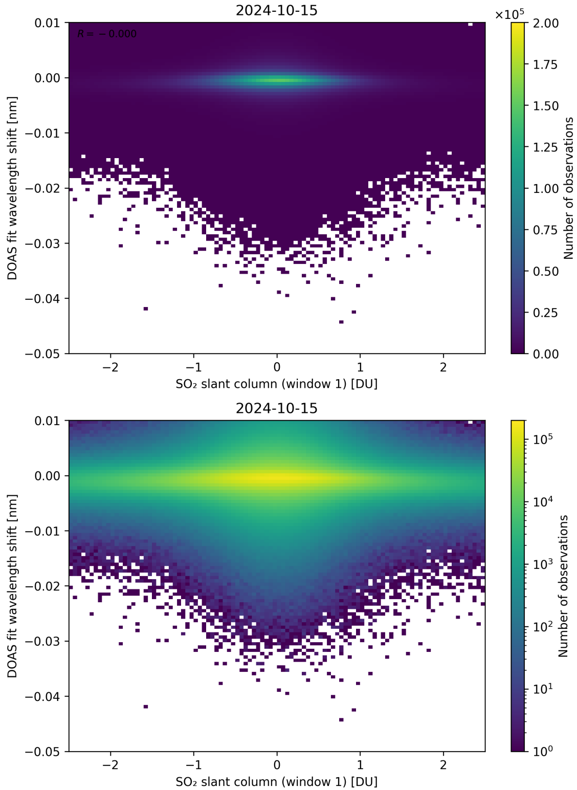
Figure 215: Scatter density plot of “SO 2 slant column (window 1)” against “DOAS fit wavelength shift” for 2024-10-14 to 2024-10-16.
