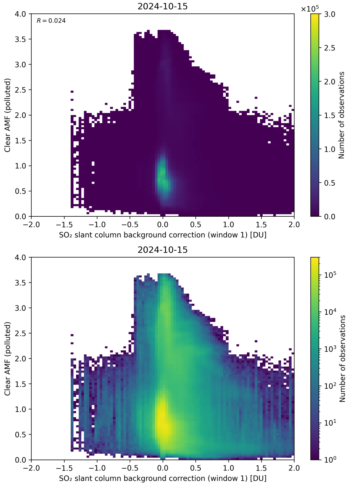
Figure 103: Scatter density plot of “SO 2 slant column background correction (window 1)” against “Clear AMF (polluted)” for 2024-10-14 to 2024-10-16.
