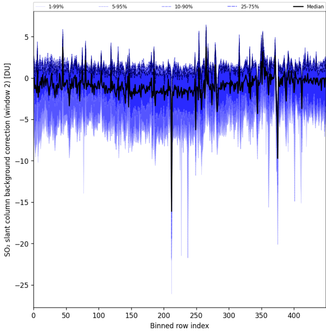
Figure 86: Along track statistics of “SO 2 slant column background correction (window 2)” for 2024-10-14 to 2024-10-16
