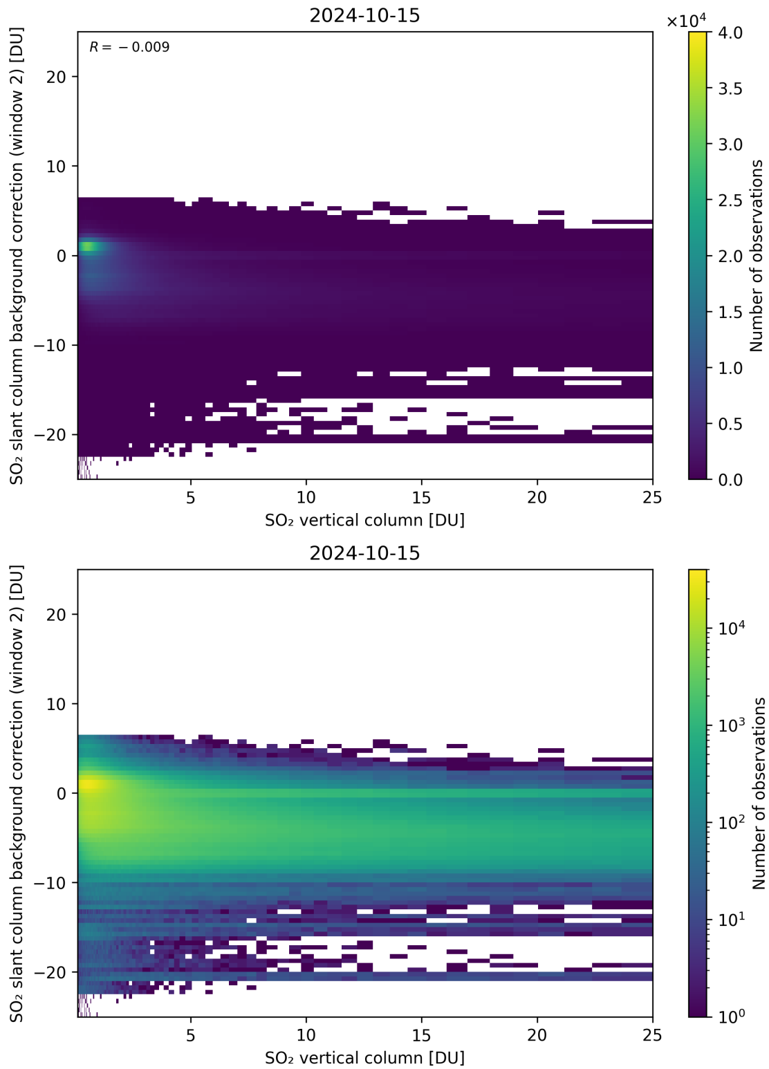
Figure 274: Scatter density plot of “SO 2 vertical column” against “SO 2 slant column background correction (window 2)” for 2024-10-14 to 2024-10-16.
