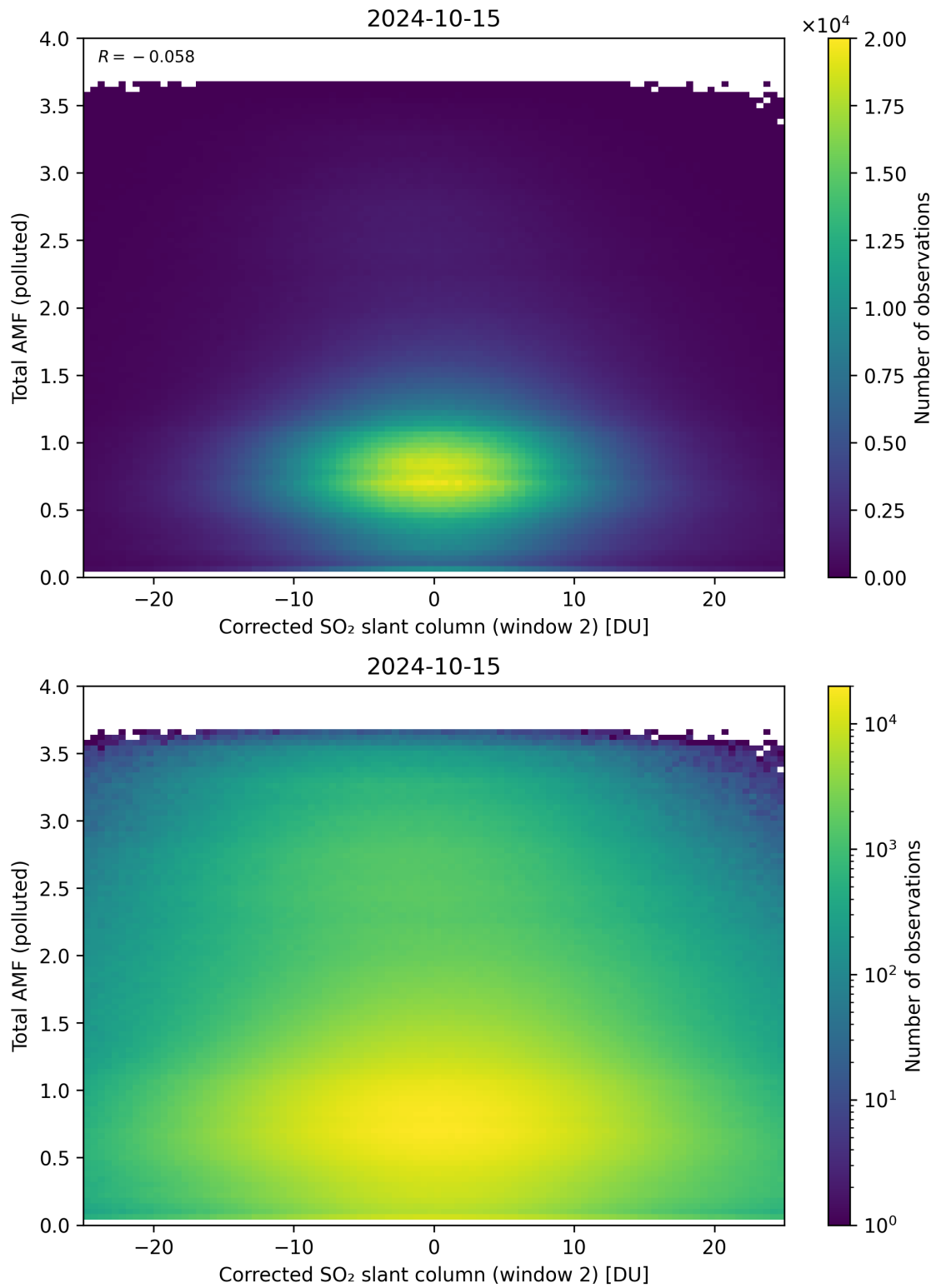
Figure 203: Scatter density plot of “Corrected SO 2 slant column (window 2)” against “Total AMF (polluted)” for 2024-10-14 to 2024-10-16.
