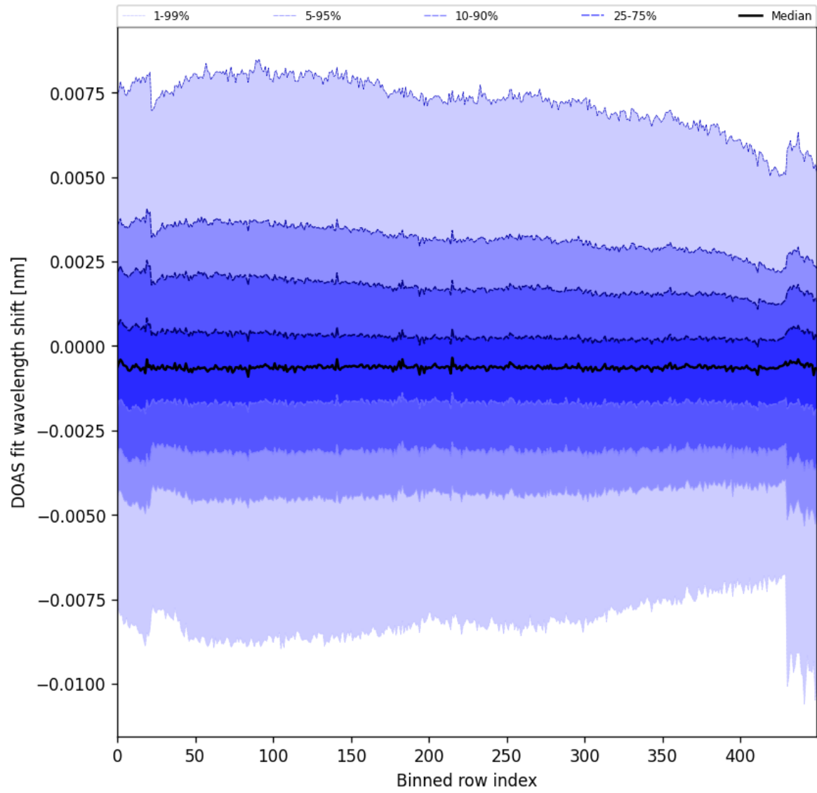
Figure 91: Along track statistics of “DOAS fit wavelength shift” for 2024-10-14 to 2024-10-16
