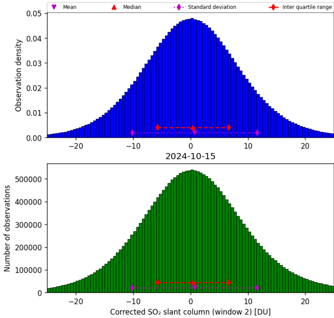
Figure 62: Histogram of “Corrected SO 2 slant column (window 2)” for 2024-10-14 to 2024-10-16
