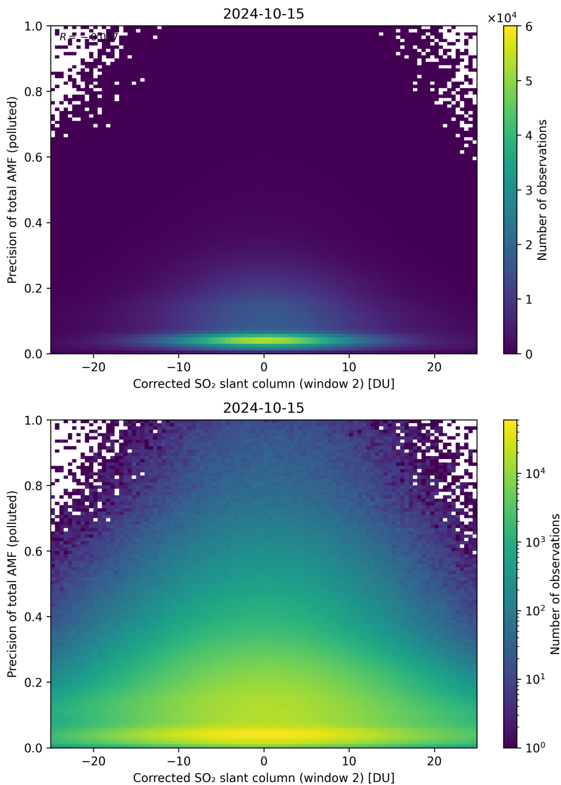
Figure 204: Scatter density plot of “Corrected SO 2 slant column (window 2)” against “Precision of total AMF (polluted)” for 2024-10-14 to 2024-10-16.
