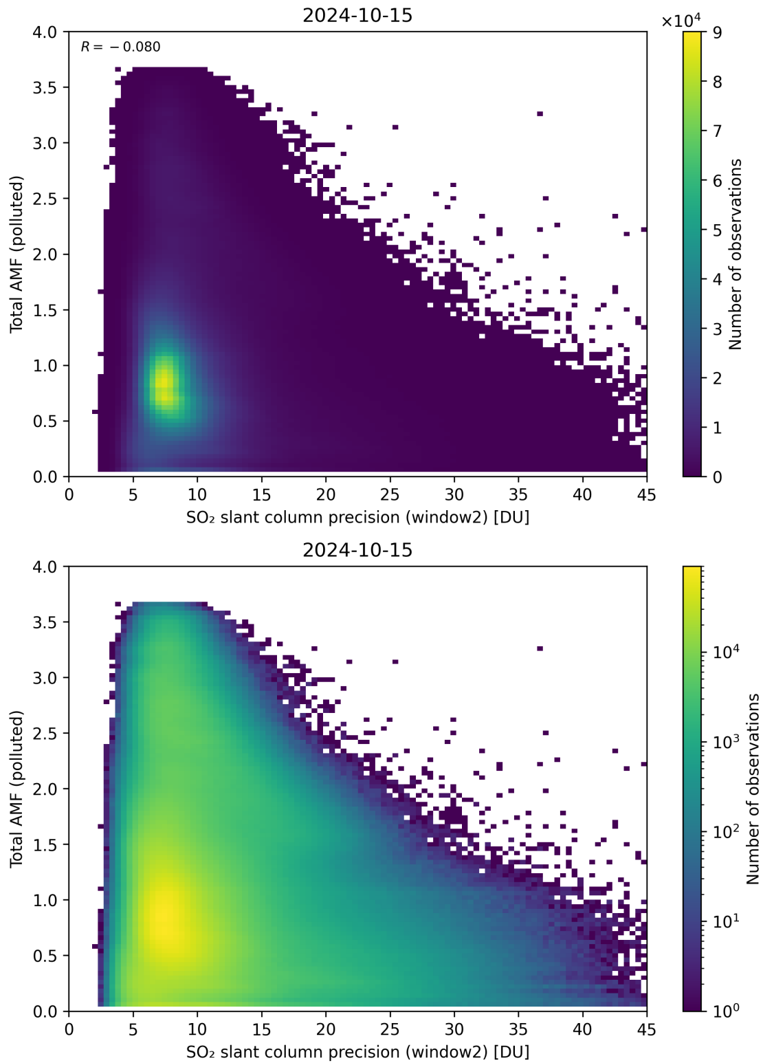
Figure 251: Scatter density plot of “SO 2 slant column precision (window2)” against “Total AMF (polluted)” for 2024-10-14 to 2024-10-16.
