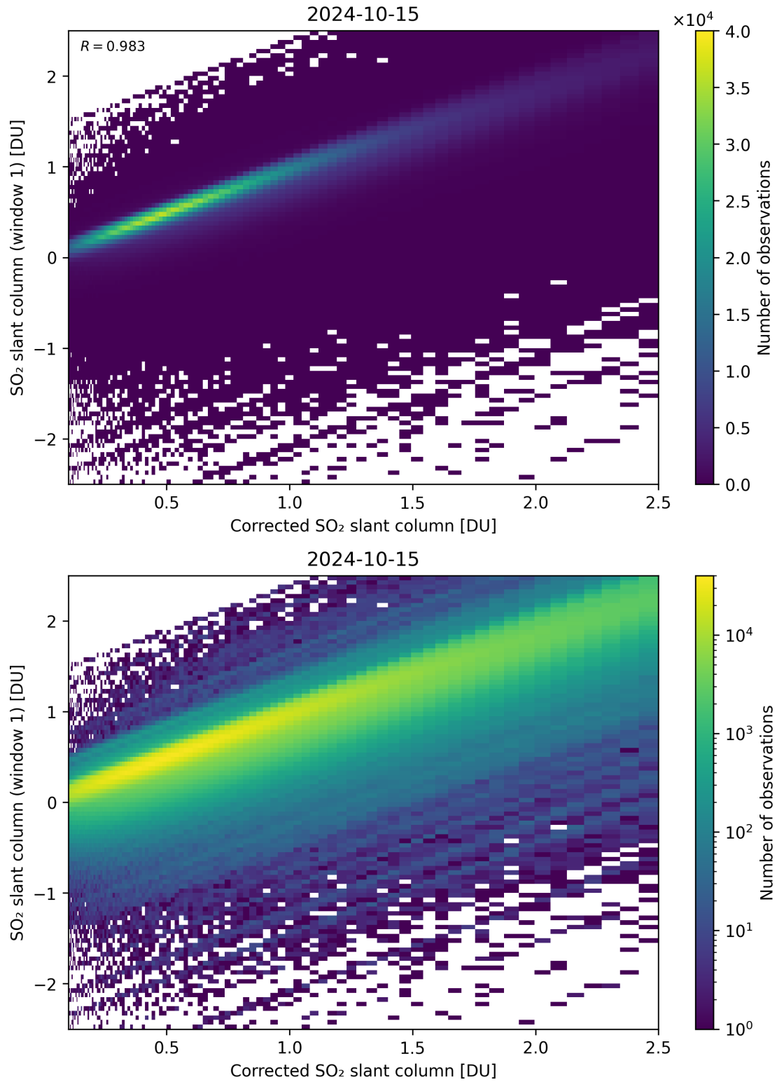
Figure 187: Scatter density plot of “Corrected SO 2 slant column” against “SO 2 slant column (window 1)” for 2024-10-14 to 2024-10-16.
