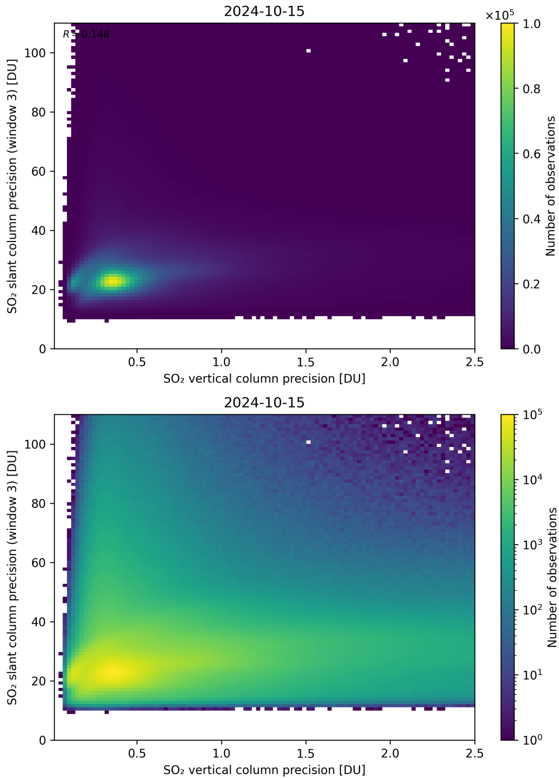
Figure 293: Scatter density plot of “SO 2 vertical column precision” against “SO 2 slant column precision (window 3)” for 2024-10-14 to 2024-10-16.
