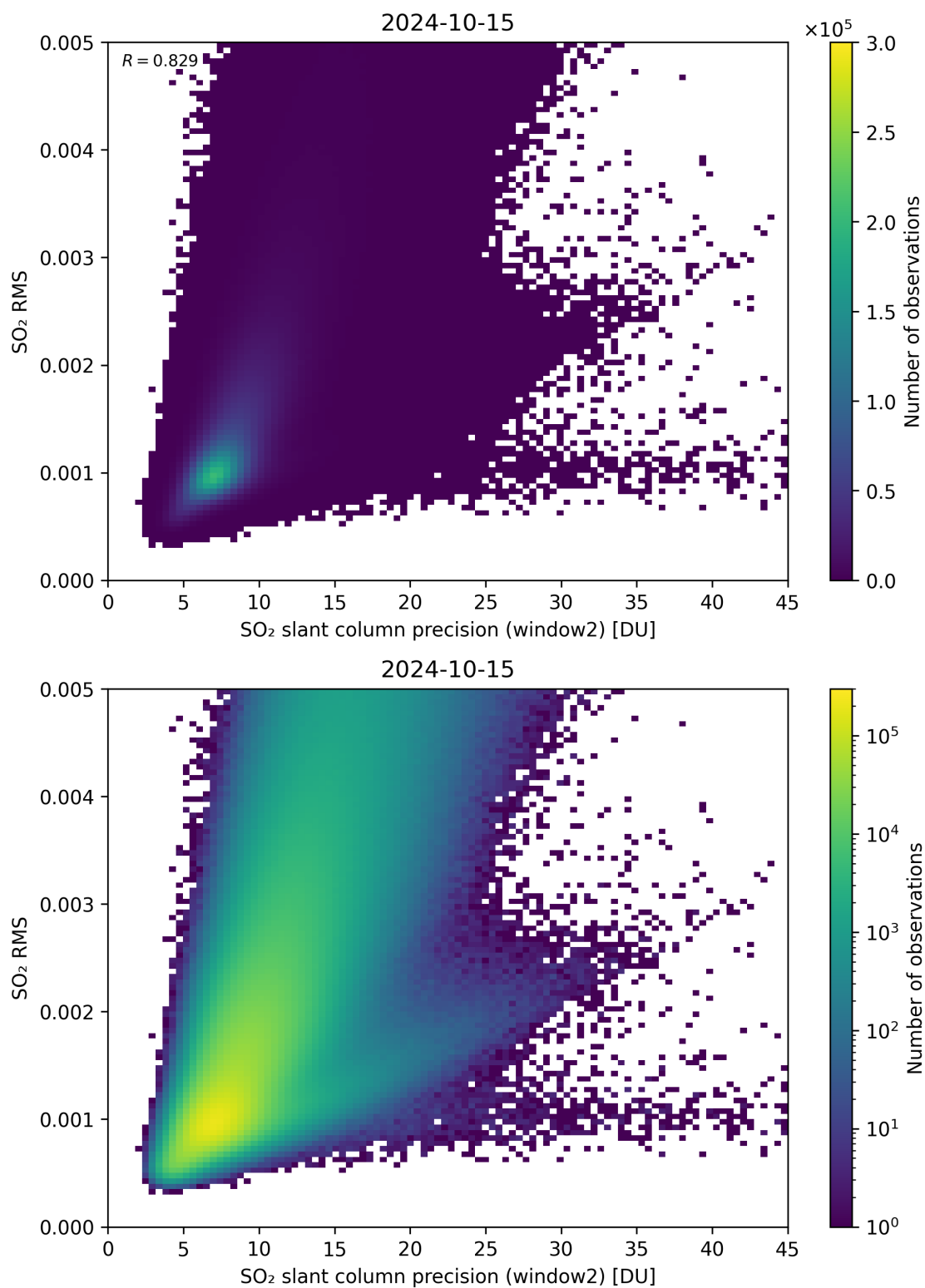
Figure 245: Scatter density plot of “SO 2 slant column precision (window2)” against “SO 2 RMS” for 2024-10-14 to 2024-10-16.
