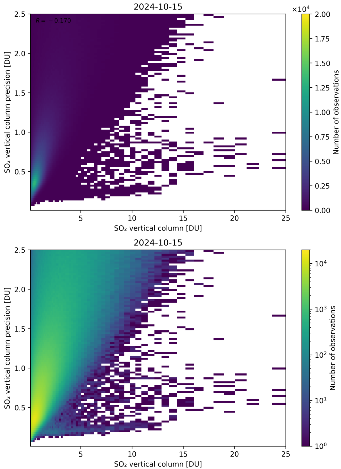
Figure 307: Scatter density plot of “SO 2 vertical column” against “SO 2 vertical column precision” for 2024-10-14 to 2024-10-16.
