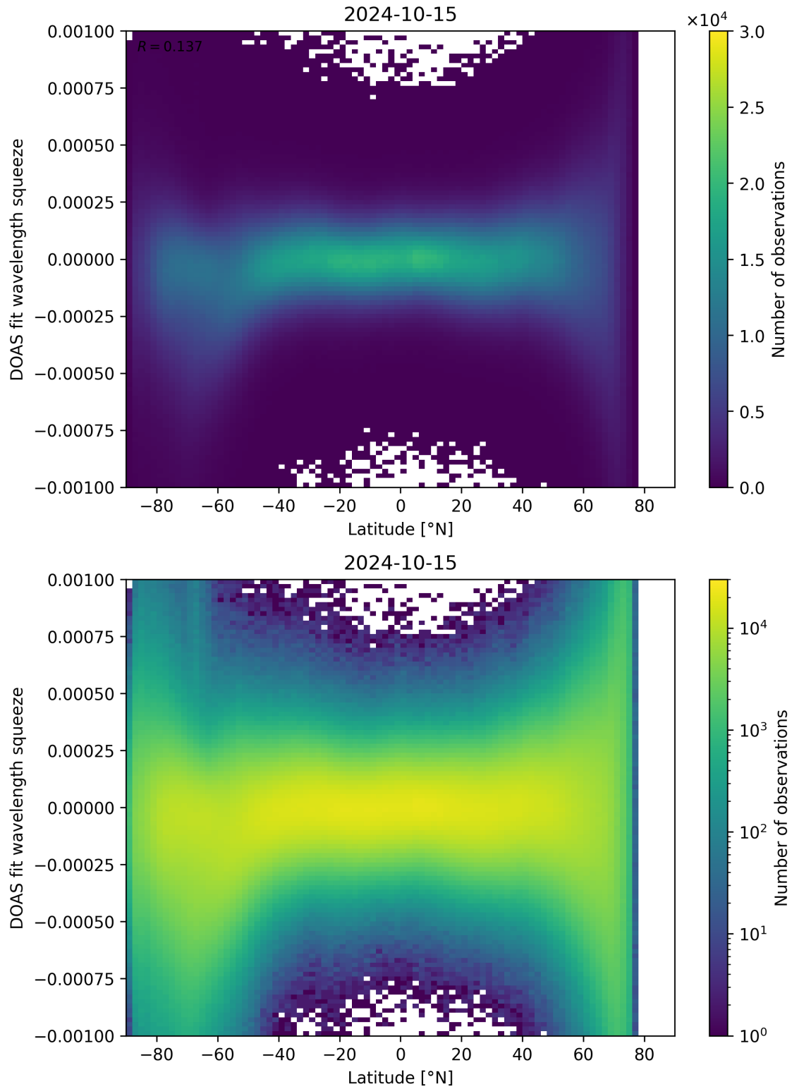
Figure 143: Scatter density plot of “Latitude” against “DOAS fit wavelength squeeze” for 2024-10-14 to 2024-10-16.
