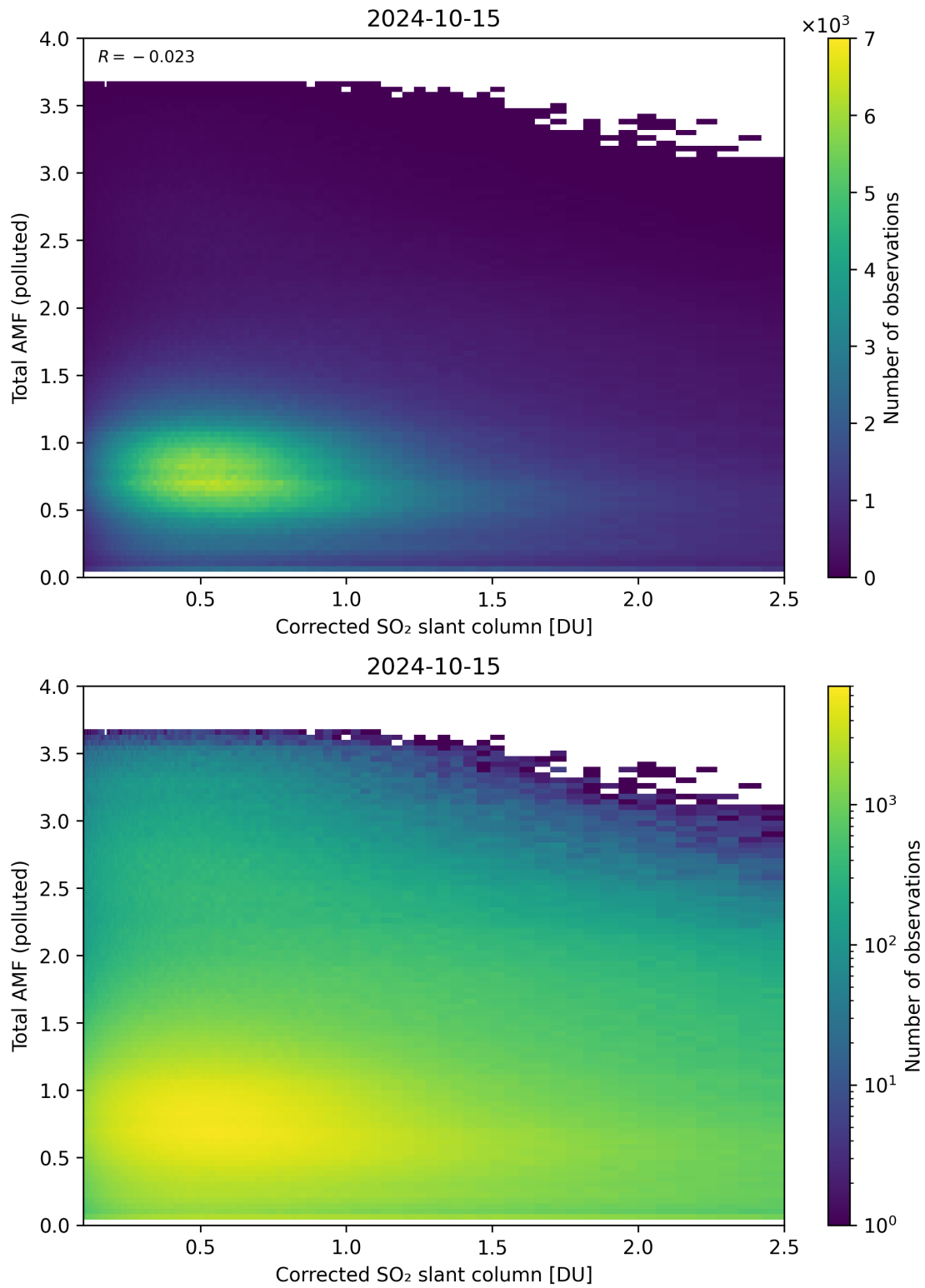
Figure 192: Scatter density plot of “Corrected SO 2 slant column” against “Total AMF (polluted)” for 2024-10-14 to 2024-10-16.
