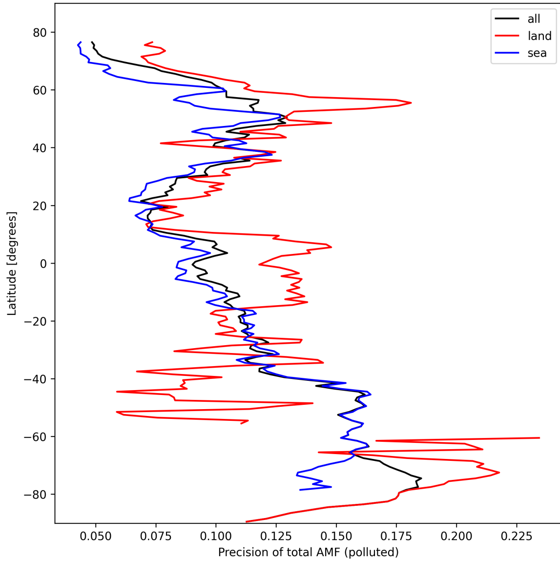
Figure 49: Zonal average of “Precision of total AMF (polluted)” for 2024-10-14 to 2024-10-16.
