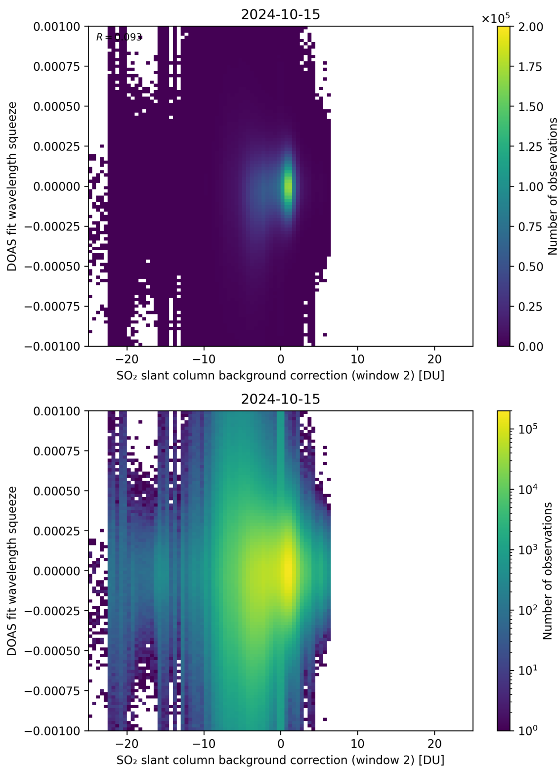
Figure 113: Scatter density plot of “SO 2 slant column background correction (window 2)” against “DOAS fit wavelength squeeze” for 2024-10-14 to 2024-10-16.
