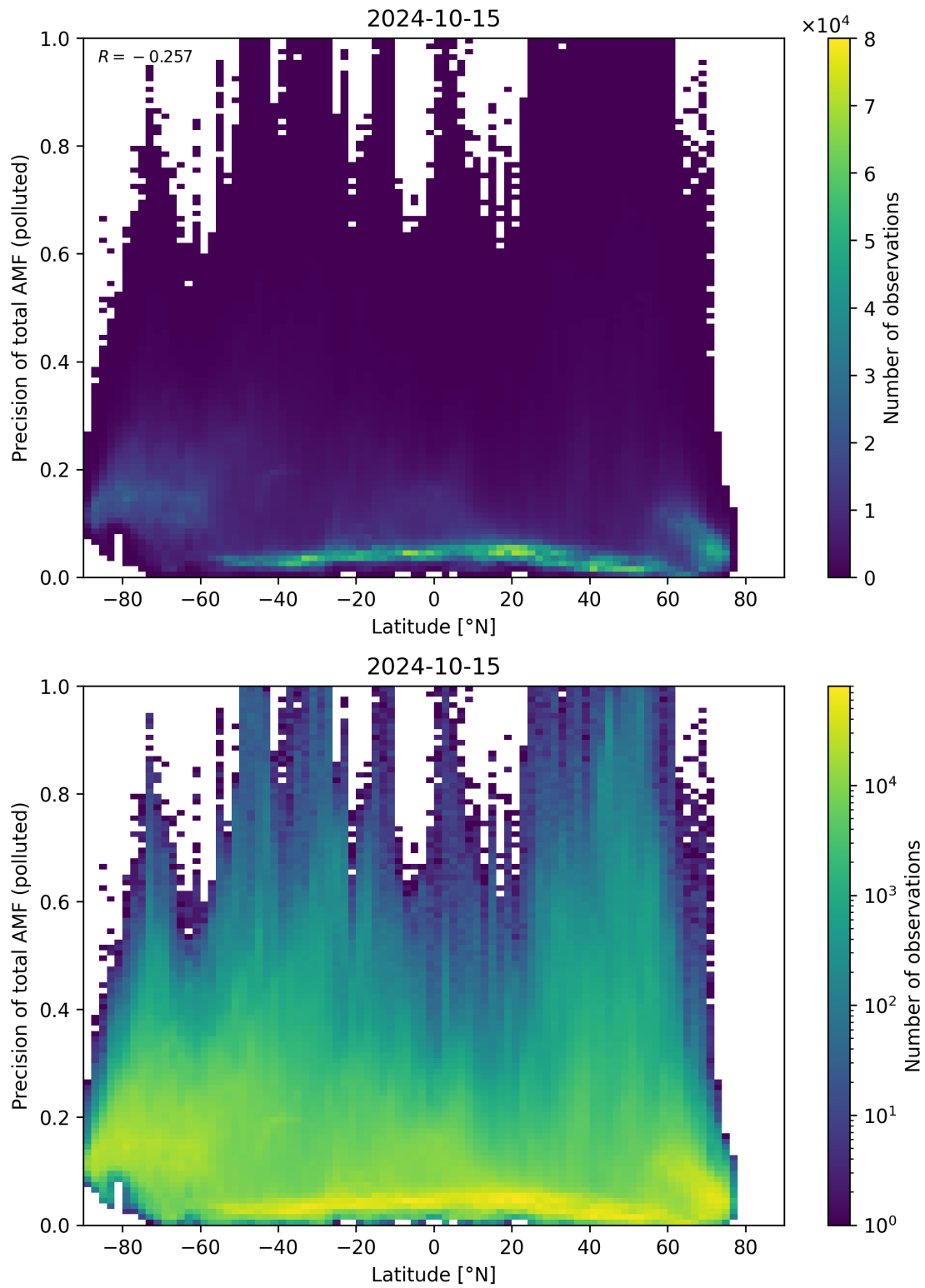
Figure 155: Scatter density plot of “Latitude” against “Precision of total AMF (polluted)” for 2024-10-14 to 2024-10-16.
