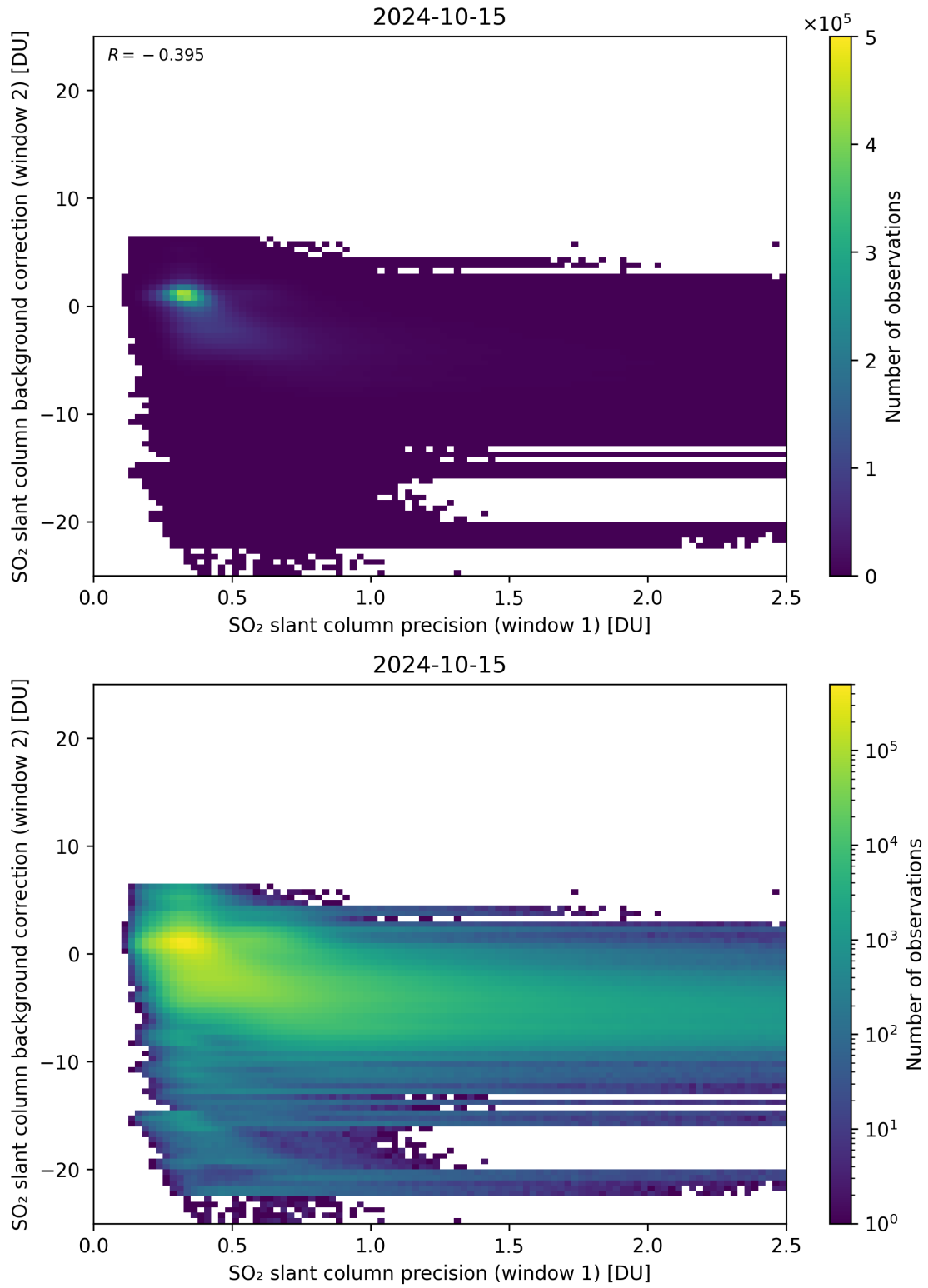
Figure 219: Scatter density plot of “SO 2 slant column precision (window 1)” against “SO 2 slant column background correction (window 2)” for 2024-10-14 to 2024-10-16.
