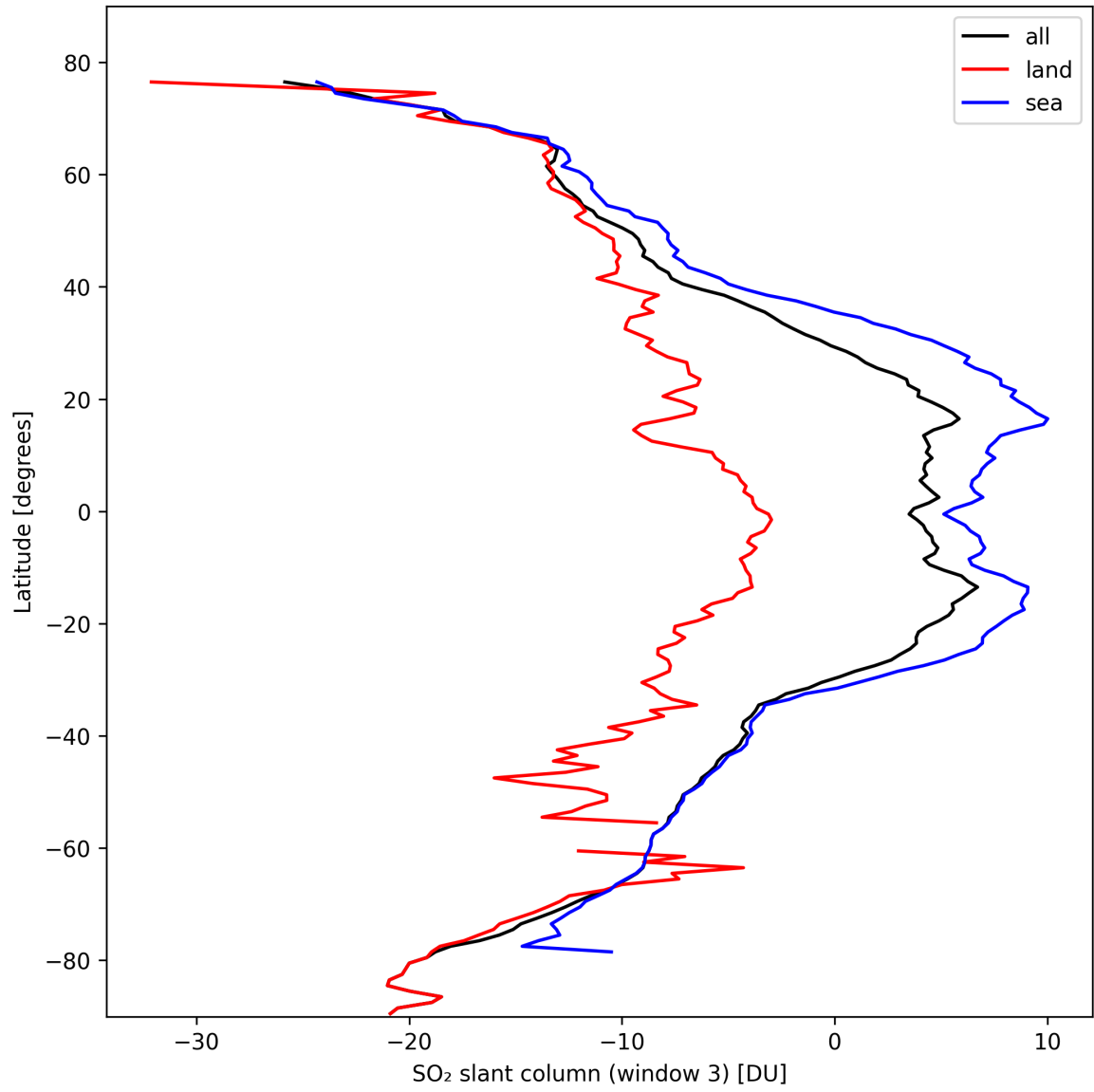
Figure 41: Zonal average of “SO 2 slant column (window 3)” for 2024-10-14 to 2024-10-16.
