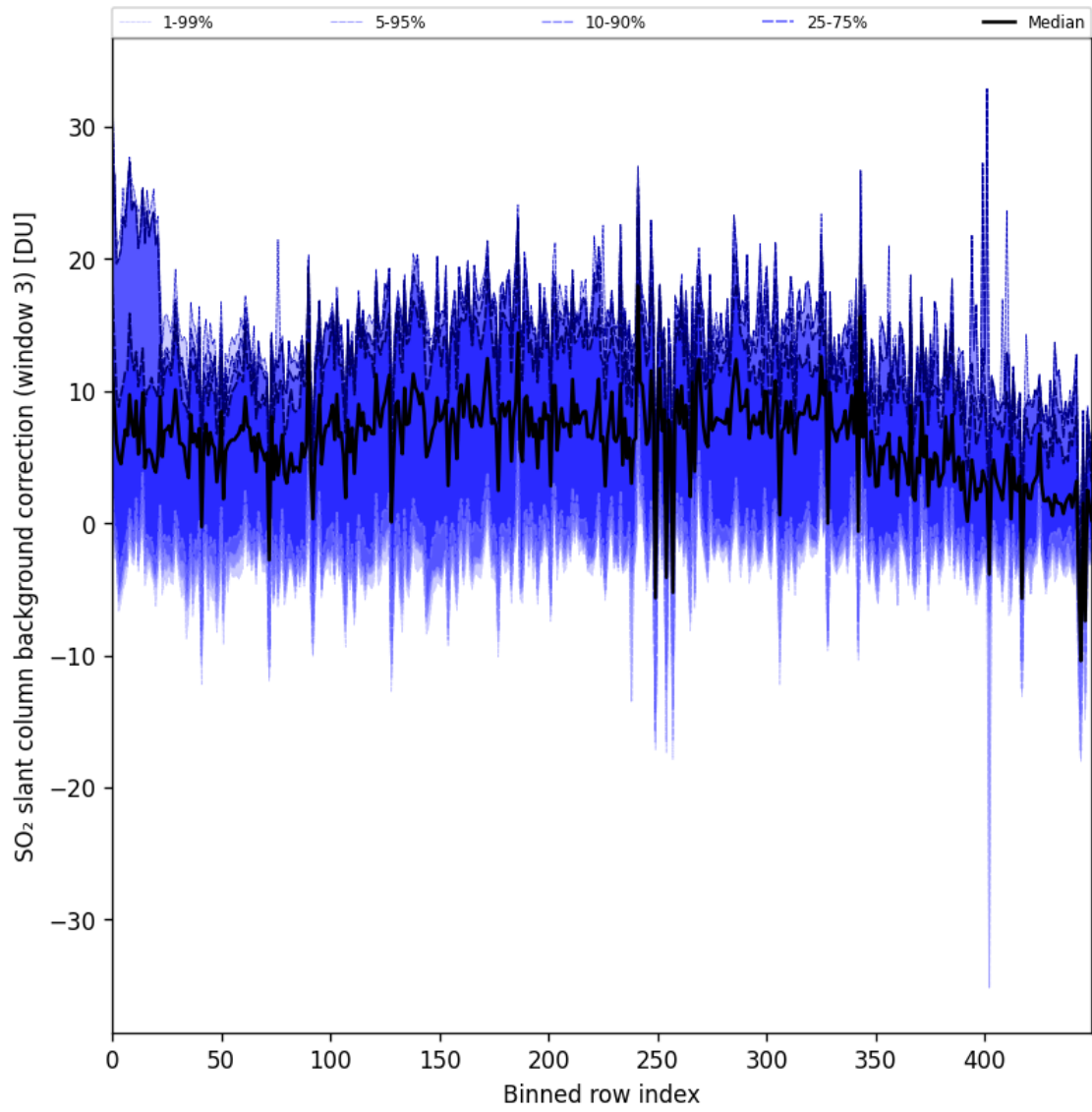
Figure 90: Along track statistics of “SO 2 slant column background correction (window 3)” for 2024-10-14 to 2024-10-16
