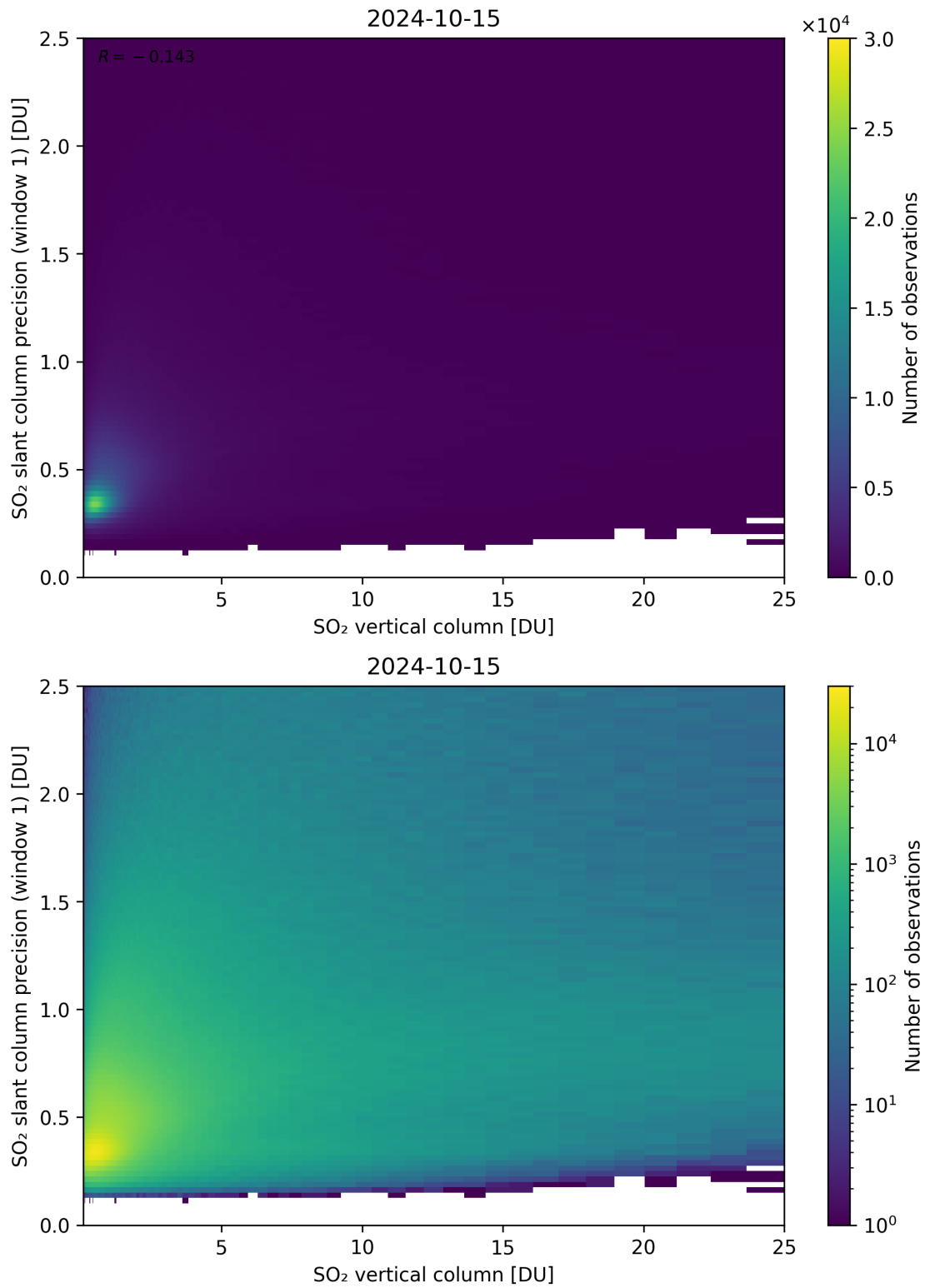
Figure 301: Scatter density plot of “SO 2 vertical column” against “SO 2 slant column precision (window 1)” for 2024-10-14 to 2024-10-16.
