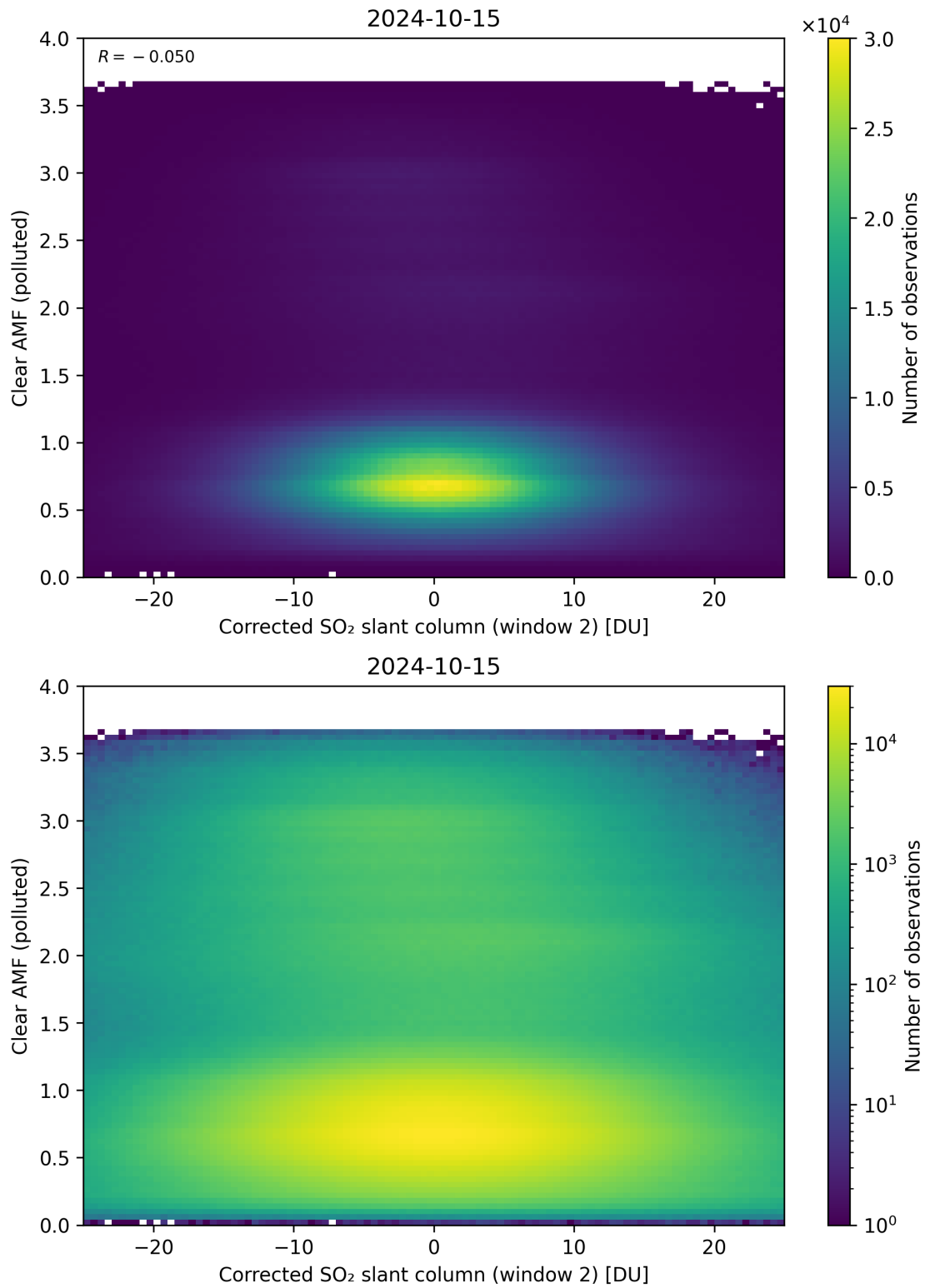
Figure 199: Scatter density plot of “Corrected SO 2 slant column (window 2)” against “Clear AMF (polluted)” for 2024-10-14 to 2024-10-16.
