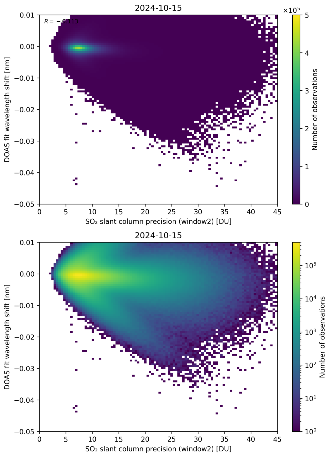
Figure 243: Scatter density plot of “SO 2 slant column precision (window2)” against “DOAS fit wavelength shift” for 2024-10-14 to 2024-10-16.
