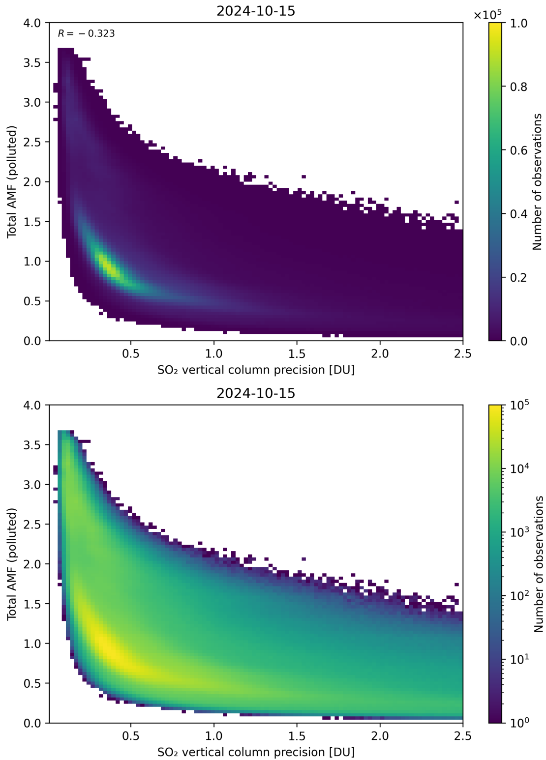
Figure 294: Scatter density plot of “SO 2 vertical column precision” against “Total AMF (polluted)” for 2024-10-14 to 2024-10-16.
