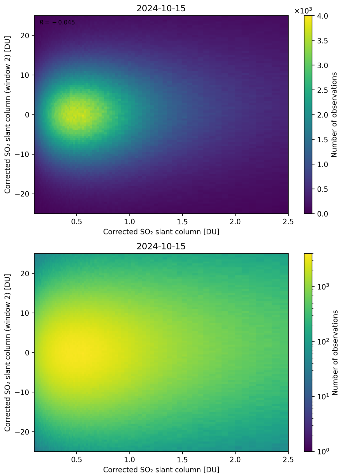
Figure 185: Scatter density plot of “Corrected SO 2 slant column” against “Corrected SO 2 slant column (window 2)” for 2024-10-14 to 2024-10-16.
