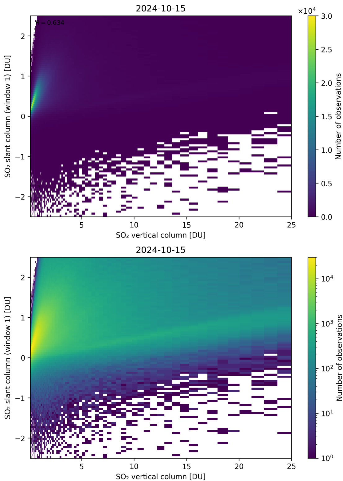
Figure 300: Scatter density plot of “SO 2 vertical column” against “SO 2 slant column (window 1)” for 2024-10-14 to 2024-10-16.
