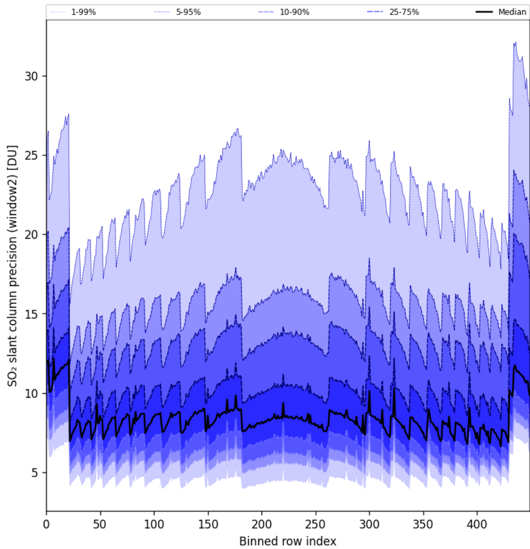
Figure 84: Along track statistics of “SO 2 slant column precision (window2)” for 2024-10-14 to 2024-10-16
