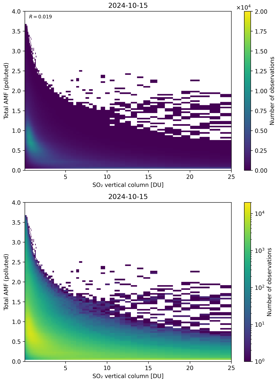
Figure 305: Scatter density plot of “SO 2 vertical column” against “Total AMF (polluted)” for 2024-10-14 to 2024-10-16.
