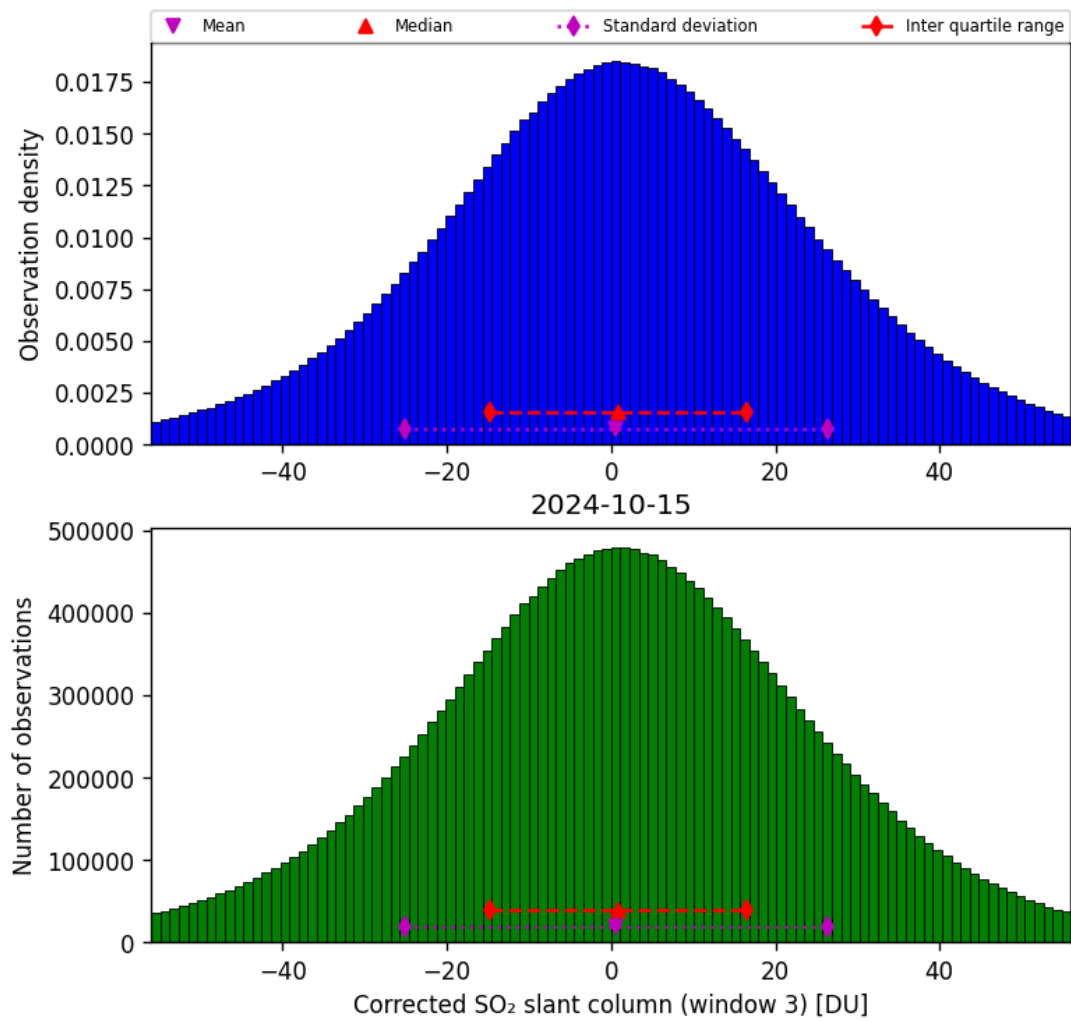
Figure 66: Histogram of “Corrected SO 2 slant column (window 3)” for 2024-10-14 to 2024-10-16
