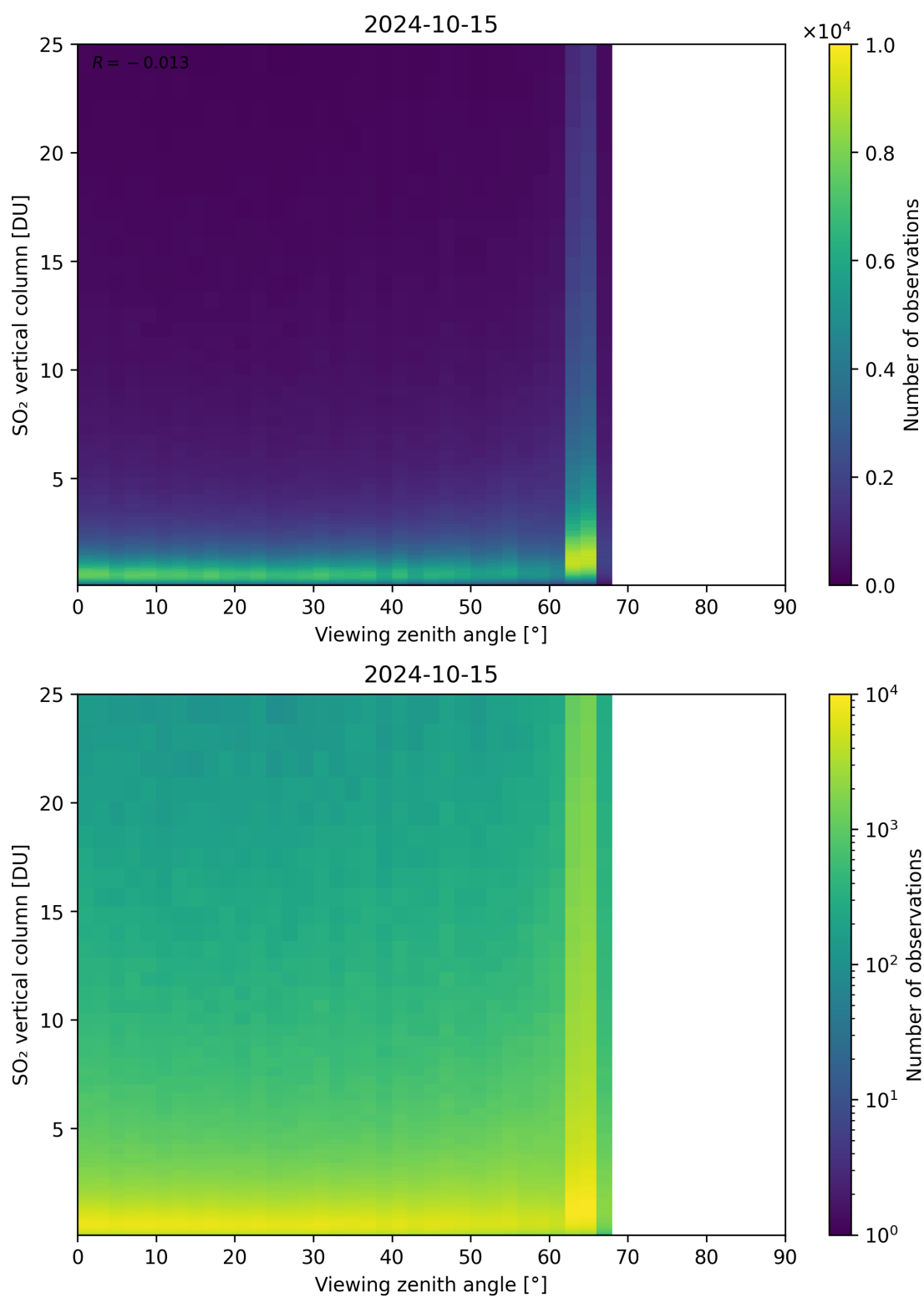
Figure 327: Scatter density plot of “Viewing zenith angle” against “SO 2 vertical column” for 2024-10-14 to 2024-10-16.
