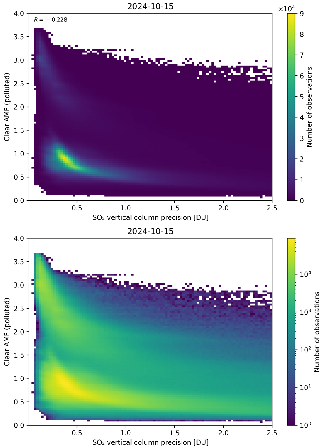
Figure 285: Scatter density plot of “SO 2 vertical column precision” against “Clear AMF (polluted)” for 2024-10-14 to 2024-10-16.
