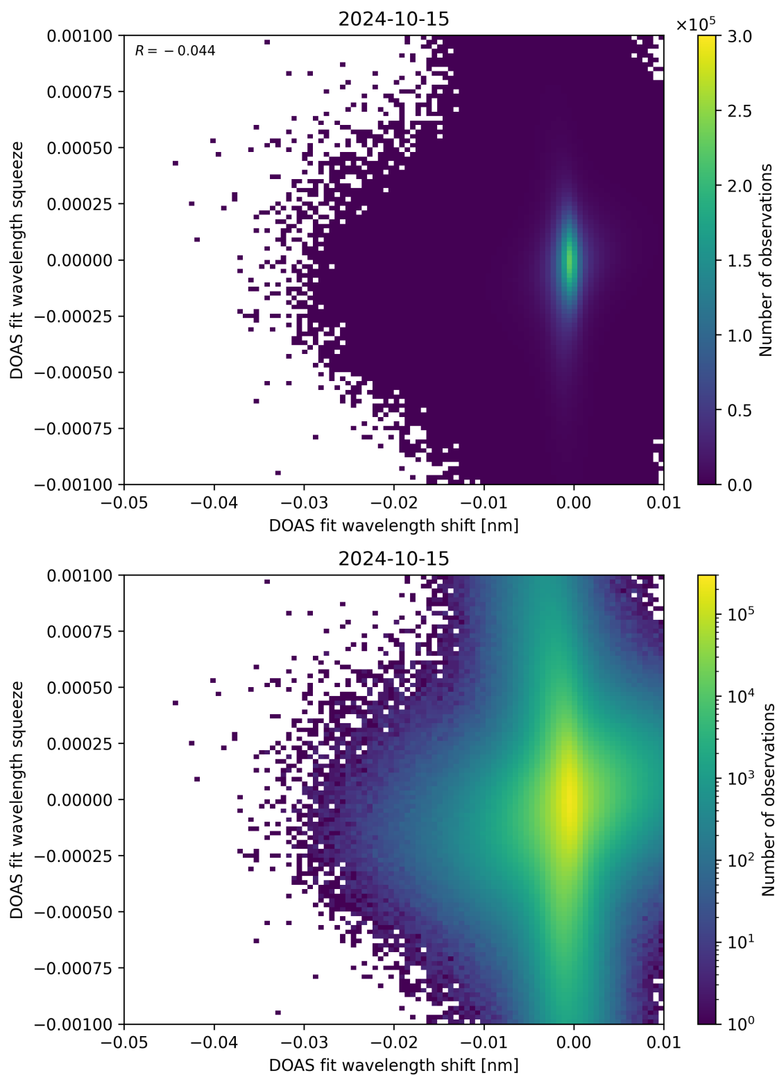
Figure 127: Scatter density plot of “DOAS fit wavelength shift” against “DOAS fit wavelength squeeze” for 2024-10-14 to 2024-10-16.
