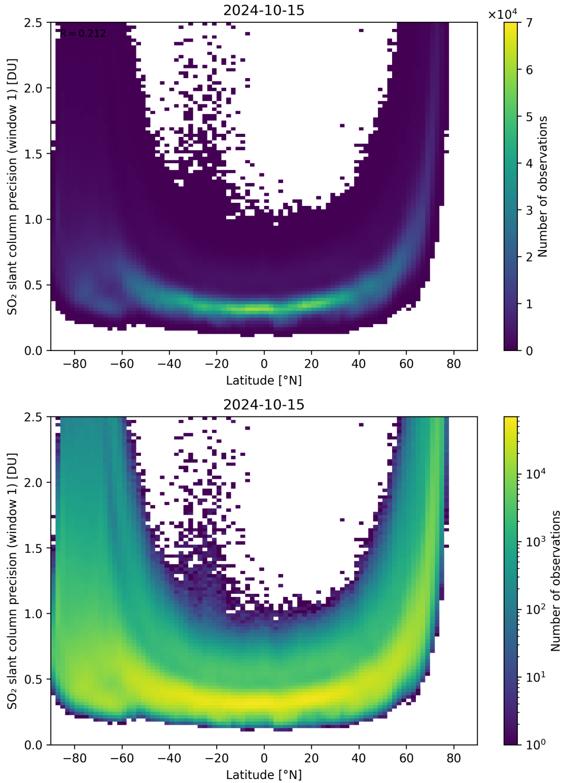
Figure 150: Scatter density plot of “Latitude” against “SO 2 slant column precision (window 1)” for 2024-10-14 to 2024-10-16.
