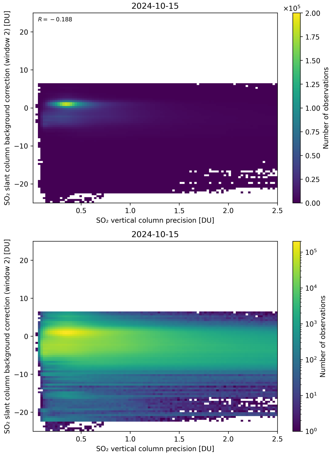
Figure 280: Scatter density plot of “SO 2 vertical column precision” against “SO 2 slant column background correction (window 2)” for 2024-10-14 to 2024-10-16.
