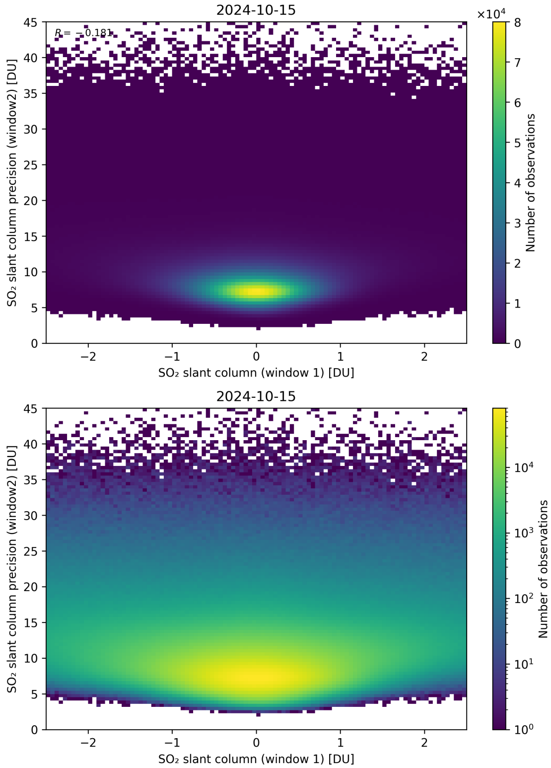
Figure 236: Scatter density plot of “SO 2 slant column (window 1)” against “SO 2 slant column precision (window2)” for 2024-10-14 to 2024-10-16.
