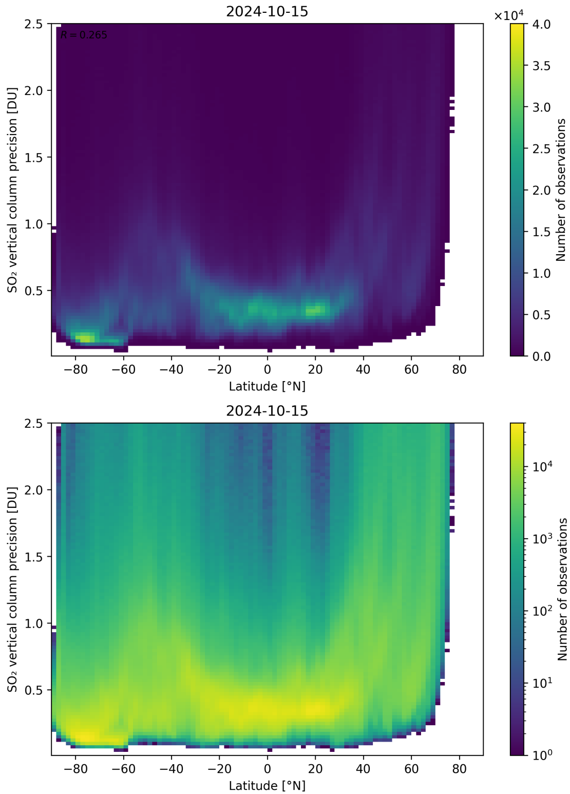
Figure 157: Scatter density plot of “Latitude” against “SO 2 vertical column precision” for 2024-10-14 to 2024-10-16.
