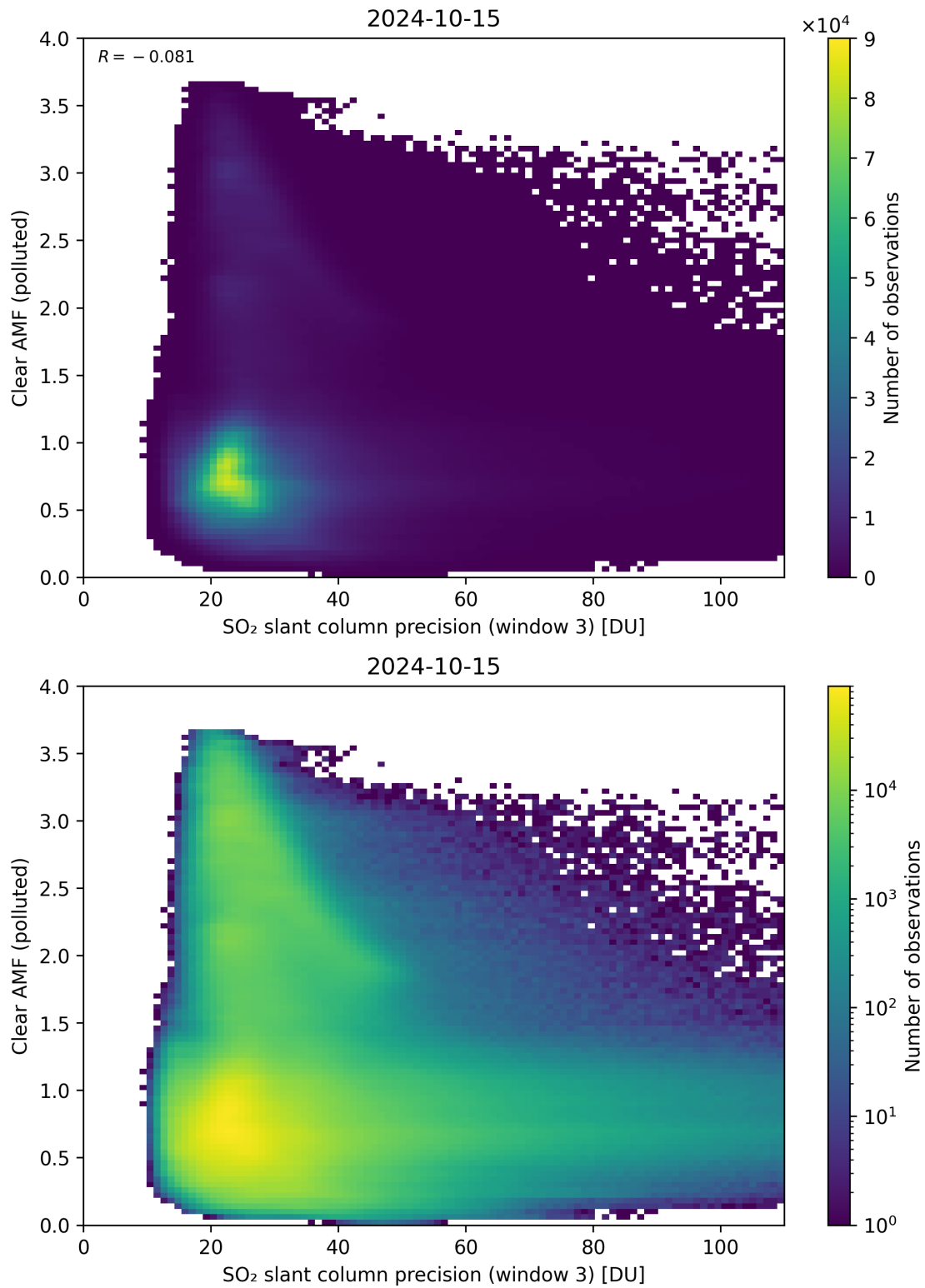
Figure 261: Scatter density plot of “SO 2 slant column precision (window 3)” against “Clear AMF (polluted)” for 2024-10-14 to 2024-10-16.
