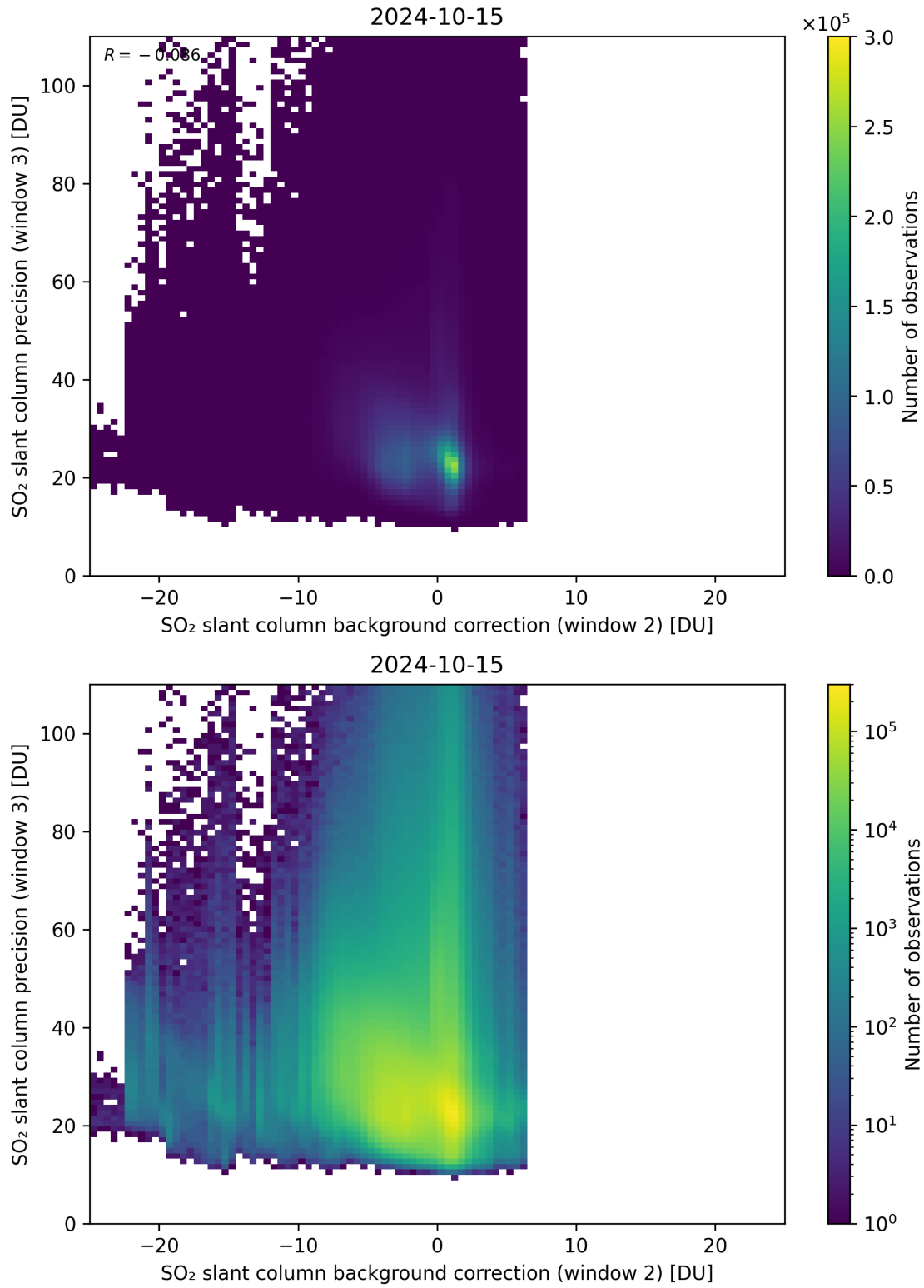
Figure 118: Scatter density plot of “SO 2 slant column background correction (window 2)” against “SO 2 slant column precision (window 3)” for 2024-10-14 to 2024-10-16.
