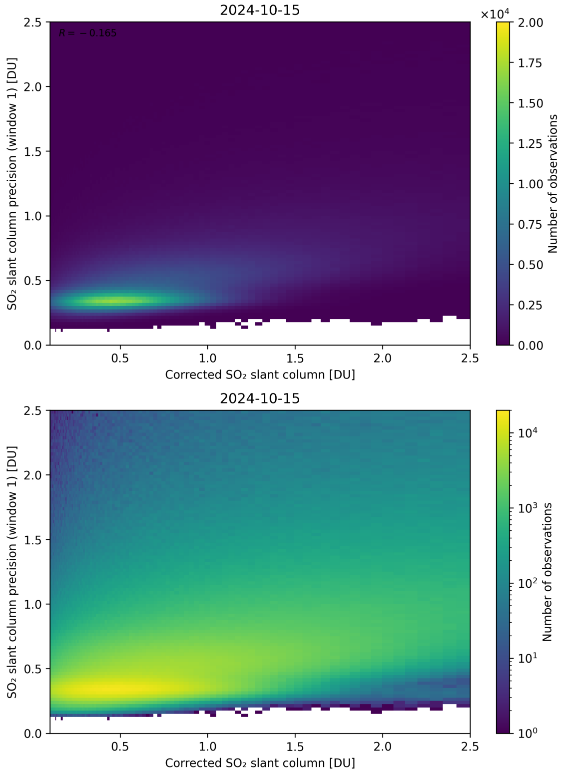
Figure 188: Scatter density plot of “Corrected SO 2 slant column” against “SO 2 slant column precision (window 1)” for 2024-10-14 to 2024-10-16.
