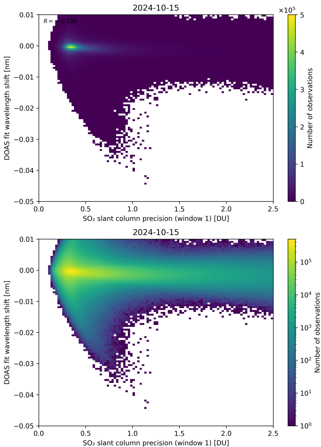
Figure 221: Scatter density plot of “SO 2 slant column precision (window 1)” against “DOAS fit wavelength shift” for 2024-10-14 to 2024-10-16.
