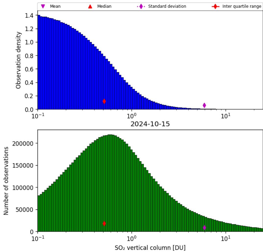
Figure 53: Histogram of “SO 2 vertical column” for 2024-10-14 to 2024-10-16
