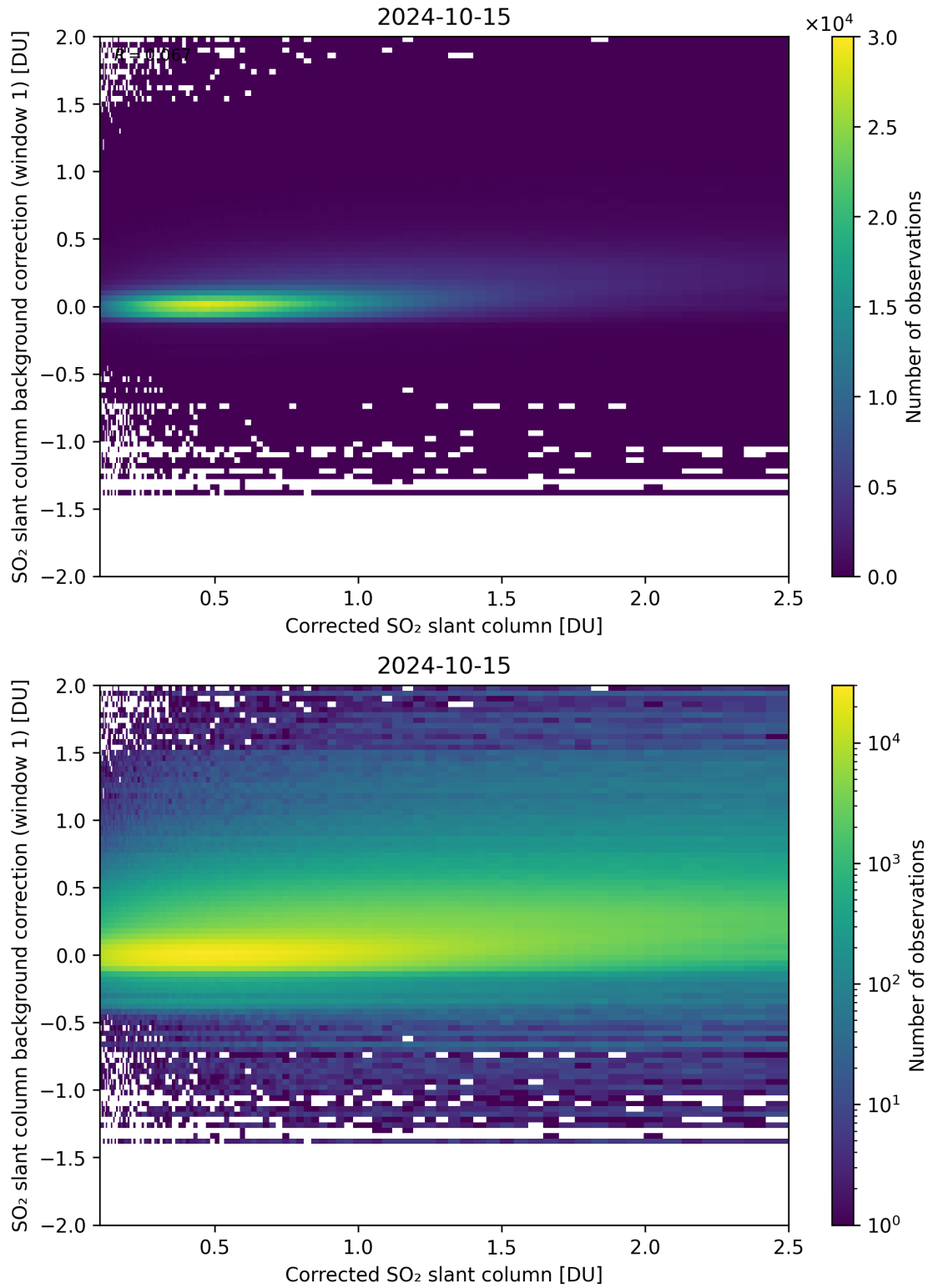
Figure 178: Scatter density plot of “Corrected SO 2 slant column” against “SO 2 slant column background correction (window 1)” for 2024-10-14 to 2024-10-16.
