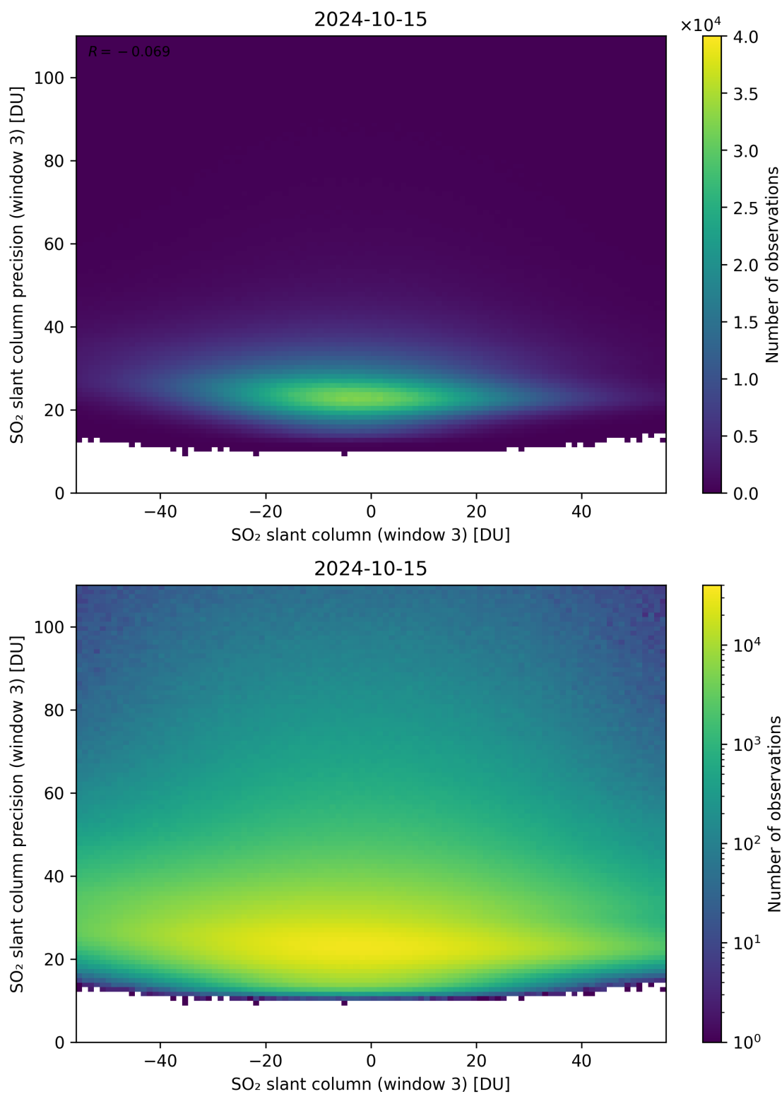
Figure 267: Scatter density plot of “SO 2 slant column (window 3)” against “SO 2 slant column precision (window 3)” for 2024-10-14 to 2024-10-16.
