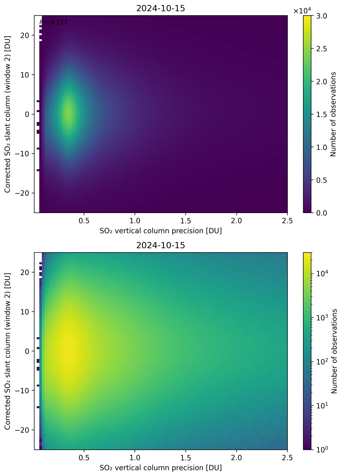
Figure 287: Scatter density plot of “SO 2 vertical column precision” against “Corrected SO 2 slant column (window 2)” for 2024-10-14 to 2024-10-16.
