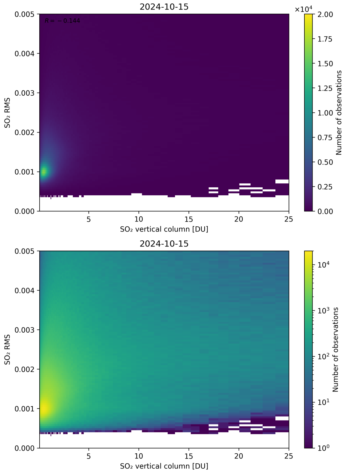
Figure 278: Scatter density plot of “SO 2 vertical column” against “SO 2 RMS” for 2024-10-14 to 2024-10-16.
