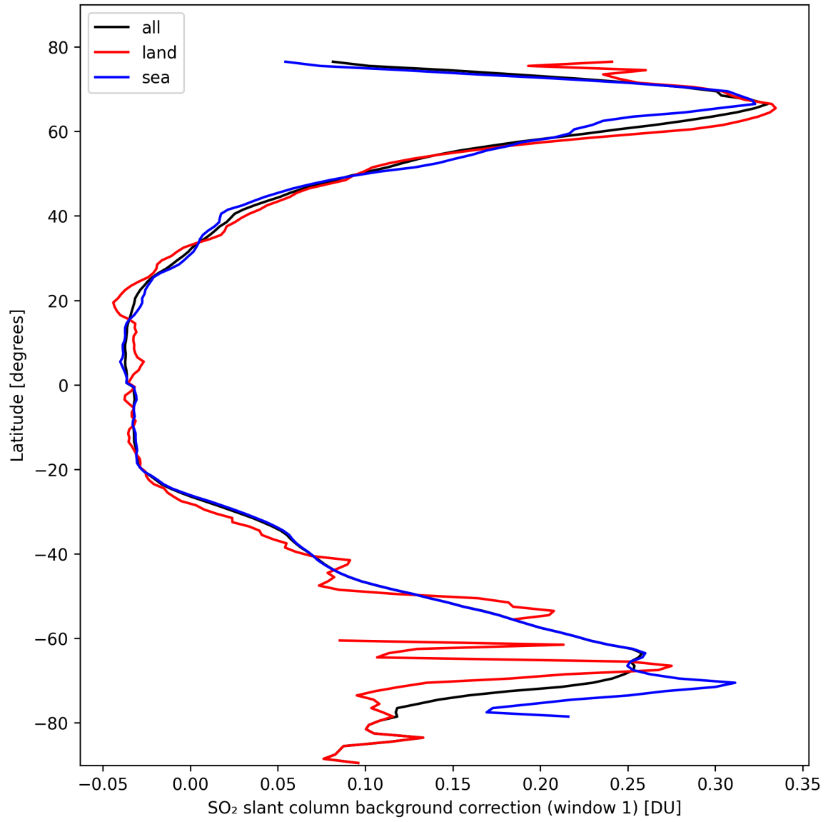
Figure 36: Zonal average of “SO 2 slant column background correction (window 1)” for 2024-10-14 to 2024-10-16.
