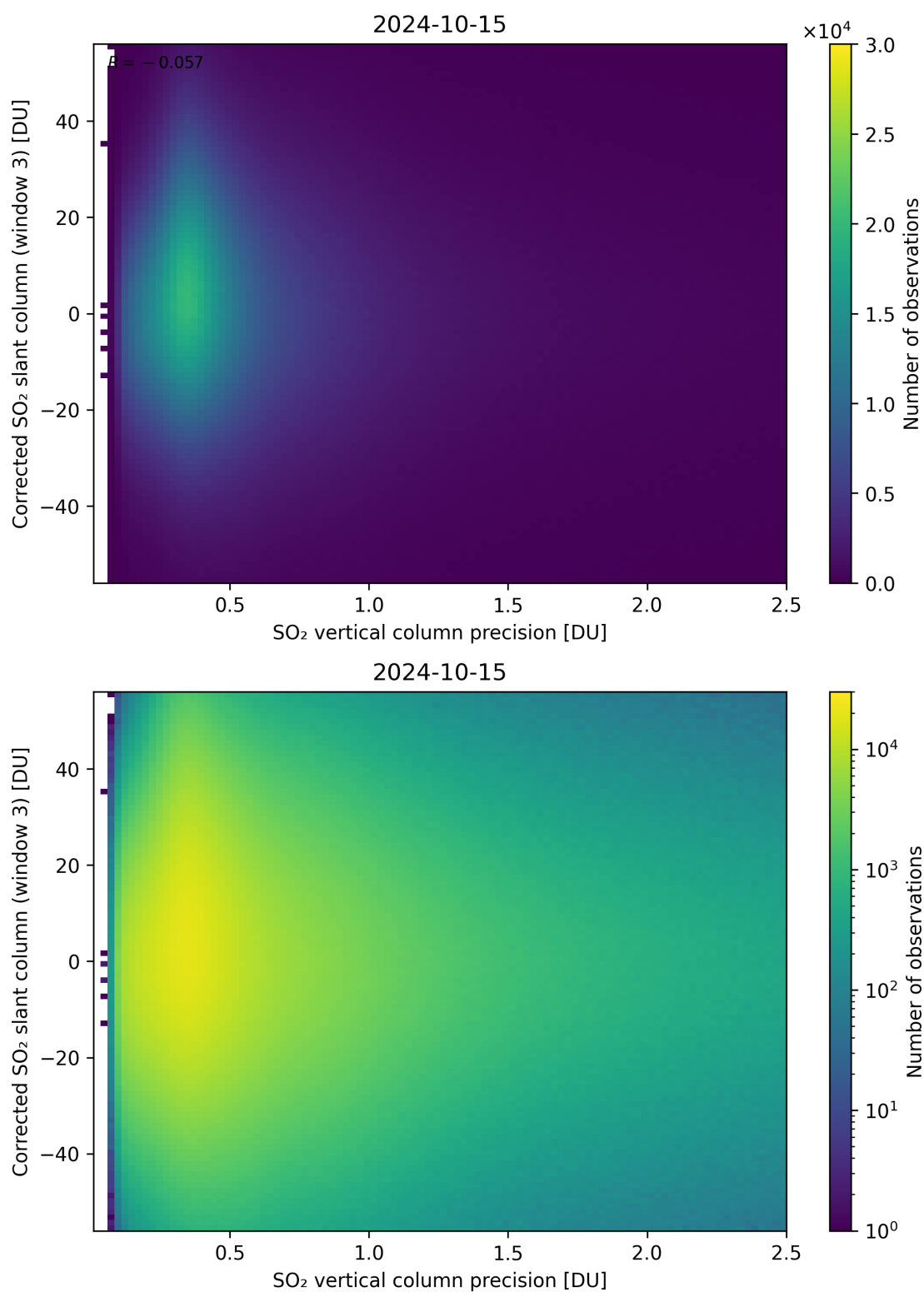
Figure 288: Scatter density plot of “SO 2 vertical column precision” against “Corrected SO 2 slant column (window 3)” for 2024-10-14 to 2024-10-16.
