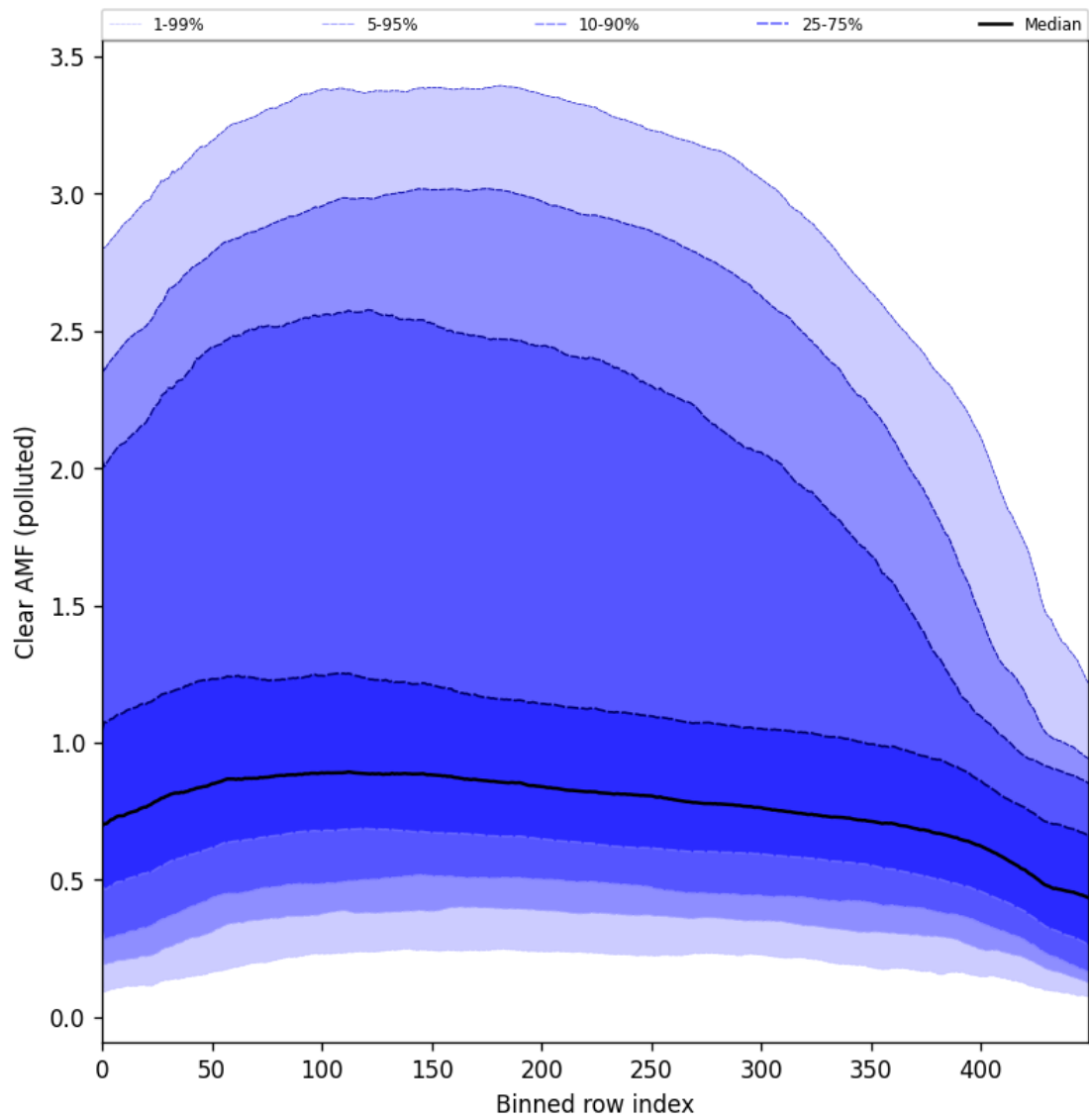
Figure 96: Along track statistics of “Clear AMF (polluted)” for 2024-10-14 to 2024-10-16
