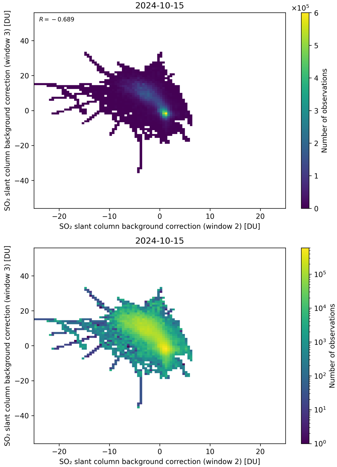
Figure 111: Scatter density plot of “SO 2 slant column background correction (window 2)” against “SO 2 slant column background correction (window 3)” for 2024-10-14 to 2024-10-16.
