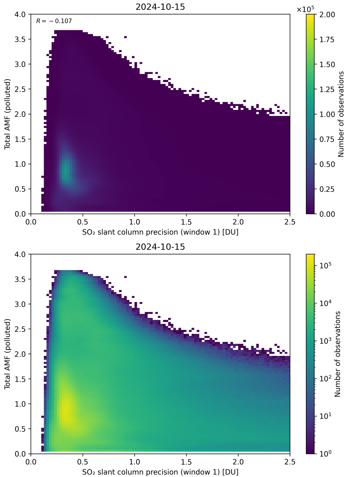
Figure 230: Scatter density plot of “SO 2 slant column precision (window 1)” against “Total AMF (polluted)” for 2024-10-14 to 2024-10-16.
