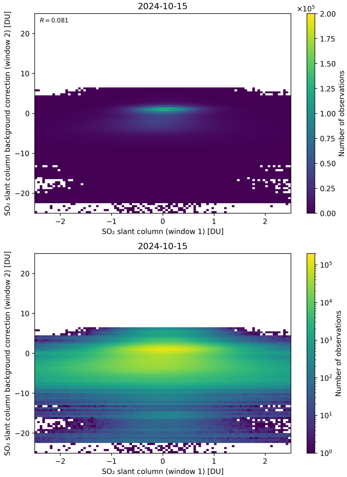
Figure 213: Scatter density plot of “SO 2 slant column (window 1)” against “SO 2 slant column background correction (window 2)” for 2024-10-14 to 2024-10-16.
