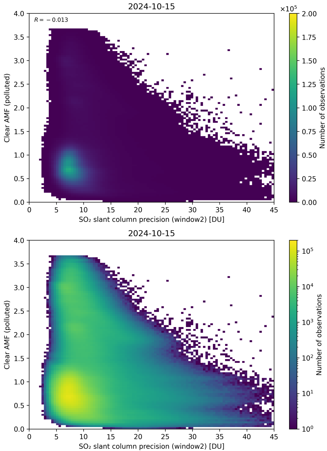
Figure 246: Scatter density plot of “SO 2 slant column precision (window2)” against “Clear AMF (polluted)” for 2024-10-14 to 2024-10-16.
