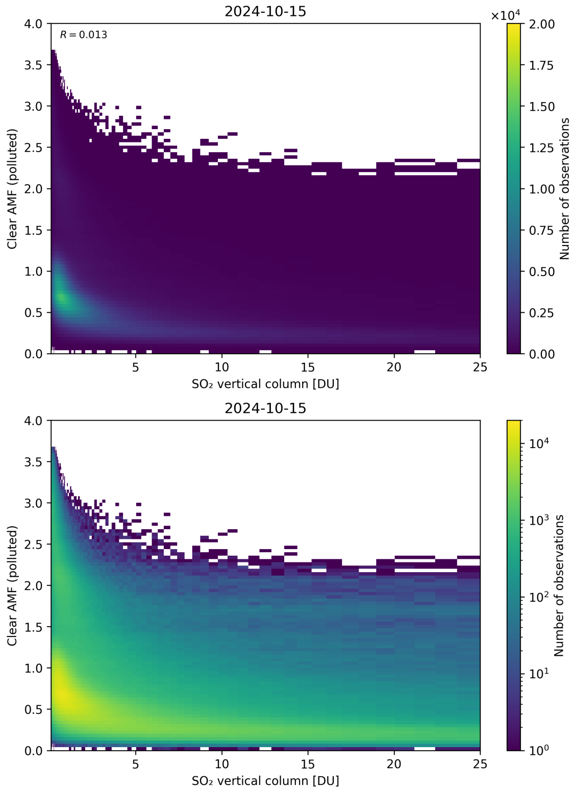
Figure 296: Scatter density plot of “SO 2 vertical column” against “Clear AMF (polluted)” for 2024-10-14 to 2024-10-16.
