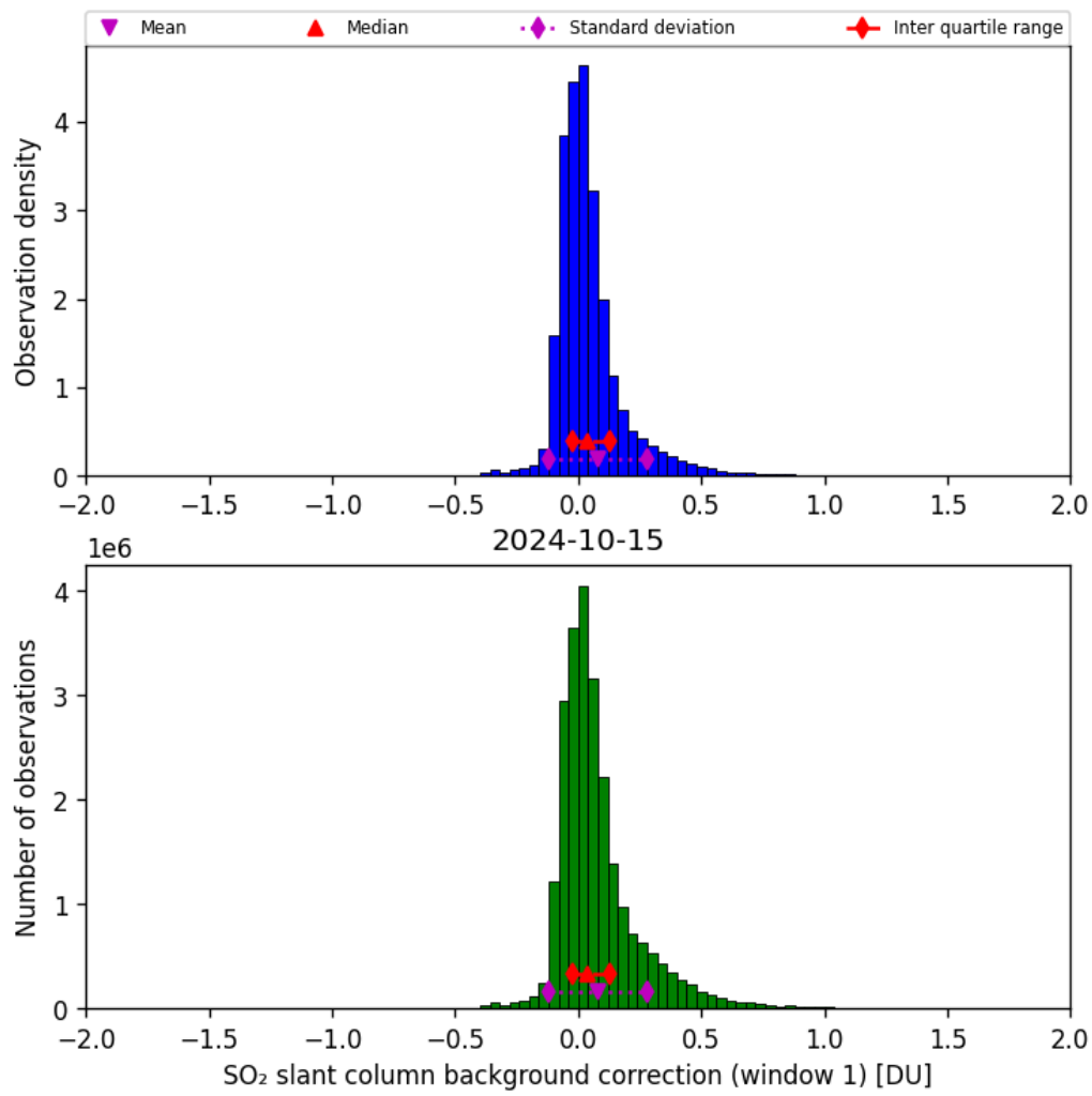
Figure 59: Histogram of “SO 2 slant column background correction (window 1)” for 2024-10-14 to 2024-10-16
