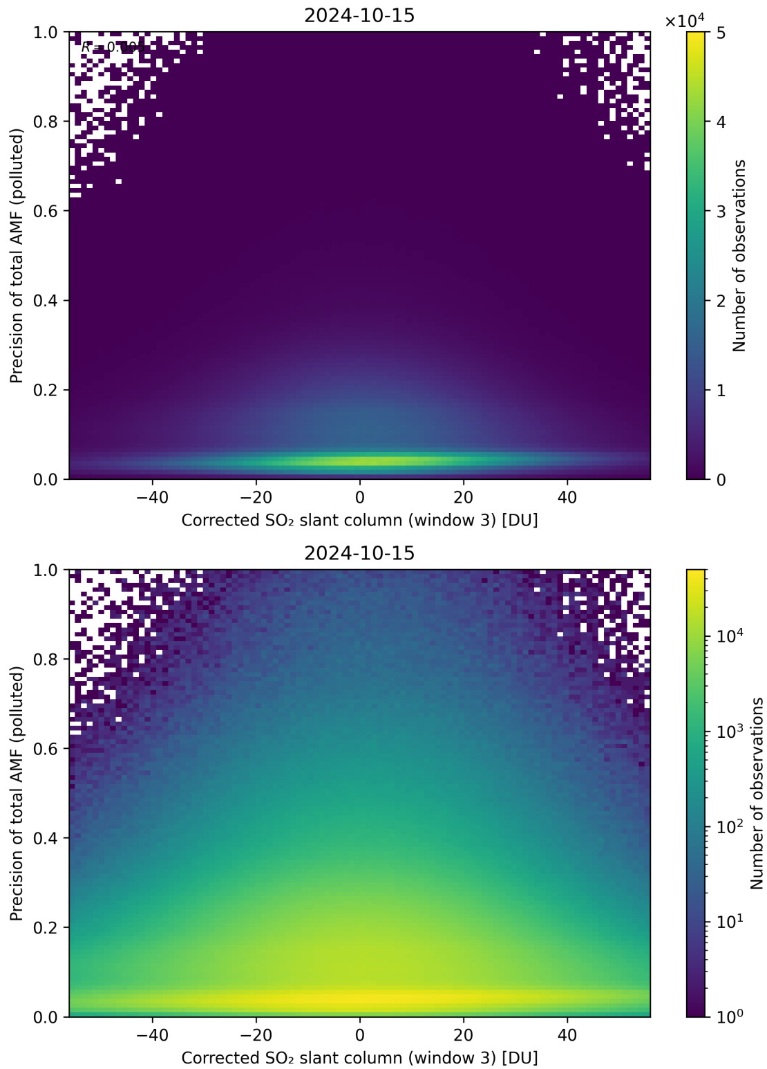
Figure 211: Scatter density plot of “Corrected SO 2 slant column (window 3)” against “Precision of total AMF (polluted)” for 2024-10-14 to 2024-10-16.
