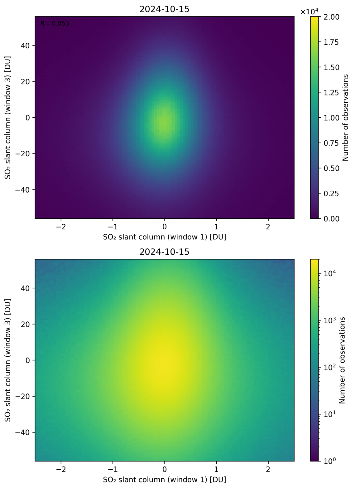
Figure 237: Scatter density plot of “SO 2 slant column (window 1)” against “SO 2 slant column (window 3)” for 2024-10-14 to 2024-10-16.
