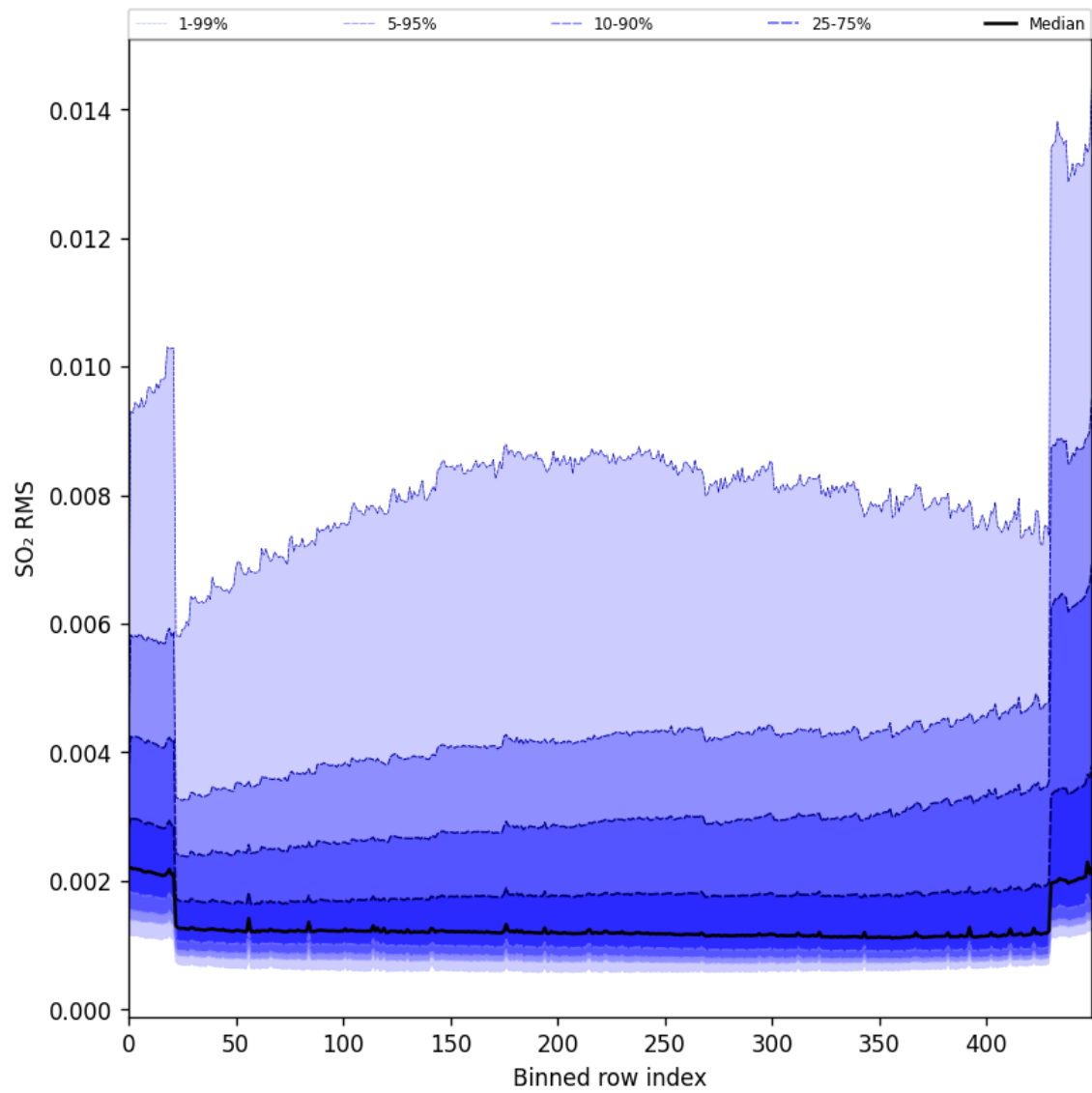
Figure 93: Along track statistics of “SO 2 RMS” for 2024-10-14 to 2024-10-16
