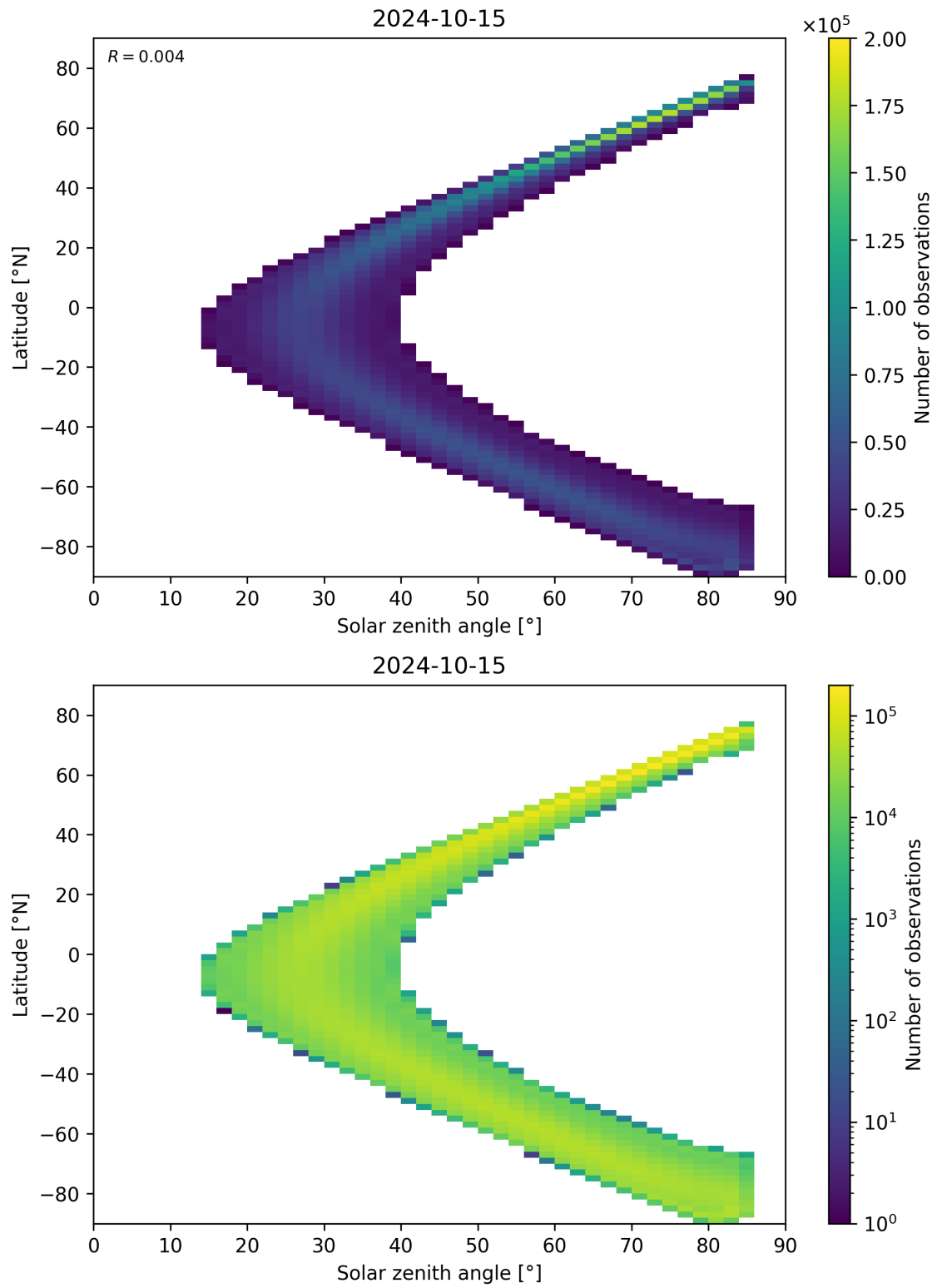
Figure 164: Scatter density plot of “Solar zenith angle” against “Latitude” for 2024-10-14 to 2024-10-16.
