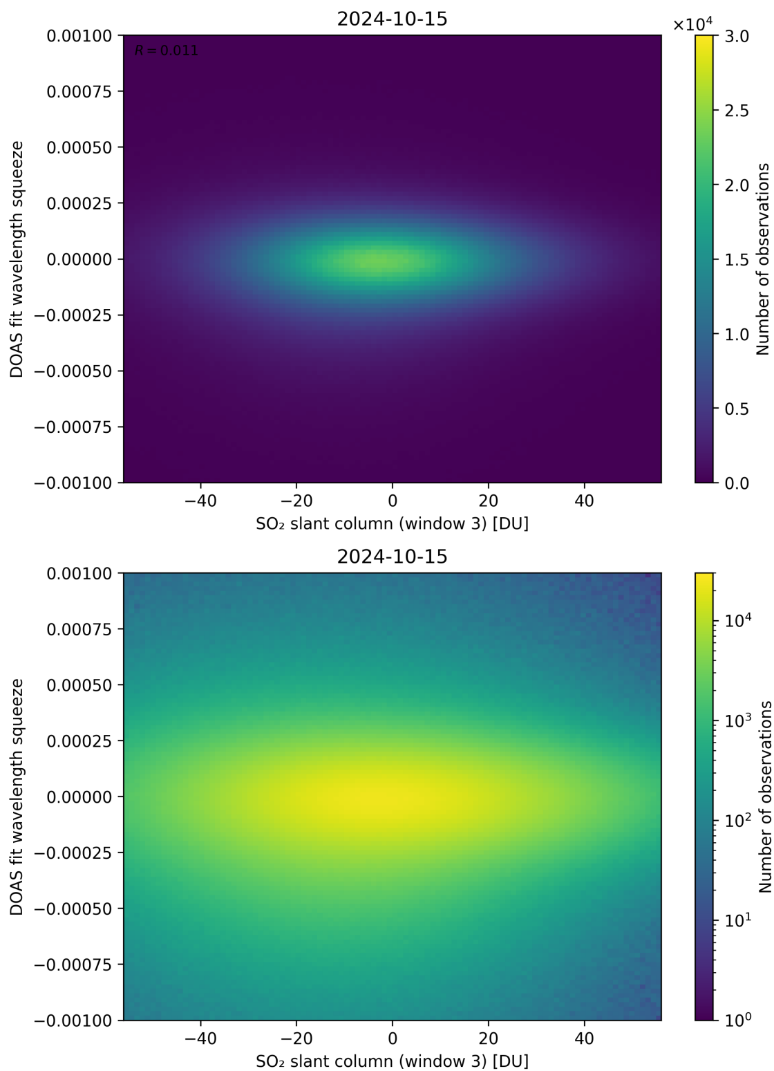
Figure 255: Scatter density plot of “SO 2 slant column (window 3)” against “DOAS fit wavelength squeeze” for 2024-10-14 to 2024-10-16.
