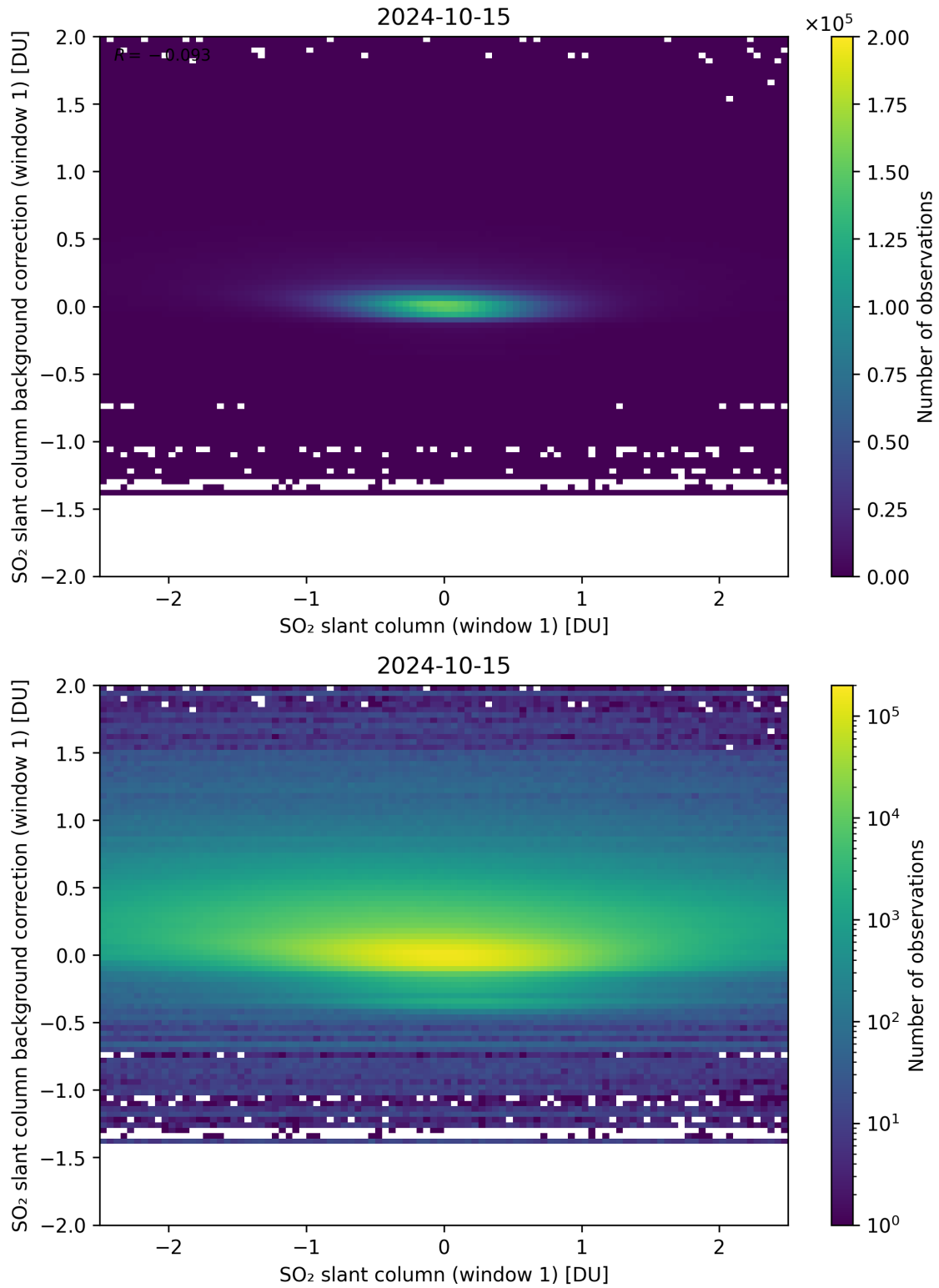
Figure 212: Scatter density plot of “SO 2 slant column (window 1)” against “SO 2 slant column background correction (window 1)” for 2024-10-14 to 2024-10-16.
