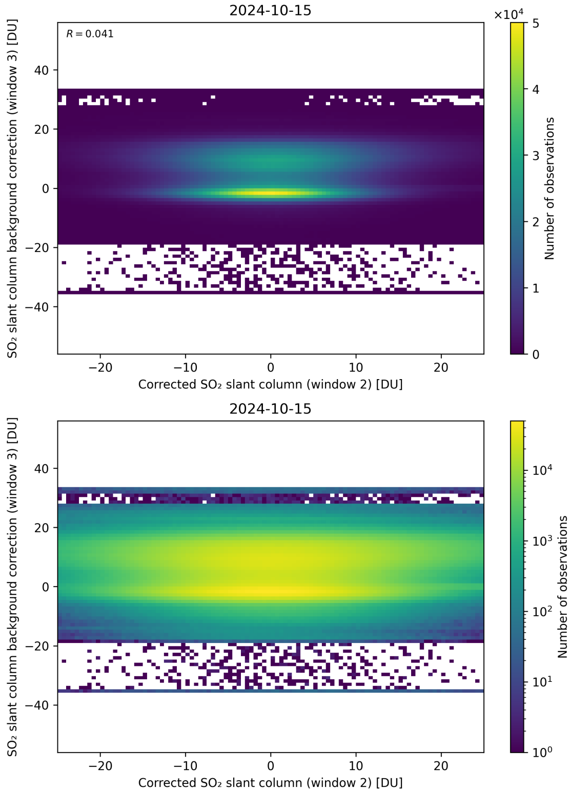
Figure 195: Scatter density plot of “Corrected SO 2 slant column (window 2)” against “SO 2 slant column background correction (window 3)” for 2024-10-14 to 2024-10-16.
