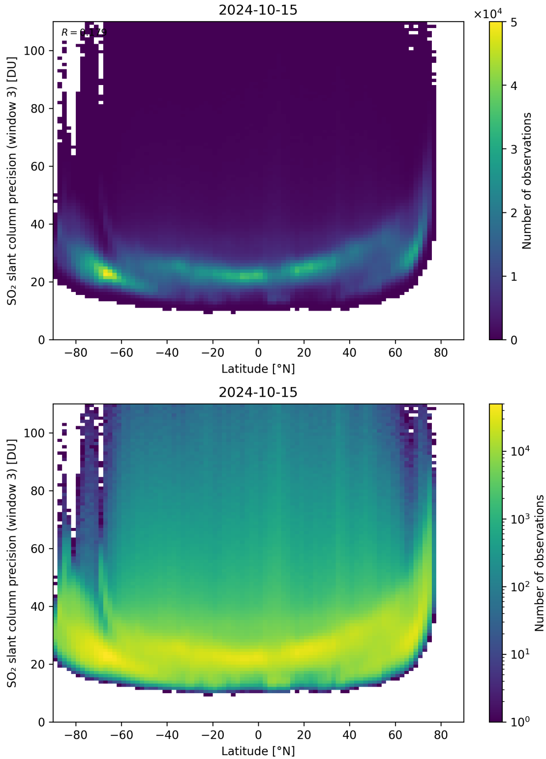
Figure 153: Scatter density plot of “Latitude” against “SO 2 slant column precision (window 3)” for 2024-10-14 to 2024-10-16.
