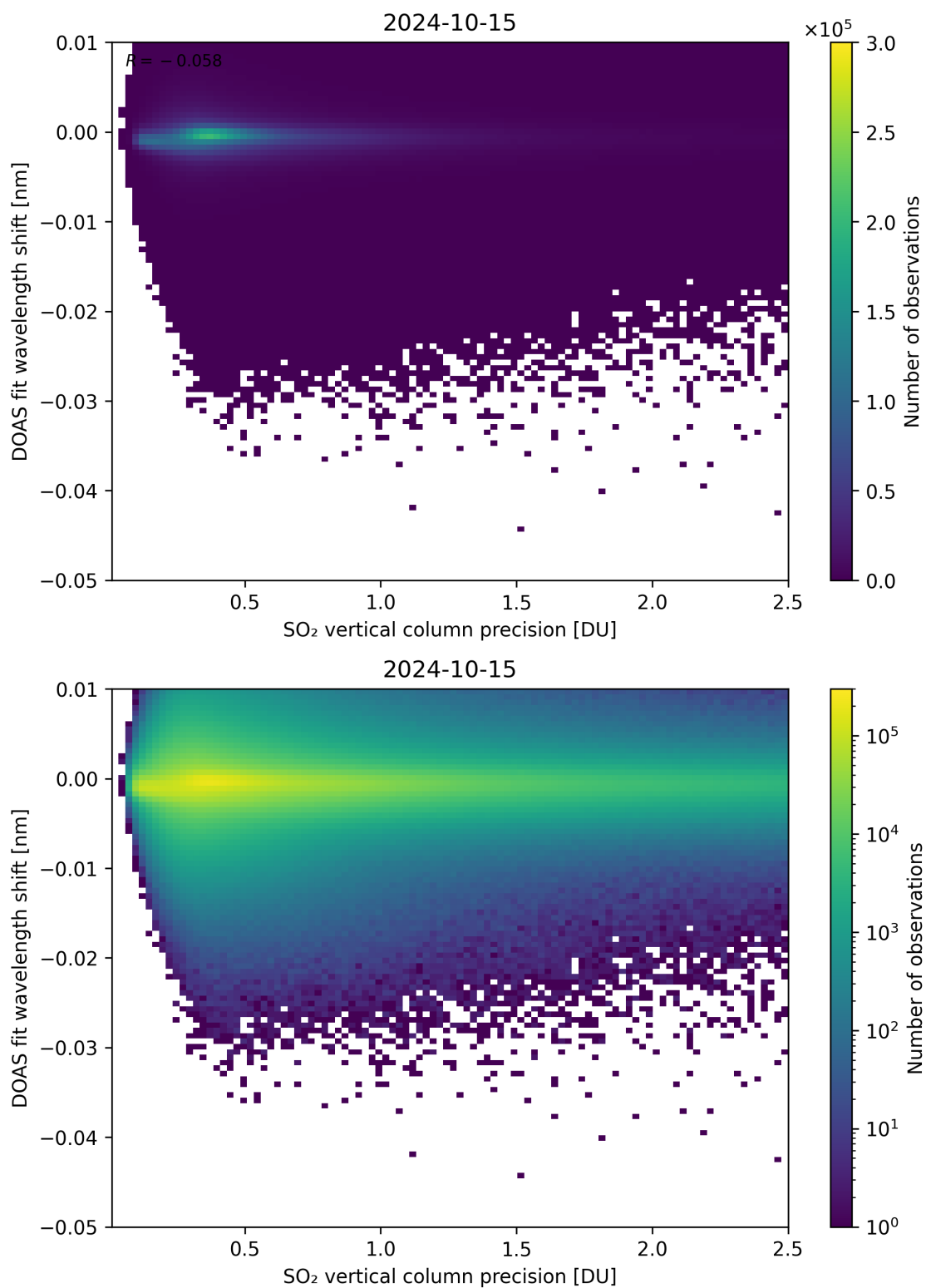
Figure 282: Scatter density plot of “SO 2 vertical column precision” against “DOAS fit wavelength shift” for 2024-10-14 to 2024-10-16.
