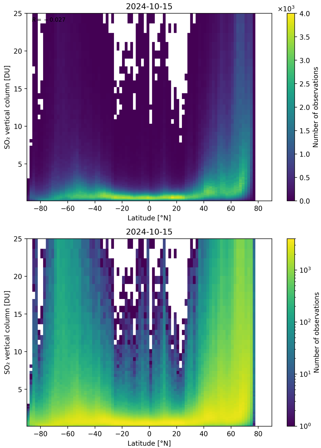
Figure 156: Scatter density plot of “Latitude” against “SO 2 vertical column” for 2024-10-14 to 2024-10-16.
