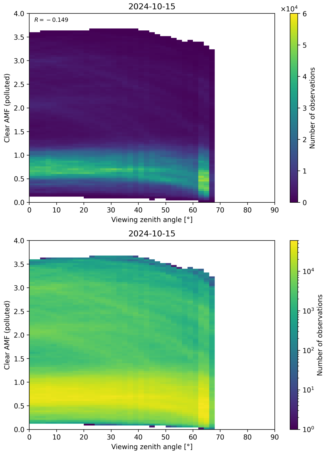
Figure 316: Scatter density plot of “Viewing zenith angle” against “Clear AMF (polluted)” for 2024-10-14 to 2024-10-16.
