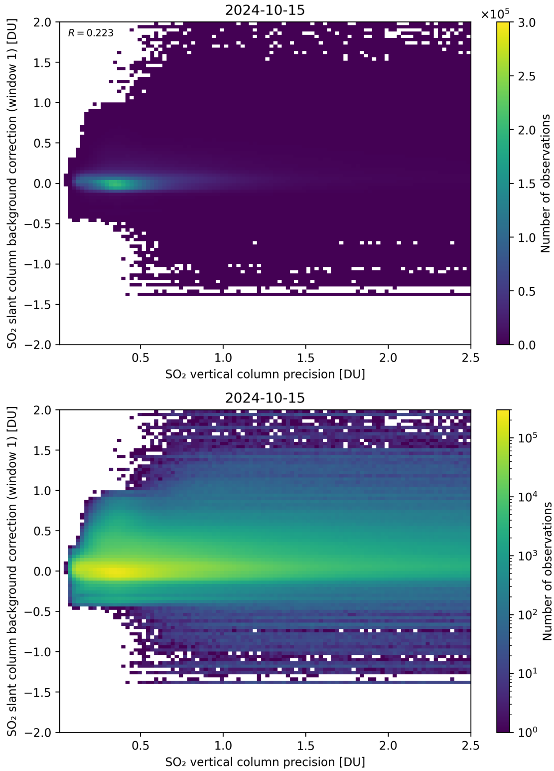
Figure 279: Scatter density plot of “SO 2 vertical column precision” against “SO 2 slant column background correction (window 1)” for 2024-10-14 to 2024-10-16.
