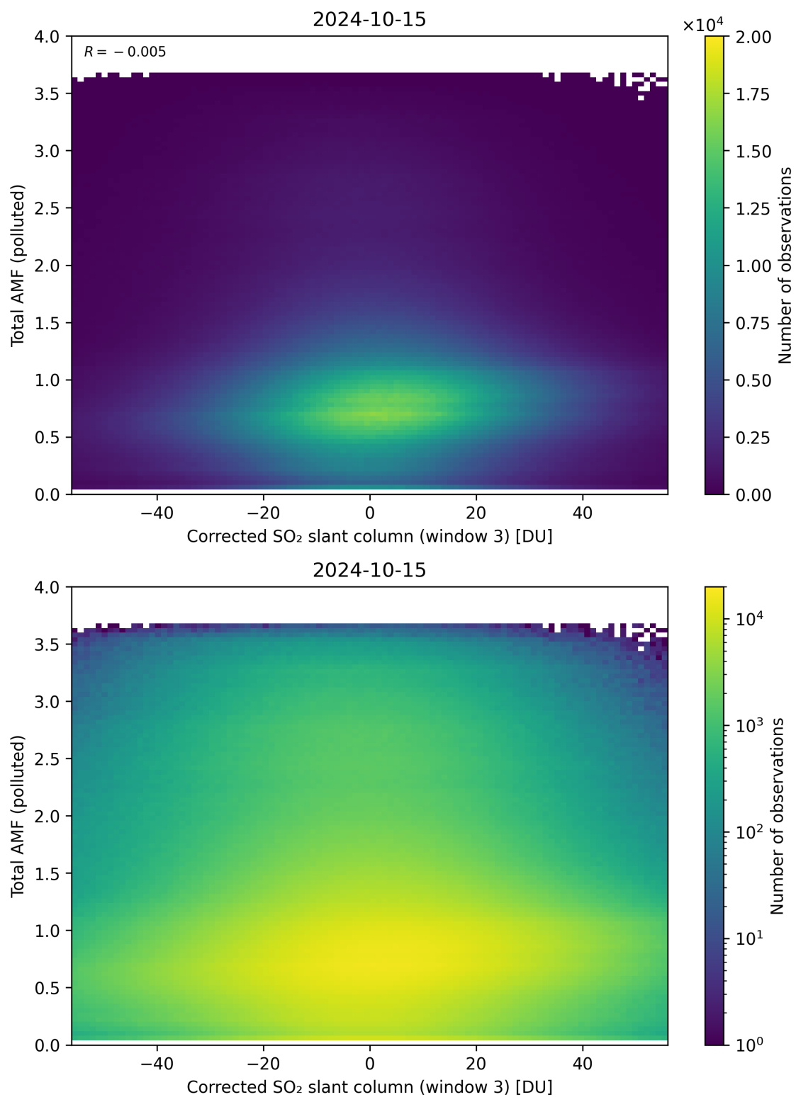
Figure 210: Scatter density plot of “Corrected SO 2 slant column (window 3)” against “Total AMF (polluted)” for 2024-10-14 to 2024-10-16.
