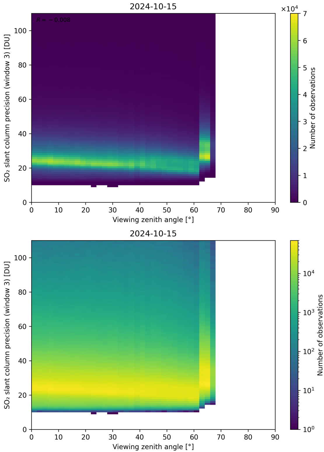
Figure 324: Scatter density plot of “Viewing zenith angle” against “SO 2 slant column precision (window 3)” for 2024-10-14 to 2024-10-16.
