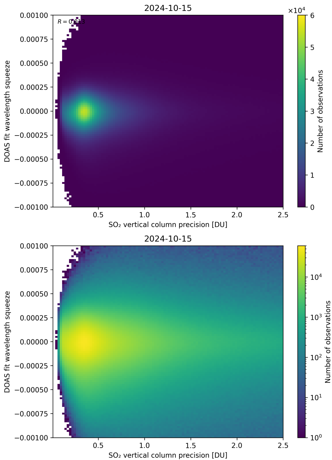
Figure 283: Scatter density plot of “SO 2 vertical column precision” against “DOAS fit wavelength squeeze” for 2024-10-14 to 2024-10-16.
