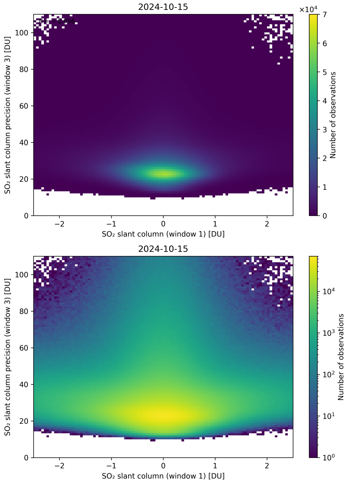
Figure 238: Scatter density plot of “SO 2 slant column (window 1)” against “SO 2 slant column precision (window 3)” for 2024-10-14 to 2024-10-16.
