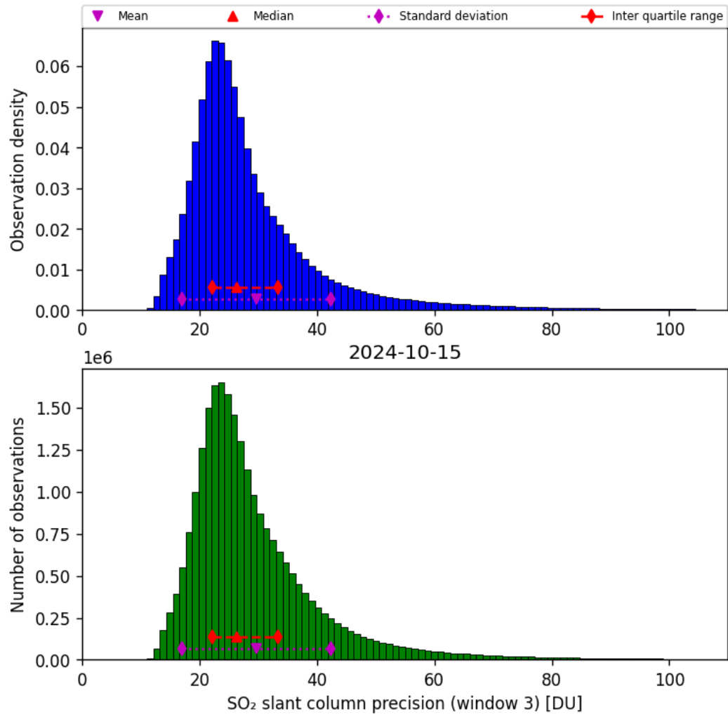
Figure 65: Histogram of “SO 2 slant column precision (window 3)” for 2024-10-14 to 2024-10-16
