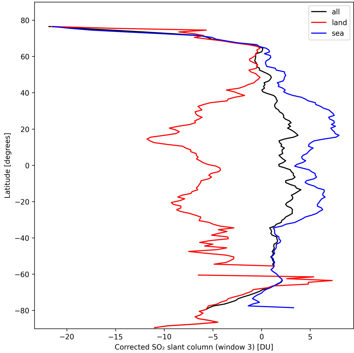
Figure 43: Zonal average of “Corrected SO 2 slant column (window 3)” for 2024-10-14 to 2024-10-16.
