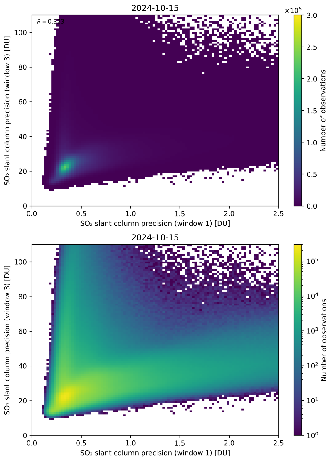
Figure 229: Scatter density plot of “SO 2 slant column precision (window 1)” against “SO 2 slant column precision (window 3)” for 2024-10-14 to 2024-10-16.
