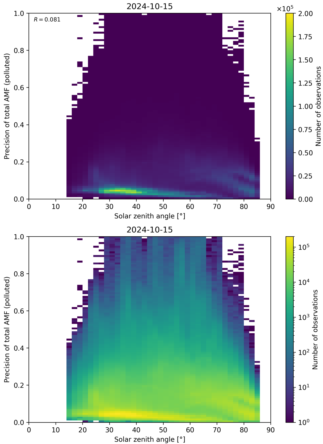
Figure 175: Scatter density plot of “Solar zenith angle” against “Precision of total AMF (polluted)” for 2024-10-14 to 2024-10-16.
