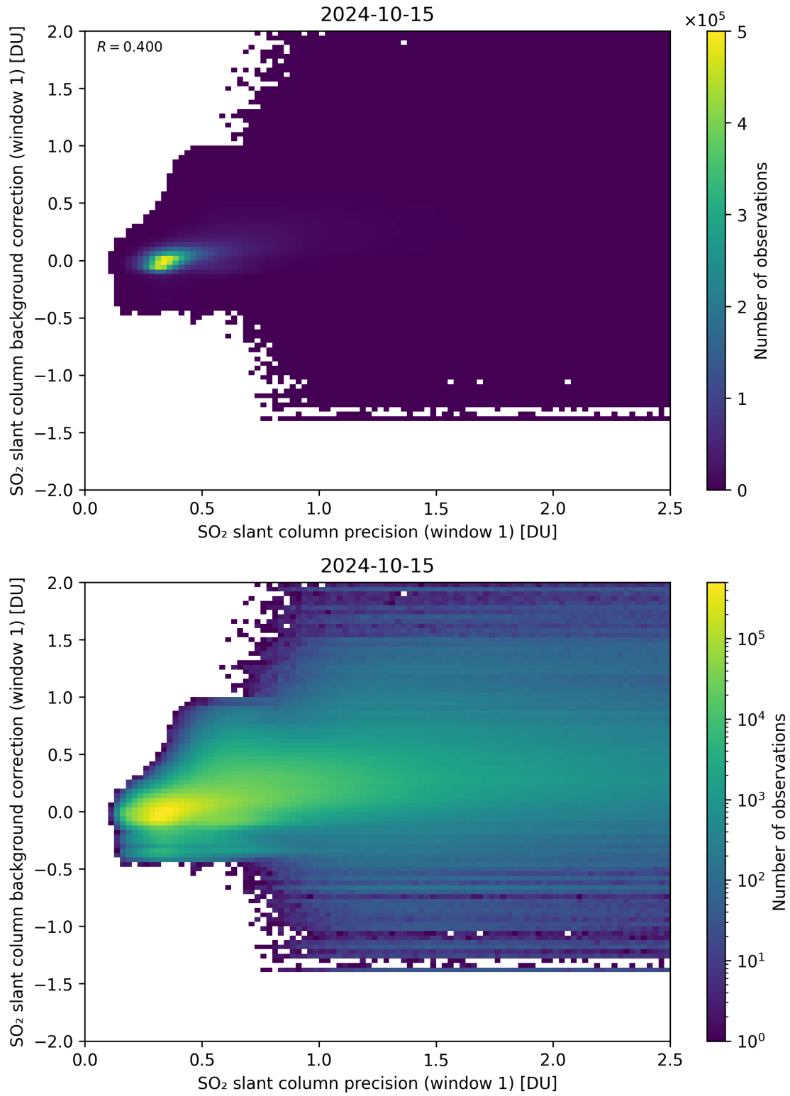
Figure 218: Scatter density plot of “SO 2 slant column precision (window 1)” against “SO 2 slant column background correction (window 1)” for 2024-10-14 to 2024-10-16.
