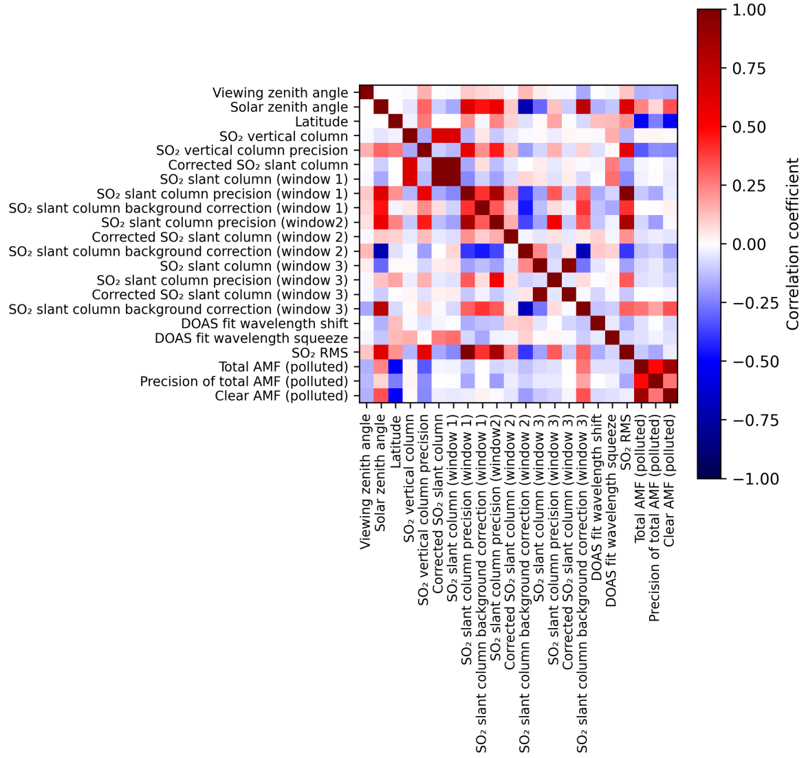
Figure 2: Map of correlation matrix for 2024-10-14 to 2024-10-16.
