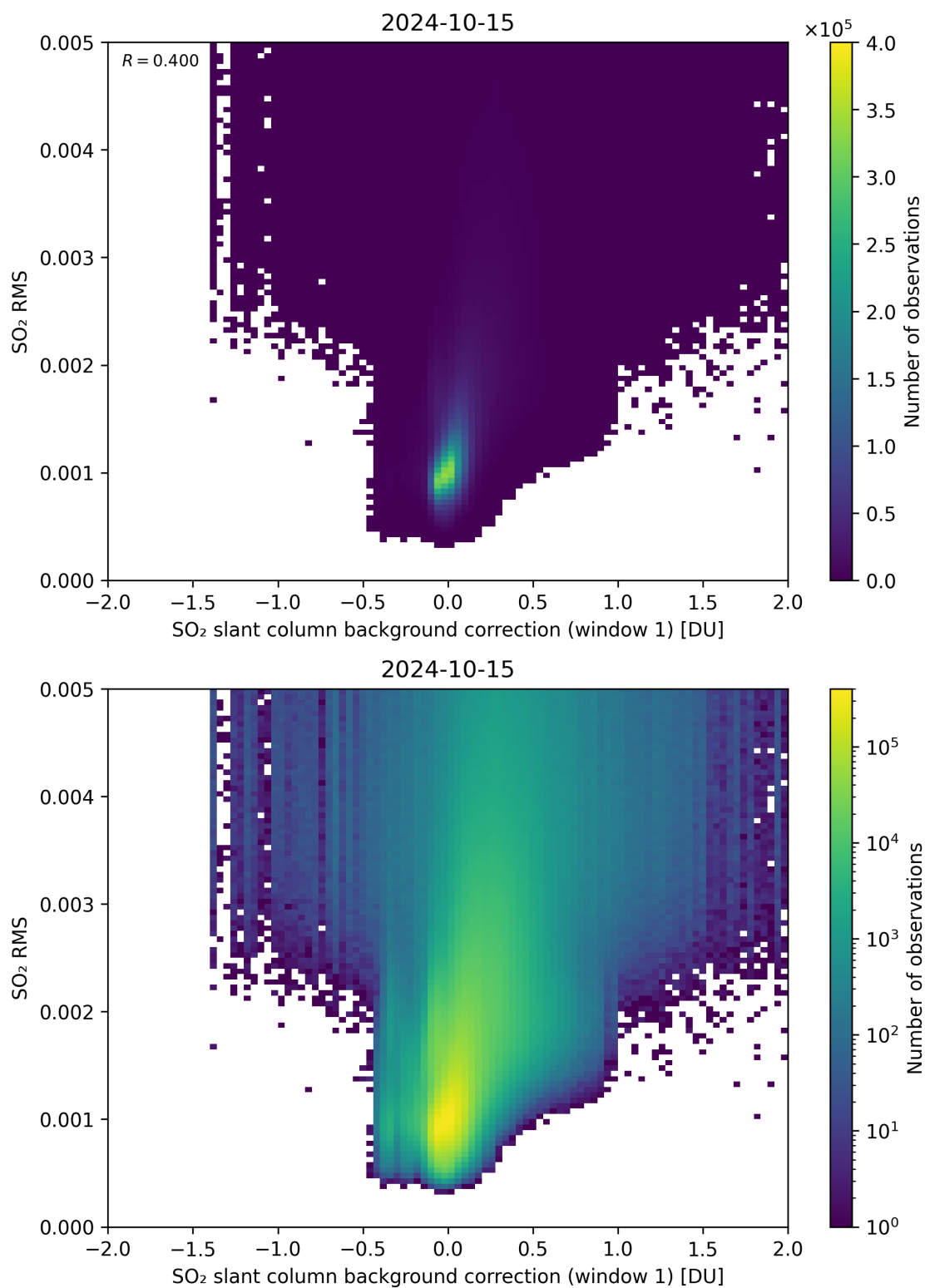
Figure 102: Scatter density plot of “SO 2 slant column background correction (window 1)” against “SO 2 RMS” for 2024-10-14 to 2024-10-16.
