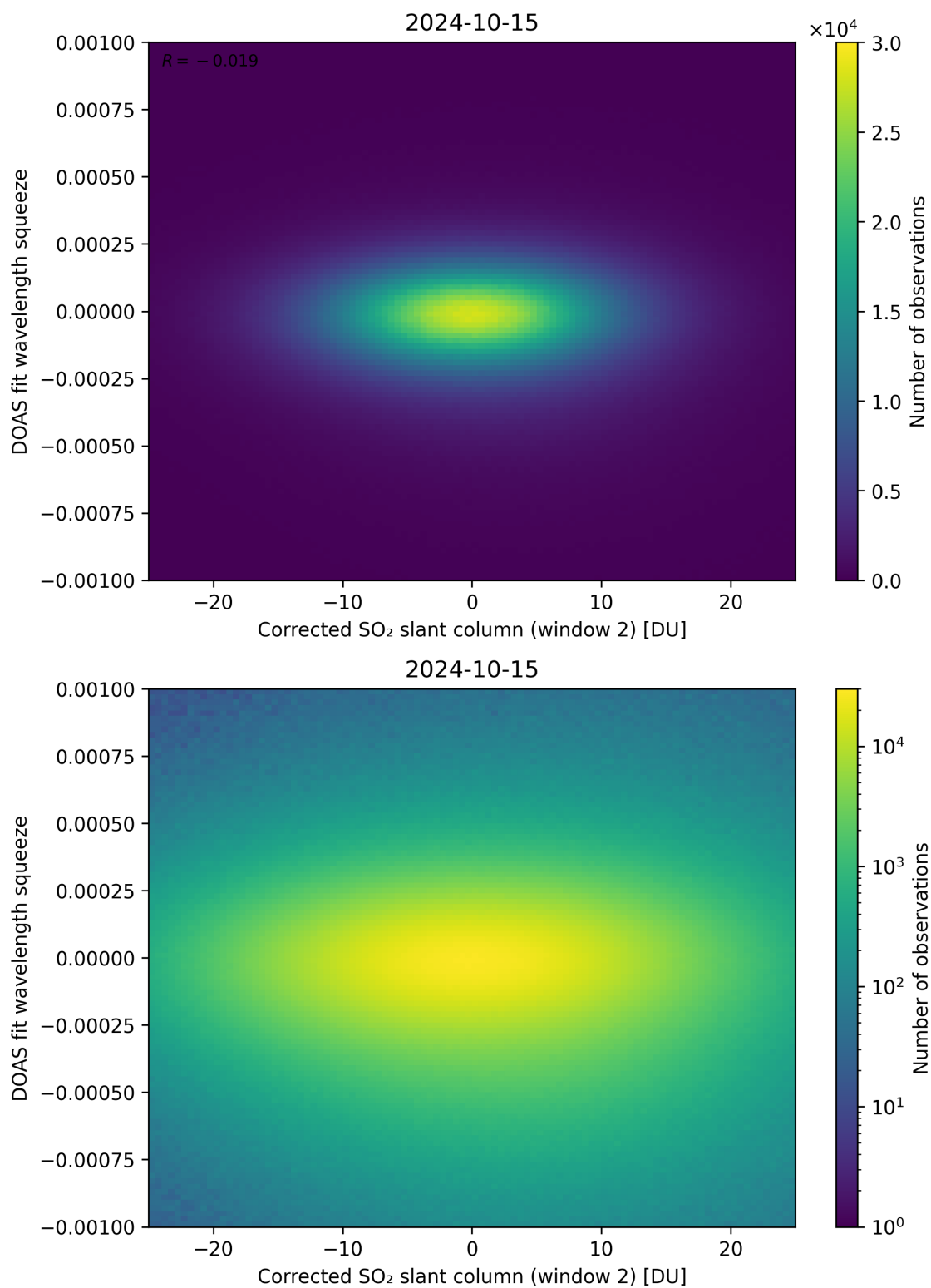
Figure 197: Scatter density plot of “Corrected SO 2 slant column (window 2)” against “DOAS fit wavelength squeeze” for 2024-10-14 to 2024-10-16.
