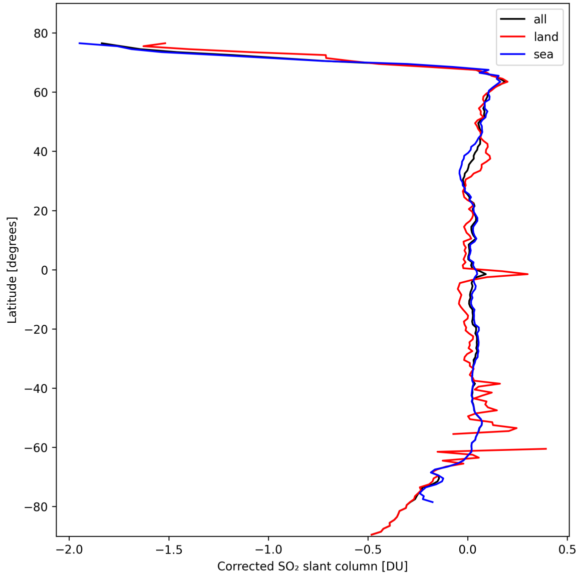
Figure 32: Zonal average of “Corrected SO 2 slant column” for 2024-10-14 to 2024-10-16.
