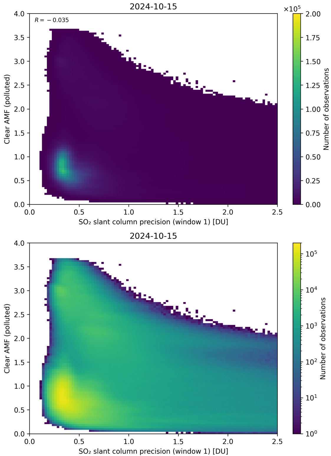
Figure 224: Scatter density plot of “SO 2 slant column precision (window 1)” against “Clear AMF (polluted)” for 2024-10-14 to 2024-10-16.
