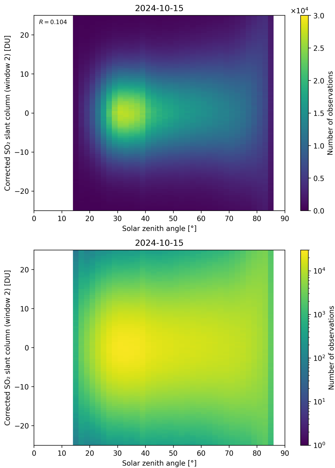
Figure 167: Scatter density plot of “Solar zenith angle” against “Corrected SO 2 slant column (window 2)” for 2024-10-14 to 2024-10-16.
