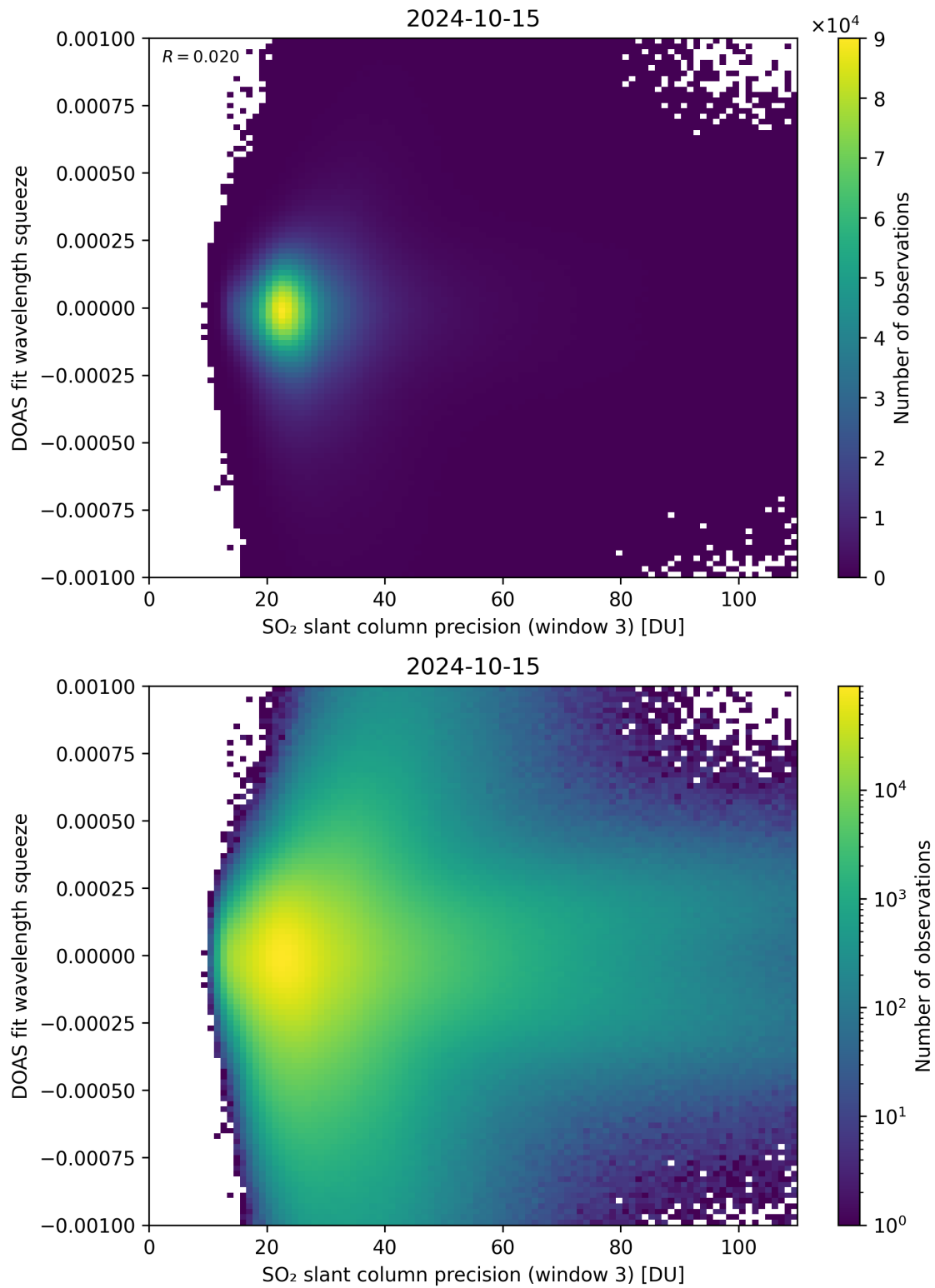
Figure 259: Scatter density plot of “SO 2 slant column precision (window 3)” against “DOAS fit wavelength squeeze” for 2024-10-14 to 2024-10-16.
