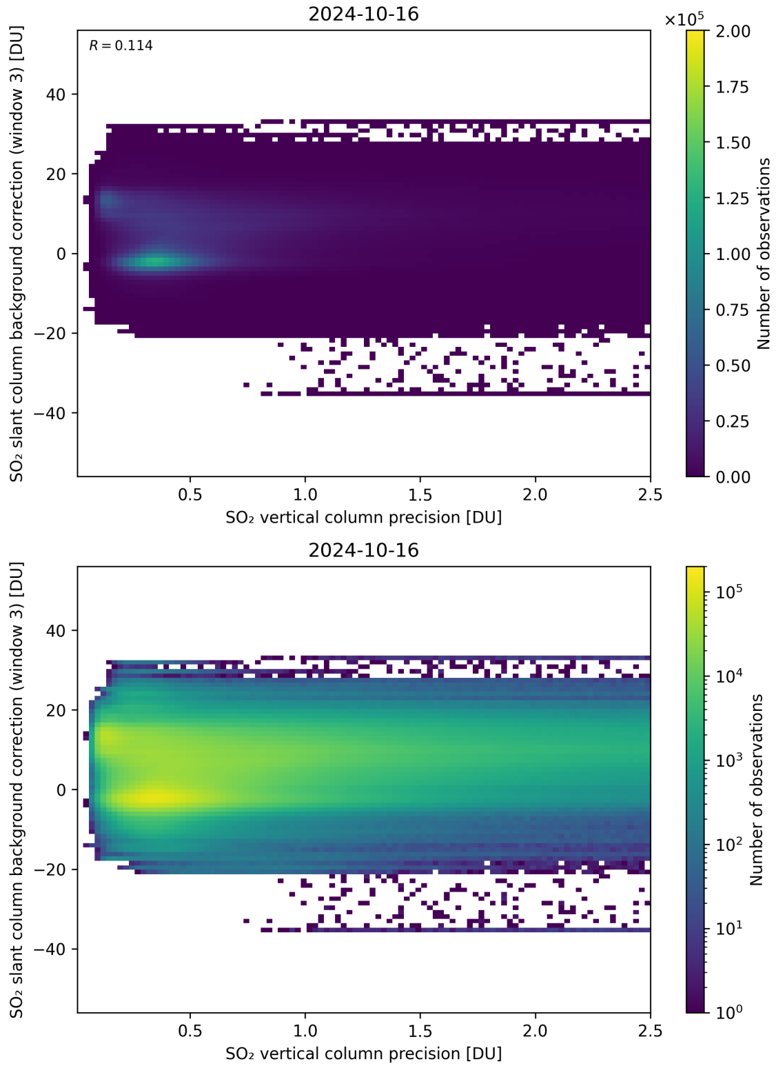
Figure 281: Scatter density plot of “SO 2 vertical column precision” against “SO 2 slant column background correction (window 3)” for 2024-10-15 to 2024-10-17.
