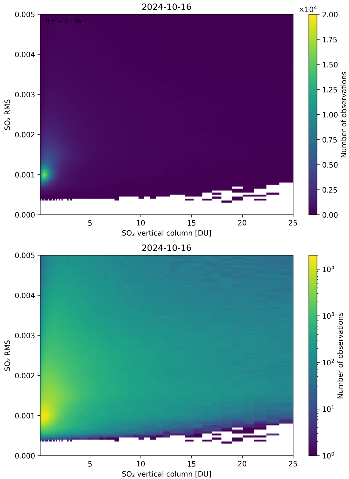
Figure 278: Scatter density plot of “SO 2 vertical column” against “SO 2 RMS” for 2024-10-15 to 2024-10-17.
