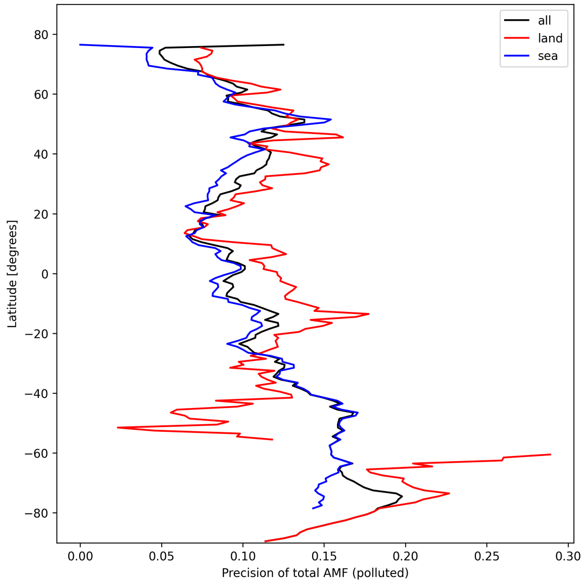
Figure 49: Zonal average of “Precision of total AMF (polluted)” for 2024-10-15 to 2024-10-17.
