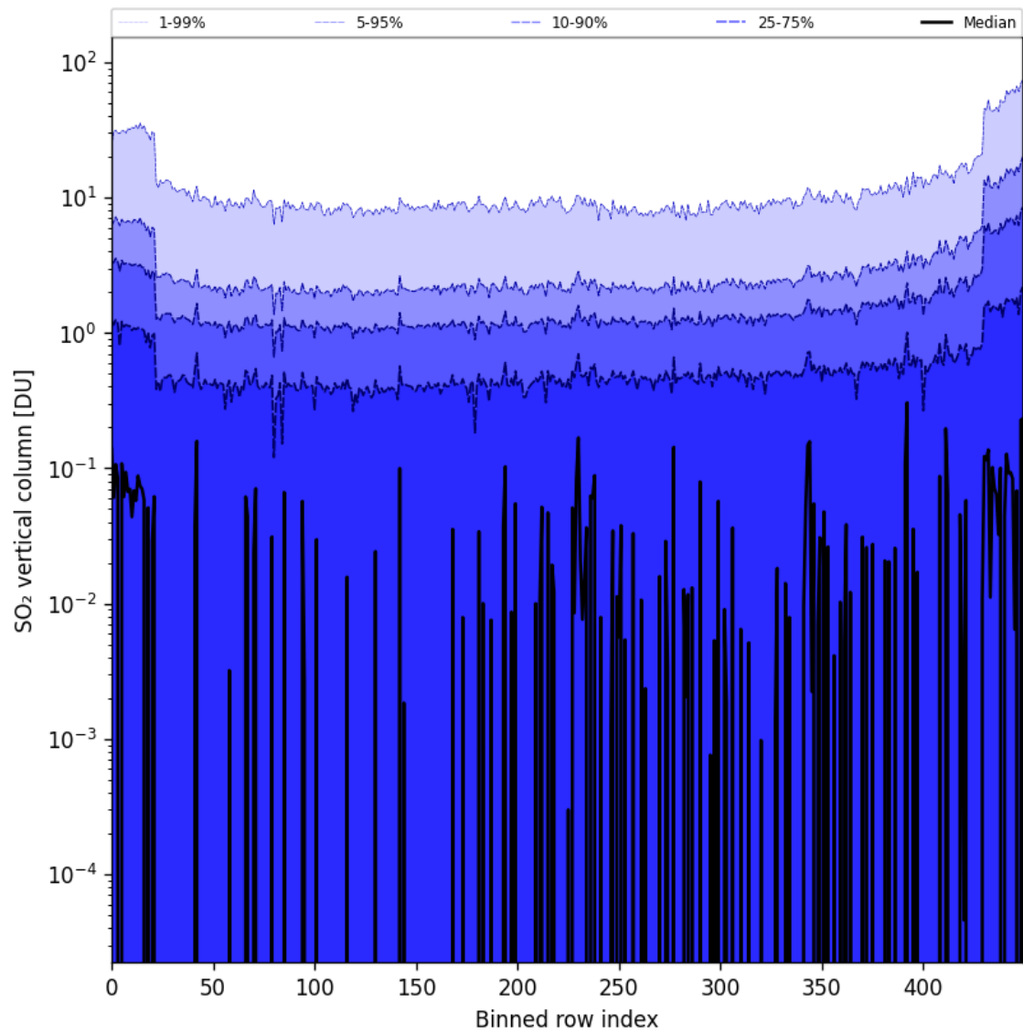
Figure 76: Along track statistics of “SO 2 vertical column” for 2024-10-15 to 2024-10-17
