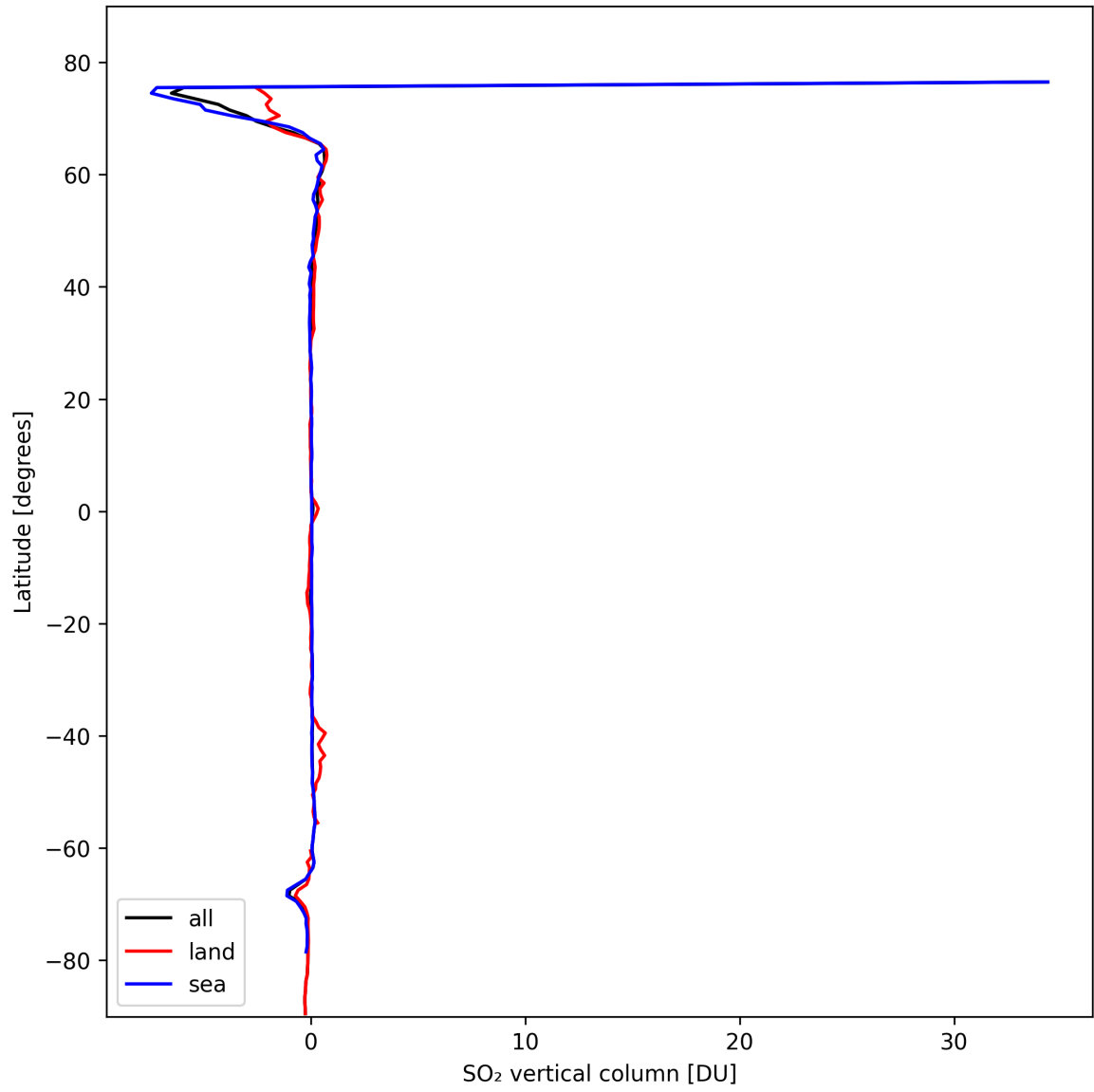
Figure 30: Zonal average of “SO 2 vertical column” for 2024-10-15 to 2024-10-17.
