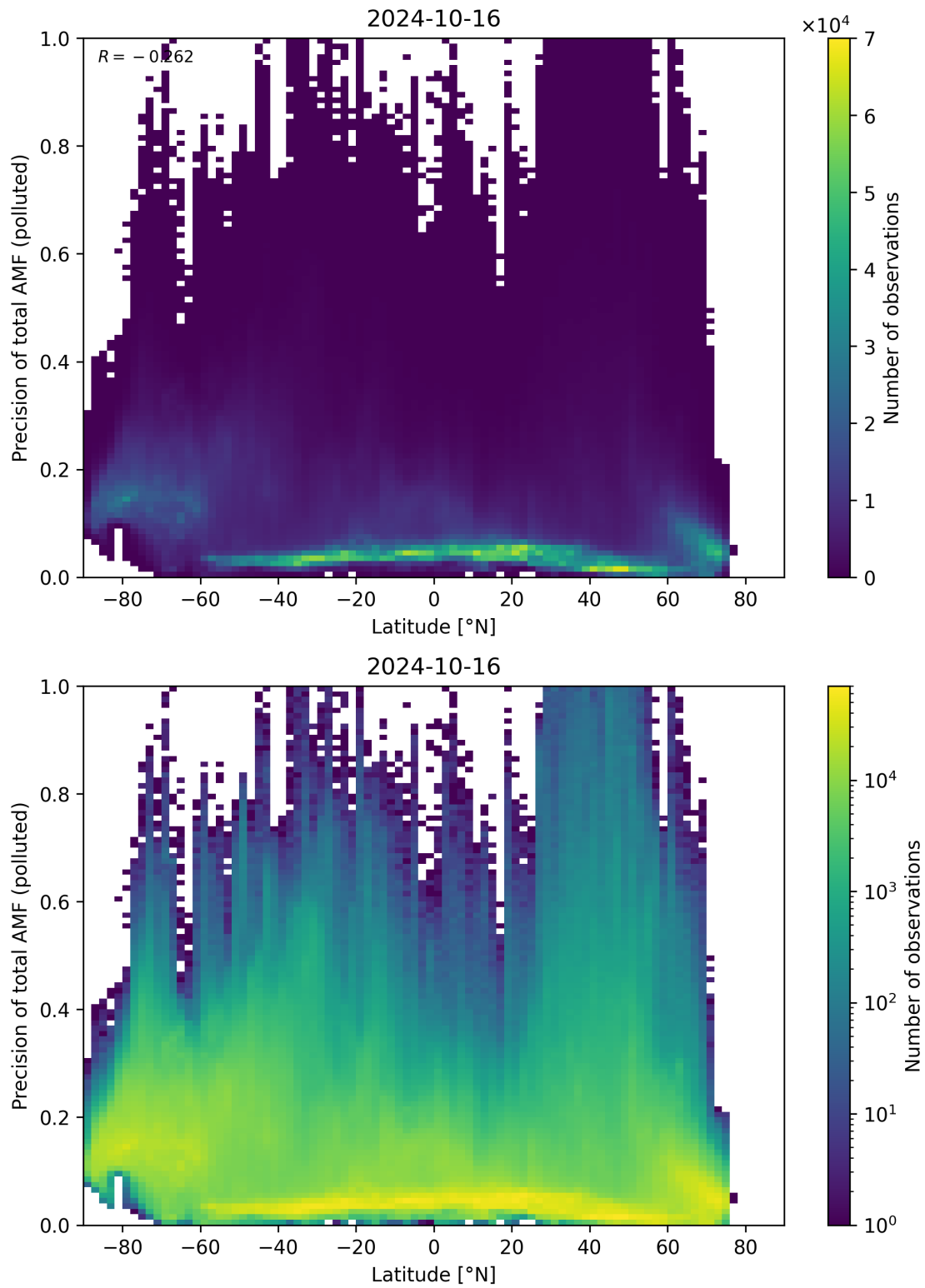
Figure 155: Scatter density plot of “Latitude” against “Precision of total AMF (polluted)” for 2024-10-15 to 2024-10-17.
