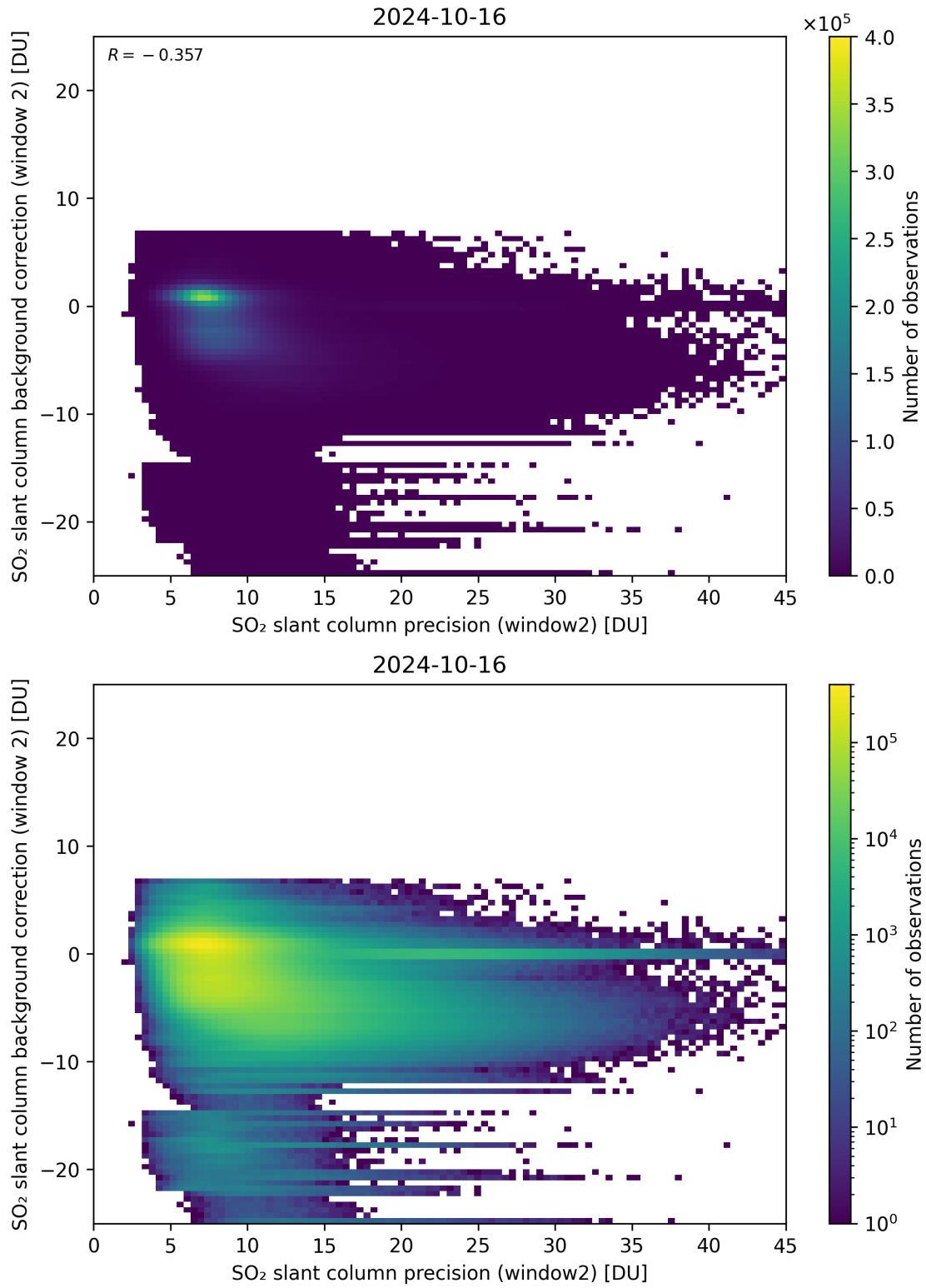
Figure 241: Scatter density plot of “SO 2 slant column precision (window2)” against “SO 2 slant column background correction (window 2)” for 2024-10-15 to 2024-10-17.
