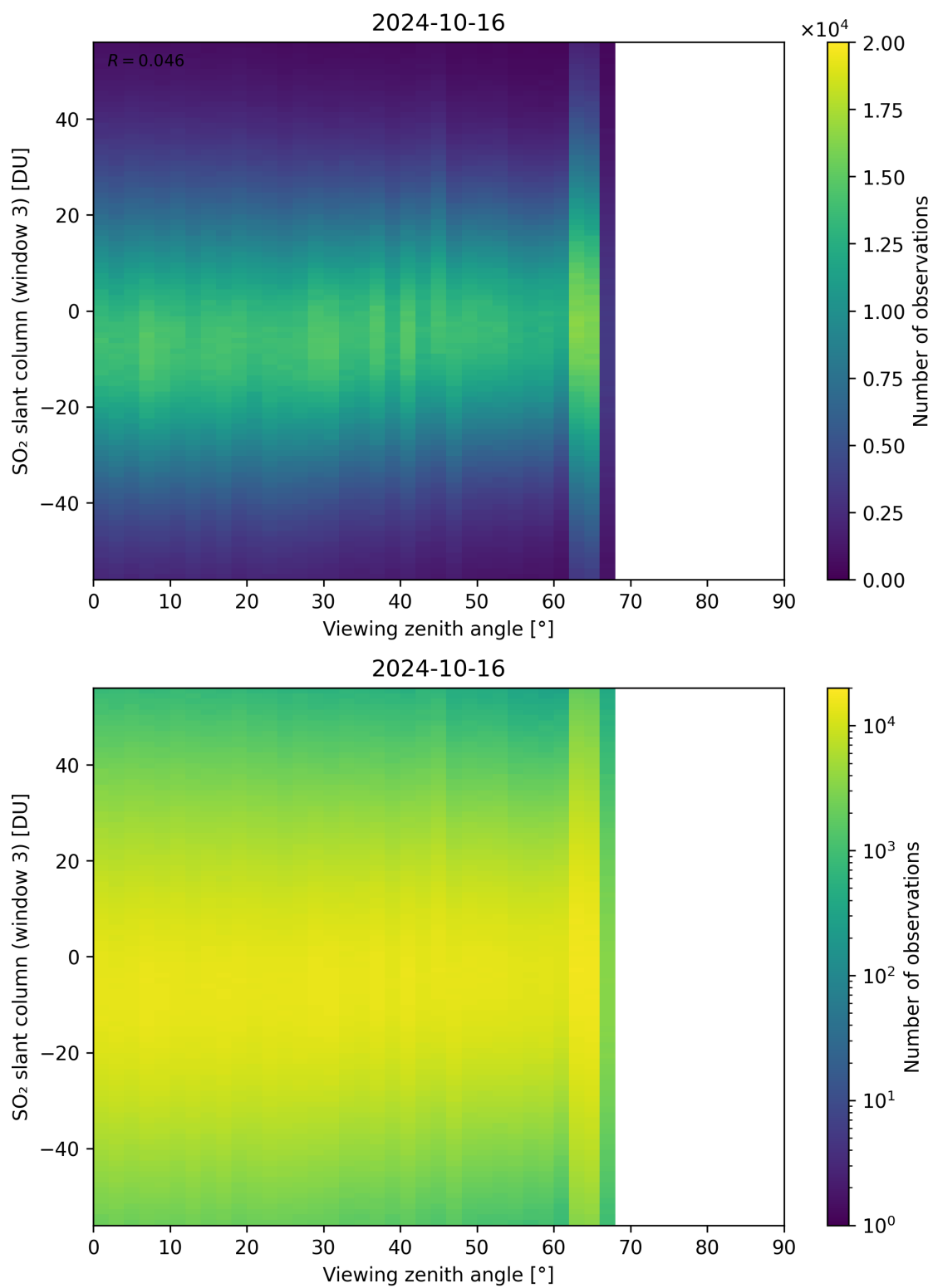
Figure 323: Scatter density plot of “Viewing zenith angle” against “SO 2 slant column (window 3)” for 2024-10-15 to 2024-10-17.
