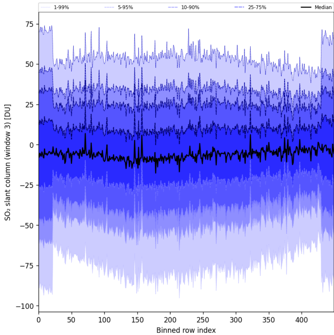
Figure 87: Along track statistics of “SO 2 slant column (window 3)” for 2024-10-15 to 2024-10-17
