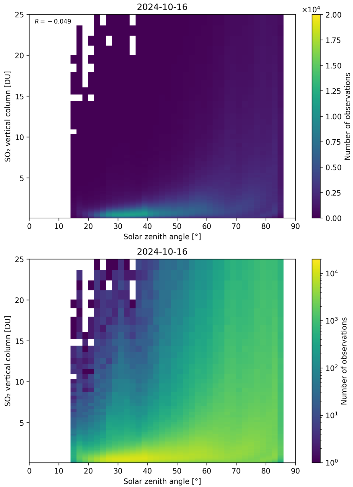
Figure 176: Scatter density plot of “Solar zenith angle” against “SO 2 vertical column” for 2024-10-15 to 2024-10-17.
