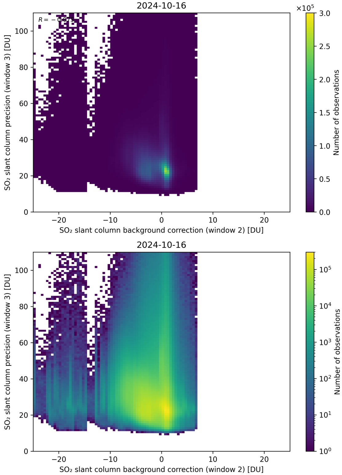
Figure 118: Scatter density plot of “SO 2 slant column background correction (window 2)” against “SO 2 slant column precision (window 3)” for 2024-10-15 to 2024-10-17.
