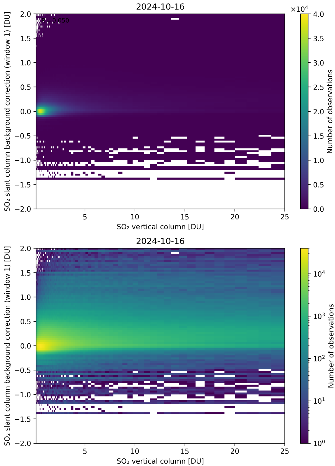
Figure 273: Scatter density plot of “SO 2 vertical column” against “SO 2 slant column background correction (window 1)” for 2024-10-15 to 2024-10-17.
