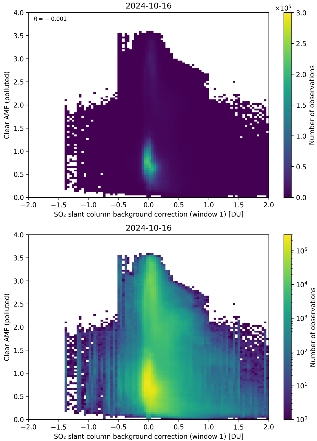
Figure 103: Scatter density plot of “SO 2 slant column background correction (window 1)” against “Clear AMF (polluted)” for 2024-10-15 to 2024-10-17.
