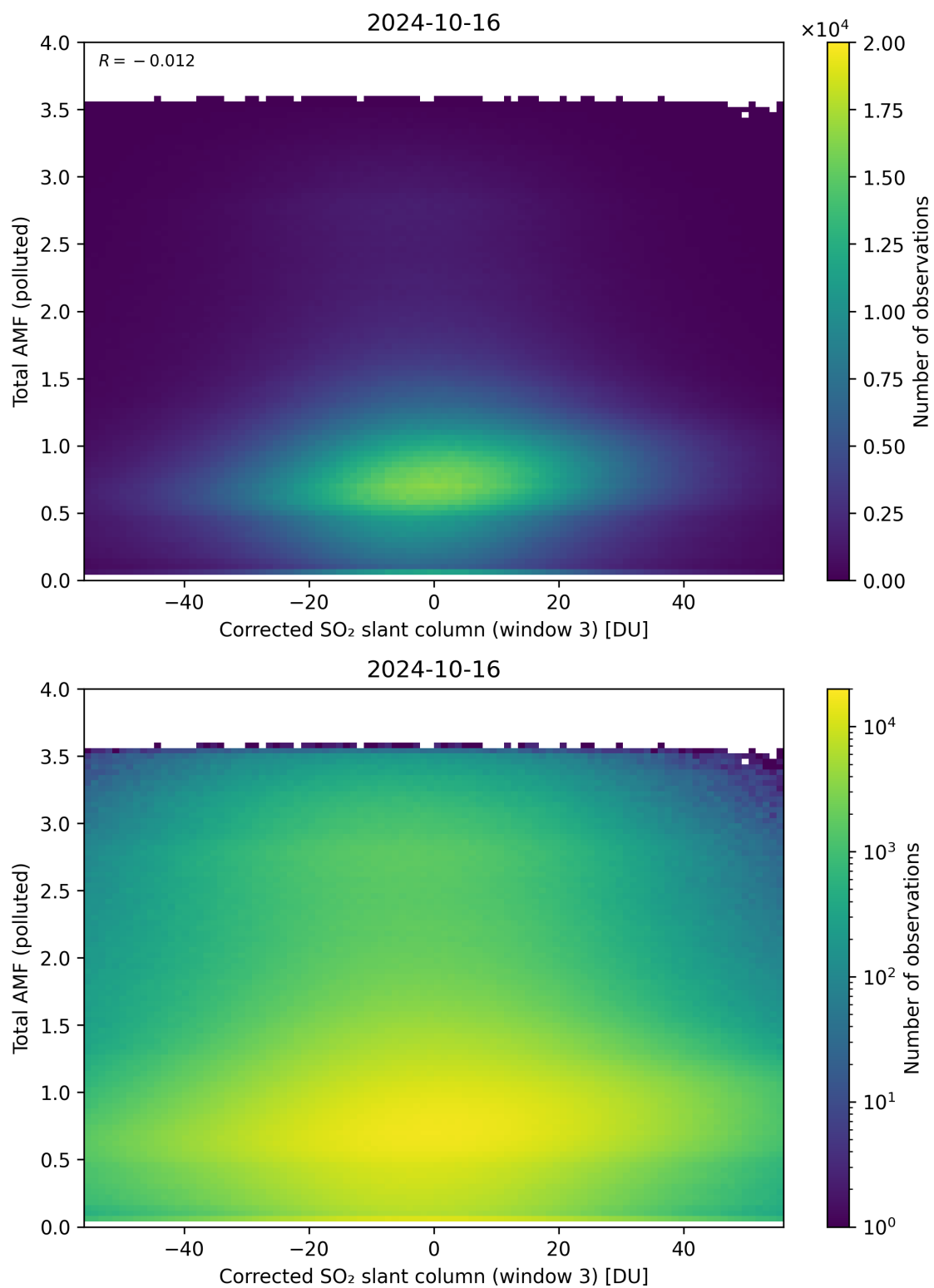
Figure 210: Scatter density plot of “Corrected SO 2 slant column (window 3)” against “Total AMF (polluted)” for 2024-10-15 to 2024-10-17.
