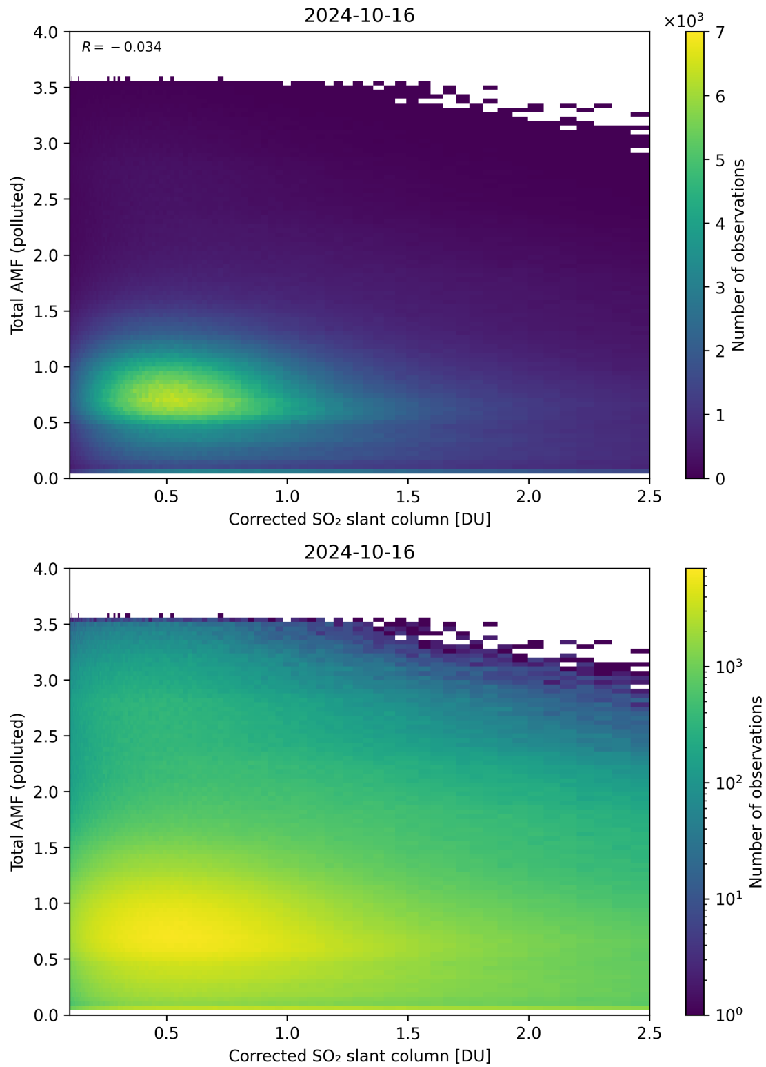
Figure 192: Scatter density plot of “Corrected SO 2 slant column” against “Total AMF (polluted)” for 2024-10-15 to 2024-10-17.
