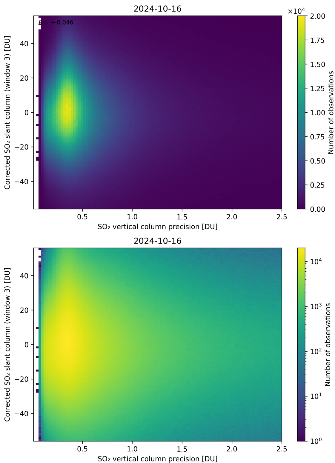
Figure 288: Scatter density plot of “SO 2 vertical column precision” against “Corrected SO 2 slant column (window 3)” for 2024-10-15 to 2024-10-17.
