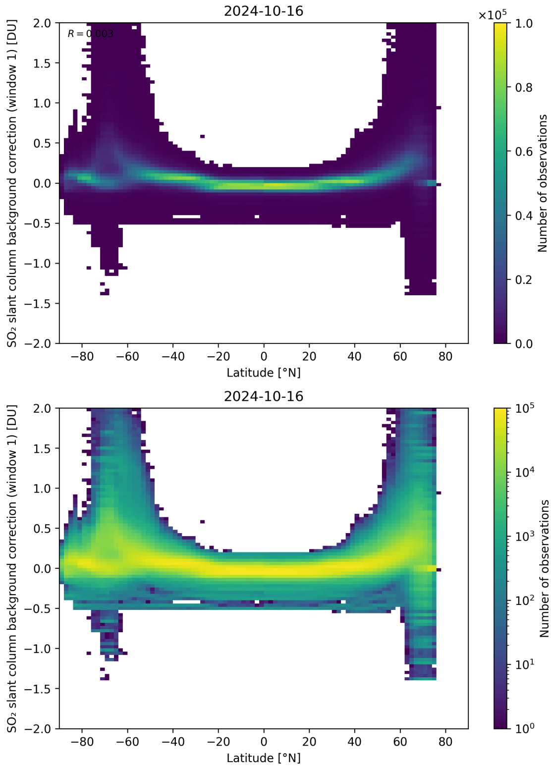
Figure 139: Scatter density plot of “Latitude” against “SO 2 slant column background correction (window 1)” for 2024-10-15 to 2024-10-17.
