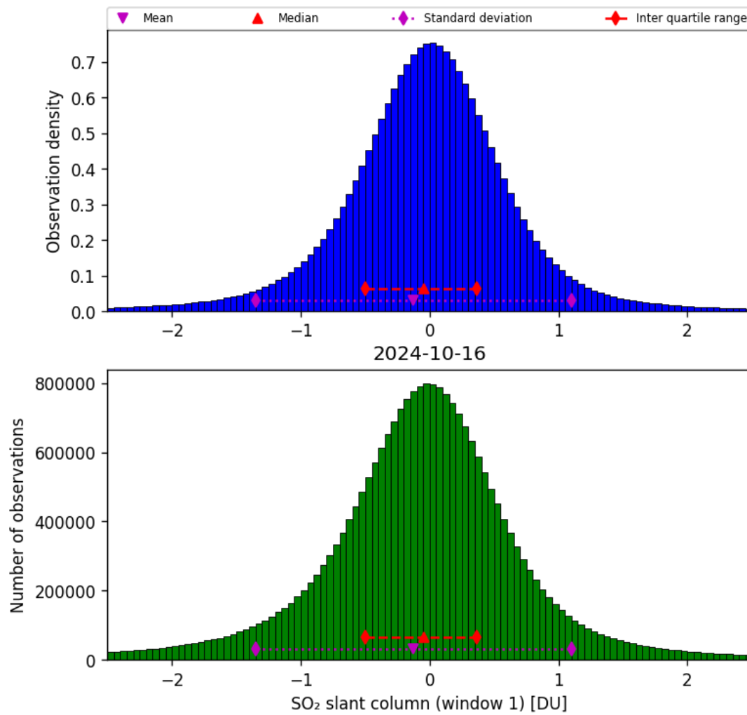
Figure 56: Histogram of “SO 2 slant column (window 1)” for 2024-10-15 to 2024-10-17
