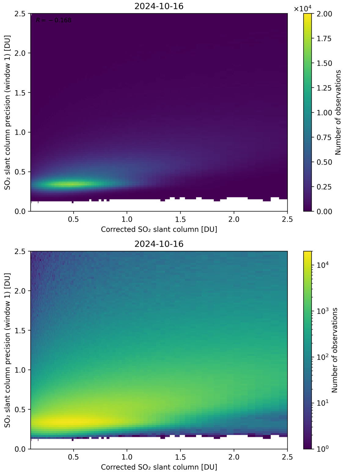
Figure 188: Scatter density plot of “Corrected SO 2 slant column” against “SO 2 slant column precision (window 1)” for 2024-10-15 to 2024-10-17.
