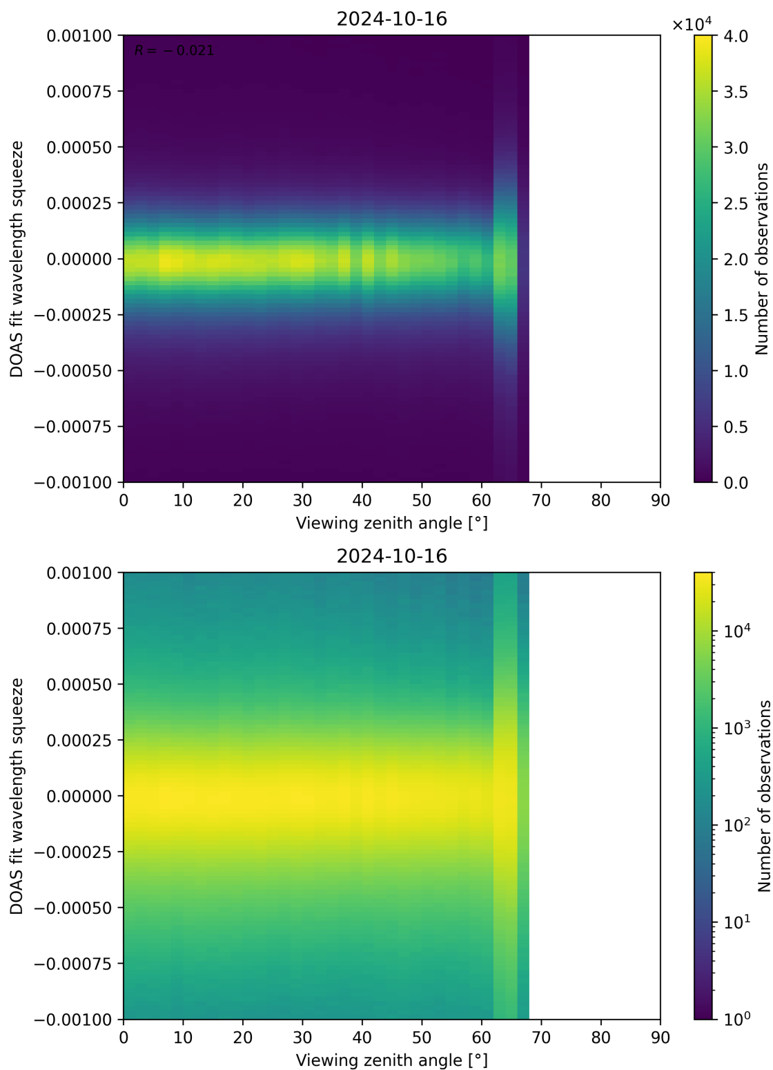
Figure 312: Scatter density plot of “Viewing zenith angle” against “DOAS fit wavelength squeeze” for 2024-10-15 to 2024-10-17.
