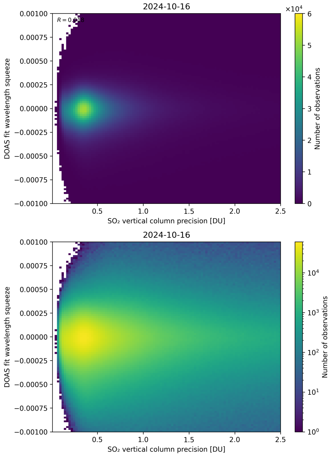
Figure 283: Scatter density plot of “SO 2 vertical column precision” against “DOAS fit wavelength squeeze” for 2024-10-15 to 2024-10-17.
