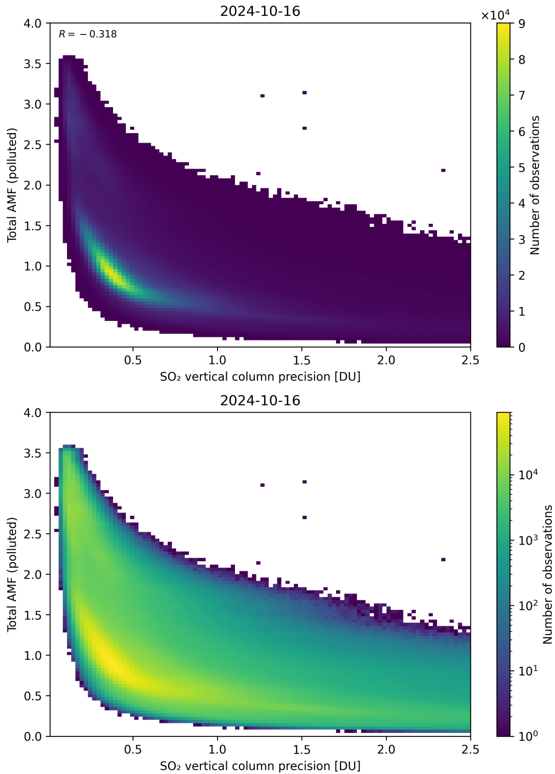
Figure 294: Scatter density plot of “SO 2 vertical column precision” against “Total AMF (polluted)” for 2024-10-15 to 2024-10-17.
