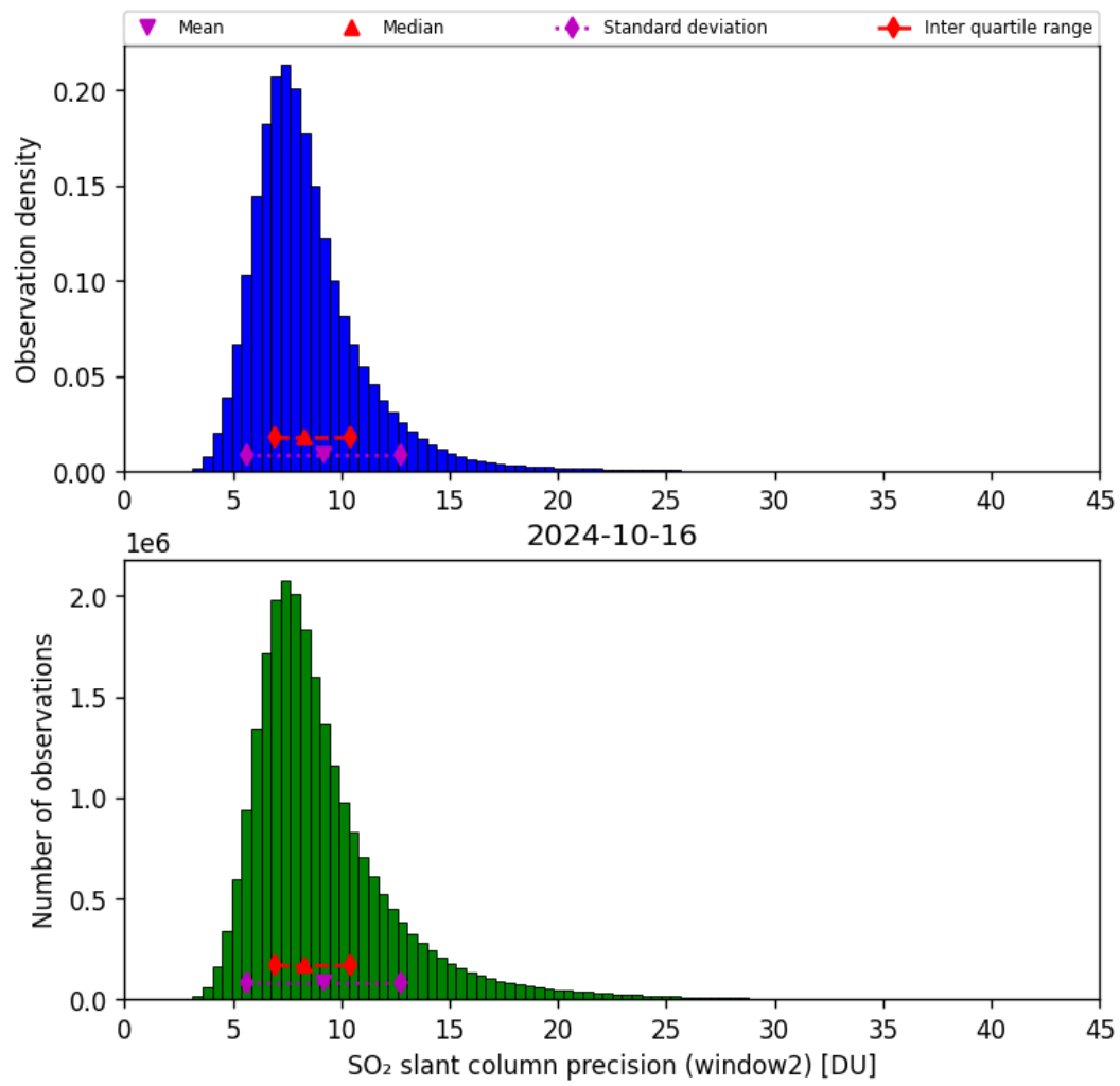
Figure 61: Histogram of “SO 2 slant column precision (window2)” for 2024-10-15 to 2024-10-17
