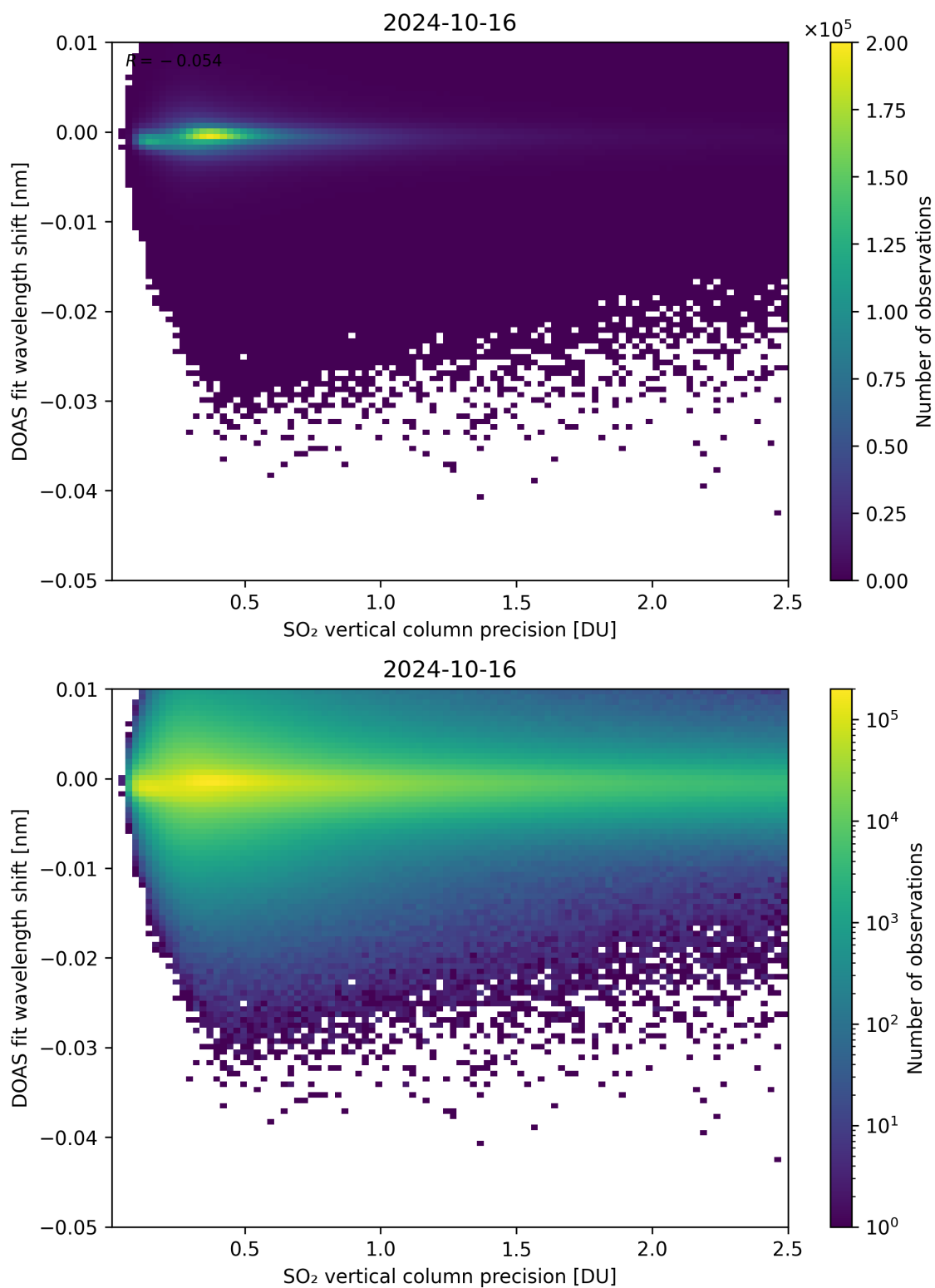
Figure 282: Scatter density plot of “SO 2 vertical column precision” against “DOAS fit wavelength shift” for 2024-10-15 to 2024-10-17.
