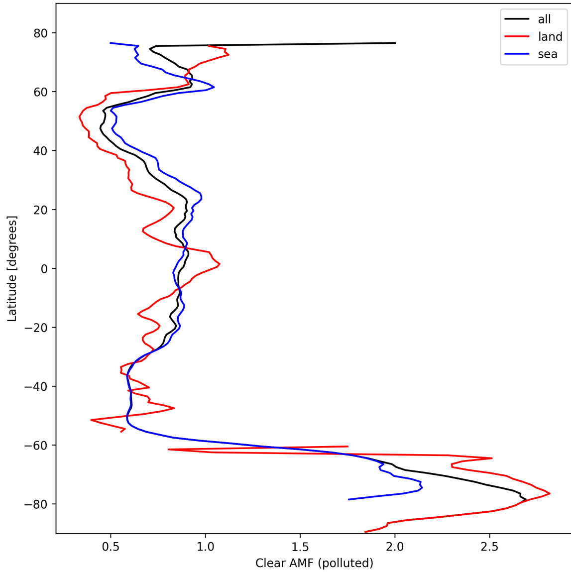
Figure 50: Zonal average of “Clear AMF (polluted)” for 2024-10-15 to 2024-10-17.
