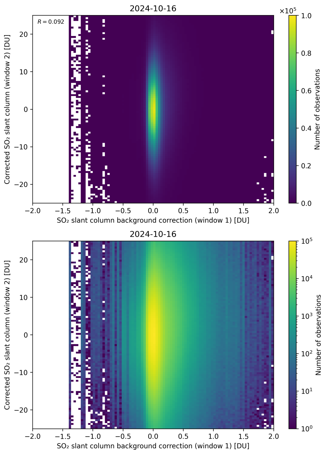
Figure 104: Scatter density plot of “SO 2 slant column background correction (window 1)” against “Corrected SO 2 slant column (window 2)” for 2024-10-15 to 2024-10-17.
