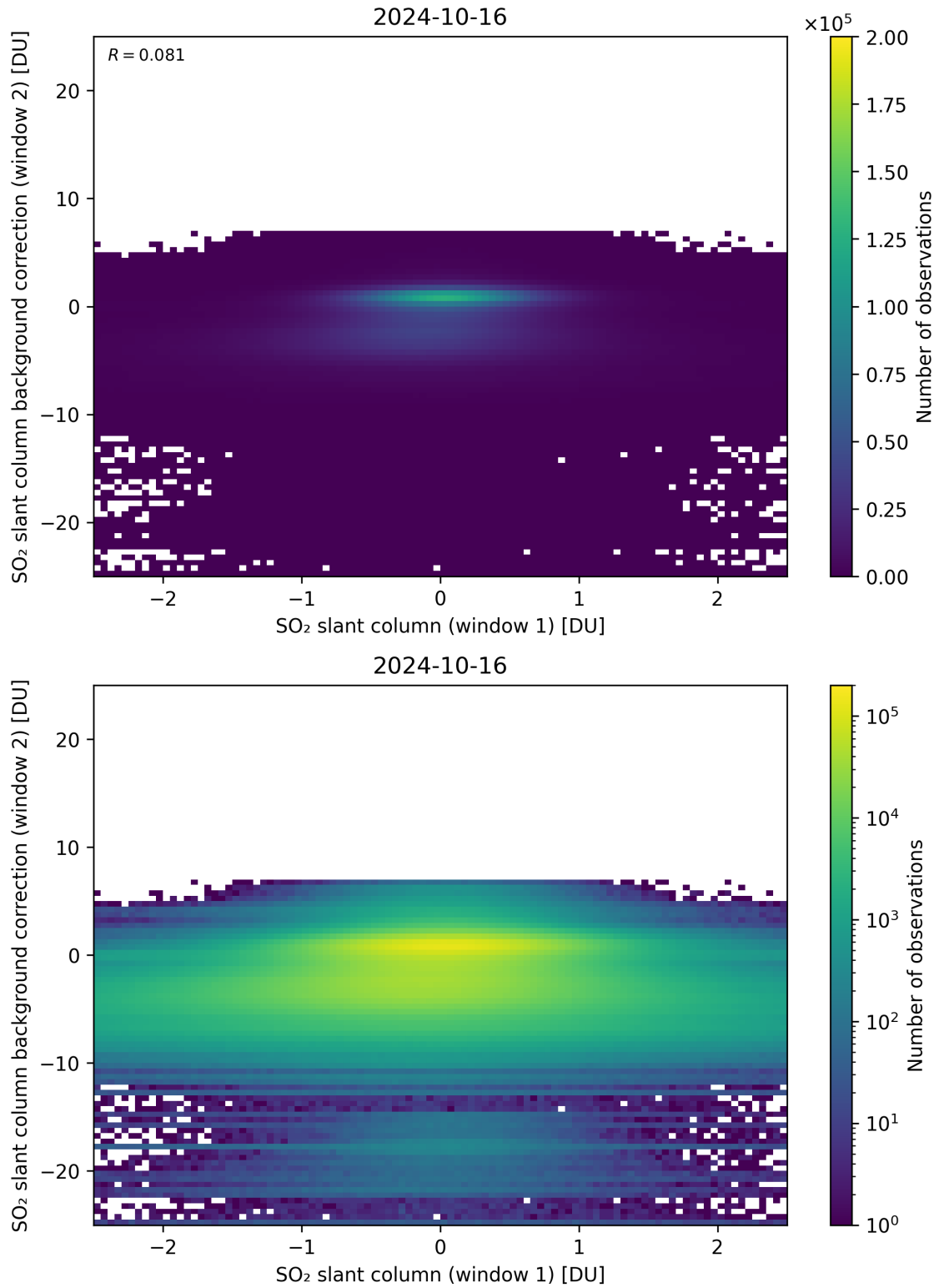
Figure 213: Scatter density plot of “SO 2 slant column (window 1)” against “SO 2 slant column background correction (window 2)” for 2024-10-15 to 2024-10-17.
