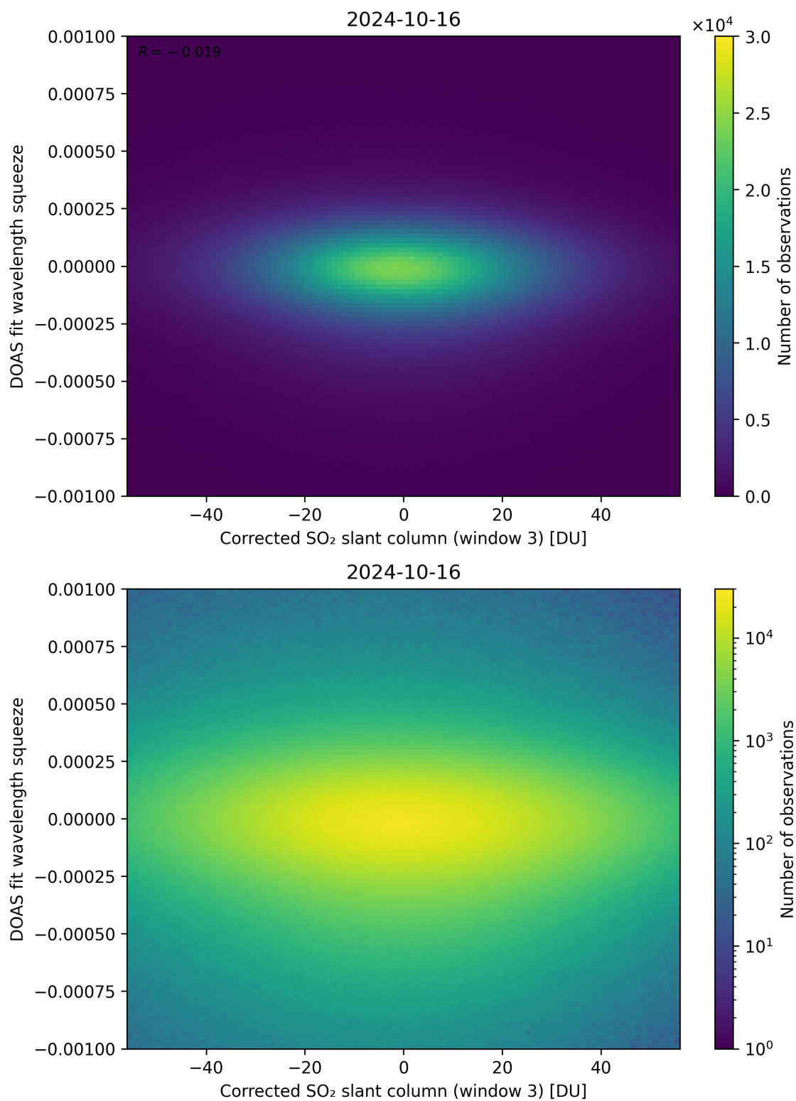
Figure 207: Scatter density plot of “Corrected SO 2 slant column (window 3)” against “DOAS fit wavelength squeeze” for 2024-10-15 to 2024-10-17.
