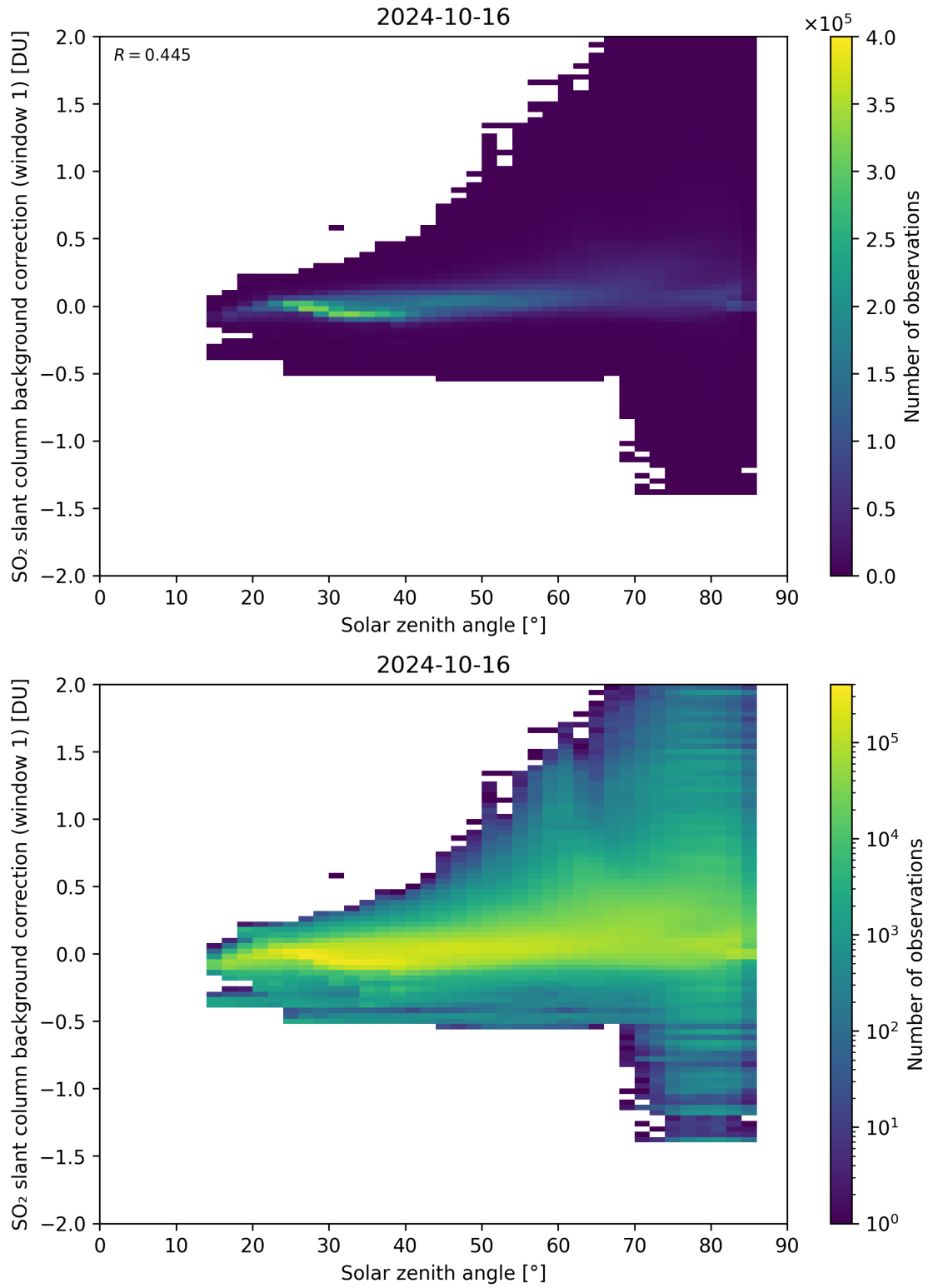
Figure 158: Scatter density plot of “Solar zenith angle” against “SO 2 slant column background correction (window 1)” for 2024-10-15 to 2024-10-17.
