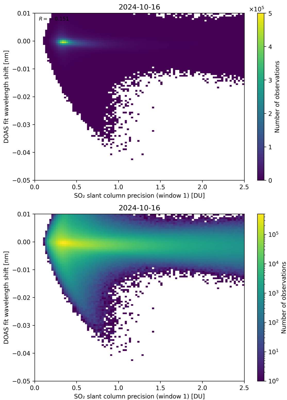
Figure 221: Scatter density plot of “SO 2 slant column precision (window 1)” against “DOAS fit wavelength shift” for 2024-10-15 to 2024-10-17.
