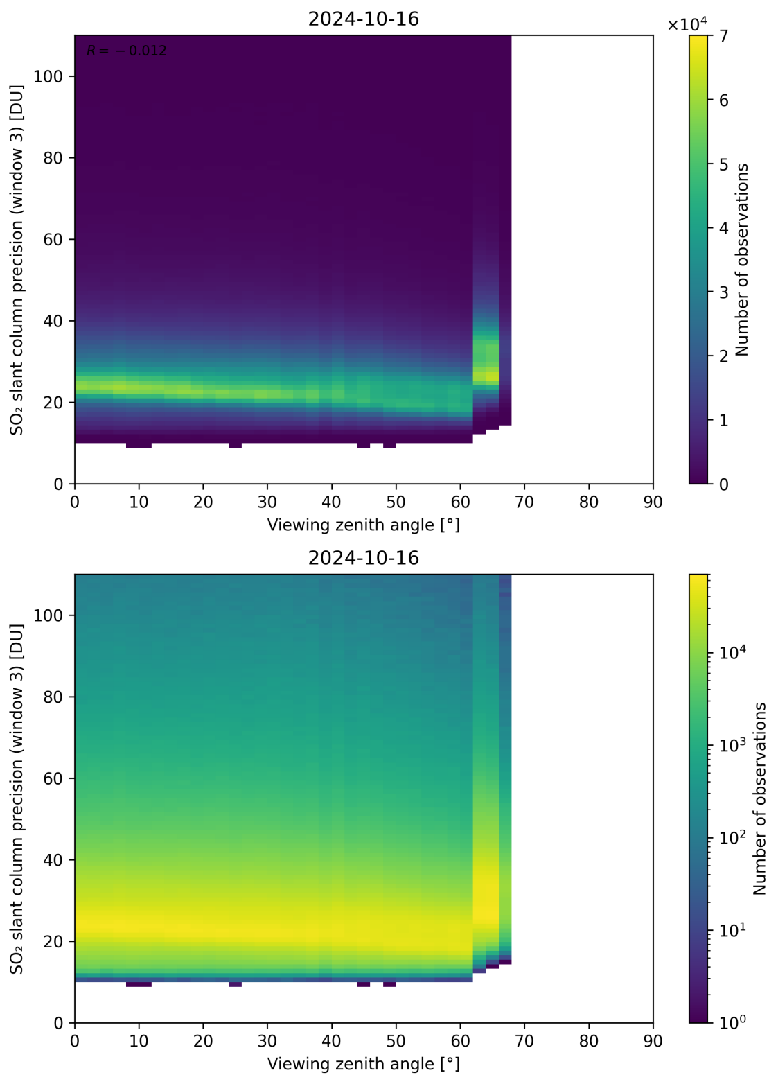
Figure 324: Scatter density plot of “Viewing zenith angle” against “SO 2 slant column precision (window 3)” for 2024-10-15 to 2024-10-17.
