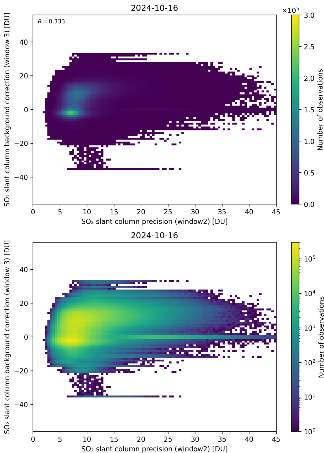
Figure 242: Scatter density plot of “SO 2 slant column precision (window2)” against “SO 2 slant column background correction (window 3)” for 2024-10-15 to 2024-10-17.
