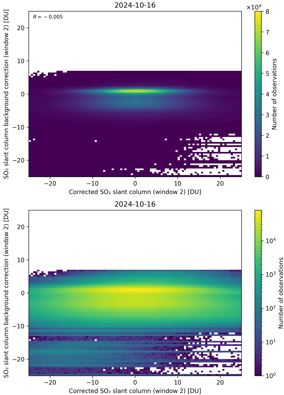
Figure 194: Scatter density plot of “Corrected SO 2 slant column (window 2)” against “SO 2 slant column background correction (window 2)” for 2024-10-15 to 2024-10-17.
