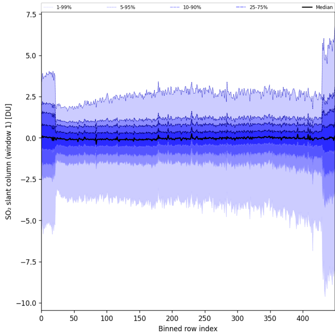
Figure 79: Along track statistics of “SO 2 slant column (window 1)” for 2024-10-15 to 2024-10-17
