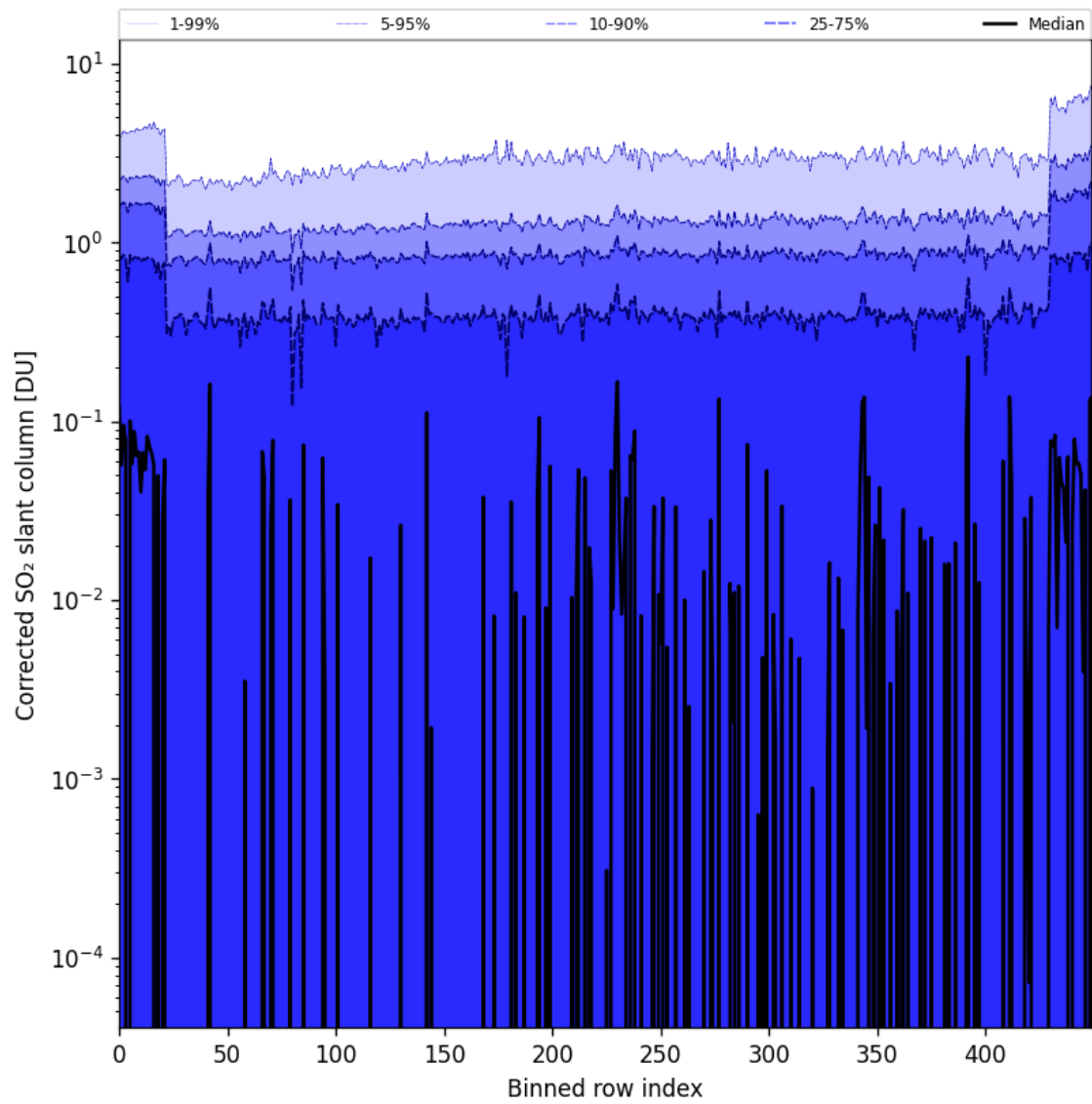
Figure 78: Along track statistics of “Corrected SO 2 slant column” for 2024-10-15 to 2024-10-17
