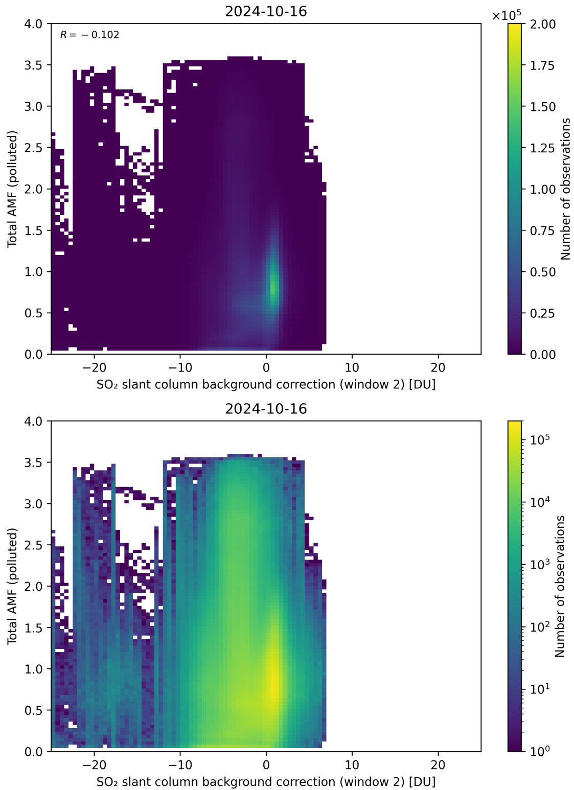
Figure 119: Scatter density plot of “SO 2 slant column background correction (window 2)” against “Total AMF (polluted)” for 2024-10-15 to 2024-10-17.
