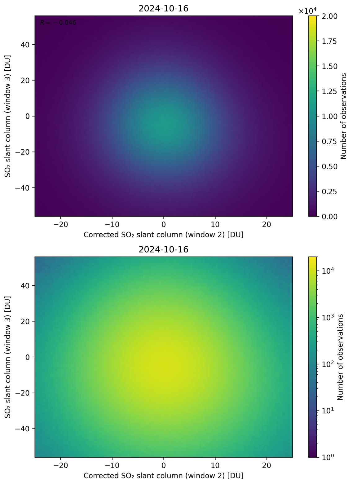
Figure 201: Scatter density plot of “Corrected SO 2 slant column (window 2)” against “SO 2 slant column (window 3)” for 2024-10-15 to 2024-10-17.
