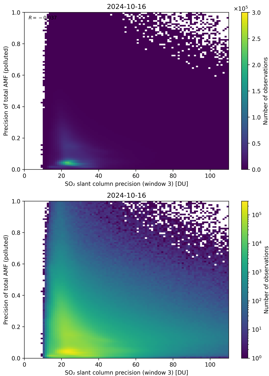
Figure 264: Scatter density plot of “SO 2 slant column precision (window 3)” against “Precision of total AMF (polluted)” for 2024-10-15 to 2024-10-17.
