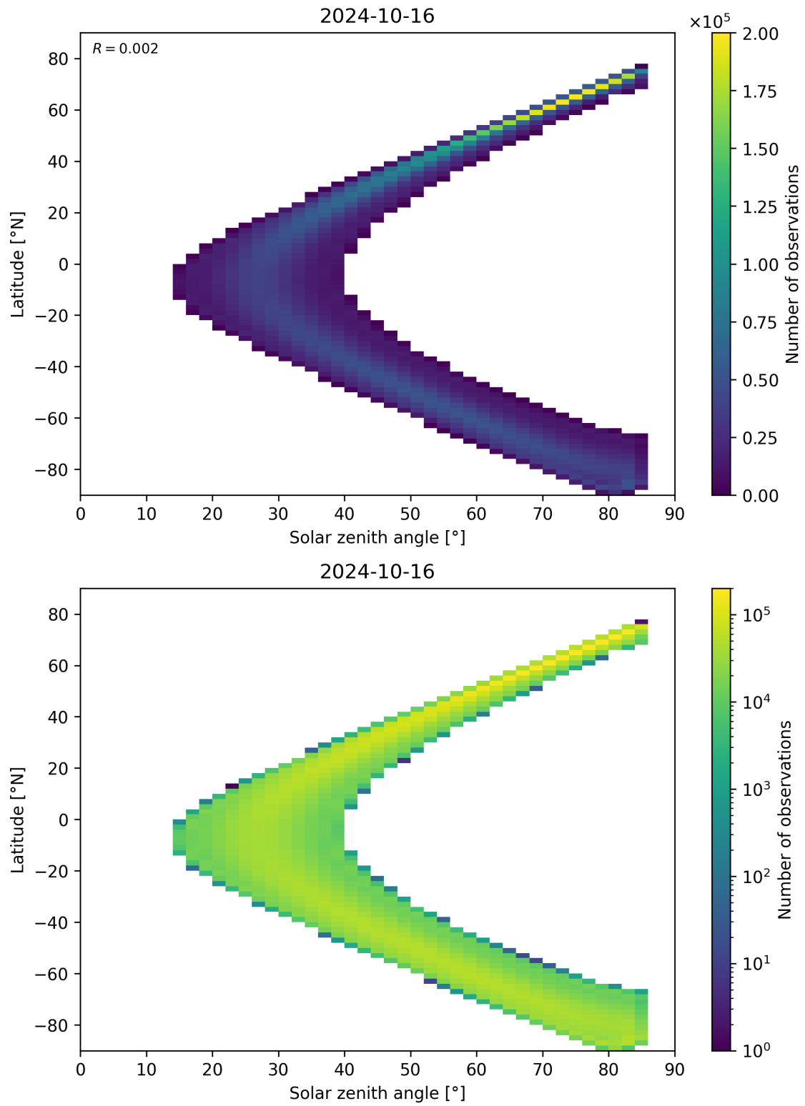
Figure 164: Scatter density plot of “Solar zenith angle” against “Latitude” for 2024-10-15 to 2024-10-17.
