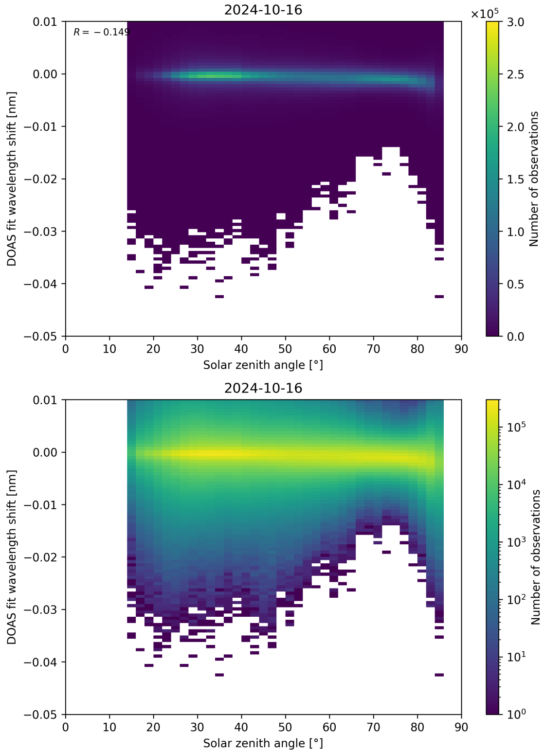
Figure 161: Scatter density plot of “Solar zenith angle” against “DOAS fit wavelength shift” for 2024-10-15 to 2024-10-17.
