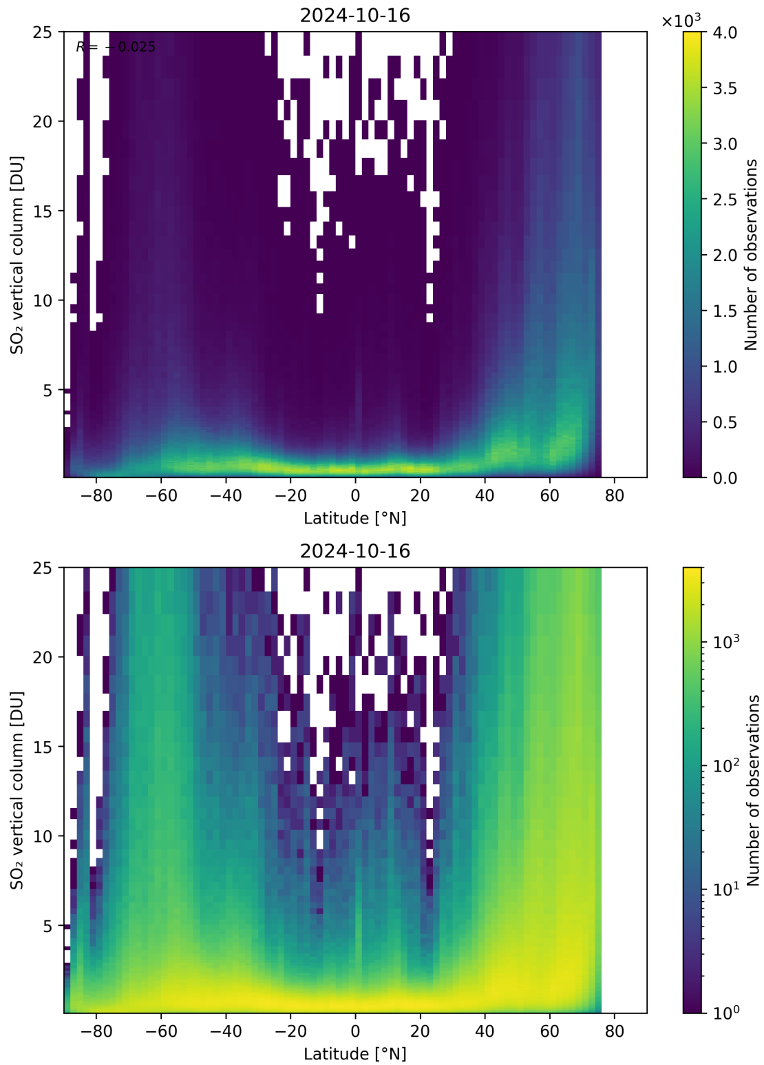
Figure 156: Scatter density plot of “Latitude” against “SO 2 vertical column” for 2024-10-15 to 2024-10-17.
