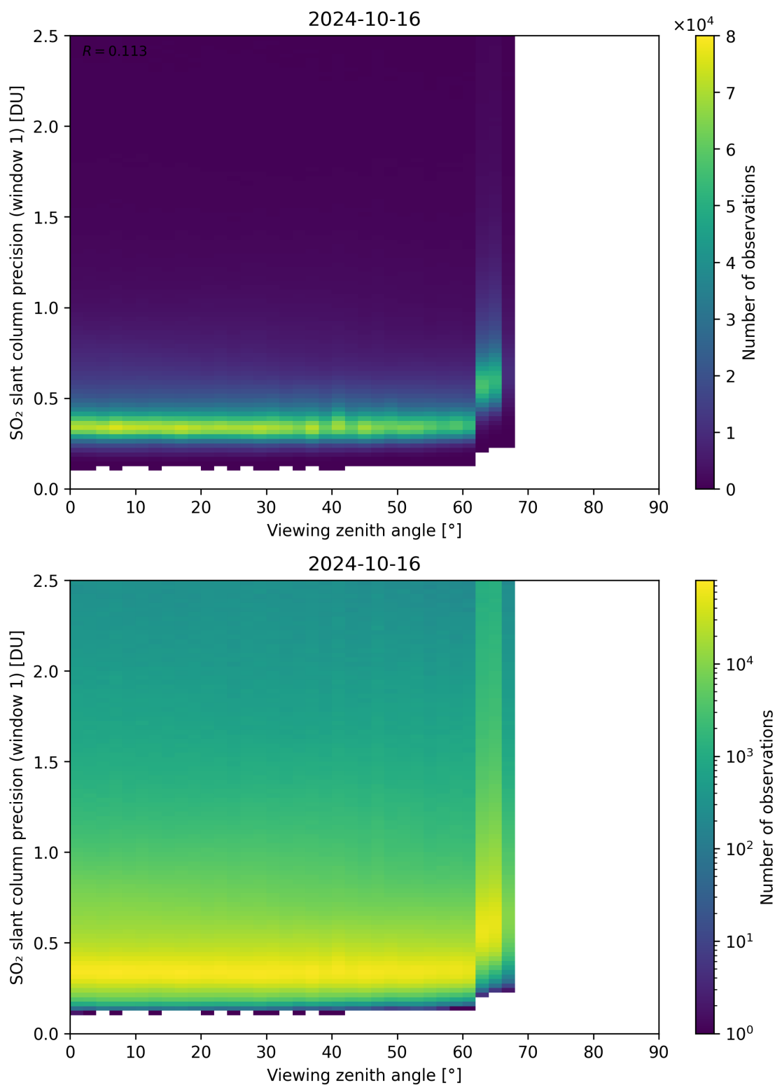
Figure 321: Scatter density plot of “Viewing zenith angle” against “SO 2 slant column precision (window 1)” for 2024-10-15 to 2024-10-17.
