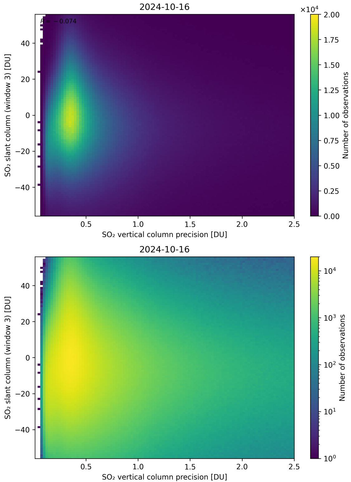
Figure 292: Scatter density plot of “SO 2 vertical column precision” against “SO 2 slant column (window 3)” for 2024-10-15 to 2024-10-17.
