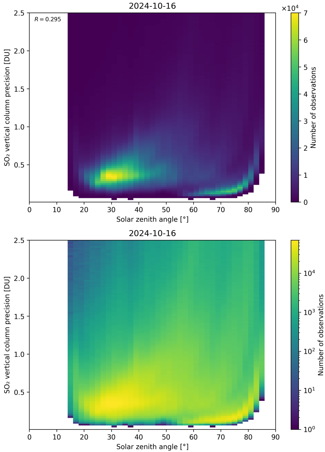
Figure 177: Scatter density plot of “Solar zenith angle” against “SO 2 vertical column precision” for 2024-10-15 to 2024-10-17.
