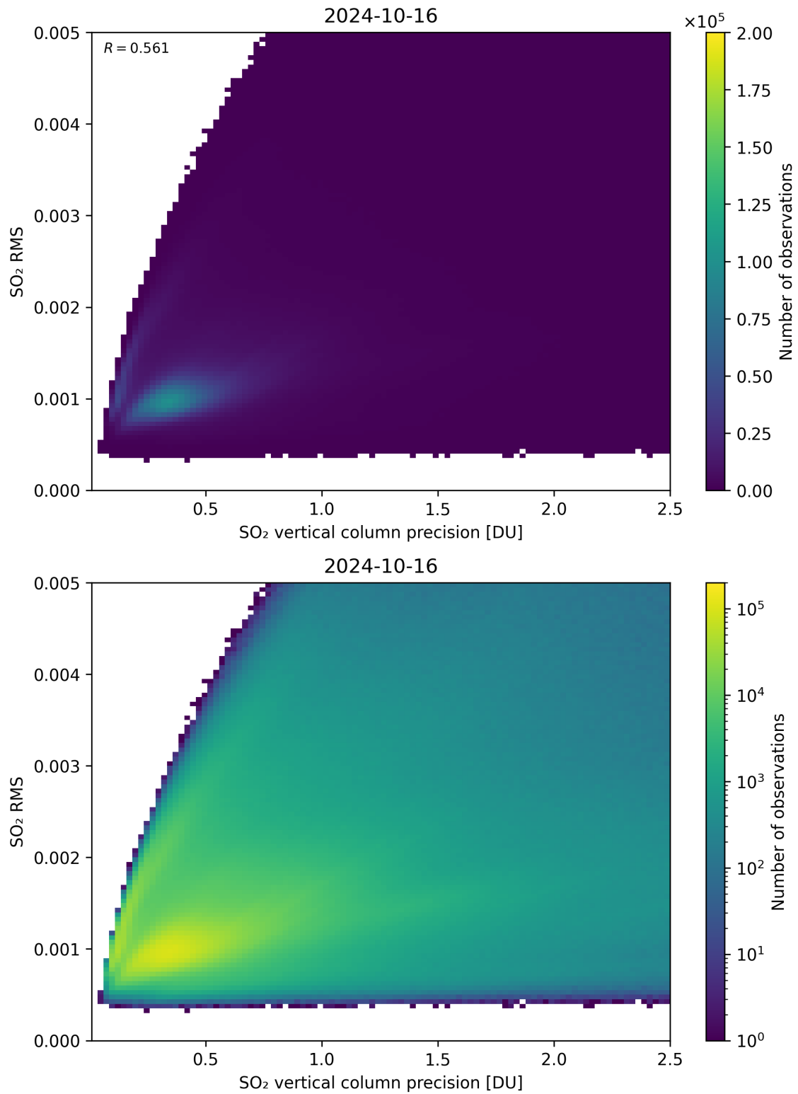
Figure 284: Scatter density plot of “SO 2 vertical column precision” against “SO 2 RMS” for 2024-10-15 to 2024-10-17.
