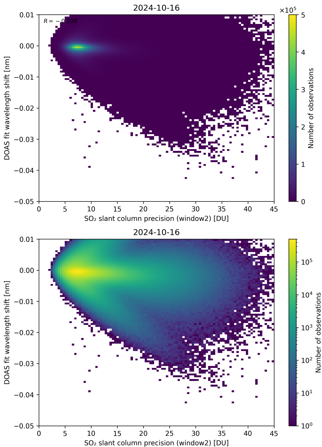
Figure 243: Scatter density plot of “SO 2 slant column precision (window2)” against “DOAS fit wavelength shift” for 2024-10-15 to 2024-10-17.
