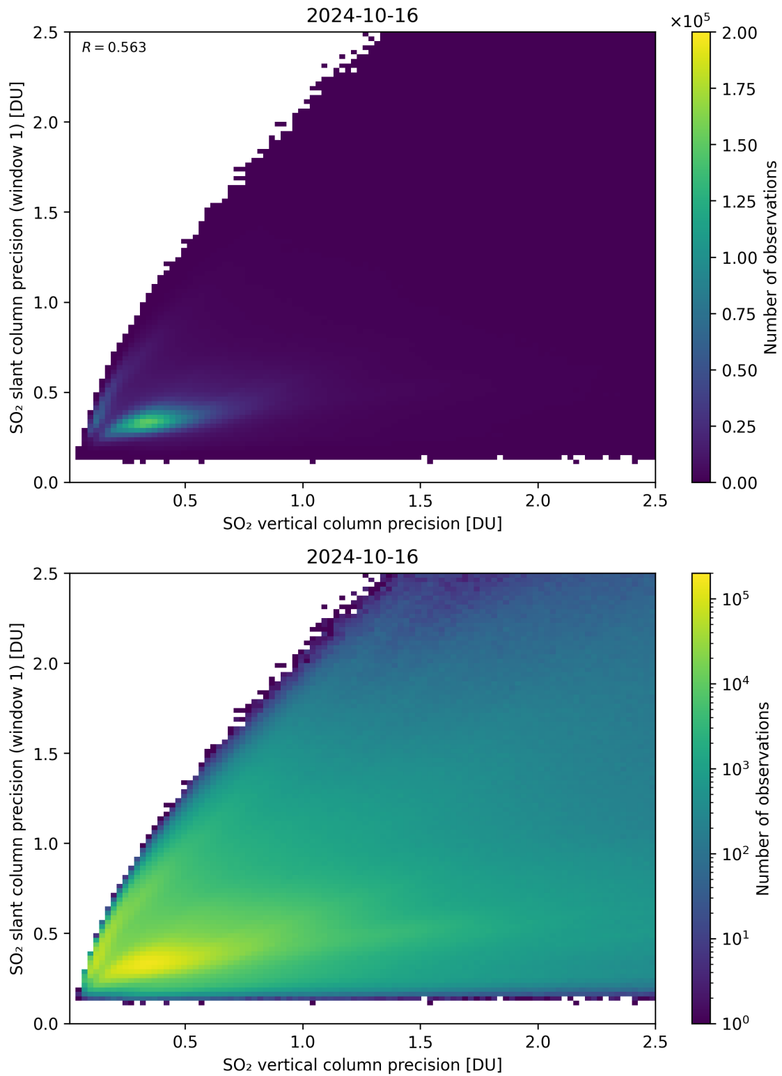
Figure 290: Scatter density plot of “SO 2 vertical column precision” against “SO 2 slant column precision (window 1)” for 2024-10-15 to 2024-10-17.
