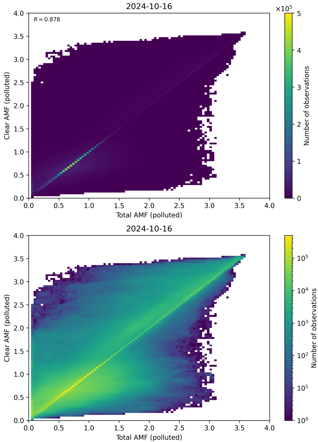
Figure 271: Scatter density plot of “Total AMF (polluted)” against “Clear AMF (polluted)” for 2024-10-15 to 2024-10-17.
