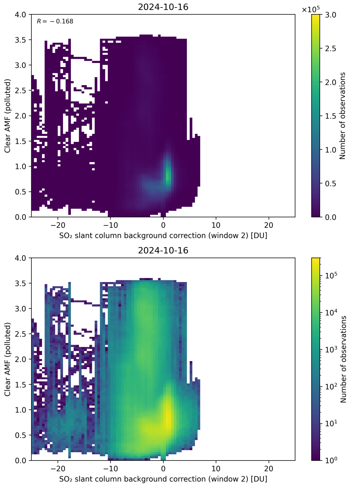
Figure 115: Scatter density plot of “SO 2 slant column background correction (window 2)” against “Clear AMF (polluted)” for 2024-10-15 to 2024-10-17.
