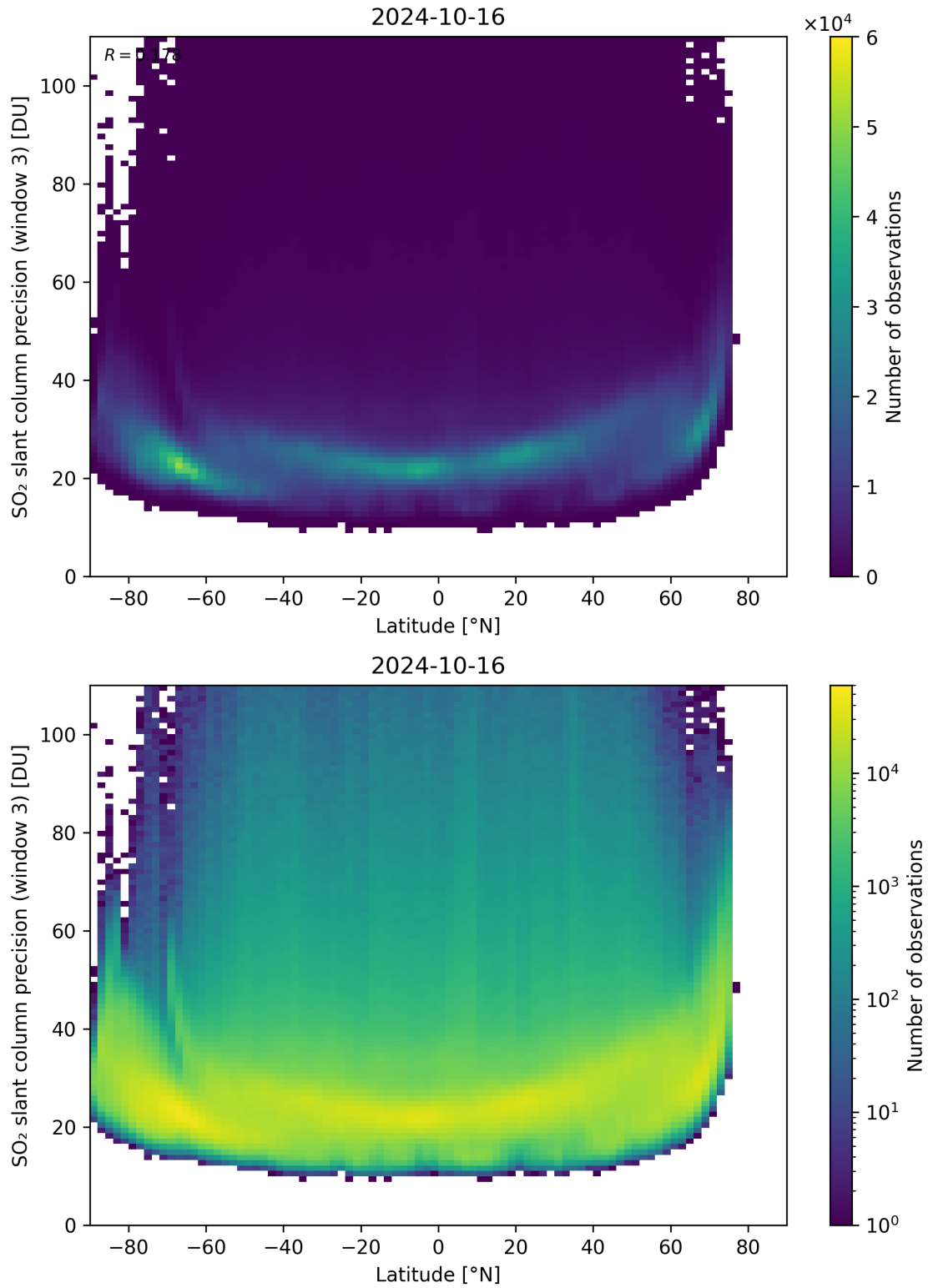
Figure 153: Scatter density plot of “Latitude” against “SO 2 slant column precision (window 3)” for 2024-10-15 to 2024-10-17.
