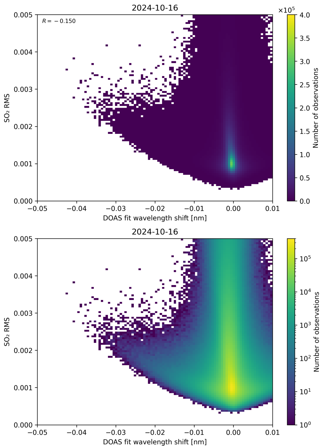
Figure 128: Scatter density plot of “DOAS fit wavelength shift” against “SO 2 RMS” for 2024-10-15 to 2024-10-17.
