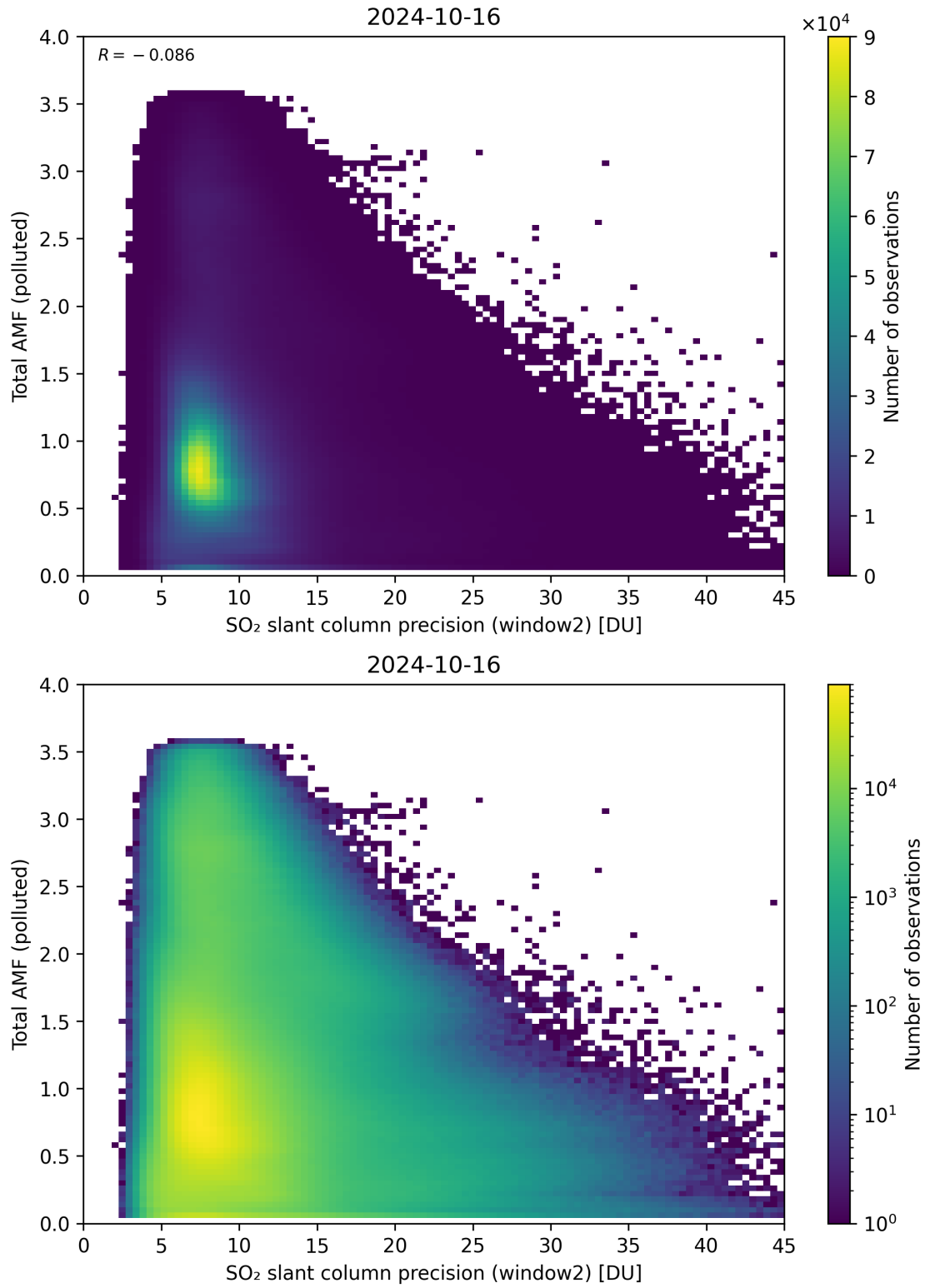
Figure 251: Scatter density plot of “SO 2 slant column precision (window2)” against “Total AMF (polluted)” for 2024-10-15 to 2024-10-17.
