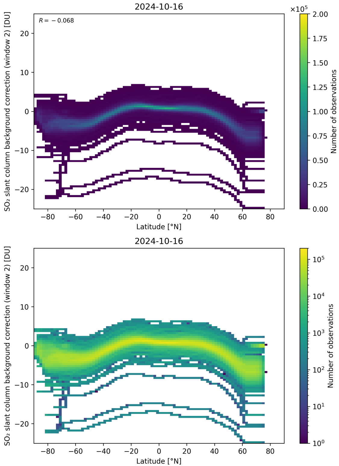
Figure 140: Scatter density plot of “Latitude” against “SO 2 slant column background correction (window 2)” for 2024-10-15 to 2024-10-17.
