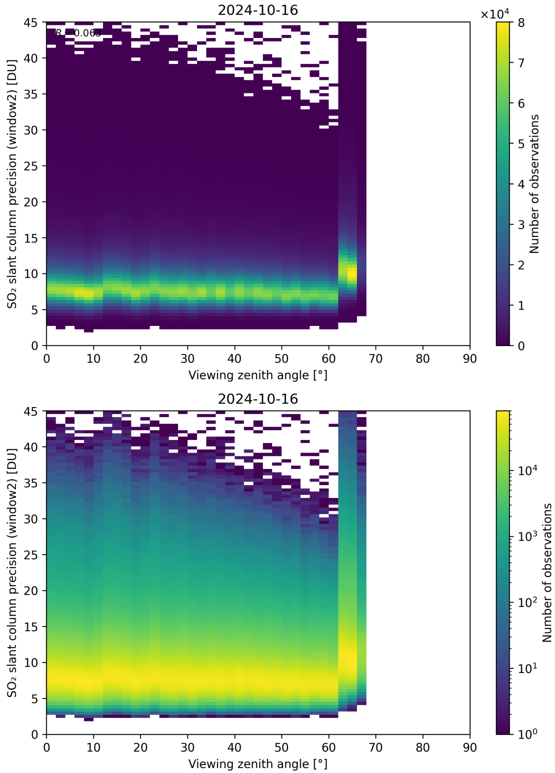
Figure 322: Scatter density plot of “Viewing zenith angle” against “SO 2 slant column precision (window2)” for 2024-10-15 to 2024-10-17.
