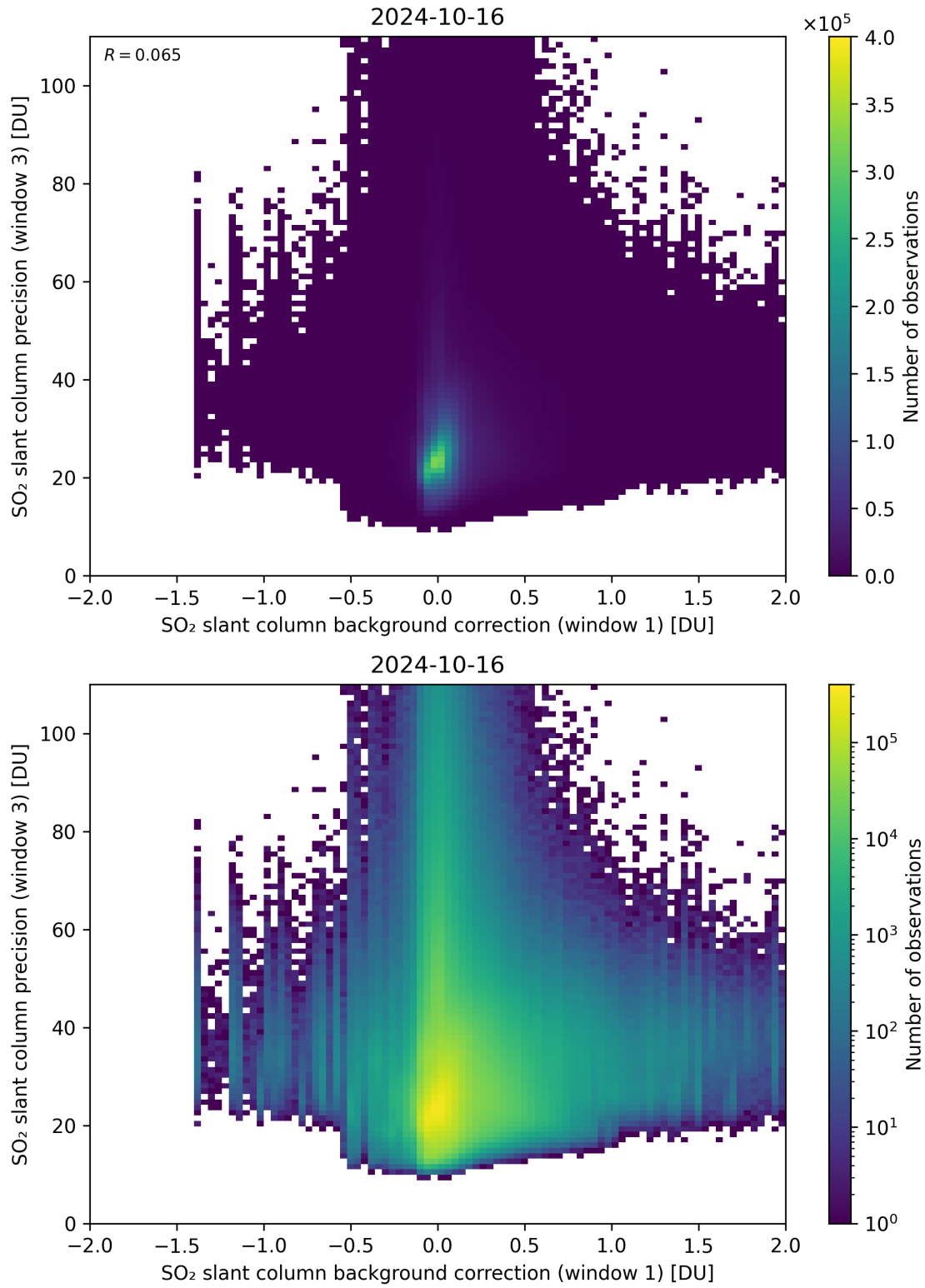
Figure 108: Scatter density plot of “SO 2 slant column background correction (window 1)” against “SO 2 slant column precision (window 3)” for 2024-10-15 to 2024-10-17.
