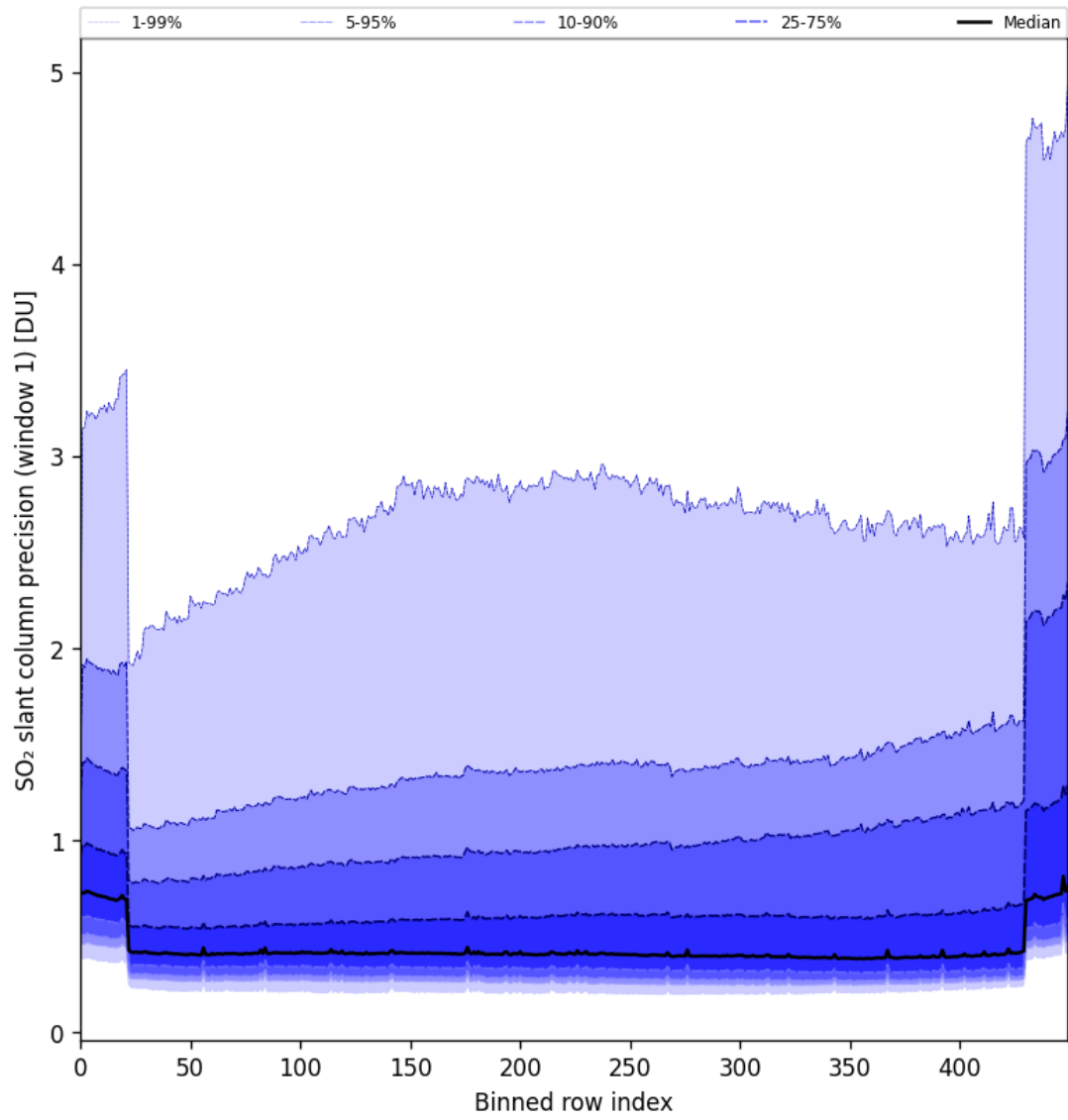
Figure 80: Along track statistics of “SO 2 slant column precision (window 1)” for 2024-10-15 to 2024-10-17
