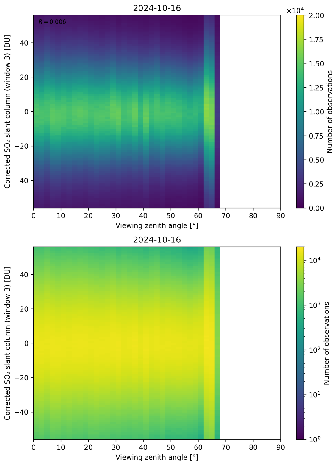
Figure 319: Scatter density plot of “Viewing zenith angle” against “Corrected SO 2 slant column (window 3)” for 2024-10-15 to 2024-10-17.
