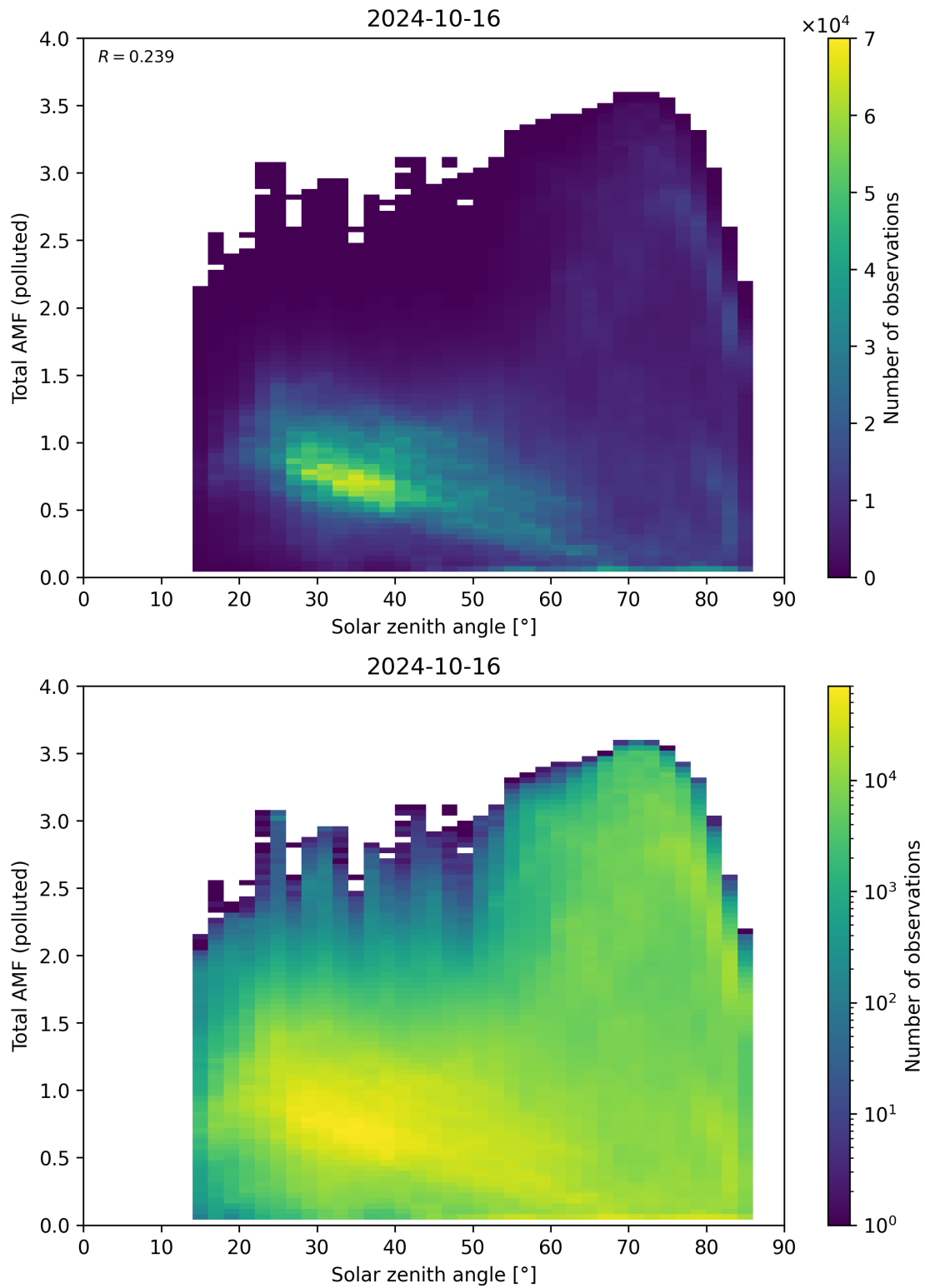
Figure 174: Scatter density plot of “Solar zenith angle” against “Total AMF (polluted)” for 2024-10-15 to 2024-10-17.
