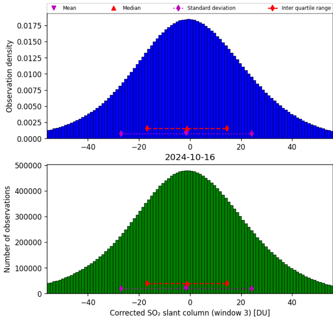
Figure 66: Histogram of “Corrected SO 2 slant column (window 3)” for 2024-10-15 to 2024-10-17
