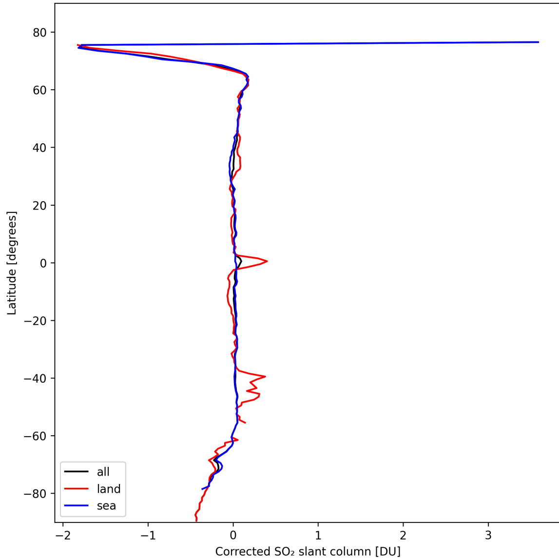
Figure 32: Zonal average of “Corrected SO 2 slant column” for 2024-10-15 to 2024-10-17.
