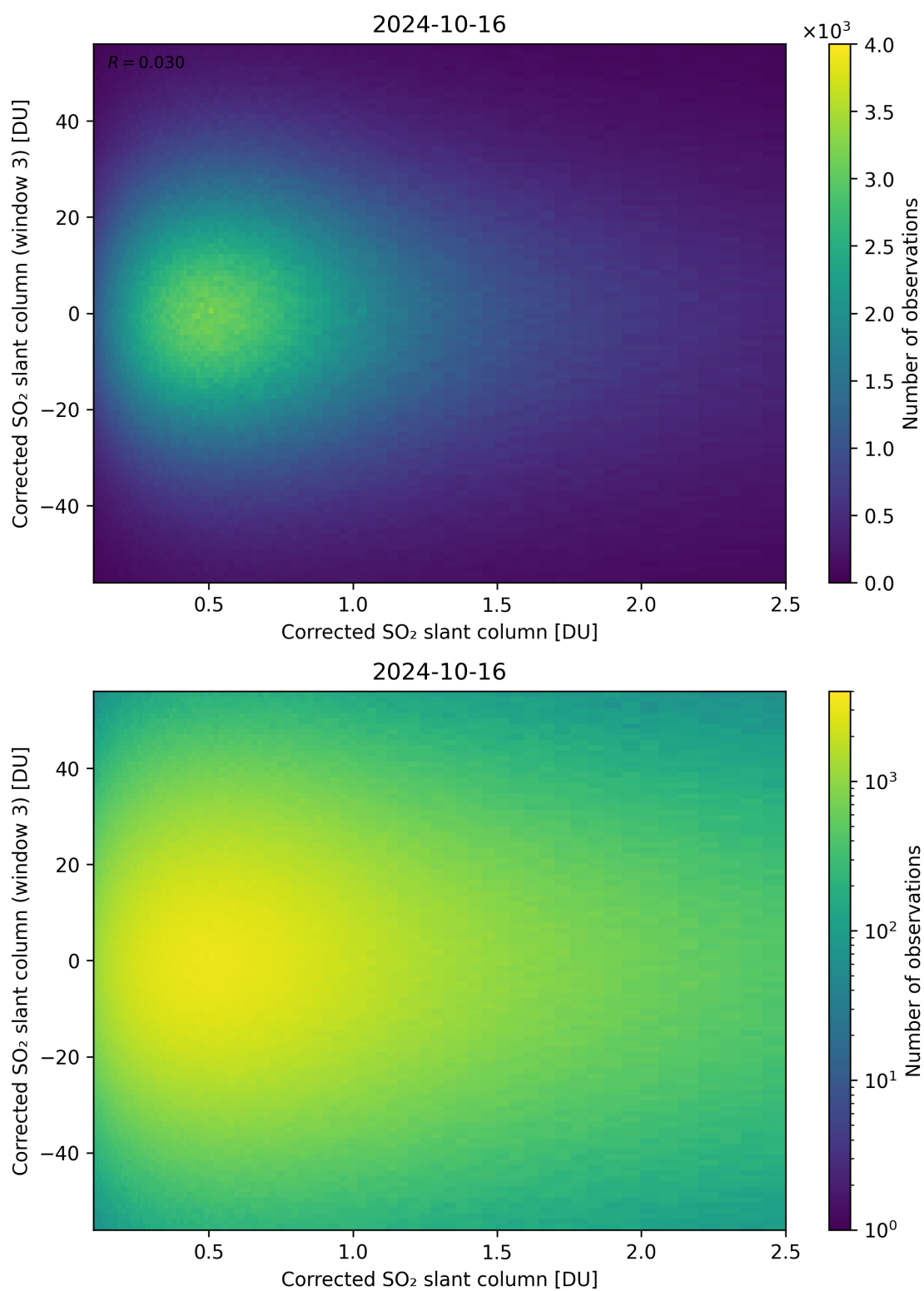
Figure 186: Scatter density plot of “Corrected SO 2 slant column” against “Corrected SO 2 slant column (window 3)” for 2024-10-15 to 2024-10-17.
