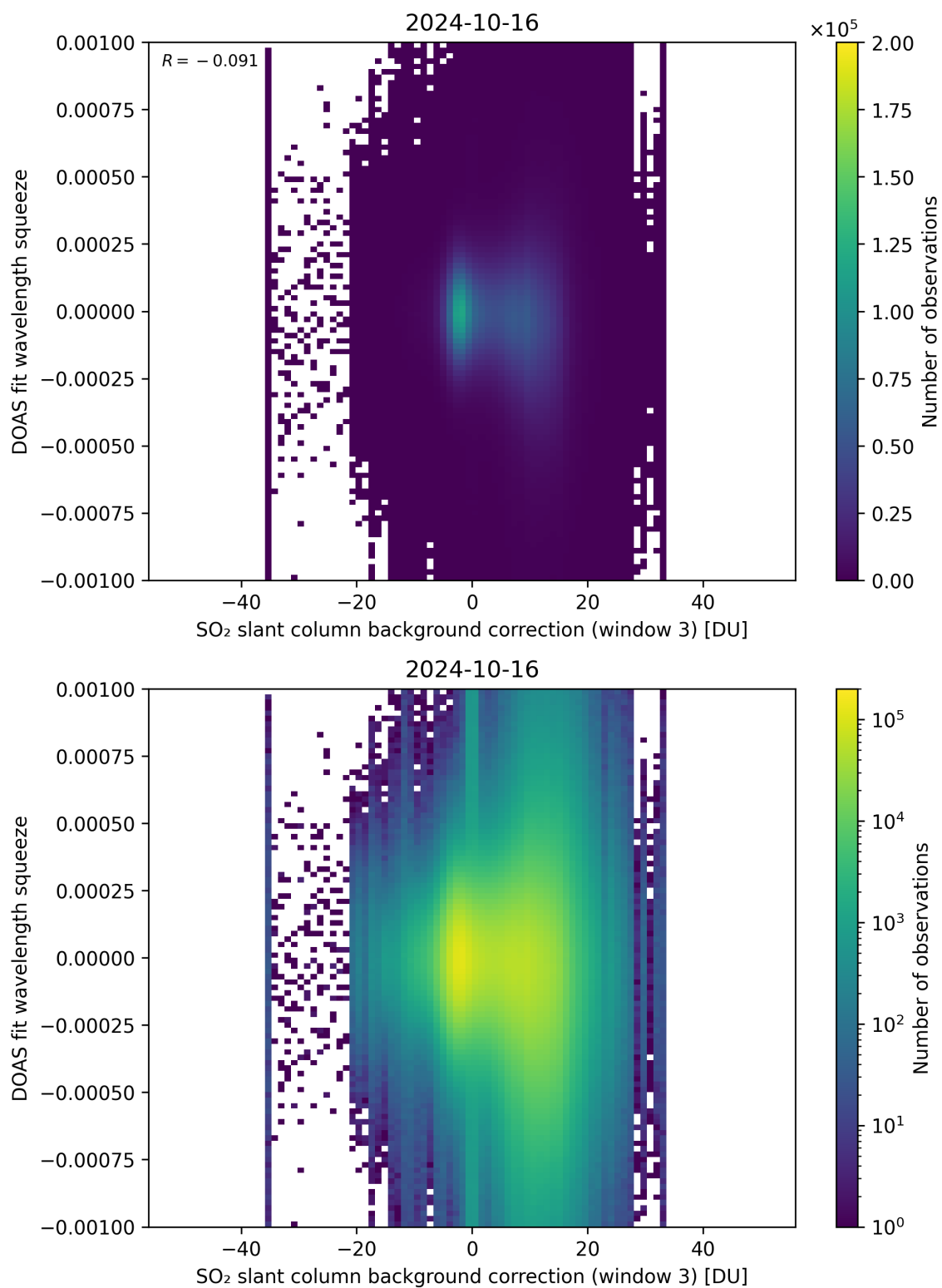
Figure 122: Scatter density plot of “SO 2 slant column background correction (window 3)” against “DOAS fit wavelength squeeze” for 2024-10-15 to 2024-10-17.
