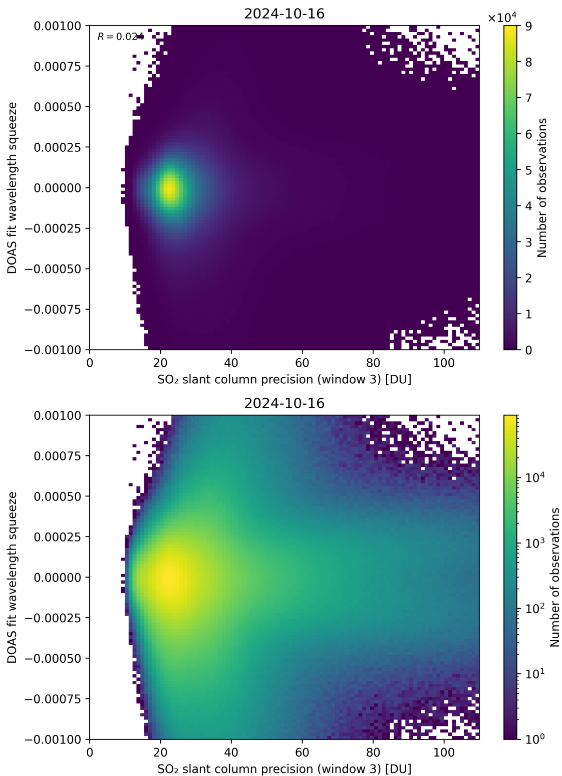
Figure 259: Scatter density plot of “SO 2 slant column precision (window 3)” against “DOAS fit wavelength squeeze” for 2024-10-15 to 2024-10-17.
