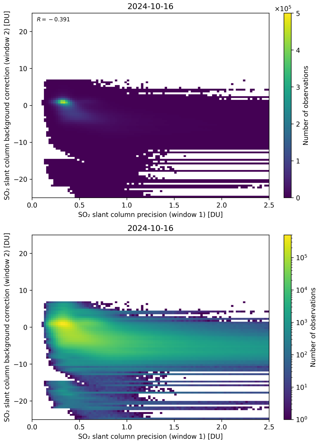
Figure 219: Scatter density plot of “SO 2 slant column precision (window 1)” against “SO 2 slant column background correction (window 2)” for 2024-10-15 to 2024-10-17.
