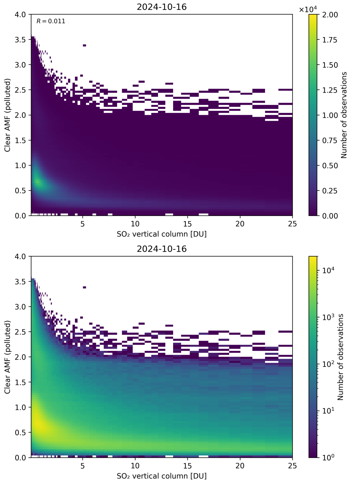
Figure 296: Scatter density plot of “SO 2 vertical column” against “Clear AMF (polluted)” for 2024-10-15 to 2024-10-17.
