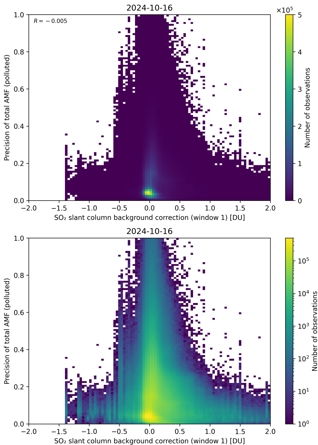
Figure 110: Scatter density plot of “SO 2 slant column background correction (window 1)” against “Precision of total AMF (polluted)” for 2024-10-15 to 2024-10-17.
