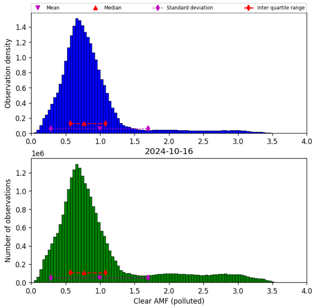
Figure 73: Histogram of “Clear AMF (polluted)” for 2024-10-15 to 2024-10-17
