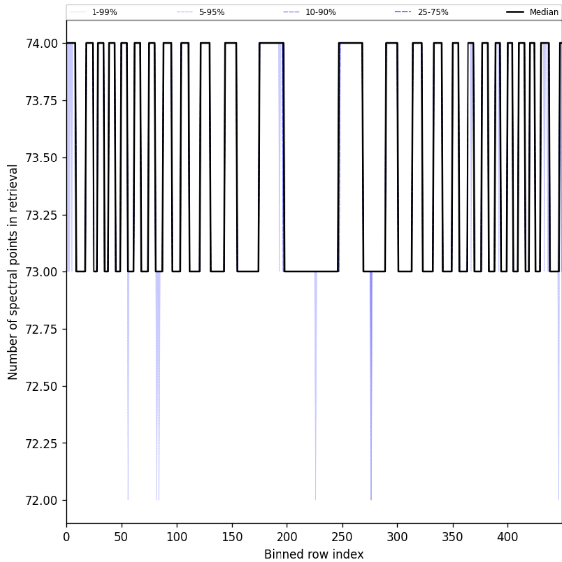
Figure 97: Along track statistics of “Number of spectral points in retrieval” for 2024-10-15 to 2024-10-17
