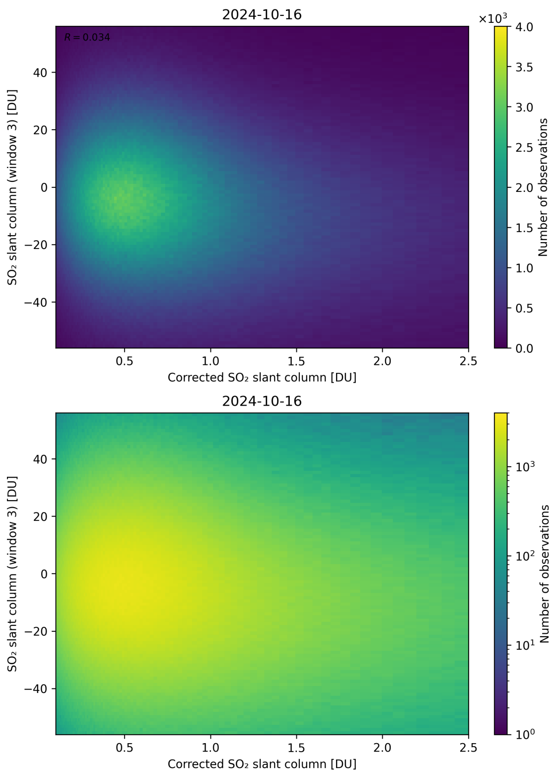
Figure 190: Scatter density plot of “Corrected SO 2 slant column” against “SO 2 slant column (window 3)” for 2024-10-15 to 2024-10-17.
