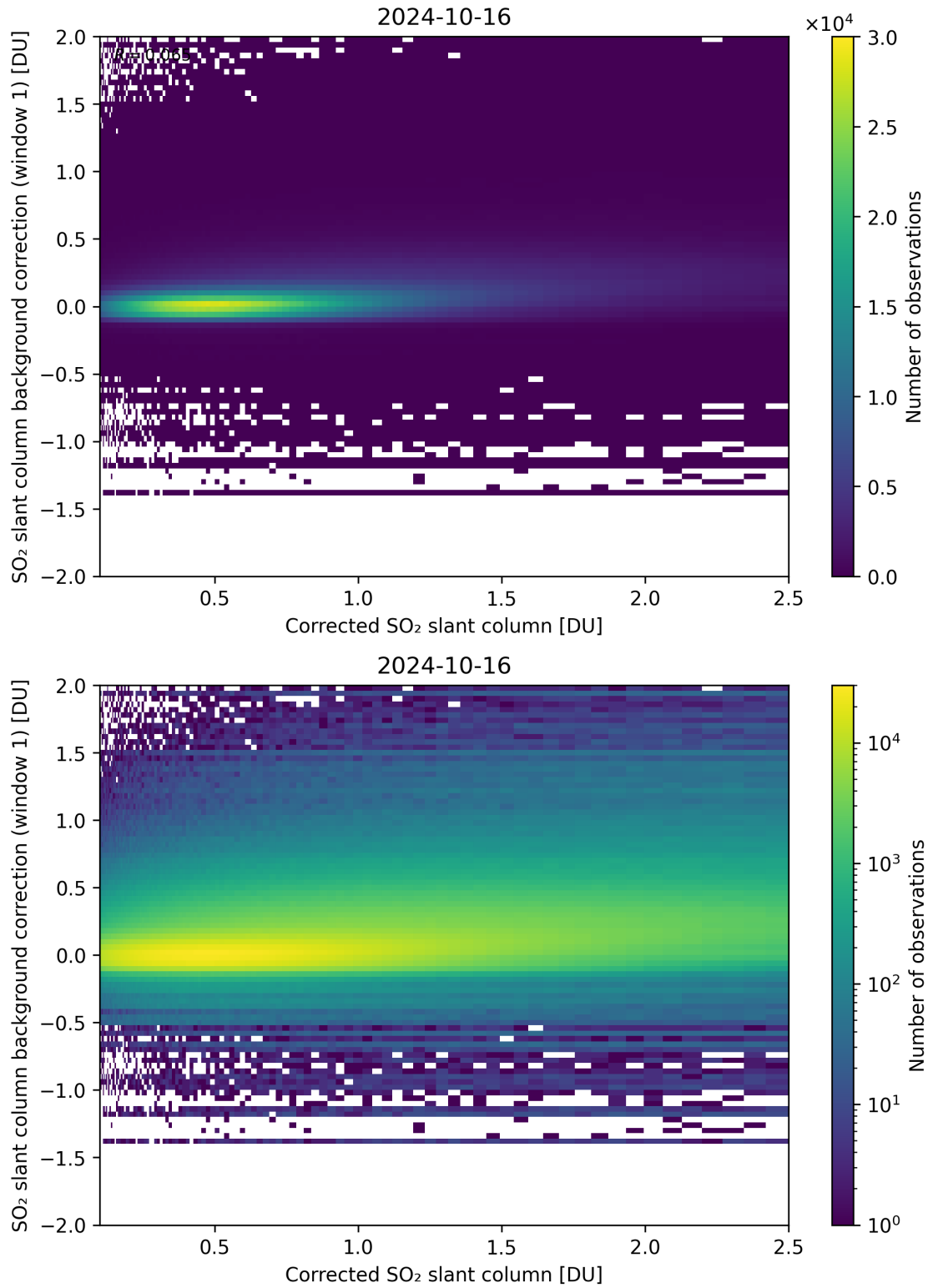
Figure 178: Scatter density plot of “Corrected SO 2 slant column” against “SO 2 slant column background correction (window 1)” for 2024-10-15 to 2024-10-17.
