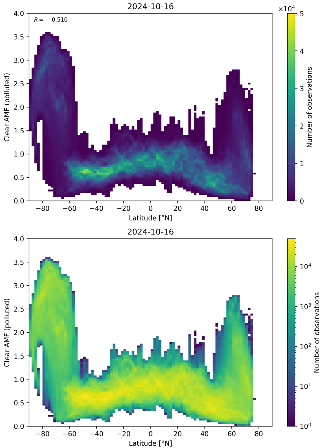
Figure 145: Scatter density plot of “Latitude” against “Clear AMF (polluted)” for 2024-10-15 to 2024-10-17.
