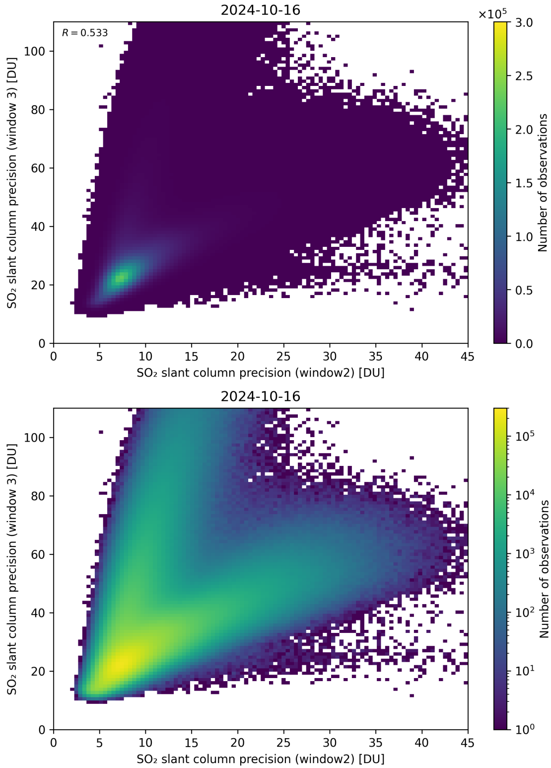
Figure 250: Scatter density plot of “SO 2 slant column precision (window2)” against “SO 2 slant column precision (window 3)” for 2024-10-15 to 2024-10-17.
