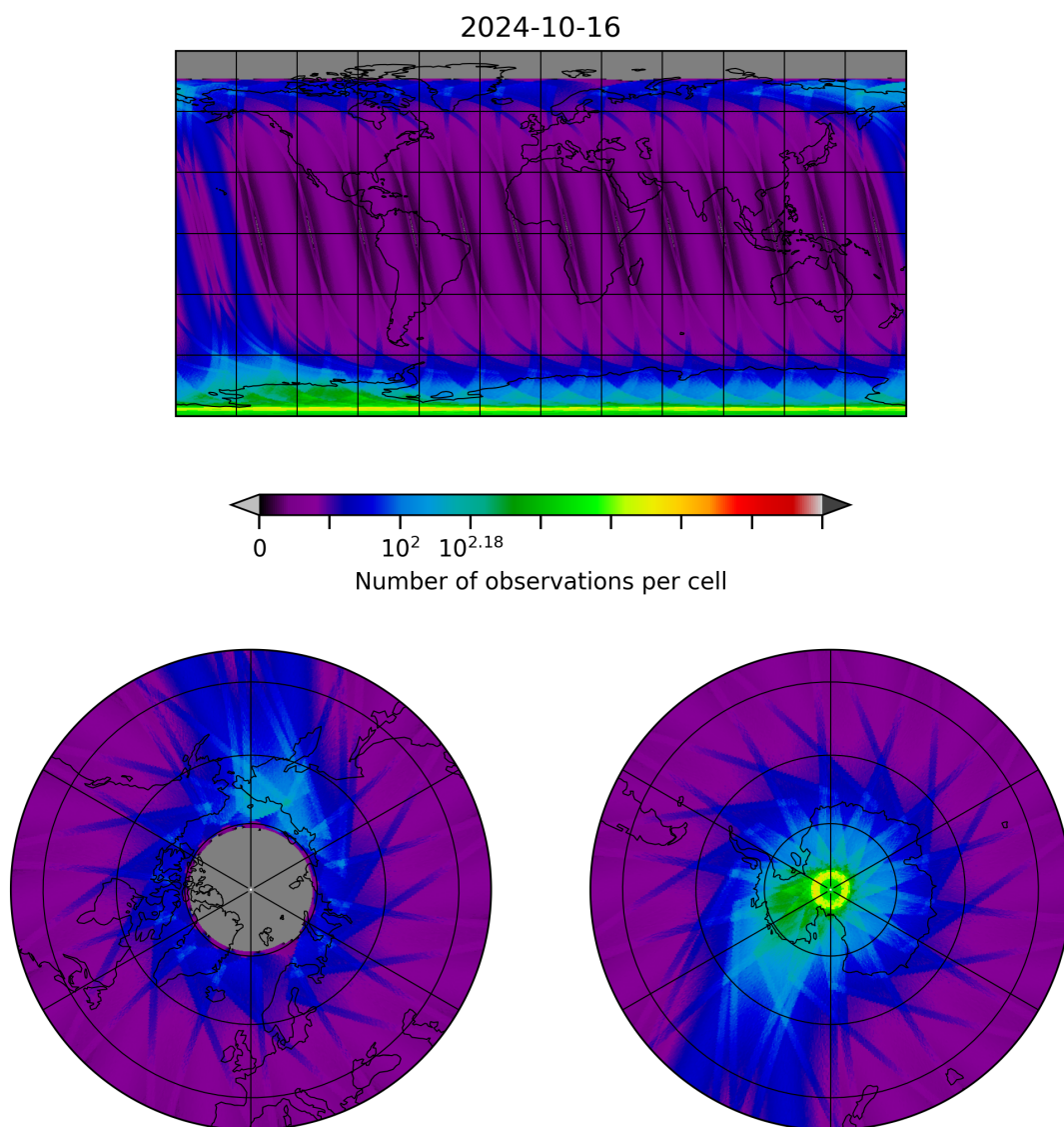
Figure 28: Map of the number of observations for 2024-10-15 to 2024-10-17
