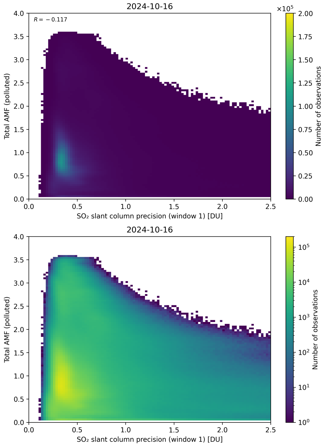
Figure 230: Scatter density plot of “SO 2 slant column precision (window 1)” against “Total AMF (polluted)” for 2024-10-15 to 2024-10-17.
