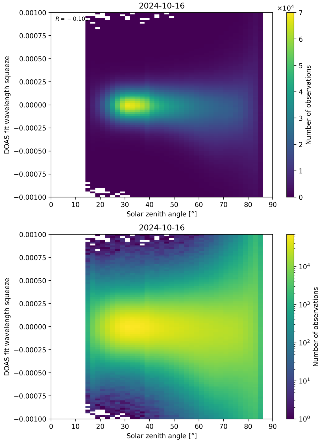
Figure 162: Scatter density plot of “Solar zenith angle” against “DOAS fit wavelength squeeze” for 2024-10-15 to 2024-10-17.
