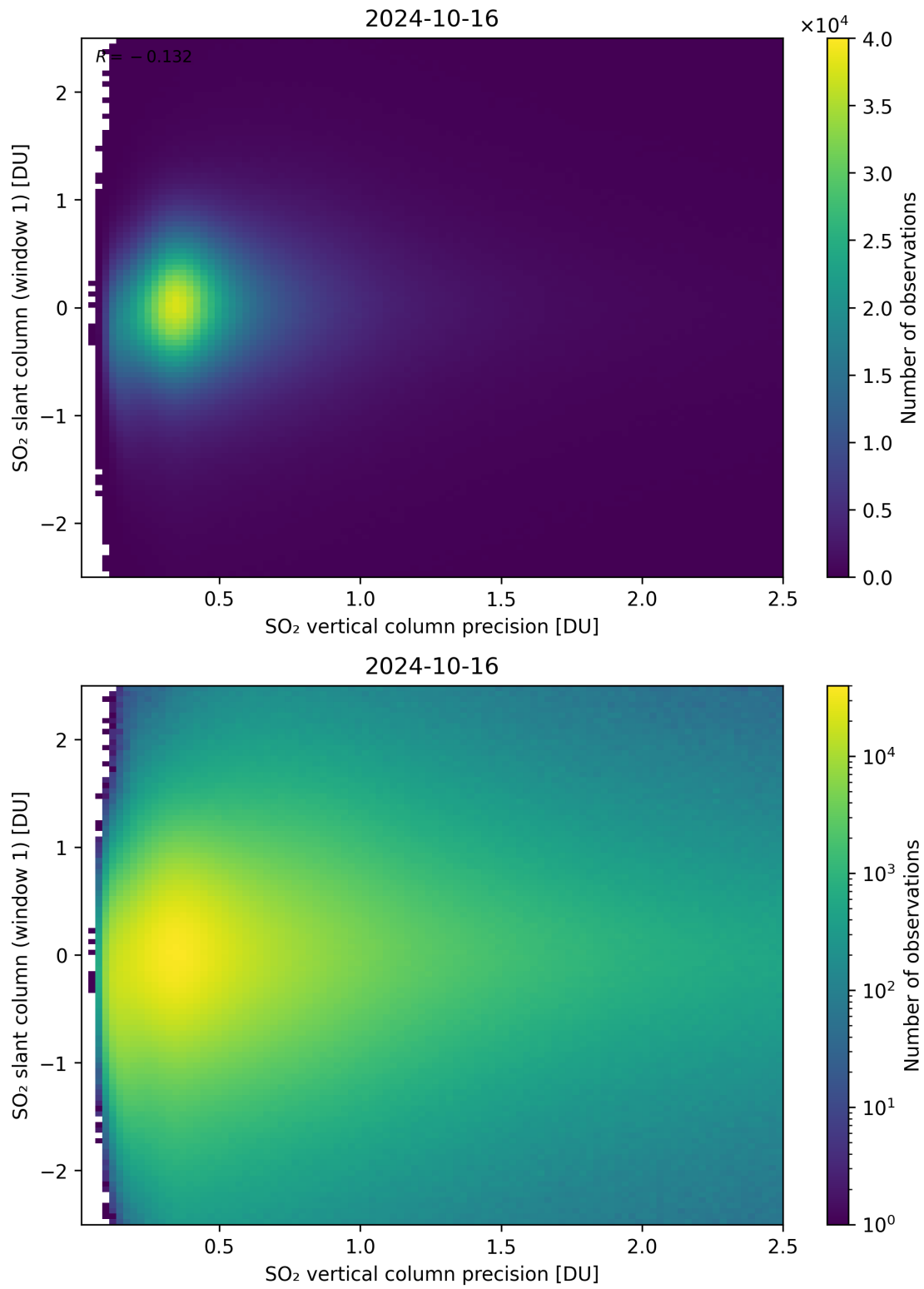
Figure 289: Scatter density plot of “SO 2 vertical column precision” against “SO 2 slant column (window 1)” for 2024-10-15 to 2024-10-17.
