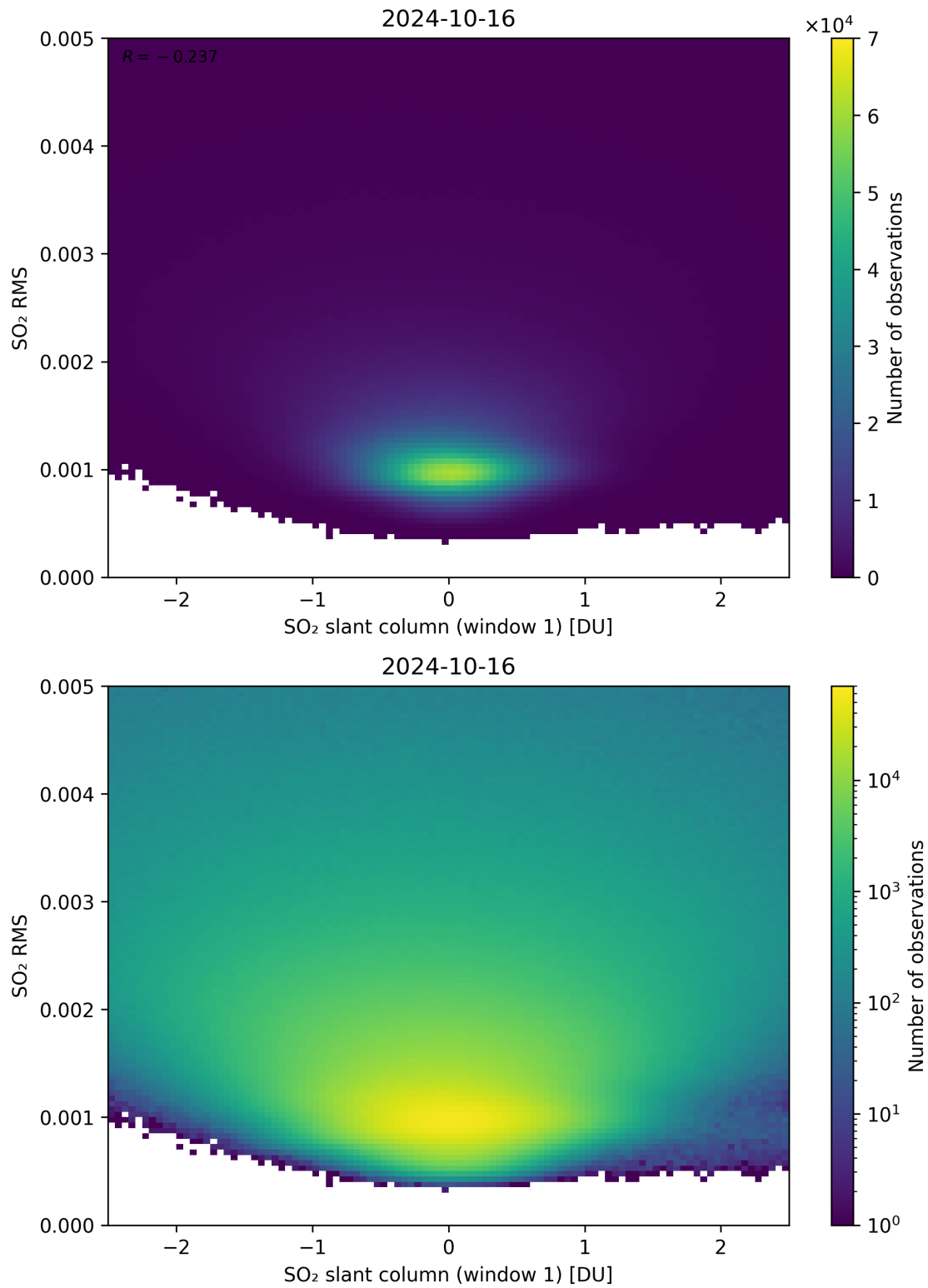
Figure 217: Scatter density plot of “SO 2 slant column (window 1)” against “SO 2 RMS” for 2024-10-15 to 2024-10-17.
