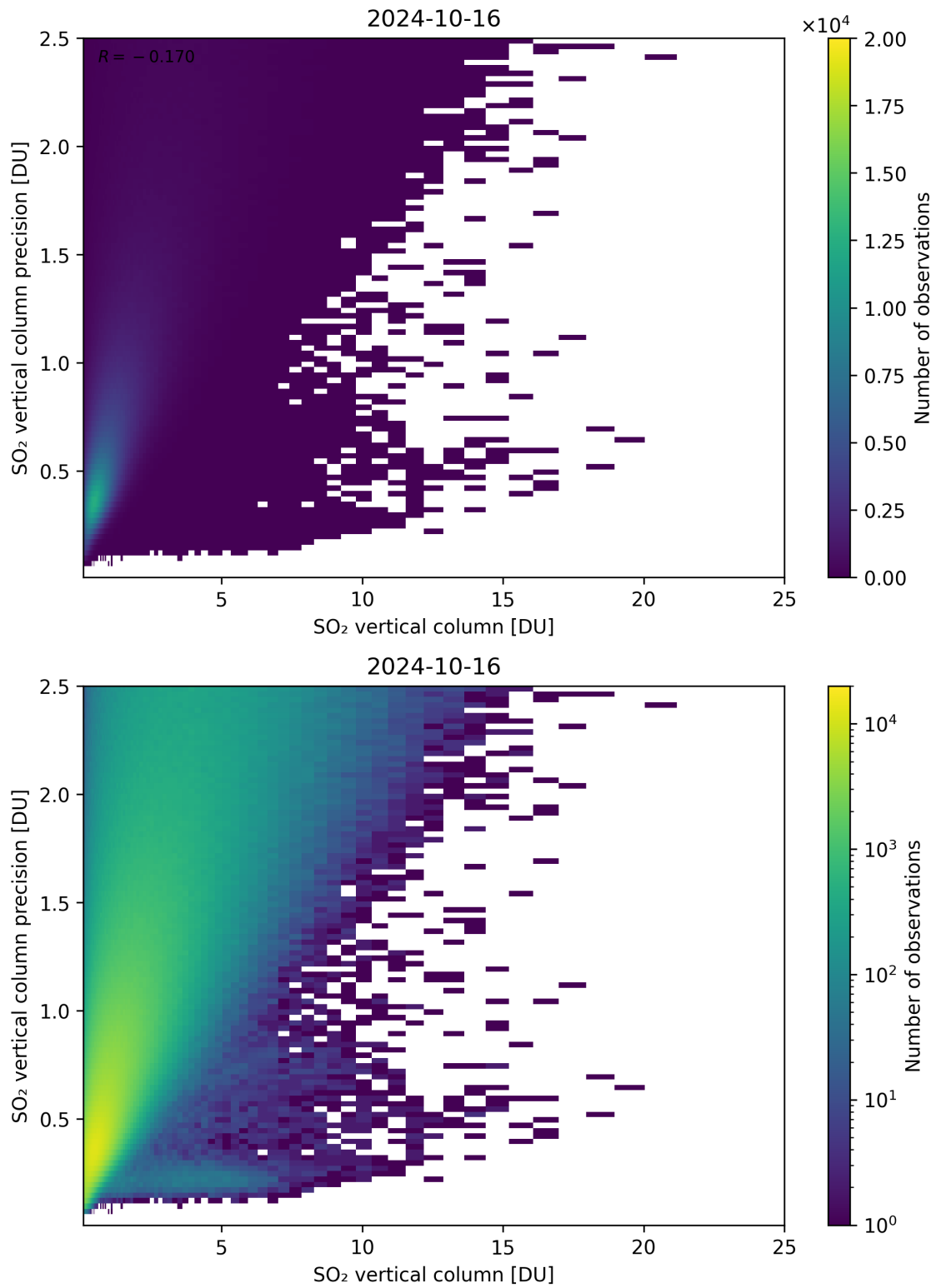
Figure 307: Scatter density plot of “SO 2 vertical column” against “SO 2 vertical column precision” for 2024-10-15 to 2024-10-17.
