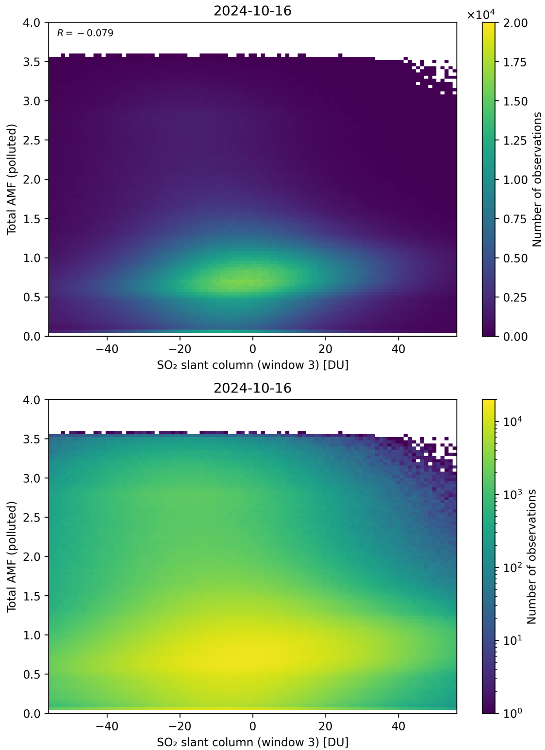
Figure 268: Scatter density plot of “SO 2 slant column (window 3)” against “Total AMF (polluted)” for 2024-10-15 to 2024-10-17.
