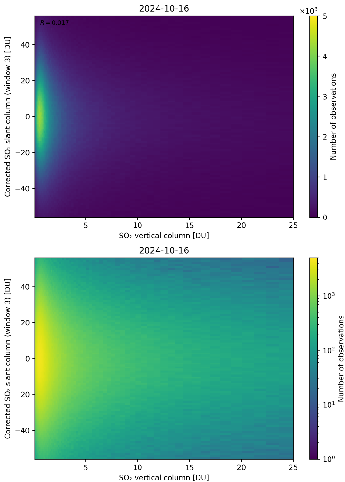
Figure 299: Scatter density plot of “SO 2 vertical column” against “Corrected SO 2 slant column (window 3)” for 2024-10-15 to 2024-10-17.
