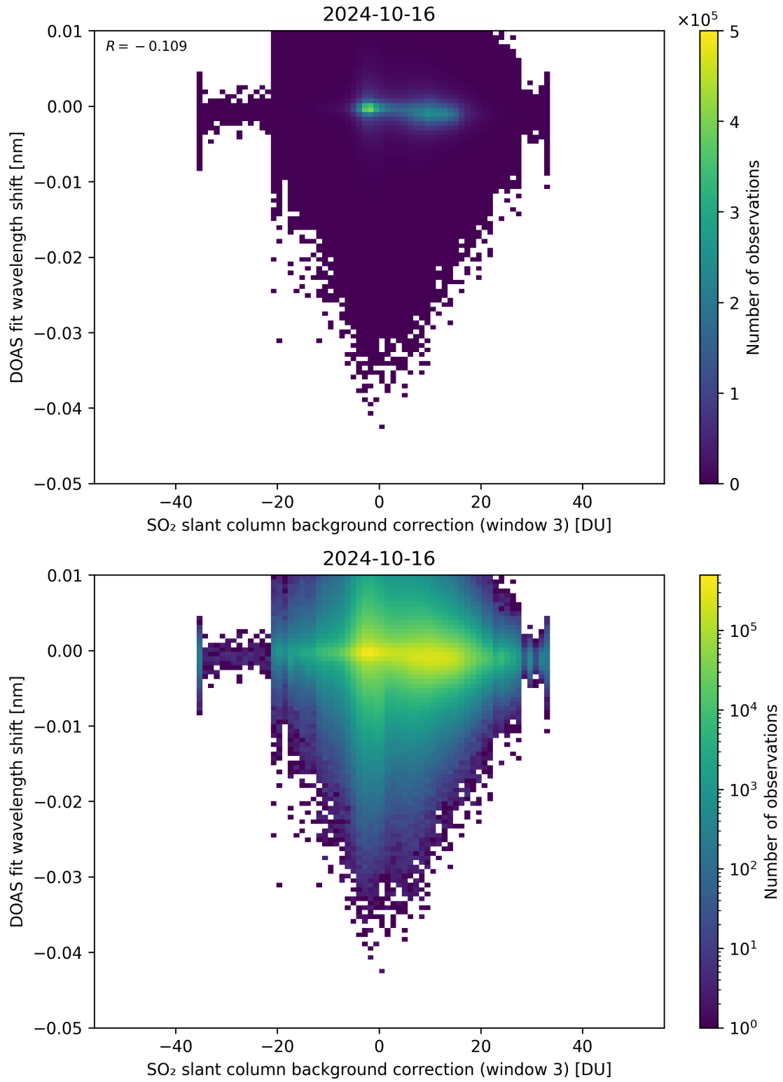
Figure 121: Scatter density plot of “SO 2 slant column background correction (window 3)” against “DOAS fit wavelength shift” for 2024-10-15 to 2024-10-17.
