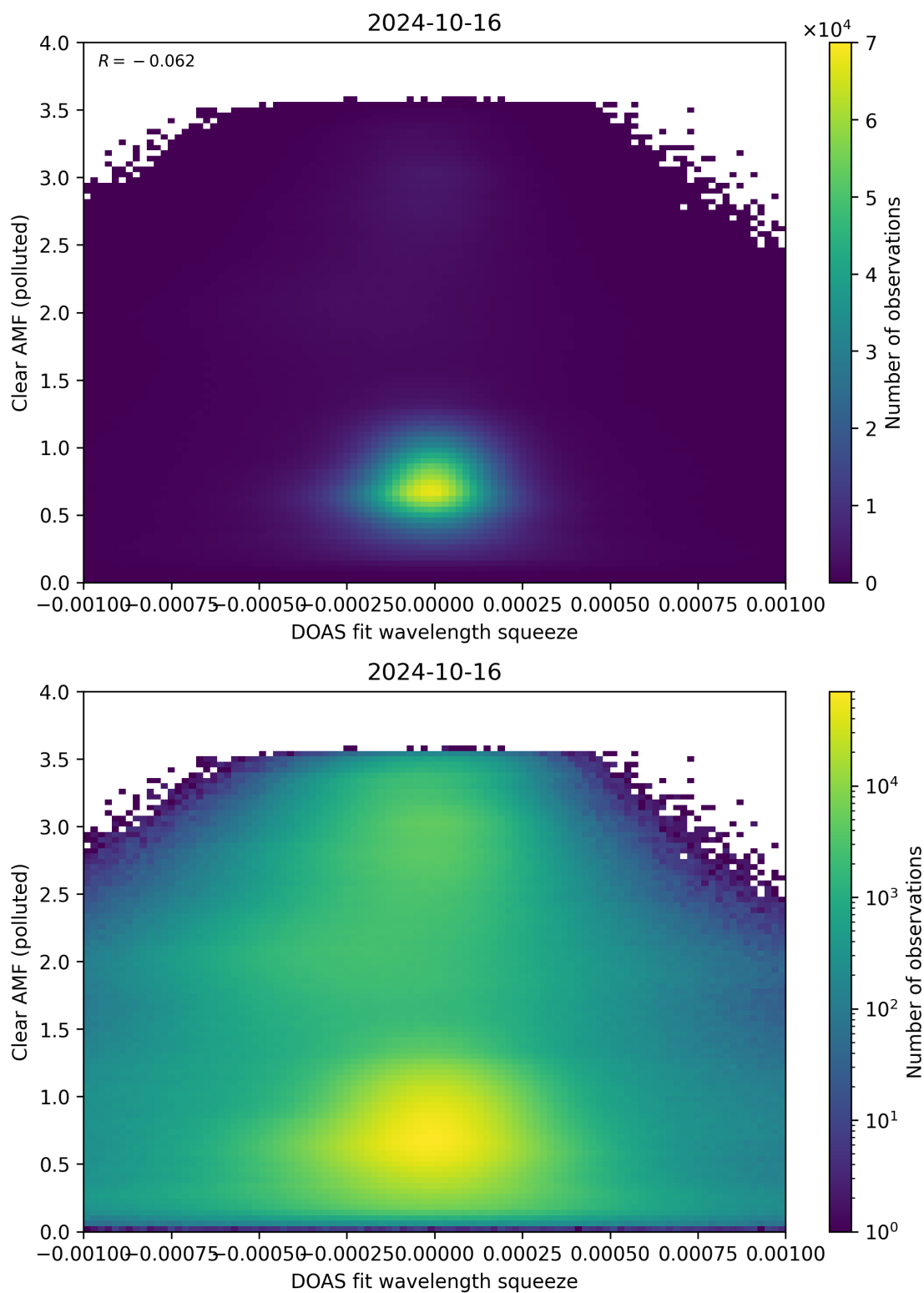
Figure 133: Scatter density plot of “DOAS fit wavelength squeeze” against “Clear AMF (polluted)” for 2024-10-15 to 2024-10-17.
