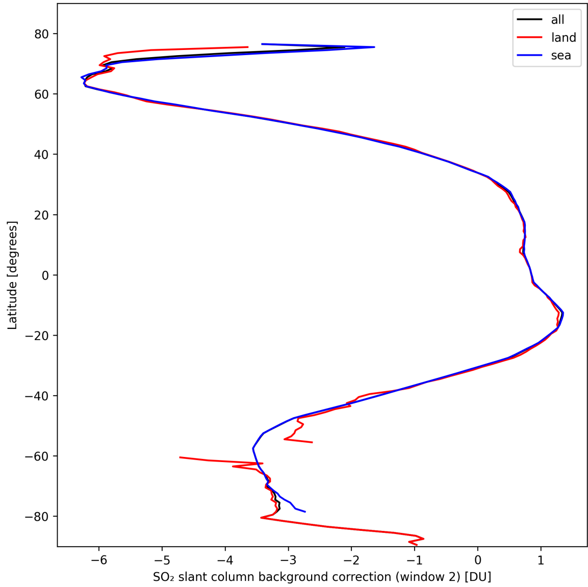
Figure 40: Zonal average of “SO 2 slant column background correction (window 2)” for 2024-10-15 to 2024-10-17.
