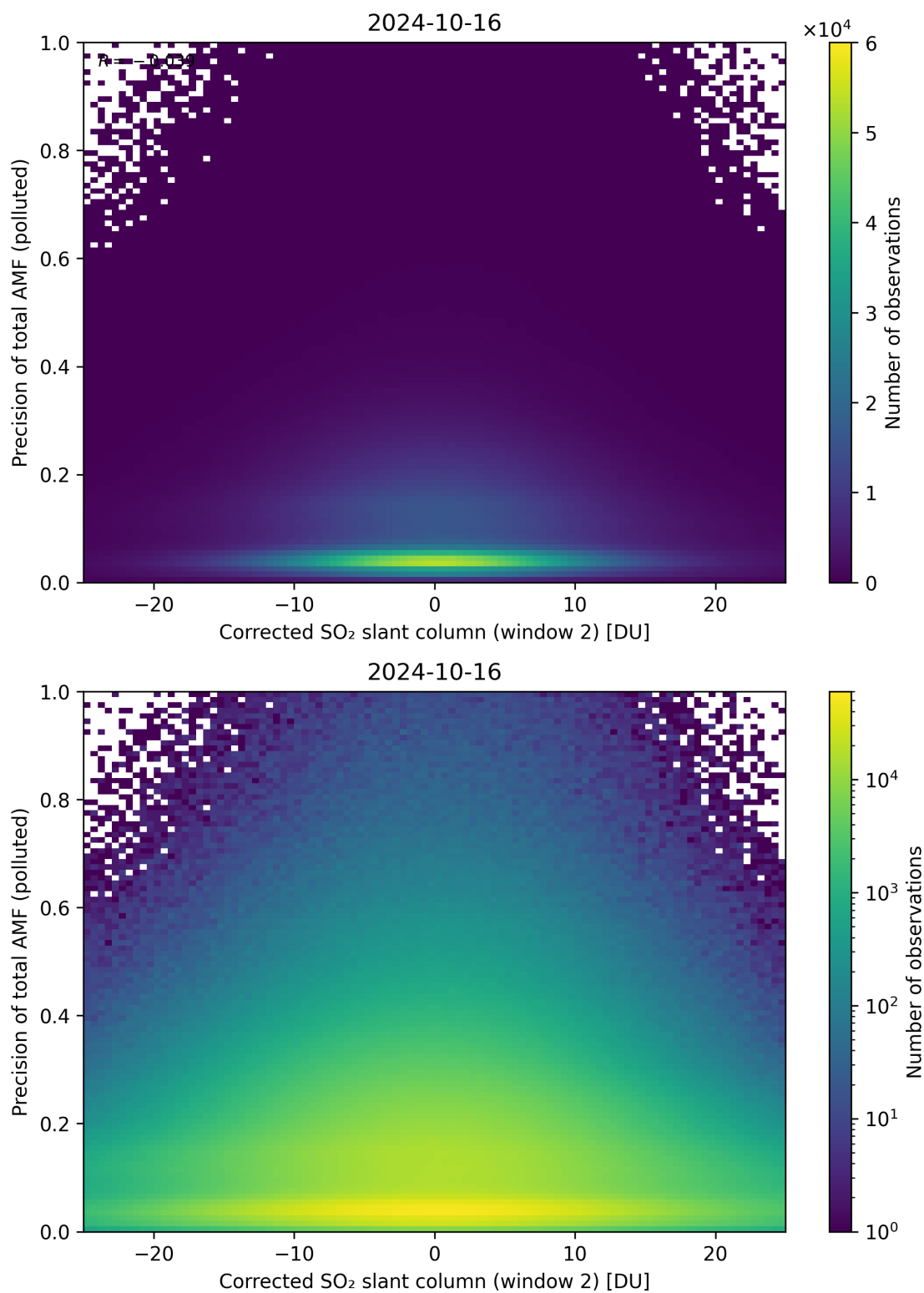
Figure 204: Scatter density plot of “Corrected SO 2 slant column (window 2)” against “Precision of total AMF (polluted)” for 2024-10-15 to 2024-10-17.
