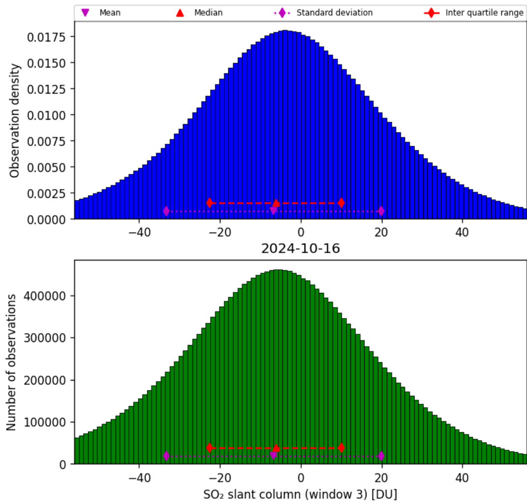
Figure 64: Histogram of “SO 2 slant column (window 3)” for 2024-10-15 to 2024-10-17
