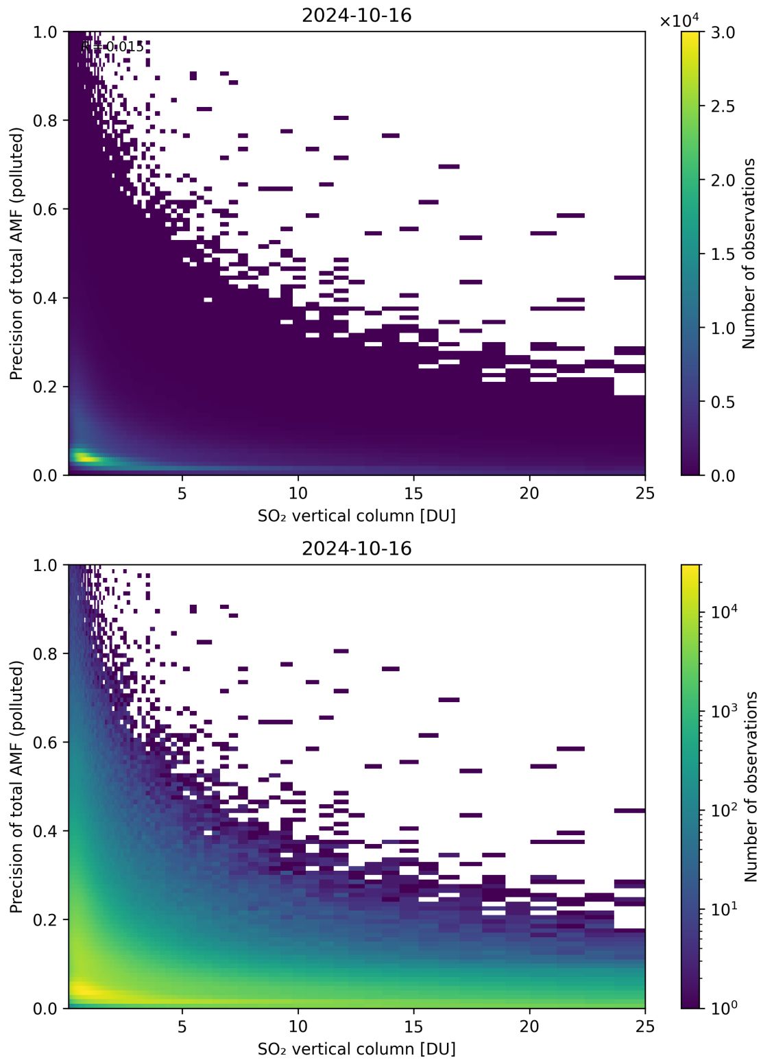
Figure 306: Scatter density plot of “SO 2 vertical column” against “Precision of total AMF (polluted)” for 2024-10-15 to 2024-10-17.
