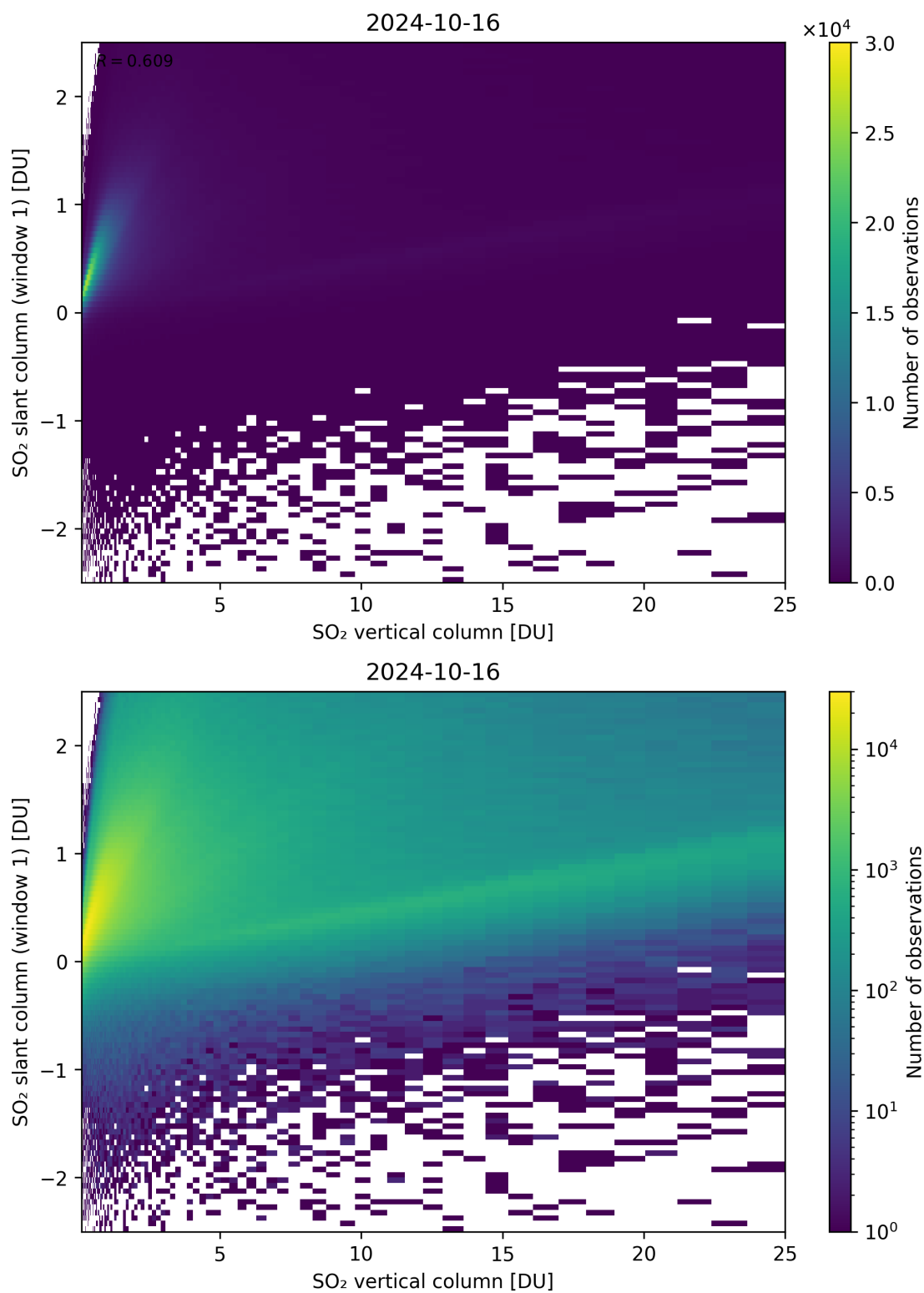
Figure 300: Scatter density plot of “SO 2 vertical column” against “SO 2 slant column (window 1)” for 2024-10-15 to 2024-10-17.
