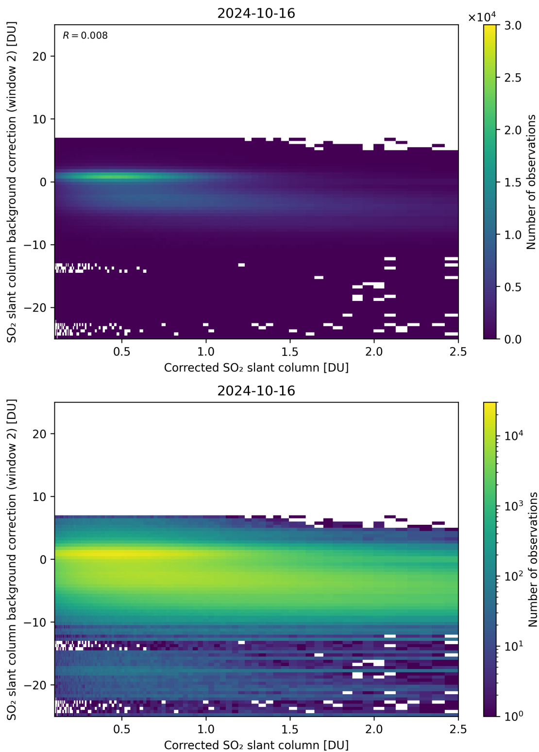
Figure 179: Scatter density plot of “Corrected SO 2 slant column” against “SO 2 slant column background correction (window 2)” for 2024-10-15 to 2024-10-17.
