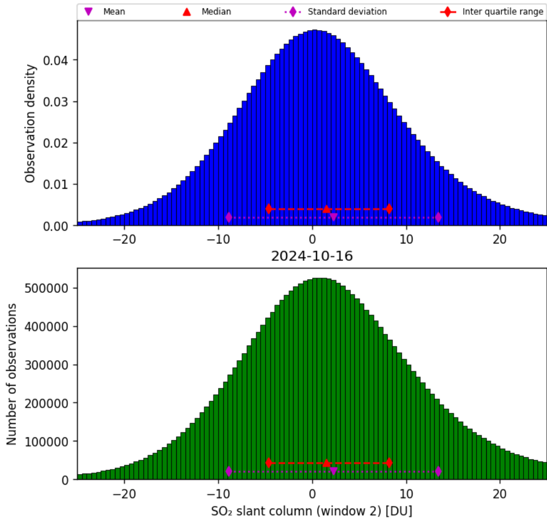
Figure 60: Histogram of “SO 2 slant column (window 2)” for 2024-10-15 to 2024-10-17
