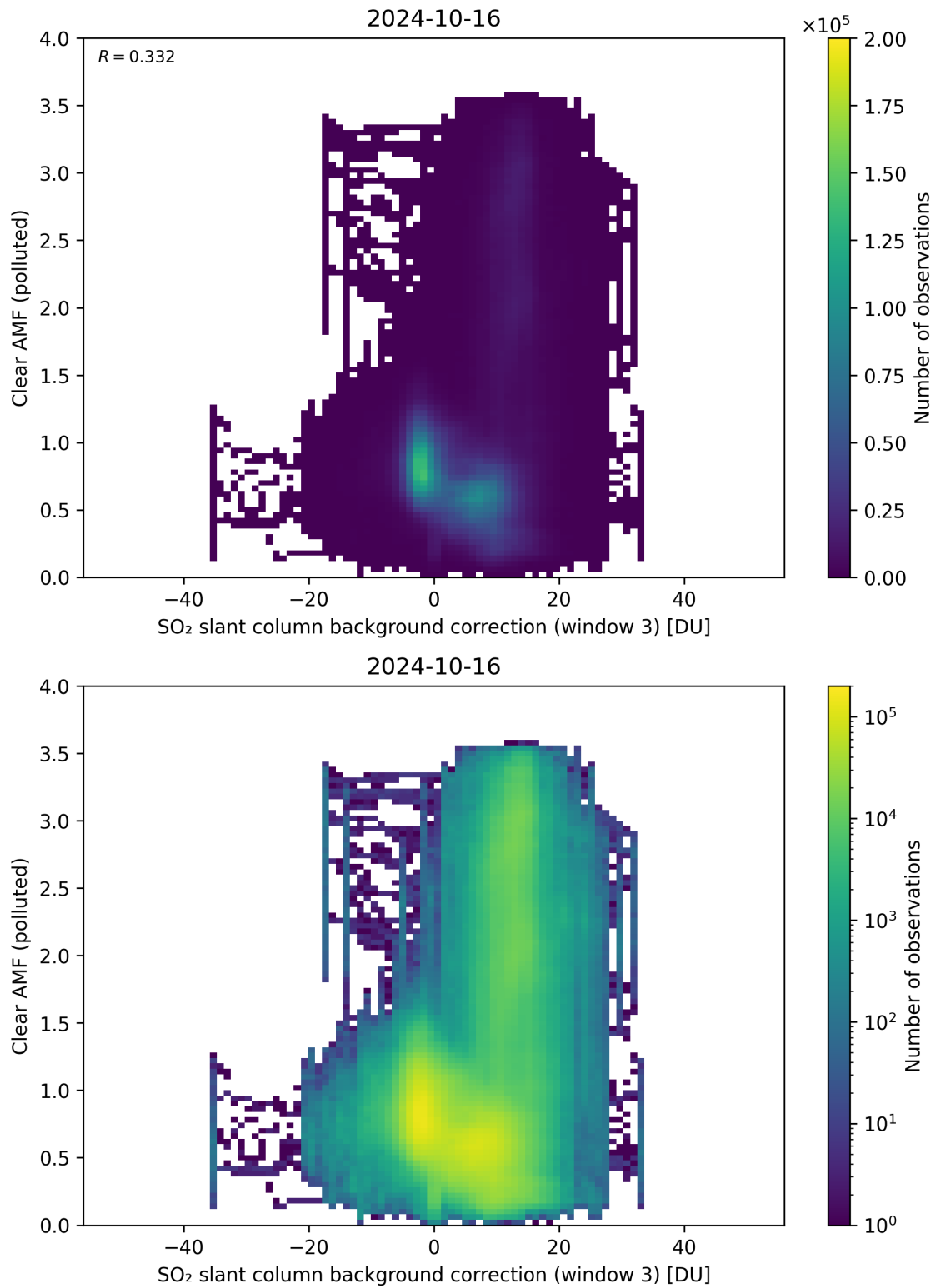
Figure 124: Scatter density plot of “SO 2 slant column background correction (window 3)” against “Clear AMF (polluted)” for 2024-10-15 to 2024-10-17.
