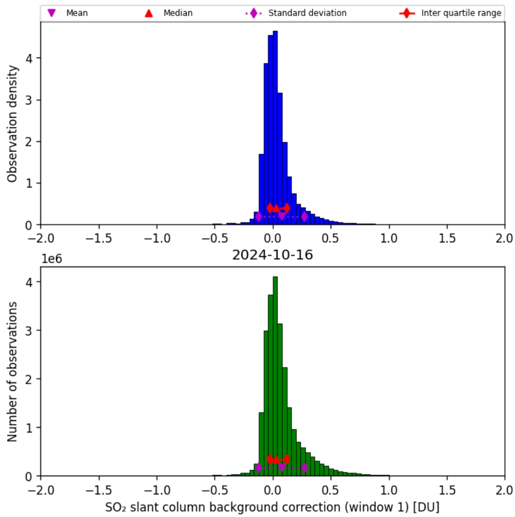
Figure 59: Histogram of “SO 2 slant column background correction (window 1)” for 2024-10-15 to 2024-10-17
