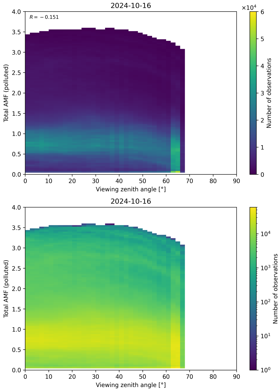
Figure 325: Scatter density plot of “Viewing zenith angle” against “Total AMF (polluted)” for 2024-10-15 to 2024-10-17.
