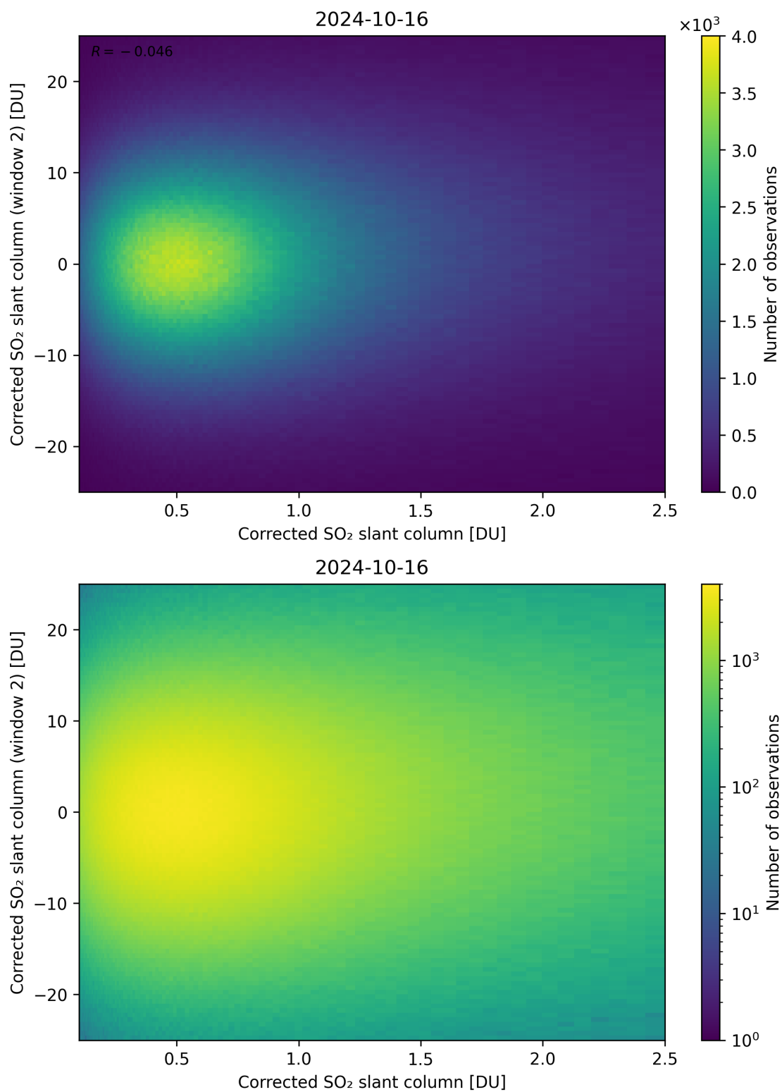
Figure 185: Scatter density plot of “Corrected SO 2 slant column” against “Corrected SO 2 slant column (window 2)” for 2024-10-15 to 2024-10-17.
