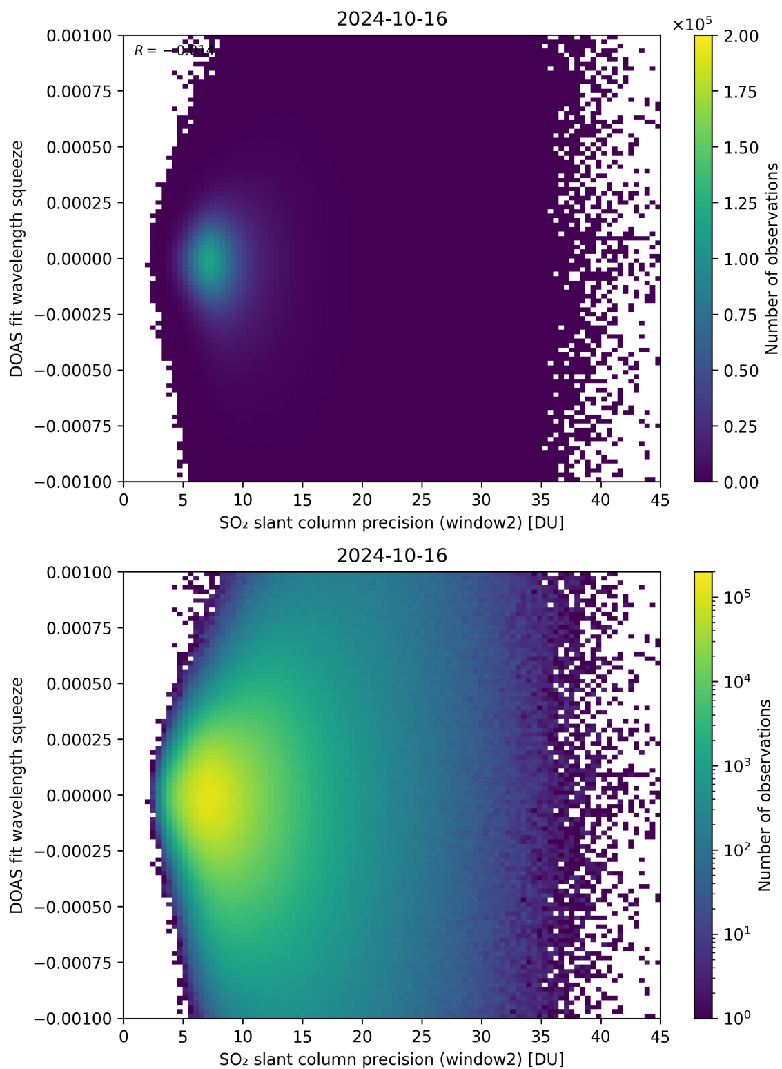
Figure 244: Scatter density plot of “SO 2 slant column precision (window2)” against “DOAS fit wavelength squeeze” for 2024-10-15 to 2024-10-17.
