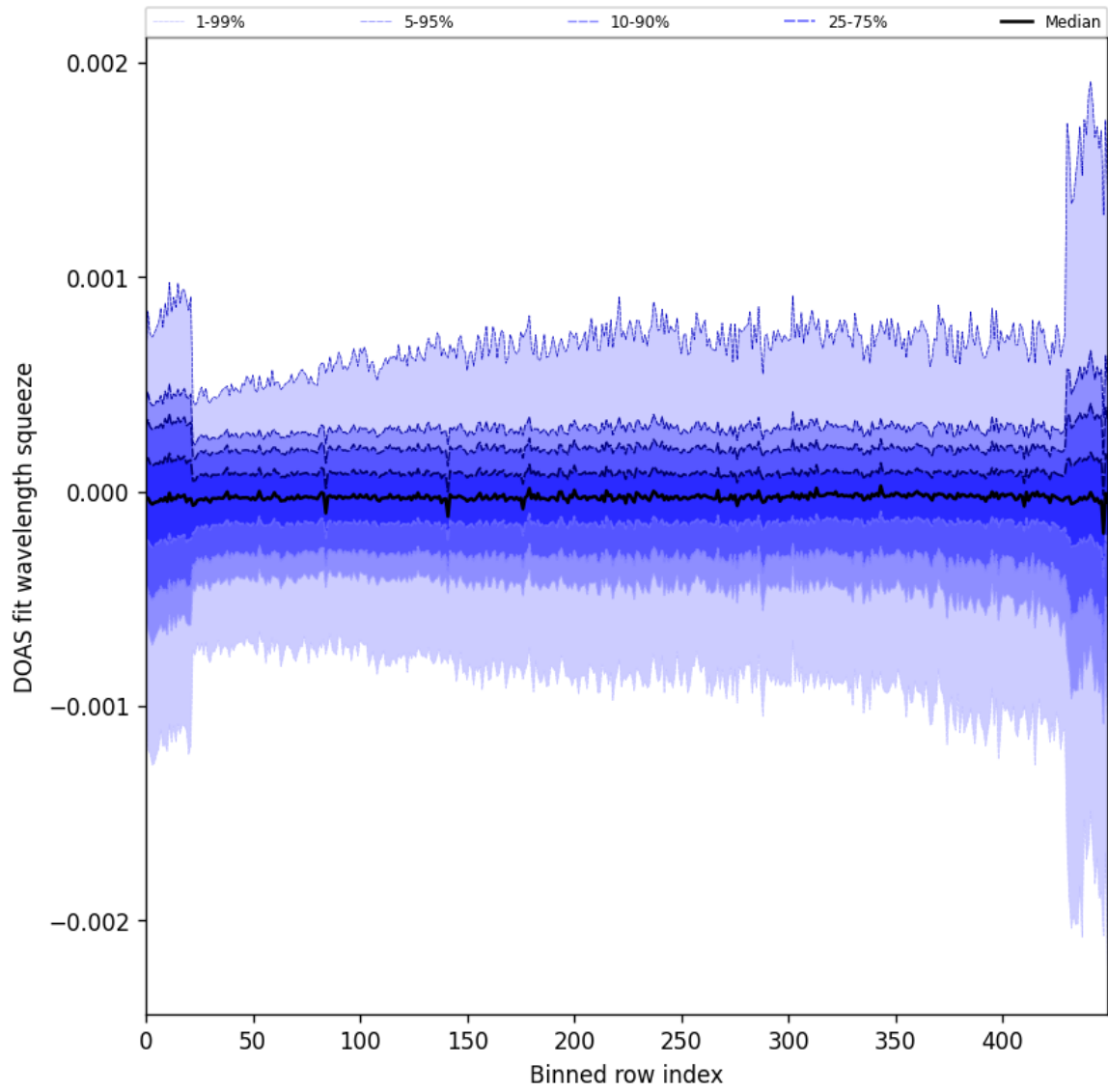
Figure 92: Along track statistics of “DOAS fit wavelength squeeze” for 2024-10-15 to 2024-10-17
