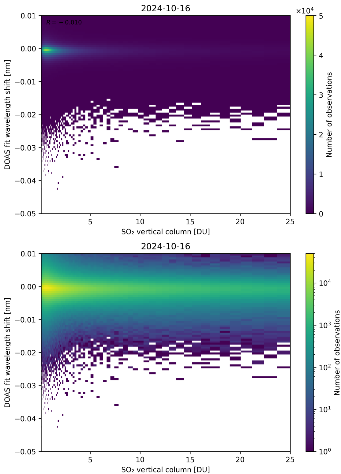
Figure 276: Scatter density plot of “SO 2 vertical column” against “DOAS fit wavelength shift” for 2024-10-15 to 2024-10-17.
