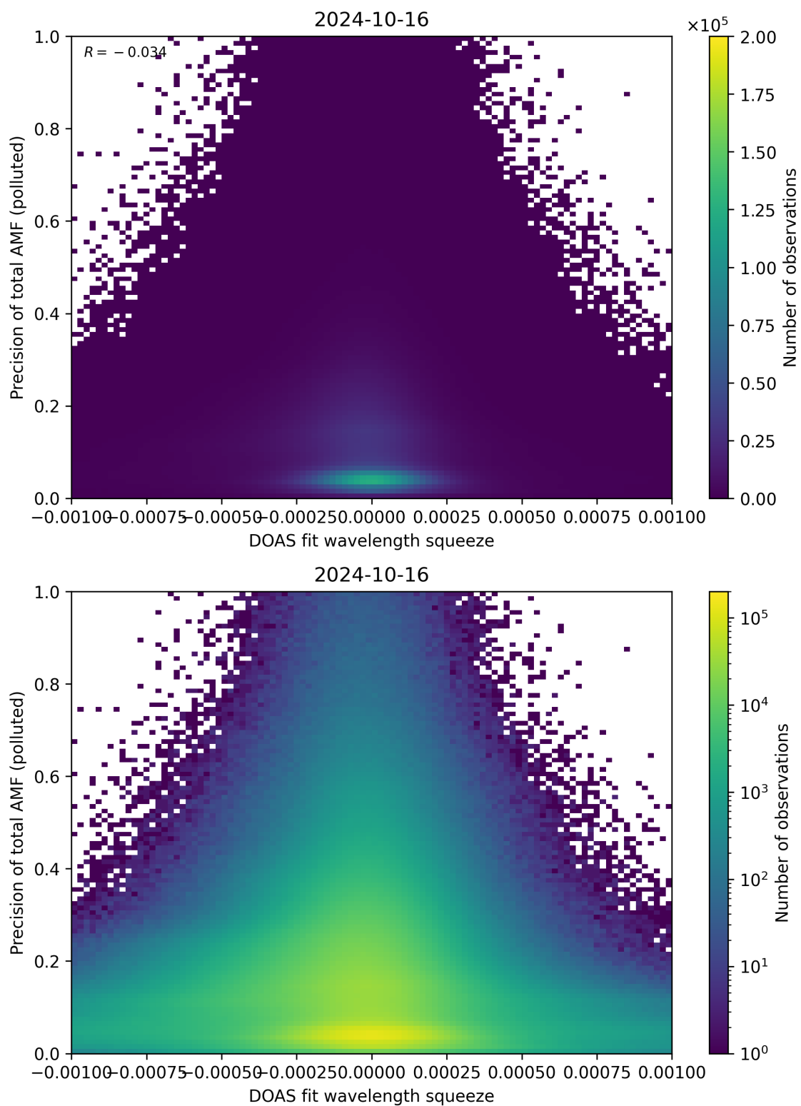
Figure 135: Scatter density plot of “DOAS fit wavelength squeeze” against “Precision of total AMF (polluted)” for 2024-10-15 to 2024-10-17.
