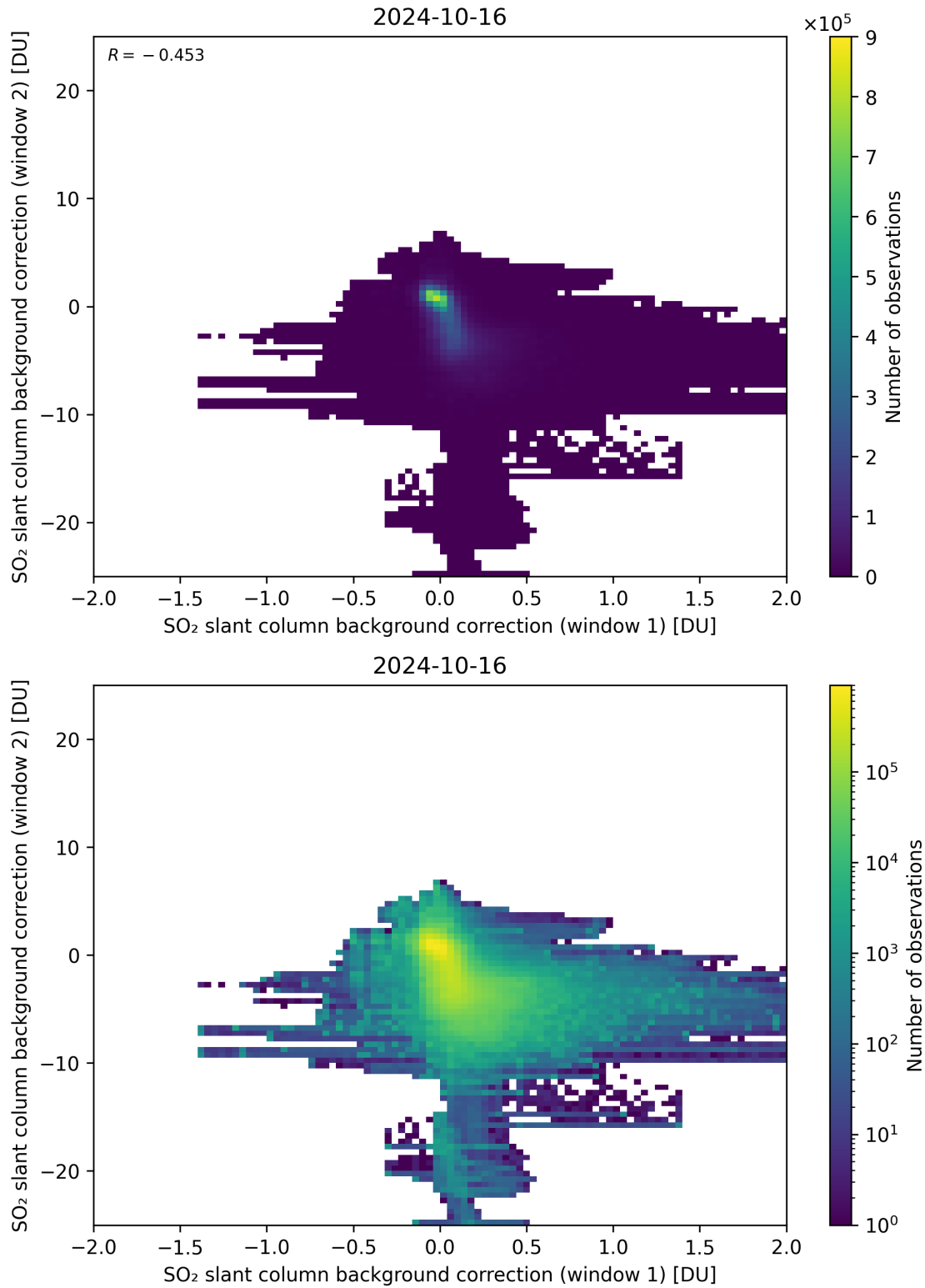
Figure 98: Scatter density plot of “SO 2 slant column background correction (window 1)” against “SO 2 slant column background correction (window 2)” for 2024-10-15 to 2024-10-17.
