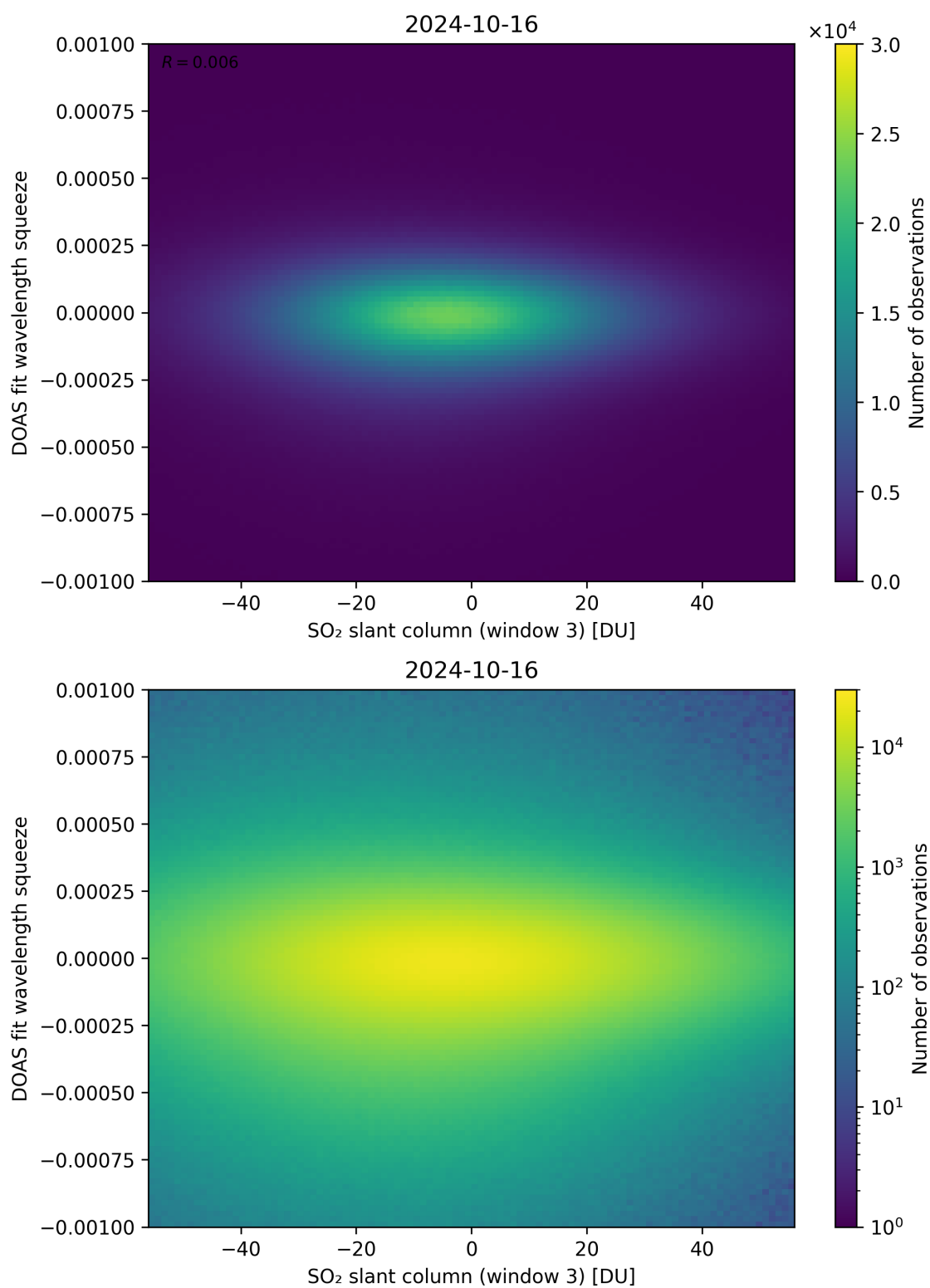
Figure 255: Scatter density plot of “SO 2 slant column (window 3)” against “DOAS fit wavelength squeeze” for 2024-10-15 to 2024-10-17.
