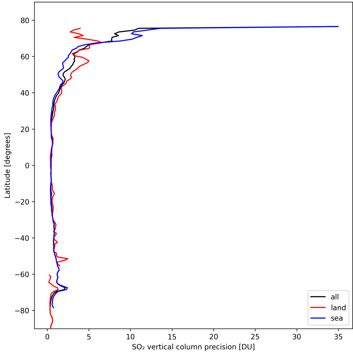
Figure 31: Zonal average of “SO 2 vertical column precision” for 2024-10-15 to 2024-10-17.
