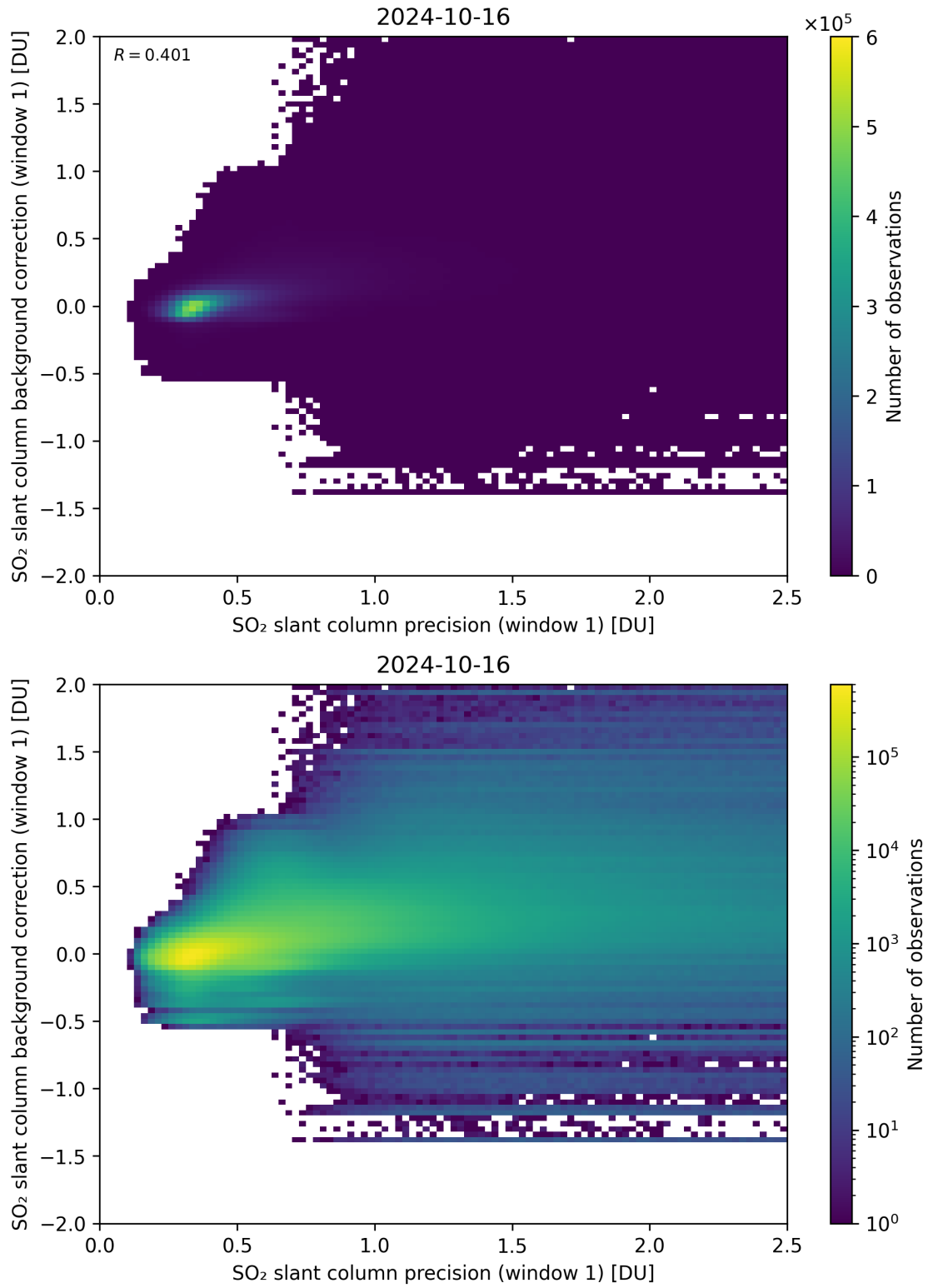
Figure 218: Scatter density plot of “SO 2 slant column precision (window 1)” against “SO 2 slant column background correction (window 1)” for 2024-10-15 to 2024-10-17.
