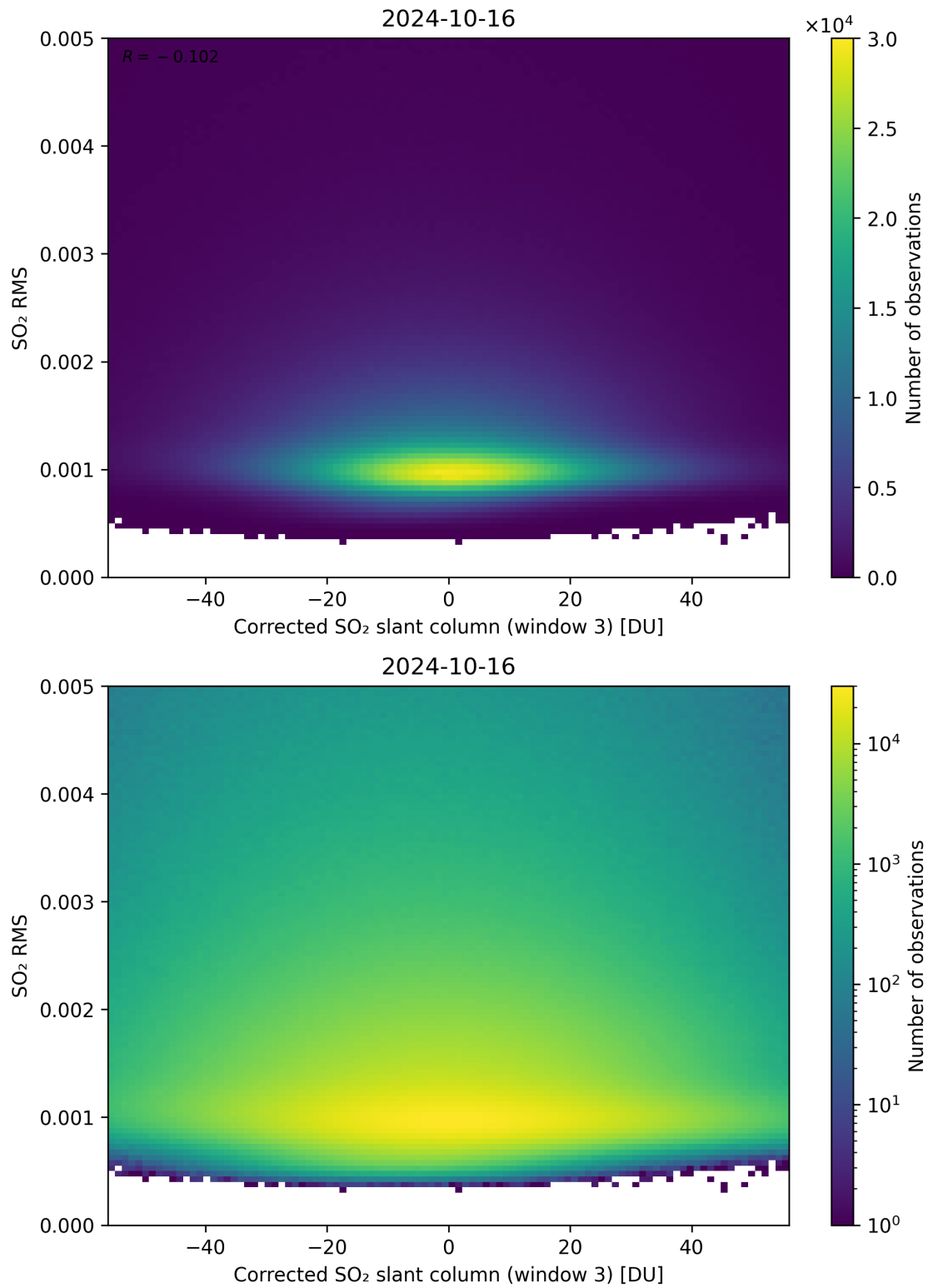
Figure 208: Scatter density plot of “Corrected SO 2 slant column (window 3)” against “SO 2 RMS” for 2024-10-15 to 2024-10-17.
