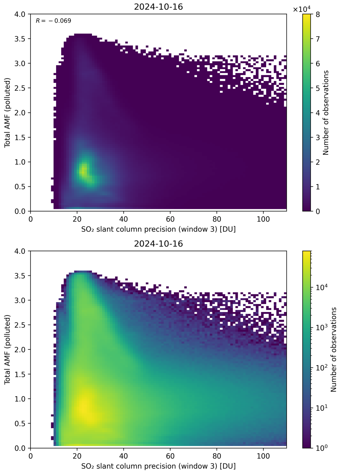
Figure 263: Scatter density plot of “SO 2 slant column precision (window 3)” against “Total AMF (polluted)” for 2024-10-15 to 2024-10-17.
