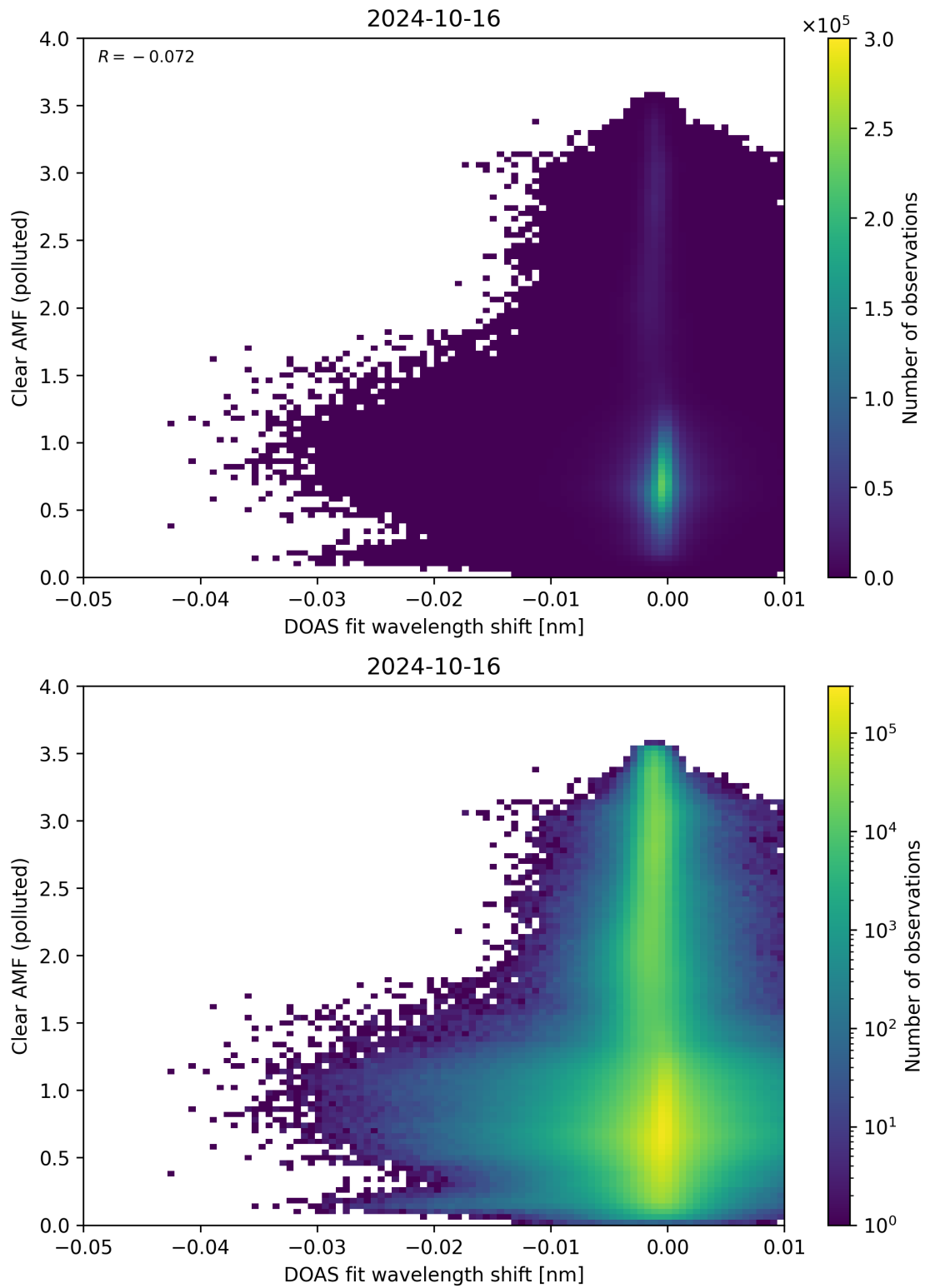
Figure 129: Scatter density plot of “DOAS fit wavelength shift” against “Clear AMF (polluted)” for 2024-10-15 to 2024-10-17.
