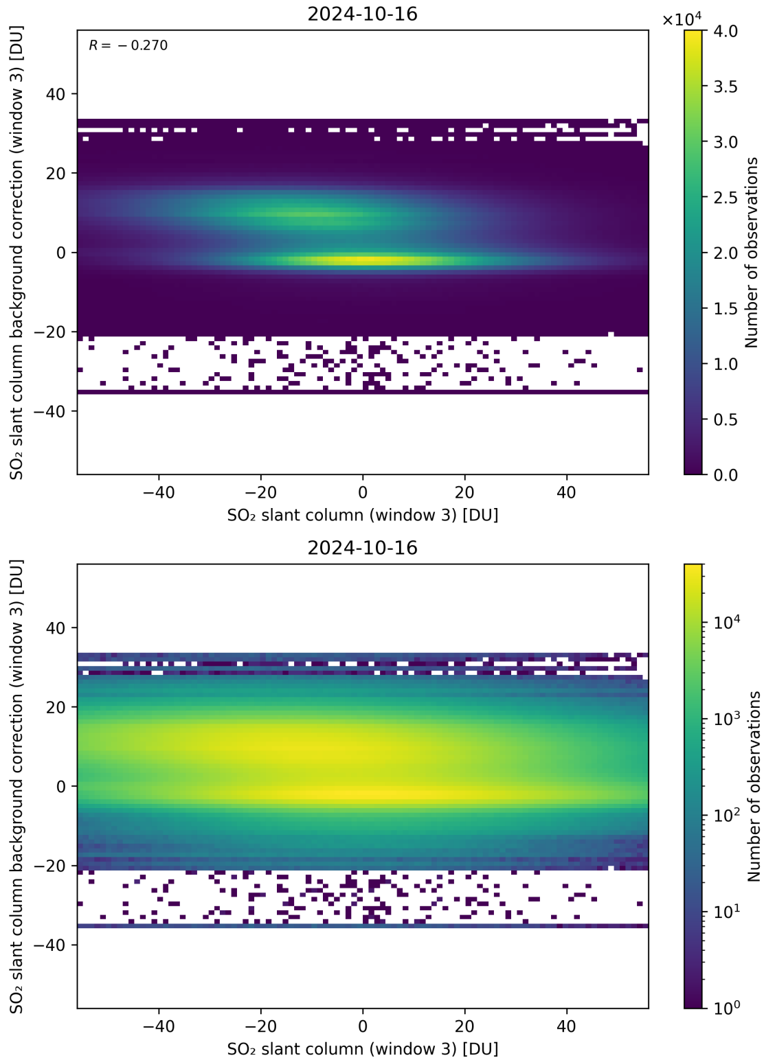
Figure 253: Scatter density plot of “SO 2 slant column (window 3)” against “SO 2 slant column background correction (window 3)” for 2024-10-15 to 2024-10-17.
