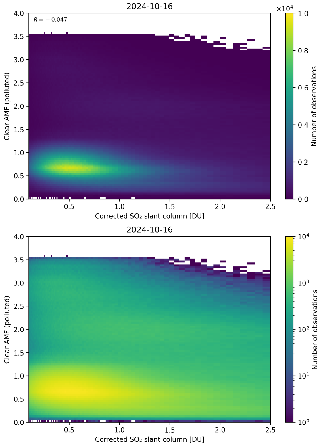
Figure 184: Scatter density plot of “Corrected SO 2 slant column” against “Clear AMF (polluted)” for 2024-10-15 to 2024-10-17.
