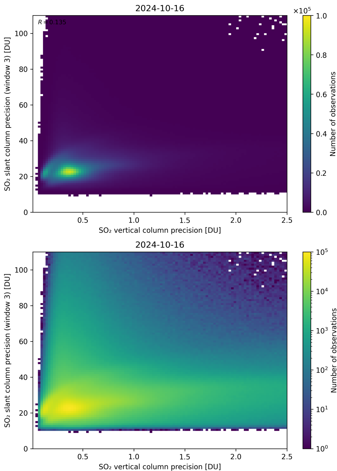
Figure 293: Scatter density plot of “SO 2 vertical column precision” against “SO 2 slant column precision (window 3)” for 2024-10-15 to 2024-10-17.
