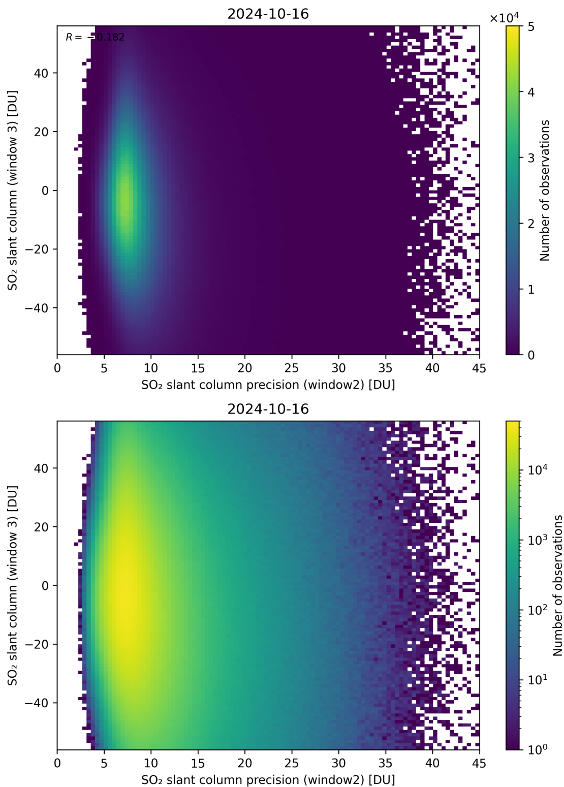
Figure 249: Scatter density plot of “SO 2 slant column precision (window2)” against “SO 2 slant column (window 3)” for 2024-10-15 to 2024-10-17.
