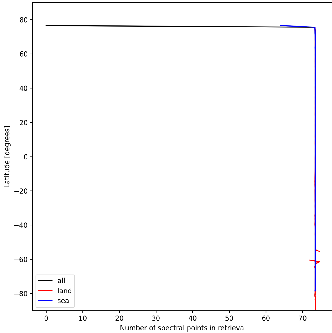
Figure 51: Zonal average of “Number of spectral points in retrieval” for 2024-10-15 to 2024-10-17.
