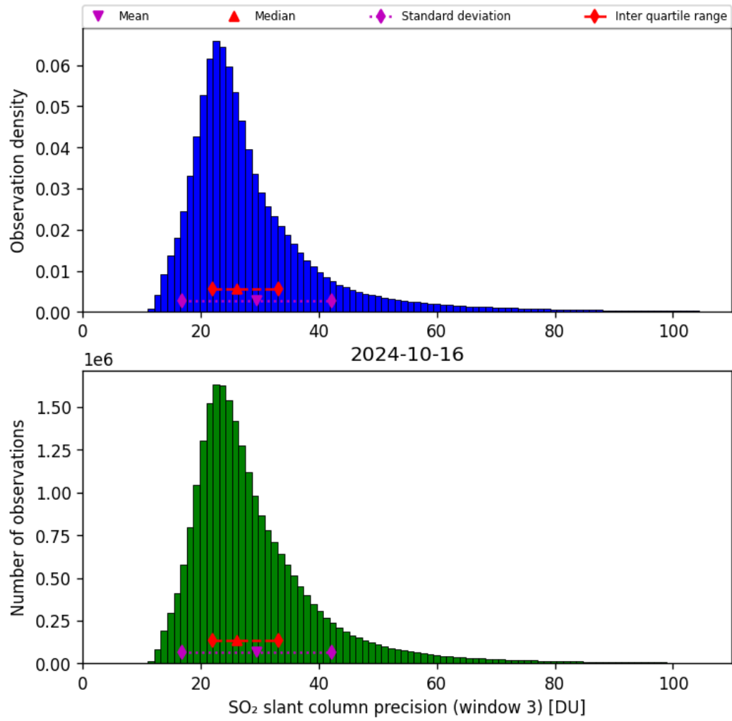
Figure 65: Histogram of “SO 2 slant column precision (window 3)” for 2024-10-15 to 2024-10-17
