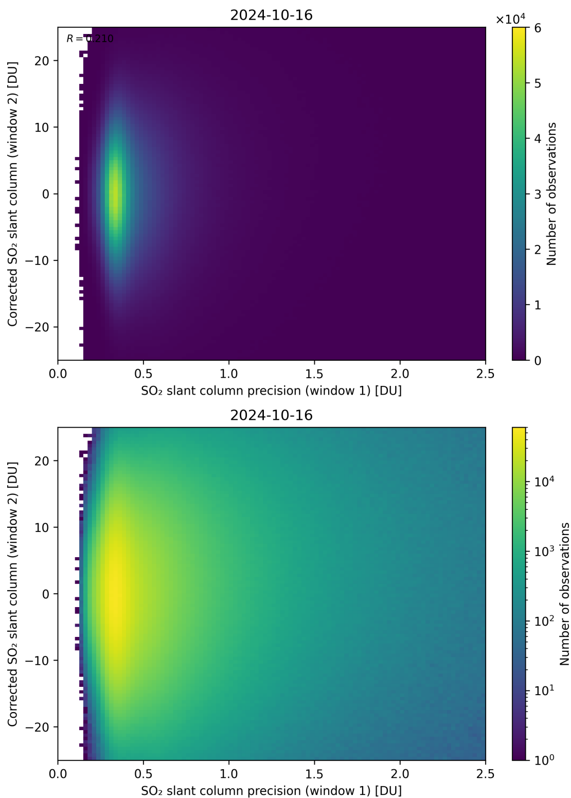
Figure 225: Scatter density plot of “SO 2 slant column precision (window 1)” against “Corrected SO 2 slant column (window 2)” for 2024-10-15 to 2024-10-17.
