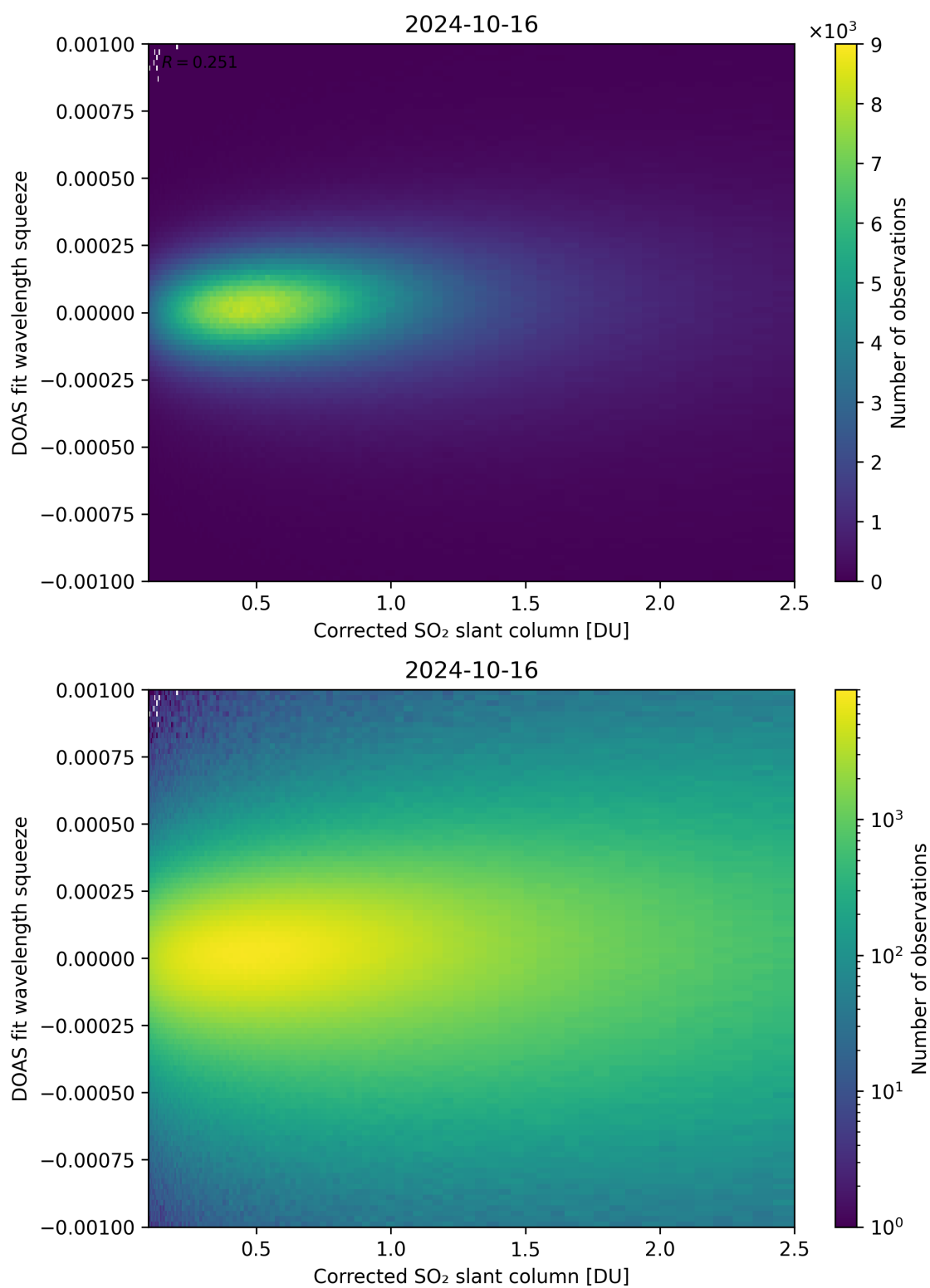
Figure 182: Scatter density plot of “Corrected SO 2 slant column” against “DOAS fit wavelength squeeze” for 2024-10-15 to 2024-10-17.
