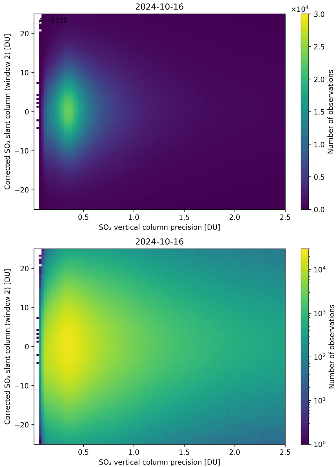
Figure 287: Scatter density plot of “SO 2 vertical column precision” against “Corrected SO 2 slant column (window 2)” for 2024-10-15 to 2024-10-17.
