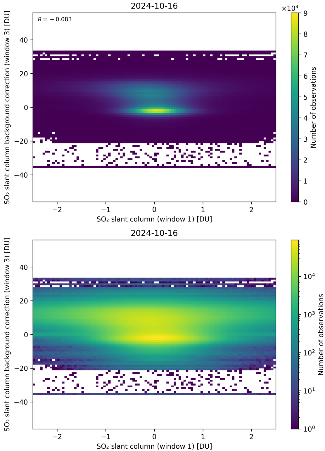
Figure 214: Scatter density plot of “SO 2 slant column (window 1)” against “SO 2 slant column background correction (window 3)” for 2024-10-15 to 2024-10-17.
