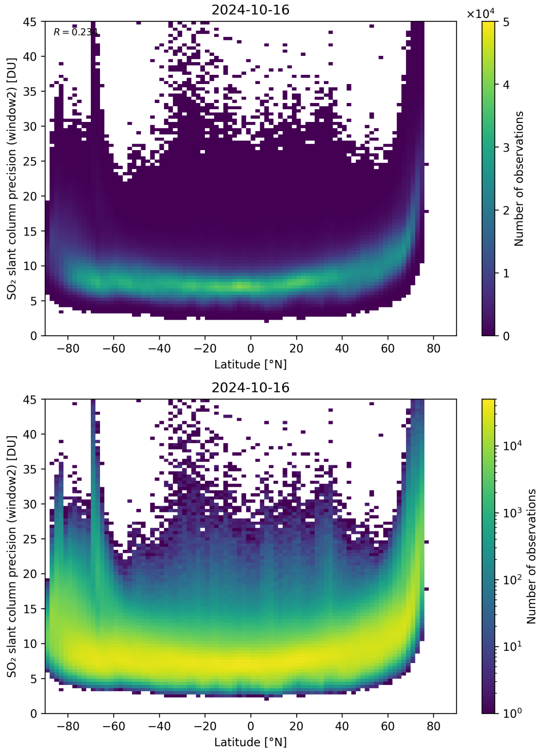
Figure 151: Scatter density plot of “Latitude” against “SO 2 slant column precision (window2)” for 2024-10-15 to 2024-10-17.
