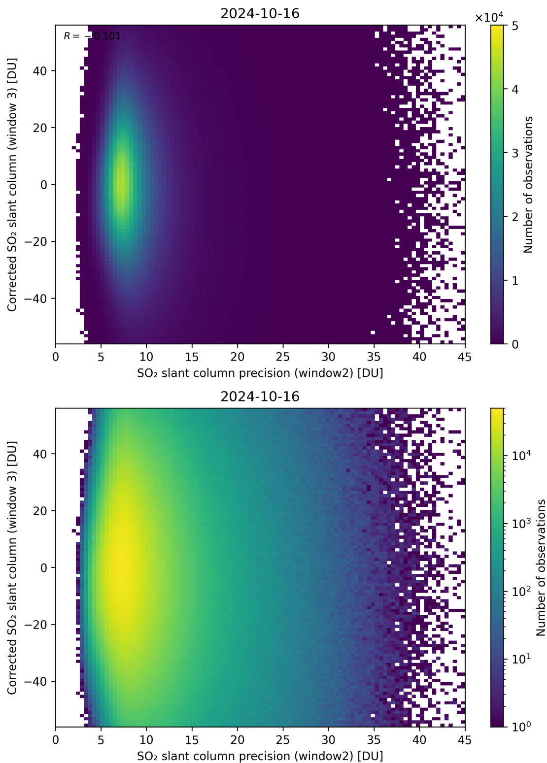
Figure 248: Scatter density plot of “SO 2 slant column precision (window2)” against “Corrected SO 2 slant column (window 3)” for 2024-10-15 to 2024-10-17.
