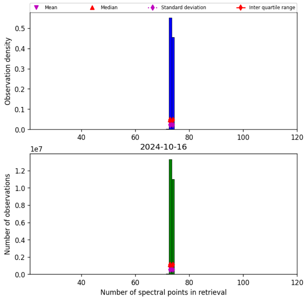
Figure 74: Histogram of “Number of spectral points in retrieval” for 2024-10-15 to 2024-10-17
