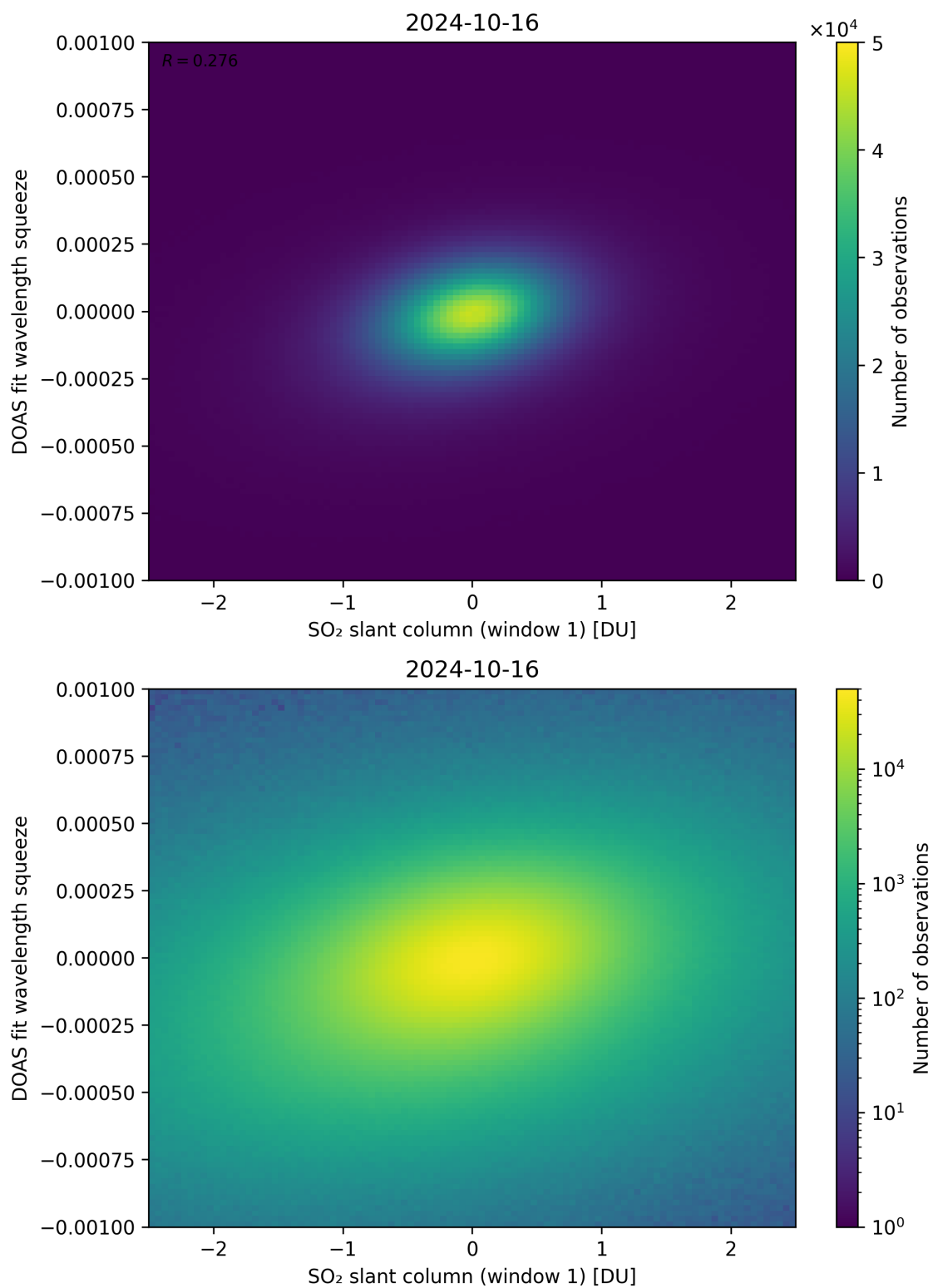
Figure 216: Scatter density plot of “SO 2 slant column (window 1)” against “DOAS fit wavelength squeeze” for 2024-10-15 to 2024-10-17.
