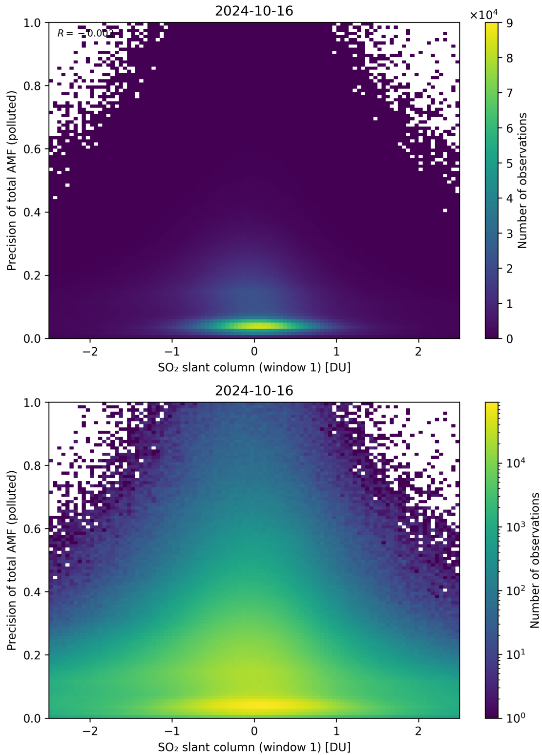
Figure 240: Scatter density plot of “SO 2 slant column (window 1)” against “Precision of total AMF (polluted)” for 2024-10-15 to 2024-10-17.
