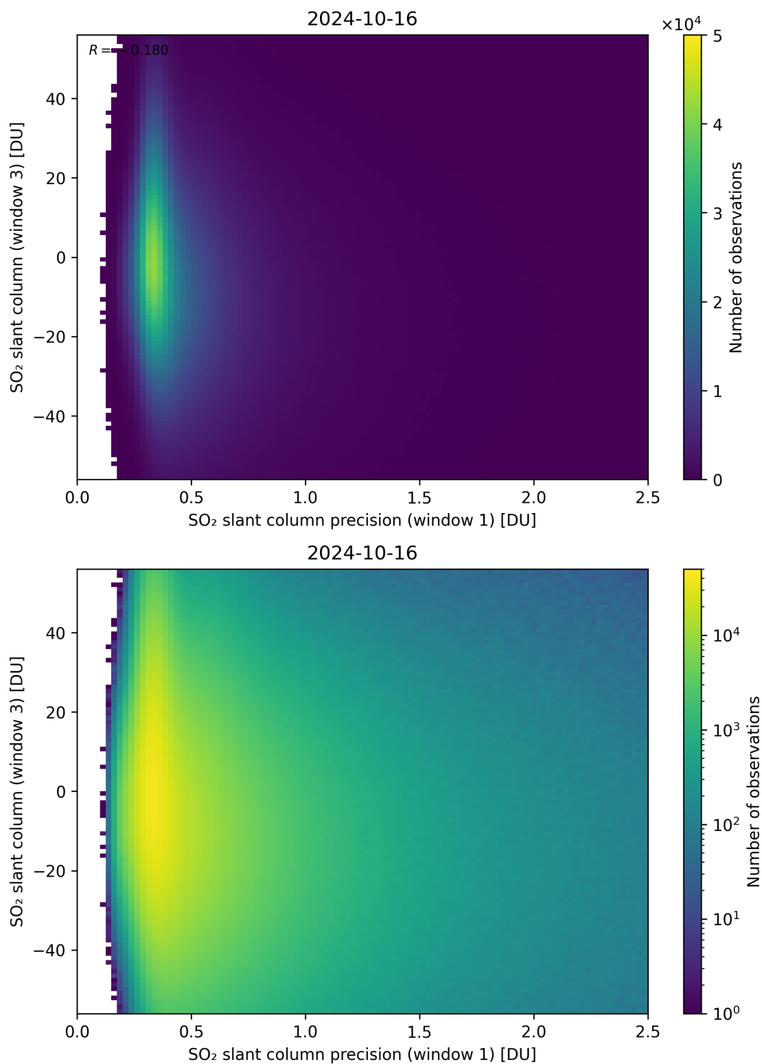
Figure 228: Scatter density plot of “SO 2 slant column precision (window 1)” against “SO 2 slant column (window 3)” for 2024-10-15 to 2024-10-17.
