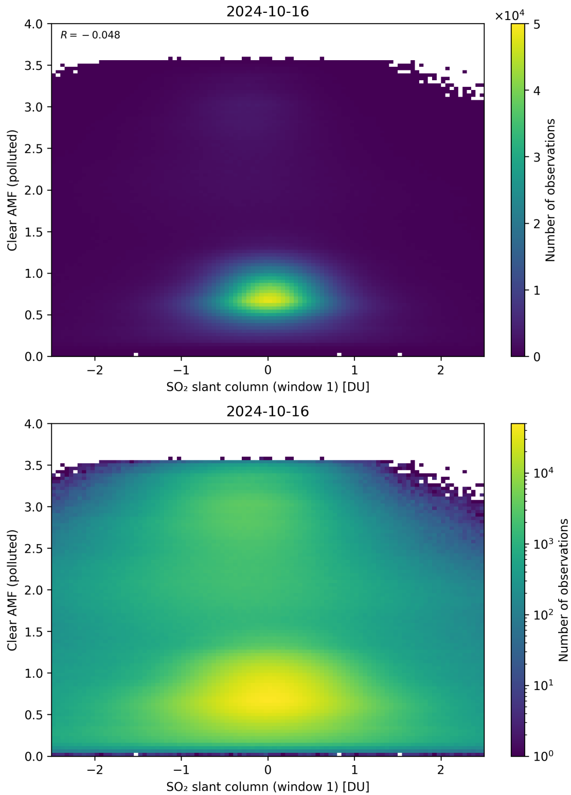
Figure 232: Scatter density plot of “SO 2 slant column (window 1)” against “Clear AMF (polluted)” for 2024-10-15 to 2024-10-17.
