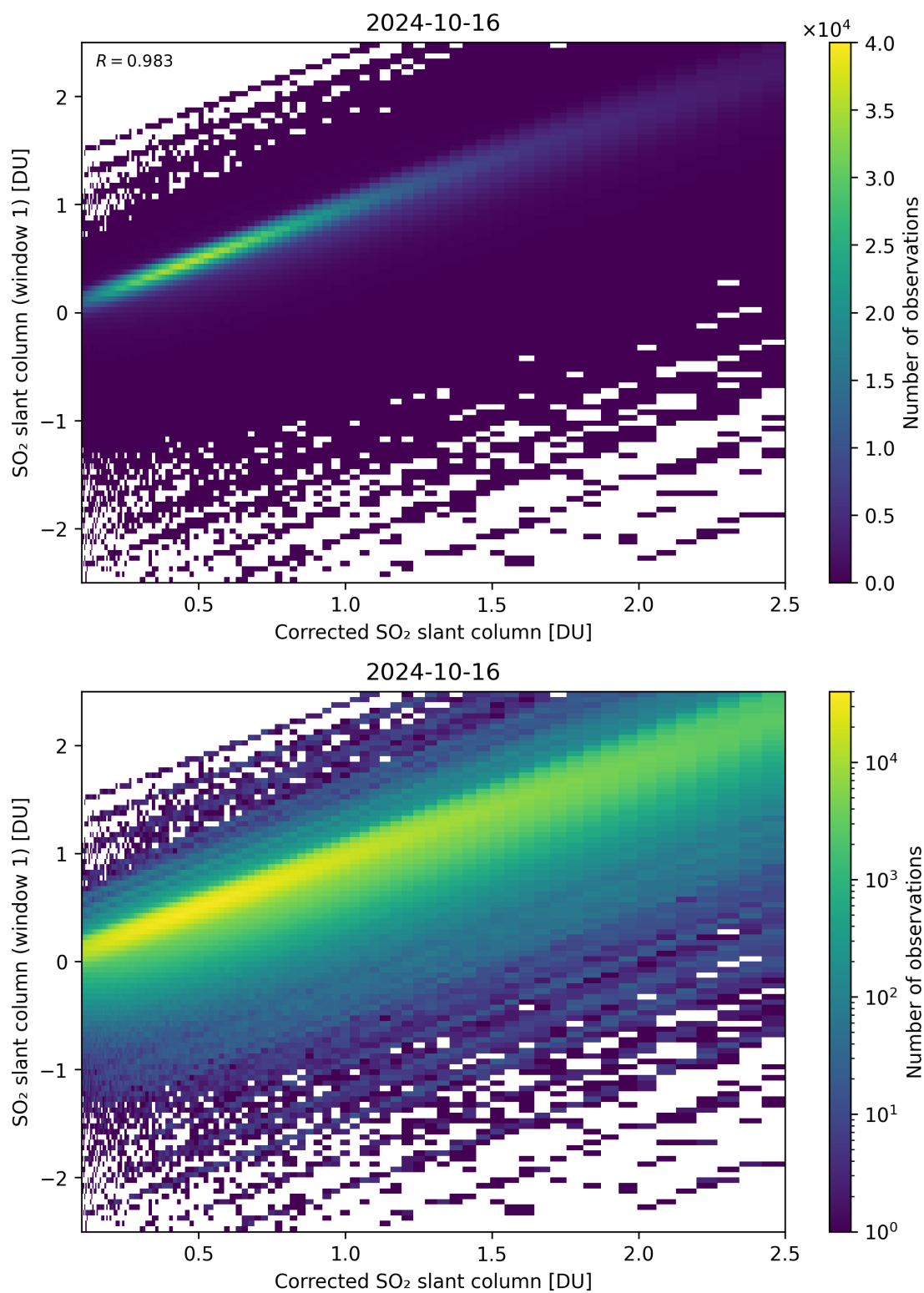
Figure 187: Scatter density plot of “Corrected SO 2 slant column” against “SO 2 slant column (window 1)” for 2024-10-15 to 2024-10-17.
