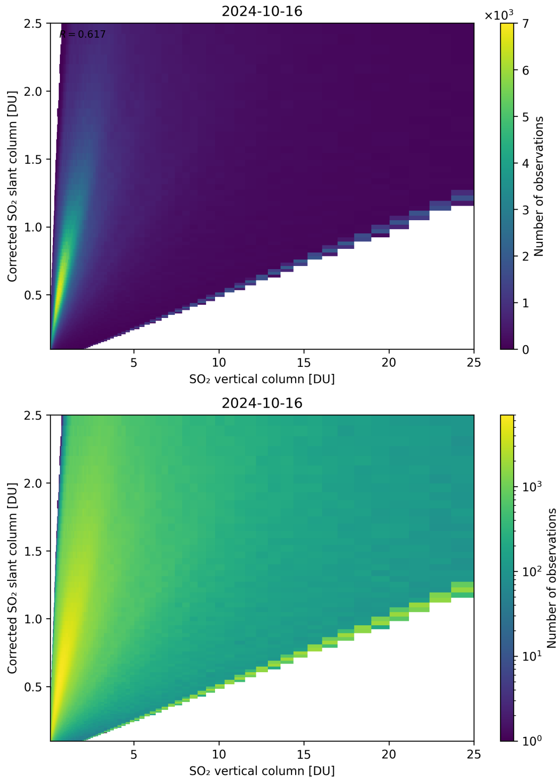
Figure 297: Scatter density plot of “SO 2 vertical column” against “Corrected SO 2 slant column” for 2024-10-15 to 2024-10-17.
