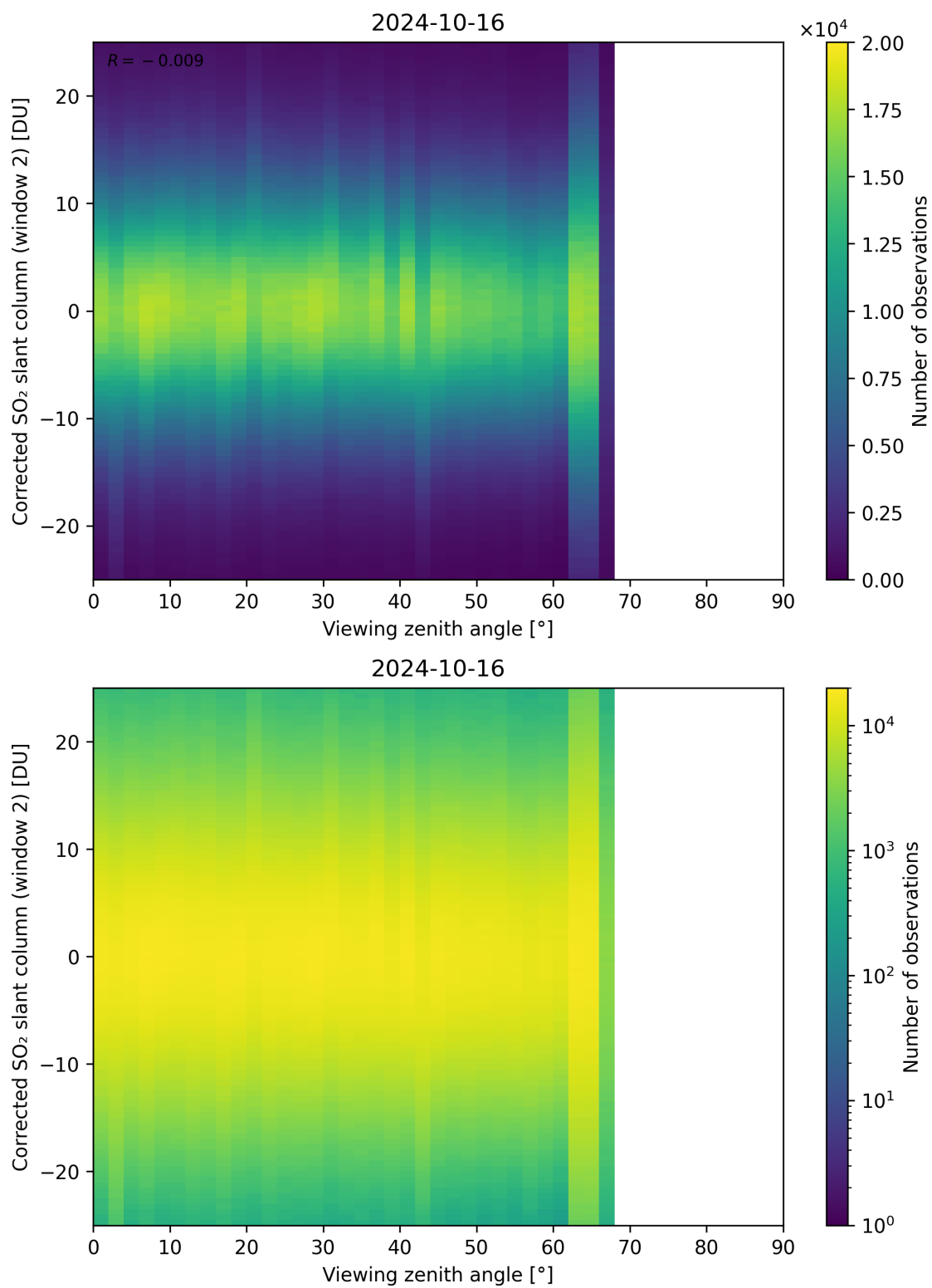
Figure 318: Scatter density plot of “Viewing zenith angle” against “Corrected SO 2 slant column (window 2)” for 2024-10-15 to 2024-10-17.
