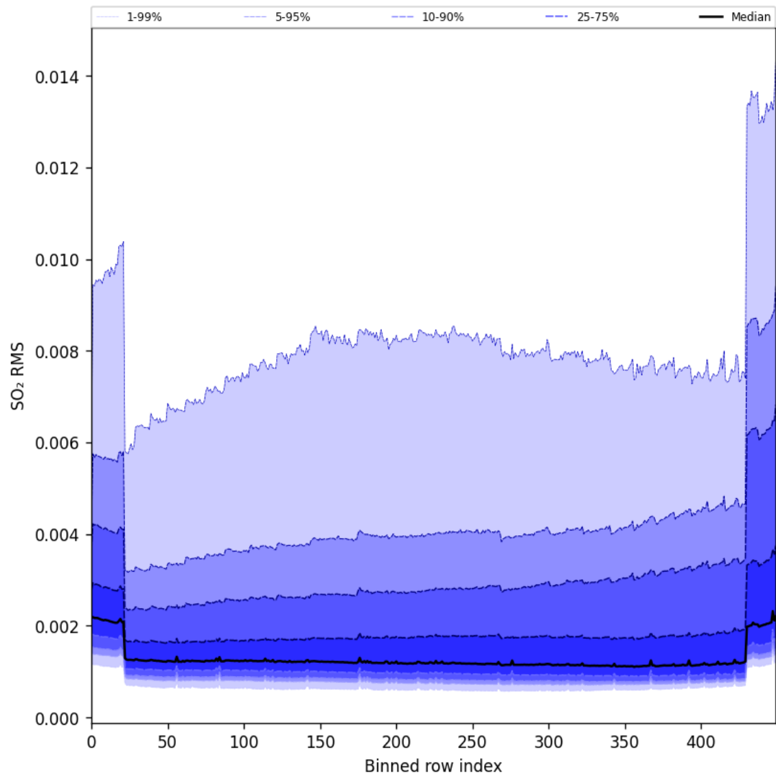
Figure 93: Along track statistics of “SO 2 RMS” for 2024-10-15 to 2024-10-17
