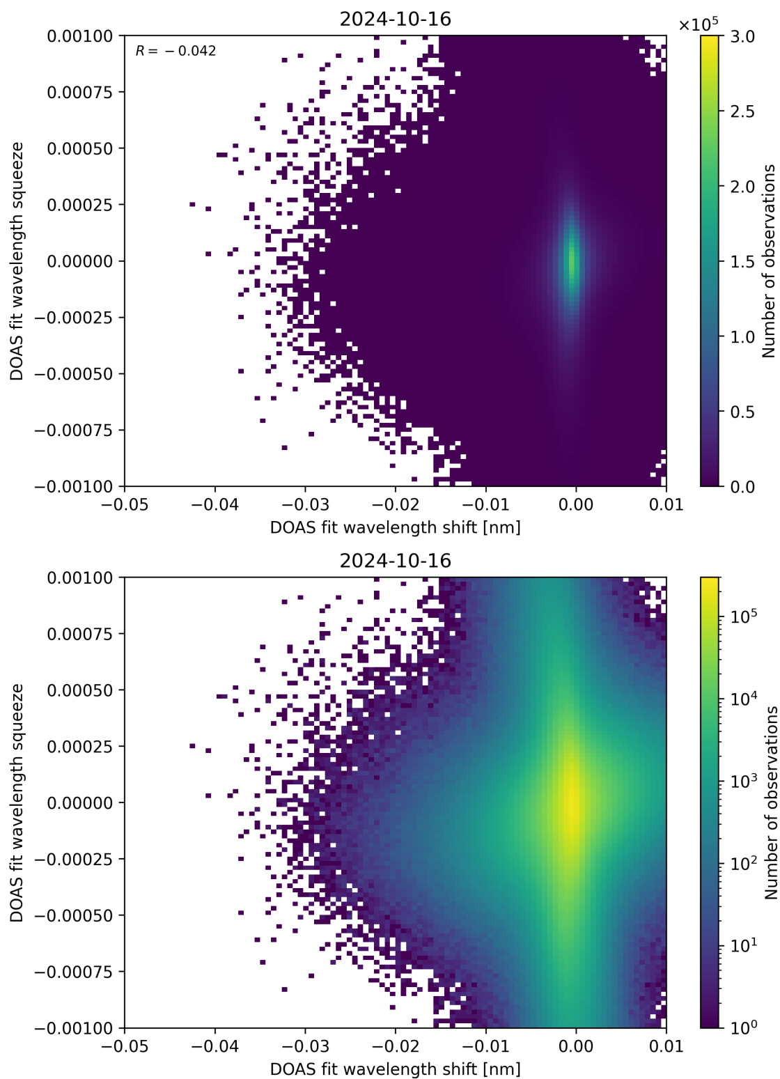
Figure 127: Scatter density plot of “DOAS fit wavelength shift” against “DOAS fit wavelength squeeze” for 2024-10-15 to 2024-10-17.
