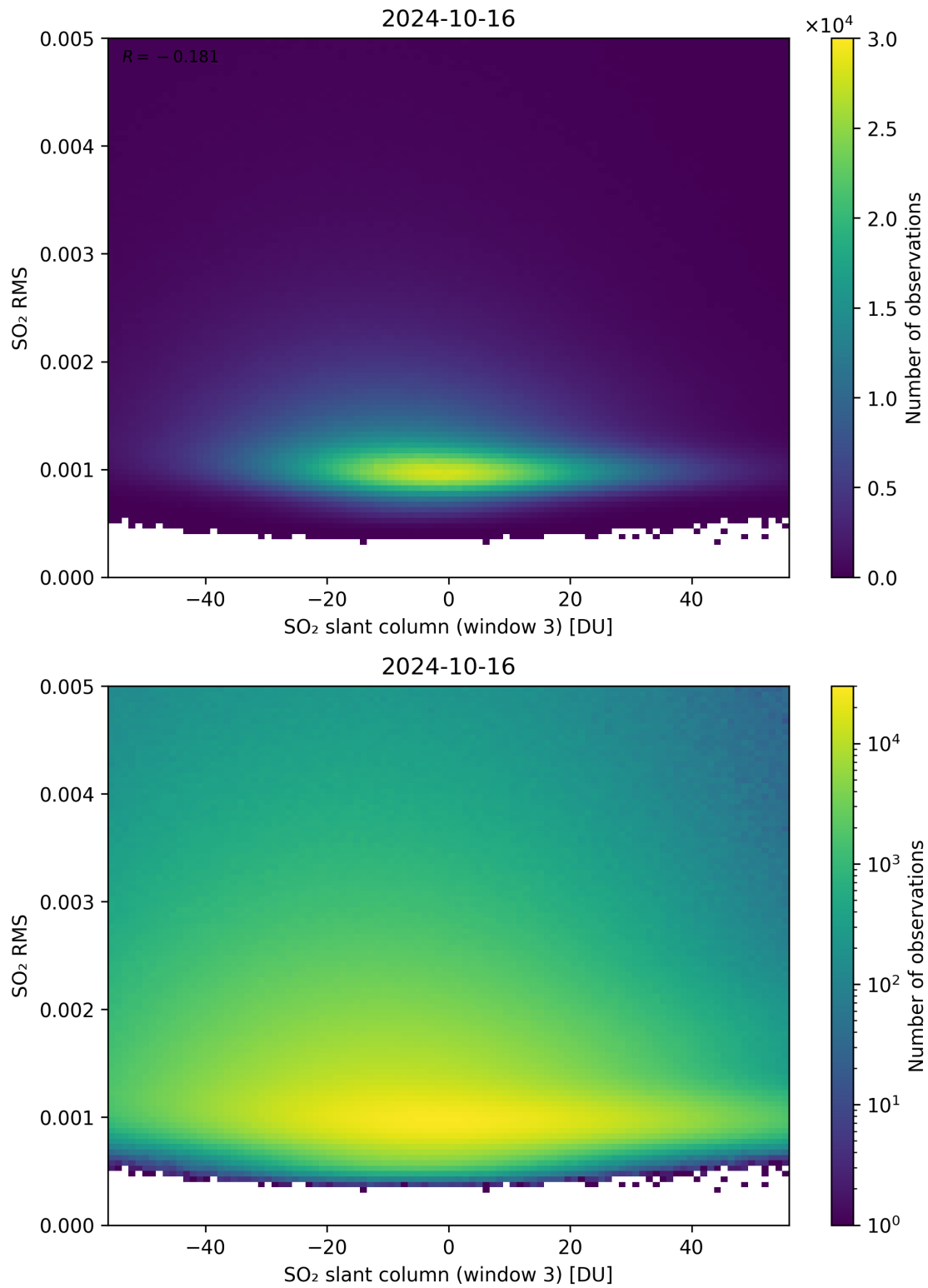
Figure 256: Scatter density plot of “SO 2 slant column (window 3)” against “SO 2 RMS” for 2024-10-15 to 2024-10-17.
