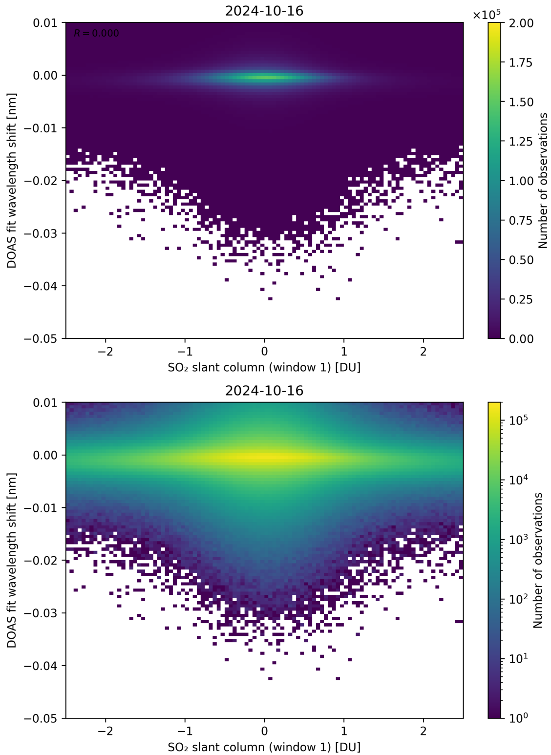
Figure 215: Scatter density plot of “SO 2 slant column (window 1)” against “DOAS fit wavelength shift” for 2024-10-15 to 2024-10-17.
