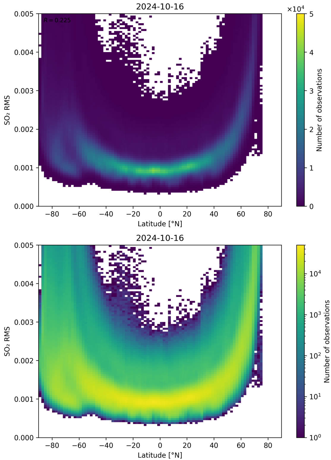
Figure 144: Scatter density plot of “Latitude” against “SO 2 RMS” for 2024-10-15 to 2024-10-17.
