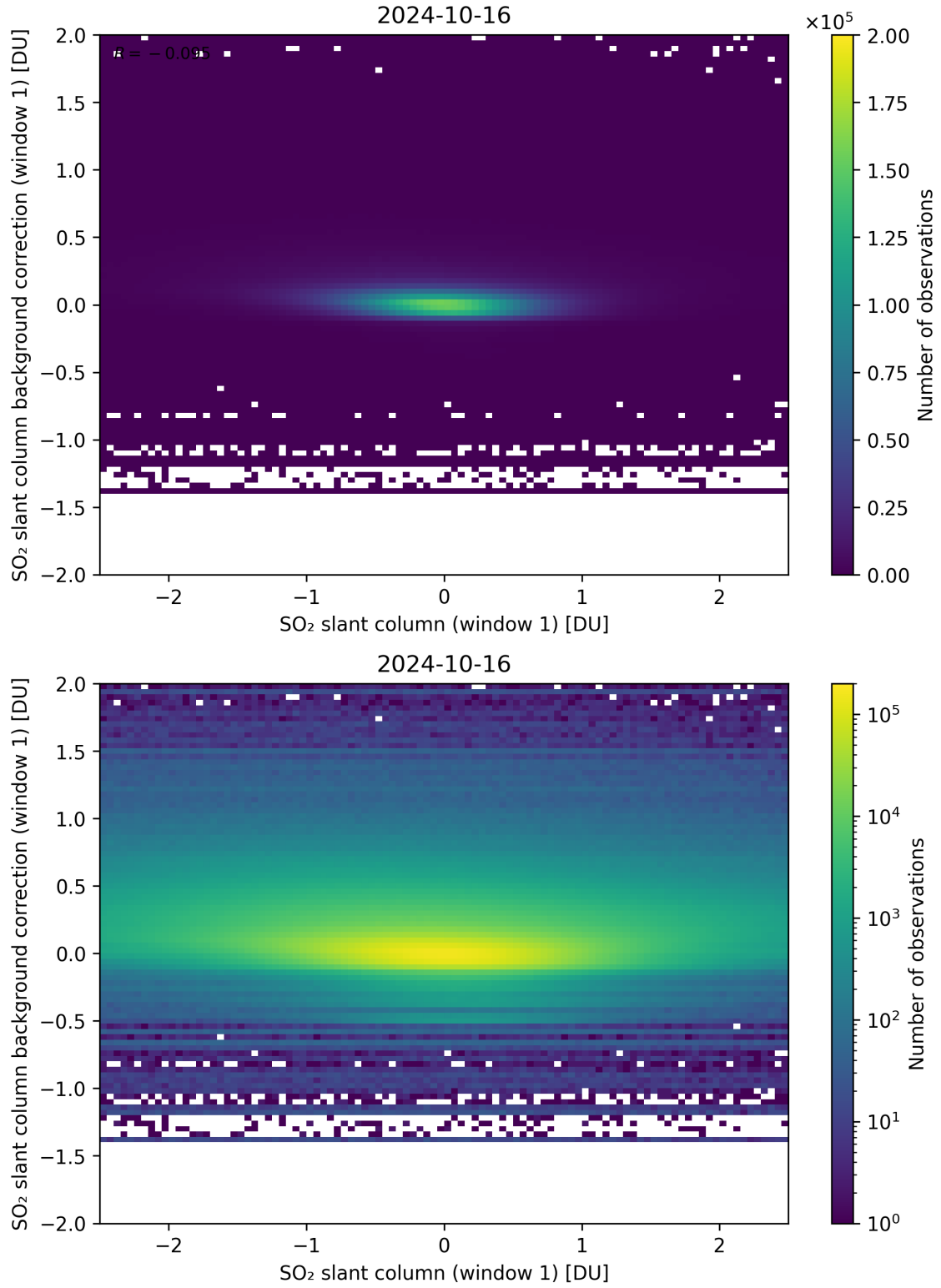
Figure 212: Scatter density plot of “SO 2 slant column (window 1)” against “SO 2 slant column background correction (window 1)” for 2024-10-15 to 2024-10-17.
