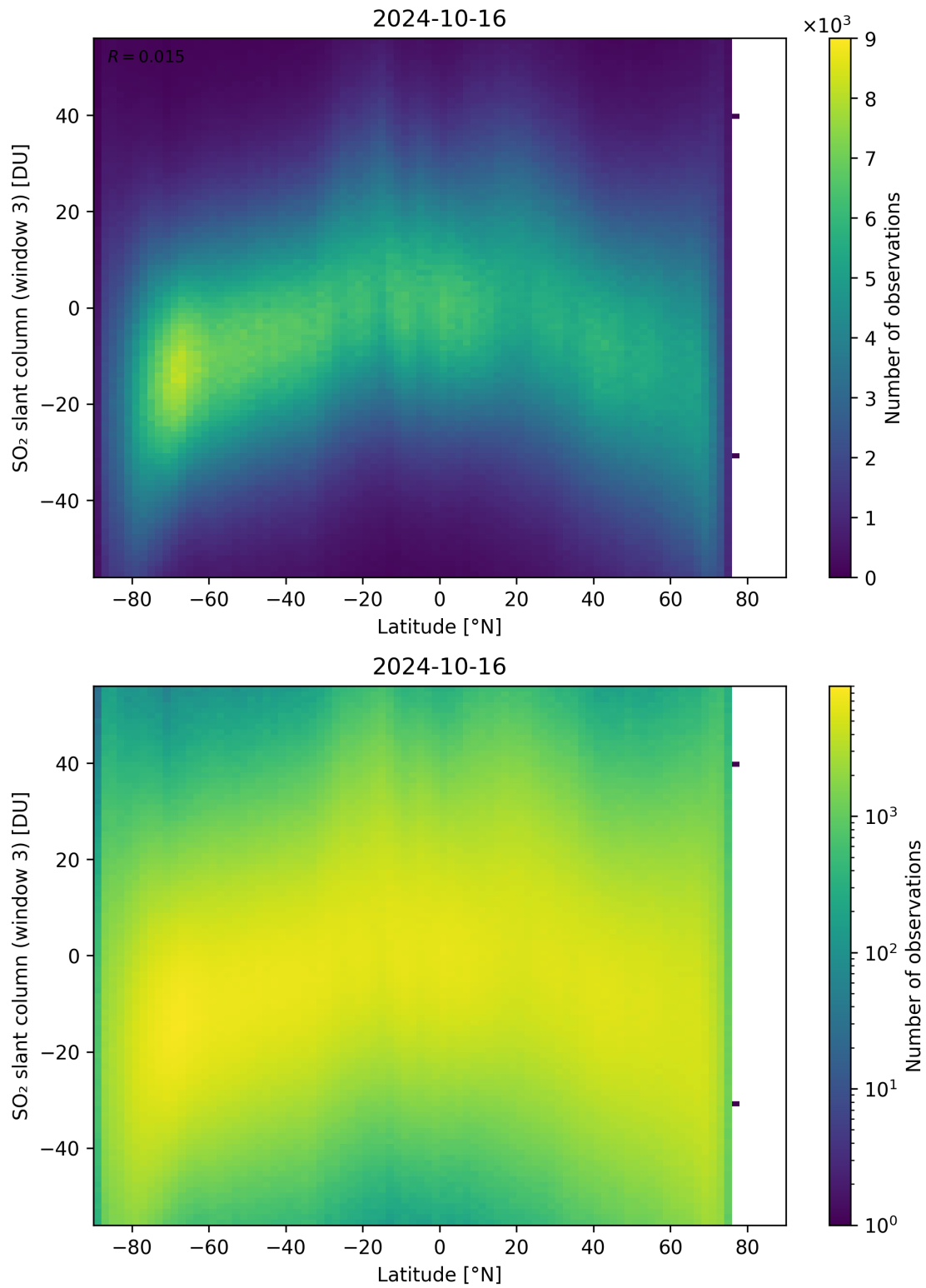
Figure 152: Scatter density plot of “Latitude” against “SO 2 slant column (window 3)” for 2024-10-15 to 2024-10-17.
