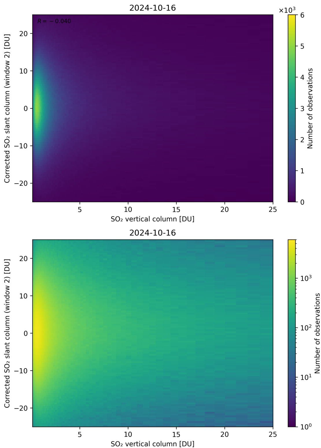
Figure 298: Scatter density plot of “SO 2 vertical column” against “Corrected SO 2 slant column (window 2)” for 2024-10-15 to 2024-10-17.
