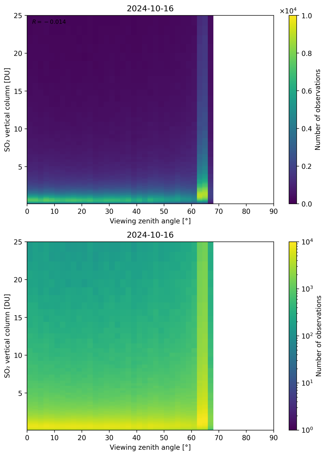
Figure 327: Scatter density plot of “Viewing zenith angle” against “SO 2 vertical column” for 2024-10-15 to 2024-10-17.
