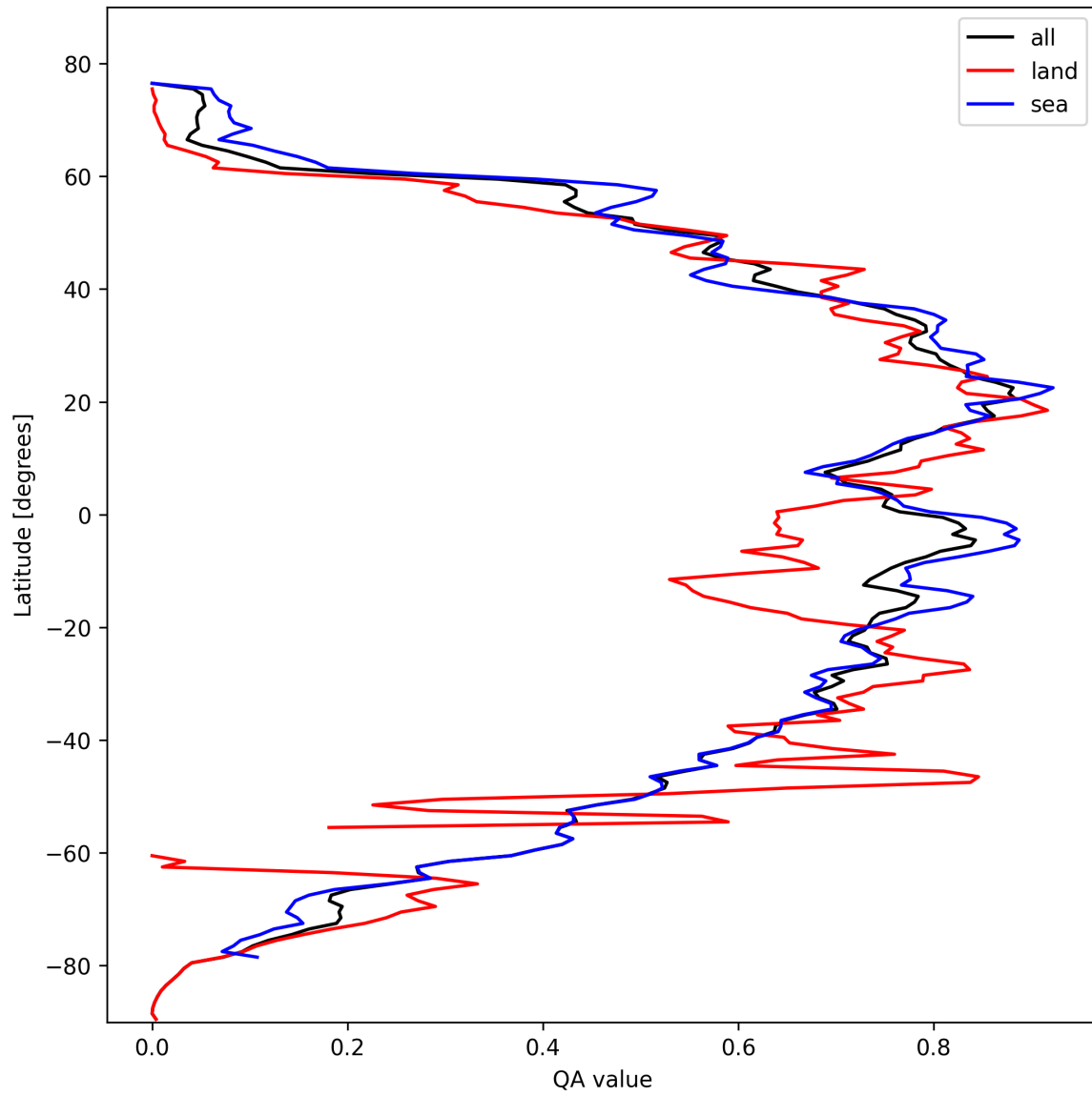
Figure 29: Zonal average of “QA value” for 2024-10-15 to 2024-10-17.
