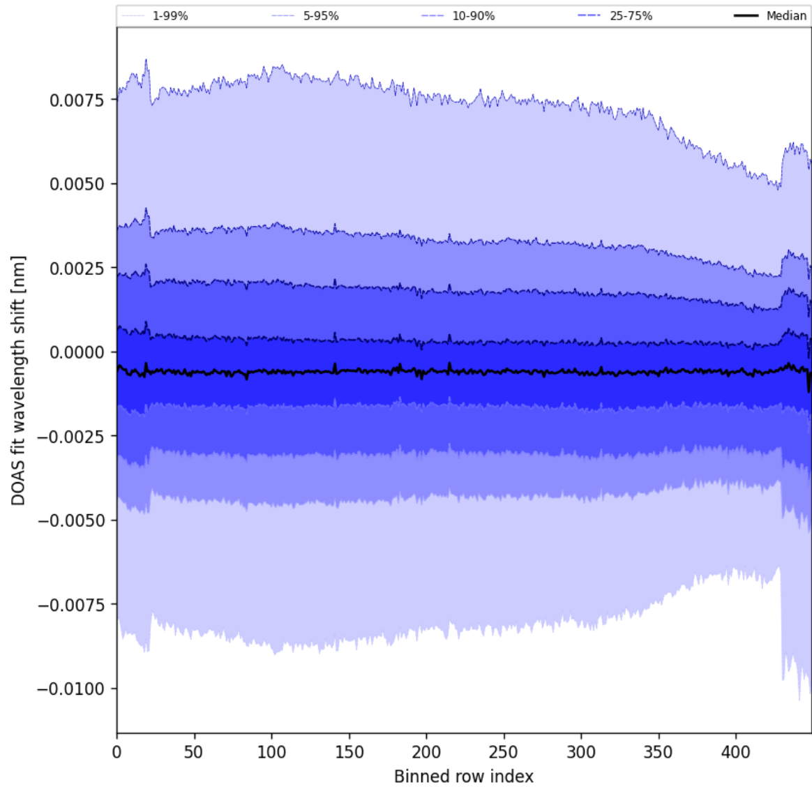
Figure 91: Along track statistics of “DOAS fit wavelength shift” for 2024-10-15 to 2024-10-17
