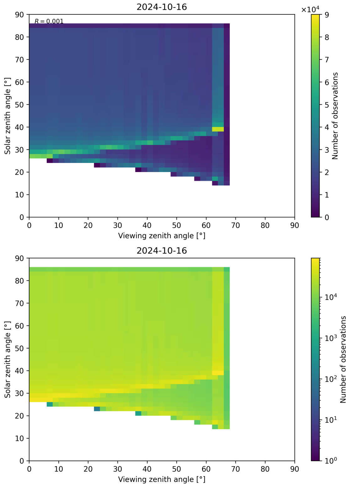
Figure 315: Scatter density plot of “Viewing zenith angle” against “Solar zenith angle” for 2024-10-15 to 2024-10-17.
