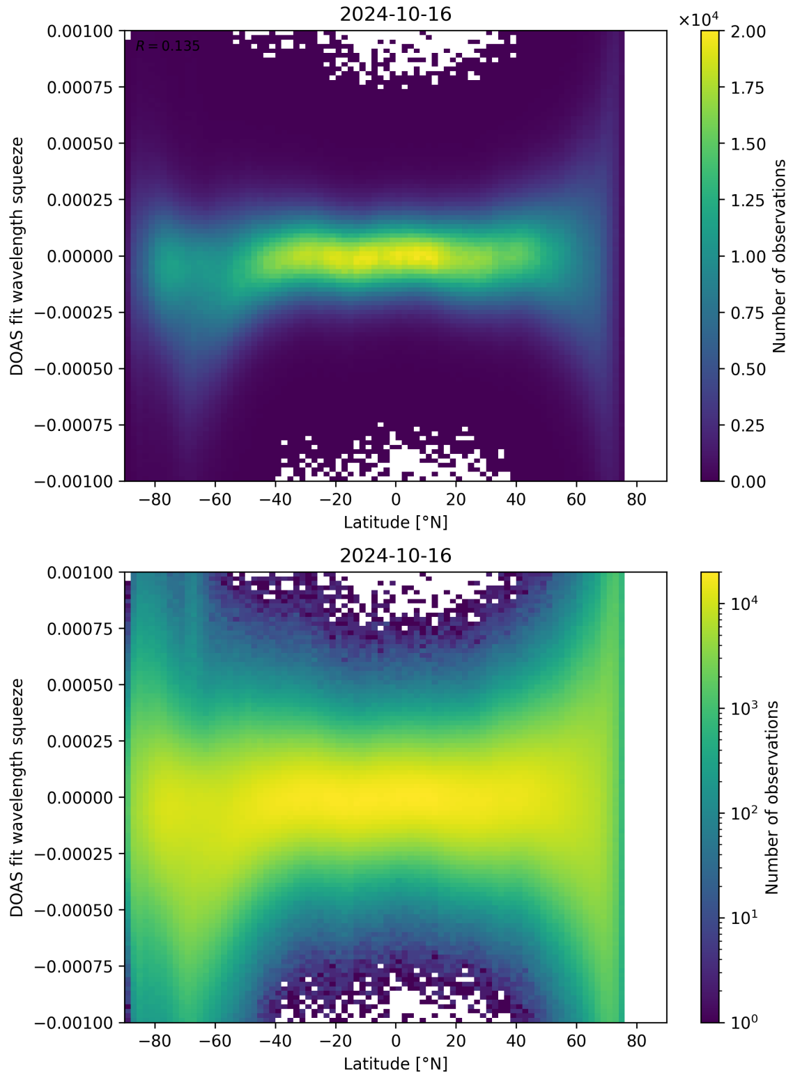
Figure 143: Scatter density plot of “Latitude” against “DOAS fit wavelength squeeze” for 2024-10-15 to 2024-10-17.
