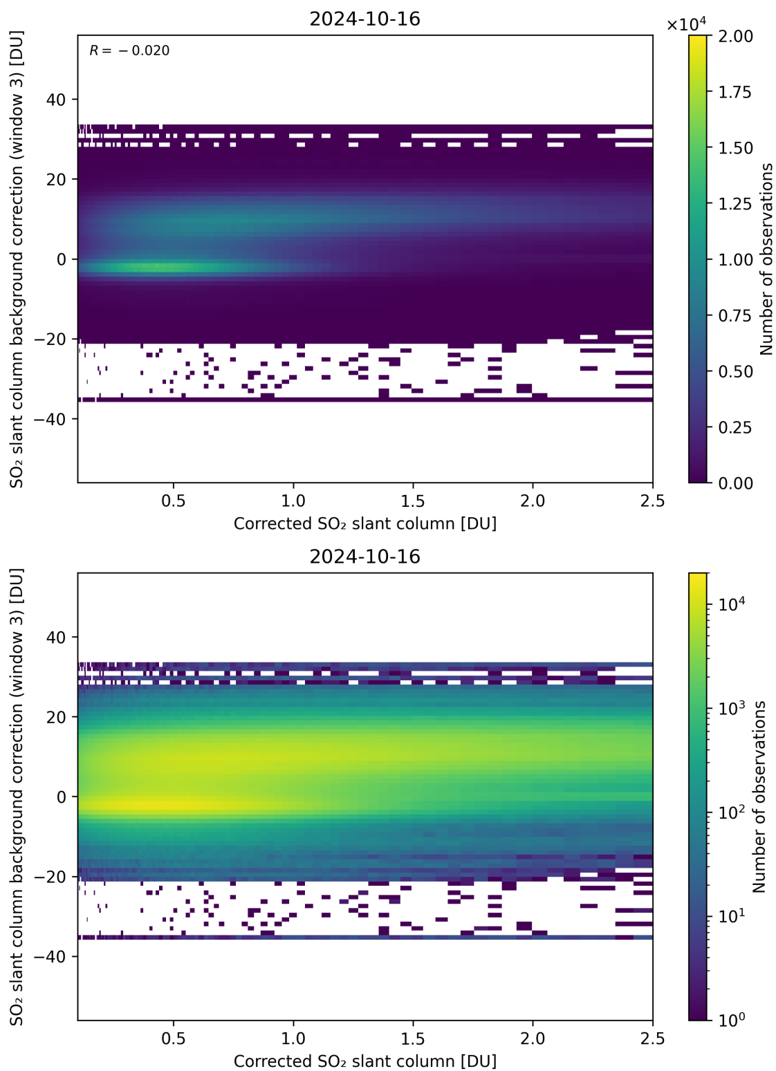
Figure 180: Scatter density plot of “Corrected SO 2 slant column” against “SO 2 slant column background correction (window 3)” for 2024-10-15 to 2024-10-17.
