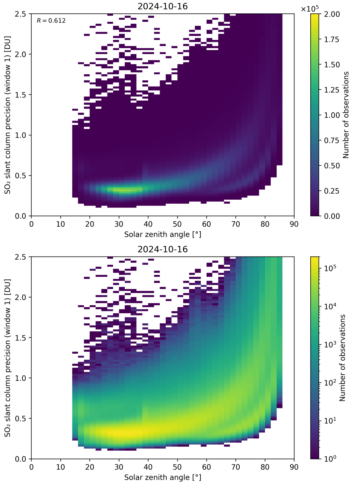
Figure 170: Scatter density plot of “Solar zenith angle” against “SO 2 slant column precision (window 1)” for 2024-10-15 to 2024-10-17.
