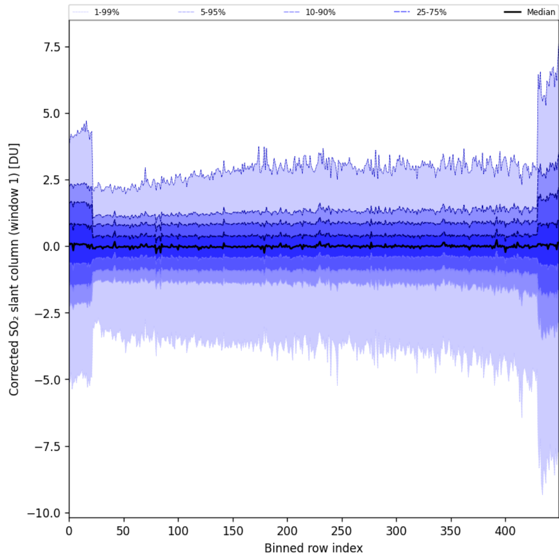
Figure 81: Along track statistics of "Corrected SO 2 slant column (window 1)" for 2024-10-15 to 2024-10-17
