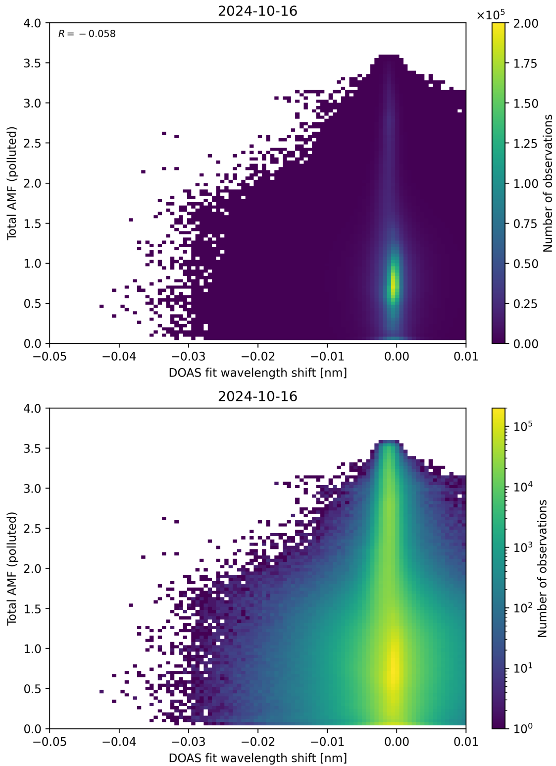
Figure 130: Scatter density plot of “DOAS fit wavelength shift” against “Total AMF (polluted)” for 2024-10-15 to 2024-10-17.
