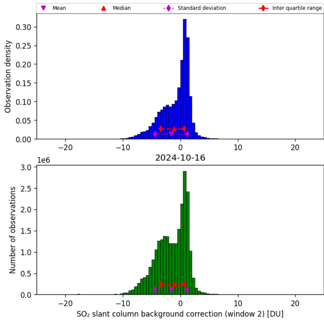
Figure 63: Histogram of “SO 2 slant column background correction (window 2)” for 2024-10-15 to 2024-10-17
