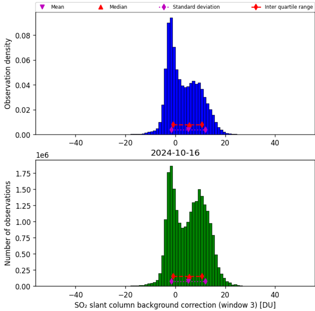
Figure 67: Histogram of “SO 2 slant column background correction (window 3)” for 2024-10-15 to 2024-10-17
