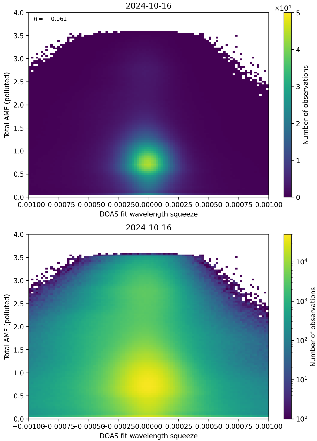
Figure 134: Scatter density plot of “DOAS fit wavelength squeeze” against “Total AMF (polluted)” for 2024-10-15 to 2024-10-17.
