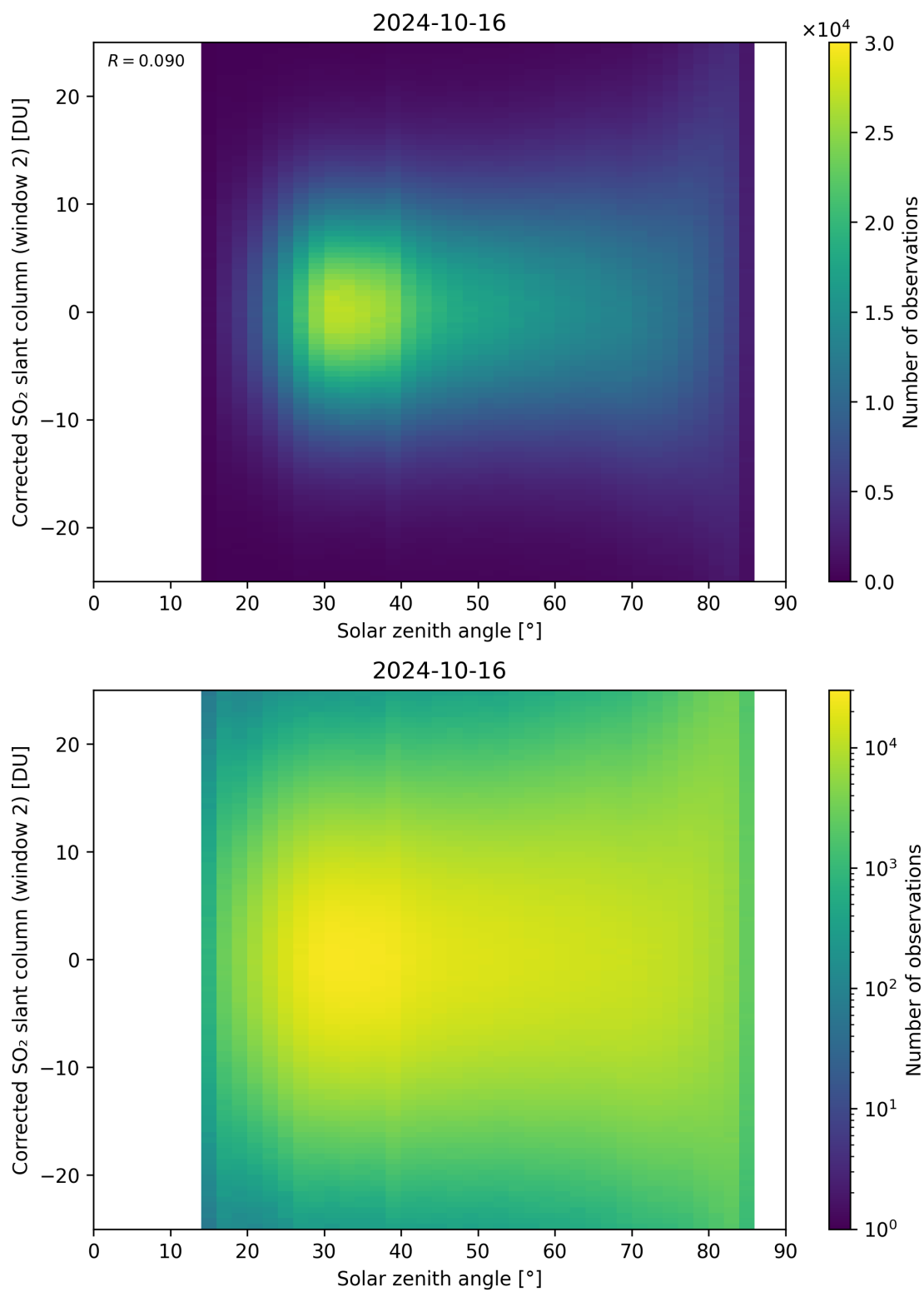
Figure 167: Scatter density plot of “Solar zenith angle” against “Corrected SO 2 slant column (window 2)” for 2024-10-15 to 2024-10-17.
