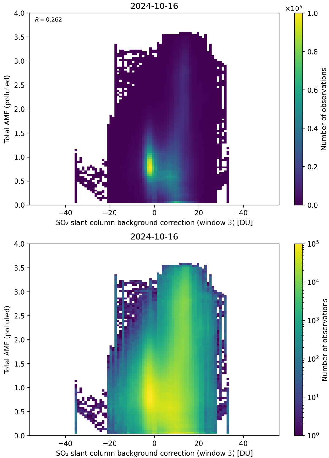
Figure 125: Scatter density plot of “SO 2 slant column background correction (window 3)” against “Total AMF (polluted)” for 2024-10-15 to 2024-10-17.
