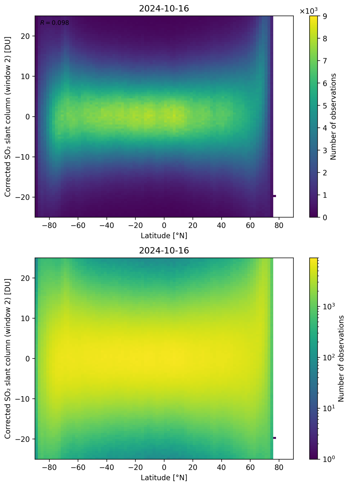
Figure 147: Scatter density plot of “Latitude” against “Corrected SO 2 slant column (window 2)” for 2024-10-15 to 2024-10-17.
