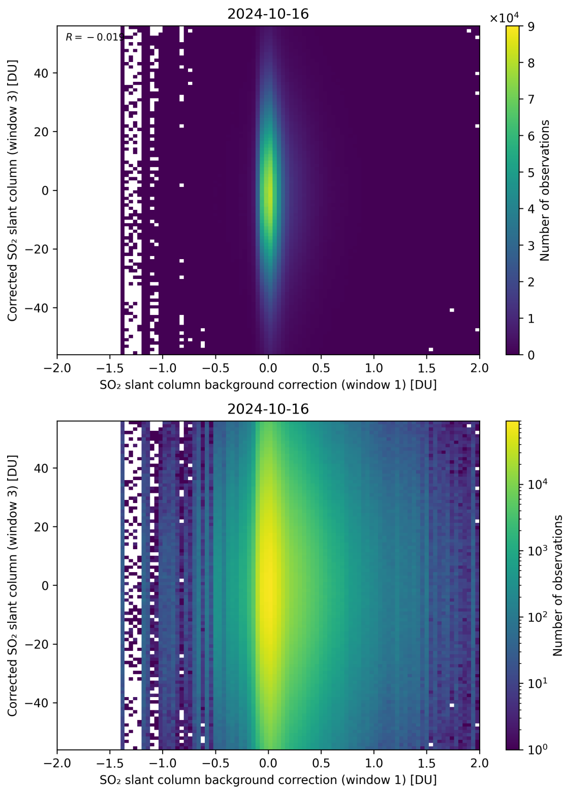
Figure 105: Scatter density plot of “SO 2 slant column background correction (window 1)” against “Corrected SO 2 slant column (window 3)” for 2024-10-15 to 2024-10-17.
