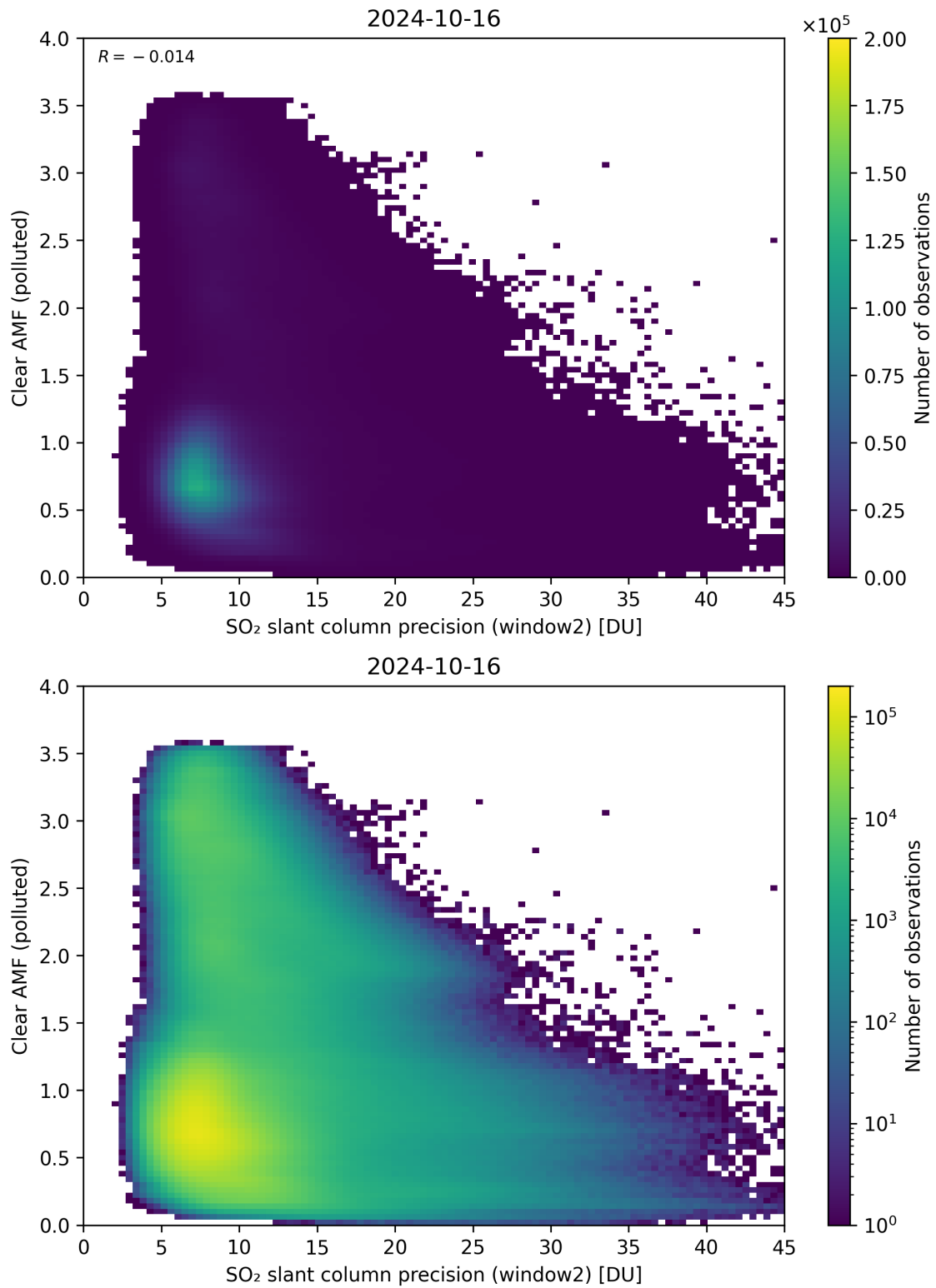
Figure 246: Scatter density plot of “SO 2 slant column precision (window2)” against “Clear AMF (polluted)” for 2024-10-15 to 2024-10-17.
