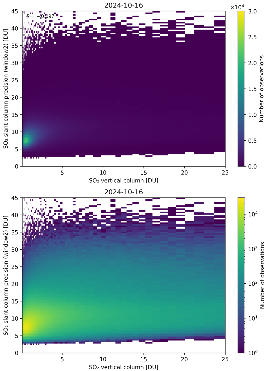
Figure 302: Scatter density plot of “SO 2 vertical column” against “SO 2 slant column precision (window2)” for 2024-10-15 to 2024-10-17.
