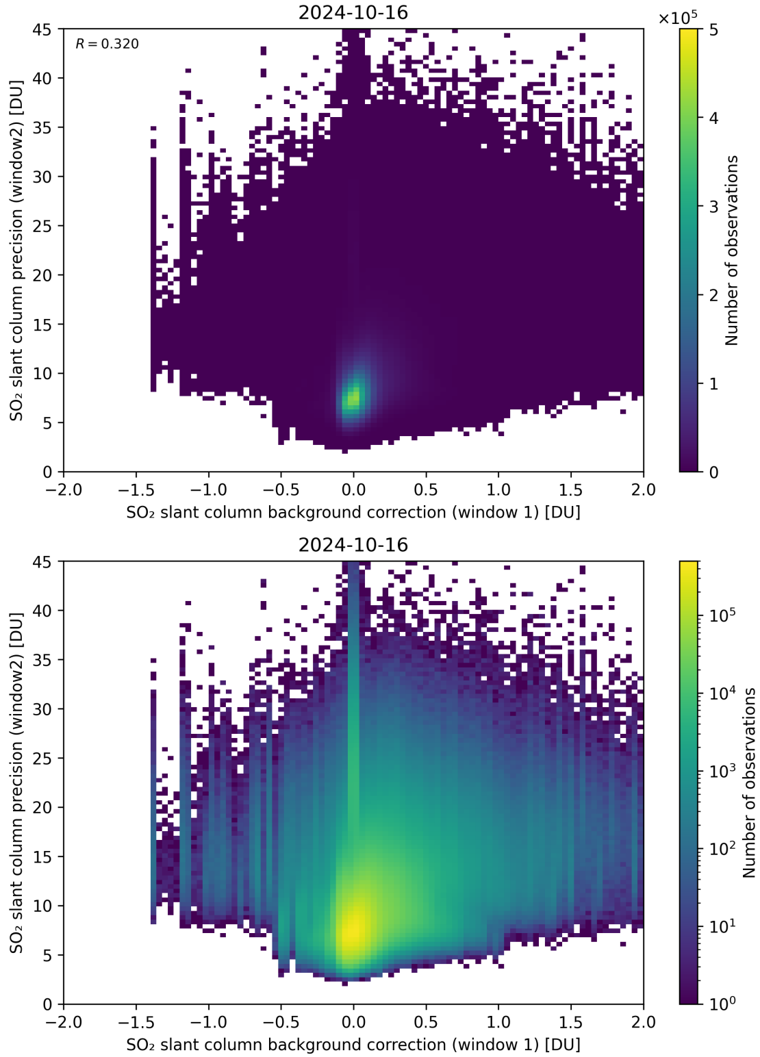
Figure 106: Scatter density plot of “SO 2 slant column background correction (window 1)” against “SO 2 slant column precision (window2)” for 2024-10-15 to 2024-10-17.
