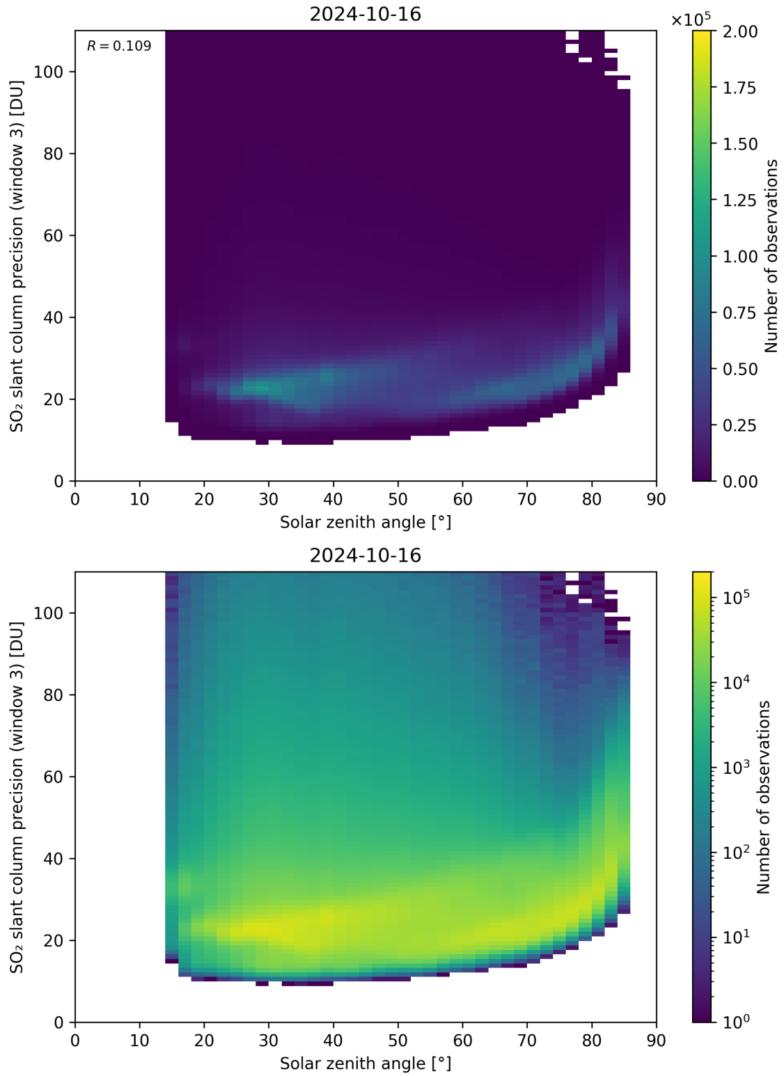
Figure 173: Scatter density plot of “Solar zenith angle” against “SO 2 slant column precision (window 3)” for 2024-10-15 to 2024-10-17.
