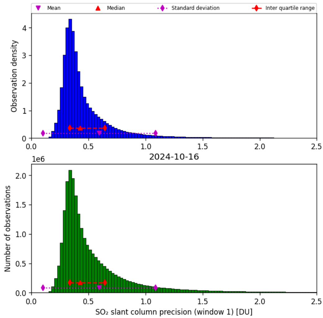
Figure 57: Histogram of “SO 2 slant column precision (window 1)” for 2024-10-15 to 2024-10-17
