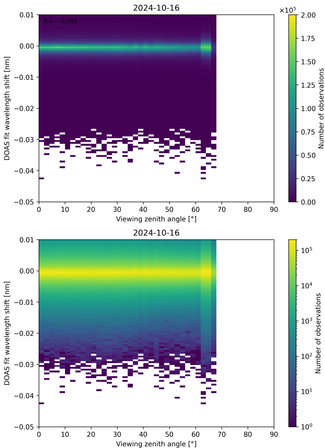
Figure 311: Scatter density plot of “Viewing zenith angle” against “DOAS fit wavelength shift” for 2024-10-15 to 2024-10-17.
