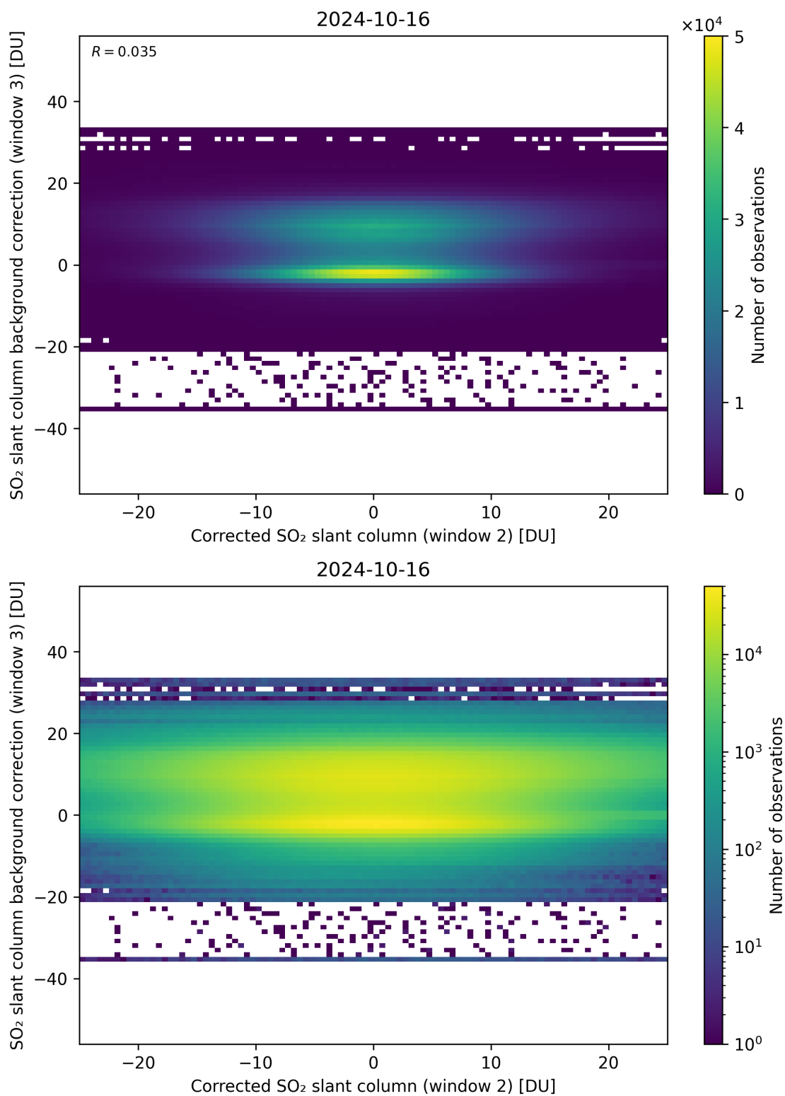
Figure 195: Scatter density plot of “Corrected SO 2 slant column (window 2)” against “SO 2 slant column background correction (window 3)” for 2024-10-15 to 2024-10-17.
