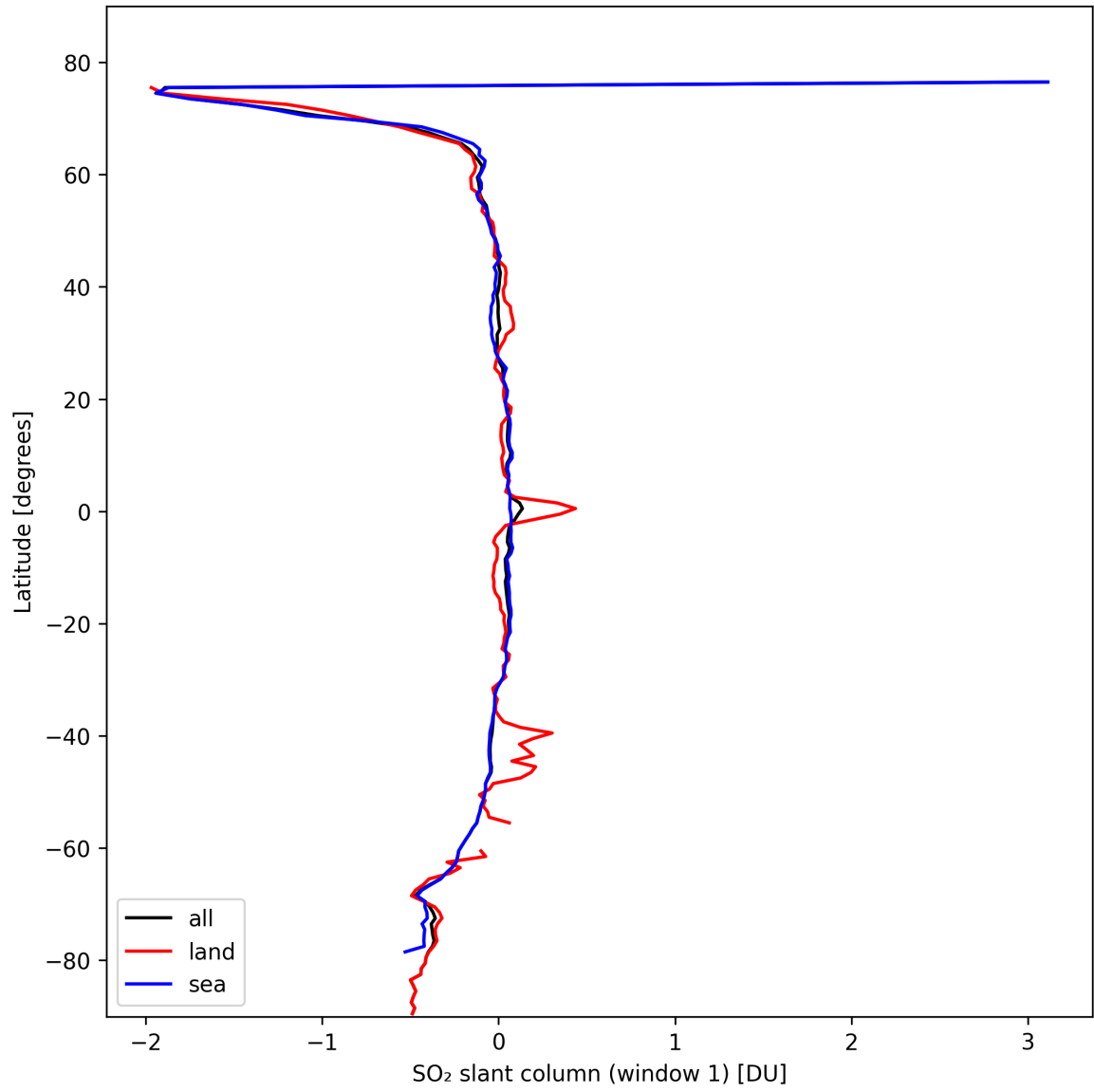
Figure 33: Zonal average of “SO 2 slant column (window 1)” for 2024-10-15 to 2024-10-17.
