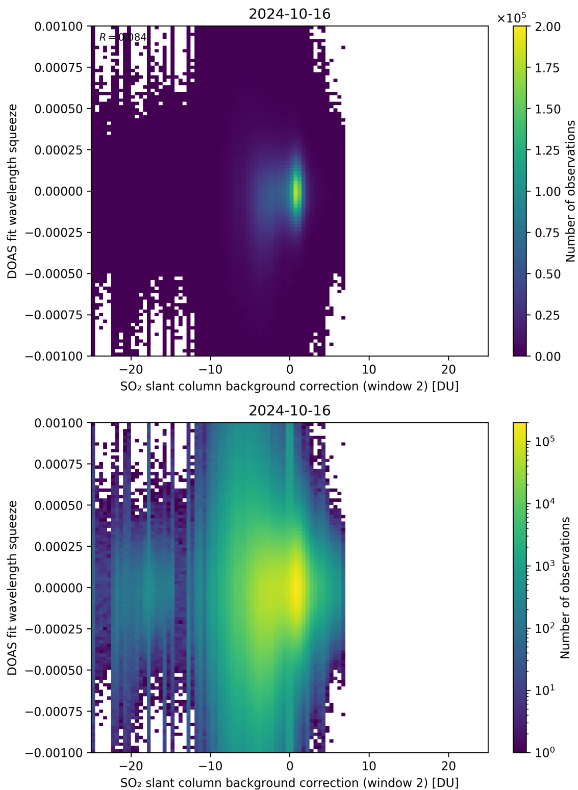
Figure 113: Scatter density plot of “SO 2 slant column background correction (window 2)” against “DOAS fit wavelength squeeze” for 2024-10-15 to 2024-10-17.
