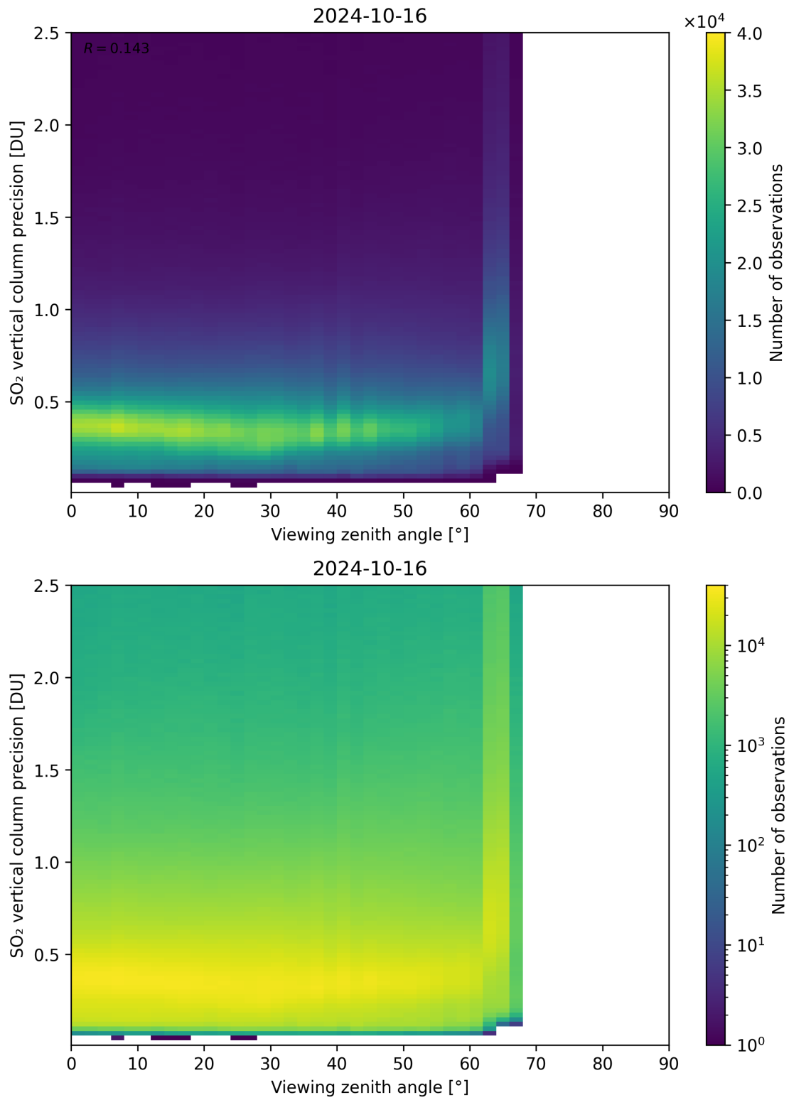
Figure 328: Scatter density plot of “Viewing zenith angle” against “SO 2 vertical column precision” for 2024-10-15 to 2024-10-17.
