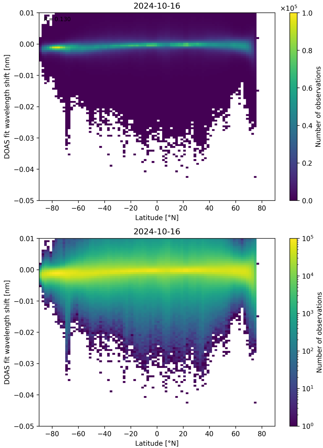
Figure 142: Scatter density plot of “Latitude” against “DOAS fit wavelength shift” for 2024-10-15 to 2024-10-17.
