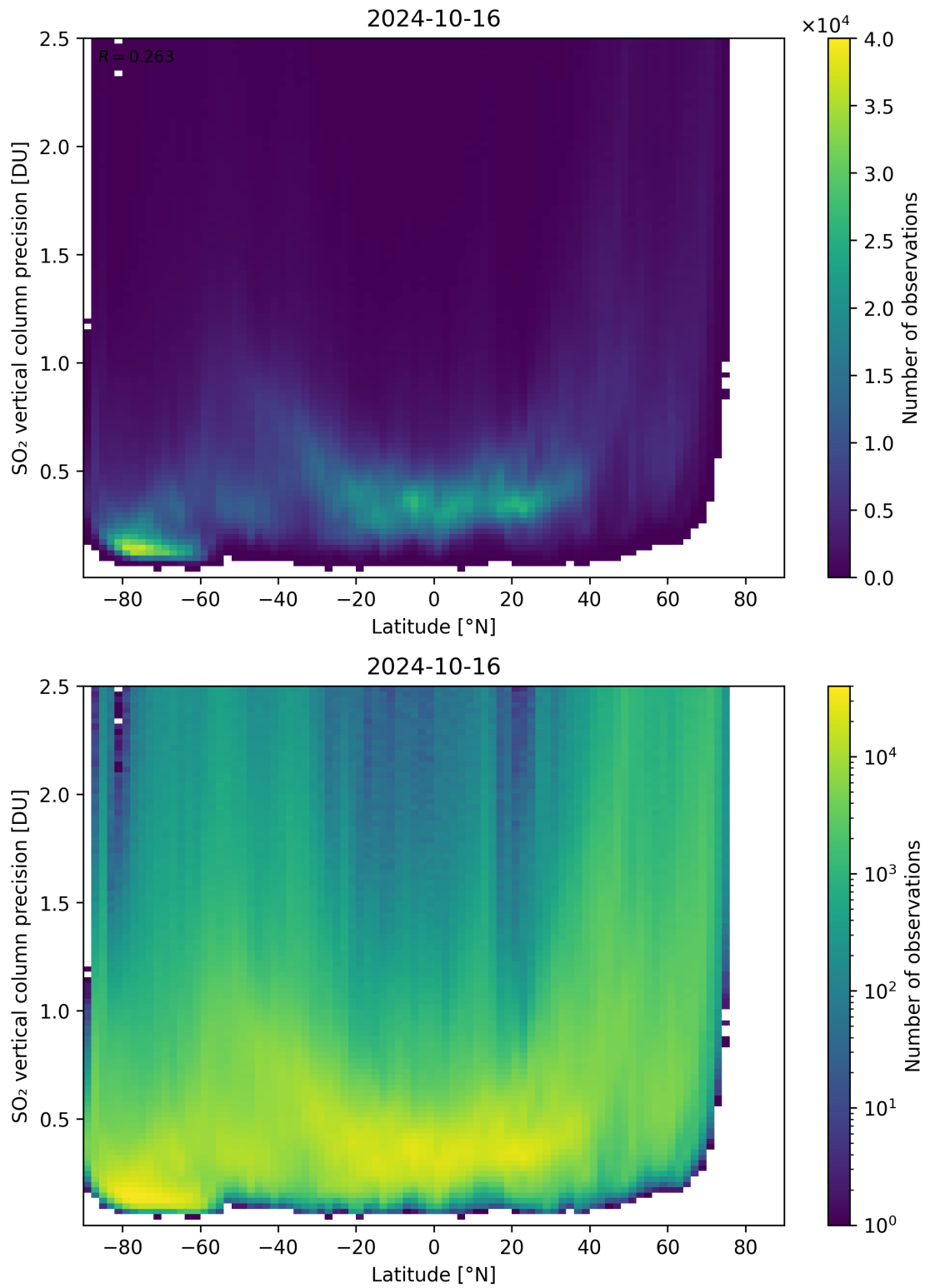
Figure 157: Scatter density plot of “Latitude” against “SO 2 vertical column precision” for 2024-10-15 to 2024-10-17.
