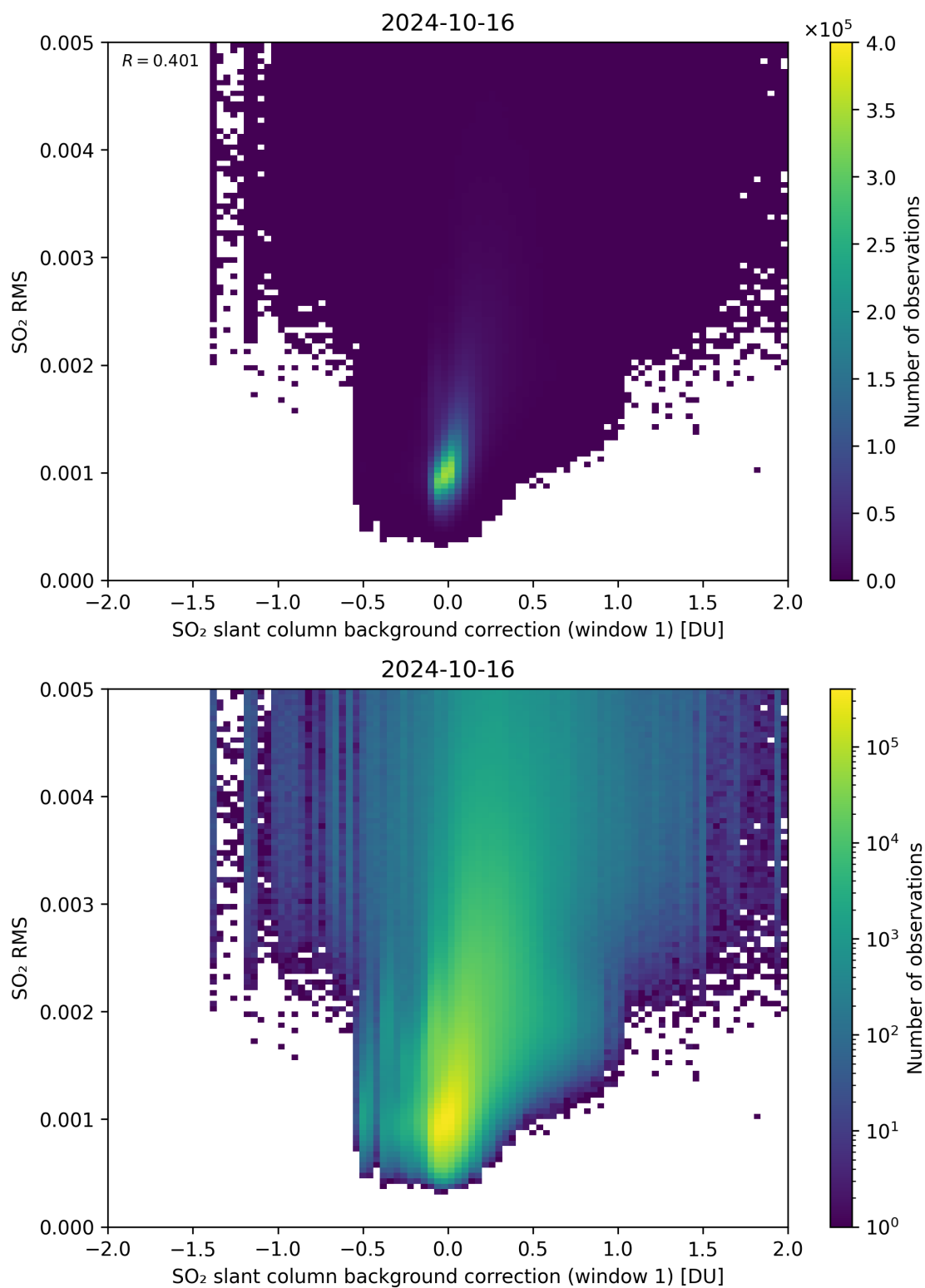
Figure 102: Scatter density plot of “SO 2 slant column background correction (window 1)” against “SO 2 RMS” for 2024-10-15 to 2024-10-17.
