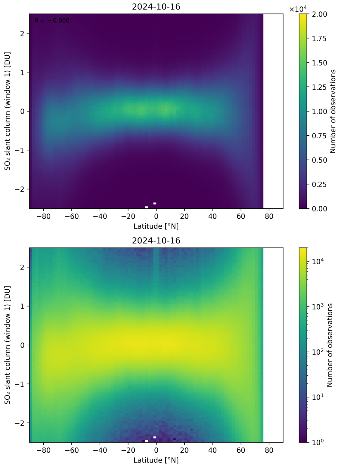
Figure 149: Scatter density plot of “Latitude” against “SO 2 slant column (window 1)” for 2024-10-15 to 2024-10-17.
