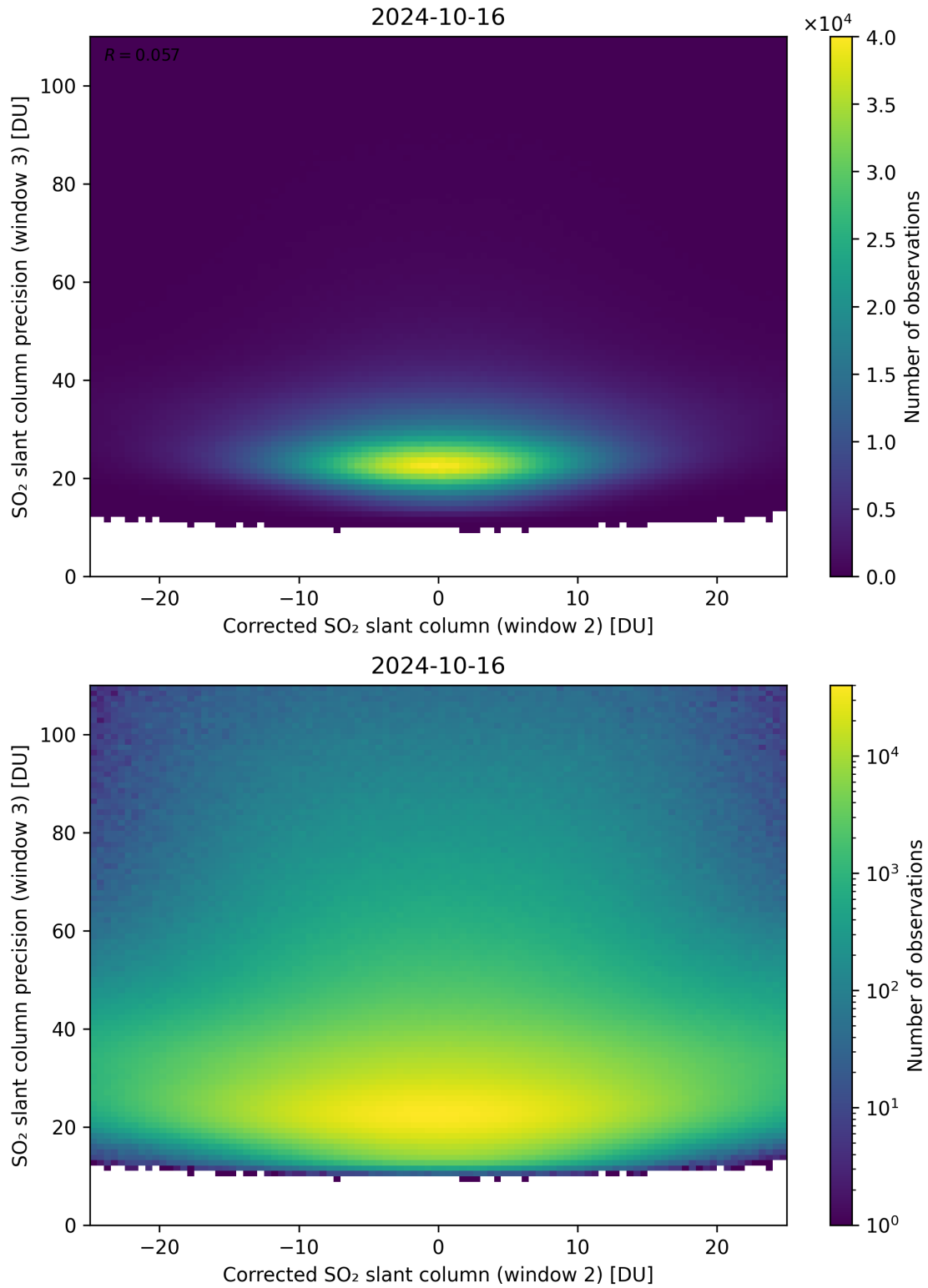
Figure 202: Scatter density plot of “Corrected SO 2 slant column (window 2)” against “SO 2 slant column precision (window 3)” for 2024-10-15 to 2024-10-17.
