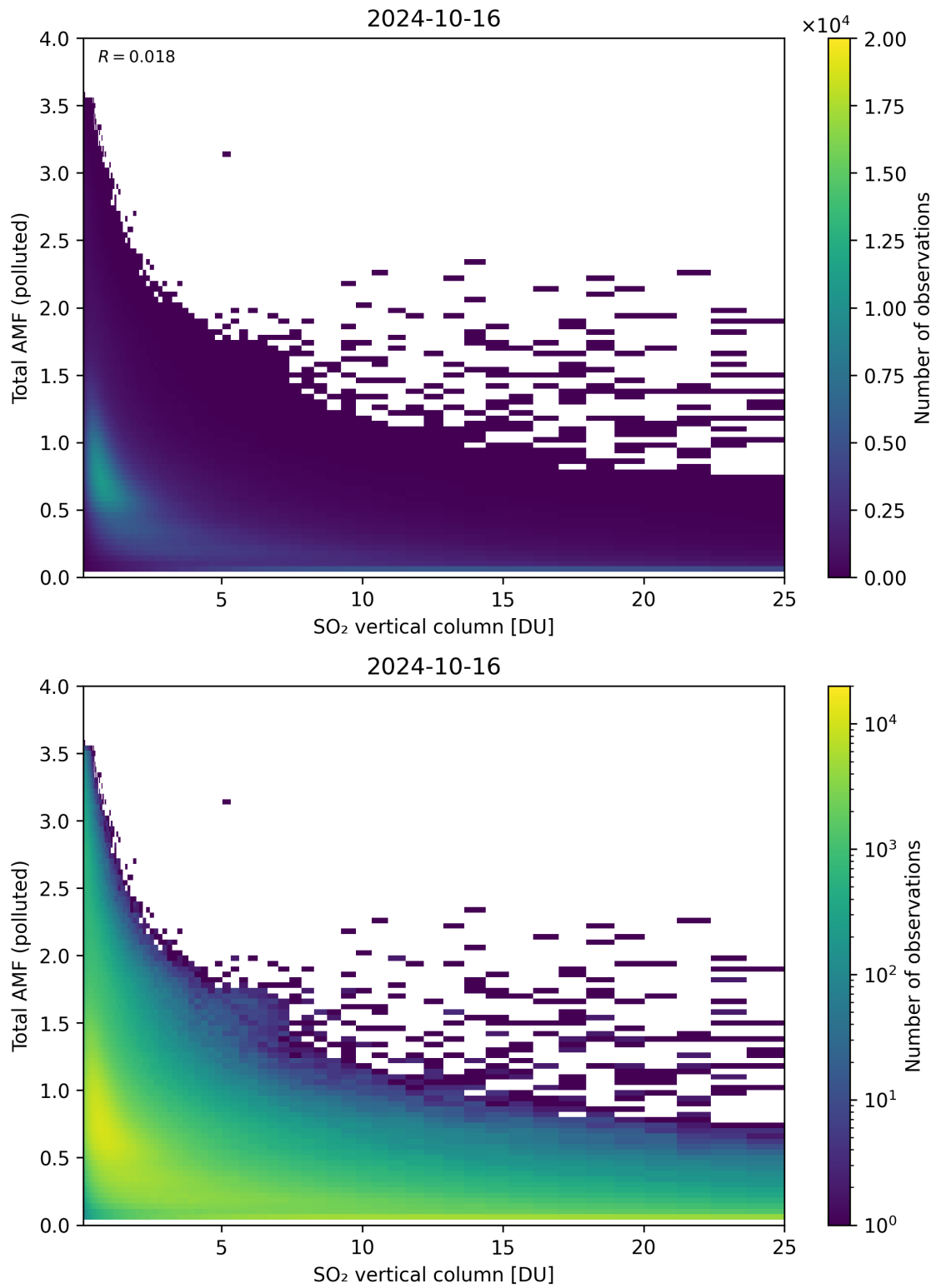
Figure 305: Scatter density plot of “SO 2 vertical column” against “Total AMF (polluted)” for 2024-10-15 to 2024-10-17.
