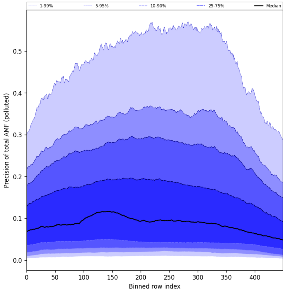
Figure 95: Along track statistics of “Precision of total AMF (polluted)” for 2024-10-15 to 2024-10-17
