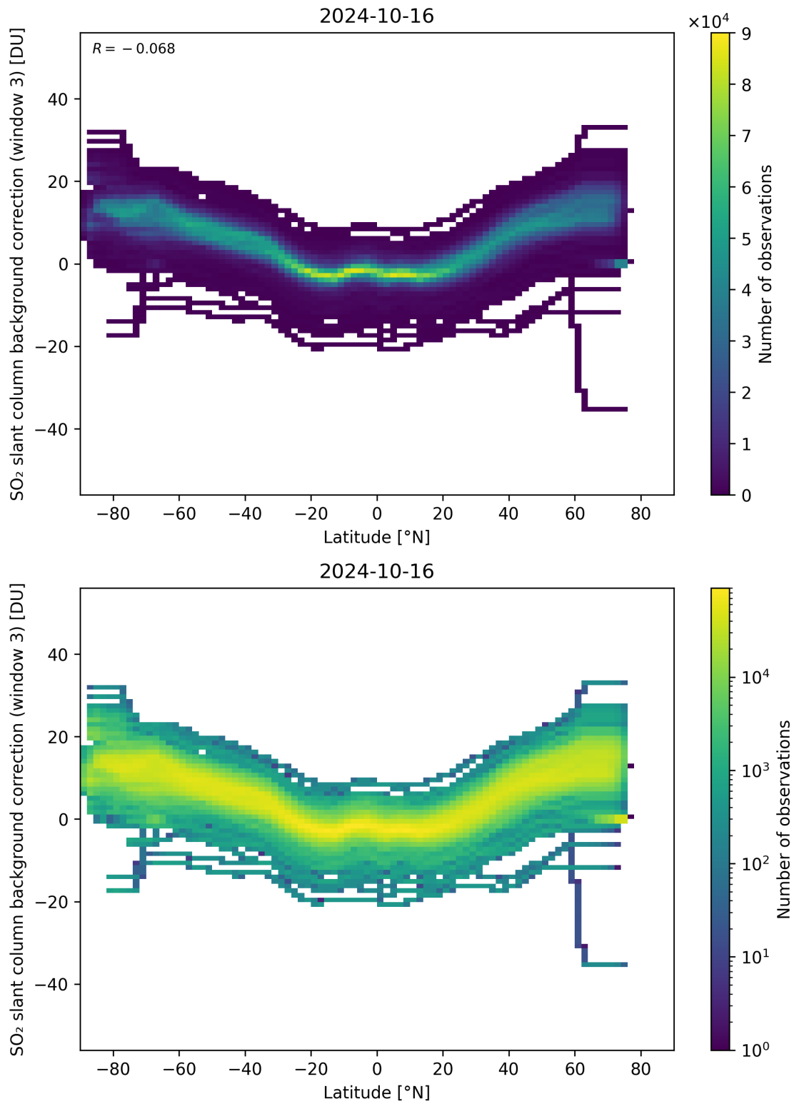
Figure 141: Scatter density plot of “Latitude” against “SO 2 slant column background correction (window 3)” for 2024-10-15 to 2024-10-17.
