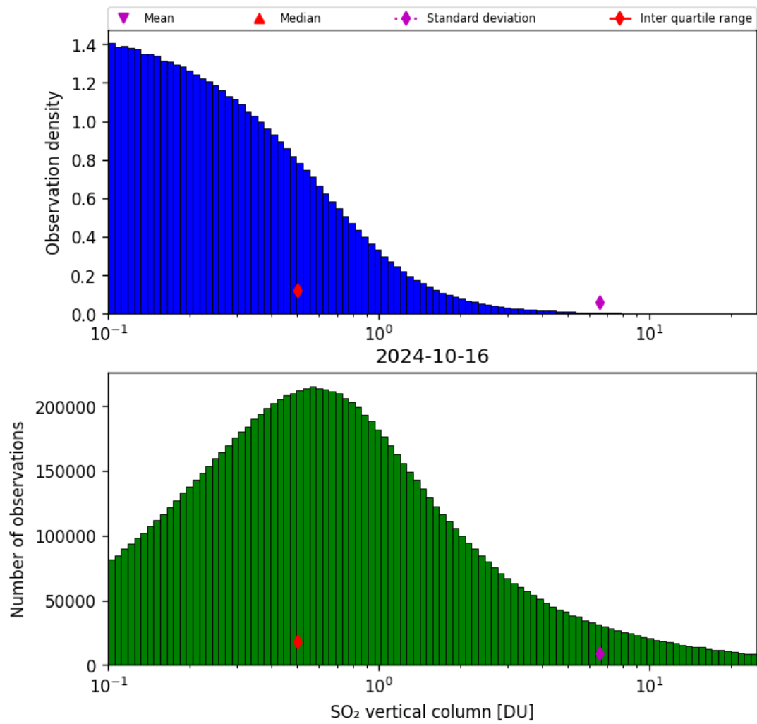
Figure 53: Histogram of “SO 2 vertical column” for 2024-10-15 to 2024-10-17
