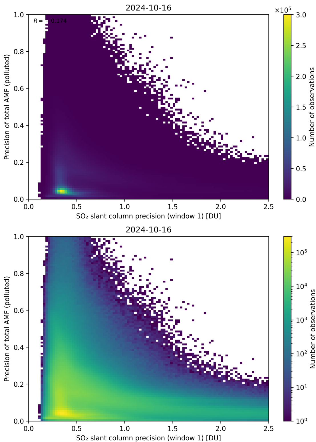
Figure 231: Scatter density plot of “SO 2 slant column precision (window 1)” against “Precision of total AMF (polluted)” for 2024-10-15 to 2024-10-17.
