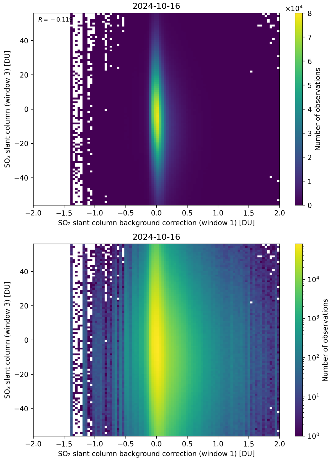
Figure 107: Scatter density plot of “SO 2 slant column background correction (window 1)” against “SO 2 slant column (window 3)” for 2024-10-15 to 2024-10-17.
