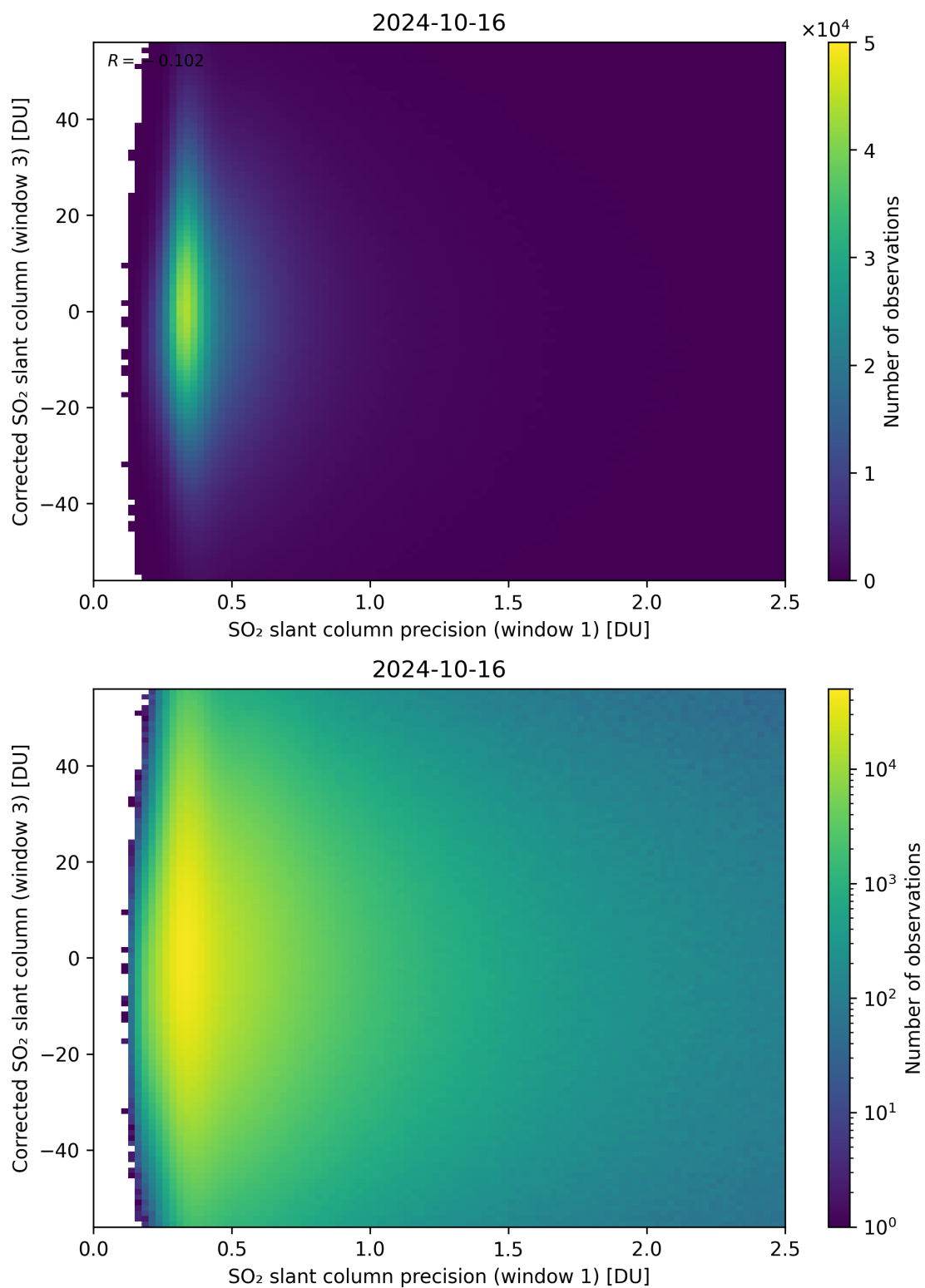
Figure 226: Scatter density plot of “SO 2 slant column precision (window 1)” against “Corrected SO 2 slant column (window 3)” for 2024-10-15 to 2024-10-17.
