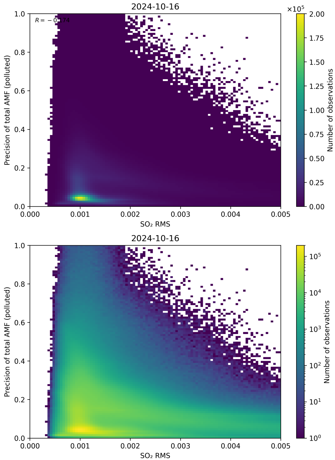
Figure 138: Scatter density plot of “SO 2 RMS” against “Precision of total AMF (polluted)” for 2024-10-15 to 2024-10-17.
