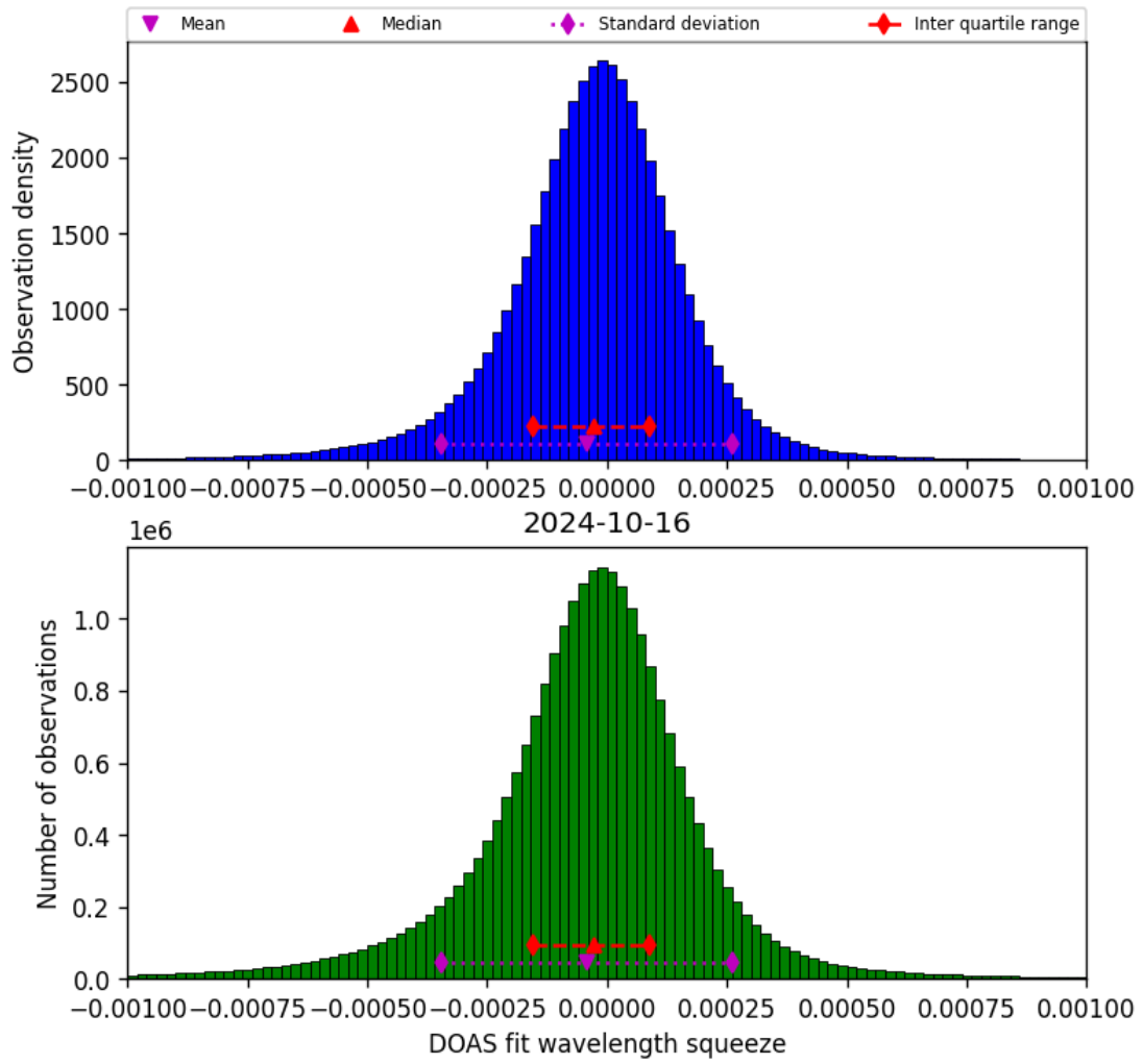
Figure 69: Histogram of “DOAS fit wavelength squeeze” for 2024-10-15 to 2024-10-17
