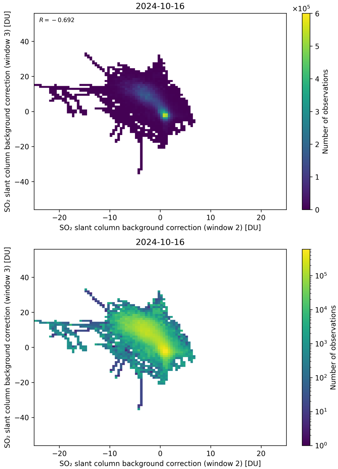
Figure 111: Scatter density plot of “SO 2 slant column background correction (window 2)” against “SO 2 slant column background correction (window 3)” for 2024-10-15 to 2024-10-17.
