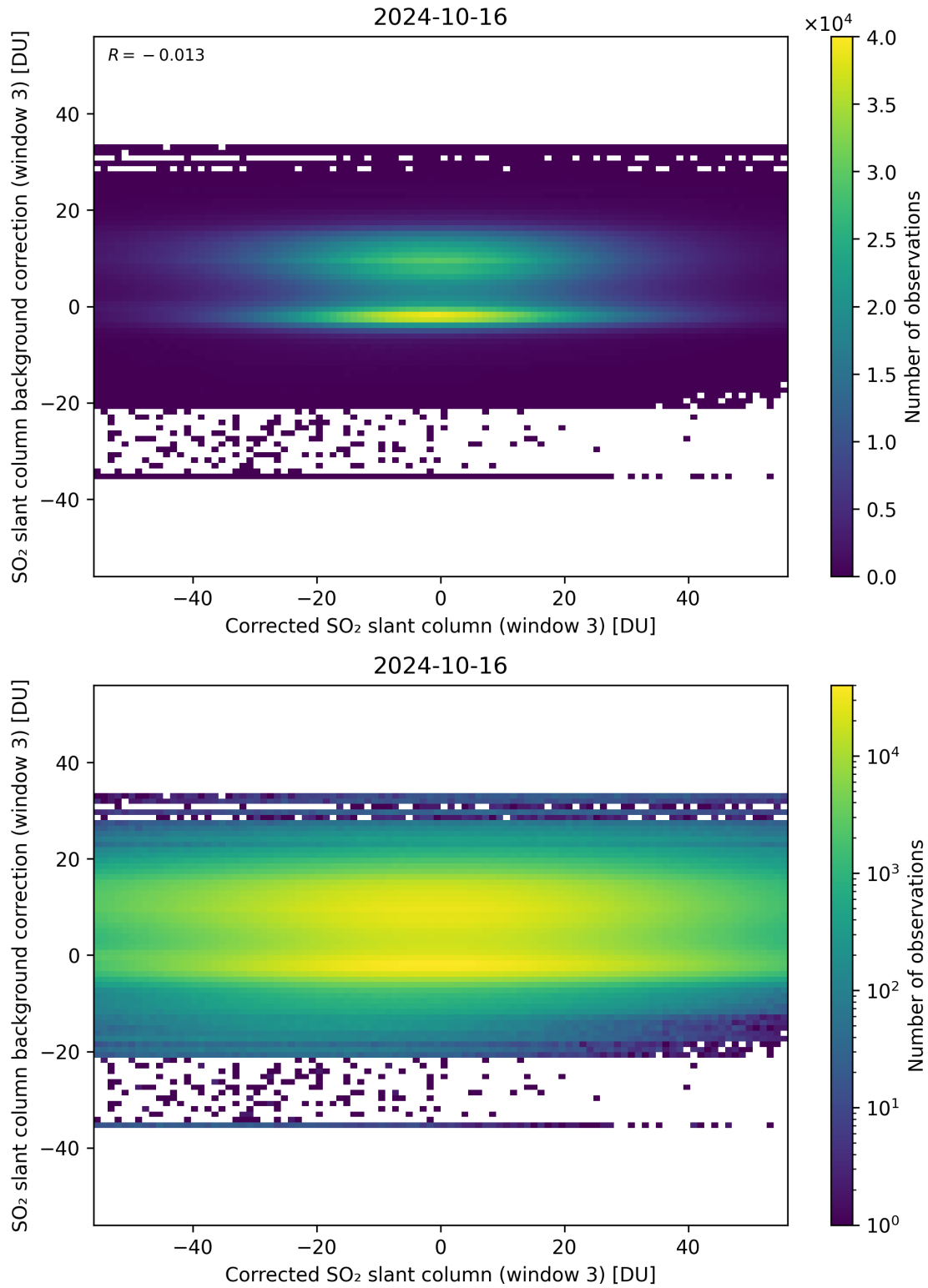
Figure 205: Scatter density plot of “Corrected SO 2 slant column (window 3)” against “SO 2 slant column background correction (window 3)” for 2024-10-15 to 2024-10-17.
