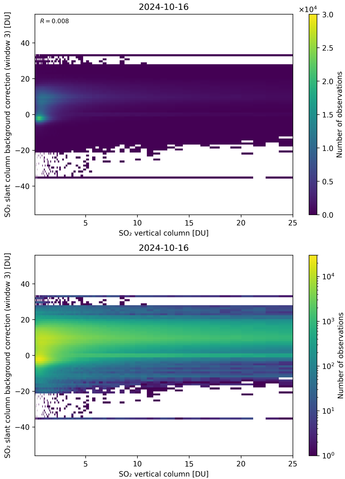
Figure 275: Scatter density plot of “SO 2 vertical column” against “SO 2 slant column background correction (window 3)” for 2024-10-15 to 2024-10-17.
