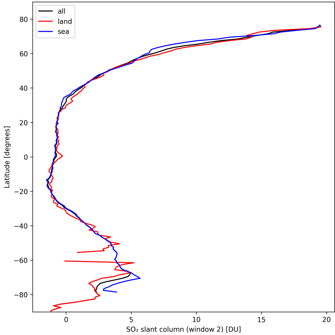
Figure 37: Zonal average of “SO 2 slant column (window 2)” for 2024-10-15 to 2024-10-17.
