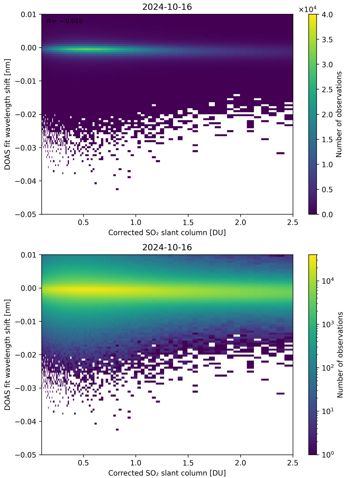
Figure 181: Scatter density plot of “Corrected SO 2 slant column” against “DOAS fit wavelength shift” for 2024-10-15 to 2024-10-17.
