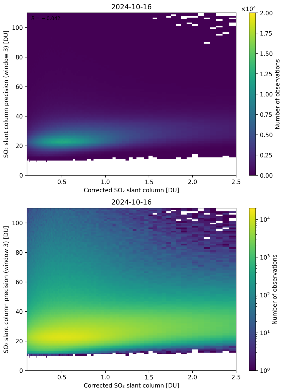
Figure 191: Scatter density plot of “Corrected SO 2 slant column” against “SO 2 slant column precision (window 3)” for 2024-10-15 to 2024-10-17.
