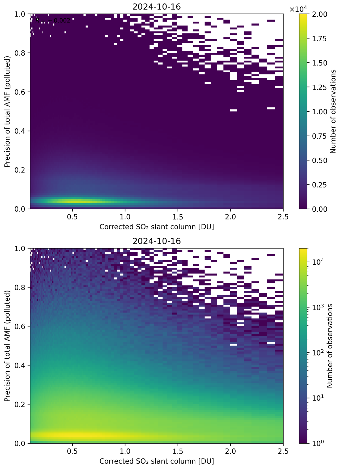
Figure 193: Scatter density plot of “Corrected SO 2 slant column” against “Precision of total AMF (polluted)” for 2024-10-15 to 2024-10-17.
