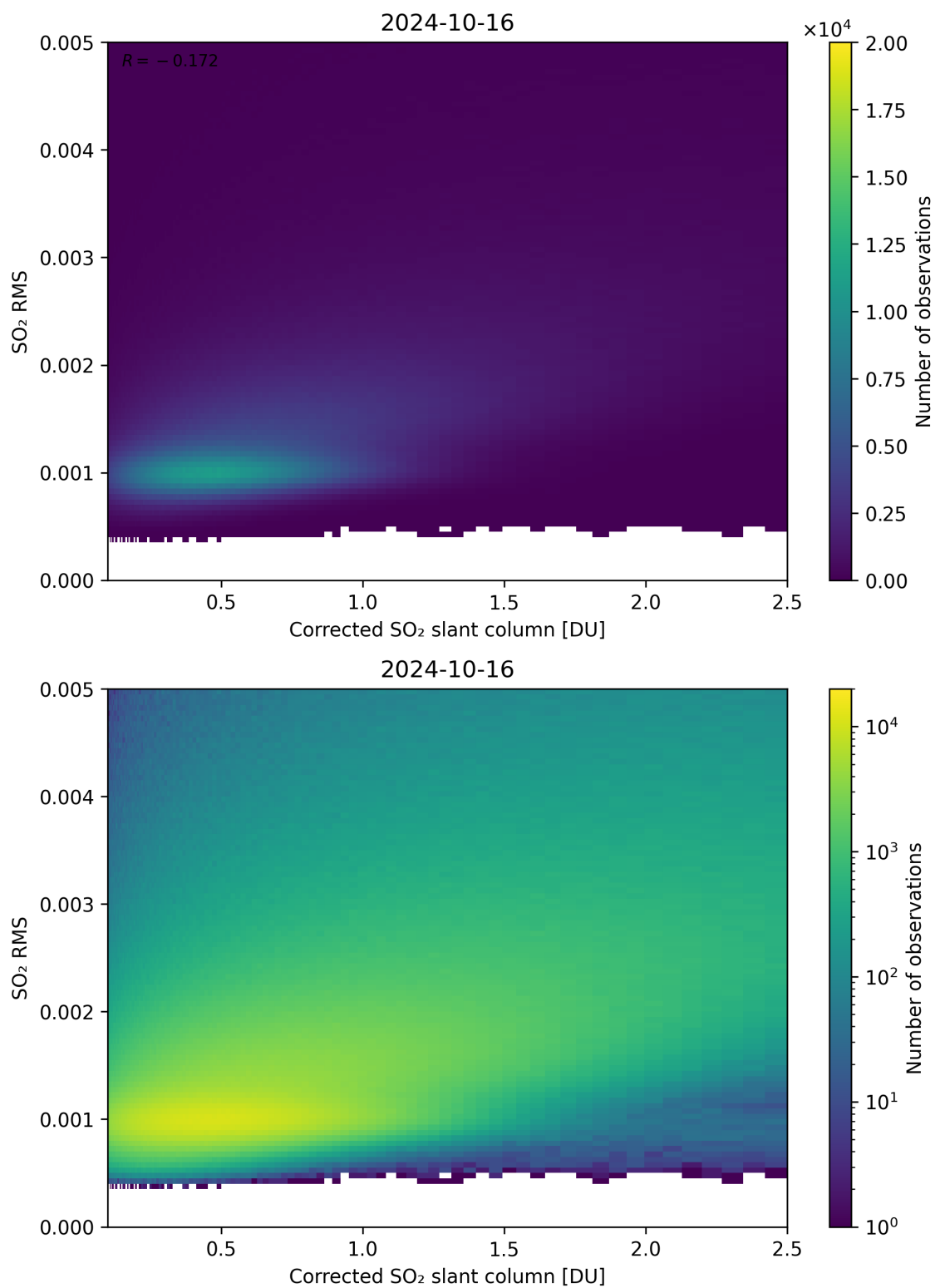
Figure 183: Scatter density plot of “Corrected SO 2 slant column” against “SO 2 RMS” for 2024-10-15 to 2024-10-17.
