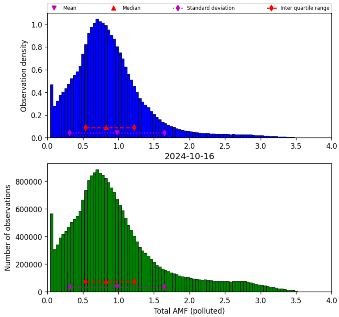
Figure 71: Histogram of “Total AMF (polluted)” for 2024-10-15 to 2024-10-17
