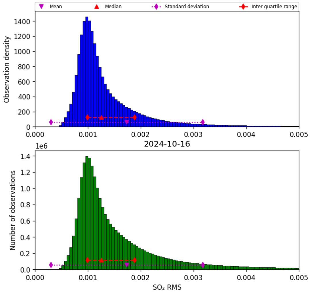
Figure 70: Histogram of “SO 2 RMS” for 2024-10-15 to 2024-10-17
