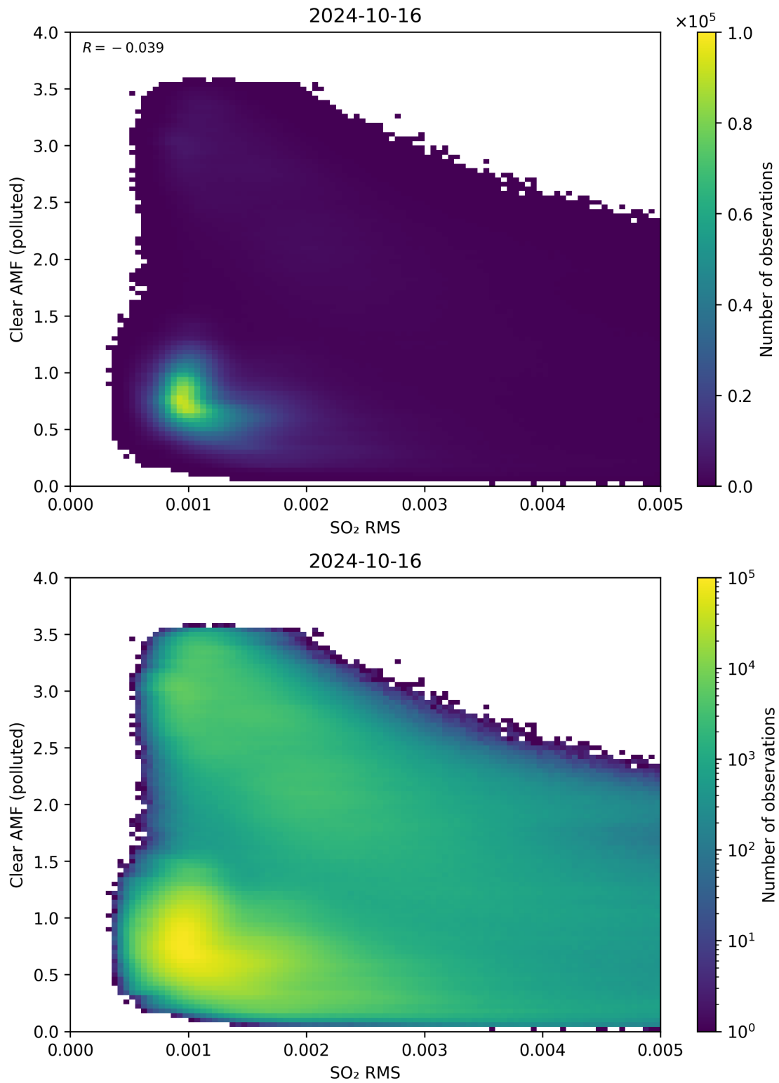
Figure 136: Scatter density plot of “SO 2 RMS” against “Clear AMF (polluted)” for 2024-10-15 to 2024-10-17.
