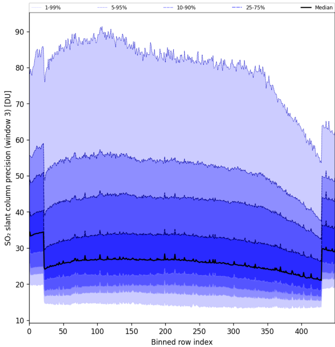
Figure 88: Along track statistics of “SO 2 slant column precision (window 3)” for 2024-10-15 to 2024-10-17
