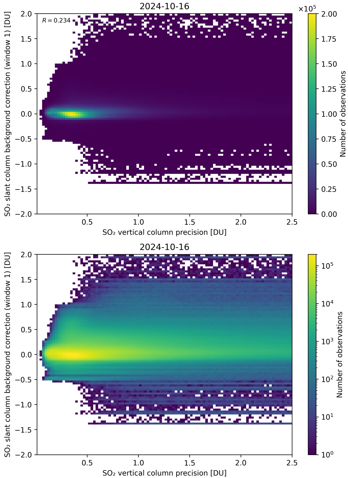
Figure 279: Scatter density plot of “SO 2 vertical column precision” against “SO 2 slant column background correction (window 1)” for 2024-10-15 to 2024-10-17.
