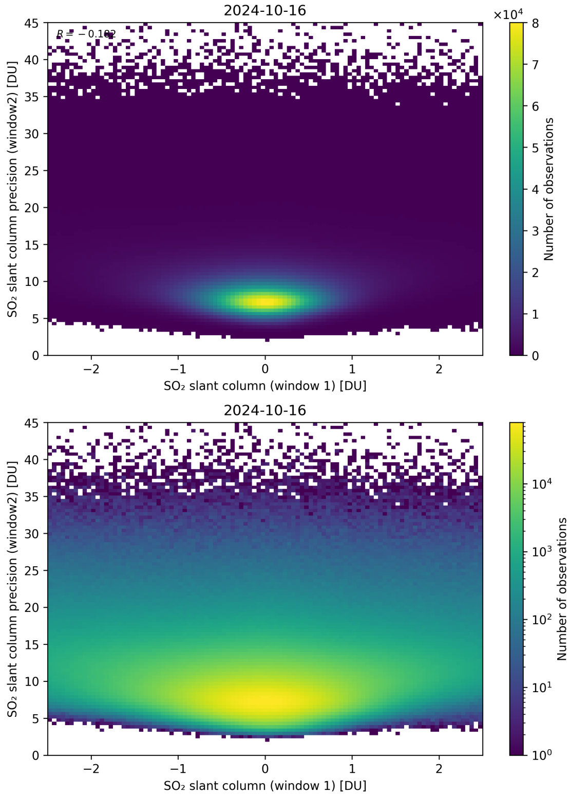
Figure 236: Scatter density plot of “SO 2 slant column (window 1)” against “SO 2 slant column precision (window2)” for 2024-10-15 to 2024-10-17.
