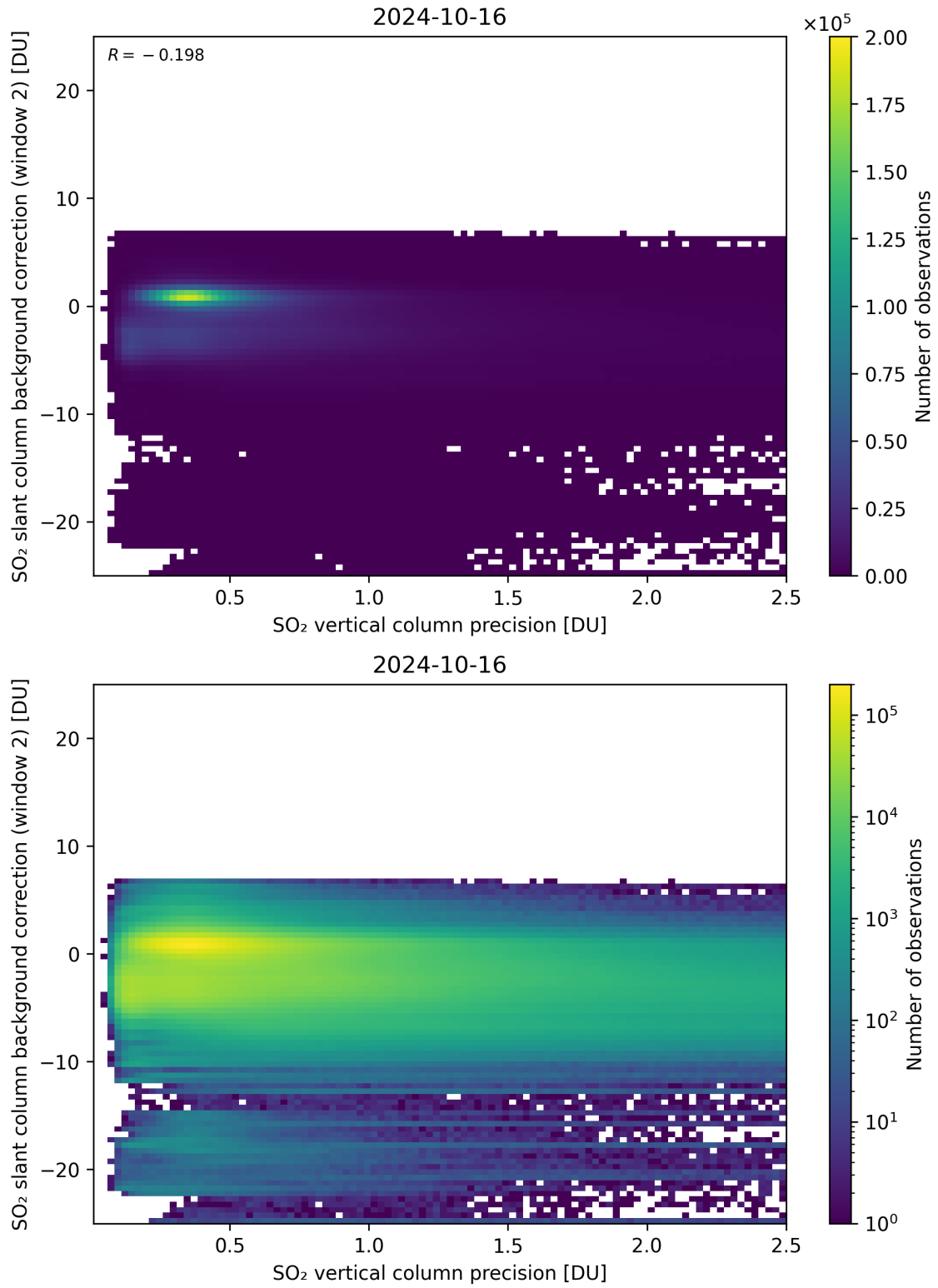
Figure 280: Scatter density plot of “SO 2 vertical column precision” against “SO 2 slant column background correction (window 2)” for 2024-10-15 to 2024-10-17.
