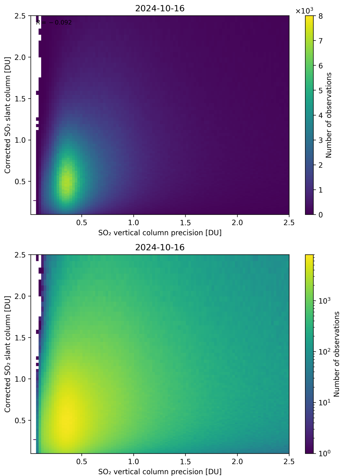
Figure 286: Scatter density plot of “SO 2 vertical column precision” against “Corrected SO 2 slant column” for 2024-10-15 to 2024-10-17.
