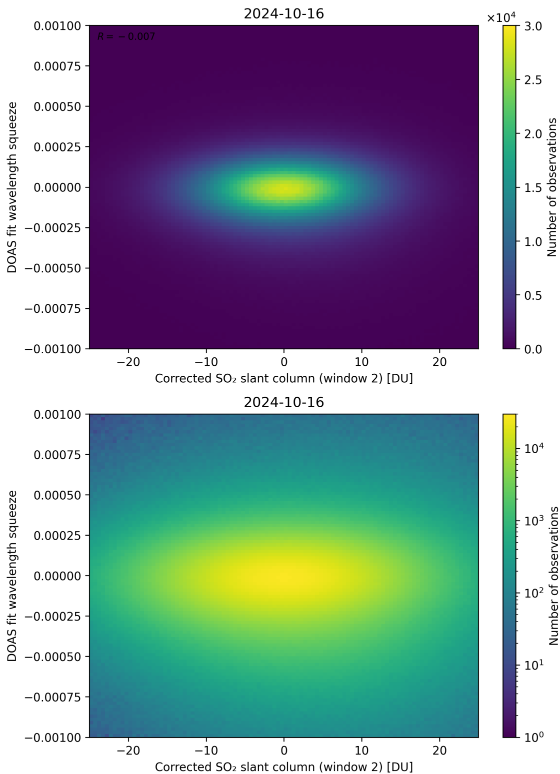
Figure 197: Scatter density plot of “Corrected SO 2 slant column (window 2)” against “DOAS fit wavelength squeeze” for 2024-10-15 to 2024-10-17.
