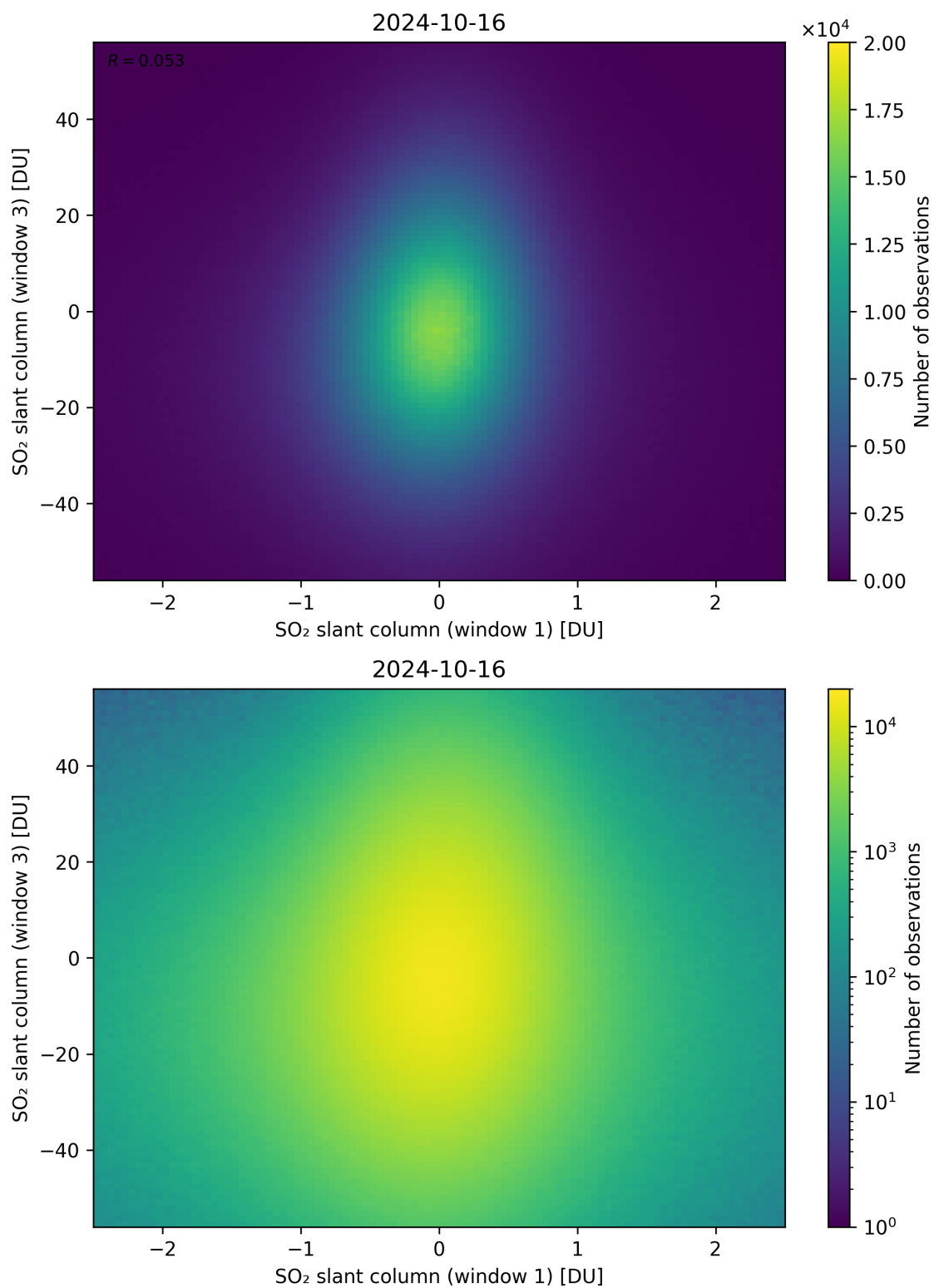
Figure 237: Scatter density plot of “SO 2 slant column (window 1)” against “SO 2 slant column (window 3)” for 2024-10-15 to 2024-10-17.
