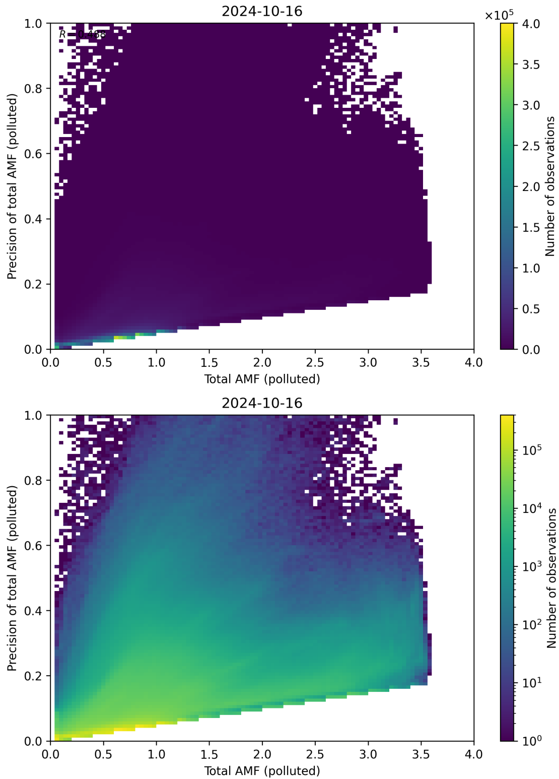
Figure 272: Scatter density plot of “Total AMF (polluted)” against “Precision of total AMF (polluted)” for 2024-10-15 to 2024-10-17.
