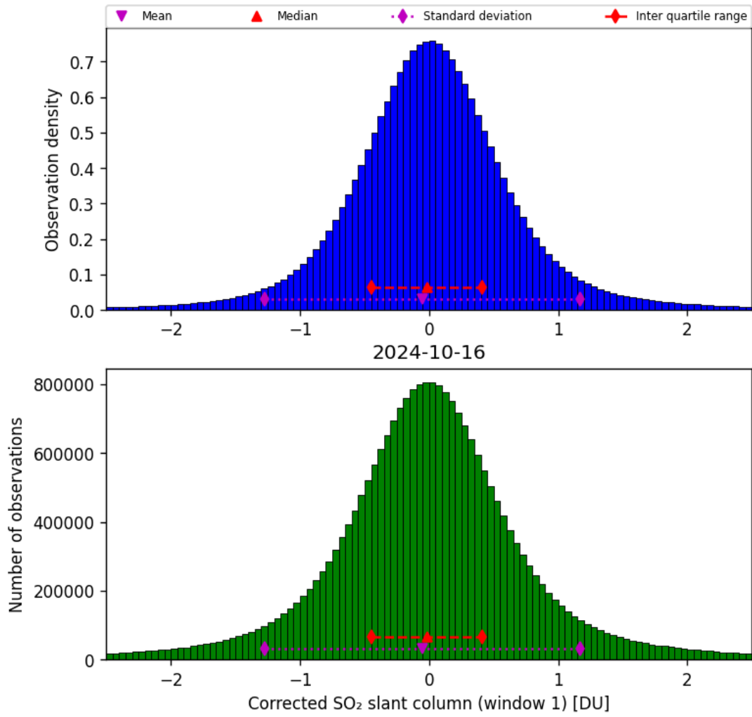
Figure 58: Histogram of “Corrected SO 2 slant column (window 1)” for 2024-10-15 to 2024-10-17
