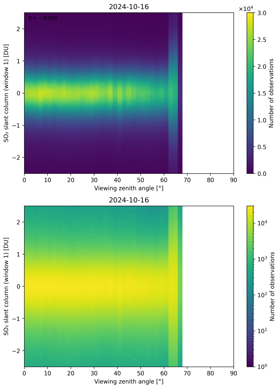
Figure 320: Scatter density plot of “Viewing zenith angle” against “SO 2 slant column (window 1)” for 2024-10-15 to 2024-10-17.
