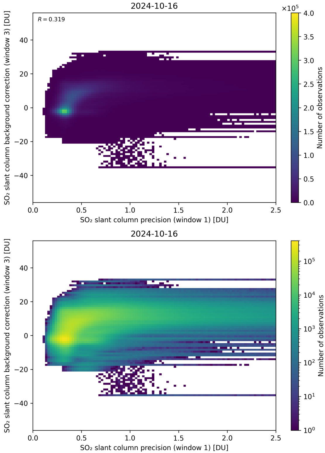
Figure 220: Scatter density plot of “SO 2 slant column precision (window 1)” against “SO 2 slant column background correction (window 3)” for 2024-10-15 to 2024-10-17.
