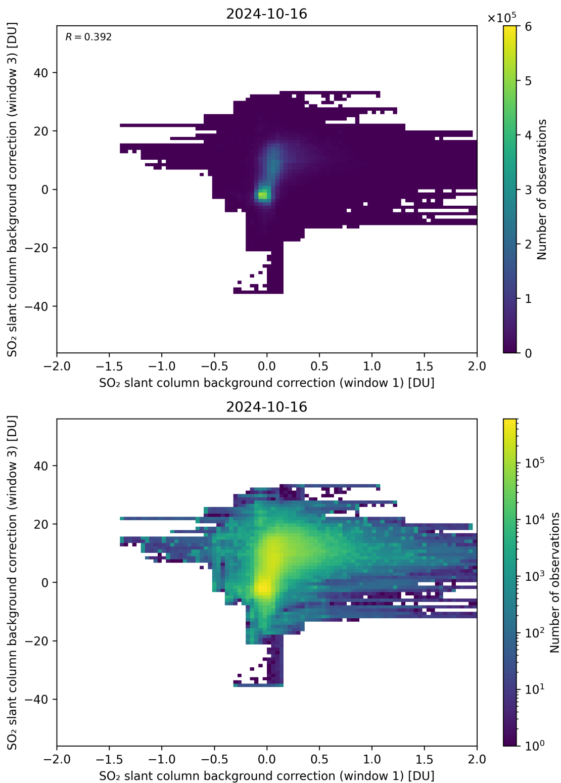
Figure 99: Scatter density plot of “SO 2 slant column background correction (window 1)” against “SO 2 slant column background correction (window 3)” for 2024-10-15 to 2024-10-17.
