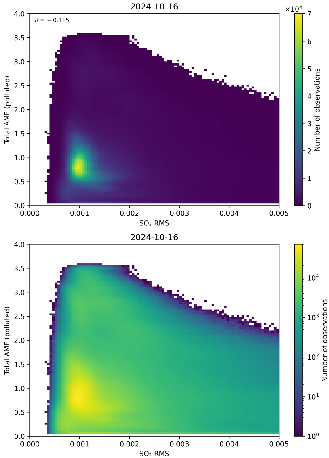
Figure 137: Scatter density plot of “SO 2 RMS” against “Total AMF (polluted)” for 2024-10-15 to 2024-10-17.
