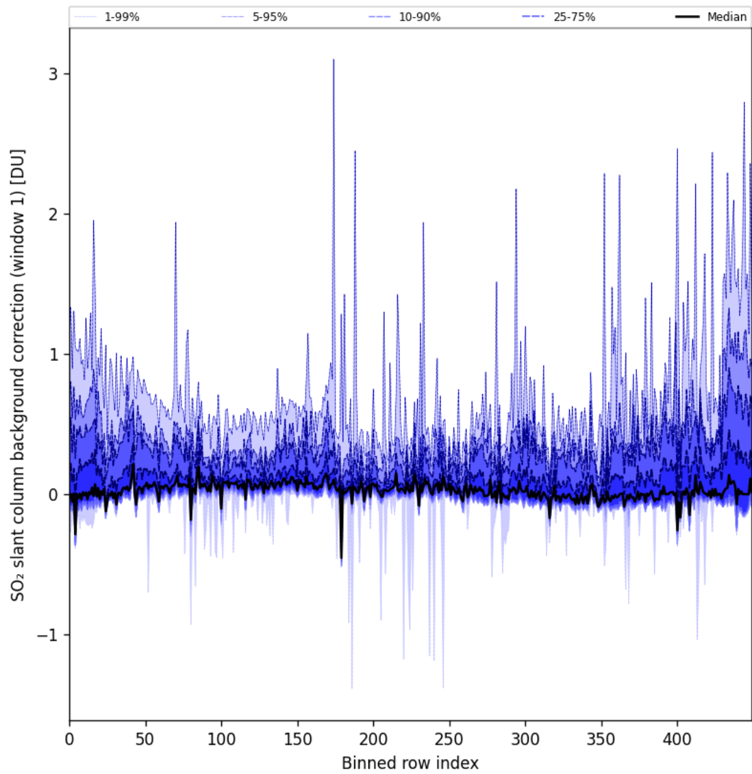
Figure 82: Along track statistics of “SO 2 slant column background correction (window 1)” for 2024-10-15 to 2024-10-17
