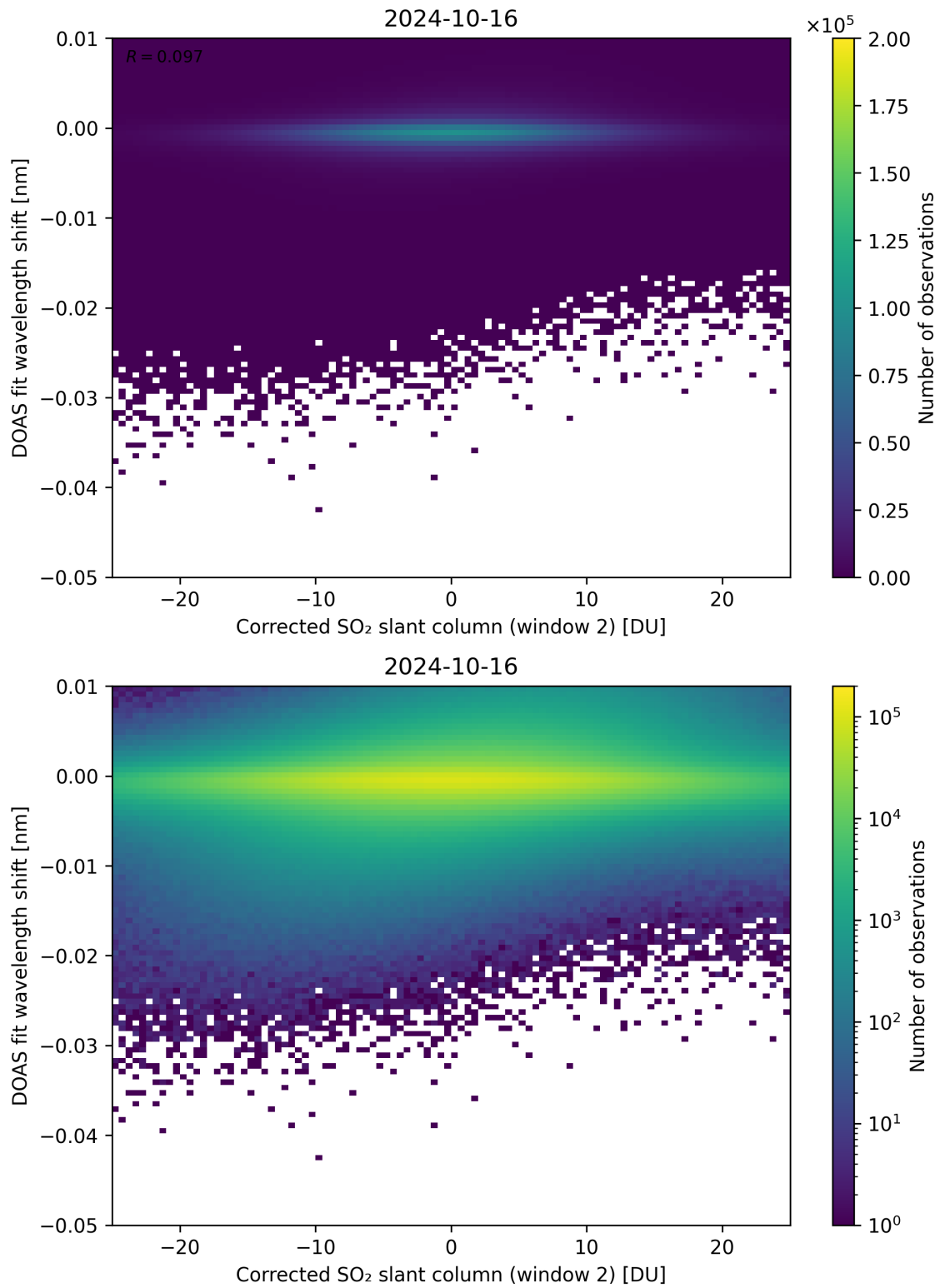
Figure 196: Scatter density plot of “Corrected SO 2 slant column (window 2)” against “DOAS fit wavelength shift” for 2024-10-15 to 2024-10-17.
