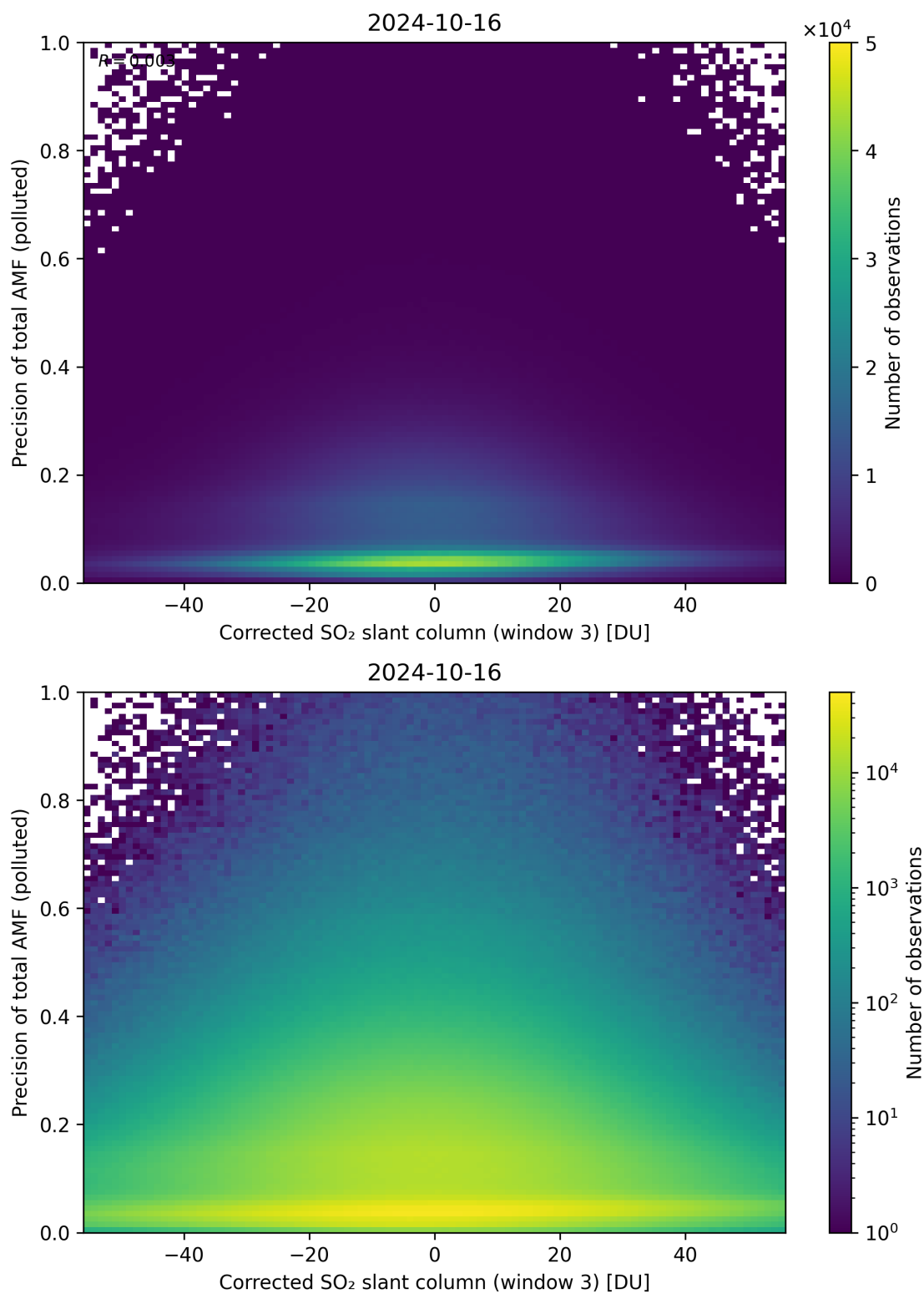
Figure 211: Scatter density plot of “Corrected SO 2 slant column (window 3)” against “Precision of total AMF (polluted)” for 2024-10-15 to 2024-10-17.
