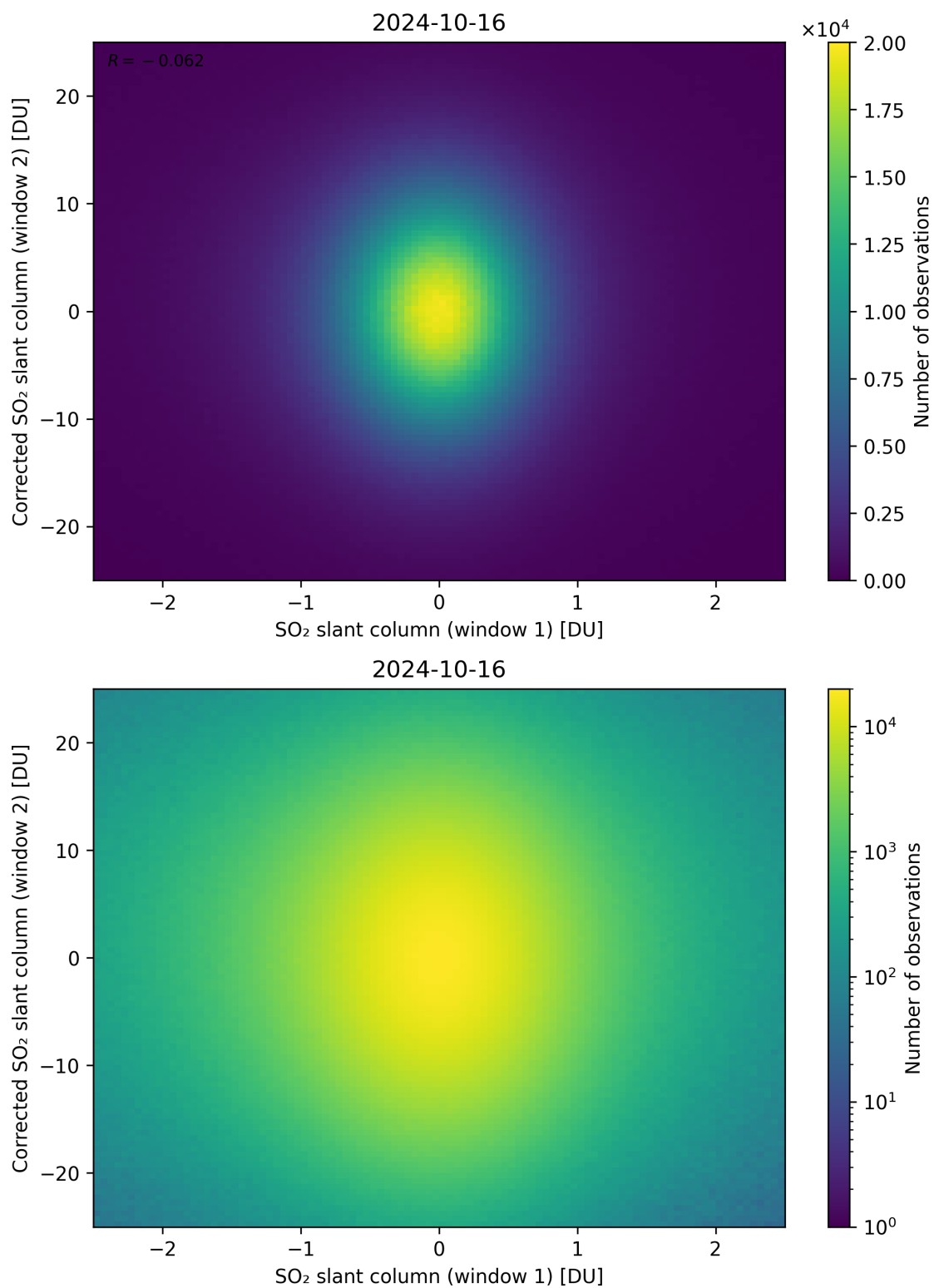
Figure 233: Scatter density plot of “SO 2 slant column (window 1)” against “Corrected SO 2 slant column (window 2)” for 2024-10-15 to 2024-10-17.
