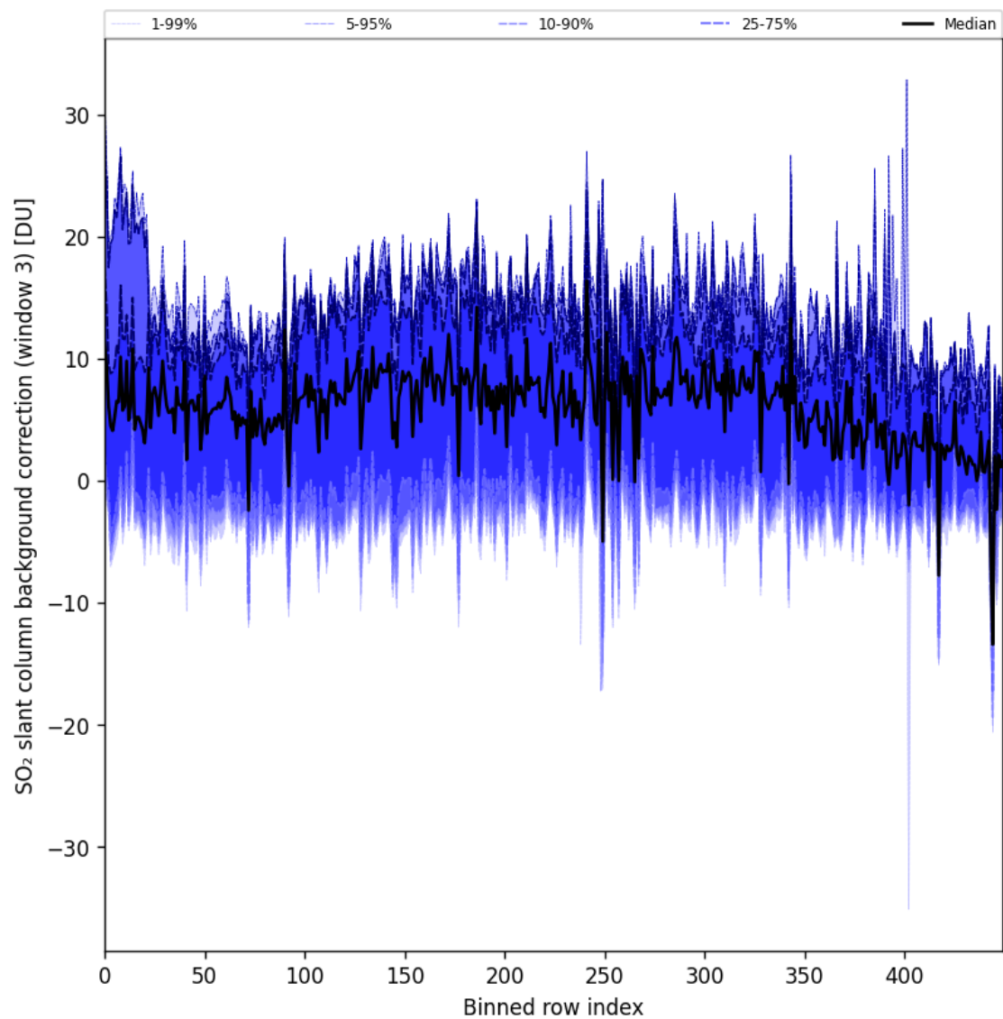
Figure 90: Along track statistics of “SO 2 slant column background correction (window 3)” for 2024-10-15 to 2024-10-17
