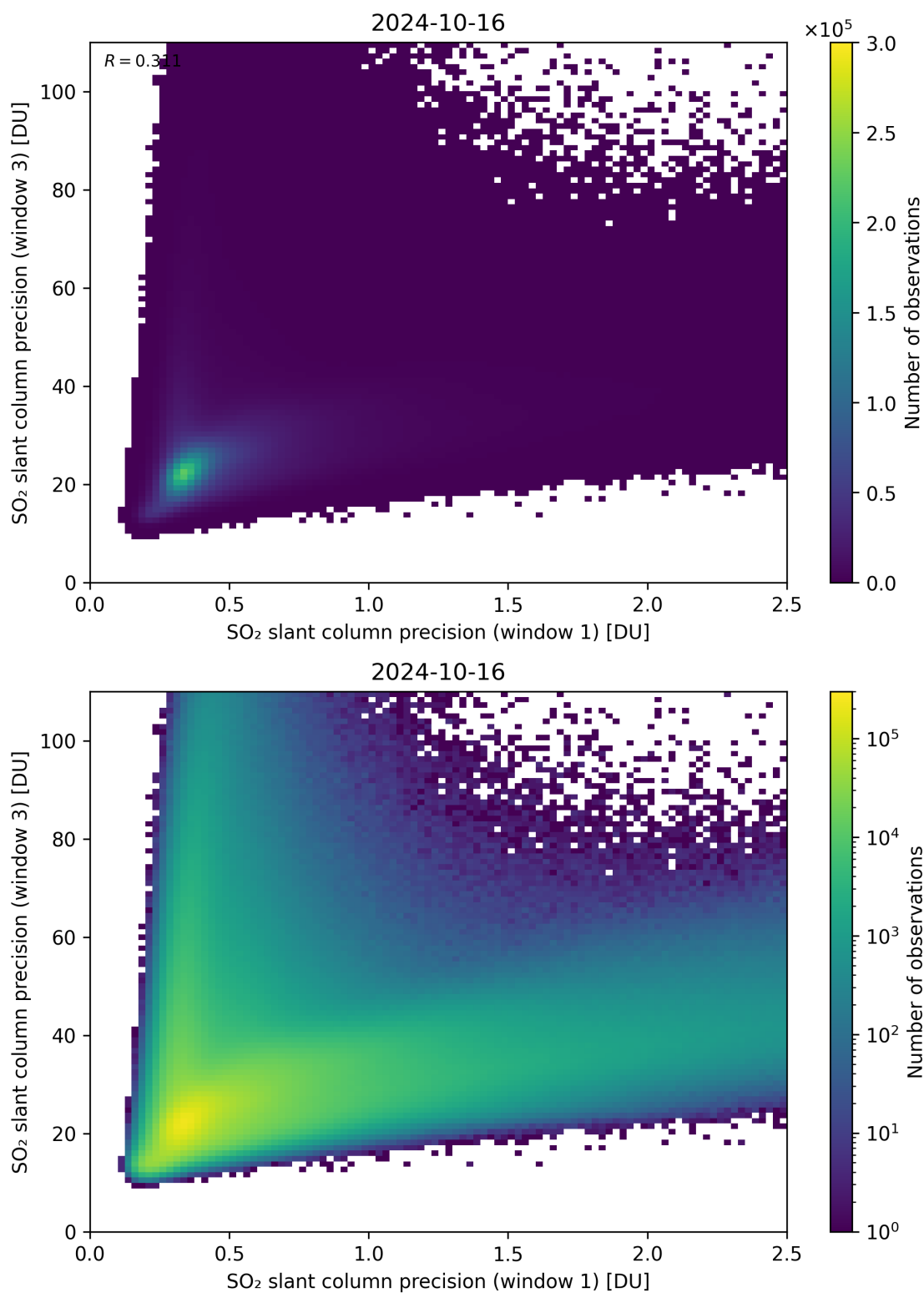
Figure 229: Scatter density plot of “SO 2 slant column precision (window 1)” against “SO 2 slant column precision (window 3)” for 2024-10-15 to 2024-10-17.
