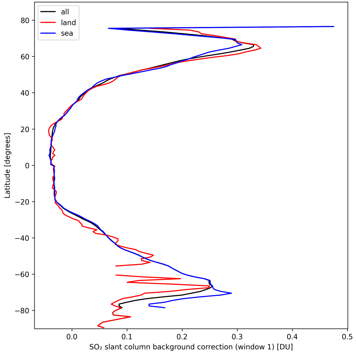
Figure 36: Zonal average of “SO 2 slant column background correction (window 1)” for 2024-10-15 to 2024-10-17.
