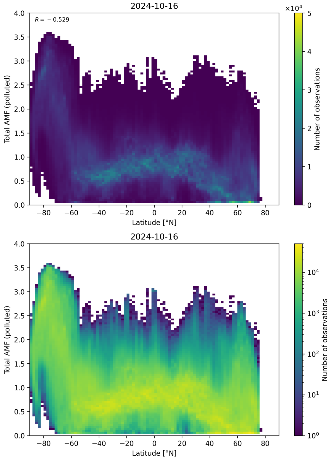
Figure 154: Scatter density plot of “Latitude” against “Total AMF (polluted)” for 2024-10-15 to 2024-10-17.
