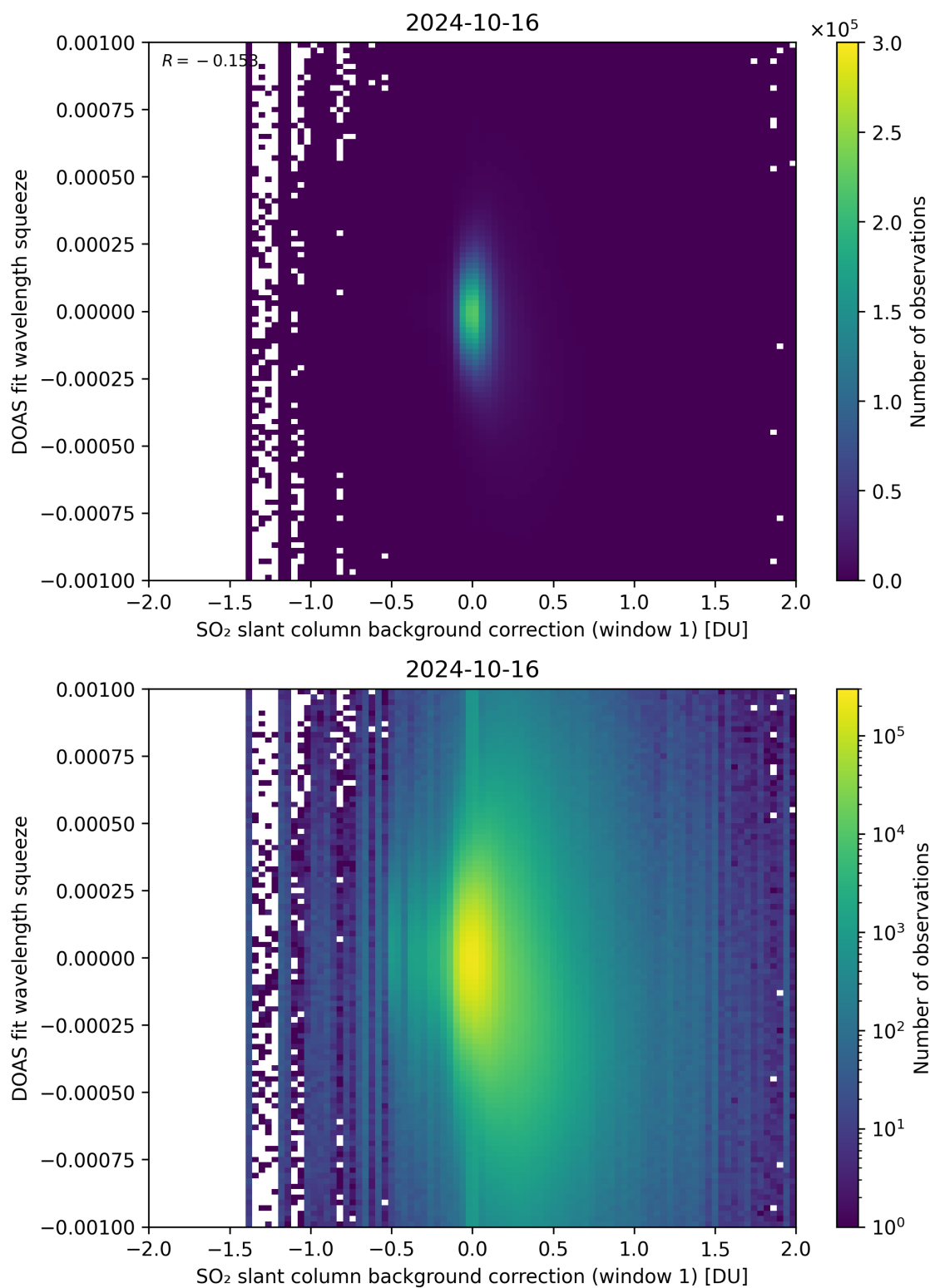
Figure 101: Scatter density plot of “SO 2 slant column background correction (window 1)” against “DOAS fit wavelength squeeze” for 2024-10-15 to 2024-10-17.
