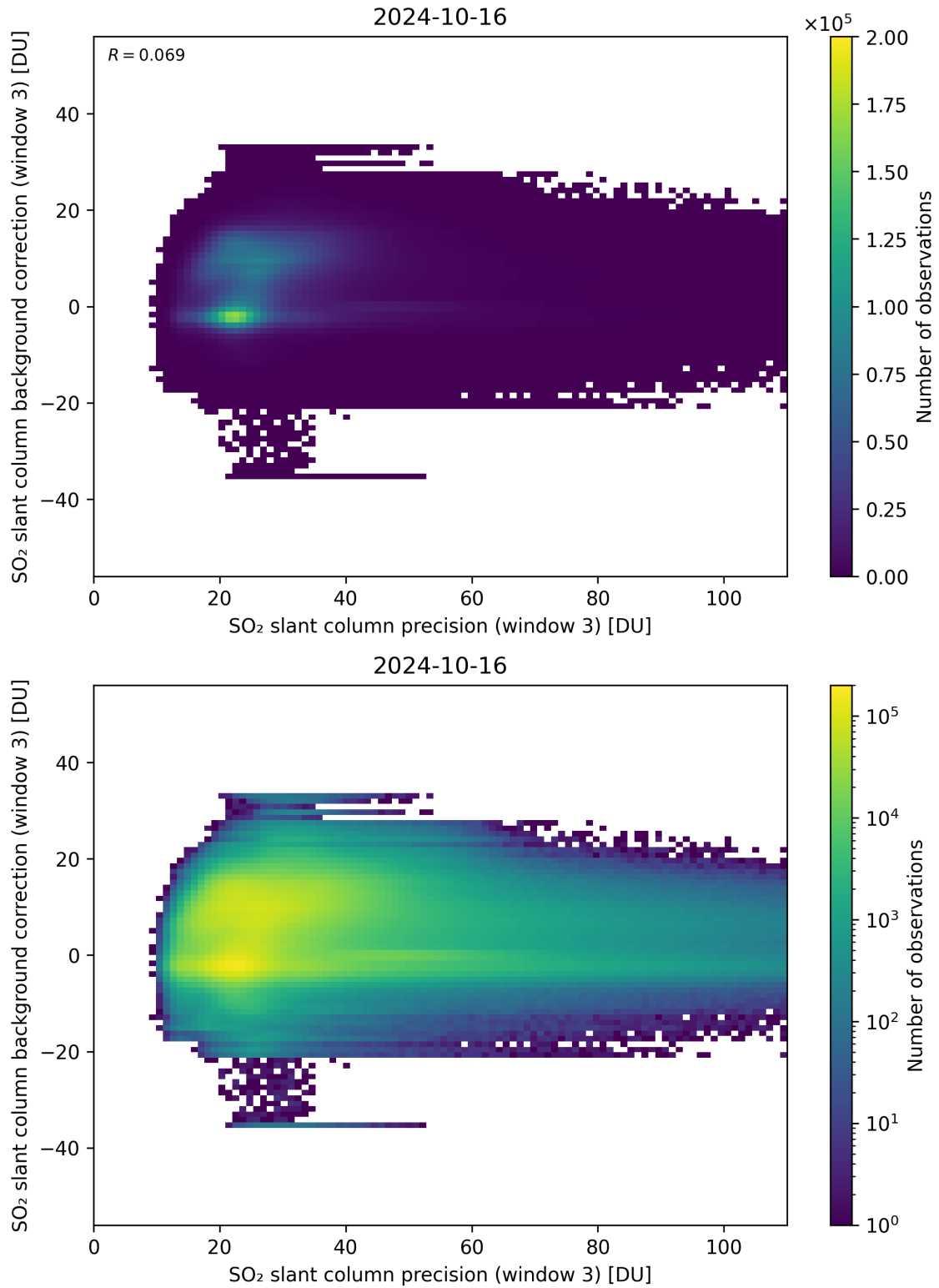
Figure 257: Scatter density plot of “SO 2 slant column precision (window 3)” against “SO 2 slant column background correction (window 3)” for 2024-10-15 to 2024-10-17.
