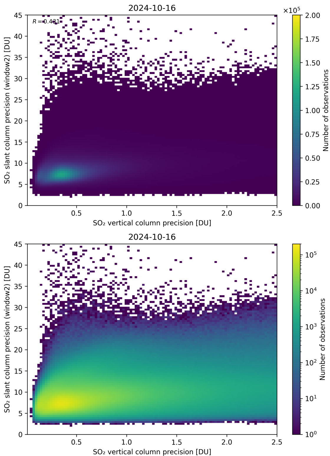
Figure 291: Scatter density plot of “SO 2 vertical column precision” against “SO 2 slant column precision (window2)” for 2024-10-15 to 2024-10-17.
