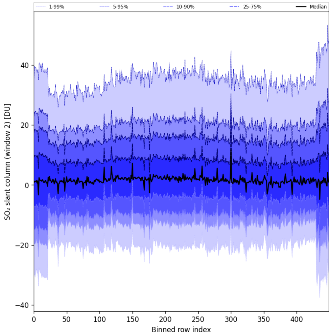
Figure 83: Along track statistics of “SO 2 slant column (window 2)” for 2024-10-15 to 2024-10-17
