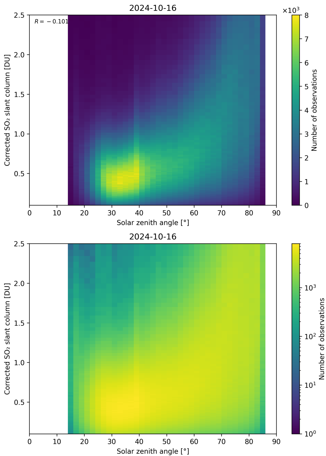
Figure 166: Scatter density plot of “Solar zenith angle” against “Corrected SO 2 slant column” for 2024-10-15 to 2024-10-17.
