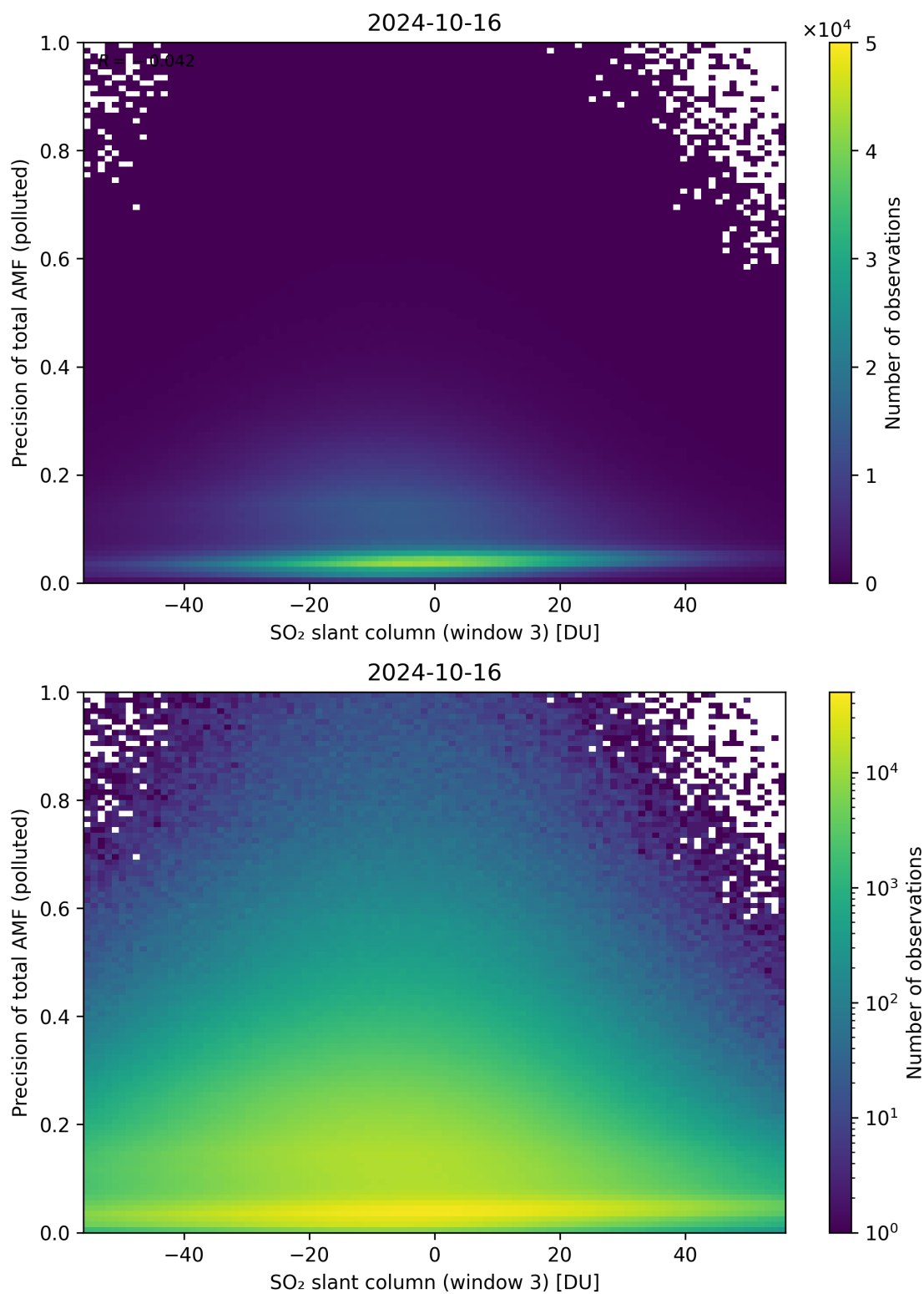
Figure 269: Scatter density plot of “SO 2 slant column (window 3)” against “Precision of total AMF (polluted)” for 2024-10-15 to 2024-10-17.
