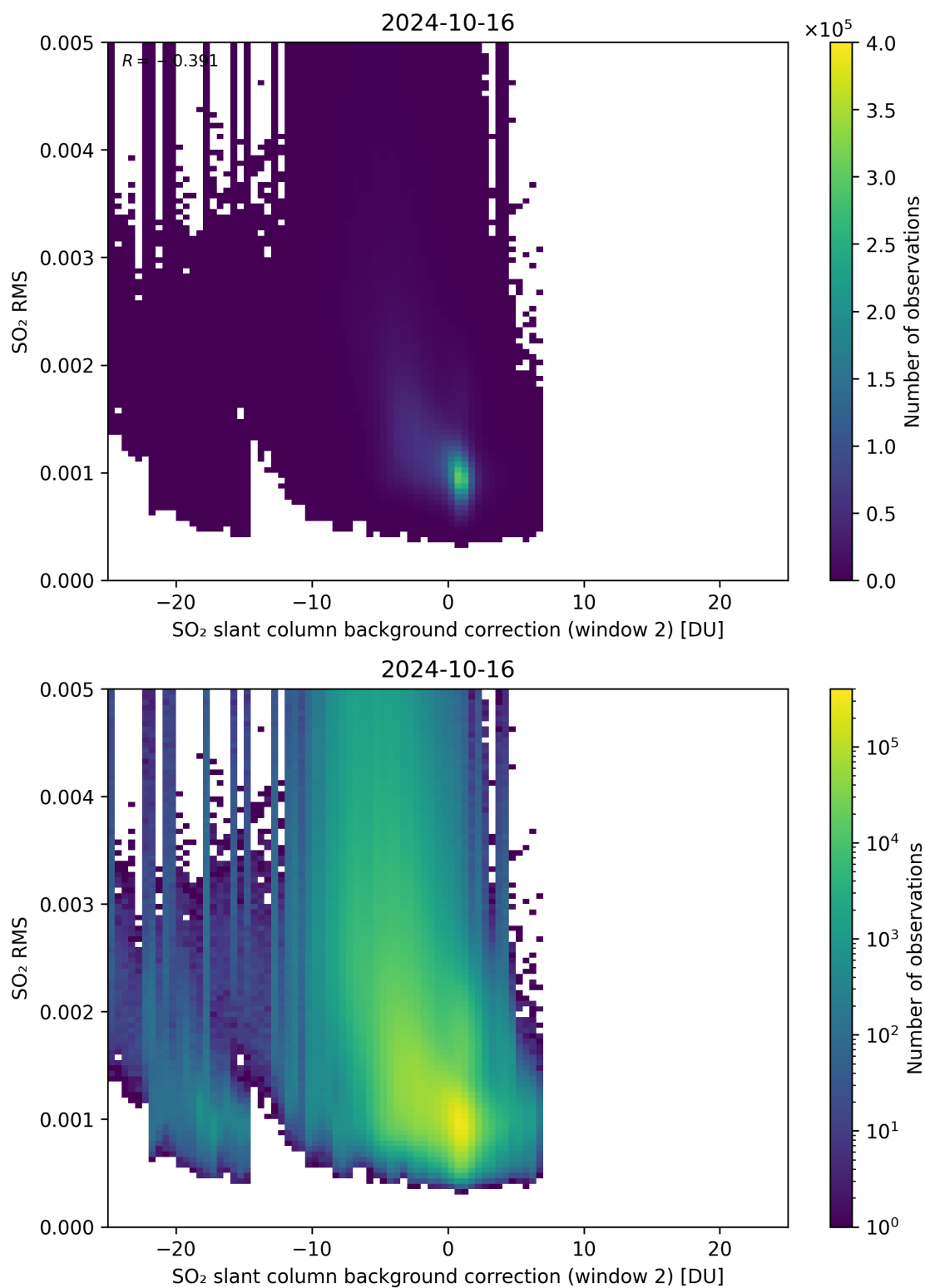
Figure 114: Scatter density plot of “SO 2 slant column background correction (window 2)” against “SO 2 RMS” for 2024-10-15 to 2024-10-17.
