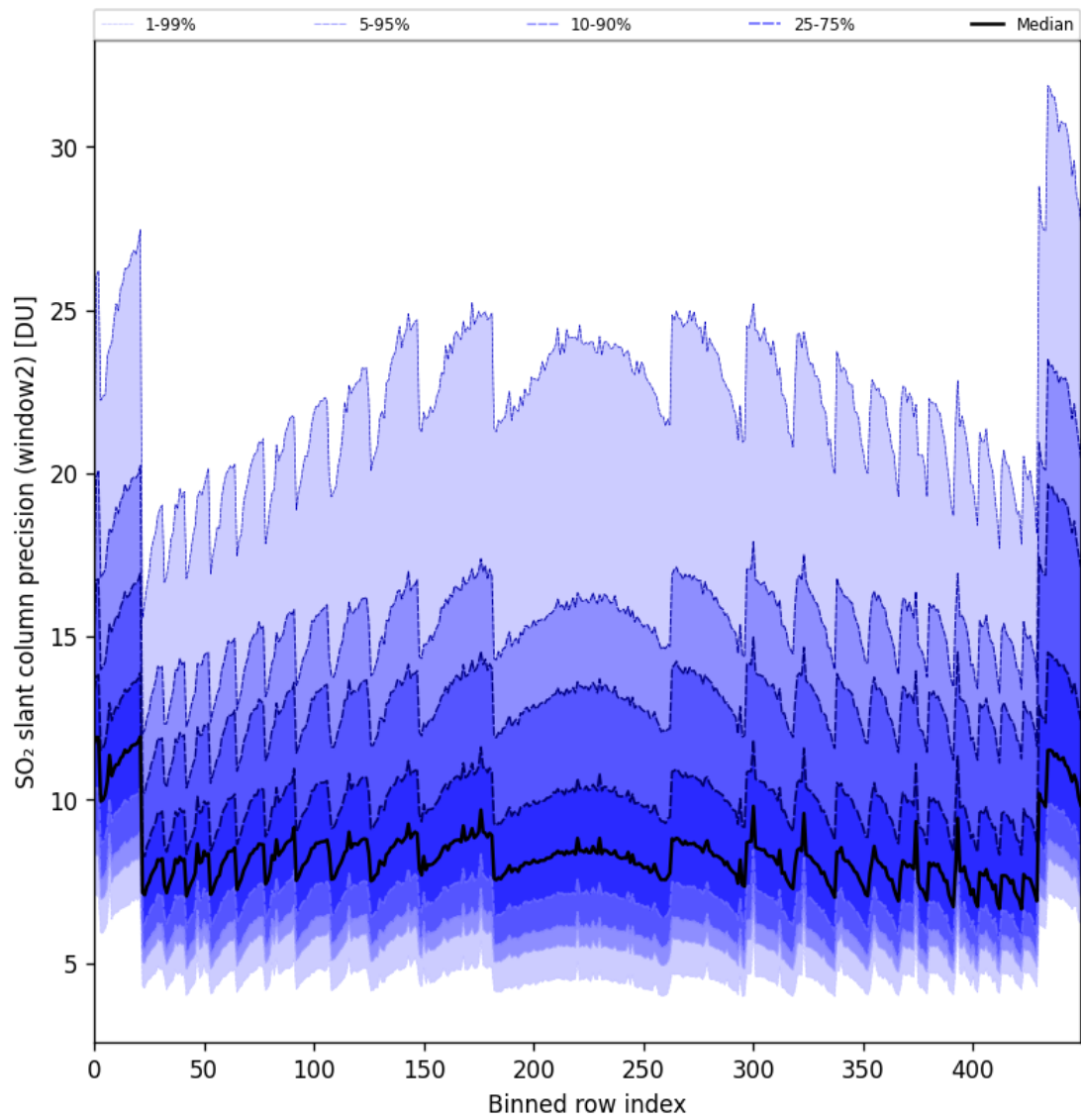
Figure 84: Along track statistics of “SO 2 slant column precision (window2)” for 2024-10-15 to 2024-10-17
