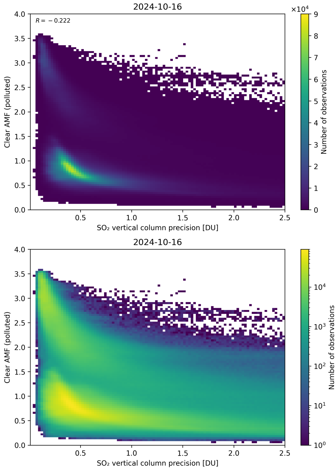
Figure 285: Scatter density plot of “SO 2 vertical column precision” against “Clear AMF (polluted)” for 2024-10-15 to 2024-10-17.
