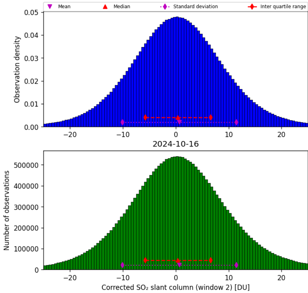
Figure 62: Histogram of “Corrected SO 2 slant column (window 2)” for 2024-10-15 to 2024-10-17
