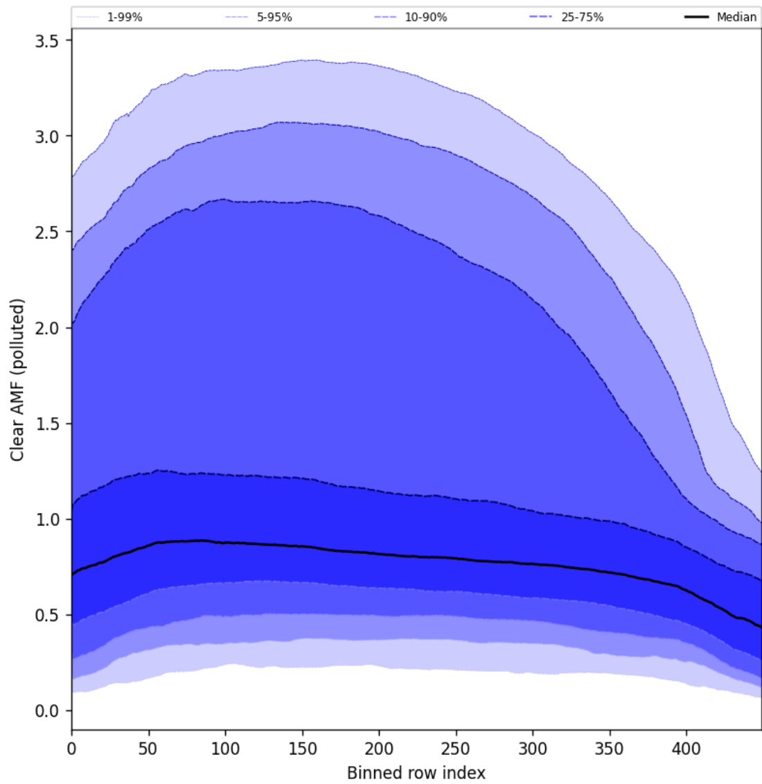
Figure 96: Along track statistics of “Clear AMF (polluted)” for 2024-10-15 to 2024-10-17
