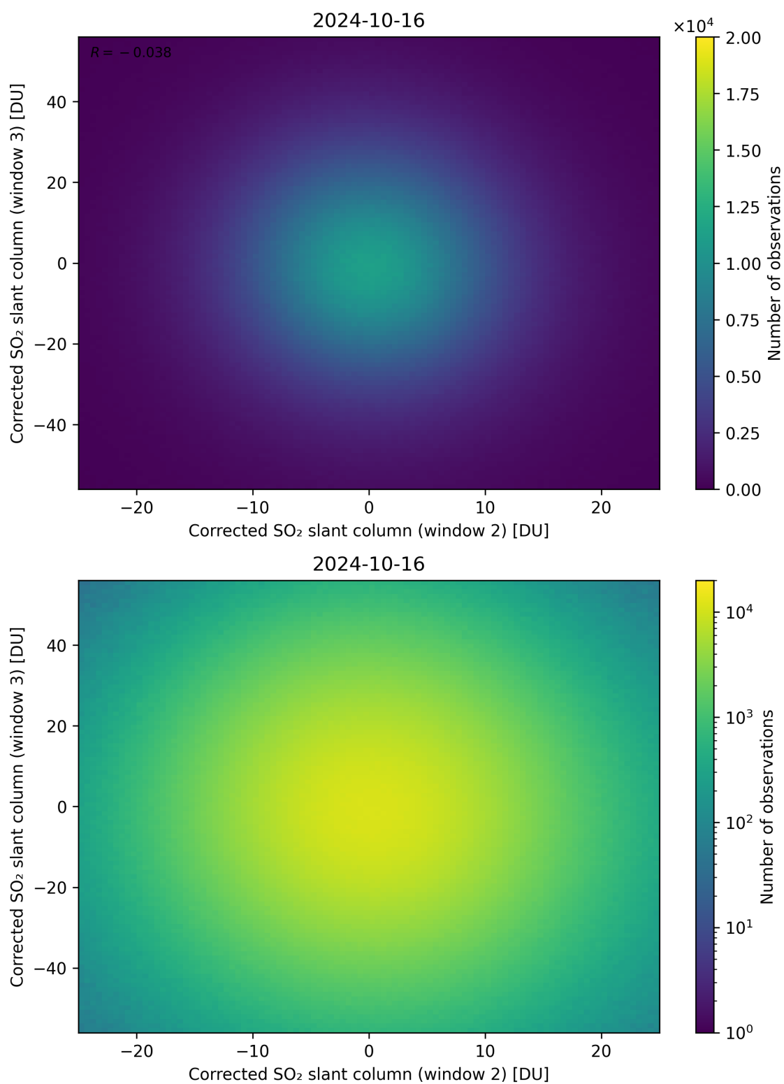
Figure 200: Scatter density plot of “Corrected SO 2 slant column (window 2)” against “Corrected SO 2 slant column (window 3)” for 2024-10-15 to 2024-10-17.
