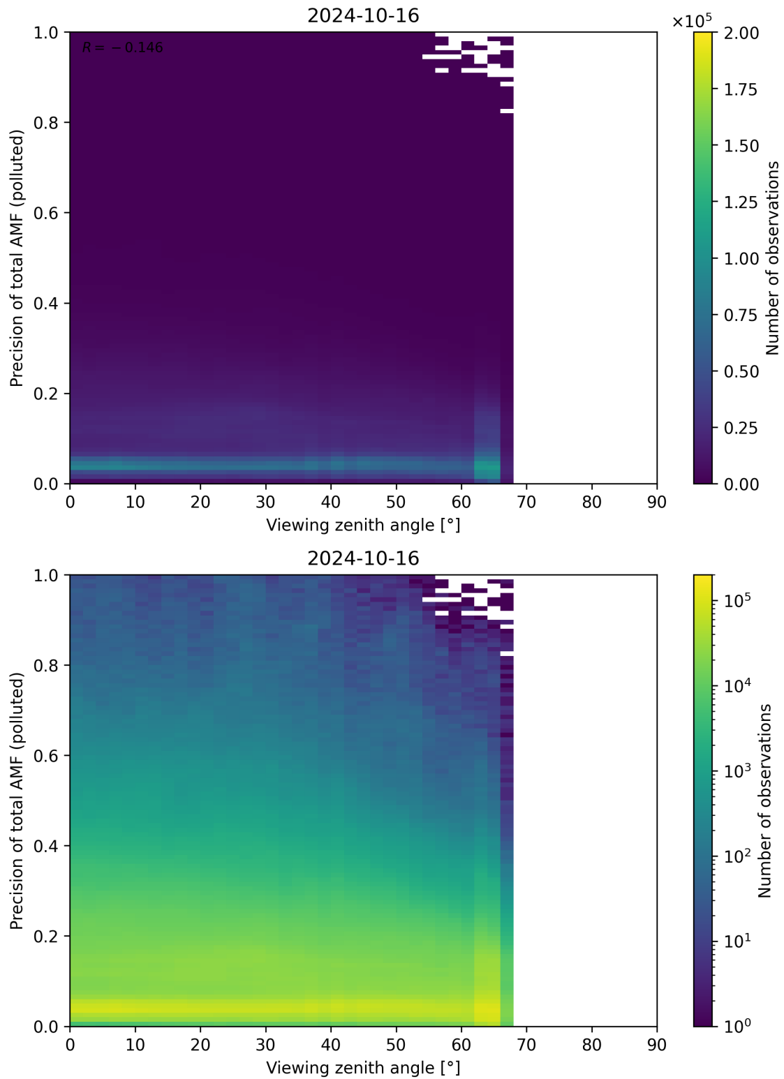
Figure 326: Scatter density plot of “Viewing zenith angle” against “Precision of total AMF (polluted)” for 2024-10-15 to 2024-10-17.
