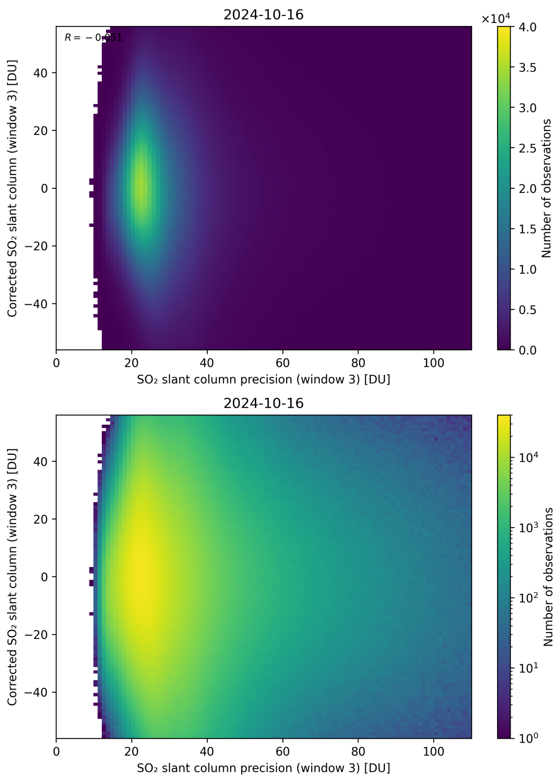
Figure 262: Scatter density plot of “SO 2 slant column precision (window 3)” against “Corrected SO 2 slant column (window 3)” for 2024-10-15 to 2024-10-17.
