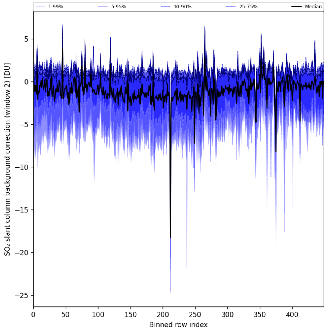
Figure 86: Along track statistics of “SO 2 slant column background correction (window 2)” for 2024-10-15 to 2024-10-17
