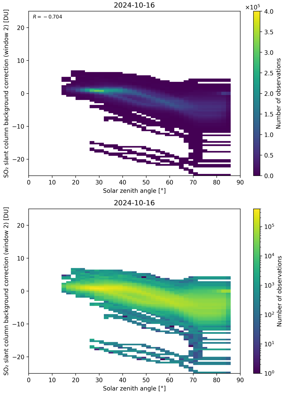
Figure 159: Scatter density plot of “Solar zenith angle” against “SO 2 slant column background correction (window 2)” for 2024-10-15 to 2024-10-17.
