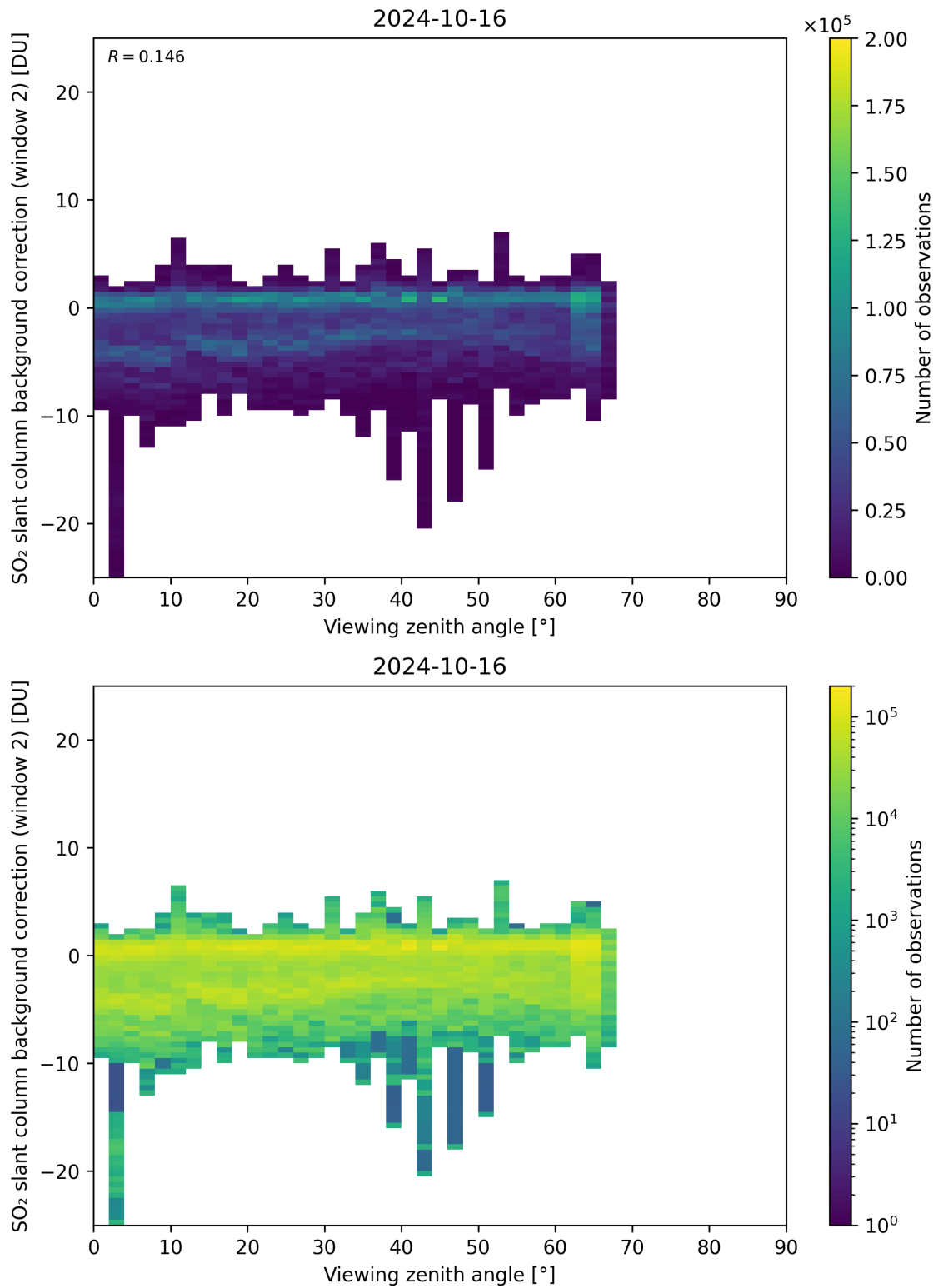
Figure 309: Scatter density plot of “Viewing zenith angle” against “SO 2 slant column background correction (window 2)” for 2024-10-15 to 2024-10-17.
