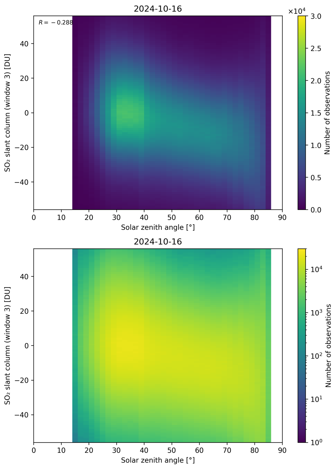
Figure 172: Scatter density plot of “Solar zenith angle” against “SO 2 slant column (window 3)” for 2024-10-15 to 2024-10-17.
