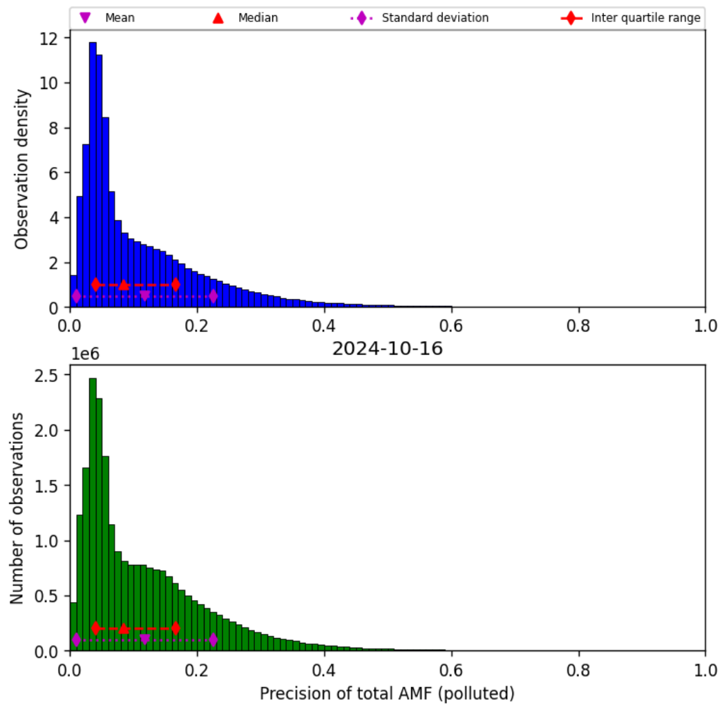
Figure 72: Histogram of “Precision of total AMF (polluted)” for 2024-10-15 to 2024-10-17
