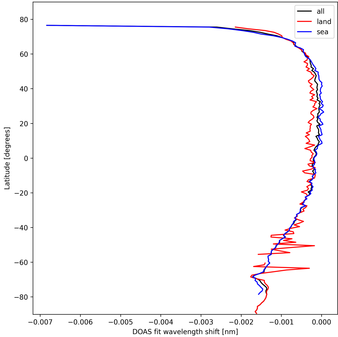
Figure 45: Zonal average of “DOAS fit wavelength shift” for 2024-10-15 to 2024-10-17.
