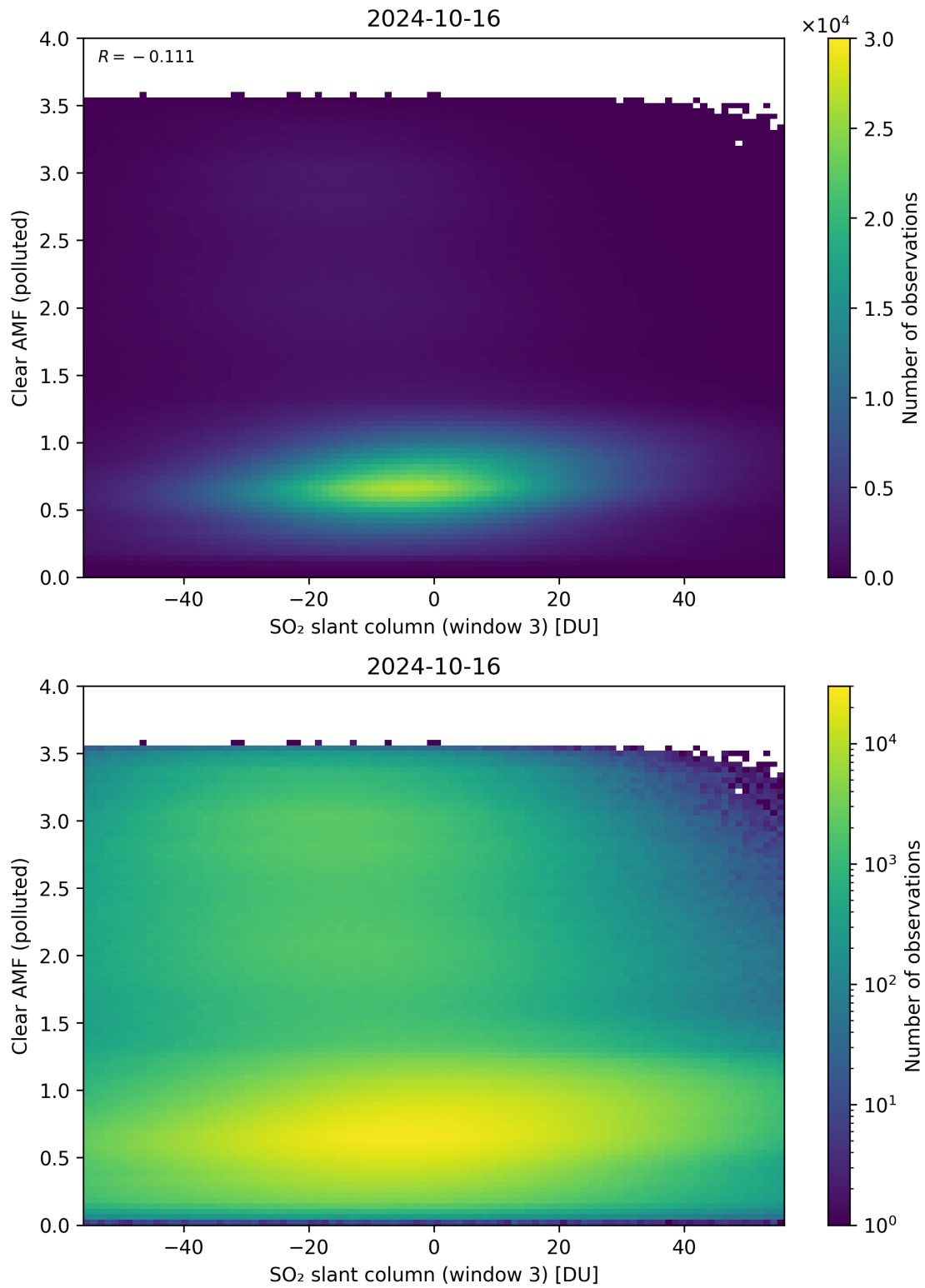
Figure 265: Scatter density plot of “SO 2 slant column (window 3)” against “Clear AMF (polluted)” for 2024-10-15 to 2024-10-17.
