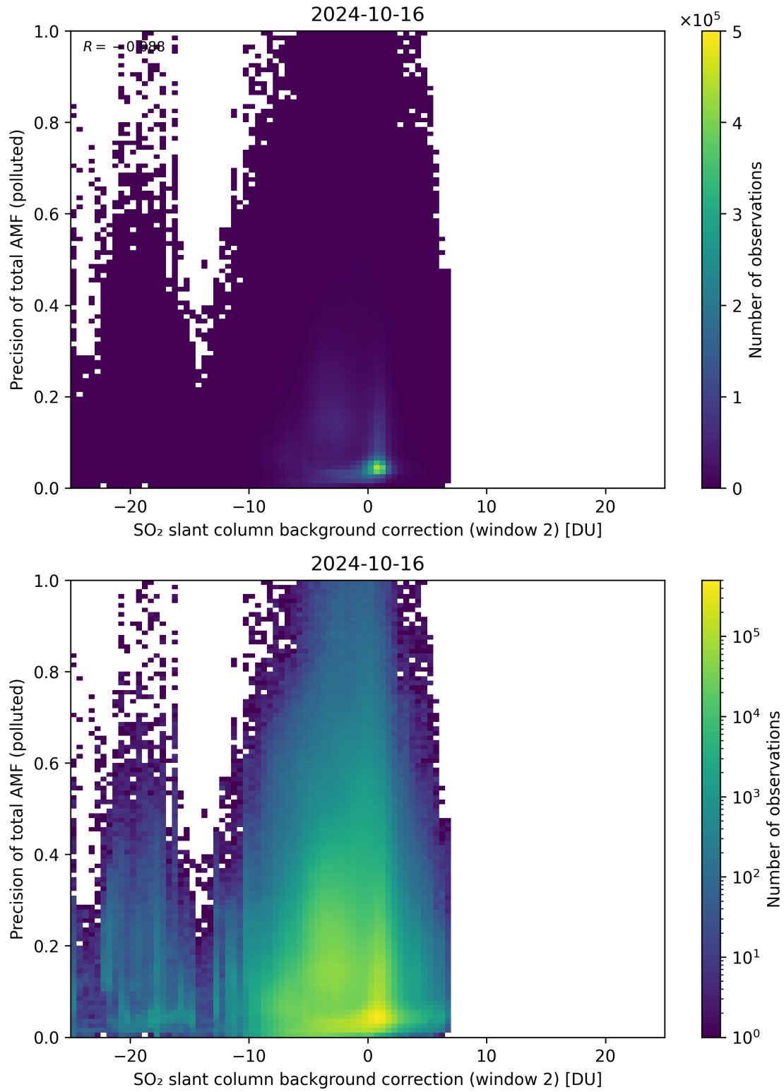
Figure 120: Scatter density plot of “SO 2 slant column background correction (window 2)” against “Precision of total AMF (polluted)” for 2024-10-15 to 2024-10-17.
