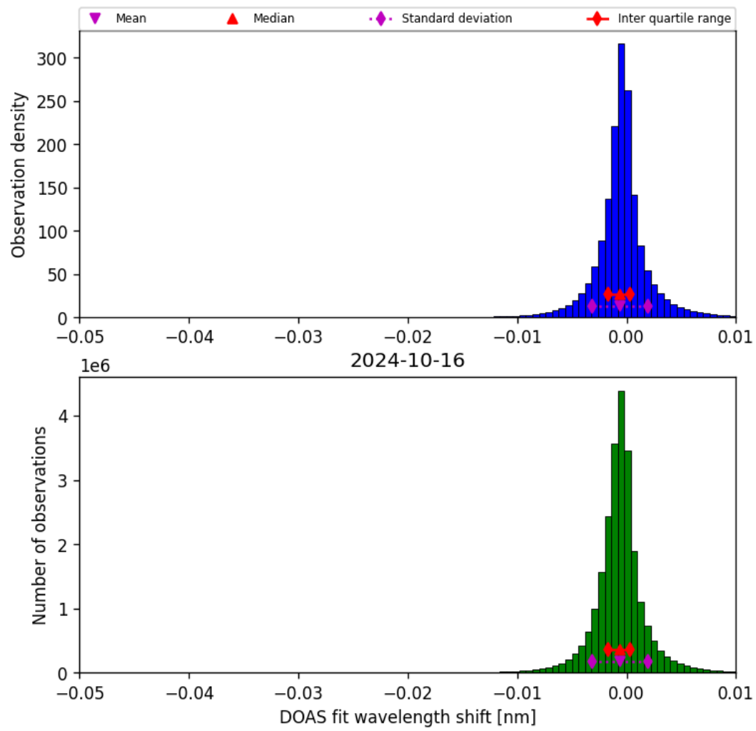
Figure 68: Histogram of “DOAS fit wavelength shift” for 2024-10-15 to 2024-10-17
