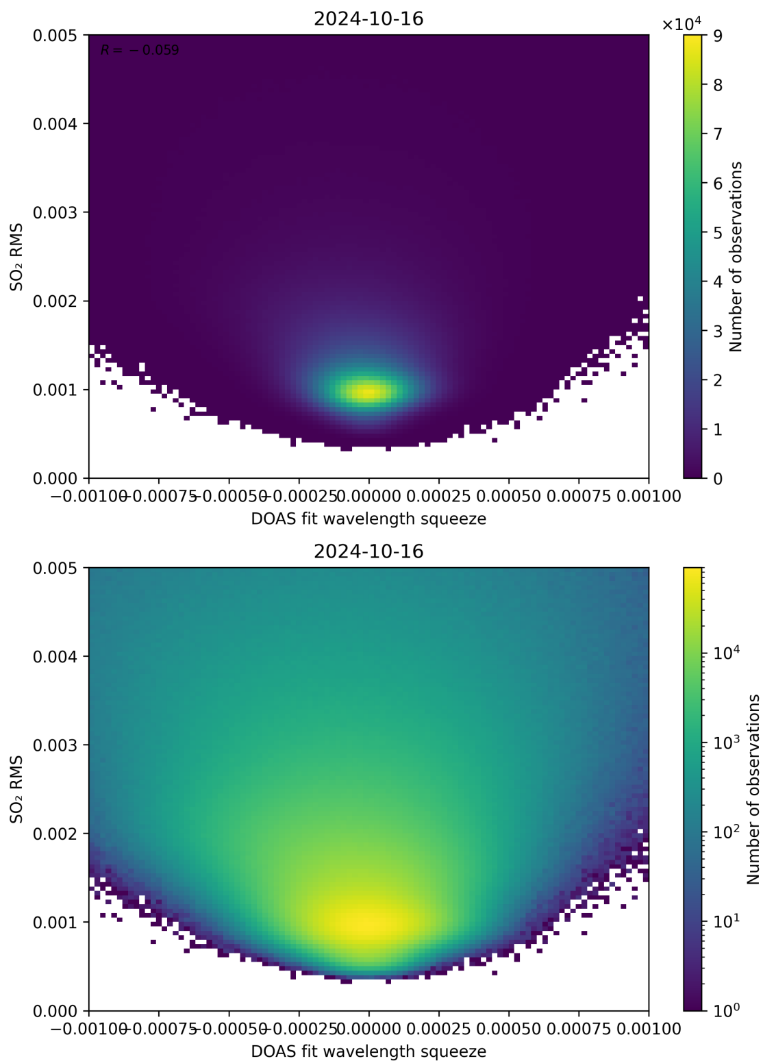
Figure 132: Scatter density plot of “DOAS fit wavelength squeeze” against “SO 2 RMS” for 2024-10-15 to 2024-10-17.
