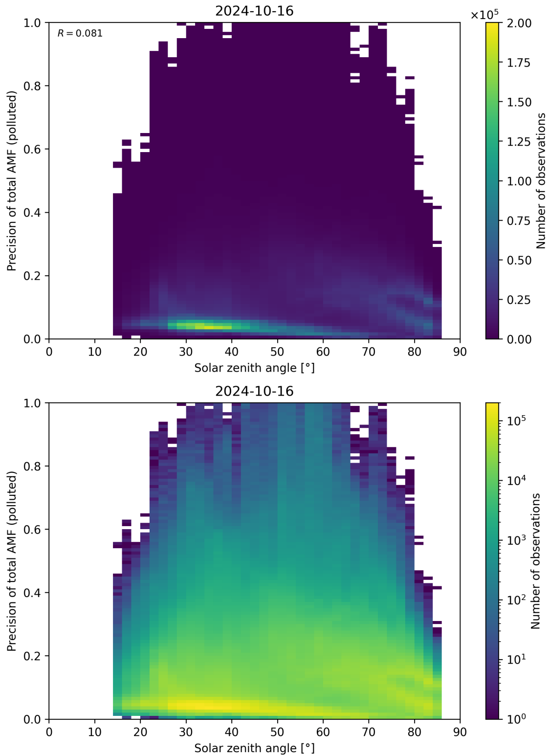
Figure 175: Scatter density plot of “Solar zenith angle” against “Precision of total AMF (polluted)” for 2024-10-15 to 2024-10-17.
