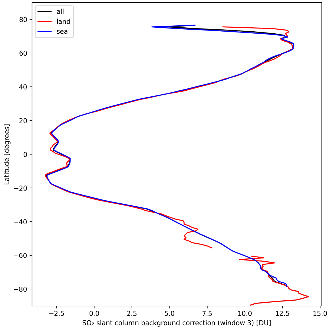
Figure 44: Zonal average of “SO 2 slant column background correction (window 3)” for 2024-10-15 to 2024-10-17.
