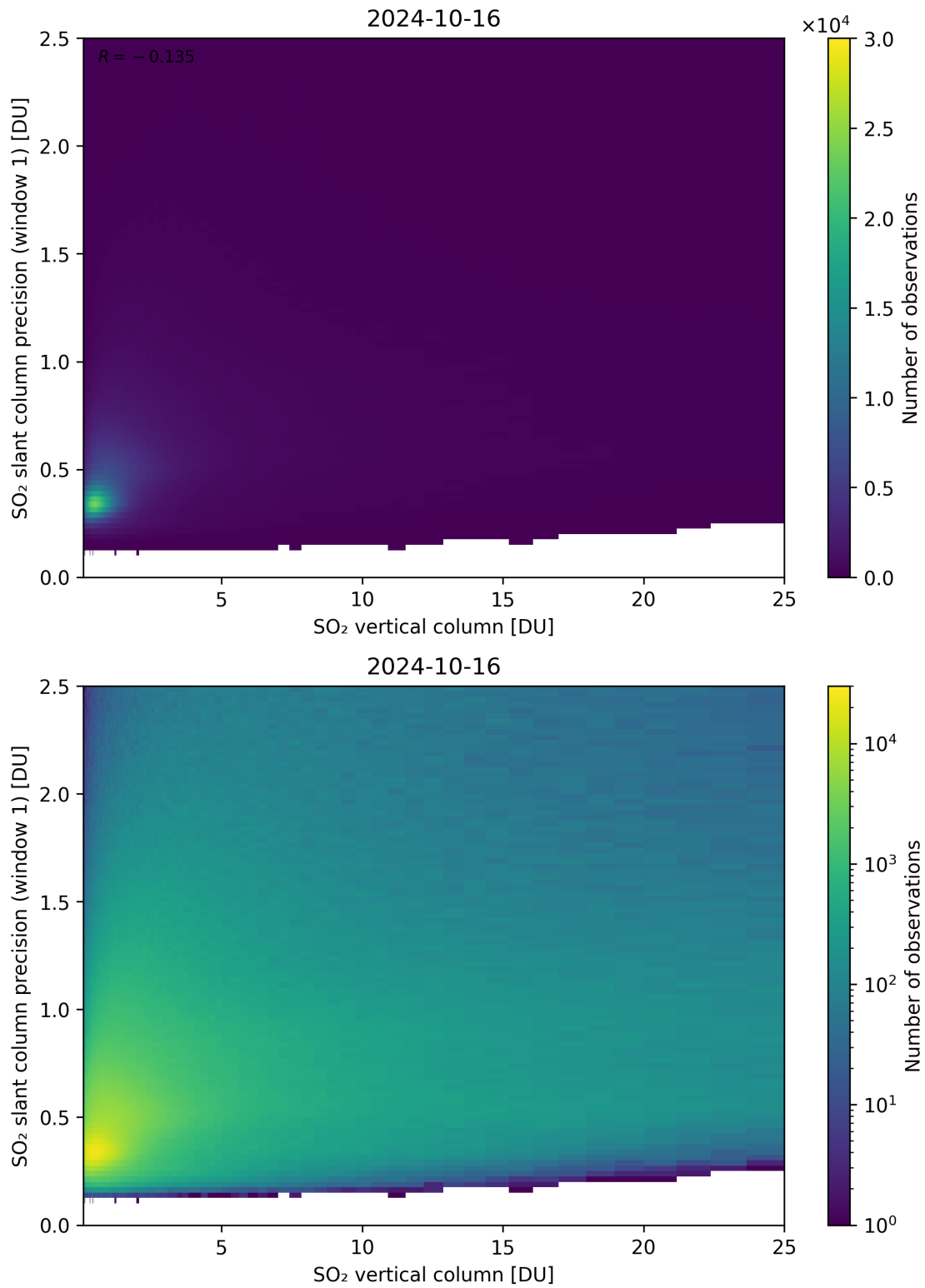
Figure 301: Scatter density plot of “SO 2 vertical column” against “SO 2 slant column precision (window 1)” for 2024-10-15 to 2024-10-17.
