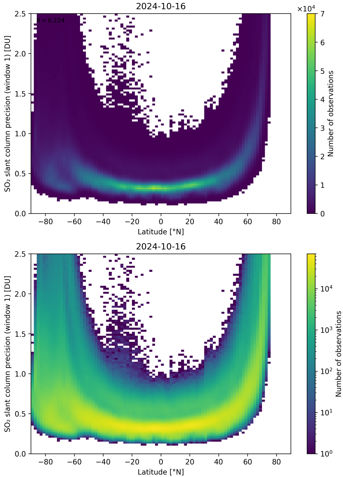
Figure 150: Scatter density plot of “Latitude” against “SO 2 slant column precision (window 1)” for 2024-10-15 to 2024-10-17.
