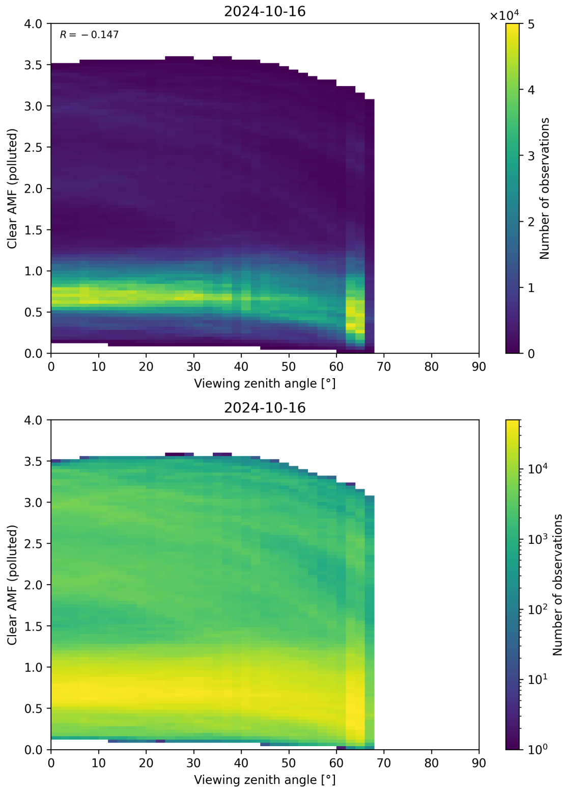
Figure 316: Scatter density plot of “Viewing zenith angle” against “Clear AMF (polluted)” for 2024-10-15 to 2024-10-17.
