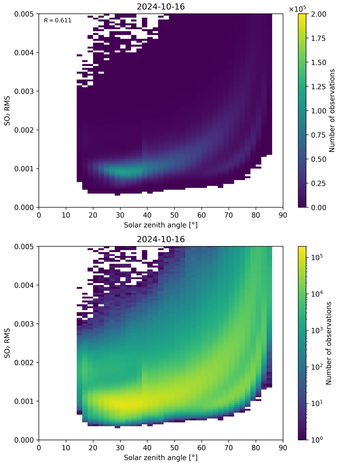
Figure 163: Scatter density plot of “Solar zenith angle” against “SO 2 RMS” for 2024-10-15 to 2024-10-17.
