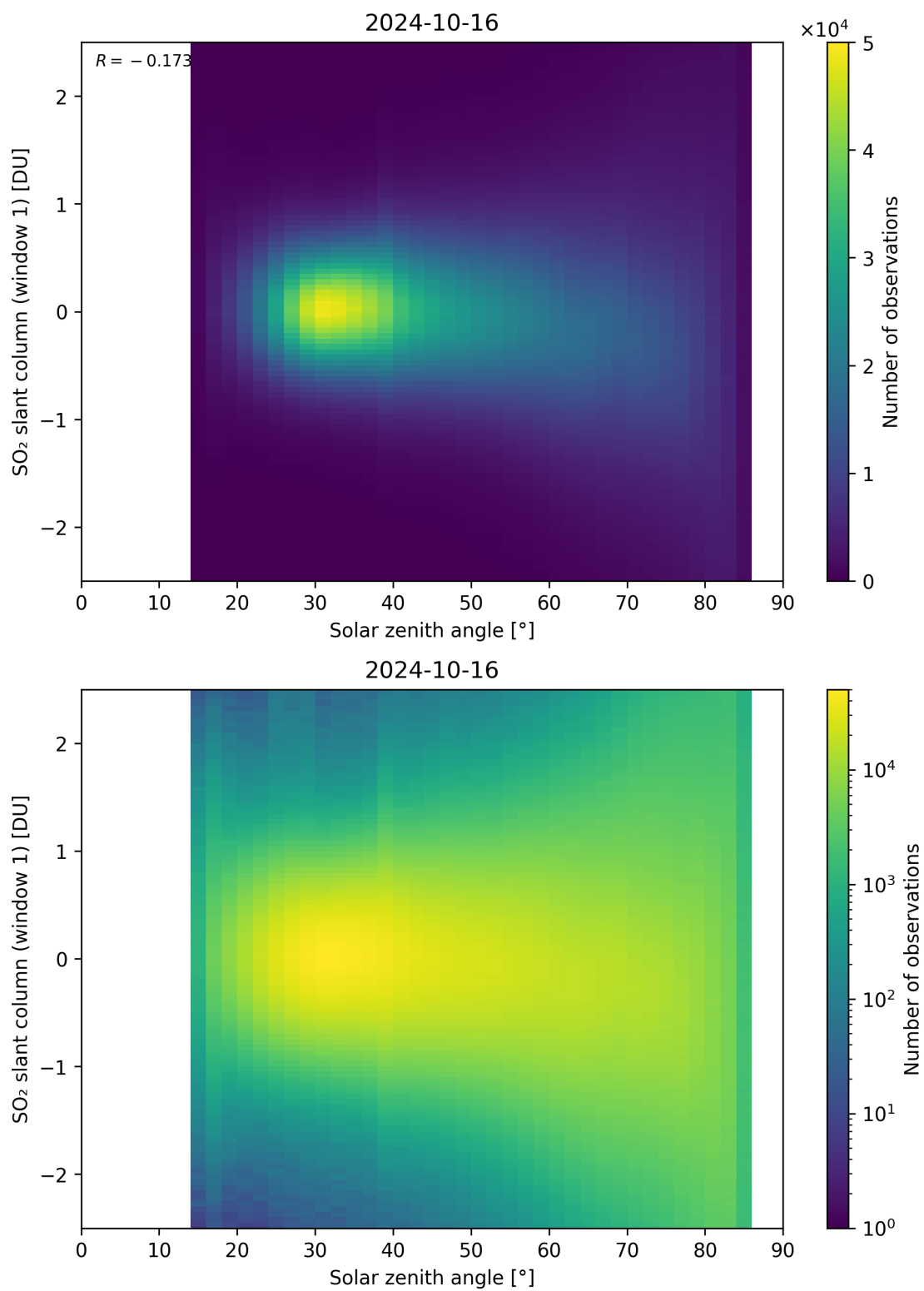
Figure 169: Scatter density plot of “Solar zenith angle” against “SO 2 slant column (window 1)” for 2024-10-15 to 2024-10-17.
