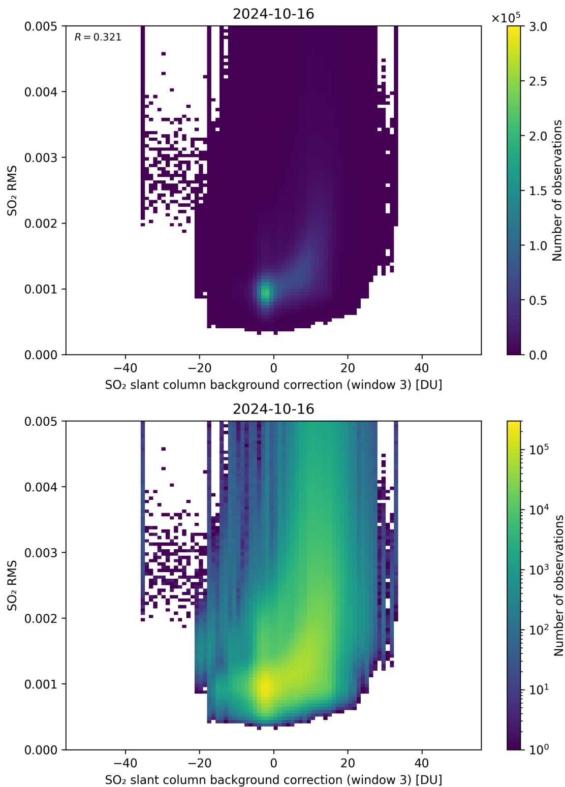
Figure 123: Scatter density plot of “SO 2 slant column background correction (window 3)” against “SO 2 RMS” for 2024-10-15 to 2024-10-17.
