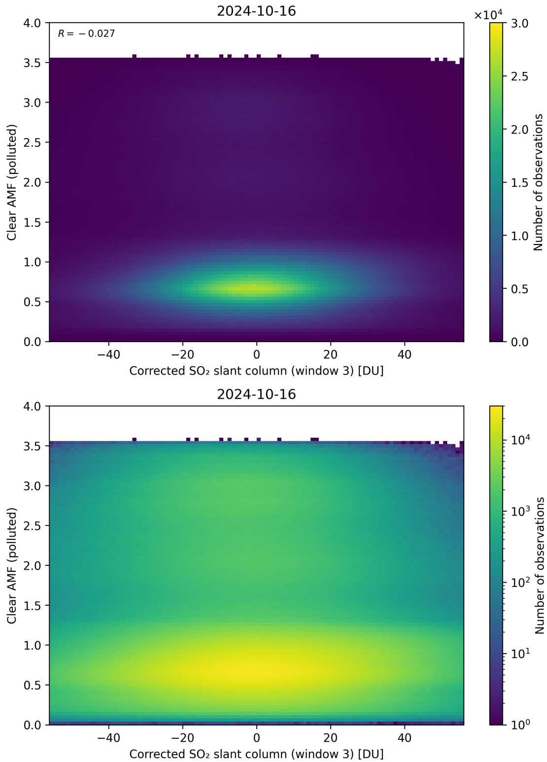
Figure 209: Scatter density plot of “Corrected SO 2 slant column (window 3)” against “Clear AMF (polluted)” for 2024-10-15 to 2024-10-17.
