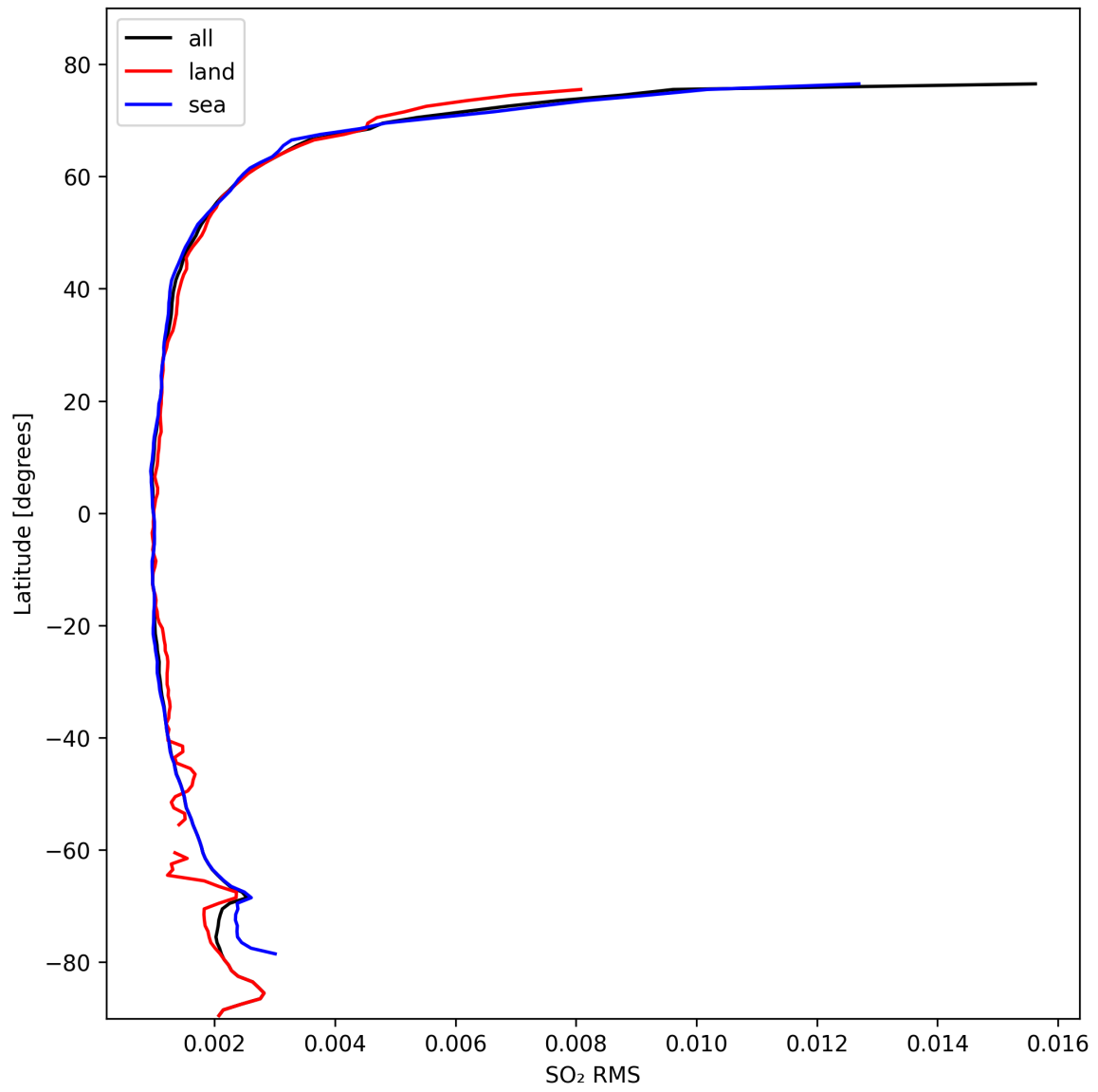
Figure 47: Zonal average of “SO 2 RMS” for 2024-10-15 to 2024-10-17.
