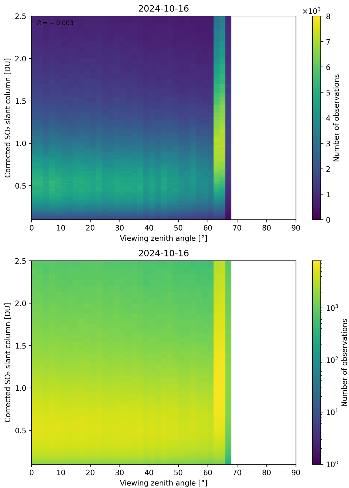
Figure 317: Scatter density plot of “Viewing zenith angle” against “Corrected SO 2 slant column” for 2024-10-15 to 2024-10-17.
