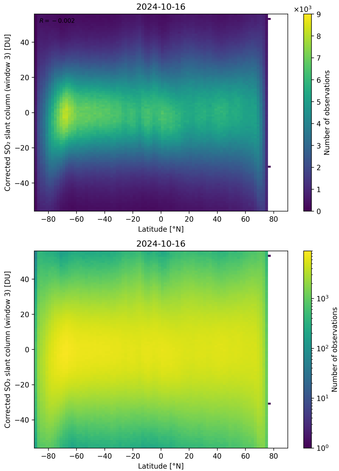
Figure 148: Scatter density plot of “Latitude” against “Corrected SO 2 slant column (window 3)” for 2024-10-15 to 2024-10-17.
