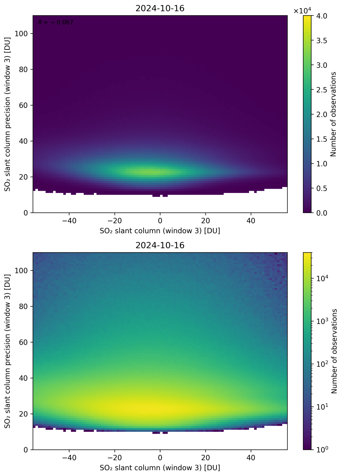
Figure 267: Scatter density plot of “SO 2 slant column (window 3)” against “SO 2 slant column precision (window 3)” for 2024-10-15 to 2024-10-17.
