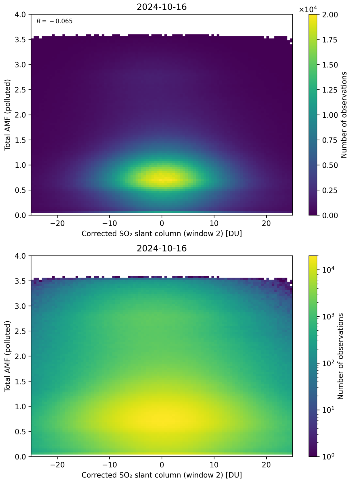
Figure 203: Scatter density plot of “Corrected SO 2 slant column (window 2)” against “Total AMF (polluted)” for 2024-10-15 to 2024-10-17.
