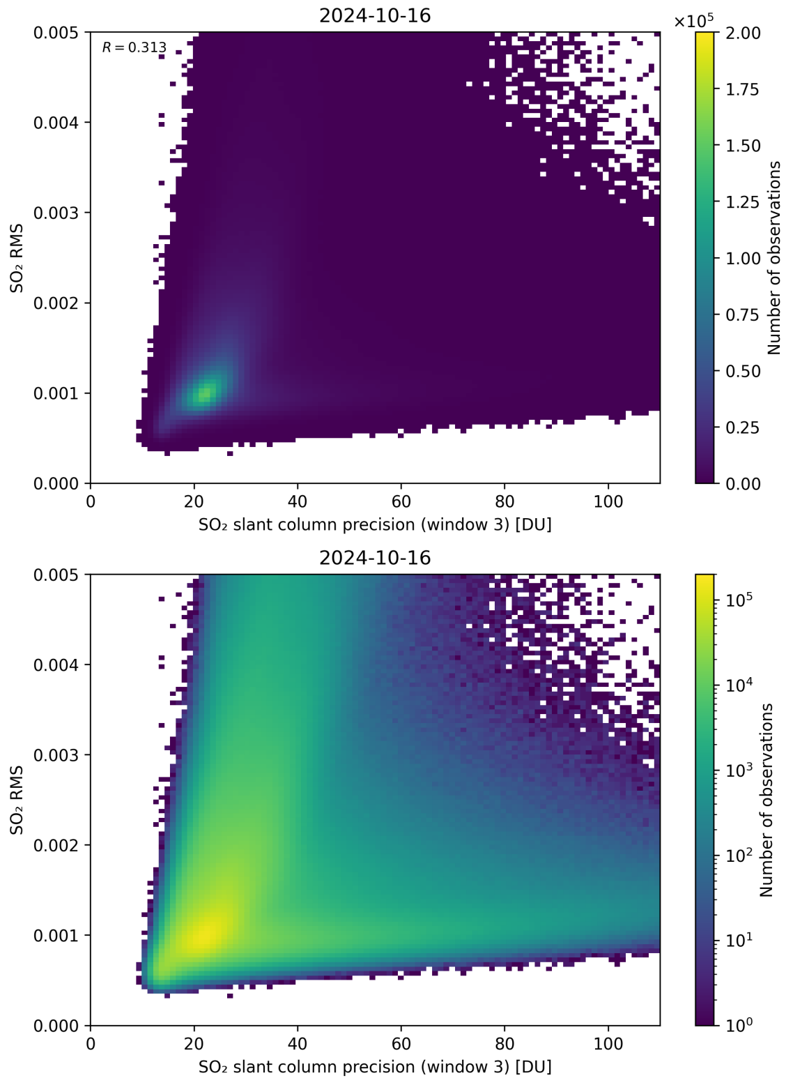
Figure 260: Scatter density plot of “SO 2 slant column precision (window 3)” against “SO 2 RMS” for 2024-10-15 to 2024-10-17.
