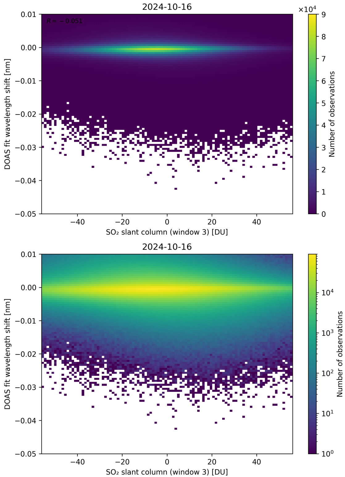
Figure 254: Scatter density plot of “SO 2 slant column (window 3)” against “DOAS fit wavelength shift” for 2024-10-15 to 2024-10-17.
