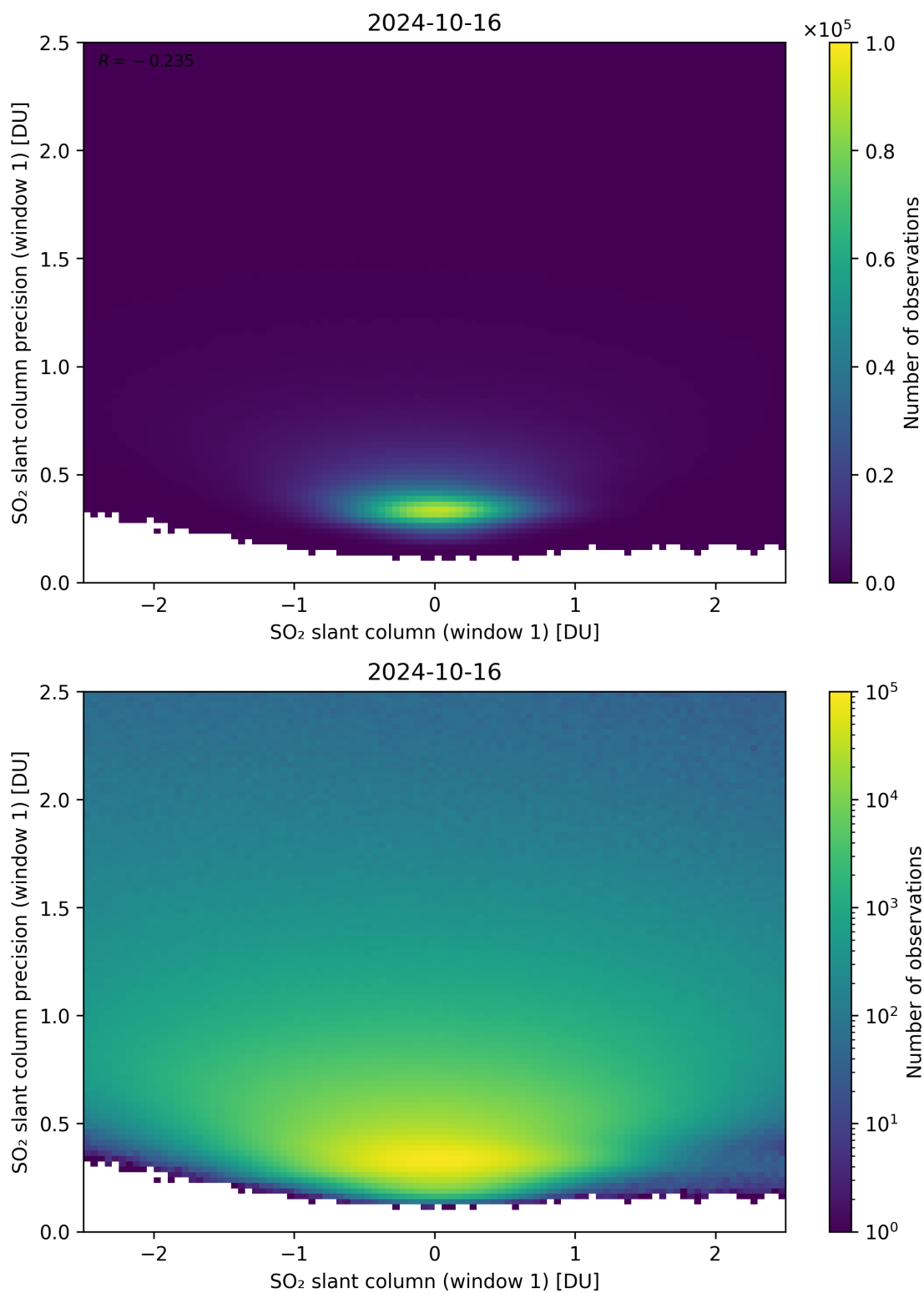
Figure 235: Scatter density plot of “SO 2 slant column (window 1)” against “SO 2 slant column precision (window 1)” for 2024-10-15 to 2024-10-17.
