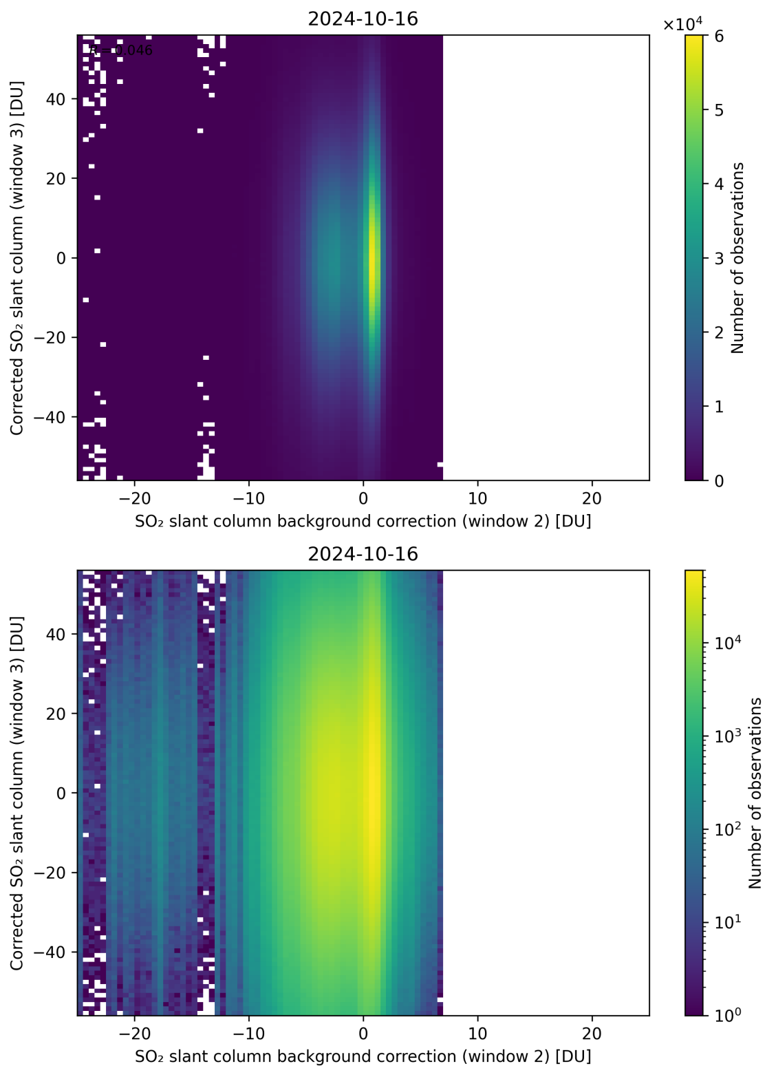
Figure 116: Scatter density plot of “SO 2 slant column background correction (window 2)” against “Corrected SO 2 slant column (window 3)” for 2024-10-15 to 2024-10-17.
