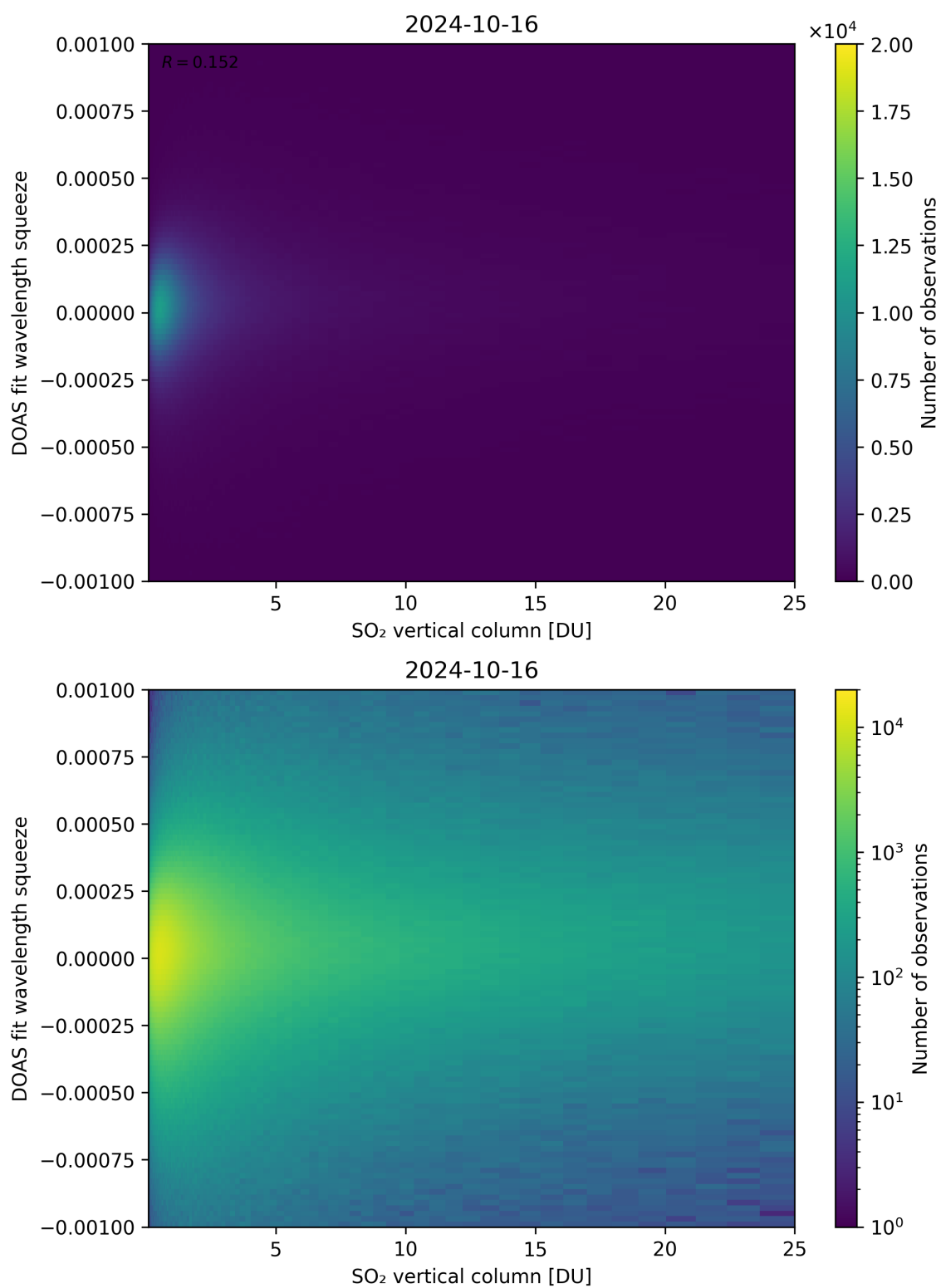
Figure 277: Scatter density plot of “SO 2 vertical column” against “DOAS fit wavelength squeeze” for 2024-10-15 to 2024-10-17.
