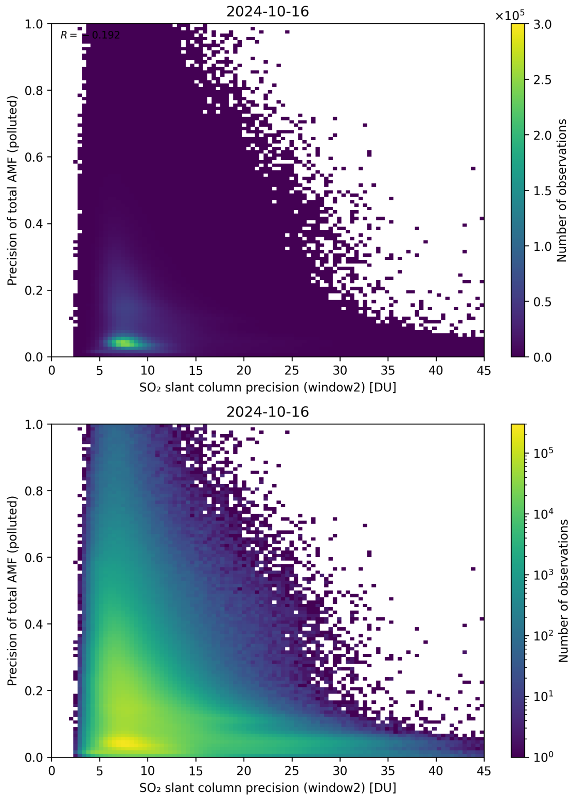
Figure 252: Scatter density plot of “SO 2 slant column precision (window2)” against “Precision of total AMF (polluted)” for 2024-10-15 to 2024-10-17.
