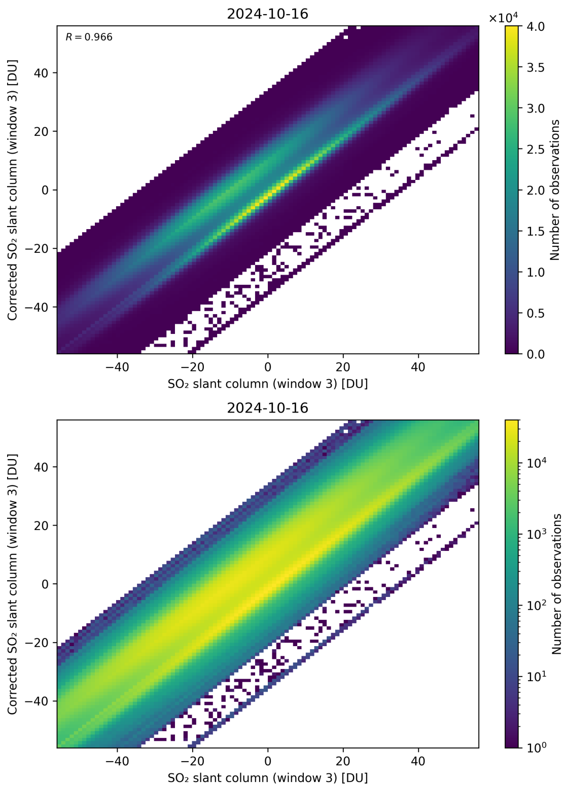
Figure 266: Scatter density plot of “SO 2 slant column (window 3)” against “Corrected SO 2 slant column (window 3)” for 2024-10-15 to 2024-10-17.
