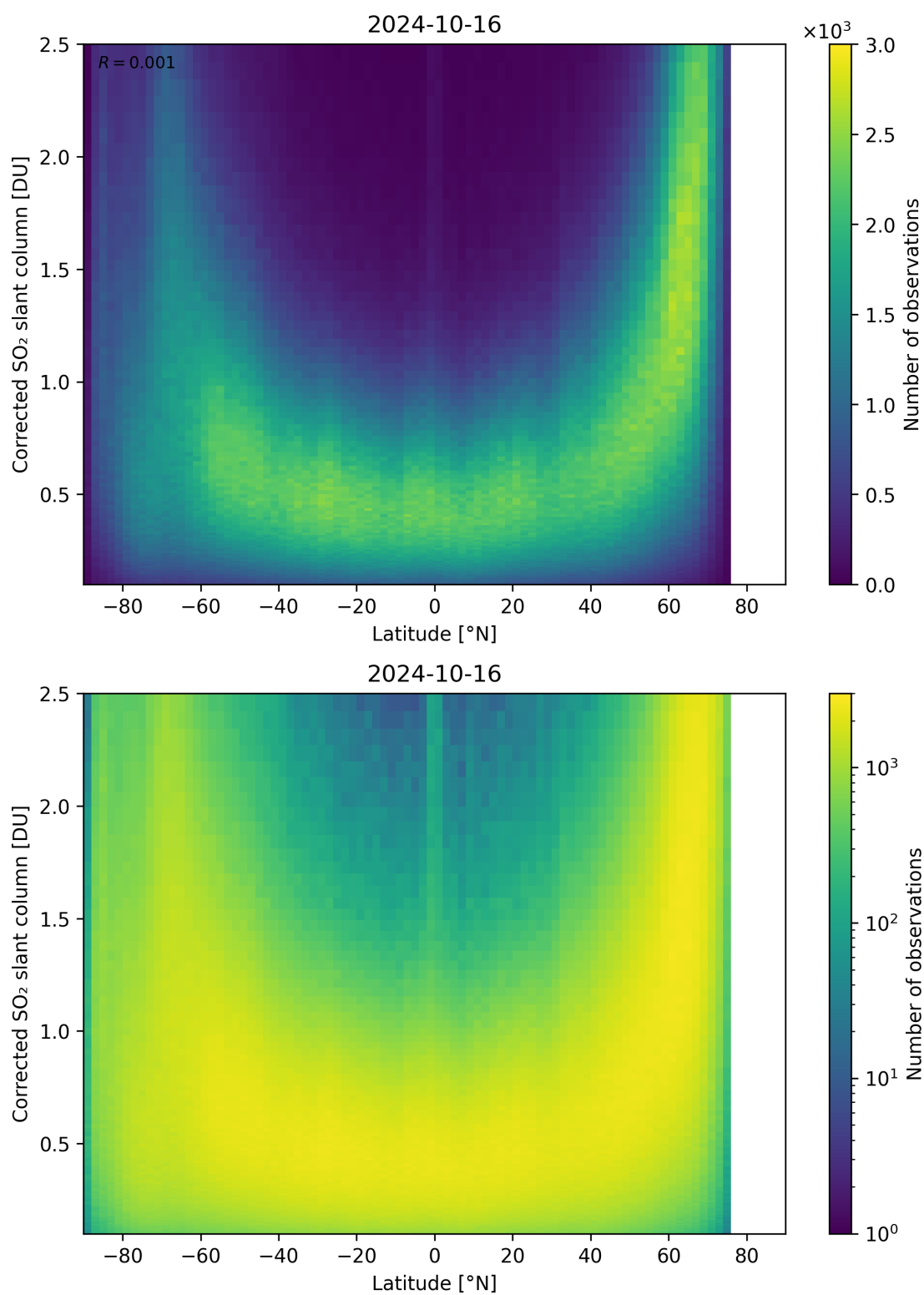
Figure 146: Scatter density plot of “Latitude” against “Corrected SO 2 slant column” for 2024-10-15 to 2024-10-17.
