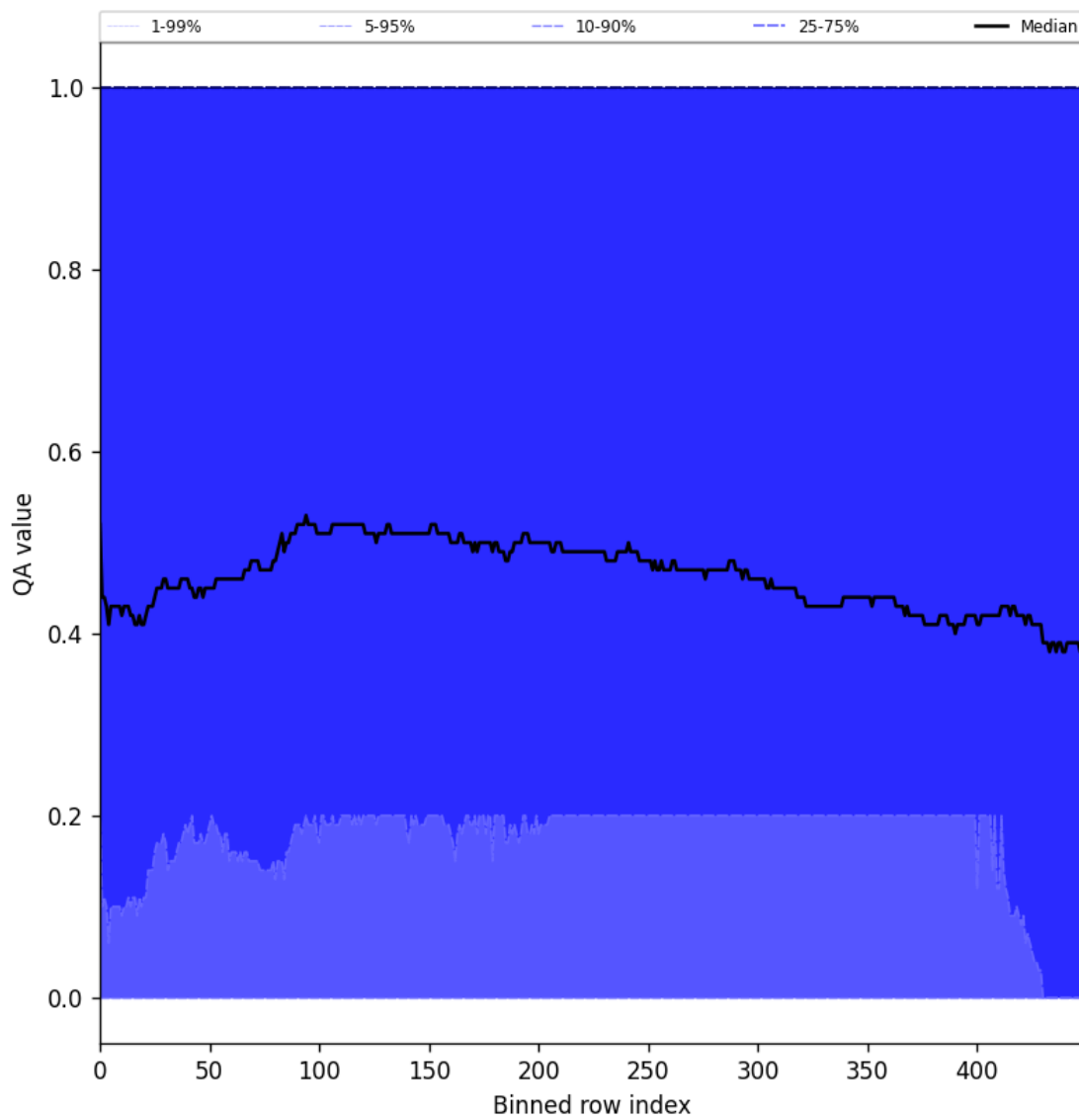
Figure 75: Along track statistics of “QA value” for 2024-10-15 to 2024-10-17
