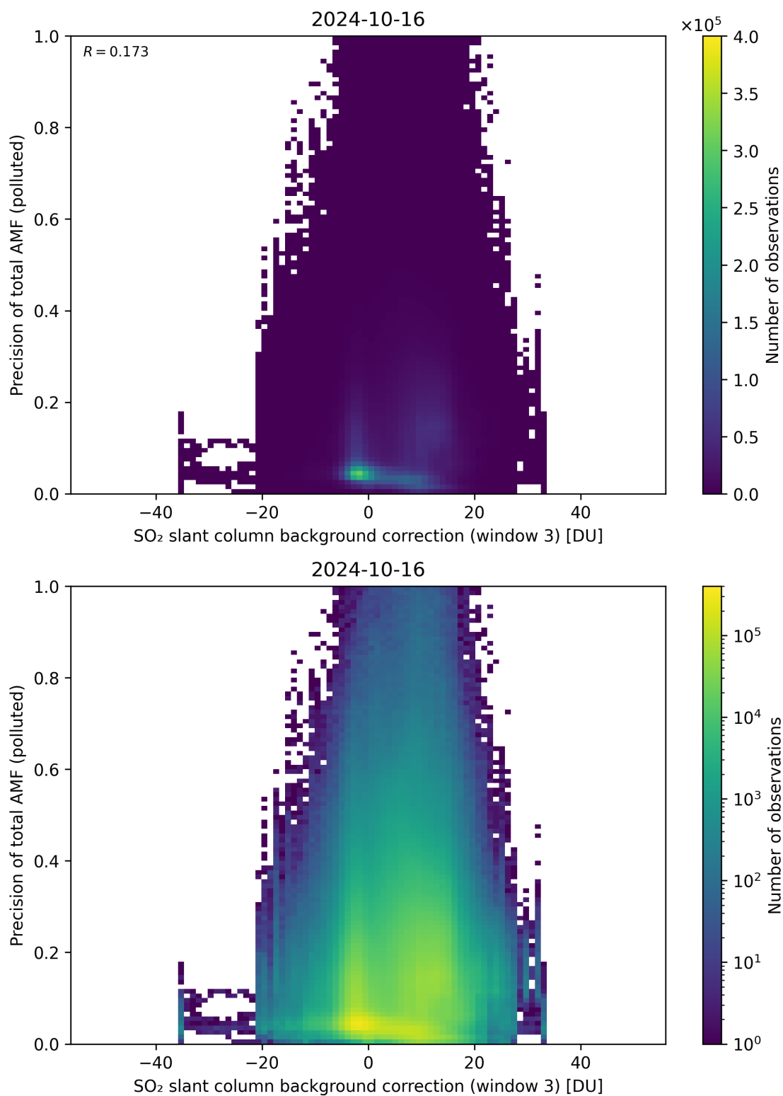
Figure 126: Scatter density plot of “SO 2 slant column background correction (window 3)” against “Precision of total AMF (polluted)” for 2024-10-15 to 2024-10-17.
