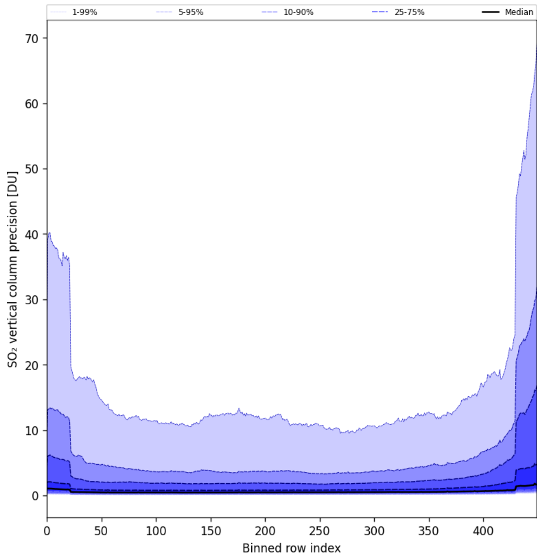
Figure 77: Along track statistics of “SO 2 vertical column precision” for 2024-10-15 to 2024-10-17
