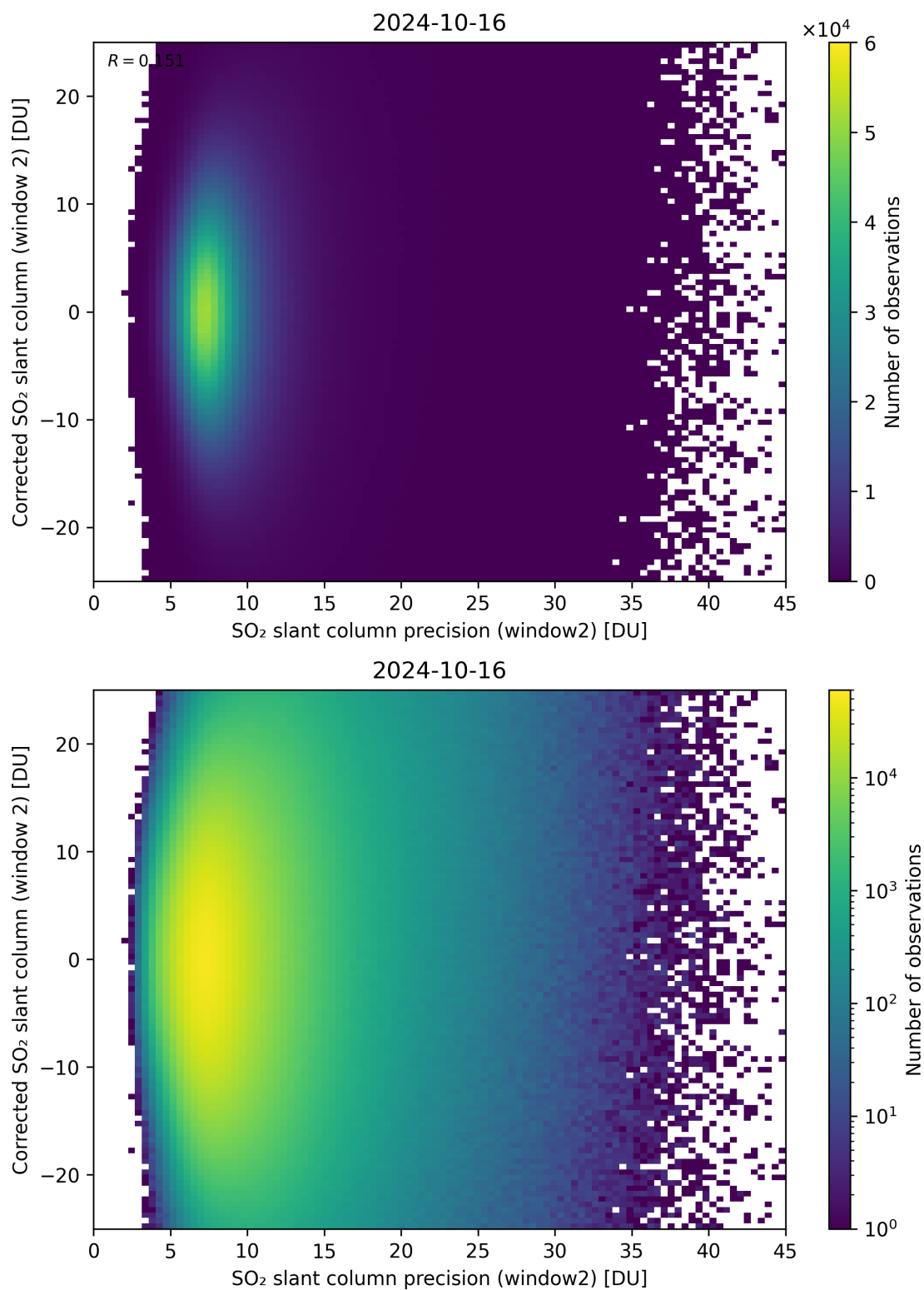
Figure 247: Scatter density plot of “SO 2 slant column precision (window2)” against “Corrected SO 2 slant column (window 2)” for 2024-10-15 to 2024-10-17.
