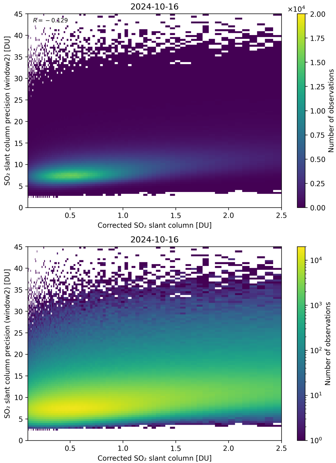
Figure 189: Scatter density plot of “Corrected SO 2 slant column” against “SO 2 slant column precision (window2)” for 2024-10-15 to 2024-10-17.
