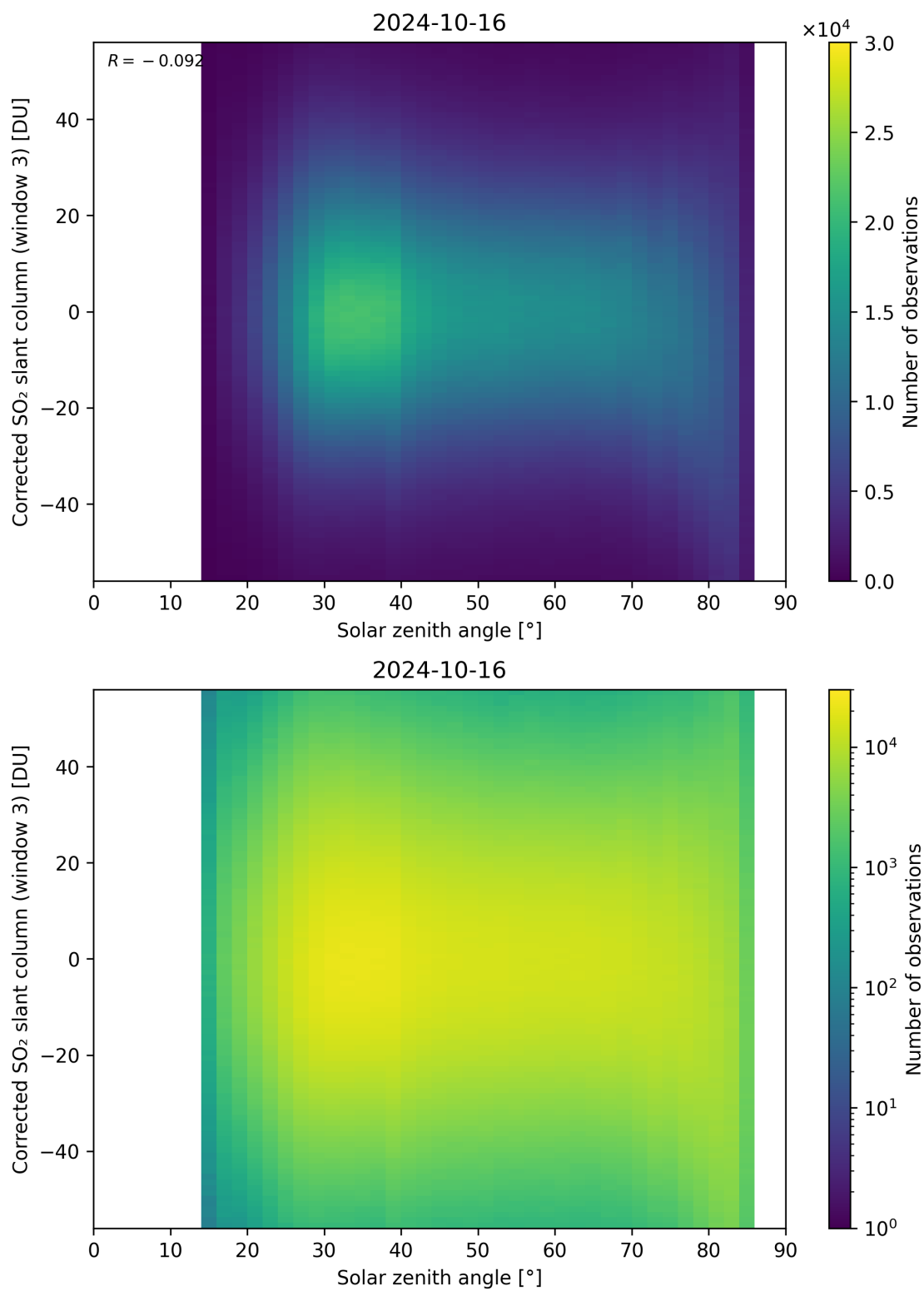
Figure 168: Scatter density plot of “Solar zenith angle” against “Corrected SO 2 slant column (window 3)” for 2024-10-15 to 2024-10-17.
