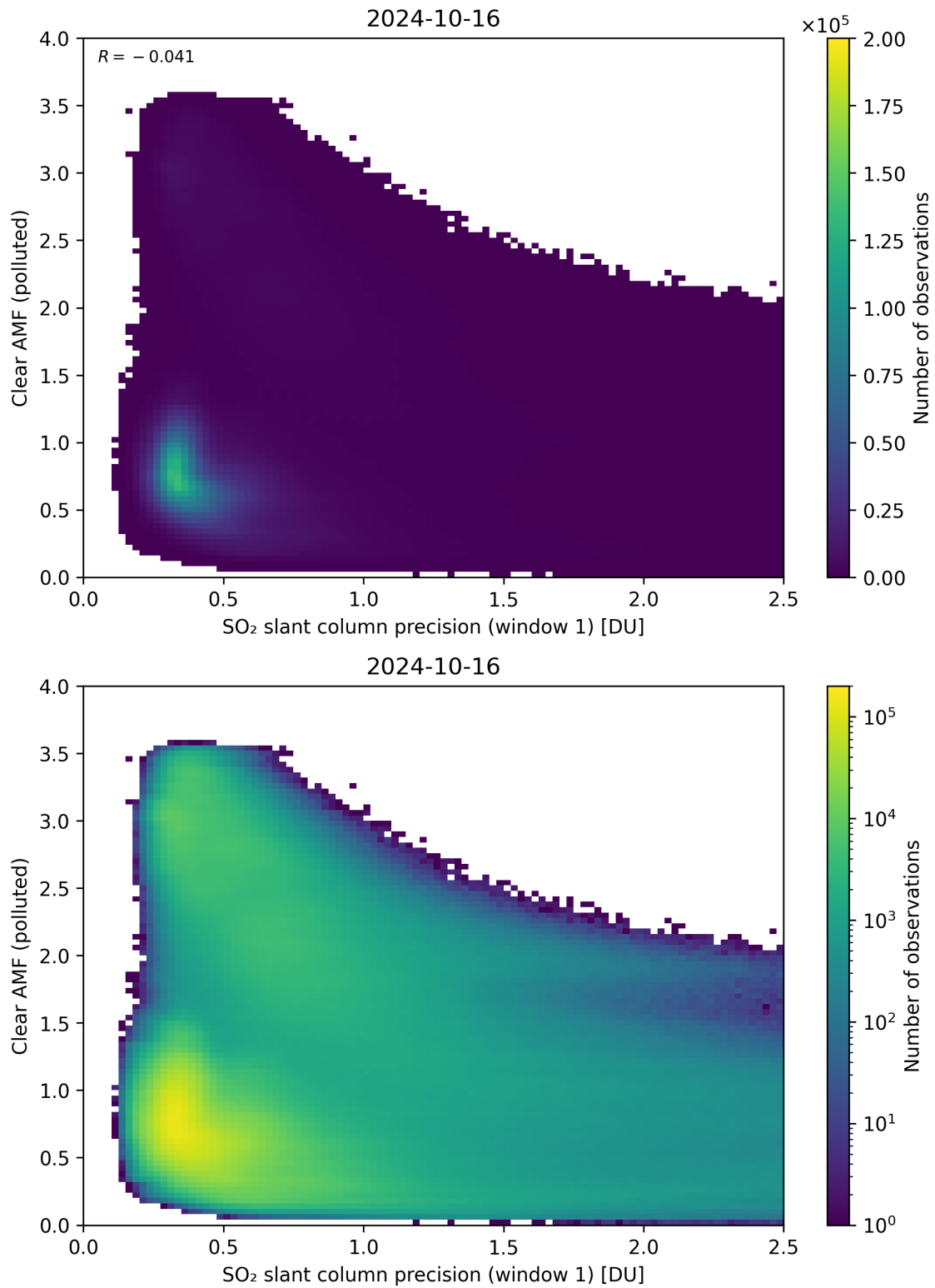
Figure 224: Scatter density plot of “SO 2 slant column precision (window 1)” against “Clear AMF (polluted)” for 2024-10-15 to 2024-10-17.
