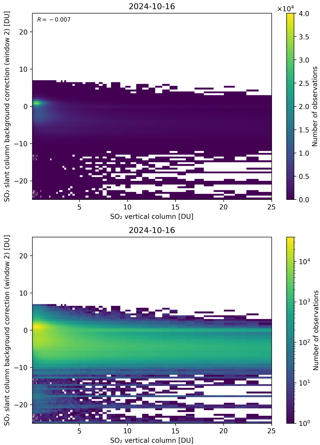
Figure 274: Scatter density plot of “SO 2 vertical column” against “SO 2 slant column background correction (window 2)” for 2024-10-15 to 2024-10-17.
