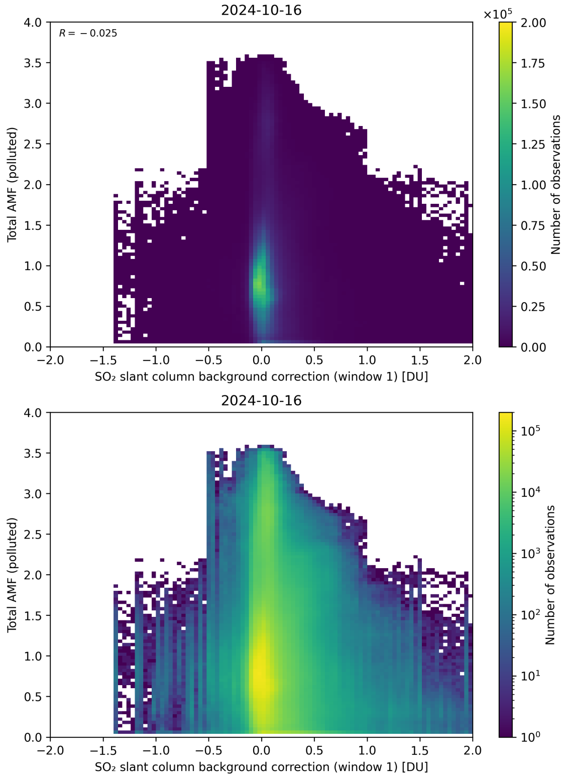
Figure 109: Scatter density plot of “SO 2 slant column background correction (window 1)” against “Total AMF (polluted)” for 2024-10-15 to 2024-10-17.
