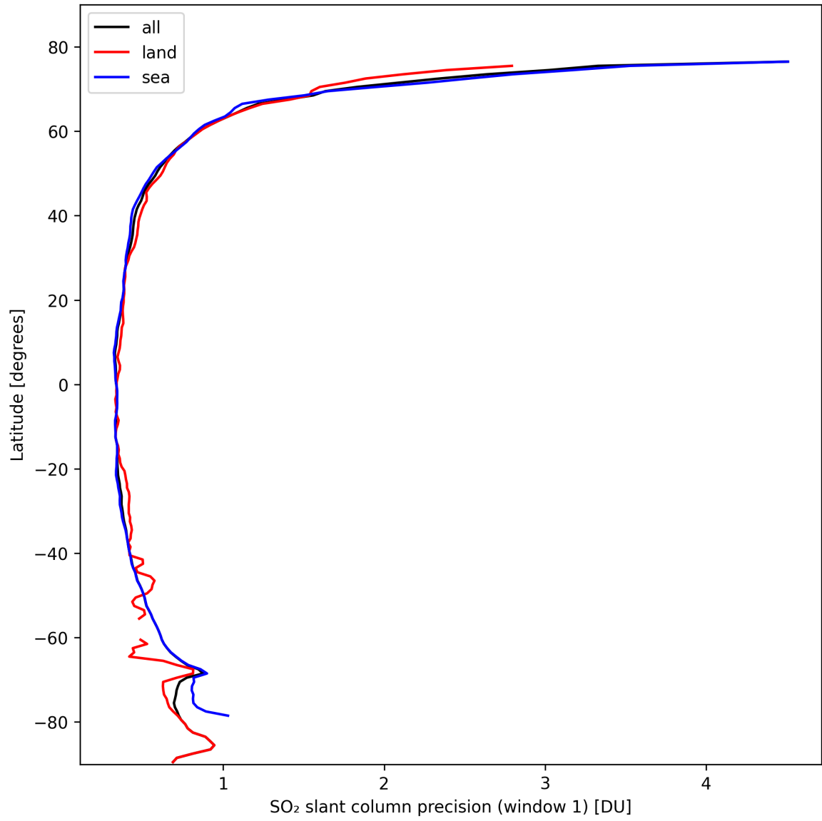
Figure 34: Zonal average of “SO 2 slant column precision (window 1)” for 2024-10-15 to 2024-10-17.
