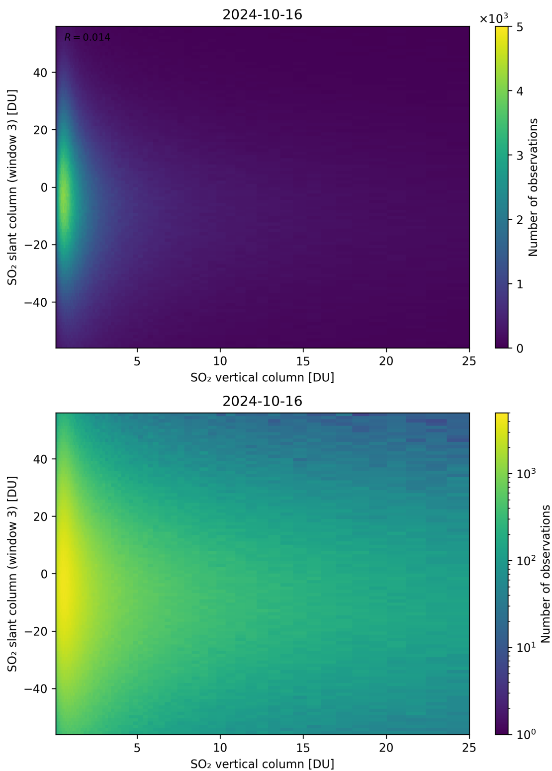
Figure 303: Scatter density plot of “SO 2 vertical column” against “SO 2 slant column (window 3)” for 2024-10-15 to 2024-10-17.
