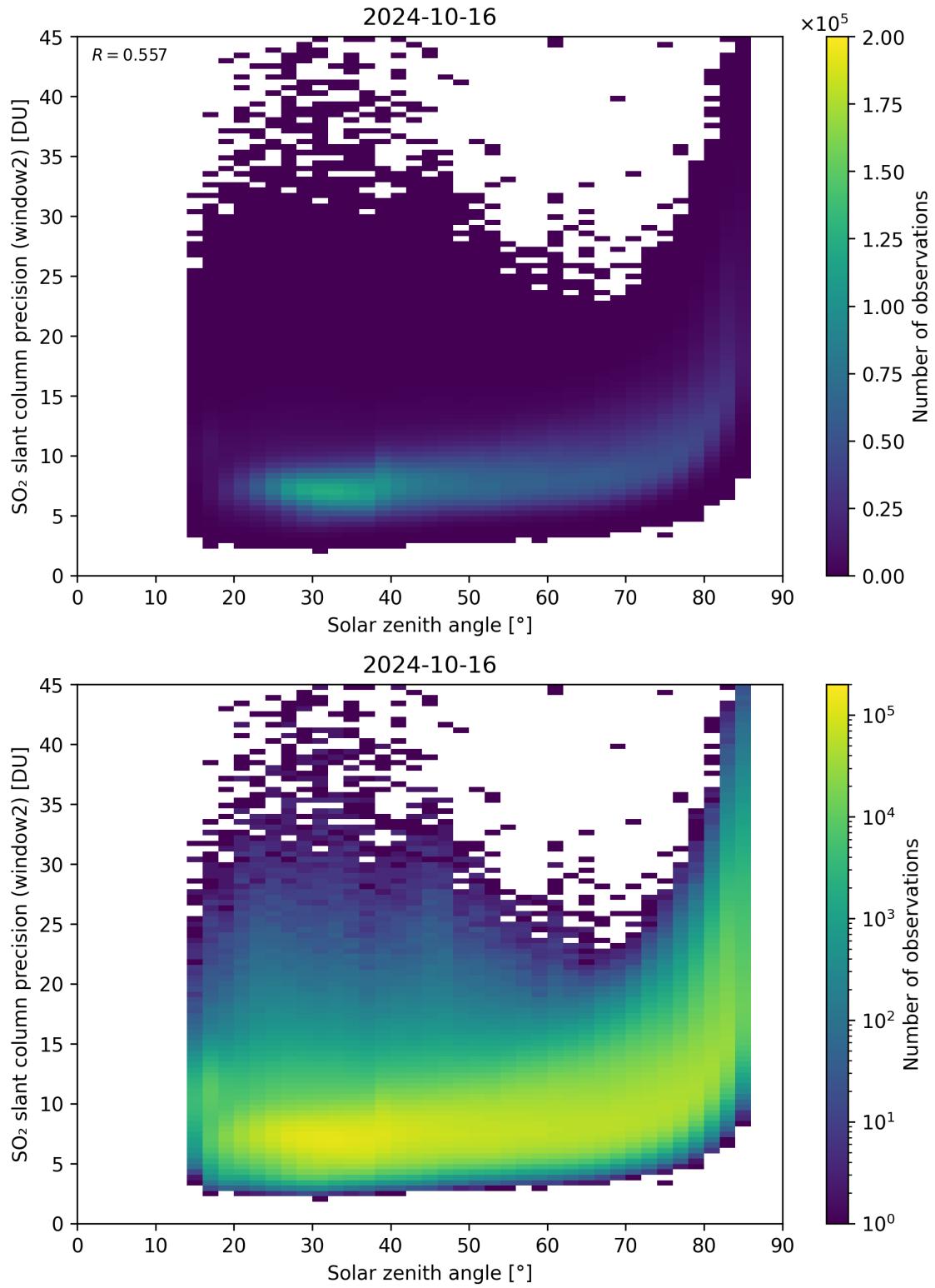
Figure 171: Scatter density plot of “Solar zenith angle” against “SO 2 slant column precision (window2)” for 2024-10-15 to 2024-10-17.
