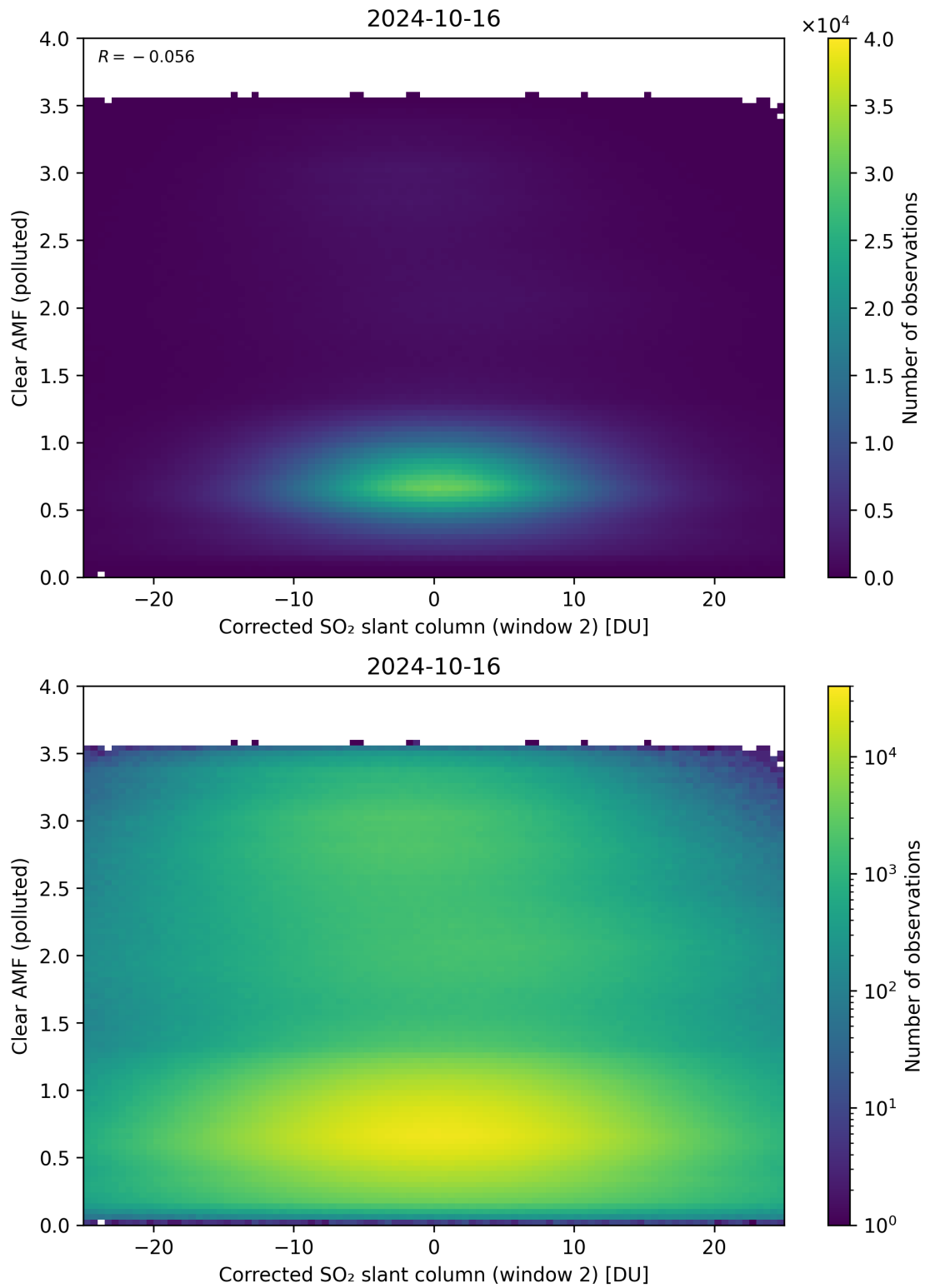
Figure 199: Scatter density plot of “Corrected SO 2 slant column (window 2)” against “Clear AMF (polluted)” for 2024-10-15 to 2024-10-17.
