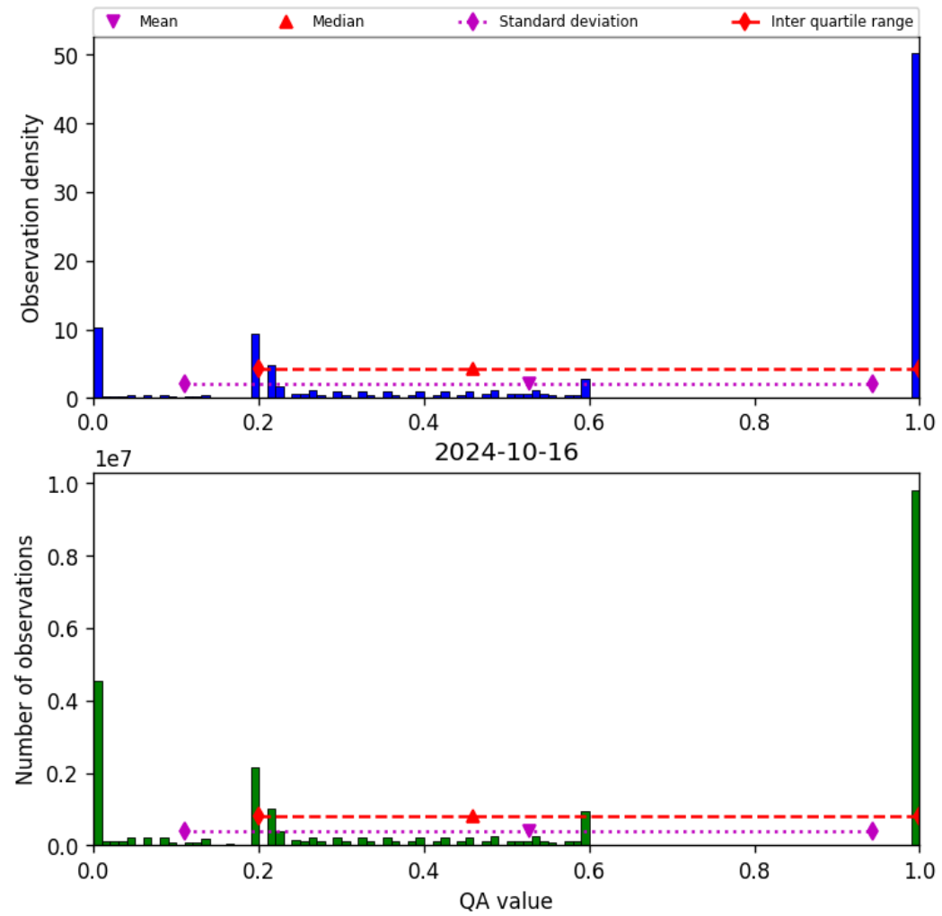
Figure 52: Histogram of “QA value” for 2024-10-15 to 2024-10-17
