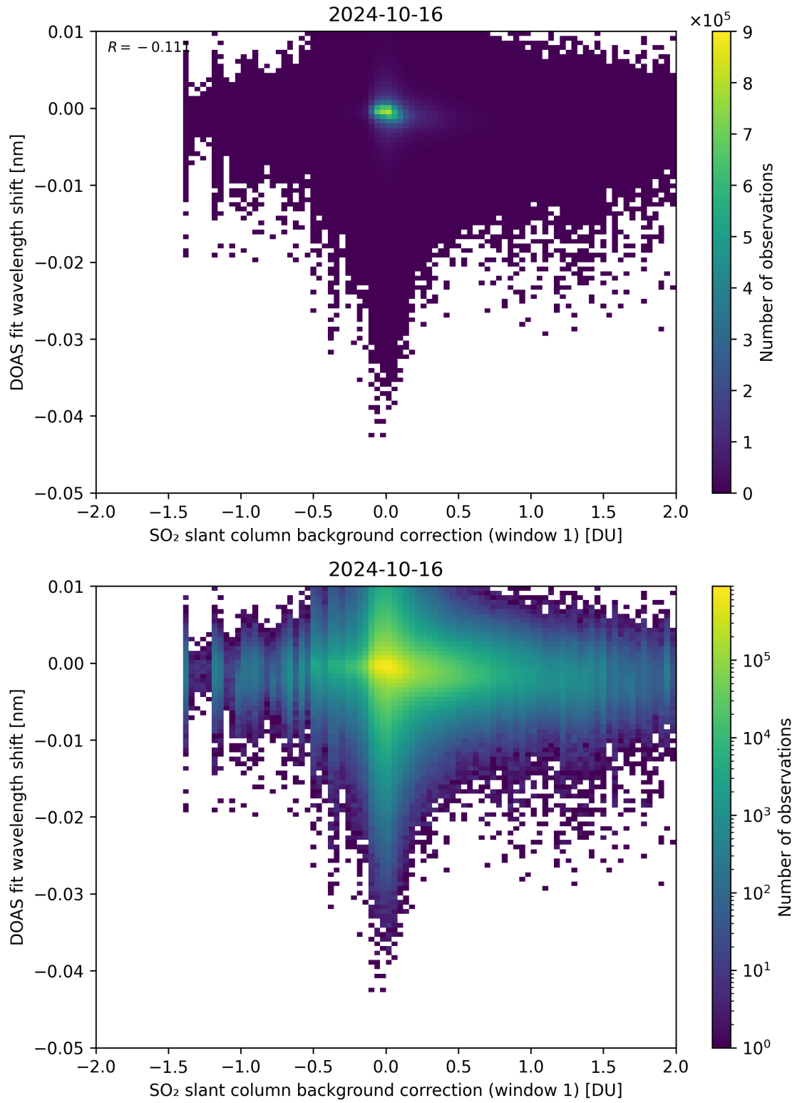
Figure 100: Scatter density plot of “SO 2 slant column background correction (window 1)” against “DOAS fit wavelength shift” for 2024-10-15 to 2024-10-17.
