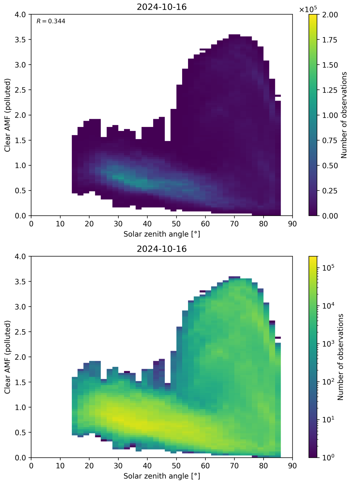
Figure 165: Scatter density plot of “Solar zenith angle” against “Clear AMF (polluted)” for 2024-10-15 to 2024-10-17.
