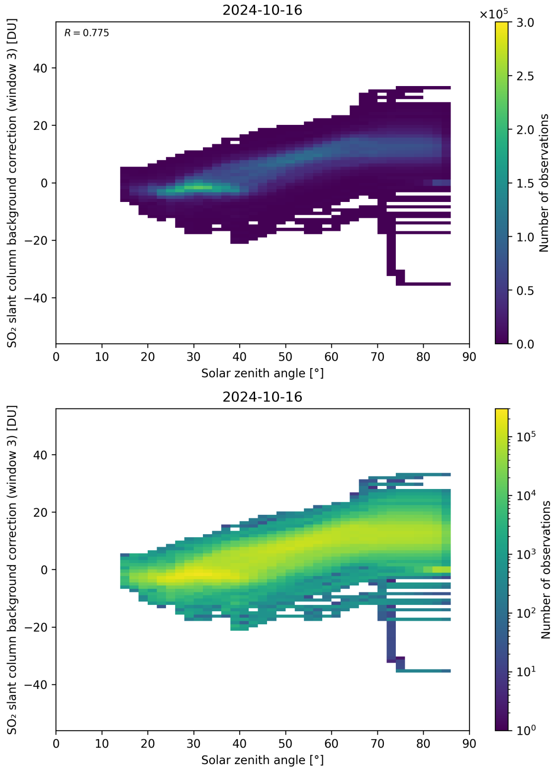
Figure 160: Scatter density plot of “Solar zenith angle” against “SO 2 slant column background correction (window 3)” for 2024-10-15 to 2024-10-17.
