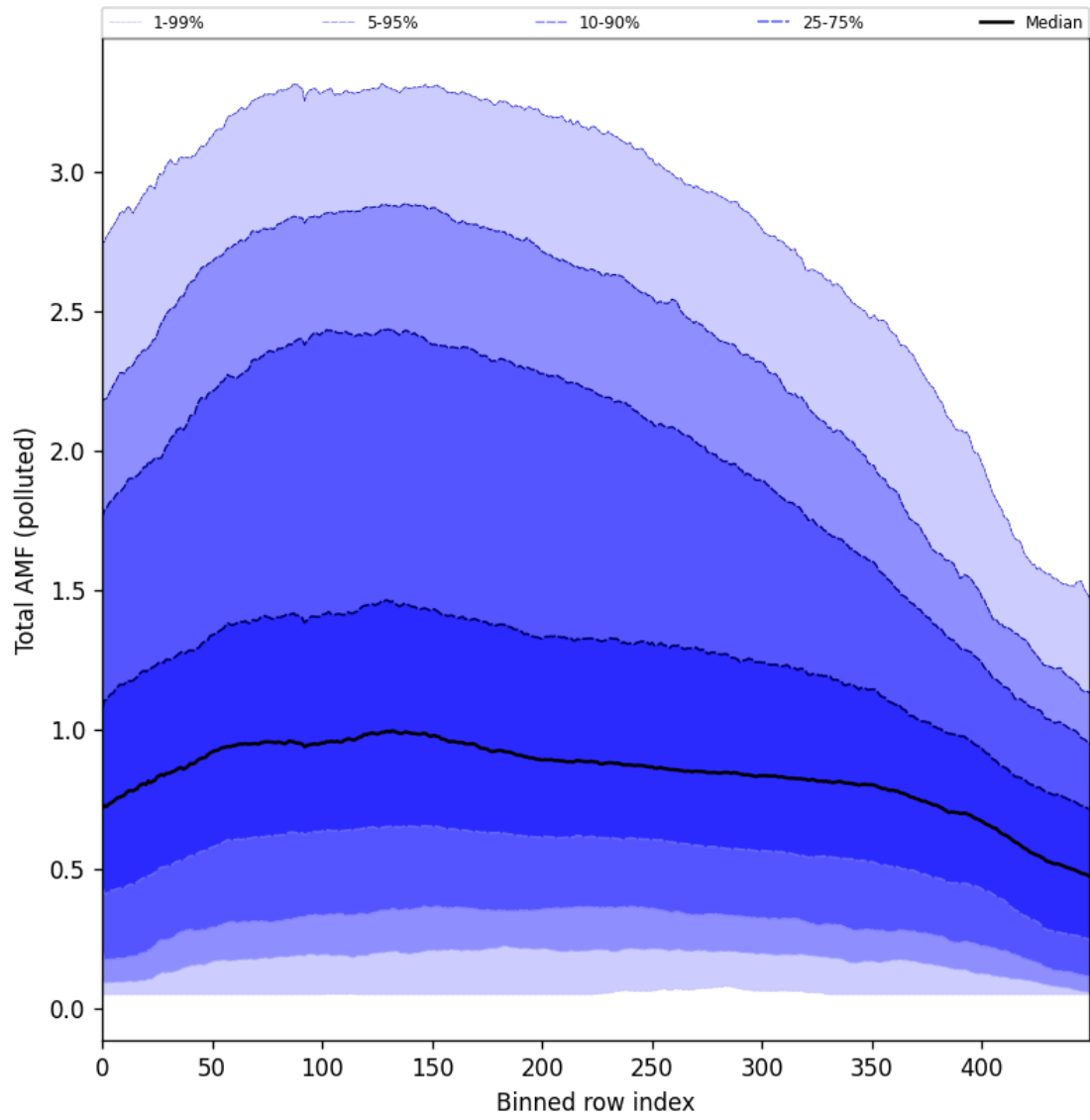
Figure 94: Along track statistics of “Total AMF (polluted)” for 2024-10-15 to 2024-10-17
