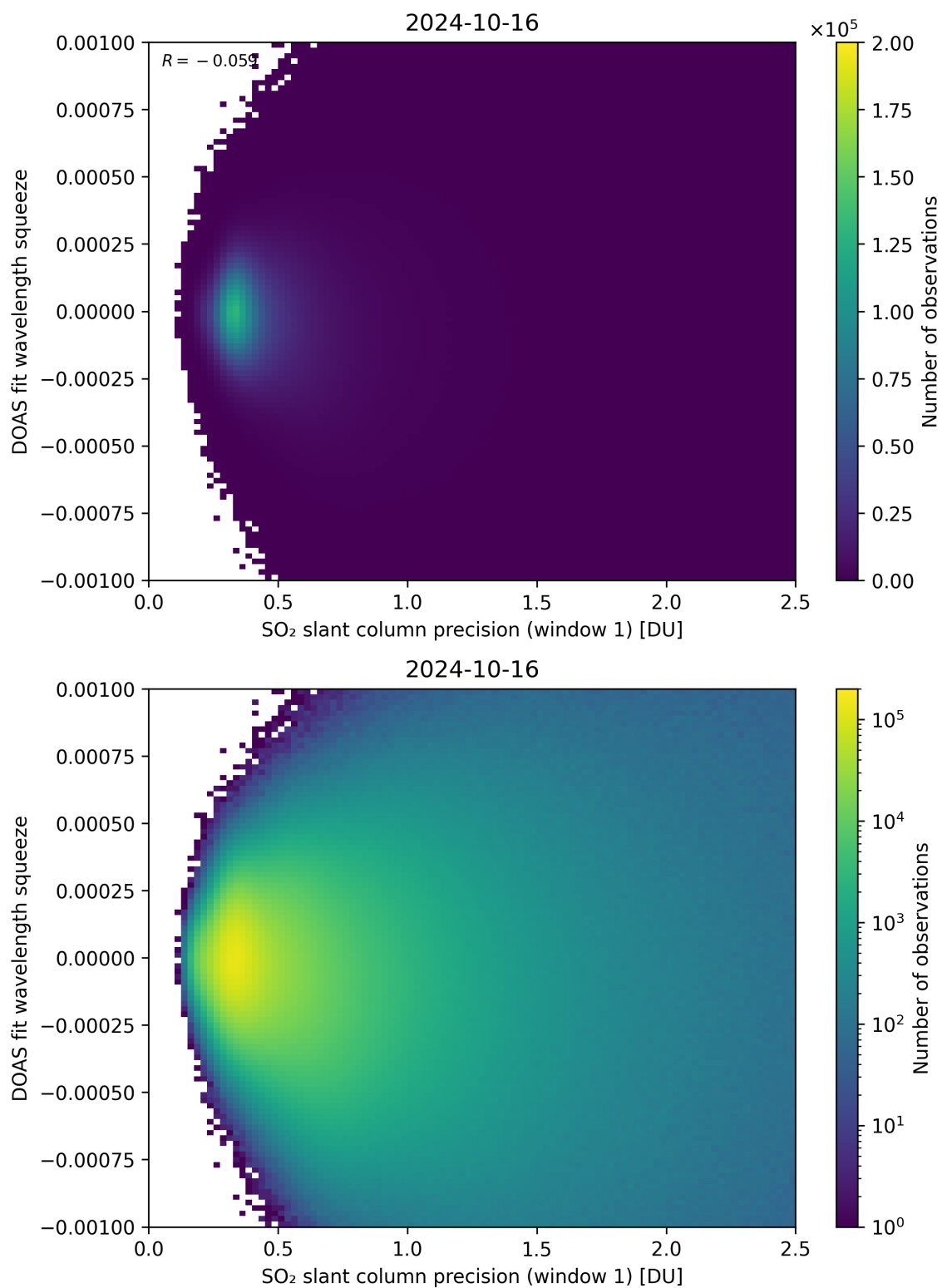
Figure 222: Scatter density plot of “SO 2 slant column precision (window 1)” against “DOAS fit wavelength squeeze” for 2024-10-15 to 2024-10-17.
