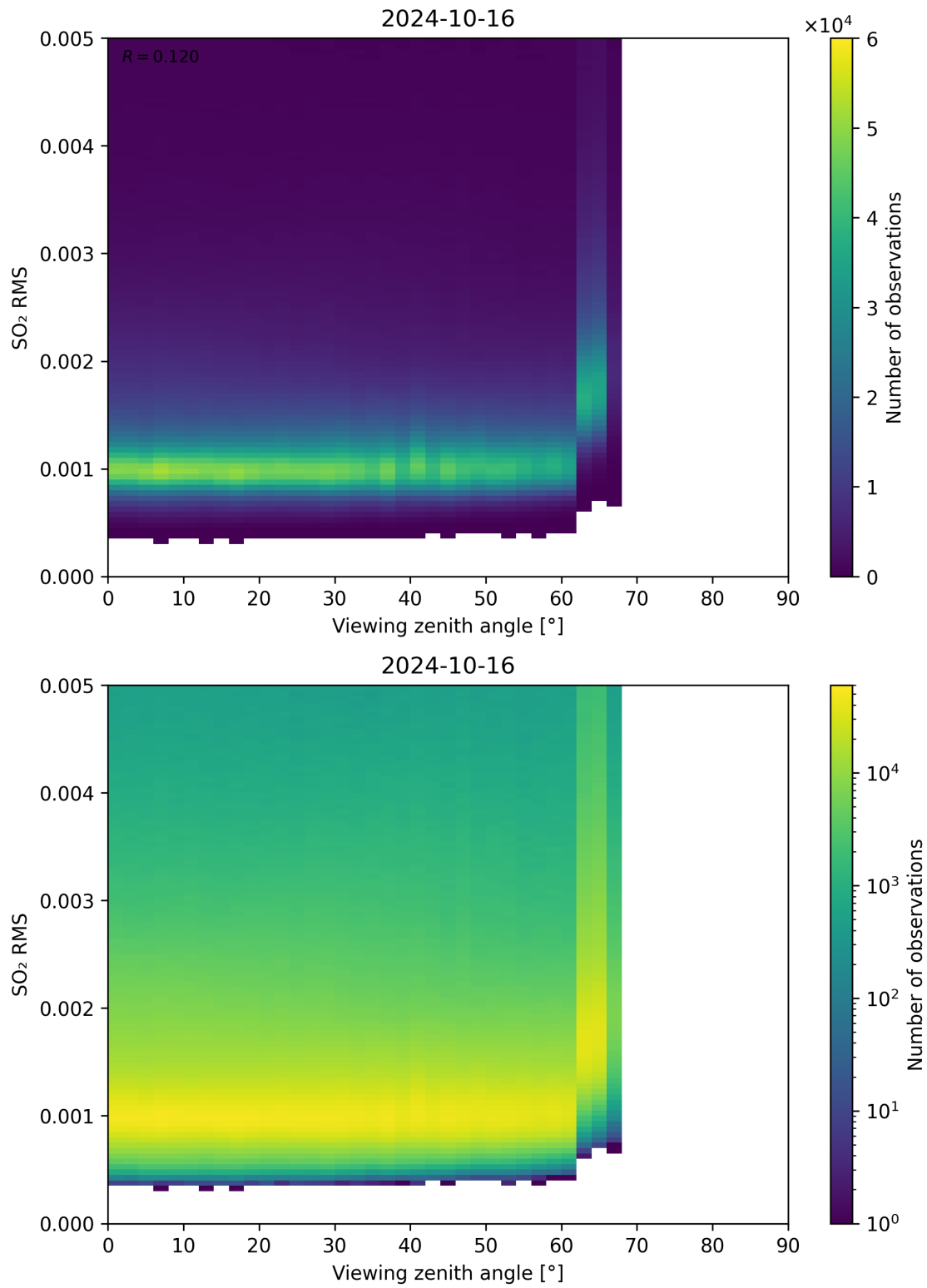
Figure 313: Scatter density plot of “Viewing zenith angle” against “SO 2 RMS” for 2024-10-15 to 2024-10-17.
