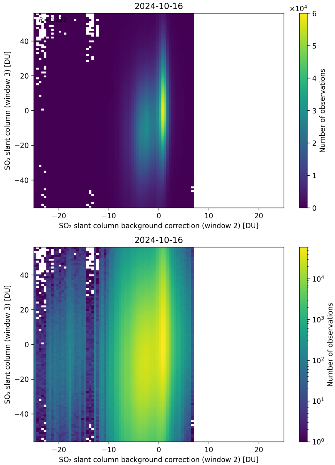
Figure 117: Scatter density plot of “SO 2 slant column background correction (window 2)” against “SO 2 slant column (window 3)” for 2024-10-15 to 2024-10-17.
