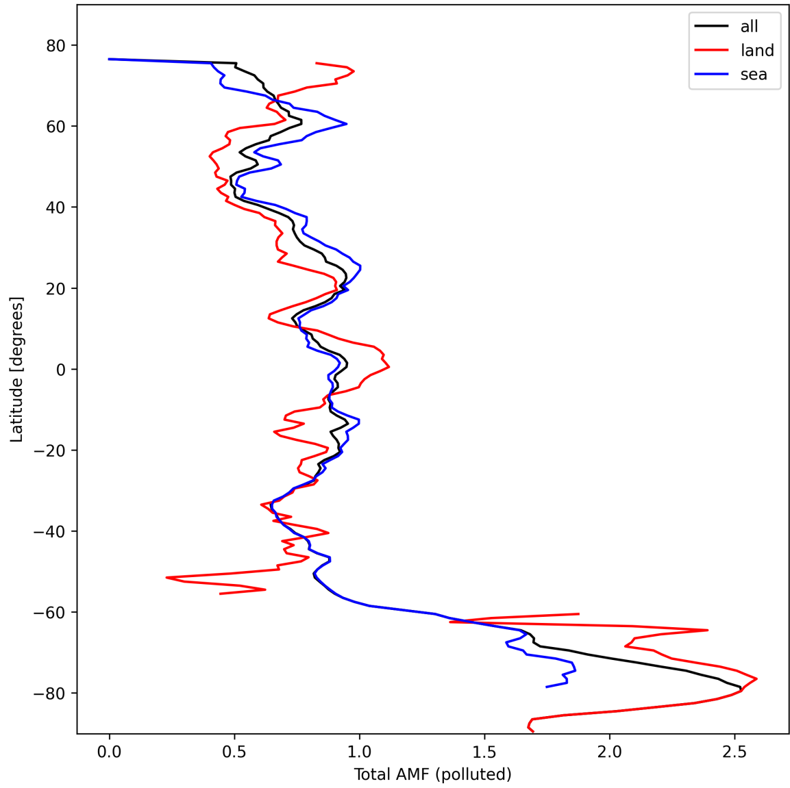
Figure 48: Zonal average of “Total AMF (polluted)” for 2024-10-15 to 2024-10-17.
