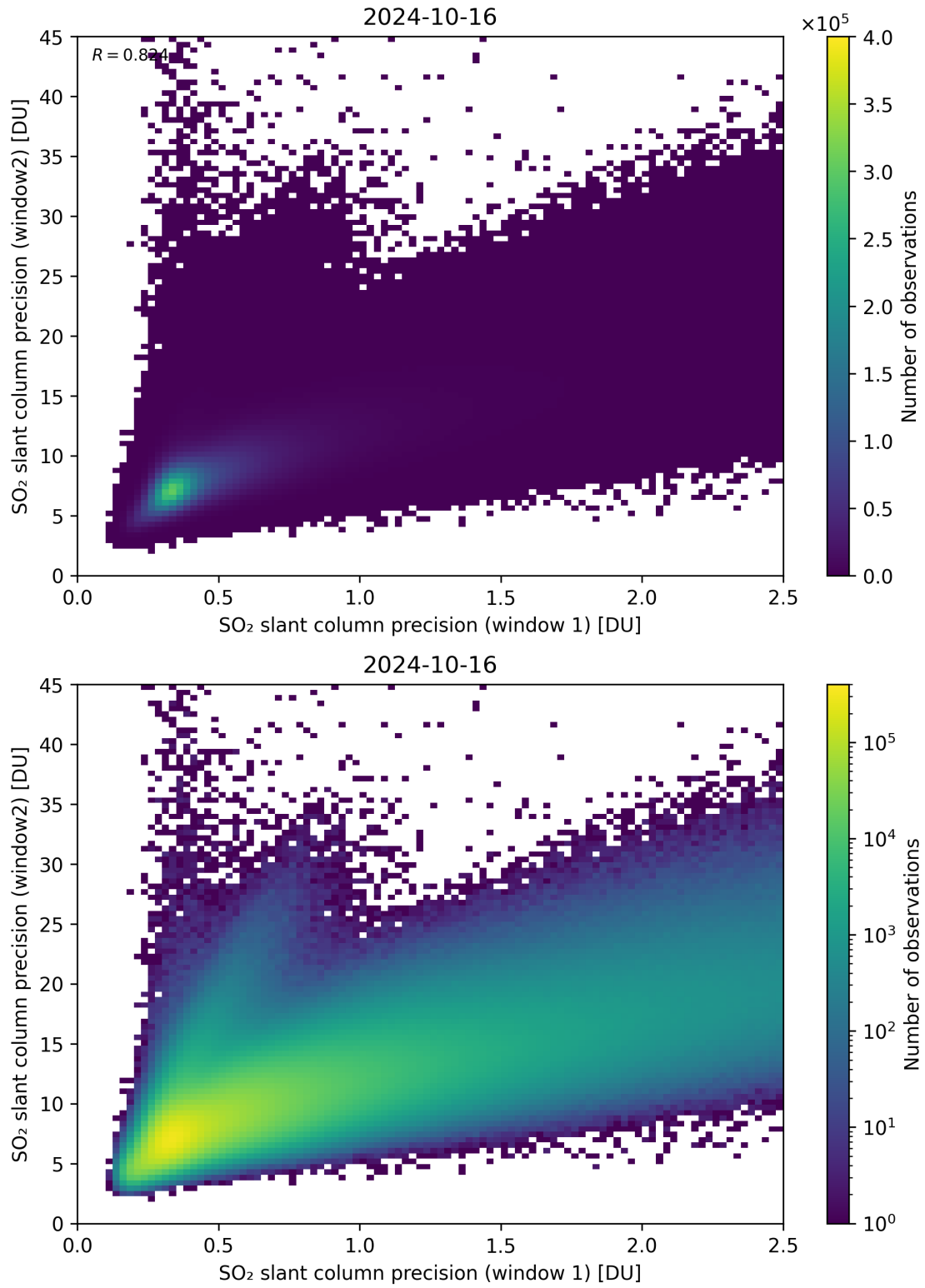
Figure 227: Scatter density plot of “SO 2 slant column precision (window 1)” against “SO 2 slant column precision (window2)” for 2024-10-15 to 2024-10-17.
