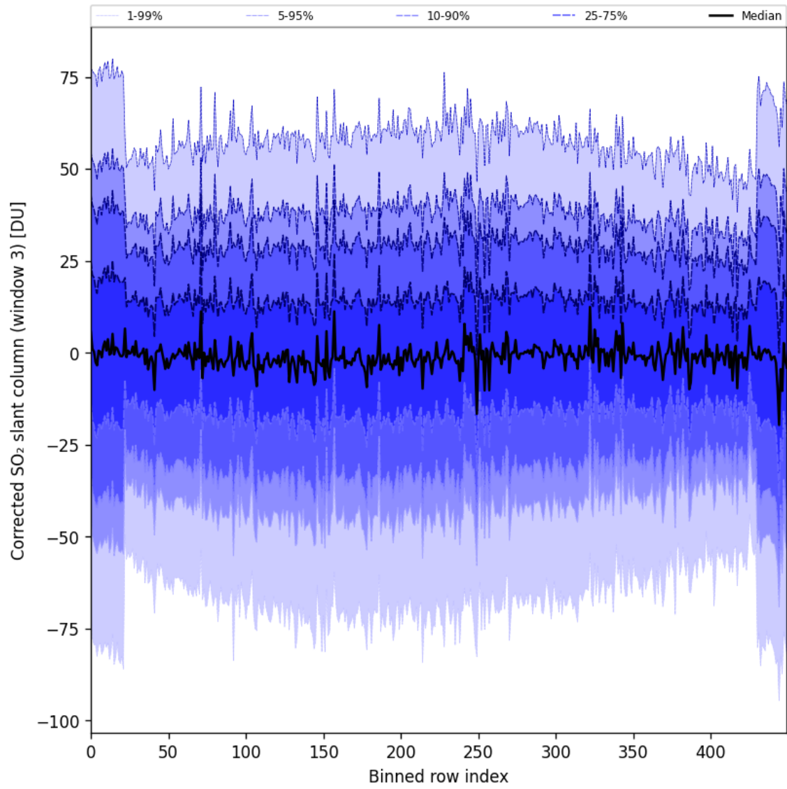
Figure 89: Along track statistics of “Corrected SO 2 slant column (window 3)” for 2024-10-15 to 2024-10-17
