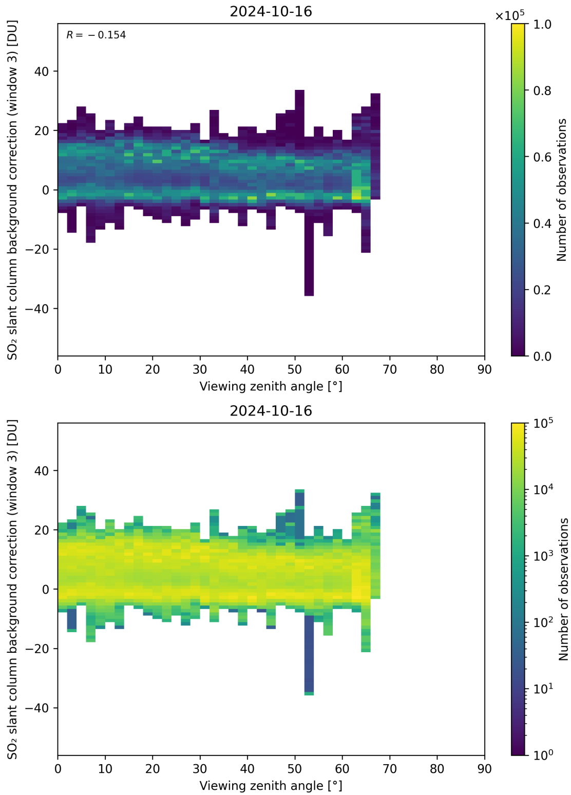
Figure 310: Scatter density plot of “Viewing zenith angle” against “SO 2 slant column background correction (window 3)” for 2024-10-15 to 2024-10-17.
