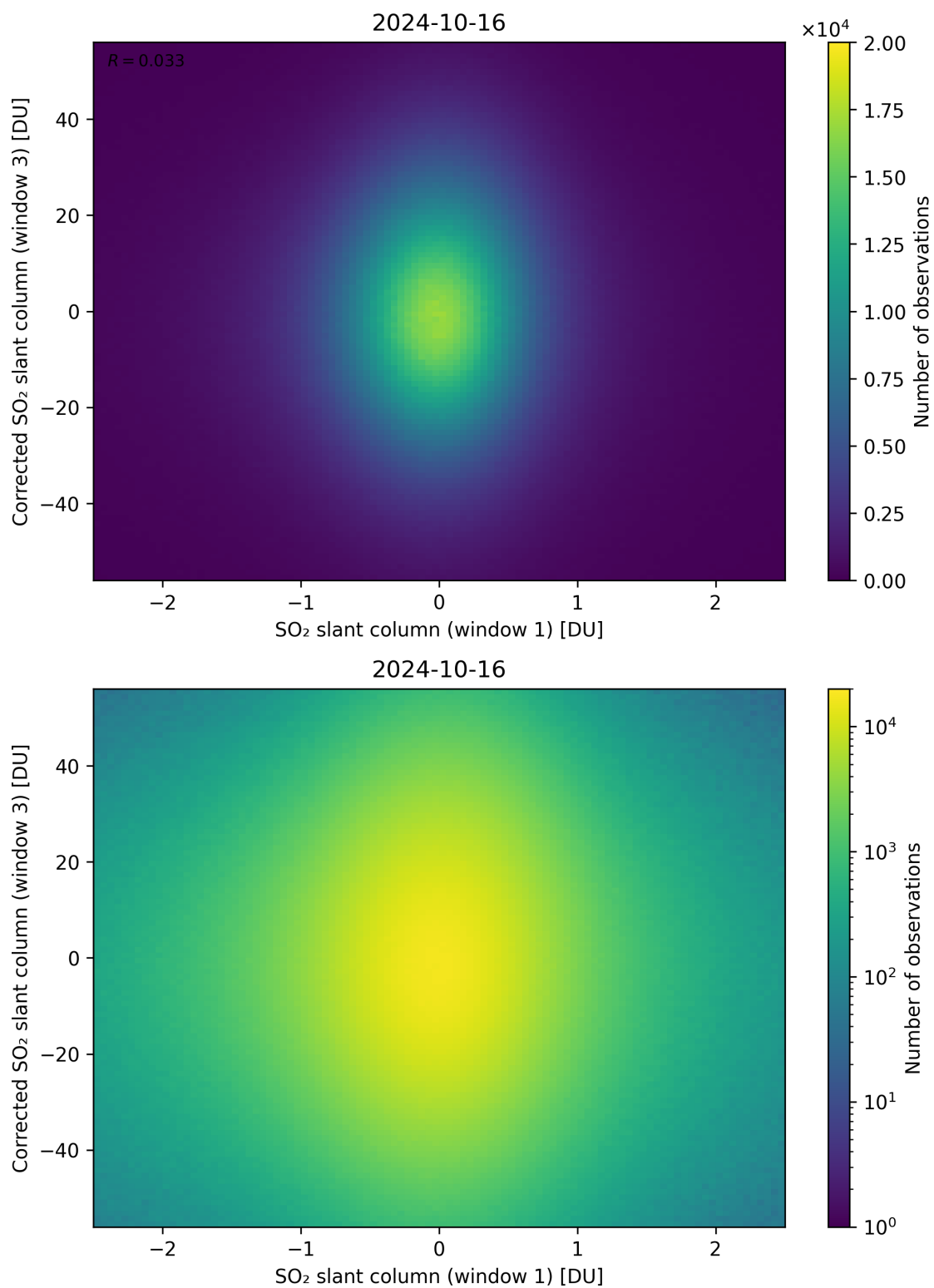
Figure 234: Scatter density plot of “SO 2 slant column (window 1)” against “Corrected SO 2 slant column (window 3)” for 2024-10-15 to 2024-10-17.
