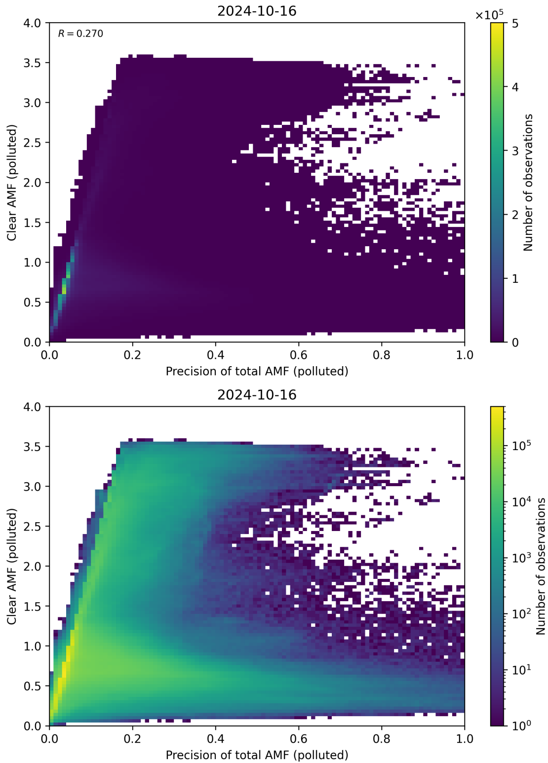
Figure 270: Scatter density plot of “Precision of total AMF (polluted)” against “Clear AMF (polluted)” for 2024-10-15 to 2024-10-17.
