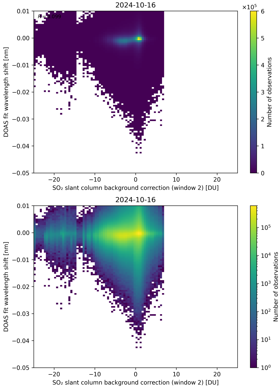
Figure 112: Scatter density plot of “SO 2 slant column background correction (window 2)” against “DOAS fit wavelength shift” for 2024-10-15 to 2024-10-17.
