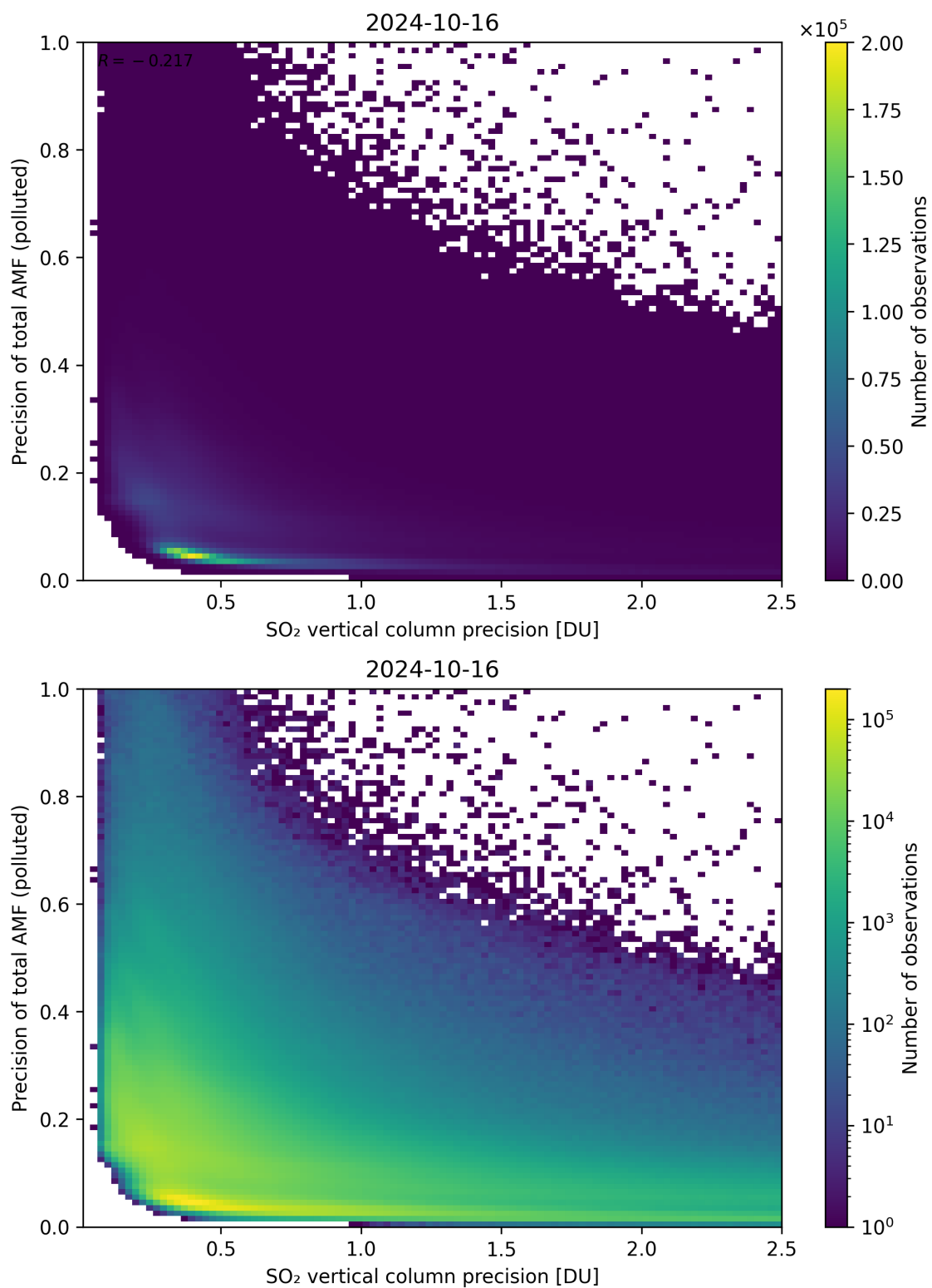
Figure 295: Scatter density plot of “SO 2 vertical column precision” against “Precision of total AMF (polluted)” for 2024-10-15 to 2024-10-17.
