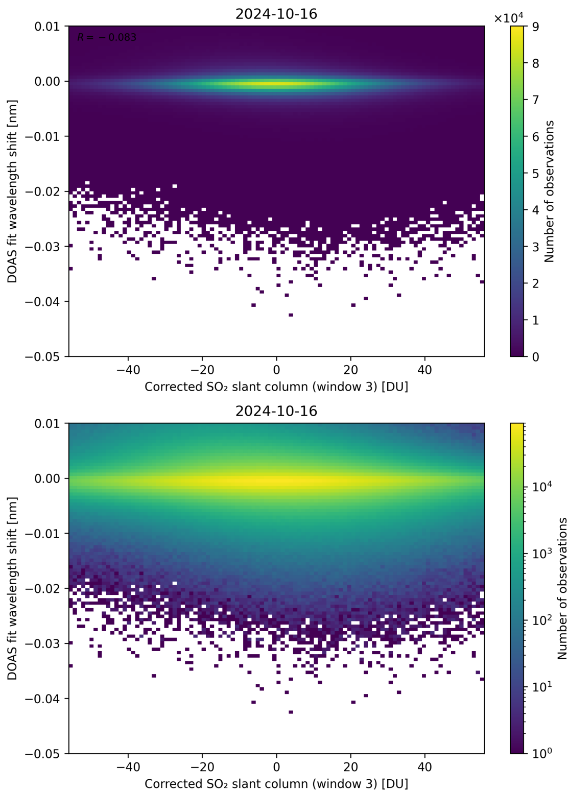
Figure 206: Scatter density plot of “Corrected SO 2 slant column (window 3)” against “DOAS fit wavelength shift” for 2024-10-15 to 2024-10-17.
