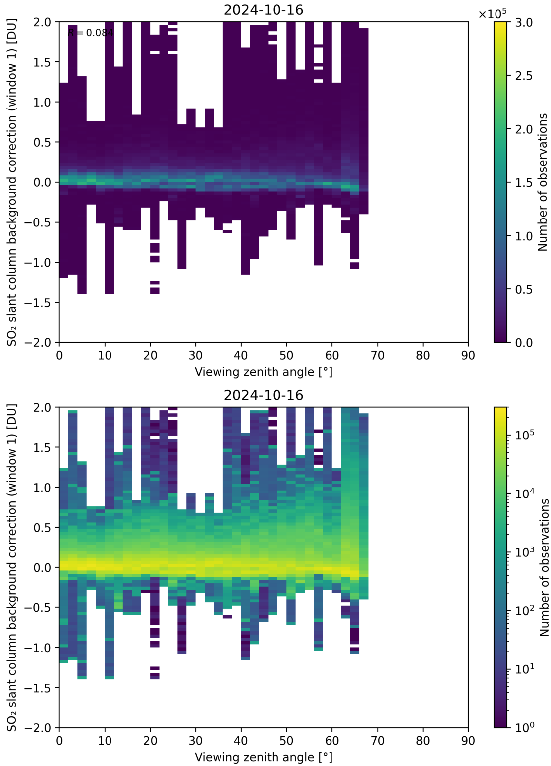
Figure 308: Scatter density plot of “Viewing zenith angle” against “SO 2 slant column background correction (window 1)” for 2024-10-15 to 2024-10-17.
