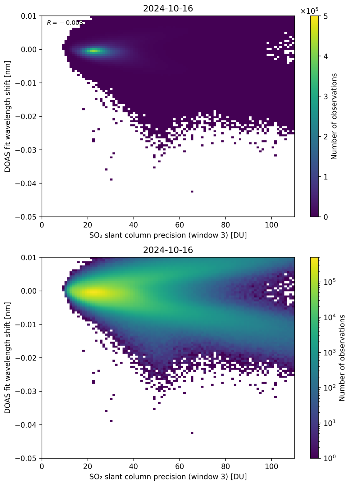
Figure 258: Scatter density plot of “SO 2 slant column precision (window 3)” against “DOAS fit wavelength shift” for 2024-10-15 to 2024-10-17.
