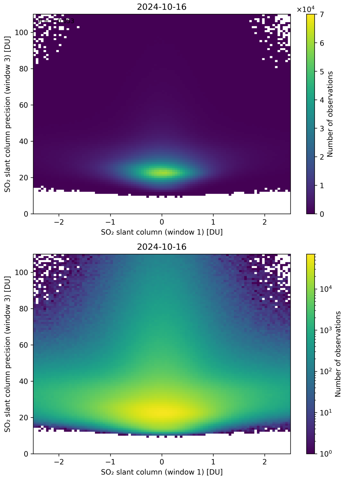
Figure 238: Scatter density plot of “SO 2 slant column (window 1)” against “SO 2 slant column precision (window 3)” for 2024-10-15 to 2024-10-17.
