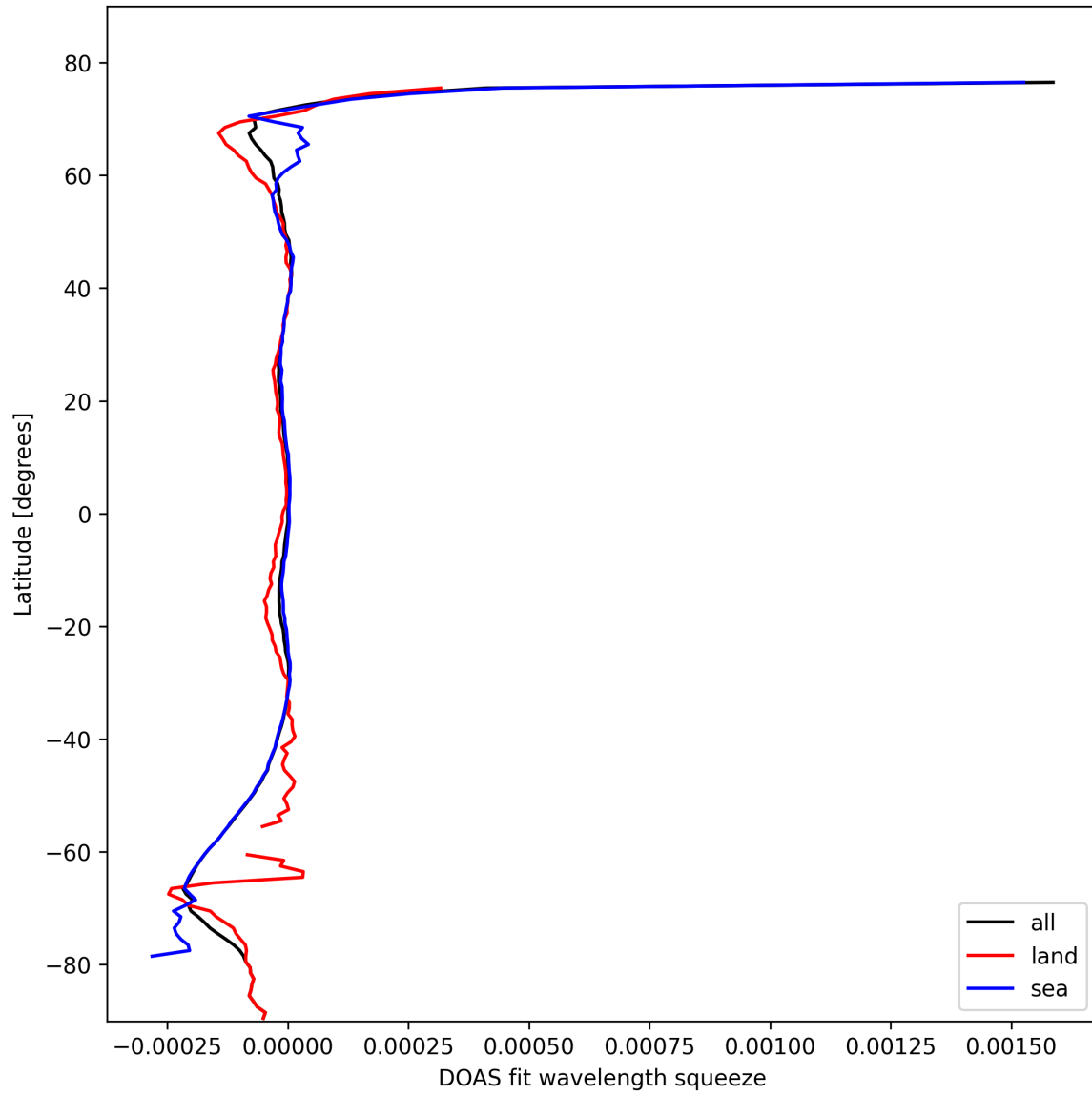
Figure 46: Zonal average of “DOAS fit wavelength squeeze” for 2024-10-15 to 2024-10-17.
