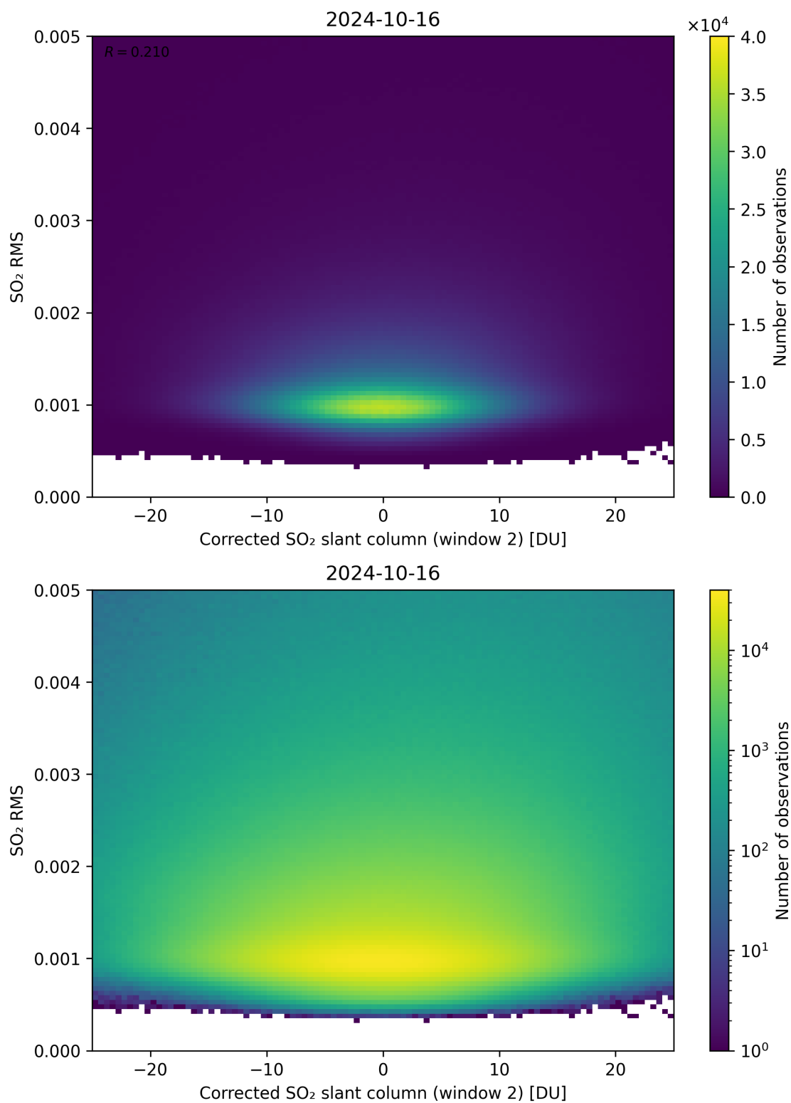
Figure 198: Scatter density plot of “Corrected SO 2 slant column (window 2)” against “SO 2 RMS” for 2024-10-15 to 2024-10-17.
