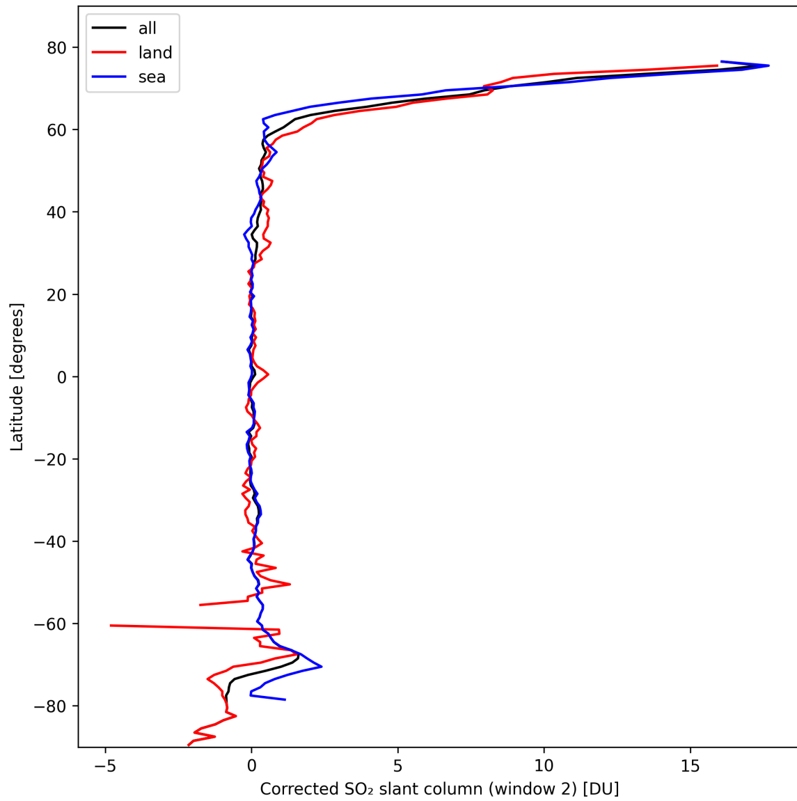
Figure 39: Zonal average of “Corrected SO 2 slant column (window 2)” for 2024-10-15 to 2024-10-17.
