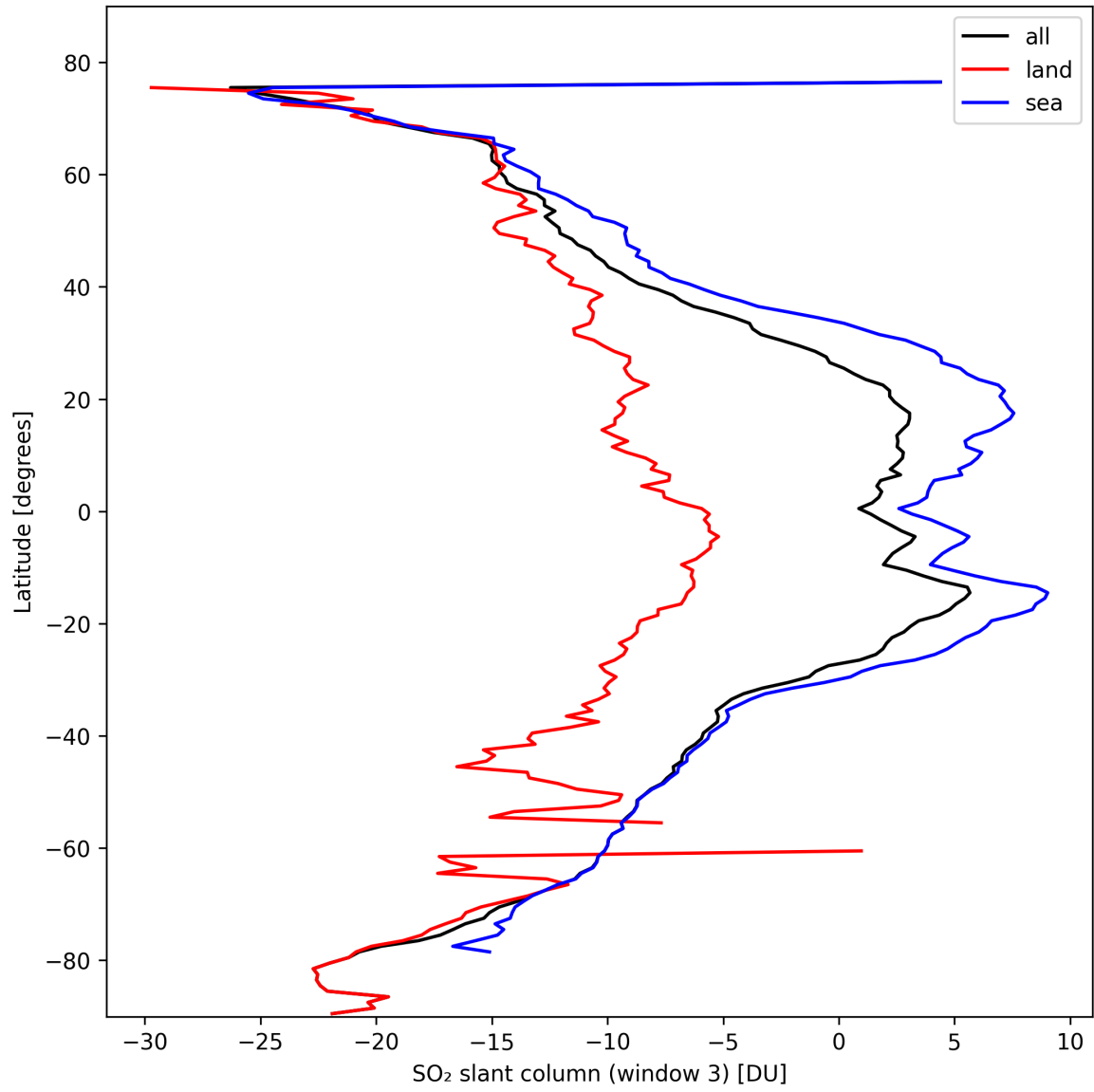
Figure 41: Zonal average of “SO 2 slant column (window 3)” for 2024-10-15 to 2024-10-17.
