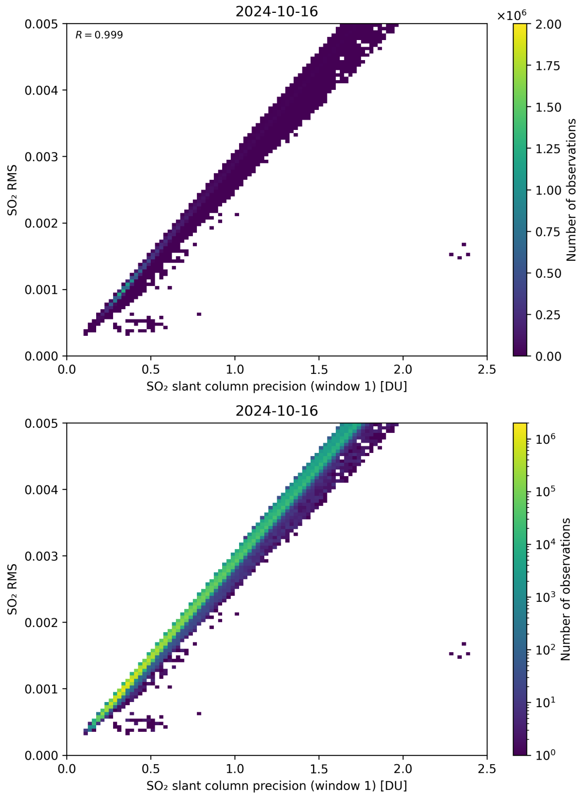
Figure 223: Scatter density plot of “SO 2 slant column precision (window 1)” against “SO 2 RMS” for 2024-10-15 to 2024-10-17.
