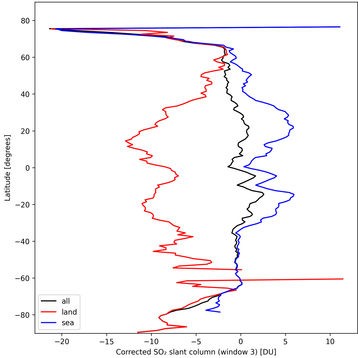
Figure 43: Zonal average of “Corrected SO 2 slant column (window 3)” for 2024-10-15 to 2024-10-17.
