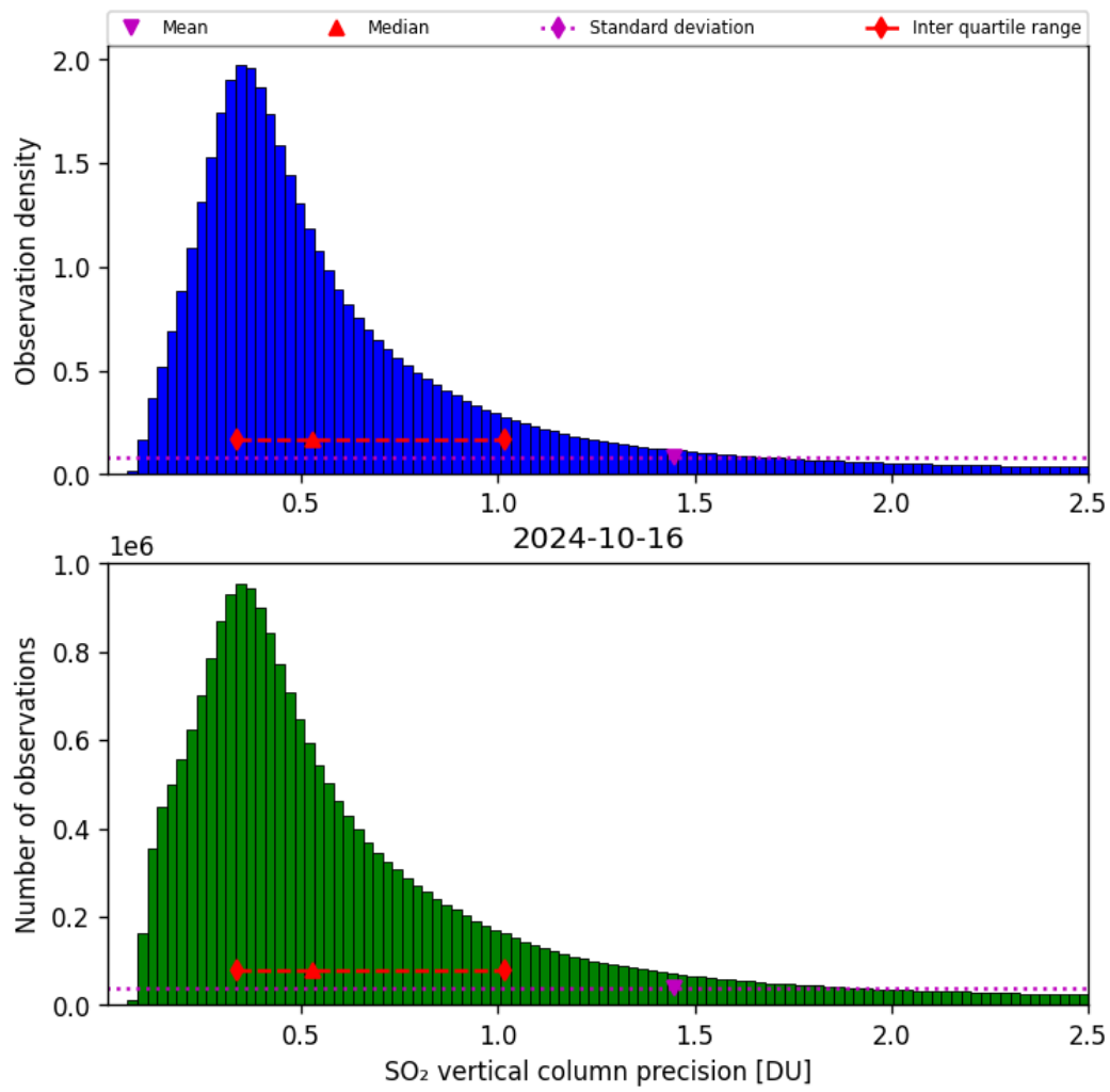
Figure 54: Histogram of “SO 2 vertical column precision” for 2024-10-15 to 2024-10-17
