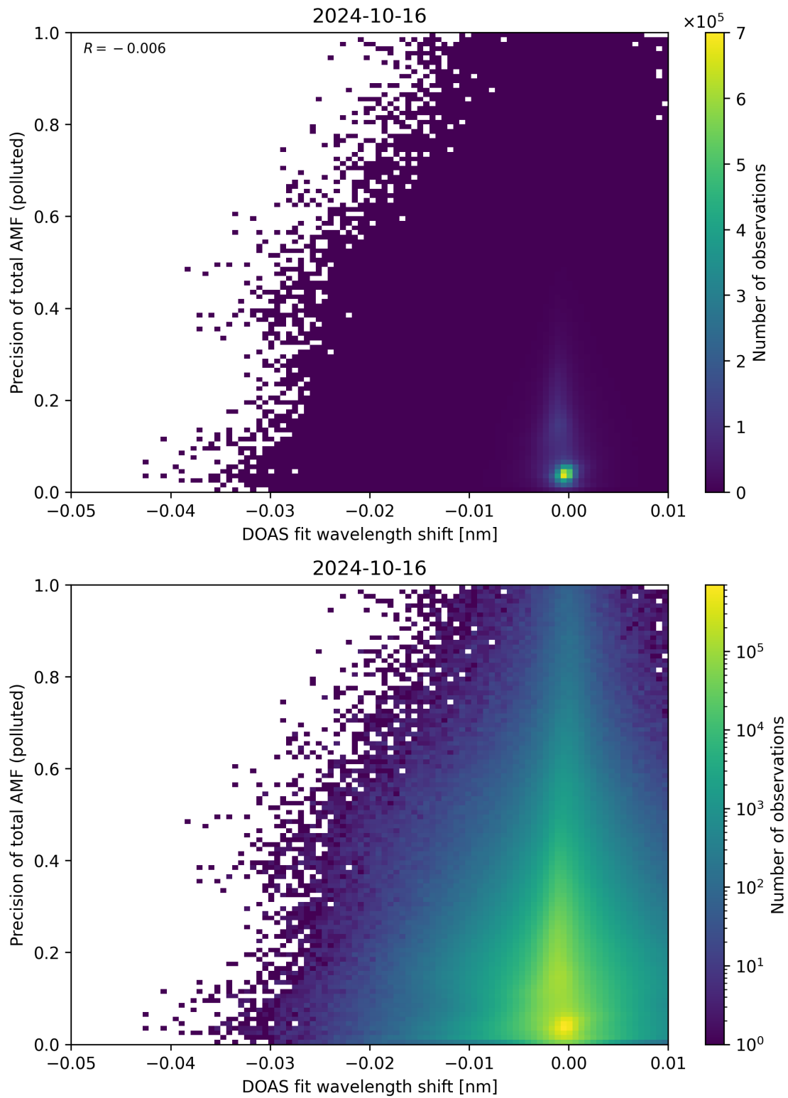
Figure 131: Scatter density plot of “DOAS fit wavelength shift” against “Precision of total AMF (polluted)” for 2024-10-15 to 2024-10-17.
