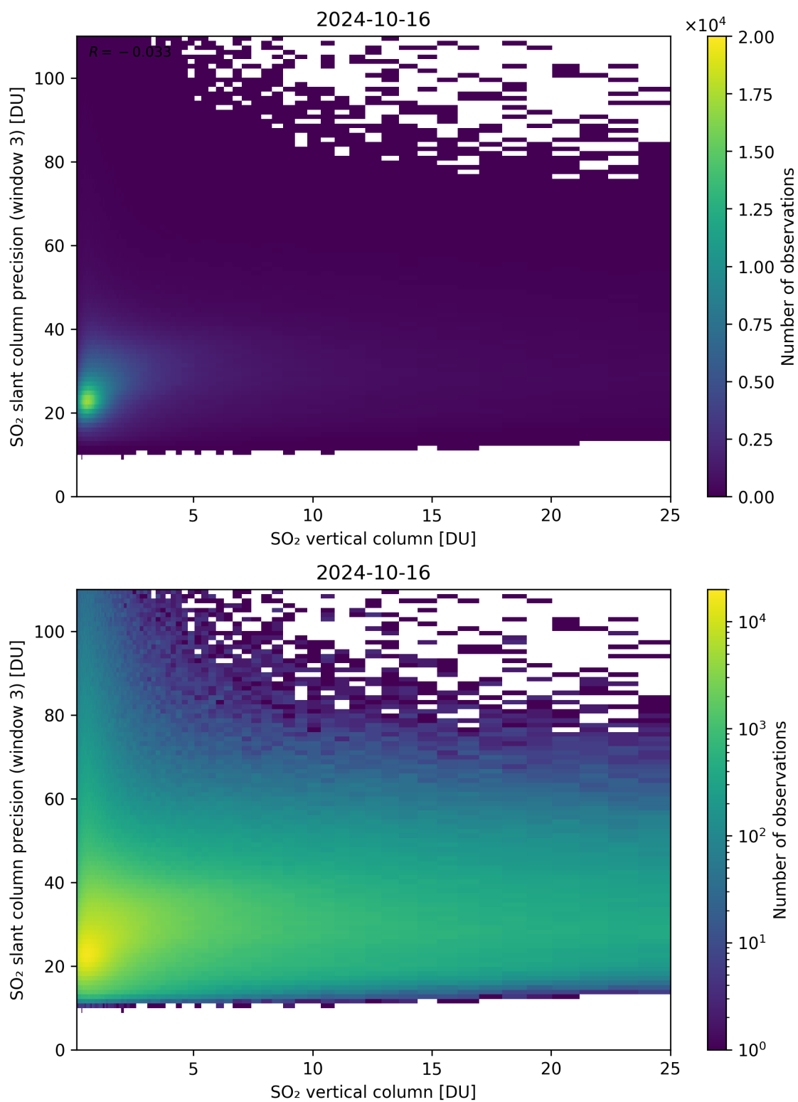
Figure 304: Scatter density plot of “SO 2 vertical column” against “SO 2 slant column precision (window 3)” for 2024-10-15 to 2024-10-17.
