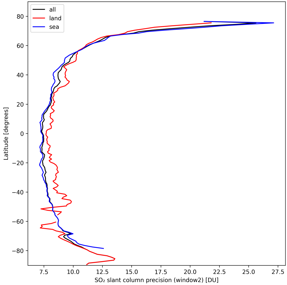
Figure 38: Zonal average of “SO 2 slant column precision (window2)” for 2024-10-15 to 2024-10-17.
