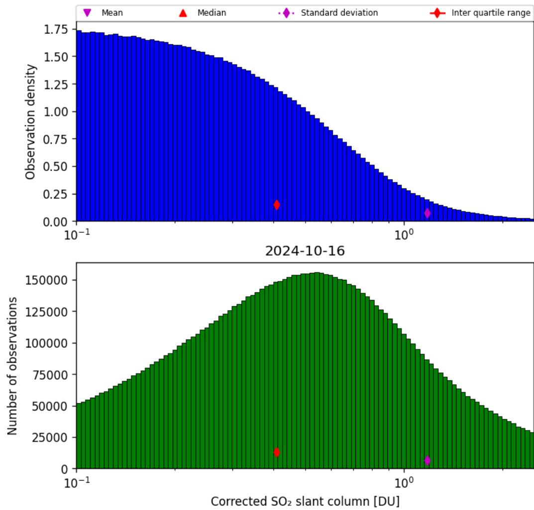
Figure 55: Histogram of “Corrected SO 2 slant column” for 2024-10-15 to 2024-10-17
