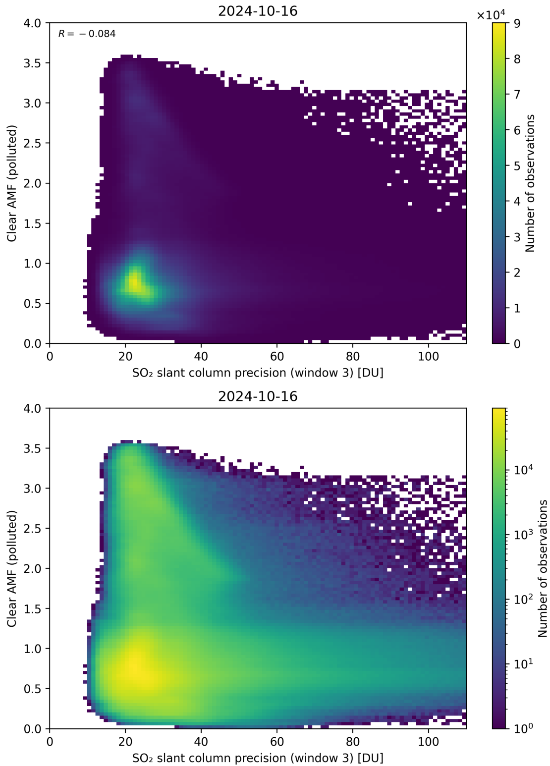
Figure 261: Scatter density plot of “SO 2 slant column precision (window 3)” against “Clear AMF (polluted)” for 2024-10-15 to 2024-10-17.
