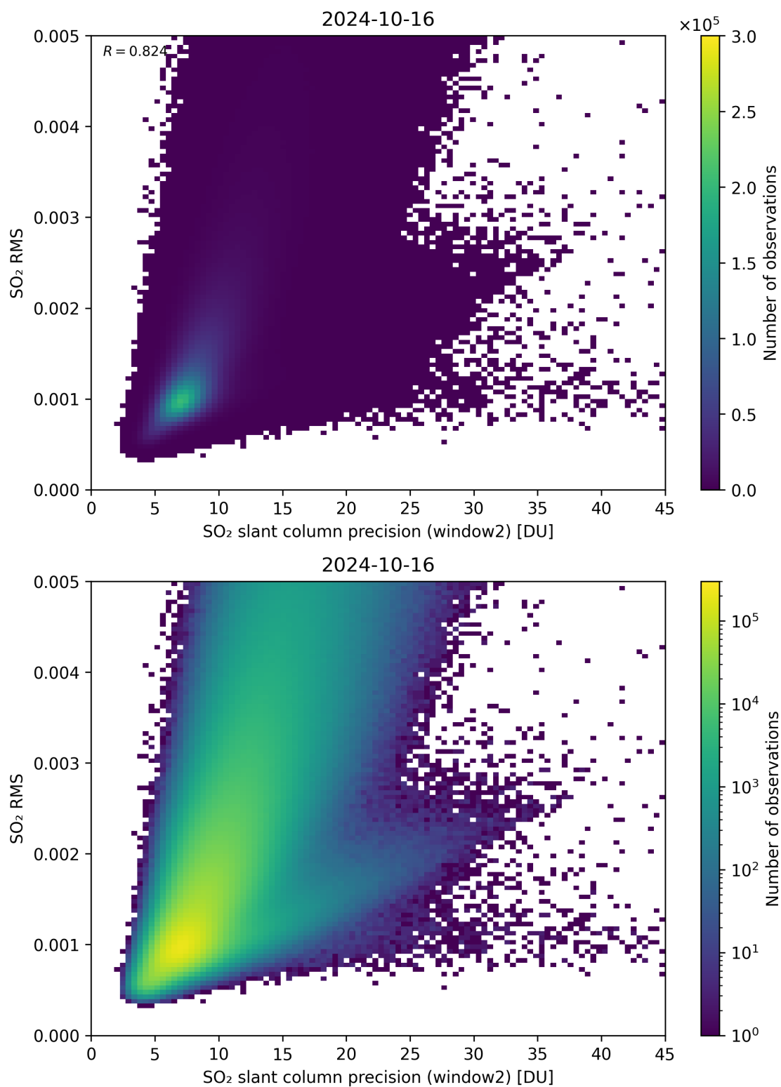
Figure 245: Scatter density plot of “SO 2 slant column precision (window2)” against “SO 2 RMS” for 2024-10-15 to 2024-10-17.
