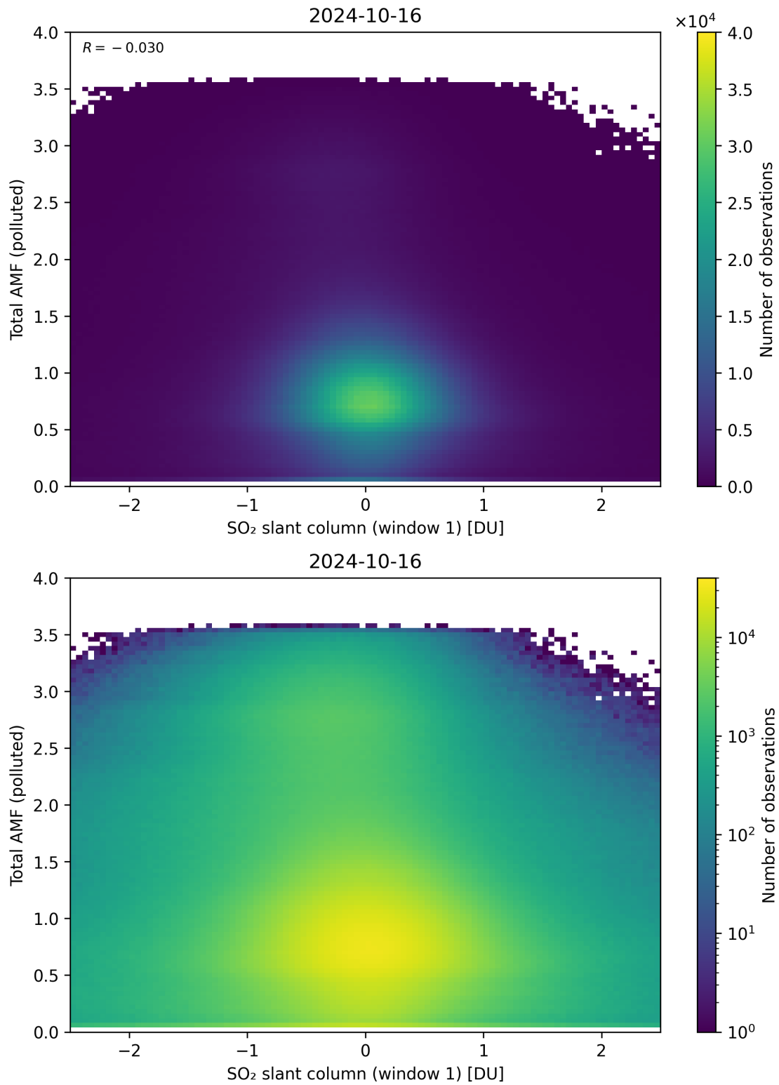
Figure 239: Scatter density plot of “SO 2 slant column (window 1)” against “Total AMF (polluted)” for 2024-10-15 to 2024-10-17.
