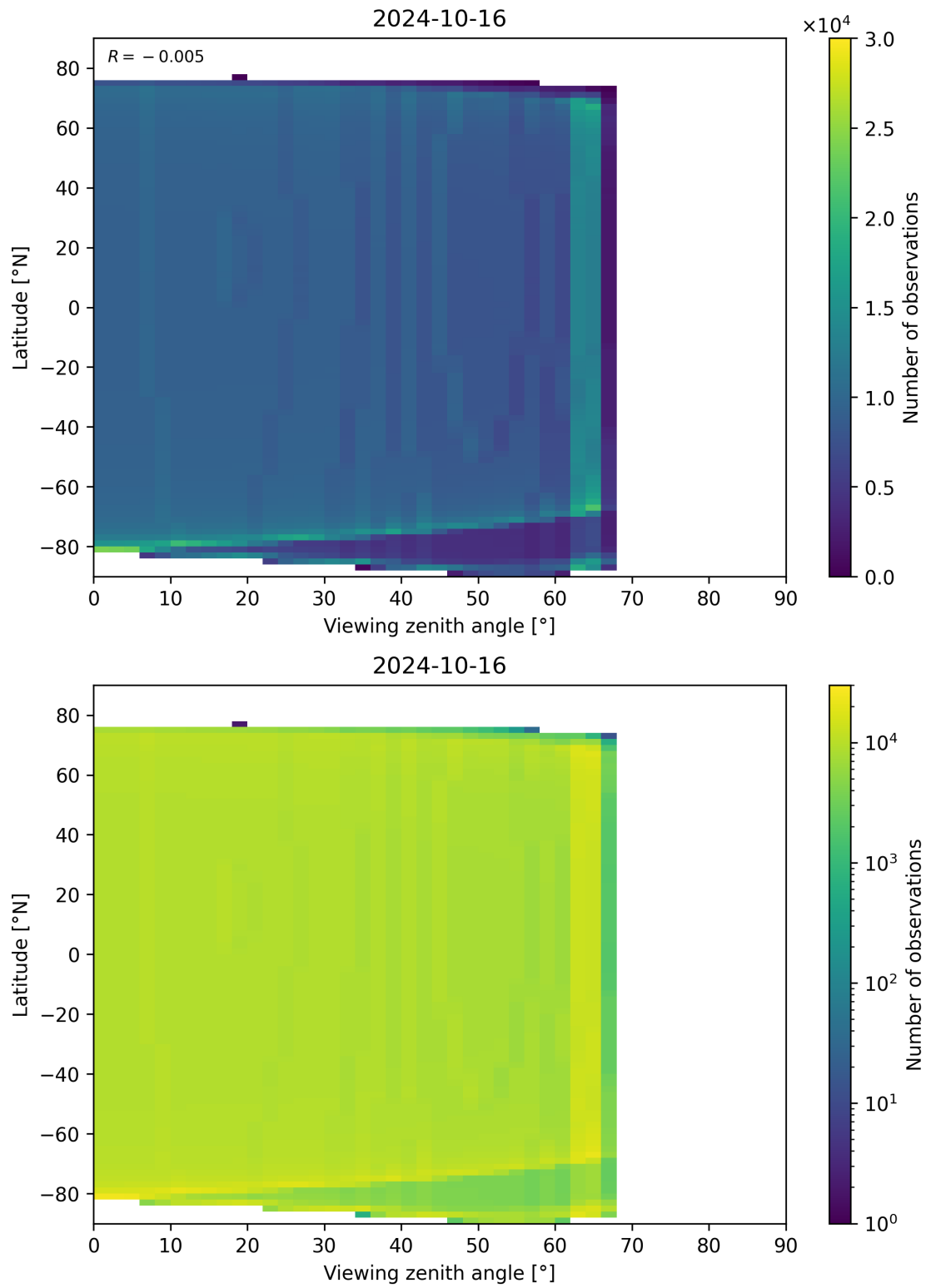
Figure 314: Scatter density plot of “Viewing zenith angle” against “Latitude” for 2024-10-15 to 2024-10-17.
