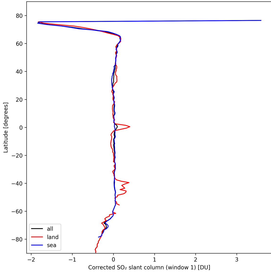
Figure 35: Zonal average of “Corrected SO 2 slant column (window 1)” for 2024-10-15 to 2024-10-17.
