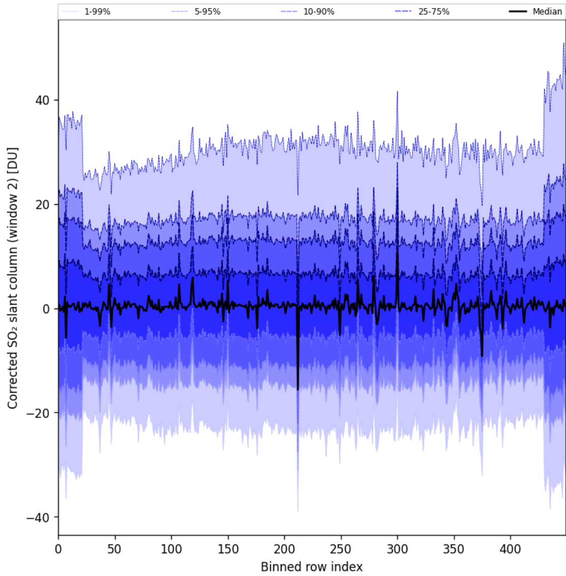
Figure 85: Along track statistics of “Corrected SO 2 slant column (window 2)” for 2024-10-15 to 2024-10-17
