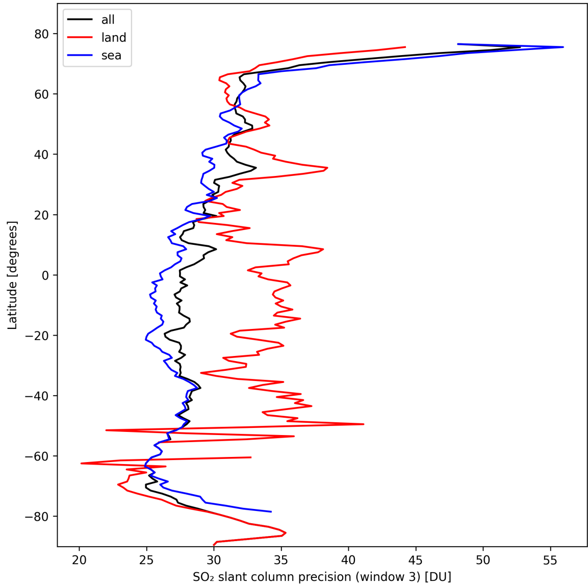
Figure 42: Zonal average of “SO 2 slant column precision (window 3)” for 2024-10-15 to 2024-10-17.
