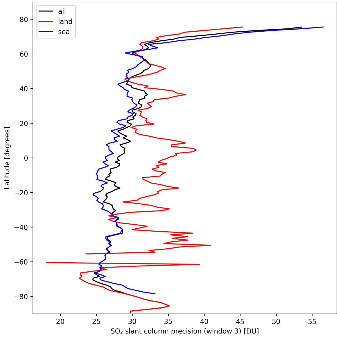
Figure 42: Zonal average of “SO 2 slant column precision (window 3)” for 2024-10-16 to 2024-10-18.
