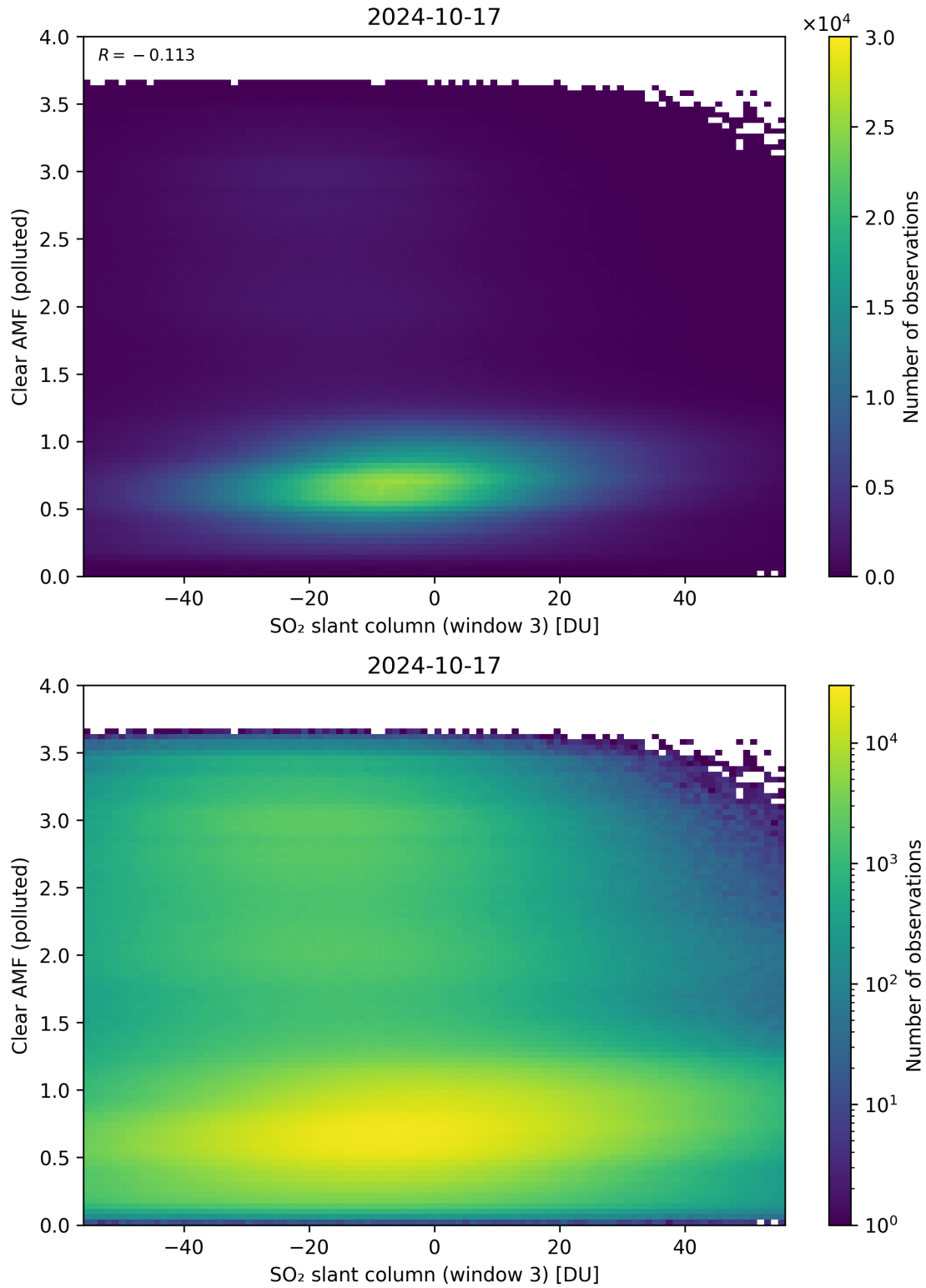
Figure 265: Scatter density plot of “SO 2 slant column (window 3)” against “Clear AMF (polluted)” for 2024-10-16 to 2024-10-18.
