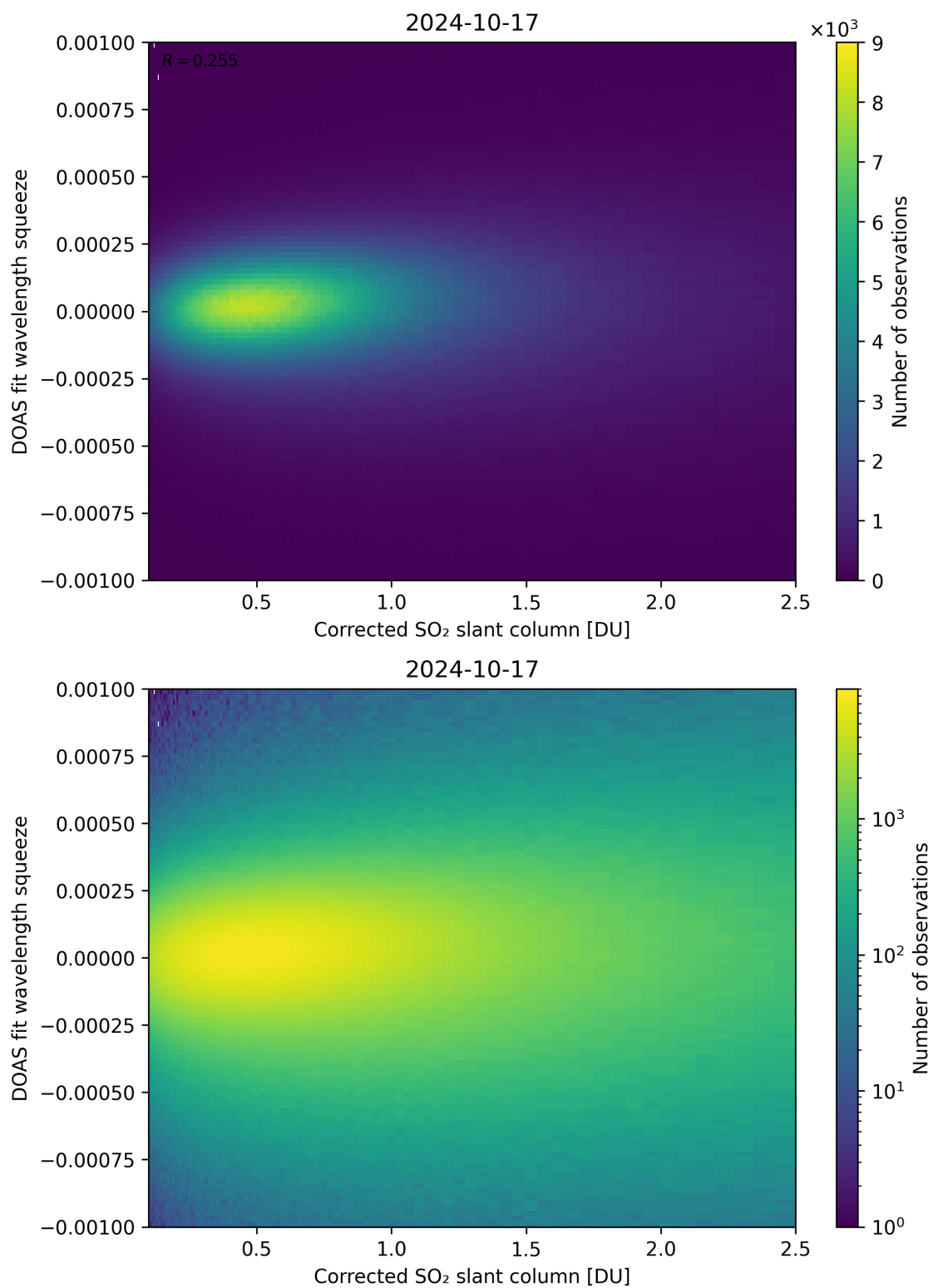
Figure 182: Scatter density plot of “Corrected SO 2 slant column” against “DOAS fit wavelength squeeze” for 2024-10-16 to 2024-10-18.
