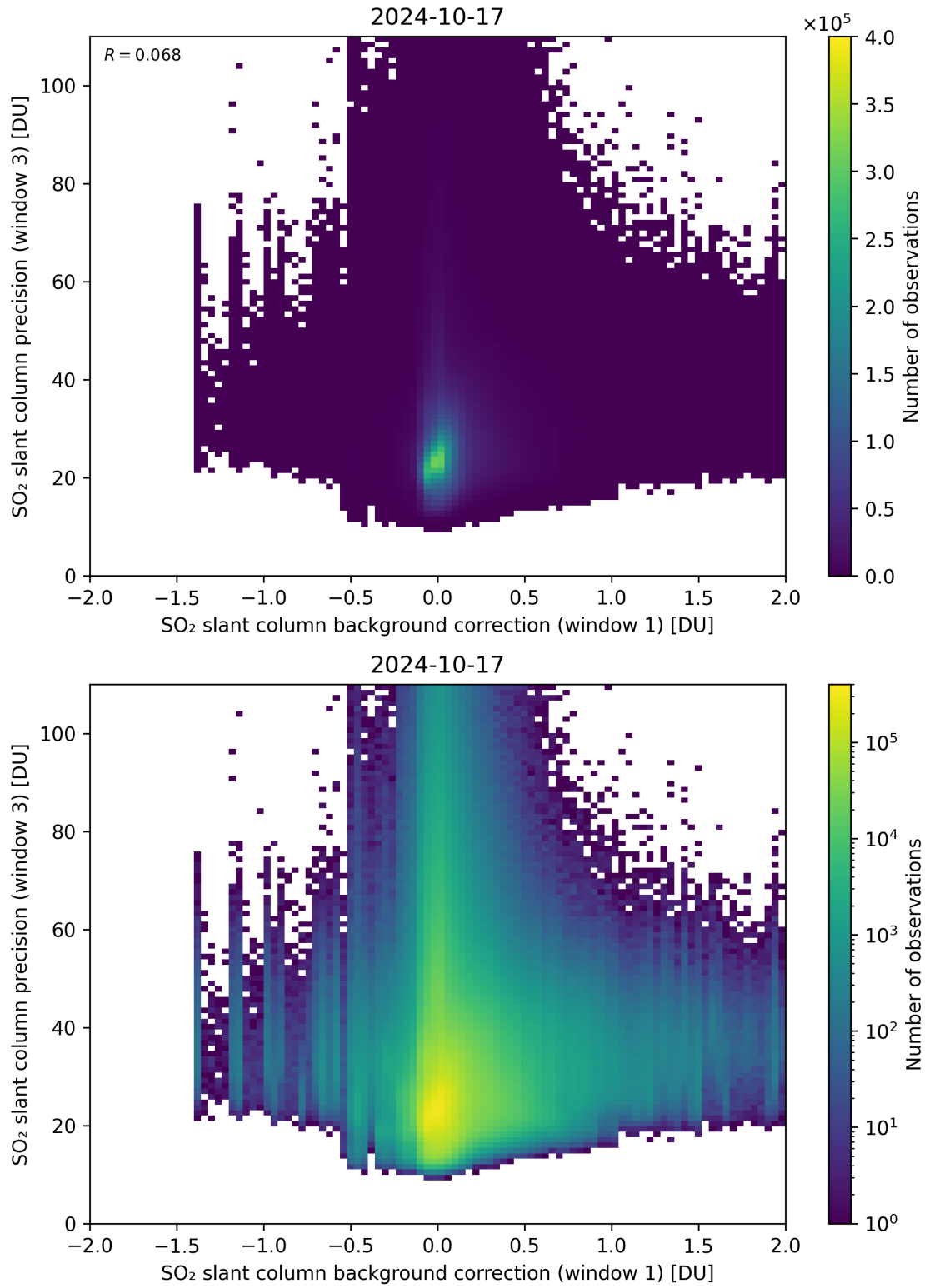
Figure 108: Scatter density plot of “SO 2 slant column background correction (window 1)” against “SO 2 slant column precision (window 3)” for 2024-10-16 to 2024-10-18.
