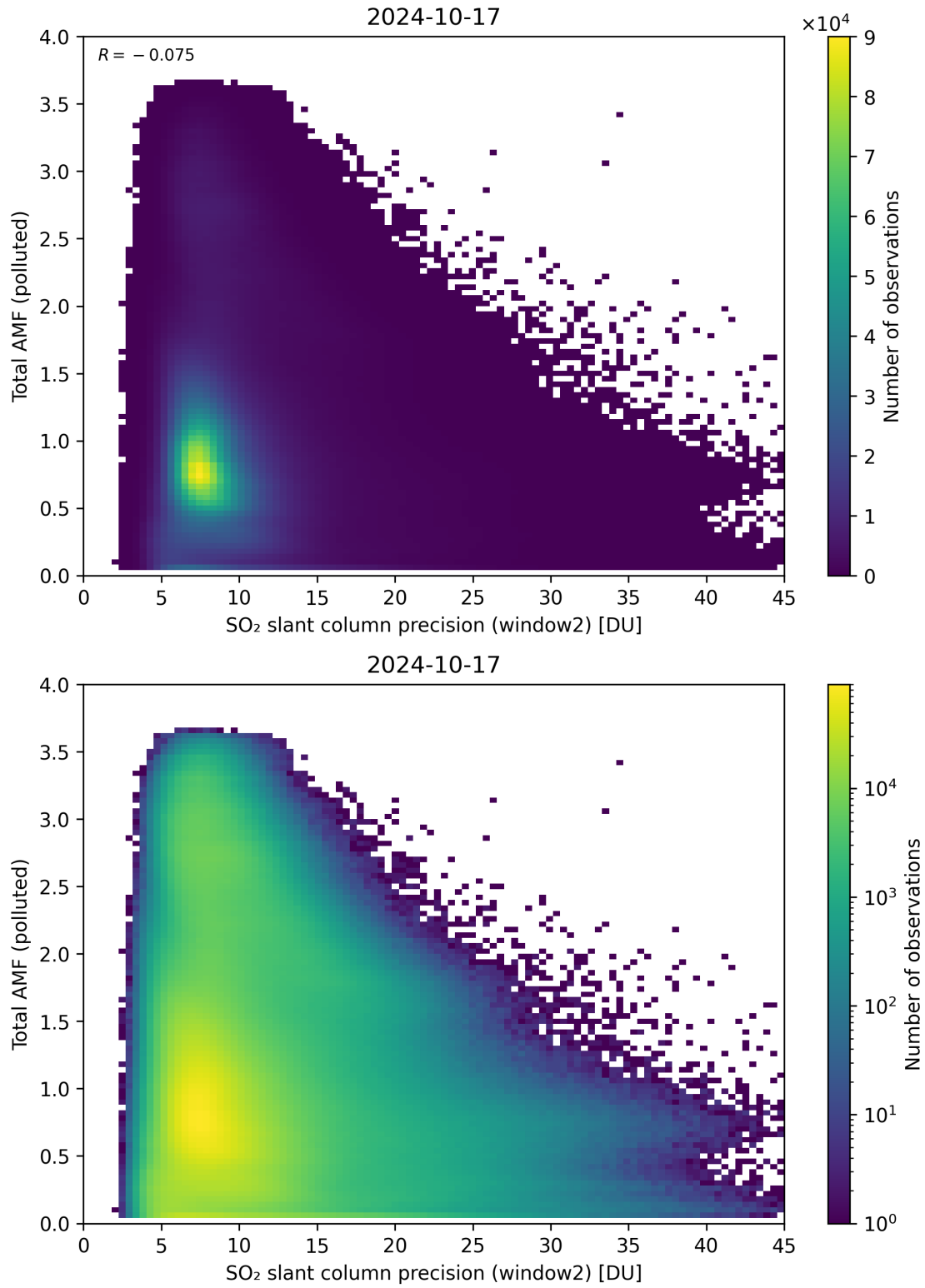
Figure 251: Scatter density plot of “SO 2 slant column precision (window2)” against “Total AMF (polluted)” for 2024-10-16 to 2024-10-18.
