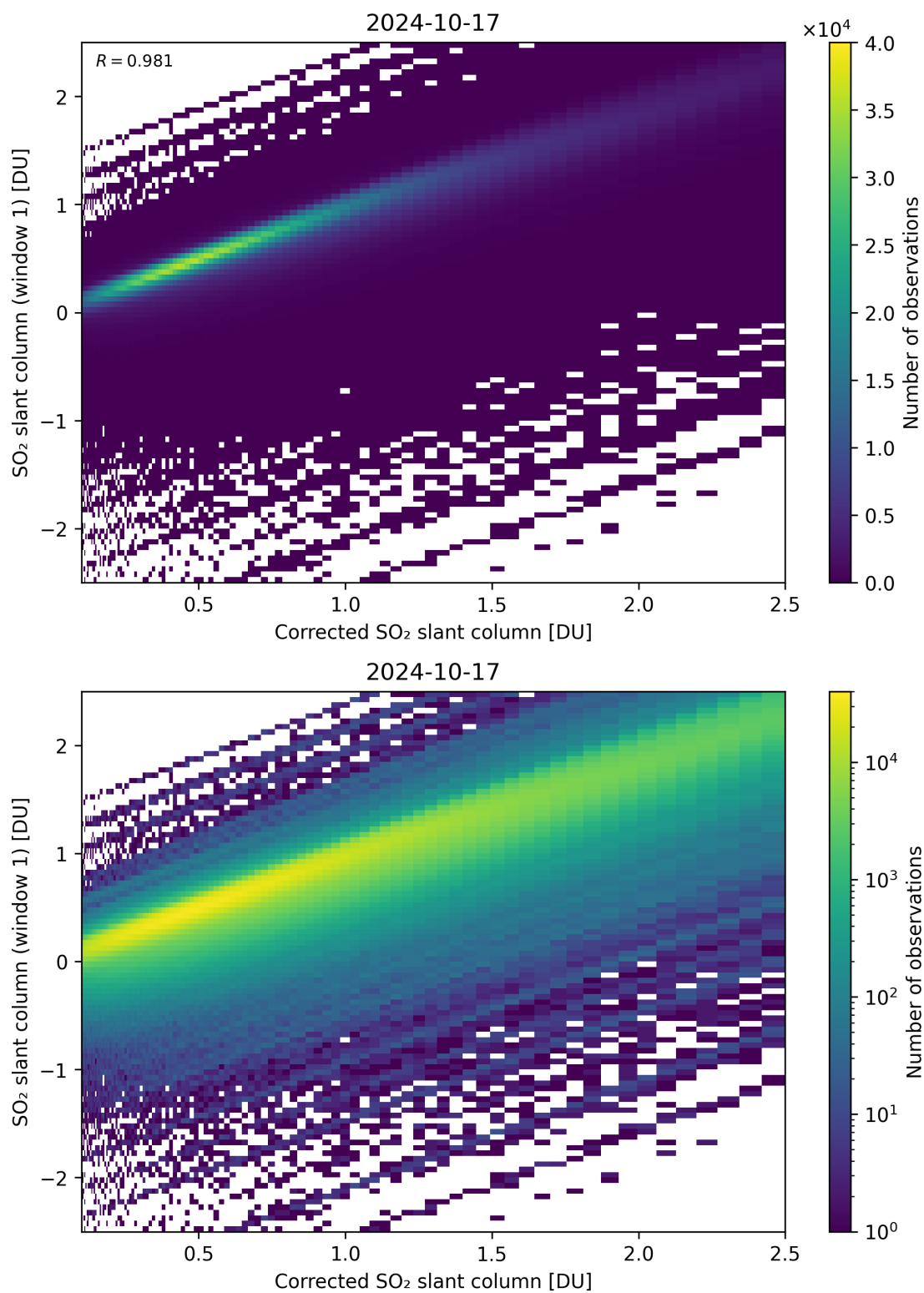
Figure 187: Scatter density plot of “Corrected SO 2 slant column” against “SO 2 slant column (window 1)” for 2024-10-16 to 2024-10-18.
