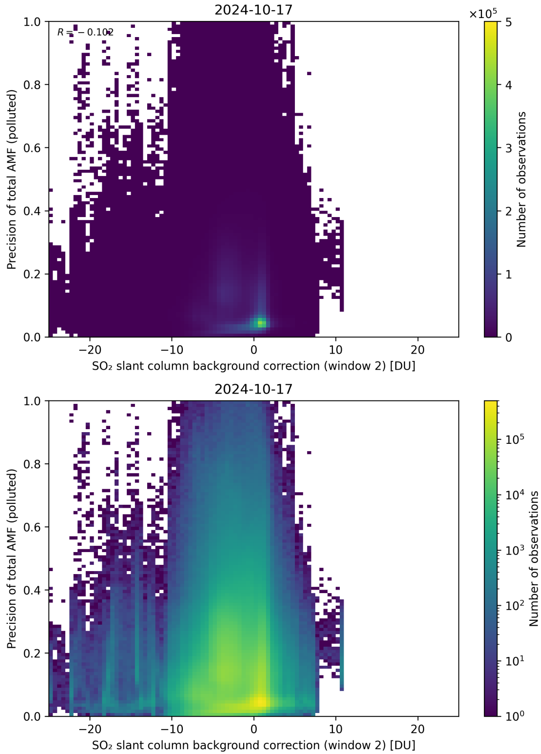
Figure 120: Scatter density plot of “SO 2 slant column background correction (window 2)” against “Precision of total AMF (polluted)” for 2024-10-16 to 2024-10-18.
