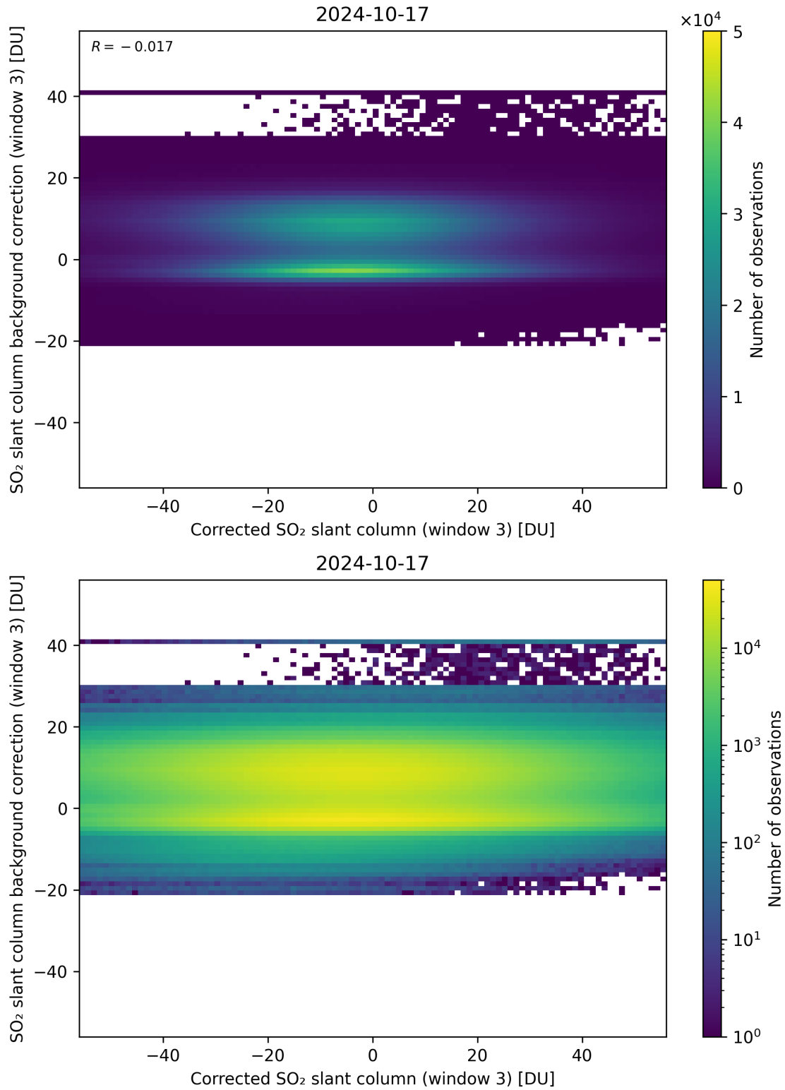
Figure 205: Scatter density plot of “Corrected SO 2 slant column (window 3)” against “SO 2 slant column background correction (window 3)” for 2024-10-16 to 2024-10-18.
