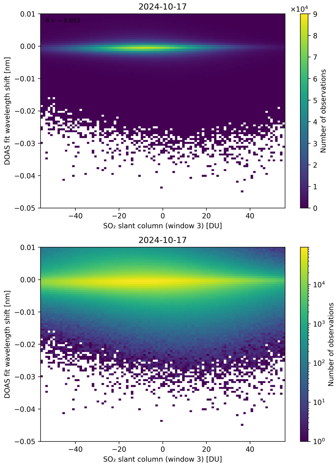
Figure 254: Scatter density plot of “SO 2 slant column (window 3)” against “DOAS fit wavelength shift” for 2024-10-16 to 2024-10-18.
