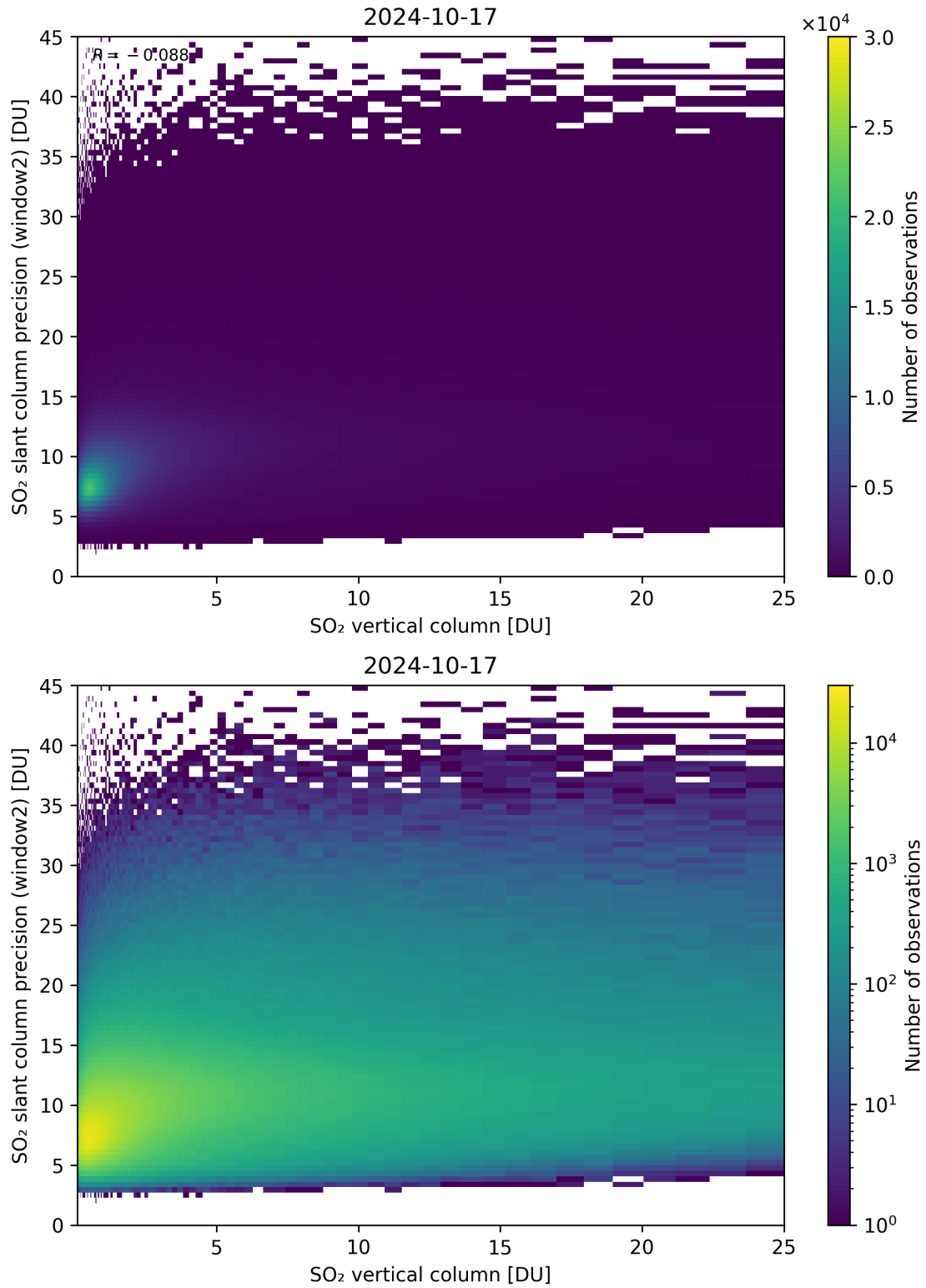
Figure 302: Scatter density plot of “SO 2 vertical column” against “SO 2 slant column precision (window2)” for 2024-10-16 to 2024-10-18.
