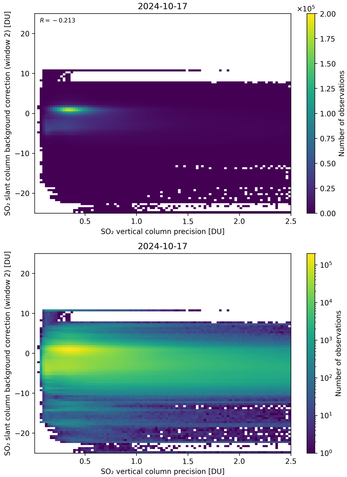
Figure 280: Scatter density plot of “SO 2 vertical column precision” against “SO 2 slant column background correction (window 2)” for 2024-10-16 to 2024-10-18.
