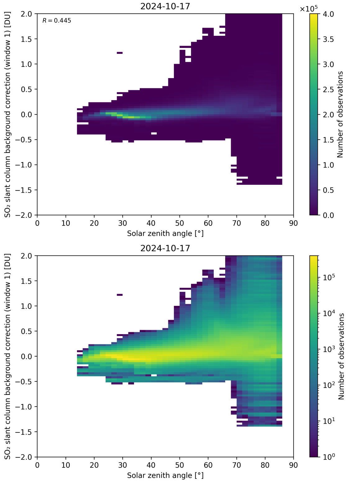
Figure 158: Scatter density plot of “Solar zenith angle” against “SO 2 slant column background correction (window 1)” for 2024-10-16 to 2024-10-18.
