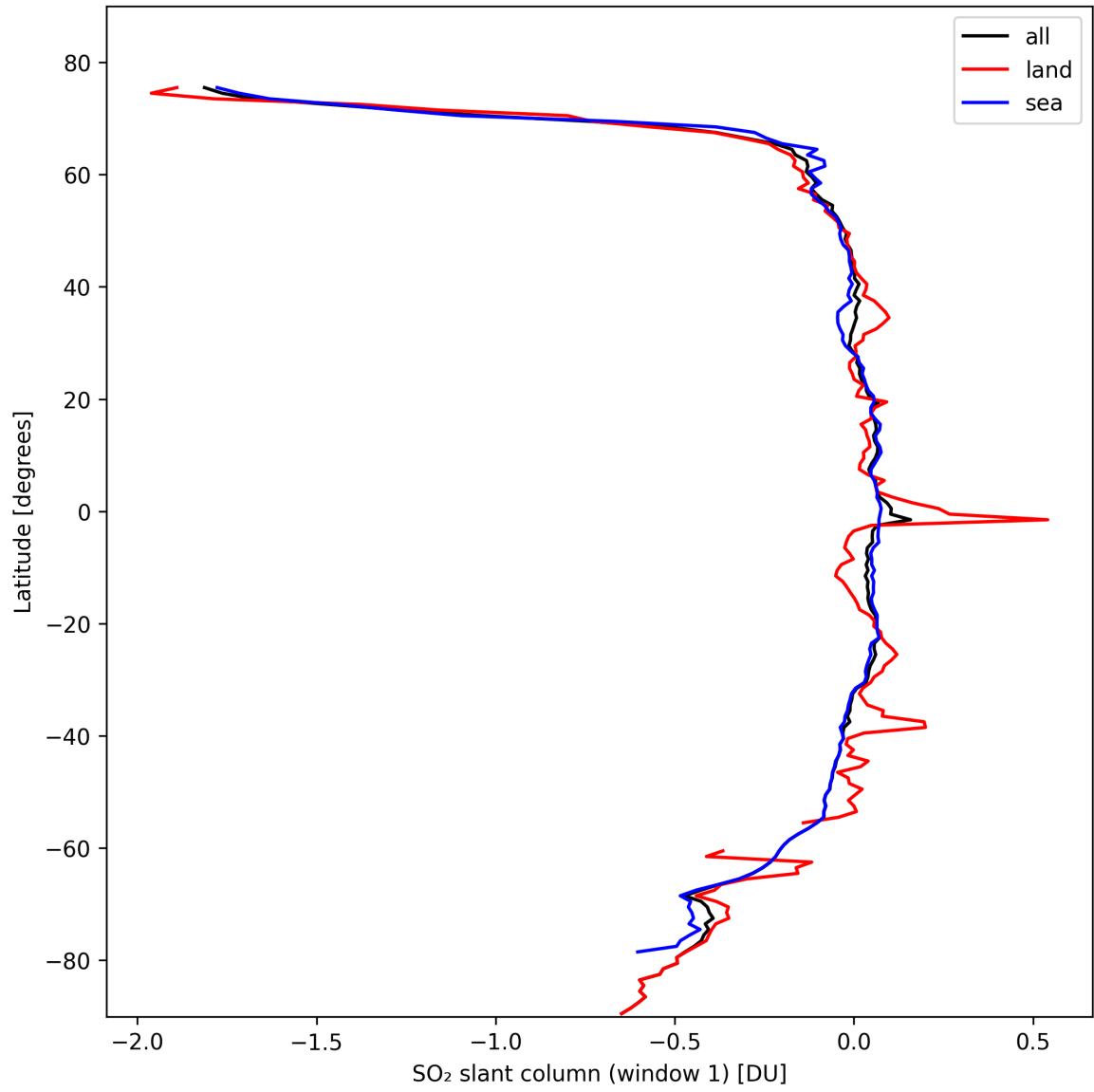
Figure 33: Zonal average of “SO 2 slant column (window 1)” for 2024-10-16 to 2024-10-18.
