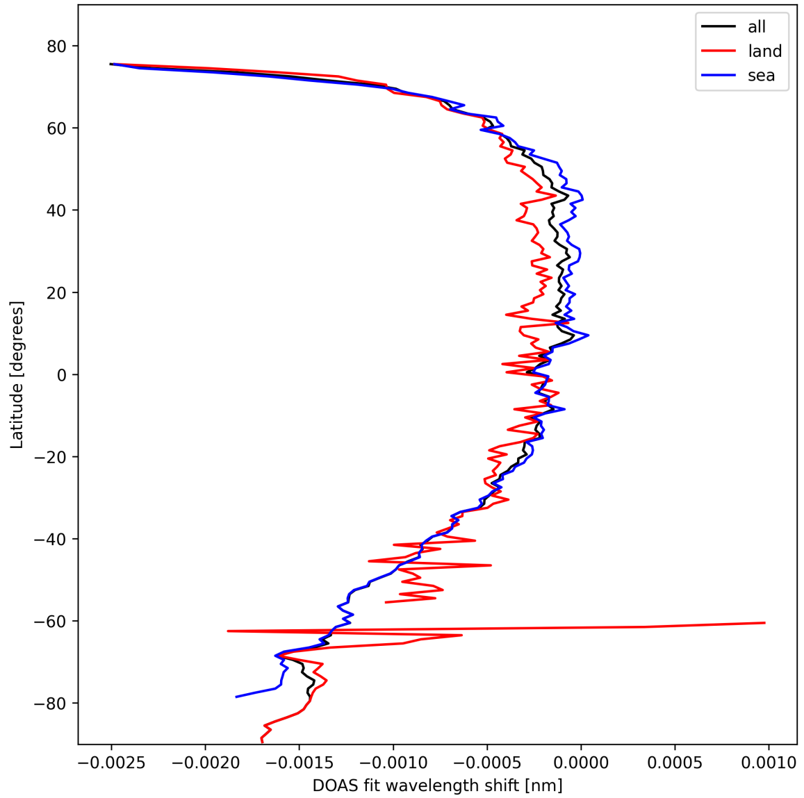
Figure 45: Zonal average of “DOAS fit wavelength shift” for 2024-10-16 to 2024-10-18.
