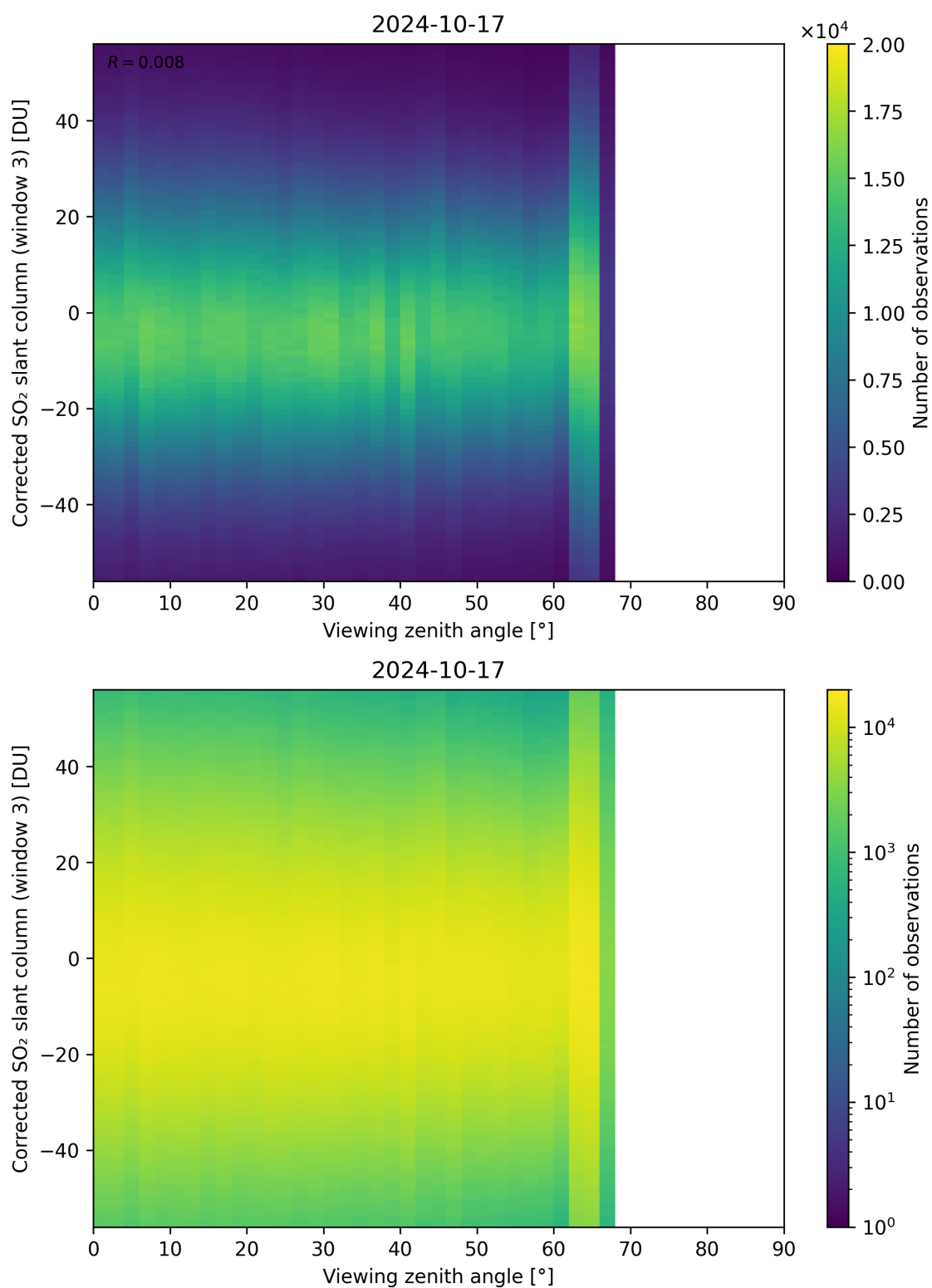
Figure 319: Scatter density plot of “Viewing zenith angle” against “Corrected SO 2 slant column (window 3)” for 2024-10-16 to 2024-10-18.
