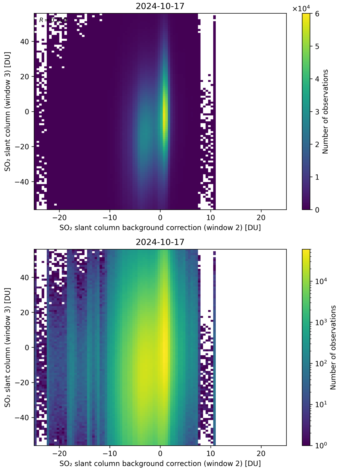
Figure 117: Scatter density plot of “SO 2 slant column background correction (window 2)” against “SO 2 slant column (window 3)” for 2024-10-16 to 2024-10-18.
