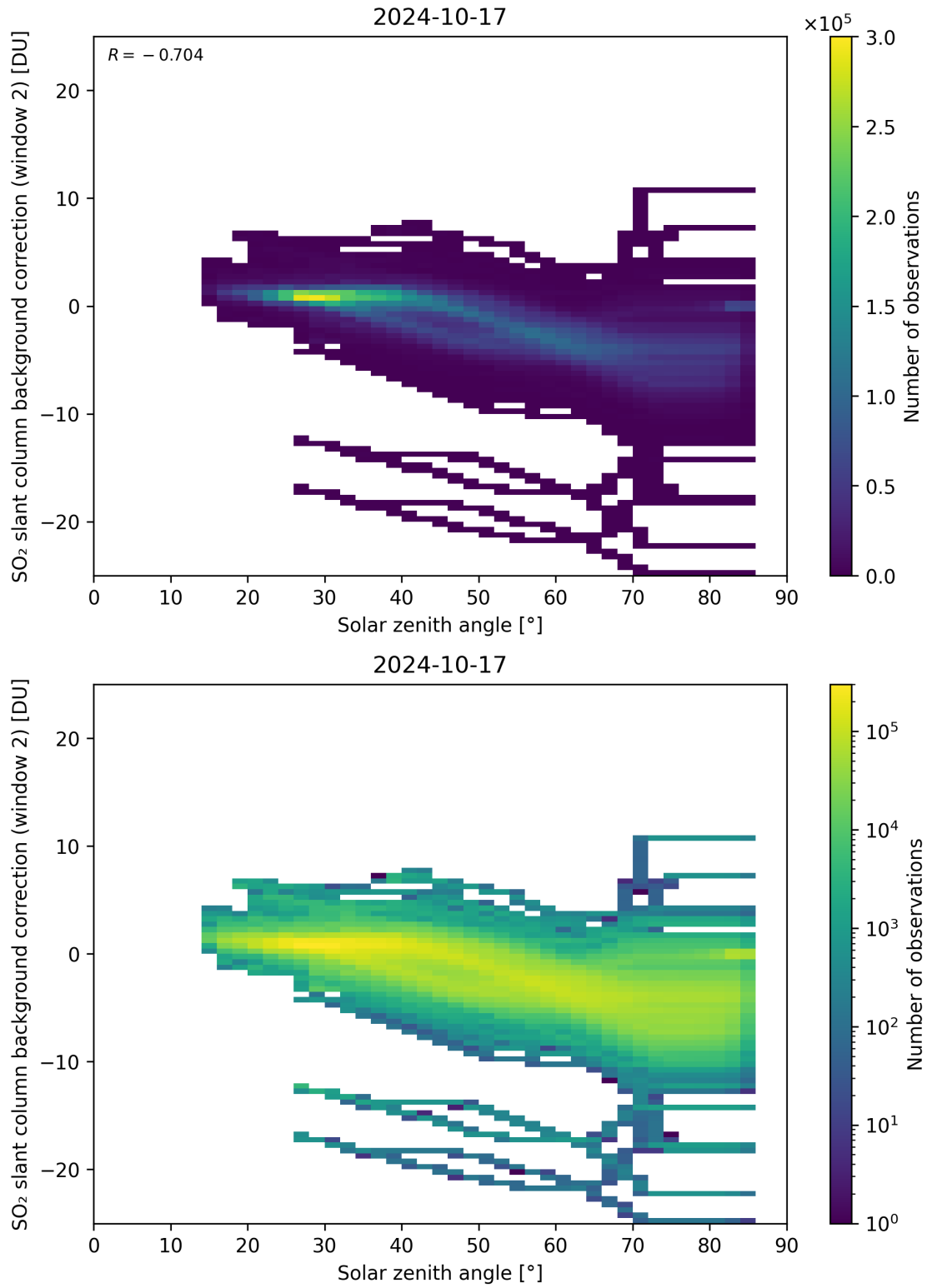
Figure 159: Scatter density plot of “Solar zenith angle” against “SO 2 slant column background correction (window 2)” for 2024-10-16 to 2024-10-18.
