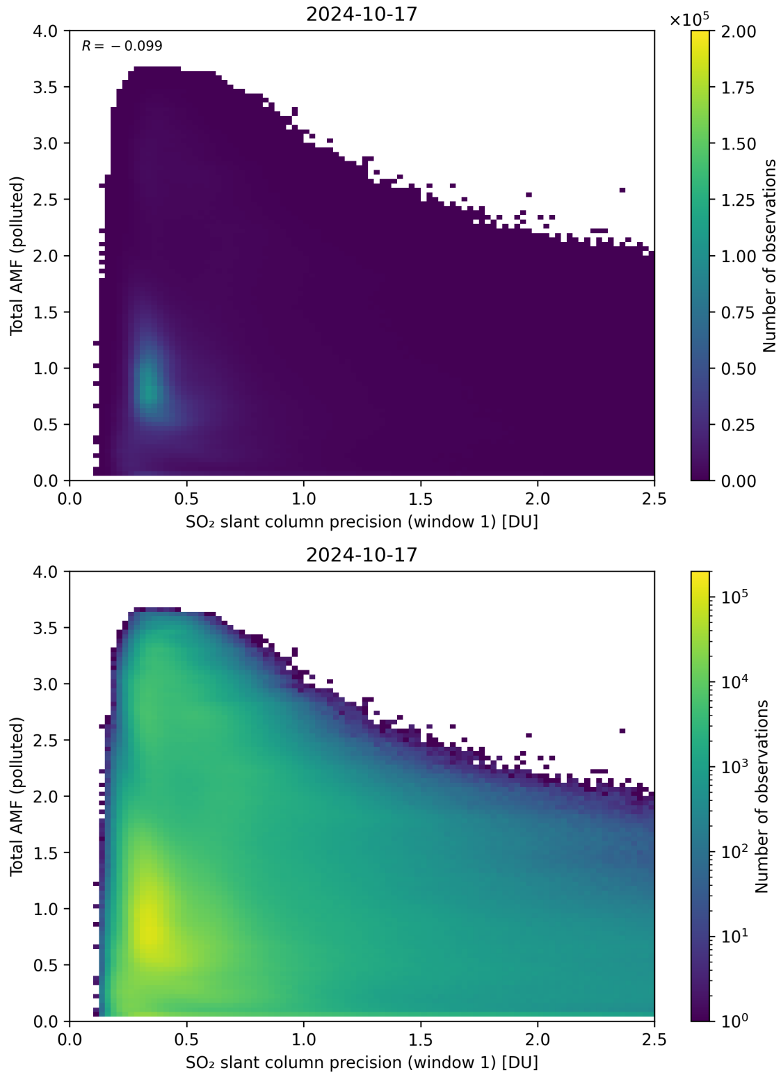
Figure 230: Scatter density plot of “SO 2 slant column precision (window 1)” against “Total AMF (polluted)” for 2024-10-16 to 2024-10-18.
