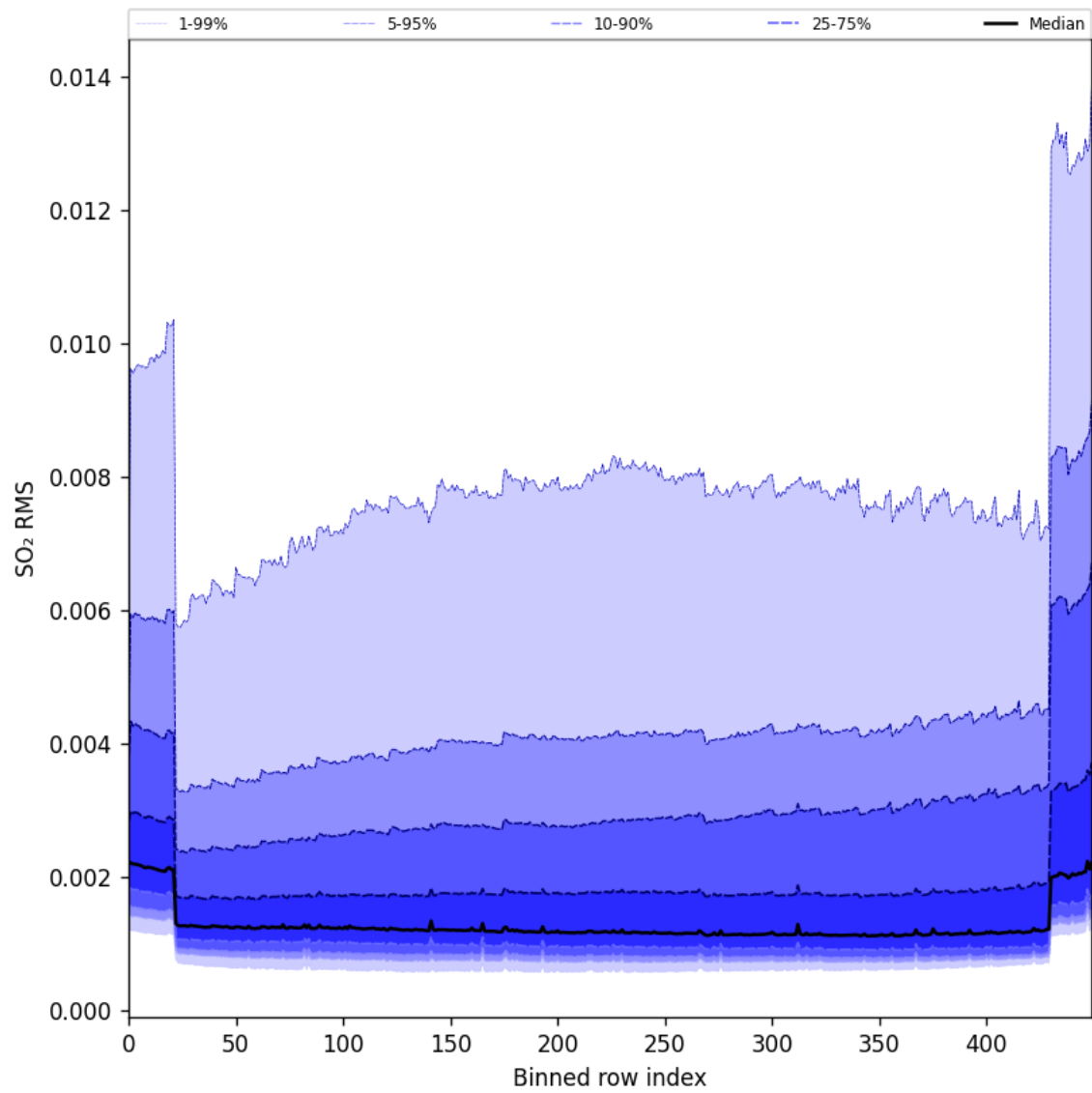
Figure 93: Along track statistics of “SO 2 RMS” for 2024-10-16 to 2024-10-18
