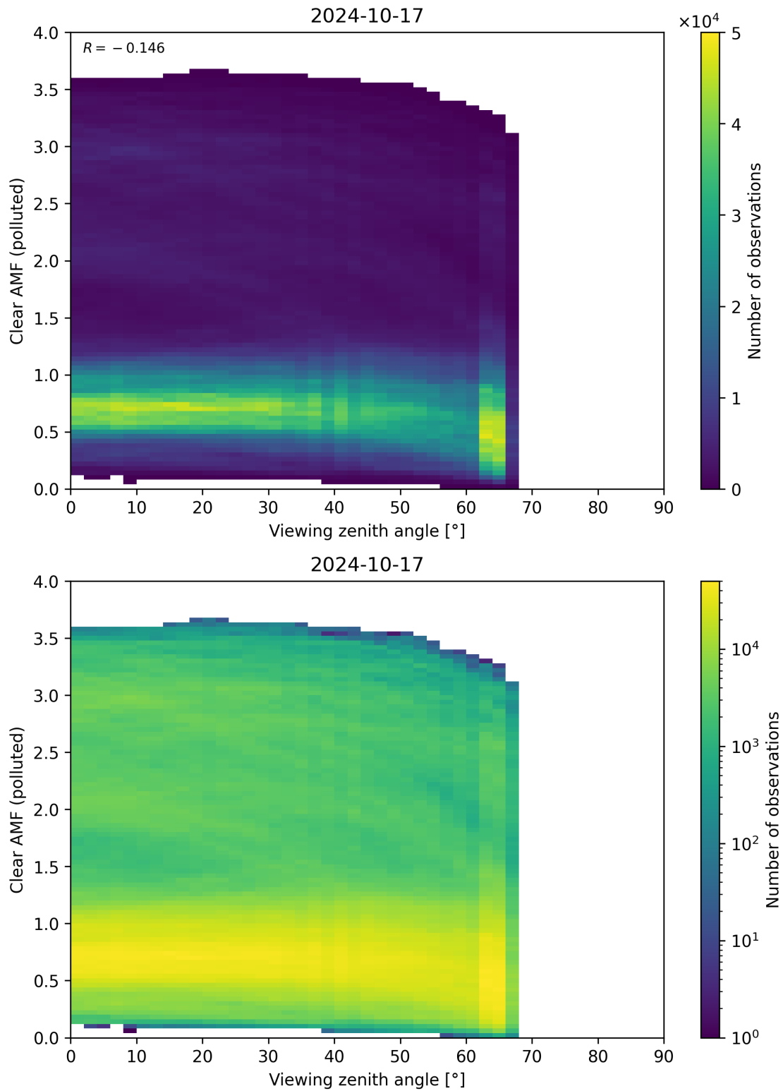
Figure 316: Scatter density plot of “Viewing zenith angle” against “Clear AMF (polluted)” for 2024-10-16 to 2024-10-18.
