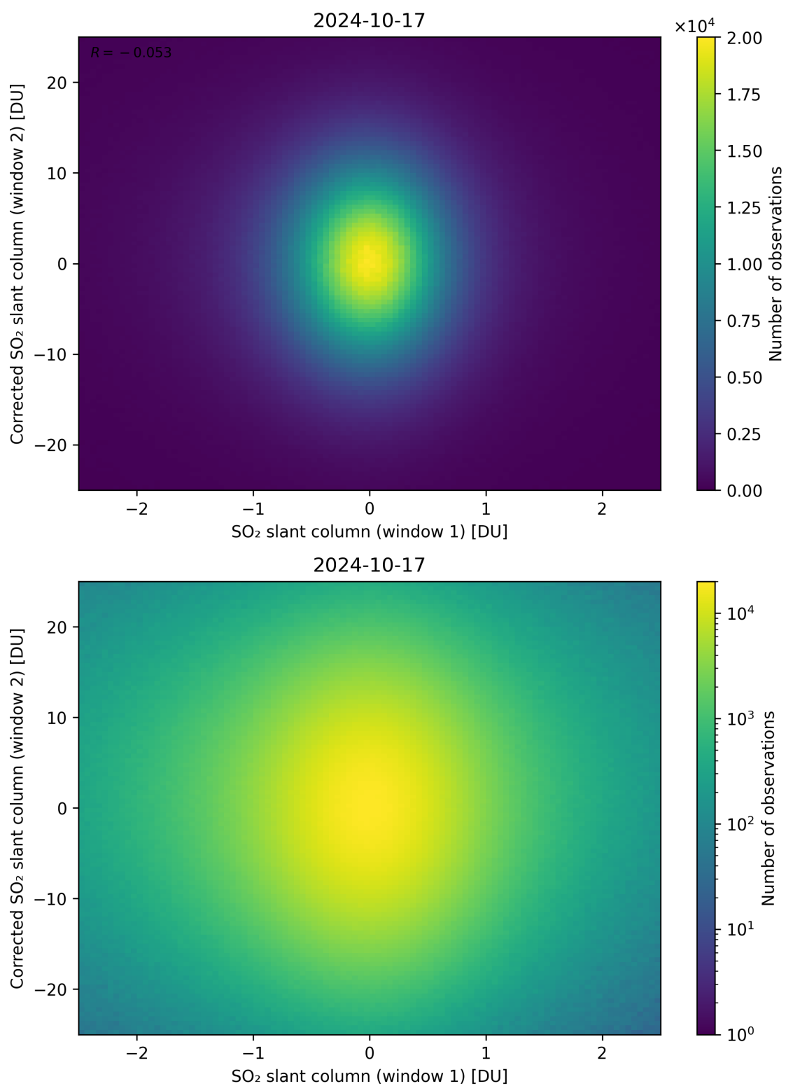
Figure 233: Scatter density plot of “SO 2 slant column (window 1)” against “Corrected SO 2 slant column (window 2)” for 2024-10-16 to 2024-10-18.
