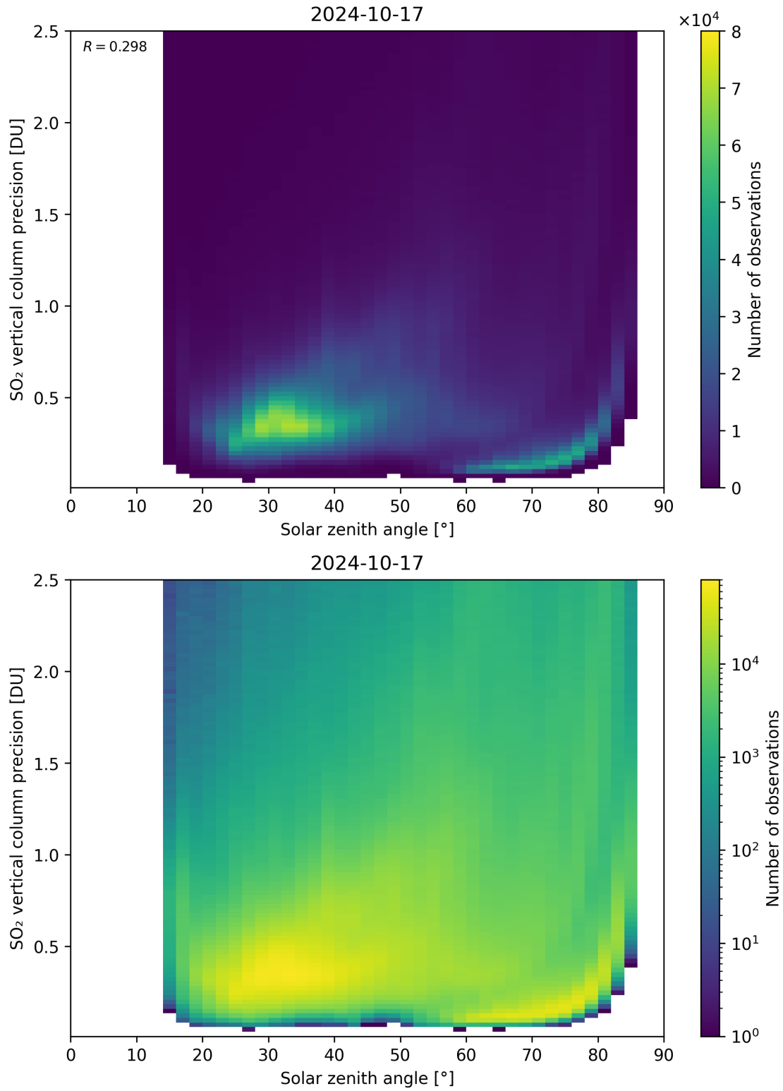
Figure 177: Scatter density plot of “Solar zenith angle” against “SO 2 vertical column precision” for 2024-10-16 to 2024-10-18.
