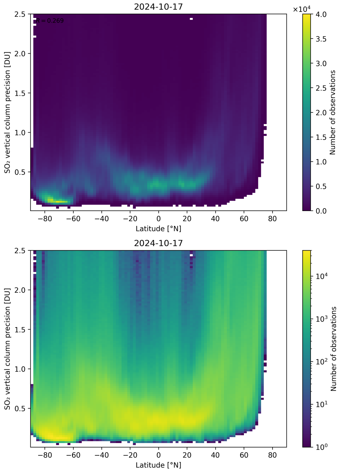
Figure 157: Scatter density plot of “Latitude” against “SO 2 vertical column precision” for 2024-10-16 to 2024-10-18.
