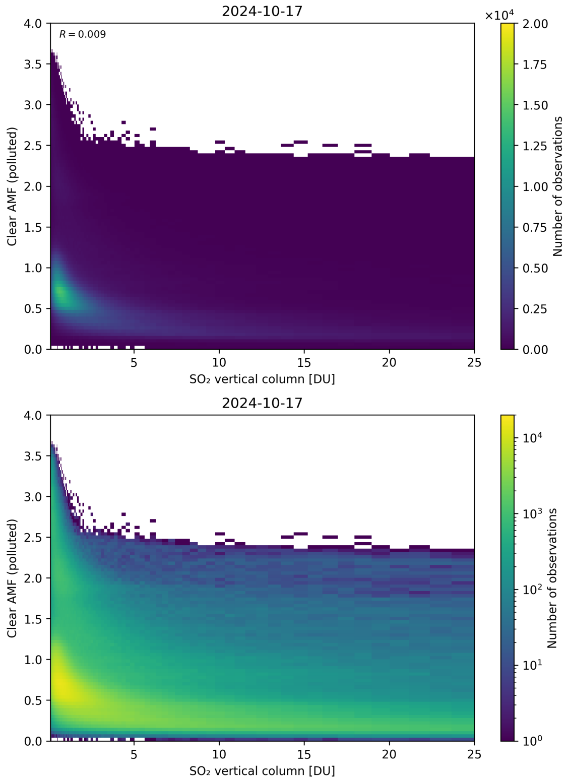
Figure 296: Scatter density plot of “SO 2 vertical column” against “Clear AMF (polluted)” for 2024-10-16 to 2024-10-18.
