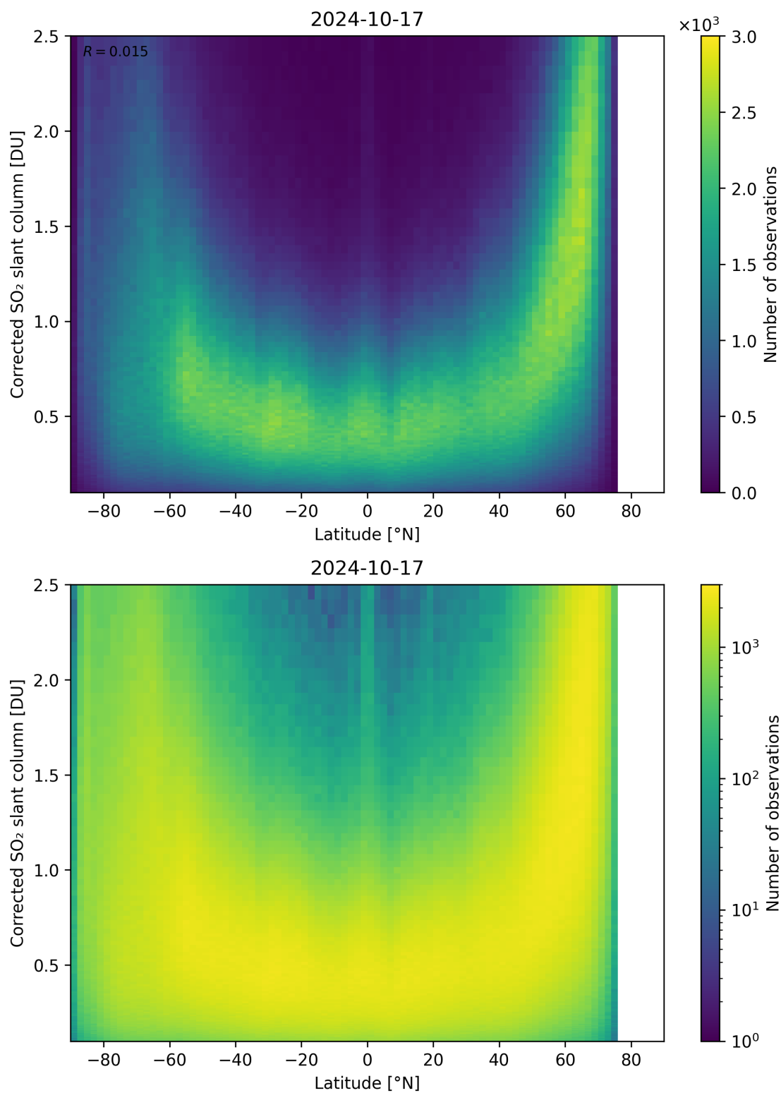
Figure 146: Scatter density plot of “Latitude” against “Corrected SO 2 slant column” for 2024-10-16 to 2024-10-18.
