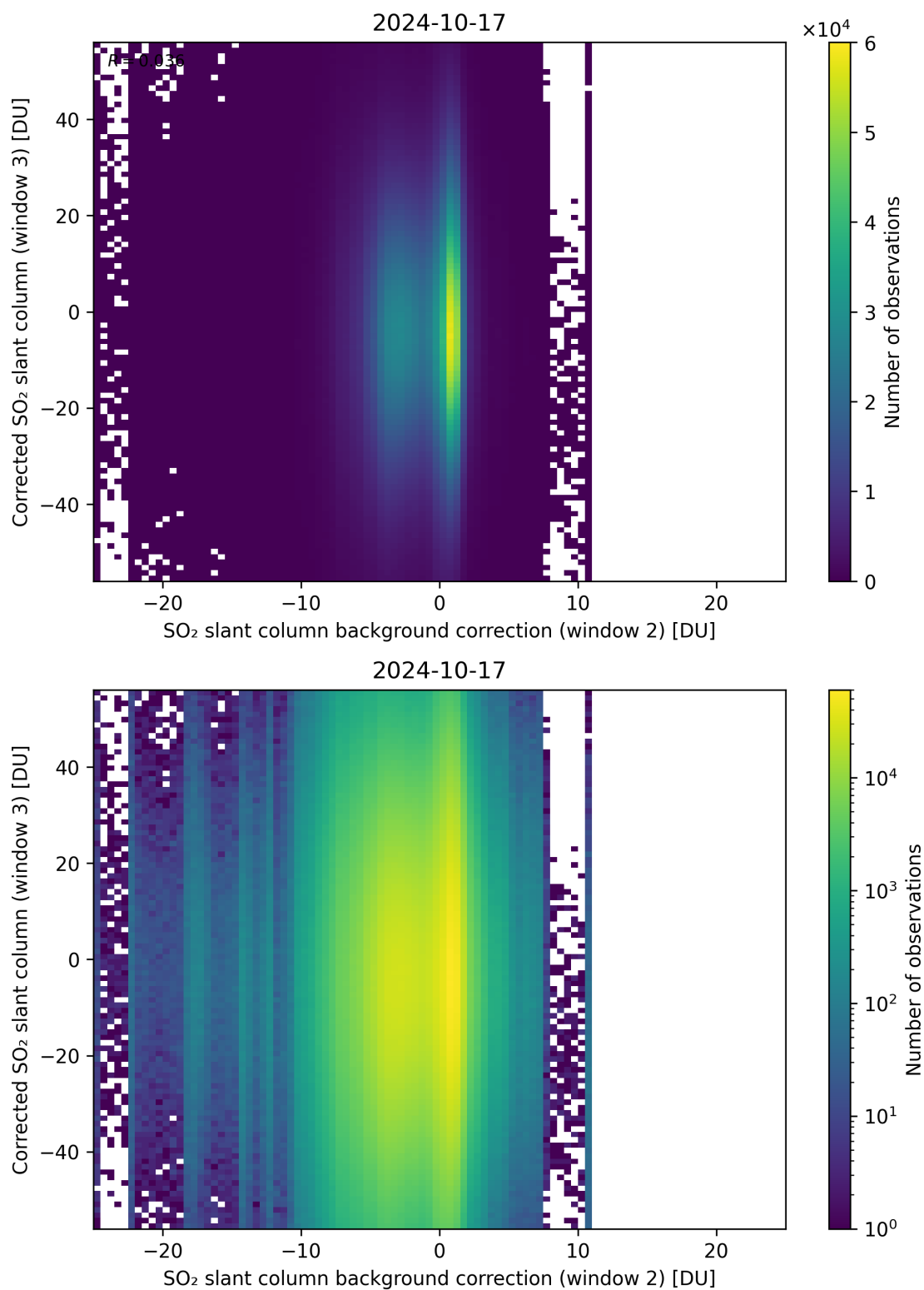
Figure 116: Scatter density plot of “SO 2 slant column background correction (window 2)” against “Corrected SO 2 slant column (window 3)” for 2024-10-16 to 2024-10-18.
