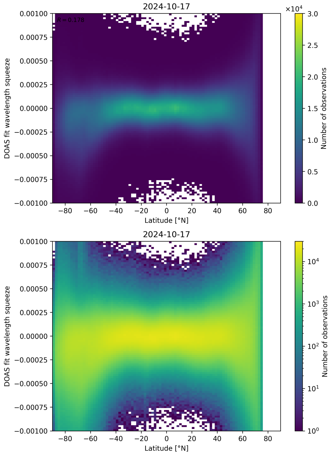
Figure 143: Scatter density plot of “Latitude” against “DOAS fit wavelength squeeze” for 2024-10-16 to 2024-10-18.
