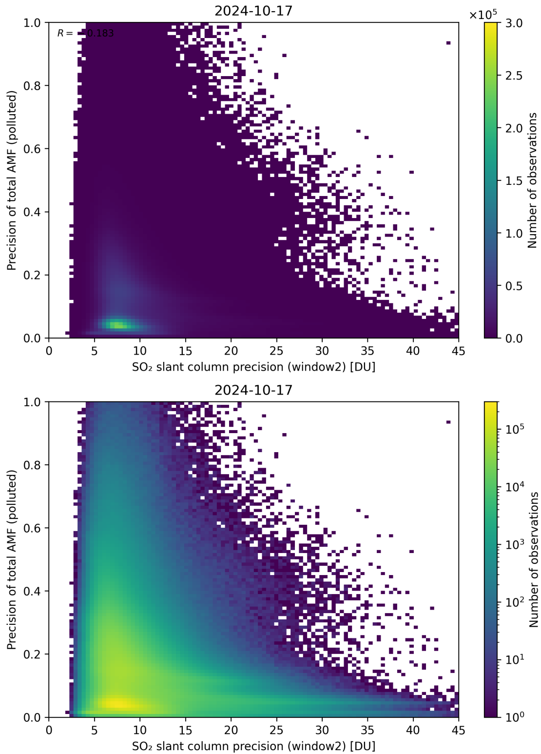
Figure 252: Scatter density plot of “SO 2 slant column precision (window2)” against “Precision of total AMF (polluted)” for 2024-10-16 to 2024-10-18.
