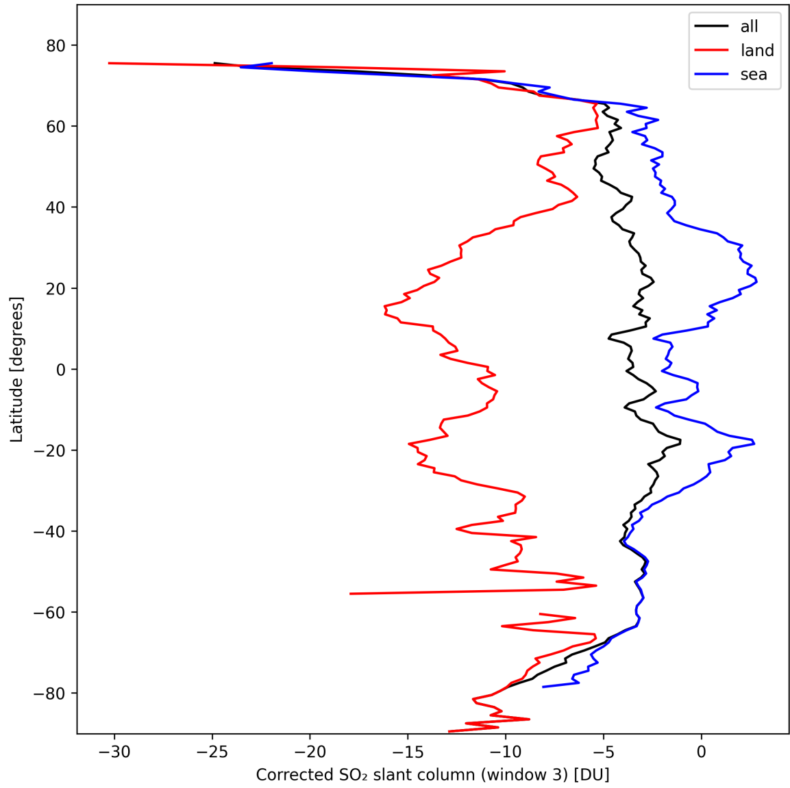
Figure 43: Zonal average of “Corrected SO 2 slant column (window 3)” for 2024-10-16 to 2024-10-18.
