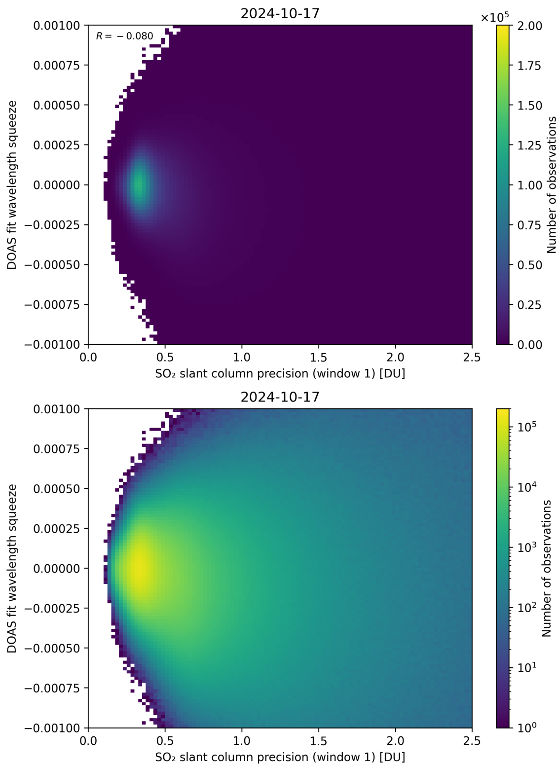
Figure 222: Scatter density plot of “SO 2 slant column precision (window 1)” against “DOAS fit wavelength squeeze” for 2024-10-16 to 2024-10-18.
