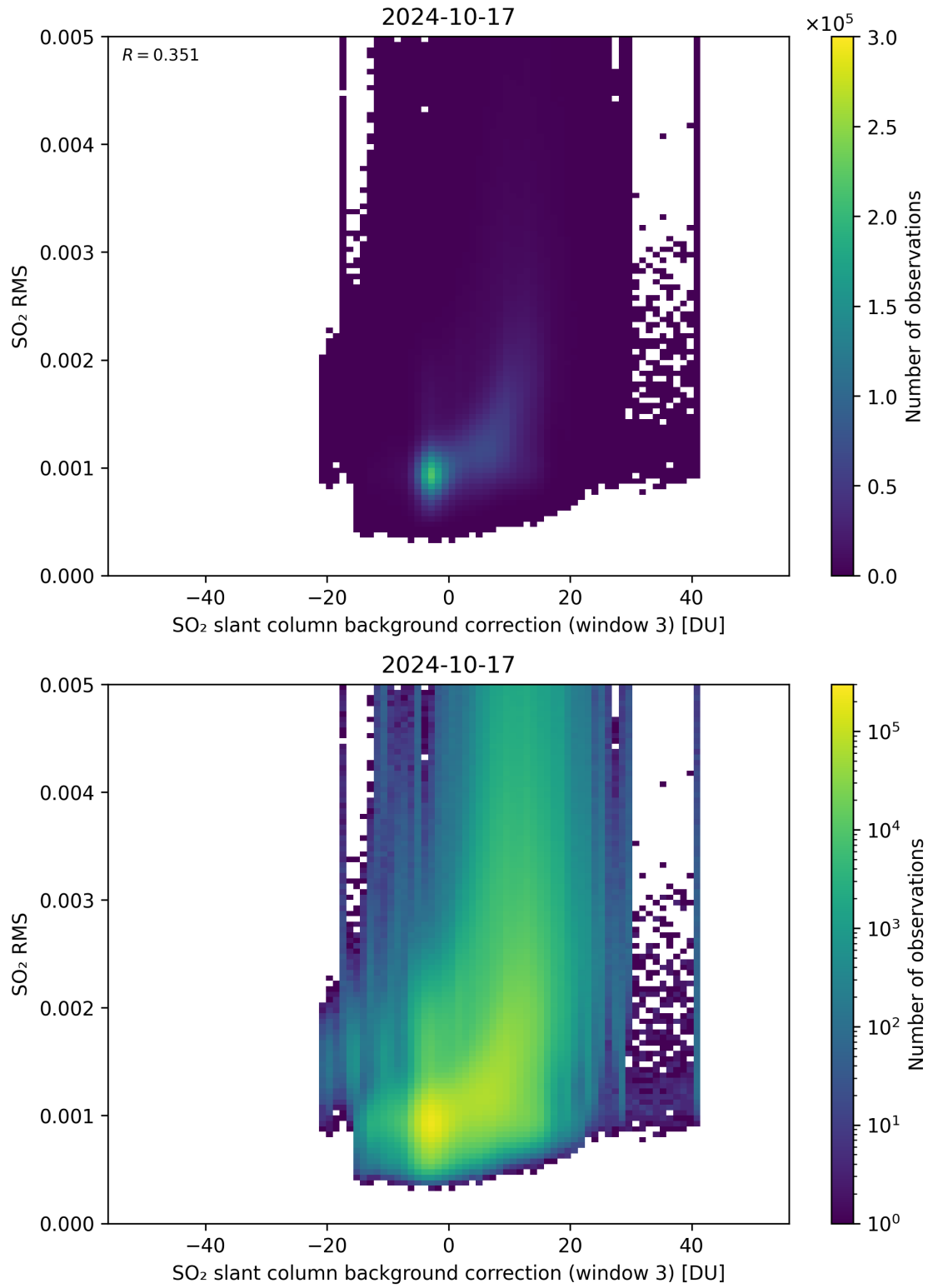
Figure 123: Scatter density plot of “SO 2 slant column background correction (window 3)” against “SO 2 RMS” for 2024-10-16 to 2024-10-18.
