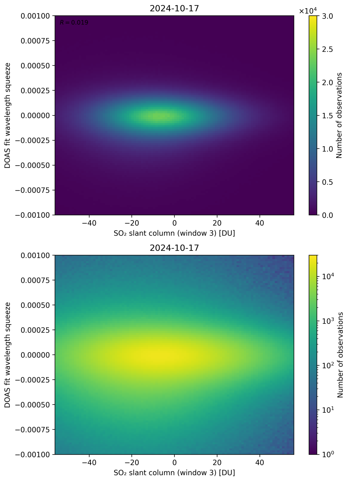
Figure 255: Scatter density plot of “SO 2 slant column (window 3)” against “DOAS fit wavelength squeeze” for 2024-10-16 to 2024-10-18.
