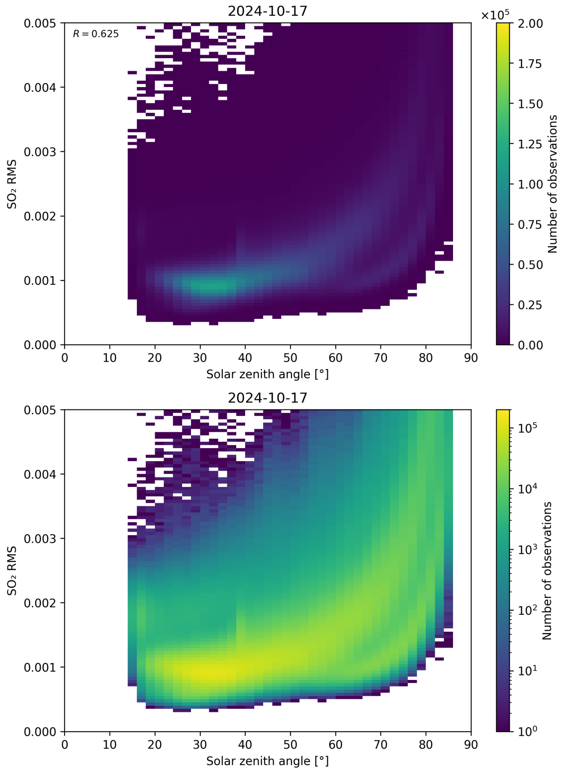
Figure 163: Scatter density plot of “Solar zenith angle” against “SO 2 RMS” for 2024-10-16 to 2024-10-18.
