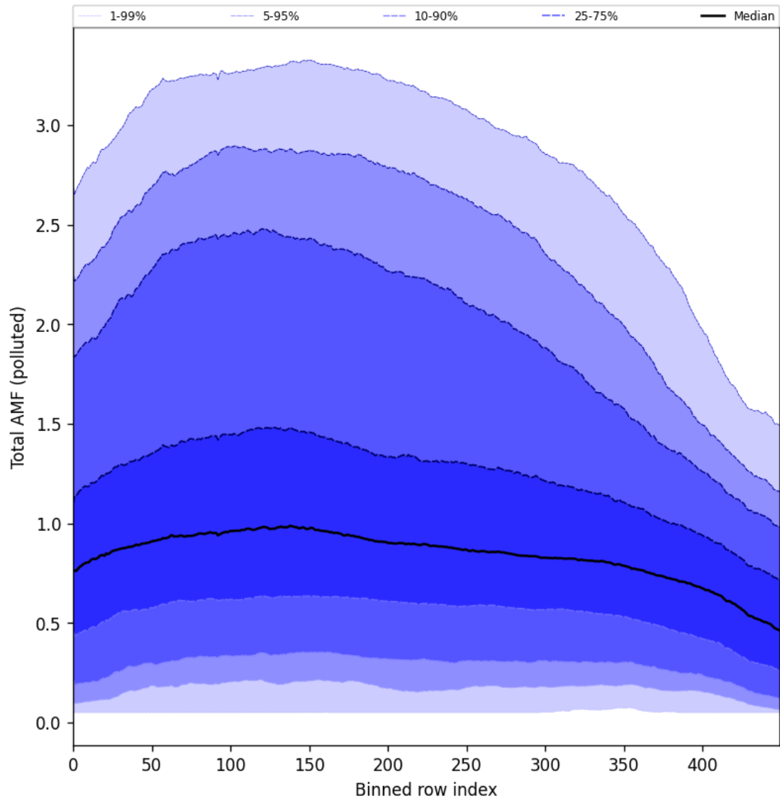
Figure 94: Along track statistics of “Total AMF (polluted)” for 2024-10-16 to 2024-10-18
