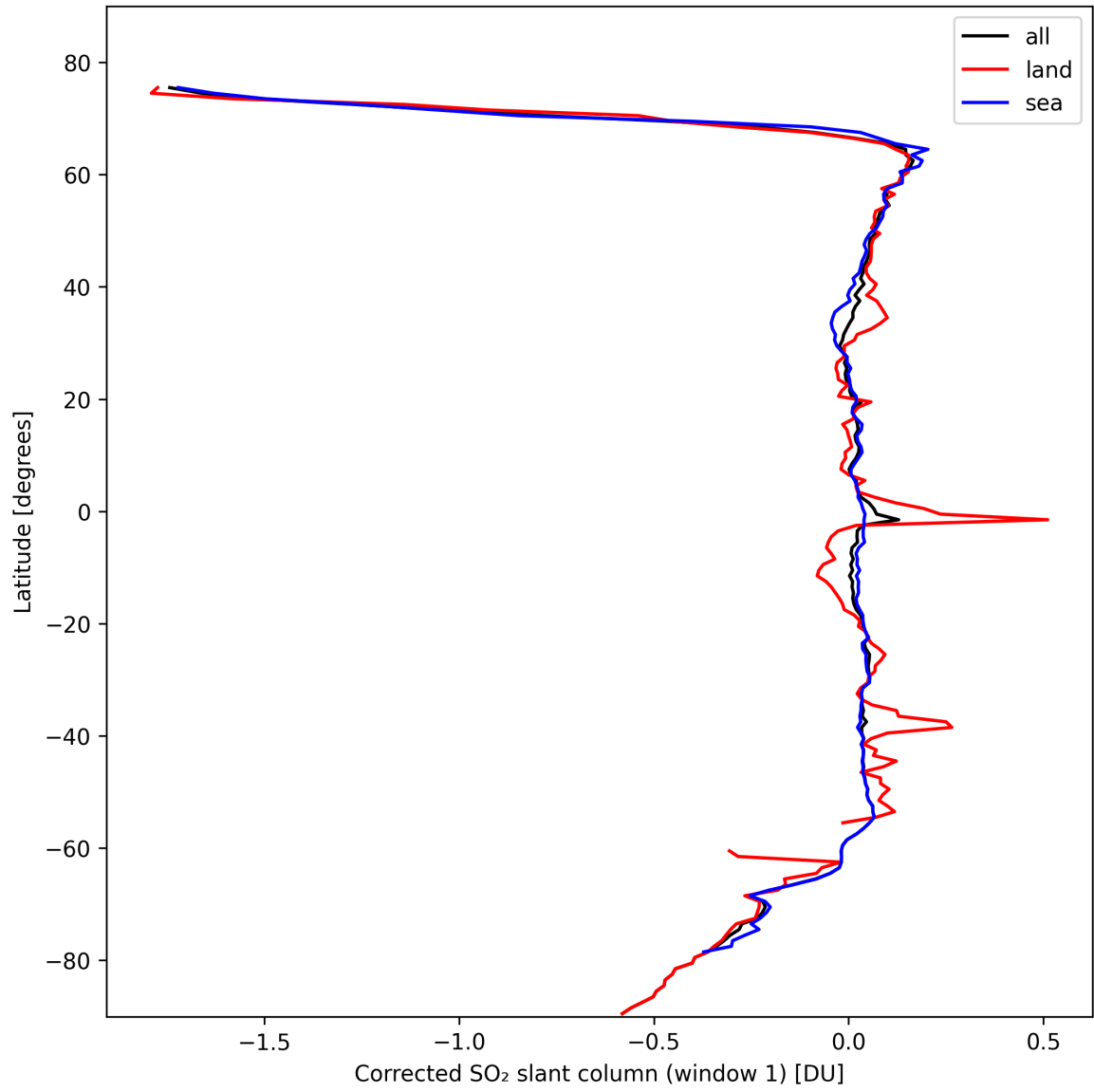
Figure 35: Zonal average of “Corrected SO 2 slant column (window 1)” for 2024-10-16 to 2024-10-18.
