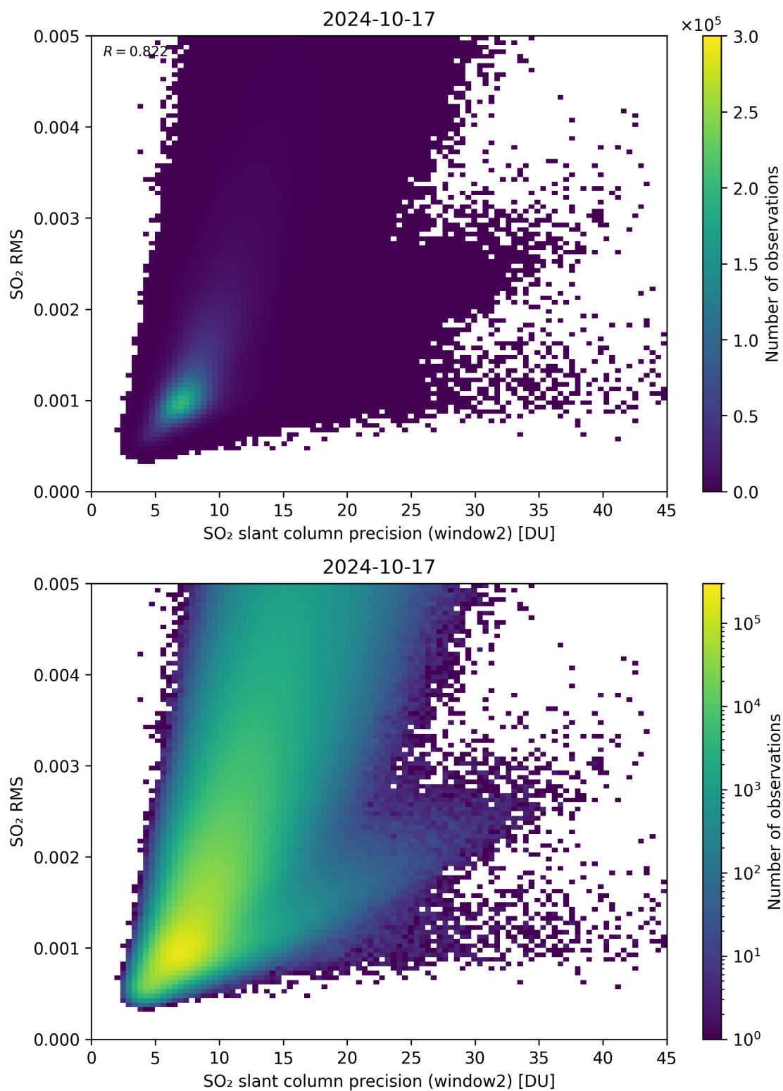
Figure 245: Scatter density plot of “SO 2 slant column precision (window2)” against “SO 2 RMS” for 2024-10-16 to 2024-10-18.
