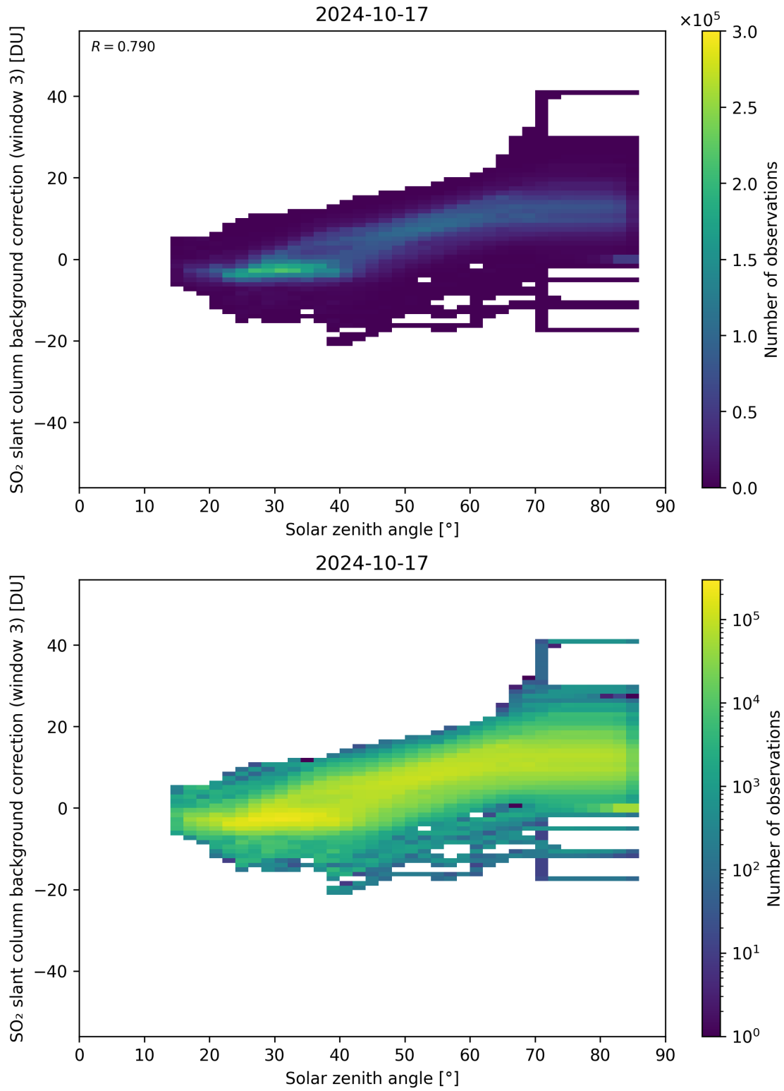
Figure 160: Scatter density plot of “Solar zenith angle” against “SO 2 slant column background correction (window 3)” for 2024-10-16 to 2024-10-18.
