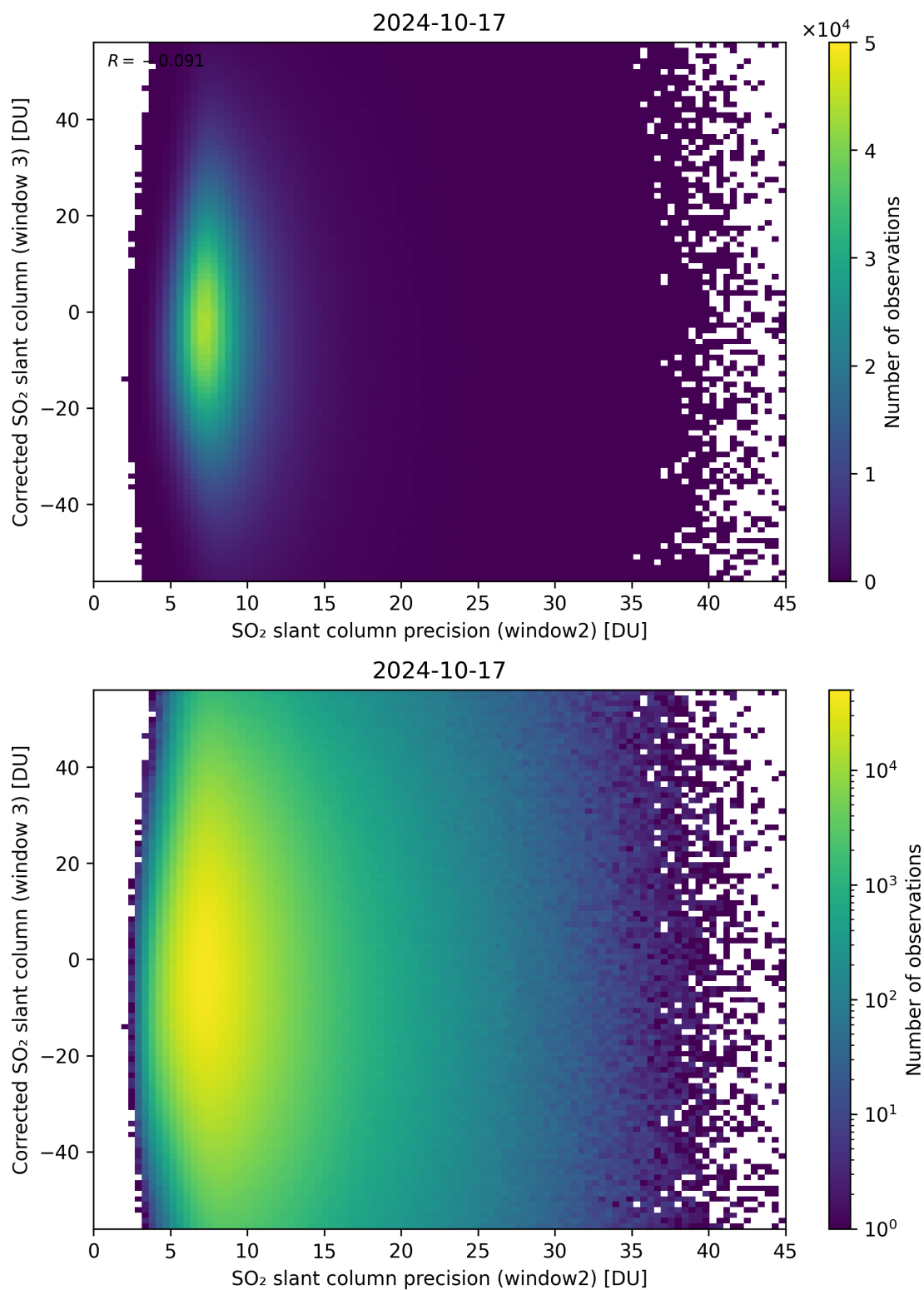
Figure 248: Scatter density plot of “SO 2 slant column precision (window2)” against “Corrected SO 2 slant column (window 3)” for 2024-10-16 to 2024-10-18.
