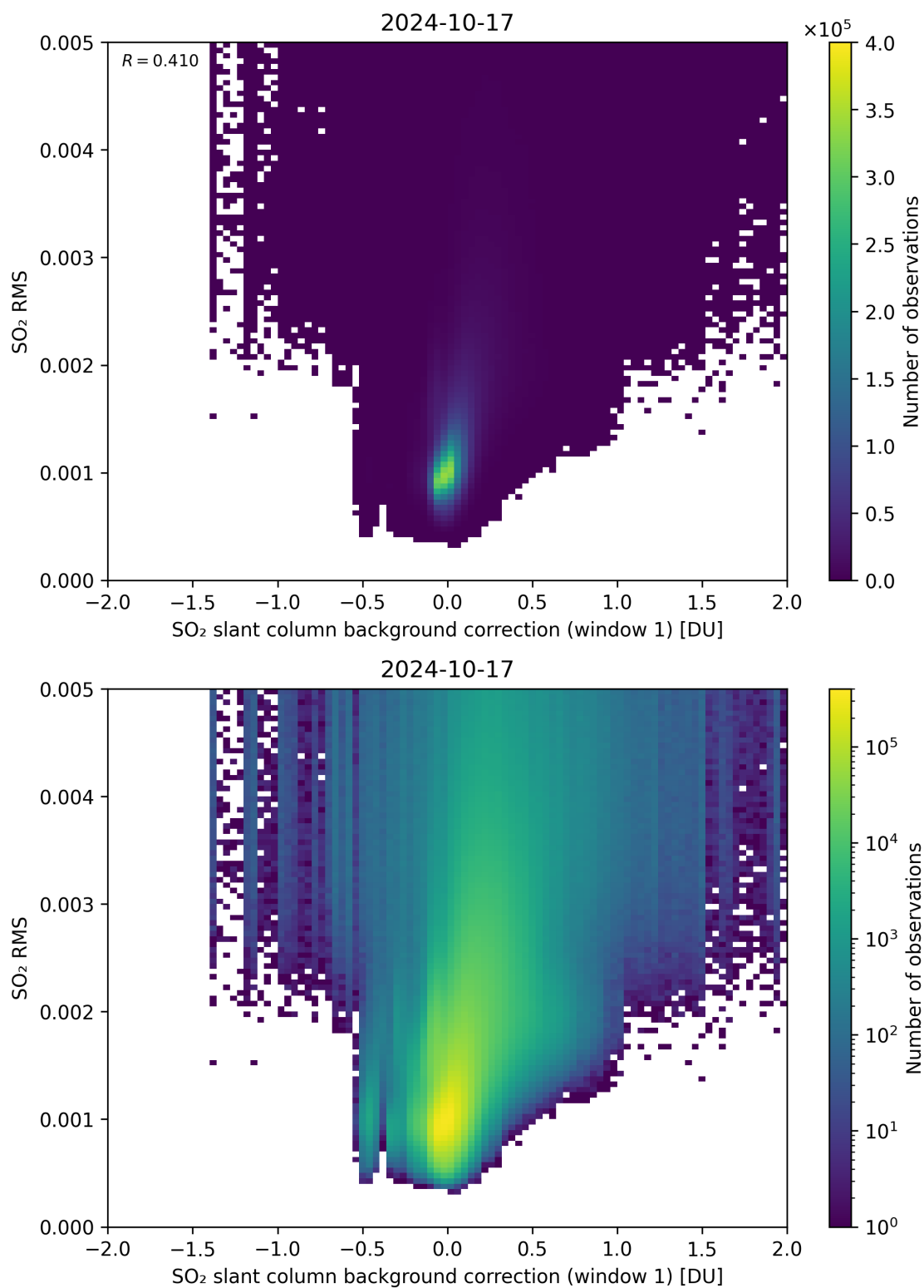
Figure 102: Scatter density plot of “SO 2 slant column background correction (window 1)” against “SO 2 RMS” for 2024-10-16 to 2024-10-18.
