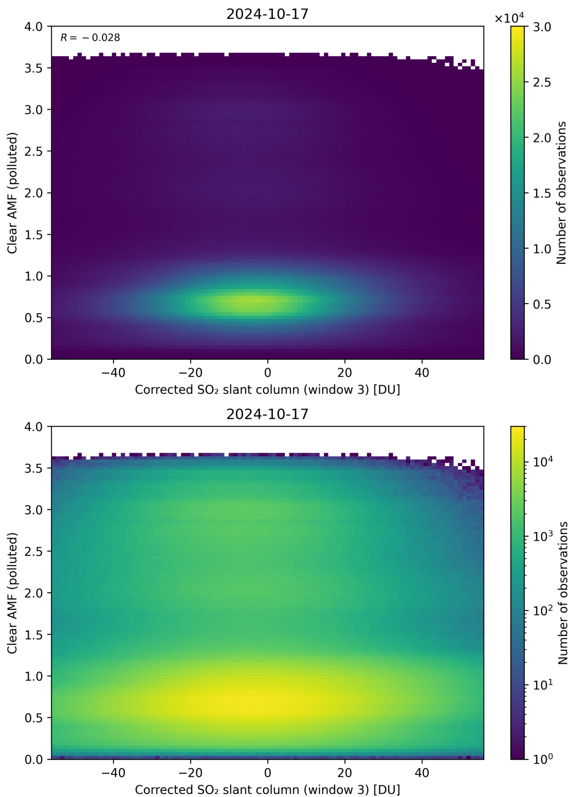
Figure 209: Scatter density plot of “Corrected SO 2 slant column (window 3)” against “Clear AMF (polluted)” for 2024-10-16 to 2024-10-18.
