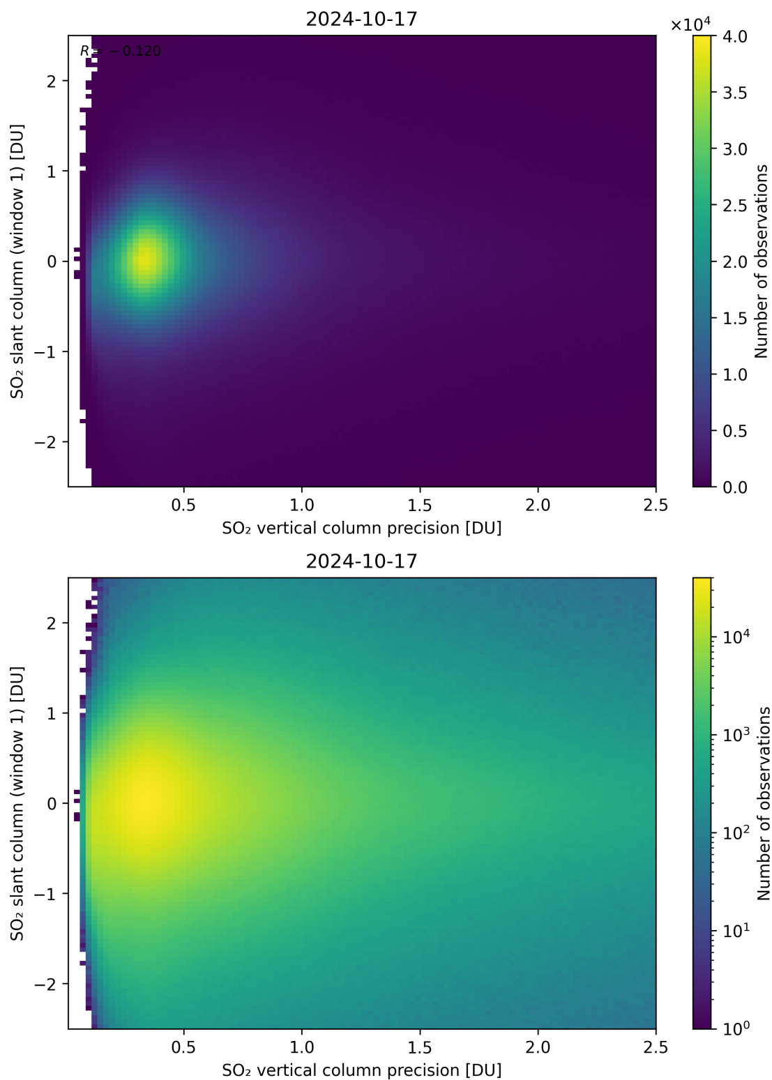
Figure 289: Scatter density plot of “SO 2 vertical column precision” against “SO 2 slant column (window 1)” for 2024-10-16 to 2024-10-18.
