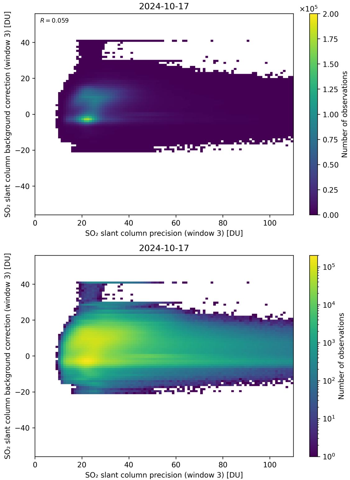
Figure 257: Scatter density plot of “SO 2 slant column precision (window 3)” against “SO 2 slant column background correction (window 3)” for 2024-10-16 to 2024-10-18.
