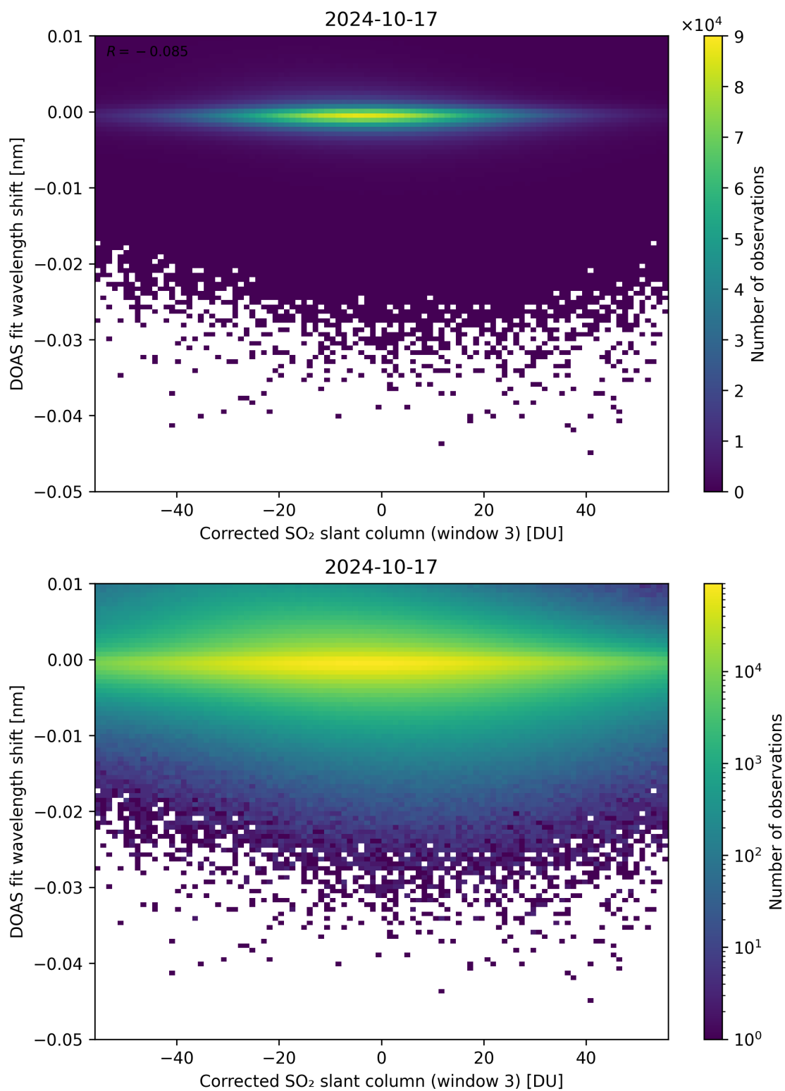
Figure 206: Scatter density plot of “Corrected SO 2 slant column (window 3)” against “DOAS fit wavelength shift” for 2024-10-16 to 2024-10-18.
