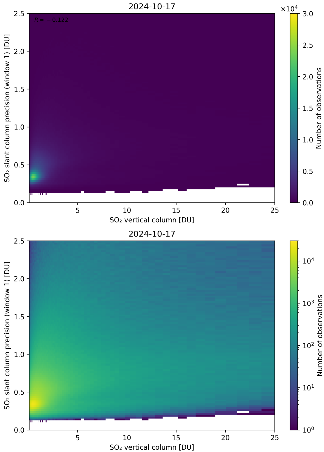
Figure 301: Scatter density plot of “SO 2 vertical column” against “SO 2 slant column precision (window 1)” for 2024-10-16 to 2024-10-18.
