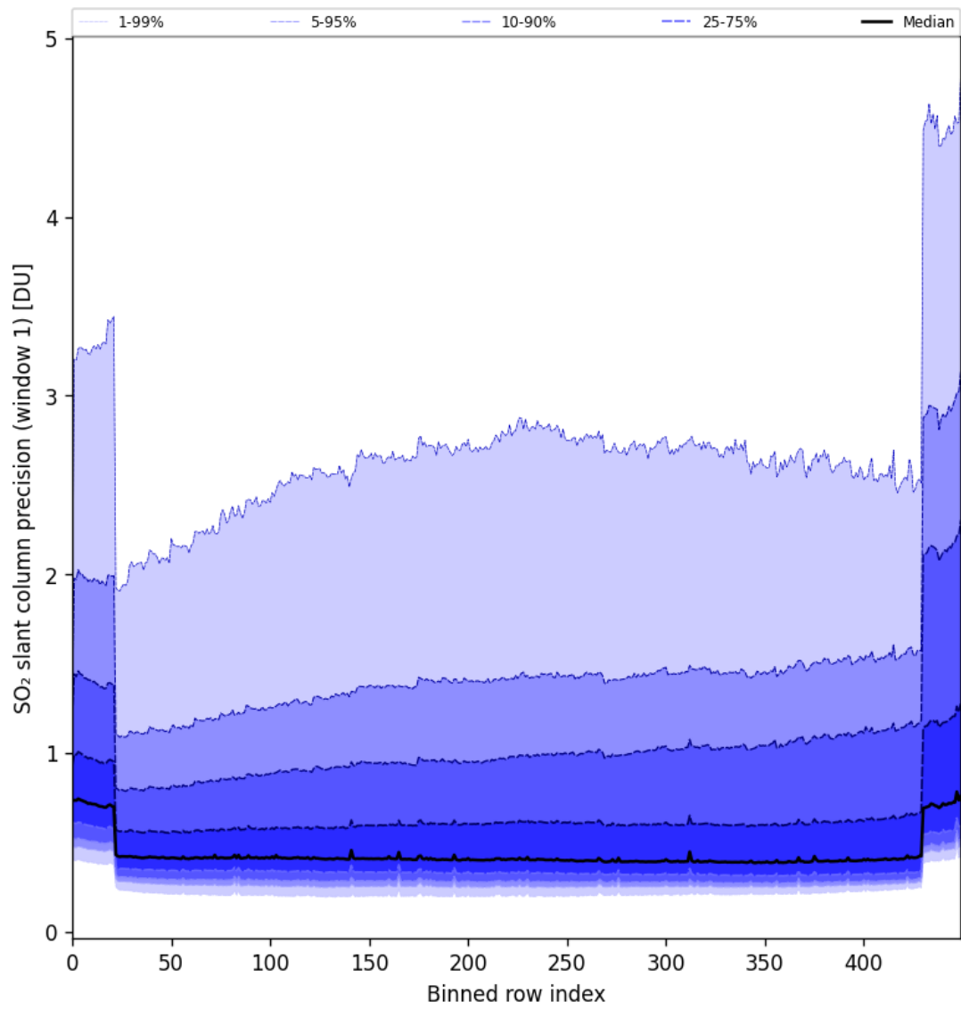
Figure 80: Along track statistics of “SO 2 slant column precision (window 1)” for 2024-10-16 to 2024-10-18
