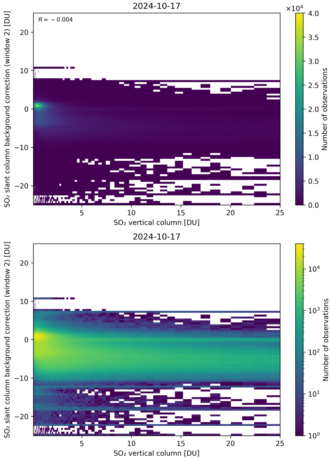
Figure 274: Scatter density plot of “SO 2 vertical column” against “SO 2 slant column background correction (window 2)” for 2024-10-16 to 2024-10-18.
