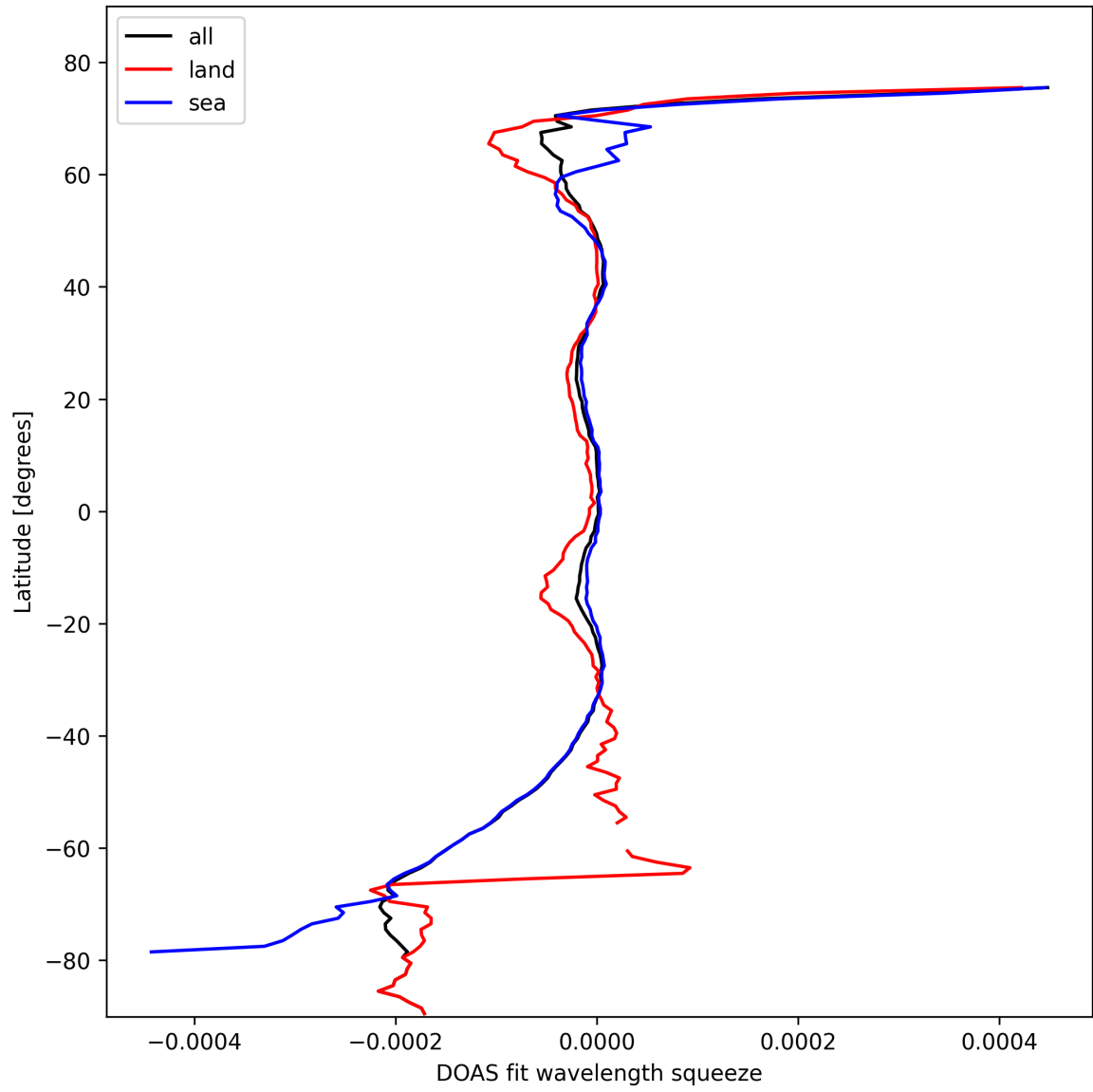
Figure 46: Zonal average of “DOAS fit wavelength squeeze” for 2024-10-16 to 2024-10-18.
