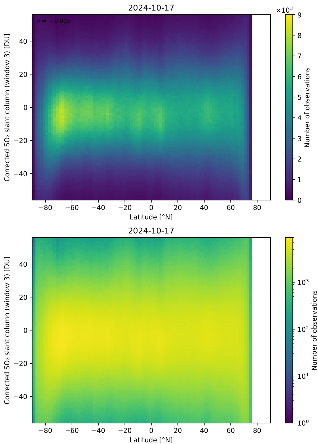
Figure 148: Scatter density plot of “Latitude” against “Corrected SO 2 slant column (window 3)” for 2024-10-16 to 2024-10-18.
