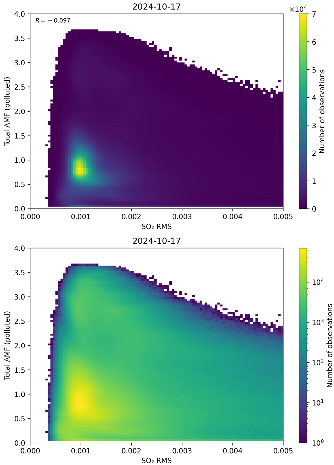
Figure 137: Scatter density plot of “SO 2 RMS” against “Total AMF (polluted)” for 2024-10-16 to 2024-10-18.
