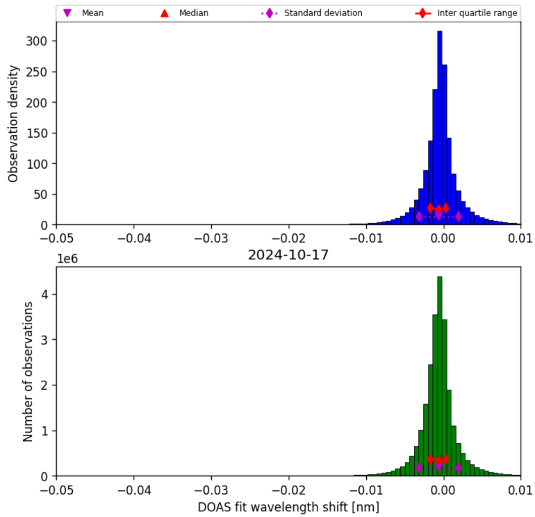
Figure 68: Histogram of “DOAS fit wavelength shift” for 2024-10-16 to 2024-10-18
