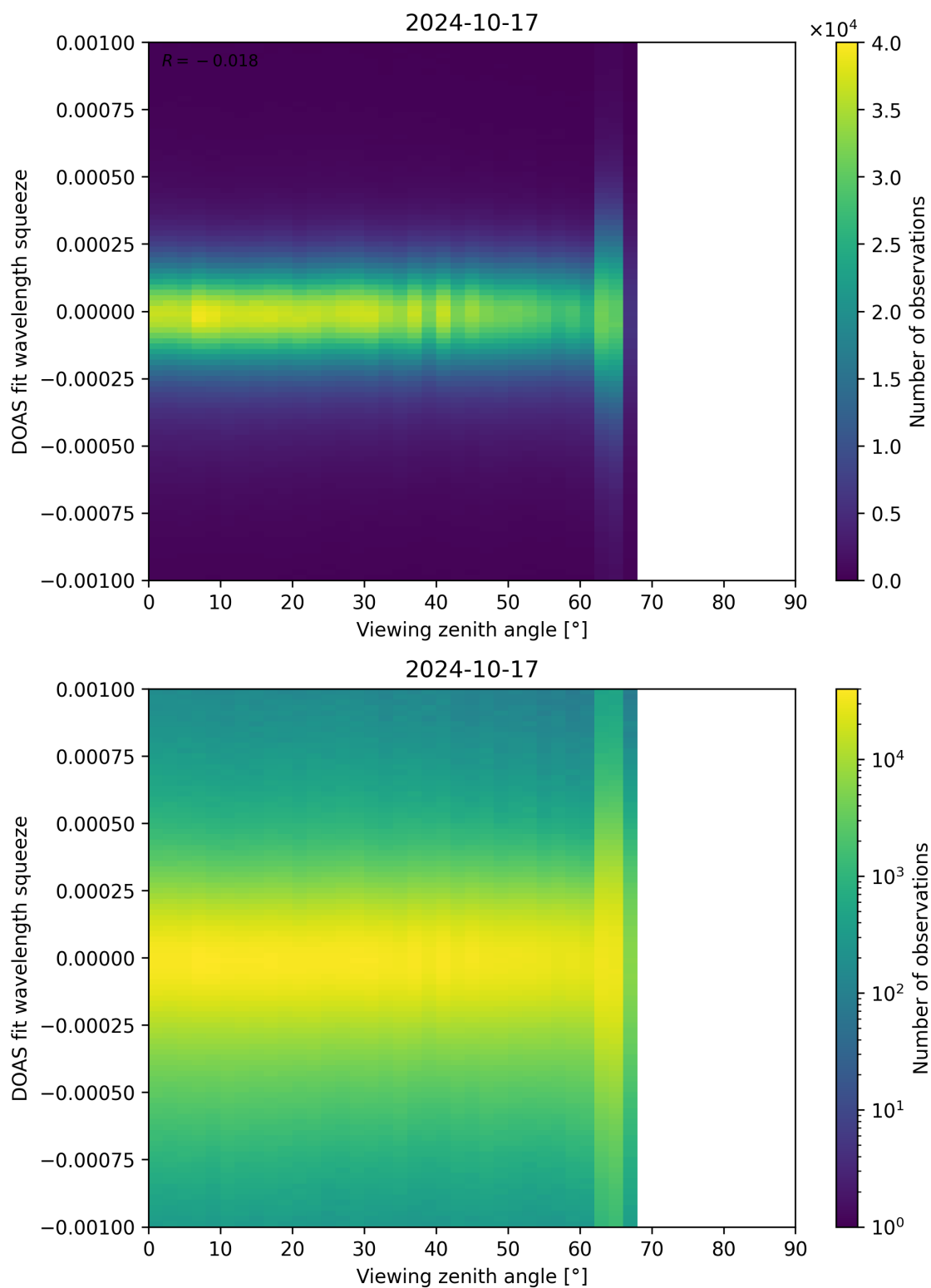
Figure 312: Scatter density plot of “Viewing zenith angle” against “DOAS fit wavelength squeeze” for 2024-10-16 to 2024-10-18.
