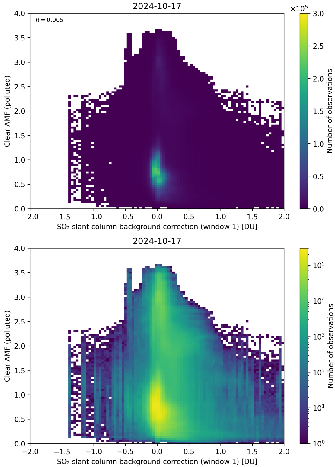
Figure 103: Scatter density plot of “SO 2 slant column background correction (window 1)” against “Clear AMF (polluted)” for 2024-10-16 to 2024-10-18.
