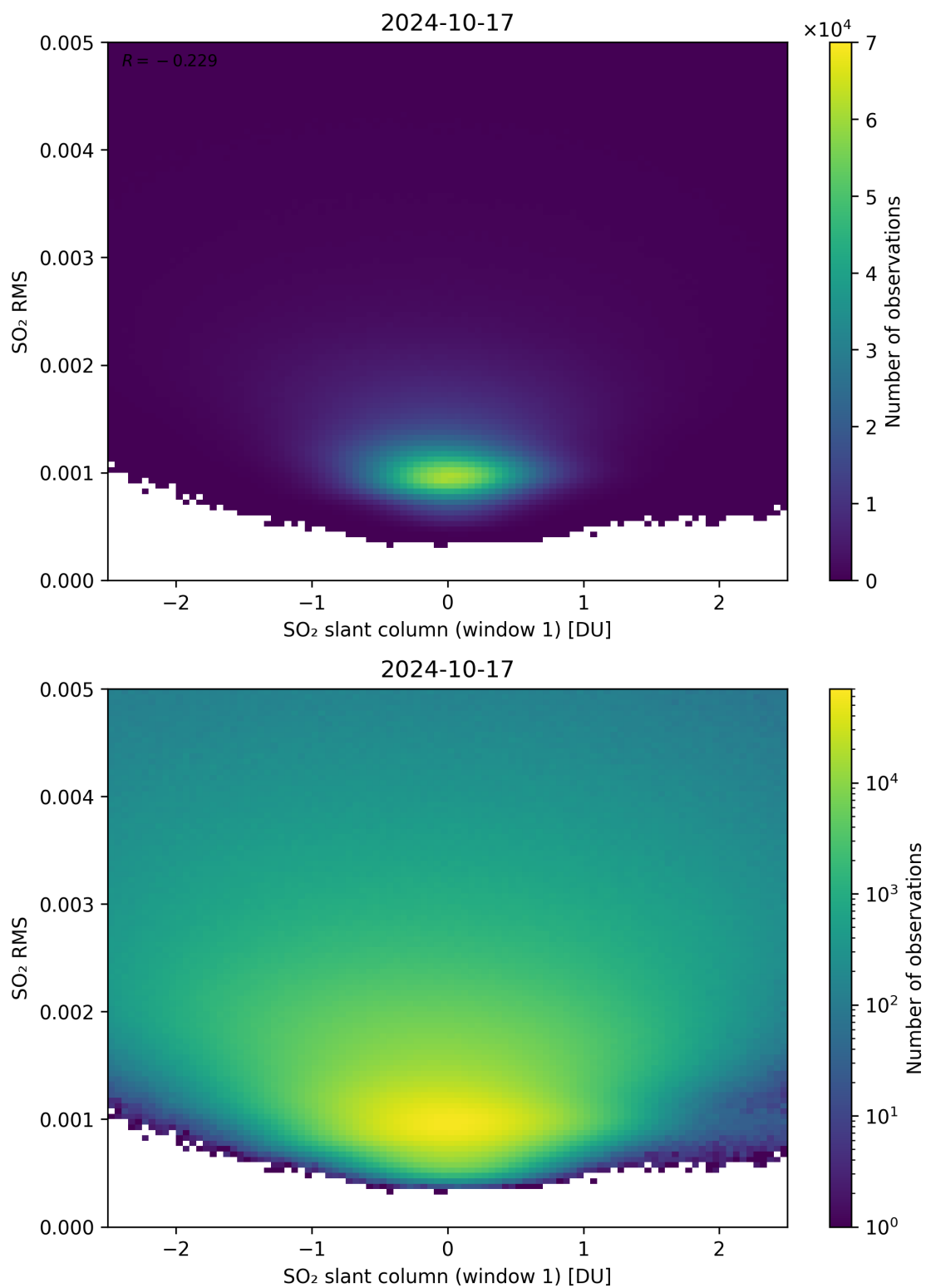
Figure 217: Scatter density plot of “SO 2 slant column (window 1)” against “SO 2 RMS” for 2024-10-16 to 2024-10-18.
