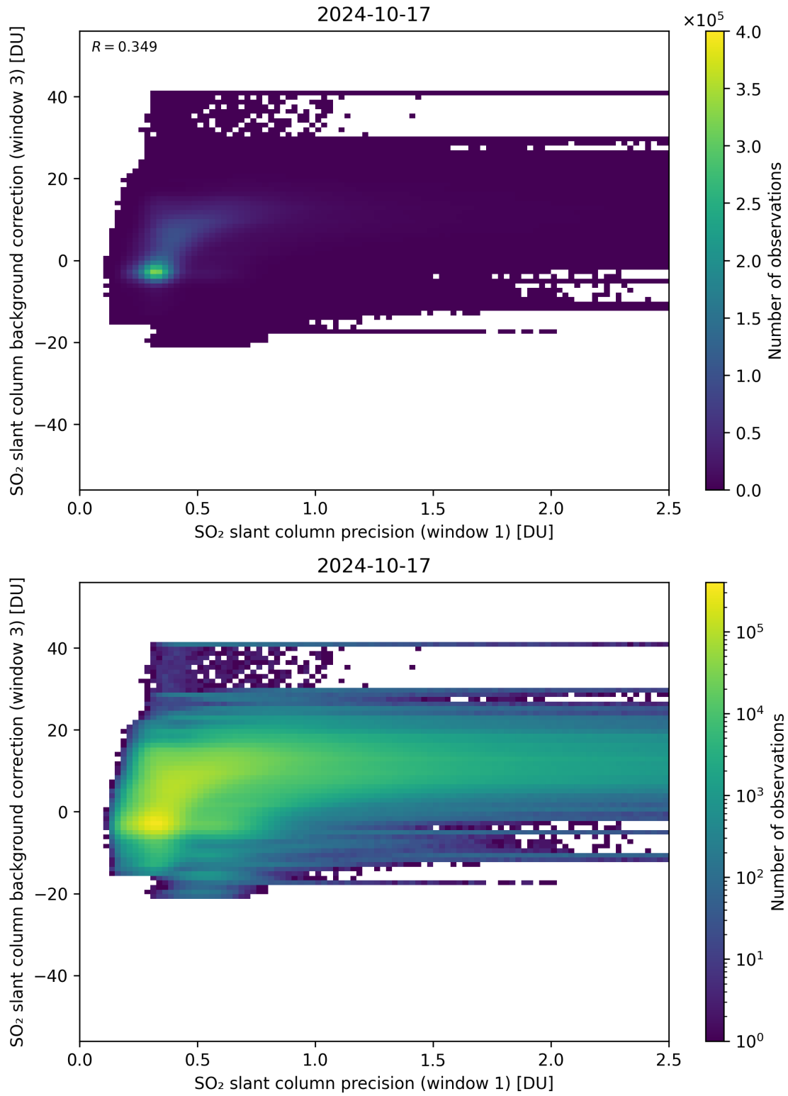
Figure 220: Scatter density plot of “SO 2 slant column precision (window 1)” against “SO 2 slant column background correction (window 3)” for 2024-10-16 to 2024-10-18.
