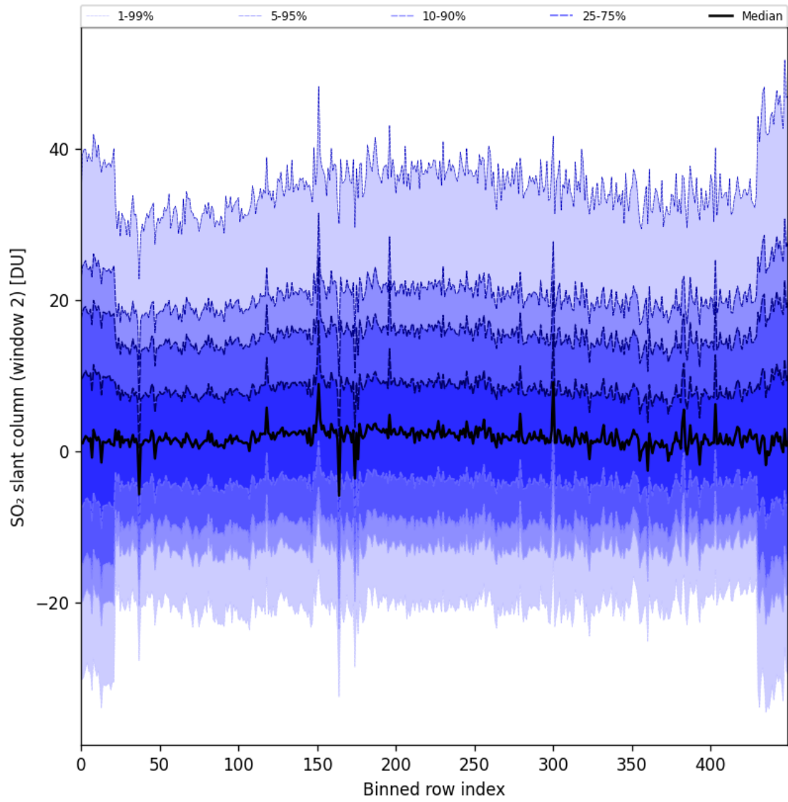
Figure 83: Along track statistics of “SO 2 slant column (window 2)” for 2024-10-16 to 2024-10-18
