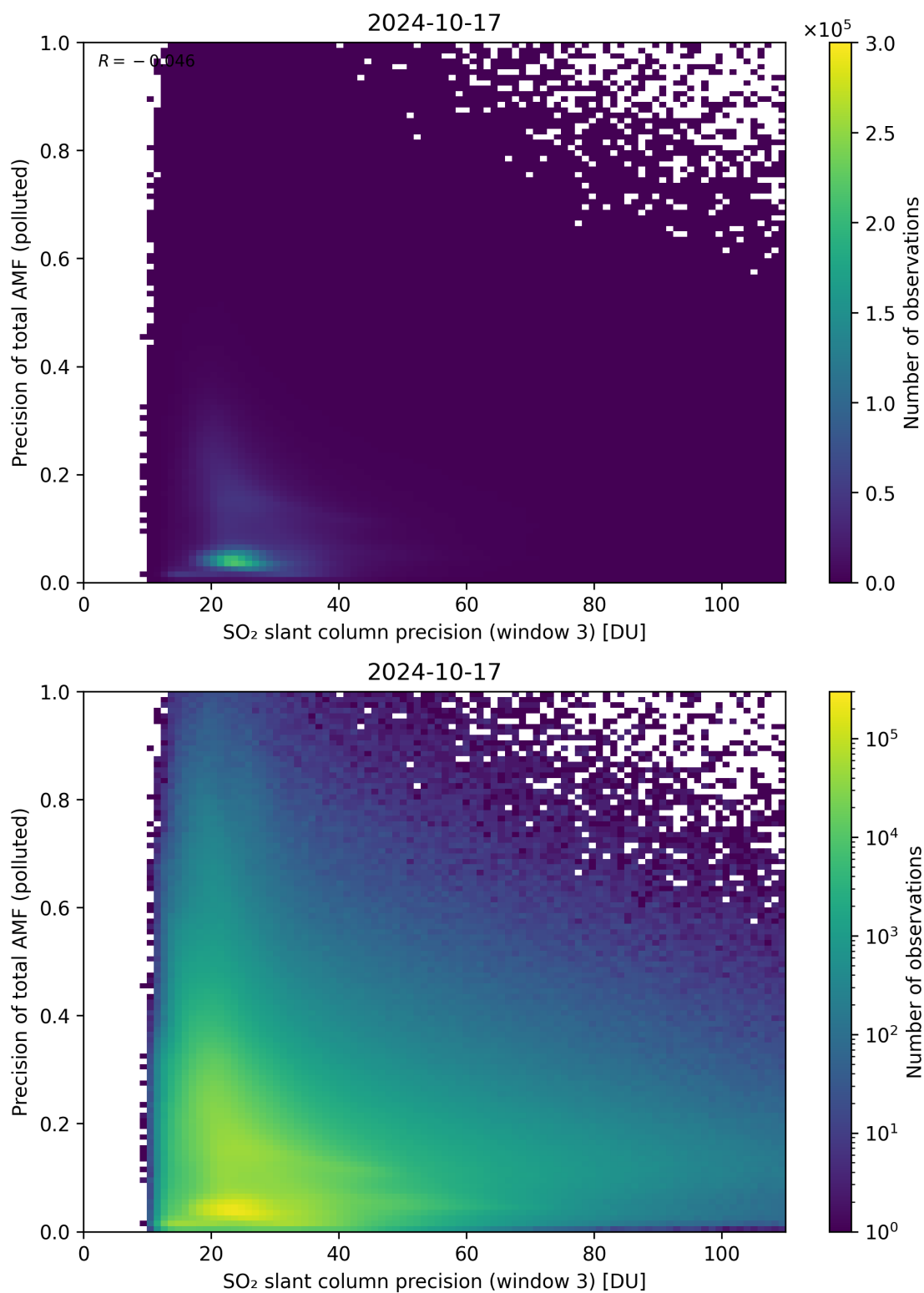
Figure 264: Scatter density plot of “SO 2 slant column precision (window 3)” against “Precision of total AMF (polluted)” for 2024-10-16 to 2024-10-18.
