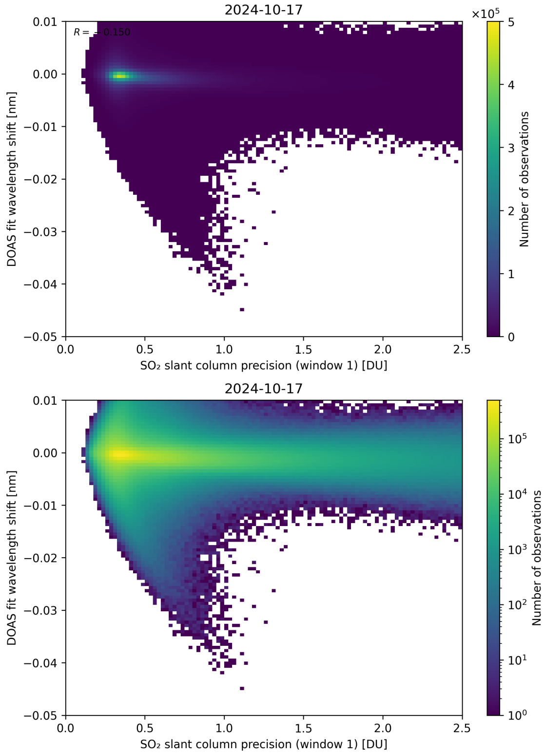
Figure 221: Scatter density plot of “SO 2 slant column precision (window 1)” against “DOAS fit wavelength shift” for 2024-10-16 to 2024-10-18.
