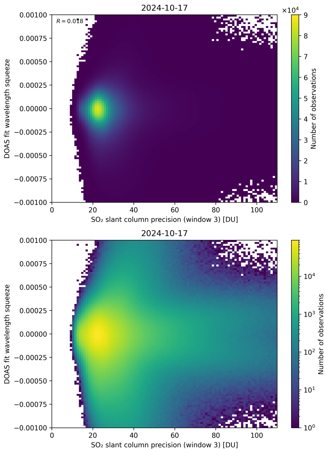
Figure 259: Scatter density plot of “SO 2 slant column precision (window 3)” against “DOAS fit wavelength squeeze” for 2024-10-16 to 2024-10-18.
