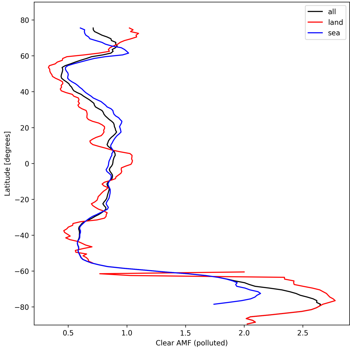
Figure 50: Zonal average of “Clear AMF (polluted)” for 2024-10-16 to 2024-10-18.
