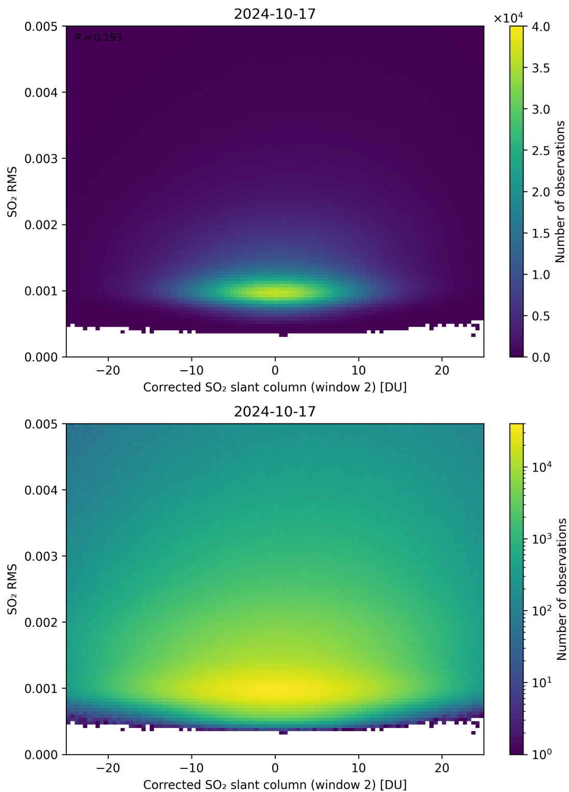
Figure 198: Scatter density plot of “Corrected SO 2 slant column (window 2)” against “SO 2 RMS” for 2024-10-16 to 2024-10-18.
