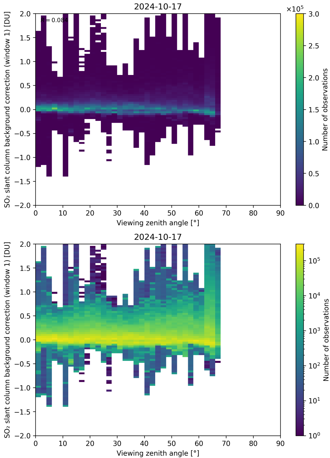
Figure 308: Scatter density plot of “Viewing zenith angle” against “SO 2 slant column background correction (window 1)” for 2024-10-16 to 2024-10-18.
