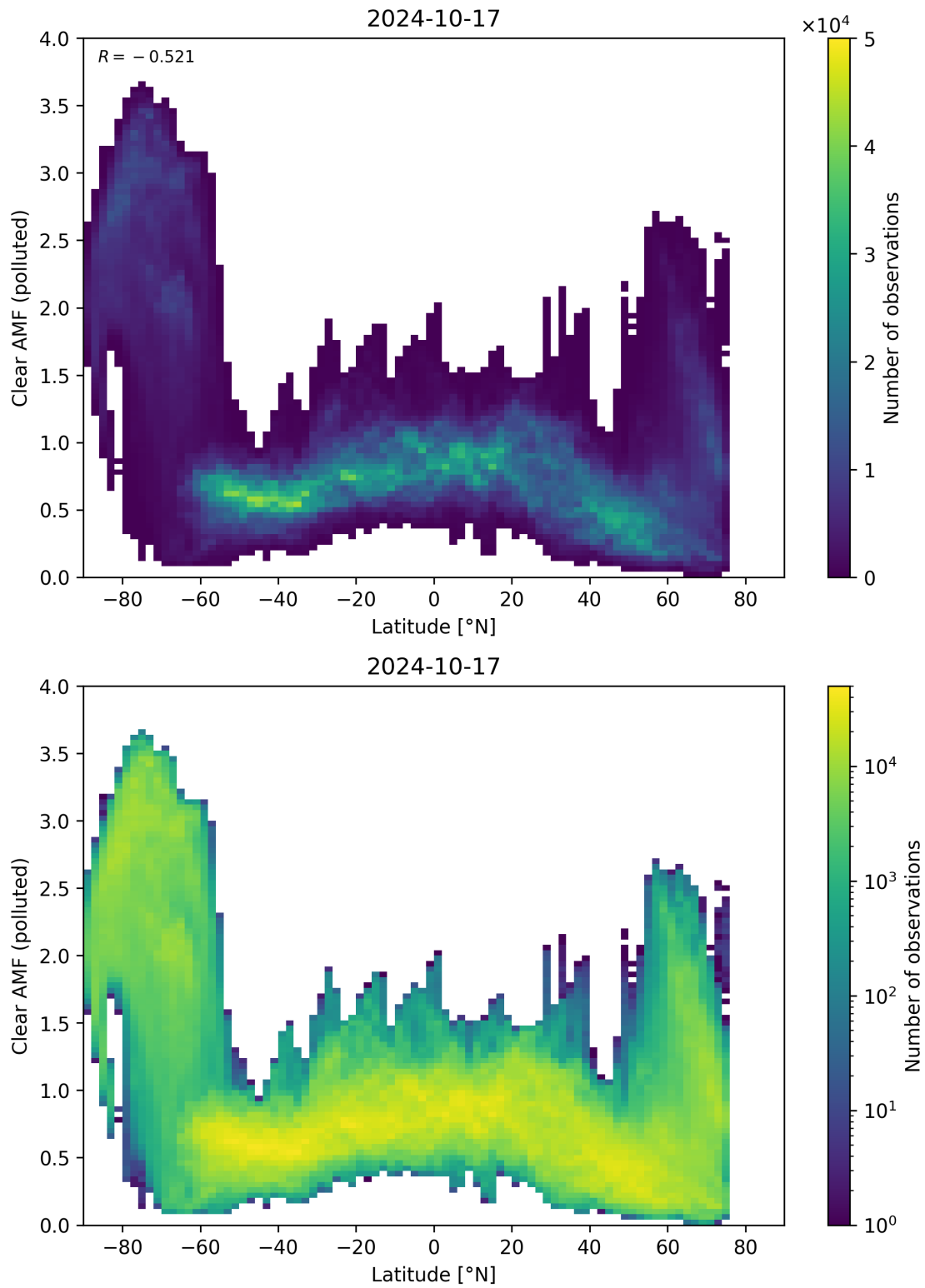
Figure 145: Scatter density plot of “Latitude” against “Clear AMF (polluted)” for 2024-10-16 to 2024-10-18.
