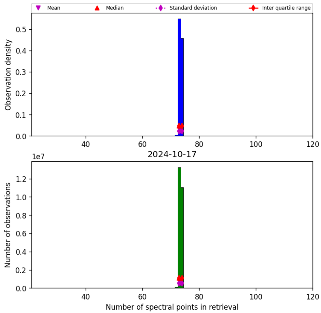
Figure 74: Histogram of “Number of spectral points in retrieval” for 2024-10-16 to 2024-10-18
