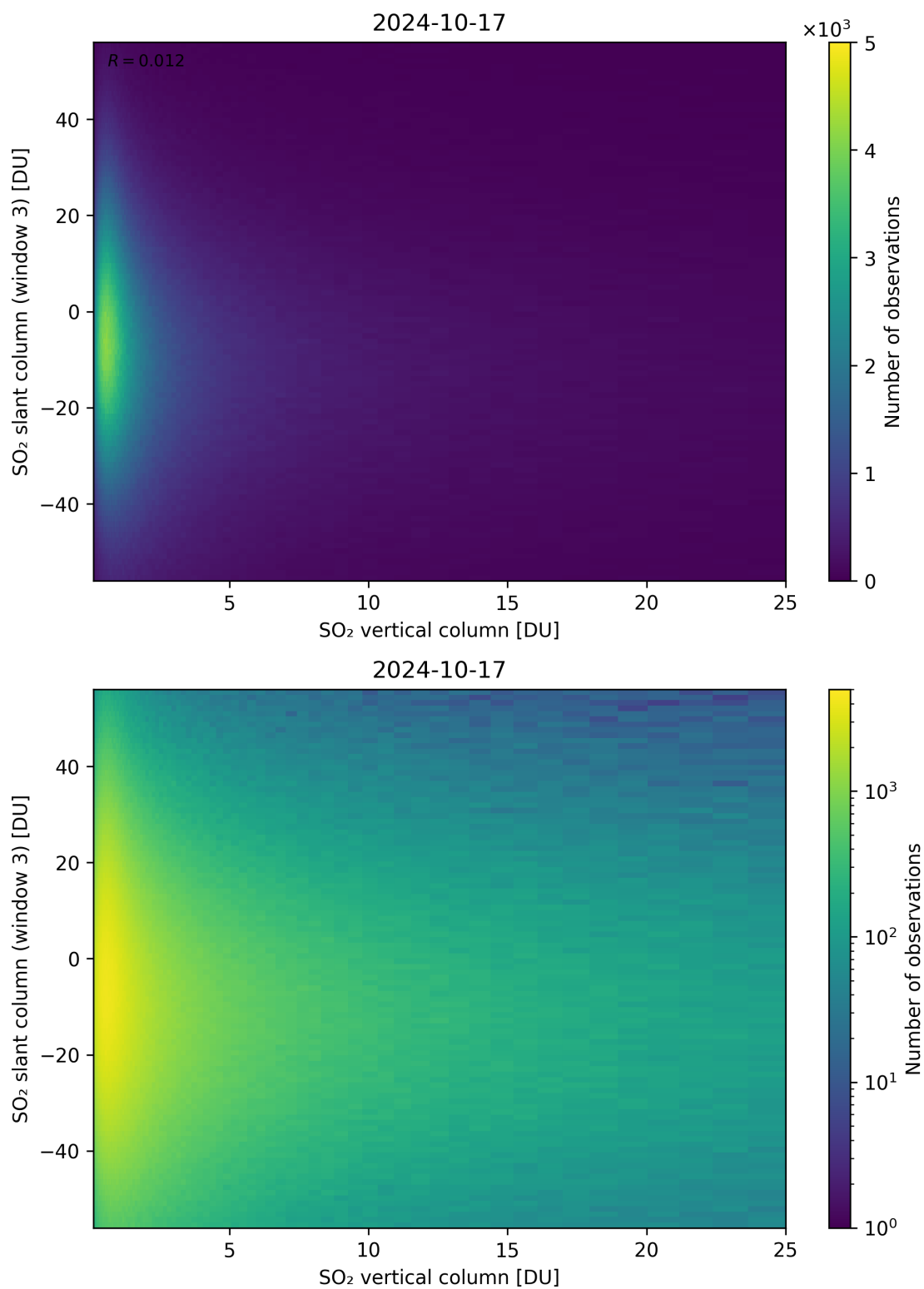
Figure 303: Scatter density plot of “SO 2 vertical column” against “SO 2 slant column (window 3)” for 2024-10-16 to 2024-10-18.
