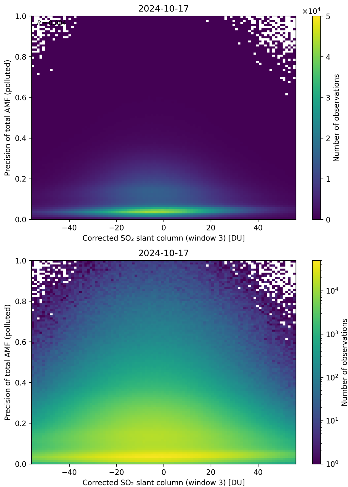
Figure 211: Scatter density plot of “Corrected SO 2 slant column (window 3)” against “Precision of total AMF (polluted)” for 2024-10-16 to 2024-10-18.
