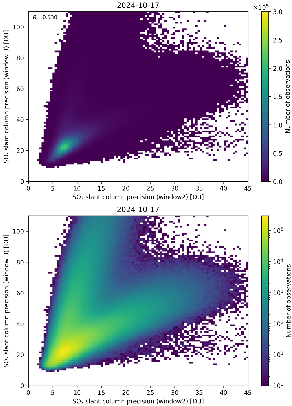
Figure 250: Scatter density plot of “SO 2 slant column precision (window2)” against “SO 2 slant column precision (window 3)” for 2024-10-16 to 2024-10-18.
