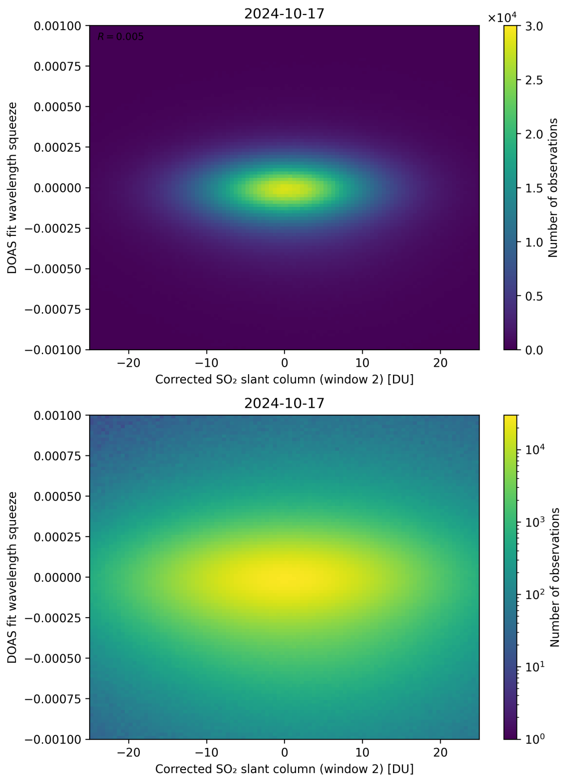
Figure 197: Scatter density plot of “Corrected SO 2 slant column (window 2)” against “DOAS fit wavelength squeeze” for 2024-10-16 to 2024-10-18.
