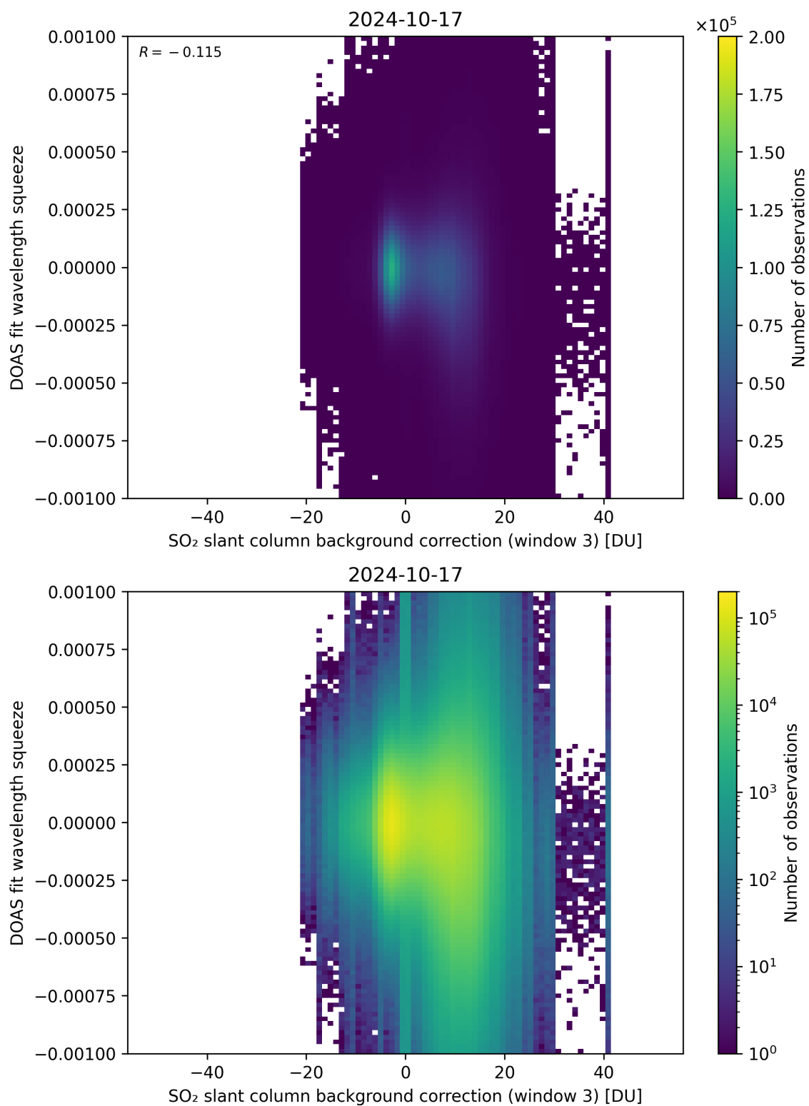
Figure 122: Scatter density plot of “SO 2 slant column background correction (window 3)” against “DOAS fit wavelength squeeze” for 2024-10-16 to 2024-10-18.
