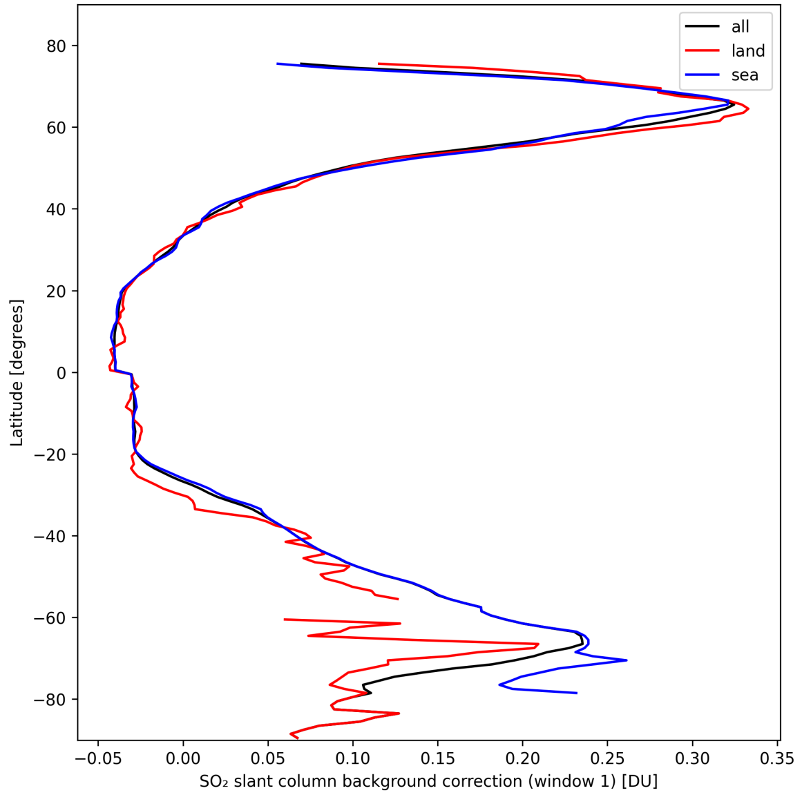
Figure 36: Zonal average of "SO 2 slant column background correction (window 1)" for 2024-10-16 to 2024-10-18.
