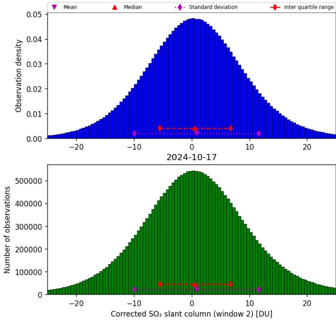
Figure 62: Histogram of “Corrected SO 2 slant column (window 2)” for 2024-10-16 to 2024-10-18
