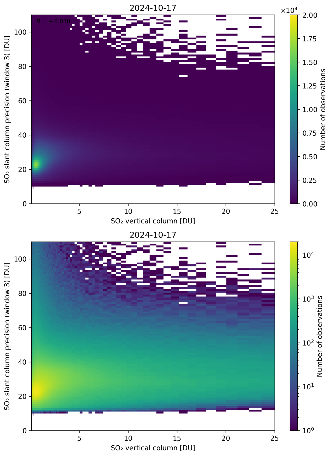
Figure 304: Scatter density plot of “SO 2 vertical column” against “SO 2 slant column precision (window 3)” for 2024-10-16 to 2024-10-18.
