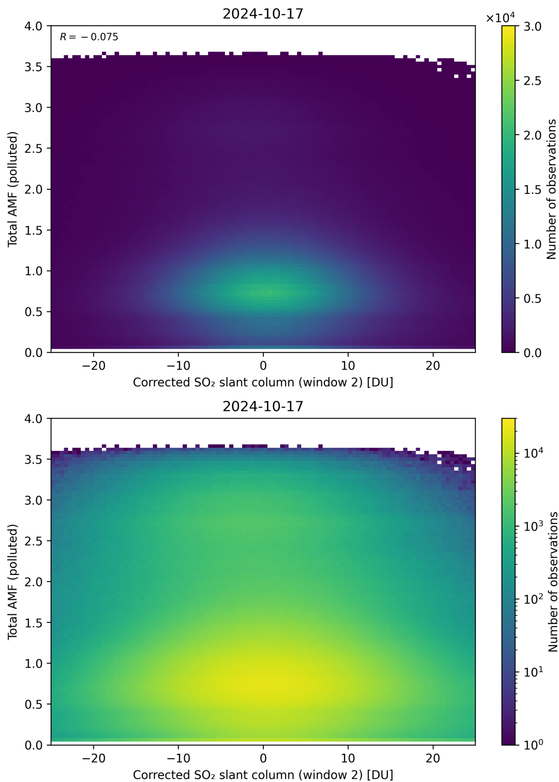
Figure 203: Scatter density plot of “Corrected SO 2 slant column (window 2)” against “Total AMF (polluted)” for 2024-10-16 to 2024-10-18.
