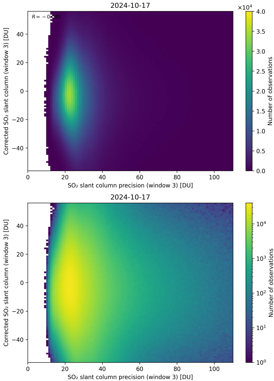
Figure 262: Scatter density plot of “SO 2 slant column precision (window 3)” against “Corrected SO 2 slant column (window 3)” for 2024-10-16 to 2024-10-18.
