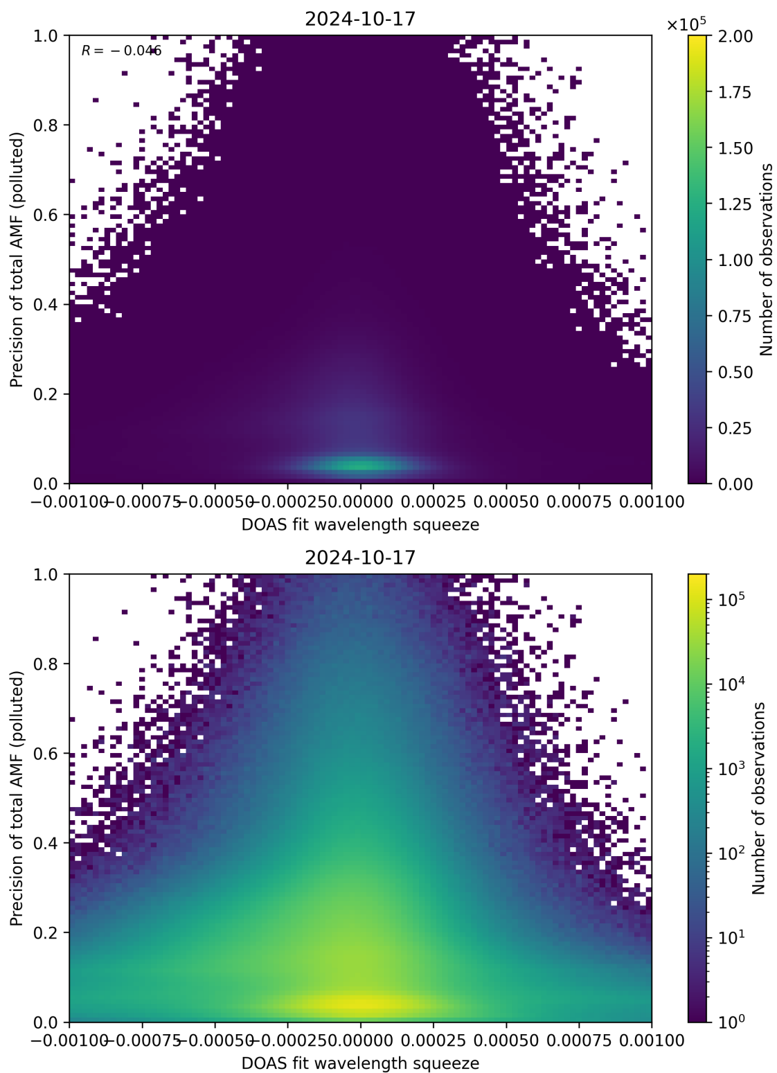
Figure 135: Scatter density plot of “DOAS fit wavelength squeeze” against “Precision of total AMF (polluted)” for 2024-10-16 to 2024-10-18.
