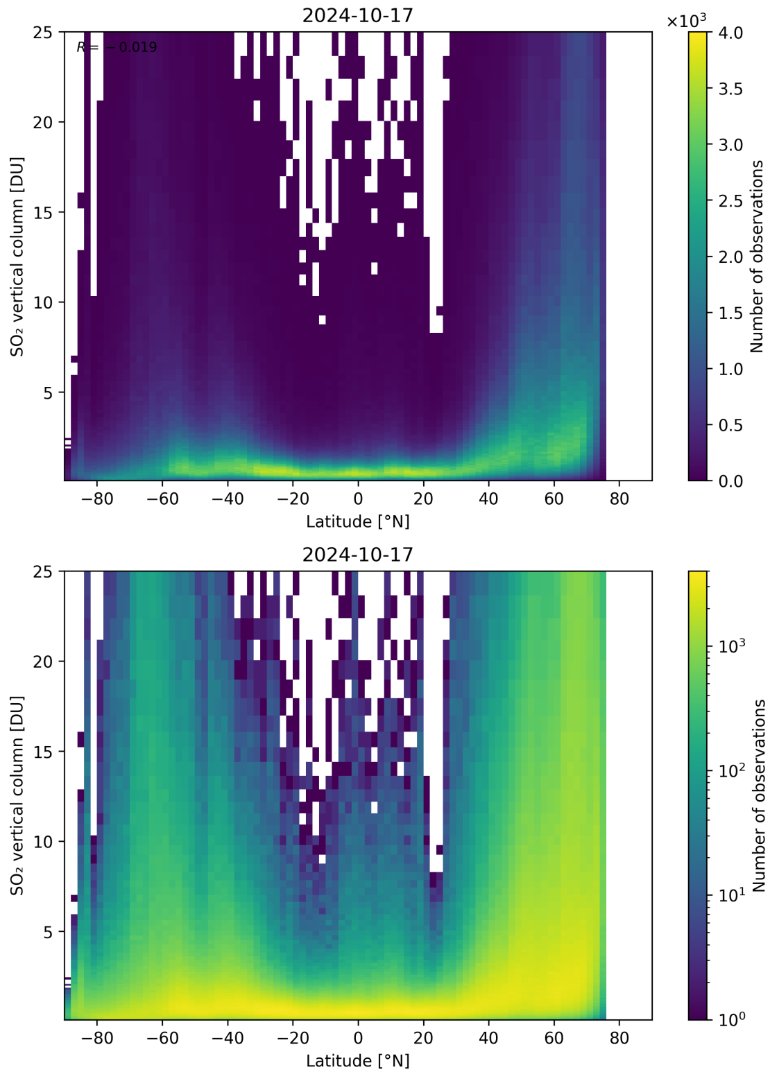
Figure 156: Scatter density plot of “Latitude” against “SO 2 vertical column” for 2024-10-16 to 2024-10-18.
