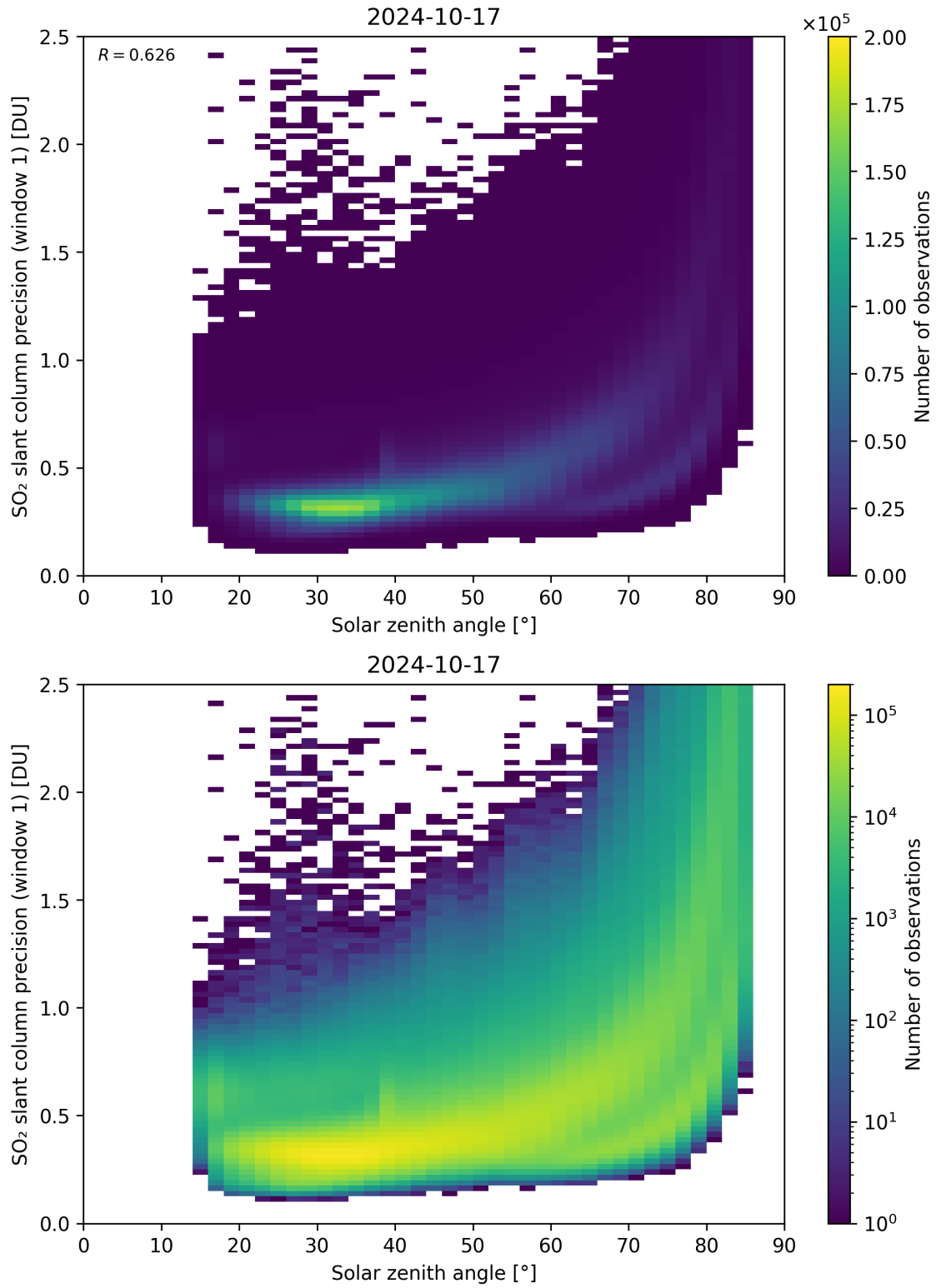
Figure 170: Scatter density plot of “Solar zenith angle” against “SO 2 slant column precision (window 1)” for 2024-10-16 to 2024-10-18.
