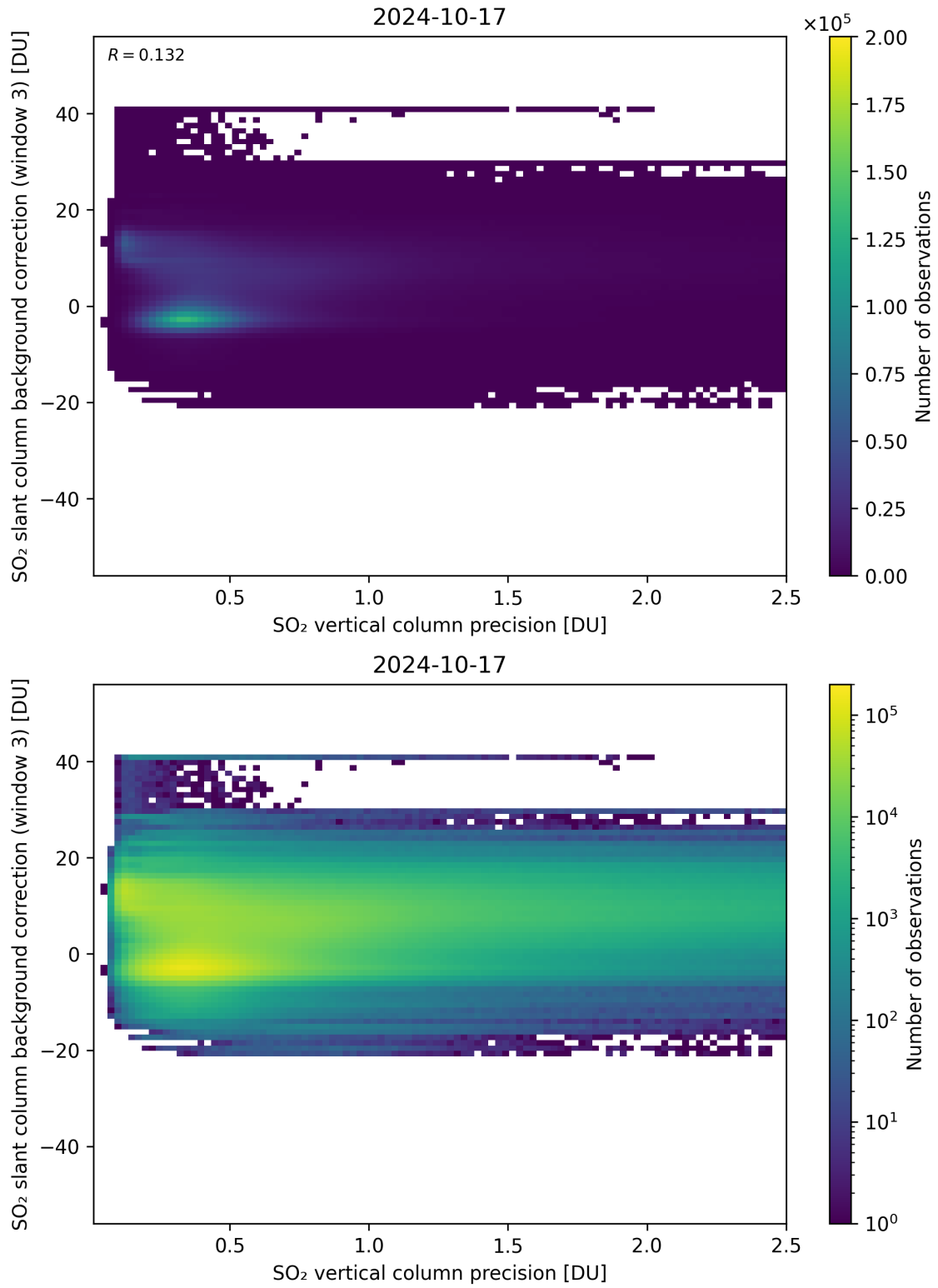
Figure 281: Scatter density plot of “SO 2 vertical column precision” against “SO 2 slant column background correction (window 3)” for 2024-10-16 to 2024-10-18.
