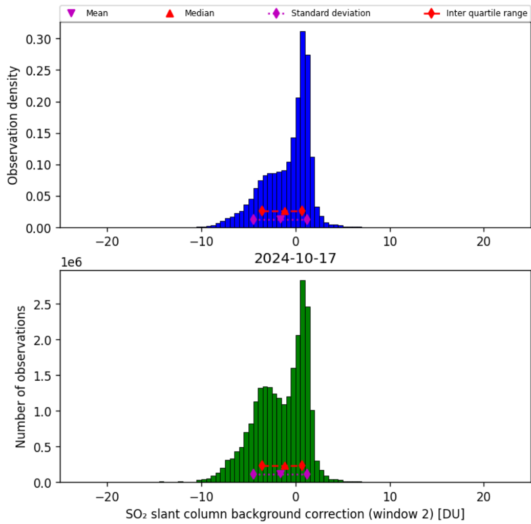
Figure 63: Histogram of “SO 2 slant column background correction (window 2)” for 2024-10-16 to 2024-10-18
