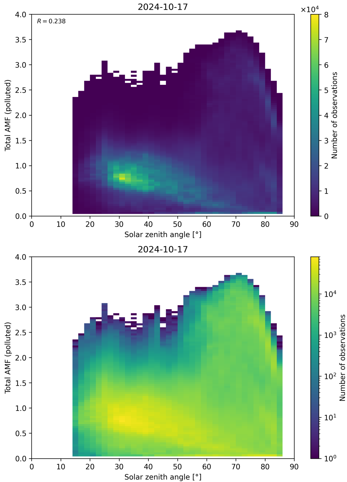
Figure 174: Scatter density plot of “Solar zenith angle” against “Total AMF (polluted)” for 2024-10-16 to 2024-10-18.
