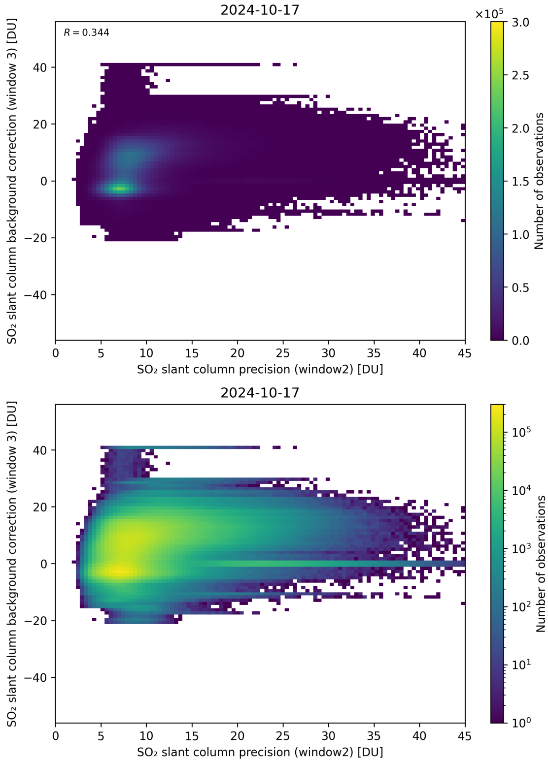
Figure 242: Scatter density plot of “SO 2 slant column precision (window2)” against “SO 2 slant column background correction (window 3)” for 2024-10-16 to 2024-10-18.
