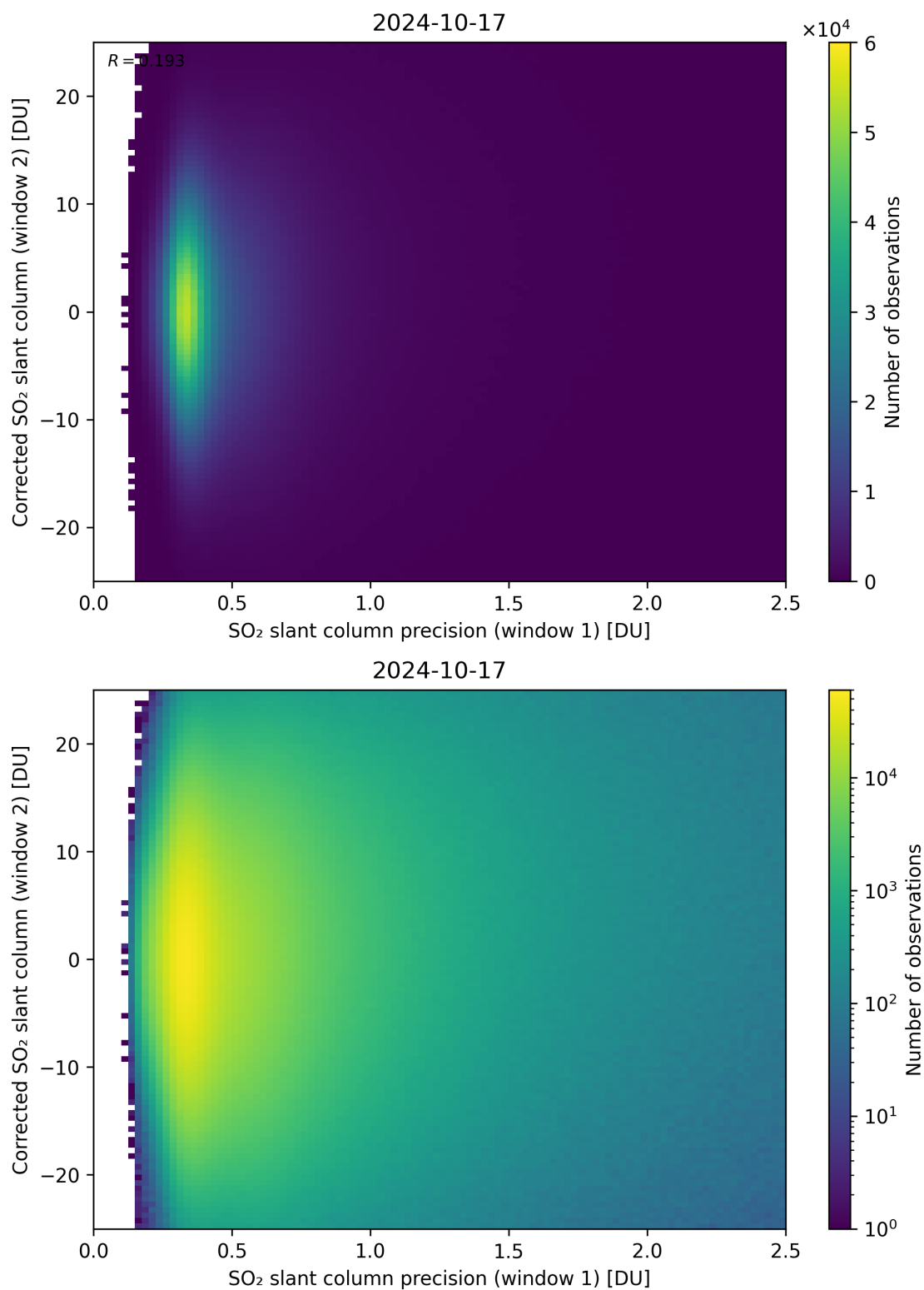
Figure 225: Scatter density plot of “SO 2 slant column precision (window 1)” against “Corrected SO 2 slant column (window 2)” for 2024-10-16 to 2024-10-18.
