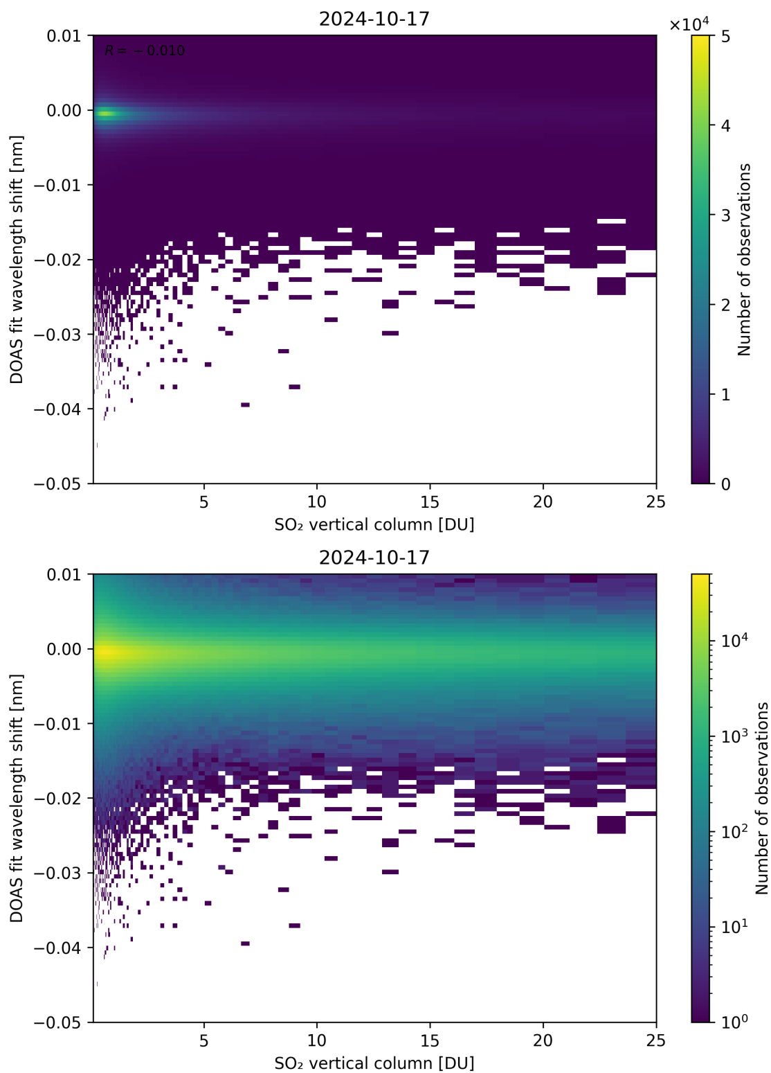
Figure 276: Scatter density plot of “SO 2 vertical column” against “DOAS fit wavelength shift” for 2024-10-16 to 2024-10-18.
