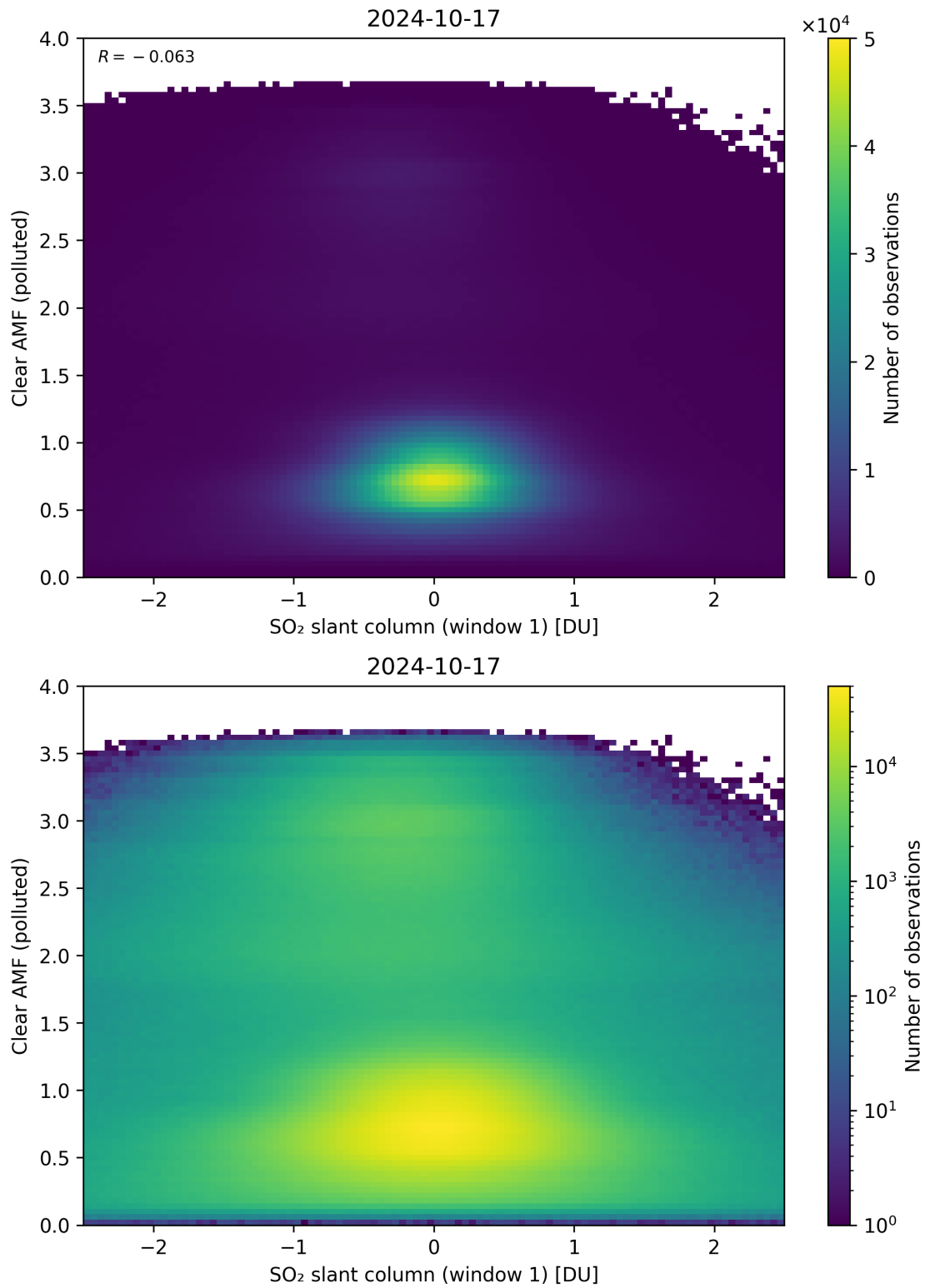
Figure 232: Scatter density plot of “SO 2 slant column (window 1)” against “Clear AMF (polluted)” for 2024-10-16 to 2024-10-18.
