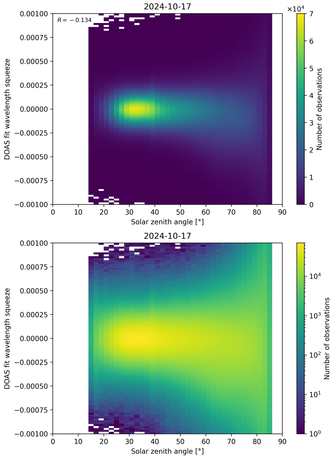
Figure 162: Scatter density plot of “Solar zenith angle” against “DOAS fit wavelength squeeze” for 2024-10-16 to 2024-10-18.
