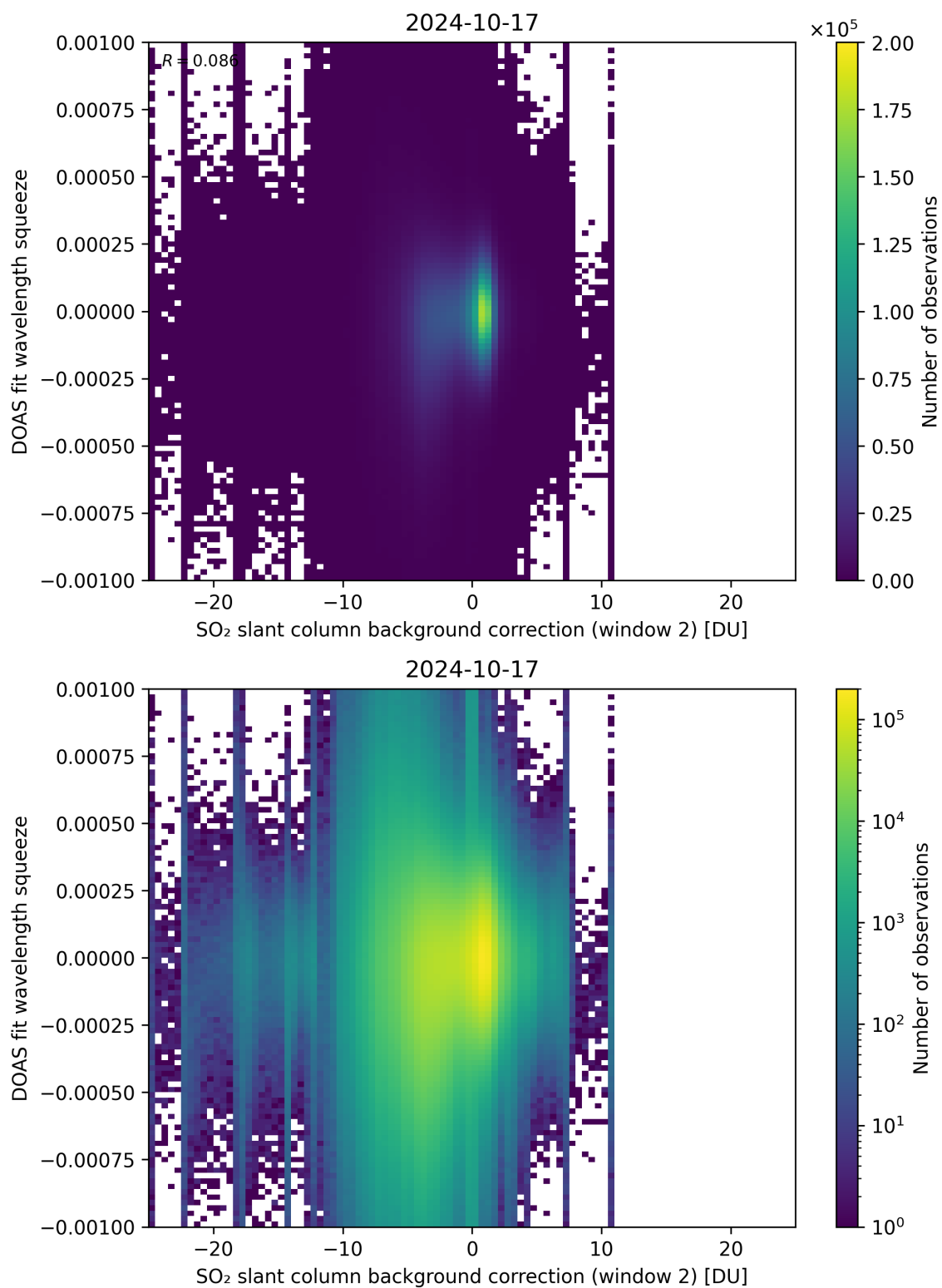
Figure 113: Scatter density plot of “SO 2 slant column background correction (window 2)” against “DOAS fit wavelength squeeze” for 2024-10-16 to 2024-10-18.
