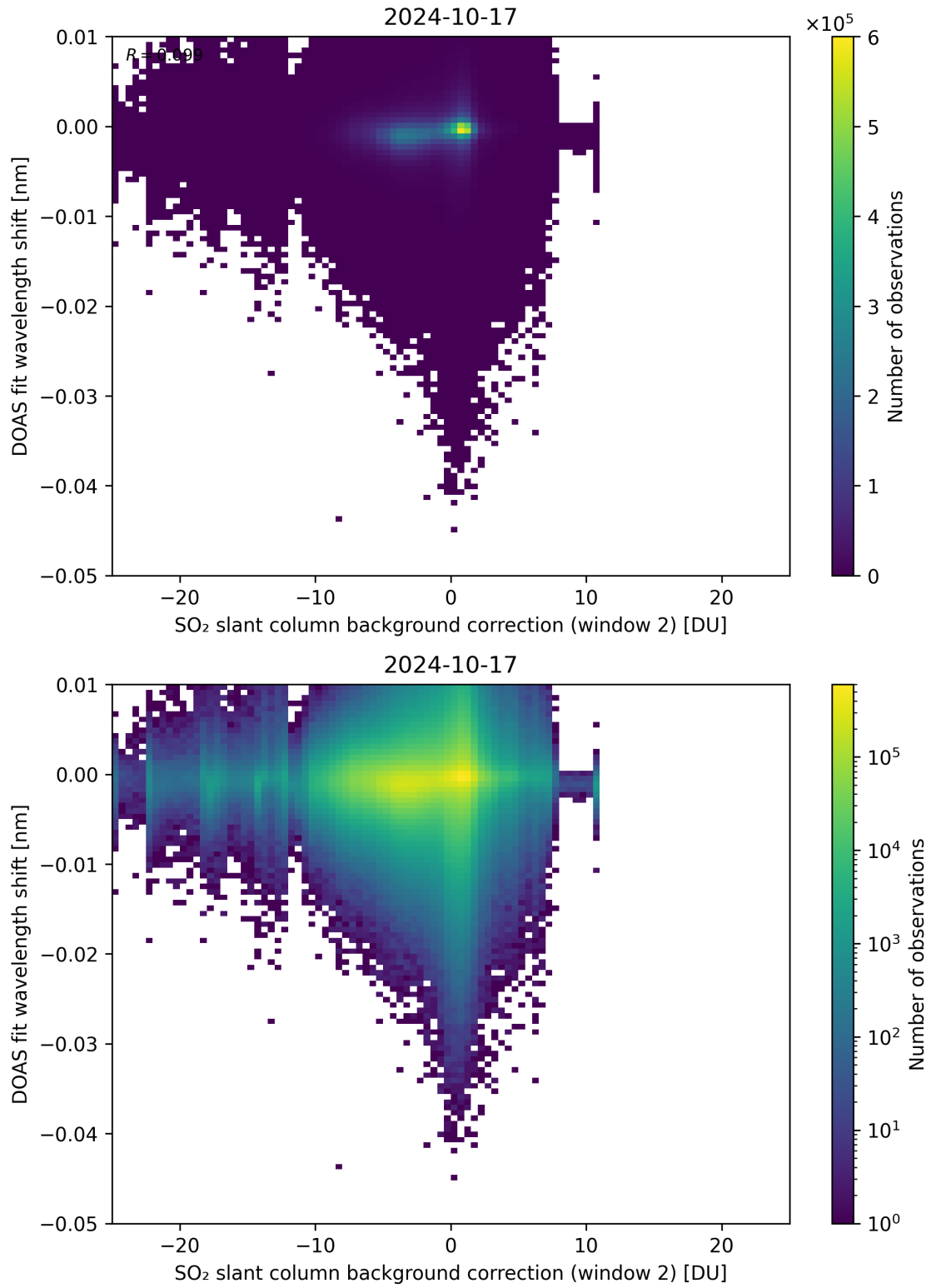
Figure 112: Scatter density plot of “SO 2 slant column background correction (window 2)” against “DOAS fit wavelength shift” for 2024-10-16 to 2024-10-18.
