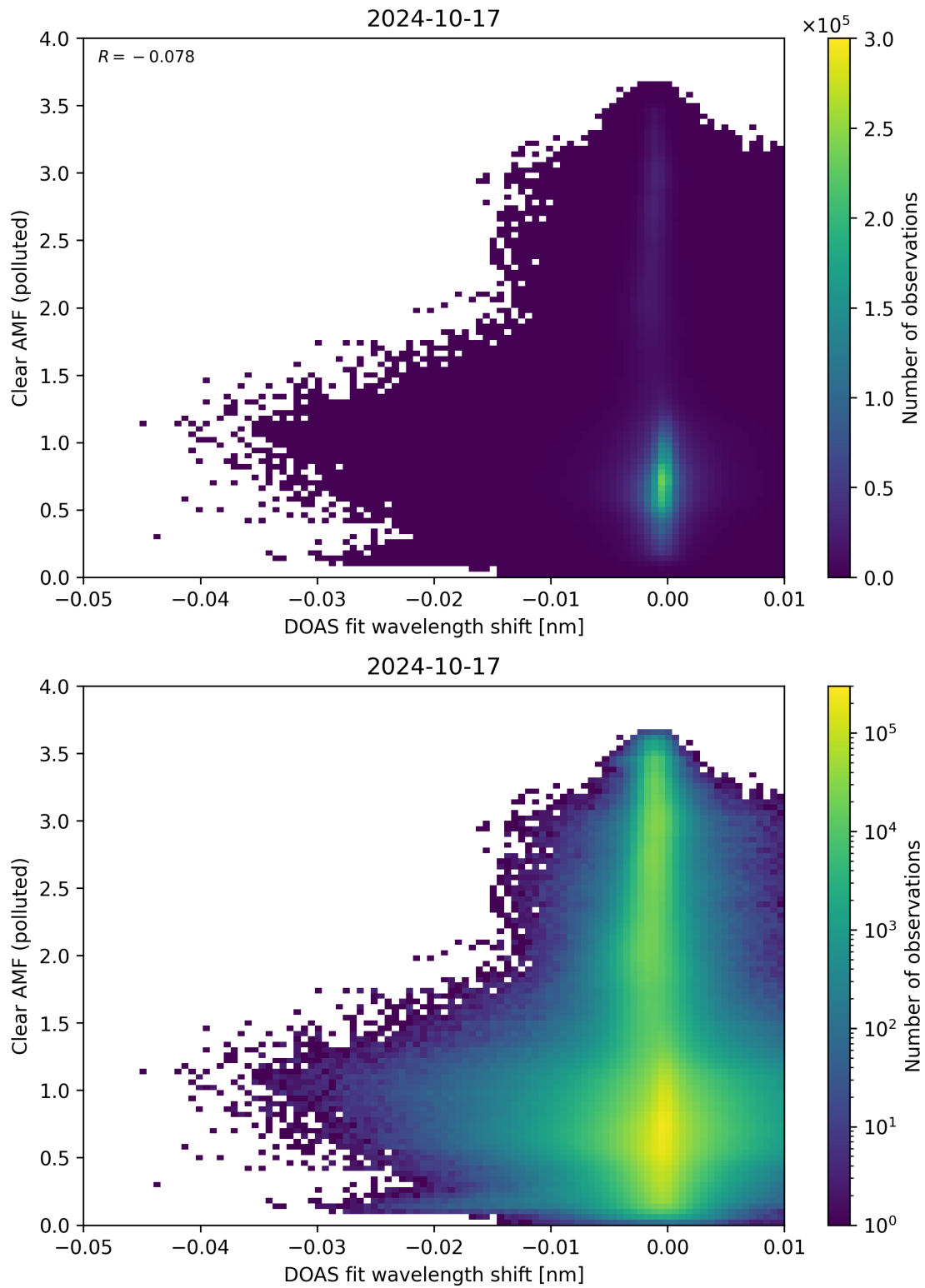
Figure 129: Scatter density plot of “DOAS fit wavelength shift” against “Clear AMF (polluted)” for 2024-10-16 to 2024-10-18.
