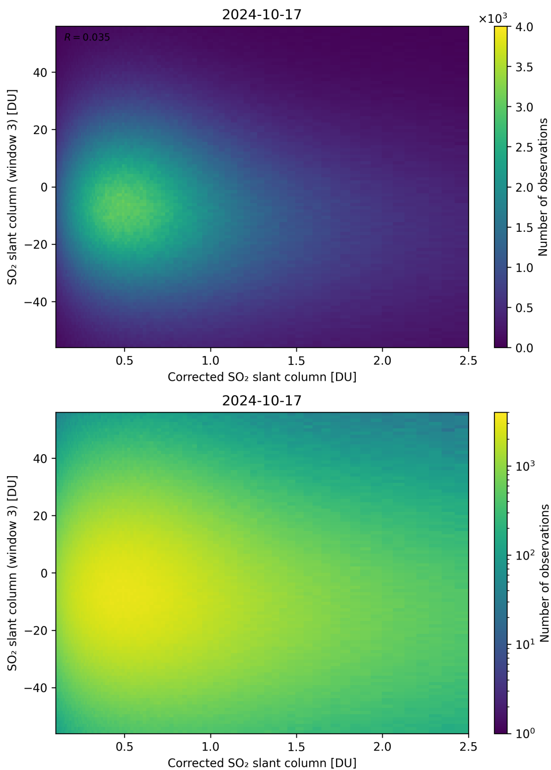
Figure 190: Scatter density plot of “Corrected SO 2 slant column” against “SO 2 slant column (window 3)” for 2024-10-16 to 2024-10-18.
