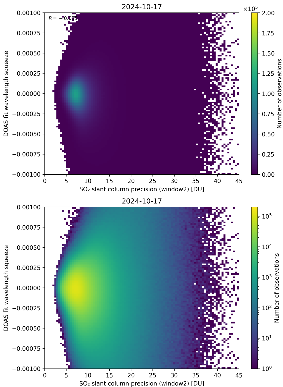
Figure 244: Scatter density plot of “SO 2 slant column precision (window2)” against “DOAS fit wavelength squeeze” for 2024-10-16 to 2024-10-18.
