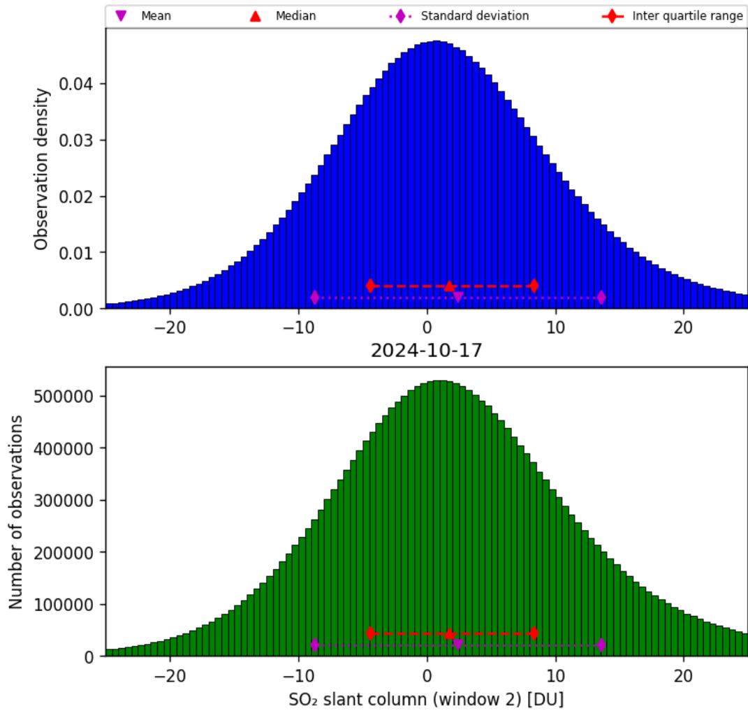
Figure 60: Histogram of “SO 2 slant column (window 2)” for 2024-10-16 to 2024-10-18
