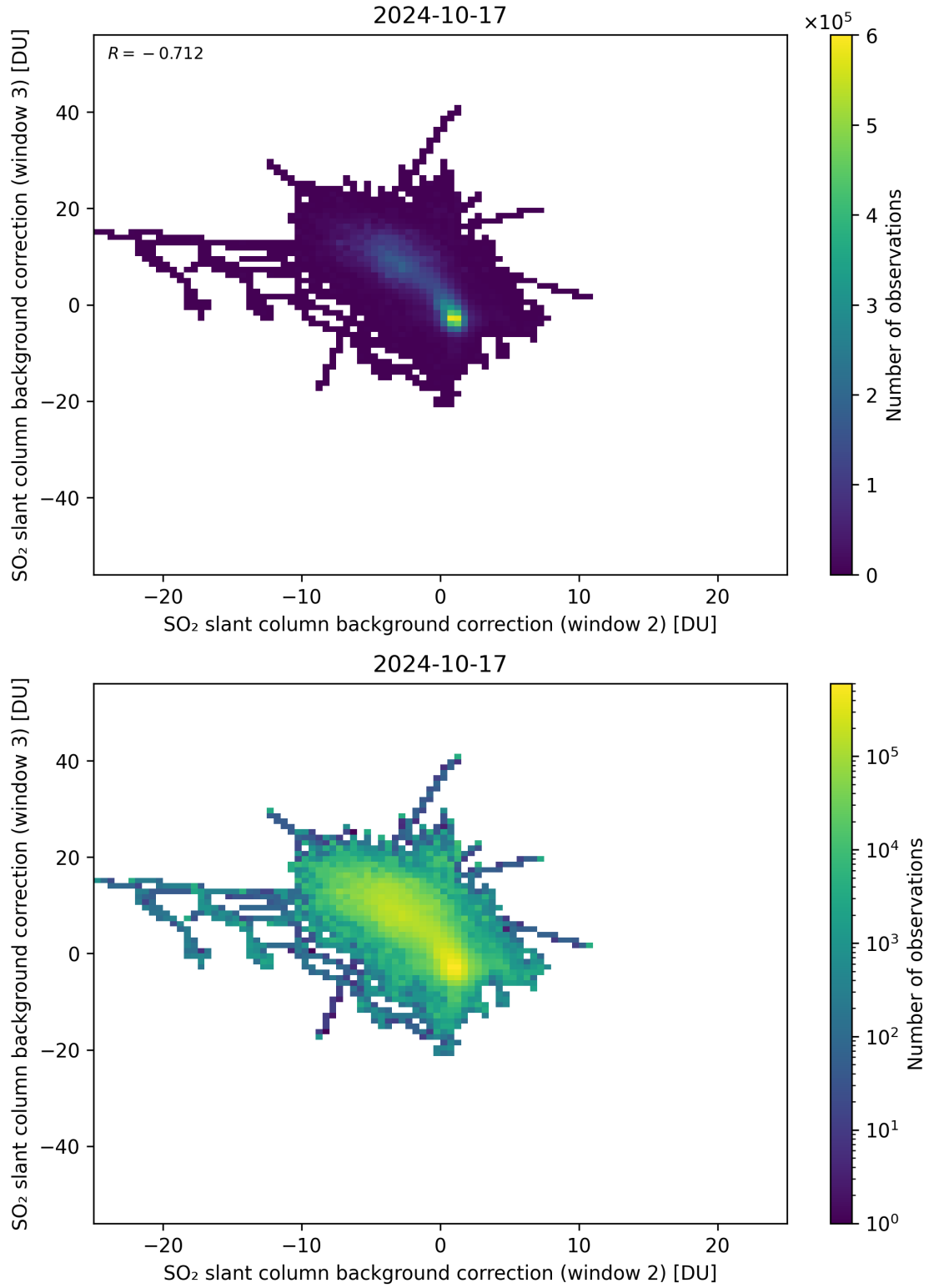
Figure 111: Scatter density plot of “SO 2 slant column background correction (window 2)” against “SO 2 slant column background correction (window 3)” for 2024-10-16 to 2024-10-18.
