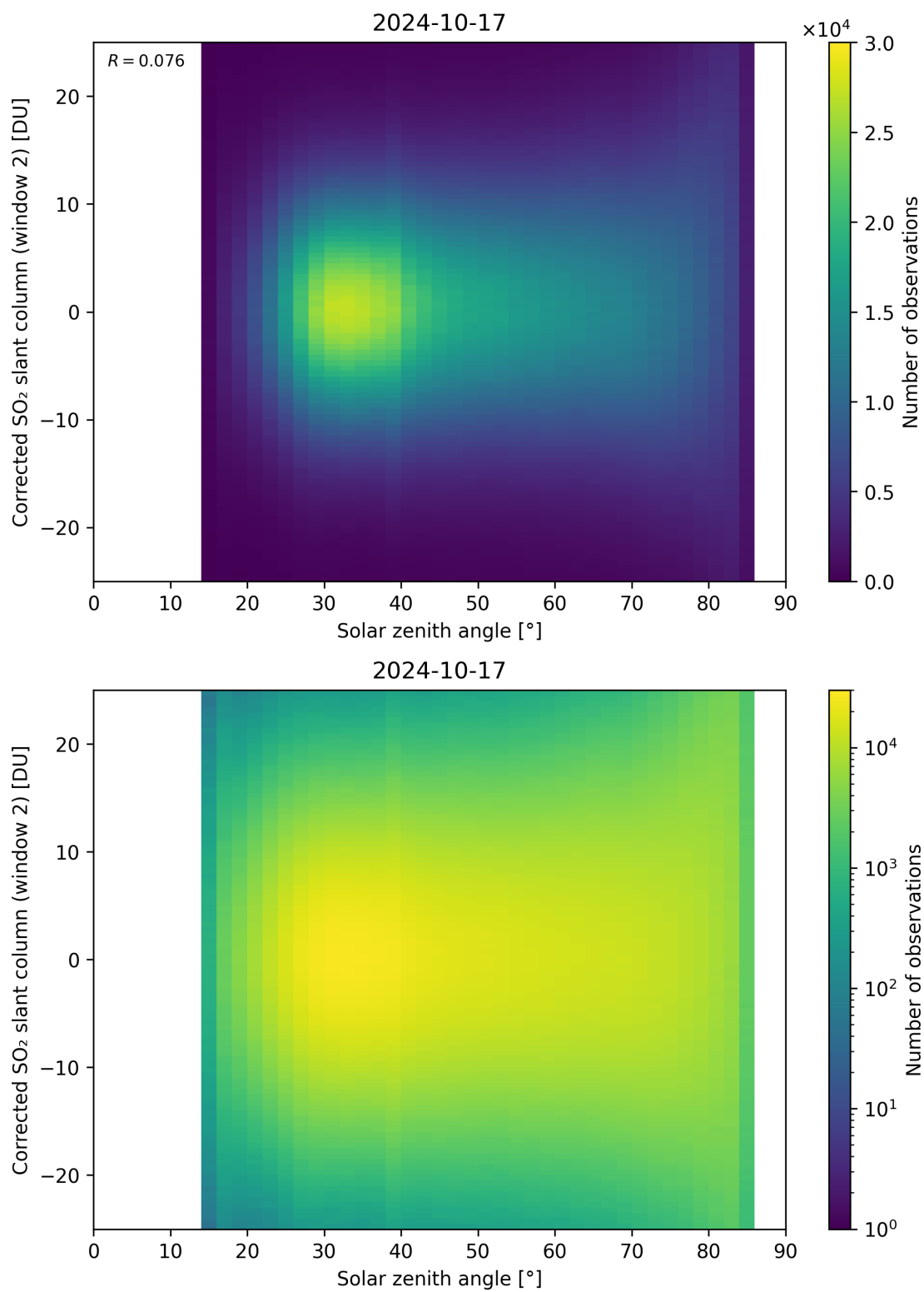
Figure 167: Scatter density plot of “Solar zenith angle” against “Corrected SO 2 slant column (window 2)” for 2024-10-16 to 2024-10-18.
