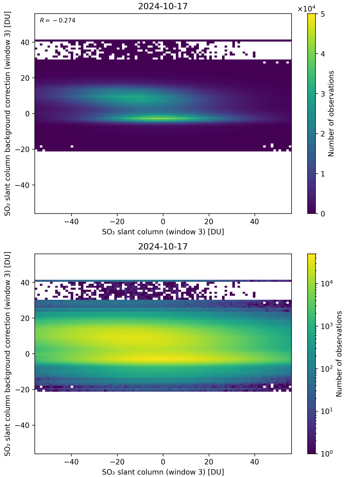
Figure 253: Scatter density plot of “SO 2 slant column (window 3)” against “SO 2 slant column background correction (window 3)” for 2024-10-16 to 2024-10-18.
