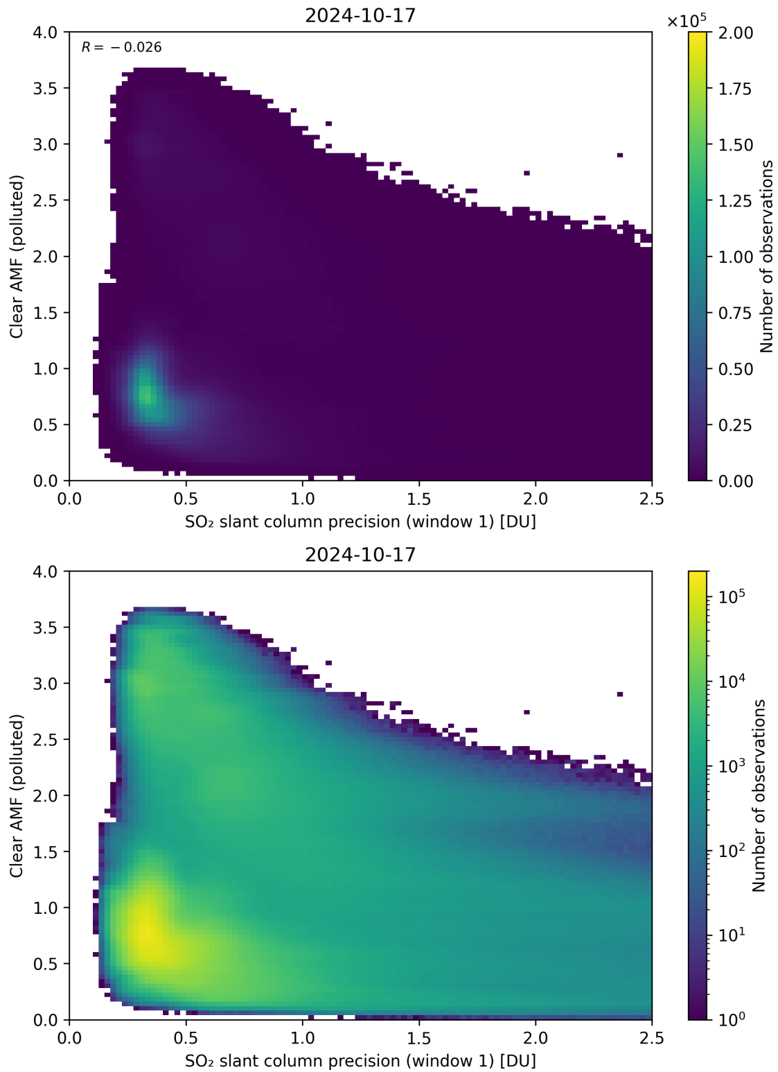
Figure 224: Scatter density plot of “SO 2 slant column precision (window 1)” against “Clear AMF (polluted)” for 2024-10-16 to 2024-10-18.
