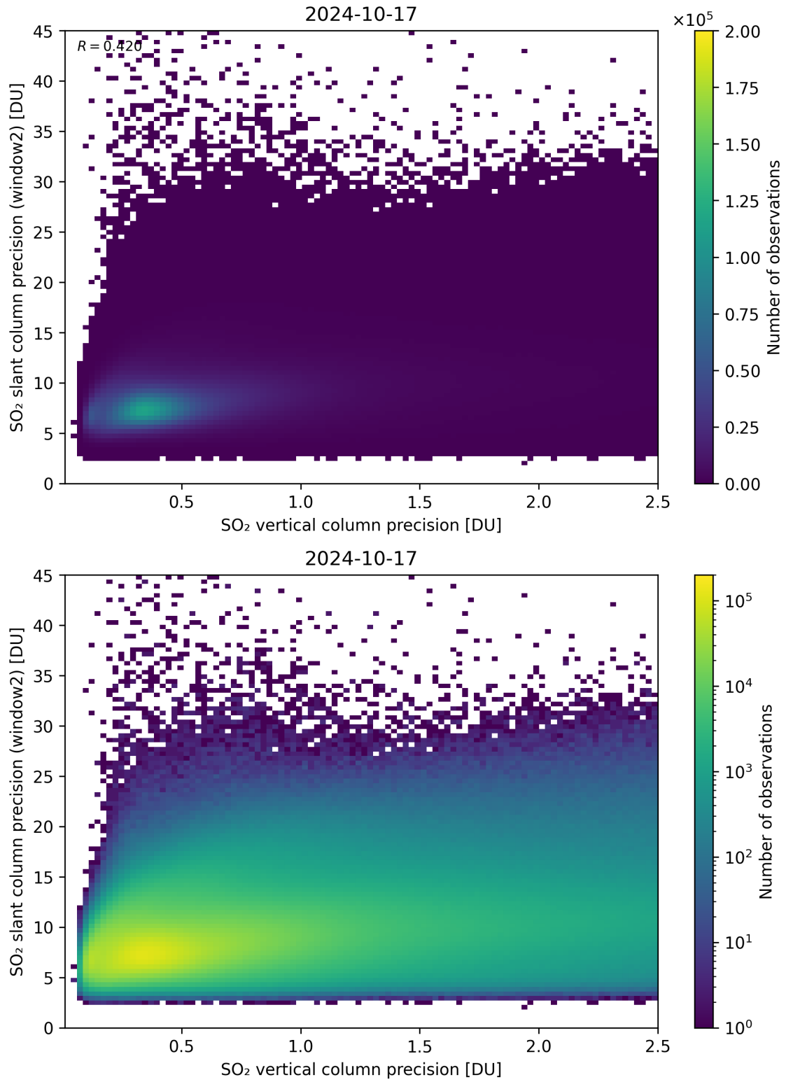
Figure 291: Scatter density plot of “SO 2 vertical column precision” against “SO 2 slant column precision (window2)” for 2024-10-16 to 2024-10-18.
