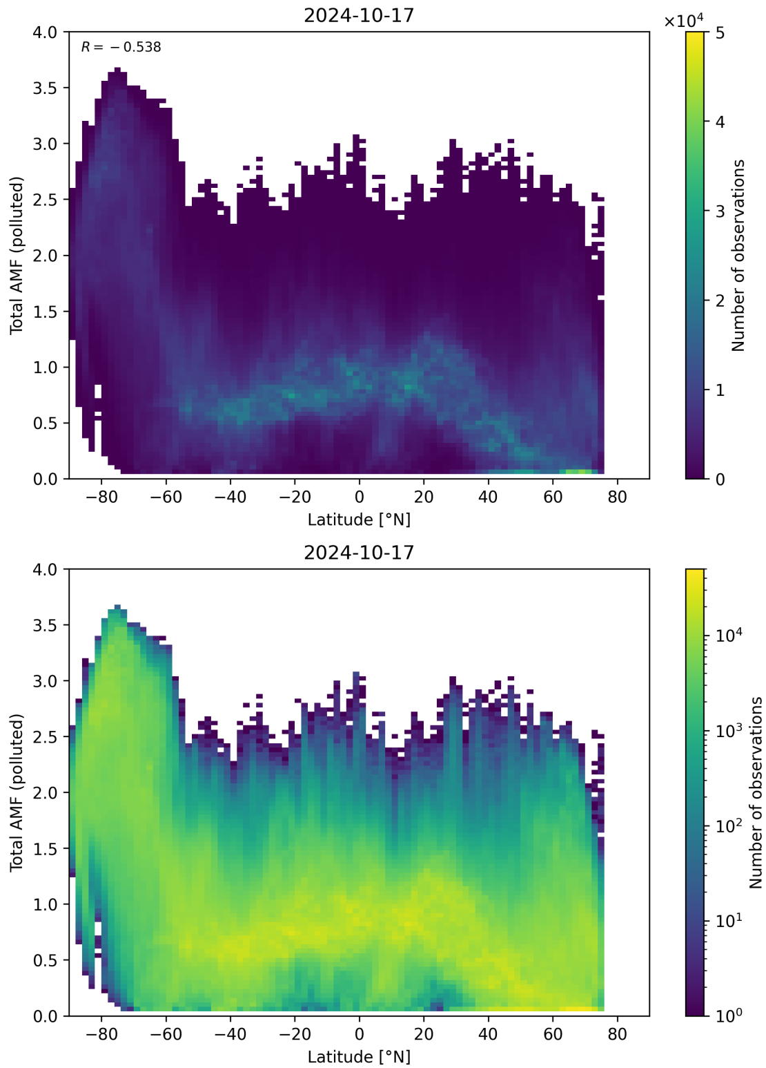
Figure 154: Scatter density plot of “Latitude” against “Total AMF (polluted)” for 2024-10-16 to 2024-10-18.
