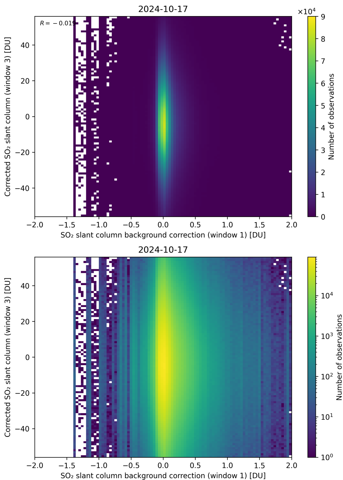
Figure 105: Scatter density plot of “SO 2 slant column background correction (window 1)” against “Corrected SO 2 slant column (window 3)” for 2024-10-16 to 2024-10-18.
