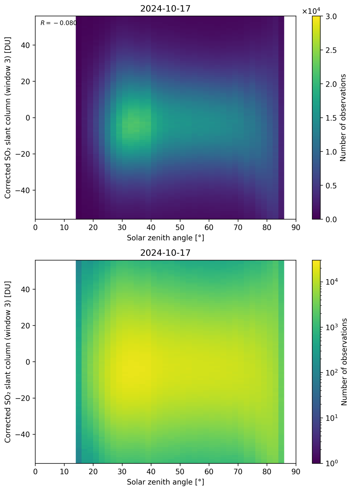
Figure 168: Scatter density plot of “Solar zenith angle” against “Corrected SO 2 slant column (window 3)” for 2024-10-16 to 2024-10-18.
