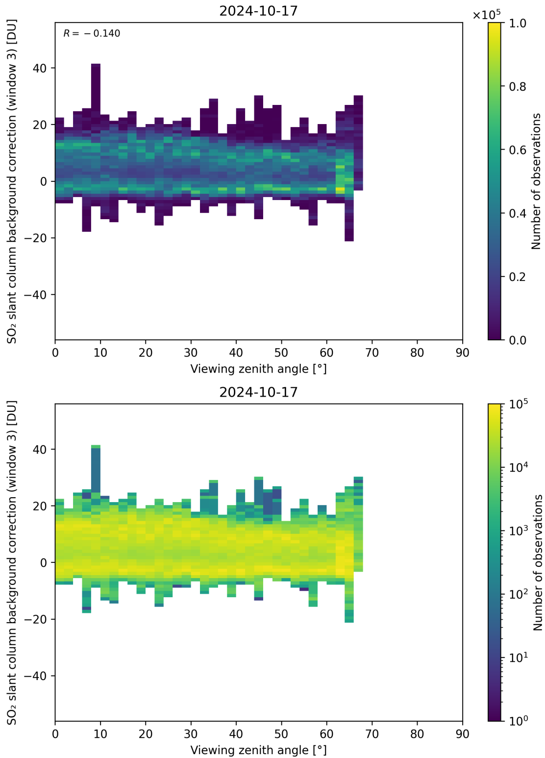
Figure 310: Scatter density plot of “Viewing zenith angle” against “SO 2 slant column background correction (window 3)” for 2024-10-16 to 2024-10-18.
