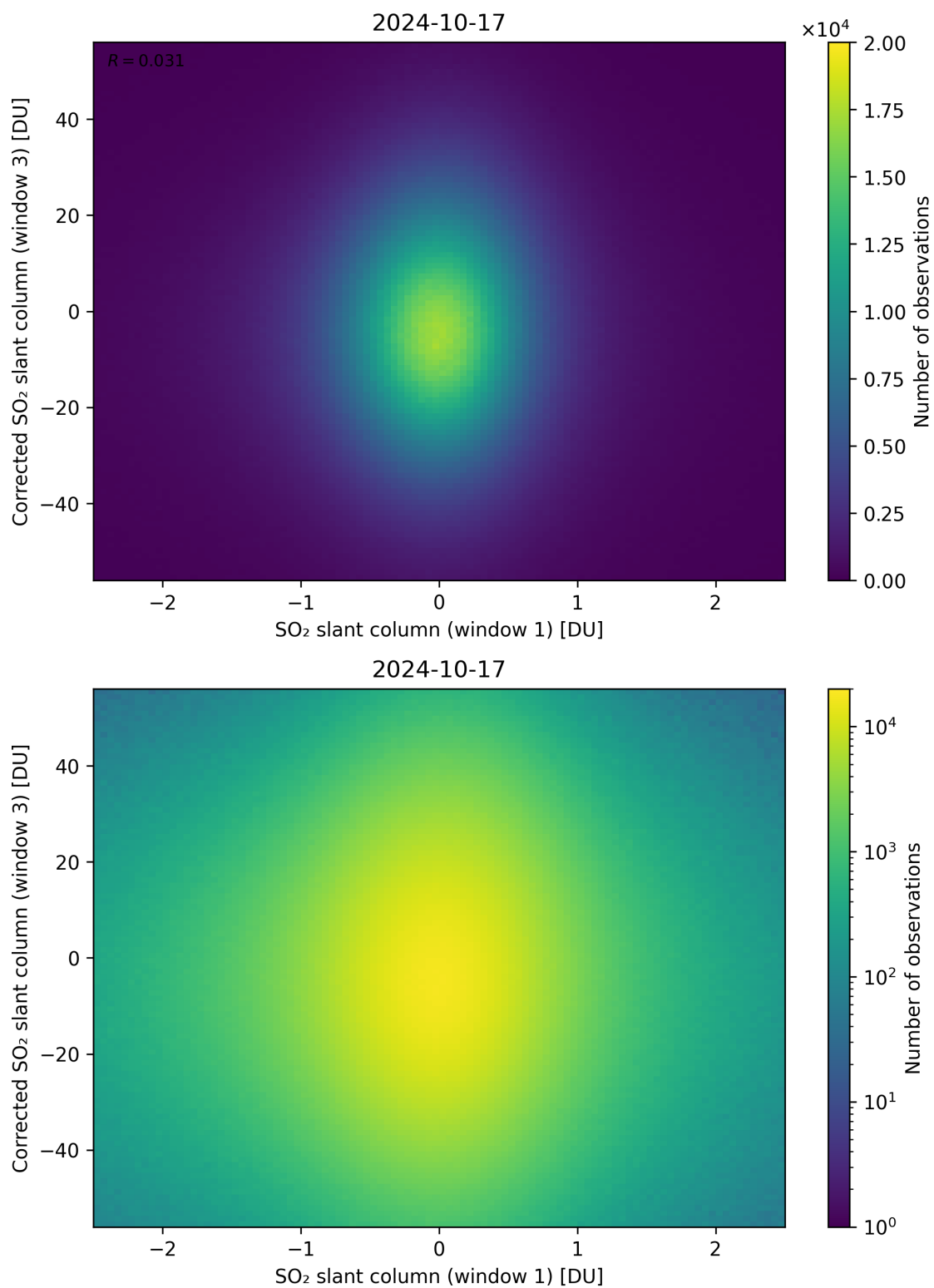
Figure 234: Scatter density plot of “SO 2 slant column (window 1)” against “Corrected SO 2 slant column (window 3)” for 2024-10-16 to 2024-10-18.
