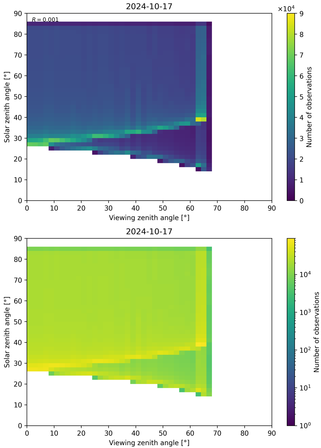
Figure 315: Scatter density plot of “Viewing zenith angle” against “Solar zenith angle” for 2024-10-16 to 2024-10-18.
