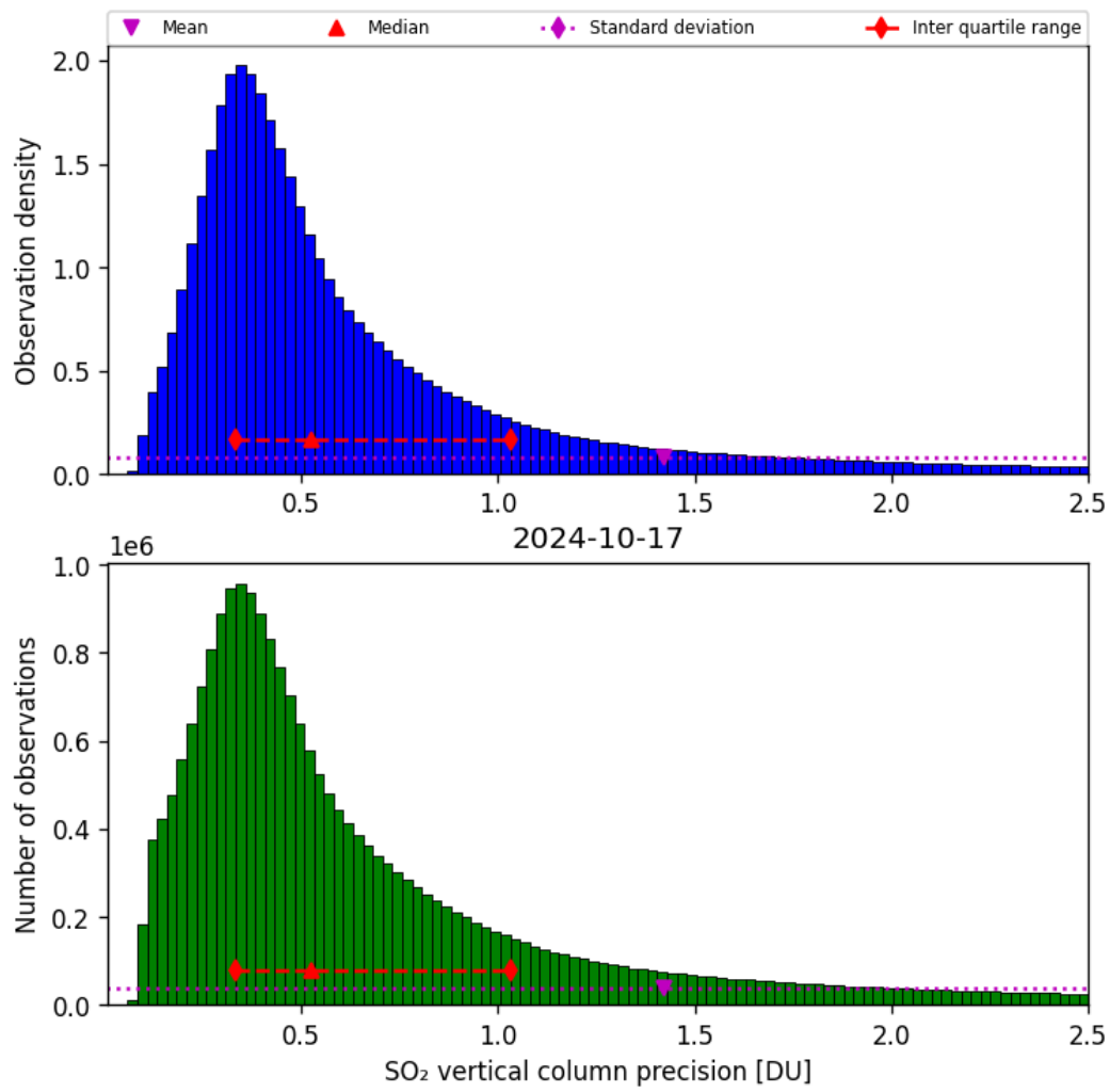
Figure 54: Histogram of “SO 2 vertical column precision” for 2024-10-16 to 2024-10-18
