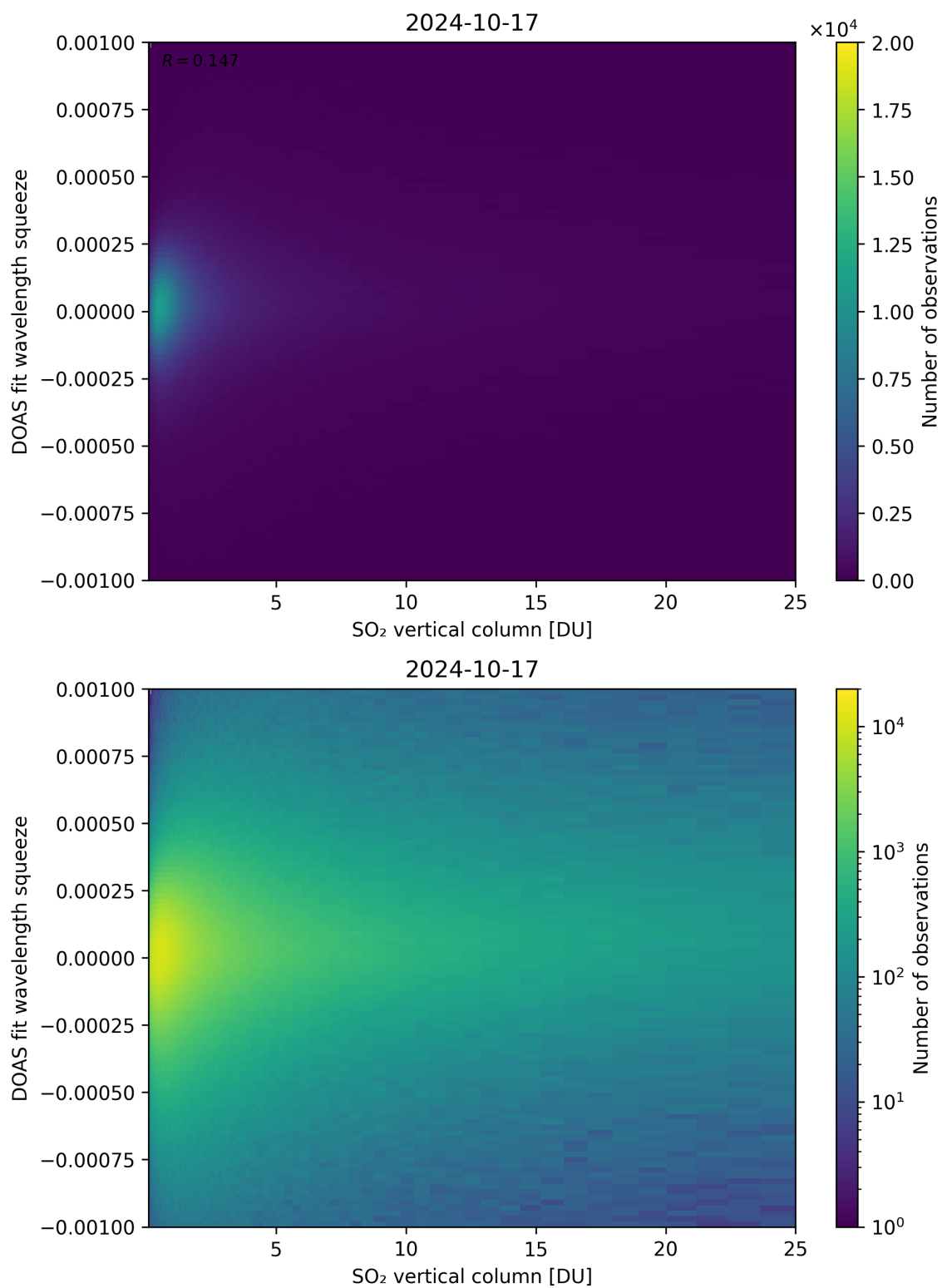
Figure 277: Scatter density plot of “SO 2 vertical column” against “DOAS fit wavelength squeeze” for 2024-10-16 to 2024-10-18.
