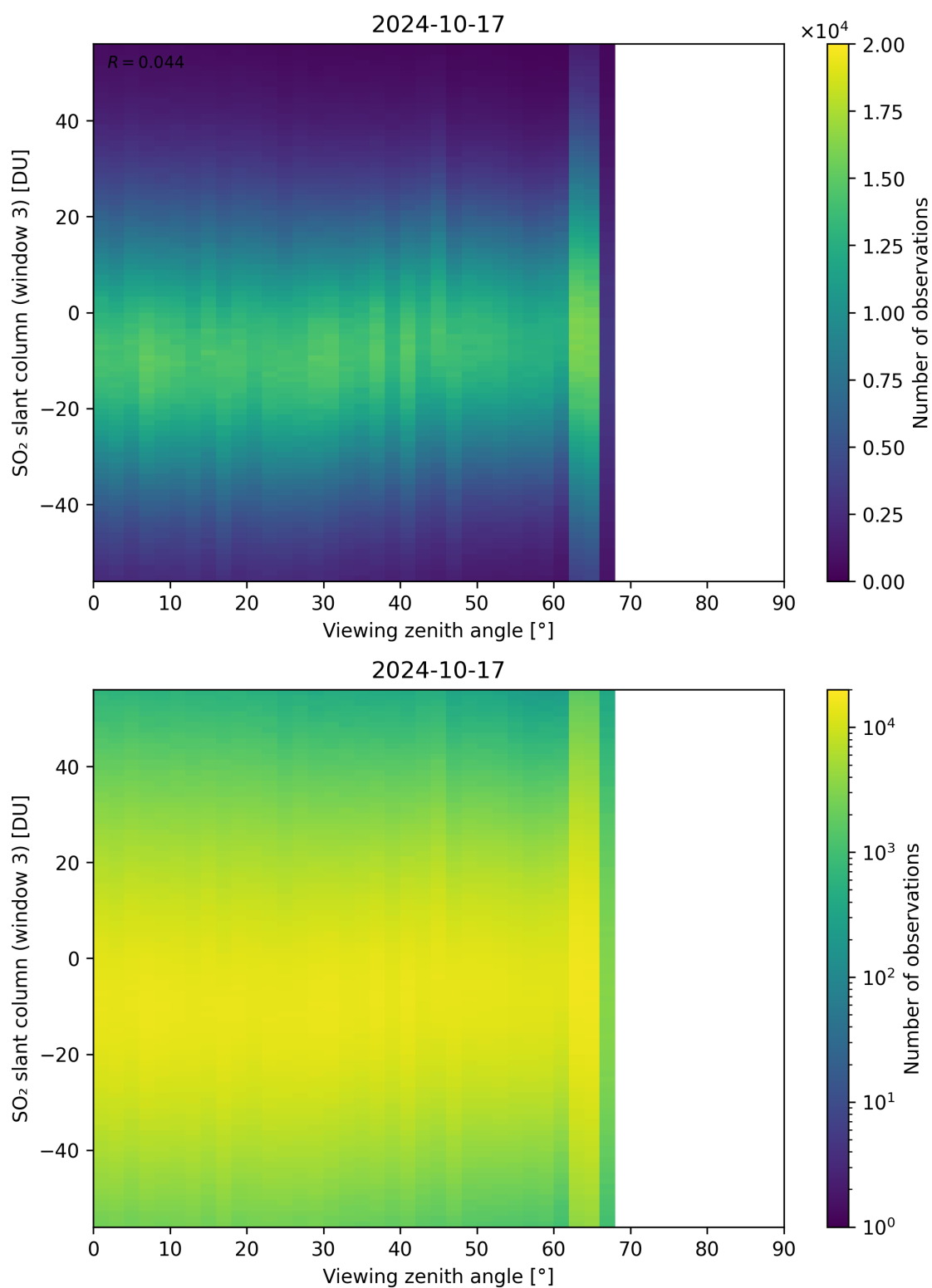
Figure 323: Scatter density plot of “Viewing zenith angle” against “SO 2 slant column (window 3)” for 2024-10-16 to 2024-10-18.
