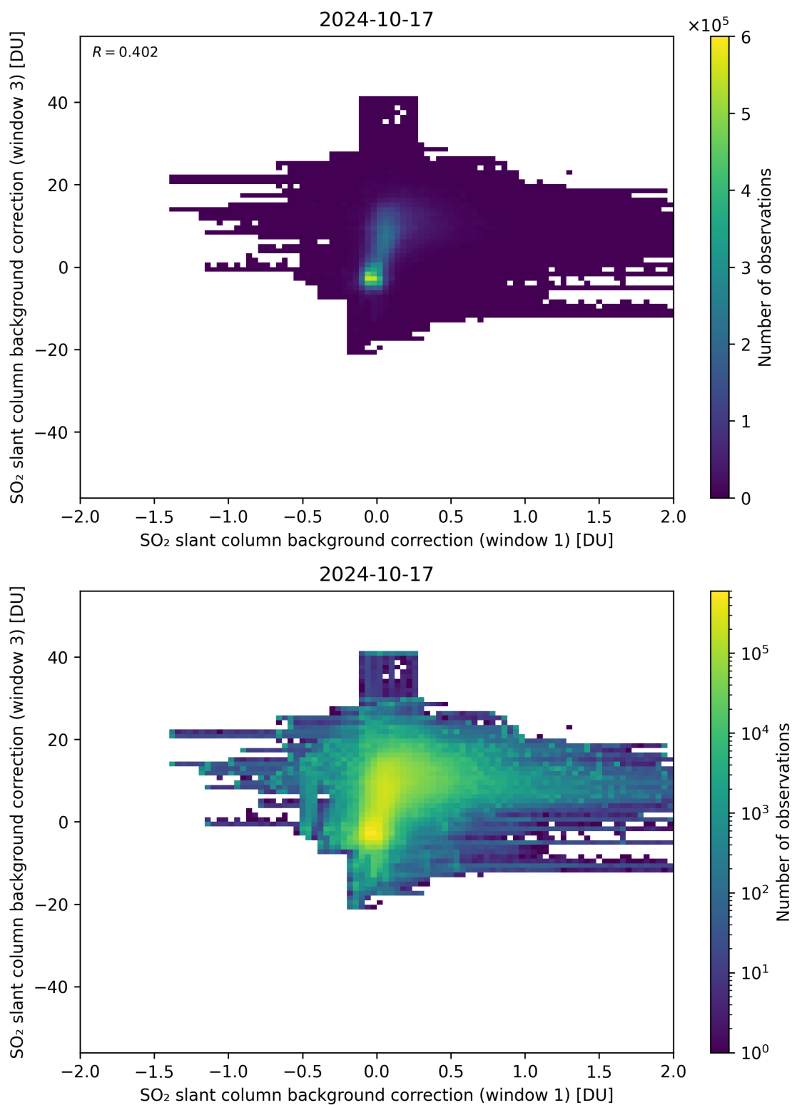
Figure 99: Scatter density plot of “SO 2 slant column background correction (window 1)” against “SO 2 slant column background correction (window 3)” for 2024-10-16 to 2024-10-18.
