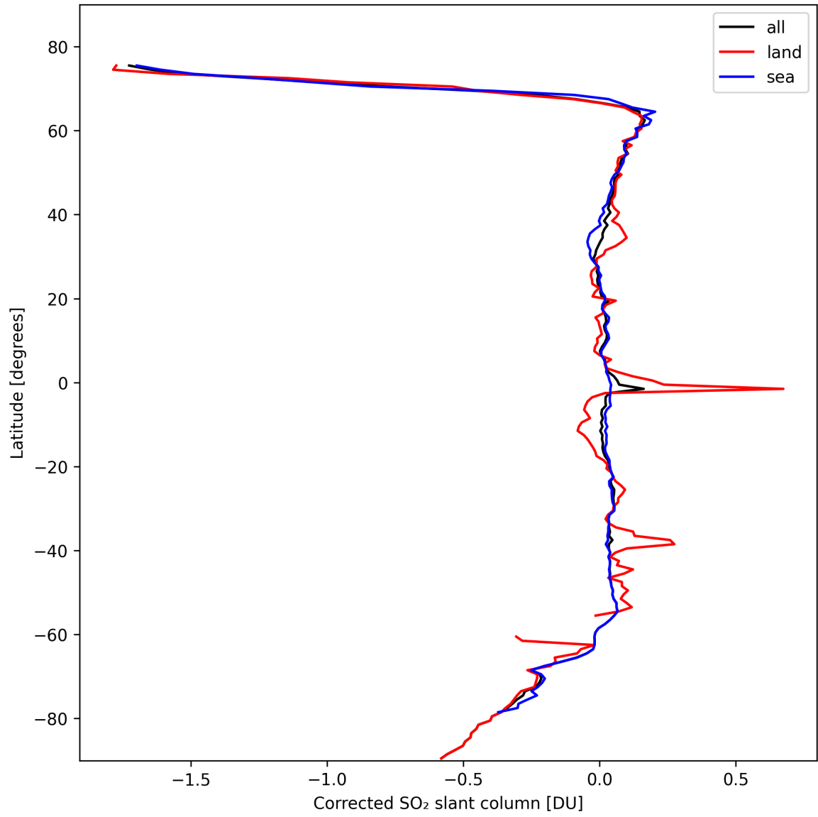
Figure 32: Zonal average of “Corrected SO 2 slant column” for 2024-10-16 to 2024-10-18.
