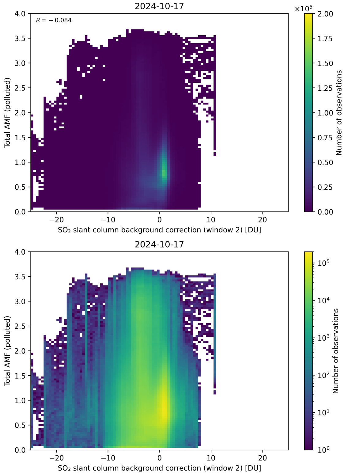
Figure 119: Scatter density plot of “SO 2 slant column background correction (window 2)” against “Total AMF (polluted)” for 2024-10-16 to 2024-10-18.
