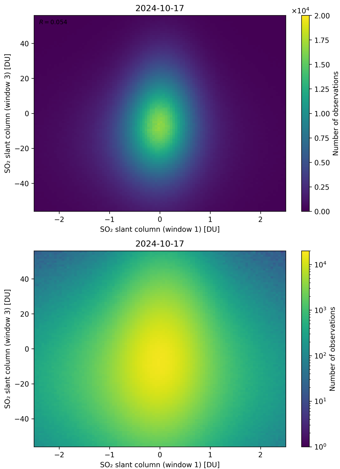
Figure 237: Scatter density plot of “SO 2 slant column (window 1)” against “SO 2 slant column (window 3)” for 2024-10-16 to 2024-10-18.
