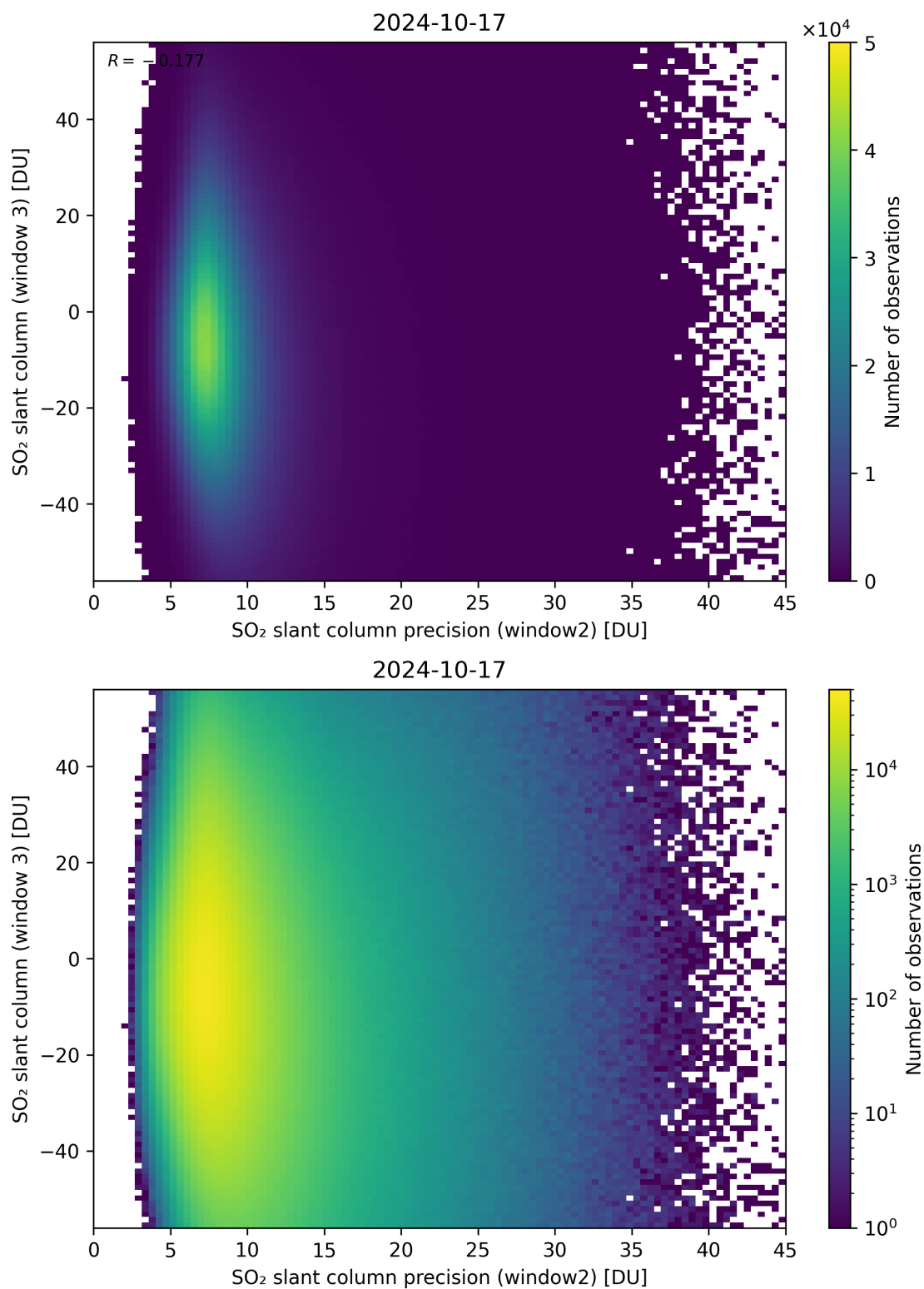
Figure 249: Scatter density plot of “SO 2 slant column precision (window2)” against “SO 2 slant column (window 3)” for 2024-10-16 to 2024-10-18.
