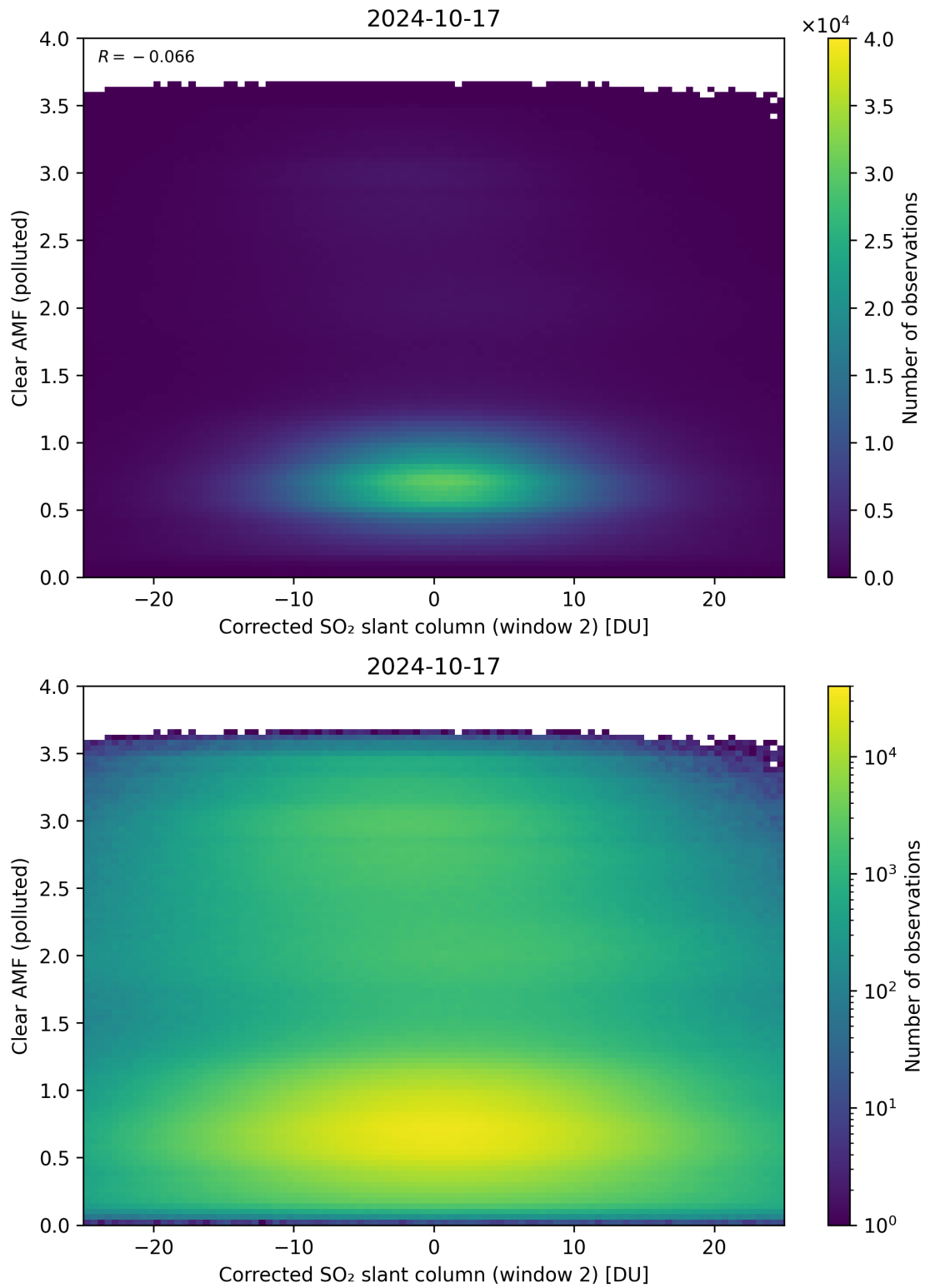
Figure 199: Scatter density plot of “Corrected SO 2 slant column (window 2)” against “Clear AMF (polluted)” for 2024-10-16 to 2024-10-18.
