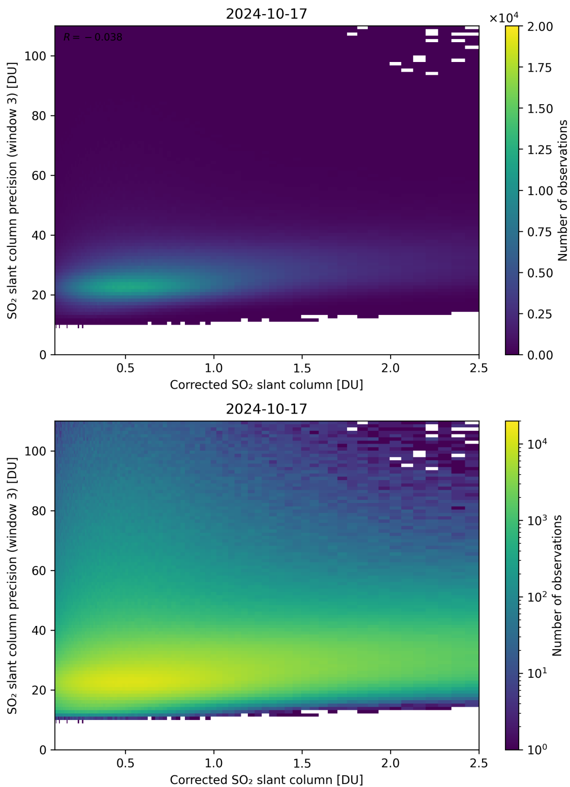
Figure 191: Scatter density plot of “Corrected SO 2 slant column” against “SO 2 slant column precision (window 3)” for 2024-10-16 to 2024-10-18.
