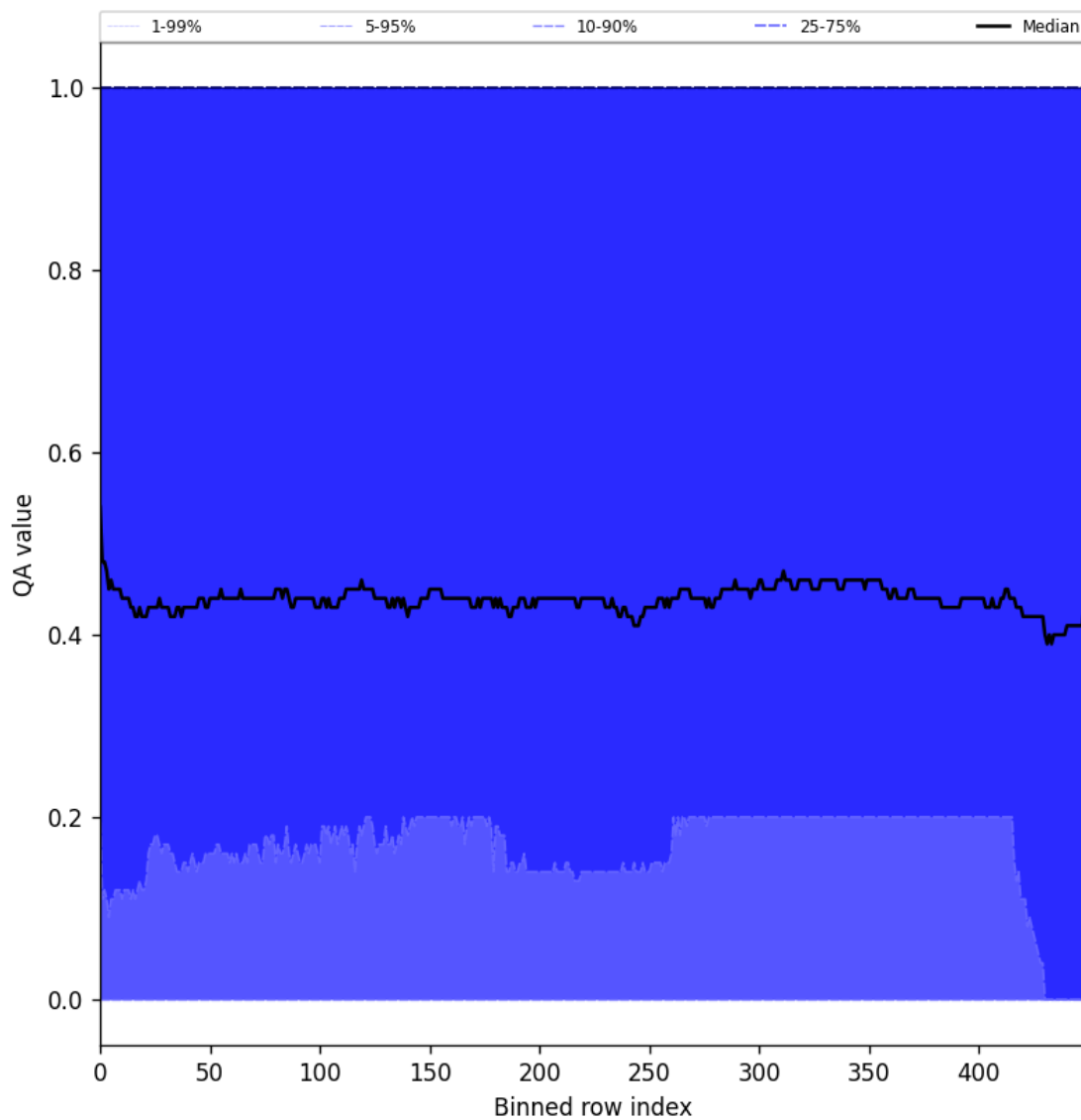
Figure 75: Along track statistics of “QA value” for 2024-10-16 to 2024-10-18
