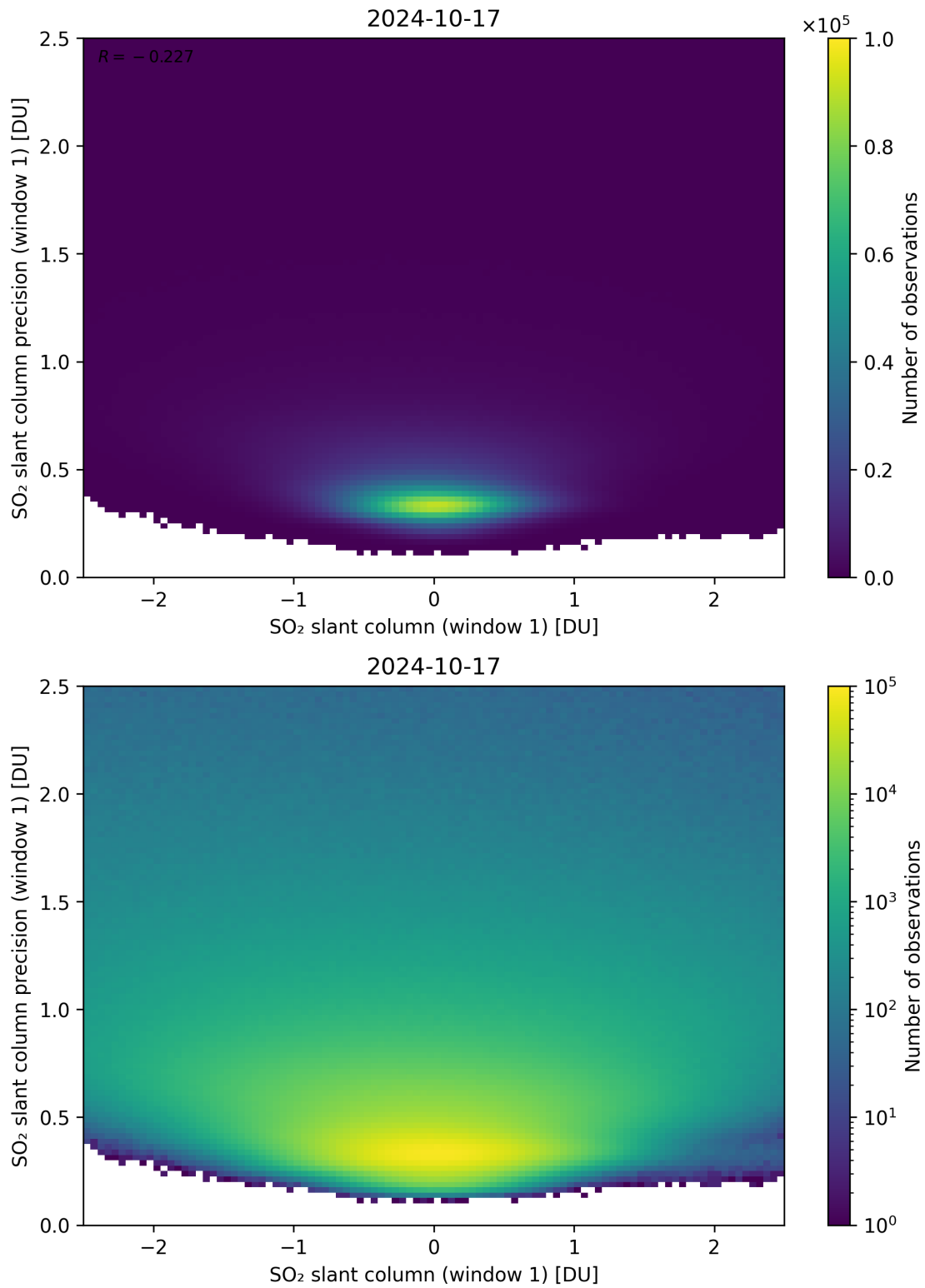
Figure 235: Scatter density plot of “SO 2 slant column (window 1)” against “SO 2 slant column precision (window 1)” for 2024-10-16 to 2024-10-18.
