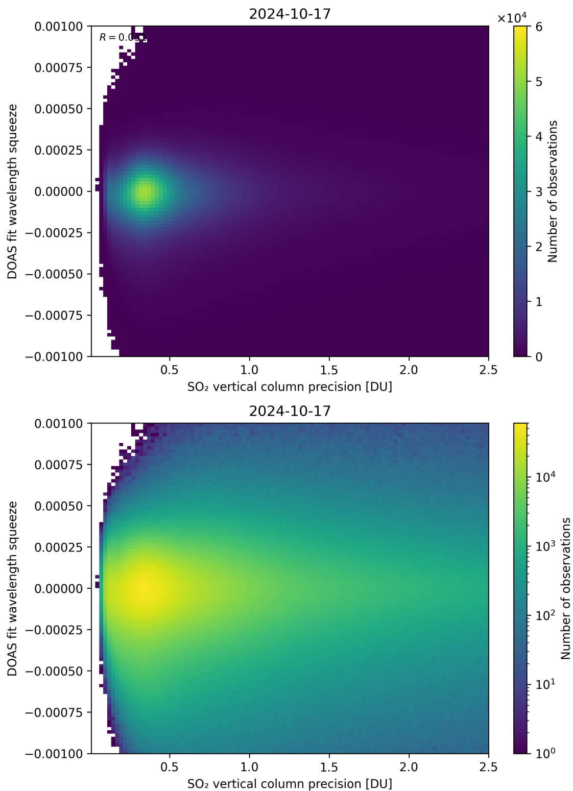
Figure 283: Scatter density plot of “SO 2 vertical column precision” against “DOAS fit wavelength squeeze” for 2024-10-16 to 2024-10-18.
