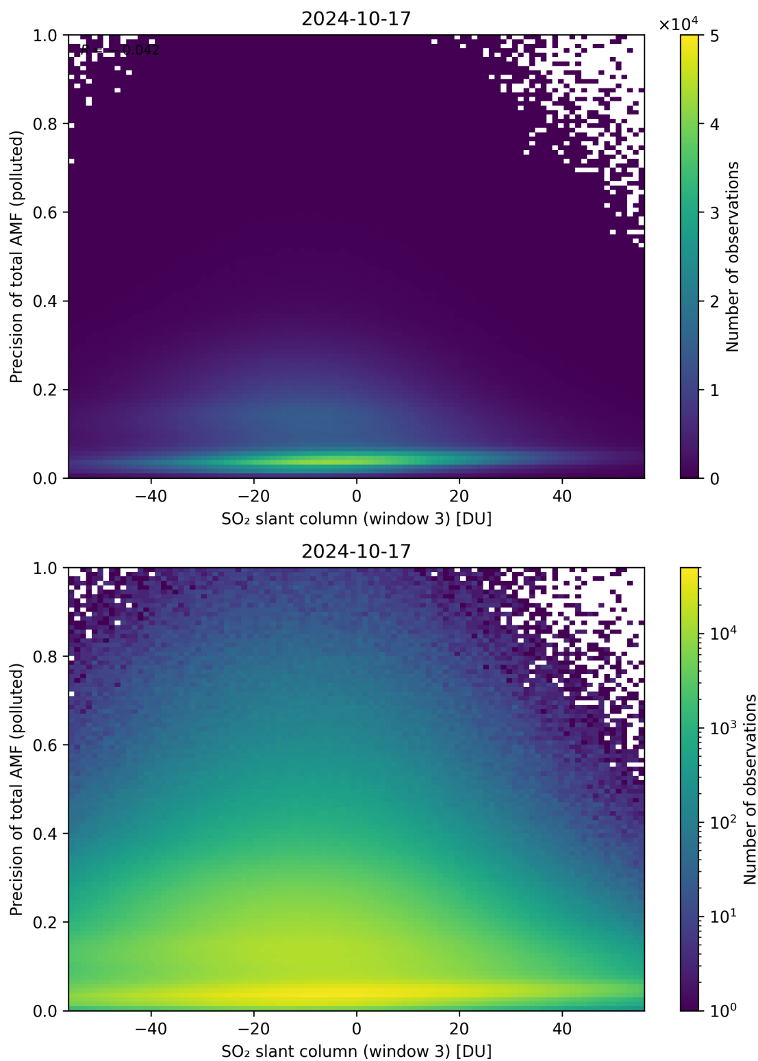
Figure 269: Scatter density plot of “SO 2 slant column (window 3)” against “Precision of total AMF (polluted)” for 2024-10-16 to 2024-10-18.
