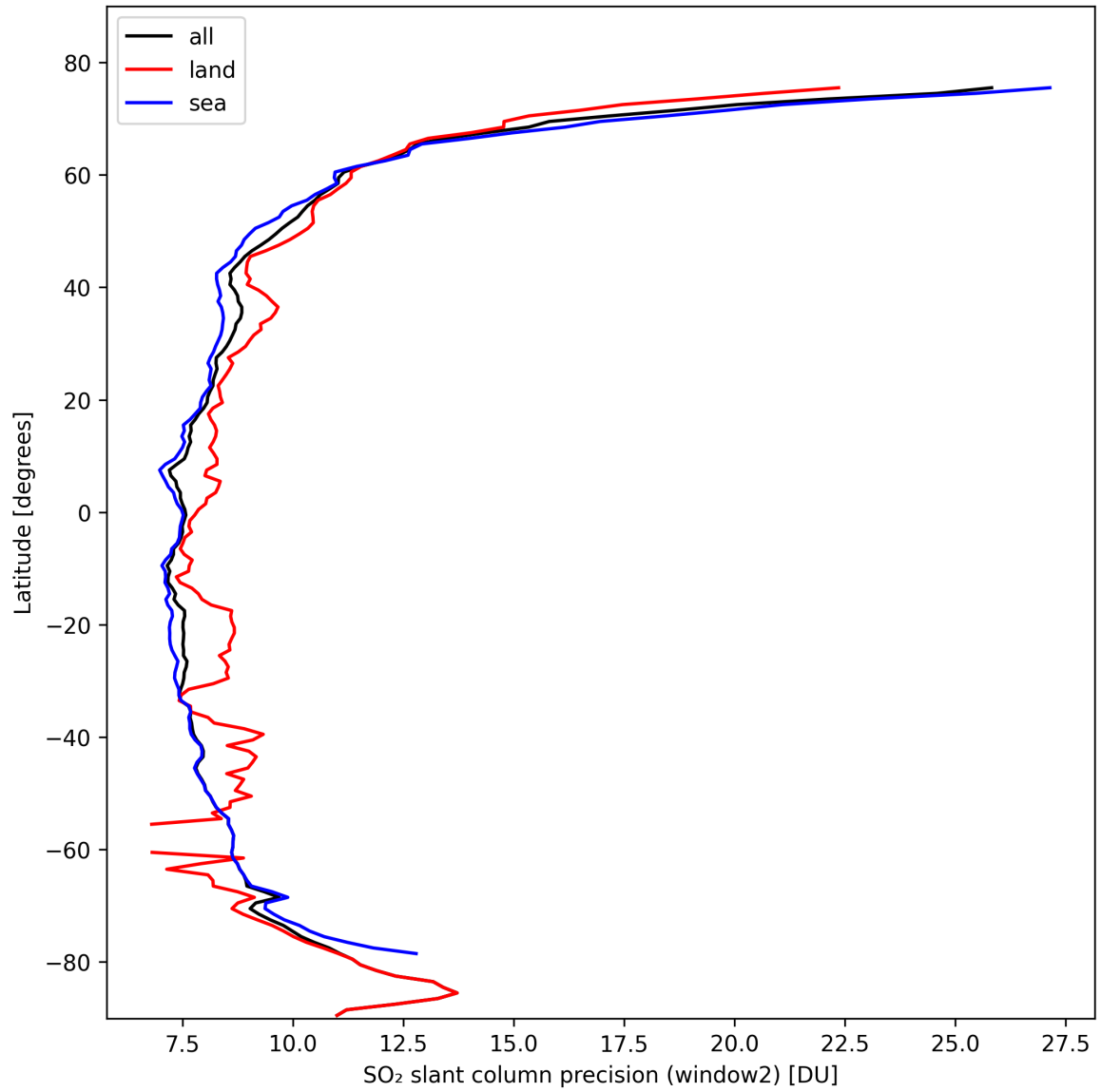
Figure 38: Zonal average of “SO 2 slant column precision (window2)” for 2024-10-16 to 2024-10-18.
