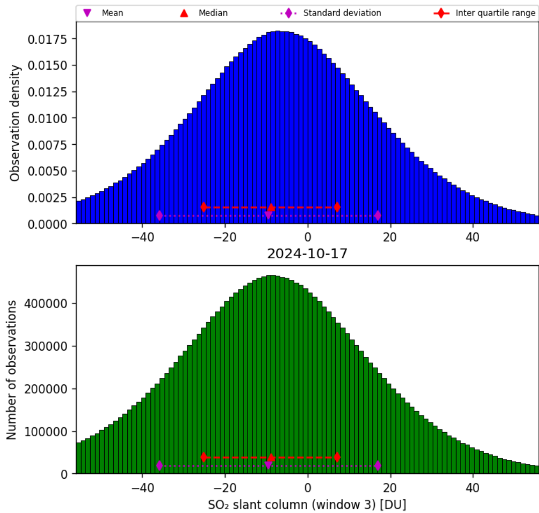
Figure 64: Histogram of “SO 2 slant column (window 3)” for 2024-10-16 to 2024-10-18
