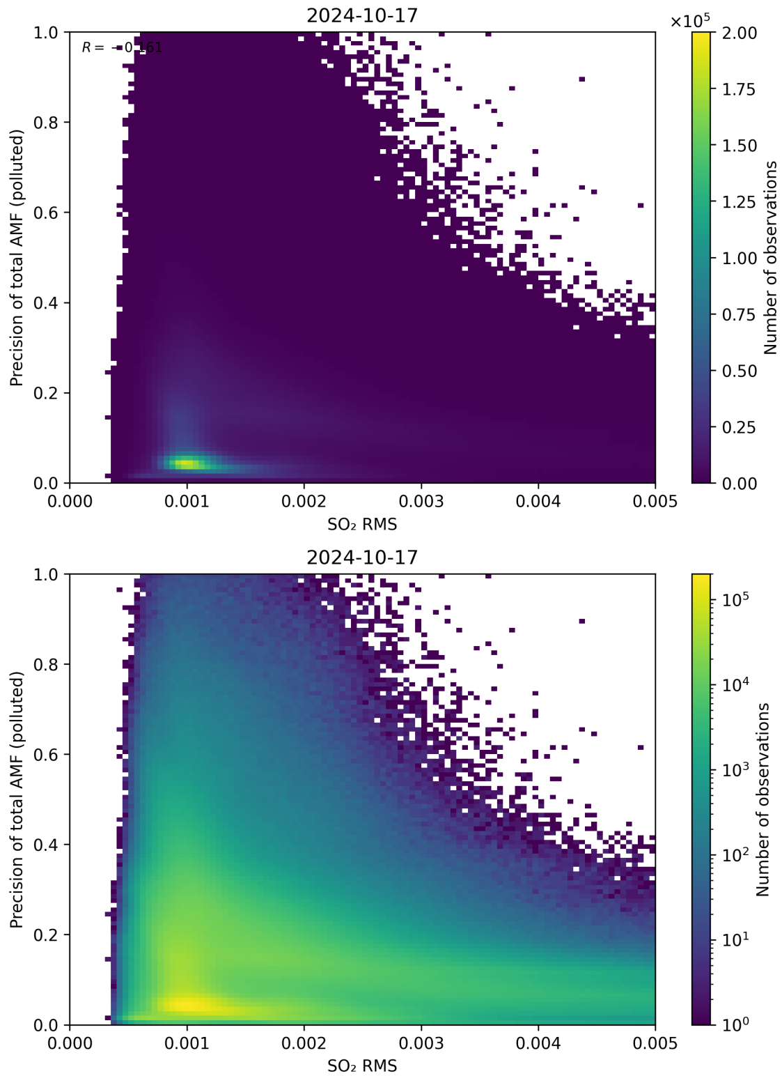
Figure 138: Scatter density plot of “SO 2 RMS” against “Precision of total AMF (polluted)” for 2024-10-16 to 2024-10-18.
