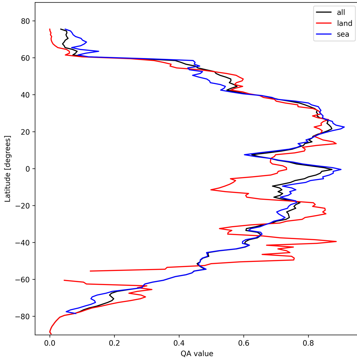
Figure 29: Zonal average of “QA value” for 2024-10-16 to 2024-10-18.
