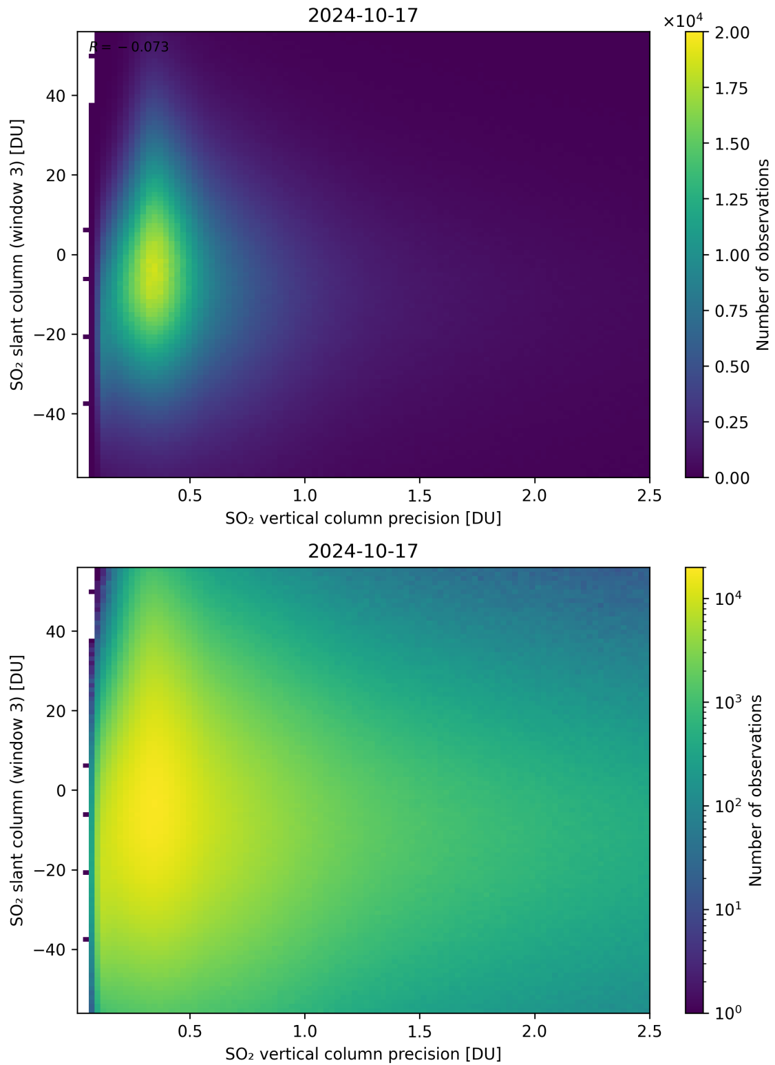
Figure 292: Scatter density plot of “SO 2 vertical column precision” against “SO 2 slant column (window 3)” for 2024-10-16 to 2024-10-18.
