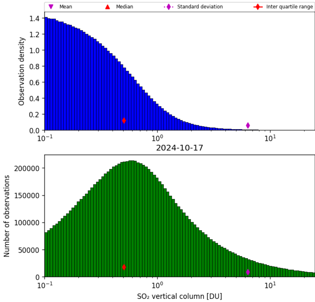
Figure 53: Histogram of “SO 2 vertical column” for 2024-10-16 to 2024-10-18
