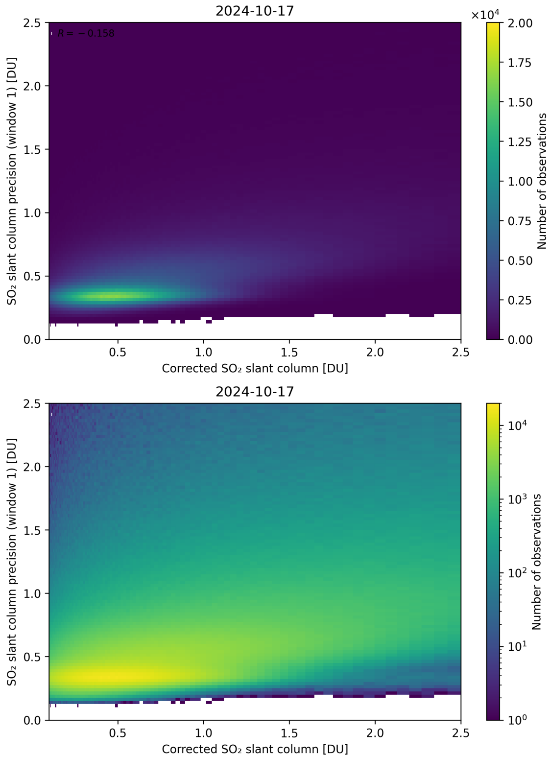
Figure 188: Scatter density plot of “Corrected SO 2 slant column” against “SO 2 slant column precision (window 1)” for 2024-10-16 to 2024-10-18.
