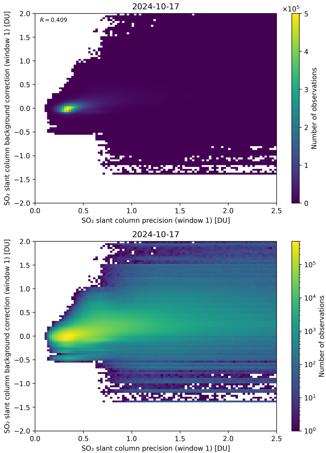
Figure 218: Scatter density plot of “SO 2 slant column precision (window 1)” against “SO 2 slant column background correction (window 1)” for 2024-10-16 to 2024-10-18.
