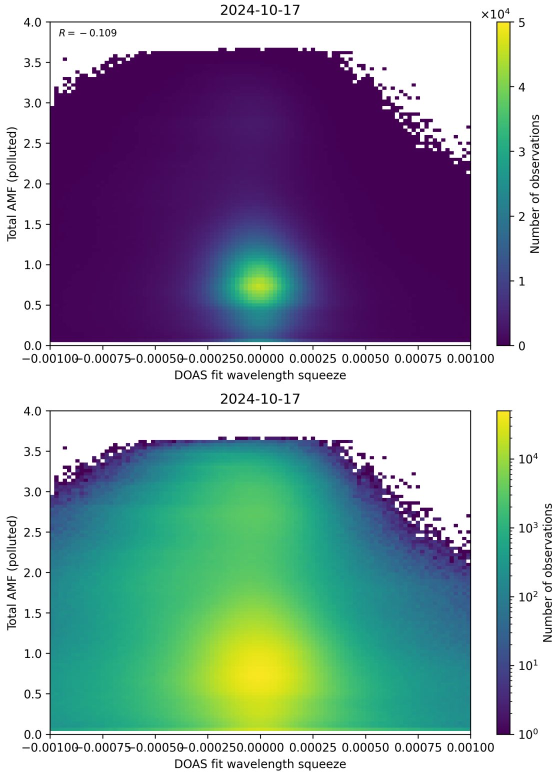
Figure 134: Scatter density plot of “DOAS fit wavelength squeeze” against “Total AMF (polluted)” for 2024-10-16 to 2024-10-18.
