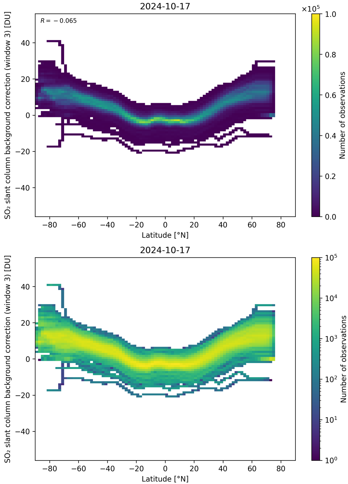
Figure 141: Scatter density plot of “Latitude” against “SO 2 slant column background correction (window 3)” for 2024-10-16 to 2024-10-18.
