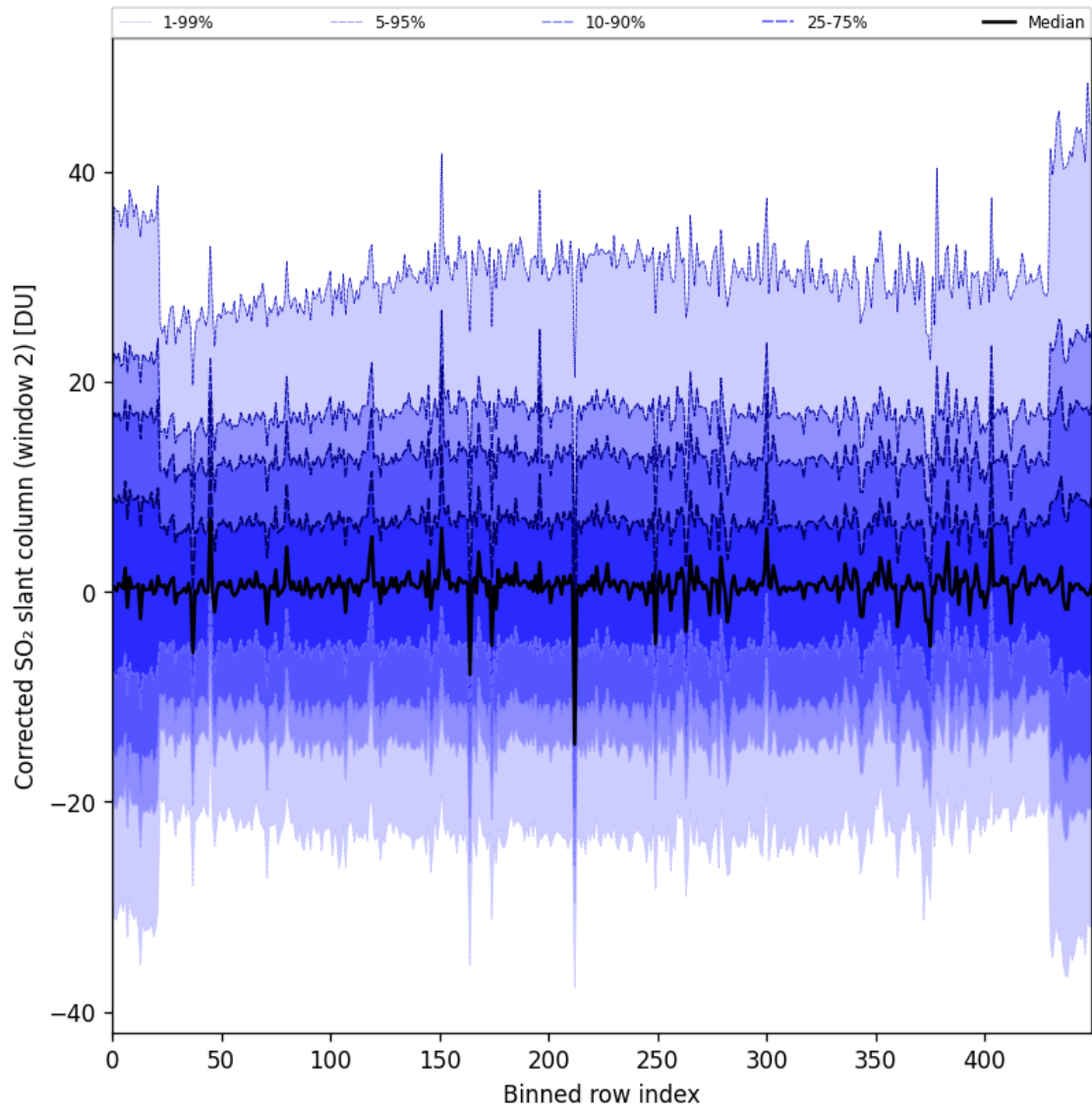
Figure 85: Along track statistics of “Corrected SO 2 slant column (window 2)” for 2024-10-16 to 2024-10-18
