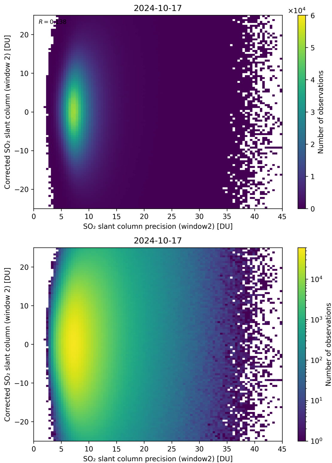
Figure 247: Scatter density plot of “SO 2 slant column precision (window2)” against “Corrected SO 2 slant column (window 2)” for 2024-10-16 to 2024-10-18.
