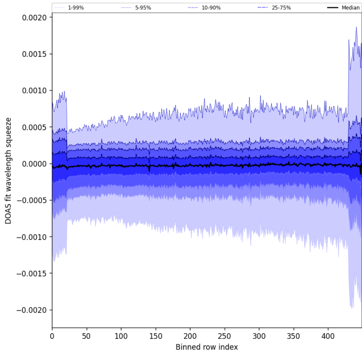
Figure 92: Along track statistics of “DOAS fit wavelength squeeze” for 2024-10-16 to 2024-10-18
