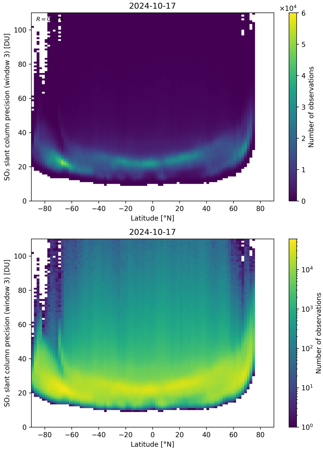
Figure 153: Scatter density plot of “Latitude” against “SO 2 slant column precision (window 3)” for 2024-10-16 to 2024-10-18.
