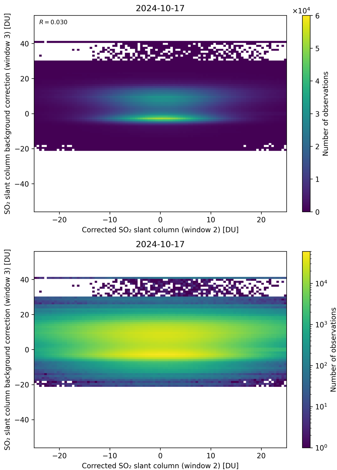
Figure 195: Scatter density plot of “Corrected SO 2 slant column (window 2)” against “SO 2 slant column background correction (window 3)” for 2024-10-16 to 2024-10-18.
