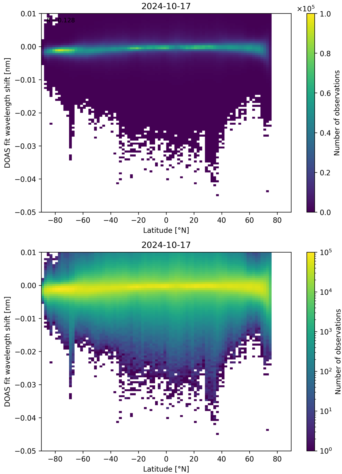
Figure 142: Scatter density plot of “Latitude” against “DOAS fit wavelength shift” for 2024-10-16 to 2024-10-18.
