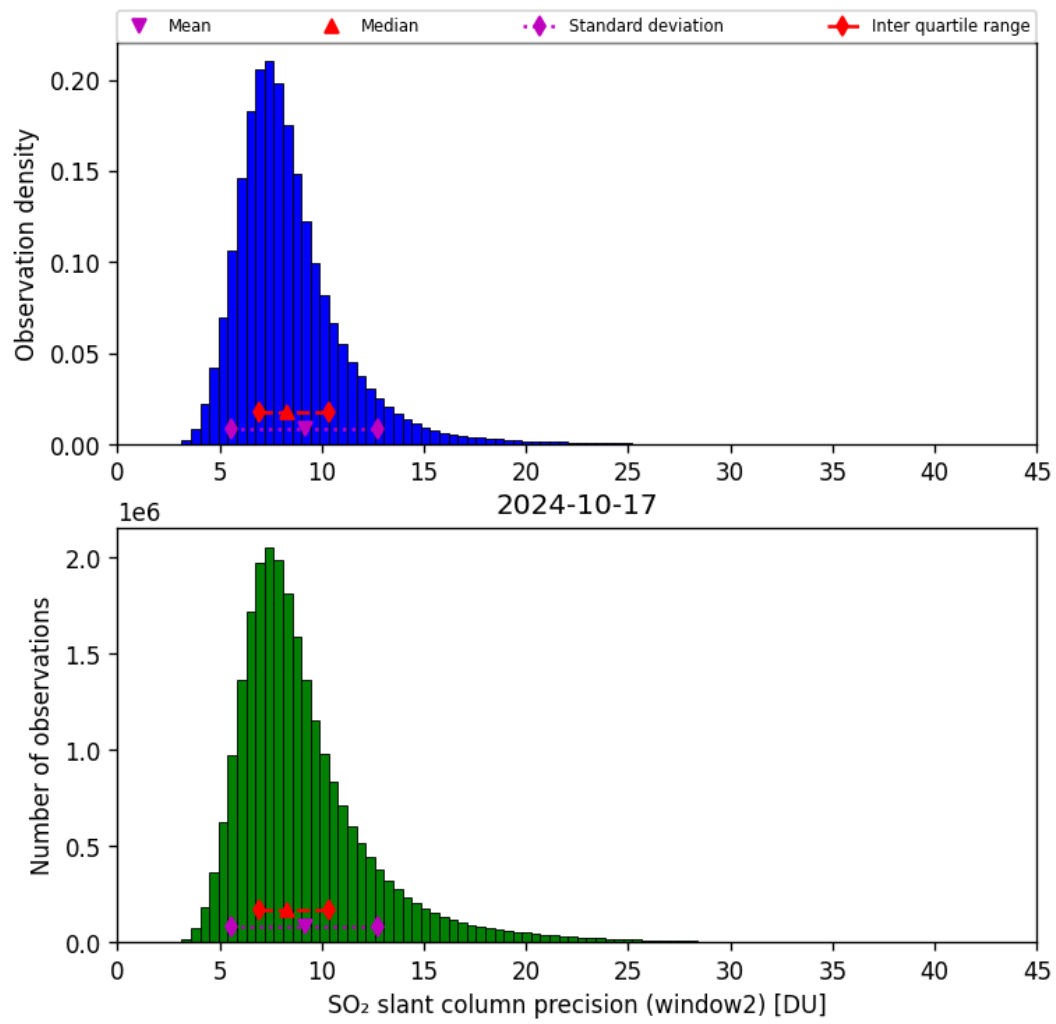
Figure 61: Histogram of “SO 2 slant column precision (window2)” for 2024-10-16 to 2024-10-18
