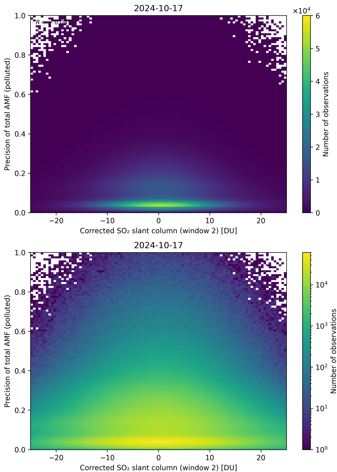
Figure 204: Scatter density plot of “Corrected SO 2 slant column (window 2)” against “Precision of total AMF (polluted)” for 2024-10-16 to 2024-10-18.
