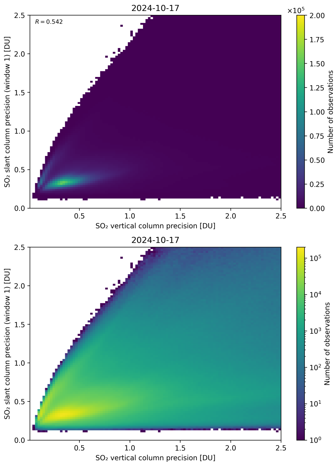
Figure 290: Scatter density plot of “SO 2 vertical column precision” against “SO 2 slant column precision (window 1)” for 2024-10-16 to 2024-10-18.
