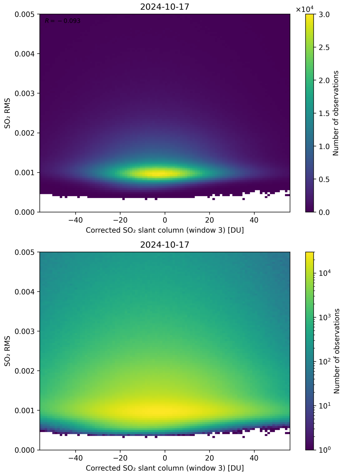
Figure 208: Scatter density plot of “Corrected SO 2 slant column (window 3)” against “SO 2 RMS” for 2024-10-16 to 2024-10-18.
