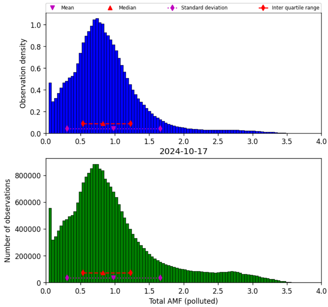
Figure 71: Histogram of “Total AMF (polluted)” for 2024-10-16 to 2024-10-18
