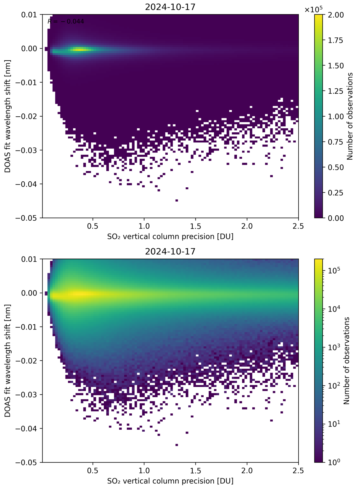
Figure 282: Scatter density plot of “SO 2 vertical column precision” against “DOAS fit wavelength shift” for 2024-10-16 to 2024-10-18.
