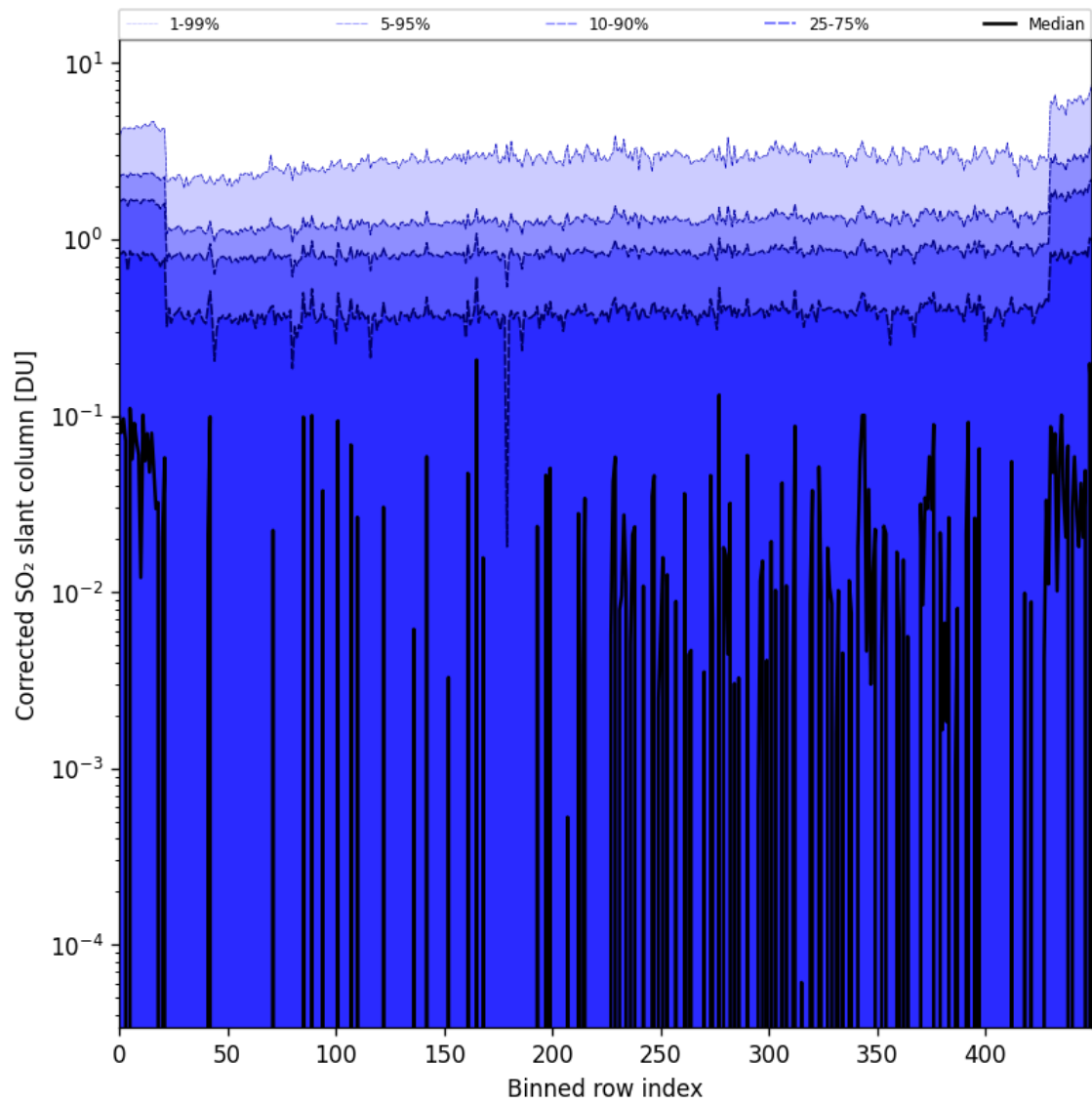
Figure 78: Along track statistics of “Corrected SO 2 slant column” for 2024-10-16 to 2024-10-18
