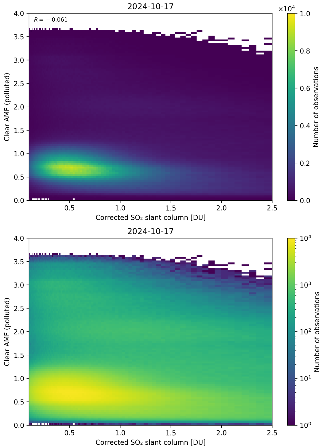
Figure 184: Scatter density plot of “Corrected SO 2 slant column” against “Clear AMF (polluted)” for 2024-10-16 to 2024-10-18.
