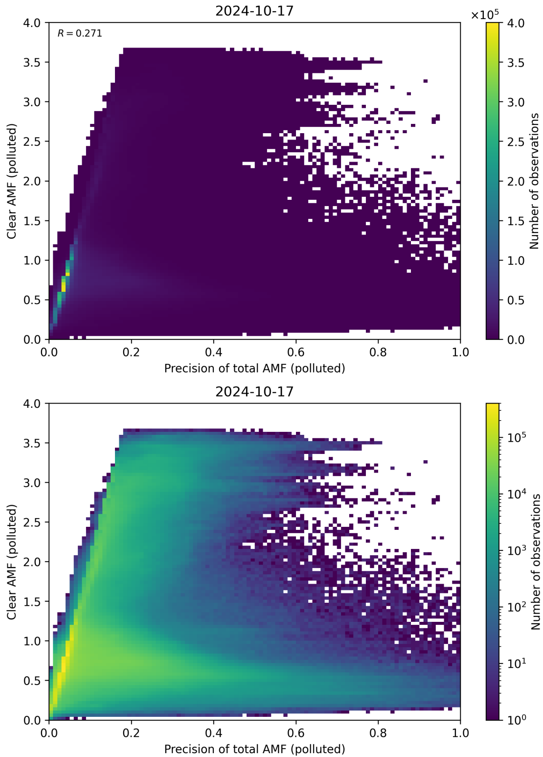
Figure 270: Scatter density plot of “Precision of total AMF (polluted)” against “Clear AMF (polluted)” for 2024-10-16 to 2024-10-18.
