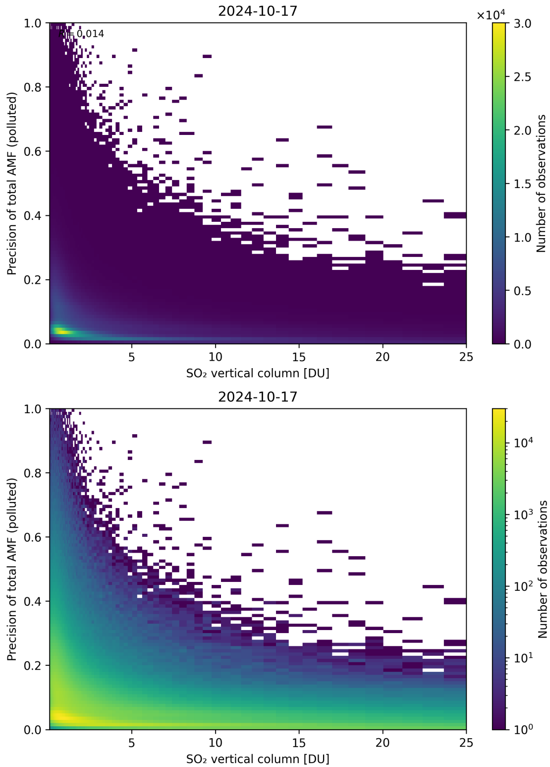
Figure 306: Scatter density plot of “SO 2 vertical column” against “Precision of total AMF (polluted)” for 2024-10-16 to 2024-10-18.
