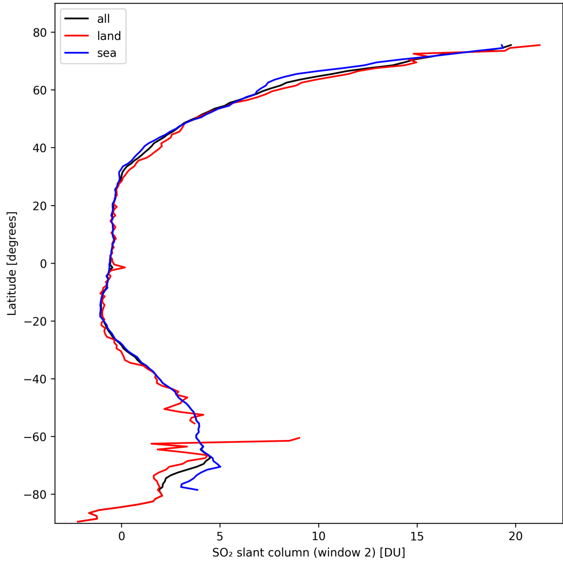
Figure 37: Zonal average of “SO 2 slant column (window 2)” for 2024-10-16 to 2024-10-18.
