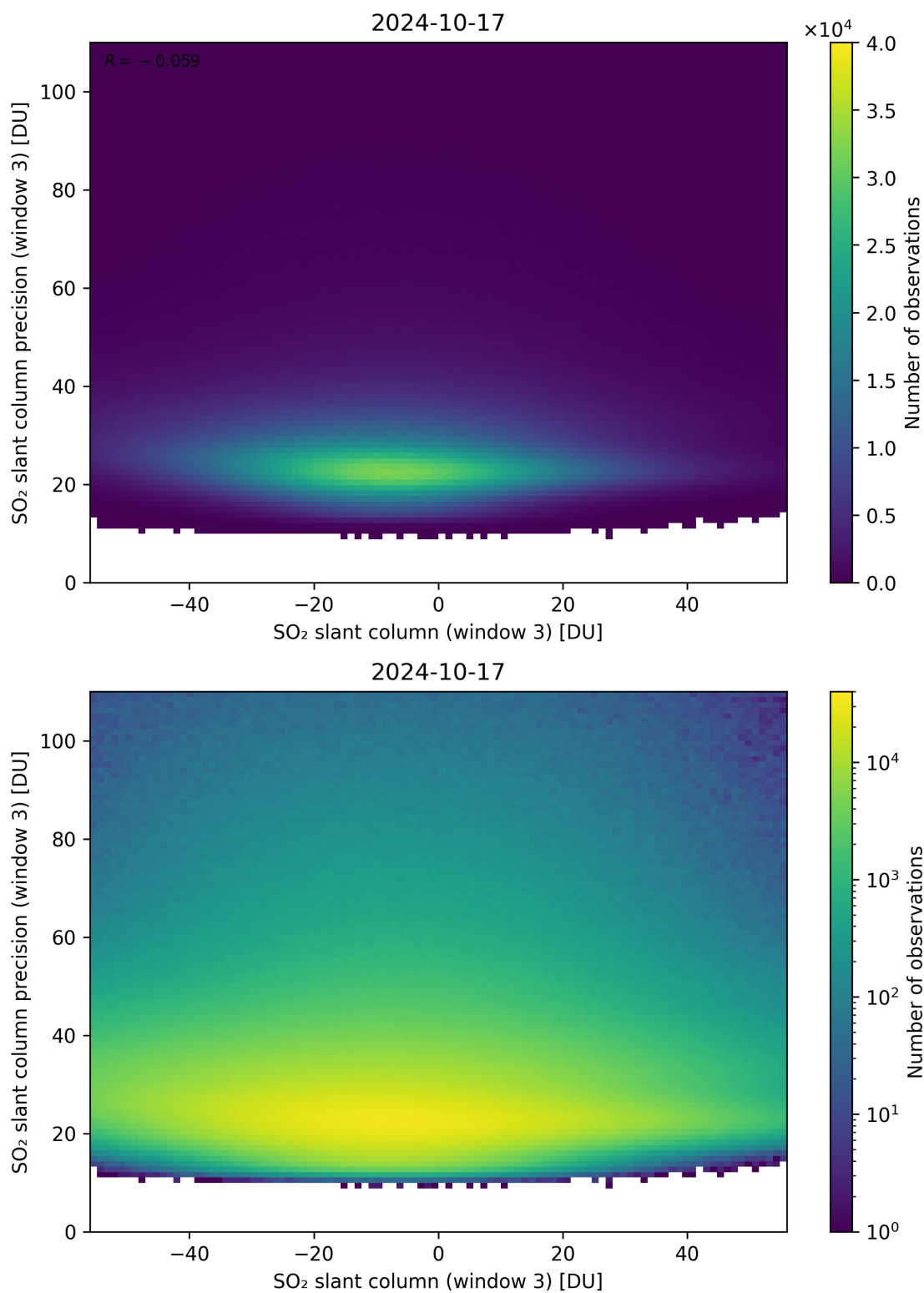
Figure 267: Scatter density plot of “SO 2 slant column (window 3)” against “SO 2 slant column precision (window 3)” for 2024-10-16 to 2024-10-18.
