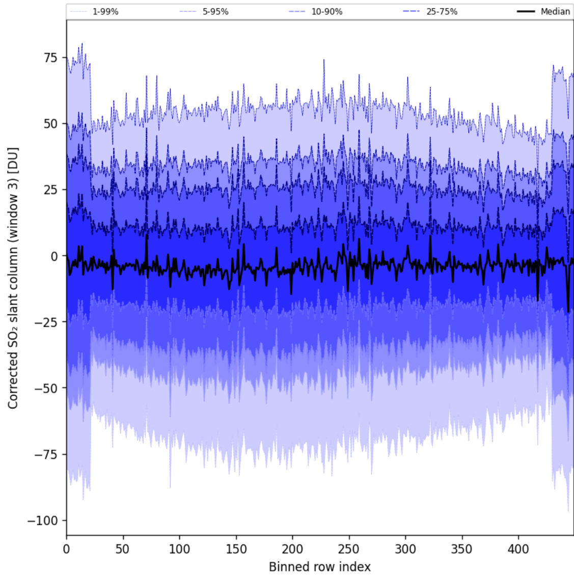
Figure 89: Along track statistics of “Corrected SO 2 slant column (window 3)” for 2024-10-16 to 2024-10-18
