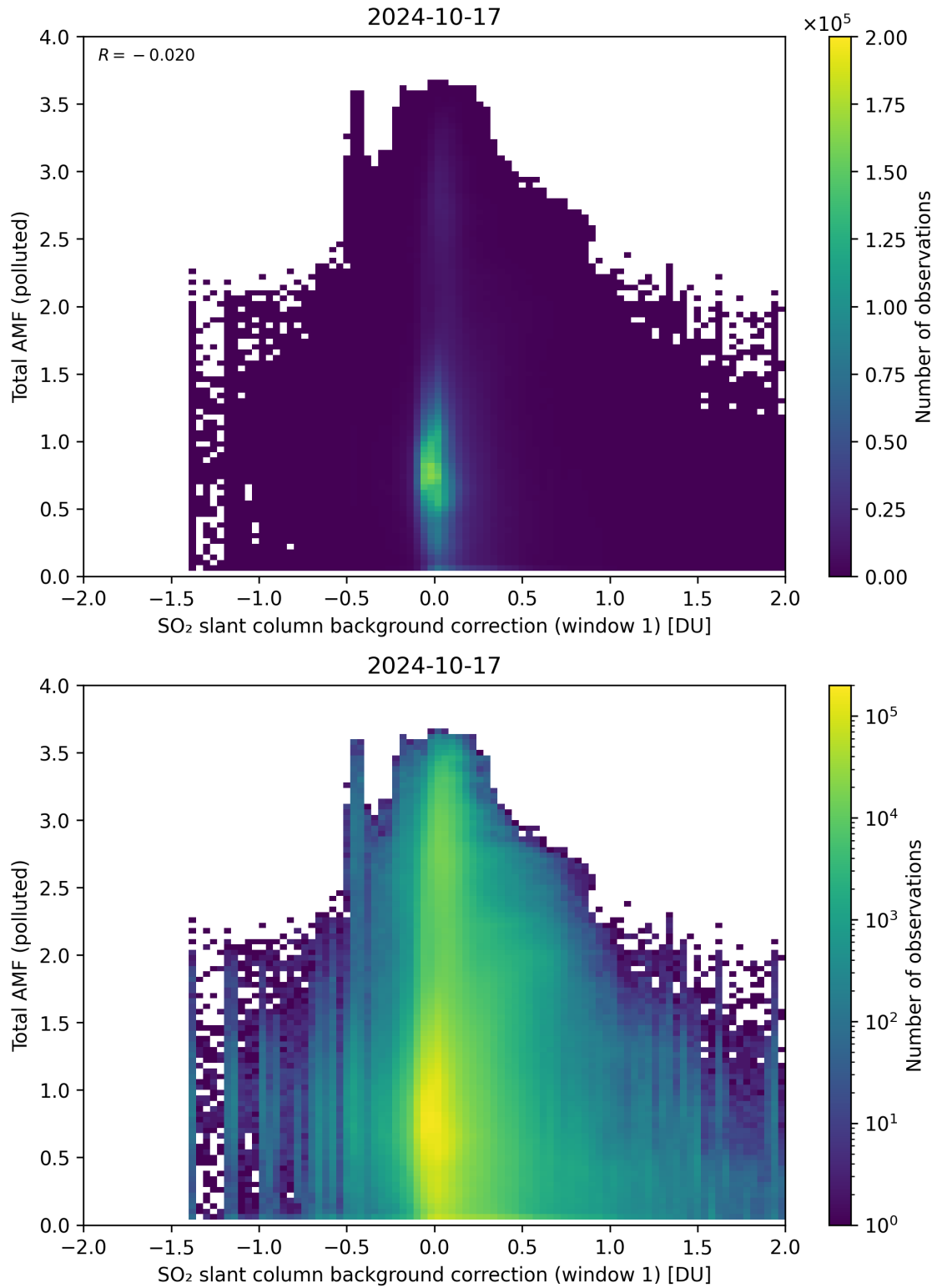
Figure 109: Scatter density plot of “SO 2 slant column background correction (window 1)” against “Total AMF (polluted)” for 2024-10-16 to 2024-10-18.
