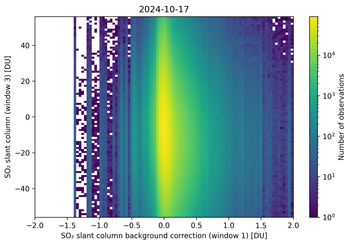
Figure 107: Scatter density plot of “SO 2 slant column background correction (window 1)” against “SO 2 slant column (window 3)” for 2024-10-16 to 2024-10-18.
