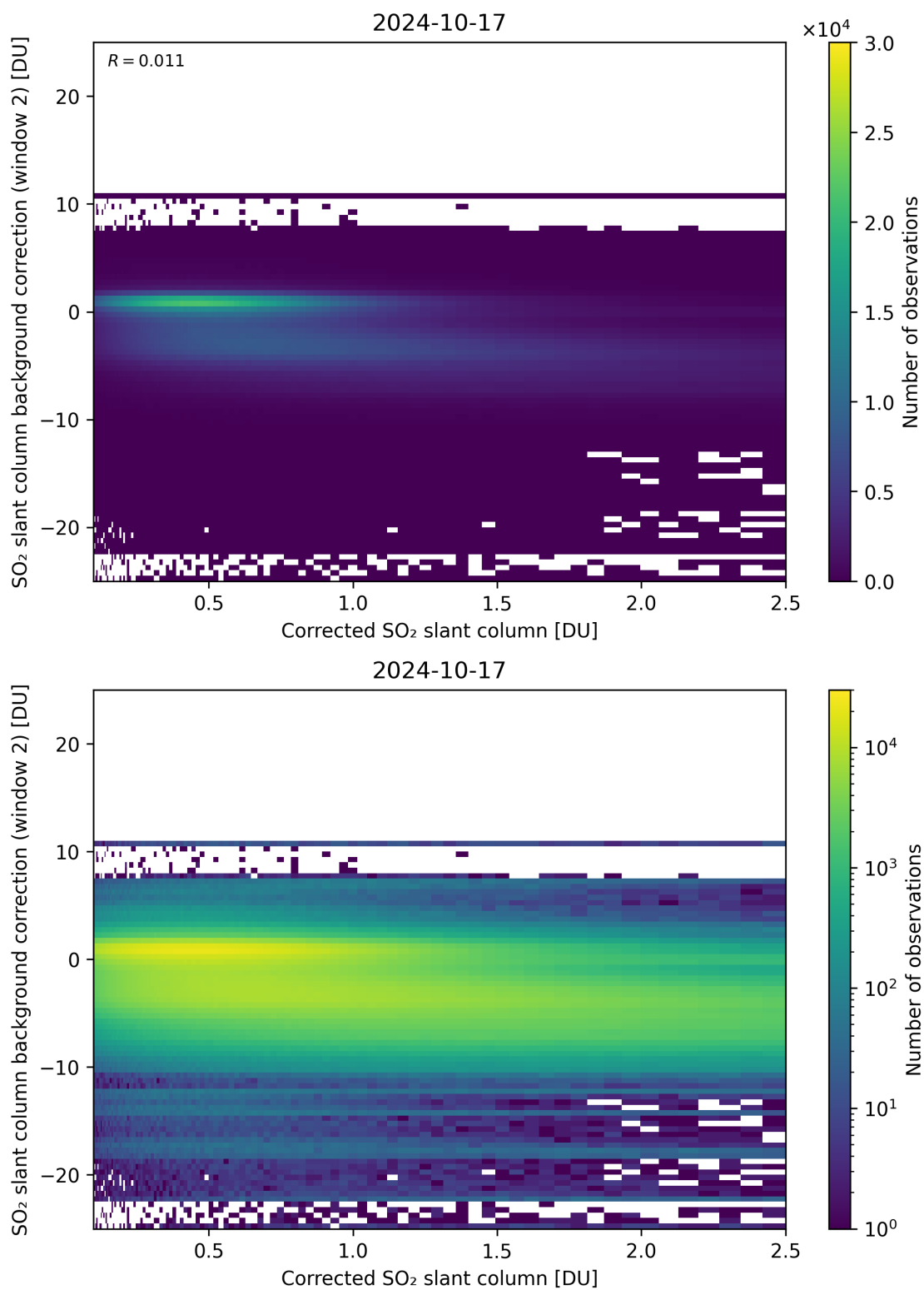
Figure 179: Scatter density plot of “Corrected SO 2 slant column” against “SO 2 slant column background correction (window 2)” for 2024-10-16 to 2024-10-18.
