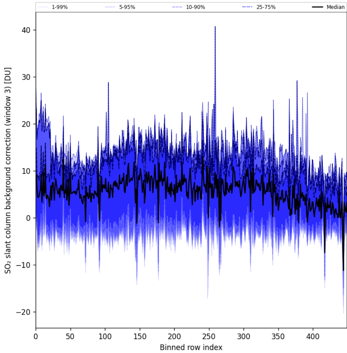
Figure 90: Along track statistics of “SO 2 slant column background correction (window 3)” for 2024-10-16 to 2024-10-18
