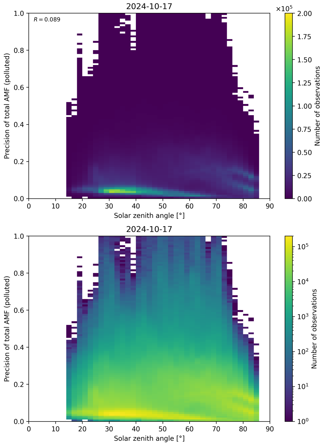
Figure 175: Scatter density plot of “Solar zenith angle” against “Precision of total AMF (polluted)” for 2024-10-16 to 2024-10-18.
