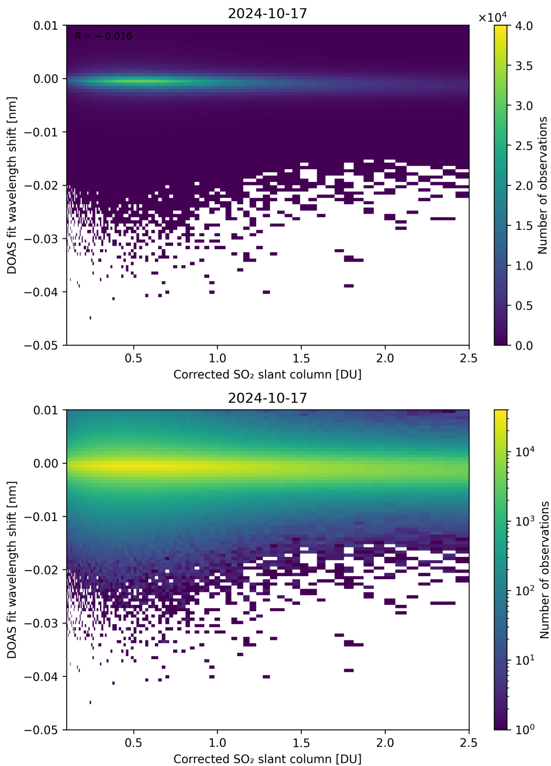
Figure 181: Scatter density plot of “Corrected SO 2 slant column” against “DOAS fit wavelength shift” for 2024-10-16 to 2024-10-18.
