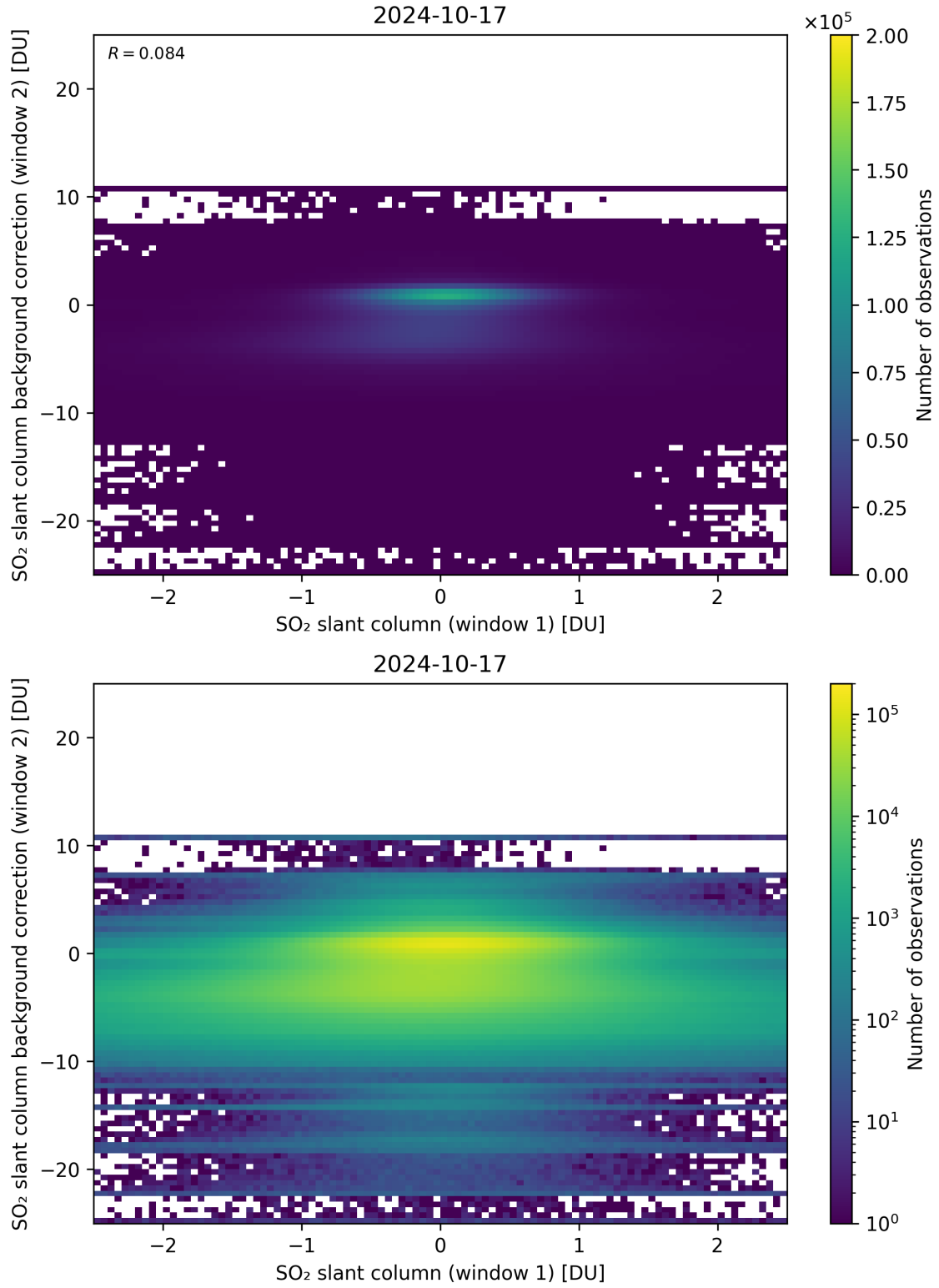
Figure 213: Scatter density plot of “SO 2 slant column (window 1)” against “SO 2 slant column background correction (window 2)” for 2024-10-16 to 2024-10-18.
