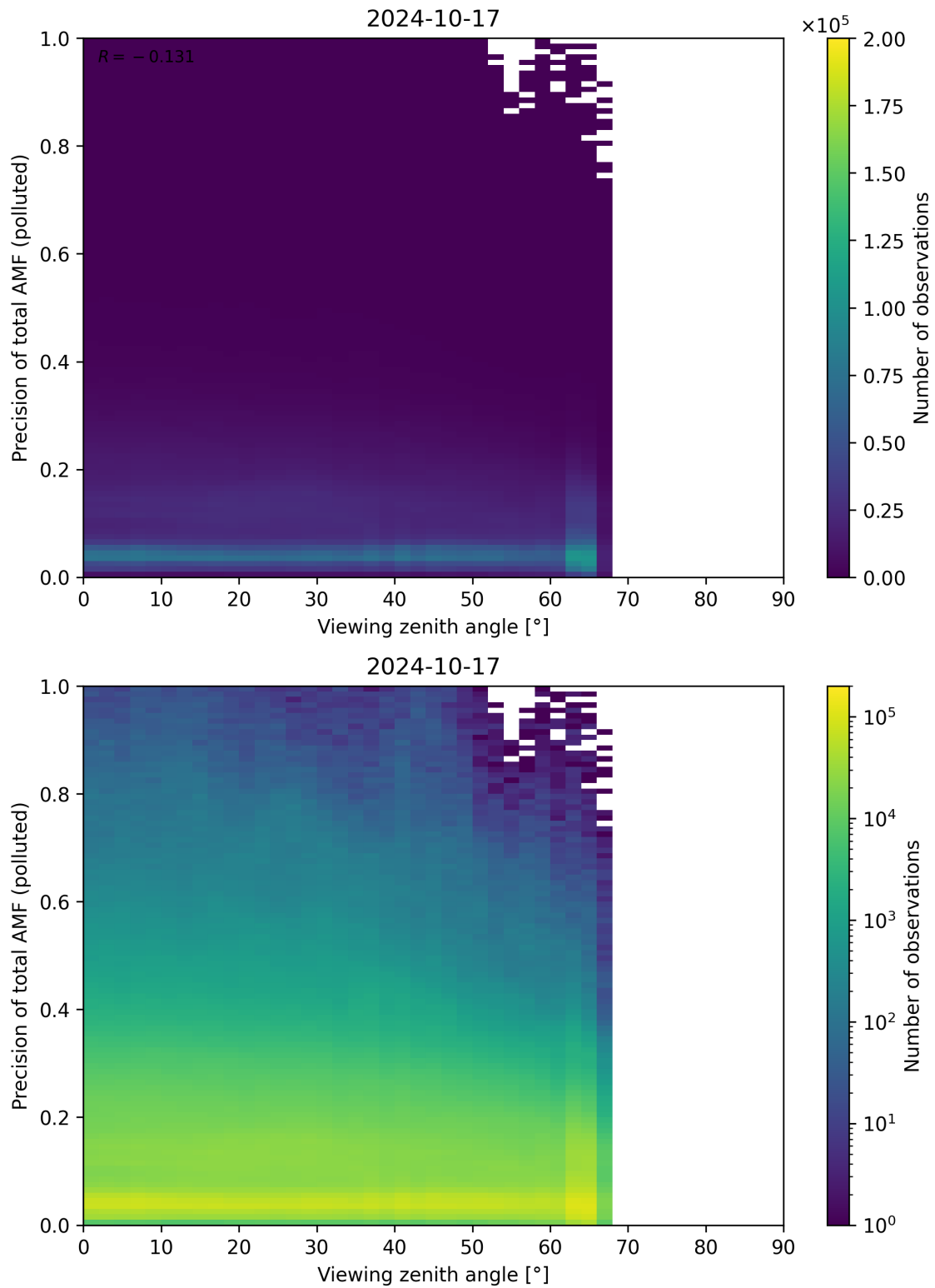
Figure 326: Scatter density plot of “Viewing zenith angle” against “Precision of total AMF (polluted)” for 2024-10-16 to 2024-10-18.
