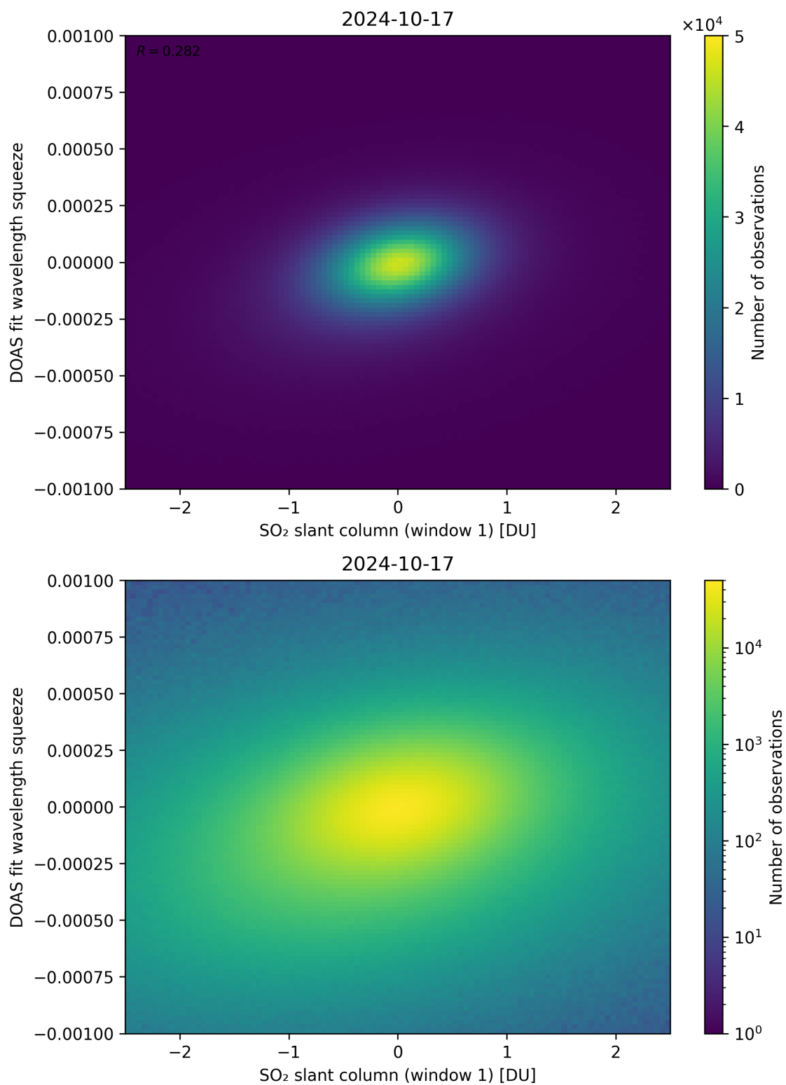
Figure 216: Scatter density plot of “SO 2 slant column (window 1)” against “DOAS fit wavelength squeeze” for 2024-10-16 to 2024-10-18.
