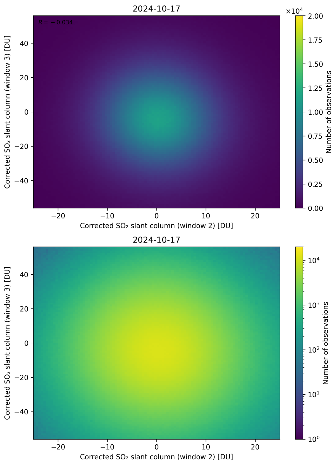
Figure 200: Scatter density plot of “Corrected SO 2 slant column (window 2)” against “Corrected SO 2 slant column (window 3)” for 2024-10-16 to 2024-10-18.
