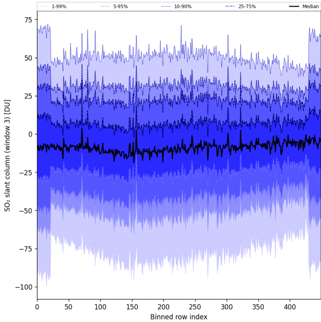
Figure 87: Along track statistics of “SO 2 slant column (window 3)” for 2024-10-16 to 2024-10-18
