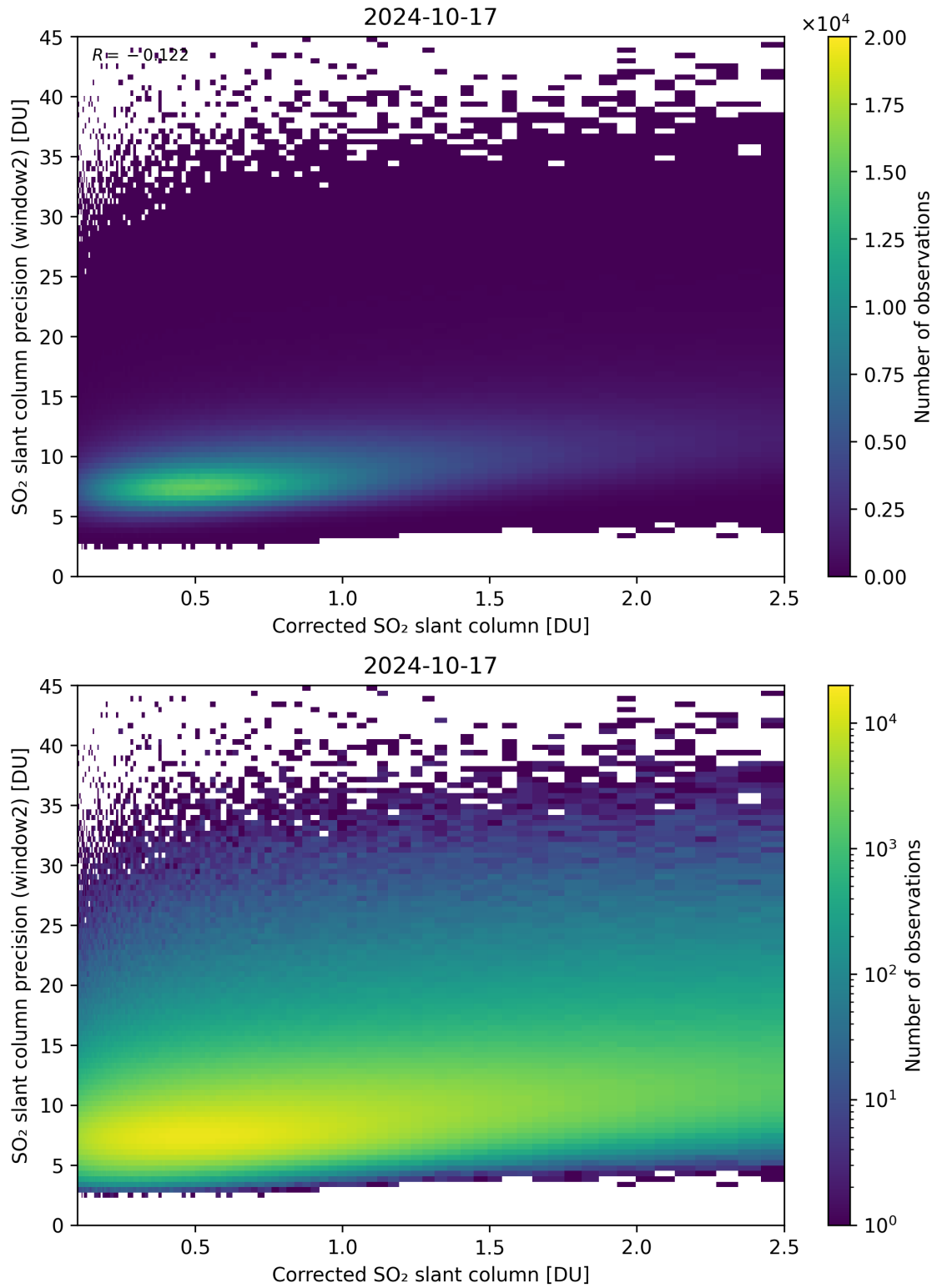
Figure 189: Scatter density plot of “Corrected SO 2 slant column” against “SO 2 slant column precision (window2)” for 2024-10-16 to 2024-10-18.
