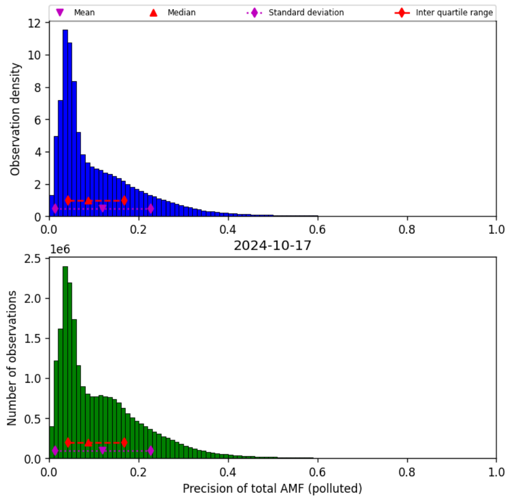
Figure 72: Histogram of “Precision of total AMF (polluted)” for 2024-10-16 to 2024-10-18
