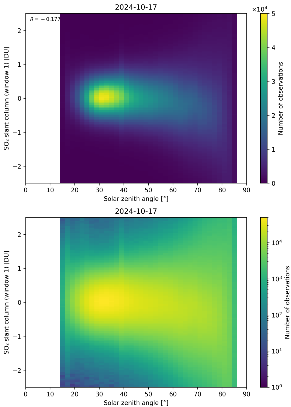
Figure 169: Scatter density plot of “Solar zenith angle” against “SO 2 slant column (window 1)” for 2024-10-16 to 2024-10-18.
