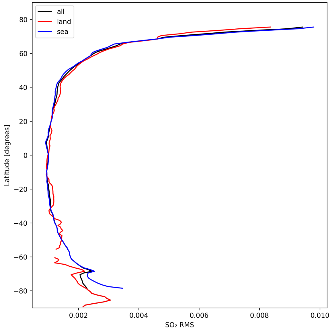
Figure 47: Zonal average of “SO 2 RMS” for 2024-10-16 to 2024-10-18.
