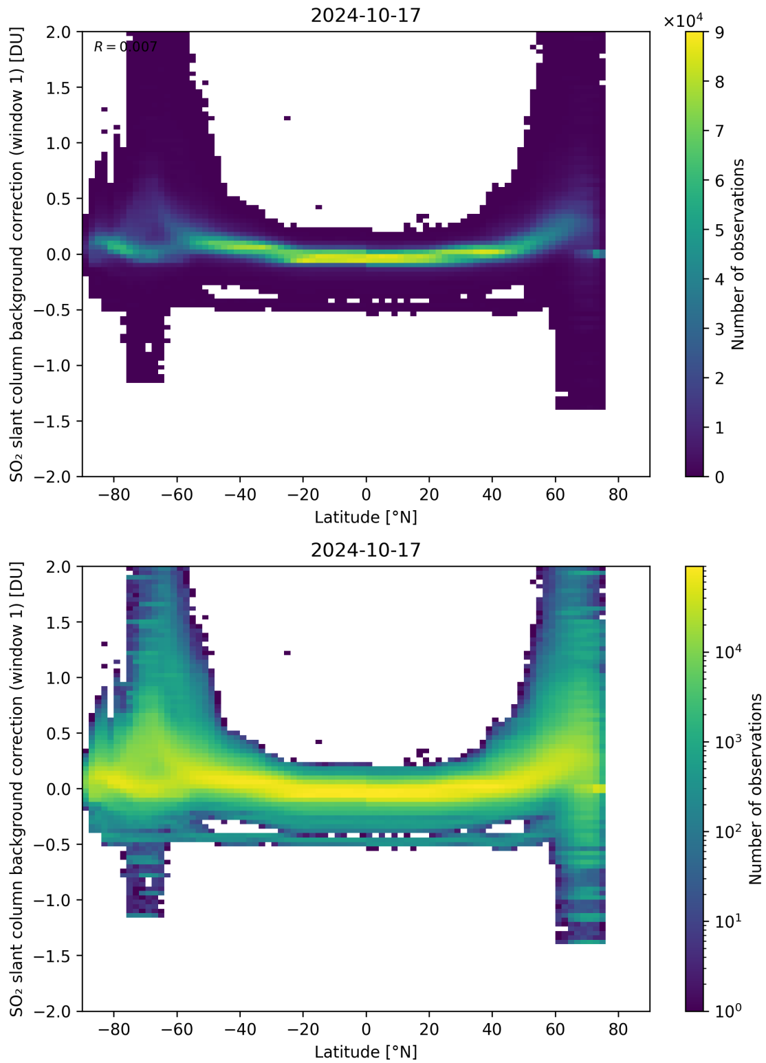
Figure 139: Scatter density plot of “Latitude” against “SO 2 slant column background correction (window 1)” for 2024-10-16 to 2024-10-18.
