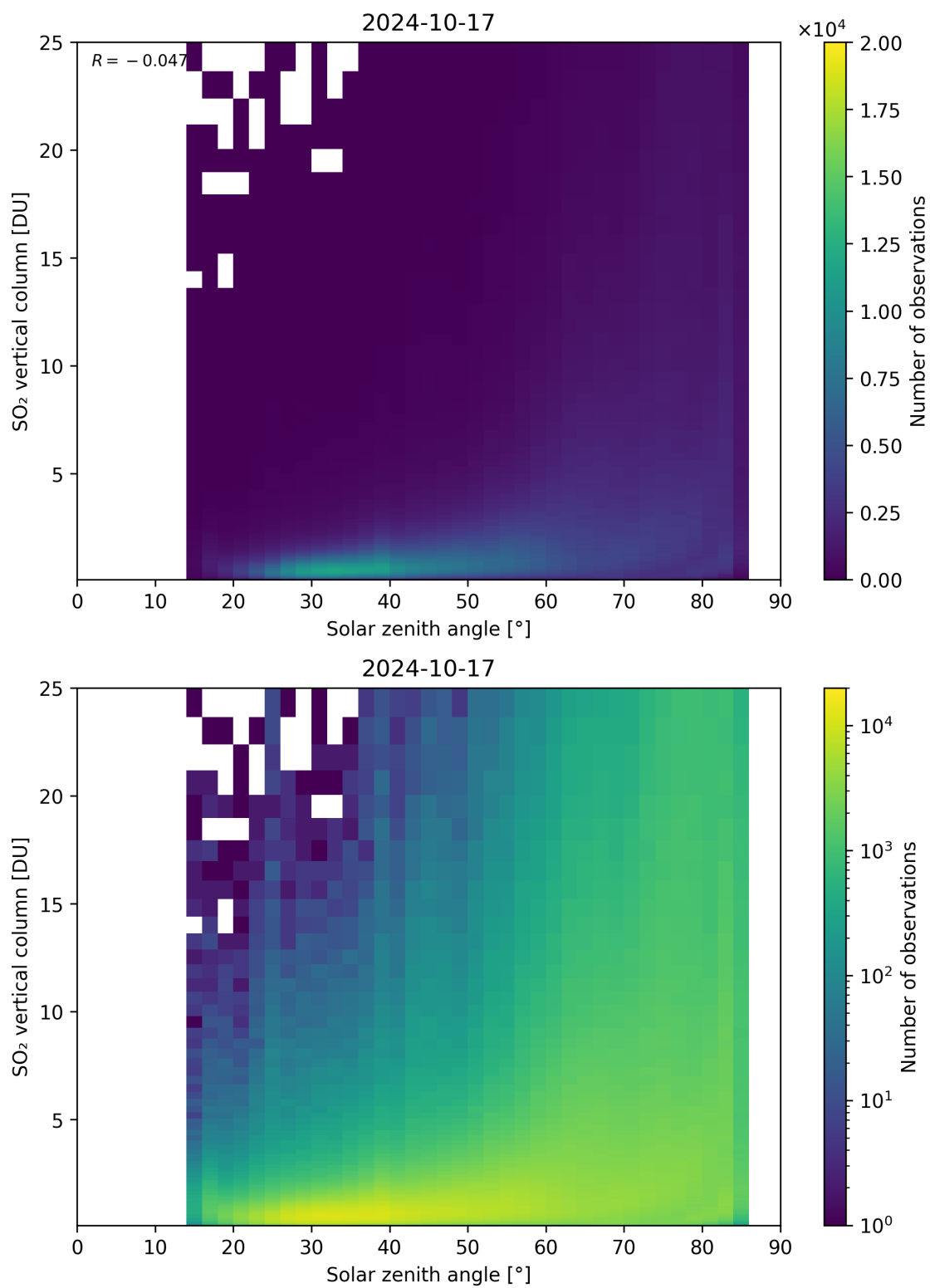
Figure 176: Scatter density plot of “Solar zenith angle” against “SO 2 vertical column” for 2024-10-16 to 2024-10-18.
