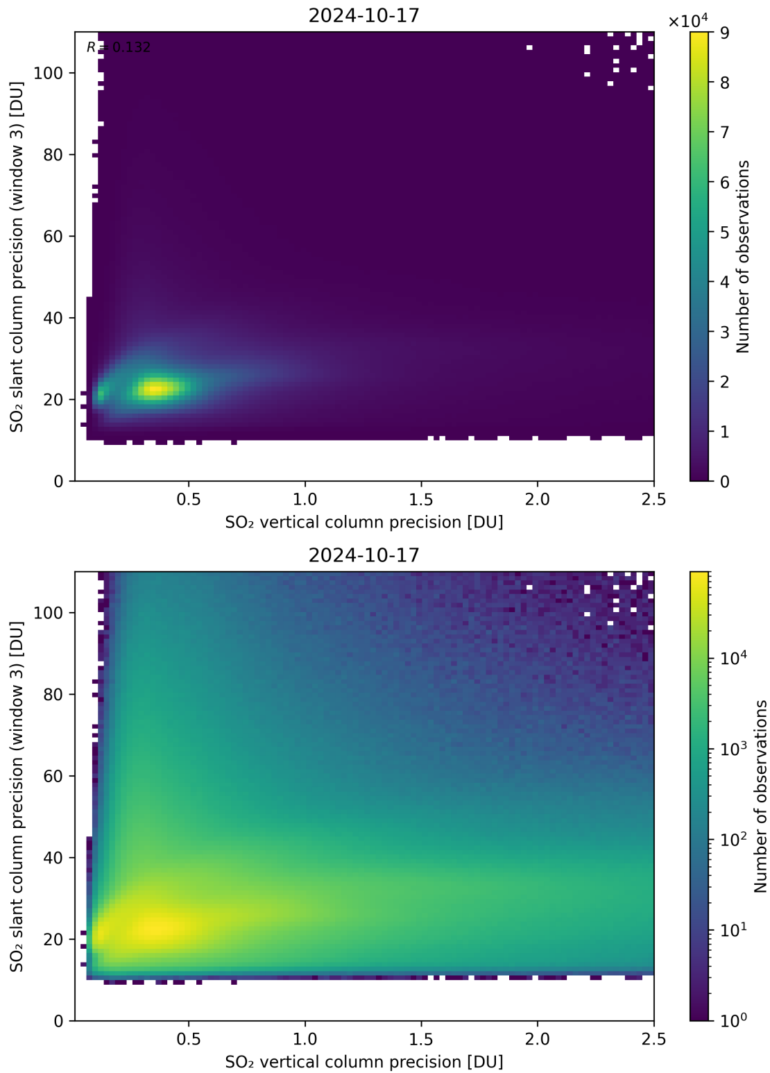
Figure 293: Scatter density plot of “SO 2 vertical column precision” against “SO 2 slant column precision (window 3)” for 2024-10-16 to 2024-10-18.
