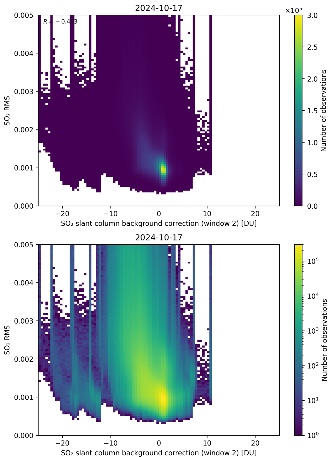
Figure 114: Scatter density plot of “SO 2 slant column background correction (window 2)” against “SO 2 RMS” for 2024-10-16 to 2024-10-18.
