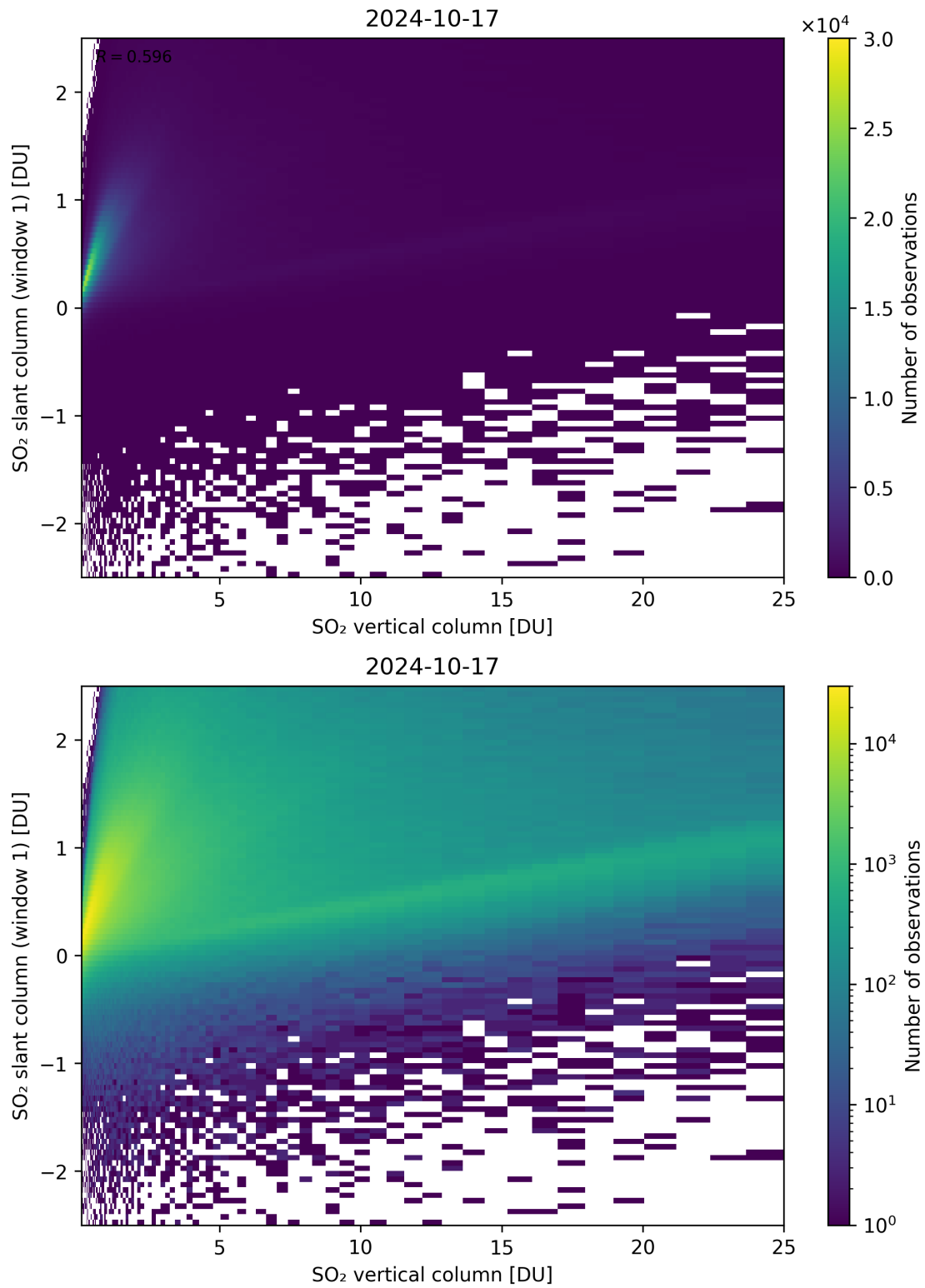
Figure 300: Scatter density plot of “SO 2 vertical column” against “SO 2 slant column (window 1)” for 2024-10-16 to 2024-10-18.
