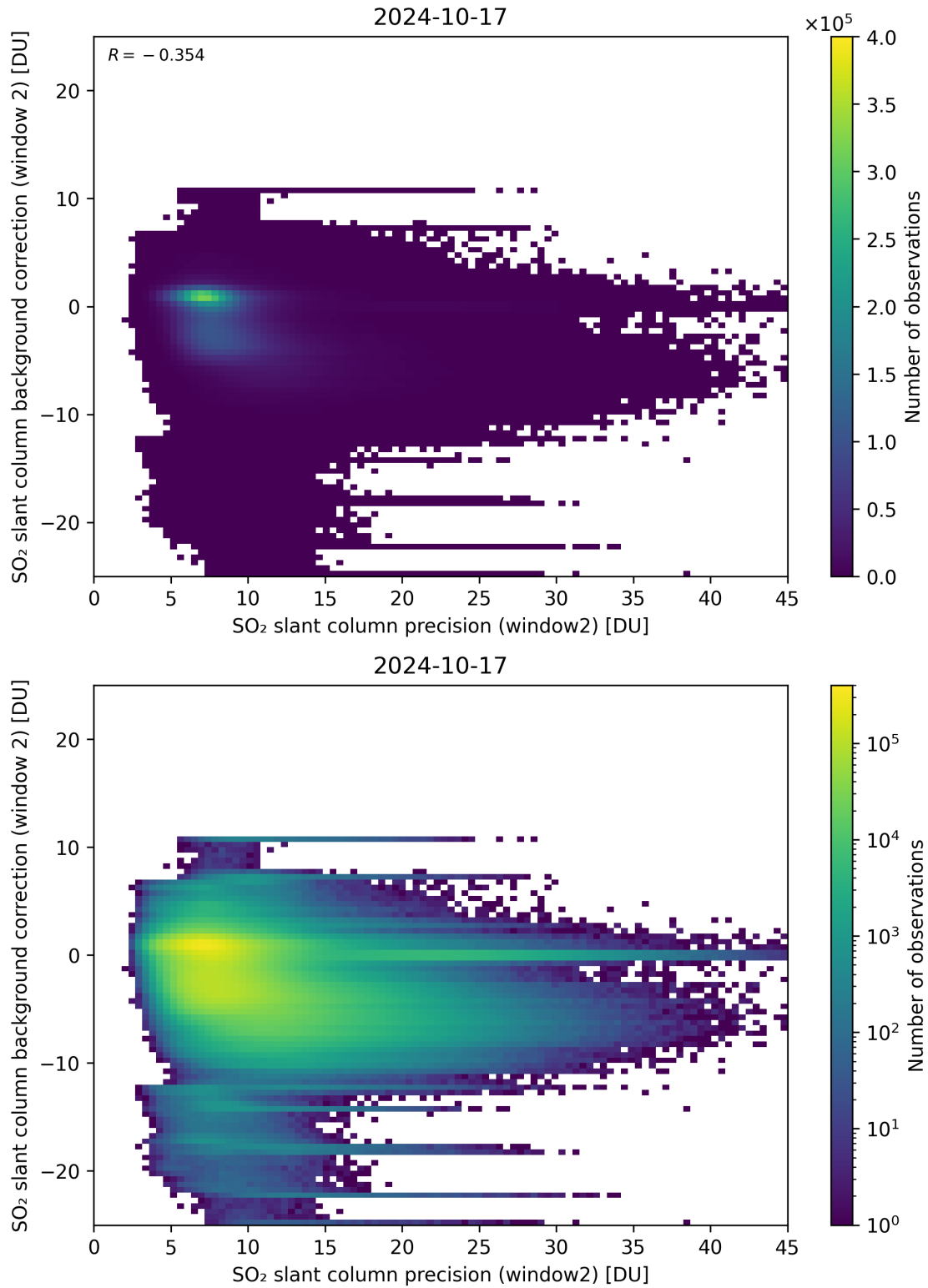
Figure 241: Scatter density plot of “SO 2 slant column precision (window2)” against “SO 2 slant column background correction (window 2)” for 2024-10-16 to 2024-10-18.
