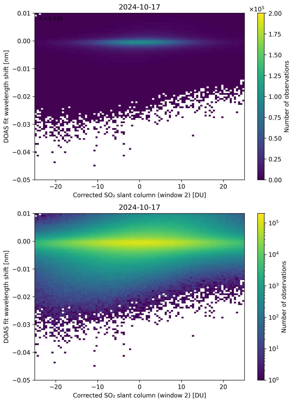
Figure 196: Scatter density plot of “Corrected SO 2 slant column (window 2)” against “DOAS fit wavelength shift” for 2024-10-16 to 2024-10-18.
