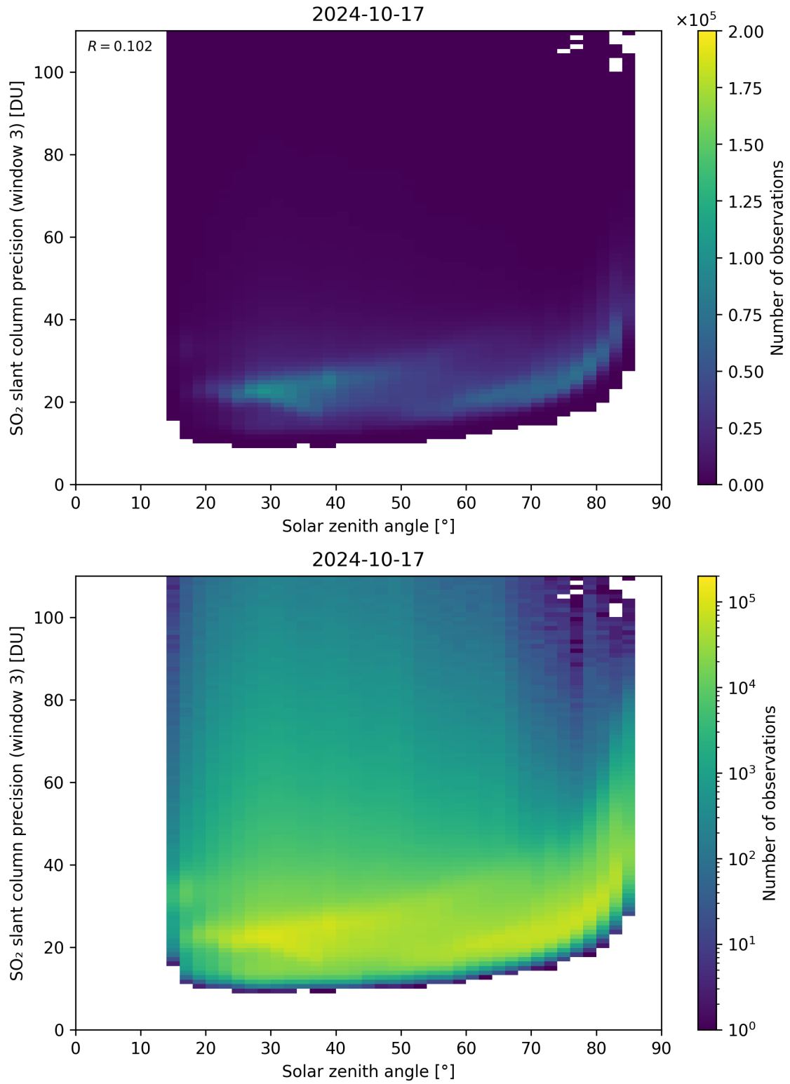
Figure 173: Scatter density plot of “Solar zenith angle” against “SO 2 slant column precision (window 3)” for 2024-10-16 to 2024-10-18.
