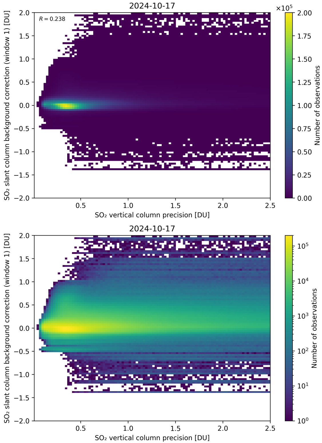
Figure 279: Scatter density plot of “SO 2 vertical column precision” against “SO 2 slant column background correction (window 1)” for 2024-10-16 to 2024-10-18.
