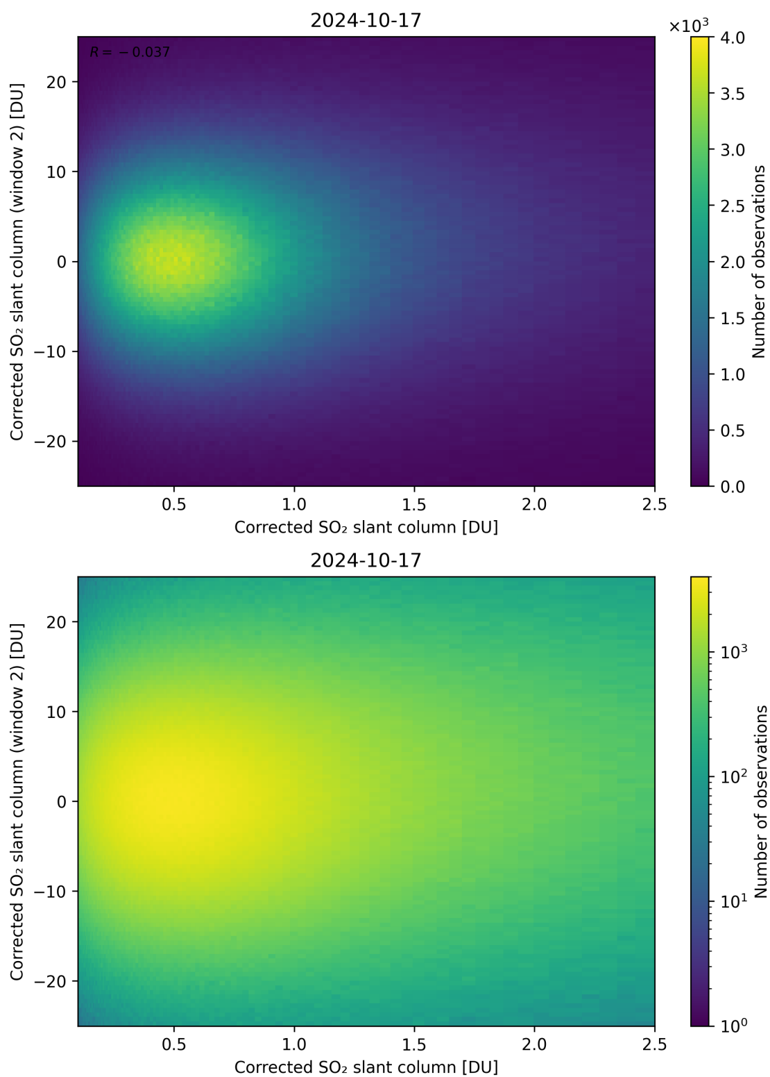
Figure 185: Scatter density plot of “Corrected SO 2 slant column” against “Corrected SO 2 slant column (window 2)” for 2024-10-16 to 2024-10-18.
