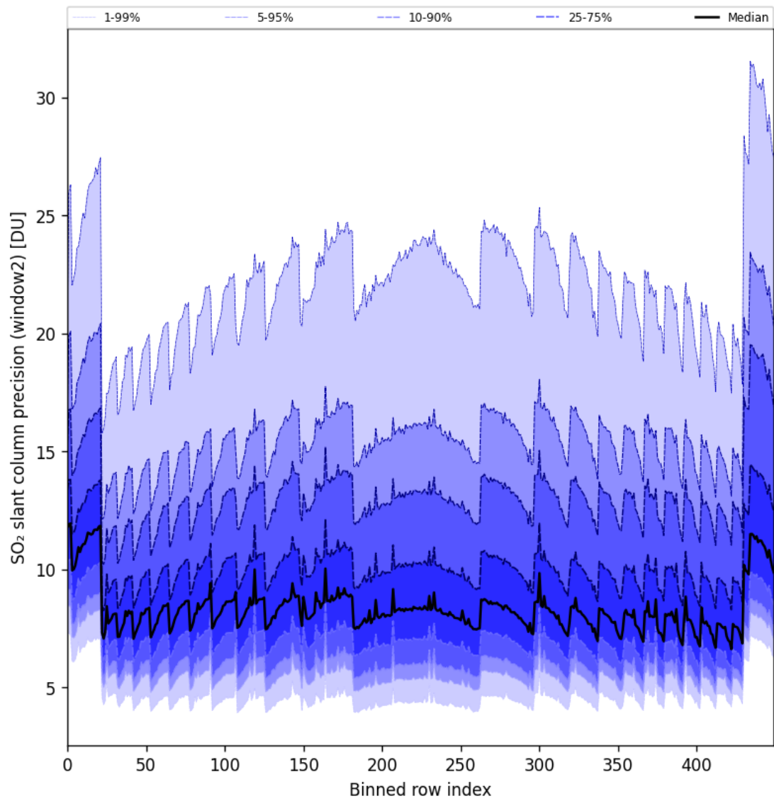
Figure 84: Along track statistics of “SO 2 slant column precision (window2)” for 2024-10-16 to 2024-10-18
