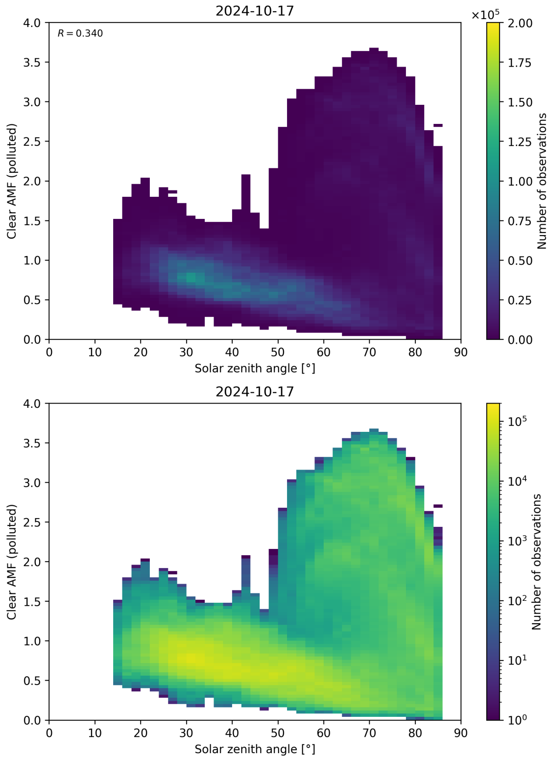
Figure 165: Scatter density plot of “Solar zenith angle” against “Clear AMF (polluted)” for 2024-10-16 to 2024-10-18.
