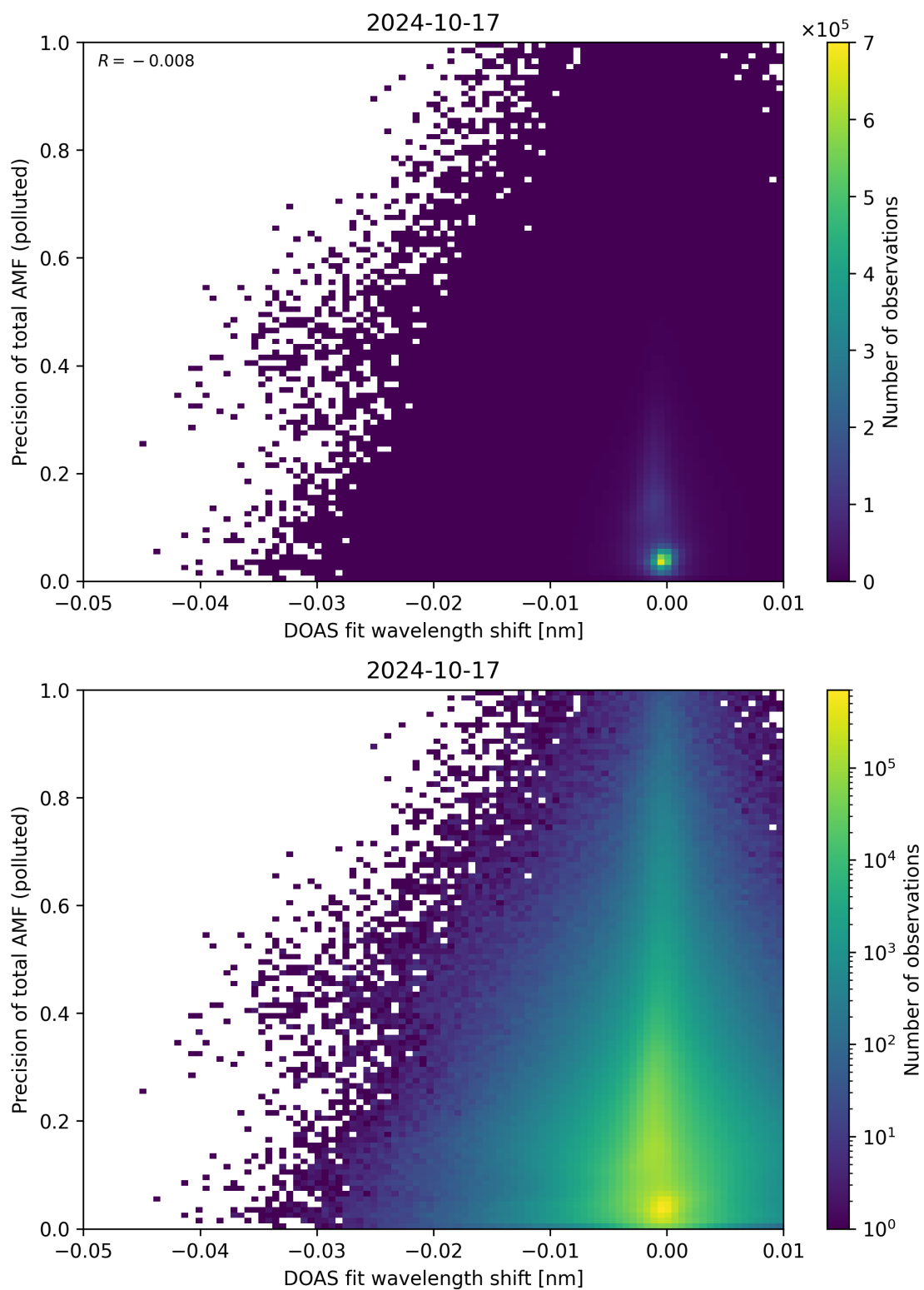
Figure 131: Scatter density plot of “DOAS fit wavelength shift” against “Precision of total AMF (polluted)” for 2024-10-16 to 2024-10-18.
