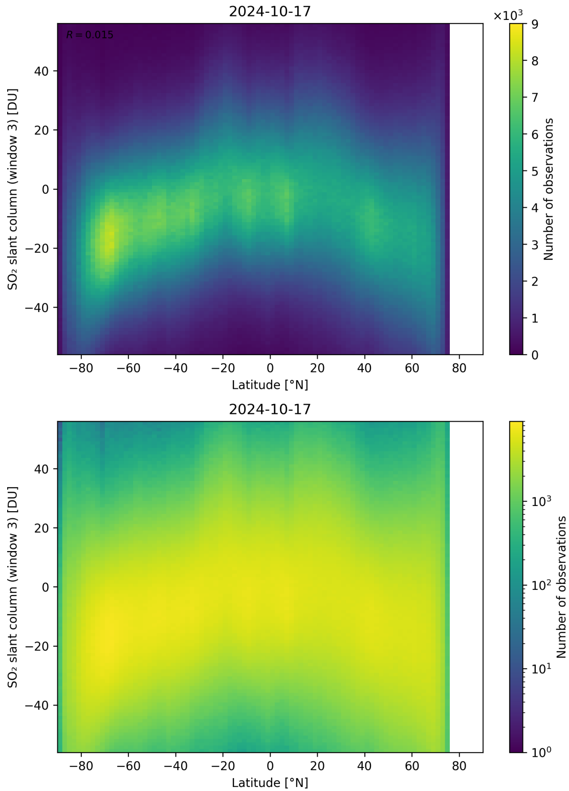
Figure 152: Scatter density plot of “Latitude” against “SO 2 slant column (window 3)” for 2024-10-16 to 2024-10-18.
