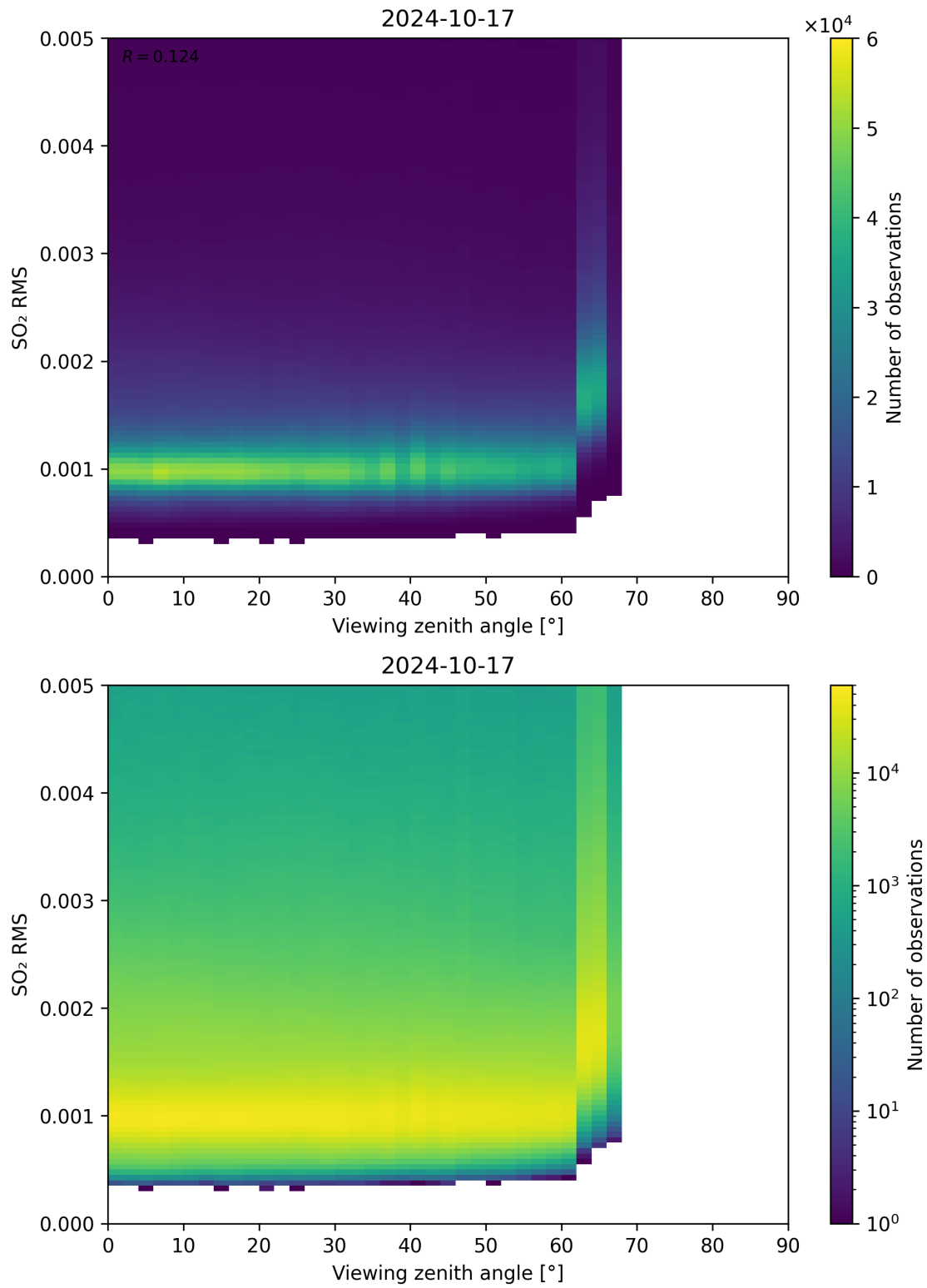
Figure 313: Scatter density plot of “Viewing zenith angle” against “SO 2 RMS” for 2024-10-16 to 2024-10-18.
