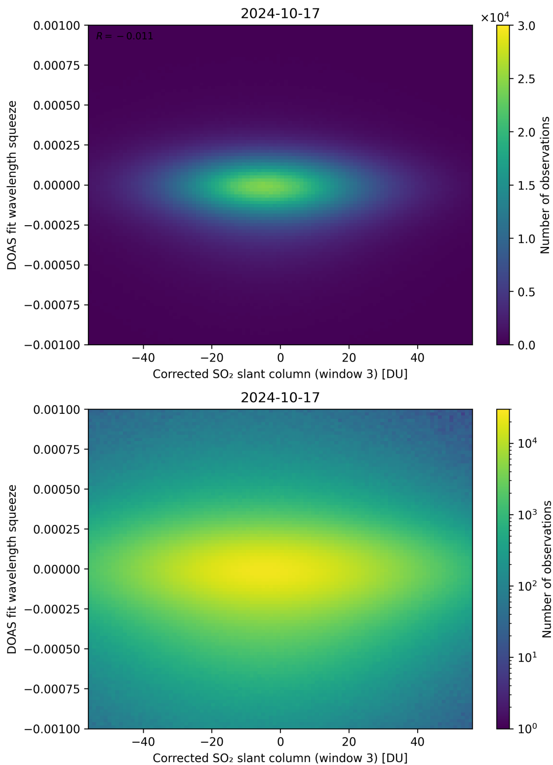
Figure 207: Scatter density plot of “Corrected SO 2 slant column (window 3)” against “DOAS fit wavelength squeeze” for 2024-10-16 to 2024-10-18.
