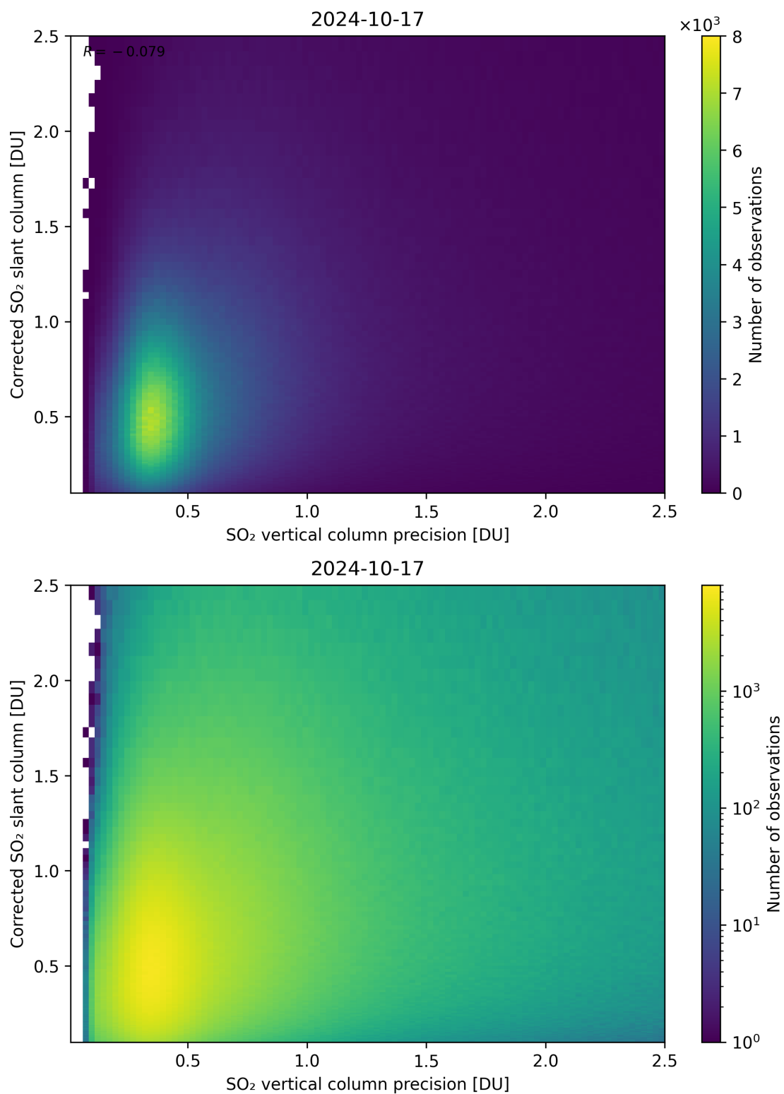
Figure 286: Scatter density plot of “SO 2 vertical column precision” against “Corrected SO 2 slant column” for 2024-10-16 to 2024-10-18.
