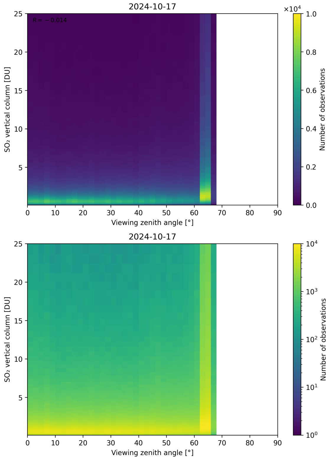
Figure 327: Scatter density plot of “Viewing zenith angle” against “SO 2 vertical column” for 2024-10-16 to 2024-10-18.
