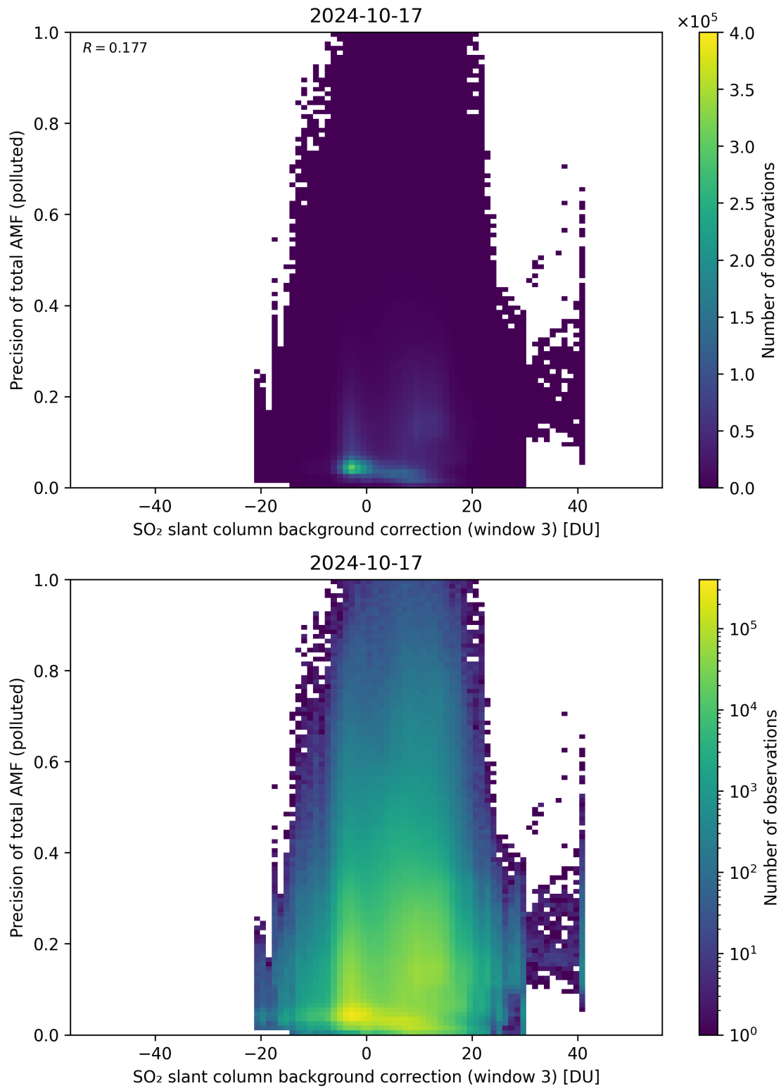
Figure 126: Scatter density plot of “SO 2 slant column background correction (window 3)” against “Precision of total AMF (polluted)” for 2024-10-16 to 2024-10-18.
