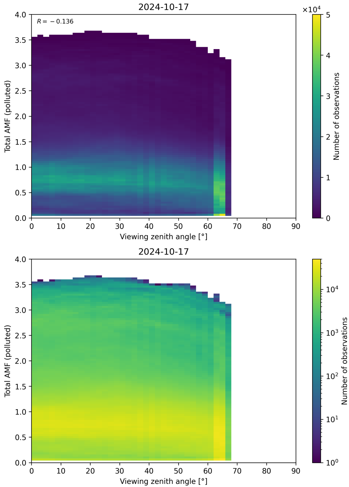
Figure 325: Scatter density plot of “Viewing zenith angle” against “Total AMF (polluted)” for 2024-10-16 to 2024-10-18.
