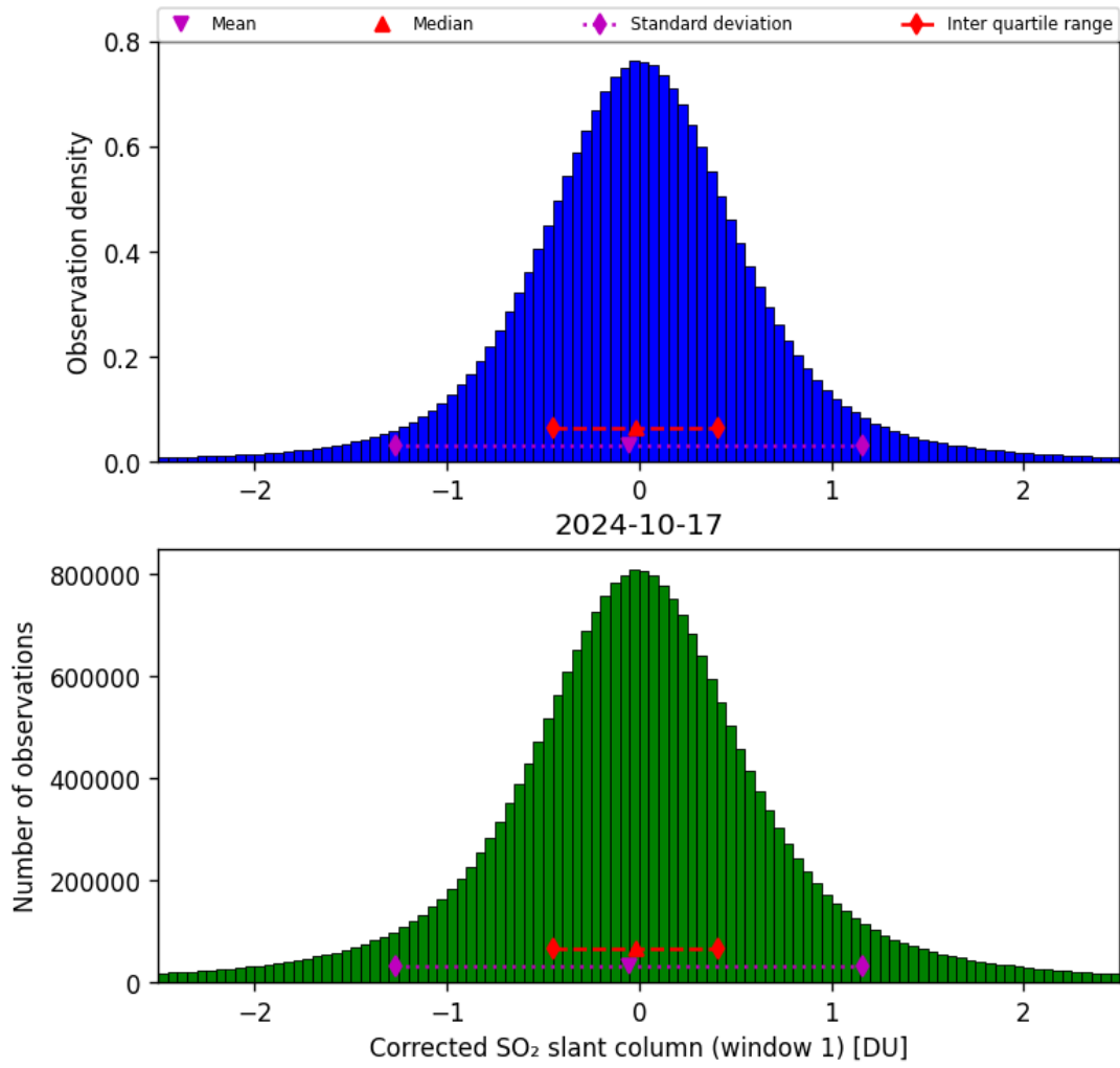
Figure 58: Histogram of “Corrected SO 2 slant column (window 1)” for 2024-10-16 to 2024-10-18
