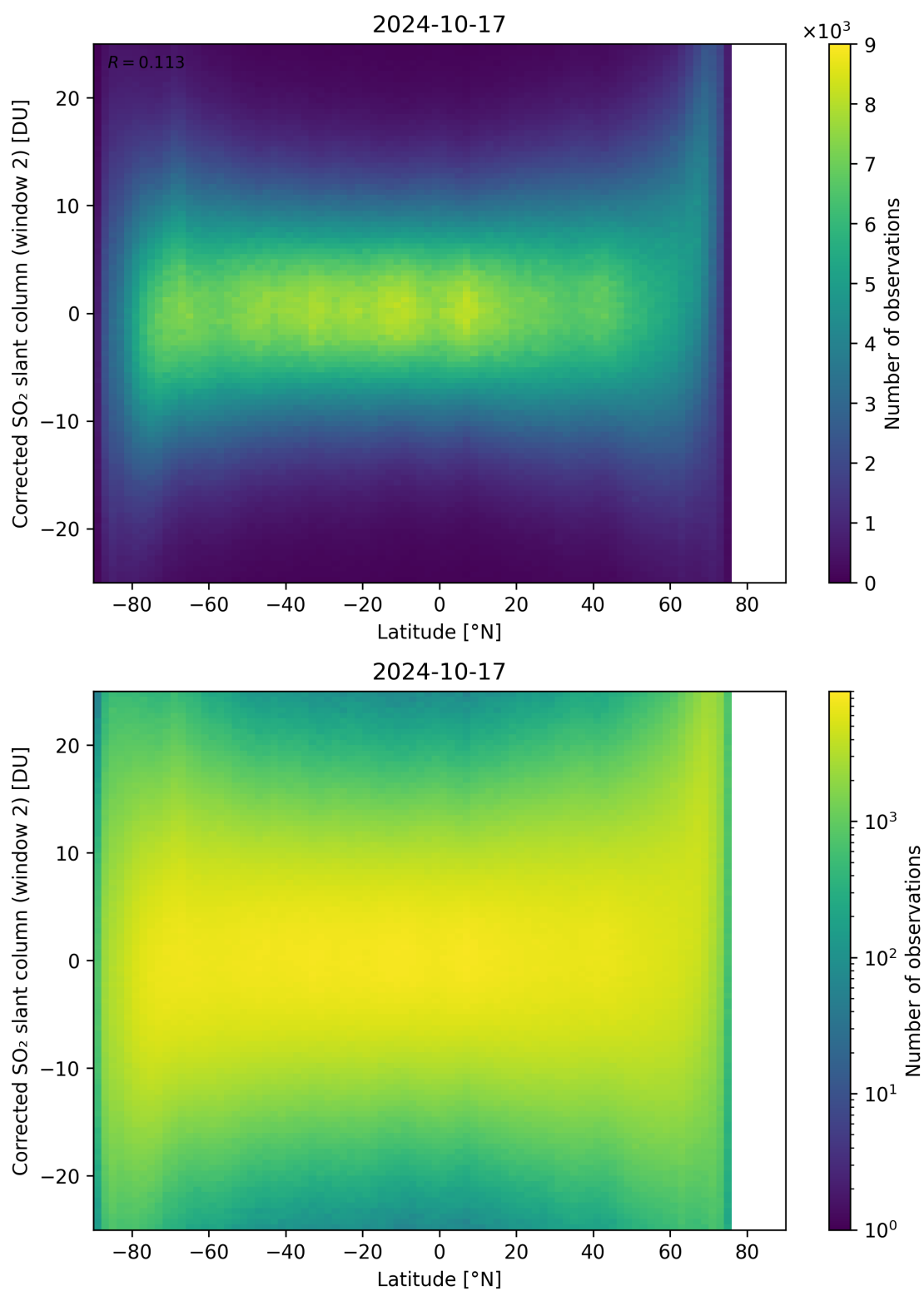
Figure 147: Scatter density plot of “Latitude” against “Corrected SO 2 slant column (window 2)” for 2024-10-16 to 2024-10-18.
