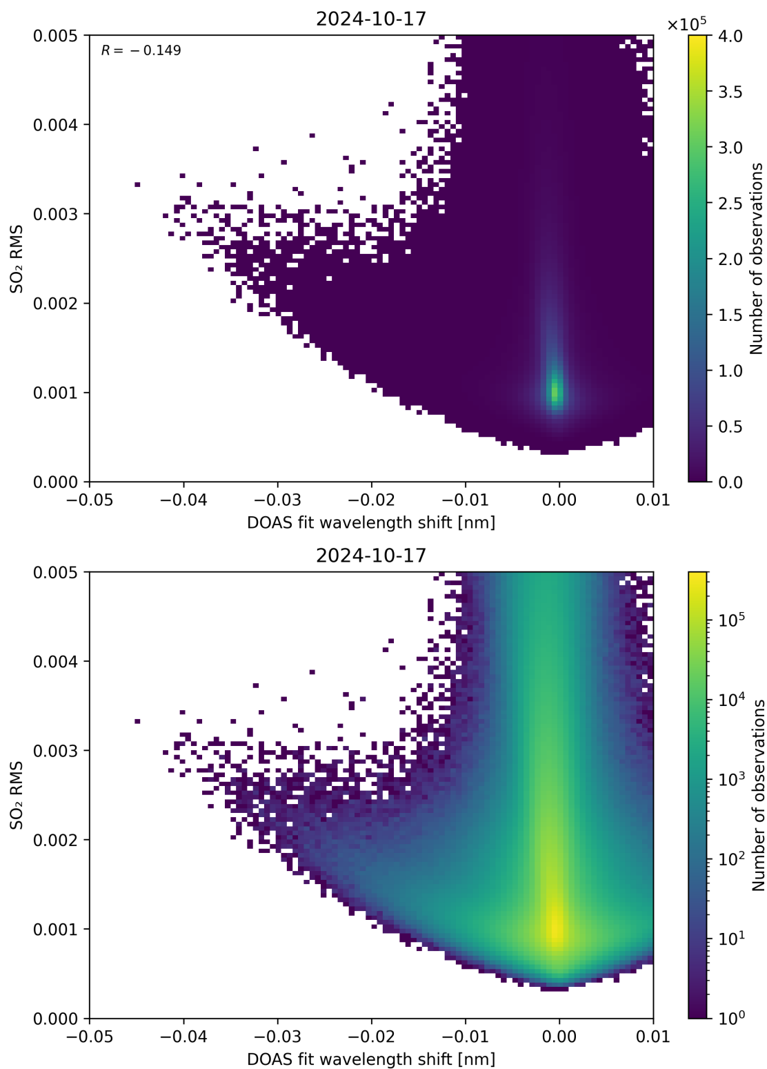
Figure 128: Scatter density plot of “DOAS fit wavelength shift” against “SO 2 RMS” for 2024-10-16 to 2024-10-18.
