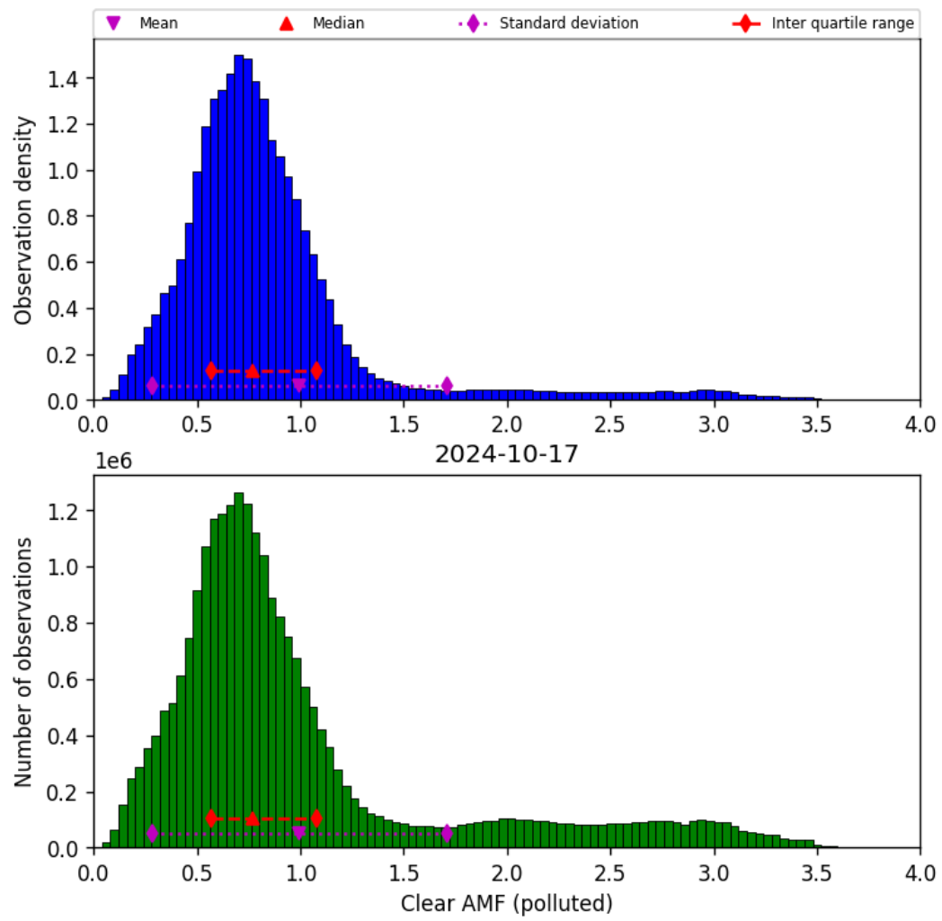
Figure 73: Histogram of “Clear AMF (polluted)” for 2024-10-16 to 2024-10-18
