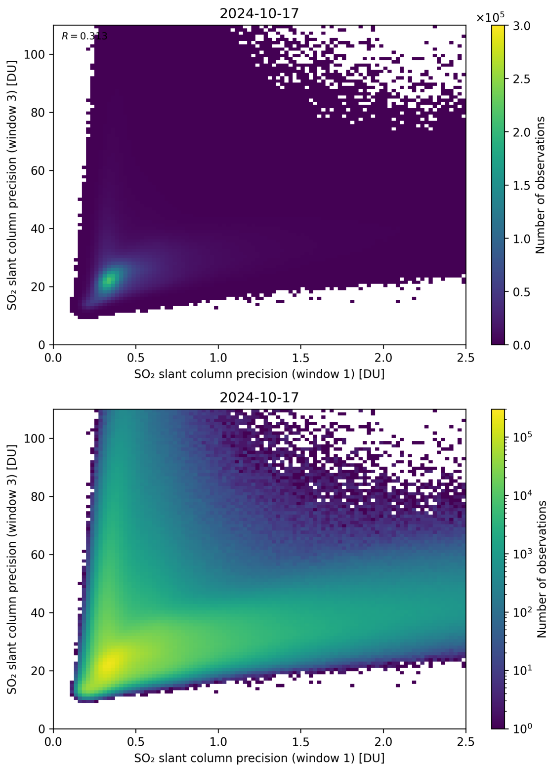
Figure 229: Scatter density plot of “SO 2 slant column precision (window 1)” against “SO 2 slant column precision (window 3)” for 2024-10-16 to 2024-10-18.
