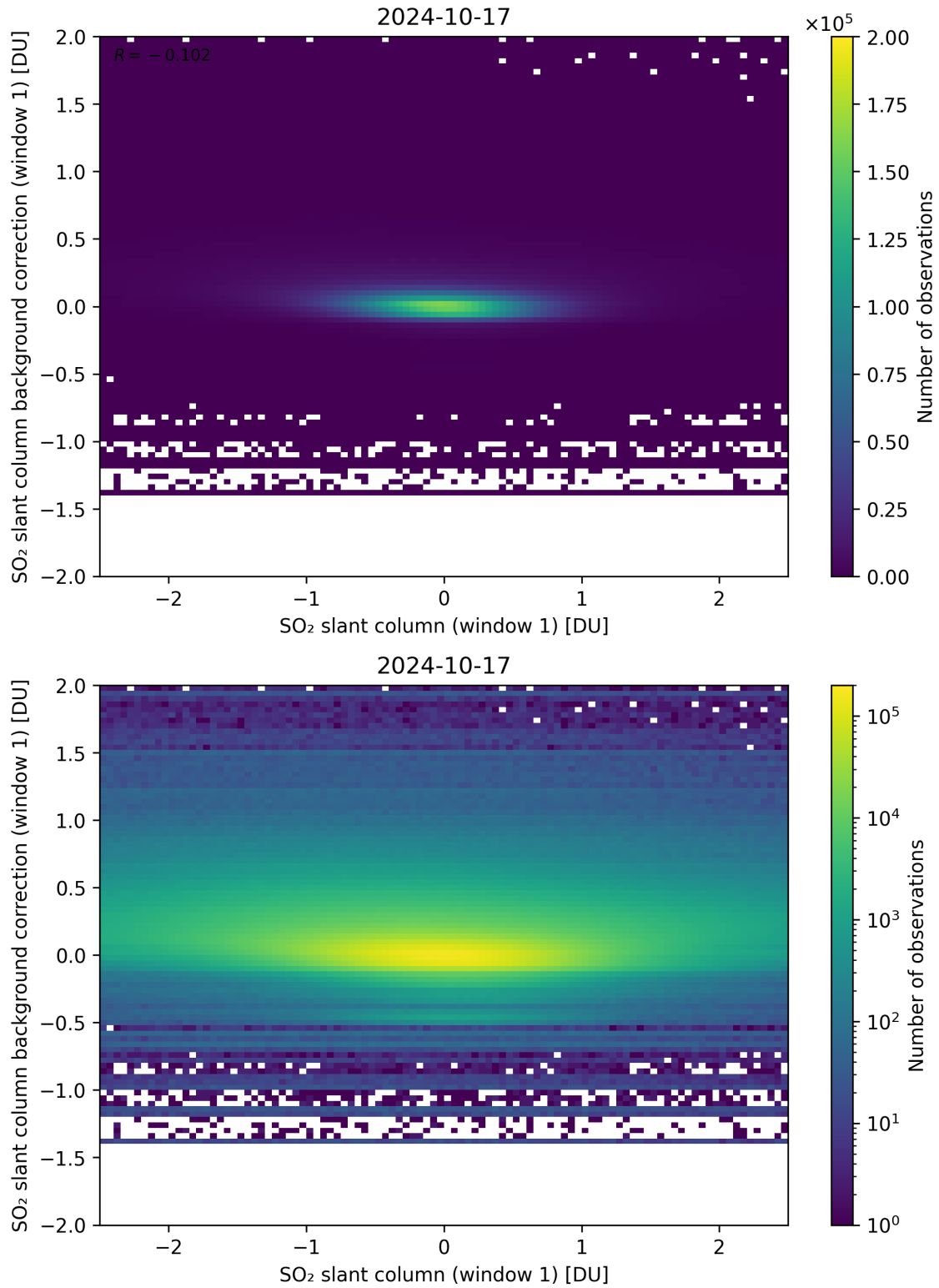
Figure 212: Scatter density plot of “SO 2 slant column (window 1)” against “SO 2 slant column background correction (window 1)” for 2024-10-16 to 2024-10-18.
