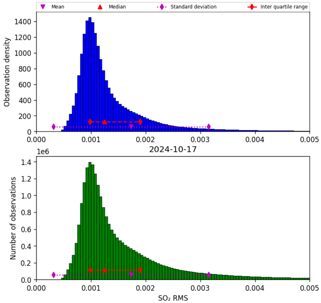
Figure 70: Histogram of “SO 2 RMS” for 2024-10-16 to 2024-10-18
