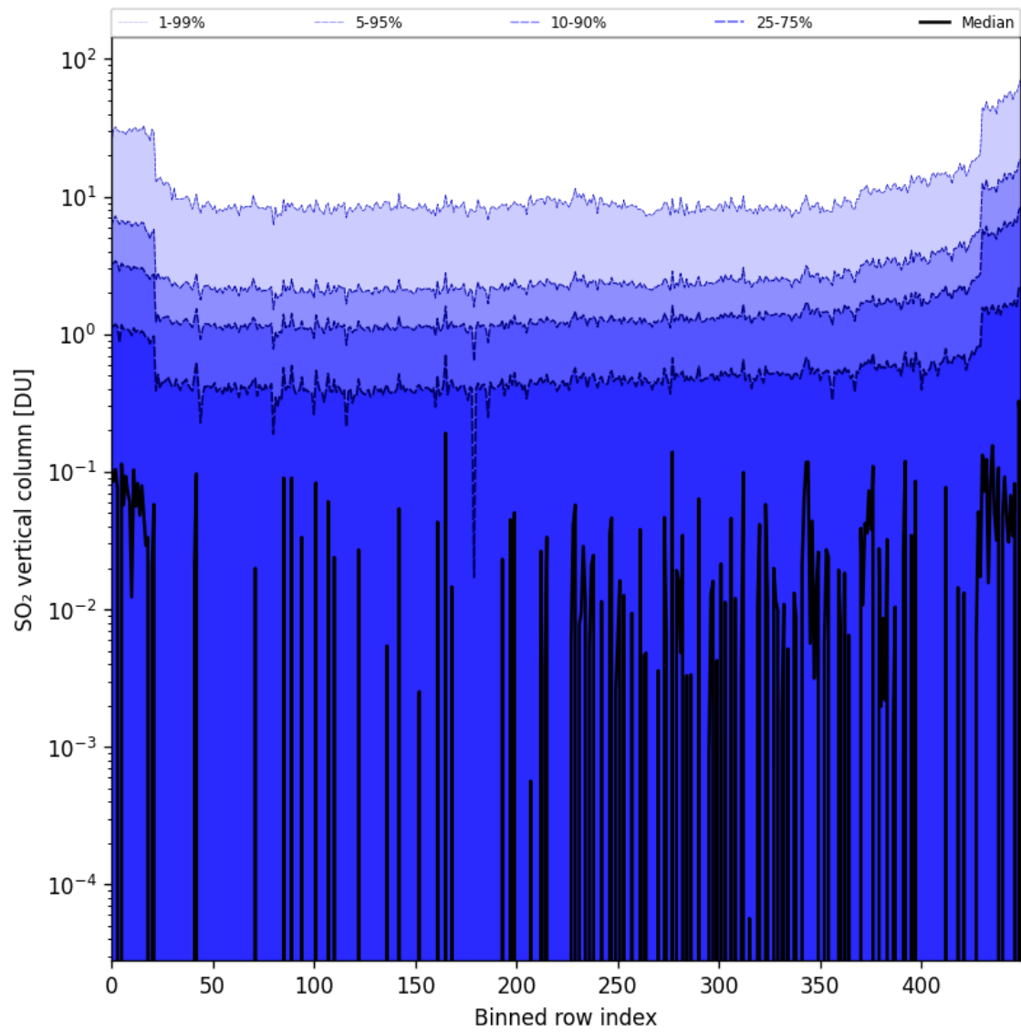
Figure 76: Along track statistics of “SO 2 vertical column” for 2024-10-16 to 2024-10-18
