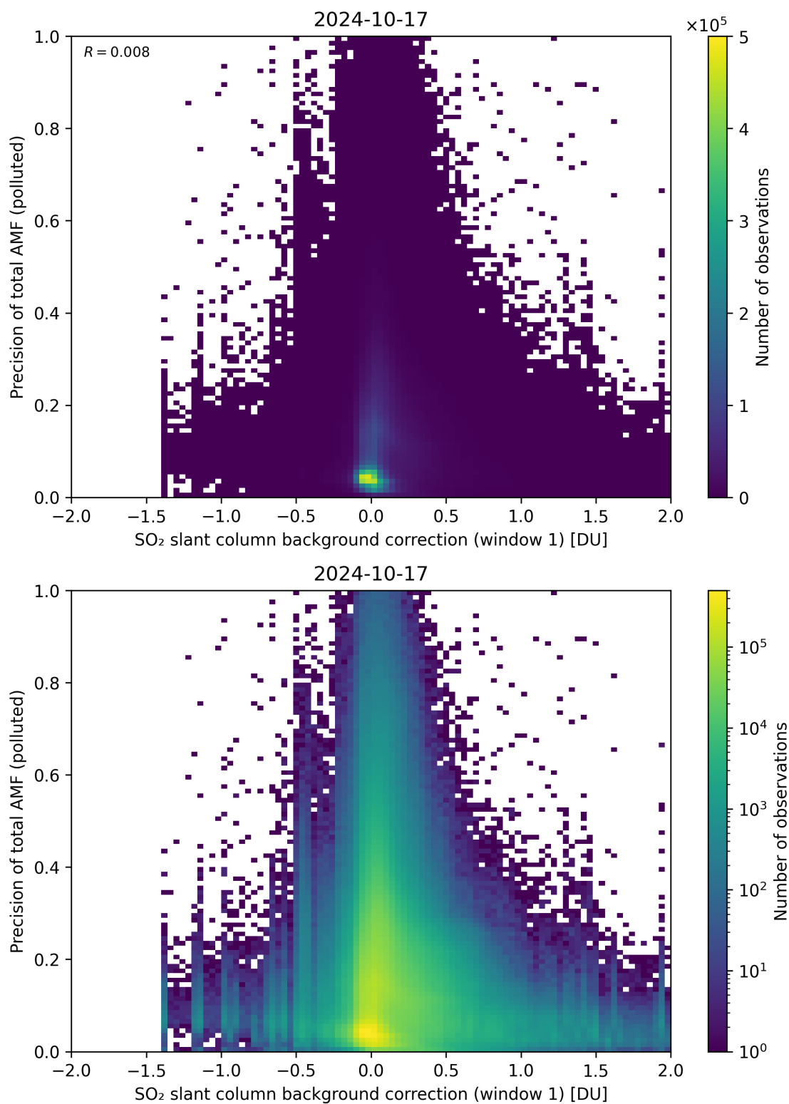
Figure 110: Scatter density plot of “SO 2 slant column background correction (window 1)” against “Precision of total AMF (polluted)” for 2024-10-16 to 2024-10-18.
