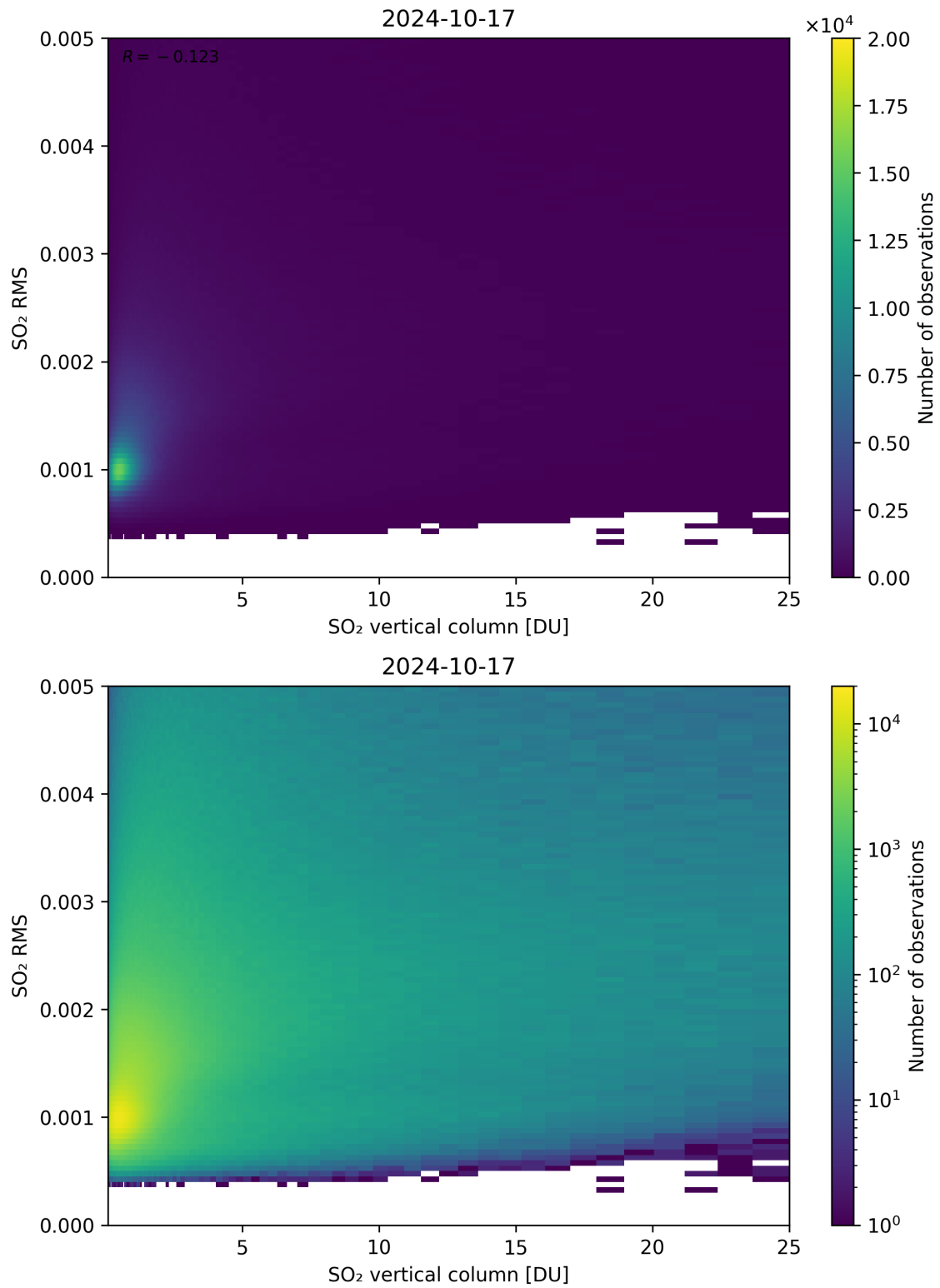
Figure 278: Scatter density plot of “SO 2 vertical column” against “SO 2 RMS” for 2024-10-16 to 2024-10-18.
