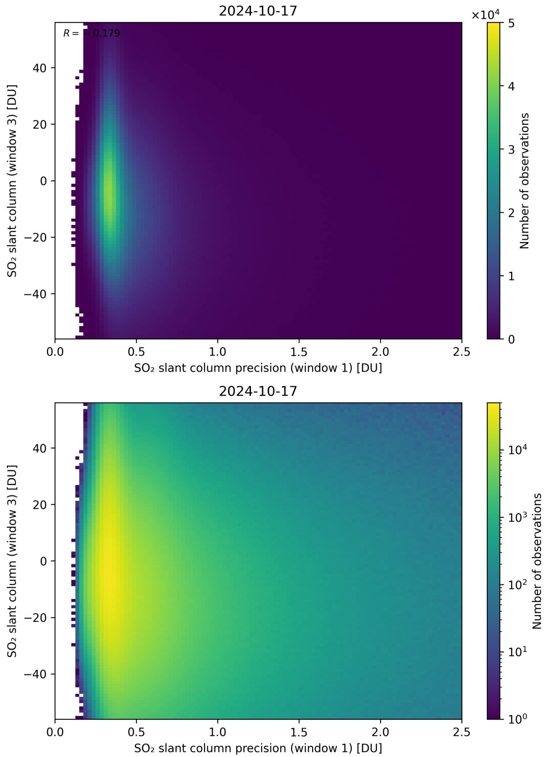
Figure 228: Scatter density plot of “SO 2 slant column precision (window 1)” against “SO 2 slant column (window 3)” for 2024-10-16 to 2024-10-18.
