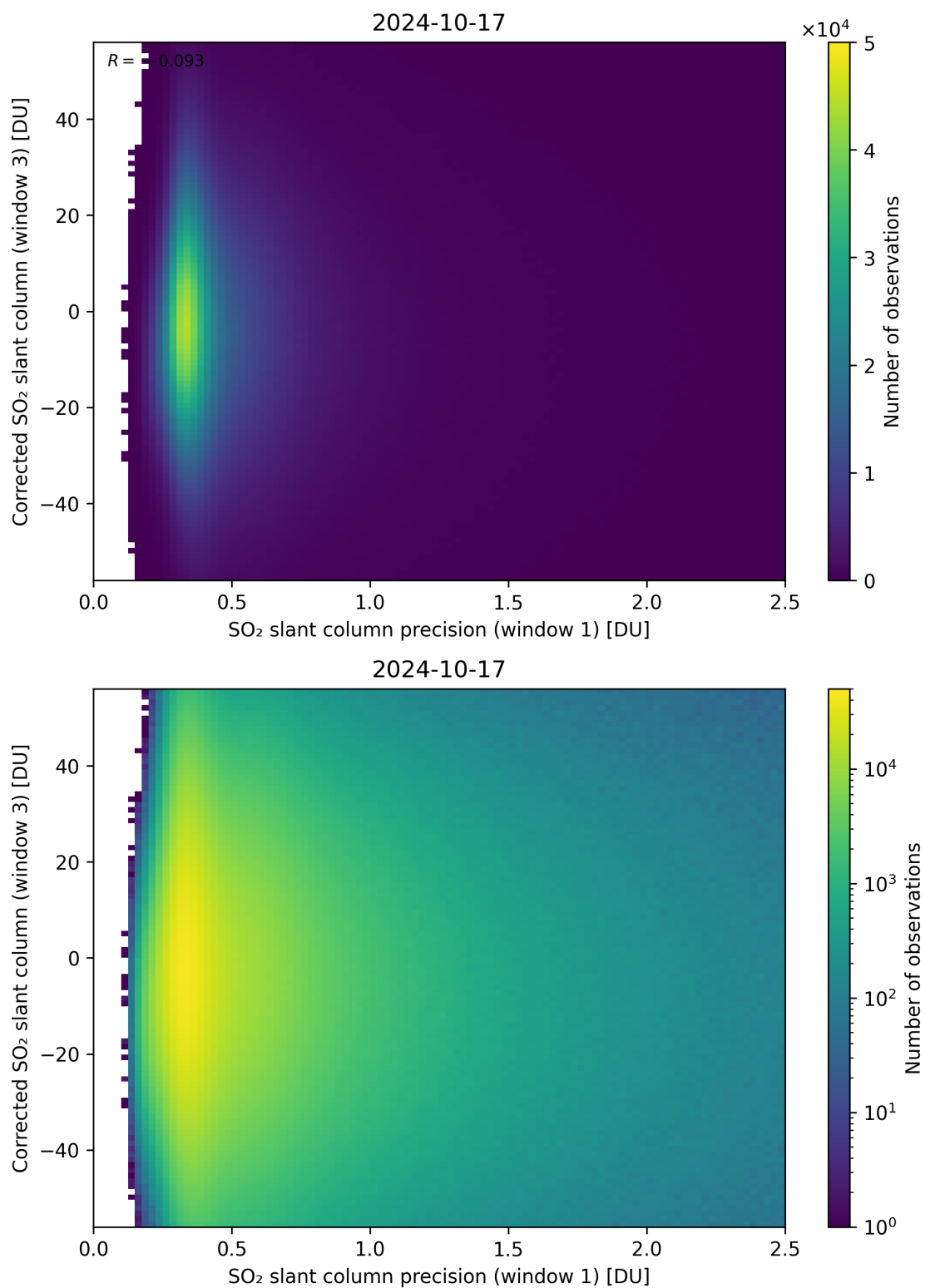
Figure 226: Scatter density plot of “SO 2 slant column precision (window 1)” against “Corrected SO 2 slant column (window 3)” for 2024-10-16 to 2024-10-18.
