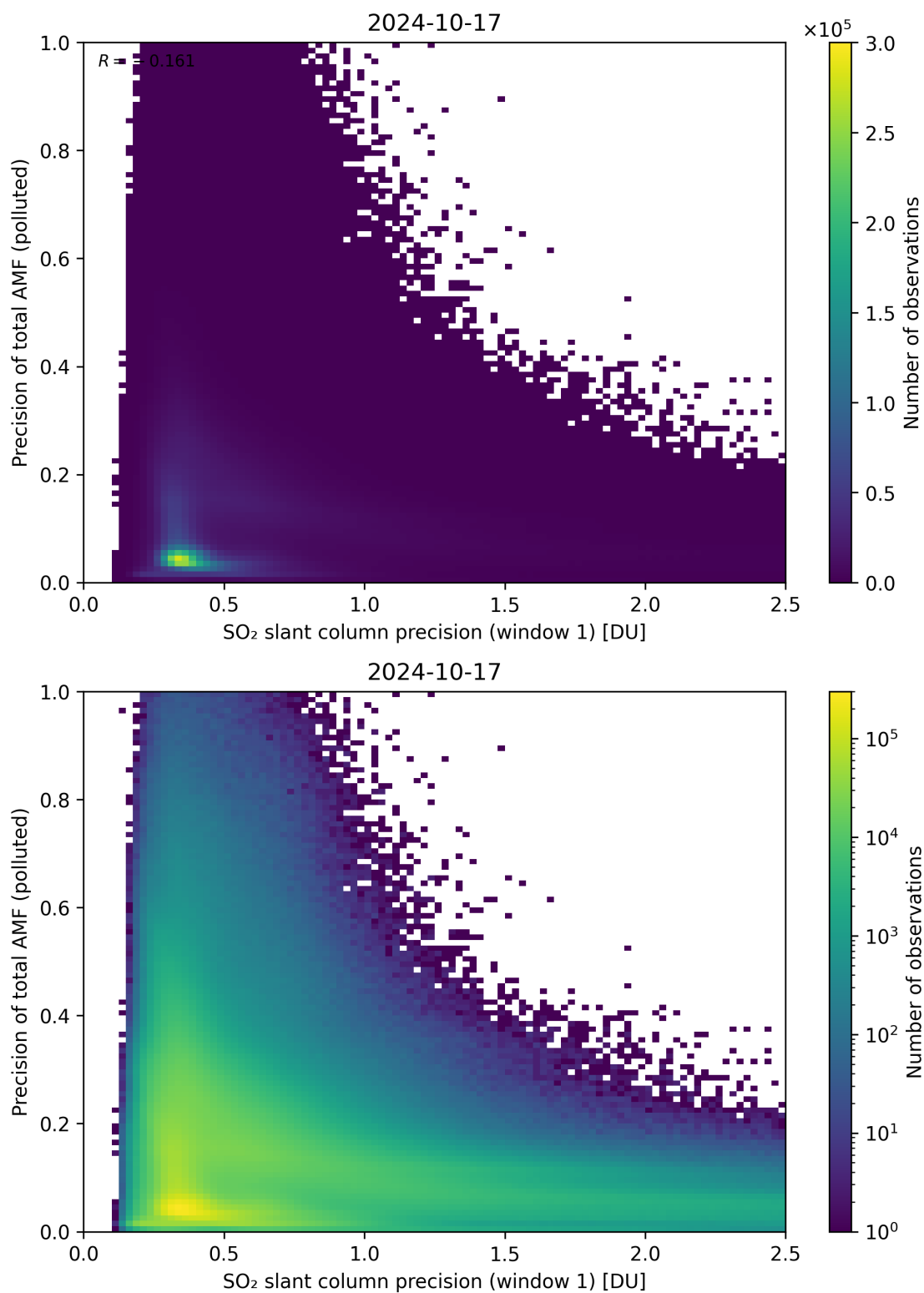
Figure 231: Scatter density plot of “SO 2 slant column precision (window 1)” against “Precision of total AMF (polluted)” for 2024-10-16 to 2024-10-18.
