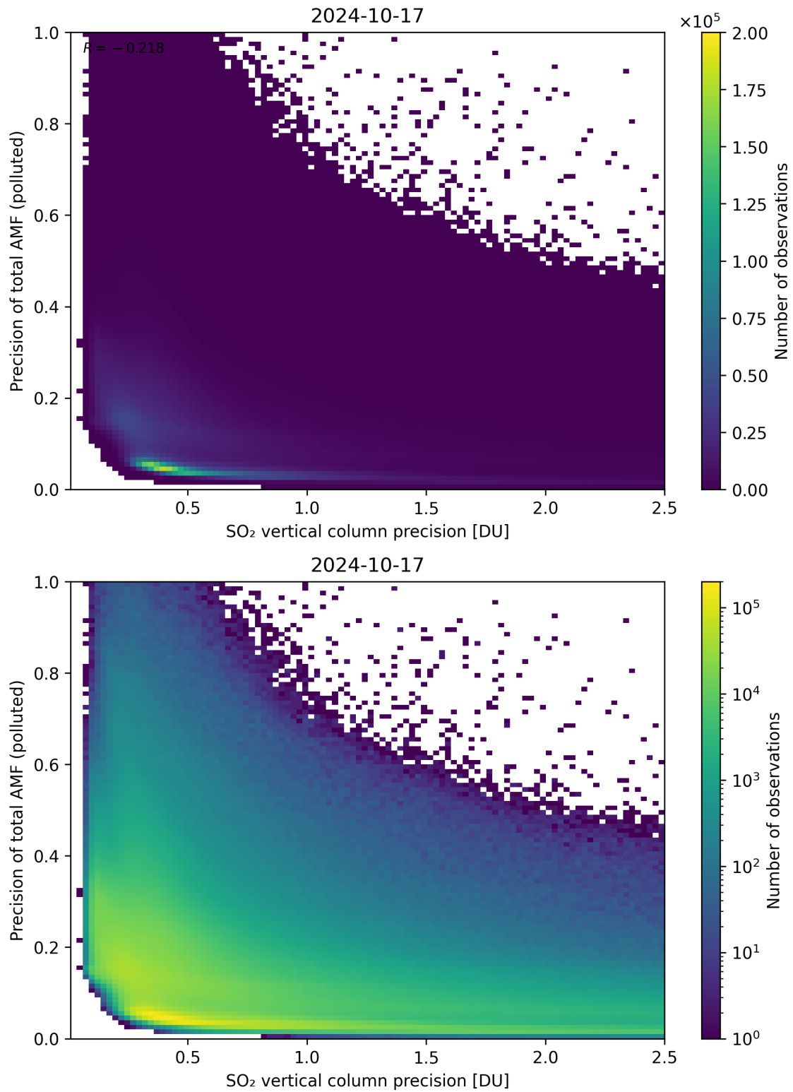
Figure 295: Scatter density plot of “SO 2 vertical column precision” against “Precision of total AMF (polluted)” for 2024-10-16 to 2024-10-18.
