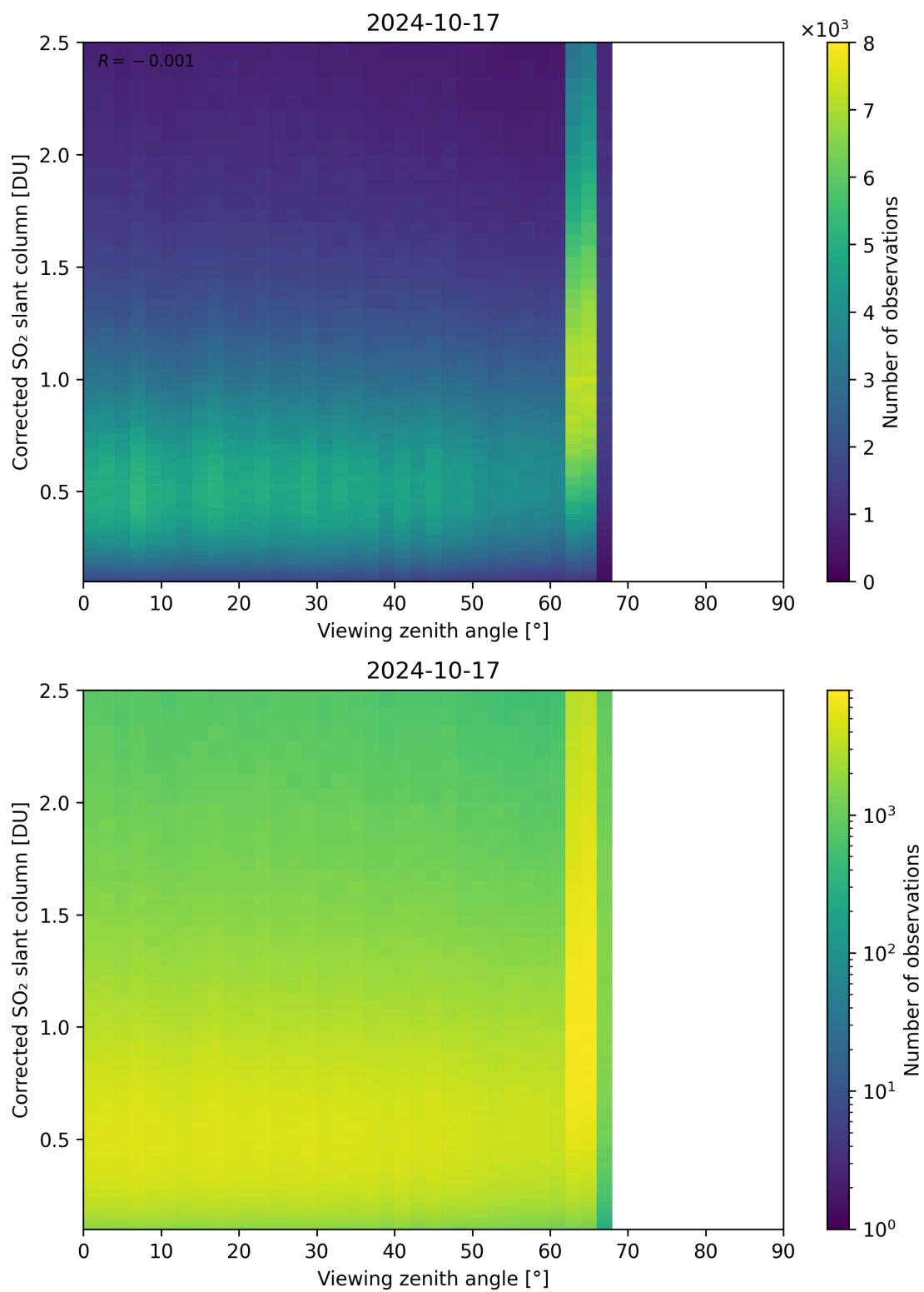
Figure 317: Scatter density plot of “Viewing zenith angle” against “Corrected SO 2 slant column” for 2024-10-16 to 2024-10-18.
