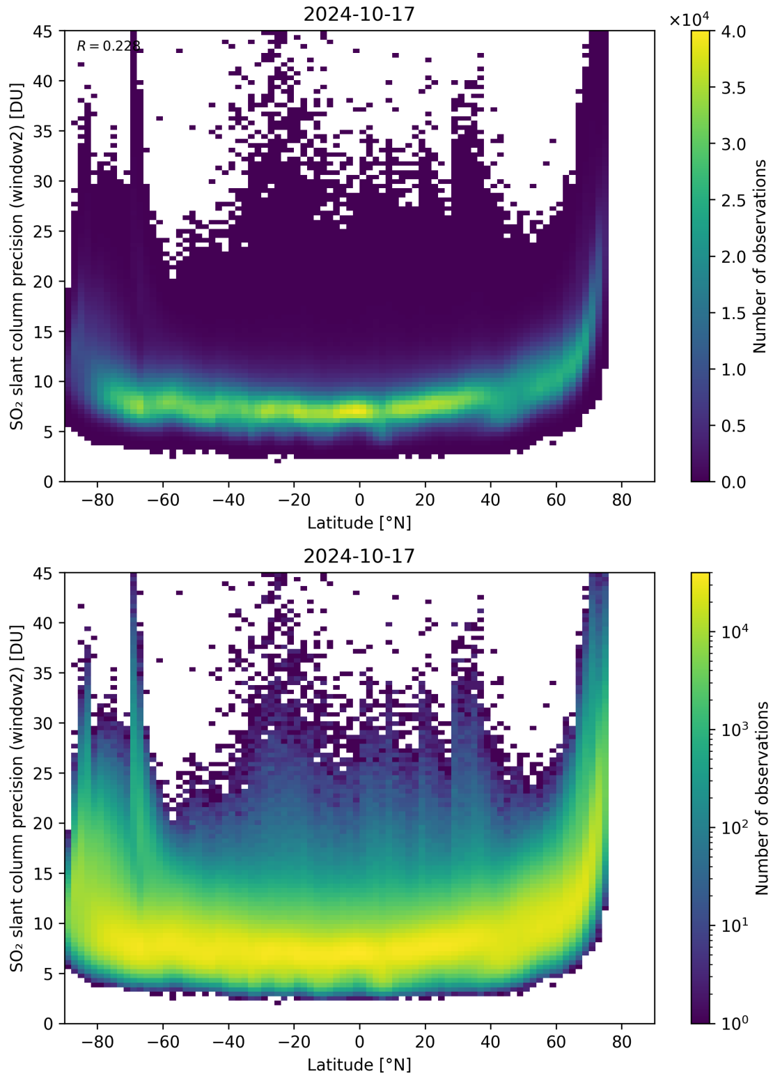
Figure 151: Scatter density plot of “Latitude” against “SO 2 slant column precision (window2)” for 2024-10-16 to 2024-10-18.
