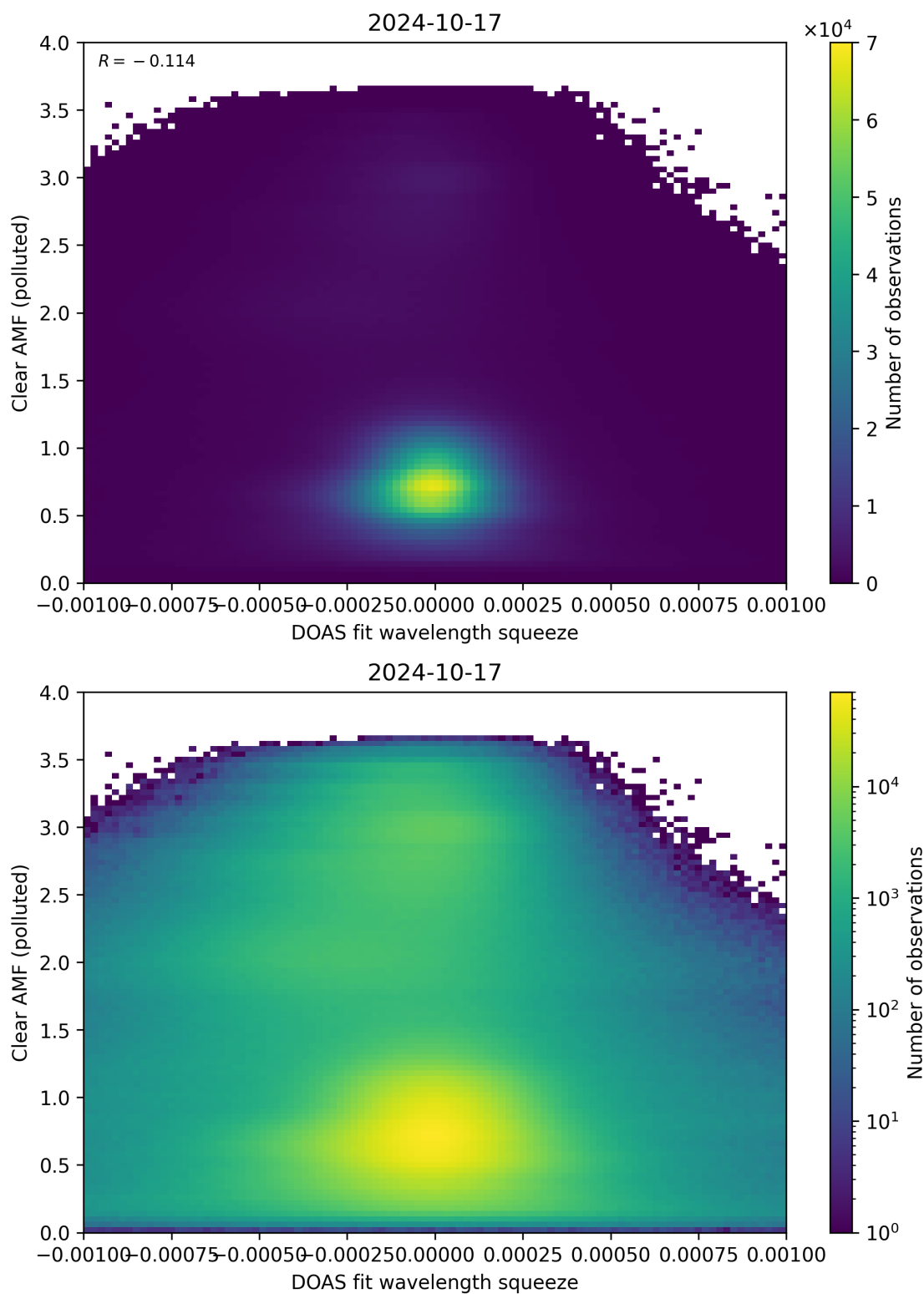
Figure 133: Scatter density plot of “DOAS fit wavelength squeeze” against “Clear AMF (polluted)” for 2024-10-16 to 2024-10-18.
