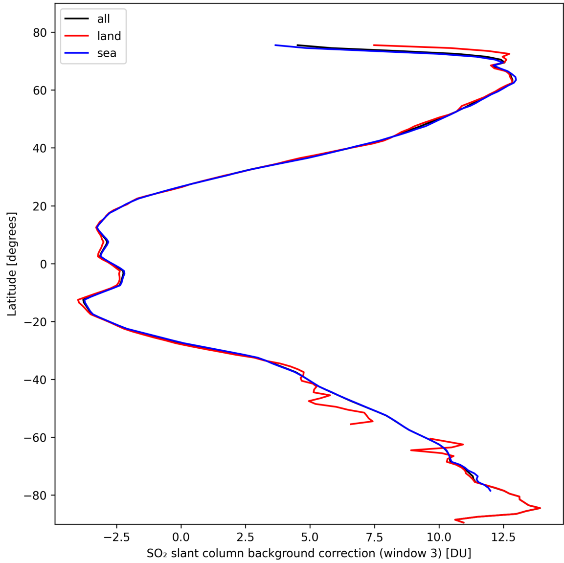
Figure 44: Zonal average of “SO 2 slant column background correction (window 3)” for 2024-10-16 to 2024-10-18.
