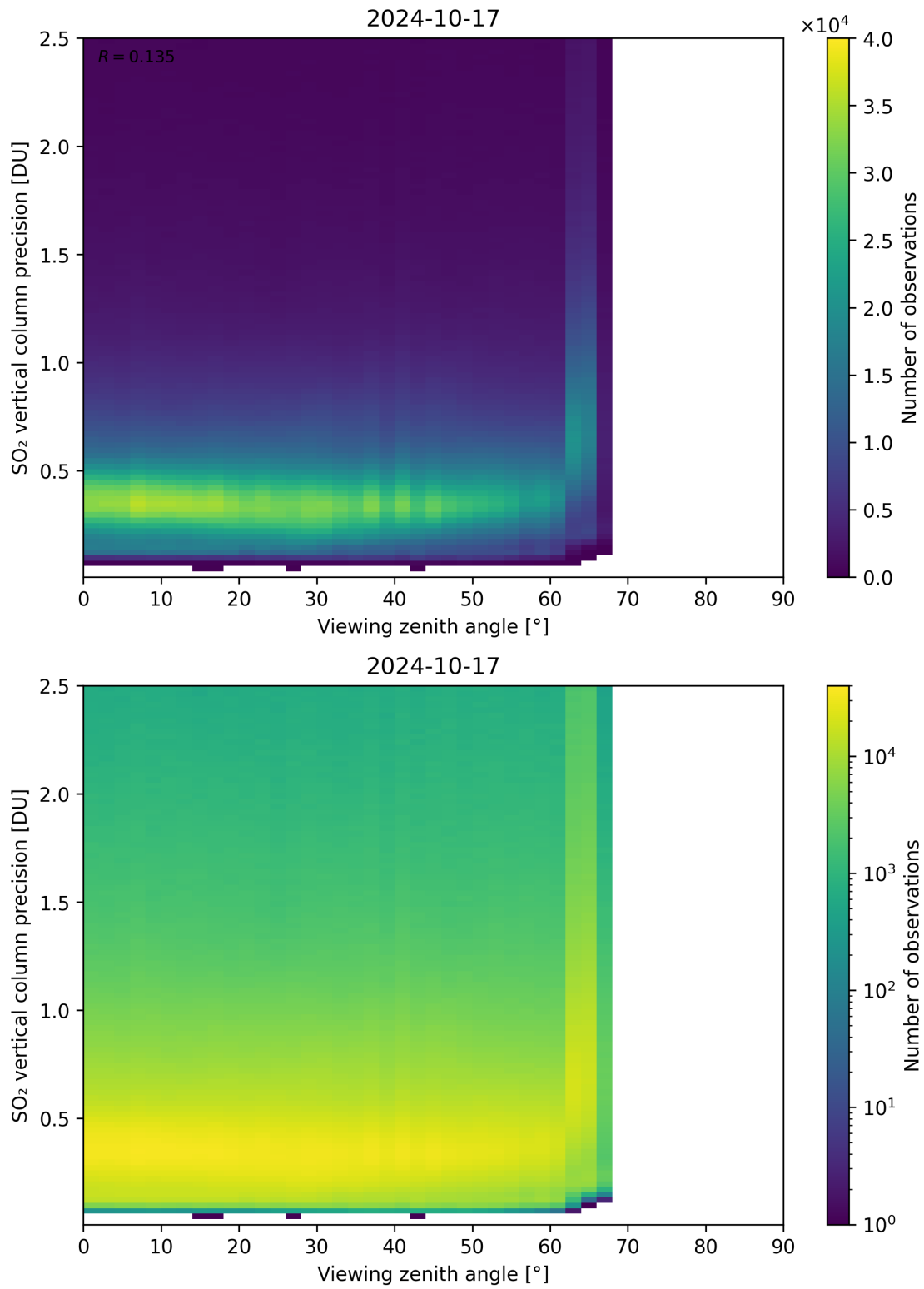
Figure 328: Scatter density plot of “Viewing zenith angle” against “SO 2 vertical column precision” for 2024-10-16 to 2024-10-18.
