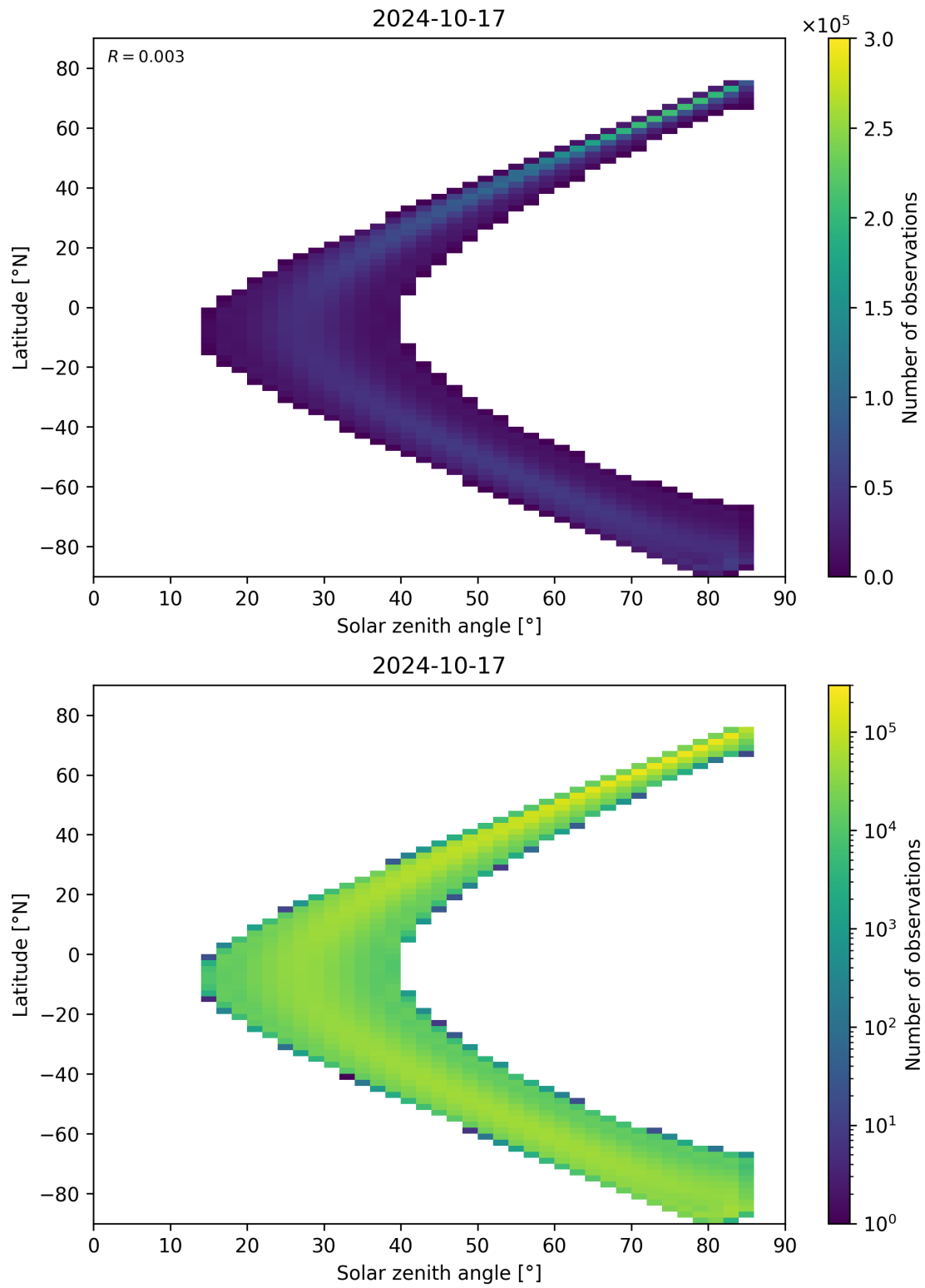
Figure 164: Scatter density plot of “Solar zenith angle” against “Latitude” for 2024-10-16 to 2024-10-18.
