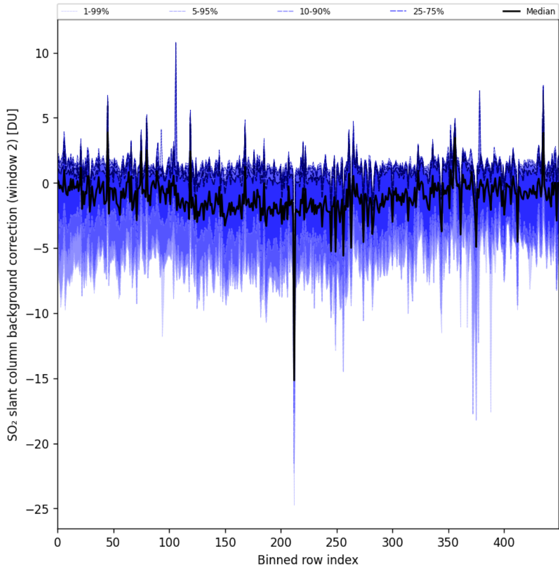
Figure 86: Along track statistics of “SO 2 slant column background correction (window 2)” for 2024-10-16 to 2024-10-18
