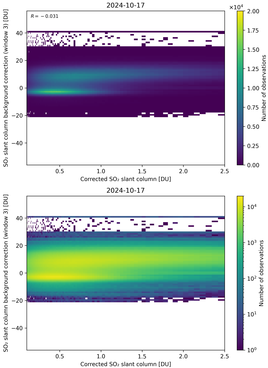
Figure 180: Scatter density plot of “Corrected SO 2 slant column” against “SO 2 slant column background correction (window 3)” for 2024-10-16 to 2024-10-18.
