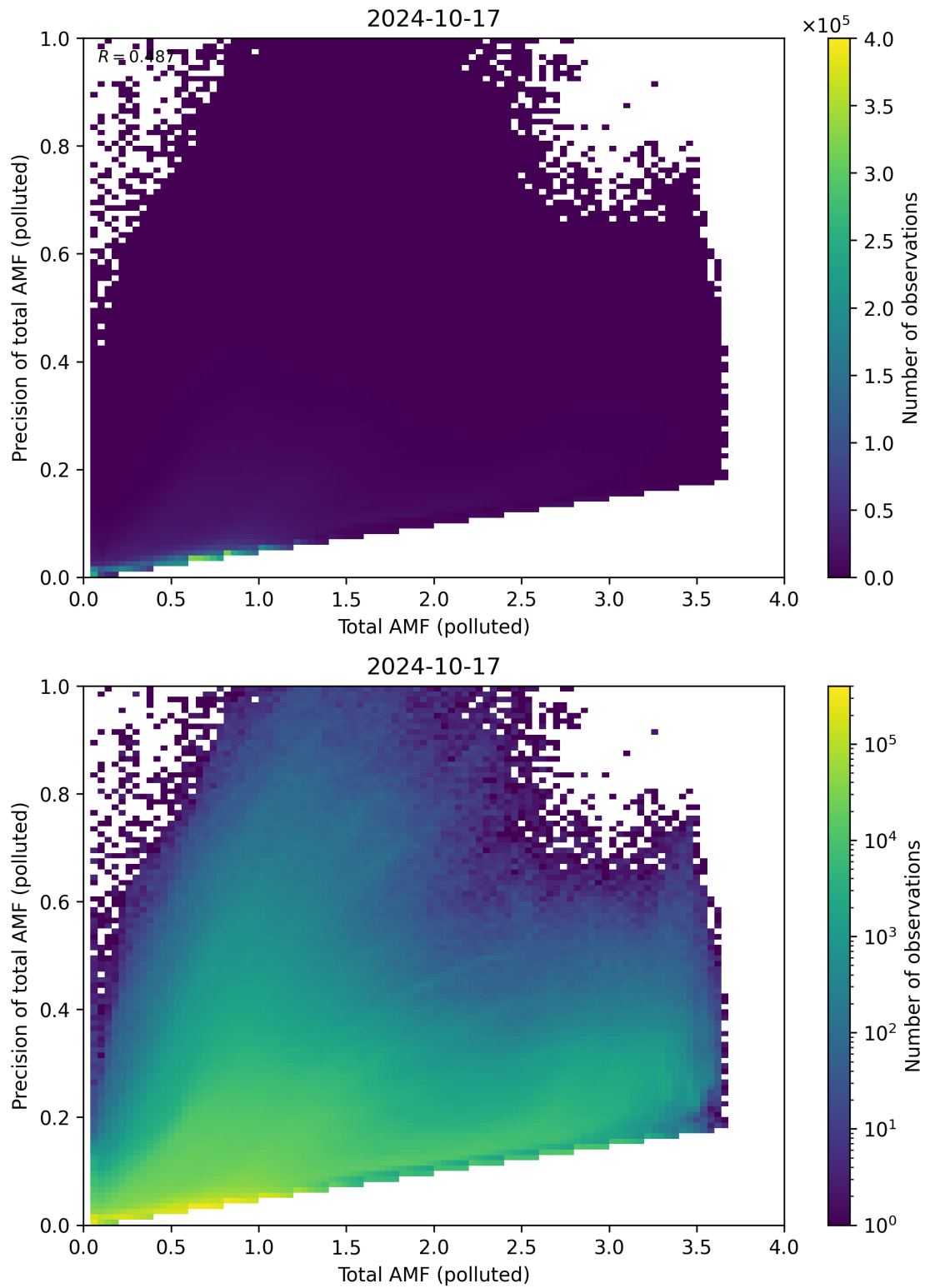
Figure 272: Scatter density plot of “Total AMF (polluted)” against “Precision of total AMF (polluted)” for 2024-10-16 to 2024-10-18.
