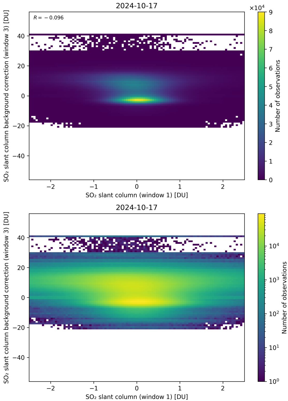
Figure 214: Scatter density plot of “SO 2 slant column (window 1)” against “SO 2 slant column background correction (window 3)” for 2024-10-16 to 2024-10-18.
