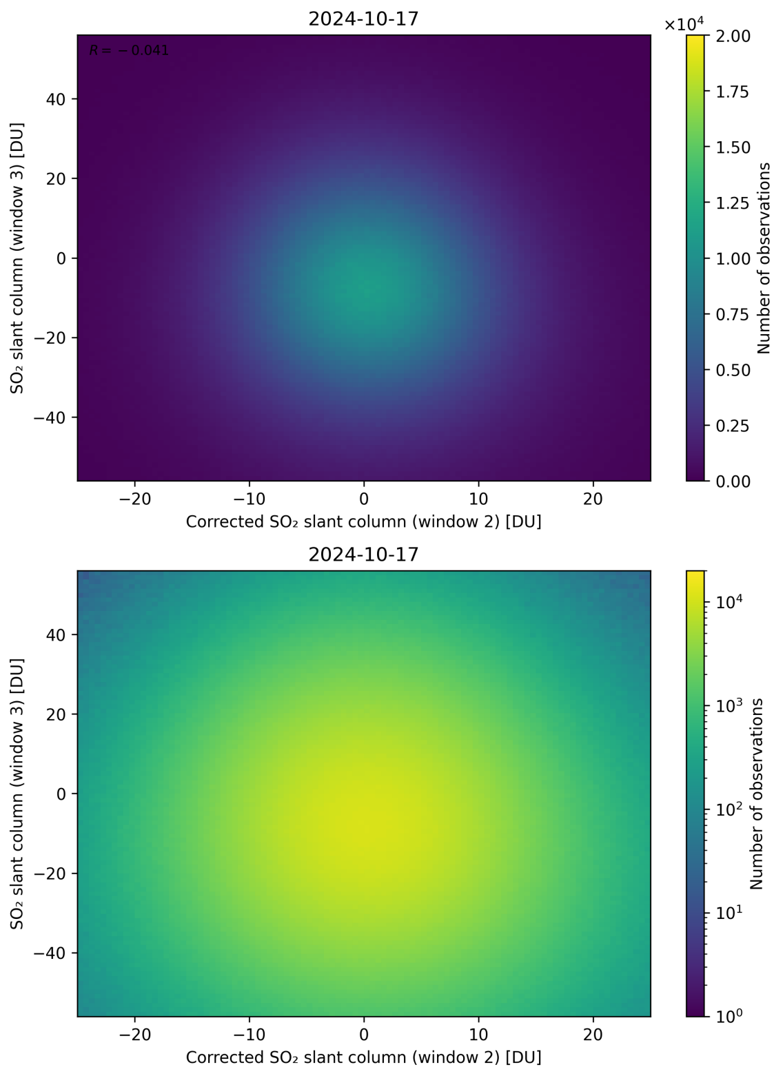
Figure 201: Scatter density plot of “Corrected SO 2 slant column (window 2)” against “SO 2 slant column (window 3)” for 2024-10-16 to 2024-10-18.
