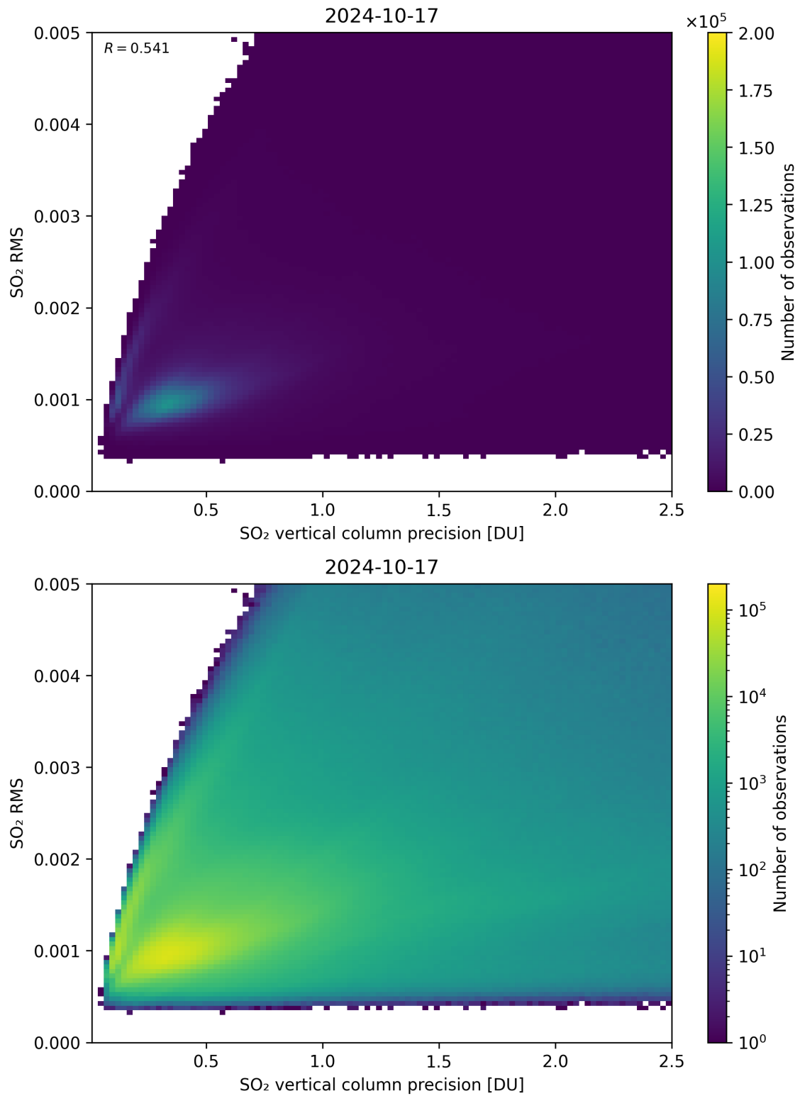
Figure 284: Scatter density plot of “SO 2 vertical column precision” against “SO 2 RMS” for 2024-10-16 to 2024-10-18.
