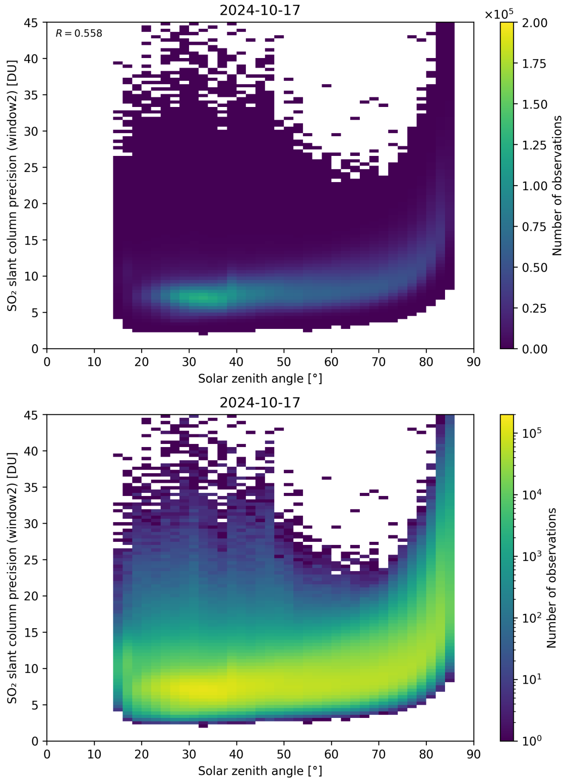
Figure 171: Scatter density plot of “Solar zenith angle” against “SO 2 slant column precision (window2)” for 2024-10-16 to 2024-10-18.
