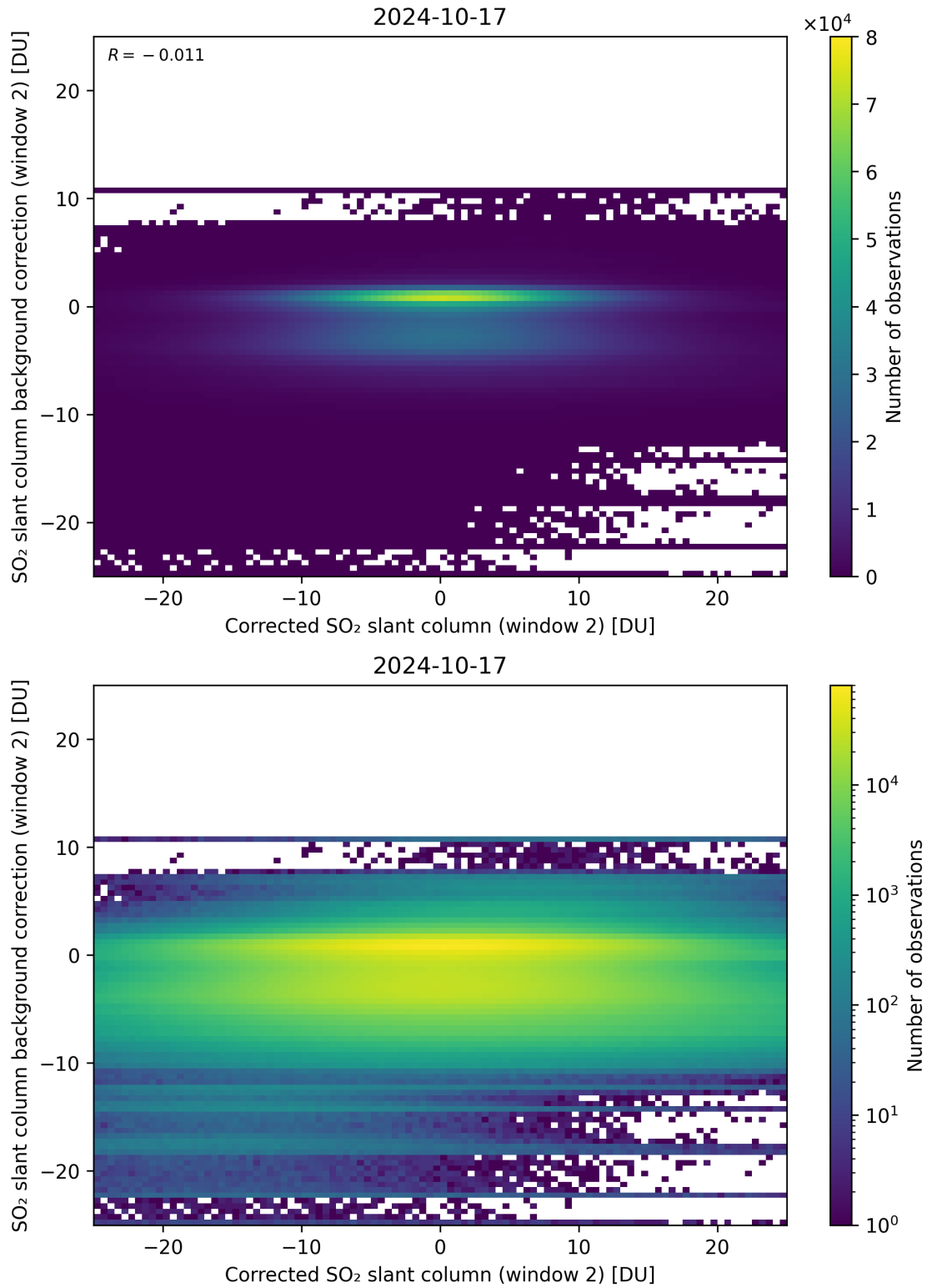
Figure 194: Scatter density plot of “Corrected SO 2 slant column (window 2)” against “SO 2 slant column background correction (window 2)” for 2024-10-16 to 2024-10-18.
