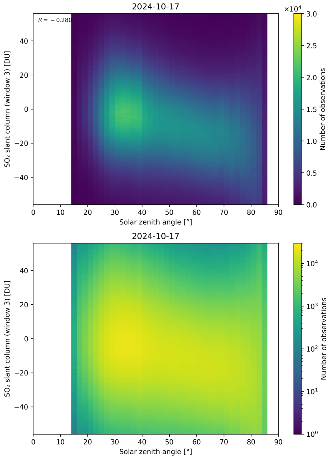
Figure 172: Scatter density plot of “Solar zenith angle” against “SO 2 slant column (window 3)” for 2024-10-16 to 2024-10-18.
