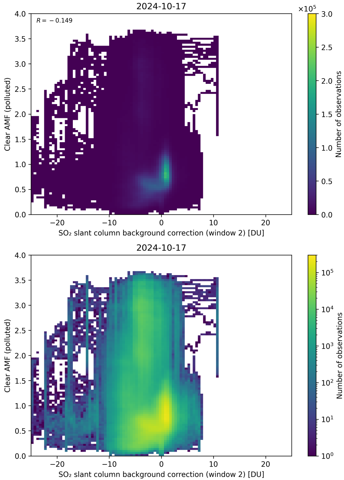
Figure 115: Scatter density plot of “SO 2 slant column background correction (window 2)” against “Clear AMF (polluted)” for 2024-10-16 to 2024-10-18.
