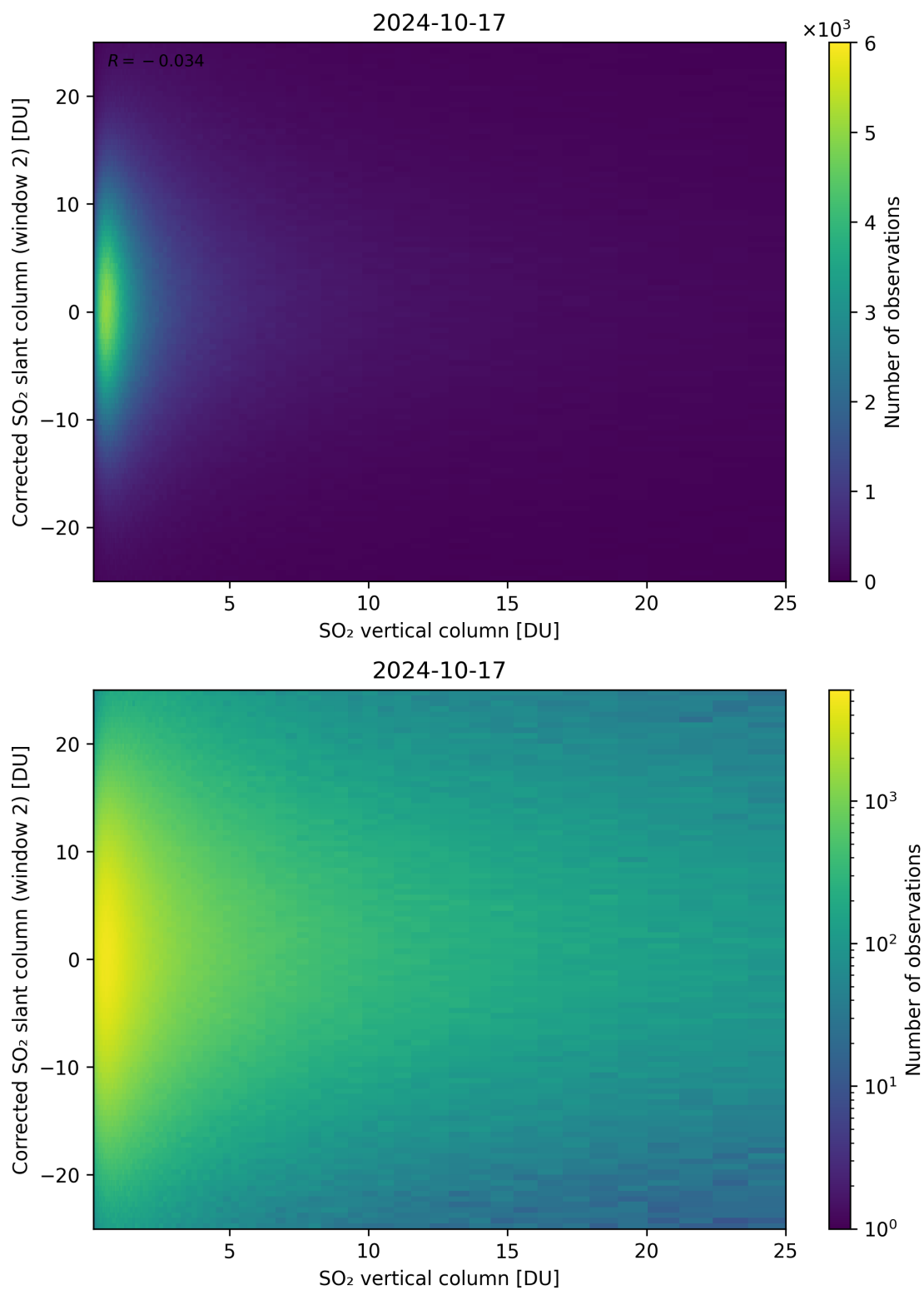
Figure 298: Scatter density plot of “SO 2 vertical column” against “Corrected SO 2 slant column (window 2)” for 2024-10-16 to 2024-10-18.
