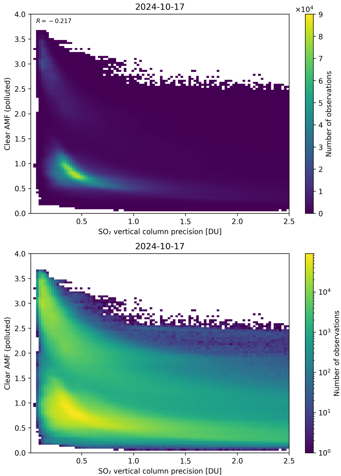
Figure 285: Scatter density plot of “SO 2 vertical column precision” against “Clear AMF (polluted)” for 2024-10-16 to 2024-10-18.
