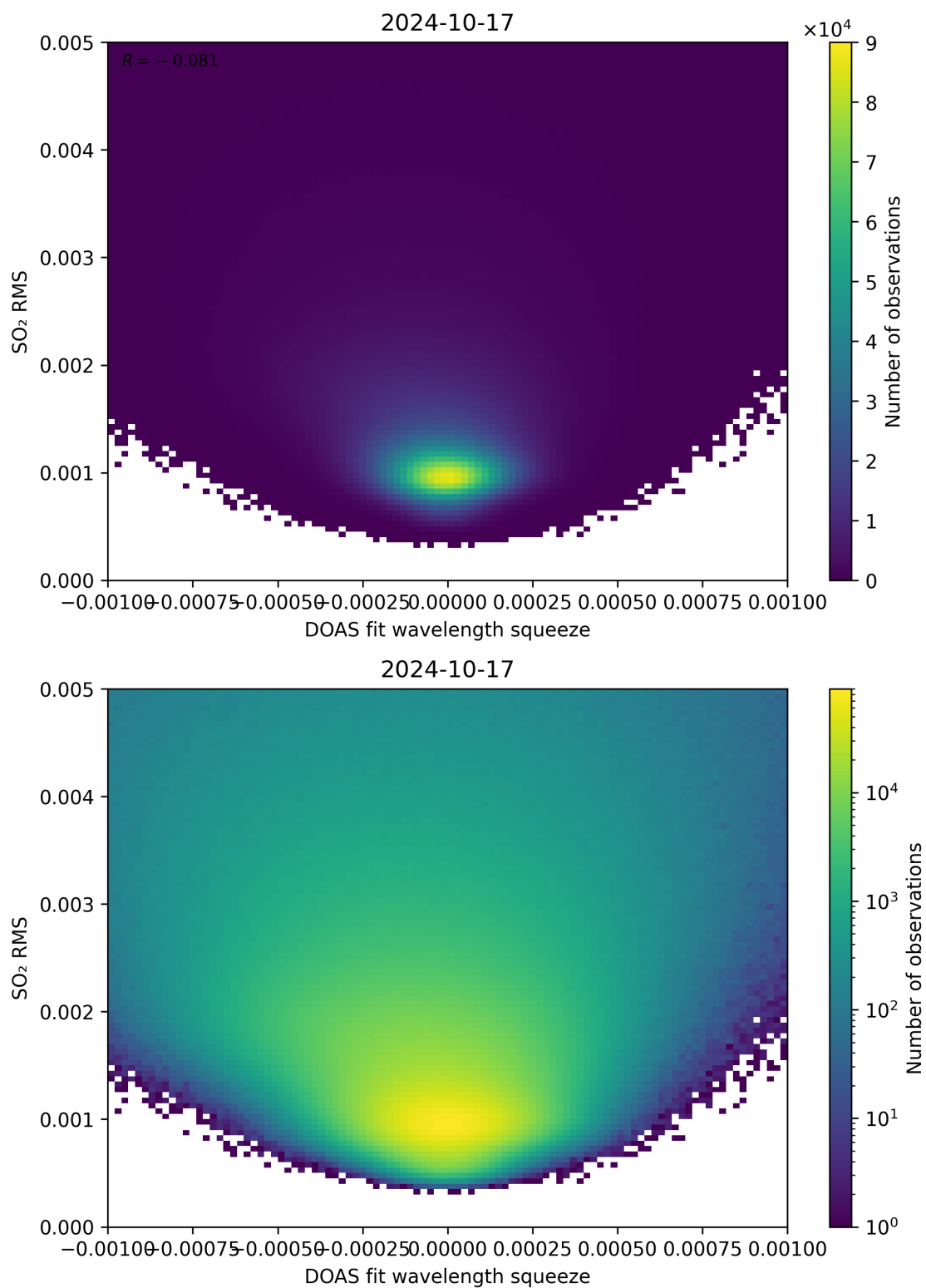
Figure 132: Scatter density plot of “DOAS fit wavelength squeeze” against “SO 2 RMS” for 2024-10-16 to 2024-10-18.
