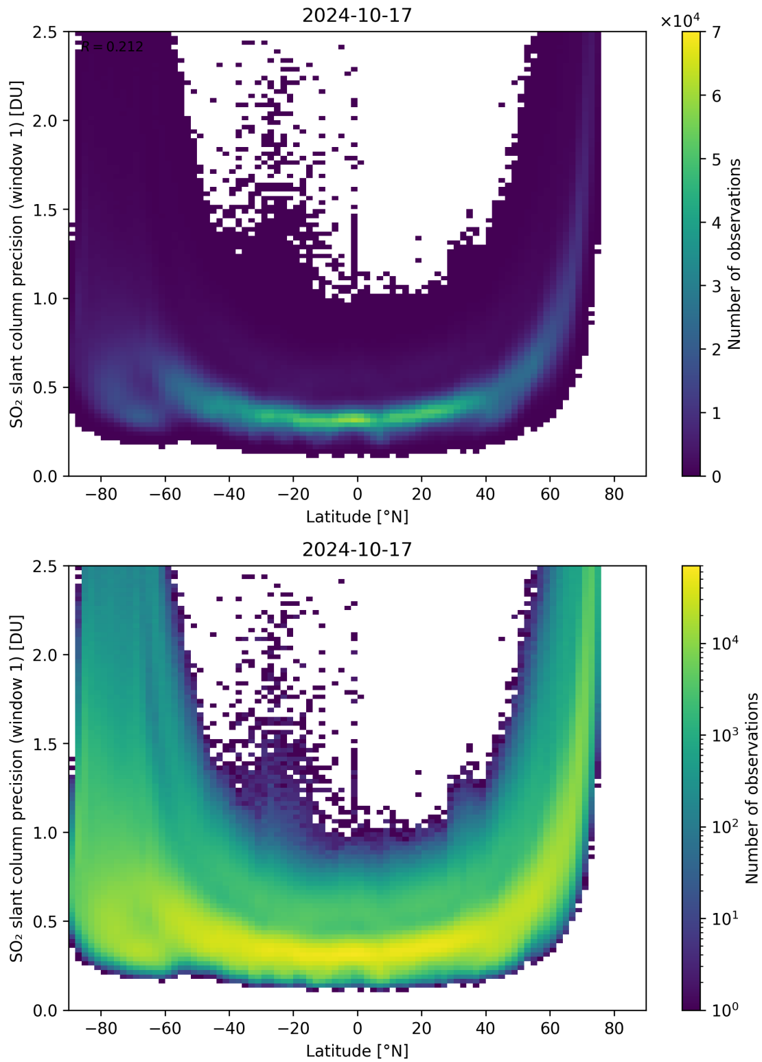
Figure 150: Scatter density plot of “Latitude” against “SO 2 slant column precision (window 1)” for 2024-10-16 to 2024-10-18.
