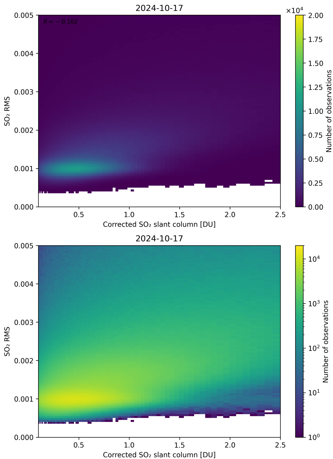
Figure 183: Scatter density plot of “Corrected SO 2 slant column” against “SO 2 RMS” for 2024-10-16 to 2024-10-18.
