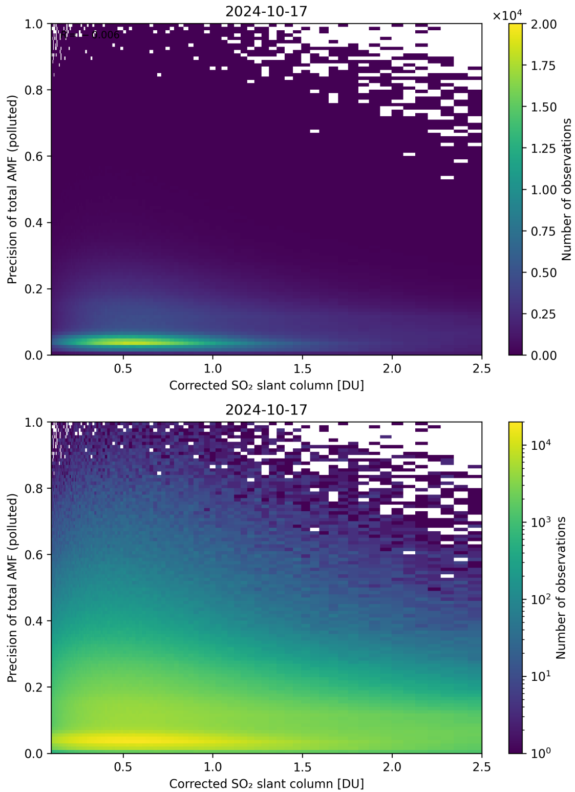
Figure 193: Scatter density plot of “Corrected SO 2 slant column” against “Precision of total AMF (polluted)” for 2024-10-16 to 2024-10-18.
