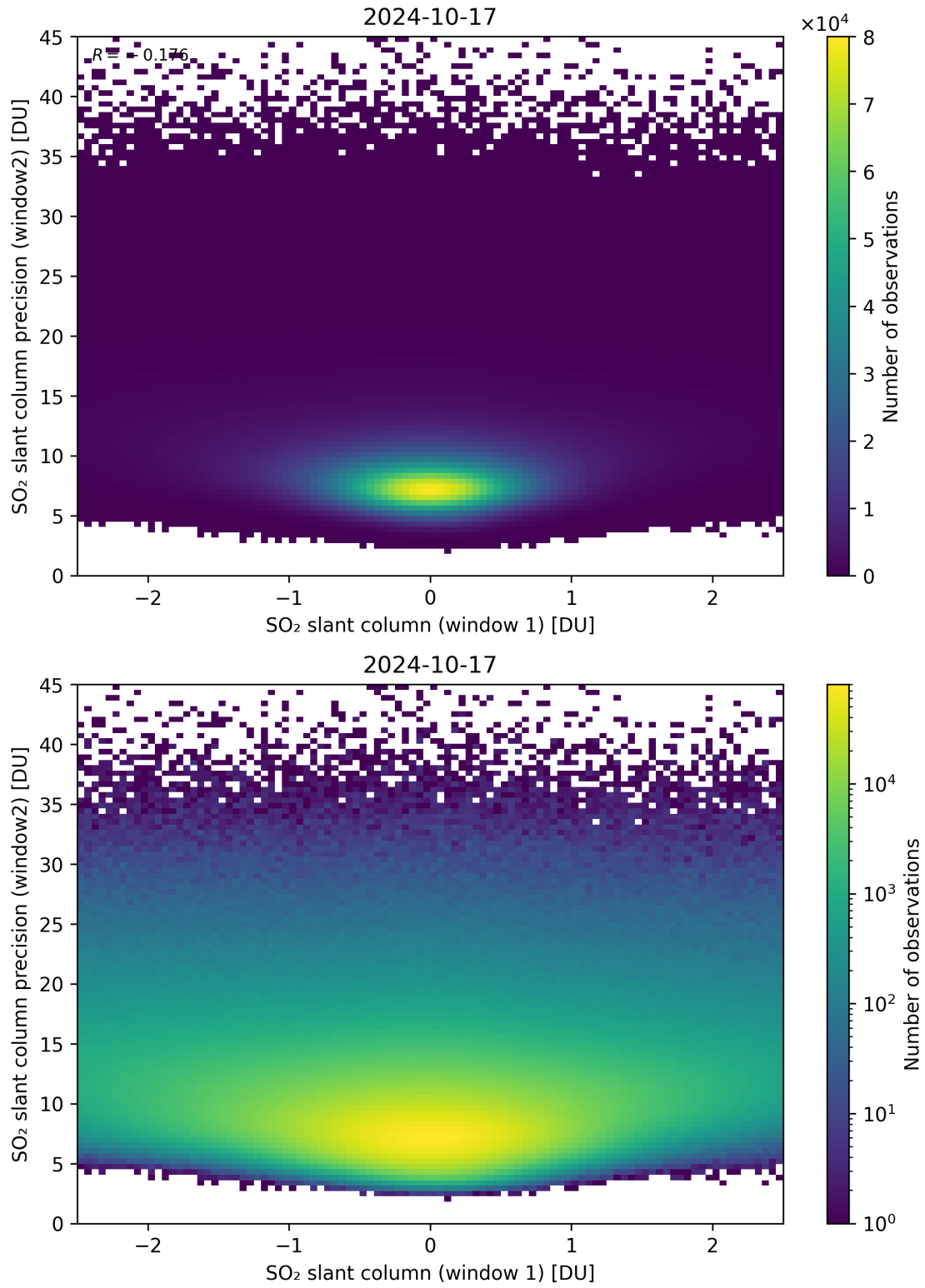
Figure 236: Scatter density plot of “SO 2 slant column (window 1)” against “SO 2 slant column precision (window2)” for 2024-10-16 to 2024-10-18.
