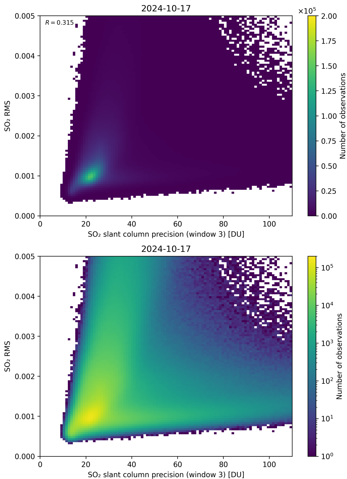
Figure 260: Scatter density plot of “SO 2 slant column precision (window 3)” against “SO 2 RMS” for 2024-10-16 to 2024-10-18.
