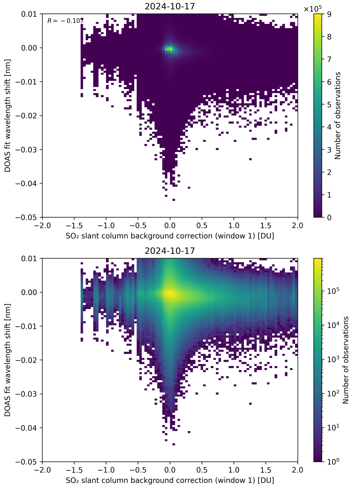
Figure 100: Scatter density plot of “SO 2 slant column background correction (window 1)” against “DOAS fit wavelength shift” for 2024-10-16 to 2024-10-18.
