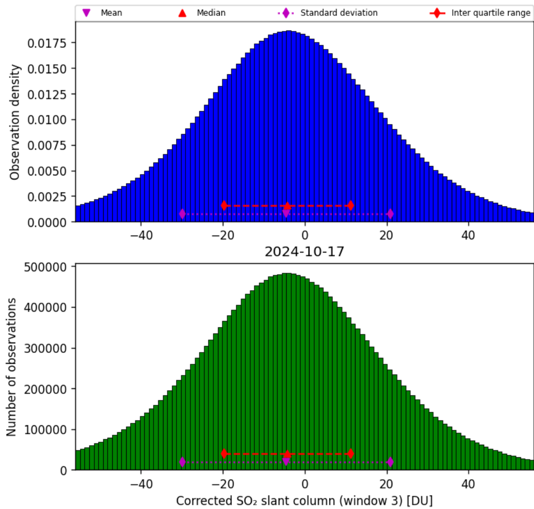
Figure 66: Histogram of “Corrected SO 2 slant column (window 3)” for 2024-10-16 to 2024-10-18
