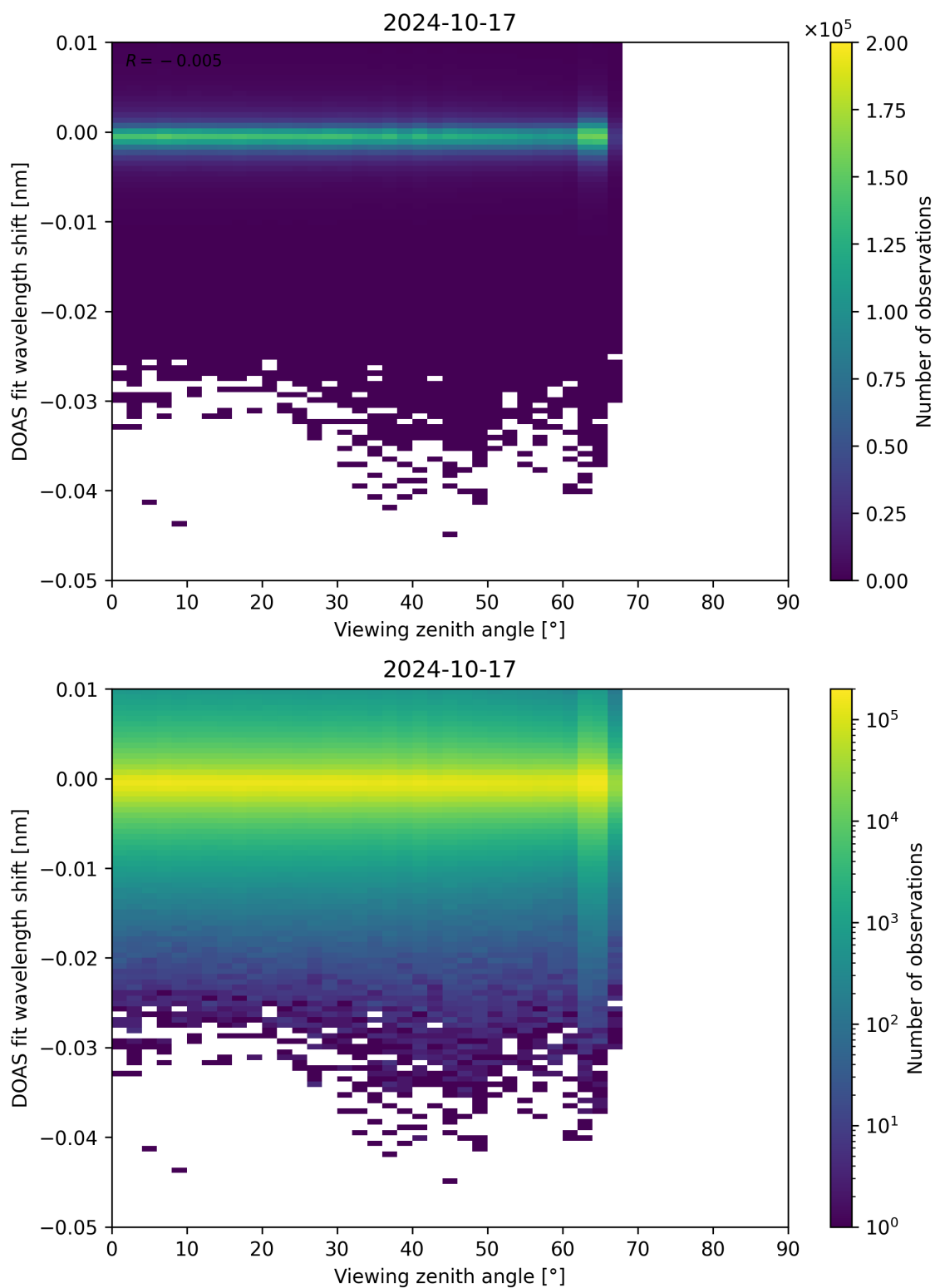
Figure 311: Scatter density plot of “Viewing zenith angle” against “DOAS fit wavelength shift” for 2024-10-16 to 2024-10-18.
