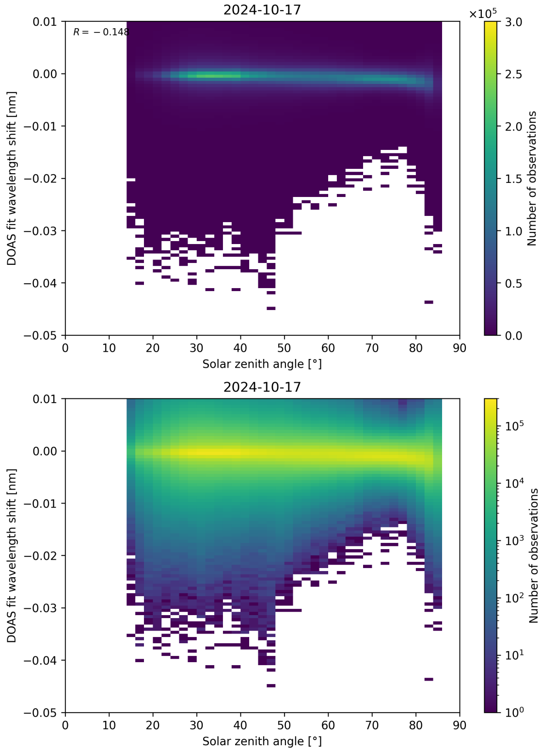
Figure 161: Scatter density plot of “Solar zenith angle” against “DOAS fit wavelength shift” for 2024-10-16 to 2024-10-18.
