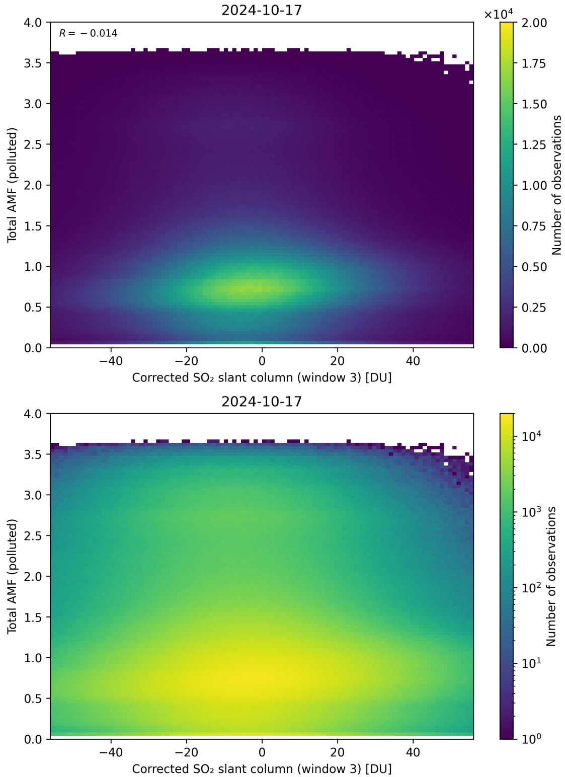
Figure 210: Scatter density plot of “Corrected SO 2 slant column (window 3)” against “Total AMF (polluted)” for 2024-10-16 to 2024-10-18.
