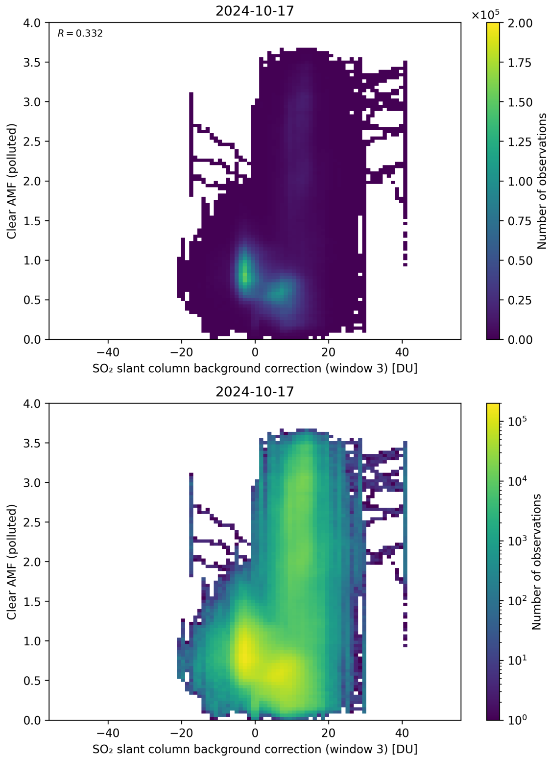
Figure 124: Scatter density plot of “SO 2 slant column background correction (window 3)” against “Clear AMF (polluted)” for 2024-10-16 to 2024-10-18.
