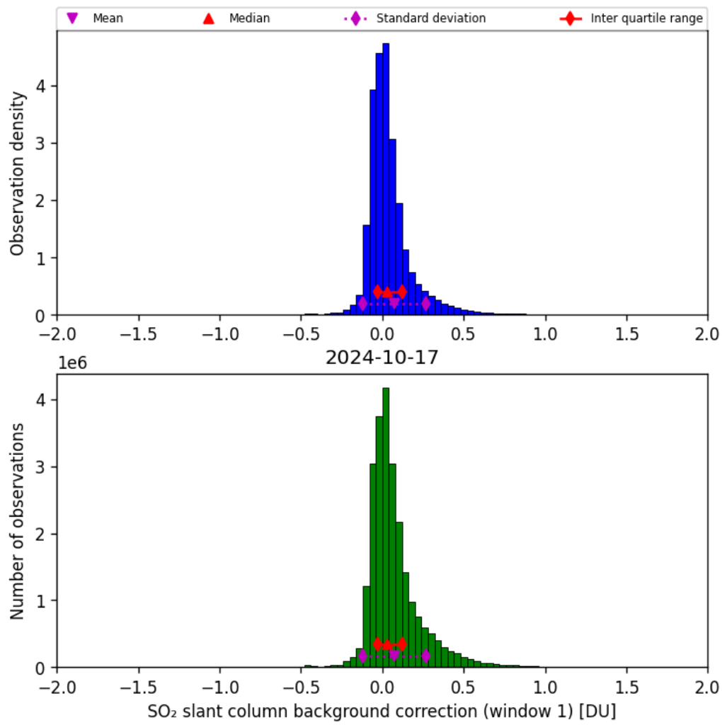
Figure 59: Histogram of “SO 2 slant column background correction (window 1)” for 2024-10-16 to 2024-10-18
