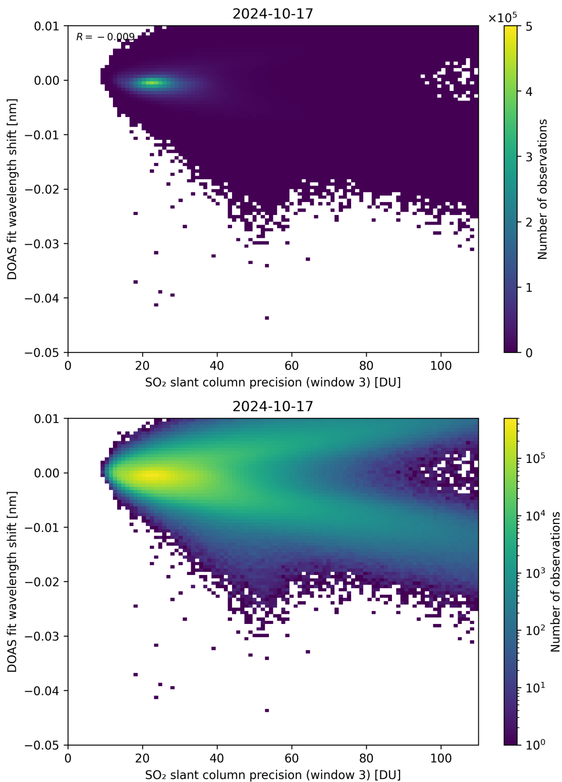
Figure 258: Scatter density plot of “SO 2 slant column precision (window 3)” against “DOAS fit wavelength shift” for 2024-10-16 to 2024-10-18.
