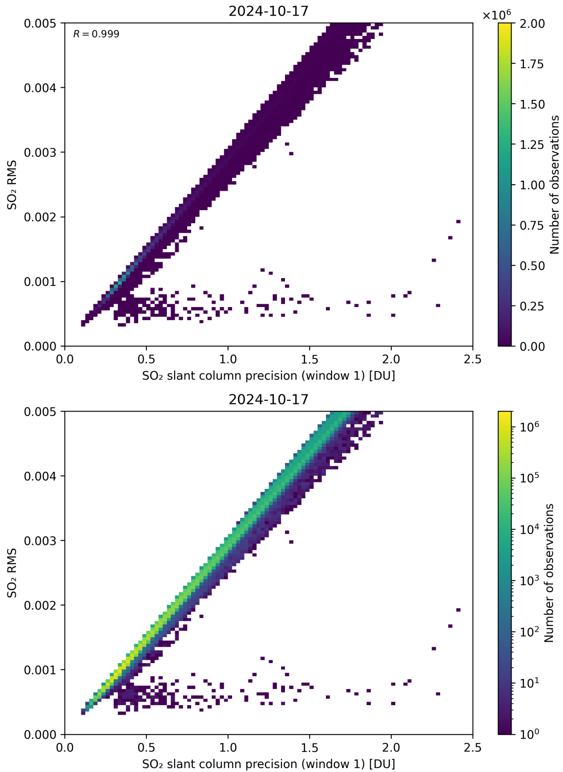
Figure 223: Scatter density plot of “SO 2 slant column precision (window 1)” against “SO 2 RMS” for 2024-10-16 to 2024-10-18.
