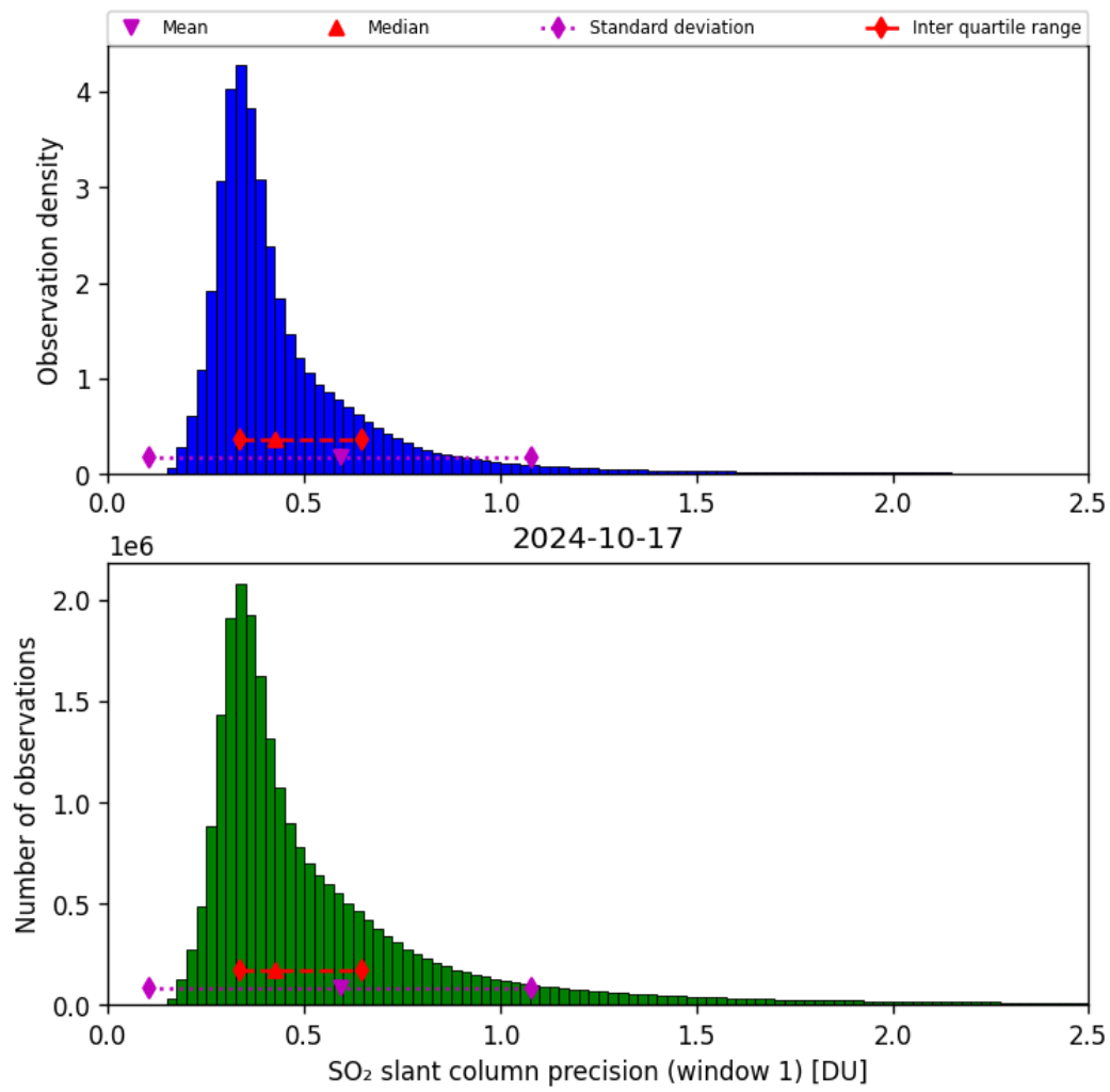
Figure 57: Histogram of “SO 2 slant column precision (window 1)” for 2024-10-16 to 2024-10-18
