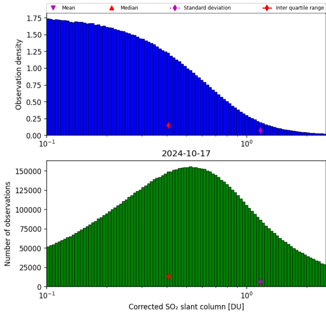
Figure 55: Histogram of “Corrected SO 2 slant column” for 2024-10-16 to 2024-10-18
