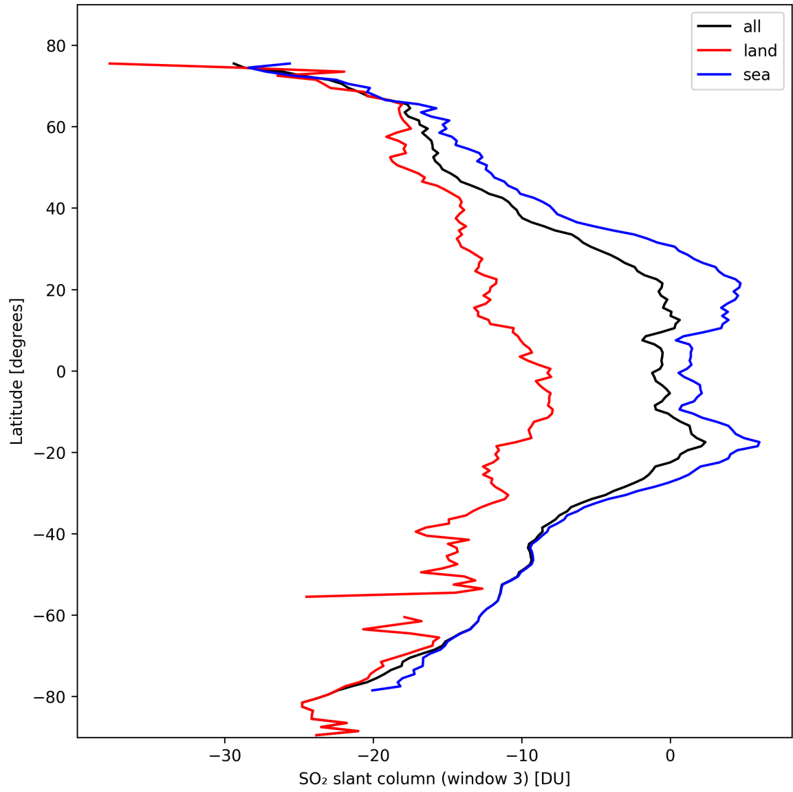
Figure 41: Zonal average of “SO 2 slant column (window 3)” for 2024-10-16 to 2024-10-18.
