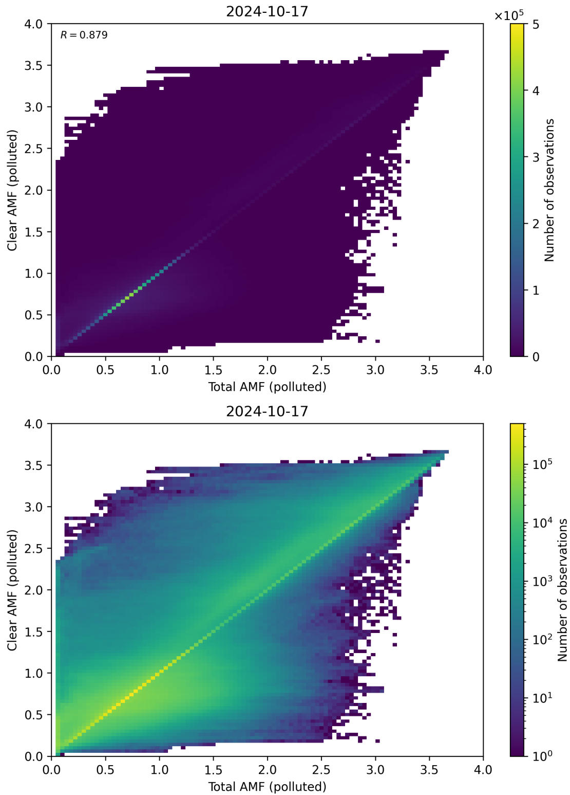
Figure 271: Scatter density plot of “Total AMF (polluted)” against “Clear AMF (polluted)” for 2024-10-16 to 2024-10-18.
