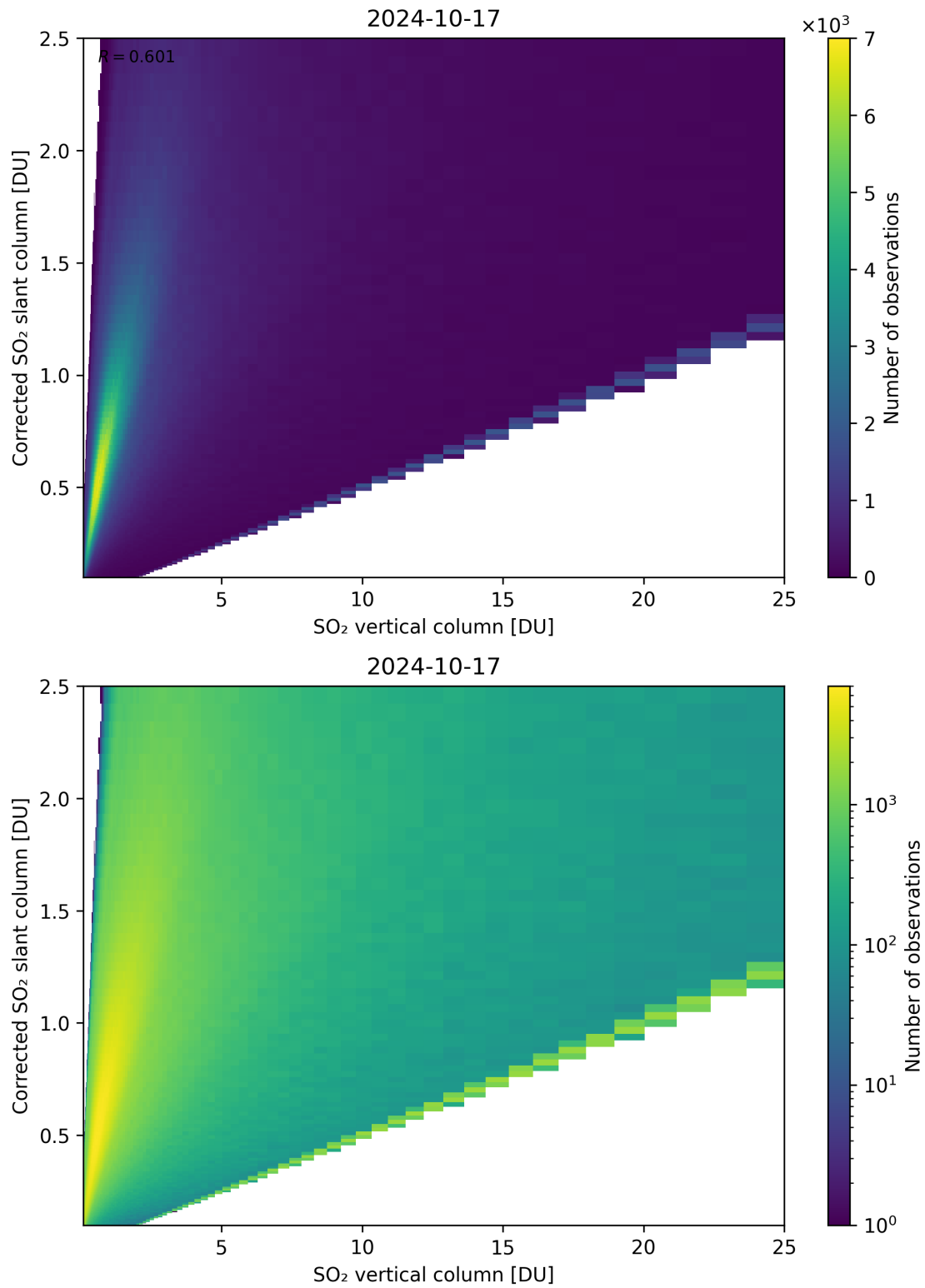
Figure 297: Scatter density plot of “SO 2 vertical column” against “Corrected SO 2 slant column” for 2024-10-16 to 2024-10-18.
