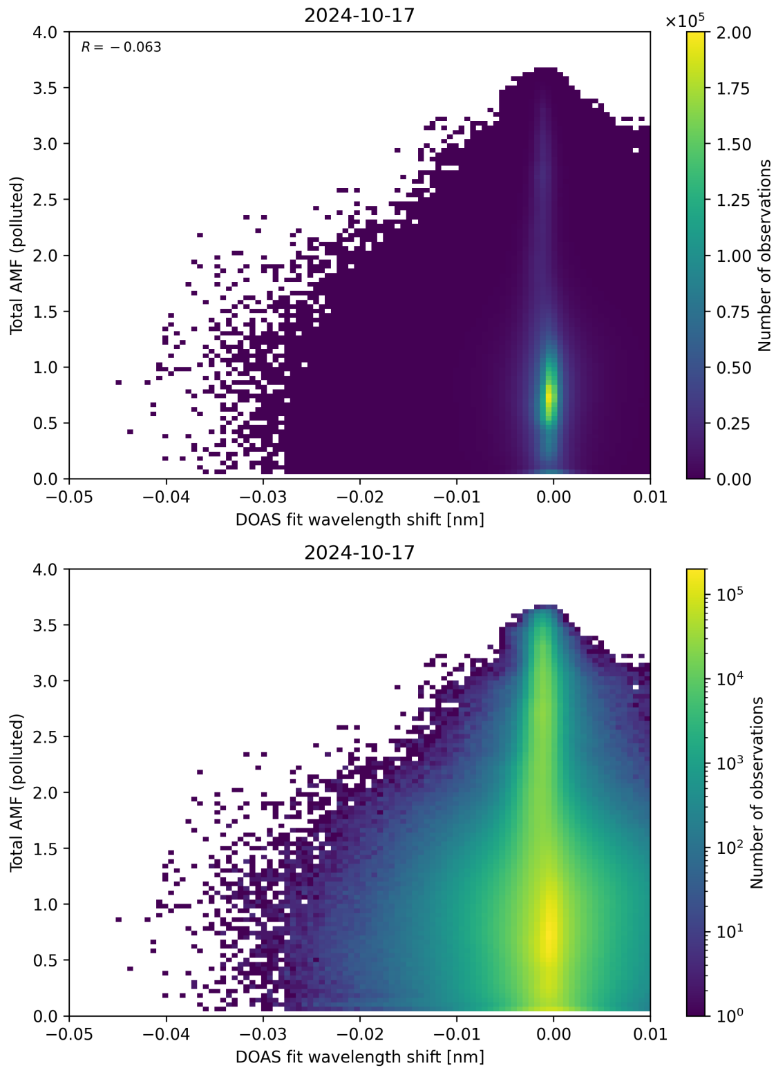
Figure 130: Scatter density plot of “DOAS fit wavelength shift” against “Total AMF (polluted)” for 2024-10-16 to 2024-10-18.
