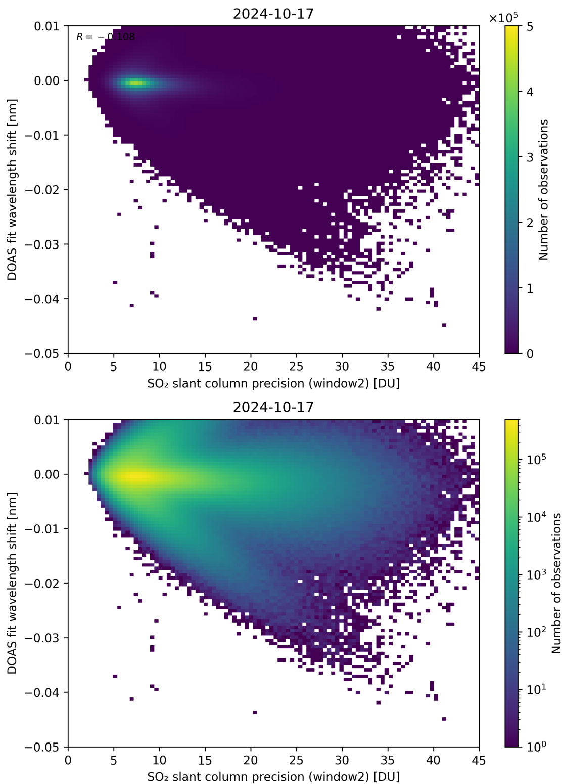
Figure 243: Scatter density plot of “SO 2 slant column precision (window2)” against “DOAS fit wavelength shift” for 2024-10-16 to 2024-10-18.
