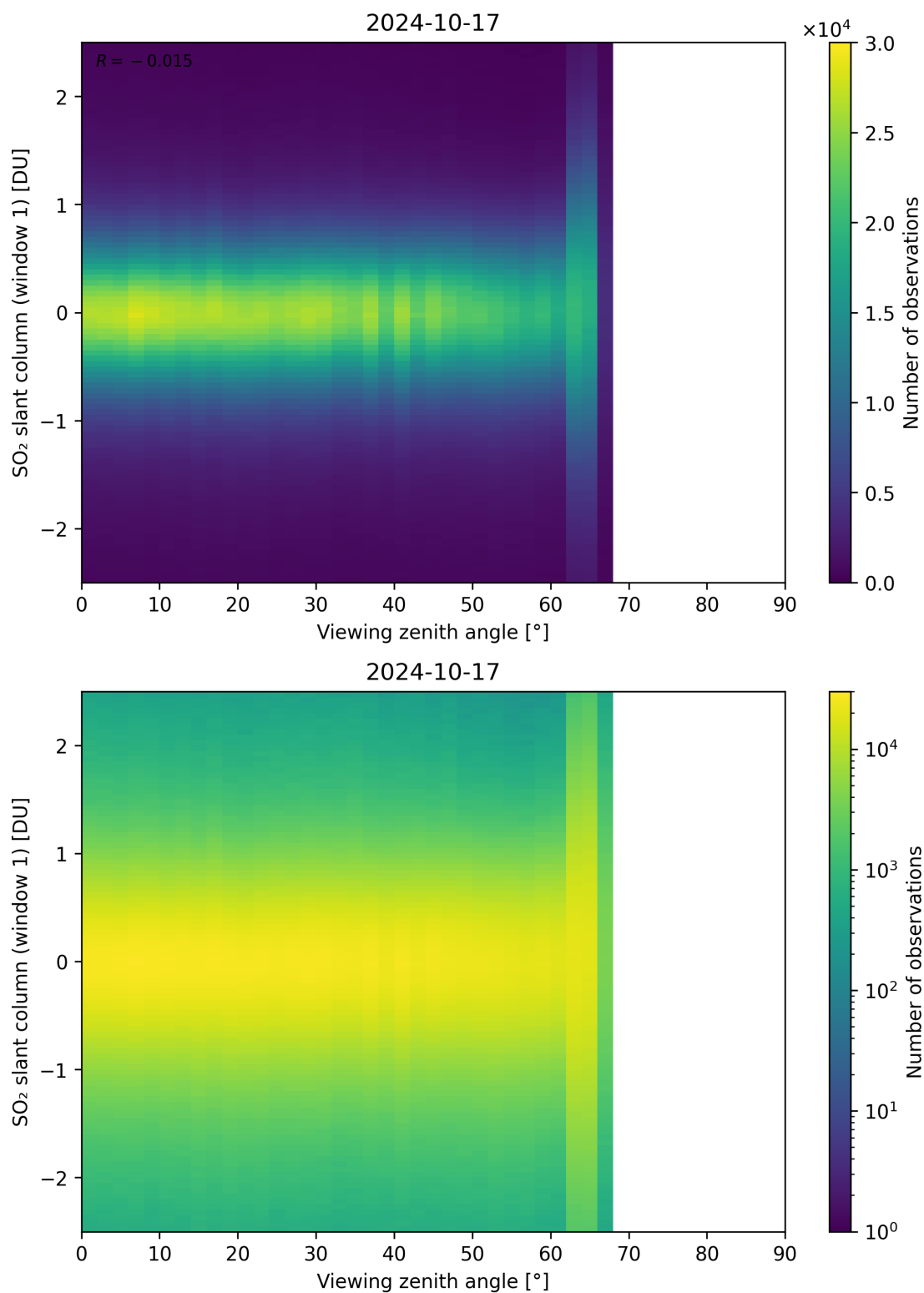
Figure 320: Scatter density plot of “Viewing zenith angle” against “SO 2 slant column (window 1)” for 2024-10-16 to 2024-10-18.
