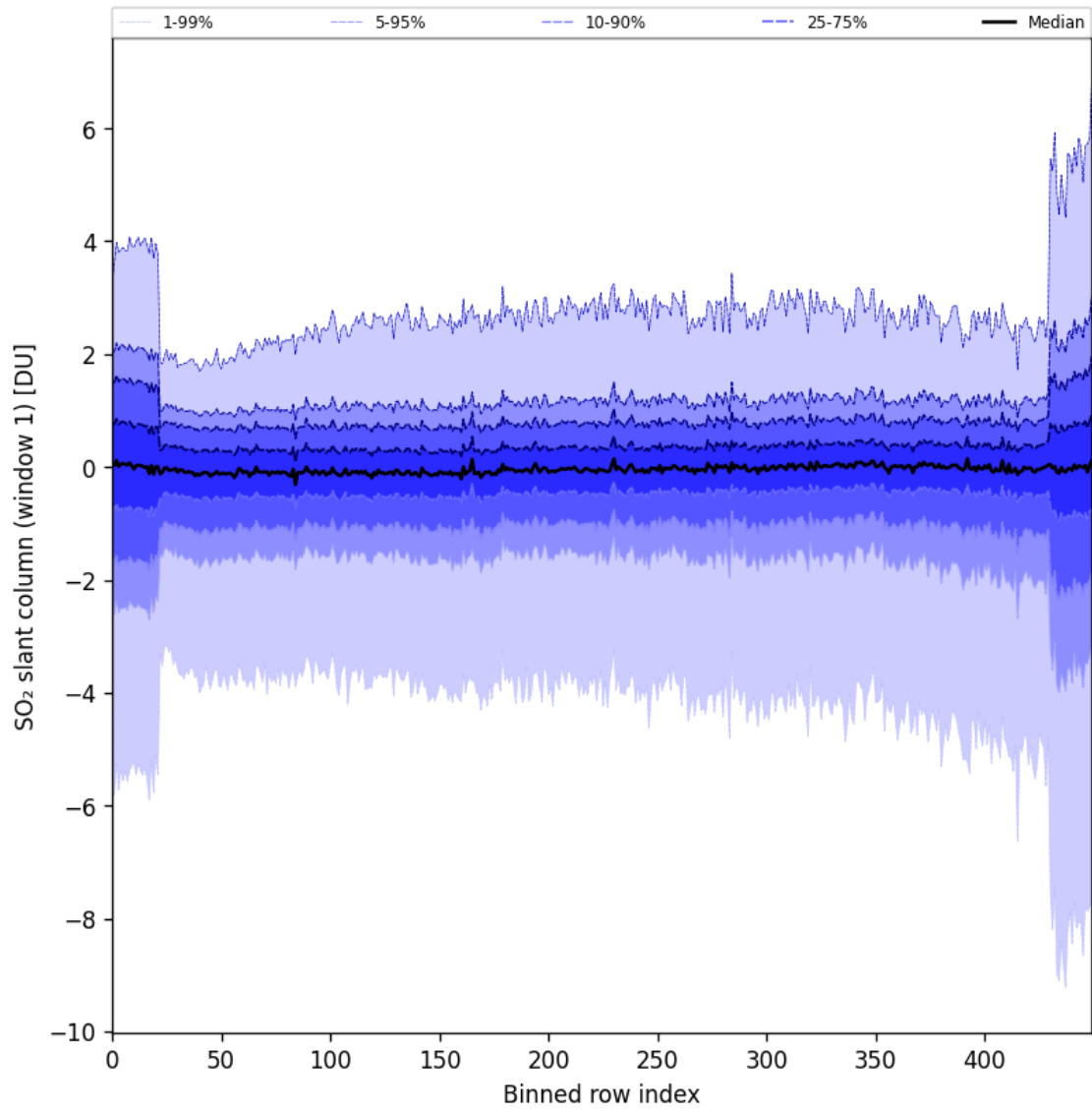
Figure 79: Along track statistics of “SO 2 slant column (window 1)” for 2024-10-16 to 2024-10-18
