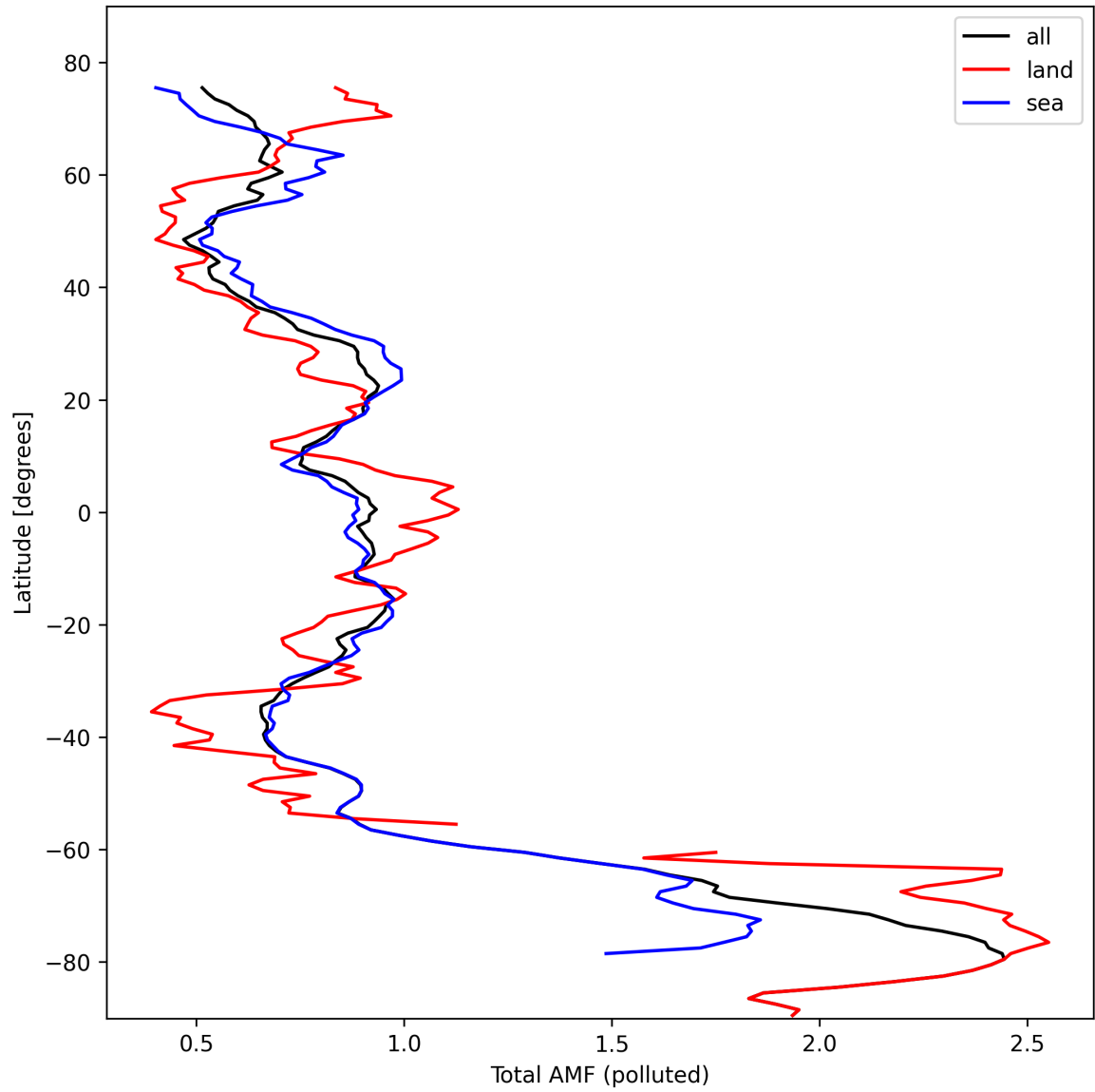
Figure 48: Zonal average of “Total AMF (polluted)” for 2024-10-16 to 2024-10-18.
