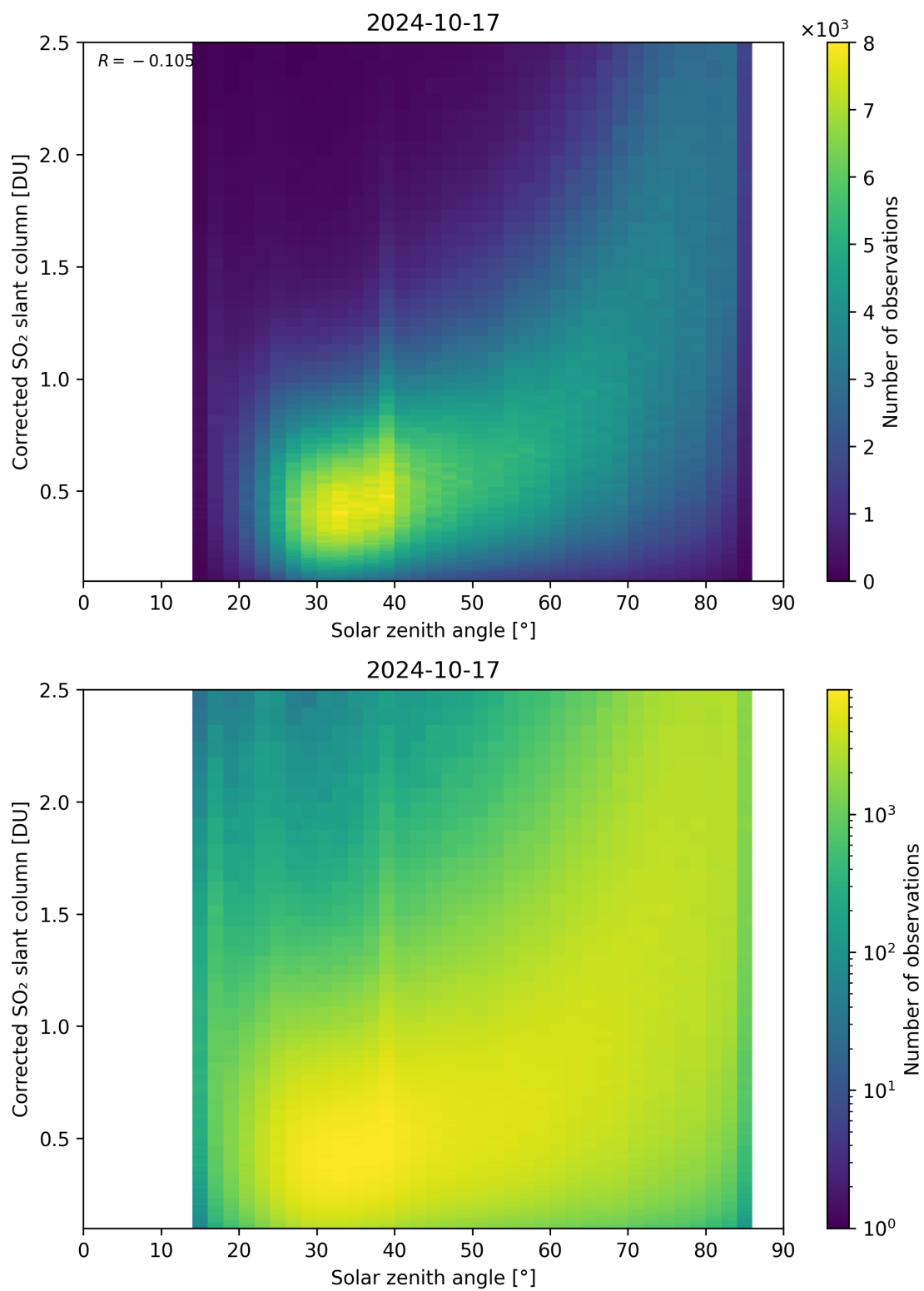
Figure 166: Scatter density plot of “Solar zenith angle” against “Corrected SO 2 slant column” for 2024-10-16 to 2024-10-18.
