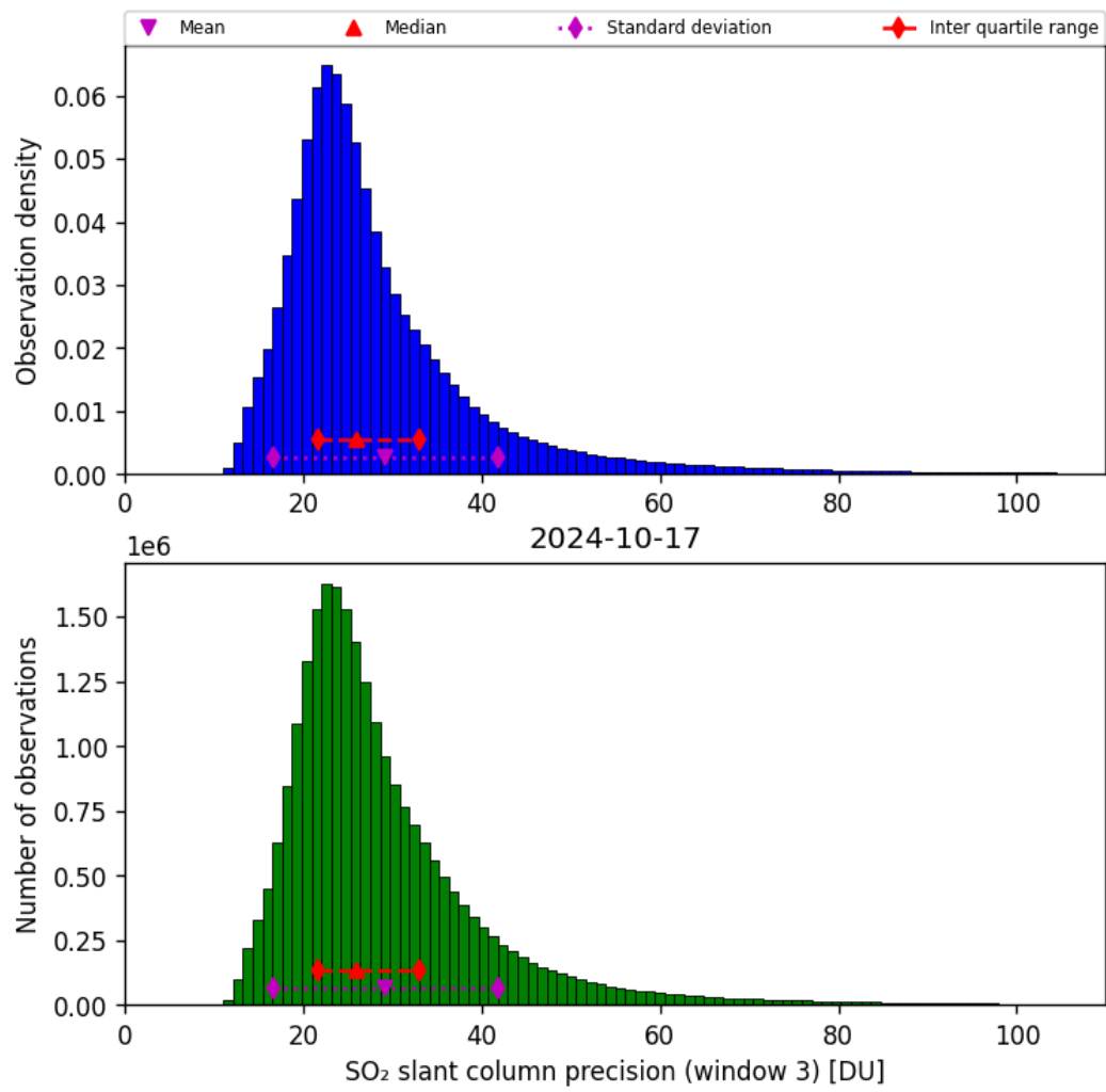
Figure 65: Histogram of “SO 2 slant column precision (window 3)” for 2024-10-16 to 2024-10-18
