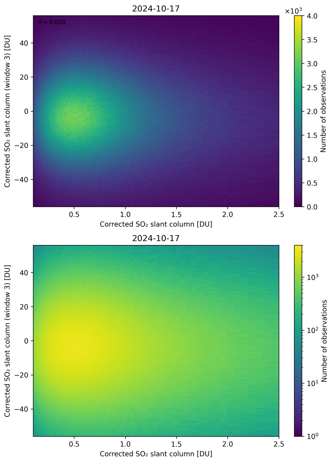
Figure 186: Scatter density plot of “Corrected SO 2 slant column” against “Corrected SO 2 slant column (window 3)” for 2024-10-16 to 2024-10-18.
