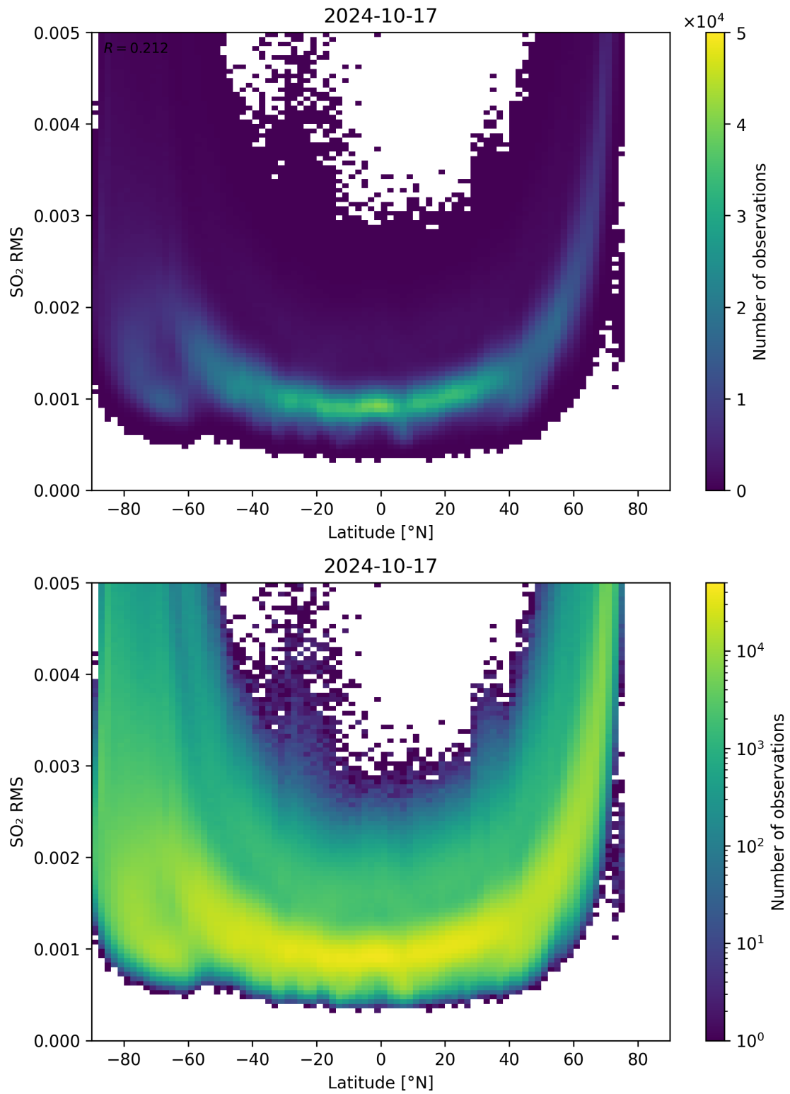
Figure 144: Scatter density plot of “Latitude” against “SO 2 RMS” for 2024-10-16 to 2024-10-18.
