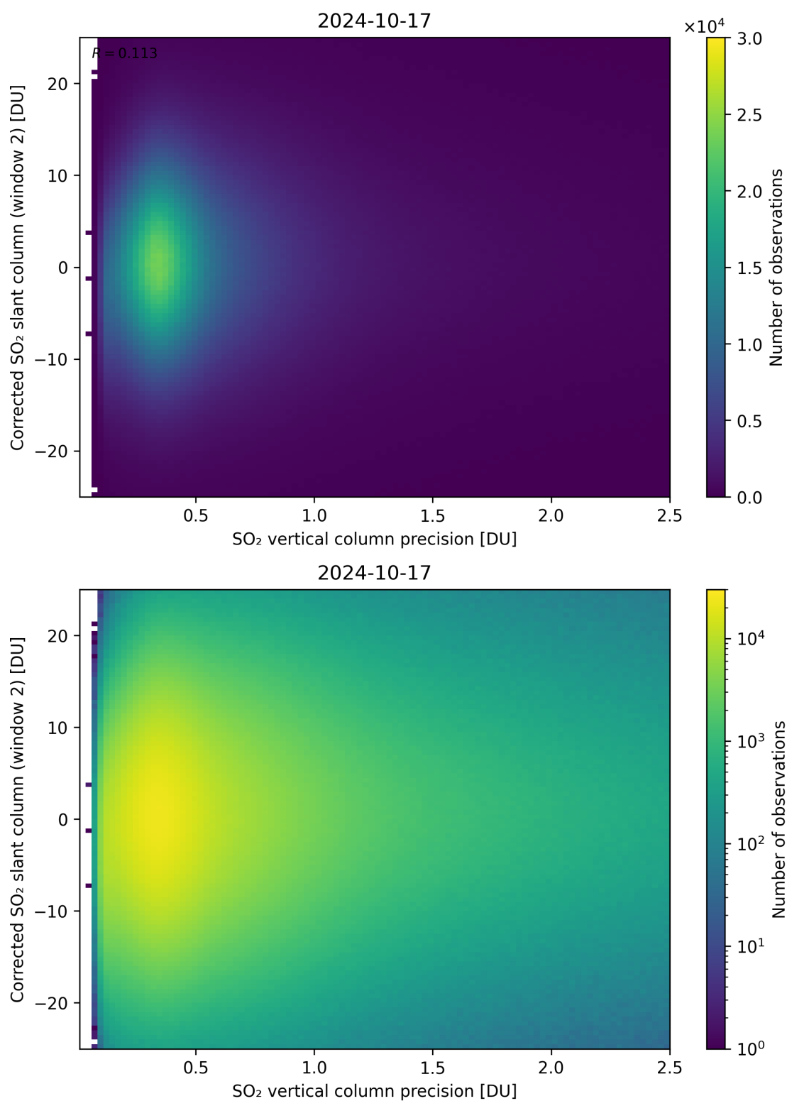
Figure 287: Scatter density plot of “SO 2 vertical column precision” against “Corrected SO 2 slant column (window 2)” for 2024-10-16 to 2024-10-18.
