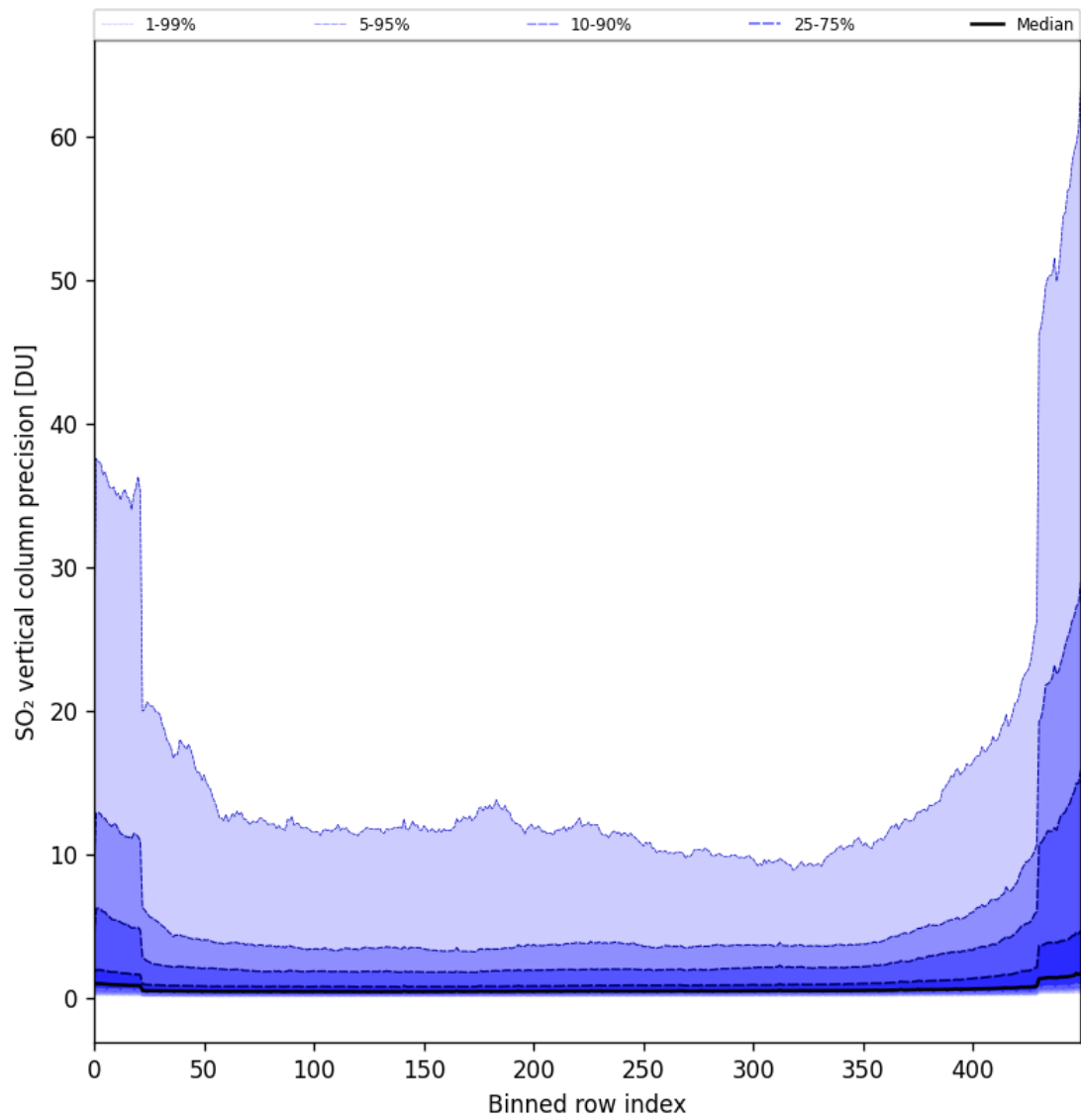
Figure 77: Along track statistics of “SO 2 vertical column precision” for 2024-10-16 to 2024-10-18
