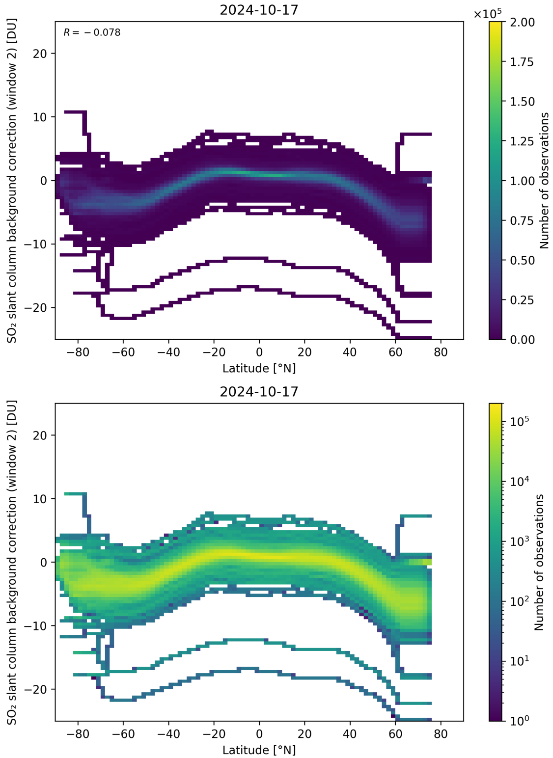
Figure 140: Scatter density plot of “Latitude” against “SO 2 slant column background correction (window 2)” for 2024-10-16 to 2024-10-18.
