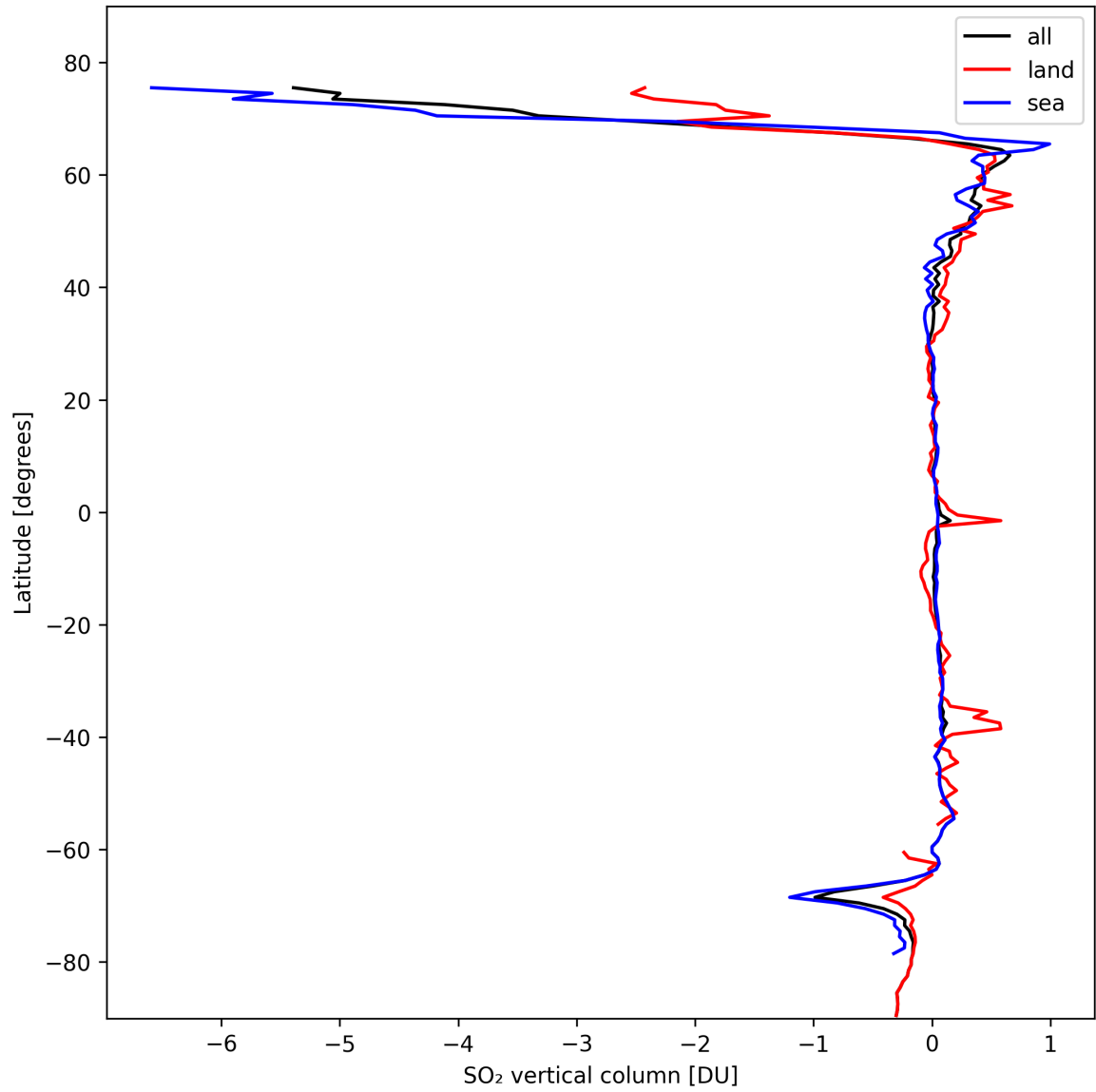
Figure 30: Zonal average of “SO 2 vertical column” for 2024-10-16 to 2024-10-18.
