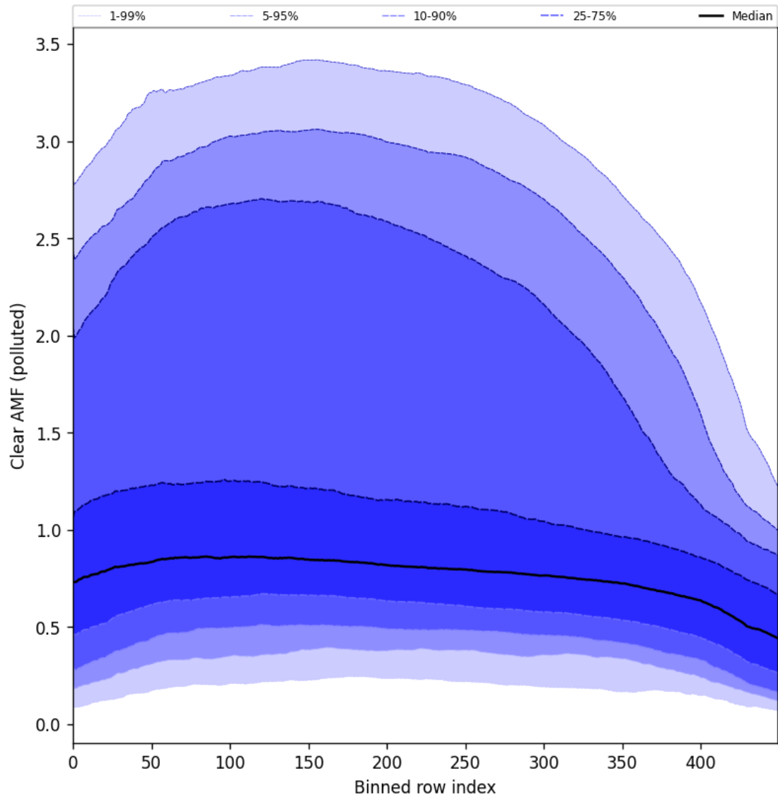
Figure 96: Along track statistics of “Clear AMF (polluted)” for 2024-10-16 to 2024-10-18
