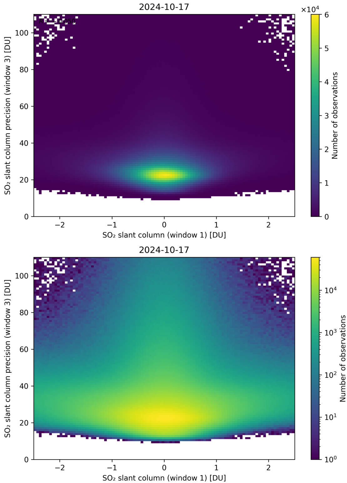
Figure 238: Scatter density plot of “SO 2 slant column (window 1)” against “SO 2 slant column precision (window 3)” for 2024-10-16 to 2024-10-18.
