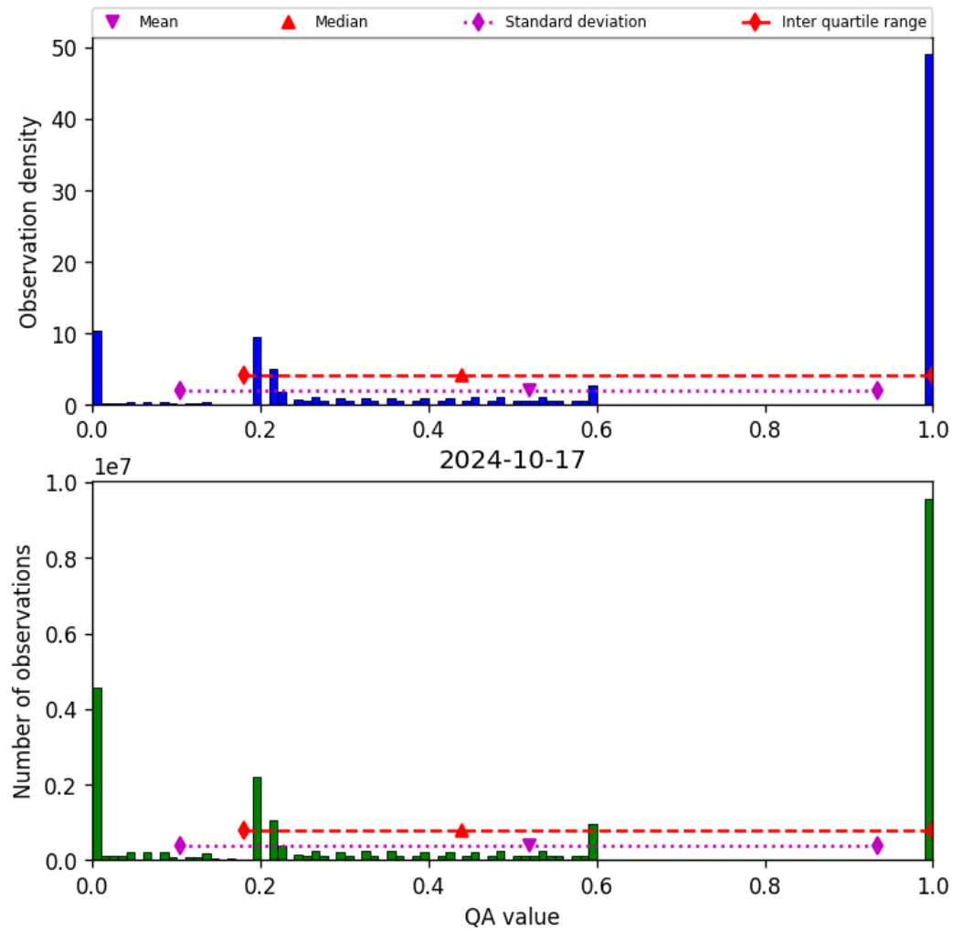
Figure 52: Histogram of “QA value” for 2024-10-16 to 2024-10-18
