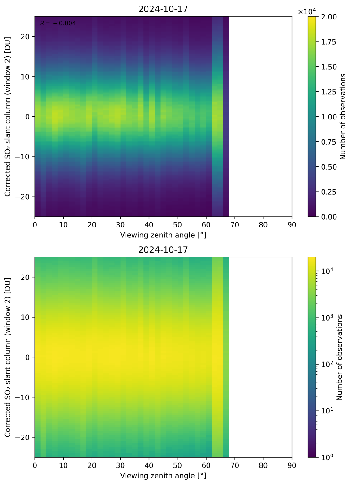
Figure 318: Scatter density plot of “Viewing zenith angle” against “Corrected SO 2 slant column (window 2)” for 2024-10-16 to 2024-10-18.
