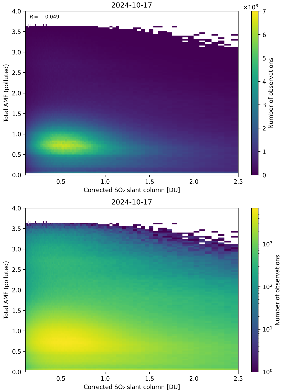
Figure 192: Scatter density plot of “Corrected SO 2 slant column” against “Total AMF (polluted)” for 2024-10-16 to 2024-10-18.
