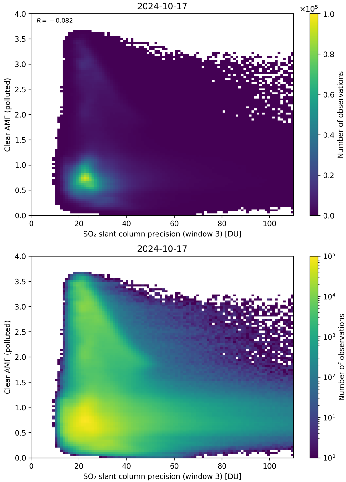
Figure 261: Scatter density plot of “SO 2 slant column precision (window 3)” against “Clear AMF (polluted)” for 2024-10-16 to 2024-10-18.
