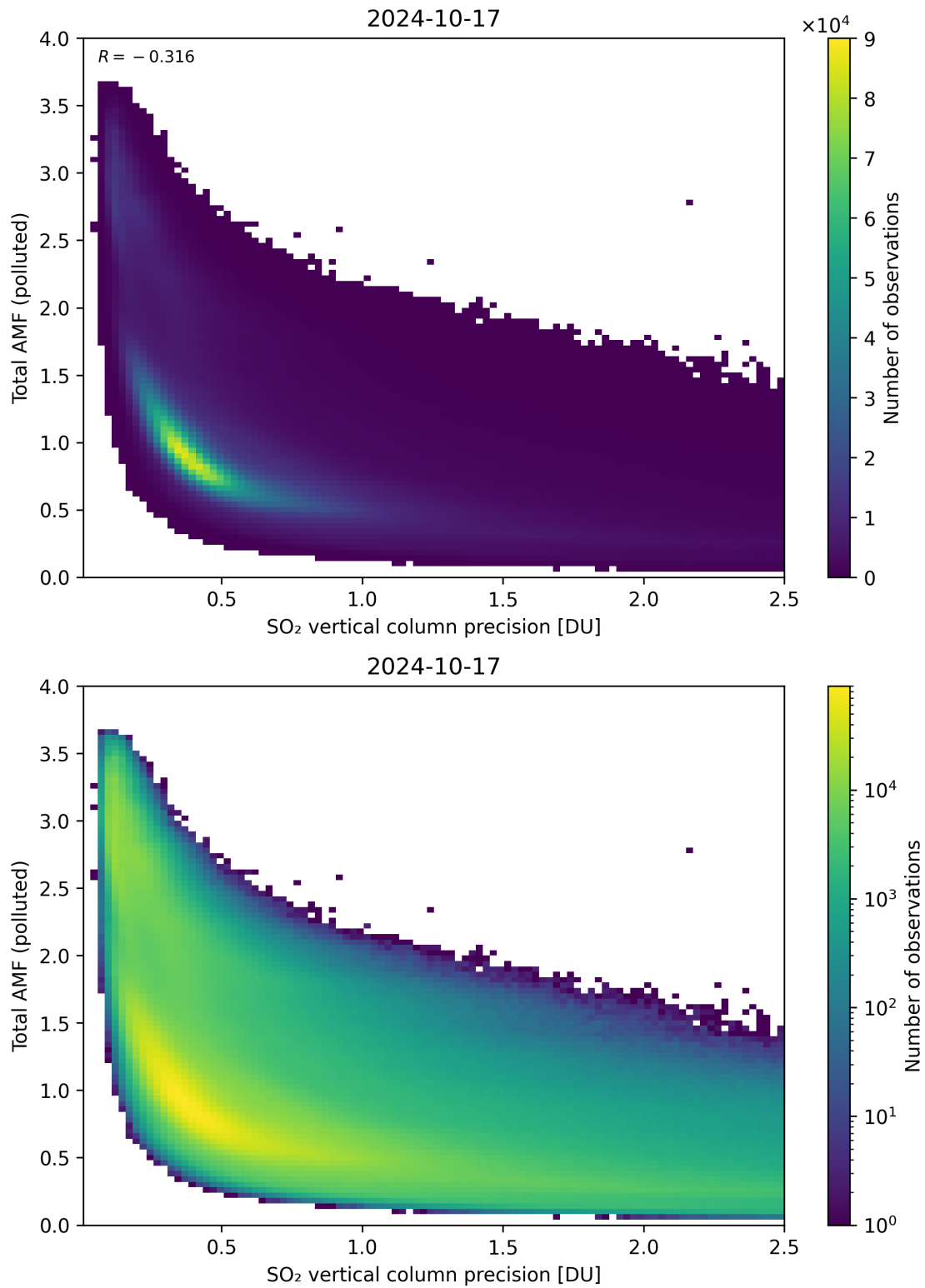
Figure 294: Scatter density plot of “SO 2 vertical column precision” against “Total AMF (polluted)” for 2024-10-16 to 2024-10-18.
