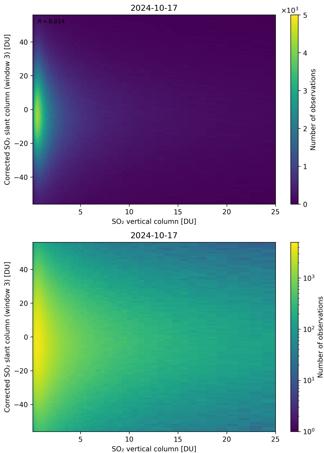
Figure 299: Scatter density plot of “SO 2 vertical column” against “Corrected SO 2 slant column (window 3)” for 2024-10-16 to 2024-10-18.
