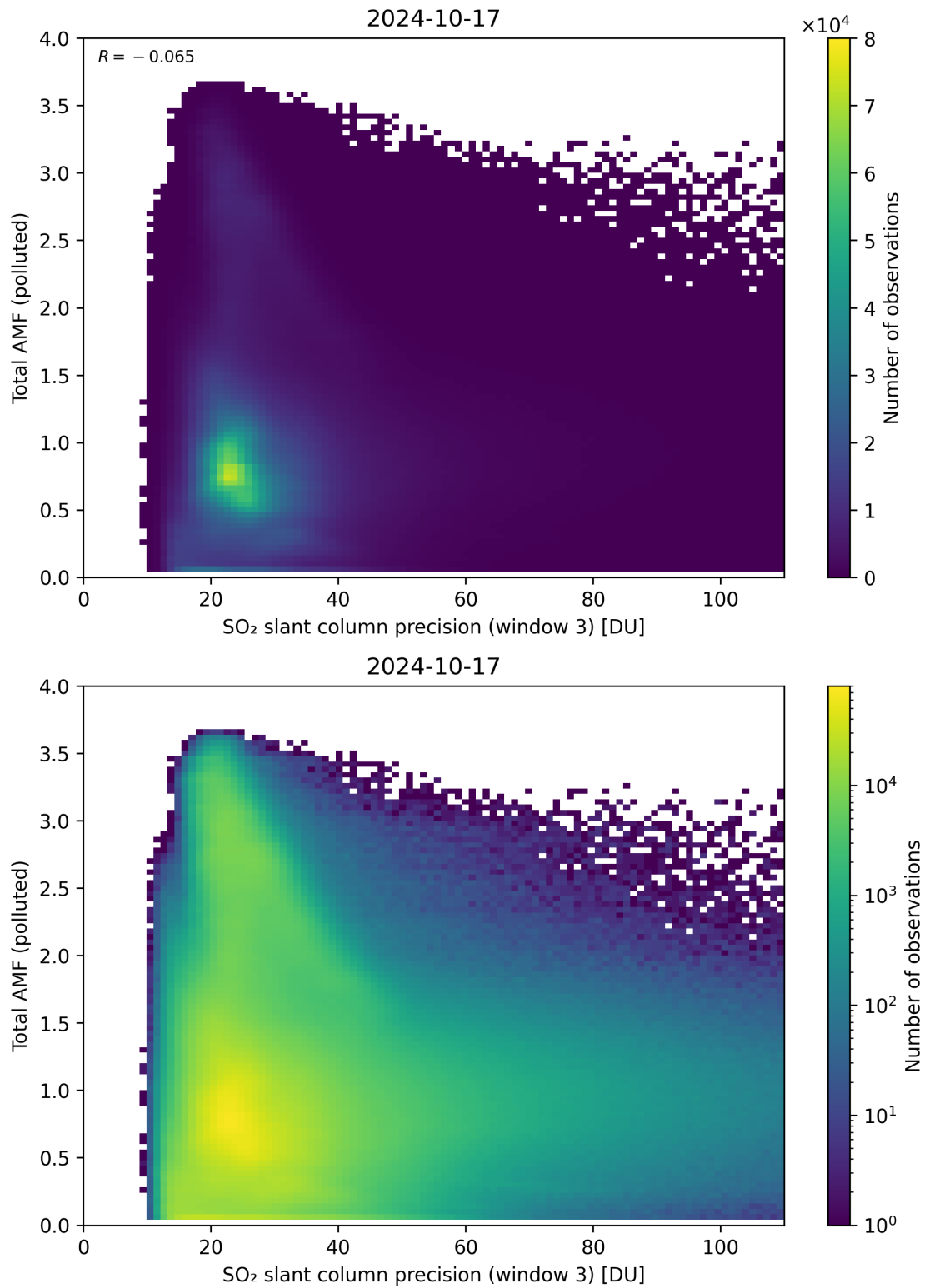
Figure 263: Scatter density plot of “SO 2 slant column precision (window 3)” against “Total AMF (polluted)” for 2024-10-16 to 2024-10-18.
