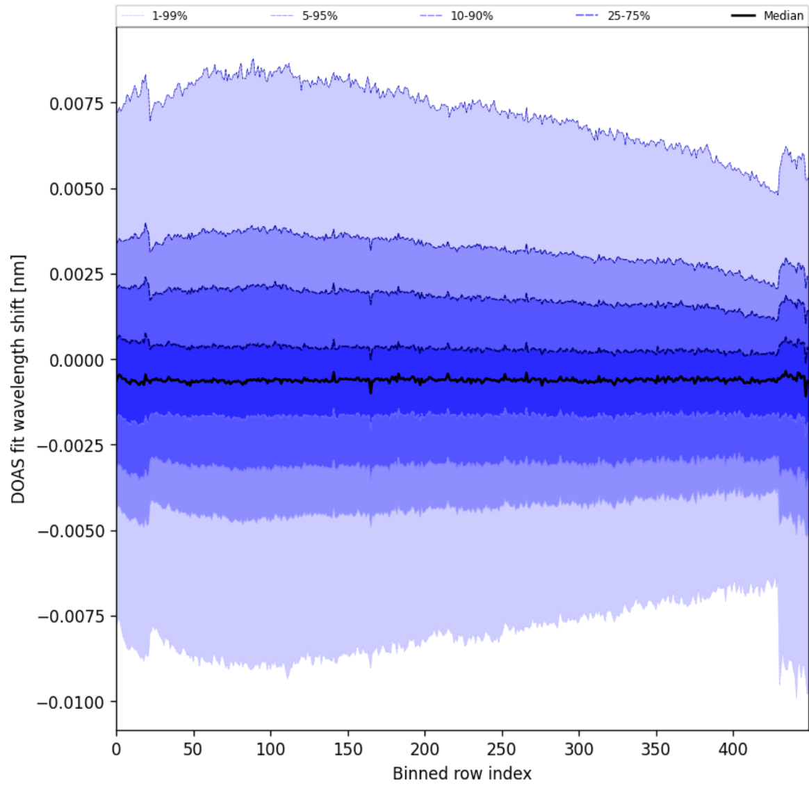
Figure 91: Along track statistics of “DOAS fit wavelength shift” for 2024-10-16 to 2024-10-18
