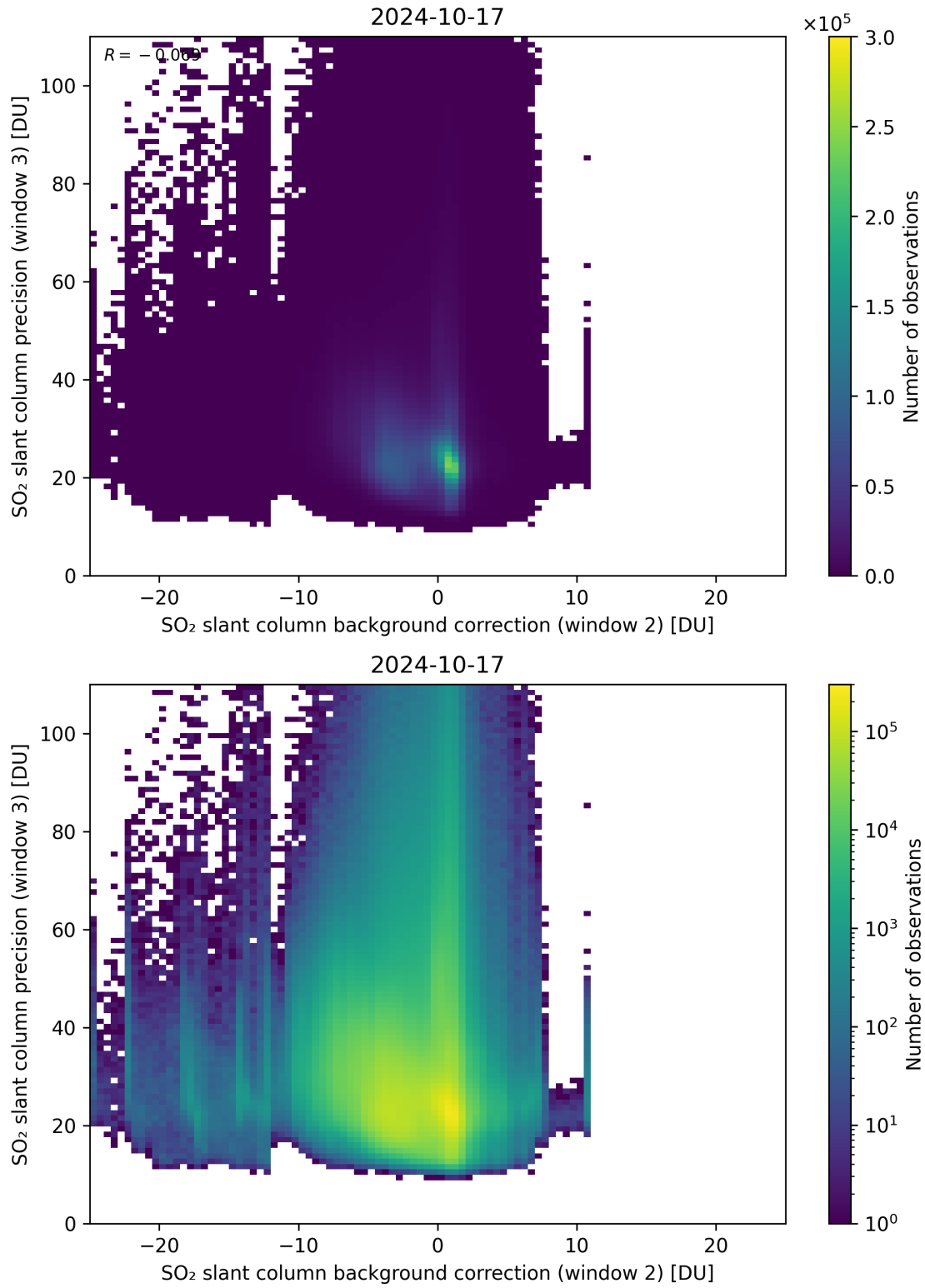
Figure 118: Scatter density plot of “SO 2 slant column background correction (window 2)” against “SO 2 slant column precision (window 3)” for 2024-10-16 to 2024-10-18.
