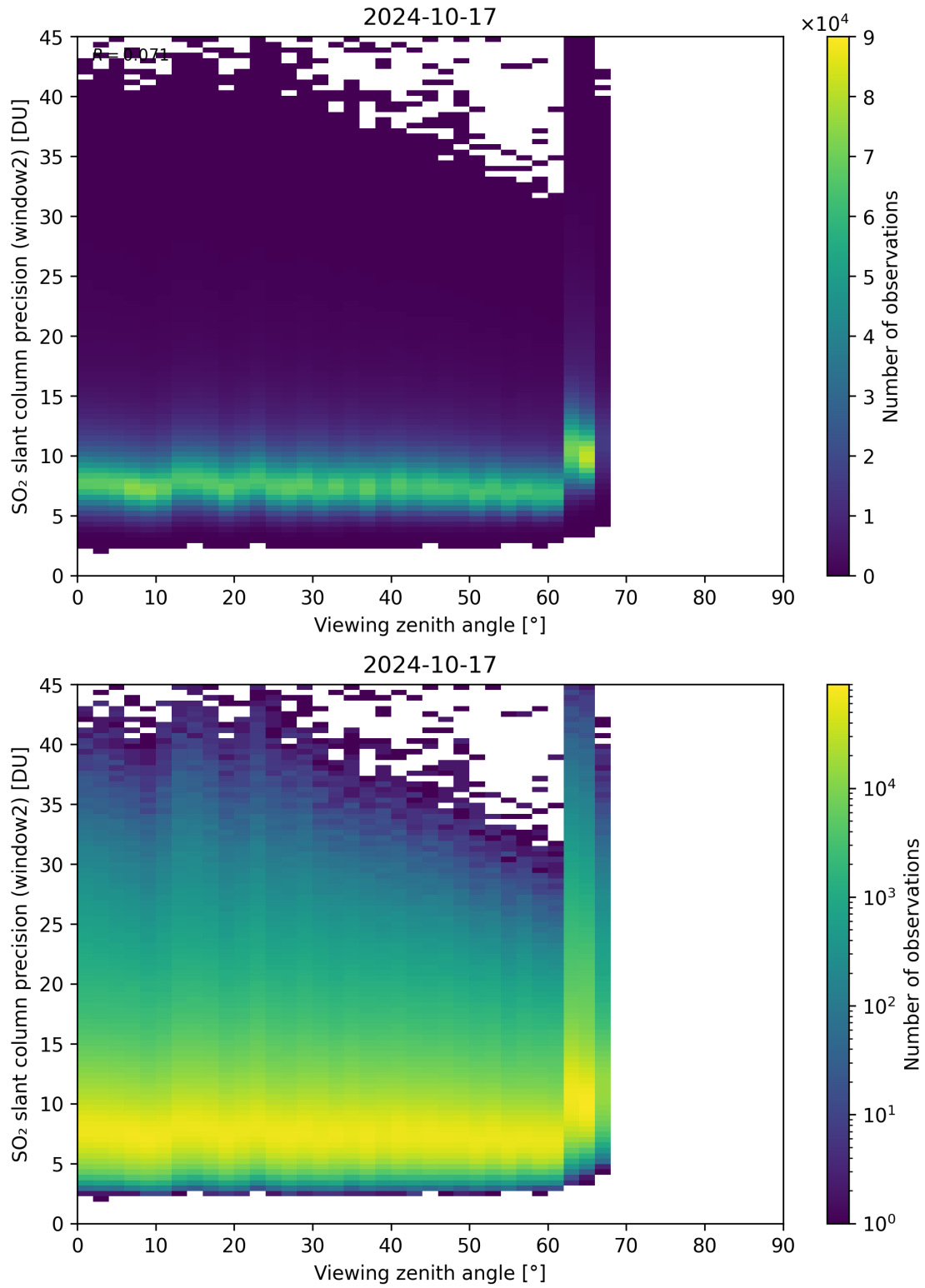
Figure 322: Scatter density plot of “Viewing zenith angle” against “SO 2 slant column precision (window2)” for 2024-10-16 to 2024-10-18.
