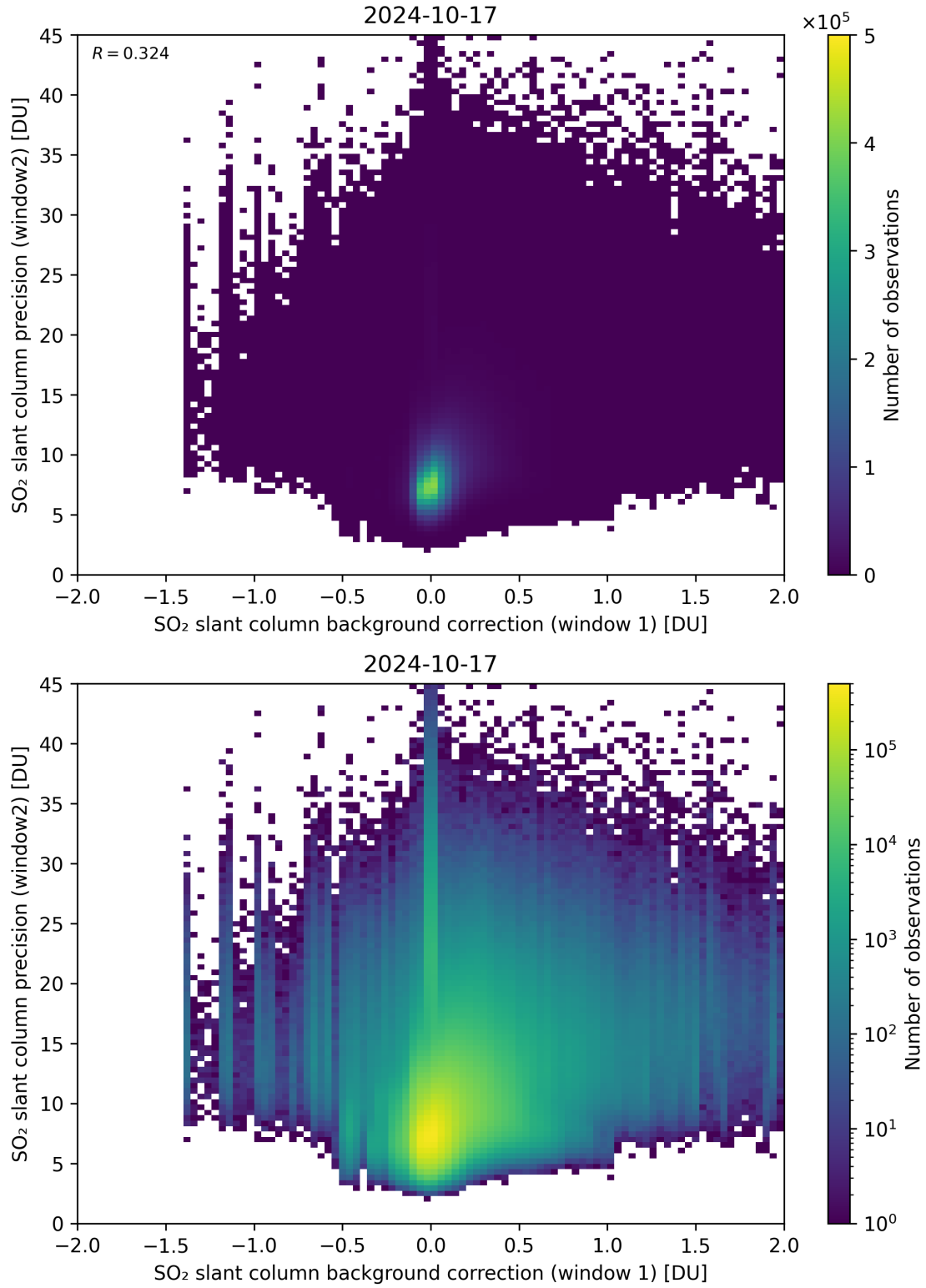
Figure 106: Scatter density plot of “SO 2 slant column background correction (window 1)” against “SO 2 slant column precision (window2)” for 2024-10-16 to 2024-10-18.
