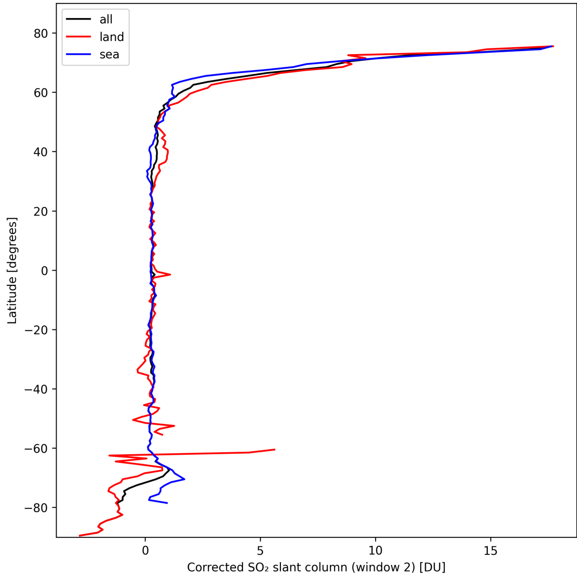
Figure 39: Zonal average of “Corrected SO 2 slant column (window 2)” for 2024-10-16 to 2024-10-18.
