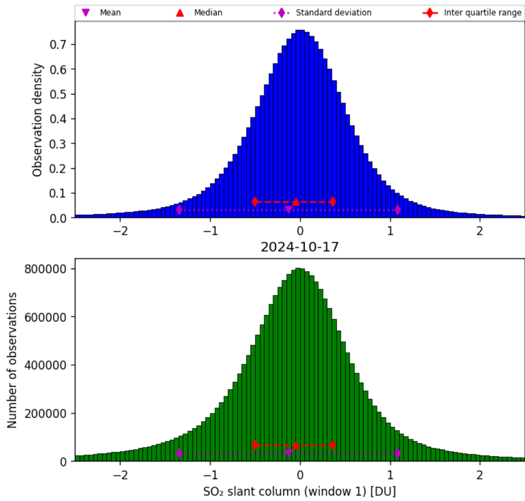
Figure 56: Histogram of “SO 2 slant column (window 1)” for 2024-10-16 to 2024-10-18
