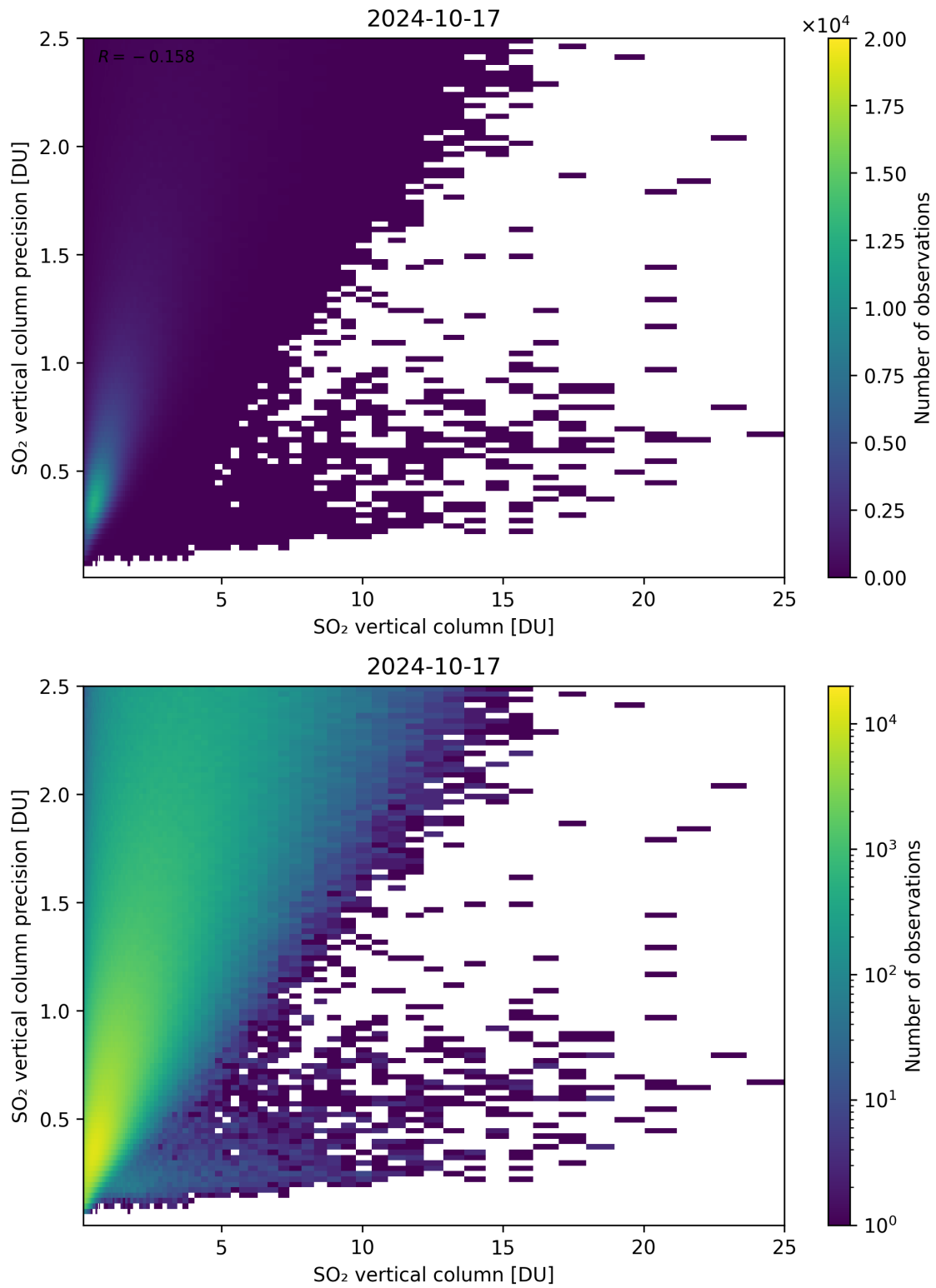
Figure 307: Scatter density plot of “SO 2 vertical column” against “SO 2 vertical column precision” for 2024-10-16 to 2024-10-18.
