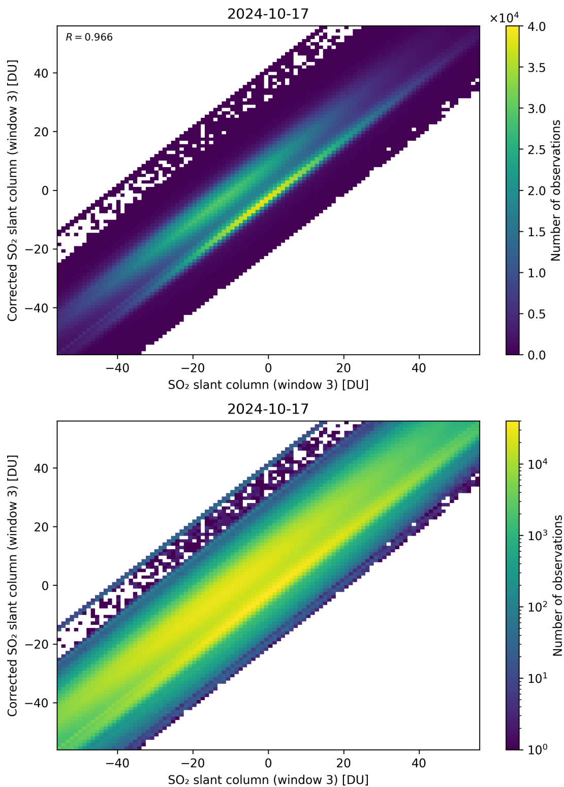
Figure 266: Scatter density plot of “SO 2 slant column (window 3)” against “Corrected SO 2 slant column (window 3)” for 2024-10-16 to 2024-10-18.
