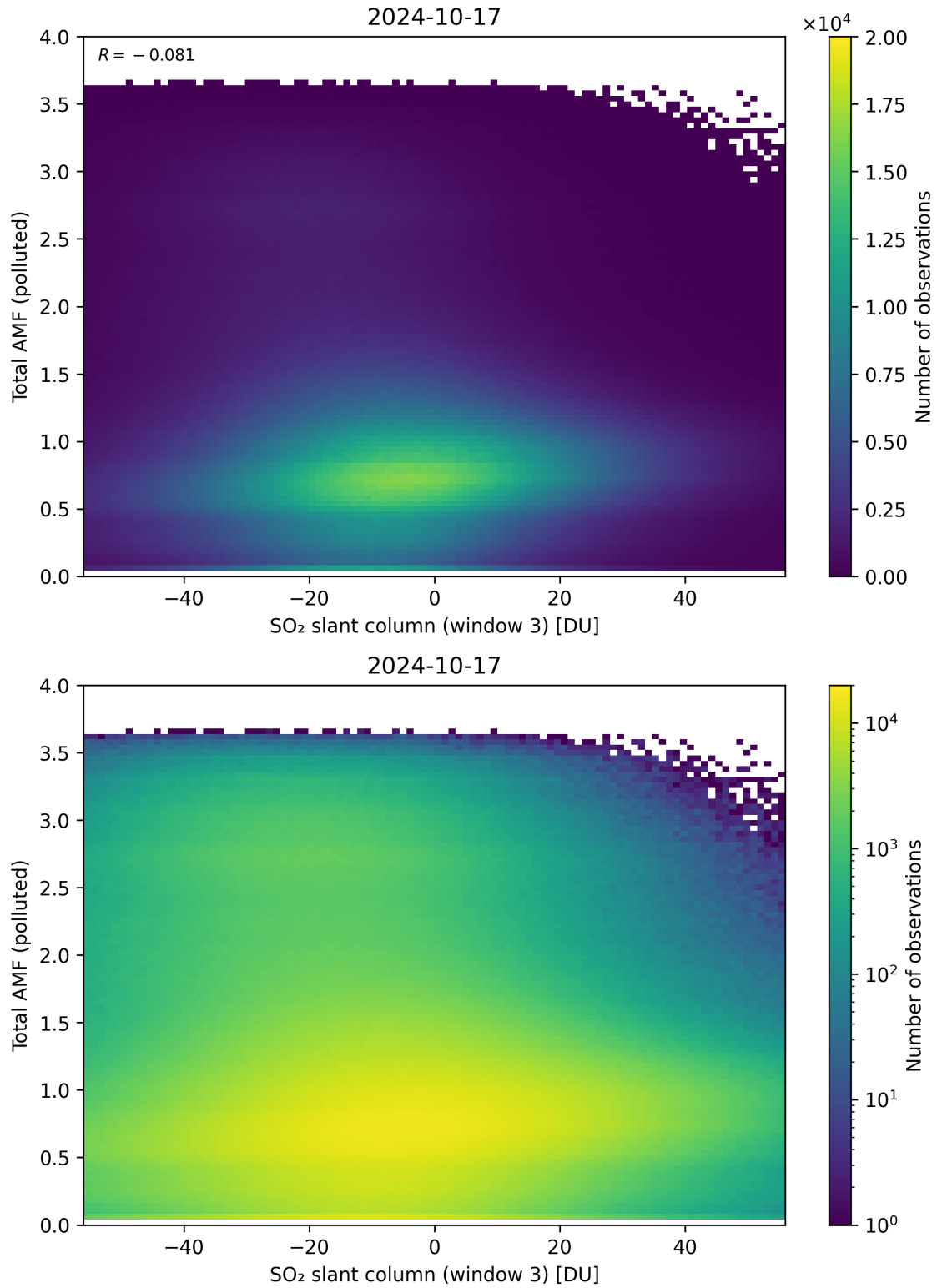
Figure 268: Scatter density plot of “SO 2 slant column (window 3)” against “Total AMF (polluted)” for 2024-10-16 to 2024-10-18.
