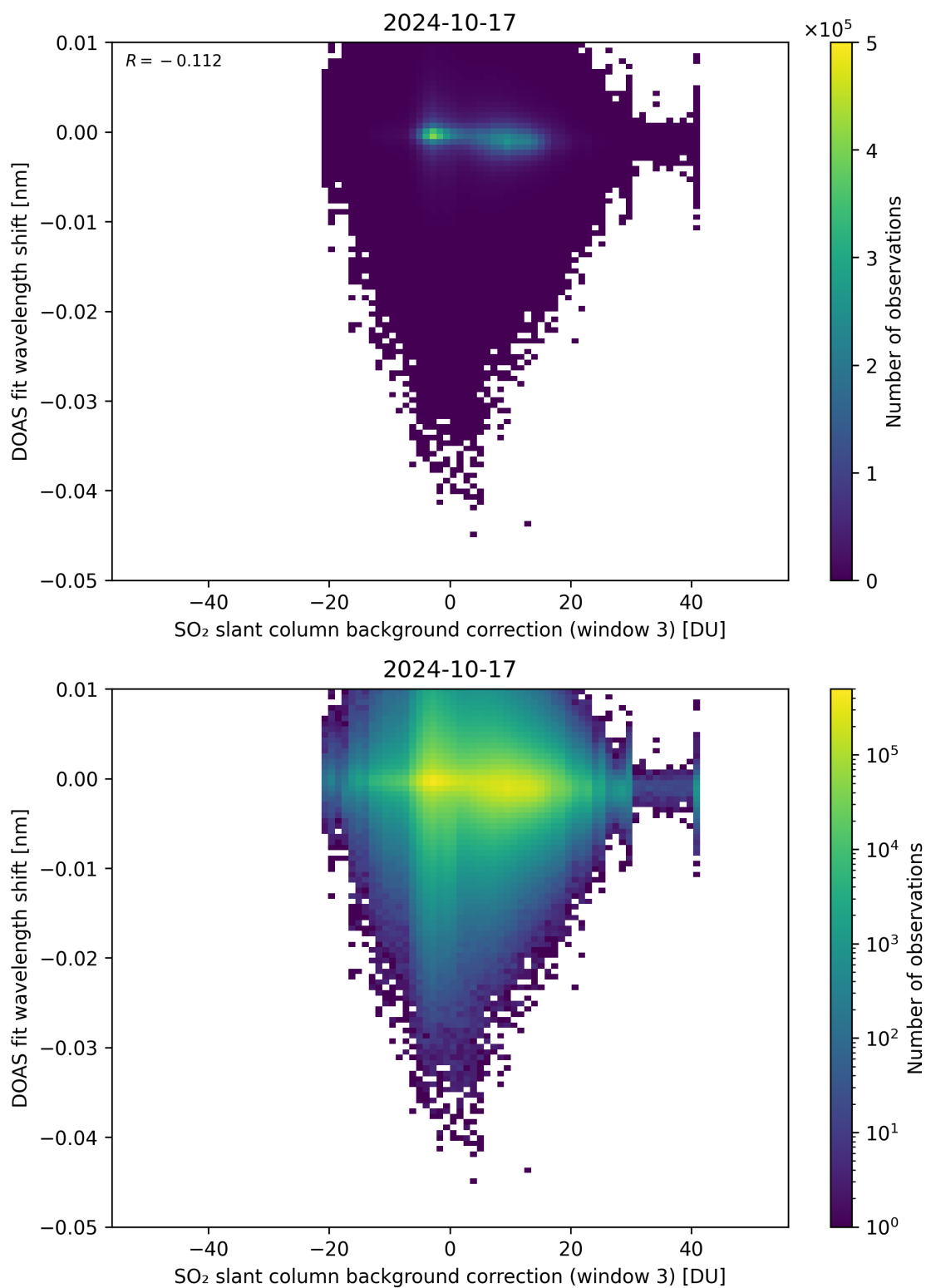
Figure 121: Scatter density plot of “SO 2 slant column background correction (window 3)” against “DOAS fit wavelength shift” for 2024-10-16 to 2024-10-18.
