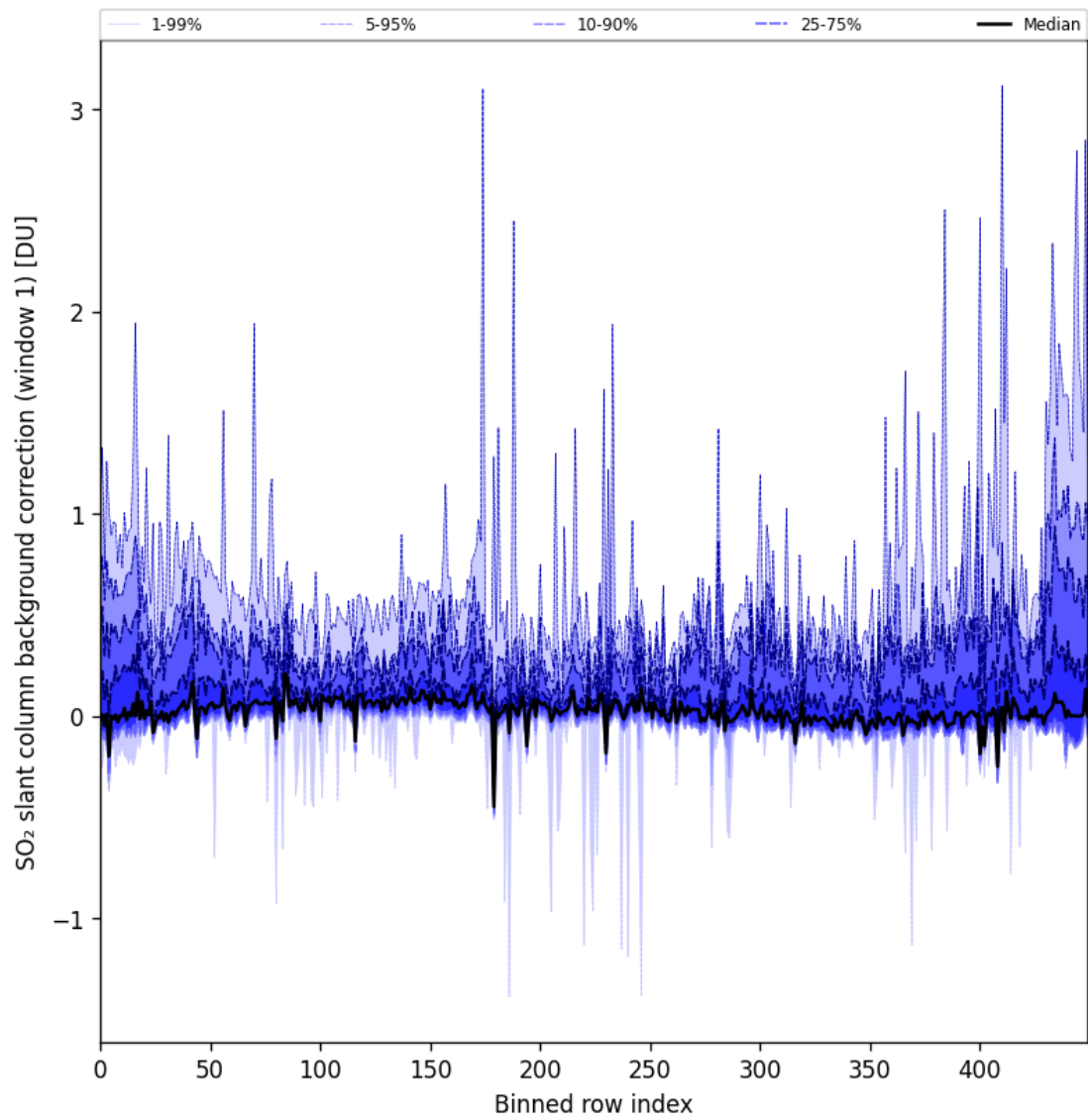
Figure 82: Along track statistics of “SO 2 slant column background correction (window 1)” for 2024-10-16 to 2024-10-18
