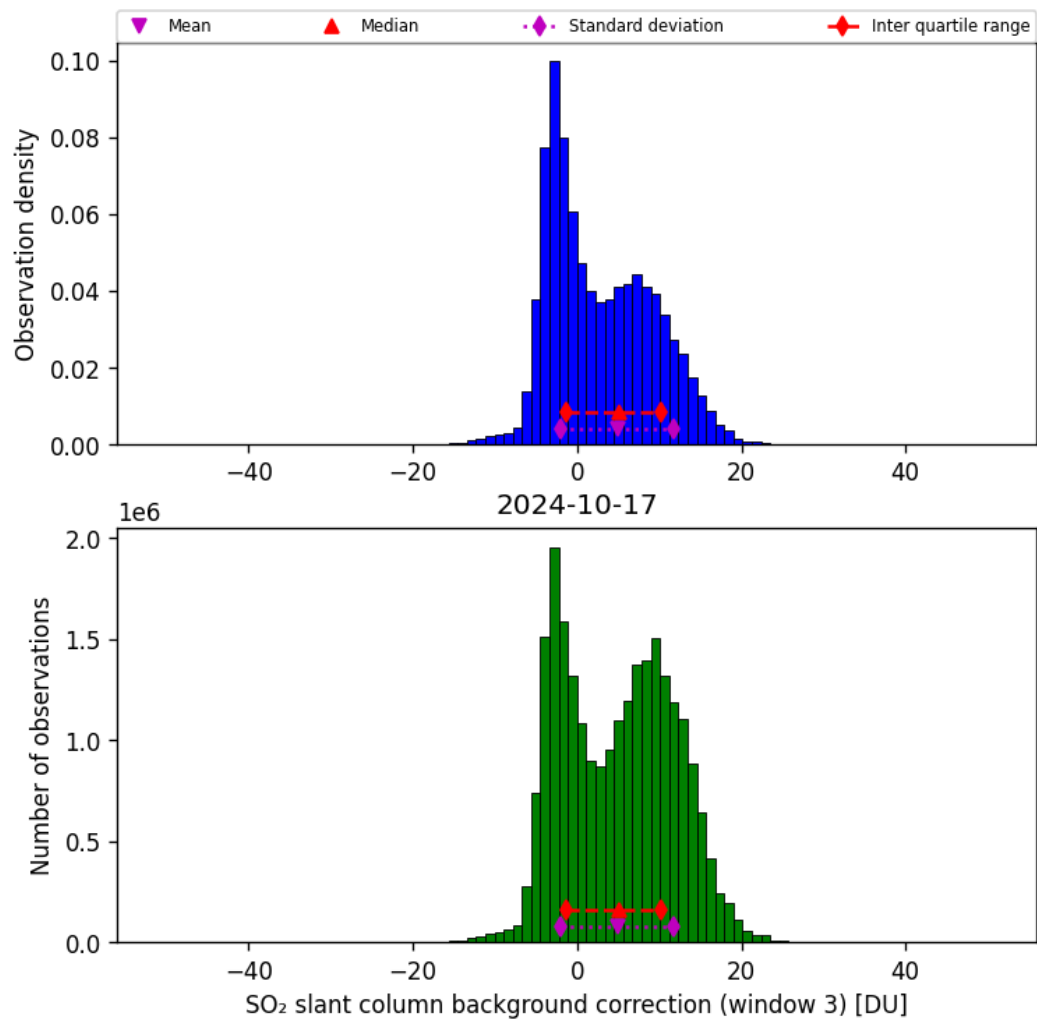
Figure 67: Histogram of “SO 2 slant column background correction (window 3)” for 2024-10-16 to 2024-10-18
