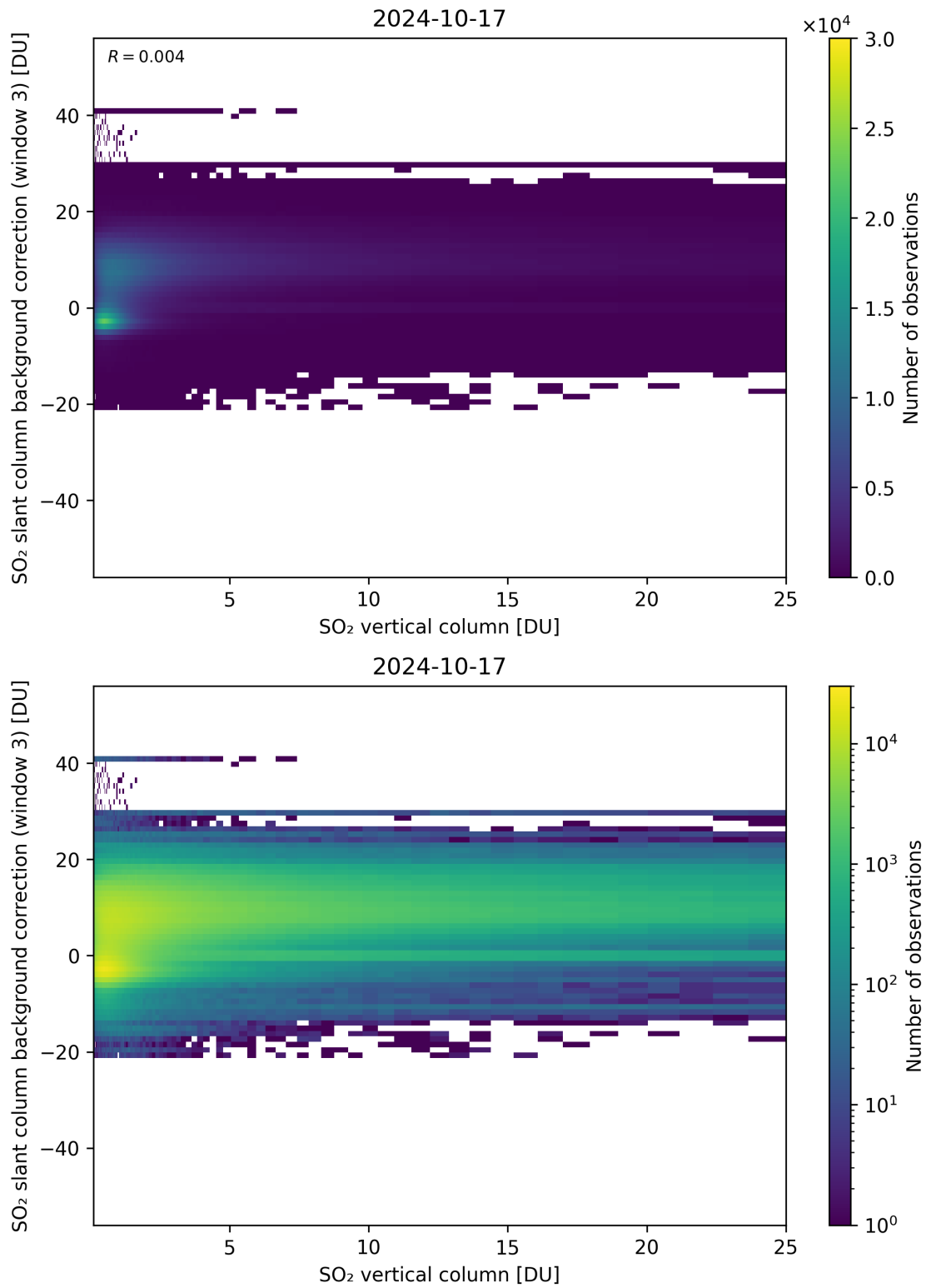
Figure 275: Scatter density plot of “SO 2 vertical column” against “SO 2 slant column background correction (window 3)” for 2024-10-16 to 2024-10-18.
