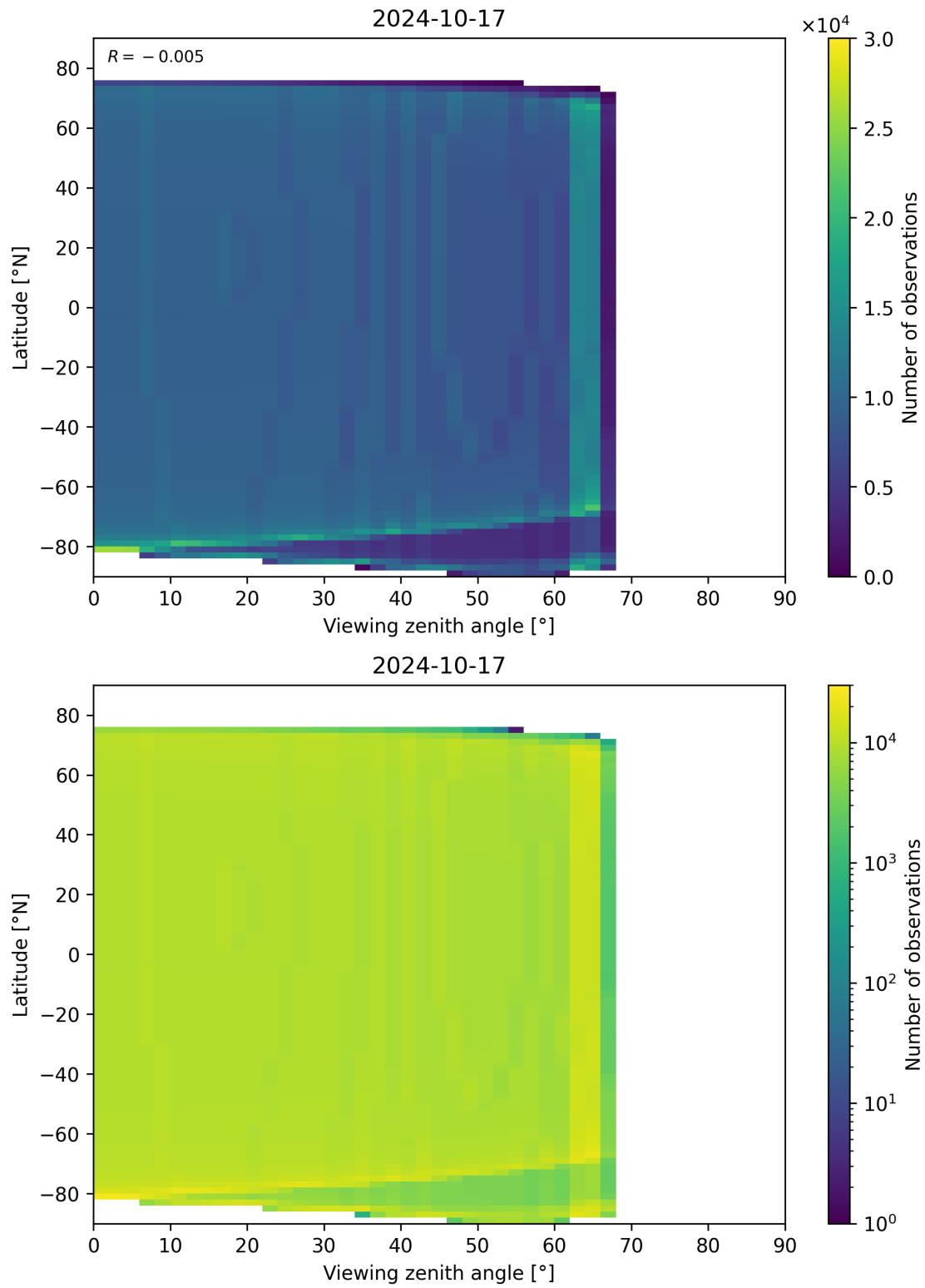
Figure 314: Scatter density plot of “Viewing zenith angle” against “Latitude” for 2024-10-16 to 2024-10-18.
