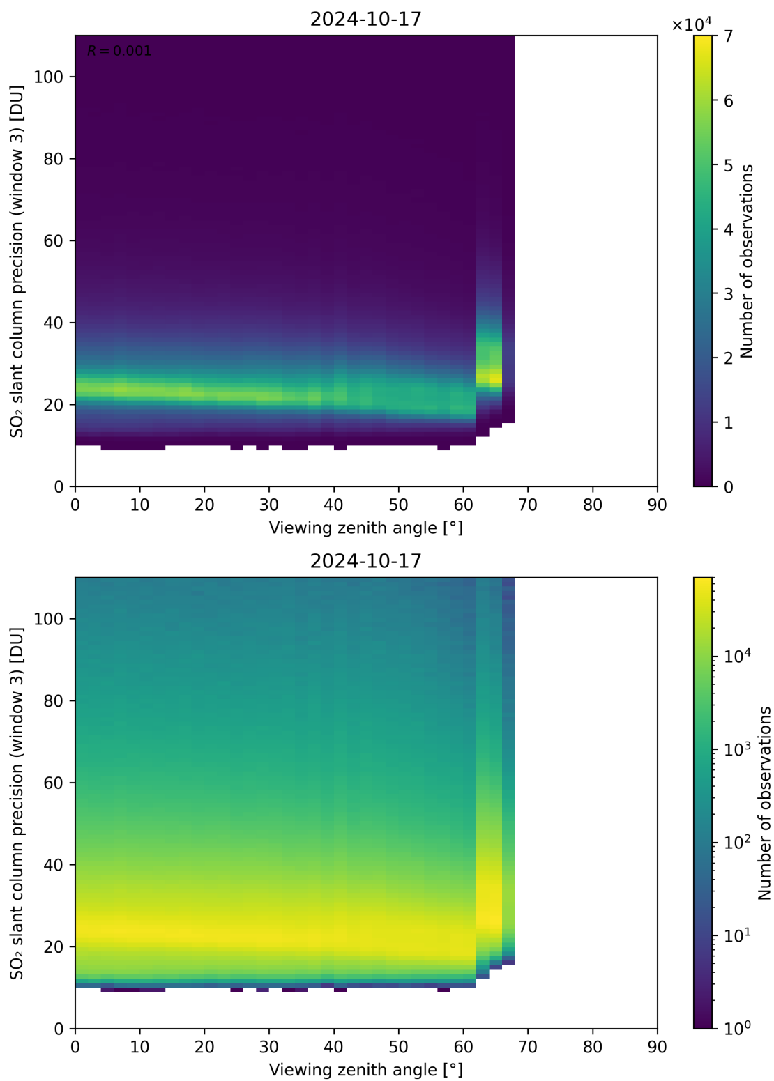
Figure 324: Scatter density plot of “Viewing zenith angle” against “SO 2 slant column precision (window 3)” for 2024-10-16 to 2024-10-18.
