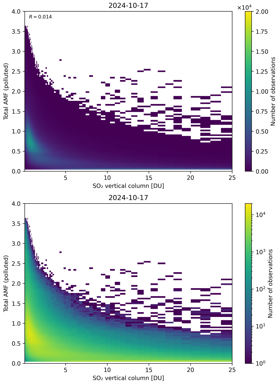
Figure 305: Scatter density plot of “SO 2 vertical column” against “Total AMF (polluted)” for 2024-10-16 to 2024-10-18.
