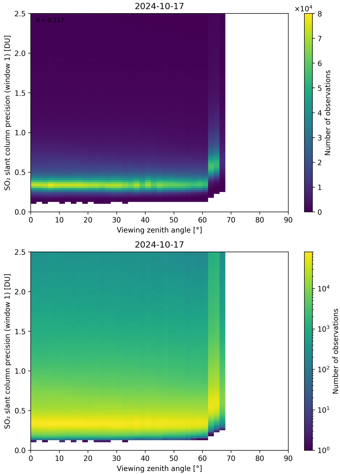
Figure 321: Scatter density plot of “Viewing zenith angle” against “SO 2 slant column precision (window 1)” for 2024-10-16 to 2024-10-18.
