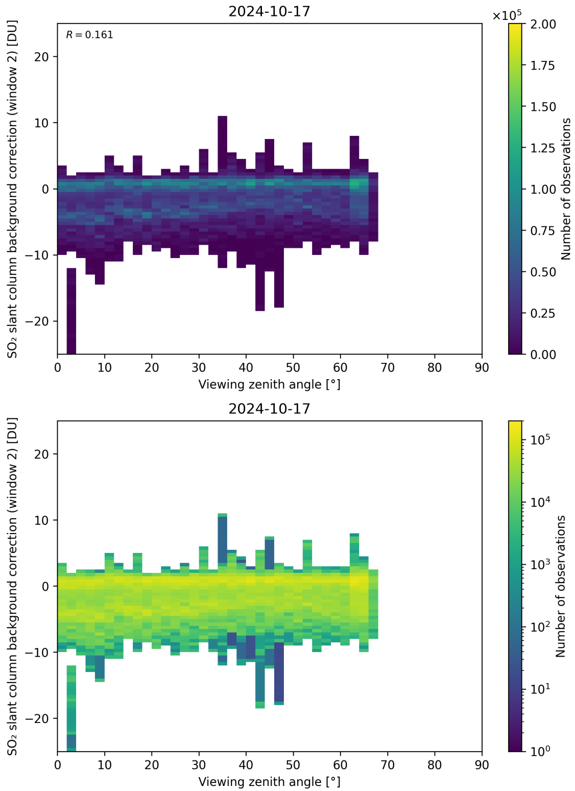
Figure 309: Scatter density plot of “Viewing zenith angle” against “SO 2 slant column background correction (window 2)” for 2024-10-16 to 2024-10-18.
