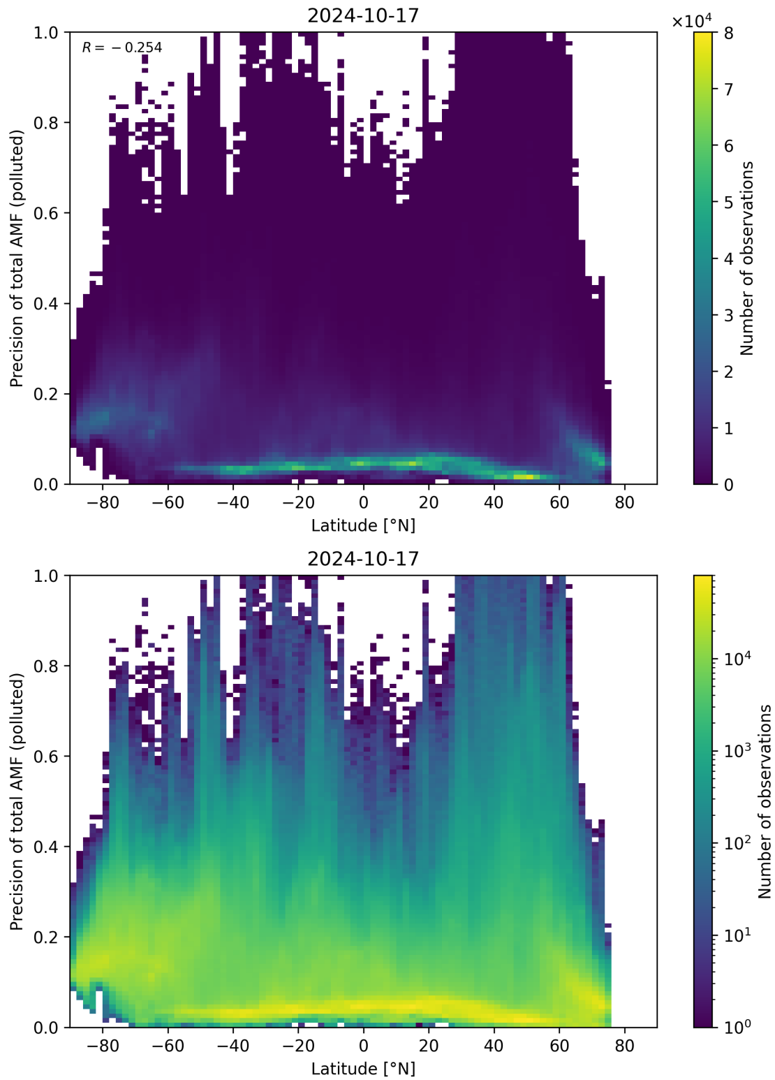
Figure 155: Scatter density plot of “Latitude” against “Precision of total AMF (polluted)” for 2024-10-16 to 2024-10-18.
