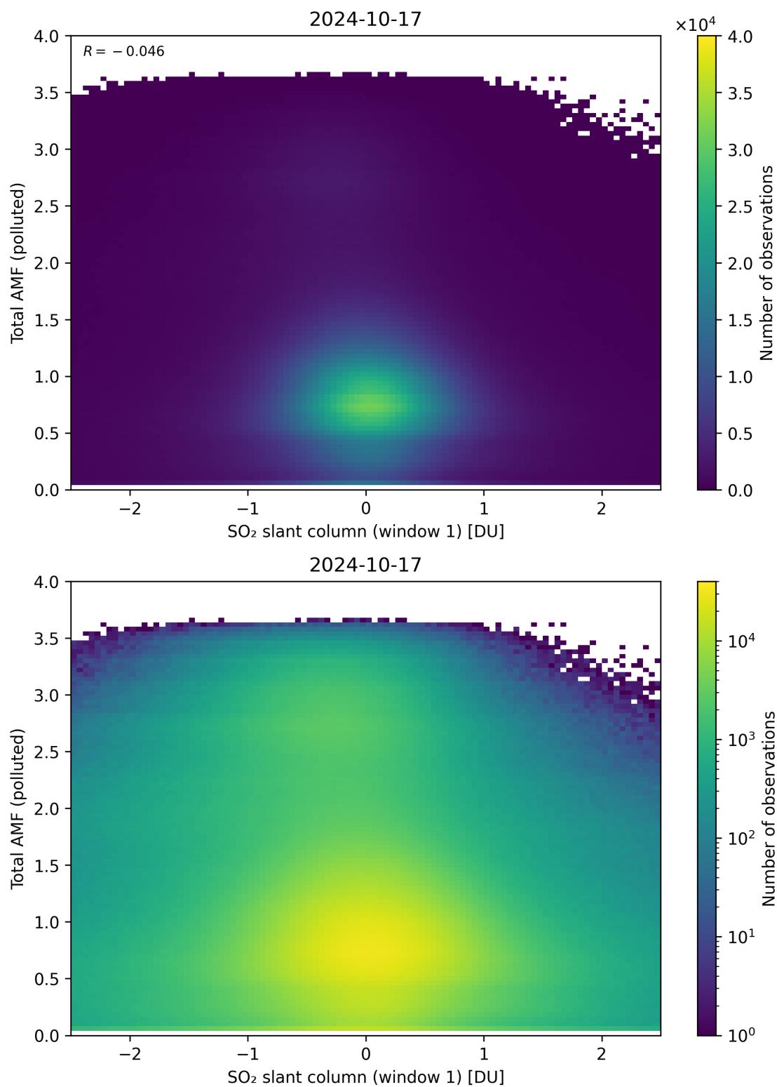
Figure 239: Scatter density plot of “SO 2 slant column (window 1)” against “Total AMF (polluted)” for 2024-10-16 to 2024-10-18.
