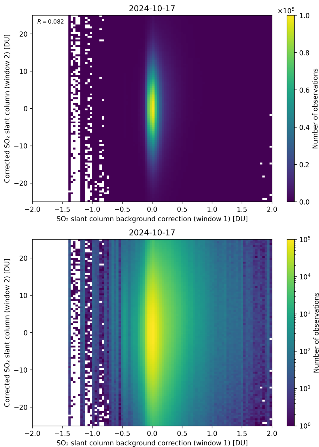
Figure 104: Scatter density plot of “SO 2 slant column background correction (window 1)” against “Corrected SO 2 slant column (window 2)” for 2024-10-16 to 2024-10-18.
