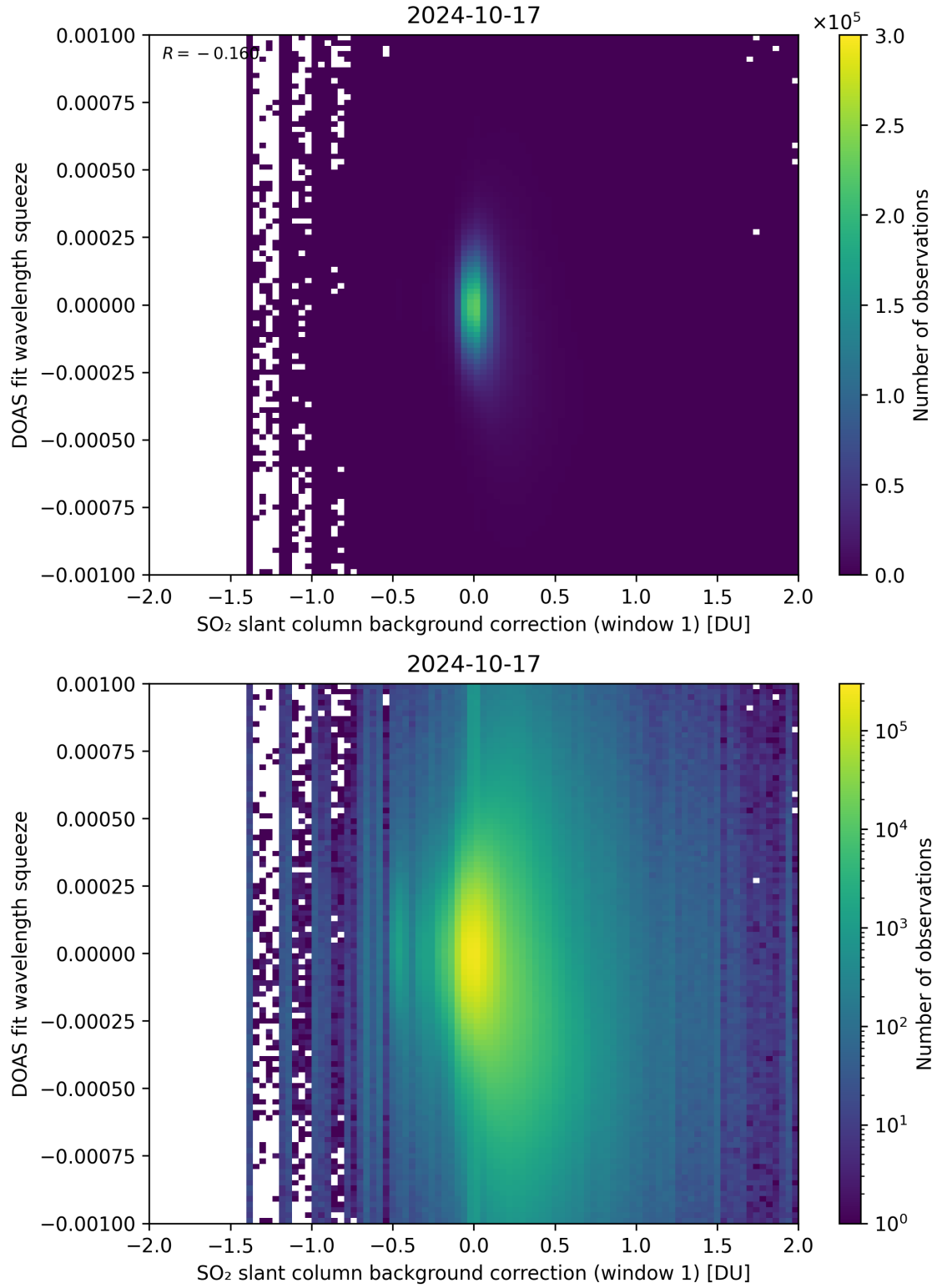
Figure 101: Scatter density plot of “SO 2 slant column background correction (window 1)” against “DOAS fit wavelength squeeze” for 2024-10-16 to 2024-10-18.
