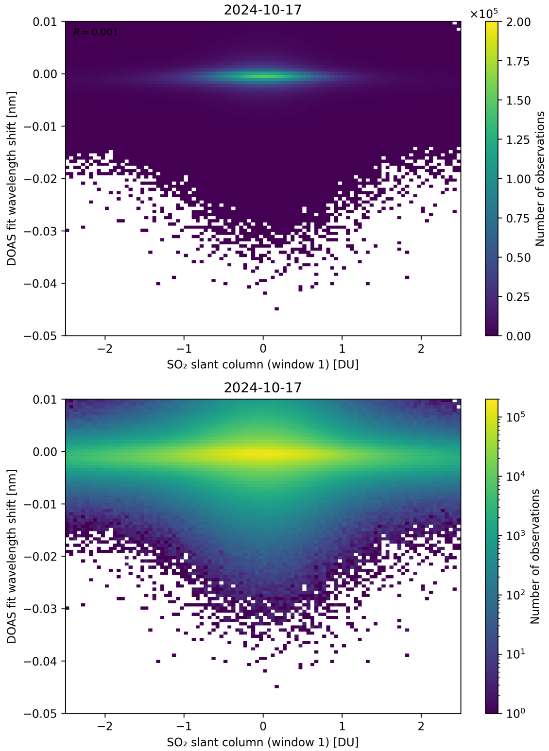
Figure 215: Scatter density plot of “SO 2 slant column (window 1)” against “DOAS fit wavelength shift” for 2024-10-16 to 2024-10-18.
