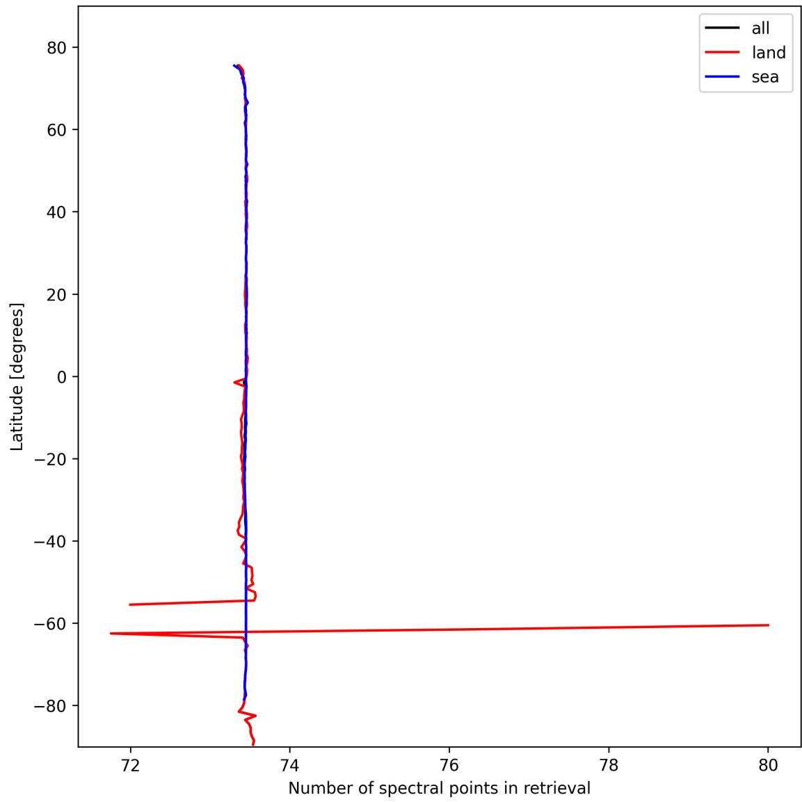
Figure 51: Zonal average of “Number of spectral points in retrieval” for 2024-10-16 to 2024-10-18.
