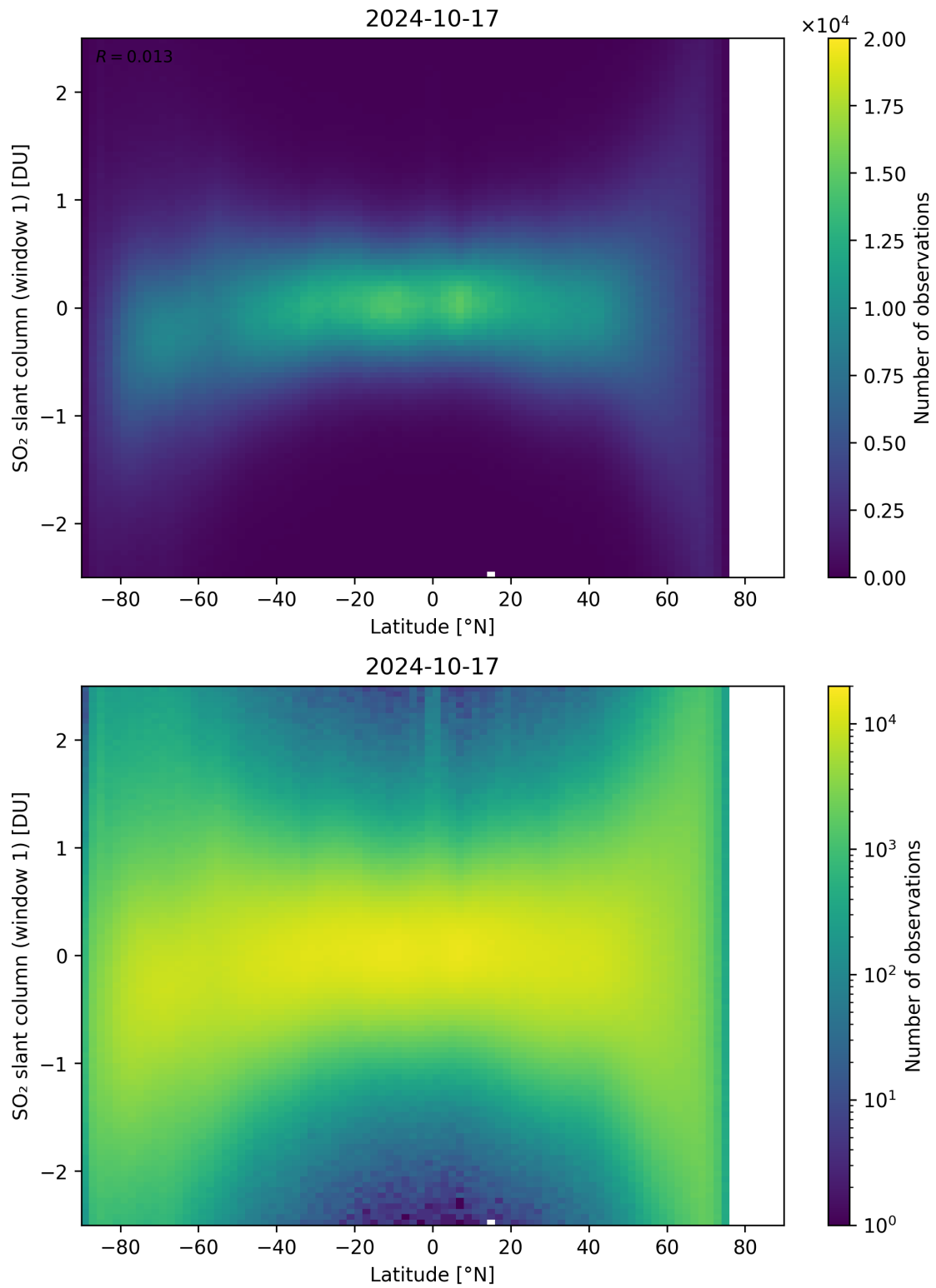
Figure 149: Scatter density plot of “Latitude” against “SO 2 slant column (window 1)” for 2024-10-16 to 2024-10-18.
