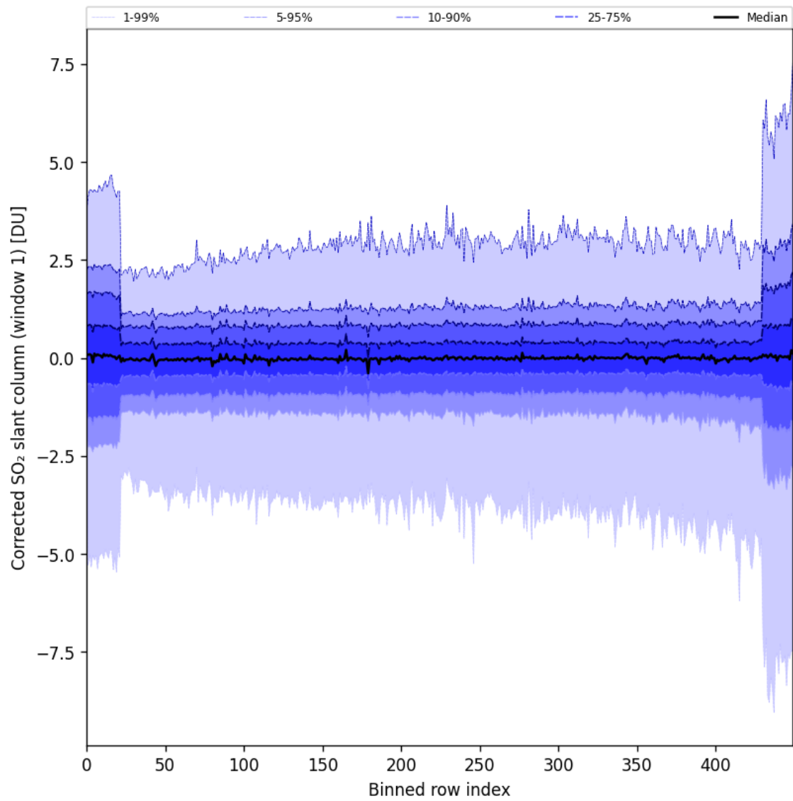
Figure 81: Along track statistics of "Corrected SO 2 slant column (window 1)" for 2024-10-16 to 2024-10-18
