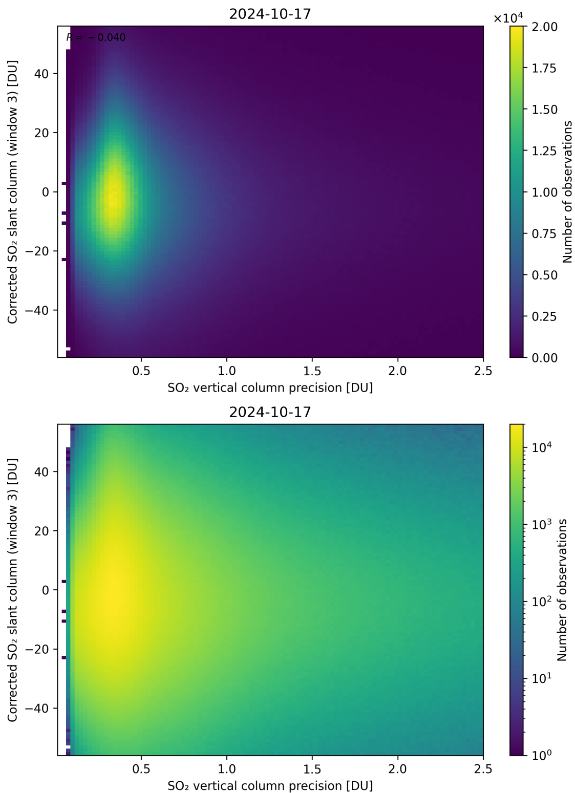
Figure 288: Scatter density plot of “SO 2 vertical column precision” against “Corrected SO 2 slant column (window 3)” for 2024-10-16 to 2024-10-18.
