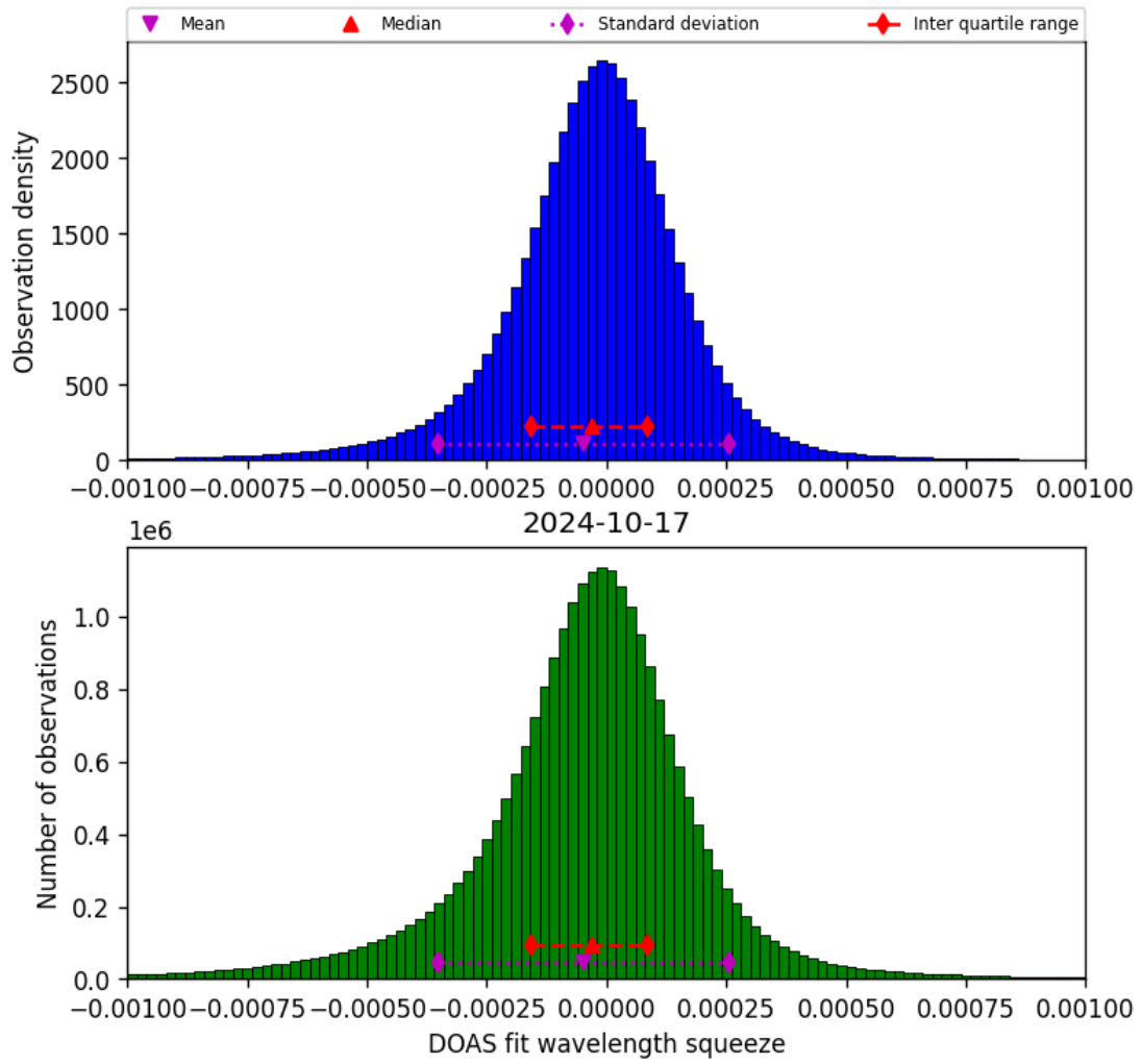
Figure 69: Histogram of “DOAS fit wavelength squeeze” for 2024-10-16 to 2024-10-18
