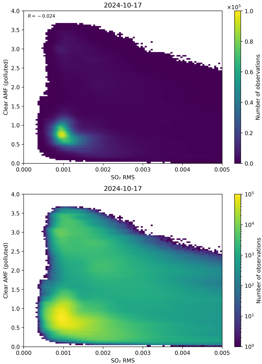
Figure 136: Scatter density plot of “SO 2 RMS” against “Clear AMF (polluted)” for 2024-10-16 to 2024-10-18.
