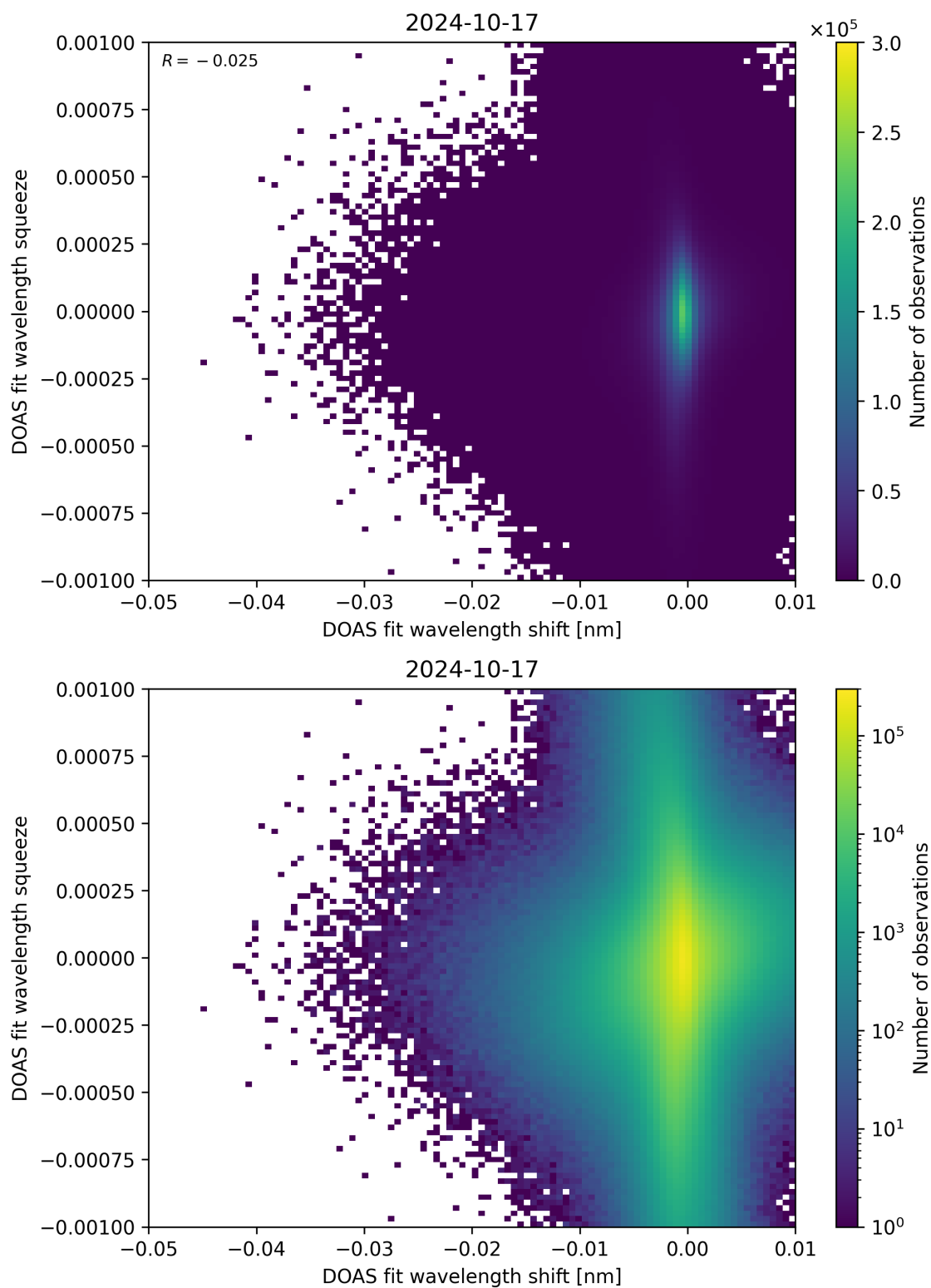
Figure 127: Scatter density plot of “DOAS fit wavelength shift” against “DOAS fit wavelength squeeze” for 2024-10-16 to 2024-10-18.
