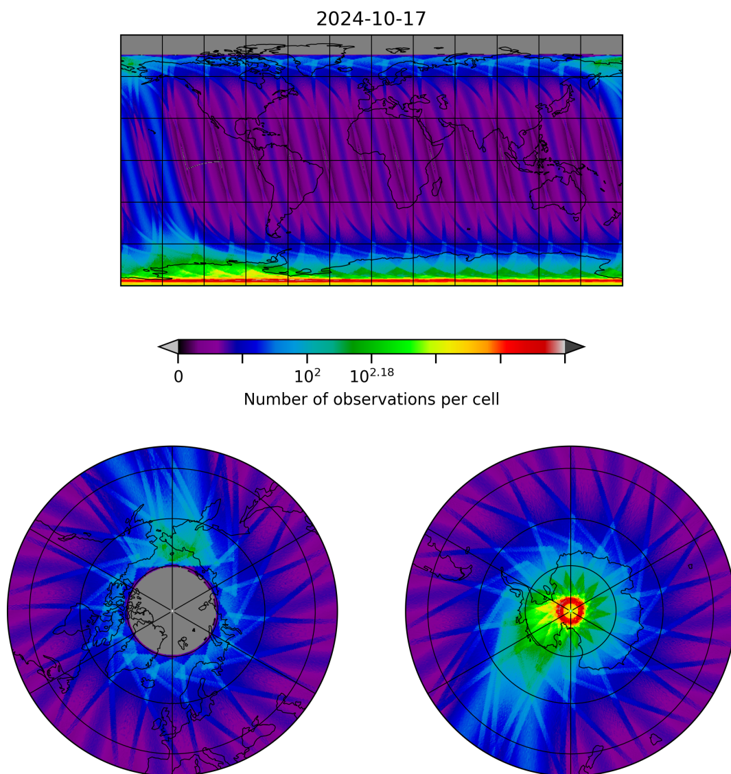
Figure 28: Map of the number of observations for 2024-10-16 to 2024-10-18
