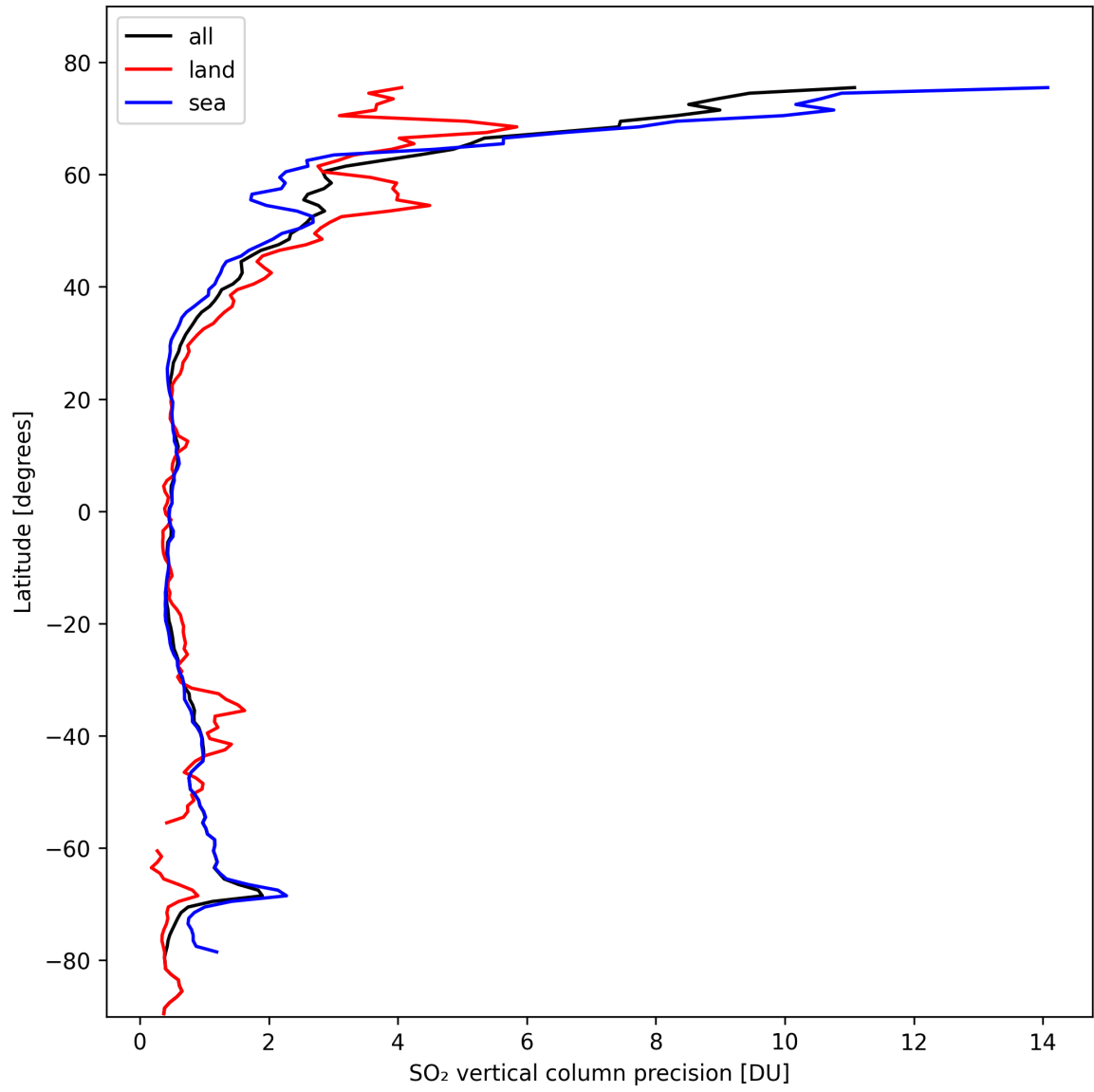
Figure 31: Zonal average of “SO 2 vertical column precision” for 2024-10-16 to 2024-10-18.
