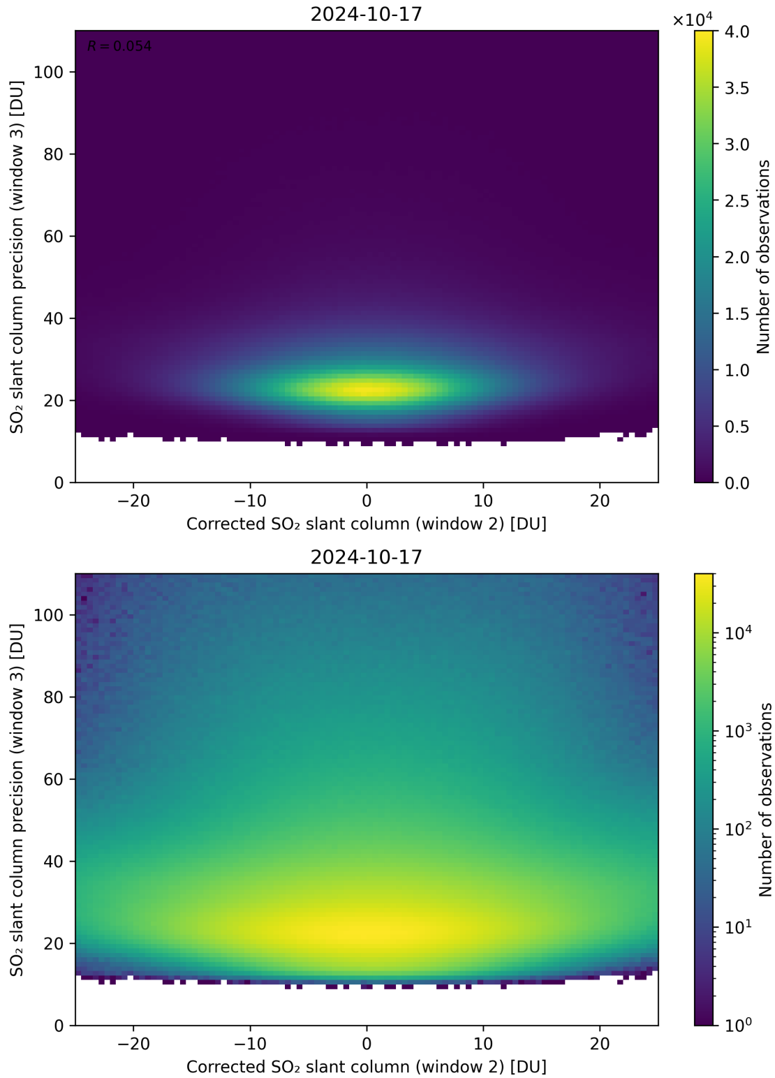
Figure 202: Scatter density plot of “Corrected SO 2 slant column (window 2)” against “SO 2 slant column precision (window 3)” for 2024-10-16 to 2024-10-18.
