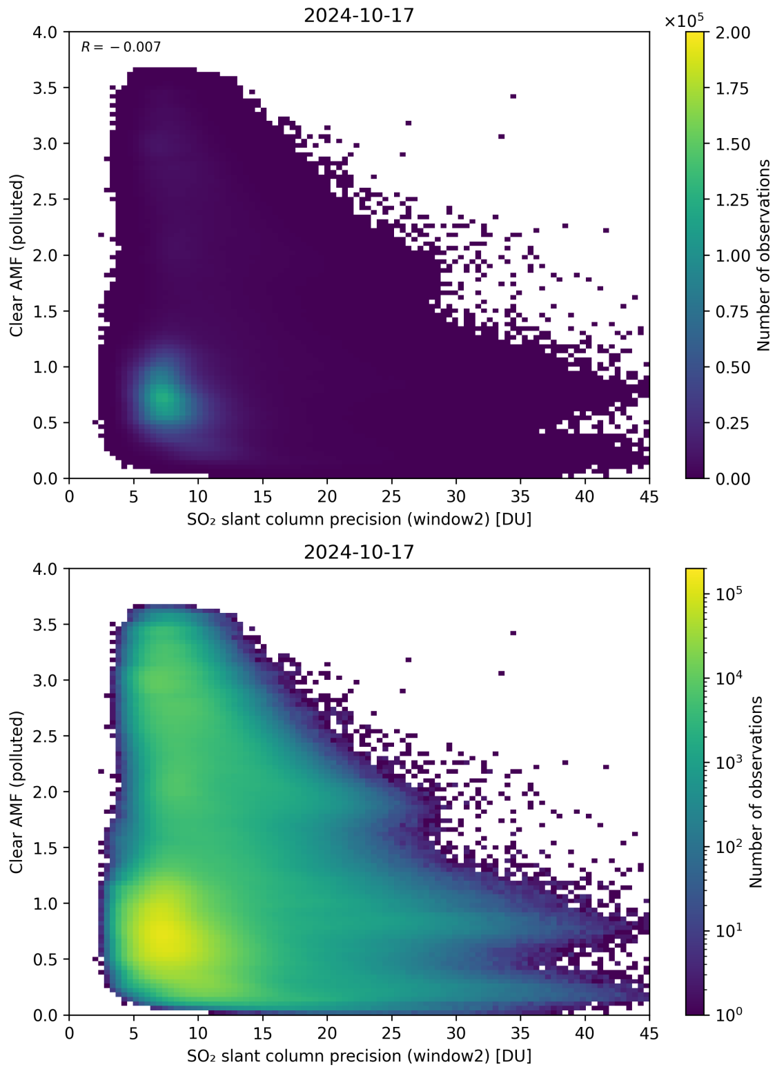
Figure 246: Scatter density plot of “SO 2 slant column precision (window2)” against “Clear AMF (polluted)” for 2024-10-16 to 2024-10-18.
