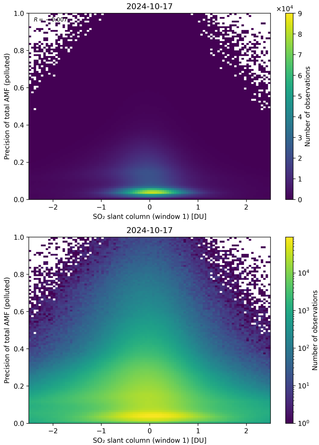
Figure 240: Scatter density plot of “SO 2 slant column (window 1)” against “Precision of total AMF (polluted)” for 2024-10-16 to 2024-10-18.
