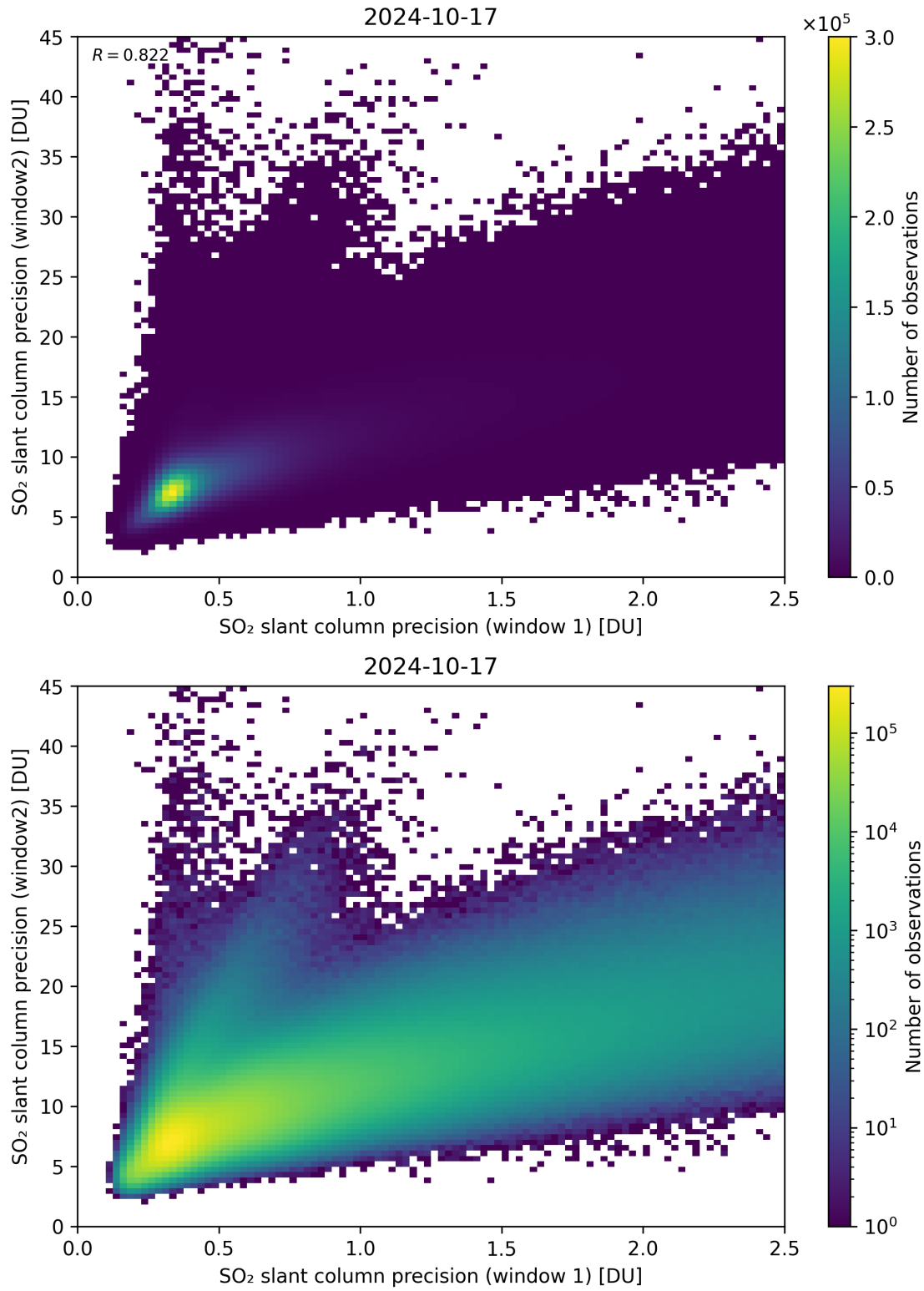
Figure 227: Scatter density plot of “SO 2 slant column precision (window 1)” against “SO 2 slant column precision (window2)” for 2024-10-16 to 2024-10-18.
