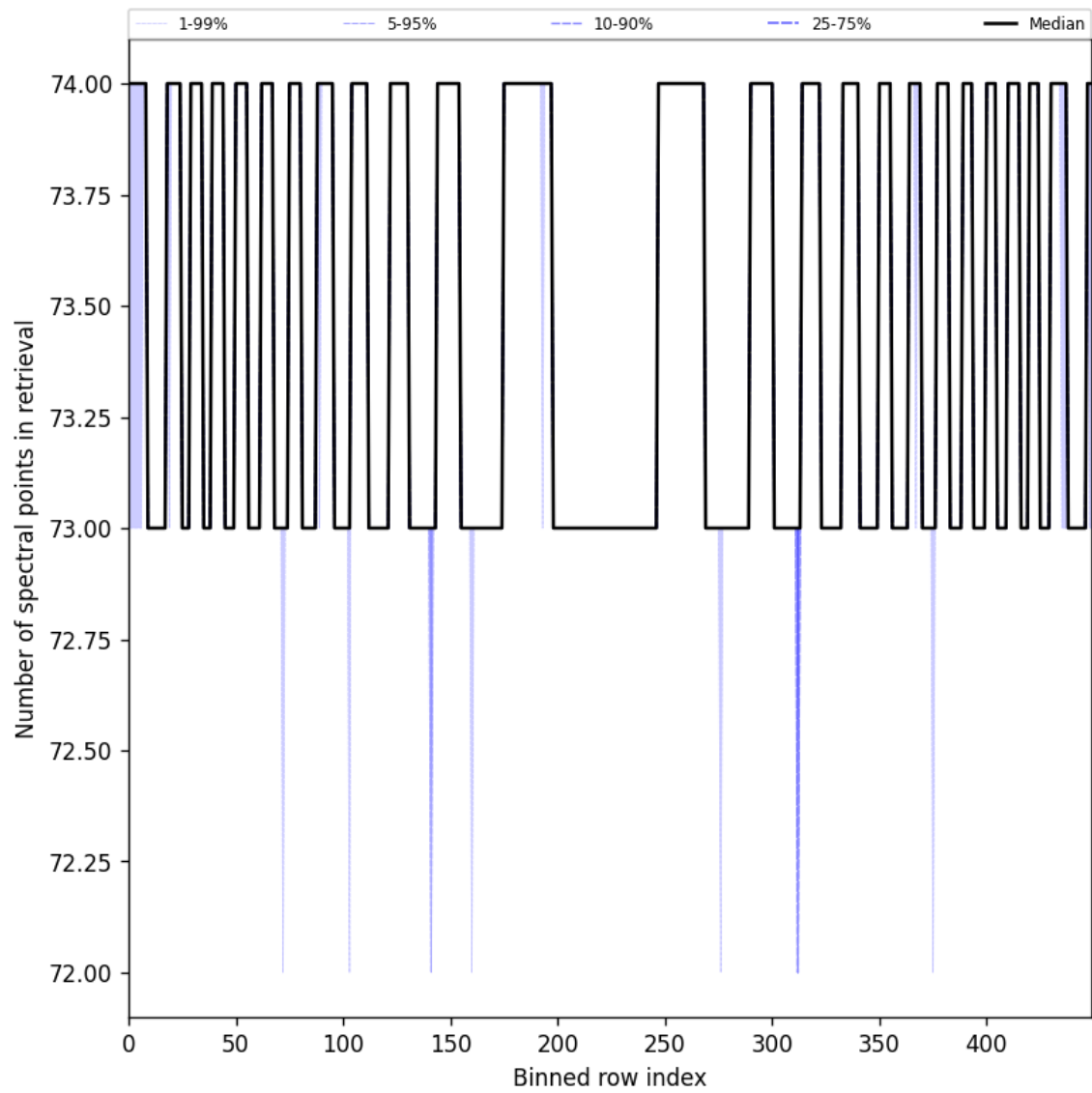
Figure 97: Along track statistics of “Number of spectral points in retrieval” for 2024-10-16 to 2024-10-18
