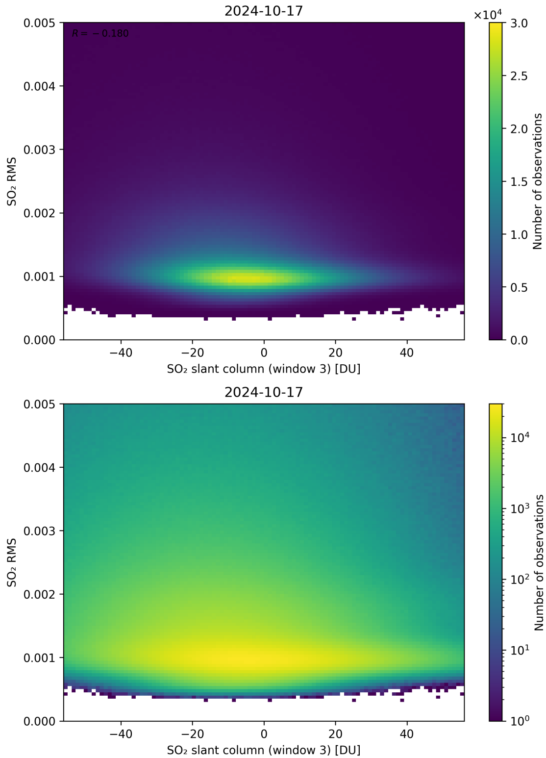
Figure 256: Scatter density plot of “SO 2 slant column (window 3)” against “SO 2 RMS” for 2024-10-16 to 2024-10-18.
