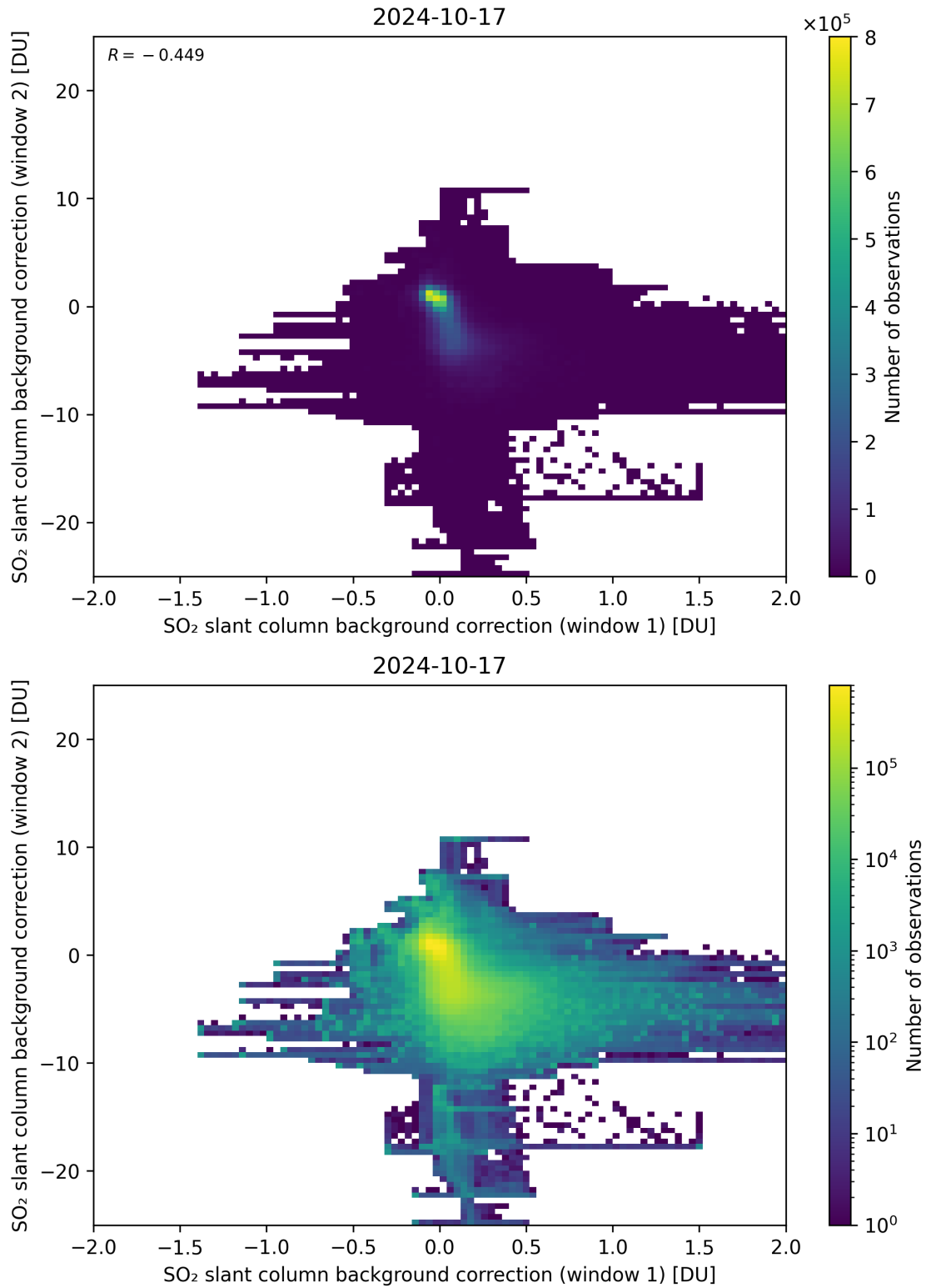
Figure 98: Scatter density plot of “SO 2 slant column background correction (window 1)” against “SO 2 slant column background correction (window 2)” for 2024-10-16 to 2024-10-18.
