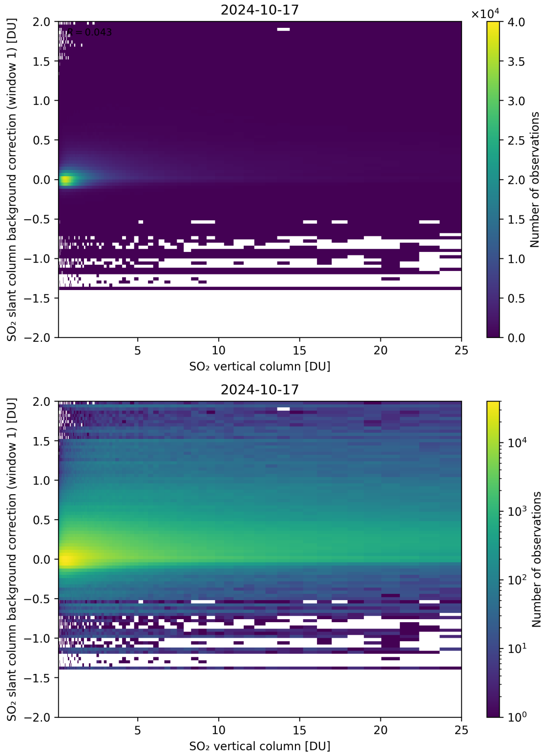
Figure 273: Scatter density plot of “SO 2 vertical column” against “SO 2 slant column background correction (window 1)” for 2024-10-16 to 2024-10-18.
