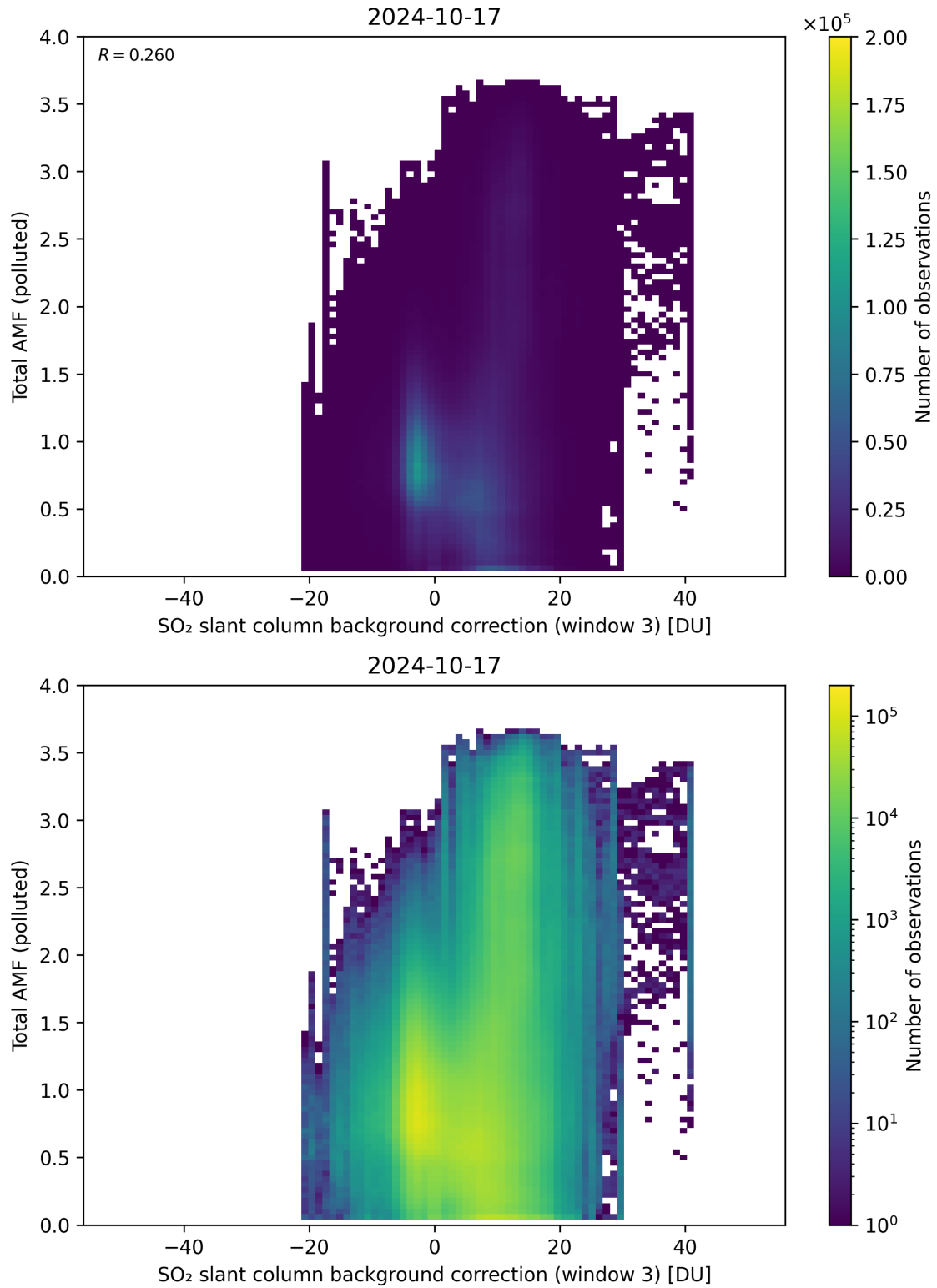
Figure 125: Scatter density plot of “SO 2 slant column background correction (window 3)” against “Total AMF (polluted)” for 2024-10-16 to 2024-10-18.
