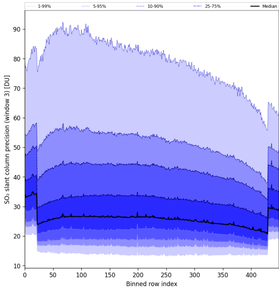
Figure 88: Along track statistics of “SO 2 slant column precision (window 3)” for 2024-10-16 to 2024-10-18
