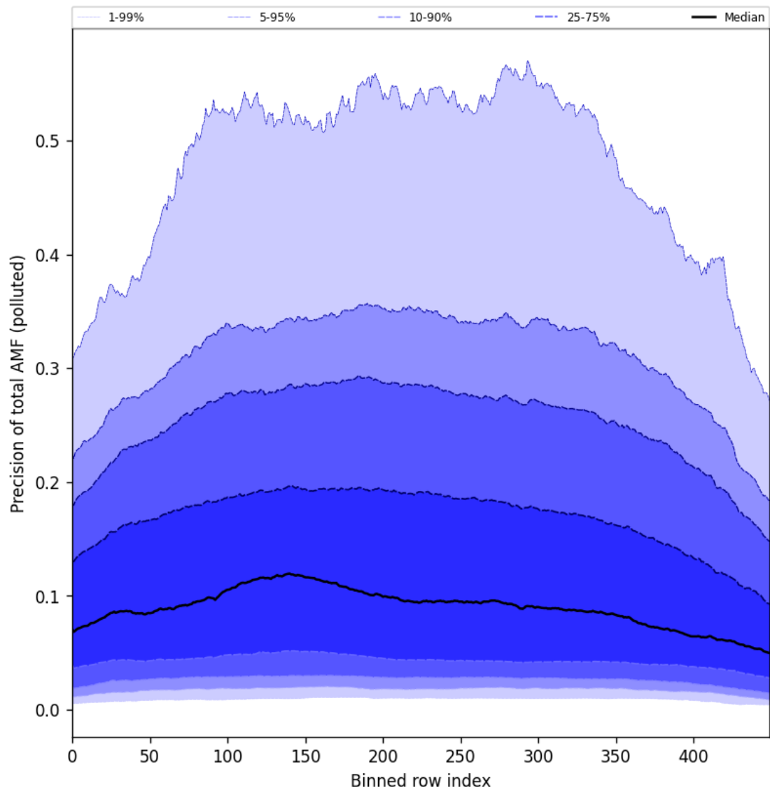
Figure 95: Along track statistics of “Precision of total AMF (polluted)” for 2024-10-16 to 2024-10-18
