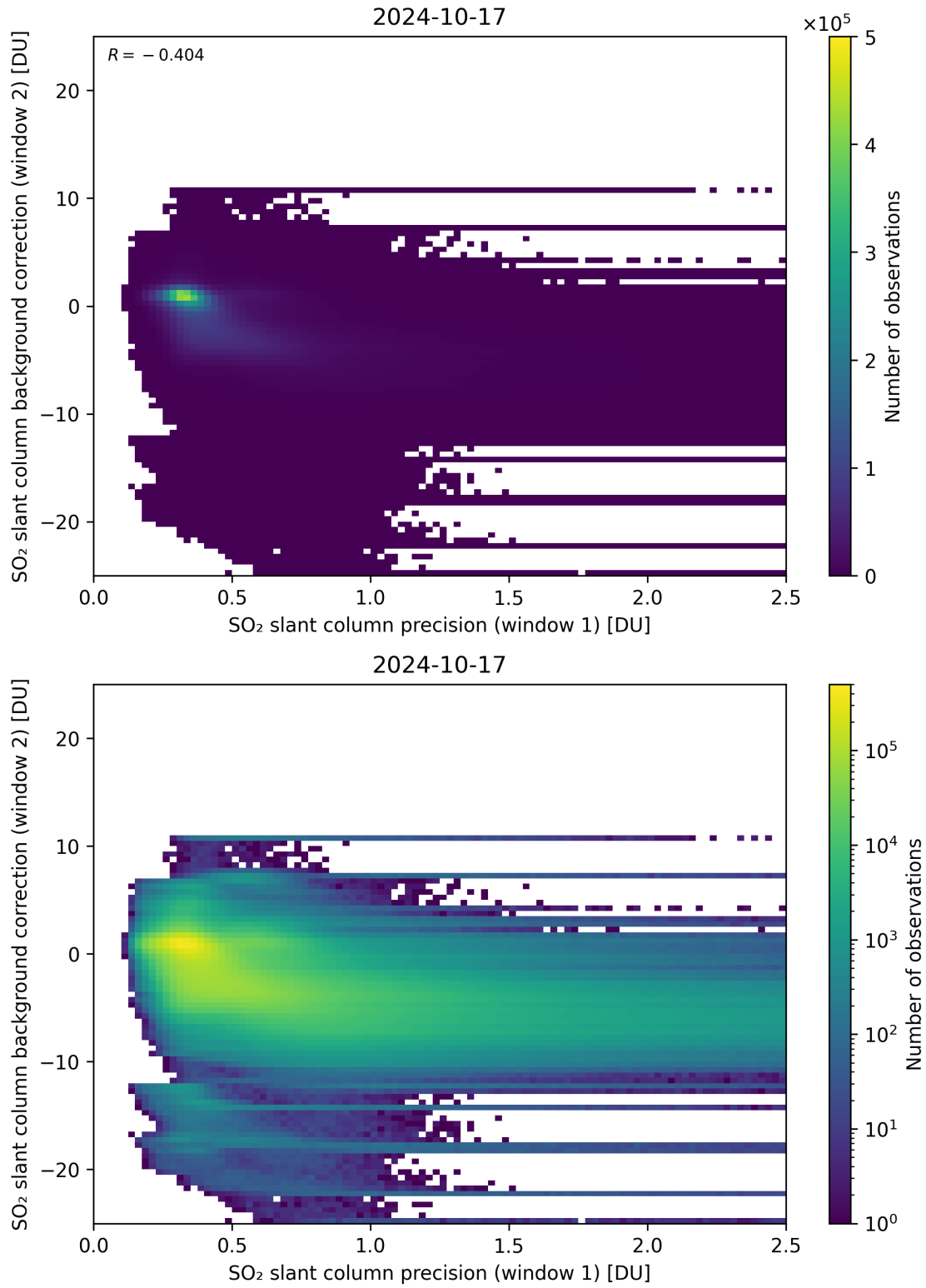
Figure 219: Scatter density plot of “SO 2 slant column precision (window 1)” against “SO 2 slant column background correction (window 2)” for 2024-10-16 to 2024-10-18.
