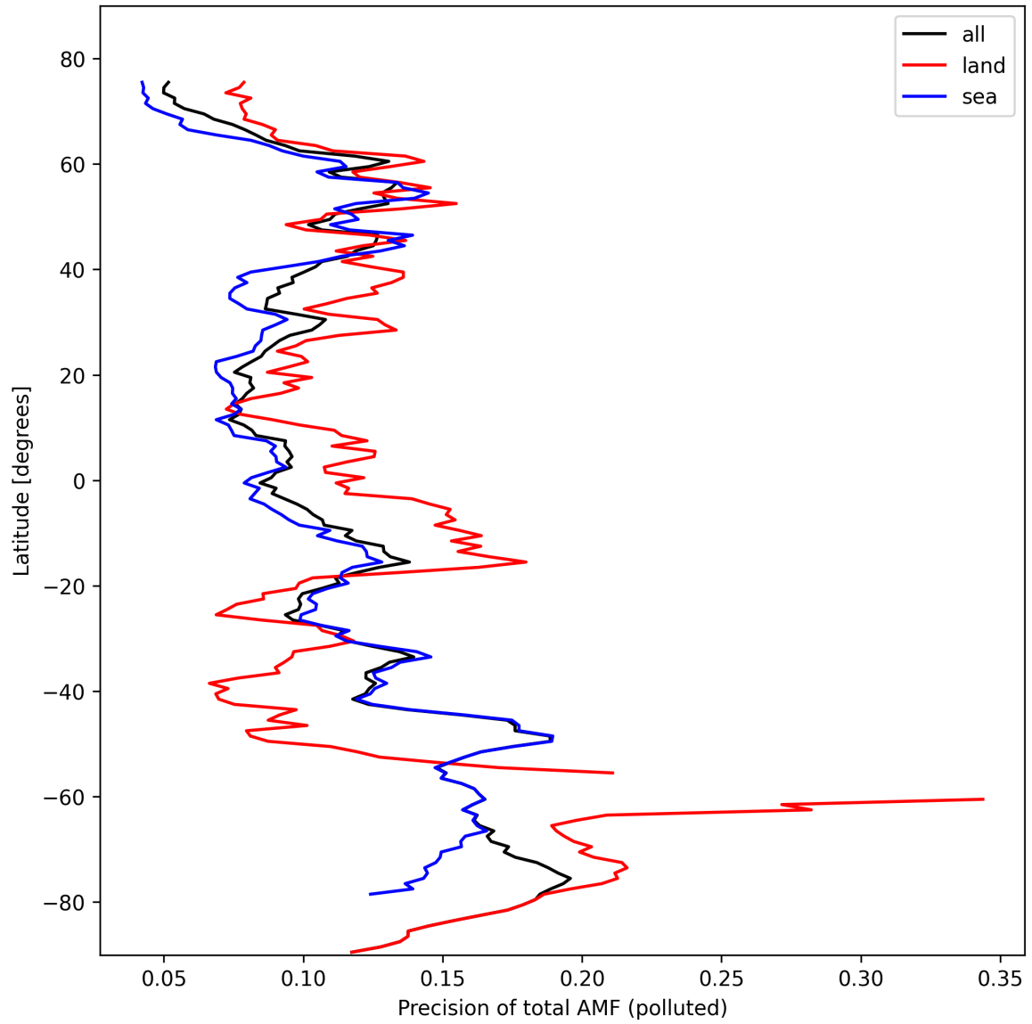
Figure 49: Zonal average of “Precision of total AMF (polluted)” for 2024-10-16 to 2024-10-18.
