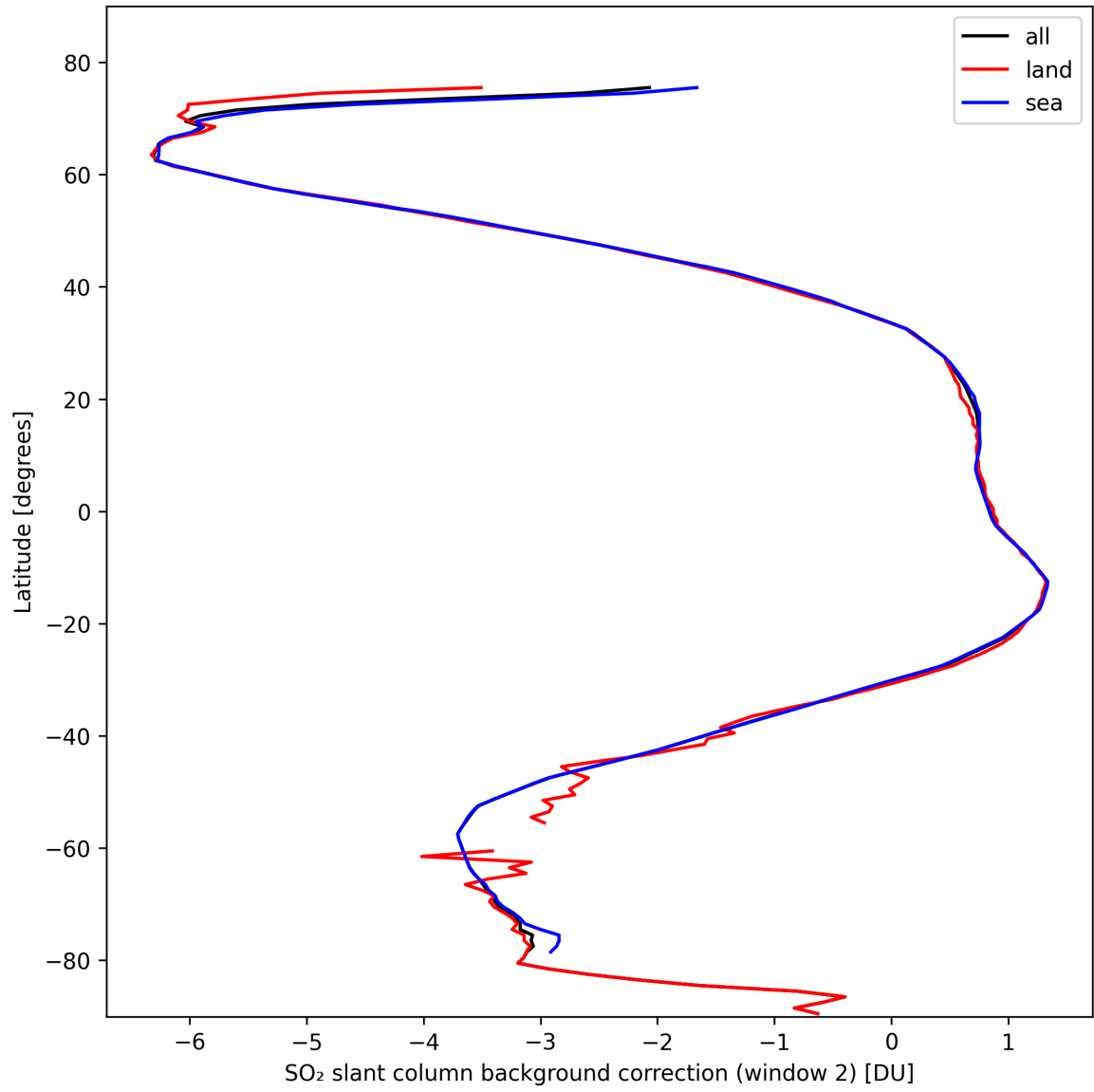
Figure 40: Zonal average of “SO 2 slant column background correction (window 2)” for 2024-10-16 to 2024-10-18.
