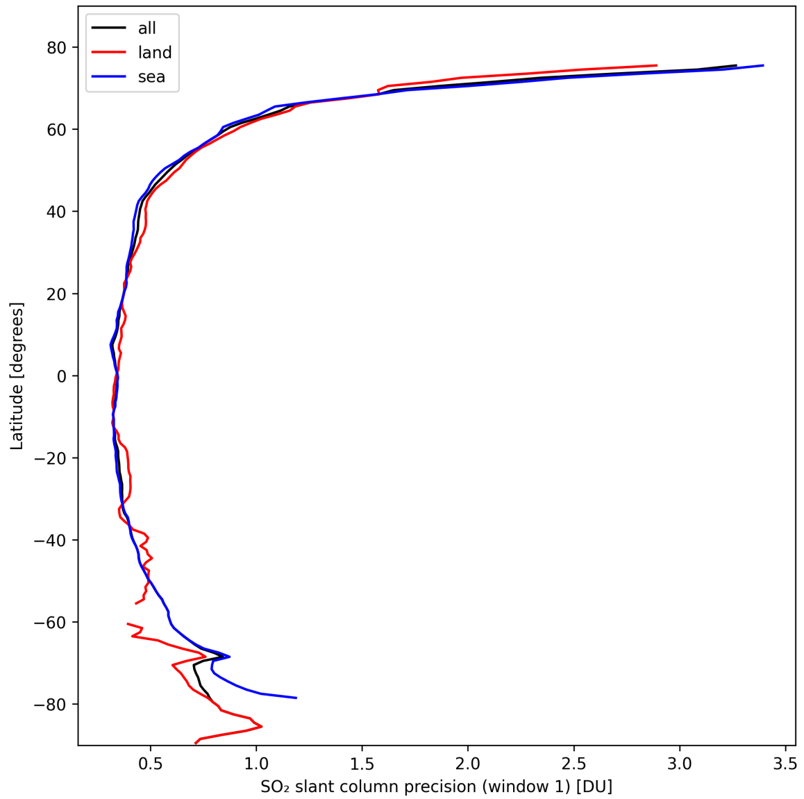
Figure 34: Zonal average of “SO 2 slant column precision (window 1)” for 2024-10-16 to 2024-10-18.
