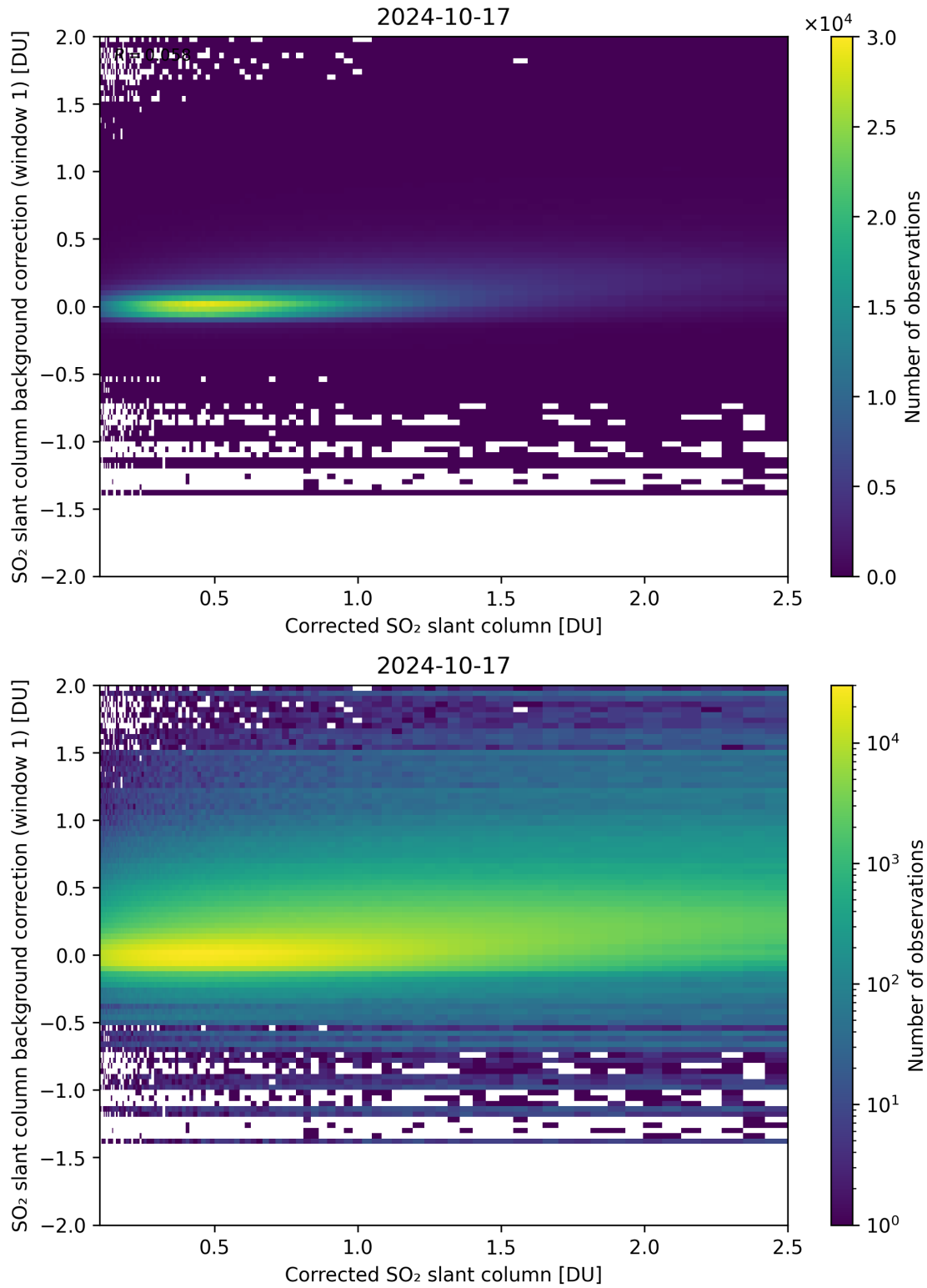
Figure 178: Scatter density plot of “Corrected SO 2 slant column” against “SO 2 slant column background correction (window 1)” for 2024-10-16 to 2024-10-18.
