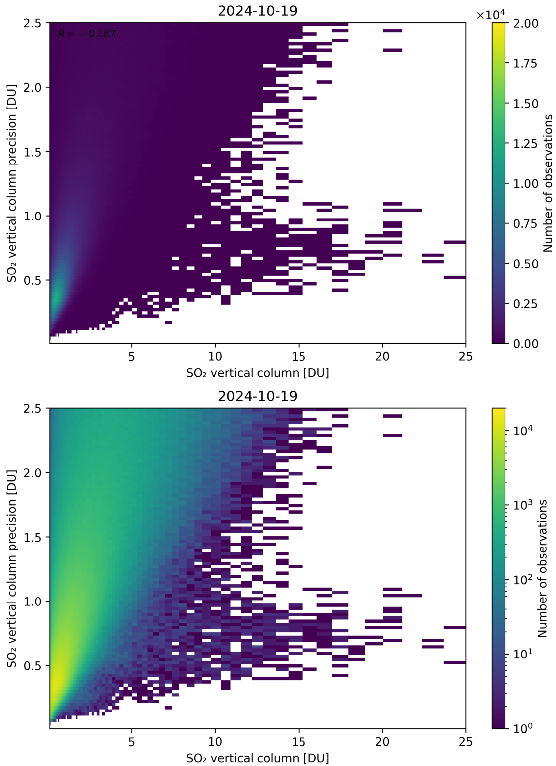
Figure 307: Scatter density plot of “SO 2 vertical column” against “SO 2 vertical column precision” for 2024-10-19 to 2024-10-20.
