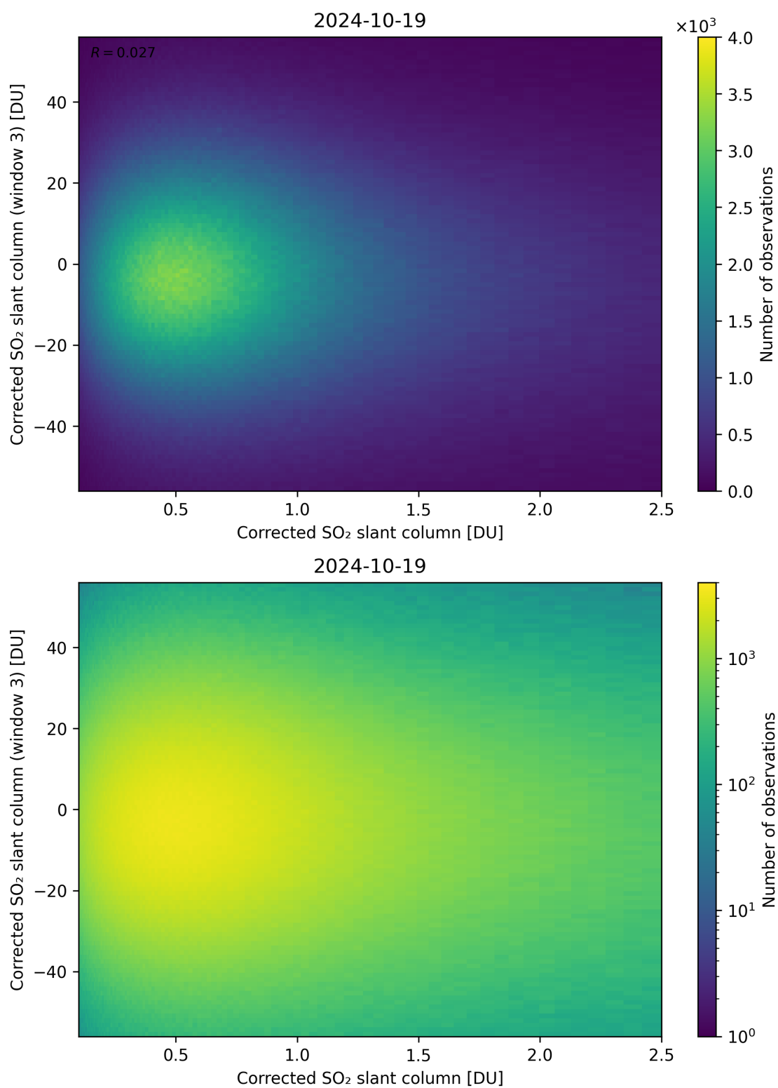
Figure 186: Scatter density plot of “Corrected SO 2 slant column” against “Corrected SO 2 slant column (window 3)” for 2024-10-19 to 2024-10-20.
