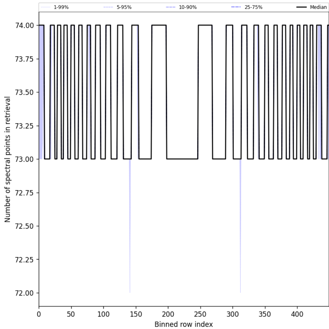
Figure 97: Along track statistics of “Number of spectral points in retrieval” for 2024-10-19 to 2024-10-20
