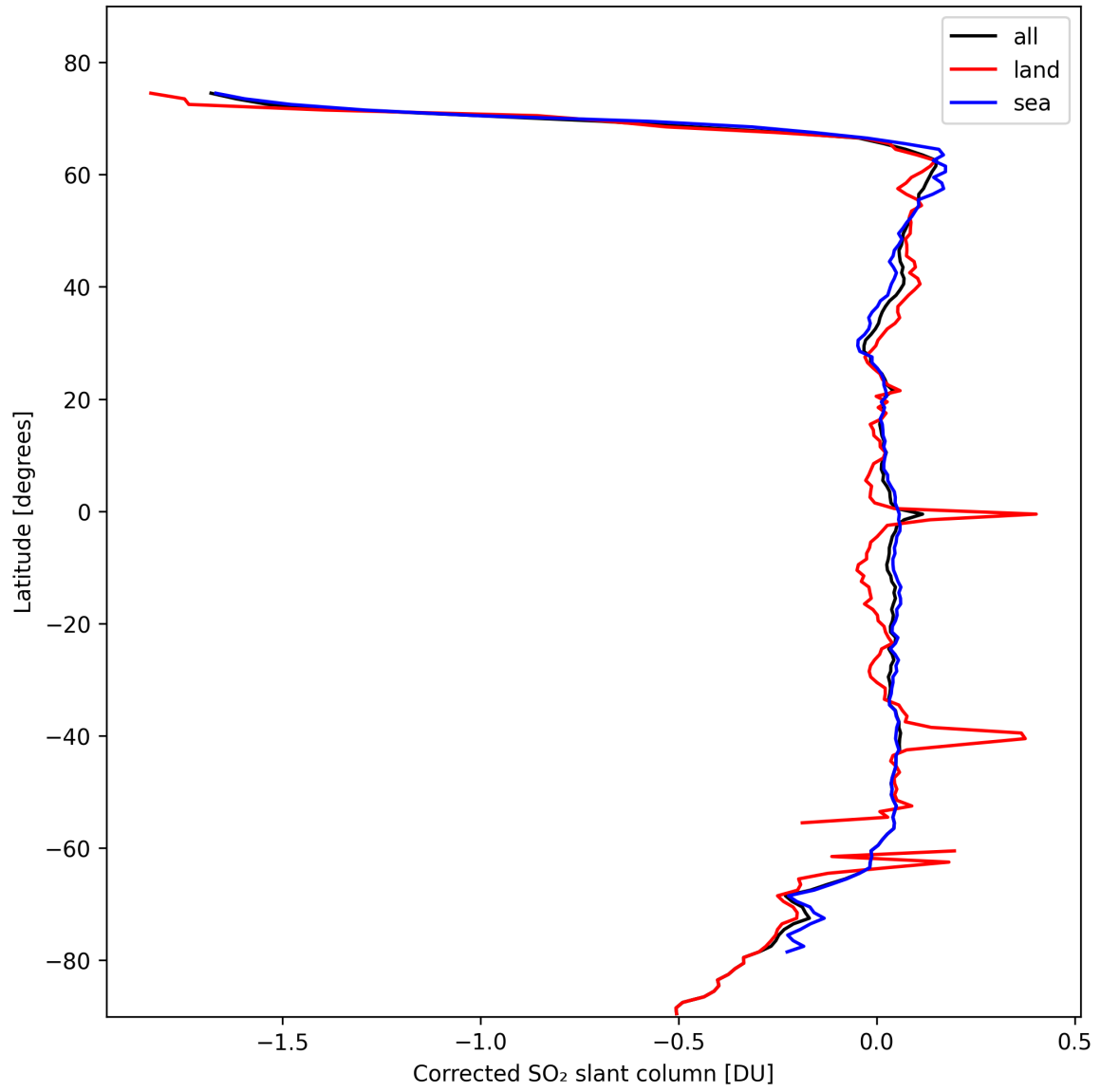
Figure 32: Zonal average of “Corrected SO 2 slant column” for 2024-10-19 to 2024-10-20.
