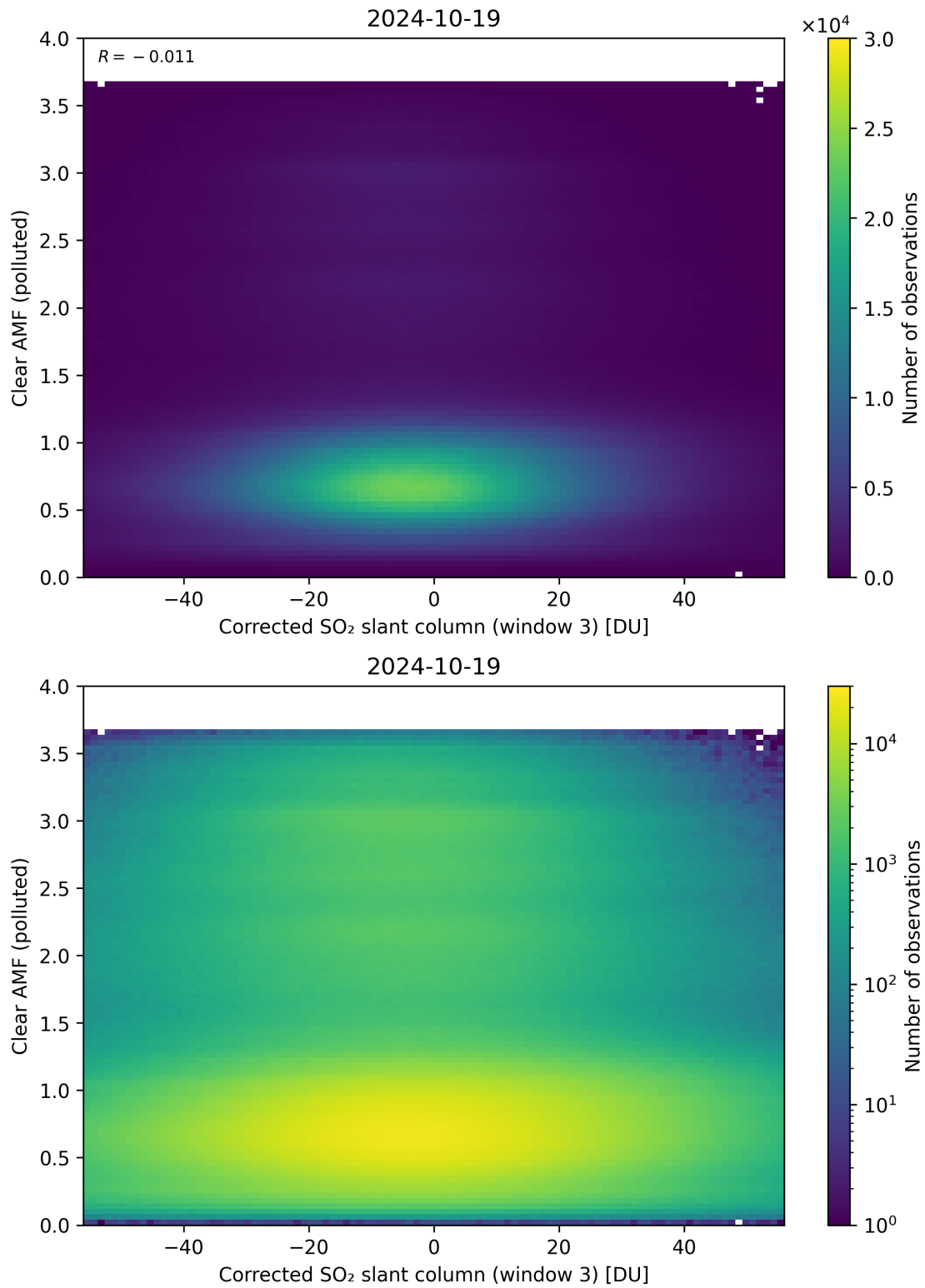
Figure 209: Scatter density plot of “Corrected SO 2 slant column (window 3)” against “Clear AMF (polluted)” for 2024-10-19 to 2024-10-20.
