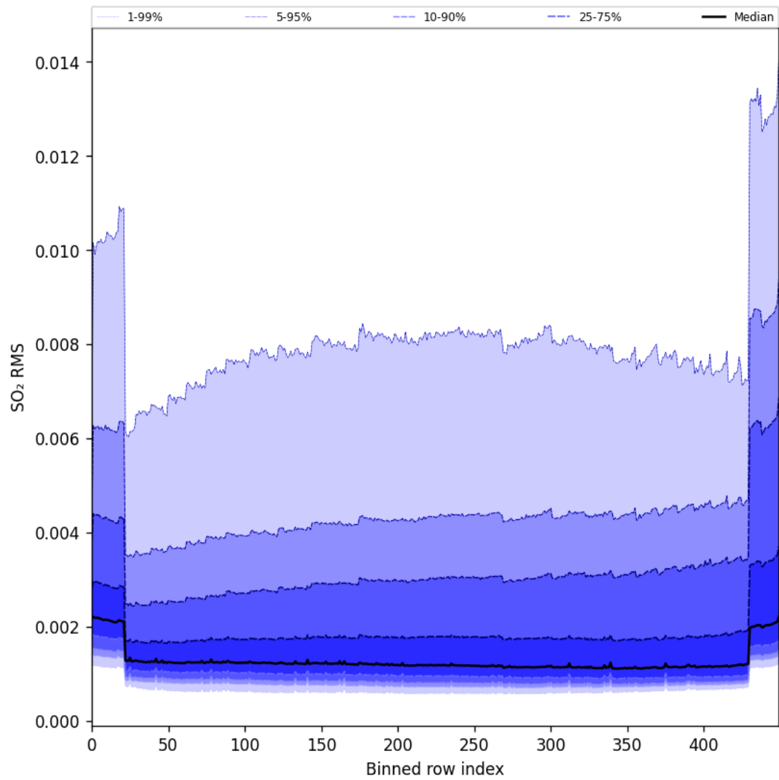
Figure 93: Along track statistics of “SO 2 RMS” for 2024-10-19 to 2024-10-20
