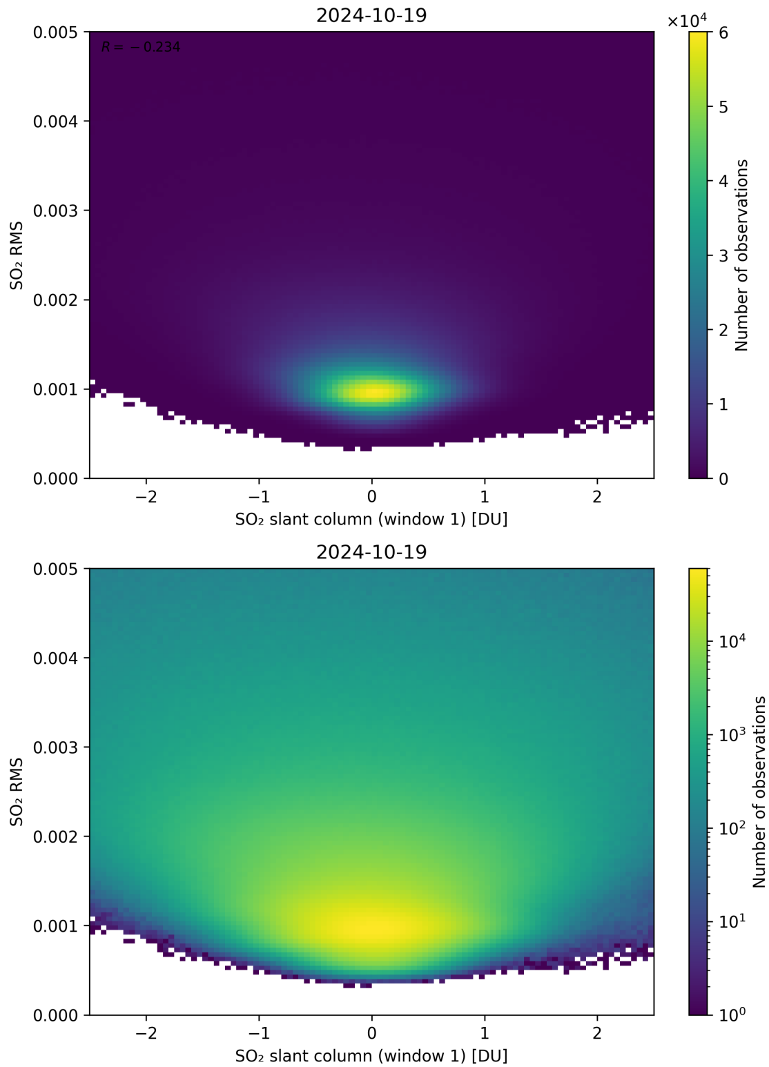
Figure 217: Scatter density plot of “SO 2 slant column (window 1)” against “SO 2 RMS” for 2024-10-19 to 2024-10-20.
