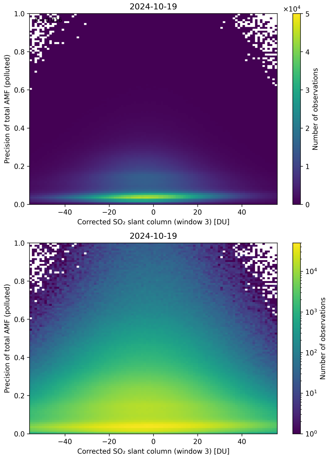
Figure 211: Scatter density plot of “Corrected SO 2 slant column (window 3)” against “Precision of total AMF (polluted)” for 2024-10-19 to 2024-10-20.
