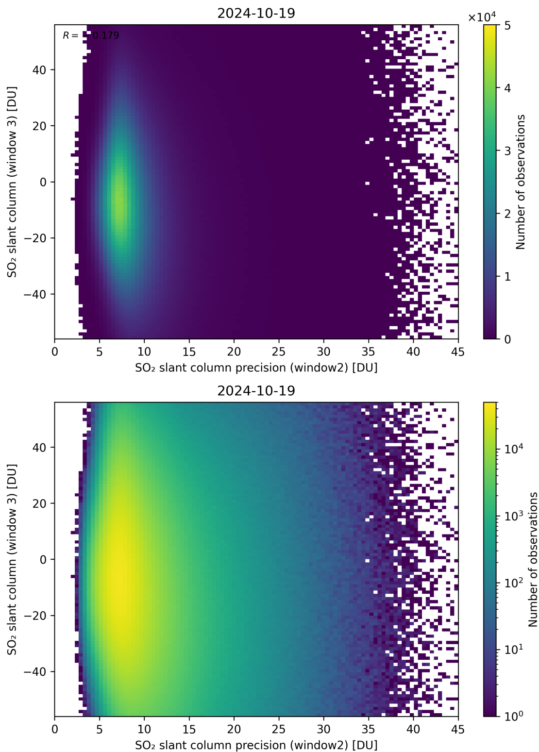
Figure 249: Scatter density plot of “SO 2 slant column precision (window2)” against “SO 2 slant column (window 3)” for 2024-10-19 to 2024-10-20.
