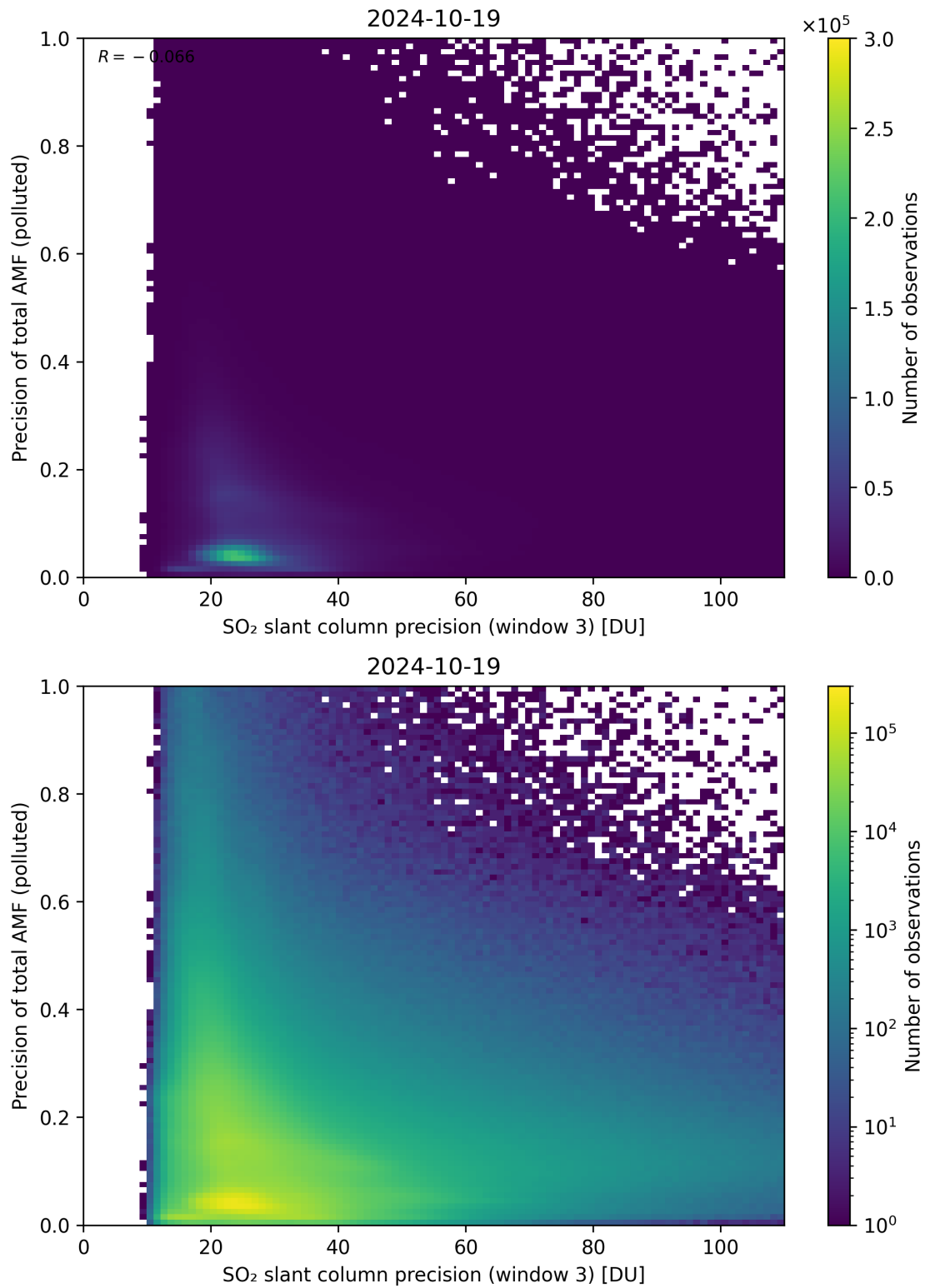
Figure 264: Scatter density plot of “SO 2 slant column precision (window 3)” against “Precision of total AMF (polluted)” for 2024-10-19 to 2024-10-20.
