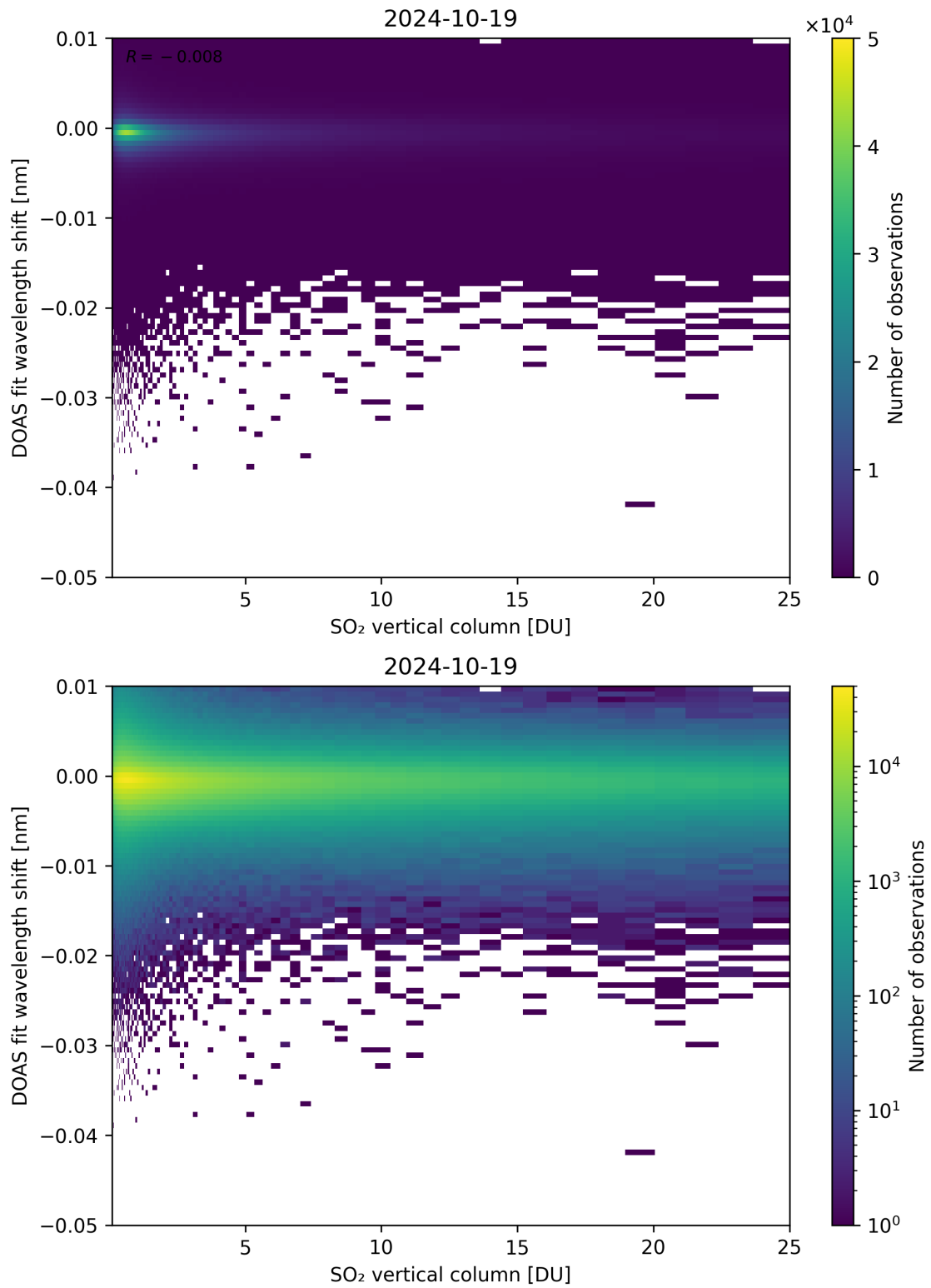
Figure 276: Scatter density plot of “SO 2 vertical column” against “DOAS fit wavelength shift” for 2024-10-19 to 2024-10-20.
