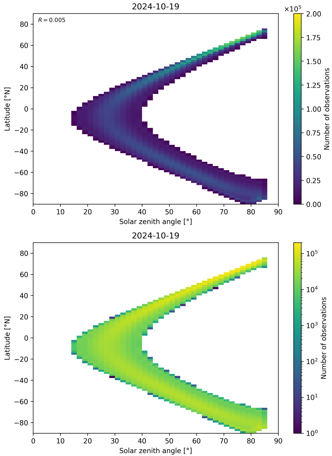
Figure 164: Scatter density plot of “Solar zenith angle” against “Latitude” for 2024-10-19 to 2024-10-20.
