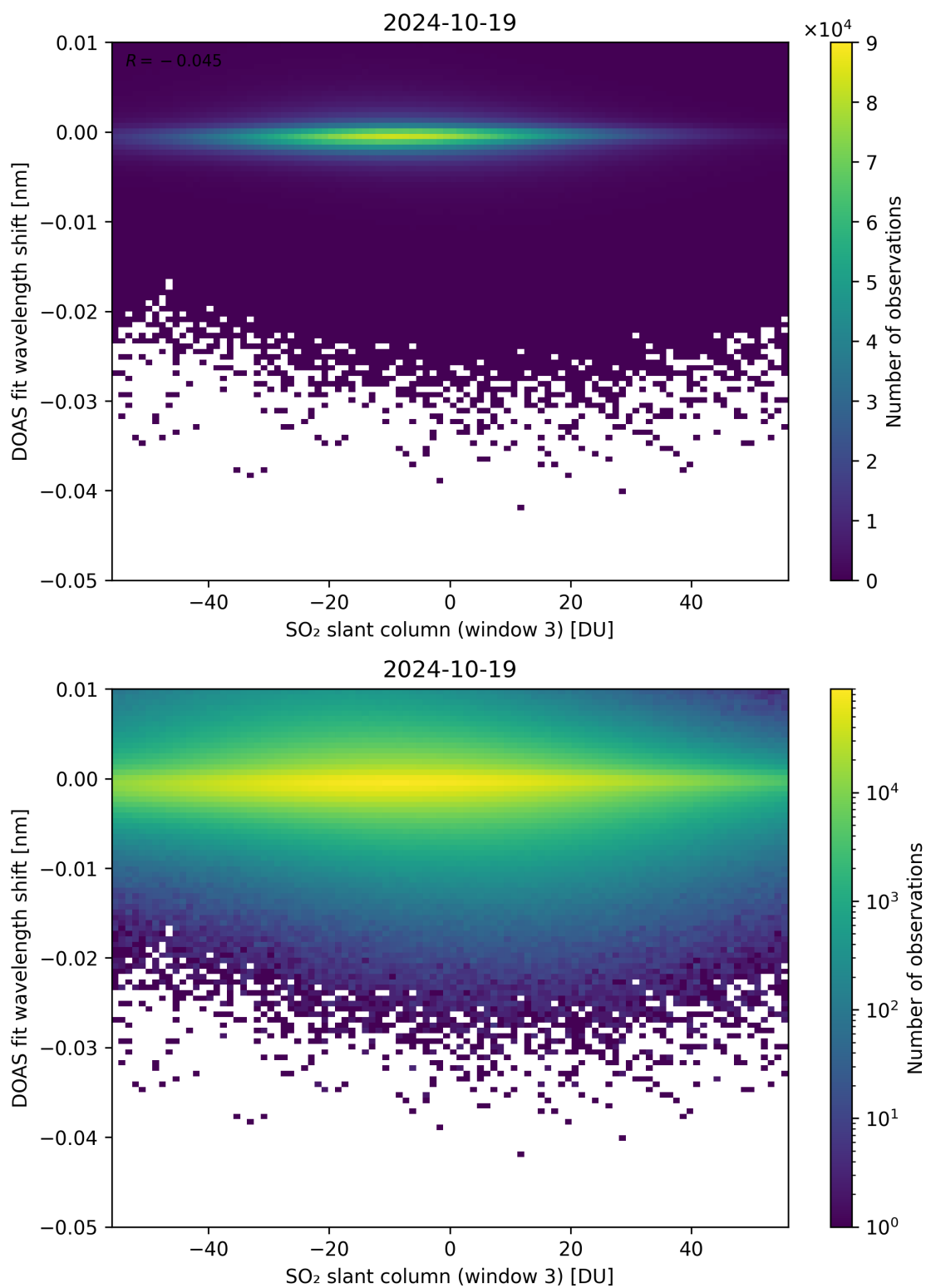
Figure 254: Scatter density plot of “SO 2 slant column (window 3)” against “DOAS fit wavelength shift” for 2024-10-19 to 2024-10-20.
