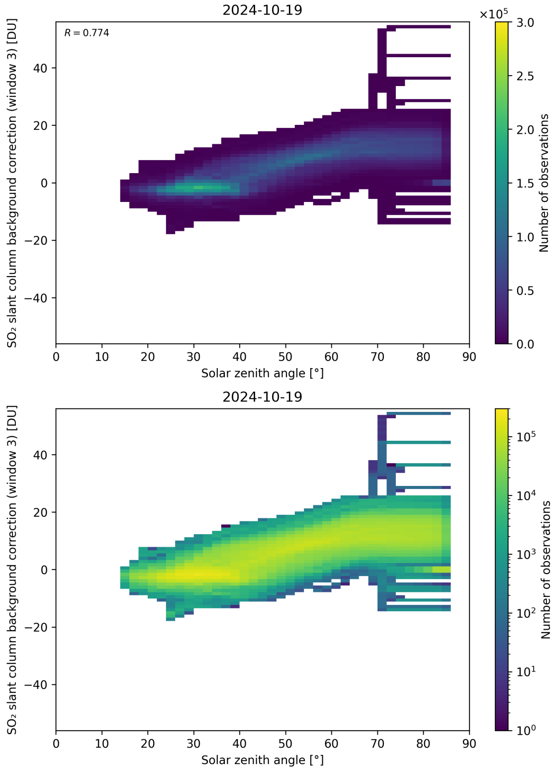
Figure 160: Scatter density plot of “Solar zenith angle” against “SO 2 slant column background correction (window 3)” for 2024-10-19 to 2024-10-20.
