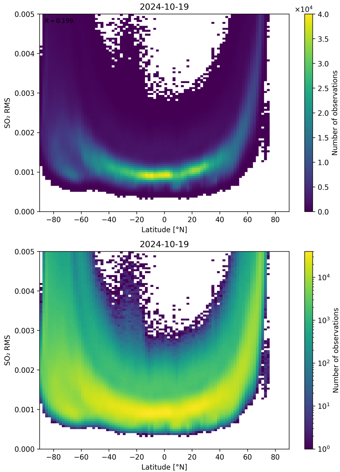
Figure 144: Scatter density plot of “Latitude” against “SO 2 RMS” for 2024-10-19 to 2024-10-20.
