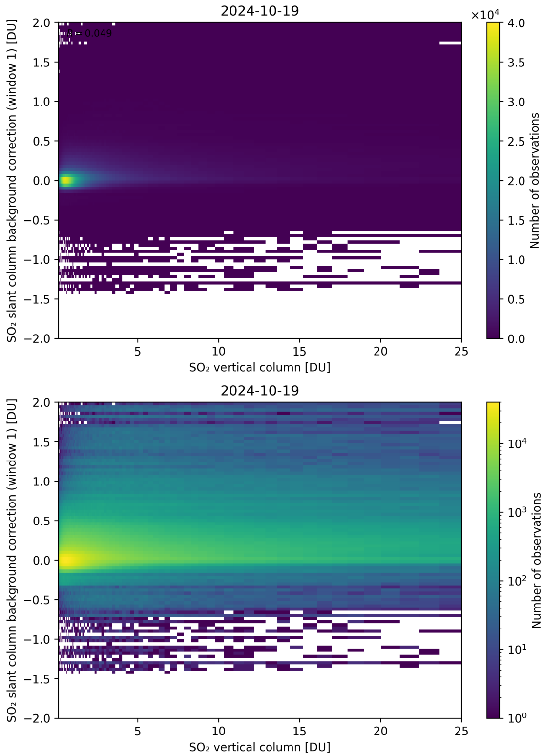
Figure 273: Scatter density plot of “SO 2 vertical column” against “SO 2 slant column background correction (window 1)” for 2024-10-19 to 2024-10-20.
