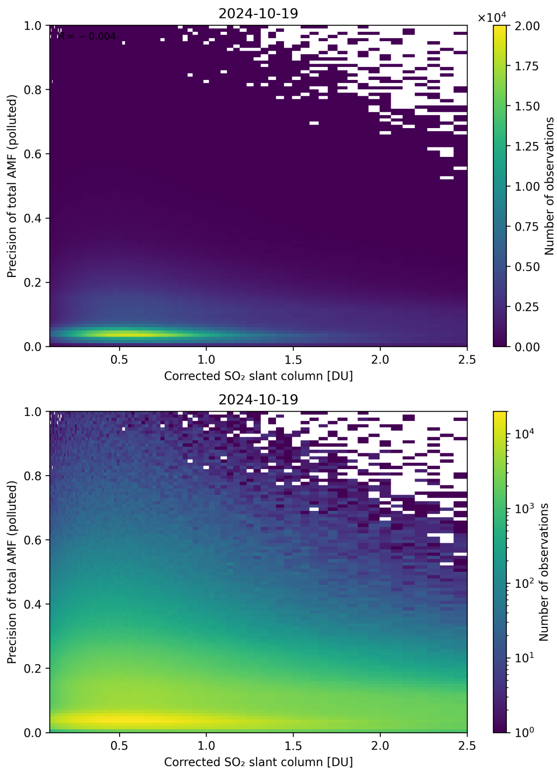
Figure 193: Scatter density plot of “Corrected SO 2 slant column” against “Precision of total AMF (polluted)” for 2024-10-19 to 2024-10-20.
