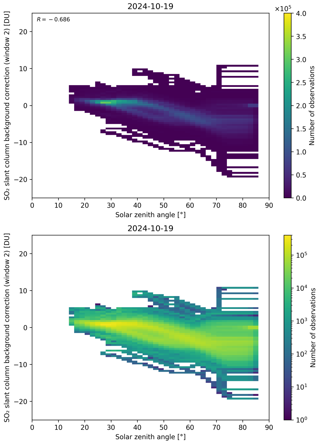
Figure 159: Scatter density plot of “Solar zenith angle” against “SO 2 slant column background correction (window 2)” for 2024-10-19 to 2024-10-20.
