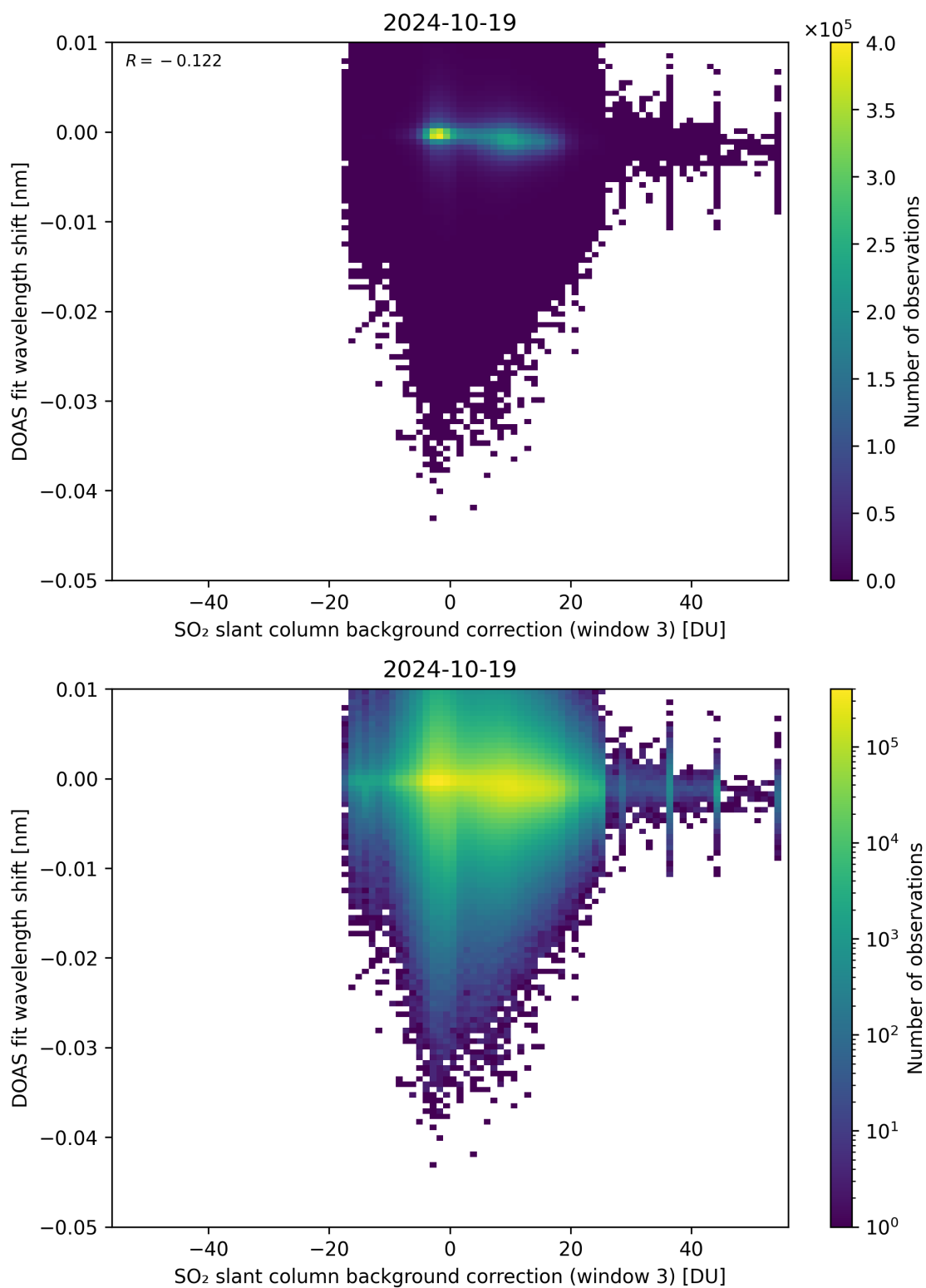
Figure 121: Scatter density plot of “SO 2 slant column background correction (window 3)” against “DOAS fit wavelength shift” for 2024-10-19 to 2024-10-20.
