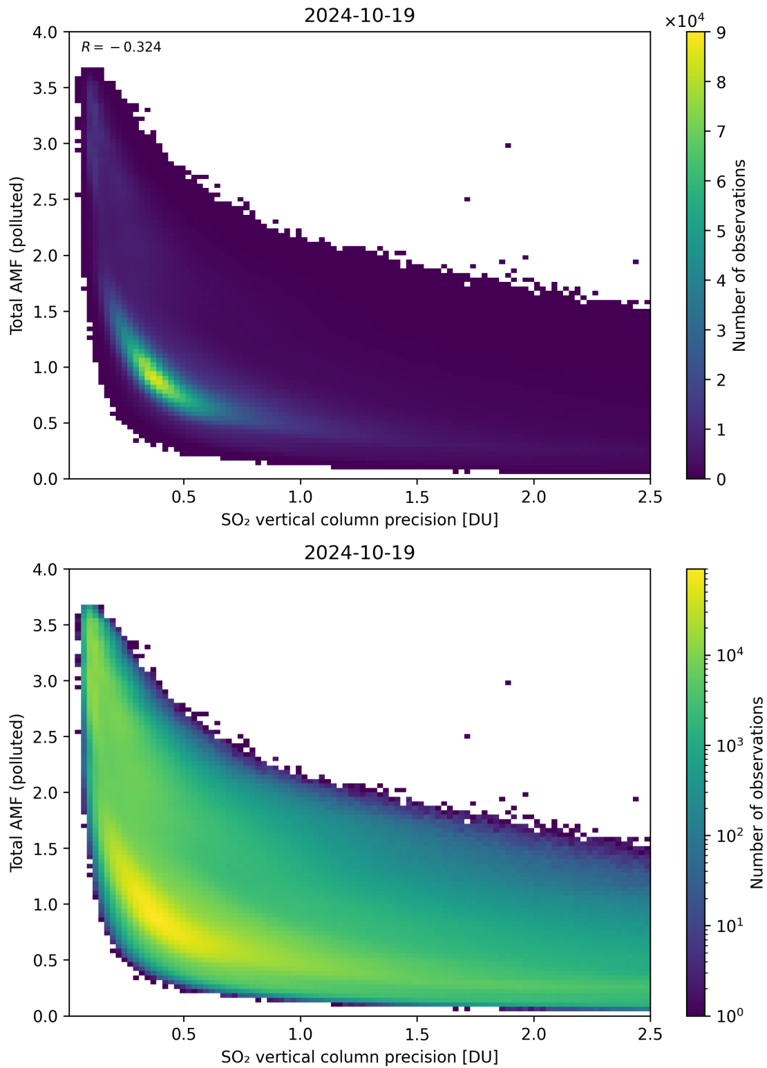
Figure 294: Scatter density plot of “SO 2 vertical column precision” against “Total AMF (polluted)” for 2024-10-19 to 2024-10-20.
