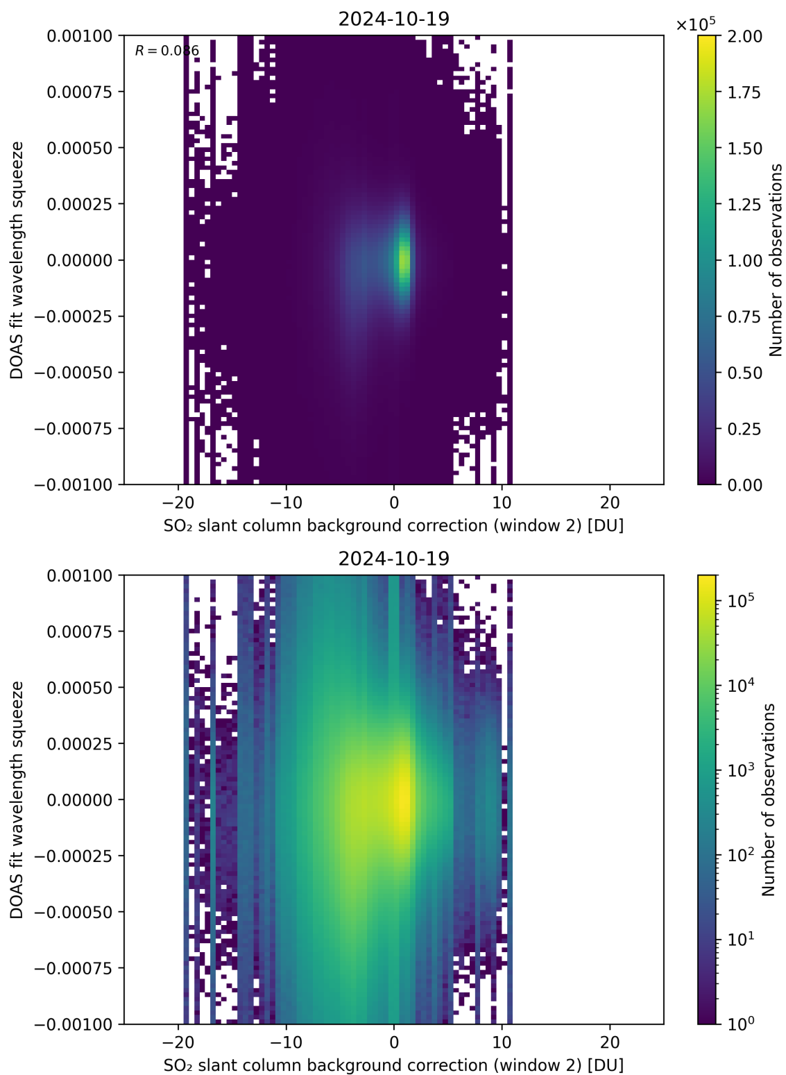
Figure 113: Scatter density plot of “SO 2 slant column background correction (window 2)” against “DOAS fit wavelength squeeze” for 2024-10-19 to 2024-10-20.
