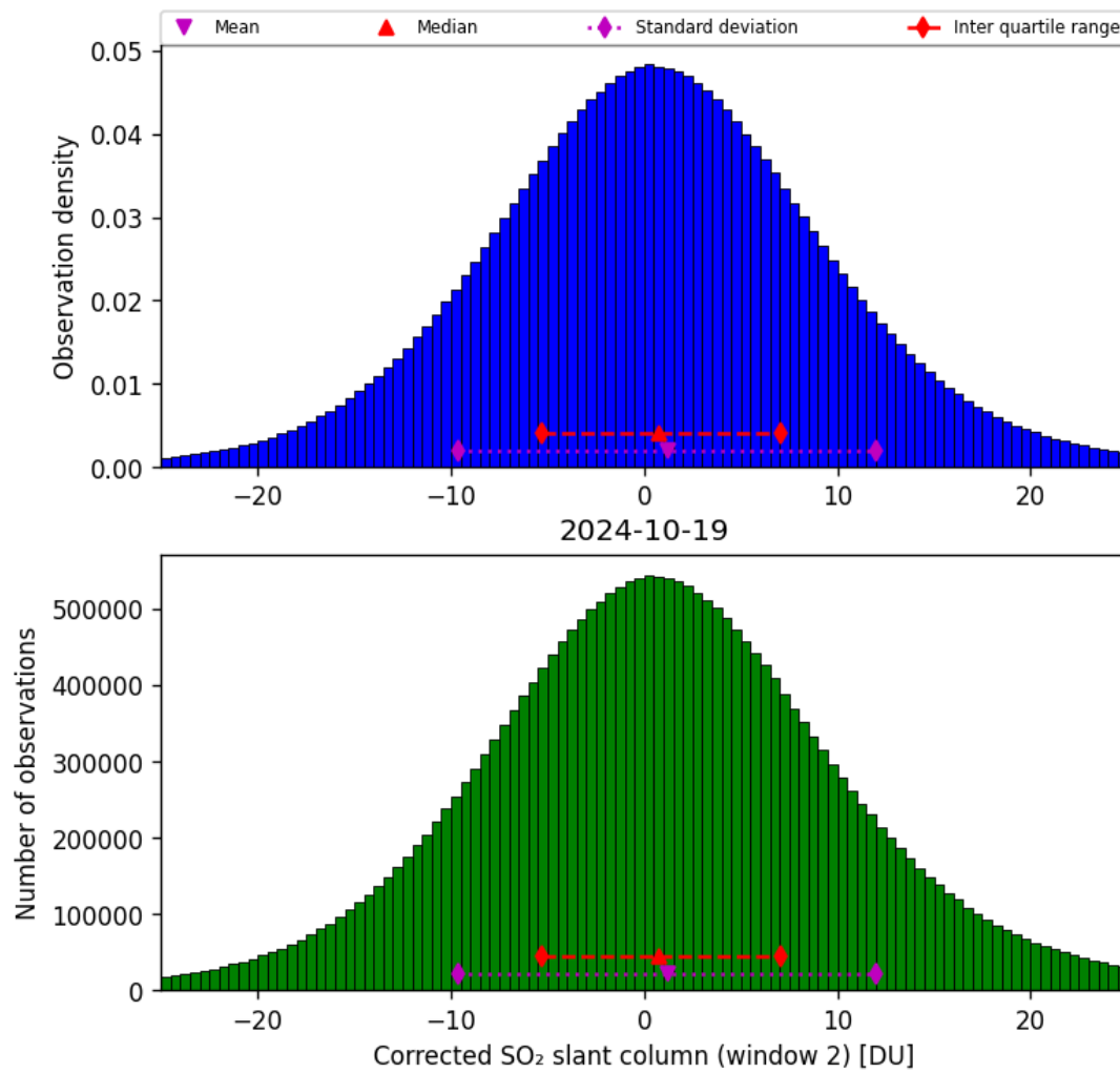
Figure 62: Histogram of “Corrected SO 2 slant column (window 2)” for 2024-10-19 to 2024-10-20
