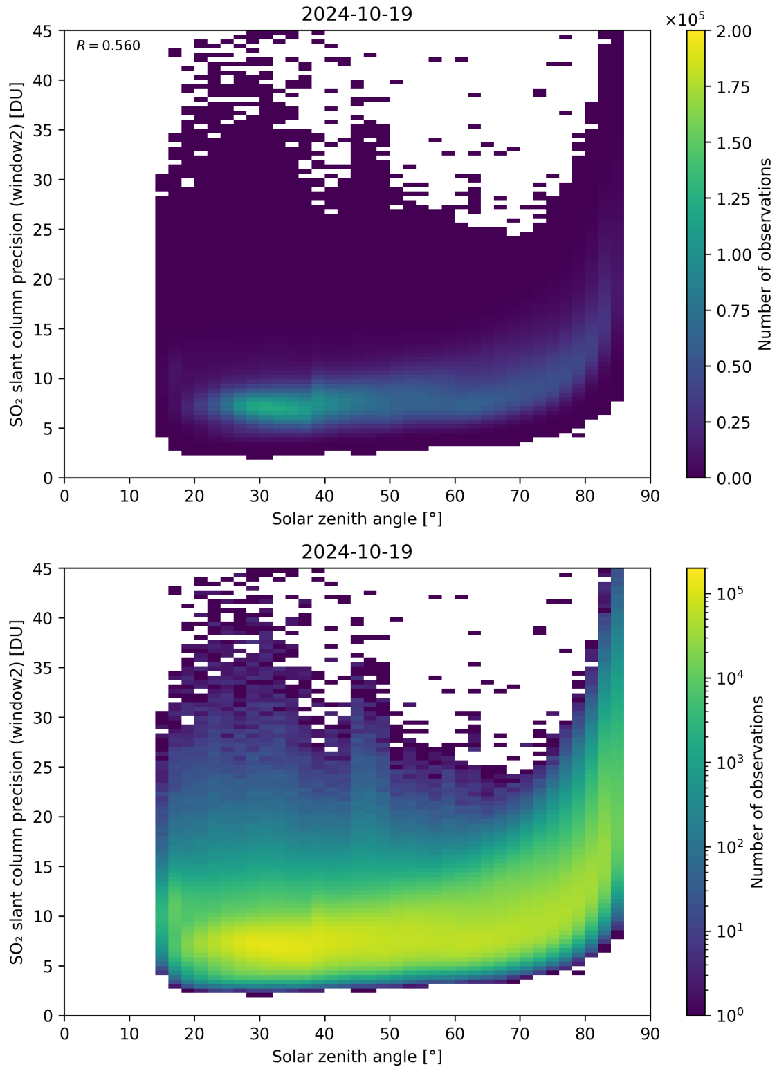
Figure 171: Scatter density plot of “Solar zenith angle” against “SO 2 slant column precision (window2)” for 2024-10-19 to 2024-10-20.
