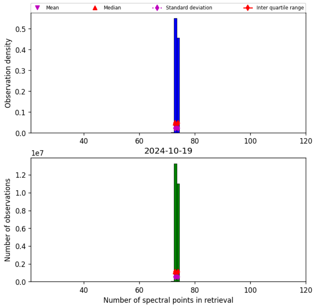
Figure 74: Histogram of “Number of spectral points in retrieval” for 2024-10-19 to 2024-10-20
