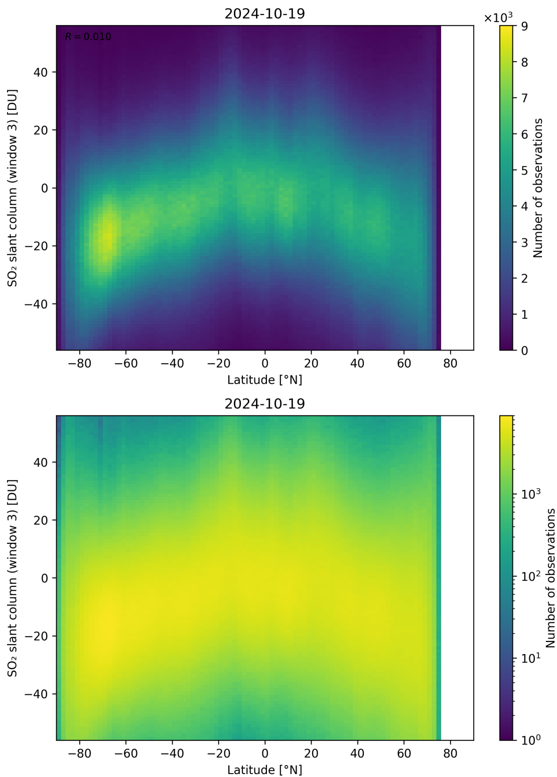
Figure 152: Scatter density plot of “Latitude” against “SO 2 slant column (window 3)” for 2024-10-19 to 2024-10-20.
