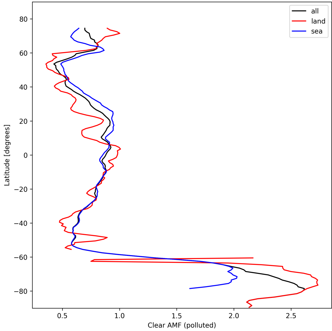
Figure 50: Zonal average of “Clear AMF (polluted)” for 2024-10-19 to 2024-10-20.
