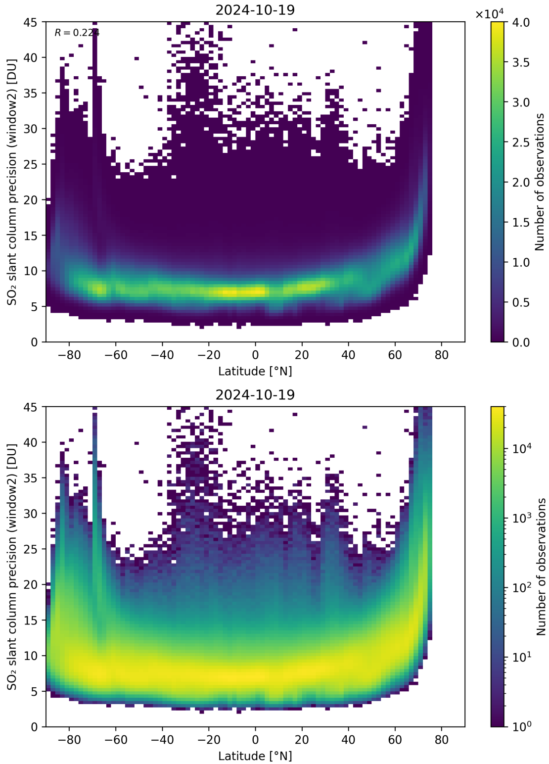
Figure 151: Scatter density plot of “Latitude” against “SO 2 slant column precision (window2)” for 2024-10-19 to 2024-10-20.
