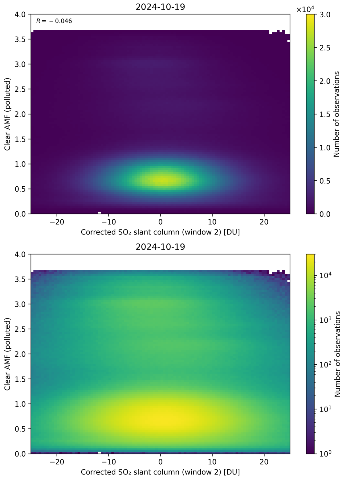
Figure 199: Scatter density plot of “Corrected SO 2 slant column (window 2)” against “Clear AMF (polluted)” for 2024-10-19 to 2024-10-20.
