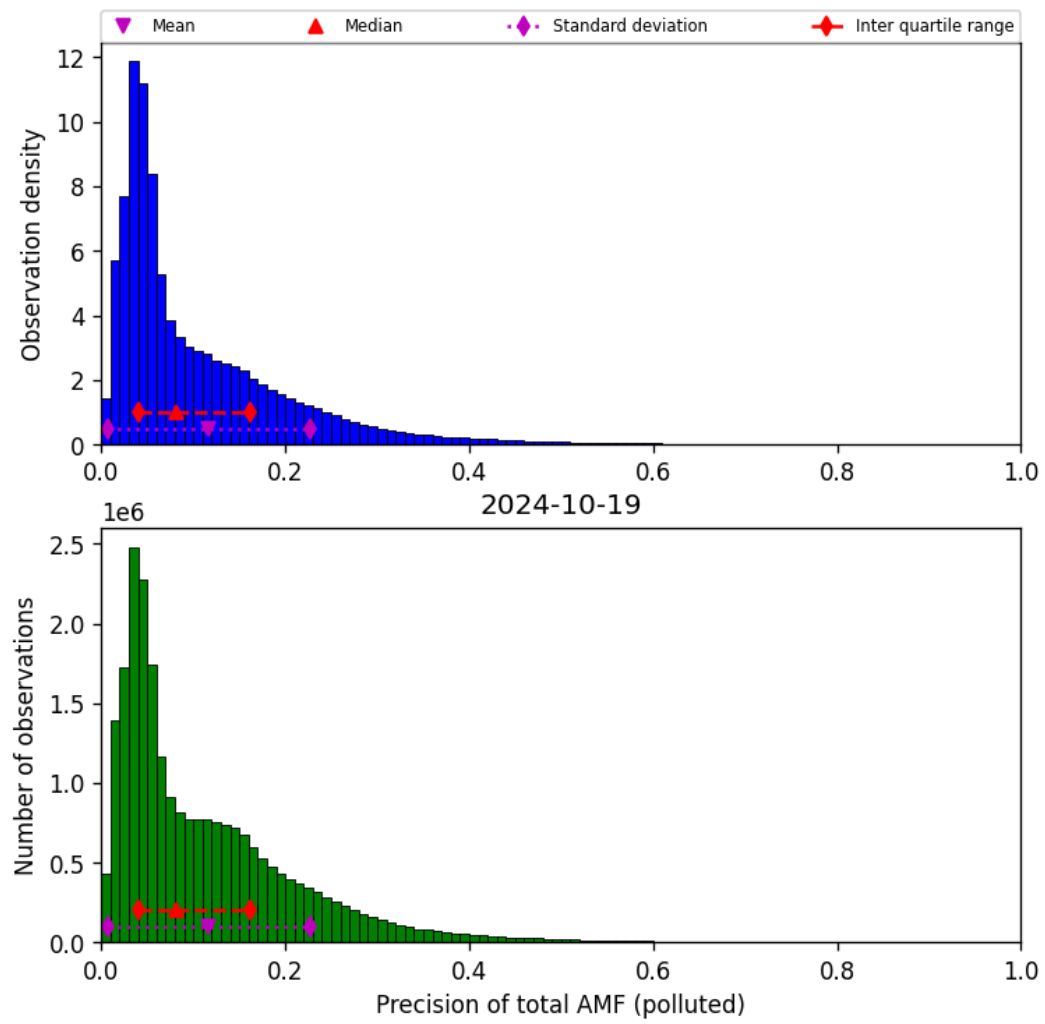
Figure 72: Histogram of “Precision of total AMF (polluted)” for 2024-10-19 to 2024-10-20
