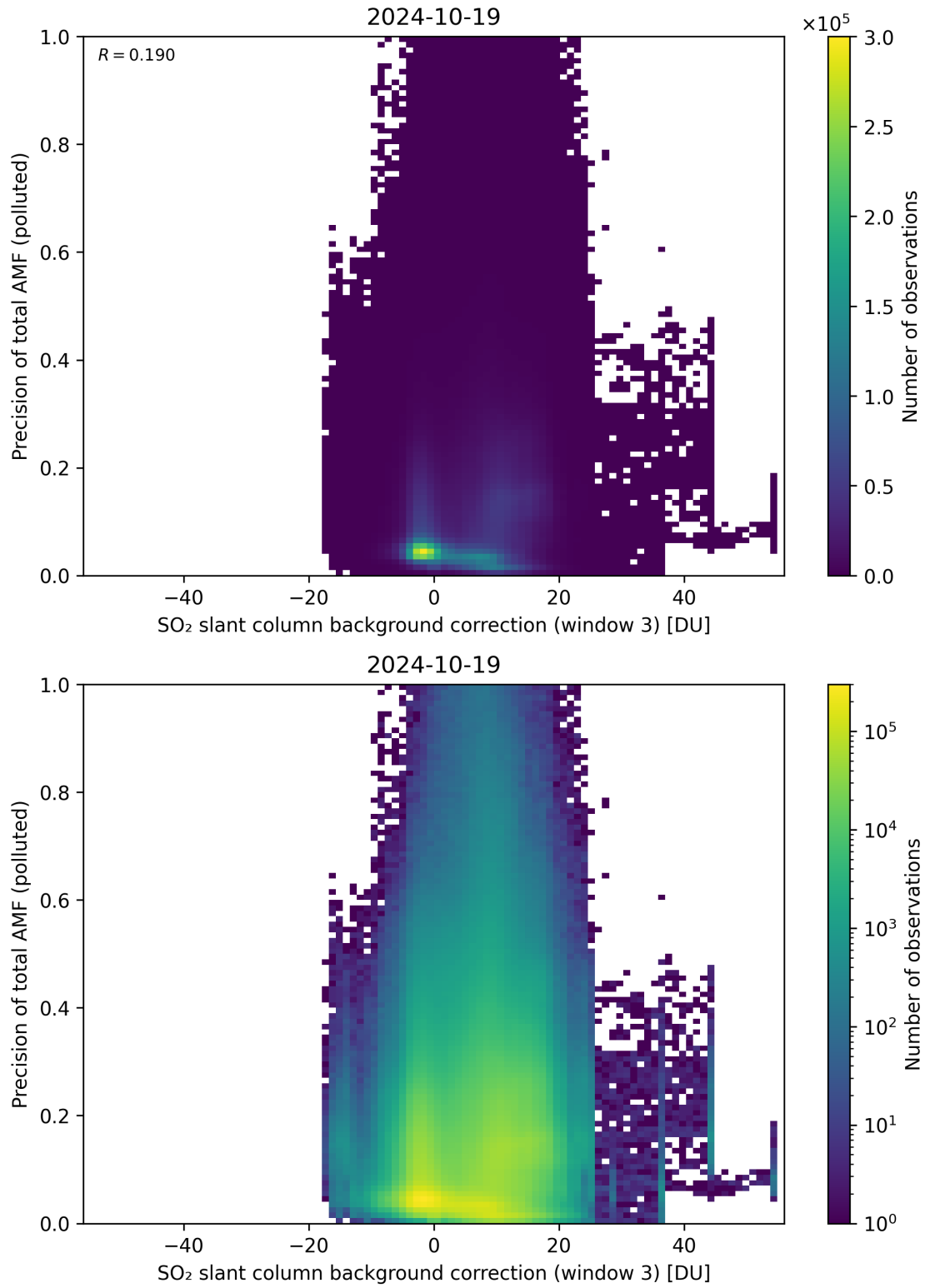
Figure 126: Scatter density plot of “SO 2 slant column background correction (window 3)” against “Precision of total AMF (polluted)” for 2024-10-19 to 2024-10-20.
