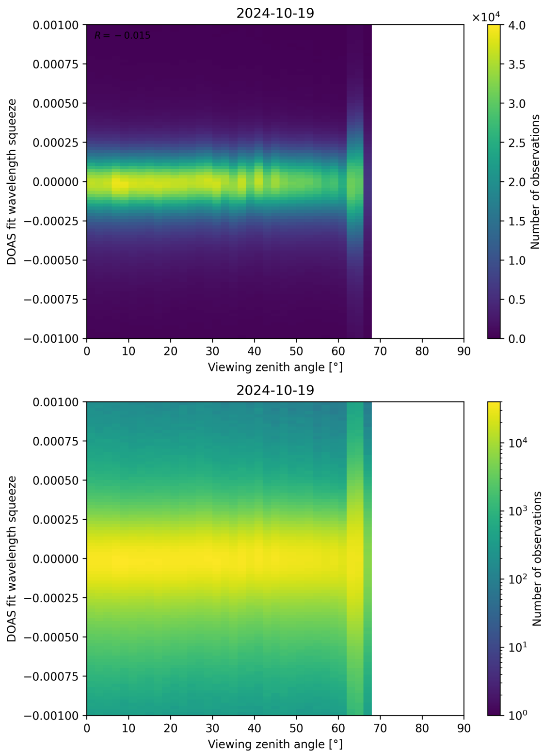
Figure 312: Scatter density plot of “Viewing zenith angle” against “DOAS fit wavelength squeeze” for 2024-10-19 to 2024-10-20.
