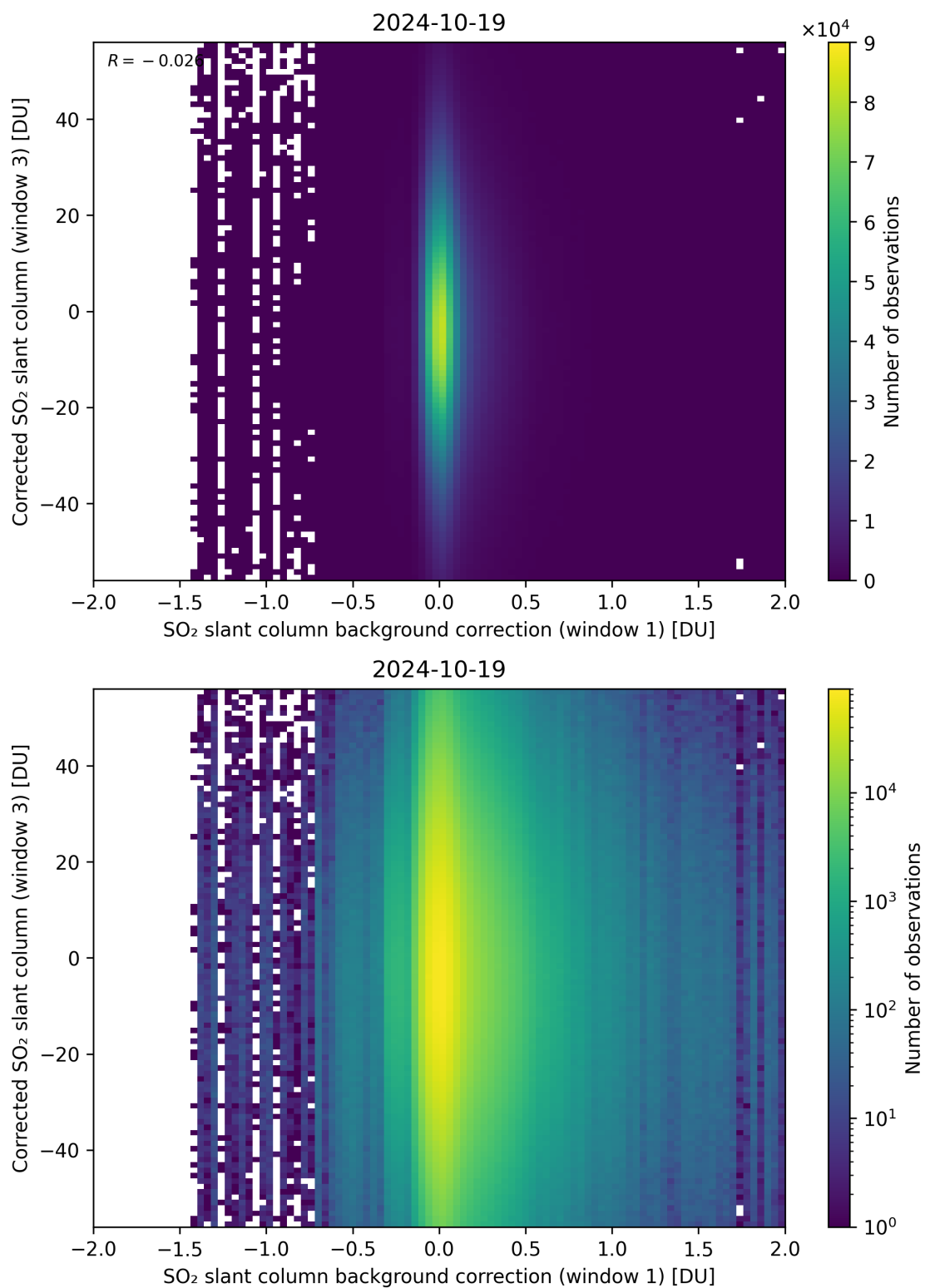
Figure 105: Scatter density plot of “SO 2 slant column background correction (window 1)” against “Corrected SO 2 slant column (window 3)” for 2024-10-19 to 2024-10-20.
