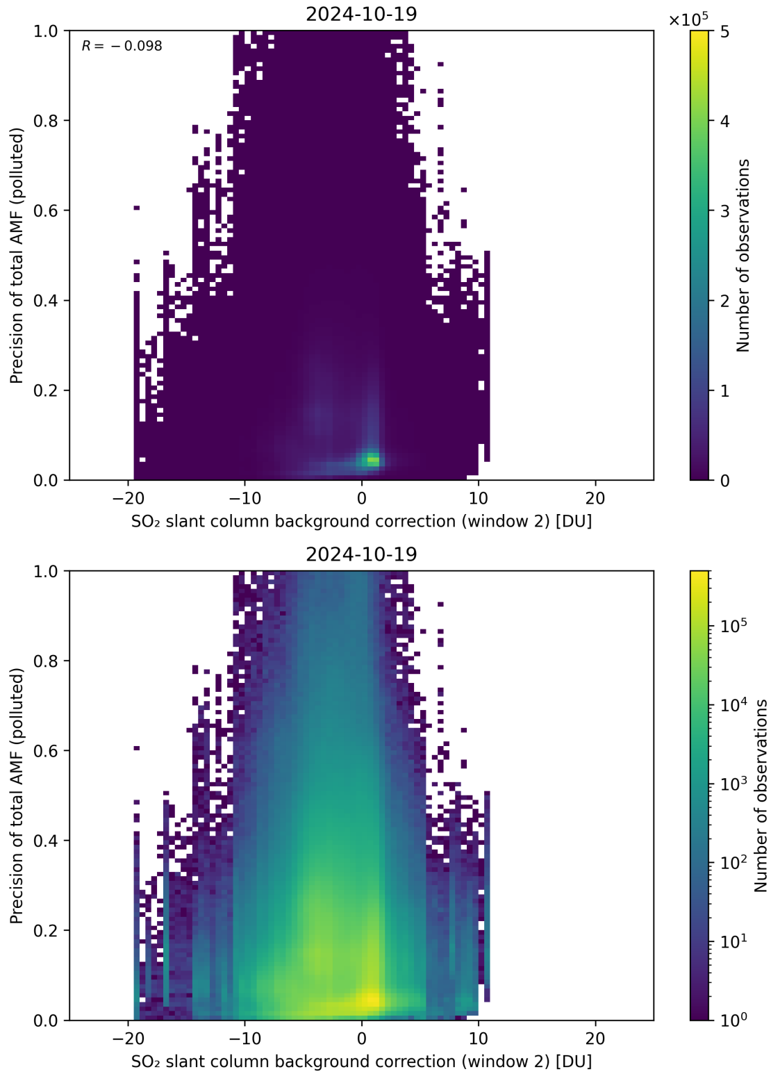
Figure 120: Scatter density plot of “SO 2 slant column background correction (window 2)” against “Precision of total AMF (polluted)” for 2024-10-19 to 2024-10-20.
