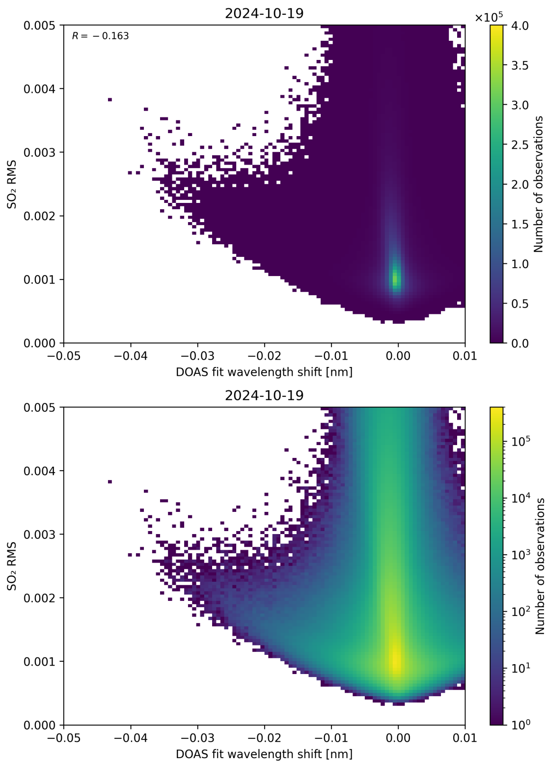
Figure 128: Scatter density plot of “DOAS fit wavelength shift” against “SO 2 RMS” for 2024-10-19 to 2024-10-20.
