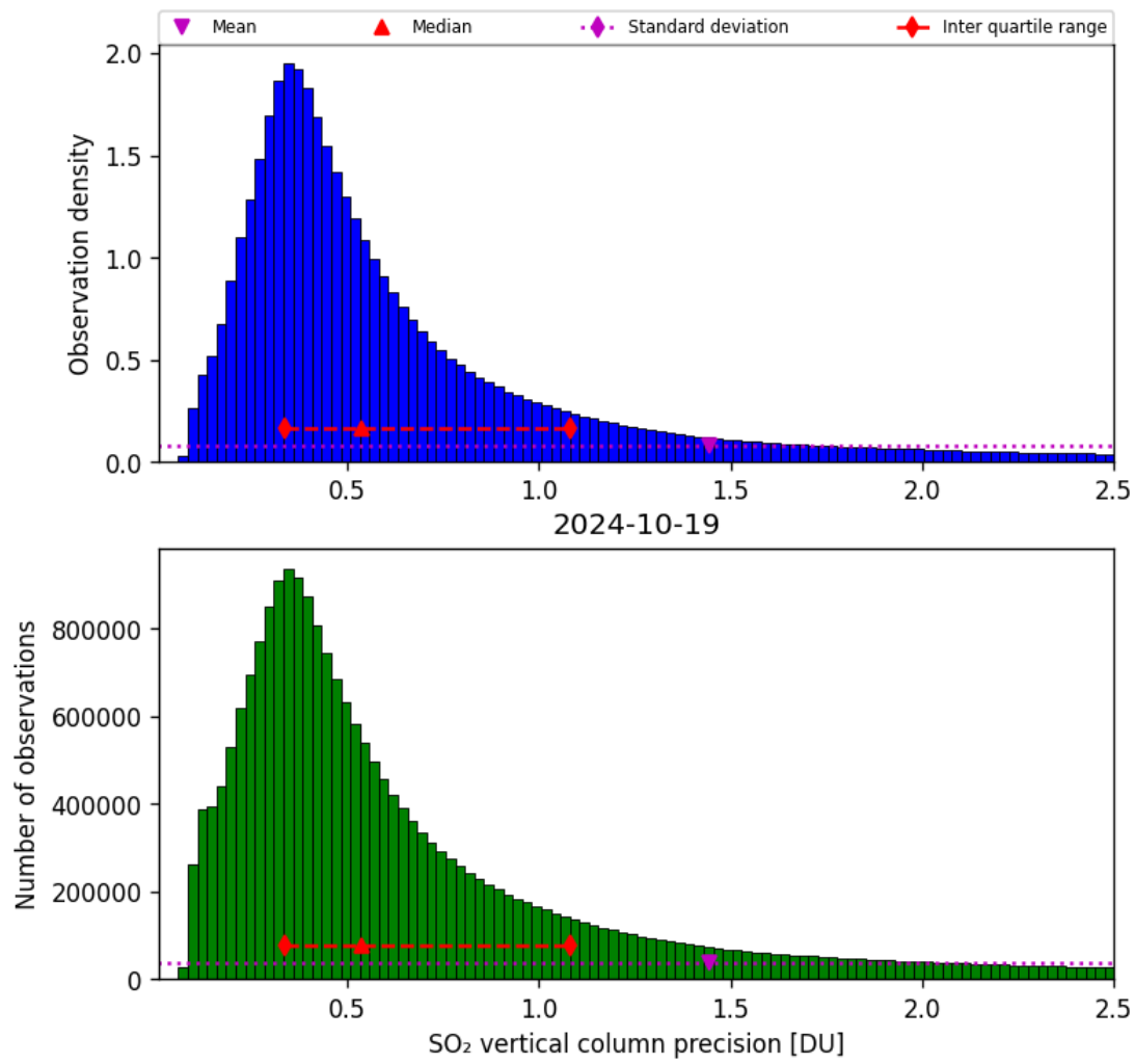
Figure 54: Histogram of “SO 2 vertical column precision” for 2024-10-19 to 2024-10-20
