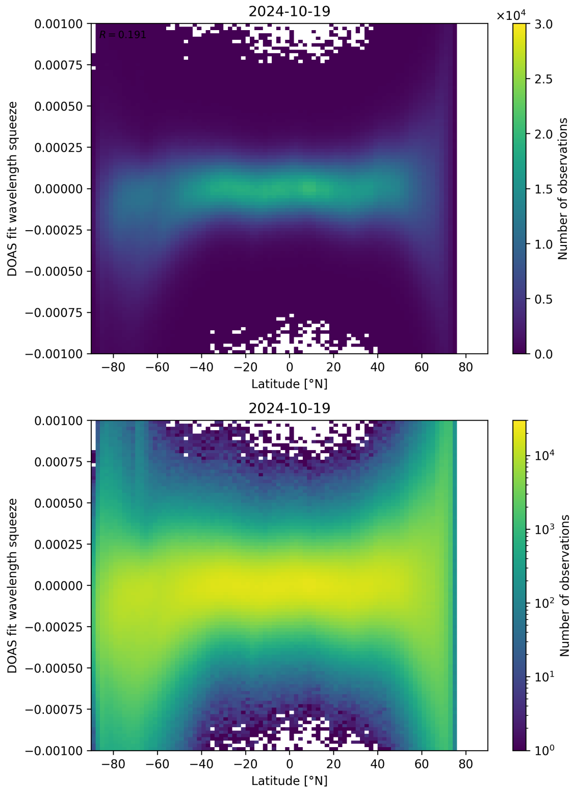
Figure 143: Scatter density plot of “Latitude” against “DOAS fit wavelength squeeze” for 2024-10-19 to 2024-10-20.
