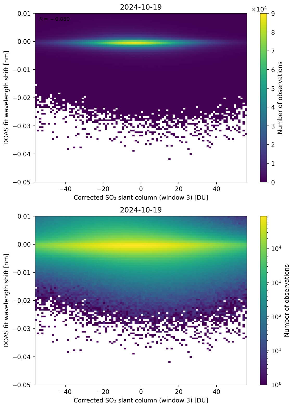
Figure 206: Scatter density plot of “Corrected SO 2 slant column (window 3)” against “DOAS fit wavelength shift” for 2024-10-19 to 2024-10-20.
