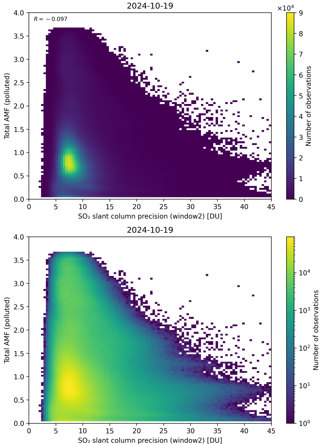
Figure 251: Scatter density plot of “SO 2 slant column precision (window2)” against “Total AMF (polluted)” for 2024-10-19 to 2024-10-20.
