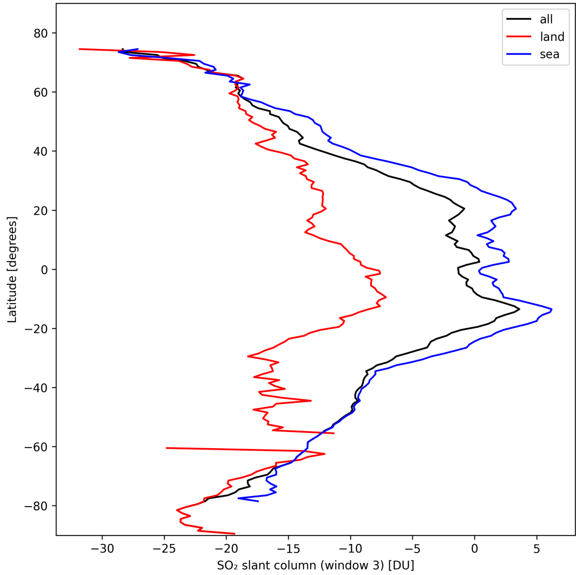
Figure 41: Zonal average of “SO 2 slant column (window 3)” for 2024-10-19 to 2024-10-20.
