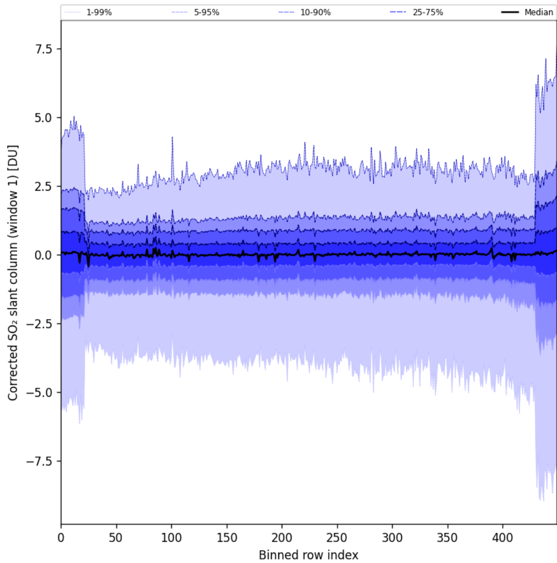
Figure 81: Along track statistics of “Corrected SO 2 slant column (window 1)” for 2024-10-19 to 2024-10-20
