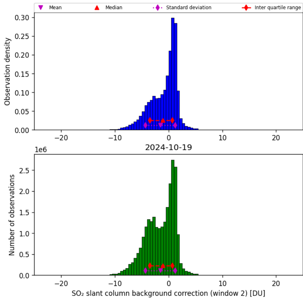
Figure 63: Histogram of “SO 2 slant column background correction (window 2)” for 2024-10-19 to 2024-10-20
