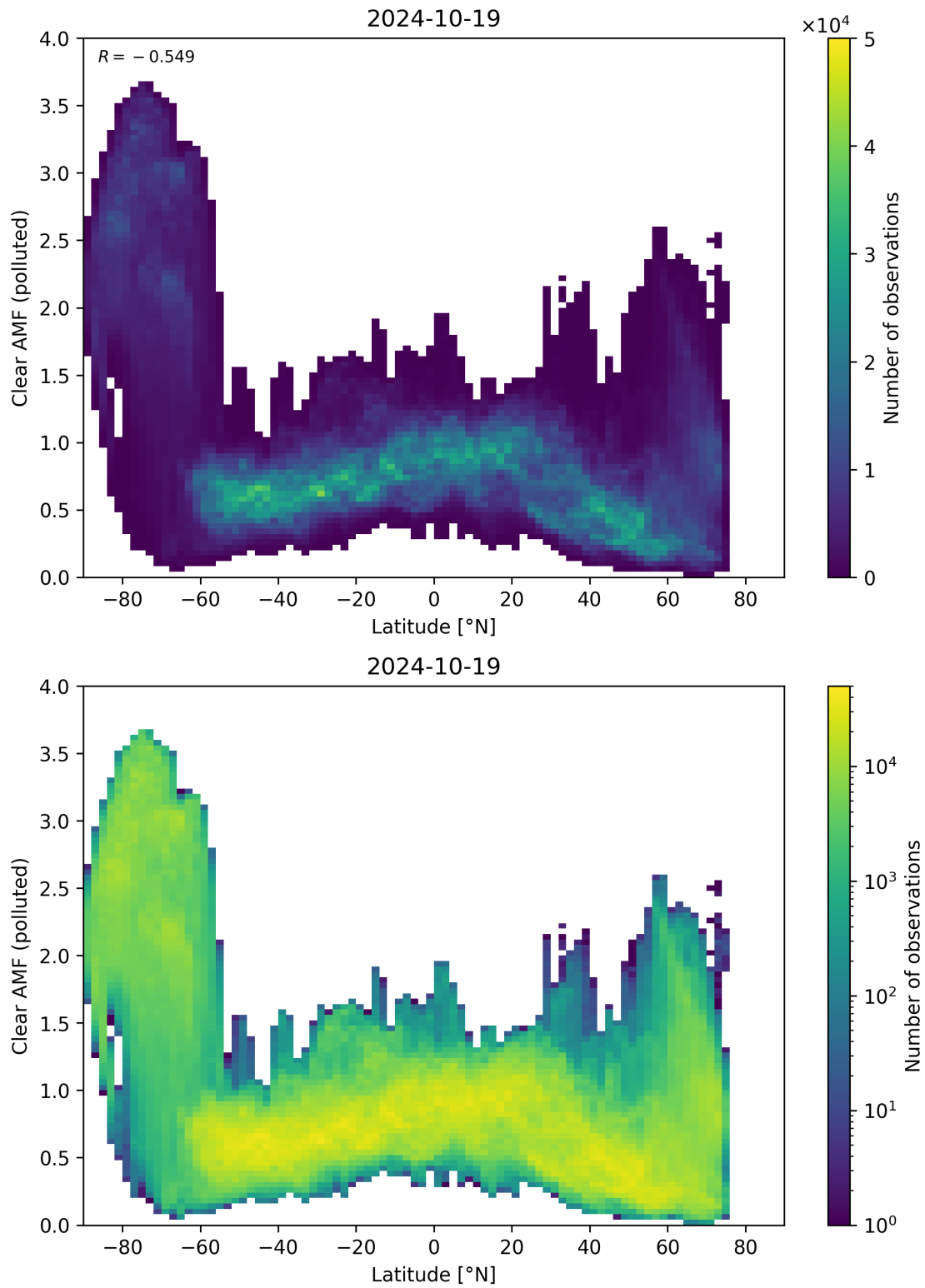
Figure 145: Scatter density plot of “Latitude” against “Clear AMF (polluted)” for 2024-10-19 to 2024-10-20.
