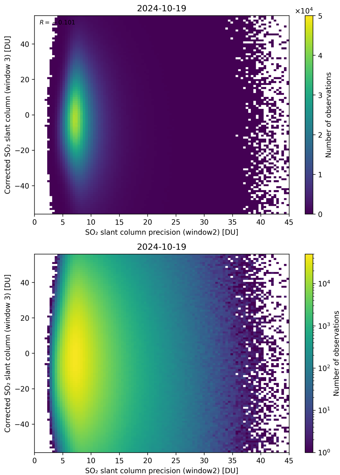
Figure 248: Scatter density plot of “SO 2 slant column precision (window2)” against “Corrected SO 2 slant column (window 3)” for 2024-10-19 to 2024-10-20.
