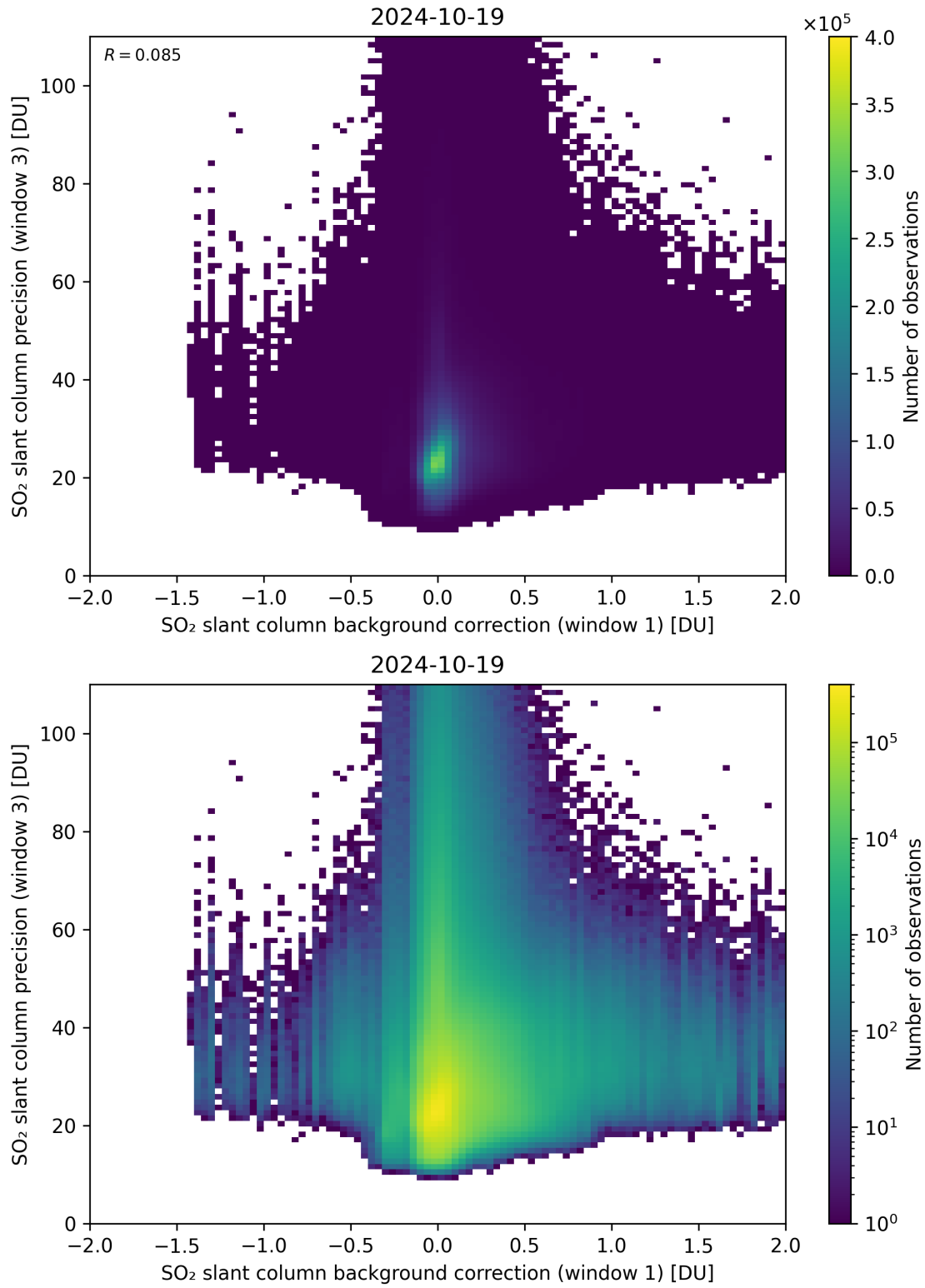
Figure 108: Scatter density plot of “SO 2 slant column background correction (window 1)” against “SO 2 slant column precision (window 3)” for 2024-10-19 to 2024-10-20.
