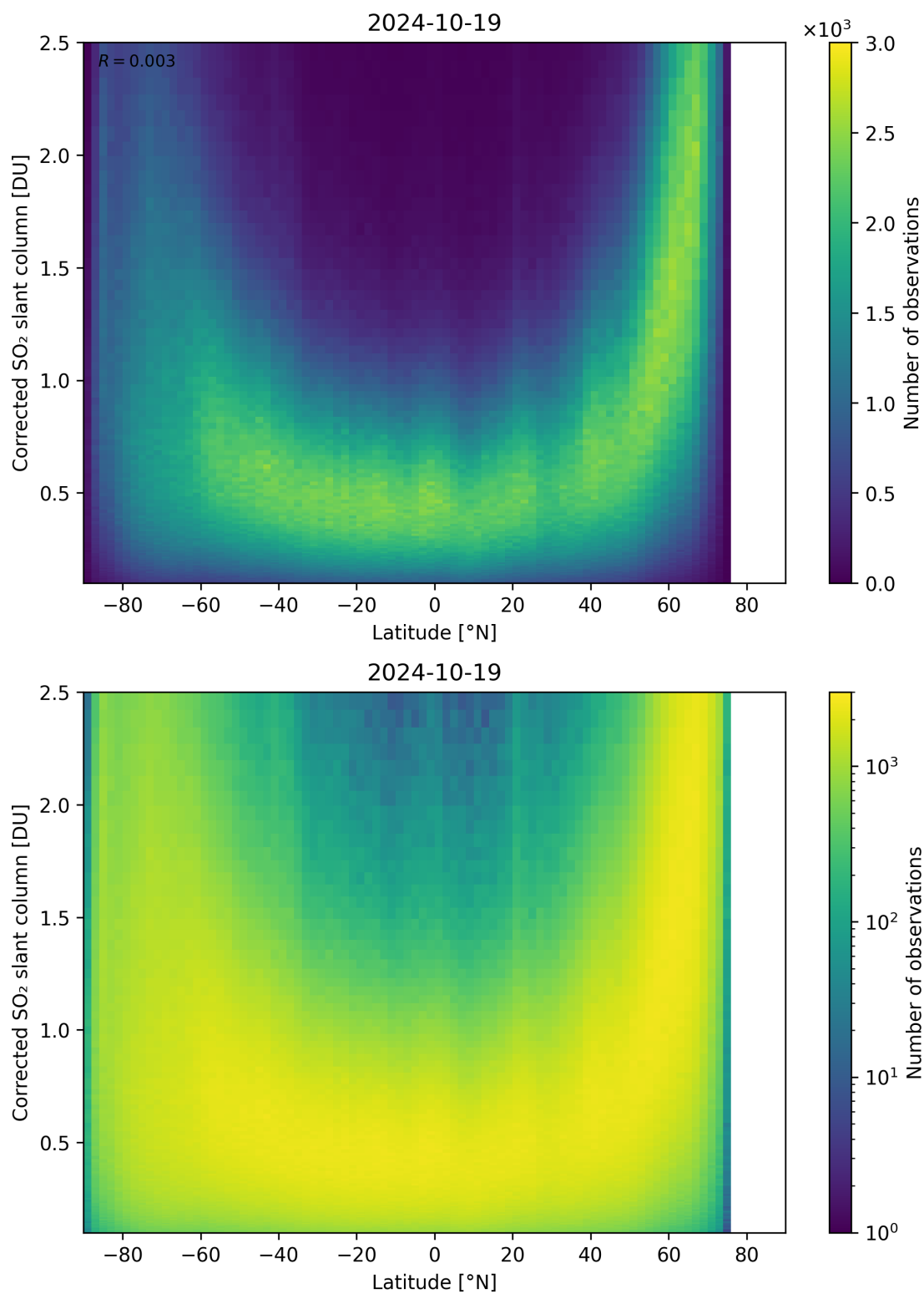
Figure 146: Scatter density plot of “Latitude” against “Corrected SO 2 slant column” for 2024-10-19 to 2024-10-20.
