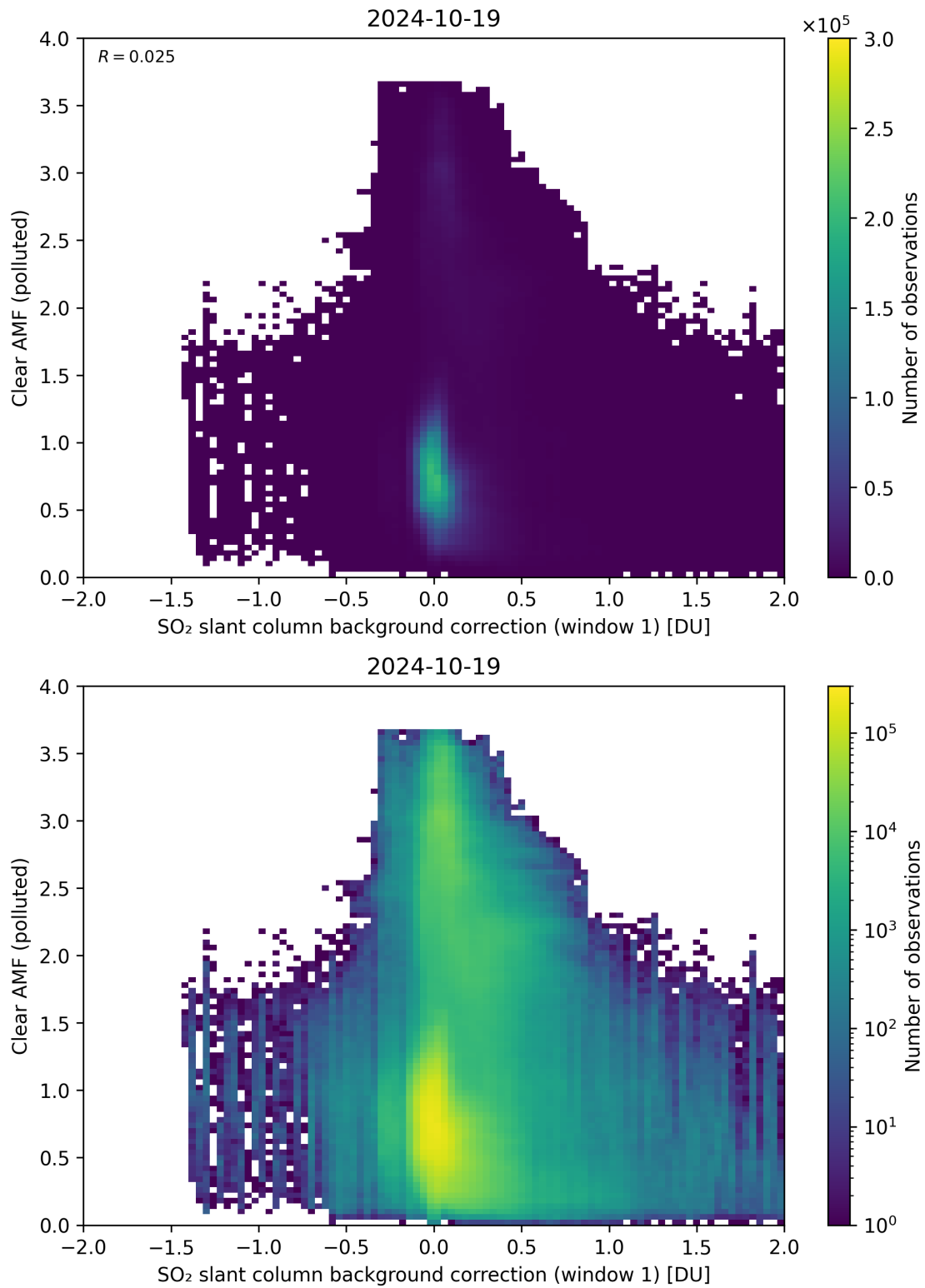
Figure 103: Scatter density plot of “SO 2 slant column background correction (window 1)” against “Clear AMF (polluted)” for 2024-10-19 to 2024-10-20.
