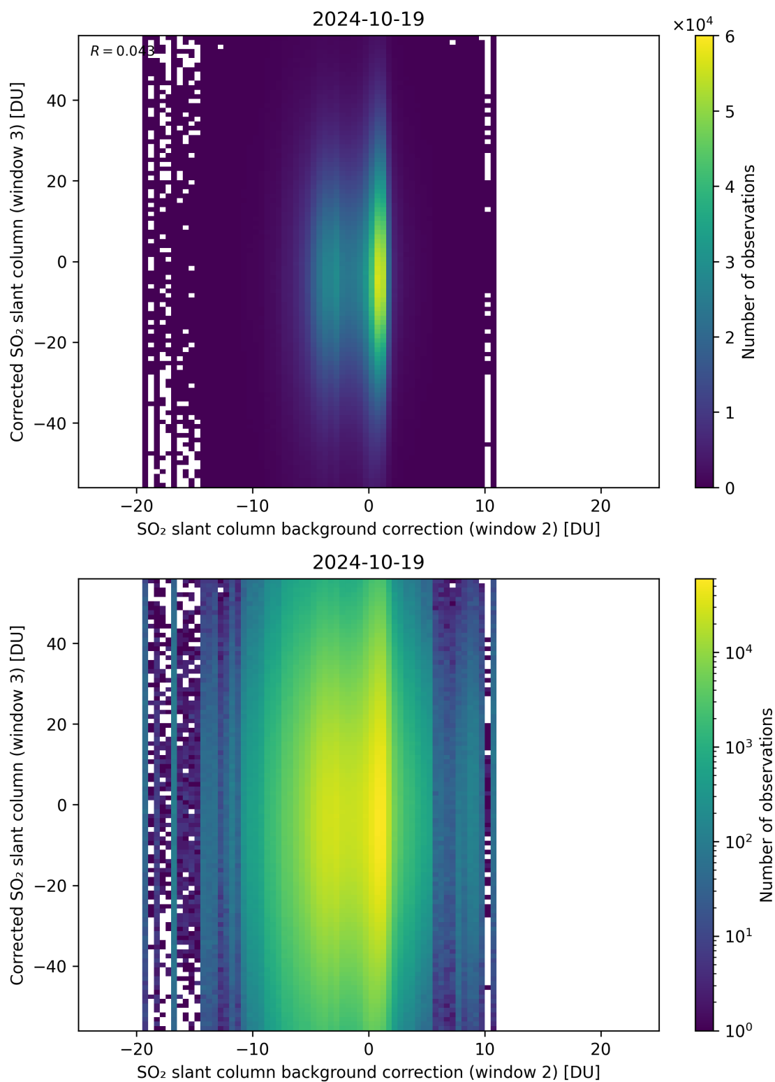
Figure 116: Scatter density plot of “SO 2 slant column background correction (window 2)” against “Corrected SO 2 slant column (window 3)” for 2024-10-19 to 2024-10-20.
