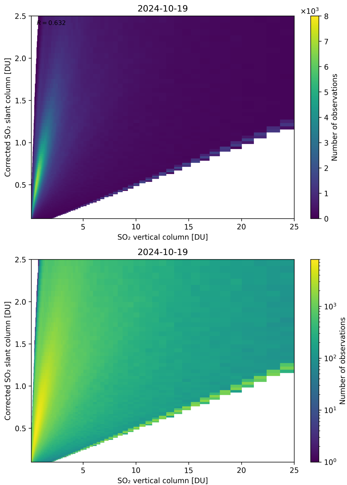
Figure 297: Scatter density plot of “SO 2 vertical column” against “Corrected SO 2 slant column” for 2024-10-19 to 2024-10-20.
