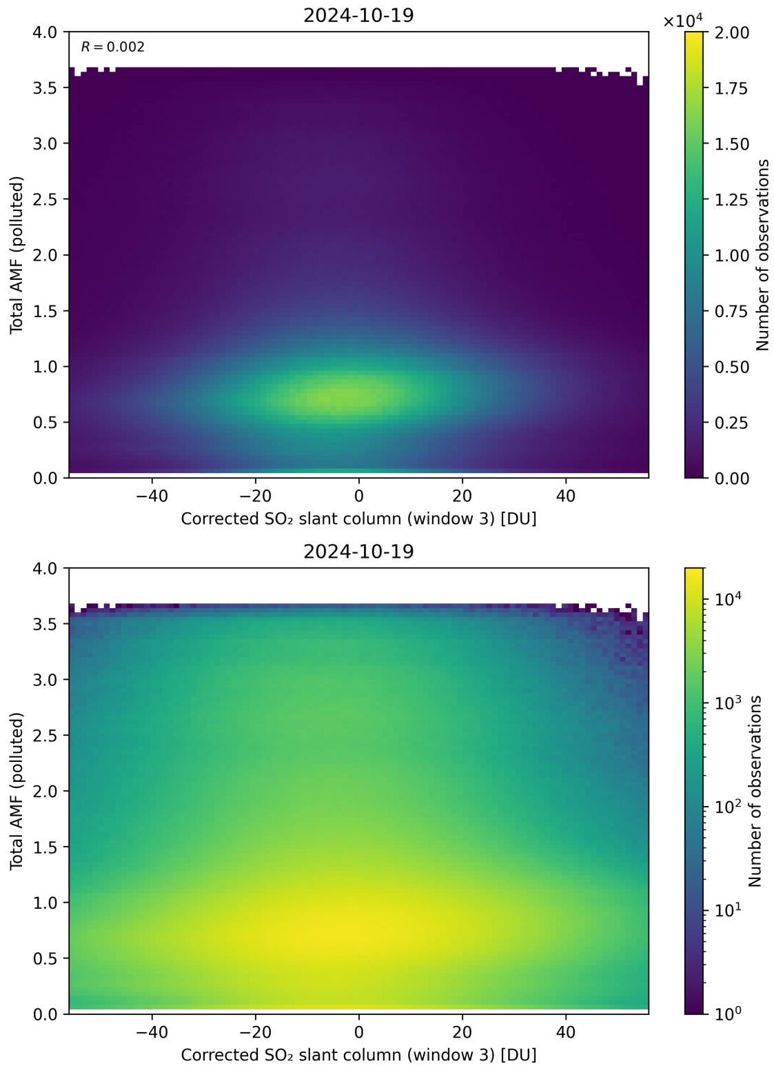
Figure 210: Scatter density plot of “Corrected SO 2 slant column (window 3)” against “Total AMF (polluted)” for 2024-10-19 to 2024-10-20.
