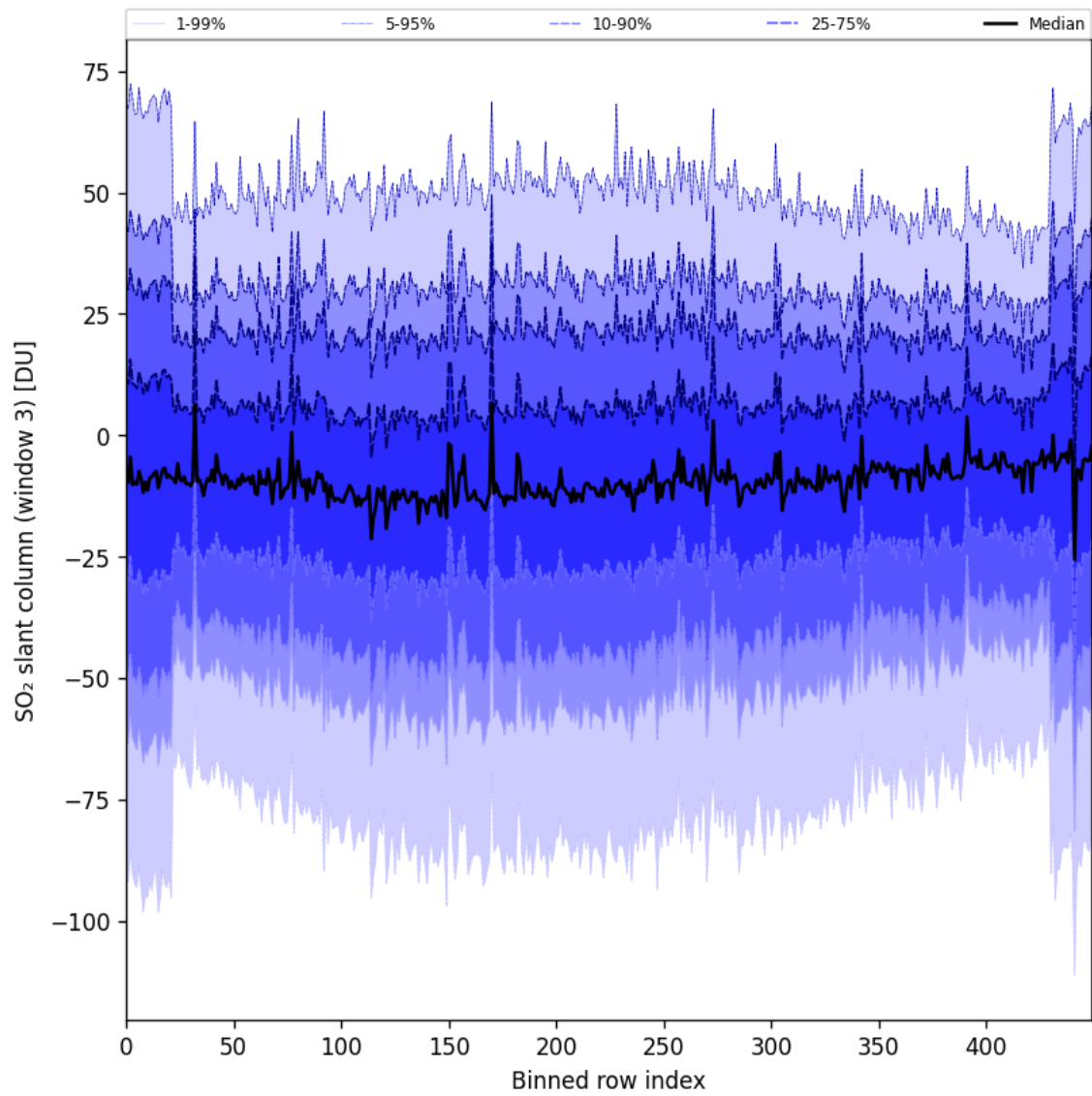
Figure 87: Along track statistics of “SO 2 slant column (window 3)” for 2024-10-19 to 2024-10-20
