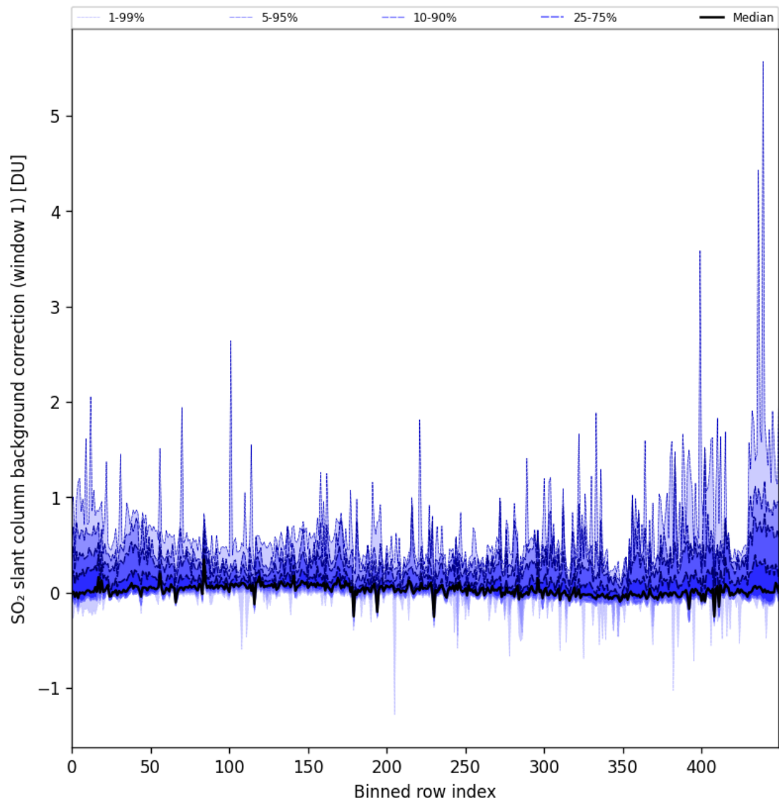
Figure 82: Along track statistics of “SO 2 slant column background correction (window 1)” for 2024-10-19 to 2024-10-20
