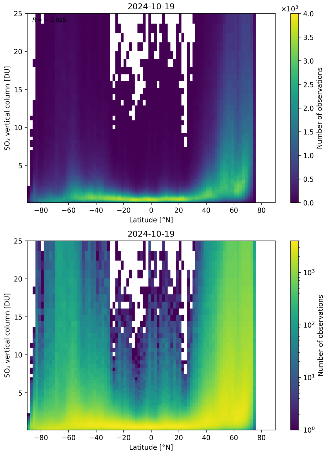
Figure 156: Scatter density plot of “Latitude” against “SO 2 vertical column” for 2024-10-19 to 2024-10-20.
