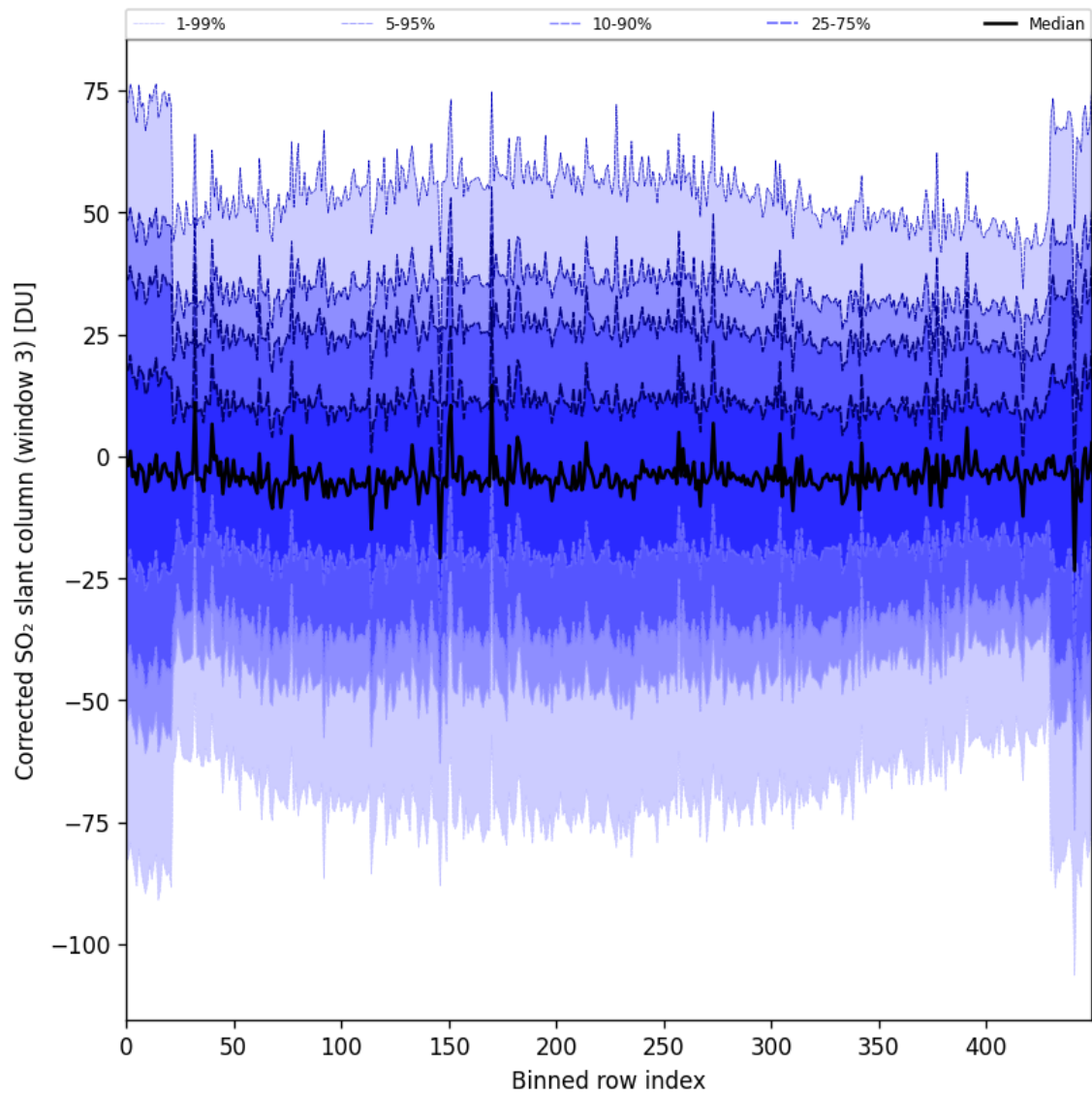
Figure 89: Along track statistics of “Corrected SO 2 slant column (window 3)” for 2024-10-19 to 2024-10-20
