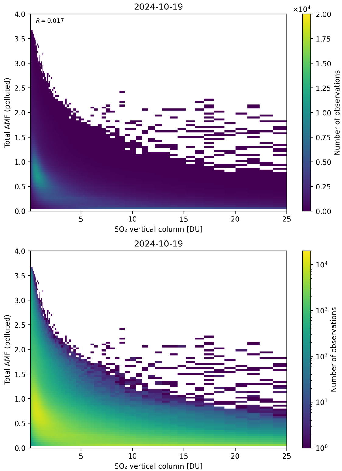
Figure 305: Scatter density plot of “SO 2 vertical column” against “Total AMF (polluted)” for 2024-10-19 to 2024-10-20.
