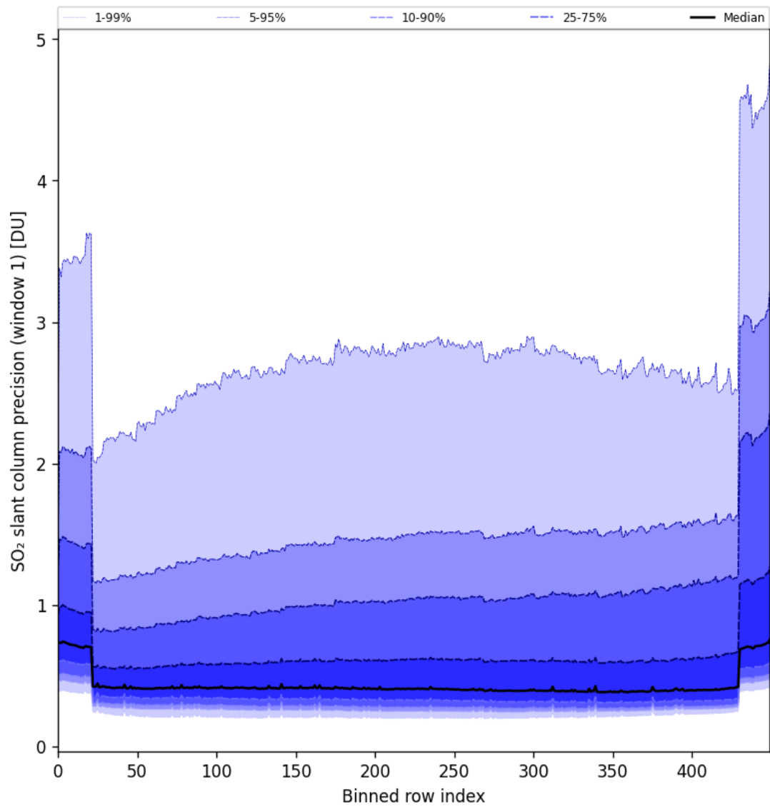
Figure 80: Along track statistics of “SO 2 slant column precision (window 1)” for 2024-10-19 to 2024-10-20
