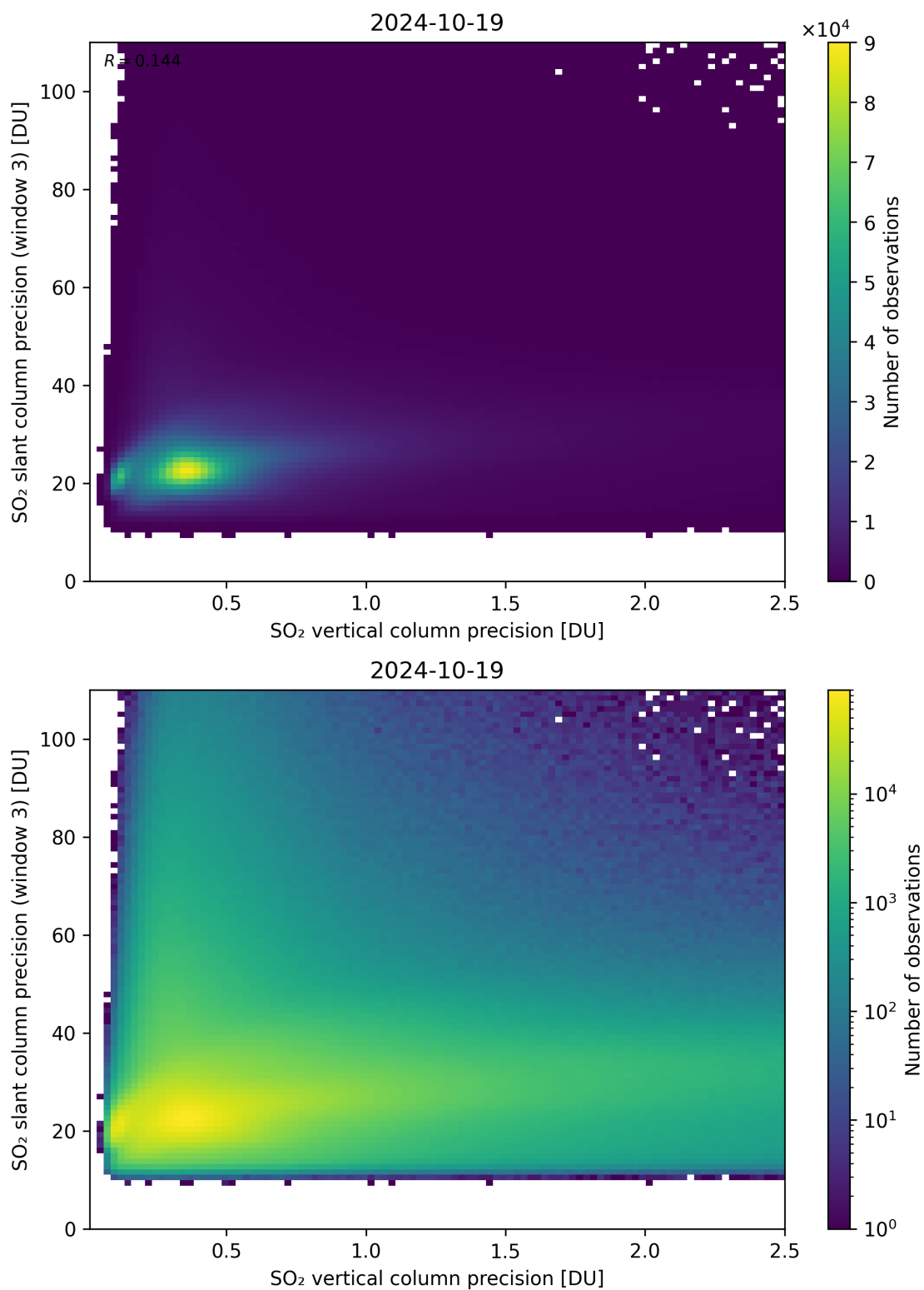
Figure 293: Scatter density plot of “SO 2 vertical column precision” against “SO 2 slant column precision (window 3)” for 2024-10-19 to 2024-10-20.
