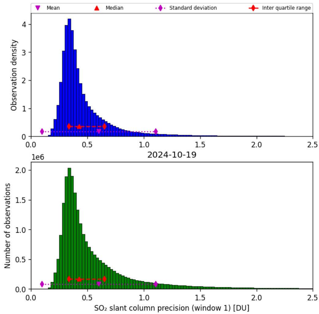
Figure 57: Histogram of “SO 2 slant column precision (window 1)” for 2024-10-19 to 2024-10-20
