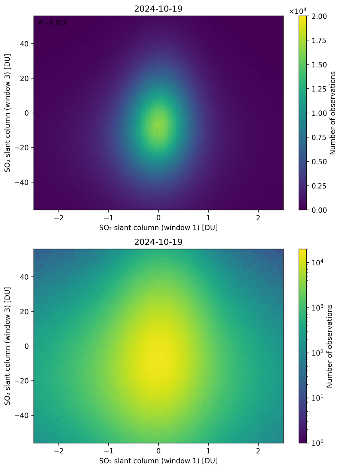
Figure 237: Scatter density plot of “SO 2 slant column (window 1)” against “SO 2 slant column (window 3)” for 2024-10-19 to 2024-10-20.
