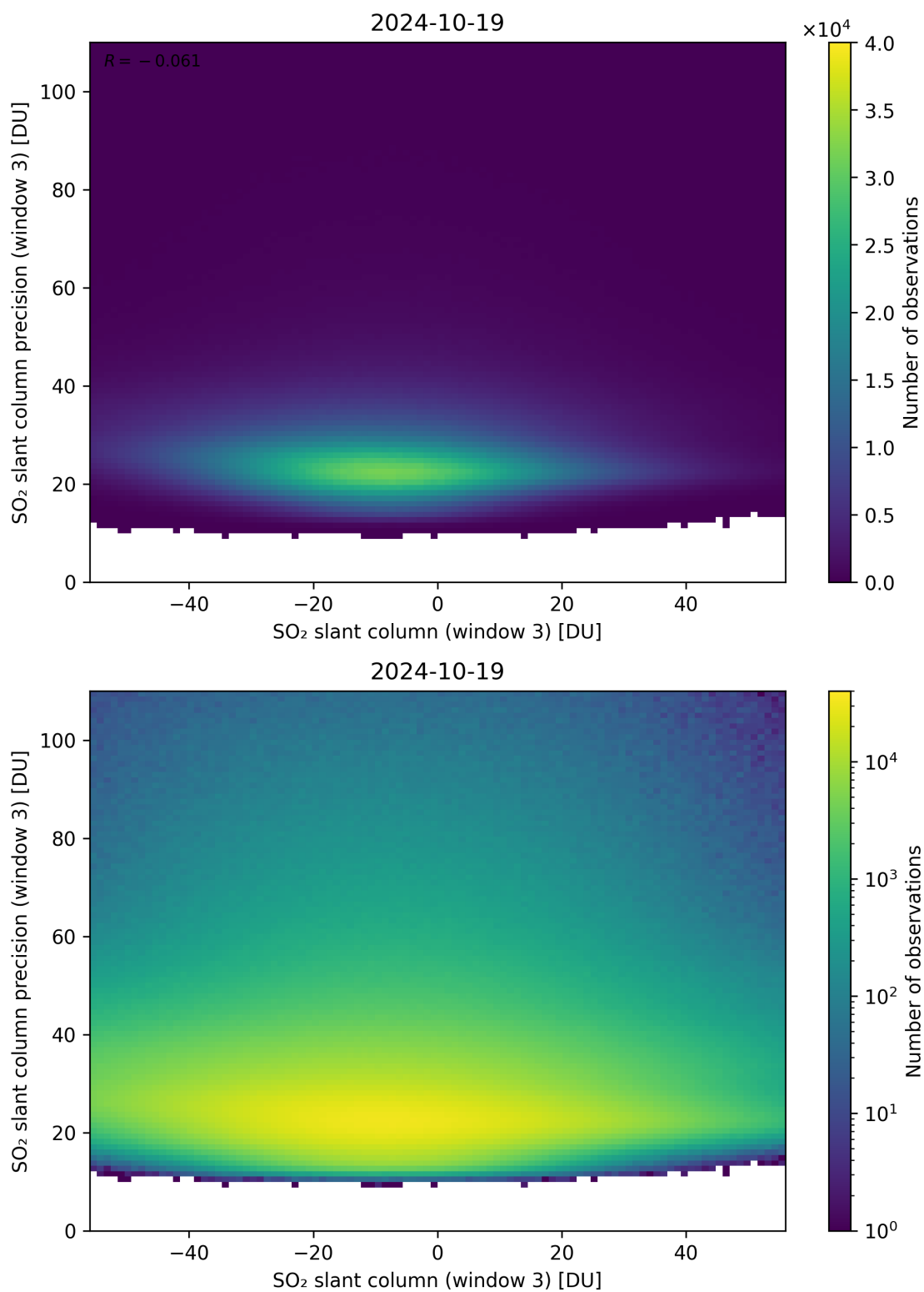
Figure 267: Scatter density plot of “SO 2 slant column (window 3)” against “SO 2 slant column precision (window 3)” for 2024-10-19 to 2024-10-20.
