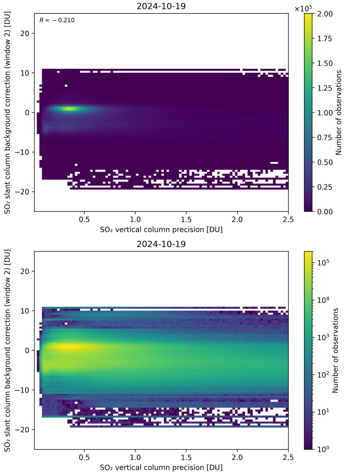
Figure 280: Scatter density plot of “SO 2 vertical column precision” against “SO 2 slant column background correction (window 2)” for 2024-10-19 to 2024-10-20.
