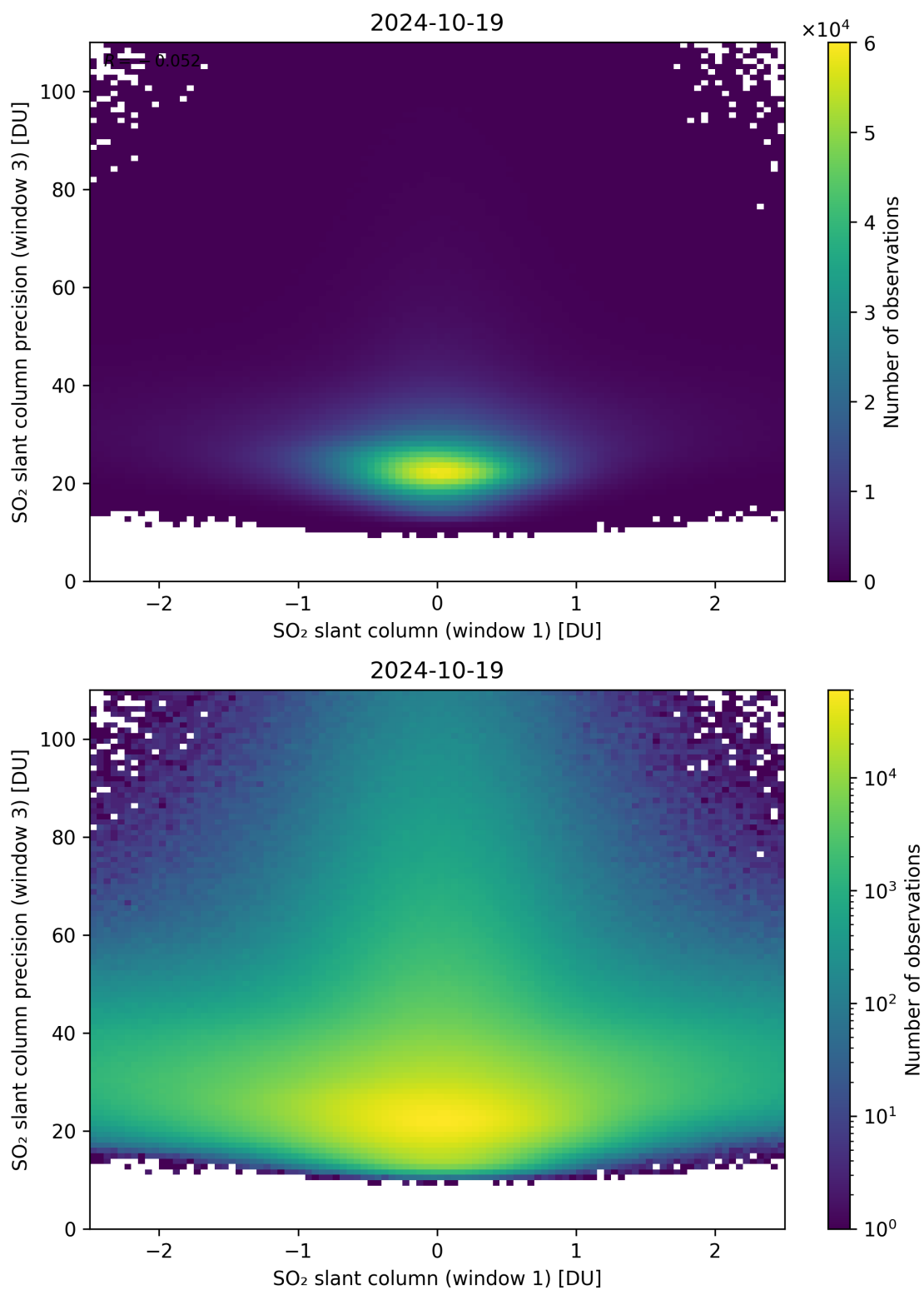
Figure 238: Scatter density plot of “SO 2 slant column (window 1)” against “SO 2 slant column precision (window 3)” for 2024-10-19 to 2024-10-20.
