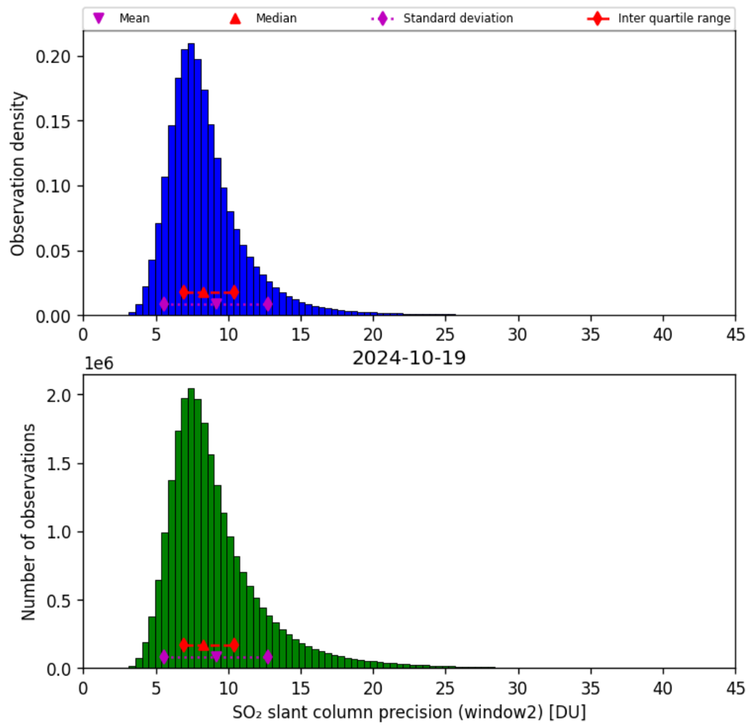
Figure 61: Histogram of “SO 2 slant column precision (window2)” for 2024-10-19 to 2024-10-20
