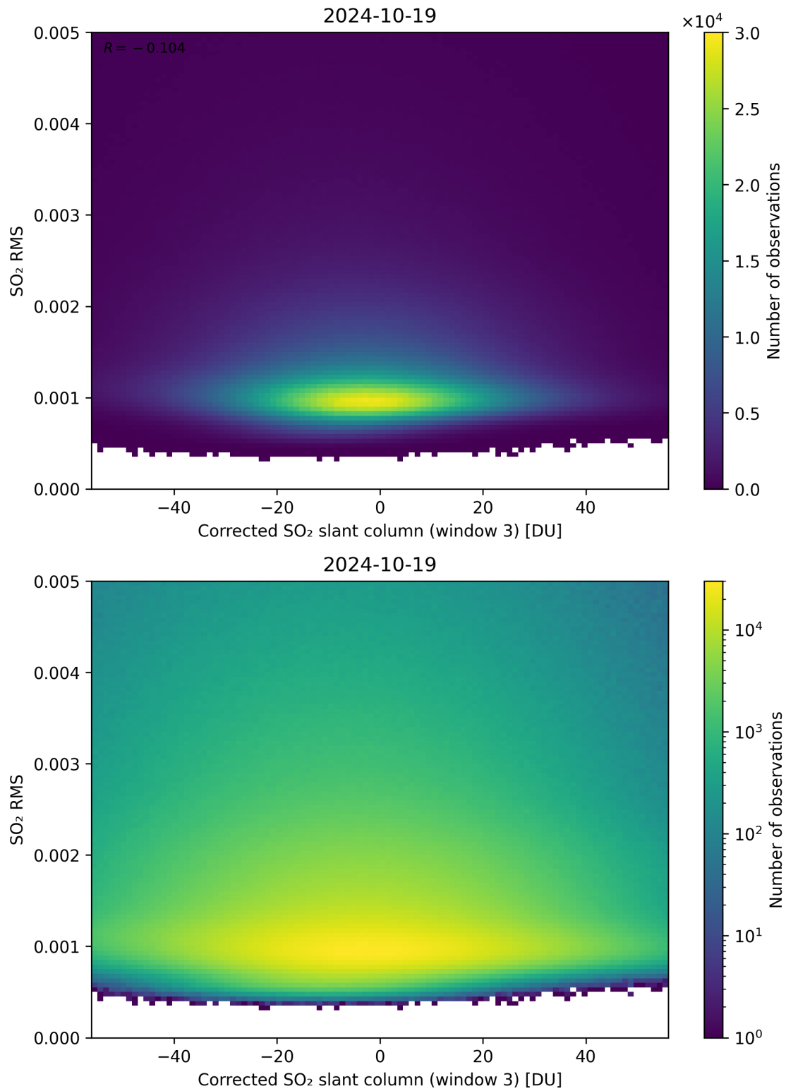
Figure 208: Scatter density plot of “Corrected SO 2 slant column (window 3)” against “SO 2 RMS” for 2024-10-19 to 2024-10-20.
