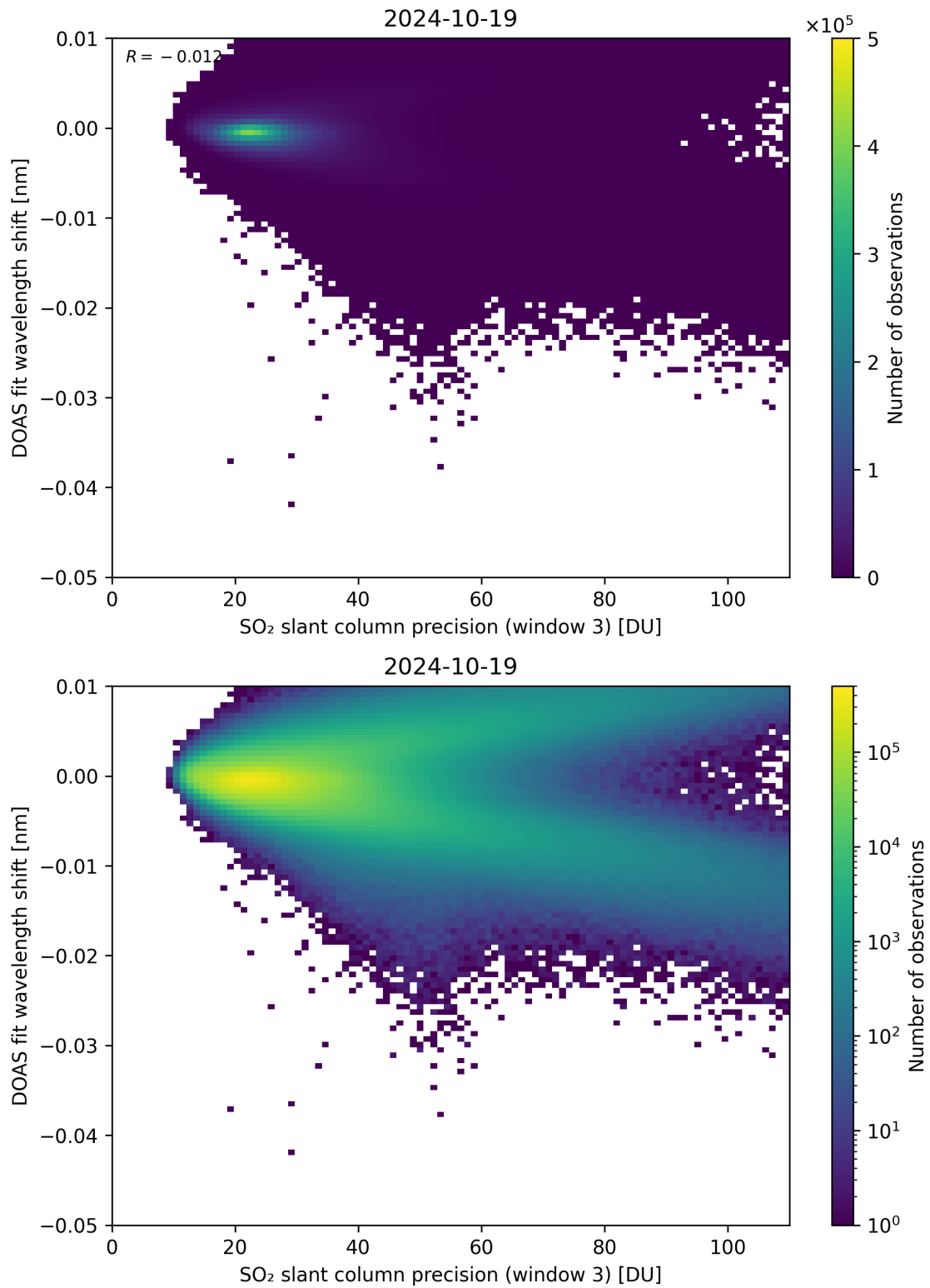
Figure 258: Scatter density plot of “SO 2 slant column precision (window 3)” against “DOAS fit wavelength shift” for 2024-10-19 to 2024-10-20.
