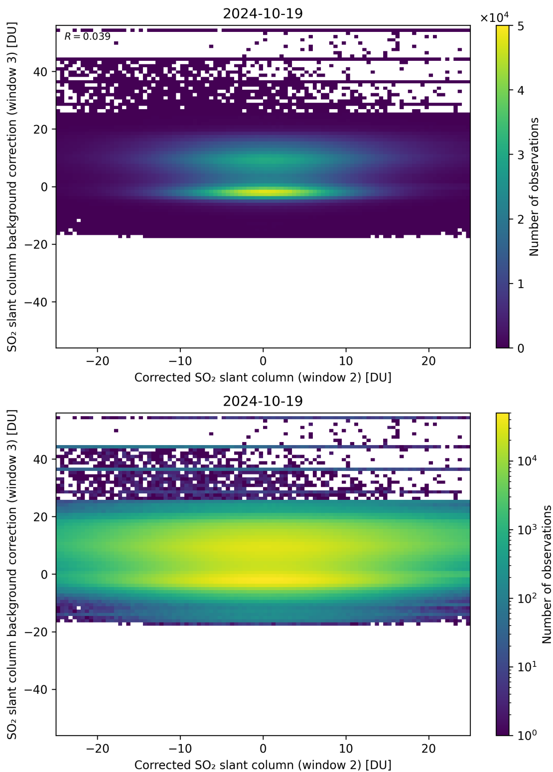
Figure 195: Scatter density plot of “Corrected SO 2 slant column (window 2)” against “SO 2 slant column background correction (window 3)” for 2024-10-19 to 2024-10-20.
