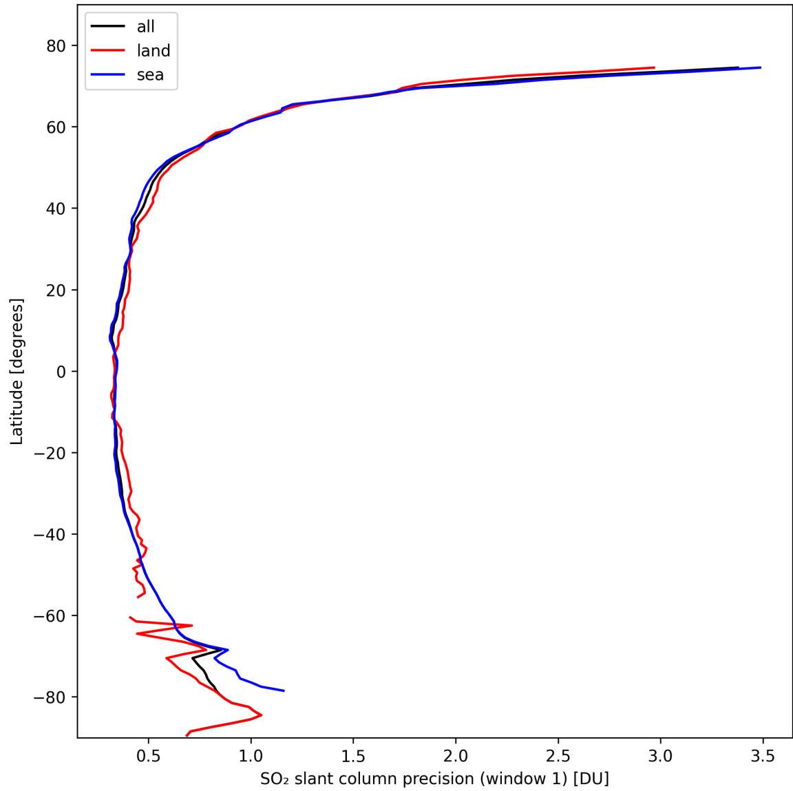
Figure 34: Zonal average of “SO 2 slant column precision (window 1)” for 2024-10-19 to 2024-10-20.
