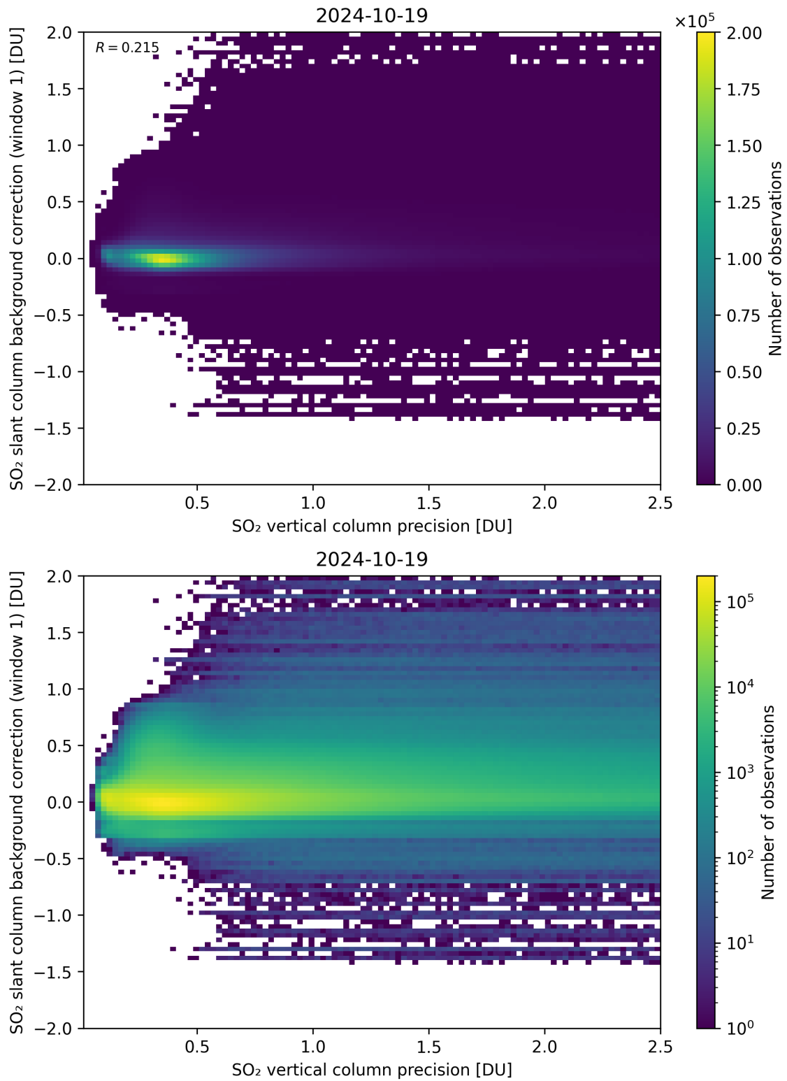
Figure 279: Scatter density plot of “SO 2 vertical column precision” against “SO 2 slant column background correction (window 1)” for 2024-10-19 to 2024-10-20.
