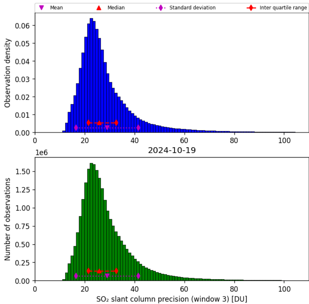
Figure 65: Histogram of “SO 2 slant column precision (window 3)” for 2024-10-19 to 2024-10-20
