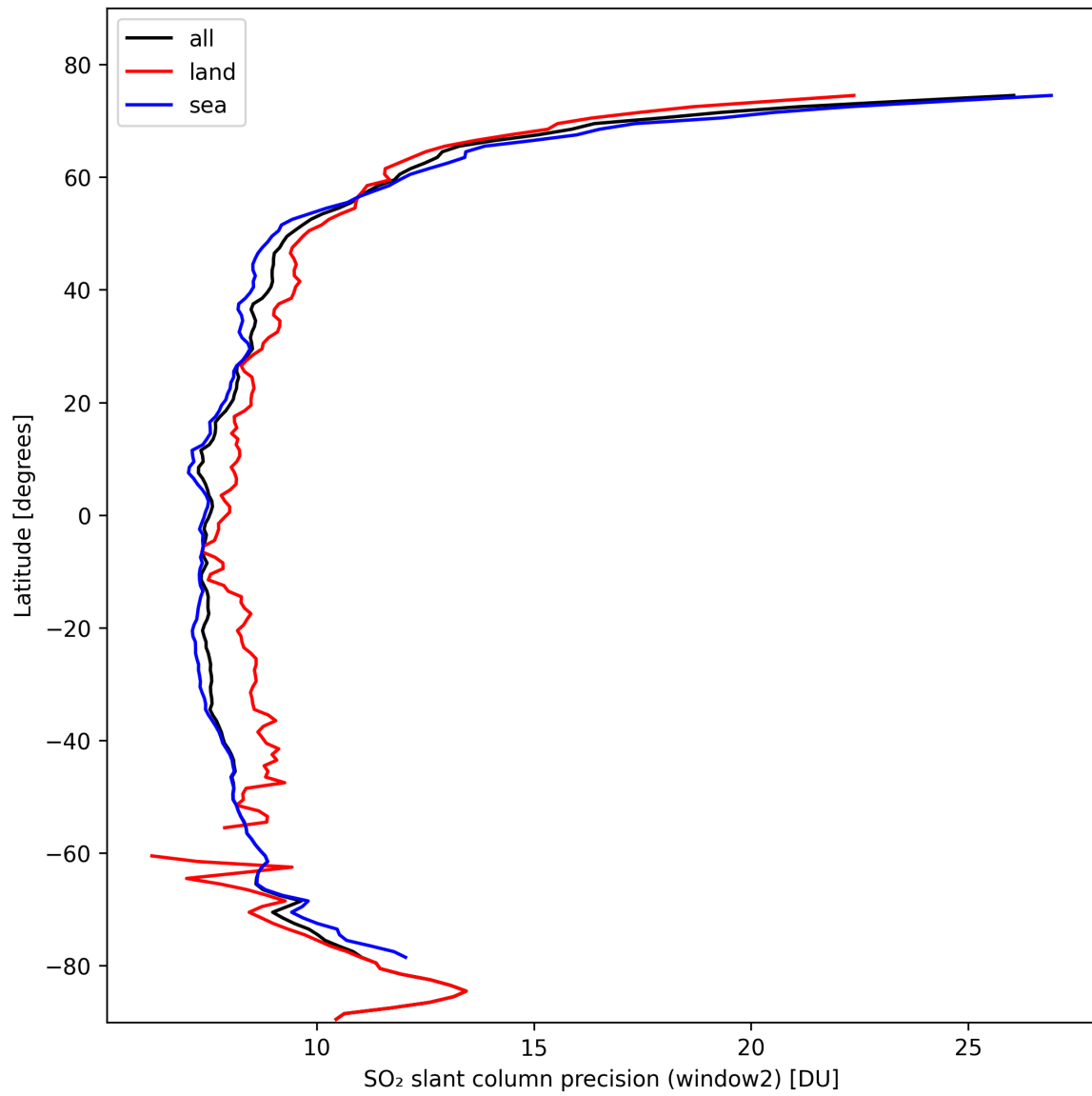
Figure 38: Zonal average of “SO 2 slant column precision (window2)” for 2024-10-19 to 2024-10-20.
