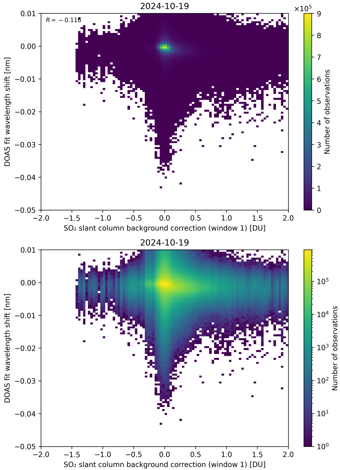
Figure 100: Scatter density plot of “SO 2 slant column background correction (window 1)” against “DOAS fit wavelength shift” for 2024-10-19 to 2024-10-20.
