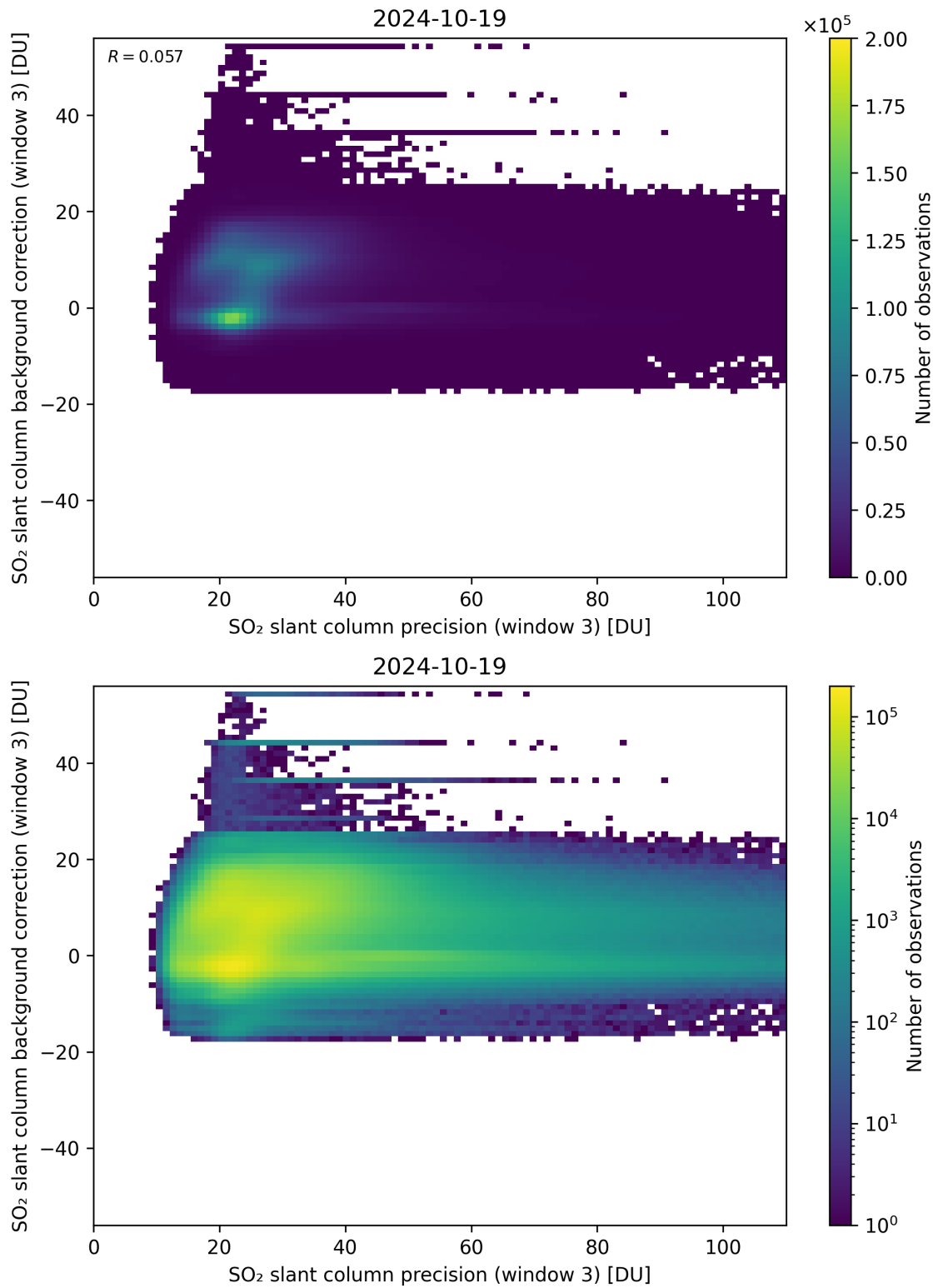
Figure 257: Scatter density plot of “SO 2 slant column precision (window 3)” against “SO 2 slant column background correction (window 3)” for 2024-10-19 to 2024-10-20.
