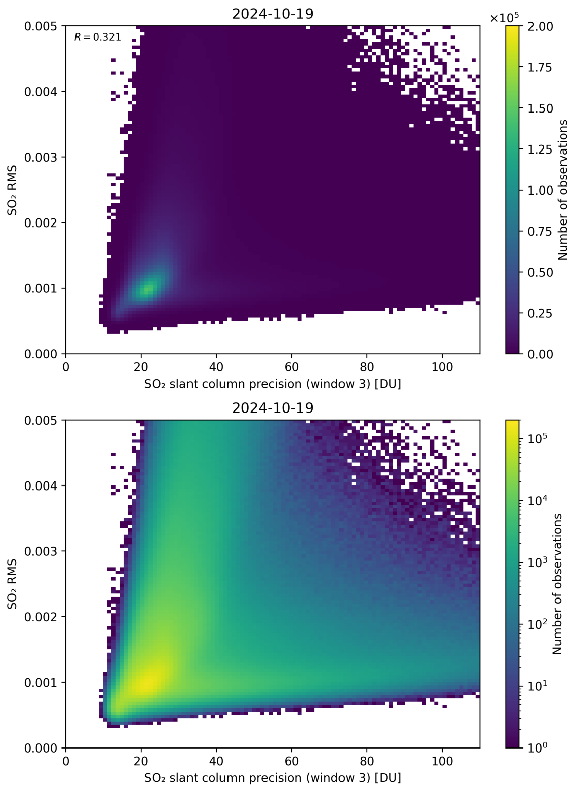
Figure 260: Scatter density plot of “SO 2 slant column precision (window 3)” against “SO 2 RMS” for 2024-10-19 to 2024-10-20.
