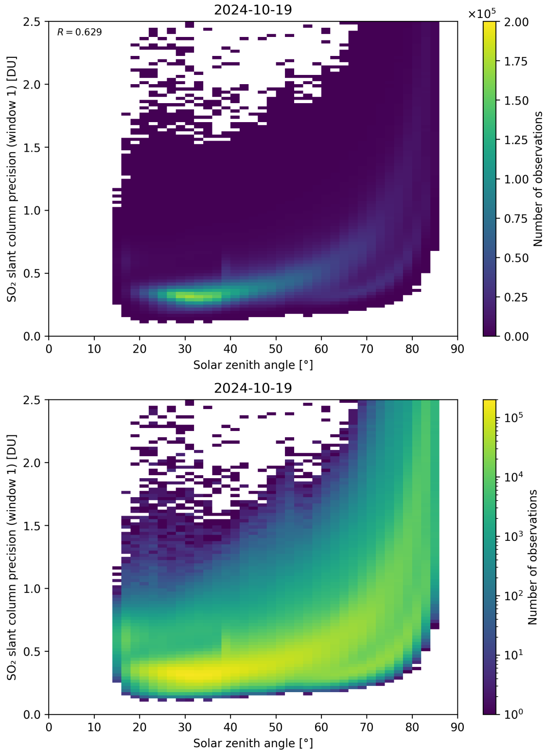
Figure 170: Scatter density plot of “Solar zenith angle” against “SO 2 slant column precision (window 1)” for 2024-10-19 to 2024-10-20.
