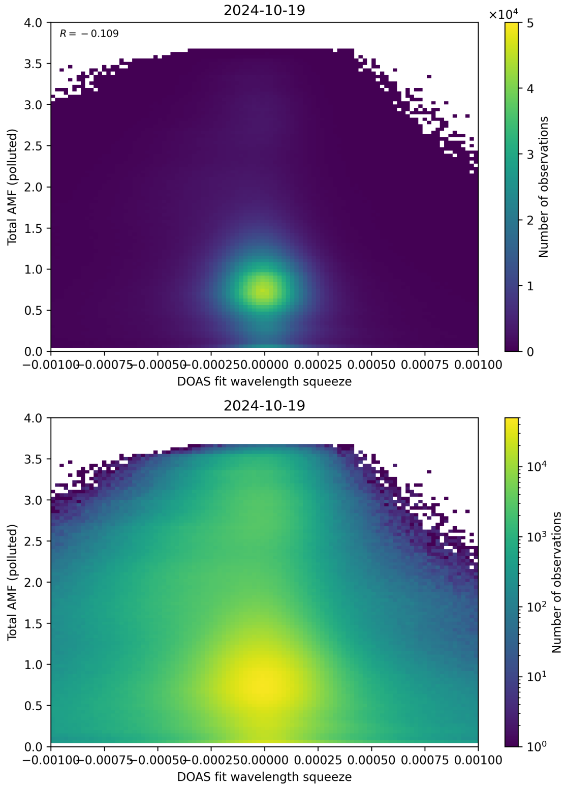
Figure 134: Scatter density plot of “DOAS fit wavelength squeeze” against “Total AMF (polluted)” for 2024-10-19 to 2024-10-20.
