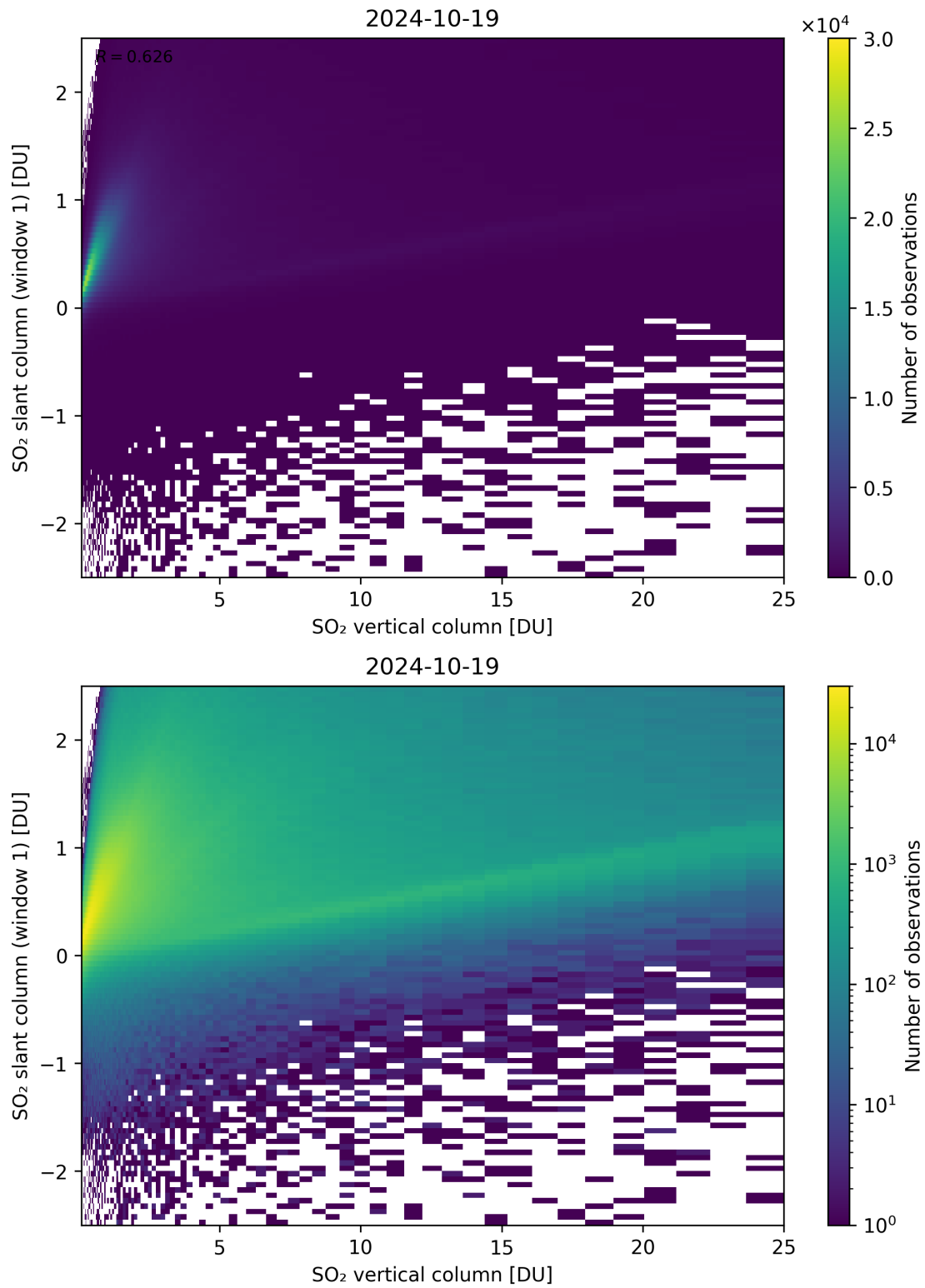
Figure 300: Scatter density plot of “SO 2 vertical column” against “SO 2 slant column (window 1)” for 2024-10-19 to 2024-10-20.
