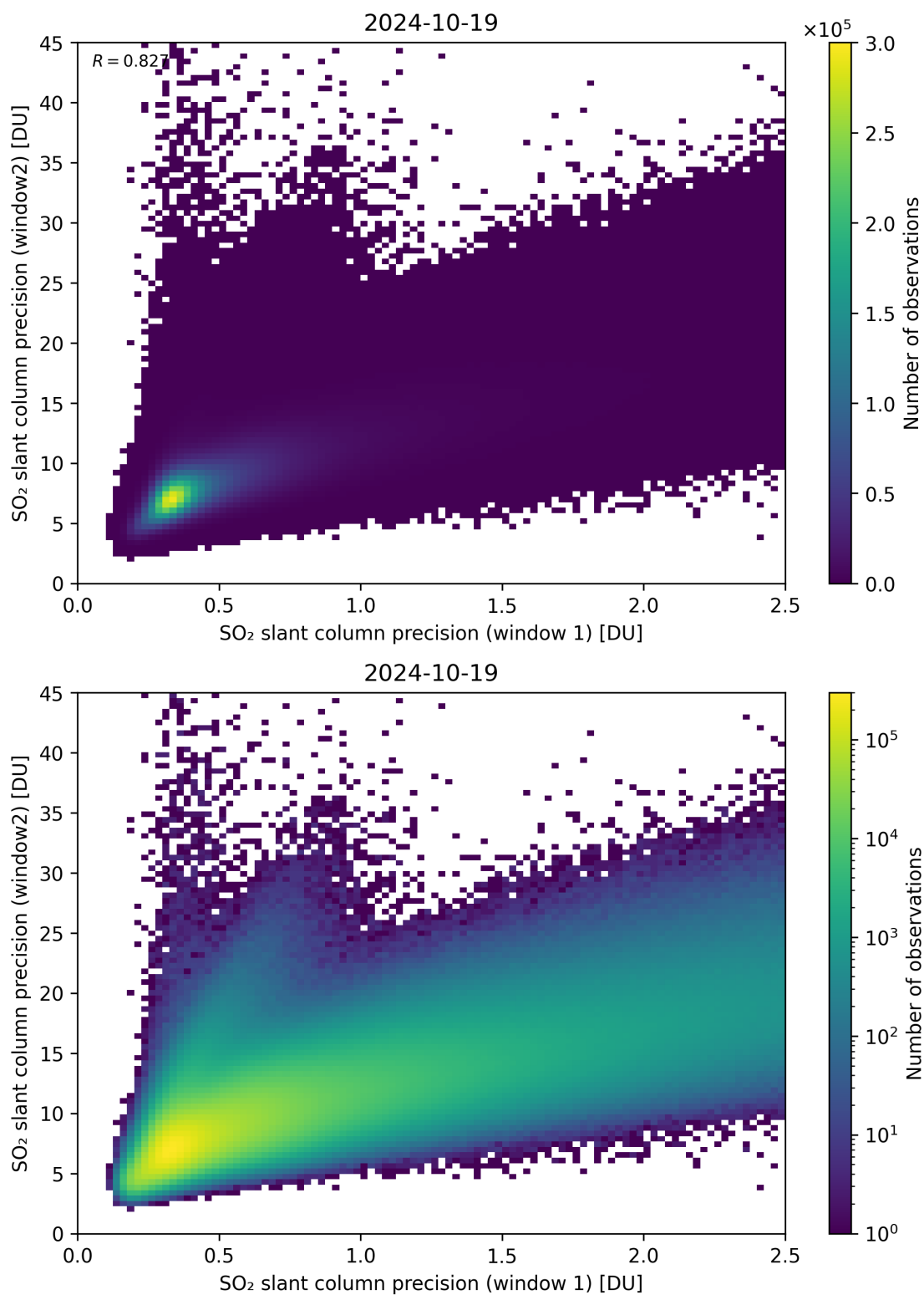
Figure 227: Scatter density plot of “SO 2 slant column precision (window 1)” against “SO 2 slant column precision (window2)” for 2024-10-19 to 2024-10-20.
