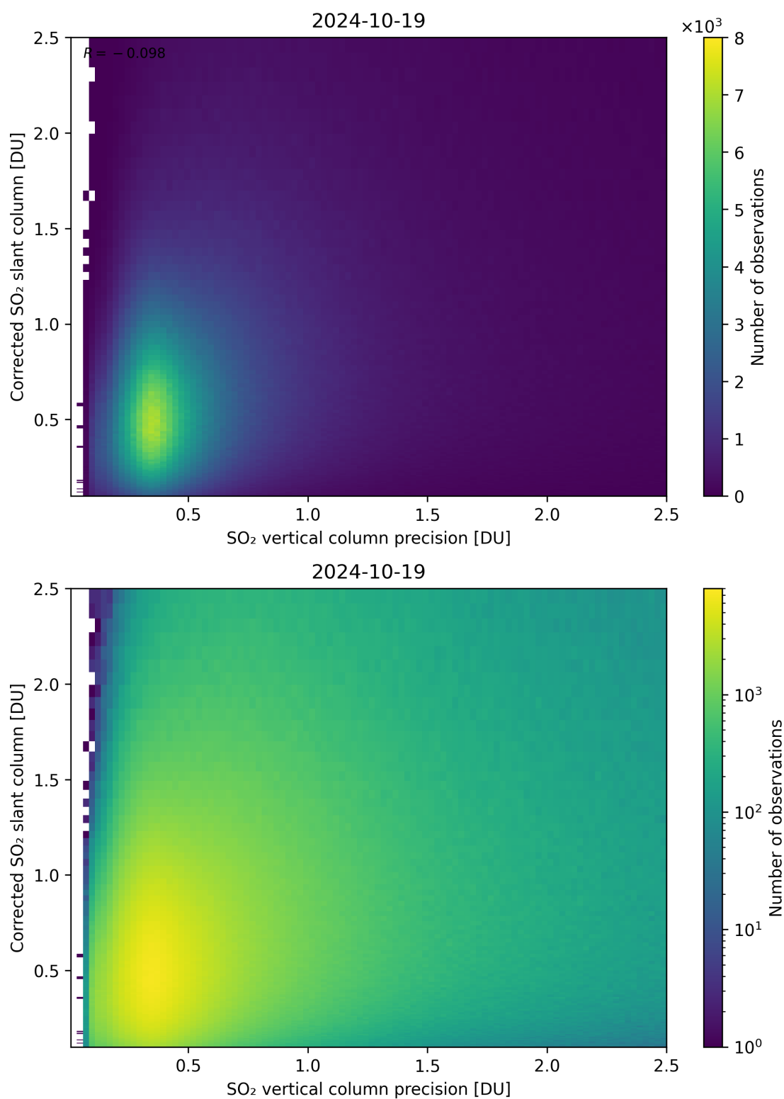
Figure 286: Scatter density plot of “SO 2 vertical column precision” against “Corrected SO 2 slant column” for 2024-10-19 to 2024-10-20.
