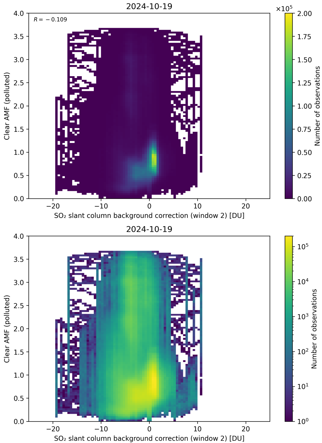
Figure 115: Scatter density plot of “SO 2 slant column background correction (window 2)” against “Clear AMF (polluted)” for 2024-10-19 to 2024-10-20.
