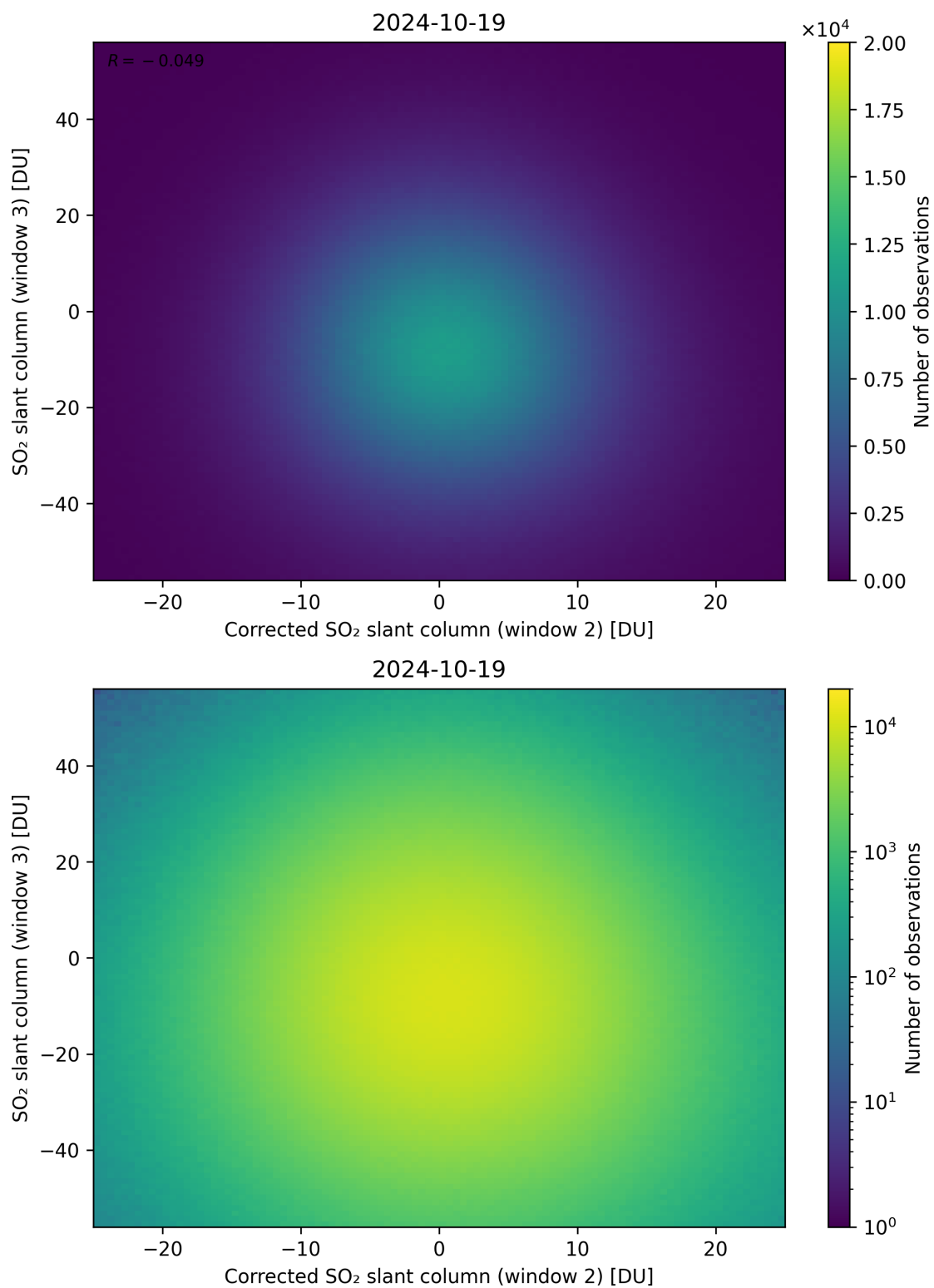
Figure 201: Scatter density plot of “Corrected SO 2 slant column (window 2)” against “SO 2 slant column (window 3)” for 2024-10-19 to 2024-10-20.
