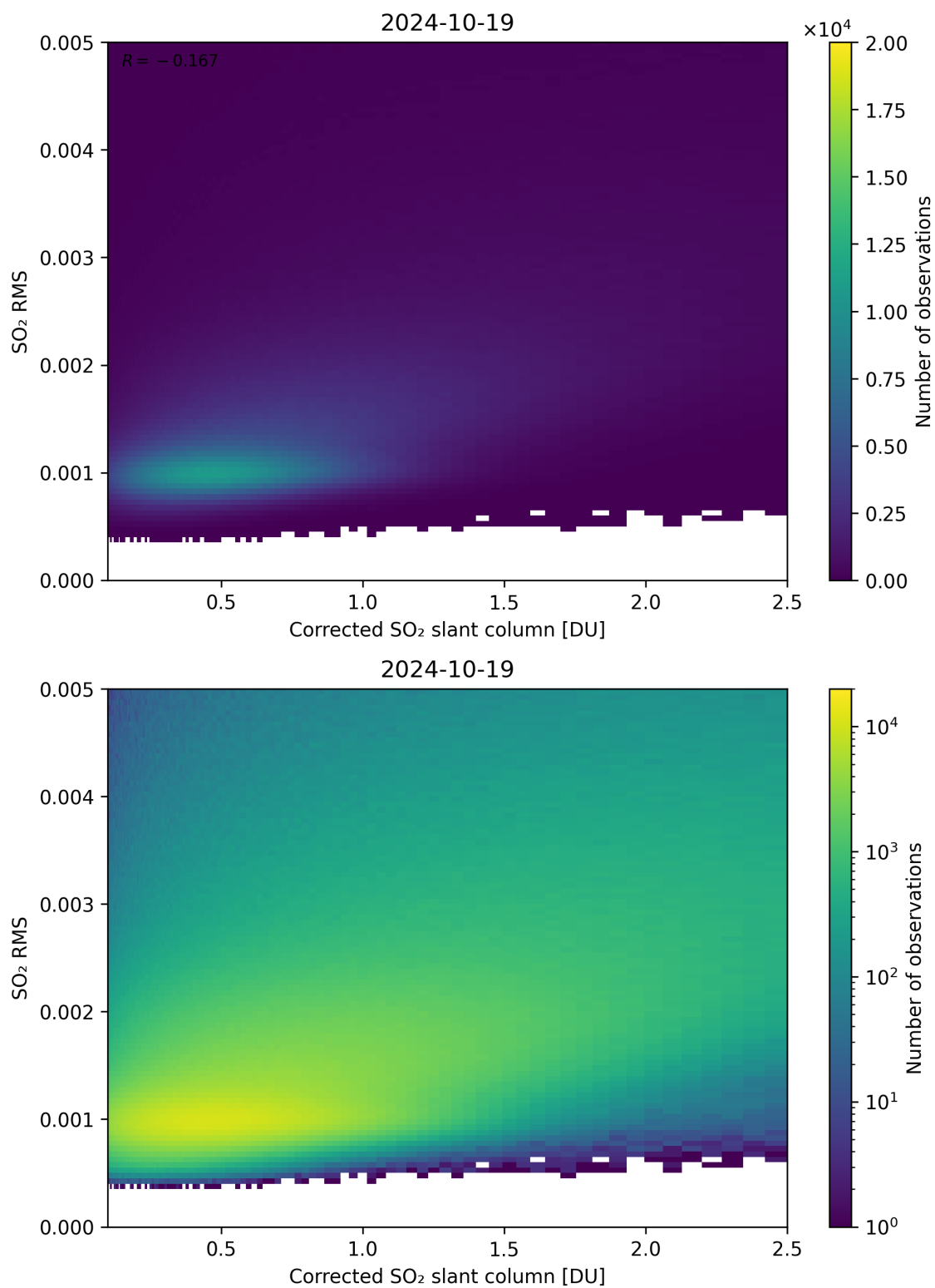
Figure 183: Scatter density plot of “Corrected SO 2 slant column” against “SO 2 RMS” for 2024-10-19 to 2024-10-20.
