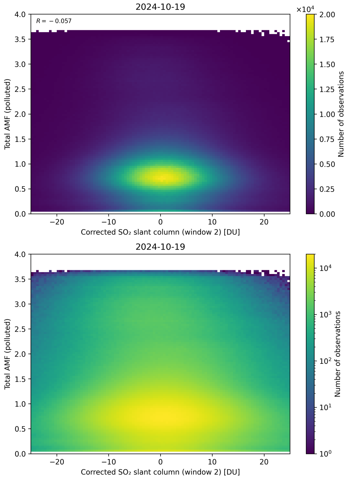
Figure 203: Scatter density plot of “Corrected SO 2 slant column (window 2)” against “Total AMF (polluted)” for 2024-10-19 to 2024-10-20.
