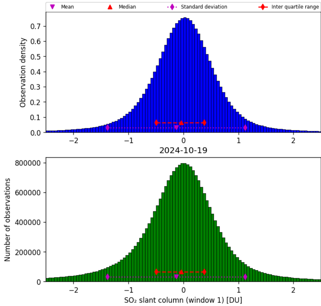
Figure 56: Histogram of “SO 2 slant column (window 1)” for 2024-10-19 to 2024-10-20
