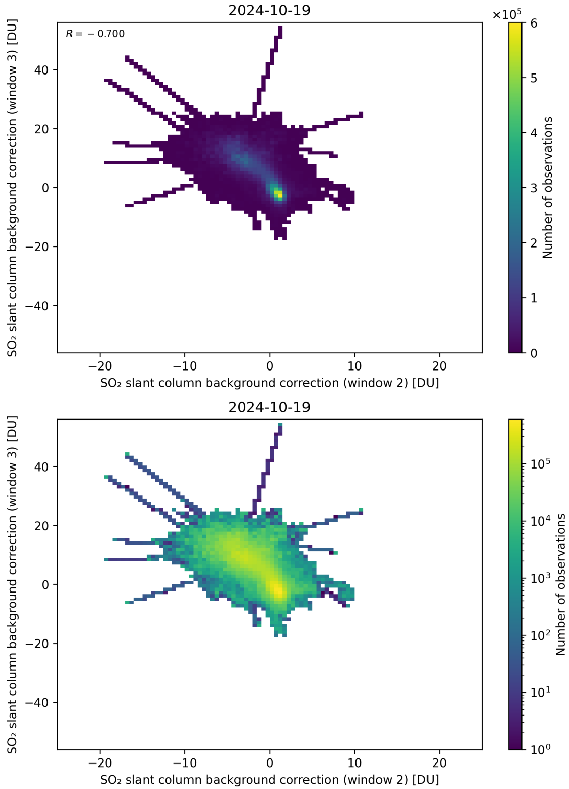
Figure 111: Scatter density plot of “SO 2 slant column background correction (window 2)” against “SO 2 slant column background correction (window 3)” for 2024-10-19 to 2024-10-20.
