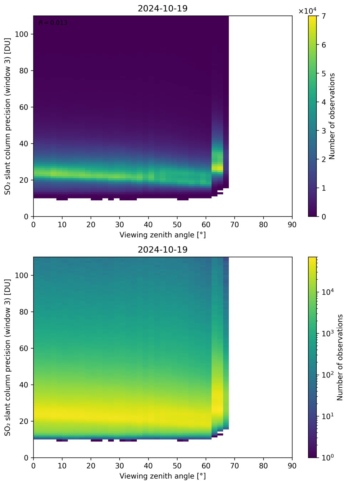
Figure 324: Scatter density plot of “Viewing zenith angle” against “SO 2 slant column precision (window 3)” for 2024-10-19 to 2024-10-20.
