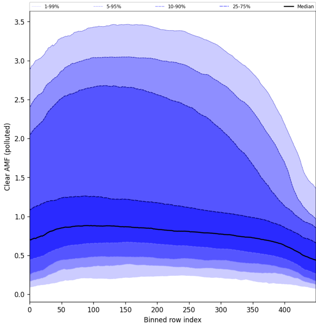
Figure 96: Along track statistics of “Clear AMF (polluted)” for 2024-10-19 to 2024-10-20
