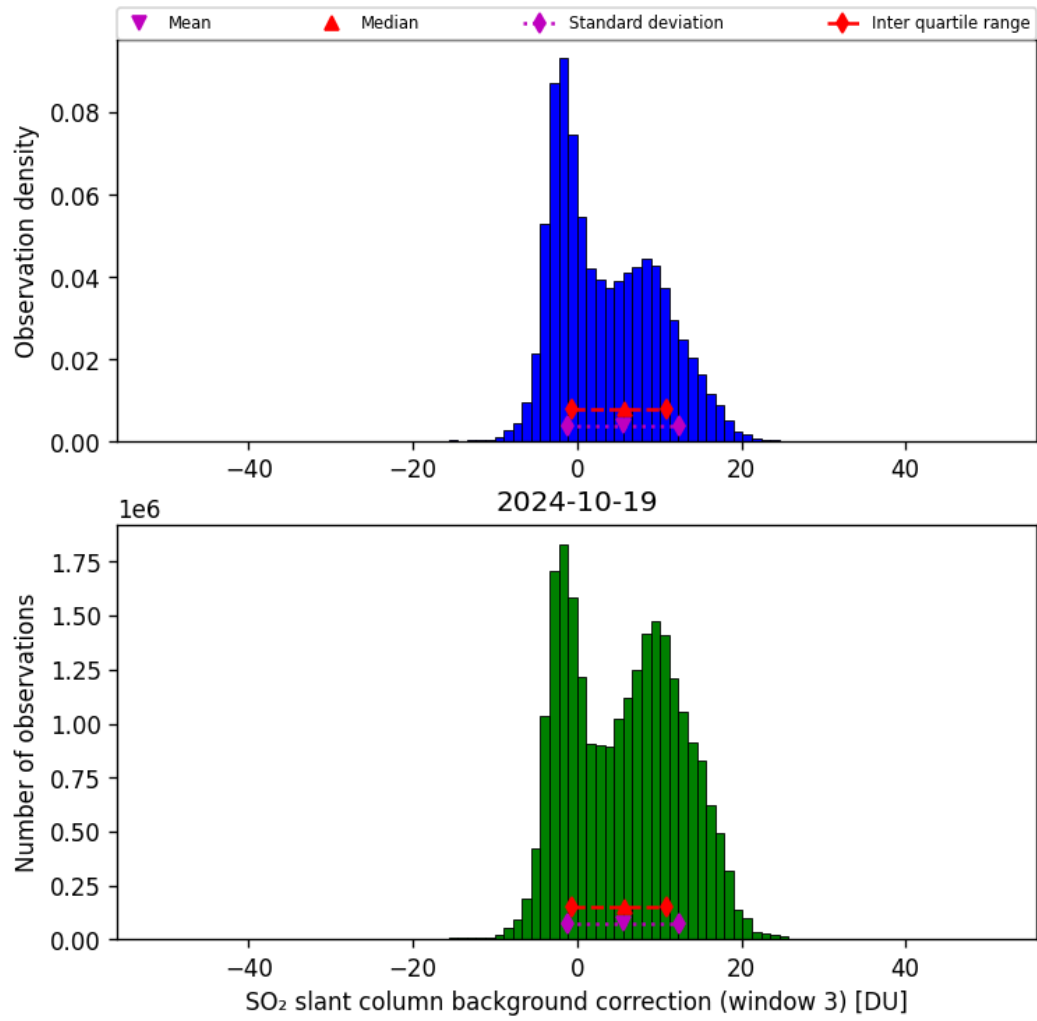
Figure 67: Histogram of “SO 2 slant column background correction (window 3)” for 2024-10-19 to 2024-10-20
