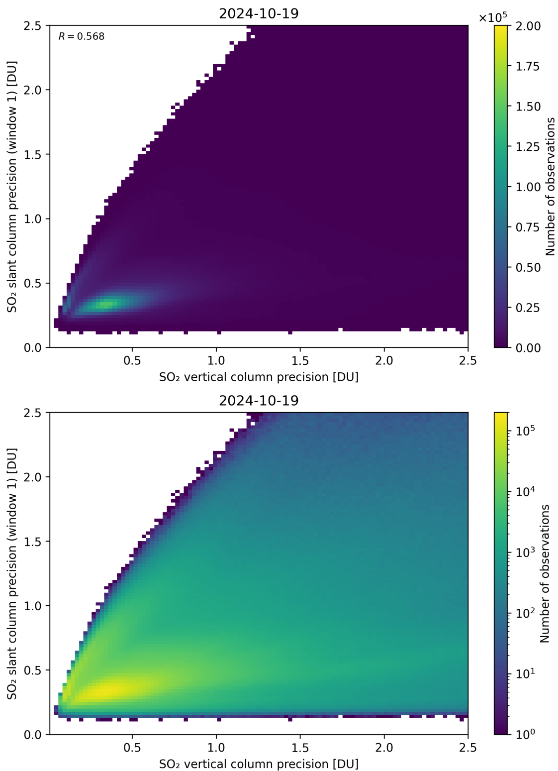
Figure 290: Scatter density plot of “SO 2 vertical column precision” against “SO 2 slant column precision (window 1)” for 2024-10-19 to 2024-10-20.
