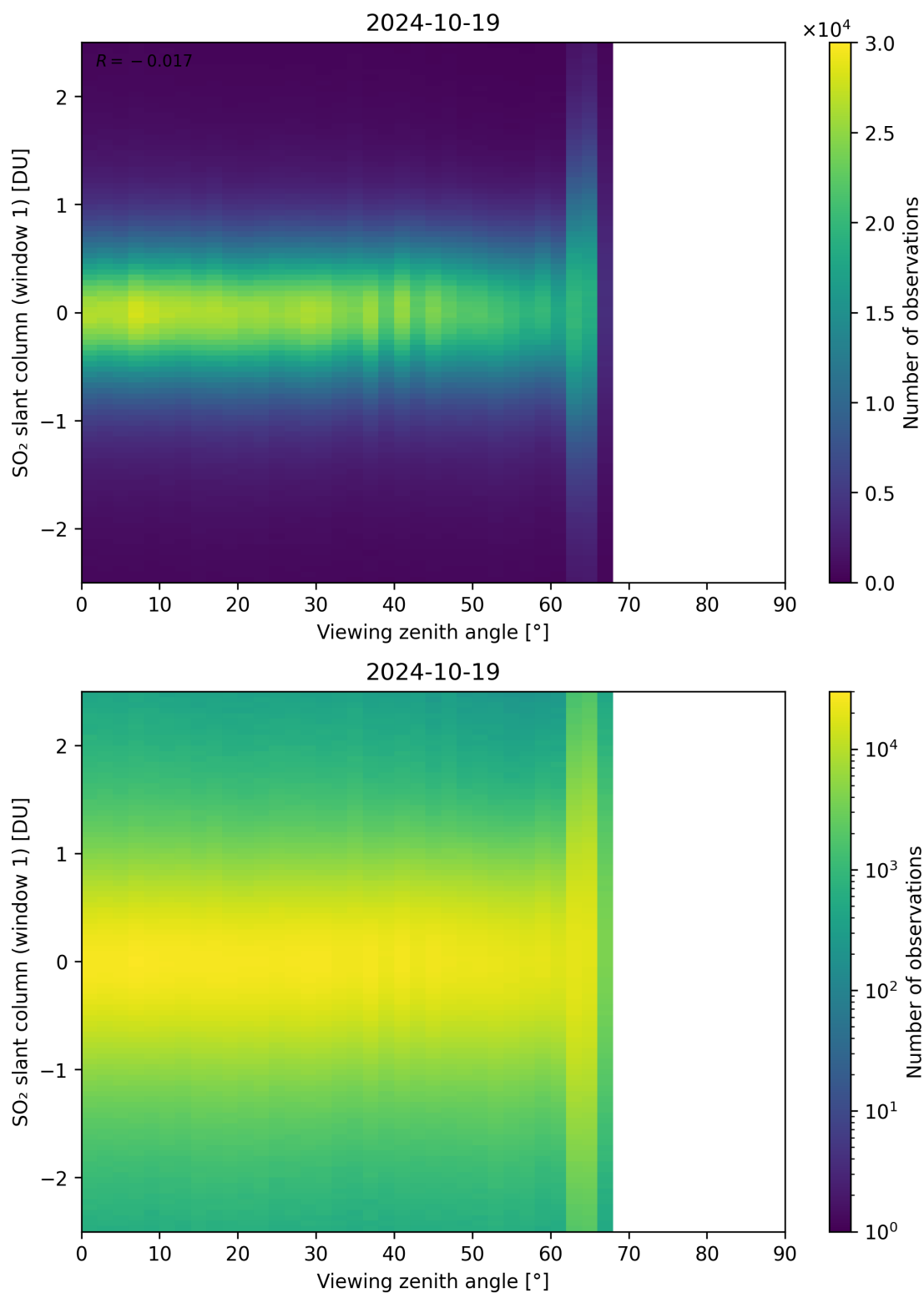
Figure 320: Scatter density plot of “Viewing zenith angle” against “SO 2 slant column (window 1)” for 2024-10-19 to 2024-10-20.
