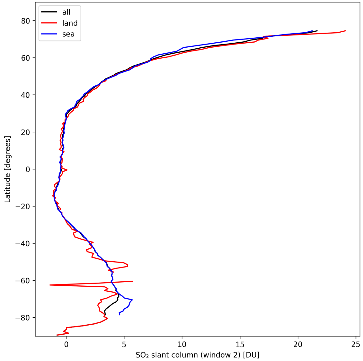
Figure 37: Zonal average of “SO 2 slant column (window 2)” for 2024-10-19 to 2024-10-20.
