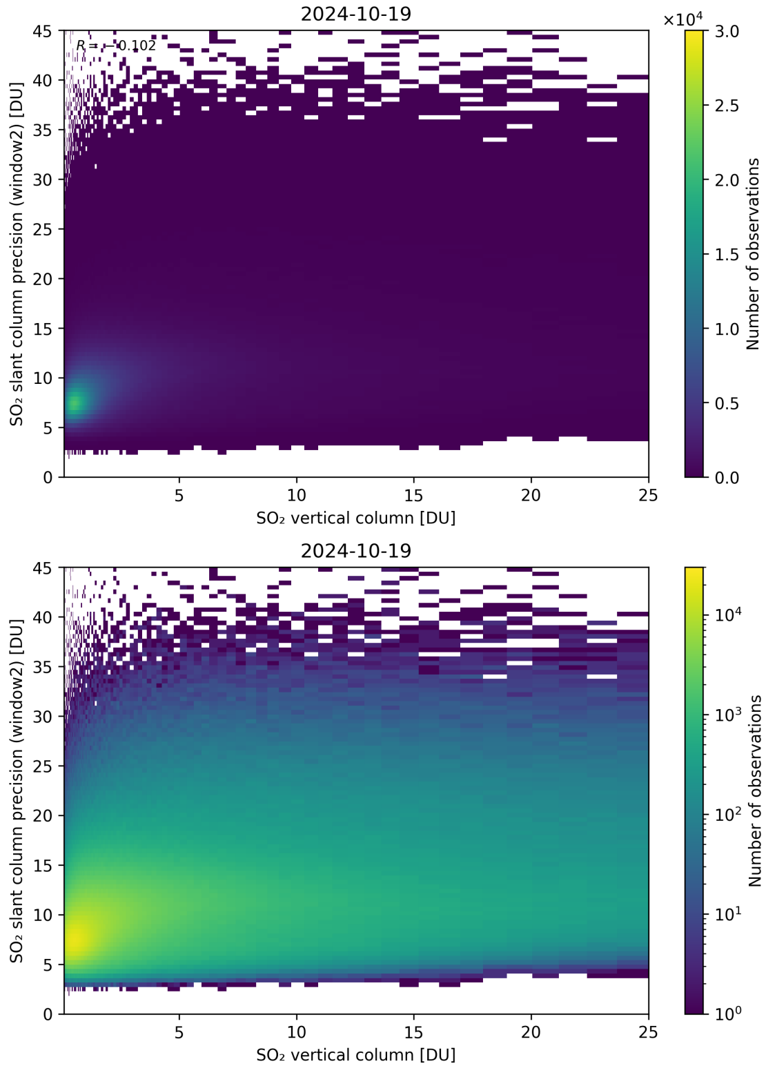
Figure 302: Scatter density plot of “SO 2 vertical column” against “SO 2 slant column precision (window2)” for 2024-10-19 to 2024-10-20.
