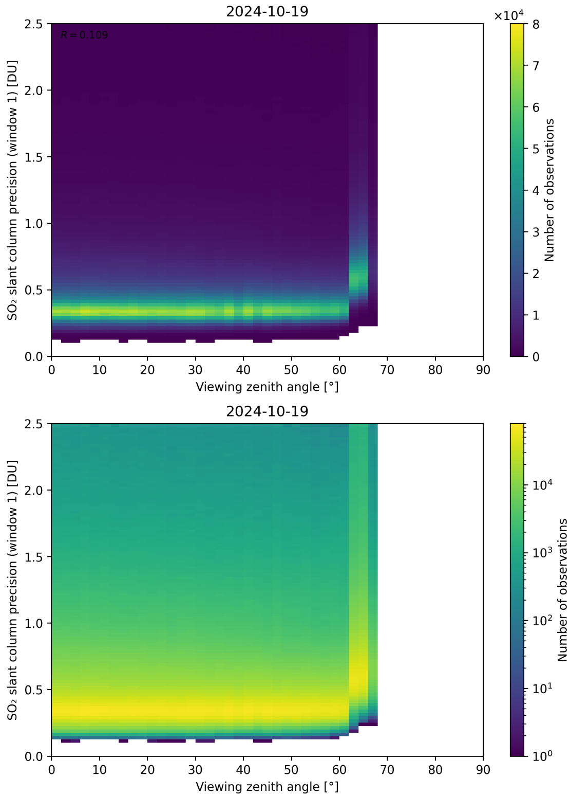
Figure 321: Scatter density plot of “Viewing zenith angle” against “SO 2 slant column precision (window 1)” for 2024-10-19 to 2024-10-20.
