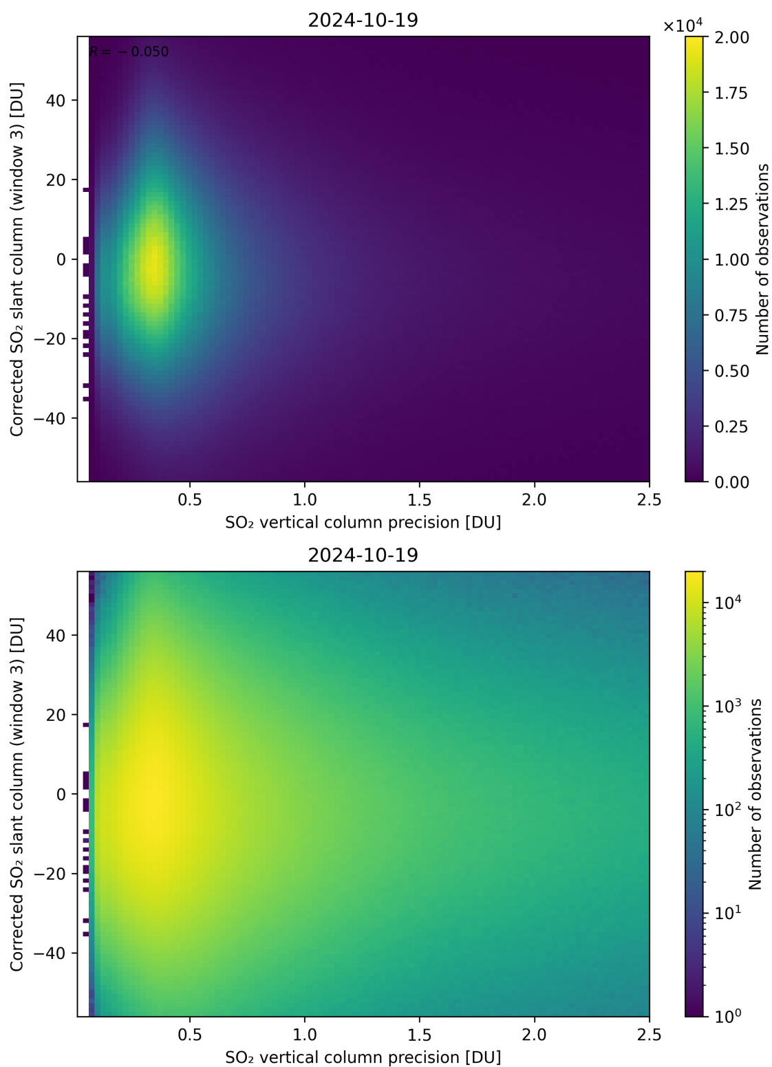
Figure 288: Scatter density plot of “SO 2 vertical column precision” against “Corrected SO 2 slant column (window 3)” for 2024-10-19 to 2024-10-20.
