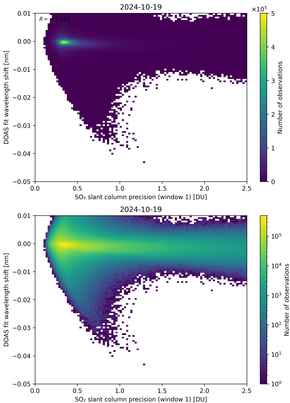
Figure 221: Scatter density plot of “SO 2 slant column precision (window 1)” against “DOAS fit wavelength shift” for 2024-10-19 to 2024-10-20.
