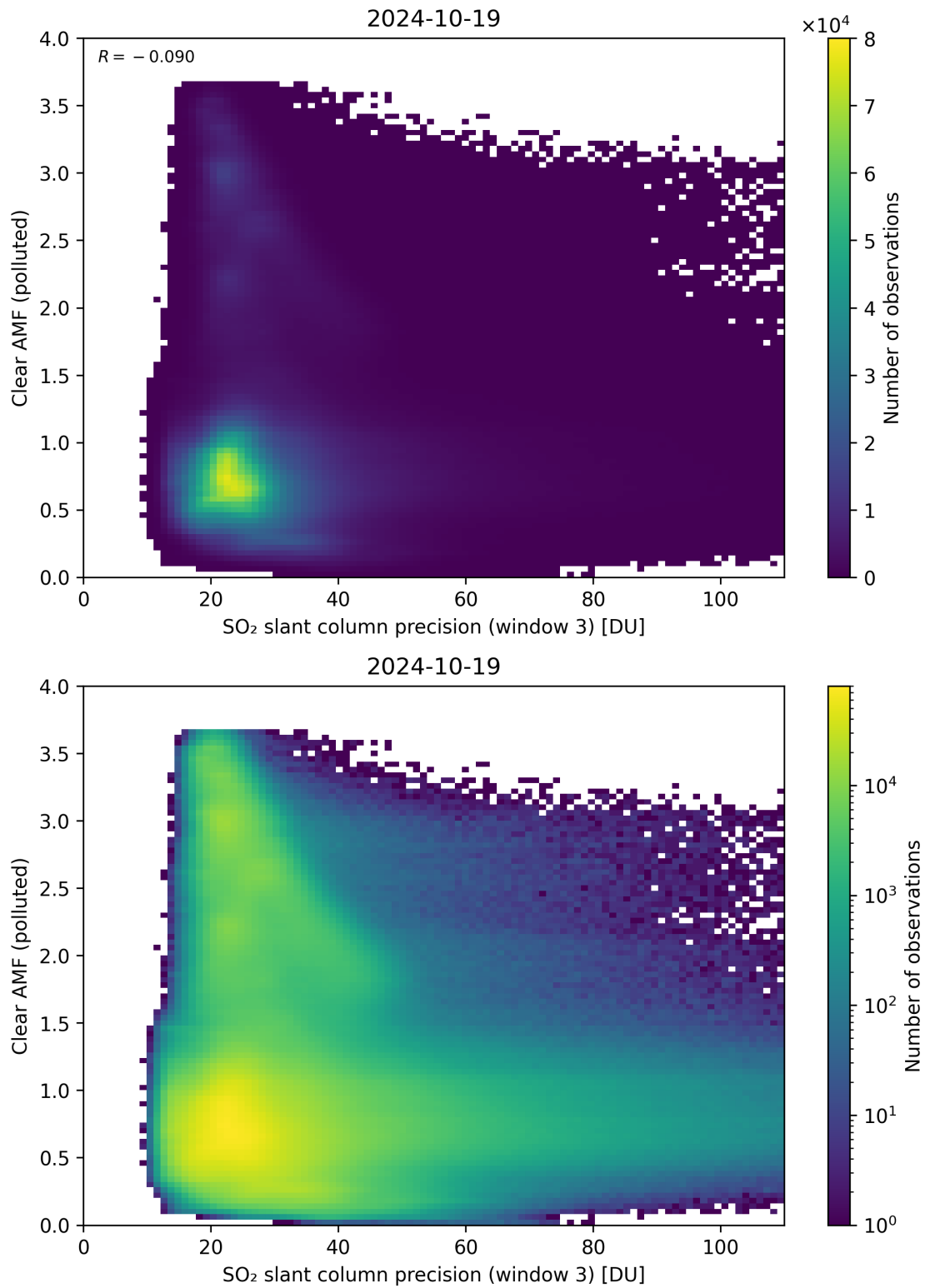
Figure 261: Scatter density plot of “SO 2 slant column precision (window 3)” against “Clear AMF (polluted)” for 2024-10-19 to 2024-10-20.
