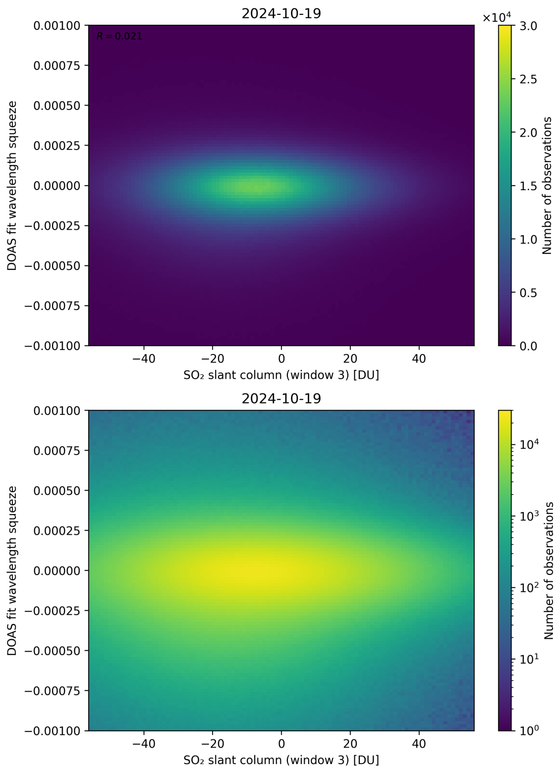
Figure 255: Scatter density plot of “SO 2 slant column (window 3)” against “DOAS fit wavelength squeeze” for 2024-10-19 to 2024-10-20.
