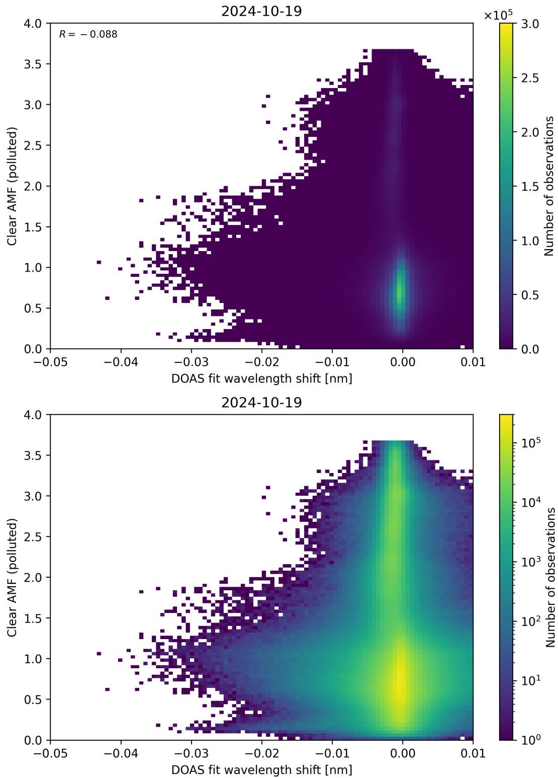
Figure 129: Scatter density plot of “DOAS fit wavelength shift” against “Clear AMF (polluted)” for 2024-10-19 to 2024-10-20.
