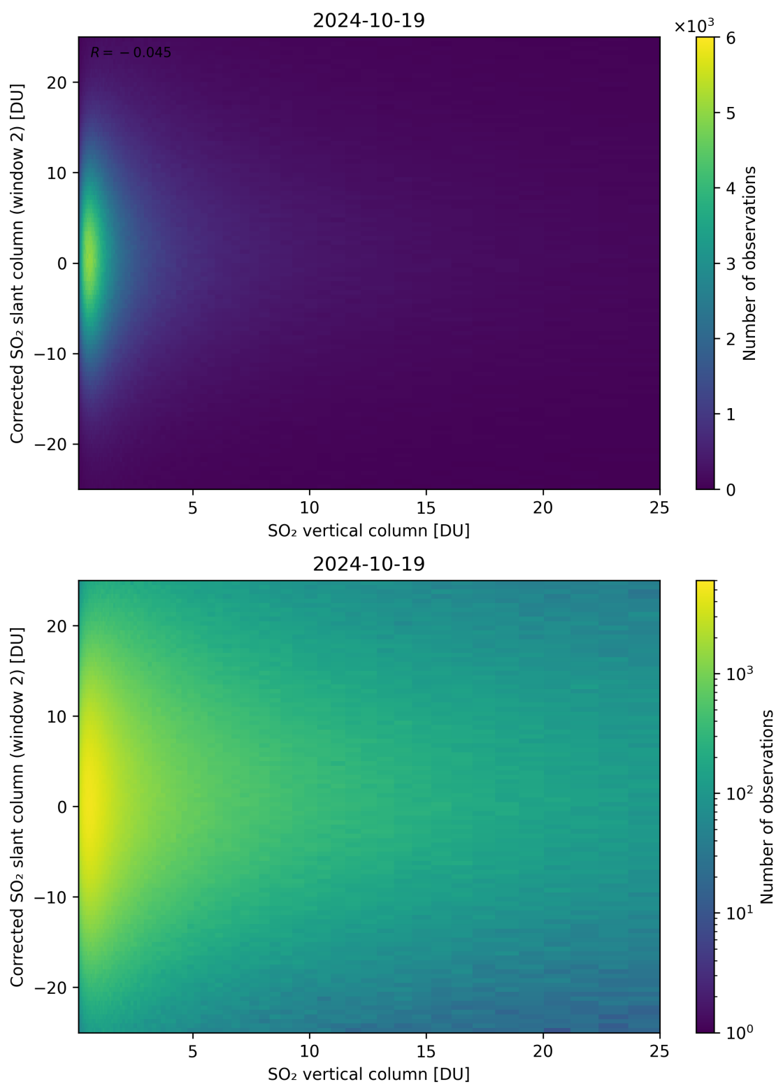
Figure 298: Scatter density plot of “SO 2 vertical column” against “Corrected SO 2 slant column (window 2)” for 2024-10-19 to 2024-10-20.
