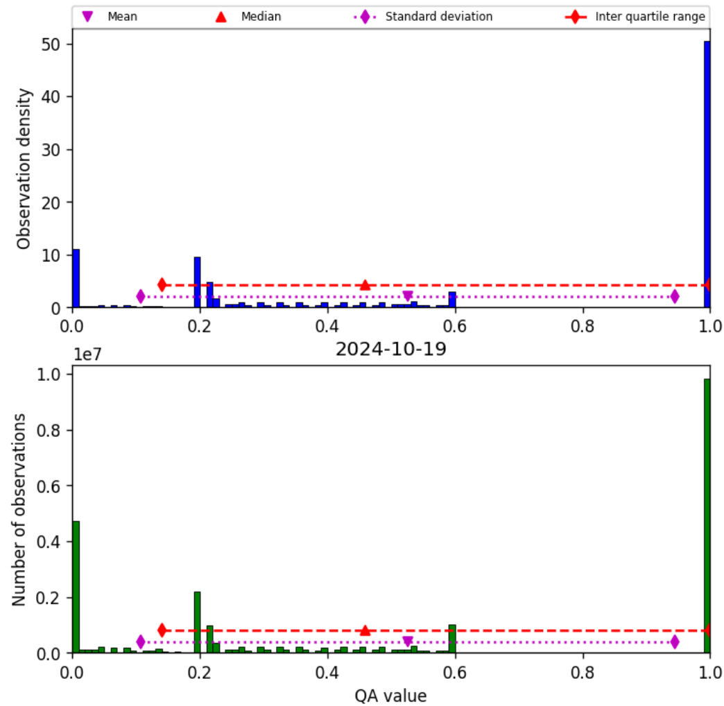
Figure 52: Histogram of “QA value” for 2024-10-19 to 2024-10-20
