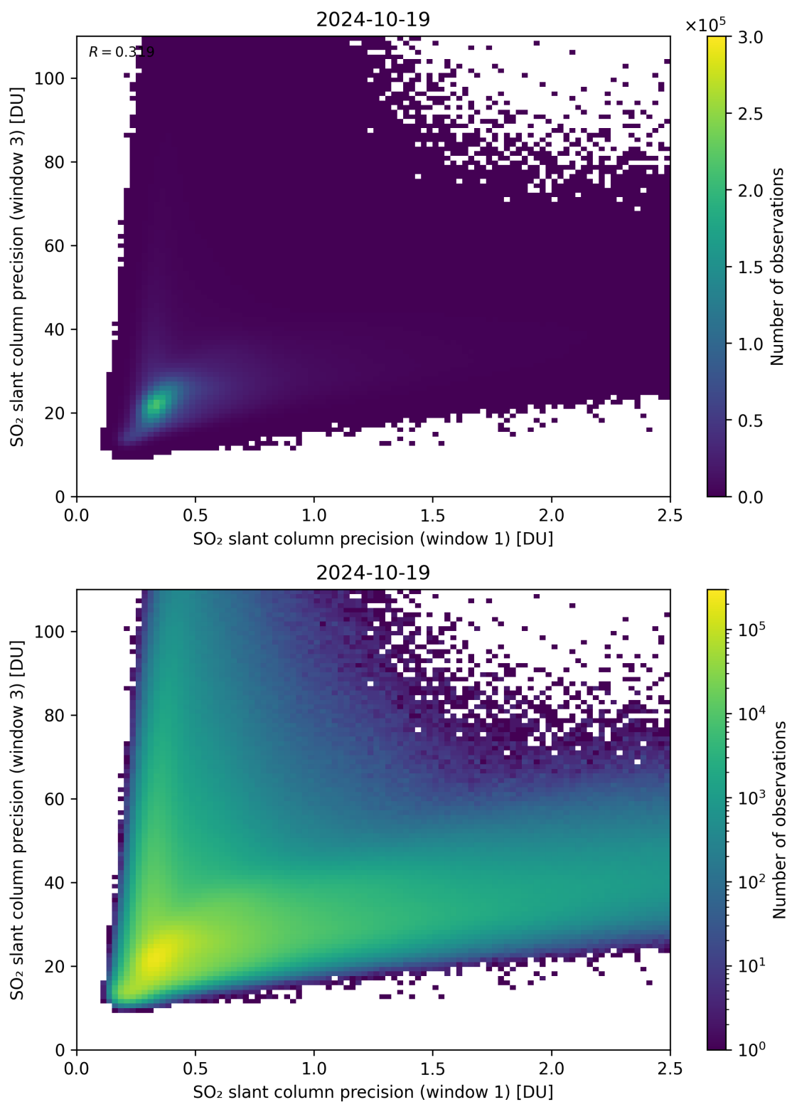
Figure 229: Scatter density plot of “SO 2 slant column precision (window 1)” against “SO 2 slant column precision (window 3)” for 2024-10-19 to 2024-10-20.
