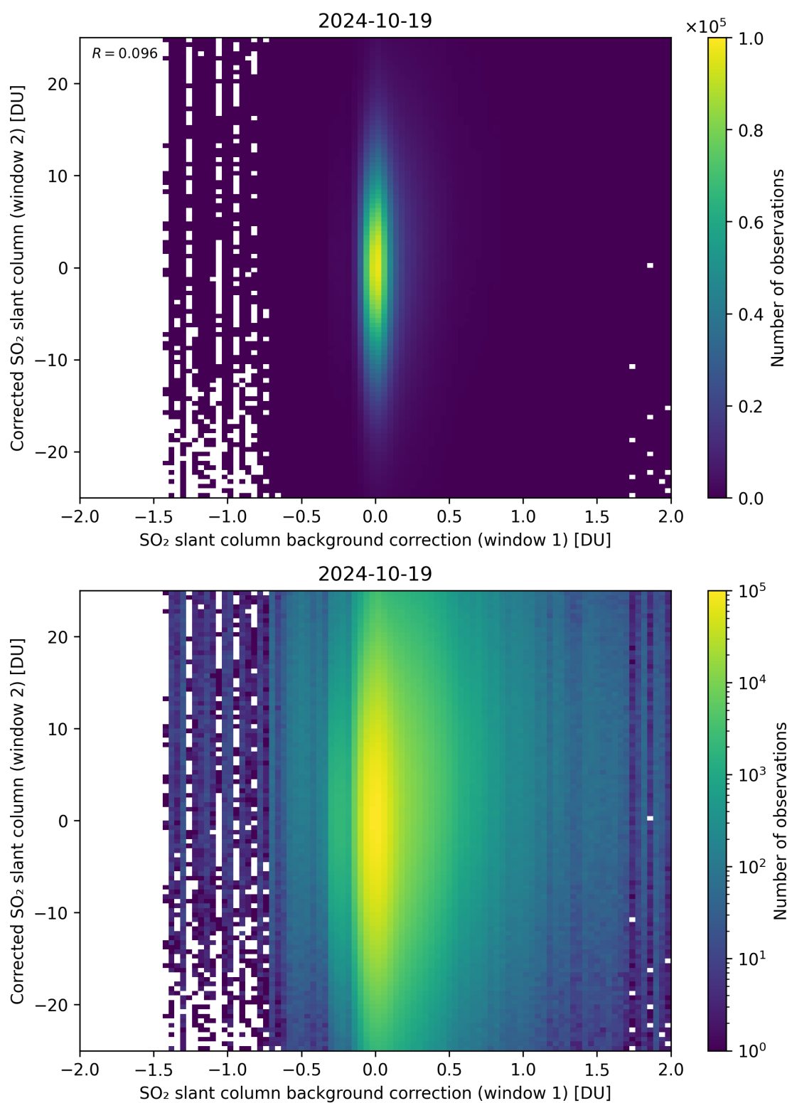
Figure 104: Scatter density plot of “SO 2 slant column background correction (window 1)” against “Corrected SO 2 slant column (window 2)” for 2024-10-19 to 2024-10-20.
