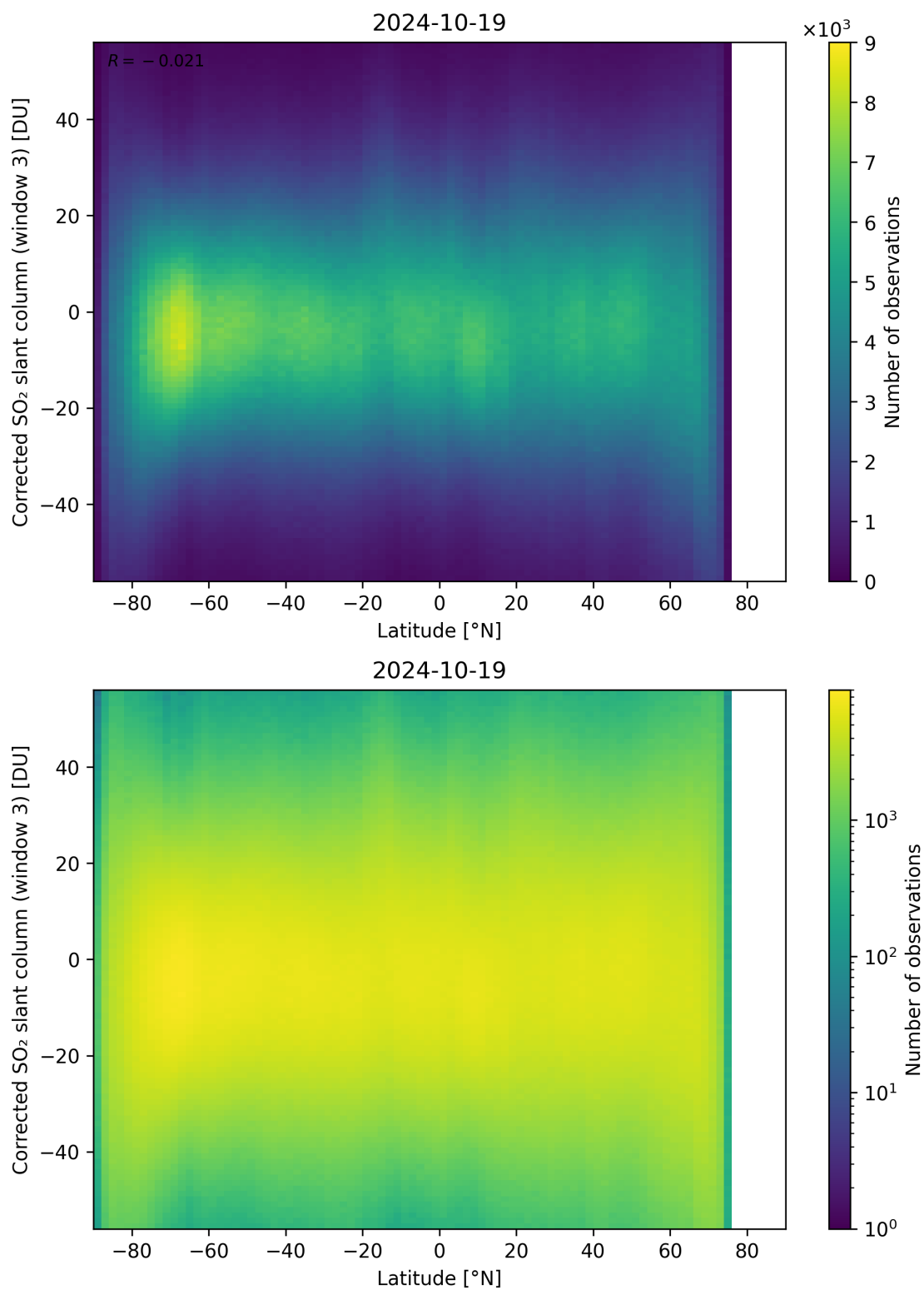
Figure 148: Scatter density plot of “Latitude” against “Corrected SO 2 slant column (window 3)” for 2024-10-19 to 2024-10-20.
