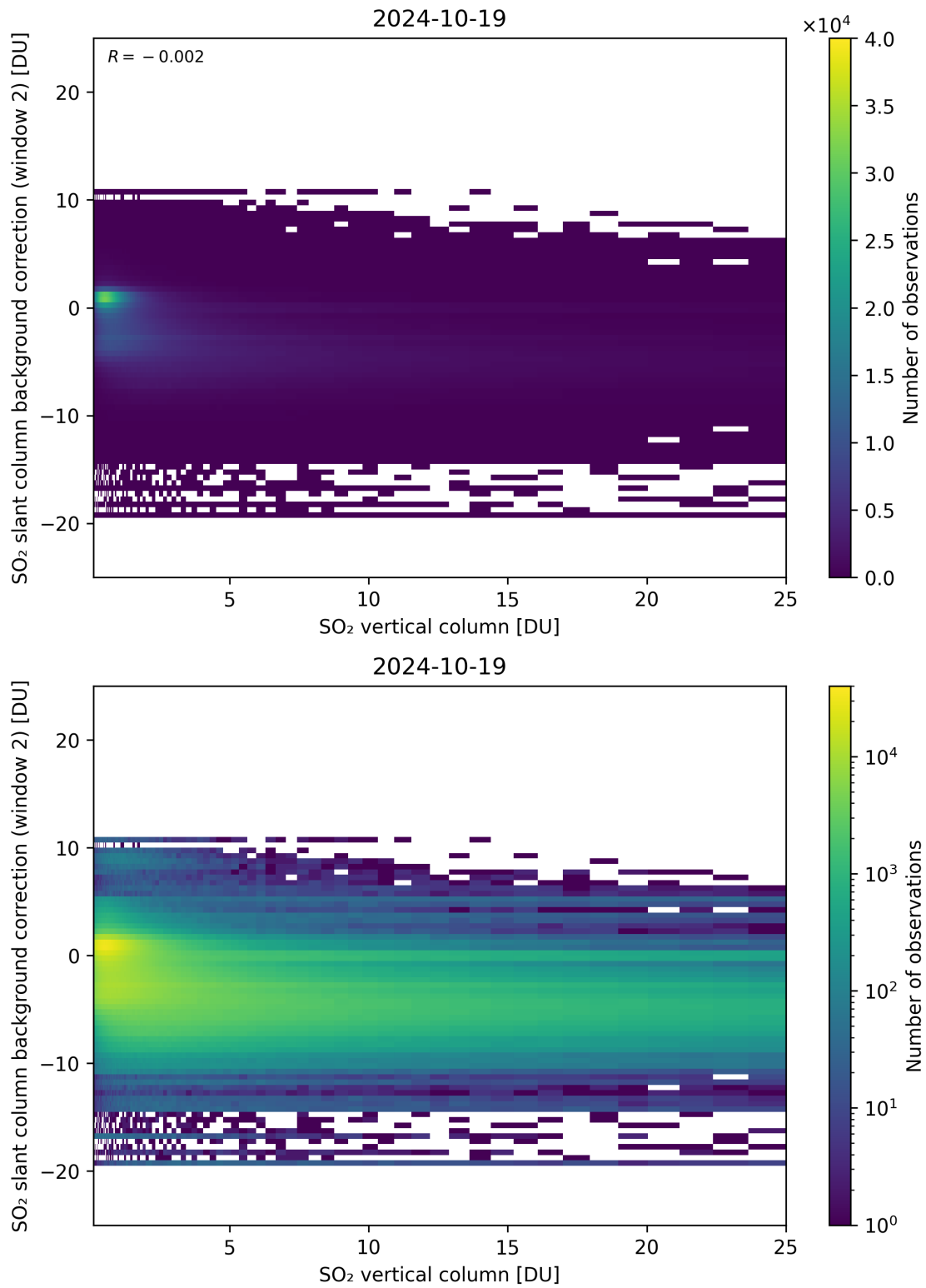
Figure 274: Scatter density plot of “SO 2 vertical column” against “SO 2 slant column background correction (window 2)” for 2024-10-19 to 2024-10-20.
