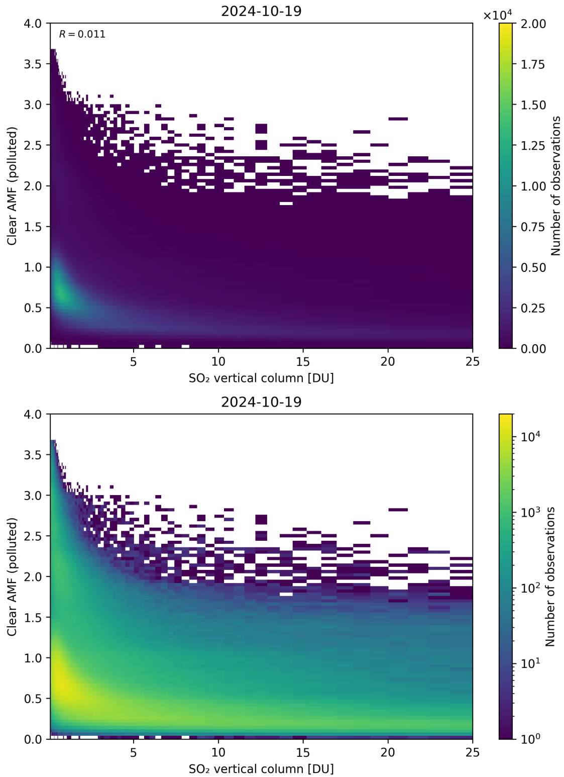
Figure 296: Scatter density plot of “SO 2 vertical column” against “Clear AMF (polluted)” for 2024-10-19 to 2024-10-20.
