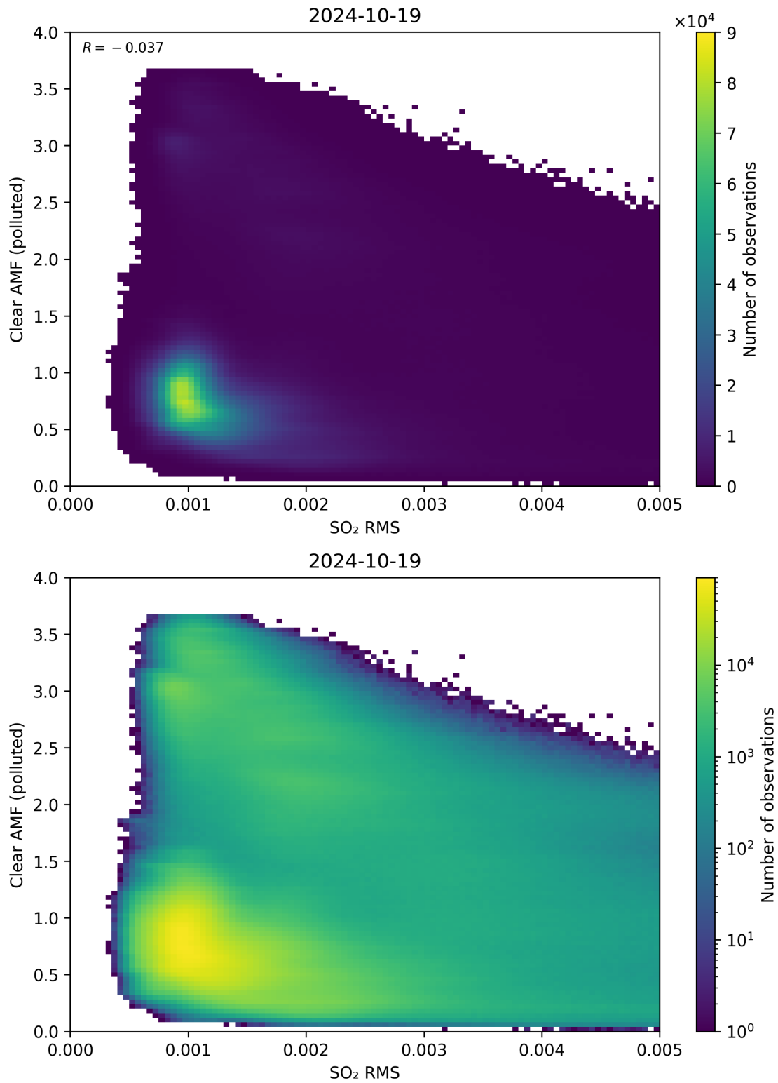
Figure 136: Scatter density plot of “SO 2 RMS” against “Clear AMF (polluted)” for 2024-10-19 to 2024-10-20.
