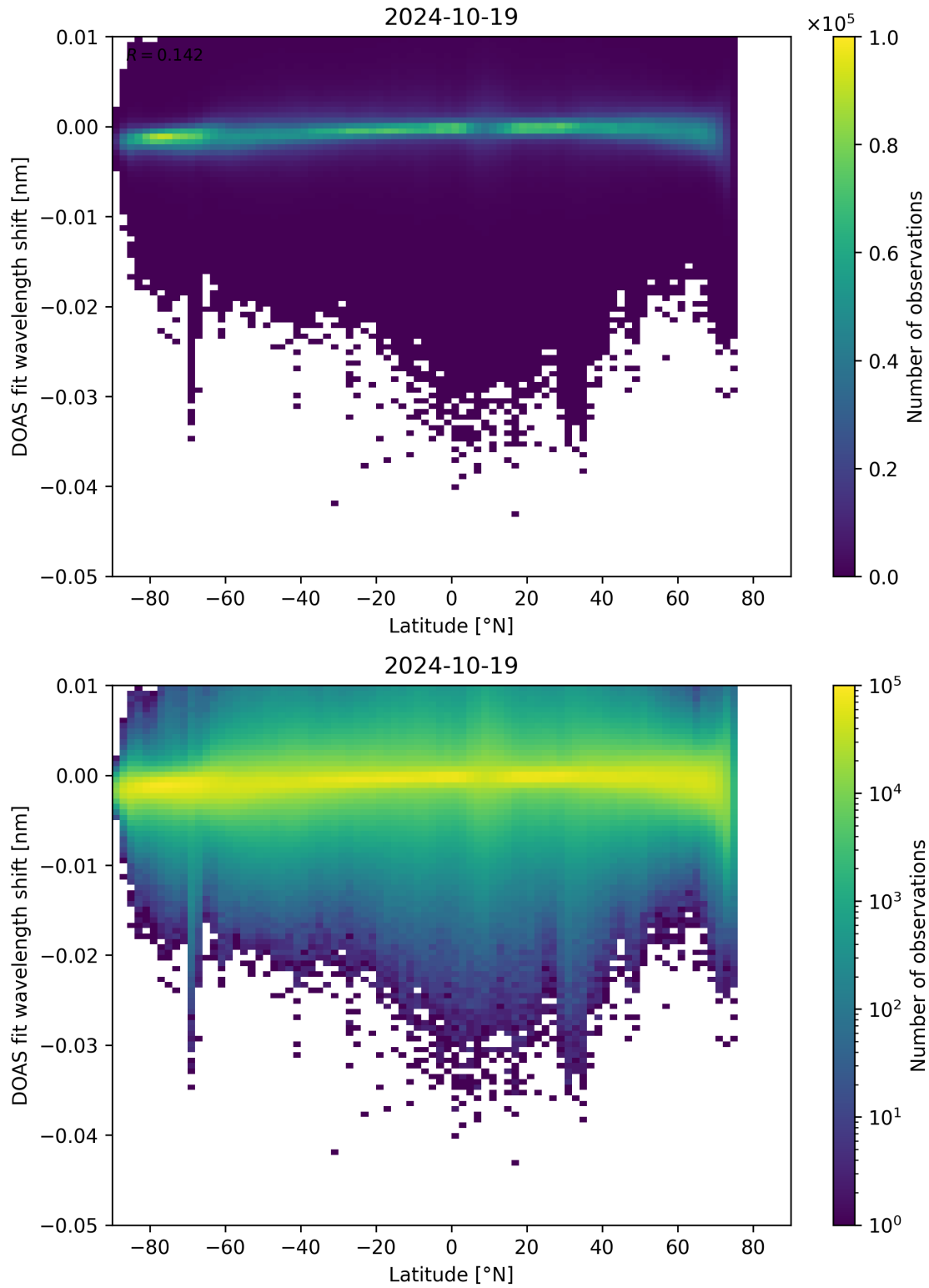
Figure 142: Scatter density plot of “Latitude” against “DOAS fit wavelength shift” for 2024-10-19 to 2024-10-20.
