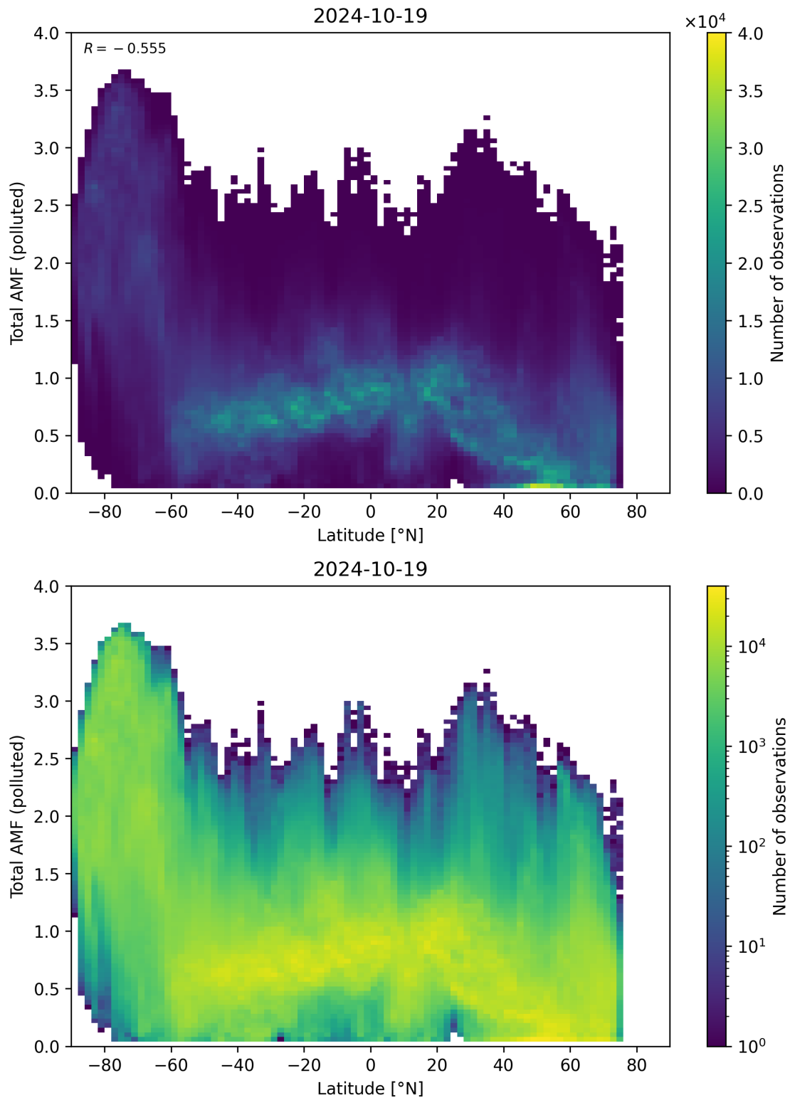
Figure 154: Scatter density plot of “Latitude” against “Total AMF (polluted)” for 2024-10-19 to 2024-10-20.
