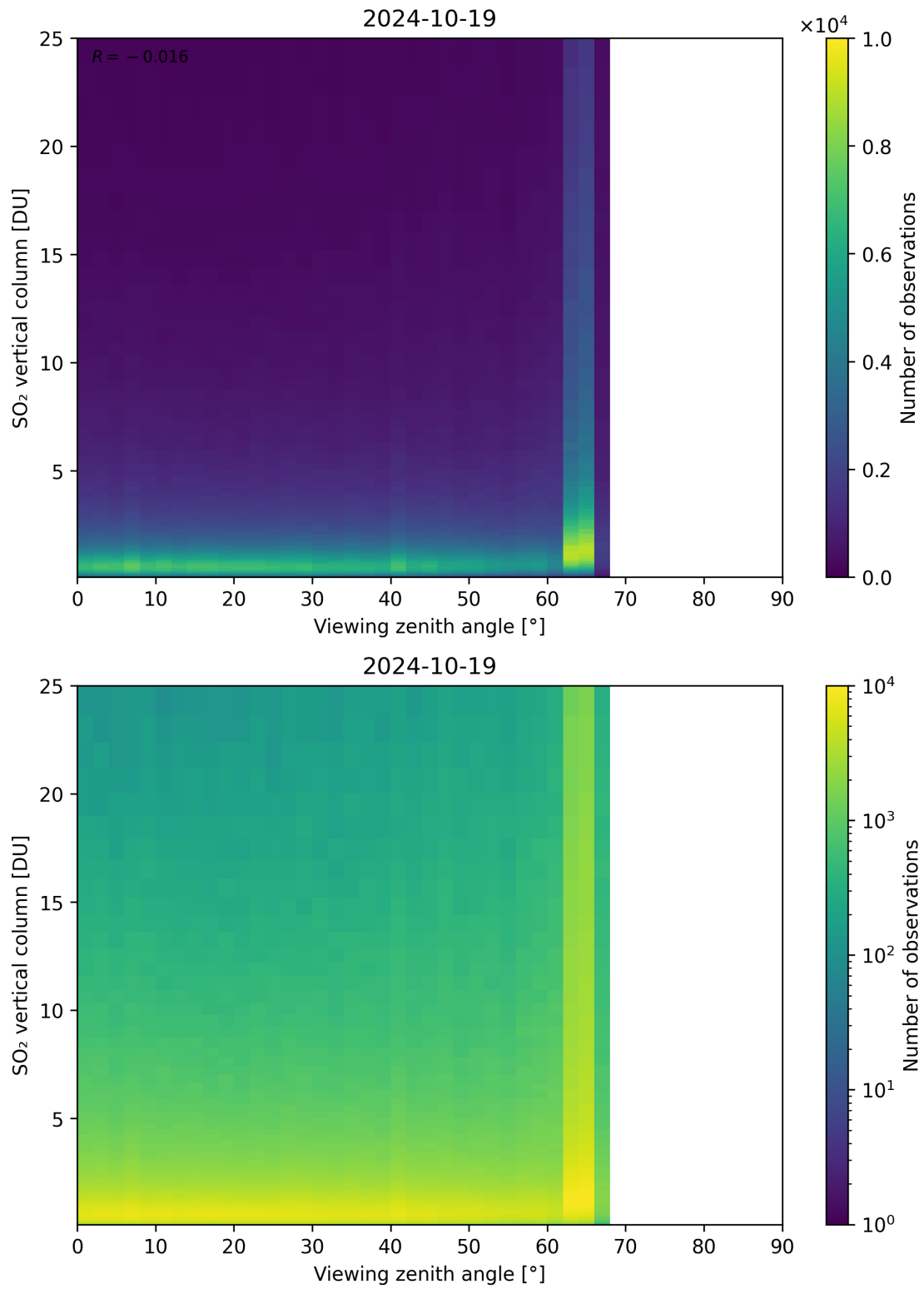
Figure 327: Scatter density plot of “Viewing zenith angle” against “SO 2 vertical column” for 2024-10-19 to 2024-10-20.
