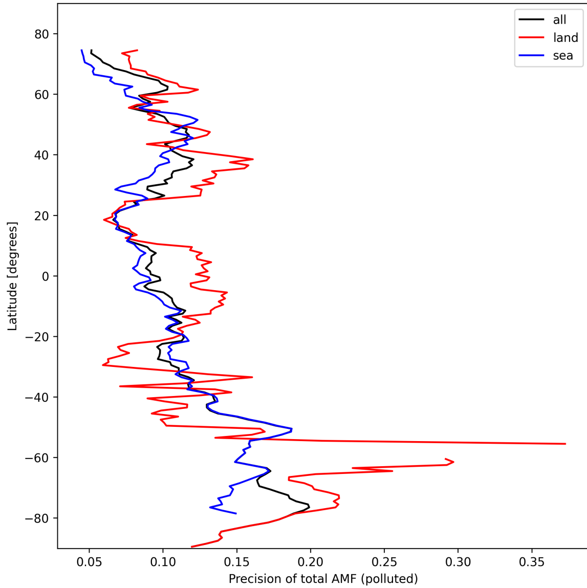
Figure 49: Zonal average of “Precision of total AMF (polluted)” for 2024-10-19 to 2024-10-20.
