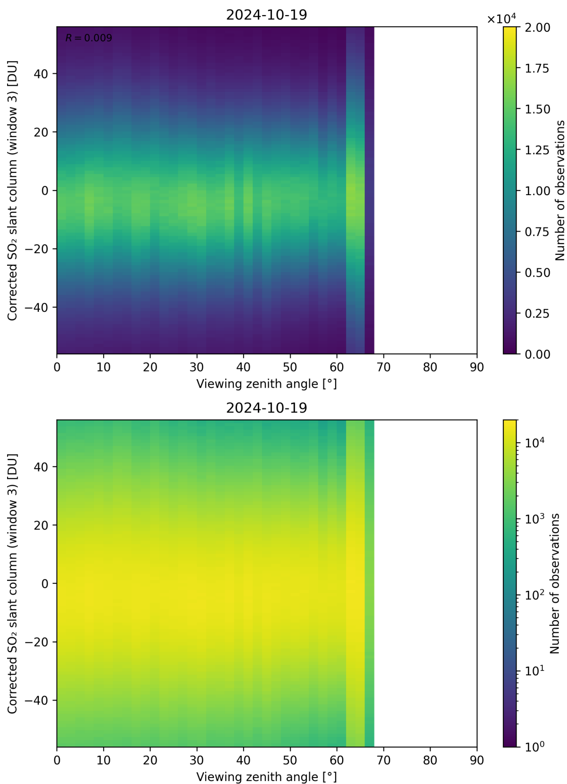
Figure 319: Scatter density plot of “Viewing zenith angle” against “Corrected SO 2 slant column (window 3)” for 2024-10-19 to 2024-10-20.
