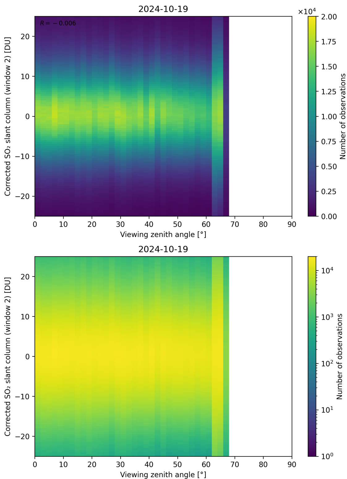
Figure 318: Scatter density plot of “Viewing zenith angle” against “Corrected SO 2 slant column (window 2)” for 2024-10-19 to 2024-10-20.
