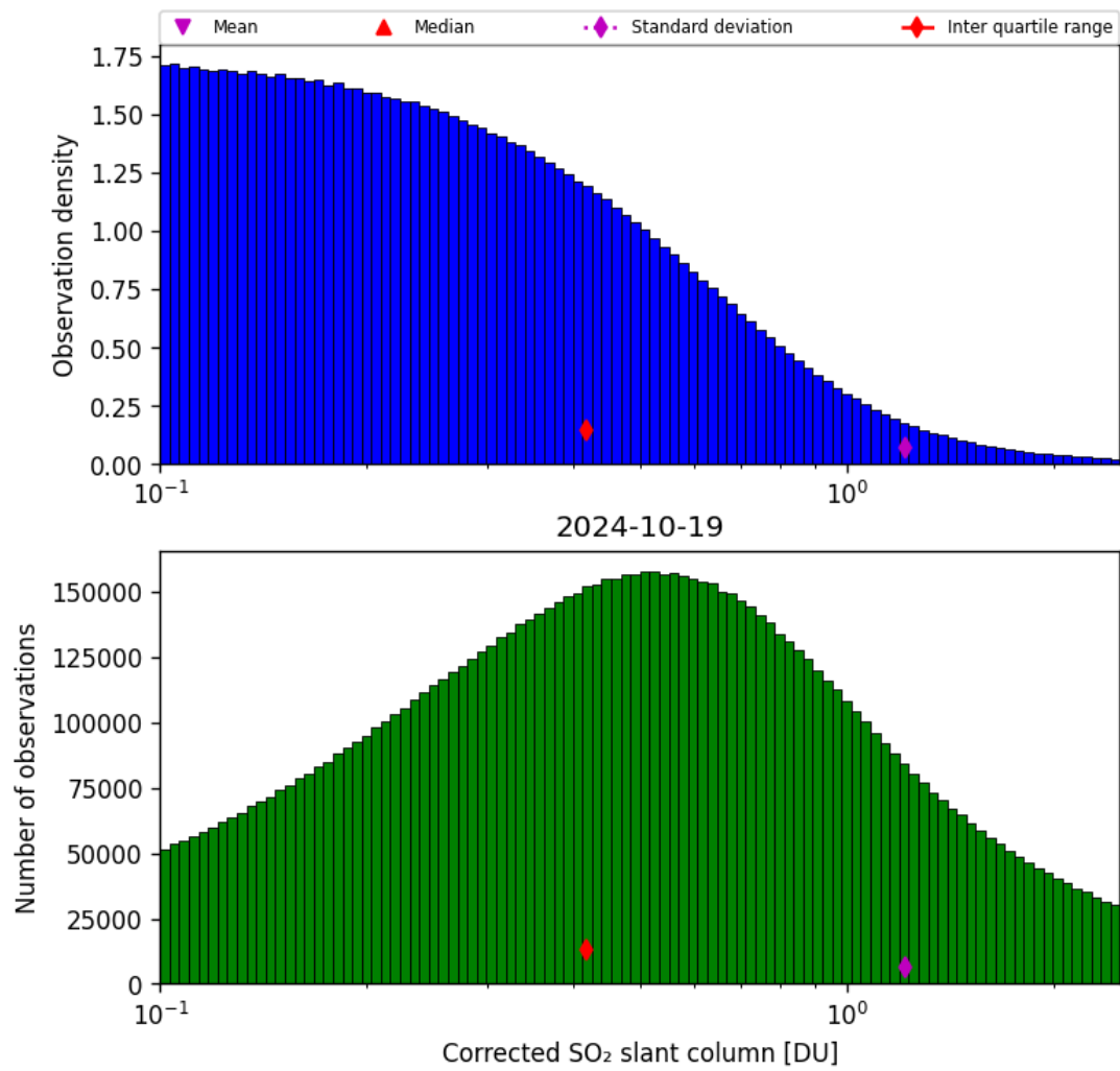
Figure 55: Histogram of “Corrected SO 2 slant column” for 2024-10-19 to 2024-10-20
