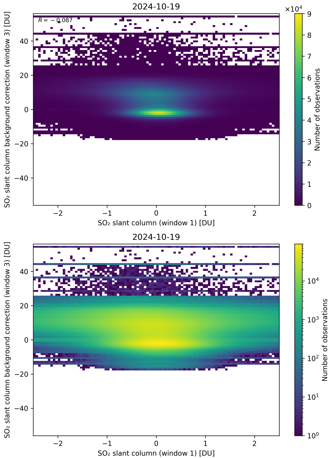
Figure 214: Scatter density plot of “SO 2 slant column (window 1)” against “SO 2 slant column background correction (window 3)” for 2024-10-19 to 2024-10-20.
