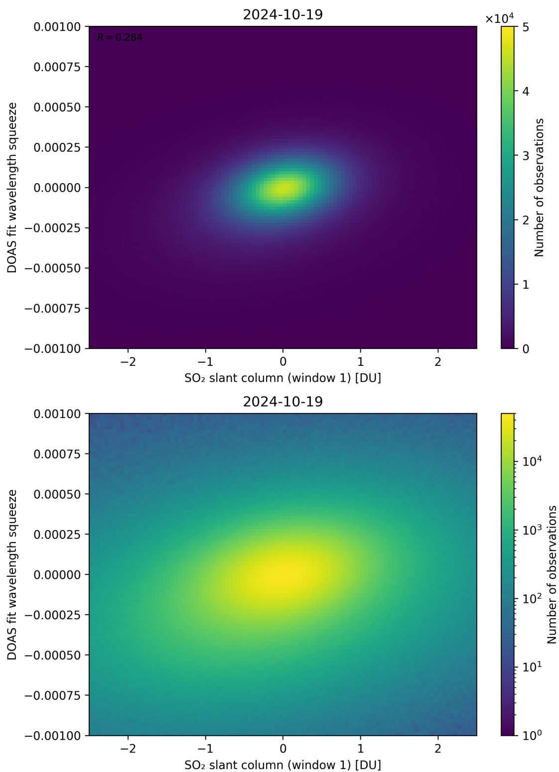
Figure 216: Scatter density plot of “SO 2 slant column (window 1)” against “DOAS fit wavelength squeeze” for 2024-10-19 to 2024-10-20.
