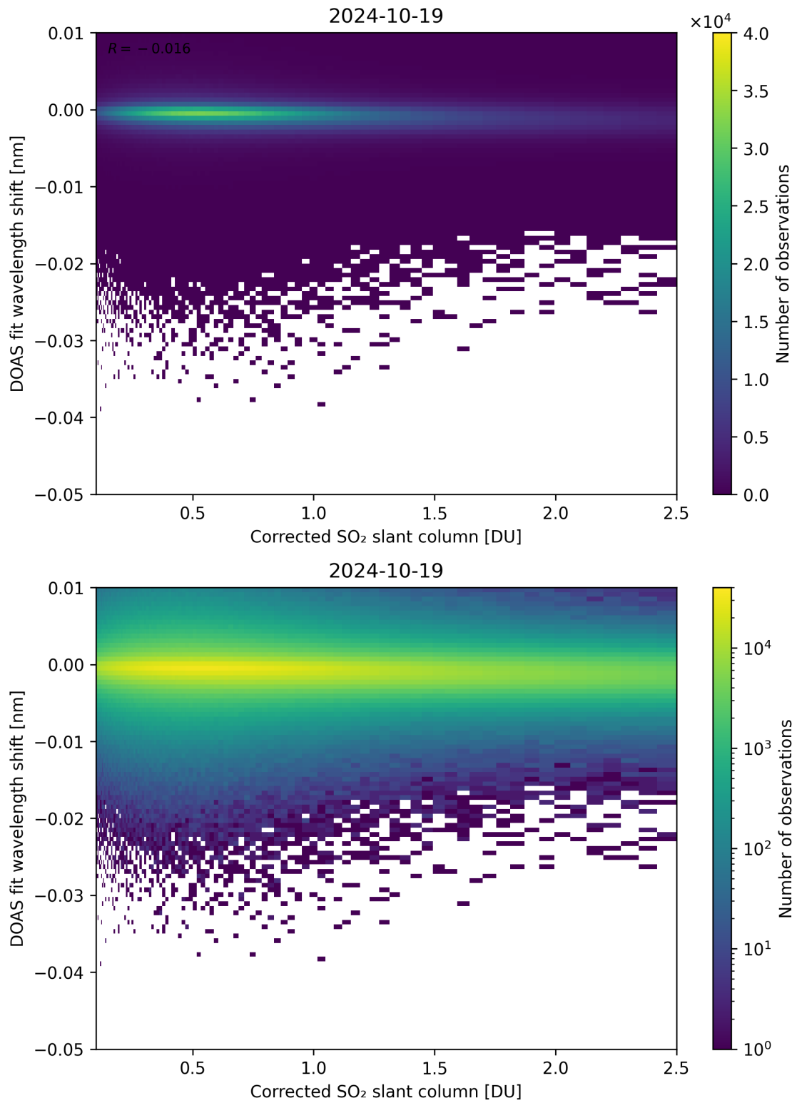
Figure 181: Scatter density plot of “Corrected SO 2 slant column” against “DOAS fit wavelength shift” for 2024-10-19 to 2024-10-20.
