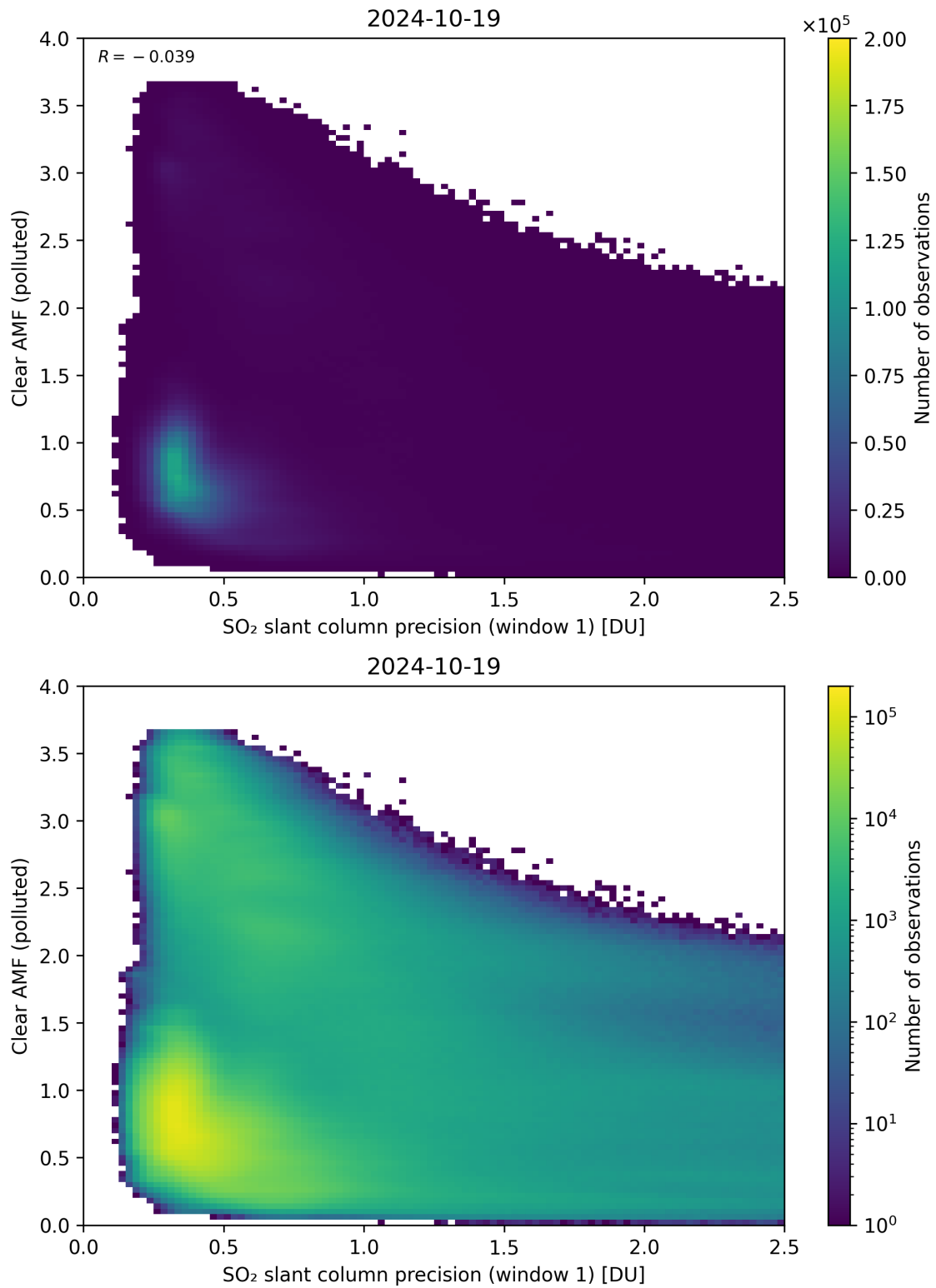
Figure 224: Scatter density plot of “SO 2 slant column precision (window 1)” against “Clear AMF (polluted)” for 2024-10-19 to 2024-10-20.
