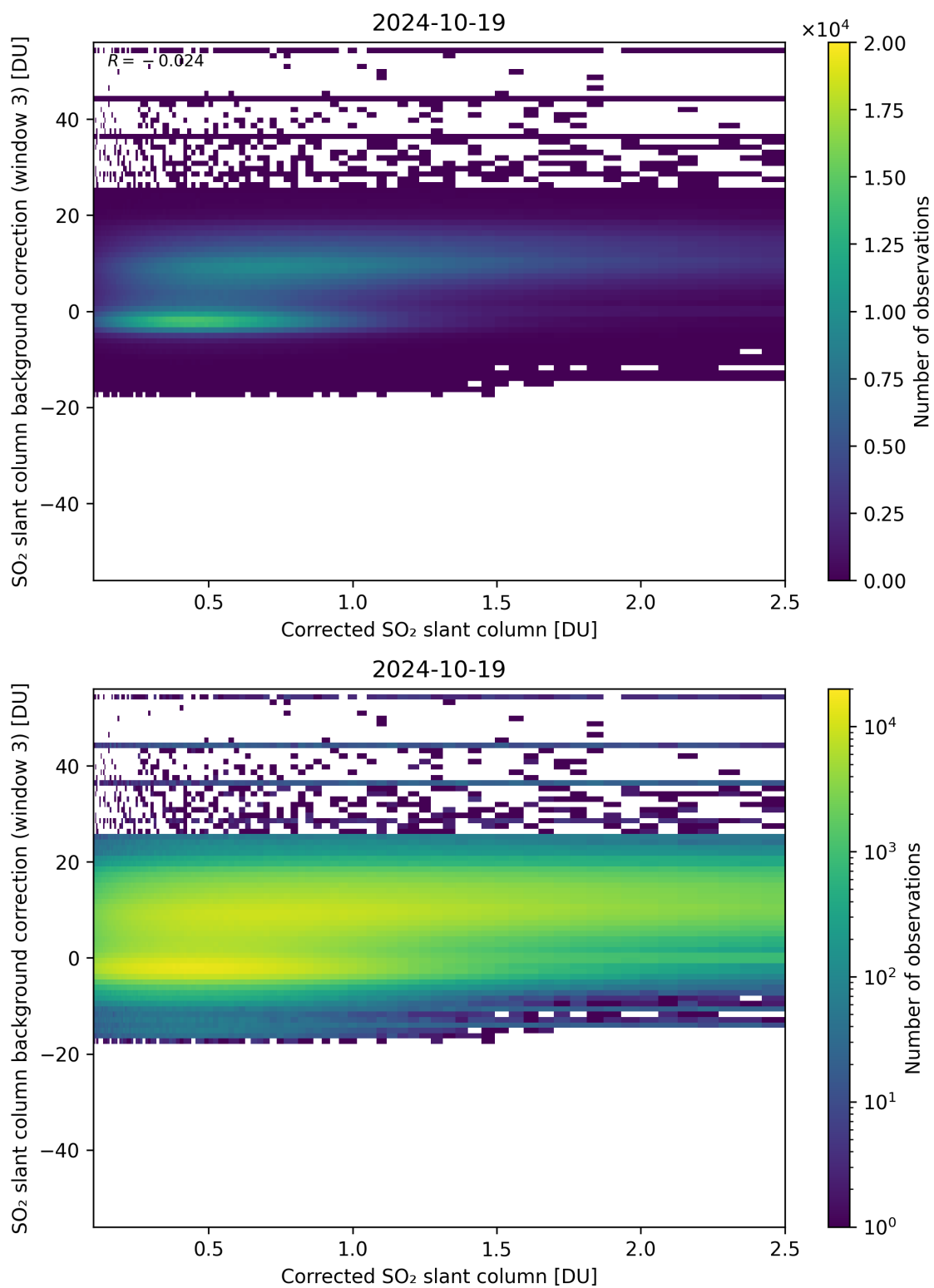
Figure 180: Scatter density plot of “Corrected SO 2 slant column” against “SO 2 slant column background correction (window 3)” for 2024-10-19 to 2024-10-20.
