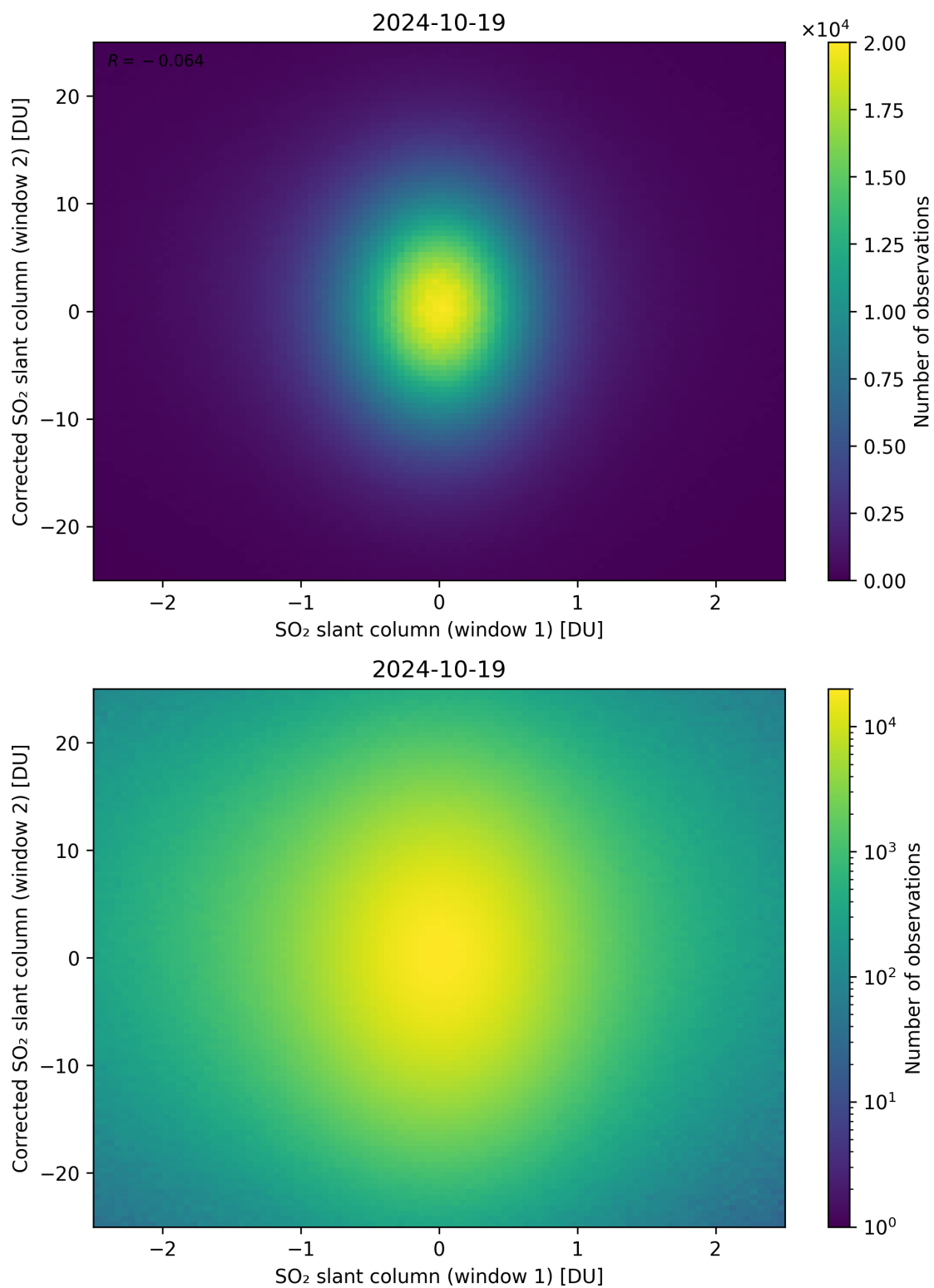
Figure 233: Scatter density plot of “SO 2 slant column (window 1)” against “Corrected SO 2 slant column (window 2)” for 2024-10-19 to 2024-10-20.
