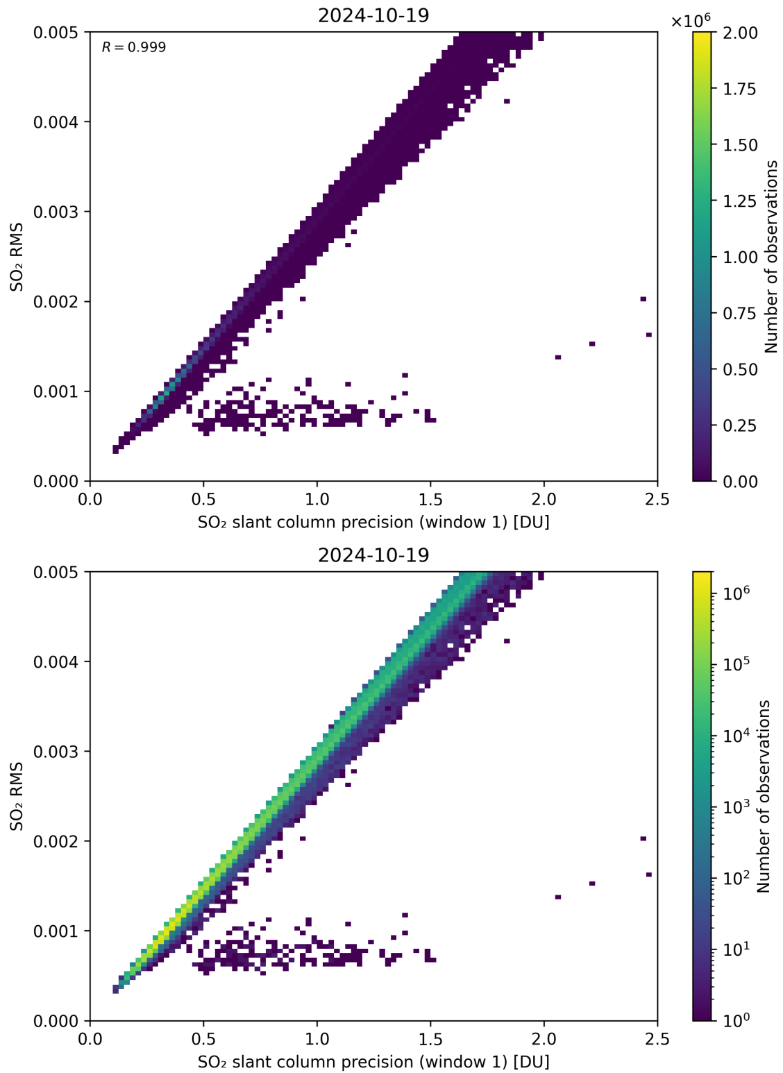
Figure 223: Scatter density plot of “SO 2 slant column precision (window 1)” against “SO 2 RMS” for 2024-10-19 to 2024-10-20.
