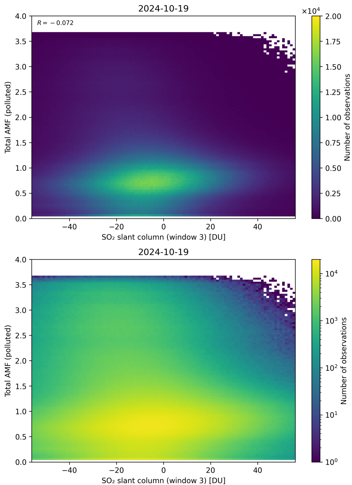
Figure 268: Scatter density plot of “SO 2 slant column (window 3)” against “Total AMF (polluted)” for 2024-10-19 to 2024-10-20.
