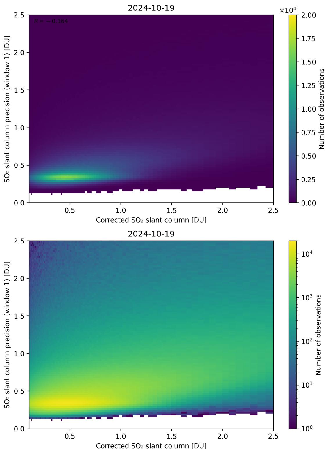
Figure 188: Scatter density plot of “Corrected SO 2 slant column” against “SO 2 slant column precision (window 1)” for 2024-10-19 to 2024-10-20.
