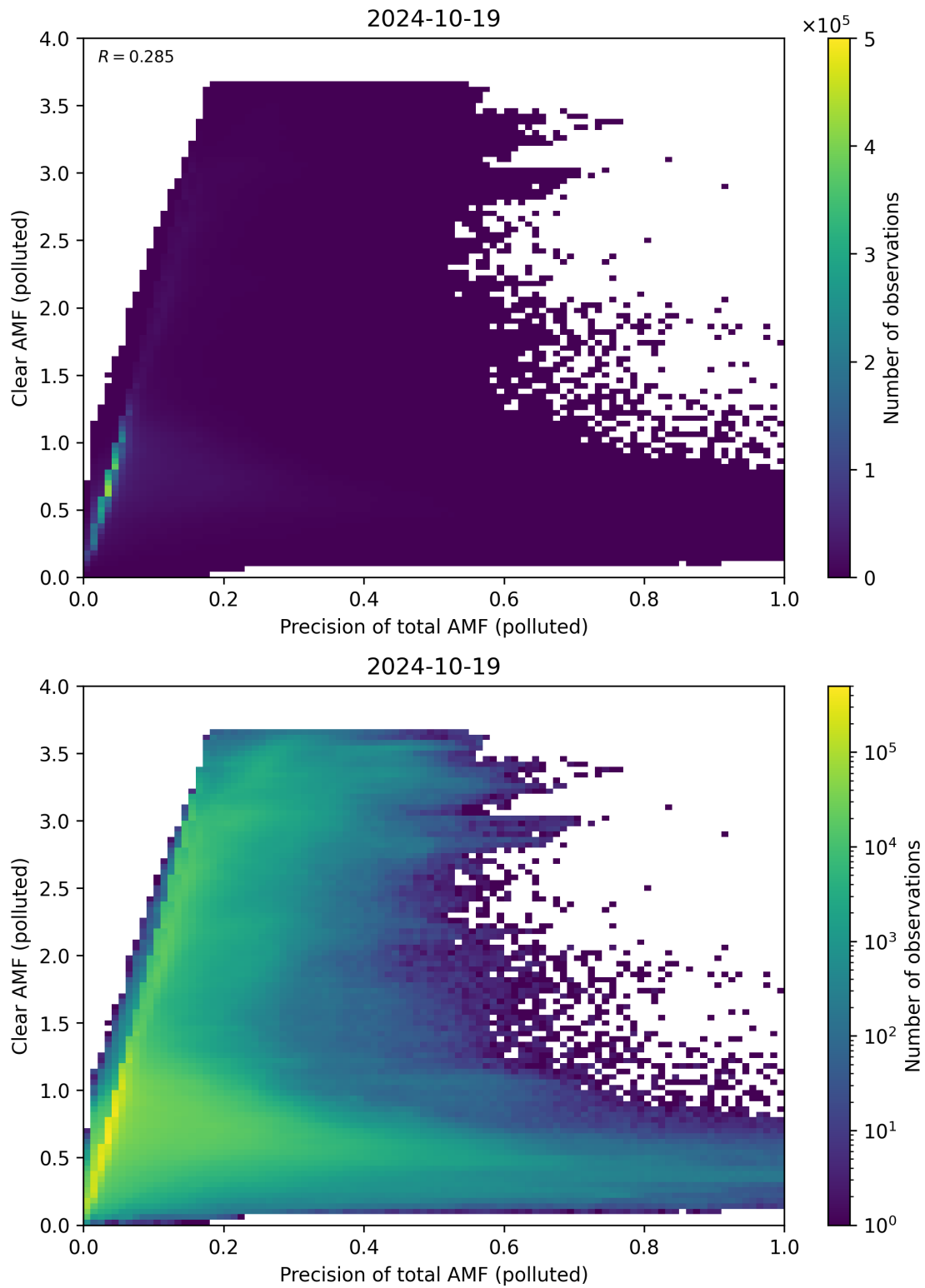
Figure 270: Scatter density plot of “Precision of total AMF (polluted)” against “Clear AMF (polluted)” for 2024-10-19 to 2024-10-20.
