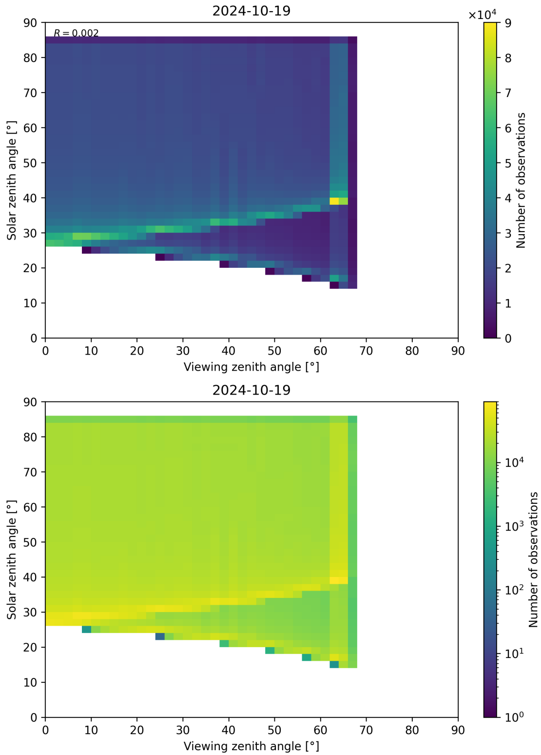
Figure 315: Scatter density plot of “Viewing zenith angle” against “Solar zenith angle” for 2024-10-19 to 2024-10-20.
