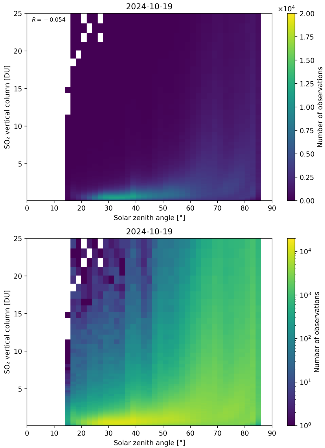
Figure 176: Scatter density plot of “Solar zenith angle” against “SO 2 vertical column” for 2024-10-19 to 2024-10-20.
