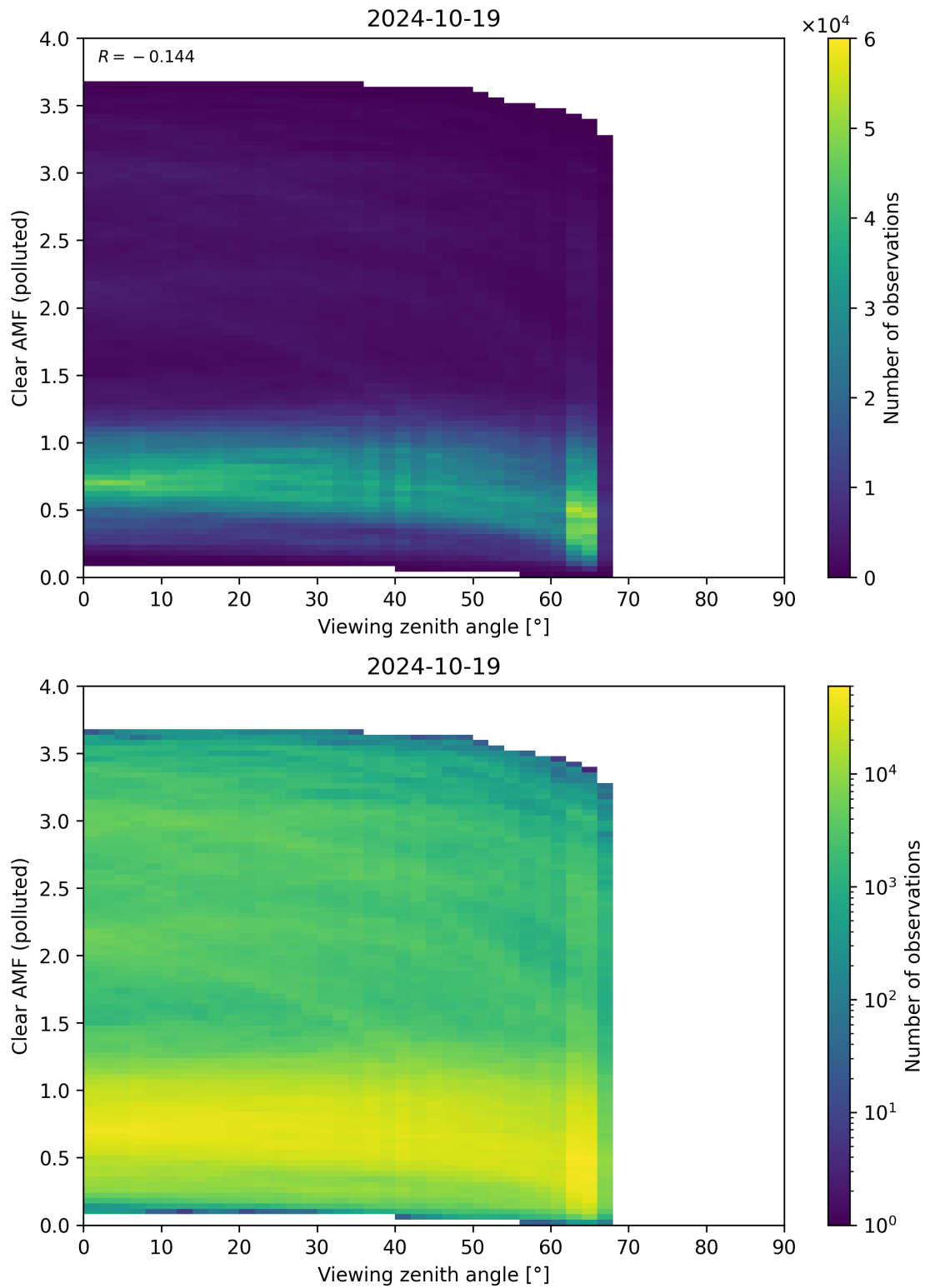
Figure 316: Scatter density plot of “Viewing zenith angle” against “Clear AMF (polluted)” for 2024-10-19 to 2024-10-20.
