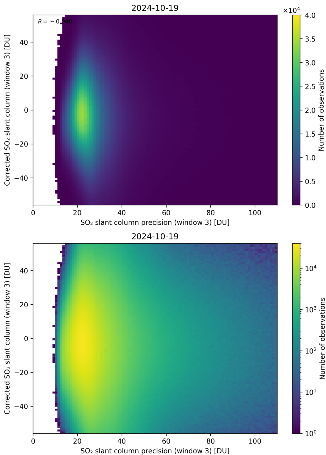
Figure 262: Scatter density plot of “SO 2 slant column precision (window 3)” against “Corrected SO 2 slant column (window 3)” for 2024-10-19 to 2024-10-20.
