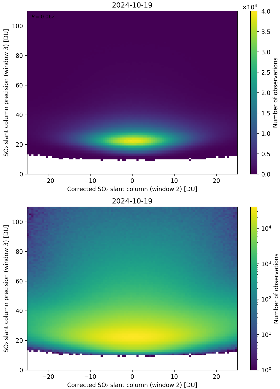
Figure 202: Scatter density plot of “Corrected SO 2 slant column (window 2)” against “SO 2 slant column precision (window 3)” for 2024-10-19 to 2024-10-20.
