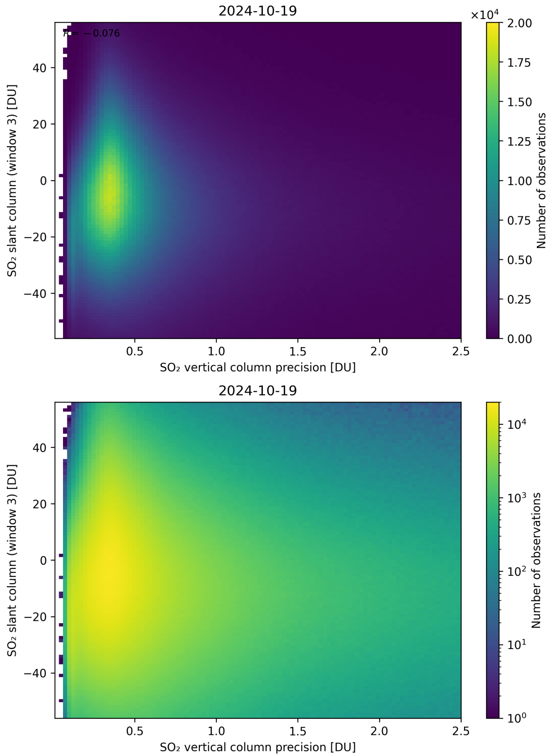
Figure 292: Scatter density plot of “SO 2 vertical column precision” against “SO 2 slant column (window 3)” for 2024-10-19 to 2024-10-20.
