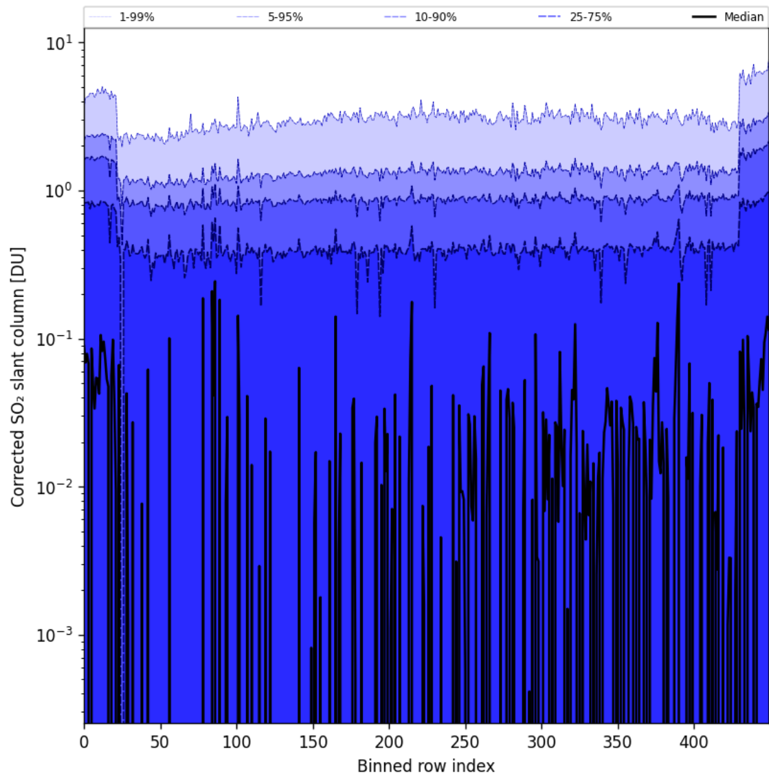
Figure 78: Along track statistics of “Corrected SO 2 slant column” for 2024-10-19 to 2024-10-20
