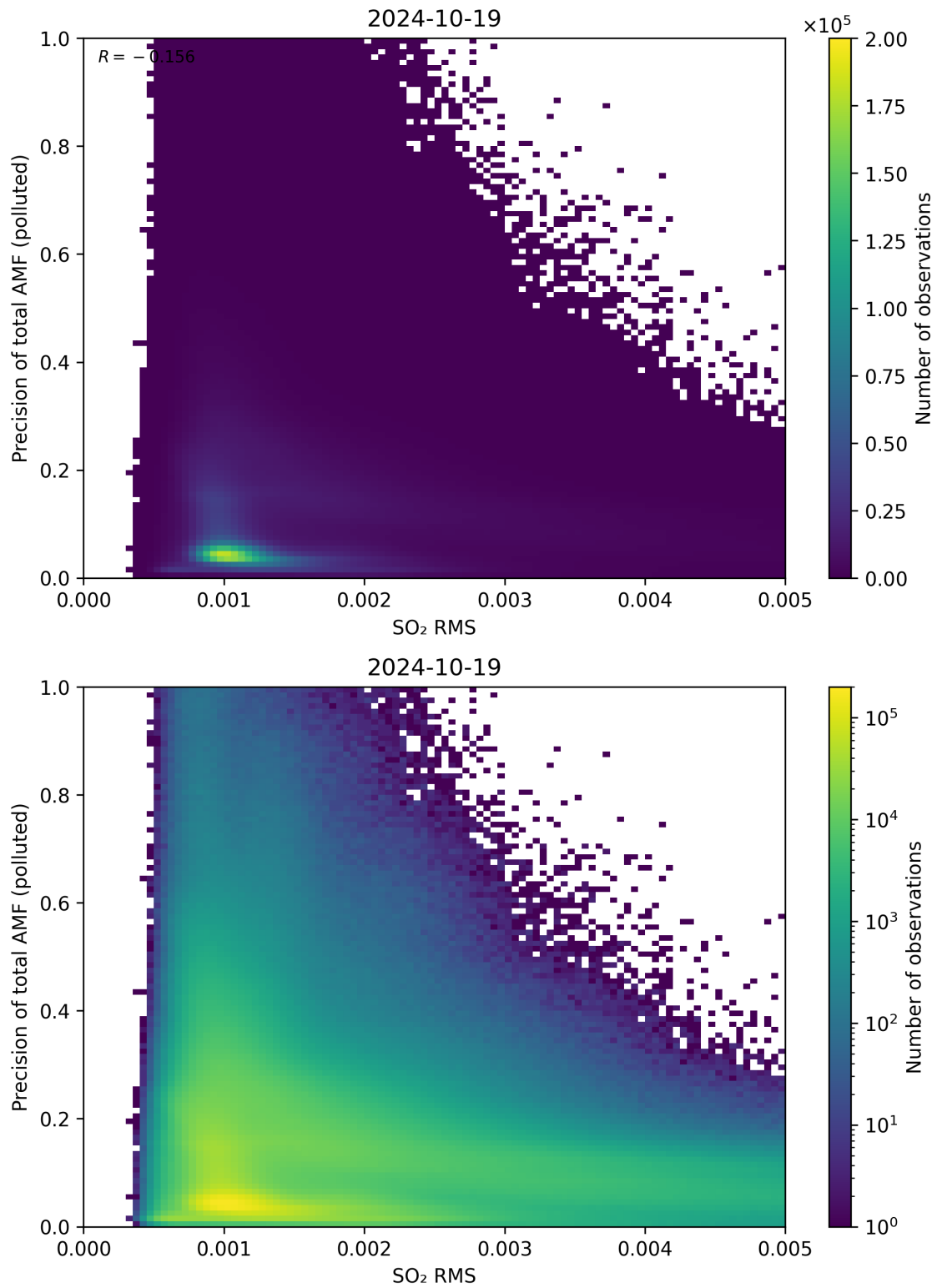
Figure 138: Scatter density plot of “SO 2 RMS” against “Precision of total AMF (polluted)” for 2024-10-19 to 2024-10-20.
