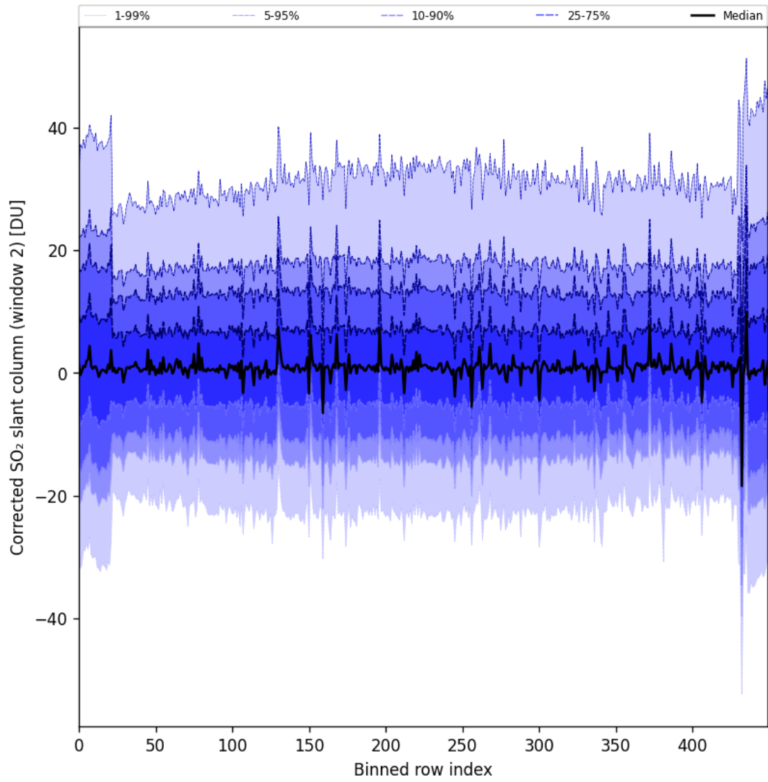
Figure 85: Along track statistics of “Corrected SO 2 slant column (window 2)” for 2024-10-19 to 2024-10-20
