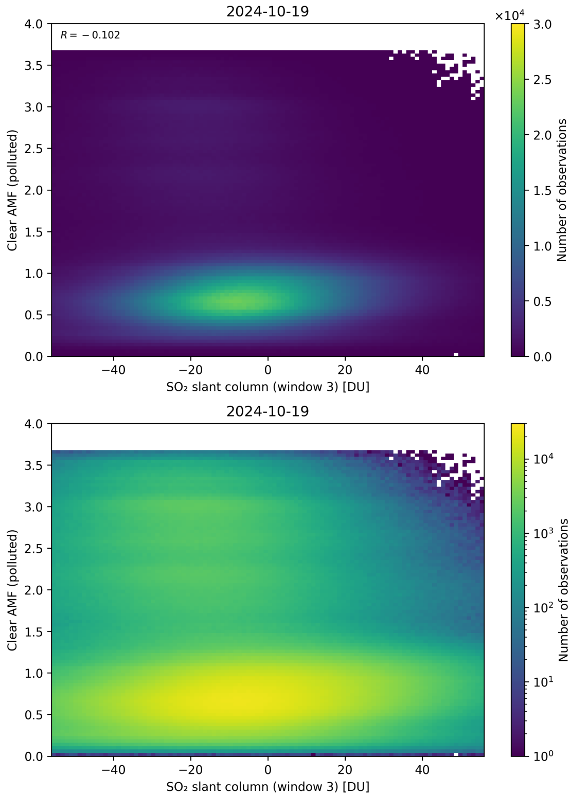
Figure 265: Scatter density plot of “SO 2 slant column (window 3)” against “Clear AMF (polluted)” for 2024-10-19 to 2024-10-20.
