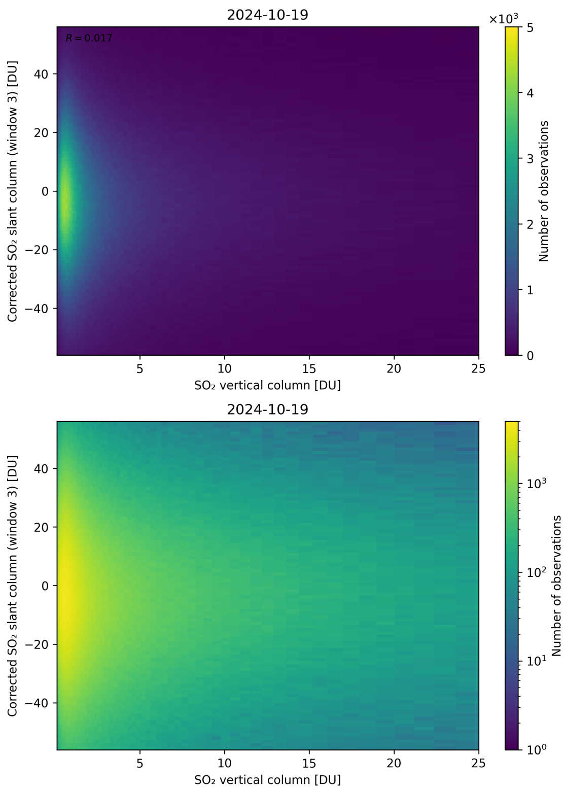
Figure 299: Scatter density plot of “SO 2 vertical column” against “Corrected SO 2 slant column (window 3)” for 2024-10-19 to 2024-10-20.
