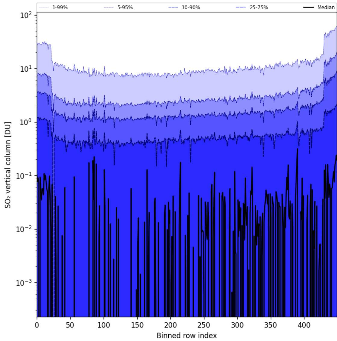
Figure 76: Along track statistics of “SO 2 vertical column” for 2024-10-19 to 2024-10-20
