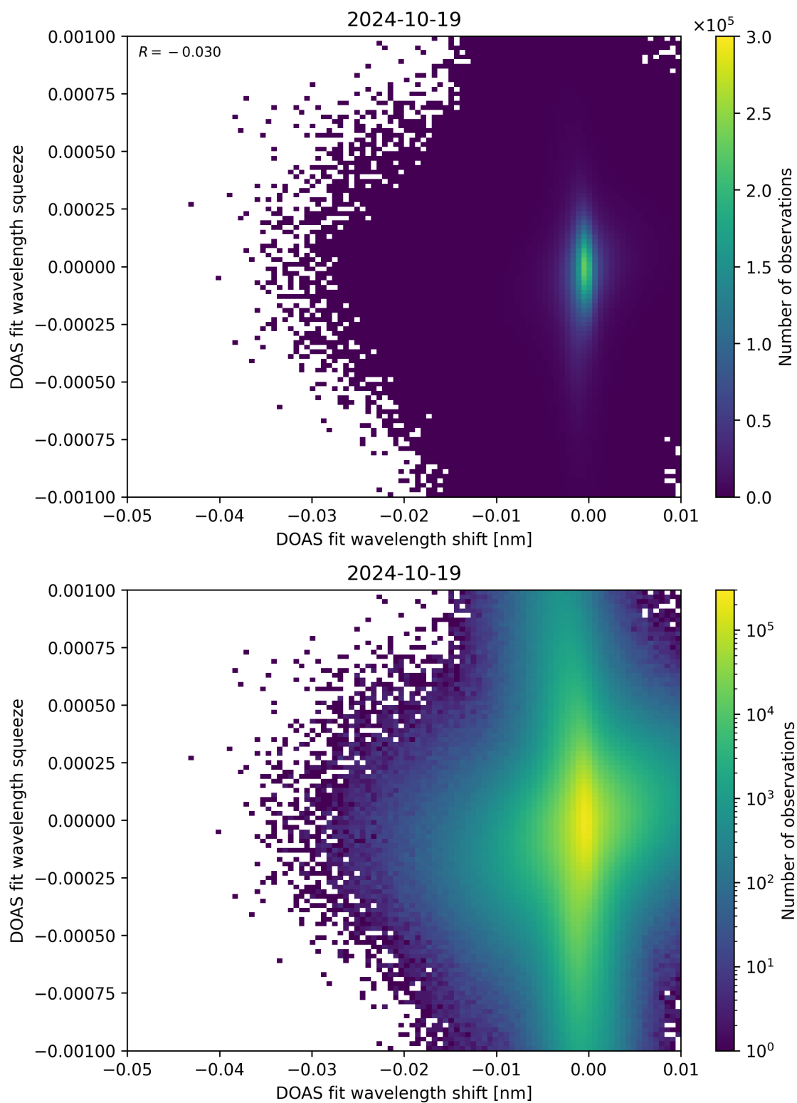
Figure 127: Scatter density plot of “DOAS fit wavelength shift” against “DOAS fit wavelength squeeze” for 2024-10-19 to 2024-10-20.
