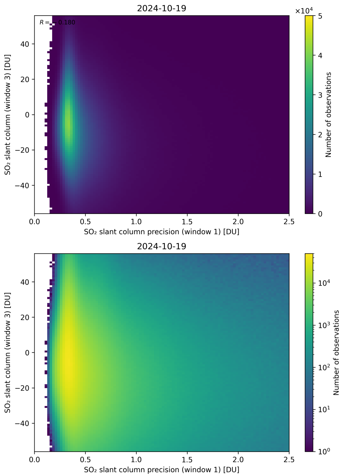
Figure 228: Scatter density plot of “SO 2 slant column precision (window 1)” against “SO 2 slant column (window 3)” for 2024-10-19 to 2024-10-20.
