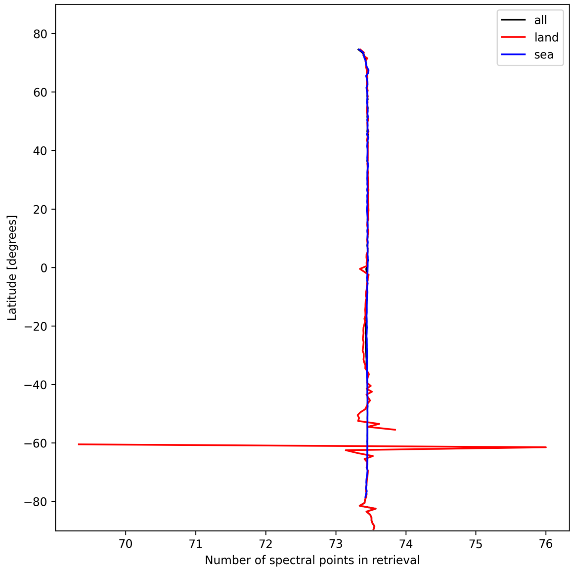
Figure 51: Zonal average of “Number of spectral points in retrieval” for 2024-10-19 to 2024-10-20.
