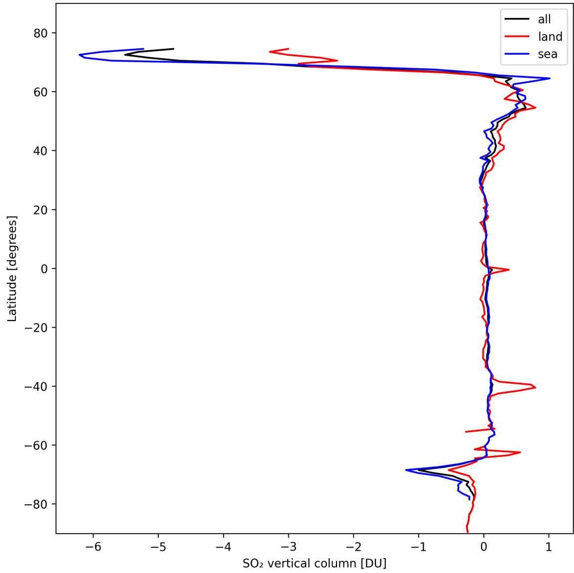
Figure 30: Zonal average of “SO 2 vertical column” for 2024-10-19 to 2024-10-20.
