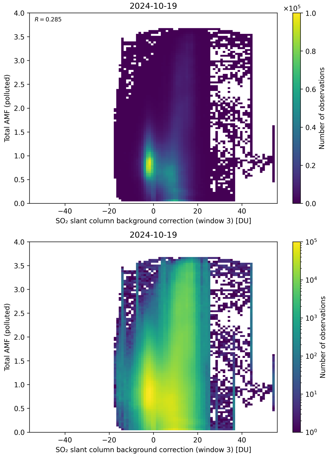
Figure 125: Scatter density plot of “SO 2 slant column background correction (window 3)” against “Total AMF (polluted)” for 2024-10-19 to 2024-10-20.
