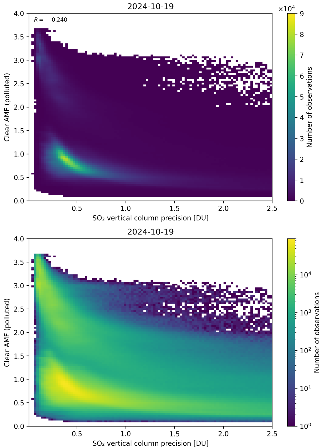
Figure 285: Scatter density plot of “SO 2 vertical column precision” against “Clear AMF (polluted)” for 2024-10-19 to 2024-10-20.
