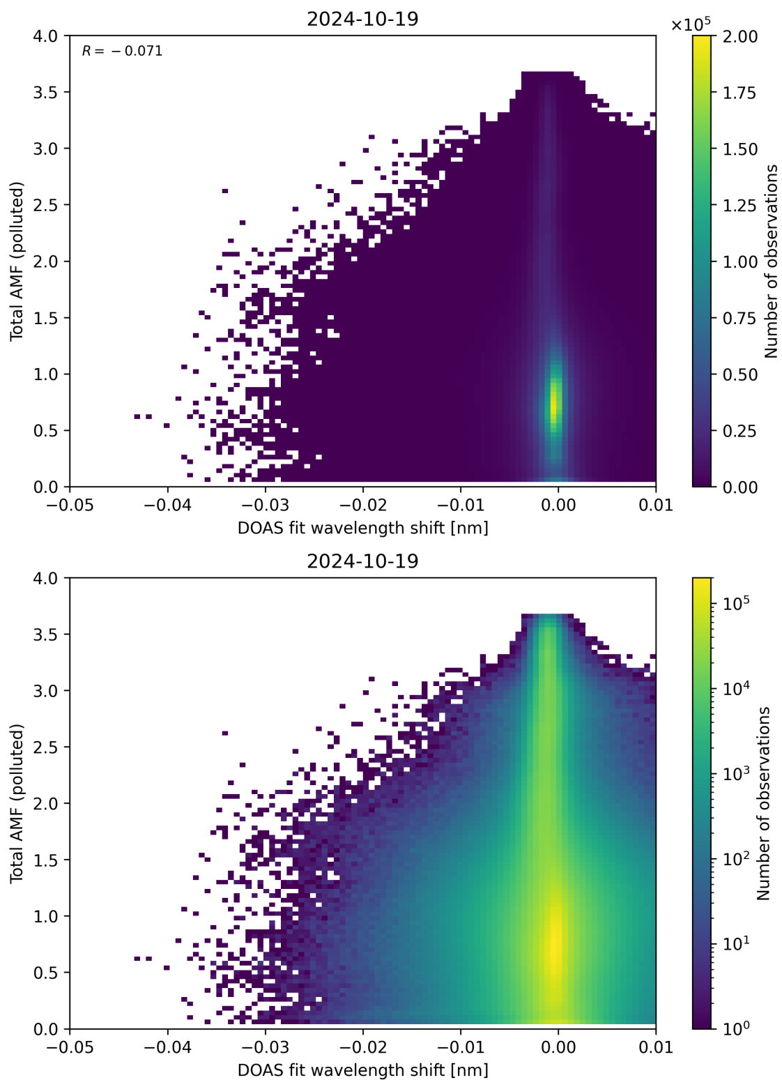
Figure 130: Scatter density plot of “DOAS fit wavelength shift” against “Total AMF (polluted)” for 2024-10-19 to 2024-10-20.
