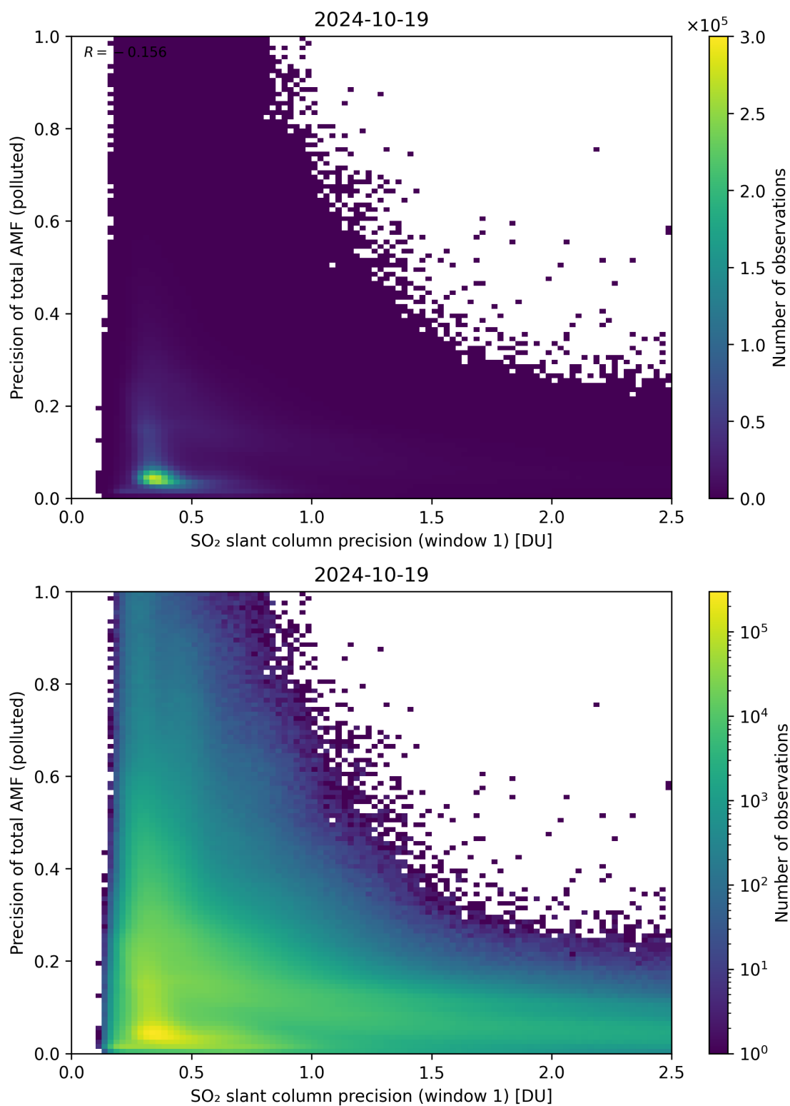
Figure 231: Scatter density plot of “SO 2 slant column precision (window 1)” against “Precision of total AMF (polluted)” for 2024-10-19 to 2024-10-20.
