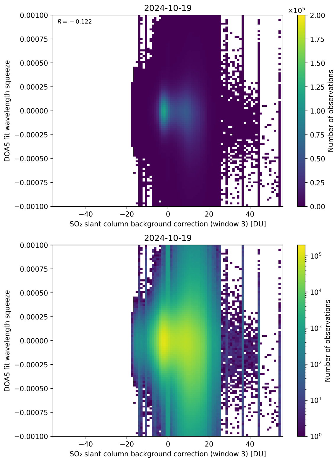
Figure 122: Scatter density plot of “SO 2 slant column background correction (window 3)” against “DOAS fit wavelength squeeze” for 2024-10-19 to 2024-10-20.
