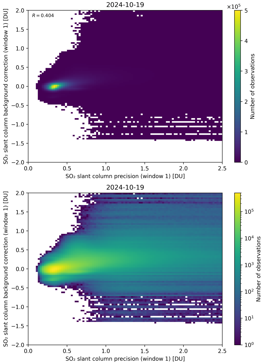
Figure 218: Scatter density plot of “SO 2 slant column precision (window 1)” against “SO 2 slant column background correction (window 1)” for 2024-10-19 to 2024-10-20.
