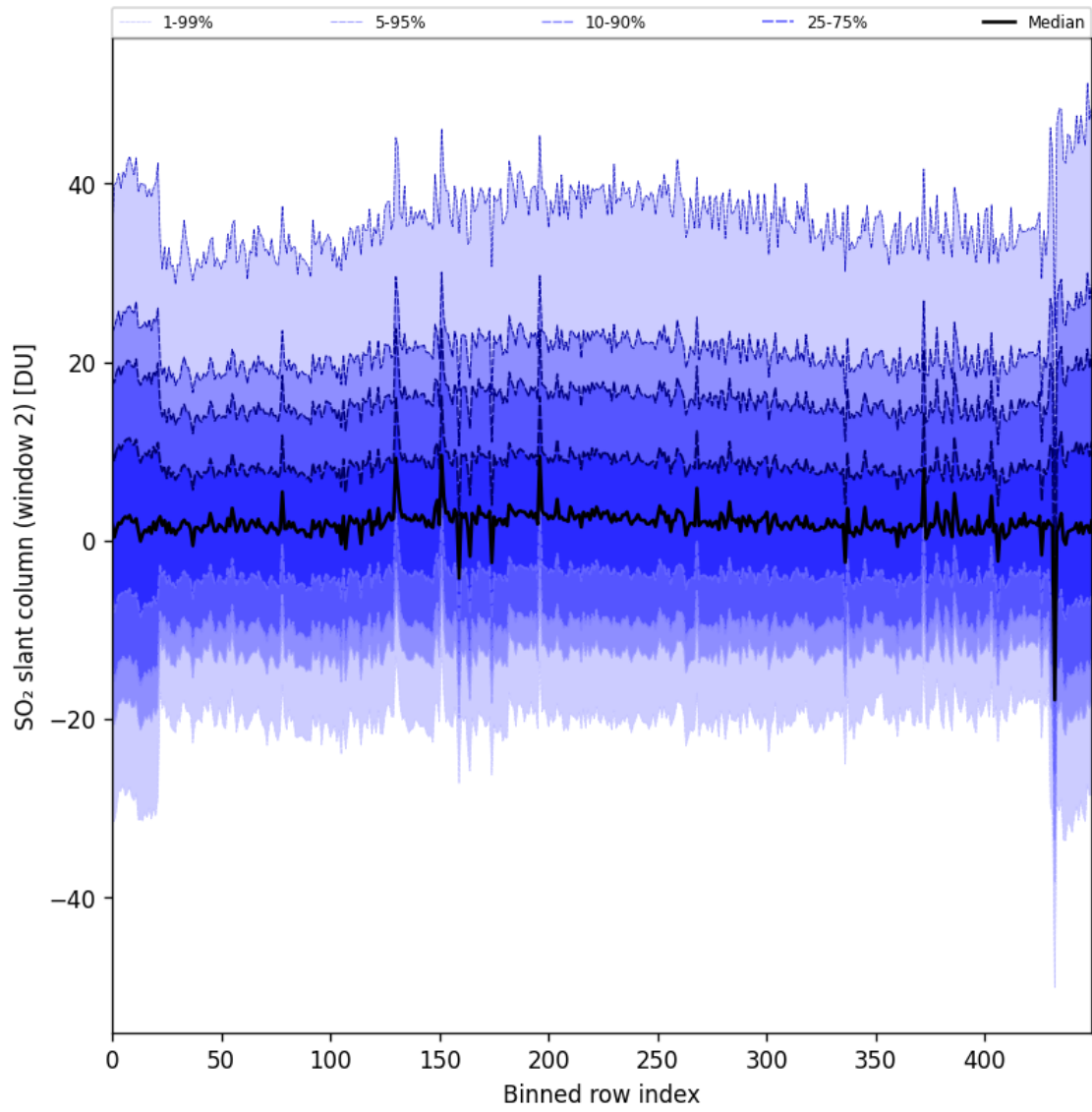
Figure 83: Along track statistics of “SO 2 slant column (window 2)” for 2024-10-19 to 2024-10-20
