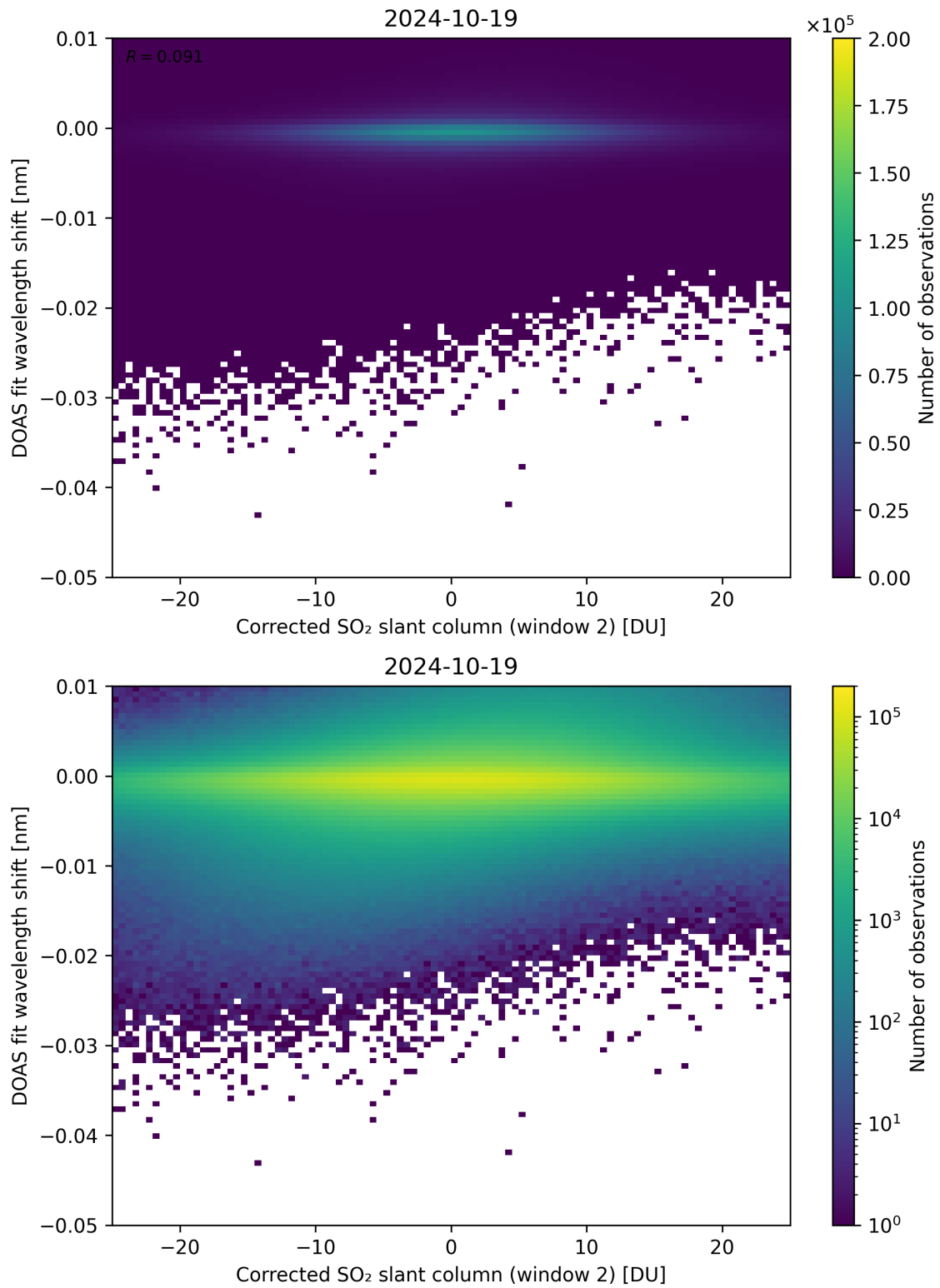
Figure 196: Scatter density plot of “Corrected SO 2 slant column (window 2)” against “DOAS fit wavelength shift” for 2024-10-19 to 2024-10-20.
