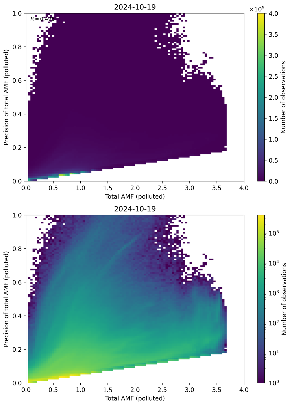
Figure 272: Scatter density plot of “Total AMF (polluted)” against “Precision of total AMF (polluted)” for 2024-10-19 to 2024-10-20.
