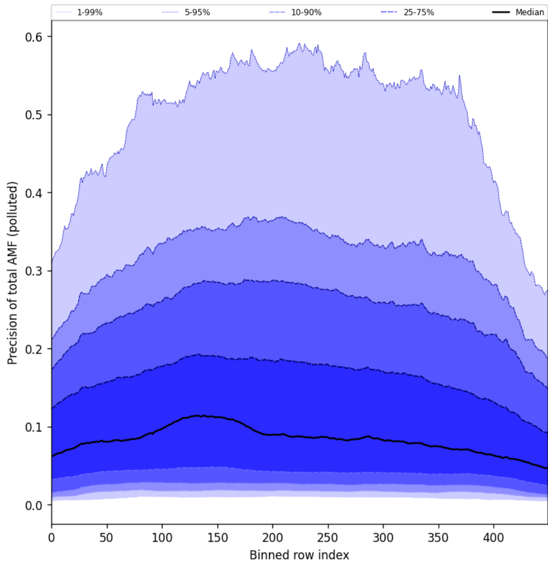
Figure 95: Along track statistics of “Precision of total AMF (polluted)” for 2024-10-19 to 2024-10-20
