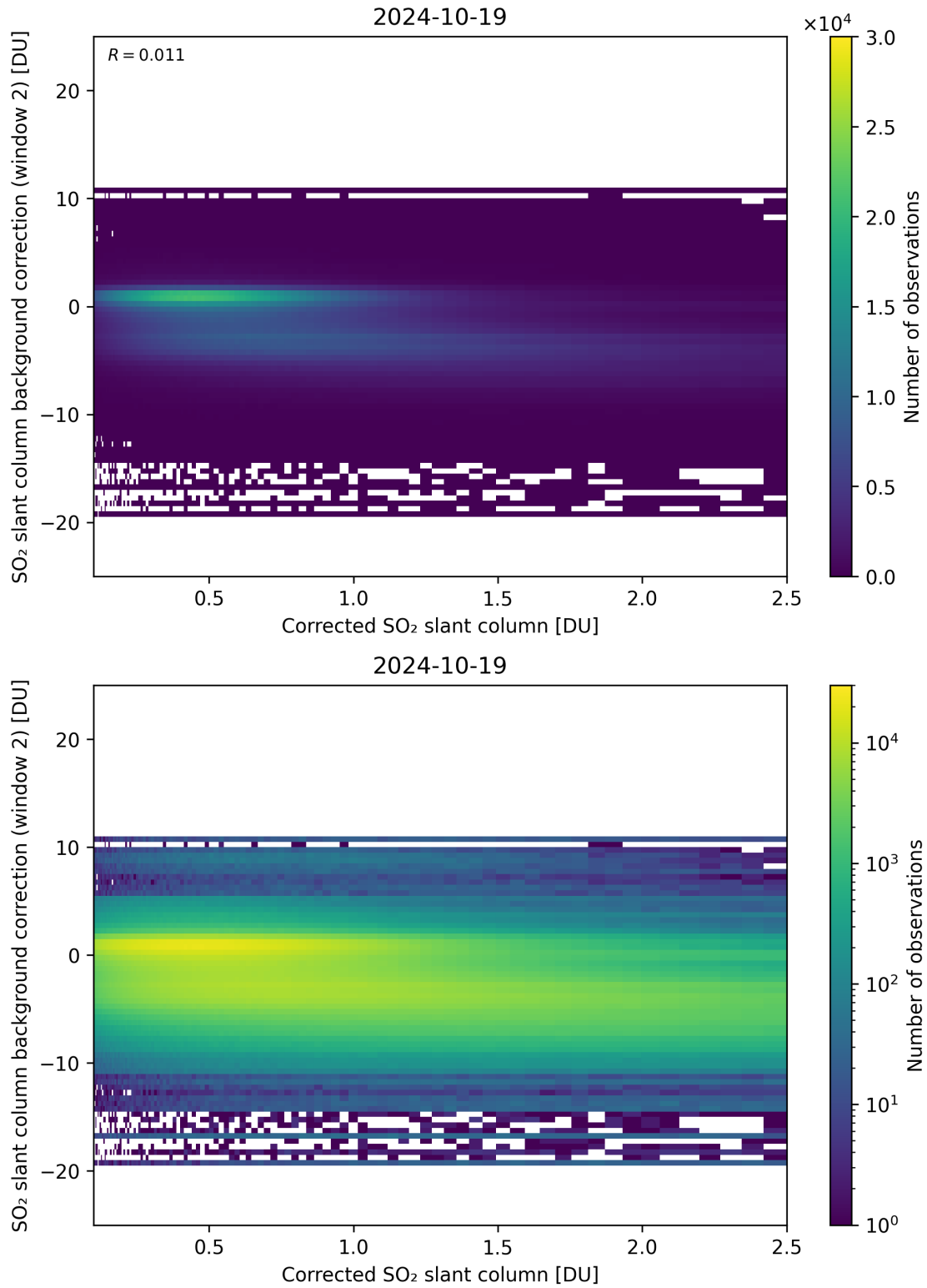
Figure 179: Scatter density plot of “Corrected SO 2 slant column” against “SO 2 slant column background correction (window 2)” for 2024-10-19 to 2024-10-20.
