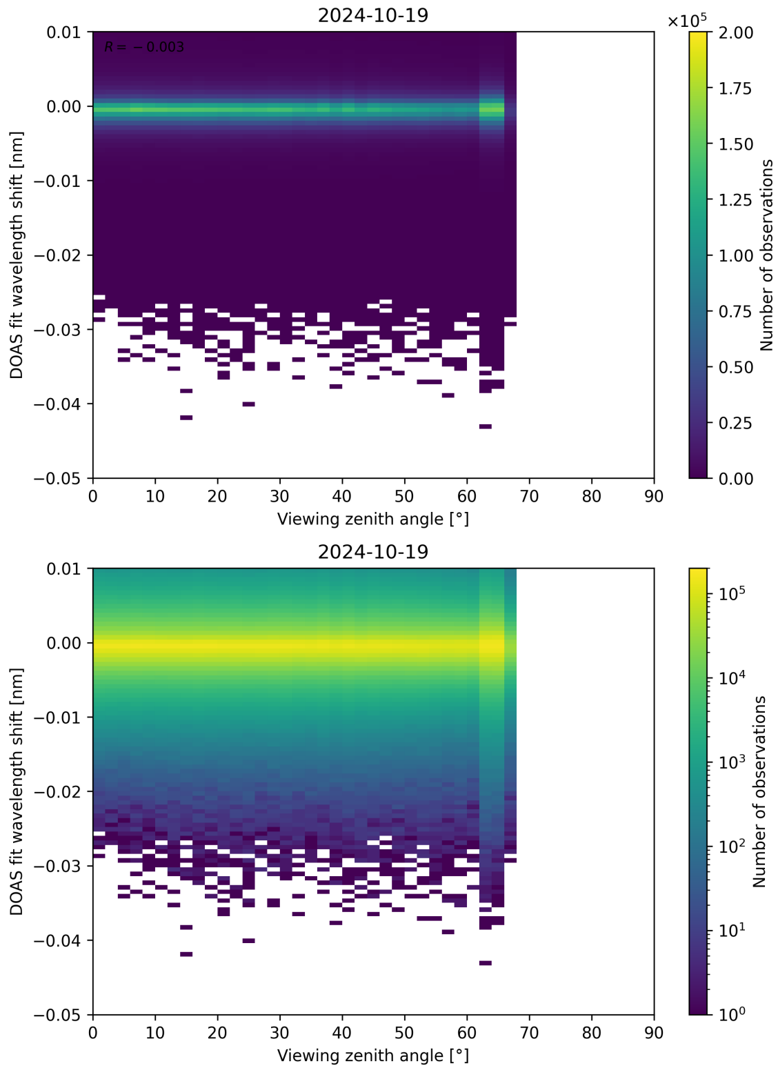
Figure 311: Scatter density plot of “Viewing zenith angle” against “DOAS fit wavelength shift” for 2024-10-19 to 2024-10-20.
