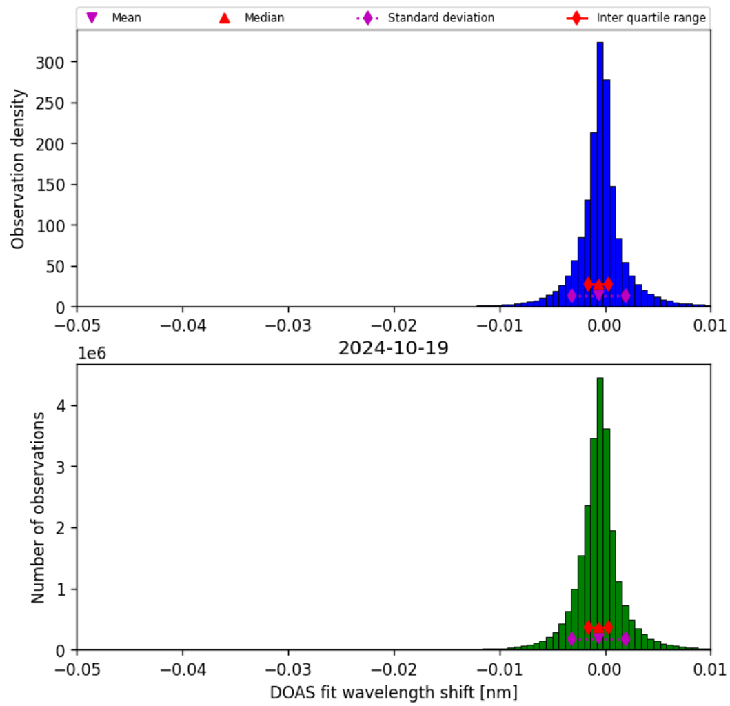
Figure 68: Histogram of “DOAS fit wavelength shift” for 2024-10-19 to 2024-10-20
