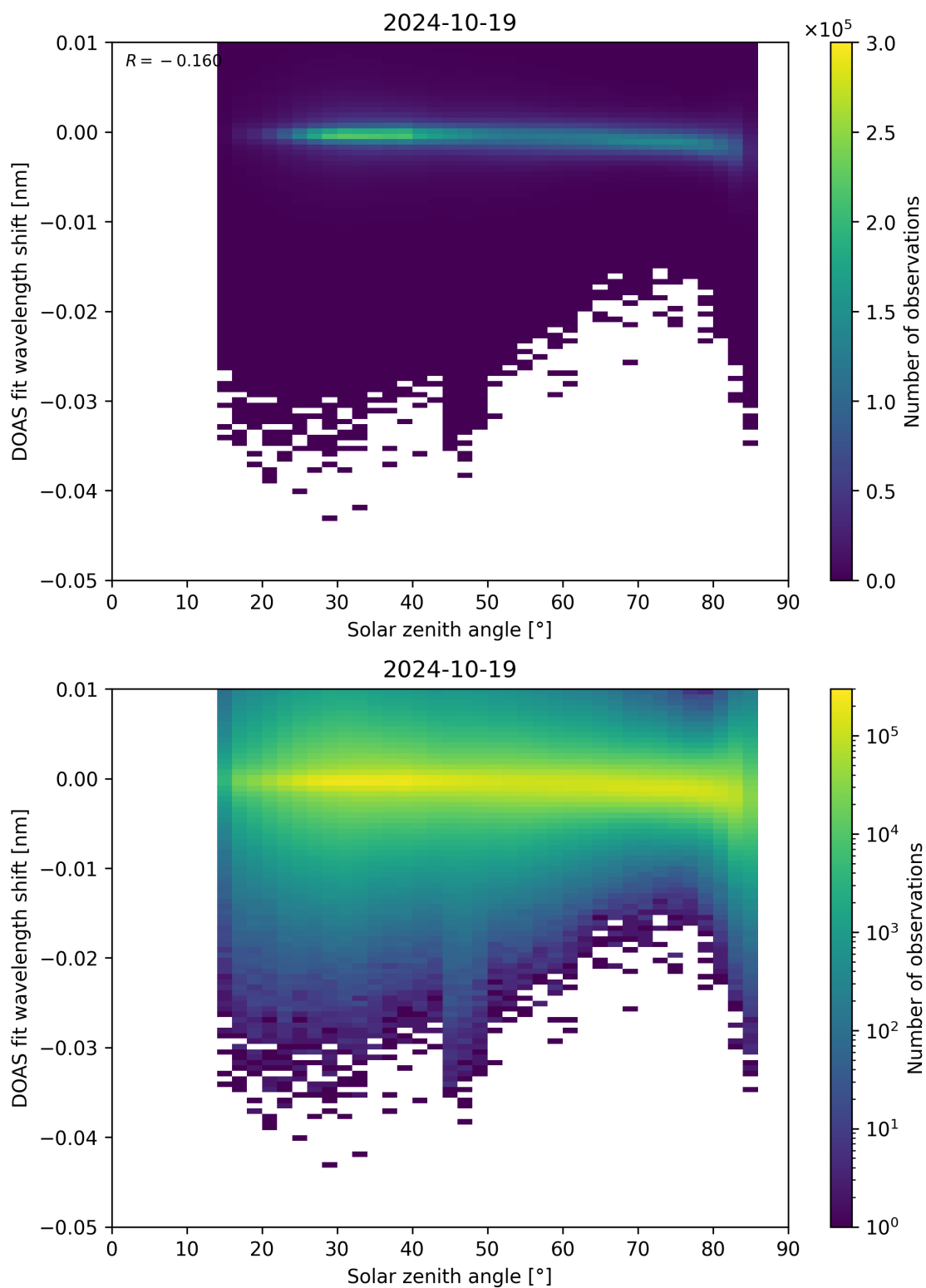
Figure 161: Scatter density plot of “Solar zenith angle” against “DOAS fit wavelength shift” for 2024-10-19 to 2024-10-20.
