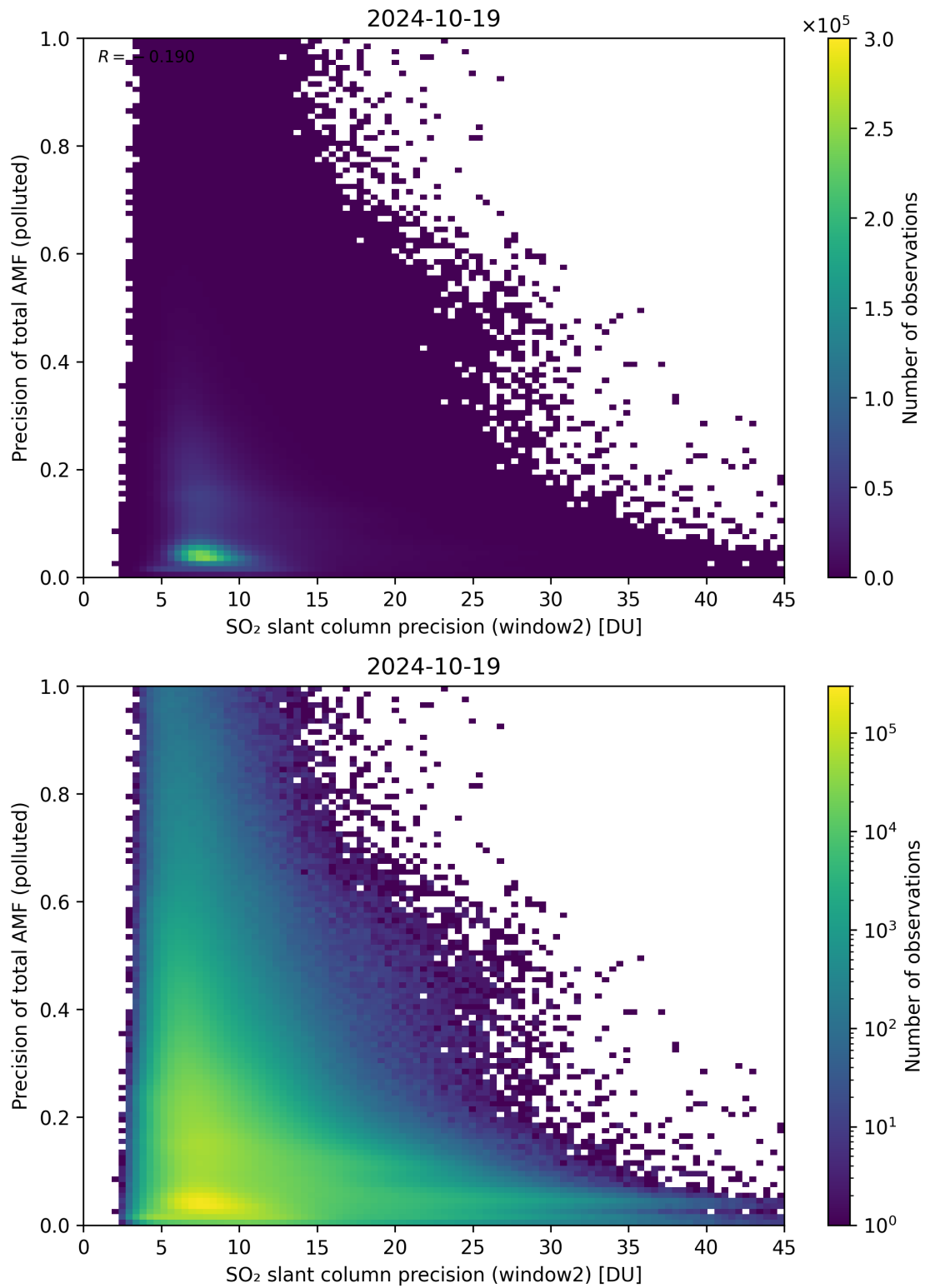
Figure 252: Scatter density plot of “SO 2 slant column precision (window2)” against “Precision of total AMF (polluted)” for 2024-10-19 to 2024-10-20.
