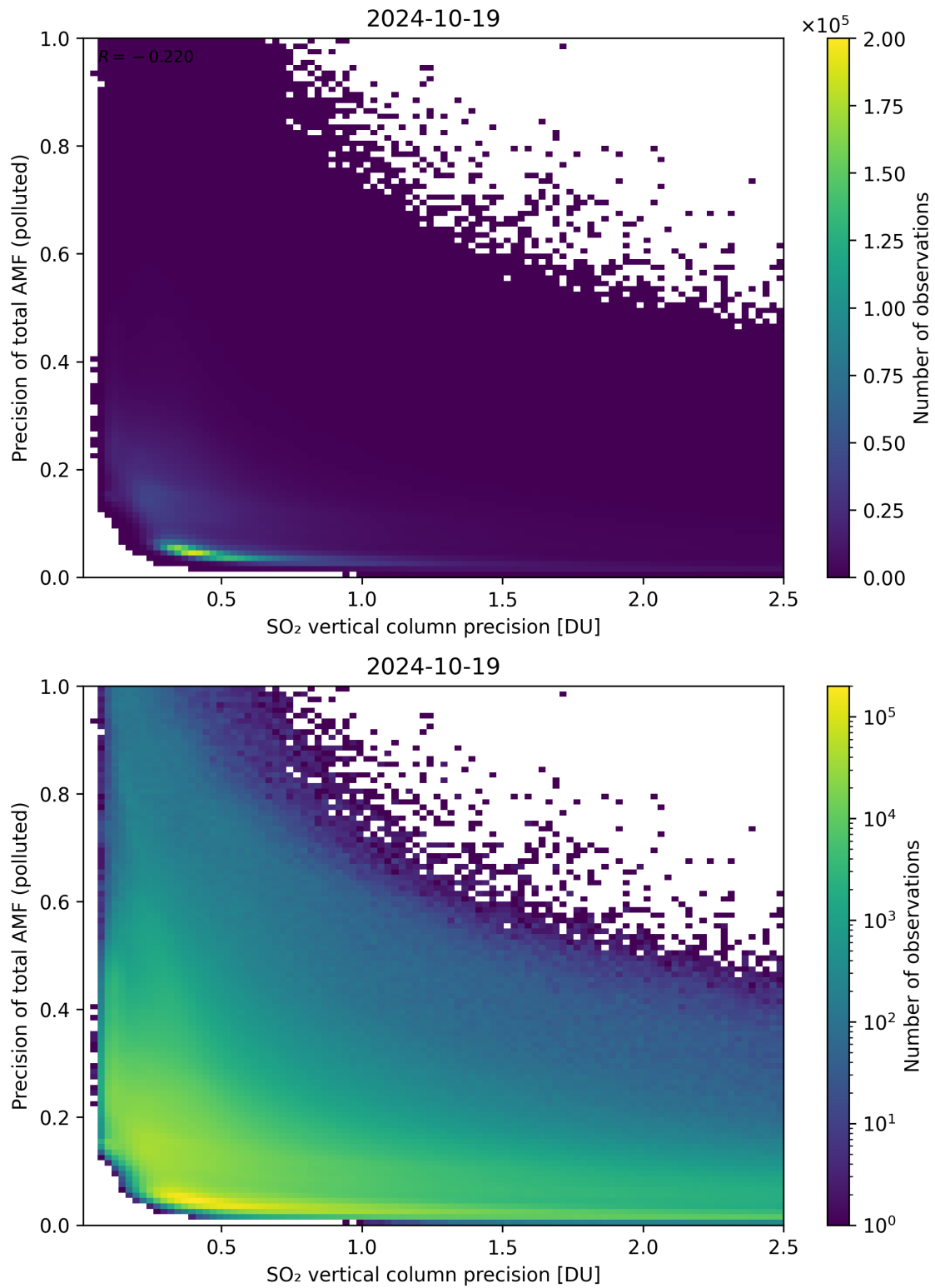
Figure 295: Scatter density plot of “SO 2 vertical column precision” against “Precision of total AMF (polluted)” for 2024-10-19 to 2024-10-20.
