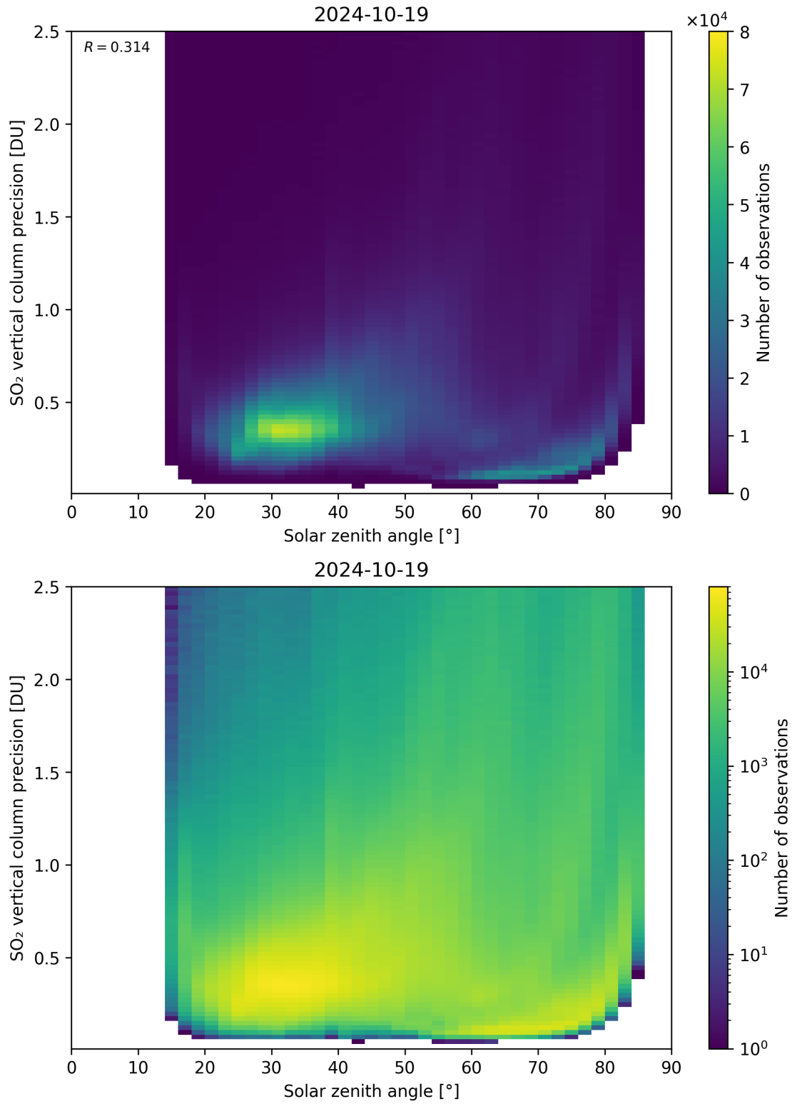
Figure 177: Scatter density plot of “Solar zenith angle” against “SO 2 vertical column precision” for 2024-10-19 to 2024-10-20.
