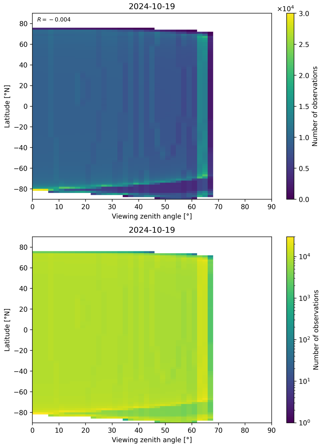
Figure 314: Scatter density plot of “Viewing zenith angle” against “Latitude” for 2024-10-19 to 2024-10-20.
