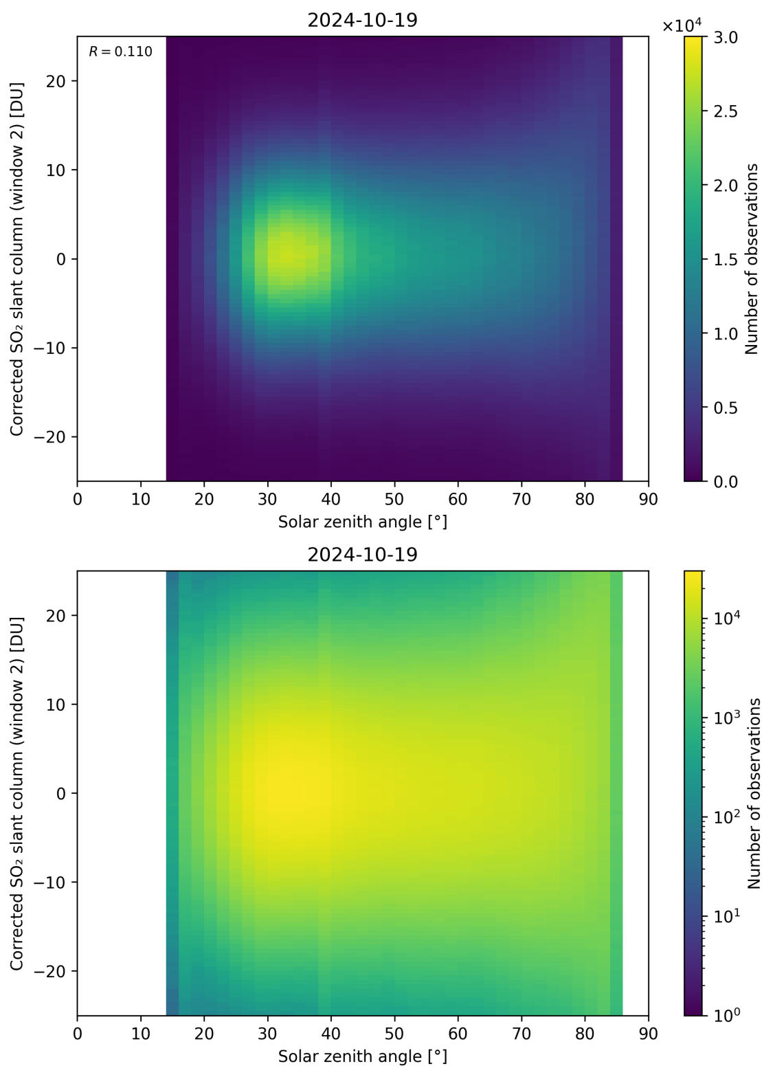
Figure 167: Scatter density plot of “Solar zenith angle” against “Corrected SO 2 slant column (window 2)” for 2024-10-19 to 2024-10-20.
