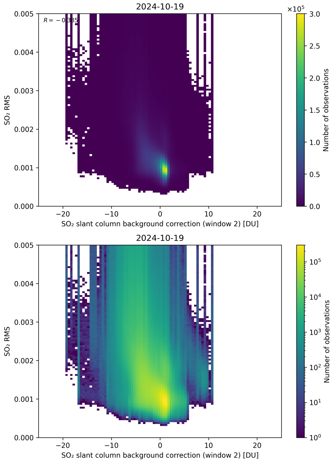
Figure 114: Scatter density plot of “SO 2 slant column background correction (window 2)” against “SO 2 RMS” for 2024-10-19 to 2024-10-20.
