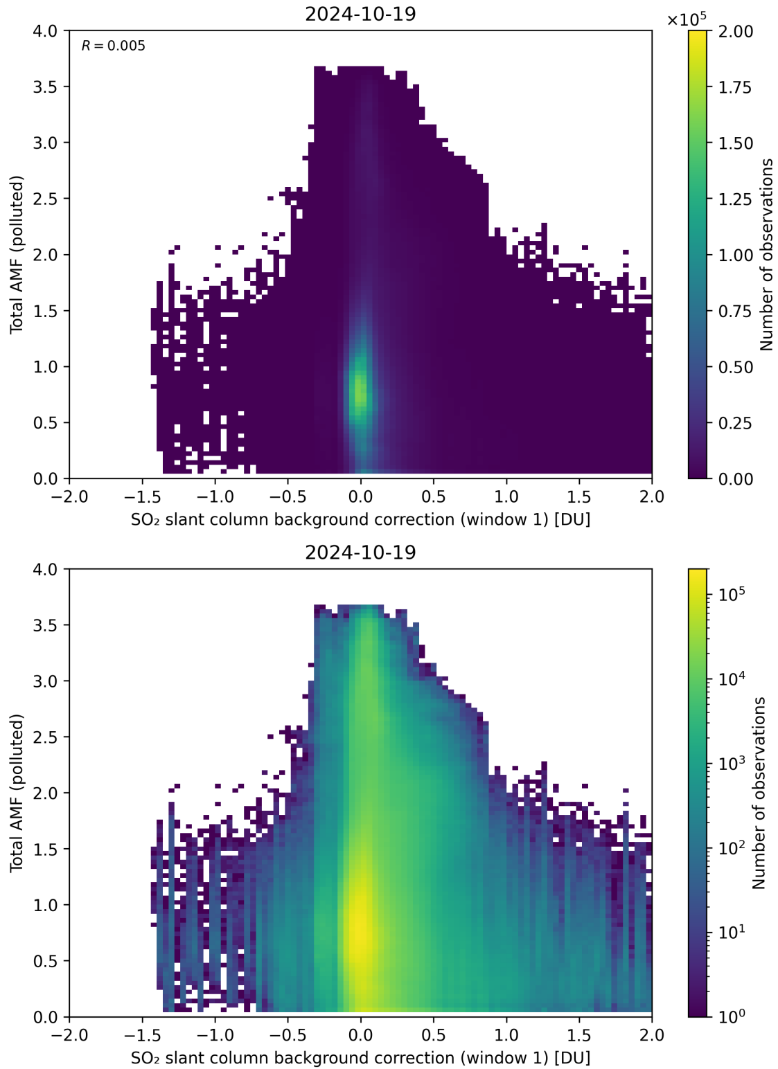
Figure 109: Scatter density plot of “SO 2 slant column background correction (window 1)” against “Total AMF (polluted)” for 2024-10-19 to 2024-10-20.
