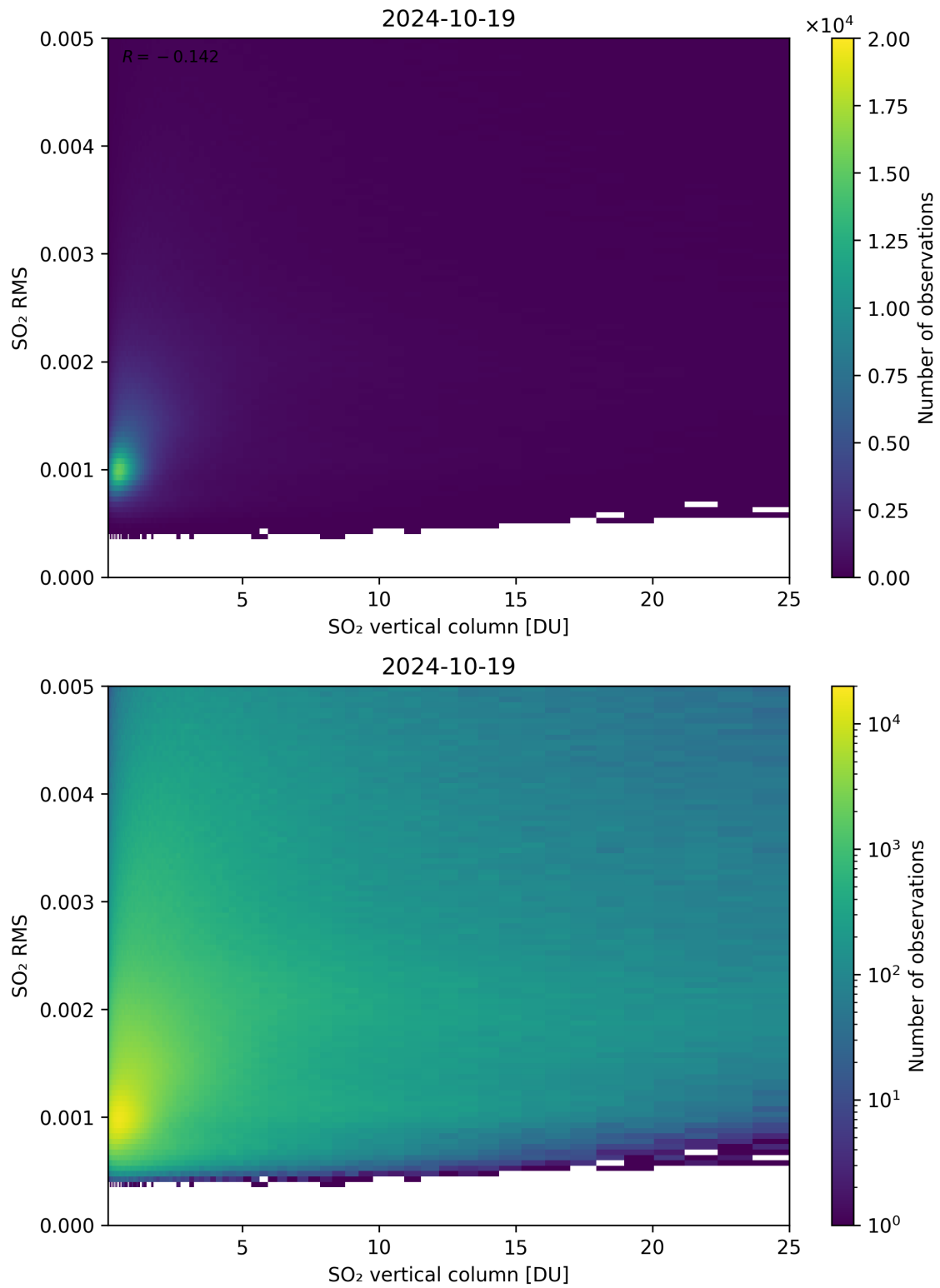
Figure 278: Scatter density plot of “SO 2 vertical column” against “SO 2 RMS” for 2024-10-19 to 2024-10-20.
