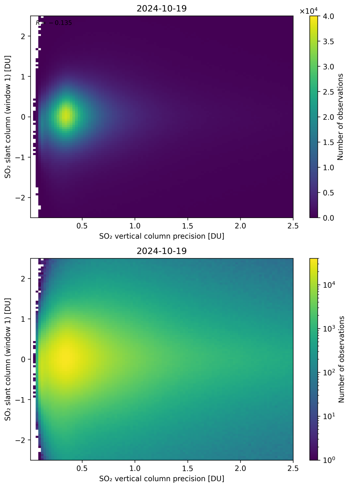
Figure 289: Scatter density plot of “SO 2 vertical column precision” against “SO 2 slant column (window 1)” for 2024-10-19 to 2024-10-20.
