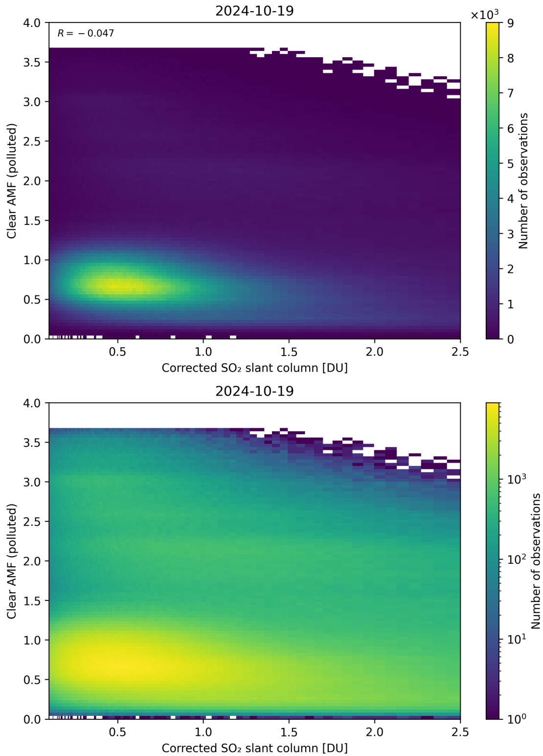
Figure 184: Scatter density plot of “Corrected SO 2 slant column” against “Clear AMF (polluted)” for 2024-10-19 to 2024-10-20.
