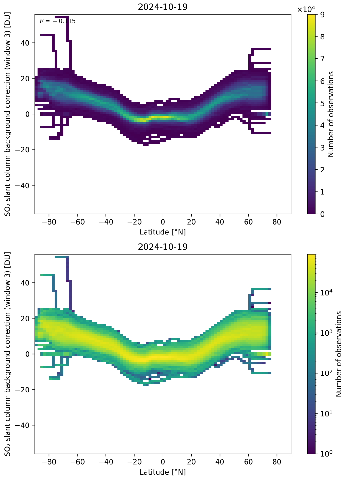
Figure 141: Scatter density plot of “Latitude” against “SO 2 slant column background correction (window 3)” for 2024-10-19 to 2024-10-20.
