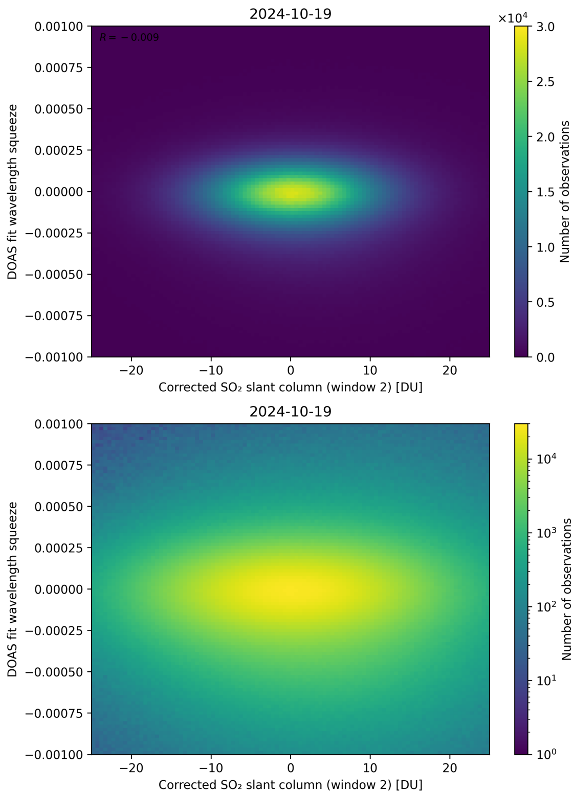
Figure 197: Scatter density plot of “Corrected SO 2 slant column (window 2)” against “DOAS fit wavelength squeeze” for 2024-10-19 to 2024-10-20.
