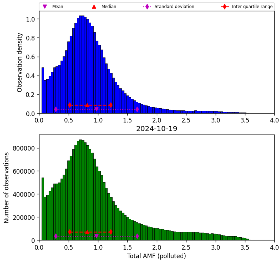
Figure 71: Histogram of “Total AMF (polluted)” for 2024-10-19 to 2024-10-20
