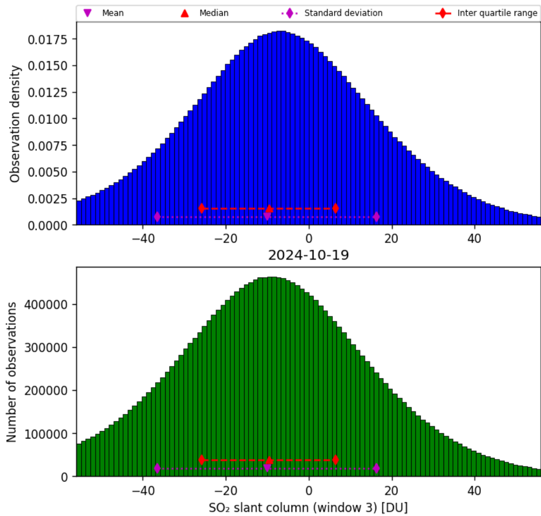
Figure 64: Histogram of “SO 2 slant column (window 3)” for 2024-10-19 to 2024-10-20
