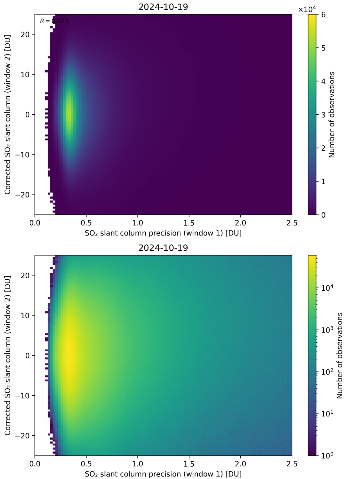
Figure 225: Scatter density plot of “SO 2 slant column precision (window 1)” against “Corrected SO 2 slant column (window 2)” for 2024-10-19 to 2024-10-20.
