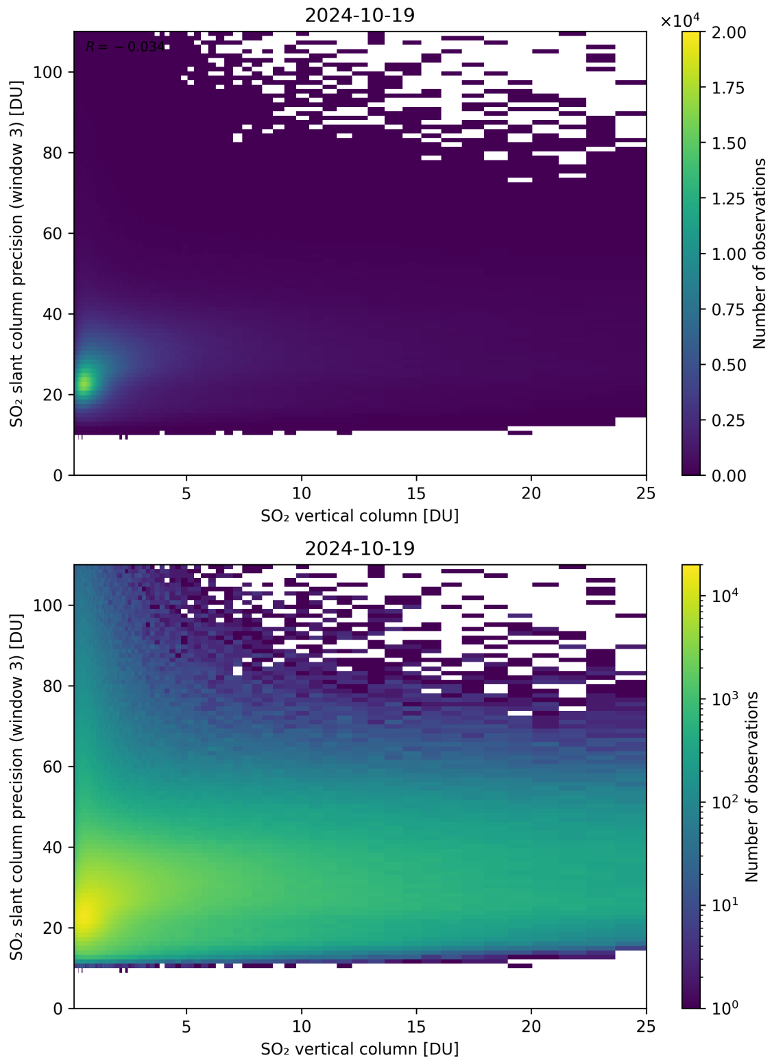
Figure 304: Scatter density plot of “SO 2 vertical column” against “SO 2 slant column precision (window 3)” for 2024-10-19 to 2024-10-20.
