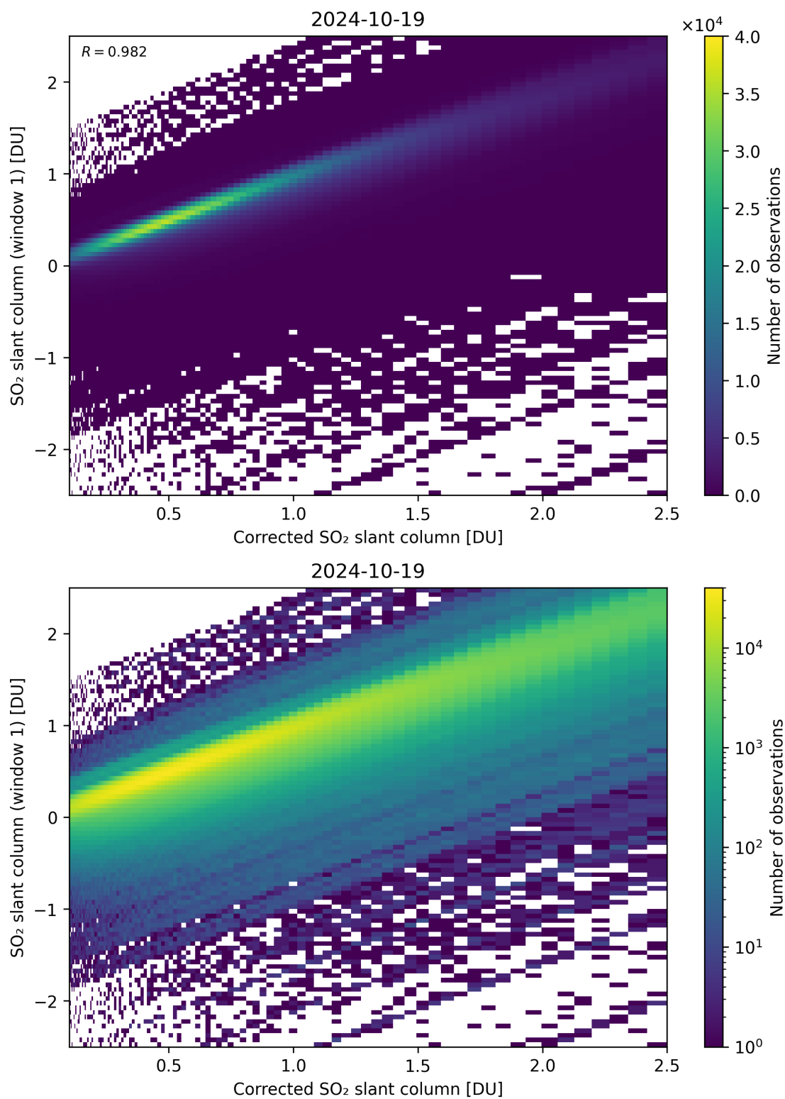
Figure 187: Scatter density plot of “Corrected SO 2 slant column” against “SO 2 slant column (window 1)” for 2024-10-19 to 2024-10-20.
