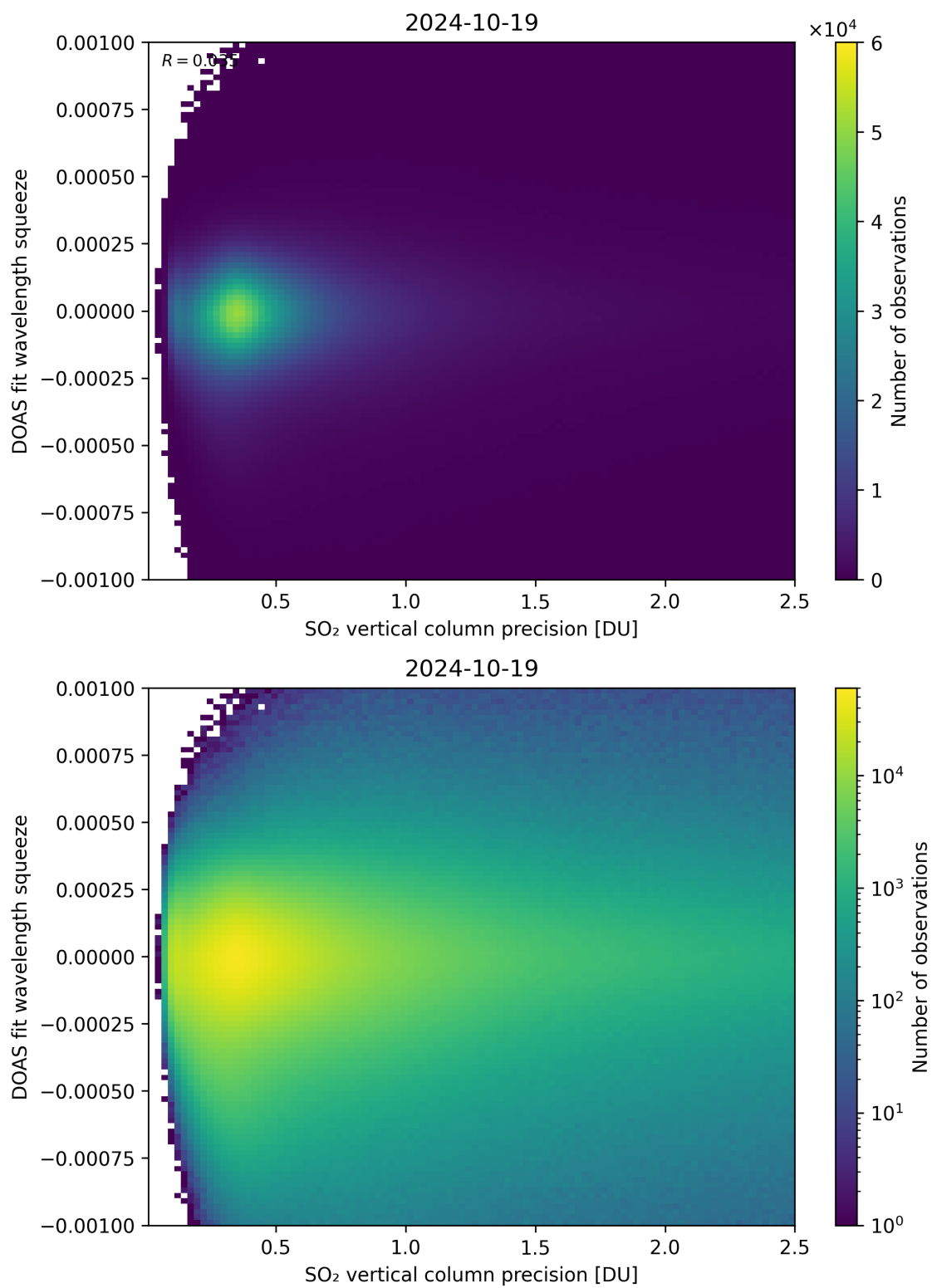
Figure 283: Scatter density plot of “SO 2 vertical column precision” against “DOAS fit wavelength squeeze” for 2024-10-19 to 2024-10-20.
