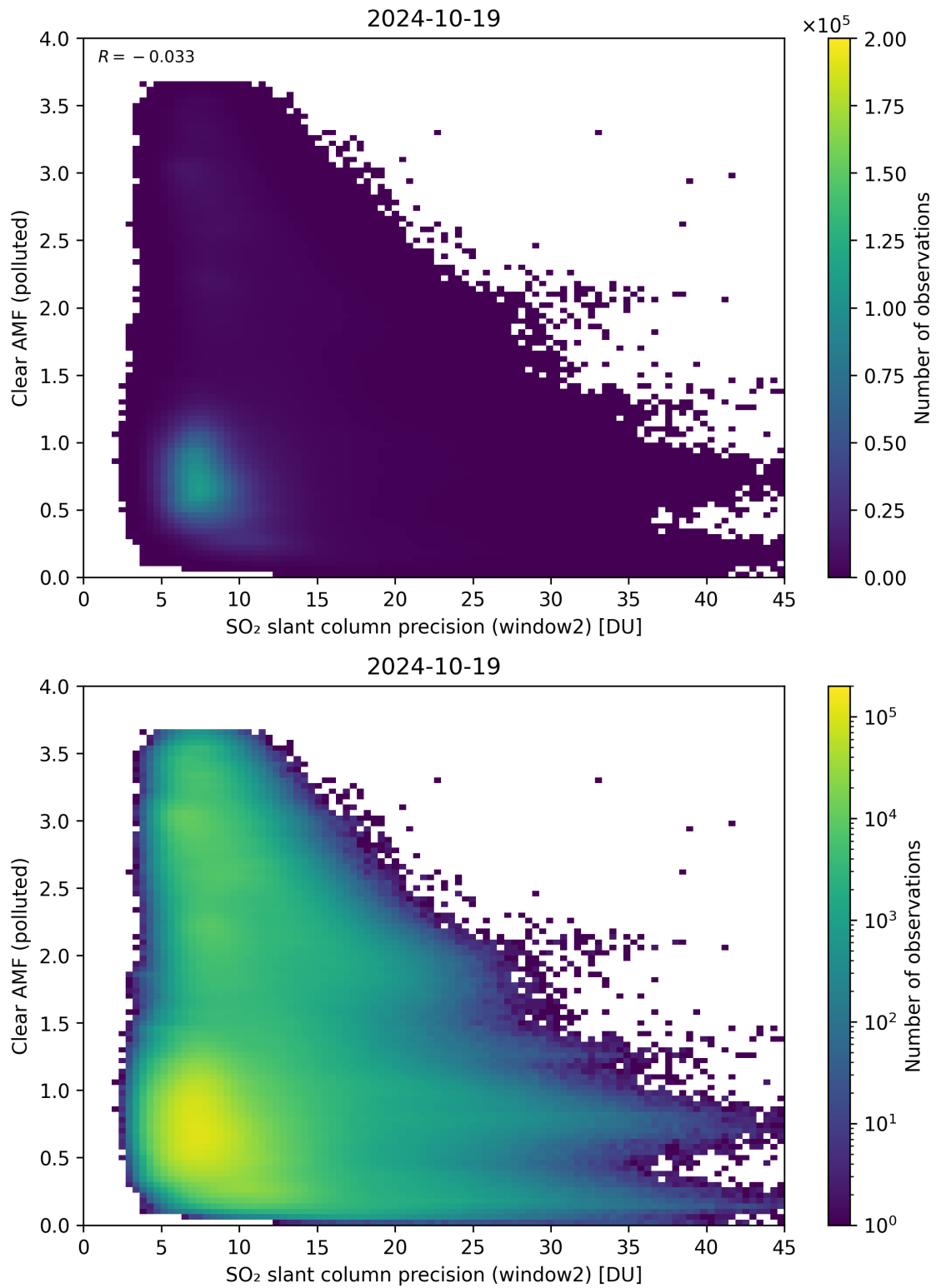
Figure 246: Scatter density plot of “SO 2 slant column precision (window2)” against “Clear AMF (polluted)” for 2024-10-19 to 2024-10-20.
