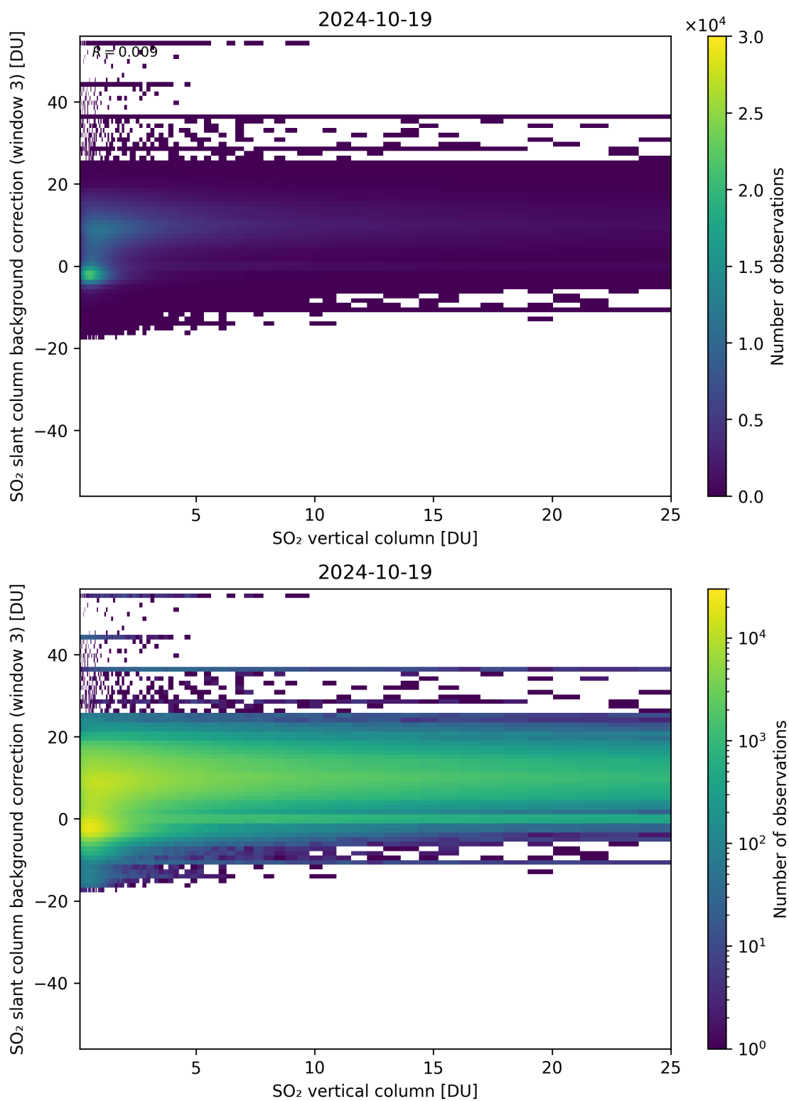
Figure 275: Scatter density plot of “SO 2 vertical column” against “SO 2 slant column background correction (window 3)” for 2024-10-19 to 2024-10-20.
