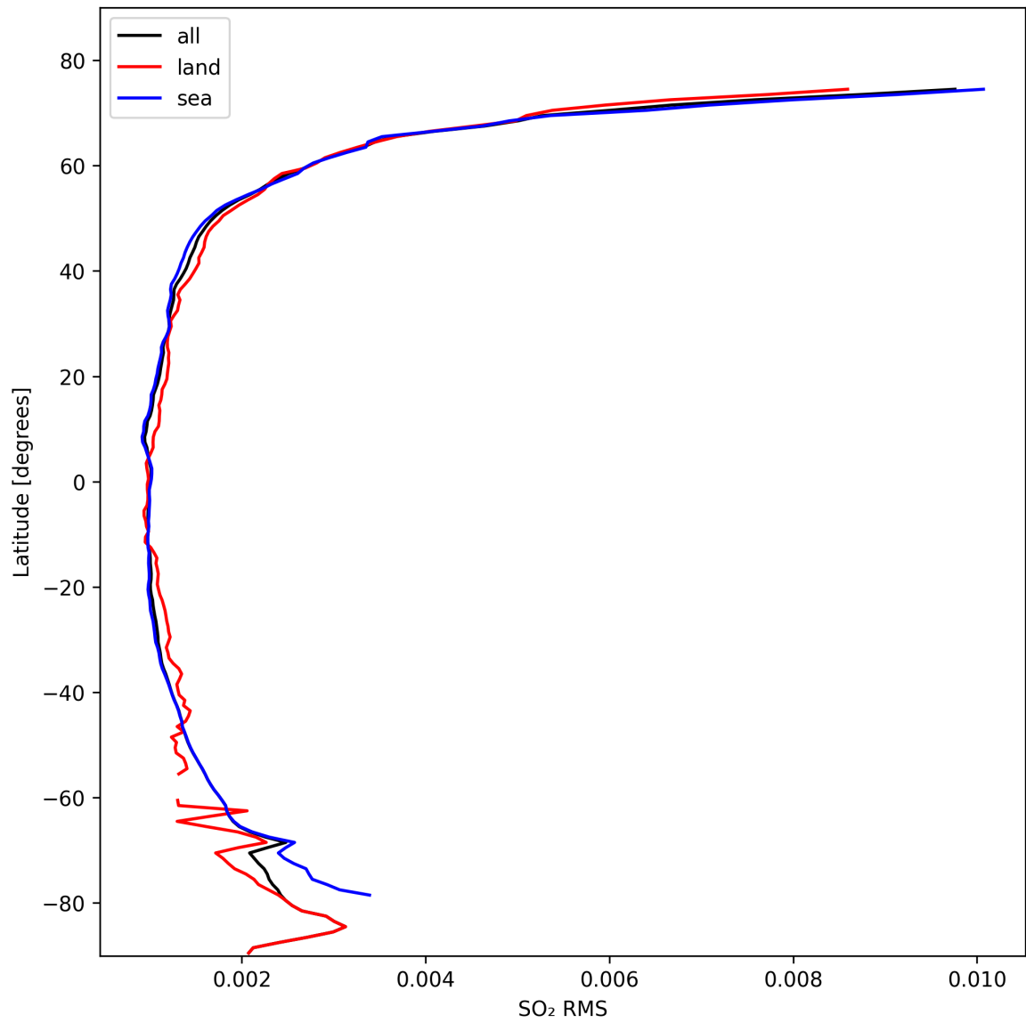
Figure 47: Zonal average of “SO 2 RMS” for 2024-10-19 to 2024-10-20.
