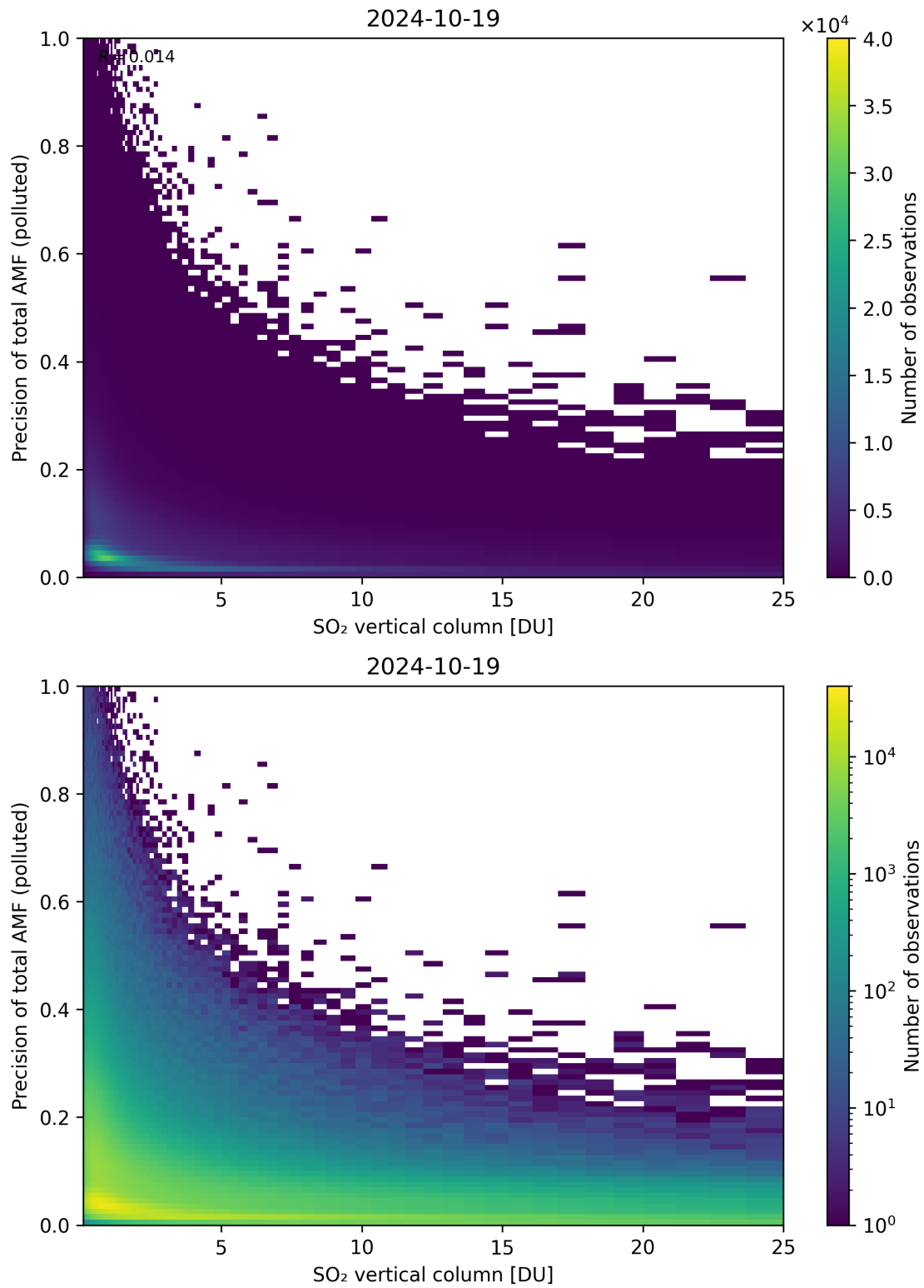
Figure 306: Scatter density plot of “SO 2 vertical column” against “Precision of total AMF (polluted)” for 2024-10-19 to 2024-10-20.
