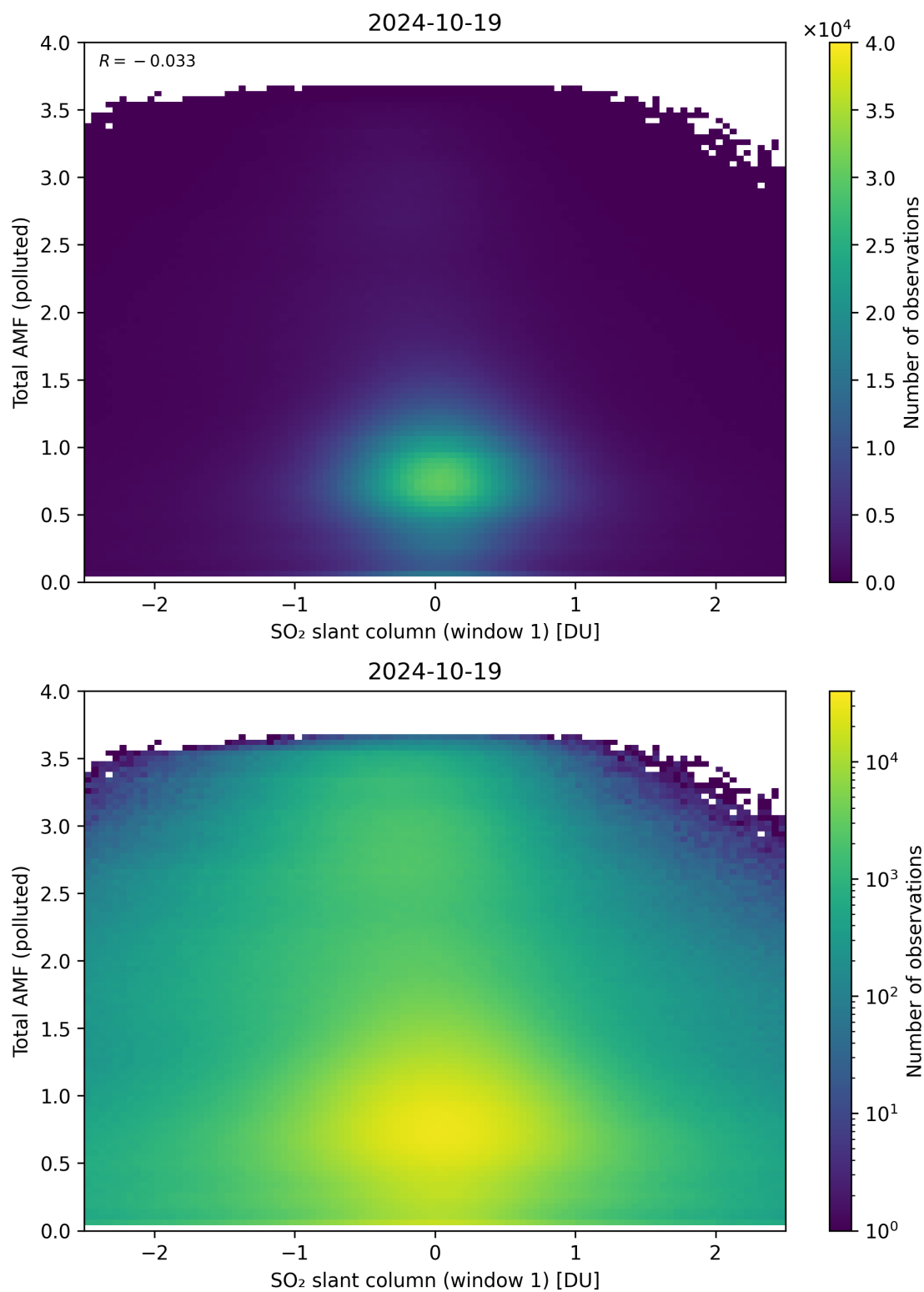
Figure 239: Scatter density plot of “SO 2 slant column (window 1)” against “Total AMF (polluted)” for 2024-10-19 to 2024-10-20.
