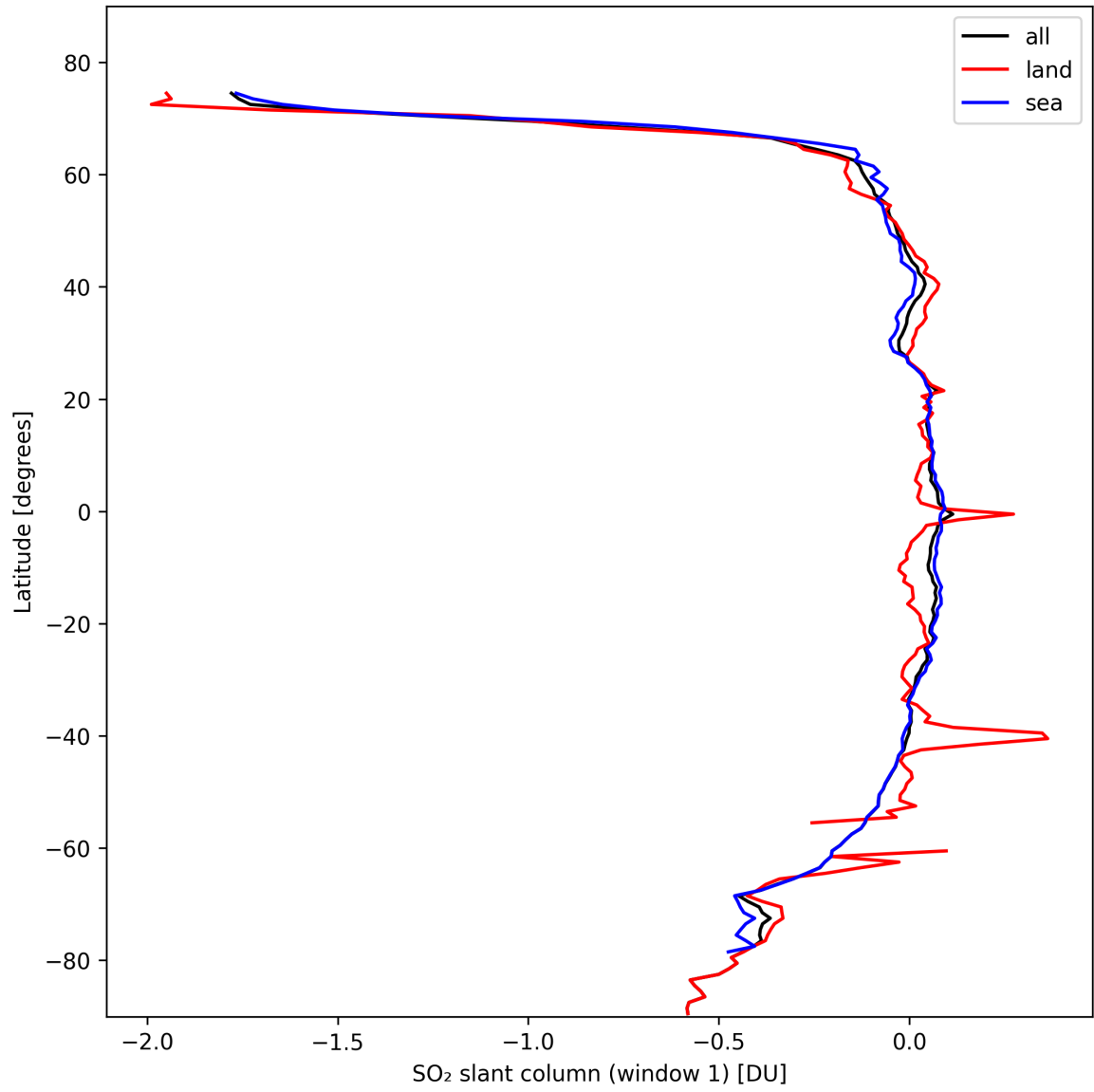
Figure 33: Zonal average of “SO 2 slant column (window 1)” for 2024-10-19 to 2024-10-20.
