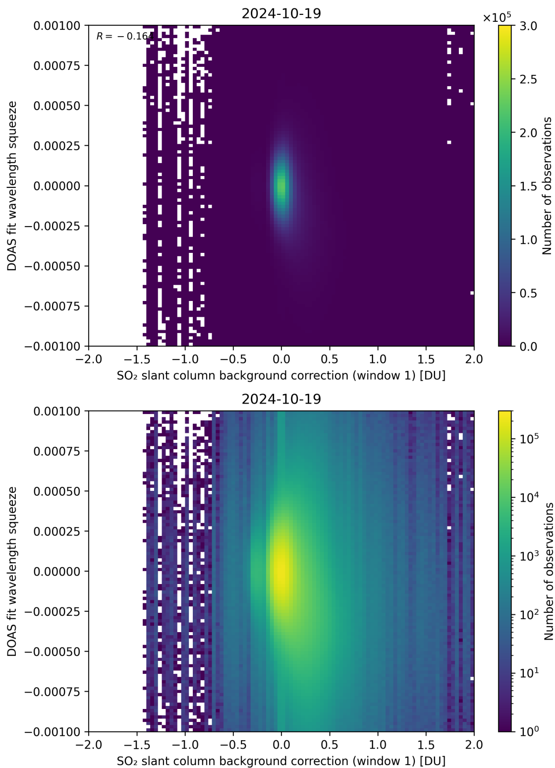
Figure 101: Scatter density plot of “SO 2 slant column background correction (window 1)” against “DOAS fit wavelength squeeze” for 2024-10-19 to 2024-10-20.
