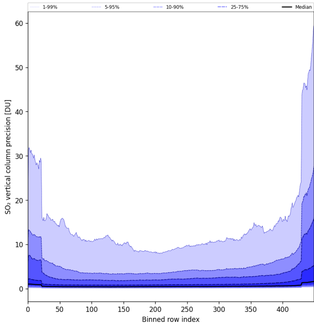
Figure 77: Along track statistics of “SO 2 vertical column precision” for 2024-10-19 to 2024-10-20
