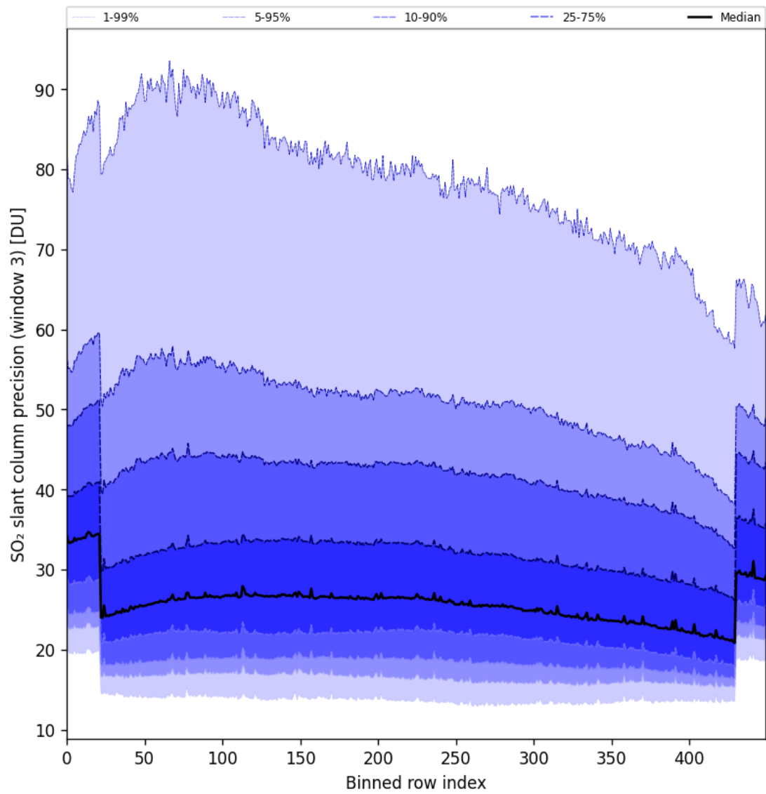
Figure 88: Along track statistics of “SO 2 slant column precision (window 3)” for 2024-10-19 to 2024-10-20
