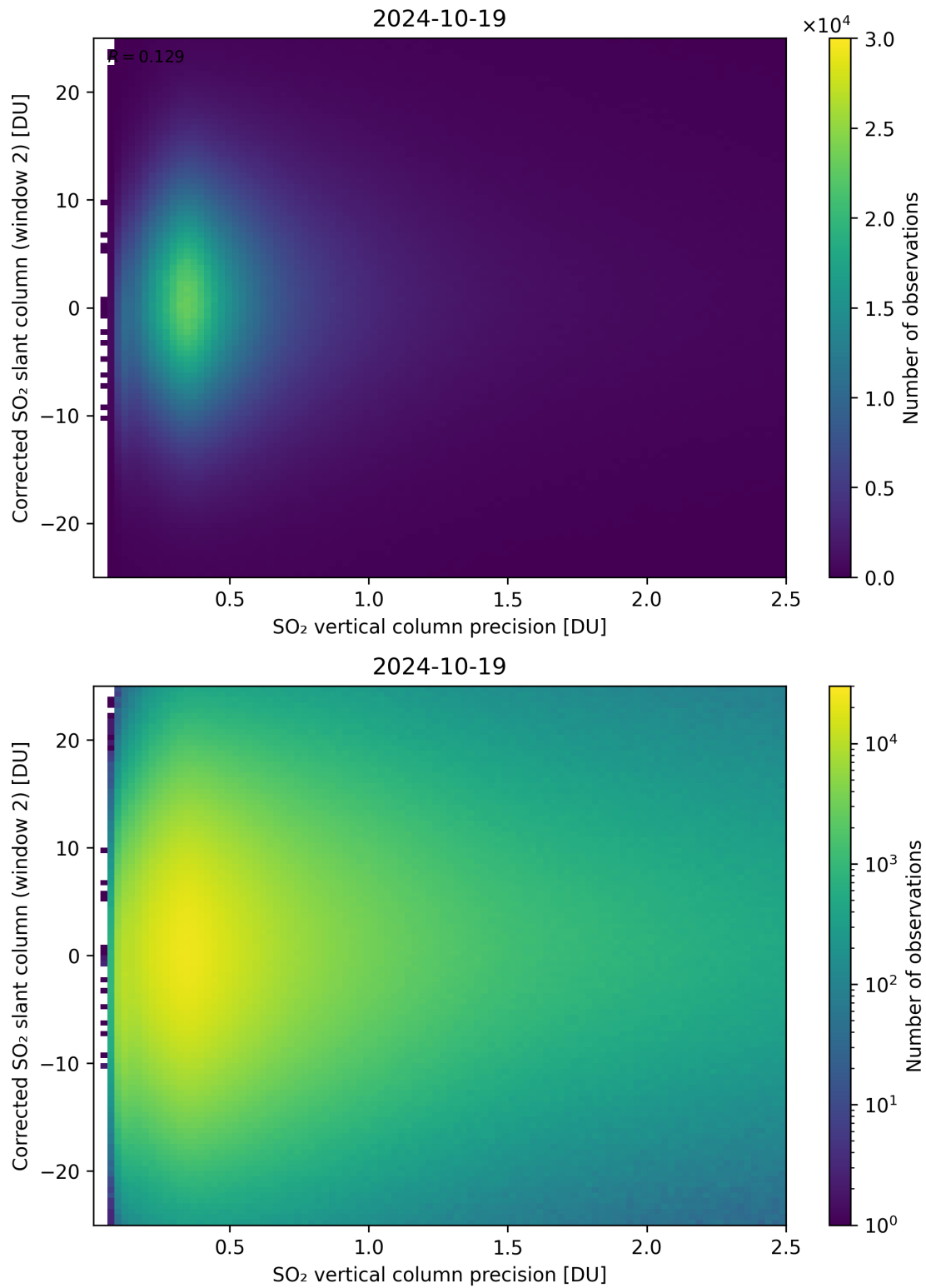
Figure 287: Scatter density plot of “SO 2 vertical column precision” against “Corrected SO 2 slant column (window 2)” for 2024-10-19 to 2024-10-20.
