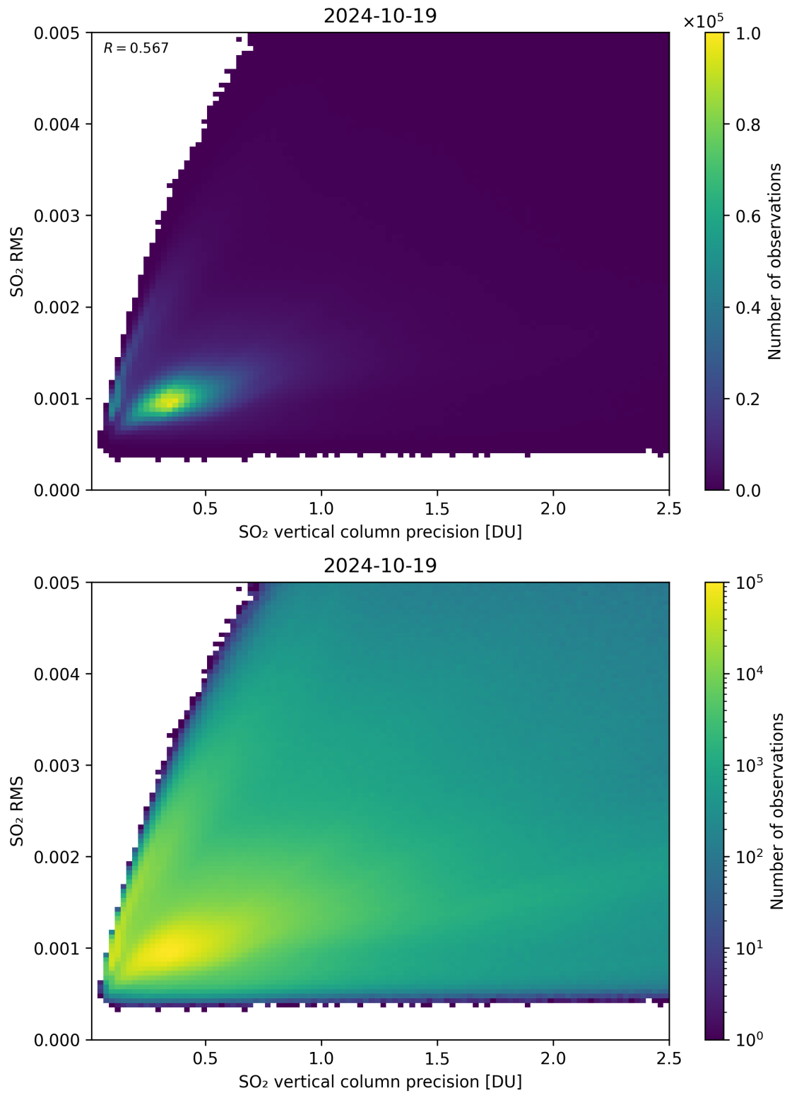
Figure 284: Scatter density plot of “SO 2 vertical column precision” against “SO 2 RMS” for 2024-10-19 to 2024-10-20.
