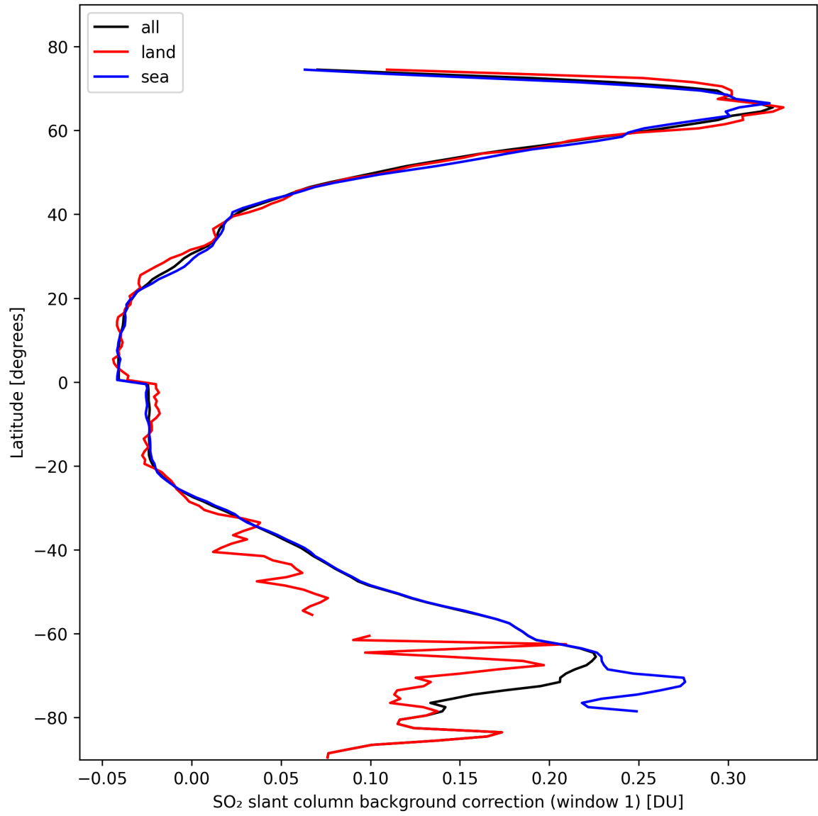
Figure 36: Zonal average of “SO 2 slant column background correction (window 1)” for 2024-10-19 to 2024-10-20.
