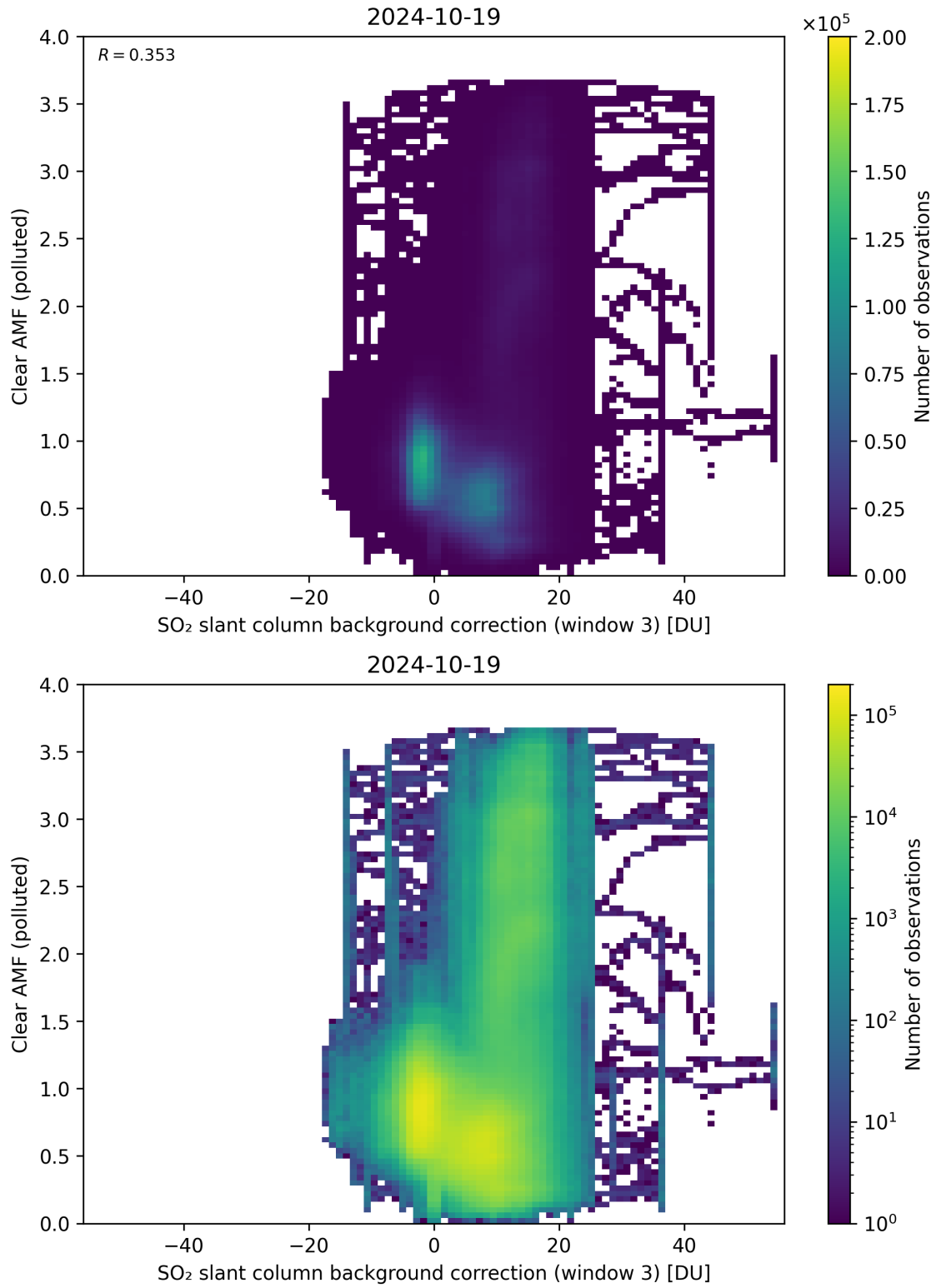
Figure 124: Scatter density plot of “SO 2 slant column background correction (window 3)” against “Clear AMF (polluted)” for 2024-10-19 to 2024-10-20.
