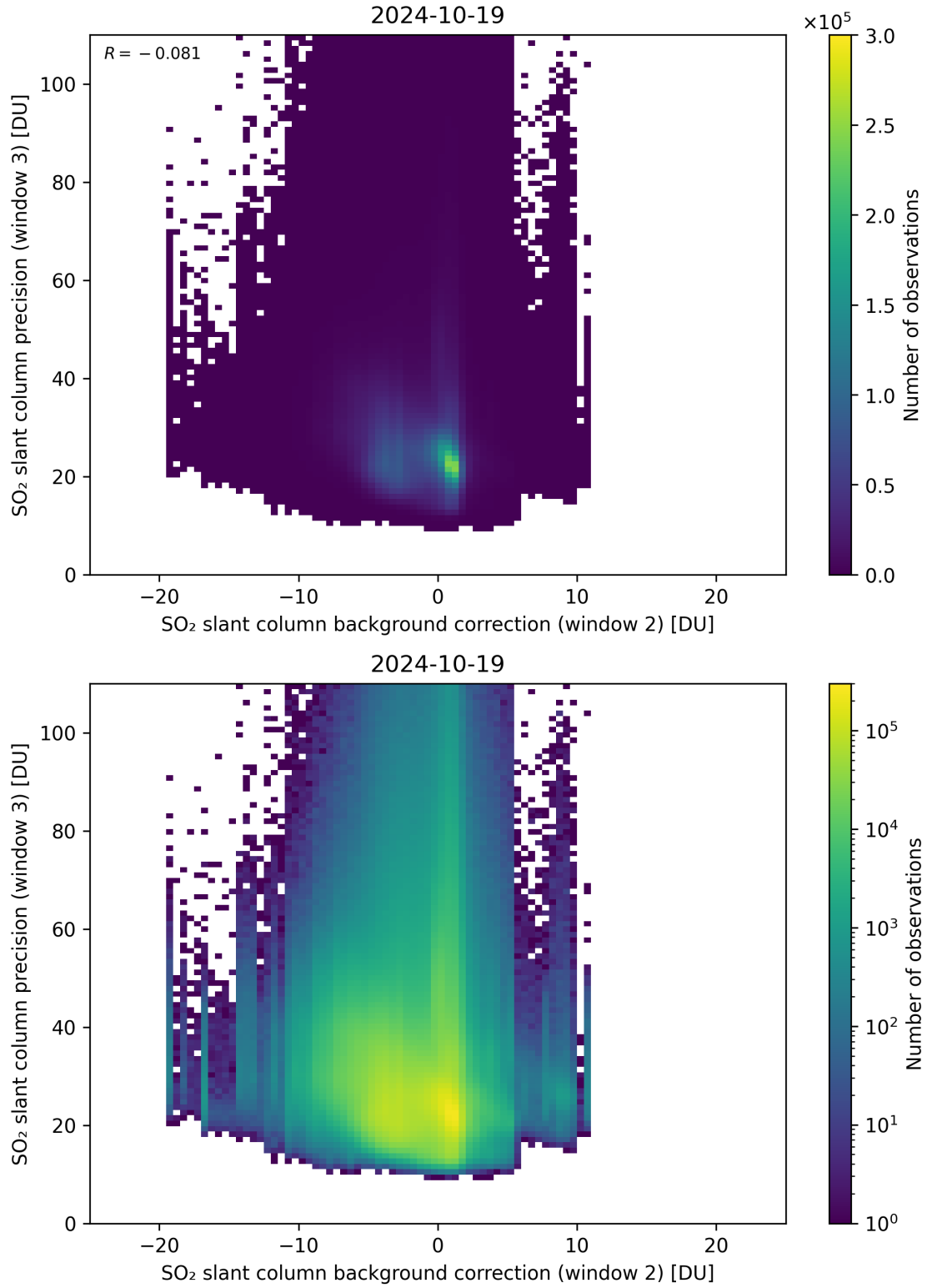
Figure 118: Scatter density plot of “SO 2 slant column background correction (window 2)” against “SO 2 slant column precision (window 3)” for 2024-10-19 to 2024-10-20.
