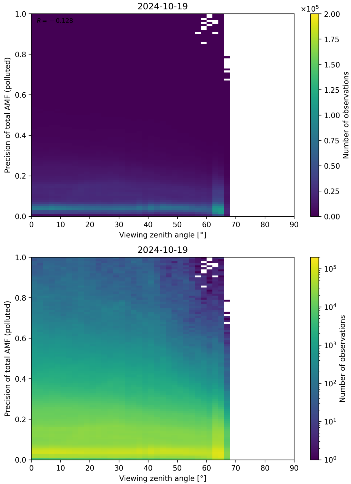
Figure 326: Scatter density plot of “Viewing zenith angle” against “Precision of total AMF (polluted)” for 2024-10-19 to 2024-10-20.
