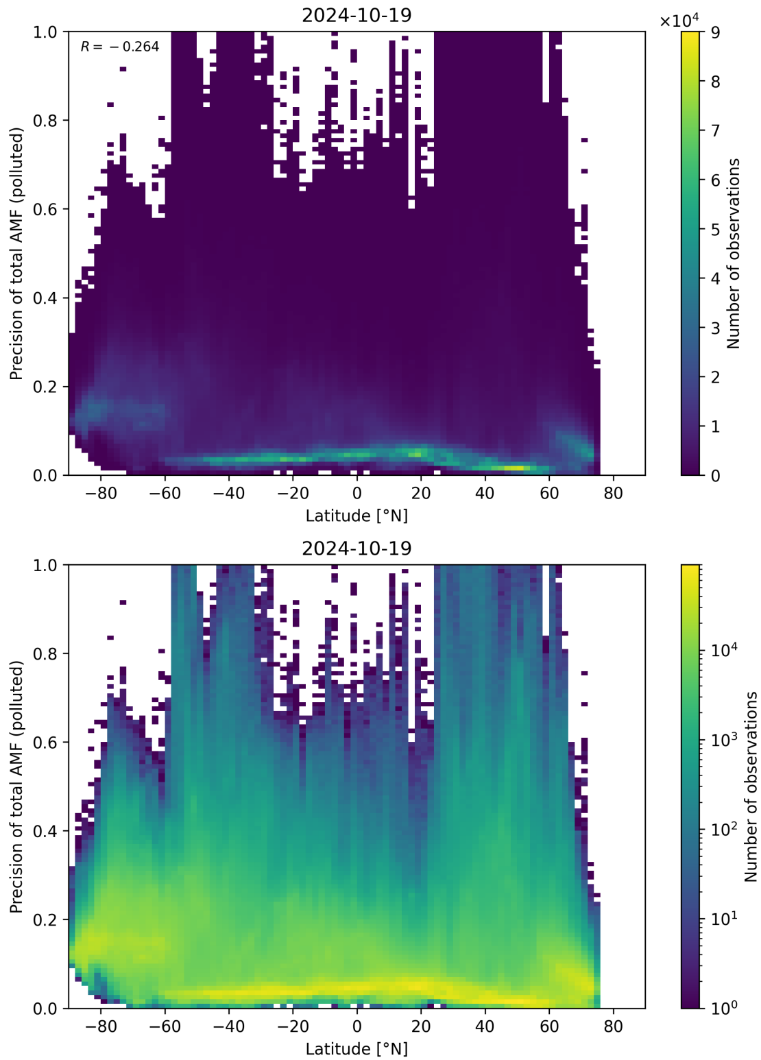
Figure 155: Scatter density plot of “Latitude” against “Precision of total AMF (polluted)” for 2024-10-19 to 2024-10-20.
