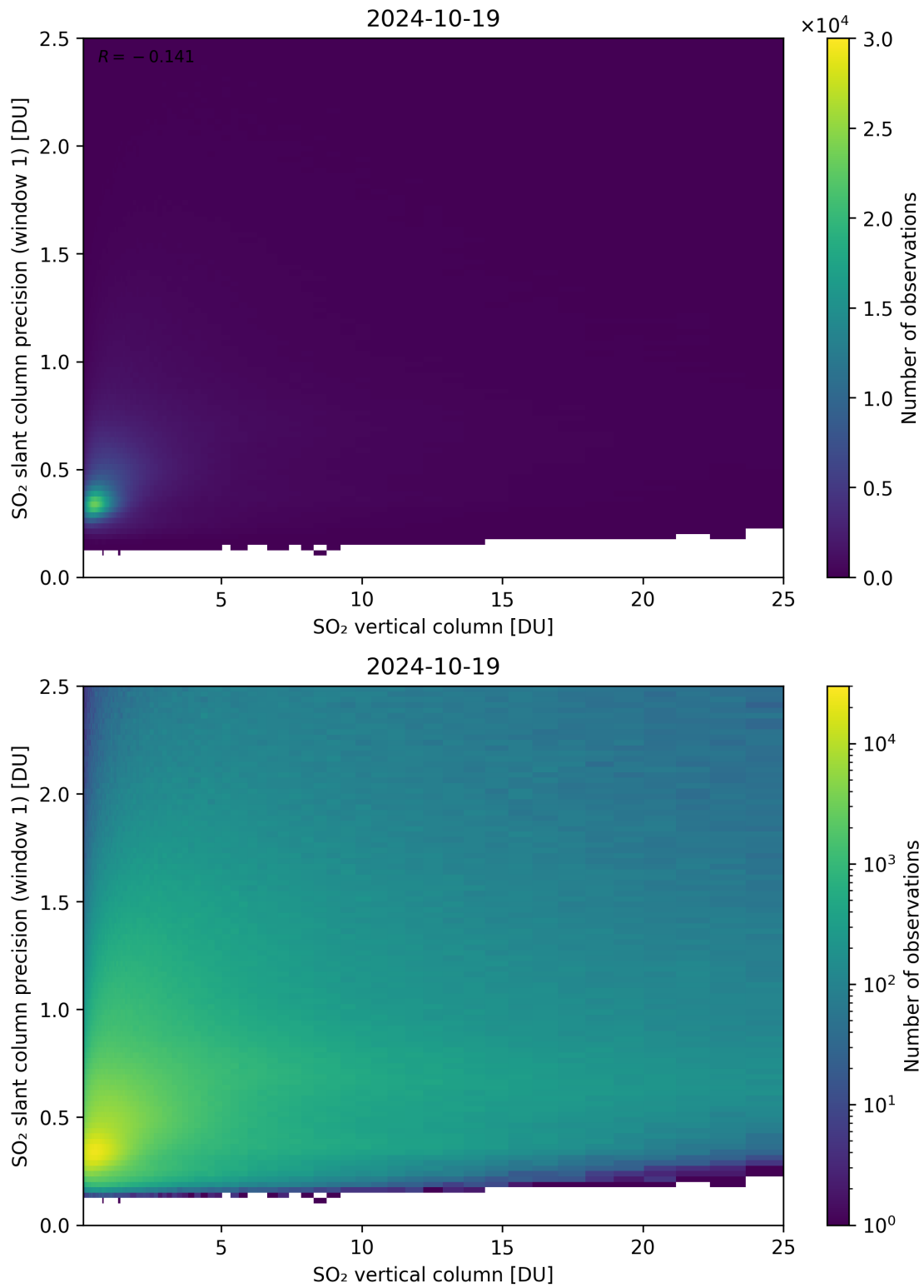
Figure 301: Scatter density plot of “SO 2 vertical column” against “SO 2 slant column precision (window 1)” for 2024-10-19 to 2024-10-20.
