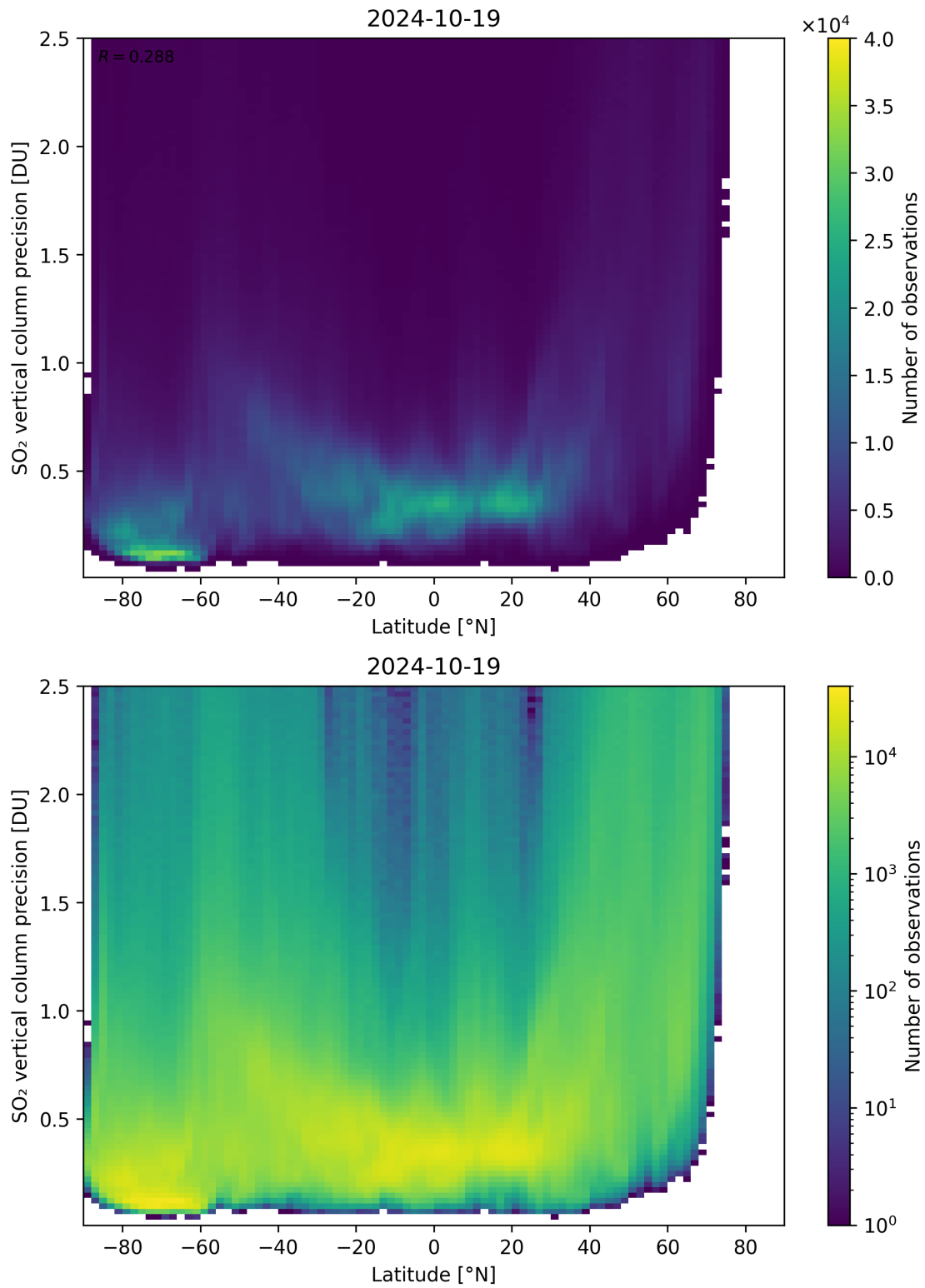
Figure 157: Scatter density plot of “Latitude” against “SO 2 vertical column precision” for 2024-10-19 to 2024-10-20.
