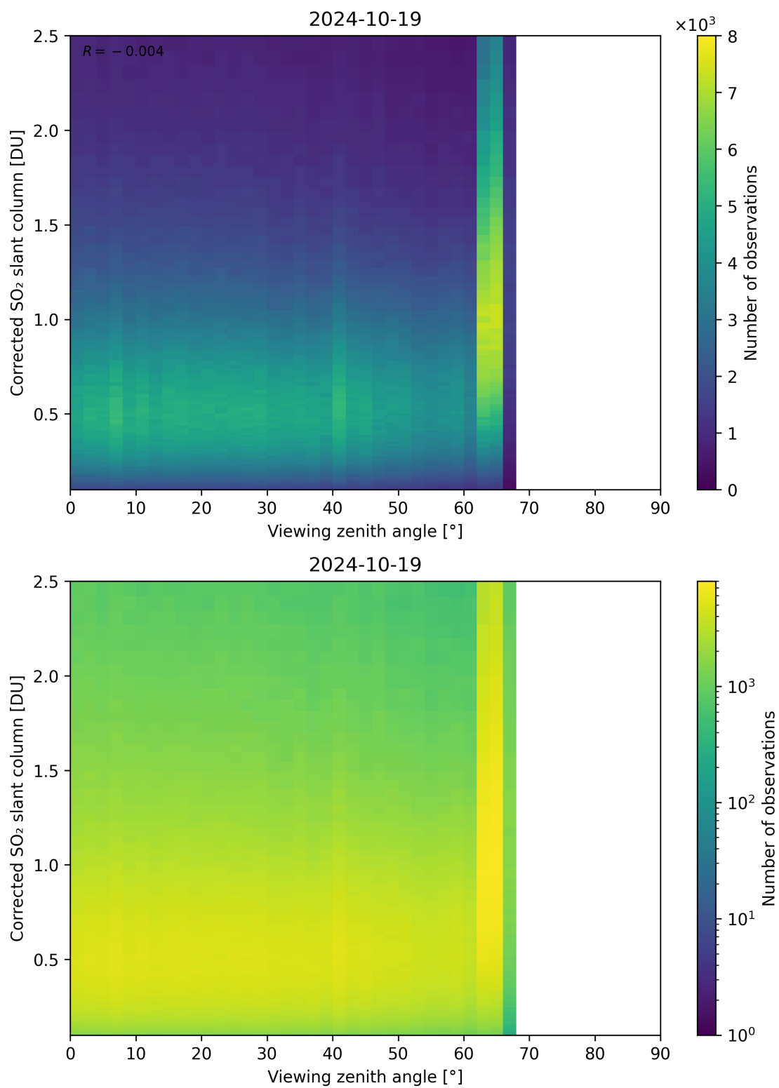
Figure 317: Scatter density plot of “Viewing zenith angle” against “Corrected SO 2 slant column” for 2024-10-19 to 2024-10-20.
