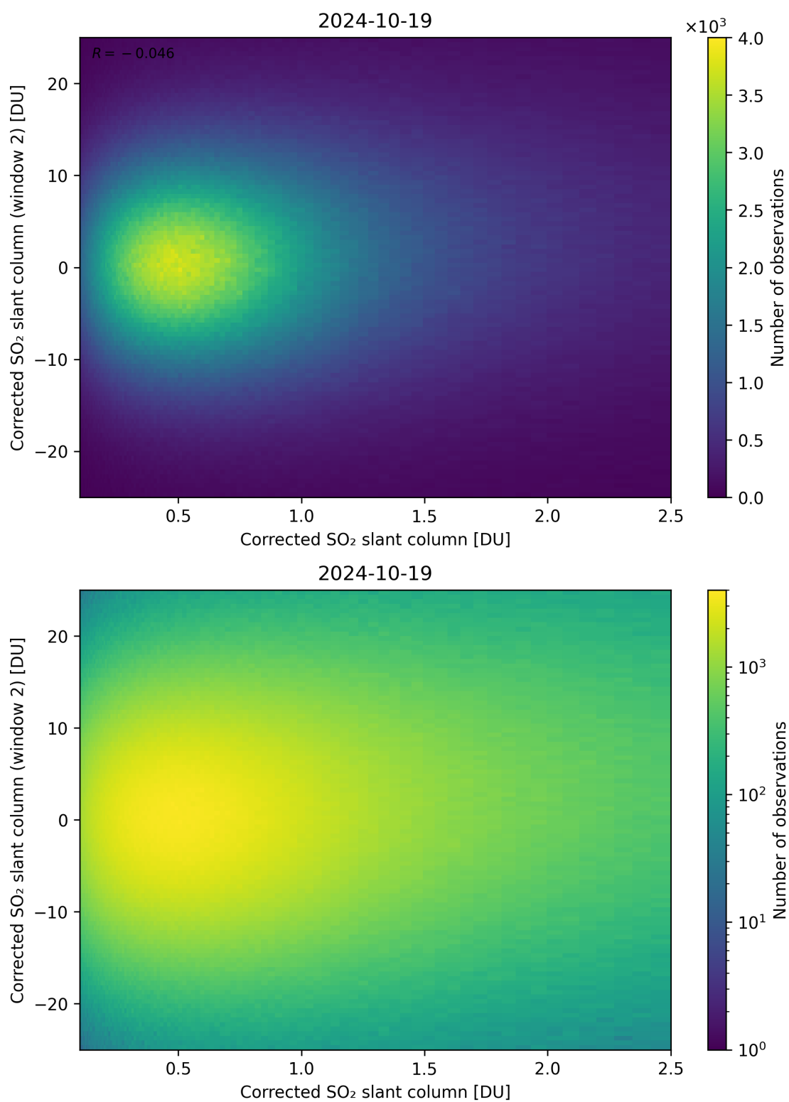
Figure 185: Scatter density plot of “Corrected SO 2 slant column” against “Corrected SO 2 slant column (window 2)” for 2024-10-19 to 2024-10-20.
