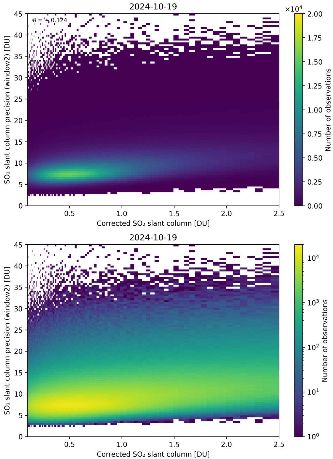
Figure 189: Scatter density plot of “Corrected SO 2 slant column” against “SO 2 slant column precision (window2)” for 2024-10-19 to 2024-10-20.
