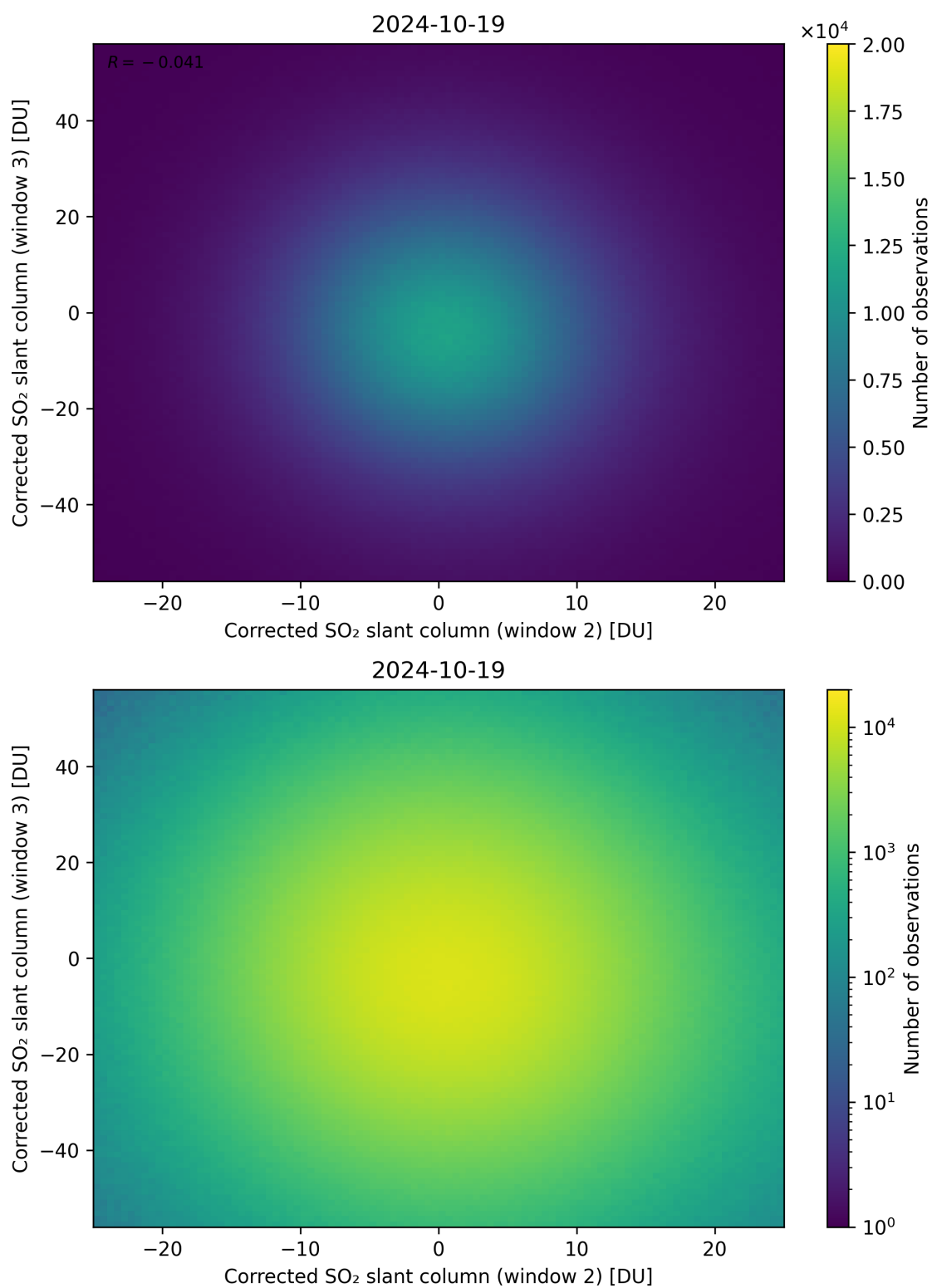
Figure 200: Scatter density plot of “Corrected SO 2 slant column (window 2)” against “Corrected SO 2 slant column (window 3)” for 2024-10-19 to 2024-10-20.
