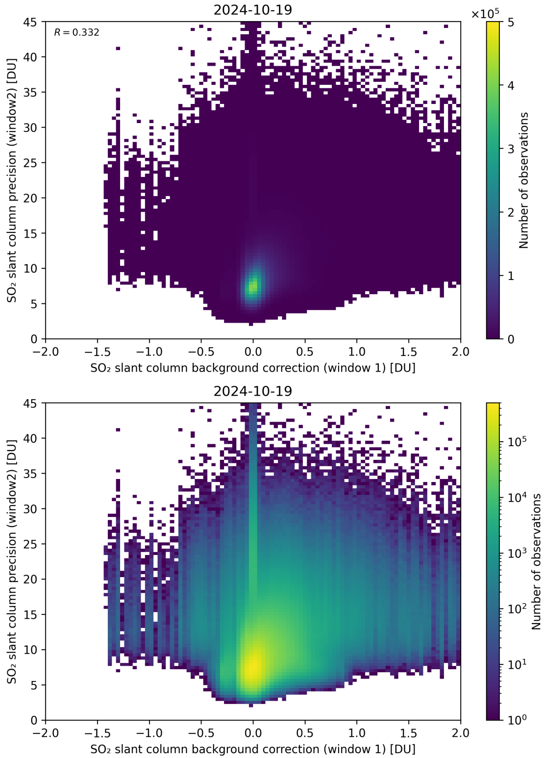
Figure 106: Scatter density plot of “SO 2 slant column background correction (window 1)” against “SO 2 slant column precision (window2)” for 2024-10-19 to 2024-10-20.
