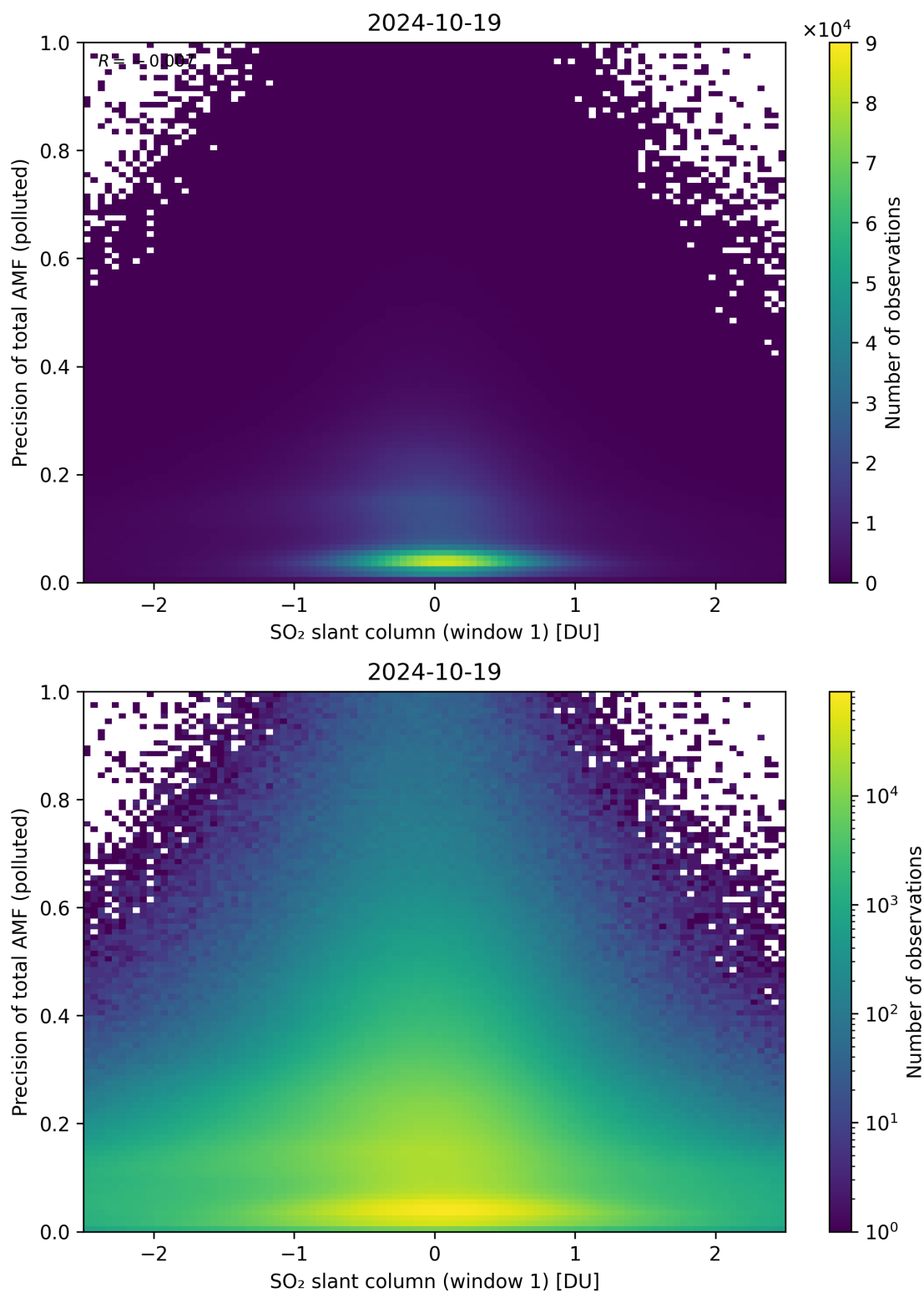
Figure 240: Scatter density plot of “SO 2 slant column (window 1)” against “Precision of total AMF (polluted)” for 2024-10-19 to 2024-10-20.
