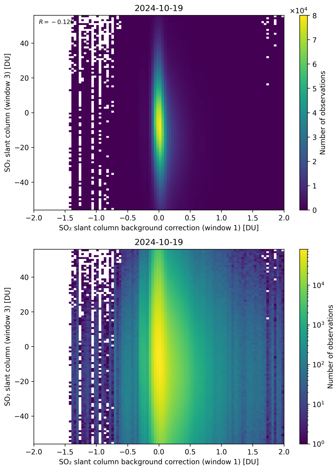
Figure 107: Scatter density plot of “SO 2 slant column background correction (window 1)” against “SO 2 slant column (window 3)” for 2024-10-19 to 2024-10-20.
