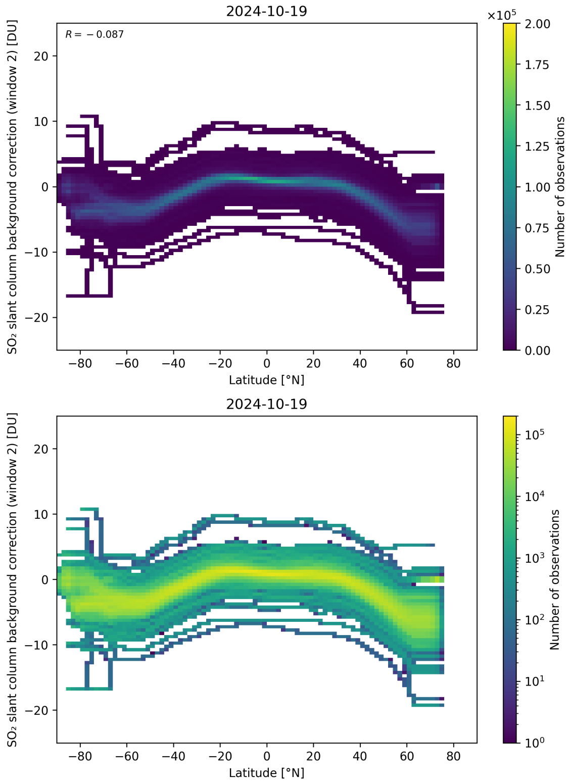
Figure 140: Scatter density plot of “Latitude” against “SO 2 slant column background correction (window 2)” for 2024-10-19 to 2024-10-20.
