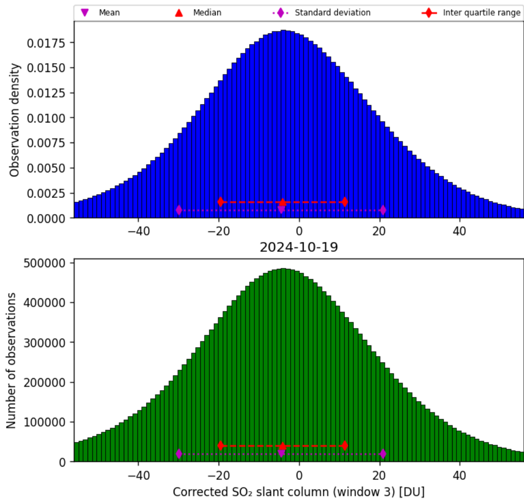
Figure 66: Histogram of “Corrected SO 2 slant column (window 3)” for 2024-10-19 to 2024-10-20
