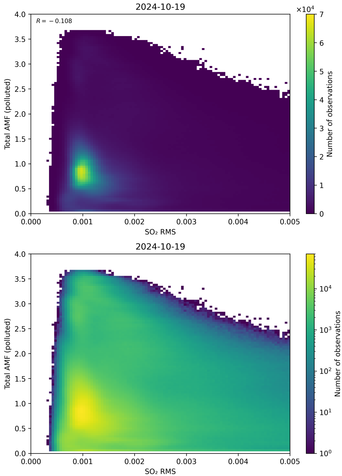
Figure 137: Scatter density plot of “SO 2 RMS” against “Total AMF (polluted)” for 2024-10-19 to 2024-10-20.
