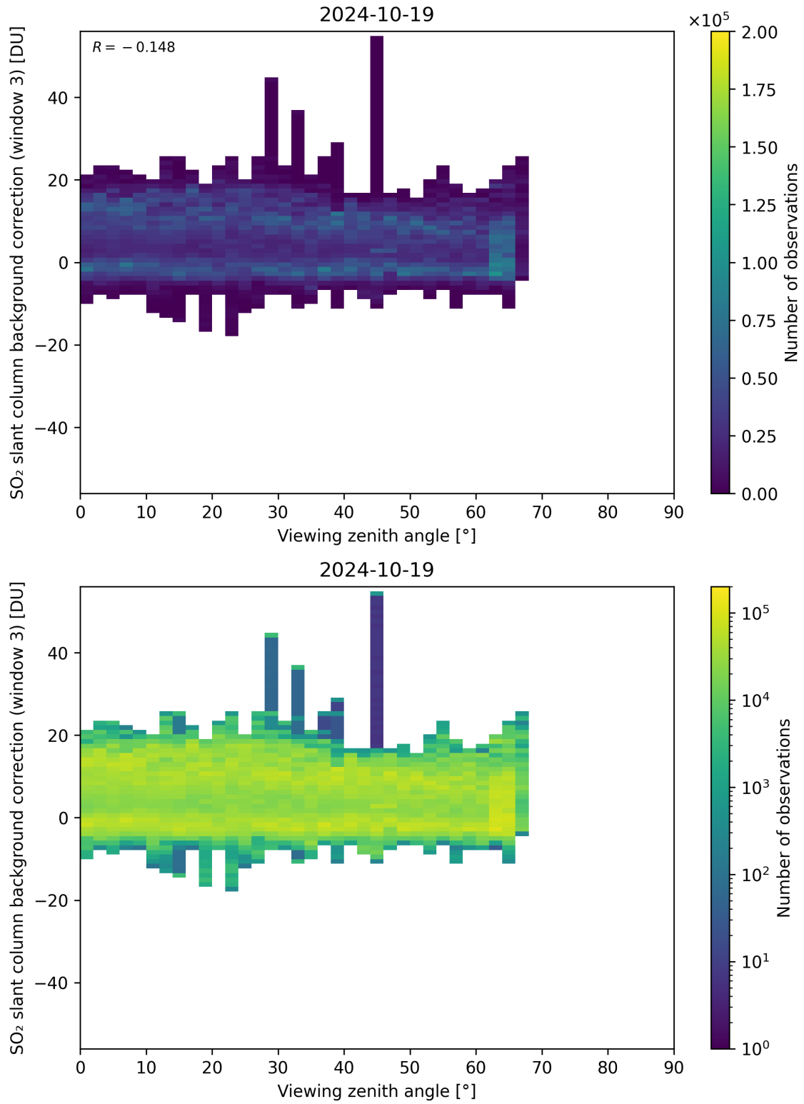
Figure 310: Scatter density plot of “Viewing zenith angle” against “SO 2 slant column background correction (window 3)” for 2024-10-19 to 2024-10-20.
