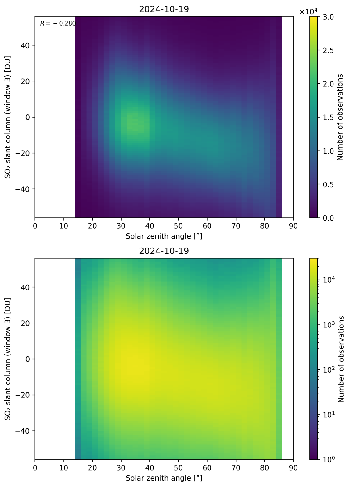
Figure 172: Scatter density plot of “Solar zenith angle” against “SO 2 slant column (window 3)” for 2024-10-19 to 2024-10-20.
