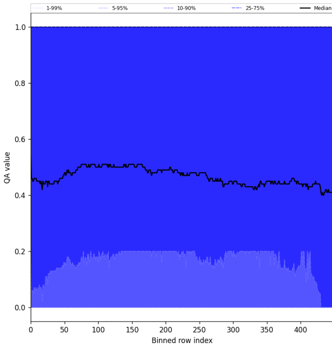
Figure 75: Along track statistics of “QA value” for 2024-10-19 to 2024-10-20
