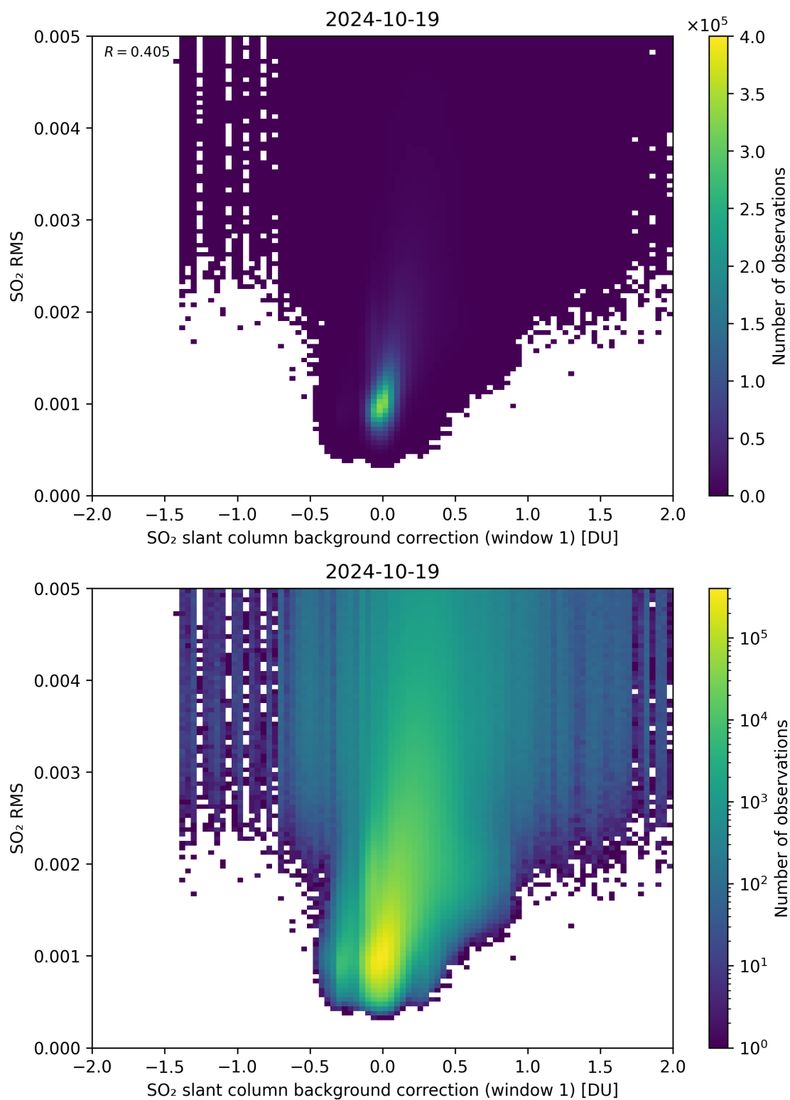
Figure 102: Scatter density plot of “SO 2 slant column background correction (window 1)” against “SO 2 RMS” for 2024-10-19 to 2024-10-20.
