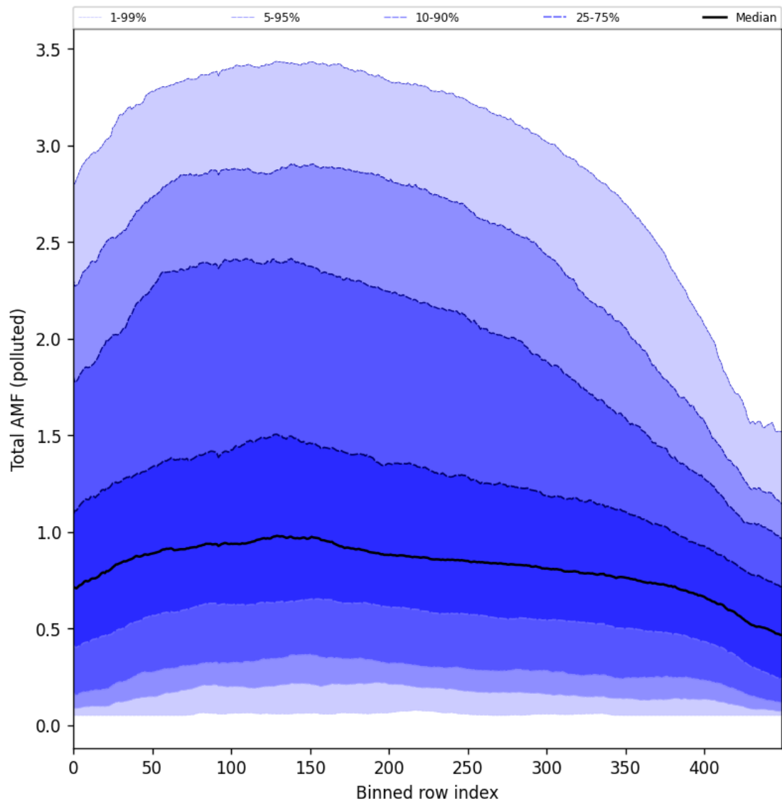
Figure 94: Along track statistics of “Total AMF (polluted)” for 2024-10-19 to 2024-10-20
