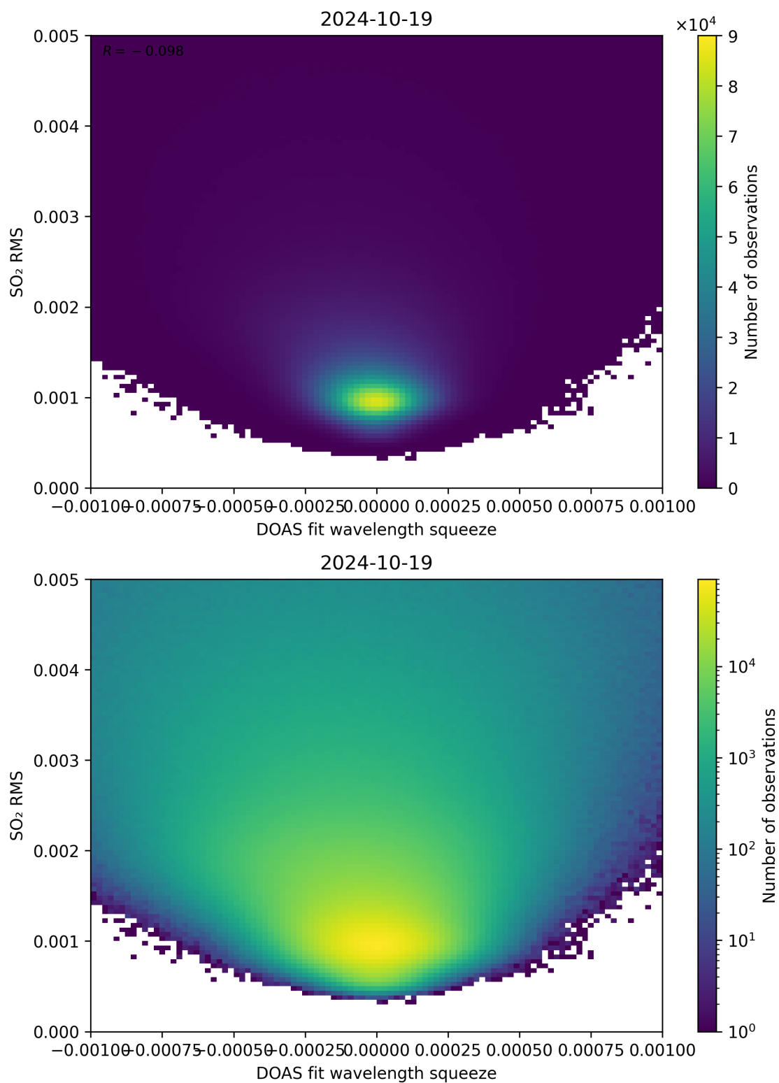
Figure 132: Scatter density plot of “DOAS fit wavelength squeeze” against “SO 2 RMS” for 2024-10-19 to 2024-10-20.
