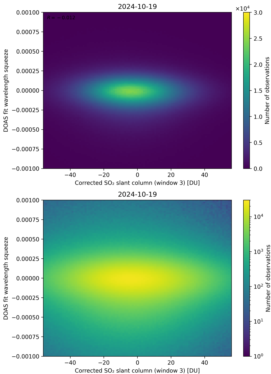
Figure 207: Scatter density plot of “Corrected SO 2 slant column (window 3)” against “DOAS fit wavelength squeeze” for 2024-10-19 to 2024-10-20.
