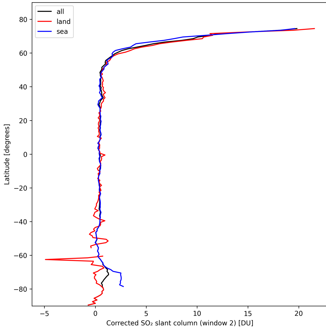
Figure 39: Zonal average of “Corrected SO 2 slant column (window 2)” for 2024-10-19 to 2024-10-20.
