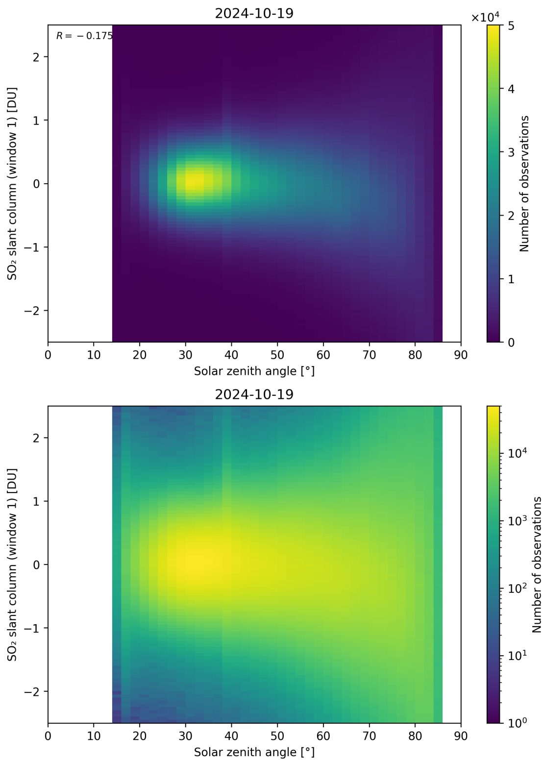
Figure 169: Scatter density plot of “Solar zenith angle” against “SO 2 slant column (window 1)” for 2024-10-19 to 2024-10-20.
