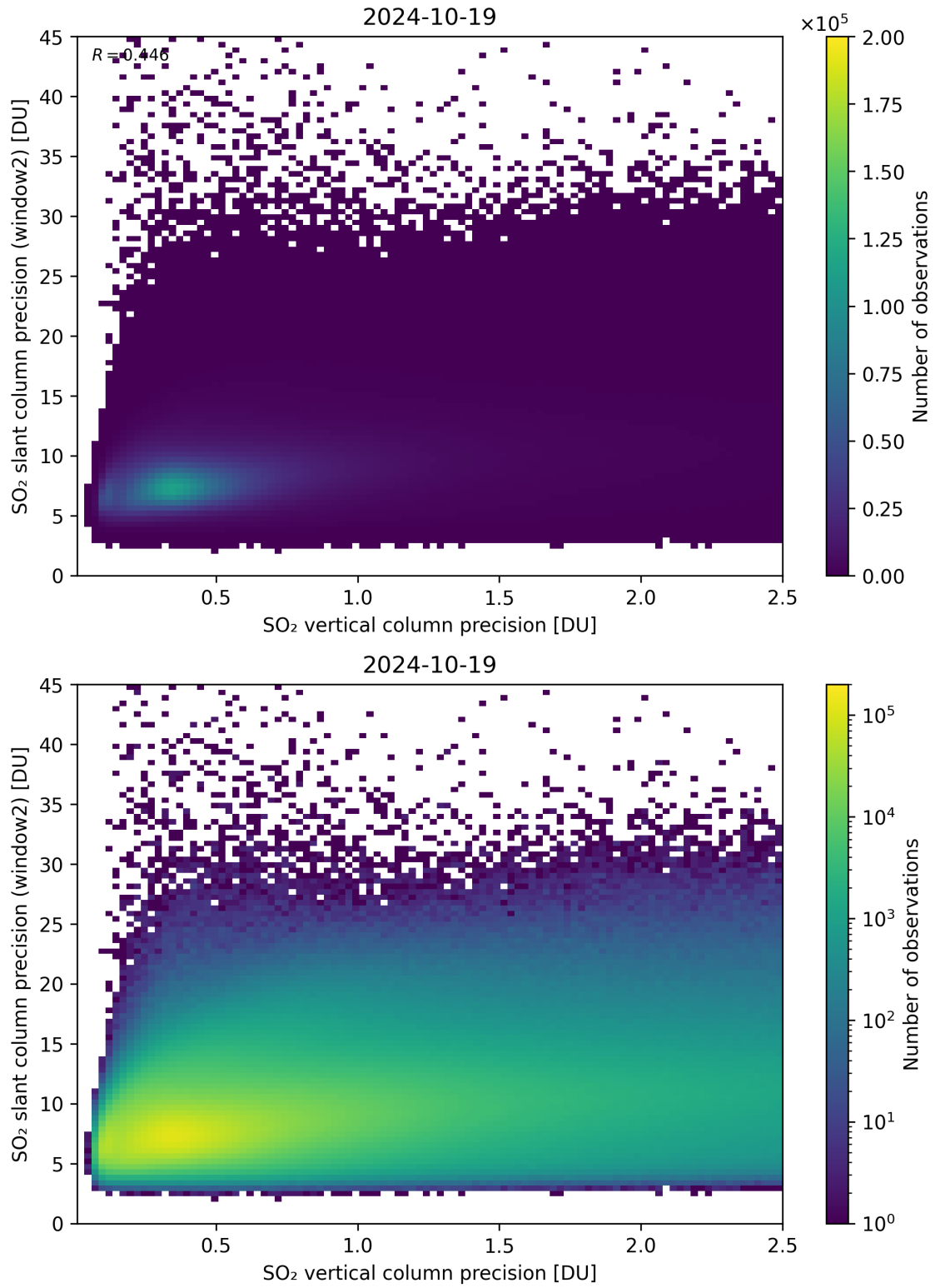
Figure 291: Scatter density plot of “SO 2 vertical column precision” against “SO 2 slant column precision (window2)” for 2024-10-19 to 2024-10-20.
