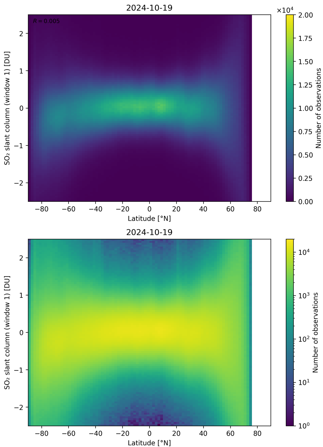
Figure 149: Scatter density plot of “Latitude” against “SO 2 slant column (window 1)” for 2024-10-19 to 2024-10-20.
