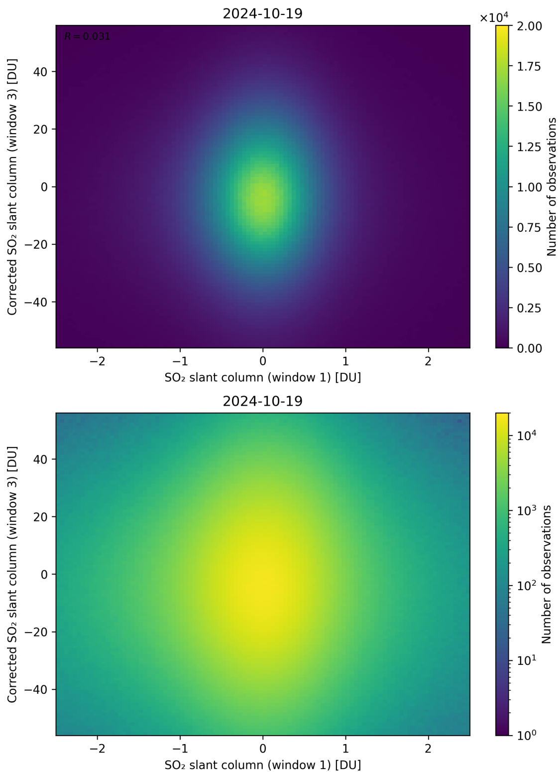
Figure 234: Scatter density plot of “SO 2 slant column (window 1)” against “Corrected SO 2 slant column (window 3)” for 2024-10-19 to 2024-10-20.
