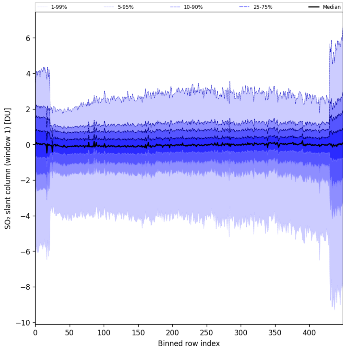
Figure 79: Along track statistics of “SO 2 slant column (window 1)” for 2024-10-19 to 2024-10-20
