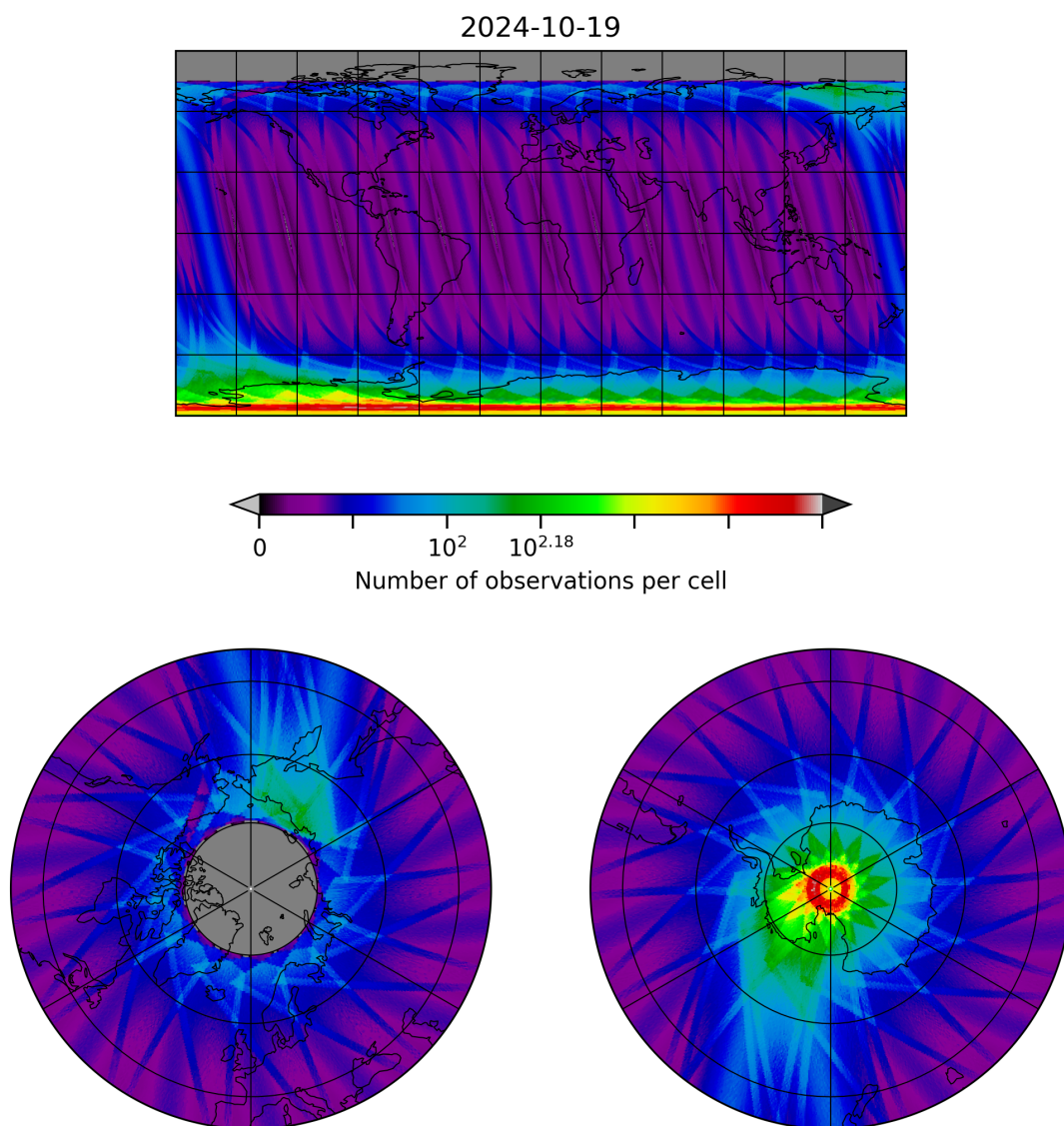
Figure 28: Map of the number of observations for 2024-10-19 to 2024-10-20
