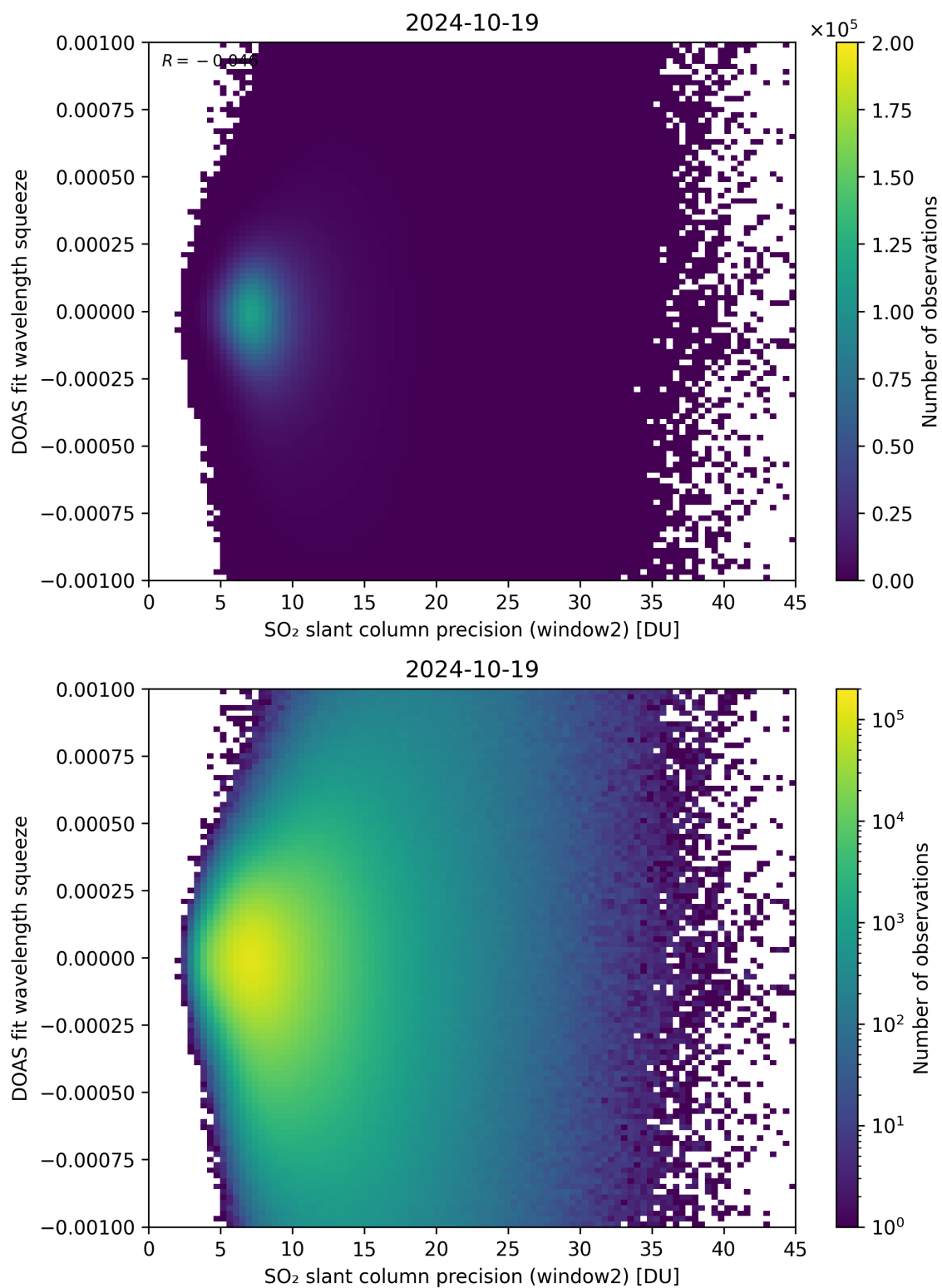
Figure 244: Scatter density plot of “SO 2 slant column precision (window2)” against “DOAS fit wavelength squeeze” for 2024-10-19 to 2024-10-20.
