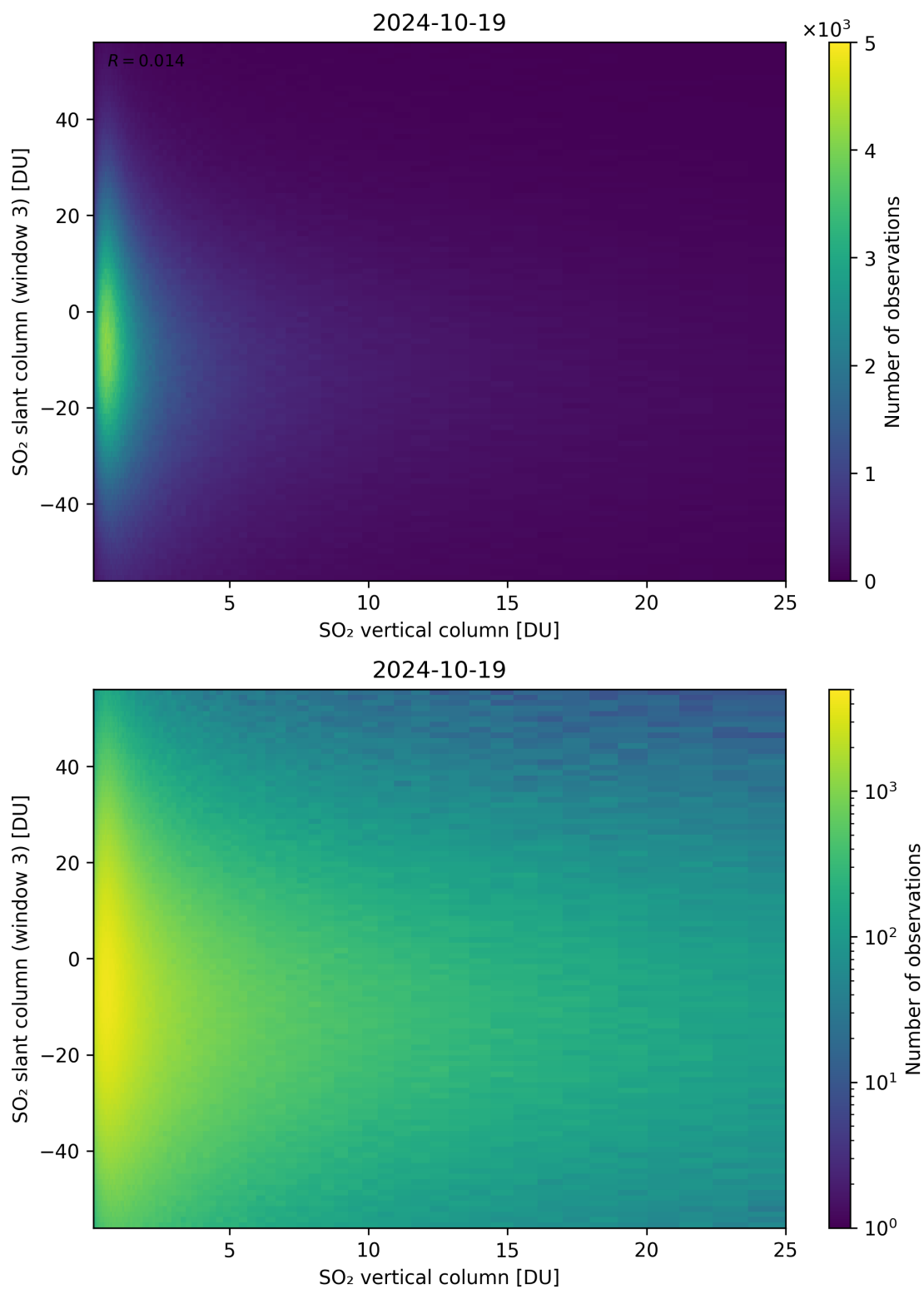
Figure 303: Scatter density plot of “SO 2 vertical column” against “SO 2 slant column (window 3)” for 2024-10-19 to 2024-10-20.
