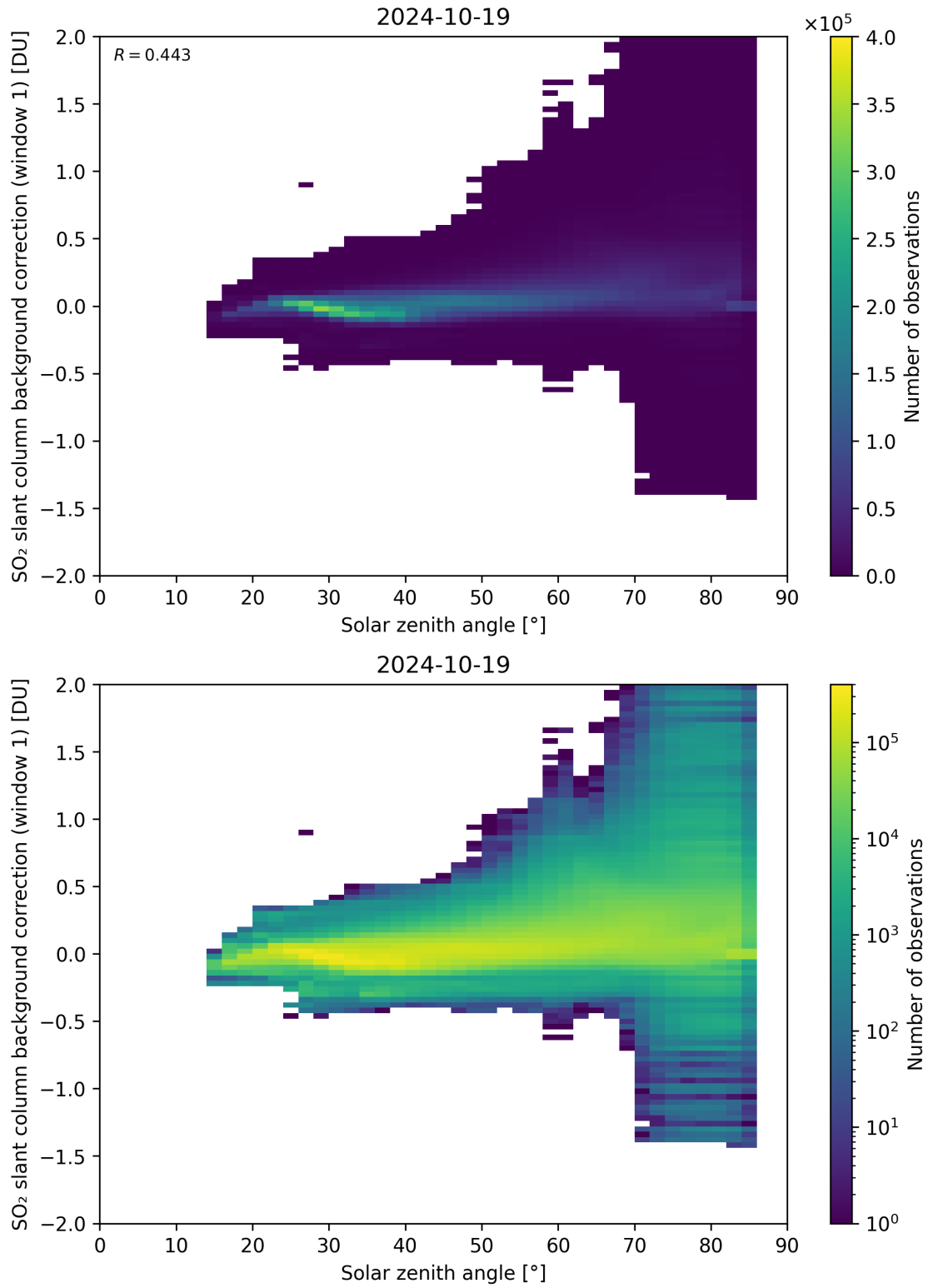
Figure 158: Scatter density plot of “Solar zenith angle” against “SO 2 slant column background correction (window 1)” for 2024-10-19 to 2024-10-20.
