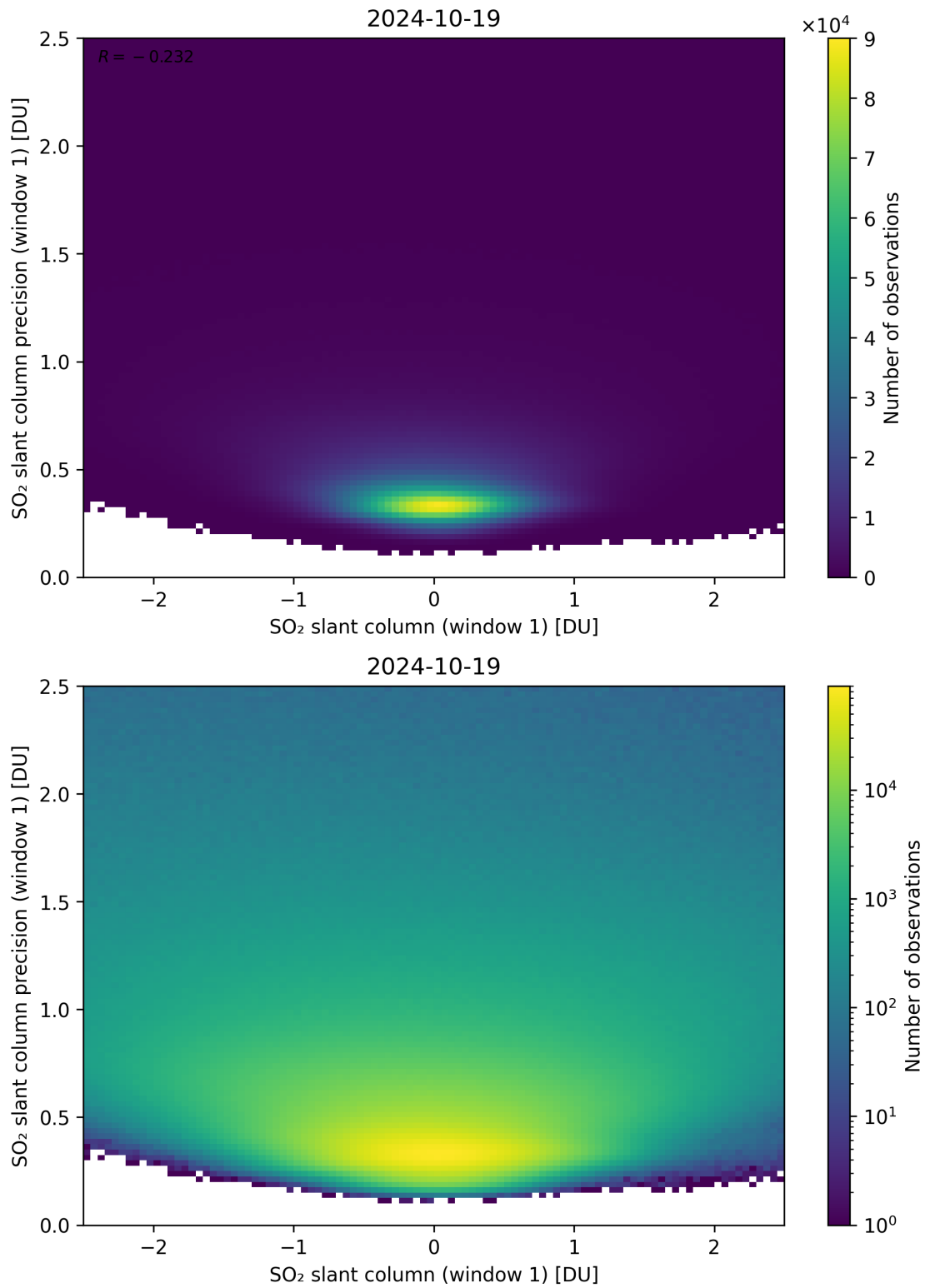
Figure 235: Scatter density plot of “SO 2 slant column (window 1)” against “SO 2 slant column precision (window 1)” for 2024-10-19 to 2024-10-20.
