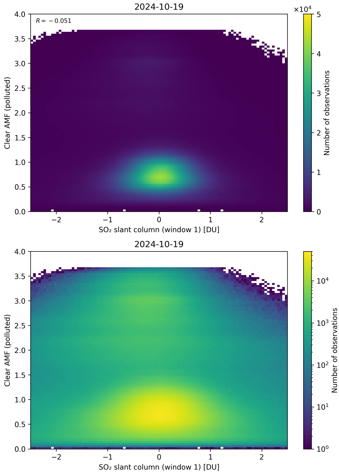
Figure 232: Scatter density plot of “SO 2 slant column (window 1)” against “Clear AMF (polluted)” for 2024-10-19 to 2024-10-20.
