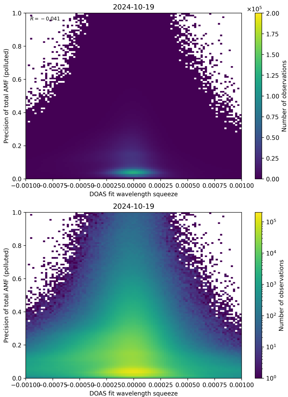
Figure 135: Scatter density plot of “DOAS fit wavelength squeeze” against “Precision of total AMF (polluted)” for 2024-10-19 to 2024-10-20.
