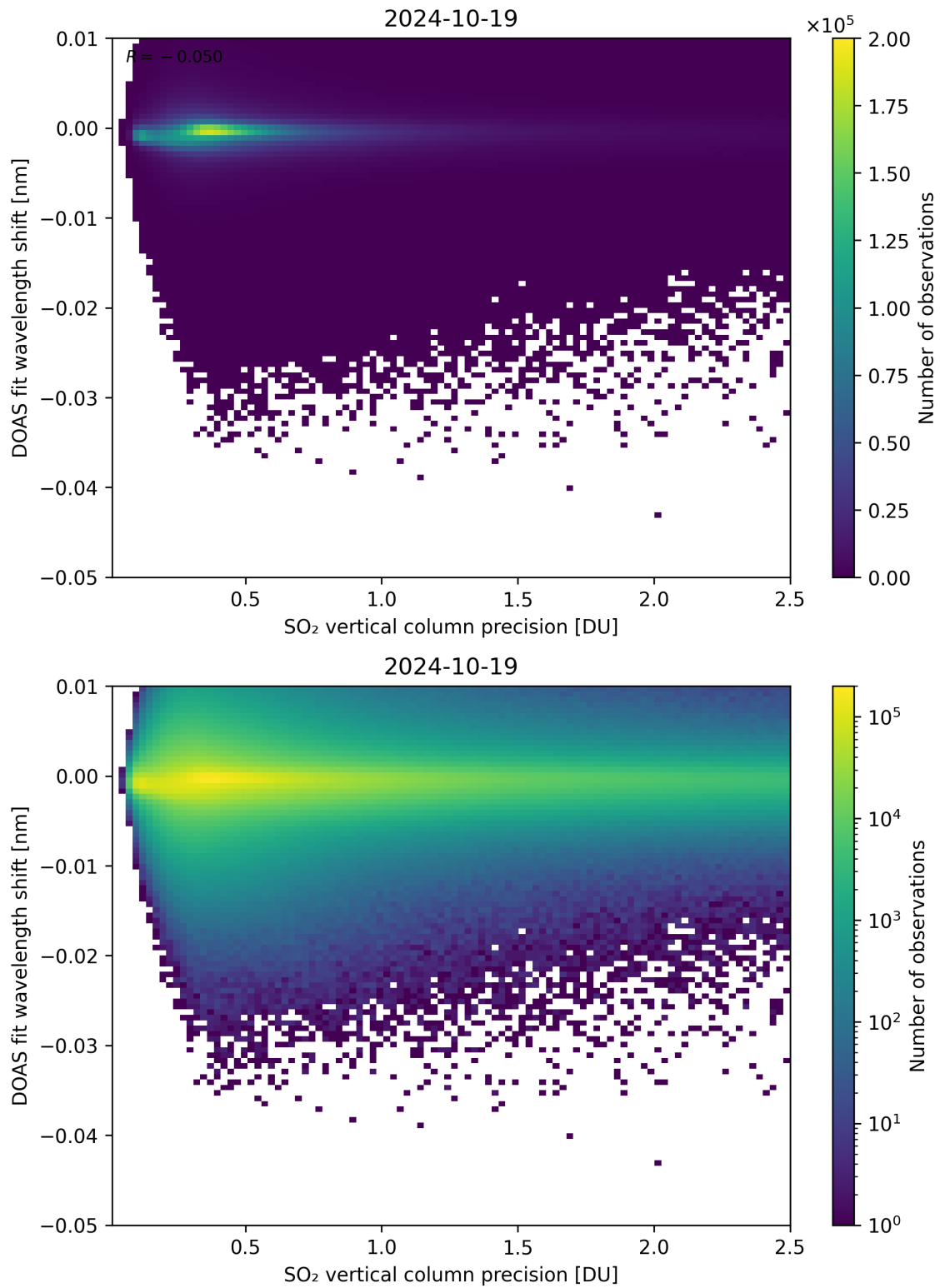
Figure 282: Scatter density plot of “SO 2 vertical column precision” against “DOAS fit wavelength shift” for 2024-10-19 to 2024-10-20.
