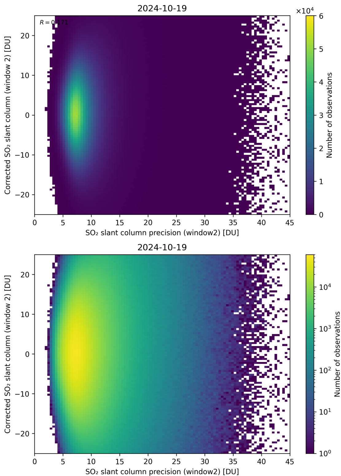
Figure 247: Scatter density plot of “SO 2 slant column precision (window2)” against “Corrected SO 2 slant column (window 2)” for 2024-10-19 to 2024-10-20.
