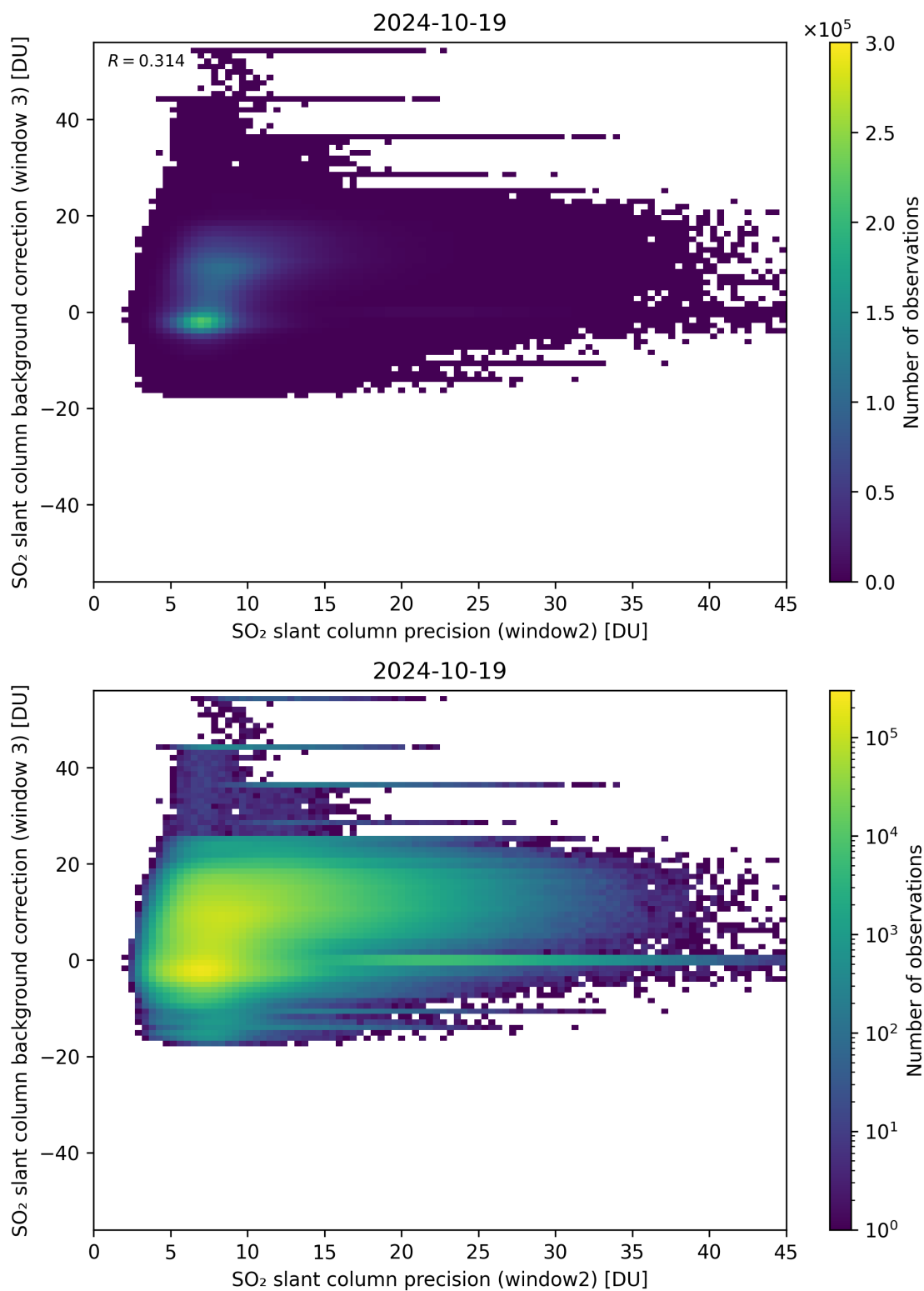
Figure 242: Scatter density plot of “SO 2 slant column precision (window2)” against “SO 2 slant column background correction (window 3)” for 2024-10-19 to 2024-10-20.
