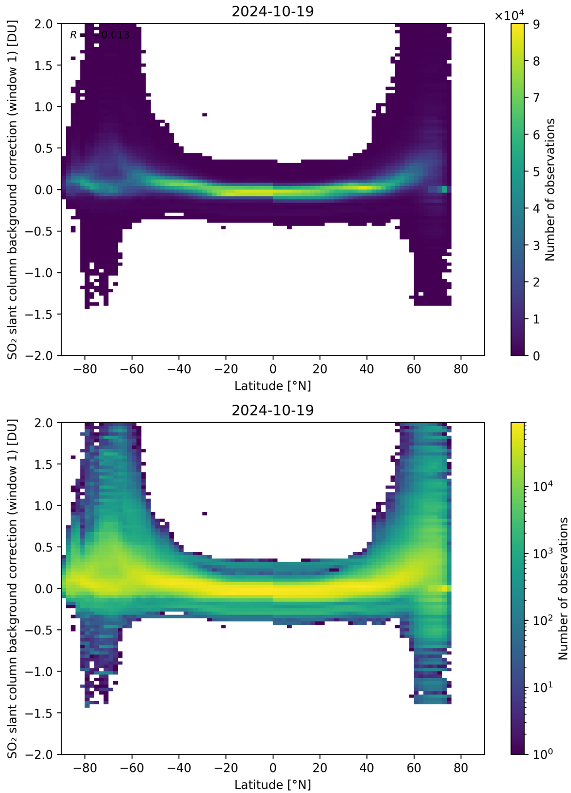
Figure 139: Scatter density plot of “Latitude” against “SO 2 slant column background correction (window 1)” for 2024-10-19 to 2024-10-20.
