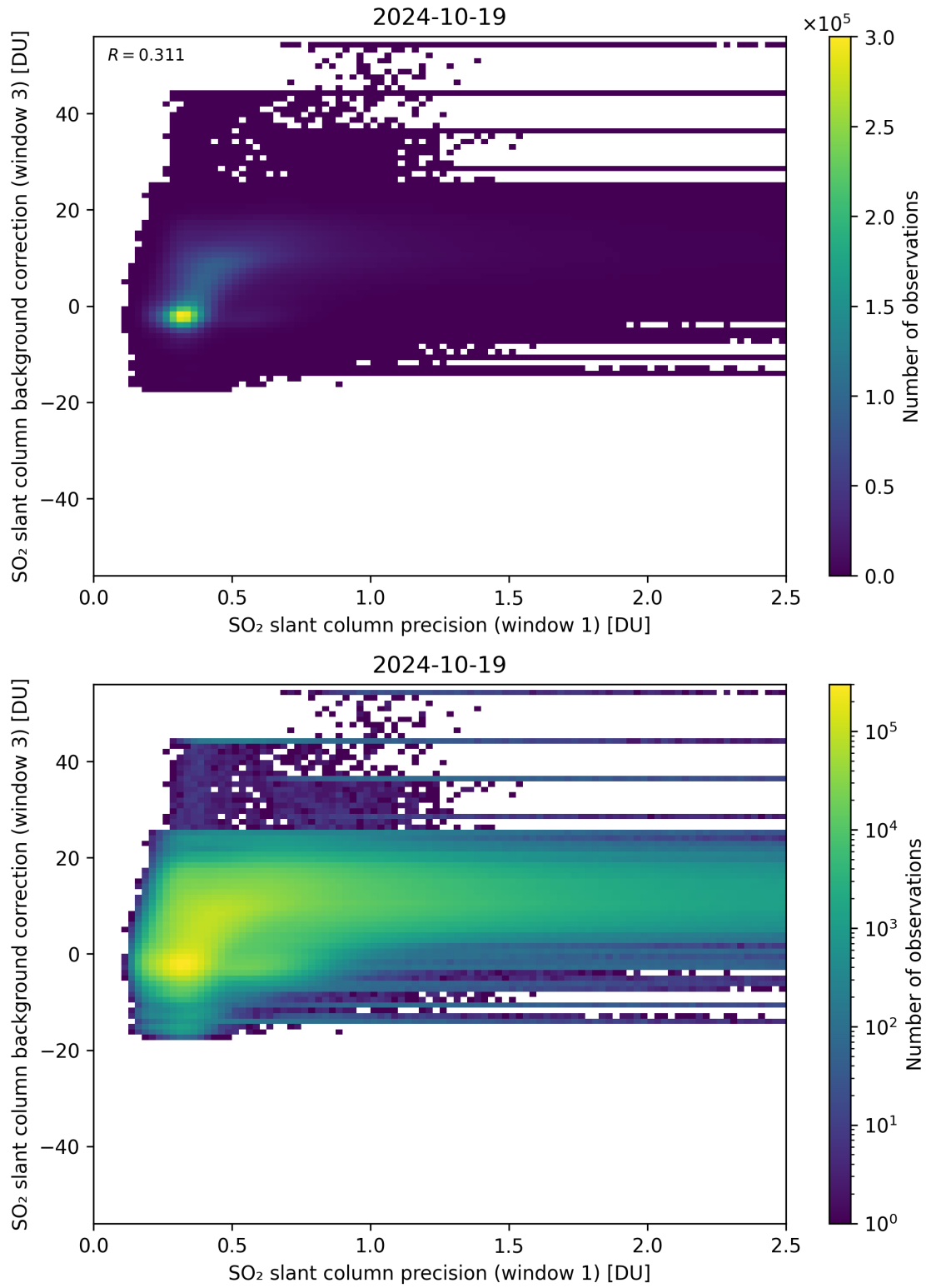
Figure 220: Scatter density plot of “SO 2 slant column precision (window 1)” against “SO 2 slant column background correction (window 3)” for 2024-10-19 to 2024-10-20.
