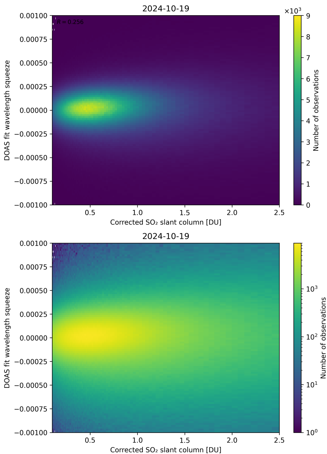
Figure 182: Scatter density plot of “Corrected SO 2 slant column” against “DOAS fit wavelength squeeze” for 2024-10-19 to 2024-10-20.
