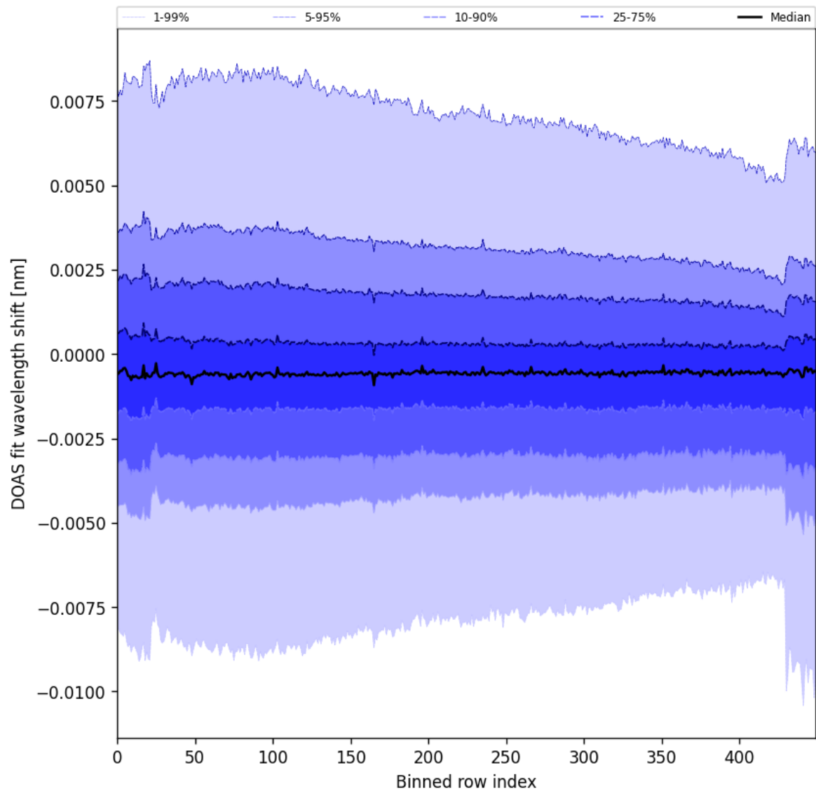
Figure 91: Along track statistics of “DOAS fit wavelength shift” for 2024-10-19 to 2024-10-20
