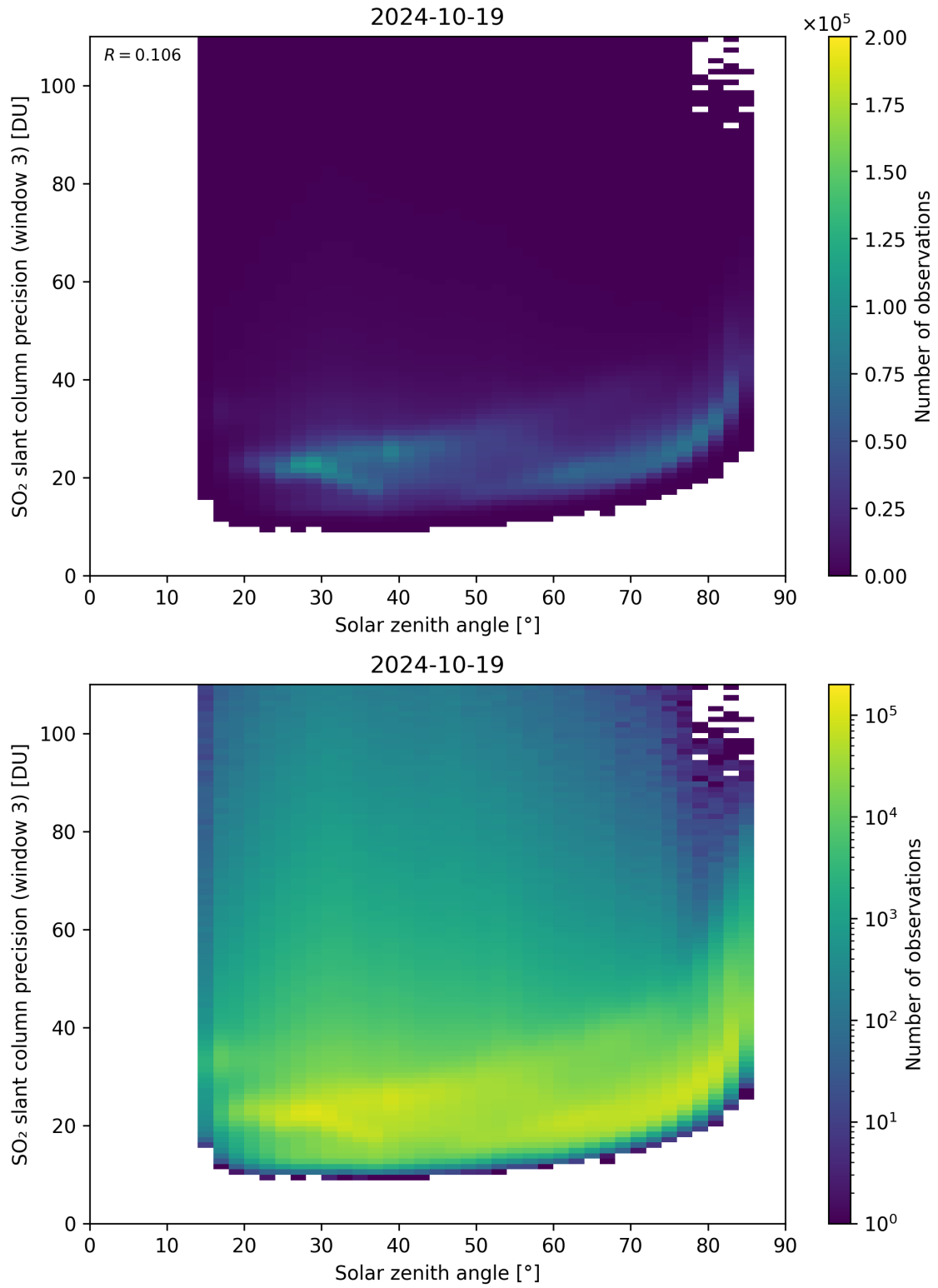
Figure 173: Scatter density plot of “Solar zenith angle” against “SO 2 slant column precision (window 3)” for 2024-10-19 to 2024-10-20.
