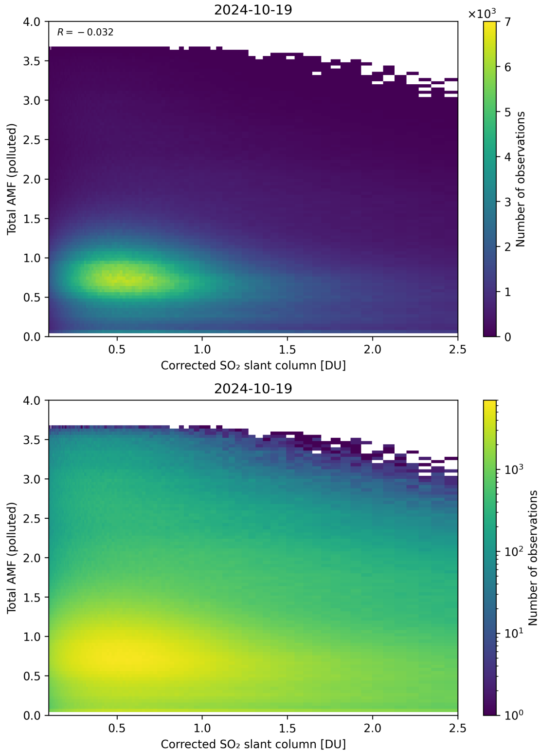
Figure 192: Scatter density plot of “Corrected SO 2 slant column” against “Total AMF (polluted)” for 2024-10-19 to 2024-10-20.
