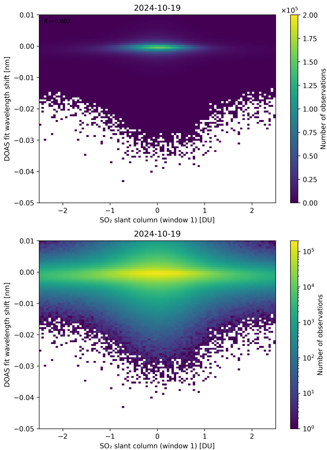
Figure 215: Scatter density plot of “SO 2 slant column (window 1)” against “DOAS fit wavelength shift” for 2024-10-19 to 2024-10-20.
