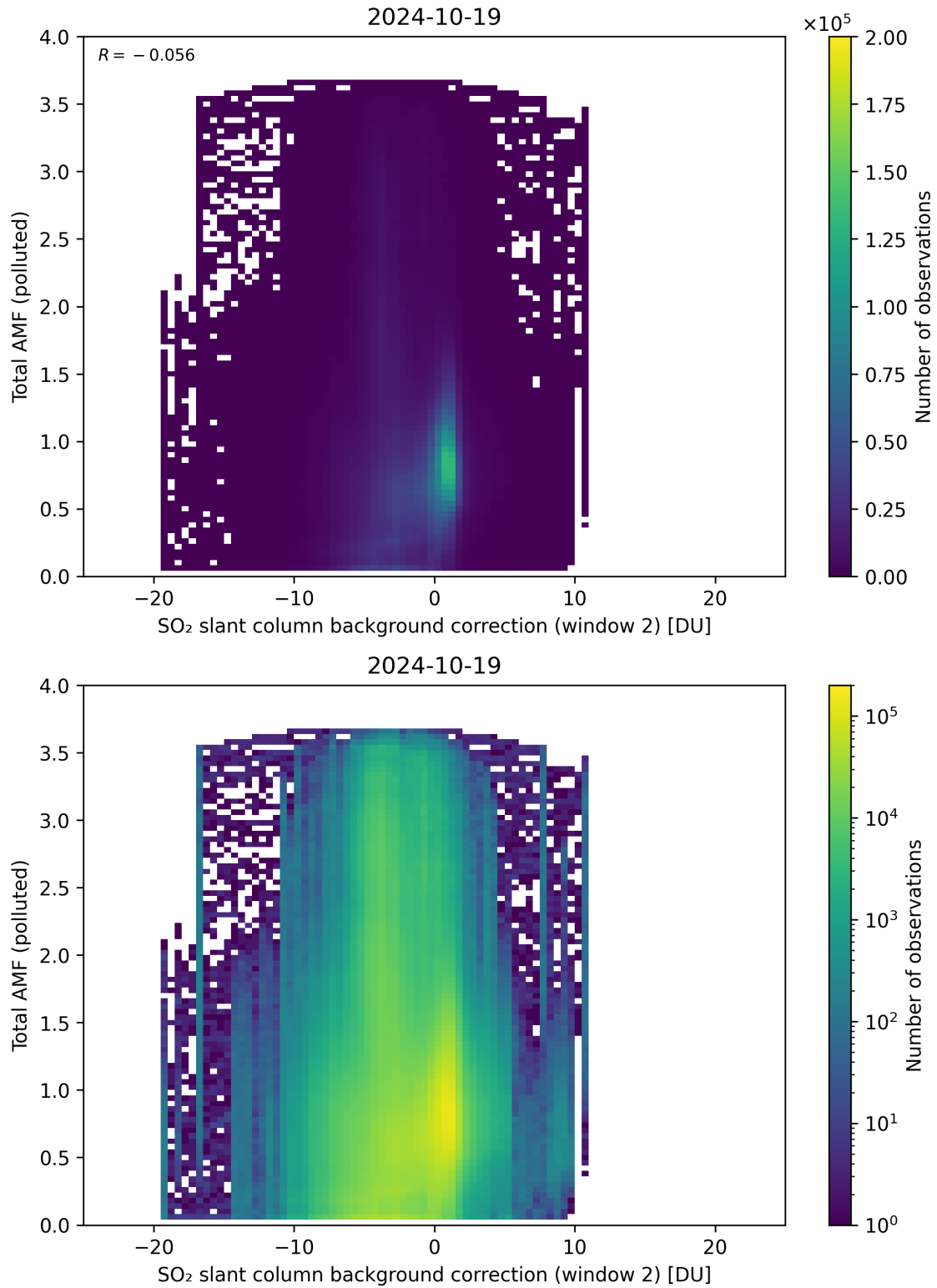
Figure 119: Scatter density plot of “SO 2 slant column background correction (window 2)” against “Total AMF (polluted)” for 2024-10-19 to 2024-10-20.
