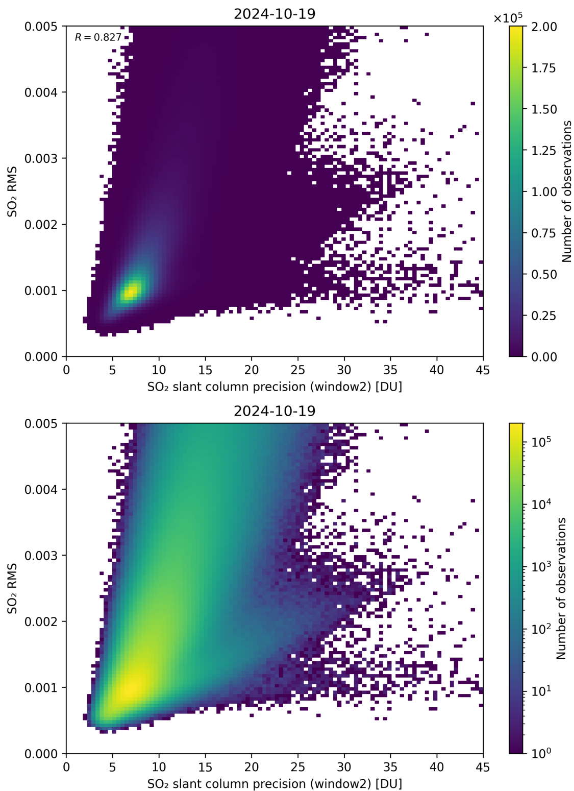
Figure 245: Scatter density plot of “SO 2 slant column precision (window2)” against “SO 2 RMS” for 2024-10-19 to 2024-10-20.
