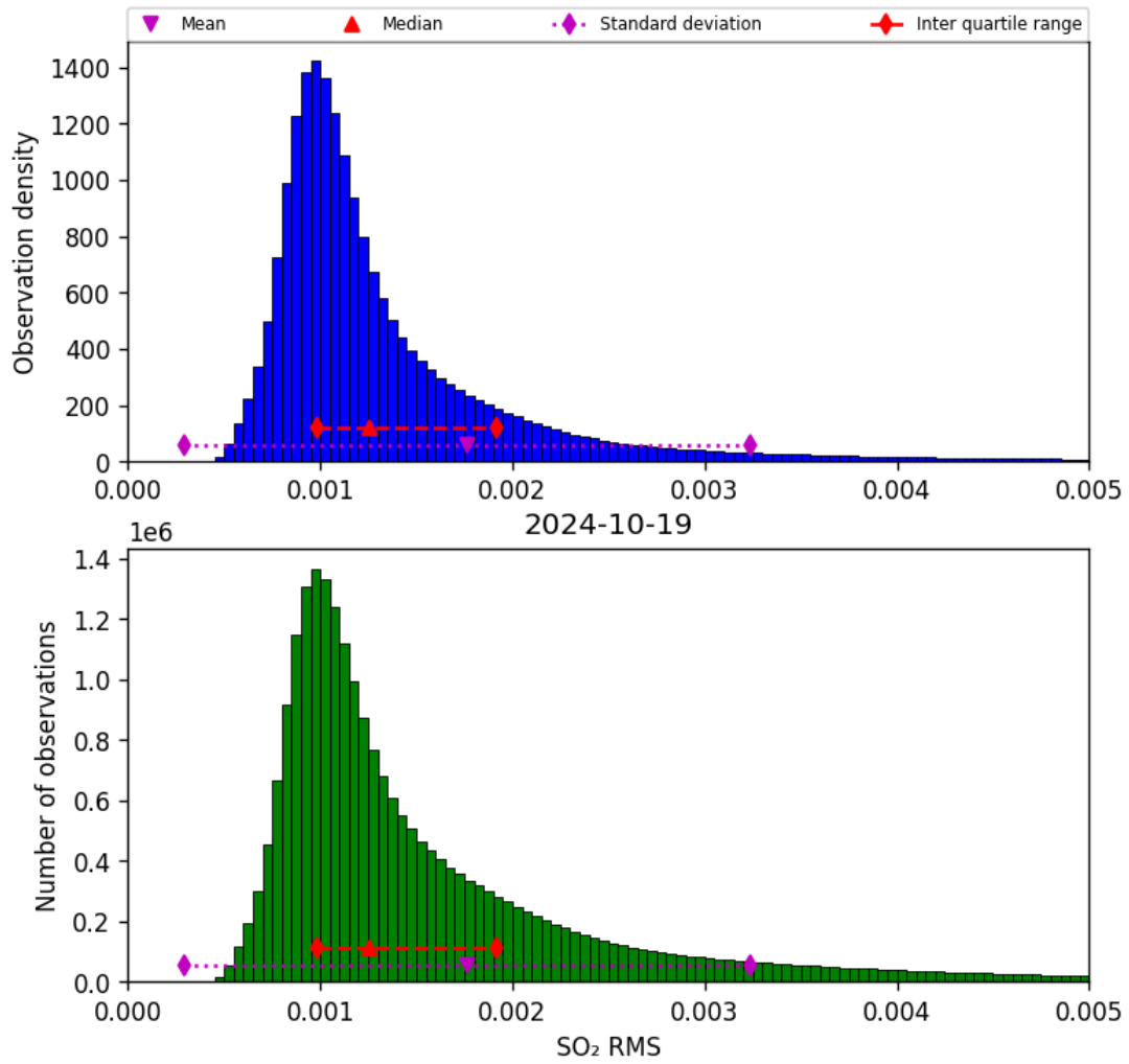
Figure 70: Histogram of “SO 2 RMS” for 2024-10-19 to 2024-10-20
