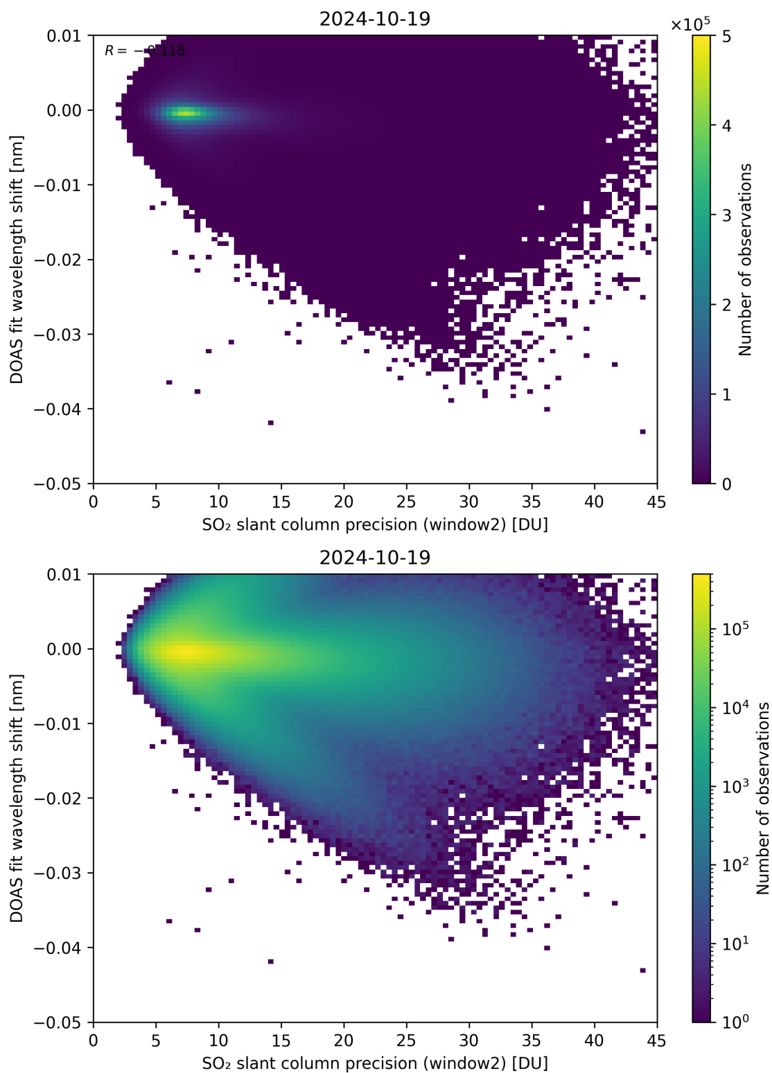
Figure 243: Scatter density plot of “SO 2 slant column precision (window2)” against “DOAS fit wavelength shift” for 2024-10-19 to 2024-10-20.
