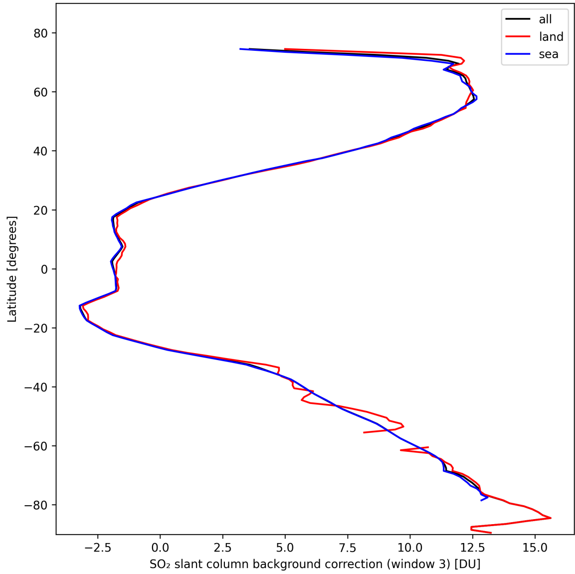
Figure 44: Zonal average of “SO 2 slant column background correction (window 3)” for 2024-10-19 to 2024-10-20.
