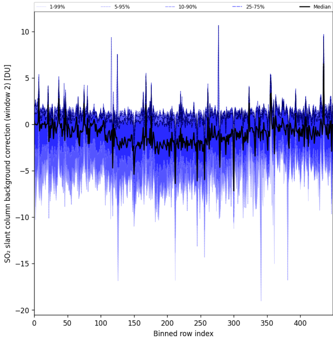
Figure 86: Along track statistics of “SO 2 slant column background correction (window 2)” for 2024-10-19 to 2024-10-20
