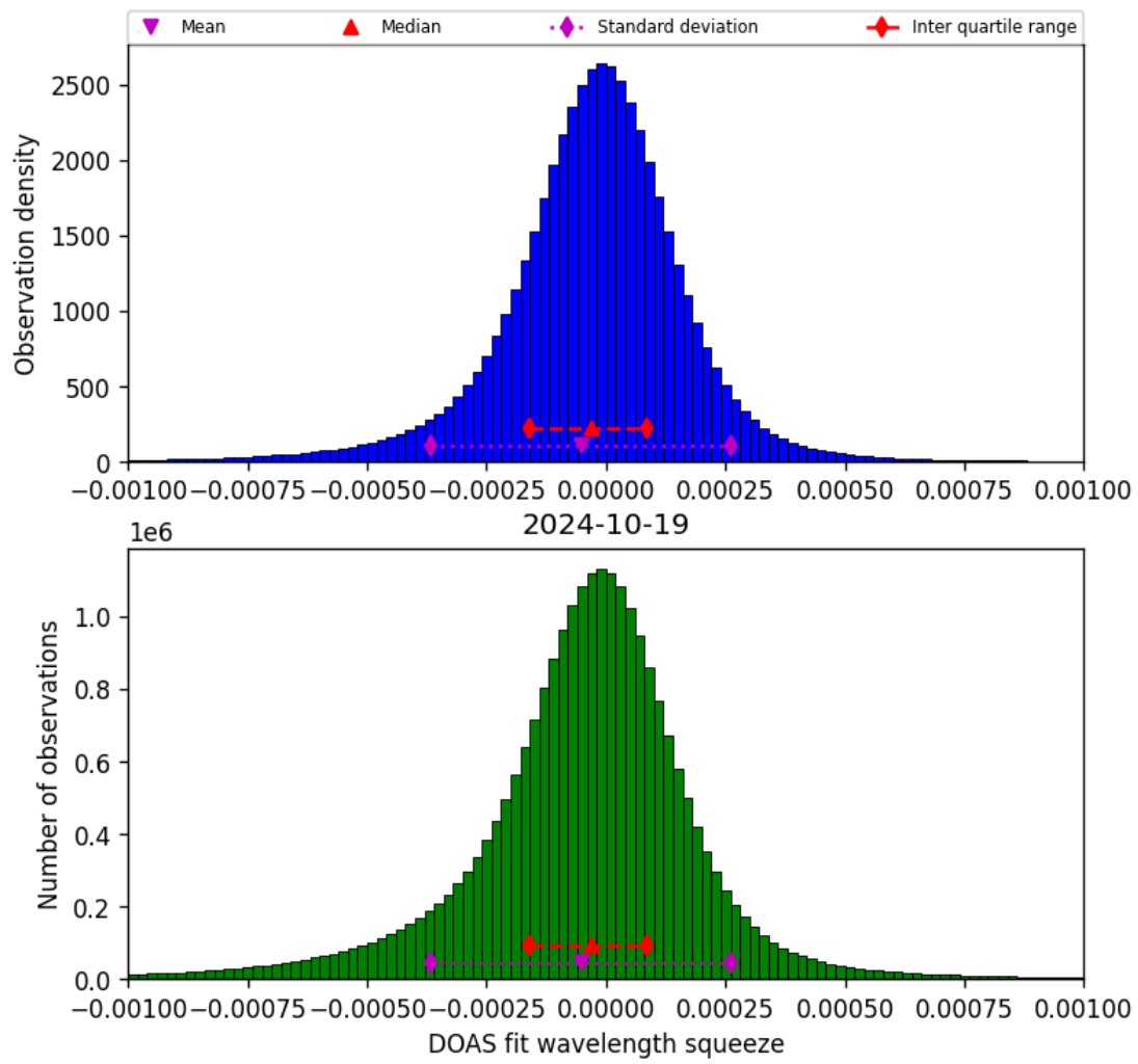
Figure 69: Histogram of “DOAS fit wavelength squeeze” for 2024-10-19 to 2024-10-20
