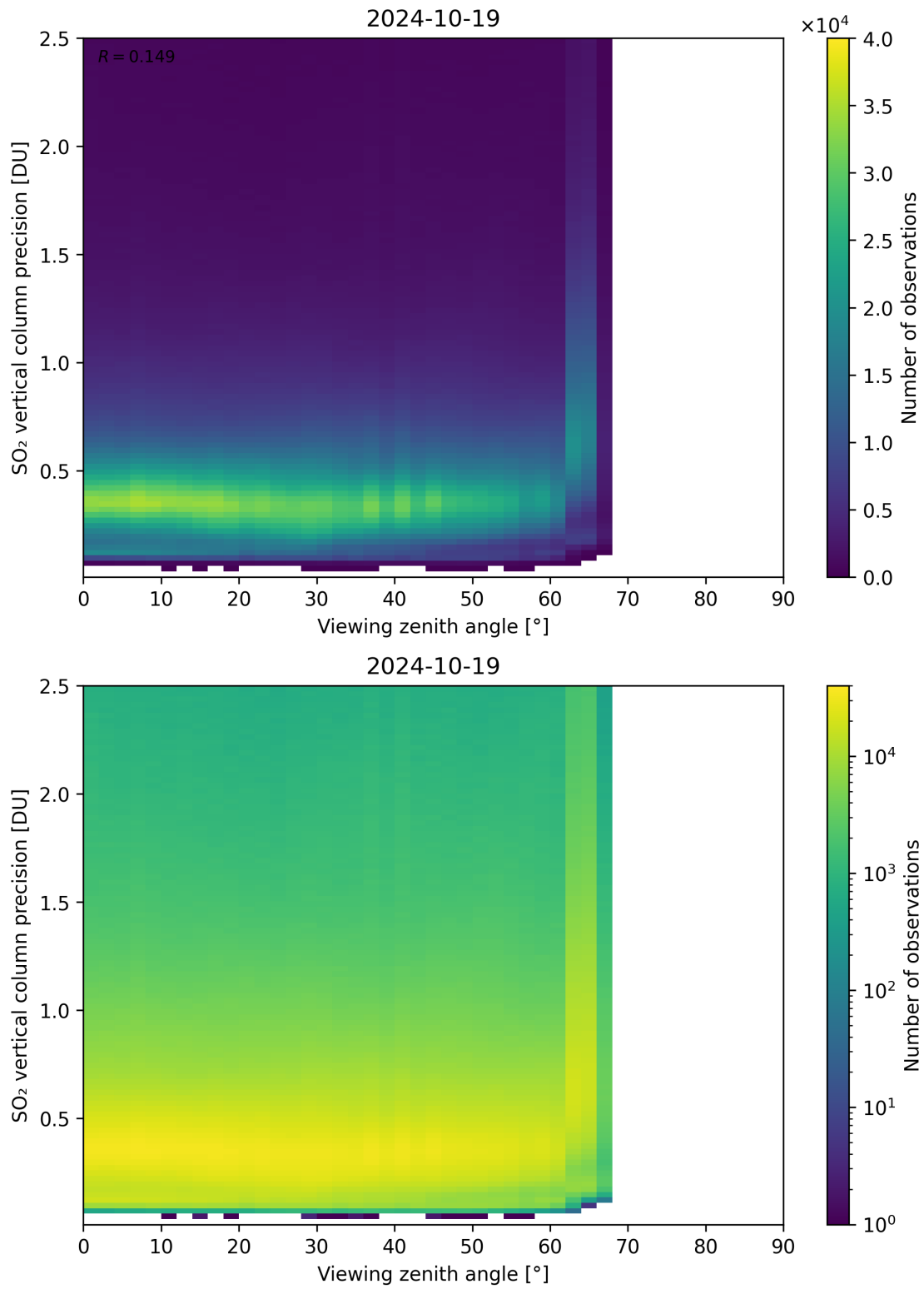
Figure 328: Scatter density plot of “Viewing zenith angle” against “SO 2 vertical column precision” for 2024-10-19 to 2024-10-20.
