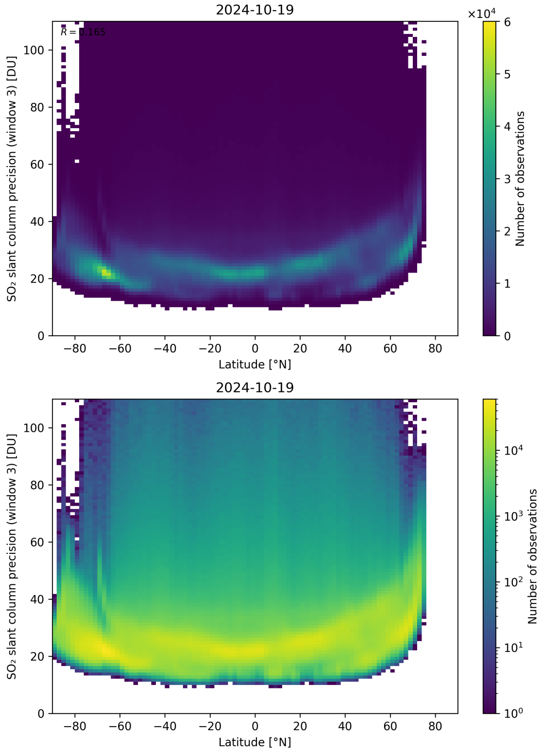
Figure 153: Scatter density plot of “Latitude” against “SO 2 slant column precision (window 3)” for 2024-10-19 to 2024-10-20.
