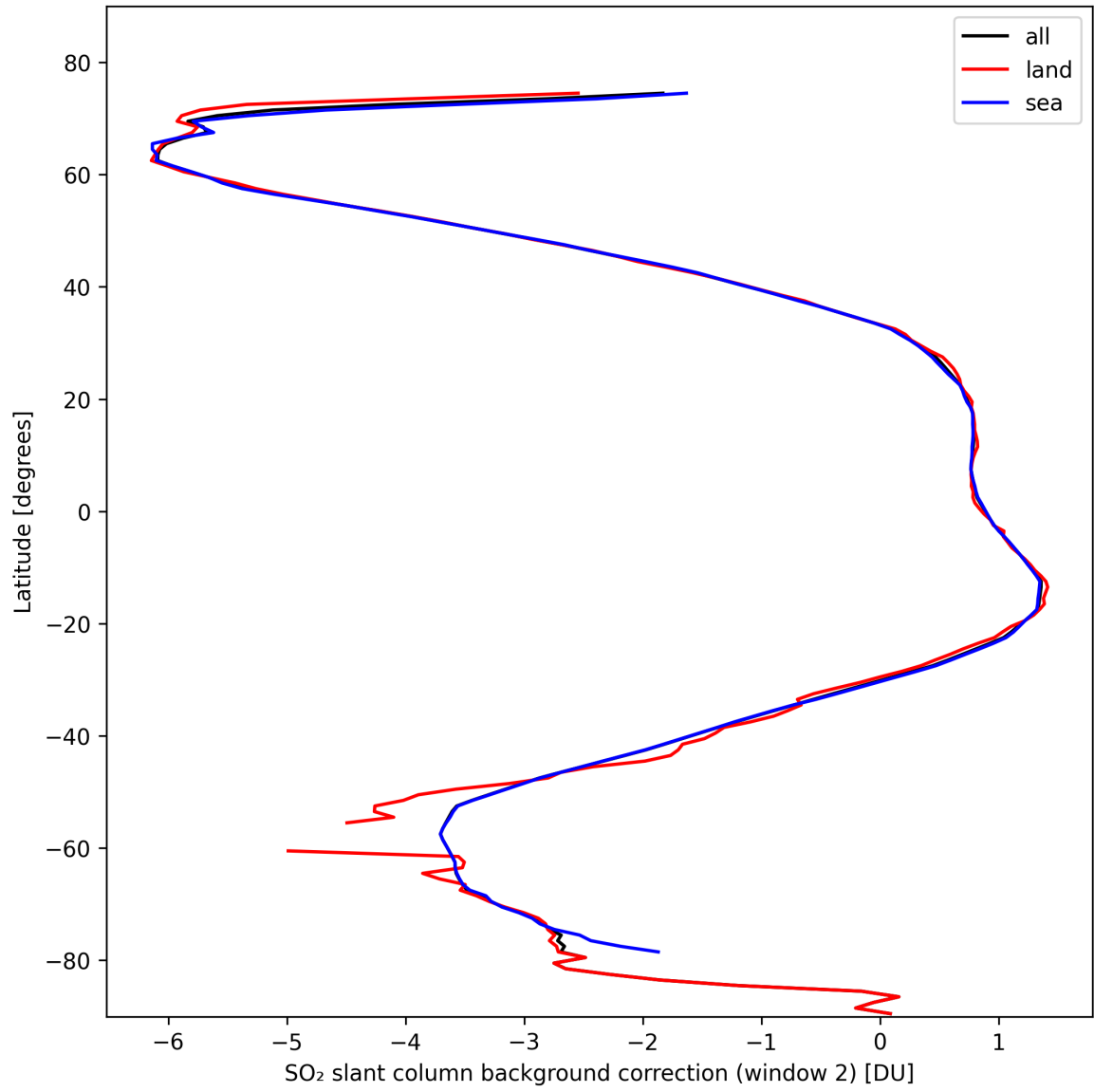
Figure 40: Zonal average of “SO 2 slant column background correction (window 2)” for 2024-10-19 to 2024-10-20.
