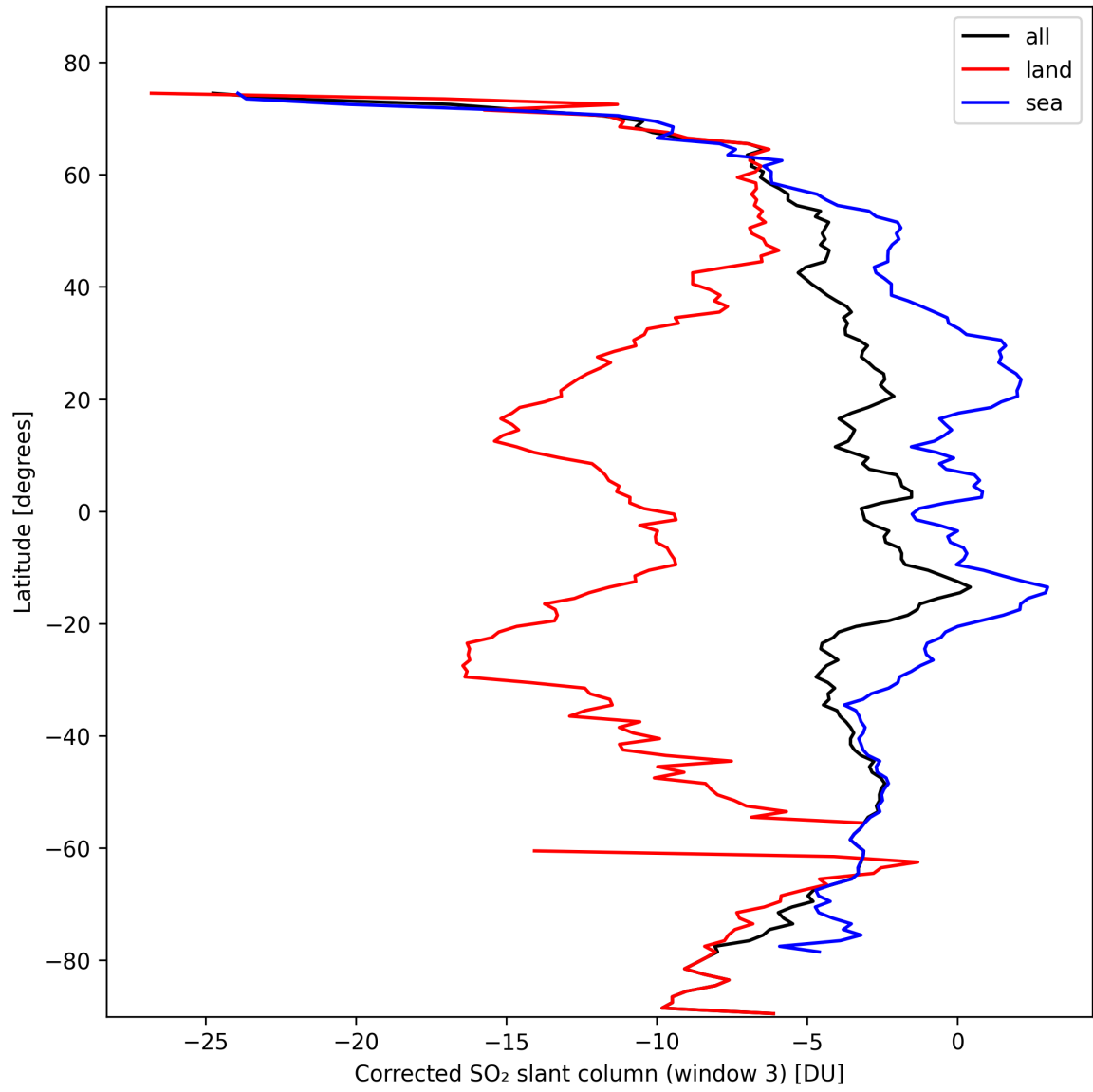
Figure 43: Zonal average of “Corrected SO 2 slant column (window 3)” for 2024-10-19 to 2024-10-20.
