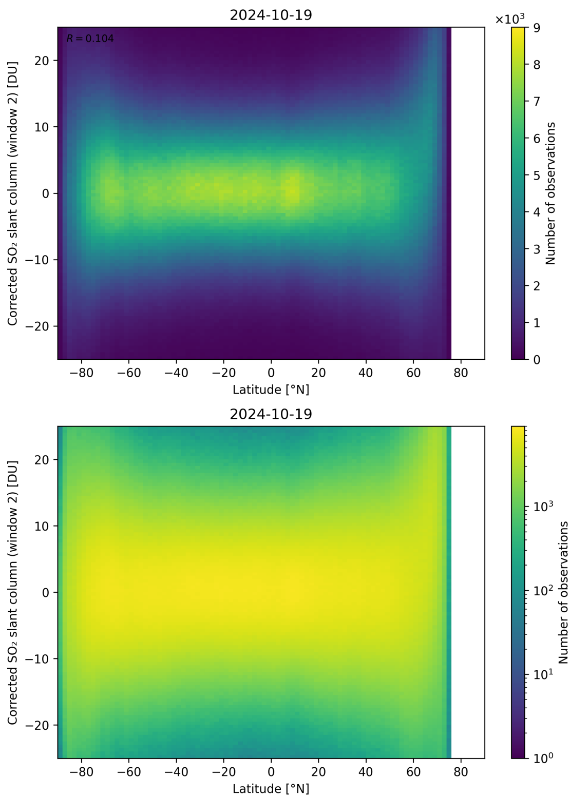
Figure 147: Scatter density plot of “Latitude” against “Corrected SO 2 slant column (window 2)” for 2024-10-19 to 2024-10-20.
