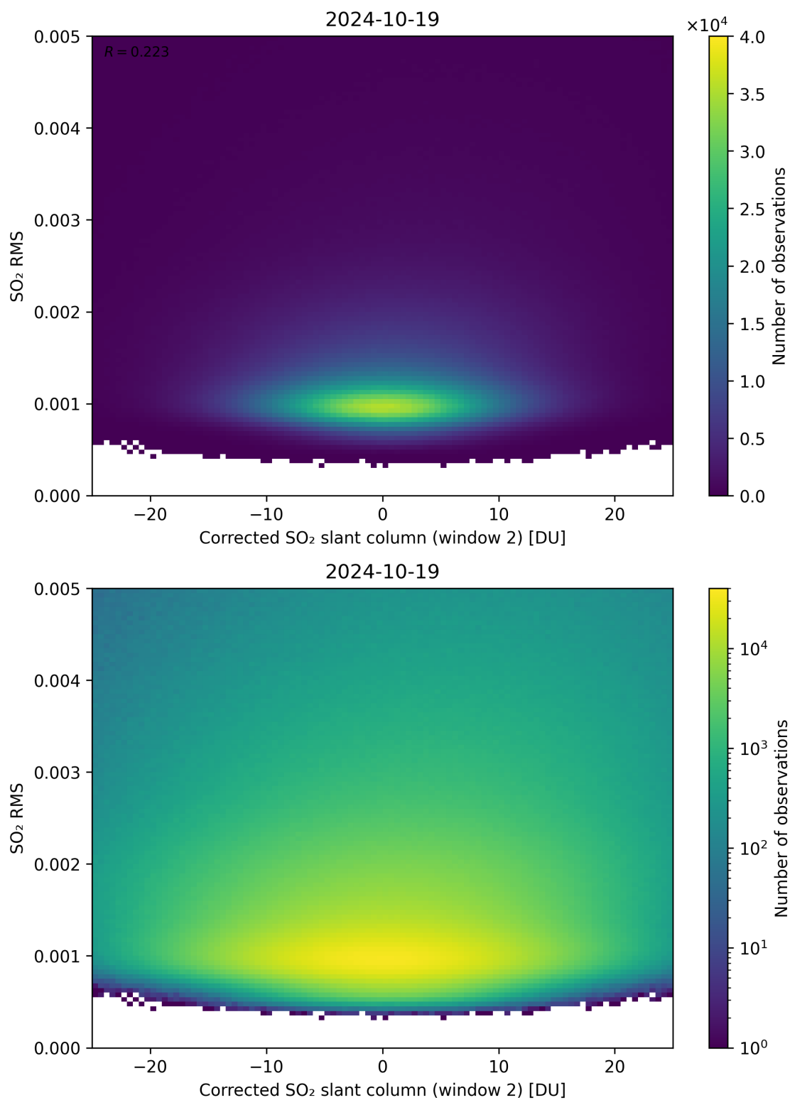
Figure 198: Scatter density plot of “Corrected SO 2 slant column (window 2)” against “SO 2 RMS” for 2024-10-19 to 2024-10-20.
