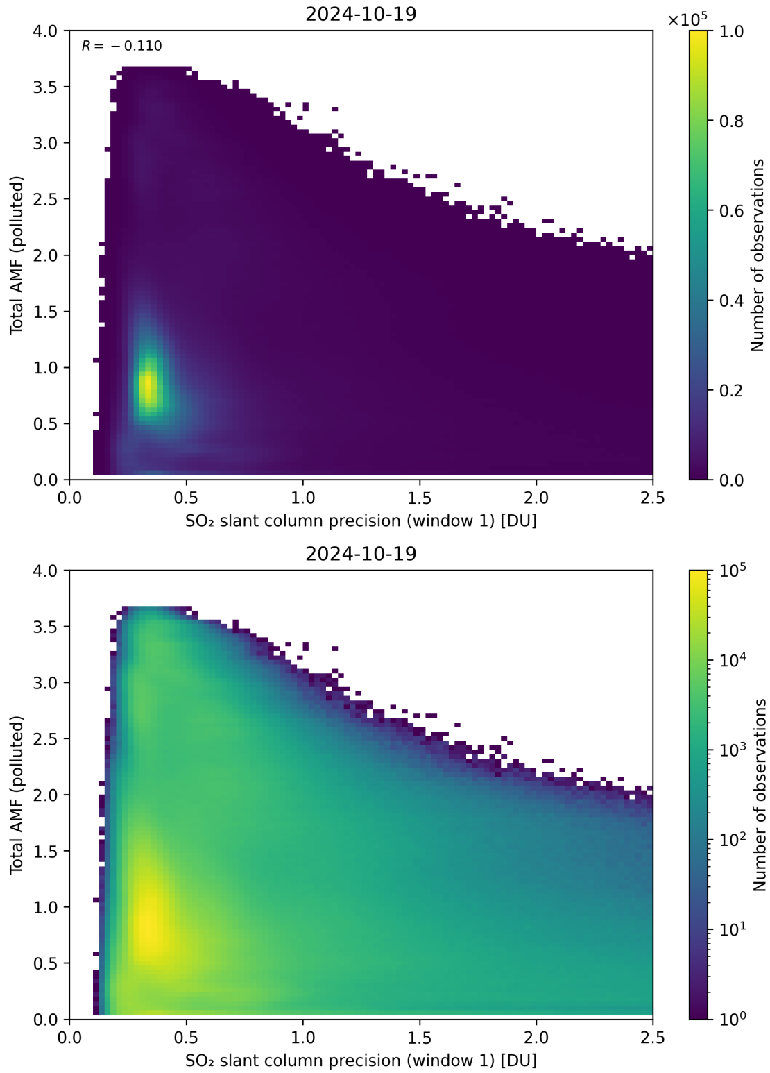
Figure 230: Scatter density plot of “SO 2 slant column precision (window 1)” against “Total AMF (polluted)” for 2024-10-19 to 2024-10-20.
