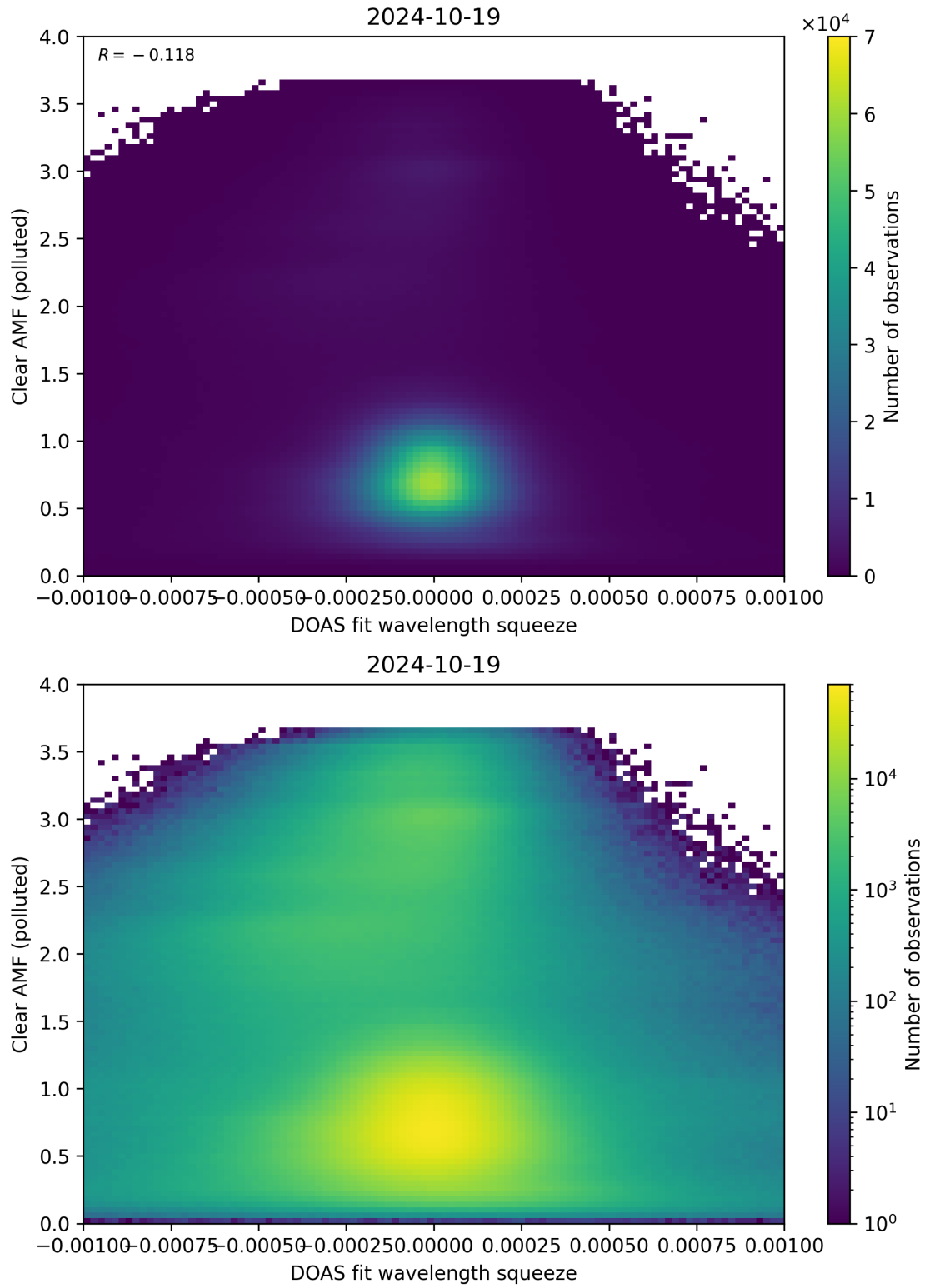
Figure 133: Scatter density plot of “DOAS fit wavelength squeeze” against “Clear AMF (polluted)” for 2024-10-19 to 2024-10-20.
