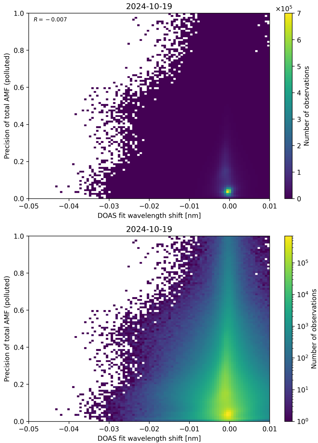
Figure 131: Scatter density plot of “DOAS fit wavelength shift” against “Precision of total AMF (polluted)” for 2024-10-19 to 2024-10-20.
