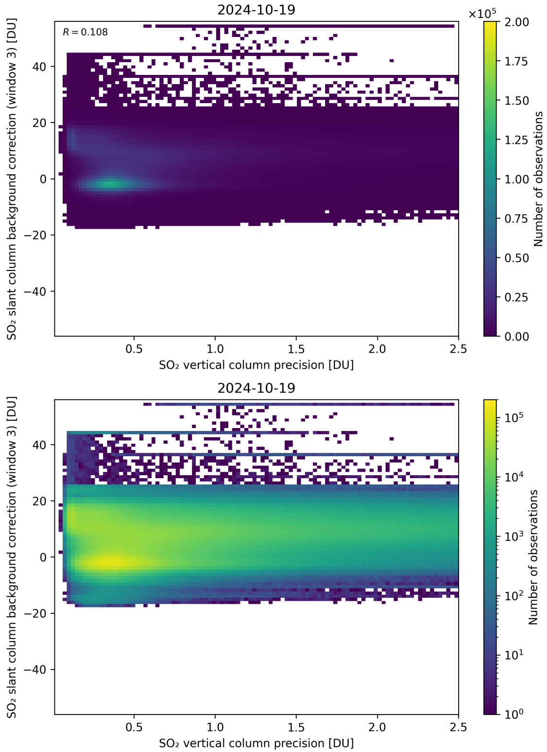
Figure 281: Scatter density plot of “SO 2 vertical column precision” against “SO 2 slant column background correction (window 3)” for 2024-10-19 to 2024-10-20.
