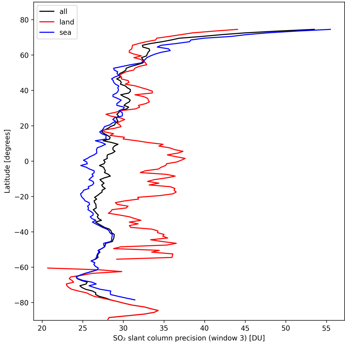
Figure 42: Zonal average of “SO 2 slant column precision (window 3)” for 2024-10-19 to 2024-10-20.
