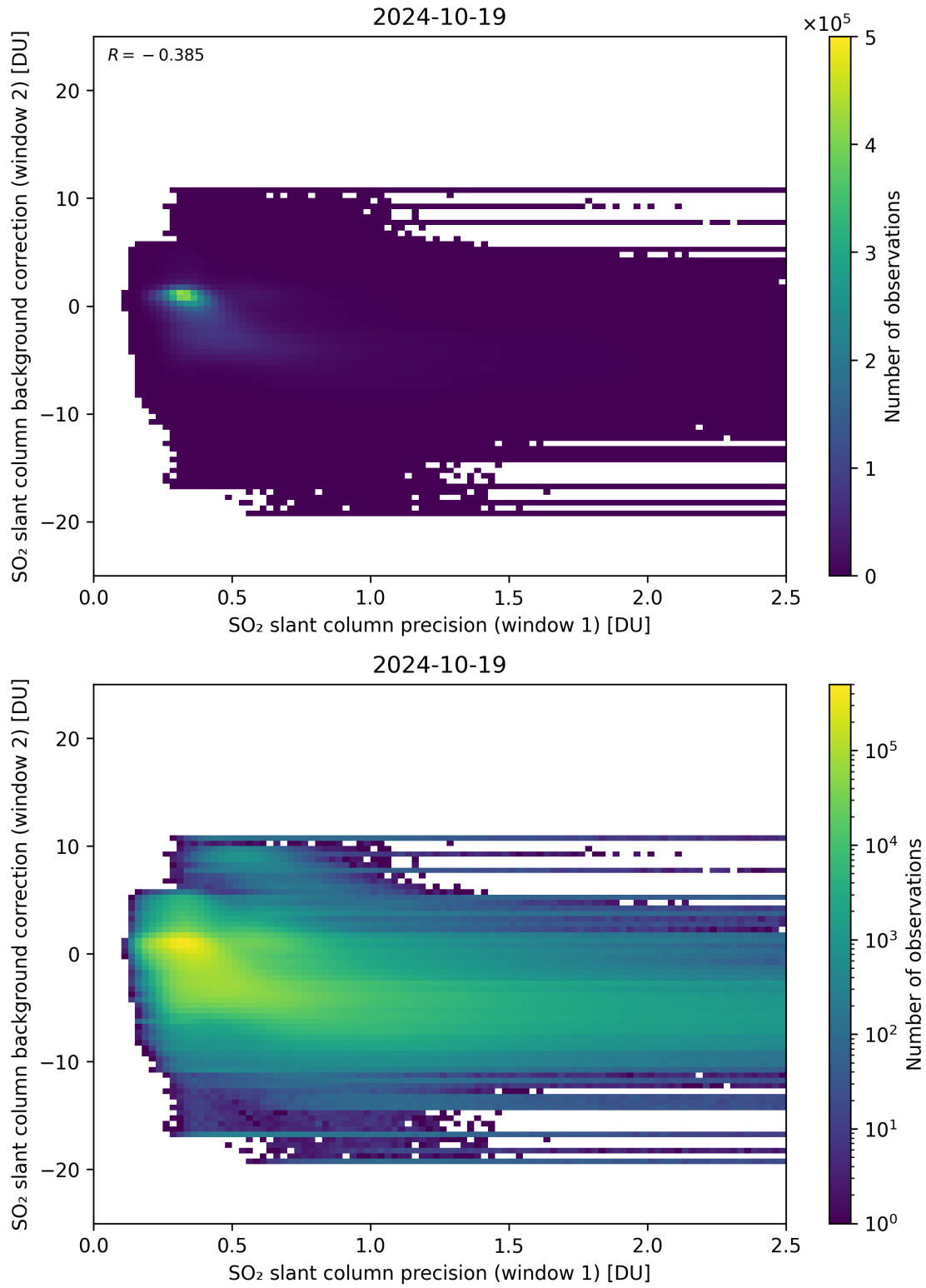
Figure 219: Scatter density plot of “SO 2 slant column precision (window 1)” against “SO 2 slant column background correction (window 2)” for 2024-10-19 to 2024-10-20.
