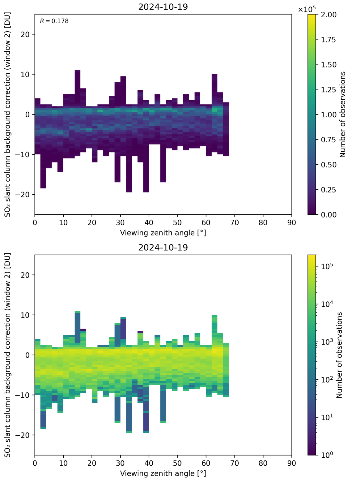
Figure 309: Scatter density plot of “Viewing zenith angle” against “SO 2 slant column background correction (window 2)” for 2024-10-19 to 2024-10-20.
