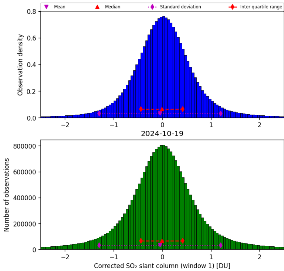
Figure 58: Histogram of “Corrected SO 2 slant column (window 1)” for 2024-10-19 to 2024-10-20
