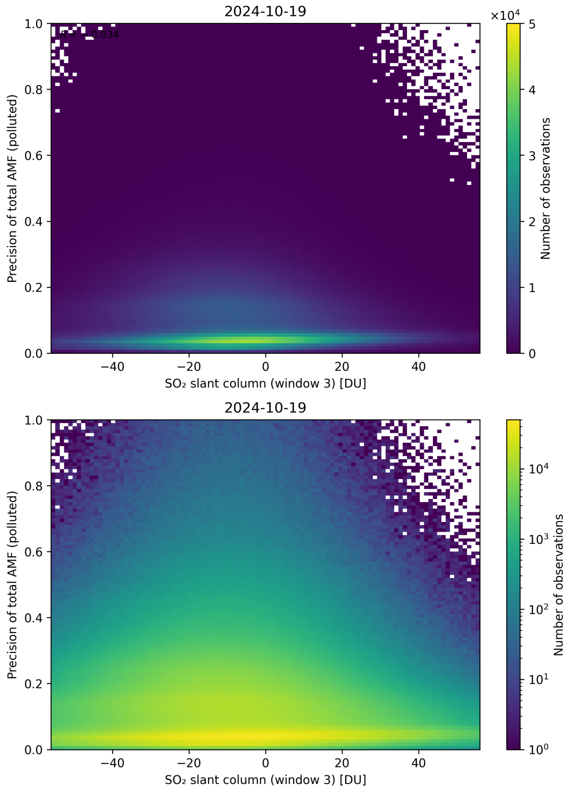
Figure 269: Scatter density plot of “SO 2 slant column (window 3)” against “Precision of total AMF (polluted)” for 2024-10-19 to 2024-10-20.
