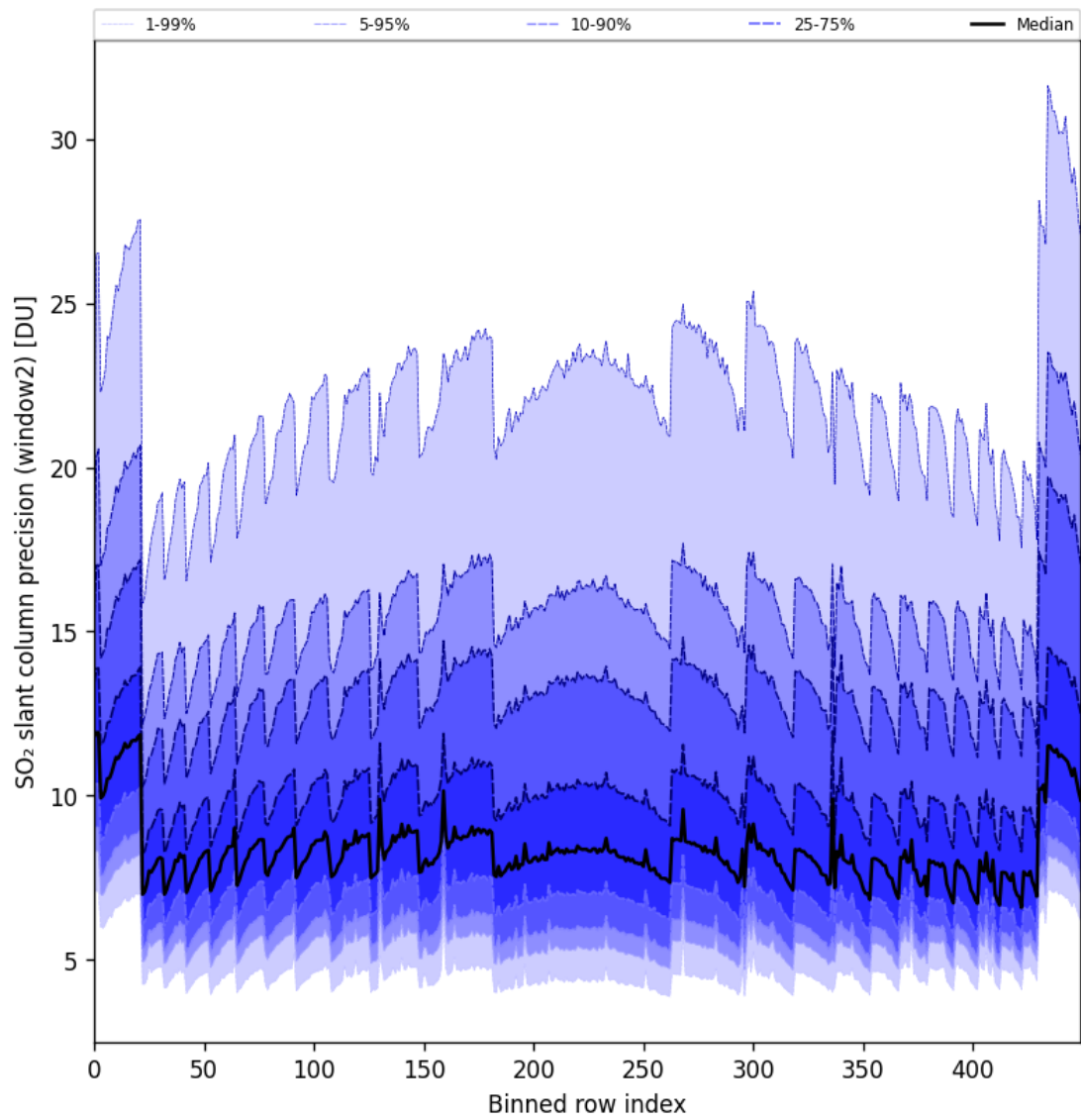
Figure 84: Along track statistics of “SO 2 slant column precision (window2)” for 2024-10-19 to 2024-10-20
