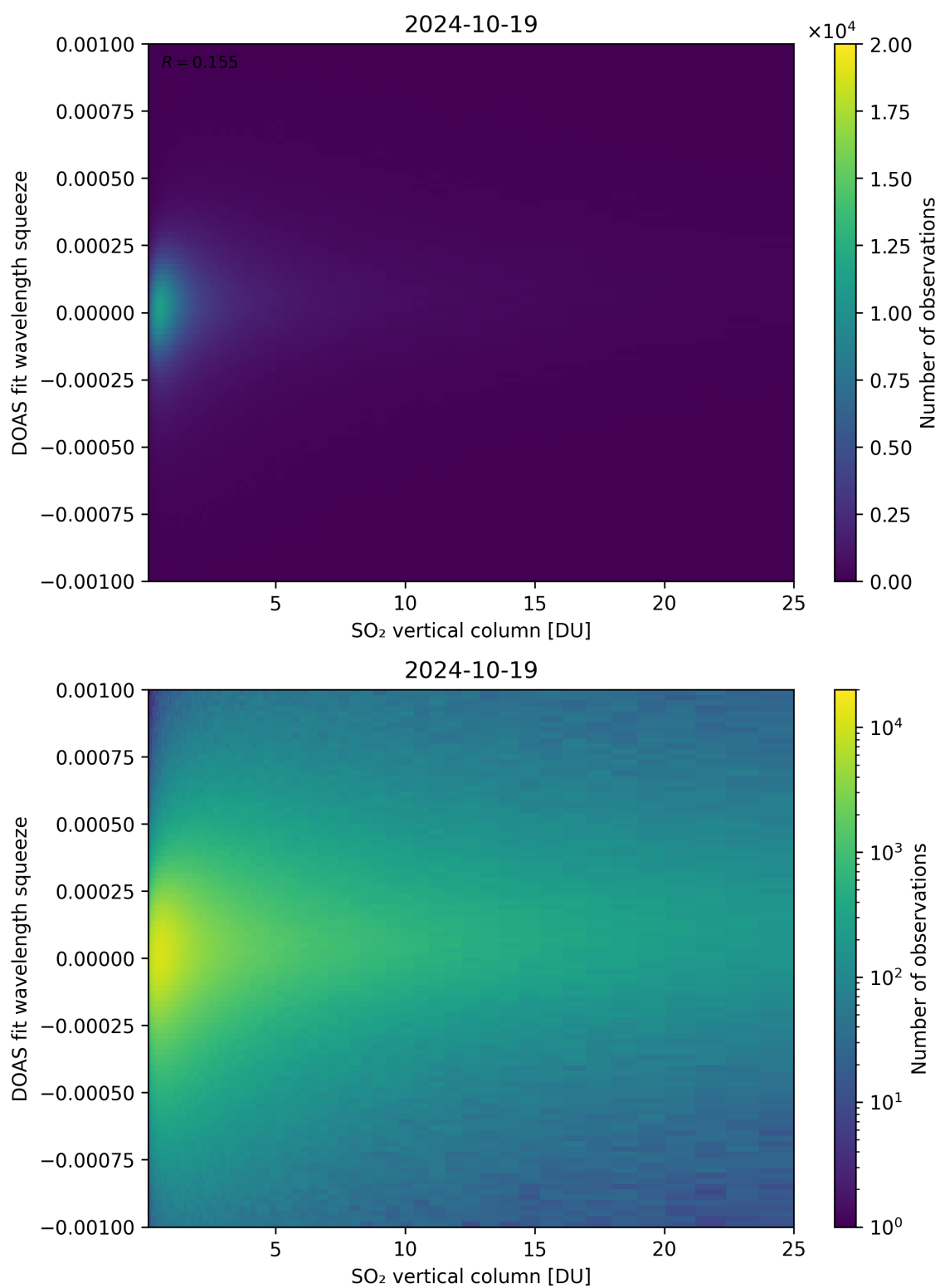
Figure 277: Scatter density plot of “SO 2 vertical column” against “DOAS fit wavelength squeeze” for 2024-10-19 to 2024-10-20.
