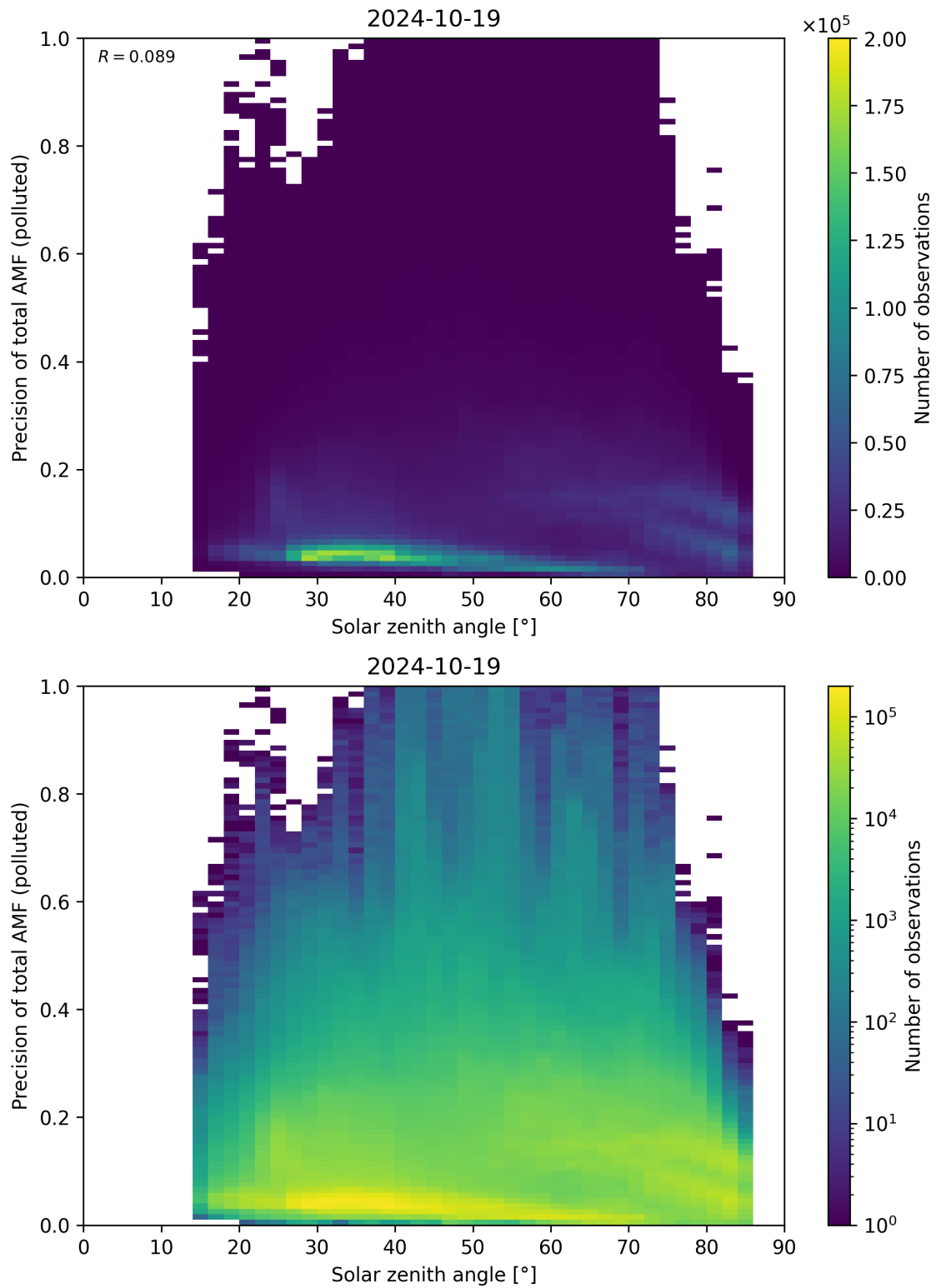
Figure 175: Scatter density plot of “Solar zenith angle” against “Precision of total AMF (polluted)” for 2024-10-19 to 2024-10-20.
