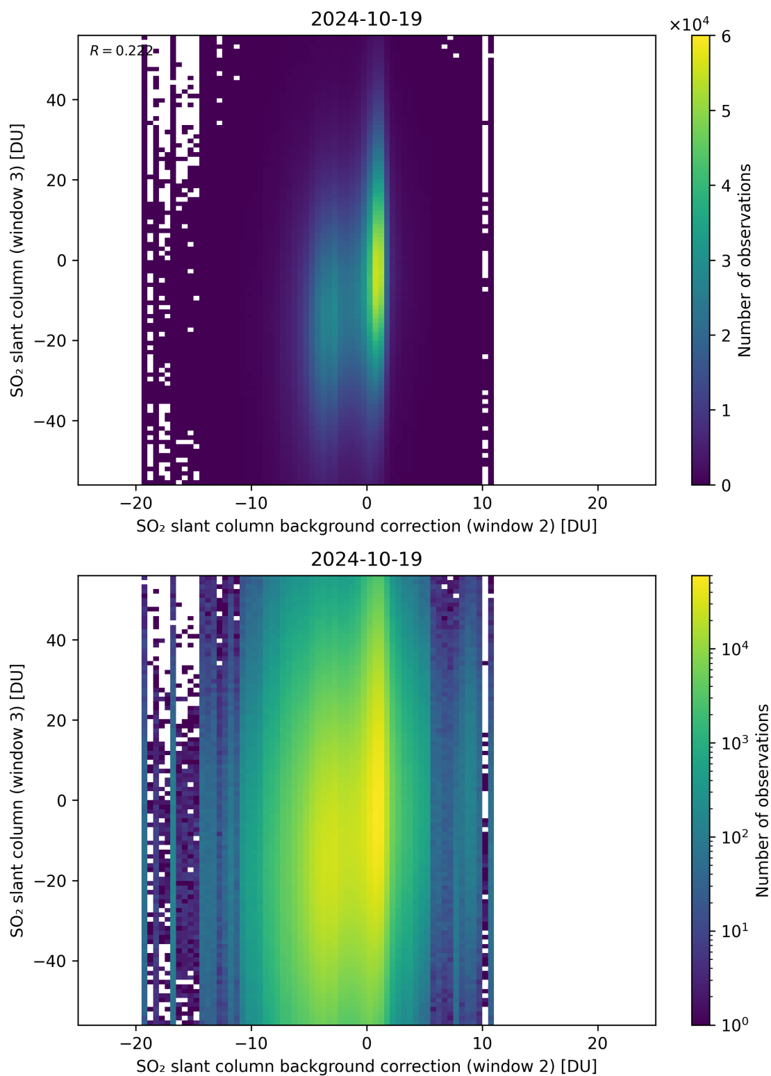
Figure 117: Scatter density plot of “SO 2 slant column background correction (window 2)” against “SO 2 slant column (window 3)” for 2024-10-19 to 2024-10-20.
