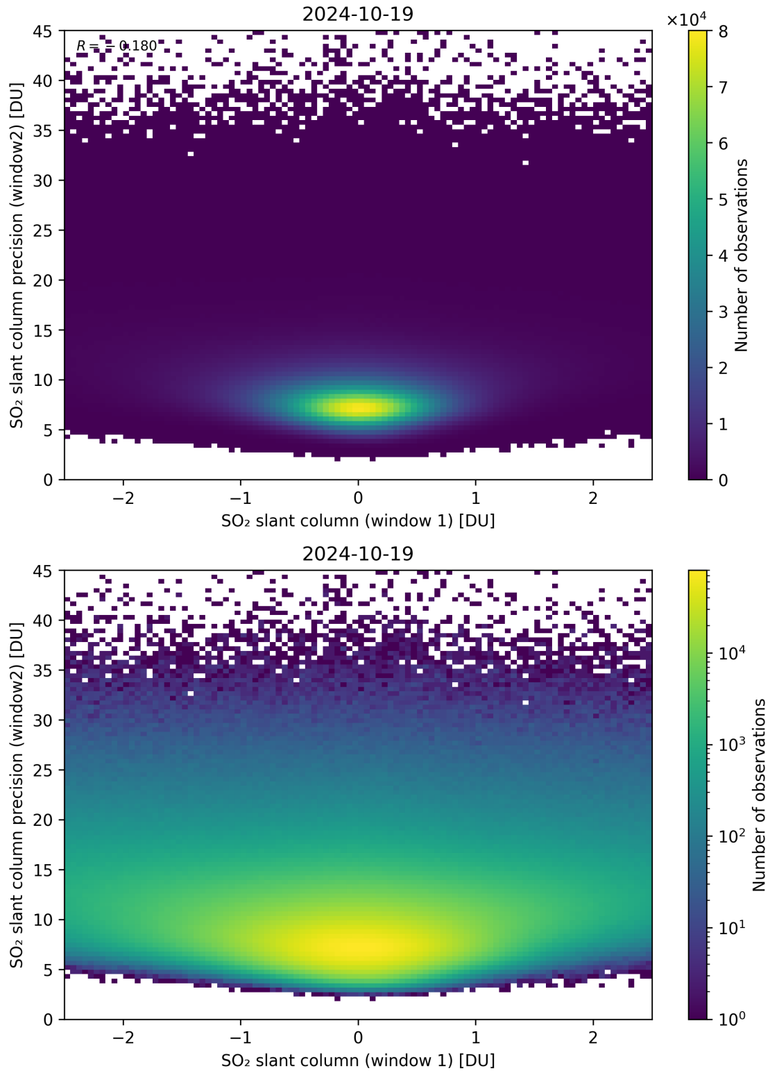
Figure 236: Scatter density plot of “SO 2 slant column (window 1)” against “SO 2 slant column precision (window2)” for 2024-10-19 to 2024-10-20.
