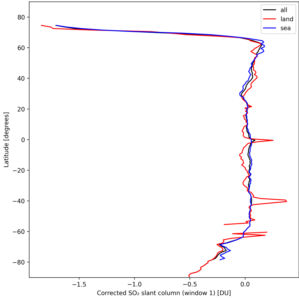
Figure 35: Zonal average of “Corrected SO 2 slant column (window 1)” for 2024-10-19 to 2024-10-20.
