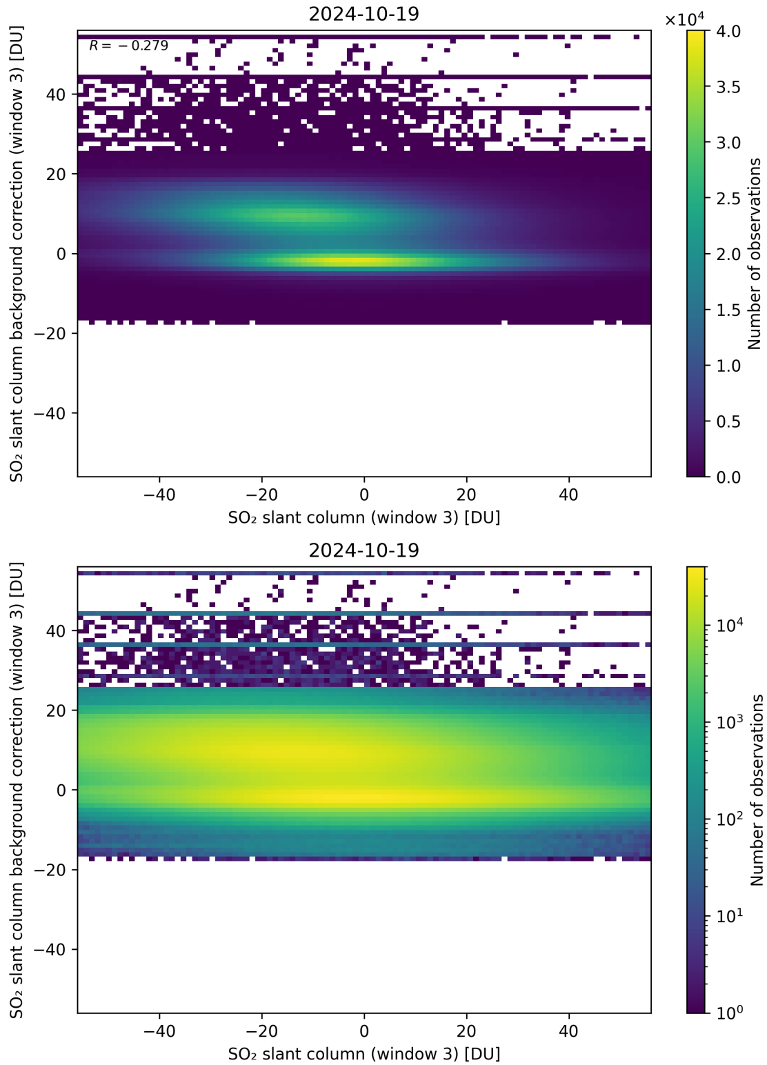
Figure 253: Scatter density plot of “SO 2 slant column (window 3)” against “SO 2 slant column background correction (window 3)” for 2024-10-19 to 2024-10-20.
