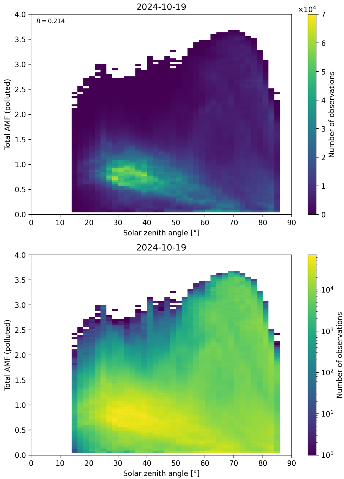
Figure 174: Scatter density plot of “Solar zenith angle” against “Total AMF (polluted)” for 2024-10-19 to 2024-10-20.
