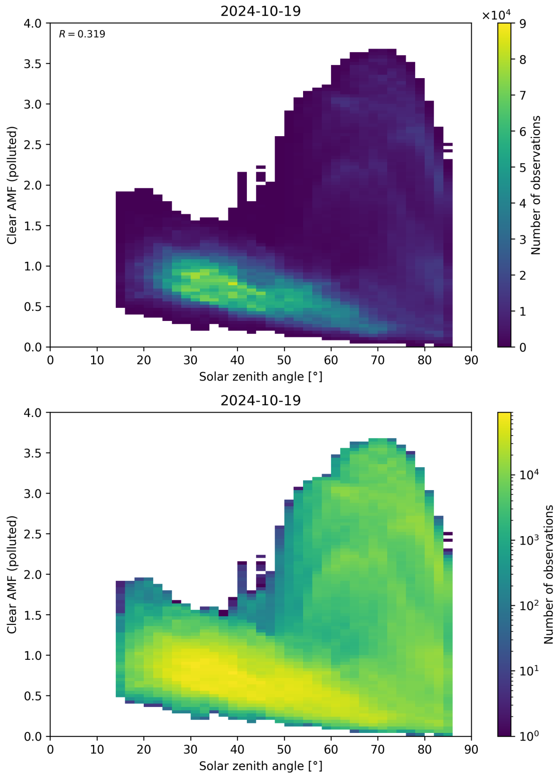
Figure 165: Scatter density plot of “Solar zenith angle” against “Clear AMF (polluted)” for 2024-10-19 to 2024-10-20.
