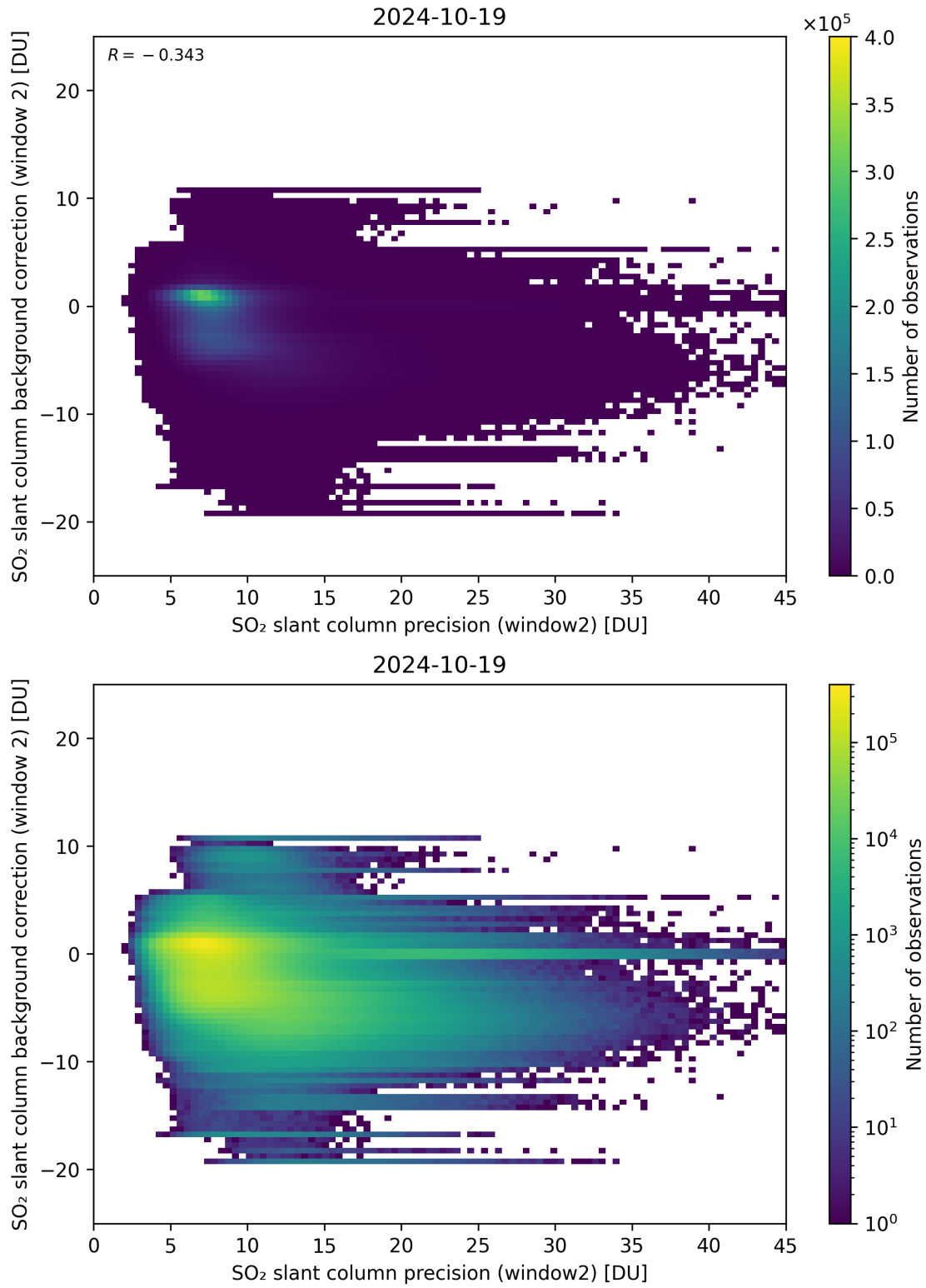
Figure 241: Scatter density plot of “SO 2 slant column precision (window2)” against “SO 2 slant column background correction (window 2)” for 2024-10-19 to 2024-10-20.
