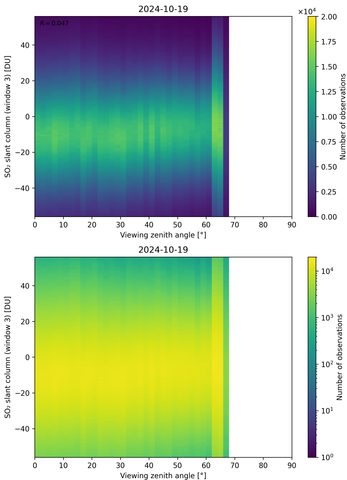
Figure 323: Scatter density plot of “Viewing zenith angle” against “SO 2 slant column (window 3)” for 2024-10-19 to 2024-10-20.
