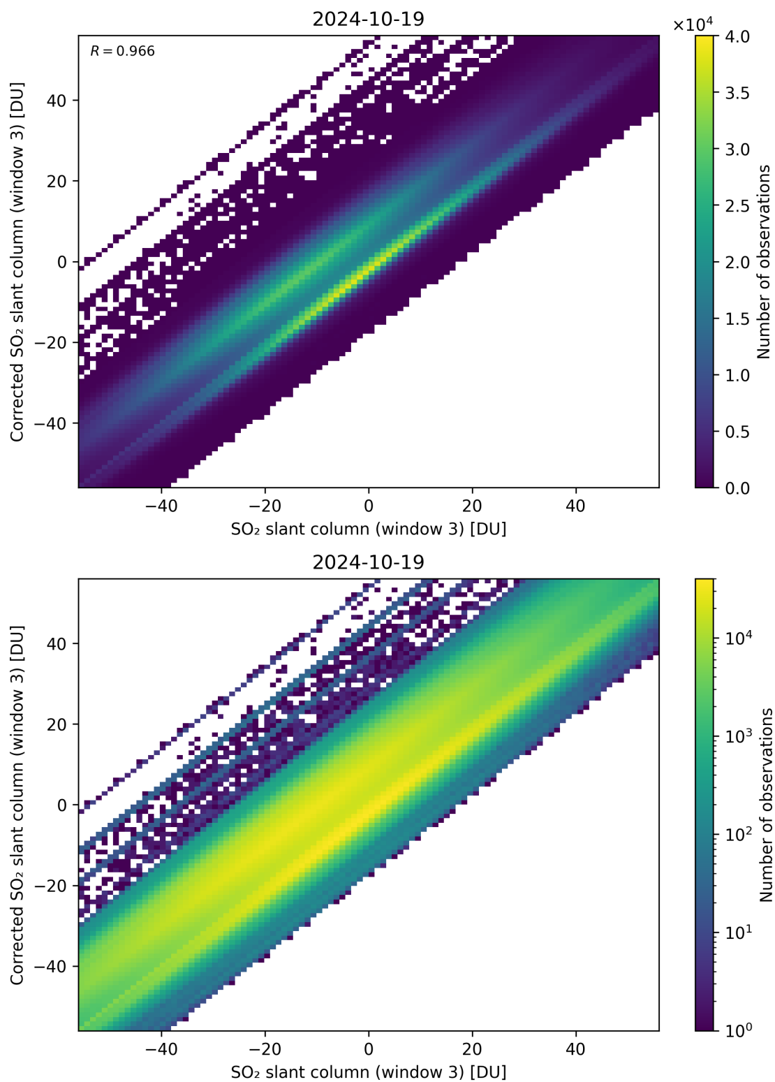
Figure 266: Scatter density plot of “SO 2 slant column (window 3)” against “Corrected SO 2 slant column (window 3)” for 2024-10-19 to 2024-10-20.
