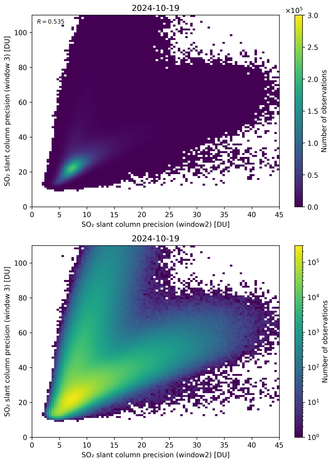
Figure 250: Scatter density plot of “SO 2 slant column precision (window2)” against “SO 2 slant column precision (window 3)” for 2024-10-19 to 2024-10-20.
