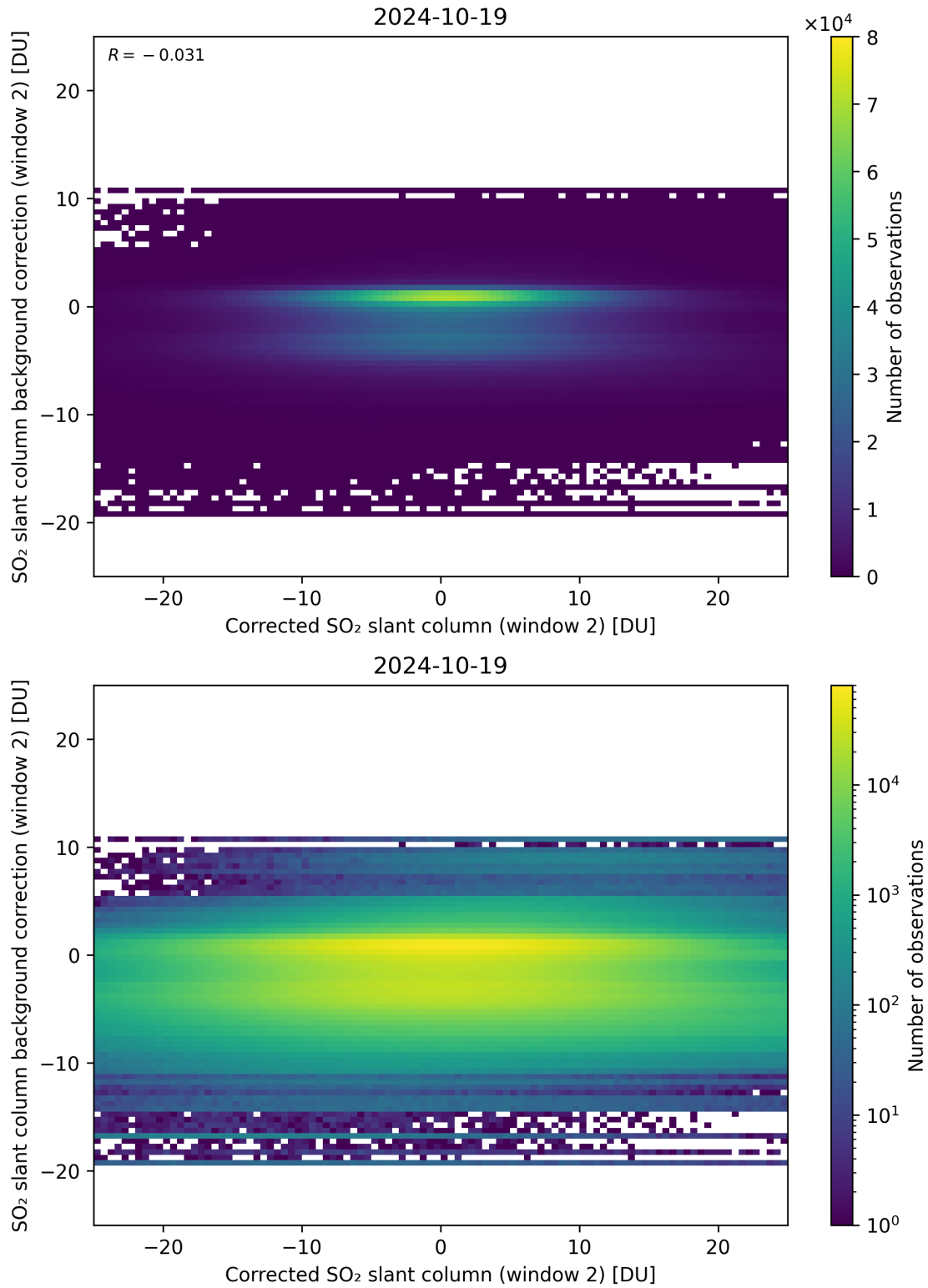
Figure 194: Scatter density plot of “Corrected SO 2 slant column (window 2)” against “SO 2 slant column background correction (window 2)” for 2024-10-19 to 2024-10-20.
