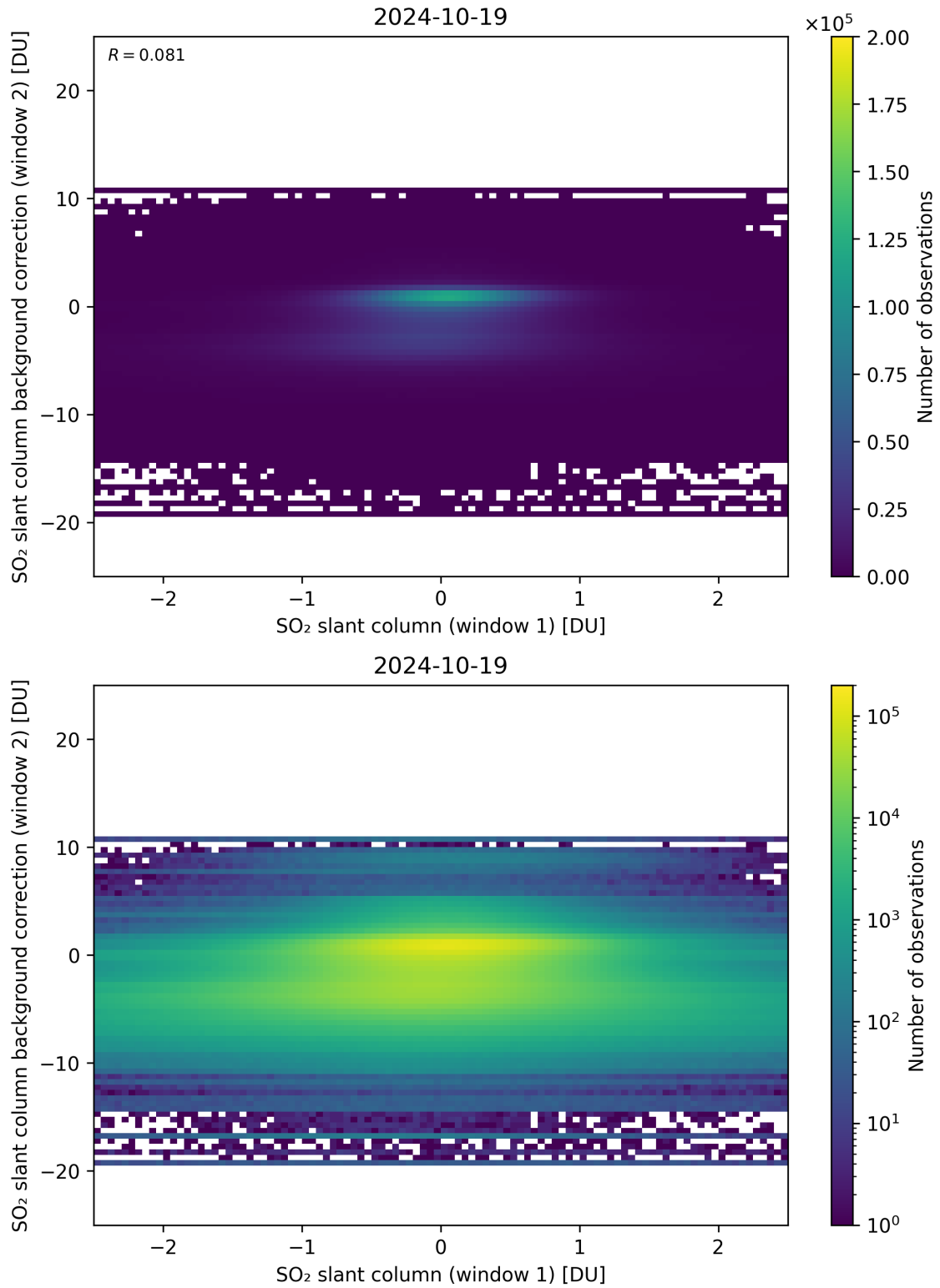
Figure 213: Scatter density plot of “SO 2 slant column (window 1)” against “SO 2 slant column background correction (window 2)” for 2024-10-19 to 2024-10-20.
