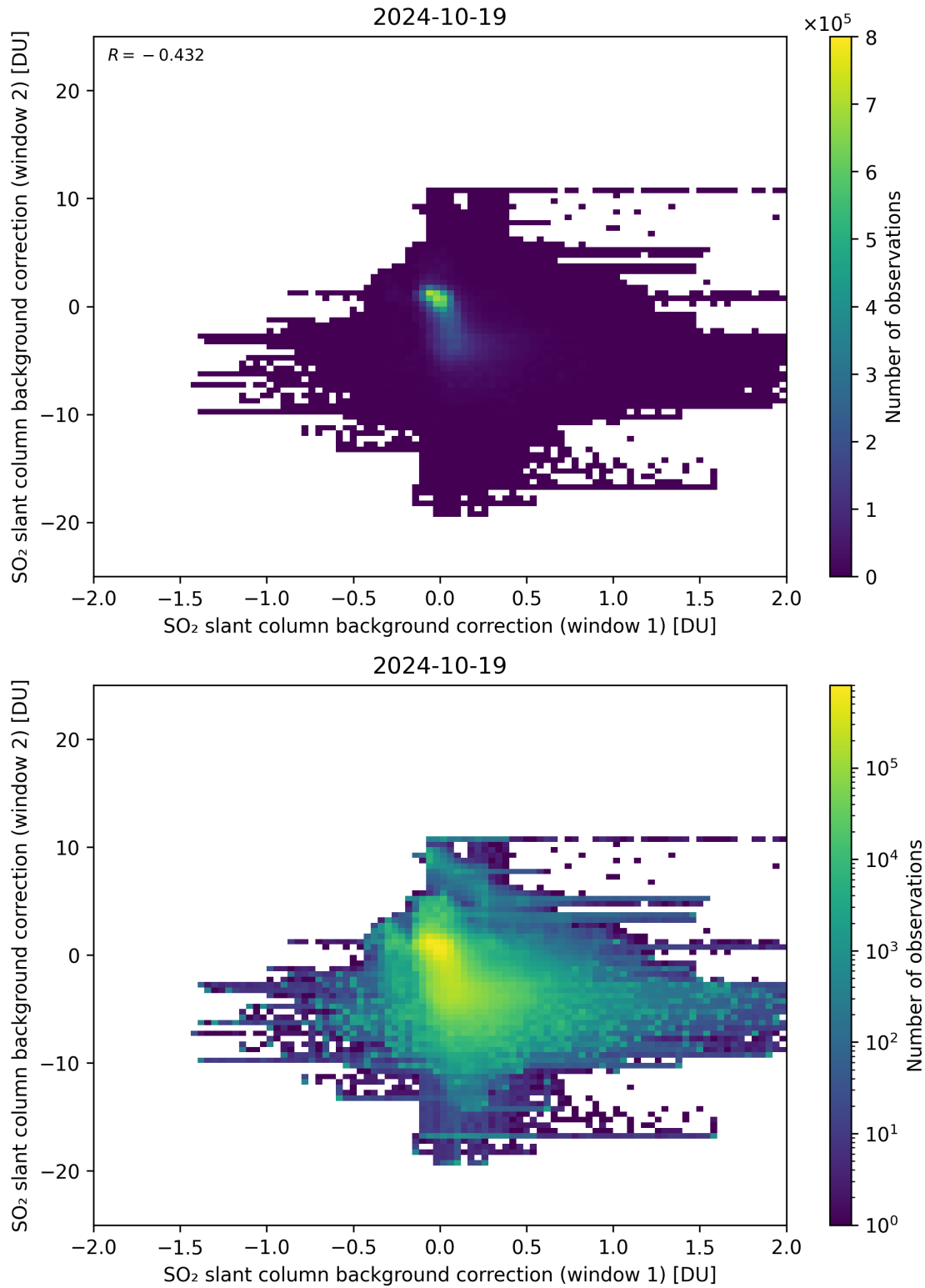
Figure 98: Scatter density plot of “SO 2 slant column background correction (window 1)” against “SO 2 slant column background correction (window 2)” for 2024-10-19 to 2024-10-20.
