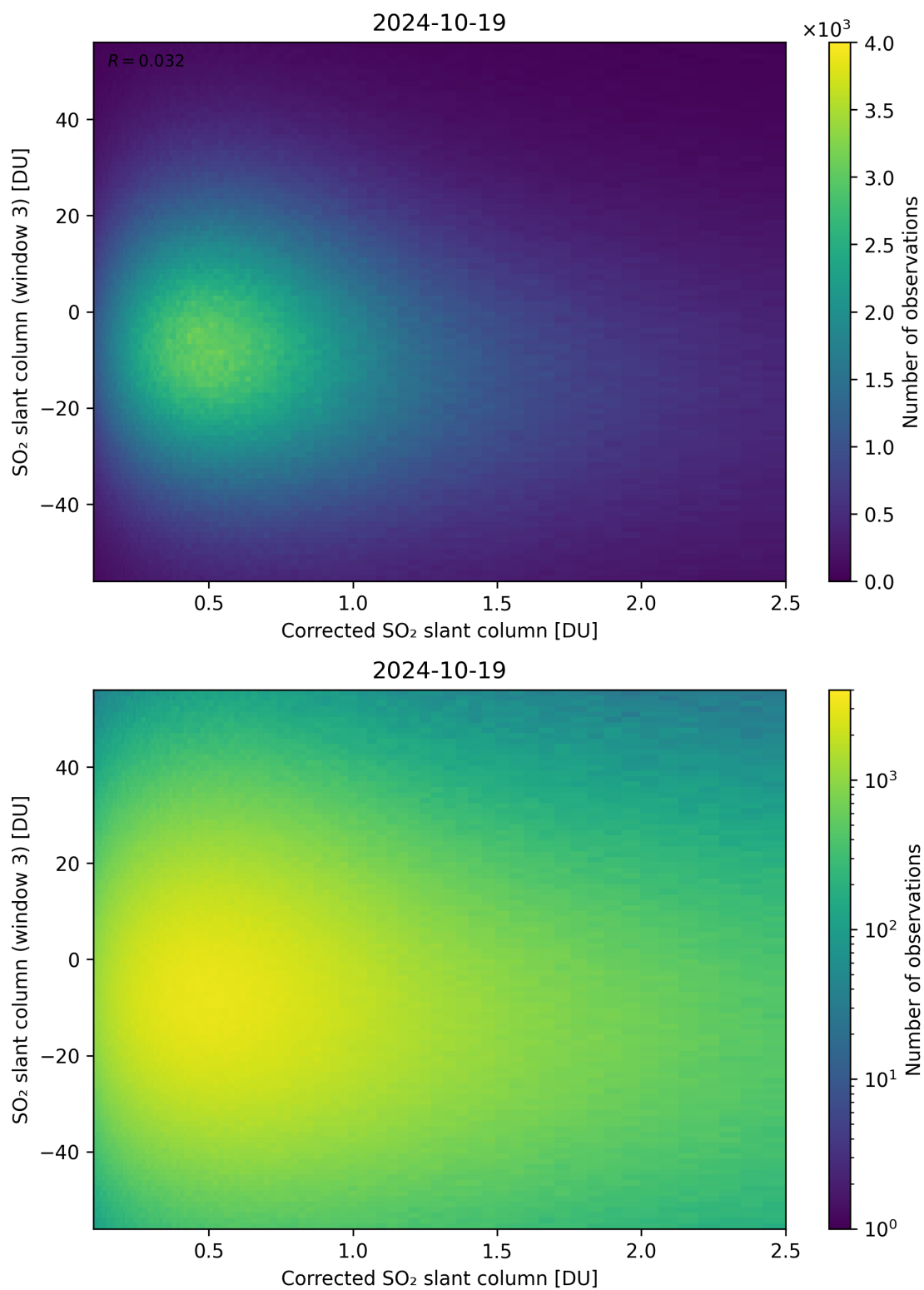
Figure 190: Scatter density plot of “Corrected SO 2 slant column” against “SO 2 slant column (window 3)” for 2024-10-19 to 2024-10-20.
