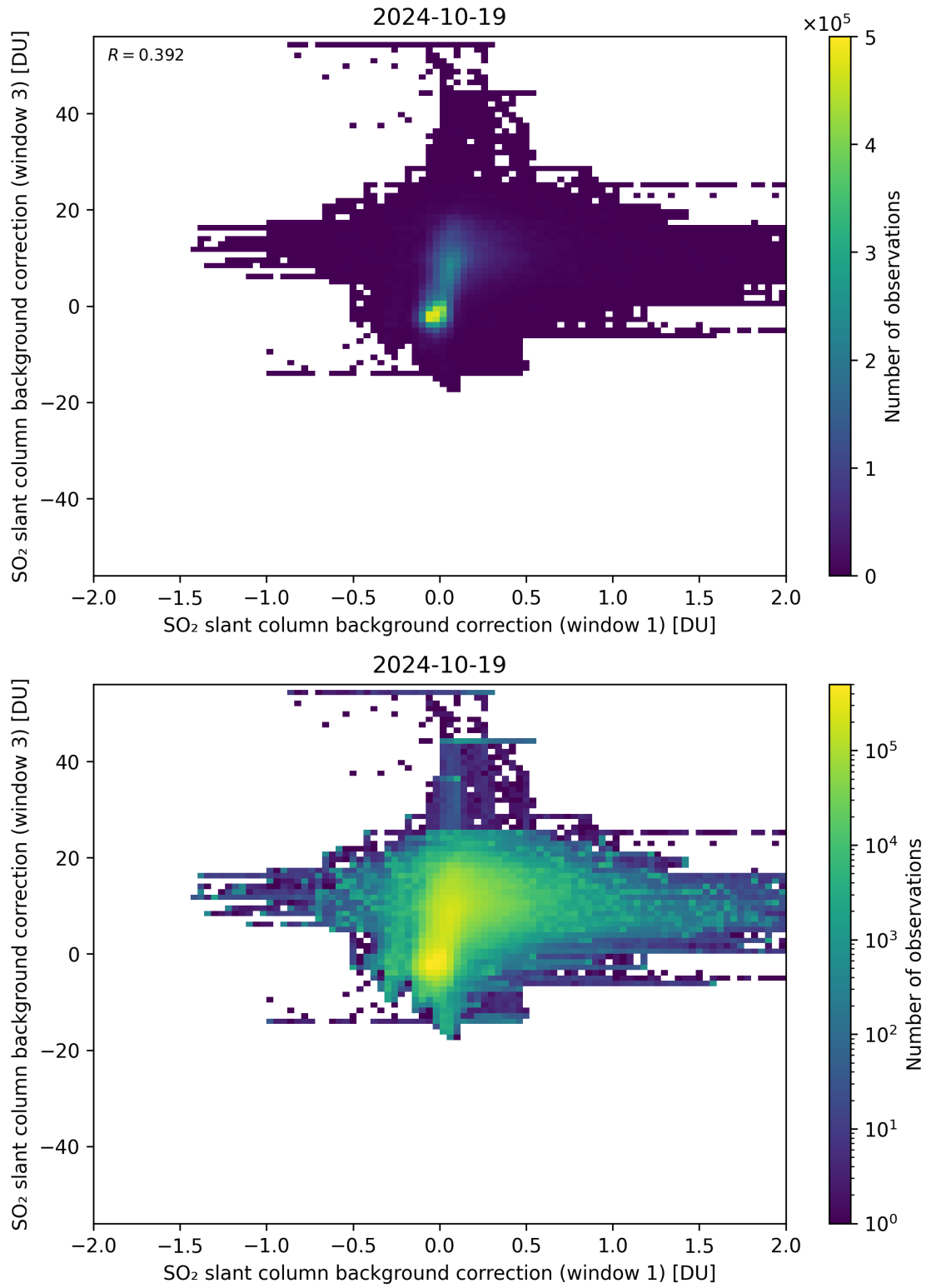
Figure 99: Scatter density plot of “SO 2 slant column background correction (window 1)” against “SO 2 slant column background correction (window 3)” for 2024-10-19 to 2024-10-20.
