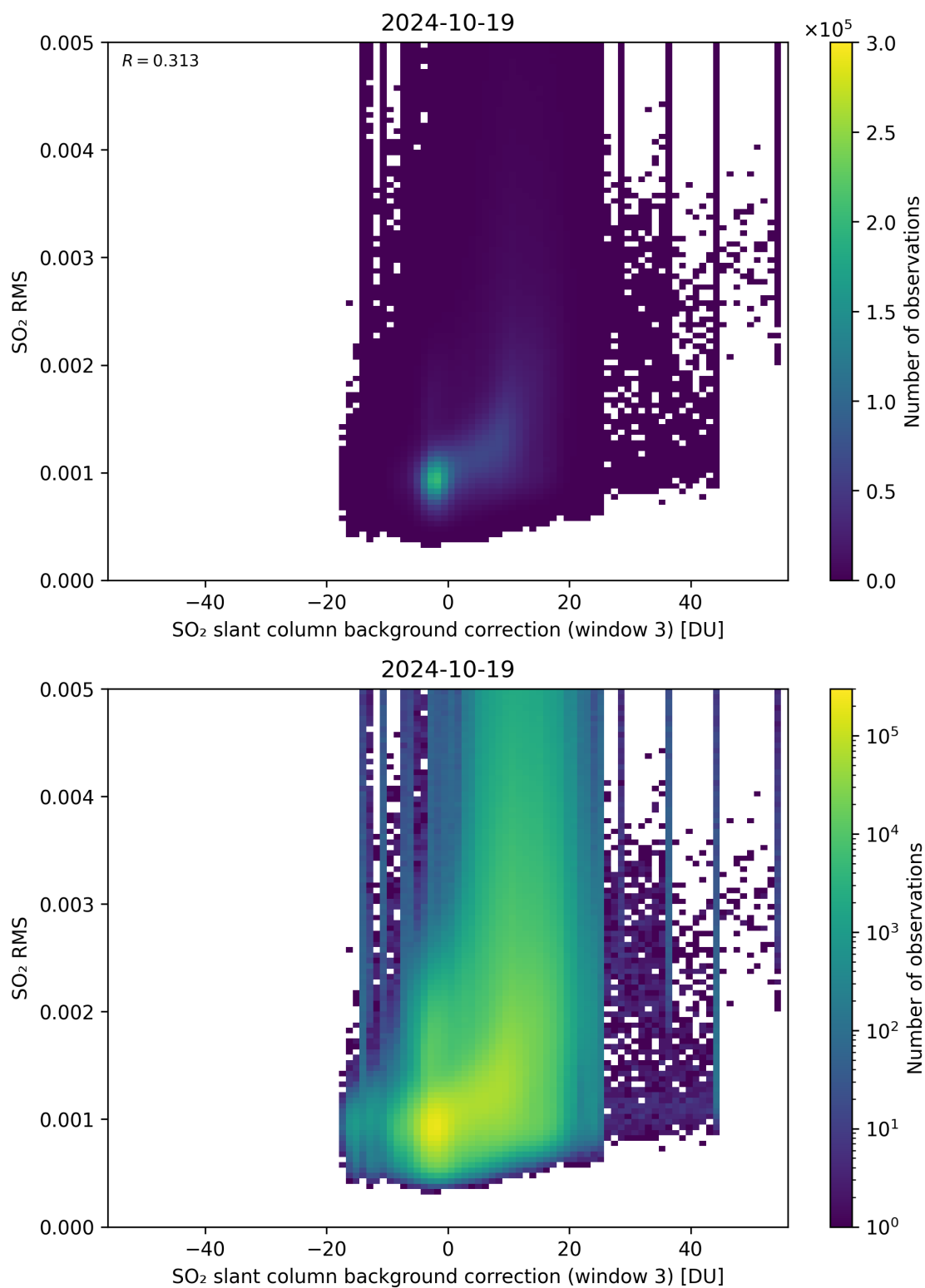
Figure 123: Scatter density plot of “SO 2 slant column background correction (window 3)” against “SO 2 RMS” for 2024-10-19 to 2024-10-20.
