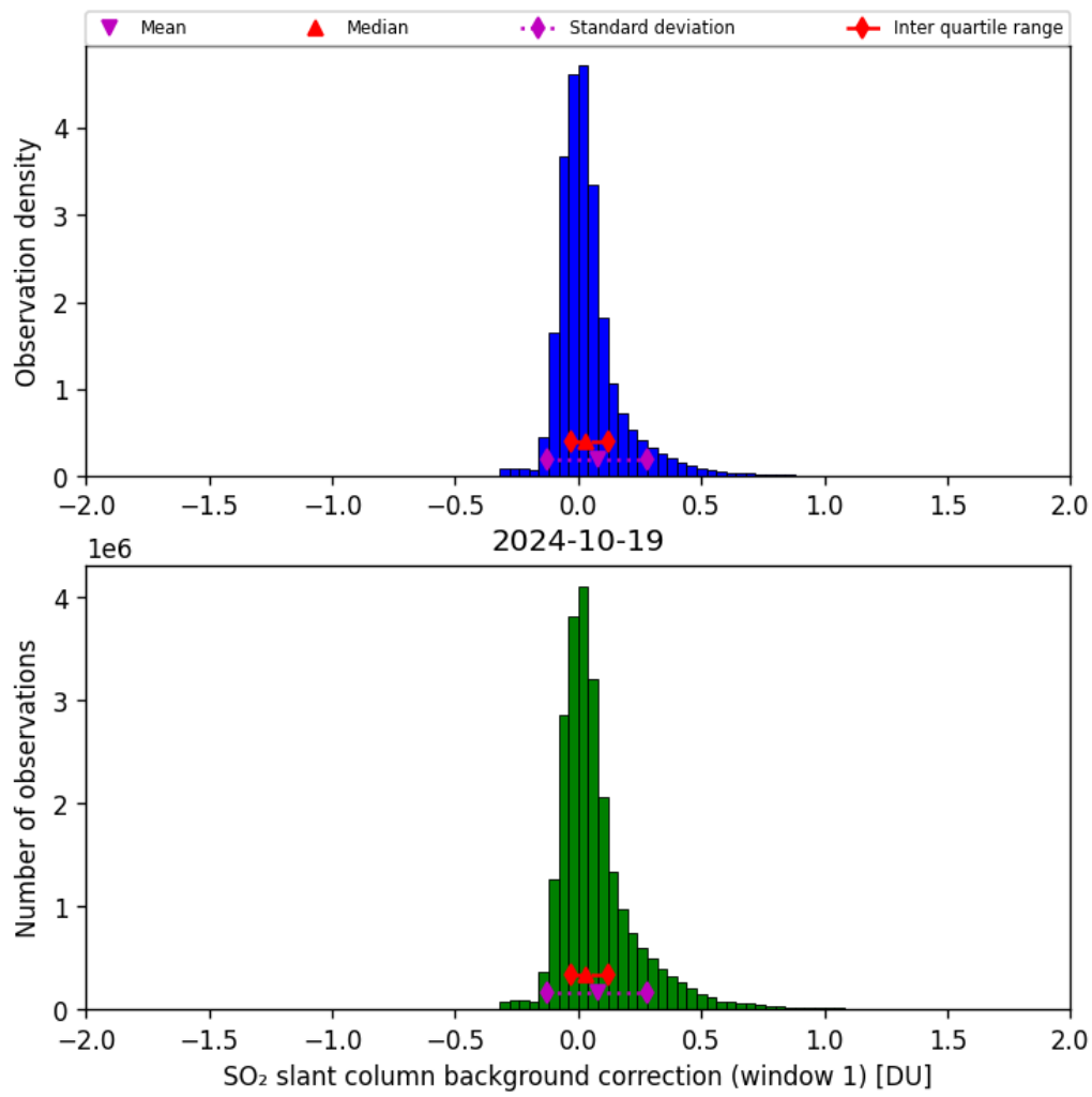
Figure 59: Histogram of “SO 2 slant column background correction (window 1)” for 2024-10-19 to 2024-10-20
