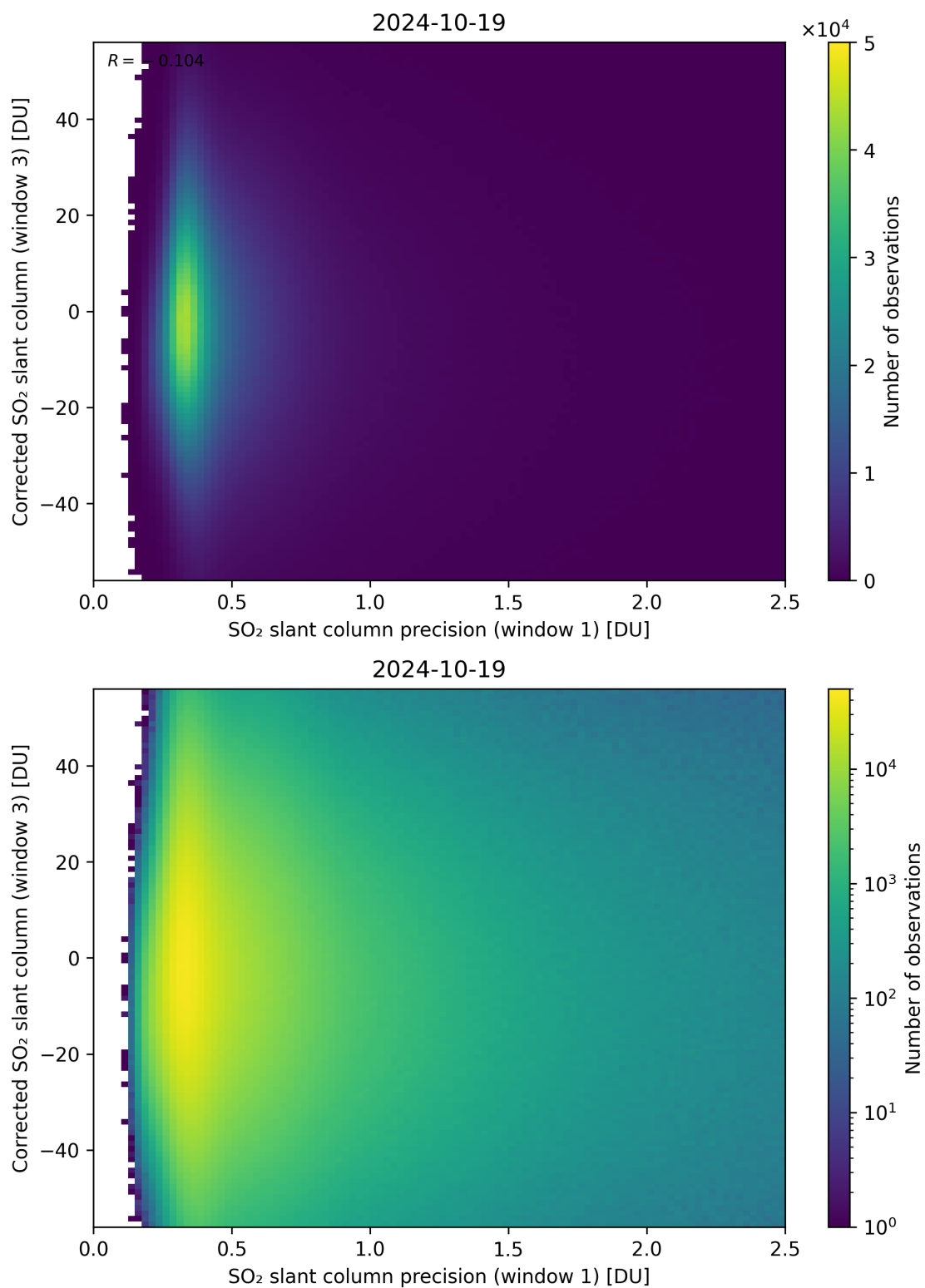
Figure 226: Scatter density plot of “SO 2 slant column precision (window 1)” against “Corrected SO 2 slant column (window 3)” for 2024-10-19 to 2024-10-20.
