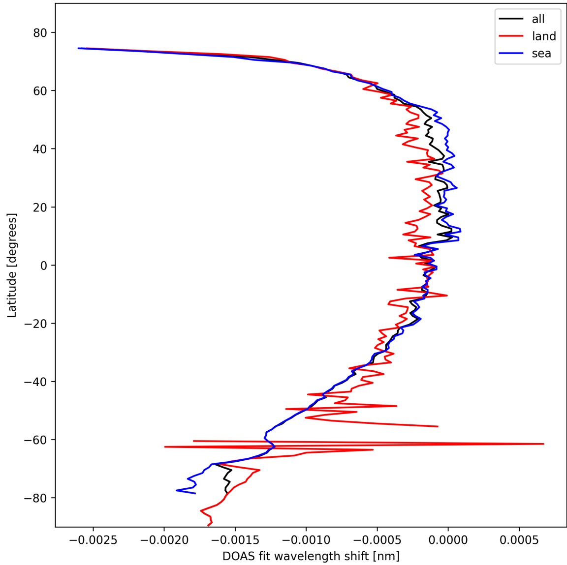
Figure 45: Zonal average of “DOAS fit wavelength shift” for 2024-10-19 to 2024-10-20.
