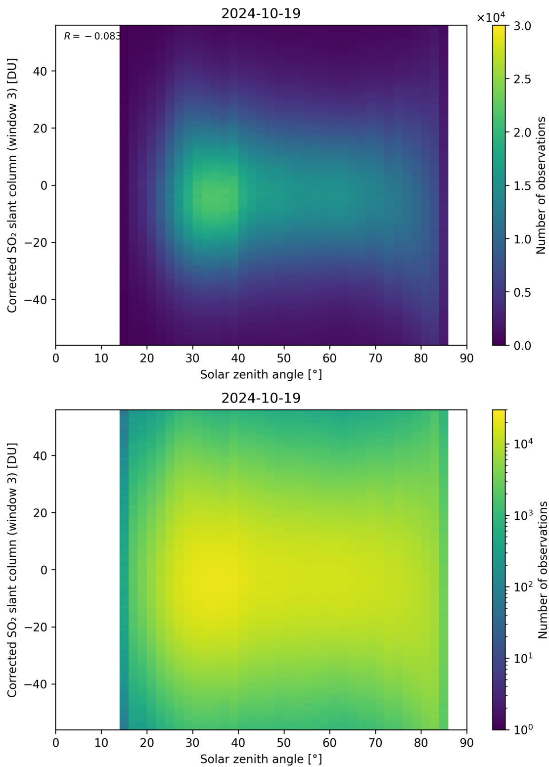
Figure 168: Scatter density plot of “Solar zenith angle” against “Corrected SO 2 slant column (window 3)” for 2024-10-19 to 2024-10-20.
