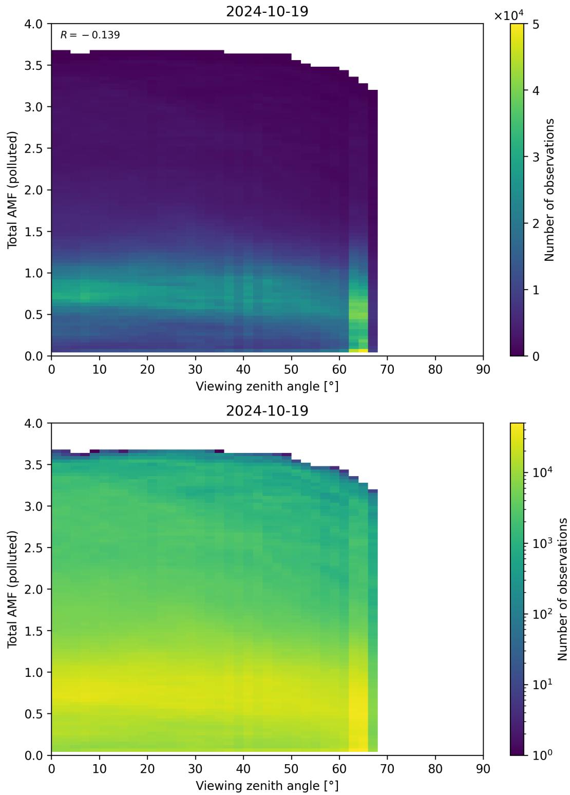
Figure 325: Scatter density plot of “Viewing zenith angle” against “Total AMF (polluted)” for 2024-10-19 to 2024-10-20.
