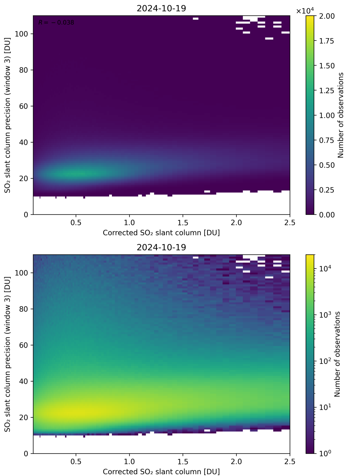
Figure 191: Scatter density plot of “Corrected SO 2 slant column” against “SO 2 slant column precision (window 3)” for 2024-10-19 to 2024-10-20.
