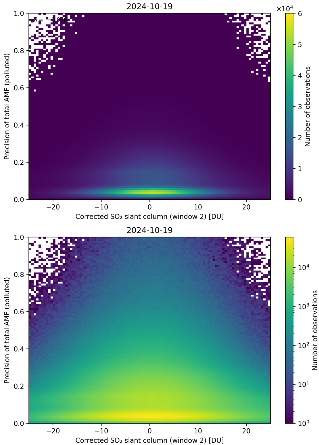
Figure 204: Scatter density plot of “Corrected SO 2 slant column (window 2)” against “Precision of total AMF (polluted)” for 2024-10-19 to 2024-10-20.
