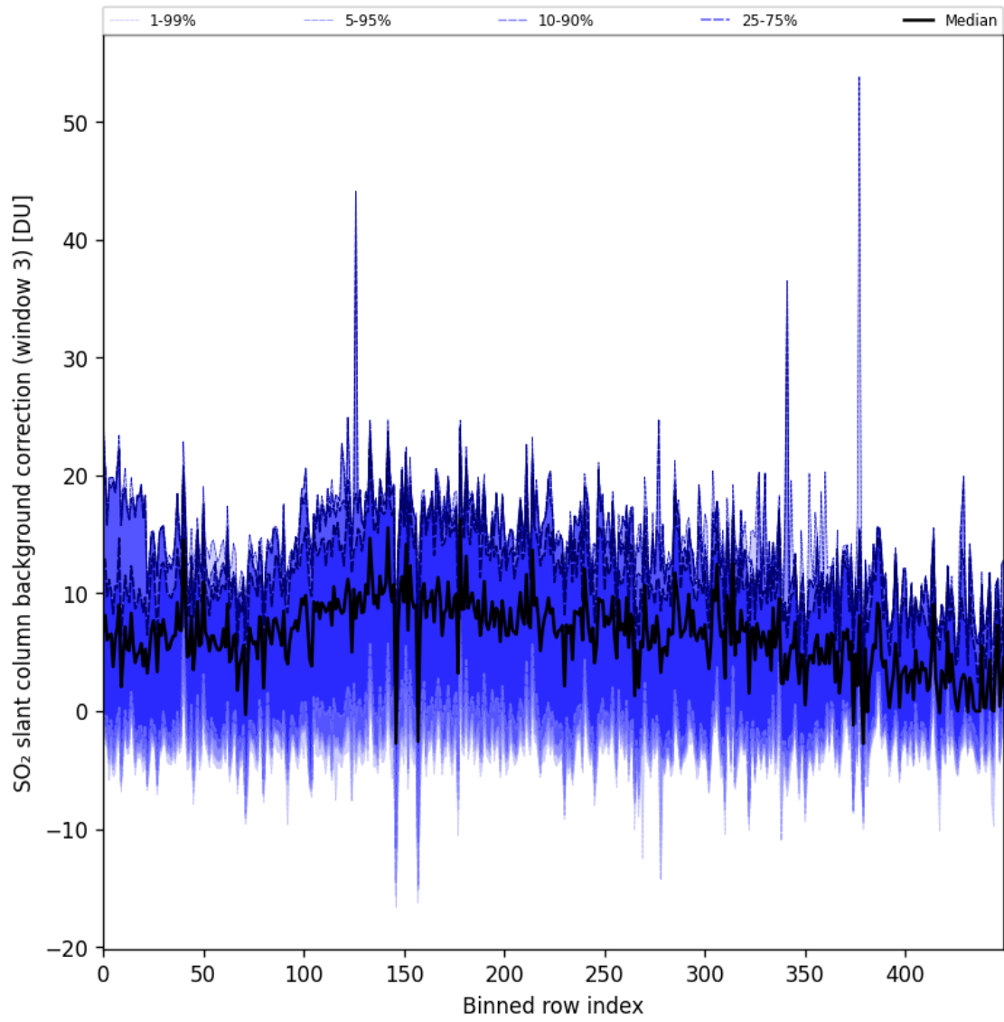
Figure 90: Along track statistics of “SO 2 slant column background correction (window 3)” for 2024-10-19 to 2024-10-20
