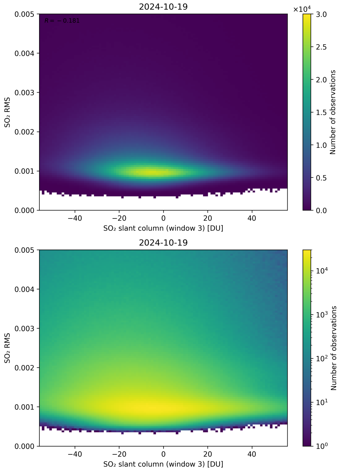
Figure 256: Scatter density plot of “SO 2 slant column (window 3)” against “SO 2 RMS” for 2024-10-19 to 2024-10-20.
