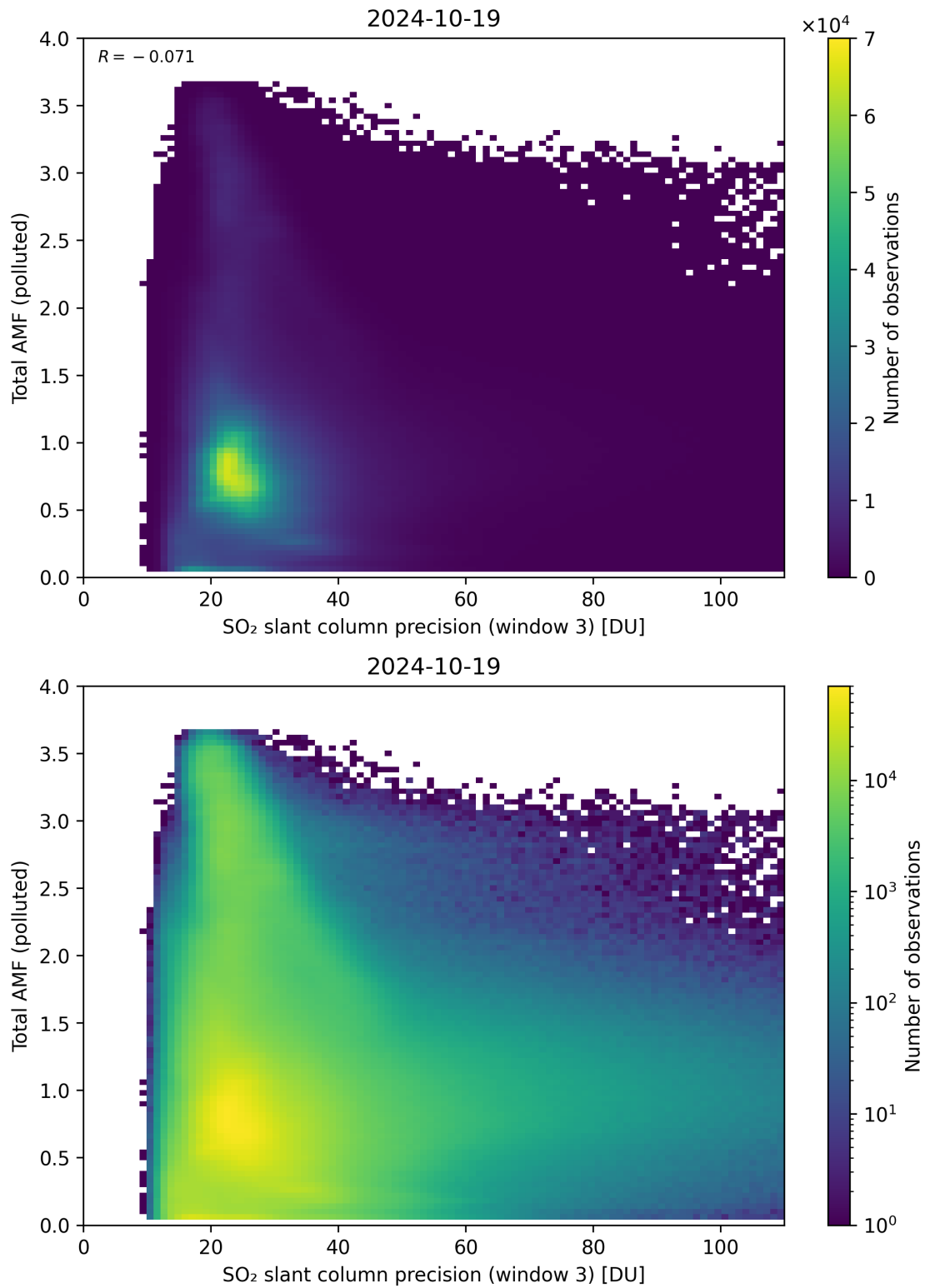
Figure 263: Scatter density plot of “SO 2 slant column precision (window 3)” against “Total AMF (polluted)” for 2024-10-19 to 2024-10-20.
