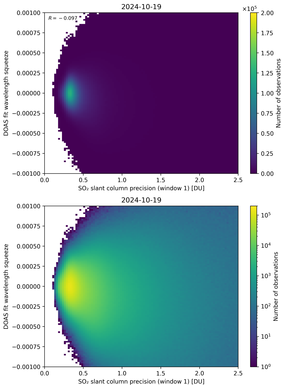
Figure 222: Scatter density plot of “SO 2 slant column precision (window 1)” against “DOAS fit wavelength squeeze” for 2024-10-19 to 2024-10-20.
