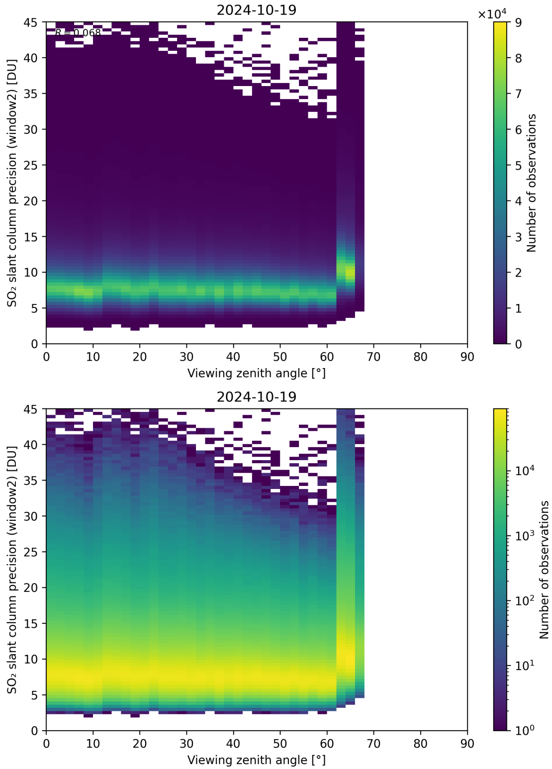
Figure 322: Scatter density plot of “Viewing zenith angle” against “SO 2 slant column precision (window2)” for 2024-10-19 to 2024-10-20.
