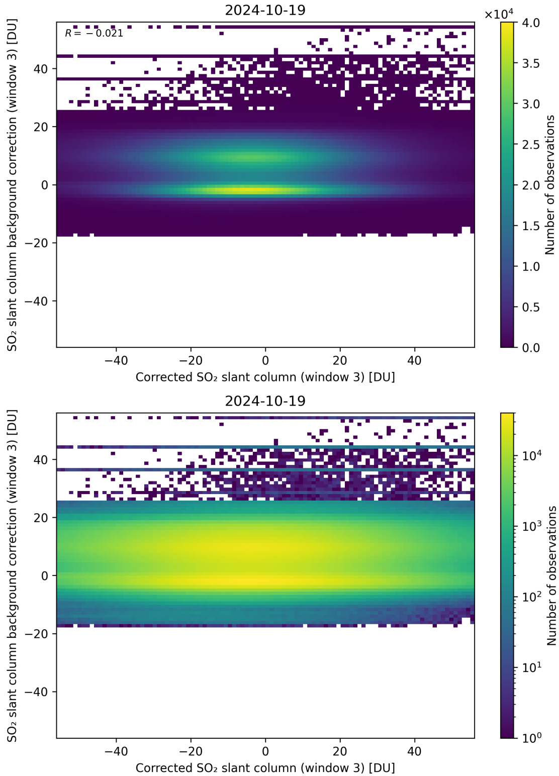
Figure 205: Scatter density plot of “Corrected SO 2 slant column (window 3)” against “SO 2 slant column background correction (window 3)” for 2024-10-19 to 2024-10-20.
