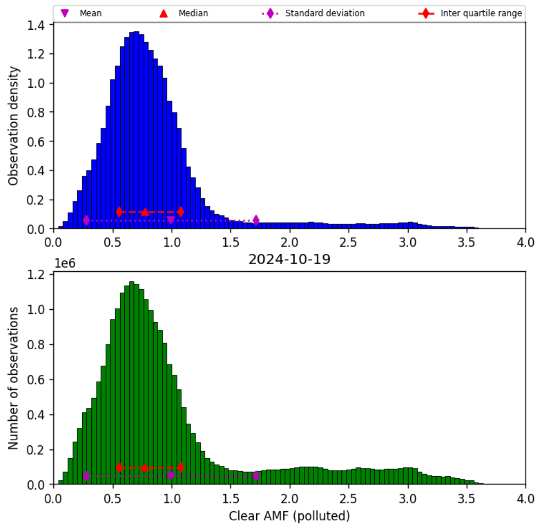
Figure 73: Histogram of “Clear AMF (polluted)” for 2024-10-19 to 2024-10-20
