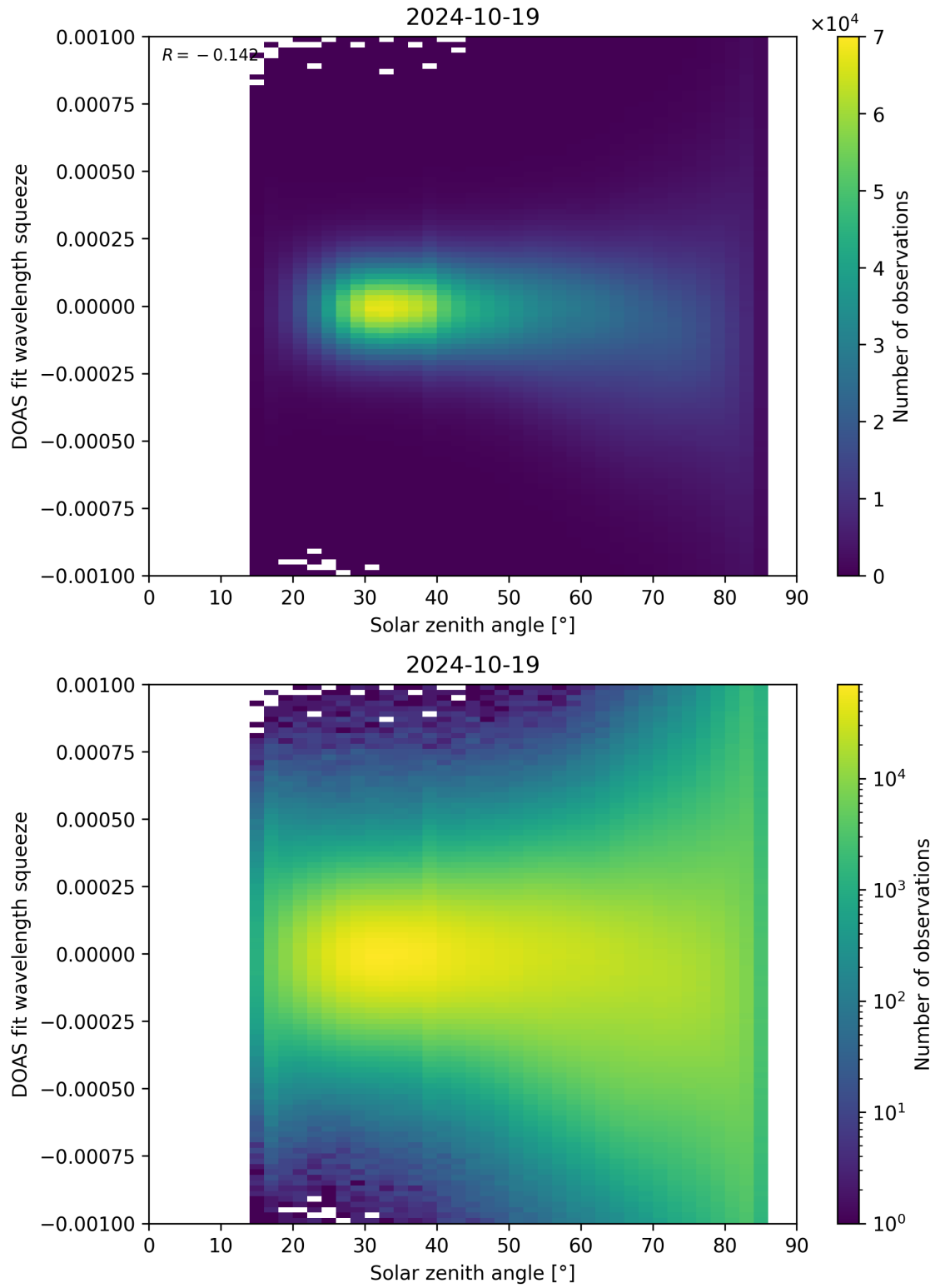
Figure 162: Scatter density plot of “Solar zenith angle” against “DOAS fit wavelength squeeze” for 2024-10-19 to 2024-10-20.
