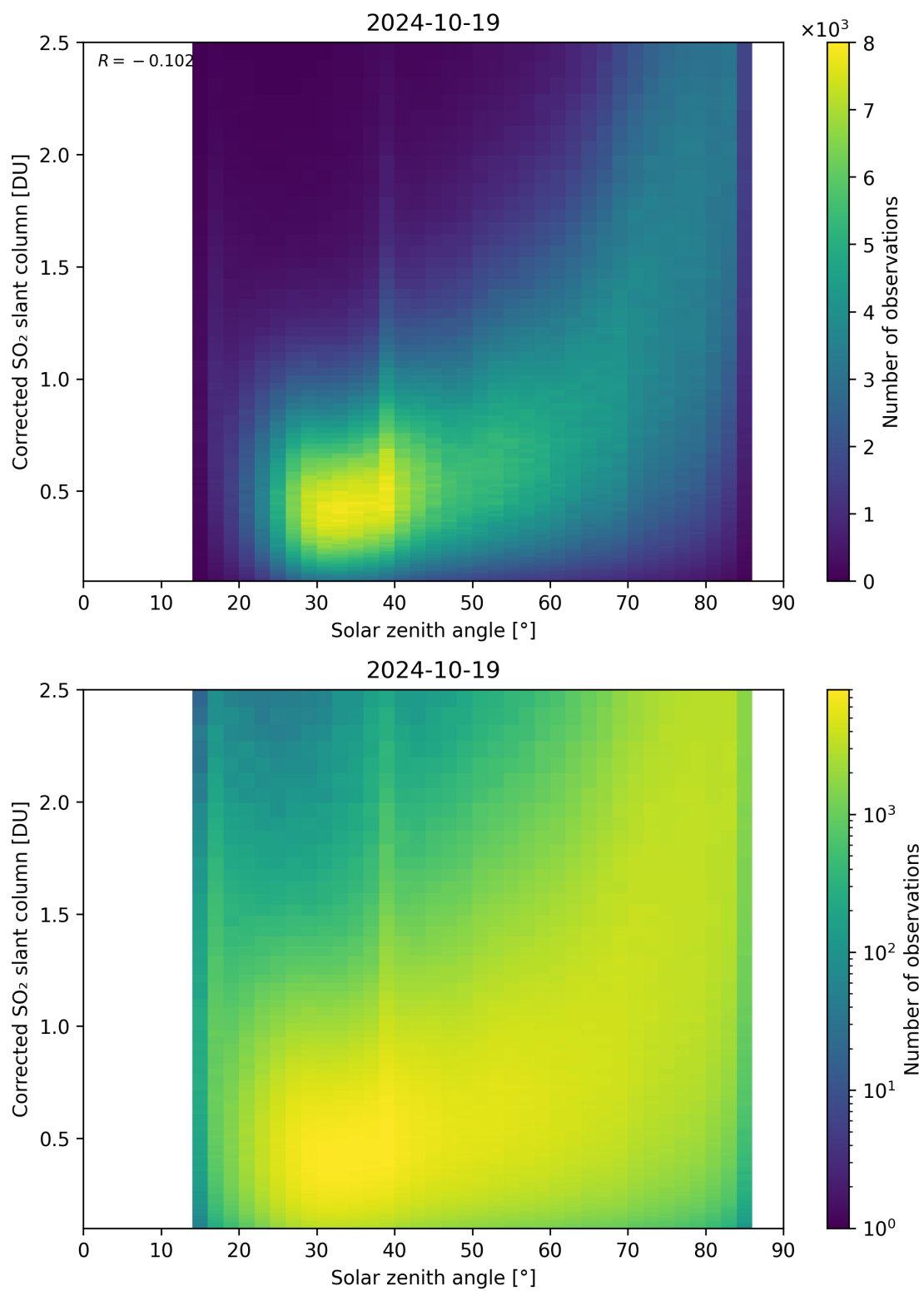
Figure 166: Scatter density plot of “Solar zenith angle” against “Corrected SO 2 slant column” for 2024-10-19 to 2024-10-20.
