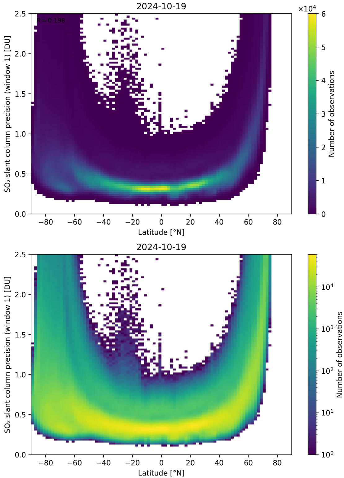
Figure 150: Scatter density plot of “Latitude” against “SO 2 slant column precision (window 1)” for 2024-10-19 to 2024-10-20.
