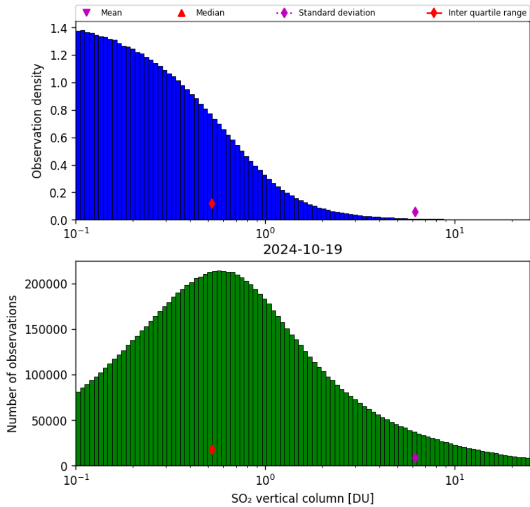
Figure 53: Histogram of “SO 2 vertical column” for 2024-10-19 to 2024-10-20
