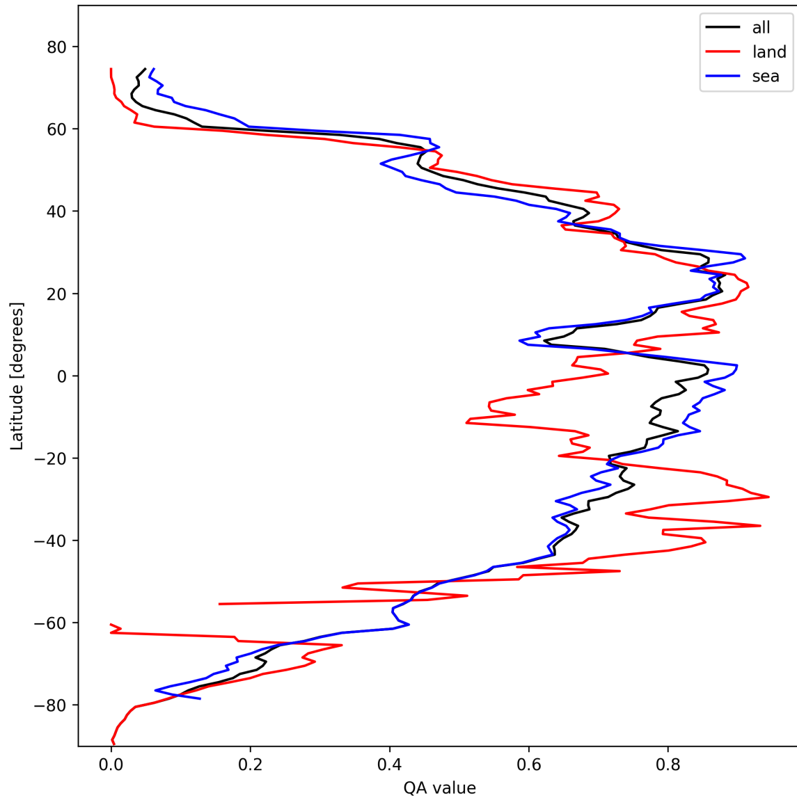
Figure 29: Zonal average of “QA value” for 2024-10-19 to 2024-10-20.
