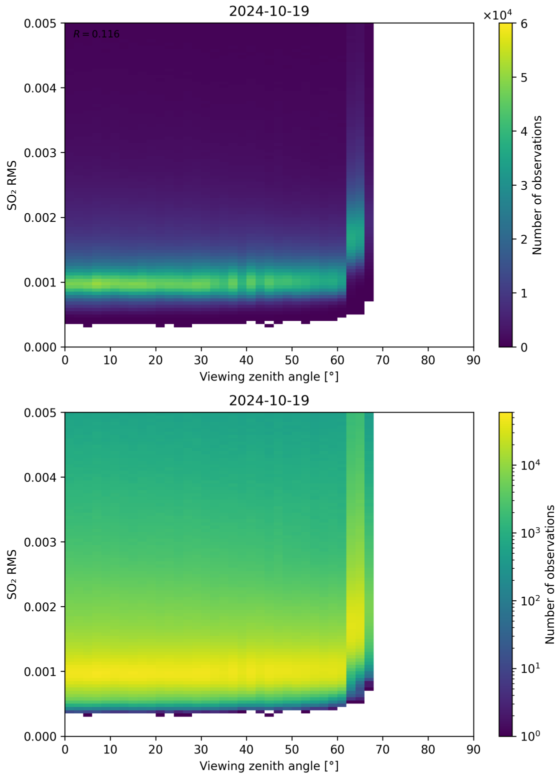
Figure 313: Scatter density plot of “Viewing zenith angle” against “SO 2 RMS” for 2024-10-19 to 2024-10-20.
