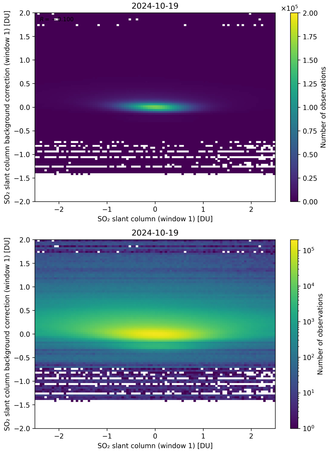
Figure 212: Scatter density plot of “SO 2 slant column (window 1)” against “SO 2 slant column background correction (window 1)” for 2024-10-19 to 2024-10-20.
