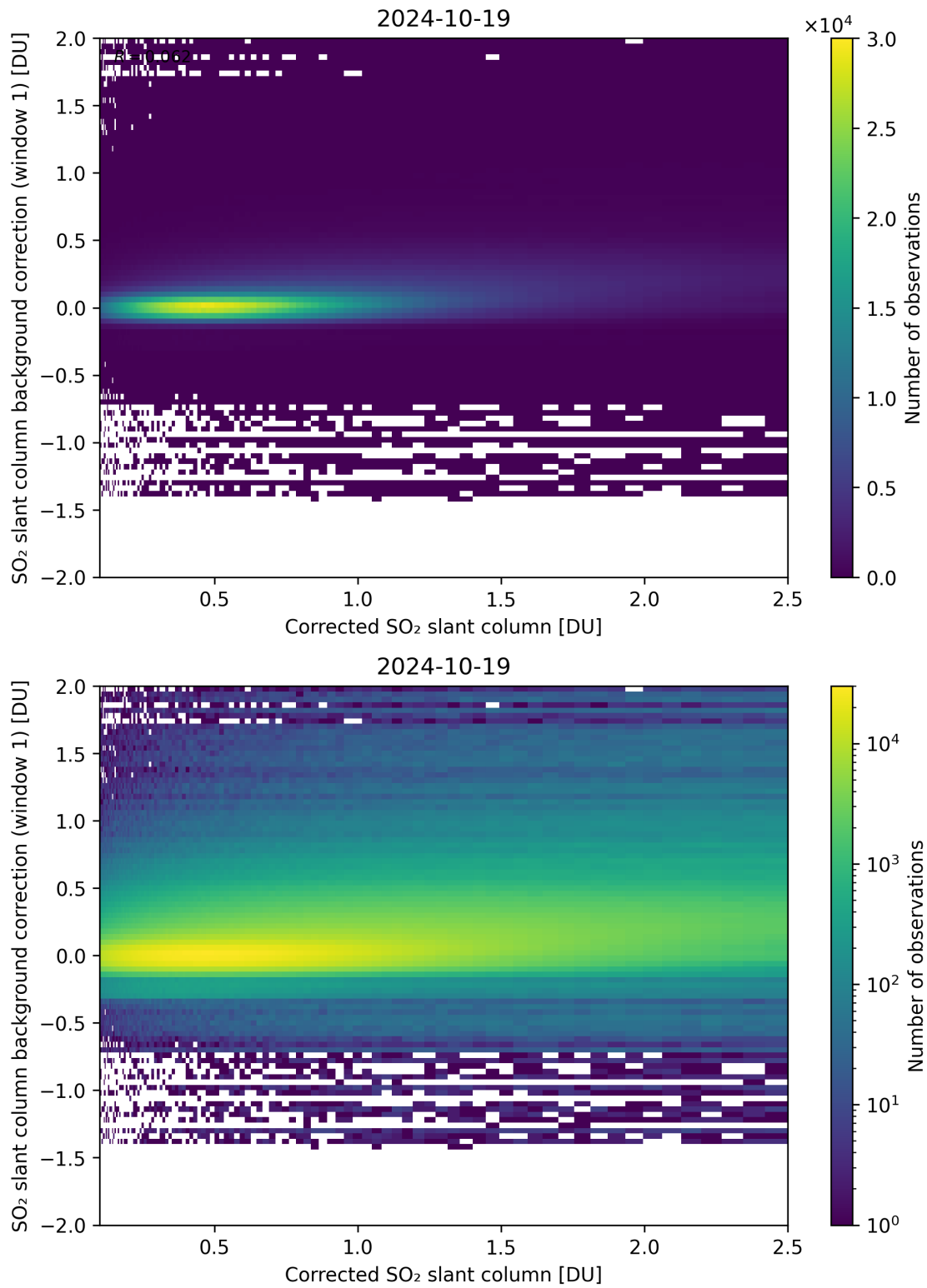
Figure 178: Scatter density plot of “Corrected SO 2 slant column” against “SO 2 slant column background correction (window 1)” for 2024-10-19 to 2024-10-20.
