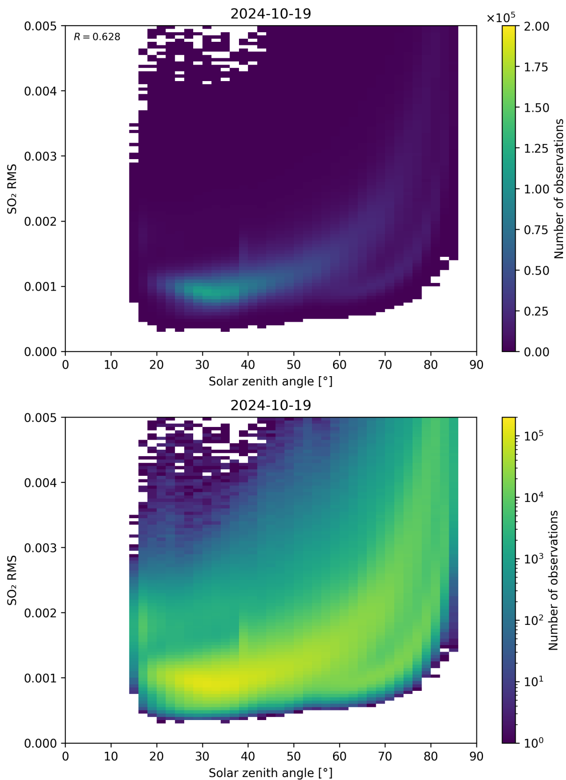
Figure 163: Scatter density plot of “Solar zenith angle” against “SO 2 RMS” for 2024-10-19 to 2024-10-20.
