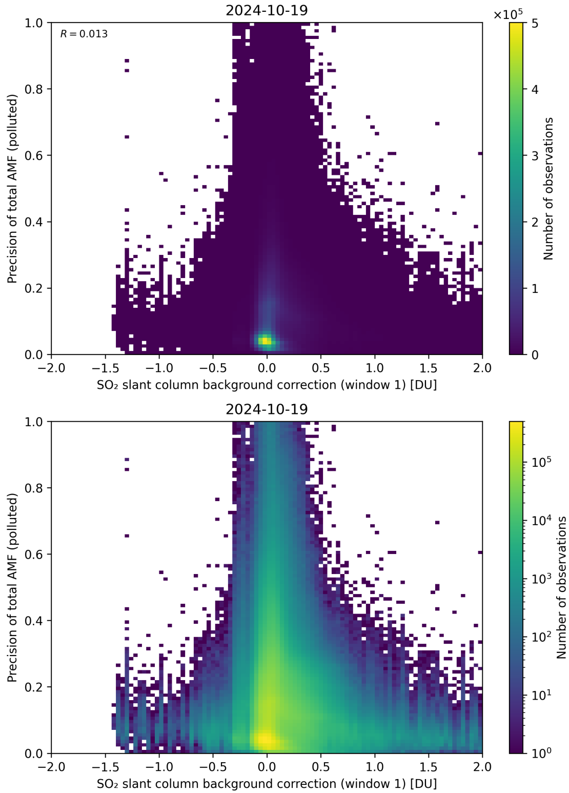
Figure 110: Scatter density plot of “SO 2 slant column background correction (window 1)” against “Precision of total AMF (polluted)” for 2024-10-19 to 2024-10-20.
