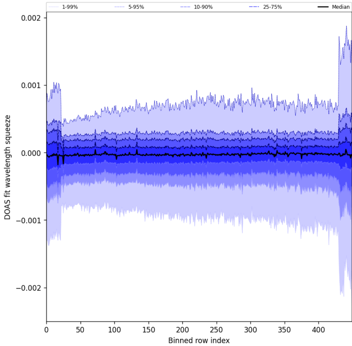
Figure 92: Along track statistics of “DOAS fit wavelength squeeze” for 2024-10-19 to 2024-10-20
