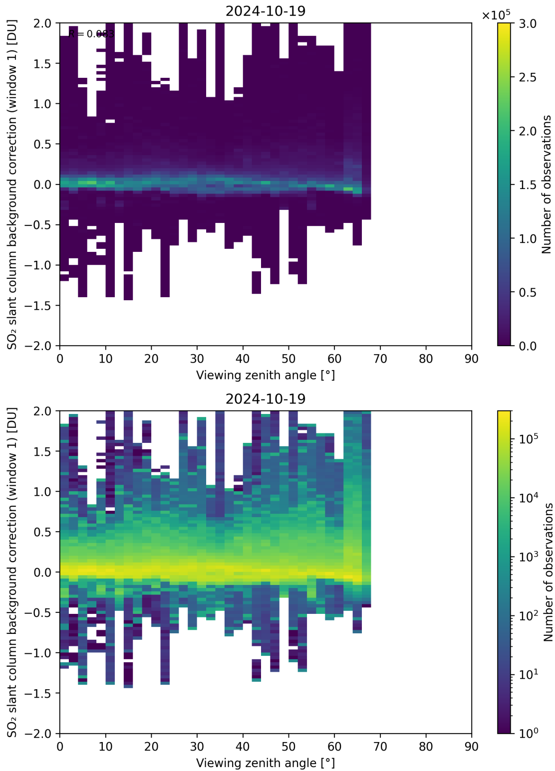
Figure 308: Scatter density plot of “Viewing zenith angle” against “SO 2 slant column background correction (window 1)” for 2024-10-19 to 2024-10-20.
