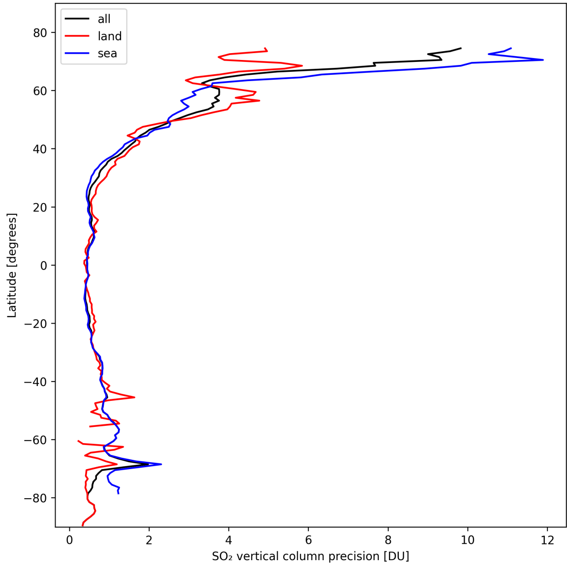
Figure 31: Zonal average of “SO 2 vertical column precision” for 2024-10-19 to 2024-10-20.
