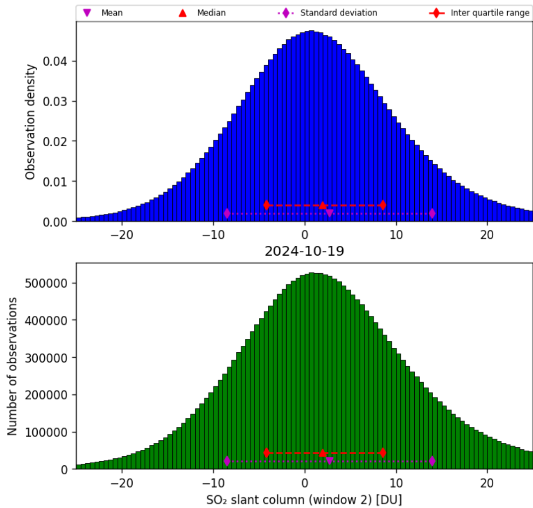
Figure 60: Histogram of “SO 2 slant column (window 2)” for 2024-10-19 to 2024-10-20
