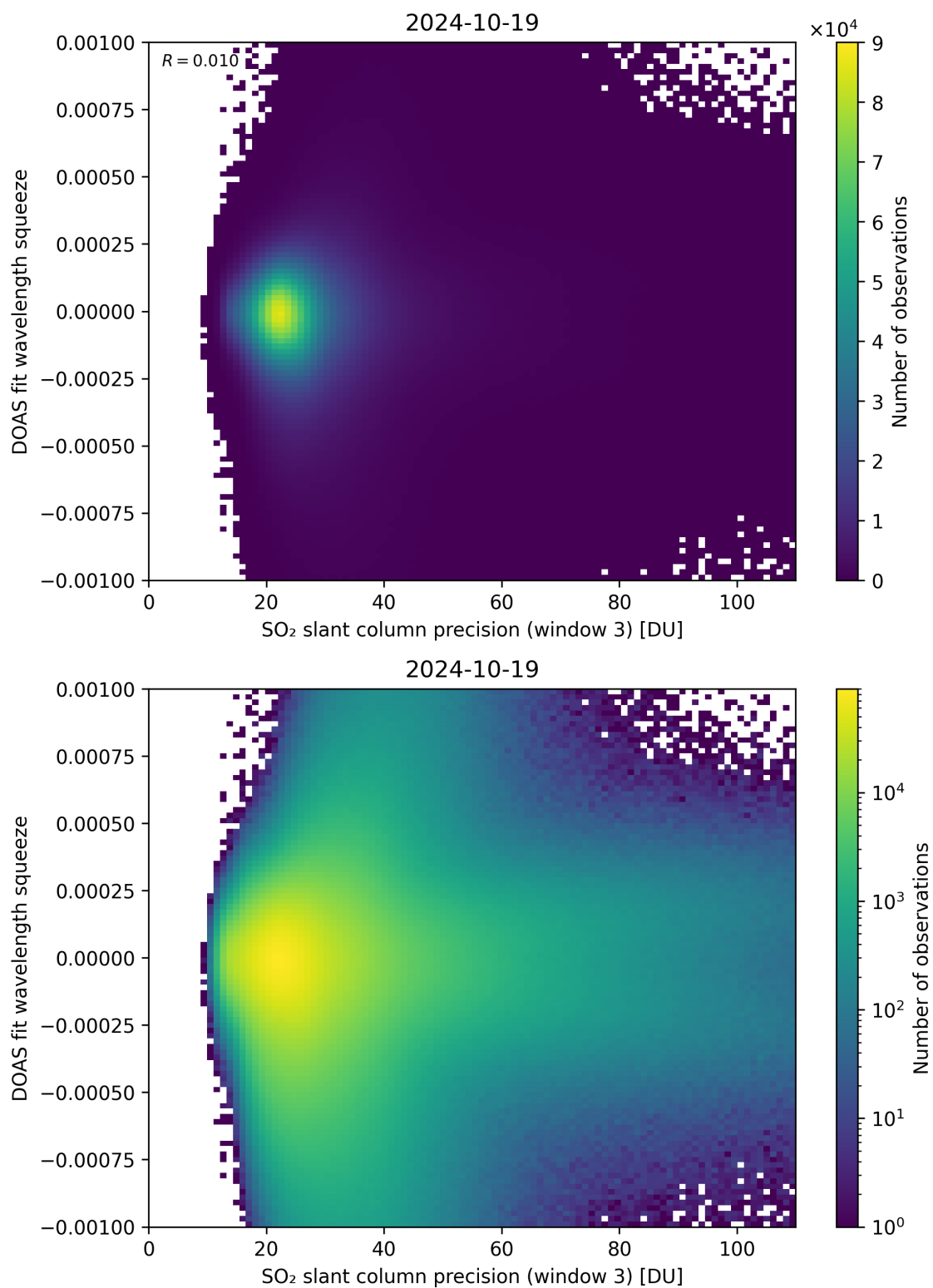
Figure 259: Scatter density plot of “SO 2 slant column precision (window 3)” against “DOAS fit wavelength squeeze” for 2024-10-19 to 2024-10-20.
