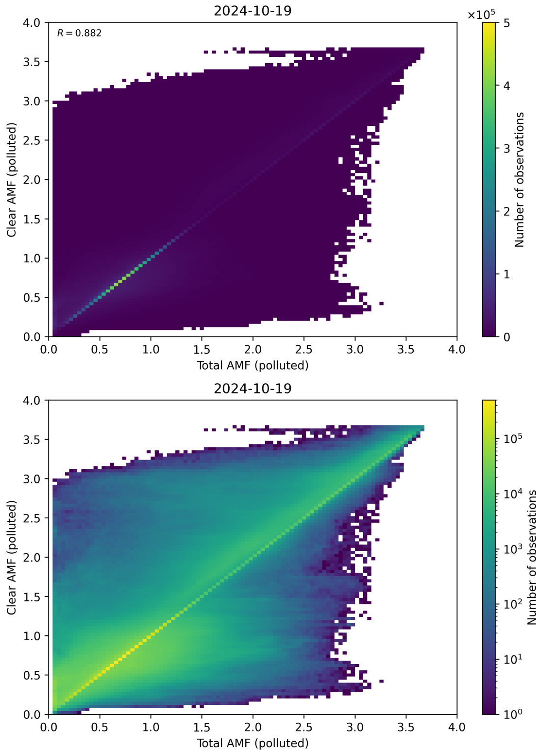
Figure 271: Scatter density plot of “Total AMF (polluted)” against “Clear AMF (polluted)” for 2024-10-19 to 2024-10-20.
