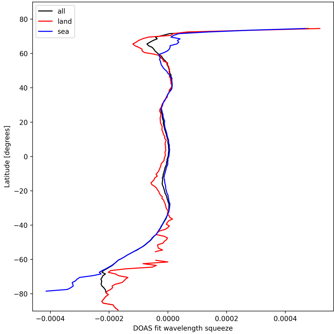
Figure 46: Zonal average of “DOAS fit wavelength squeeze” for 2024-10-19 to 2024-10-20.
