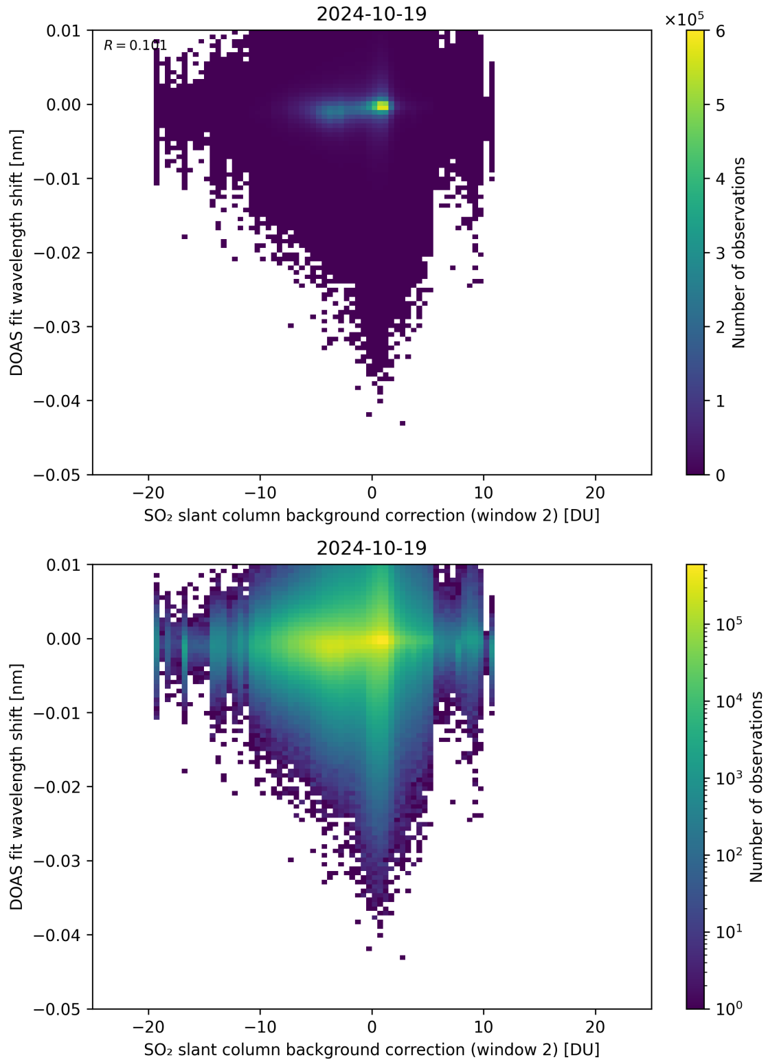
Figure 112: Scatter density plot of “SO 2 slant column background correction (window 2)” against “DOAS fit wavelength shift” for 2024-10-19 to 2024-10-20.
