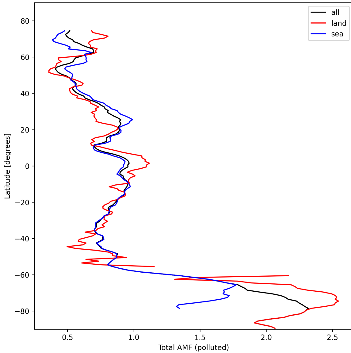
Figure 48: Zonal average of “Total AMF (polluted)” for 2024-10-19 to 2024-10-20.
