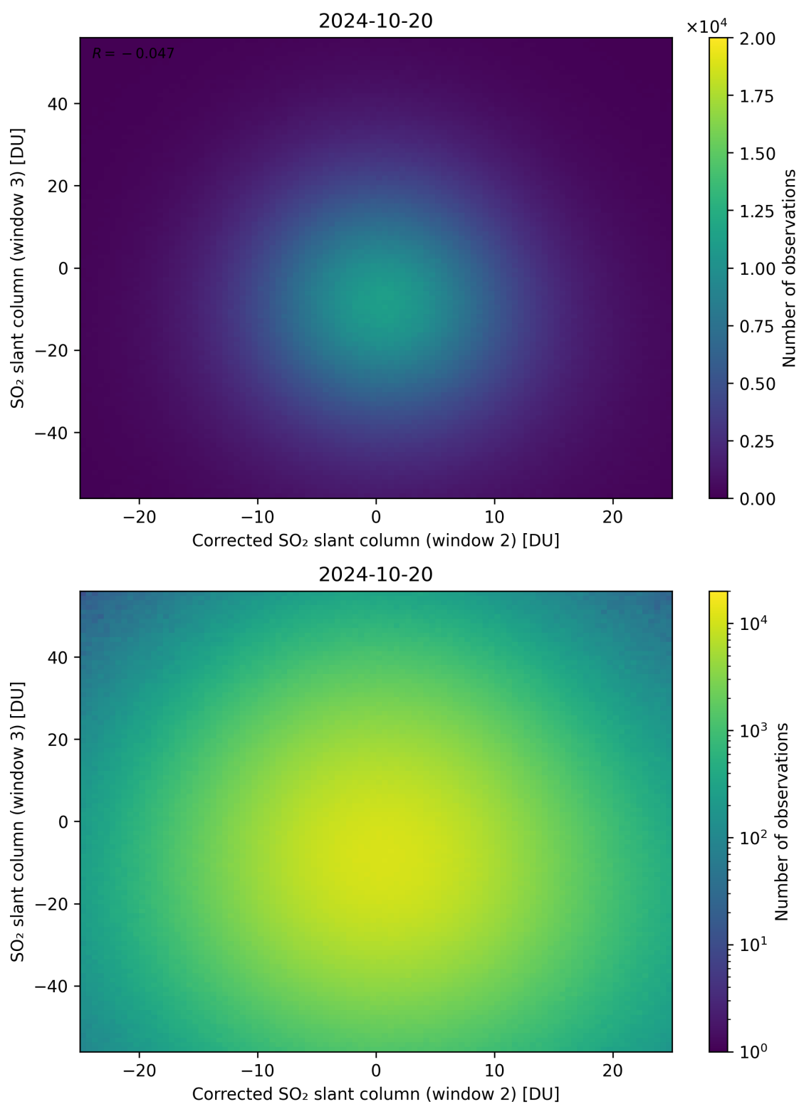
Figure 201: Scatter density plot of “Corrected SO 2 slant column (window 2)” against “SO 2 slant column (window 3)” for 2024-10-19 to 2024-10-21.
