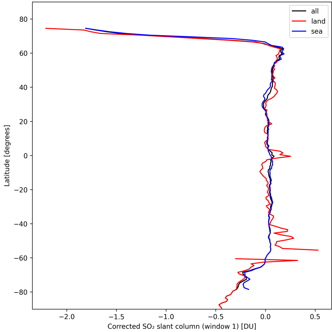
Figure 35: Zonal average of “Corrected SO 2 slant column (window 1)” for 2024-10-19 to 2024-10-21.
