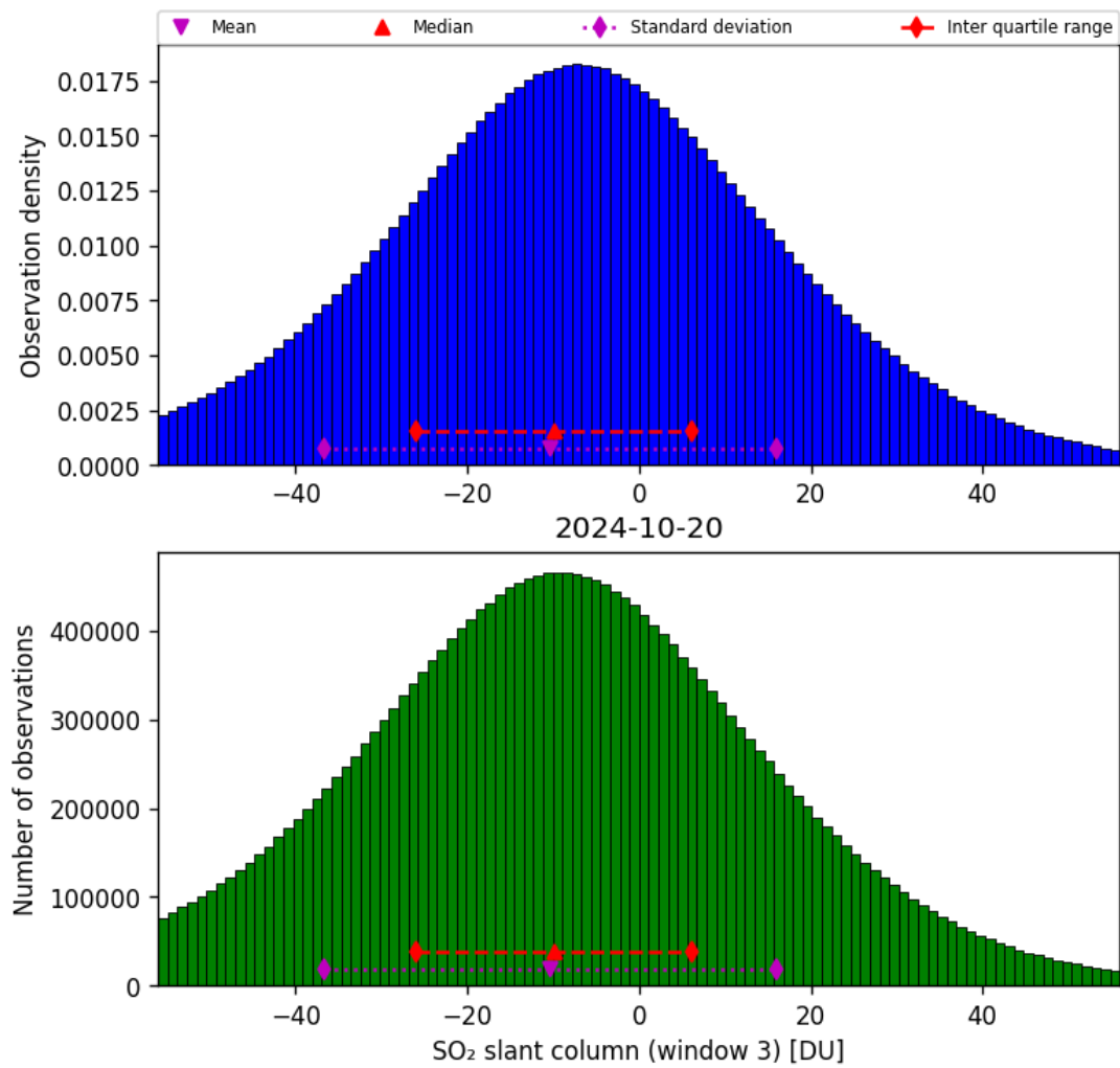
Figure 64: Histogram of “SO 2 slant column (window 3)” for 2024-10-19 to 2024-10-21
