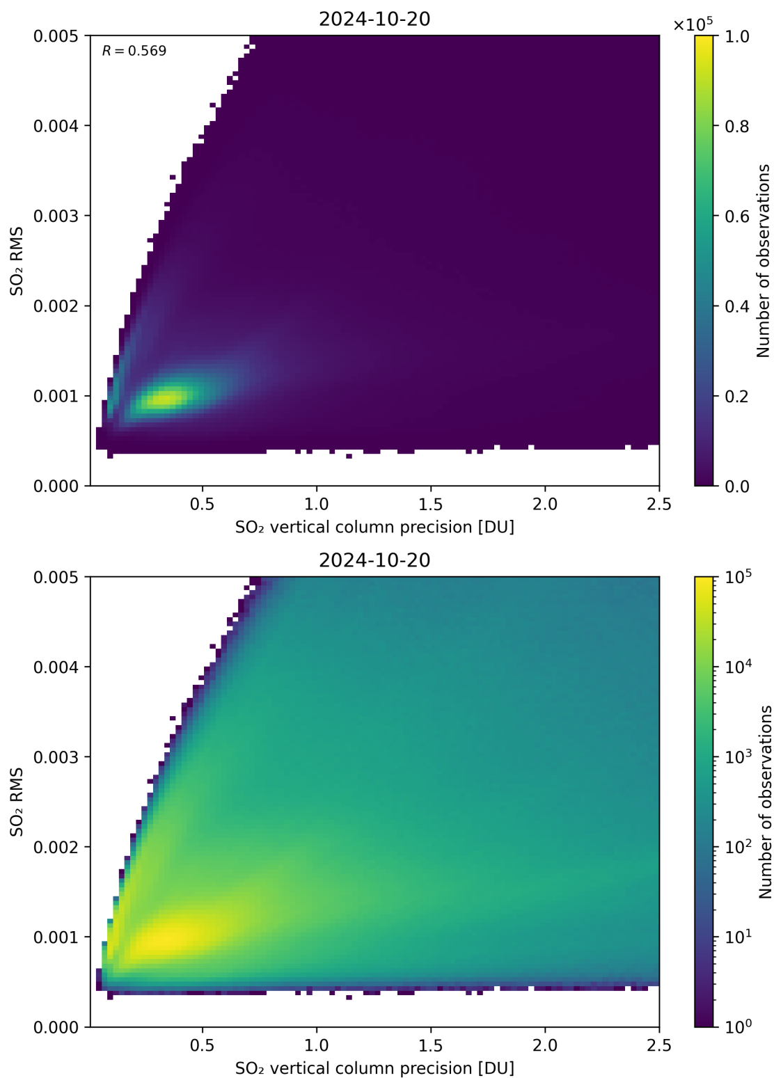
Figure 284: Scatter density plot of “SO 2 vertical column precision” against “SO 2 RMS” for 2024-10-19 to 2024-10-21.
