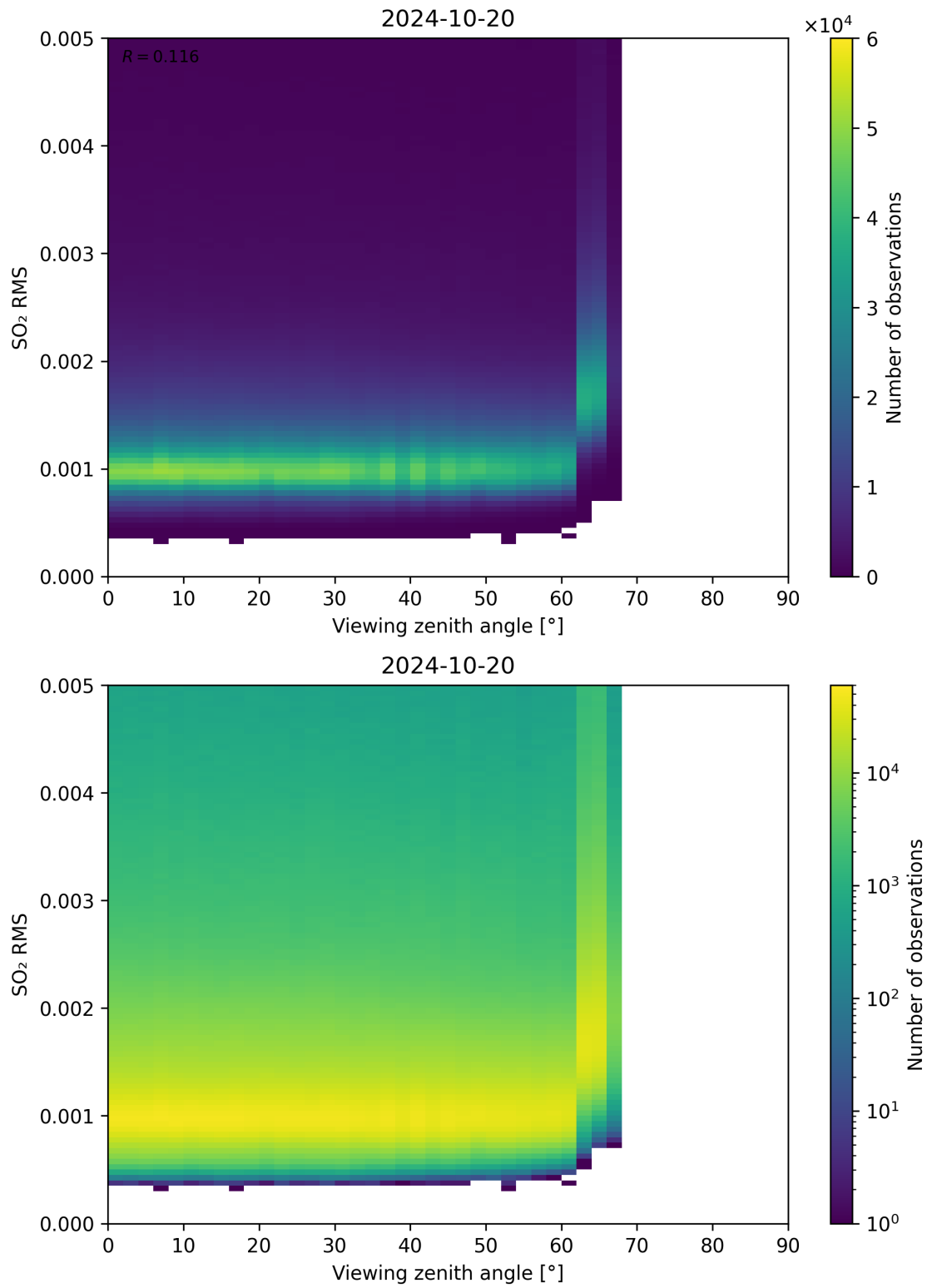
Figure 313: Scatter density plot of “Viewing zenith angle” against “SO 2 RMS” for 2024-10-19 to 2024-10-21.
