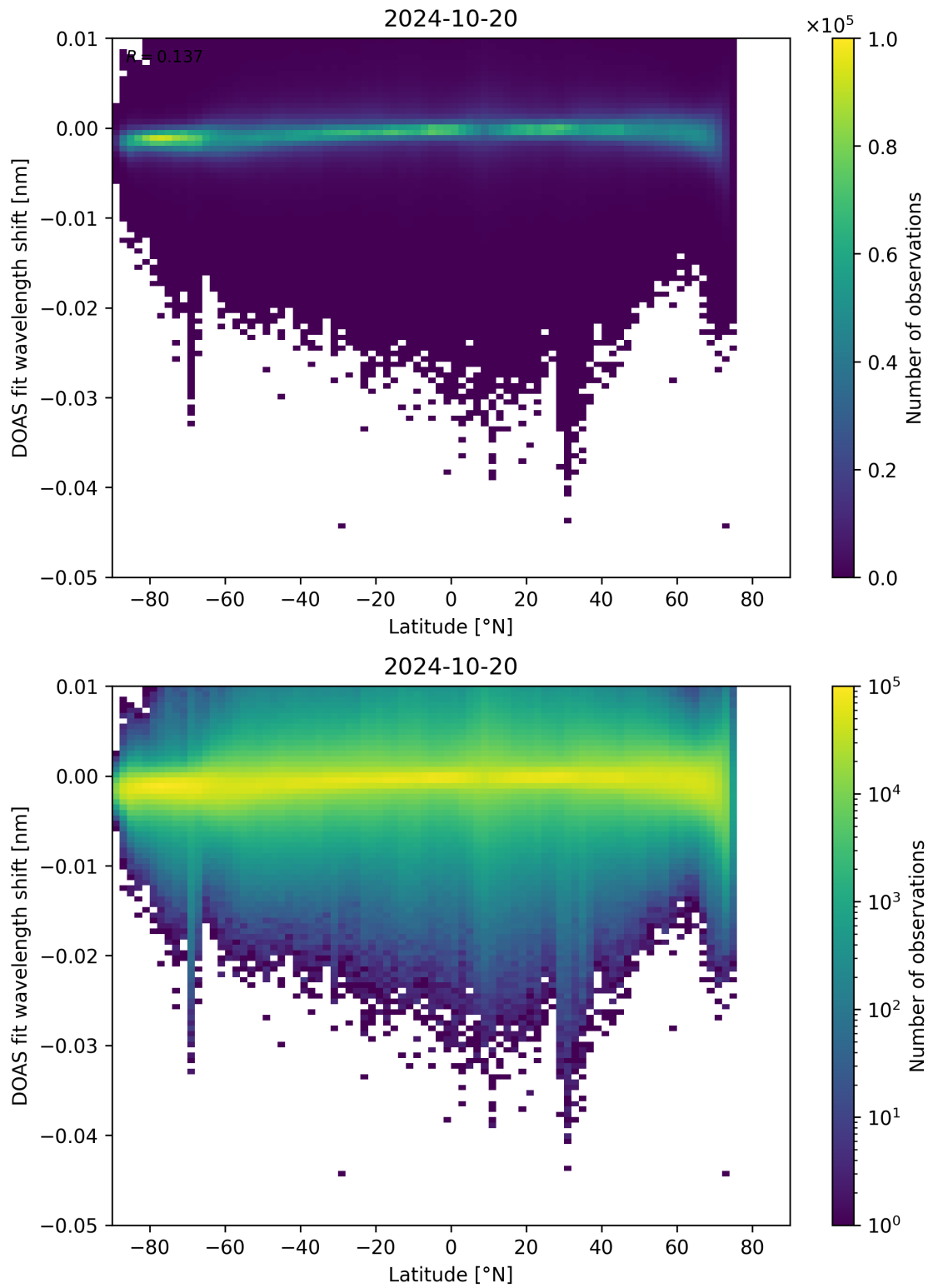
Figure 142: Scatter density plot of “Latitude” against “DOAS fit wavelength shift” for 2024-10-19 to 2024-10-21.
