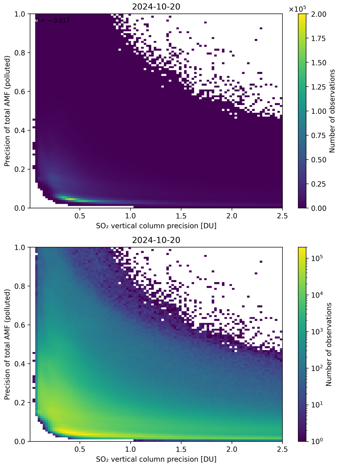
Figure 295: Scatter density plot of “SO 2 vertical column precision” against “Precision of total AMF (polluted)” for 2024-10-19 to 2024-10-21.
