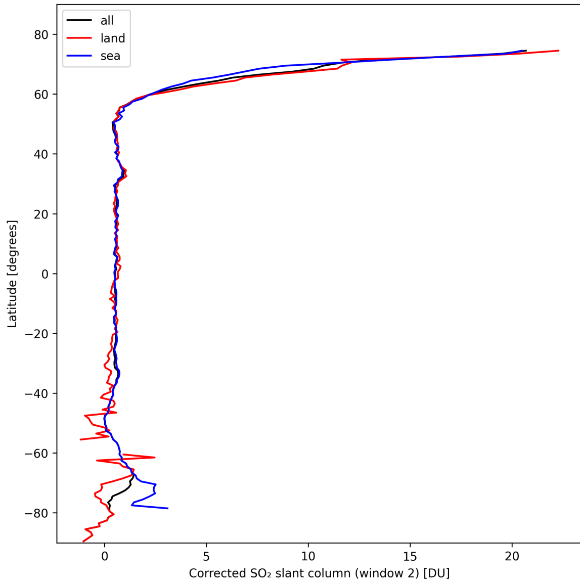
Figure 39: Zonal average of “Corrected SO 2 slant column (window 2)” for 2024-10-19 to 2024-10-21.
