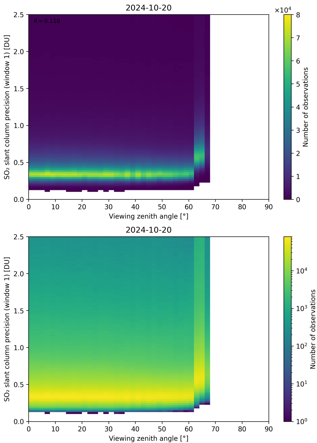
Figure 321: Scatter density plot of “Viewing zenith angle” against “SO 2 slant column precision (window 1)” for 2024-10-19 to 2024-10-21.
