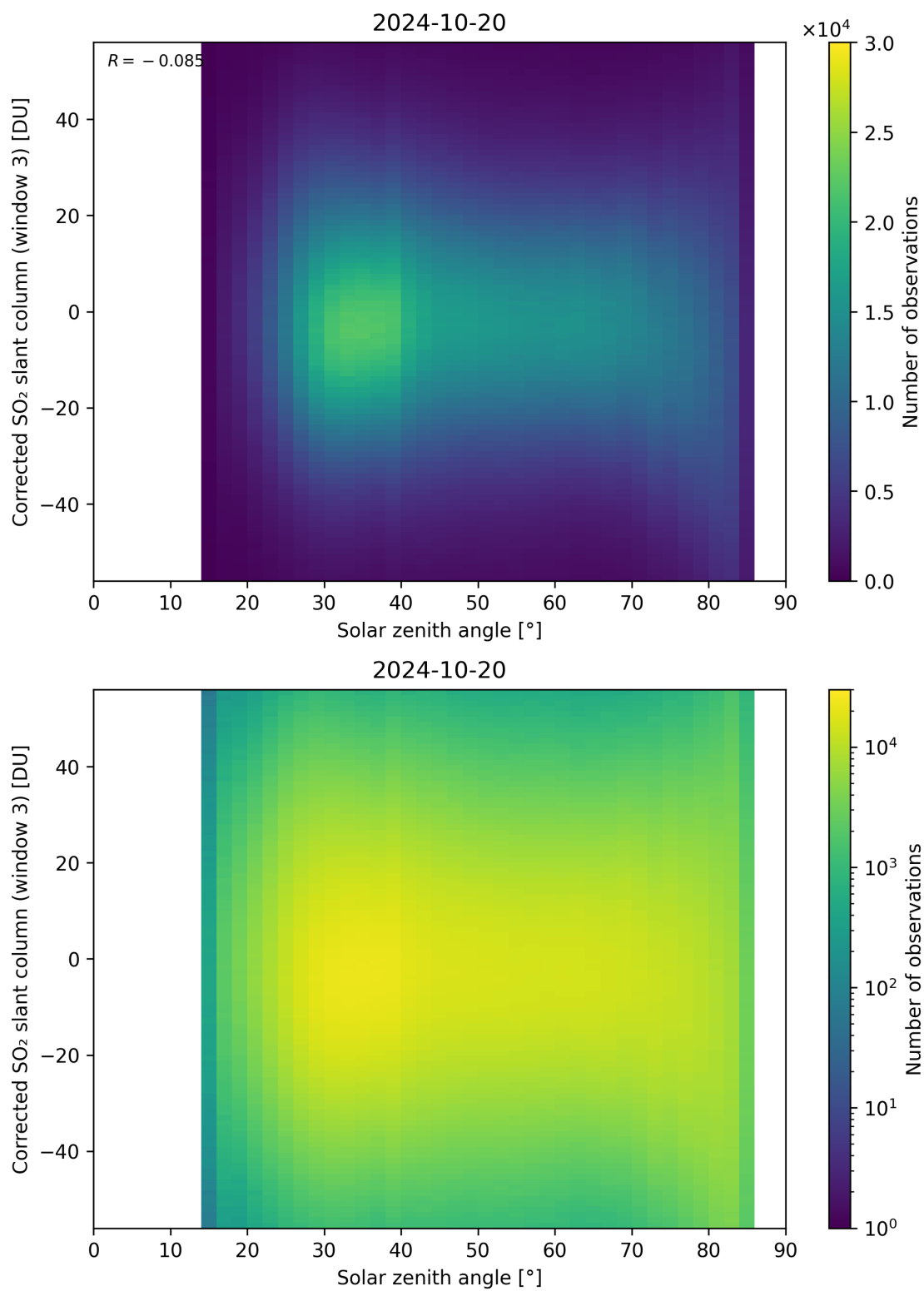
Figure 168: Scatter density plot of “Solar zenith angle” against “Corrected SO 2 slant column (window 3)” for 2024-10-19 to 2024-10-21.
