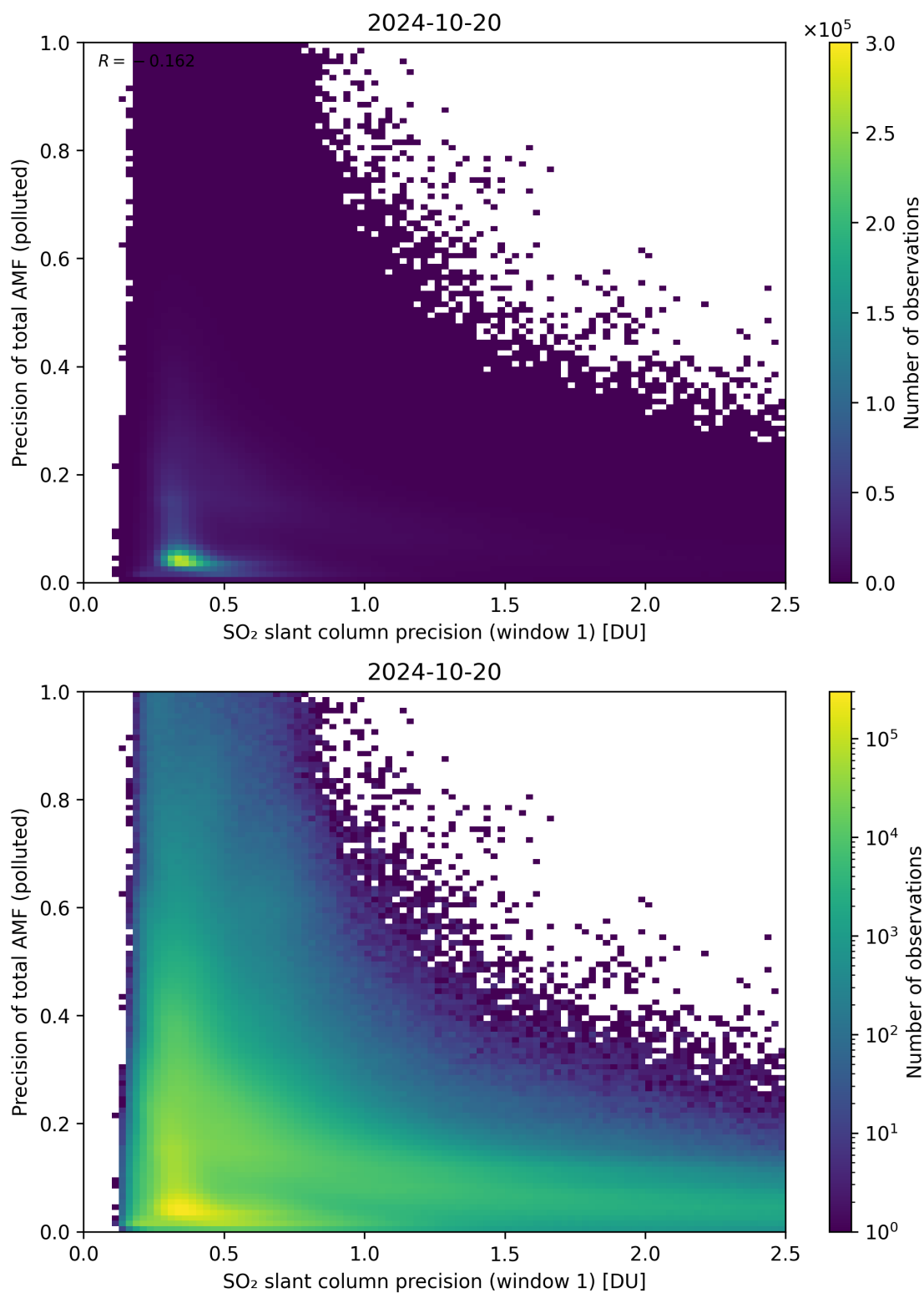
Figure 231: Scatter density plot of “SO 2 slant column precision (window 1)” against “Precision of total AMF (polluted)” for 2024-10-19 to 2024-10-21.
