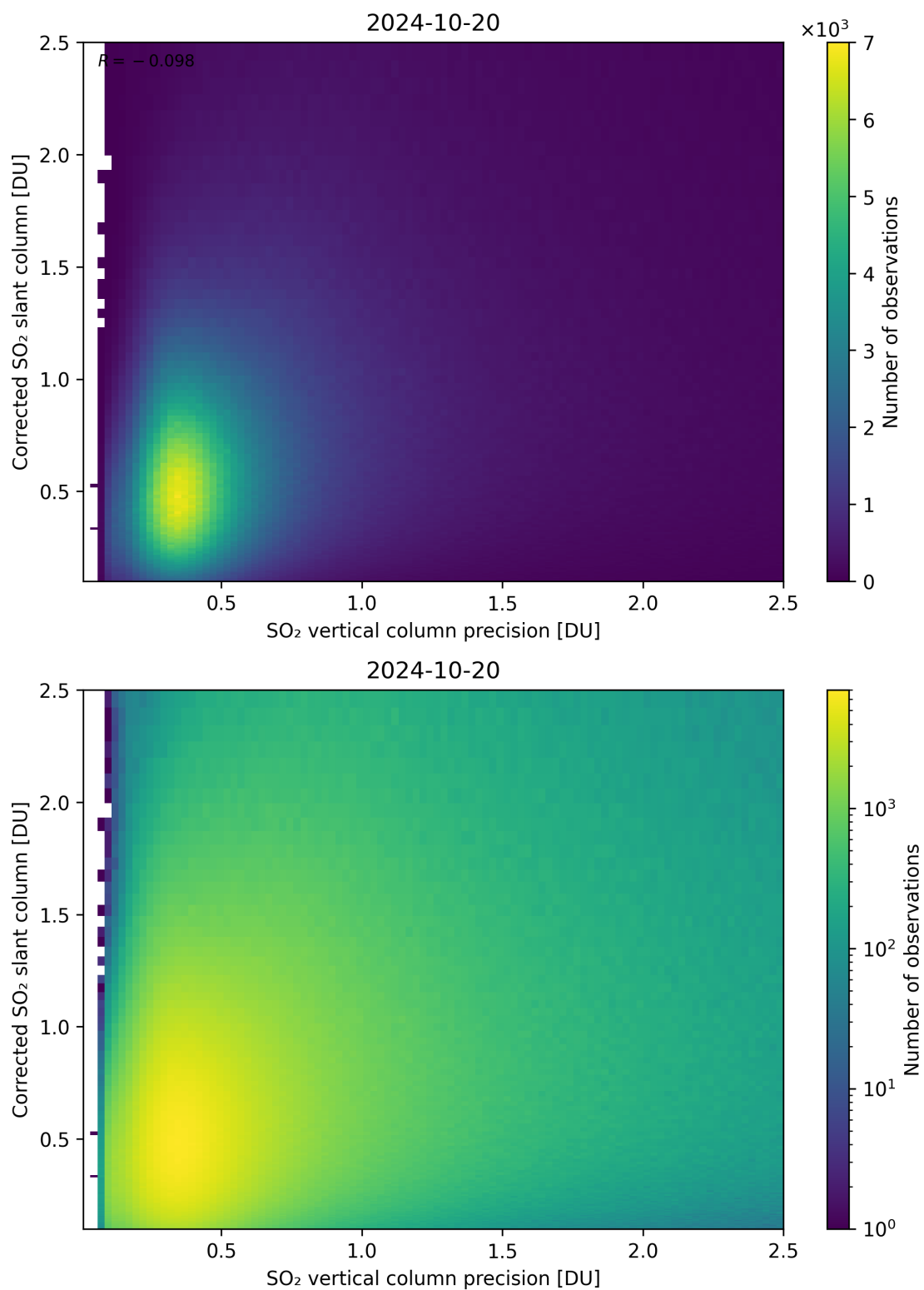
Figure 286: Scatter density plot of “SO 2 vertical column precision” against “Corrected SO 2 slant column” for 2024-10-19 to 2024-10-21.
