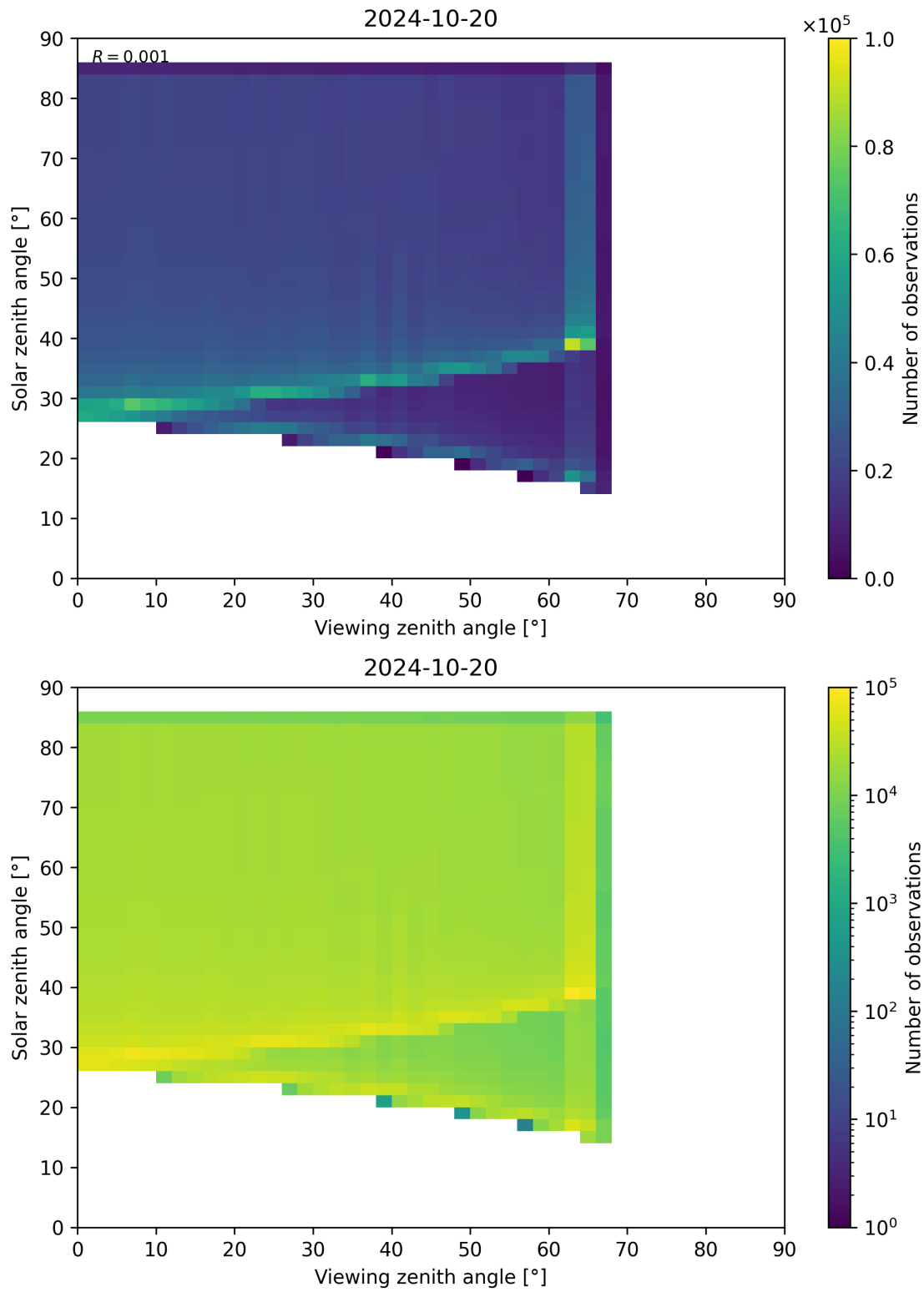
Figure 315: Scatter density plot of “Viewing zenith angle” against “Solar zenith angle” for 2024-10-19 to 2024-10-21.
