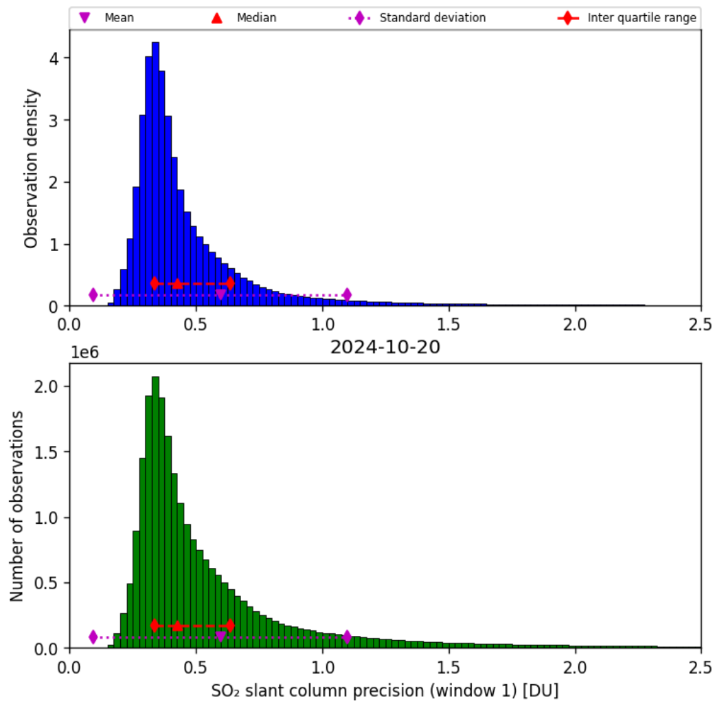
Figure 57: Histogram of “SO 2 slant column precision (window 1)” for 2024-10-19 to 2024-10-21
