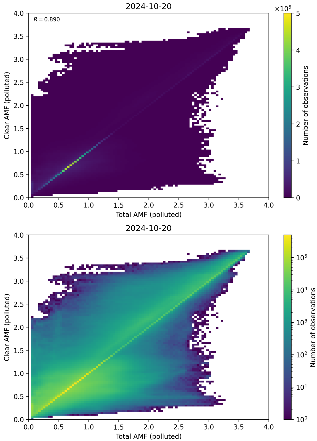
Figure 271: Scatter density plot of “Total AMF (polluted)” against “Clear AMF (polluted)” for 2024-10-19 to 2024-10-21.
