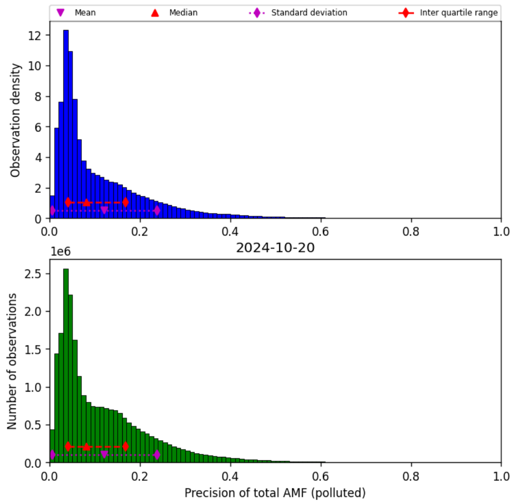
Figure 72: Histogram of “Precision of total AMF (polluted)” for 2024-10-19 to 2024-10-21
