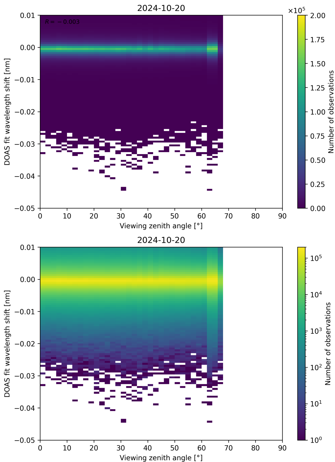
Figure 311: Scatter density plot of “Viewing zenith angle” against “DOAS fit wavelength shift” for 2024-10-19 to 2024-10-21.
