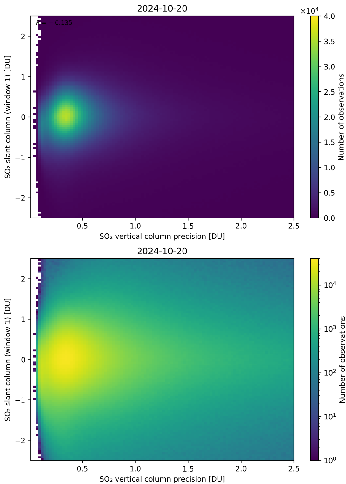
Figure 289: Scatter density plot of “SO 2 vertical column precision” against “SO 2 slant column (window 1)” for 2024-10-19 to 2024-10-21.
