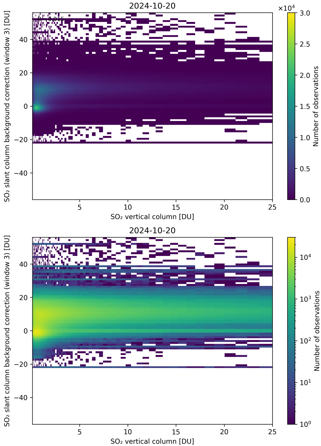
Figure 275: Scatter density plot of “SO 2 vertical column” against “SO 2 slant column background correction (window 3)” for 2024-10-19 to 2024-10-21.
