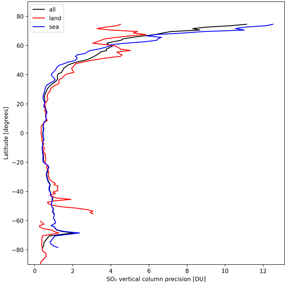
Figure 31: Zonal average of “SO 2 vertical column precision” for 2024-10-19 to 2024-10-21.
