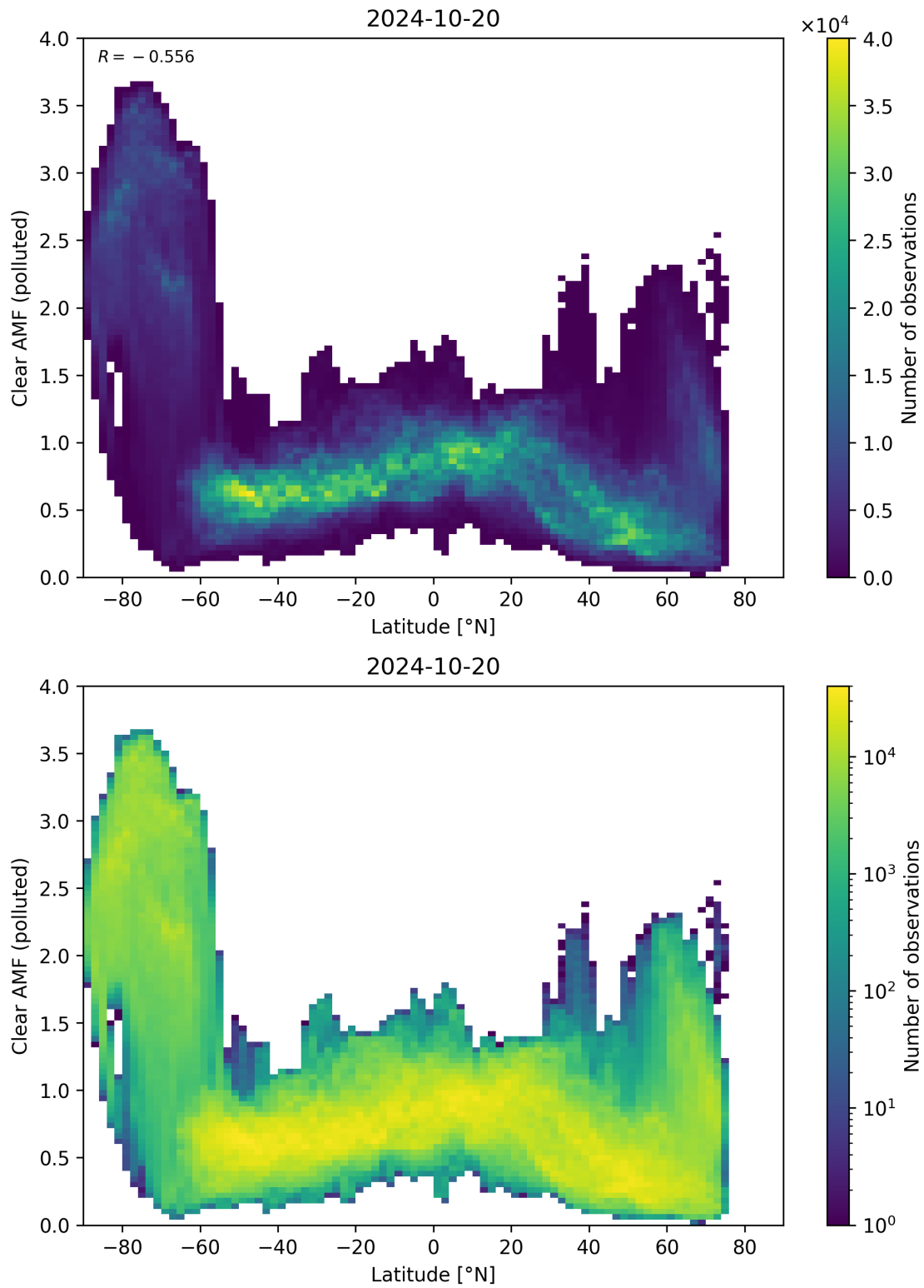
Figure 145: Scatter density plot of “Latitude” against “Clear AMF (polluted)” for 2024-10-19 to 2024-10-21.
