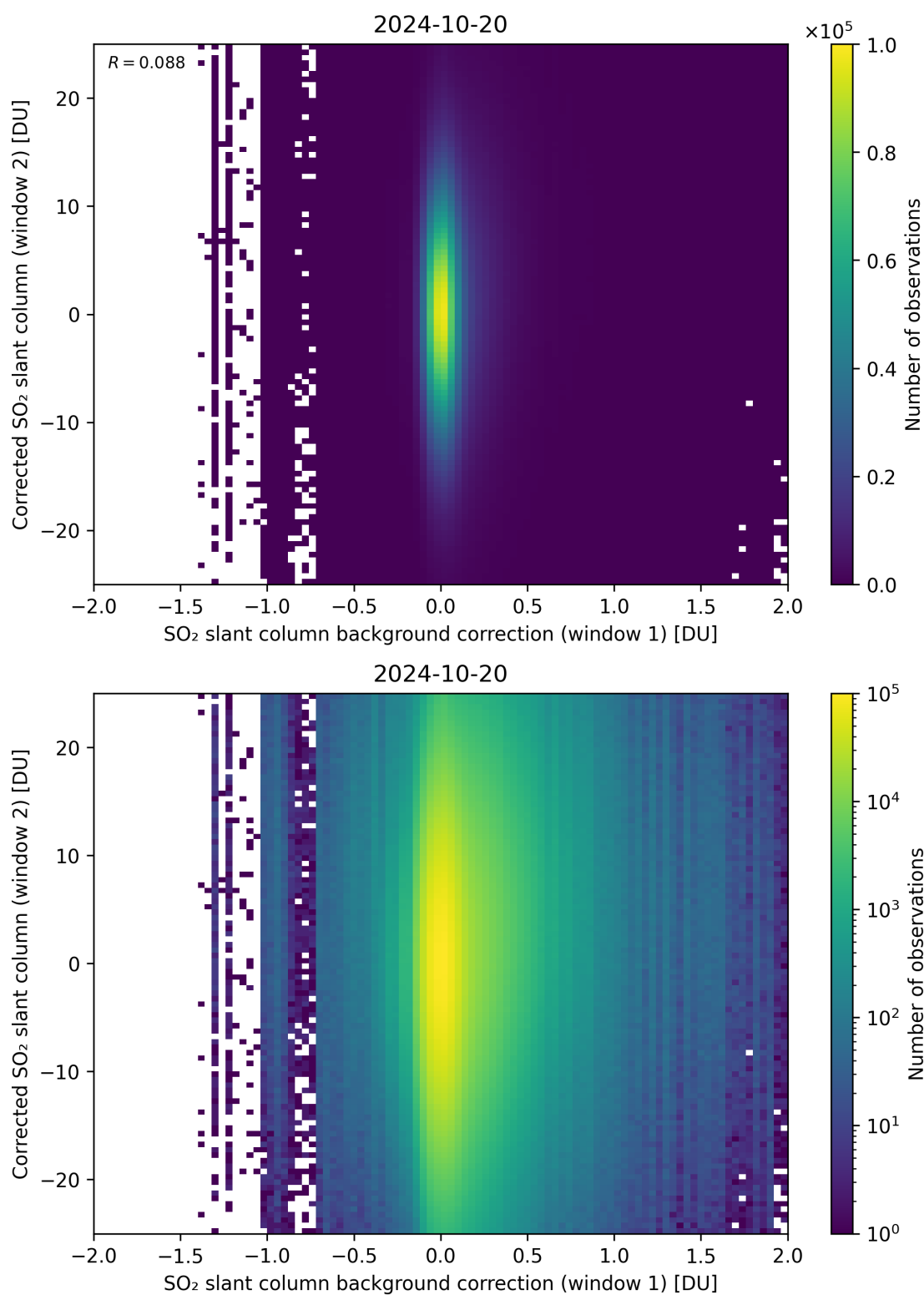
Figure 104: Scatter density plot of “SO 2 slant column background correction (window 1)” against “Corrected SO 2 slant column (window 2)” for 2024-10-19 to 2024-10-21.
