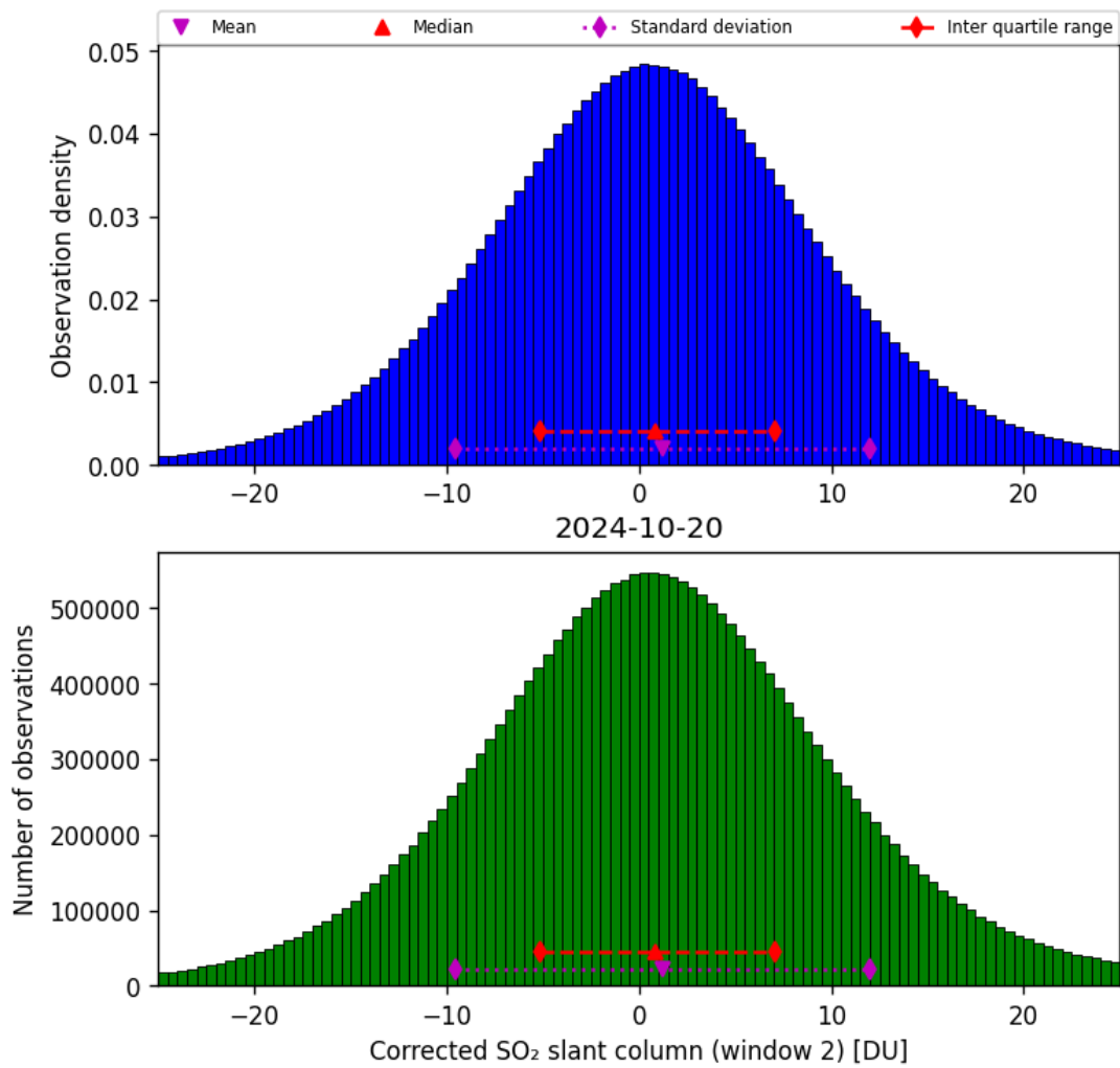
Figure 62: Histogram of “Corrected SO 2 slant column (window 2)” for 2024-10-19 to 2024-10-21
