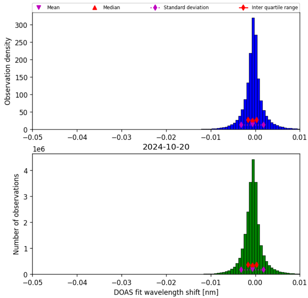
Figure 68: Histogram of “DOAS fit wavelength shift” for 2024-10-19 to 2024-10-21
