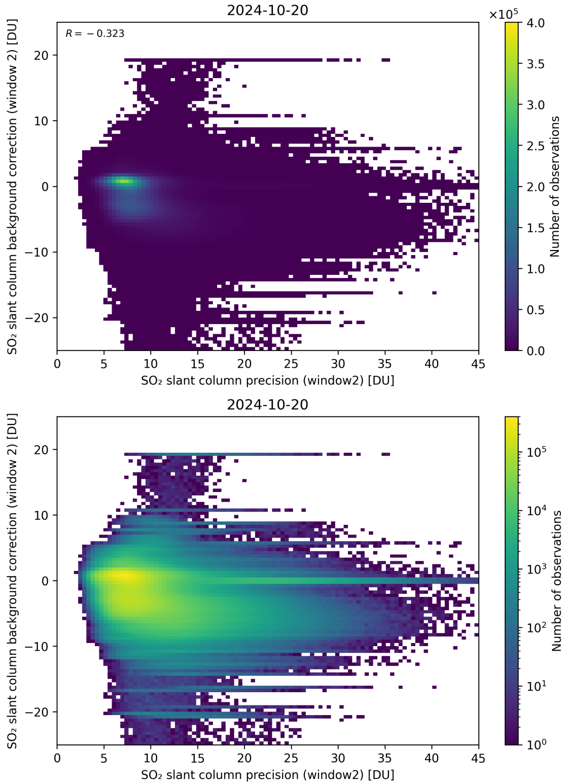
Figure 241: Scatter density plot of “SO 2 slant column precision (window2)” against “SO 2 slant column background correction (window 2)” for 2024-10-19 to 2024-10-21.
