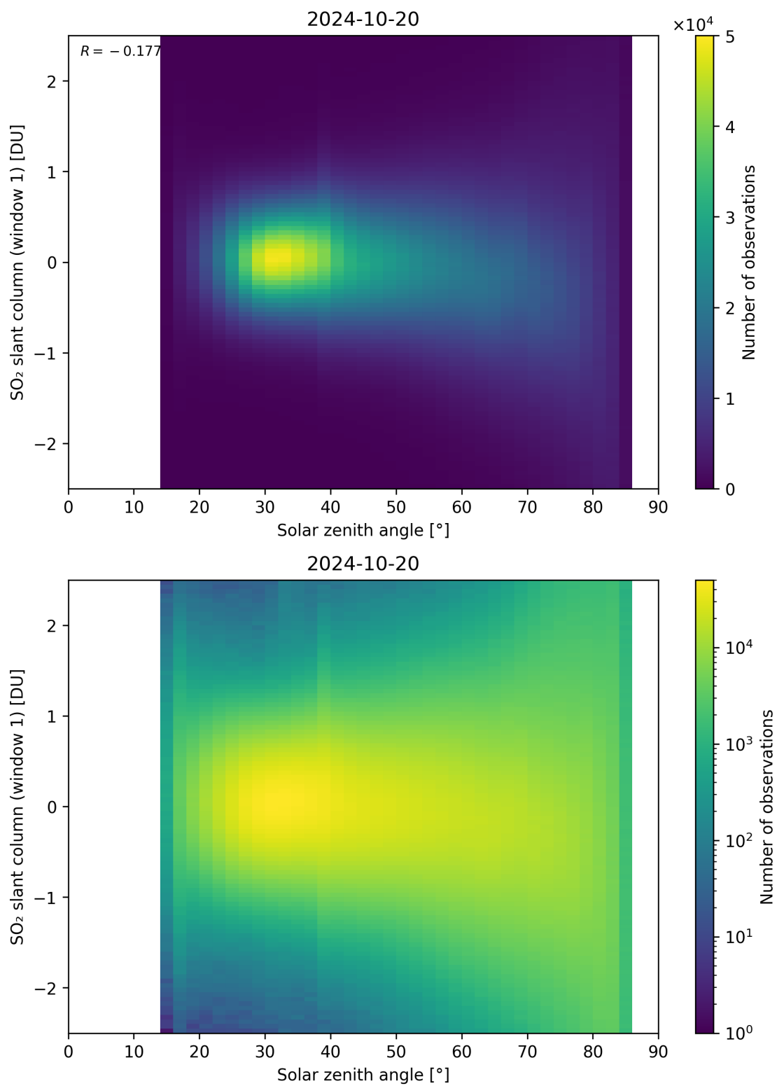
Figure 169: Scatter density plot of “Solar zenith angle” against “SO 2 slant column (window 1)” for 2024-10-19 to 2024-10-21.
