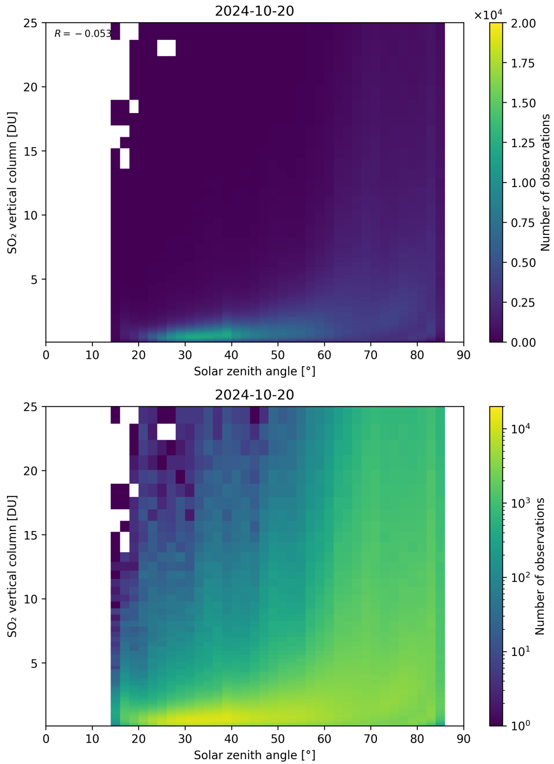
Figure 176: Scatter density plot of “Solar zenith angle” against “SO 2 vertical column” for 2024-10-19 to 2024-10-21.
