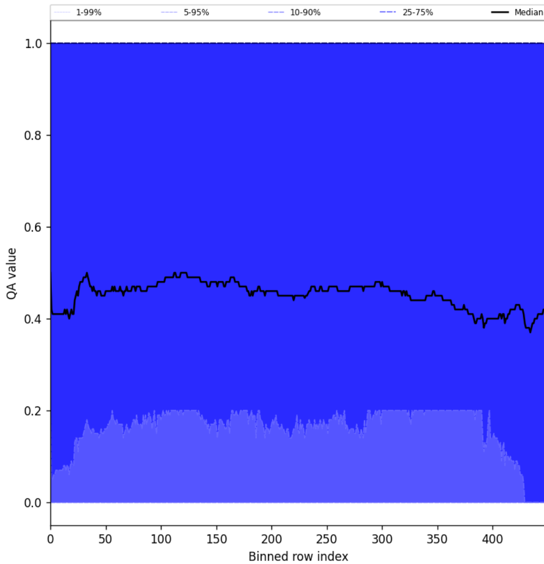
Figure 75: Along track statistics of “QA value” for 2024-10-19 to 2024-10-21
