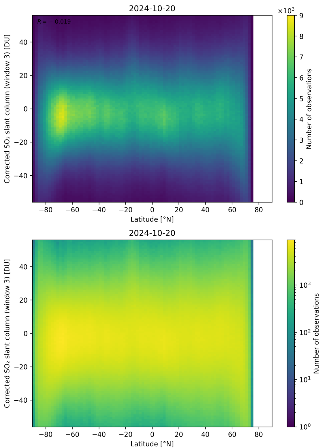
Figure 148: Scatter density plot of “Latitude” against “Corrected SO 2 slant column (window 3)” for 2024-10-19 to 2024-10-21.
