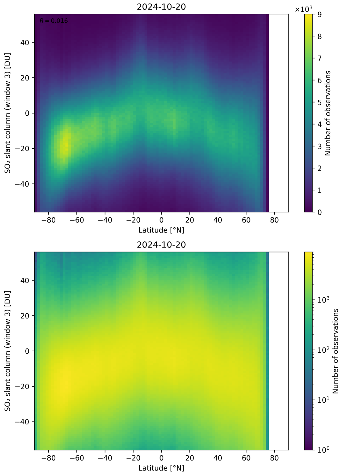
Figure 152: Scatter density plot of “Latitude” against “SO 2 slant column (window 3)” for 2024-10-19 to 2024-10-21.
