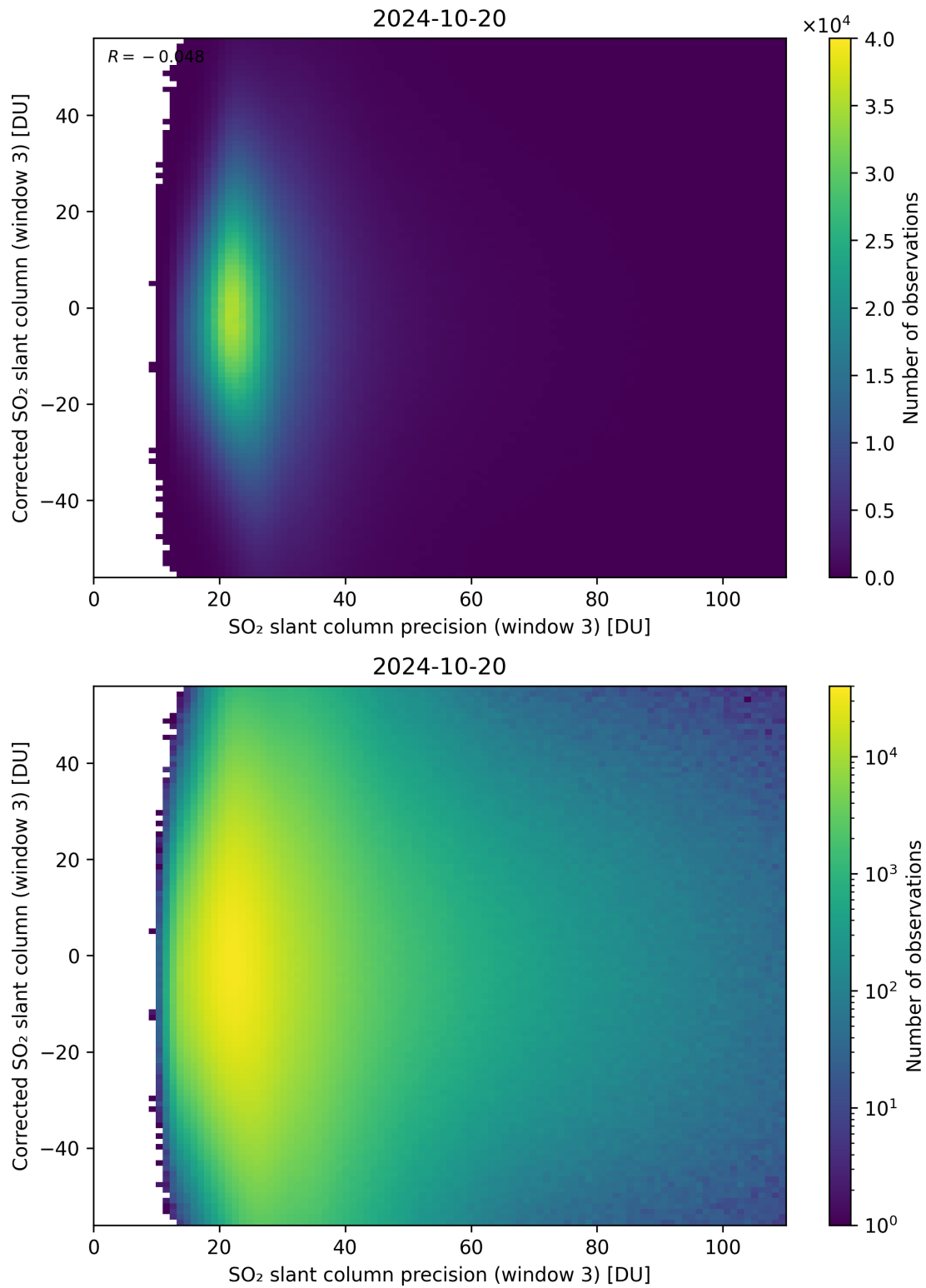
Figure 262: Scatter density plot of “SO 2 slant column precision (window 3)” against “Corrected SO 2 slant column (window 3)” for 2024-10-19 to 2024-10-21.
