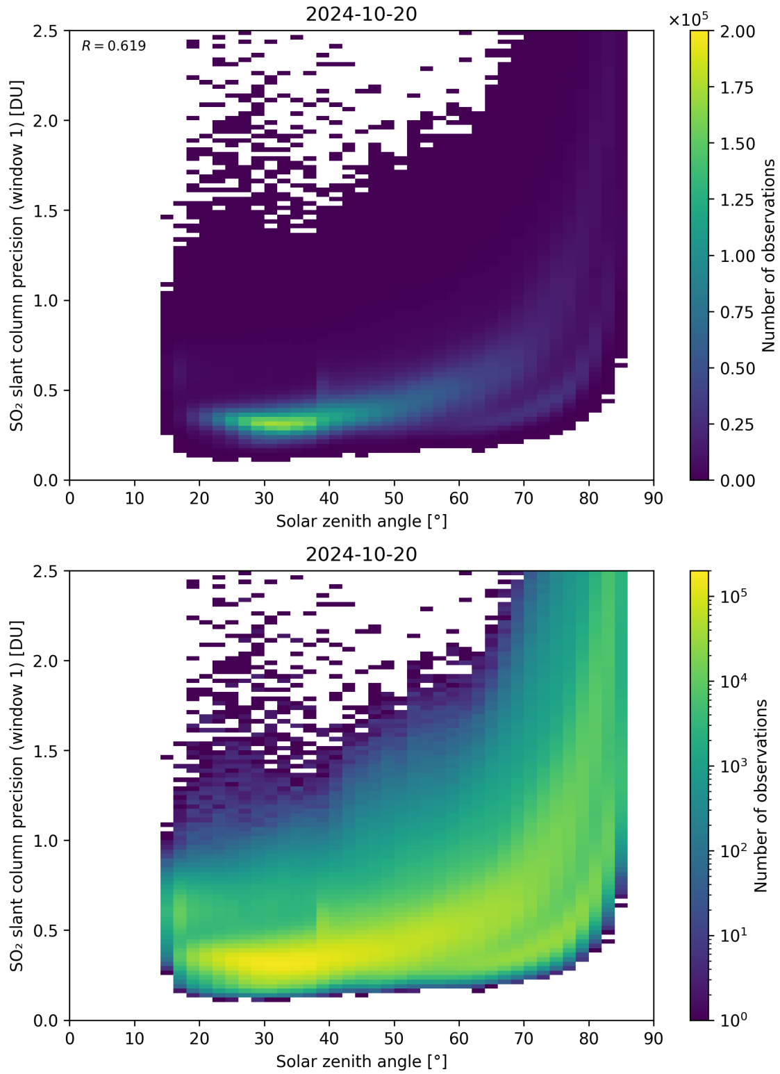
Figure 170: Scatter density plot of “Solar zenith angle” against “SO 2 slant column precision (window 1)” for 2024-10-19 to 2024-10-21.
