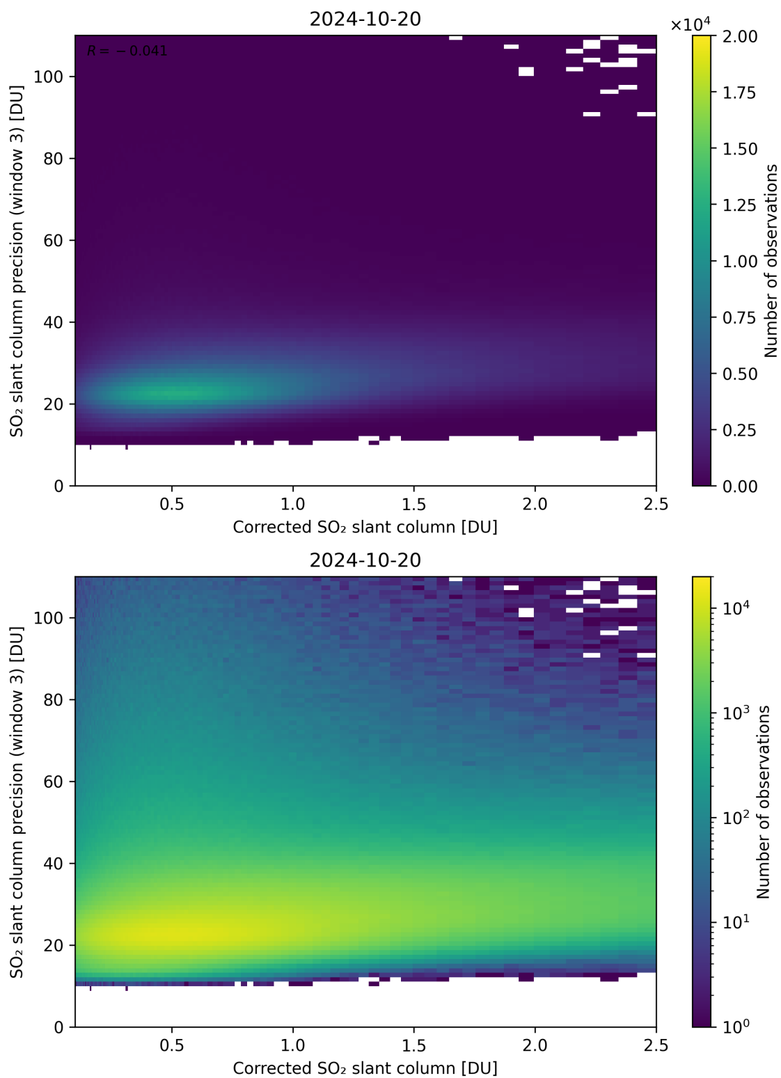
Figure 191: Scatter density plot of “Corrected SO 2 slant column” against “SO 2 slant column precision (window 3)” for 2024-10-19 to 2024-10-21.
