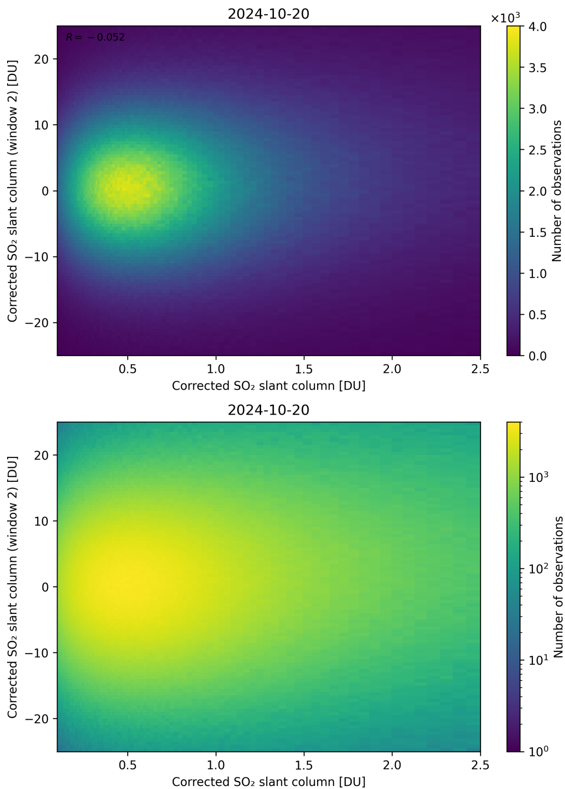
Figure 185: Scatter density plot of “Corrected SO 2 slant column” against “Corrected SO 2 slant column (window 2)” for 2024-10-19 to 2024-10-21.
