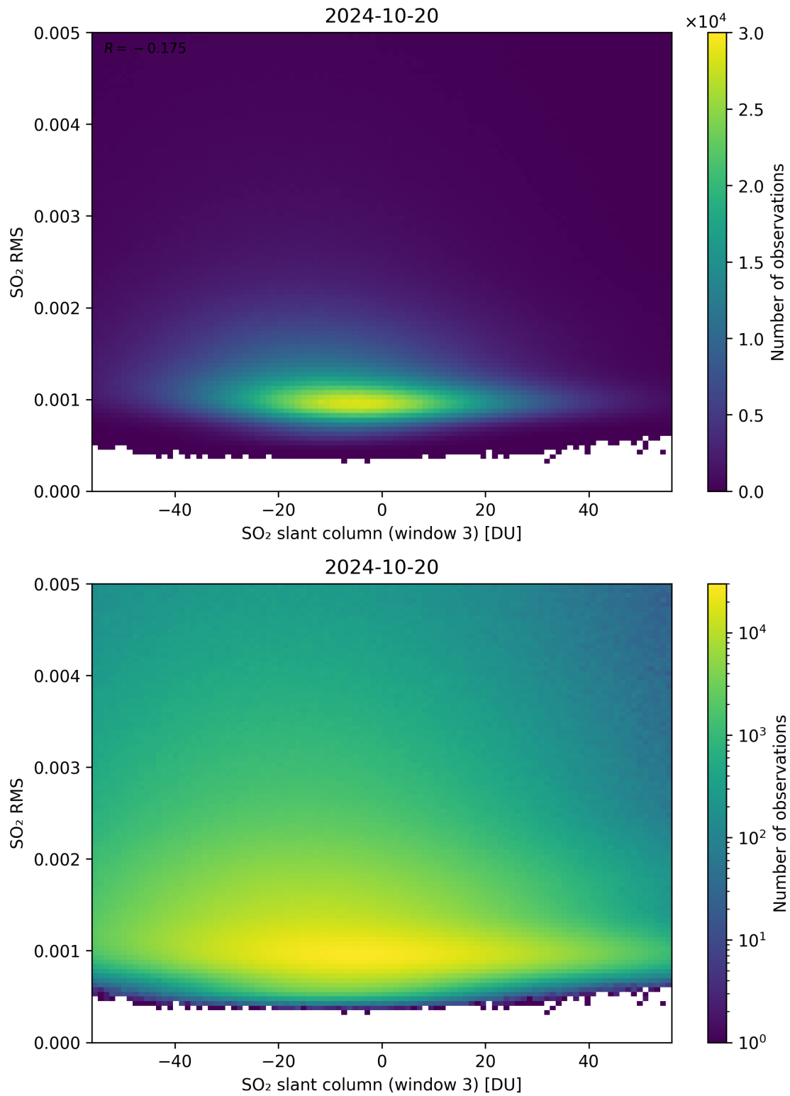
Figure 256: Scatter density plot of “SO 2 slant column (window 3)” against “SO 2 RMS” for 2024-10-19 to 2024-10-21.
