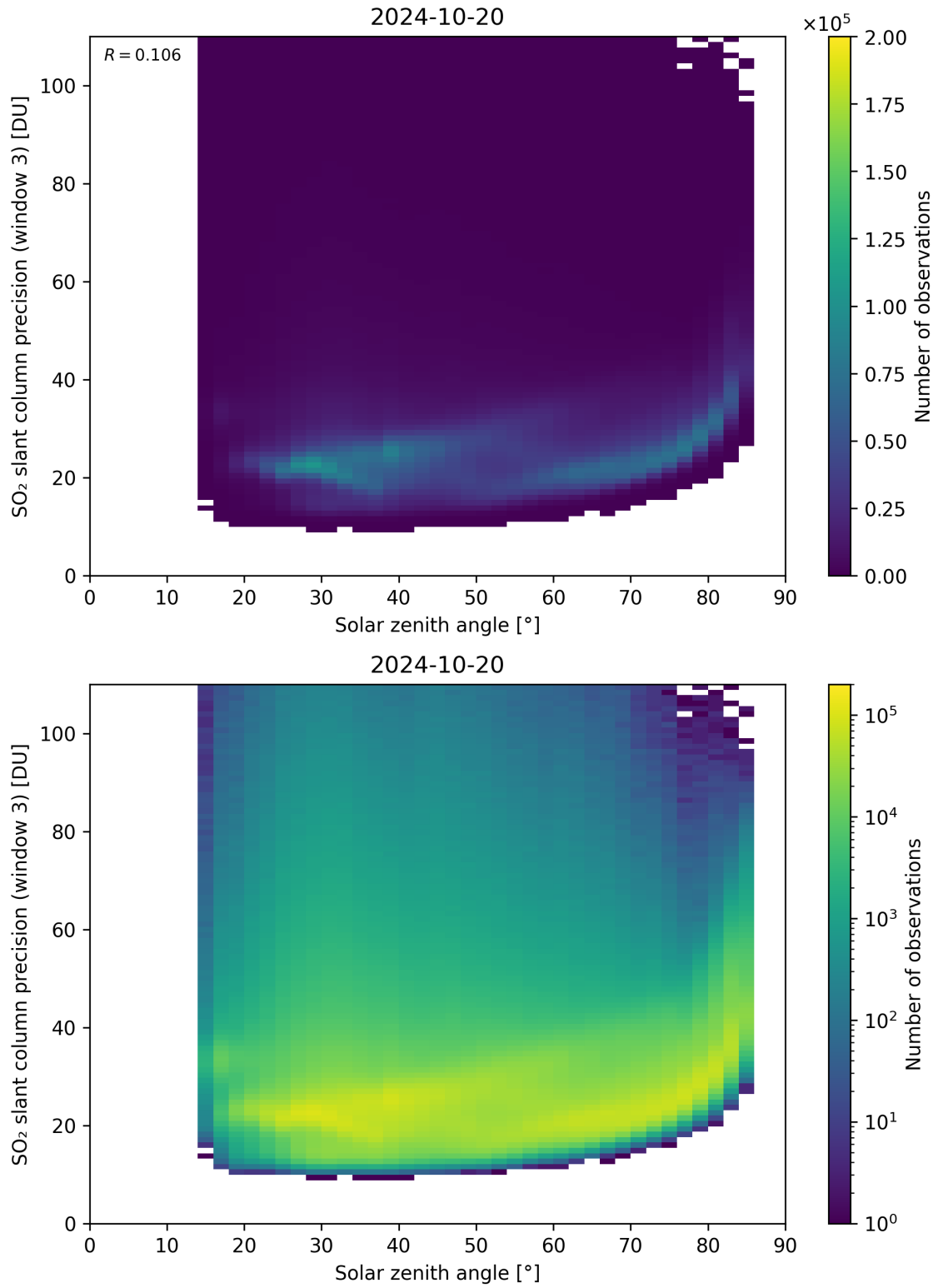
Figure 173: Scatter density plot of “Solar zenith angle” against “SO 2 slant column precision (window 3)” for 2024-10-19 to 2024-10-21.
