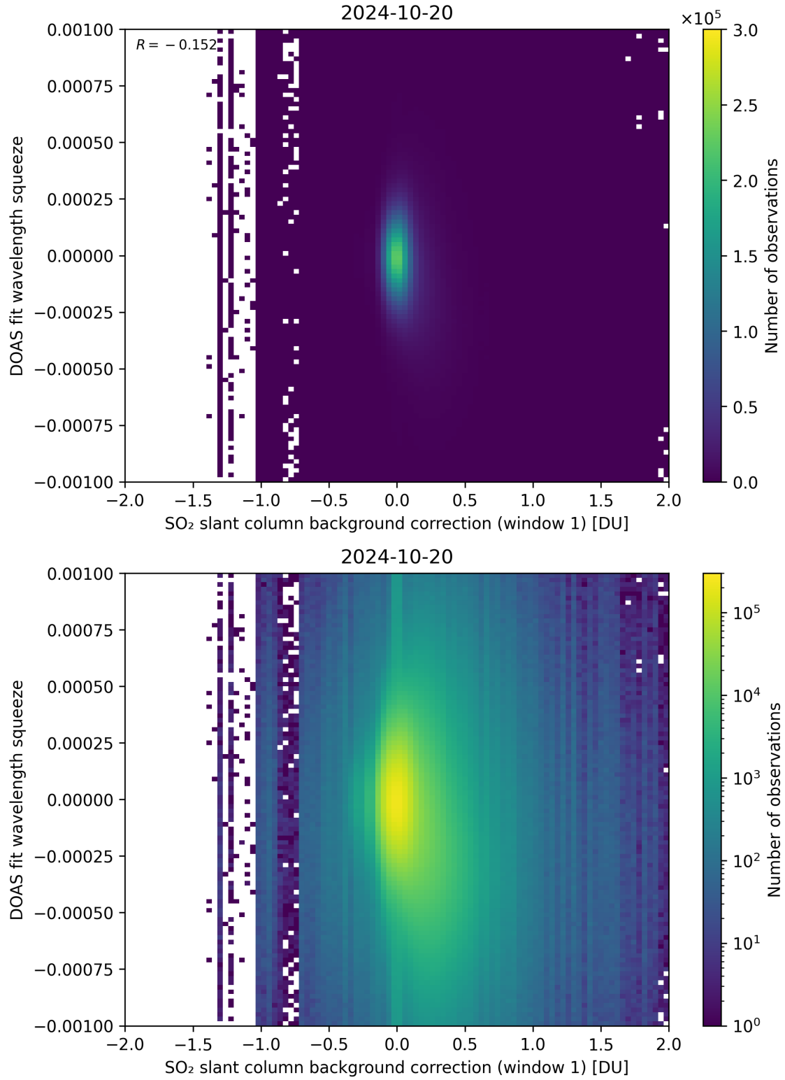
Figure 101: Scatter density plot of “SO 2 slant column background correction (window 1)” against “DOAS fit wavelength squeeze” for 2024-10-19 to 2024-10-21.
