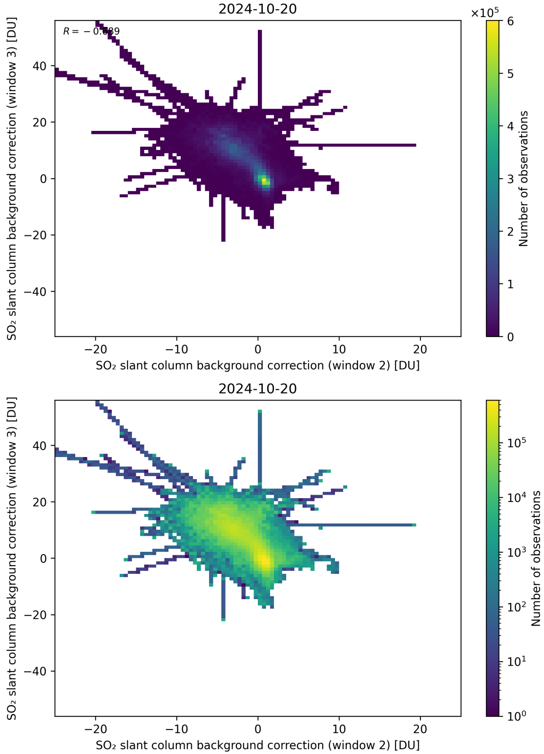
Figure 111: Scatter density plot of “SO 2 slant column background correction (window 2)” against “SO 2 slant column background correction (window 3)” for 2024-10-19 to 2024-10-21.
