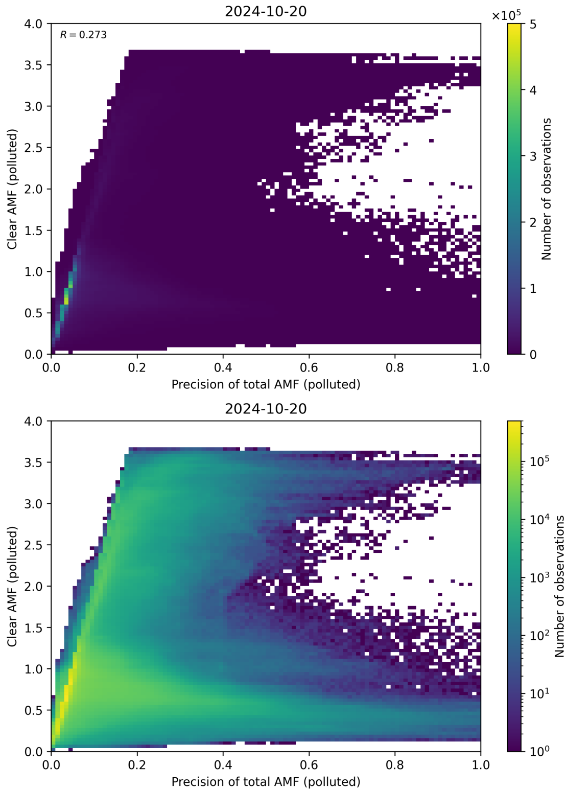
Figure 270: Scatter density plot of “Precision of total AMF (polluted)” against “Clear AMF (polluted)” for 2024-10-19 to 2024-10-21.
