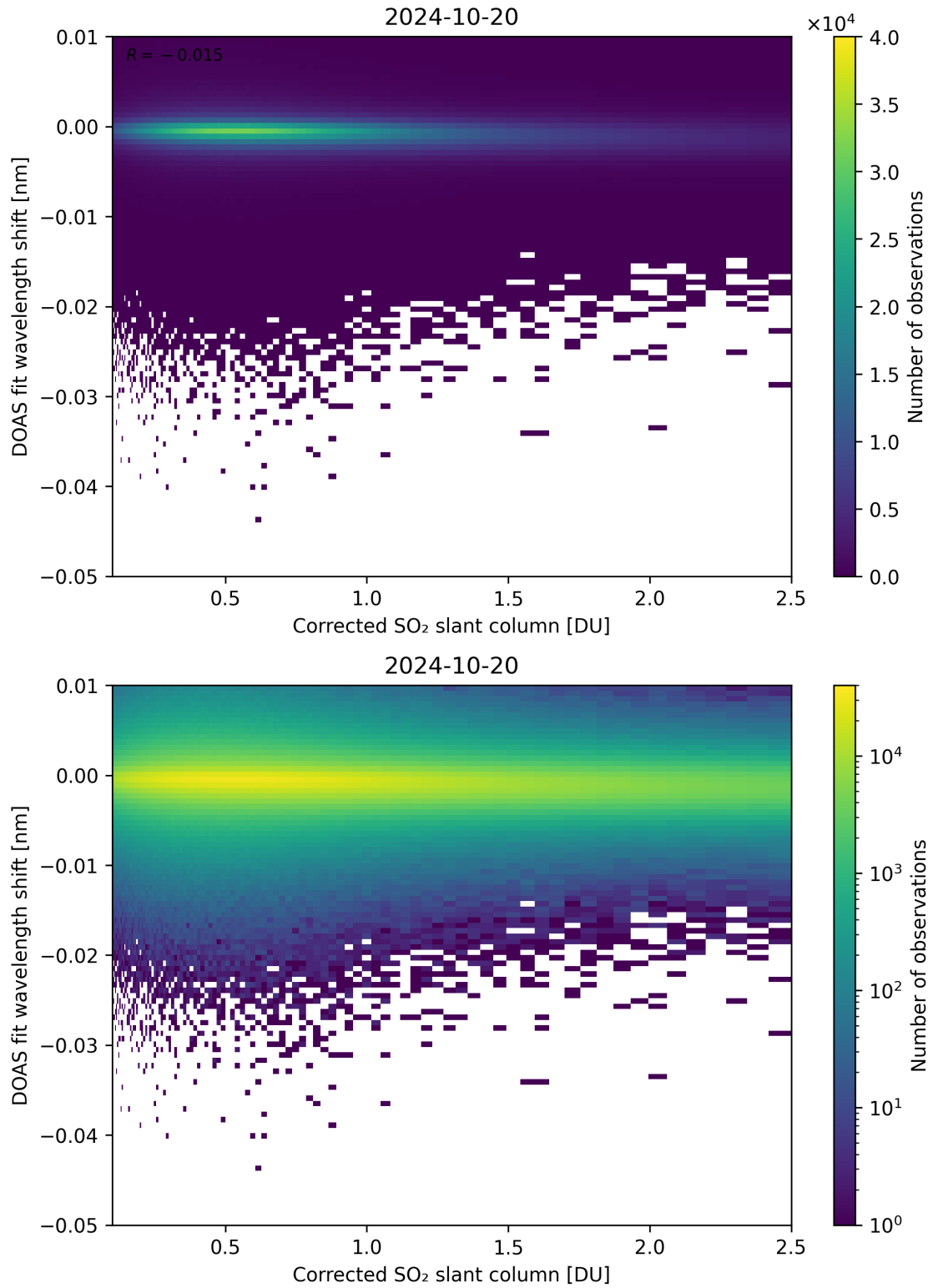
Figure 181: Scatter density plot of “Corrected SO 2 slant column” against “DOAS fit wavelength shift” for 2024-10-19 to 2024-10-21.
