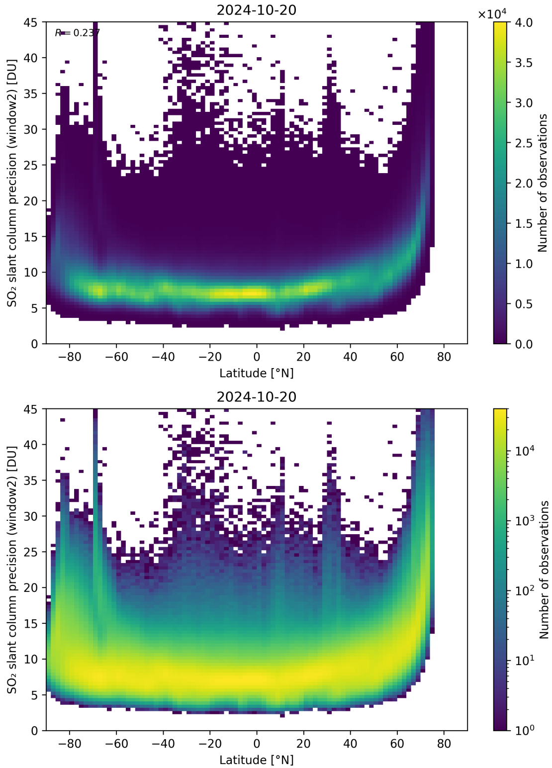
Figure 151: Scatter density plot of “Latitude” against “SO 2 slant column precision (window2)” for 2024-10-19 to 2024-10-21.
