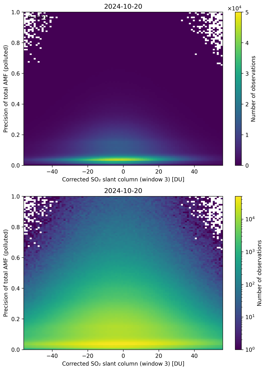
Figure 211: Scatter density plot of “Corrected SO 2 slant column (window 3)” against “Precision of total AMF (polluted)” for 2024-10-19 to 2024-10-21.
