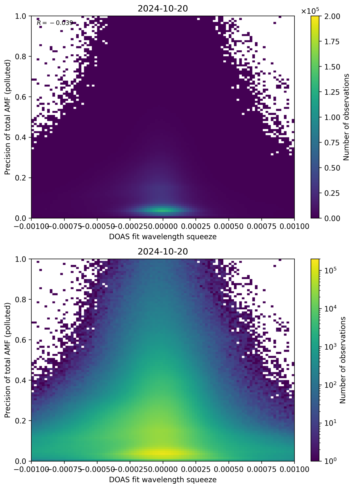
Figure 135: Scatter density plot of “DOAS fit wavelength squeeze” against “Precision of total AMF (polluted)” for 2024-10-19 to 2024-10-21.
