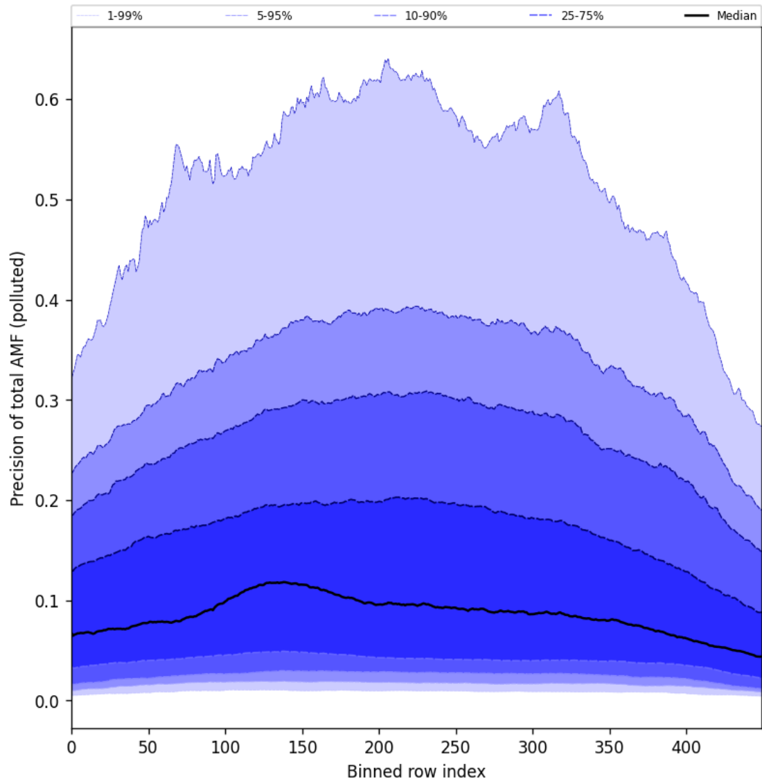
Figure 95: Along track statistics of “Precision of total AMF (polluted)” for 2024-10-19 to 2024-10-21
