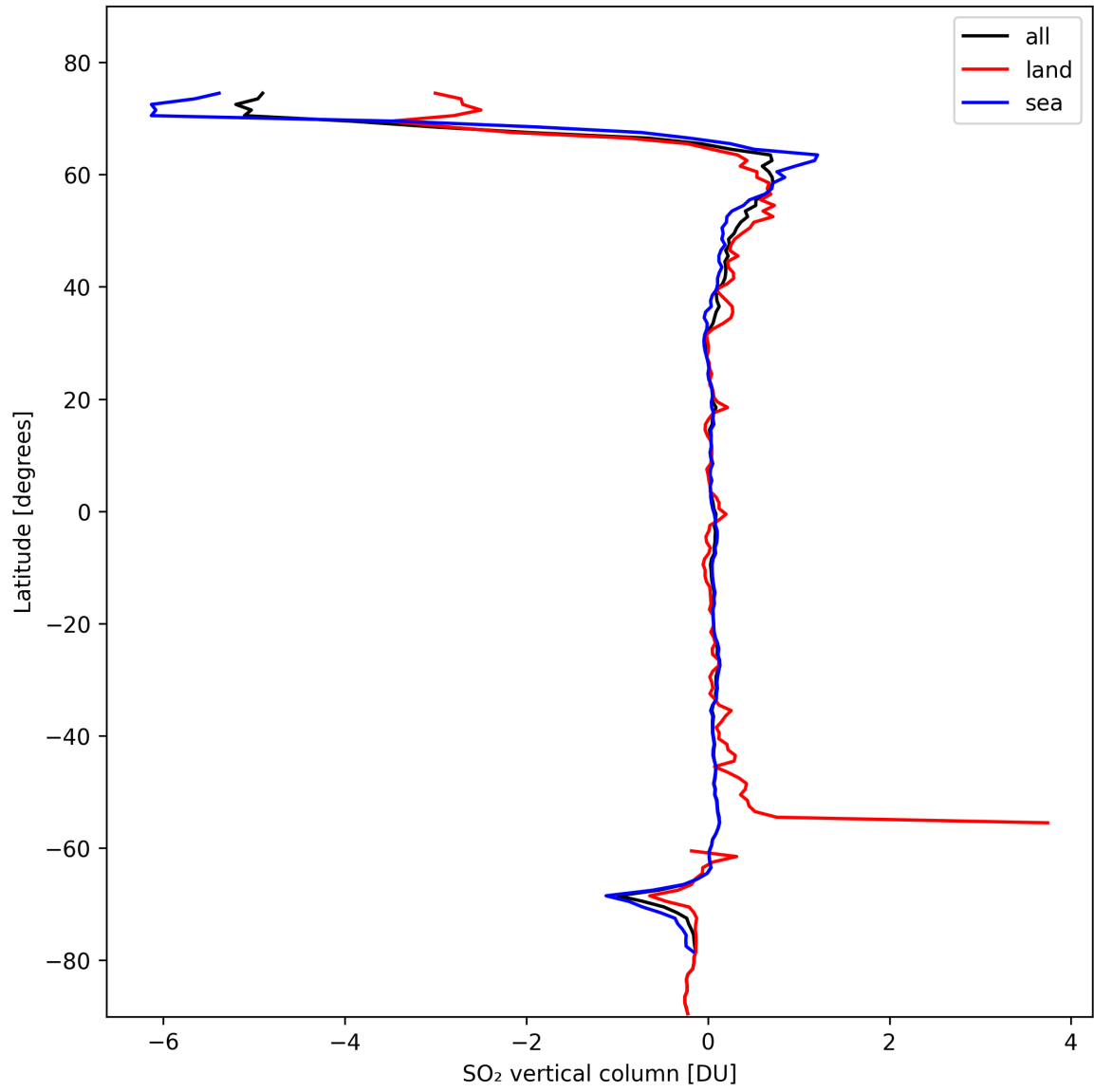
Figure 30: Zonal average of “SO 2 vertical column” for 2024-10-19 to 2024-10-21.
