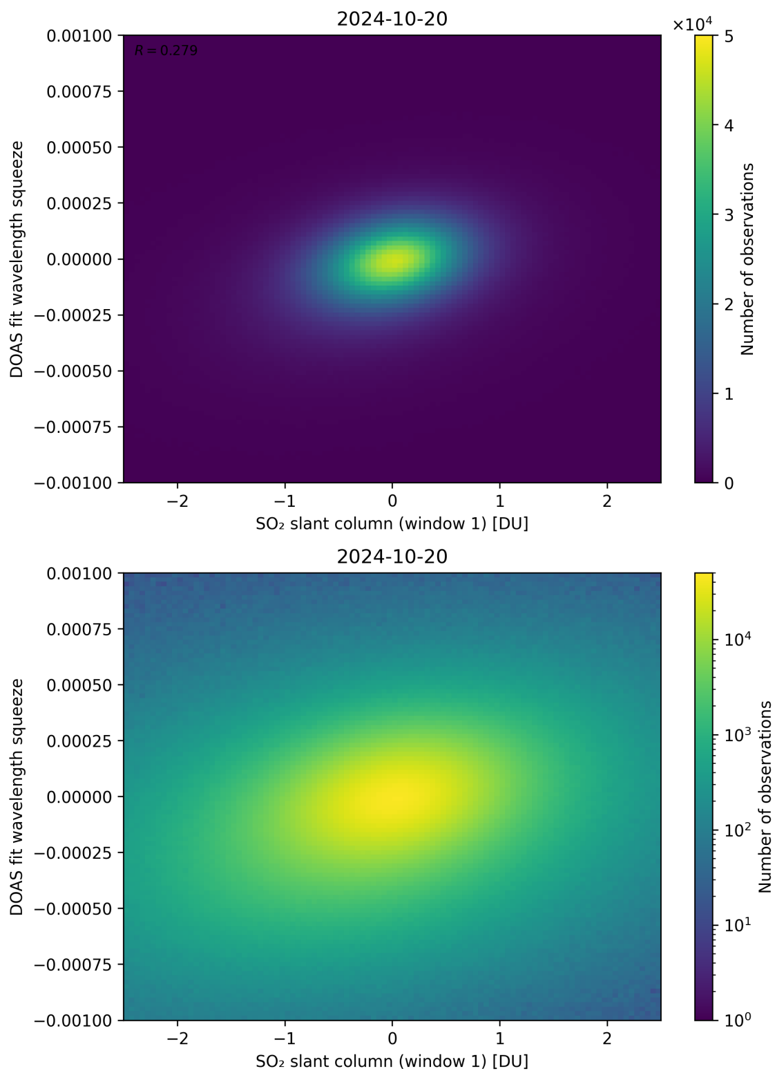
Figure 216: Scatter density plot of “SO 2 slant column (window 1)” against “DOAS fit wavelength squeeze” for 2024-10-19 to 2024-10-21.
