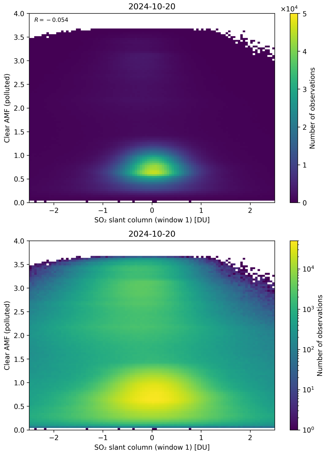
Figure 232: Scatter density plot of “SO 2 slant column (window 1)” against “Clear AMF (polluted)” for 2024-10-19 to 2024-10-21.
