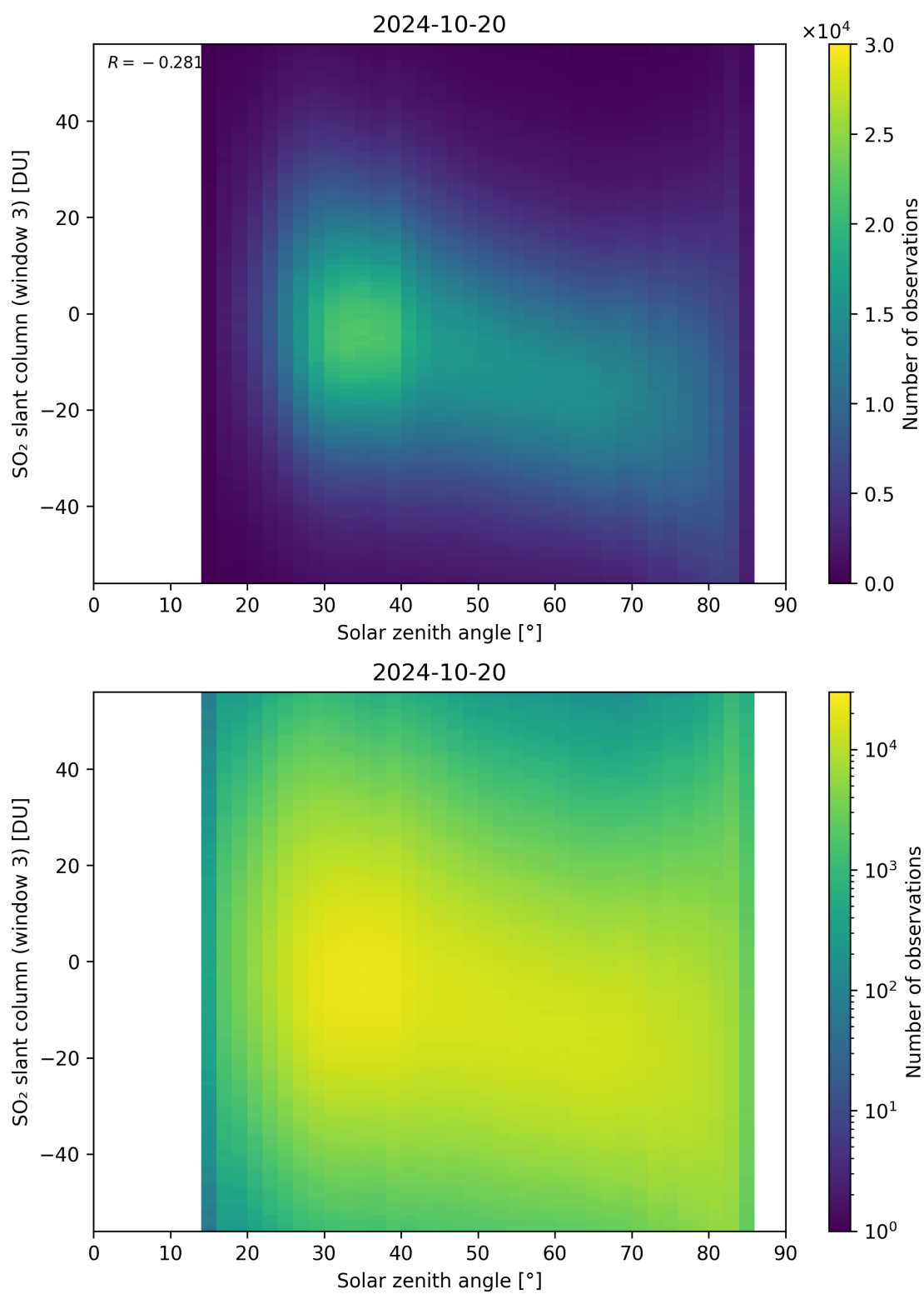
Figure 172: Scatter density plot of “Solar zenith angle” against “SO 2 slant column (window 3)” for 2024-10-19 to 2024-10-21.
