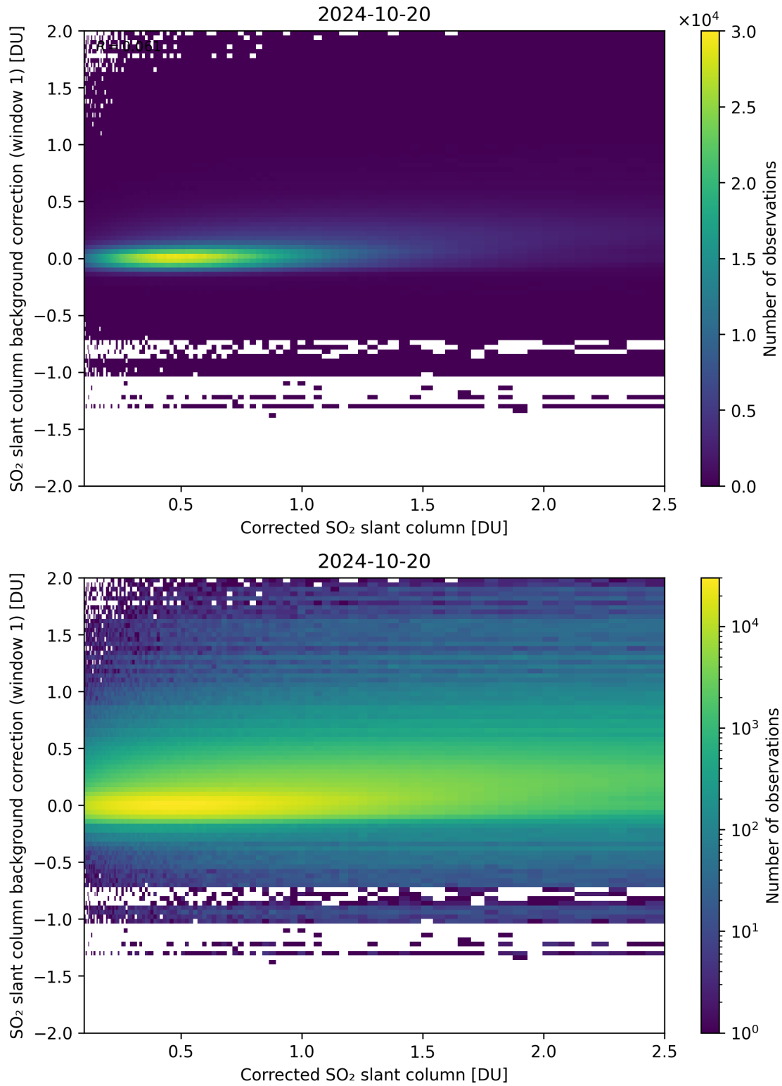
Figure 178: Scatter density plot of “Corrected SO 2 slant column” against “SO 2 slant column background correction (window 1)” for 2024-10-19 to 2024-10-21.
