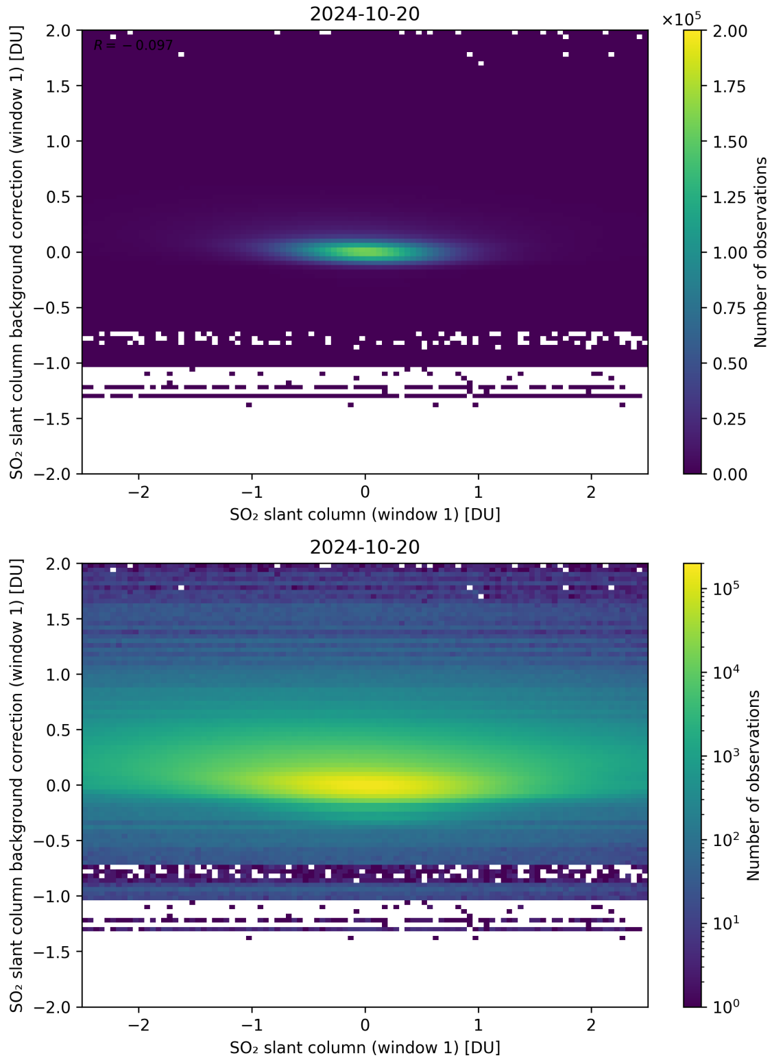
Figure 212: Scatter density plot of “SO 2 slant column (window 1)” against “SO 2 slant column background correction (window 1)” for 2024-10-19 to 2024-10-21.
