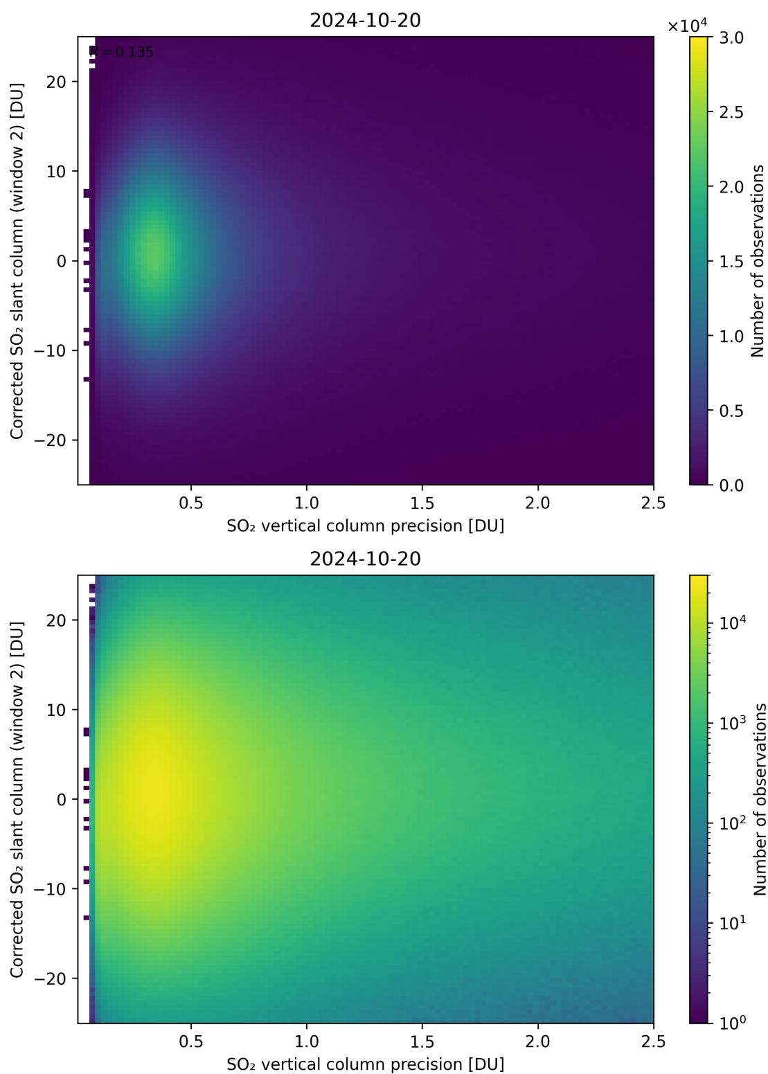
Figure 287: Scatter density plot of “SO 2 vertical column precision” against “Corrected SO 2 slant column (window 2)” for 2024-10-19 to 2024-10-21.
