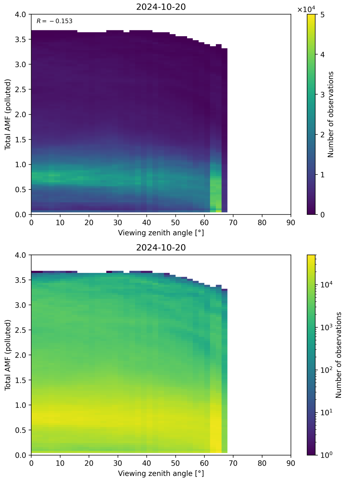
Figure 325: Scatter density plot of “Viewing zenith angle” against “Total AMF (polluted)” for 2024-10-19 to 2024-10-21.
