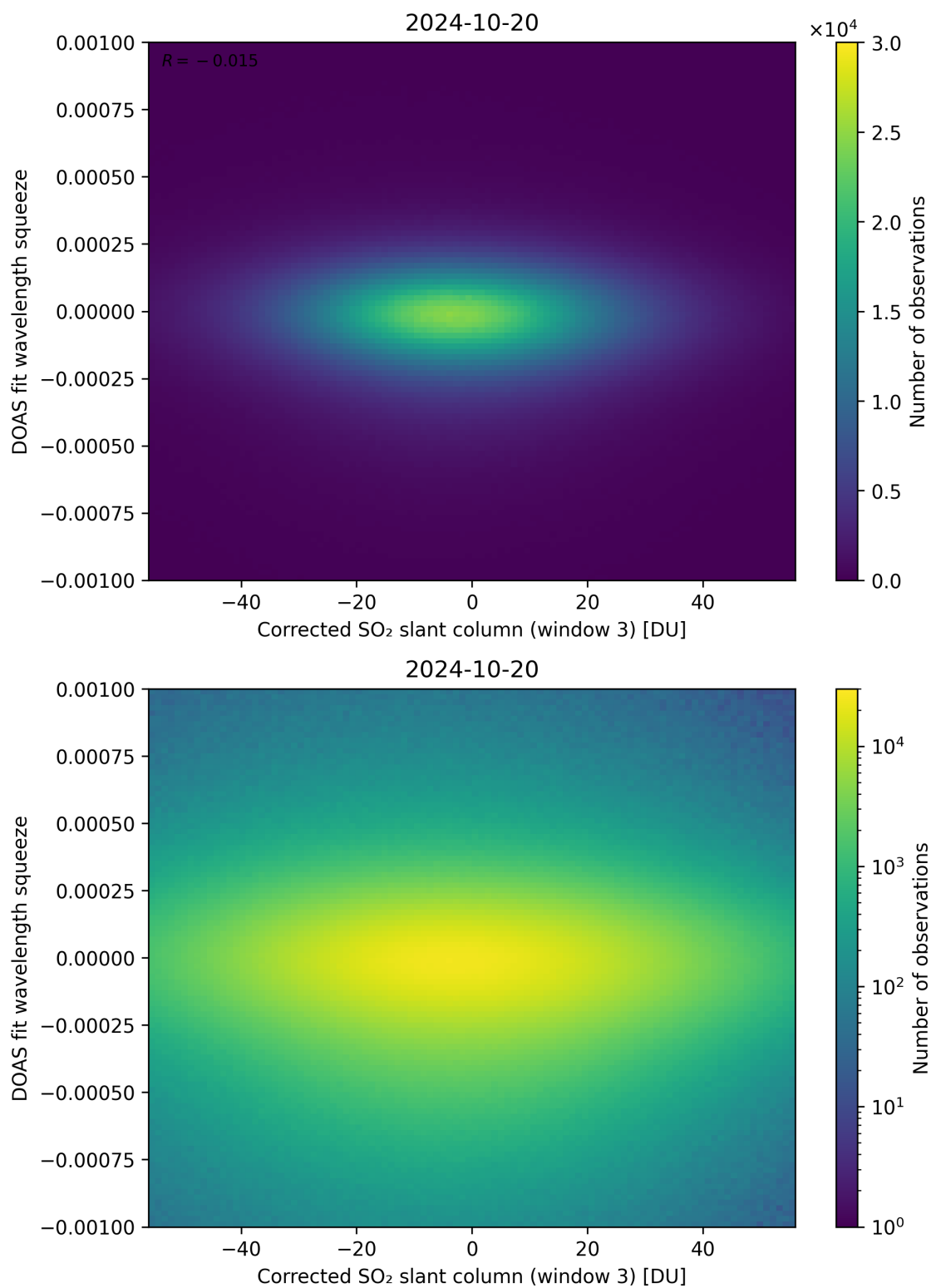
Figure 207: Scatter density plot of “Corrected SO 2 slant column (window 3)” against “DOAS fit wavelength squeeze” for 2024-10-19 to 2024-10-21.
