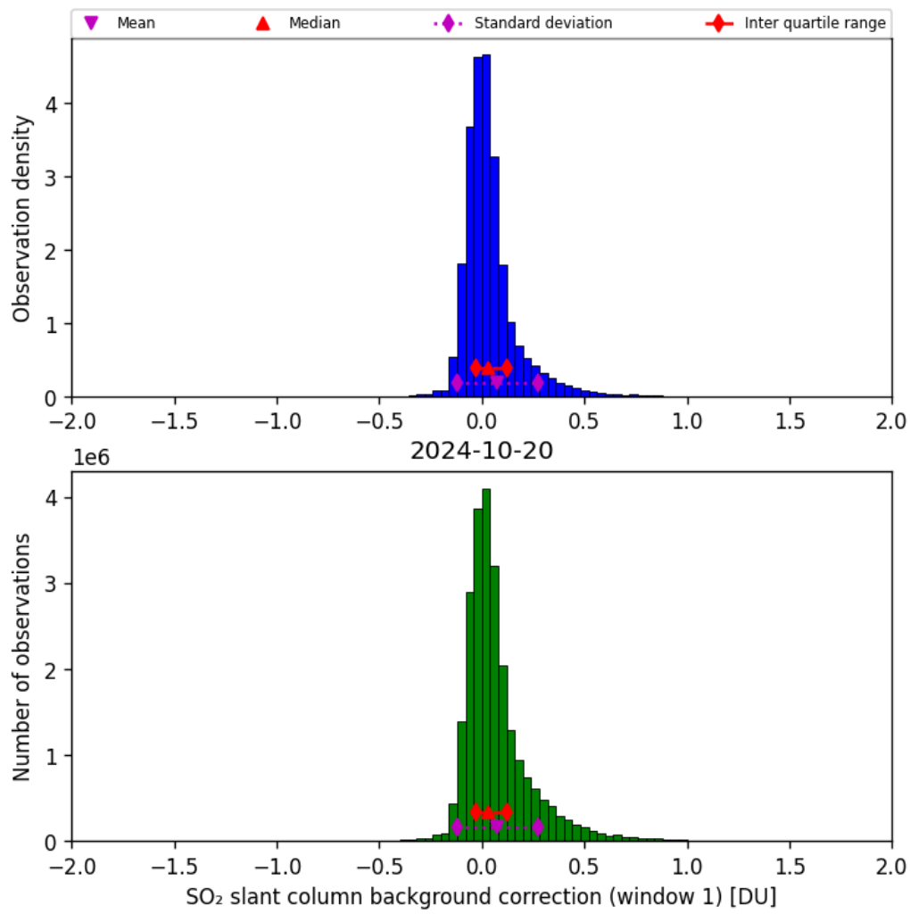
Figure 59: Histogram of “SO 2 slant column background correction (window 1)” for 2024-10-19 to 2024-10-21
