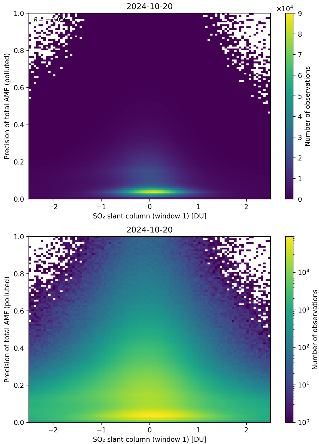
Figure 240: Scatter density plot of “SO 2 slant column (window 1)” against “Precision of total AMF (polluted)” for 2024-10-19 to 2024-10-21.
