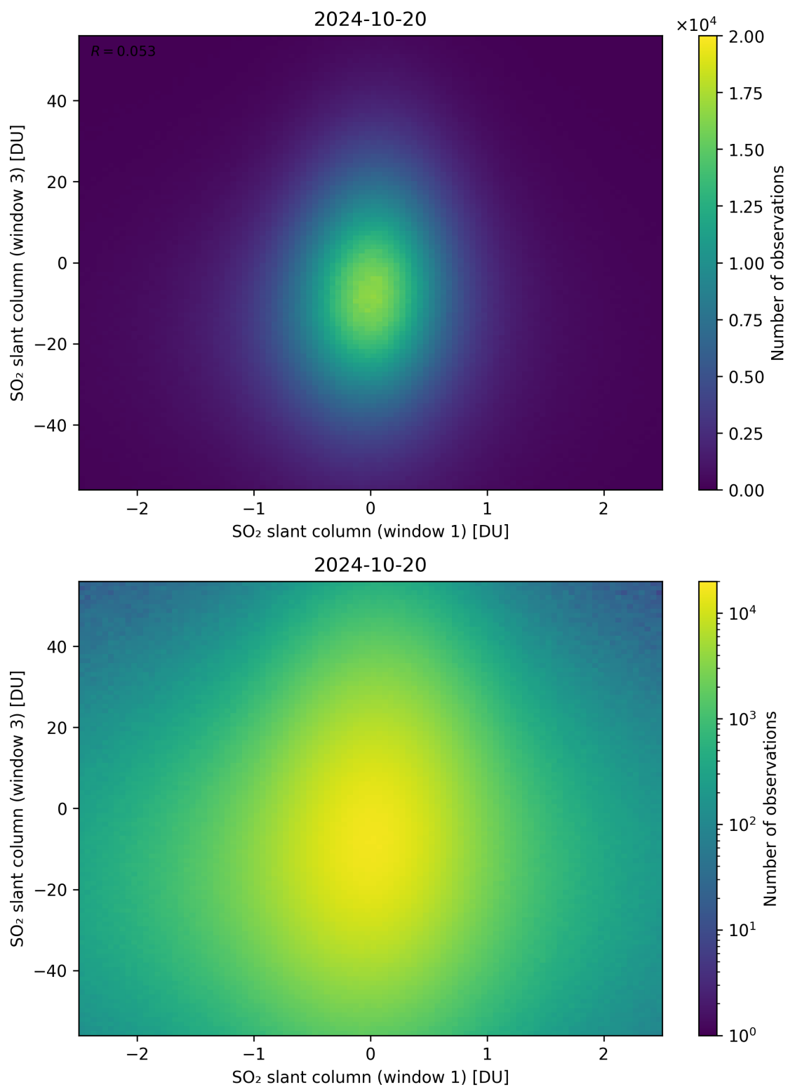
Figure 237: Scatter density plot of “SO 2 slant column (window 1)” against “SO 2 slant column (window 3)” for 2024-10-19 to 2024-10-21.
