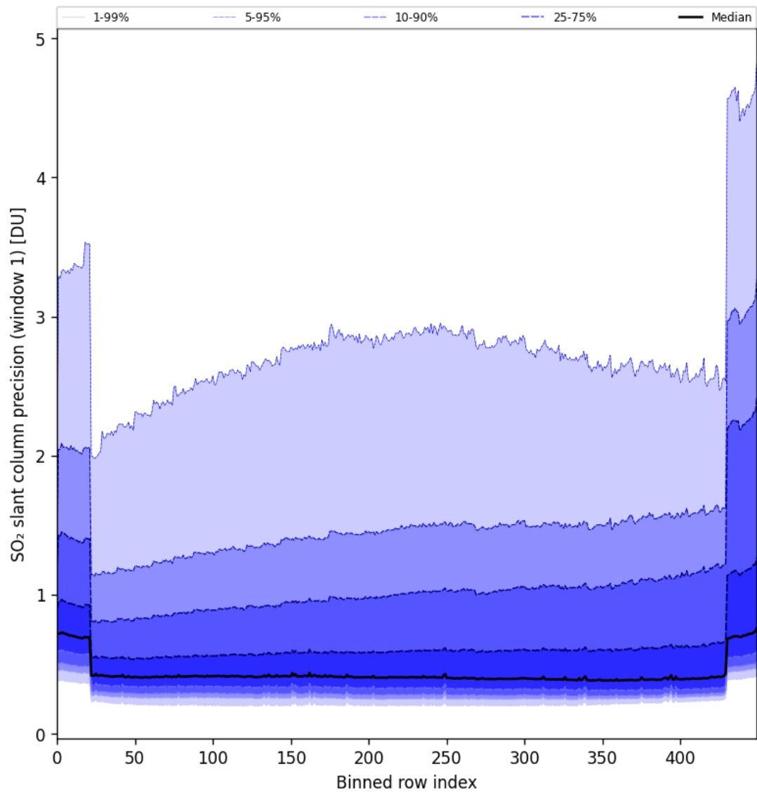
Figure 80: Along track statistics of “SO 2 slant column precision (window 1)” for 2024-10-19 to 2024-10-21
