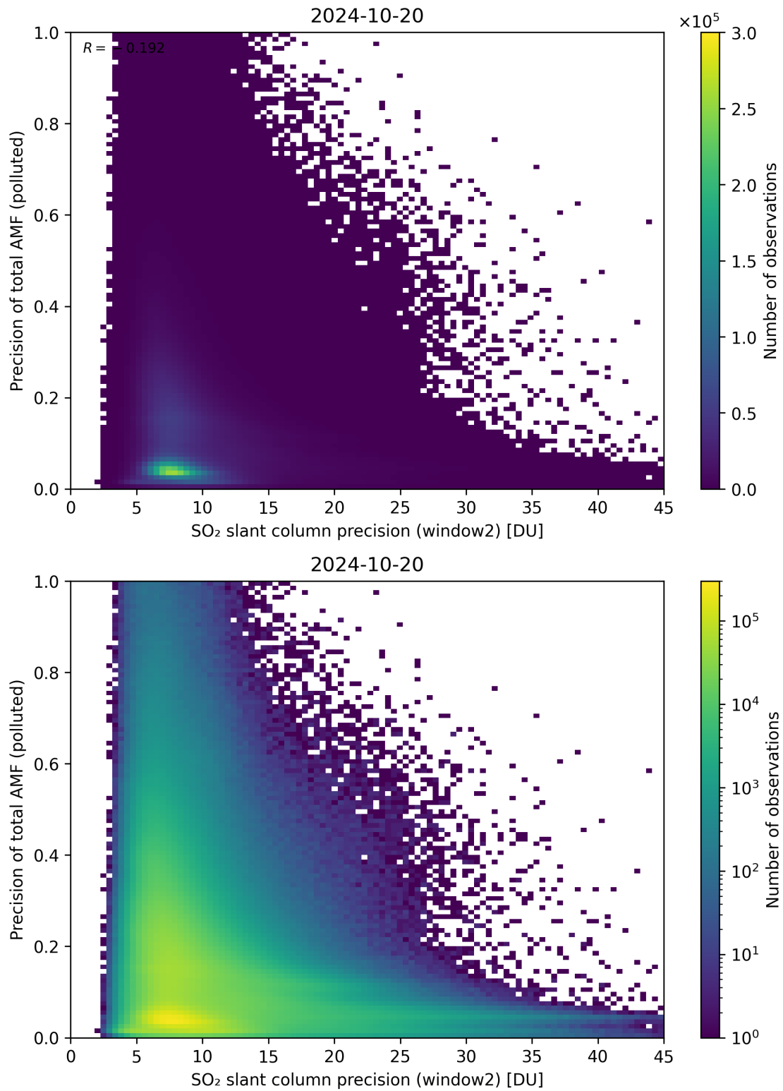
Figure 252: Scatter density plot of “SO 2 slant column precision (window2)” against “Precision of total AMF (polluted)” for 2024-10-19 to 2024-10-21.
