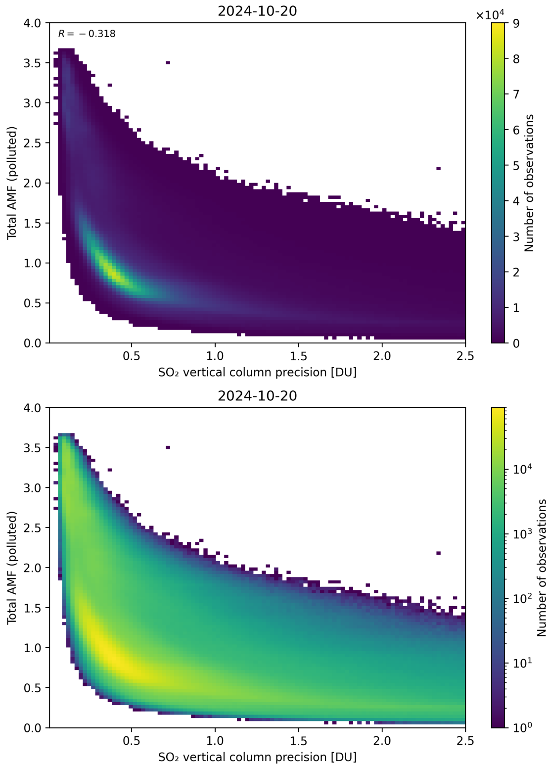
Figure 294: Scatter density plot of “SO 2 vertical column precision” against “Total AMF (polluted)” for 2024-10-19 to 2024-10-21.
