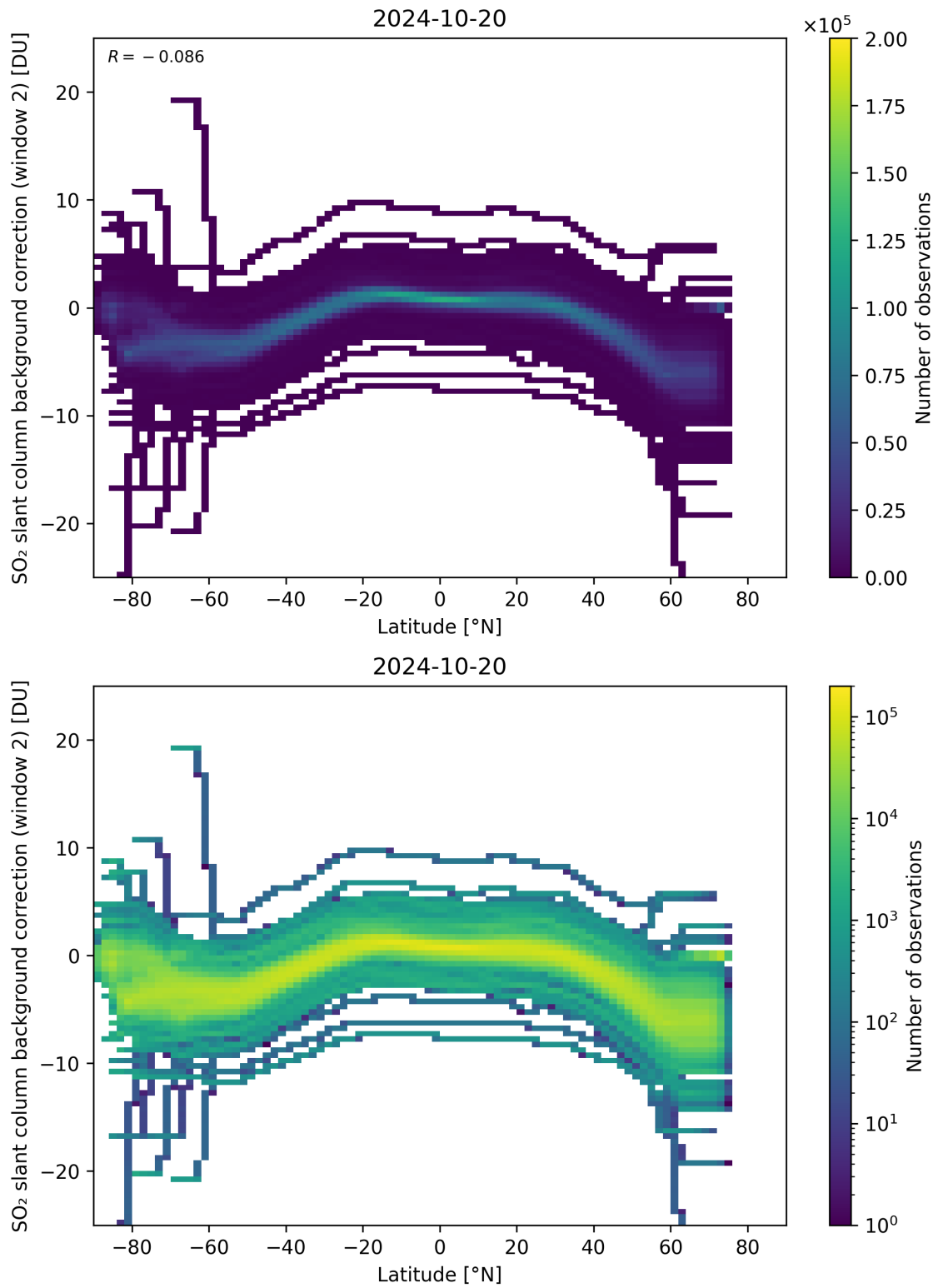
Figure 140: Scatter density plot of “Latitude” against “SO 2 slant column background correction (window 2)” for 2024-10-19 to 2024-10-21.
