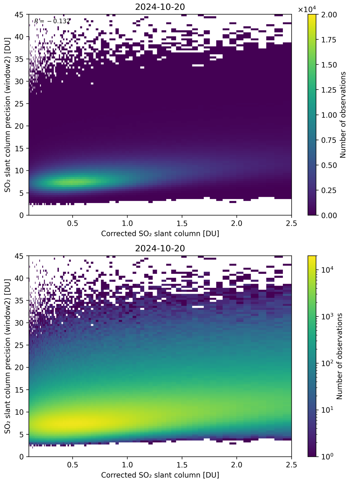
Figure 189: Scatter density plot of “Corrected SO 2 slant column” against “SO 2 slant column precision (window2)” for 2024-10-19 to 2024-10-21.
