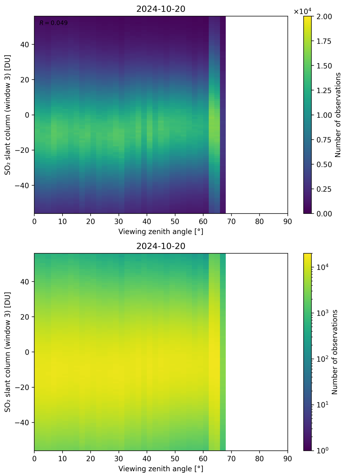
Figure 323: Scatter density plot of “Viewing zenith angle” against “SO 2 slant column (window 3)” for 2024-10-19 to 2024-10-21.
