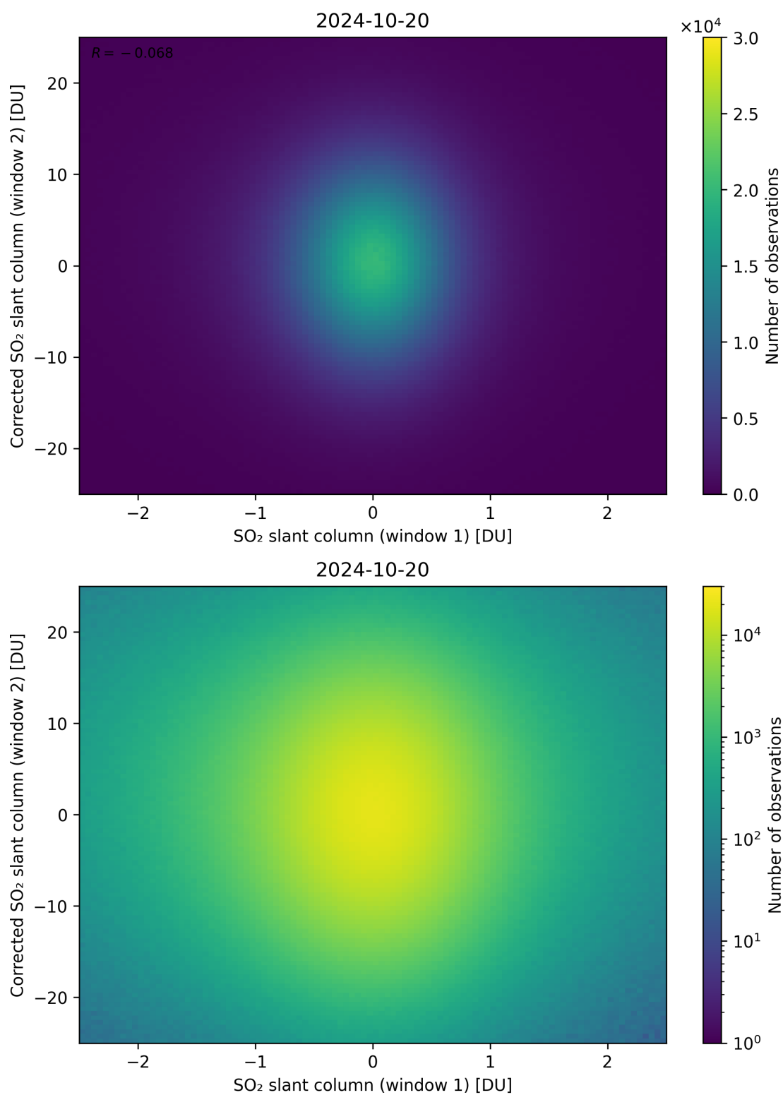
Figure 233: Scatter density plot of “SO 2 slant column (window 1)” against “Corrected SO 2 slant column (window 2)” for 2024-10-19 to 2024-10-21.
