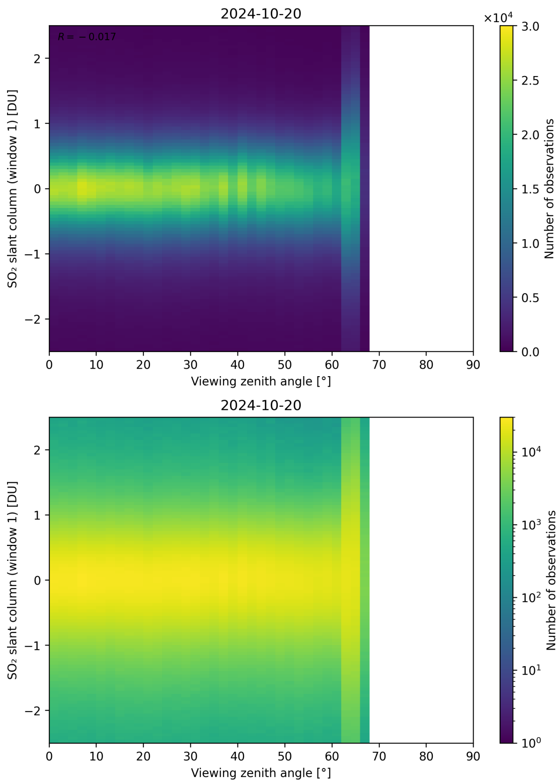
Figure 320: Scatter density plot of “Viewing zenith angle” against “SO 2 slant column (window 1)” for 2024-10-19 to 2024-10-21.
