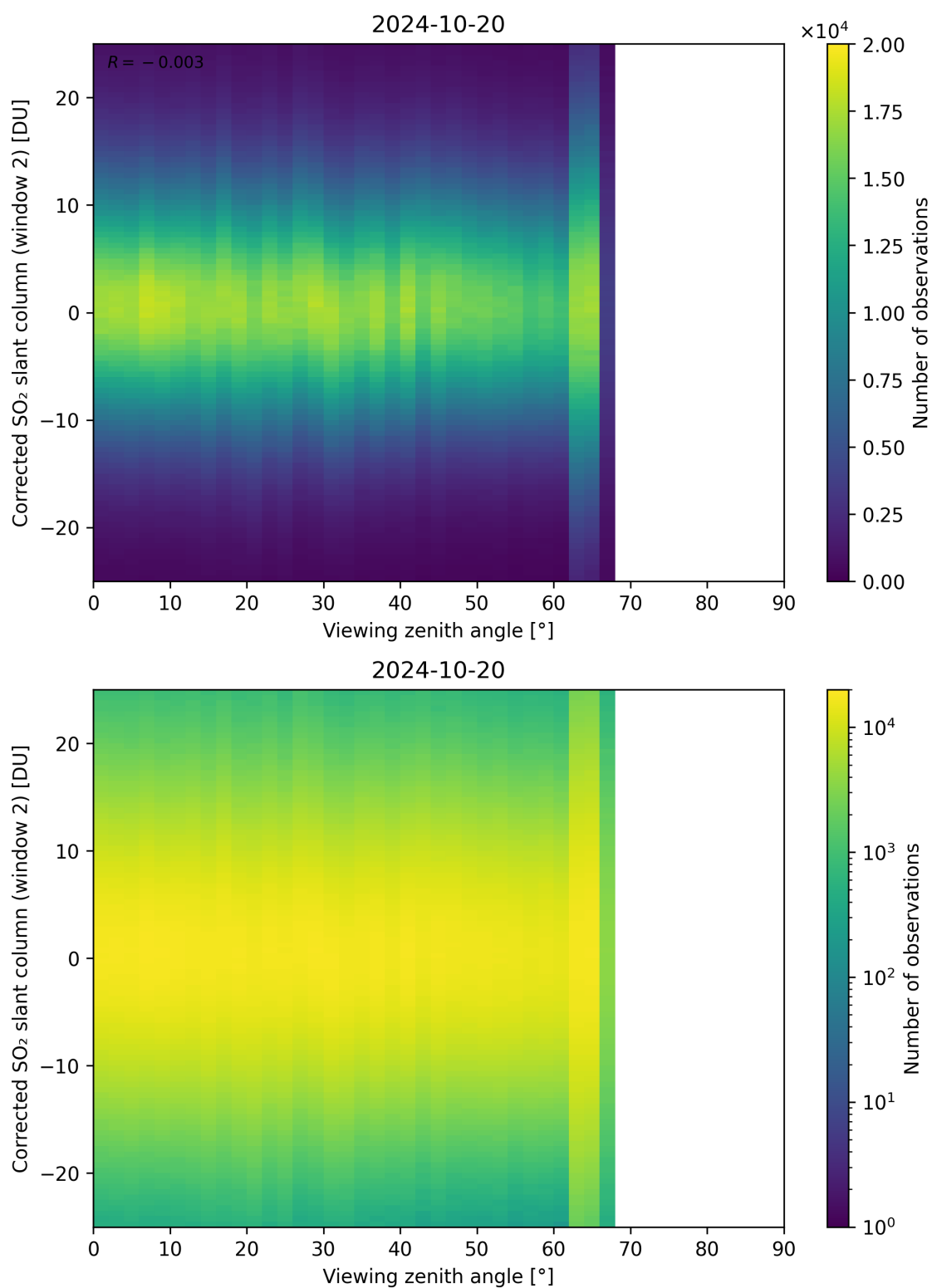
Figure 318: Scatter density plot of “Viewing zenith angle” against “Corrected SO 2 slant column (window 2)” for 2024-10-19 to 2024-10-21.
