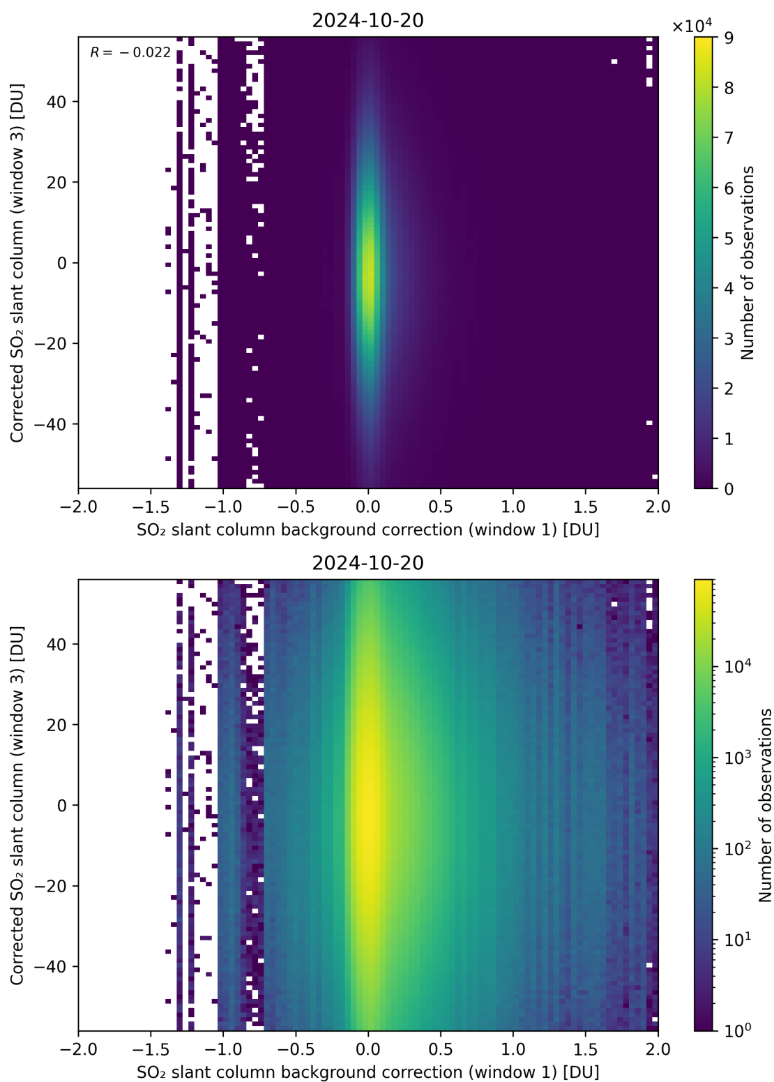
Figure 105: Scatter density plot of “SO 2 slant column background correction (window 1)” against “Corrected SO 2 slant column (window 3)” for 2024-10-19 to 2024-10-21.
