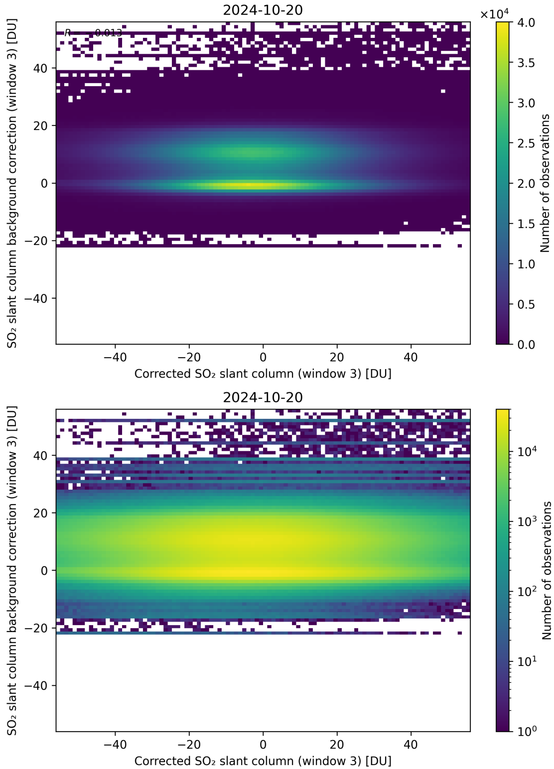
Figure 205: Scatter density plot of “Corrected SO 2 slant column (window 3)” against “SO 2 slant column background correction (window 3)” for 2024-10-19 to 2024-10-21.
