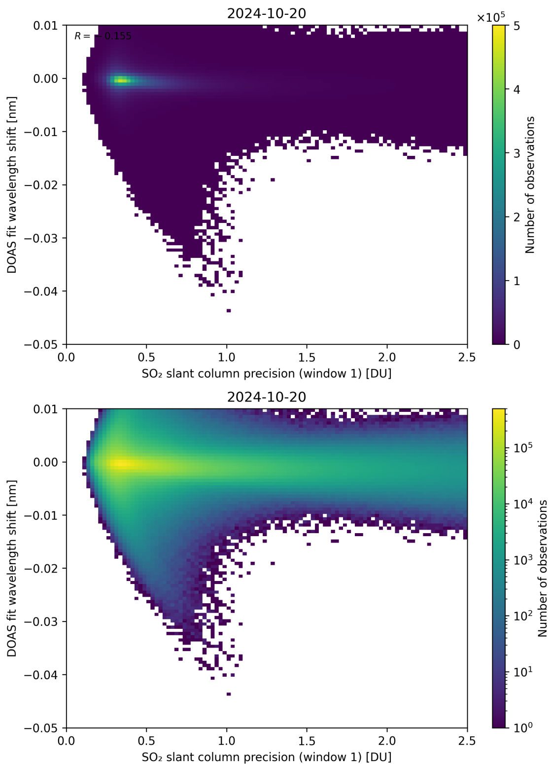
Figure 221: Scatter density plot of “SO 2 slant column precision (window 1)” against “DOAS fit wavelength shift” for 2024-10-19 to 2024-10-21.
