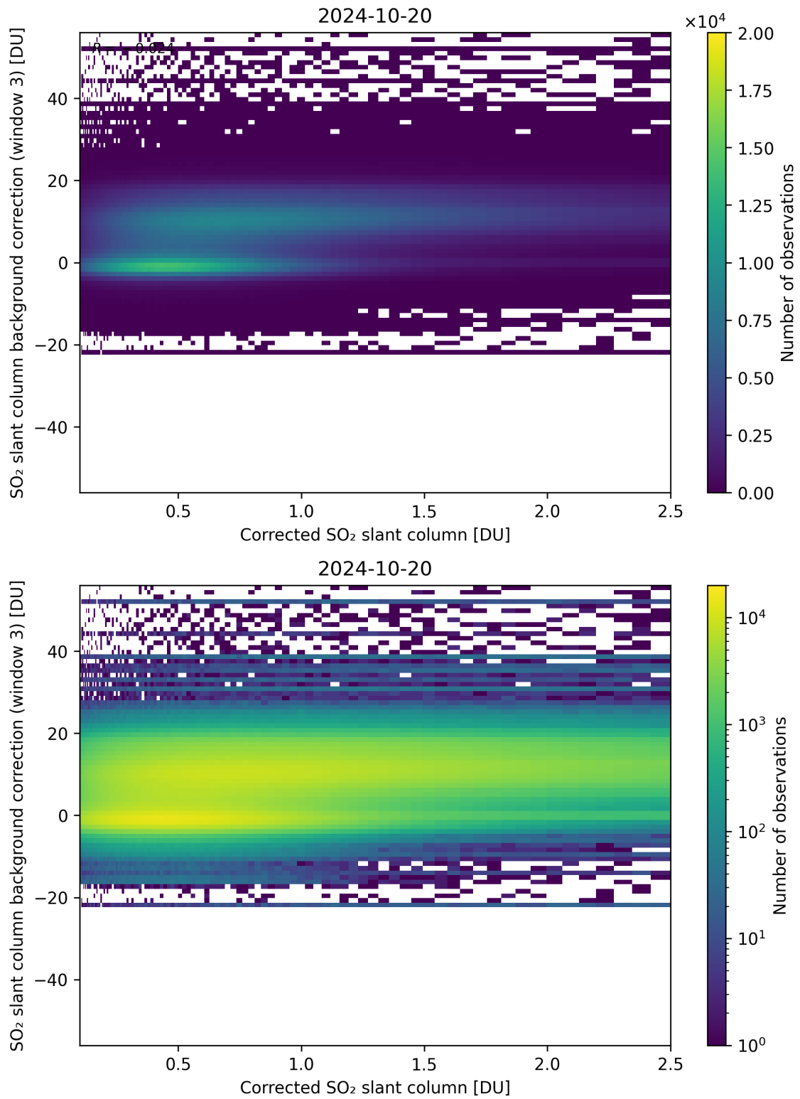
Figure 180: Scatter density plot of “Corrected SO 2 slant column” against “SO 2 slant column background correction (window 3)” for 2024-10-19 to 2024-10-21.
