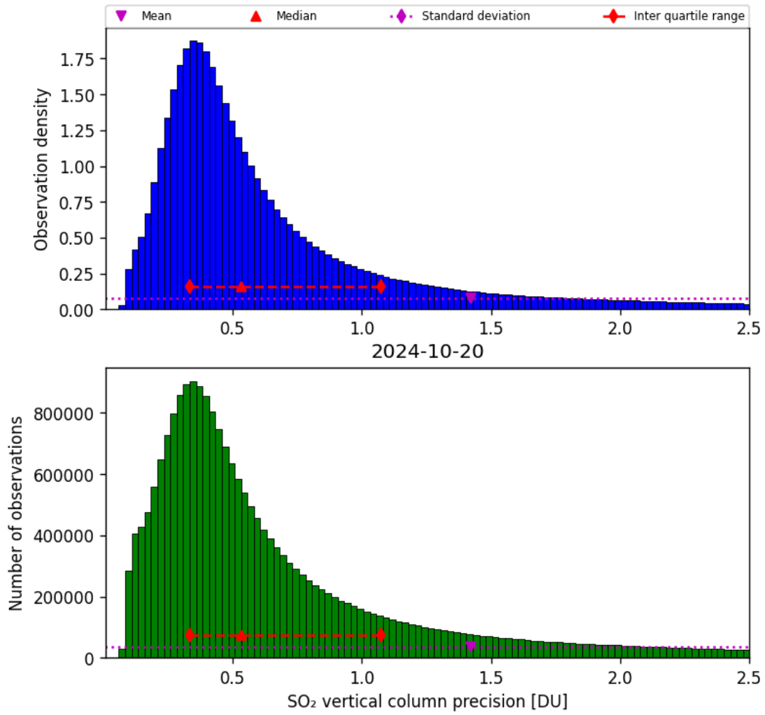
Figure 54: Histogram of “SO 2 vertical column precision” for 2024-10-19 to 2024-10-21
