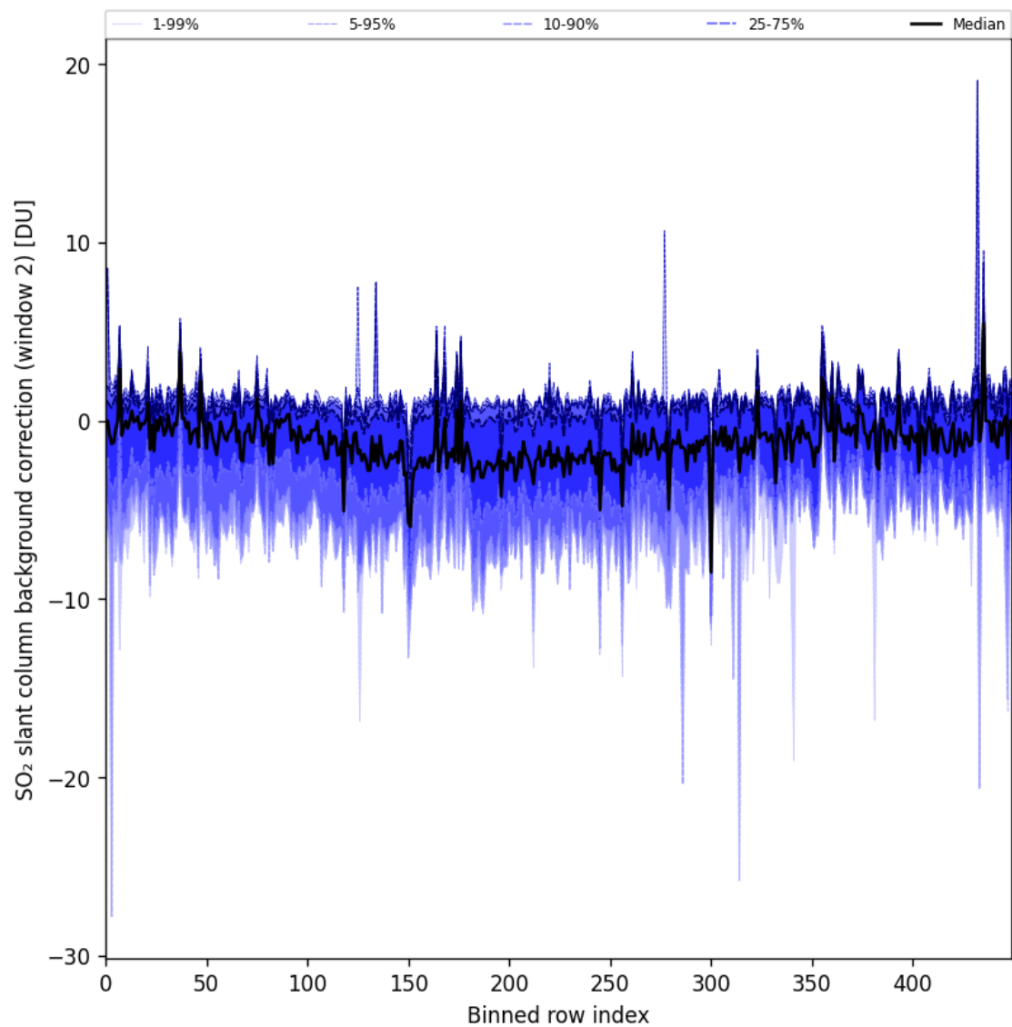
Figure 86: Along track statistics of “SO 2 slant column background correction (window 2)” for 2024-10-19 to 2024-10-21
