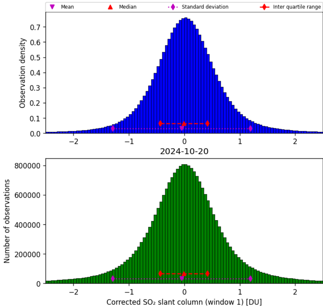
Figure 58: Histogram of “Corrected SO 2 slant column (window 1)” for 2024-10-19 to 2024-10-21
