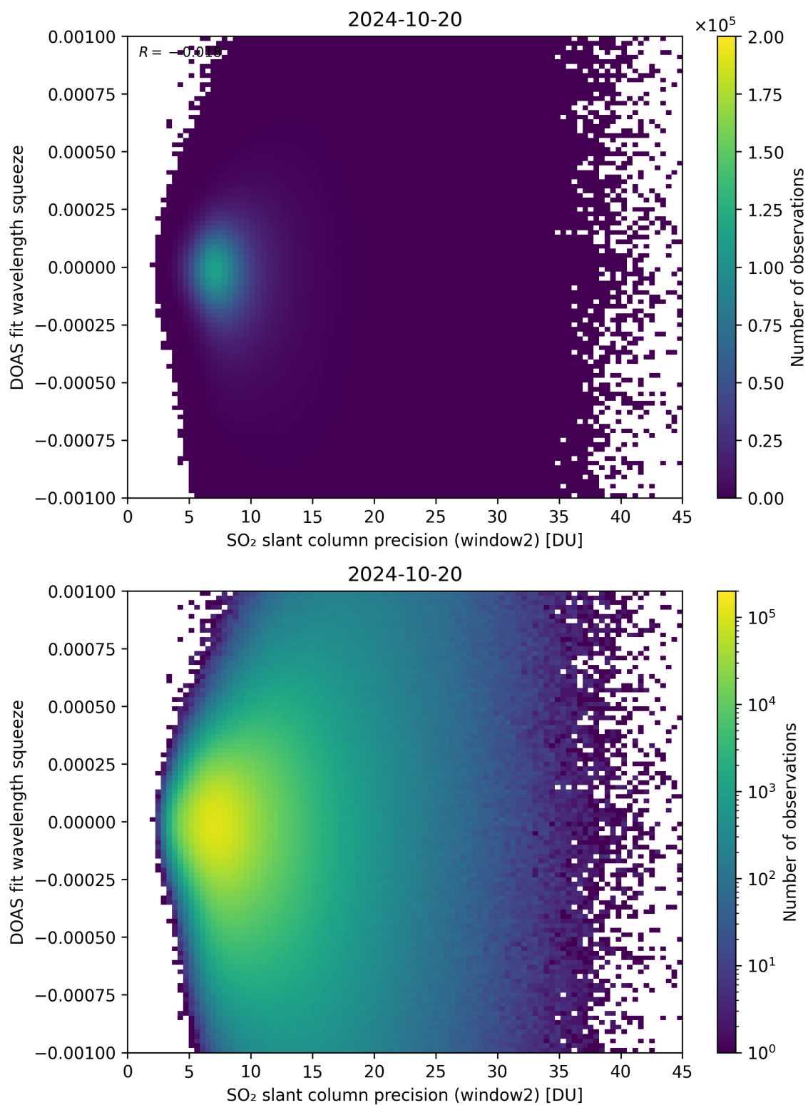
Figure 244: Scatter density plot of “SO 2 slant column precision (window2)” against “DOAS fit wavelength squeeze” for 2024-10-19 to 2024-10-21.
