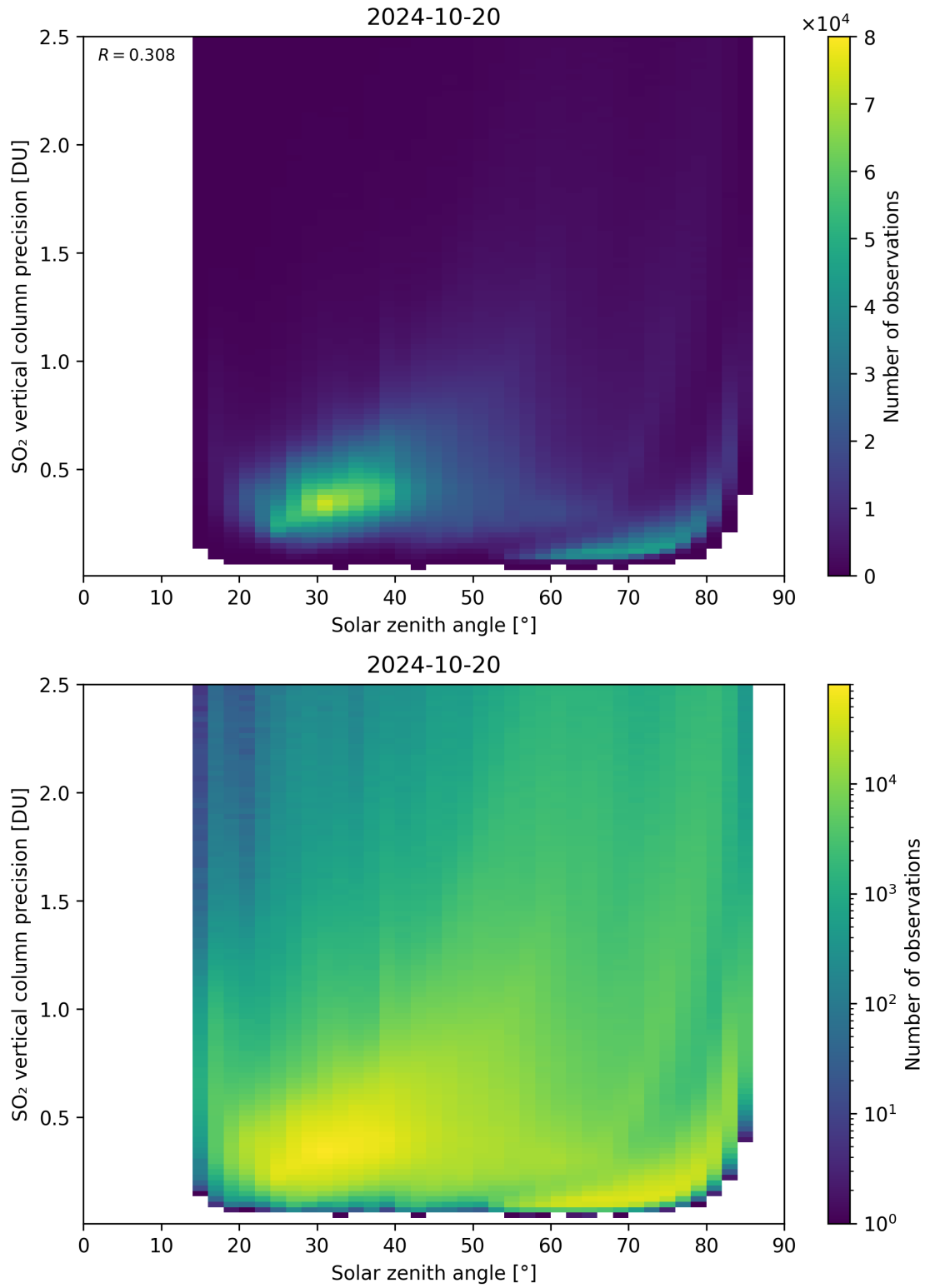
Figure 177: Scatter density plot of “Solar zenith angle” against “SO 2 vertical column precision” for 2024-10-19 to 2024-10-21.
