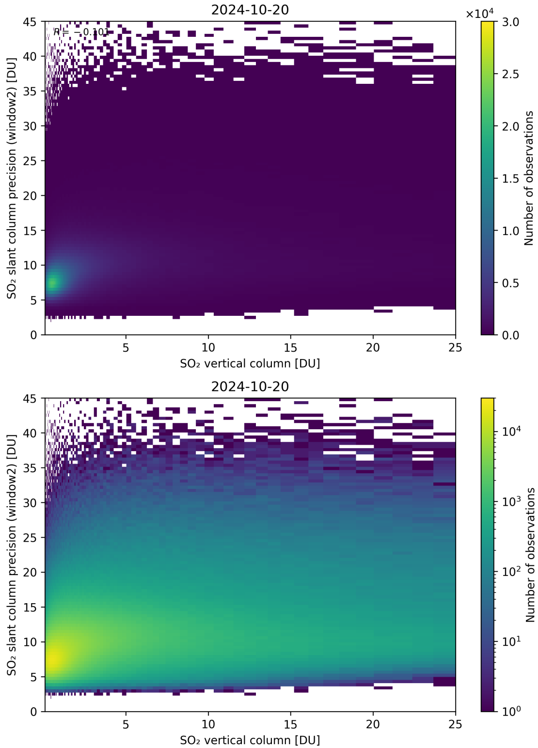
Figure 302: Scatter density plot of “SO 2 vertical column” against “SO 2 slant column precision (window2)” for 2024-10-19 to 2024-10-21.
