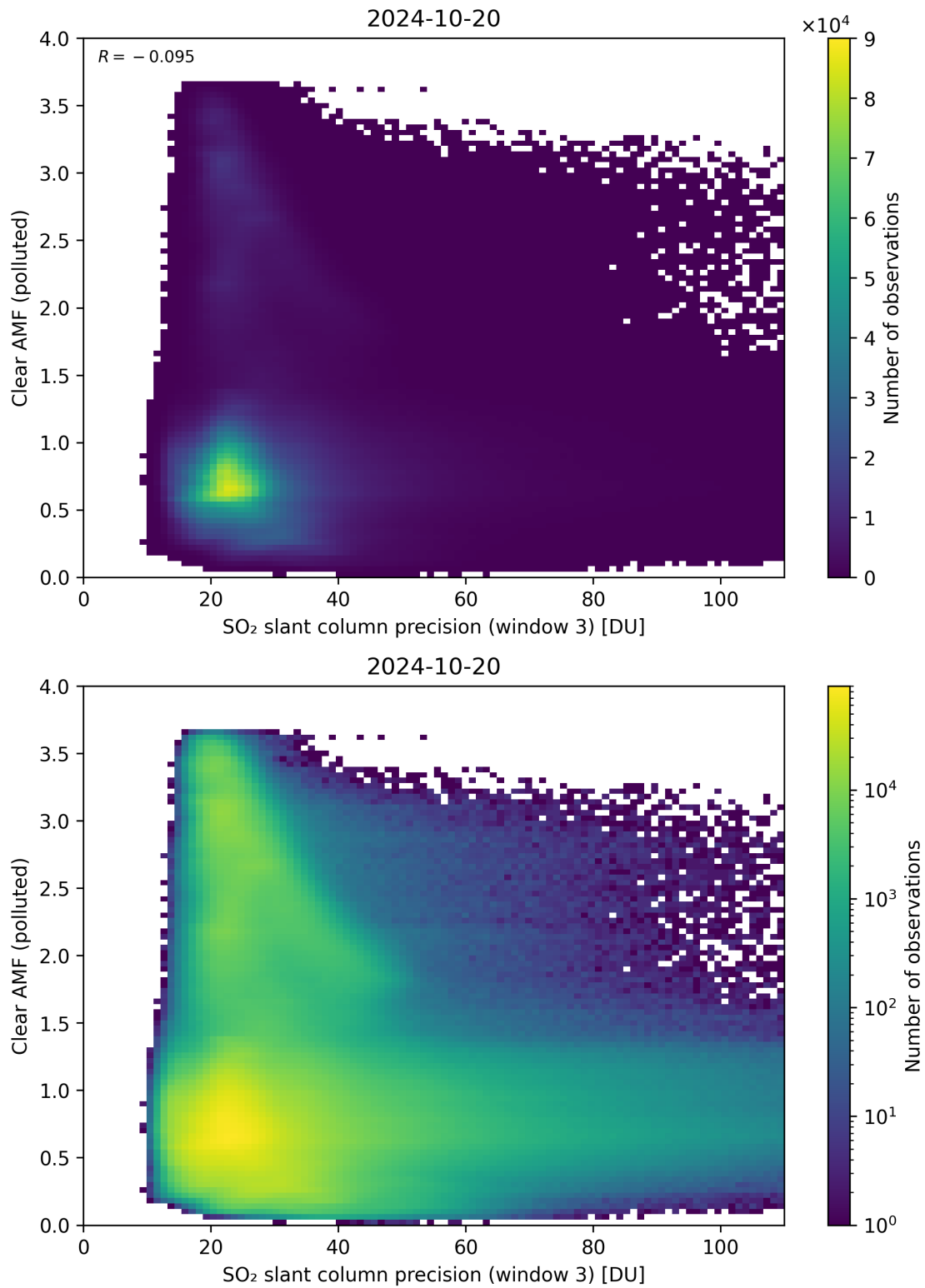
Figure 261: Scatter density plot of “SO 2 slant column precision (window 3)” against “Clear AMF (polluted)” for 2024-10-19 to 2024-10-21.
