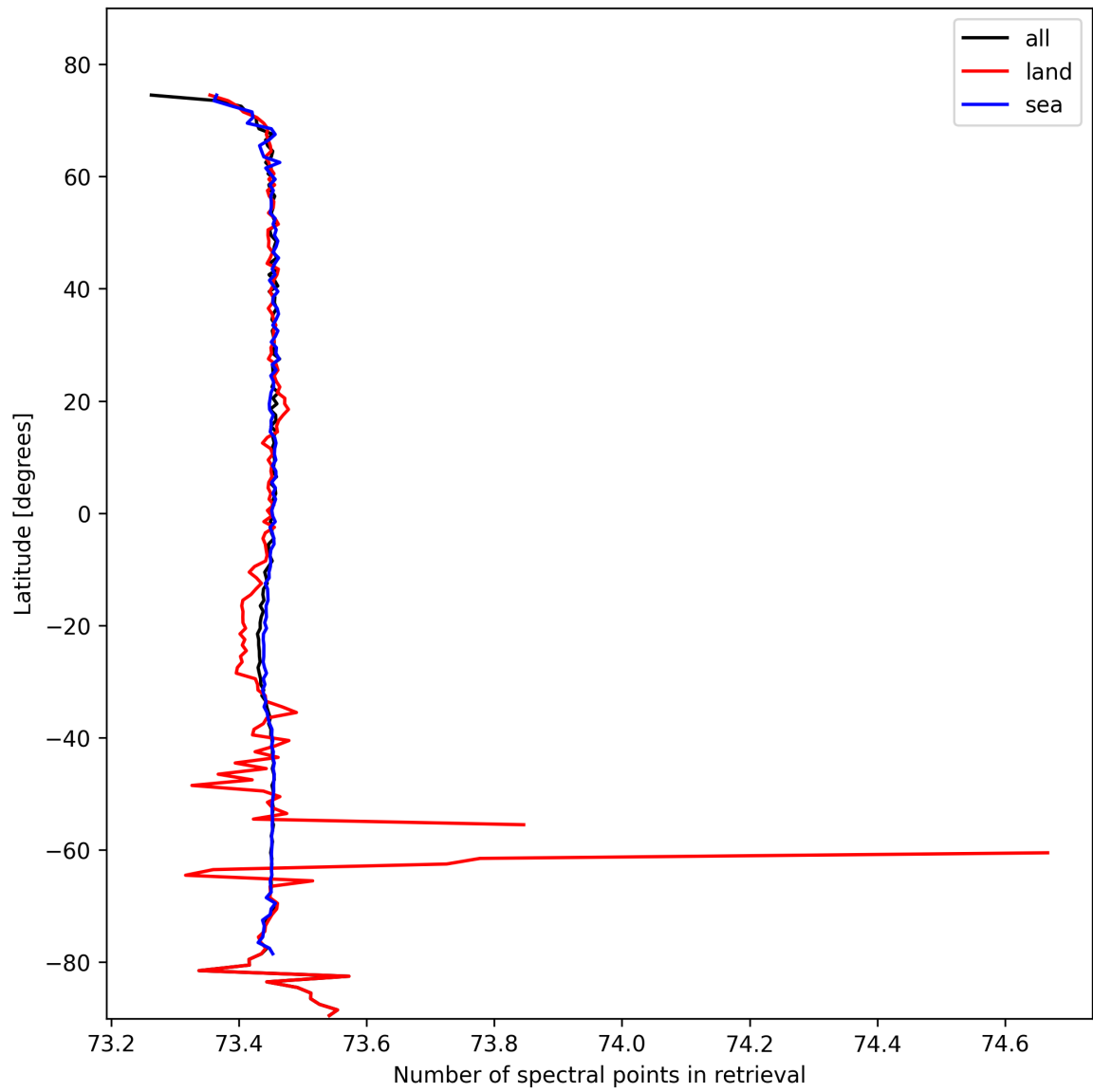
Figure 51: Zonal average of “Number of spectral points in retrieval” for 2024-10-19 to 2024-10-21.
