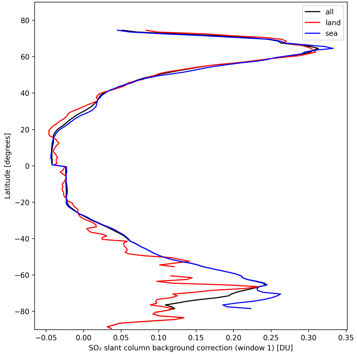
Figure 36: Zonal average of “SO 2 slant column background correction (window 1)” for 2024-10-19 to 2024-10-21.
