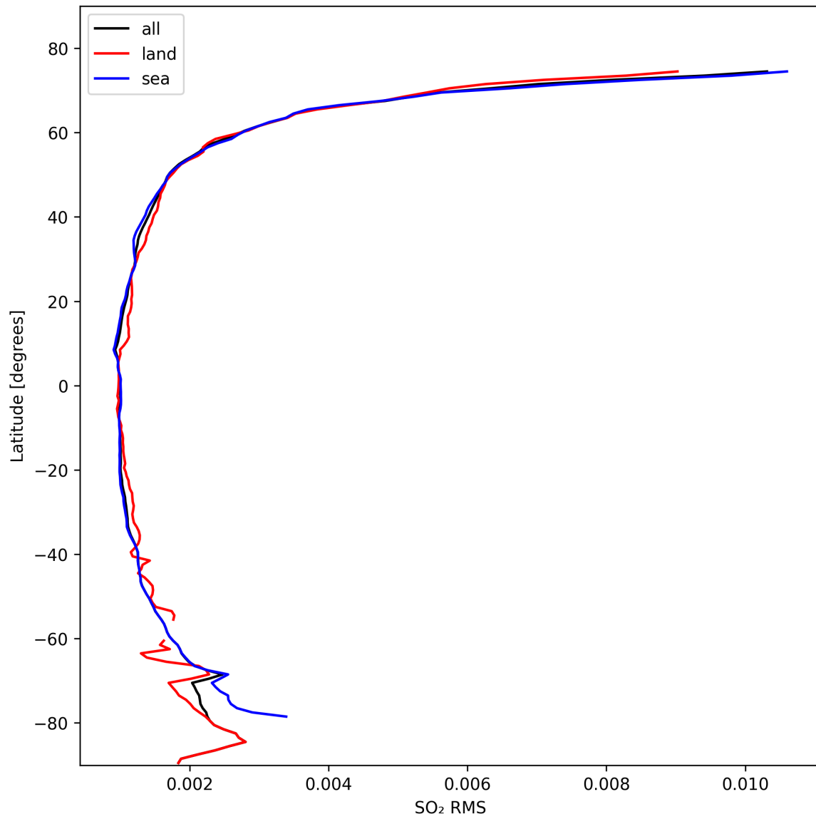
Figure 47: Zonal average of “SO 2 RMS” for 2024-10-19 to 2024-10-21.
