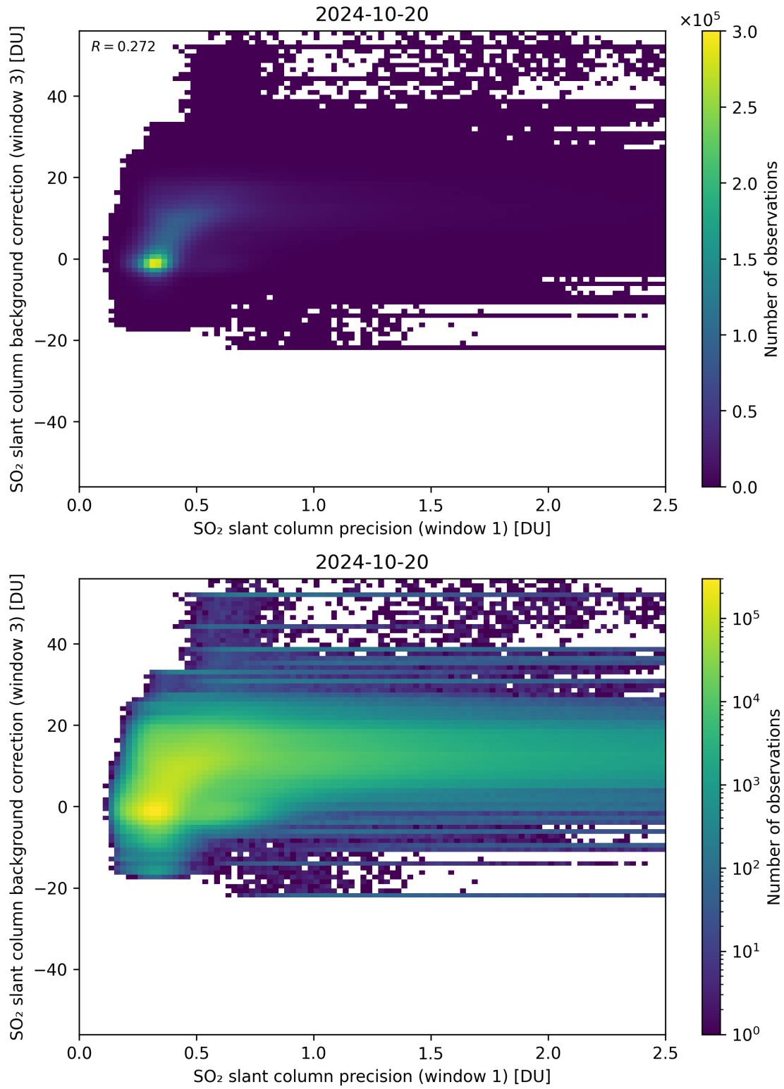
Figure 220: Scatter density plot of “SO 2 slant column precision (window 1)” against “SO 2 slant column background correction (window 3)” for 2024-10-19 to 2024-10-21.
