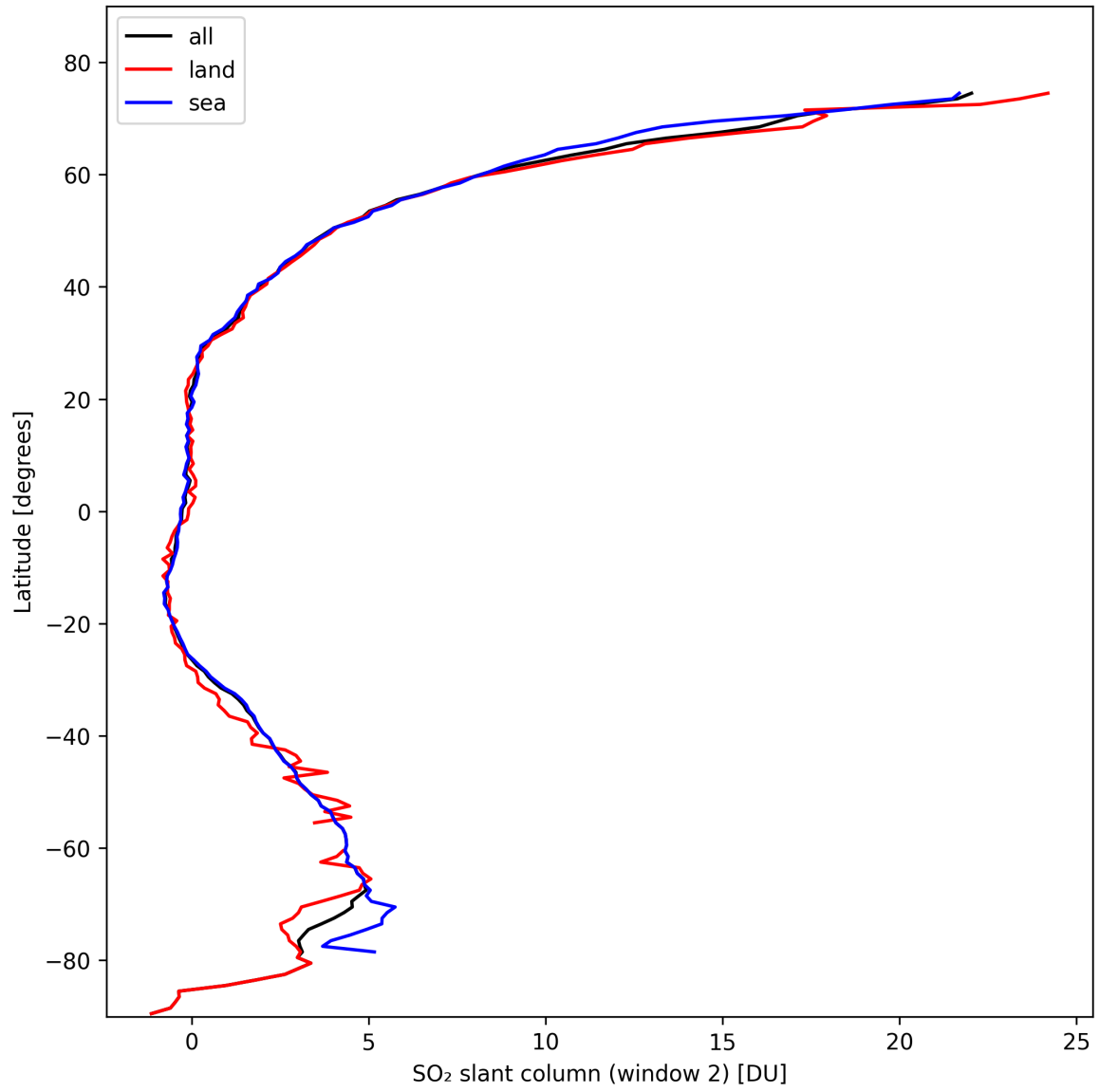
Figure 37: Zonal average of “SO 2 slant column (window 2)” for 2024-10-19 to 2024-10-21.
