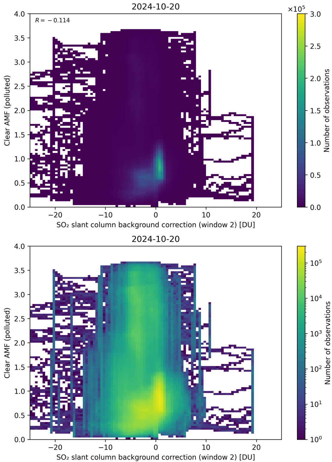
Figure 115: Scatter density plot of “SO 2 slant column background correction (window 2)” against “Clear AMF (polluted)” for 2024-10-19 to 2024-10-21.
