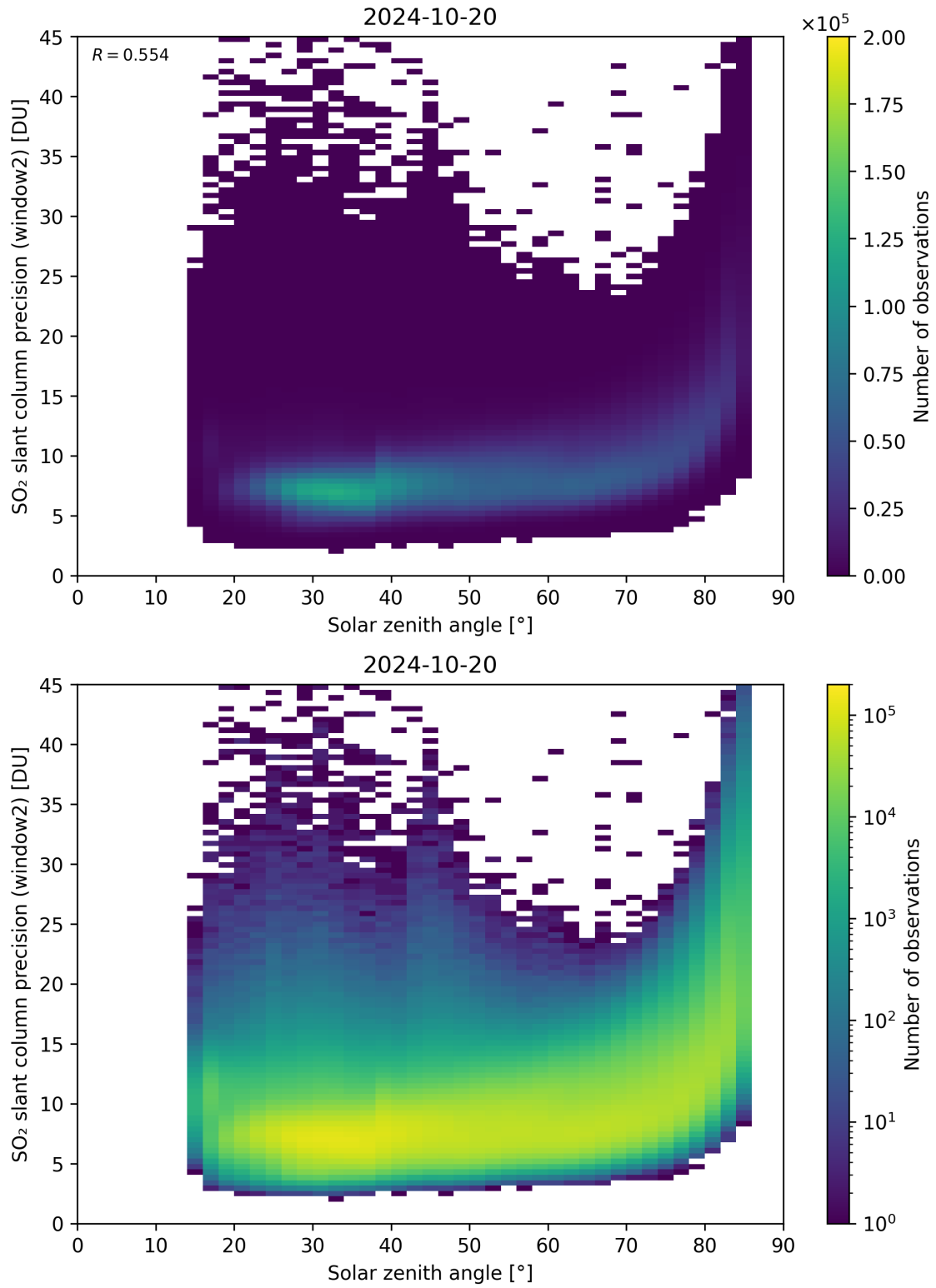
Figure 171: Scatter density plot of “Solar zenith angle” against “SO 2 slant column precision (window2)” for 2024-10-19 to 2024-10-21.
