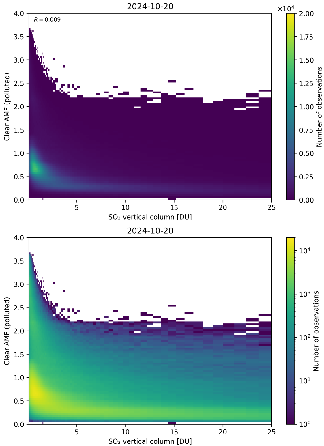
Figure 296: Scatter density plot of “SO 2 vertical column” against “Clear AMF (polluted)” for 2024-10-19 to 2024-10-21.
