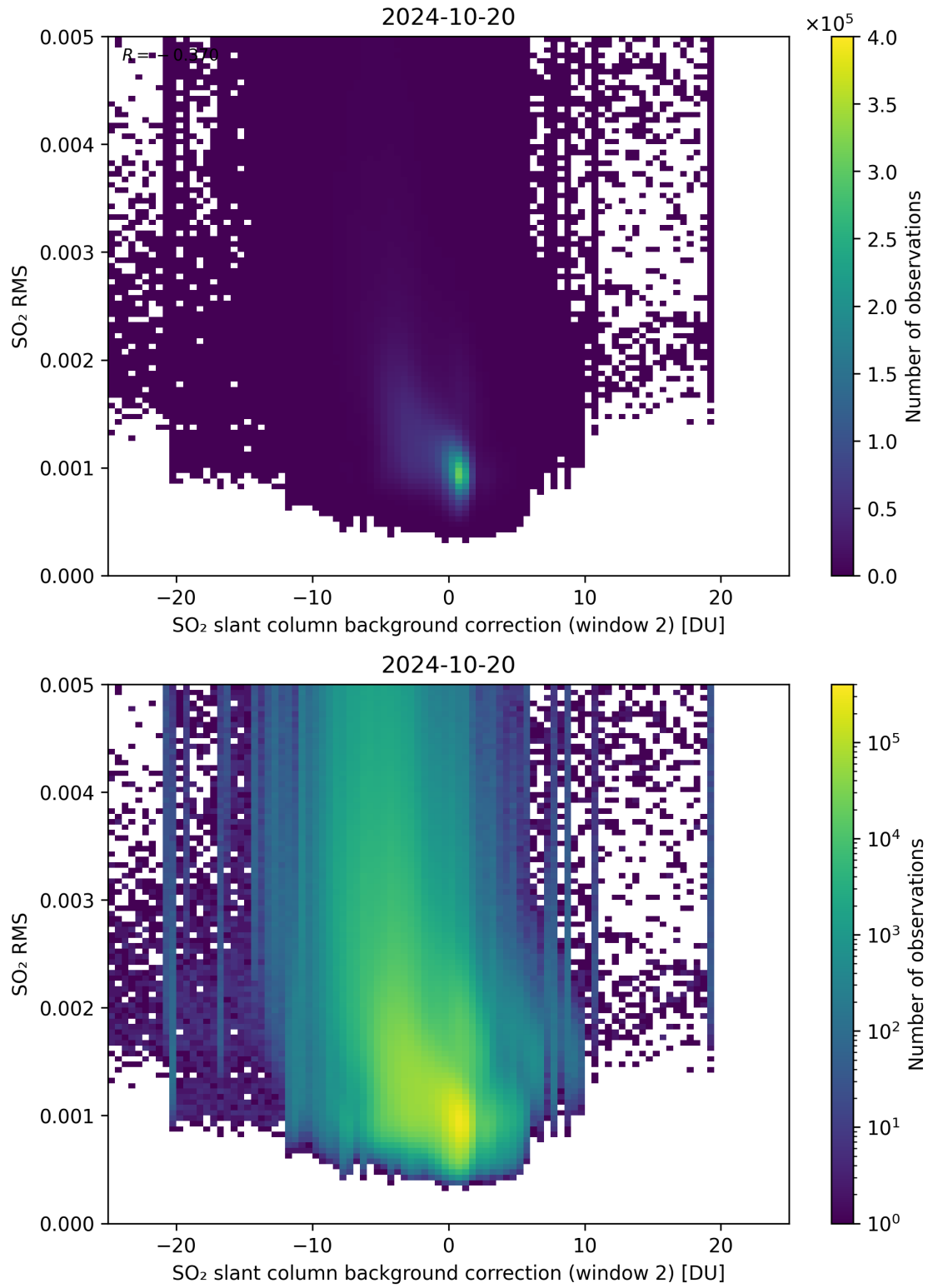
Figure 114: Scatter density plot of “SO 2 slant column background correction (window 2)” against “SO 2 RMS” for 2024-10-19 to 2024-10-21.
