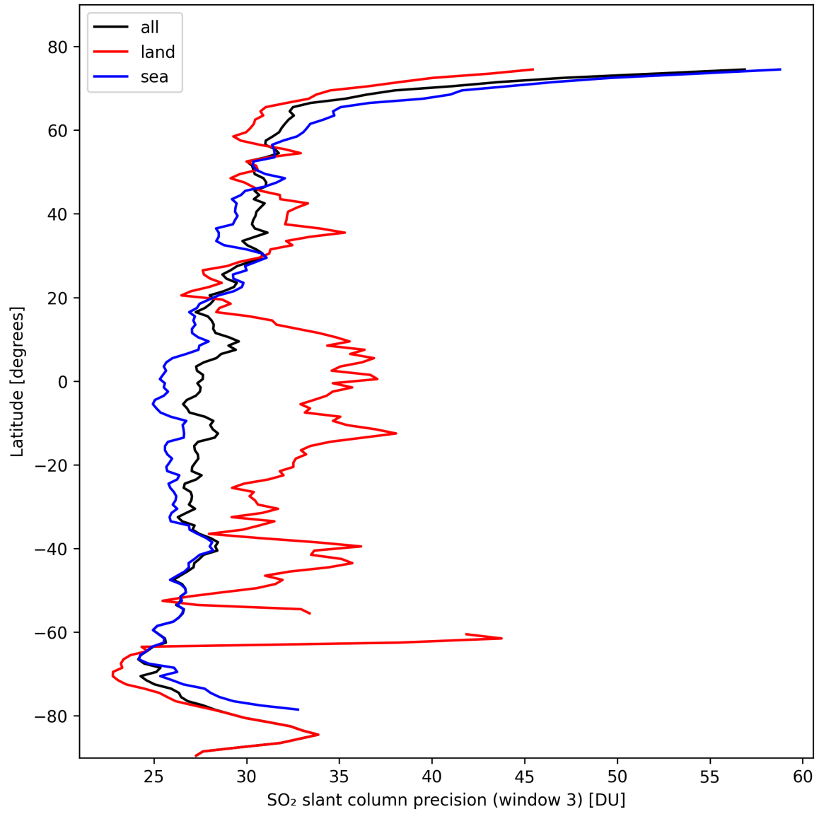
Figure 42: Zonal average of “SO 2 slant column precision (window 3)” for 2024-10-19 to 2024-10-21.
