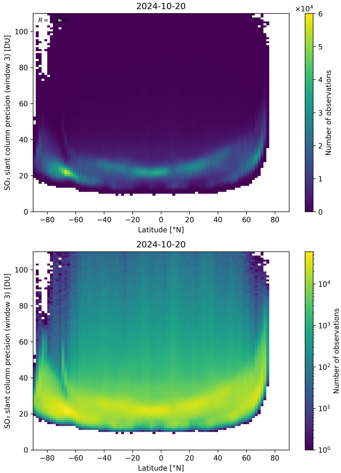
Figure 153: Scatter density plot of “Latitude” against “SO 2 slant column precision (window 3)” for 2024-10-19 to 2024-10-21.
