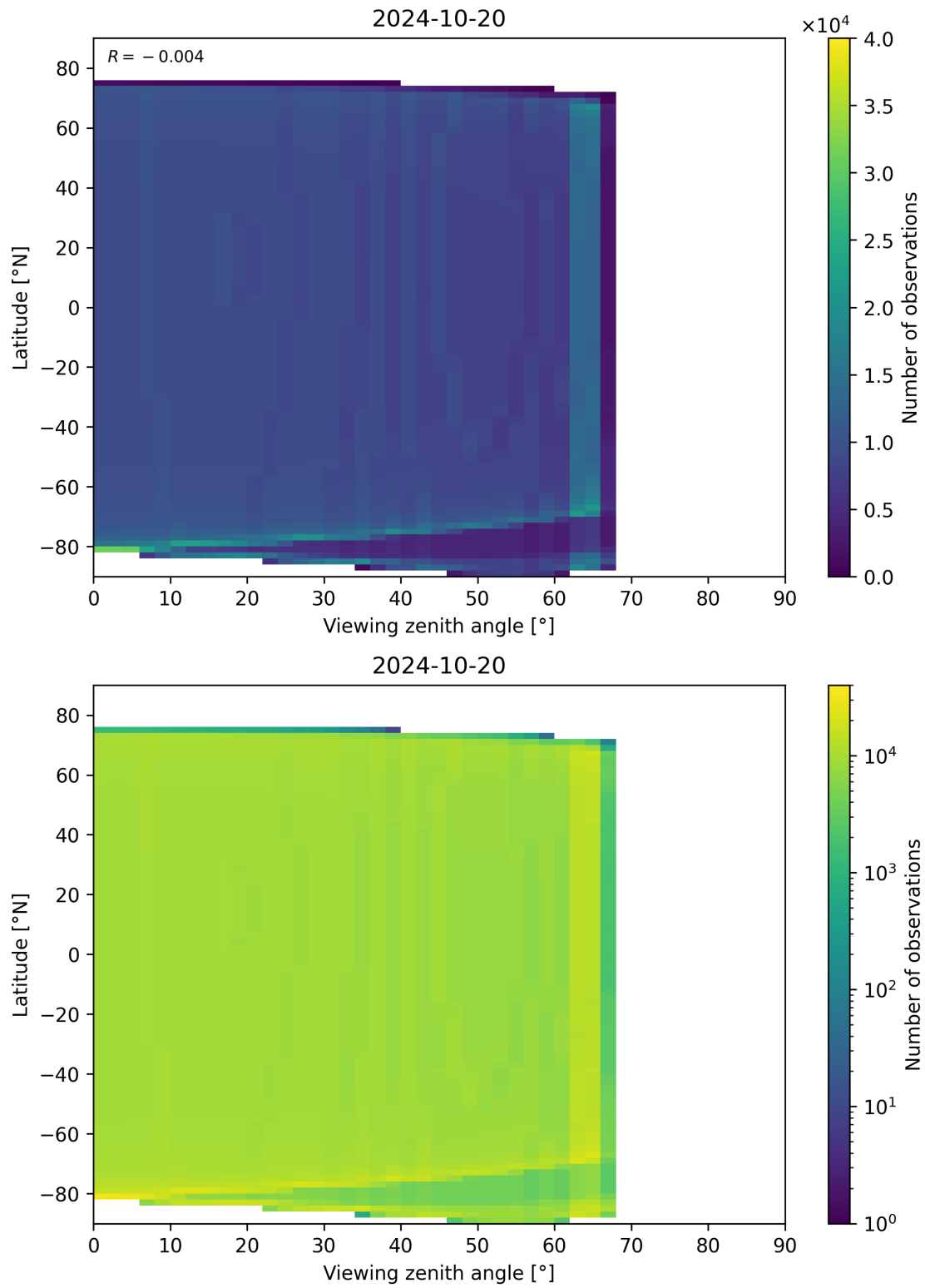
Figure 314: Scatter density plot of “Viewing zenith angle” against “Latitude” for 2024-10-19 to 2024-10-21.
