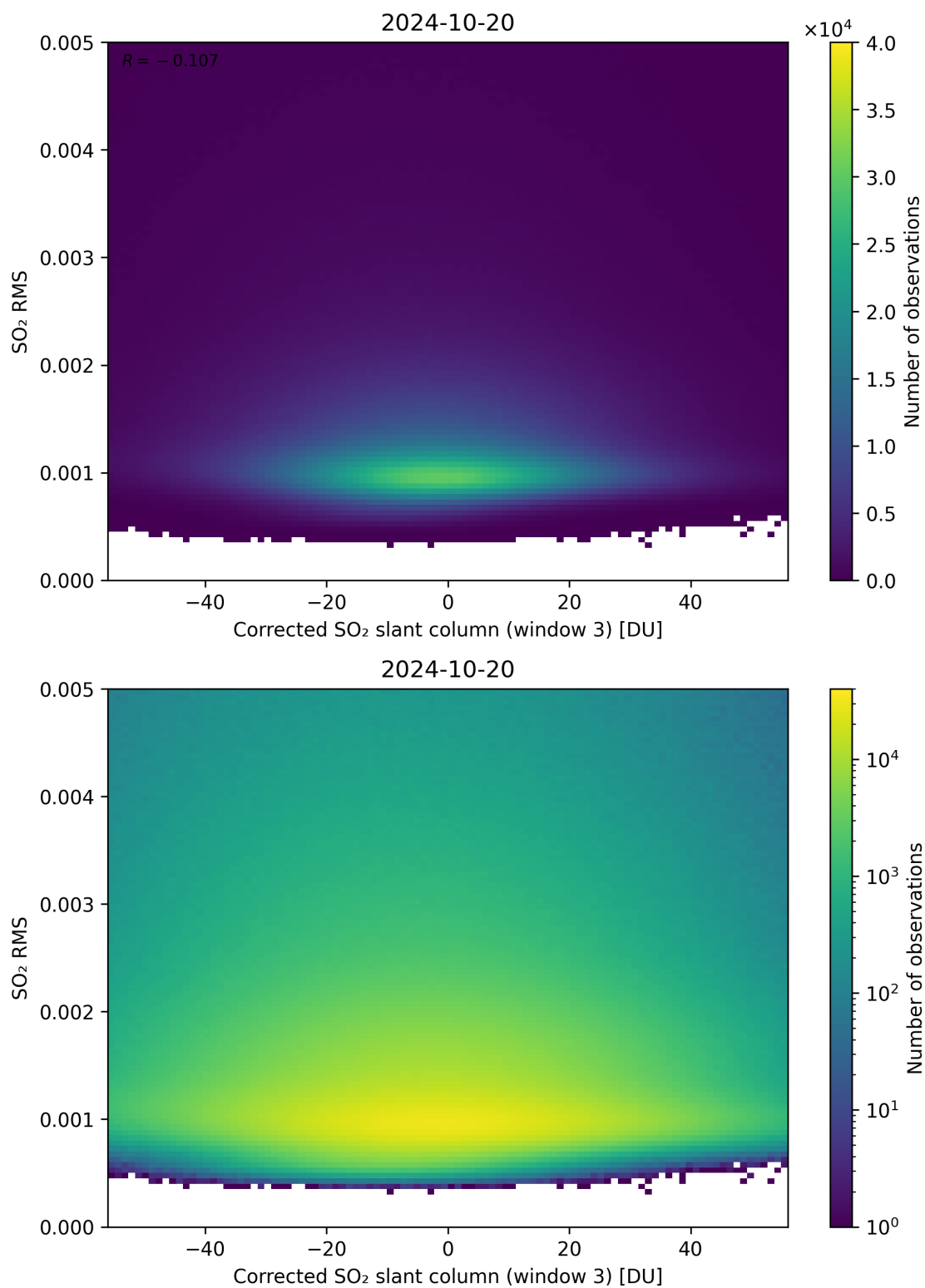
Figure 208: Scatter density plot of “Corrected SO 2 slant column (window 3)” against “SO 2 RMS” for 2024-10-19 to 2024-10-21.
