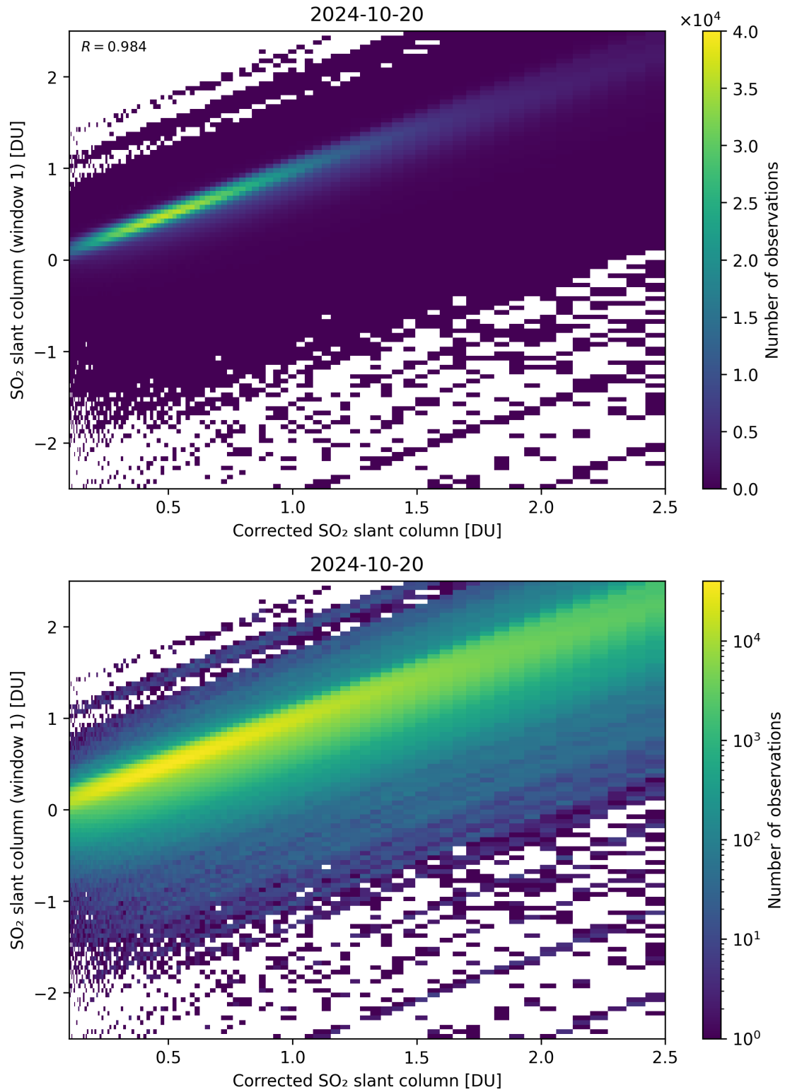
Figure 187: Scatter density plot of “Corrected SO 2 slant column” against “SO 2 slant column (window 1)” for 2024-10-19 to 2024-10-21.
