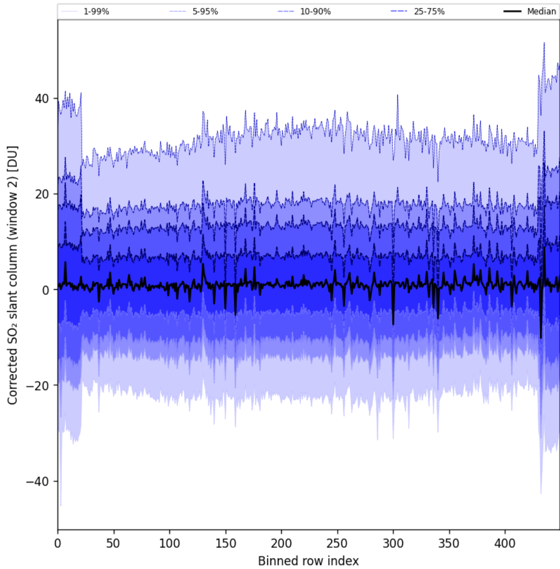
Figure 85: Along track statistics of “Corrected SO 2 slant column (window 2)” for 2024-10-19 to 2024-10-21
