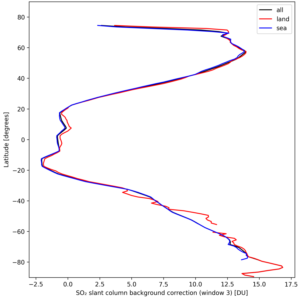
Figure 44: Zonal average of “SO 2 slant column background correction (window 3)” for 2024-10-19 to 2024-10-21.
