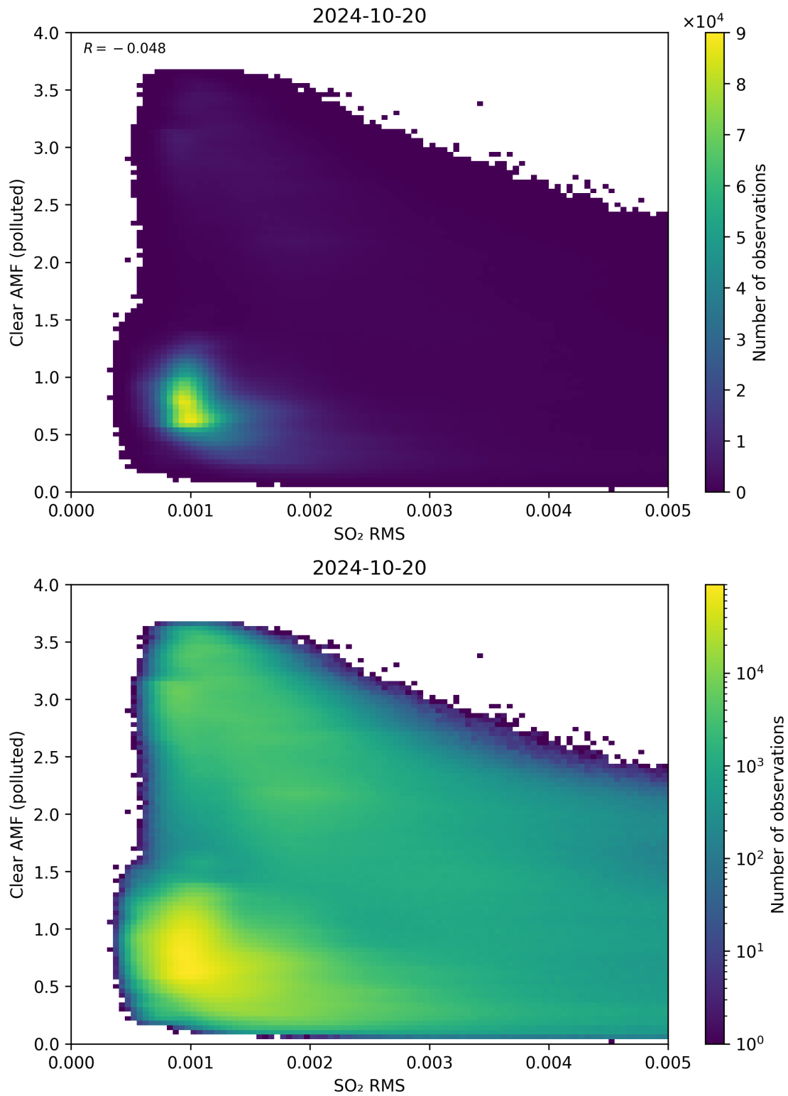
Figure 136: Scatter density plot of “SO 2 RMS” against “Clear AMF (polluted)” for 2024-10-19 to 2024-10-21.
