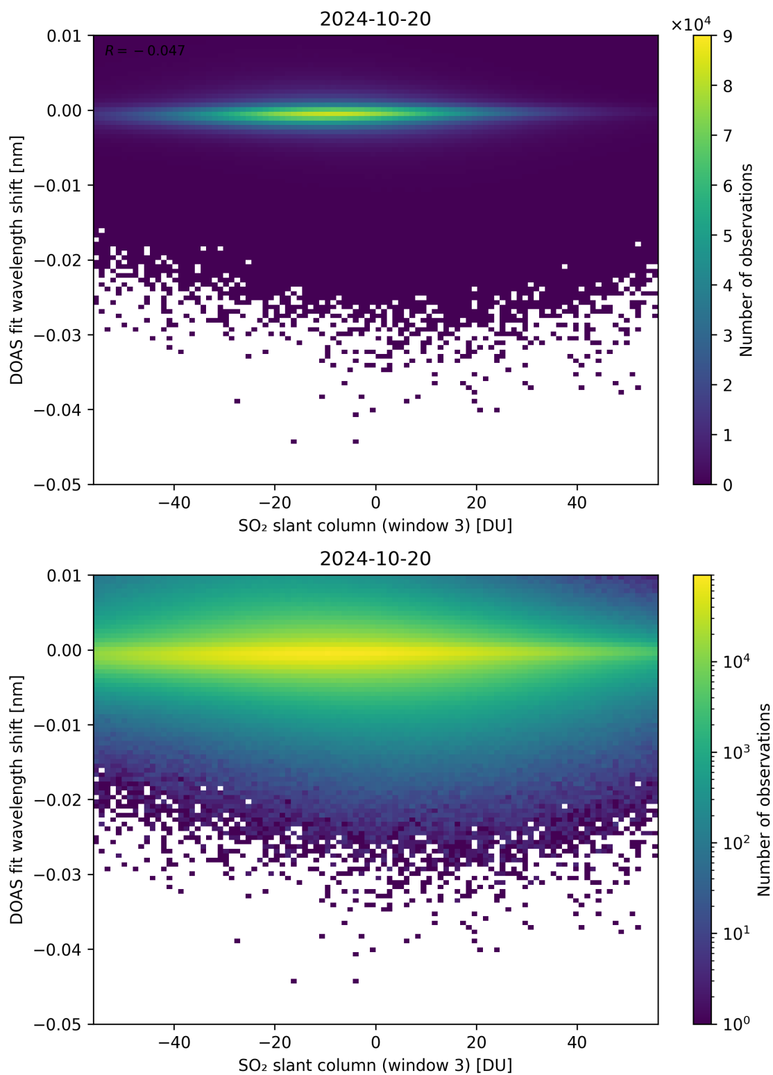
Figure 254: Scatter density plot of “SO 2 slant column (window 3)” against “DOAS fit wavelength shift” for 2024-10-19 to 2024-10-21.
