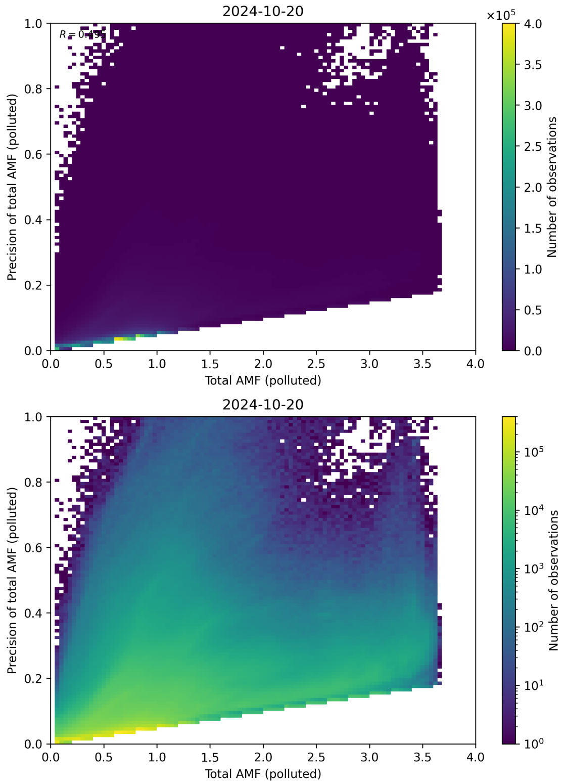
Figure 272: Scatter density plot of “Total AMF (polluted)” against “Precision of total AMF (polluted)” for 2024-10-19 to 2024-10-21.
