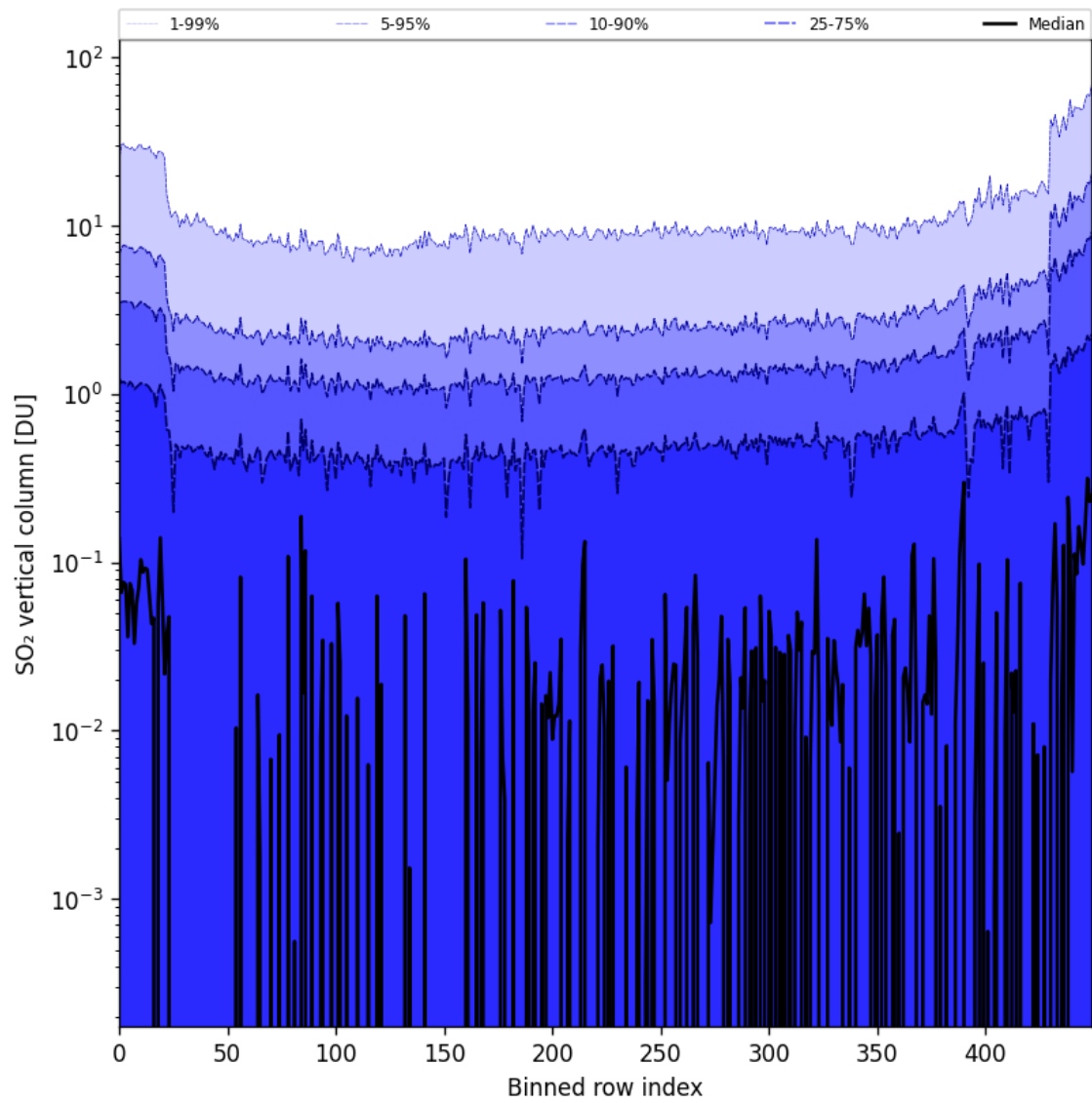
Figure 76: Along track statistics of “SO 2 vertical column” for 2024-10-19 to 2024-10-21
