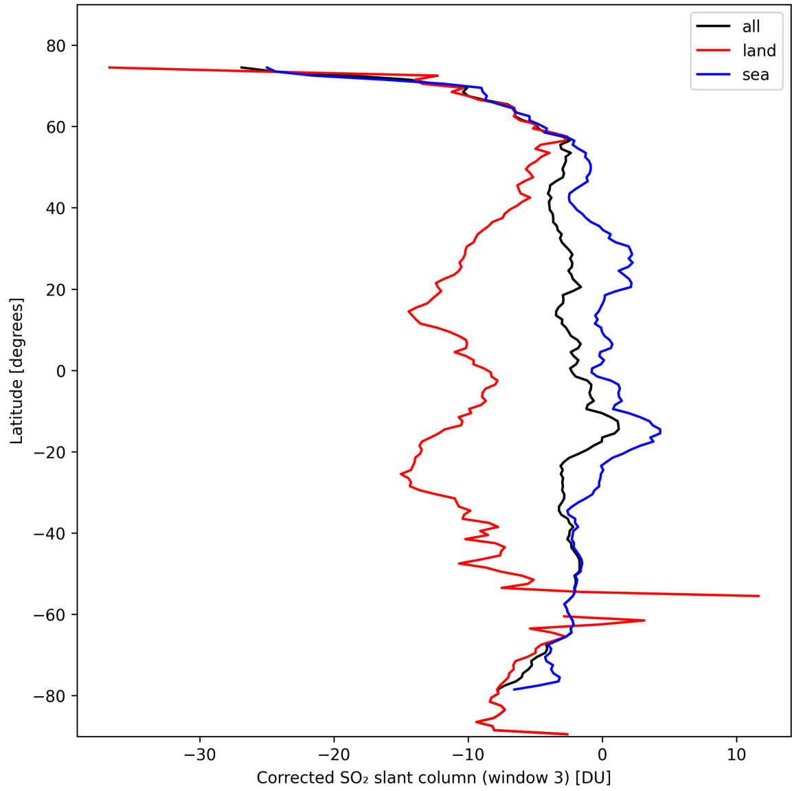
Figure 43: Zonal average of “Corrected SO 2 slant column (window 3)” for 2024-10-19 to 2024-10-21.
