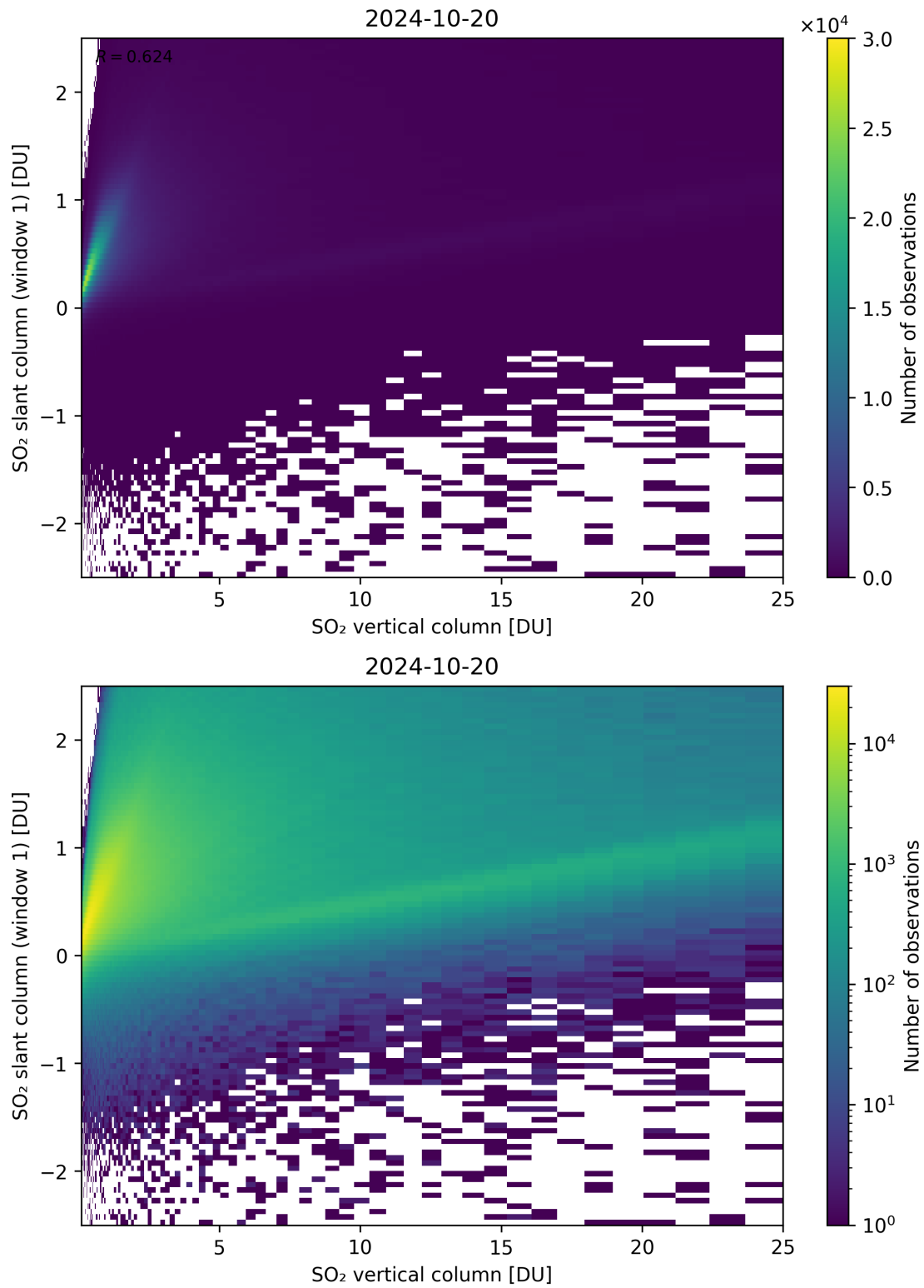
Figure 300: Scatter density plot of “SO 2 vertical column” against “SO 2 slant column (window 1)” for 2024-10-19 to 2024-10-21.
