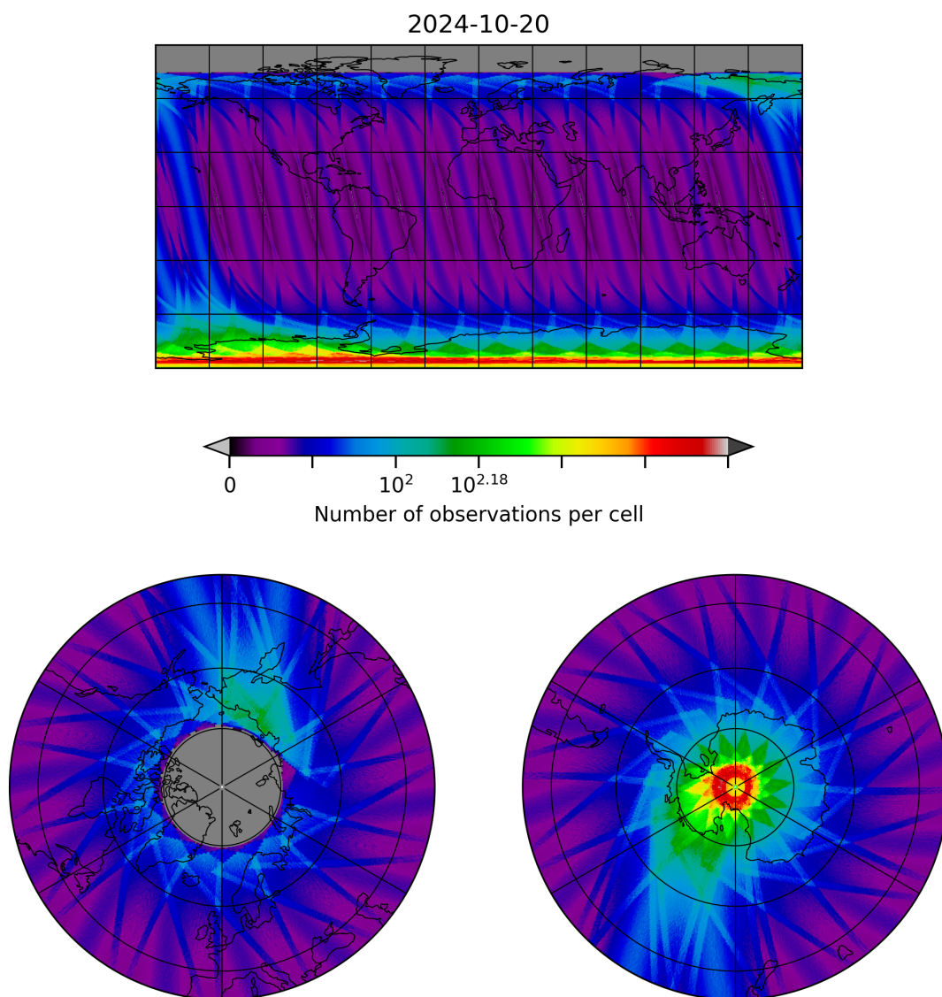
Figure 28: Map of the number of observations for 2024-10-19 to 2024-10-21
