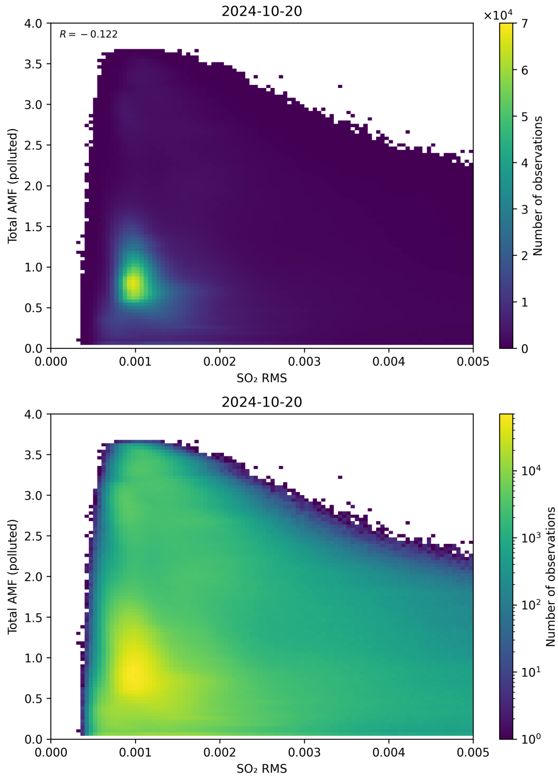
Figure 137: Scatter density plot of “SO 2 RMS” against “Total AMF (polluted)” for 2024-10-19 to 2024-10-21.
