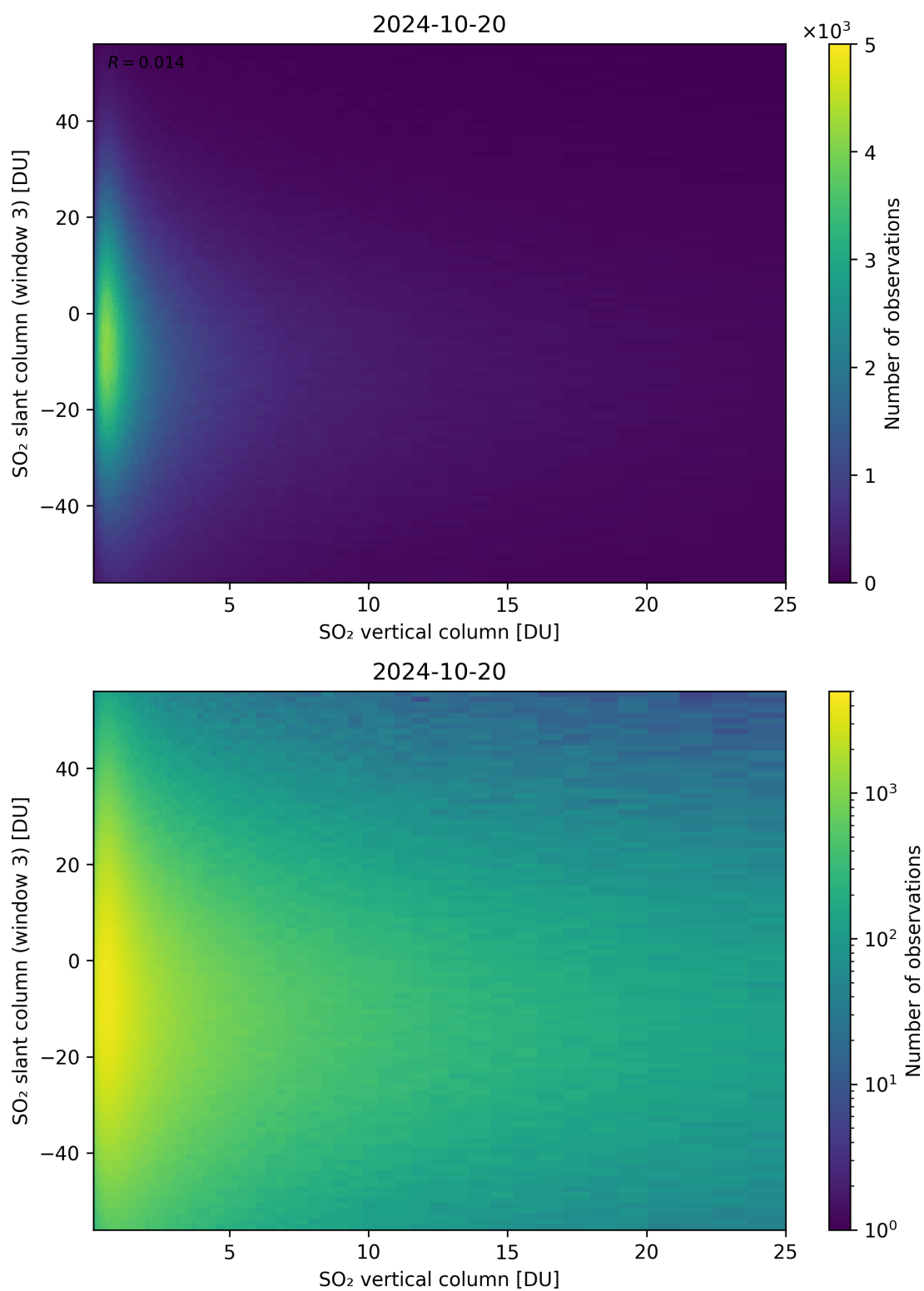
Figure 303: Scatter density plot of “SO 2 vertical column” against “SO 2 slant column (window 3)” for 2024-10-19 to 2024-10-21.
