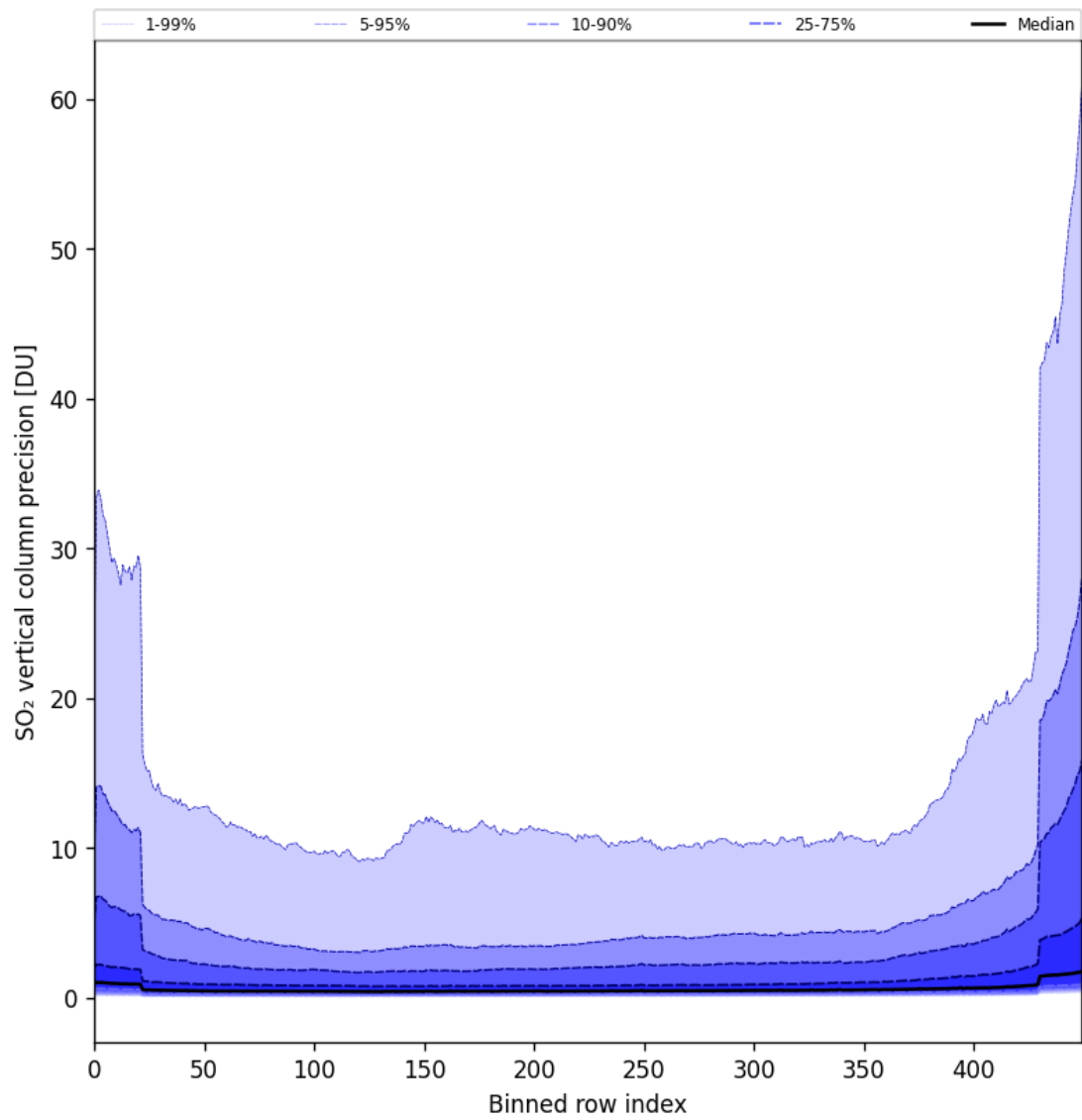
Figure 77: Along track statistics of “SO 2 vertical column precision” for 2024-10-19 to 2024-10-21
