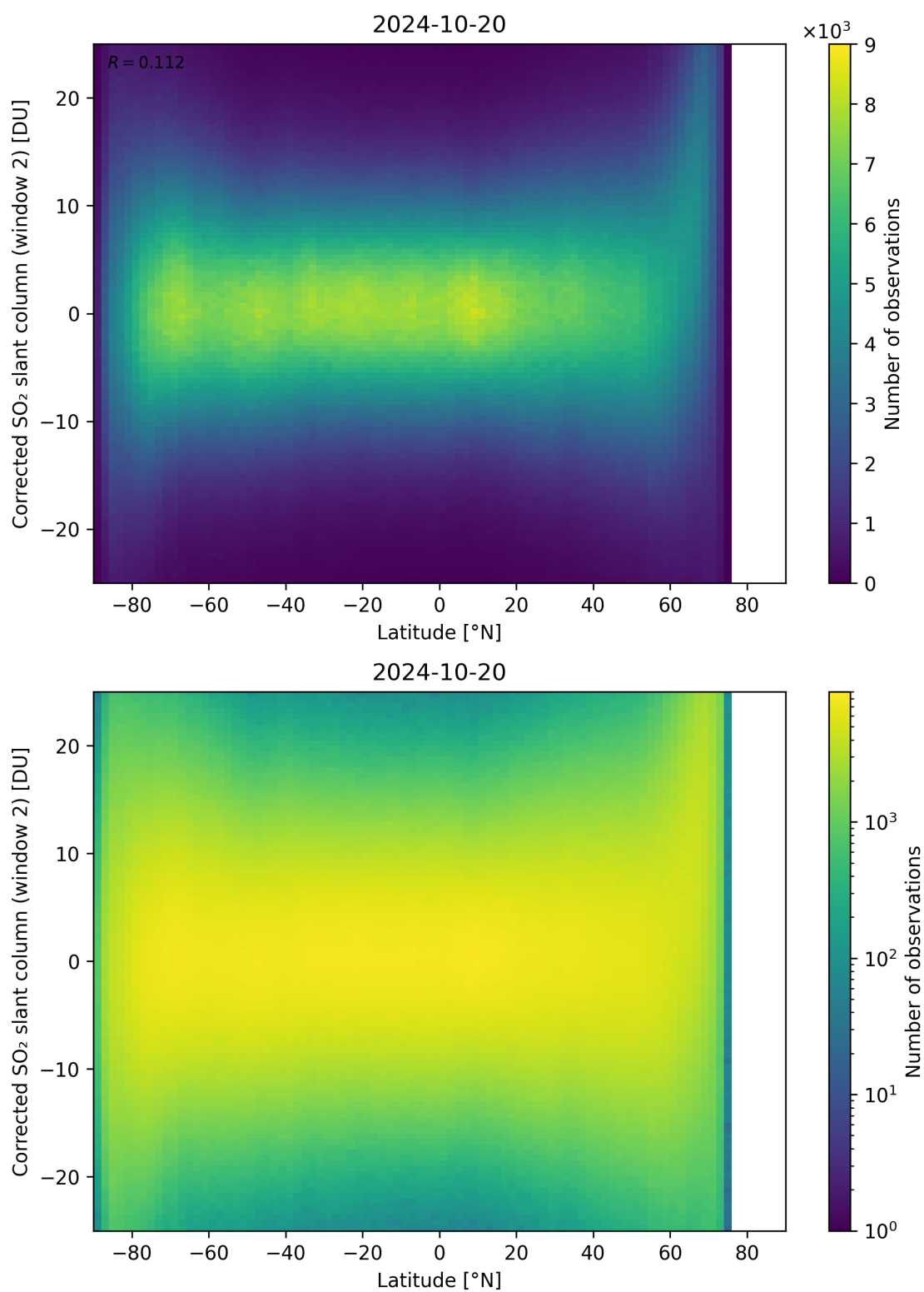
Figure 147: Scatter density plot of “Latitude” against “Corrected SO 2 slant column (window 2)” for 2024-10-19 to 2024-10-21.
