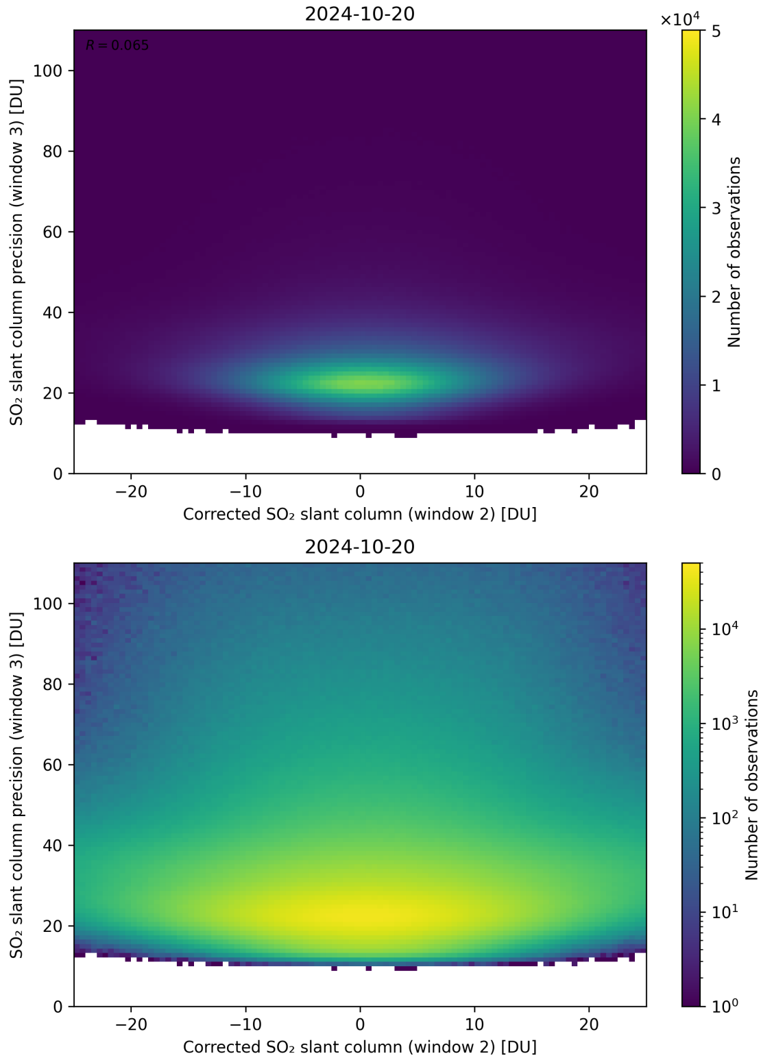
Figure 202: Scatter density plot of “Corrected SO 2 slant column (window 2)” against “SO 2 slant column precision (window 3)” for 2024-10-19 to 2024-10-21.
