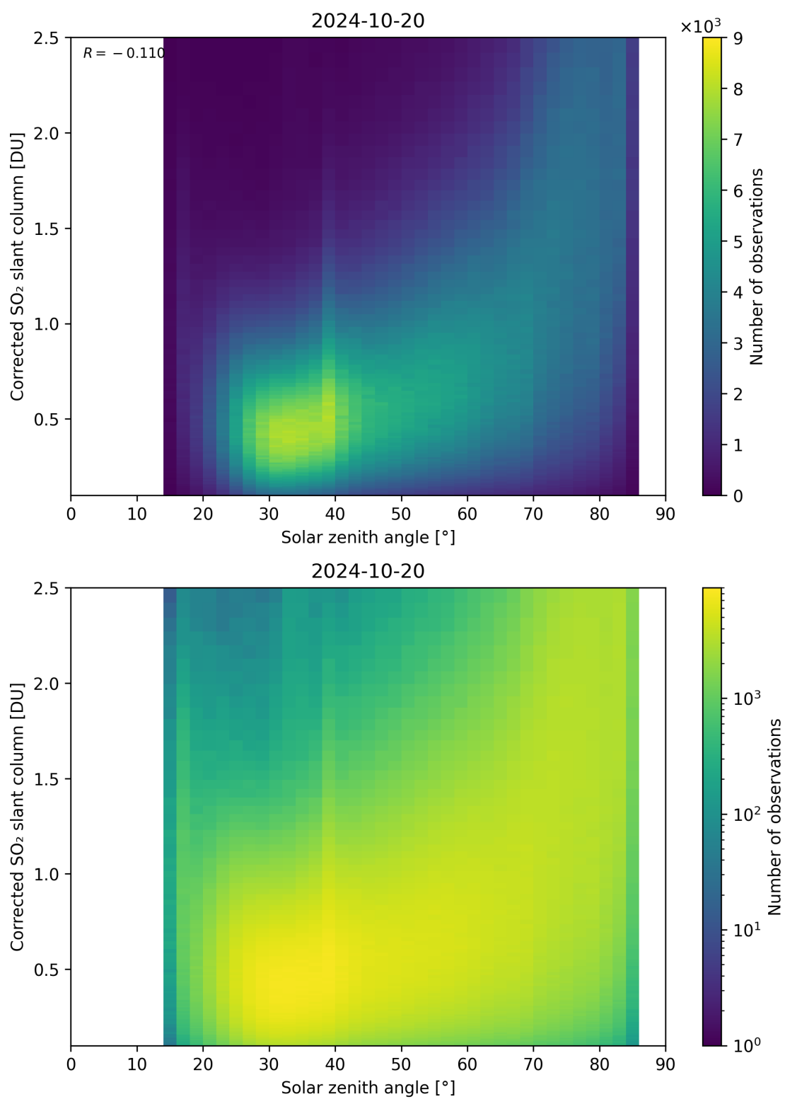
Figure 166: Scatter density plot of “Solar zenith angle” against “Corrected SO 2 slant column” for 2024-10-19 to 2024-10-21.
