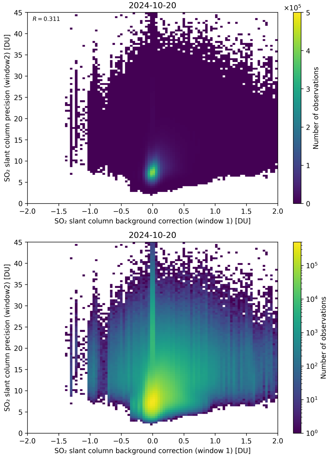
Figure 106: Scatter density plot of “SO 2 slant column background correction (window 1)” against “SO 2 slant column precision (window2)” for 2024-10-19 to 2024-10-21.
