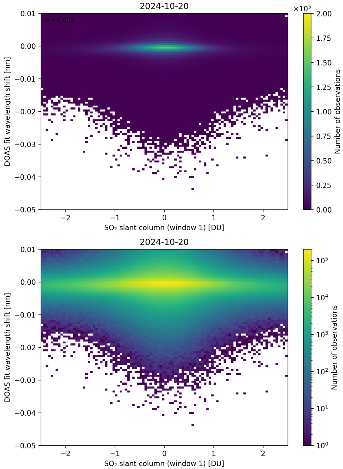
Figure 215: Scatter density plot of “SO 2 slant column (window 1)” against “DOAS fit wavelength shift” for 2024-10-19 to 2024-10-21.
