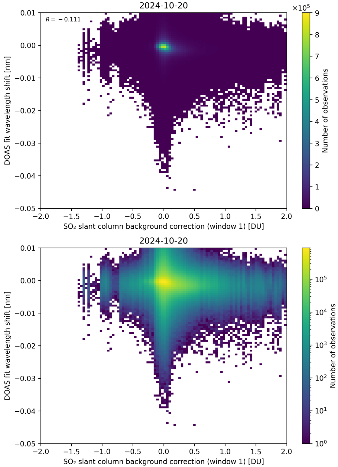
Figure 100: Scatter density plot of “SO 2 slant column background correction (window 1)” against “DOAS fit wavelength shift” for 2024-10-19 to 2024-10-21.
