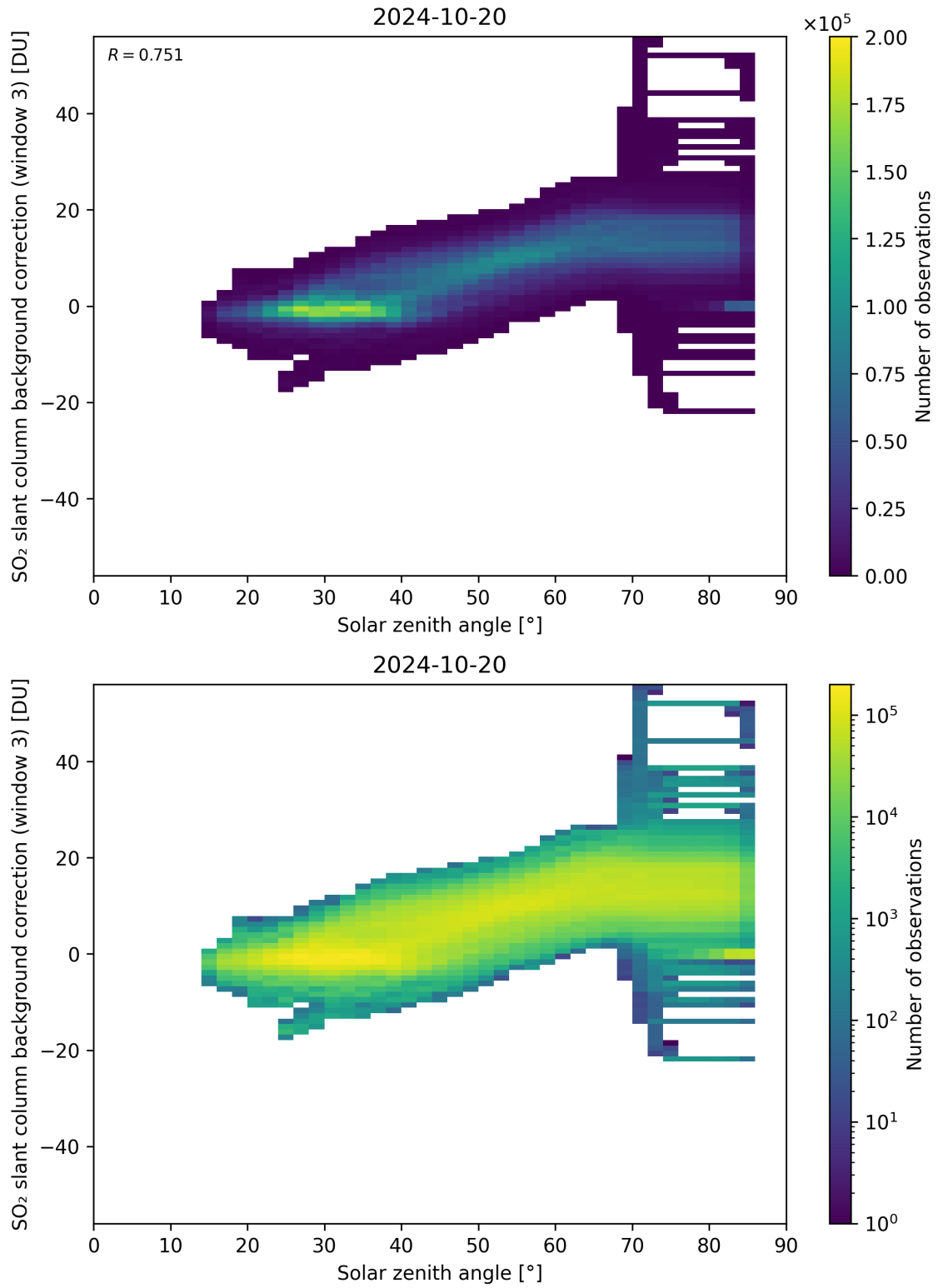
Figure 160: Scatter density plot of “Solar zenith angle” against “SO 2 slant column background correction (window 3)” for 2024-10-19 to 2024-10-21.
