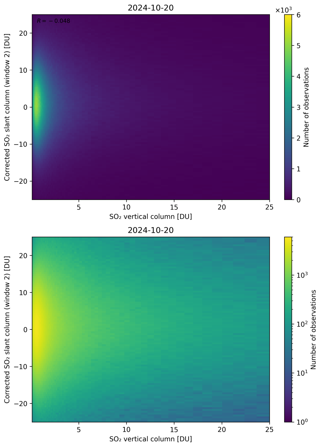
Figure 298: Scatter density plot of “SO 2 vertical column” against “Corrected SO 2 slant column (window 2)” for 2024-10-19 to 2024-10-21.
