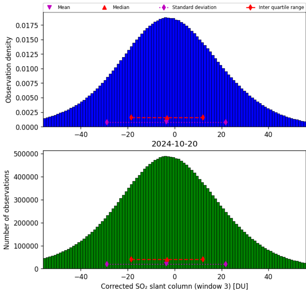
Figure 66: Histogram of “Corrected SO 2 slant column (window 3)” for 2024-10-19 to 2024-10-21
