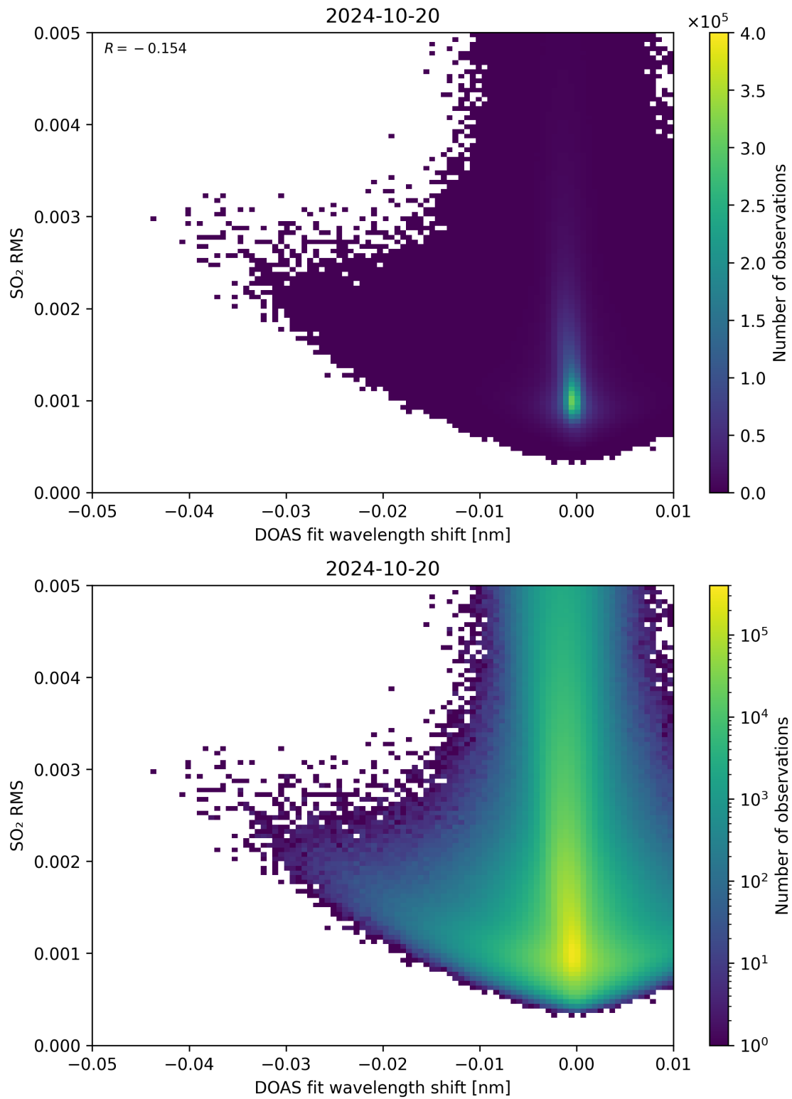
Figure 128: Scatter density plot of “DOAS fit wavelength shift” against “SO 2 RMS” for 2024-10-19 to 2024-10-21.
