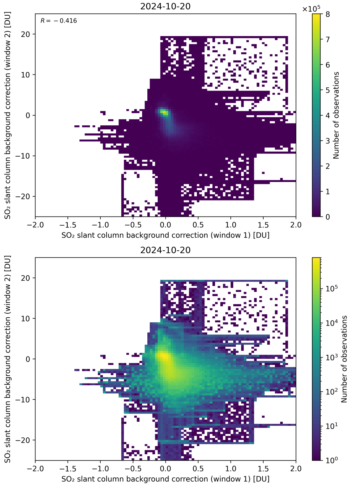
Figure 98: Scatter density plot of “SO 2 slant column background correction (window 1)” against “SO 2 slant column background correction (window 2)” for 2024-10-19 to 2024-10-21.
