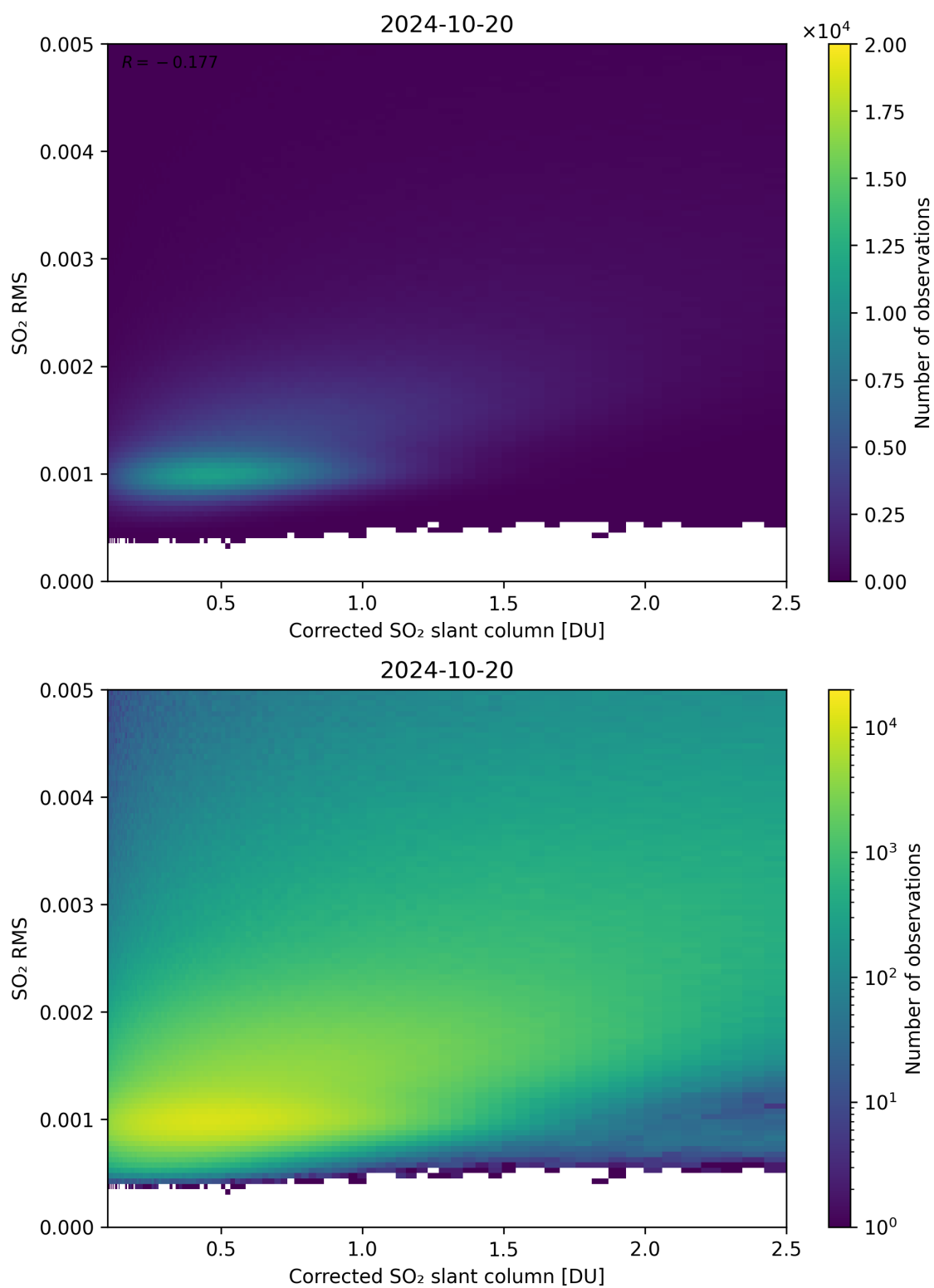
Figure 183: Scatter density plot of “Corrected SO 2 slant column” against “SO 2 RMS” for 2024-10-19 to 2024-10-21.
