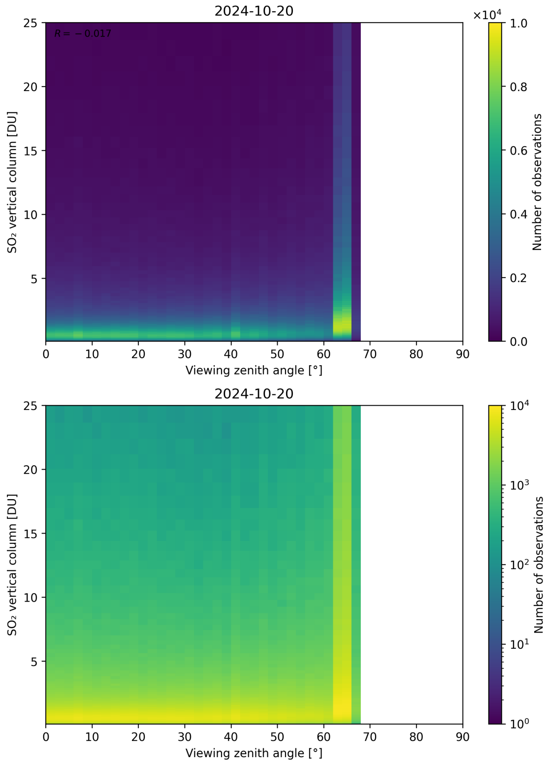
Figure 327: Scatter density plot of “Viewing zenith angle” against “SO 2 vertical column” for 2024-10-19 to 2024-10-21.
