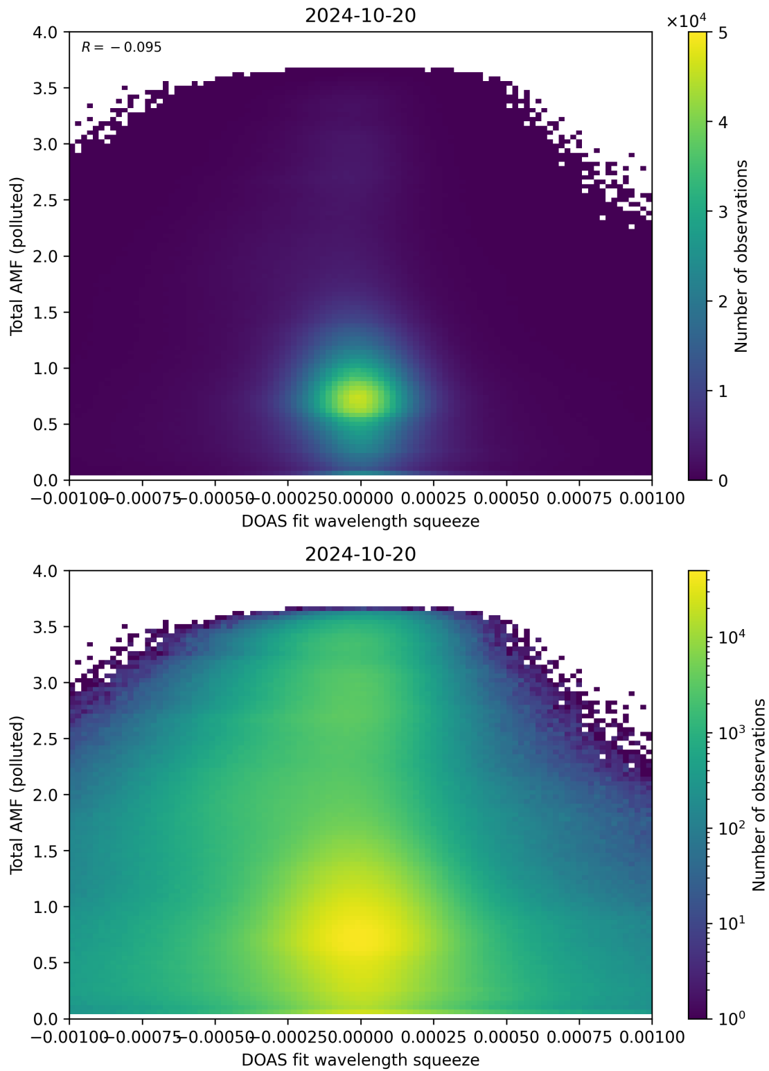
Figure 134: Scatter density plot of “DOAS fit wavelength squeeze” against “Total AMF (polluted)” for 2024-10-19 to 2024-10-21.
