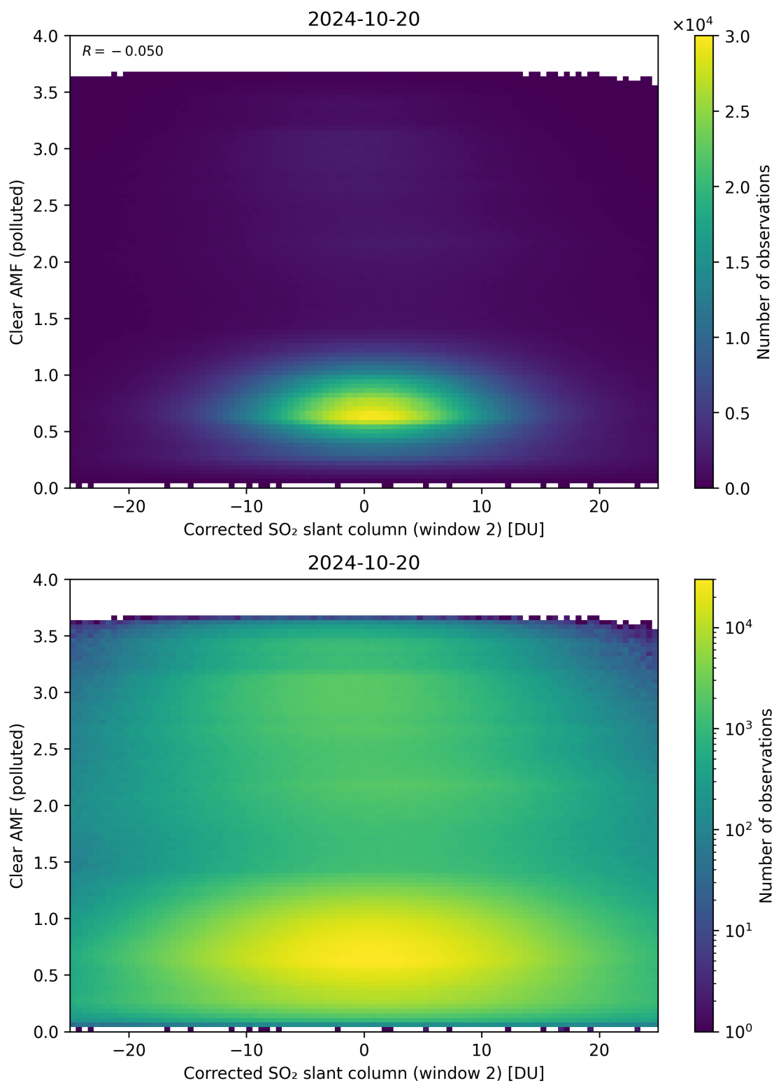
Figure 199: Scatter density plot of “Corrected SO 2 slant column (window 2)” against “Clear AMF (polluted)” for 2024-10-19 to 2024-10-21.
