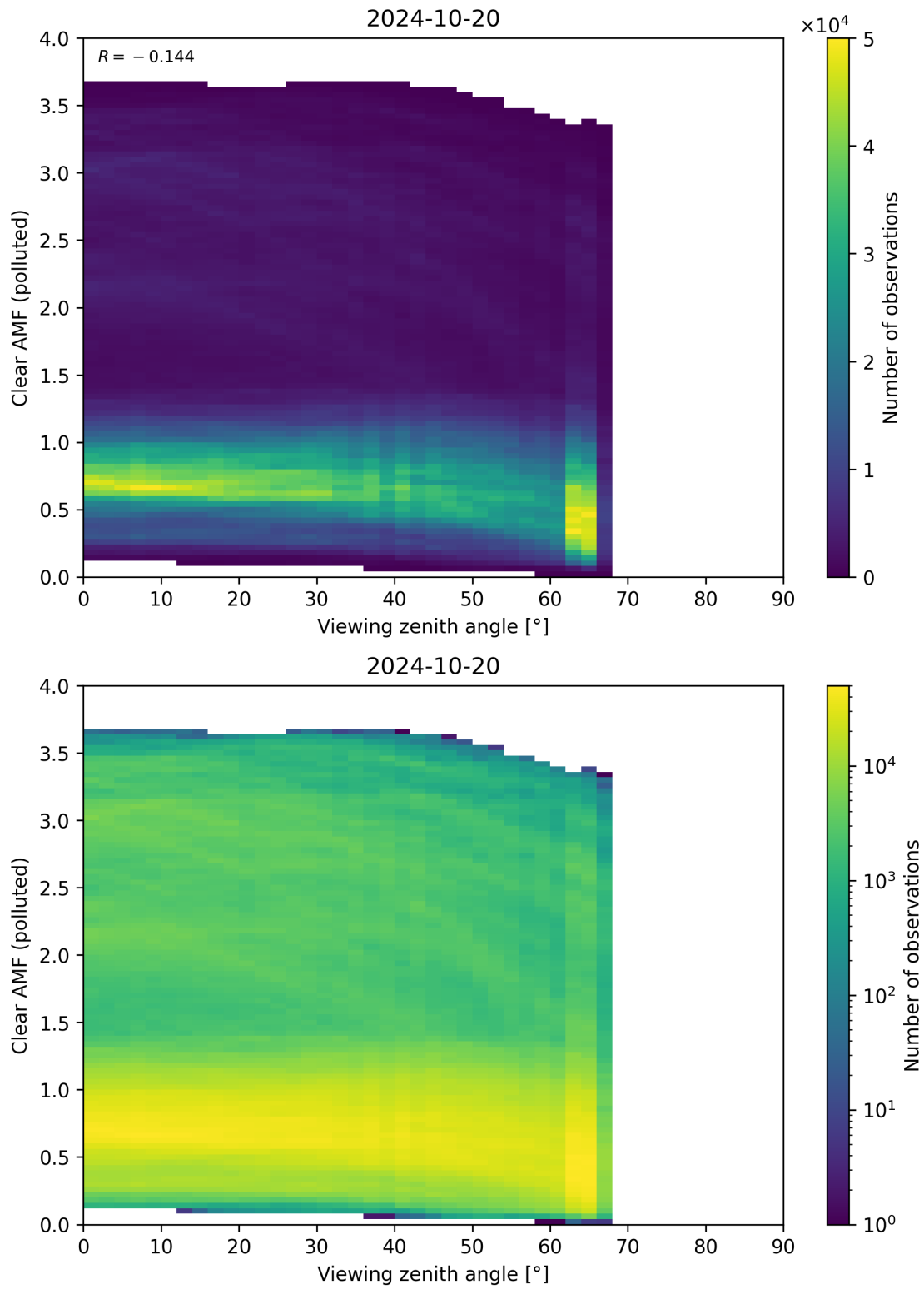
Figure 316: Scatter density plot of “Viewing zenith angle” against “Clear AMF (polluted)” for 2024-10-19 to 2024-10-21.
