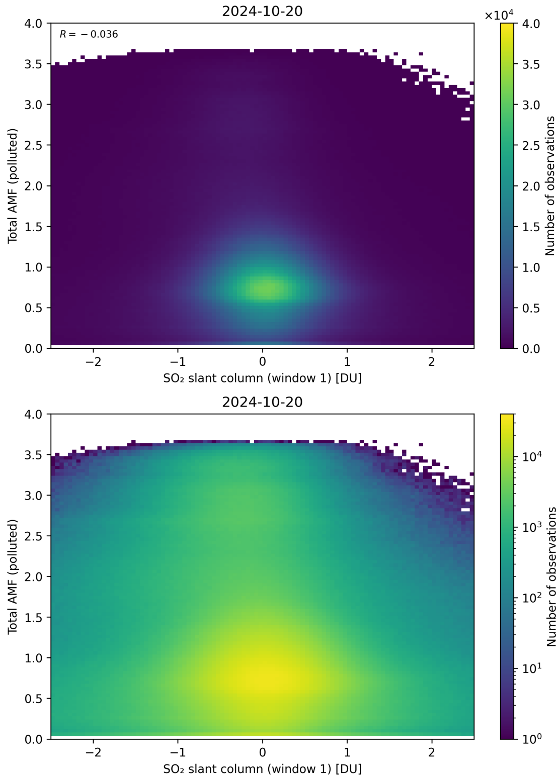
Figure 239: Scatter density plot of “SO 2 slant column (window 1)” against “Total AMF (polluted)” for 2024-10-19 to 2024-10-21.
