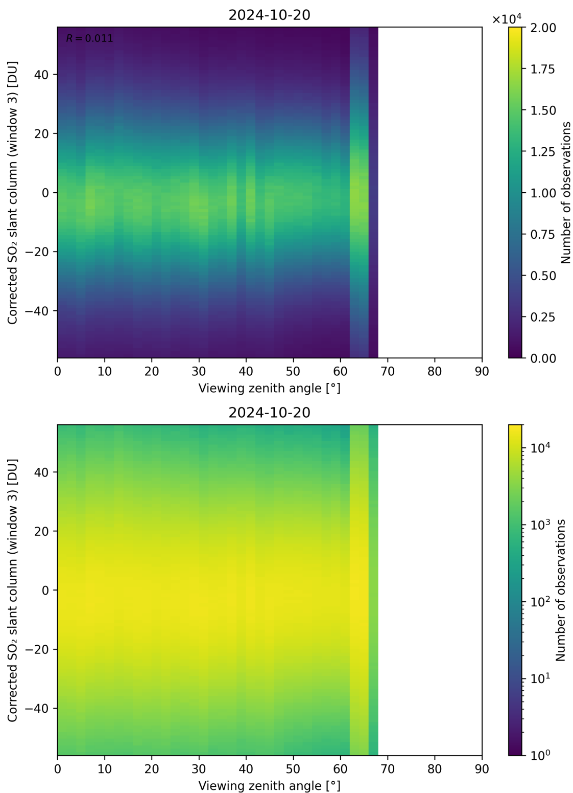
Figure 319: Scatter density plot of “Viewing zenith angle” against “Corrected SO 2 slant column (window 3)” for 2024-10-19 to 2024-10-21.
