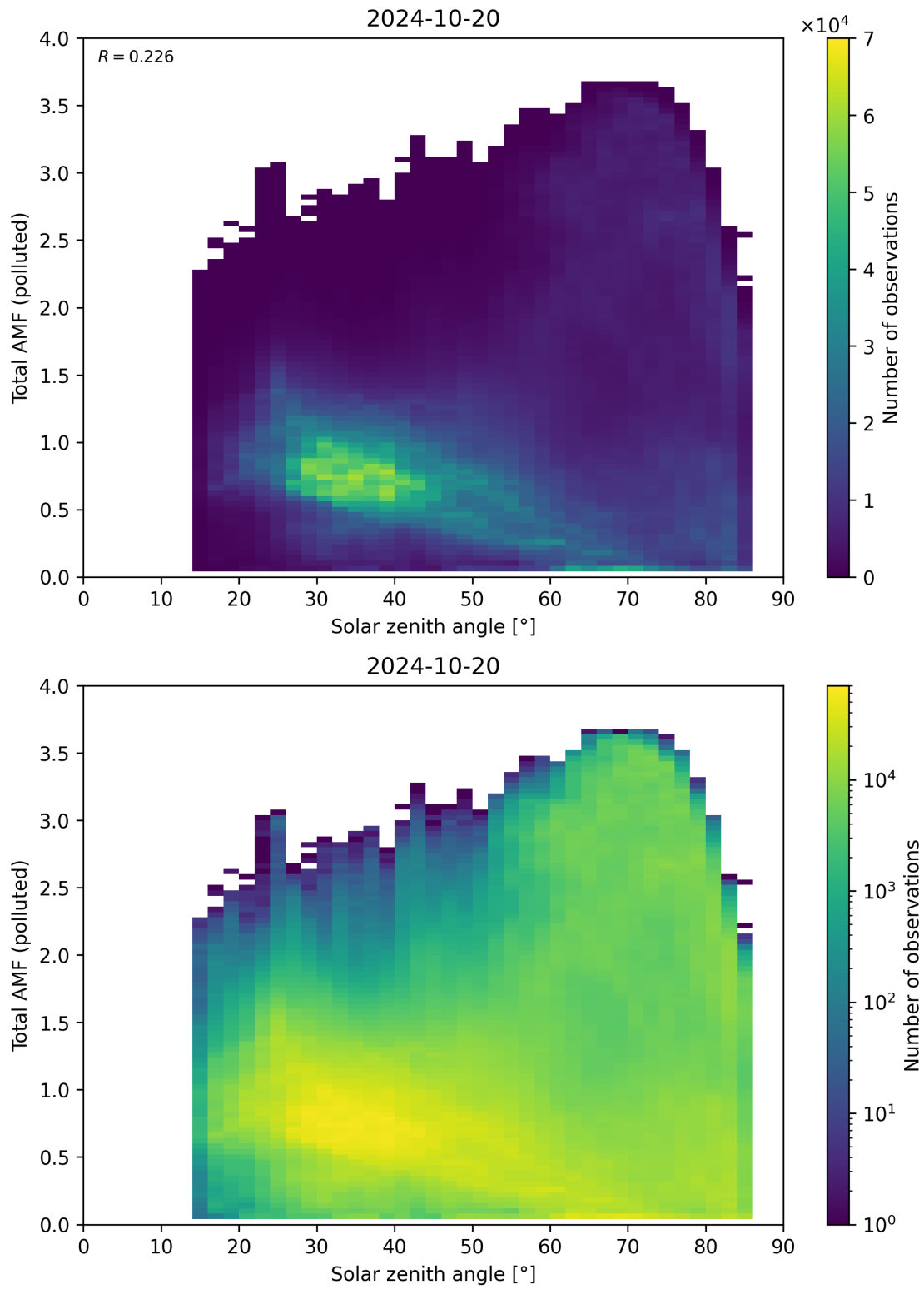
Figure 174: Scatter density plot of “Solar zenith angle” against “Total AMF (polluted)” for 2024-10-19 to 2024-10-21.
