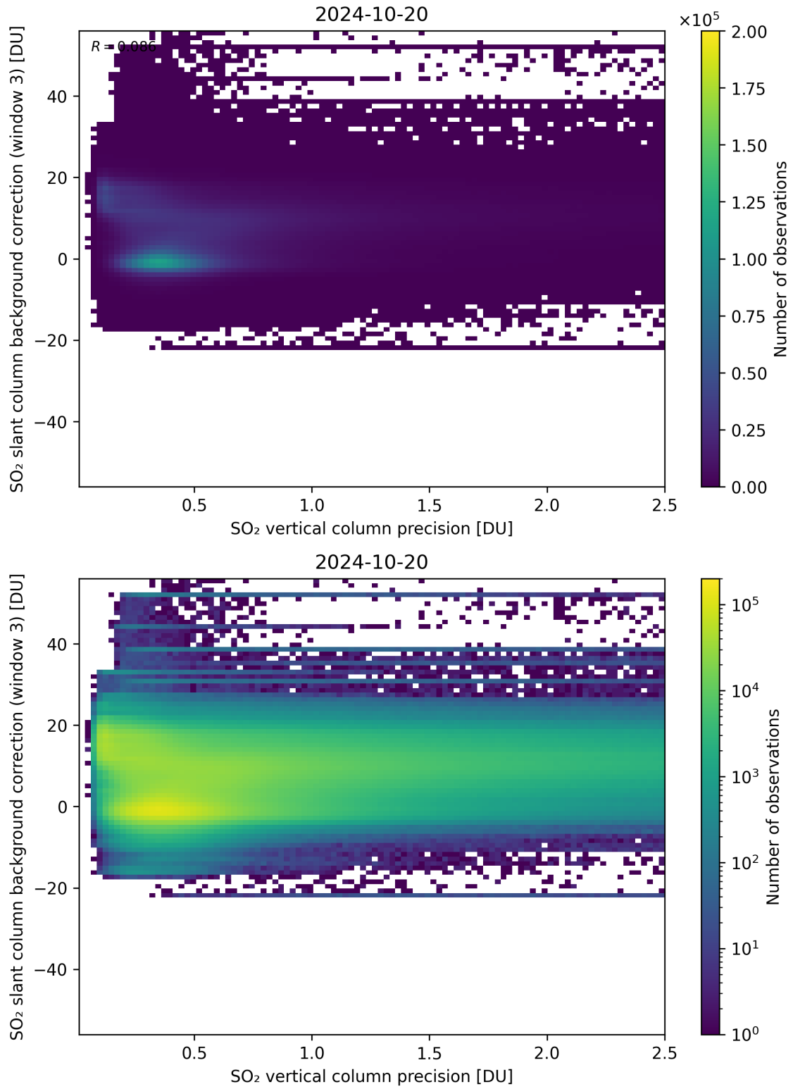
Figure 281: Scatter density plot of “SO 2 vertical column precision” against “SO 2 slant column background correction (window 3)” for 2024-10-19 to 2024-10-21.
