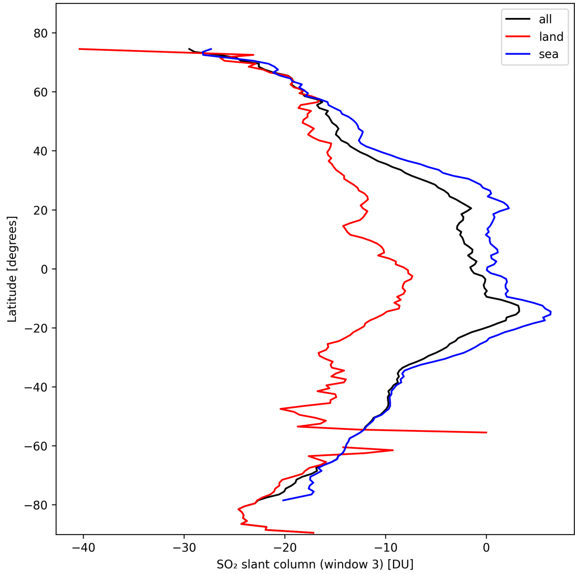
Figure 41: Zonal average of “SO 2 slant column (window 3)” for 2024-10-19 to 2024-10-21.
