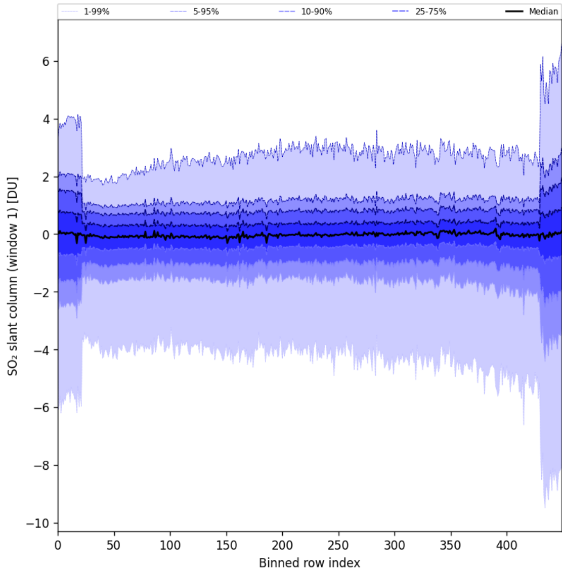
Figure 79: Along track statistics of “SO 2 slant column (window 1)” for 2024-10-19 to 2024-10-21
