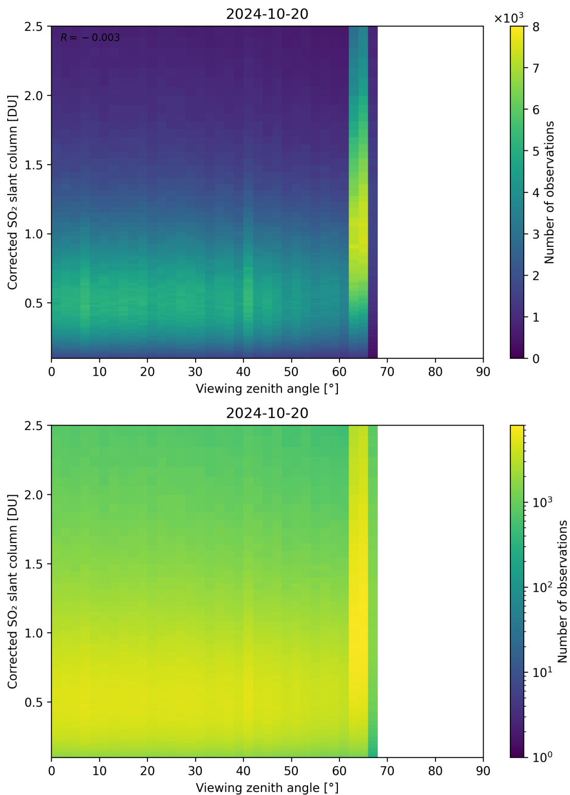
Figure 317: Scatter density plot of “Viewing zenith angle” against “Corrected SO 2 slant column” for 2024-10-19 to 2024-10-21.
