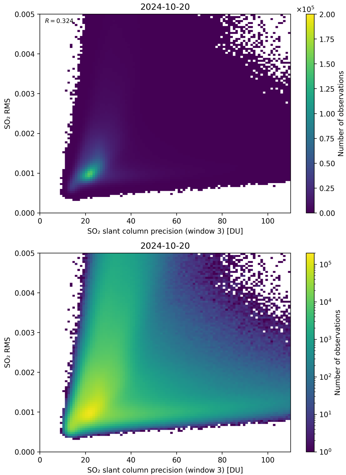
Figure 260: Scatter density plot of “SO 2 slant column precision (window 3)” against “SO 2 RMS” for 2024-10-19 to 2024-10-21.
