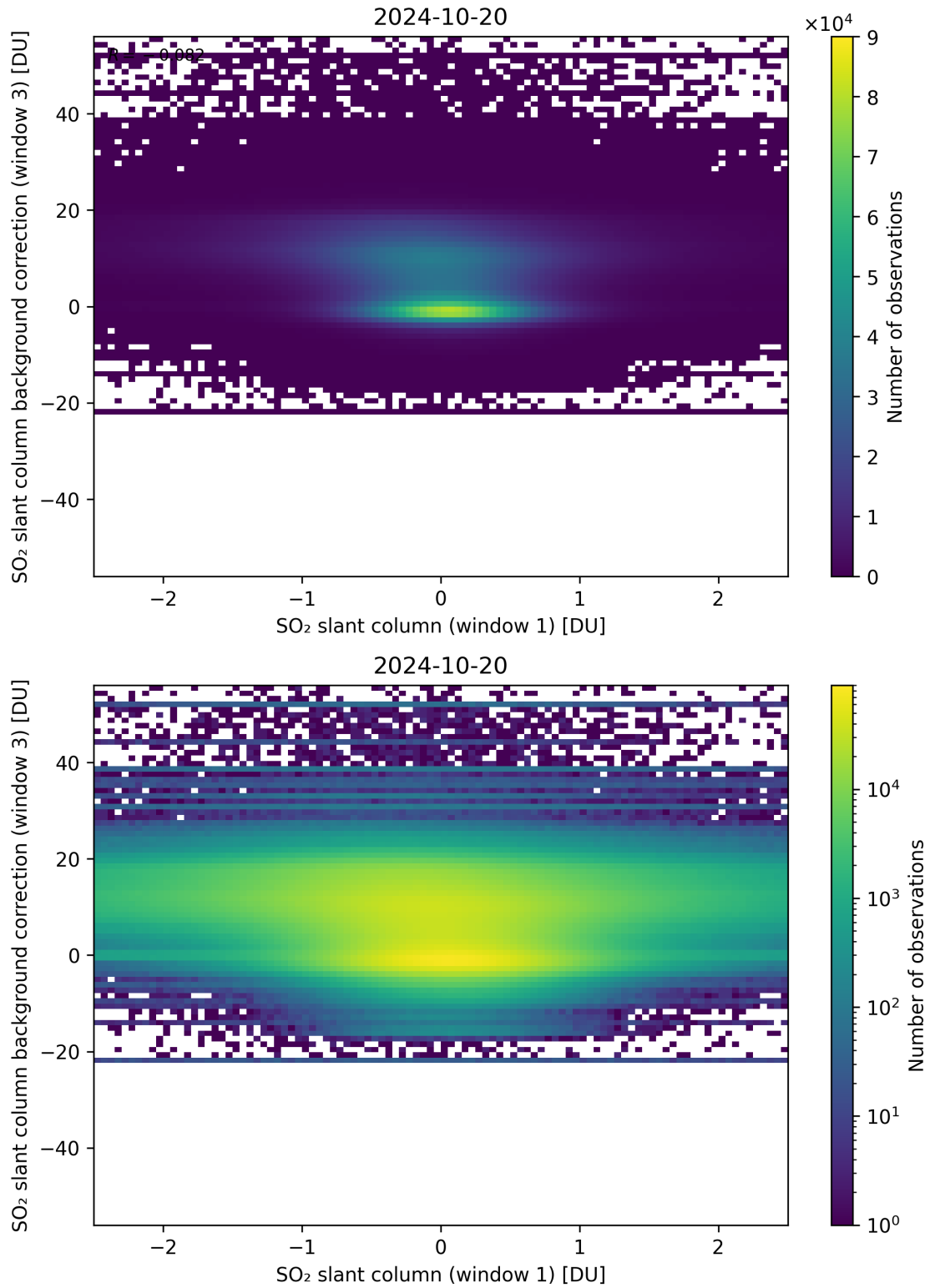
Figure 214: Scatter density plot of “SO 2 slant column (window 1)” against “SO 2 slant column background correction (window 3)” for 2024-10-19 to 2024-10-21.
