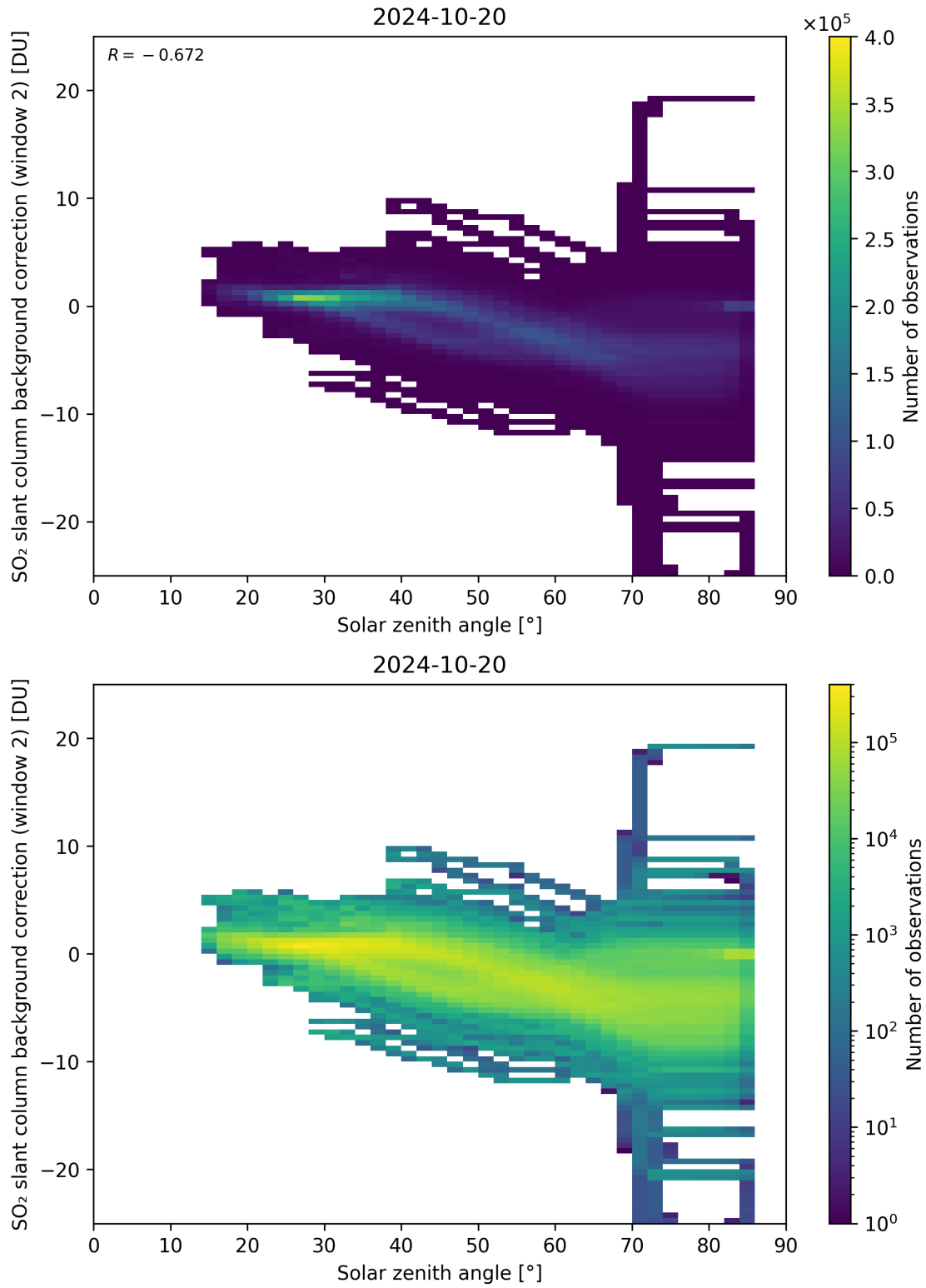
Figure 159: Scatter density plot of “Solar zenith angle” against “SO 2 slant column background correction (window 2)” for 2024-10-19 to 2024-10-21.
