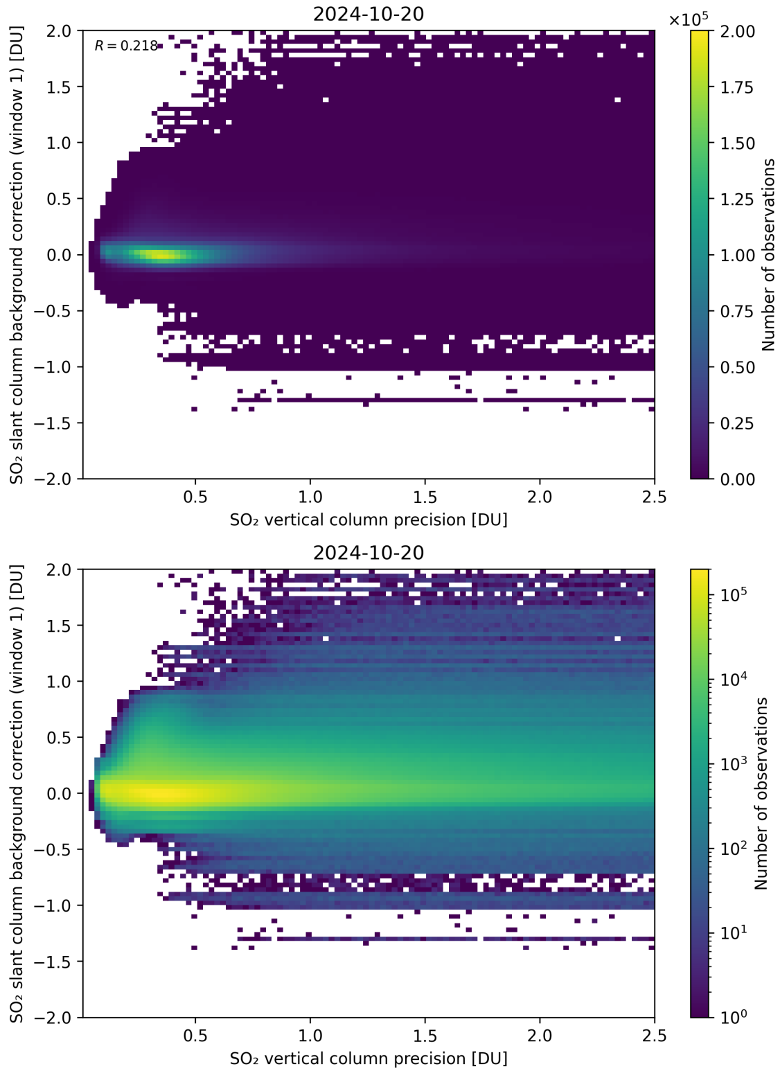
Figure 279: Scatter density plot of “SO 2 vertical column precision” against “SO 2 slant column background correction (window 1)” for 2024-10-19 to 2024-10-21.
