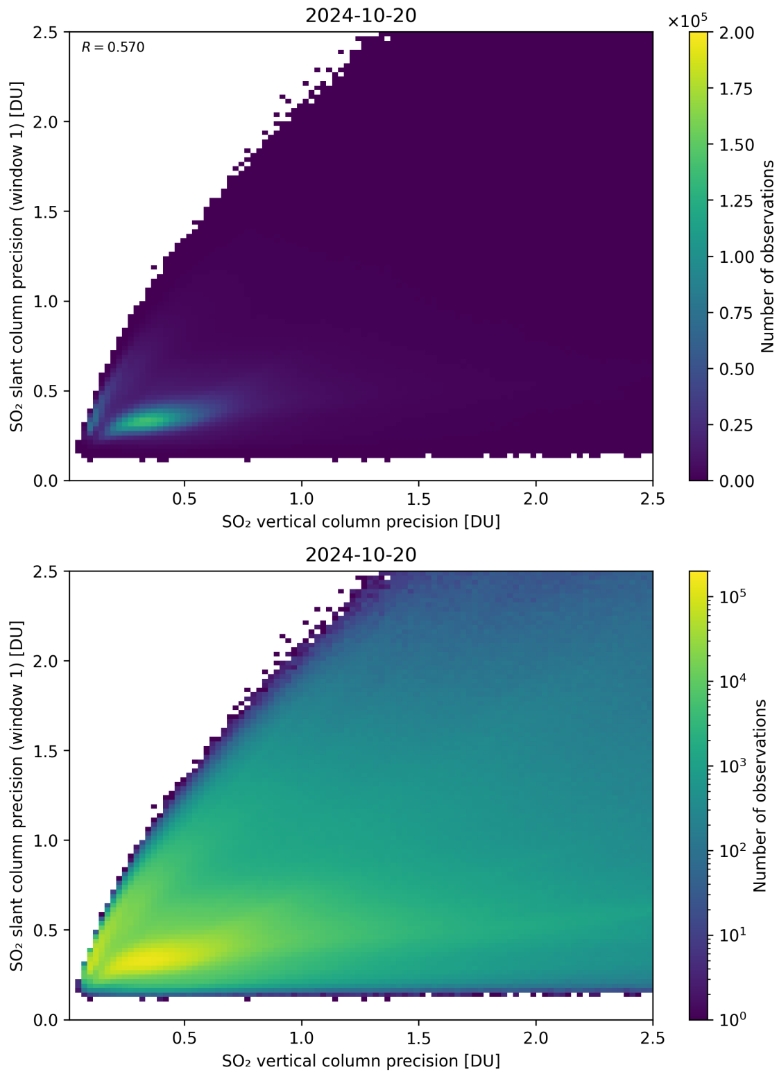
Figure 290: Scatter density plot of “SO 2 vertical column precision” against “SO 2 slant column precision (window 1)” for 2024-10-19 to 2024-10-21.
