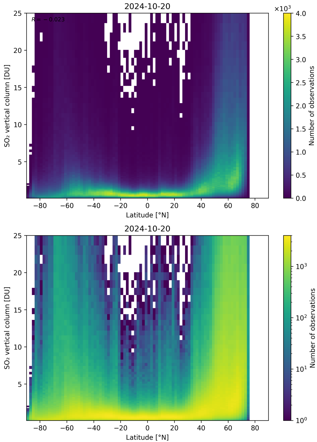
Figure 156: Scatter density plot of “Latitude” against “SO 2 vertical column” for 2024-10-19 to 2024-10-21.
