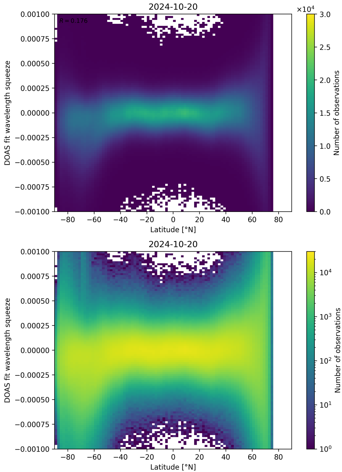
Figure 143: Scatter density plot of “Latitude” against “DOAS fit wavelength squeeze” for 2024-10-19 to 2024-10-21.
