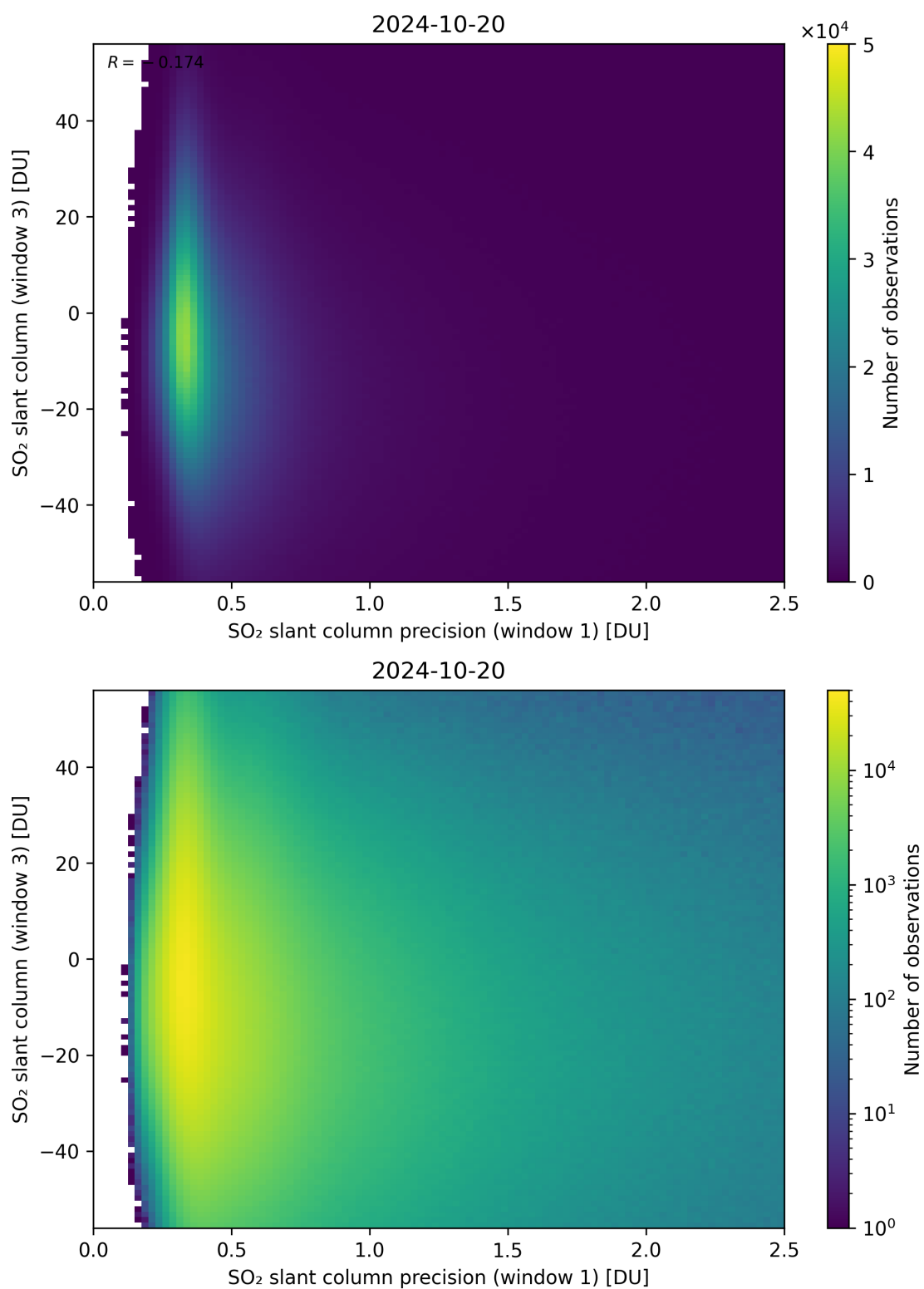
Figure 228: Scatter density plot of “SO 2 slant column precision (window 1)” against “SO 2 slant column (window 3)” for 2024-10-19 to 2024-10-21.
