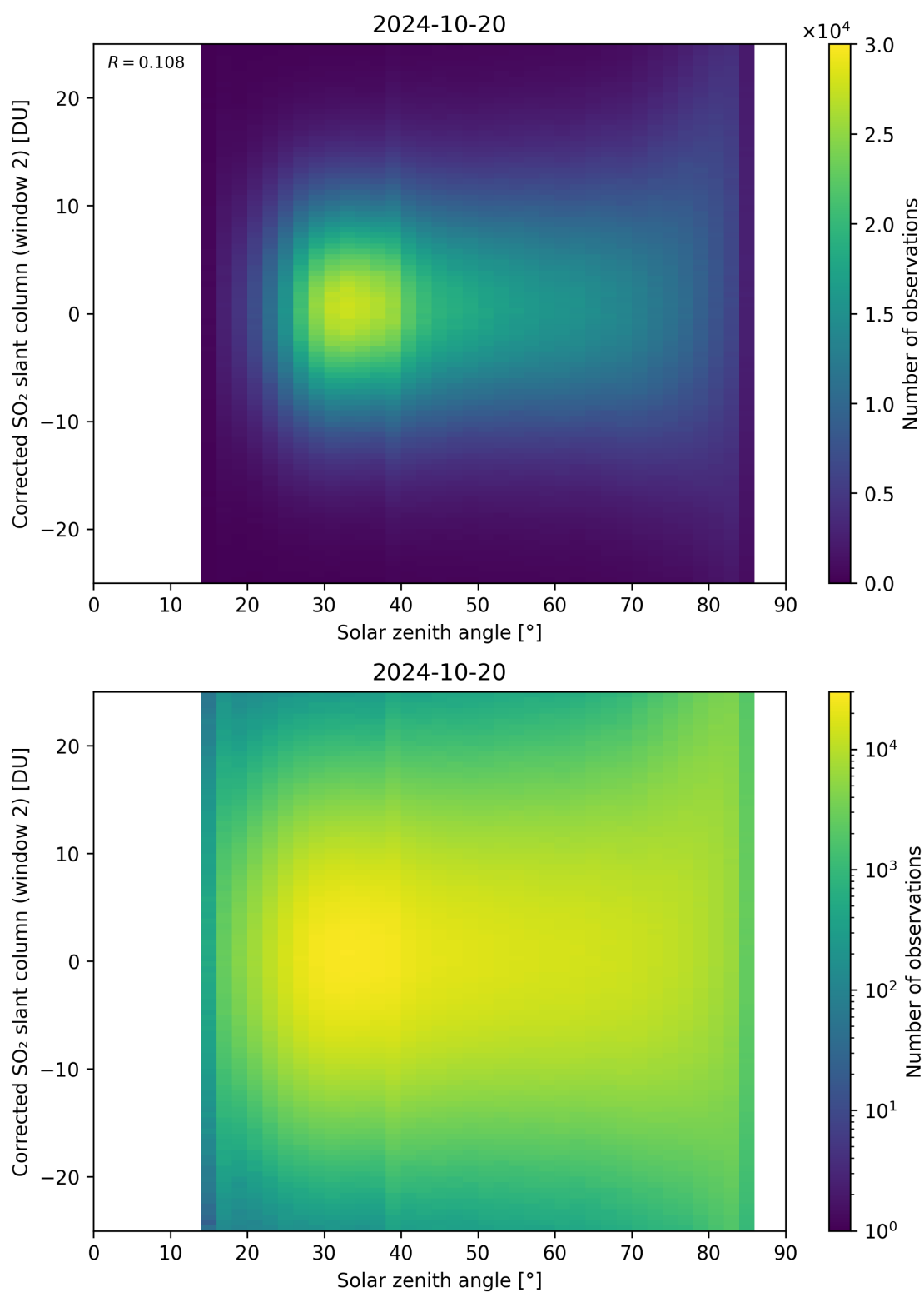
Figure 167: Scatter density plot of “Solar zenith angle” against “Corrected SO 2 slant column (window 2)” for 2024-10-19 to 2024-10-21.
