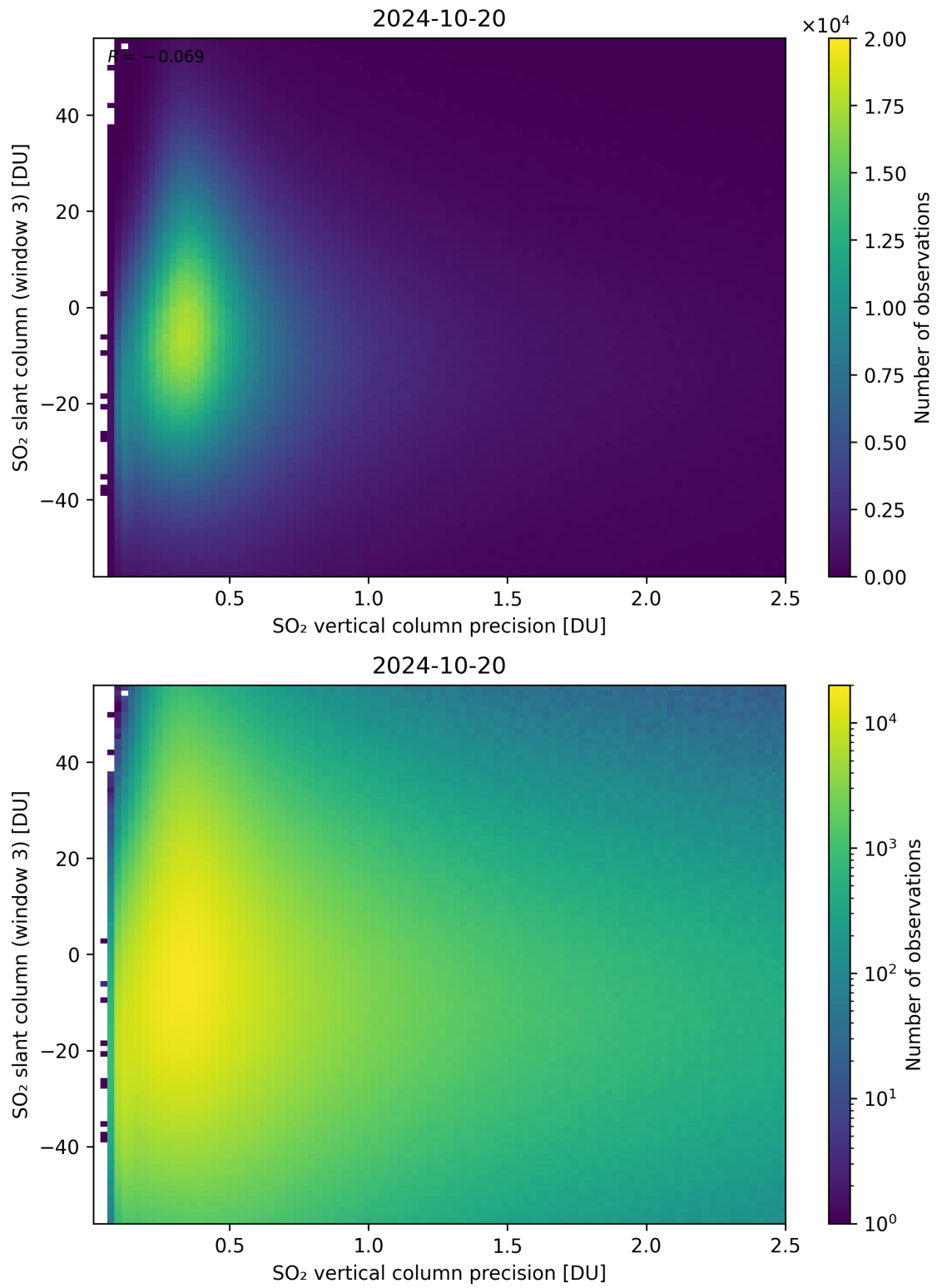
Figure 292: Scatter density plot of “SO 2 vertical column precision” against “SO 2 slant column (window 3)” for 2024-10-19 to 2024-10-21.
