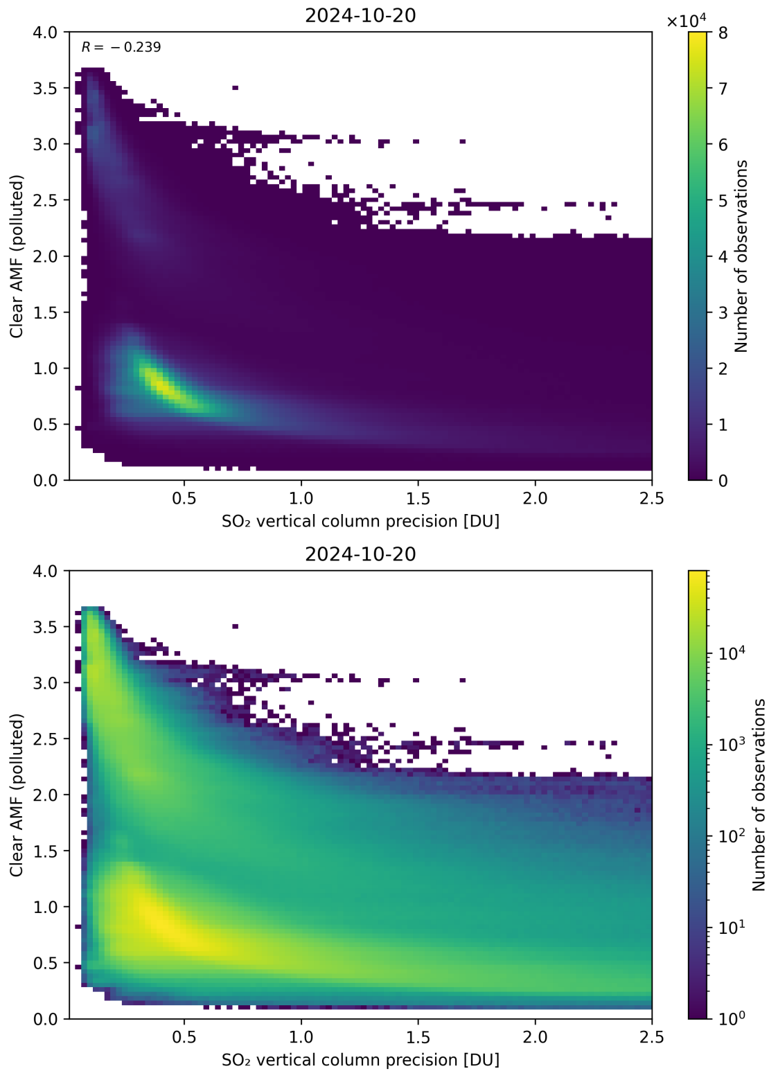
Figure 285: Scatter density plot of “SO 2 vertical column precision” against “Clear AMF (polluted)” for 2024-10-19 to 2024-10-21.
