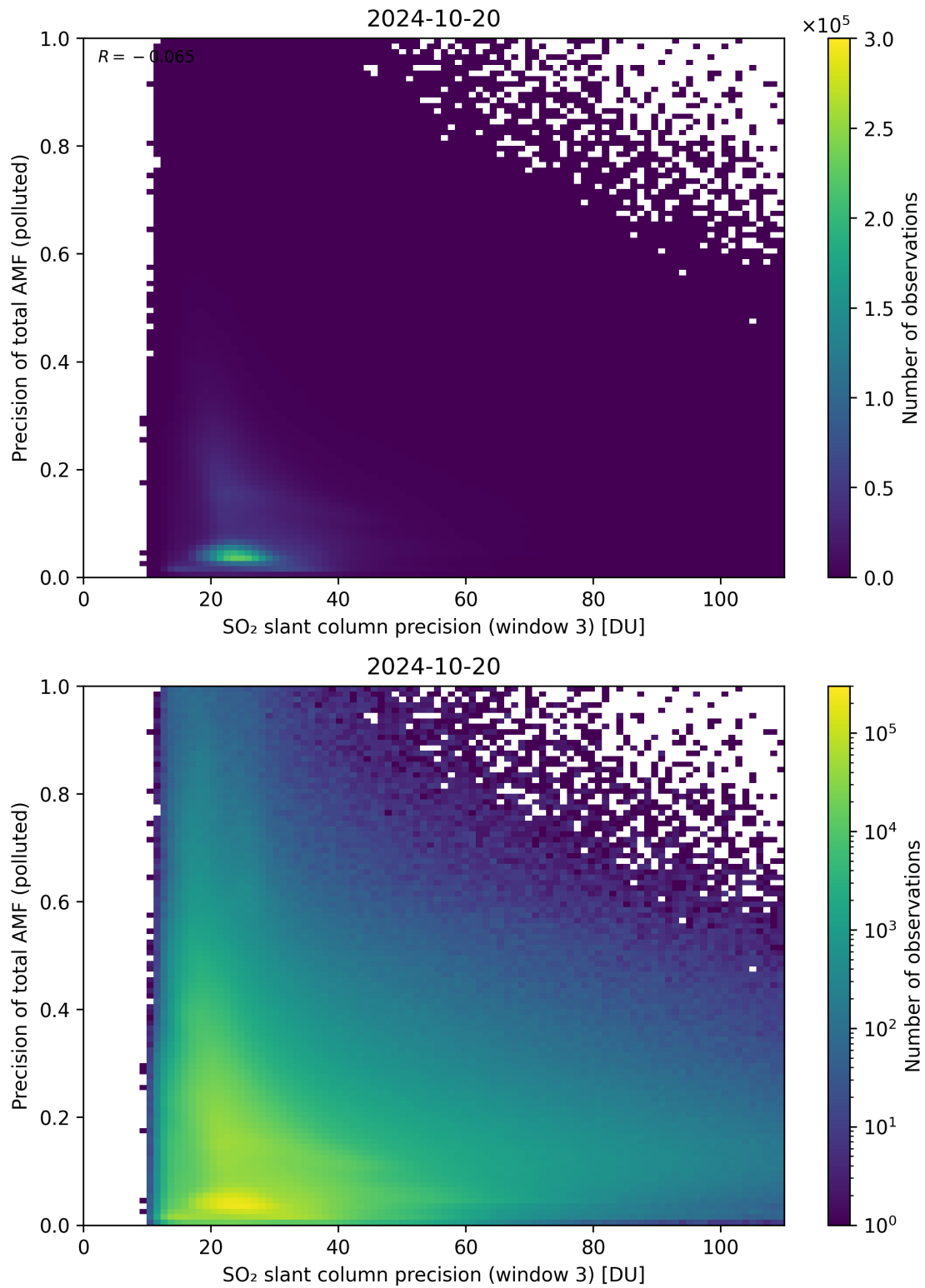
Figure 264: Scatter density plot of “SO 2 slant column precision (window 3)” against “Precision of total AMF (polluted)” for 2024-10-19 to 2024-10-21.
