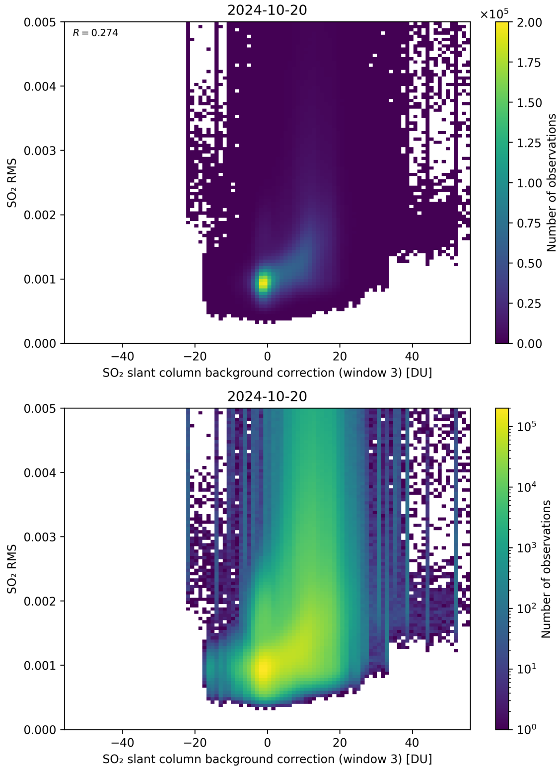
Figure 123: Scatter density plot of “SO 2 slant column background correction (window 3)” against “SO 2 RMS” for 2024-10-19 to 2024-10-21.
