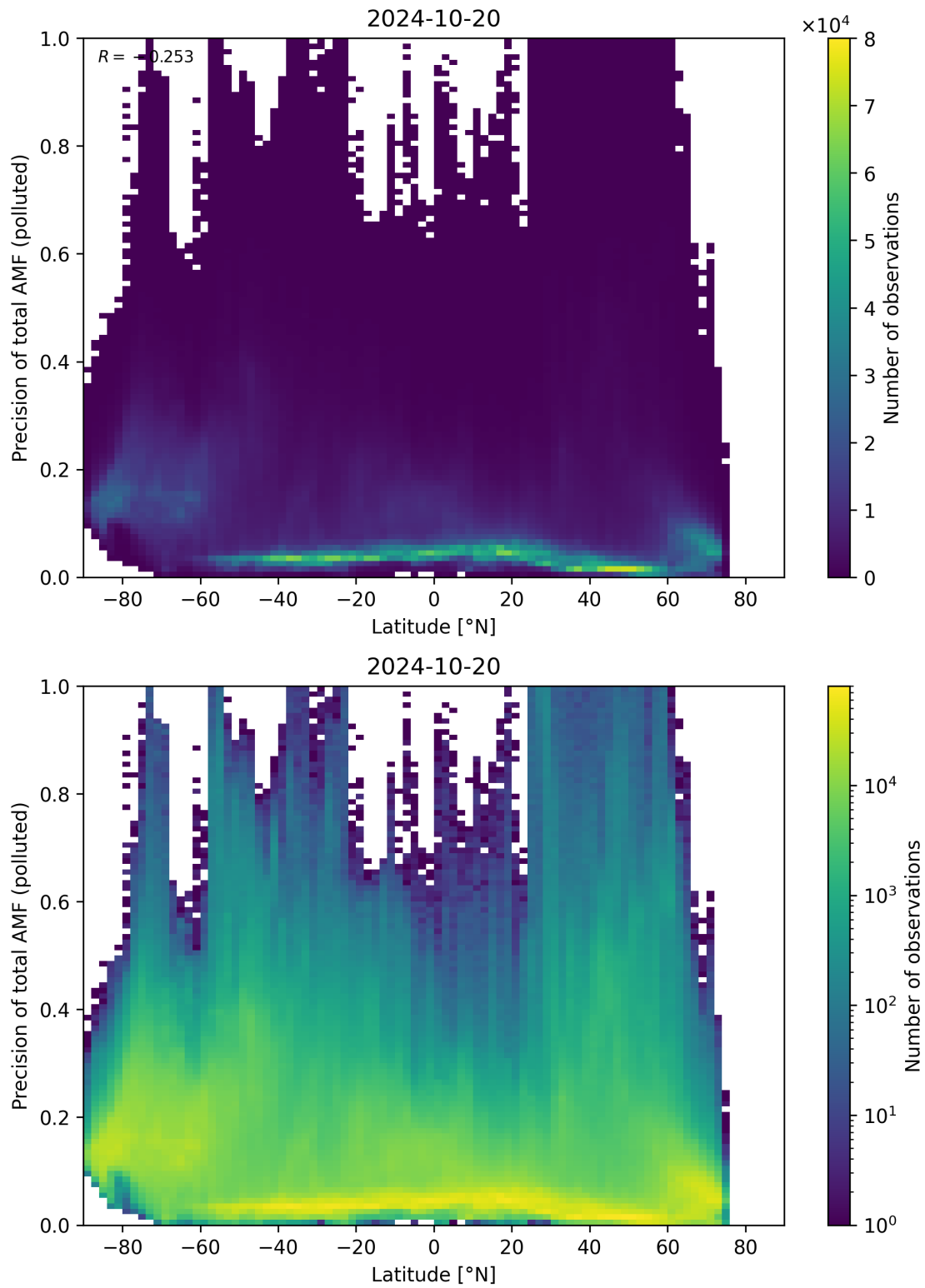
Figure 155: Scatter density plot of “Latitude” against “Precision of total AMF (polluted)” for 2024-10-19 to 2024-10-21.
