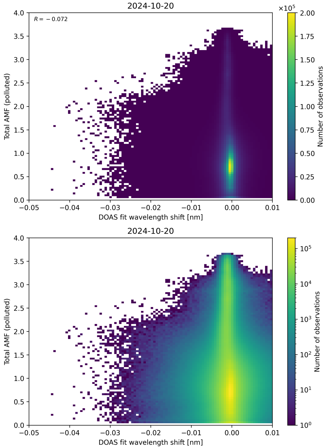
Figure 130: Scatter density plot of “DOAS fit wavelength shift” against “Total AMF (polluted)” for 2024-10-19 to 2024-10-21.
