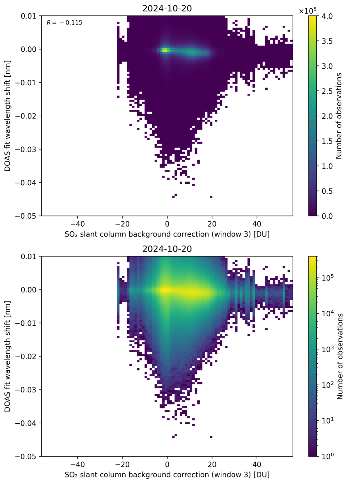
Figure 121: Scatter density plot of “SO 2 slant column background correction (window 3)” against “DOAS fit wavelength shift” for 2024-10-19 to 2024-10-21.
