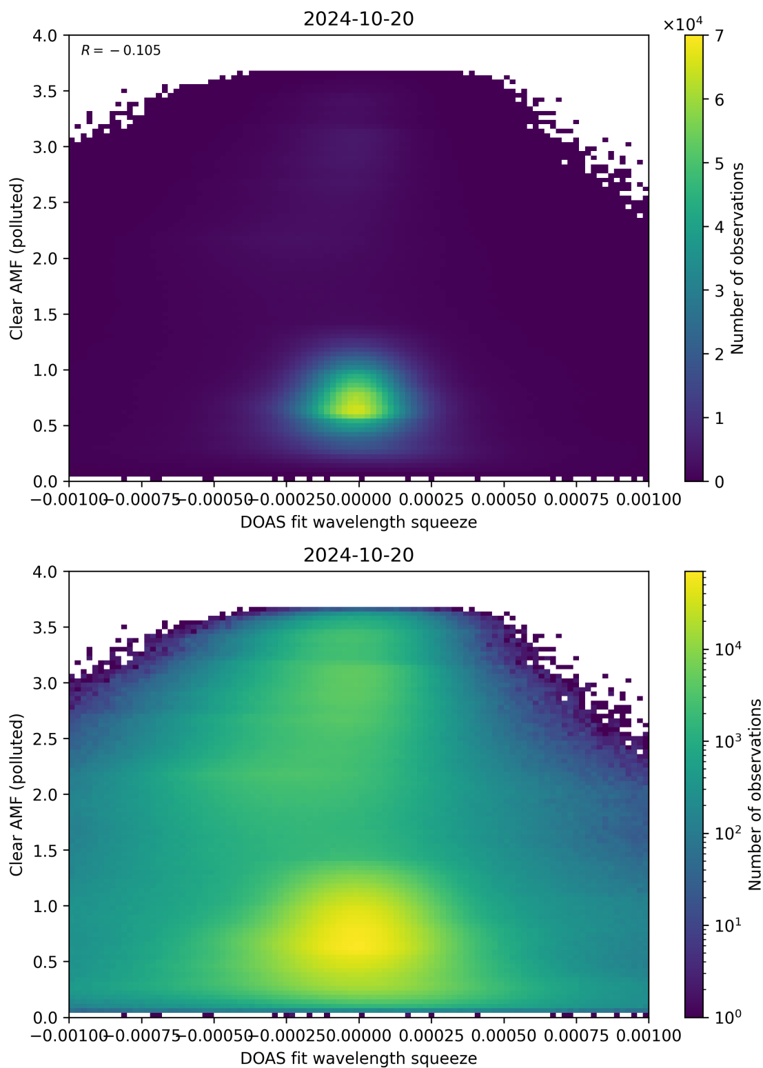
Figure 133: Scatter density plot of “DOAS fit wavelength squeeze” against “Clear AMF (polluted)” for 2024-10-19 to 2024-10-21.
