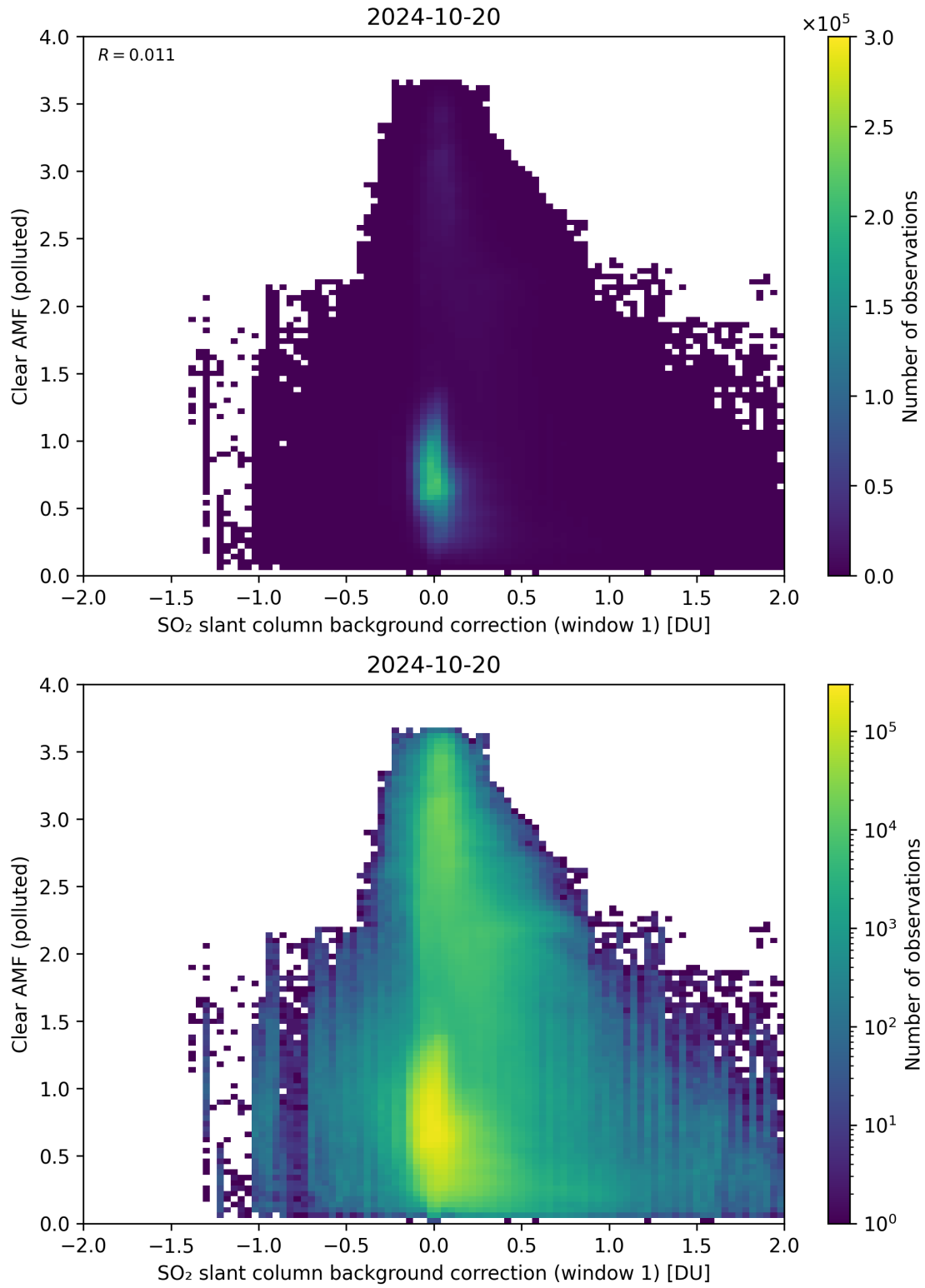
Figure 103: Scatter density plot of “SO 2 slant column background correction (window 1)” against “Clear AMF (polluted)” for 2024-10-19 to 2024-10-21.
