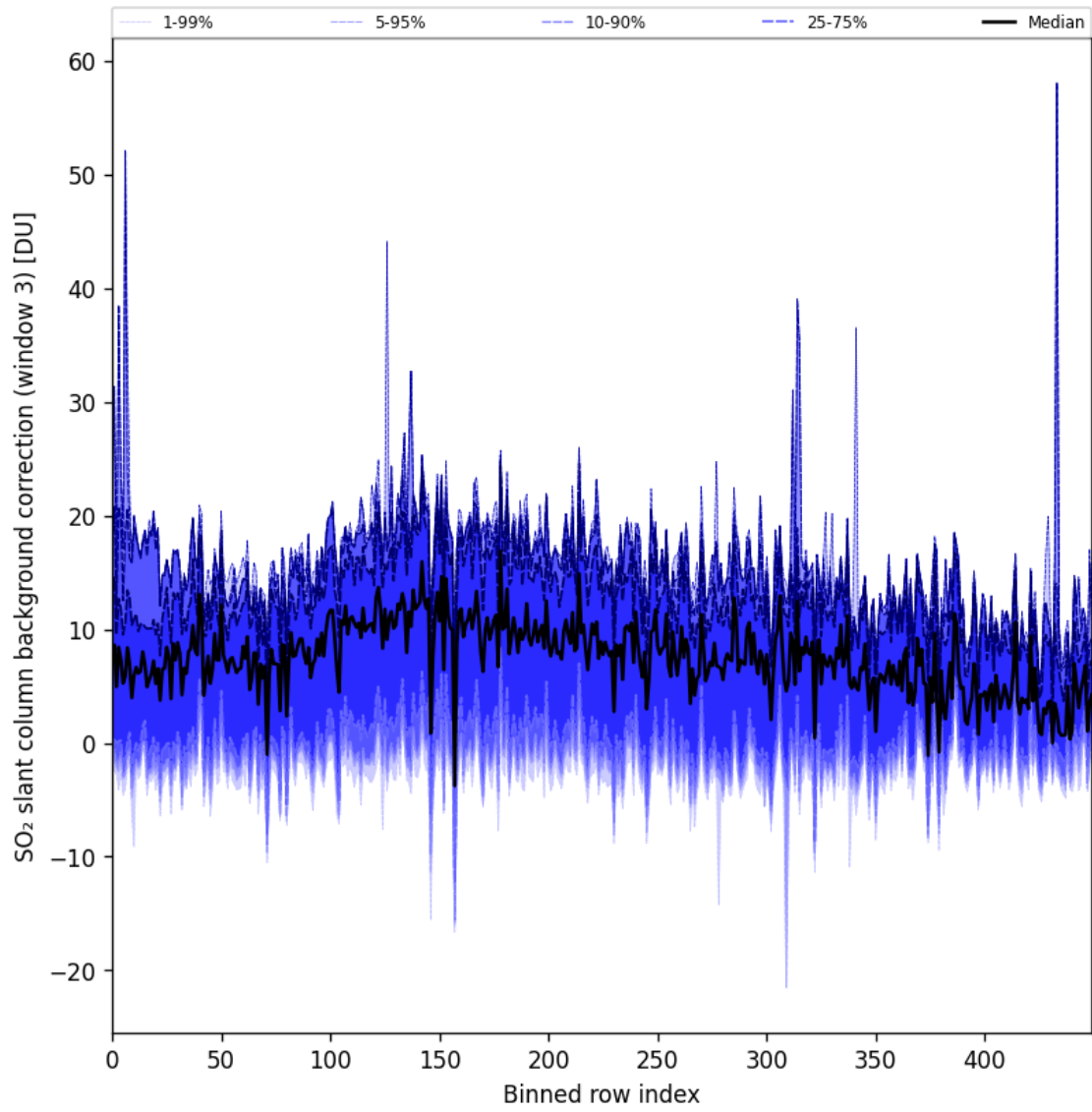
Figure 90: Along track statistics of “SO 2 slant column background correction (window 3)” for 2024-10-19 to 2024-10-21
