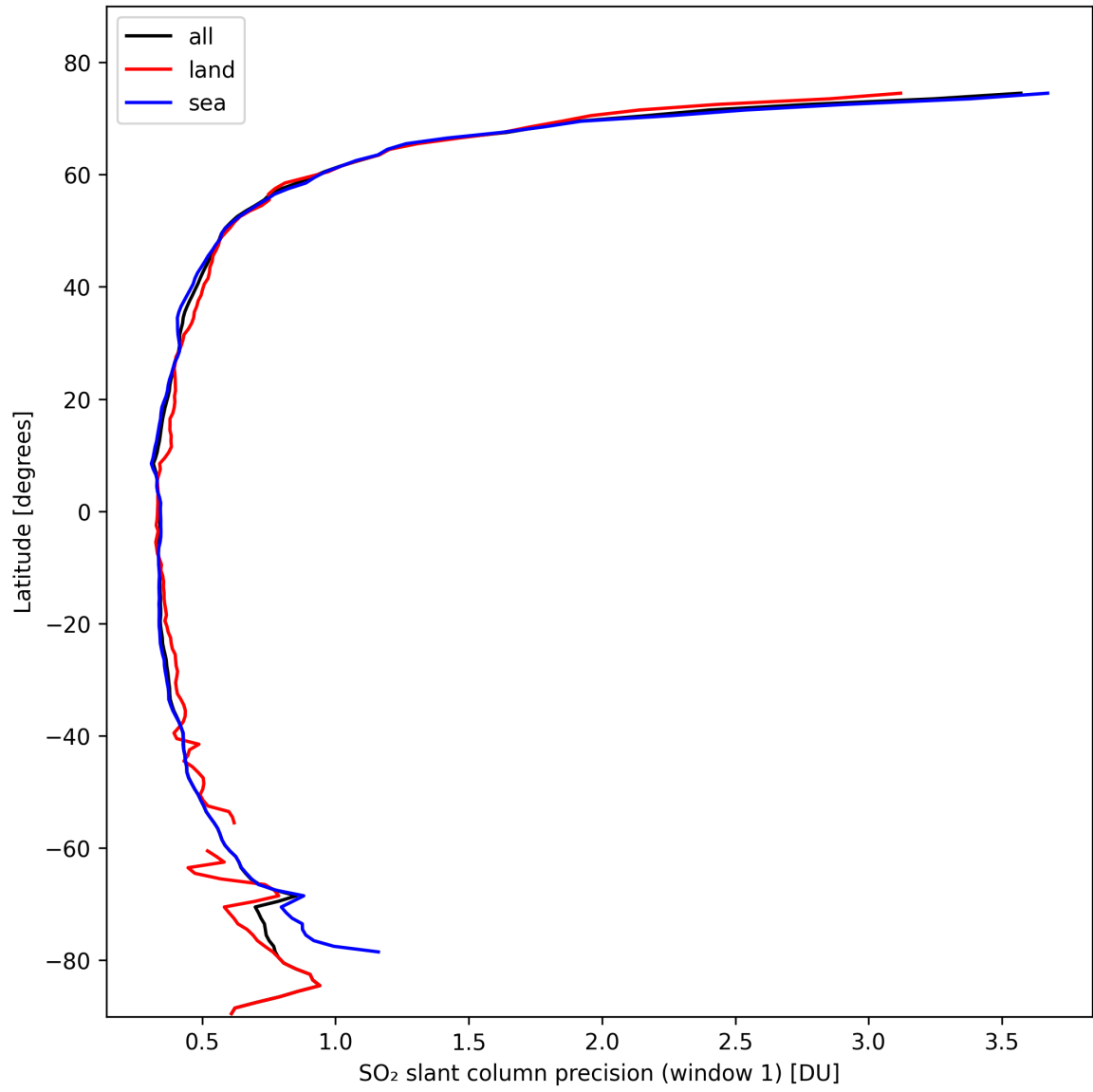
Figure 34: Zonal average of “SO 2 slant column precision (window 1)” for 2024-10-19 to 2024-10-21.
