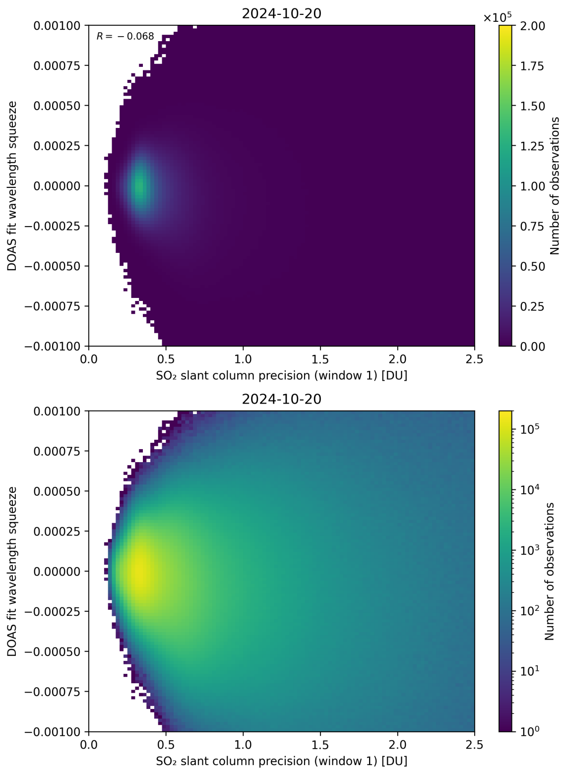
Figure 222: Scatter density plot of “SO 2 slant column precision (window 1)” against “DOAS fit wavelength squeeze” for 2024-10-19 to 2024-10-21.
