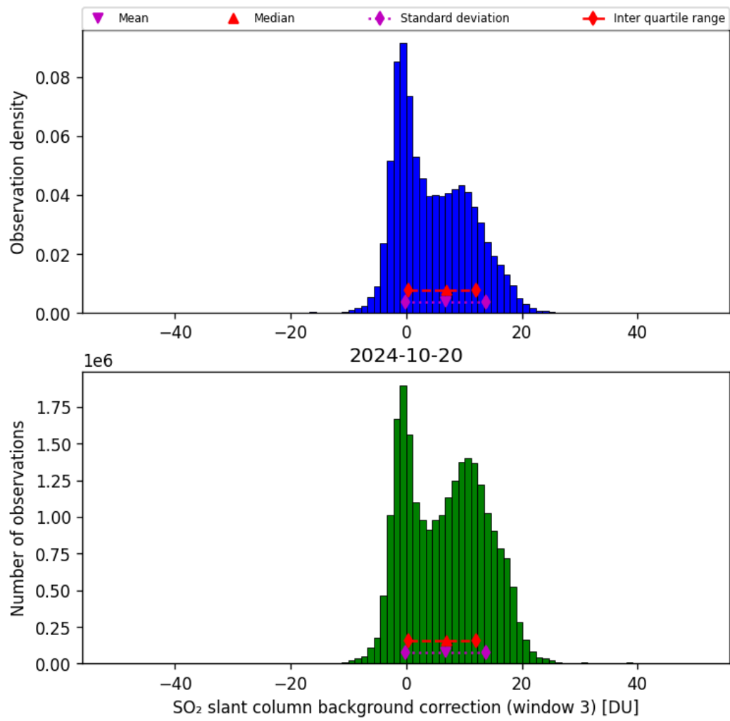
Figure 67: Histogram of “SO 2 slant column background correction (window 3)” for 2024-10-19 to 2024-10-21
