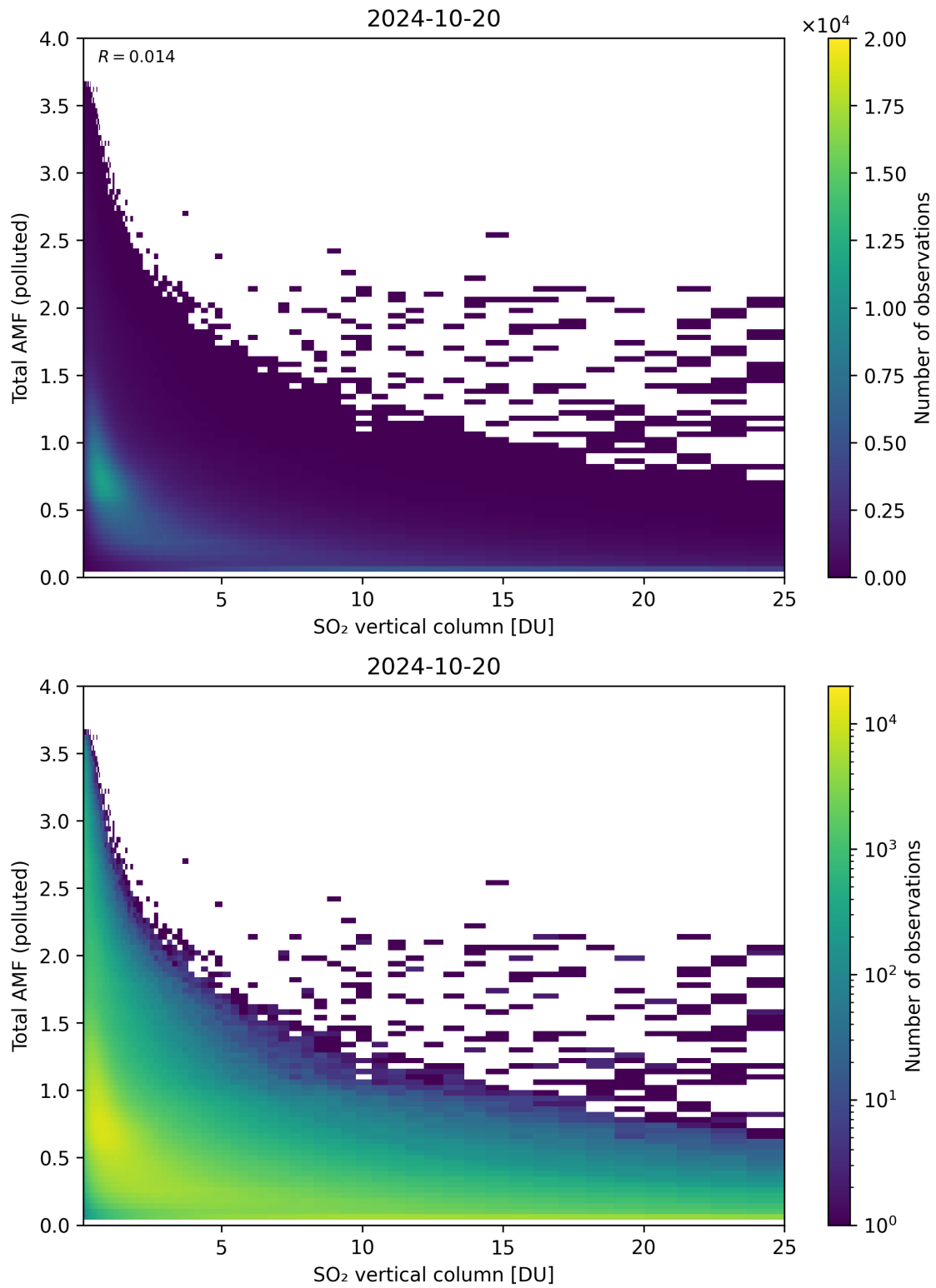
Figure 305: Scatter density plot of “SO 2 vertical column” against “Total AMF (polluted)” for 2024-10-19 to 2024-10-21.
