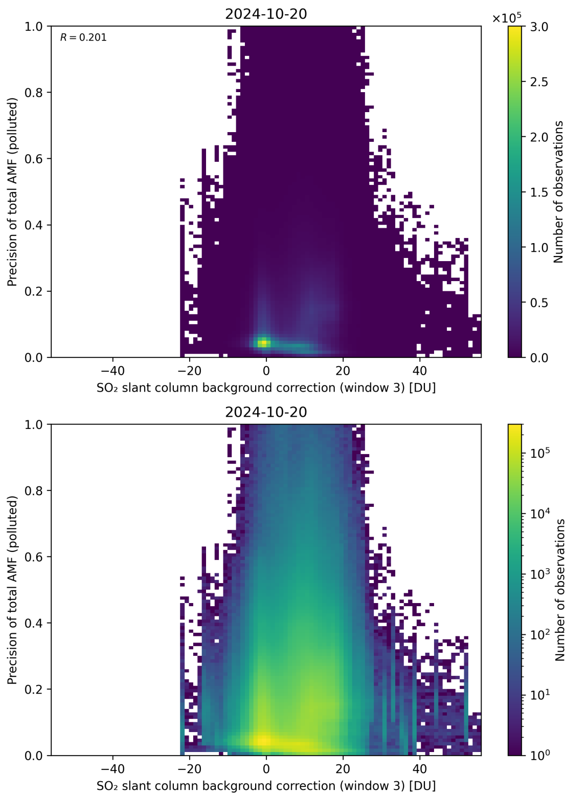
Figure 126: Scatter density plot of “SO 2 slant column background correction (window 3)” against “Precision of total AMF (polluted)” for 2024-10-19 to 2024-10-21.
