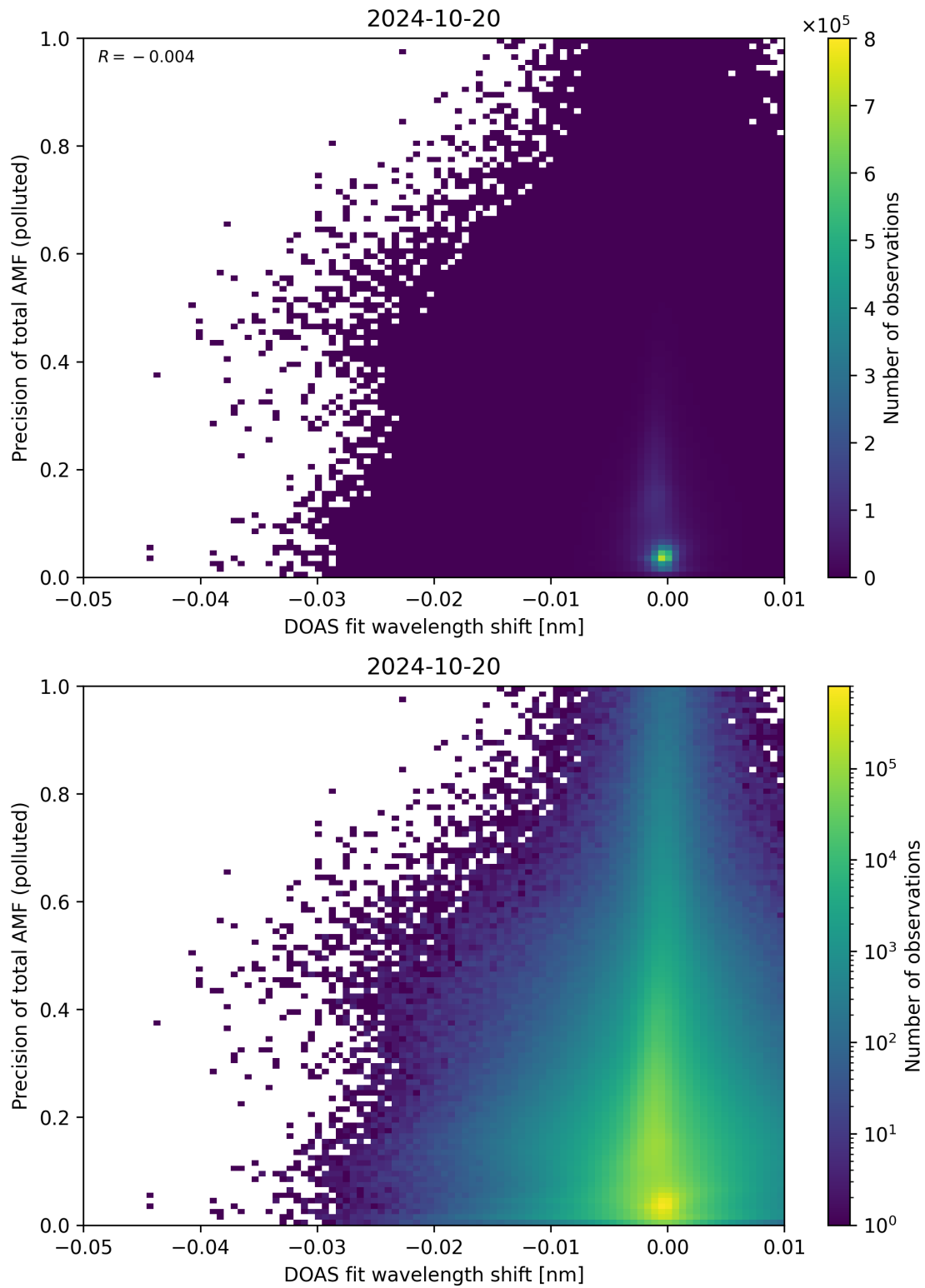
Figure 131: Scatter density plot of “DOAS fit wavelength shift” against “Precision of total AMF (polluted)” for 2024-10-19 to 2024-10-21.
