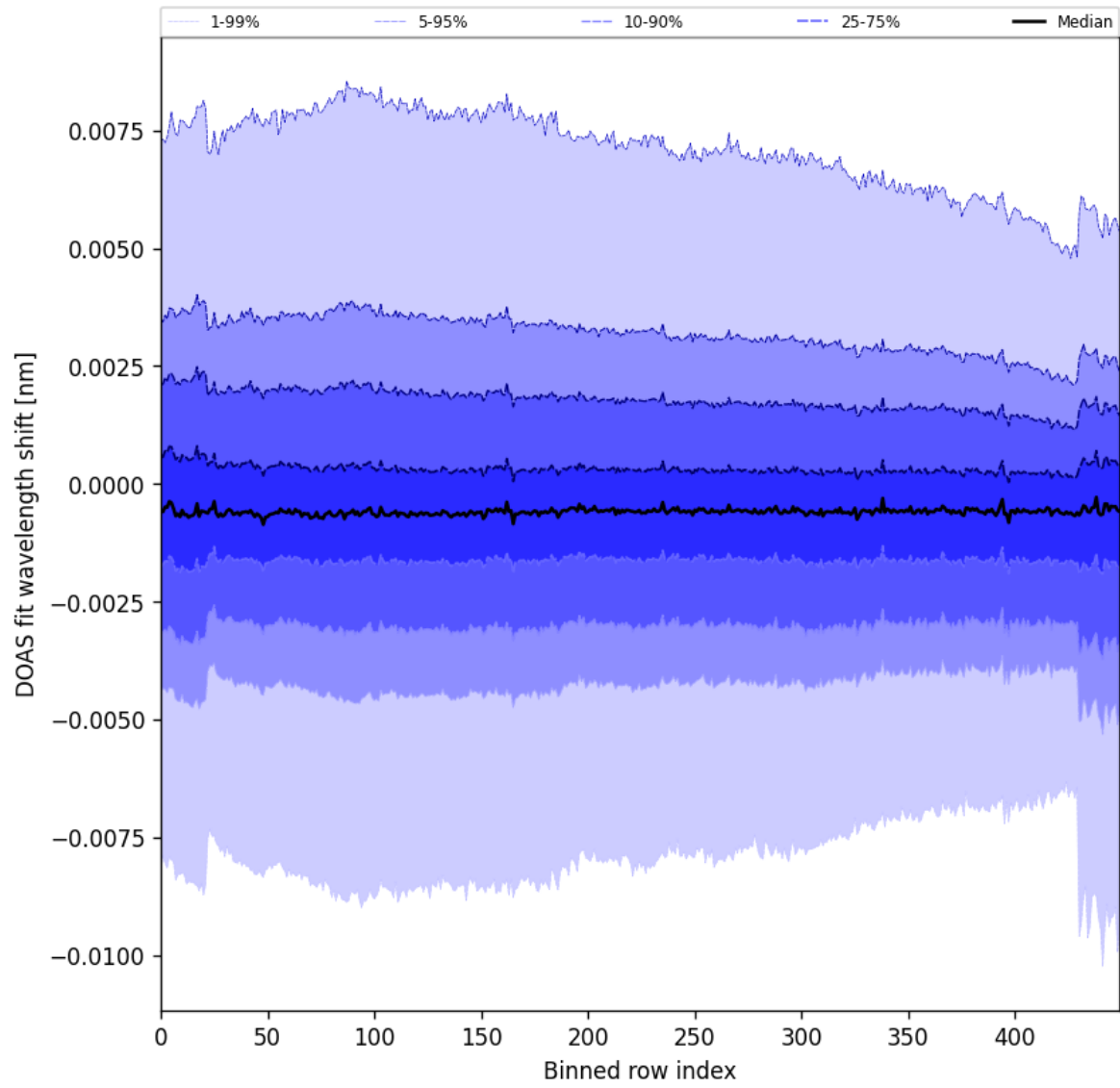
Figure 91: Along track statistics of “DOAS fit wavelength shift” for 2024-10-19 to 2024-10-21
