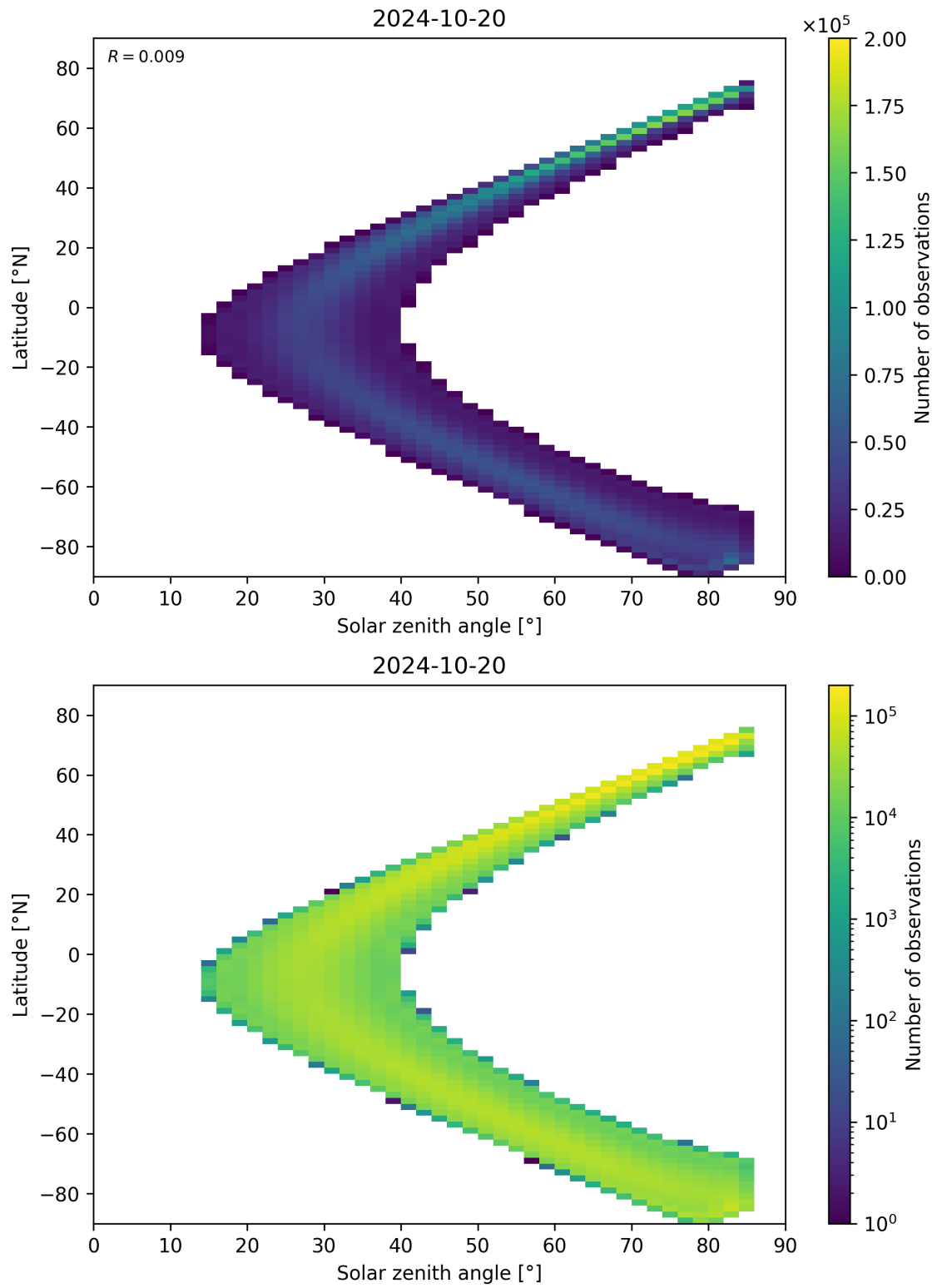
Figure 164: Scatter density plot of “Solar zenith angle” against “Latitude” for 2024-10-19 to 2024-10-21.
