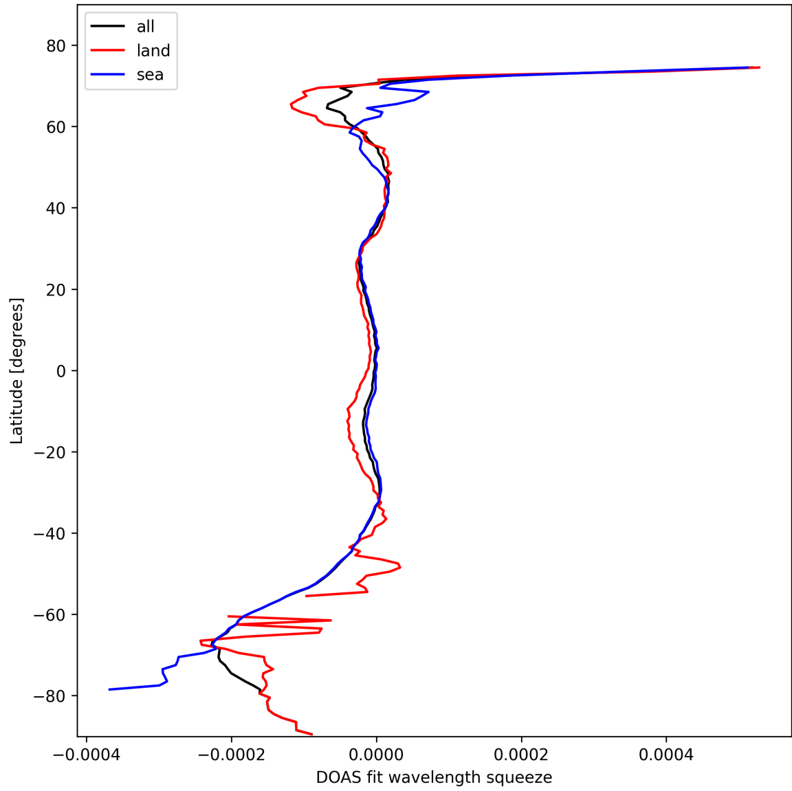
Figure 46: Zonal average of “DOAS fit wavelength squeeze” for 2024-10-19 to 2024-10-21.
