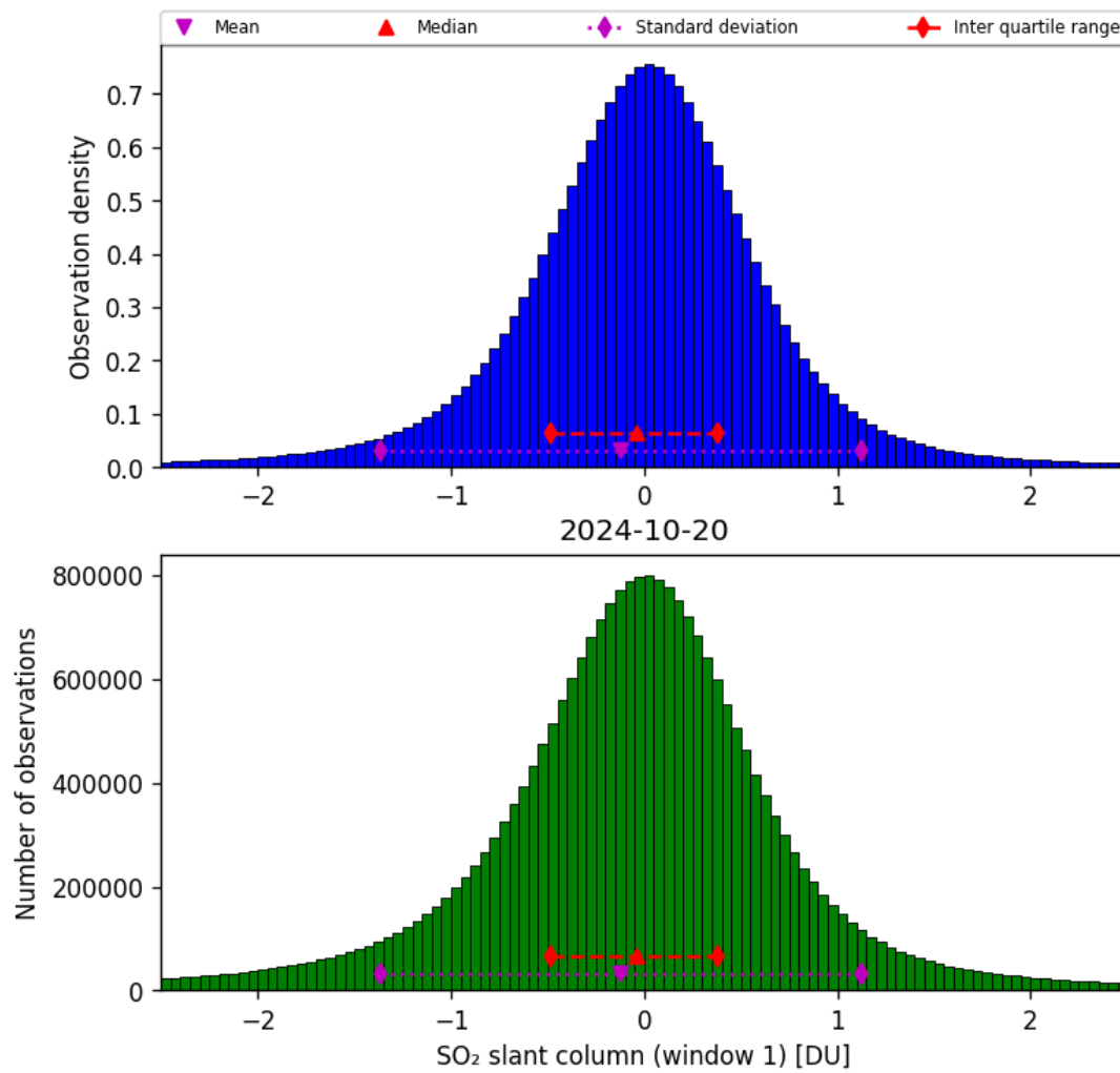
Figure 56: Histogram of “SO 2 slant column (window 1)” for 2024-10-19 to 2024-10-21
