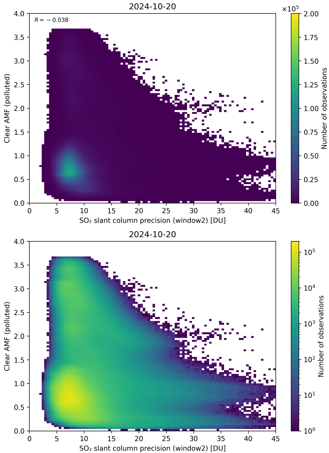
Figure 246: Scatter density plot of “SO 2 slant column precision (window2)” against “Clear AMF (polluted)” for 2024-10-19 to 2024-10-21.
