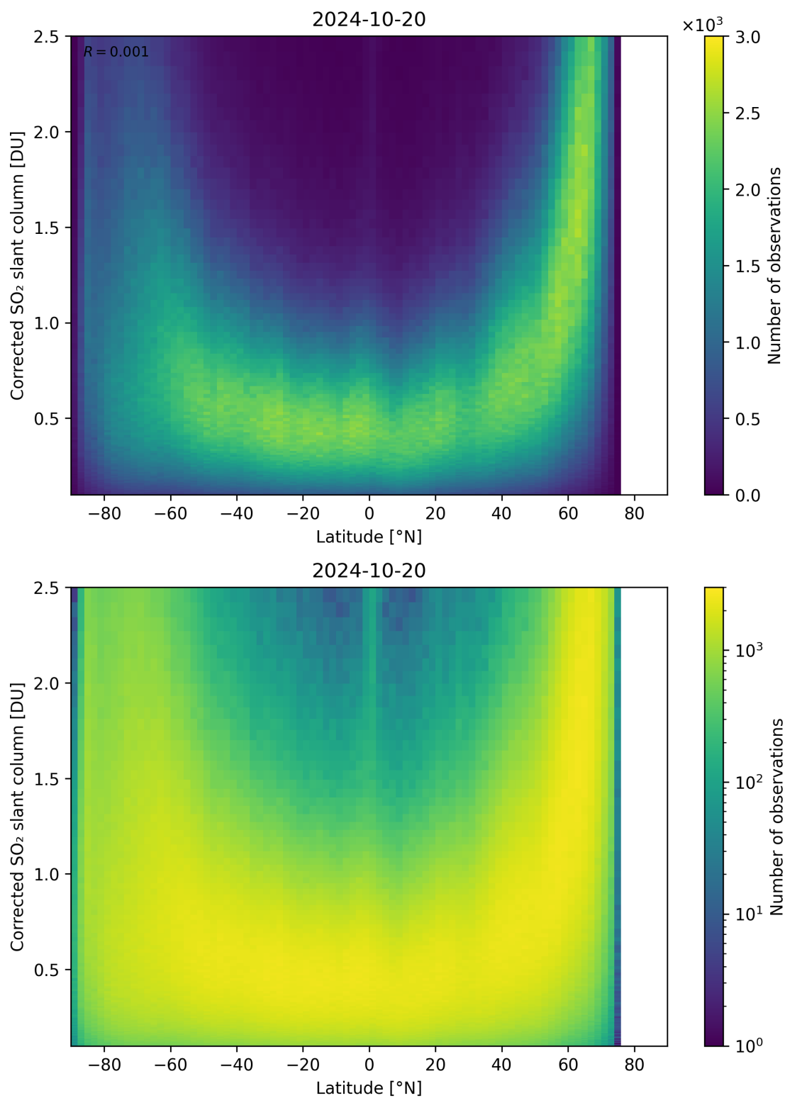
Figure 146: Scatter density plot of “Latitude” against “Corrected SO 2 slant column” for 2024-10-19 to 2024-10-21.
