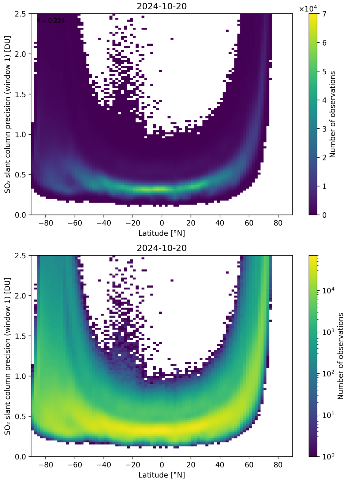
Figure 150: Scatter density plot of “Latitude” against “SO 2 slant column precision (window 1)” for 2024-10-19 to 2024-10-21.
