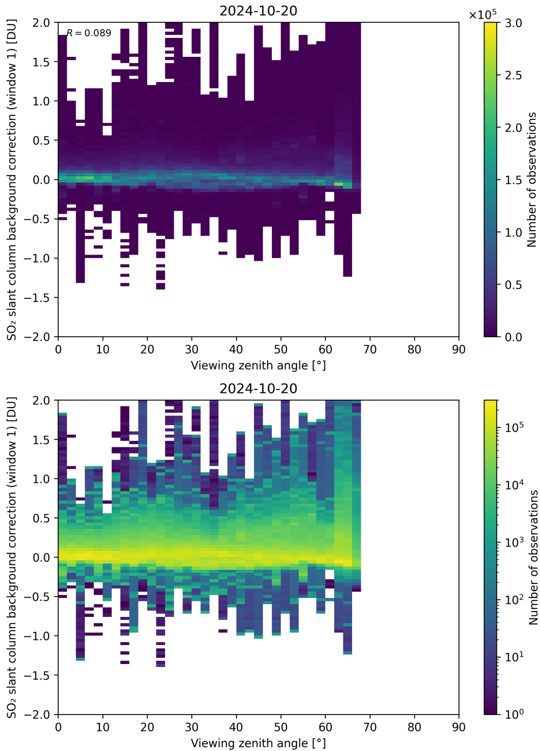
Figure 308: Scatter density plot of “Viewing zenith angle” against “SO 2 slant column background correction (window 1)” for 2024-10-19 to 2024-10-21.
