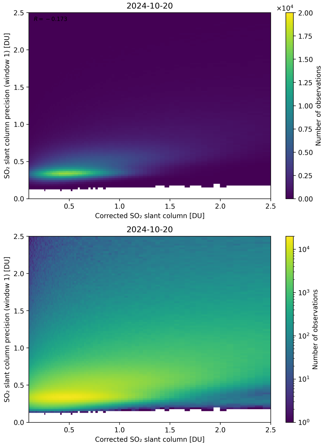
Figure 188: Scatter density plot of “Corrected SO 2 slant column” against “SO 2 slant column precision (window 1)” for 2024-10-19 to 2024-10-21.
