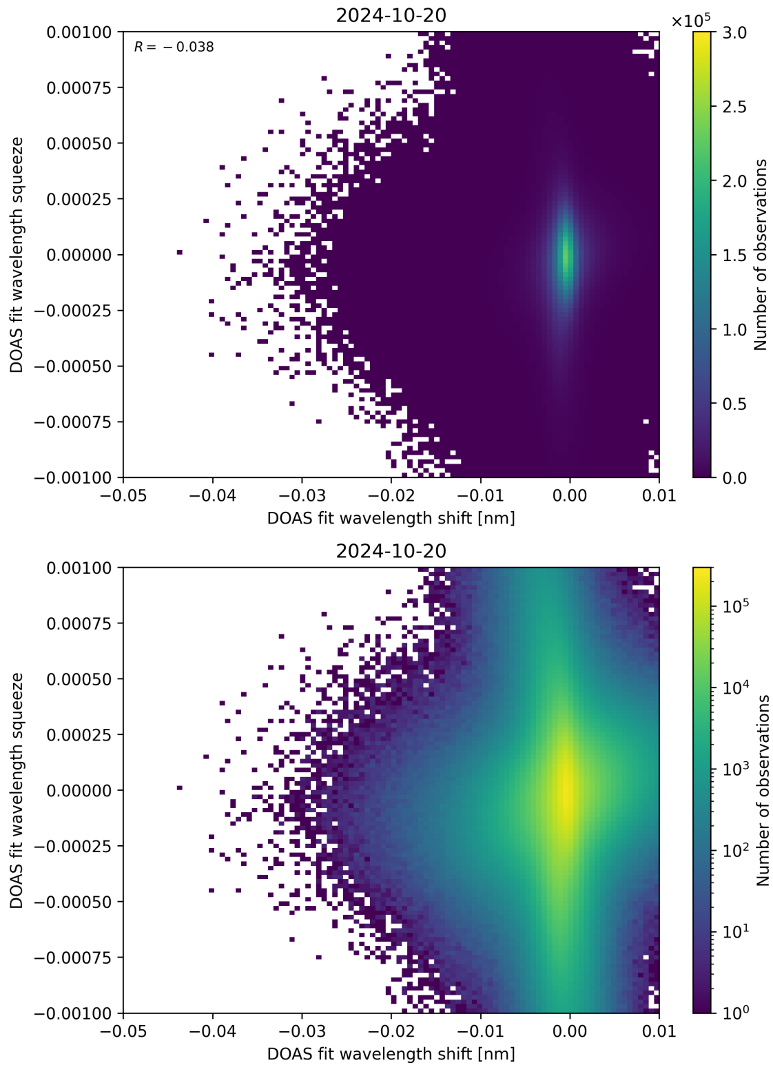
Figure 127: Scatter density plot of “DOAS fit wavelength shift” against “DOAS fit wavelength squeeze” for 2024-10-19 to 2024-10-21.
