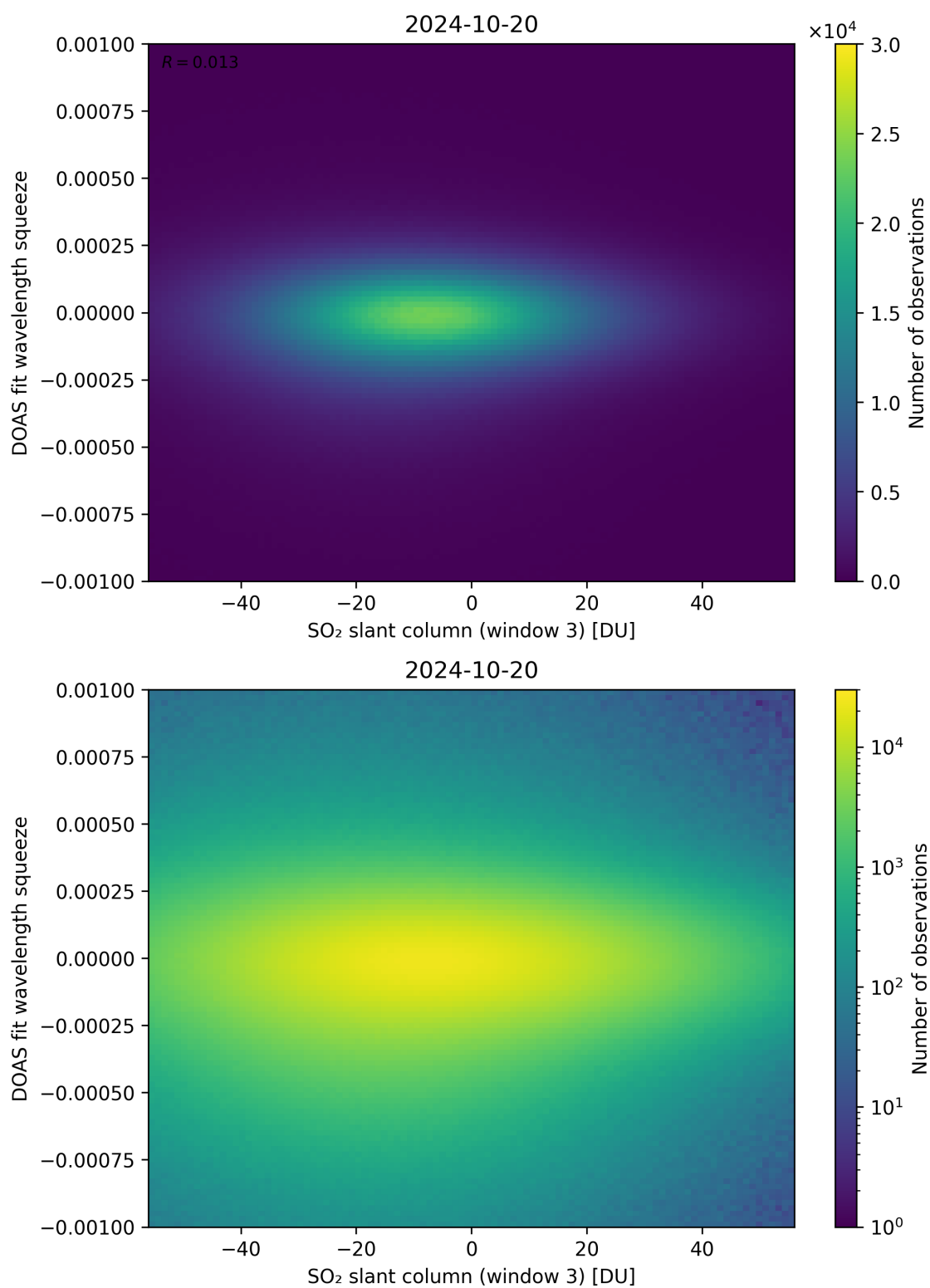
Figure 255: Scatter density plot of “SO 2 slant column (window 3)” against “DOAS fit wavelength squeeze” for 2024-10-19 to 2024-10-21.
