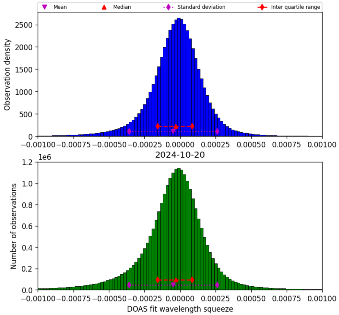
Figure 69: Histogram of “DOAS fit wavelength squeeze” for 2024-10-19 to 2024-10-21
