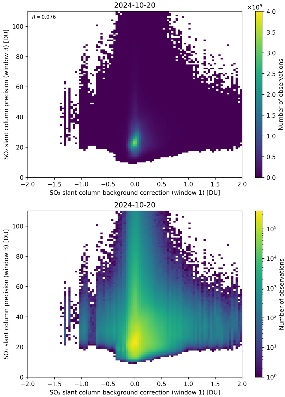
Figure 108: Scatter density plot of “SO 2 slant column background correction (window 1)” against “SO 2 slant column precision (window 3)” for 2024-10-19 to 2024-10-21.
