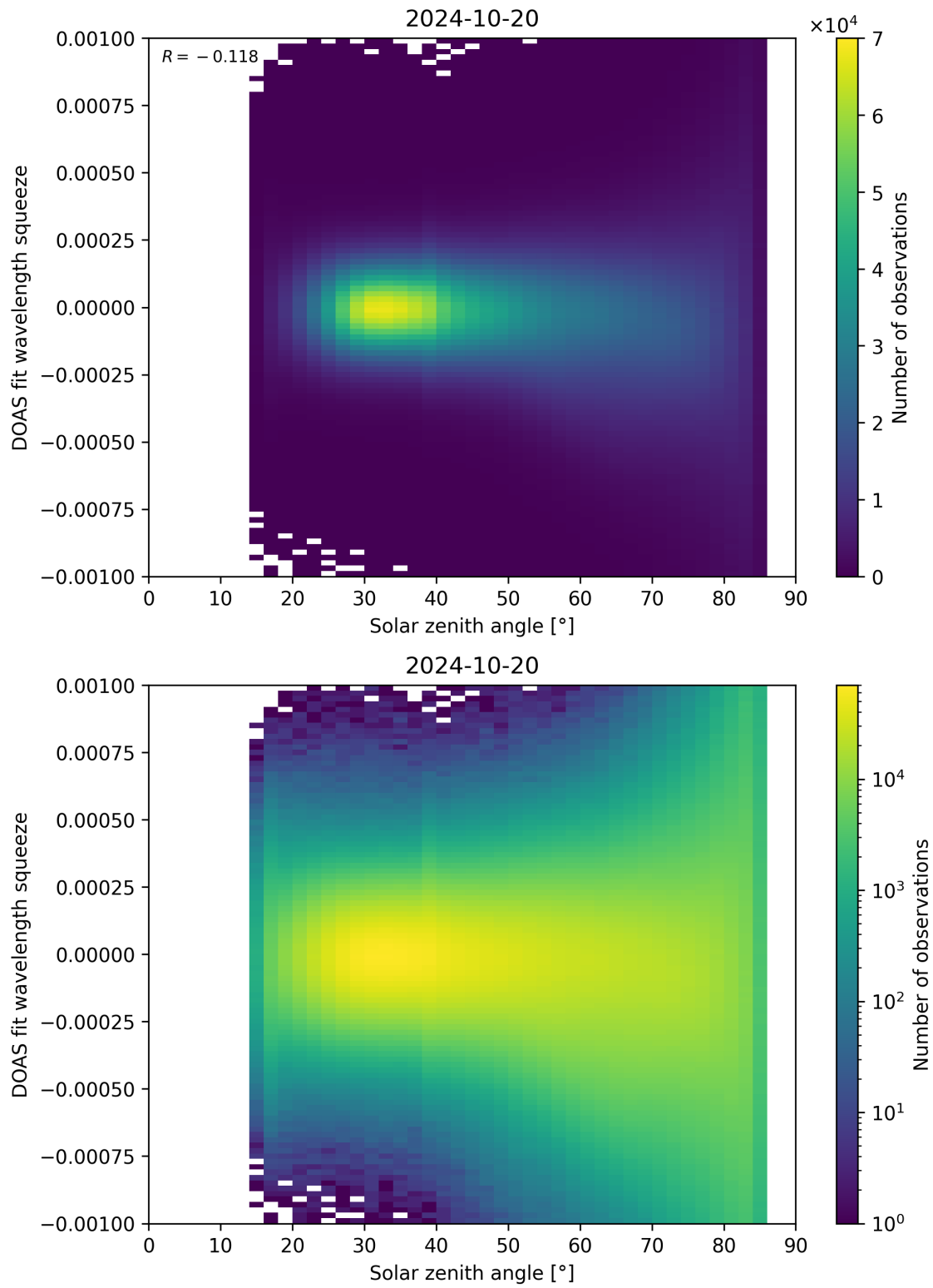
Figure 162: Scatter density plot of “Solar zenith angle” against “DOAS fit wavelength squeeze” for 2024-10-19 to 2024-10-21.
