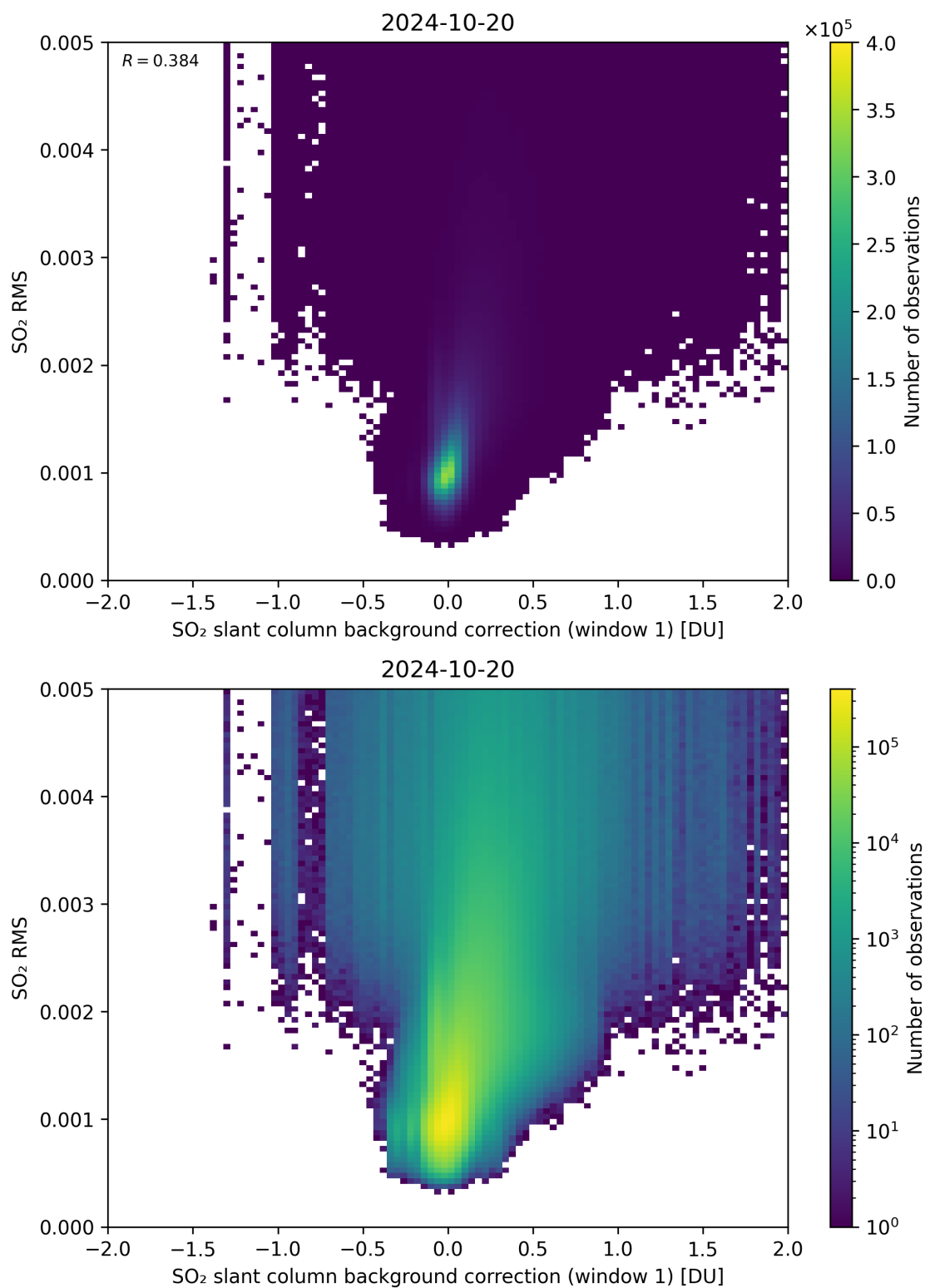
Figure 102: Scatter density plot of “SO 2 slant column background correction (window 1)” against “SO 2 RMS” for 2024-10-19 to 2024-10-21.
