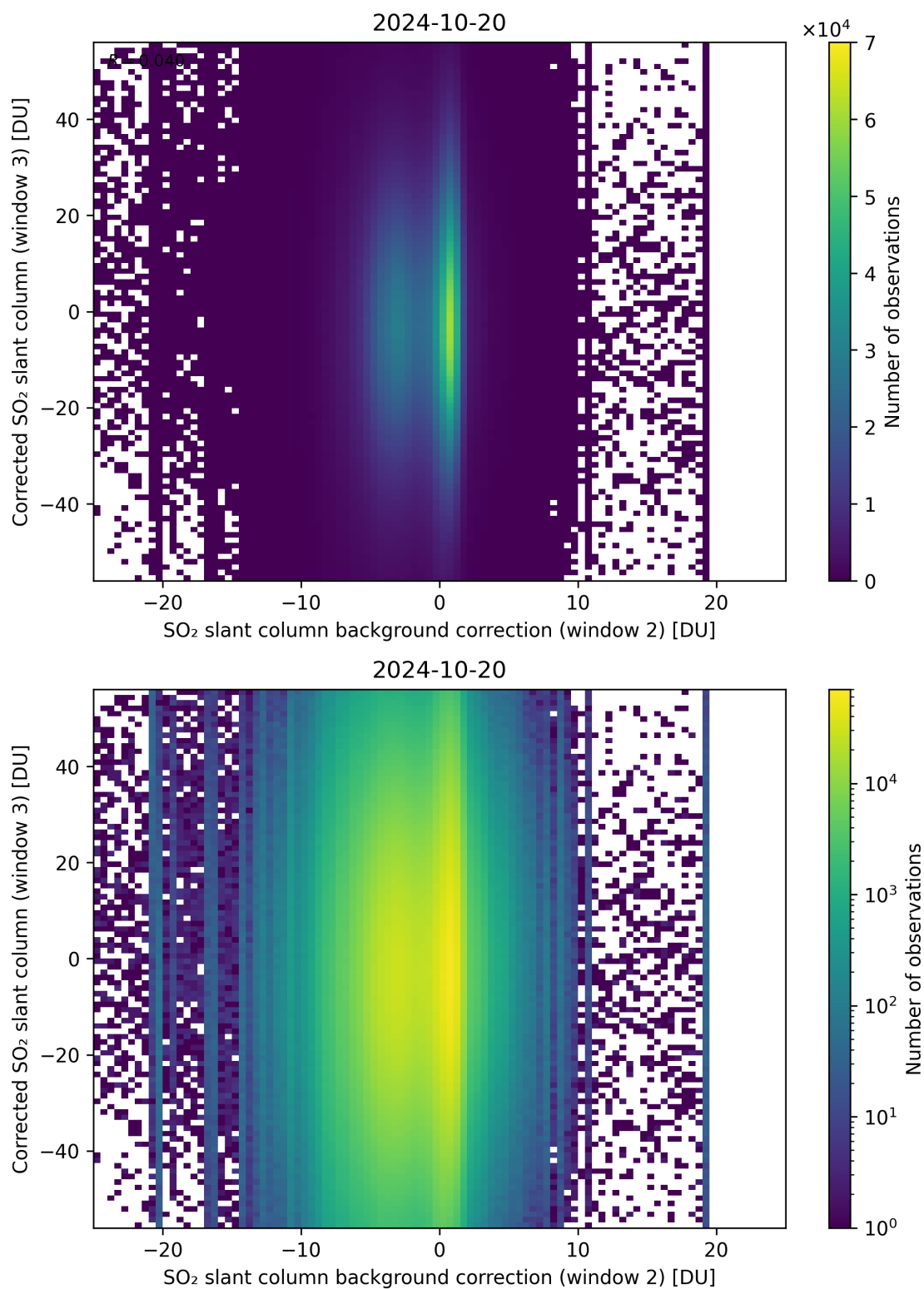
Figure 116: Scatter density plot of “SO 2 slant column background correction (window 2)” against “Corrected SO 2 slant column (window 3)” for 2024-10-19 to 2024-10-21.
