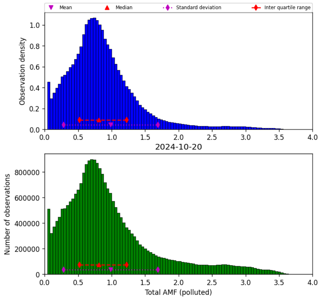
Figure 71: Histogram of “Total AMF (polluted)” for 2024-10-19 to 2024-10-21
