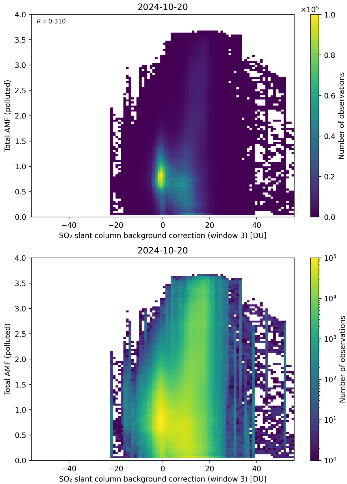
Figure 125: Scatter density plot of “SO 2 slant column background correction (window 3)” against “Total AMF (polluted)” for 2024-10-19 to 2024-10-21.
