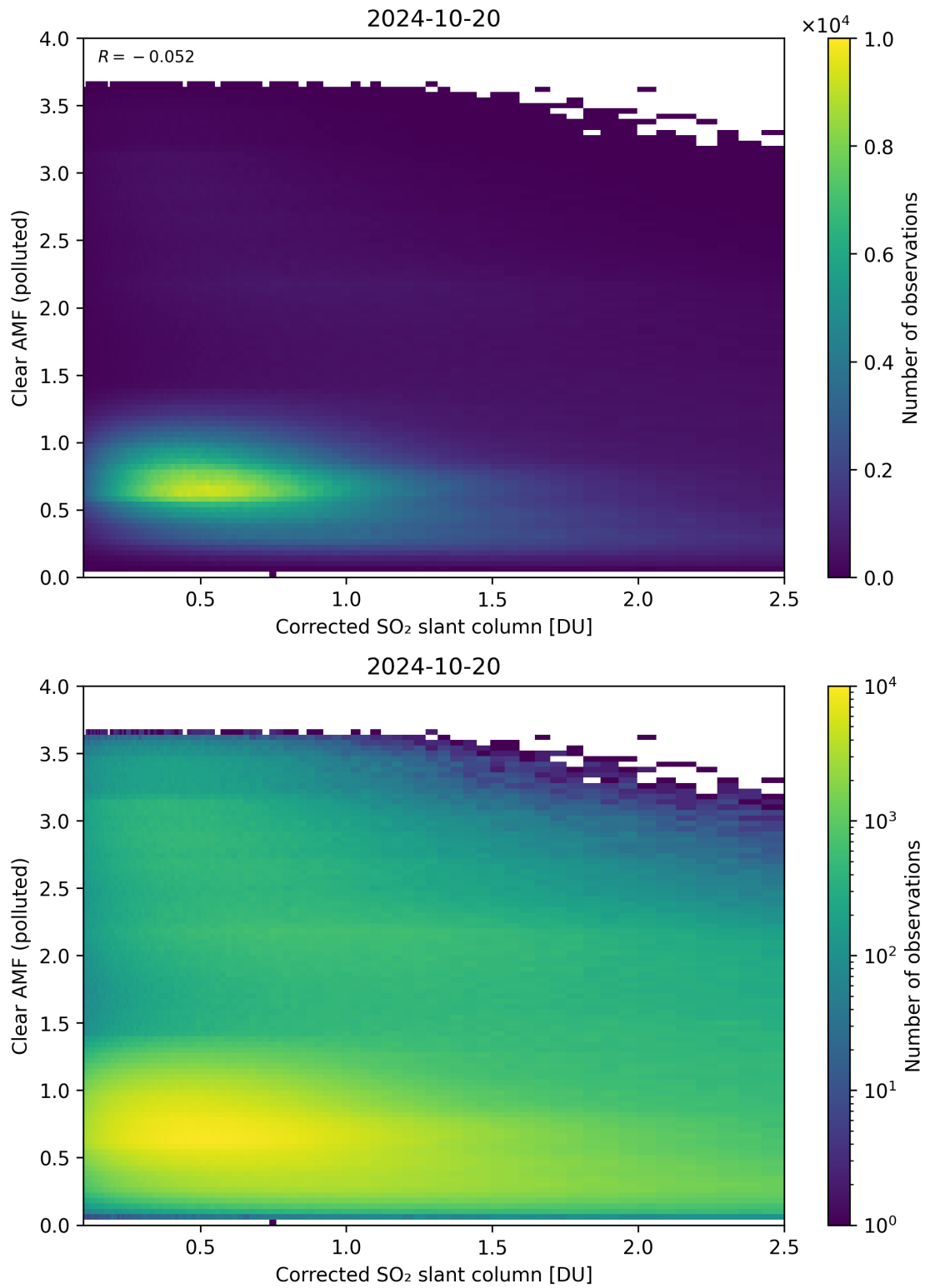
Figure 184: Scatter density plot of “Corrected SO 2 slant column” against “Clear AMF (polluted)” for 2024-10-19 to 2024-10-21.
