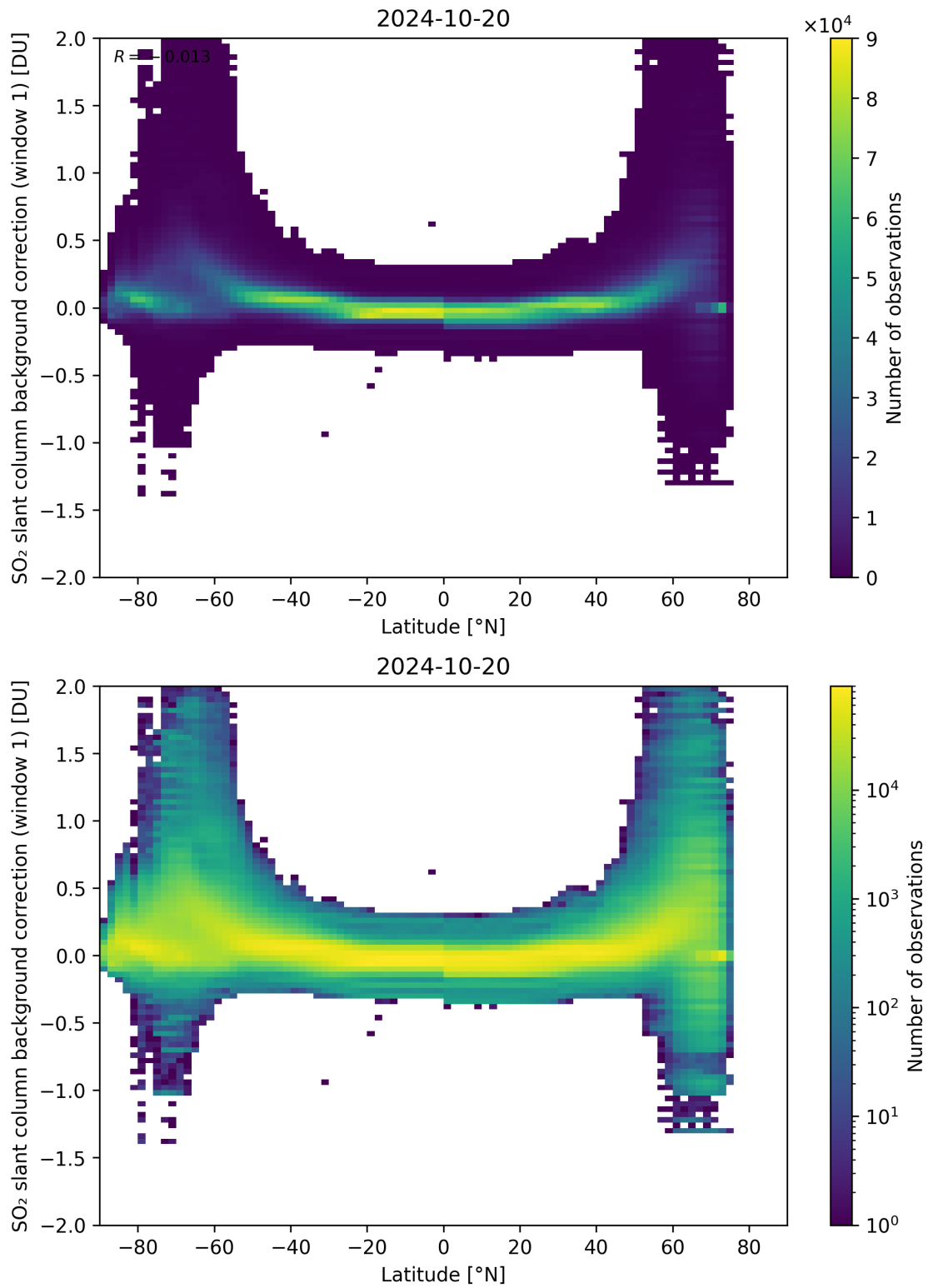
Figure 139: Scatter density plot of “Latitude” against “SO 2 slant column background correction (window 1)” for 2024-10-19 to 2024-10-21.
