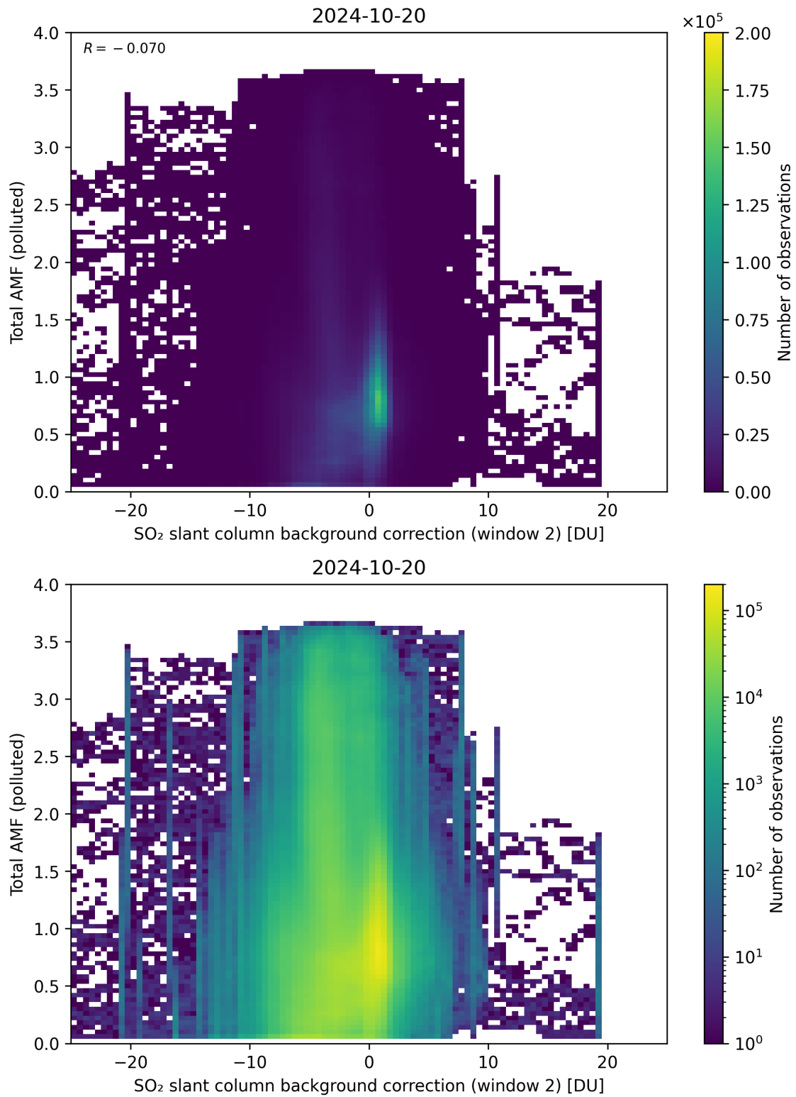
Figure 119: Scatter density plot of “SO 2 slant column background correction (window 2)” against “Total AMF (polluted)” for 2024-10-19 to 2024-10-21.
