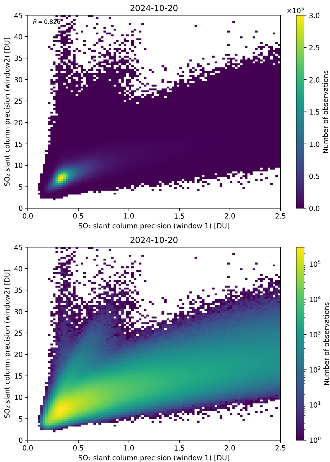
Figure 227: Scatter density plot of “SO 2 slant column precision (window 1)” against “SO 2 slant column precision (window2)” for 2024-10-19 to 2024-10-21.
