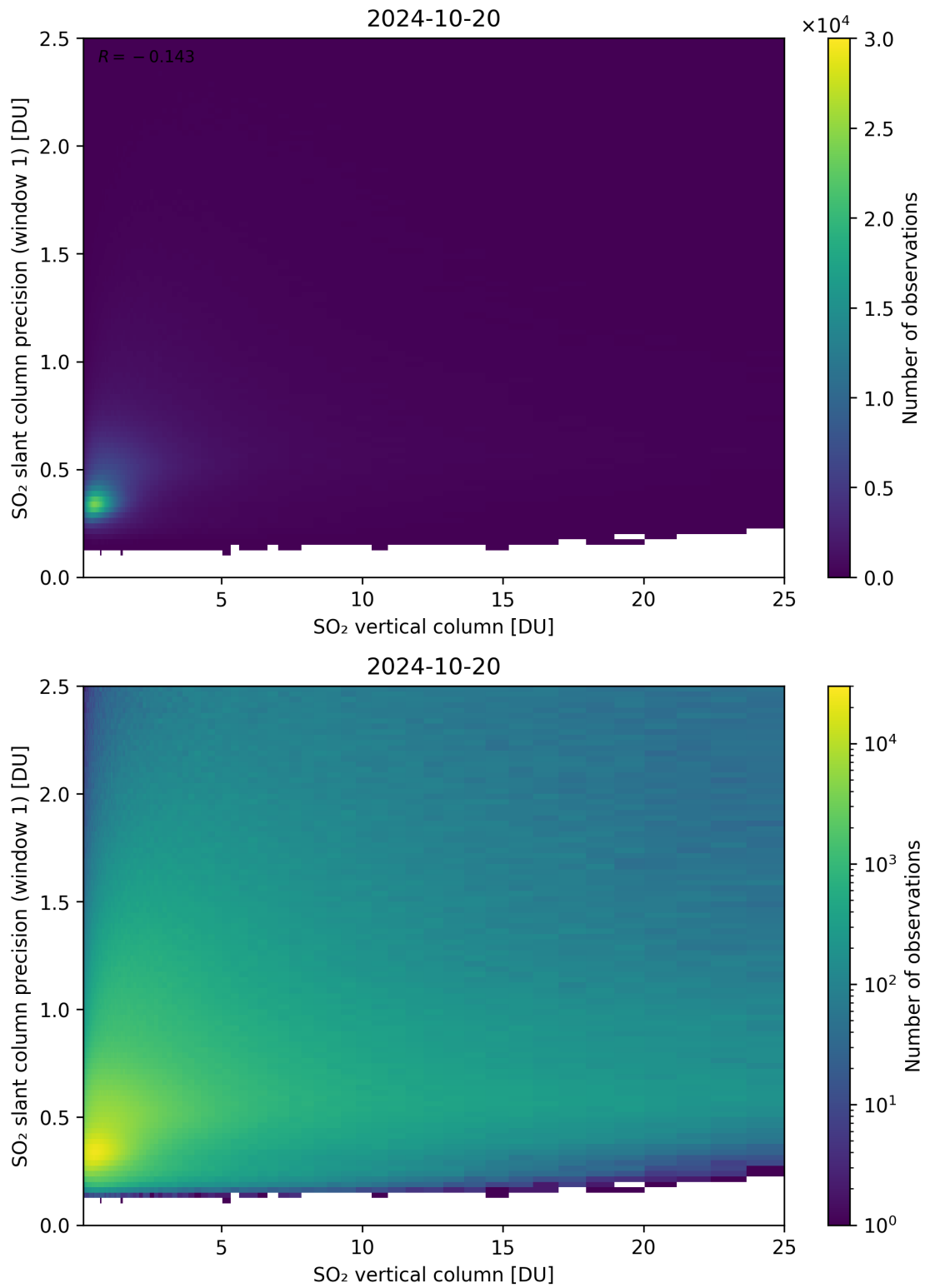
Figure 301: Scatter density plot of “SO 2 vertical column” against “SO 2 slant column precision (window 1)” for 2024-10-19 to 2024-10-21.
