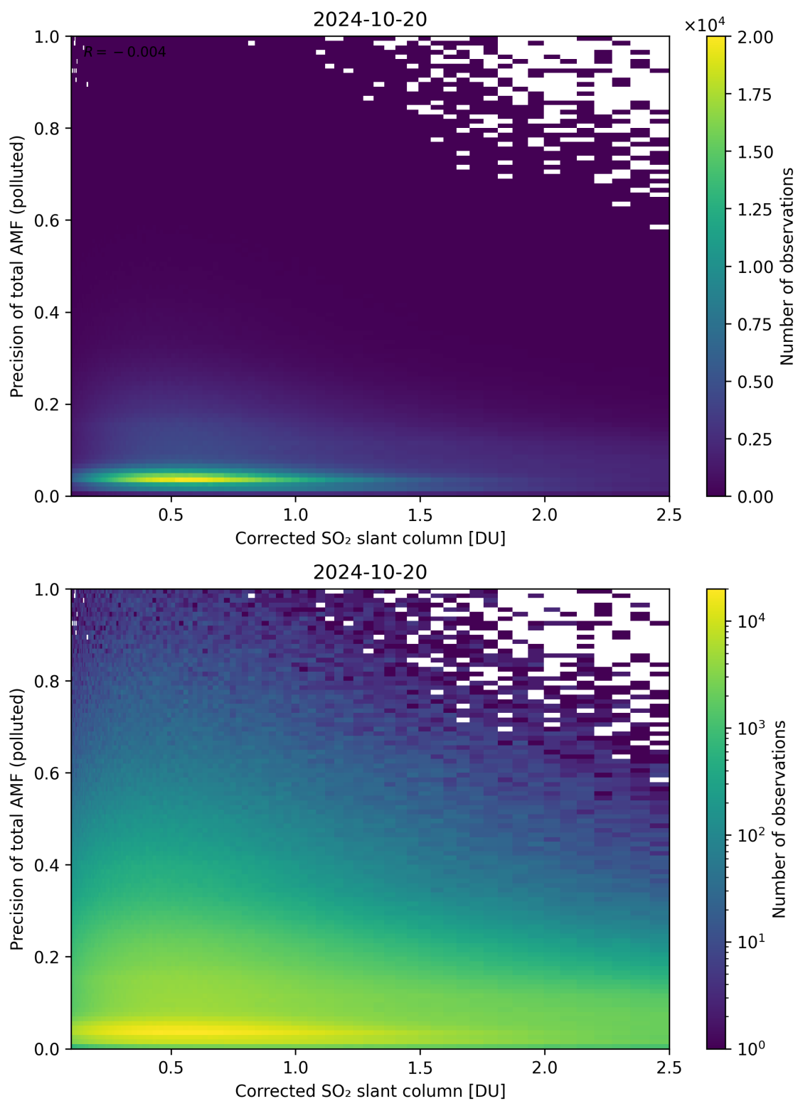
Figure 193: Scatter density plot of “Corrected SO 2 slant column” against “Precision of total AMF (polluted)” for 2024-10-19 to 2024-10-21.
