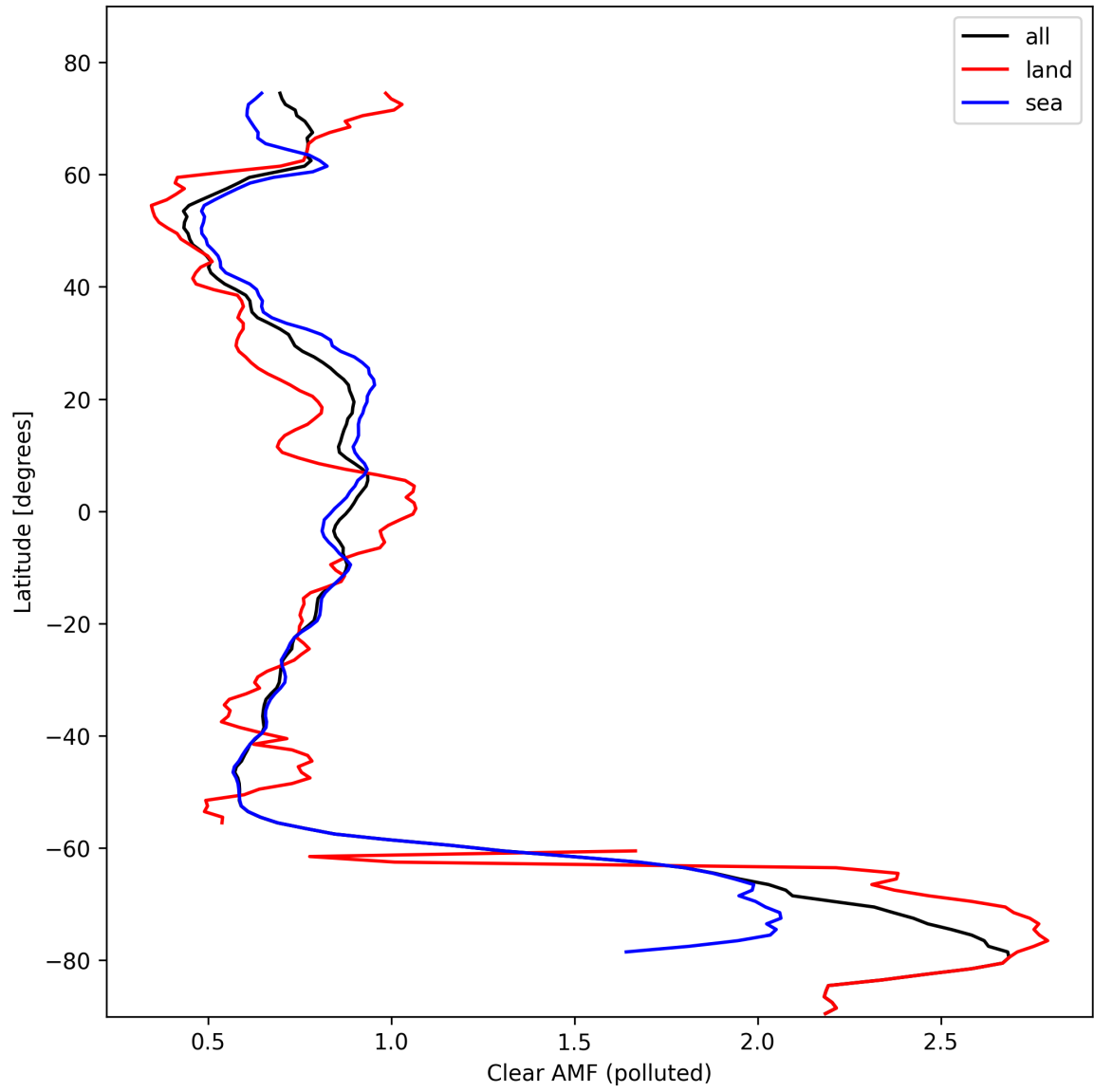
Figure 50: Zonal average of “Clear AMF (polluted)” for 2024-10-19 to 2024-10-21.
