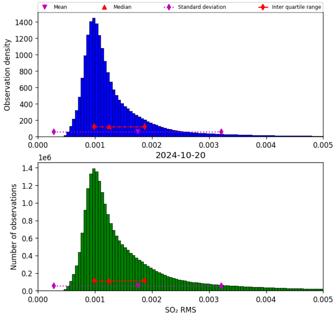
Figure 70: Histogram of “SO 2 RMS” for 2024-10-19 to 2024-10-21
