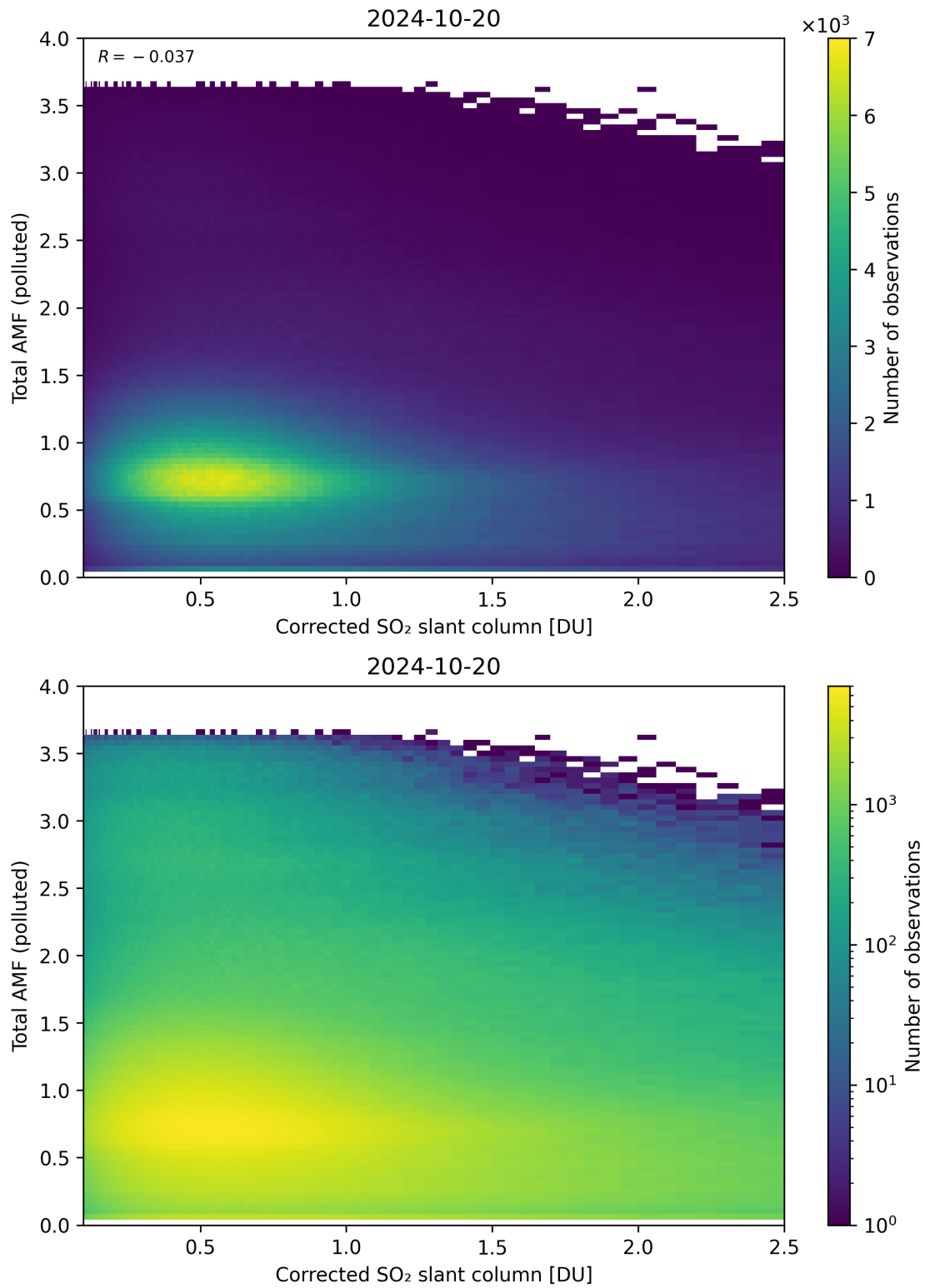
Figure 192: Scatter density plot of “Corrected SO 2 slant column” against “Total AMF (polluted)” for 2024-10-19 to 2024-10-21.
