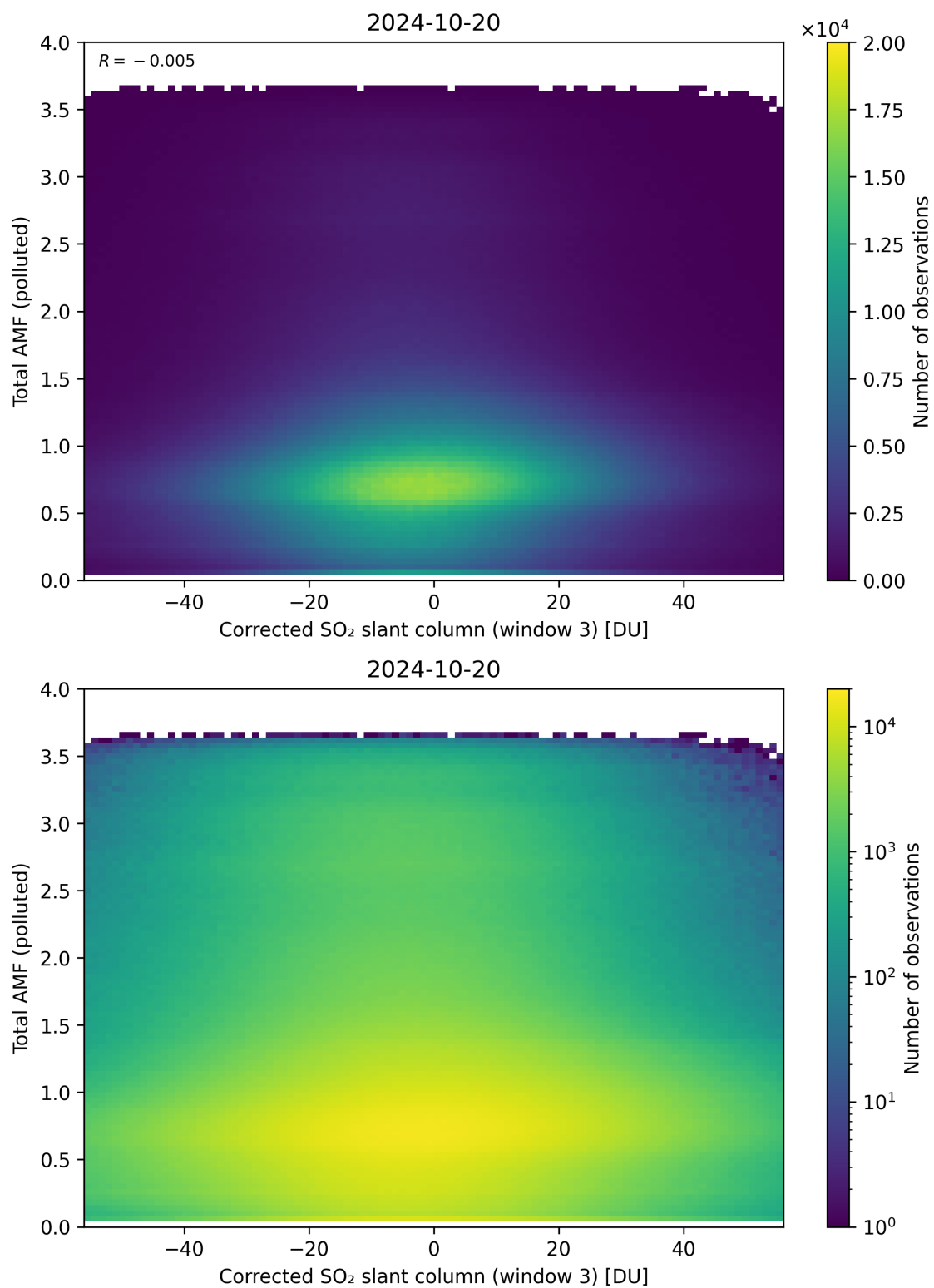
Figure 210: Scatter density plot of “Corrected SO 2 slant column (window 3)” against “Total AMF (polluted)” for 2024-10-19 to 2024-10-21.
