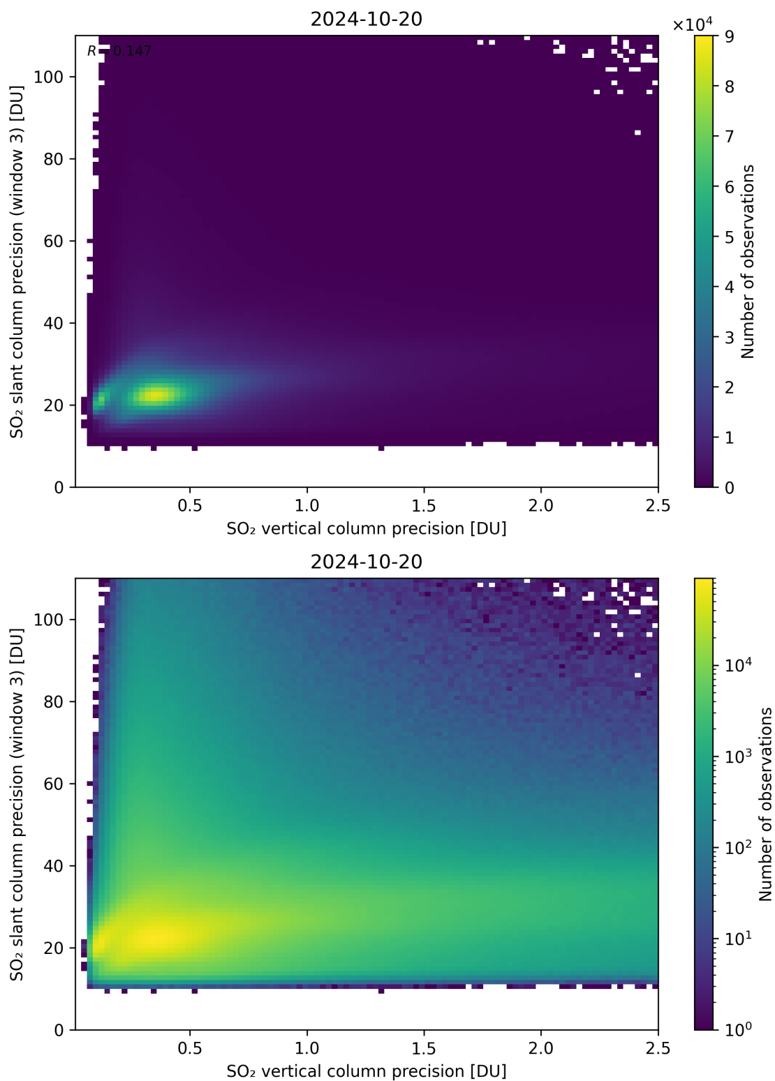
Figure 293: Scatter density plot of “SO 2 vertical column precision” against “SO 2 slant column precision (window 3)” for 2024-10-19 to 2024-10-21.
