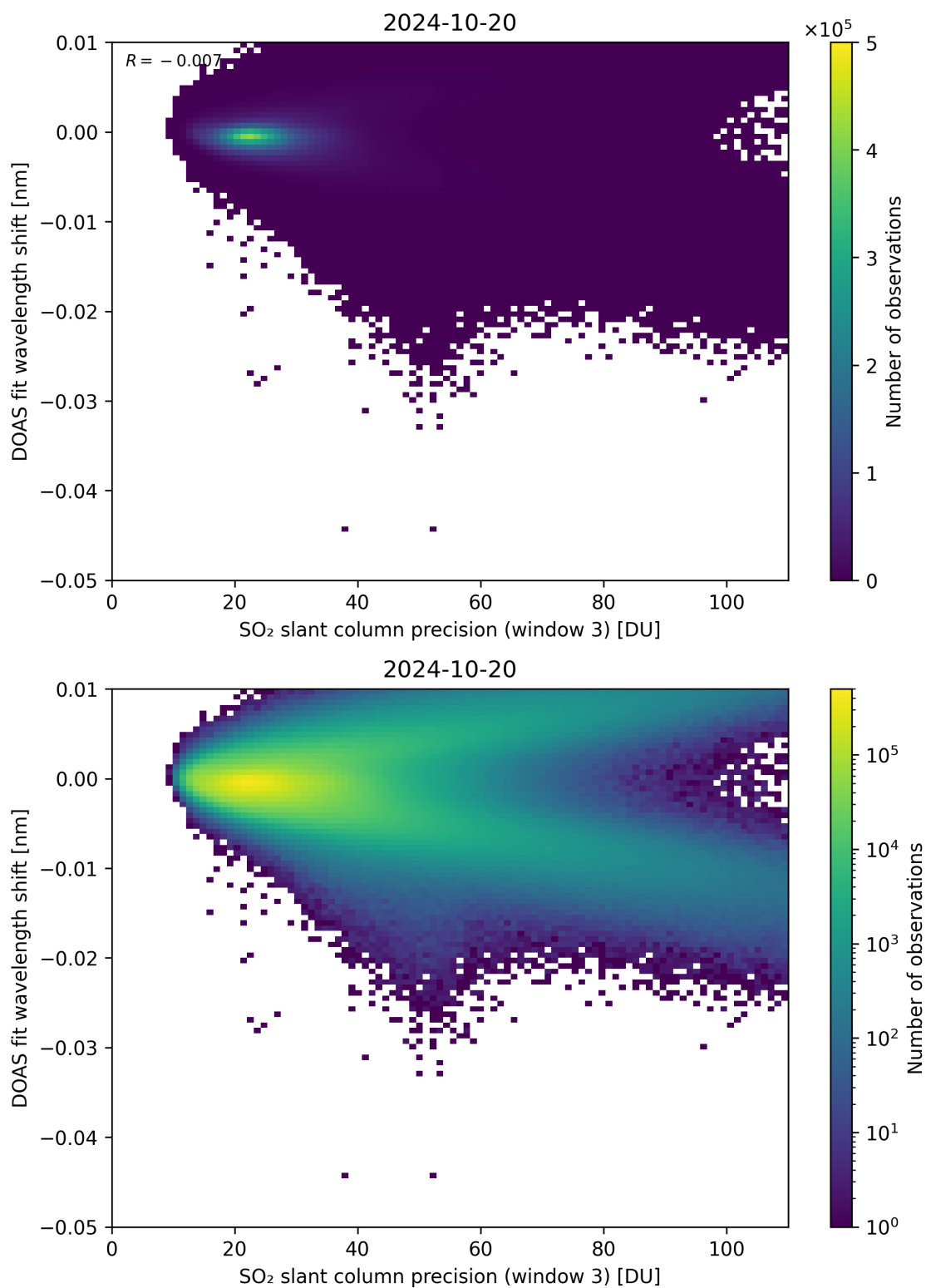
Figure 258: Scatter density plot of “SO 2 slant column precision (window 3)” against “DOAS fit wavelength shift” for 2024-10-19 to 2024-10-21.
