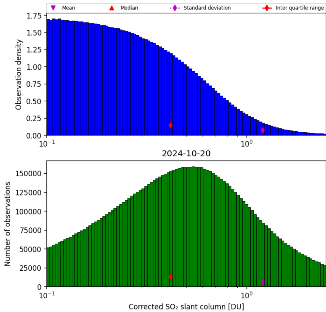
Figure 55: Histogram of “Corrected SO 2 slant column” for 2024-10-19 to 2024-10-21
