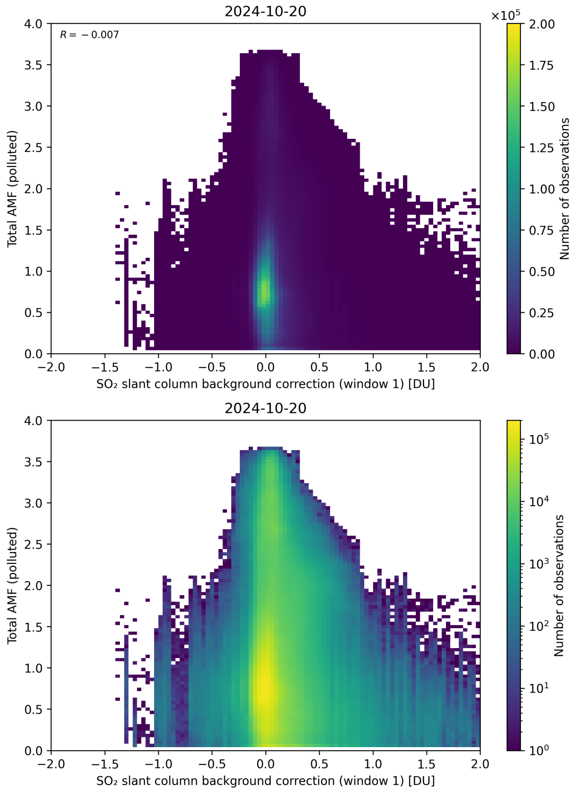
Figure 109: Scatter density plot of “SO 2 slant column background correction (window 1)” against “Total AMF (polluted)” for 2024-10-19 to 2024-10-21.
