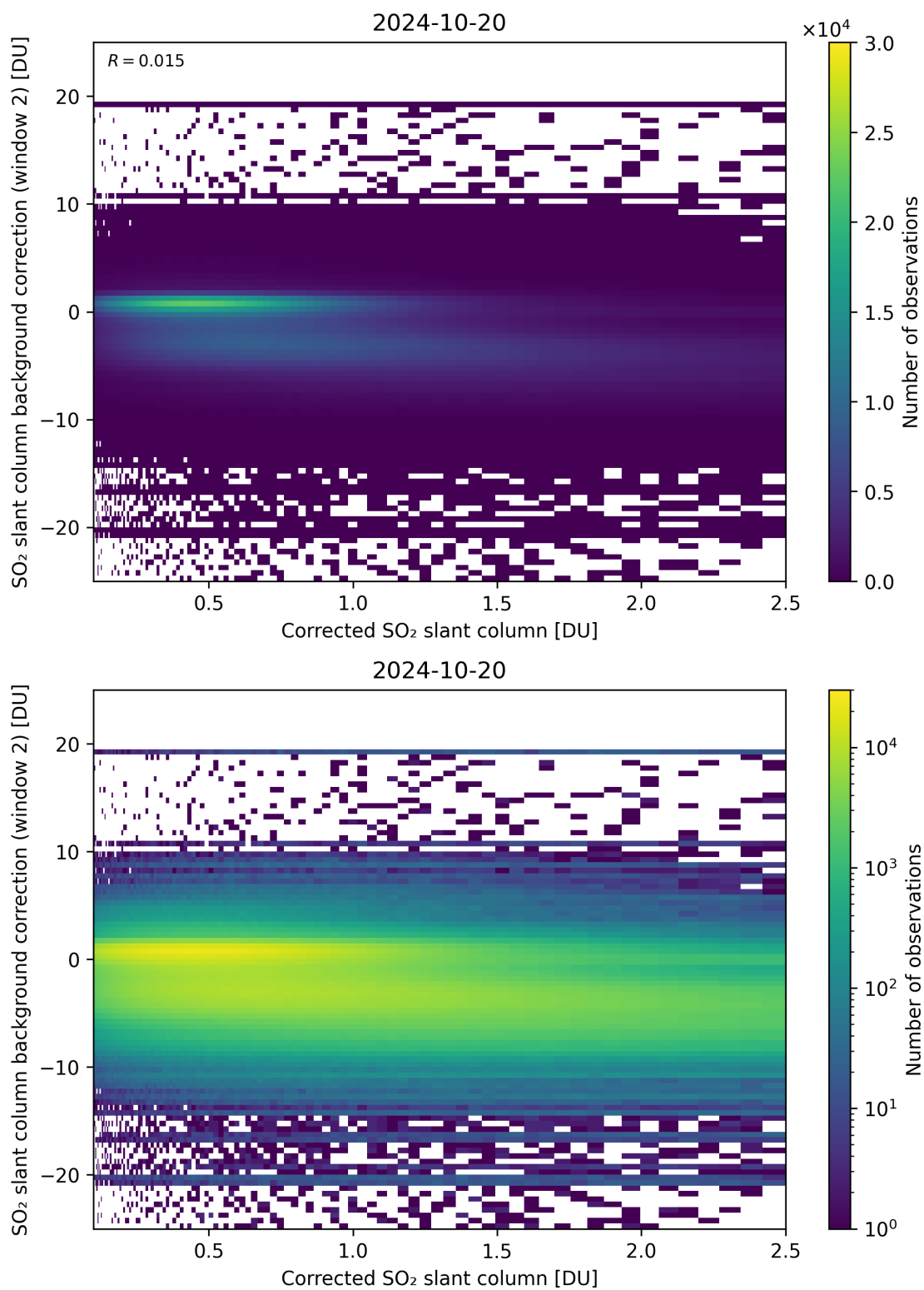
Figure 179: Scatter density plot of “Corrected SO 2 slant column” against “SO 2 slant column background correction (window 2)” for 2024-10-19 to 2024-10-21.
