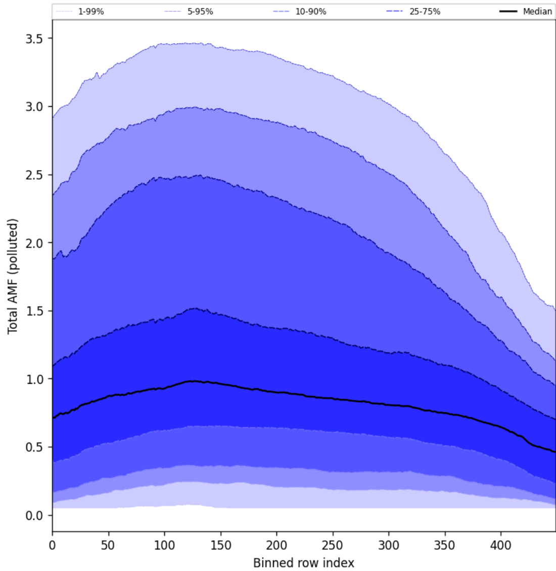
Figure 94: Along track statistics of “Total AMF (polluted)” for 2024-10-19 to 2024-10-21
