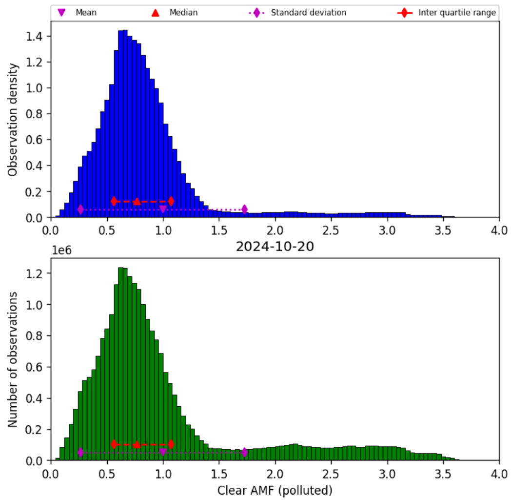
Figure 73: Histogram of “Clear AMF (polluted)” for 2024-10-19 to 2024-10-21
