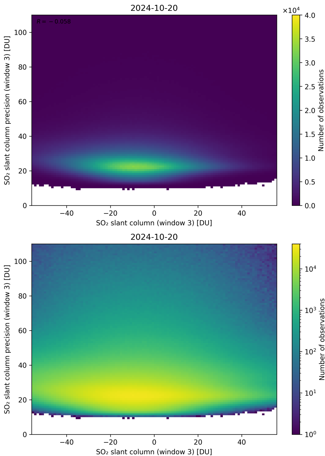
Figure 267: Scatter density plot of “SO 2 slant column (window 3)” against “SO 2 slant column precision (window 3)” for 2024-10-19 to 2024-10-21.
