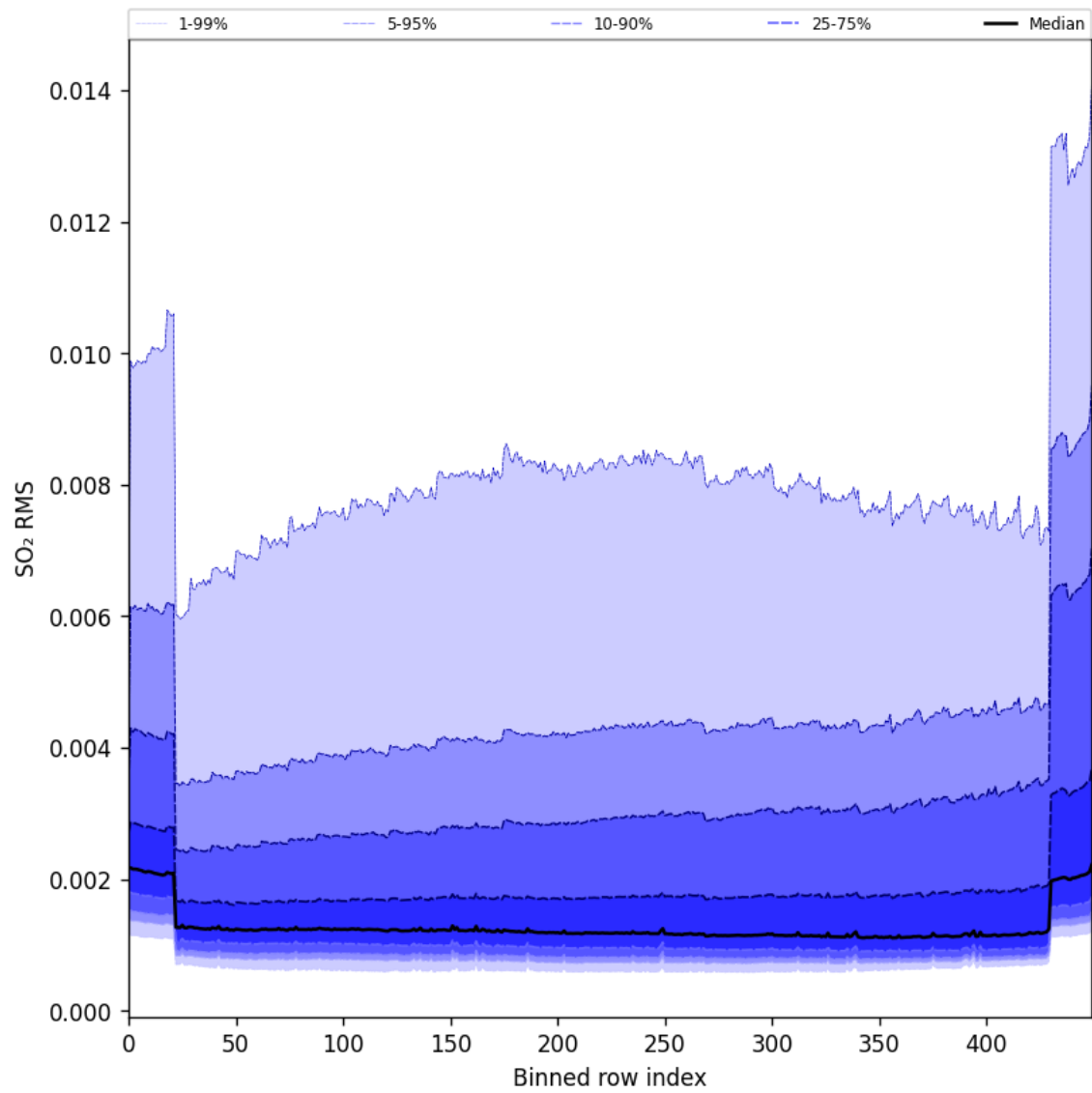
Figure 93: Along track statistics of “SO 2 RMS” for 2024-10-19 to 2024-10-21
