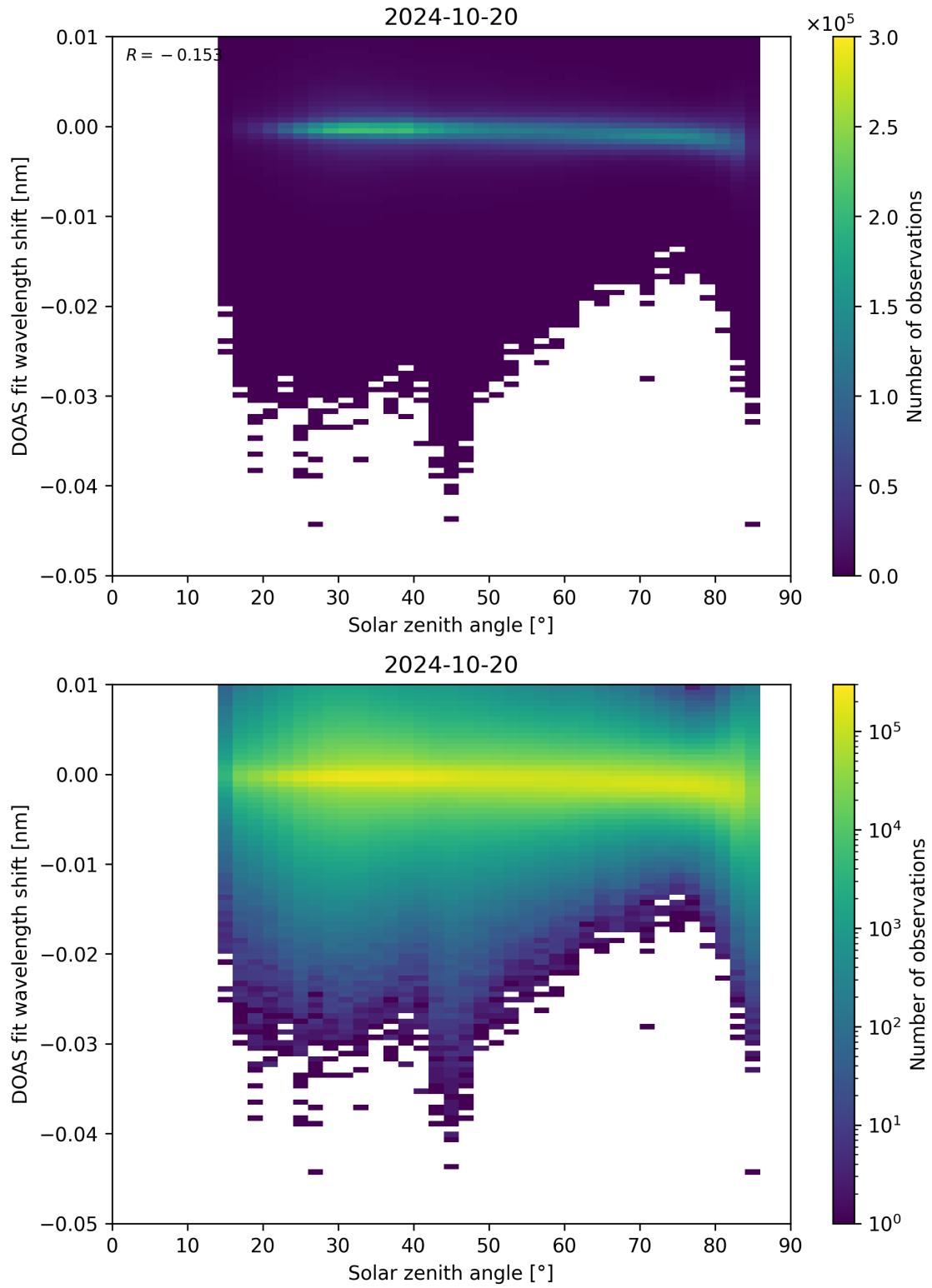
Figure 161: Scatter density plot of “Solar zenith angle” against “DOAS fit wavelength shift” for 2024-10-19 to 2024-10-21.
