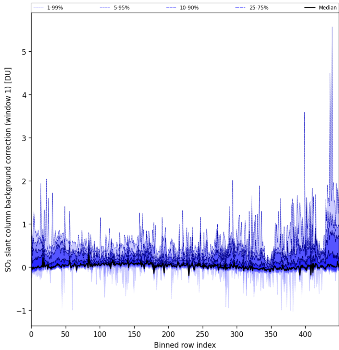
Figure 82: Along track statistics of “SO 2 slant column background correction (window 1)” for 2024-10-19 to 2024-10-21
