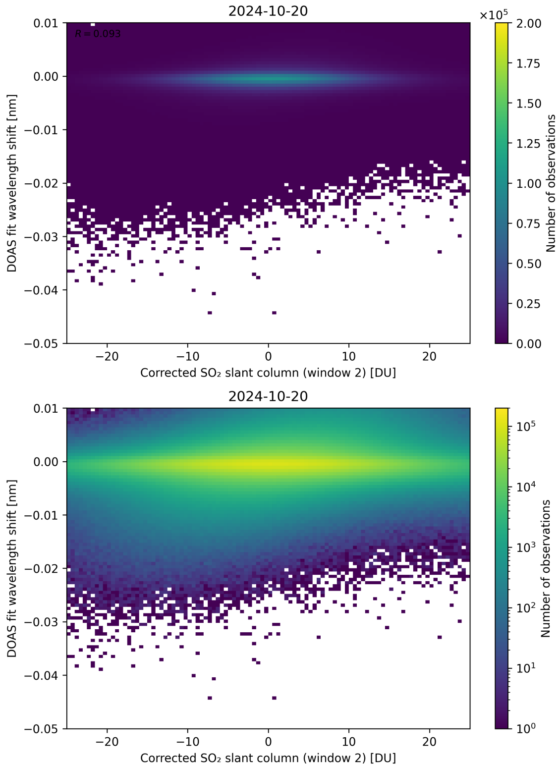
Figure 196: Scatter density plot of “Corrected SO 2 slant column (window 2)” against “DOAS fit wavelength shift” for 2024-10-19 to 2024-10-21.
