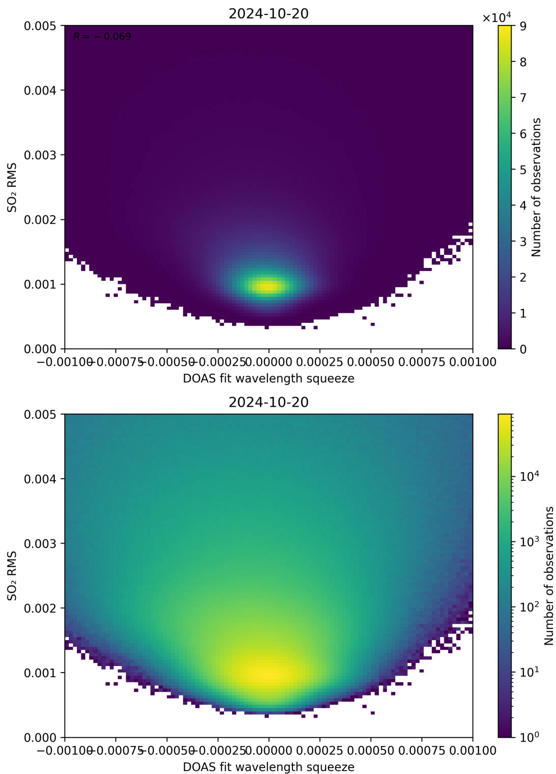
Figure 132: Scatter density plot of “DOAS fit wavelength squeeze” against “SO 2 RMS” for 2024-10-19 to 2024-10-21.
