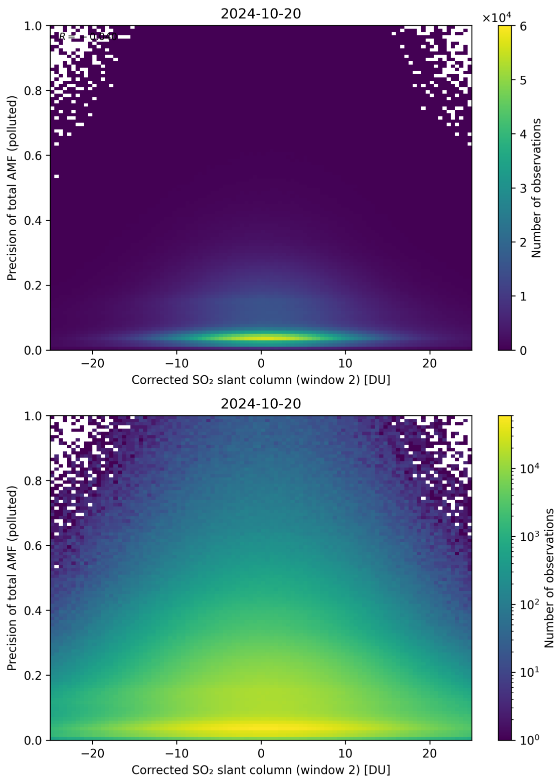
Figure 204: Scatter density plot of “Corrected SO 2 slant column (window 2)” against “Precision of total AMF (polluted)” for 2024-10-19 to 2024-10-21.
