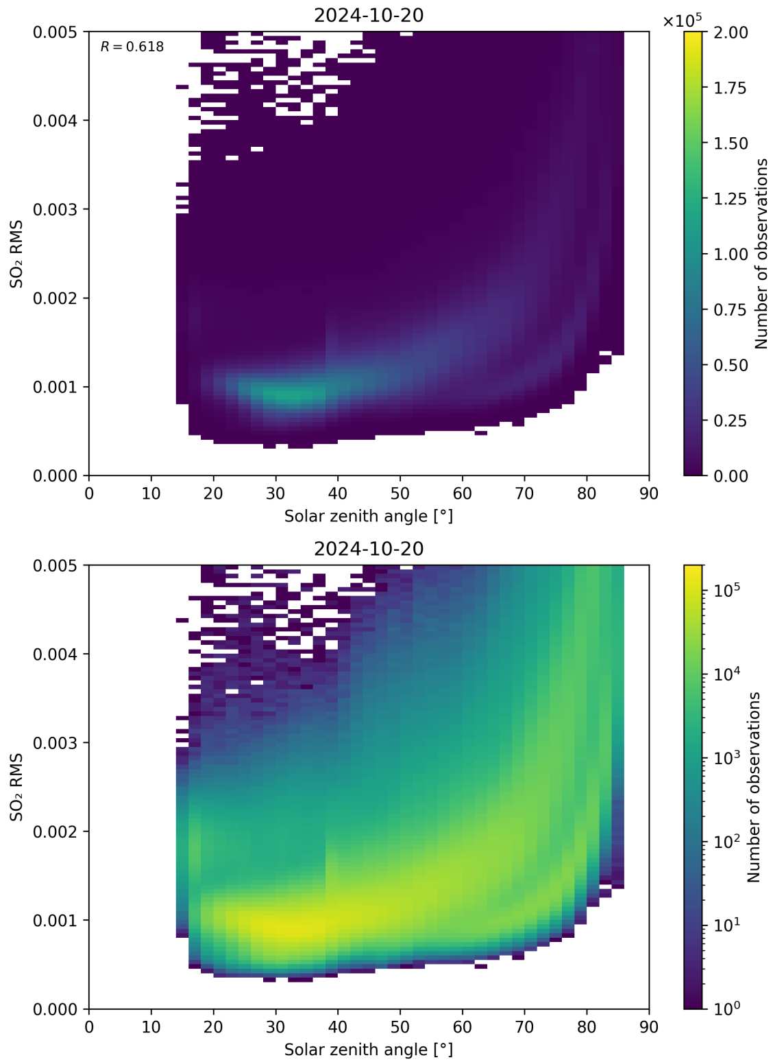
Figure 163: Scatter density plot of “Solar zenith angle” against “SO 2 RMS” for 2024-10-19 to 2024-10-21.
