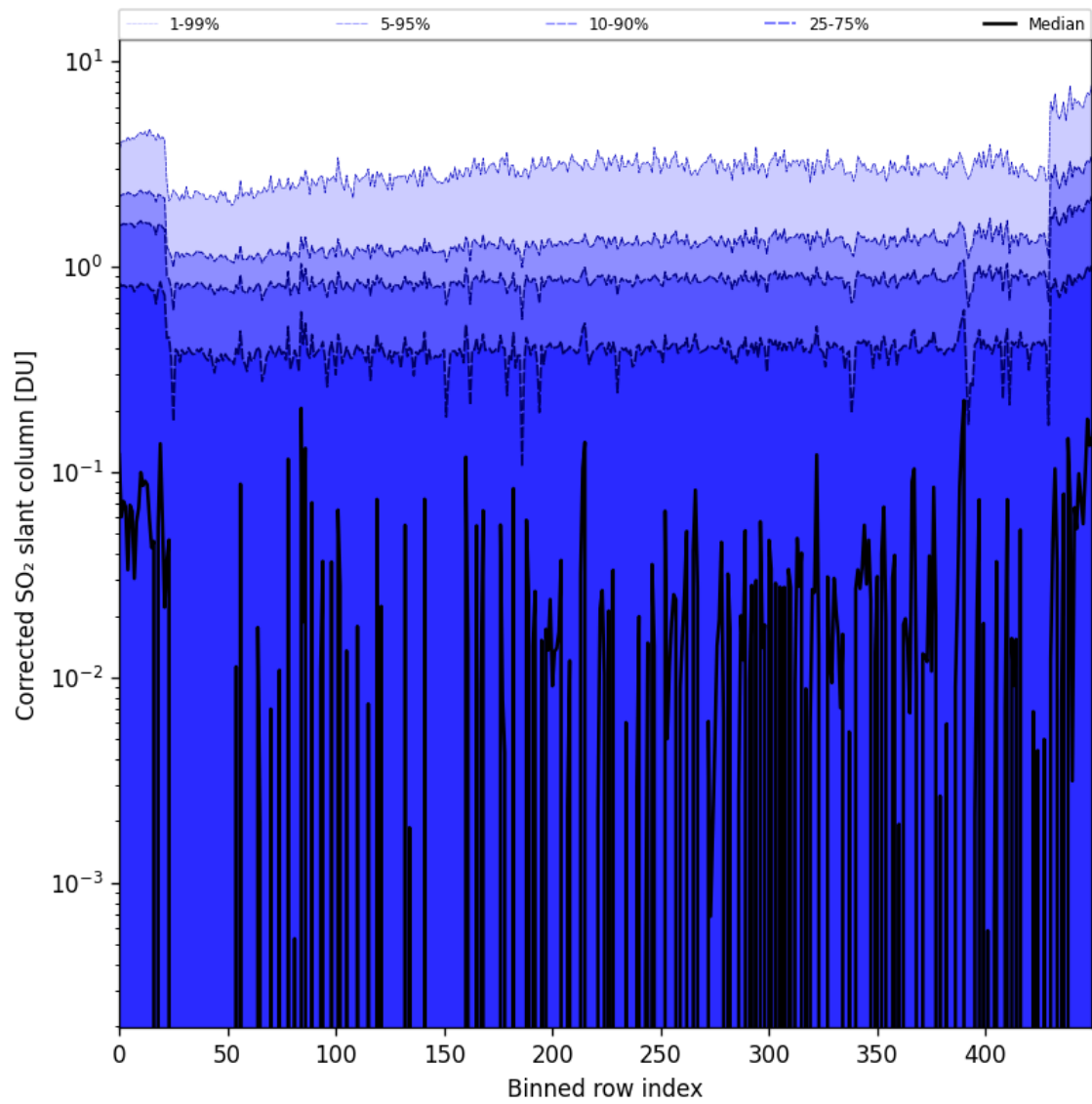
Figure 78: Along track statistics of “Corrected SO 2 slant column” for 2024-10-19 to 2024-10-21
