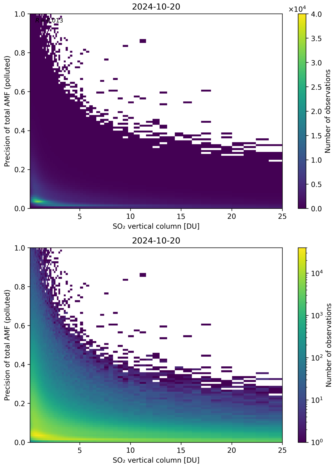
Figure 306: Scatter density plot of “SO 2 vertical column” against “Precision of total AMF (polluted)” for 2024-10-19 to 2024-10-21.
