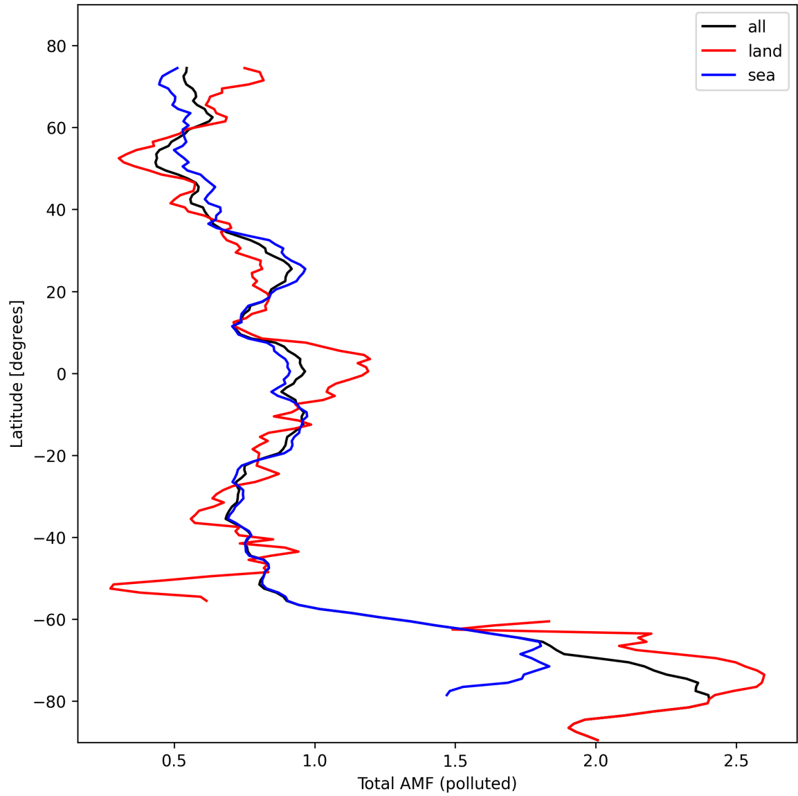
Figure 48: Zonal average of “Total AMF (polluted)” for 2024-10-19 to 2024-10-21.
