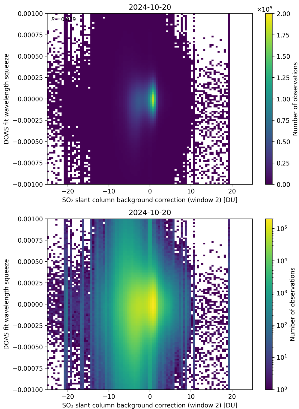
Figure 113: Scatter density plot of “SO 2 slant column background correction (window 2)” against “DOAS fit wavelength squeeze” for 2024-10-19 to 2024-10-21.
