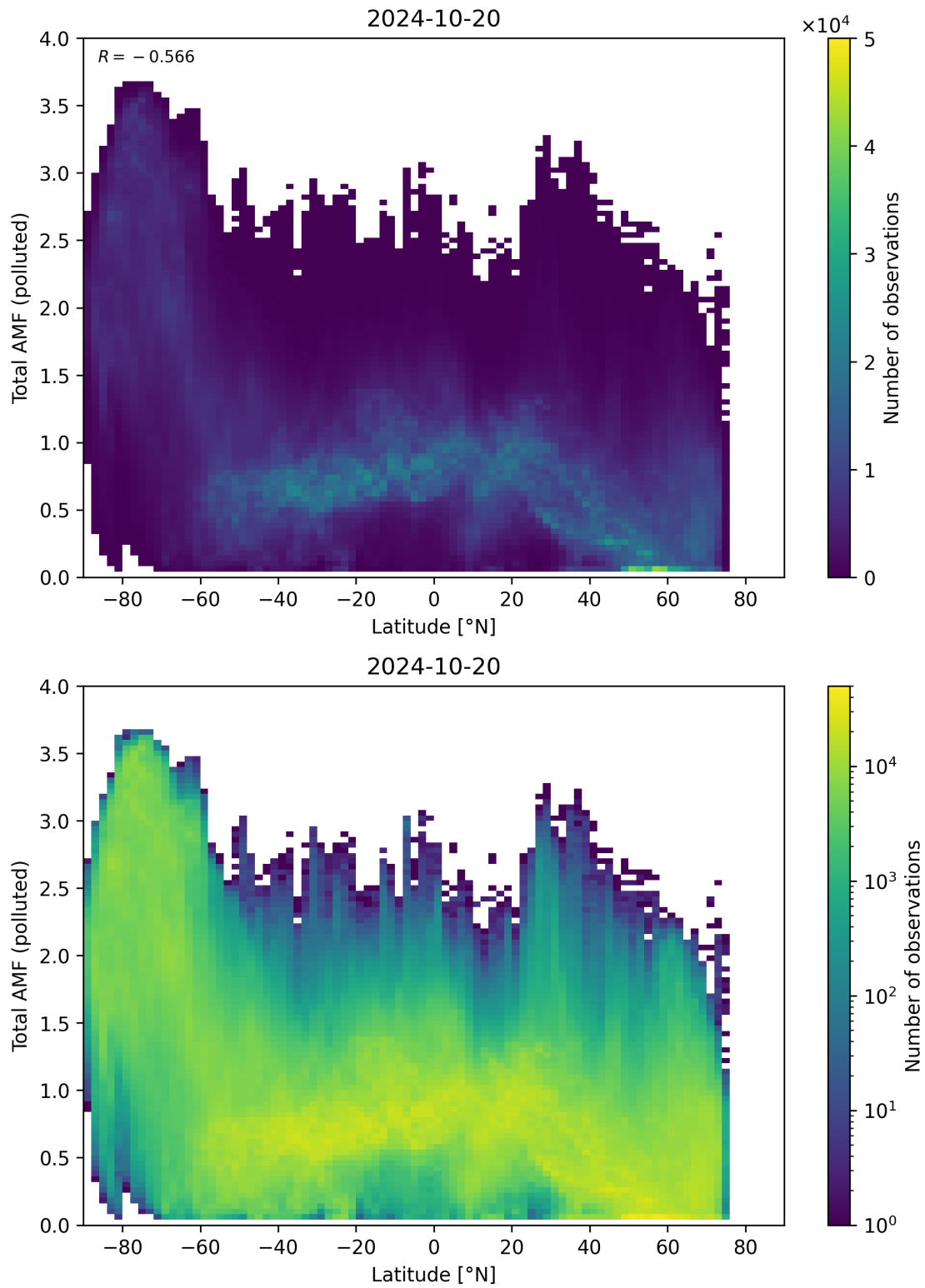
Figure 154: Scatter density plot of “Latitude” against “Total AMF (polluted)” for 2024-10-19 to 2024-10-21.
