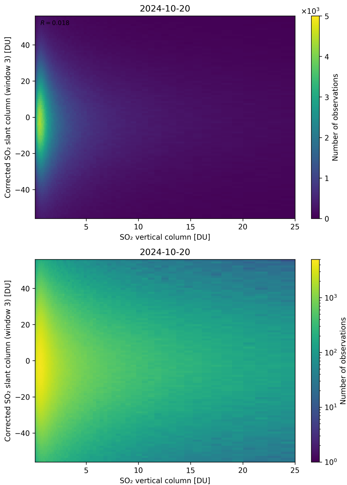
Figure 299: Scatter density plot of “SO 2 vertical column” against “Corrected SO 2 slant column (window 3)” for 2024-10-19 to 2024-10-21.
