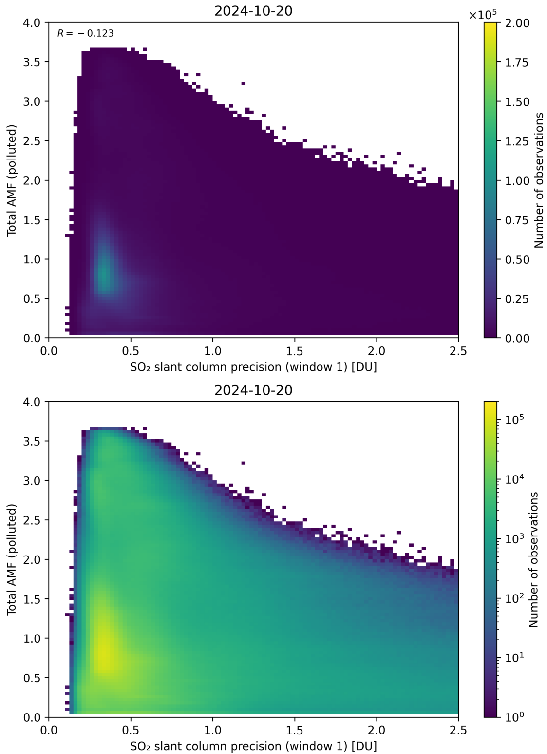
Figure 230: Scatter density plot of “SO 2 slant column precision (window 1)” against “Total AMF (polluted)” for 2024-10-19 to 2024-10-21.
