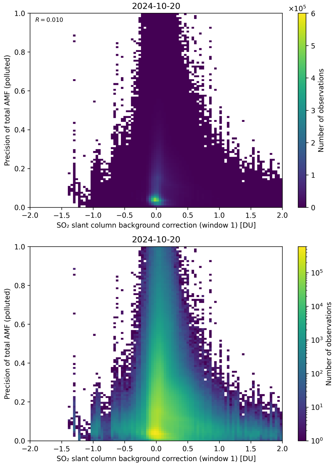
Figure 110: Scatter density plot of “SO 2 slant column background correction (window 1)” against “Precision of total AMF (polluted)” for 2024-10-19 to 2024-10-21.
