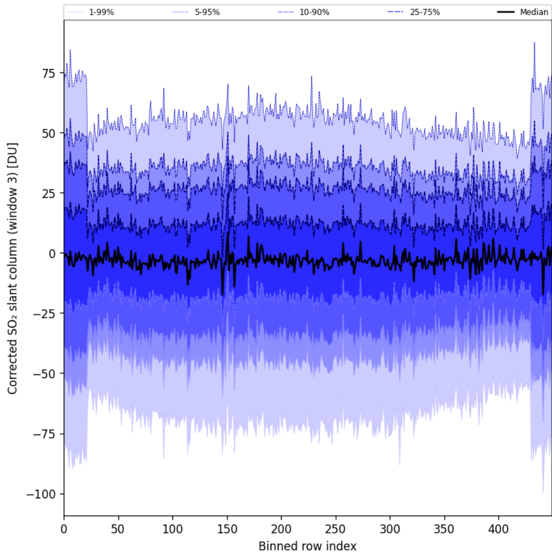
Figure 89: Along track statistics of “Corrected SO 2 slant column (window 3)” for 2024-10-19 to 2024-10-21
