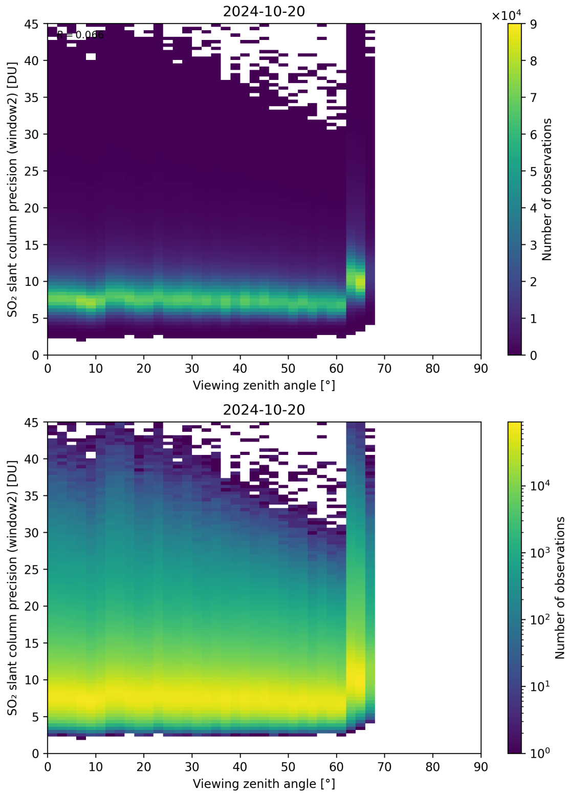
Figure 322: Scatter density plot of “Viewing zenith angle” against “SO 2 slant column precision (window2)” for 2024-10-19 to 2024-10-21.
