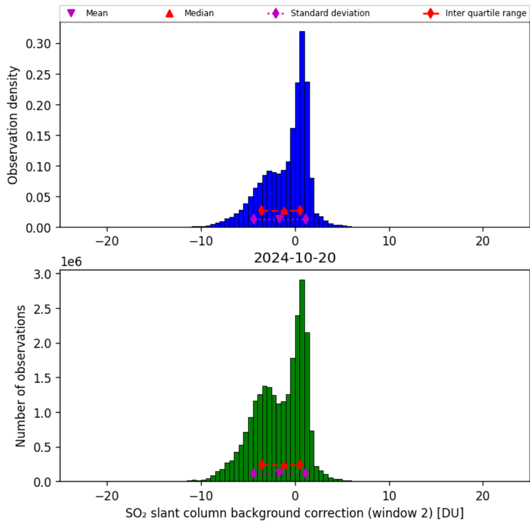
Figure 63: Histogram of “SO 2 slant column background correction (window 2)” for 2024-10-19 to 2024-10-21
