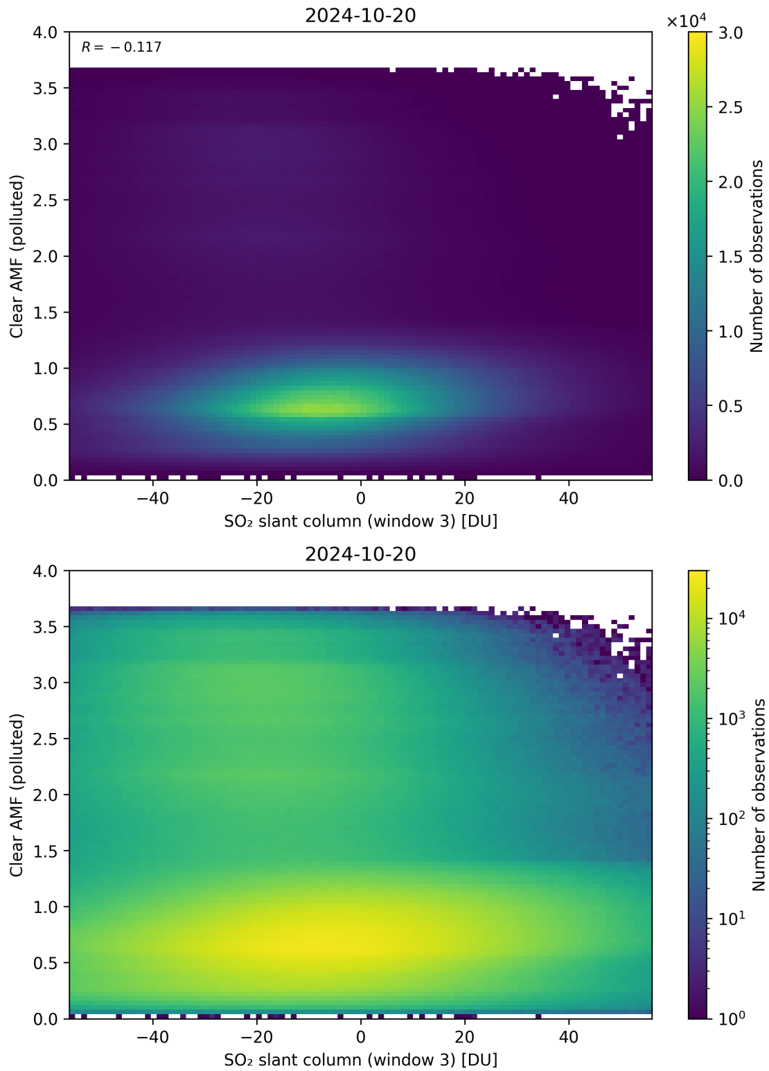
Figure 265: Scatter density plot of “SO 2 slant column (window 3)” against “Clear AMF (polluted)” for 2024-10-19 to 2024-10-21.
