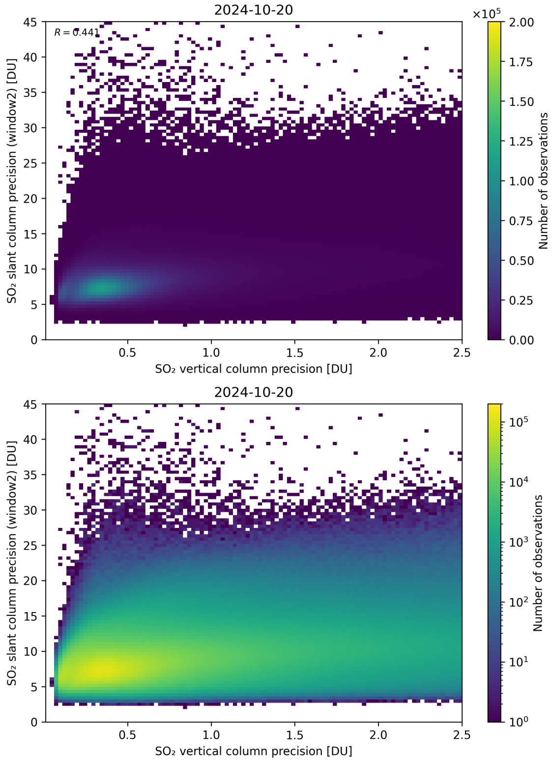
Figure 291: Scatter density plot of “SO 2 vertical column precision” against “SO 2 slant column precision (window2)” for 2024-10-19 to 2024-10-21.
