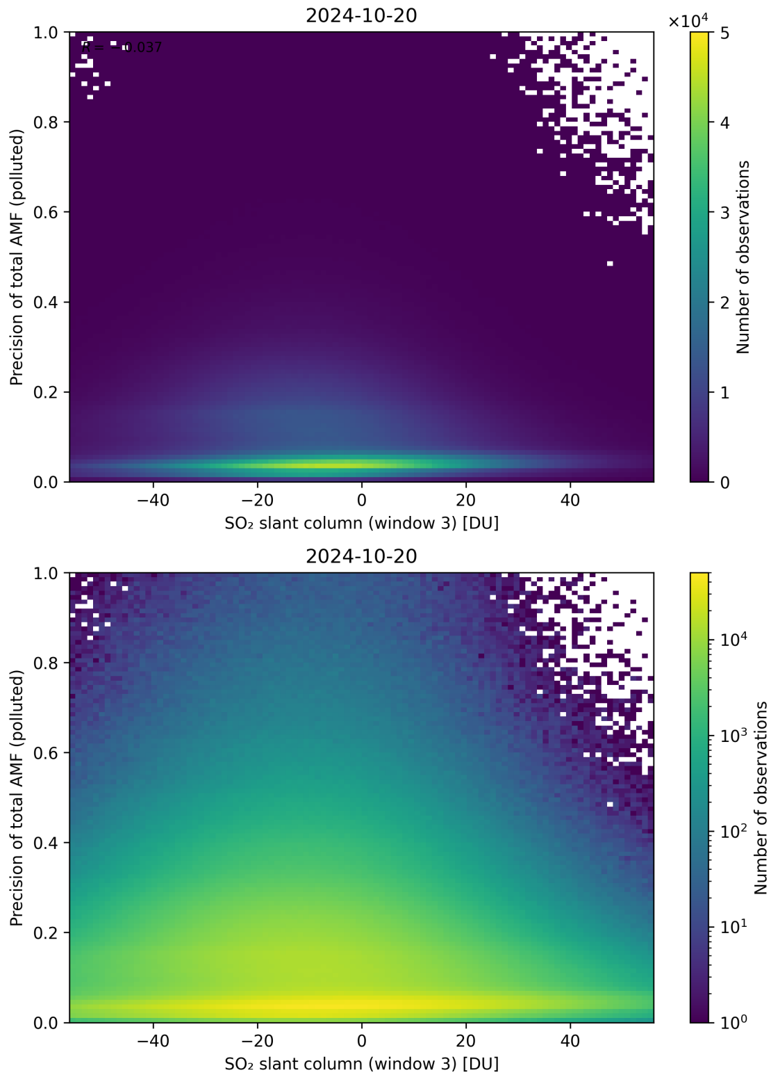
Figure 269: Scatter density plot of “SO 2 slant column (window 3)” against “Precision of total AMF (polluted)” for 2024-10-19 to 2024-10-21.
