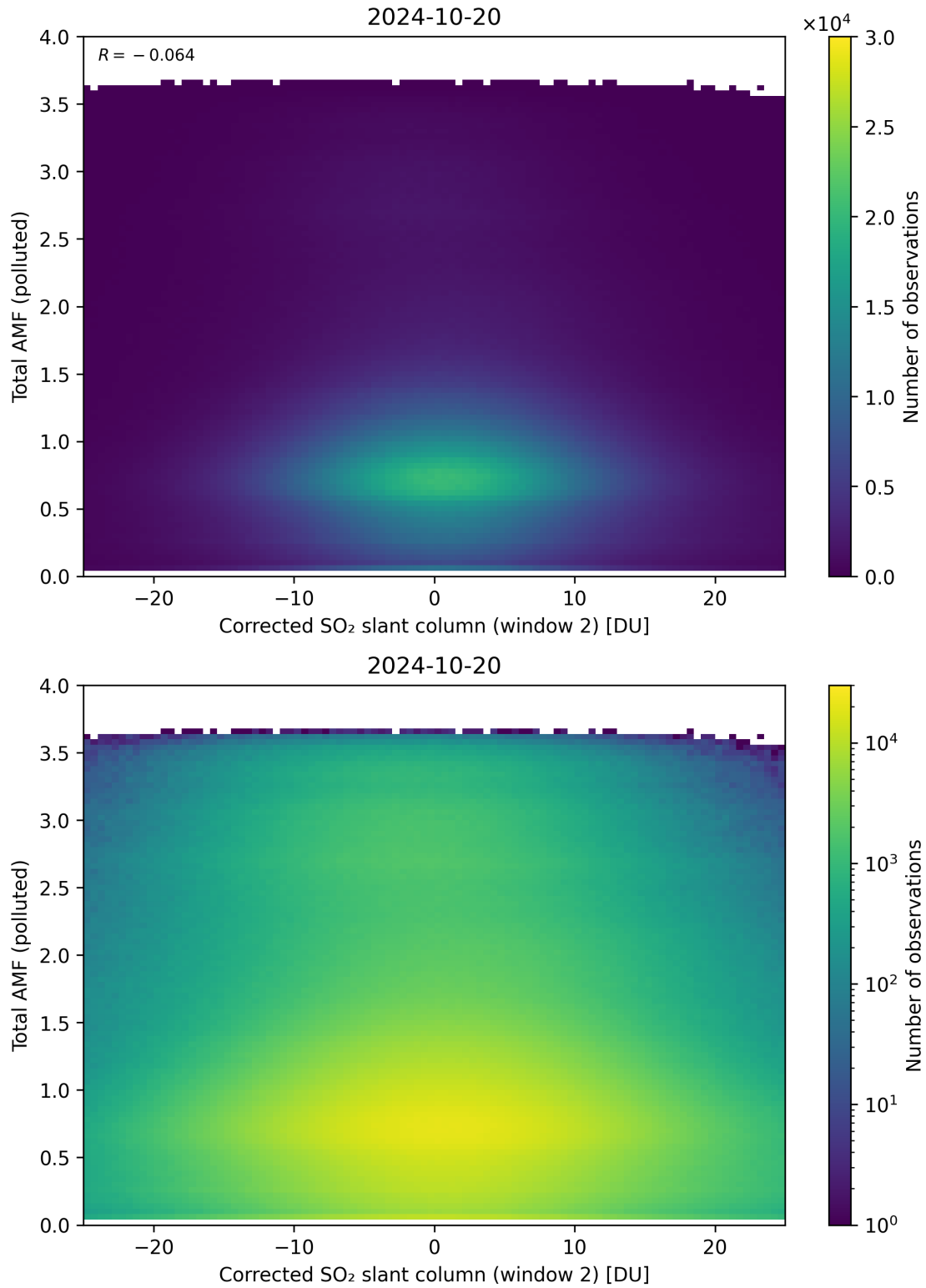
Figure 203: Scatter density plot of “Corrected SO 2 slant column (window 2)” against “Total AMF (polluted)” for 2024-10-19 to 2024-10-21.
