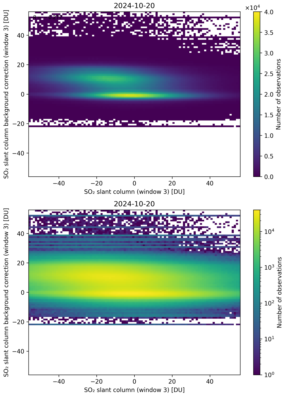
Figure 253: Scatter density plot of “SO 2 slant column (window 3)” against “SO 2 slant column background correction (window 3)” for 2024-10-19 to 2024-10-21.
