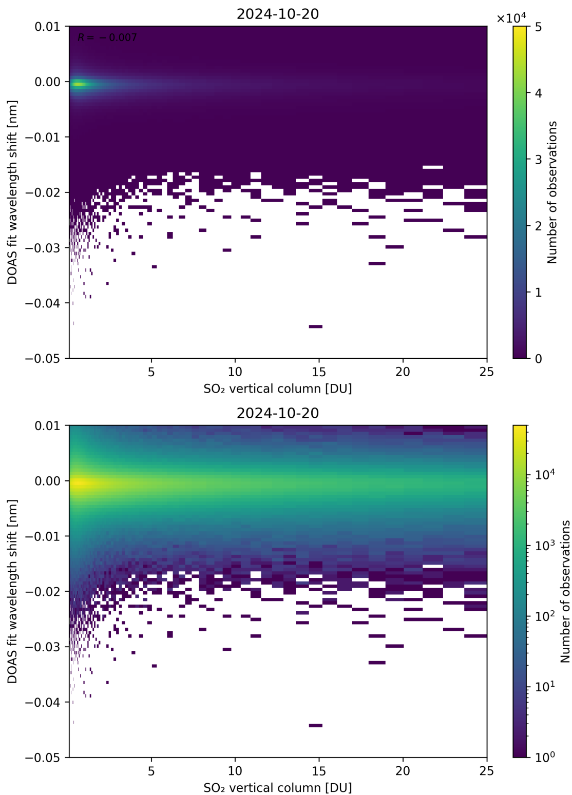
Figure 276: Scatter density plot of “SO 2 vertical column” against “DOAS fit wavelength shift” for 2024-10-19 to 2024-10-21.
