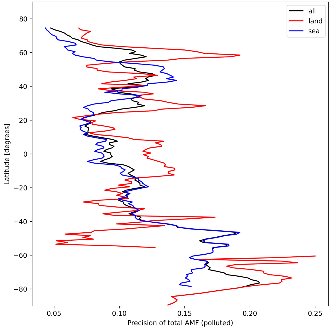
Figure 49: Zonal average of “Precision of total AMF (polluted)” for 2024-10-19 to 2024-10-21.
