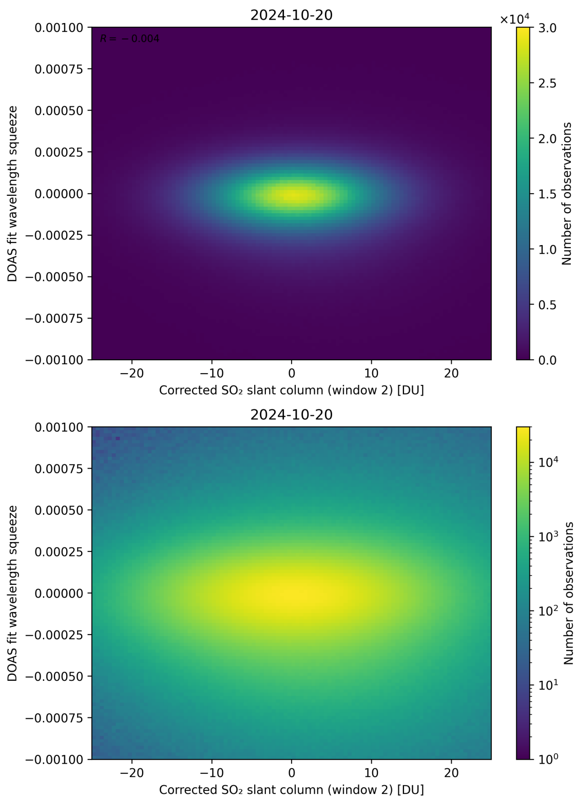
Figure 197: Scatter density plot of “Corrected SO 2 slant column (window 2)” against “DOAS fit wavelength squeeze” for 2024-10-19 to 2024-10-21.
