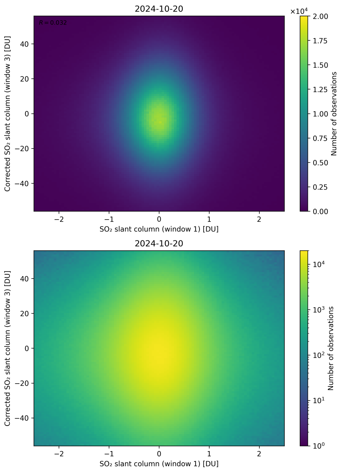
Figure 234: Scatter density plot of “SO 2 slant column (window 1)” against “Corrected SO 2 slant column (window 3)” for 2024-10-19 to 2024-10-21.
