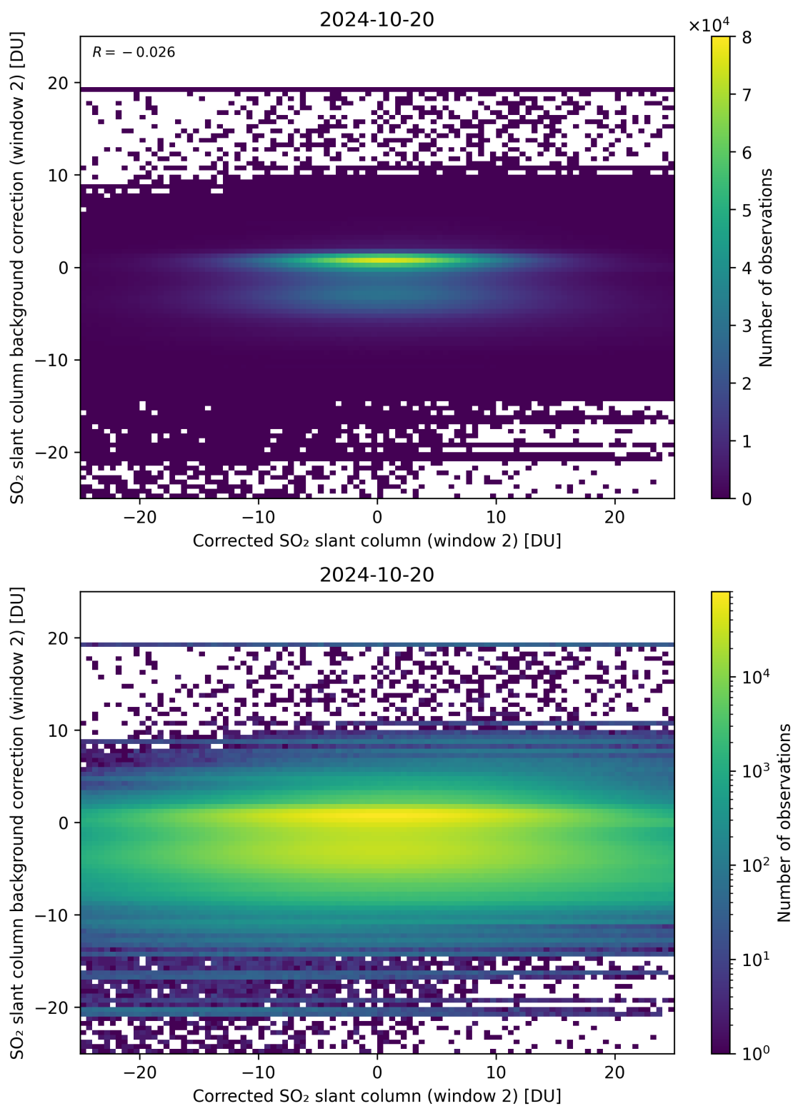
Figure 194: Scatter density plot of “Corrected SO 2 slant column (window 2)” against “SO 2 slant column background correction (window 2)” for 2024-10-19 to 2024-10-21.
