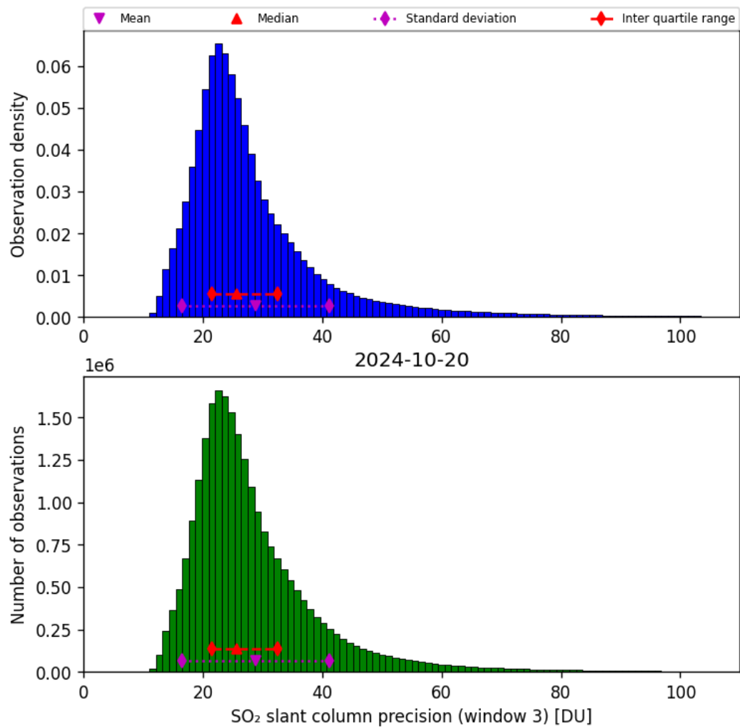
Figure 65: Histogram of “SO 2 slant column precision (window 3)” for 2024-10-19 to 2024-10-21
