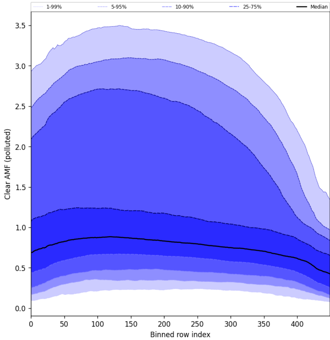
Figure 96: Along track statistics of “Clear AMF (polluted)” for 2024-10-19 to 2024-10-21
