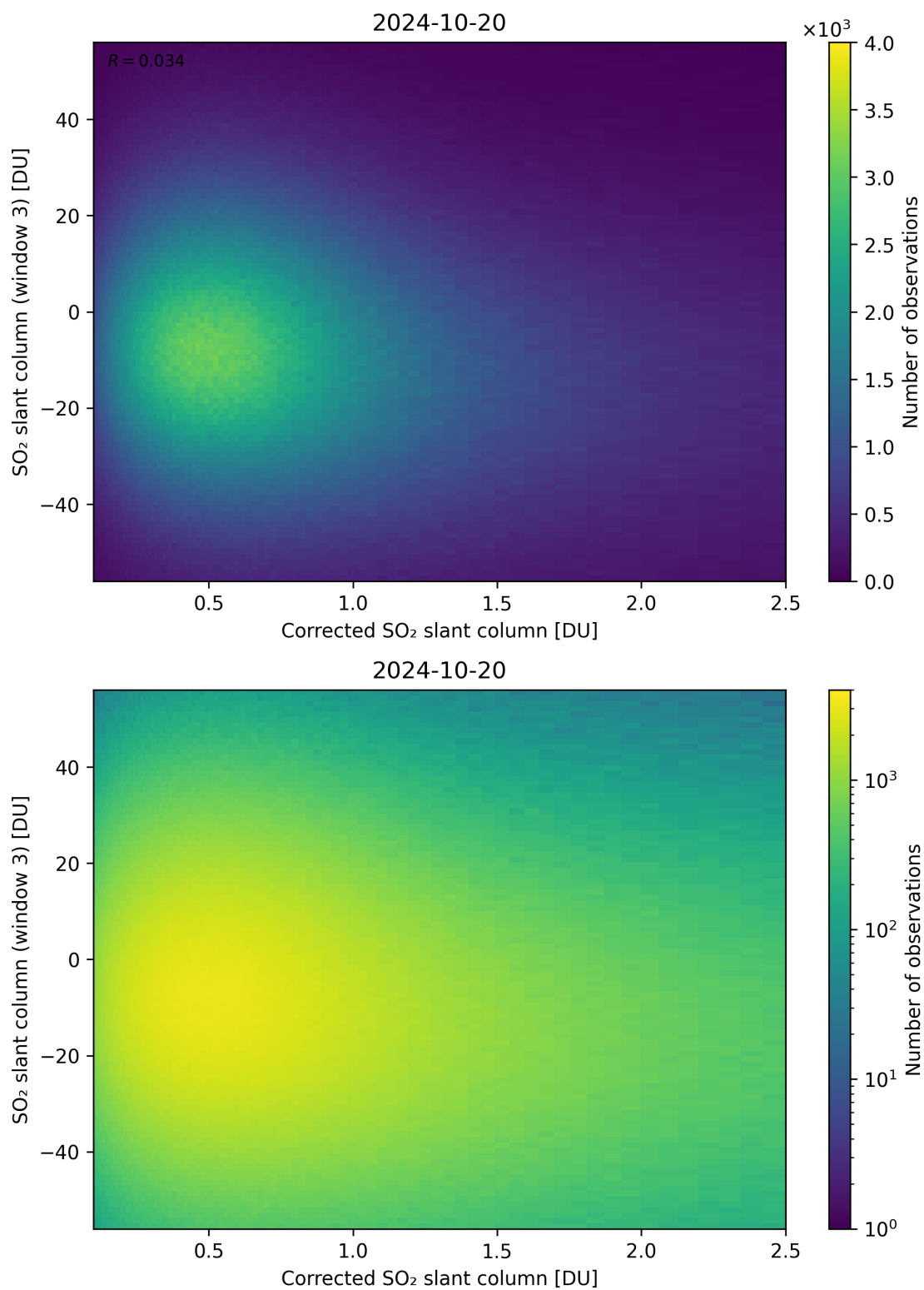
Figure 190: Scatter density plot of “Corrected SO 2 slant column” against “SO 2 slant column (window 3)” for 2024-10-19 to 2024-10-21.
