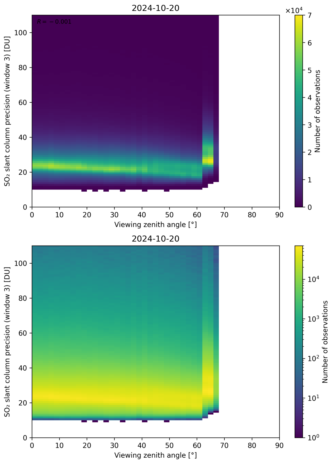
Figure 324: Scatter density plot of “Viewing zenith angle” against “SO 2 slant column precision (window 3)” for 2024-10-19 to 2024-10-21.
