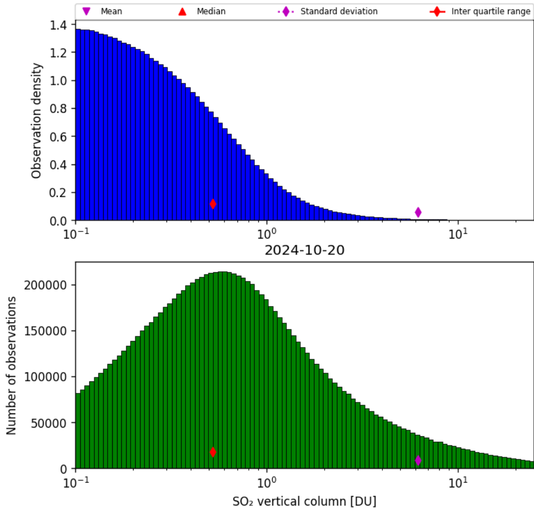
Figure 53: Histogram of “SO 2 vertical column” for 2024-10-19 to 2024-10-21
