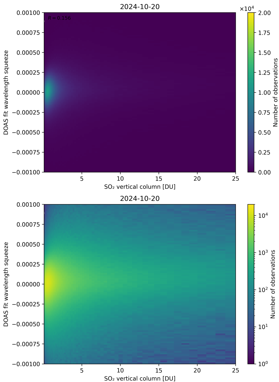
Figure 277: Scatter density plot of “SO 2 vertical column” against “DOAS fit wavelength squeeze” for 2024-10-19 to 2024-10-21.
