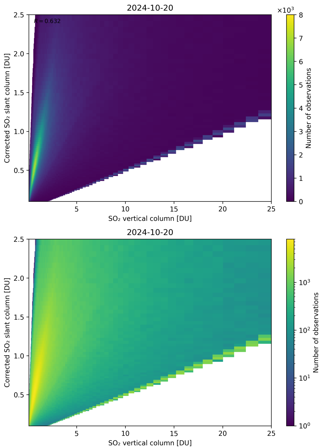
Figure 297: Scatter density plot of “SO 2 vertical column” against “Corrected SO 2 slant column” for 2024-10-19 to 2024-10-21.
