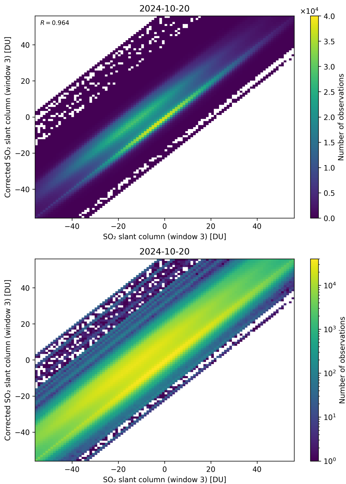
Figure 266: Scatter density plot of “SO 2 slant column (window 3)” against “Corrected SO 2 slant column (window 3)” for 2024-10-19 to 2024-10-21.
