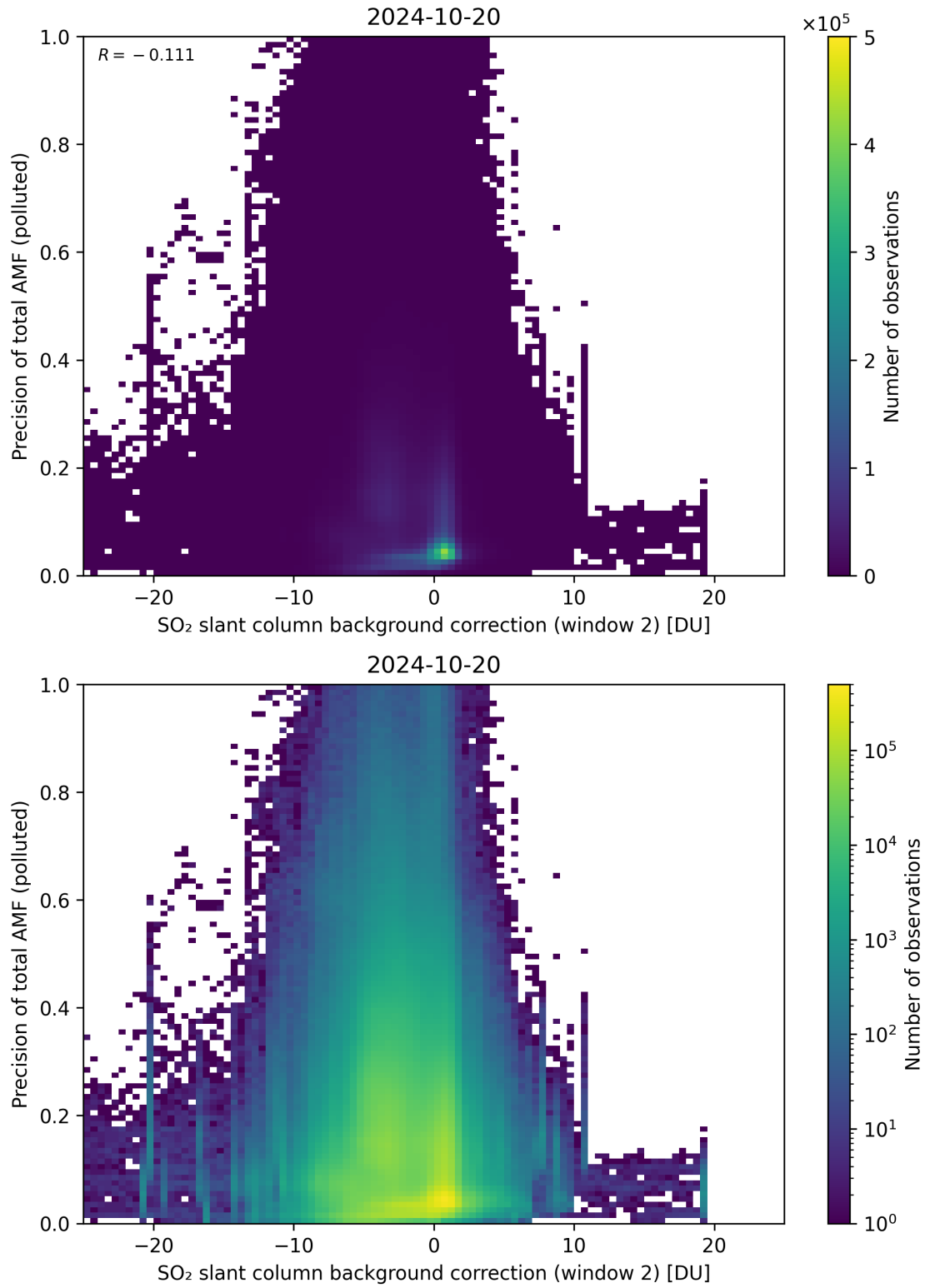
Figure 120: Scatter density plot of “SO 2 slant column background correction (window 2)” against “Precision of total AMF (polluted)” for 2024-10-19 to 2024-10-21.
