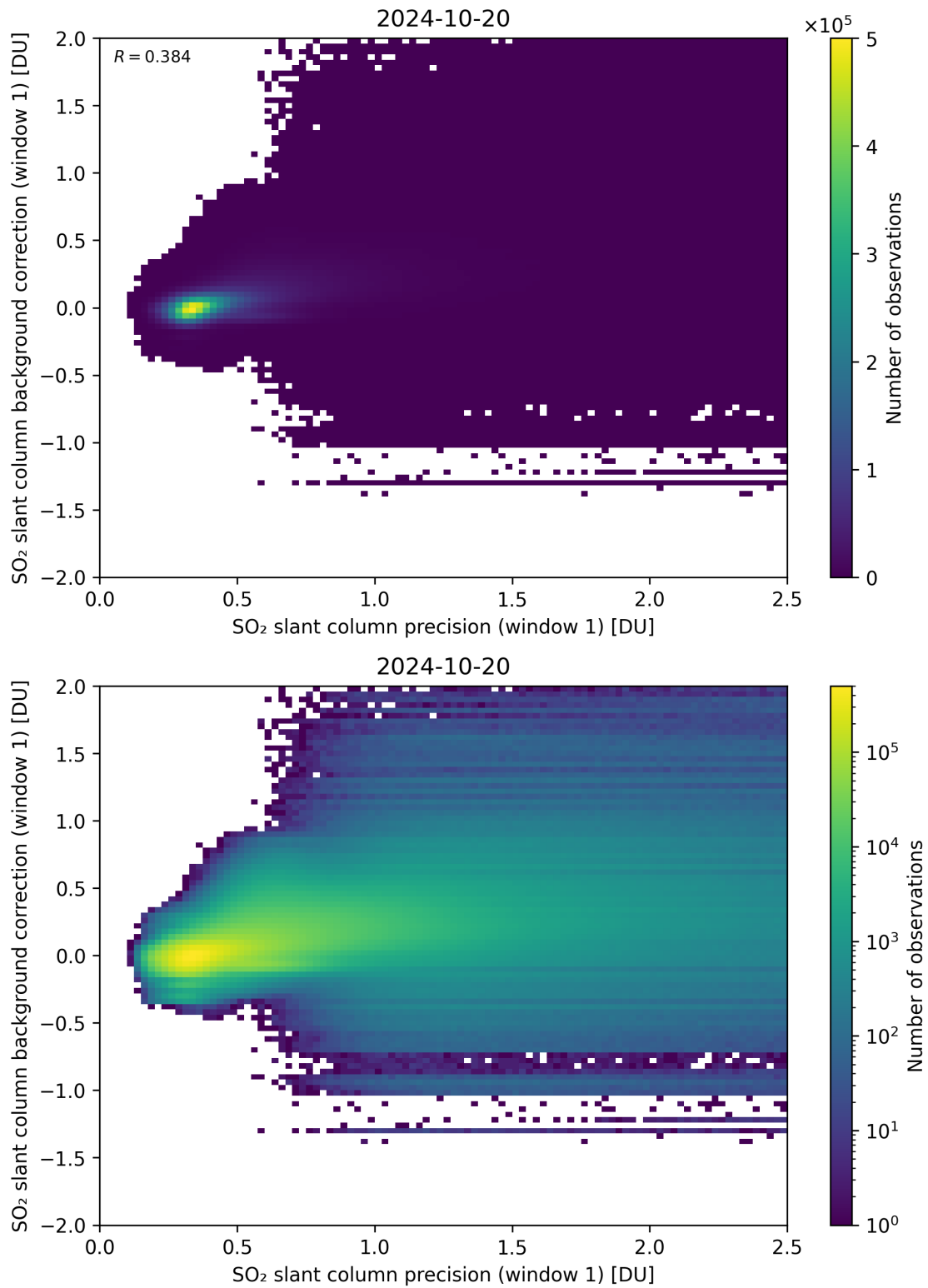
Figure 218: Scatter density plot of “SO 2 slant column precision (window 1)” against “SO 2 slant column background correction (window 1)” for 2024-10-19 to 2024-10-21.
