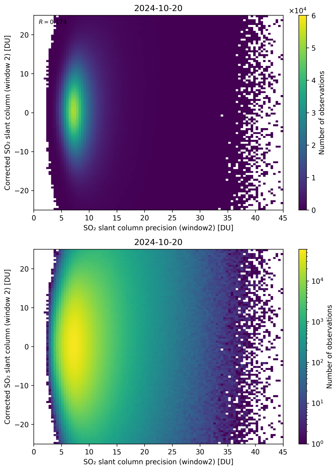
Figure 247: Scatter density plot of “SO 2 slant column precision (window2)” against “Corrected SO 2 slant column (window 2)” for 2024-10-19 to 2024-10-21.
