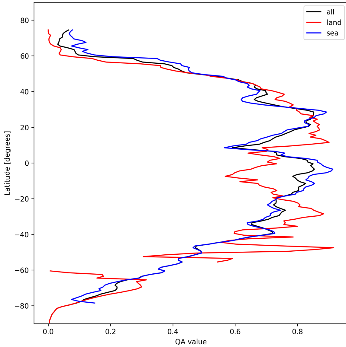
Figure 29: Zonal average of “QA value” for 2024-10-19 to 2024-10-21.
