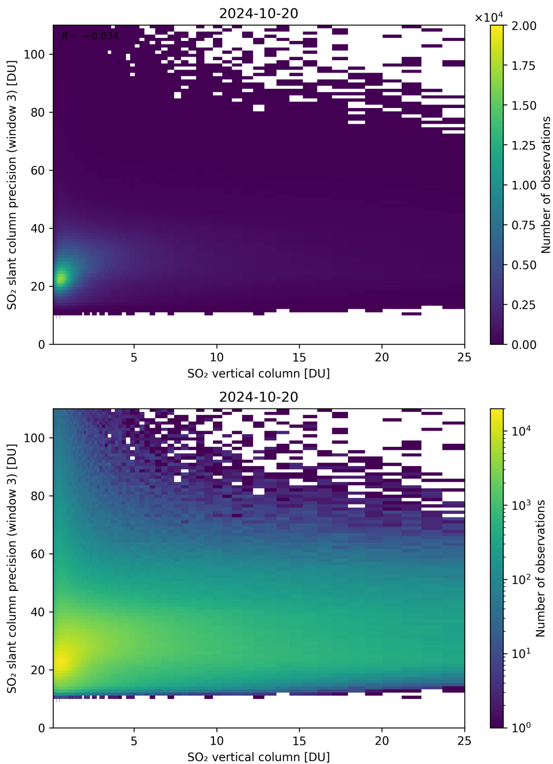
Figure 304: Scatter density plot of “SO 2 vertical column” against “SO 2 slant column precision (window 3)” for 2024-10-19 to 2024-10-21.
