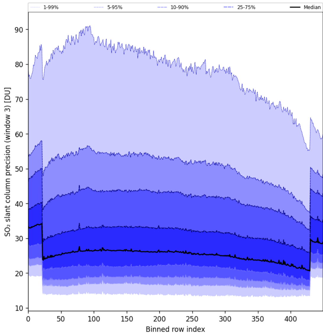
Figure 88: Along track statistics of “SO 2 slant column precision (window 3)” for 2024-10-19 to 2024-10-21
