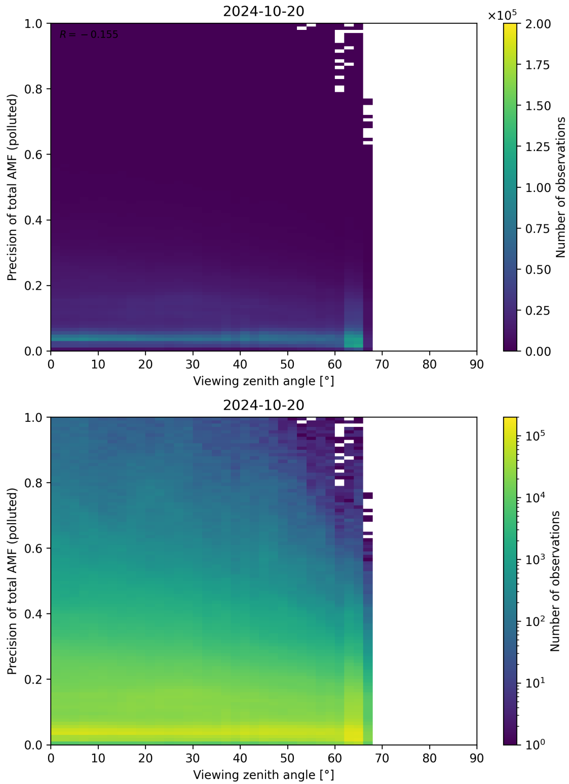
Figure 326: Scatter density plot of “Viewing zenith angle” against “Precision of total AMF (polluted)” for 2024-10-19 to 2024-10-21.
