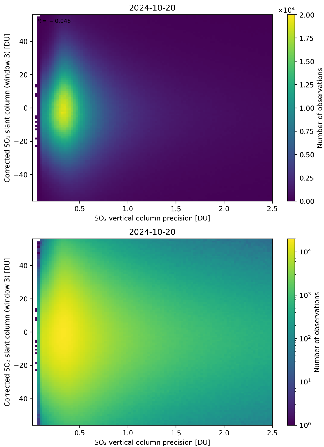
Figure 288: Scatter density plot of “SO 2 vertical column precision” against “Corrected SO 2 slant column (window 3)” for 2024-10-19 to 2024-10-21.
