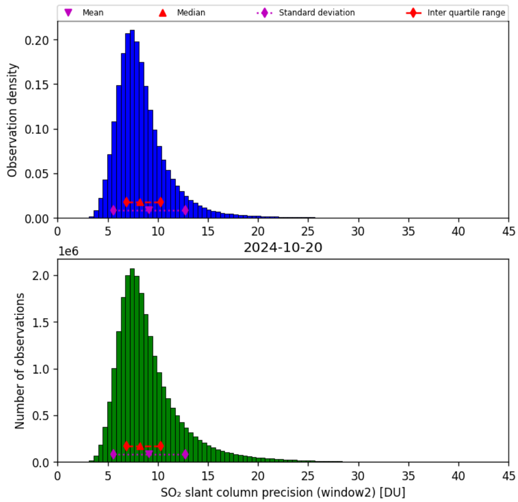
Figure 61: Histogram of “SO 2 slant column precision (window2)” for 2024-10-19 to 2024-10-21
