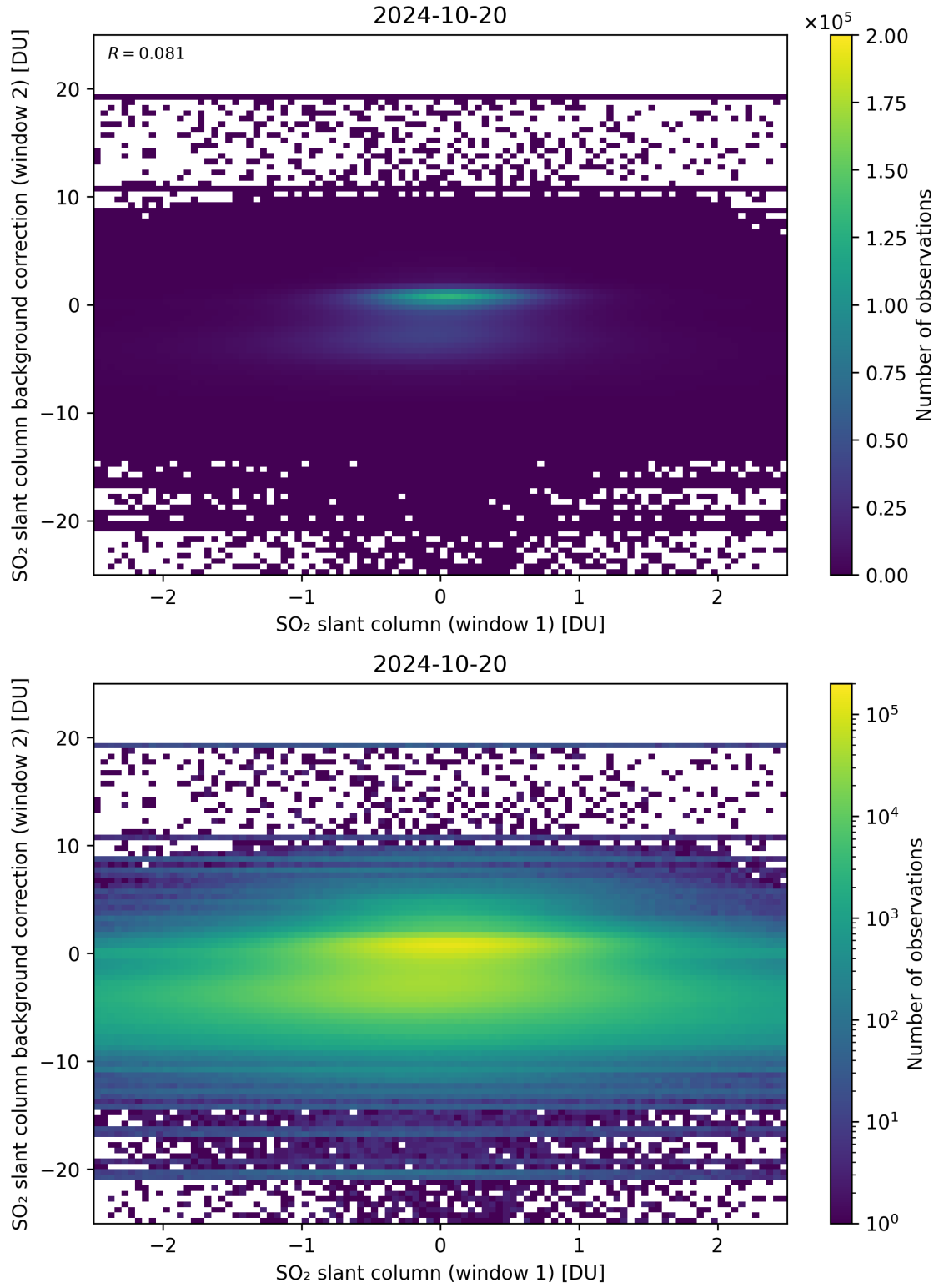
Figure 213: Scatter density plot of “SO 2 slant column (window 1)” against “SO 2 slant column background correction (window 2)” for 2024-10-19 to 2024-10-21.
