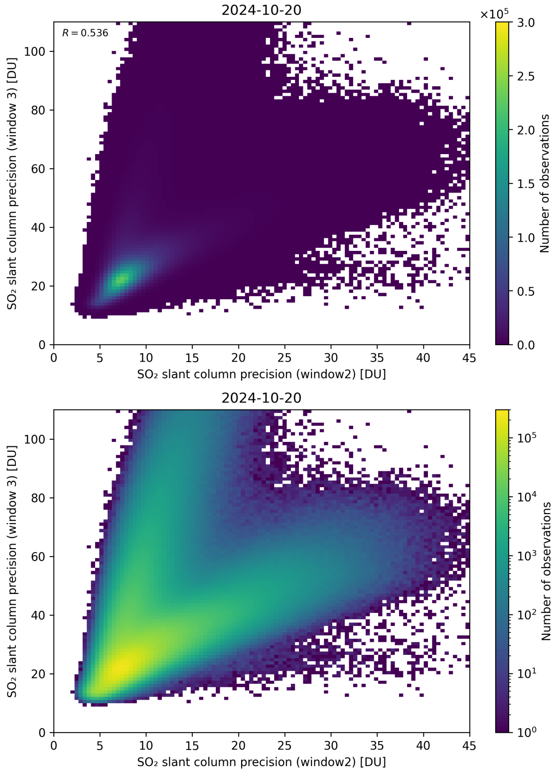
Figure 250: Scatter density plot of “SO 2 slant column precision (window2)” against “SO 2 slant column precision (window 3)” for 2024-10-19 to 2024-10-21.
