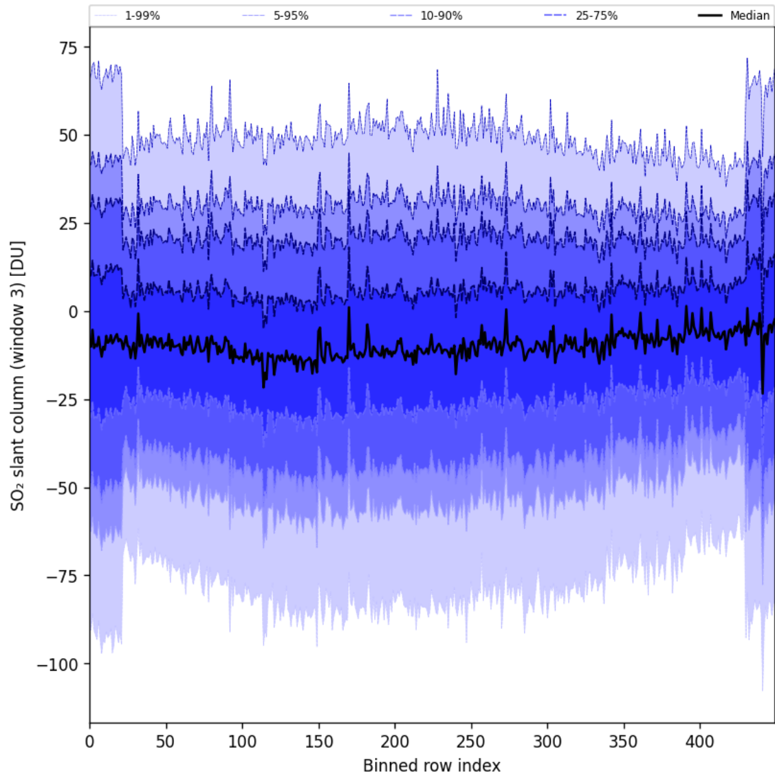
Figure 87: Along track statistics of “SO 2 slant column (window 3)” for 2024-10-19 to 2024-10-21
