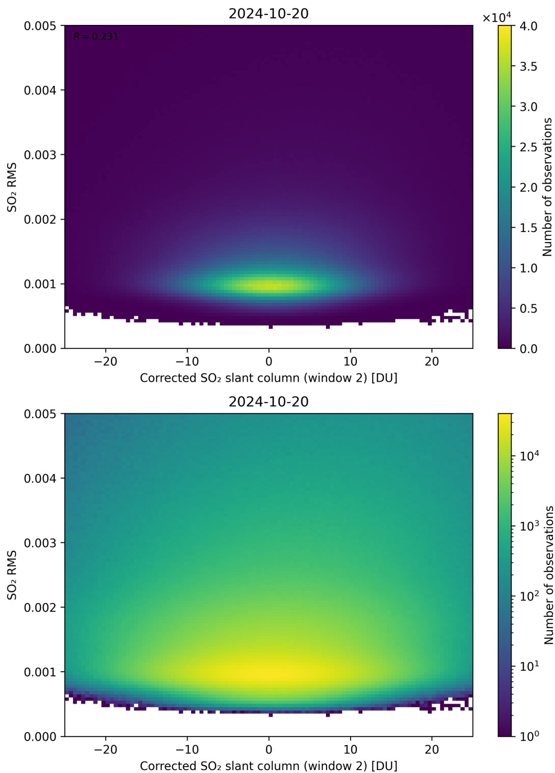
Figure 198: Scatter density plot of “Corrected SO 2 slant column (window 2)” against “SO 2 RMS” for 2024-10-19 to 2024-10-21.
