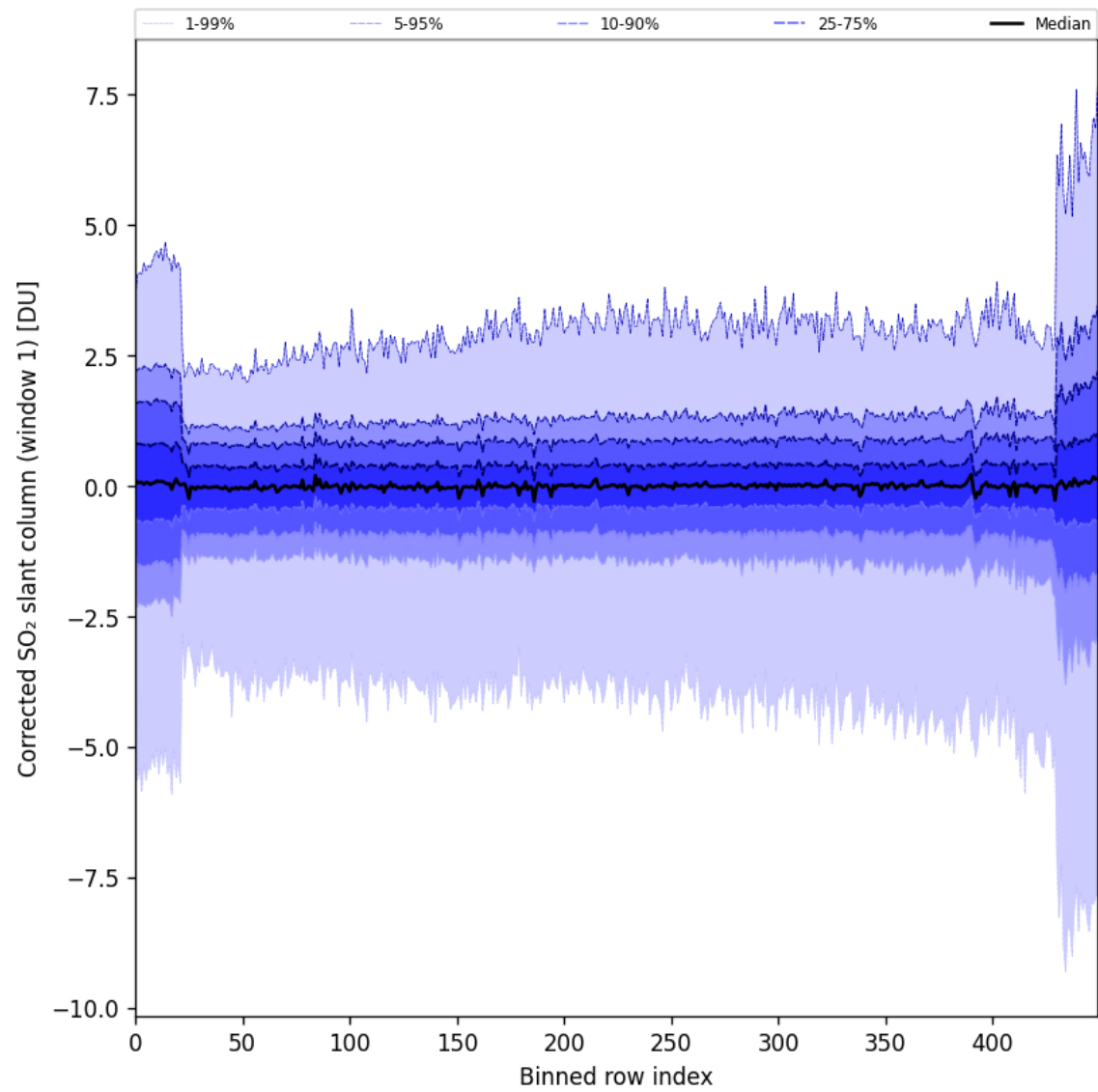
Figure 81: Along track statistics of “Corrected SO 2 slant column (window 1)” for 2024-10-19 to 2024-10-21
