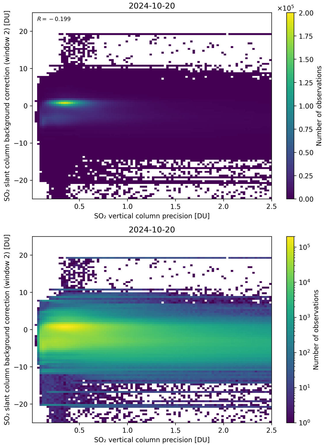
Figure 280: Scatter density plot of “SO 2 vertical column precision” against “SO 2 slant column background correction (window 2)” for 2024-10-19 to 2024-10-21.
