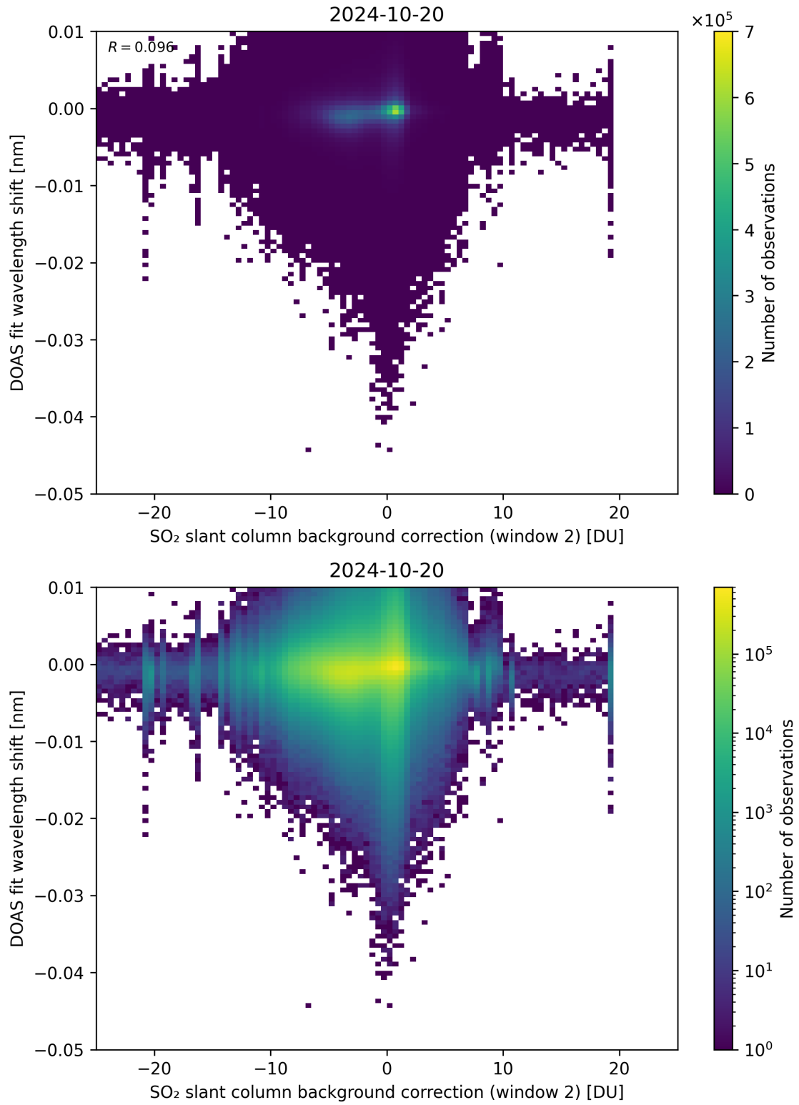
Figure 112: Scatter density plot of “SO 2 slant column background correction (window 2)” against “DOAS fit wavelength shift” for 2024-10-19 to 2024-10-21.
