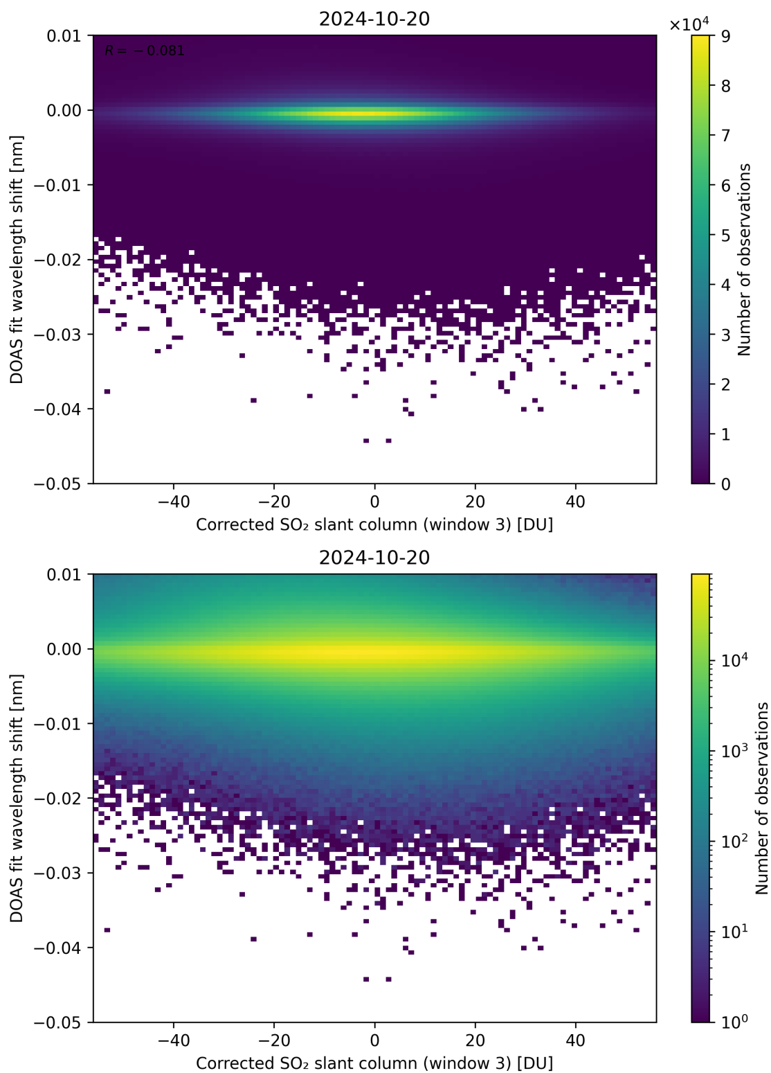
Figure 206: Scatter density plot of “Corrected SO 2 slant column (window 3)” against “DOAS fit wavelength shift” for 2024-10-19 to 2024-10-21.
