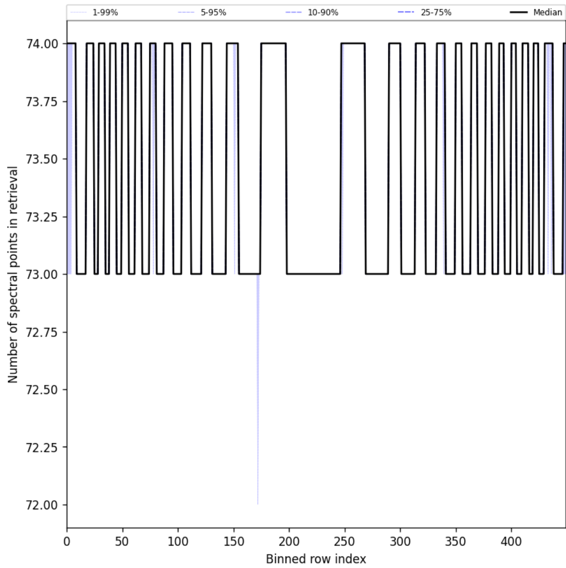
Figure 97: Along track statistics of “Number of spectral points in retrieval” for 2024-10-19 to 2024-10-21
