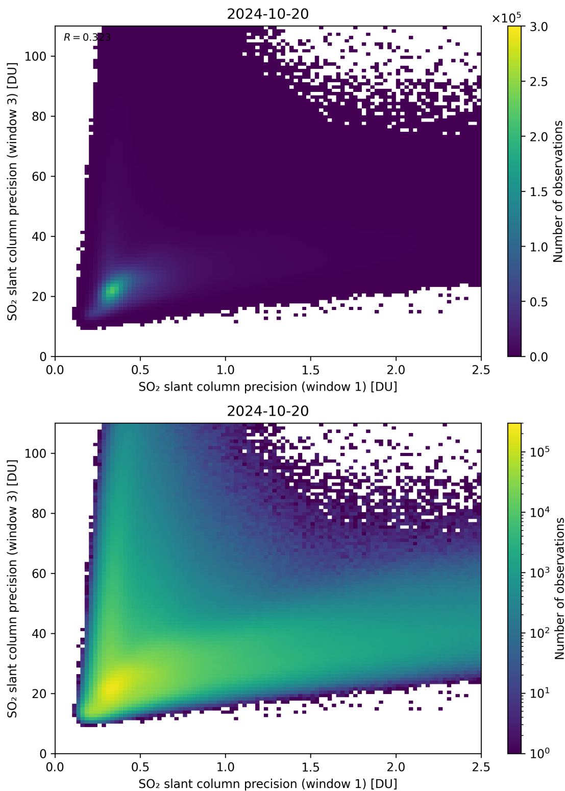
Figure 229: Scatter density plot of “SO 2 slant column precision (window 1)” against “SO 2 slant column precision (window 3)” for 2024-10-19 to 2024-10-21.
