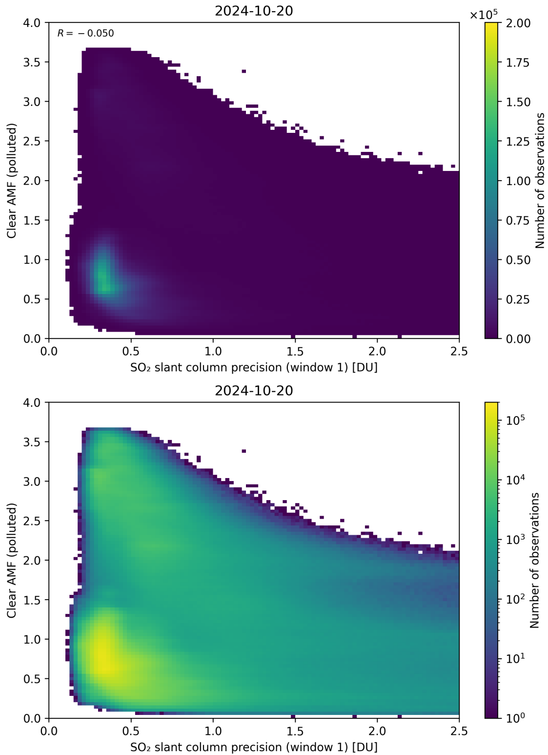
Figure 224: Scatter density plot of “SO 2 slant column precision (window 1)” against “Clear AMF (polluted)” for 2024-10-19 to 2024-10-21.
