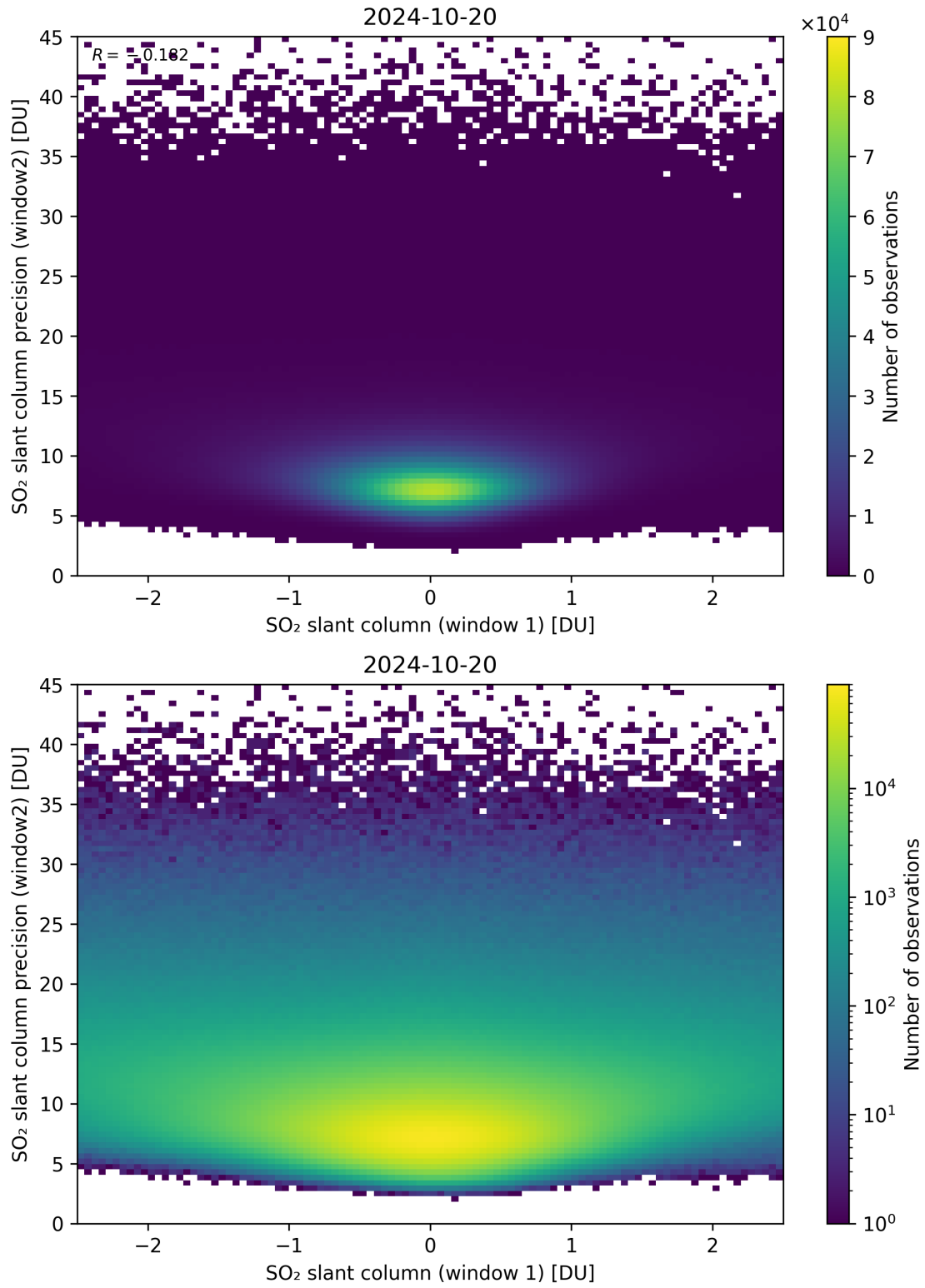
Figure 236: Scatter density plot of “SO 2 slant column (window 1)” against “SO 2 slant column precision (window2)” for 2024-10-19 to 2024-10-21.
