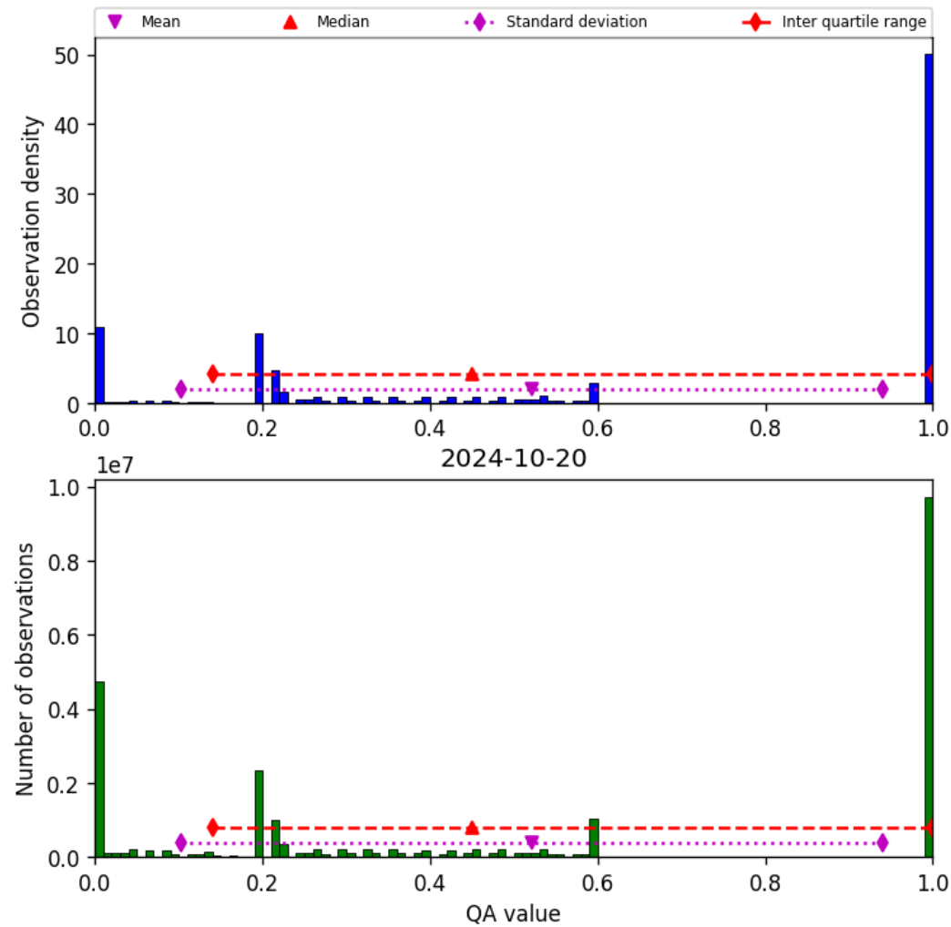
Figure 52: Histogram of “QA value” for 2024-10-19 to 2024-10-21
