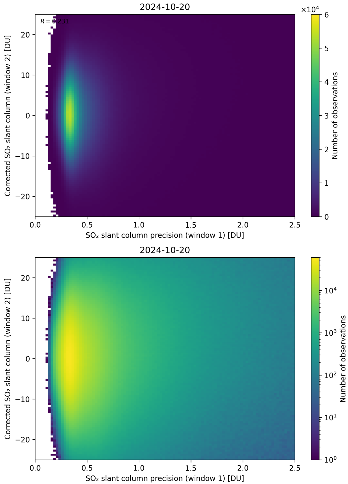
Figure 225: Scatter density plot of “SO 2 slant column precision (window 1)” against “Corrected SO 2 slant column (window 2)” for 2024-10-19 to 2024-10-21.
