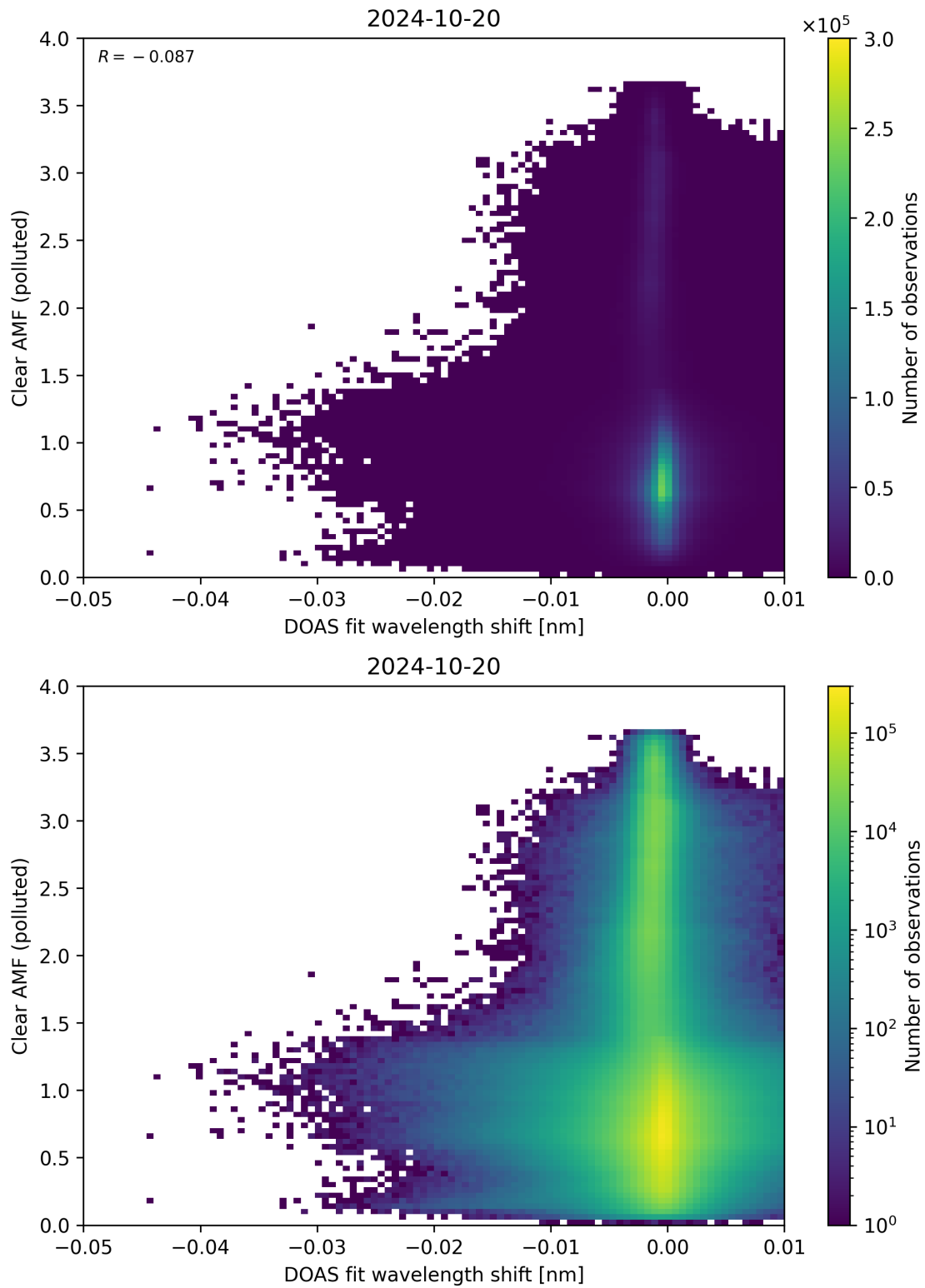
Figure 129: Scatter density plot of “DOAS fit wavelength shift” against “Clear AMF (polluted)” for 2024-10-19 to 2024-10-21.
