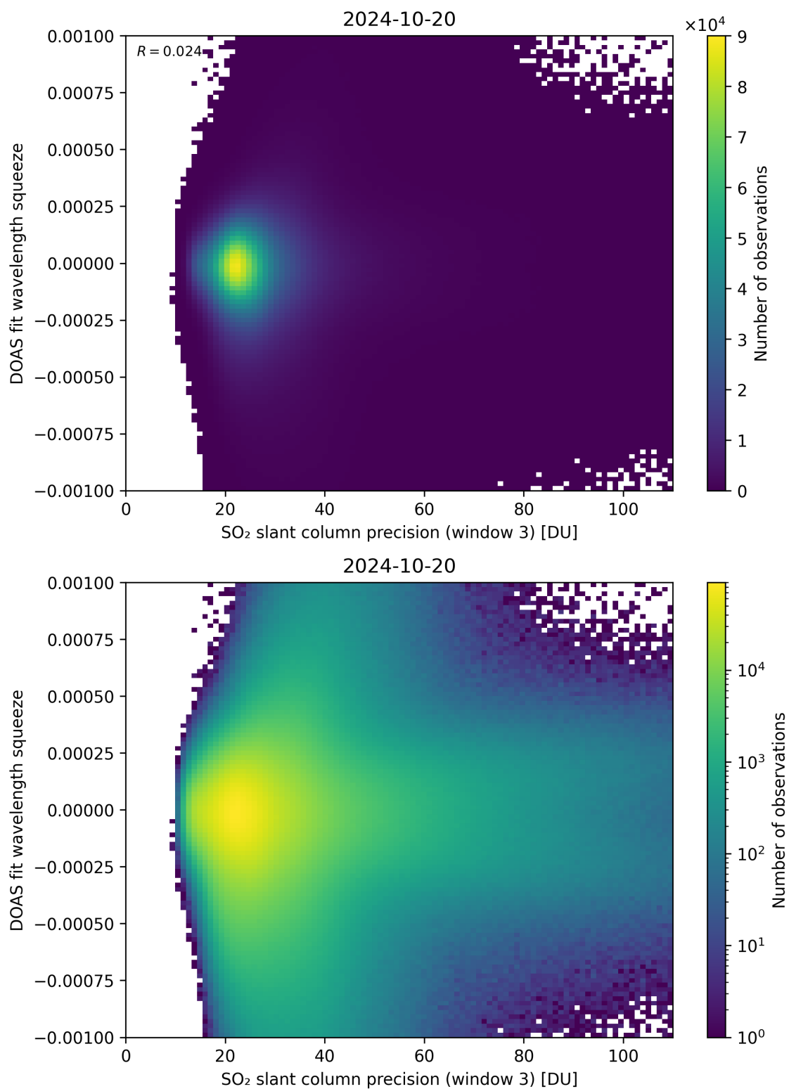
Figure 259: Scatter density plot of “SO 2 slant column precision (window 3)” against “DOAS fit wavelength squeeze” for 2024-10-19 to 2024-10-21.
