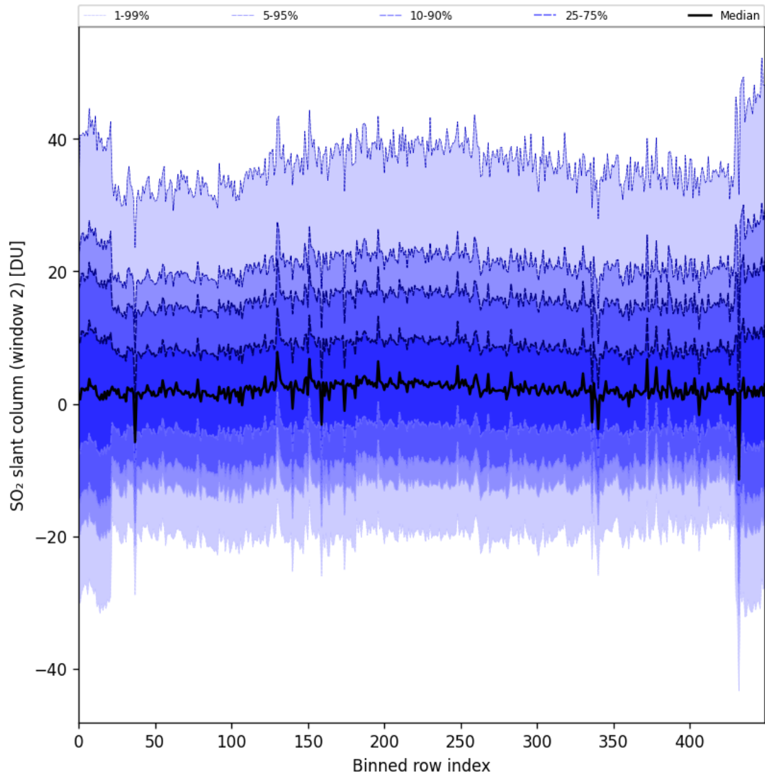
Figure 83: Along track statistics of “SO 2 slant column (window 2)” for 2024-10-19 to 2024-10-21
