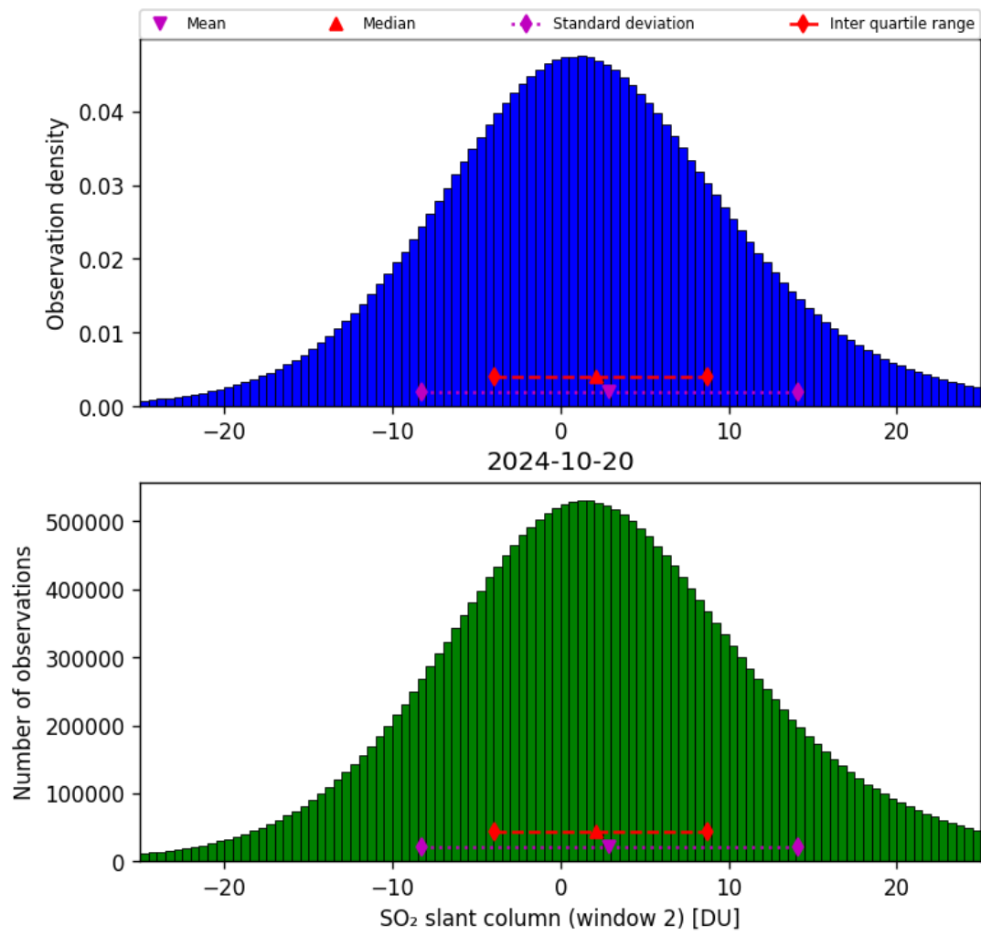
Figure 60: Histogram of “SO 2 slant column (window 2)” for 2024-10-19 to 2024-10-21
