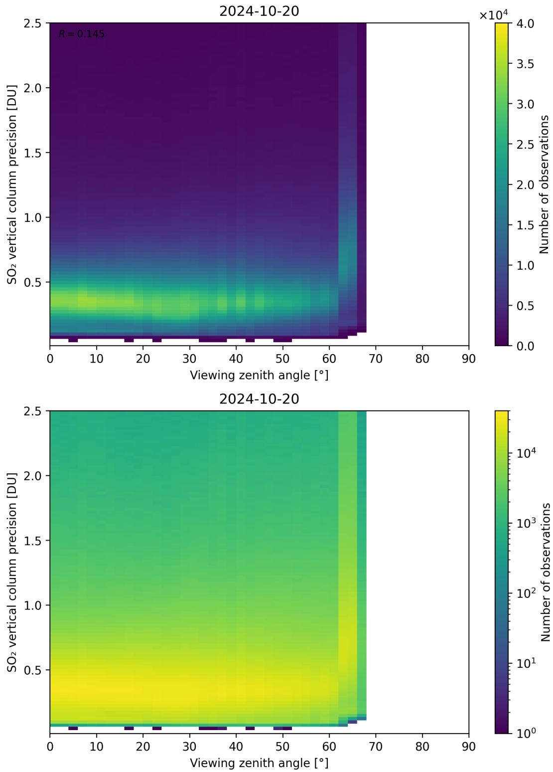
Figure 328: Scatter density plot of “Viewing zenith angle” against “SO 2 vertical column precision” for 2024-10-19 to 2024-10-21.
