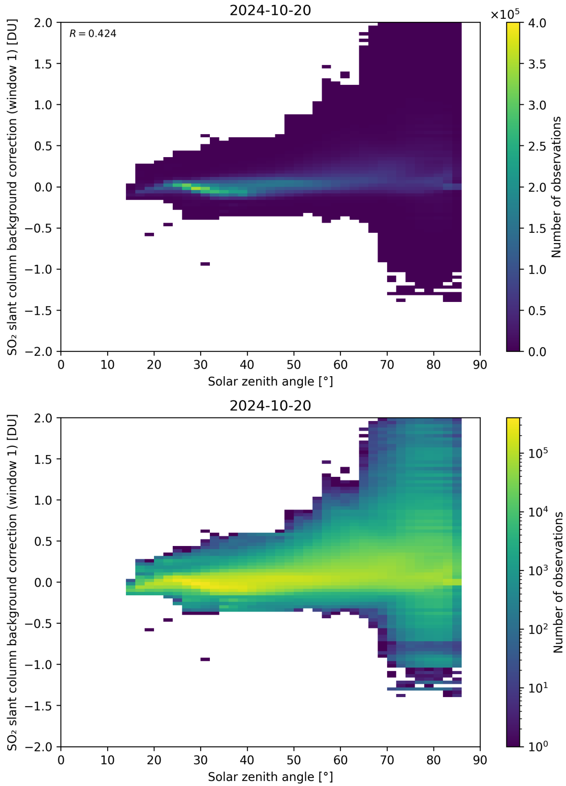
Figure 158: Scatter density plot of “Solar zenith angle” against “SO 2 slant column background correction (window 1)” for 2024-10-19 to 2024-10-21.
