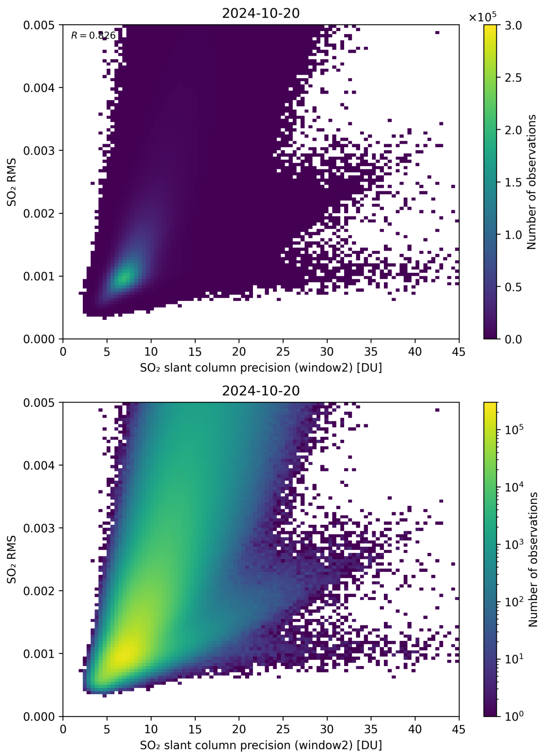
Figure 245: Scatter density plot of “SO 2 slant column precision (window2)” against “SO 2 RMS” for 2024-10-19 to 2024-10-21.
