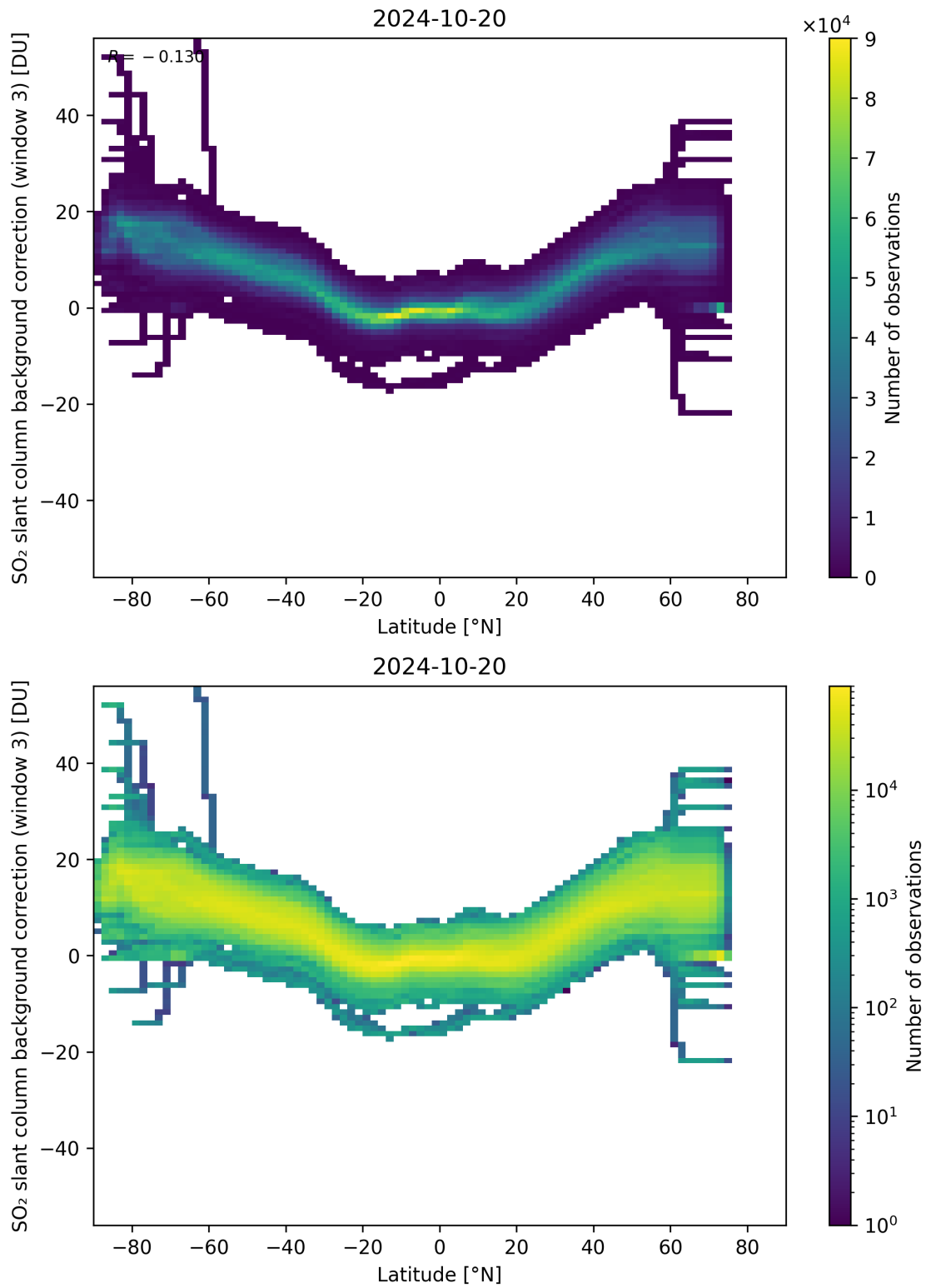
Figure 141: Scatter density plot of “Latitude” against “SO 2 slant column background correction (window 3)” for 2024-10-19 to 2024-10-21.
