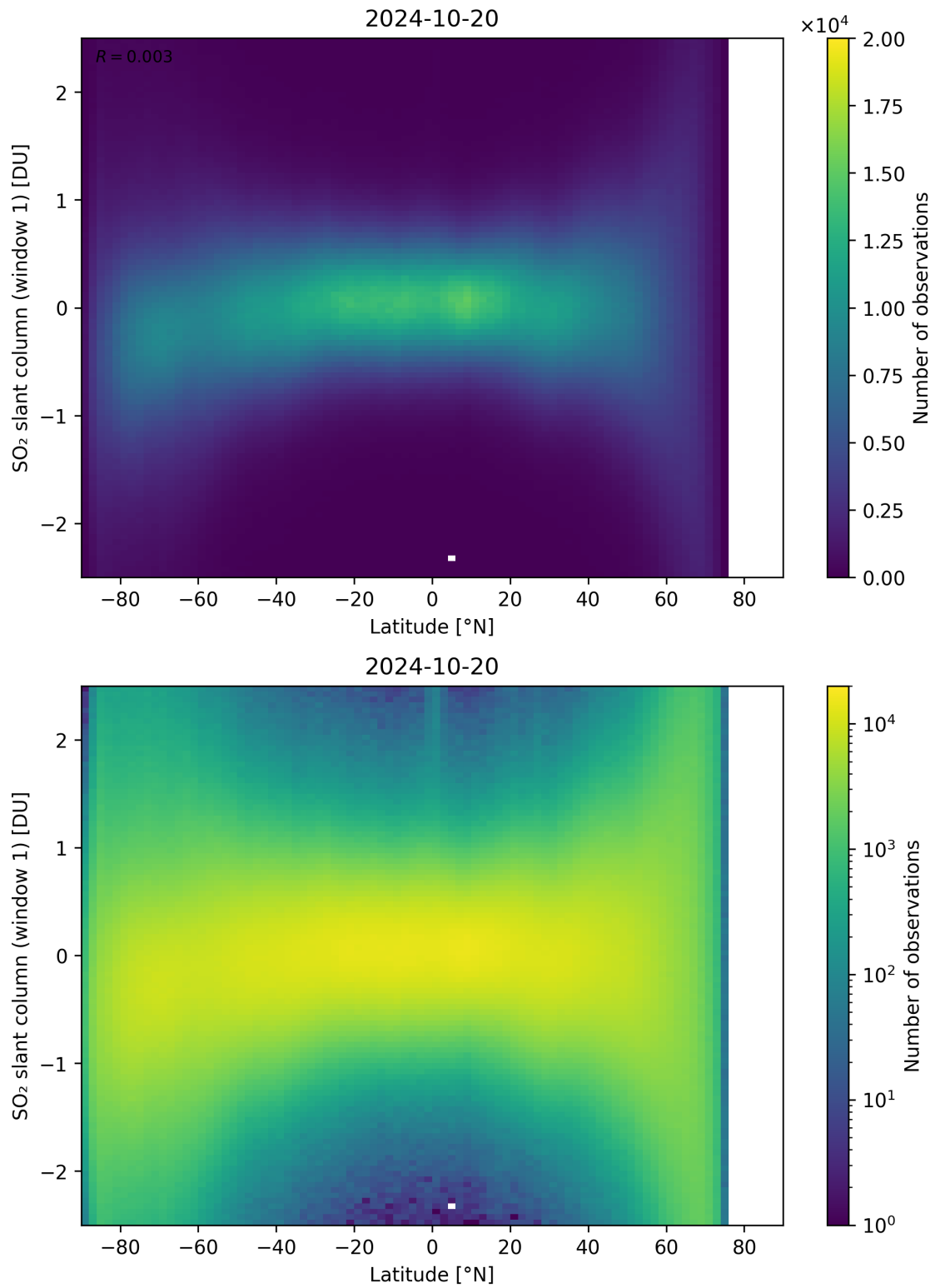
Figure 149: Scatter density plot of “Latitude” against “SO 2 slant column (window 1)” for 2024-10-19 to 2024-10-21.
