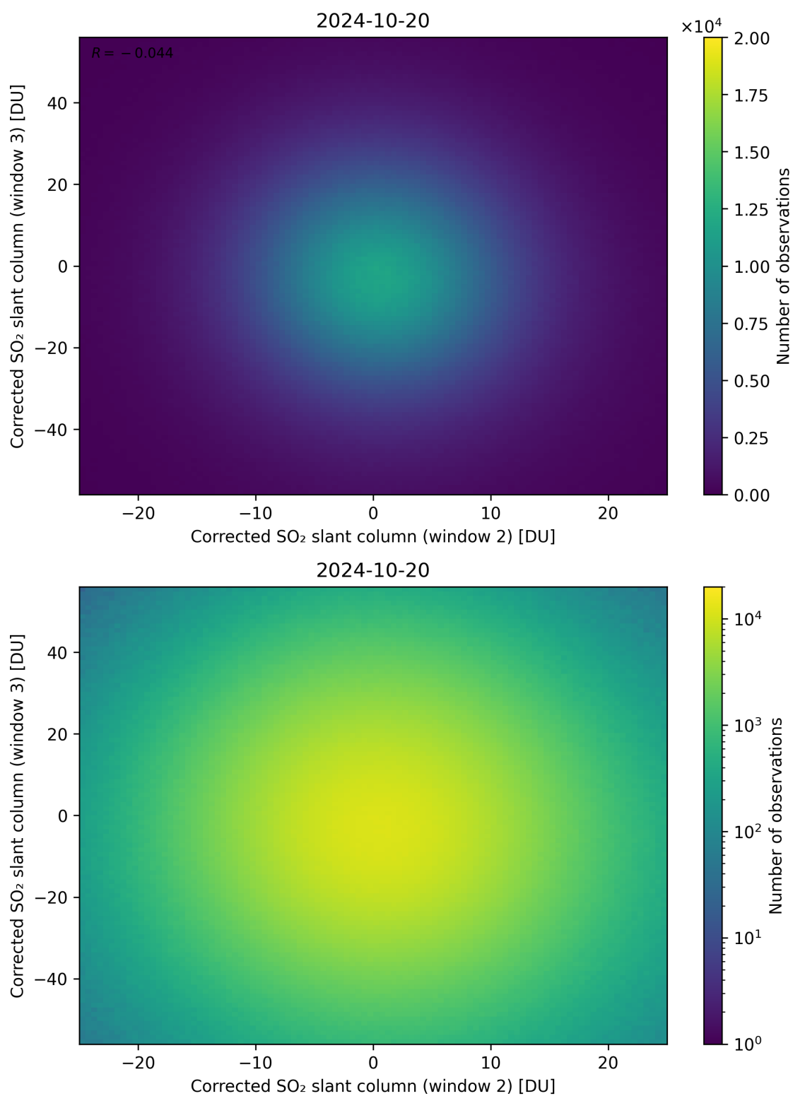
Figure 200: Scatter density plot of “Corrected SO 2 slant column (window 2)” against “Corrected SO 2 slant column (window 3)” for 2024-10-19 to 2024-10-21.
