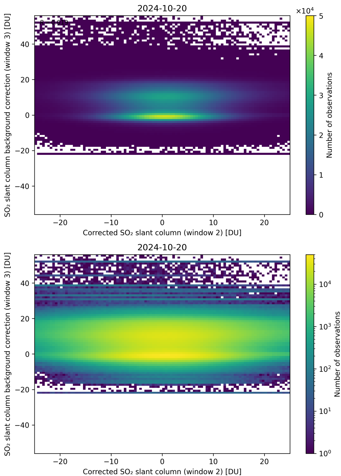
Figure 195: Scatter density plot of “Corrected SO 2 slant column (window 2)” against “SO 2 slant column background correction (window 3)” for 2024-10-19 to 2024-10-21.
