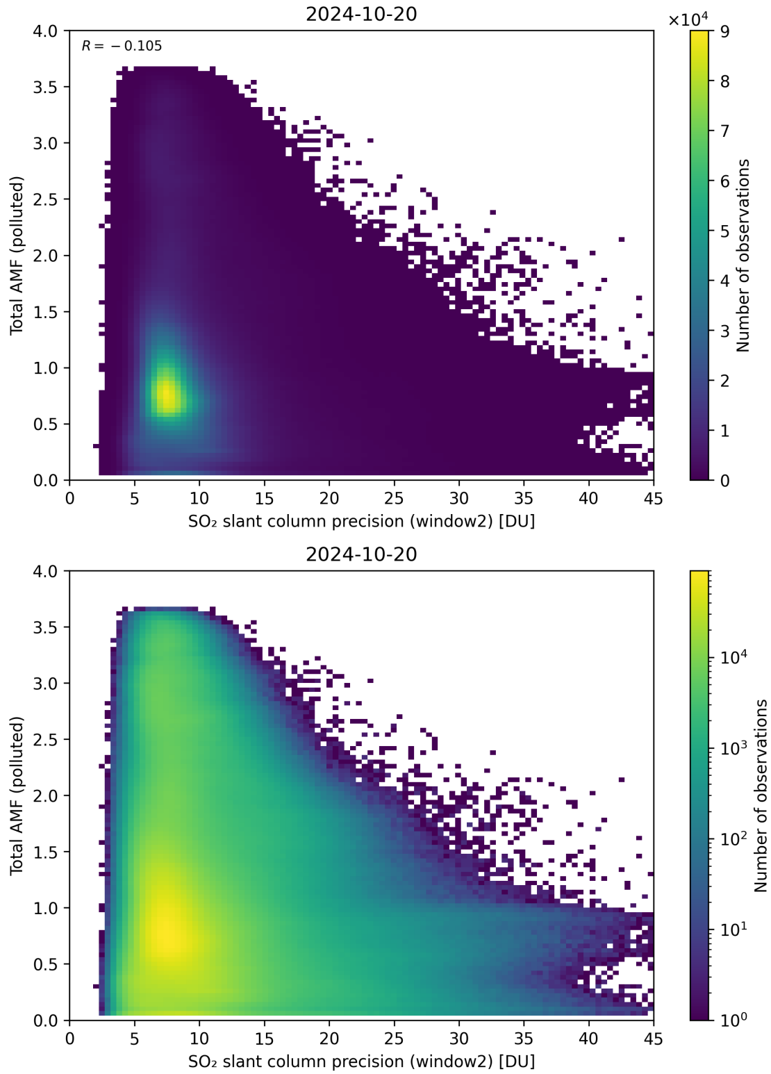
Figure 251: Scatter density plot of “SO 2 slant column precision (window2)” against “Total AMF (polluted)” for 2024-10-19 to 2024-10-21.
