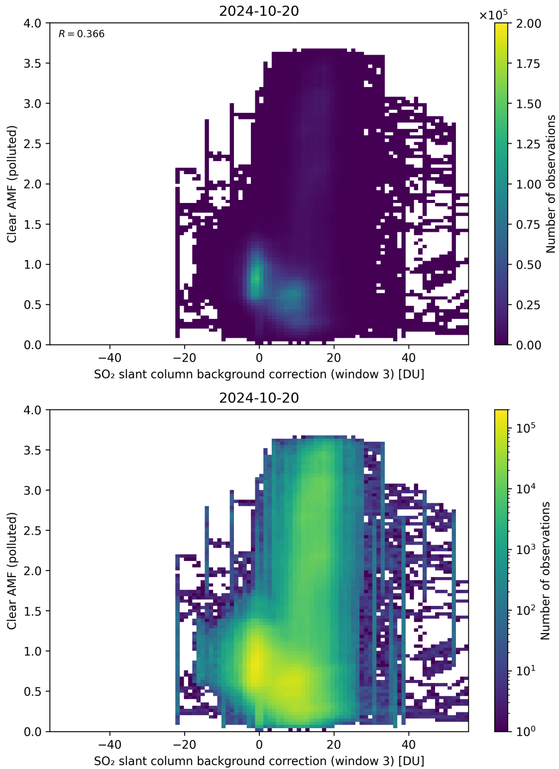
Figure 124: Scatter density plot of “SO 2 slant column background correction (window 3)” against “Clear AMF (polluted)” for 2024-10-19 to 2024-10-21.
