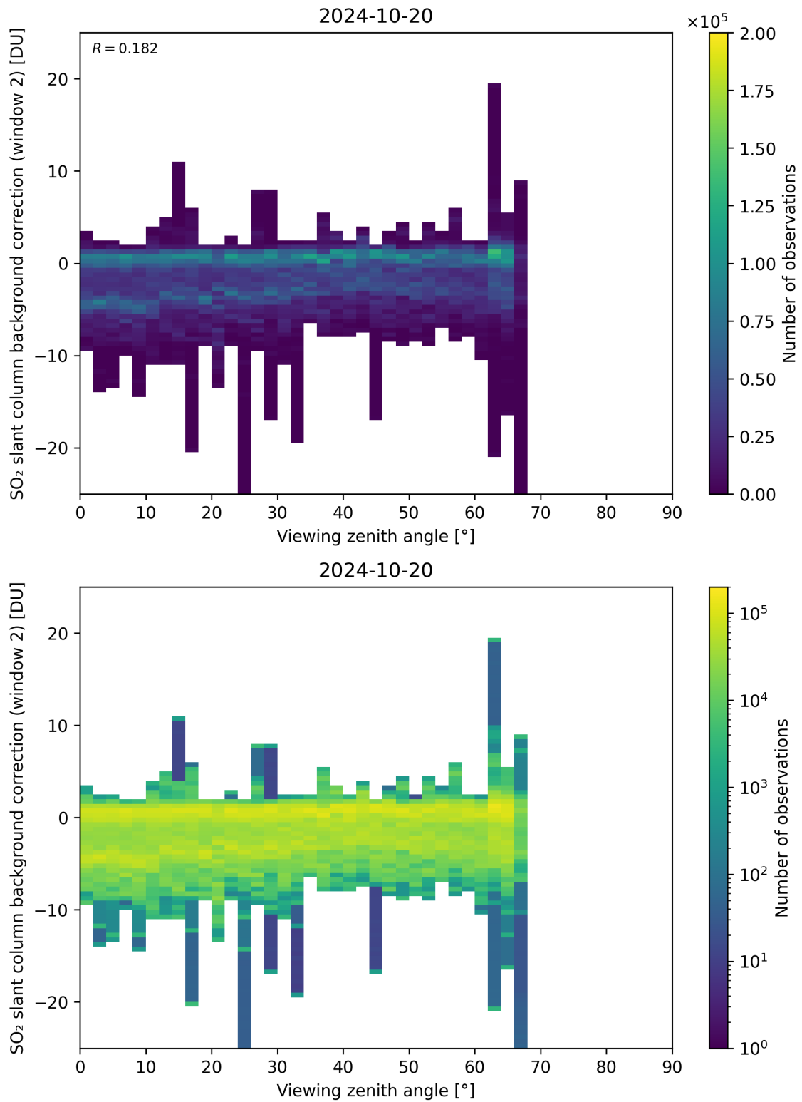
Figure 309: Scatter density plot of “Viewing zenith angle” against “SO 2 slant column background correction (window 2)” for 2024-10-19 to 2024-10-21.
