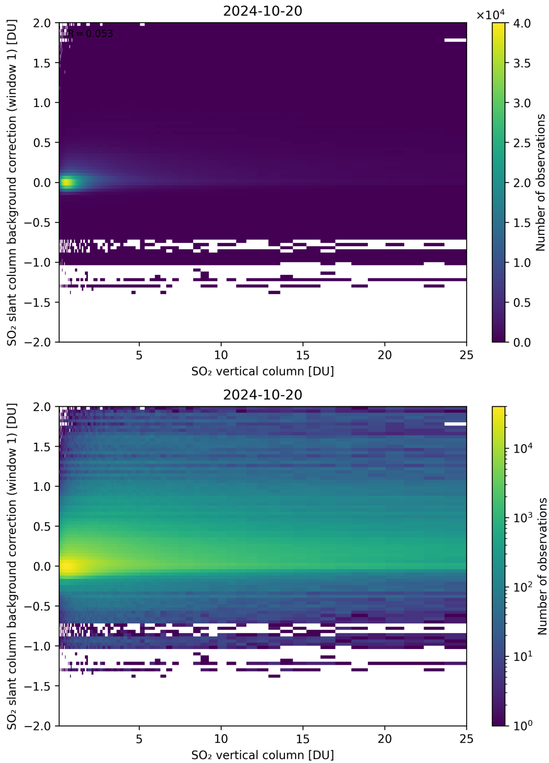
Figure 273: Scatter density plot of “SO 2 vertical column” against “SO 2 slant column background correction (window 1)” for 2024-10-19 to 2024-10-21.
