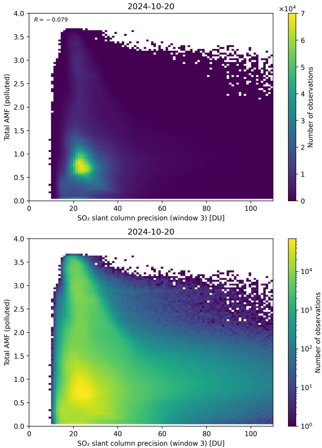
Figure 263: Scatter density plot of “SO 2 slant column precision (window 3)” against “Total AMF (polluted)” for 2024-10-19 to 2024-10-21.
