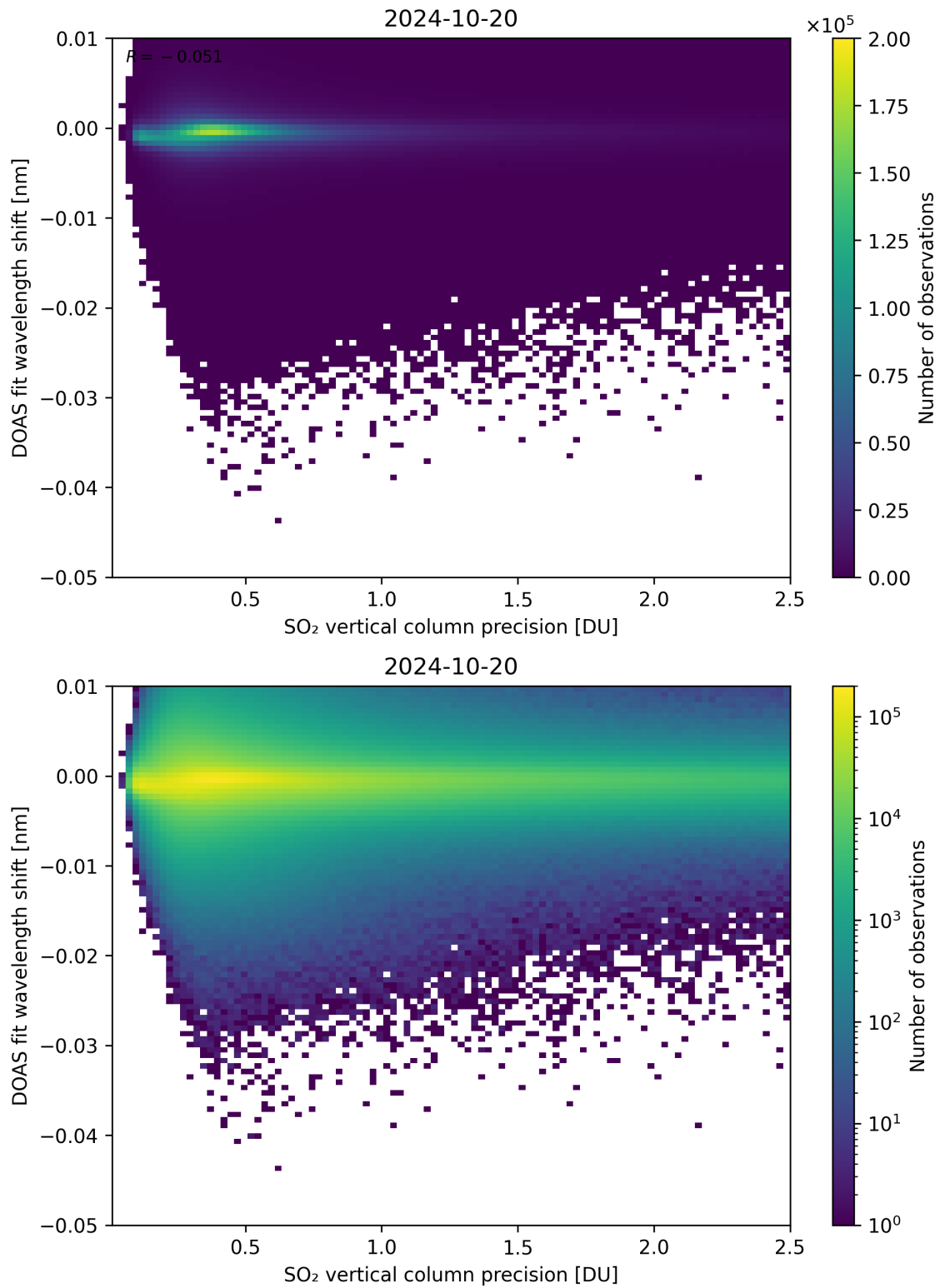
Figure 282: Scatter density plot of “SO 2 vertical column precision” against “DOAS fit wavelength shift” for 2024-10-19 to 2024-10-21.
