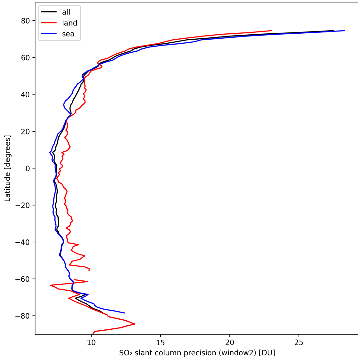
Figure 38: Zonal average of “SO 2 slant column precision (window2)” for 2024-10-19 to 2024-10-21.
