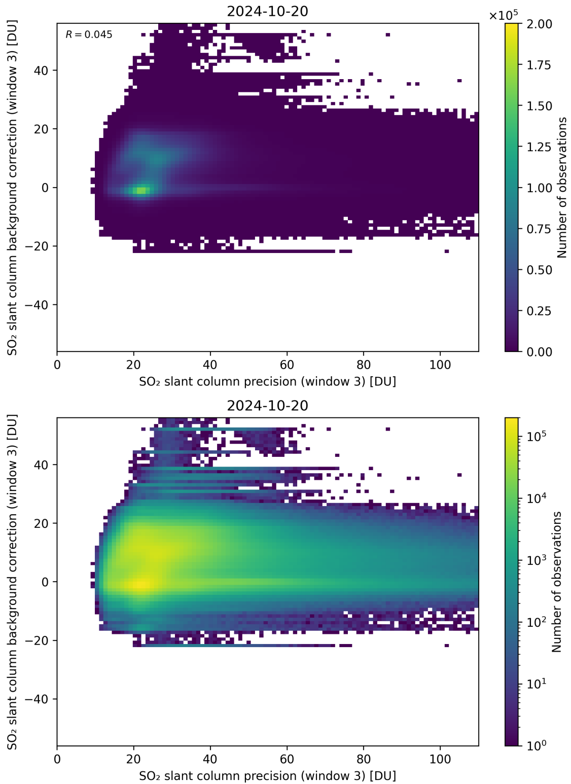
Figure 257: Scatter density plot of “SO 2 slant column precision (window 3)” against “SO 2 slant column background correction (window 3)” for 2024-10-19 to 2024-10-21.
