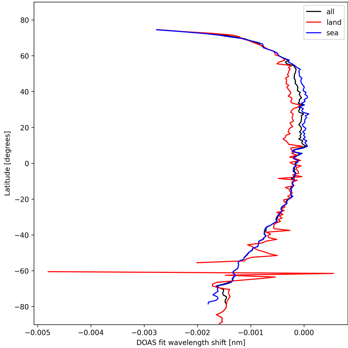
Figure 45: Zonal average of “DOAS fit wavelength shift” for 2024-10-19 to 2024-10-21.
