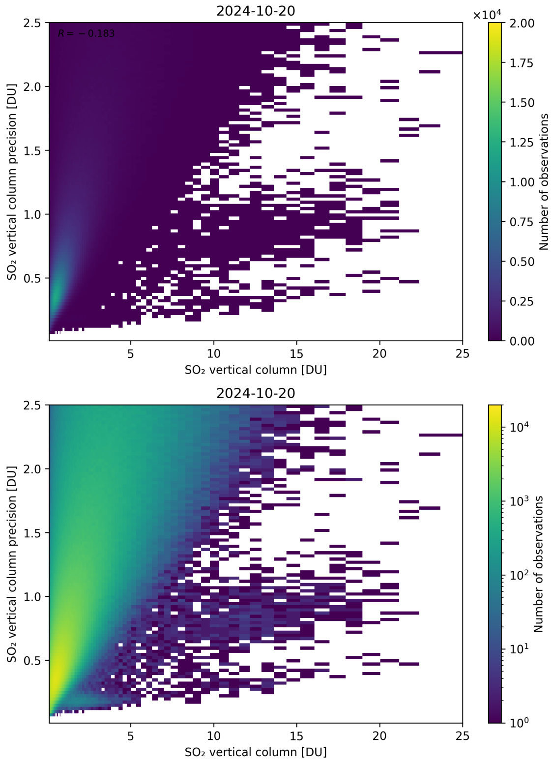
Figure 307: Scatter density plot of “SO 2 vertical column” against “SO 2 vertical column precision” for 2024-10-19 to 2024-10-21.
