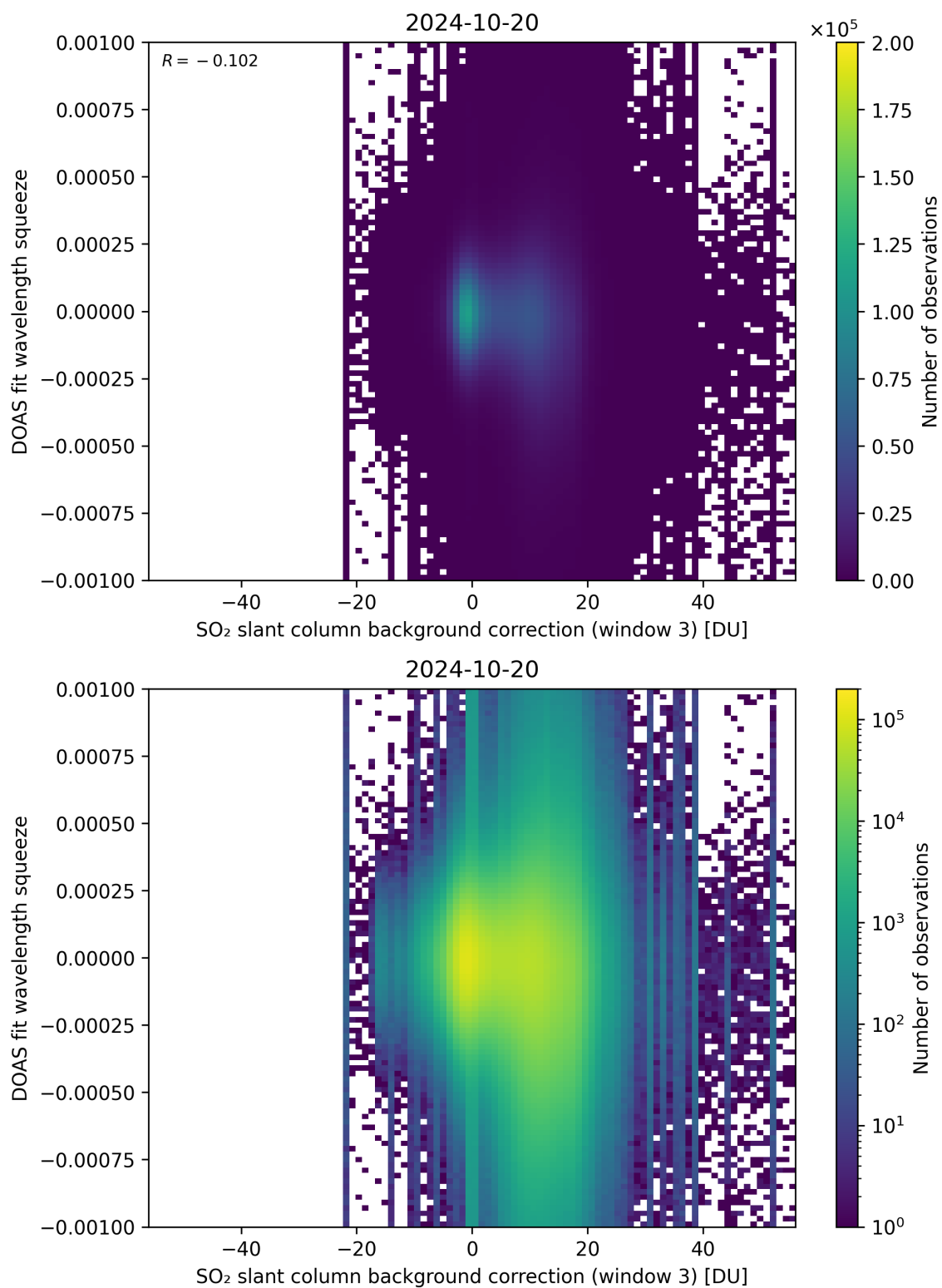
Figure 122: Scatter density plot of “SO 2 slant column background correction (window 3)” against “DOAS fit wavelength squeeze” for 2024-10-19 to 2024-10-21.
