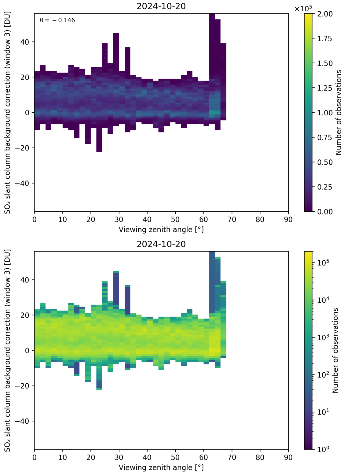
Figure 310: Scatter density plot of “Viewing zenith angle” against “SO 2 slant column background correction (window 3)” for 2024-10-19 to 2024-10-21.
