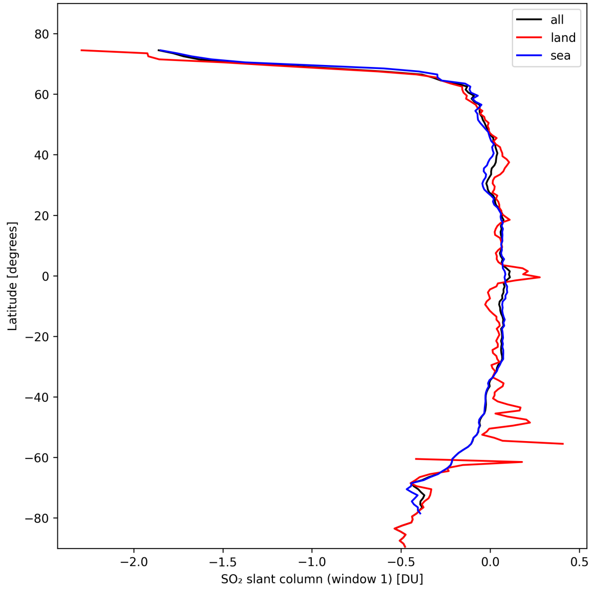
Figure 33: Zonal average of “SO 2 slant column (window 1)” for 2024-10-19 to 2024-10-21.
