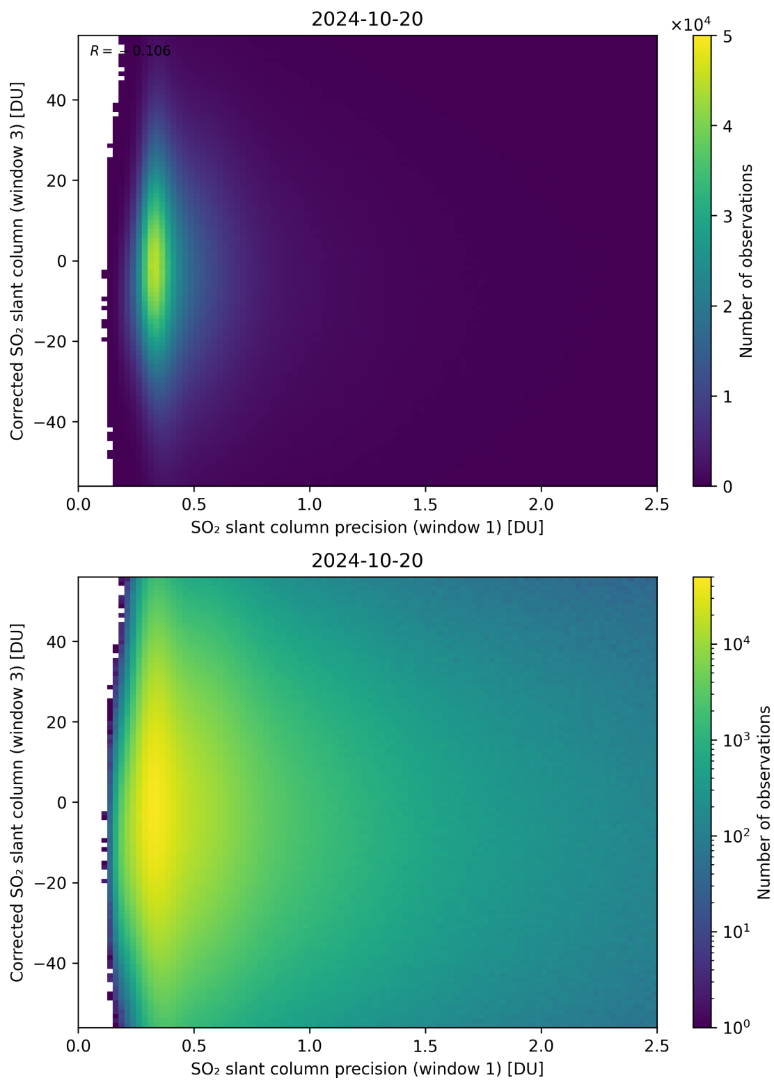
Figure 226: Scatter density plot of “SO 2 slant column precision (window 1)” against “Corrected SO 2 slant column (window 3)” for 2024-10-19 to 2024-10-21.
