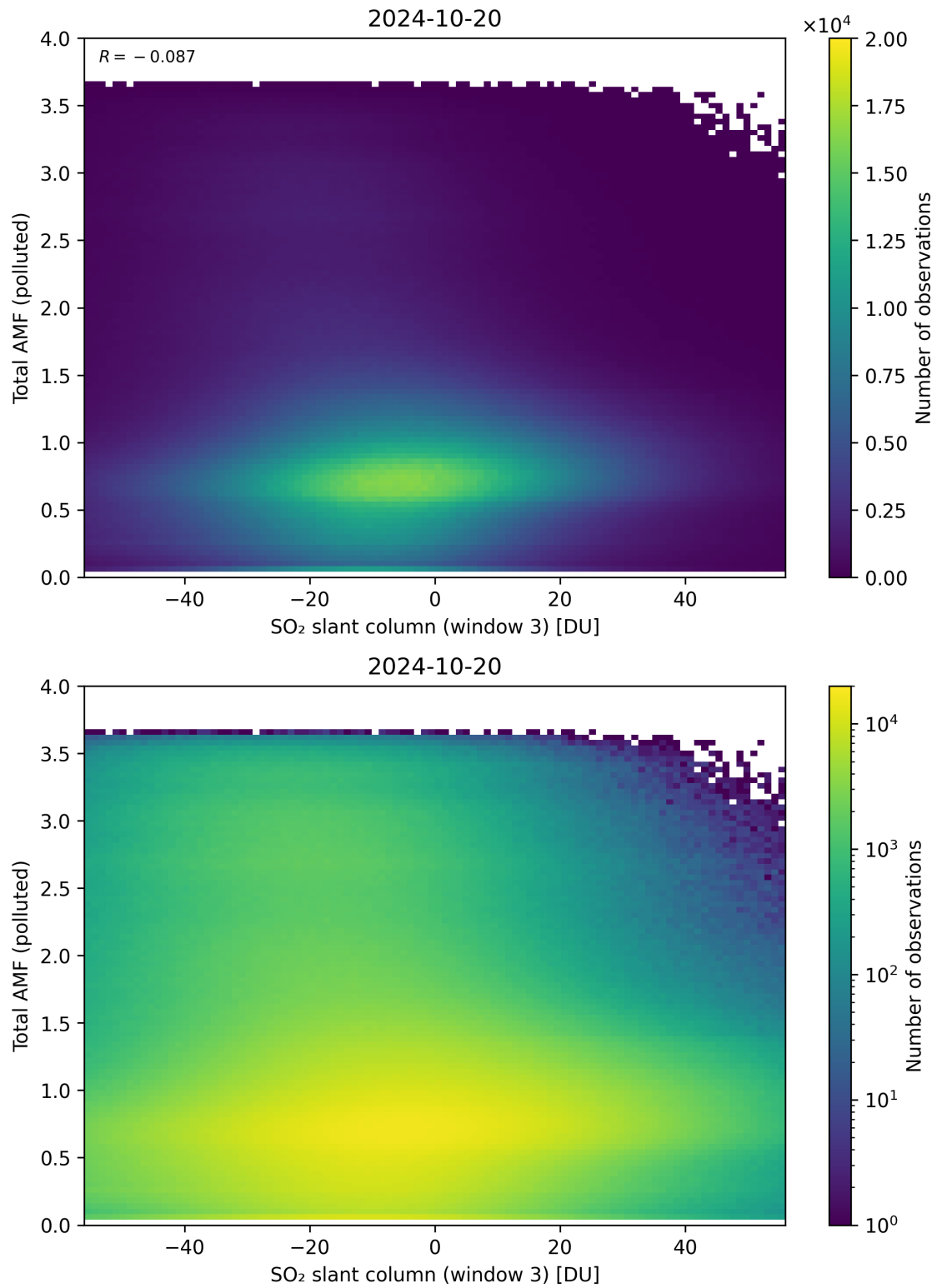
Figure 268: Scatter density plot of “SO 2 slant column (window 3)” against “Total AMF (polluted)” for 2024-10-19 to 2024-10-21.
