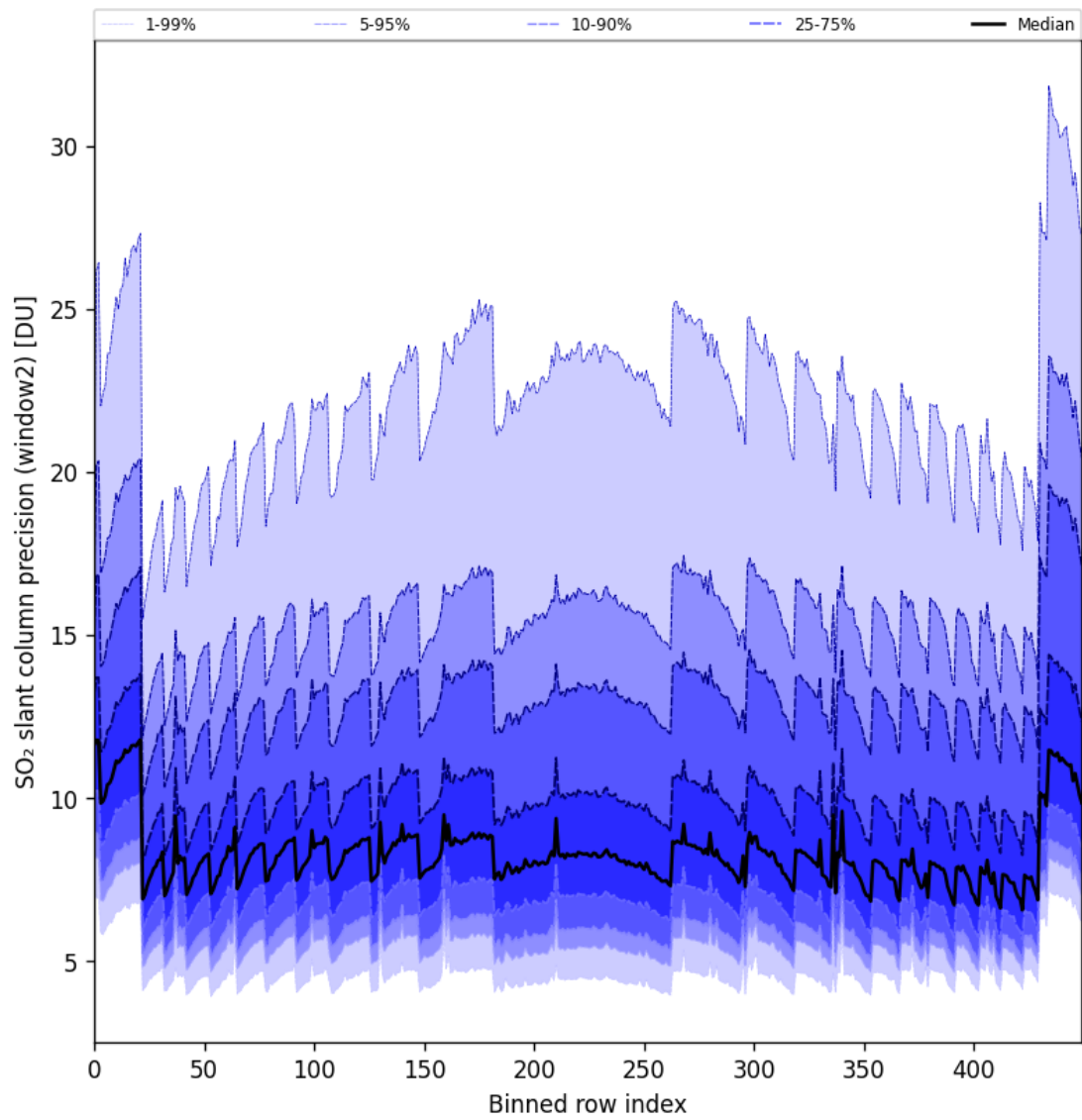
Figure 84: Along track statistics of “SO 2 slant column precision (window2)” for 2024-10-19 to 2024-10-21
