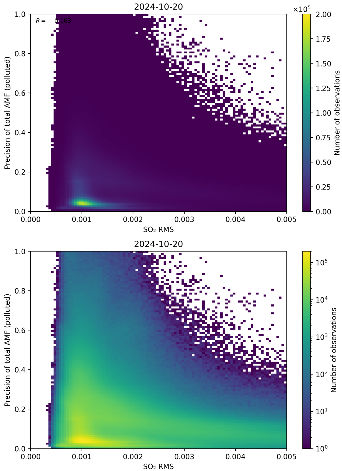
Figure 138: Scatter density plot of “SO 2 RMS” against “Precision of total AMF (polluted)” for 2024-10-19 to 2024-10-21.
