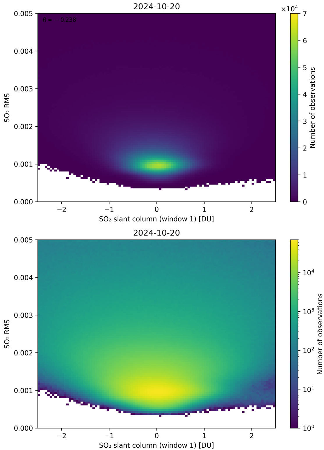
Figure 217: Scatter density plot of “SO 2 slant column (window 1)” against “SO 2 RMS” for 2024-10-19 to 2024-10-21.
