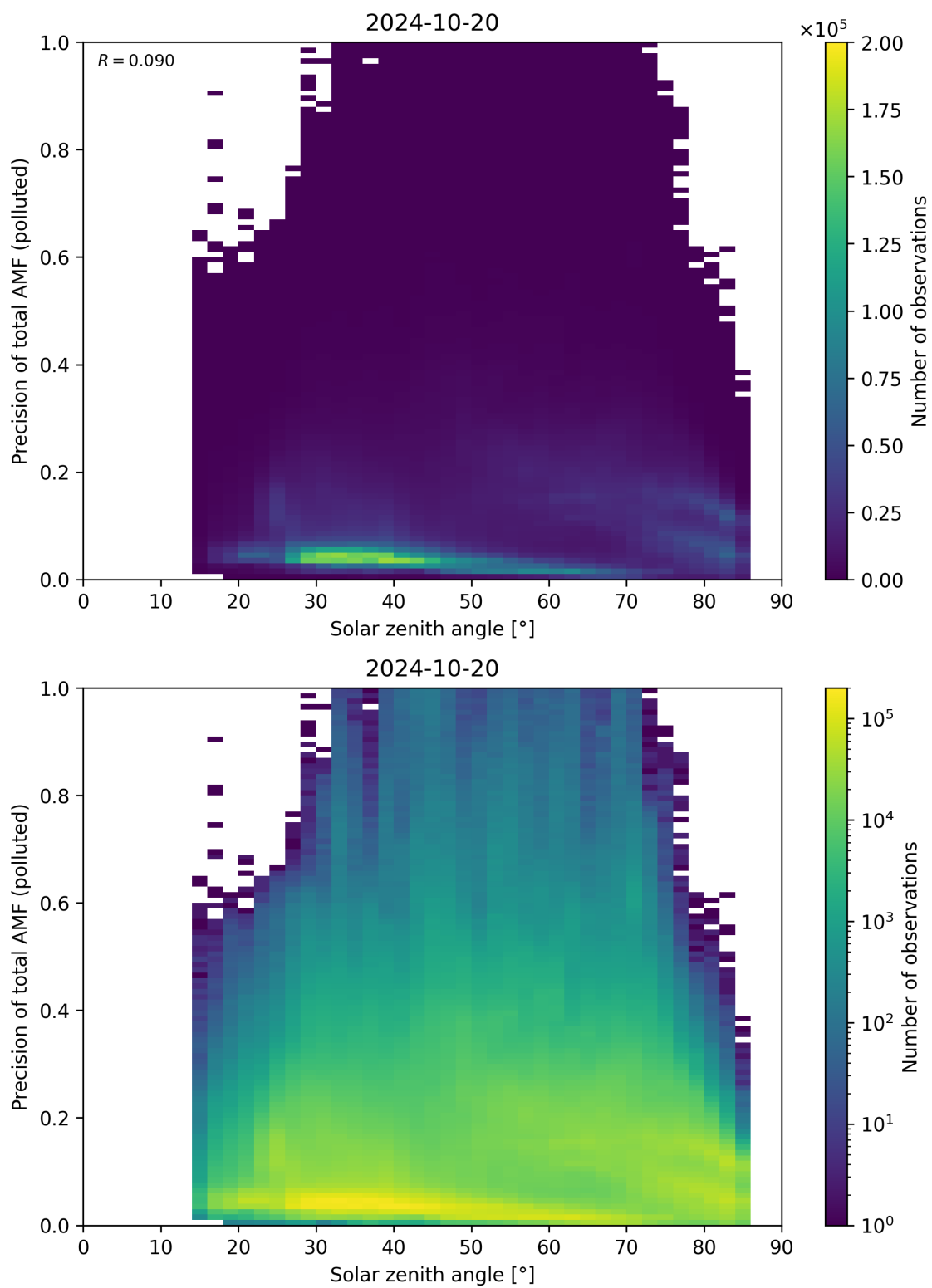
Figure 175: Scatter density plot of “Solar zenith angle” against “Precision of total AMF (polluted)” for 2024-10-19 to 2024-10-21.
