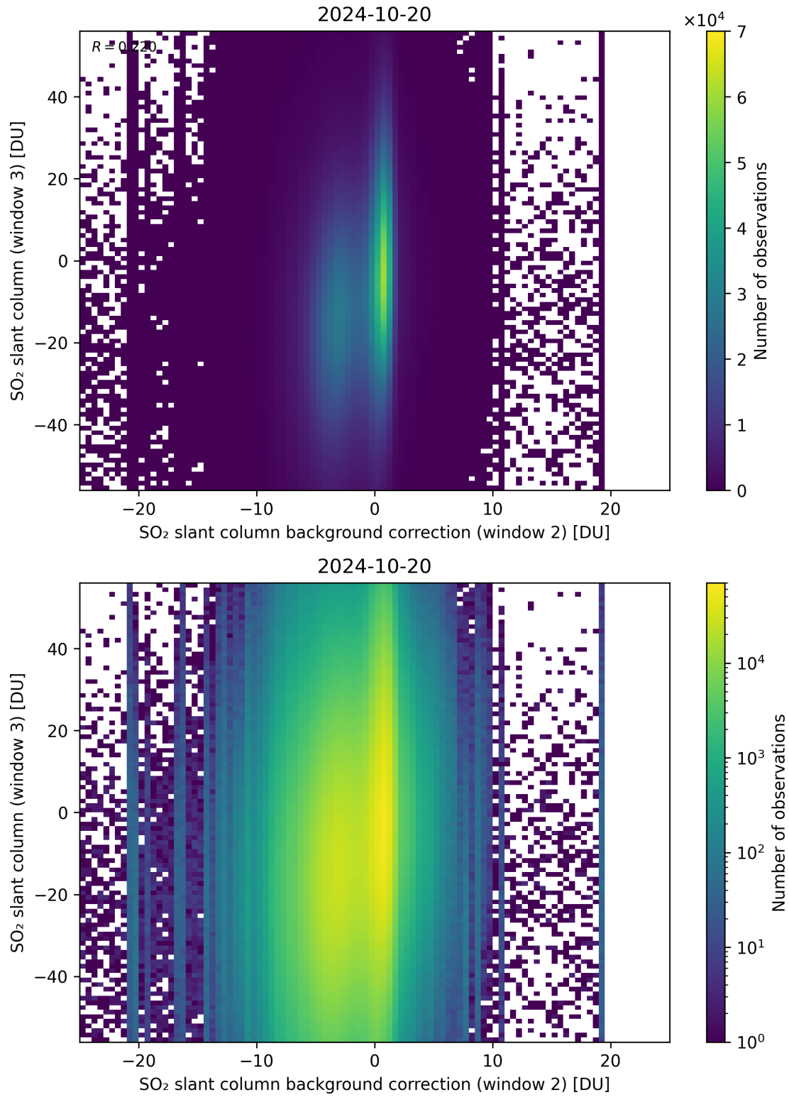
Figure 117: Scatter density plot of “SO 2 slant column background correction (window 2)” against “SO 2 slant column (window 3)” for 2024-10-19 to 2024-10-21.
