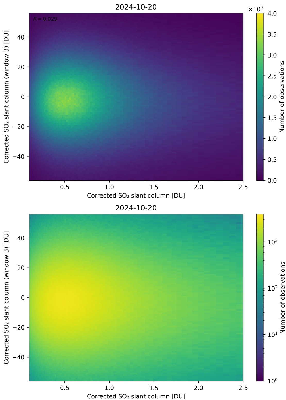
Figure 186: Scatter density plot of “Corrected SO 2 slant column” against “Corrected SO 2 slant column (window 3)” for 2024-10-19 to 2024-10-21.
