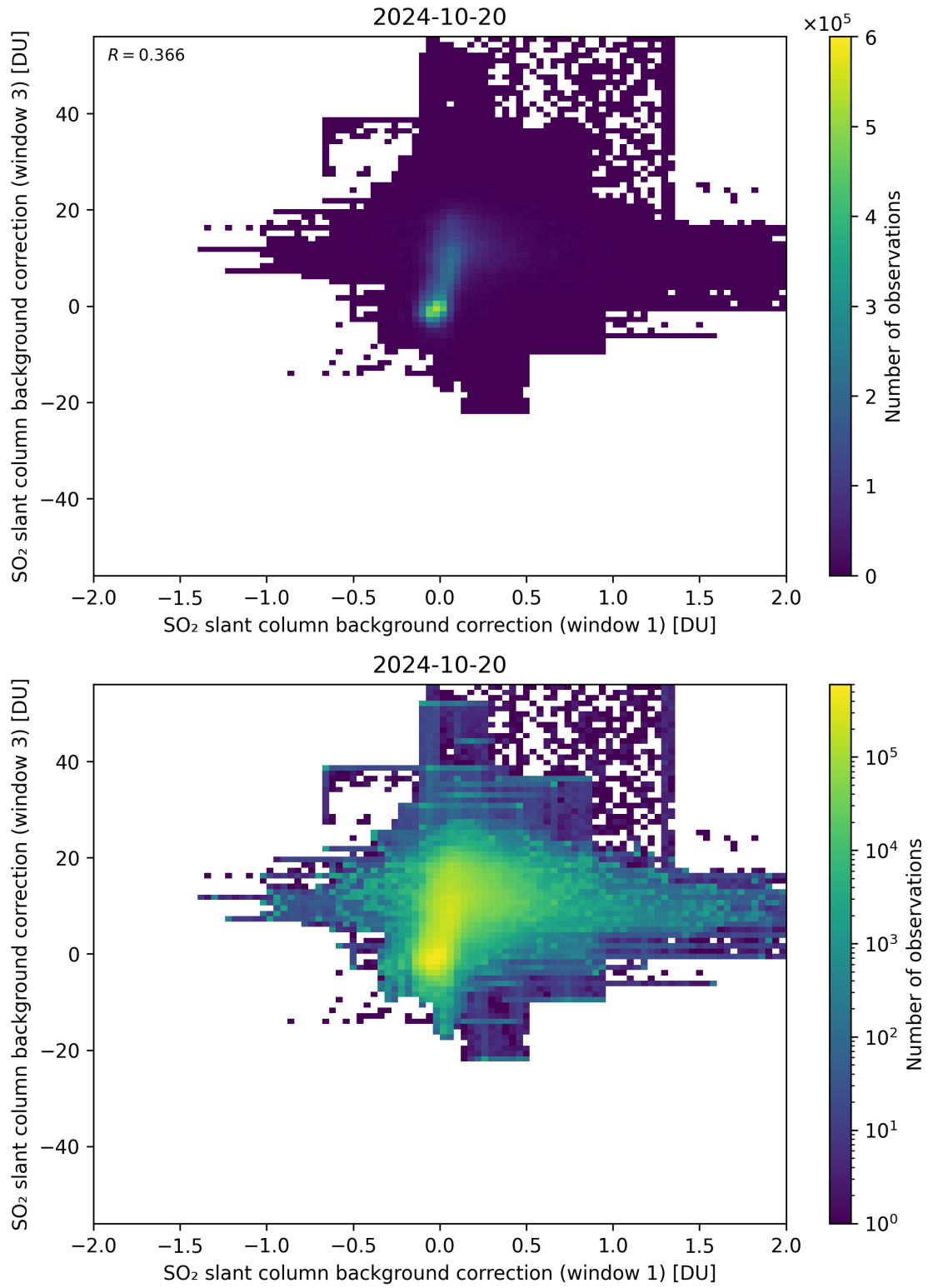
Figure 99: Scatter density plot of “SO 2 slant column background correction (window 1)” against “SO 2 slant column background correction (window 3)” for 2024-10-19 to 2024-10-21.
