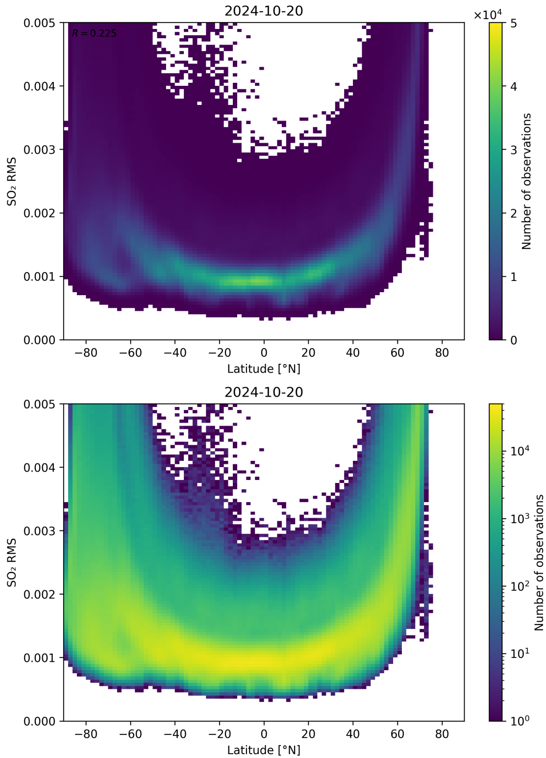
Figure 144: Scatter density plot of “Latitude” against “SO 2 RMS” for 2024-10-19 to 2024-10-21.
