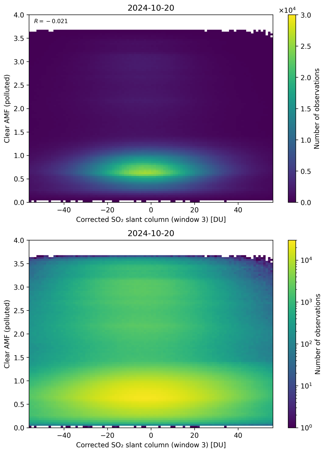
Figure 209: Scatter density plot of “Corrected SO 2 slant column (window 3)” against “Clear AMF (polluted)” for 2024-10-19 to 2024-10-21.
