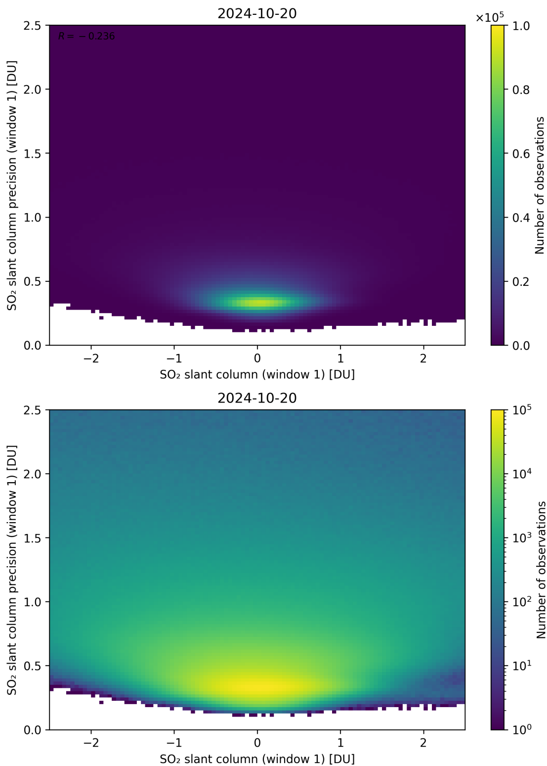
Figure 235: Scatter density plot of “SO 2 slant column (window 1)” against “SO 2 slant column precision (window 1)” for 2024-10-19 to 2024-10-21.
