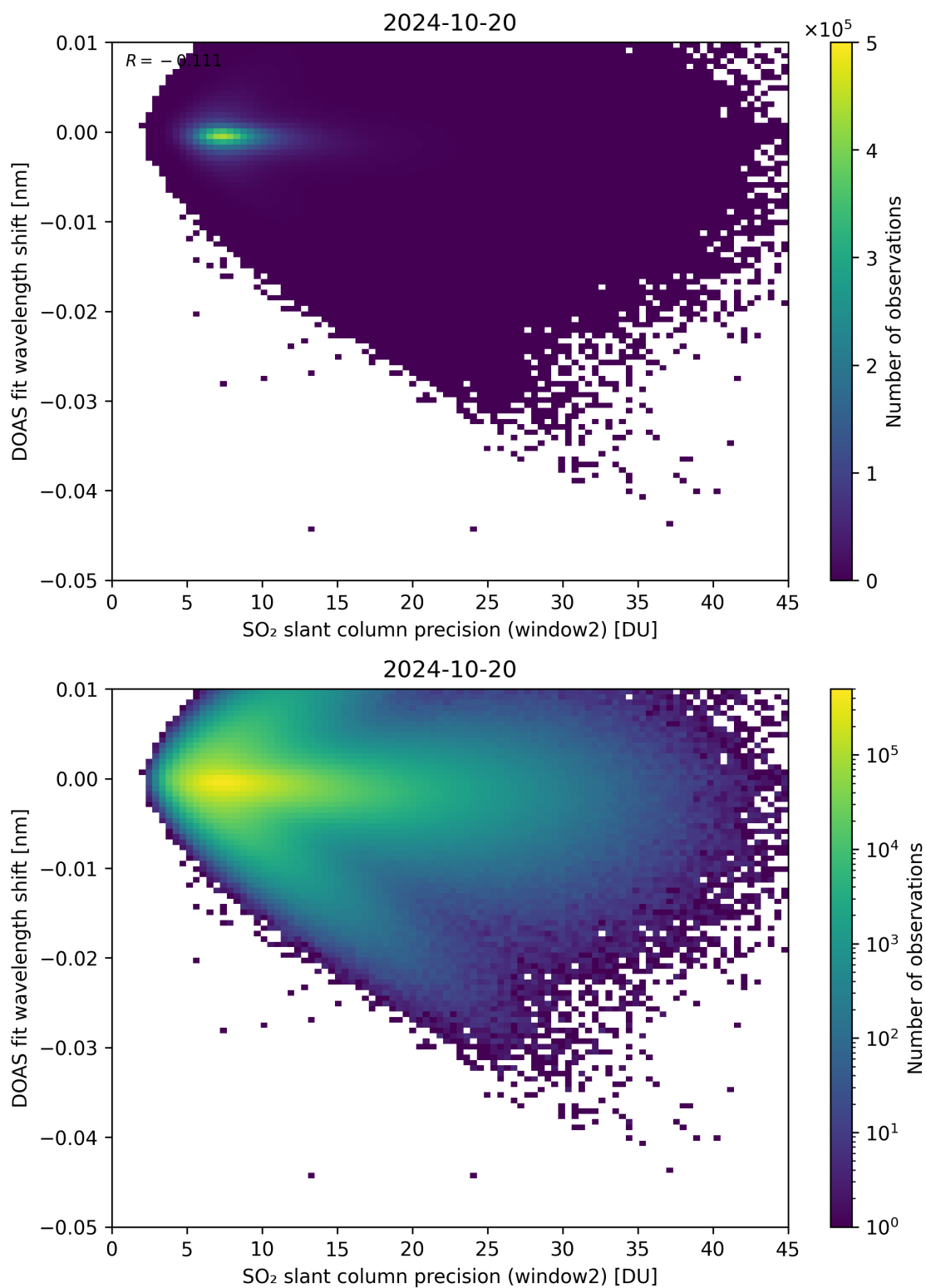
Figure 243: Scatter density plot of “SO 2 slant column precision (window2)” against “DOAS fit wavelength shift” for 2024-10-19 to 2024-10-21.
