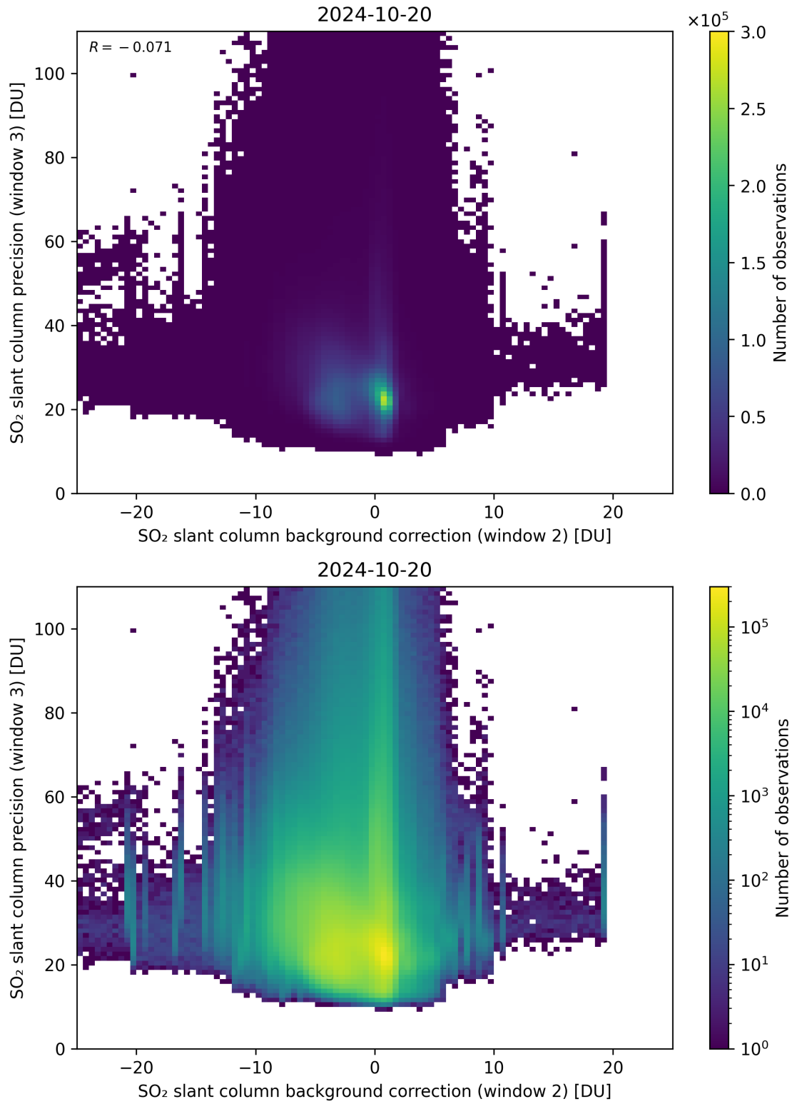
Figure 118: Scatter density plot of “SO 2 slant column background correction (window 2)” against “SO 2 slant column precision (window 3)” for 2024-10-19 to 2024-10-21.
