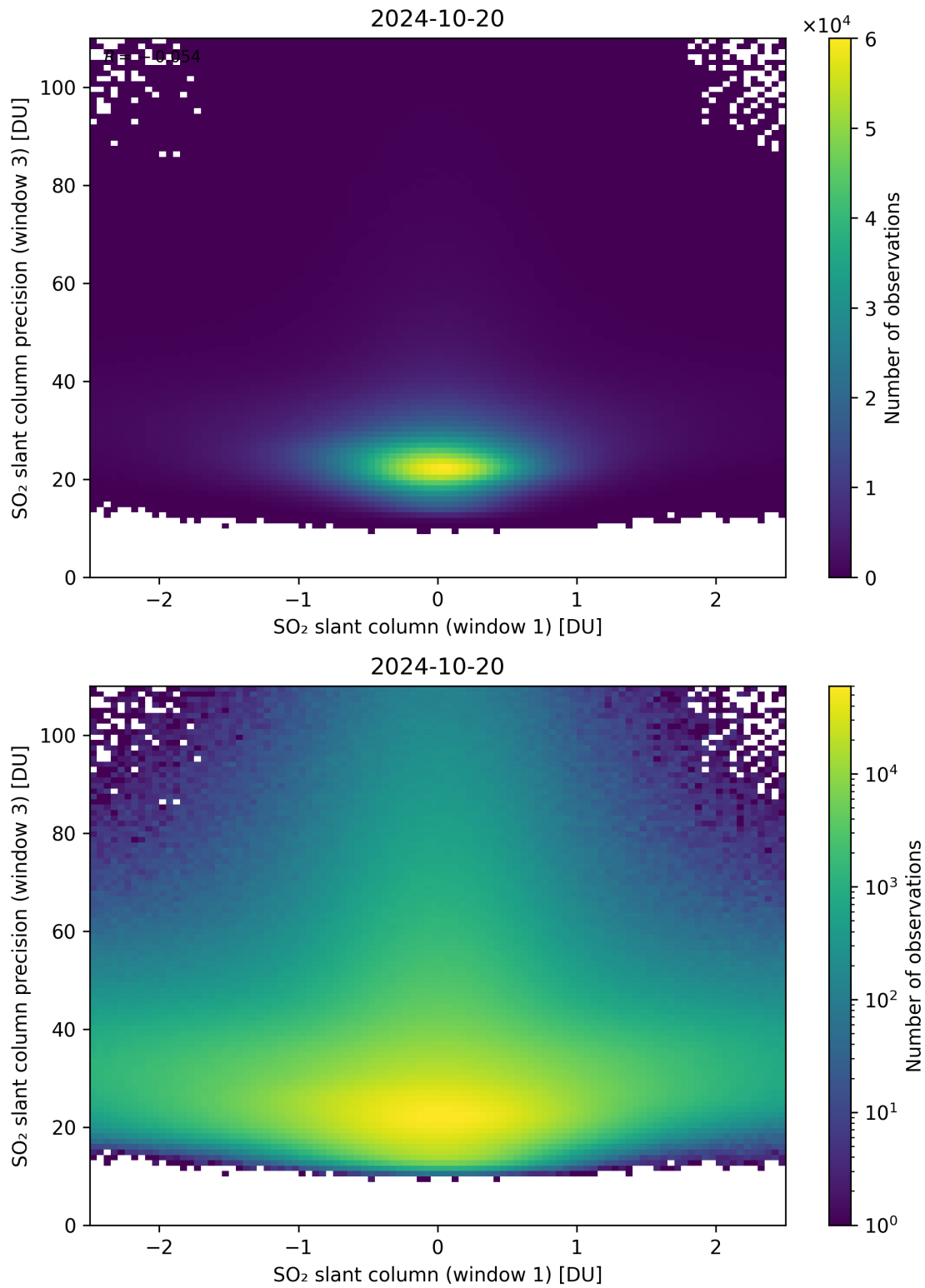
Figure 238: Scatter density plot of “SO 2 slant column (window 1)” against “SO 2 slant column precision (window 3)” for 2024-10-19 to 2024-10-21.
