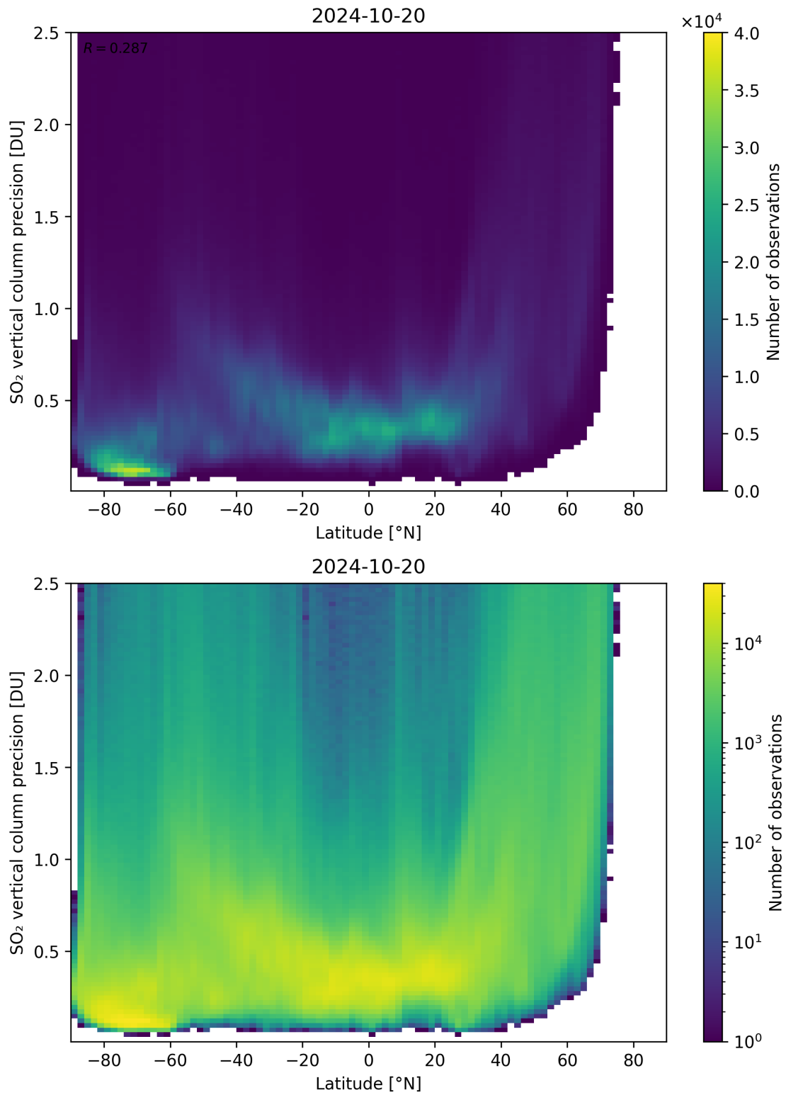
Figure 157: Scatter density plot of “Latitude” against “SO 2 vertical column precision” for 2024-10-19 to 2024-10-21.
