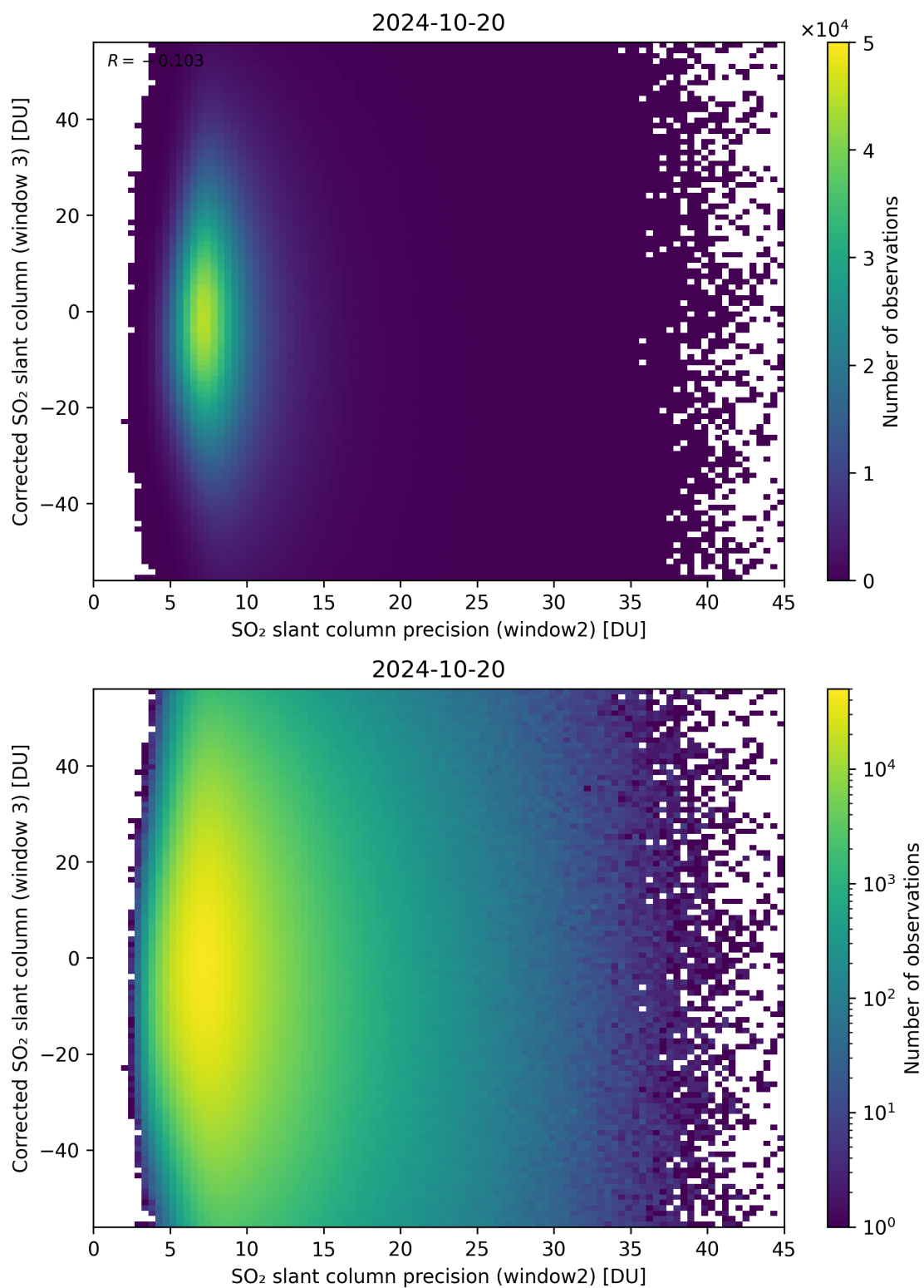
Figure 248: Scatter density plot of “SO 2 slant column precision (window2)” against “Corrected SO 2 slant column (window 3)” for 2024-10-19 to 2024-10-21.
