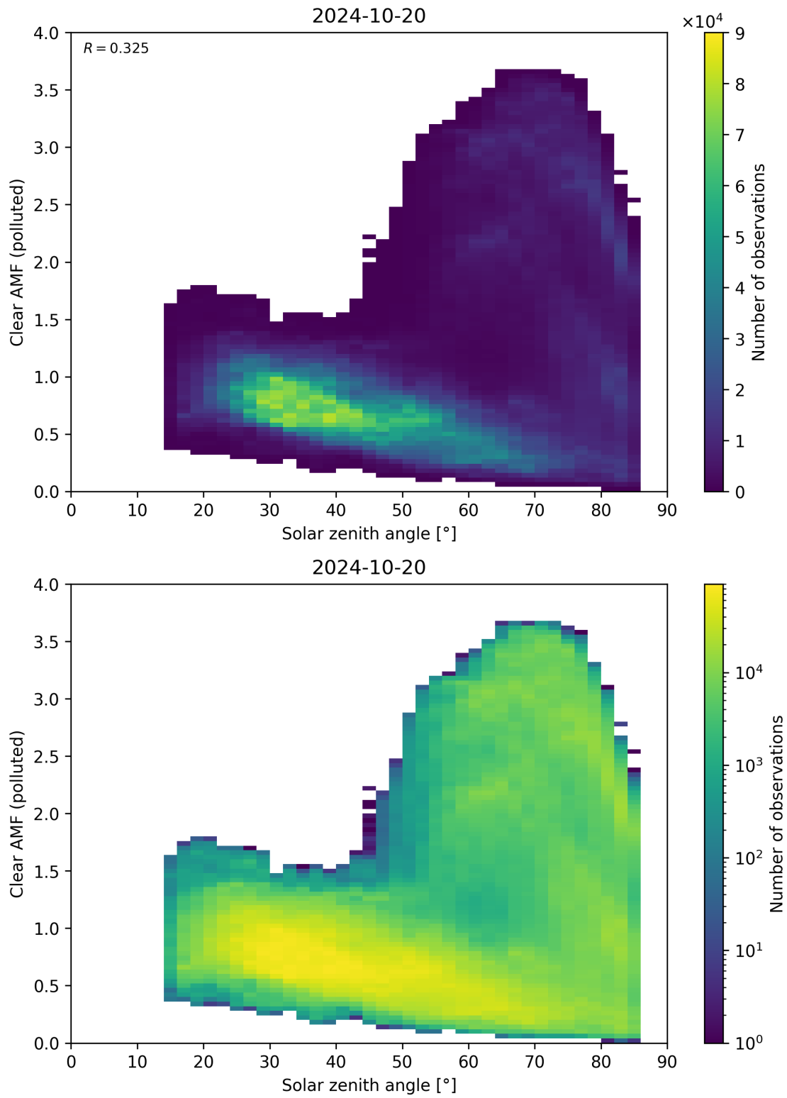
Figure 165: Scatter density plot of “Solar zenith angle” against “Clear AMF (polluted)” for 2024-10-19 to 2024-10-21.
