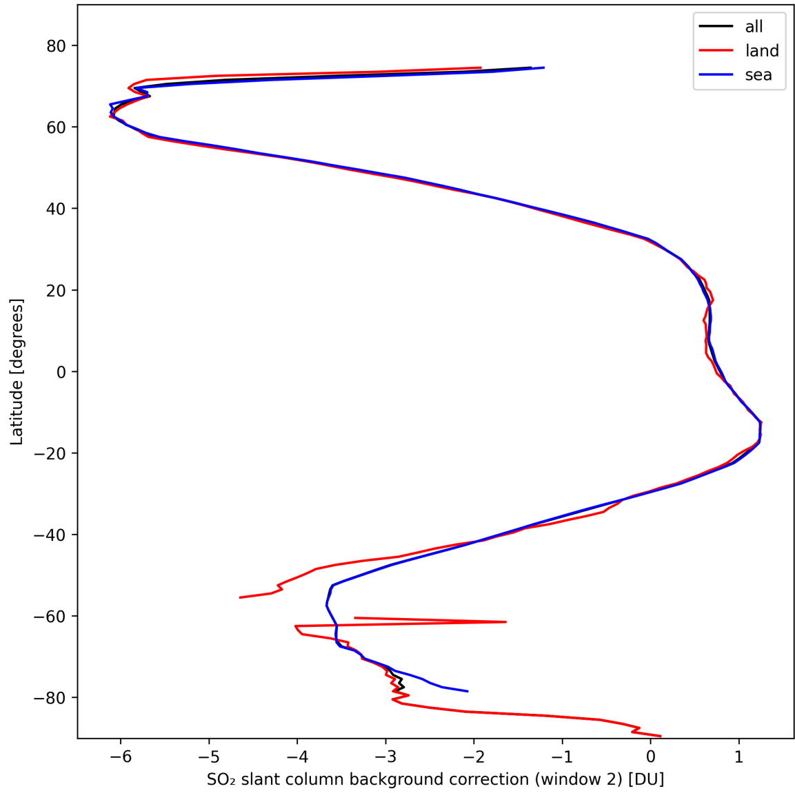
Figure 40: Zonal average of “SO 2 slant column background correction (window 2)” for 2024-10-19 to 2024-10-21.
