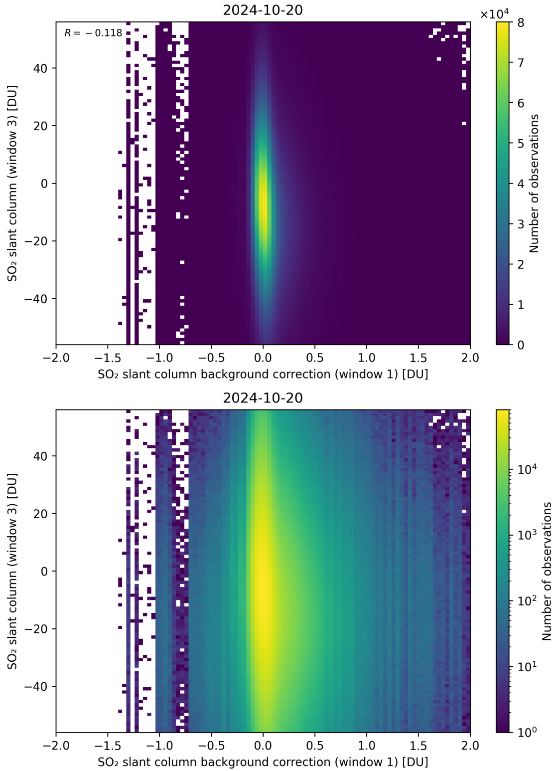
Figure 107: Scatter density plot of “SO 2 slant column background correction (window 1)” against “SO 2 slant column (window 3)” for 2024-10-19 to 2024-10-21.
