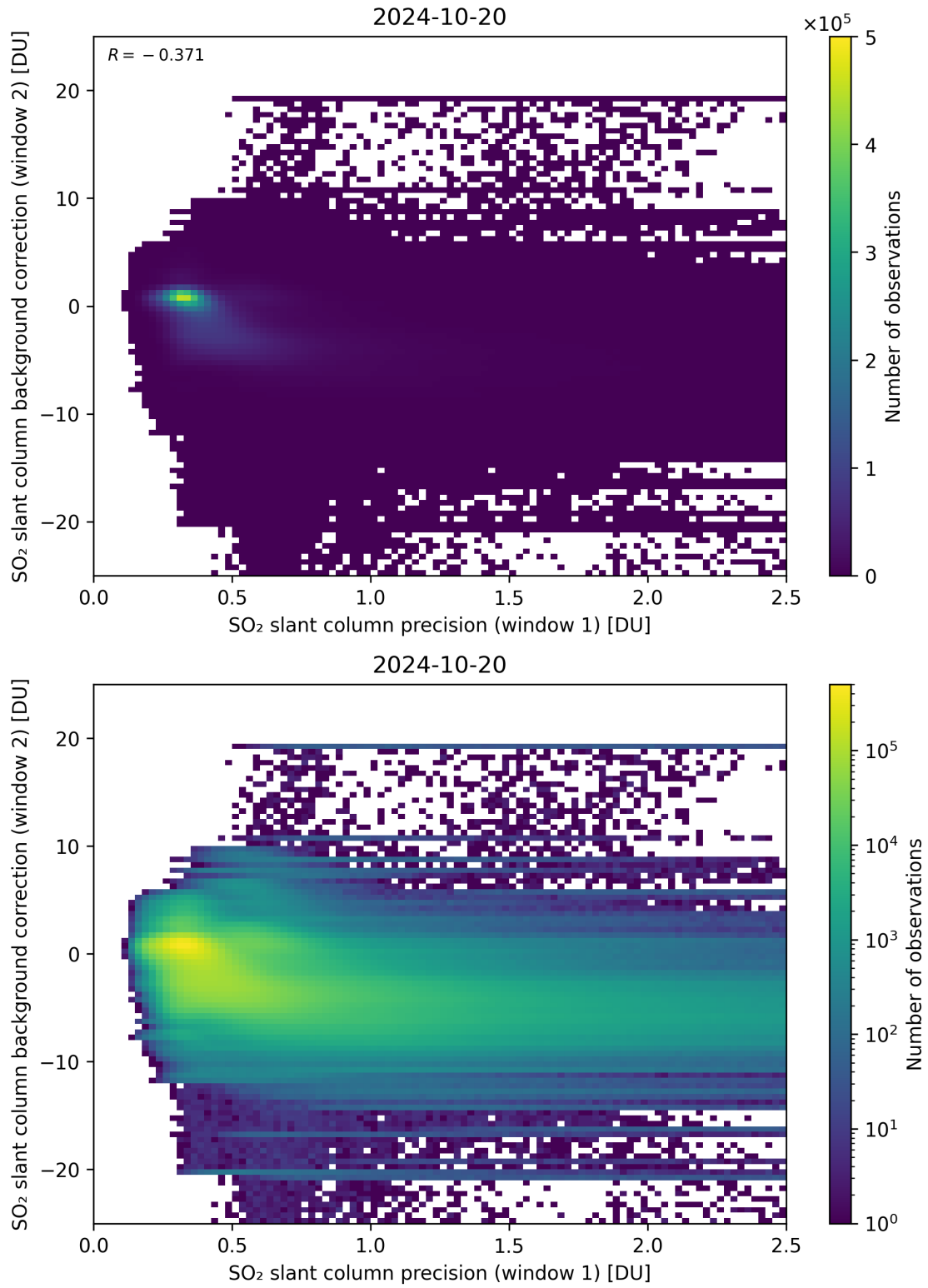
Figure 219: Scatter density plot of “SO 2 slant column precision (window 1)” against “SO 2 slant column background correction (window 2)” for 2024-10-19 to 2024-10-21.
