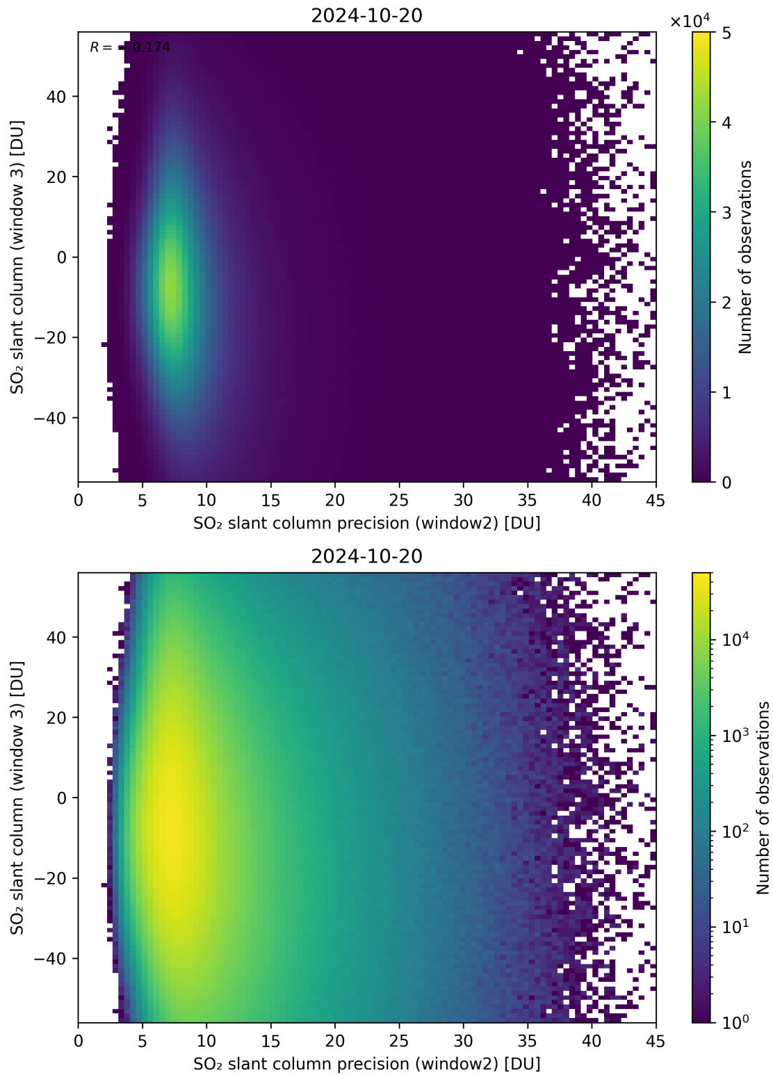
Figure 249: Scatter density plot of “SO 2 slant column precision (window2)” against “SO 2 slant column (window 3)” for 2024-10-19 to 2024-10-21.
