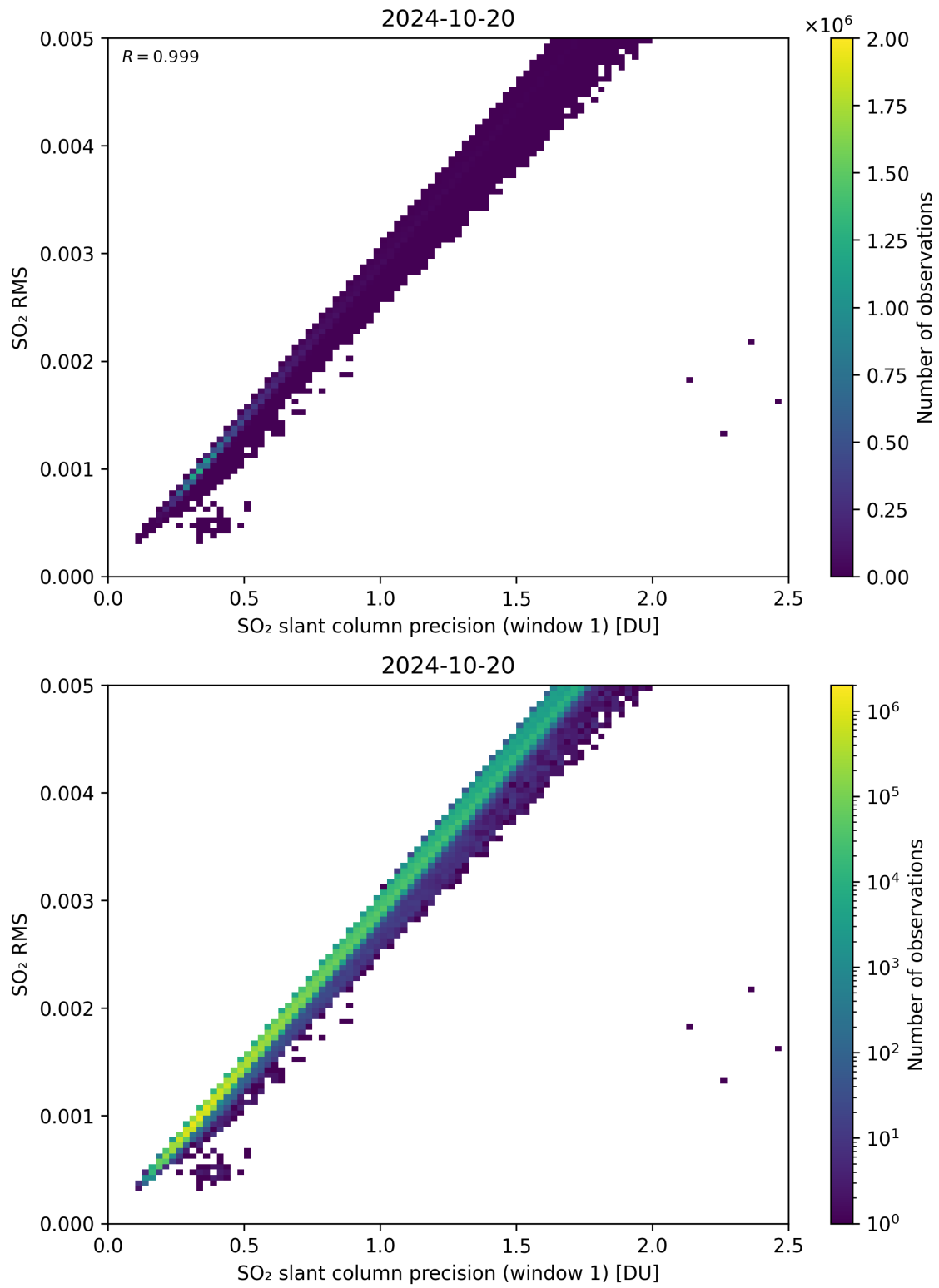
Figure 223: Scatter density plot of “SO 2 slant column precision (window 1)” against “SO 2 RMS” for 2024-10-19 to 2024-10-21.
