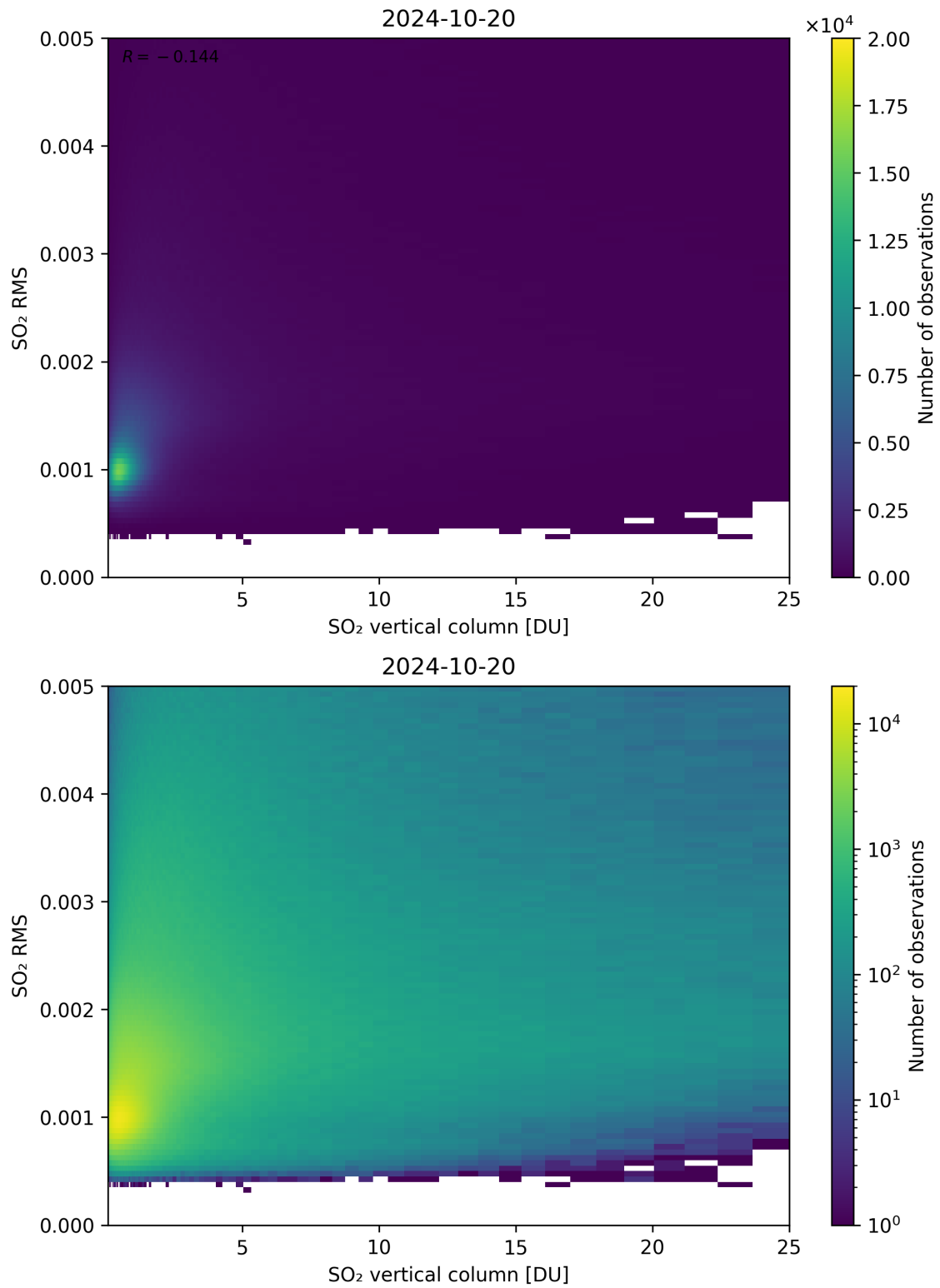
Figure 278: Scatter density plot of “SO 2 vertical column” against “SO 2 RMS” for 2024-10-19 to 2024-10-21.
