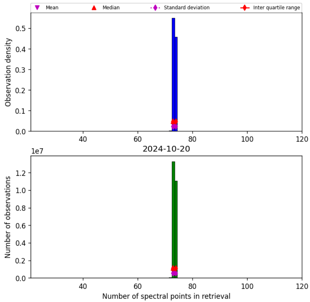
Figure 74: Histogram of “Number of spectral points in retrieval” for 2024-10-19 to 2024-10-21
