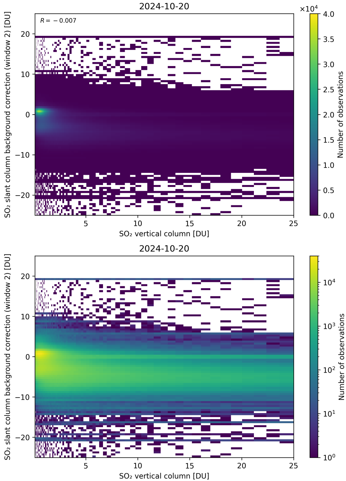
Figure 274: Scatter density plot of “SO 2 vertical column” against “SO 2 slant column background correction (window 2)” for 2024-10-19 to 2024-10-21.
