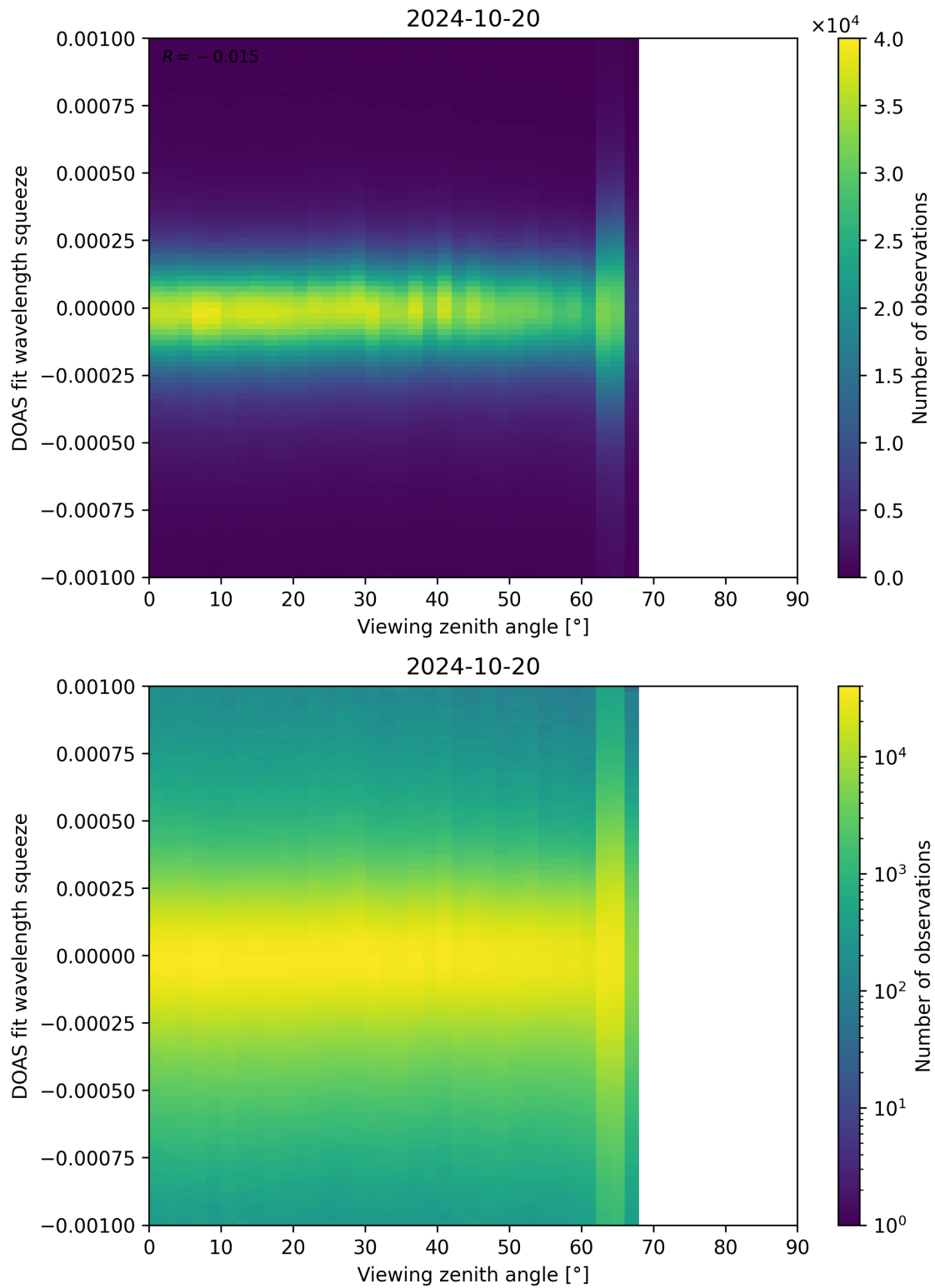
Figure 312: Scatter density plot of “Viewing zenith angle” against “DOAS fit wavelength squeeze” for 2024-10-19 to 2024-10-21.
