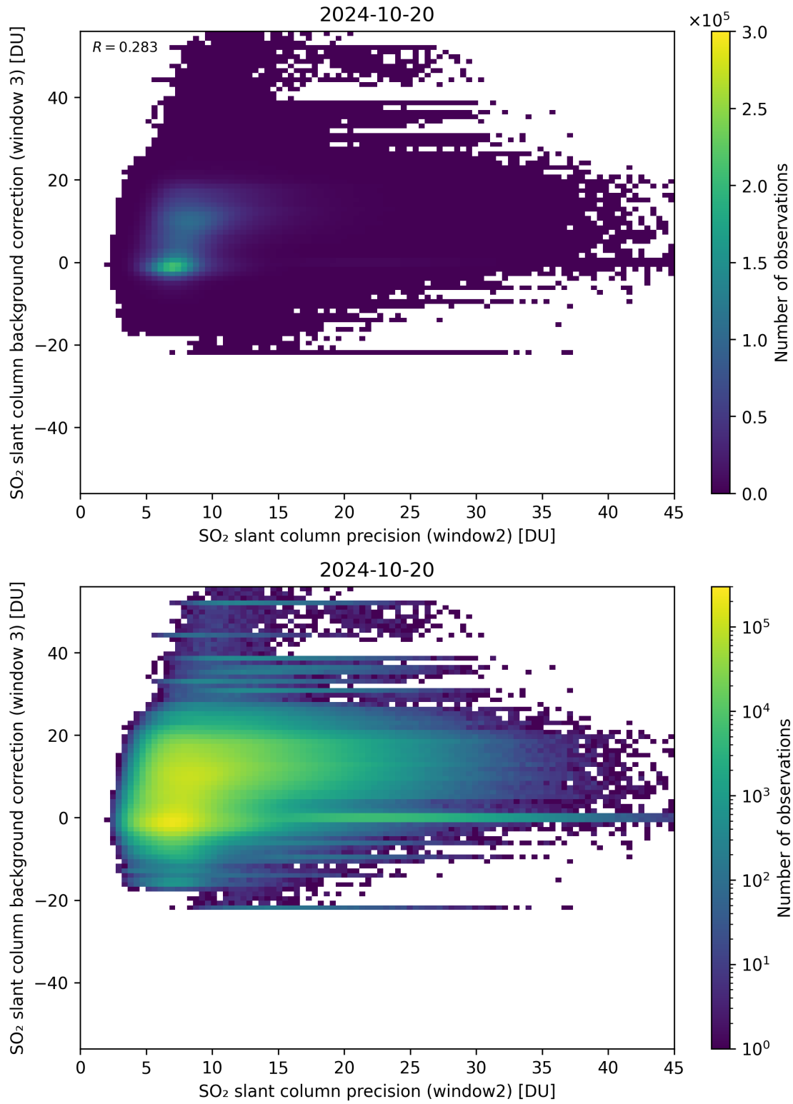
Figure 242: Scatter density plot of “SO 2 slant column precision (window2)” against “SO 2 slant column background correction (window 3)” for 2024-10-19 to 2024-10-21.
