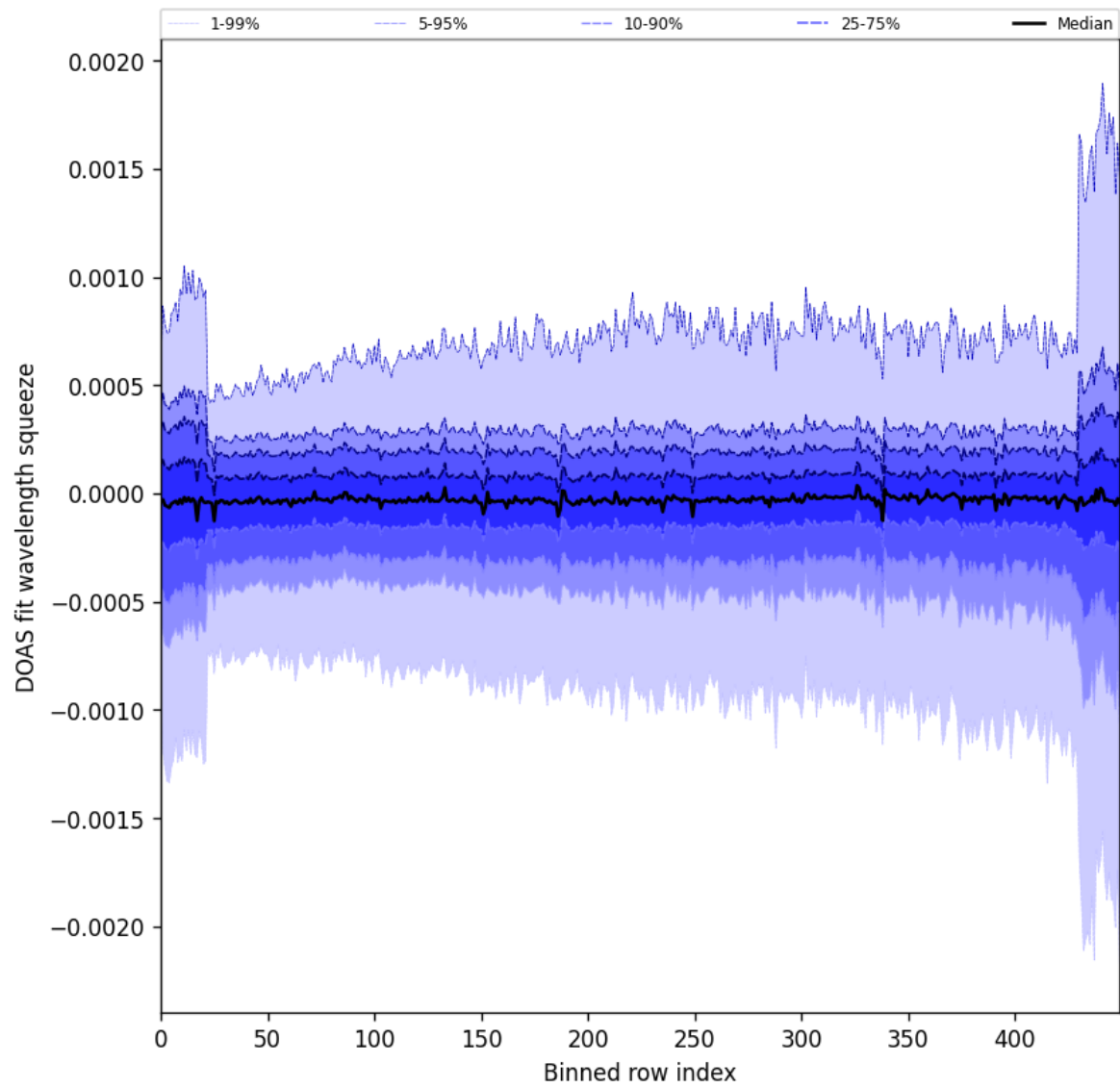
Figure 92: Along track statistics of “DOAS fit wavelength squeeze” for 2024-10-19 to 2024-10-21
