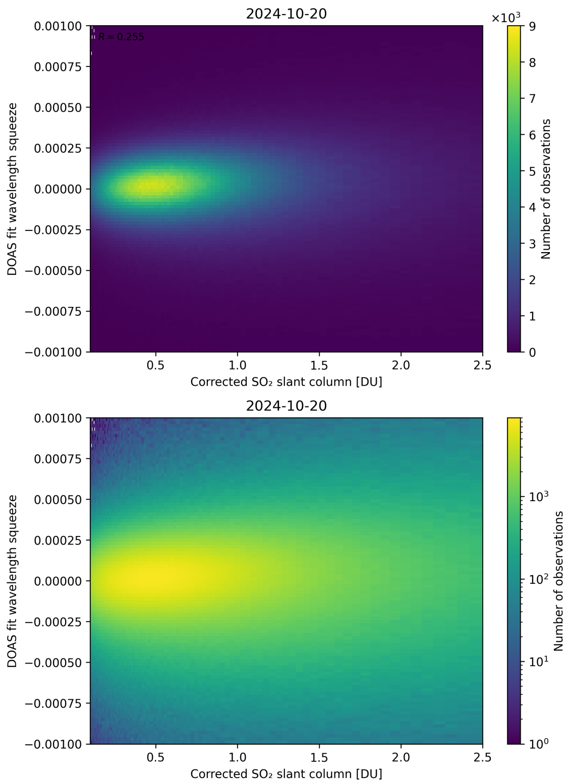
Figure 182: Scatter density plot of “Corrected SO 2 slant column” against “DOAS fit wavelength squeeze” for 2024-10-19 to 2024-10-21.
