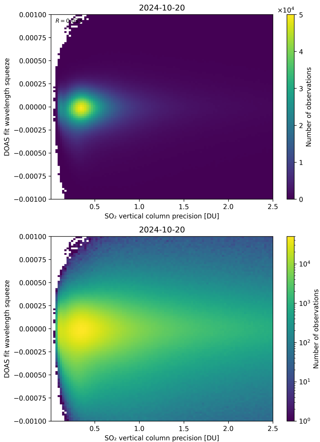
Figure 283: Scatter density plot of “SO 2 vertical column precision” against “DOAS fit wavelength squeeze” for 2024-10-19 to 2024-10-21.
