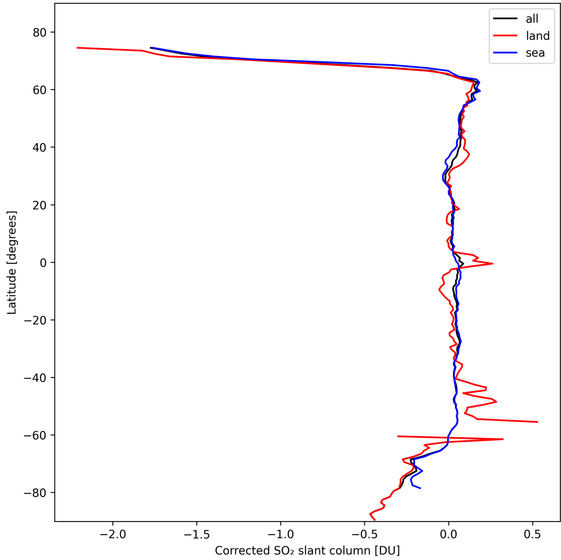
Figure 32: Zonal average of “Corrected SO 2 slant column” for 2024-10-19 to 2024-10-21.
