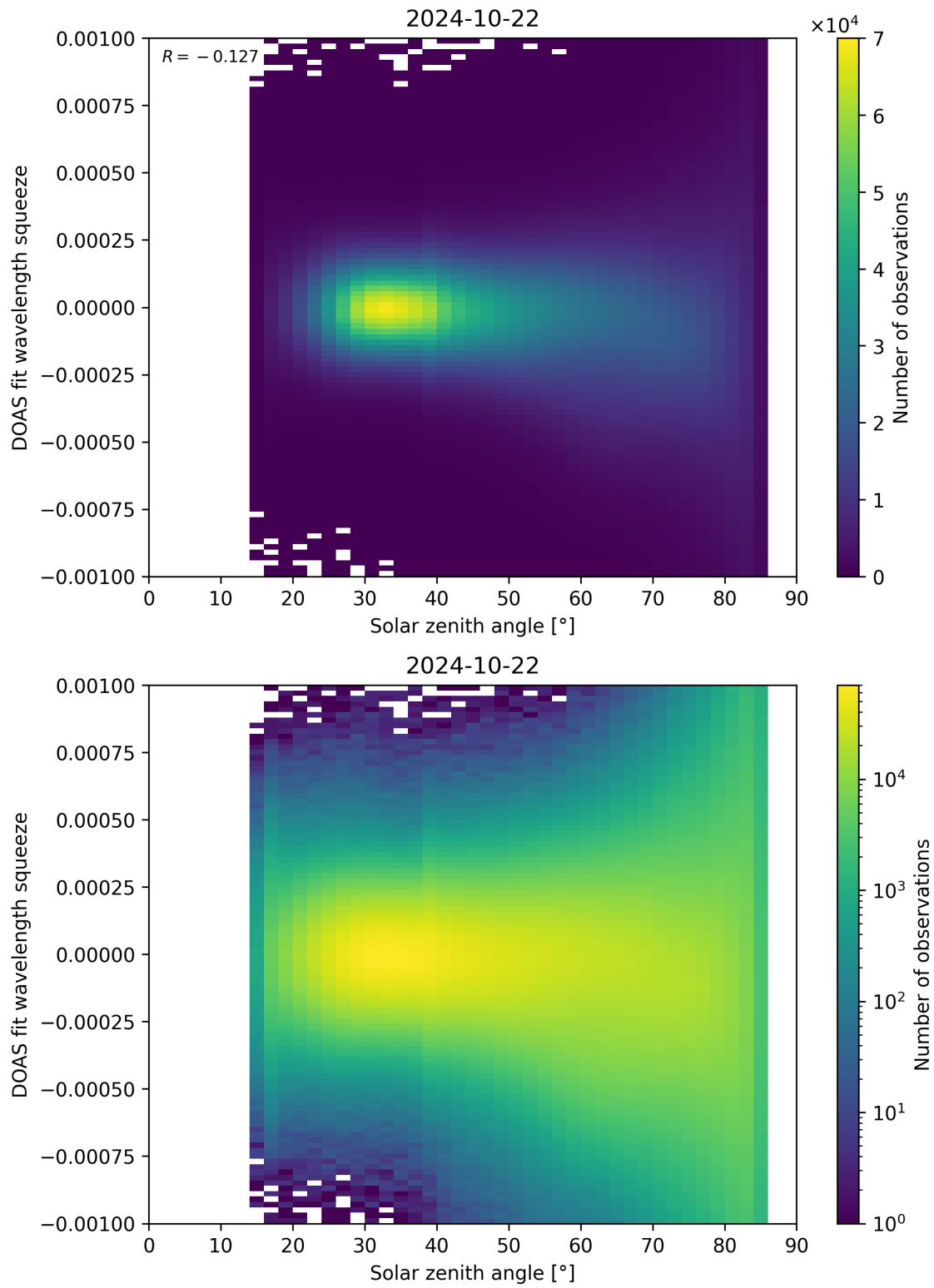
Figure 162: Scatter density plot of “Solar zenith angle” against “DOAS fit wavelength squeeze” for 2024-10-21 to 2024-10-23.
