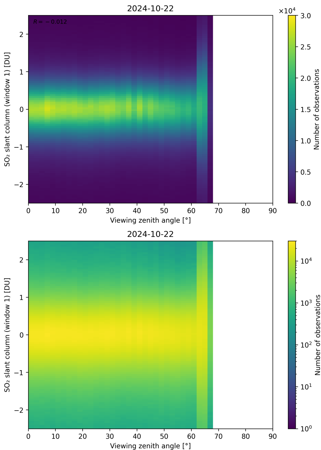
Figure 320: Scatter density plot of “Viewing zenith angle” against “SO 2 slant column (window 1)” for 2024-10-21 to 2024-10-23.
