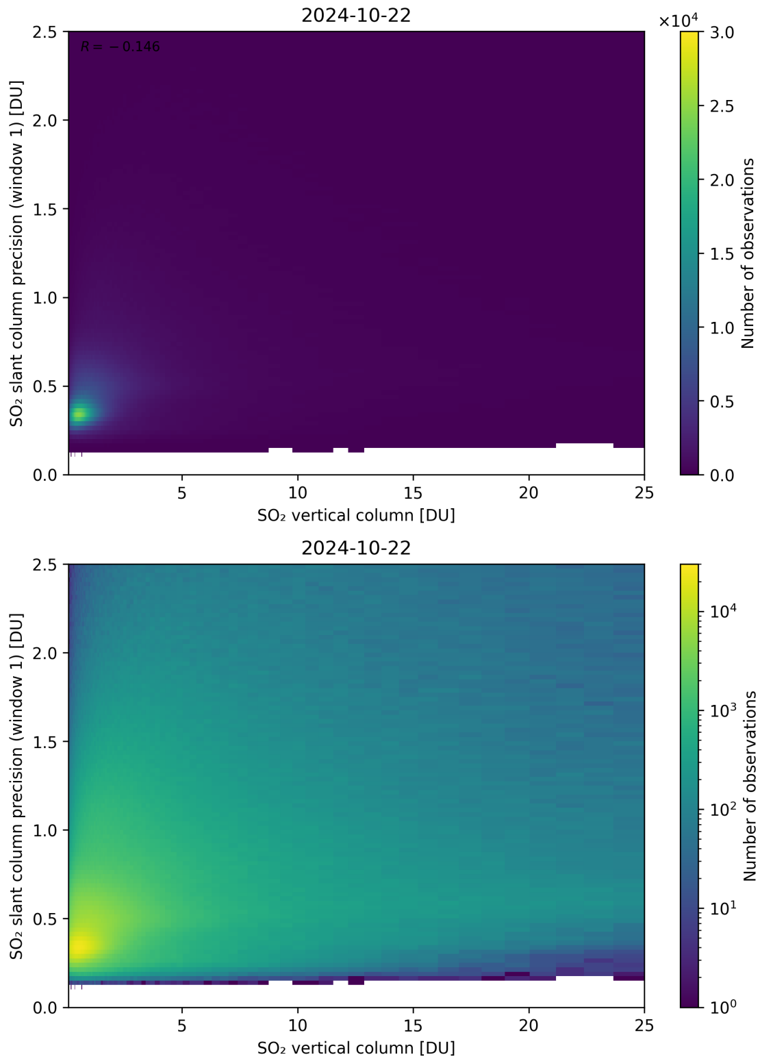
Figure 301: Scatter density plot of “SO 2 vertical column” against “SO 2 slant column precision (window 1)” for 2024-10-21 to 2024-10-23.
