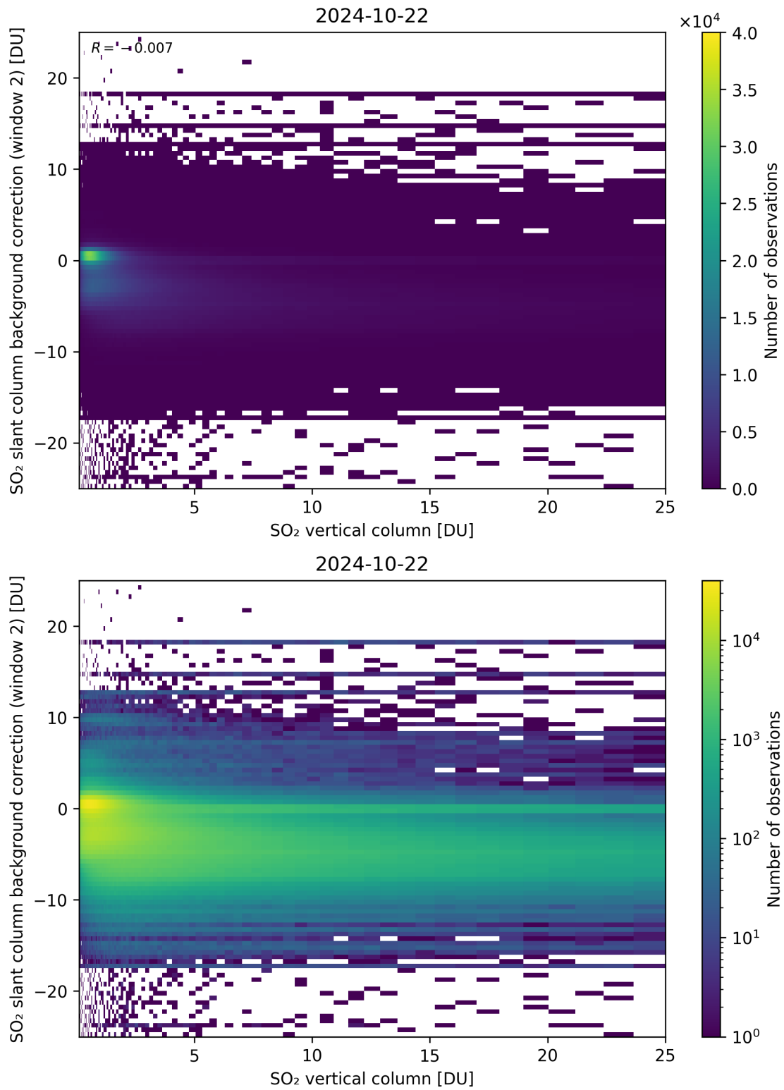
Figure 274: Scatter density plot of “SO 2 vertical column” against “SO 2 slant column background correction (window 2)” for 2024-10-21 to 2024-10-23.
