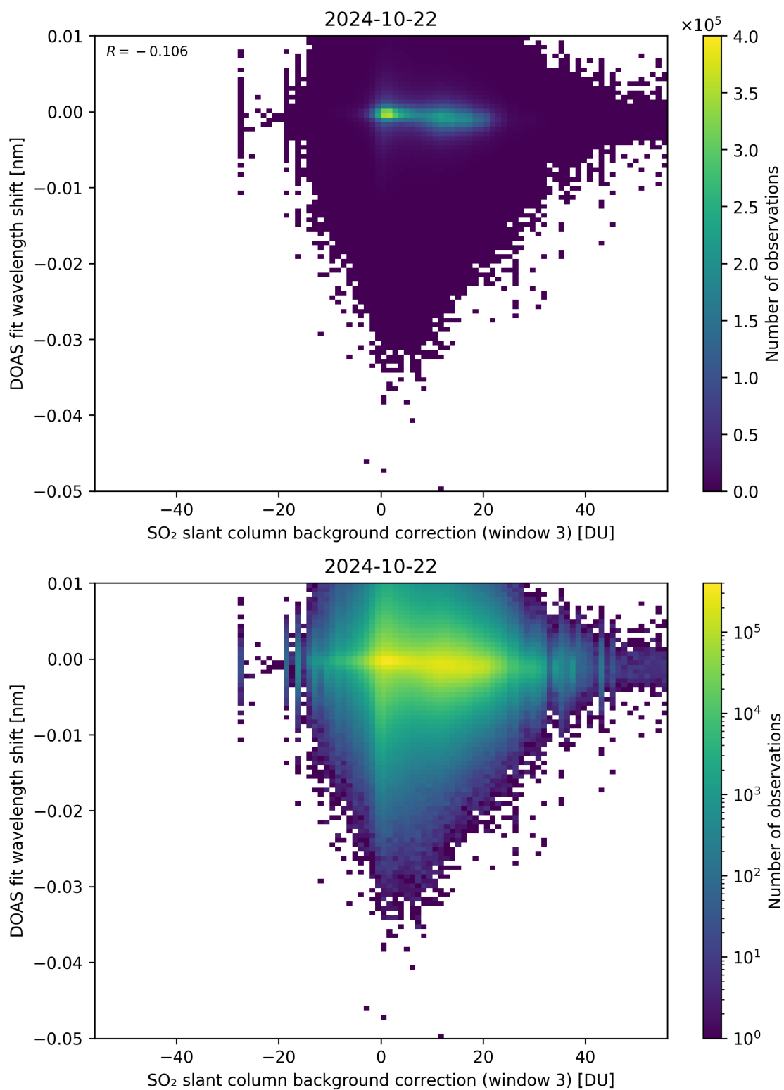
Figure 121: Scatter density plot of “SO 2 slant column background correction (window 3)” against “DOAS fit wavelength shift” for 2024-10-21 to 2024-10-23.
