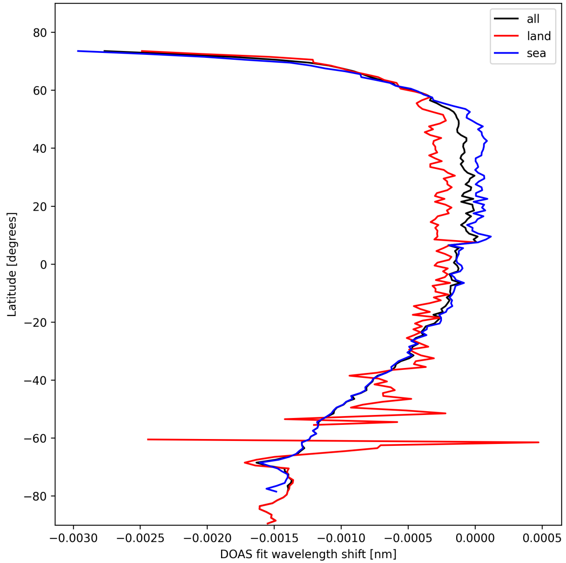
Figure 45: Zonal average of “DOAS fit wavelength shift” for 2024-10-21 to 2024-10-23.
