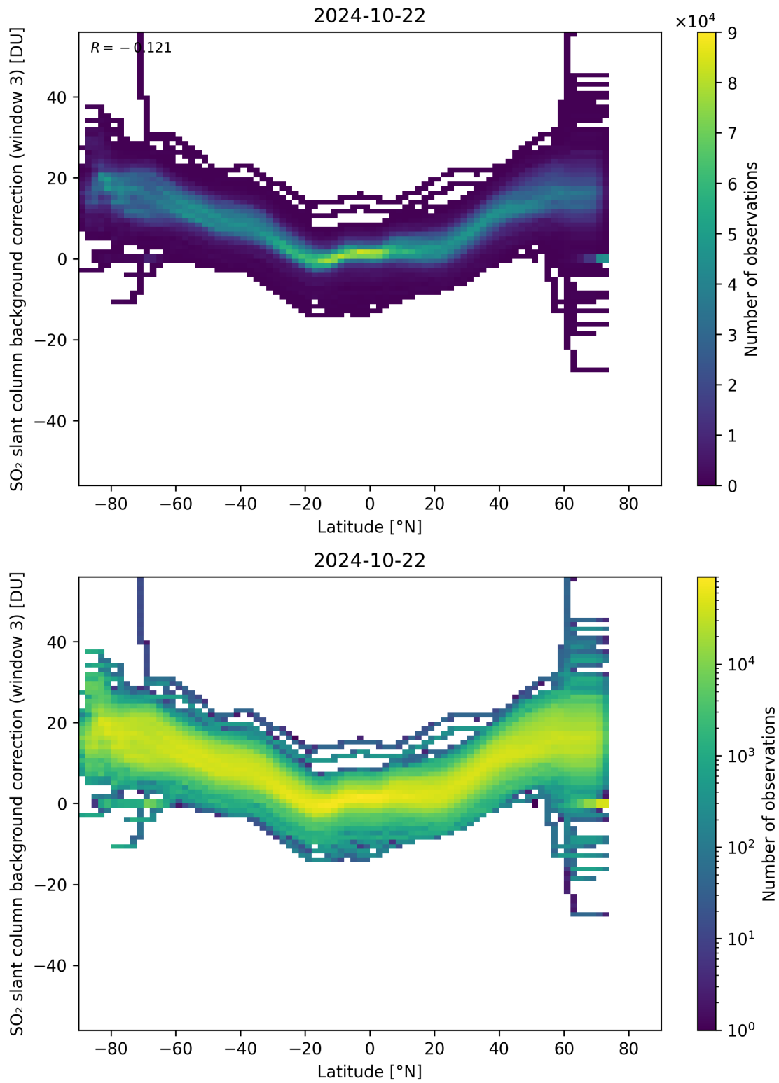
Figure 141: Scatter density plot of “Latitude” against “SO 2 slant column background correction (window 3)” for 2024-10-21 to 2024-10-23.
