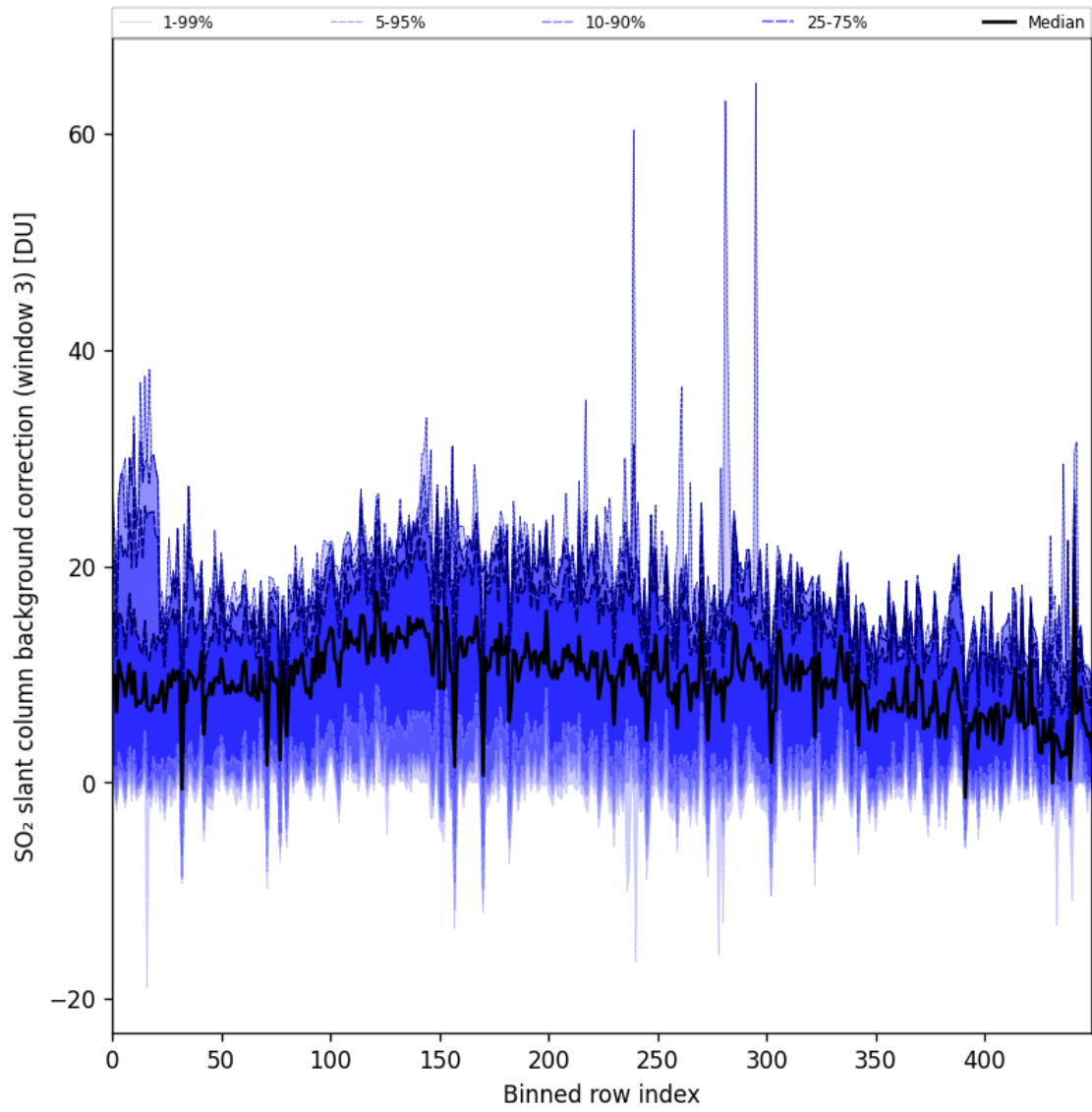
Figure 90: Along track statistics of “SO 2 slant column background correction (window 3)” for 2024-10-21 to 2024-10-23
