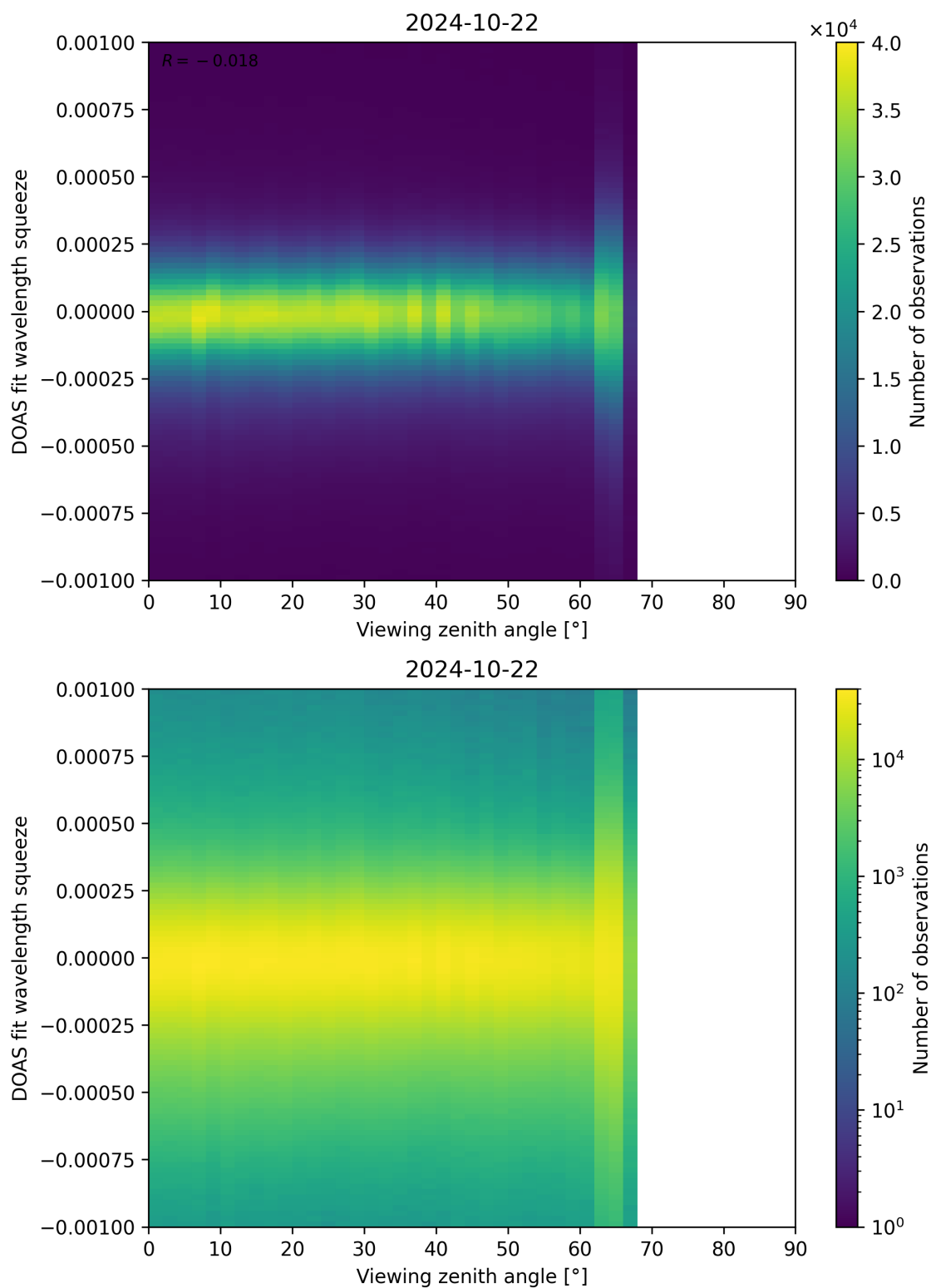
Figure 312: Scatter density plot of “Viewing zenith angle” against “DOAS fit wavelength squeeze” for 2024-10-21 to 2024-10-23.
