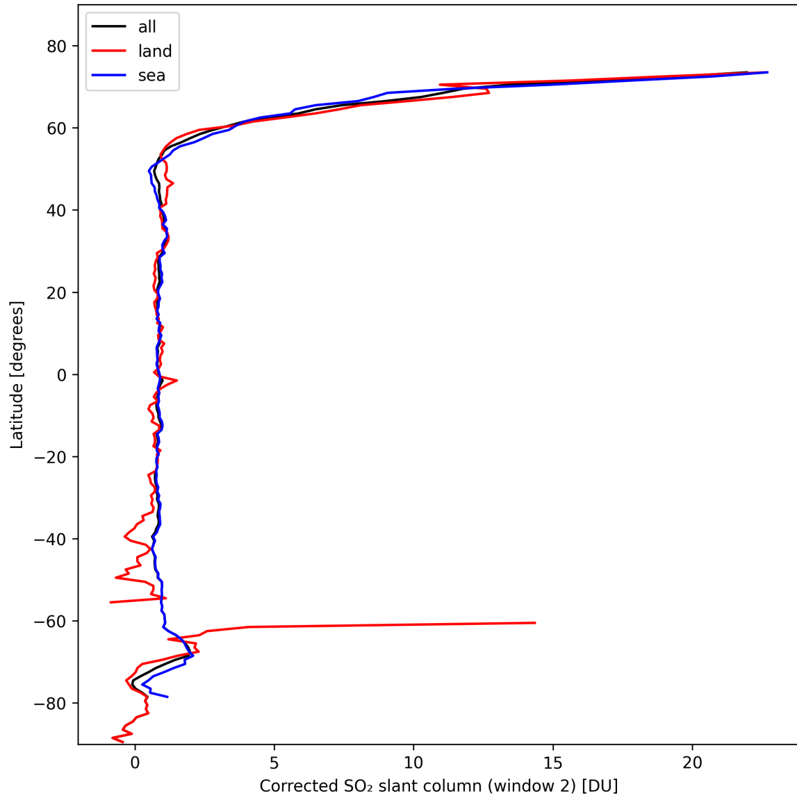
Figure 39: Zonal average of “Corrected SO 2 slant column (window 2)” for 2024-10-21 to 2024-10-23.
