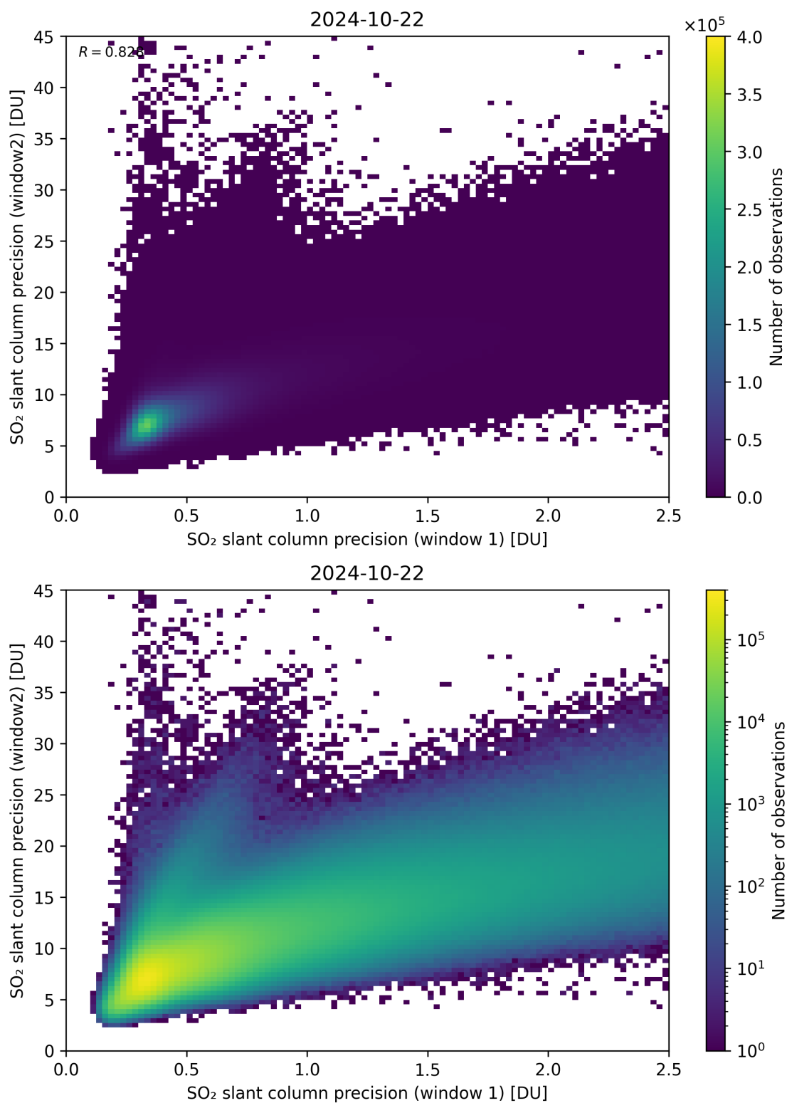
Figure 227: Scatter density plot of “SO 2 slant column precision (window 1)” against “SO 2 slant column precision (window2)” for 2024-10-21 to 2024-10-23.
