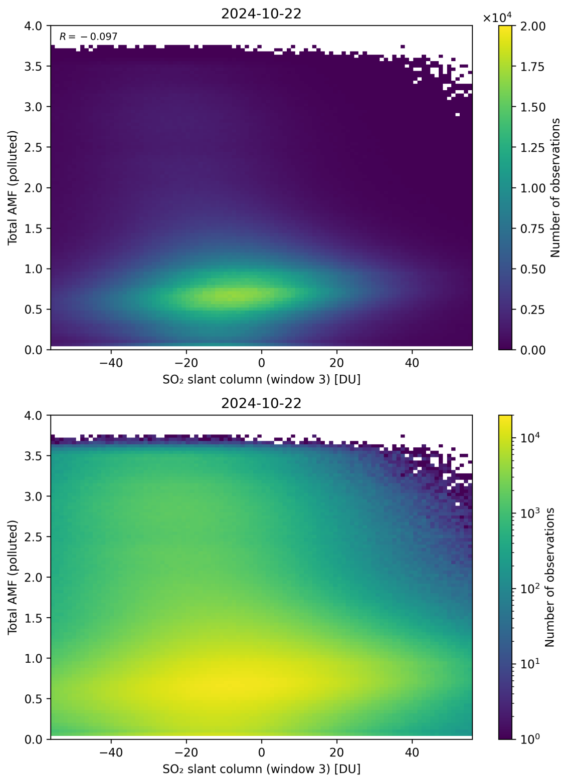
Figure 268: Scatter density plot of “SO 2 slant column (window 3)” against “Total AMF (polluted)” for 2024-10-21 to 2024-10-23.
