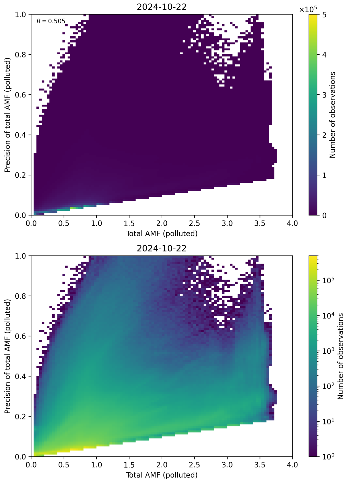
Figure 272: Scatter density plot of “Total AMF (polluted)” against “Precision of total AMF (polluted)” for 2024-10-21 to 2024-10-23.
