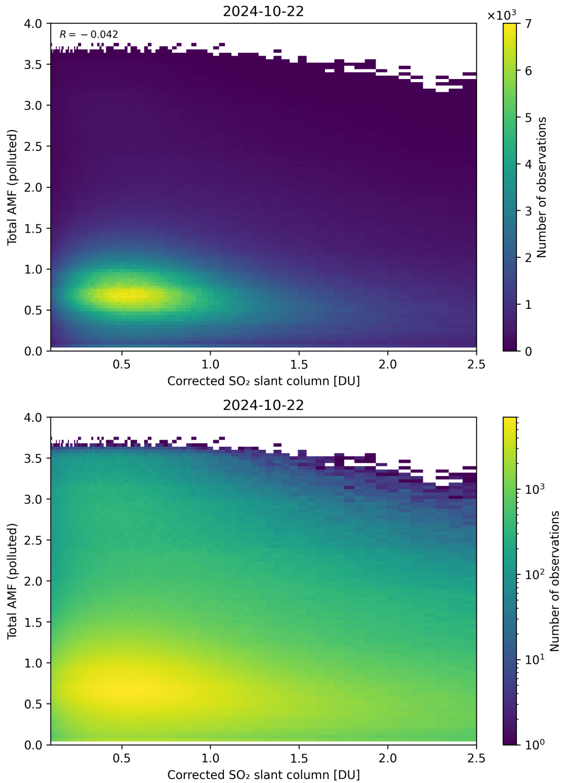
Figure 192: Scatter density plot of “Corrected SO 2 slant column” against “Total AMF (polluted)” for 2024-10-21 to 2024-10-23.
