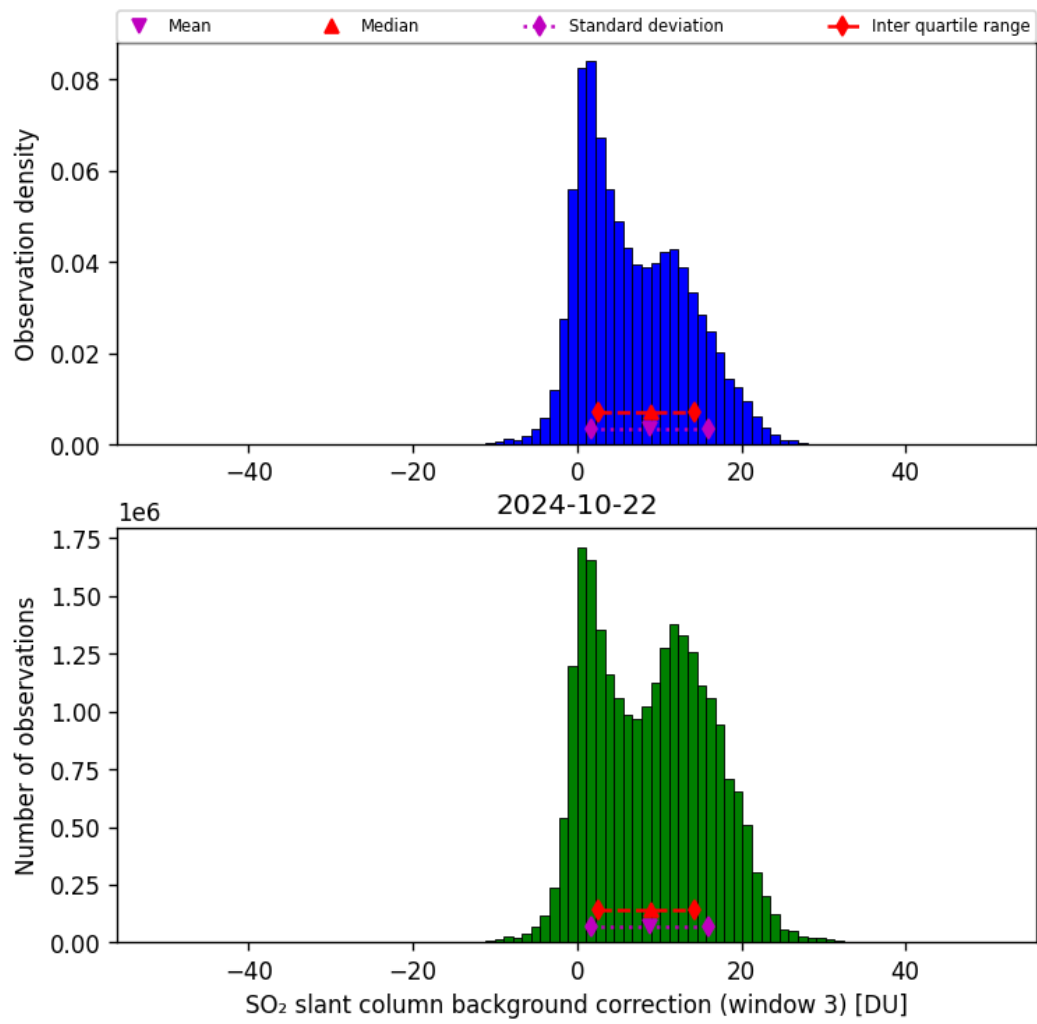
Figure 67: Histogram of “SO 2 slant column background correction (window 3)” for 2024-10-21 to 2024-10-23
