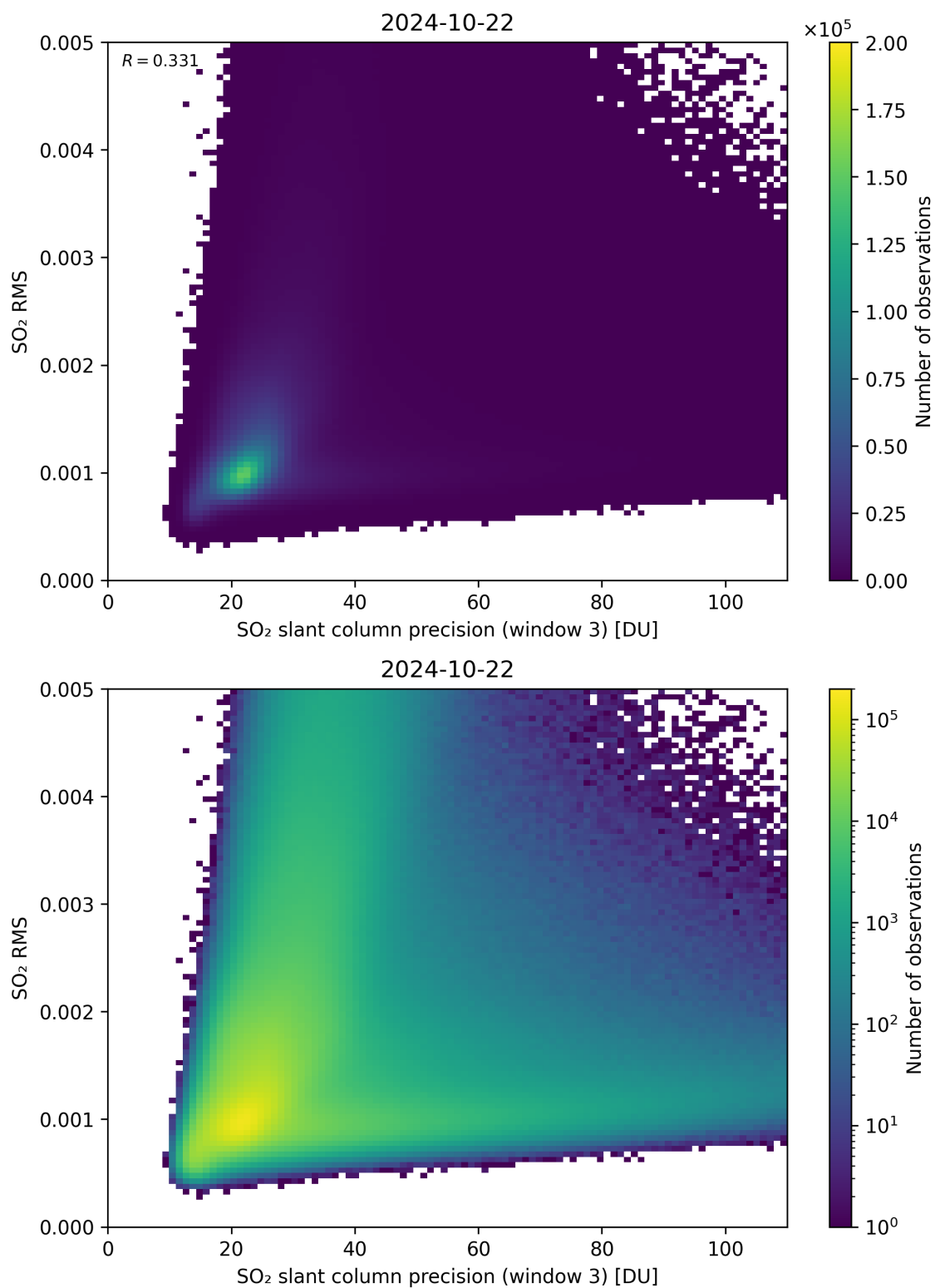
Figure 260: Scatter density plot of “SO 2 slant column precision (window 3)” against “SO 2 RMS” for 2024-10-21 to 2024-10-23.
