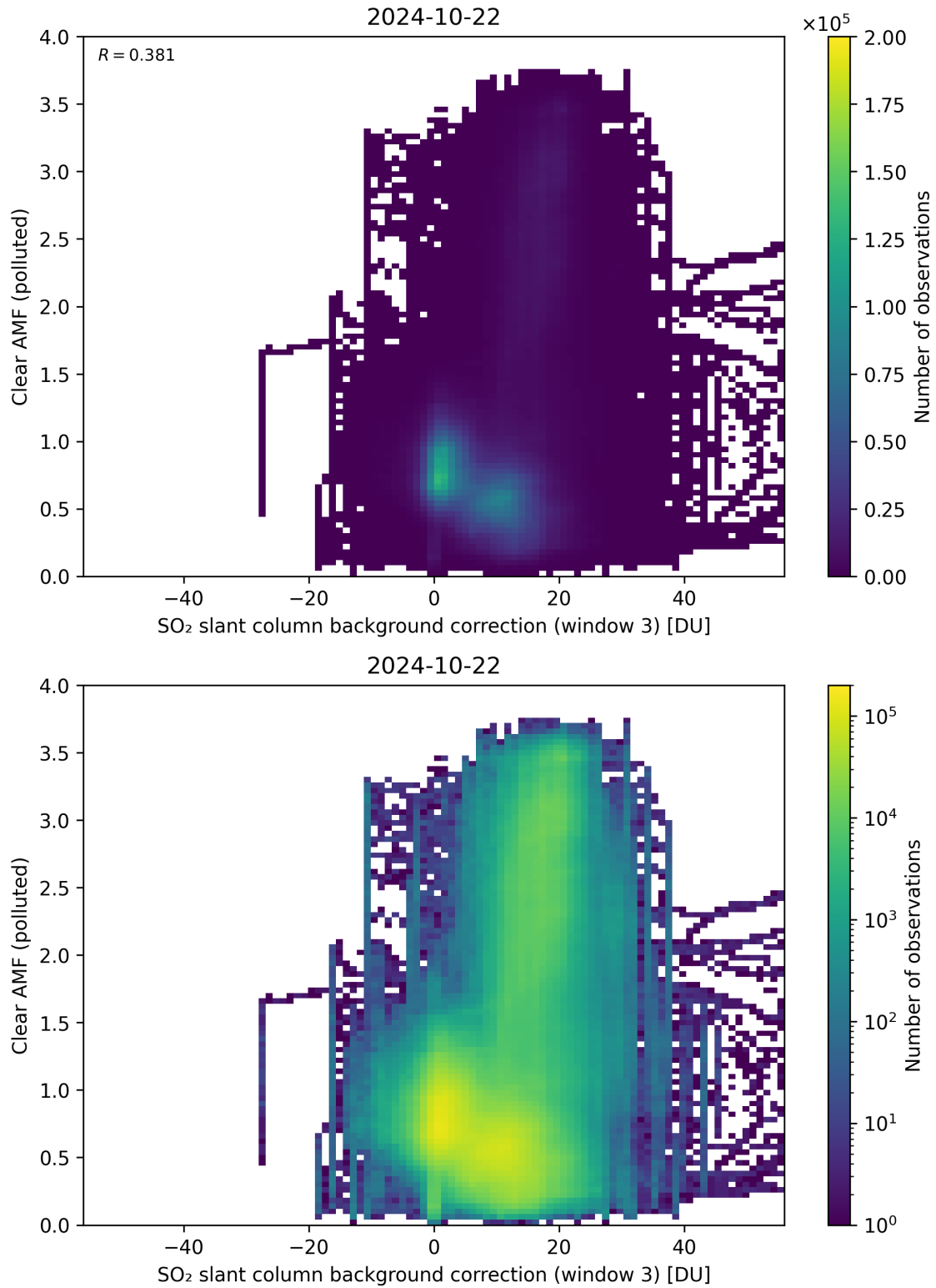
Figure 124: Scatter density plot of “SO 2 slant column background correction (window 3)” against “Clear AMF (polluted)” for 2024-10-21 to 2024-10-23.
