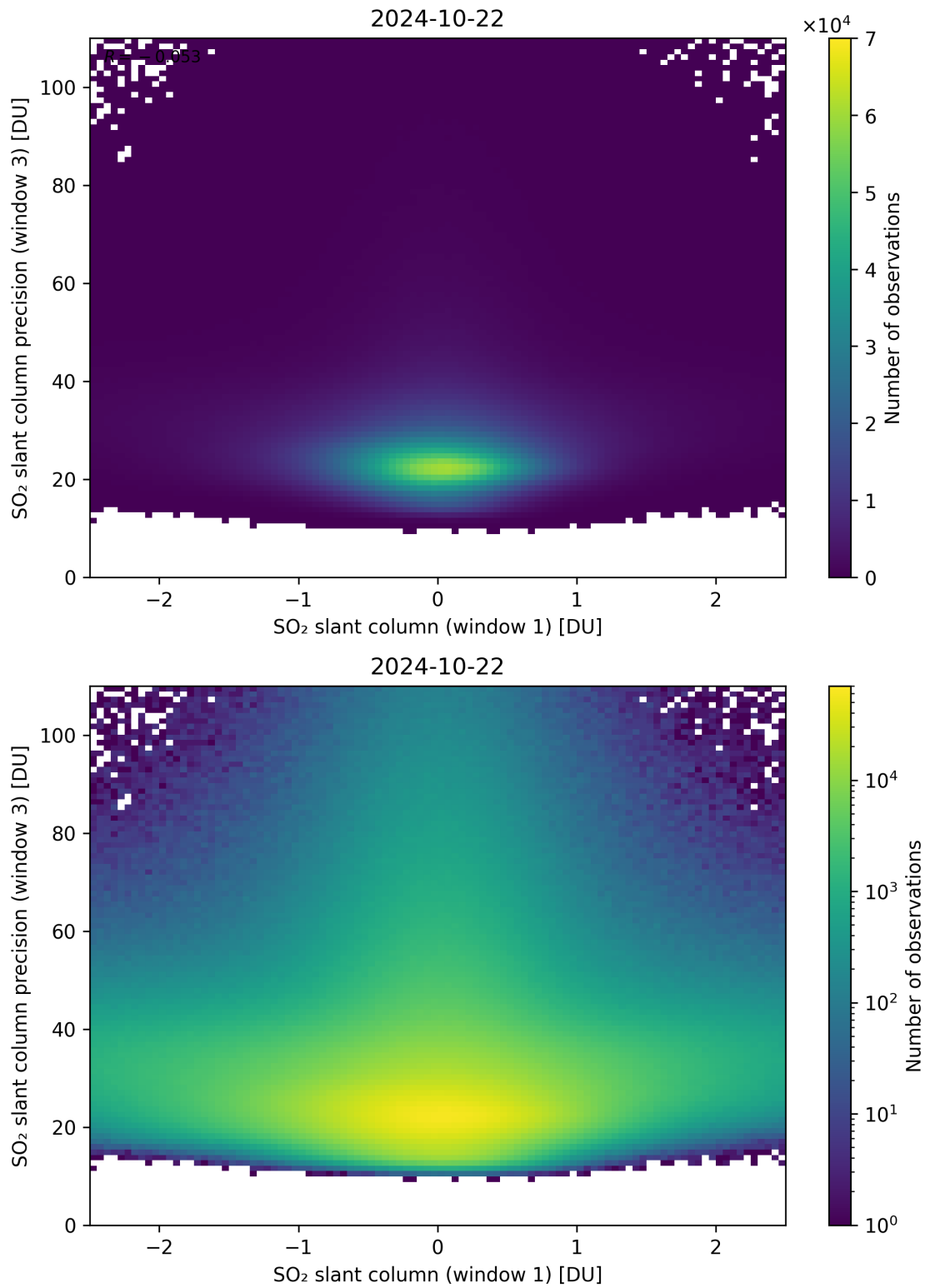
Figure 238: Scatter density plot of “SO 2 slant column (window 1)” against “SO 2 slant column precision (window 3)” for 2024-10-21 to 2024-10-23.
