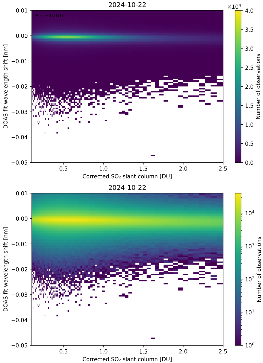
Figure 181: Scatter density plot of “Corrected SO 2 slant column” against “DOAS fit wavelength shift” for 2024-10-21 to 2024-10-23.
