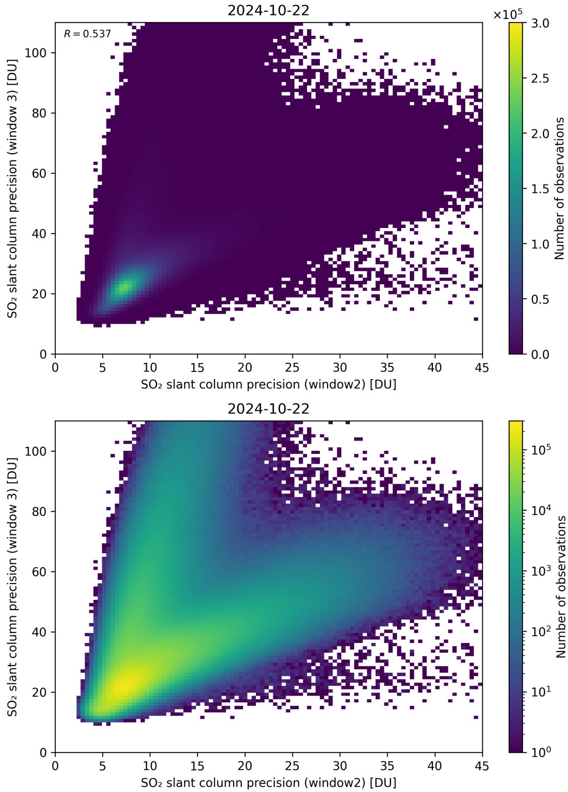
Figure 250: Scatter density plot of “SO 2 slant column precision (window2)” against “SO 2 slant column precision (window 3)” for 2024-10-21 to 2024-10-23.
