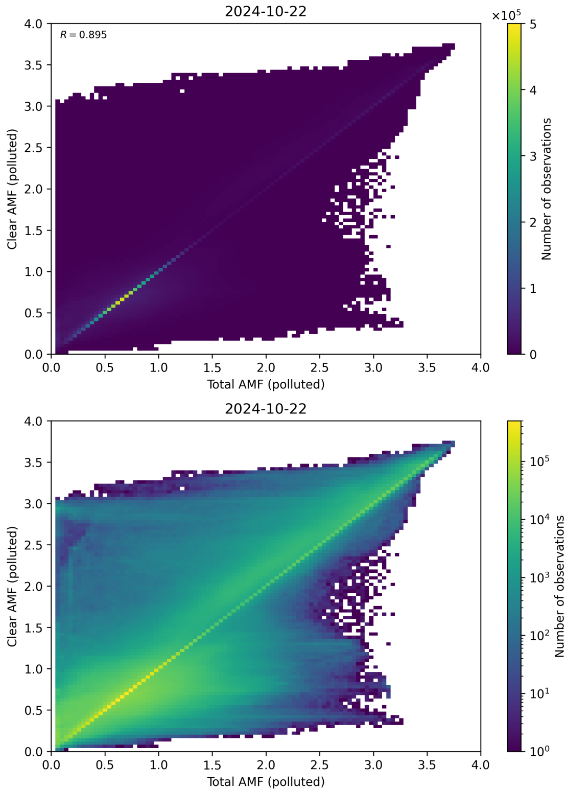
Figure 271: Scatter density plot of “Total AMF (polluted)” against “Clear AMF (polluted)” for 2024-10-21 to 2024-10-23.
