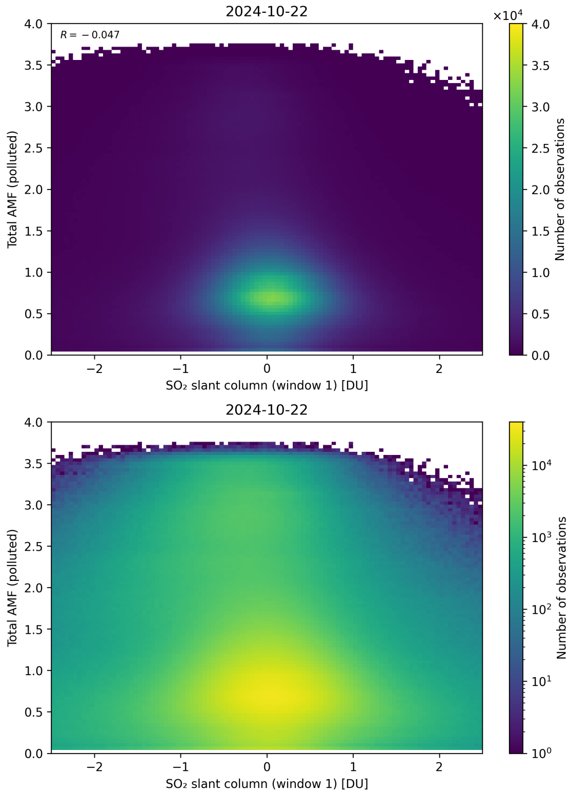
Figure 239: Scatter density plot of “SO 2 slant column (window 1)” against “Total AMF (polluted)” for 2024-10-21 to 2024-10-23.
