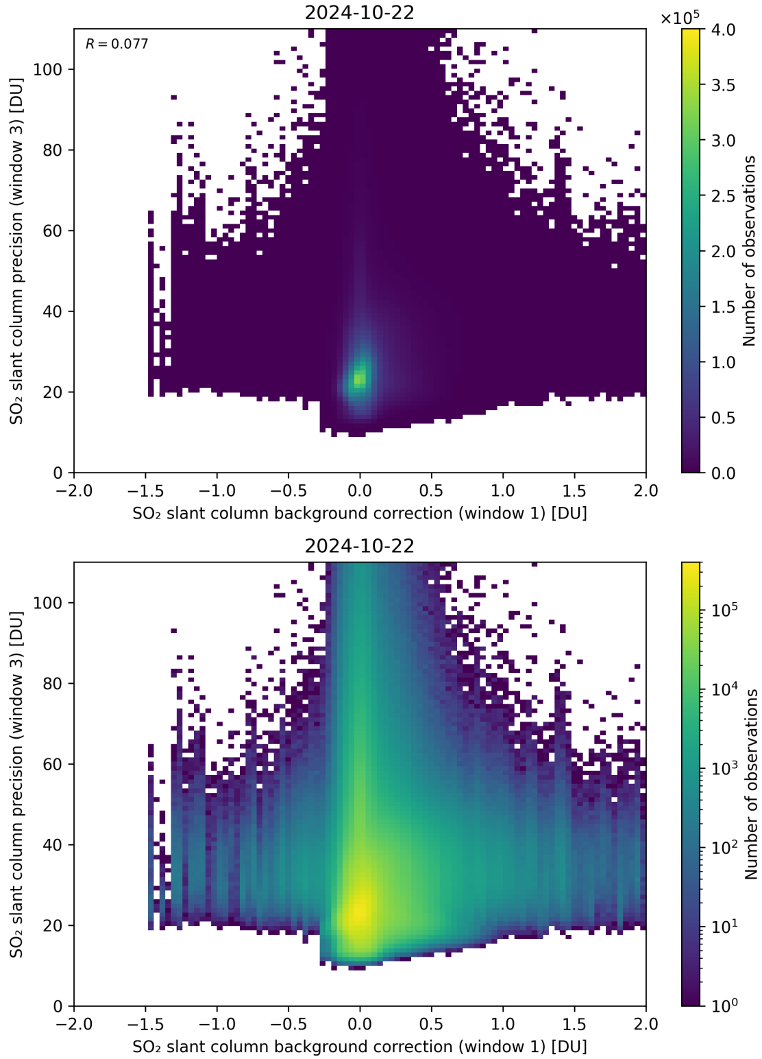
Figure 108: Scatter density plot of “SO 2 slant column background correction (window 1)” against “SO 2 slant column precision (window 3)” for 2024-10-21 to 2024-10-23.
