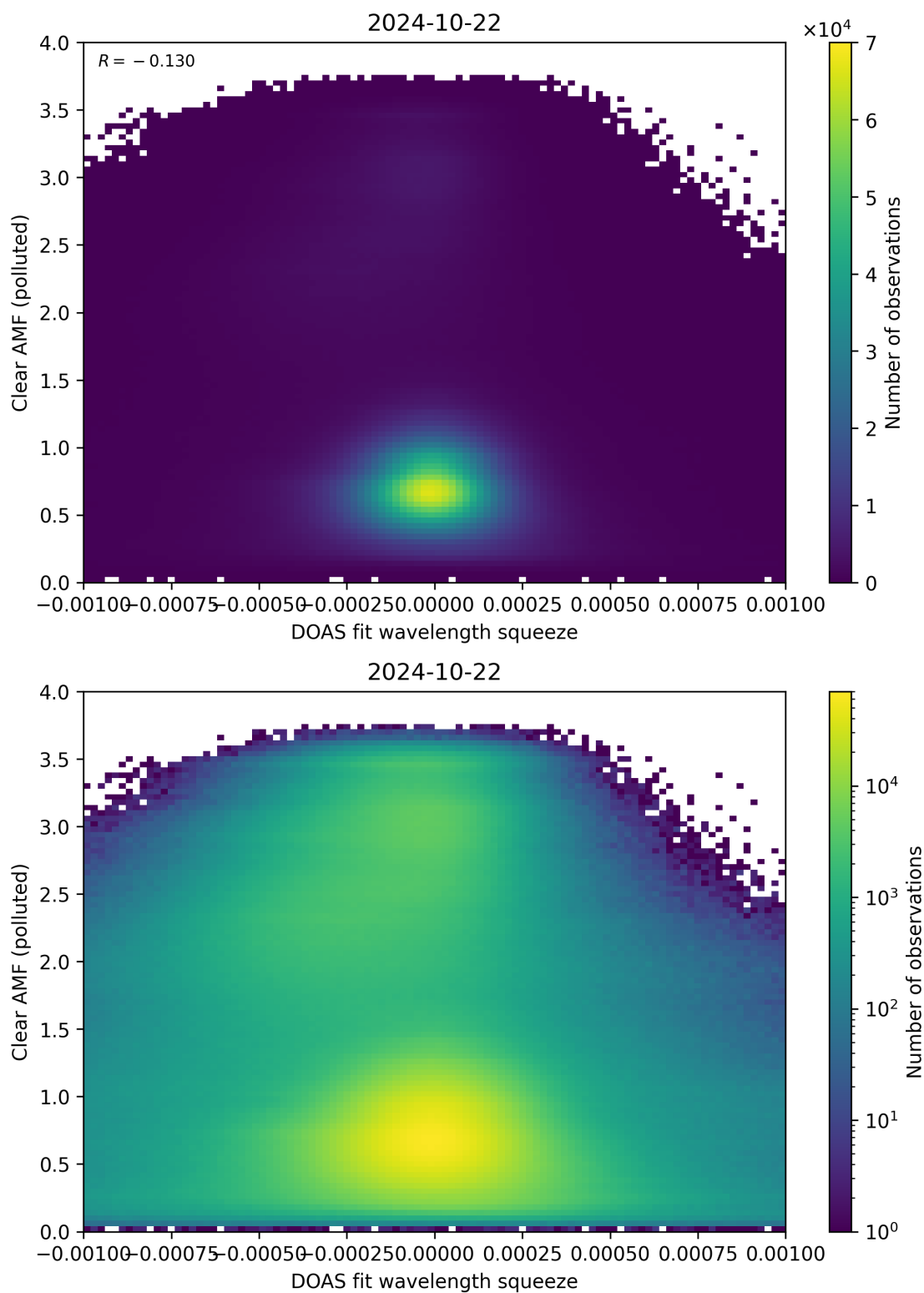
Figure 133: Scatter density plot of “DOAS fit wavelength squeeze” against “Clear AMF (polluted)” for 2024-10-21 to 2024-10-23.
