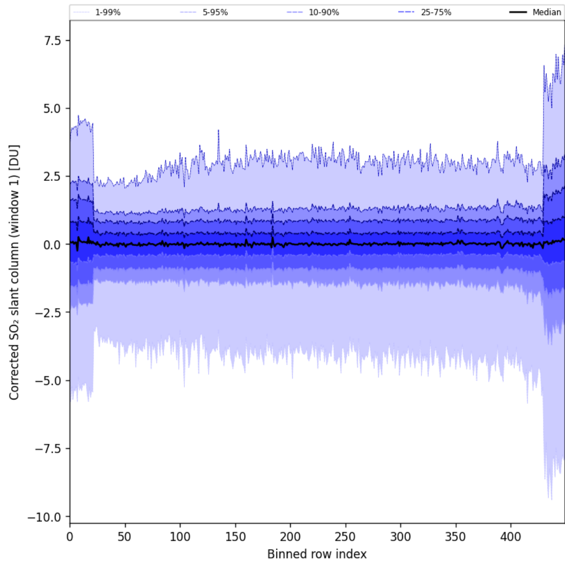
Figure 81: Along track statistics of “Corrected SO 2 slant column (window 1)” for 2024-10-21 to 2024-10-23
