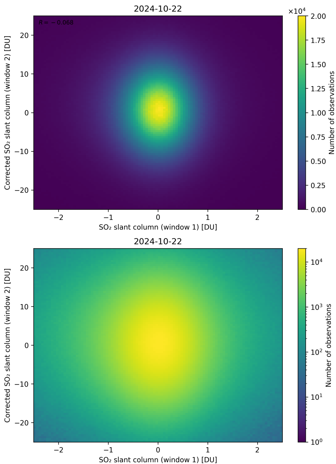
Figure 233: Scatter density plot of “SO 2 slant column (window 1)” against “Corrected SO 2 slant column (window 2)” for 2024-10-21 to 2024-10-23.
