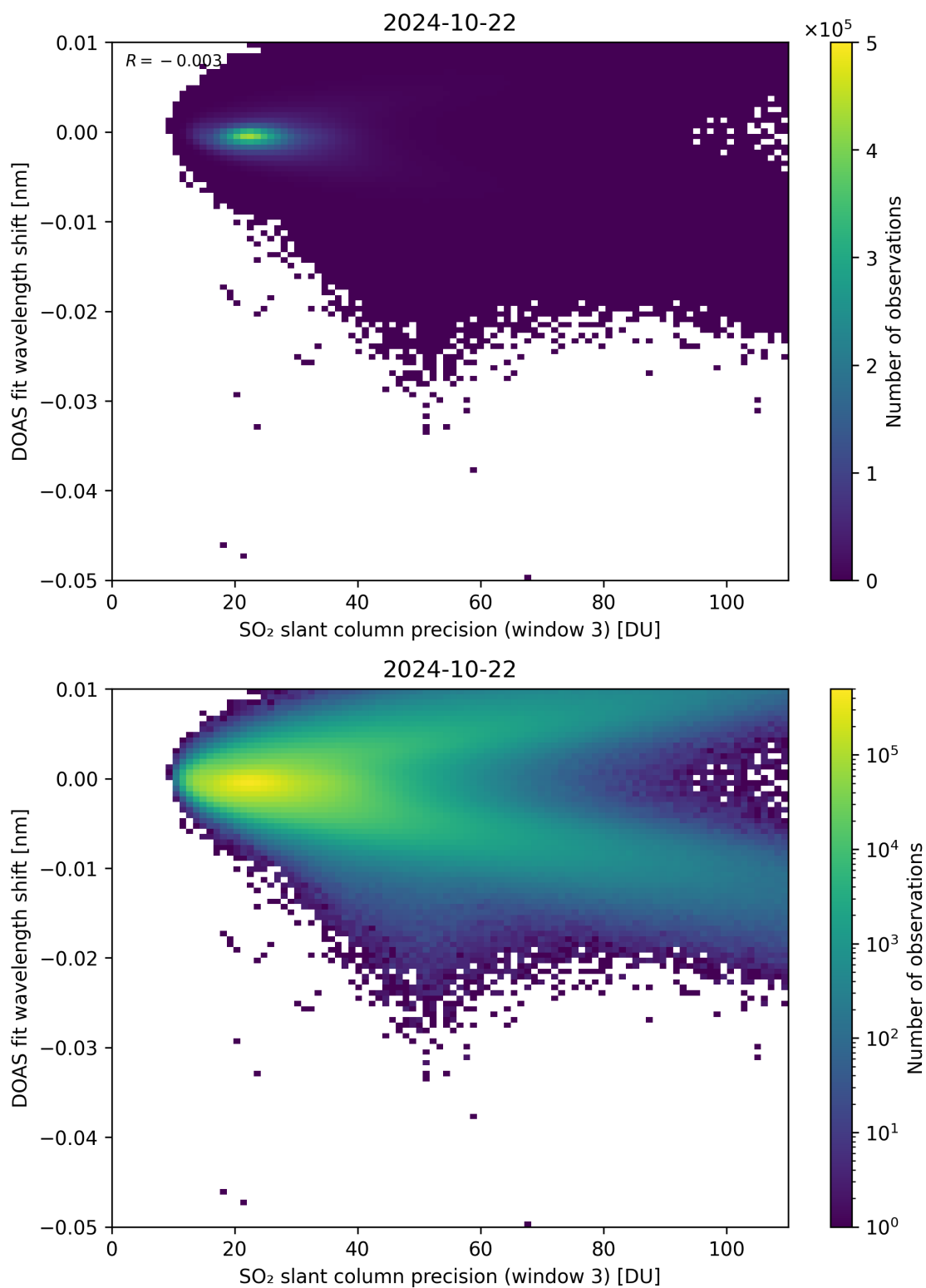
Figure 258: Scatter density plot of “SO 2 slant column precision (window 3)” against “DOAS fit wavelength shift” for 2024-10-21 to 2024-10-23.
