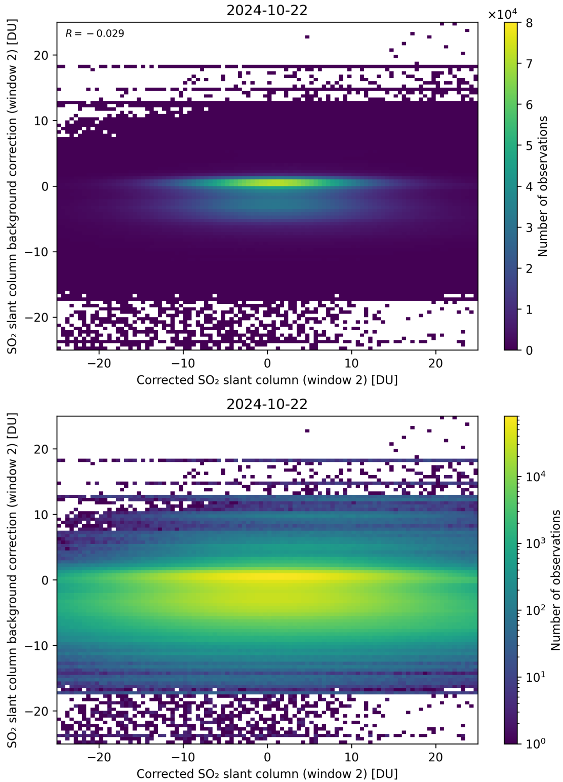
Figure 194: Scatter density plot of “Corrected SO 2 slant column (window 2)” against “SO 2 slant column background correction (window 2)” for 2024-10-21 to 2024-10-23.
