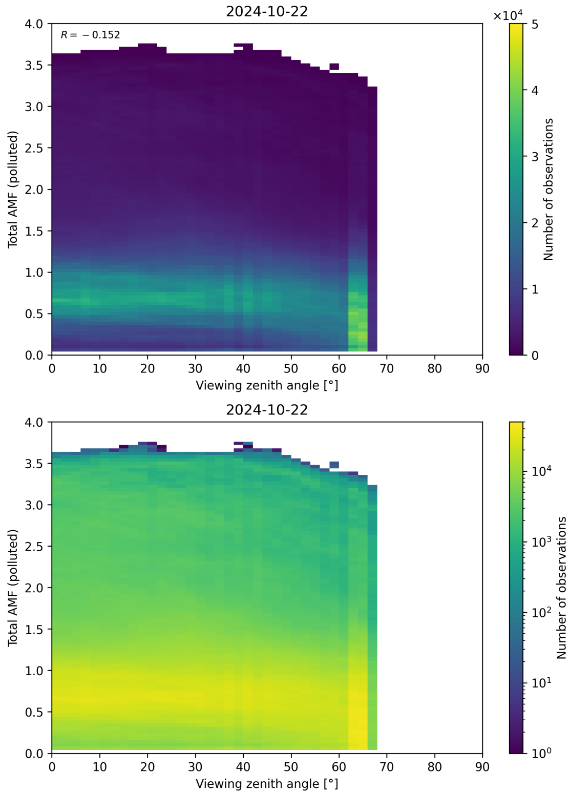
Figure 325: Scatter density plot of “Viewing zenith angle” against “Total AMF (polluted)” for 2024-10-21 to 2024-10-23.
