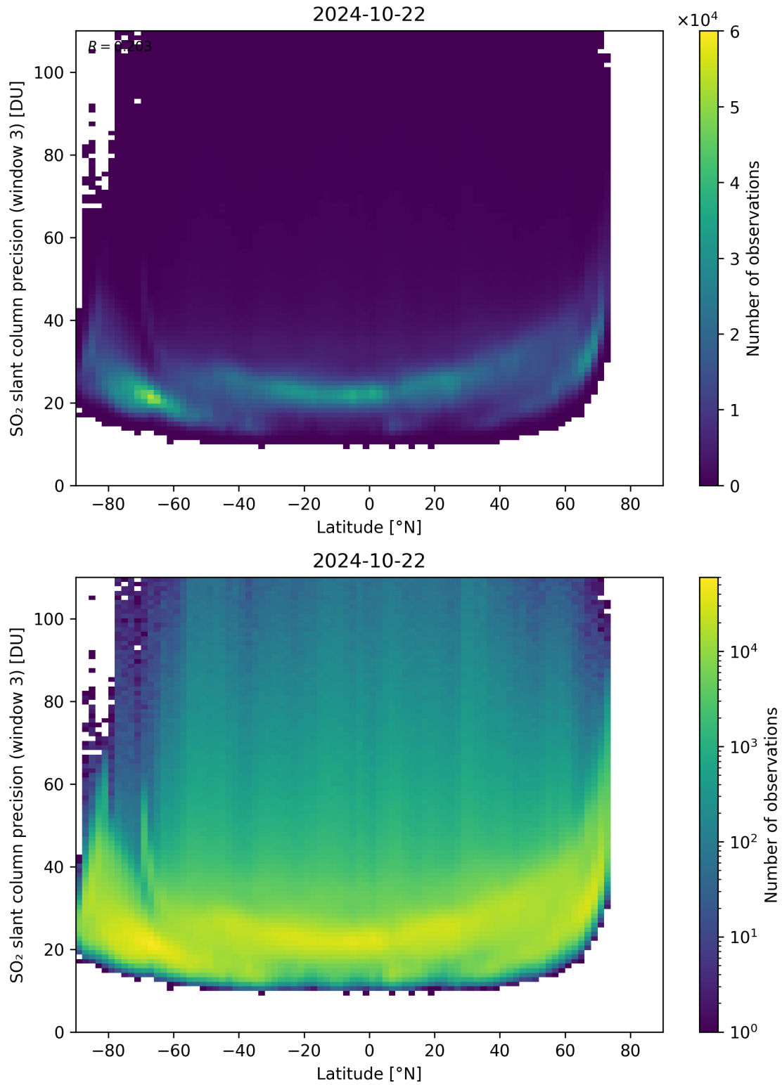
Figure 153: Scatter density plot of “Latitude” against “SO 2 slant column precision (window 3)” for 2024-10-21 to 2024-10-23.
