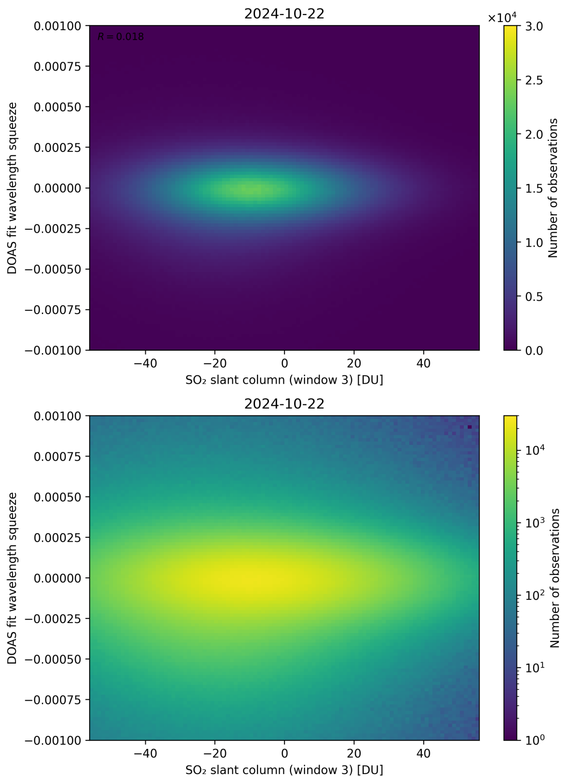
Figure 255: Scatter density plot of “SO 2 slant column (window 3)” against “DOAS fit wavelength squeeze” for 2024-10-21 to 2024-10-23.
