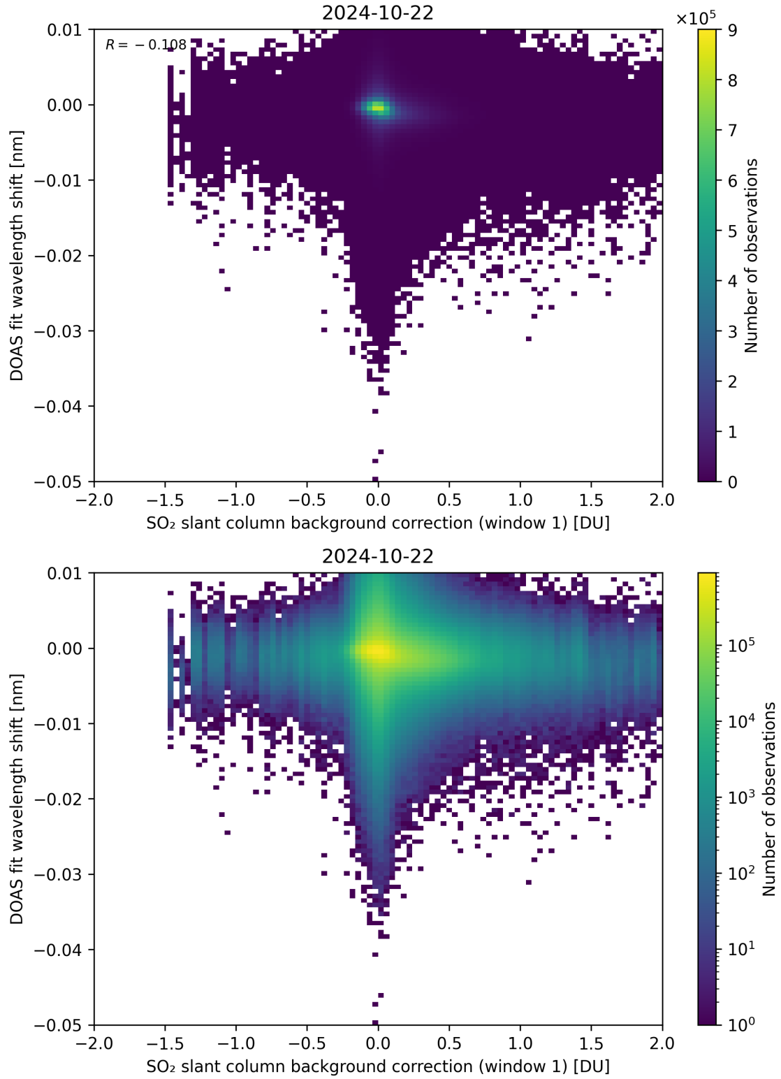
Figure 100: Scatter density plot of “SO 2 slant column background correction (window 1)” against “DOAS fit wavelength shift” for 2024-10-21 to 2024-10-23.
