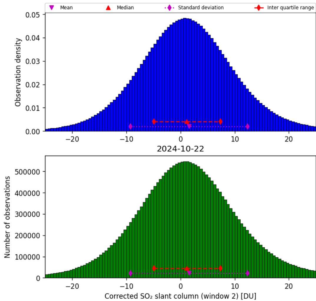
Figure 62: Histogram of “Corrected SO 2 slant column (window 2)” for 2024-10-21 to 2024-10-23
