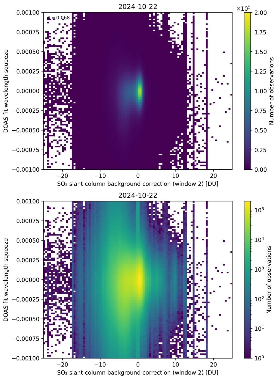
Figure 113: Scatter density plot of “SO 2 slant column background correction (window 2)” against “DOAS fit wavelength squeeze” for 2024-10-21 to 2024-10-23.
