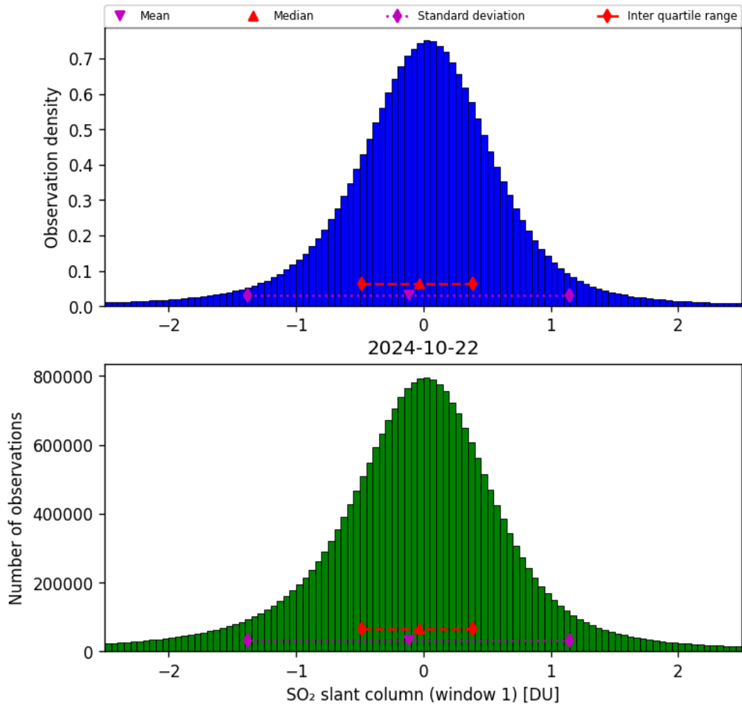
Figure 56: Histogram of “SO 2 slant column (window 1)” for 2024-10-21 to 2024-10-23
