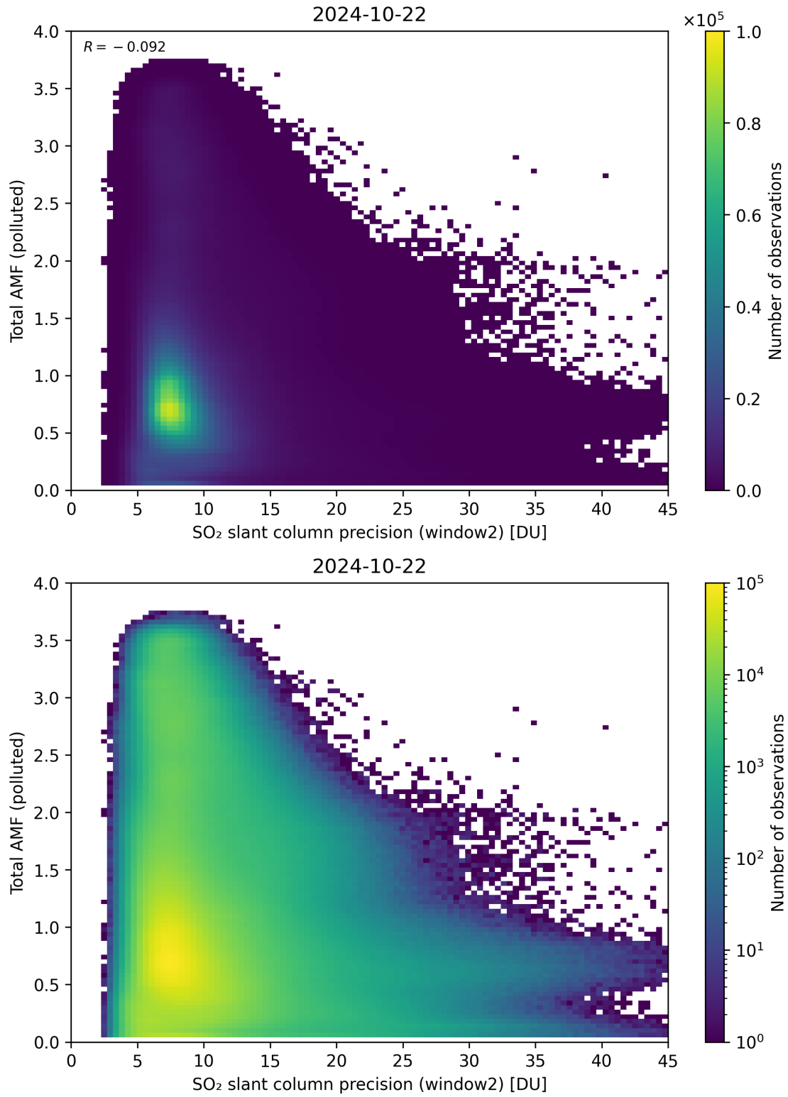
Figure 251: Scatter density plot of “SO 2 slant column precision (window2)” against “Total AMF (polluted)” for 2024-10-21 to 2024-10-23.
