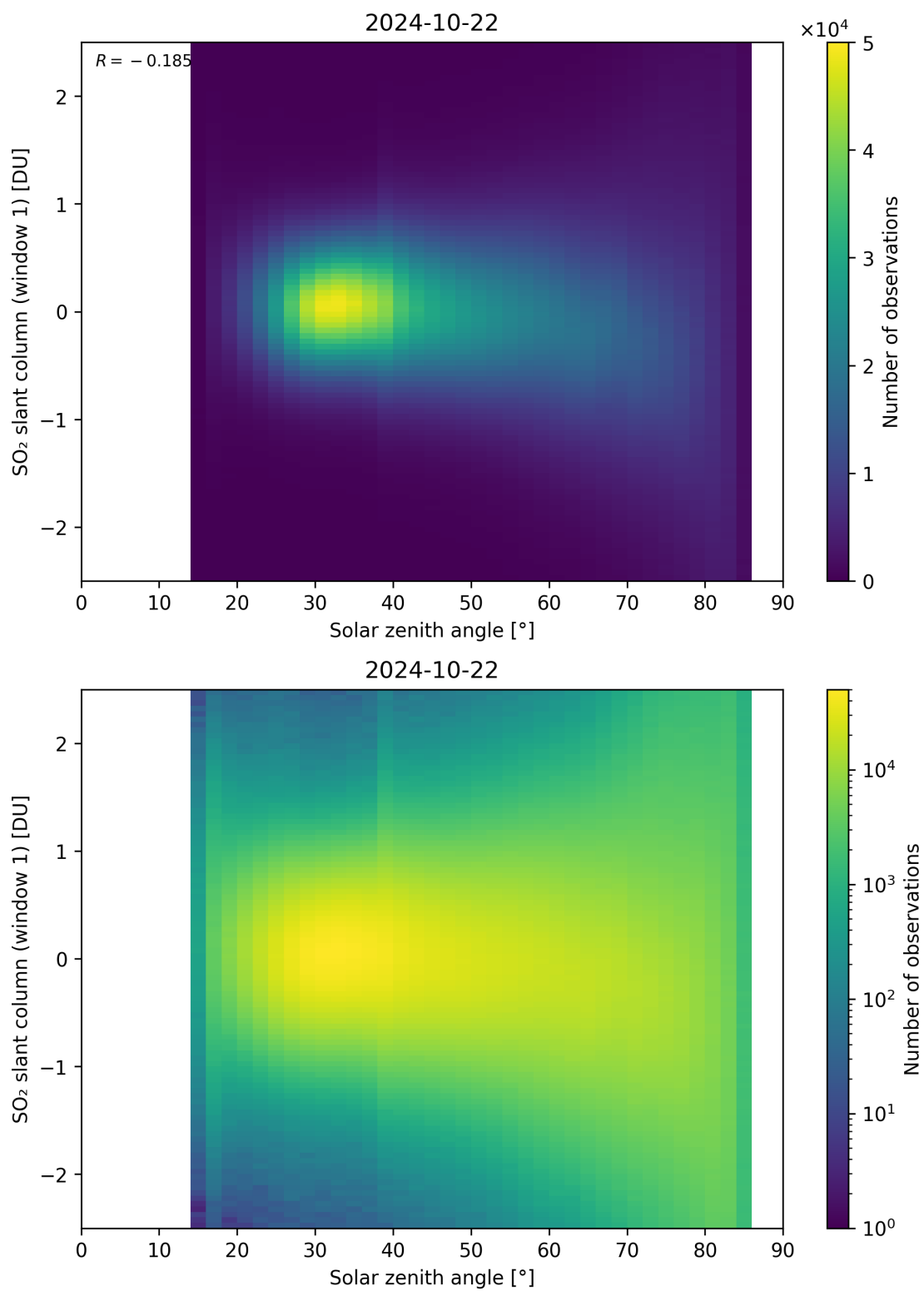
Figure 169: Scatter density plot of “Solar zenith angle” against “SO 2 slant column (window 1)” for 2024-10-21 to 2024-10-23.
