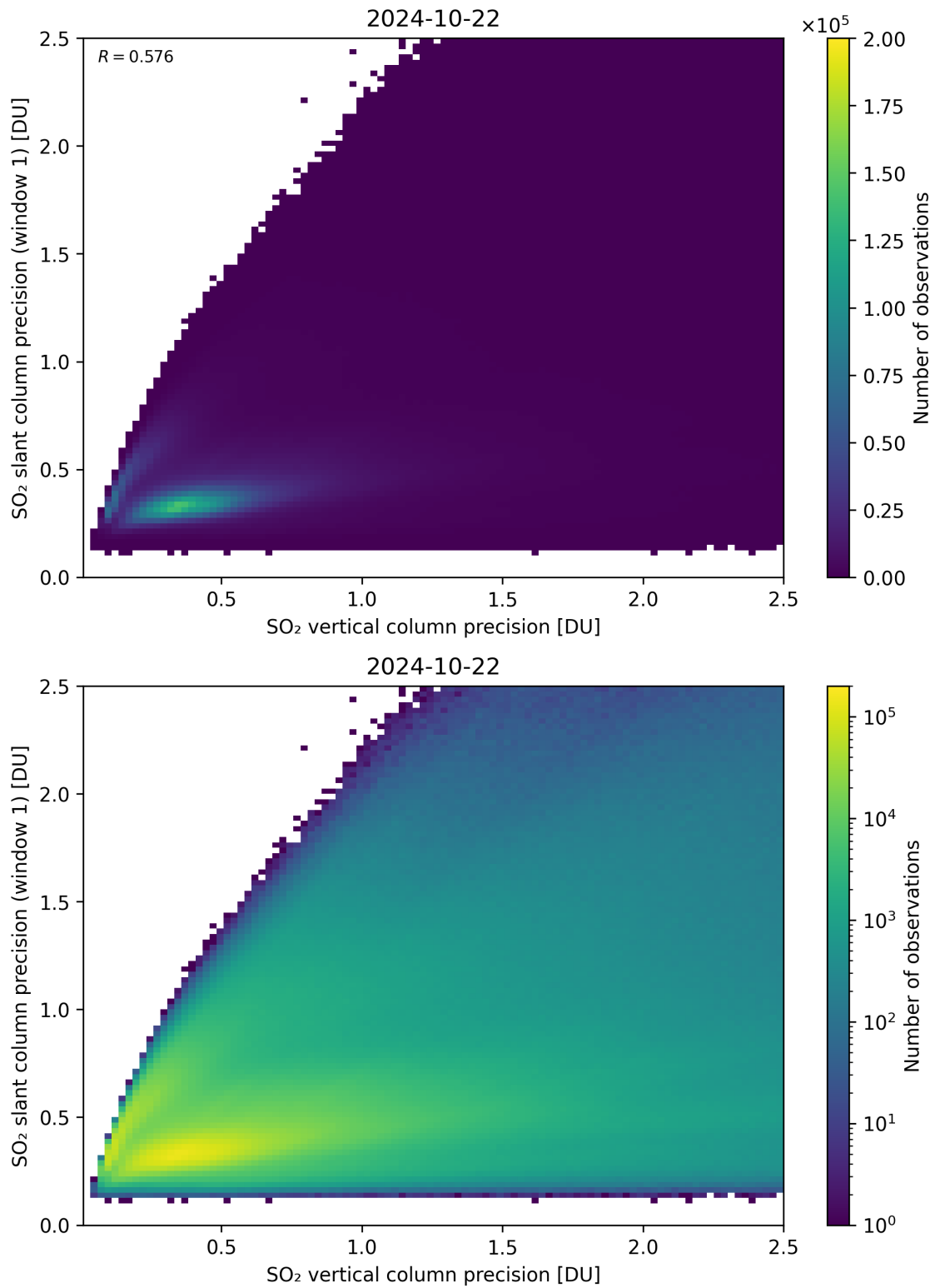
Figure 290: Scatter density plot of “SO 2 vertical column precision” against “SO 2 slant column precision (window 1)” for 2024-10-21 to 2024-10-23.
