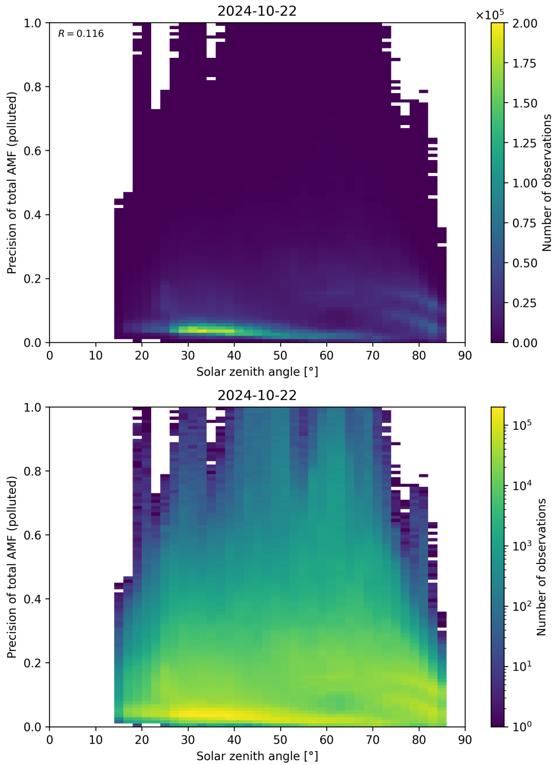
Figure 175: Scatter density plot of “Solar zenith angle” against “Precision of total AMF (polluted)” for 2024-10-21 to 2024-10-23.
