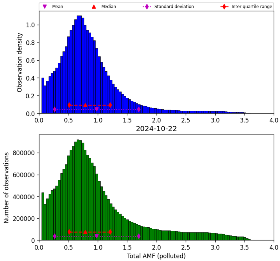
Figure 71: Histogram of “Total AMF (polluted)” for 2024-10-21 to 2024-10-23
