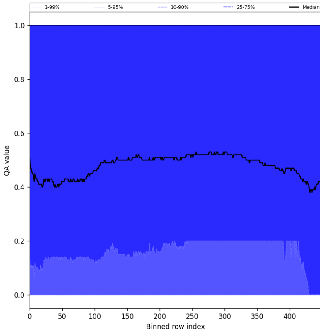
Figure 75: Along track statistics of “QA value” for 2024-10-21 to 2024-10-23
