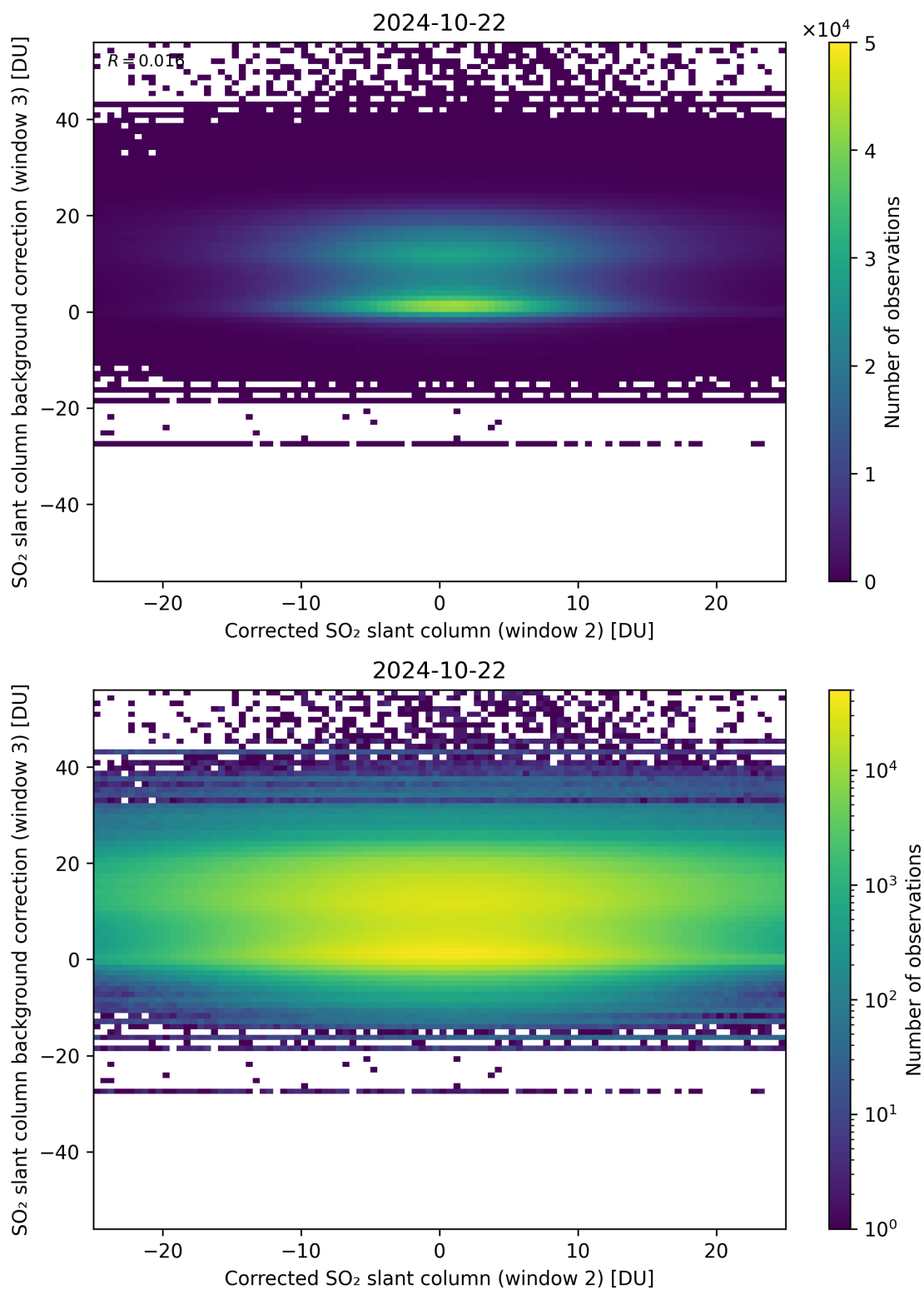
Figure 195: Scatter density plot of “Corrected SO 2 slant column (window 2)” against “SO 2 slant column background correction (window 3)” for 2024-10-21 to 2024-10-23.
