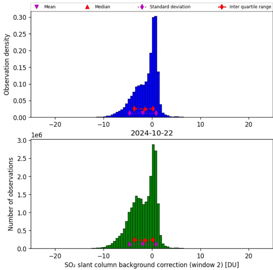
Figure 63: Histogram of “SO 2 slant column background correction (window 2)” for 2024-10-21 to 2024-10-23
