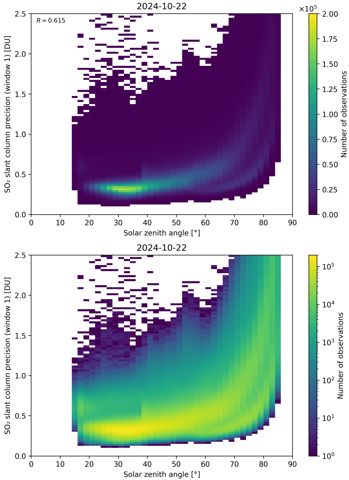
Figure 170: Scatter density plot of “Solar zenith angle” against “SO 2 slant column precision (window 1)” for 2024-10-21 to 2024-10-23.
