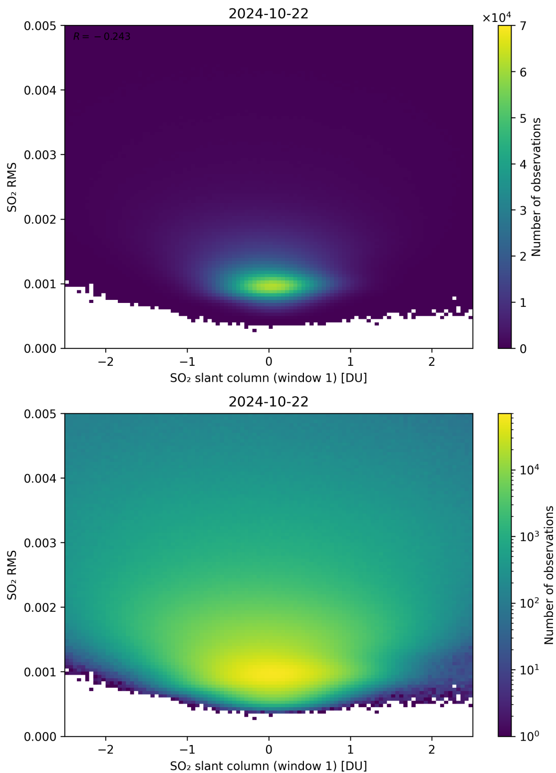
Figure 217: Scatter density plot of “SO 2 slant column (window 1)” against “SO 2 RMS” for 2024-10-21 to 2024-10-23.
