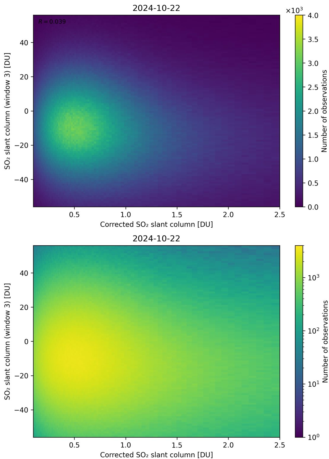
Figure 190: Scatter density plot of “Corrected SO 2 slant column” against “SO 2 slant column (window 3)” for 2024-10-21 to 2024-10-23.
