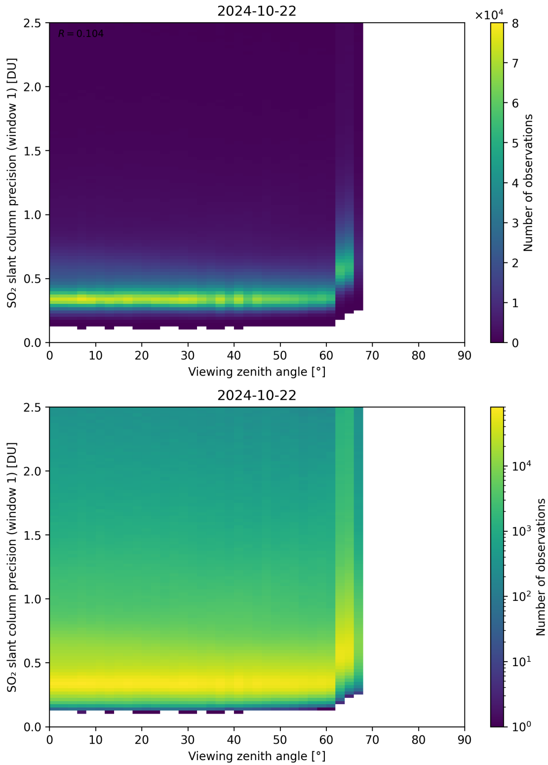
Figure 321: Scatter density plot of “Viewing zenith angle” against “SO 2 slant column precision (window 1)” for 2024-10-21 to 2024-10-23.
