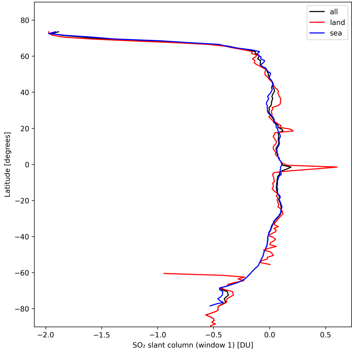
Figure 33: Zonal average of “SO 2 slant column (window 1)” for 2024-10-21 to 2024-10-23.
