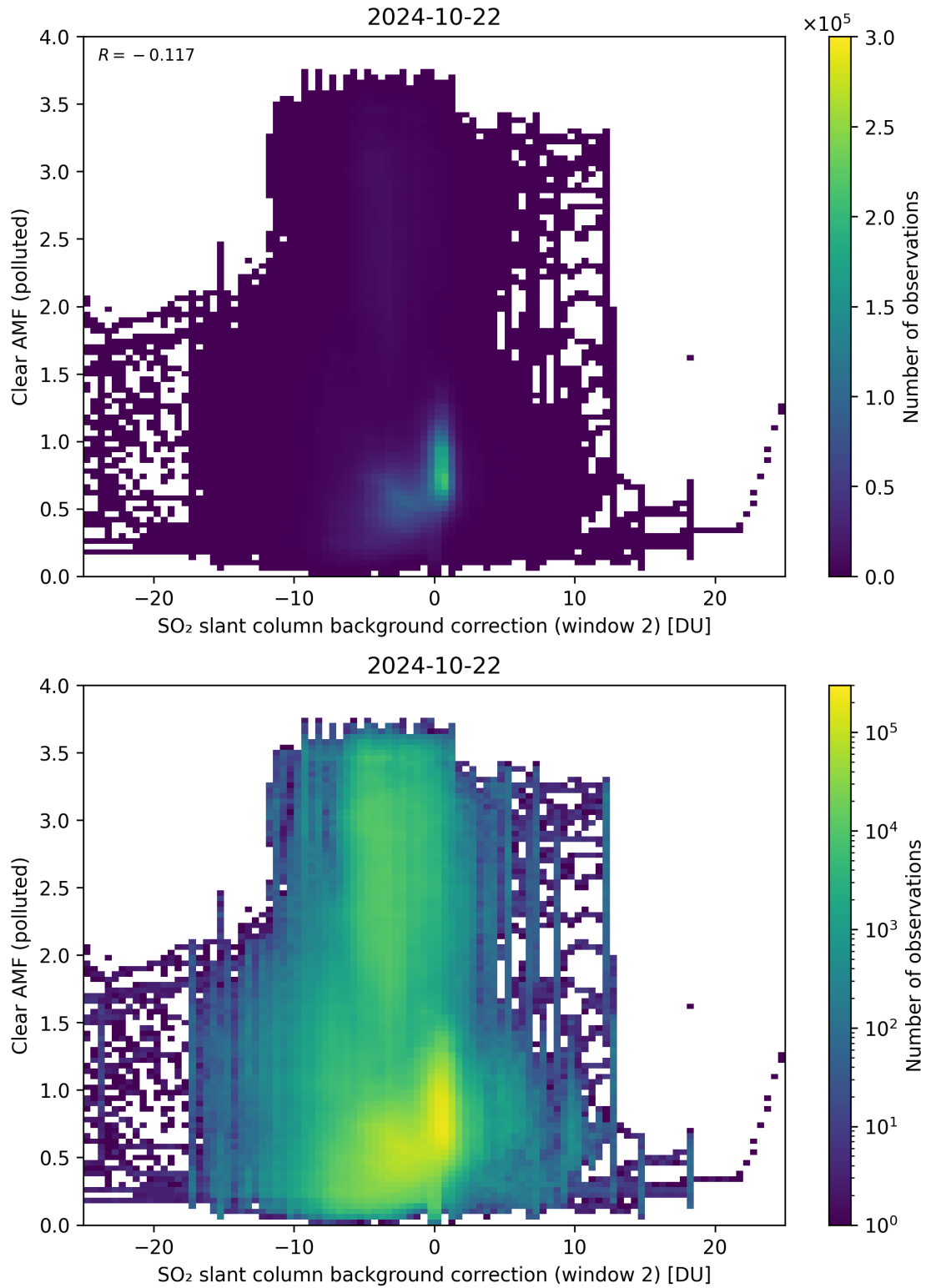
Figure 115: Scatter density plot of “SO 2 slant column background correction (window 2)” against “Clear AMF (polluted)” for 2024-10-21 to 2024-10-23.
