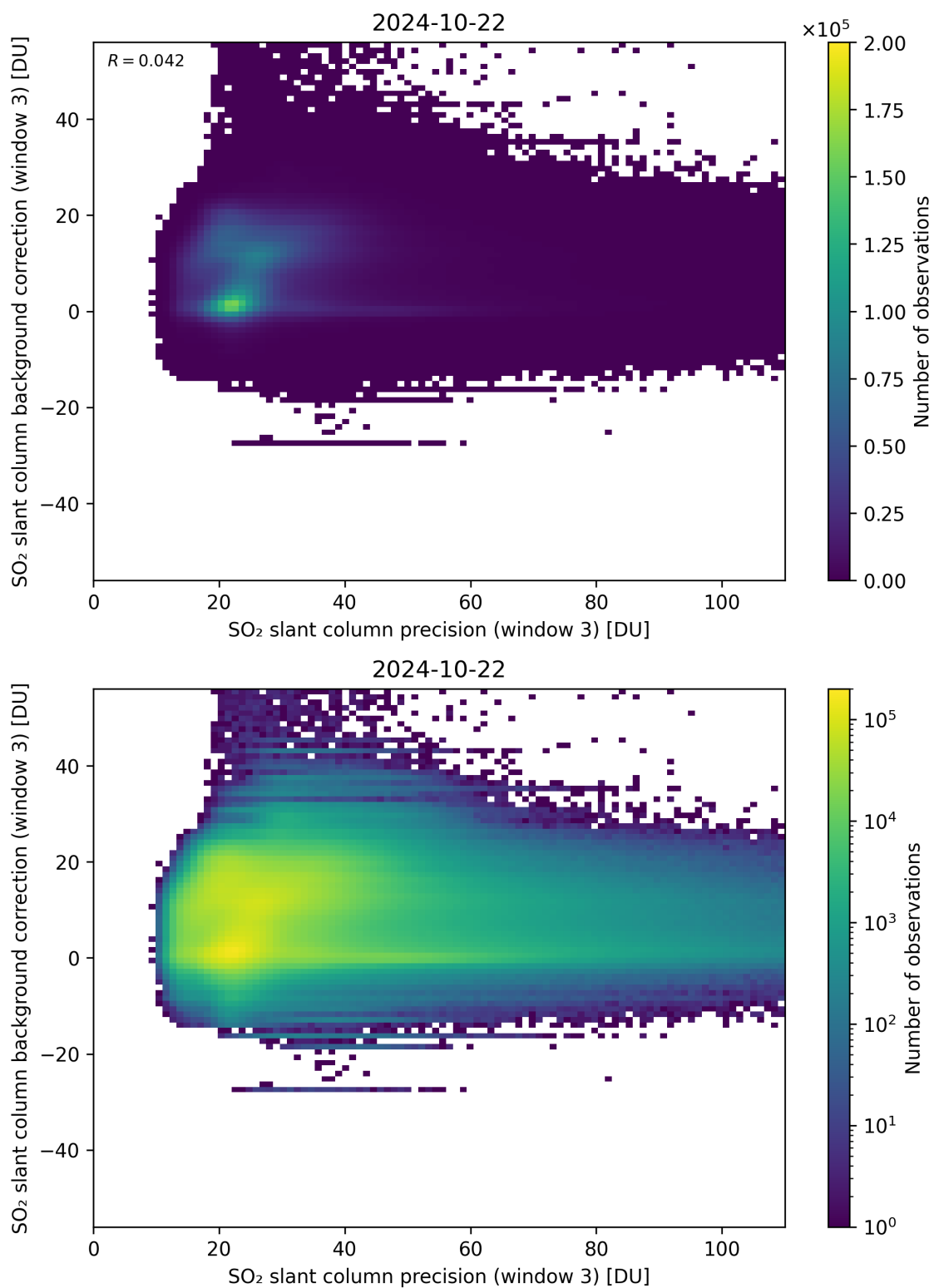
Figure 257: Scatter density plot of “SO 2 slant column precision (window 3)” against “SO 2 slant column background correction (window 3)” for 2024-10-21 to 2024-10-23.
