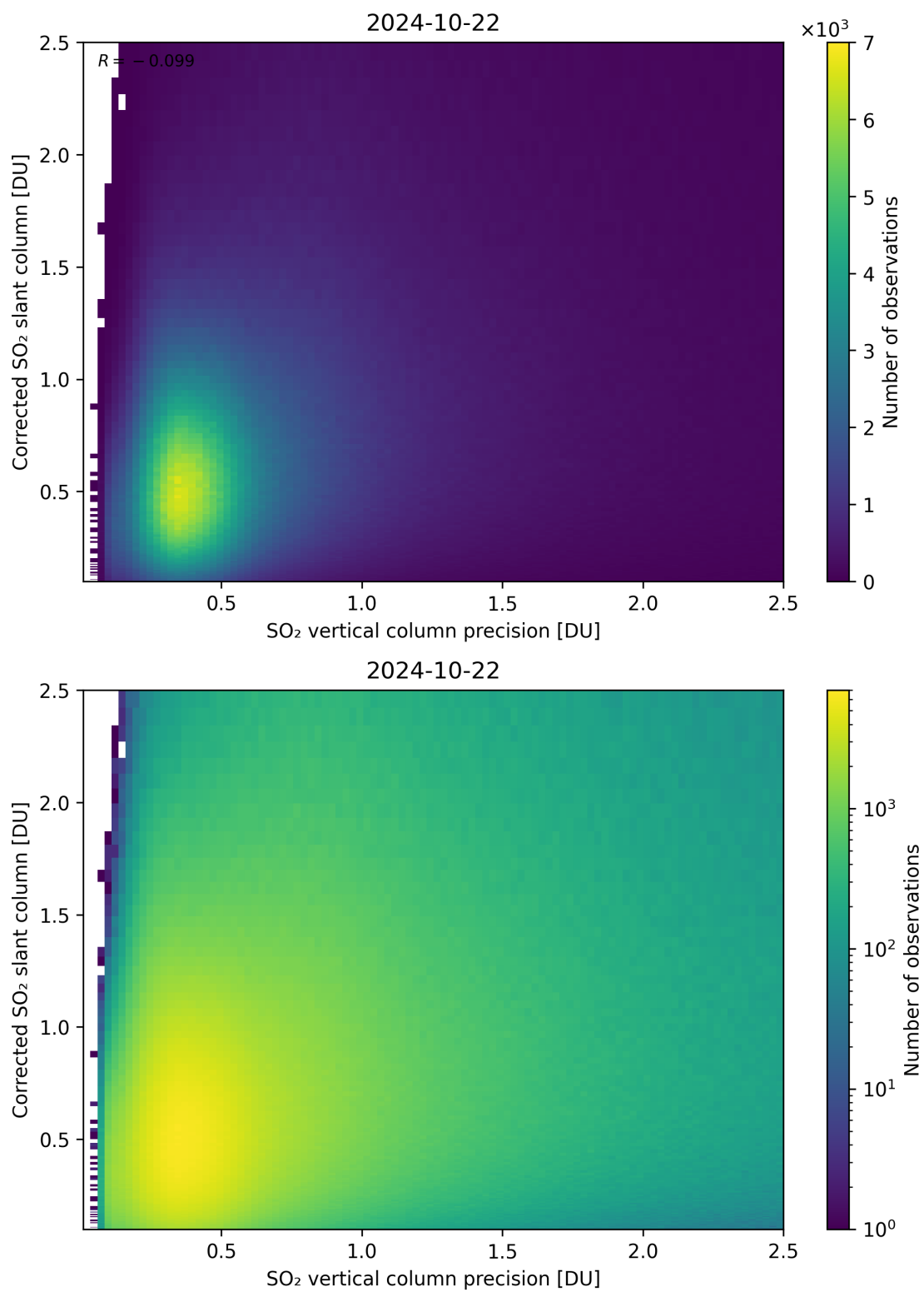
Figure 286: Scatter density plot of “SO 2 vertical column precision” against “Corrected SO 2 slant column” for 2024-10-21 to 2024-10-23.
