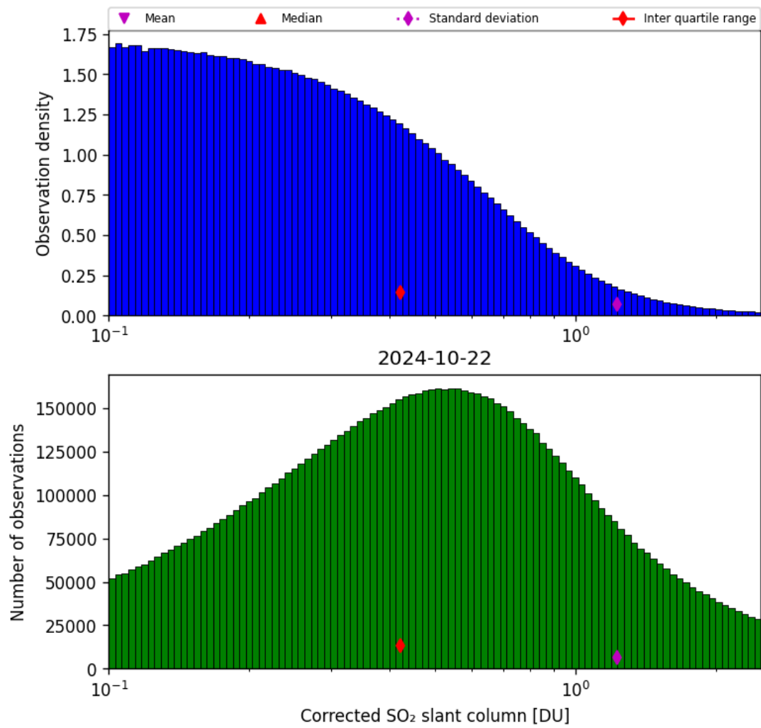
Figure 55: Histogram of “Corrected SO 2 slant column” for 2024-10-21 to 2024-10-23
