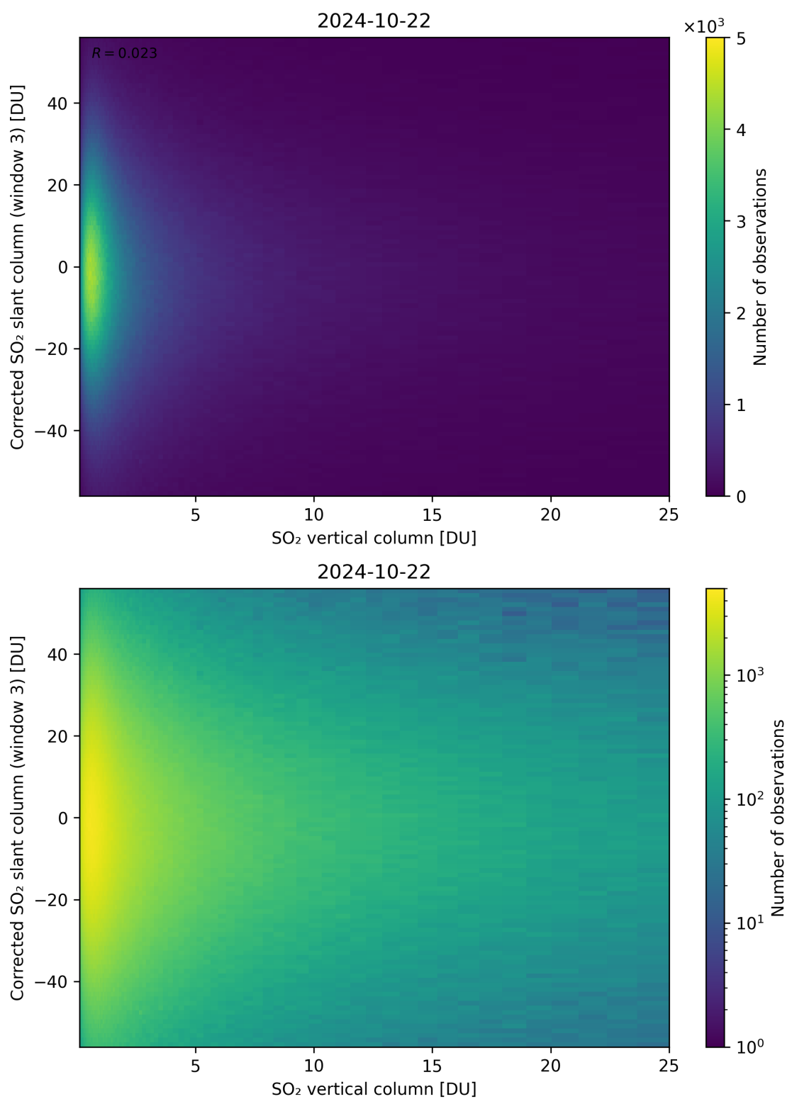
Figure 299: Scatter density plot of “SO 2 vertical column” against “Corrected SO 2 slant column (window 3)” for 2024-10-21 to 2024-10-23.
