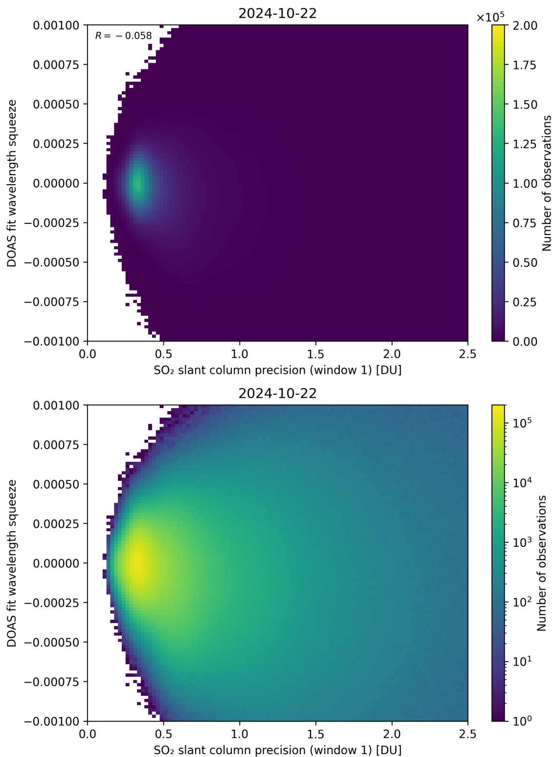
Figure 222: Scatter density plot of “SO 2 slant column precision (window 1)” against “DOAS fit wavelength squeeze” for 2024-10-21 to 2024-10-23.
