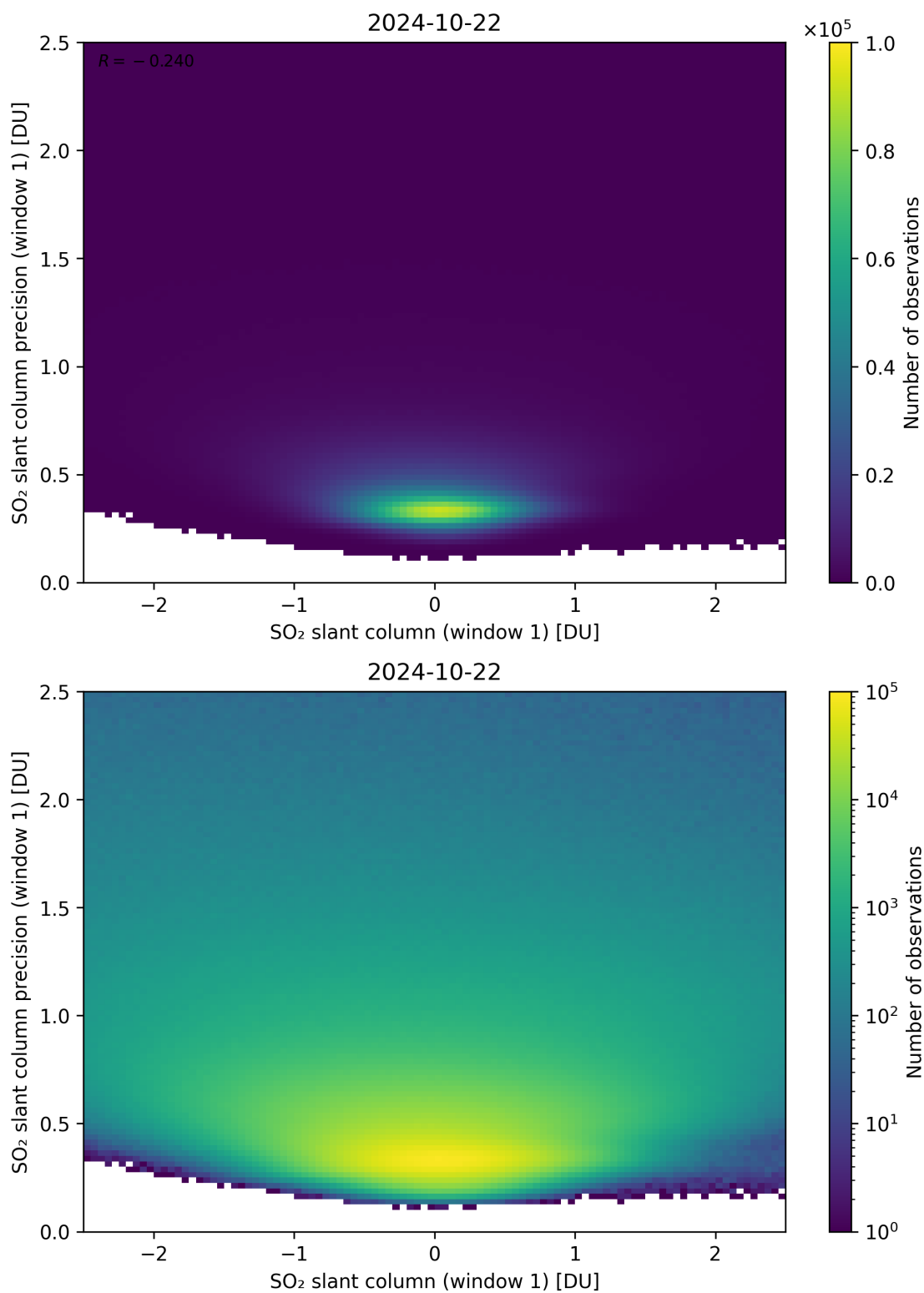
Figure 235: Scatter density plot of “SO 2 slant column (window 1)” against “SO 2 slant column precision (window 1)” for 2024-10-21 to 2024-10-23.
