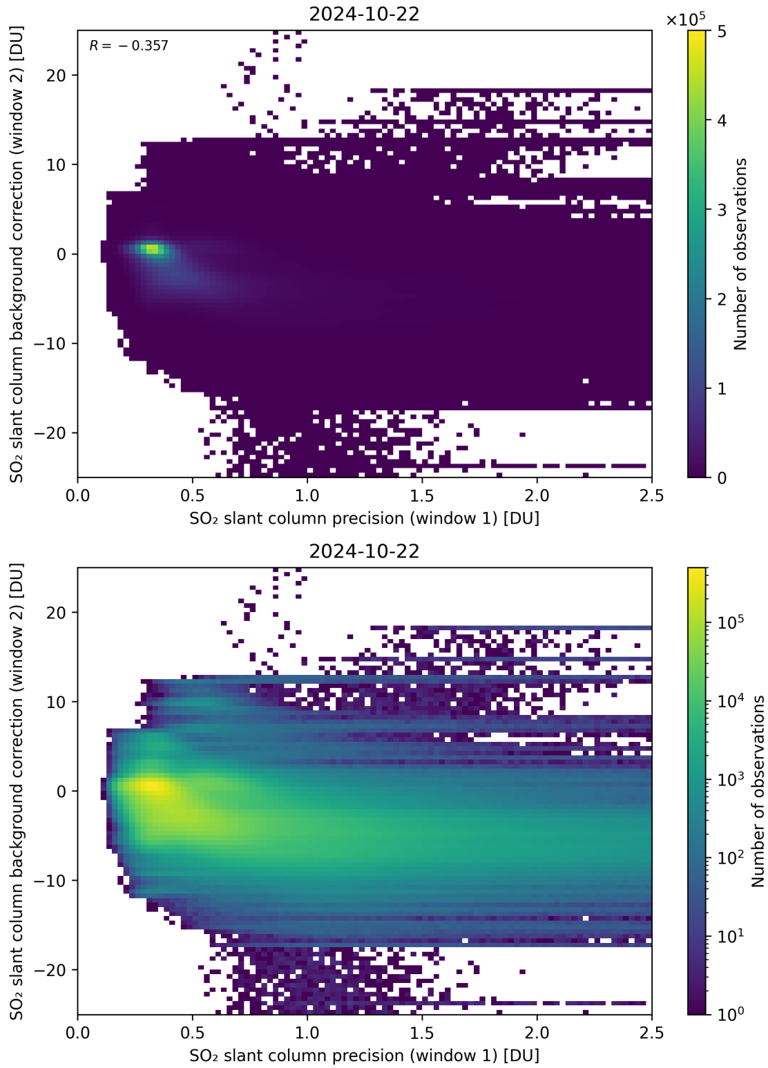
Figure 219: Scatter density plot of “SO 2 slant column precision (window 1)” against “SO 2 slant column background correction (window 2)” for 2024-10-21 to 2024-10-23.
