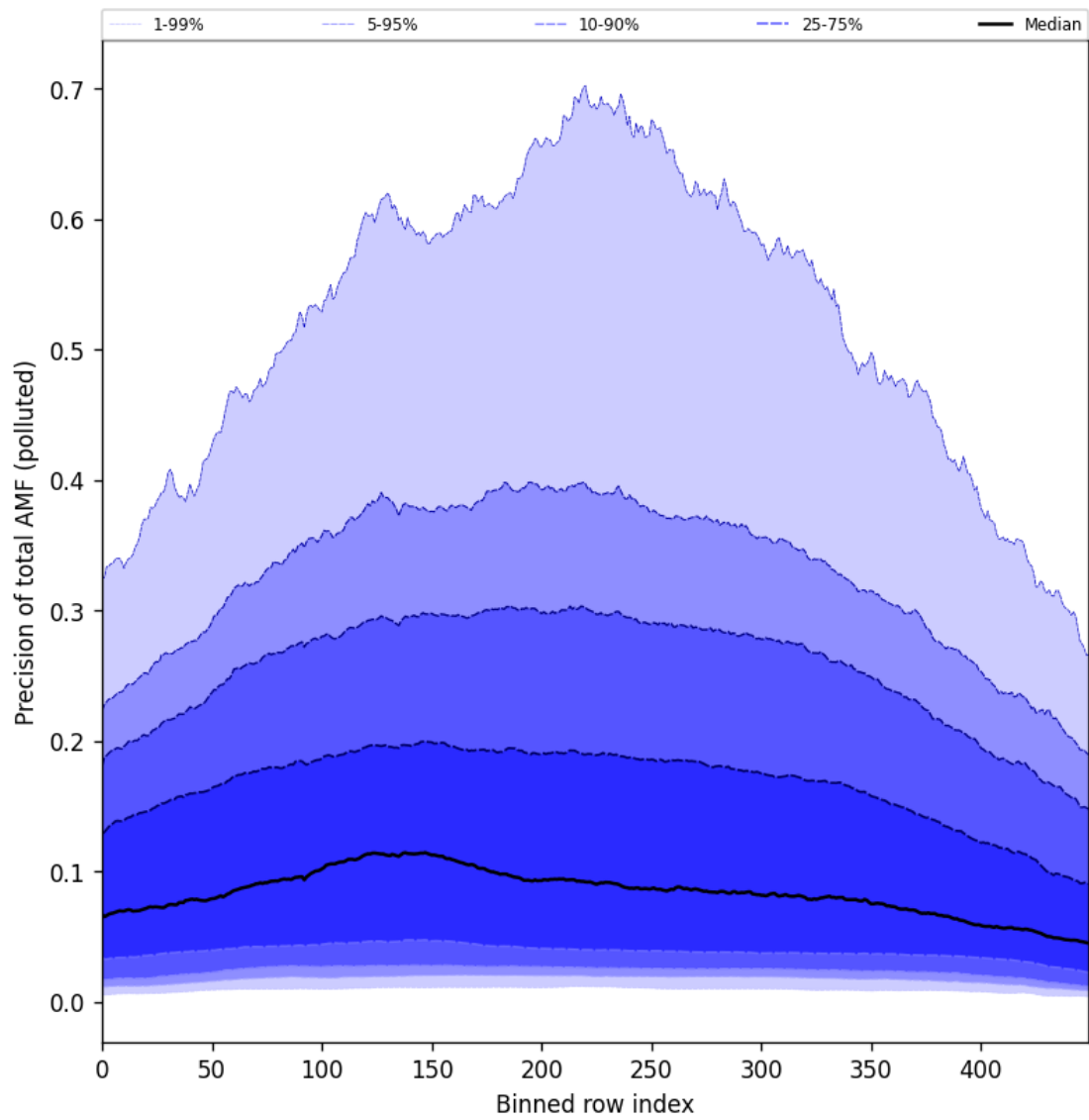
Figure 95: Along track statistics of “Precision of total AMF (polluted)” for 2024-10-21 to 2024-10-23
