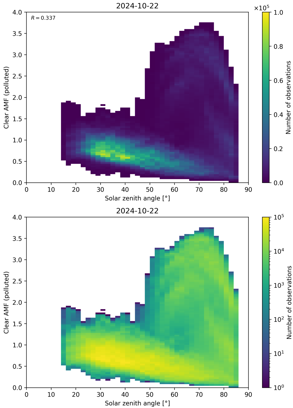
Figure 165: Scatter density plot of “Solar zenith angle” against “Clear AMF (polluted)” for 2024-10-21 to 2024-10-23.
