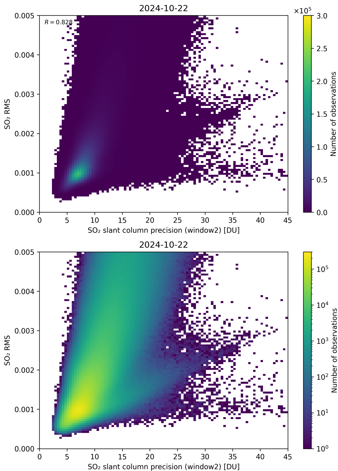
Figure 245: Scatter density plot of “SO 2 slant column precision (window2)” against “SO 2 RMS” for 2024-10-21 to 2024-10-23.
