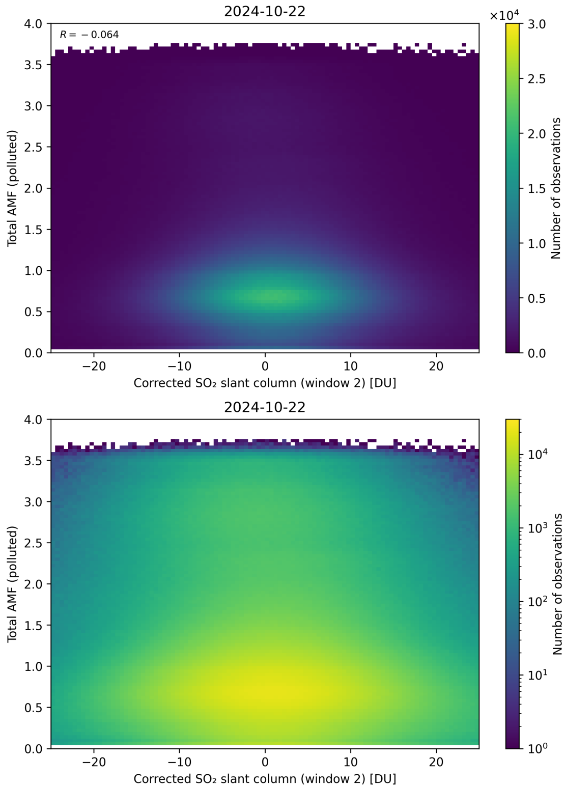
Figure 203: Scatter density plot of “Corrected SO 2 slant column (window 2)” against “Total AMF (polluted)” for 2024-10-21 to 2024-10-23.
