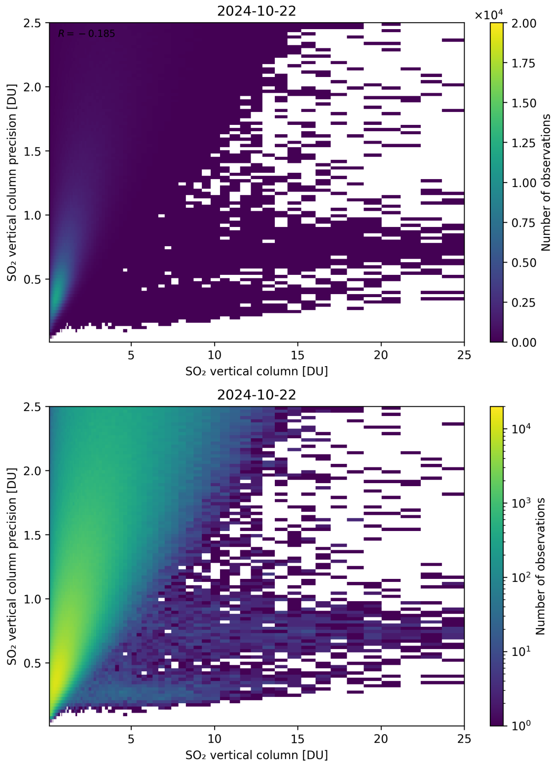
Figure 307: Scatter density plot of “SO 2 vertical column” against “SO 2 vertical column precision” for 2024-10-21 to 2024-10-23.
