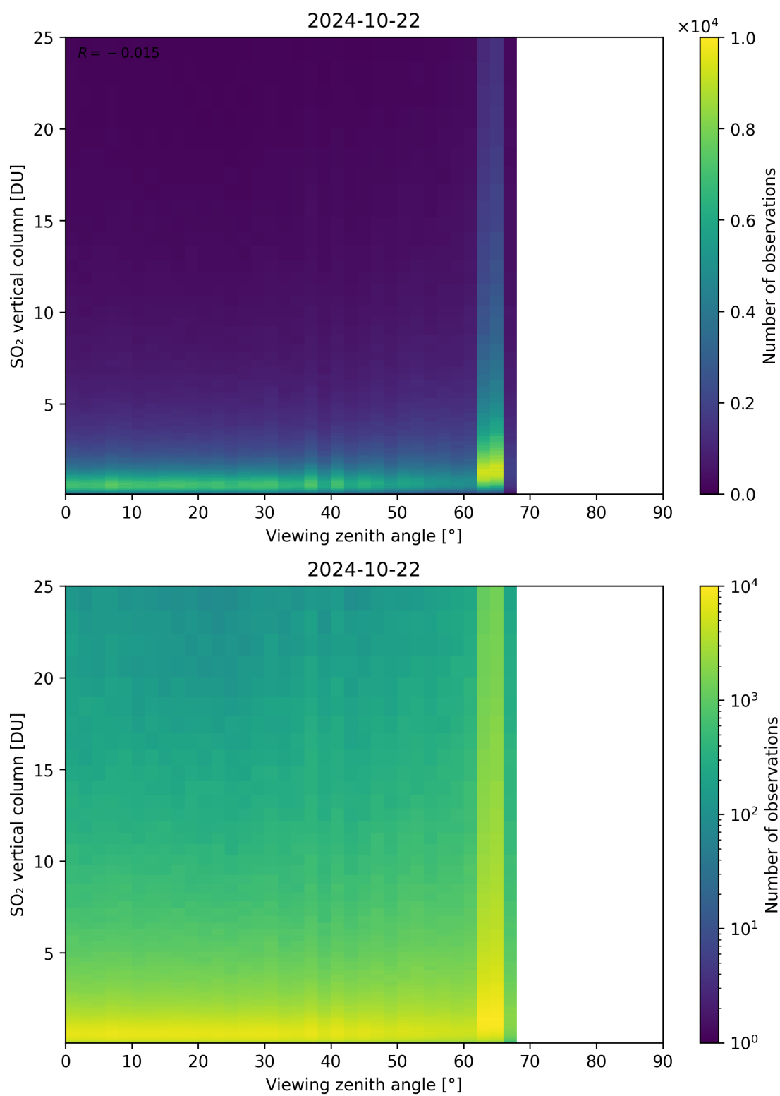
Figure 327: Scatter density plot of “Viewing zenith angle” against “SO 2 vertical column” for 2024-10-21 to 2024-10-23.
