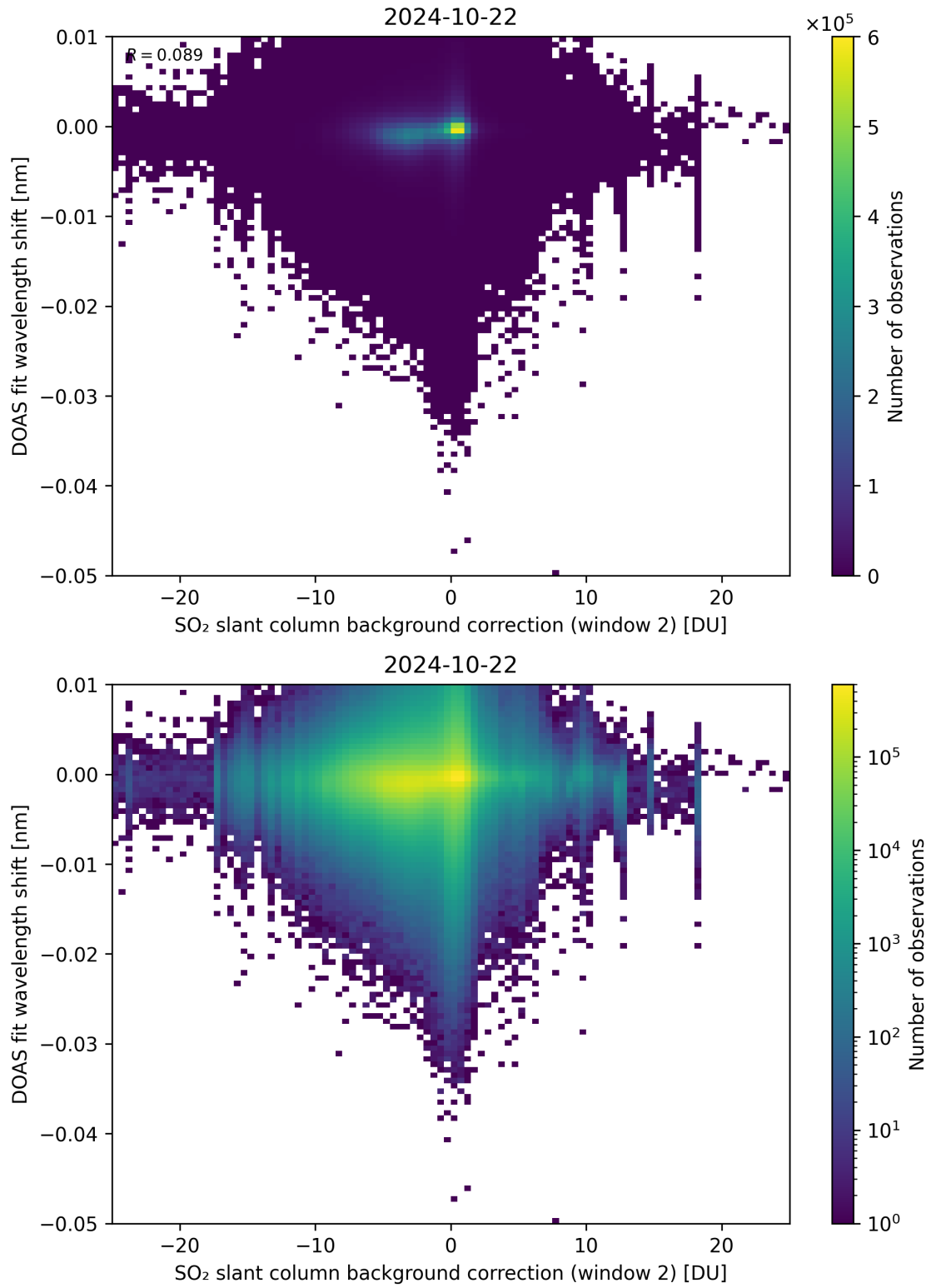
Figure 112: Scatter density plot of “SO 2 slant column background correction (window 2)” against “DOAS fit wavelength shift” for 2024-10-21 to 2024-10-23.
