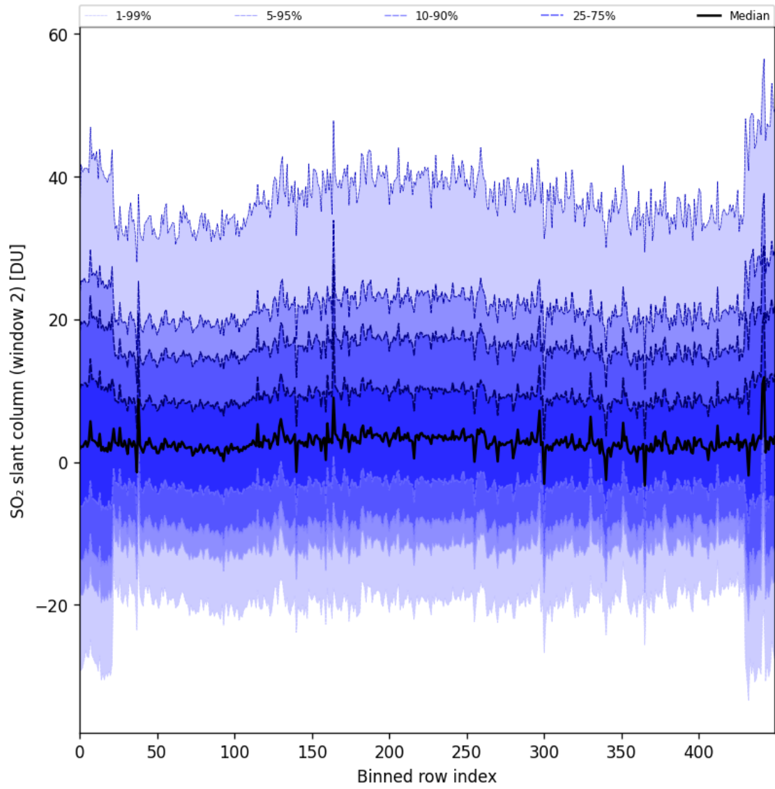
Figure 83: Along track statistics of “SO 2 slant column (window 2)” for 2024-10-21 to 2024-10-23
