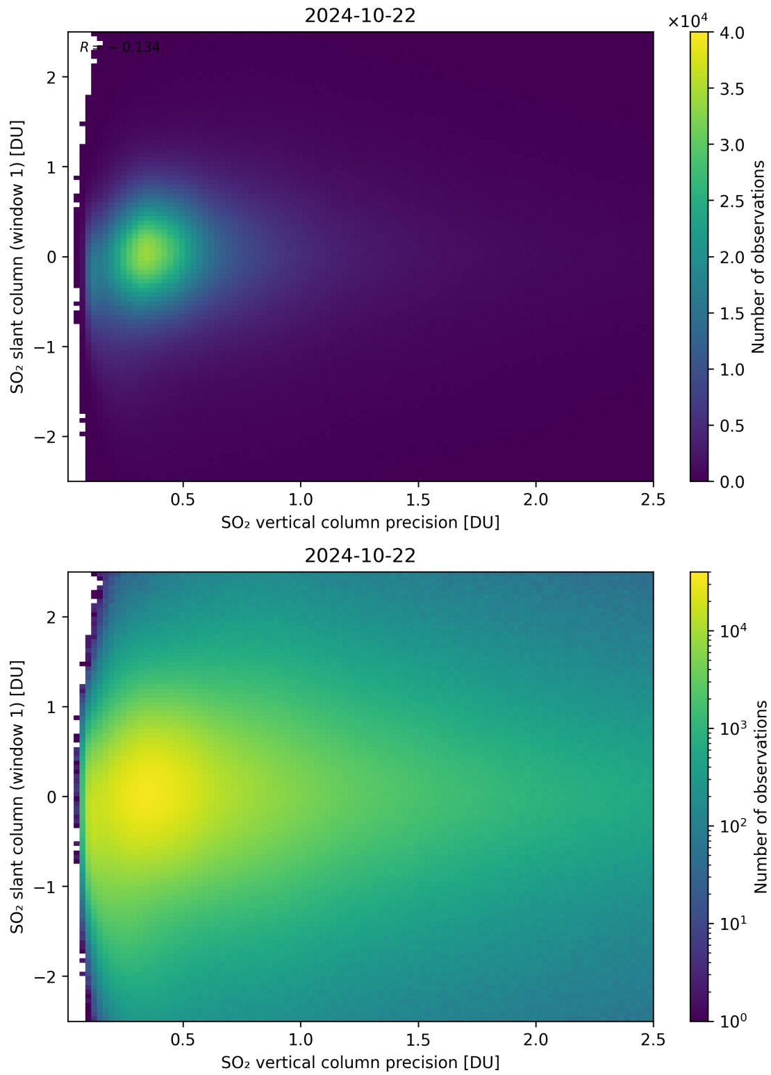
Figure 289: Scatter density plot of “SO 2 vertical column precision” against “SO 2 slant column (window 1)” for 2024-10-21 to 2024-10-23.
