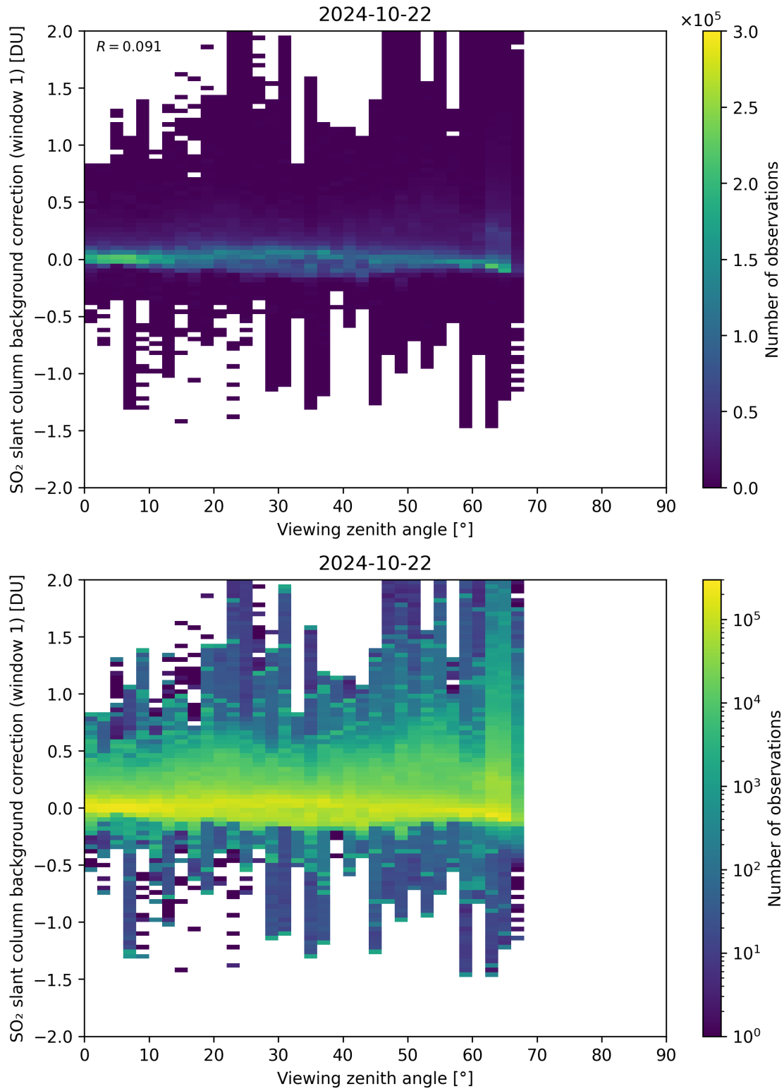
Figure 308: Scatter density plot of “Viewing zenith angle” against “SO 2 slant column background correction (window 1)” for 2024-10-21 to 2024-10-23.
