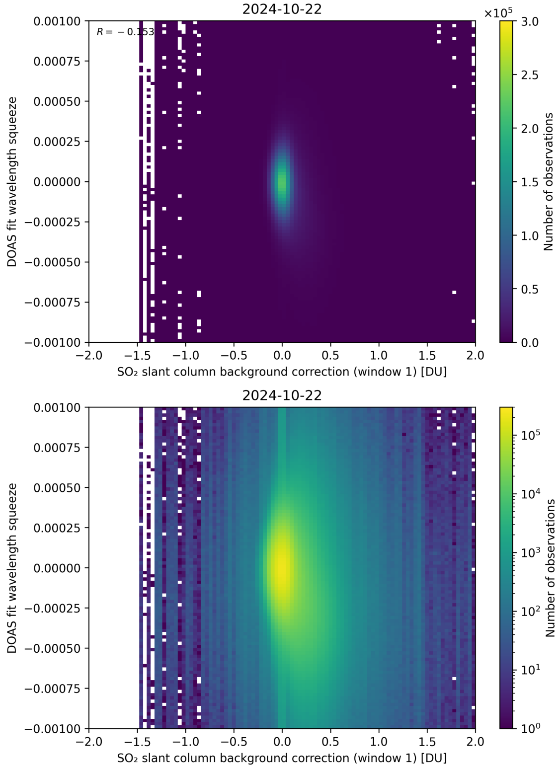
Figure 101: Scatter density plot of “SO 2 slant column background correction (window 1)” against “DOAS fit wavelength squeeze” for 2024-10-21 to 2024-10-23.
