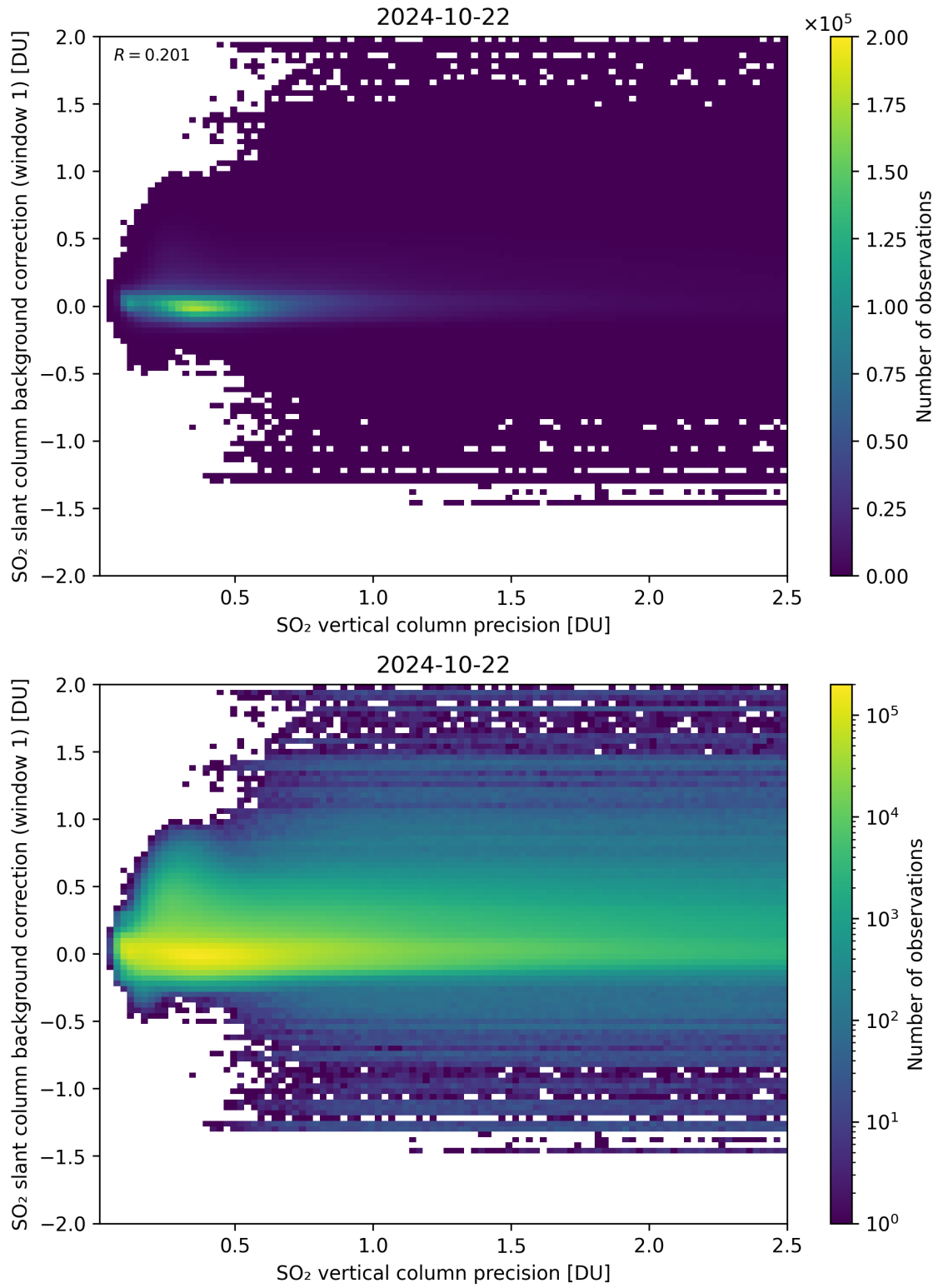
Figure 279: Scatter density plot of “SO 2 vertical column precision” against “SO 2 slant column background correction (window 1)” for 2024-10-21 to 2024-10-23.
