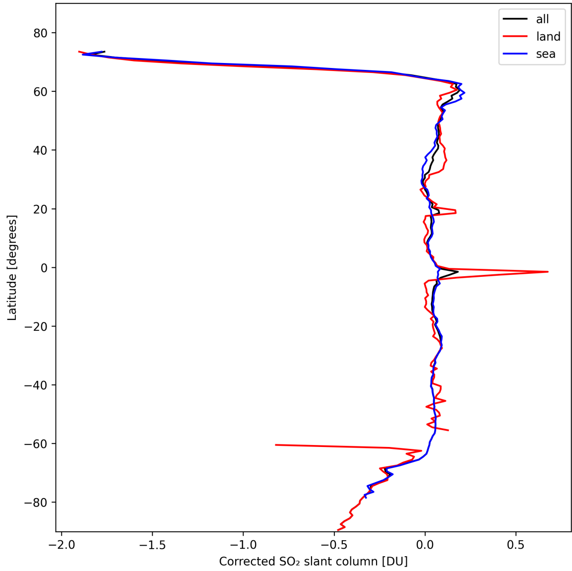
Figure 32: Zonal average of “Corrected SO 2 slant column” for 2024-10-21 to 2024-10-23.
