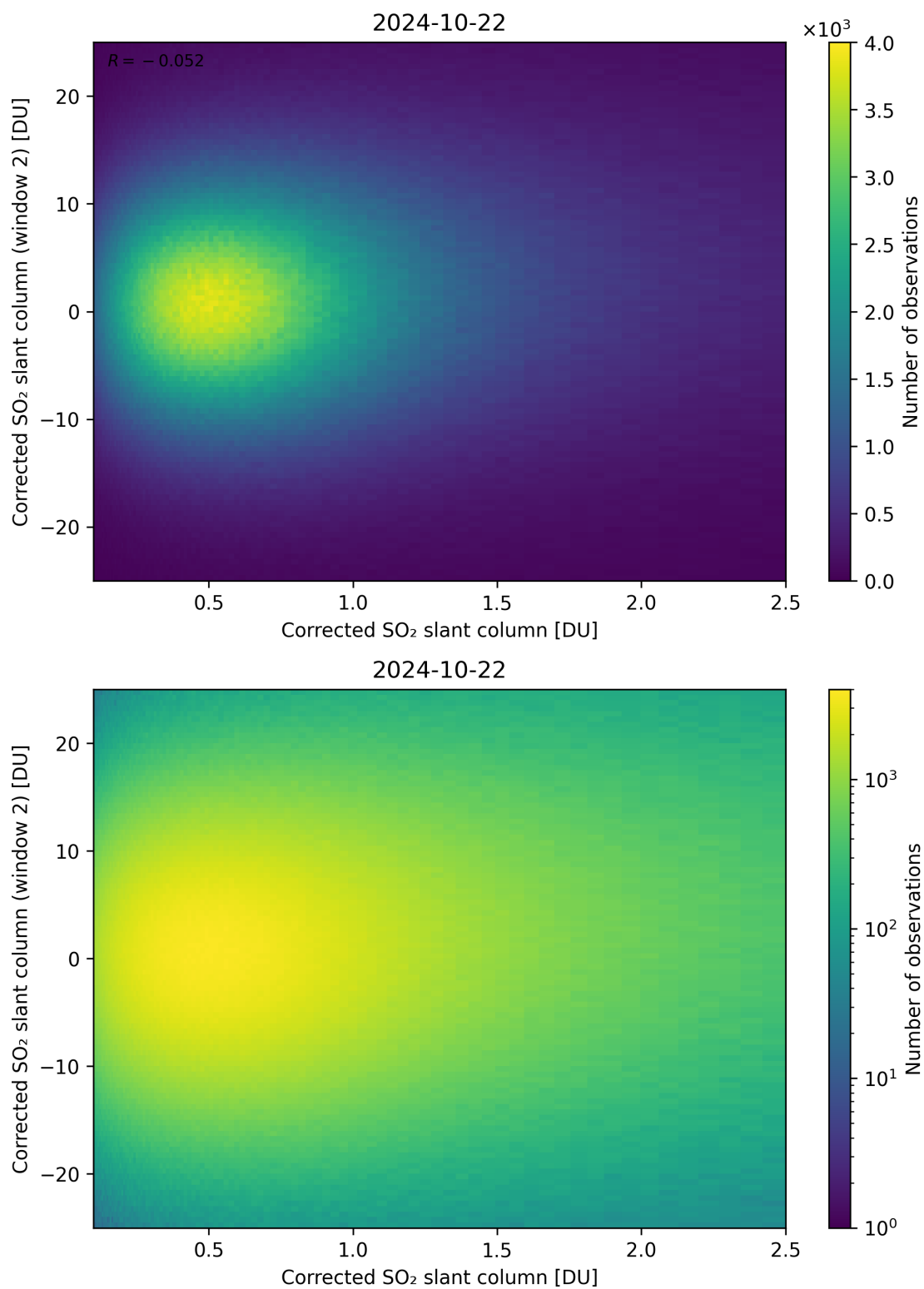
Figure 185: Scatter density plot of “Corrected SO 2 slant column” against “Corrected SO 2 slant column (window 2)” for 2024-10-21 to 2024-10-23.
