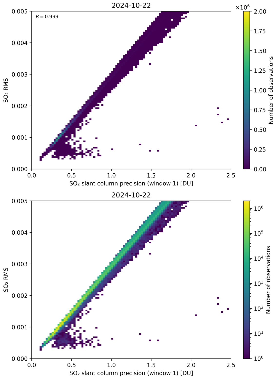
Figure 223: Scatter density plot of “SO 2 slant column precision (window 1)” against “SO 2 RMS” for 2024-10-21 to 2024-10-23.
