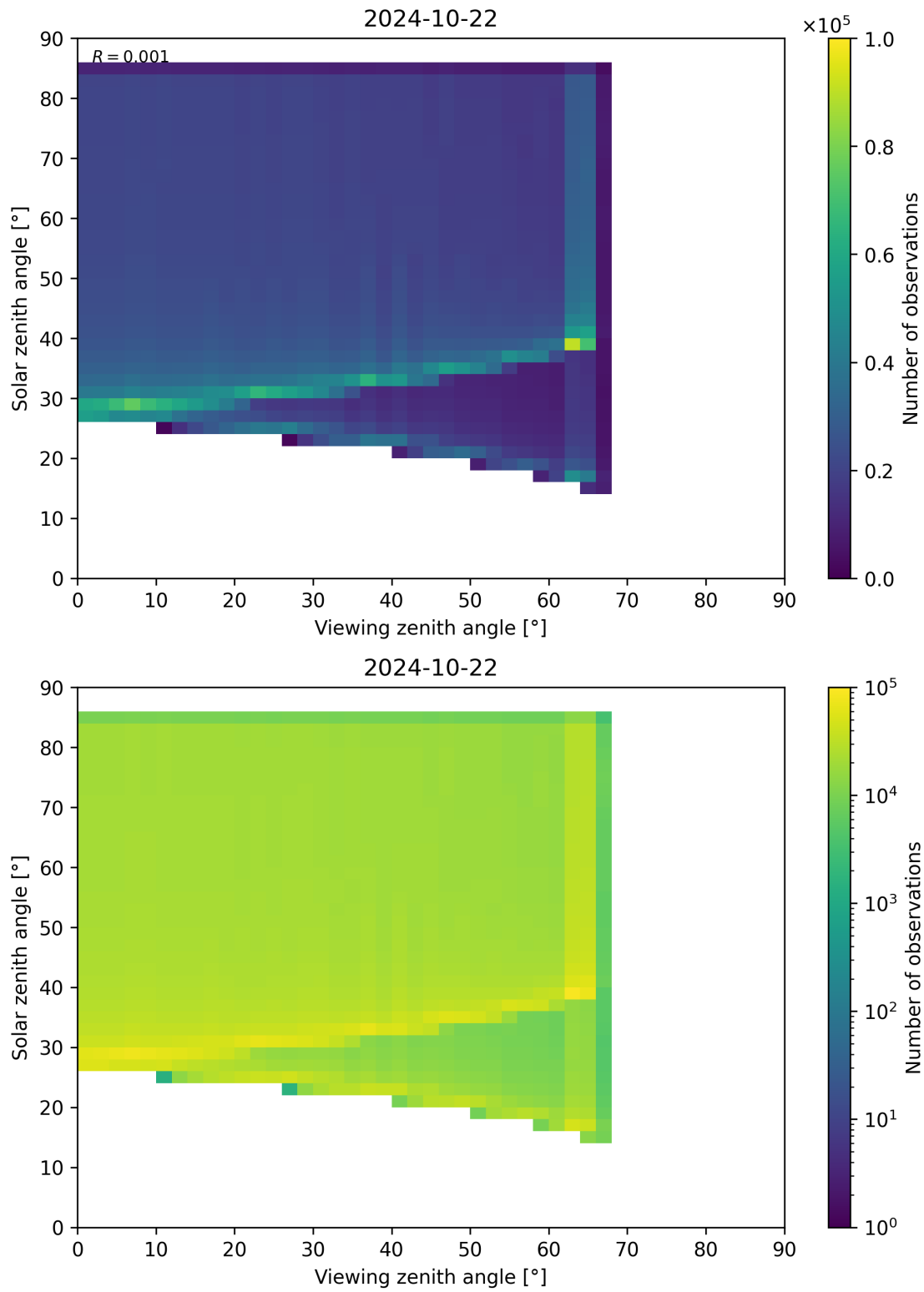
Figure 315: Scatter density plot of “Viewing zenith angle” against “Solar zenith angle” for 2024-10-21 to 2024-10-23.
