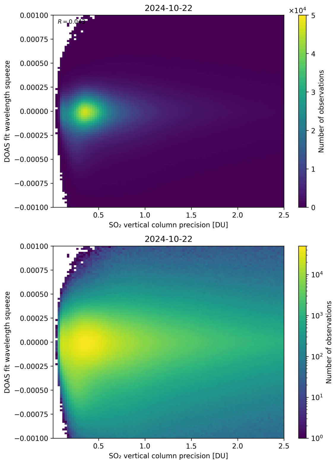
Figure 283: Scatter density plot of “SO 2 vertical column precision” against “DOAS fit wavelength squeeze” for 2024-10-21 to 2024-10-23.
