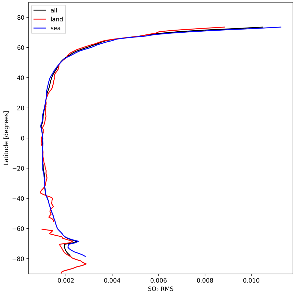
Figure 47: Zonal average of “SO 2 RMS” for 2024-10-21 to 2024-10-23.
