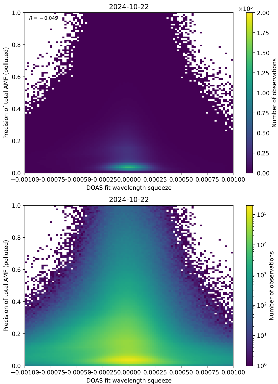
Figure 135: Scatter density plot of “DOAS fit wavelength squeeze” against “Precision of total AMF (polluted)” for 2024-10-21 to 2024-10-23.
