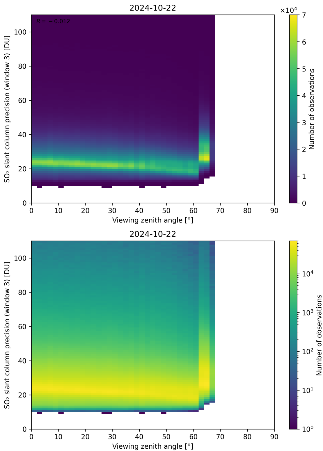
Figure 324: Scatter density plot of “Viewing zenith angle” against “SO 2 slant column precision (window 3)” for 2024-10-21 to 2024-10-23.
