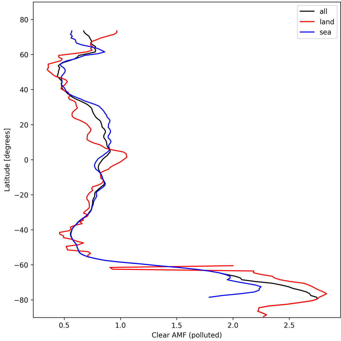
Figure 50: Zonal average of “Clear AMF (polluted)” for 2024-10-21 to 2024-10-23.
