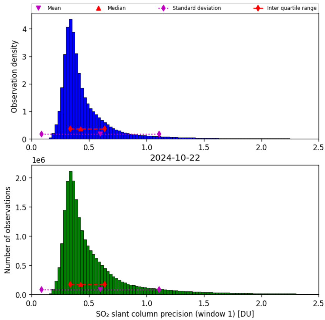
Figure 57: Histogram of “SO 2 slant column precision (window 1)” for 2024-10-21 to 2024-10-23
