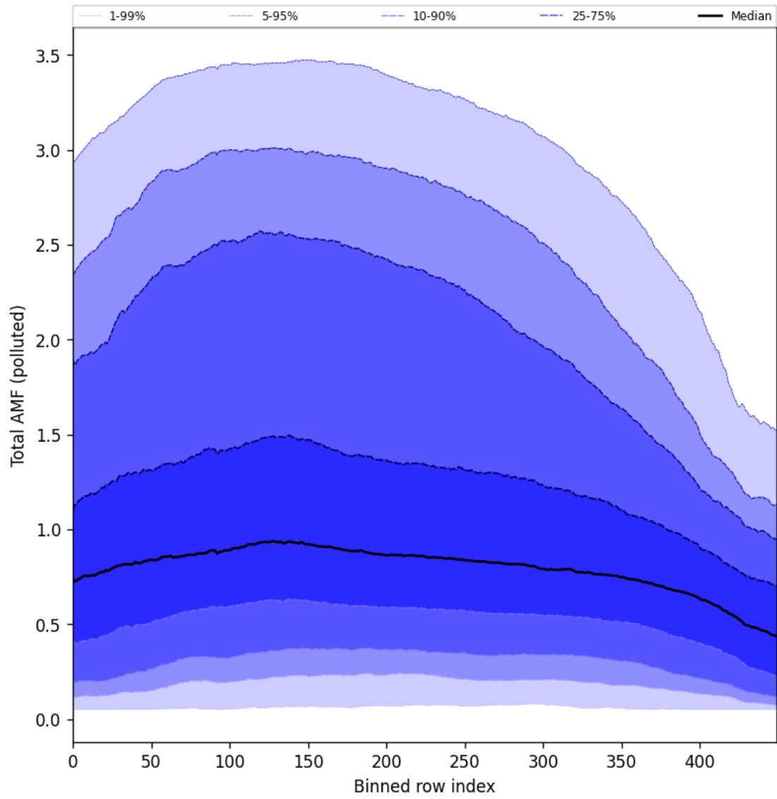
Figure 94: Along track statistics of “Total AMF (polluted)” for 2024-10-21 to 2024-10-23
