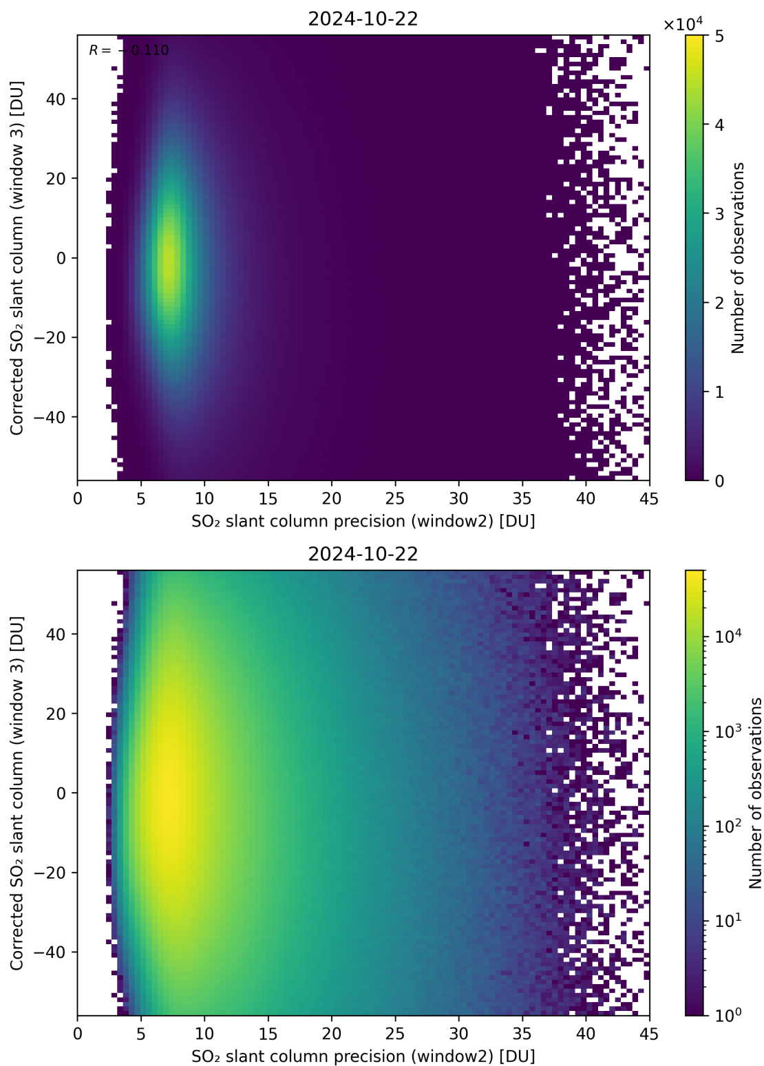
Figure 248: Scatter density plot of “SO 2 slant column precision (window2)” against “Corrected SO 2 slant column (window 3)” for 2024-10-21 to 2024-10-23.
