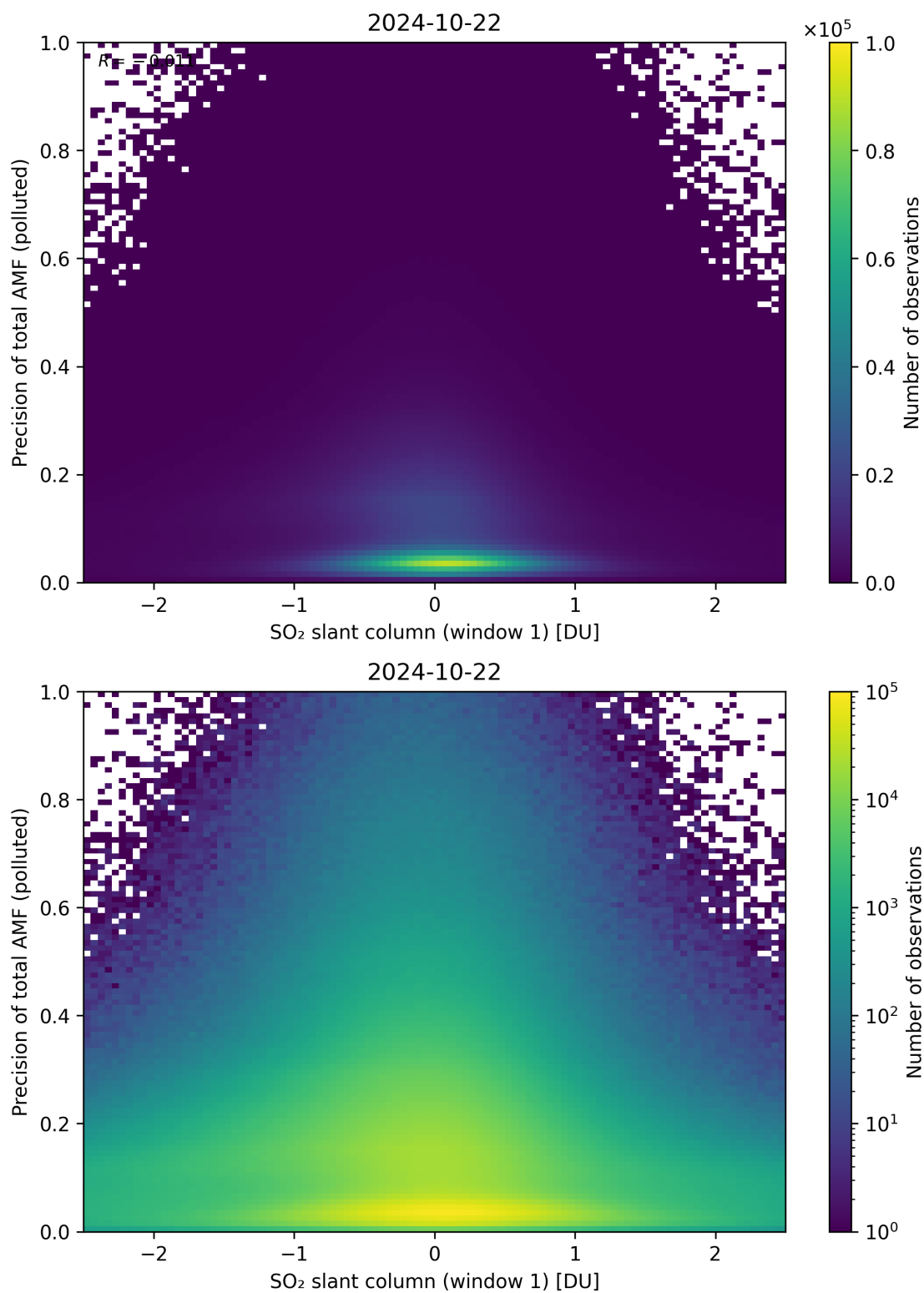
Figure 240: Scatter density plot of “SO 2 slant column (window 1)” against “Precision of total AMF (polluted)” for 2024-10-21 to 2024-10-23.
