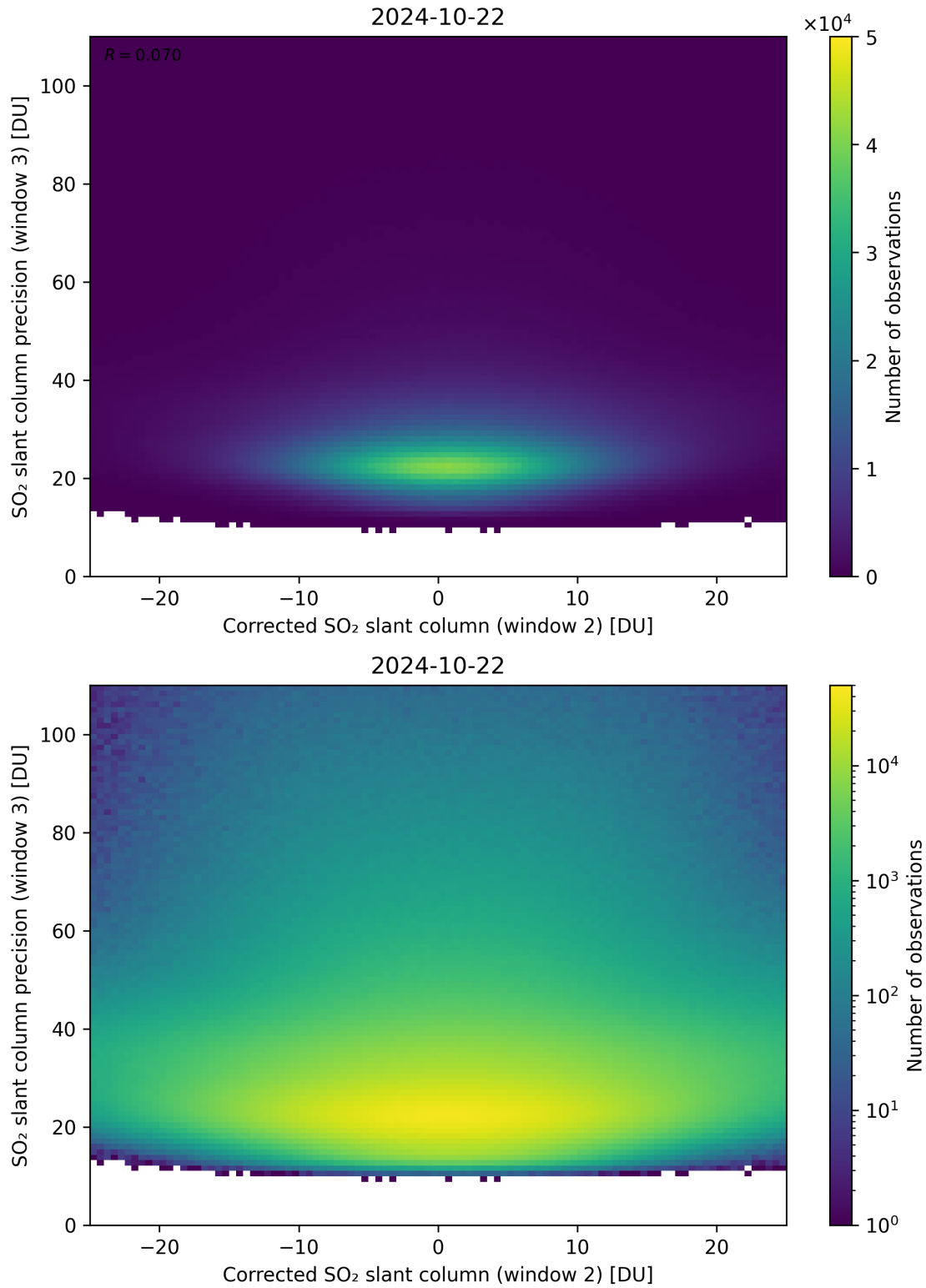
Figure 202: Scatter density plot of “Corrected SO 2 slant column (window 2)” against “SO 2 slant column precision (window 3)” for 2024-10-21 to 2024-10-23.
