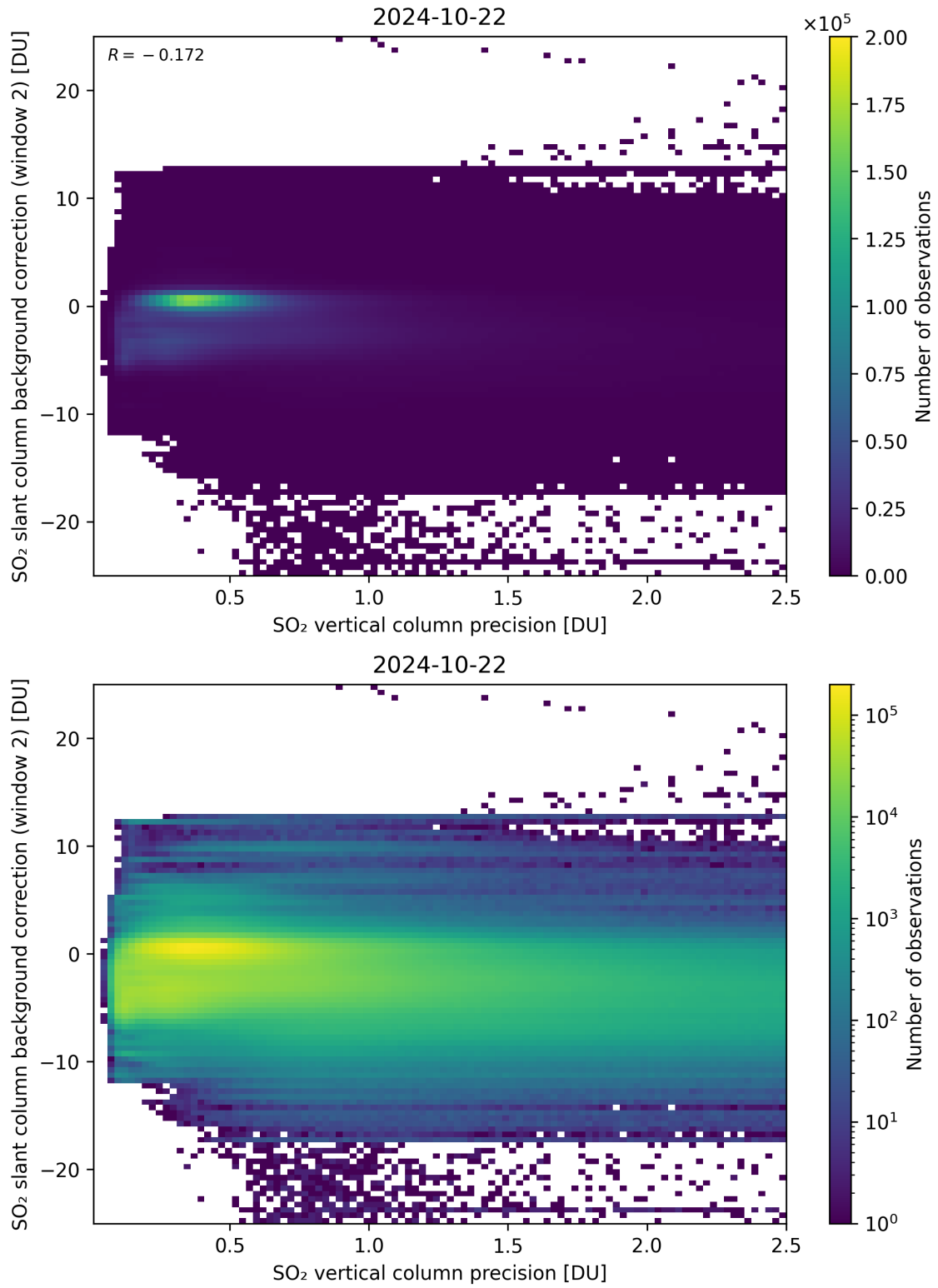
Figure 280: Scatter density plot of “SO 2 vertical column precision” against “SO 2 slant column background correction (window 2)” for 2024-10-21 to 2024-10-23.
