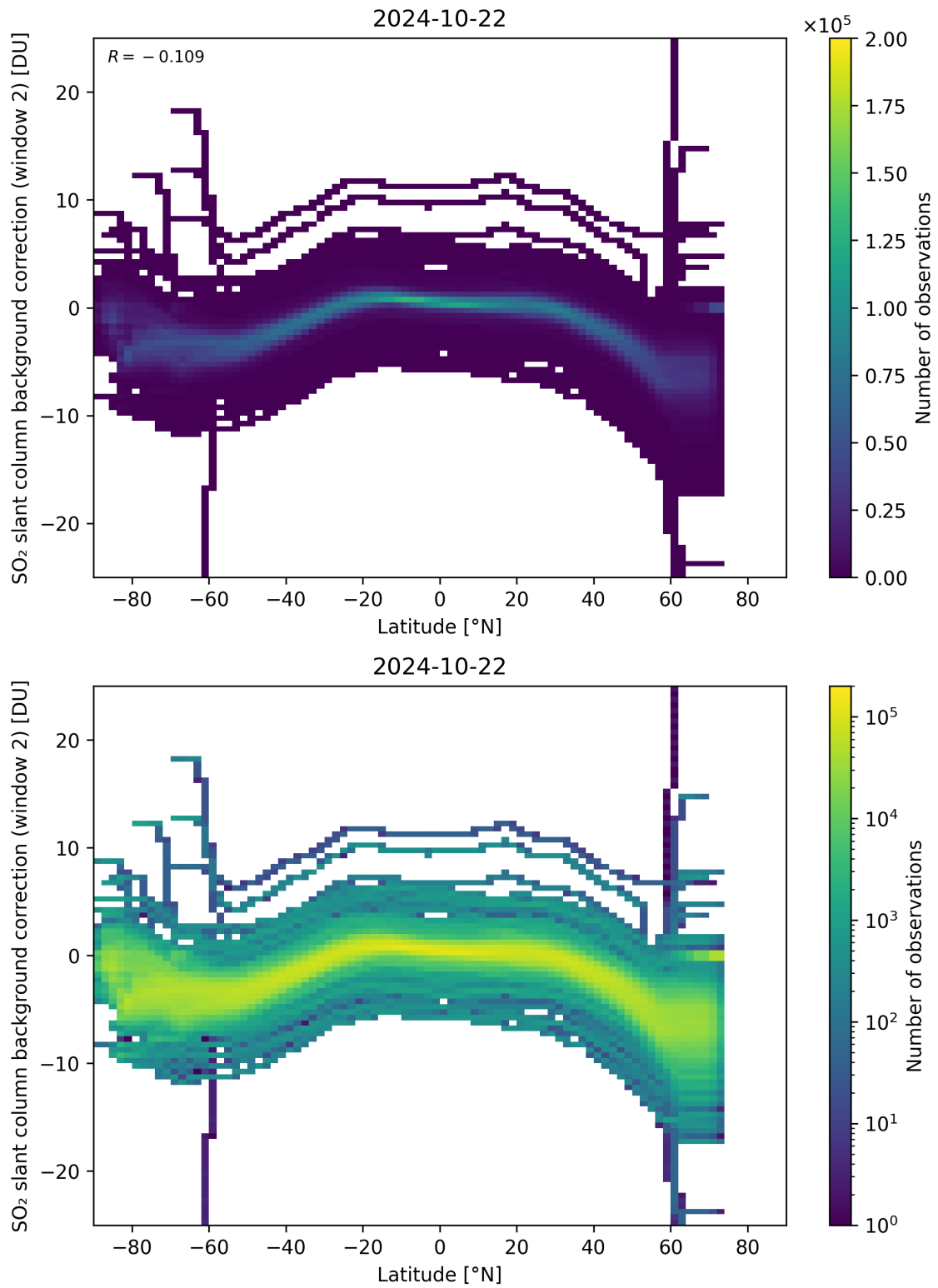
Figure 140: Scatter density plot of “Latitude” against “SO 2 slant column background correction (window 2)” for 2024-10-21 to 2024-10-23.
