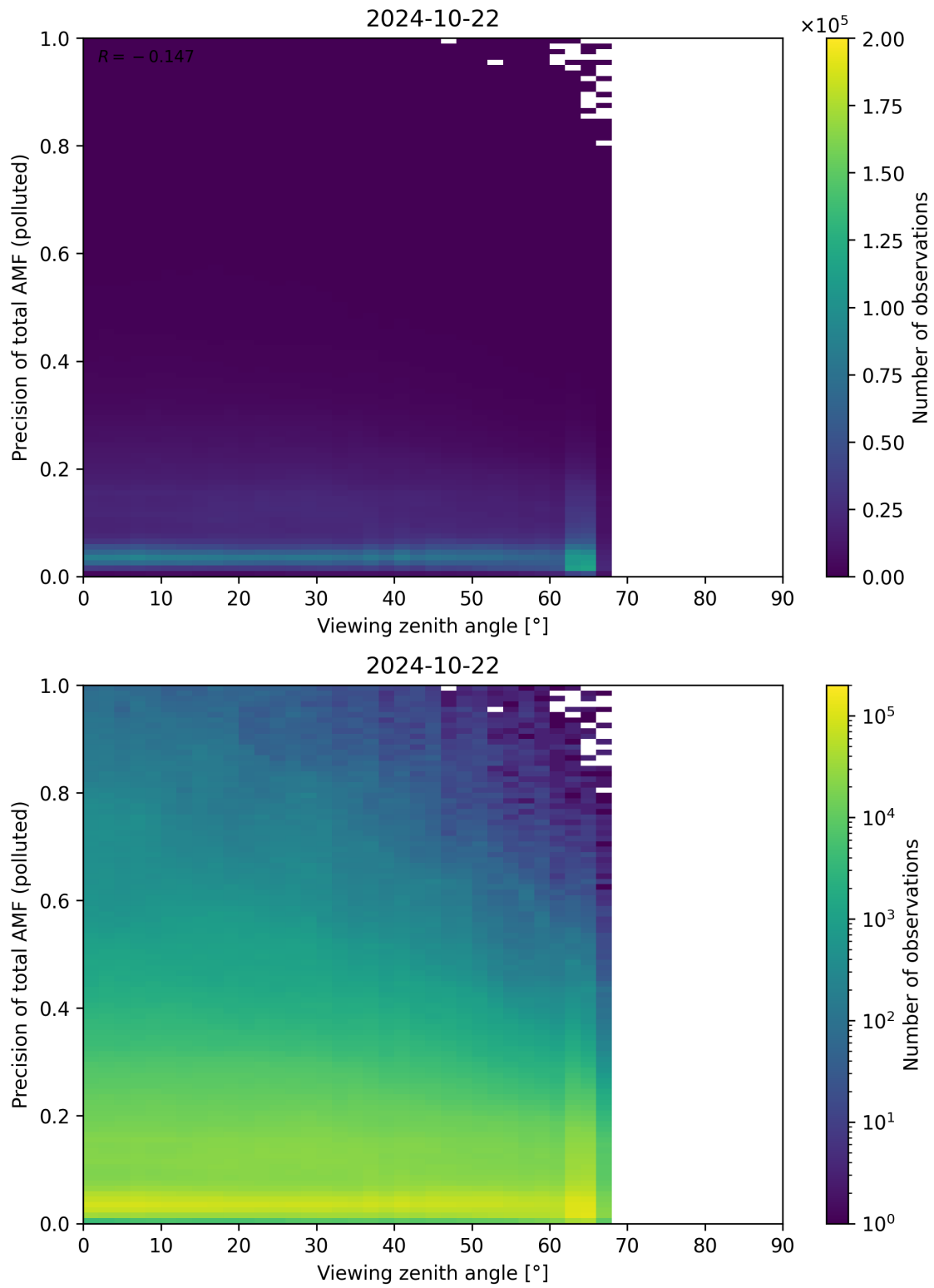
Figure 326: Scatter density plot of “Viewing zenith angle” against “Precision of total AMF (polluted)” for 2024-10-21 to 2024-10-23.
