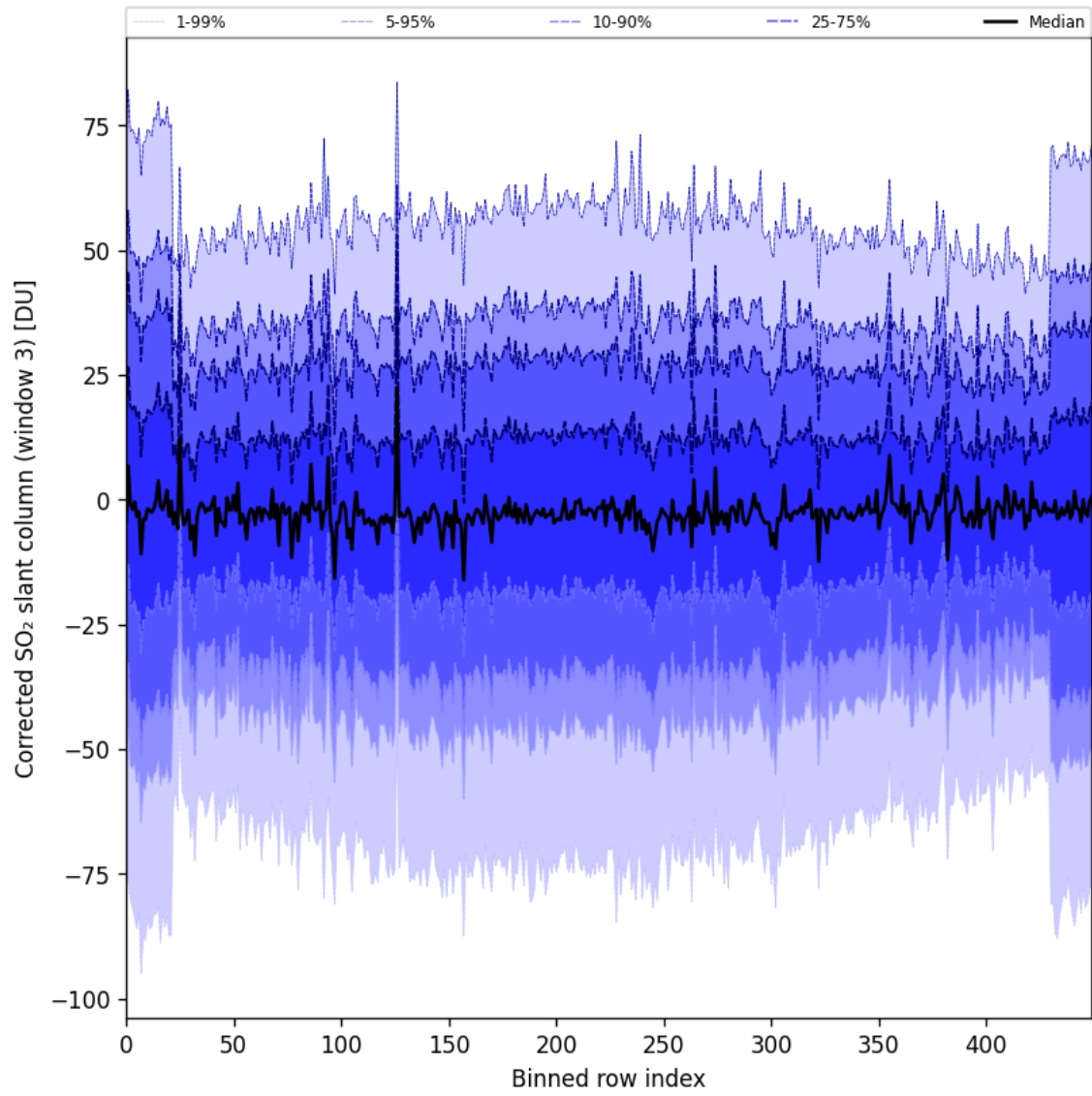
Figure 89: Along track statistics of “Corrected SO 2 slant column (window 3)” for 2024-10-21 to 2024-10-23
