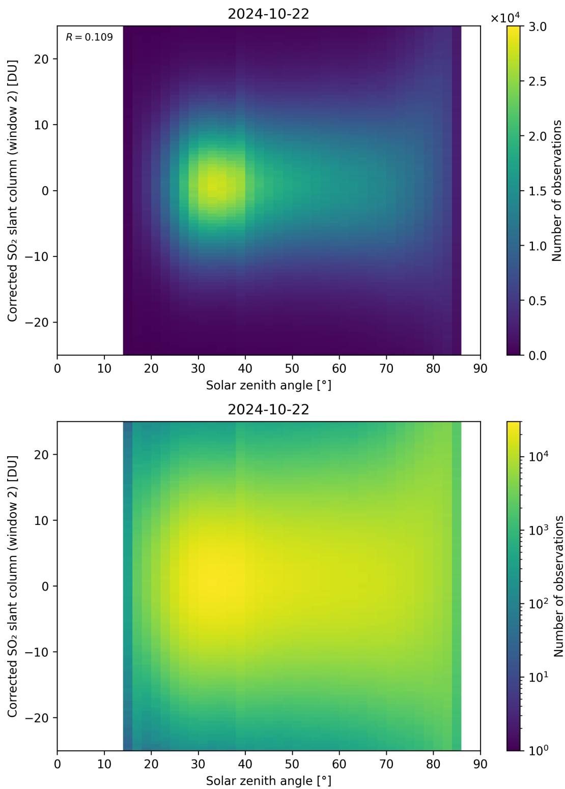
Figure 167: Scatter density plot of “Solar zenith angle” against “Corrected SO 2 slant column (window 2)” for 2024-10-21 to 2024-10-23.
