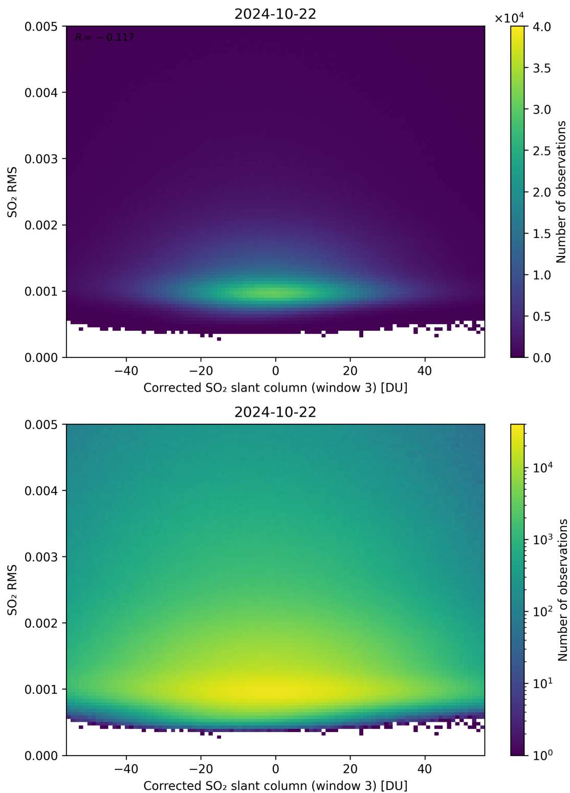
Figure 208: Scatter density plot of “Corrected SO 2 slant column (window 3)” against “SO 2 RMS” for 2024-10-21 to 2024-10-23.
