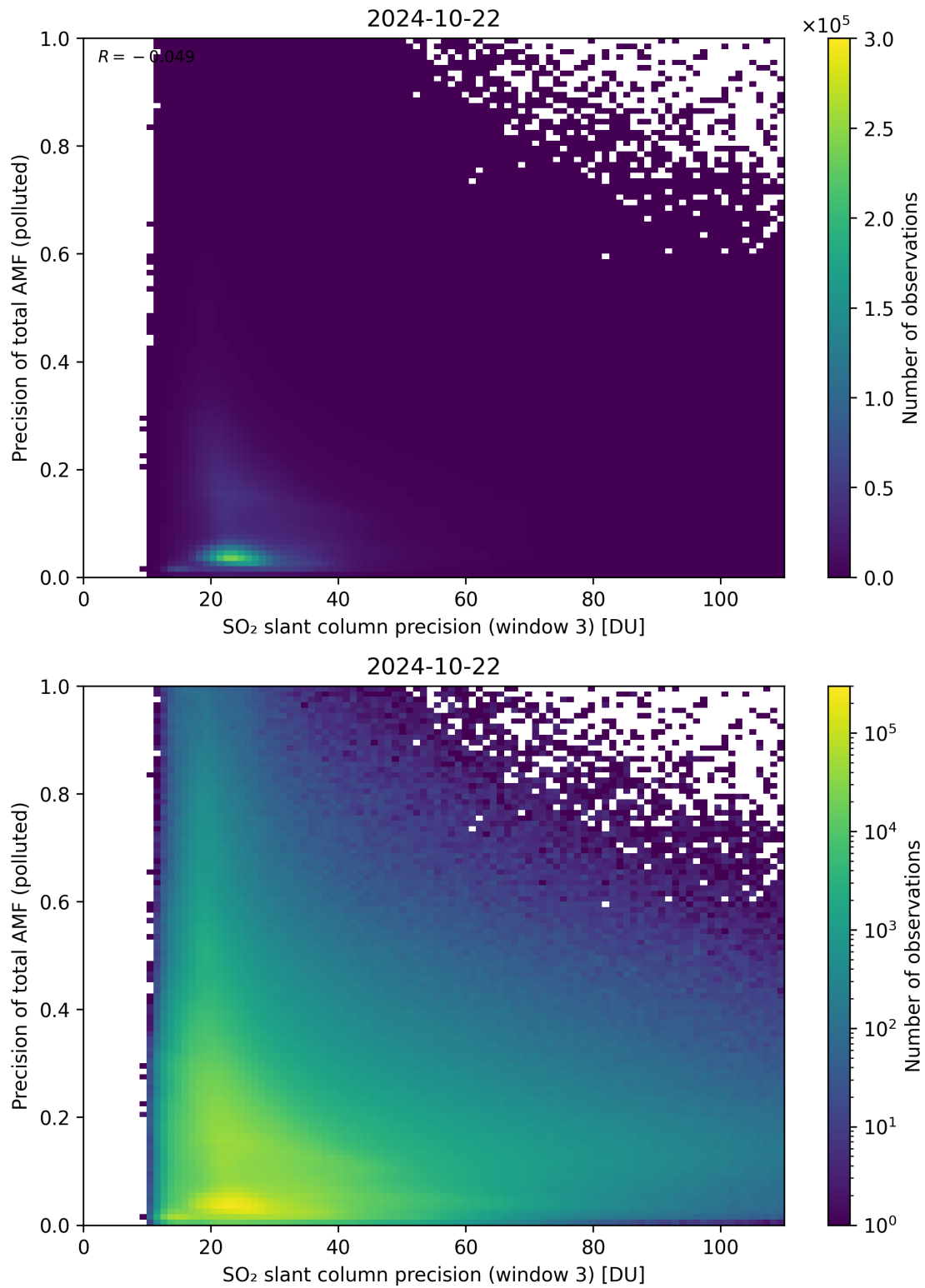
Figure 264: Scatter density plot of “SO 2 slant column precision (window 3)” against “Precision of total AMF (polluted)” for 2024-10-21 to 2024-10-23.
