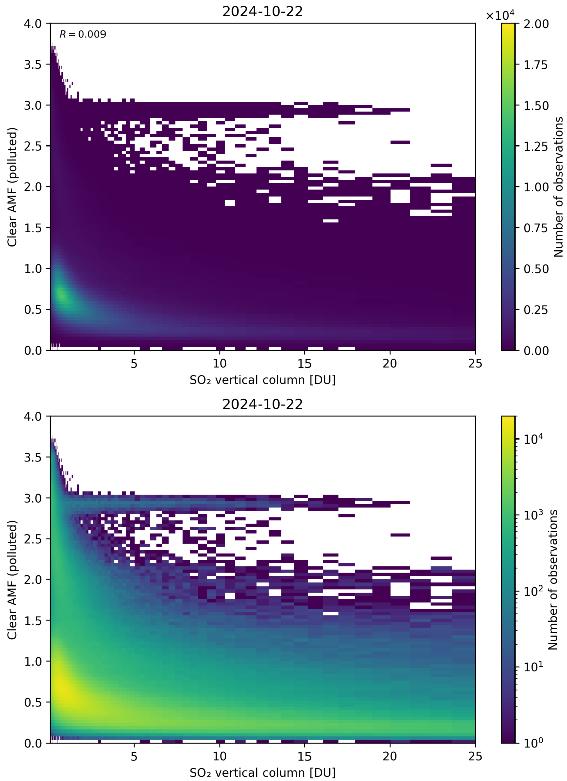
Figure 296: Scatter density plot of “SO 2 vertical column” against “Clear AMF (polluted)” for 2024-10-21 to 2024-10-23.
