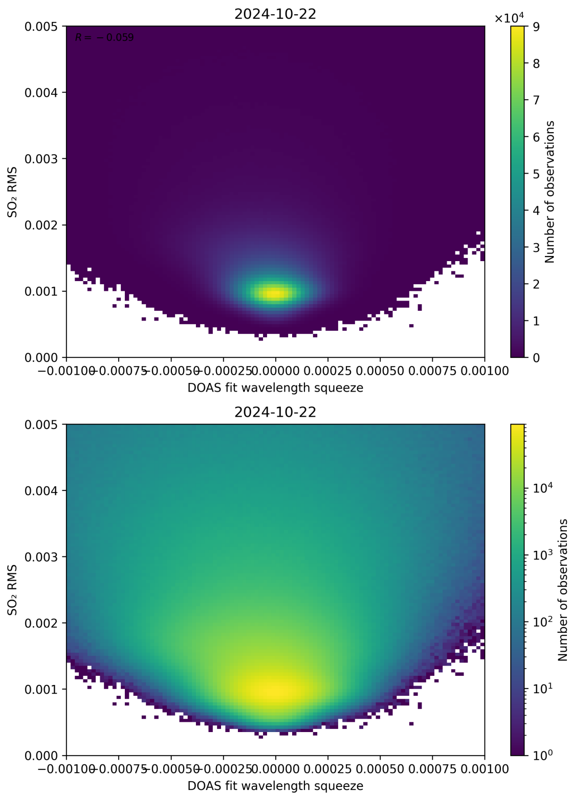
Figure 132: Scatter density plot of “DOAS fit wavelength squeeze” against “SO 2 RMS” for 2024-10-21 to 2024-10-23.
