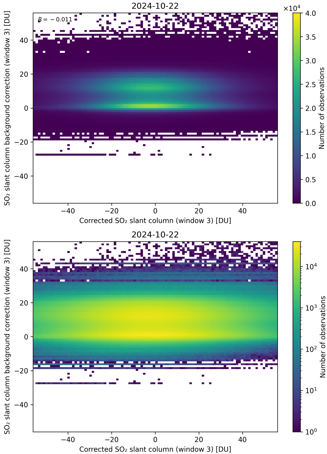
Figure 205: Scatter density plot of “Corrected SO 2 slant column (window 3)” against “SO 2 slant column background correction (window 3)” for 2024-10-21 to 2024-10-23.
