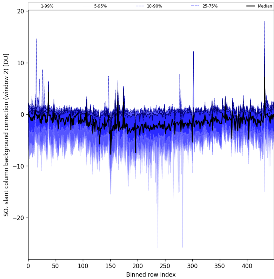
Figure 86: Along track statistics of “SO 2 slant column background correction (window 2)” for 2024-10-21 to 2024-10-23
