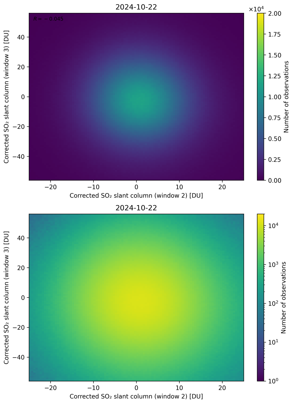
Figure 200: Scatter density plot of “Corrected SO 2 slant column (window 2)” against “Corrected SO 2 slant column (window 3)” for 2024-10-21 to 2024-10-23.
