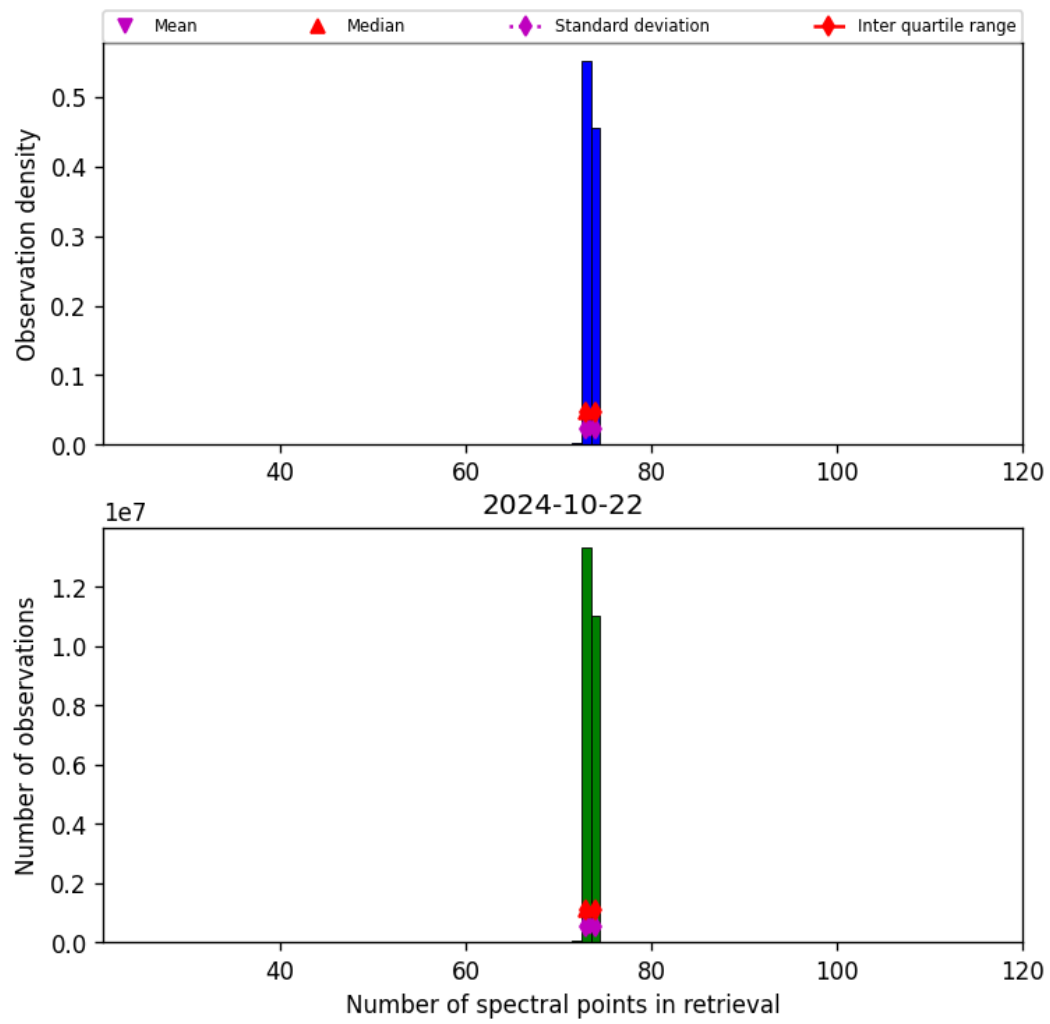
Figure 74: Histogram of “Number of spectral points in retrieval” for 2024-10-21 to 2024-10-23
