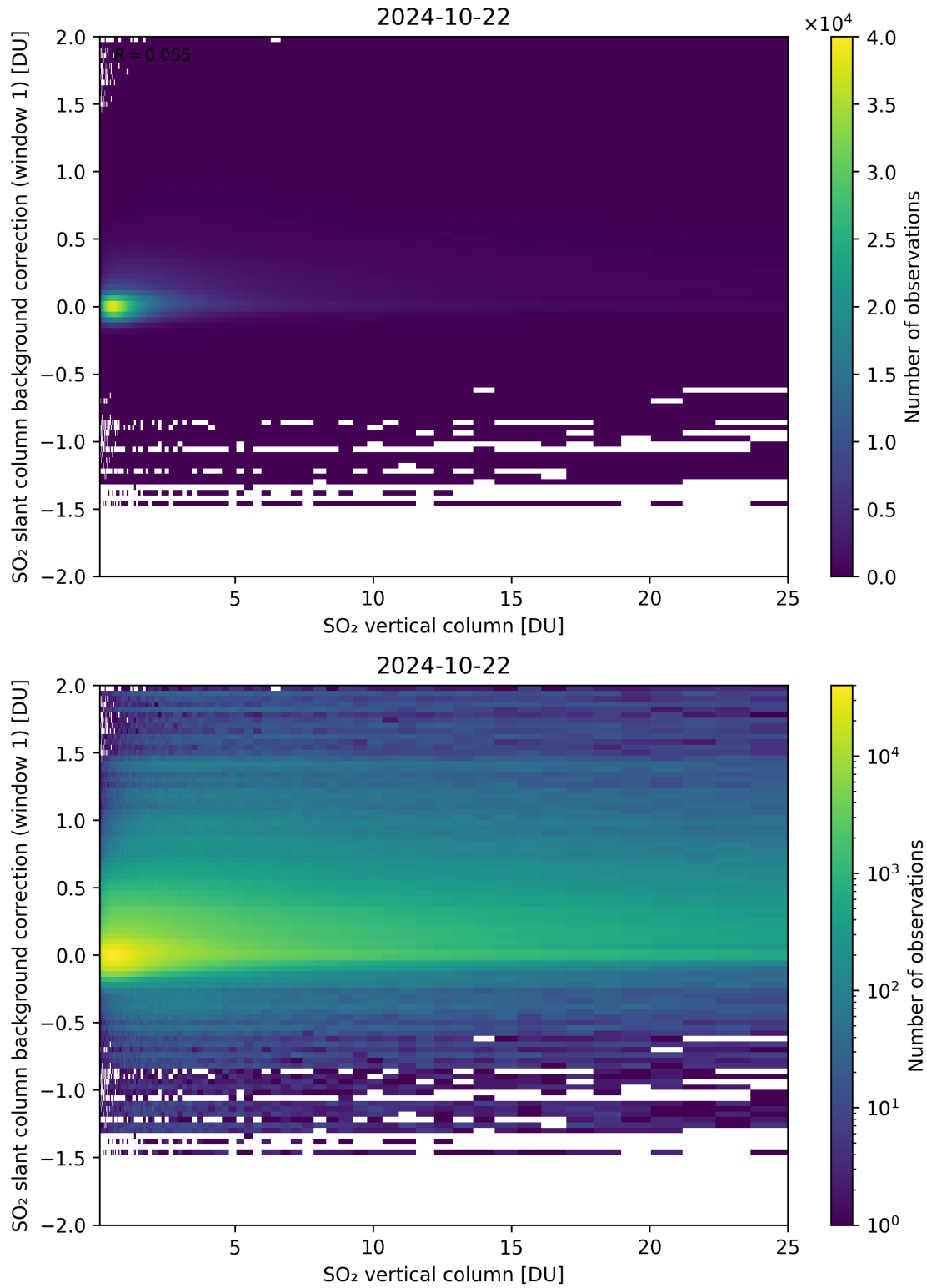
Figure 273: Scatter density plot of “SO 2 vertical column” against “SO 2 slant column background correction (window 1)” for 2024-10-21 to 2024-10-23.
