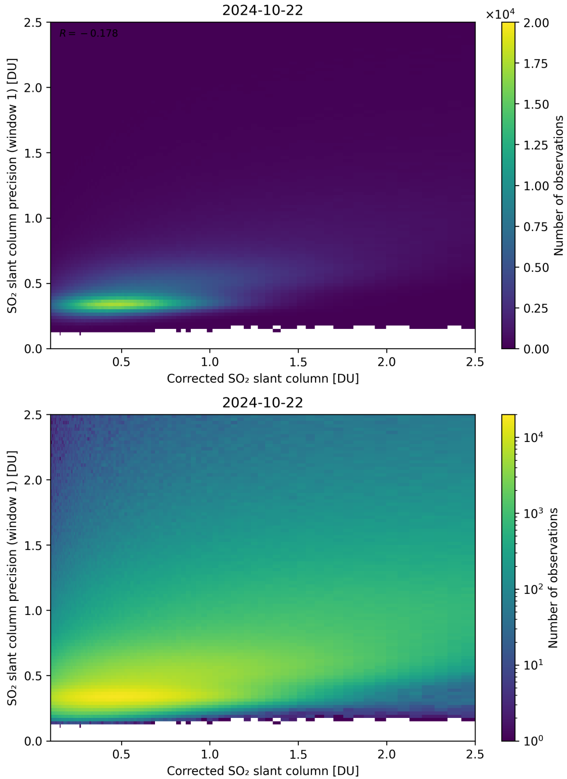
Figure 188: Scatter density plot of “Corrected SO 2 slant column” against “SO 2 slant column precision (window 1)” for 2024-10-21 to 2024-10-23.
