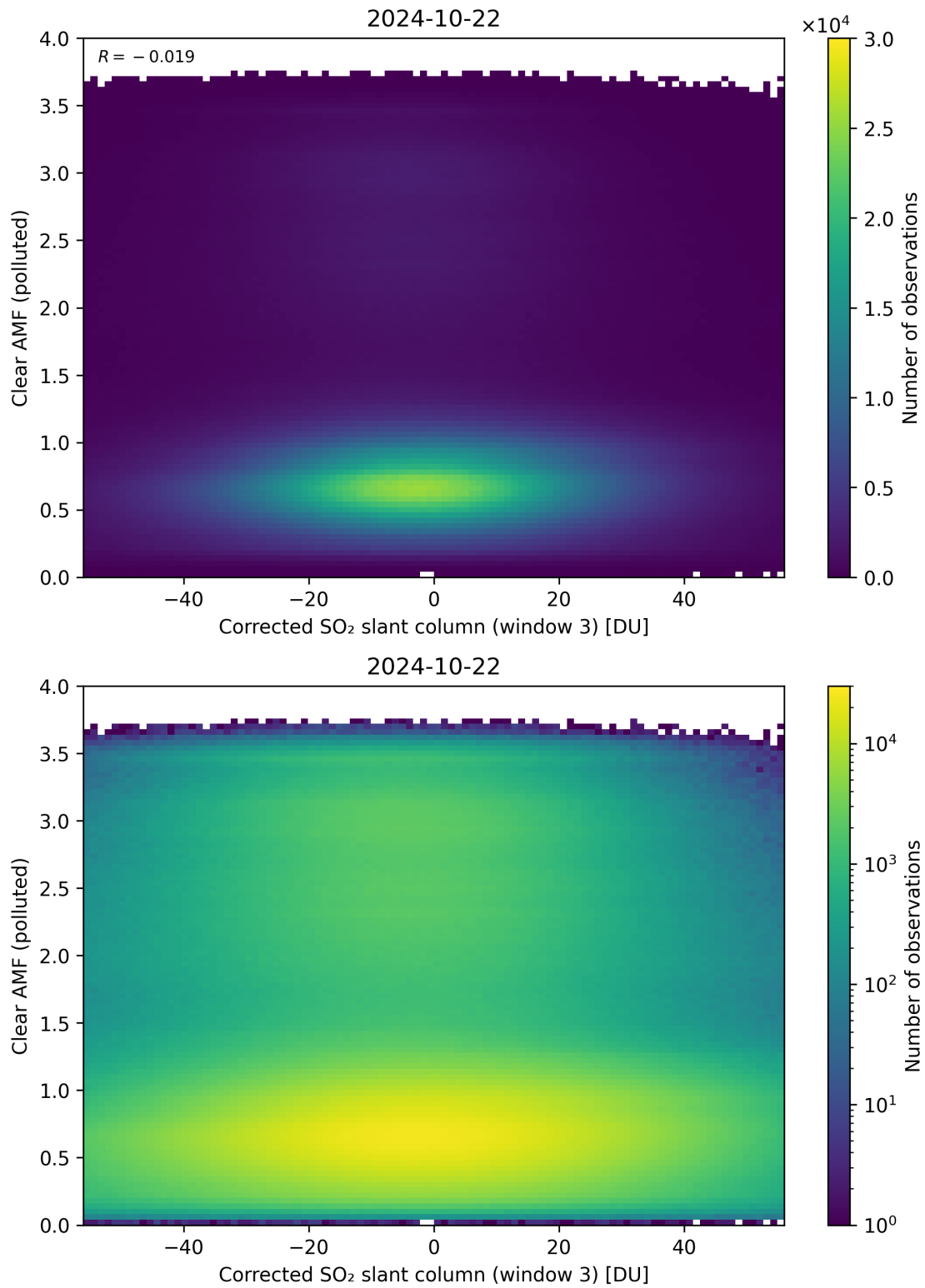
Figure 209: Scatter density plot of “Corrected SO 2 slant column (window 3)” against “Clear AMF (polluted)” for 2024-10-21 to 2024-10-23.
