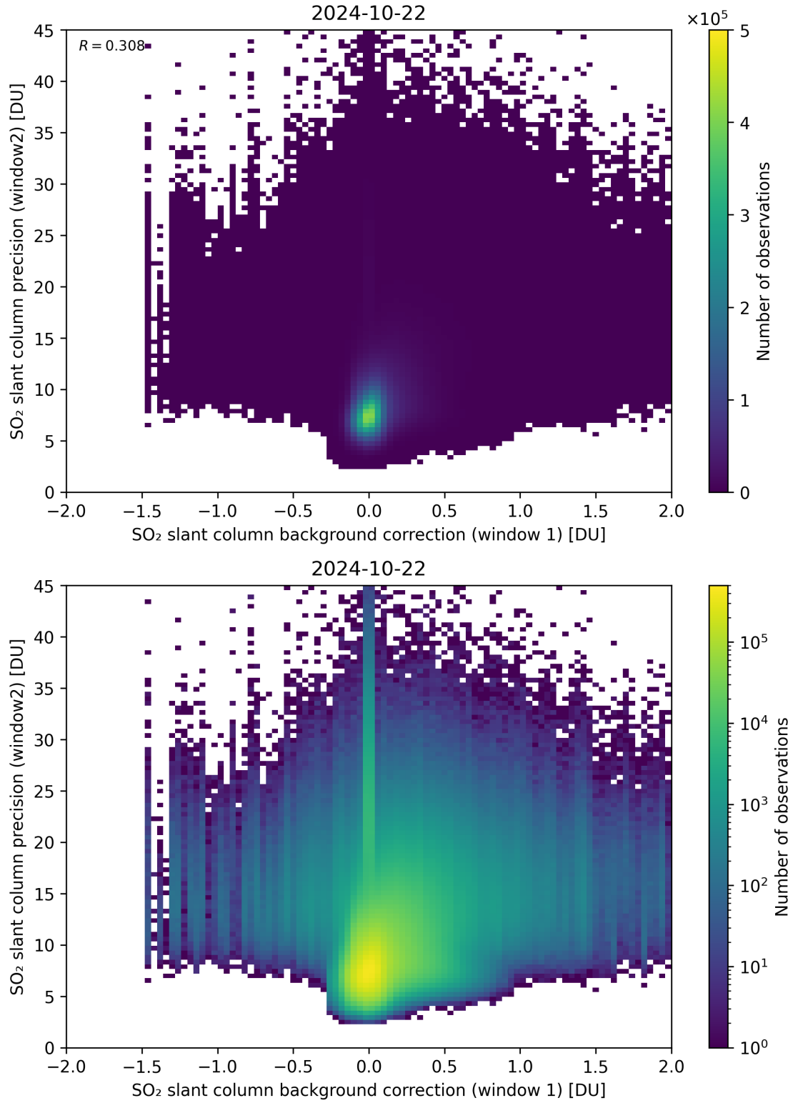
Figure 106: Scatter density plot of “SO 2 slant column background correction (window 1)” against “SO 2 slant column precision (window2)” for 2024-10-21 to 2024-10-23.
