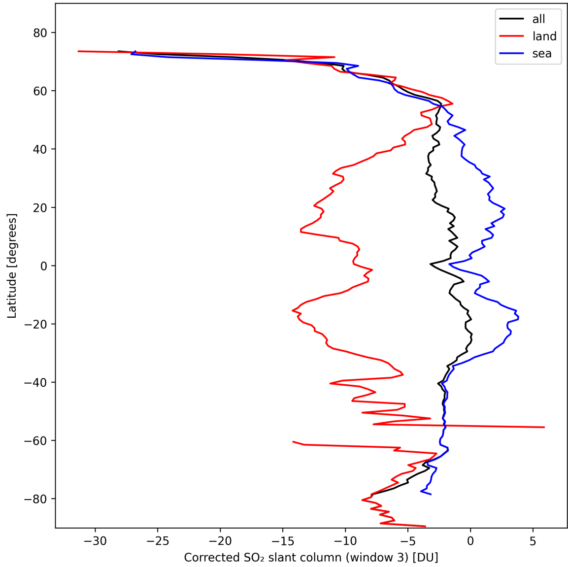
Figure 43: Zonal average of “Corrected SO 2 slant column (window 3)” for 2024-10-21 to 2024-10-23.
