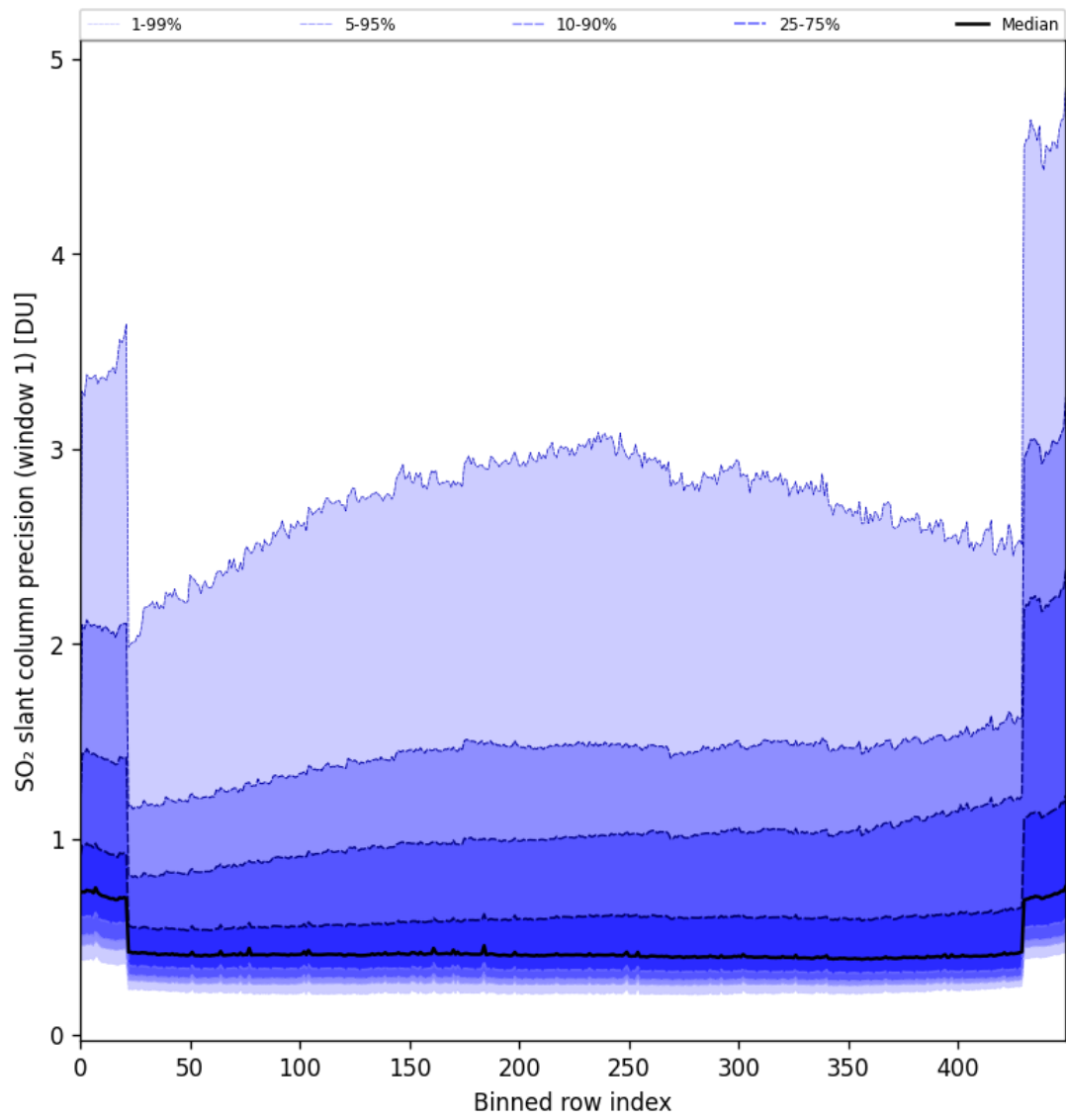
Figure 80: Along track statistics of “SO 2 slant column precision (window 1)” for 2024-10-21 to 2024-10-23
