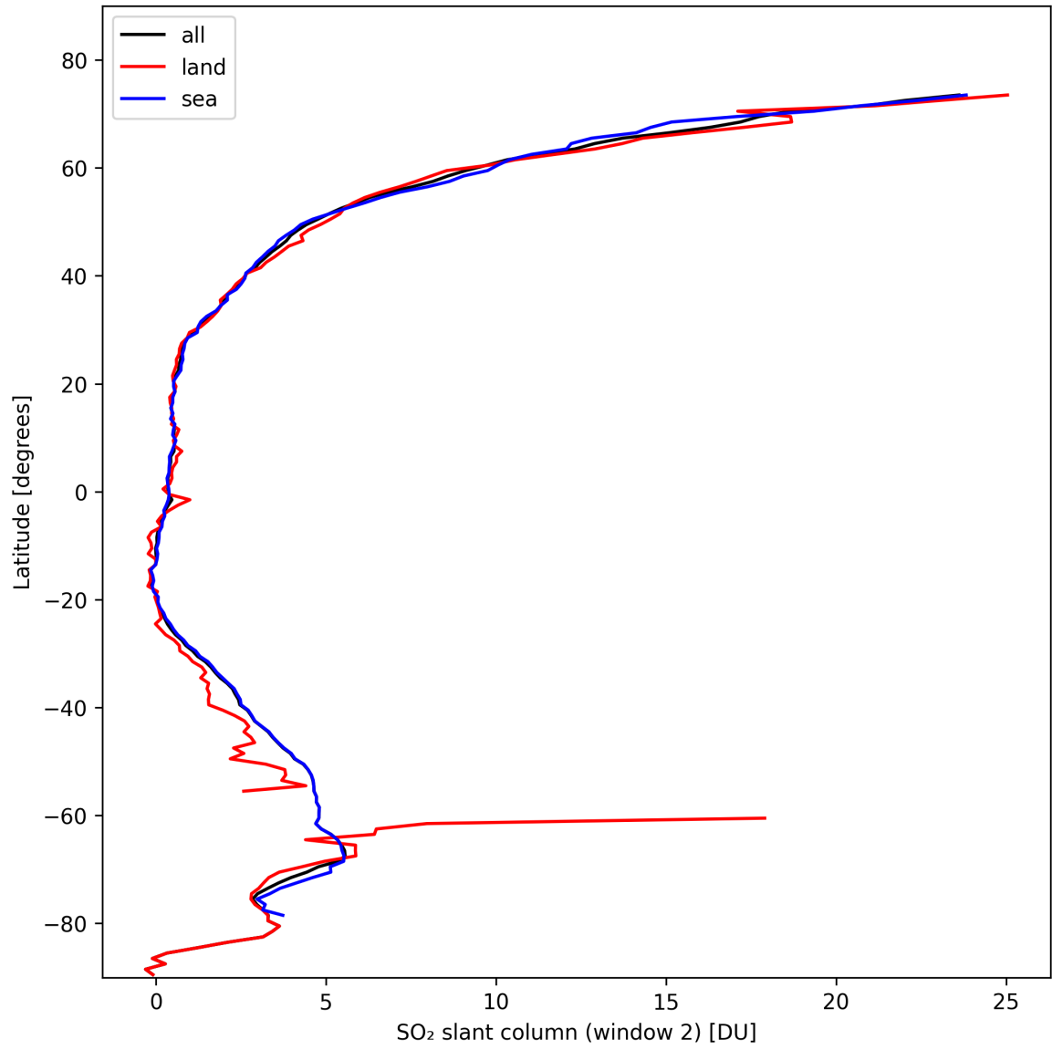
Figure 37: Zonal average of “SO 2 slant column (window 2)” for 2024-10-21 to 2024-10-23.
