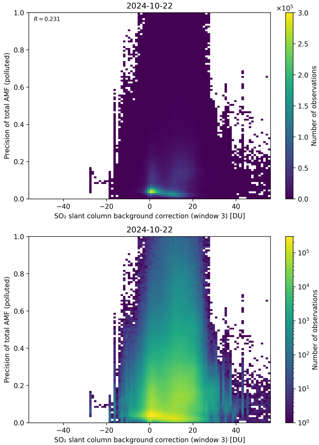
Figure 126: Scatter density plot of “SO 2 slant column background correction (window 3)” against “Precision of total AMF (polluted)” for 2024-10-21 to 2024-10-23.
