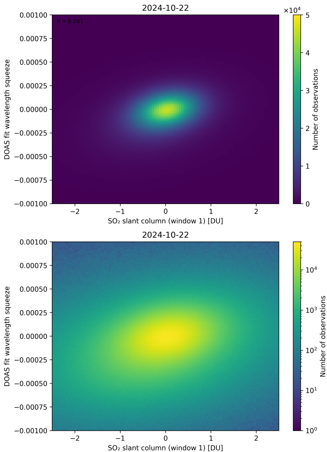
Figure 216: Scatter density plot of “SO 2 slant column (window 1)” against “DOAS fit wavelength squeeze” for 2024-10-21 to 2024-10-23.
