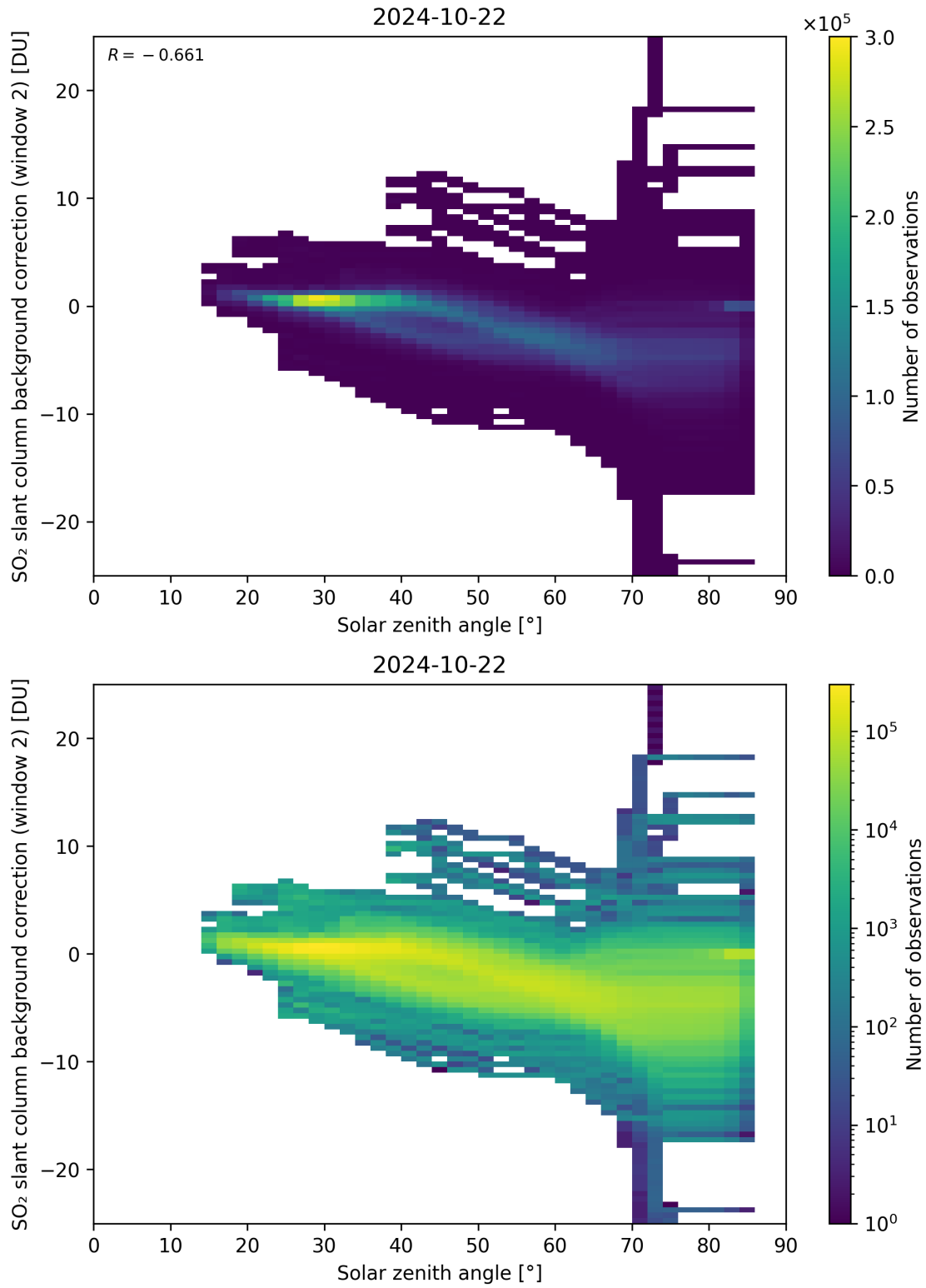
Figure 159: Scatter density plot of “Solar zenith angle” against “SO 2 slant column background correction (window 2)” for 2024-10-21 to 2024-10-23.
