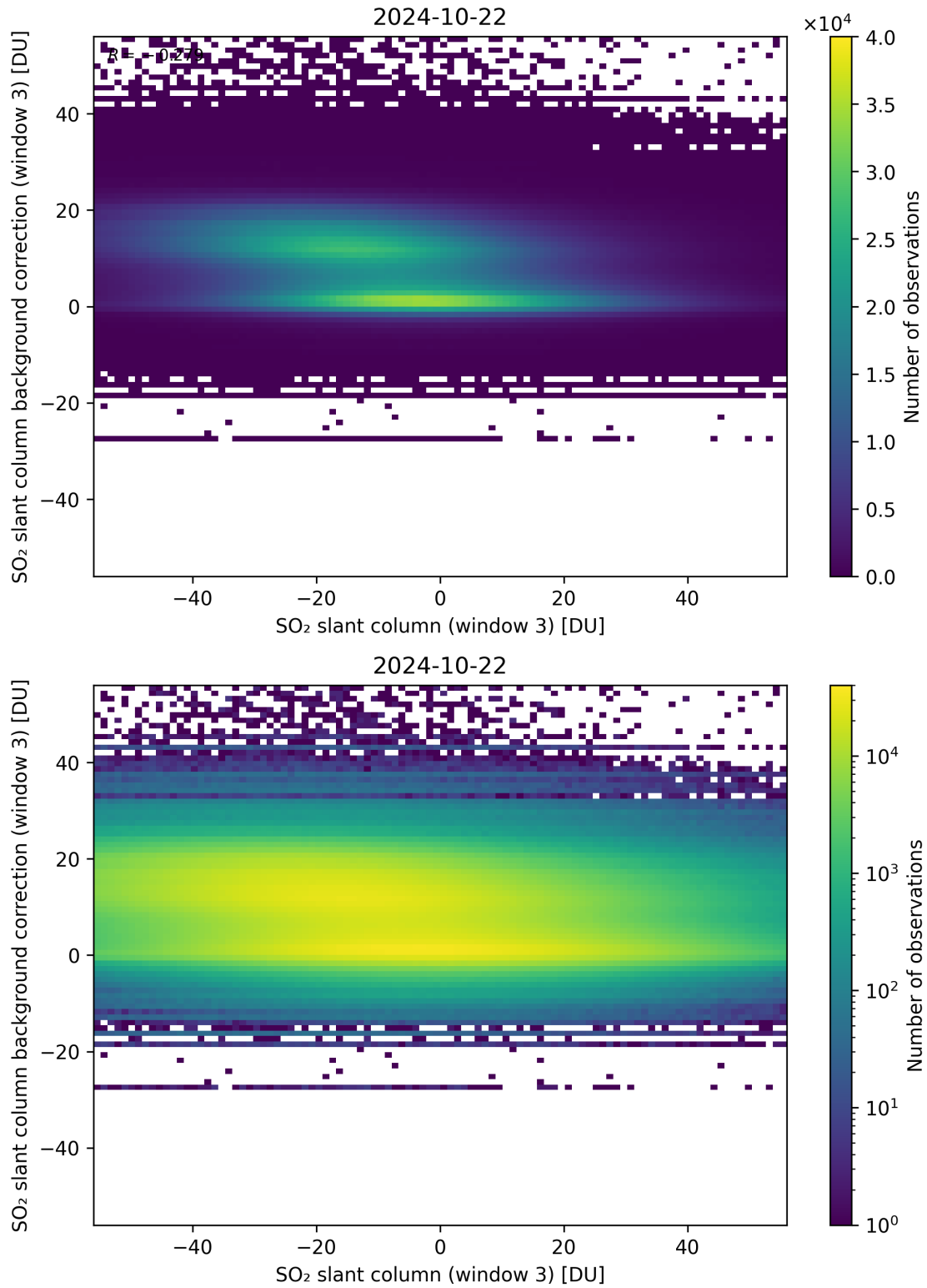
Figure 253: Scatter density plot of “SO 2 slant column (window 3)” against “SO 2 slant column background correction (window 3)” for 2024-10-21 to 2024-10-23.
