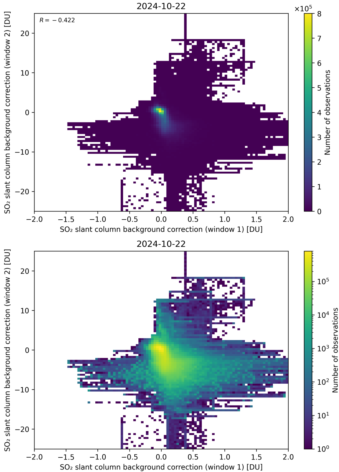
Figure 98: Scatter density plot of “SO 2 slant column background correction (window 1)” against “SO 2 slant column background correction (window 2)” for 2024-10-21 to 2024-10-23.
