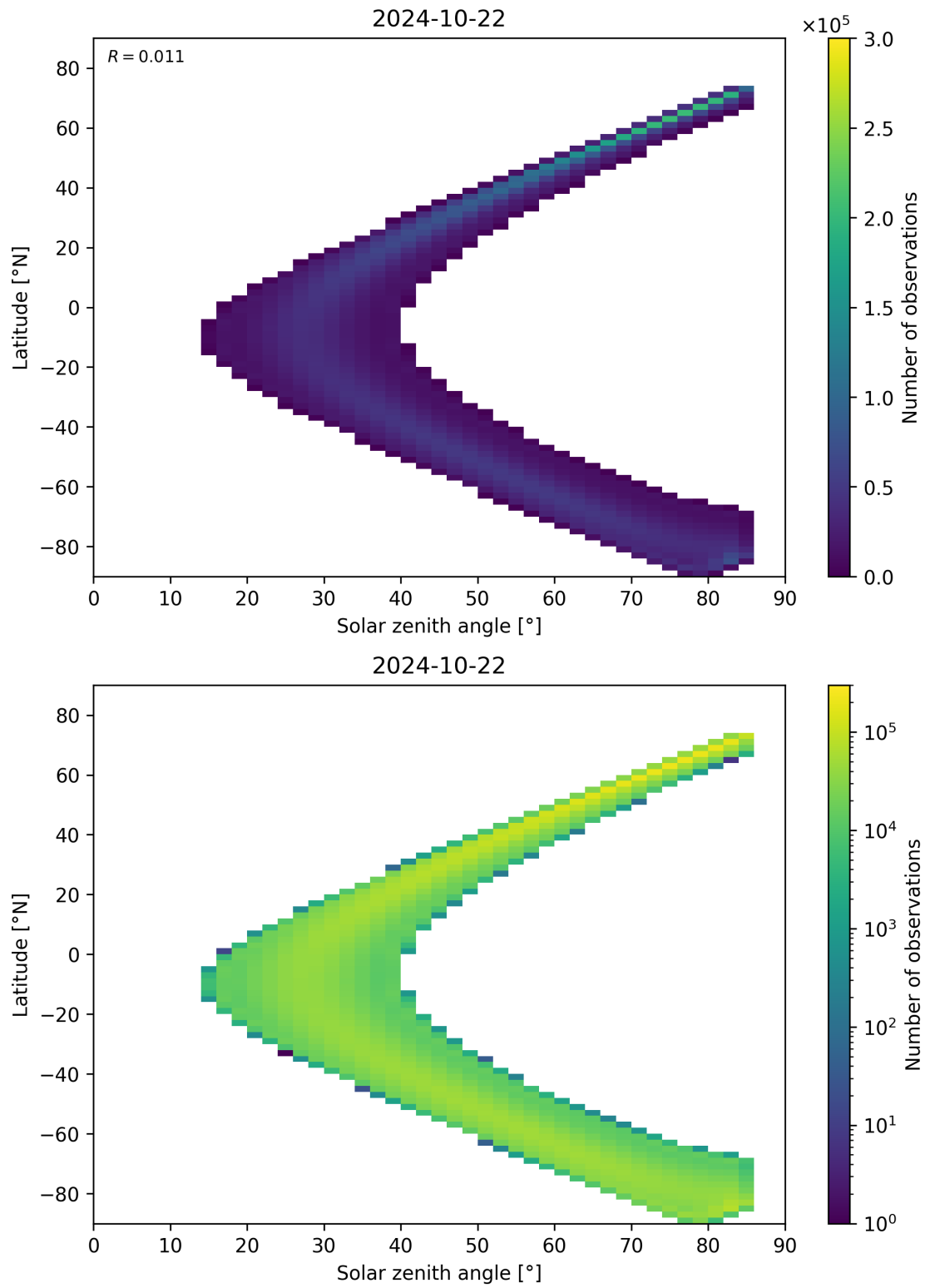
Figure 164: Scatter density plot of “Solar zenith angle” against “Latitude” for 2024-10-21 to 2024-10-23.
