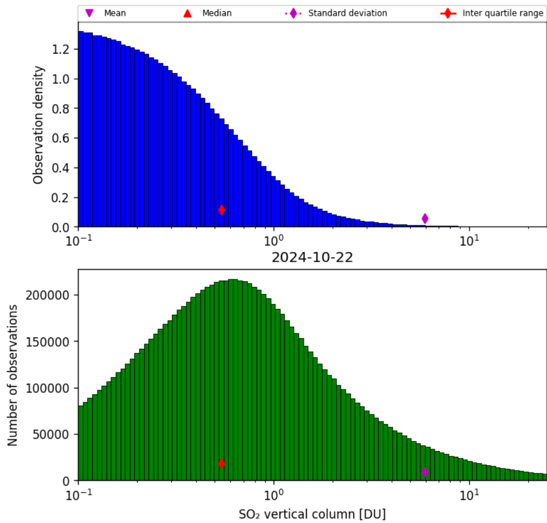
Figure 53: Histogram of “SO 2 vertical column” for 2024-10-21 to 2024-10-23
