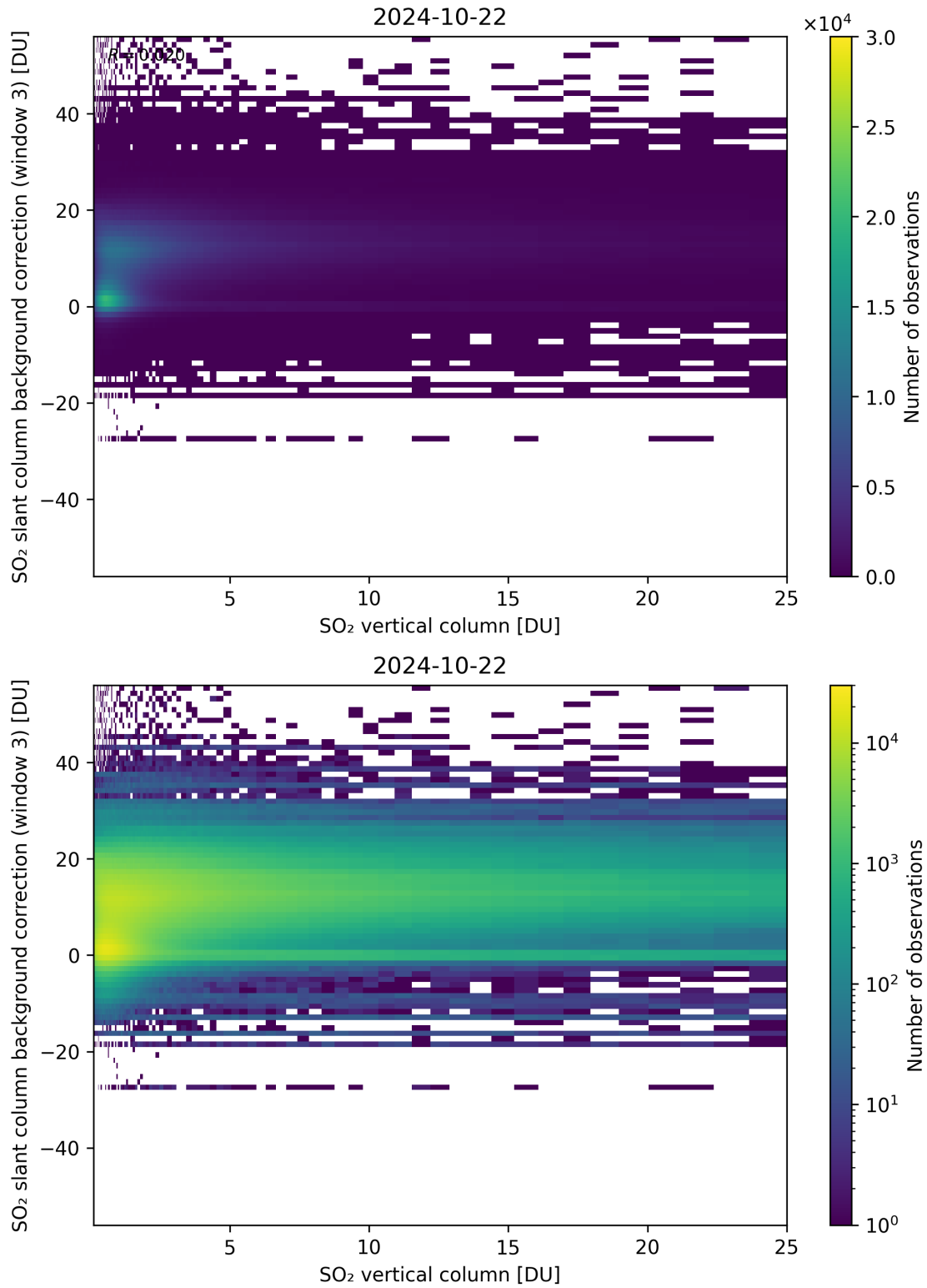
Figure 275: Scatter density plot of “SO 2 vertical column” against “SO 2 slant column background correction (window 3)” for 2024-10-21 to 2024-10-23.
