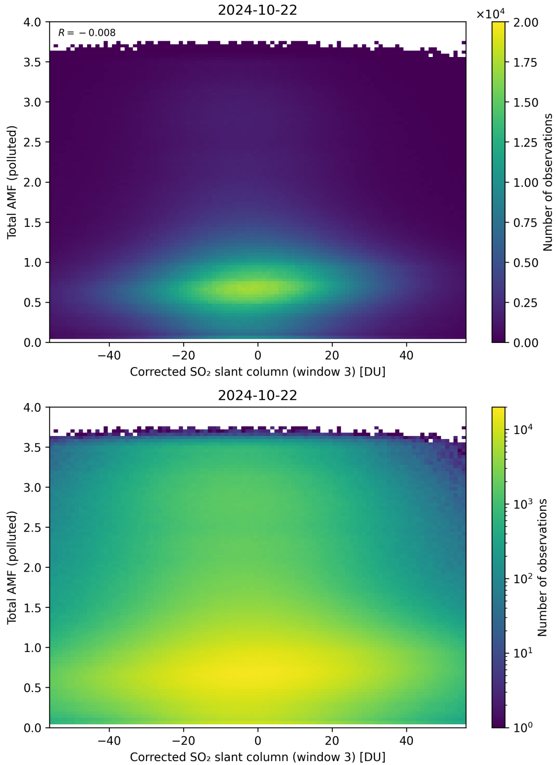
Figure 210: Scatter density plot of “Corrected SO 2 slant column (window 3)” against “Total AMF (polluted)” for 2024-10-21 to 2024-10-23.
