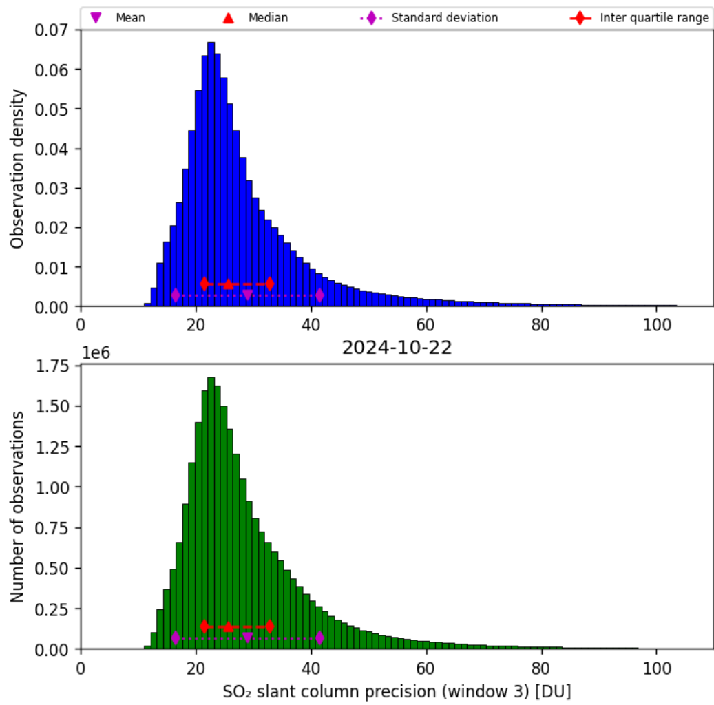
Figure 65: Histogram of “SO 2 slant column precision (window 3)” for 2024-10-21 to 2024-10-23
