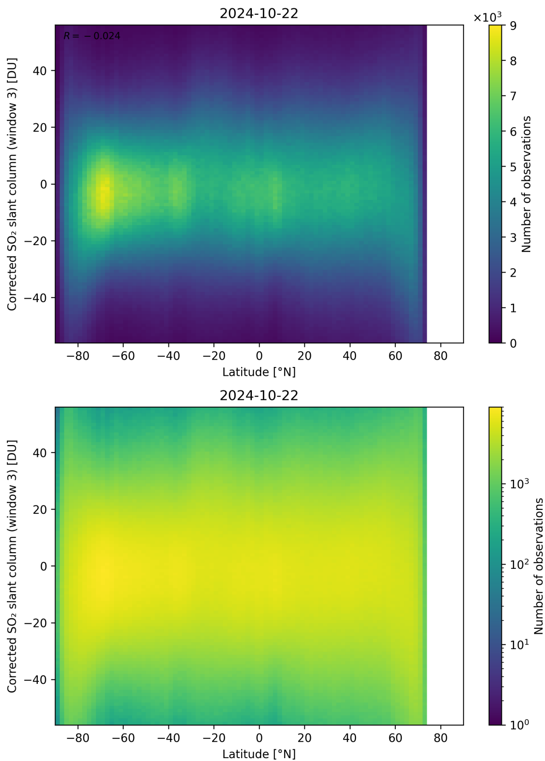
Figure 148: Scatter density plot of “Latitude” against “Corrected SO 2 slant column (window 3)” for 2024-10-21 to 2024-10-23.
