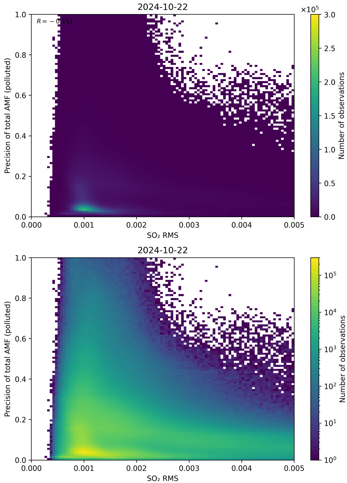
Figure 138: Scatter density plot of “SO 2 RMS” against “Precision of total AMF (polluted)” for 2024-10-21 to 2024-10-23.
