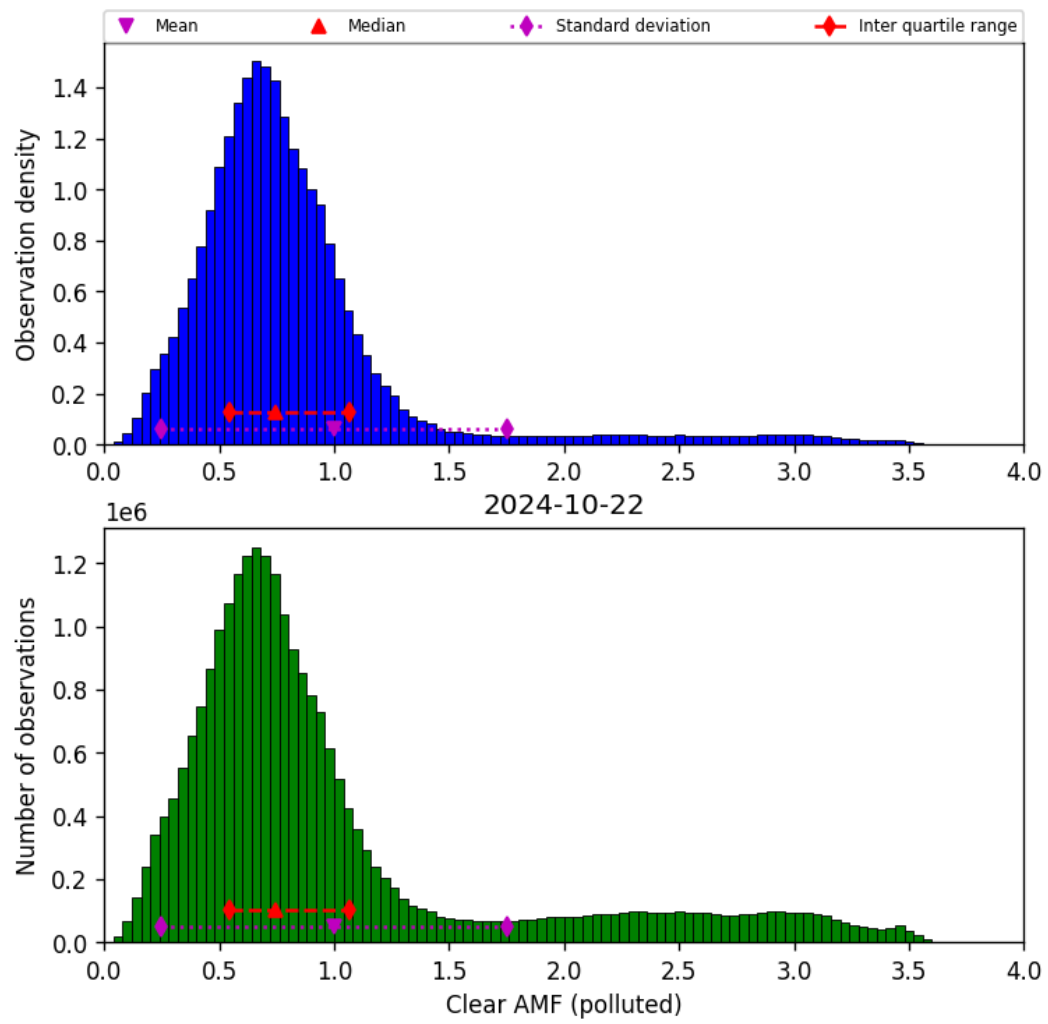
Figure 73: Histogram of “Clear AMF (polluted)” for 2024-10-21 to 2024-10-23
