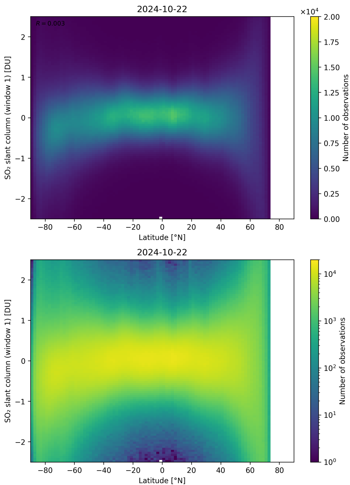
Figure 149: Scatter density plot of “Latitude” against “SO 2 slant column (window 1)” for 2024-10-21 to 2024-10-23.
