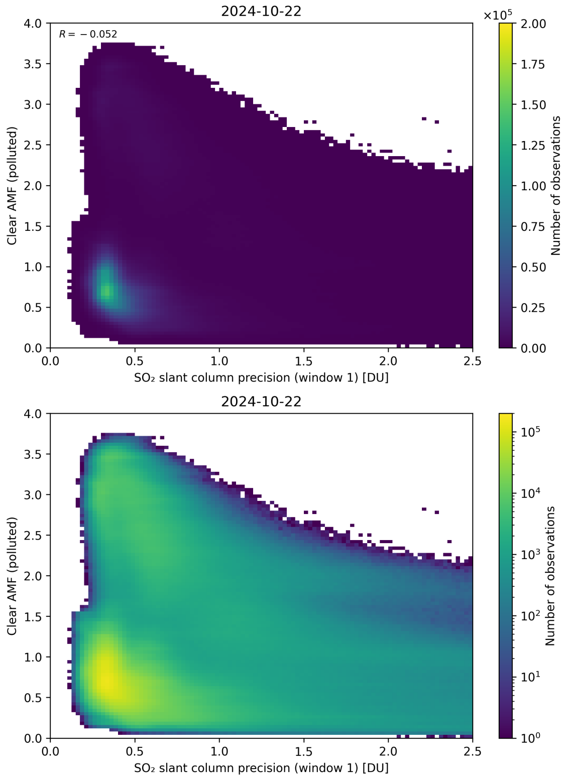
Figure 224: Scatter density plot of “SO 2 slant column precision (window 1)” against “Clear AMF (polluted)” for 2024-10-21 to 2024-10-23.
