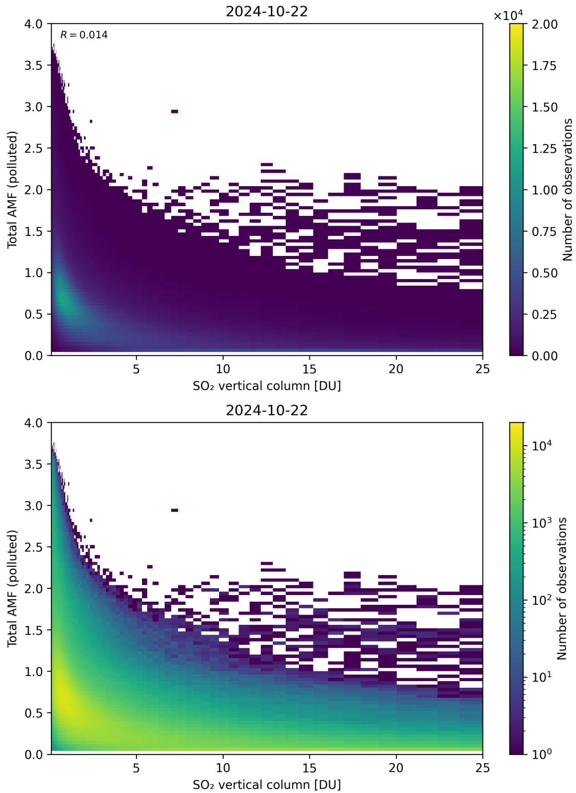
Figure 305: Scatter density plot of “SO 2 vertical column” against “Total AMF (polluted)” for 2024-10-21 to 2024-10-23.
