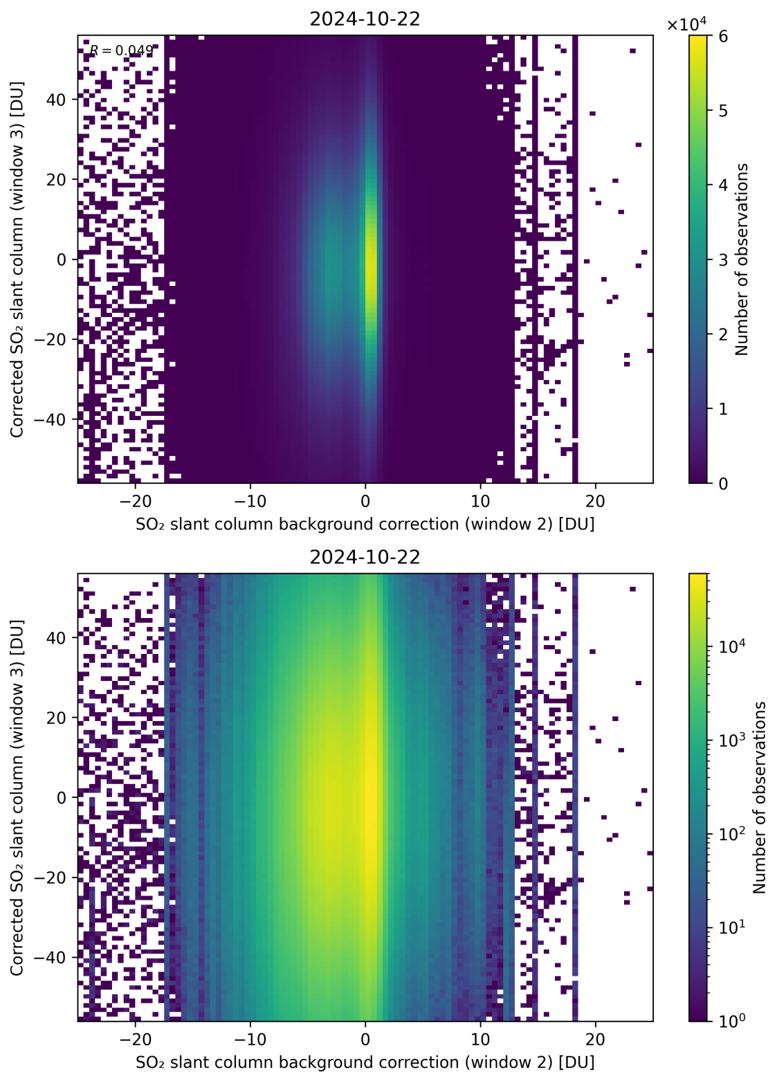
Figure 116: Scatter density plot of “SO 2 slant column background correction (window 2)” against “Corrected SO 2 slant column (window 3)” for 2024-10-21 to 2024-10-23.
