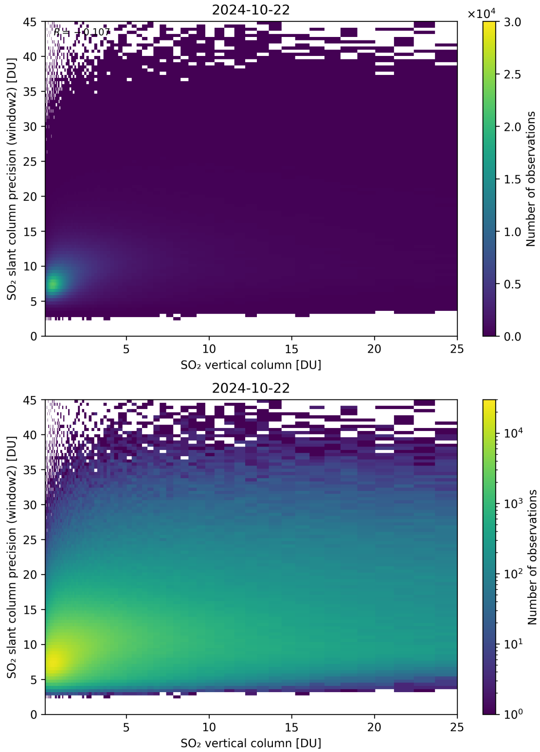
Figure 302: Scatter density plot of “SO 2 vertical column” against “SO 2 slant column precision (window2)” for 2024-10-21 to 2024-10-23.
