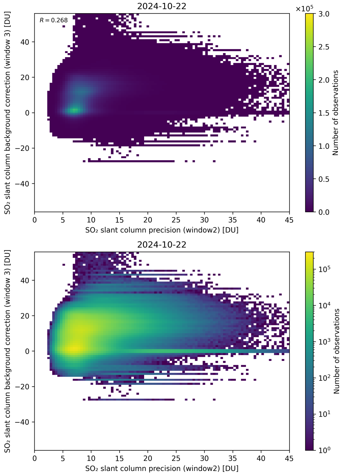
Figure 242: Scatter density plot of “SO 2 slant column precision (window2)” against “SO 2 slant column background correction (window 3)” for 2024-10-21 to 2024-10-23.
