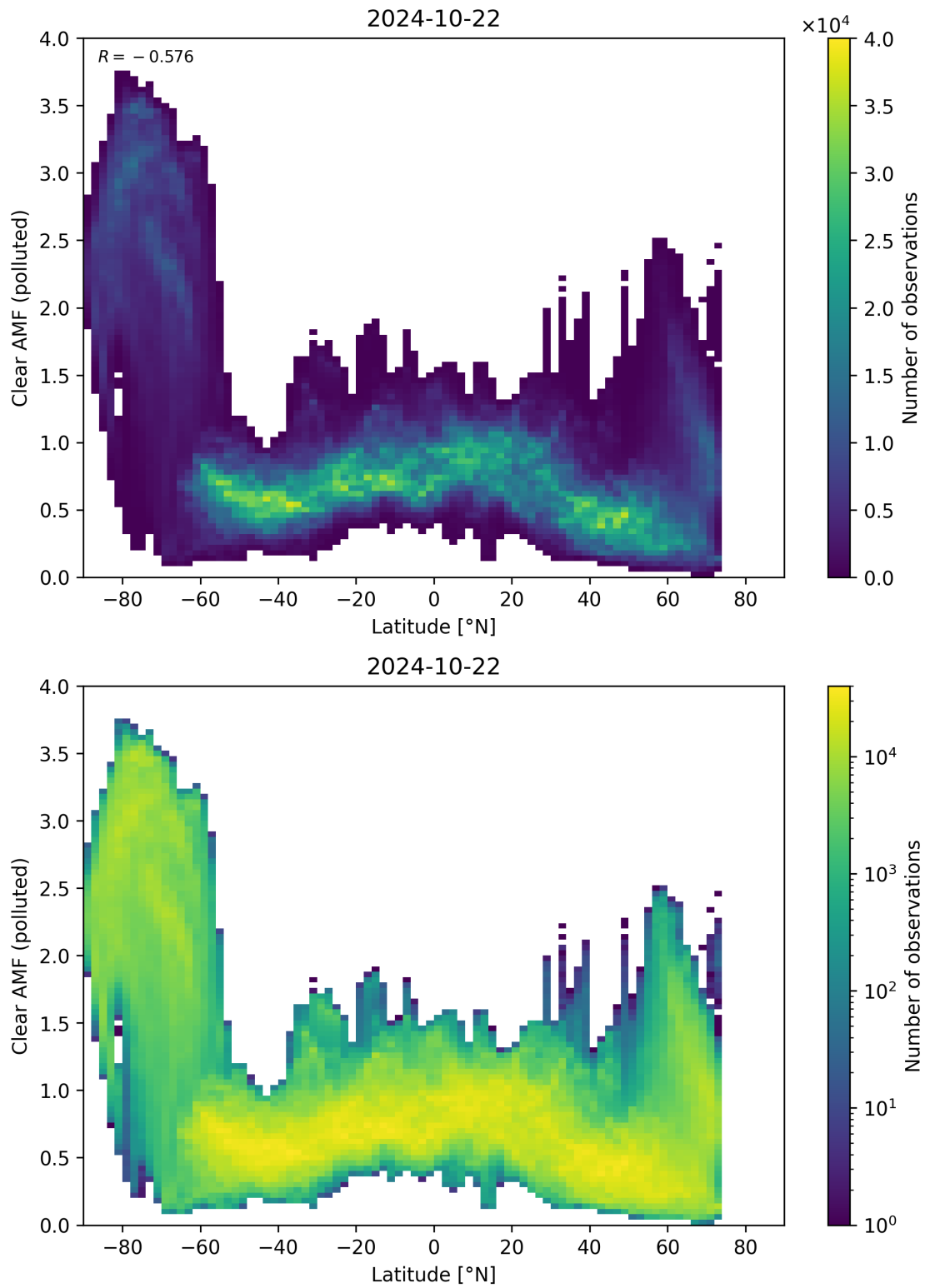
Figure 145: Scatter density plot of “Latitude” against “Clear AMF (polluted)” for 2024-10-21 to 2024-10-23.
