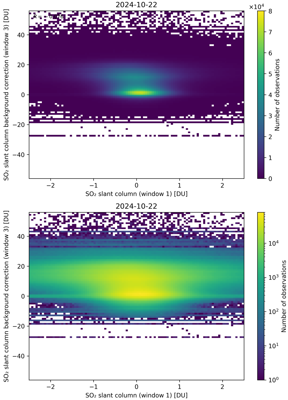
Figure 214: Scatter density plot of “SO 2 slant column (window 1)” against “SO 2 slant column background correction (window 3)” for 2024-10-21 to 2024-10-23.
