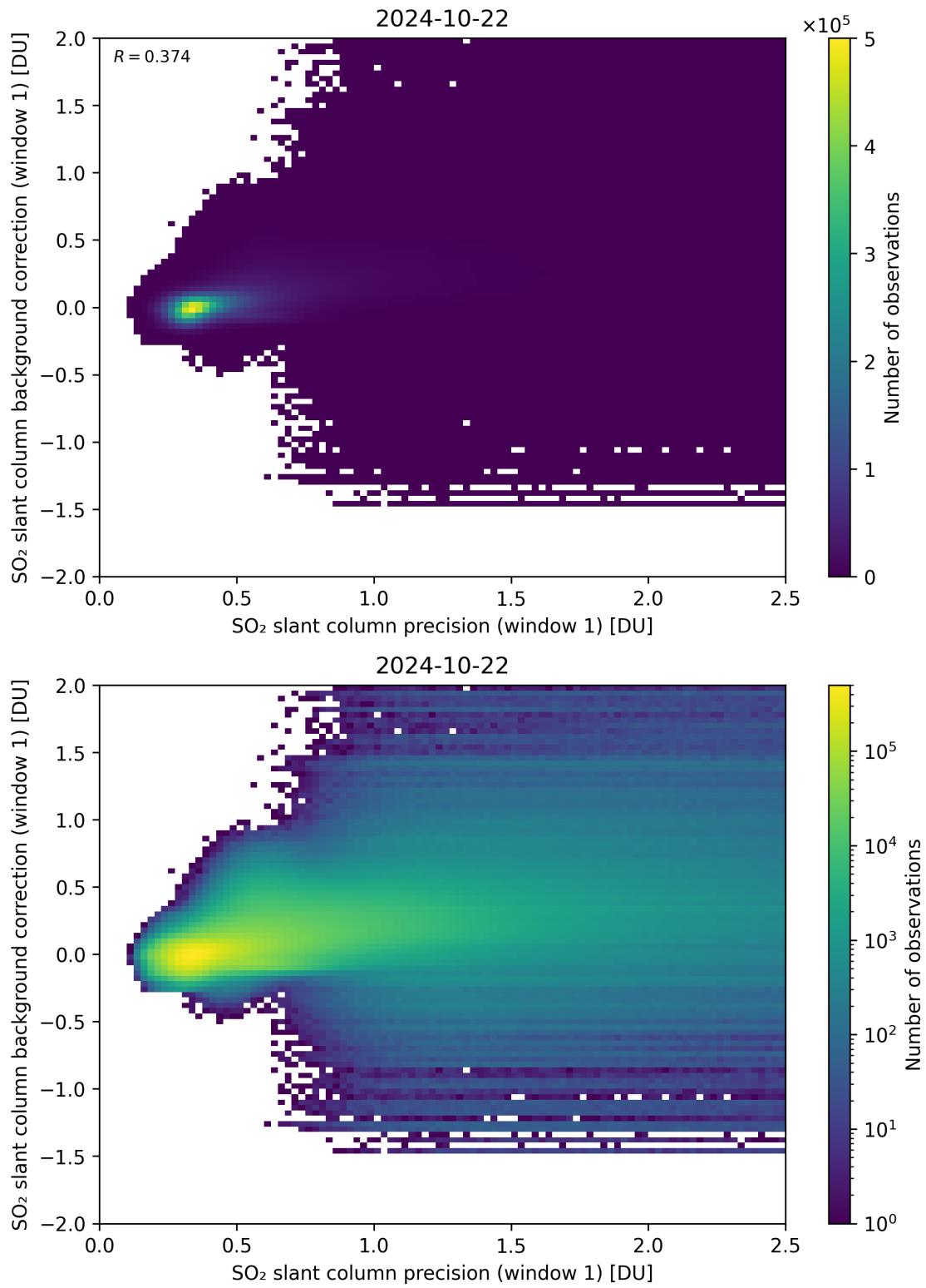
Figure 218: Scatter density plot of “SO 2 slant column precision (window 1)” against “SO 2 slant column background correction (window 1)” for 2024-10-21 to 2024-10-23.
