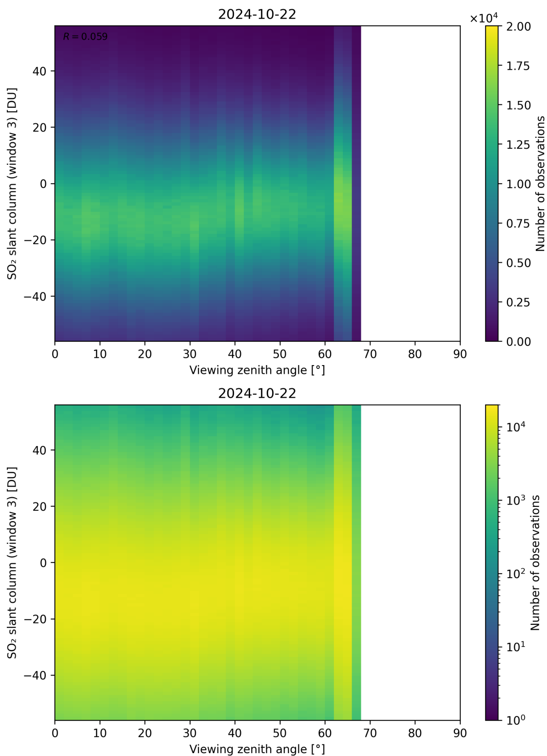
Figure 323: Scatter density plot of “Viewing zenith angle” against “SO 2 slant column (window 3)” for 2024-10-21 to 2024-10-23.
