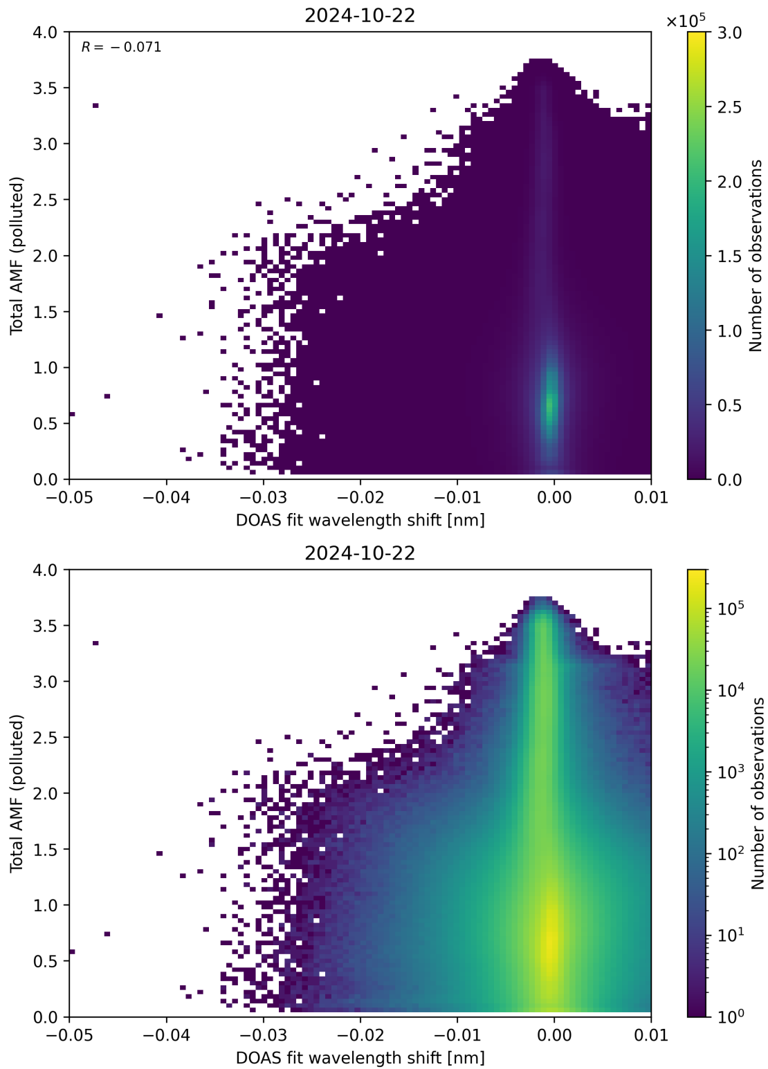
Figure 130: Scatter density plot of “DOAS fit wavelength shift” against “Total AMF (polluted)” for 2024-10-21 to 2024-10-23.
