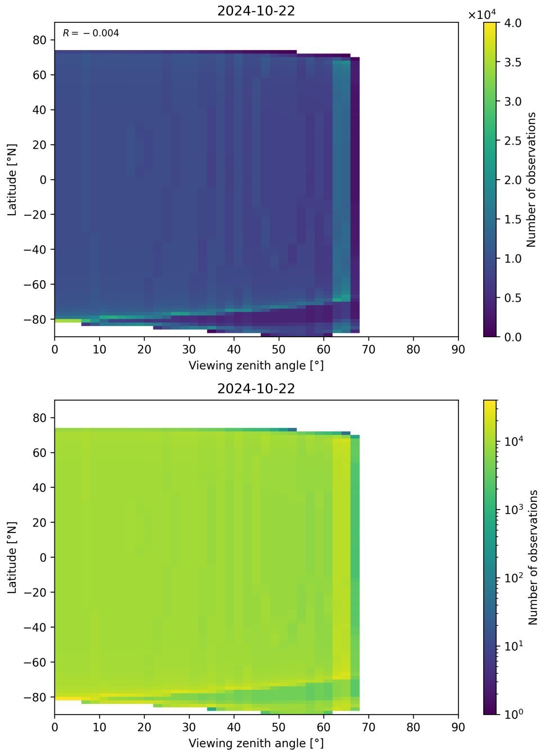
Figure 314: Scatter density plot of “Viewing zenith angle” against “Latitude” for 2024-10-21 to 2024-10-23.
