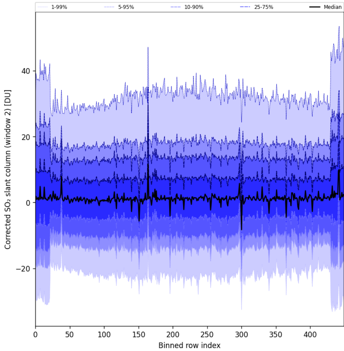
Figure 85: Along track statistics of “Corrected SO 2 slant column (window 2)” for 2024-10-21 to 2024-10-23
