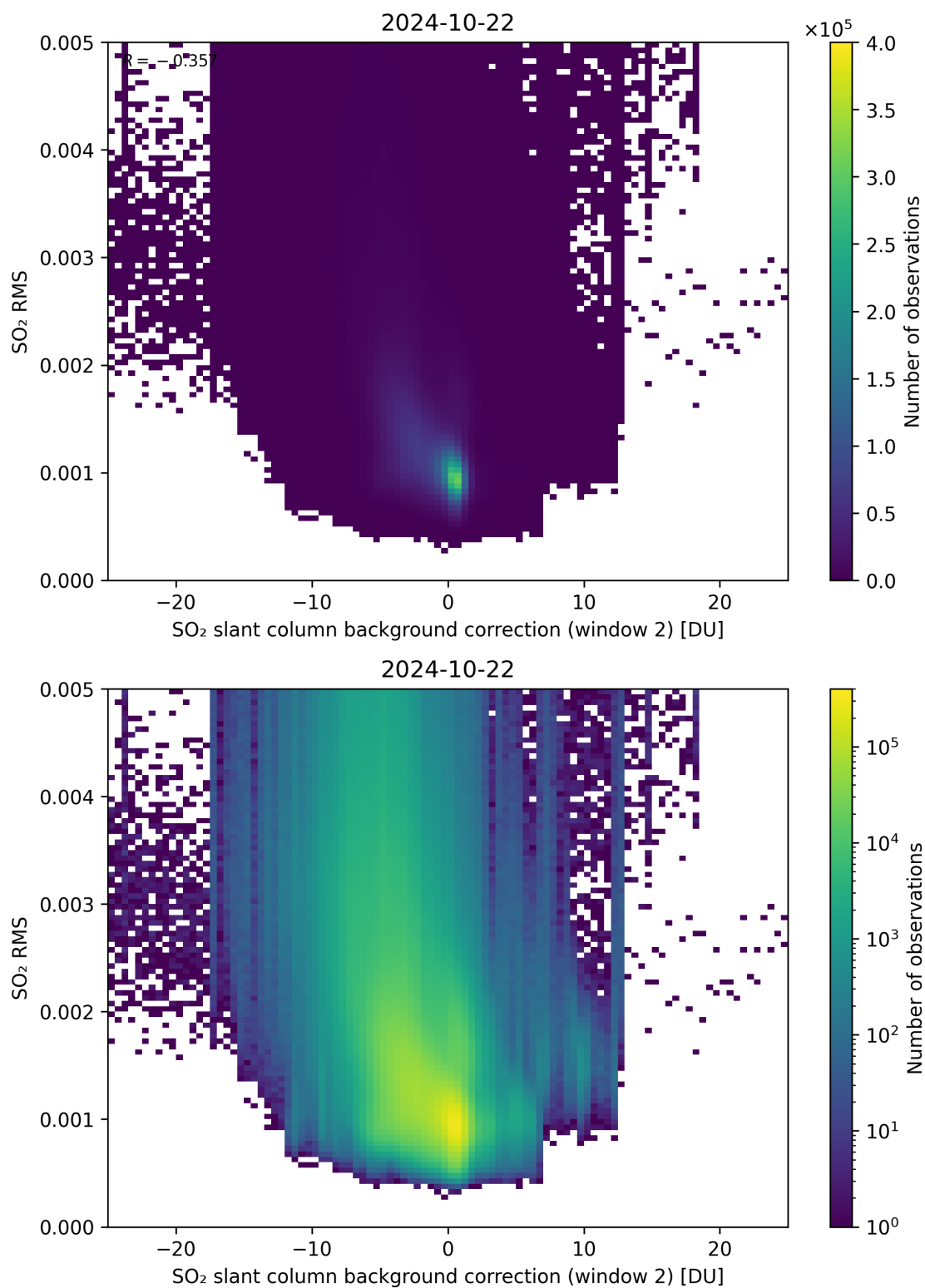
Figure 114: Scatter density plot of “SO 2 slant column background correction (window 2)” against “SO 2 RMS” for 2024-10-21 to 2024-10-23.
