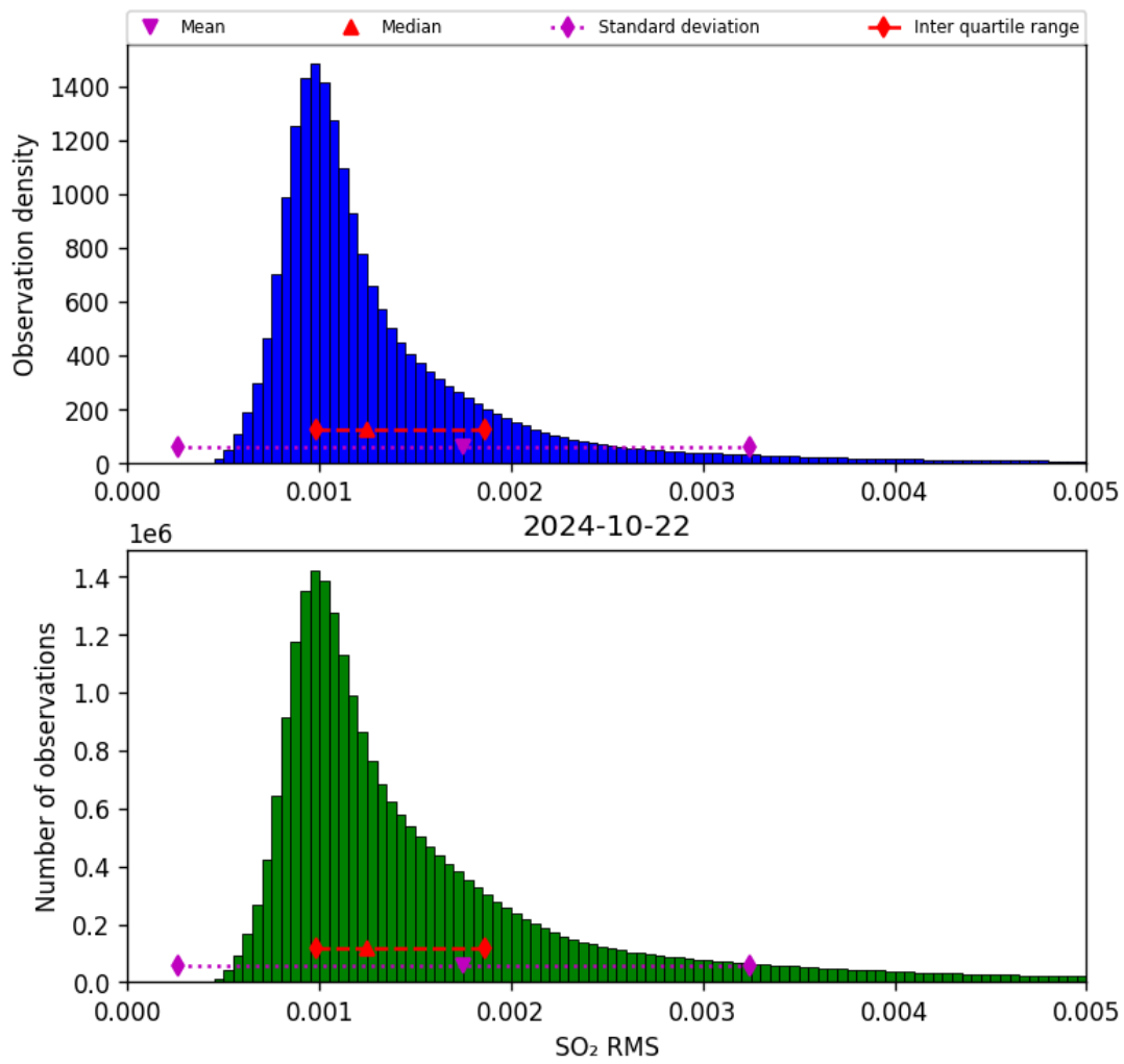
Figure 70: Histogram of “SO 2 RMS” for 2024-10-21 to 2024-10-23
