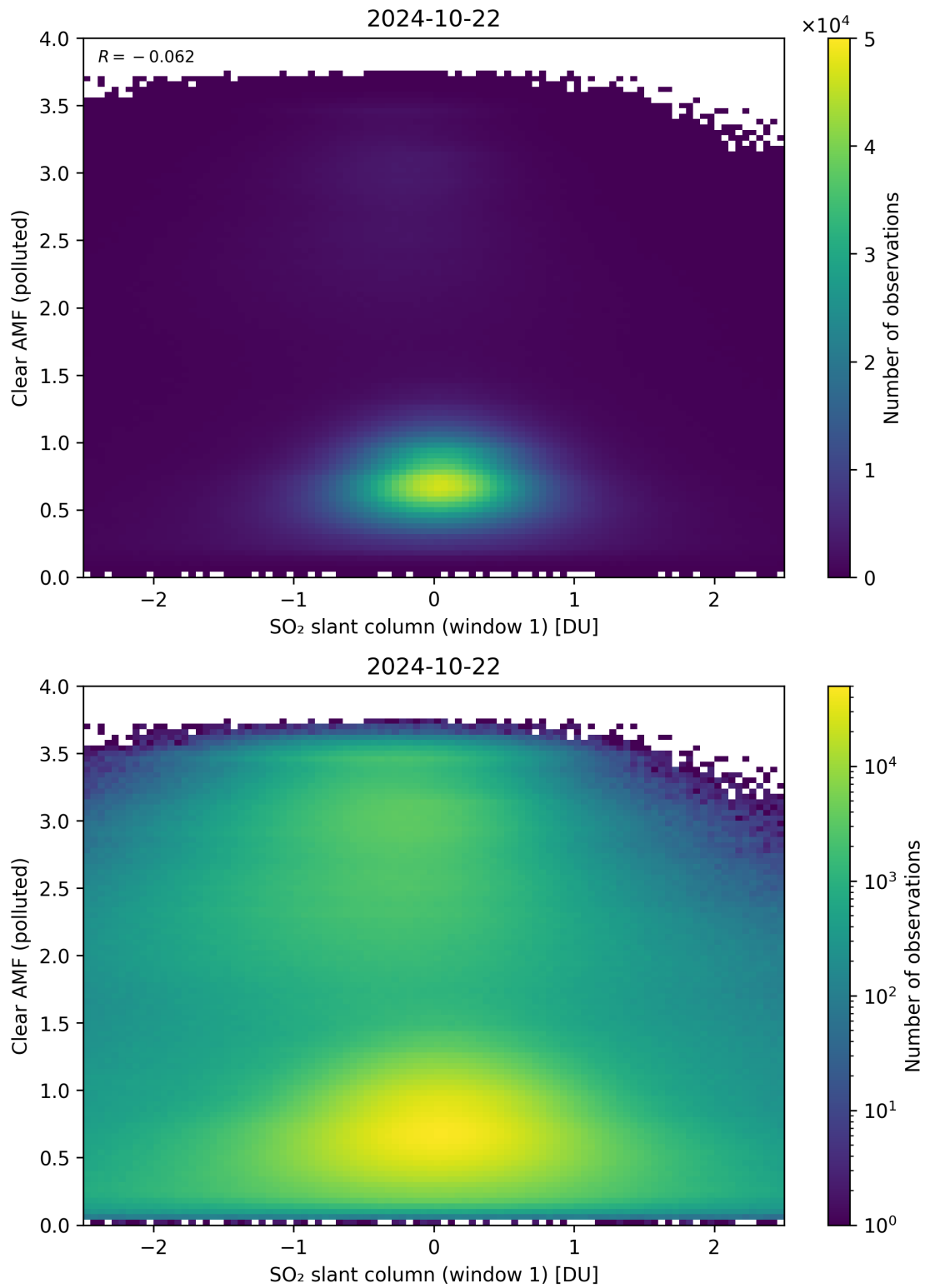
Figure 232: Scatter density plot of “SO 2 slant column (window 1)” against “Clear AMF (polluted)” for 2024-10-21 to 2024-10-23.
