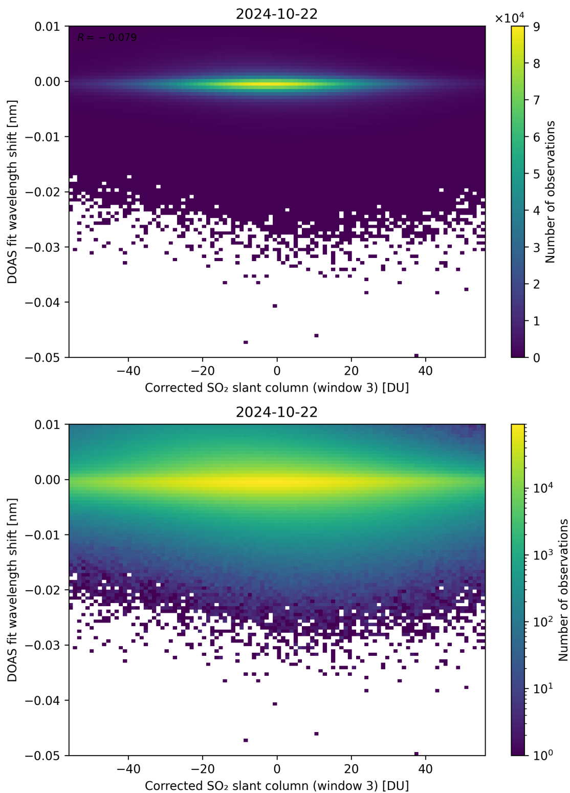
Figure 206: Scatter density plot of “Corrected SO 2 slant column (window 3)” against “DOAS fit wavelength shift” for 2024-10-21 to 2024-10-23.
