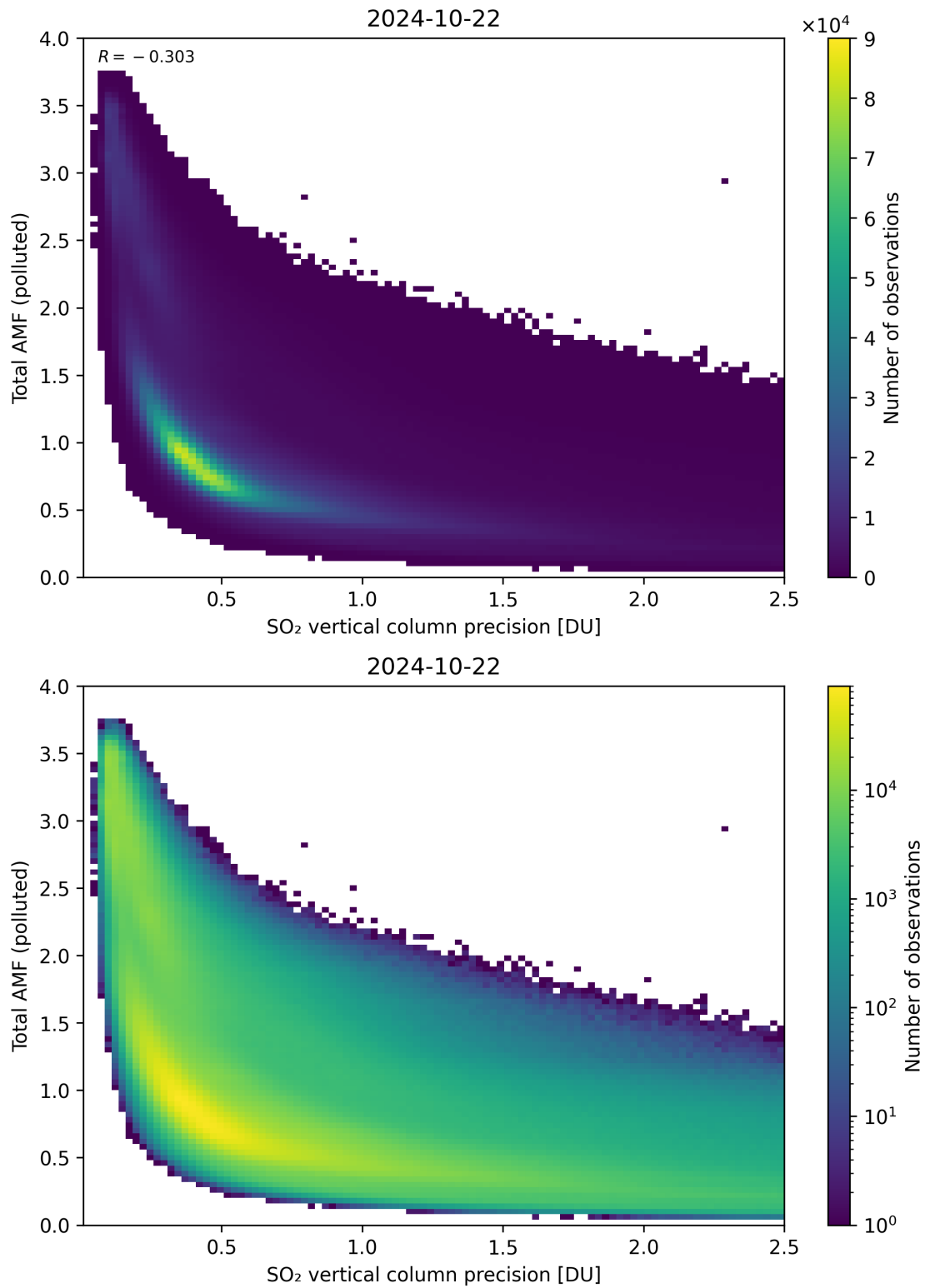
Figure 294: Scatter density plot of “SO 2 vertical column precision” against “Total AMF (polluted)” for 2024-10-21 to 2024-10-23.
