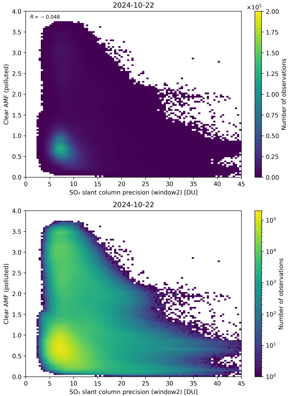
Figure 246: Scatter density plot of “SO 2 slant column precision (window2)” against “Clear AMF (polluted)” for 2024-10-21 to 2024-10-23.
