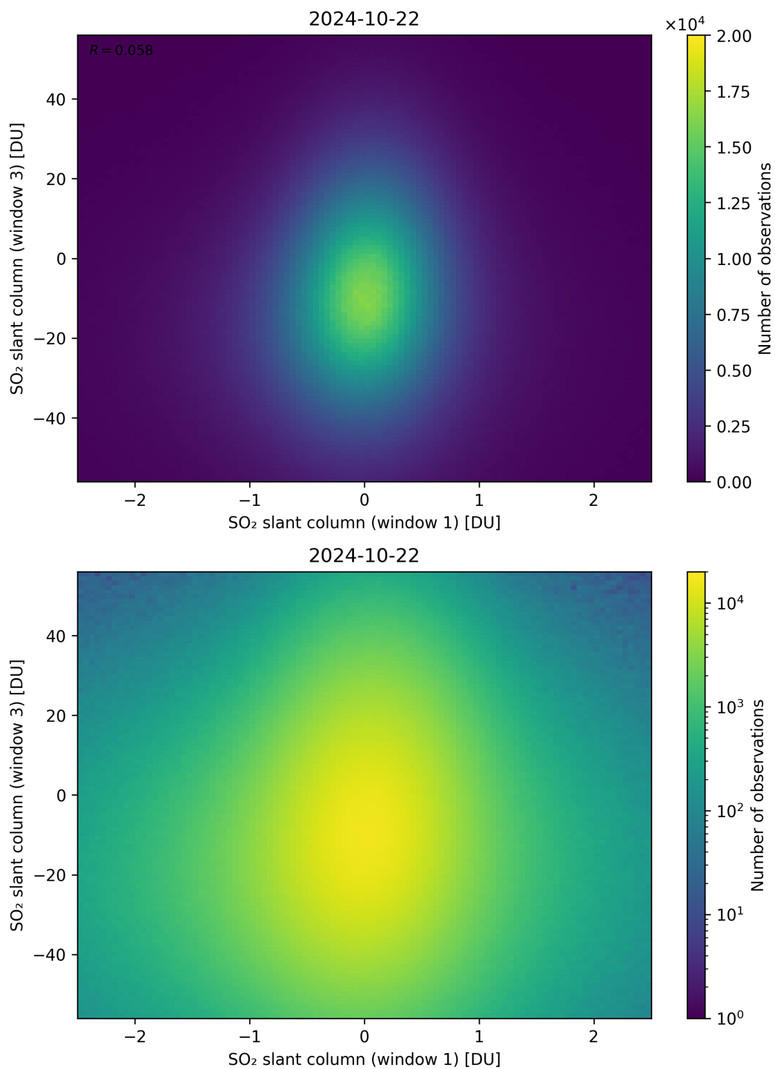
Figure 237: Scatter density plot of “SO 2 slant column (window 1)” against “SO 2 slant column (window 3)” for 2024-10-21 to 2024-10-23.
