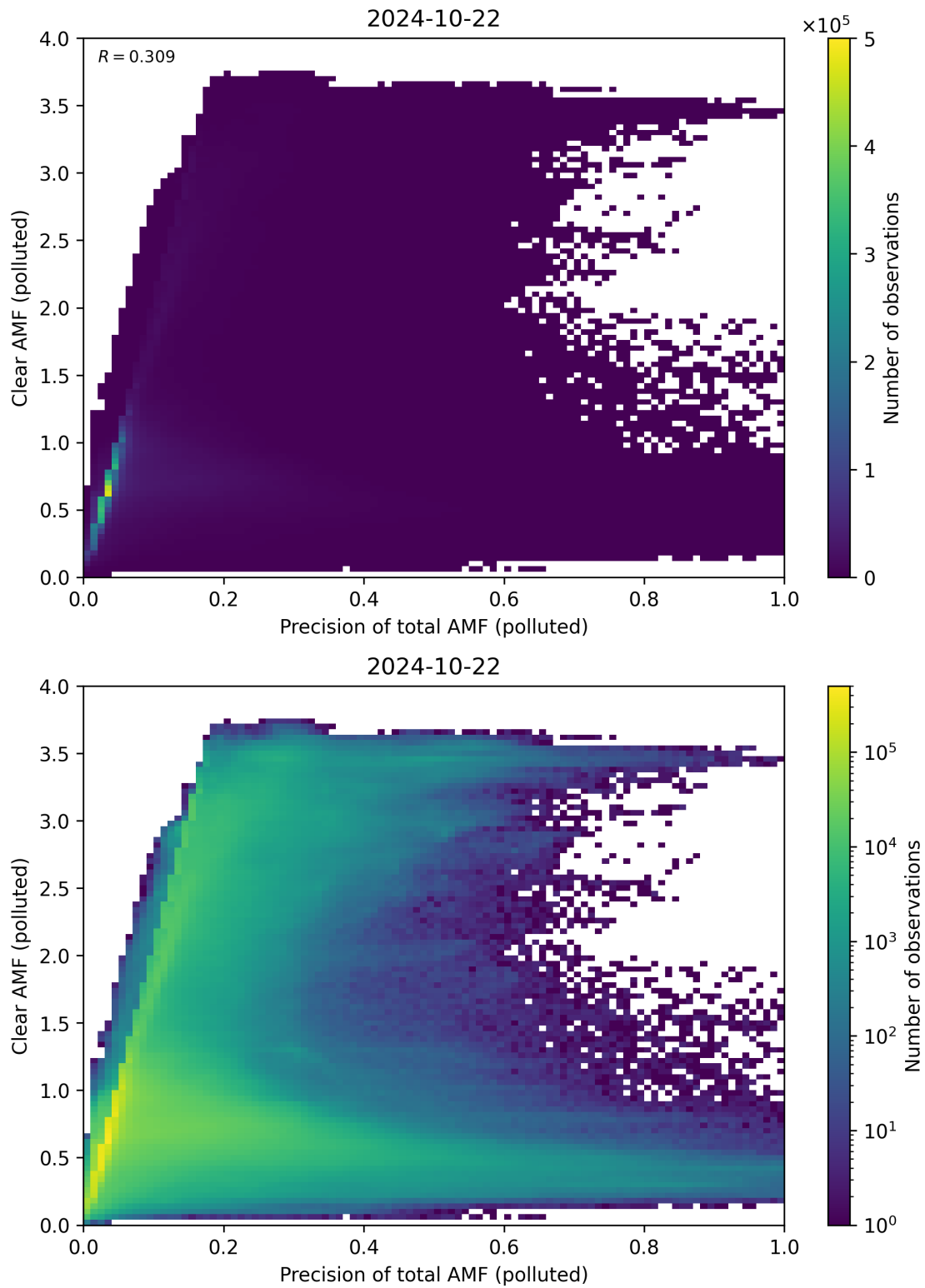
Figure 270: Scatter density plot of “Precision of total AMF (polluted)” against “Clear AMF (polluted)” for 2024-10-21 to 2024-10-23.
