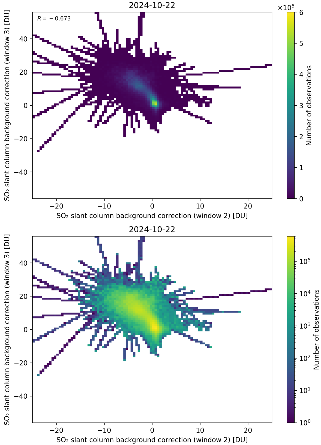
Figure 111: Scatter density plot of “SO 2 slant column background correction (window 2)” against “SO 2 slant column background correction (window 3)” for 2024-10-21 to 2024-10-23.
