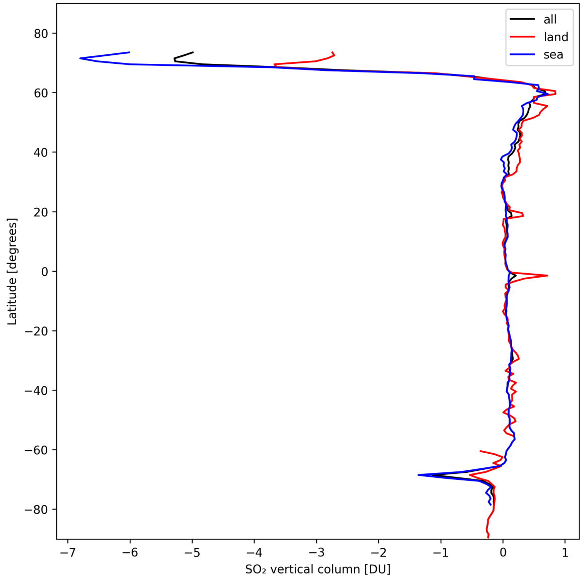
Figure 30: Zonal average of “SO 2 vertical column” for 2024-10-21 to 2024-10-23.
