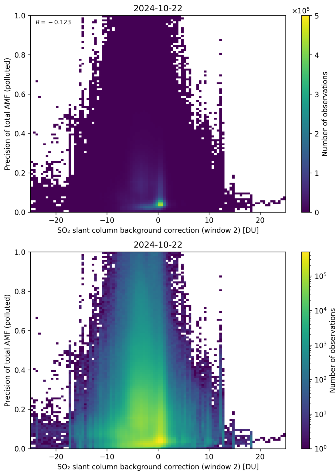
Figure 120: Scatter density plot of “SO 2 slant column background correction (window 2)” against “Precision of total AMF (polluted)” for 2024-10-21 to 2024-10-23.
