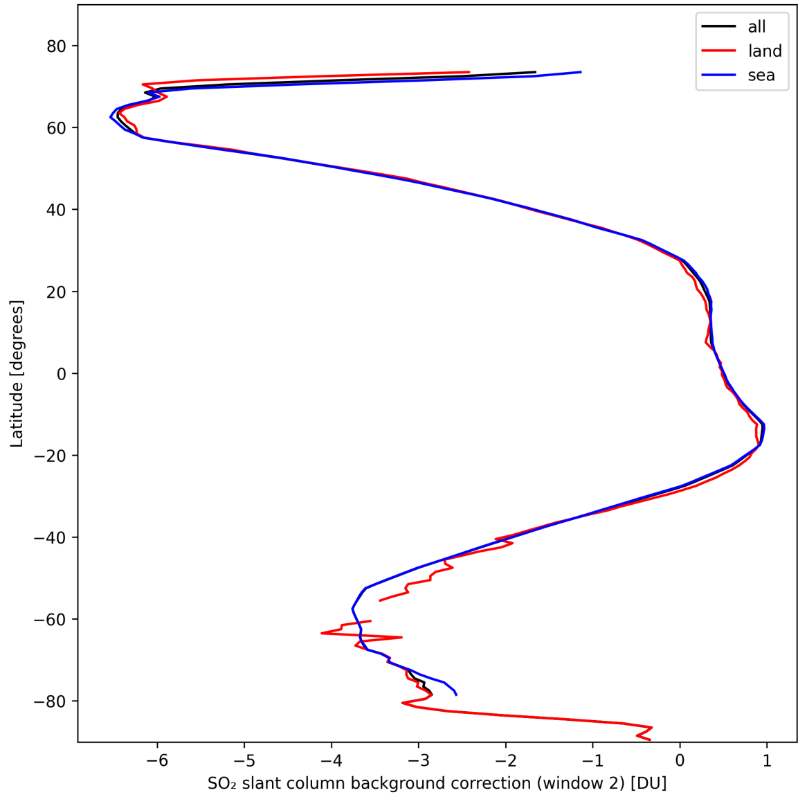
Figure 40: Zonal average of “SO 2 slant column background correction (window 2)” for 2024-10-21 to 2024-10-23.
