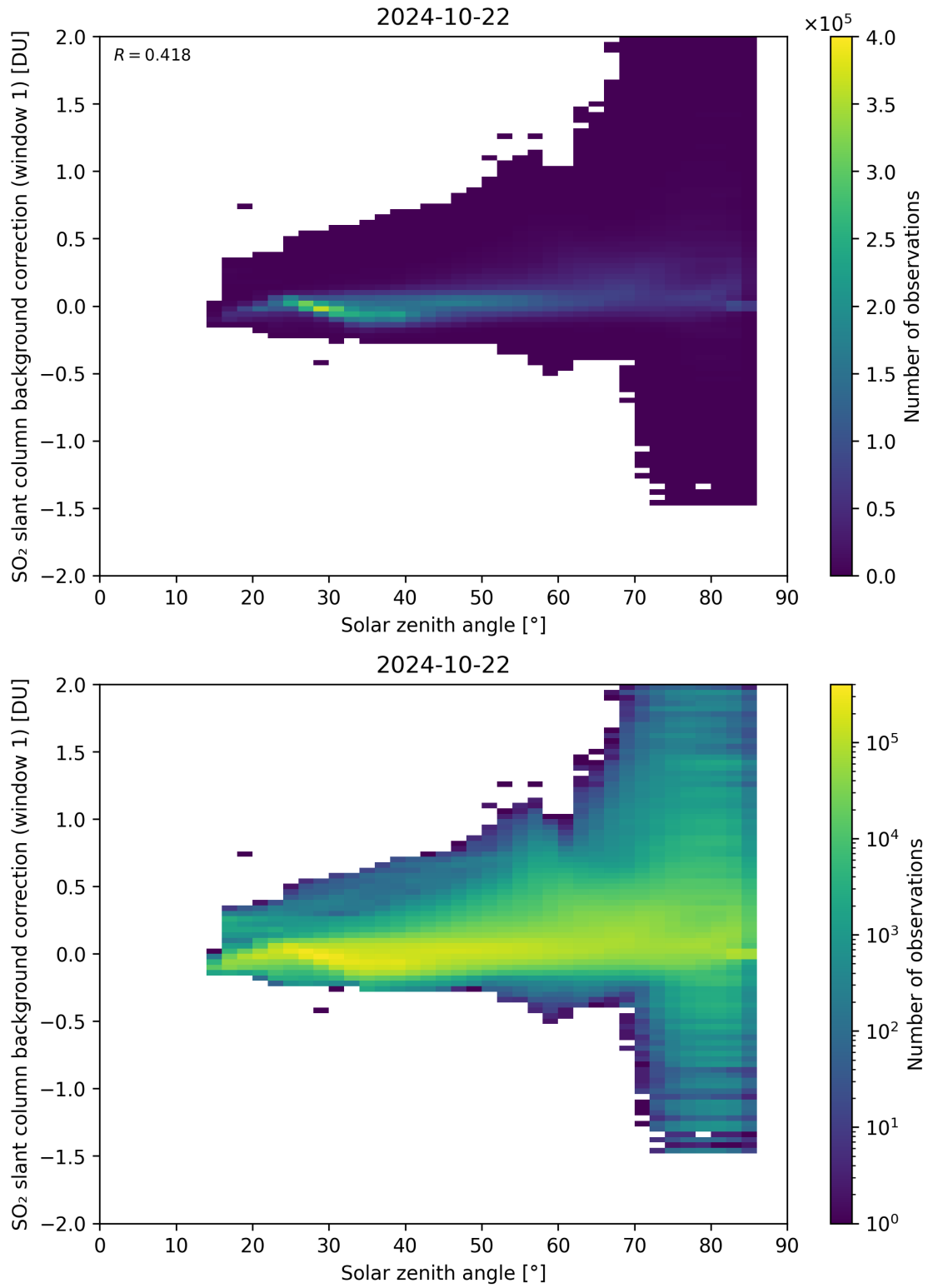
Figure 158: Scatter density plot of “Solar zenith angle” against “SO 2 slant column background correction (window 1)” for 2024-10-21 to 2024-10-23.
