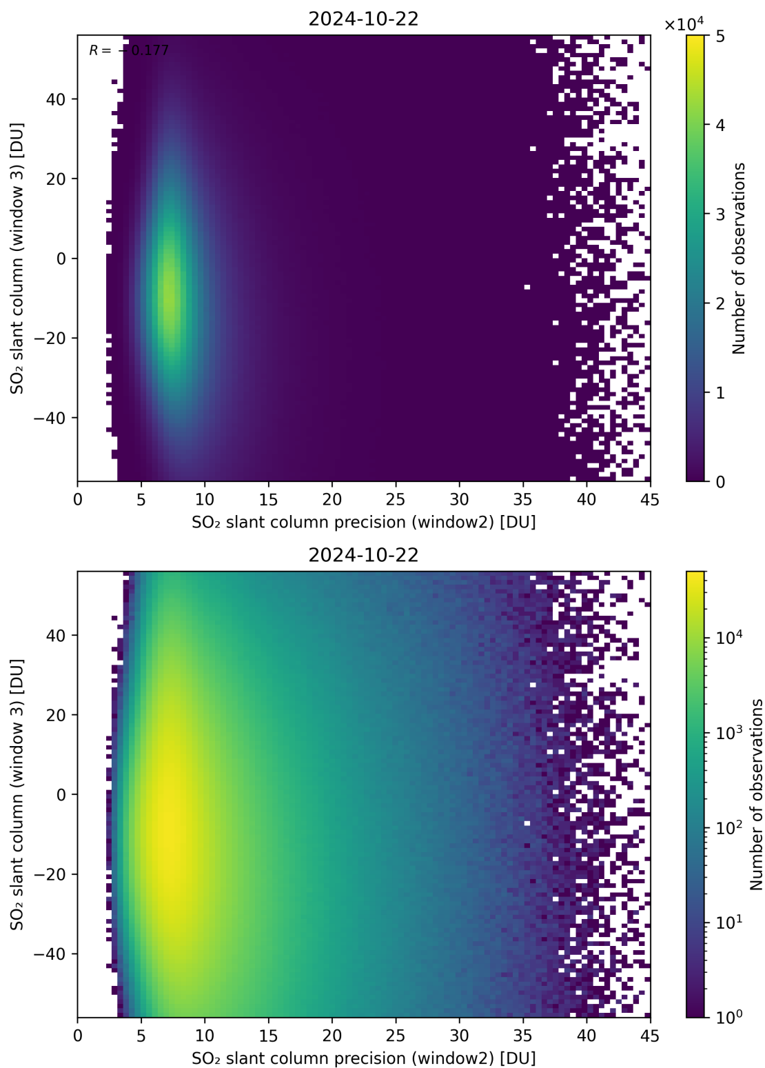
Figure 249: Scatter density plot of “SO 2 slant column precision (window2)” against “SO 2 slant column (window 3)” for 2024-10-21 to 2024-10-23.
