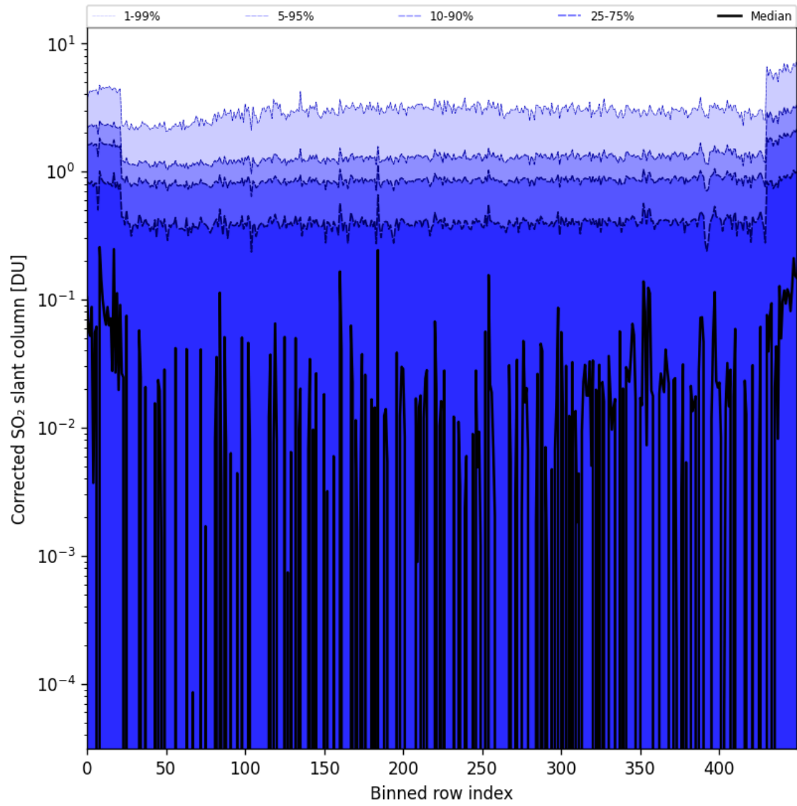
Figure 78: Along track statistics of “Corrected SO 2 slant column” for 2024-10-21 to 2024-10-23
