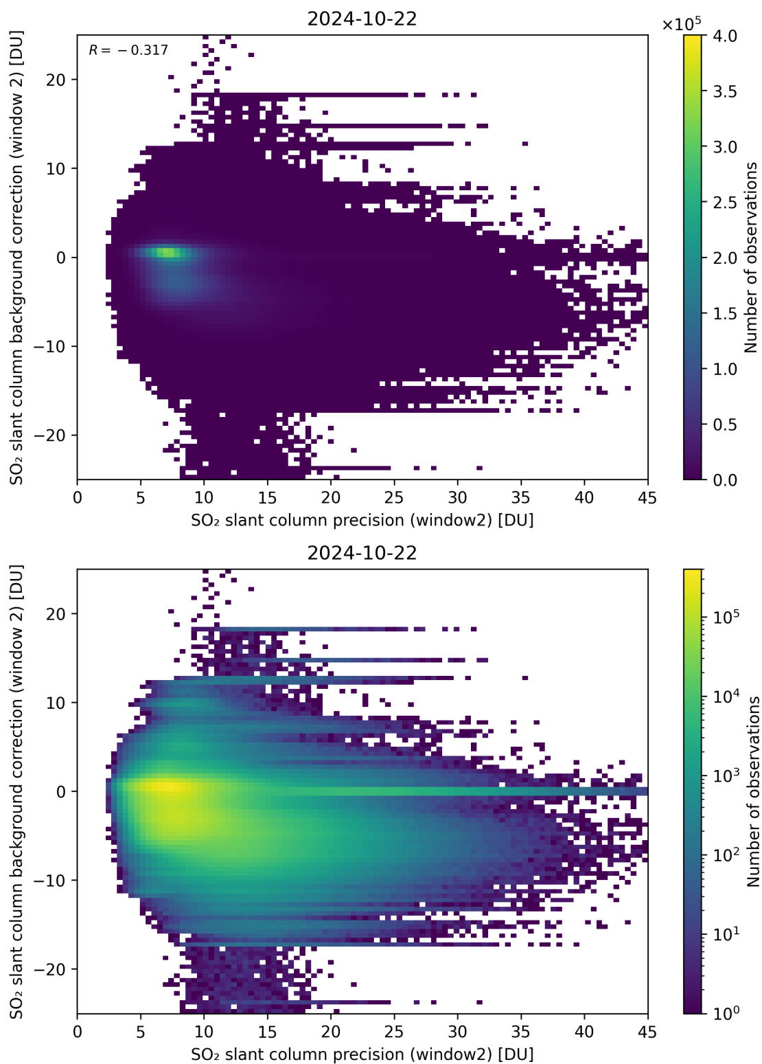
Figure 241: Scatter density plot of “SO 2 slant column precision (window2)” against “SO 2 slant column background correction (window 2)” for 2024-10-21 to 2024-10-23.
