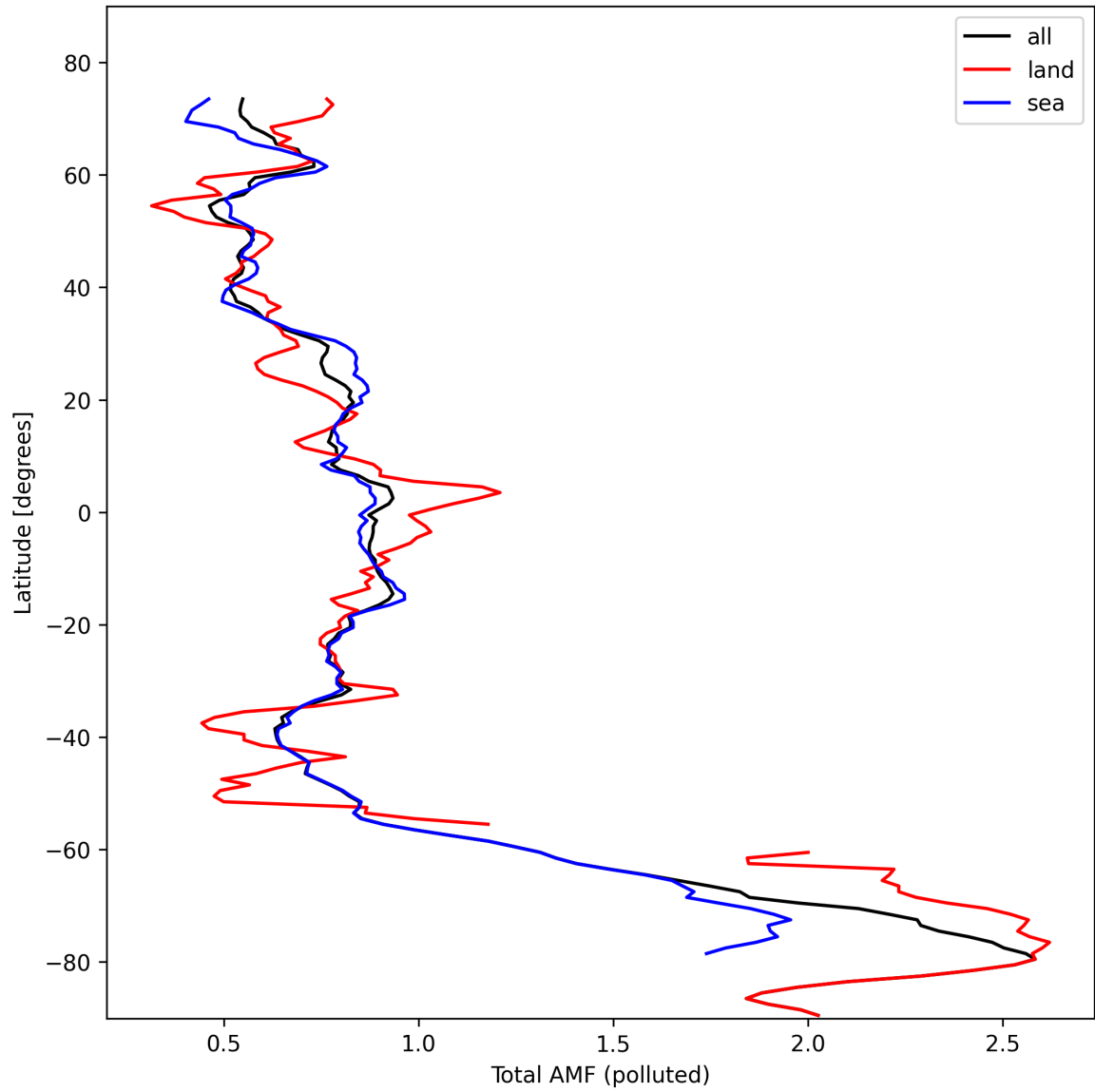
Figure 48: Zonal average of “Total AMF (polluted)” for 2024-10-21 to 2024-10-23.
