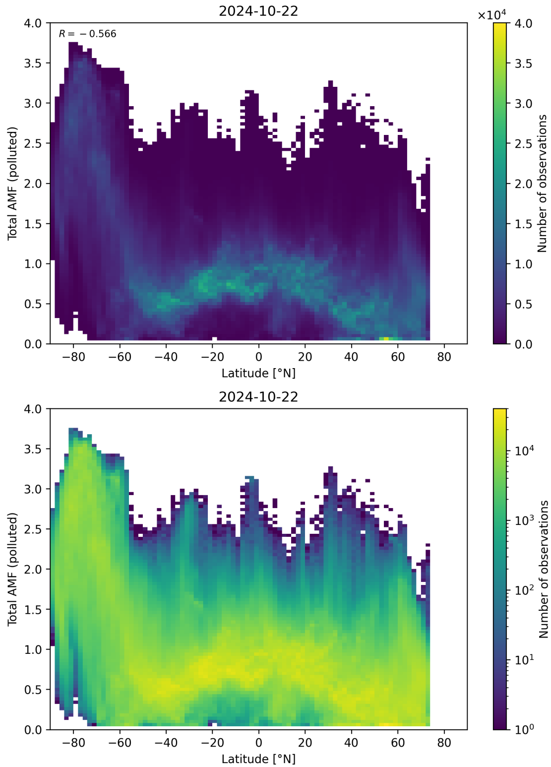
Figure 154: Scatter density plot of “Latitude” against “Total AMF (polluted)” for 2024-10-21 to 2024-10-23.
