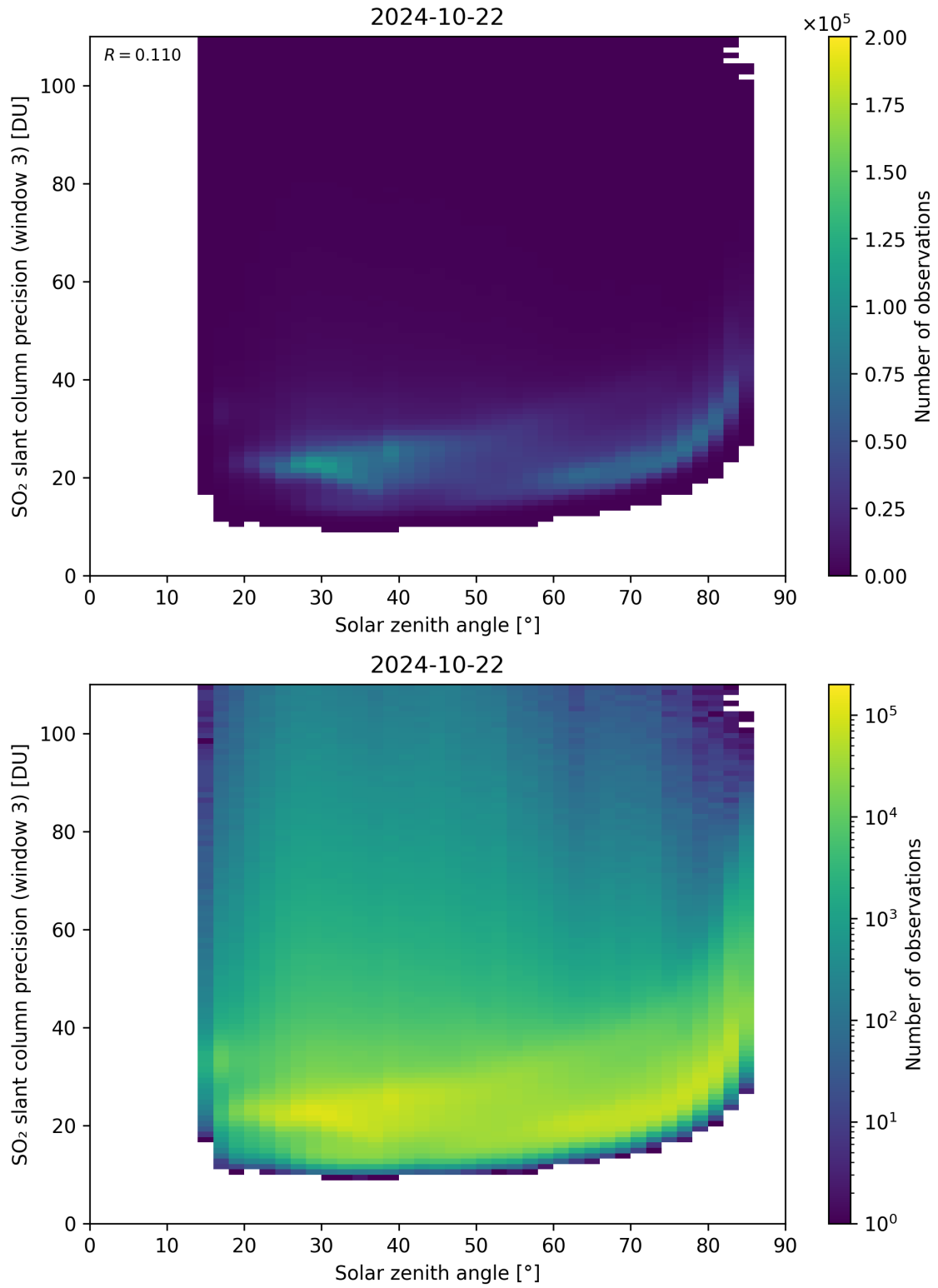
Figure 173: Scatter density plot of “Solar zenith angle” against “SO 2 slant column precision (window 3)” for 2024-10-21 to 2024-10-23.
