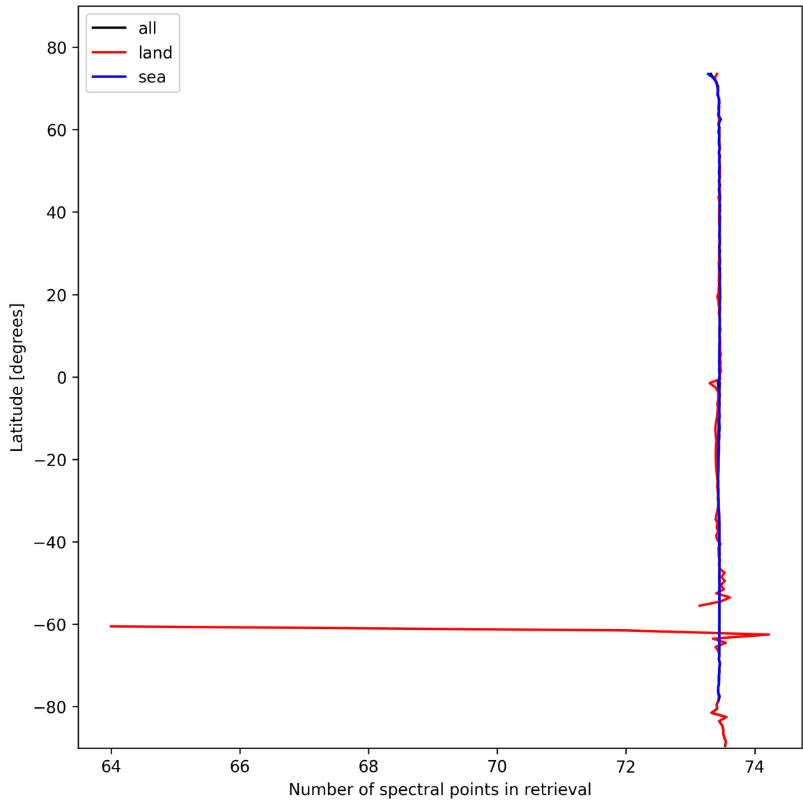
Figure 51: Zonal average of “Number of spectral points in retrieval” for 2024-10-21 to 2024-10-23.
