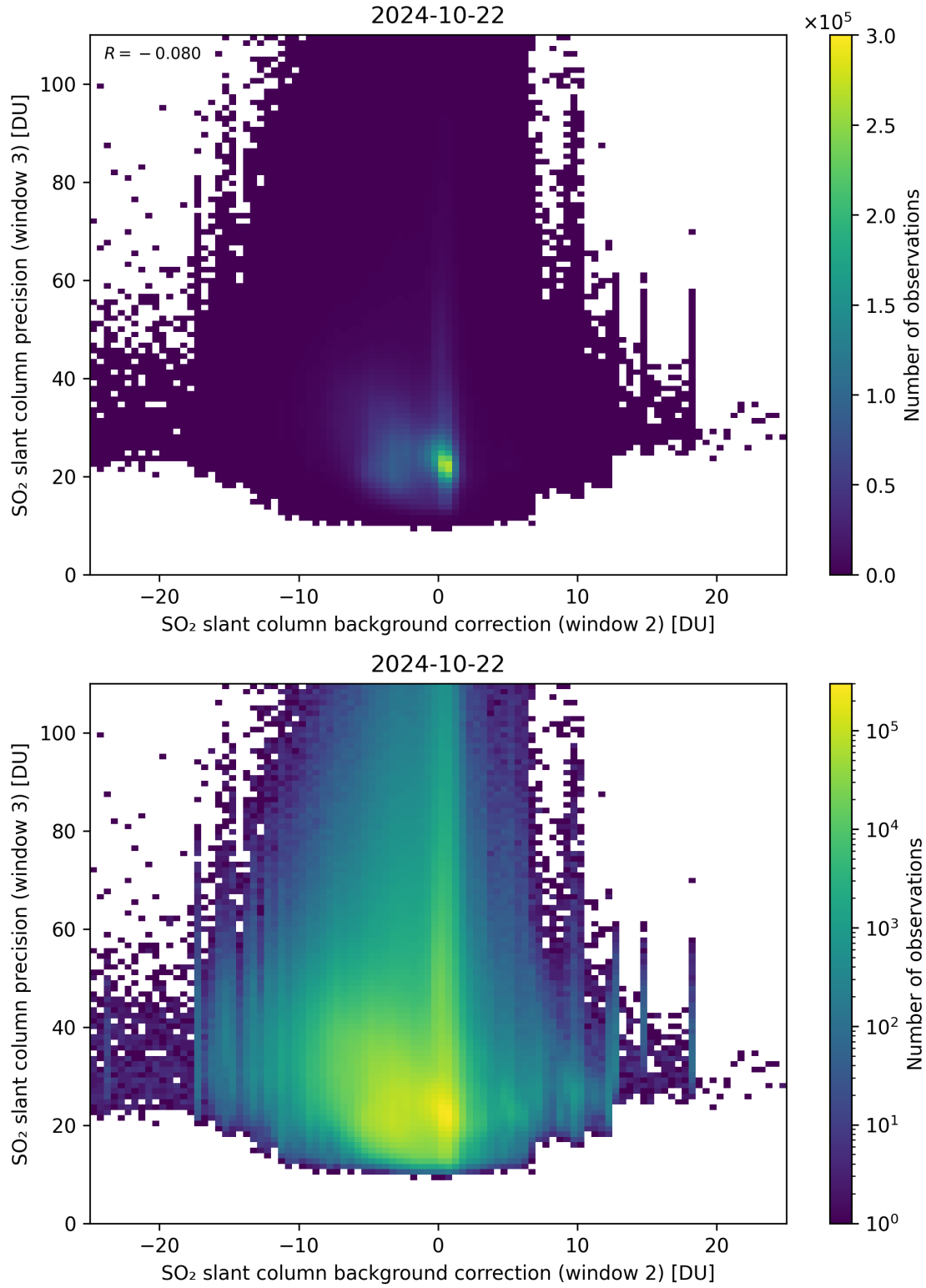
Figure 118: Scatter density plot of “SO 2 slant column background correction (window 2)” against “SO 2 slant column precision (window 3)” for 2024-10-21 to 2024-10-23.
