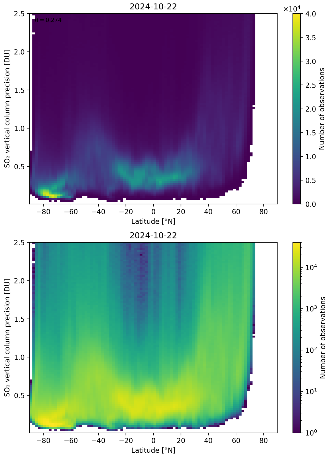
Figure 157: Scatter density plot of “Latitude” against “SO 2 vertical column precision” for 2024-10-21 to 2024-10-23.
