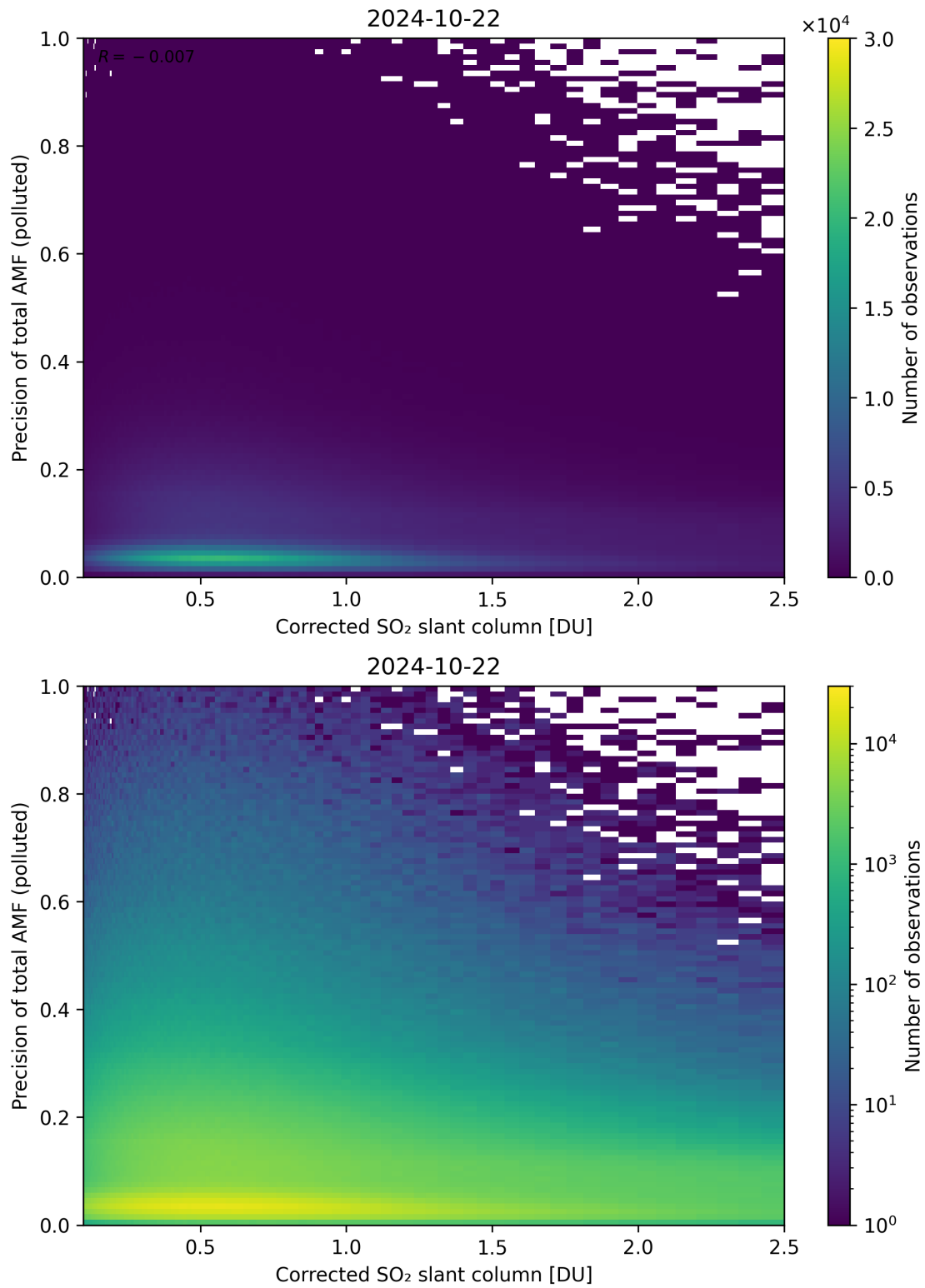
Figure 193: Scatter density plot of “Corrected SO 2 slant column” against “Precision of total AMF (polluted)” for 2024-10-21 to 2024-10-23.
