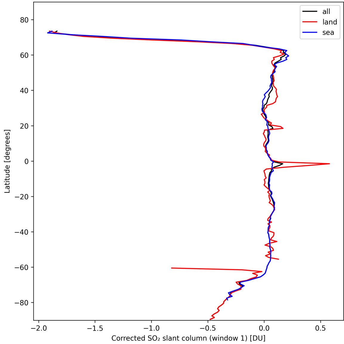
Figure 35: Zonal average of “Corrected SO 2 slant column (window 1)” for 2024-10-21 to 2024-10-23.
