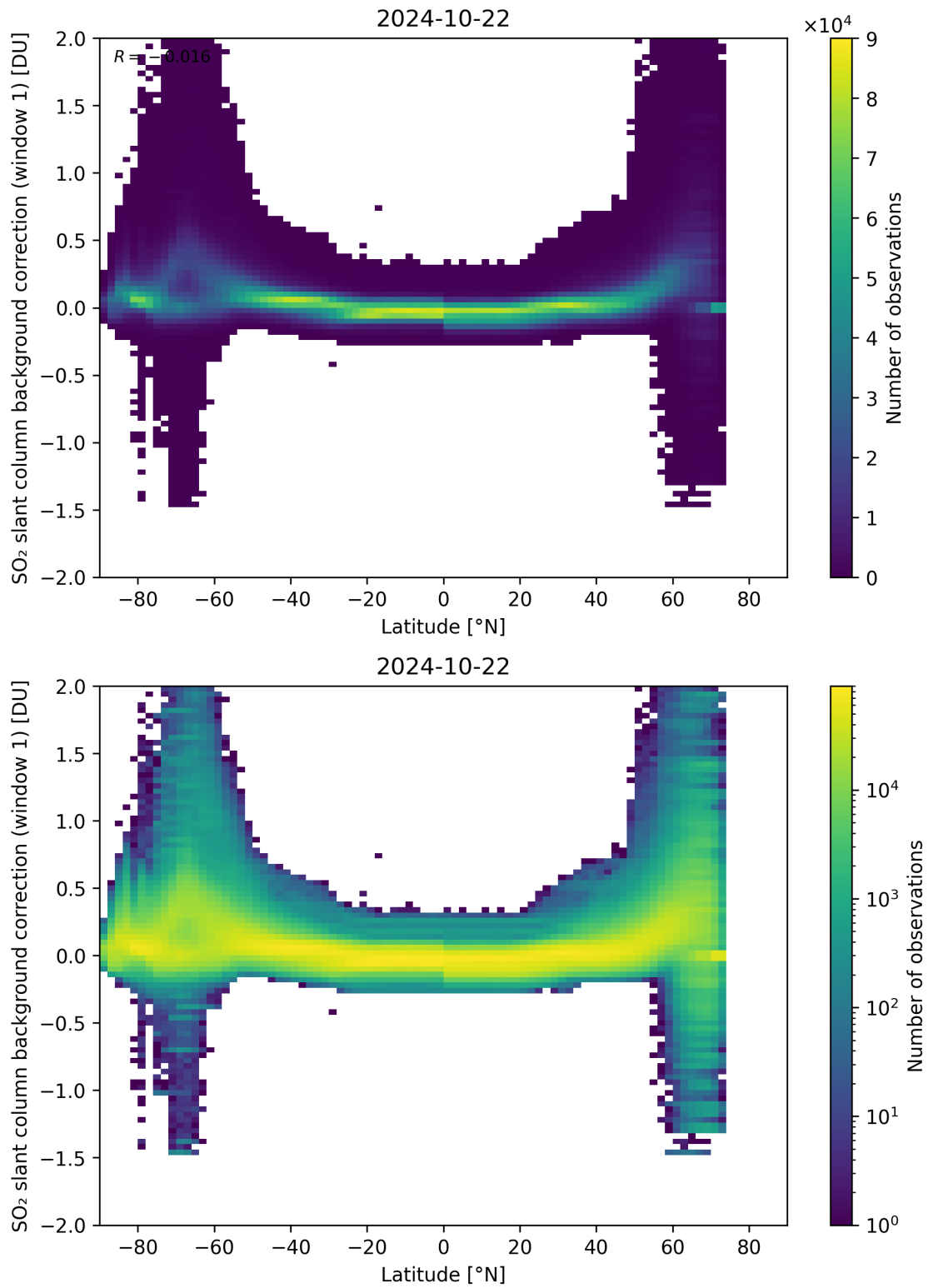
Figure 139: Scatter density plot of “Latitude” against “SO 2 slant column background correction (window 1)” for 2024-10-21 to 2024-10-23.
