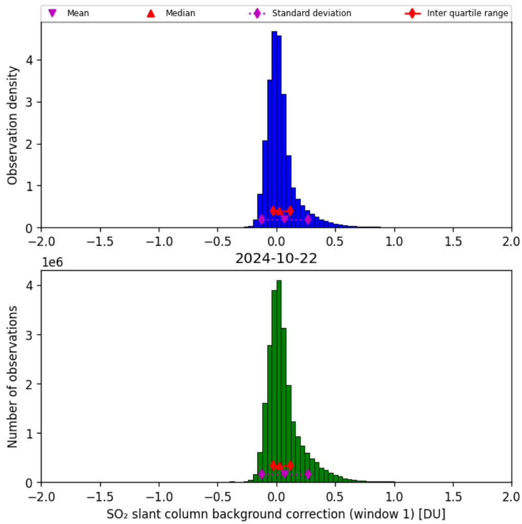
Figure 59: Histogram of “SO 2 slant column background correction (window 1)” for 2024-10-21 to 2024-10-23
