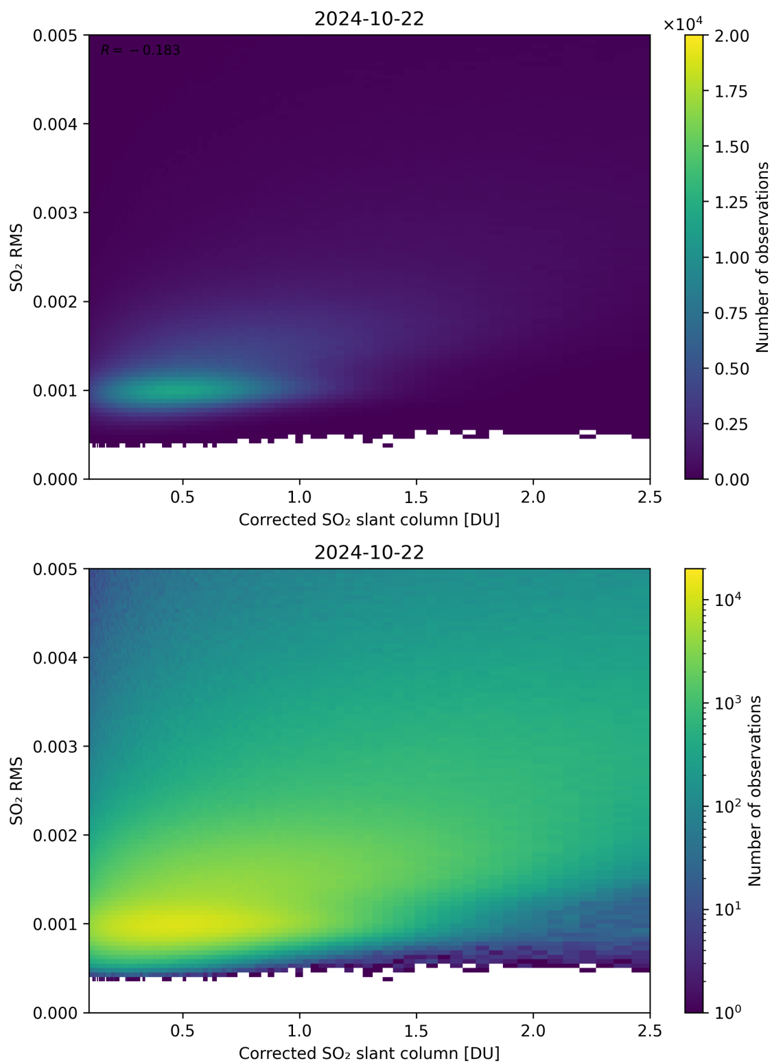
Figure 183: Scatter density plot of “Corrected SO 2 slant column” against “SO 2 RMS” for 2024-10-21 to 2024-10-23.
