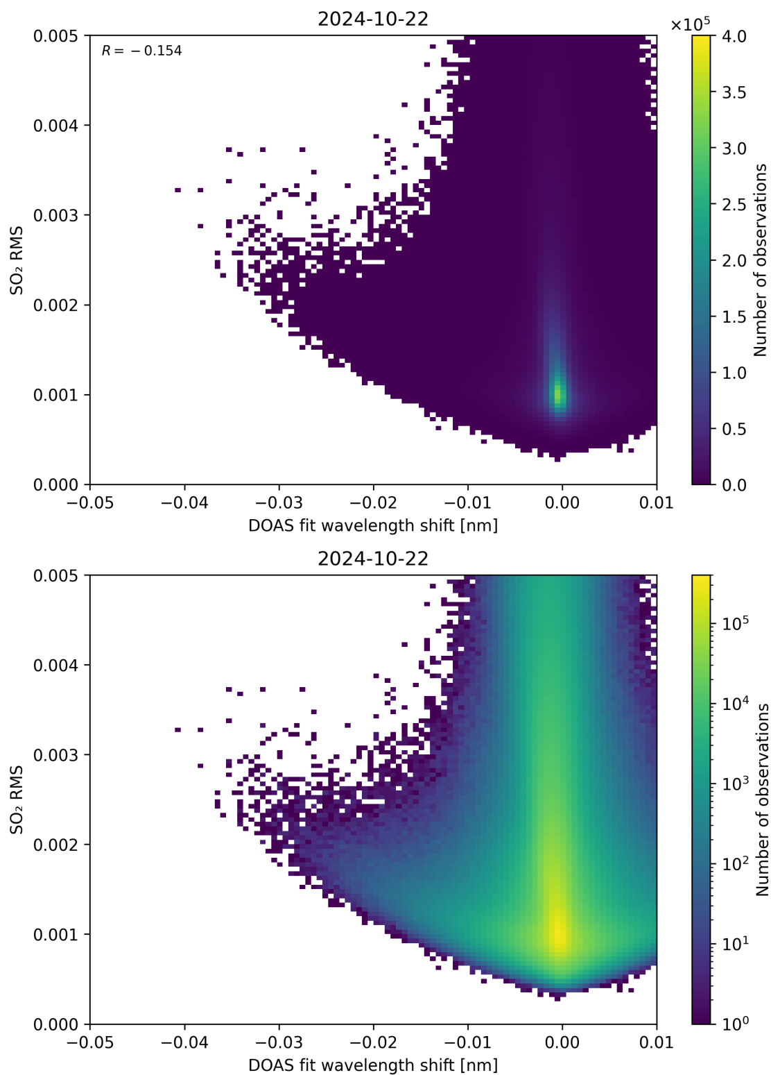
Figure 128: Scatter density plot of “DOAS fit wavelength shift” against “SO 2 RMS” for 2024-10-21 to 2024-10-23.
