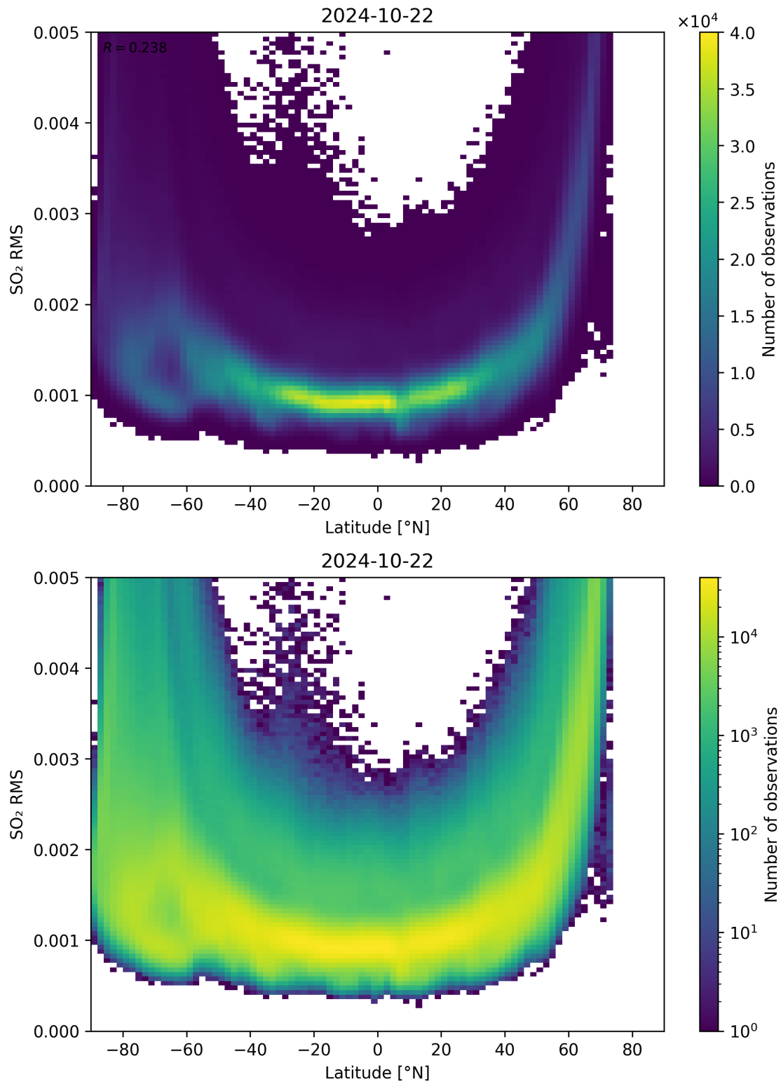
Figure 144: Scatter density plot of “Latitude” against “SO 2 RMS” for 2024-10-21 to 2024-10-23.
