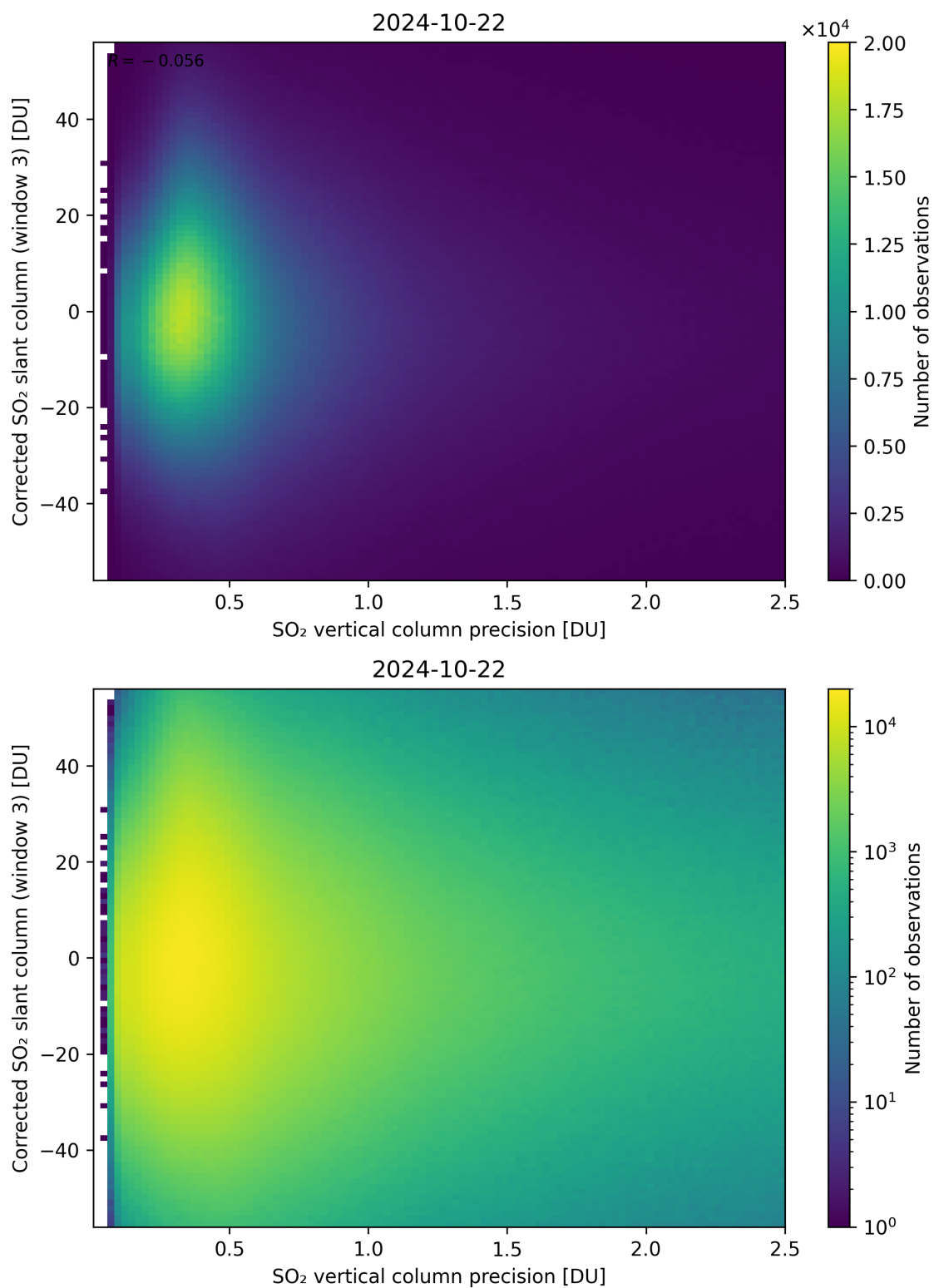
Figure 288: Scatter density plot of “SO 2 vertical column precision” against “Corrected SO 2 slant column (window 3)” for 2024-10-21 to 2024-10-23.
