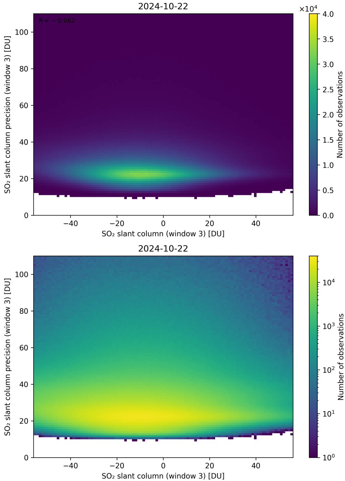
Figure 267: Scatter density plot of “SO 2 slant column (window 3)” against “SO 2 slant column precision (window 3)” for 2024-10-21 to 2024-10-23.
