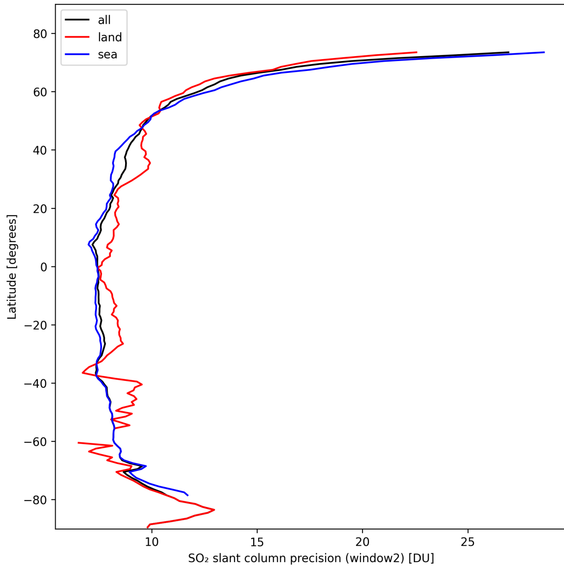
Figure 38: Zonal average of “SO 2 slant column precision (window2)” for 2024-10-21 to 2024-10-23.
