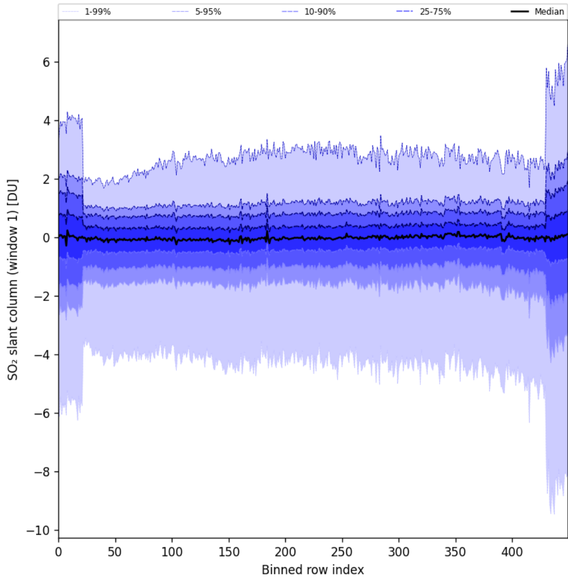
Figure 79: Along track statistics of “SO 2 slant column (window 1)” for 2024-10-21 to 2024-10-23
