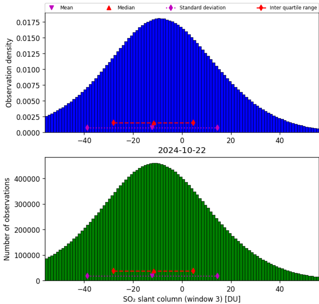
Figure 64: Histogram of “SO 2 slant column (window 3)” for 2024-10-21 to 2024-10-23
