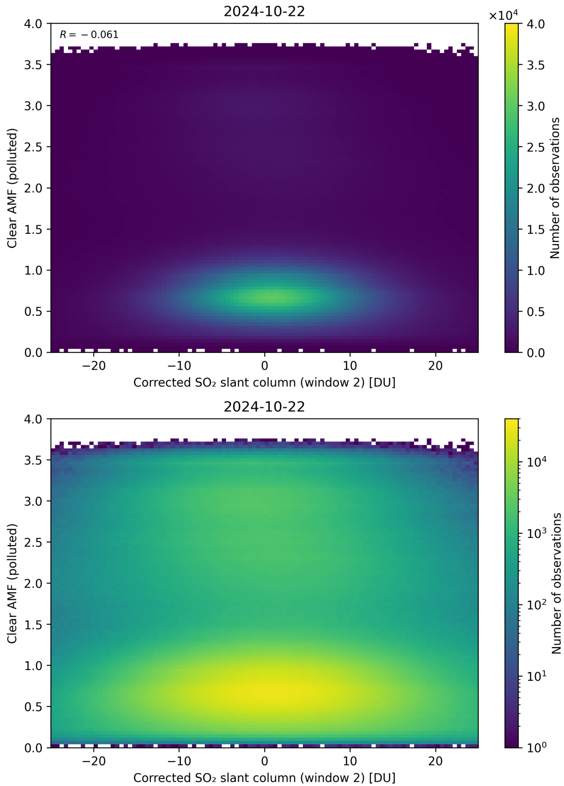
Figure 199: Scatter density plot of “Corrected SO 2 slant column (window 2)” against “Clear AMF (polluted)” for 2024-10-21 to 2024-10-23.
