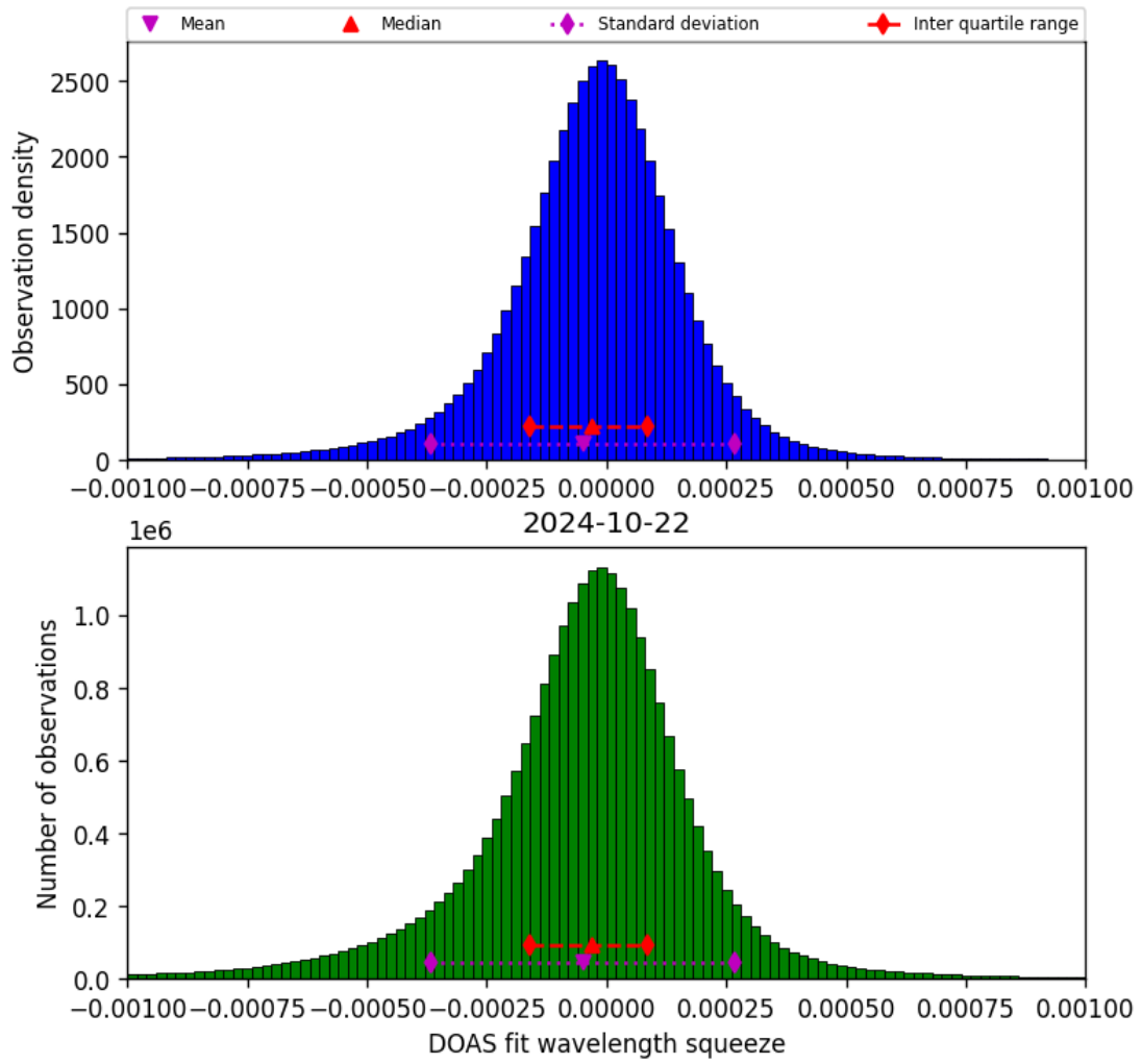
Figure 69: Histogram of “DOAS fit wavelength squeeze” for 2024-10-21 to 2024-10-23
