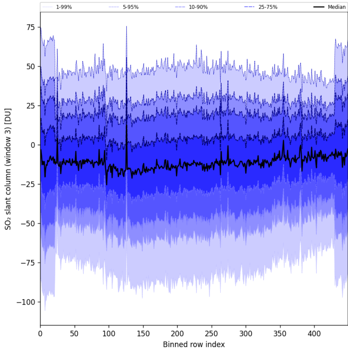
Figure 87: Along track statistics of “SO 2 slant column (window 3)” for 2024-10-21 to 2024-10-23
