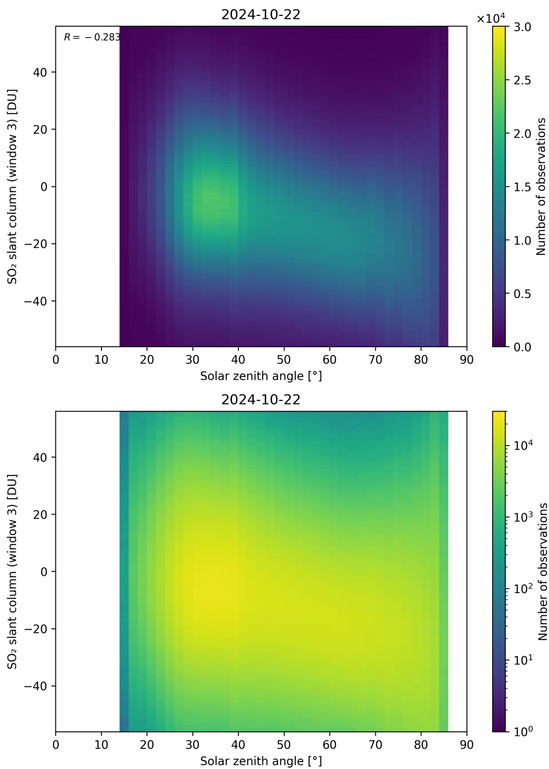
Figure 172: Scatter density plot of “Solar zenith angle” against “SO 2 slant column (window 3)” for 2024-10-21 to 2024-10-23.
