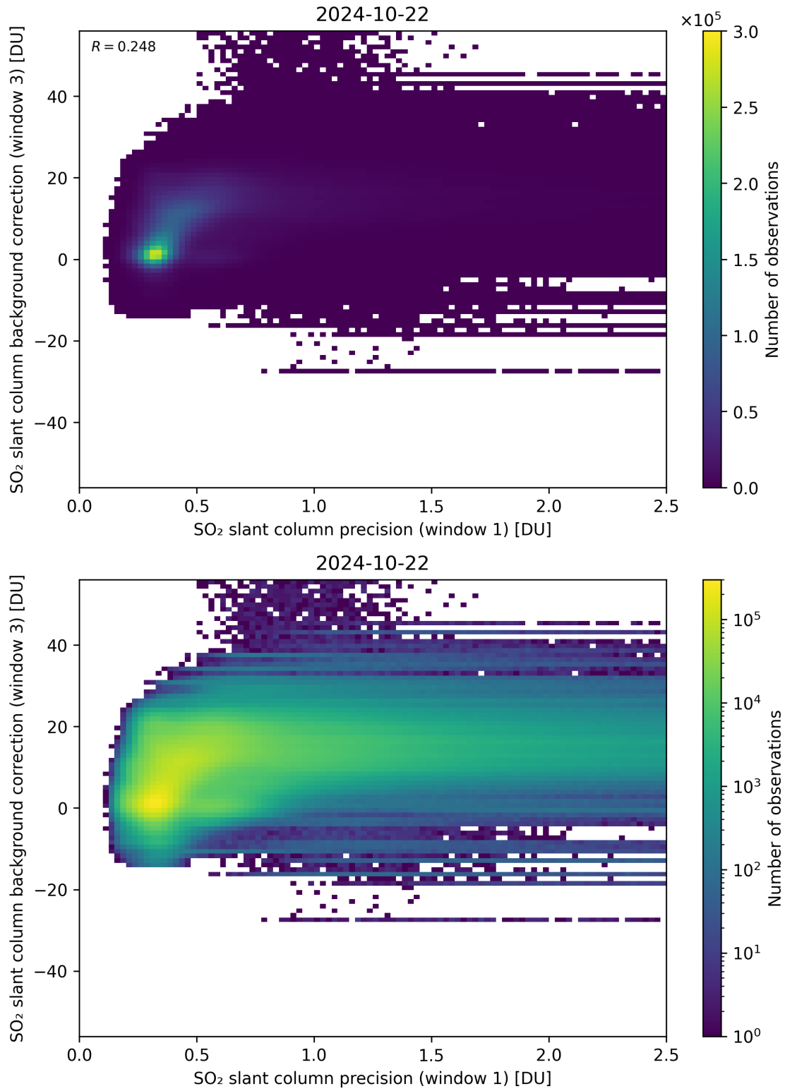
Figure 220: Scatter density plot of “SO 2 slant column precision (window 1)” against “SO 2 slant column background correction (window 3)” for 2024-10-21 to 2024-10-23.
