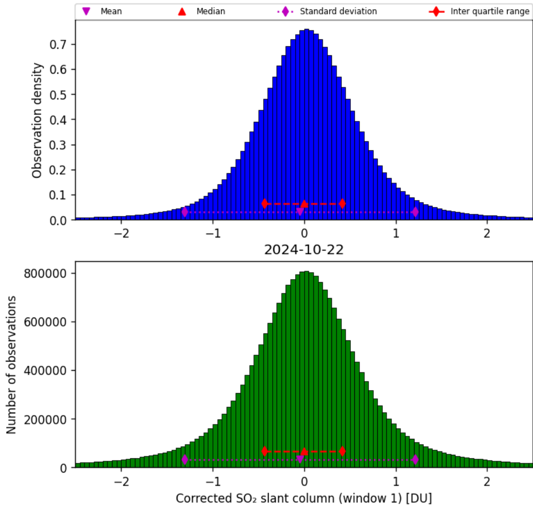
Figure 58: Histogram of “Corrected SO 2 slant column (window 1)” for 2024-10-21 to 2024-10-23
