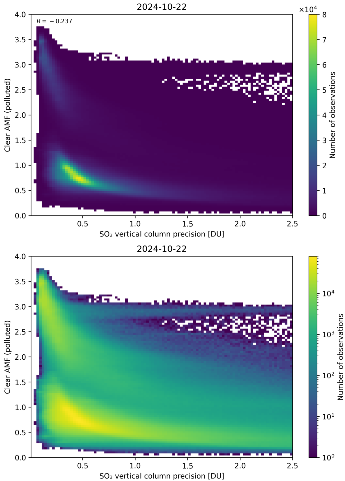
Figure 285: Scatter density plot of “SO 2 vertical column precision” against “Clear AMF (polluted)” for 2024-10-21 to 2024-10-23.
