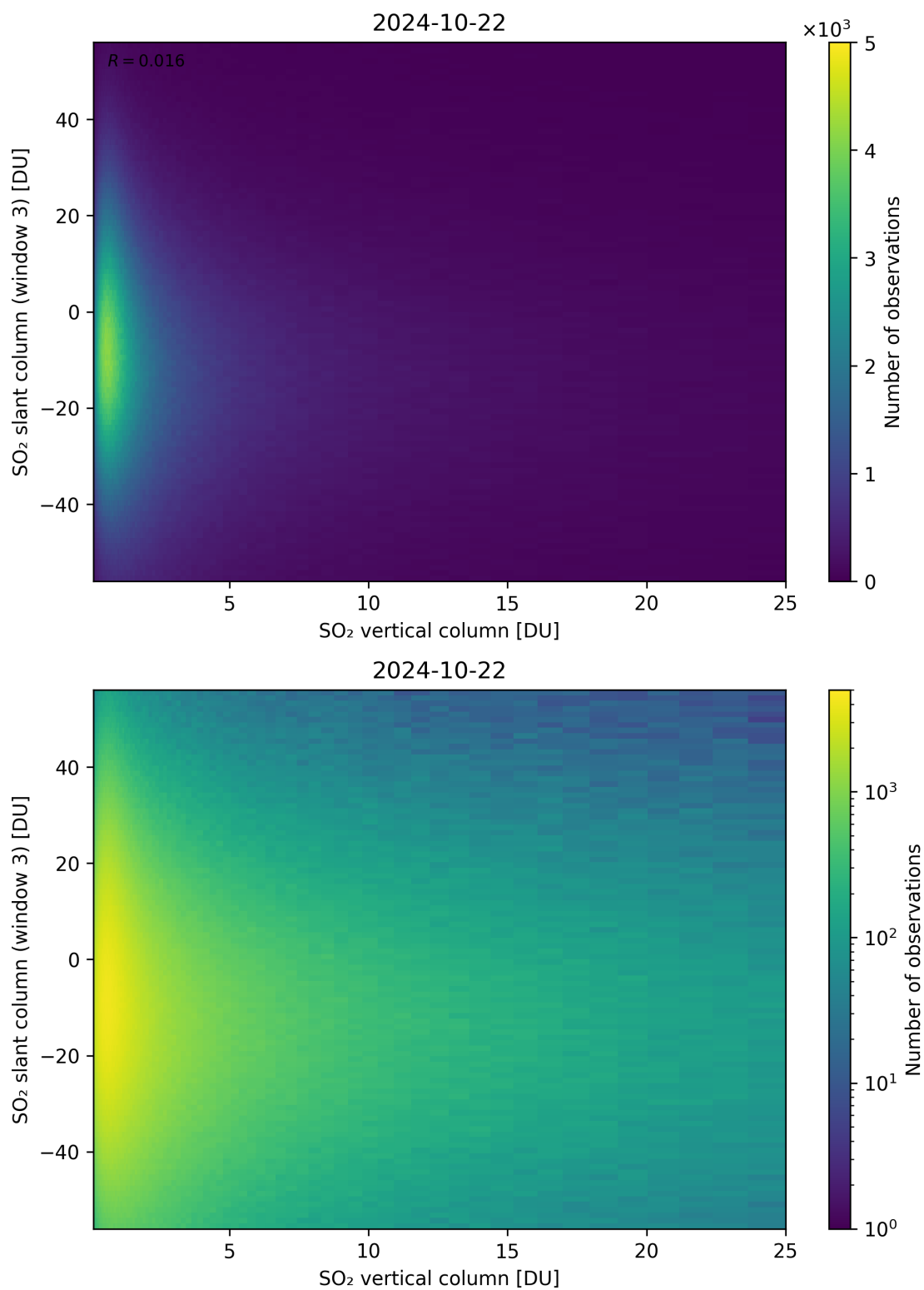
Figure 303: Scatter density plot of “SO 2 vertical column” against “SO 2 slant column (window 3)” for 2024-10-21 to 2024-10-23.
