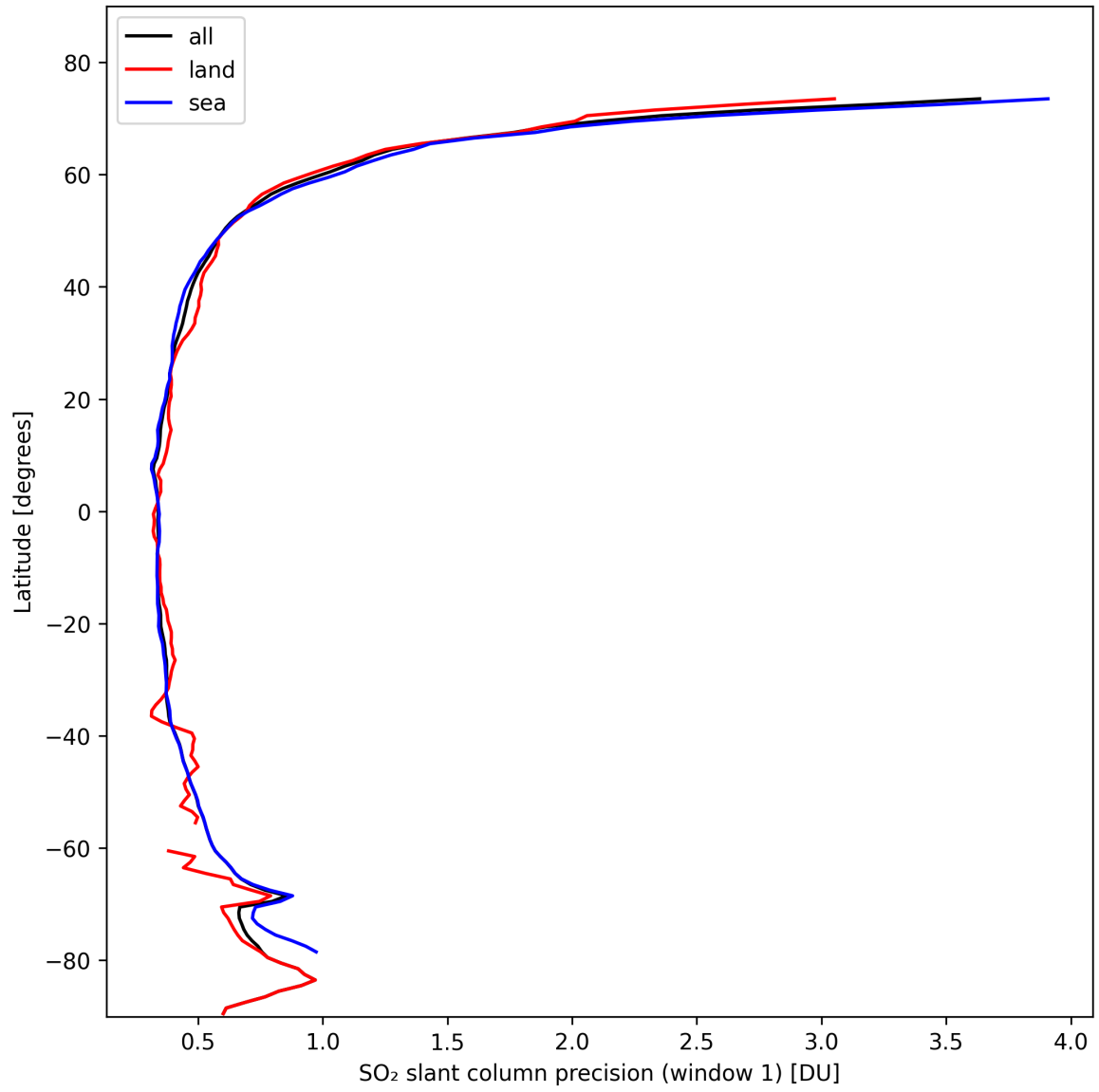
Figure 34: Zonal average of “SO 2 slant column precision (window 1)” for 2024-10-21 to 2024-10-23.
