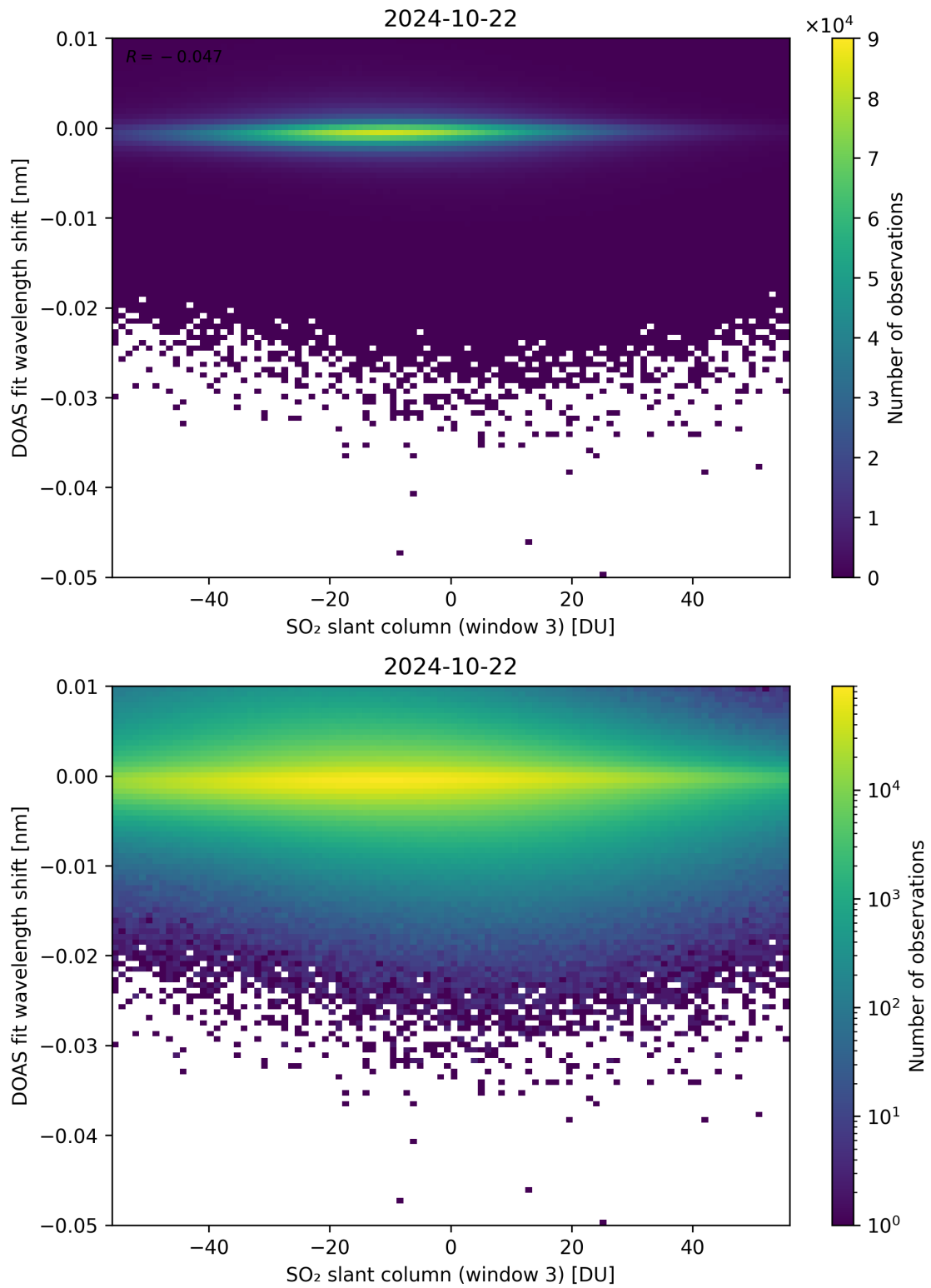
Figure 254: Scatter density plot of “SO 2 slant column (window 3)” against “DOAS fit wavelength shift” for 2024-10-21 to 2024-10-23.
