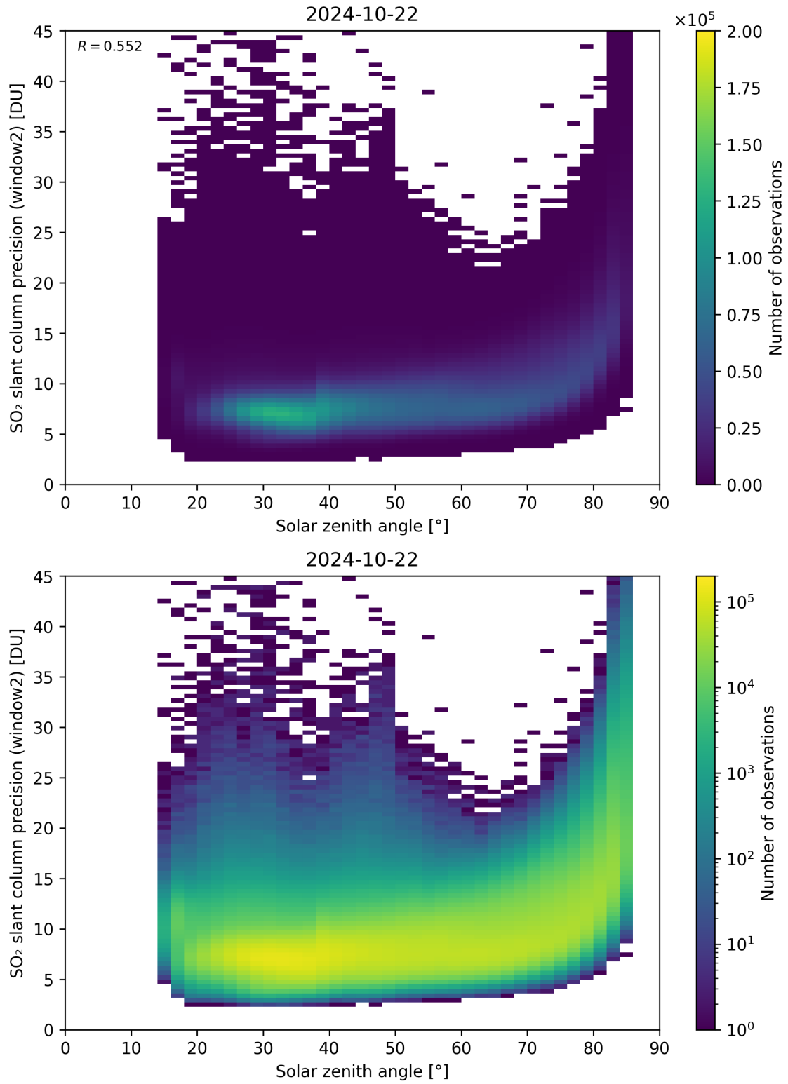
Figure 171: Scatter density plot of “Solar zenith angle” against “SO 2 slant column precision (window2)” for 2024-10-21 to 2024-10-23.
