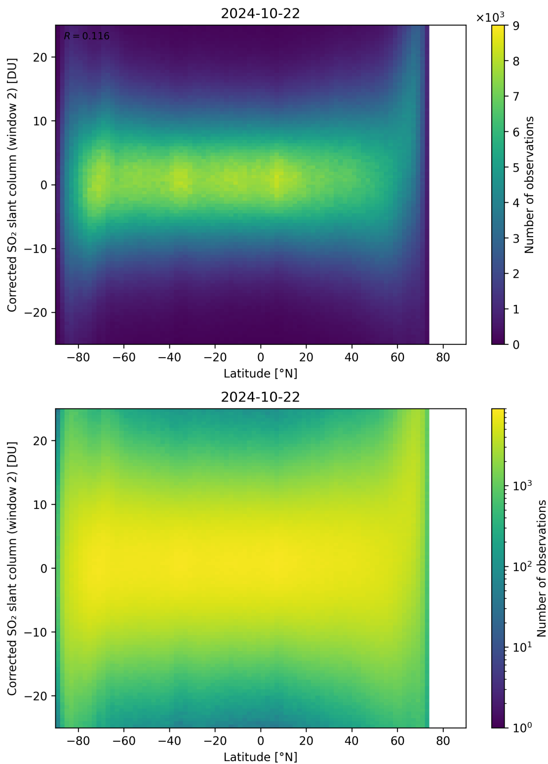
Figure 147: Scatter density plot of “Latitude” against “Corrected SO 2 slant column (window 2)” for 2024-10-21 to 2024-10-23.
