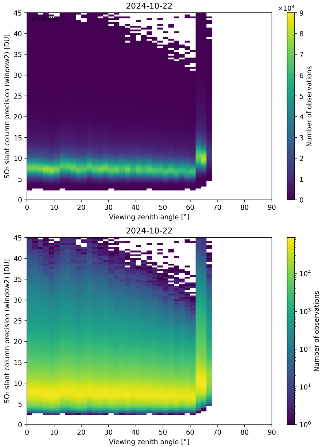
Figure 322: Scatter density plot of “Viewing zenith angle” against “SO 2 slant column precision (window2)” for 2024-10-21 to 2024-10-23.
