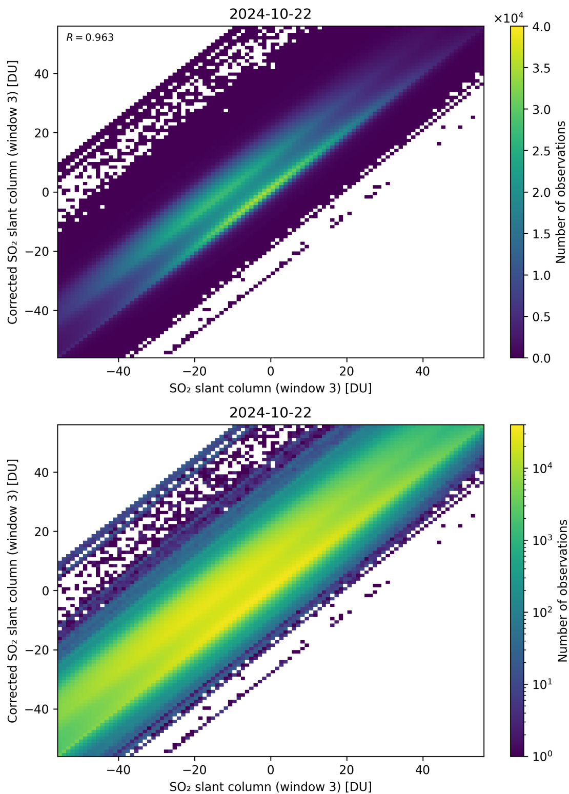
Figure 266: Scatter density plot of “SO 2 slant column (window 3)” against “Corrected SO 2 slant column (window 3)” for 2024-10-21 to 2024-10-23.
