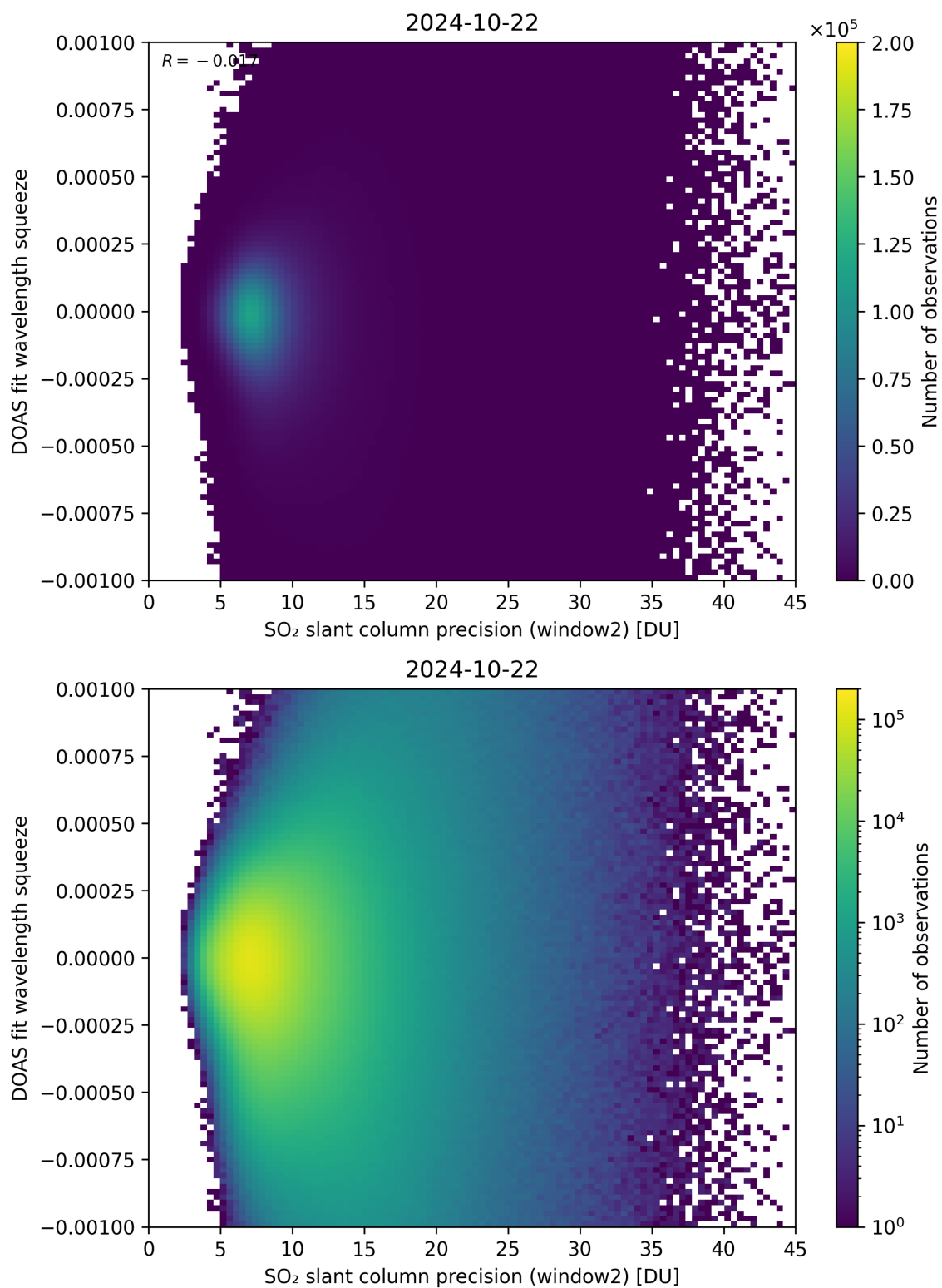
Figure 244: Scatter density plot of “SO 2 slant column precision (window2)” against “DOAS fit wavelength squeeze” for 2024-10-21 to 2024-10-23.
