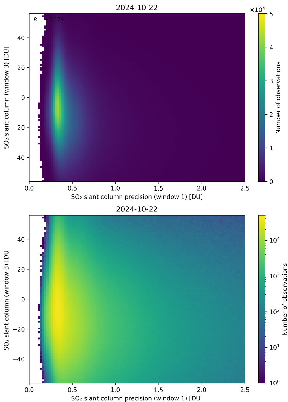
Figure 228: Scatter density plot of “SO 2 slant column precision (window 1)” against “SO 2 slant column (window 3)” for 2024-10-21 to 2024-10-23.
