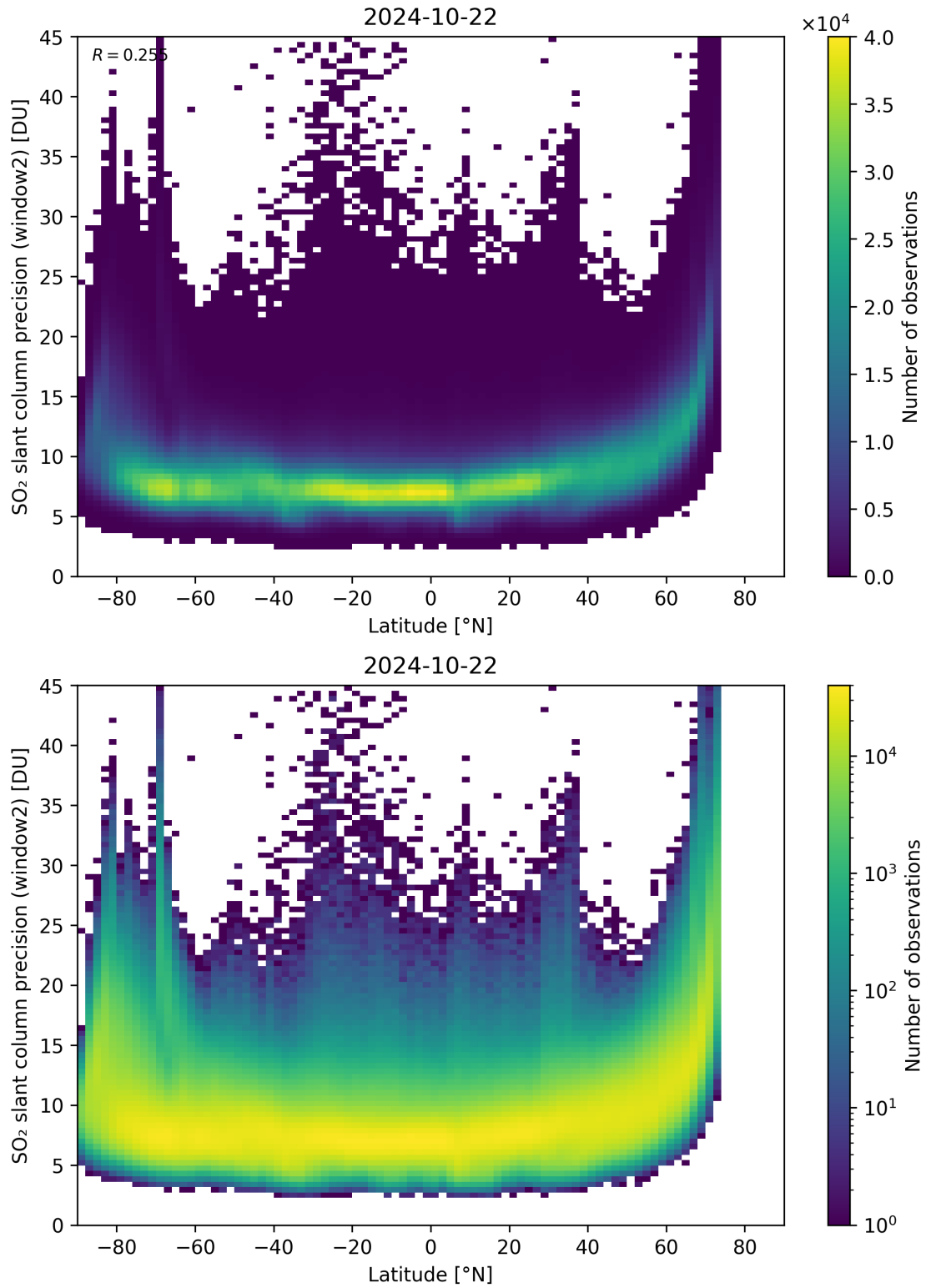
Figure 151: Scatter density plot of “Latitude” against “SO 2 slant column precision (window2)” for 2024-10-21 to 2024-10-23.
