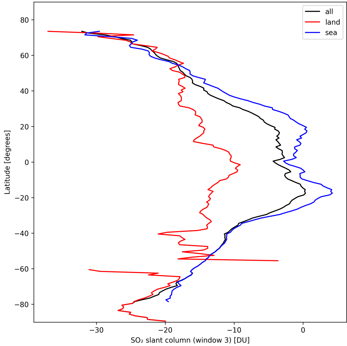
Figure 41: Zonal average of “SO 2 slant column (window 3)” for 2024-10-21 to 2024-10-23.
