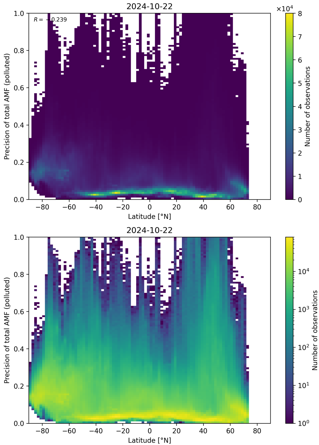
Figure 155: Scatter density plot of “Latitude” against “Precision of total AMF (polluted)” for 2024-10-21 to 2024-10-23.
