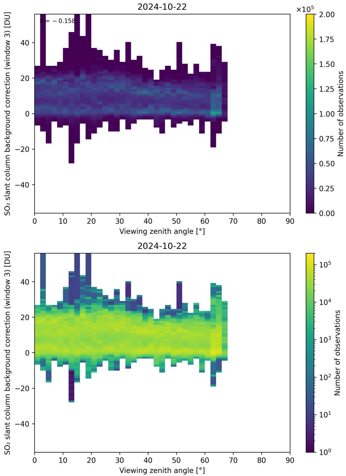
Figure 310: Scatter density plot of “Viewing zenith angle” against “SO 2 slant column background correction (window 3)” for 2024-10-21 to 2024-10-23.
