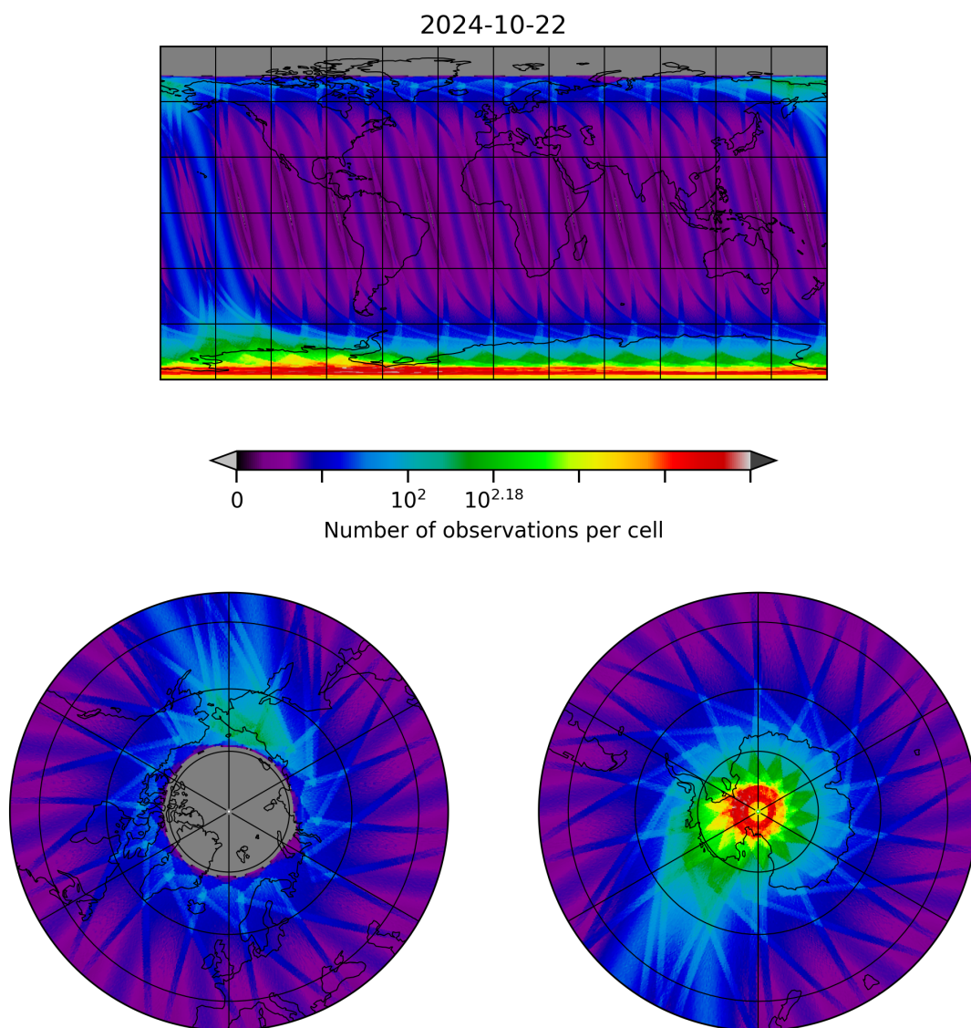
Figure 28: Map of the number of observations for 2024-10-21 to 2024-10-23
