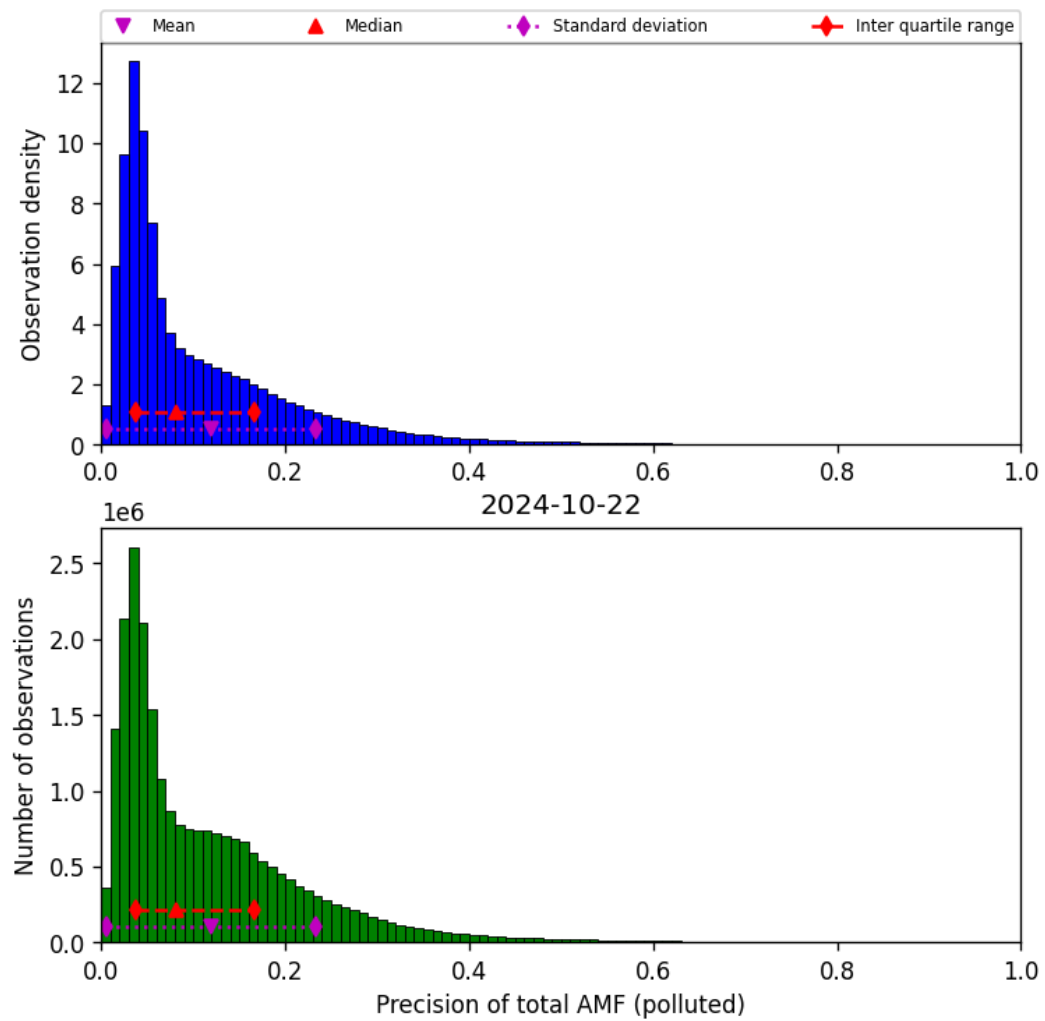
Figure 72: Histogram of “Precision of total AMF (polluted)” for 2024-10-21 to 2024-10-23
