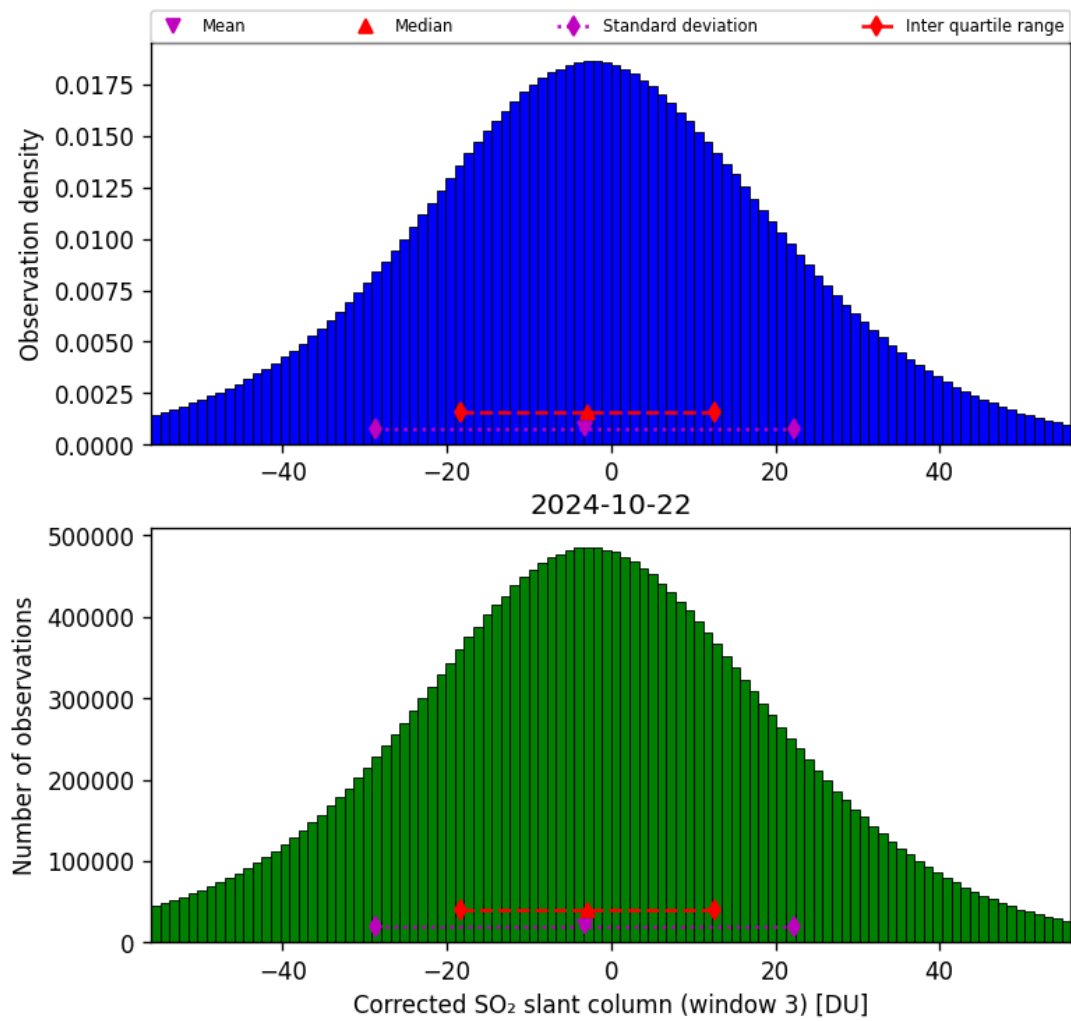
Figure 66: Histogram of “Corrected SO 2 slant column (window 3)” for 2024-10-21 to 2024-10-23
