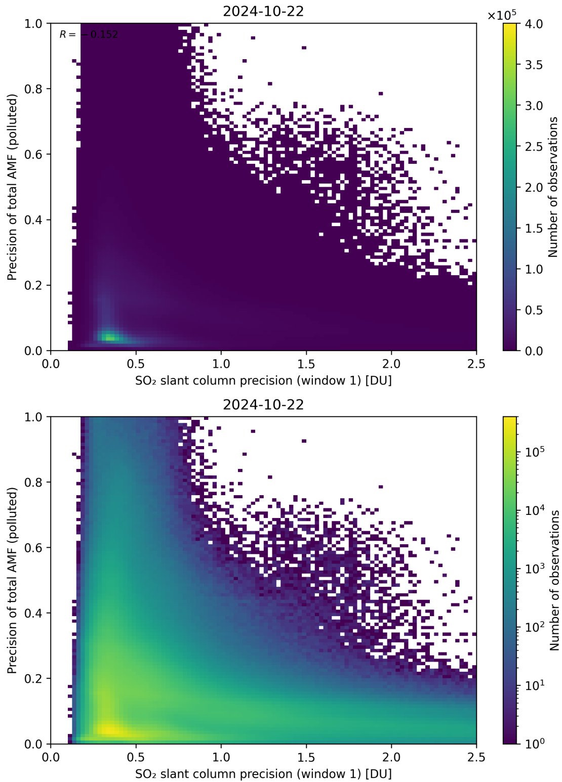
Figure 231: Scatter density plot of “SO 2 slant column precision (window 1)” against “Precision of total AMF (polluted)” for 2024-10-21 to 2024-10-23.
