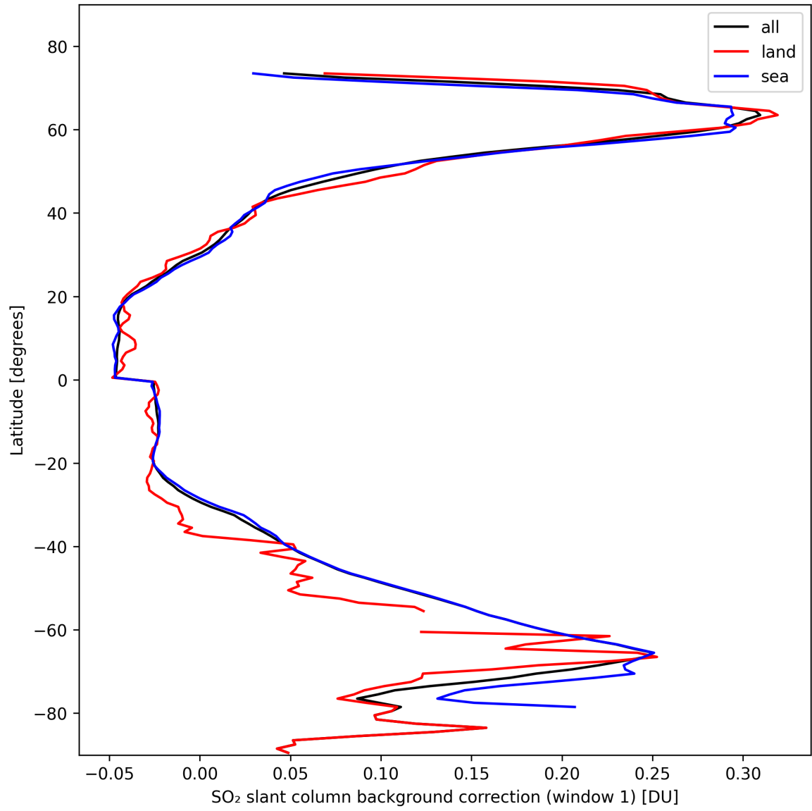
Figure 36: Zonal average of “SO 2 slant column background correction (window 1)” for 2024-10-21 to 2024-10-23.
