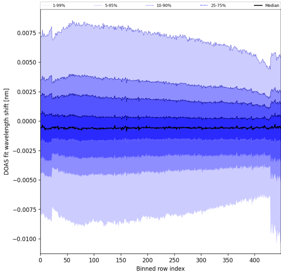
Figure 91: Along track statistics of “DOAS fit wavelength shift” for 2024-10-21 to 2024-10-23
