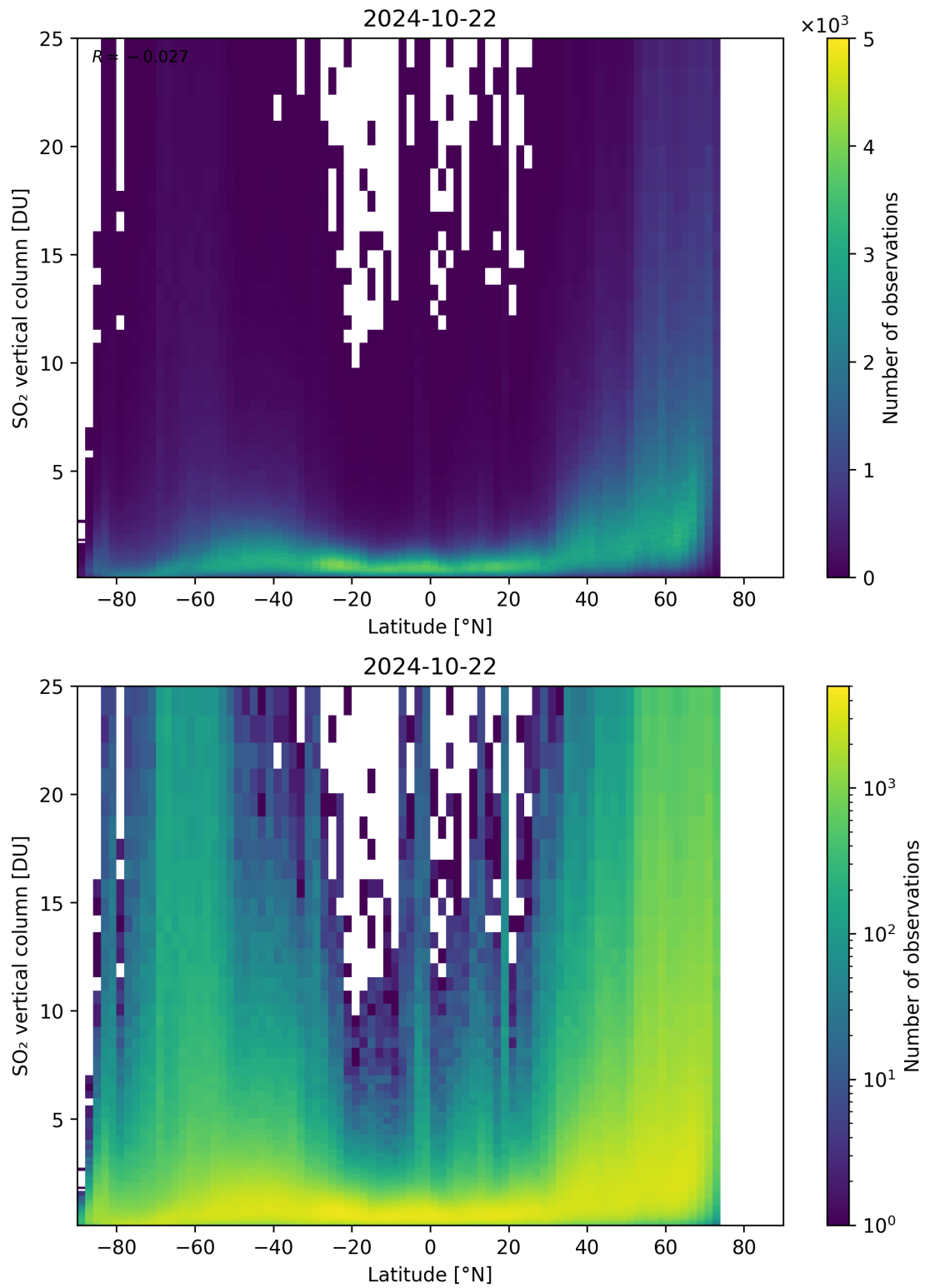
Figure 156: Scatter density plot of “Latitude” against “SO 2 vertical column” for 2024-10-21 to 2024-10-23.
