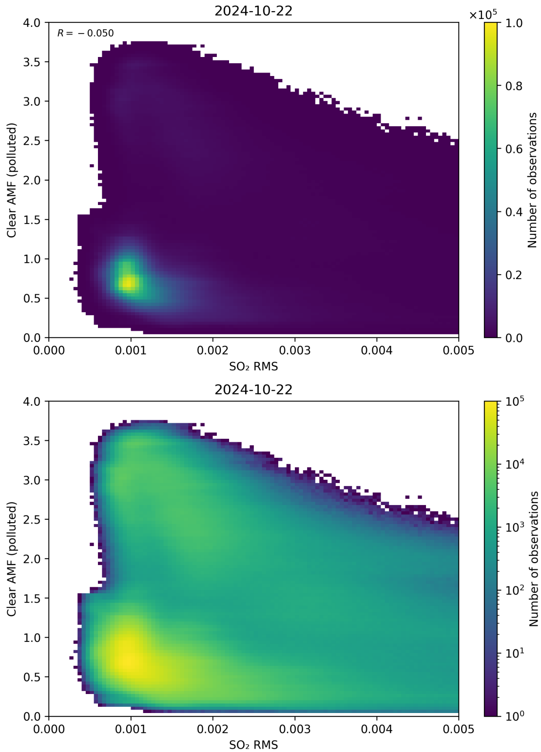
Figure 136: Scatter density plot of “SO 2 RMS” against “Clear AMF (polluted)” for 2024-10-21 to 2024-10-23.
