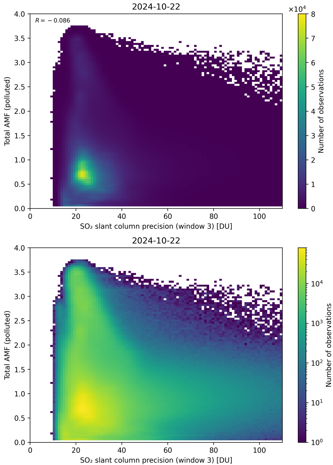
Figure 263: Scatter density plot of “SO 2 slant column precision (window 3)” against “Total AMF (polluted)” for 2024-10-21 to 2024-10-23.
