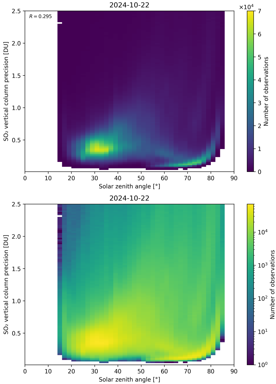
Figure 177: Scatter density plot of “Solar zenith angle” against “SO 2 vertical column precision” for 2024-10-21 to 2024-10-23.
