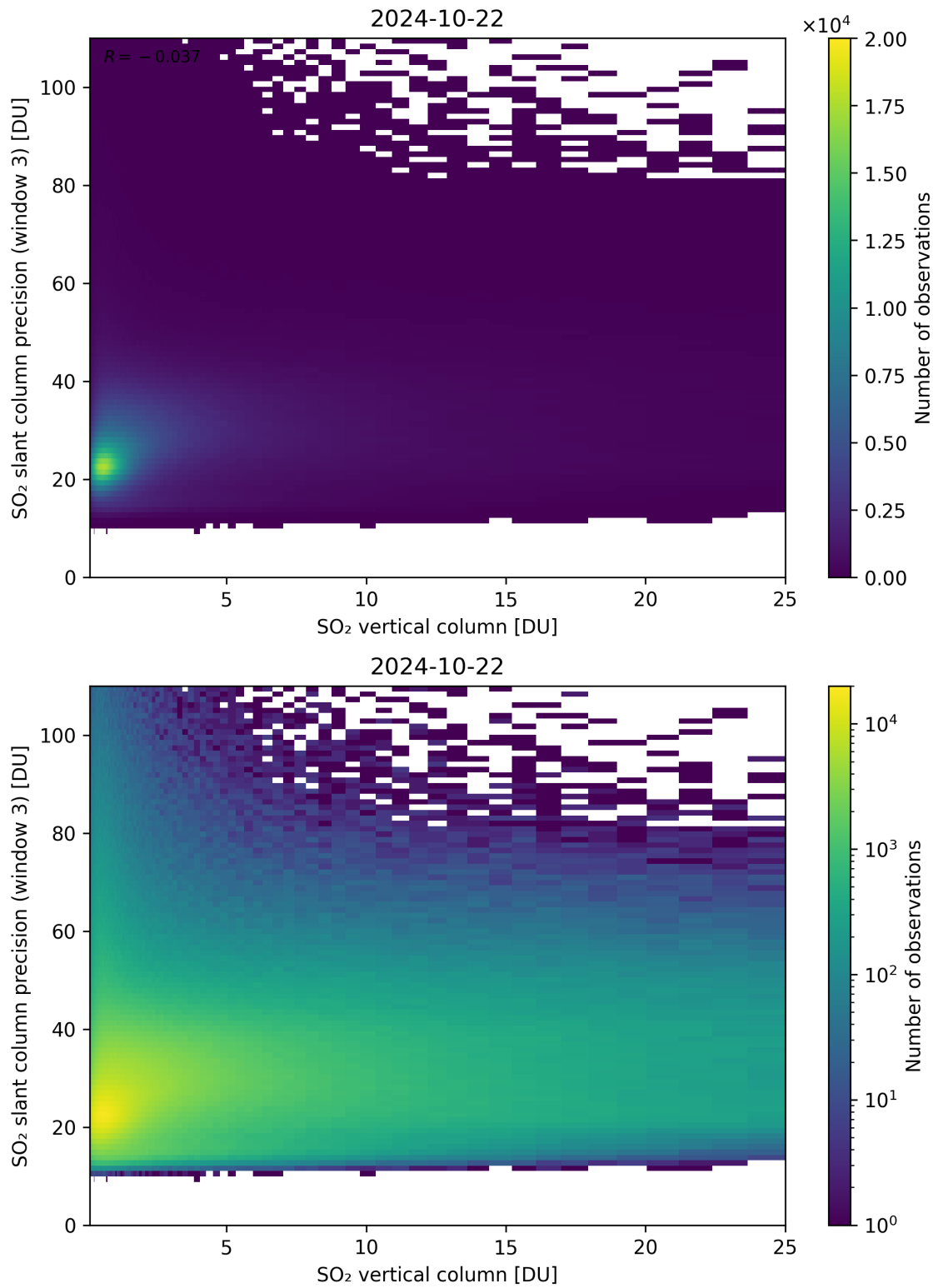
Figure 304: Scatter density plot of “SO 2 vertical column” against “SO 2 slant column precision (window 3)” for 2024-10-21 to 2024-10-23.
