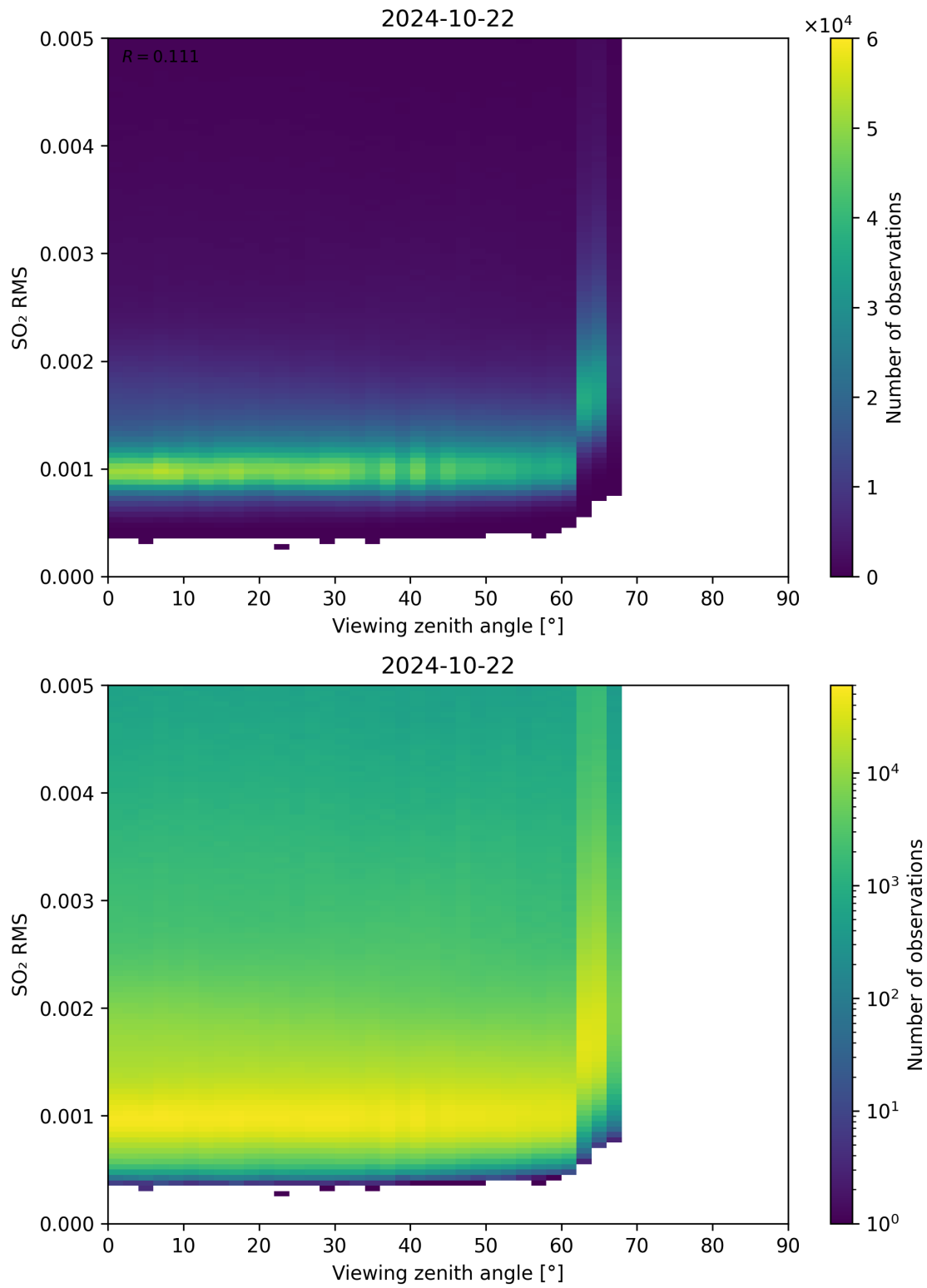
Figure 313: Scatter density plot of “Viewing zenith angle” against “SO 2 RMS” for 2024-10-21 to 2024-10-23.
