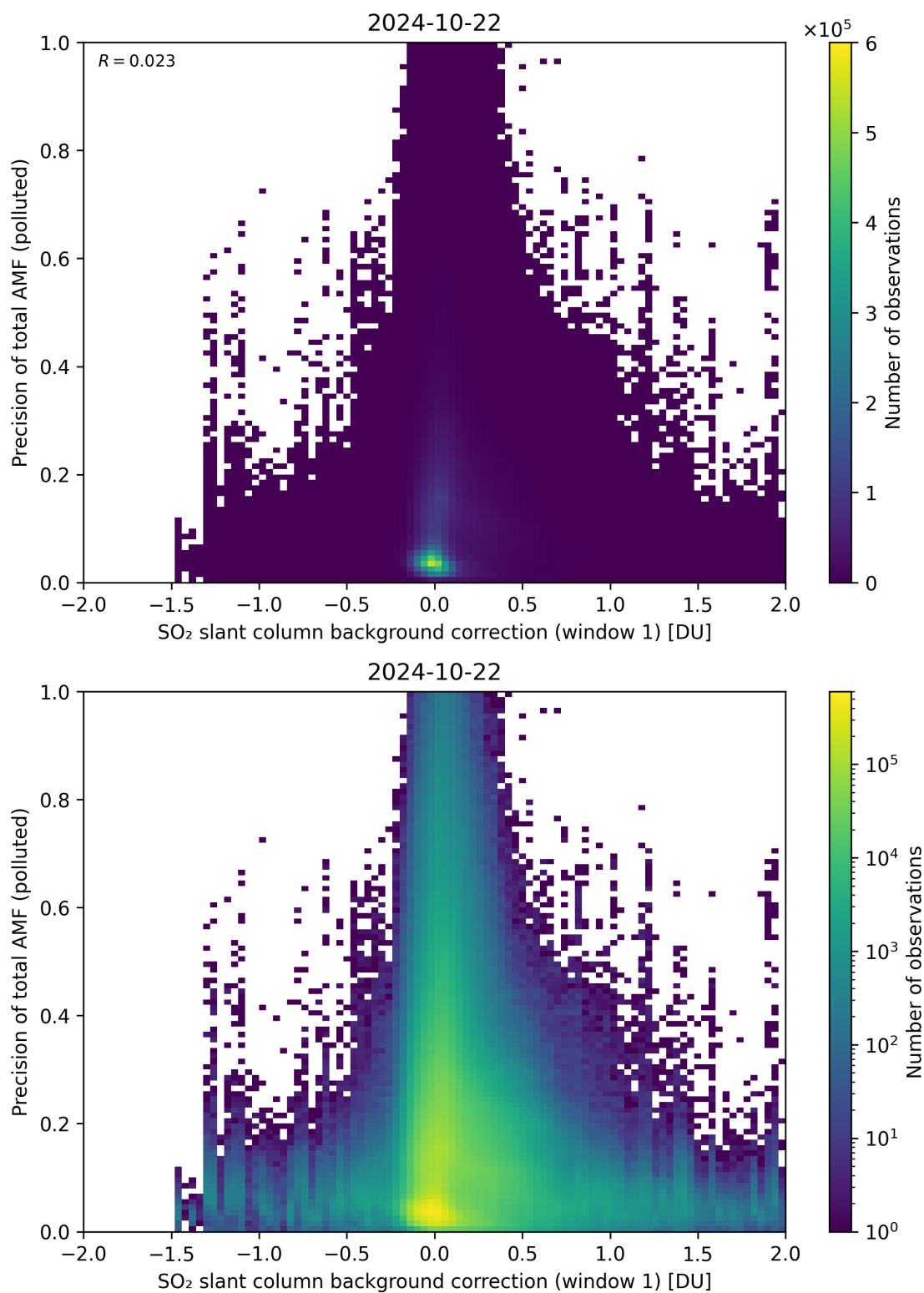
Figure 110: Scatter density plot of “SO 2 slant column background correction (window 1)” against “Precision of total AMF (polluted)” for 2024-10-21 to 2024-10-23.
