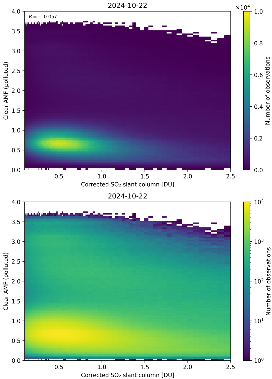
Figure 184: Scatter density plot of “Corrected SO 2 slant column” against “Clear AMF (polluted)” for 2024-10-21 to 2024-10-23.
