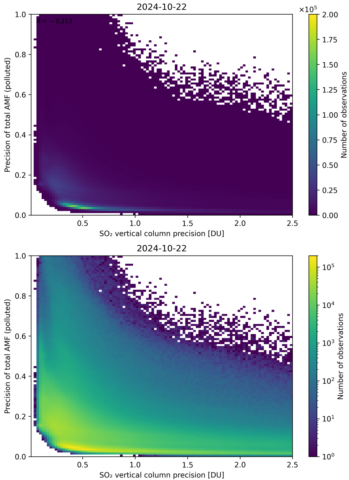
Figure 295: Scatter density plot of “SO 2 vertical column precision” against “Precision of total AMF (polluted)” for 2024-10-21 to 2024-10-23.
