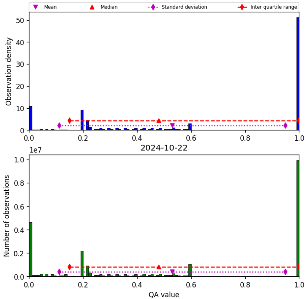
Figure 52: Histogram of “QA value” for 2024-10-21 to 2024-10-23
