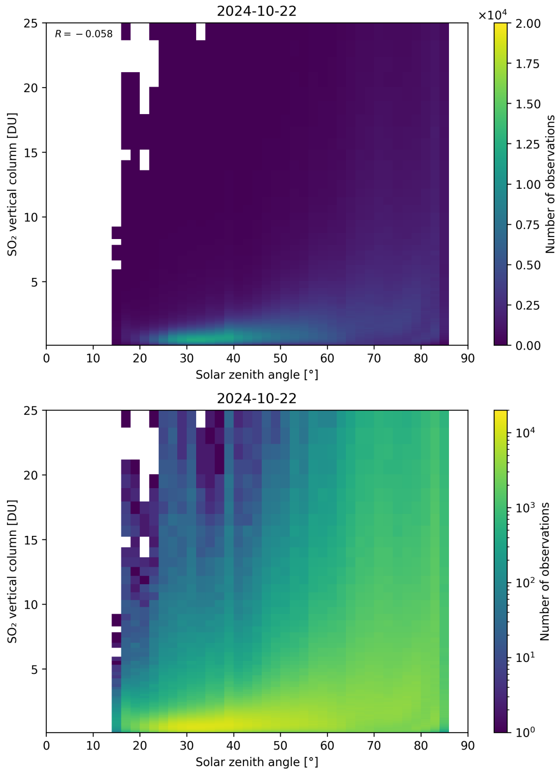
Figure 176: Scatter density plot of “Solar zenith angle” against “SO 2 vertical column” for 2024-10-21 to 2024-10-23.
