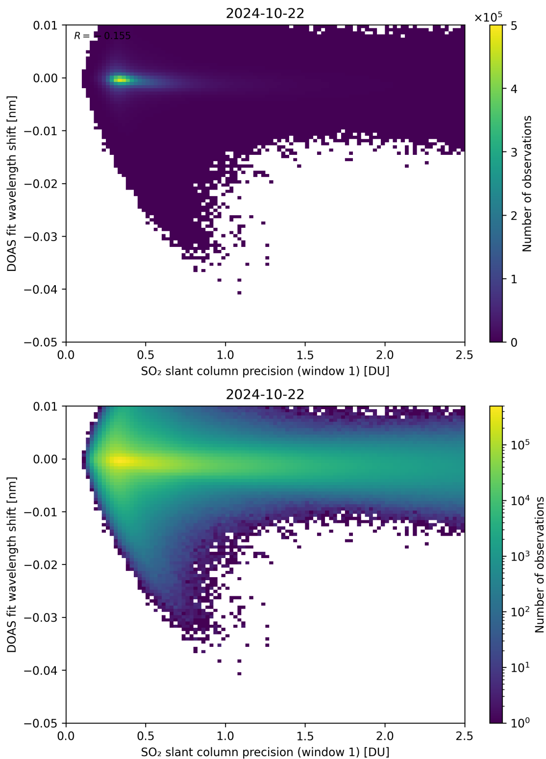
Figure 221: Scatter density plot of “SO 2 slant column precision (window 1)” against “DOAS fit wavelength shift” for 2024-10-21 to 2024-10-23.
