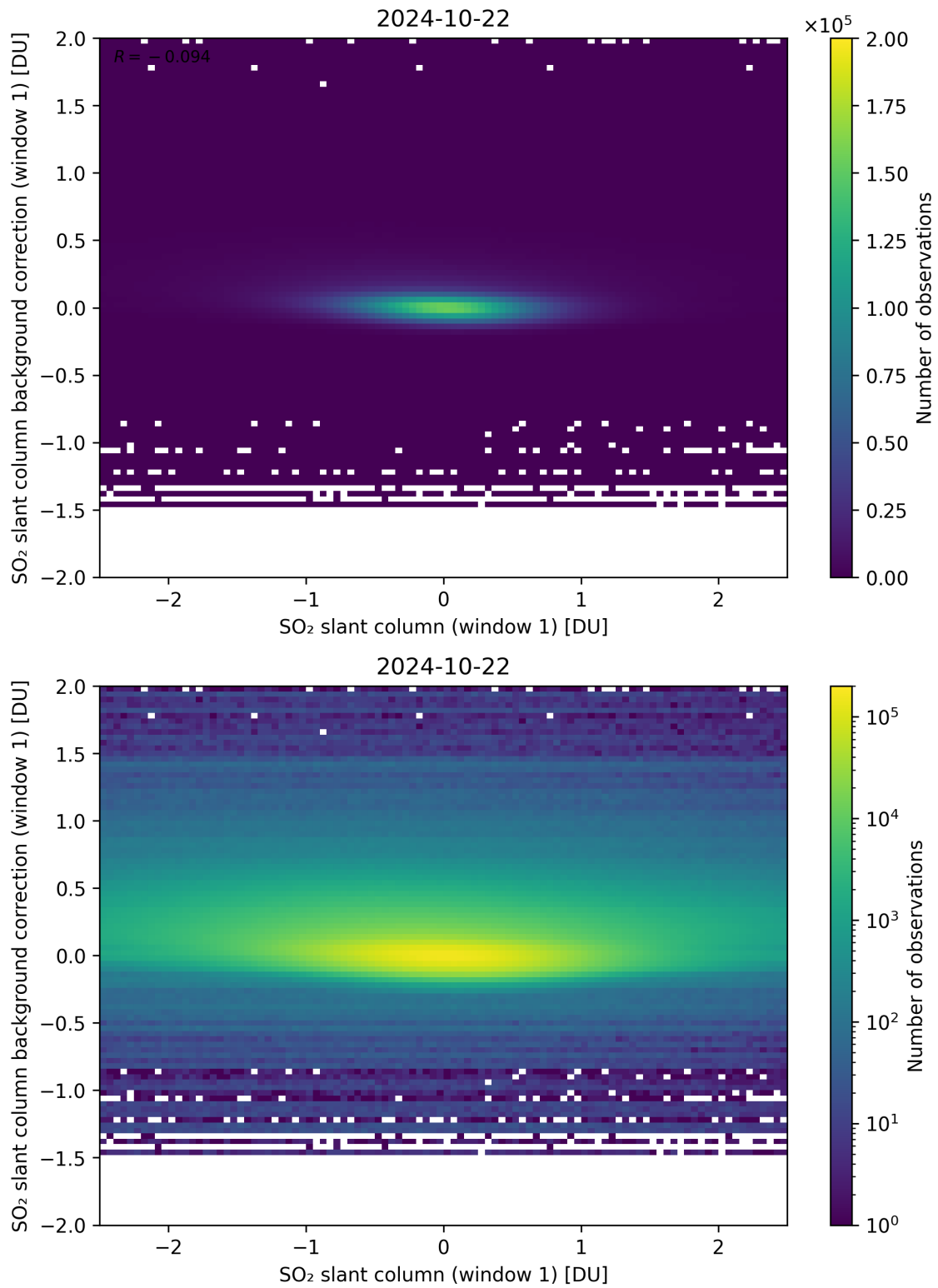
Figure 212: Scatter density plot of “SO 2 slant column (window 1)” against “SO 2 slant column background correction (window 1)” for 2024-10-21 to 2024-10-23.
