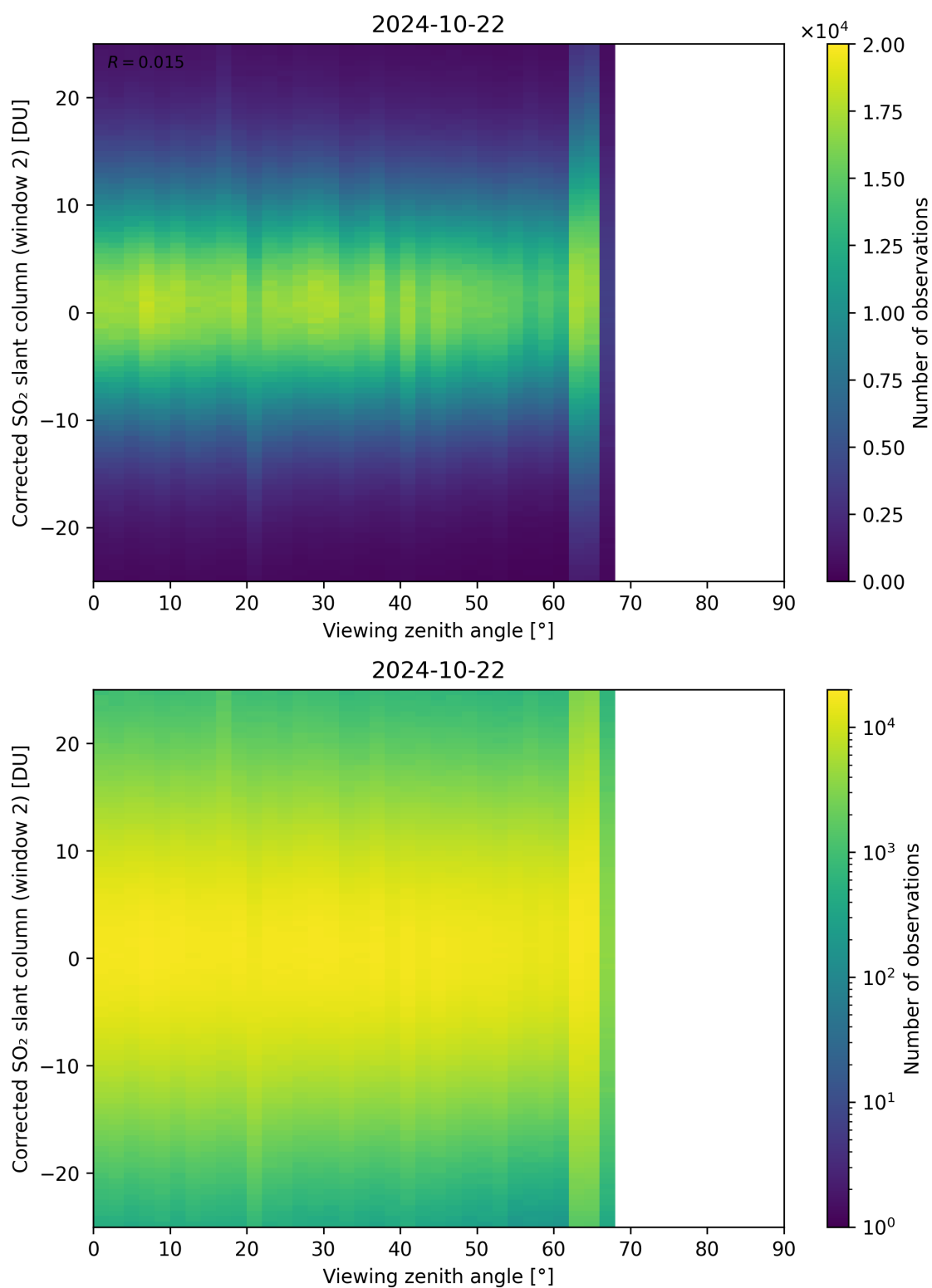
Figure 318: Scatter density plot of “Viewing zenith angle” against “Corrected SO 2 slant column (window 2)” for 2024-10-21 to 2024-10-23.
