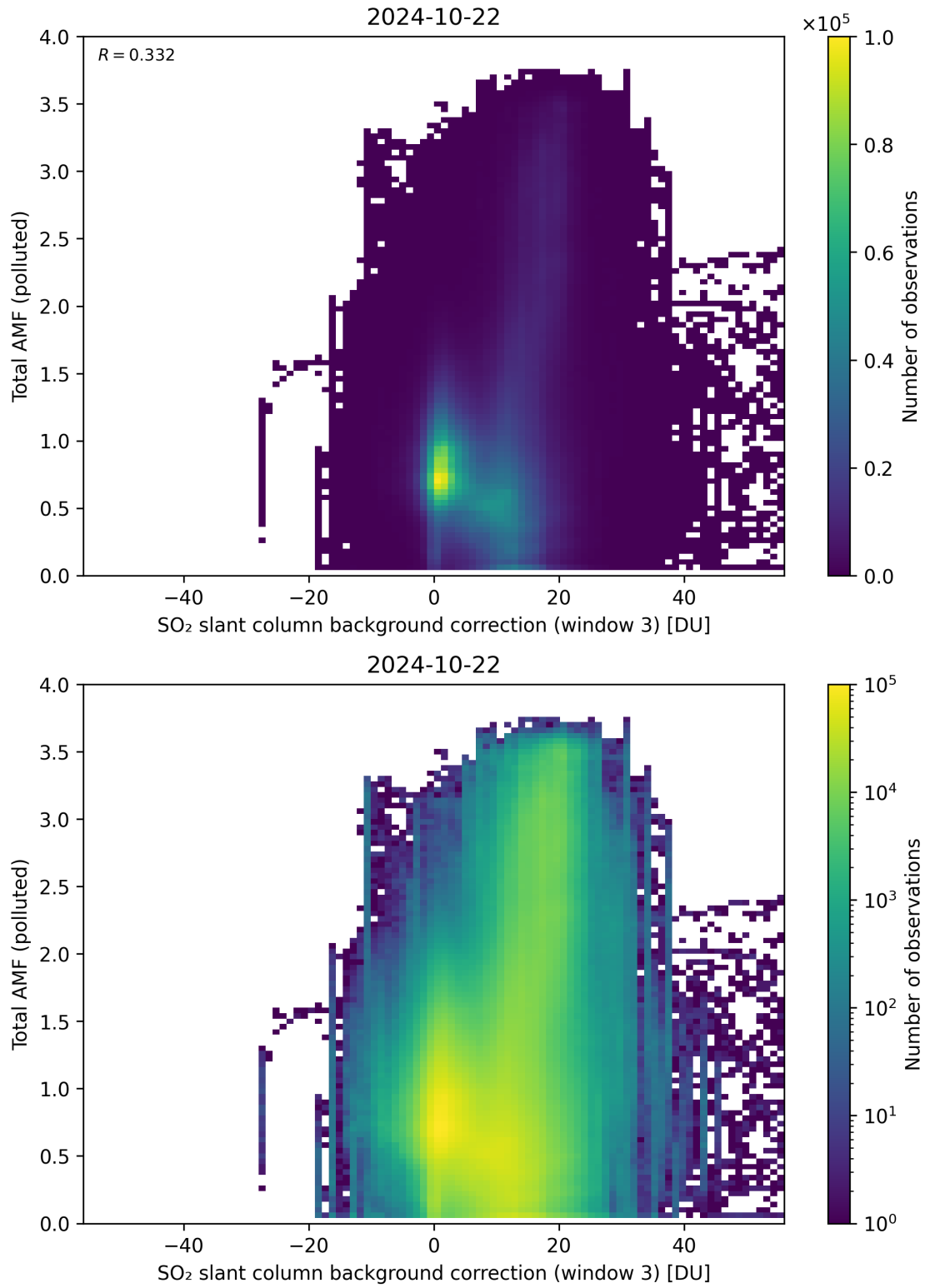
Figure 125: Scatter density plot of “SO 2 slant column background correction (window 3)” against “Total AMF (polluted)” for 2024-10-21 to 2024-10-23.
