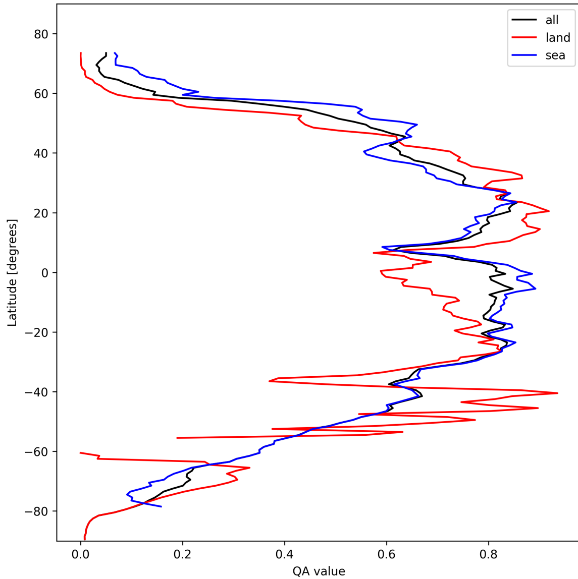
Figure 29: Zonal average of “QA value” for 2024-10-21 to 2024-10-23.
