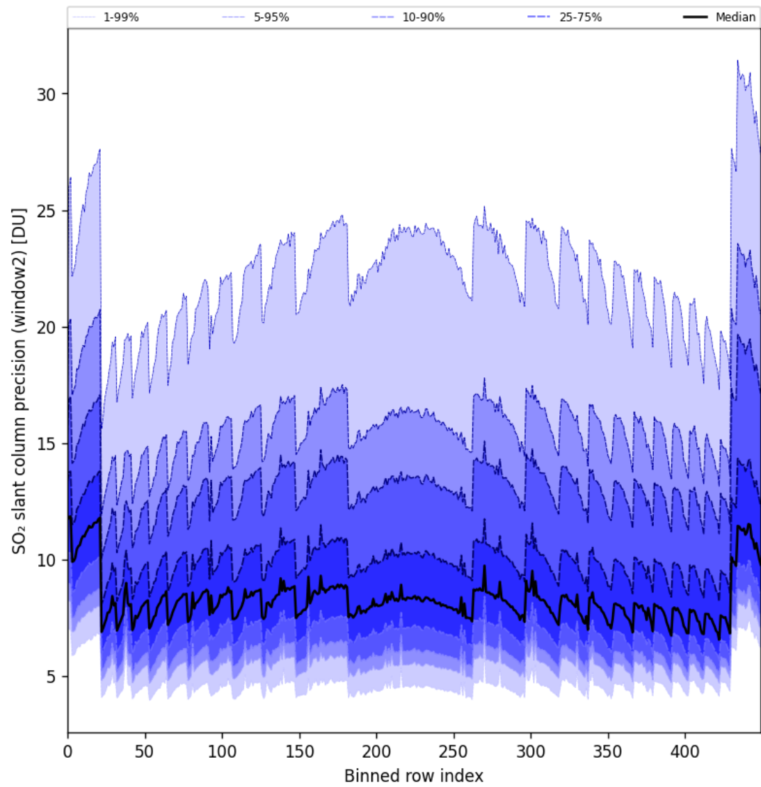
Figure 84: Along track statistics of “SO 2 slant column precision (window2)” for 2024-10-21 to 2024-10-23
