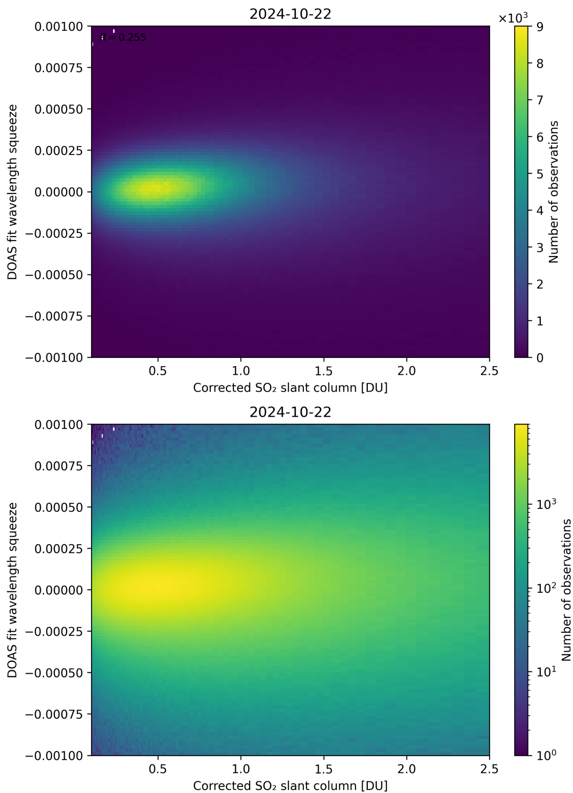
Figure 182: Scatter density plot of “Corrected SO 2 slant column” against “DOAS fit wavelength squeeze” for 2024-10-21 to 2024-10-23.
