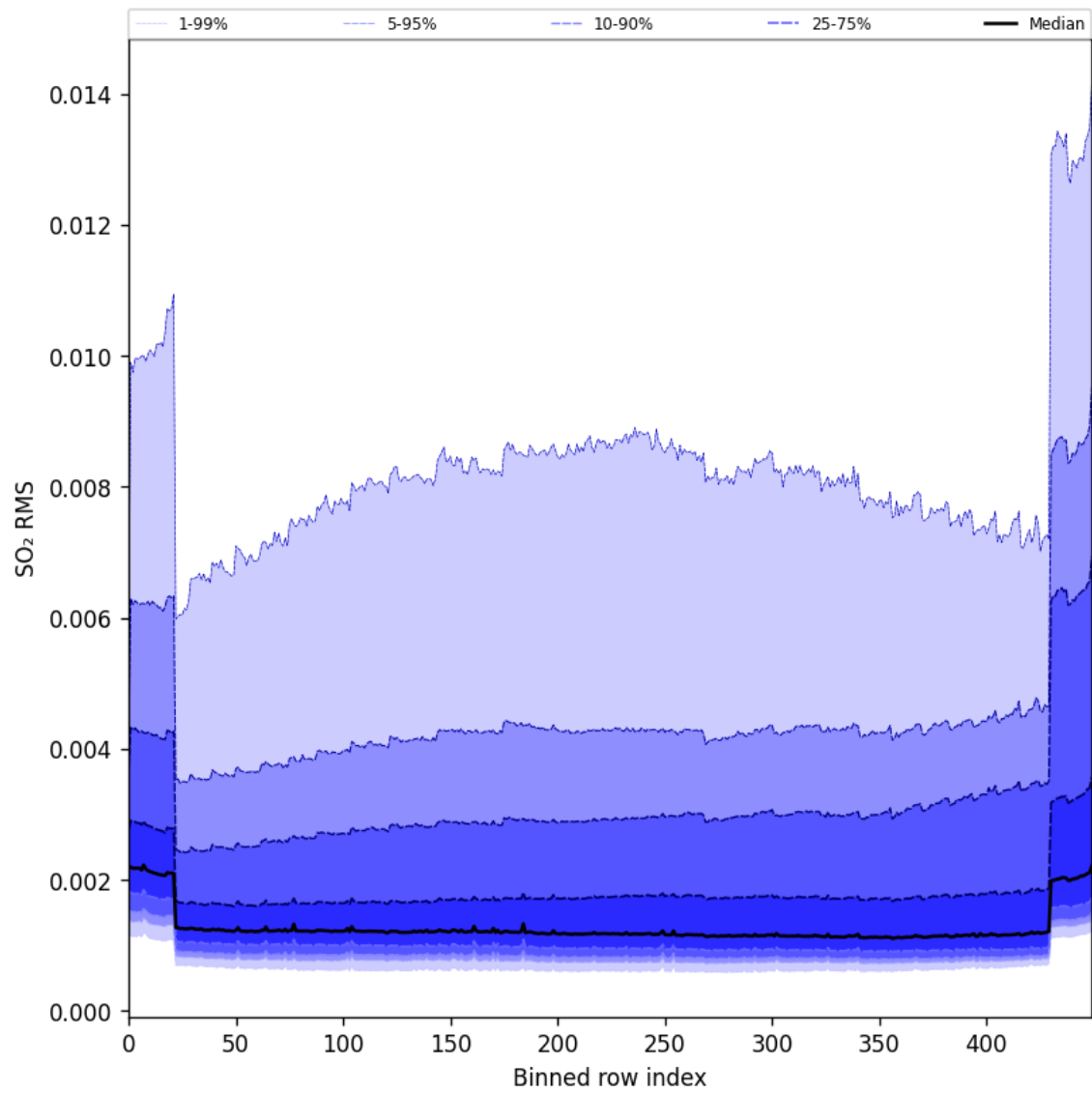
Figure 93: Along track statistics of “SO 2 RMS” for 2024-10-21 to 2024-10-23
