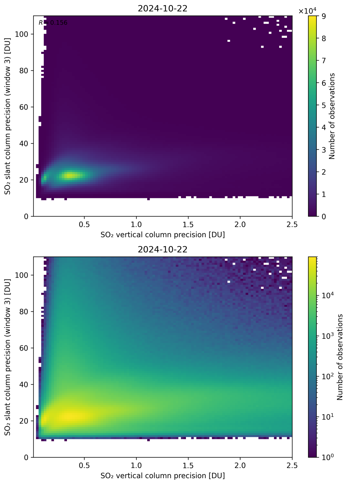
Figure 293: Scatter density plot of “SO 2 vertical column precision” against “SO 2 slant column precision (window 3)” for 2024-10-21 to 2024-10-23.
