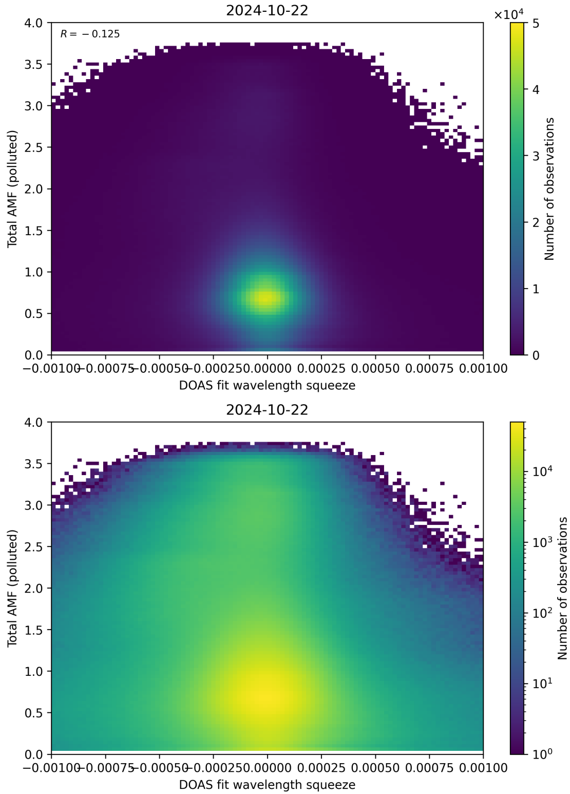
Figure 134: Scatter density plot of “DOAS fit wavelength squeeze” against “Total AMF (polluted)” for 2024-10-21 to 2024-10-23.
