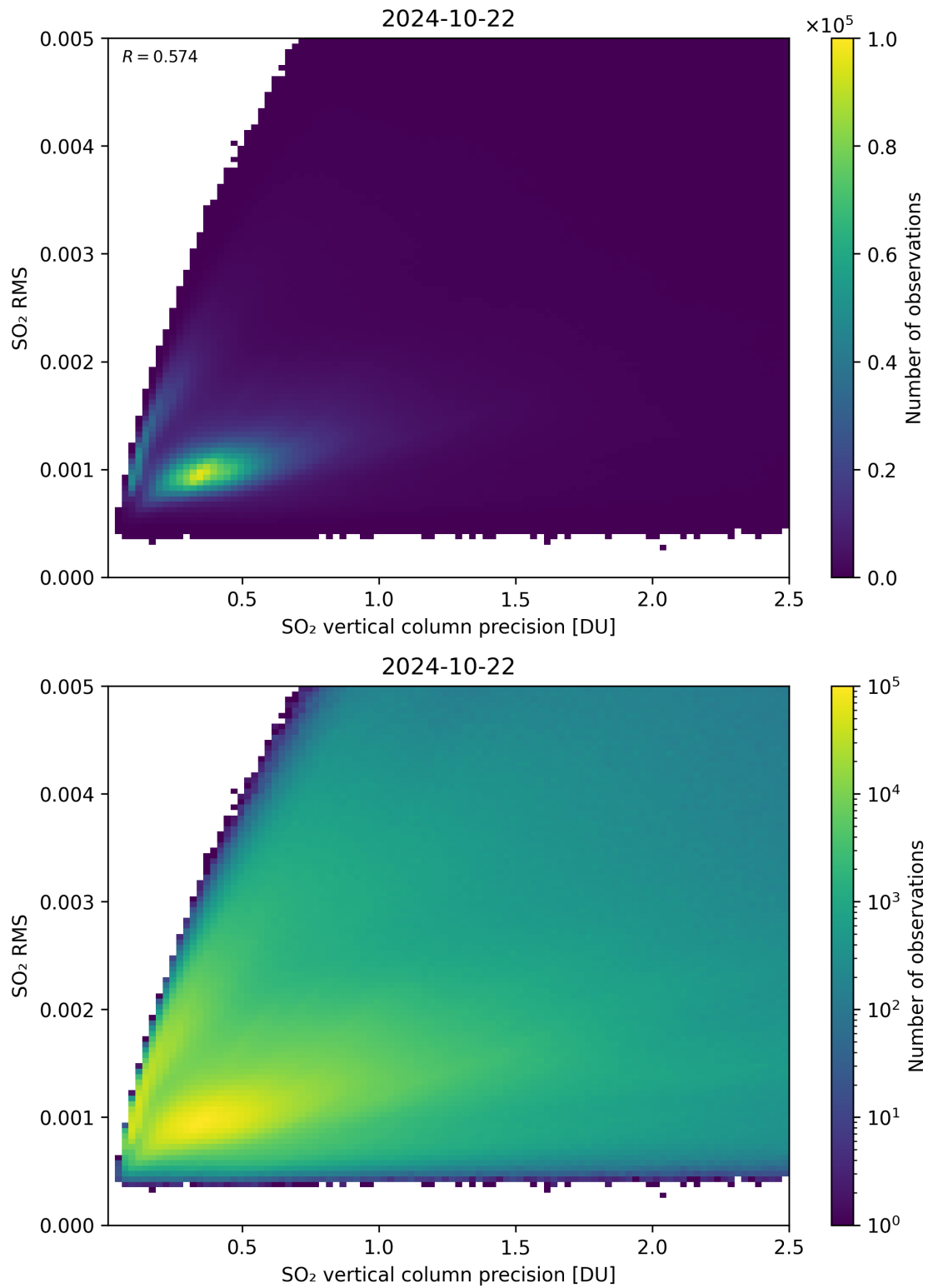
Figure 284: Scatter density plot of “SO 2 vertical column precision” against “SO 2 RMS” for 2024-10-21 to 2024-10-23.
