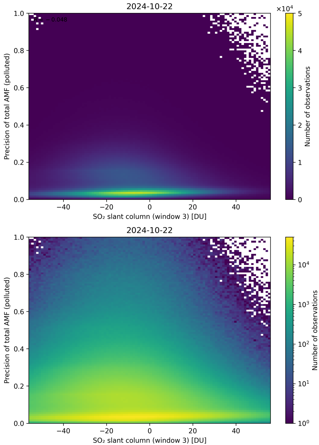
Figure 269: Scatter density plot of “SO 2 slant column (window 3)” against “Precision of total AMF (polluted)” for 2024-10-21 to 2024-10-23.
