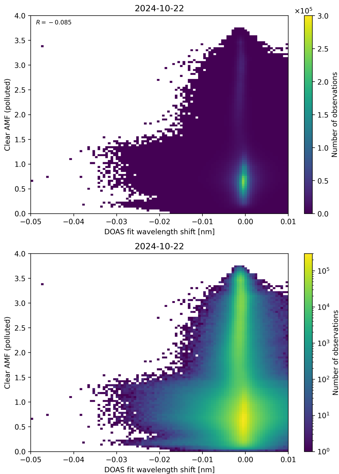
Figure 129: Scatter density plot of “DOAS fit wavelength shift” against “Clear AMF (polluted)” for 2024-10-21 to 2024-10-23.
