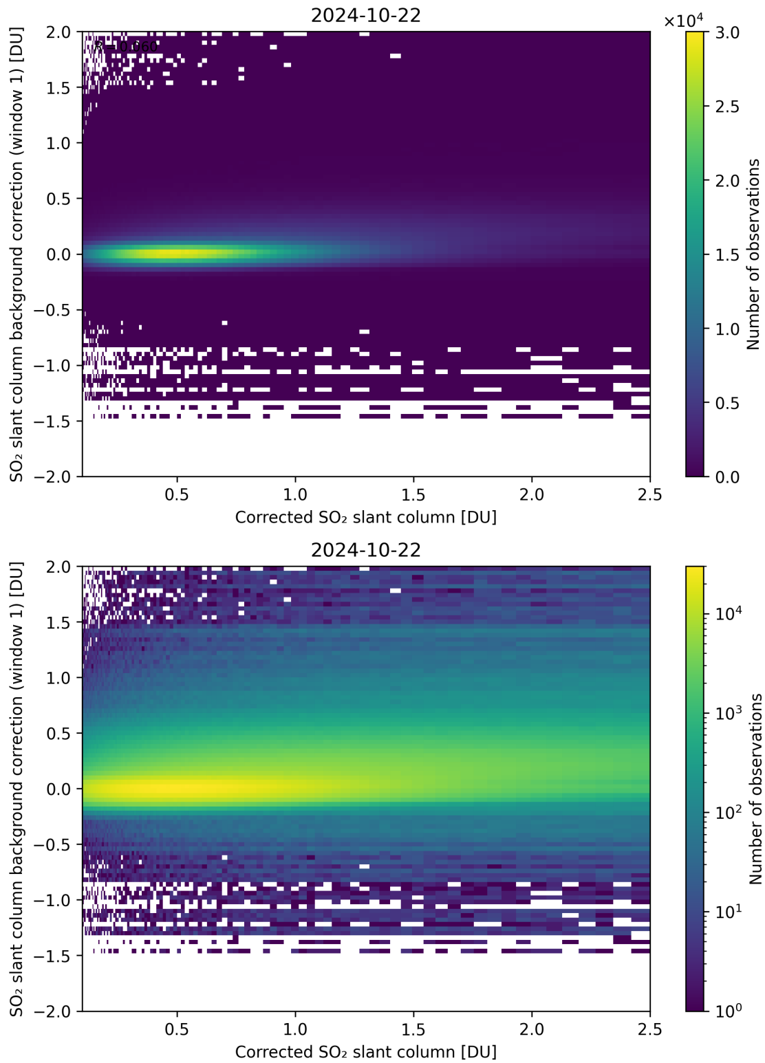
Figure 178: Scatter density plot of “Corrected SO 2 slant column” against “SO 2 slant column background correction (window 1)” for 2024-10-21 to 2024-10-23.
