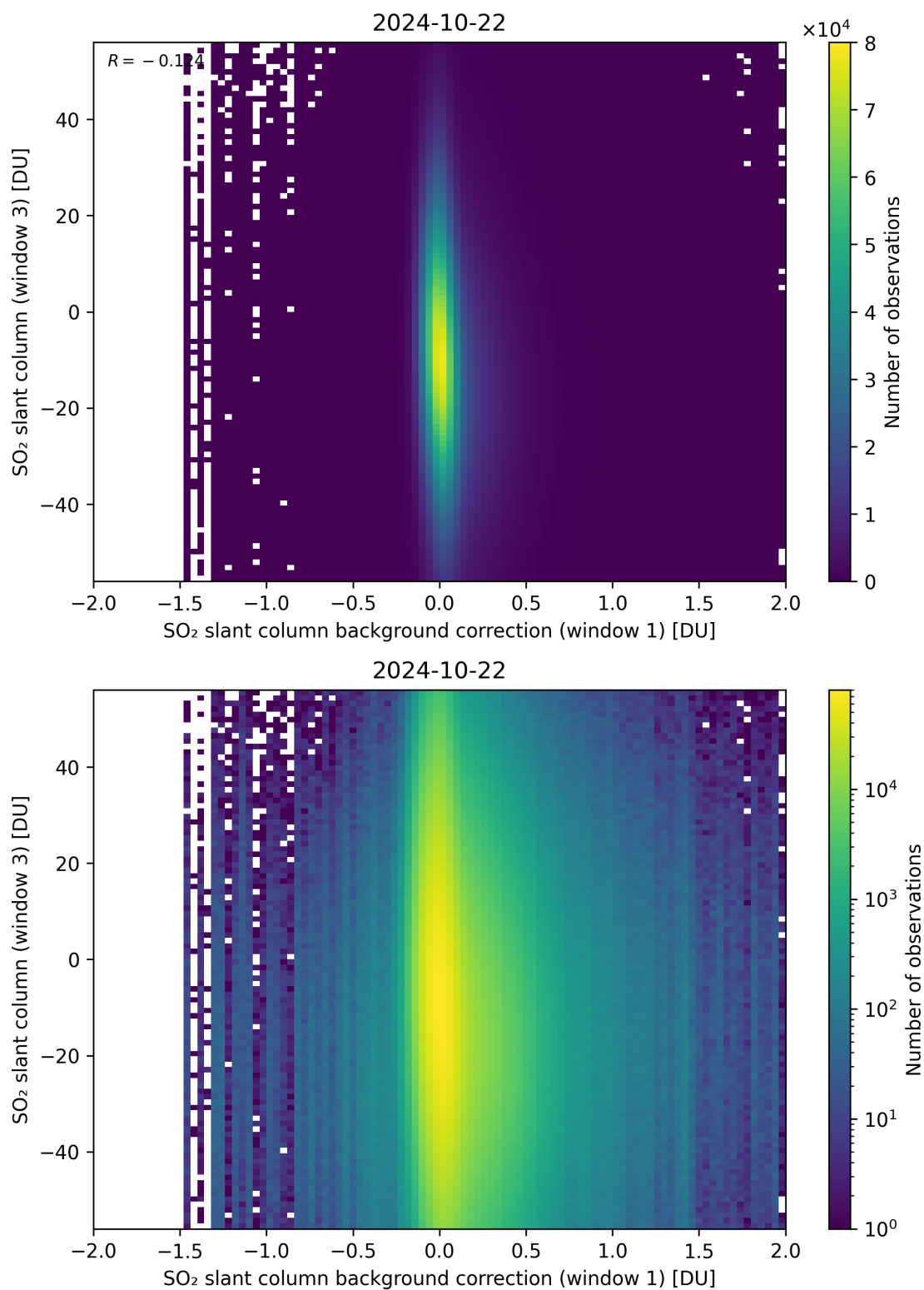
Figure 107: Scatter density plot of “SO 2 slant column background correction (window 1)” against “SO 2 slant column (window 3)” for 2024-10-21 to 2024-10-23.
