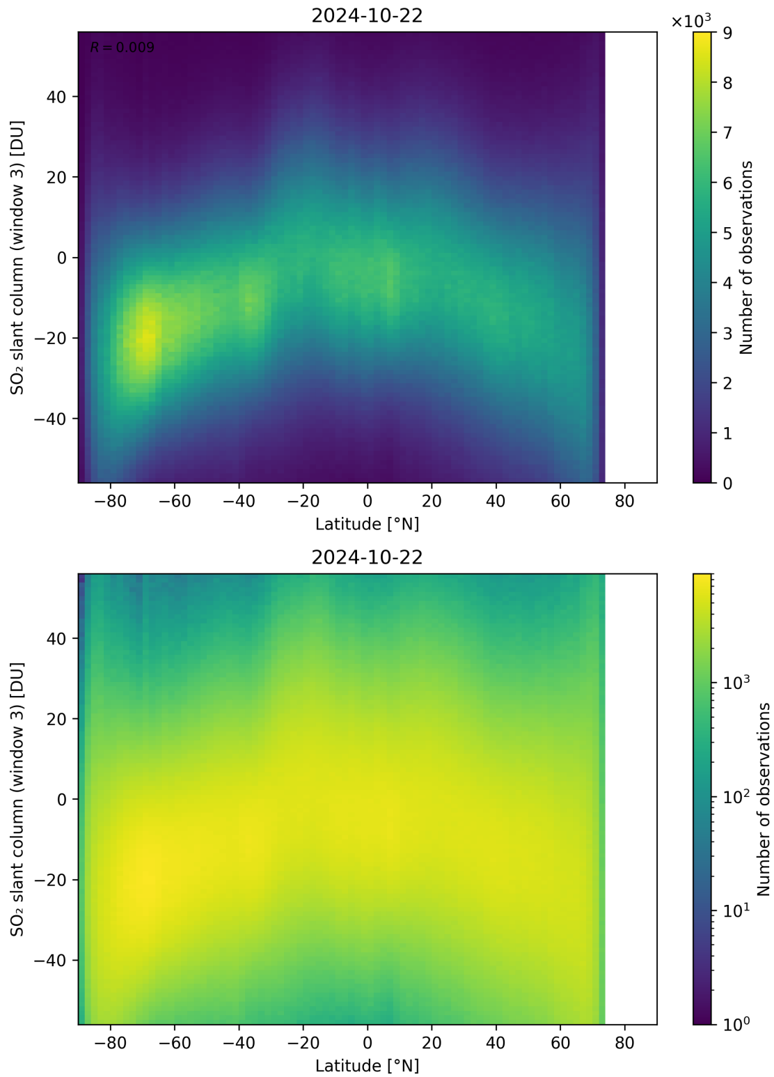
Figure 152: Scatter density plot of “Latitude” against “SO 2 slant column (window 3)” for 2024-10-21 to 2024-10-23.
