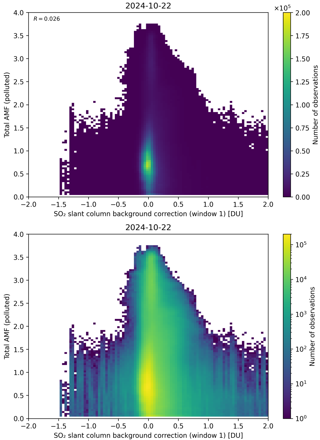
Figure 109: Scatter density plot of “SO 2 slant column background correction (window 1)” against “Total AMF (polluted)” for 2024-10-21 to 2024-10-23.
