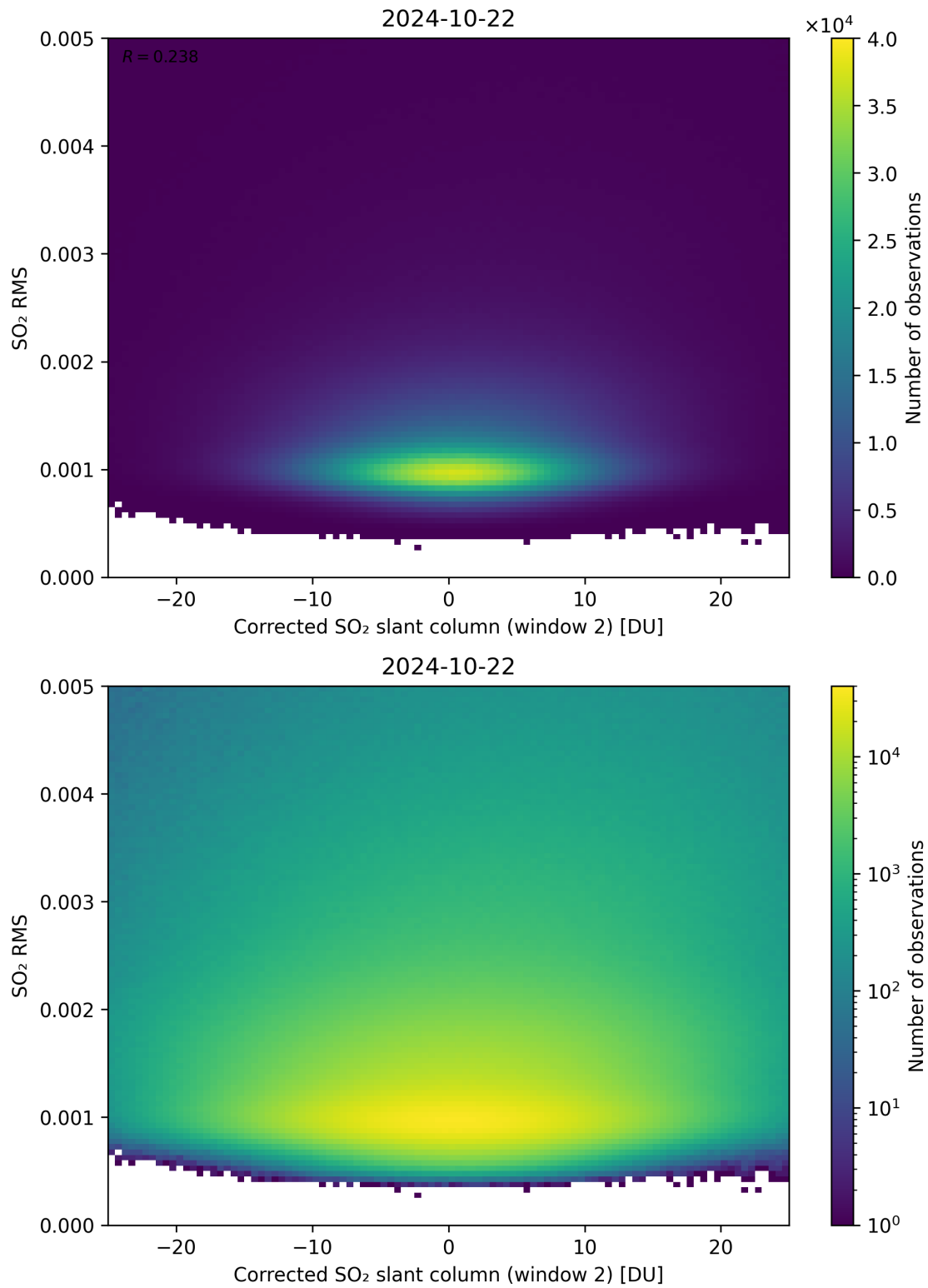
Figure 198: Scatter density plot of “Corrected SO 2 slant column (window 2)” against “SO 2 RMS” for 2024-10-21 to 2024-10-23.
