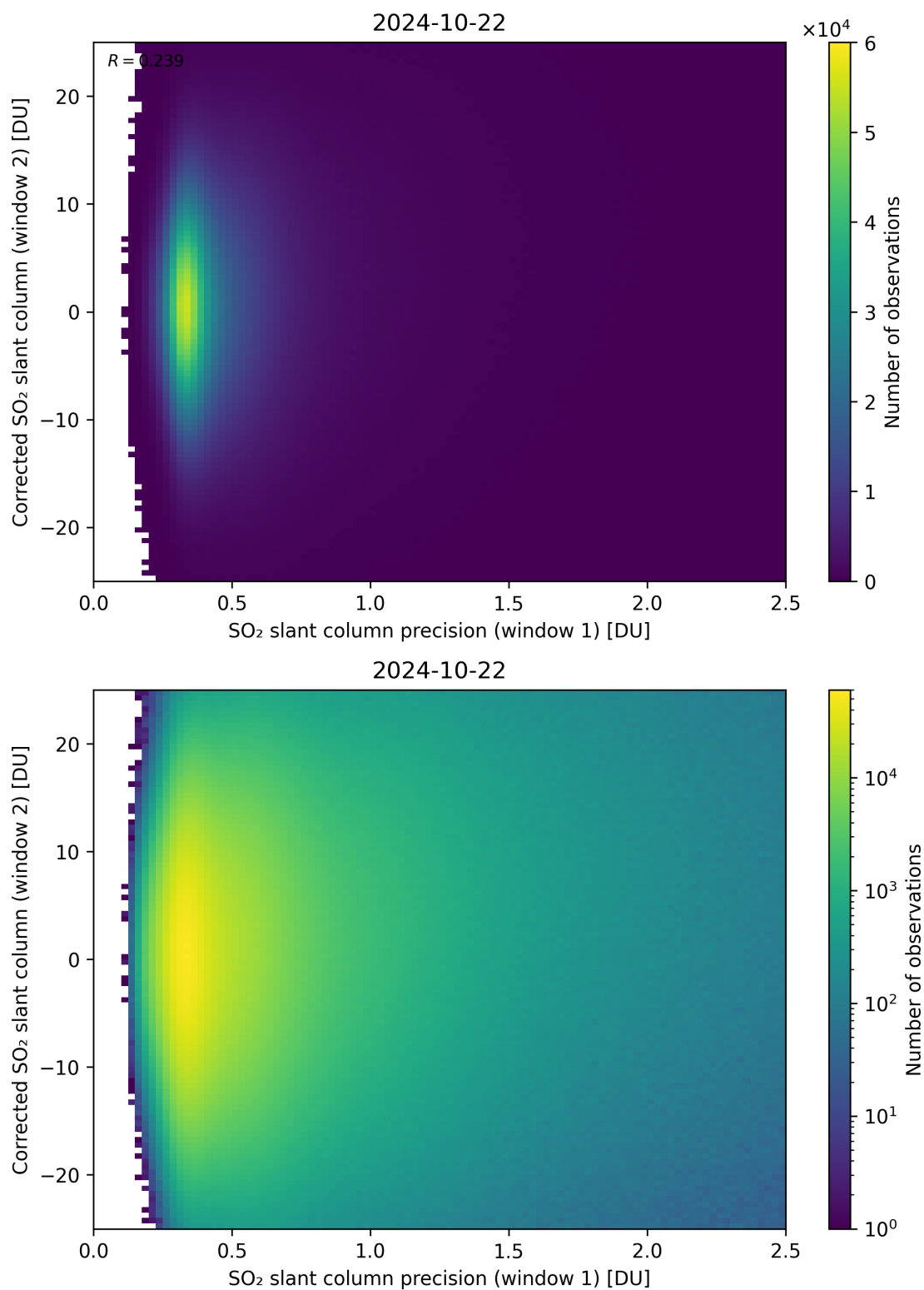
Figure 225: Scatter density plot of “SO 2 slant column precision (window 1)” against “Corrected SO 2 slant column (window 2)” for 2024-10-21 to 2024-10-23.
