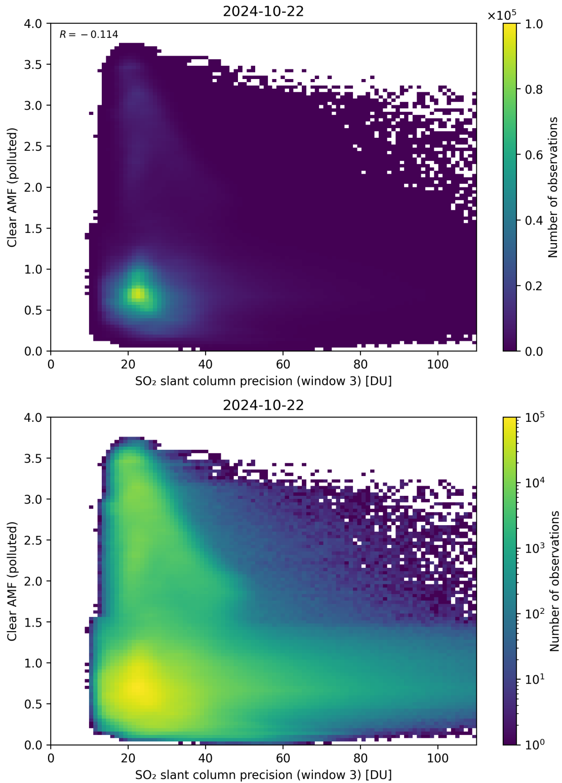
Figure 261: Scatter density plot of “SO 2 slant column precision (window 3)” against “Clear AMF (polluted)” for 2024-10-21 to 2024-10-23.
