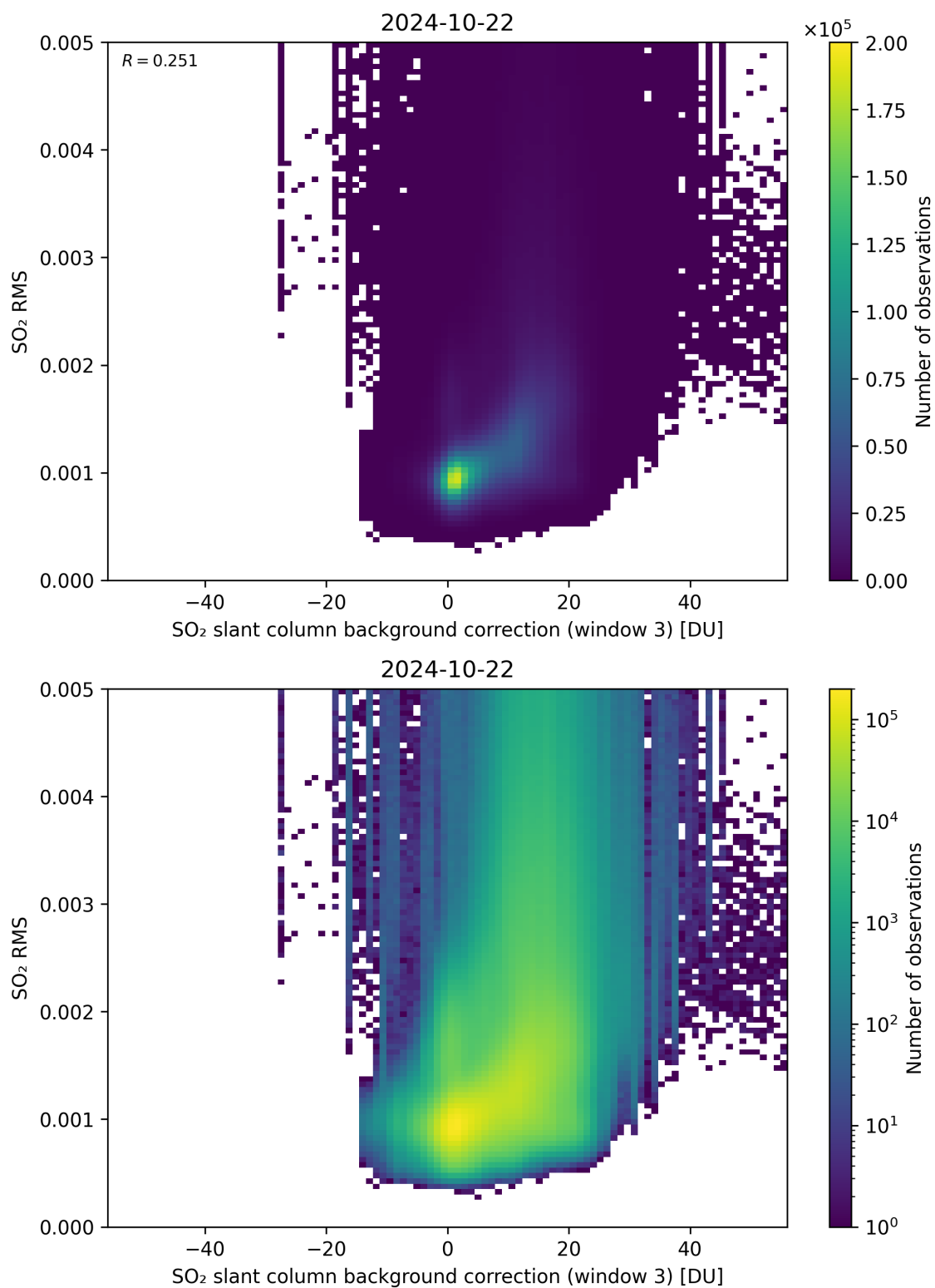
Figure 123: Scatter density plot of “SO 2 slant column background correction (window 3)” against “SO 2 RMS” for 2024-10-21 to 2024-10-23.
