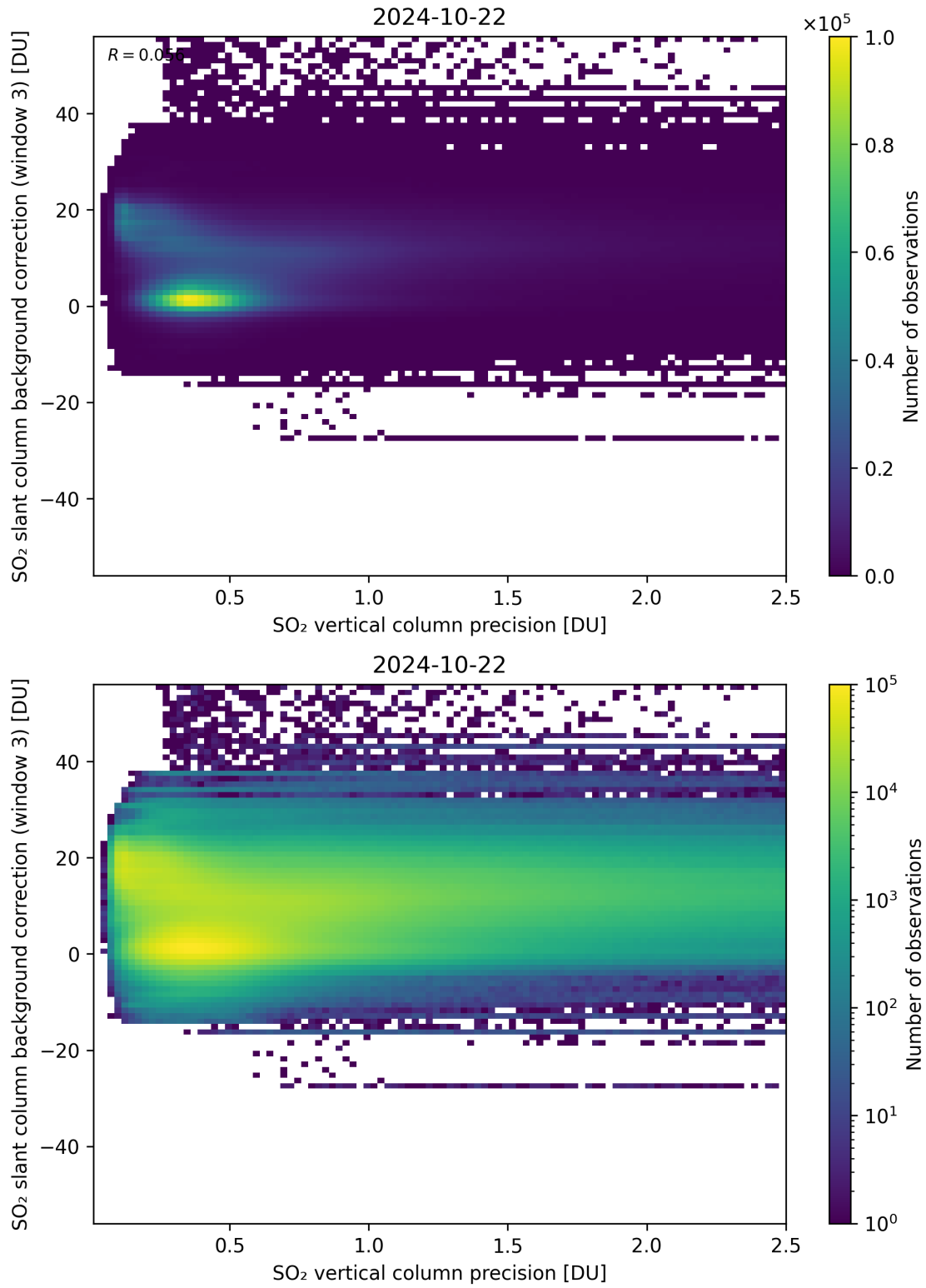
Figure 281: Scatter density plot of “SO 2 vertical column precision” against “SO 2 slant column background correction (window 3)” for 2024-10-21 to 2024-10-23.
