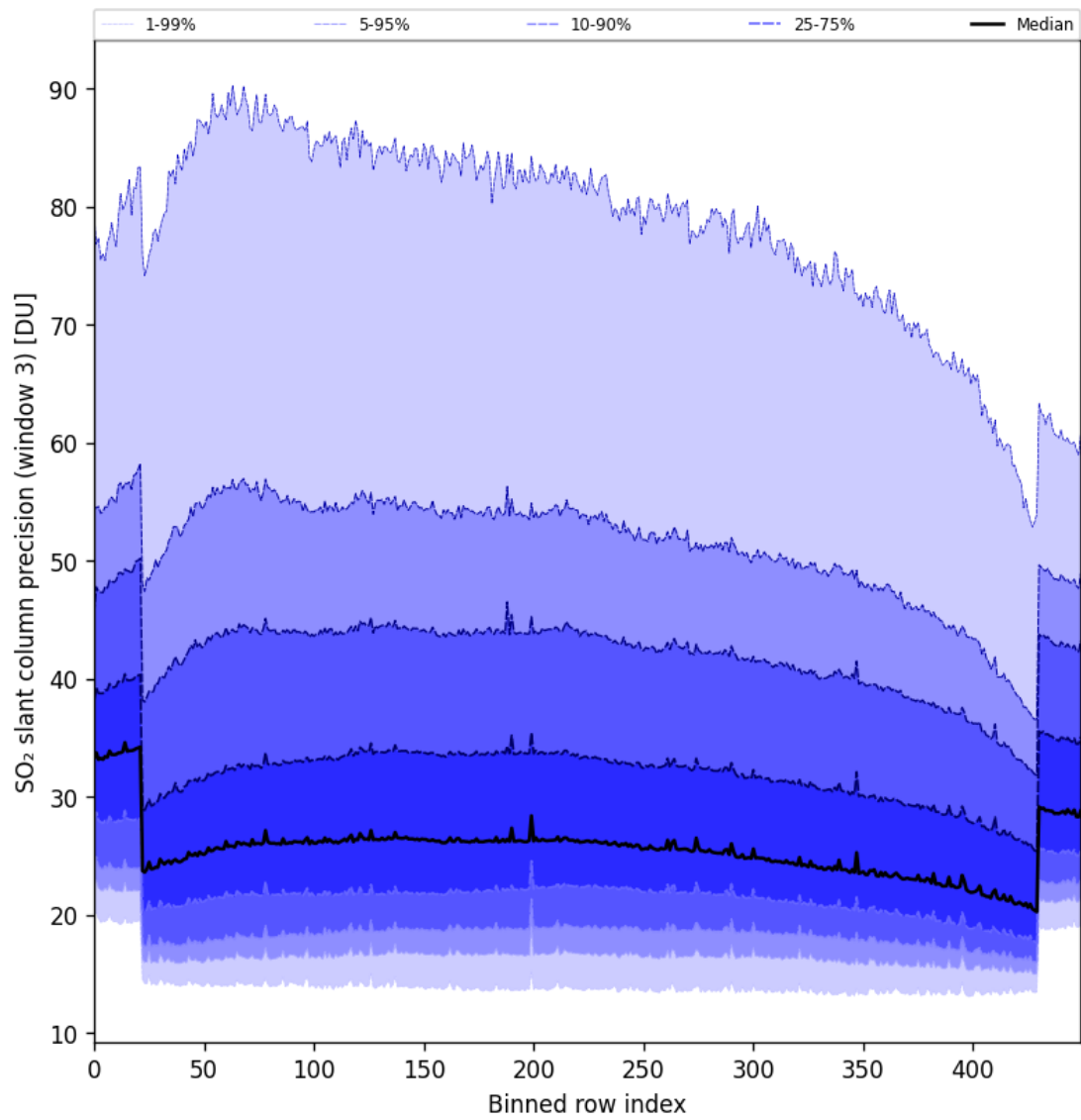
Figure 88: Along track statistics of “SO 2 slant column precision (window 3)” for 2024-10-21 to 2024-10-23
