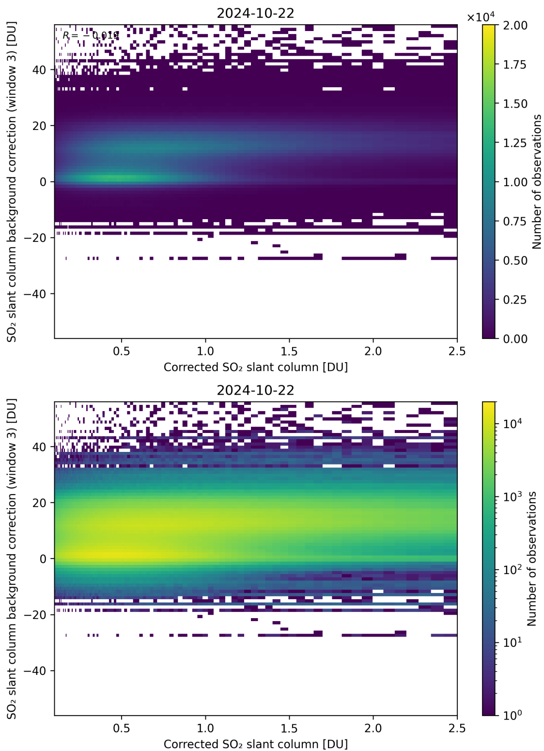
Figure 180: Scatter density plot of “Corrected SO 2 slant column” against “SO 2 slant column background correction (window 3)” for 2024-10-21 to 2024-10-23.
