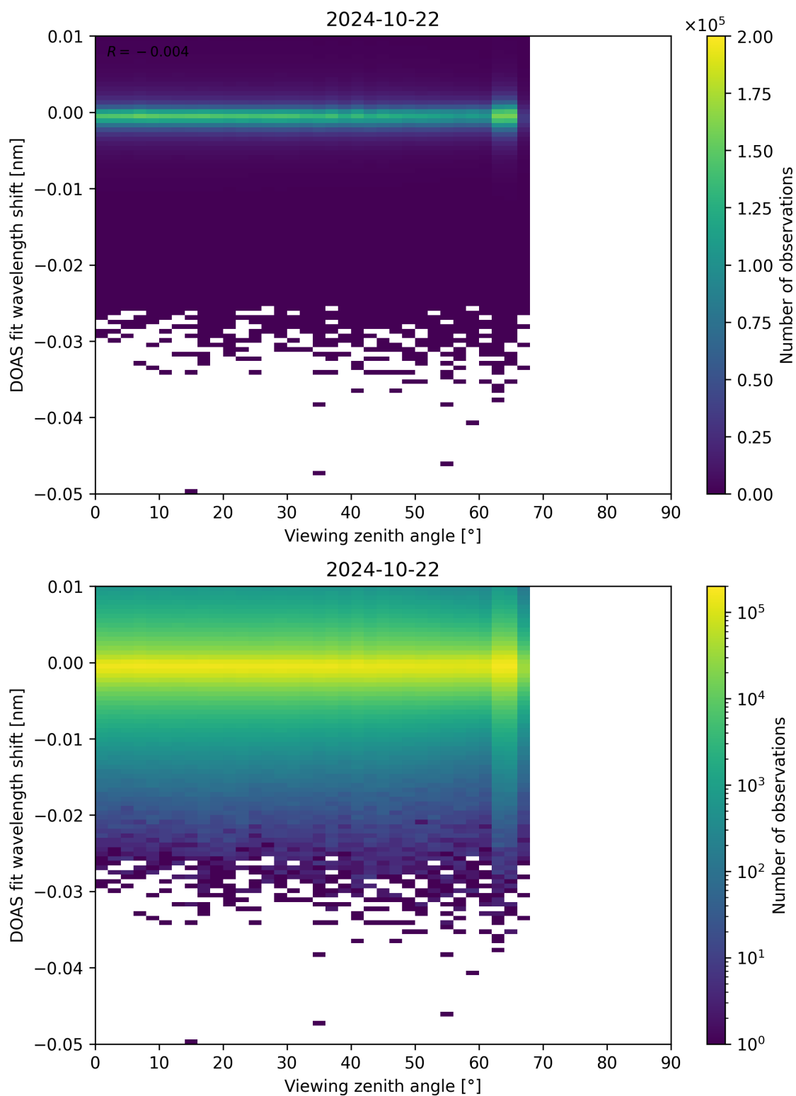
Figure 311: Scatter density plot of “Viewing zenith angle” against “DOAS fit wavelength shift” for 2024-10-21 to 2024-10-23.
