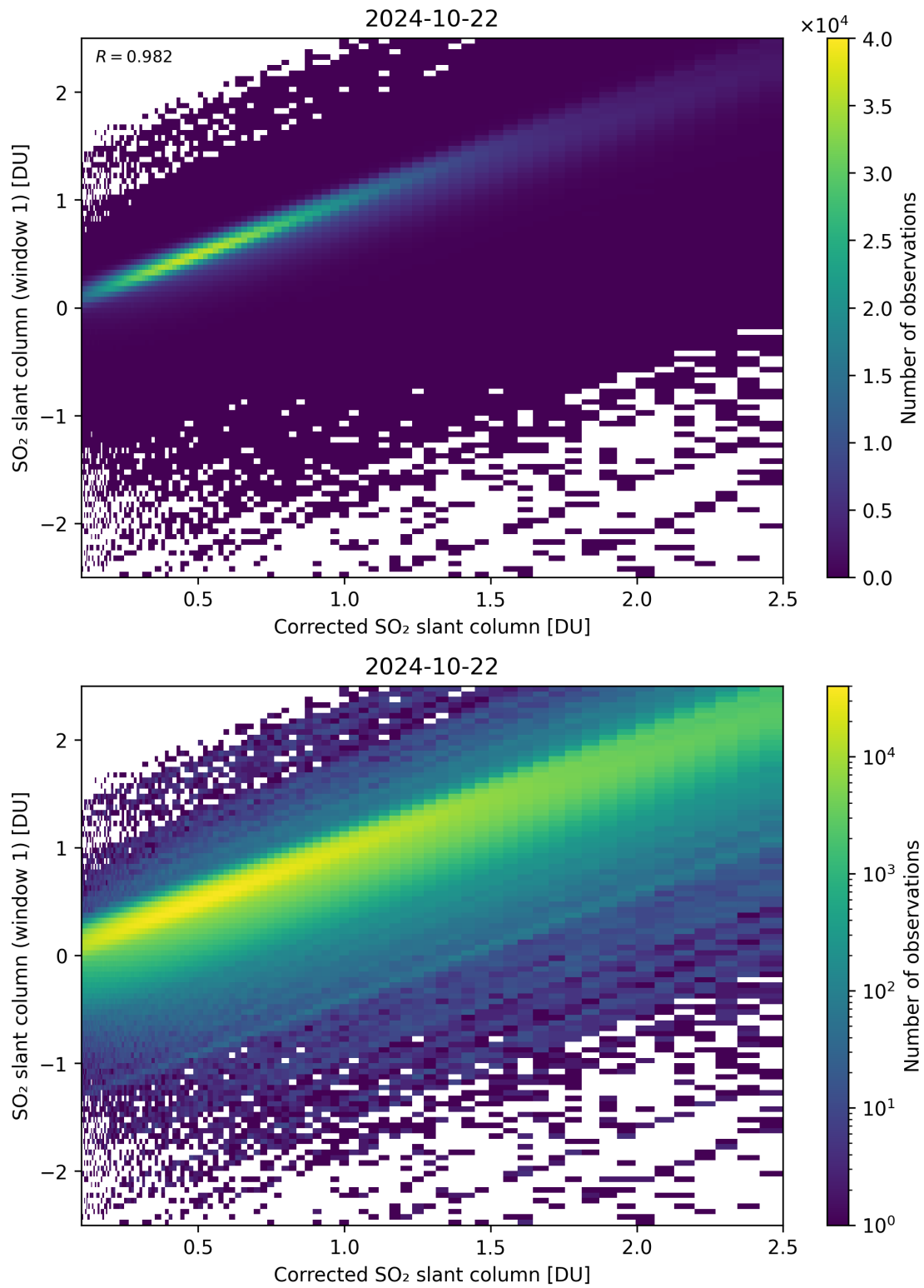
Figure 187: Scatter density plot of “Corrected SO 2 slant column” against “SO 2 slant column (window 1)” for 2024-10-21 to 2024-10-23.
