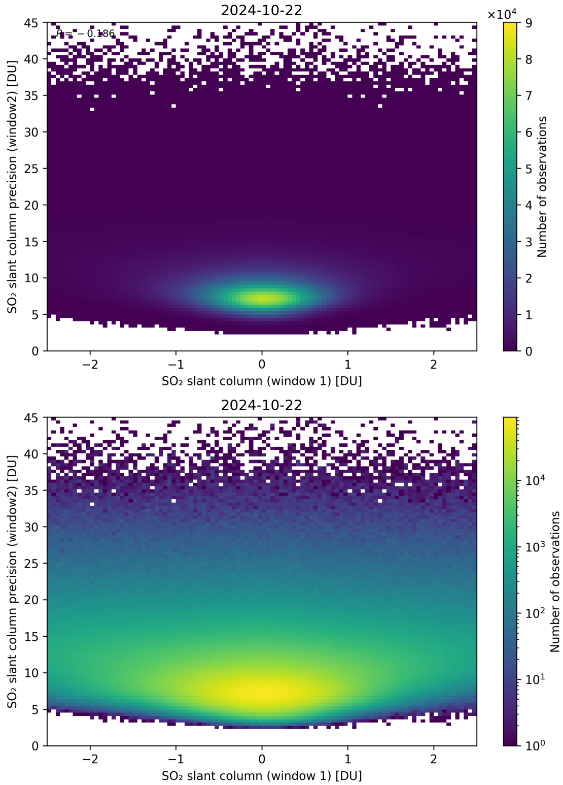
Figure 236: Scatter density plot of “SO 2 slant column (window 1)” against “SO 2 slant column precision (window2)” for 2024-10-21 to 2024-10-23.
