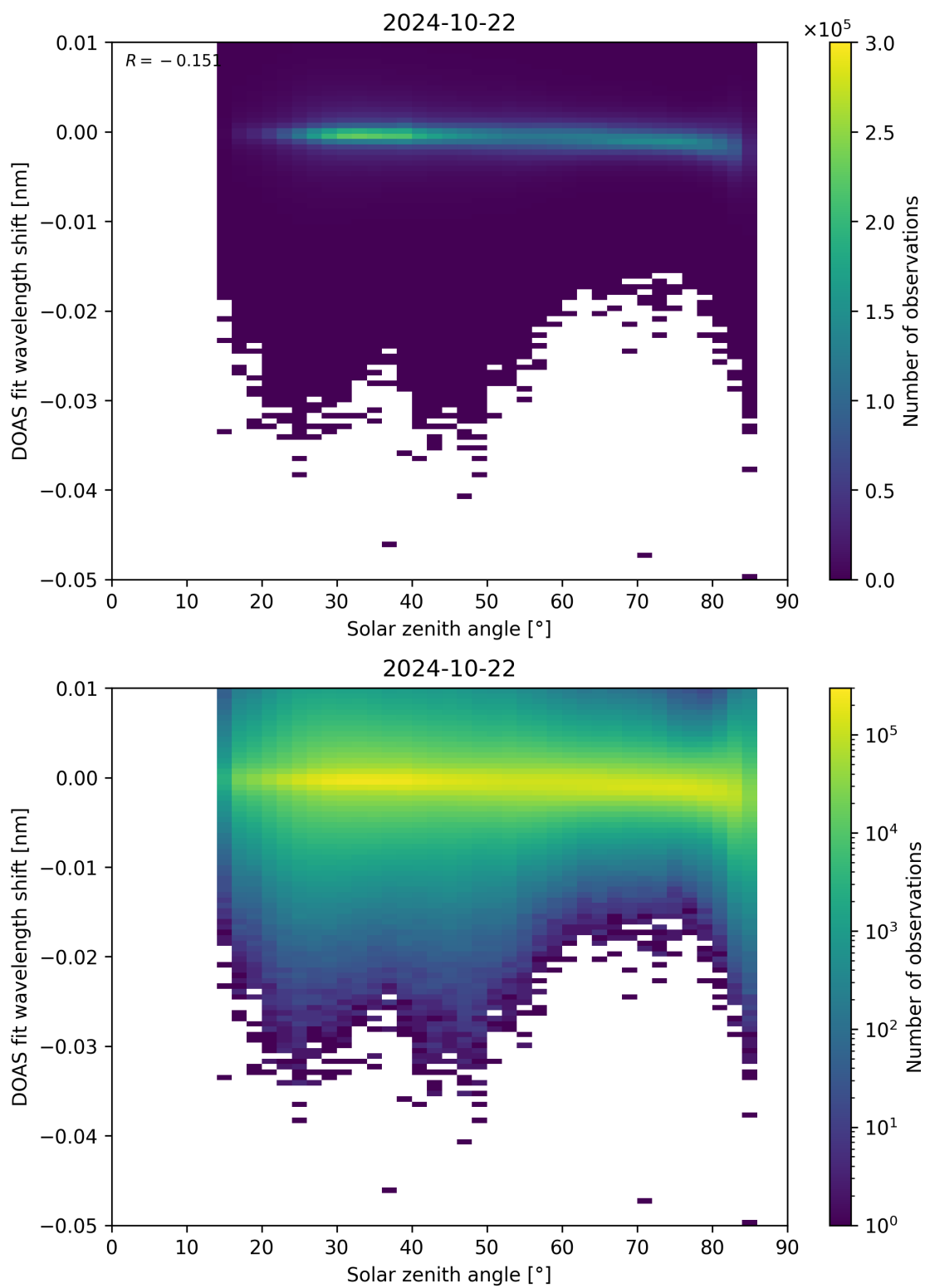
Figure 161: Scatter density plot of “Solar zenith angle” against “DOAS fit wavelength shift” for 2024-10-21 to 2024-10-23.
