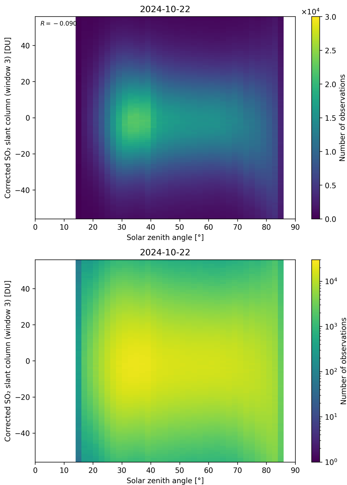
Figure 168: Scatter density plot of “Solar zenith angle” against “Corrected SO 2 slant column (window 3)” for 2024-10-21 to 2024-10-23.
