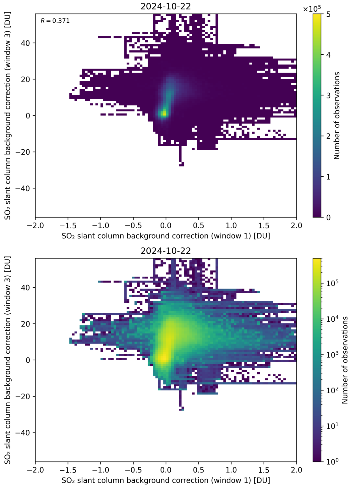
Figure 99: Scatter density plot of “SO 2 slant column background correction (window 1)” against “SO 2 slant column background correction (window 3)” for 2024-10-21 to 2024-10-23.
