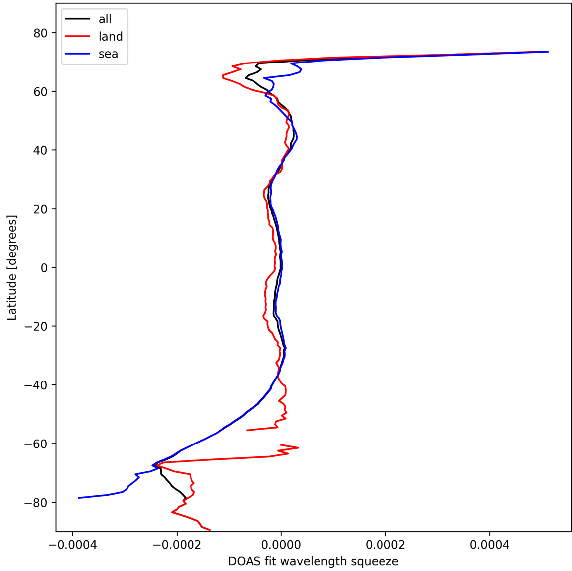
Figure 46: Zonal average of “DOAS fit wavelength squeeze” for 2024-10-21 to 2024-10-23.
