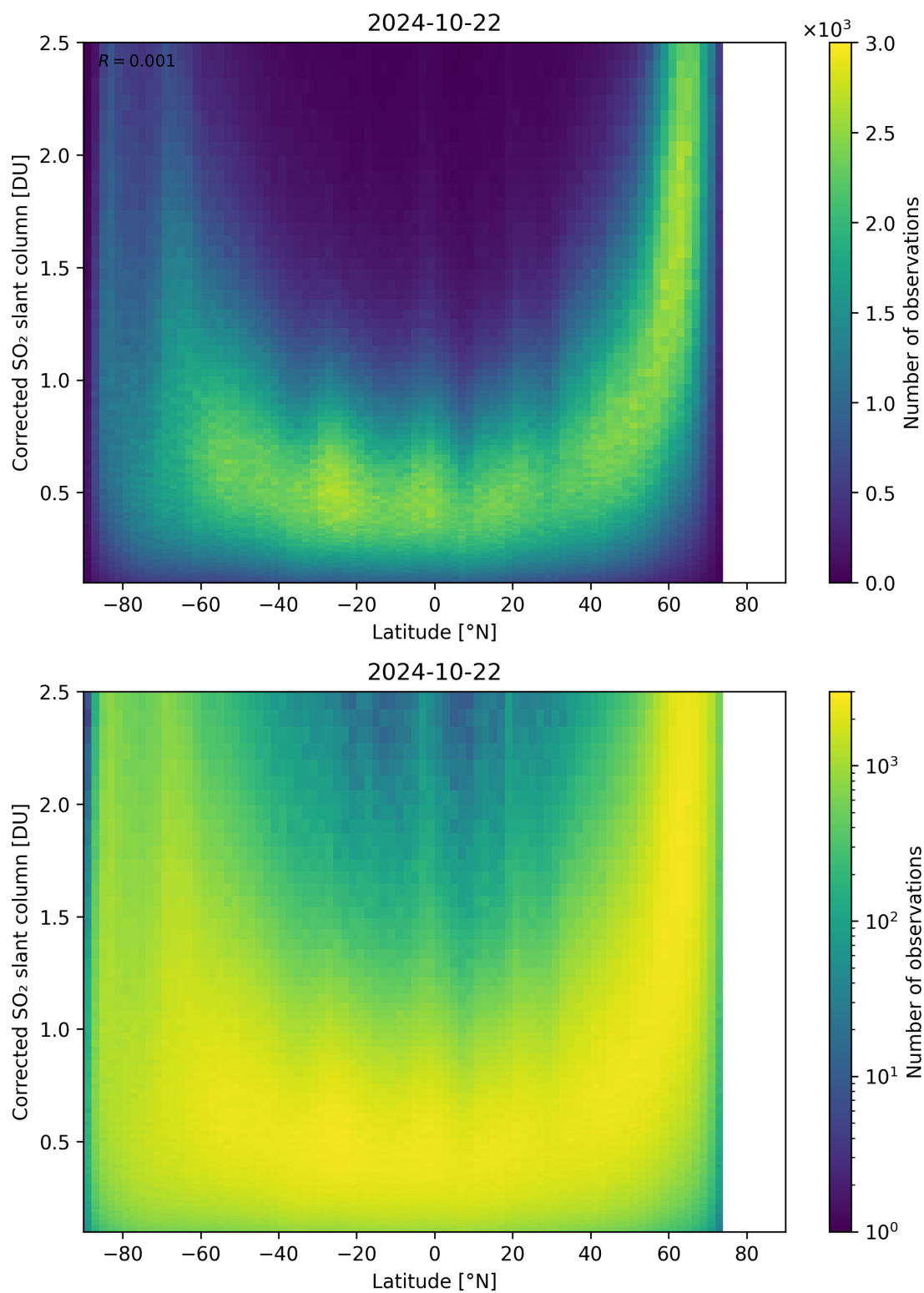
Figure 146: Scatter density plot of “Latitude” against “Corrected SO 2 slant column” for 2024-10-21 to 2024-10-23.
