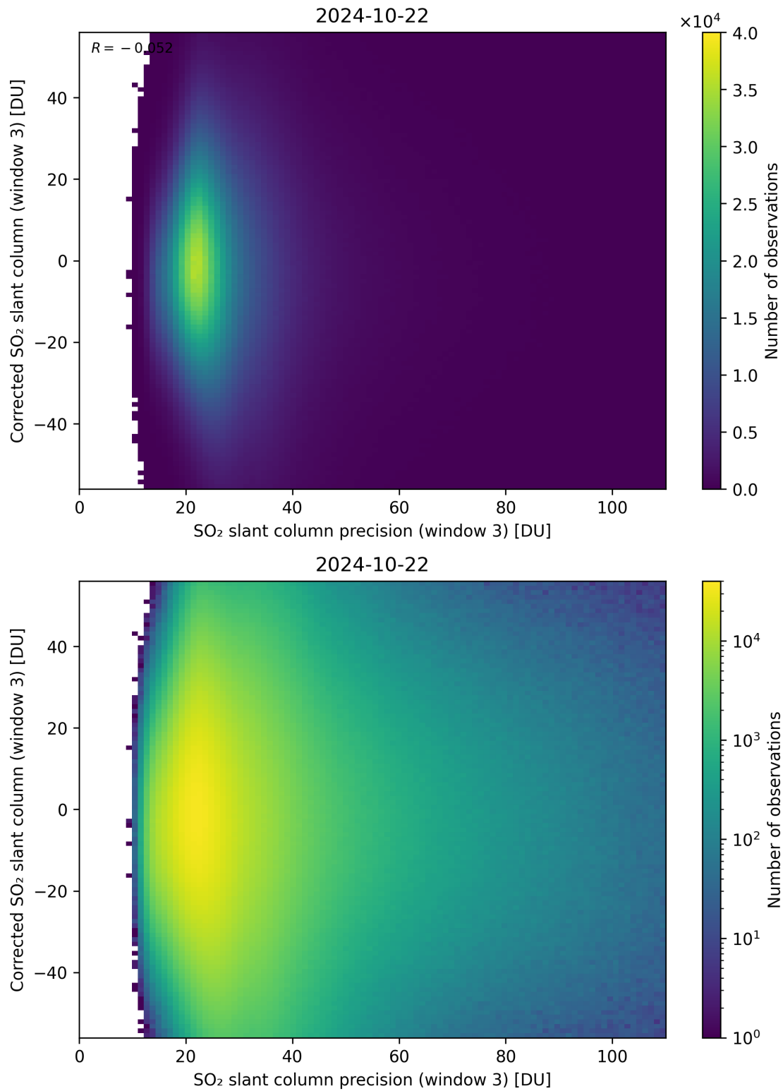
Figure 262: Scatter density plot of “SO 2 slant column precision (window 3)” against “Corrected SO 2 slant column (window 3)” for 2024-10-21 to 2024-10-23.
