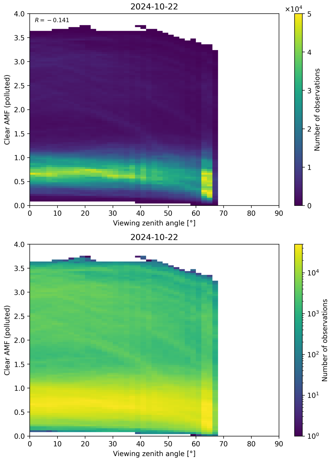
Figure 316: Scatter density plot of “Viewing zenith angle” against “Clear AMF (polluted)” for 2024-10-21 to 2024-10-23.
