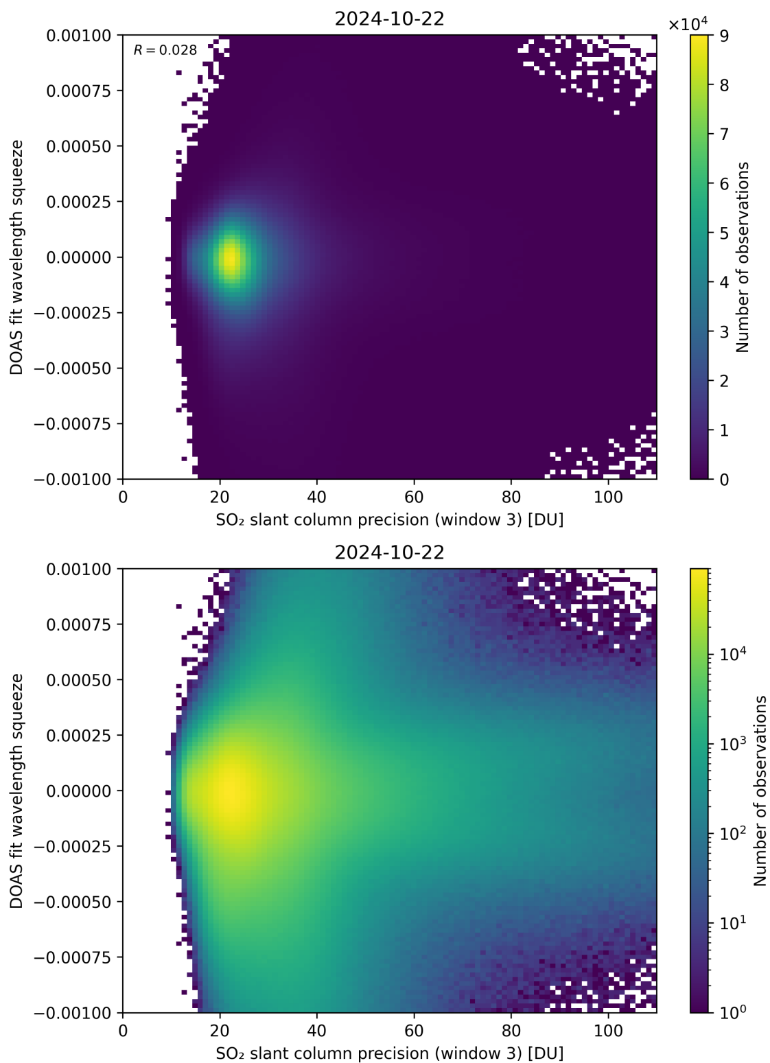
Figure 259: Scatter density plot of “SO 2 slant column precision (window 3)” against “DOAS fit wavelength squeeze” for 2024-10-21 to 2024-10-23.
