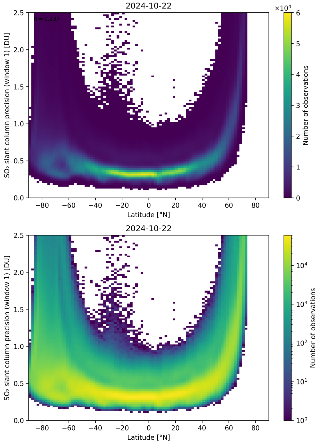
Figure 150: Scatter density plot of “Latitude” against “SO 2 slant column precision (window 1)” for 2024-10-21 to 2024-10-23.
