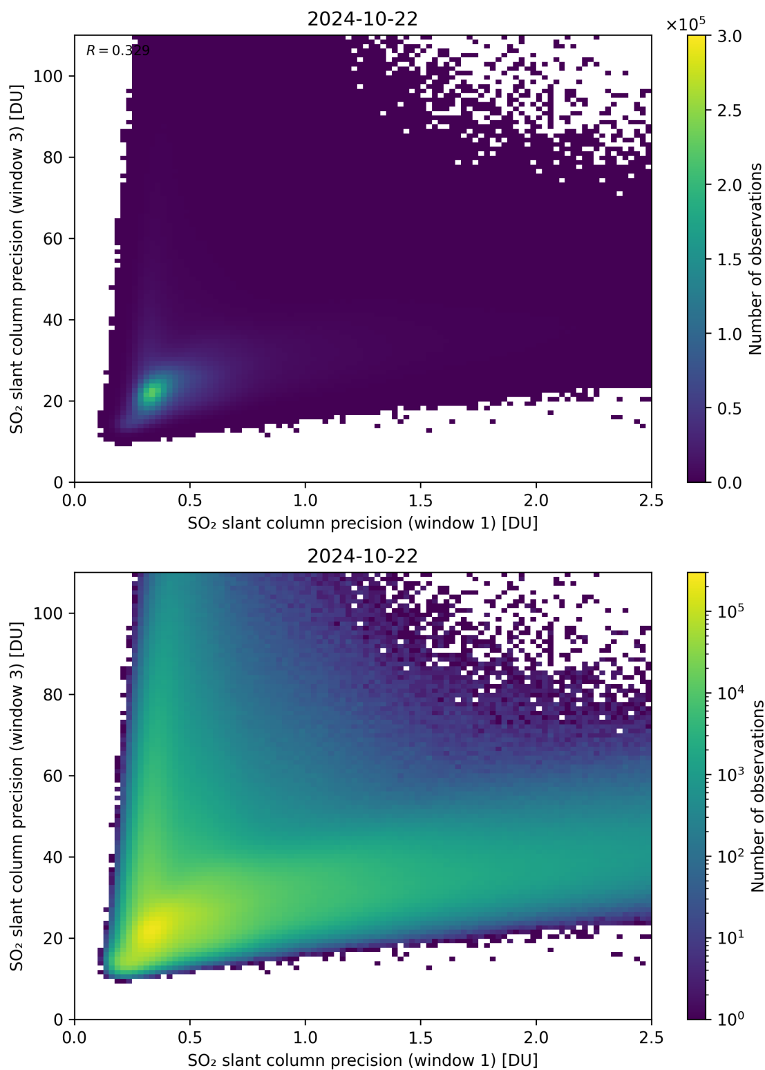
Figure 229: Scatter density plot of “SO 2 slant column precision (window 1)” against “SO 2 slant column precision (window 3)” for 2024-10-21 to 2024-10-23.
