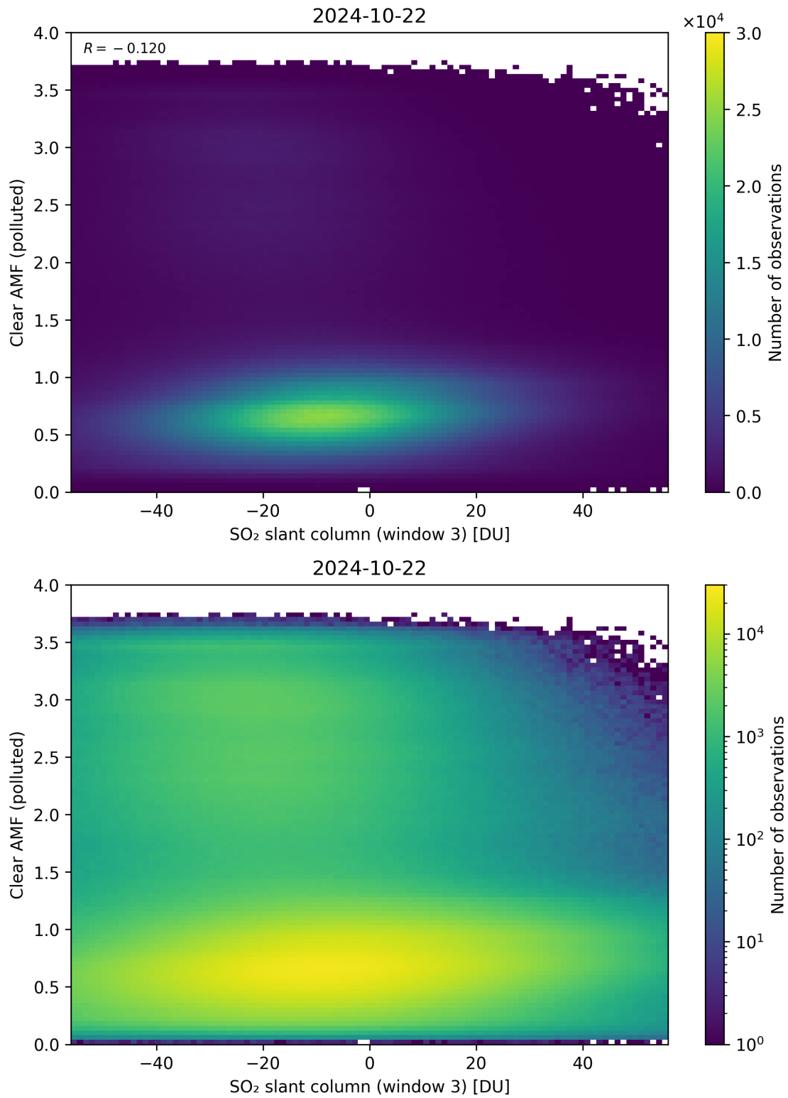
Figure 265: Scatter density plot of “SO 2 slant column (window 3)” against “Clear AMF (polluted)” for 2024-10-21 to 2024-10-23.
