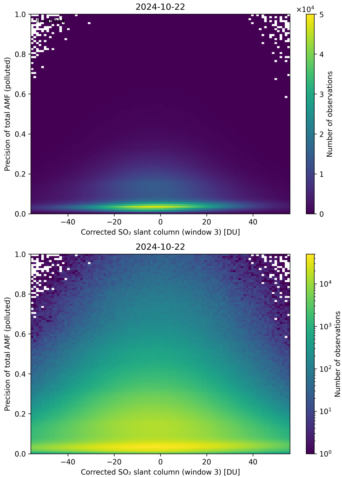
Figure 211: Scatter density plot of “Corrected SO 2 slant column (window 3)” against “Precision of total AMF (polluted)” for 2024-10-21 to 2024-10-23.
