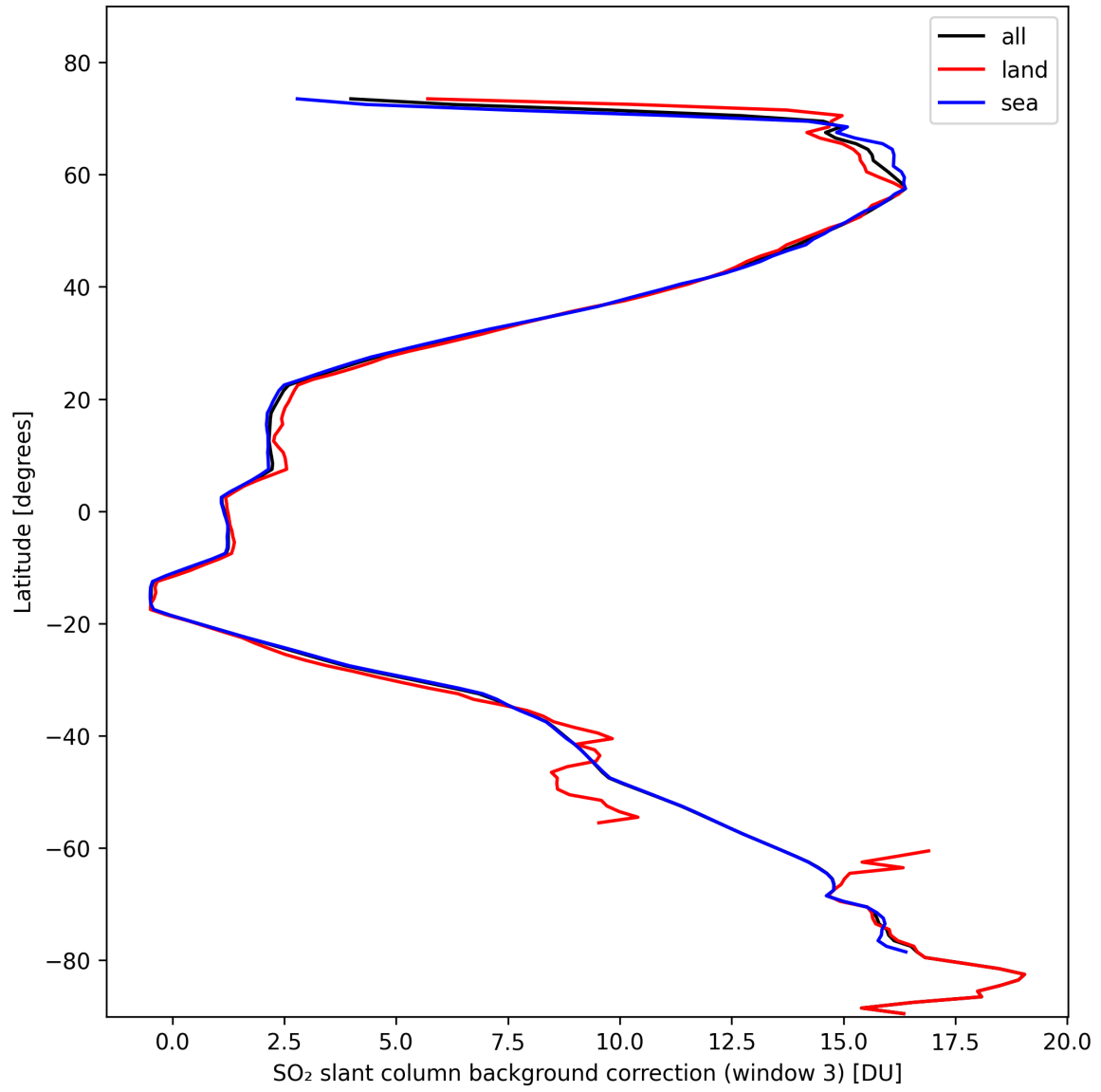
Figure 44: Zonal average of “SO 2 slant column background correction (window 3)” for 2024-10-21 to 2024-10-23.
