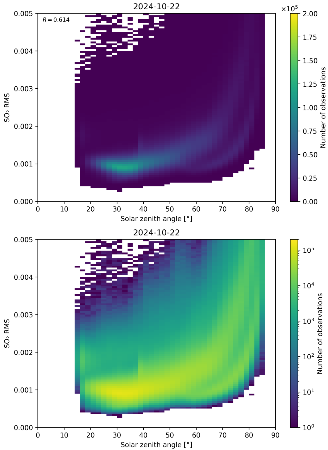
Figure 163: Scatter density plot of “Solar zenith angle” against “SO 2 RMS” for 2024-10-21 to 2024-10-23.
