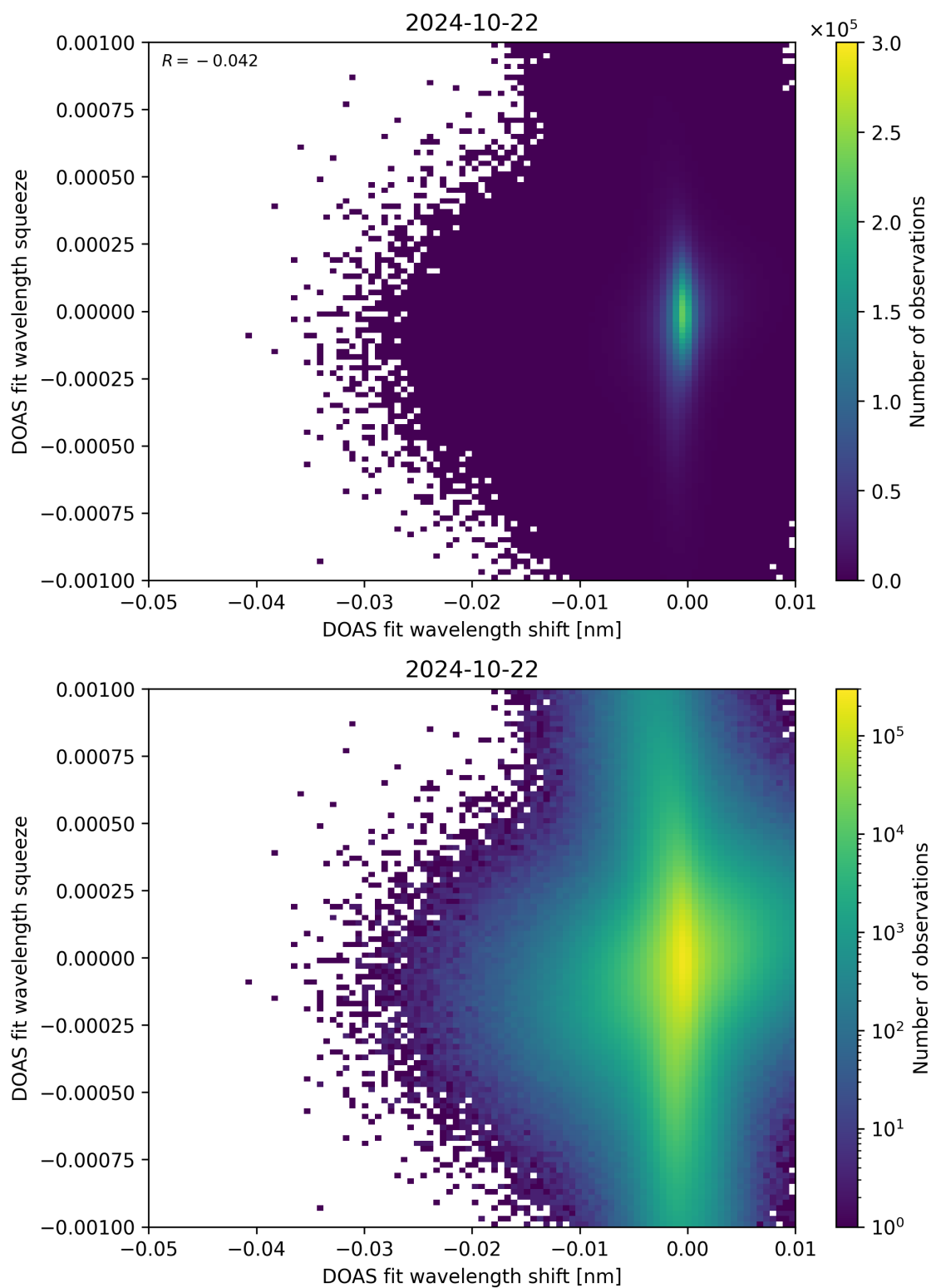
Figure 127: Scatter density plot of “DOAS fit wavelength shift” against “DOAS fit wavelength squeeze” for 2024-10-21 to 2024-10-23.
