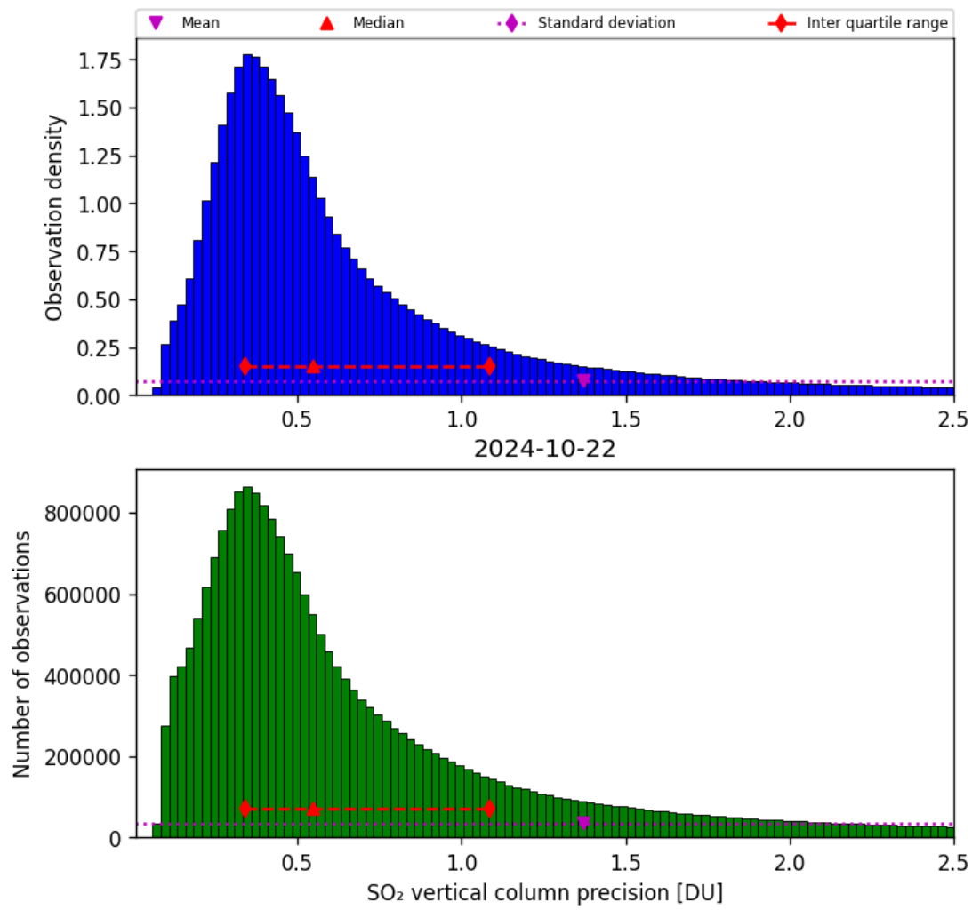
Figure 54: Histogram of “SO 2 vertical column precision” for 2024-10-21 to 2024-10-23
