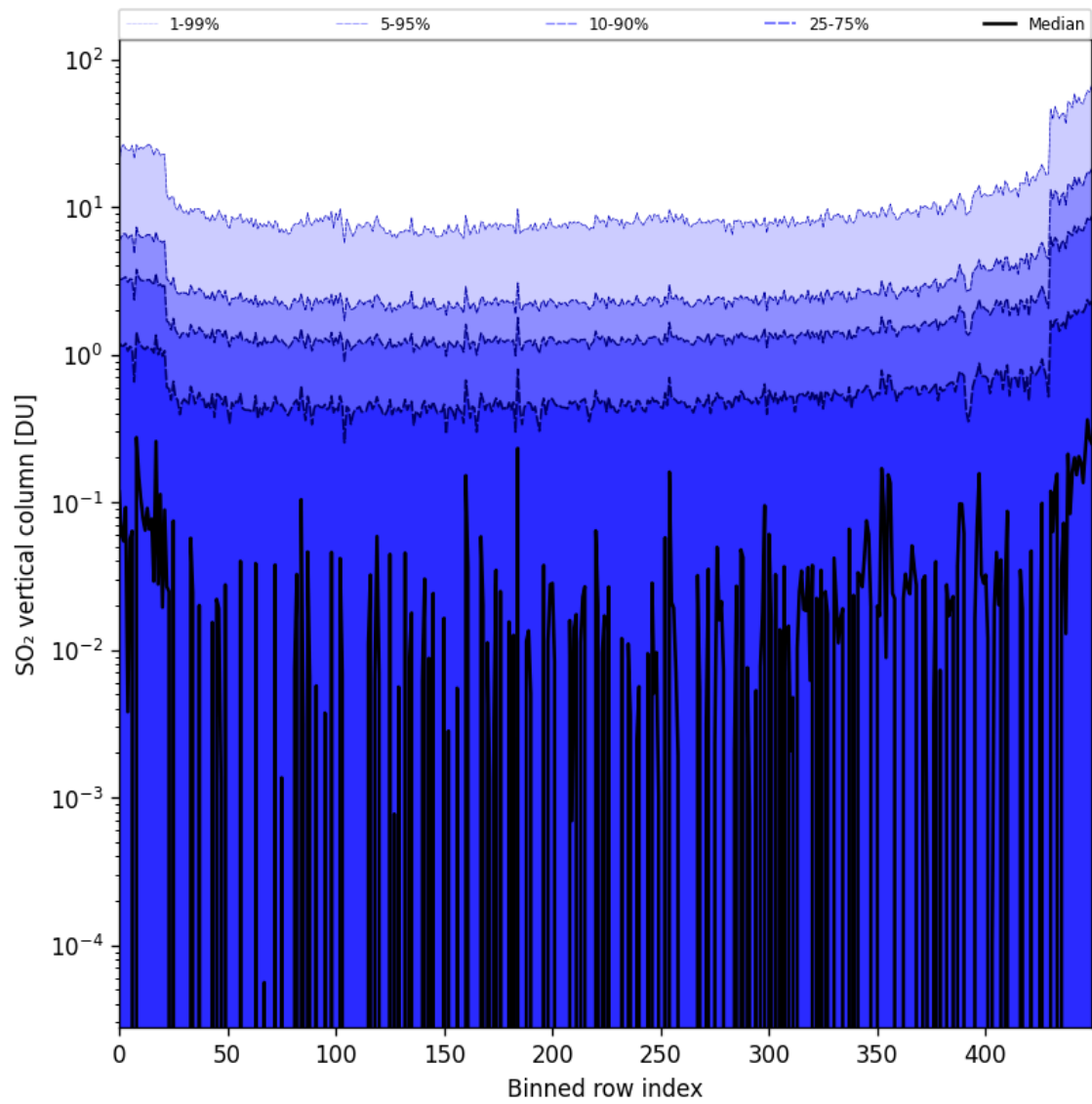
Figure 76: Along track statistics of “SO 2 vertical column” for 2024-10-21 to 2024-10-23
