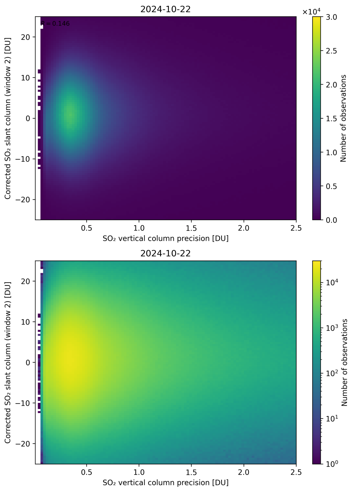
Figure 287: Scatter density plot of “SO 2 vertical column precision” against “Corrected SO 2 slant column (window 2)” for 2024-10-21 to 2024-10-23.
