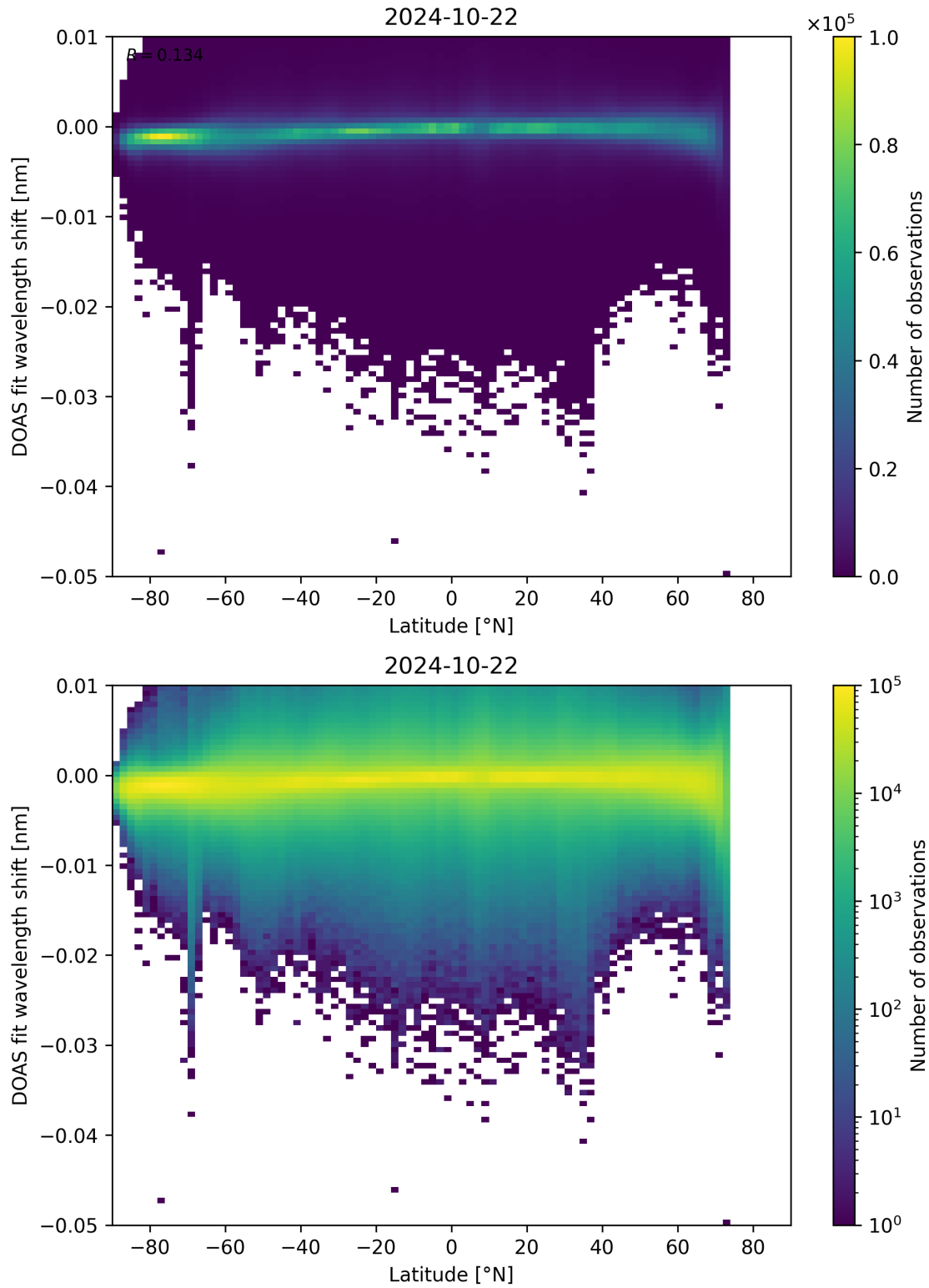
Figure 142: Scatter density plot of “Latitude” against “DOAS fit wavelength shift” for 2024-10-21 to 2024-10-23.
