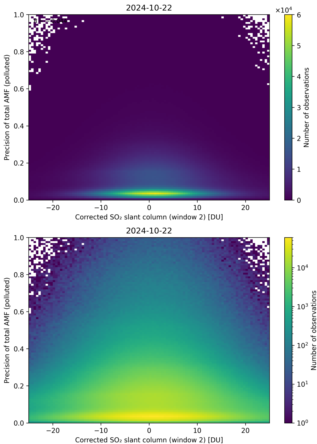
Figure 204: Scatter density plot of “Corrected SO 2 slant column (window 2)” against “Precision of total AMF (polluted)” for 2024-10-21 to 2024-10-23.
