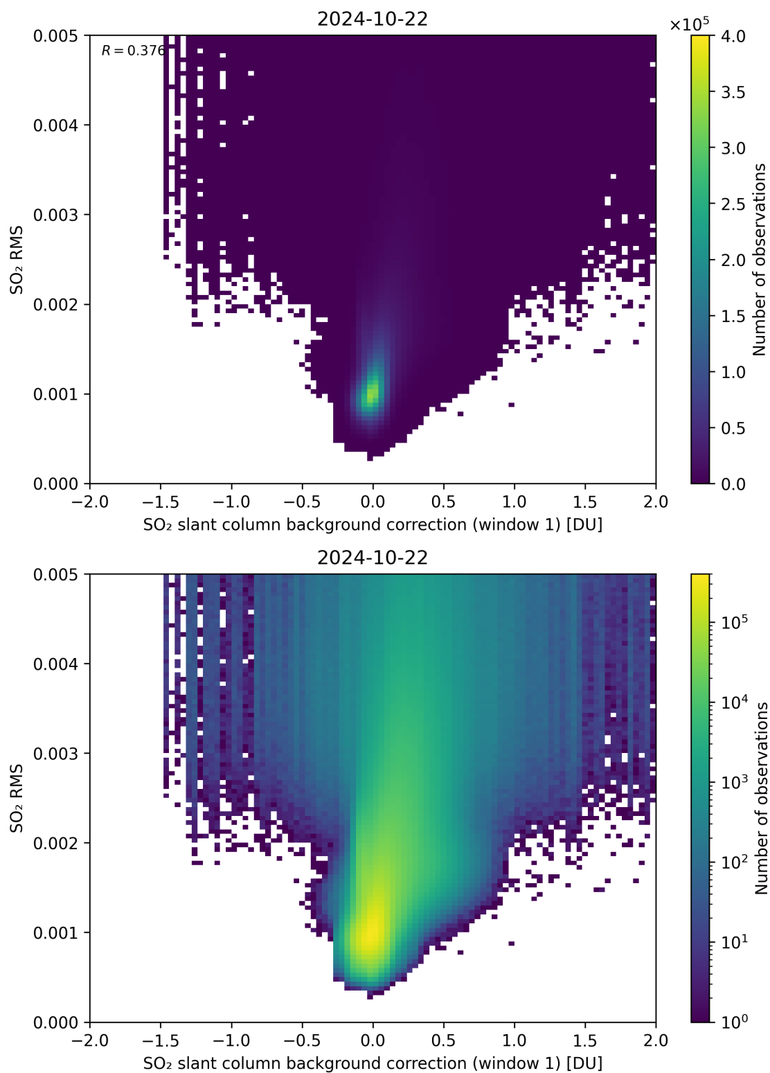
Figure 102: Scatter density plot of “SO 2 slant column background correction (window 1)” against “SO 2 RMS” for 2024-10-21 to 2024-10-23.
