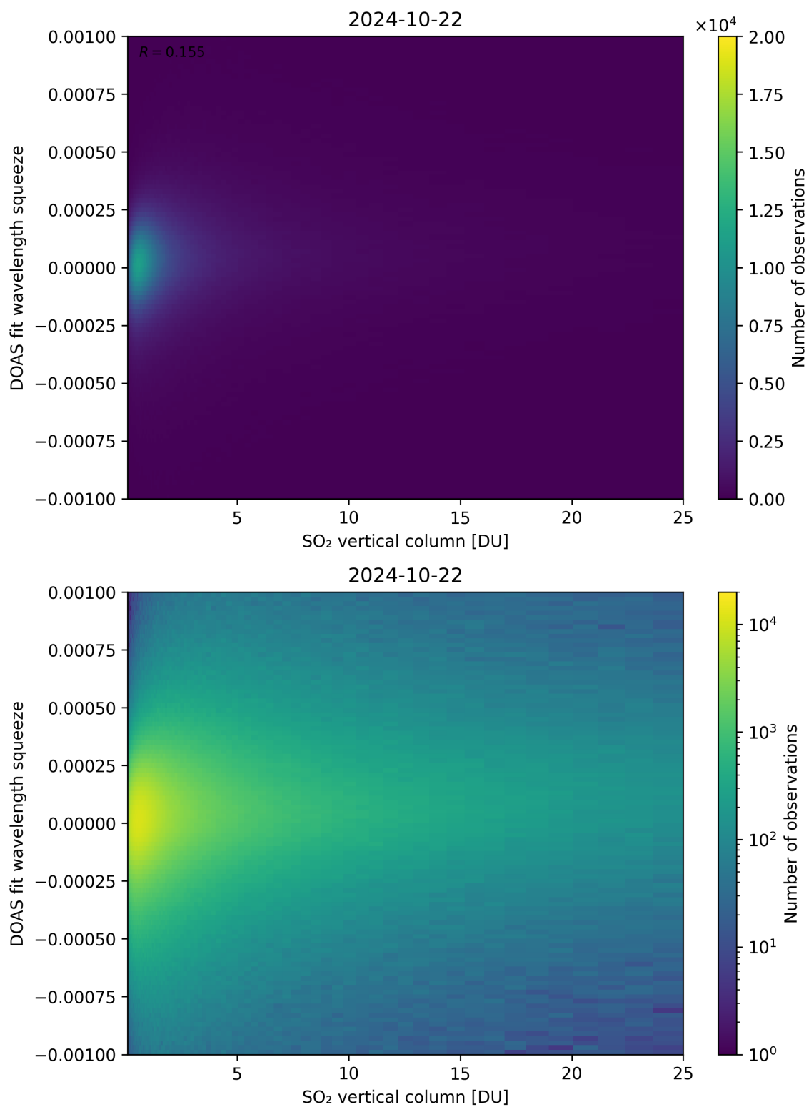
Figure 277: Scatter density plot of “SO 2 vertical column” against “DOAS fit wavelength squeeze” for 2024-10-21 to 2024-10-23.
