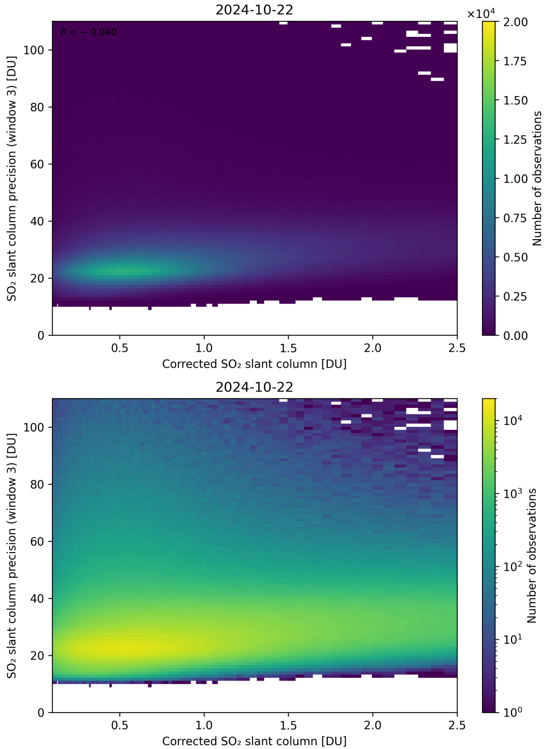
Figure 191: Scatter density plot of “Corrected SO 2 slant column” against “SO 2 slant column precision (window 3)” for 2024-10-21 to 2024-10-23.
