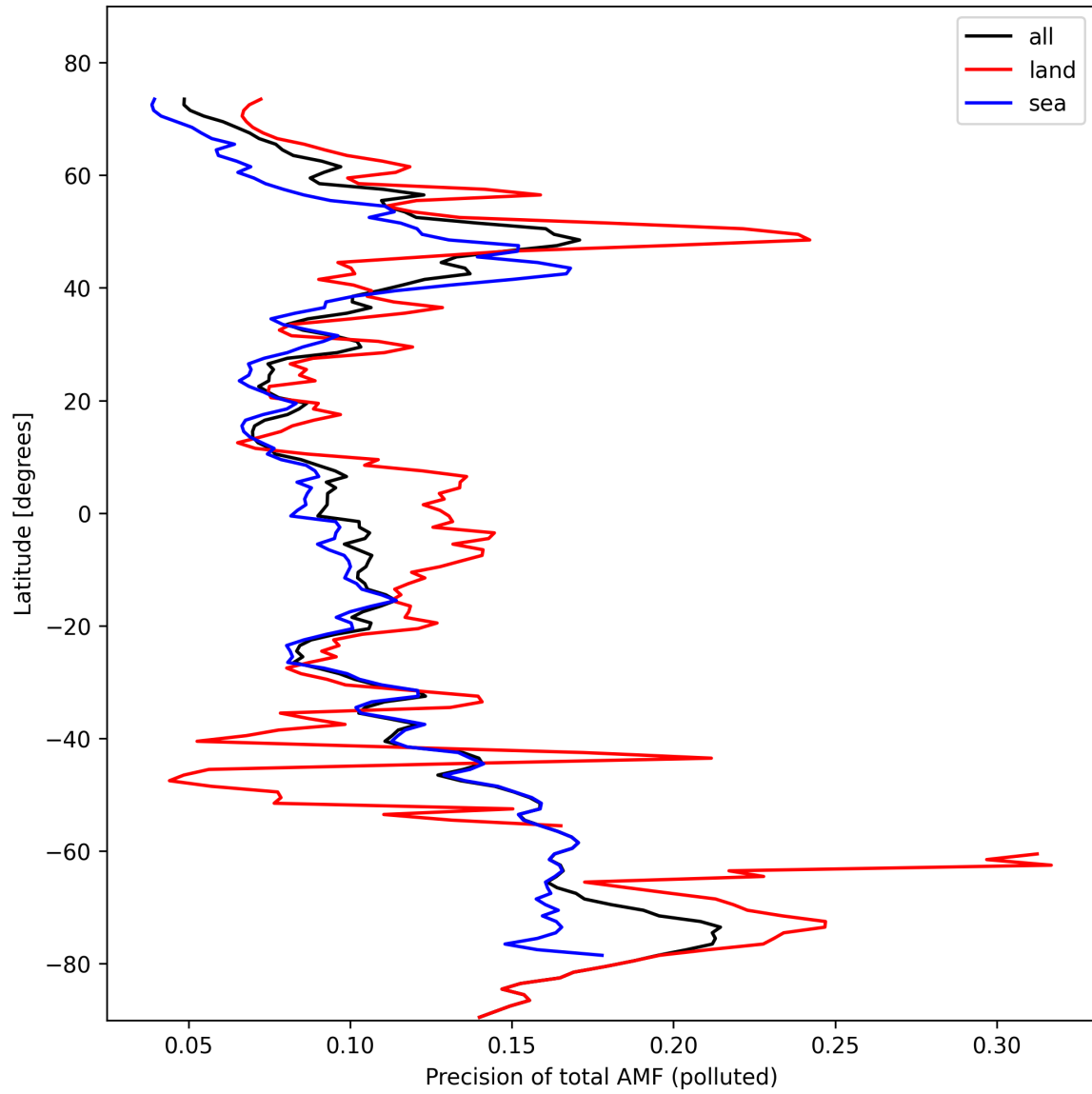
Figure 49: Zonal average of “Precision of total AMF (polluted)” for 2024-10-21 to 2024-10-23.
