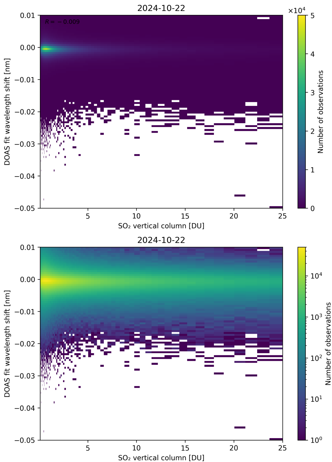
Figure 276: Scatter density plot of “SO 2 vertical column” against “DOAS fit wavelength shift” for 2024-10-21 to 2024-10-23.
