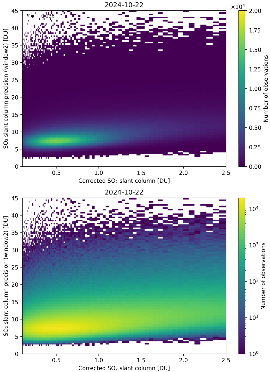
Figure 189: Scatter density plot of “Corrected SO 2 slant column” against “SO 2 slant column precision (window2)” for 2024-10-21 to 2024-10-23.
