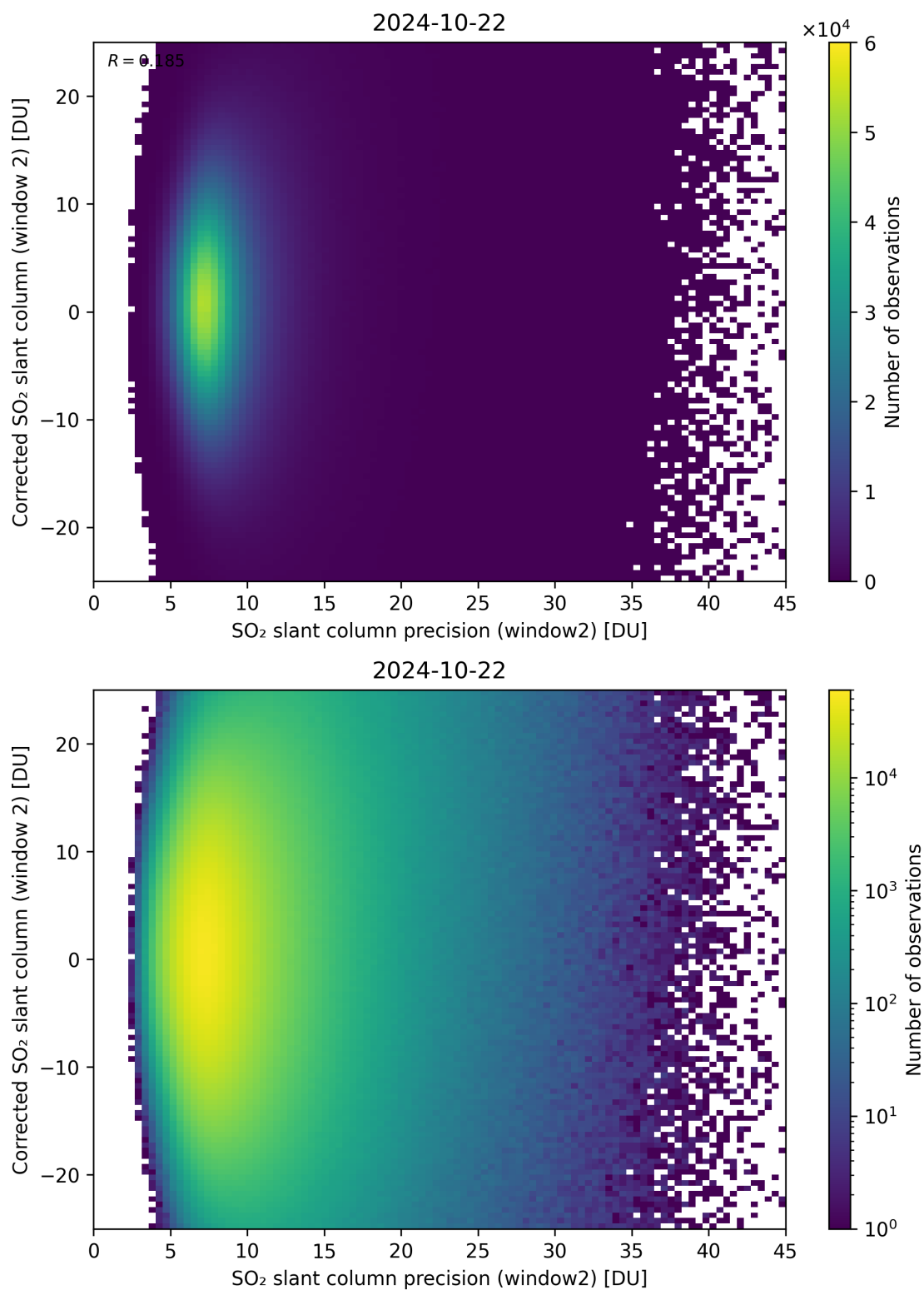
Figure 247: Scatter density plot of “SO 2 slant column precision (window2)” against “Corrected SO 2 slant column (window 2)” for 2024-10-21 to 2024-10-23.
