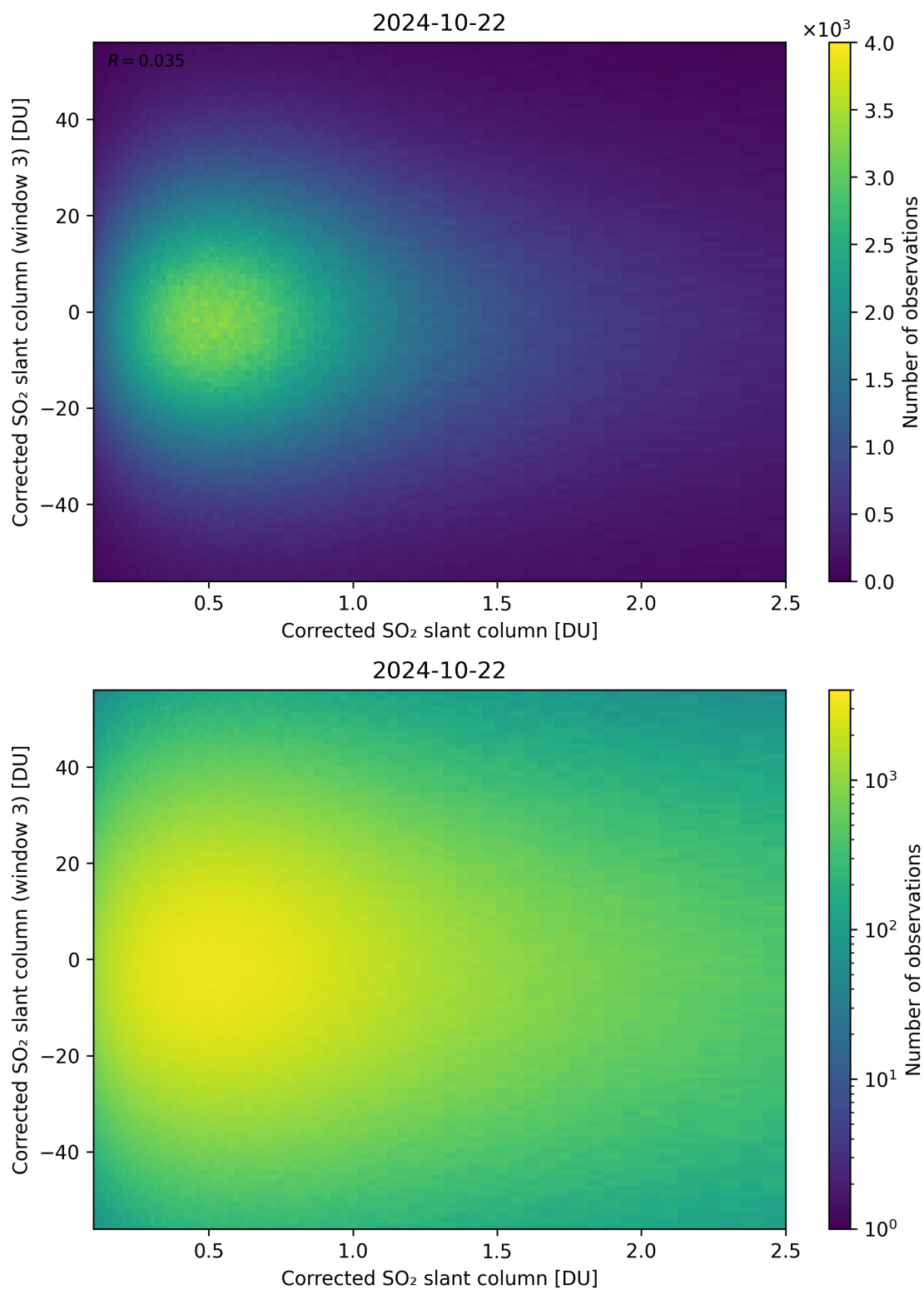
Figure 186: Scatter density plot of “Corrected SO 2 slant column” against “Corrected SO 2 slant column (window 3)” for 2024-10-21 to 2024-10-23.
