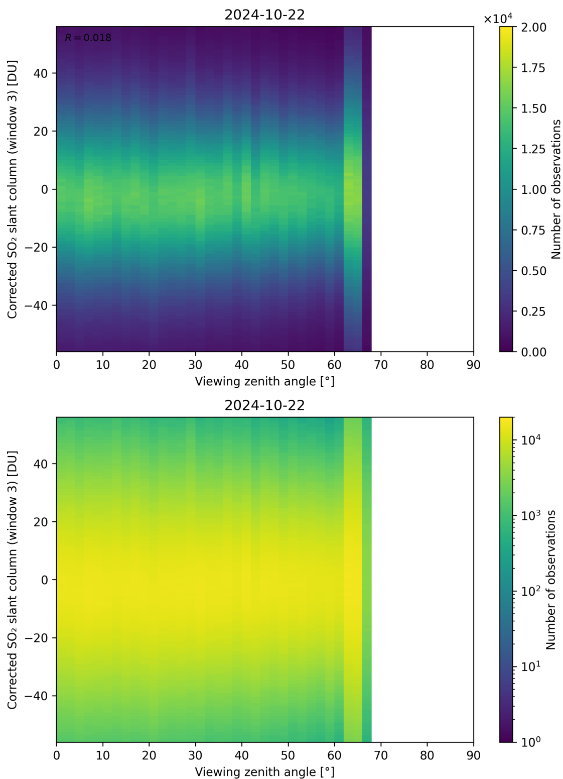
Figure 319: Scatter density plot of “Viewing zenith angle” against “Corrected SO 2 slant column (window 3)” for 2024-10-21 to 2024-10-23.
