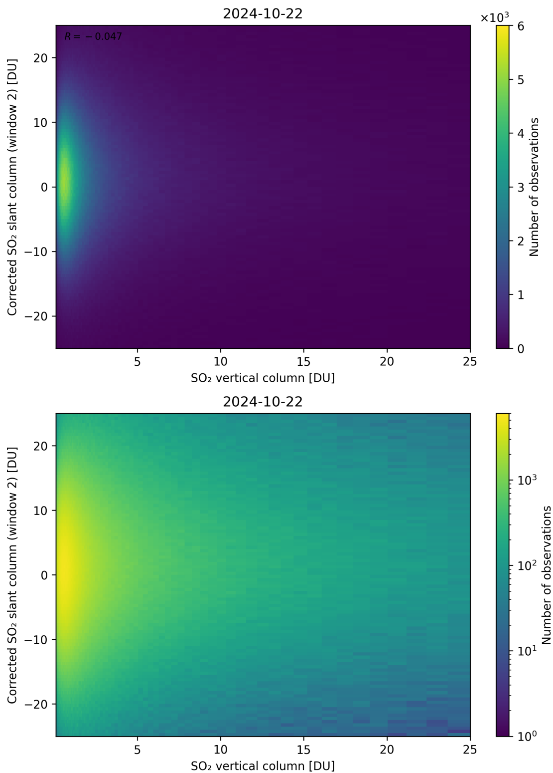
Figure 298: Scatter density plot of “SO 2 vertical column” against “Corrected SO 2 slant column (window 2)” for 2024-10-21 to 2024-10-23.
