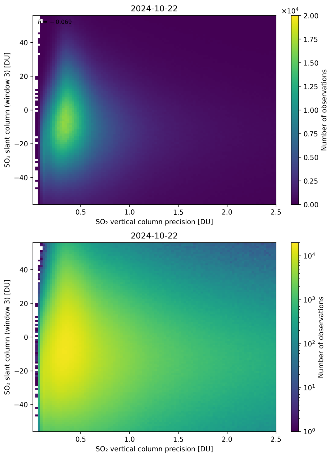
Figure 292: Scatter density plot of “SO 2 vertical column precision” against “SO 2 slant column (window 3)” for 2024-10-21 to 2024-10-23.
