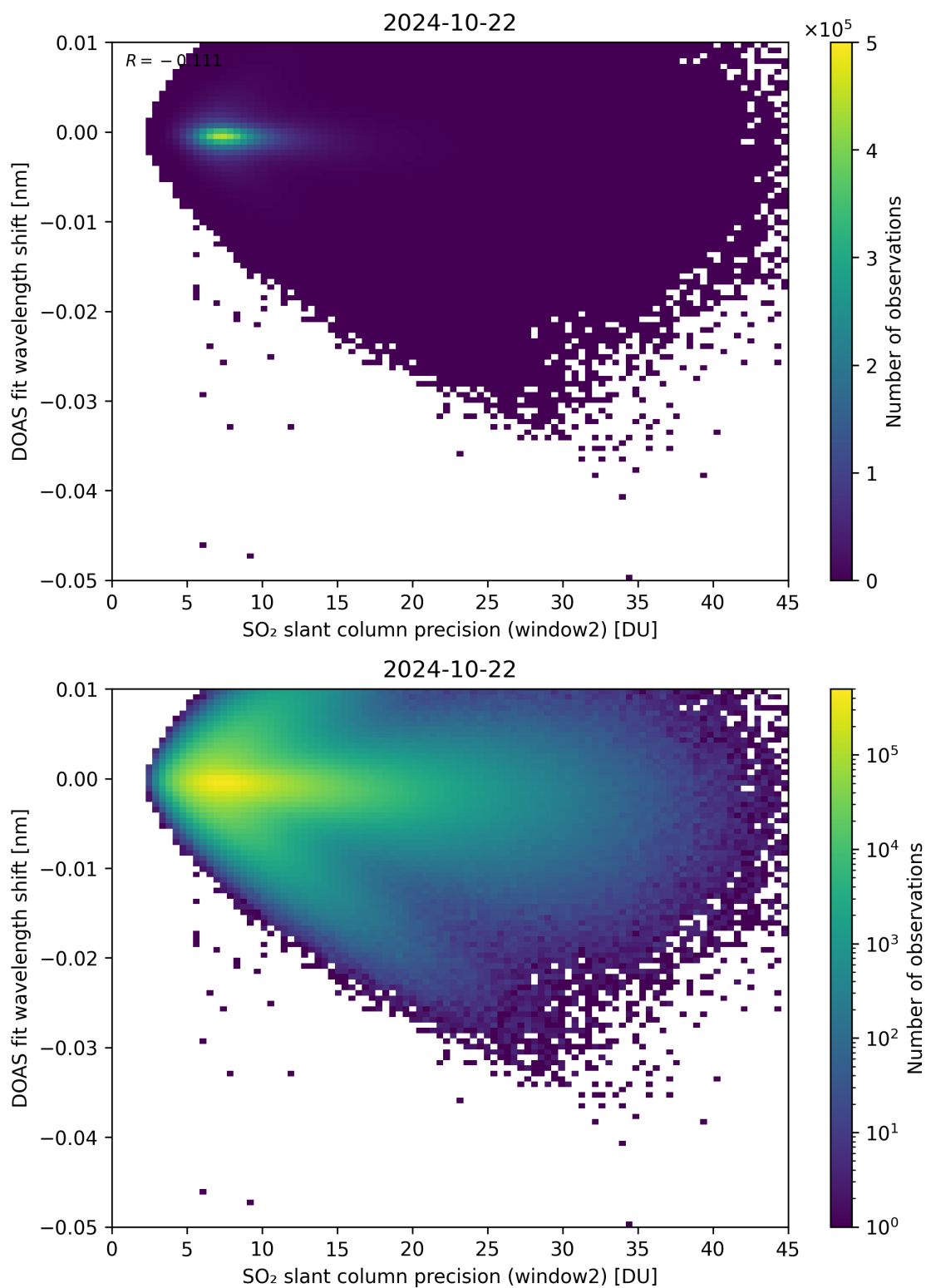
Figure 243: Scatter density plot of “SO 2 slant column precision (window2)” against “DOAS fit wavelength shift” for 2024-10-21 to 2024-10-23.
