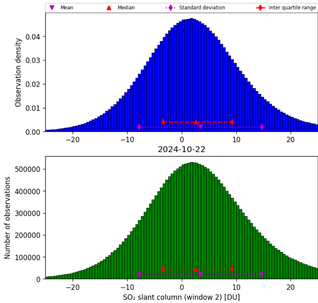
Figure 60: Histogram of “SO 2 slant column (window 2)” for 2024-10-21 to 2024-10-23
