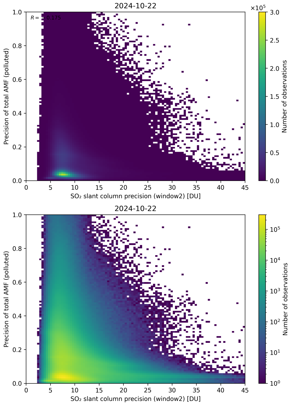
Figure 252: Scatter density plot of “SO 2 slant column precision (window2)” against “Precision of total AMF (polluted)” for 2024-10-21 to 2024-10-23.
