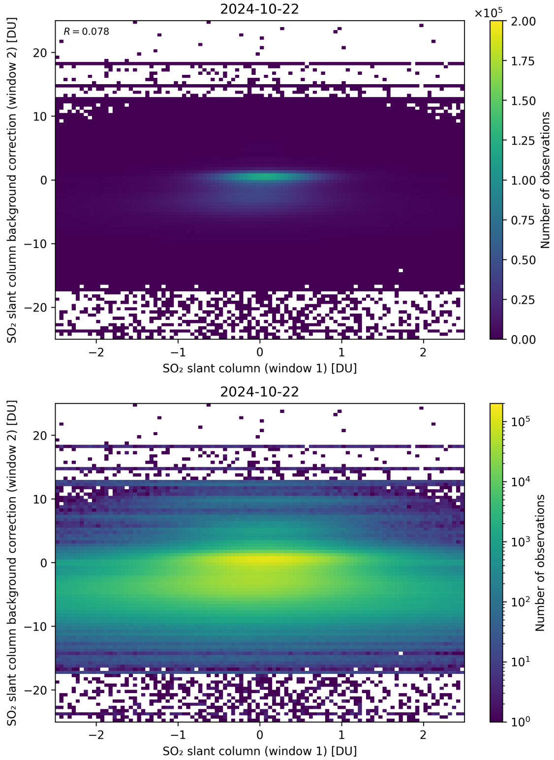
Figure 213: Scatter density plot of “SO 2 slant column (window 1)” against “SO 2 slant column background correction (window 2)” for 2024-10-21 to 2024-10-23.
