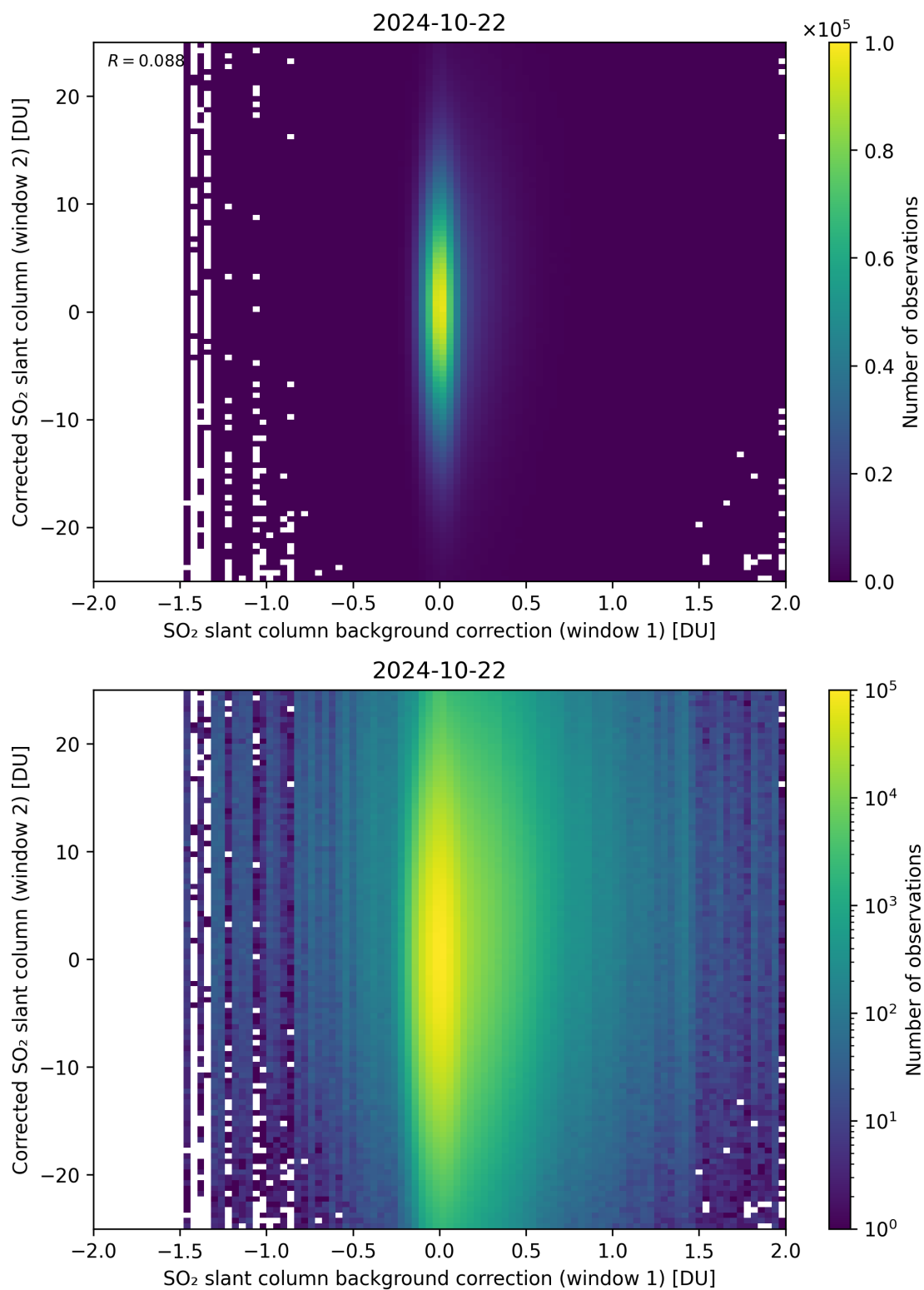
Figure 104: Scatter density plot of “SO 2 slant column background correction (window 1)” against “Corrected SO 2 slant column (window 2)” for 2024-10-21 to 2024-10-23.
