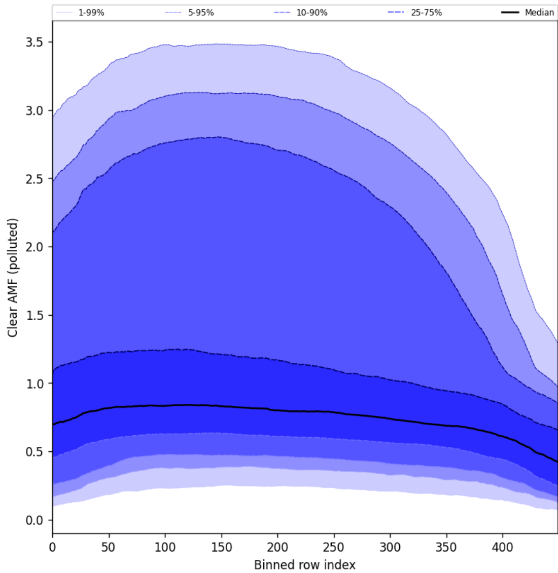
Figure 96: Along track statistics of “Clear AMF (polluted)” for 2024-10-21 to 2024-10-23
