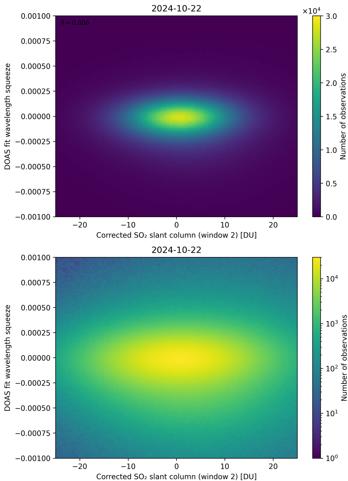
Figure 197: Scatter density plot of “Corrected SO 2 slant column (window 2)” against “DOAS fit wavelength squeeze” for 2024-10-21 to 2024-10-23.
