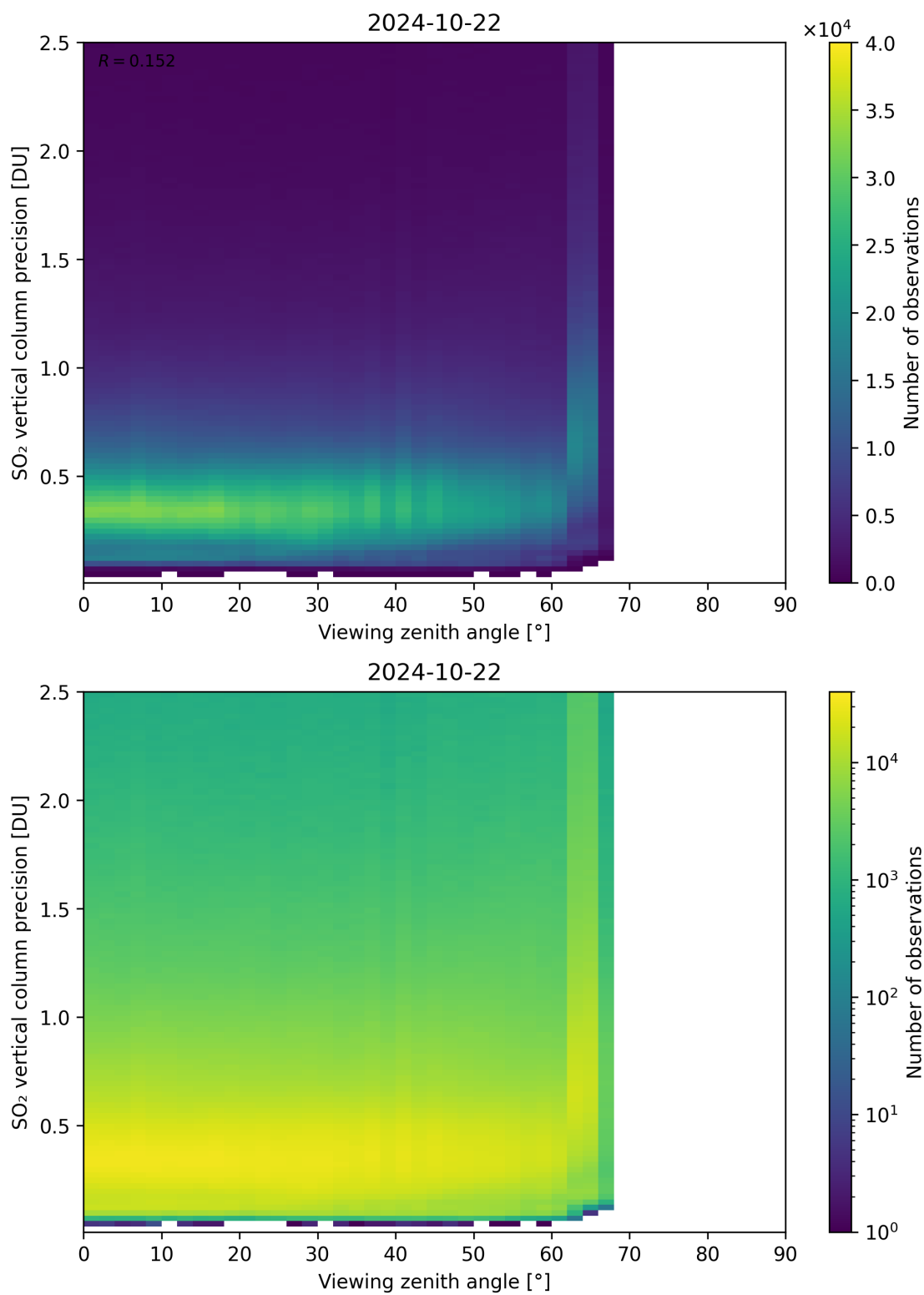
Figure 328: Scatter density plot of “Viewing zenith angle” against “SO 2 vertical column precision” for 2024-10-21 to 2024-10-23.
