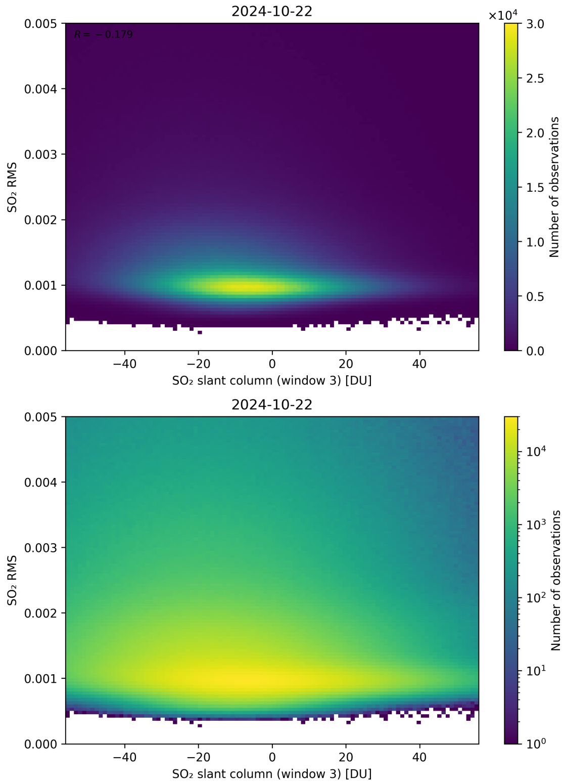
Figure 256: Scatter density plot of “SO 2 slant column (window 3)” against “SO 2 RMS” for 2024-10-21 to 2024-10-23.
