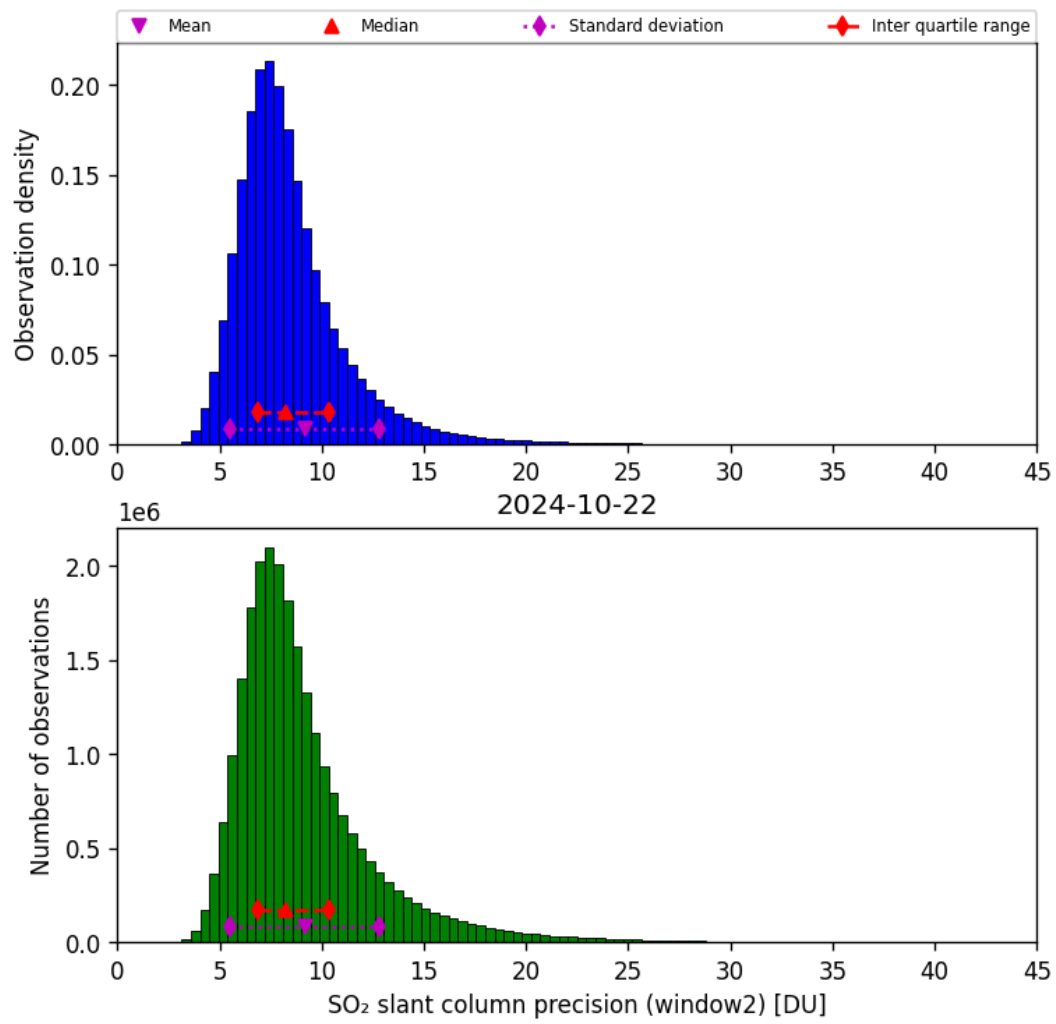
Figure 61: Histogram of “SO 2 slant column precision (window2)” for 2024-10-21 to 2024-10-23
