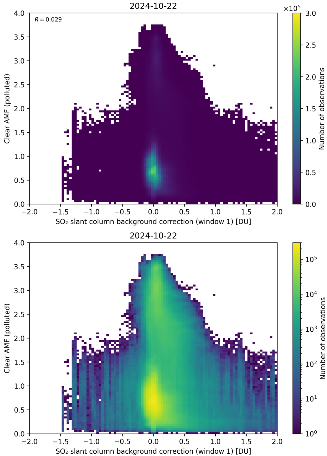
Figure 103: Scatter density plot of “SO 2 slant column background correction (window 1)” against “Clear AMF (polluted)” for 2024-10-21 to 2024-10-23.
