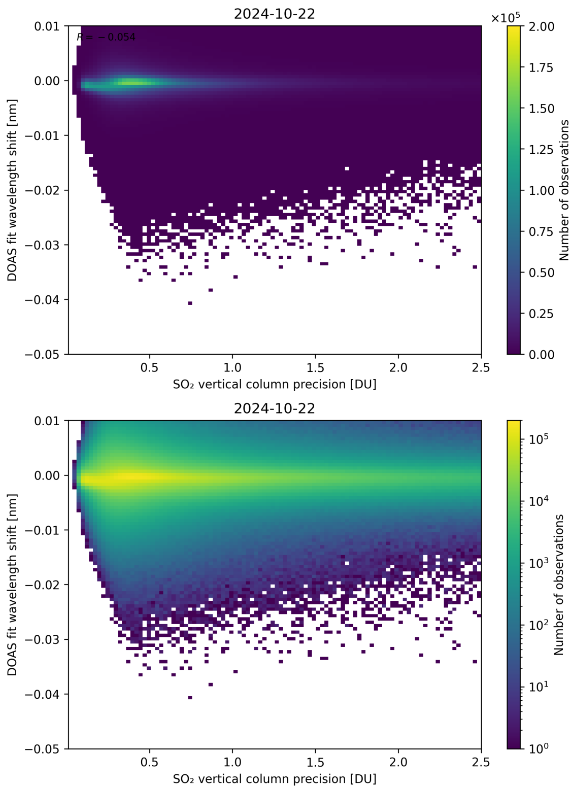
Figure 282: Scatter density plot of “SO 2 vertical column precision” against “DOAS fit wavelength shift” for 2024-10-21 to 2024-10-23.
