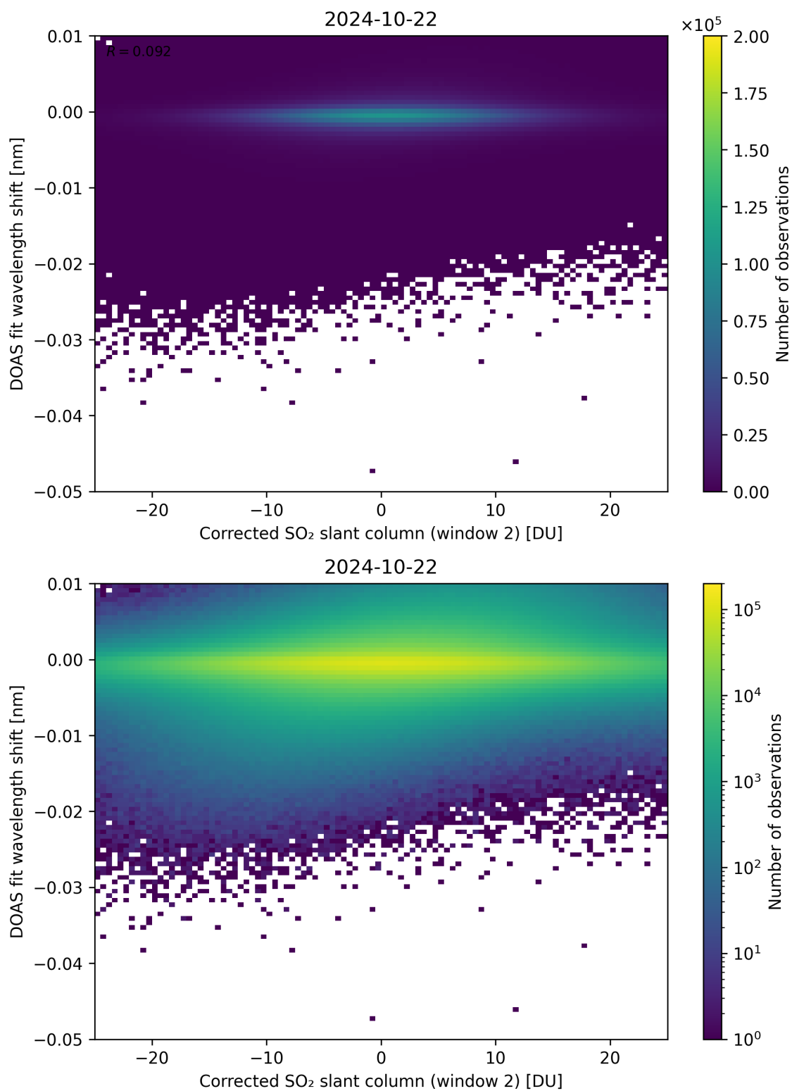
Figure 196: Scatter density plot of “Corrected SO 2 slant column (window 2)” against “DOAS fit wavelength shift” for 2024-10-21 to 2024-10-23.
