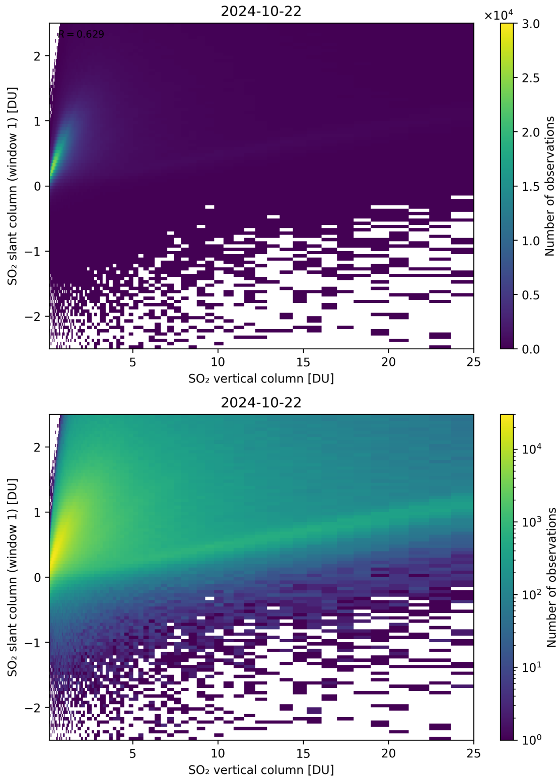
Figure 300: Scatter density plot of “SO 2 vertical column” against “SO 2 slant column (window 1)” for 2024-10-21 to 2024-10-23.
