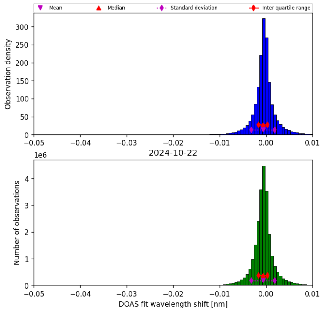
Figure 68: Histogram of “DOAS fit wavelength shift” for 2024-10-21 to 2024-10-23
