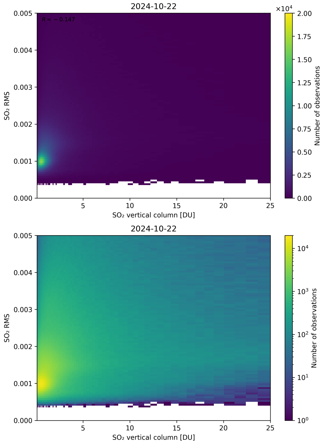
Figure 278: Scatter density plot of “SO 2 vertical column” against “SO 2 RMS” for 2024-10-21 to 2024-10-23.
