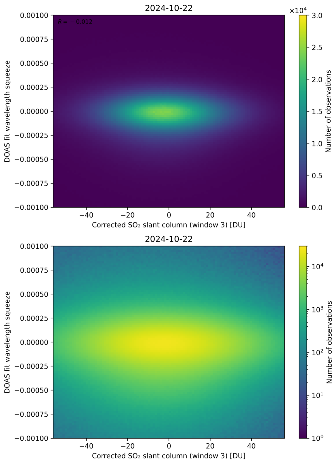
Figure 207: Scatter density plot of “Corrected SO 2 slant column (window 3)” against “DOAS fit wavelength squeeze” for 2024-10-21 to 2024-10-23.
