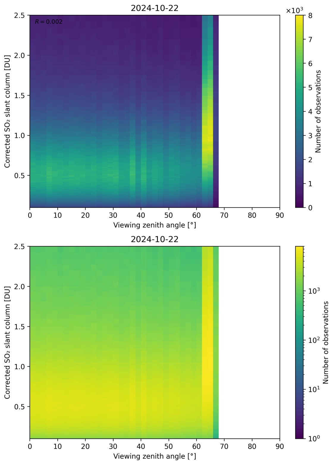
Figure 317: Scatter density plot of “Viewing zenith angle” against “Corrected SO 2 slant column” for 2024-10-21 to 2024-10-23.
