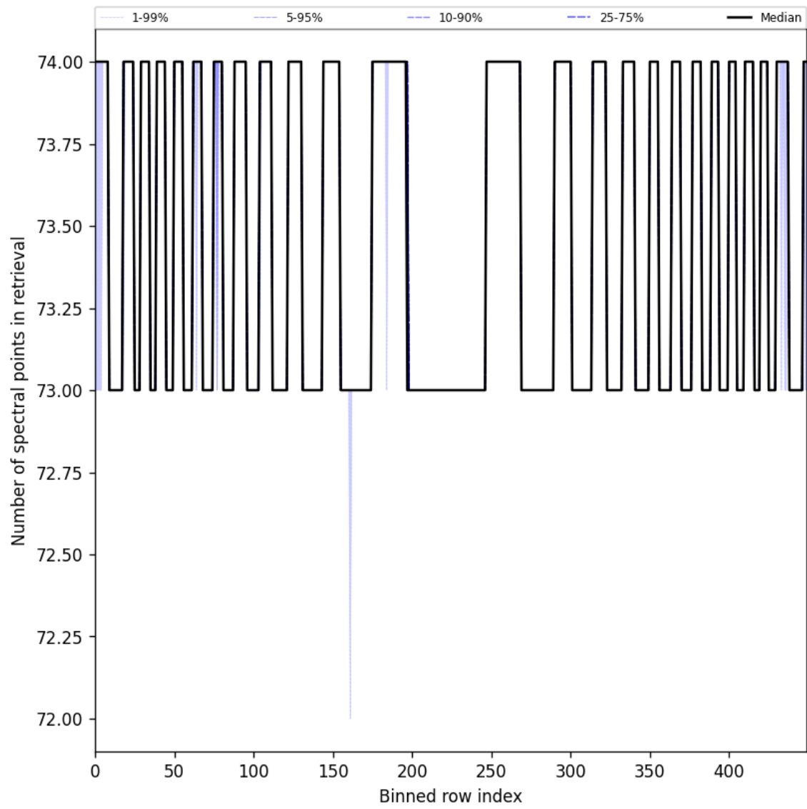
Figure 97: Along track statistics of “Number of spectral points in retrieval” for 2024-10-21 to 2024-10-23
