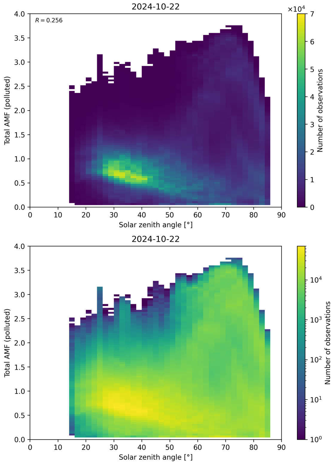
Figure 174: Scatter density plot of “Solar zenith angle” against “Total AMF (polluted)” for 2024-10-21 to 2024-10-23.
