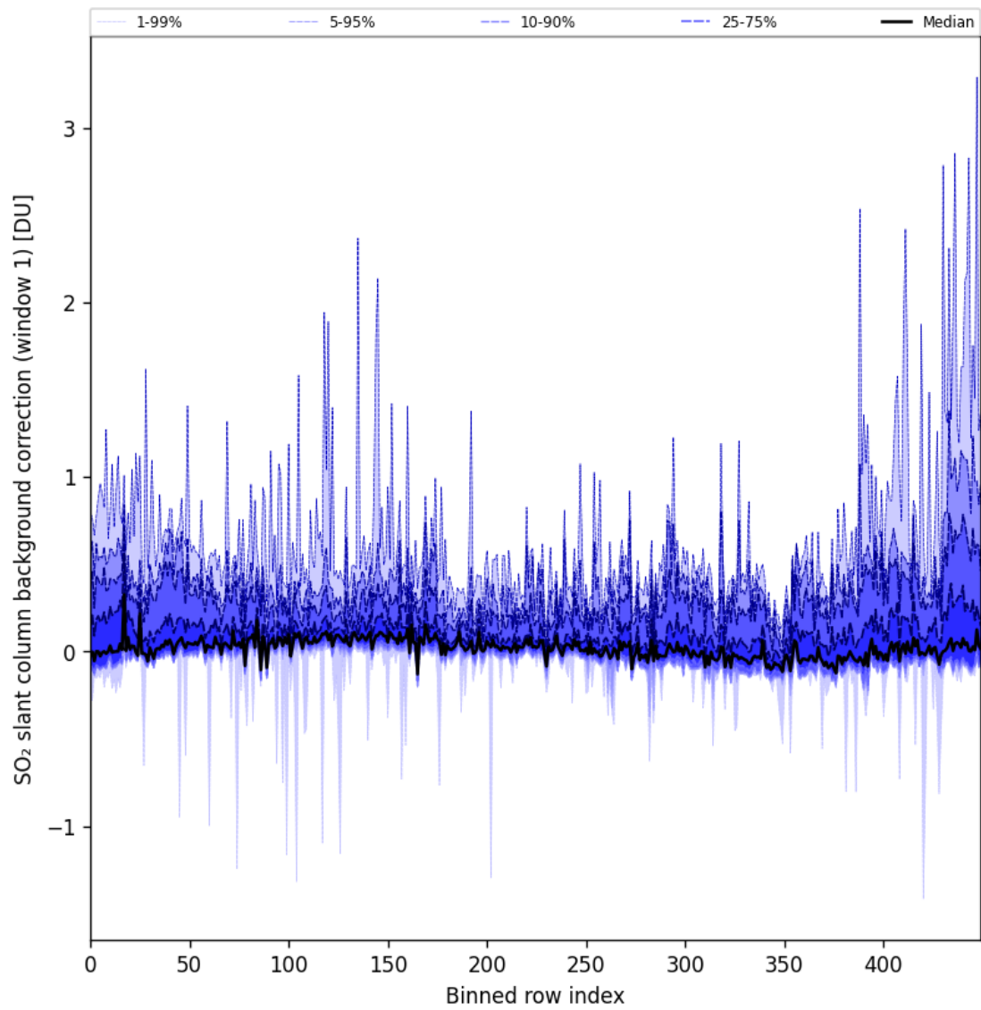
Figure 82: Along track statistics of “SO 2 slant column background correction (window 1)” for 2024-10-21 to 2024-10-23
