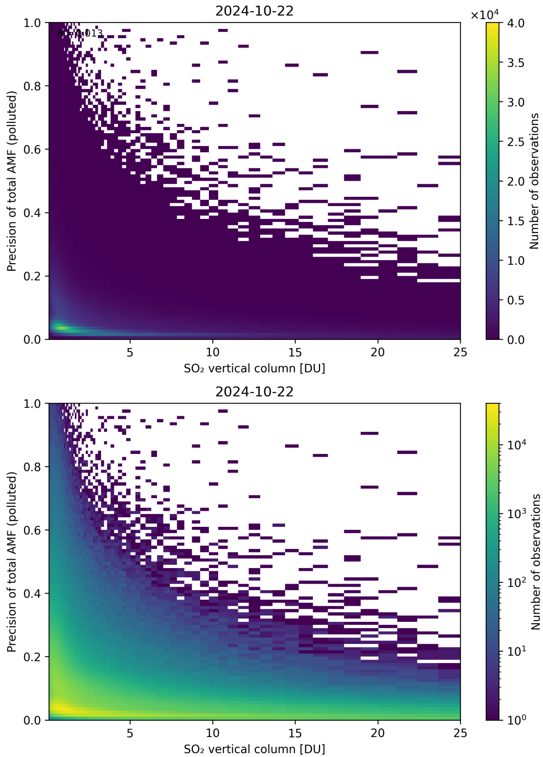
Figure 306: Scatter density plot of “SO 2 vertical column” against “Precision of total AMF (polluted)” for 2024-10-21 to 2024-10-23.
