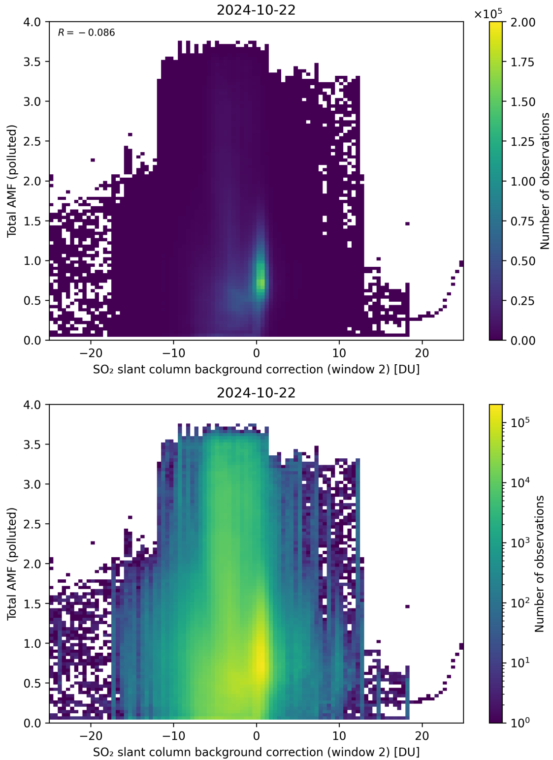
Figure 119: Scatter density plot of “SO 2 slant column background correction (window 2)” against “Total AMF (polluted)” for 2024-10-21 to 2024-10-23.
