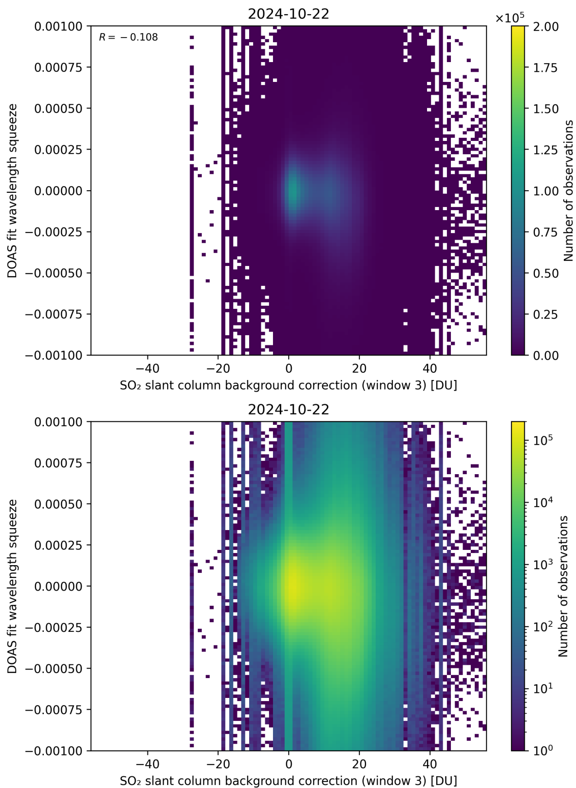
Figure 122: Scatter density plot of “SO 2 slant column background correction (window 3)” against “DOAS fit wavelength squeeze” for 2024-10-21 to 2024-10-23.
