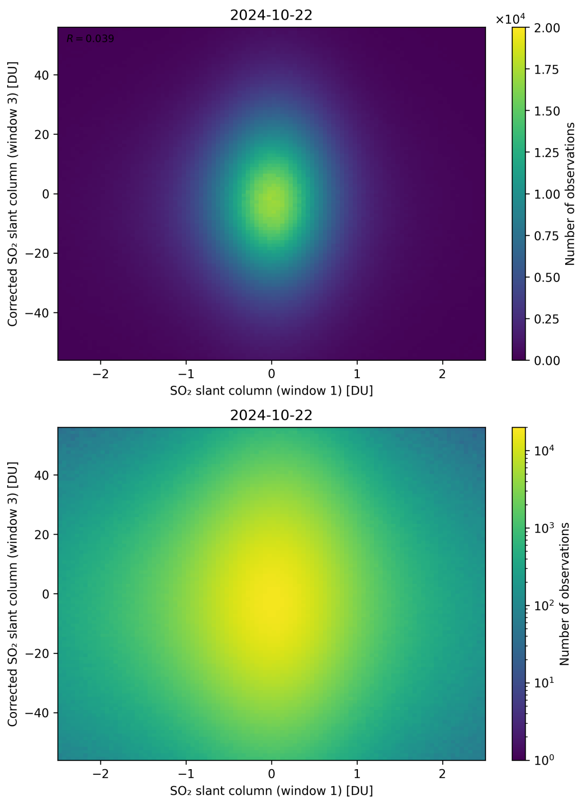
Figure 234: Scatter density plot of “SO 2 slant column (window 1)” against “Corrected SO 2 slant column (window 3)” for 2024-10-21 to 2024-10-23.
