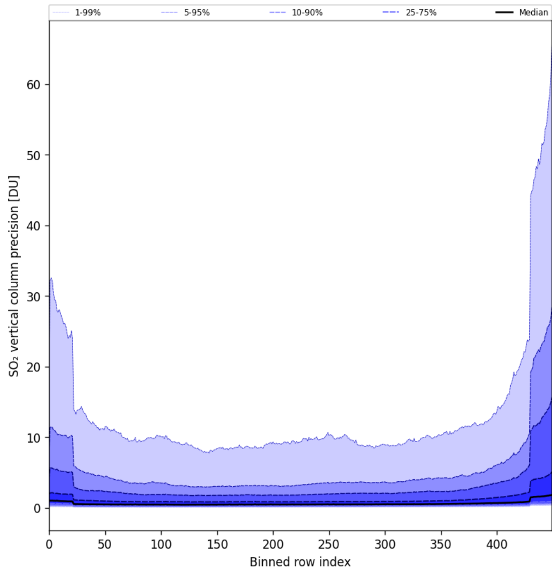
Figure 77: Along track statistics of “SO 2 vertical column precision” for 2024-10-21 to 2024-10-23
