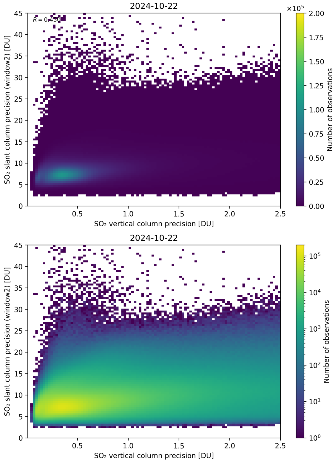
Figure 291: Scatter density plot of “SO 2 vertical column precision” against “SO 2 slant column precision (window2)” for 2024-10-21 to 2024-10-23.
