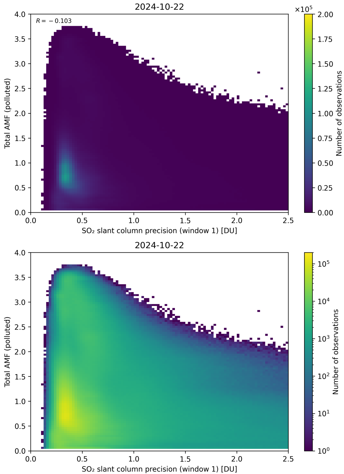
Figure 230: Scatter density plot of “SO 2 slant column precision (window 1)” against “Total AMF (polluted)” for 2024-10-21 to 2024-10-23.
