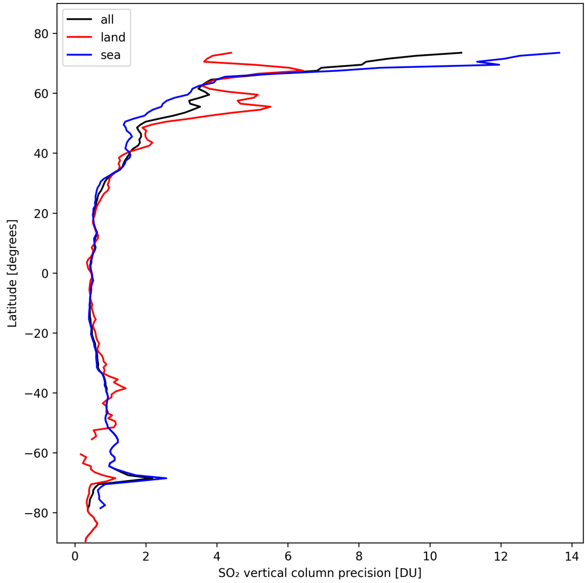
Figure 31: Zonal average of “SO 2 vertical column precision” for 2024-10-21 to 2024-10-23.
