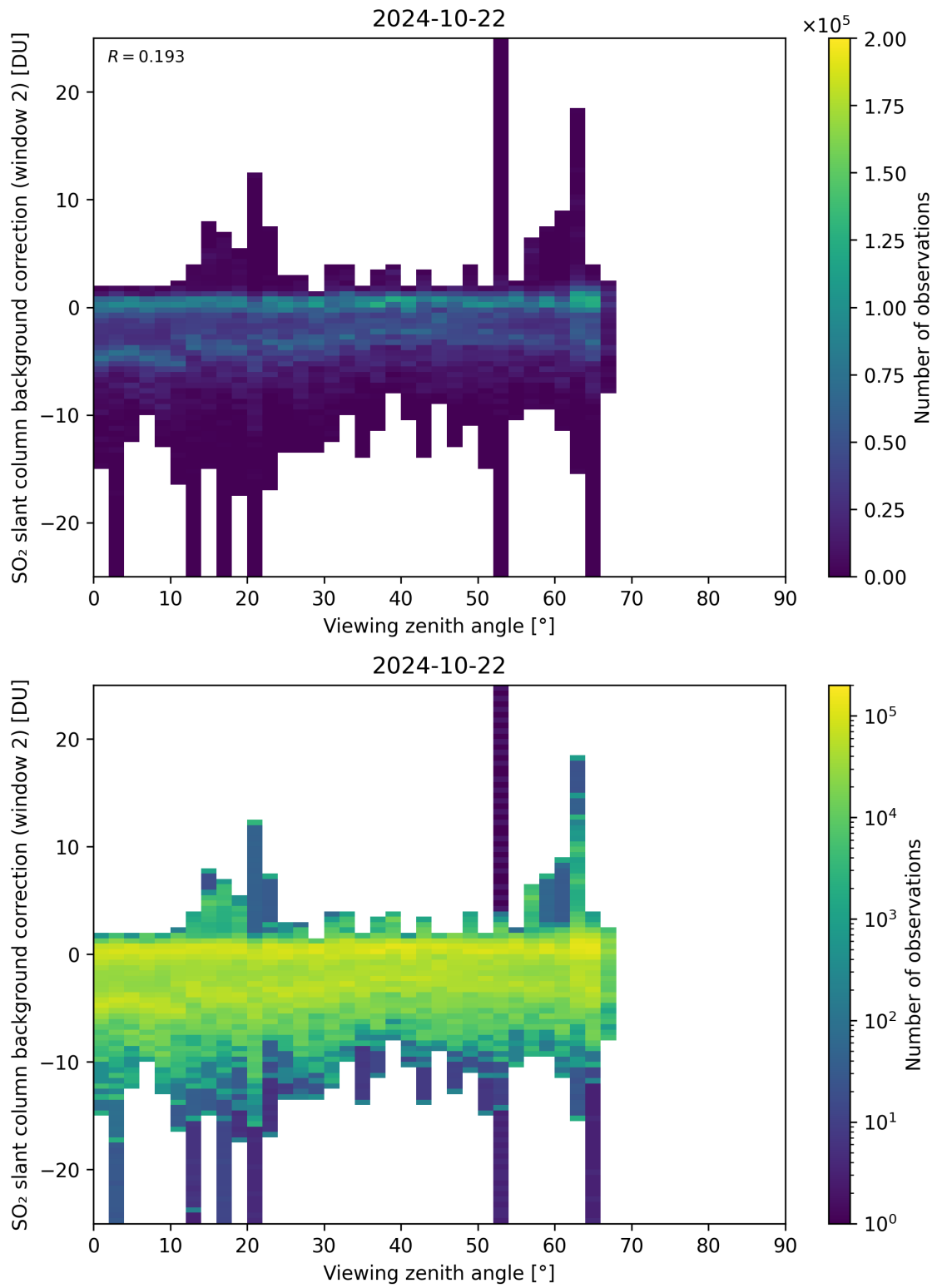
Figure 309: Scatter density plot of “Viewing zenith angle” against “SO 2 slant column background correction (window 2)” for 2024-10-21 to 2024-10-23.
