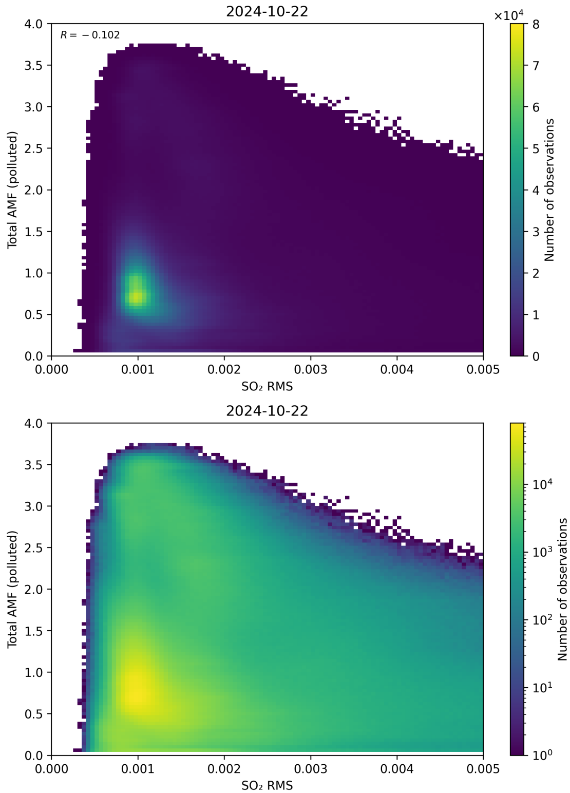
Figure 137: Scatter density plot of “SO 2 RMS” against “Total AMF (polluted)” for 2024-10-21 to 2024-10-23.
