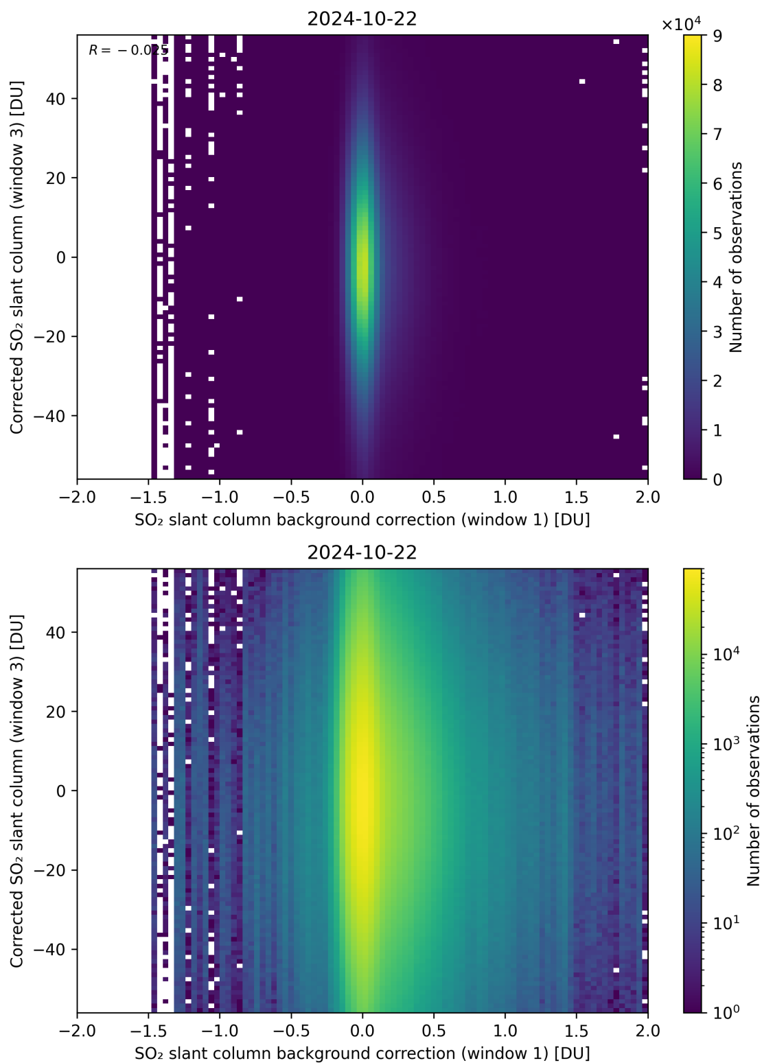
Figure 105: Scatter density plot of “SO 2 slant column background correction (window 1)” against “Corrected SO 2 slant column (window 3)” for 2024-10-21 to 2024-10-23.
