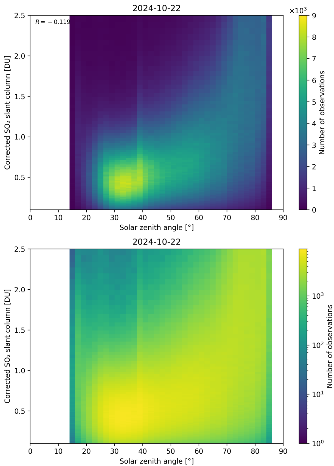
Figure 166: Scatter density plot of “Solar zenith angle” against “Corrected SO 2 slant column” for 2024-10-21 to 2024-10-23.
