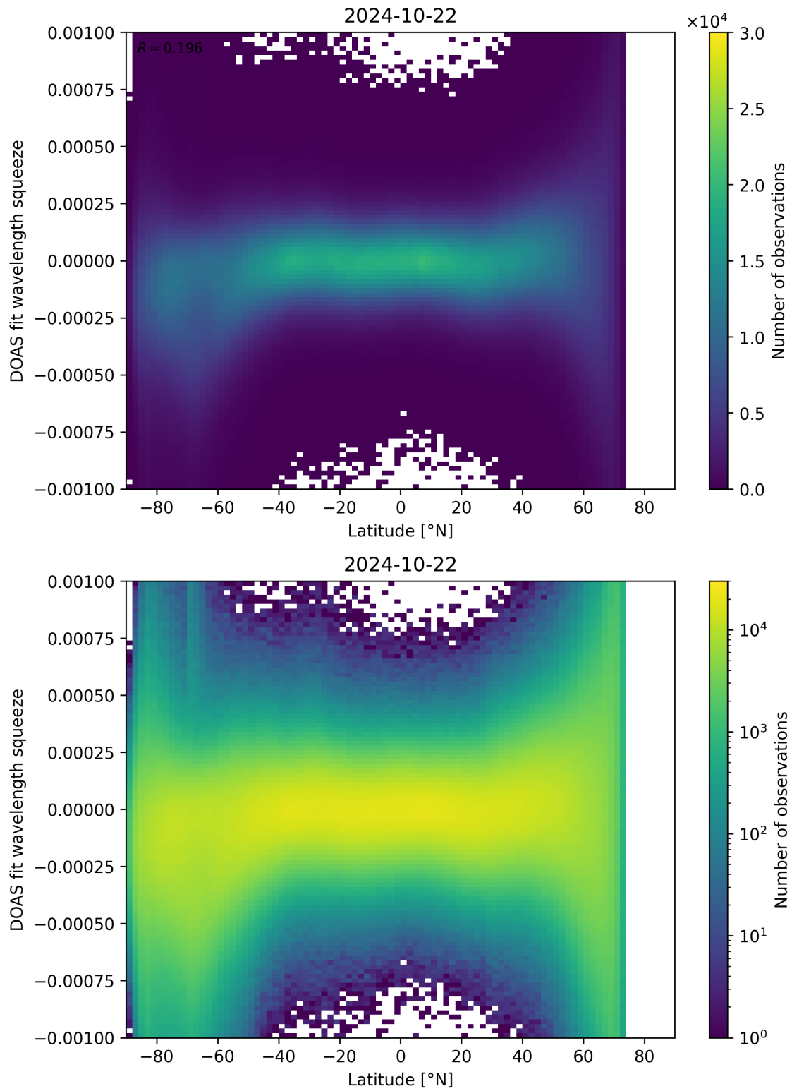
Figure 143: Scatter density plot of “Latitude” against “DOAS fit wavelength squeeze” for 2024-10-21 to 2024-10-23.
