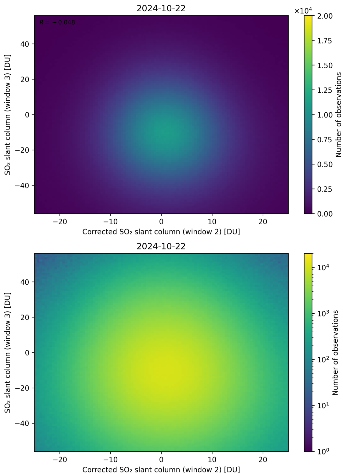
Figure 201: Scatter density plot of “Corrected SO 2 slant column (window 2)” against “SO 2 slant column (window 3)” for 2024-10-21 to 2024-10-23.
