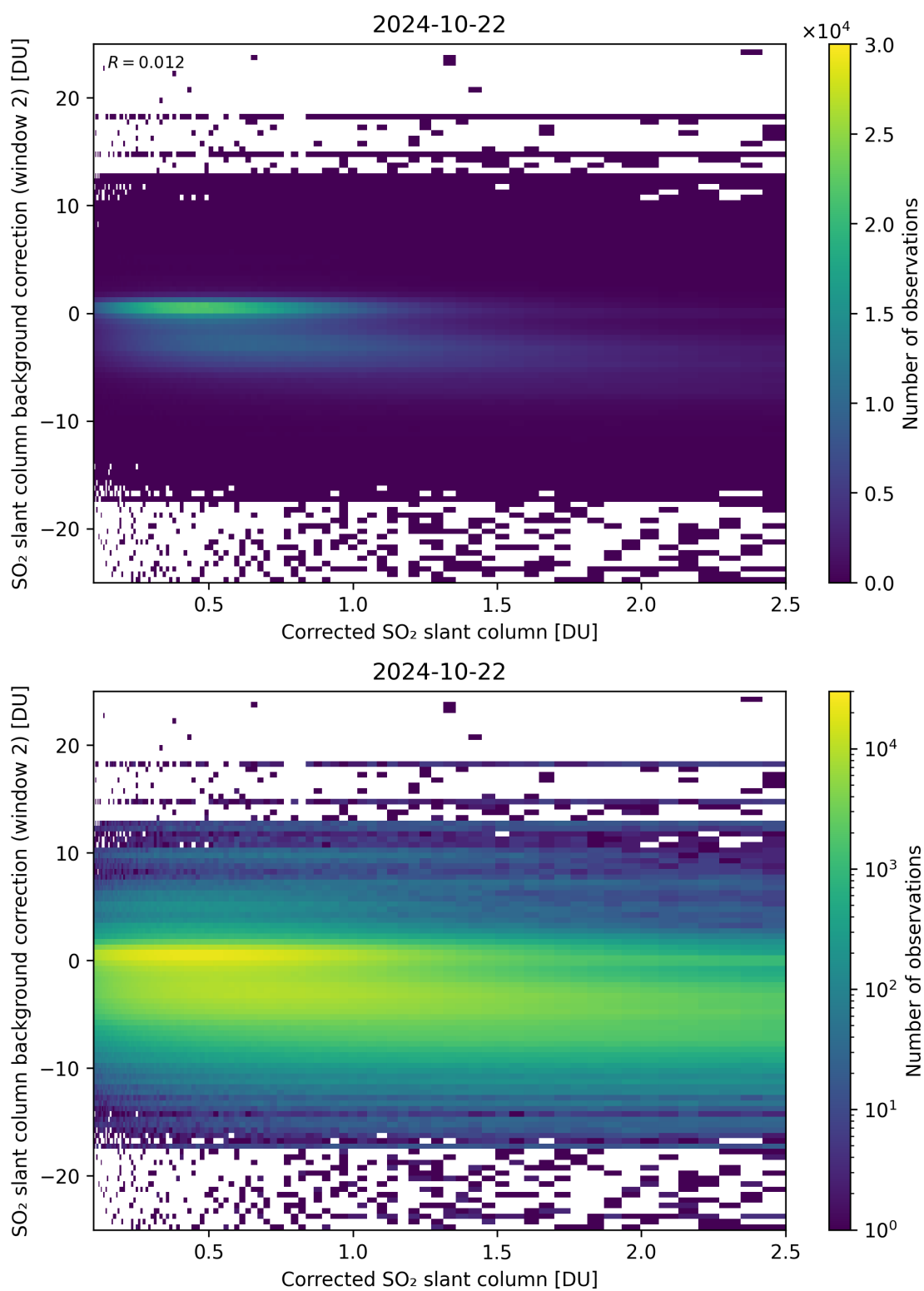
Figure 179: Scatter density plot of “Corrected SO 2 slant column” against “SO 2 slant column background correction (window 2)” for 2024-10-21 to 2024-10-23.
