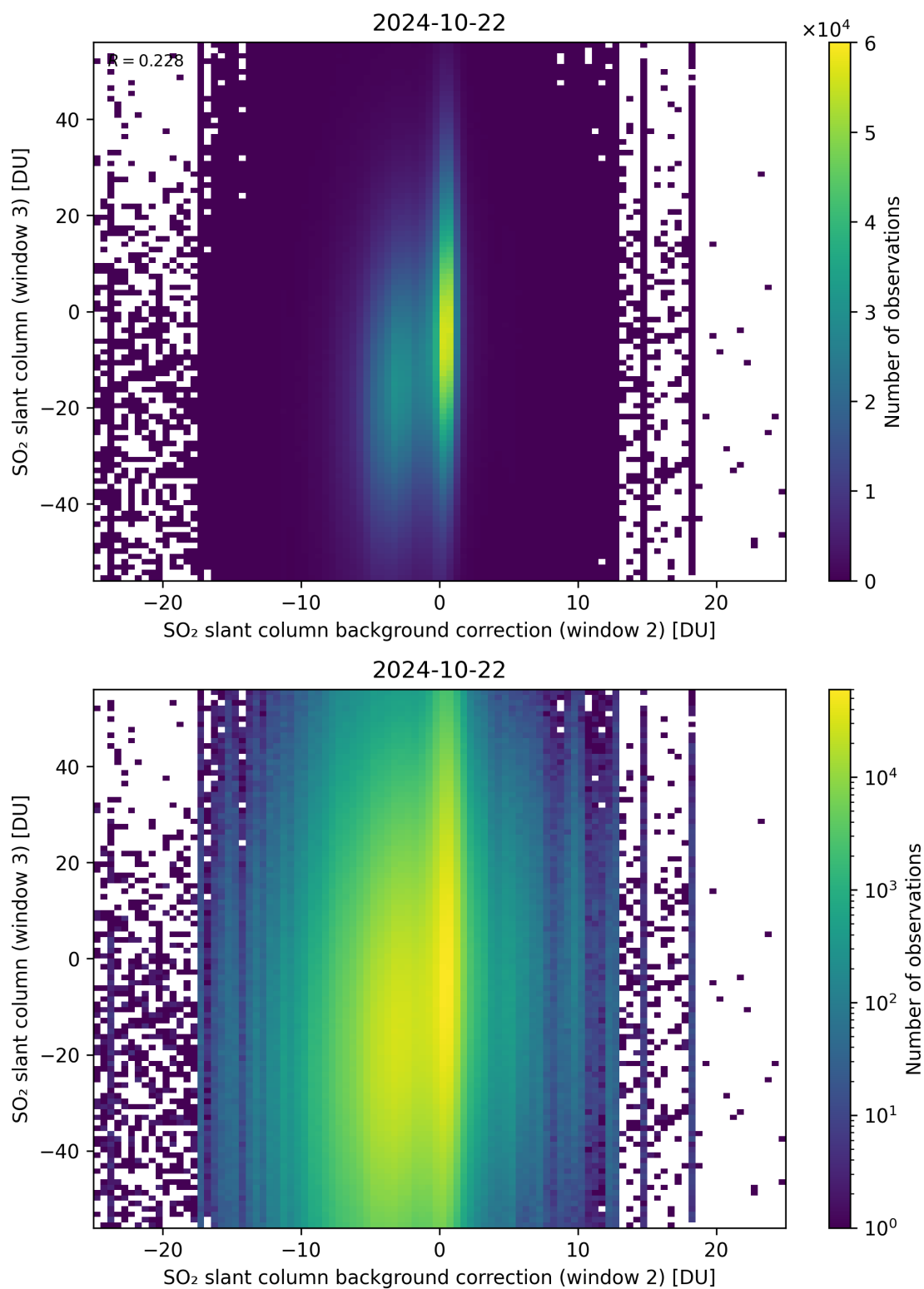
Figure 117: Scatter density plot of “SO 2 slant column background correction (window 2)” against “SO 2 slant column (window 3)” for 2024-10-21 to 2024-10-23.
