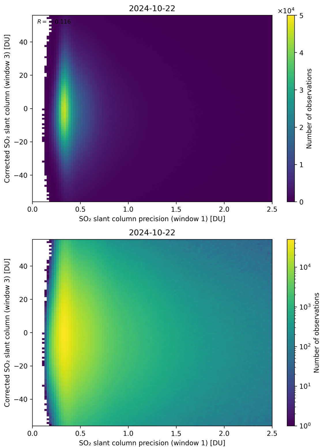
Figure 226: Scatter density plot of “SO 2 slant column precision (window 1)” against “Corrected SO 2 slant column (window 3)” for 2024-10-21 to 2024-10-23.
