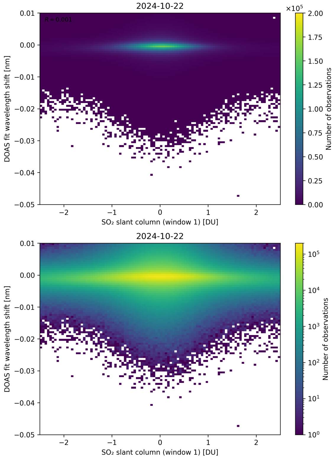
Figure 215: Scatter density plot of “SO 2 slant column (window 1)” against “DOAS fit wavelength shift” for 2024-10-21 to 2024-10-23.
