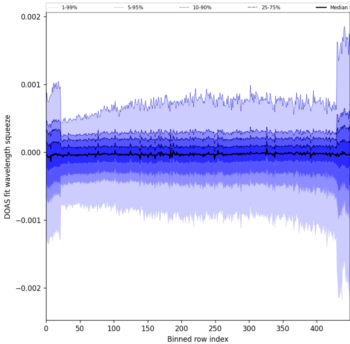
Figure 92: Along track statistics of “DOAS fit wavelength squeeze” for 2024-10-21 to 2024-10-23
