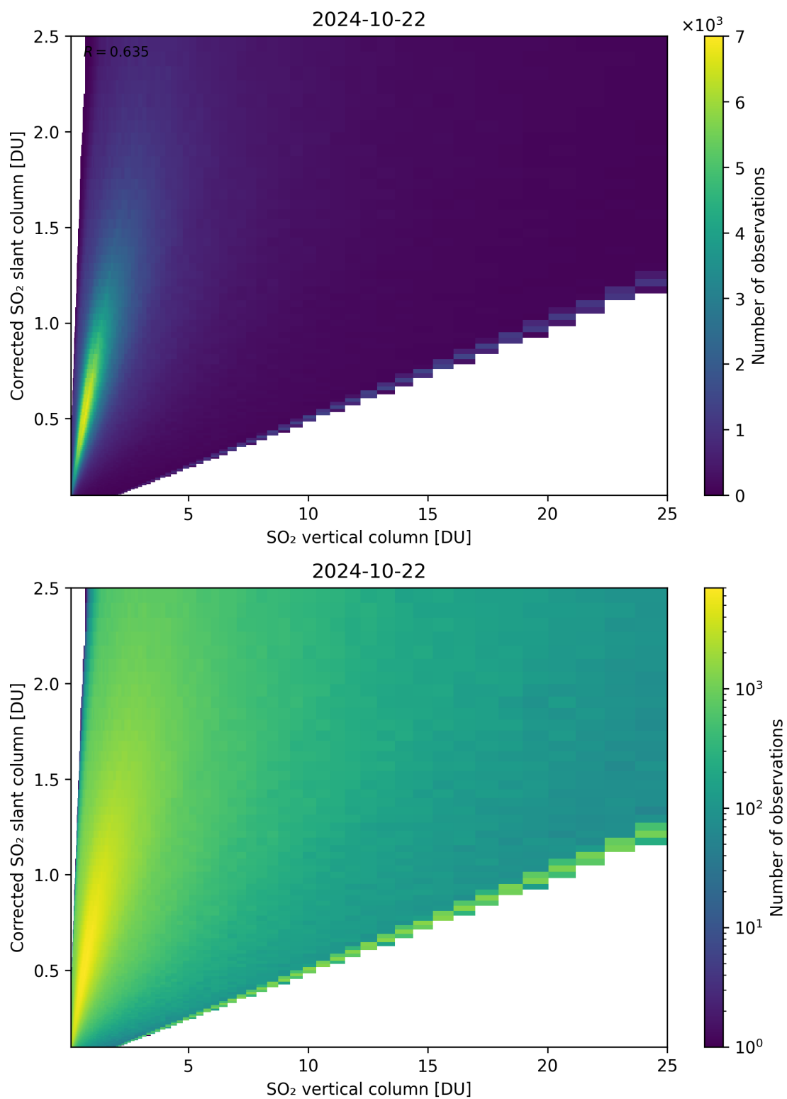
Figure 297: Scatter density plot of “SO 2 vertical column” against “Corrected SO 2 slant column” for 2024-10-21 to 2024-10-23.
