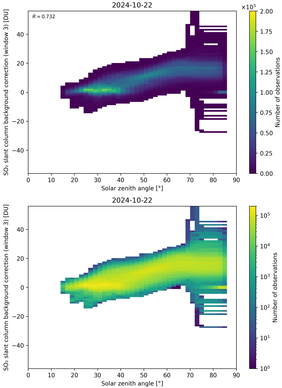
Figure 160: Scatter density plot of “Solar zenith angle” against “SO 2 slant column background correction (window 3)” for 2024-10-21 to 2024-10-23.
