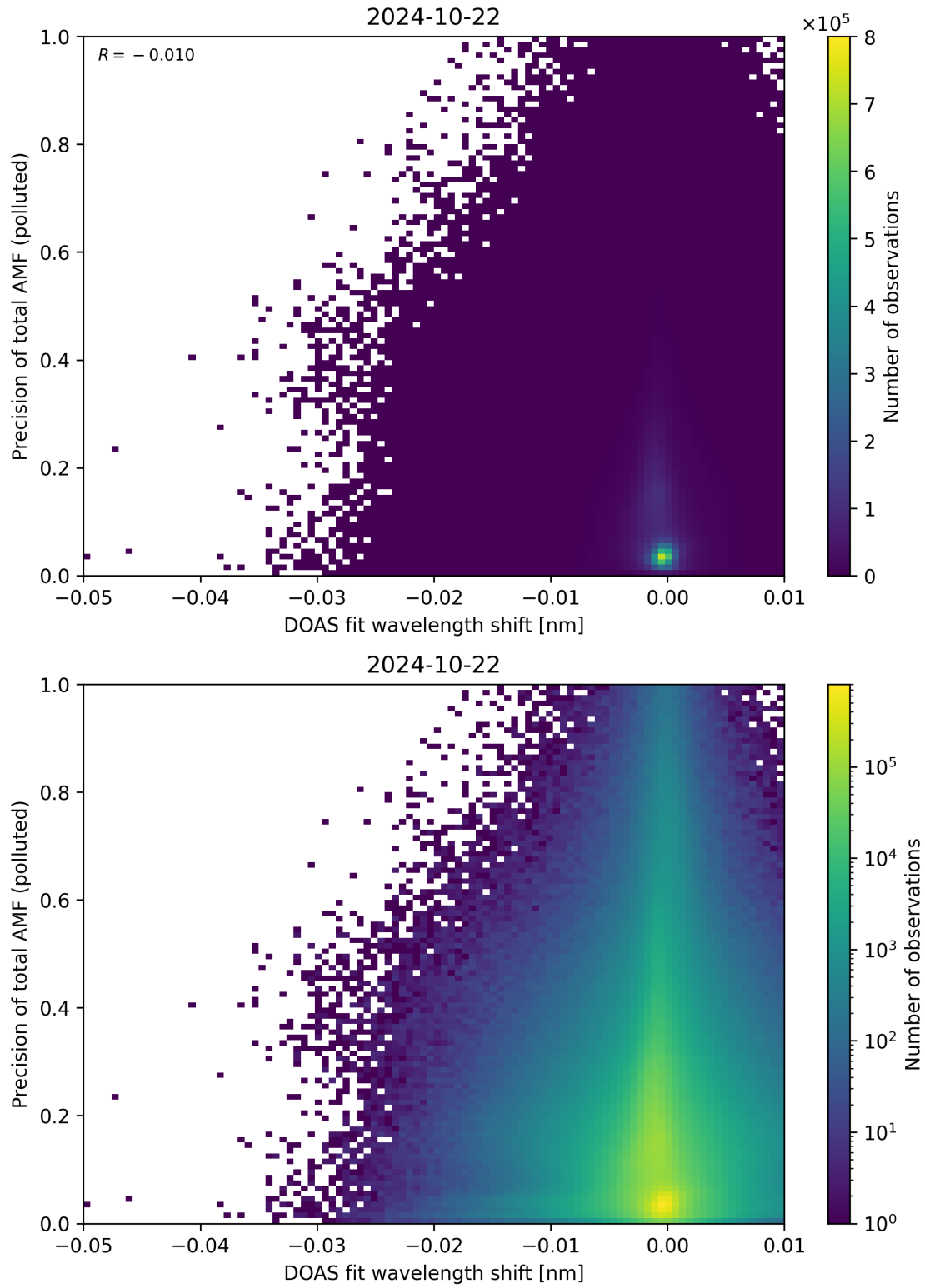
Figure 131: Scatter density plot of “DOAS fit wavelength shift” against “Precision of total AMF (polluted)” for 2024-10-21 to 2024-10-23.
