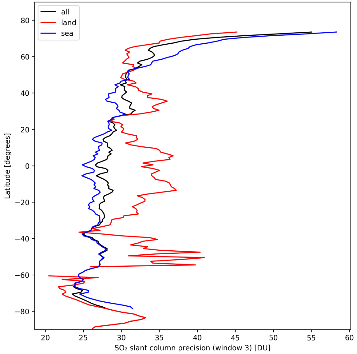
Figure 42: Zonal average of “SO 2 slant column precision (window 3)” for 2024-10-21 to 2024-10-23.
