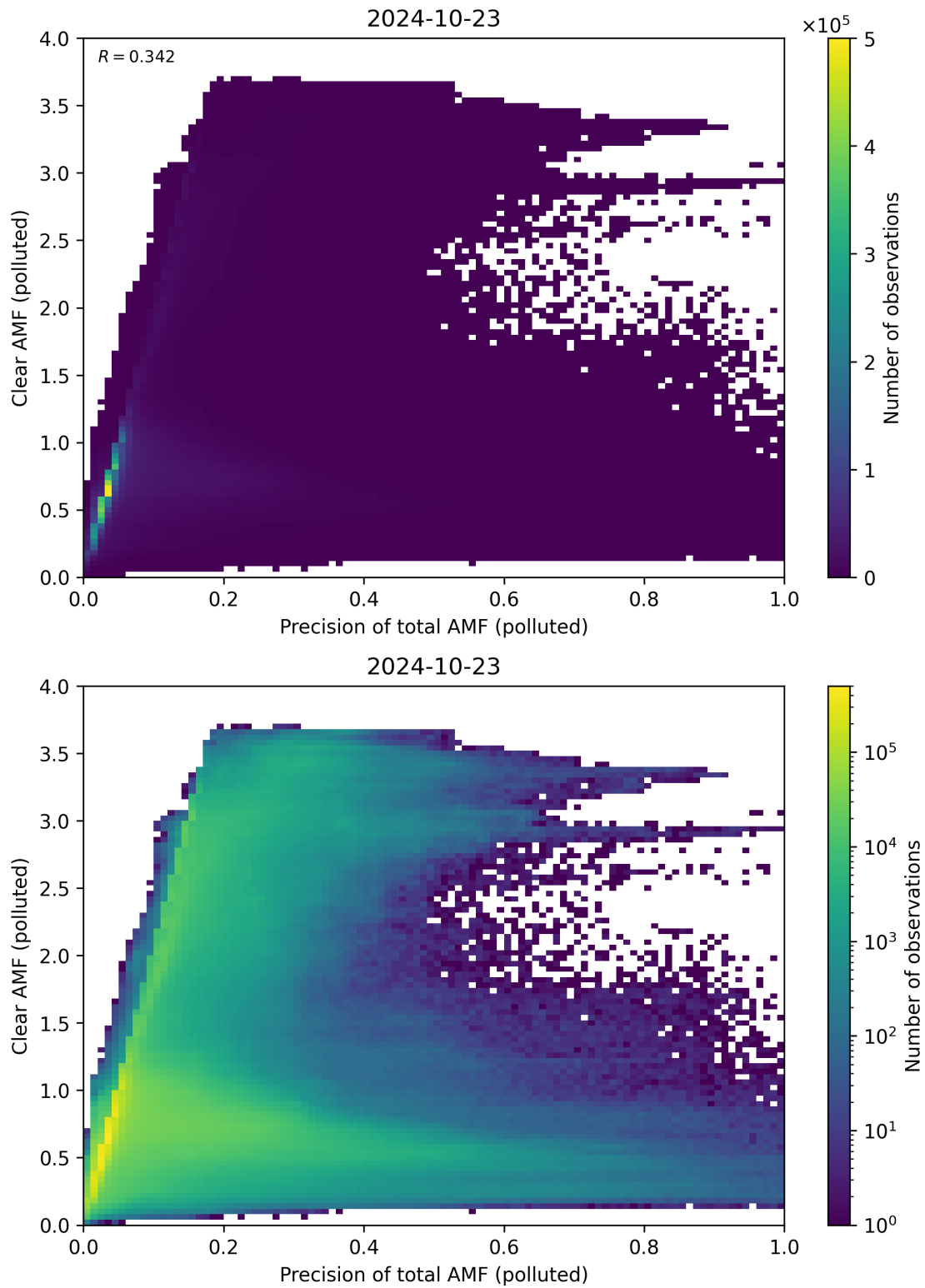
Figure 270: Scatter density plot of “Precision of total AMF (polluted)” against “Clear AMF (polluted)” for 2024-10-22 to 2024-10-24.
