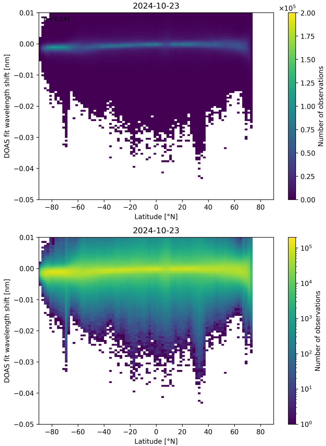
Figure 142: Scatter density plot of “Latitude” against “DOAS fit wavelength shift” for 2024-10-22 to 2024-10-24.
