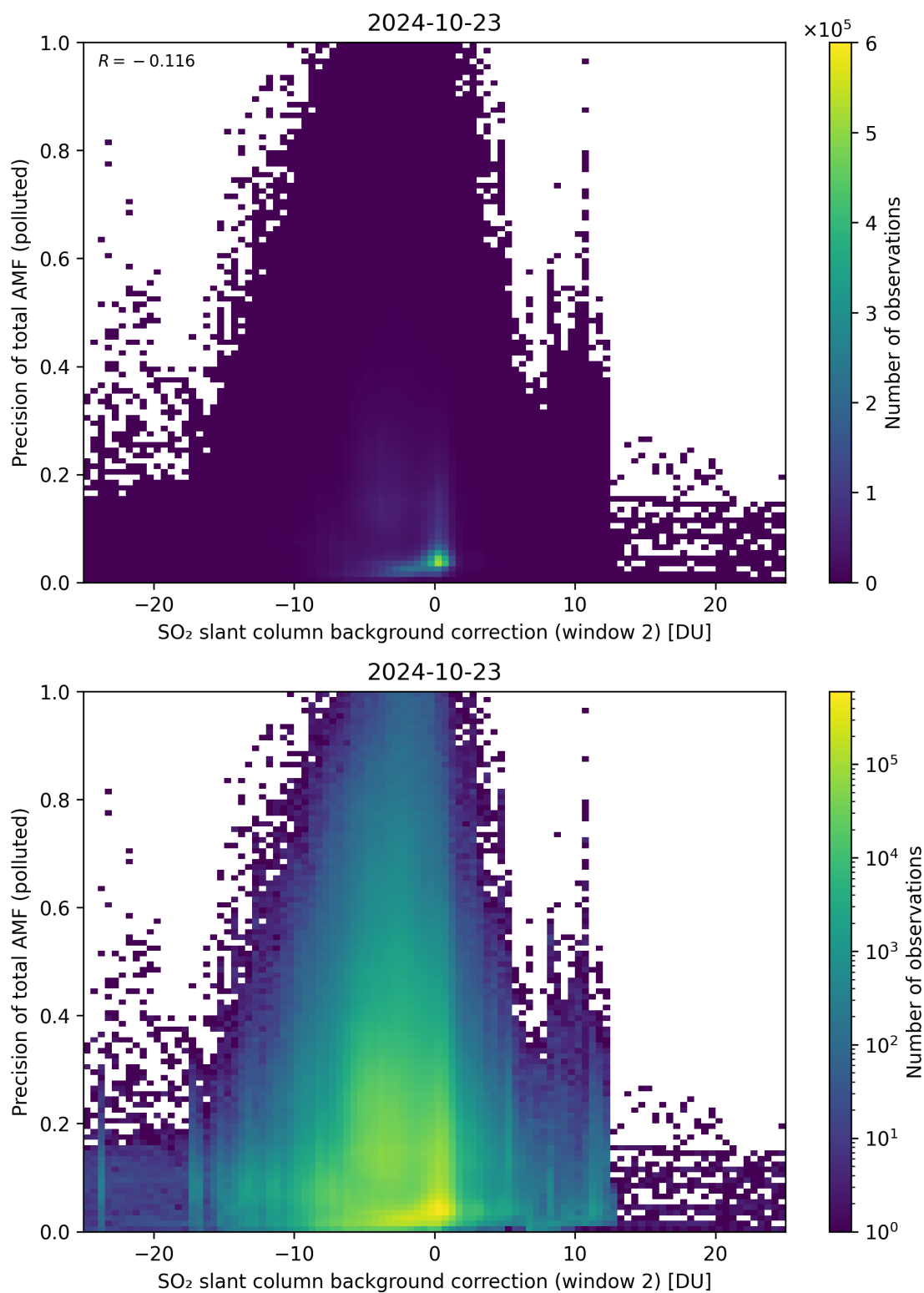
Figure 120: Scatter density plot of “SO 2 slant column background correction (window 2)” against “Precision of total AMF (polluted)” for 2024-10-22 to 2024-10-24.
