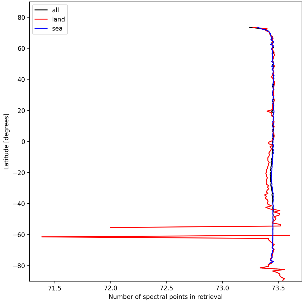
Figure 51: Zonal average of “Number of spectral points in retrieval” for 2024-10-22 to 2024-10-24.
