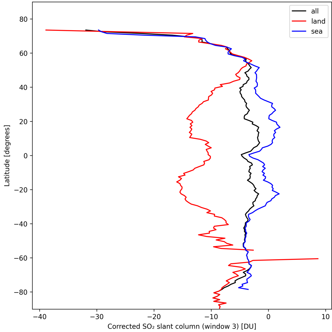
Figure 43: Zonal average of “Corrected SO 2 slant column (window 3)” for 2024-10-22 to 2024-10-24.
