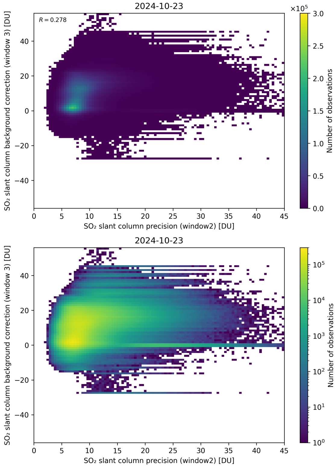
Figure 242: Scatter density plot of “SO 2 slant column precision (window2)” against “SO 2 slant column background correction (window 3)” for 2024-10-22 to 2024-10-24.
