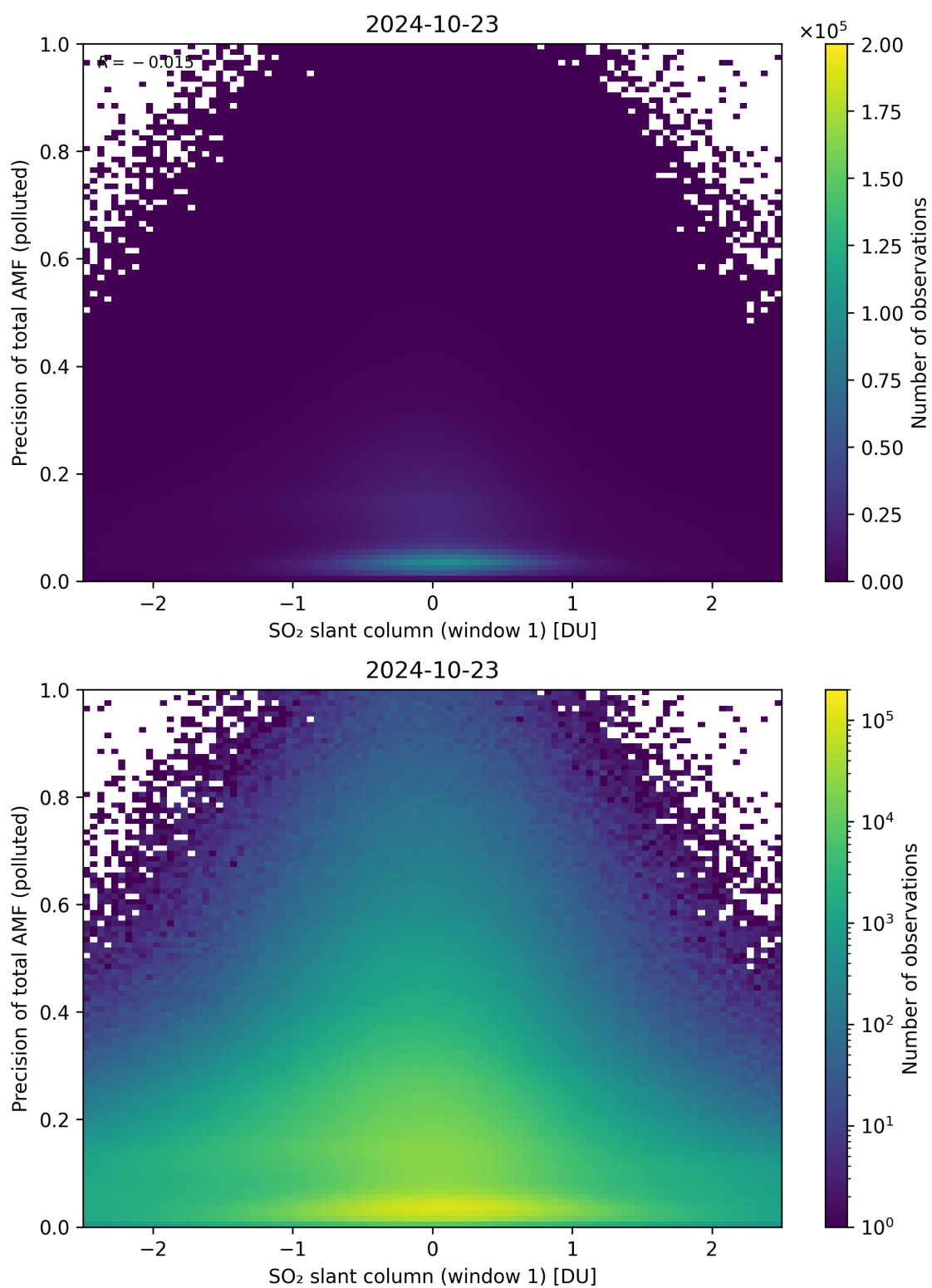
Figure 240: Scatter density plot of “SO 2 slant column (window 1)” against “Precision of total AMF (polluted)” for 2024-10-22 to 2024-10-24.
