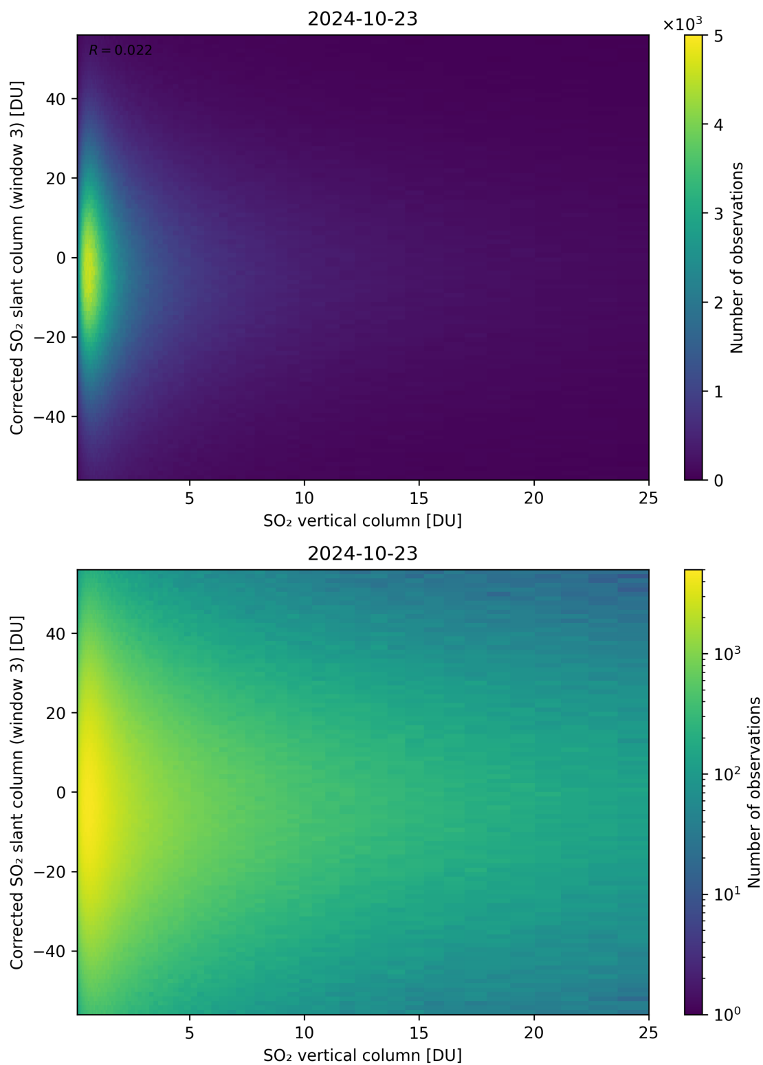
Figure 299: Scatter density plot of “SO 2 vertical column” against “Corrected SO 2 slant column (window 3)” for 2024-10-22 to 2024-10-24.
