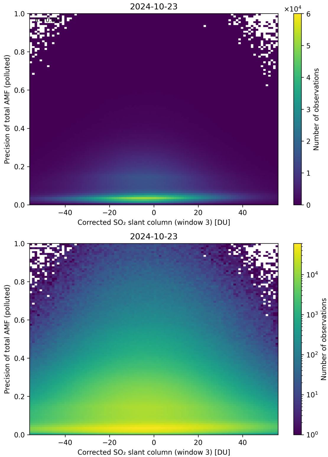
Figure 211: Scatter density plot of “Corrected SO 2 slant column (window 3)” against “Precision of total AMF (polluted)” for 2024-10-22 to 2024-10-24.
