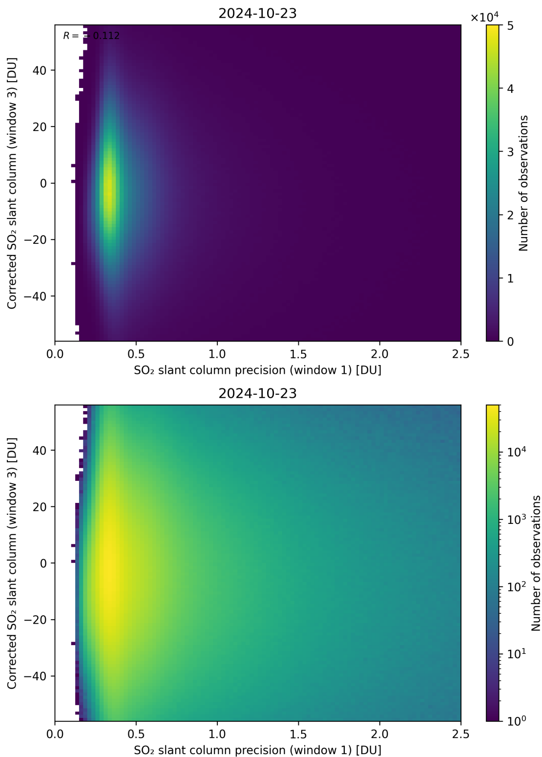
Figure 226: Scatter density plot of “SO 2 slant column precision (window 1)” against “Corrected SO 2 slant column (window 3)” for 2024-10-22 to 2024-10-24.
