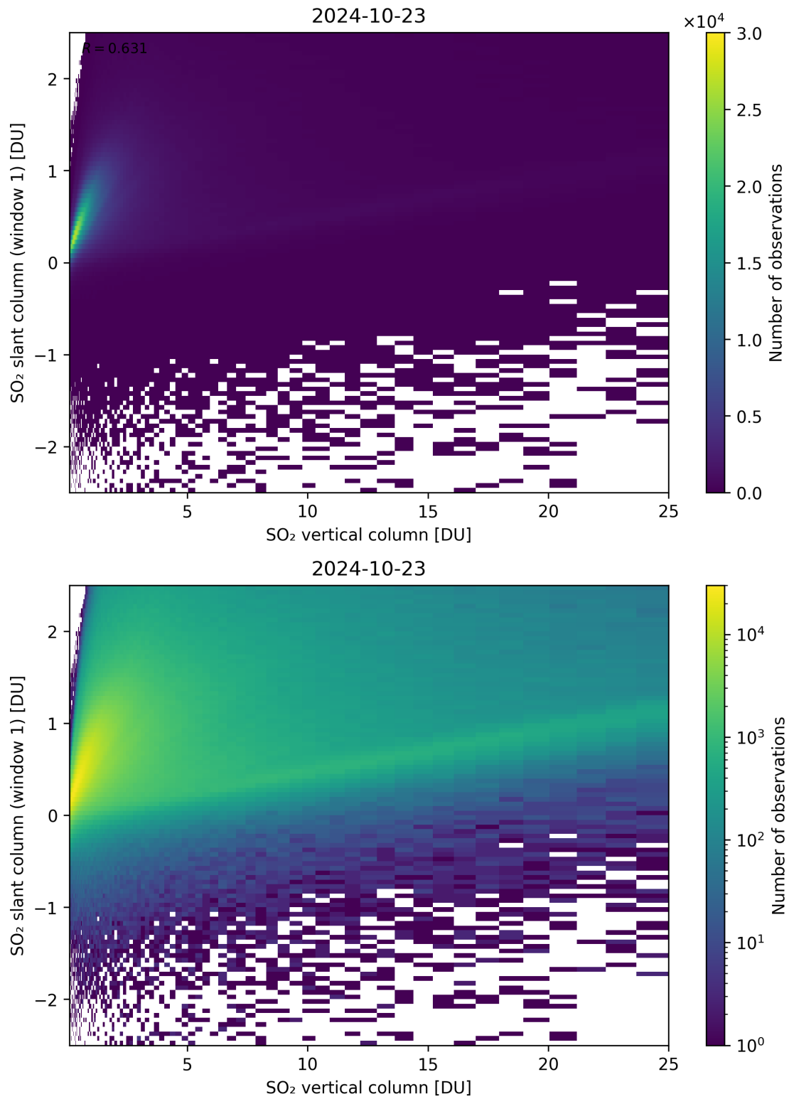
Figure 300: Scatter density plot of “SO 2 vertical column” against “SO 2 slant column (window 1)” for 2024-10-22 to 2024-10-24.
