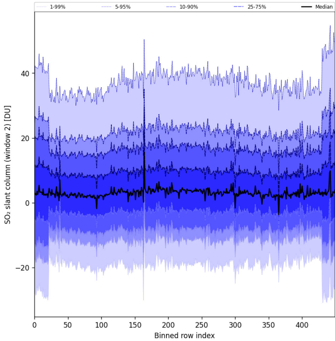
Figure 83: Along track statistics of “SO 2 slant column (window 2)” for 2024-10-22 to 2024-10-24
