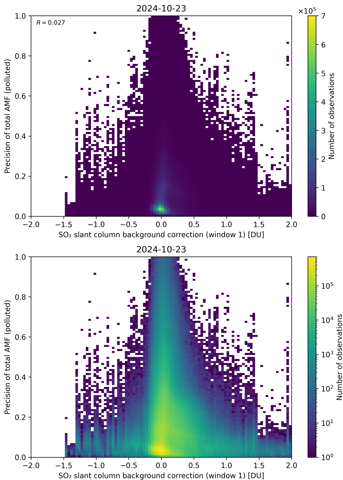
Figure 110: Scatter density plot of “SO 2 slant column background correction (window 1)” against “Precision of total AMF (polluted)” for 2024-10-22 to 2024-10-24.
