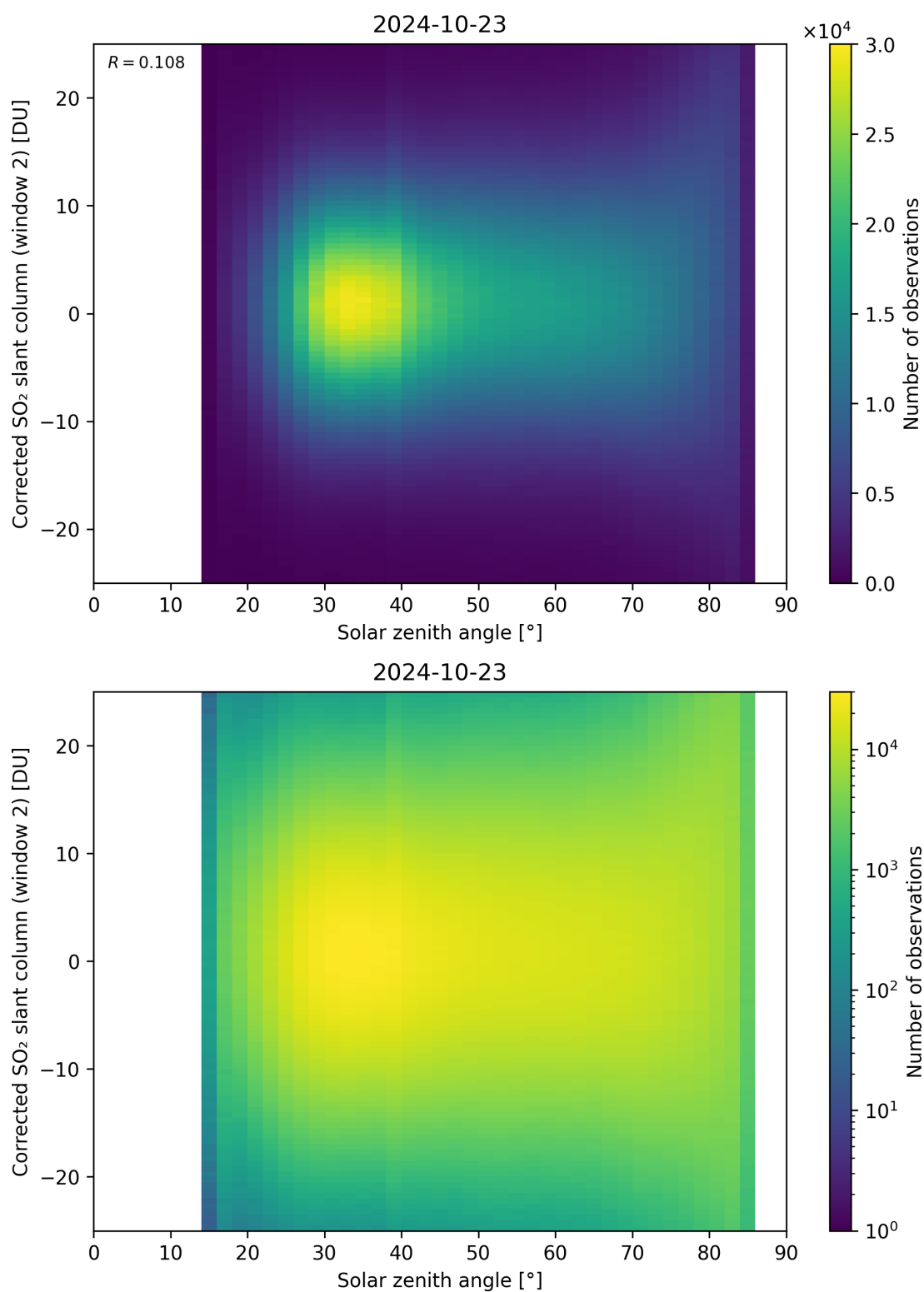
Figure 167: Scatter density plot of “Solar zenith angle” against “Corrected SO 2 slant column (window 2)” for 2024-10-22 to 2024-10-24.
