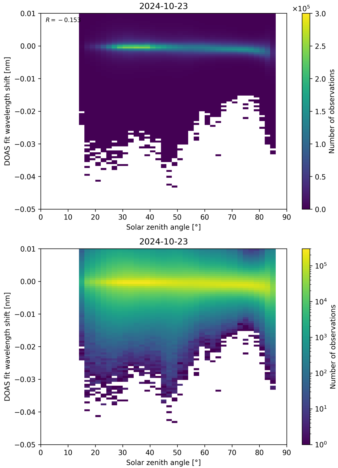
Figure 161: Scatter density plot of “Solar zenith angle” against “DOAS fit wavelength shift” for 2024-10-22 to 2024-10-24.
