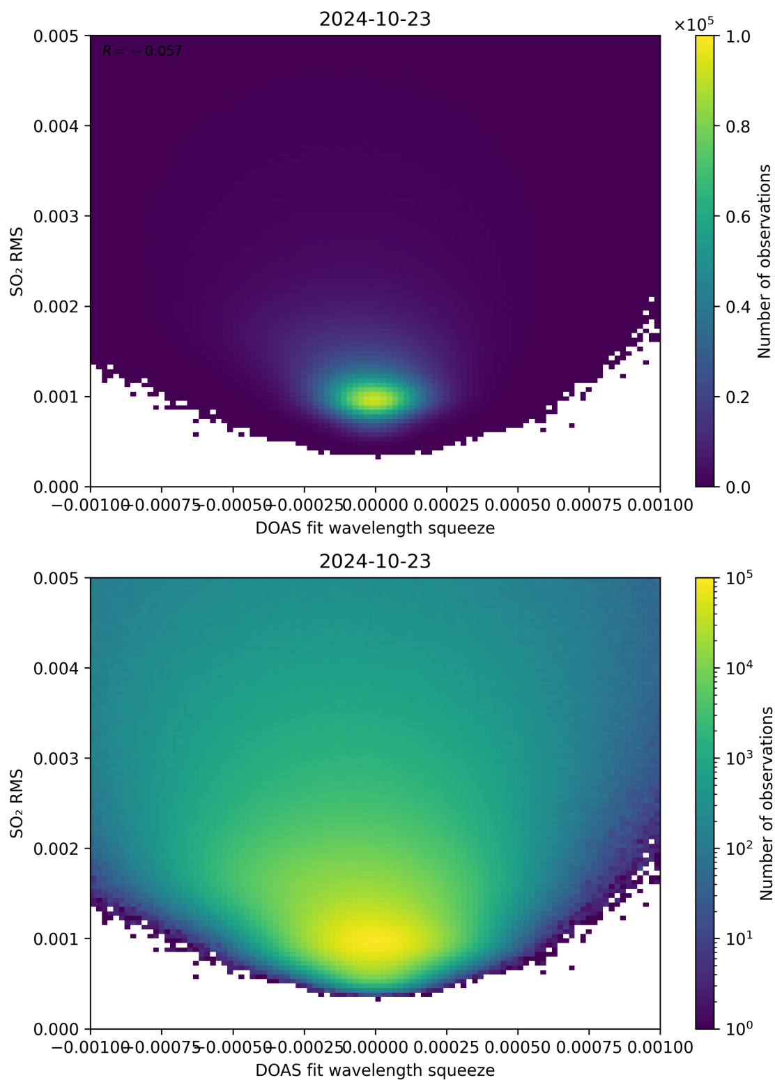
Figure 132: Scatter density plot of “DOAS fit wavelength squeeze” against “SO 2 RMS” for 2024-10-22 to 2024-10-24.
