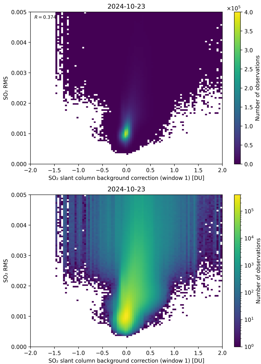
Figure 102: Scatter density plot of “SO 2 slant column background correction (window 1)” against “SO 2 RMS” for 2024-10-22 to 2024-10-24.
