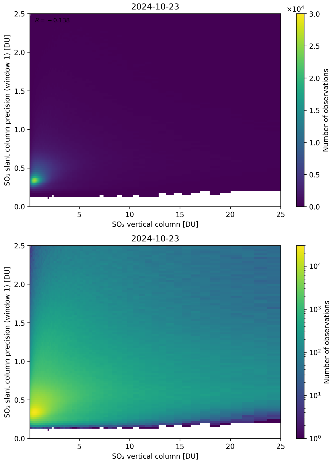
Figure 301: Scatter density plot of “SO 2 vertical column” against “SO 2 slant column precision (window 1)” for 2024-10-22 to 2024-10-24.
