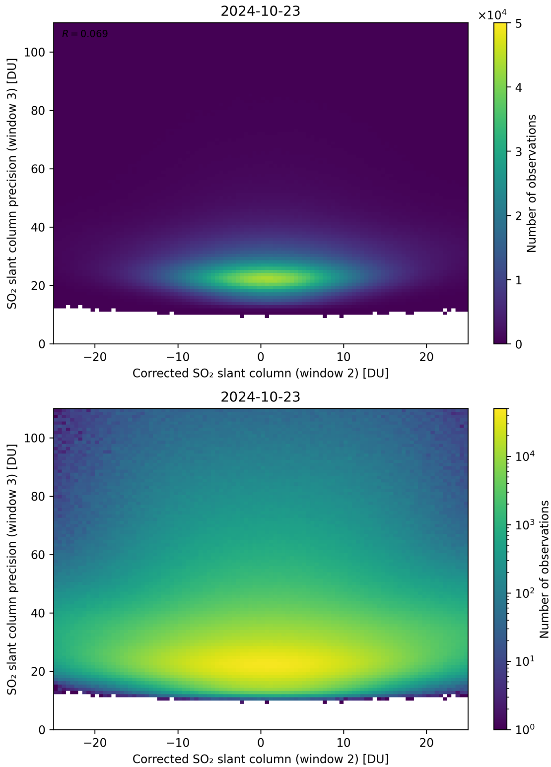
Figure 202: Scatter density plot of “Corrected SO 2 slant column (window 2)” against “SO 2 slant column precision (window 3)” for 2024-10-22 to 2024-10-24.
