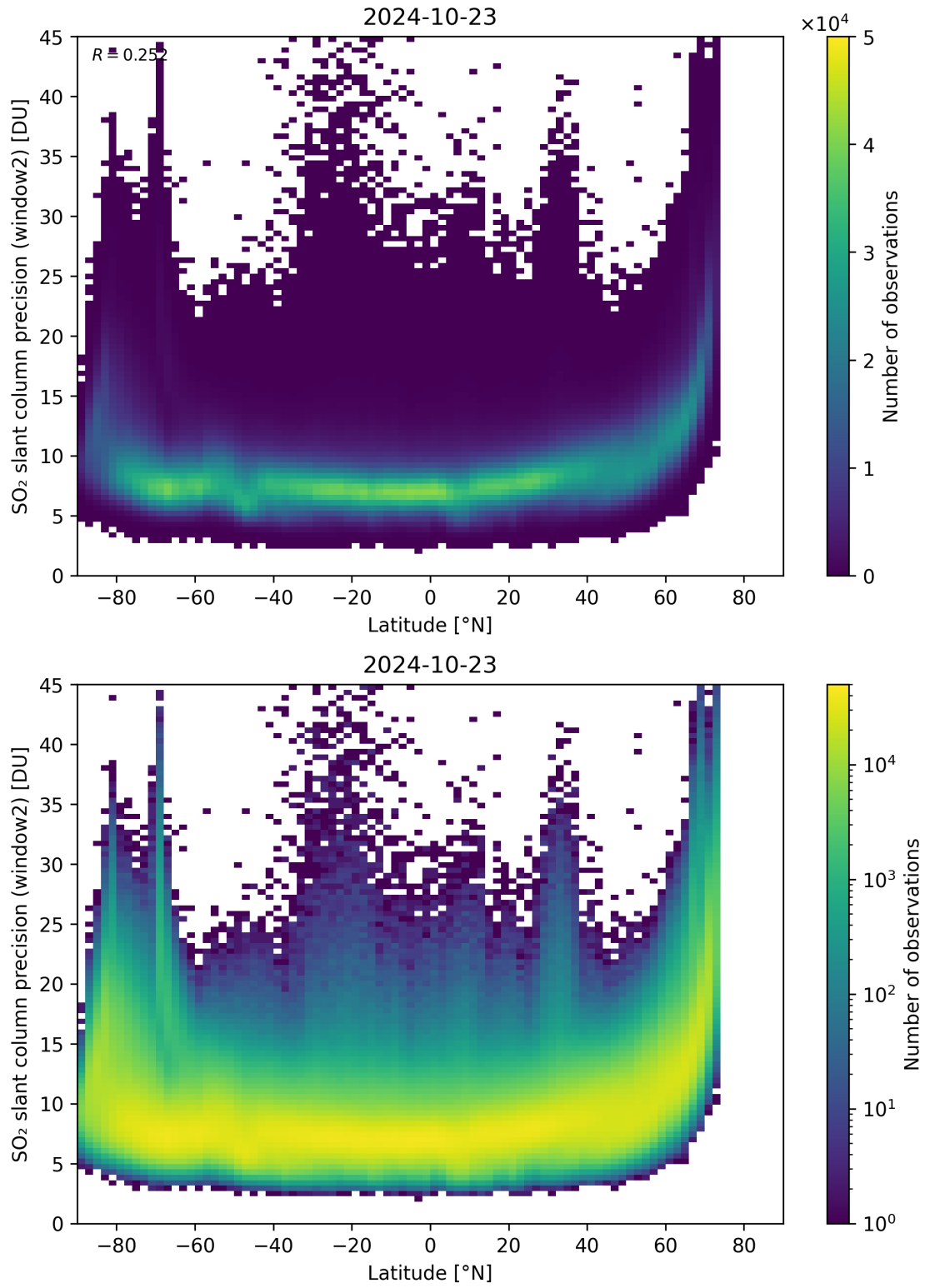
Figure 151: Scatter density plot of “Latitude” against “SO 2 slant column precision (window2)” for 2024-10-22 to 2024-10-24.
