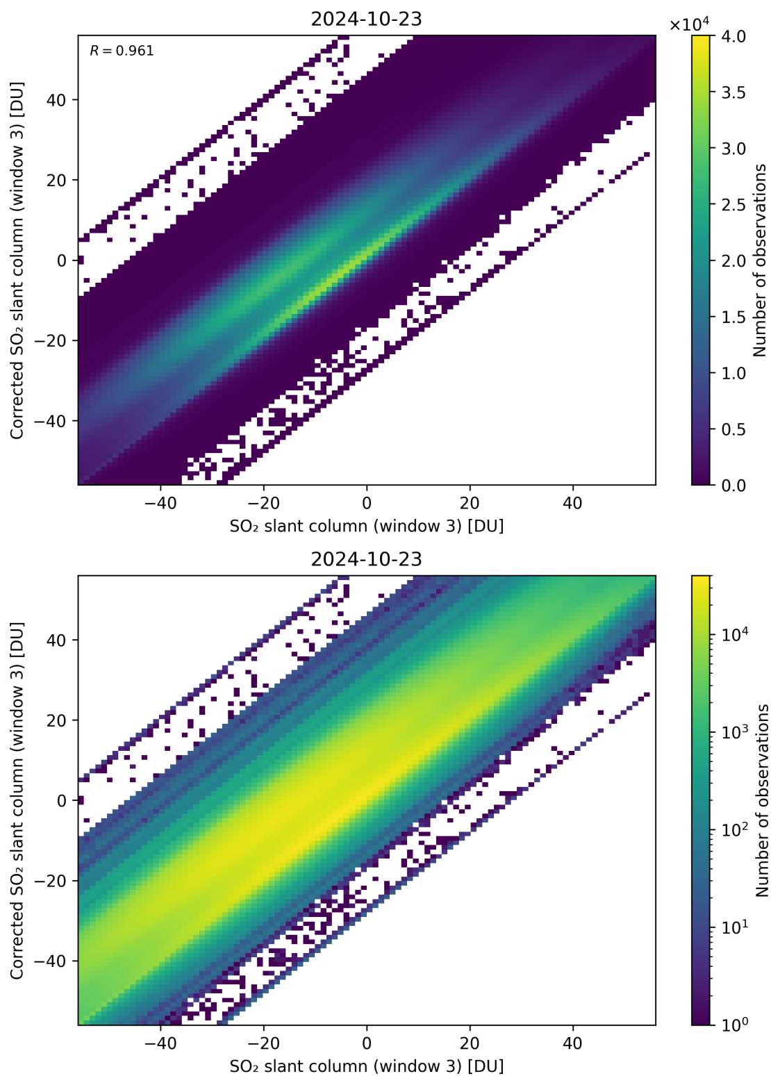
Figure 266: Scatter density plot of “SO 2 slant column (window 3)” against “Corrected SO 2 slant column (window 3)” for 2024-10-22 to 2024-10-24.
