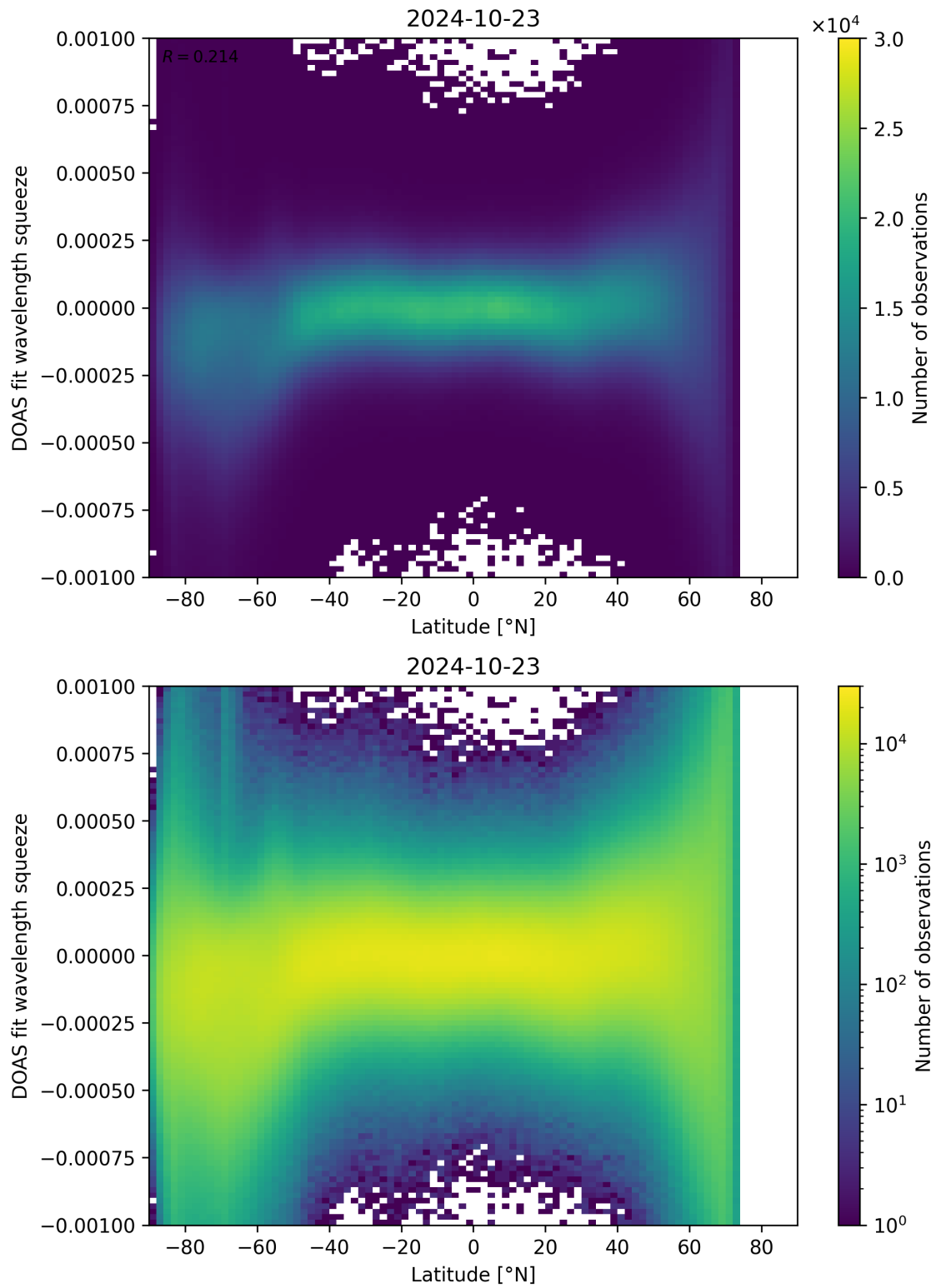
Figure 143: Scatter density plot of “Latitude” against “DOAS fit wavelength squeeze” for 2024-10-22 to 2024-10-24.
