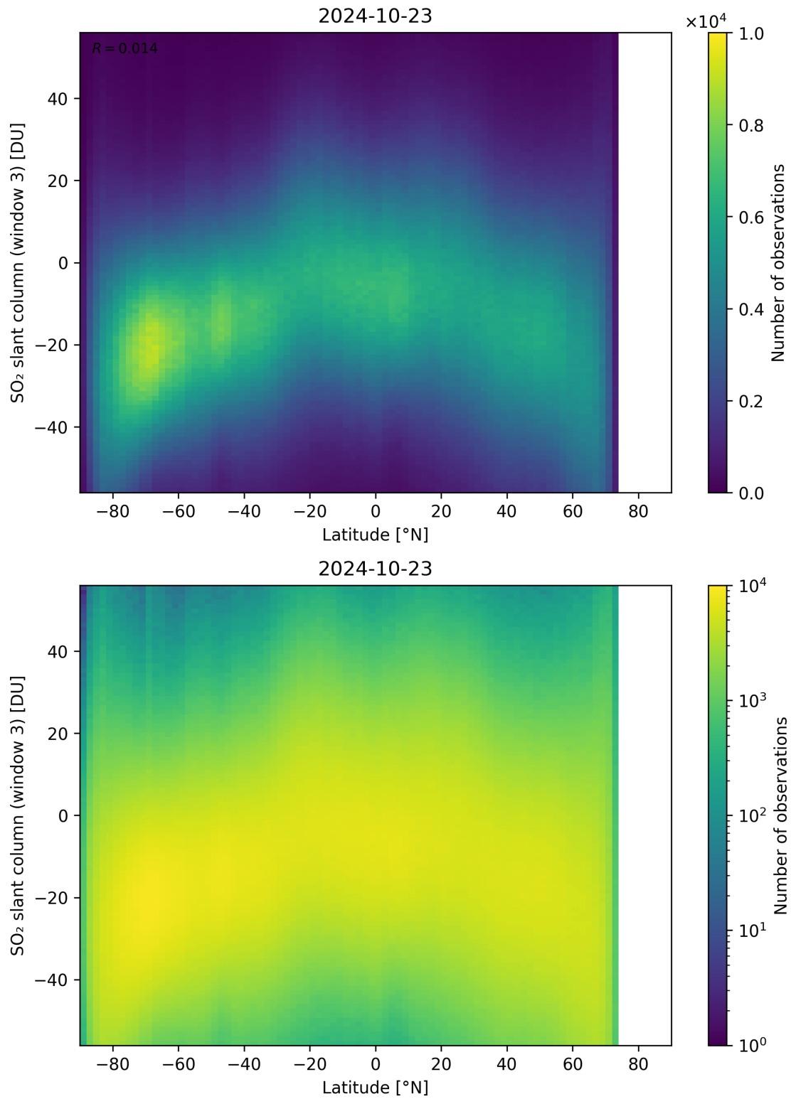
Figure 152: Scatter density plot of “Latitude” against “SO 2 slant column (window 3)” for 2024-10-22 to 2024-10-24.
