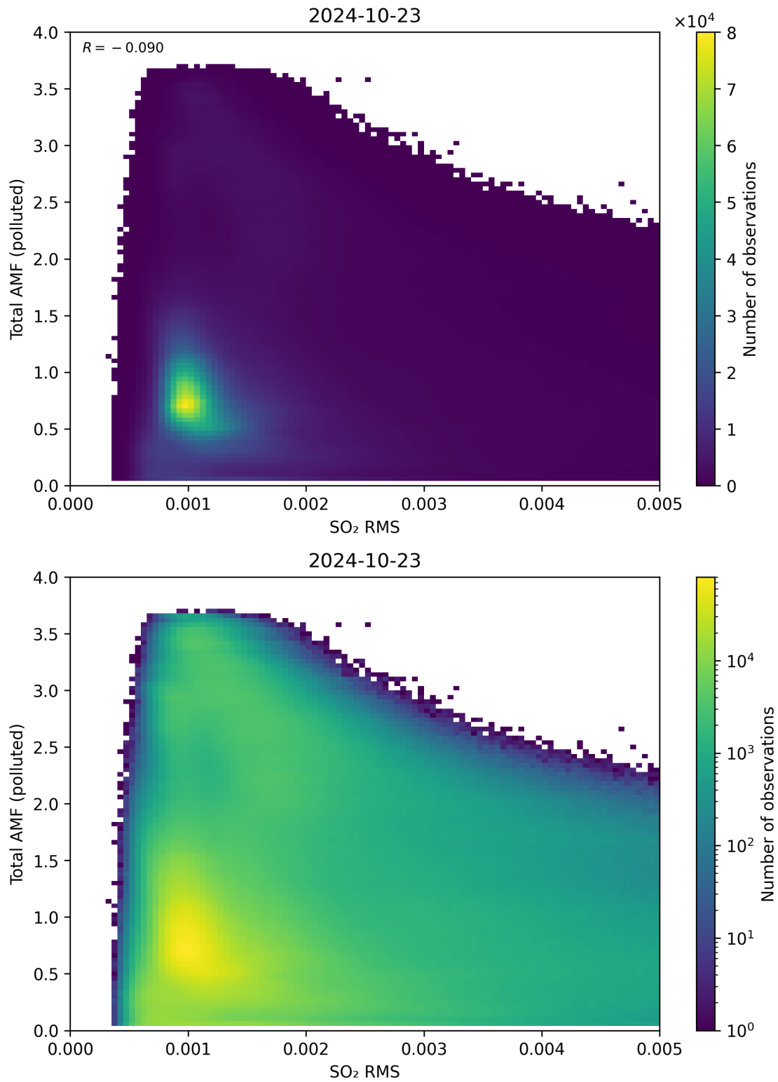
Figure 137: Scatter density plot of “SO 2 RMS” against “Total AMF (polluted)” for 2024-10-22 to 2024-10-24.
