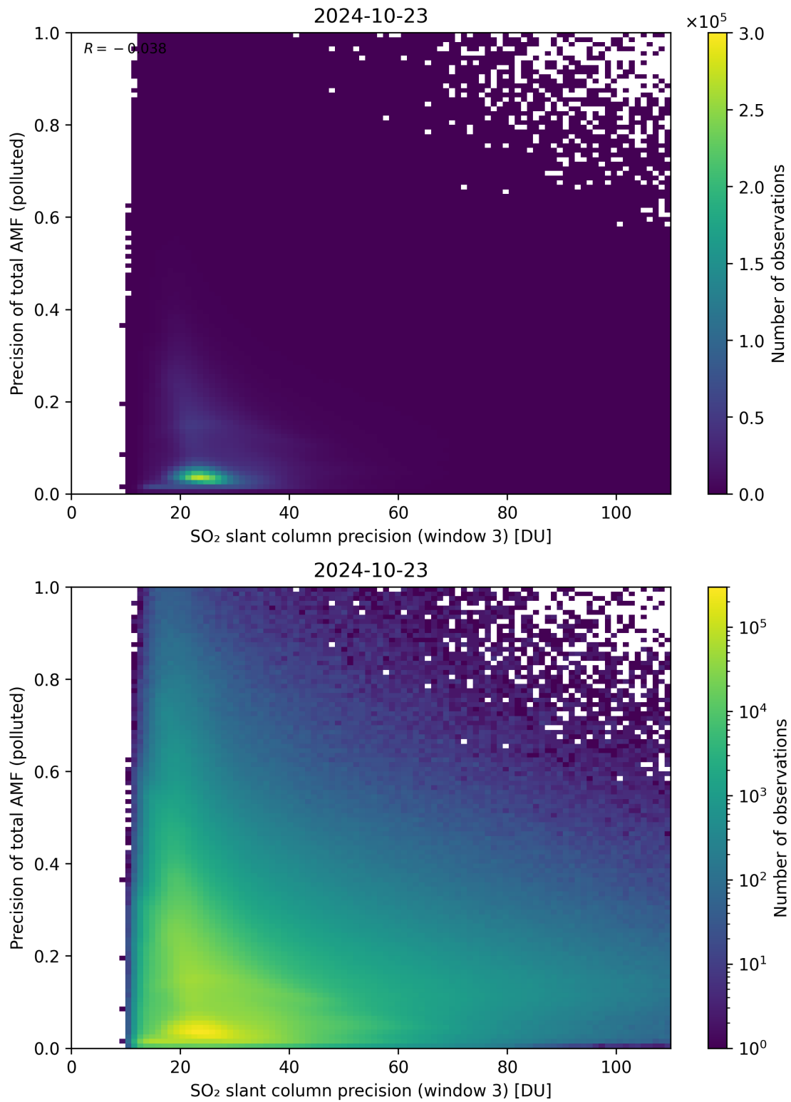
Figure 264: Scatter density plot of “SO 2 slant column precision (window 3)” against “Precision of total AMF (polluted)” for 2024-10-22 to 2024-10-24.
