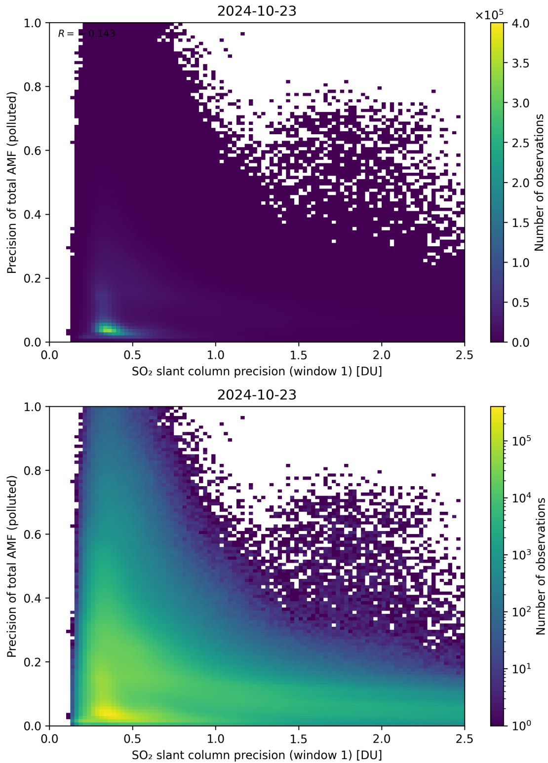
Figure 231: Scatter density plot of “SO 2 slant column precision (window 1)” against “Precision of total AMF (polluted)” for 2024-10-22 to 2024-10-24.
