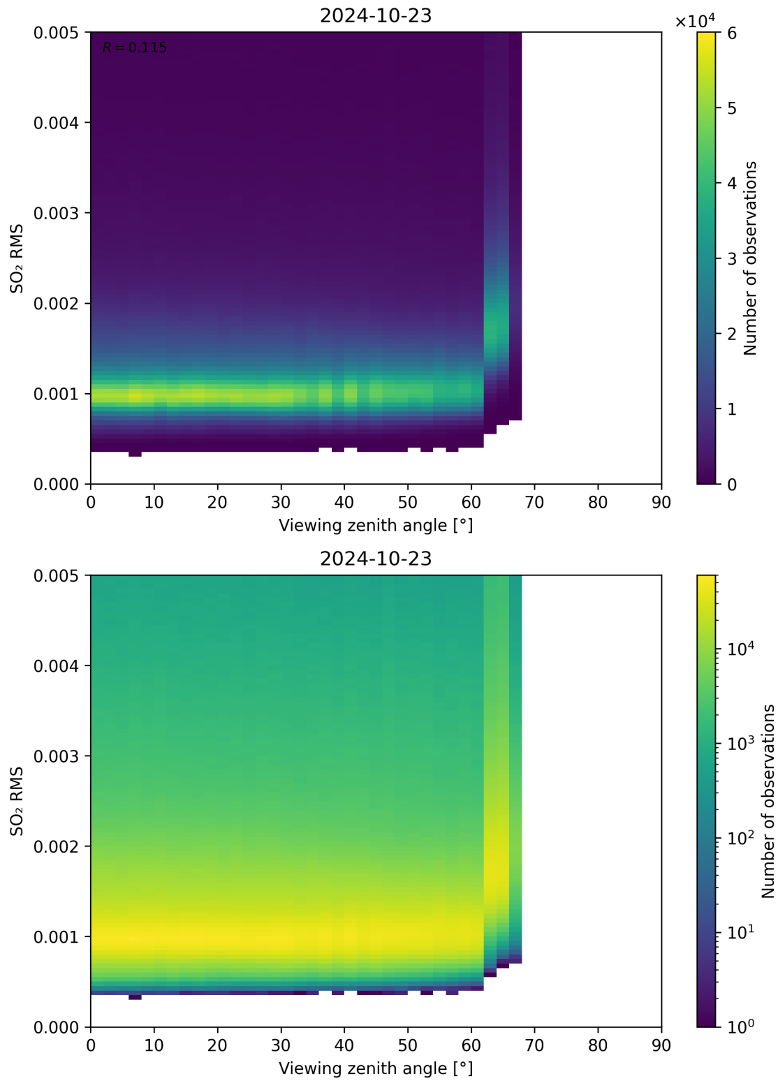
Figure 313: Scatter density plot of “Viewing zenith angle” against “SO 2 RMS” for 2024-10-22 to 2024-10-24.
