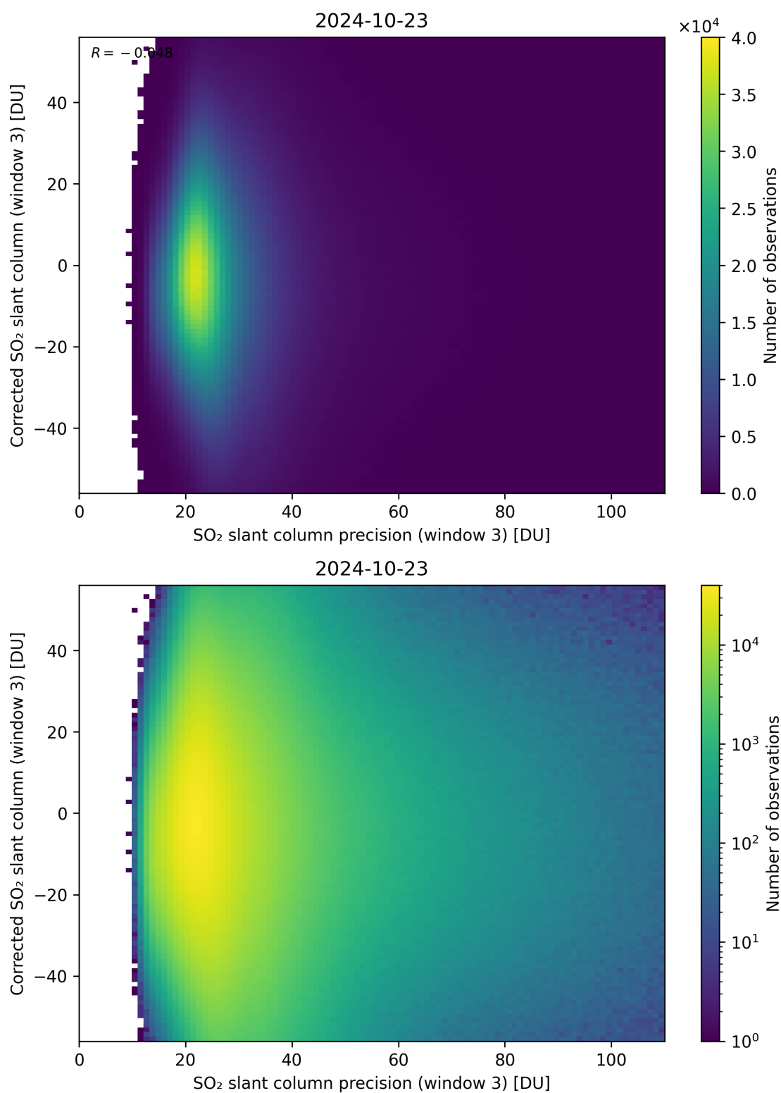
Figure 262: Scatter density plot of “SO 2 slant column precision (window 3)” against “Corrected SO 2 slant column (window 3)” for 2024-10-22 to 2024-10-24.
