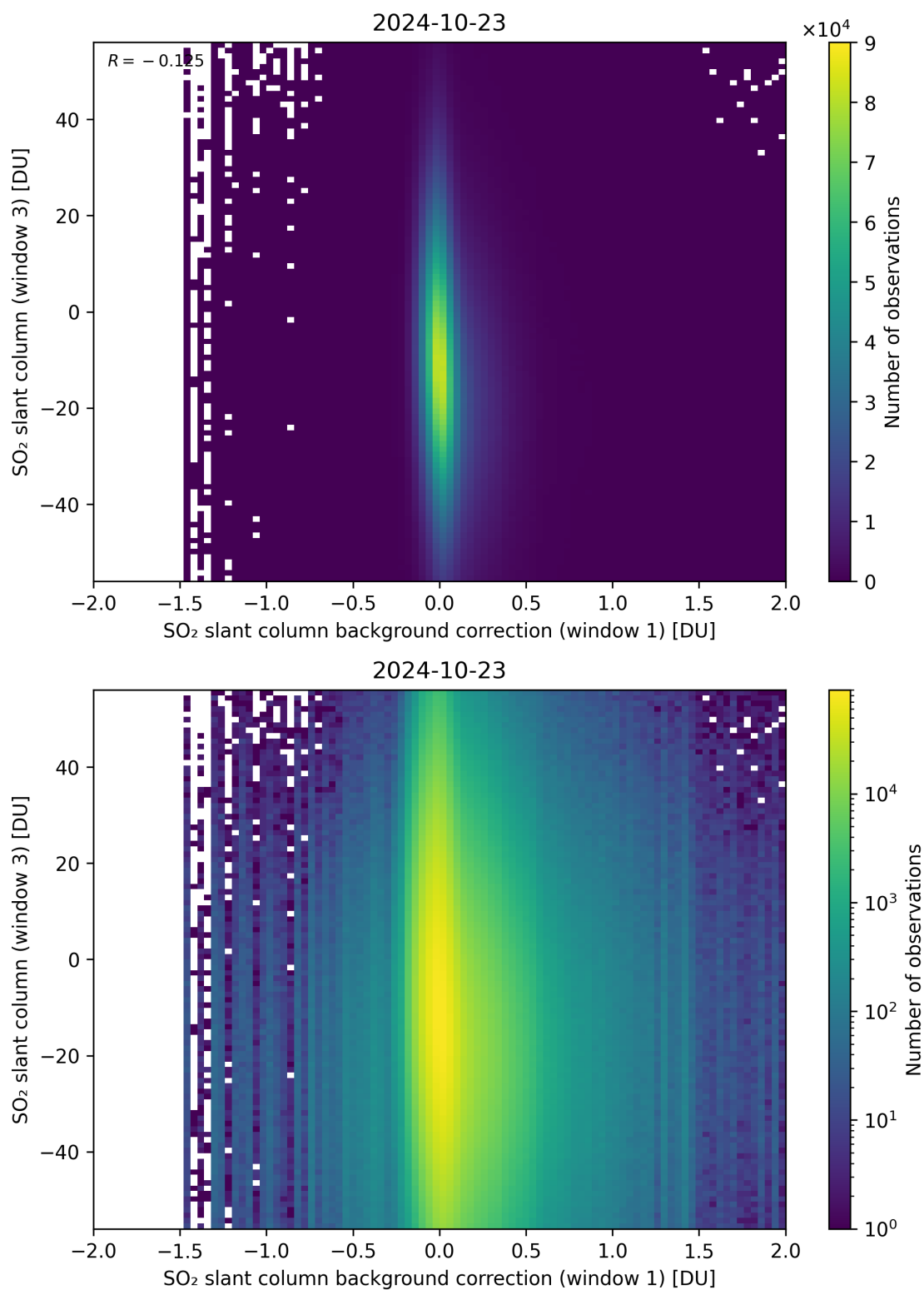
Figure 107: Scatter density plot of “SO 2 slant column background correction (window 1)” against “SO 2 slant column (window 3)” for 2024-10-22 to 2024-10-24.
