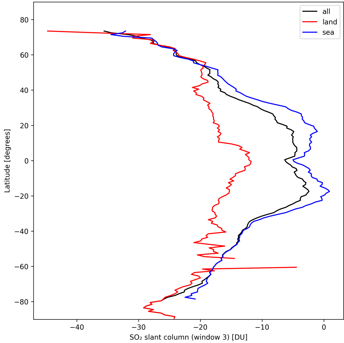
Figure 41: Zonal average of “SO 2 slant column (window 3)” for 2024-10-22 to 2024-10-24.
