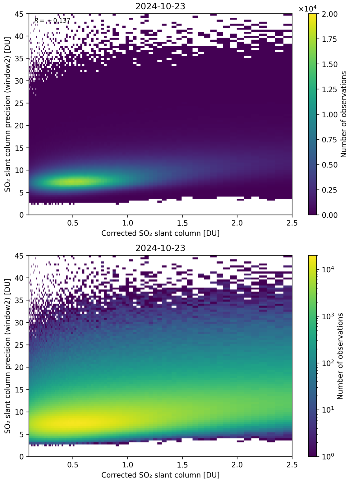
Figure 189: Scatter density plot of “Corrected SO 2 slant column” against “SO 2 slant column precision (window2)” for 2024-10-22 to 2024-10-24.
