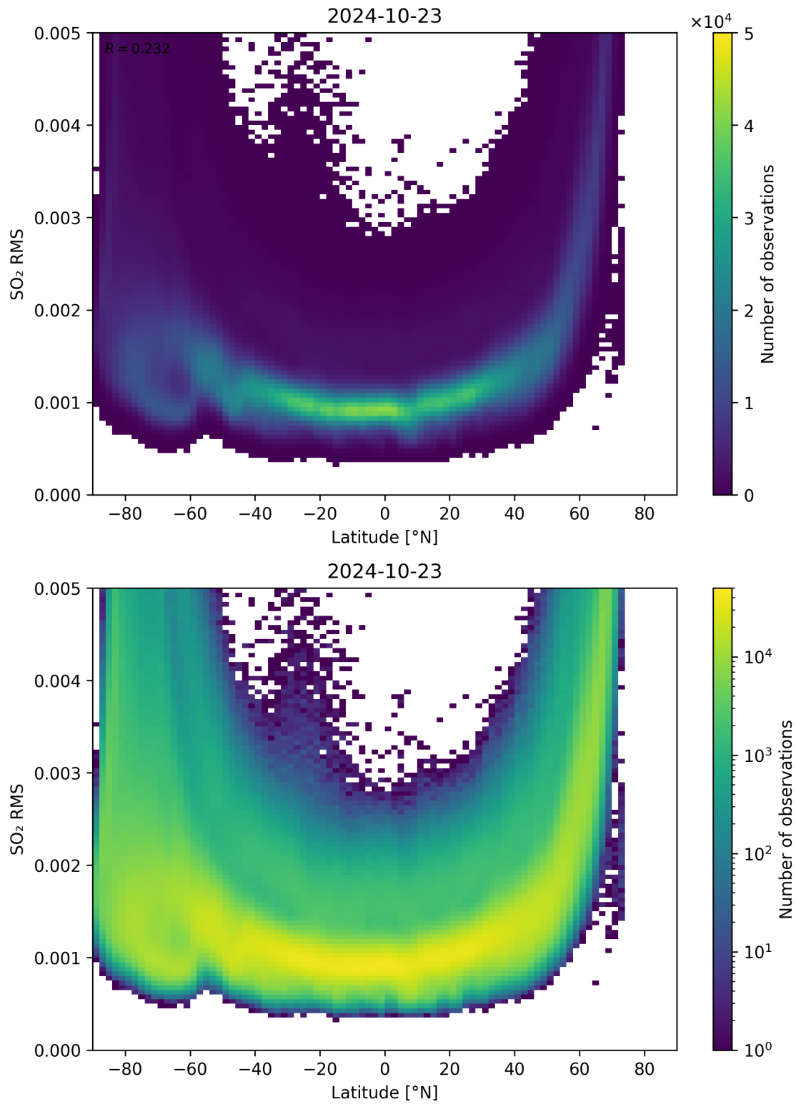
Figure 144: Scatter density plot of “Latitude” against “SO 2 RMS” for 2024-10-22 to 2024-10-24.
