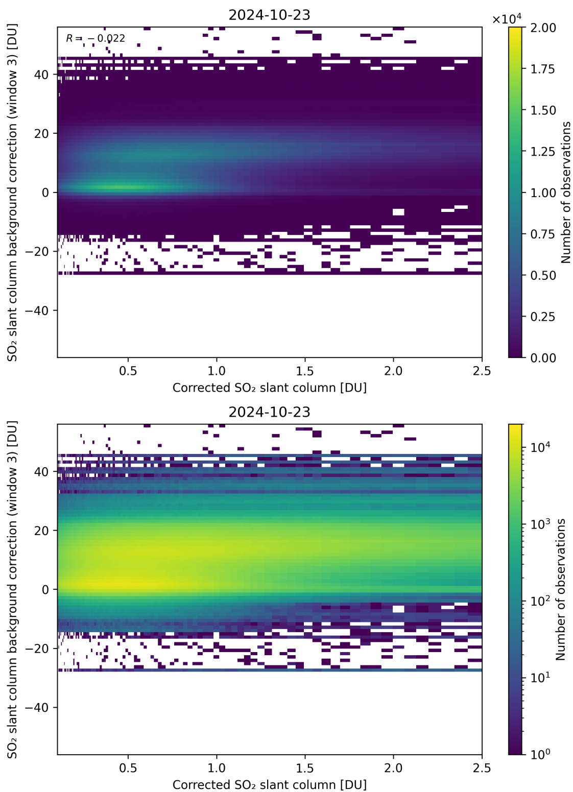
Figure 180: Scatter density plot of “Corrected SO 2 slant column” against “SO 2 slant column background correction (window 3)” for 2024-10-22 to 2024-10-24.
