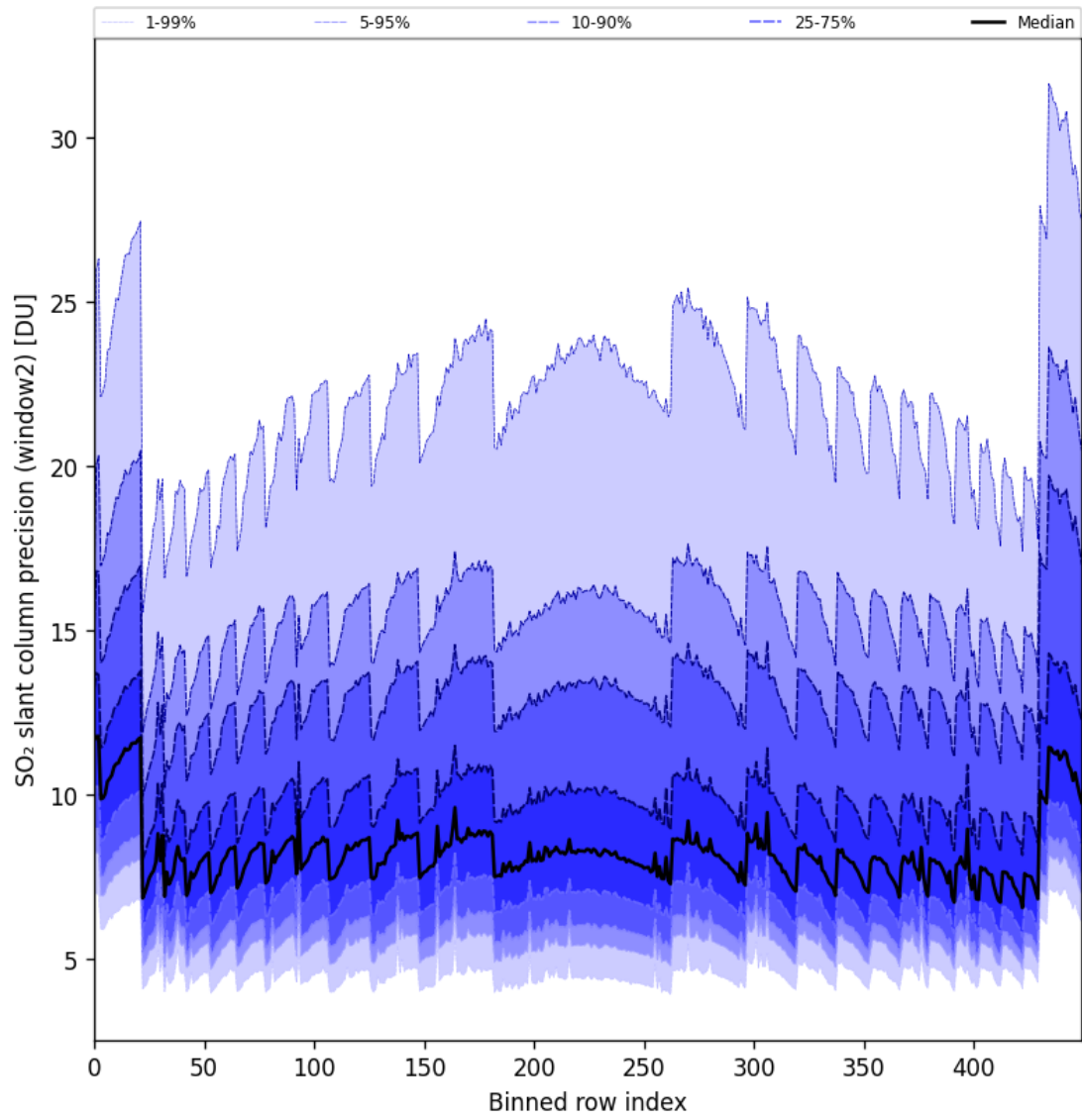
Figure 84: Along track statistics of “SO 2 slant column precision (window2)” for 2024-10-22 to 2024-10-24
