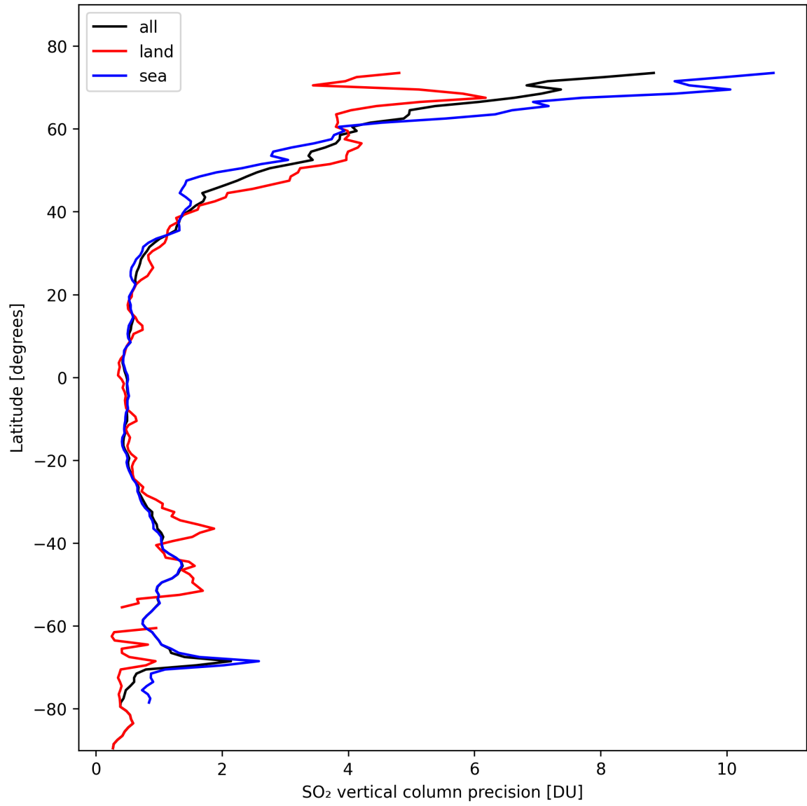
Figure 31: Zonal average of “SO 2 vertical column precision” for 2024-10-22 to 2024-10-24.
