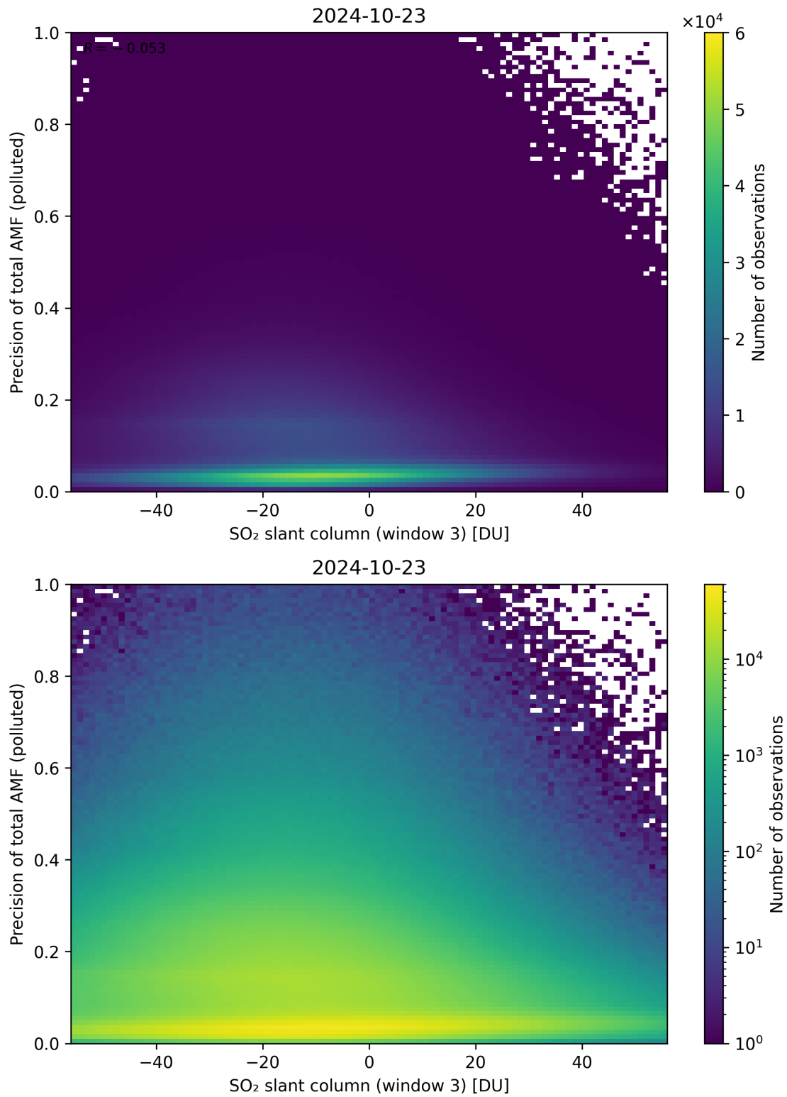
Figure 269: Scatter density plot of “SO 2 slant column (window 3)” against “Precision of total AMF (polluted)” for 2024-10-22 to 2024-10-24.
