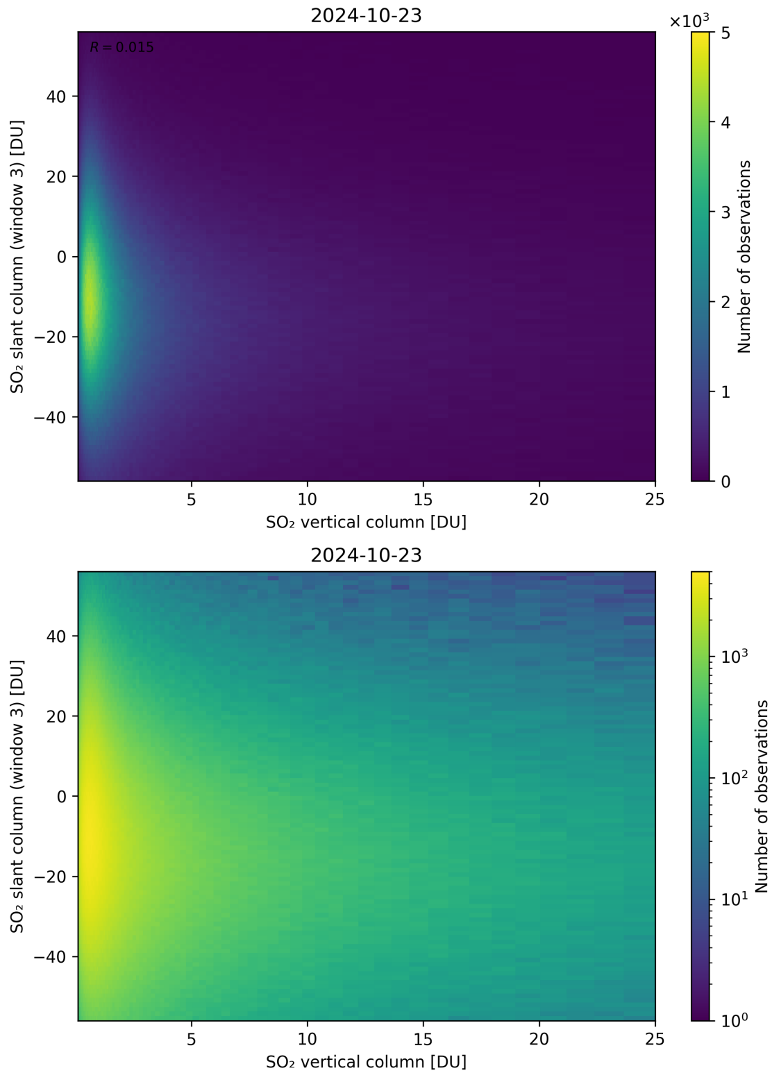
Figure 303: Scatter density plot of “SO 2 vertical column” against “SO 2 slant column (window 3)” for 2024-10-22 to 2024-10-24.
