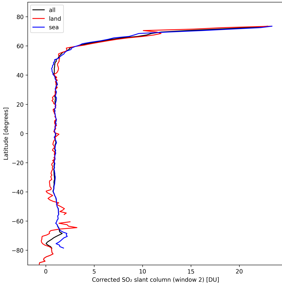
Figure 39: Zonal average of “Corrected SO 2 slant column (window 2)” for 2024-10-22 to 2024-10-24.
