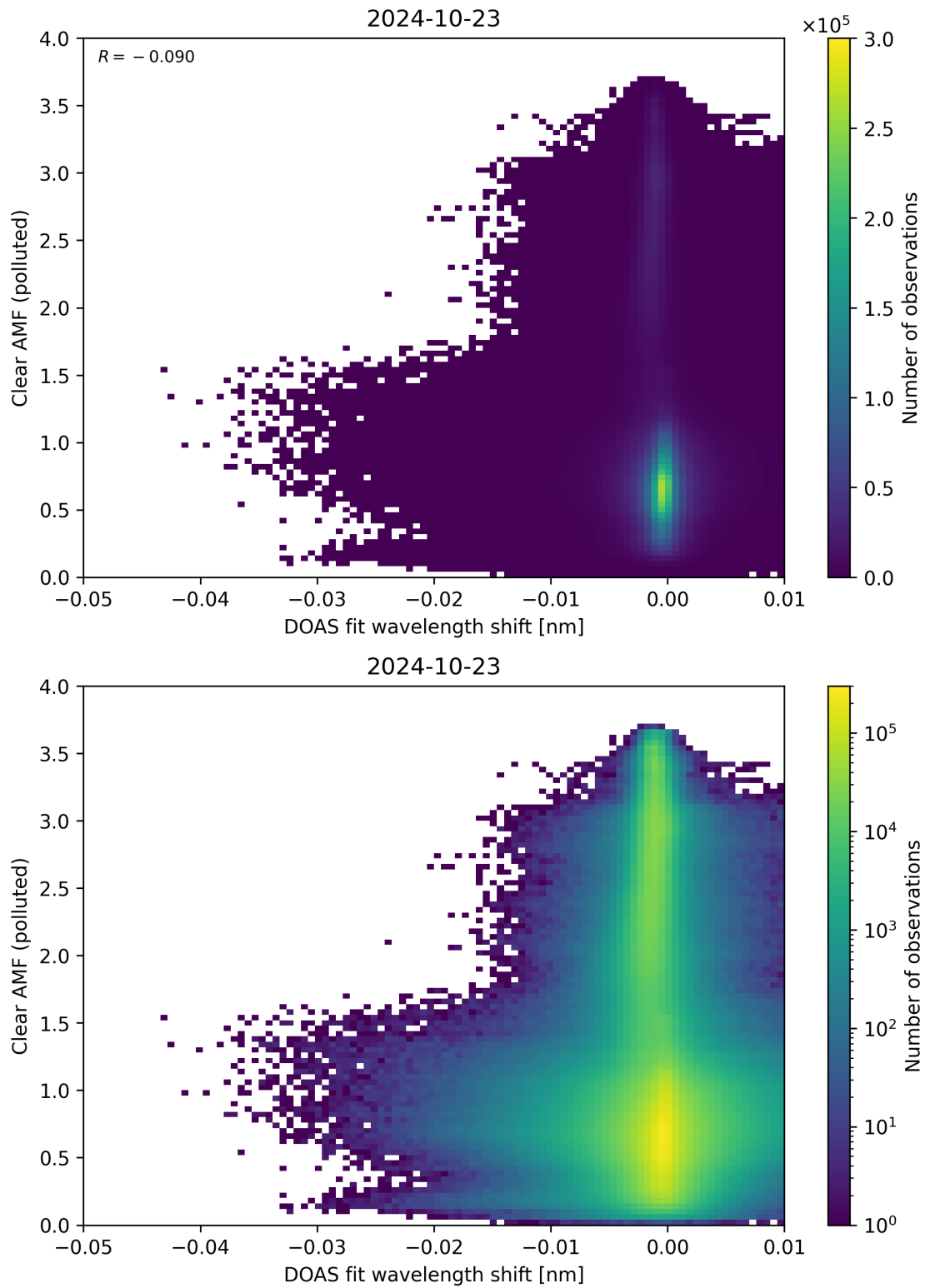
Figure 129: Scatter density plot of “DOAS fit wavelength shift” against “Clear AMF (polluted)” for 2024-10-22 to 2024-10-24.
