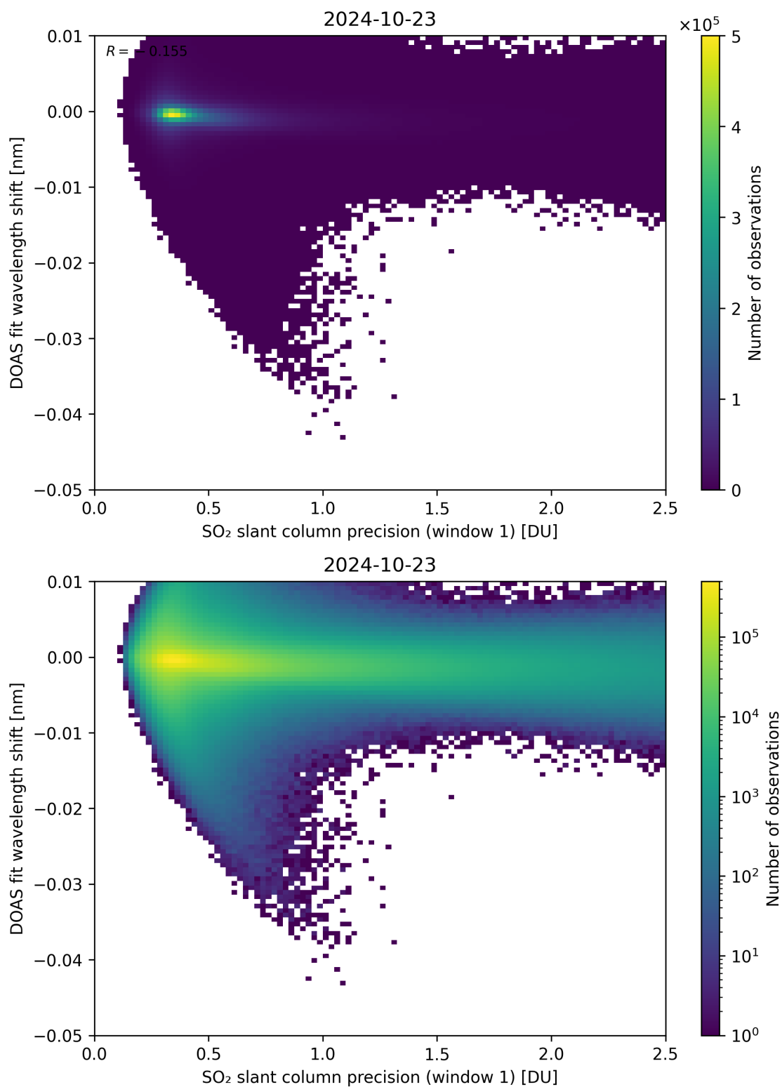
Figure 221: Scatter density plot of “SO 2 slant column precision (window 1)” against “DOAS fit wavelength shift” for 2024-10-22 to 2024-10-24.
