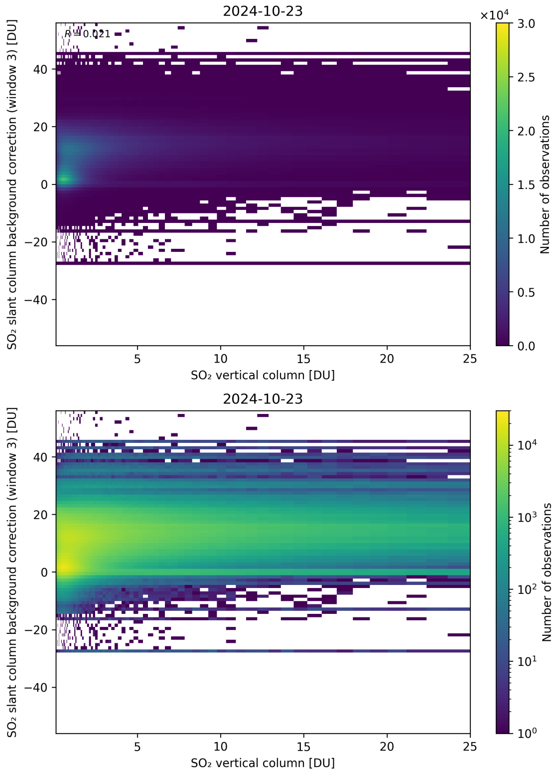
Figure 275: Scatter density plot of “SO 2 vertical column” against “SO 2 slant column background correction (window 3)” for 2024-10-22 to 2024-10-24.
