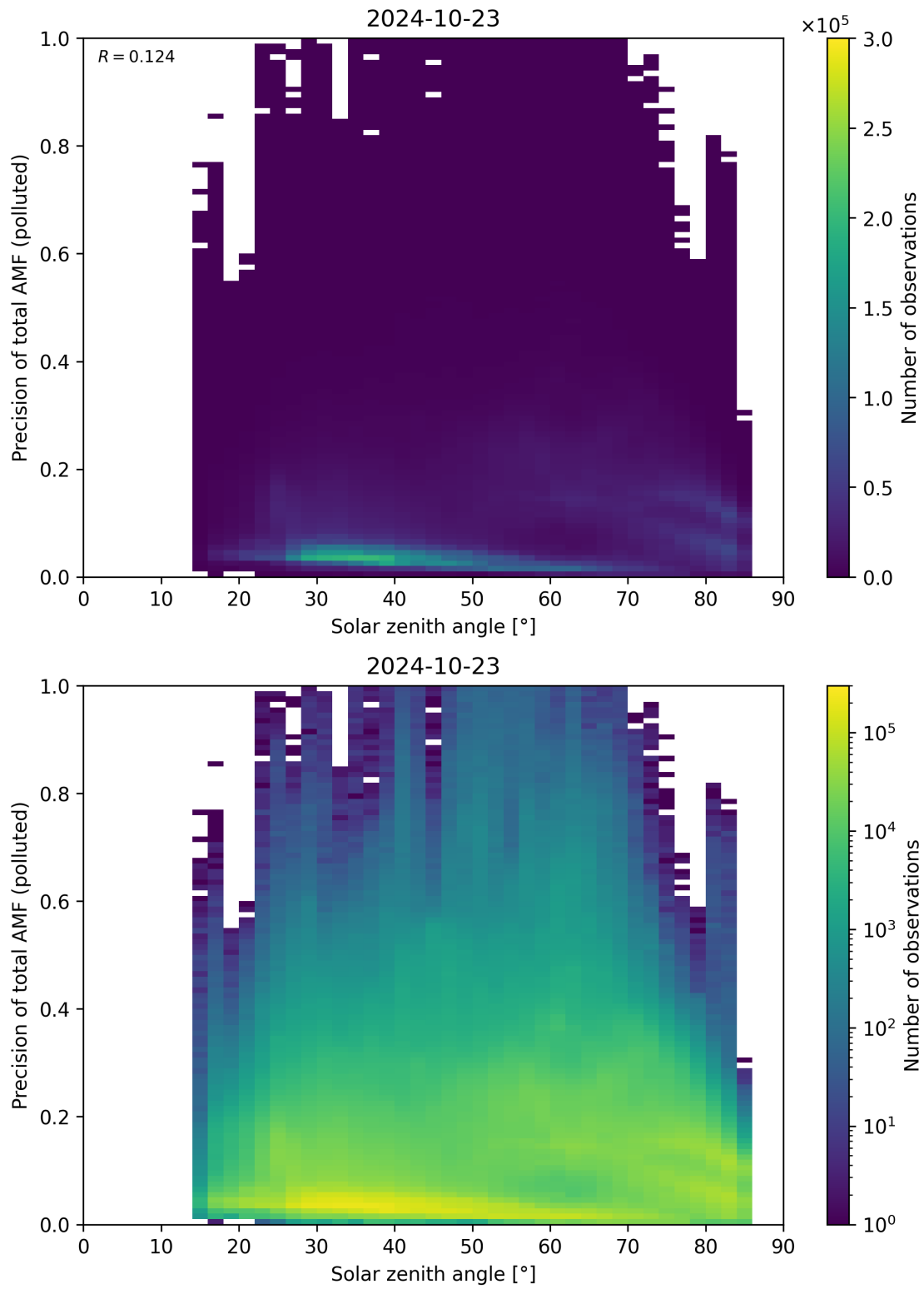
Figure 175: Scatter density plot of “Solar zenith angle” against “Precision of total AMF (polluted)” for 2024-10-22 to 2024-10-24.
