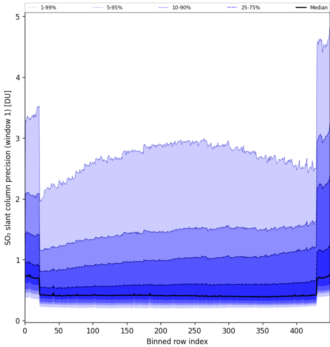
Figure 80: Along track statistics of “SO 2 slant column precision (window 1)” for 2024-10-22 to 2024-10-24
