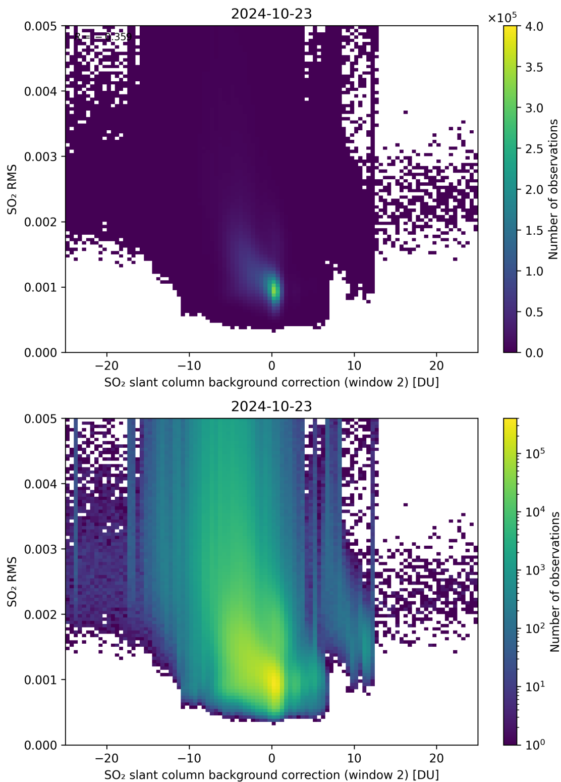
Figure 114: Scatter density plot of “SO 2 slant column background correction (window 2)” against “SO 2 RMS” for 2024-10-22 to 2024-10-24.
