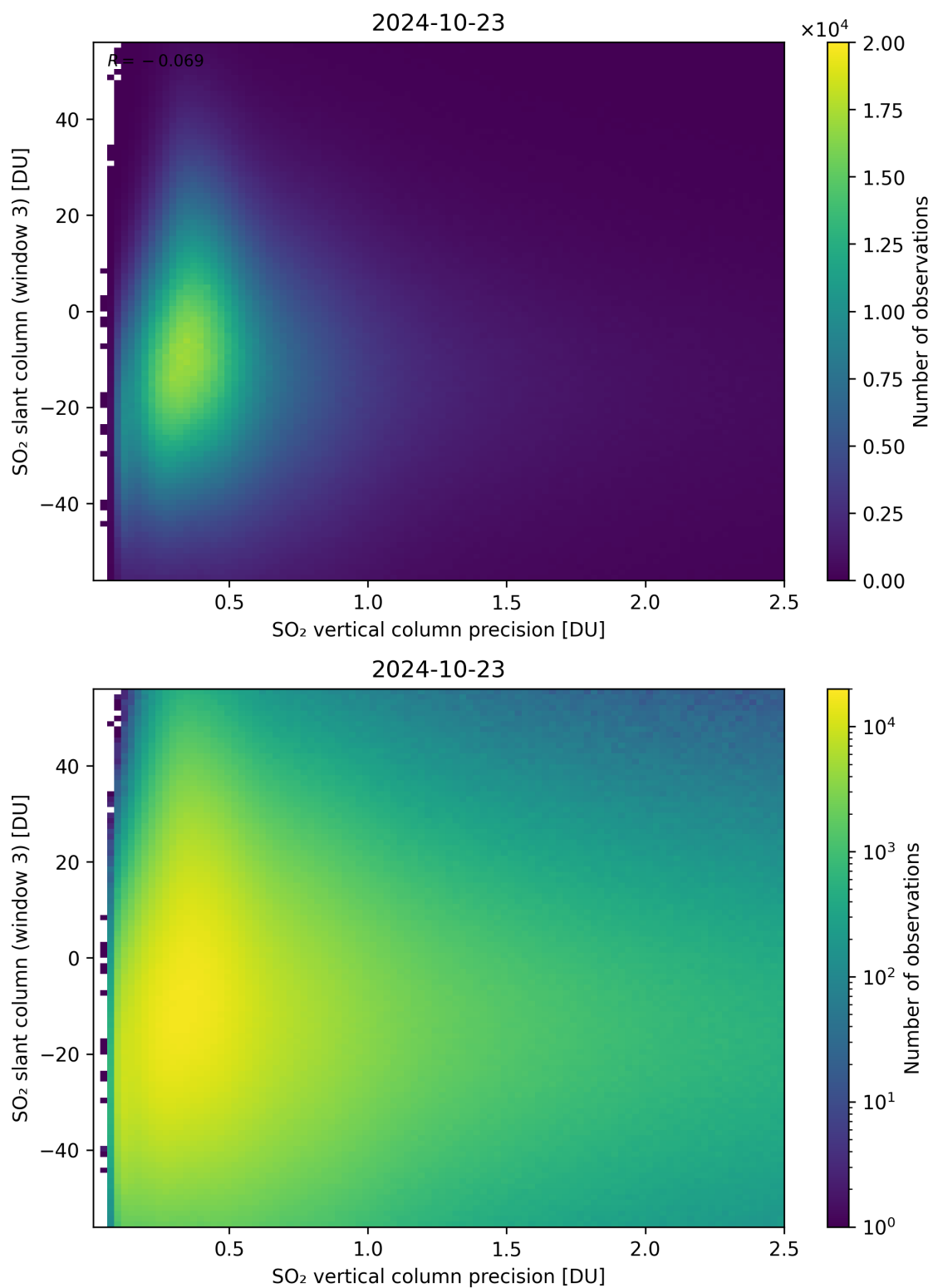
Figure 292: Scatter density plot of “SO 2 vertical column precision” against “SO 2 slant column (window 3)” for 2024-10-22 to 2024-10-24.
