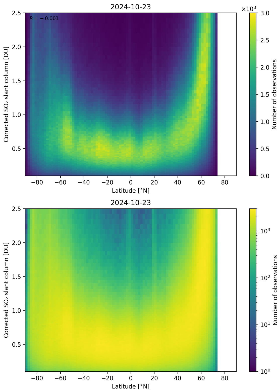
Figure 146: Scatter density plot of “Latitude” against “Corrected SO 2 slant column” for 2024-10-22 to 2024-10-24.
