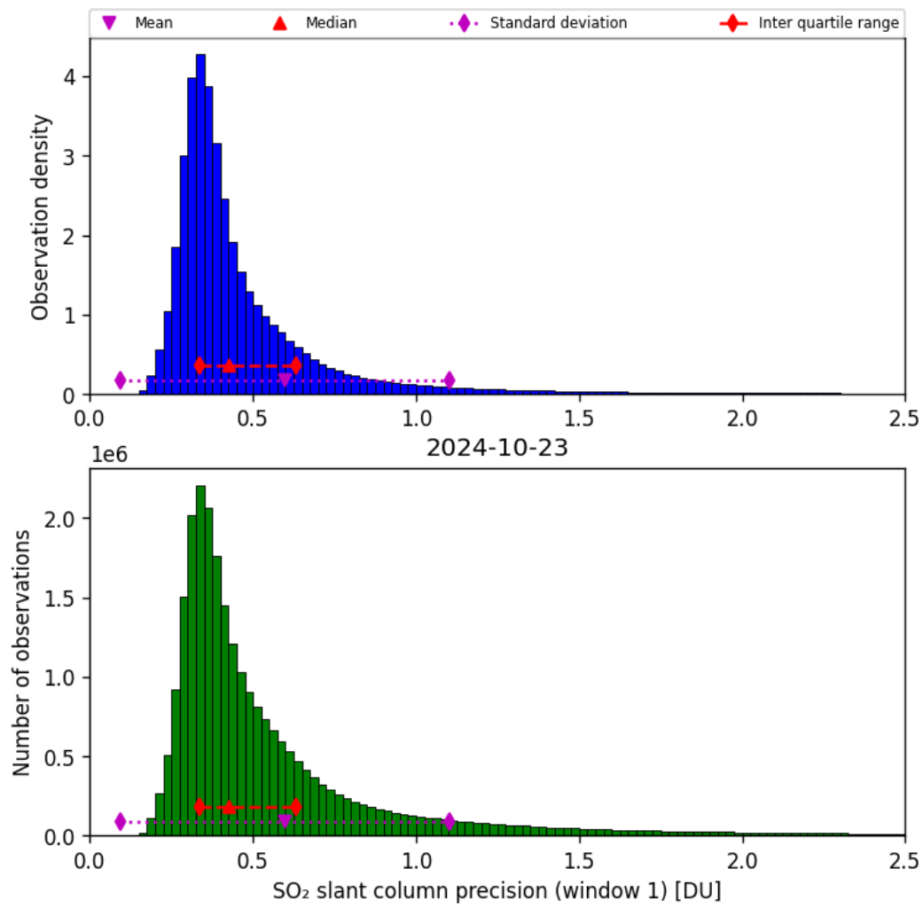
Figure 57: Histogram of “SO 2 slant column precision (window 1)” for 2024-10-22 to 2024-10-24
