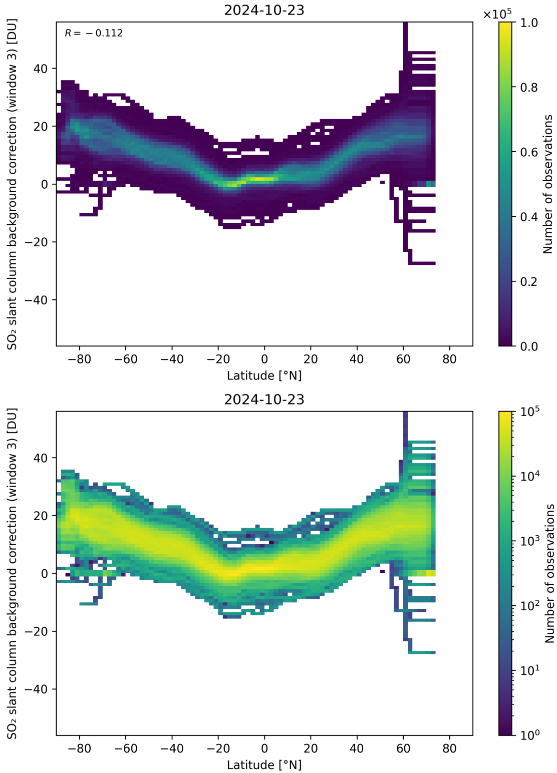
Figure 141: Scatter density plot of “Latitude” against “SO 2 slant column background correction (window 3)” for 2024-10-22 to 2024-10-24.
