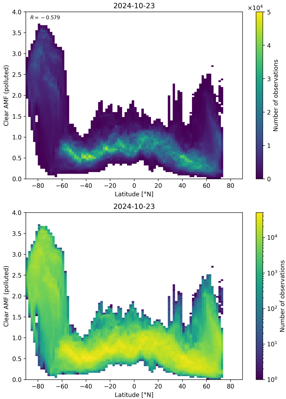
Figure 145: Scatter density plot of “Latitude” against “Clear AMF (polluted)” for 2024-10-22 to 2024-10-24.
