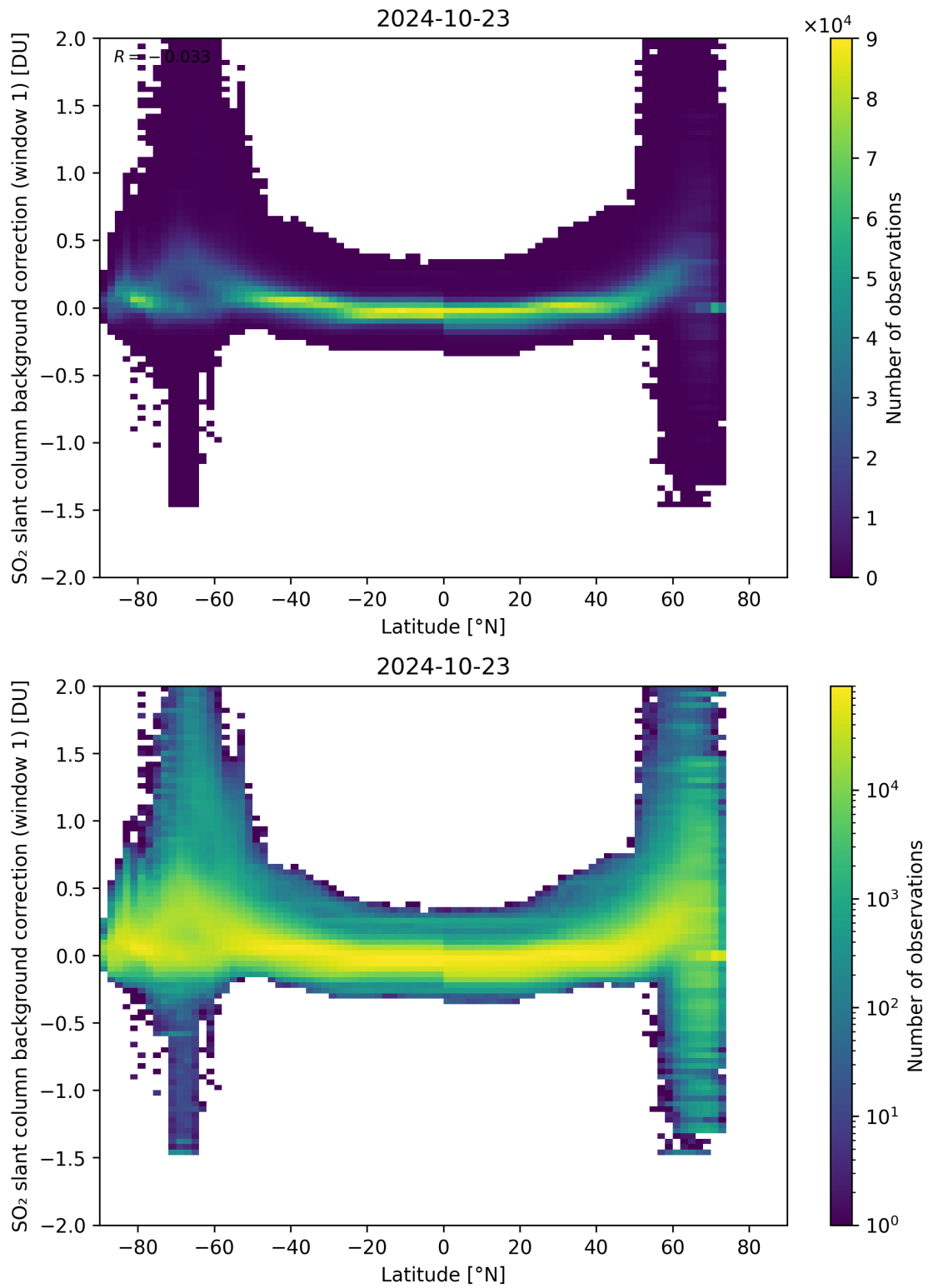
Figure 139: Scatter density plot of “Latitude” against “SO 2 slant column background correction (window 1)” for 2024-10-22 to 2024-10-24.
