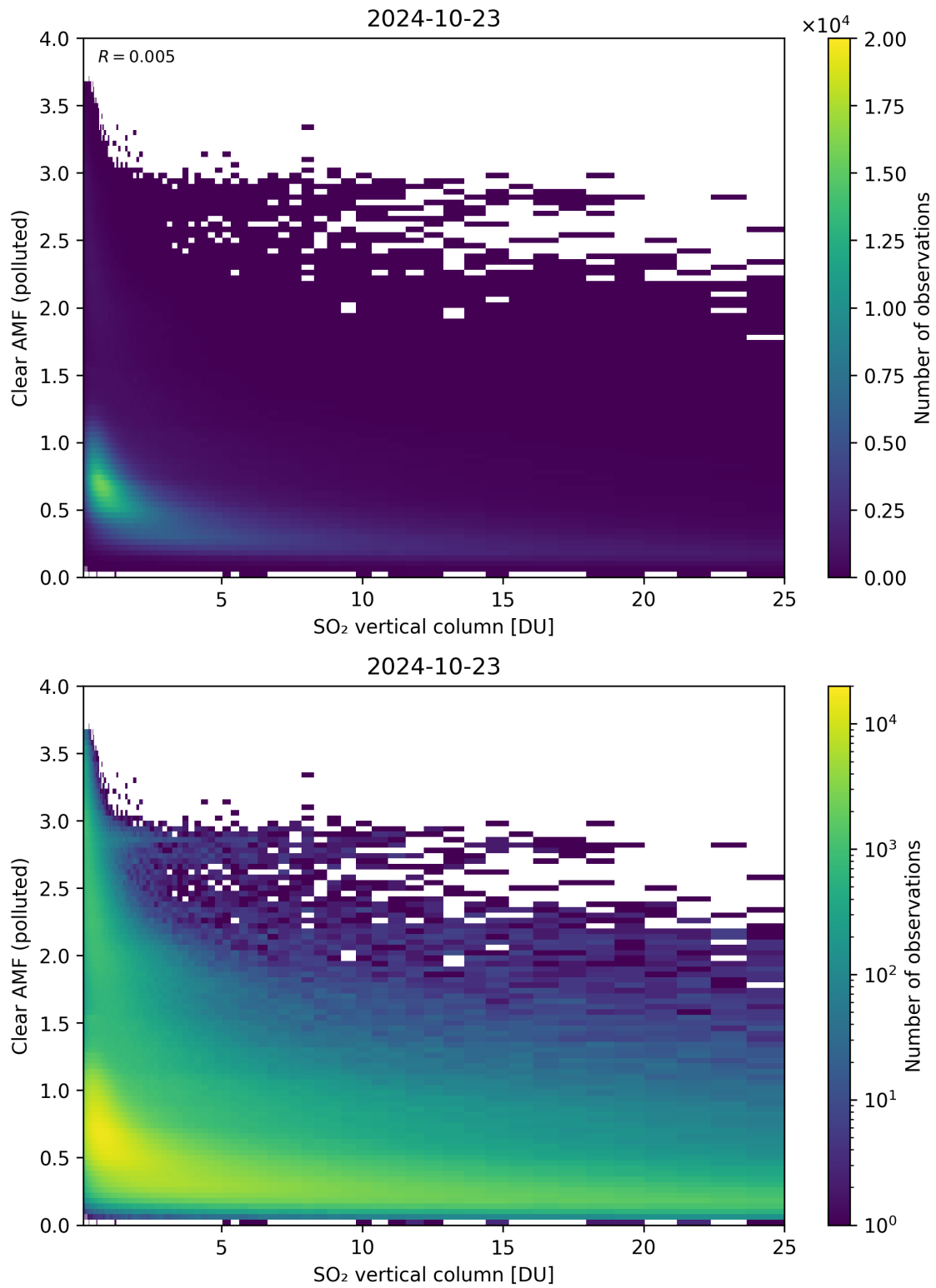
Figure 296: Scatter density plot of “SO 2 vertical column” against “Clear AMF (polluted)” for 2024-10-22 to 2024-10-24.
