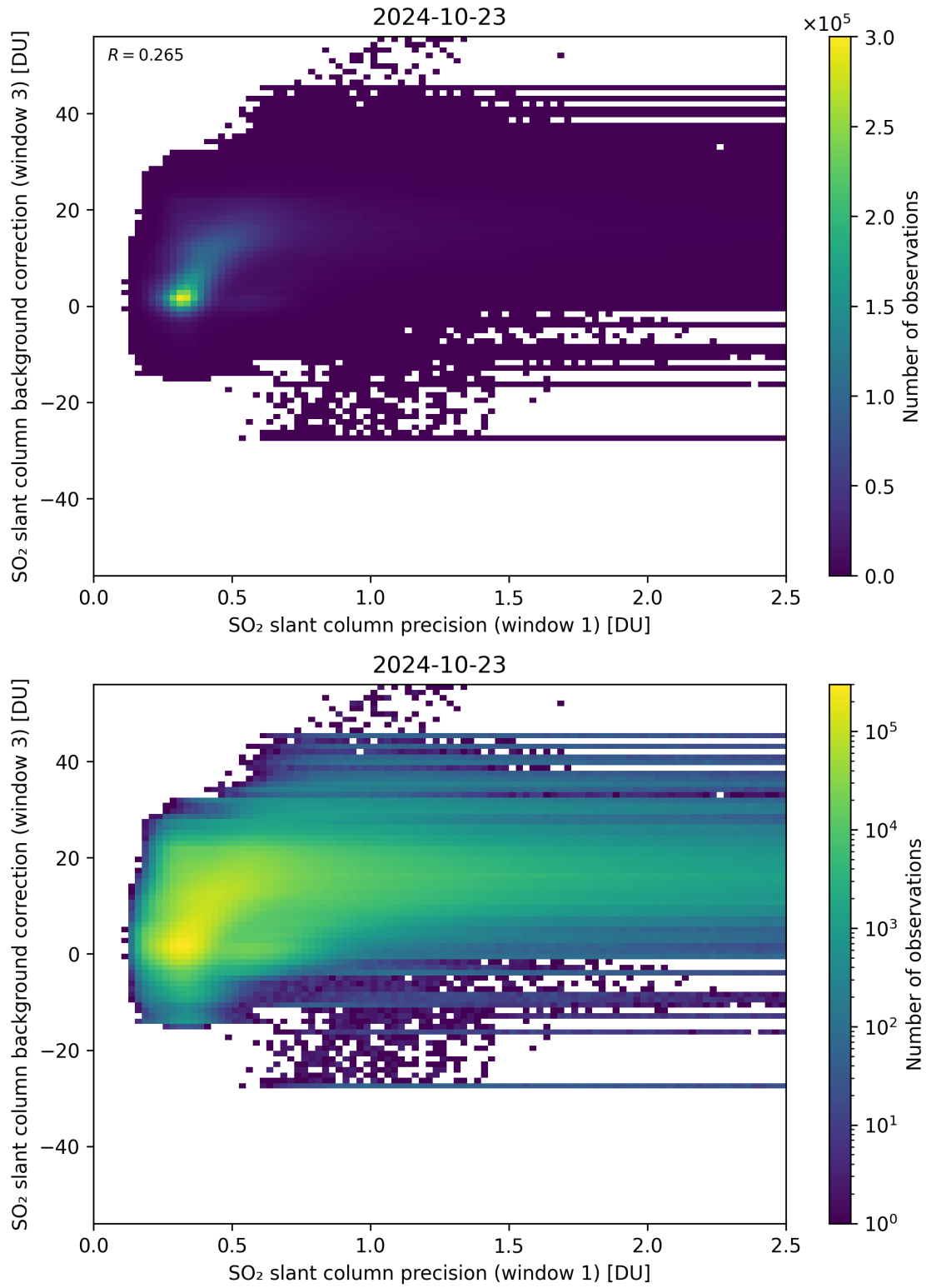
Figure 220: Scatter density plot of “SO 2 slant column precision (window 1)” against “SO 2 slant column background correction (window 3)” for 2024-10-22 to 2024-10-24.
