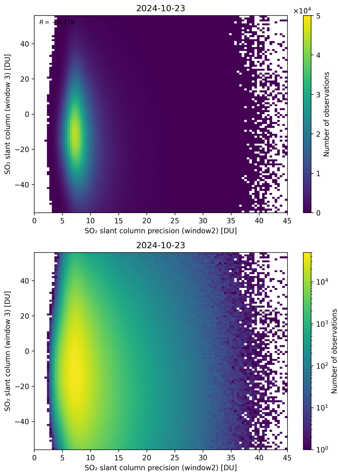
Figure 249: Scatter density plot of “SO 2 slant column precision (window2)” against “SO 2 slant column (window 3)” for 2024-10-22 to 2024-10-24.
