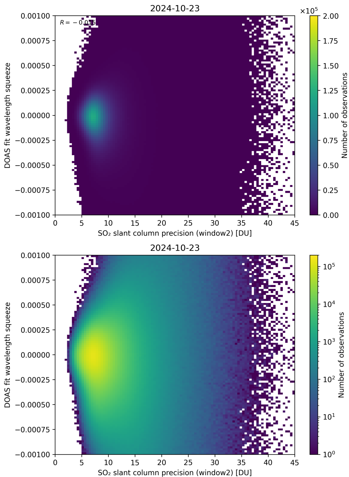
Figure 244: Scatter density plot of “SO 2 slant column precision (window2)” against “DOAS fit wavelength squeeze” for 2024-10-22 to 2024-10-24.
