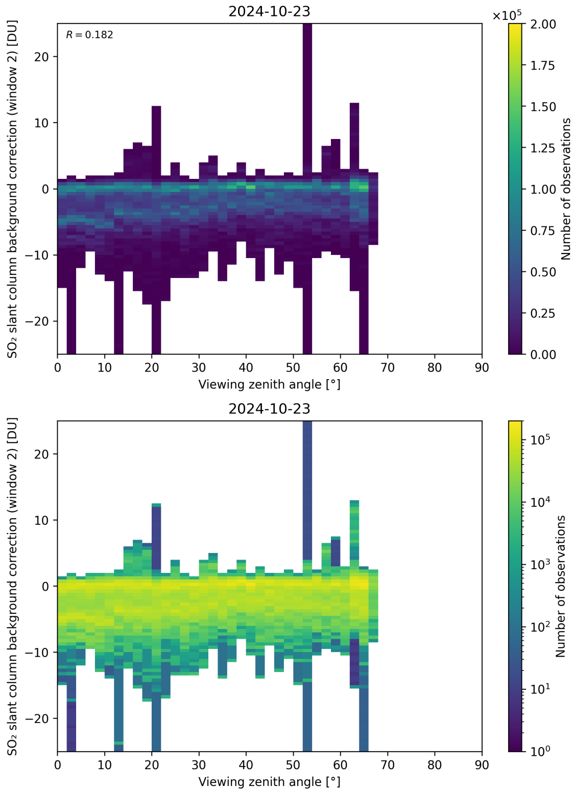
Figure 309: Scatter density plot of “Viewing zenith angle” against “SO 2 slant column background correction (window 2)” for 2024-10-22 to 2024-10-24.
