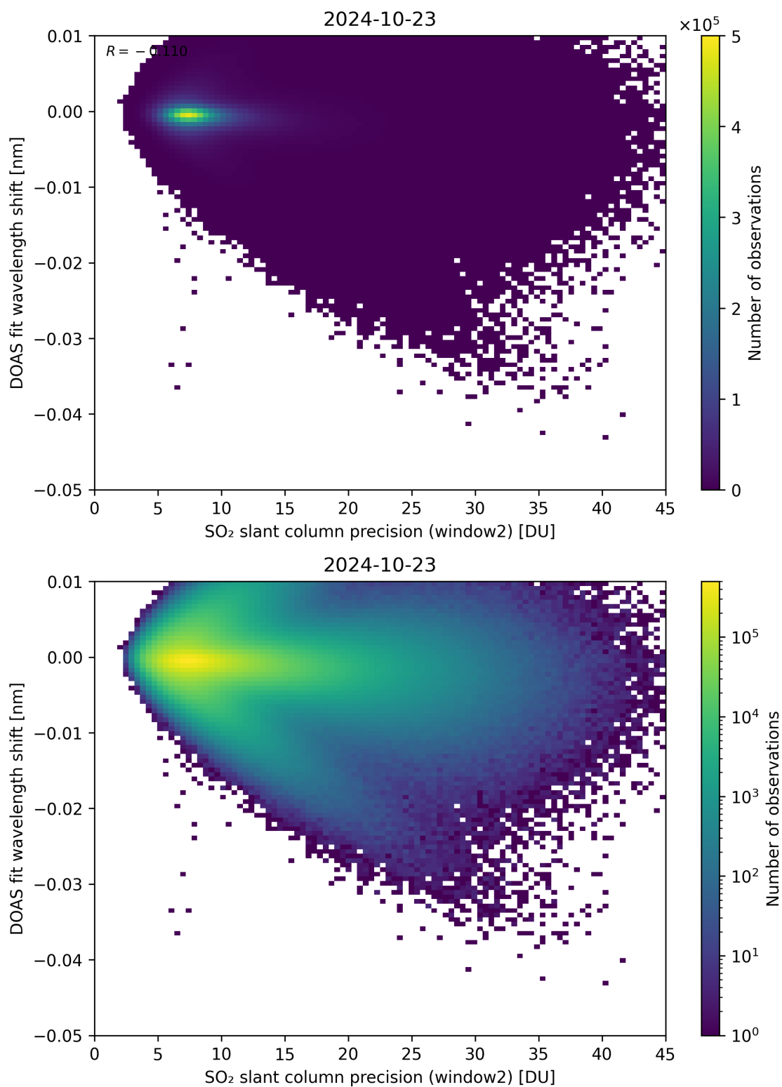
Figure 243: Scatter density plot of “SO 2 slant column precision (window2)” against “DOAS fit wavelength shift” for 2024-10-22 to 2024-10-24.
