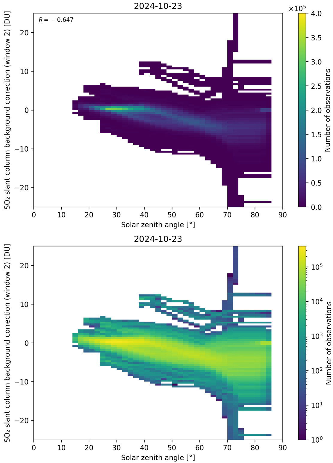
Figure 159: Scatter density plot of “Solar zenith angle” against “SO 2 slant column background correction (window 2)” for 2024-10-22 to 2024-10-24.
