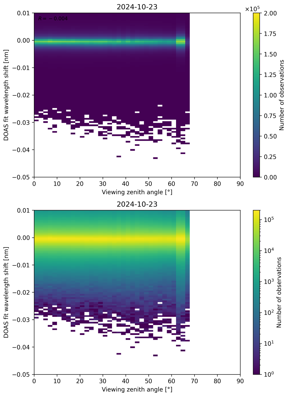
Figure 311: Scatter density plot of “Viewing zenith angle” against “DOAS fit wavelength shift” for 2024-10-22 to 2024-10-24.
