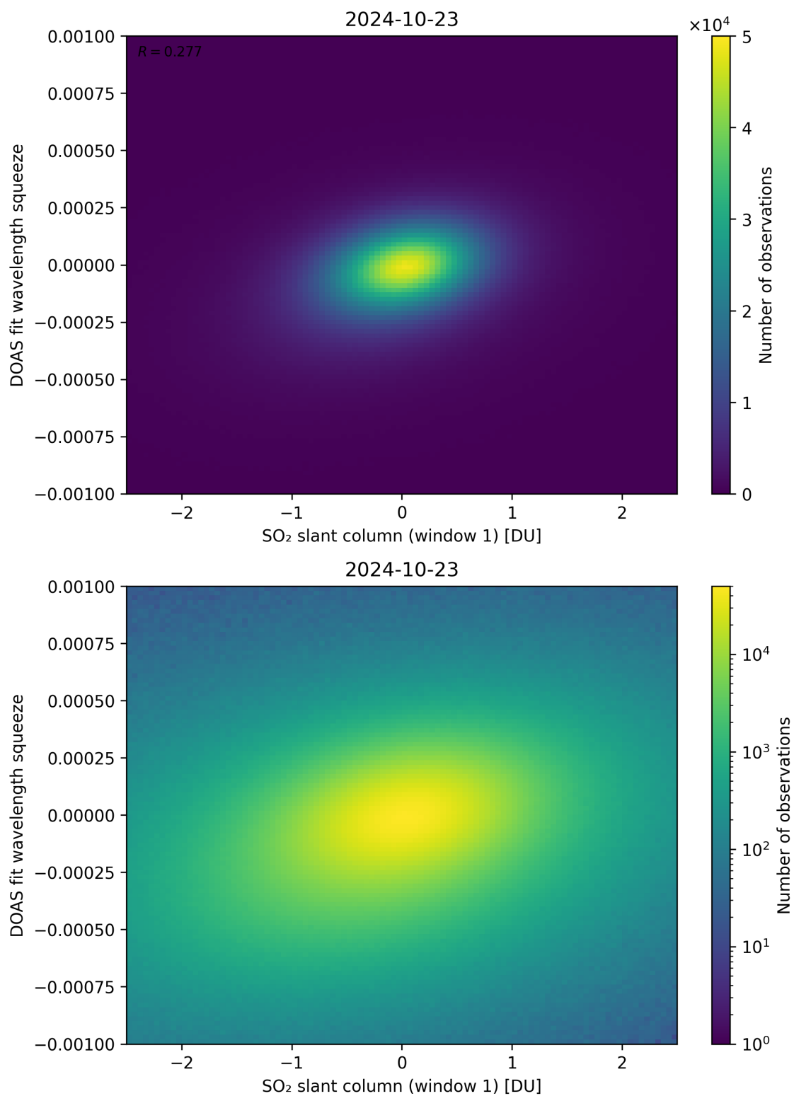
Figure 216: Scatter density plot of “SO 2 slant column (window 1)” against “DOAS fit wavelength squeeze” for 2024-10-22 to 2024-10-24.
