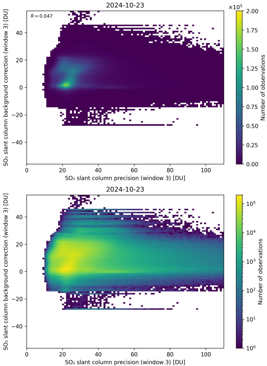
Figure 257: Scatter density plot of “SO 2 slant column precision (window 3)” against “SO 2 slant column background correction (window 3)” for 2024-10-22 to 2024-10-24.
