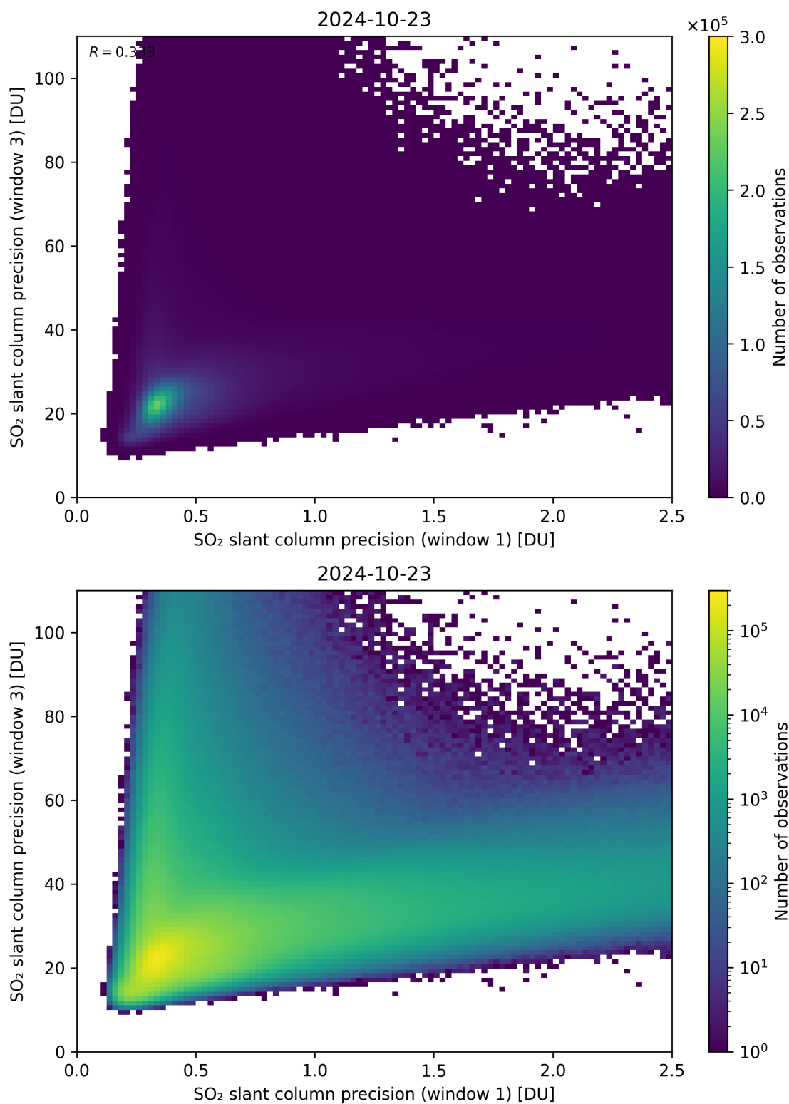
Figure 229: Scatter density plot of “SO 2 slant column precision (window 1)” against “SO 2 slant column precision (window 3)” for 2024-10-22 to 2024-10-24.
