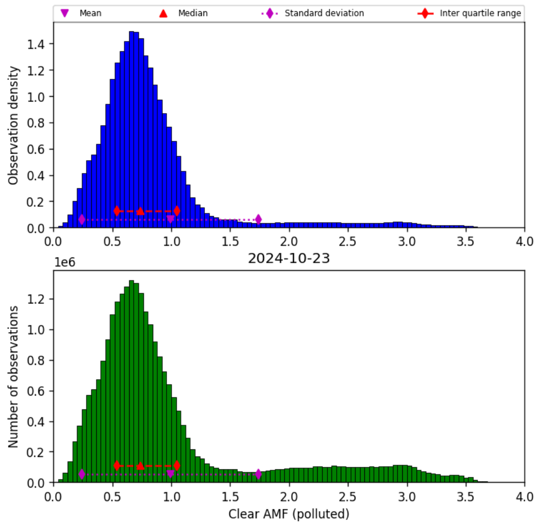
Figure 73: Histogram of “Clear AMF (polluted)” for 2024-10-22 to 2024-10-24
