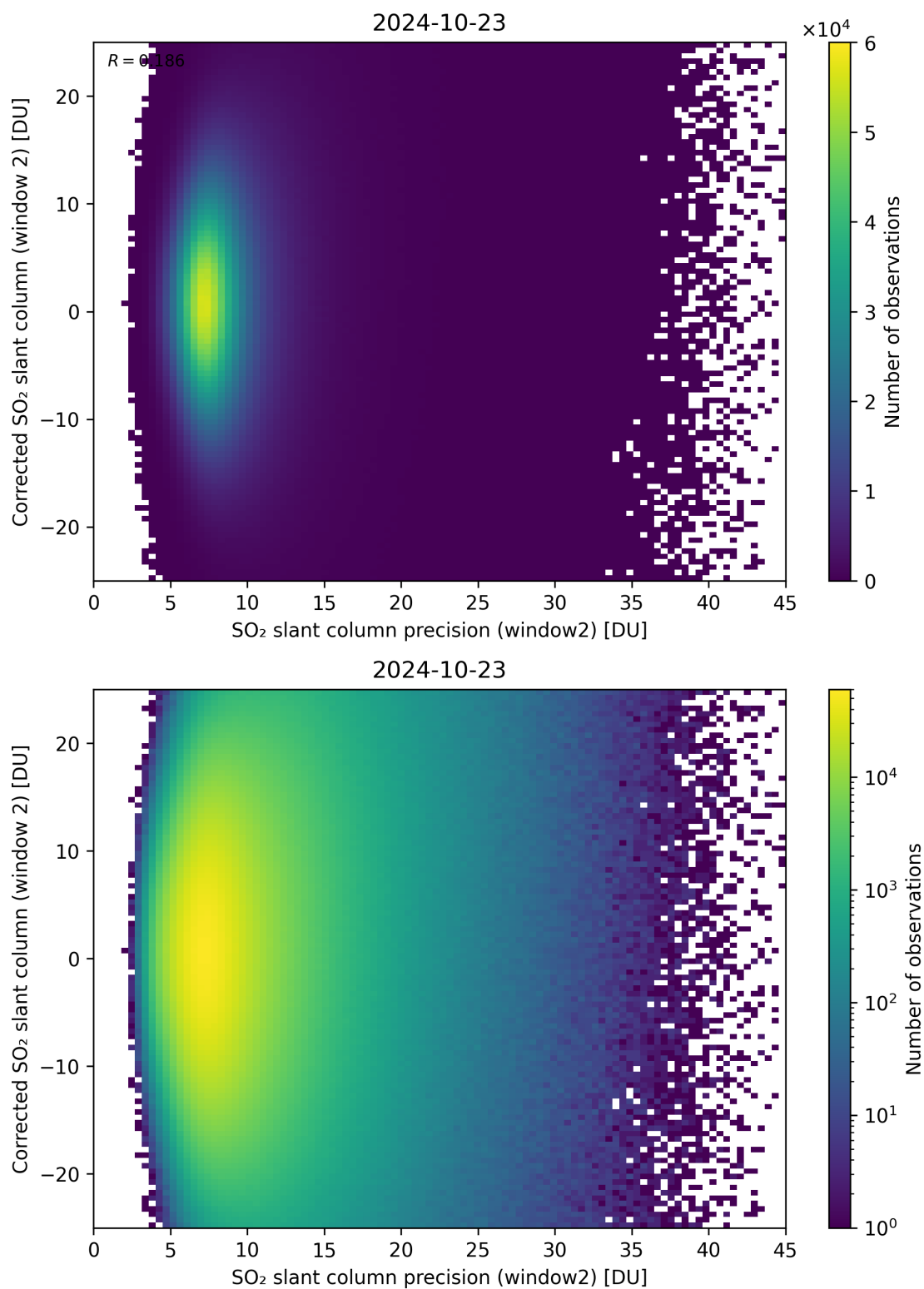
Figure 247: Scatter density plot of “SO 2 slant column precision (window2)” against “Corrected SO 2 slant column (window 2)” for 2024-10-22 to 2024-10-24.
