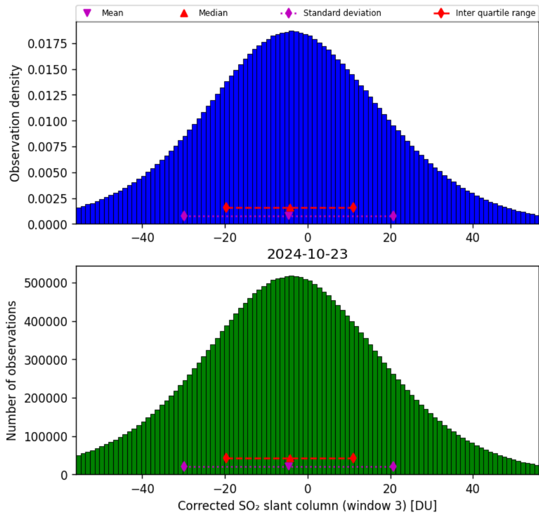
Figure 66: Histogram of “Corrected SO 2 slant column (window 3)” for 2024-10-22 to 2024-10-24
