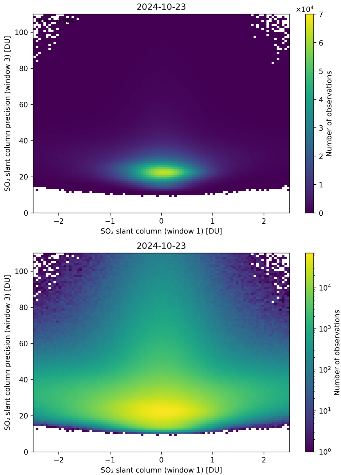
Figure 238: Scatter density plot of “SO 2 slant column (window 1)” against “SO 2 slant column precision (window 3)” for 2024-10-22 to 2024-10-24.
