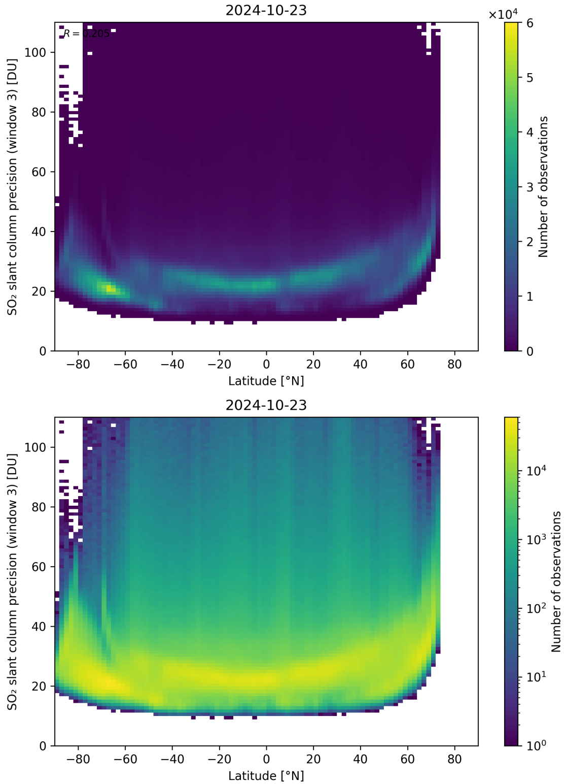
Figure 153: Scatter density plot of “Latitude” against “SO 2 slant column precision (window 3)” for 2024-10-22 to 2024-10-24.
