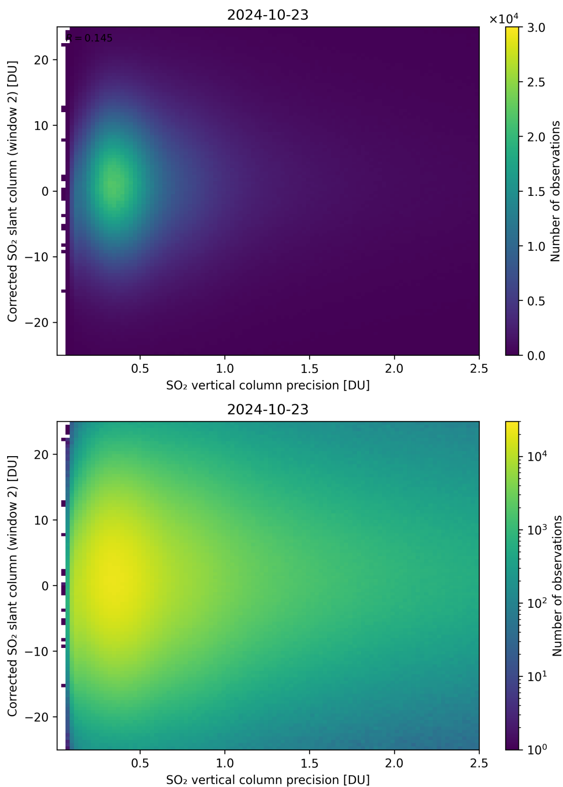
Figure 287: Scatter density plot of “SO 2 vertical column precision” against “Corrected SO 2 slant column (window 2)” for 2024-10-22 to 2024-10-24.
