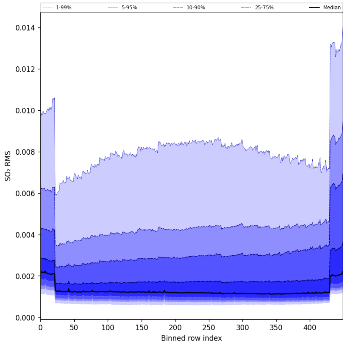
Figure 93: Along track statistics of “SO 2 RMS” for 2024-10-22 to 2024-10-24
