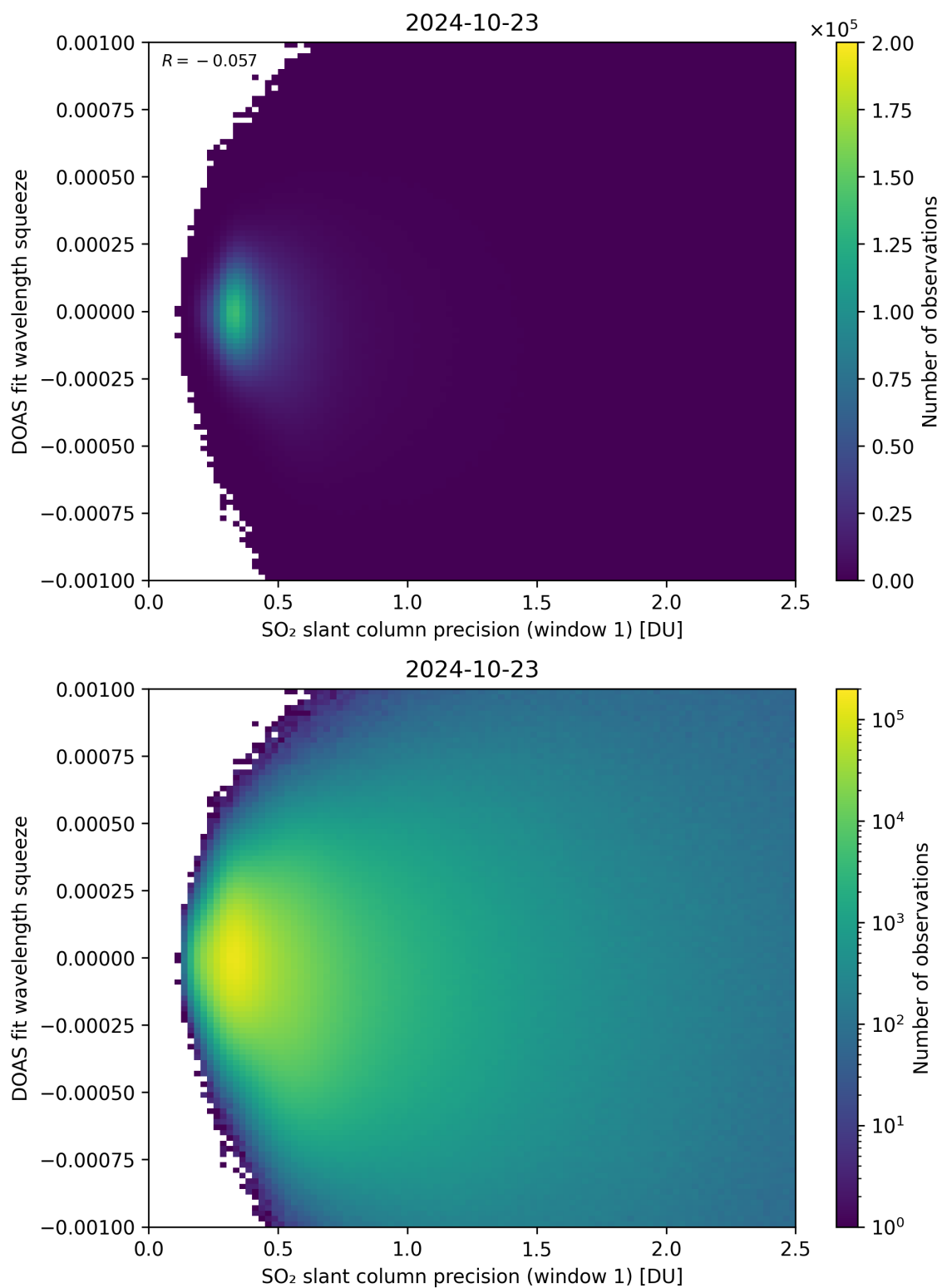
Figure 222: Scatter density plot of “SO 2 slant column precision (window 1)” against “DOAS fit wavelength squeeze” for 2024-10-22 to 2024-10-24.
