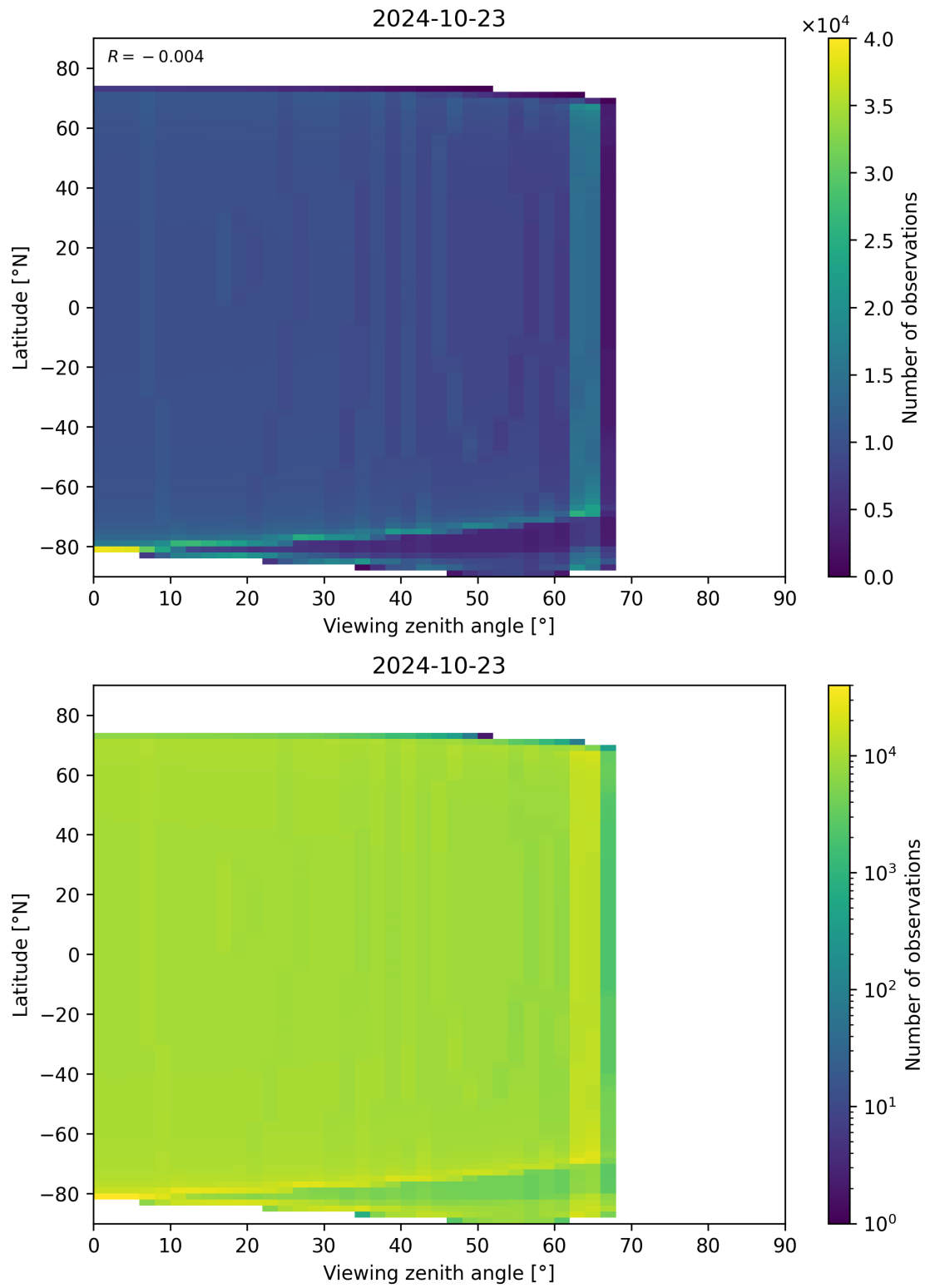
Figure 314: Scatter density plot of “Viewing zenith angle” against “Latitude” for 2024-10-22 to 2024-10-24.
