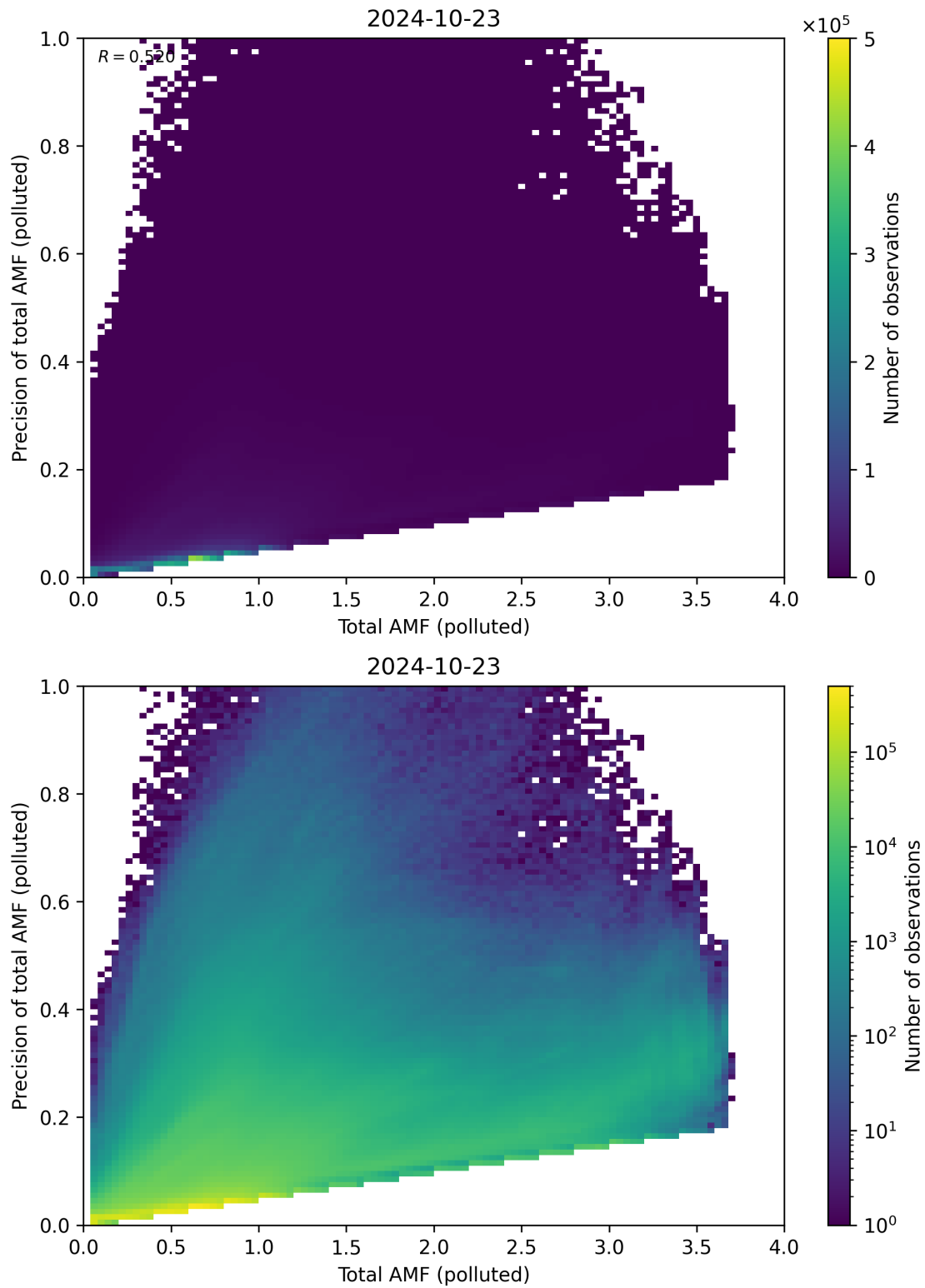
Figure 272: Scatter density plot of “Total AMF (polluted)” against “Precision of total AMF (polluted)” for 2024-10-22 to 2024-10-24.
