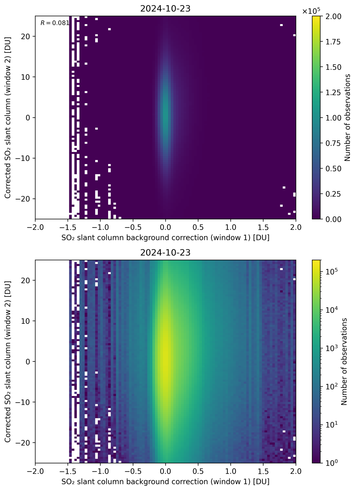
Figure 104: Scatter density plot of “SO 2 slant column background correction (window 1)” against “Corrected SO 2 slant column (window 2)” for 2024-10-22 to 2024-10-24.
