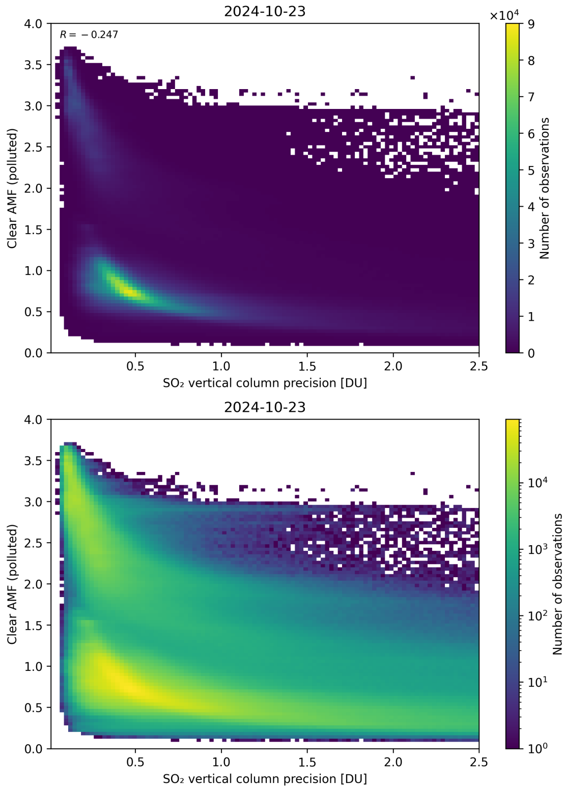
Figure 285: Scatter density plot of “SO 2 vertical column precision” against “Clear AMF (polluted)” for 2024-10-22 to 2024-10-24.
