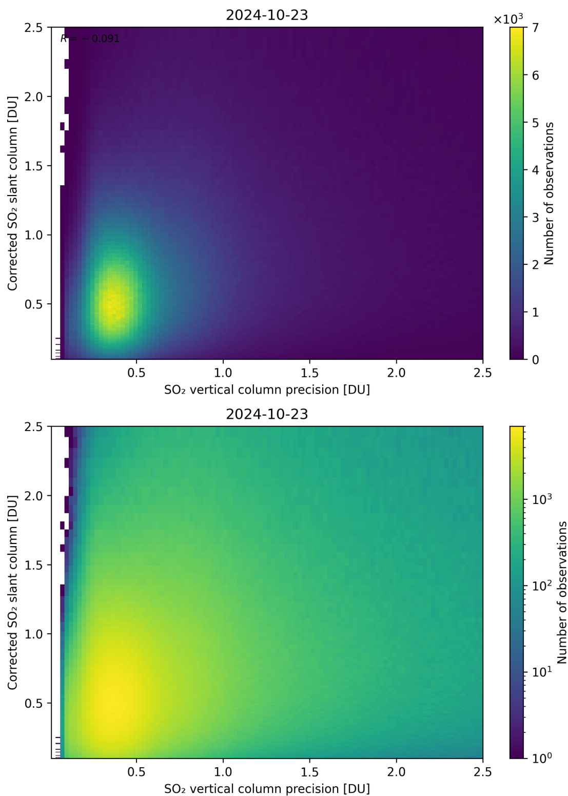
Figure 286: Scatter density plot of “SO 2 vertical column precision” against “Corrected SO 2 slant column” for 2024-10-22 to 2024-10-24.
