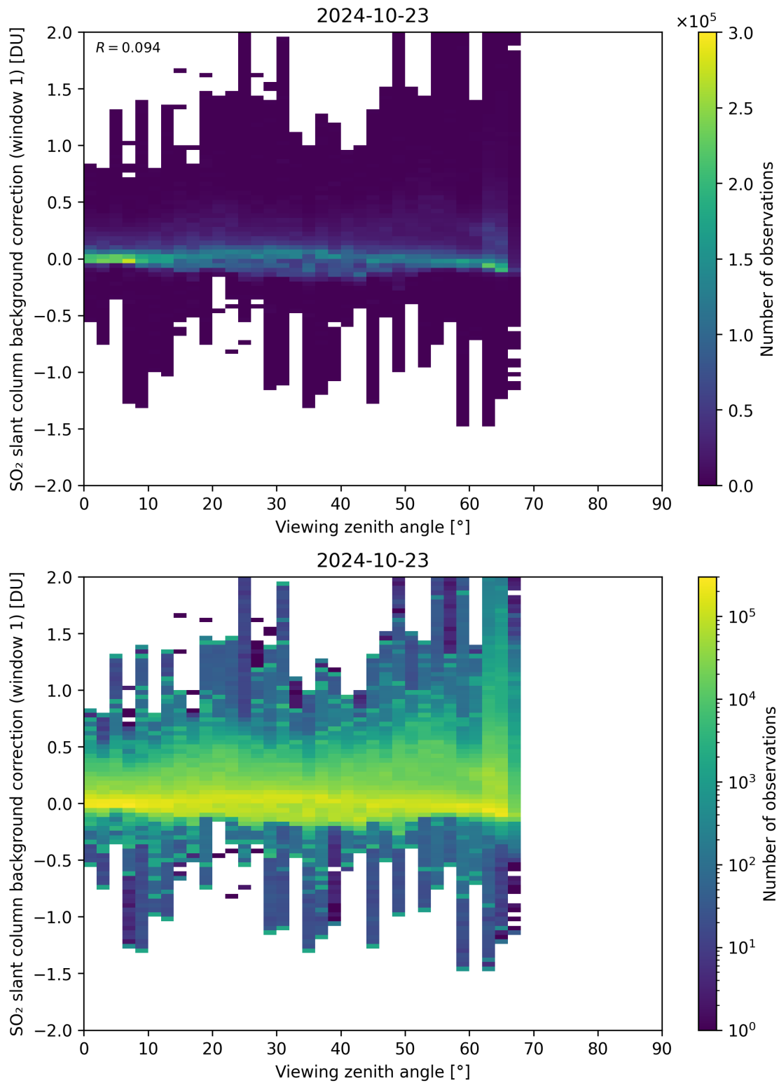
Figure 308: Scatter density plot of “Viewing zenith angle” against “SO 2 slant column background correction (window 1)” for 2024-10-22 to 2024-10-24.
