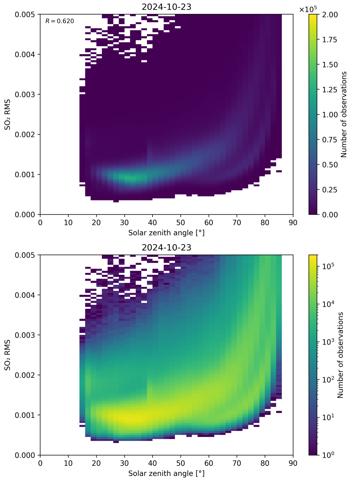
Figure 163: Scatter density plot of “Solar zenith angle” against “SO 2 RMS” for 2024-10-22 to 2024-10-24.
