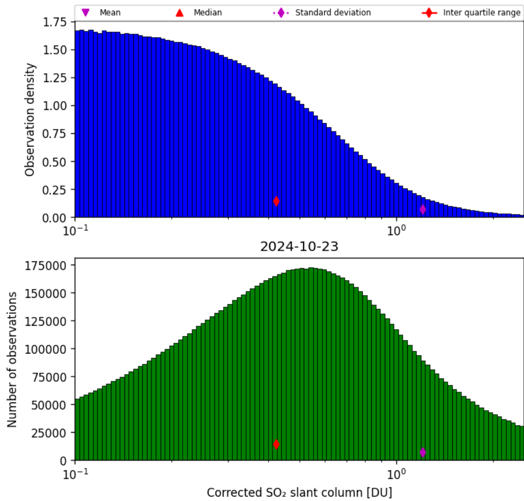
Figure 55: Histogram of “Corrected SO 2 slant column” for 2024-10-22 to 2024-10-24
