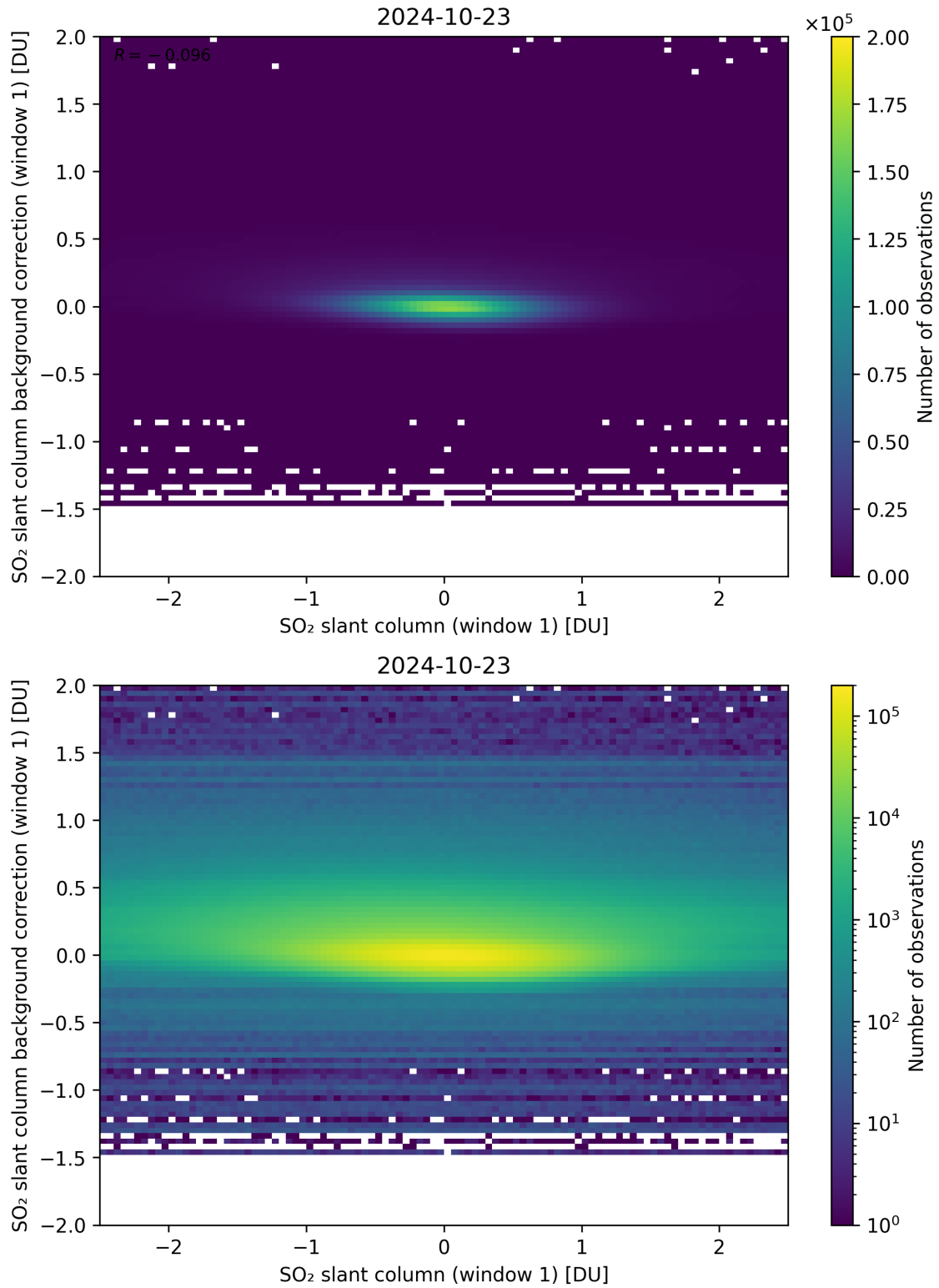
Figure 212: Scatter density plot of “SO 2 slant column (window 1)” against “SO 2 slant column background correction (window 1)” for 2024-10-22 to 2024-10-24.
