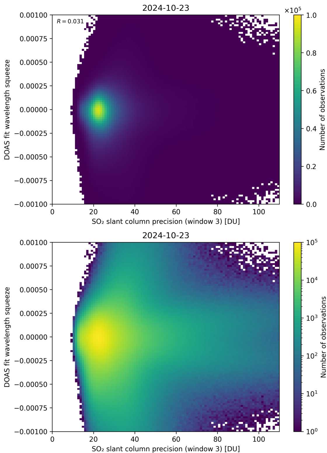
Figure 259: Scatter density plot of “SO 2 slant column precision (window 3)” against “DOAS fit wavelength squeeze” for 2024-10-22 to 2024-10-24.
