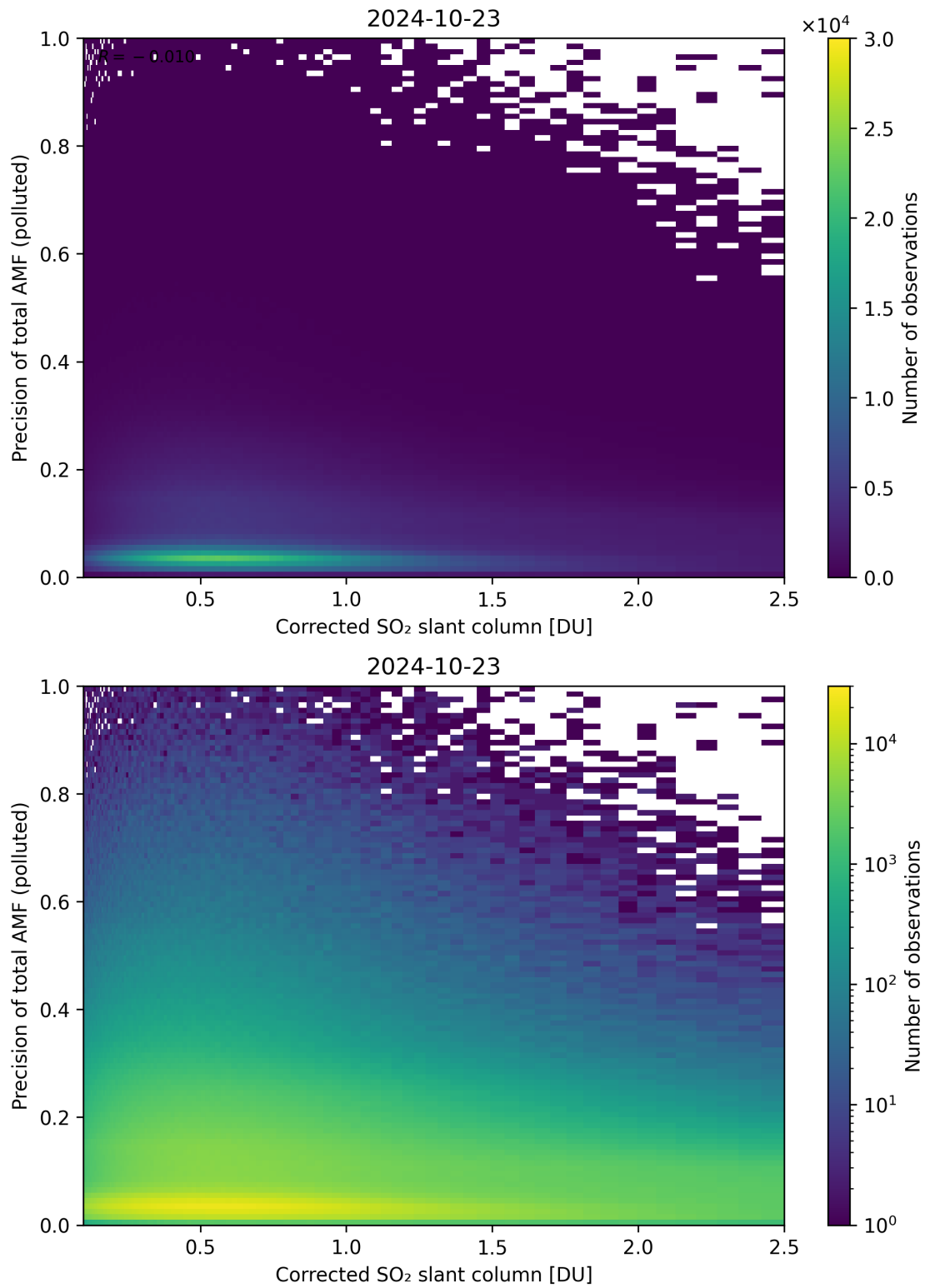
Figure 193: Scatter density plot of “Corrected SO 2 slant column” against “Precision of total AMF (polluted)” for 2024-10-22 to 2024-10-24.
