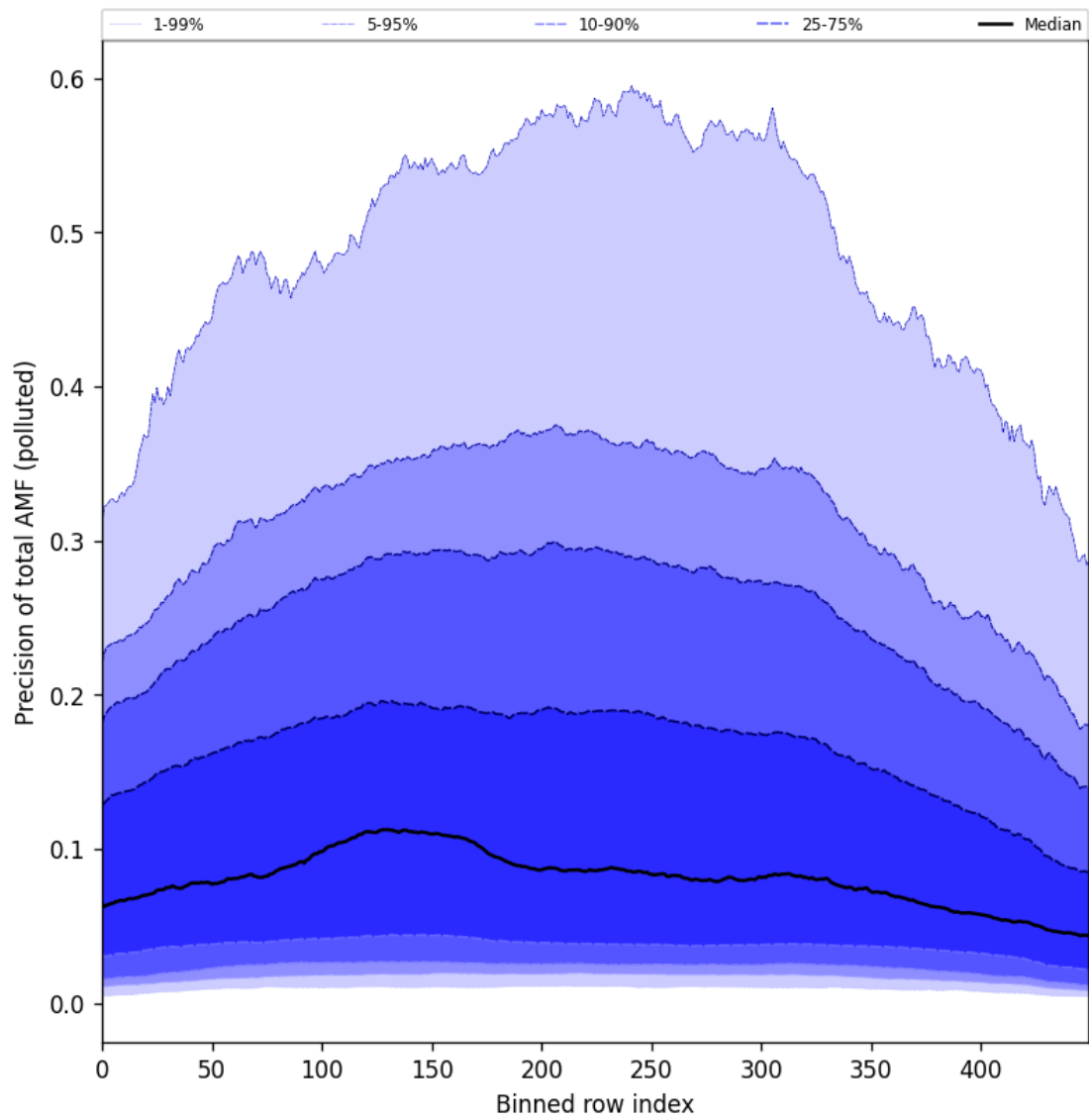
Figure 95: Along track statistics of “Precision of total AMF (polluted)” for 2024-10-22 to 2024-10-24
