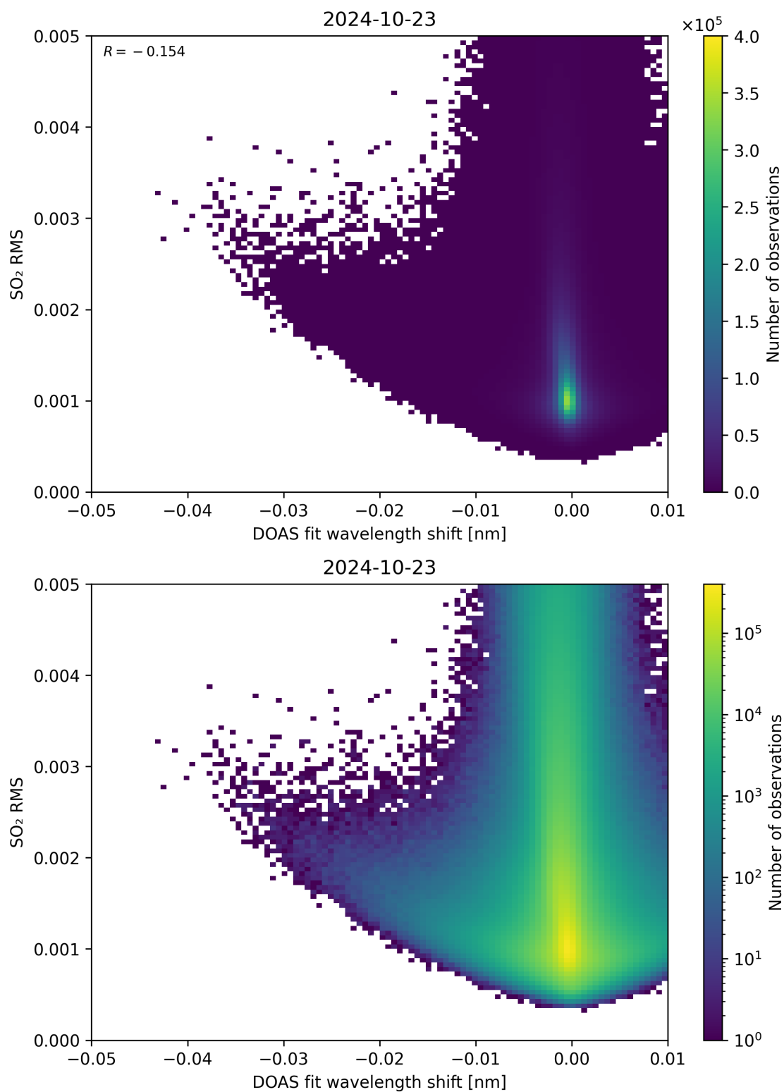
Figure 128: Scatter density plot of “DOAS fit wavelength shift” against “SO 2 RMS” for 2024-10-22 to 2024-10-24.
