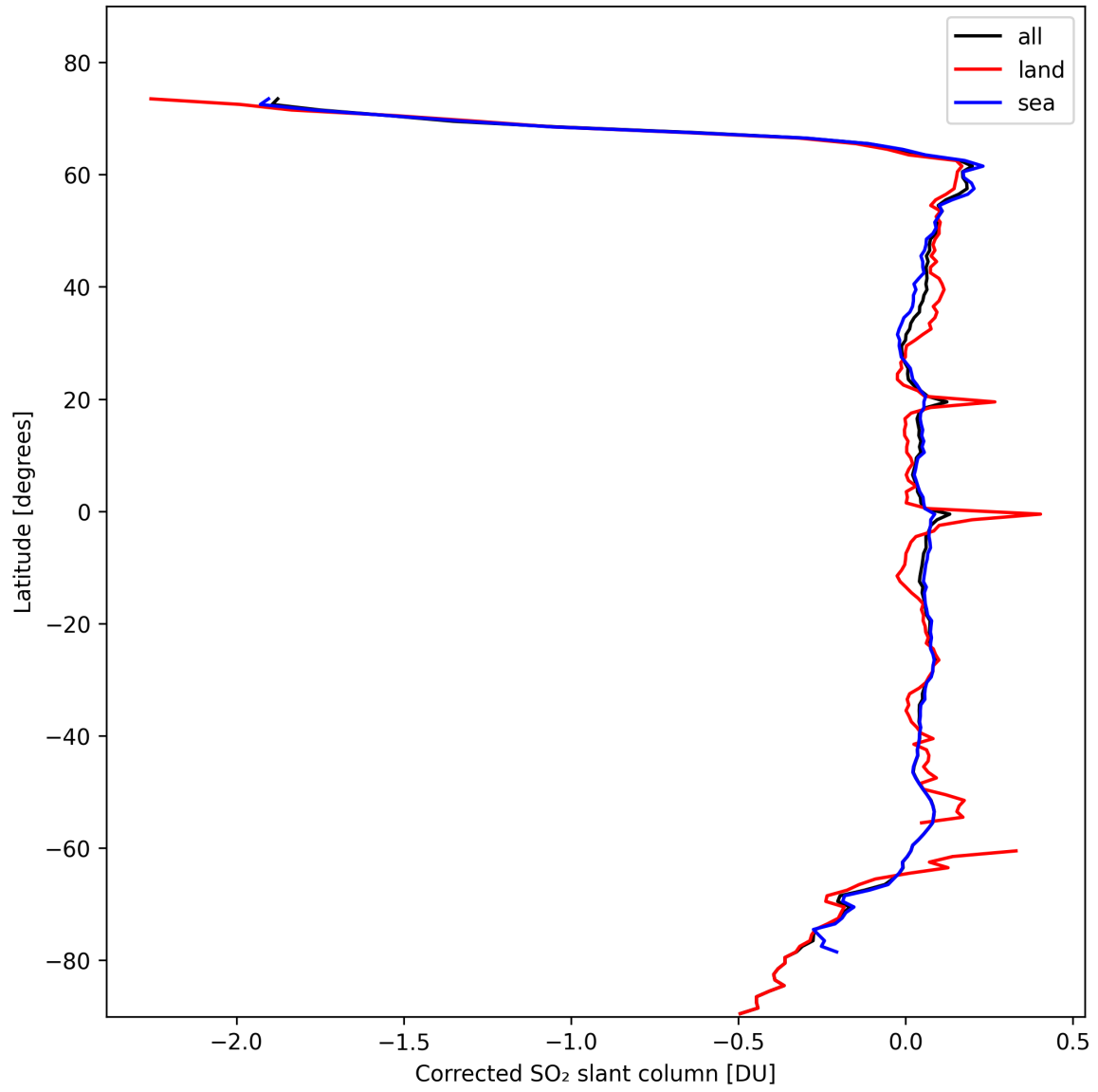
Figure 32: Zonal average of “Corrected SO 2 slant column” for 2024-10-22 to 2024-10-24.
