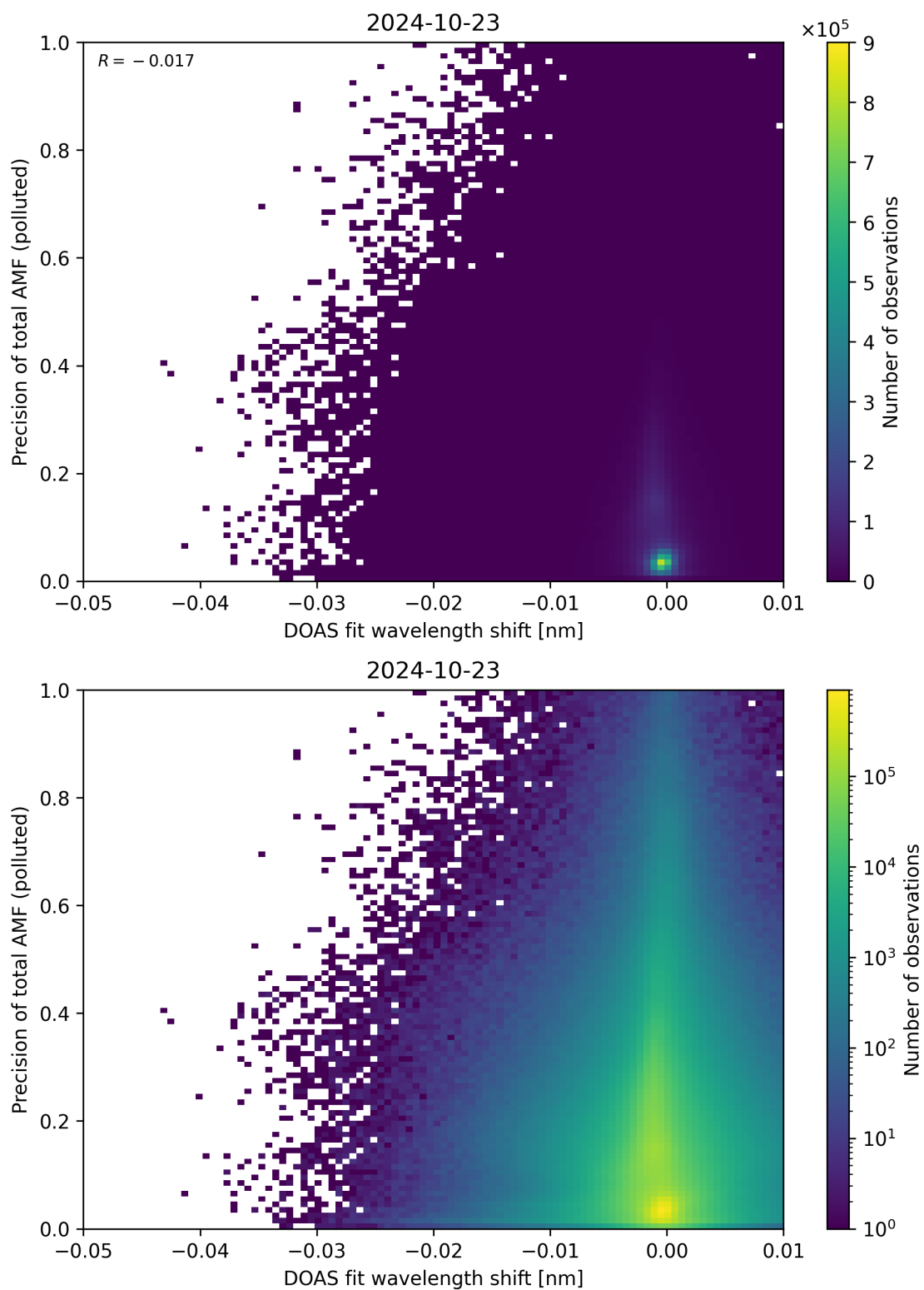
Figure 131: Scatter density plot of “DOAS fit wavelength shift” against “Precision of total AMF (polluted)” for 2024-10-22 to 2024-10-24.
