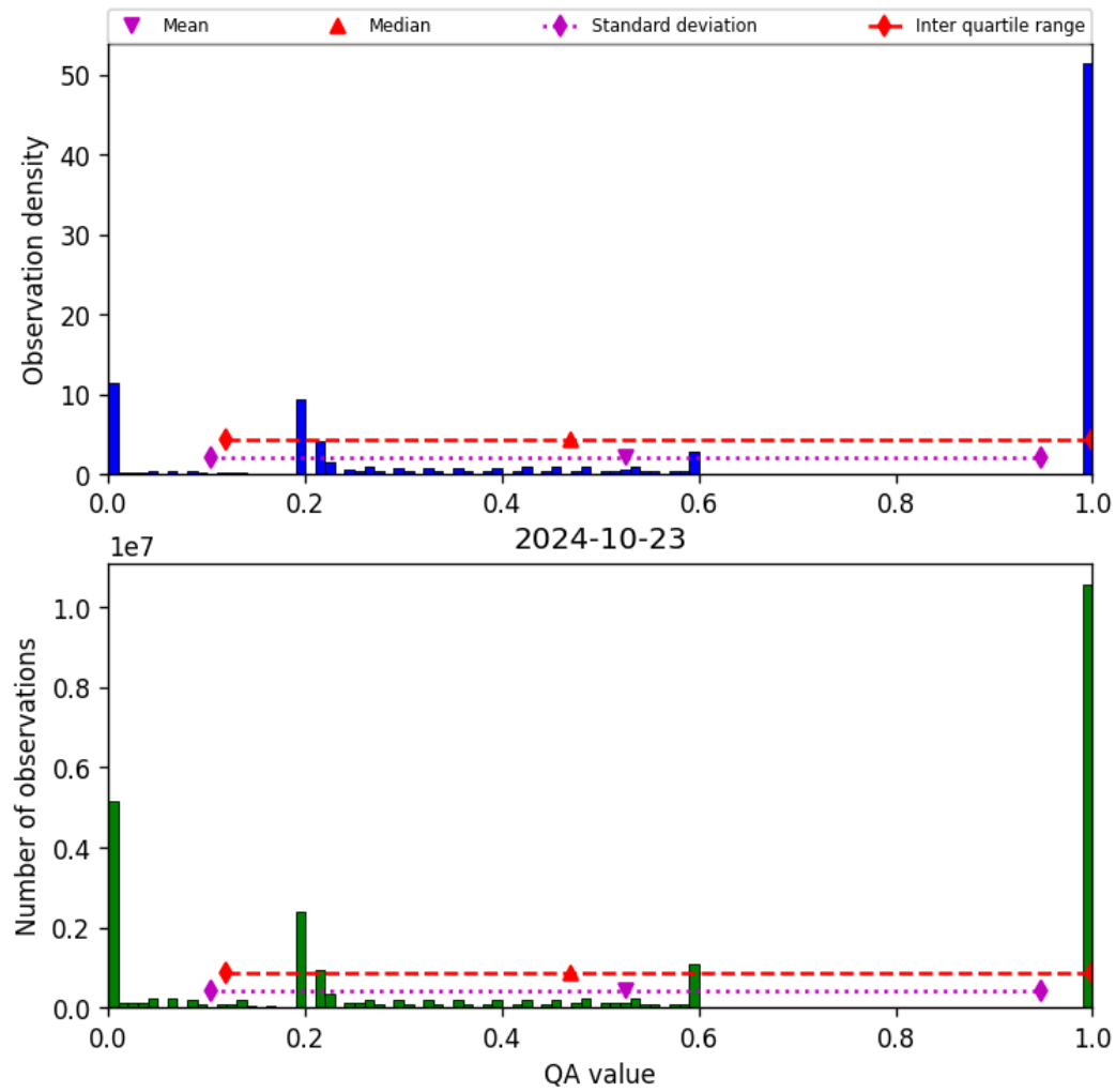
Figure 52: Histogram of “QA value” for 2024-10-22 to 2024-10-24
