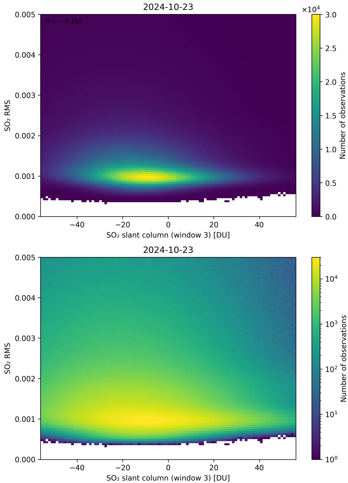
Figure 256: Scatter density plot of “SO 2 slant column (window 3)” against “SO 2 RMS” for 2024-10-22 to 2024-10-24.
