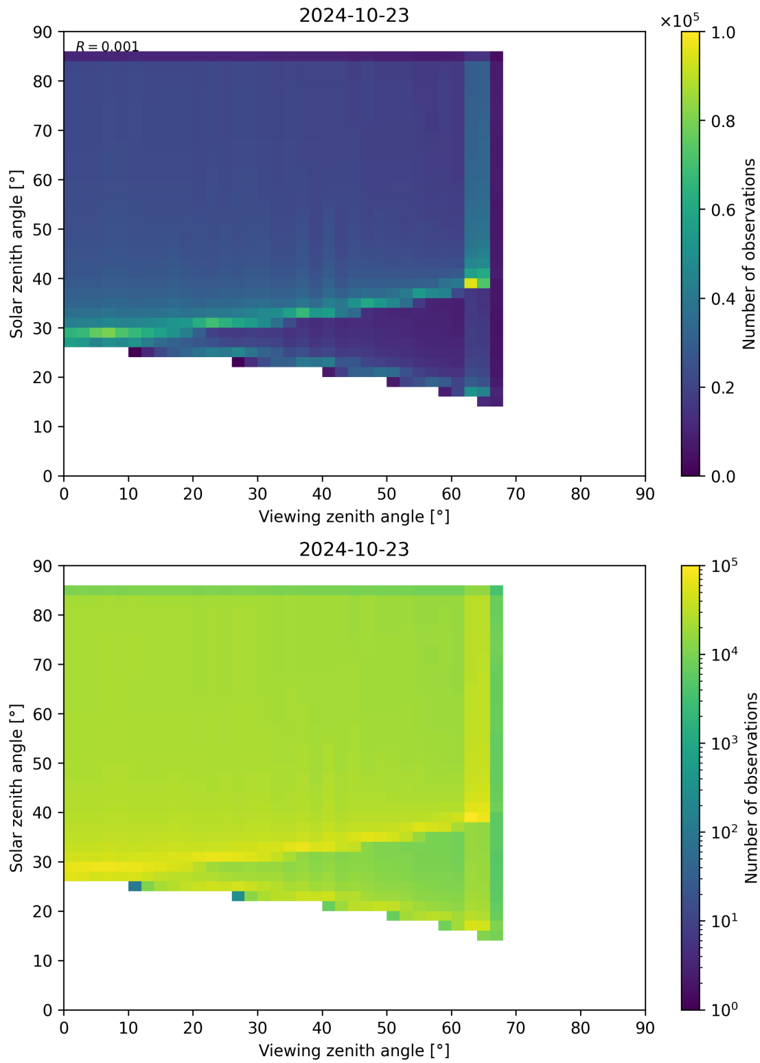
Figure 315: Scatter density plot of “Viewing zenith angle” against “Solar zenith angle” for 2024-10-22 to 2024-10-24.
