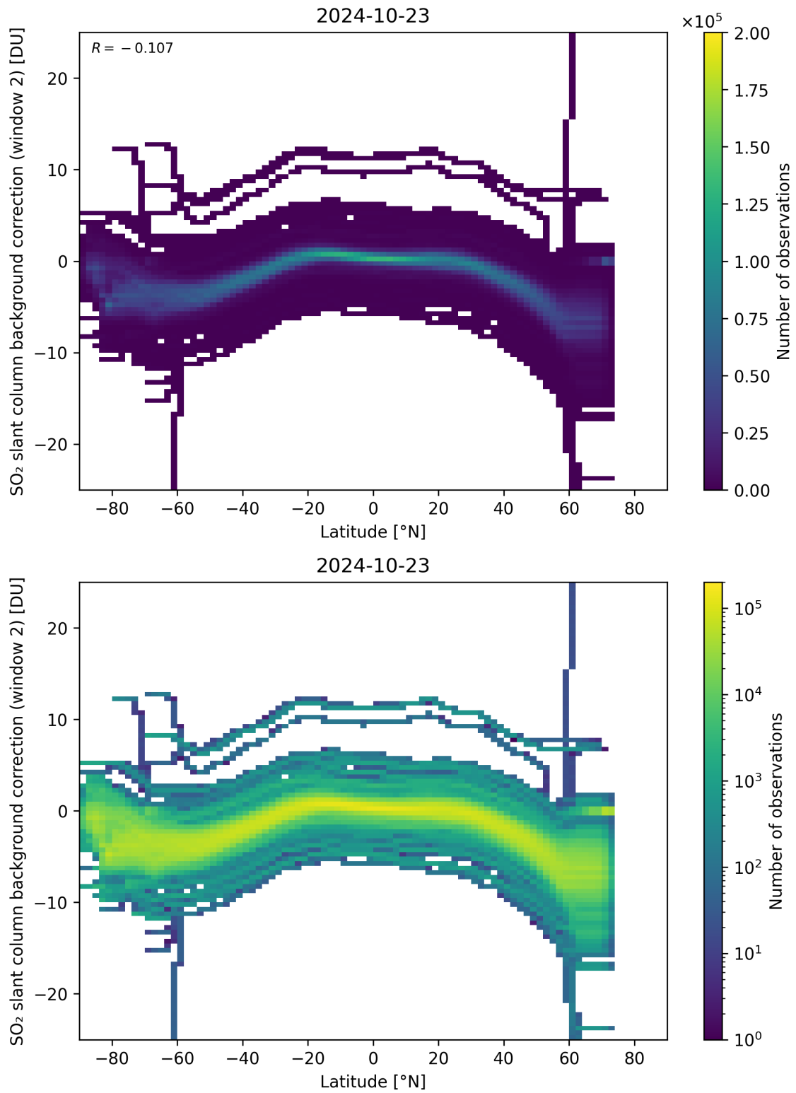
Figure 140: Scatter density plot of “Latitude” against “SO 2 slant column background correction (window 2)” for 2024-10-22 to 2024-10-24.
