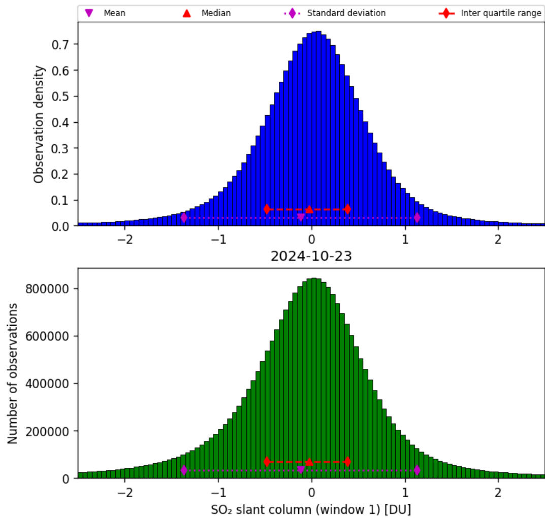
Figure 56: Histogram of “SO 2 slant column (window 1)” for 2024-10-22 to 2024-10-24
