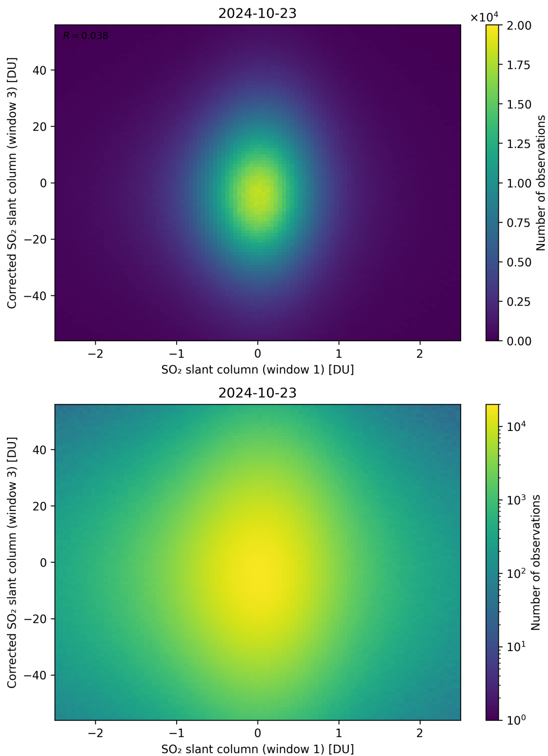
Figure 234: Scatter density plot of “SO 2 slant column (window 1)” against “Corrected SO 2 slant column (window 3)” for 2024-10-22 to 2024-10-24.
