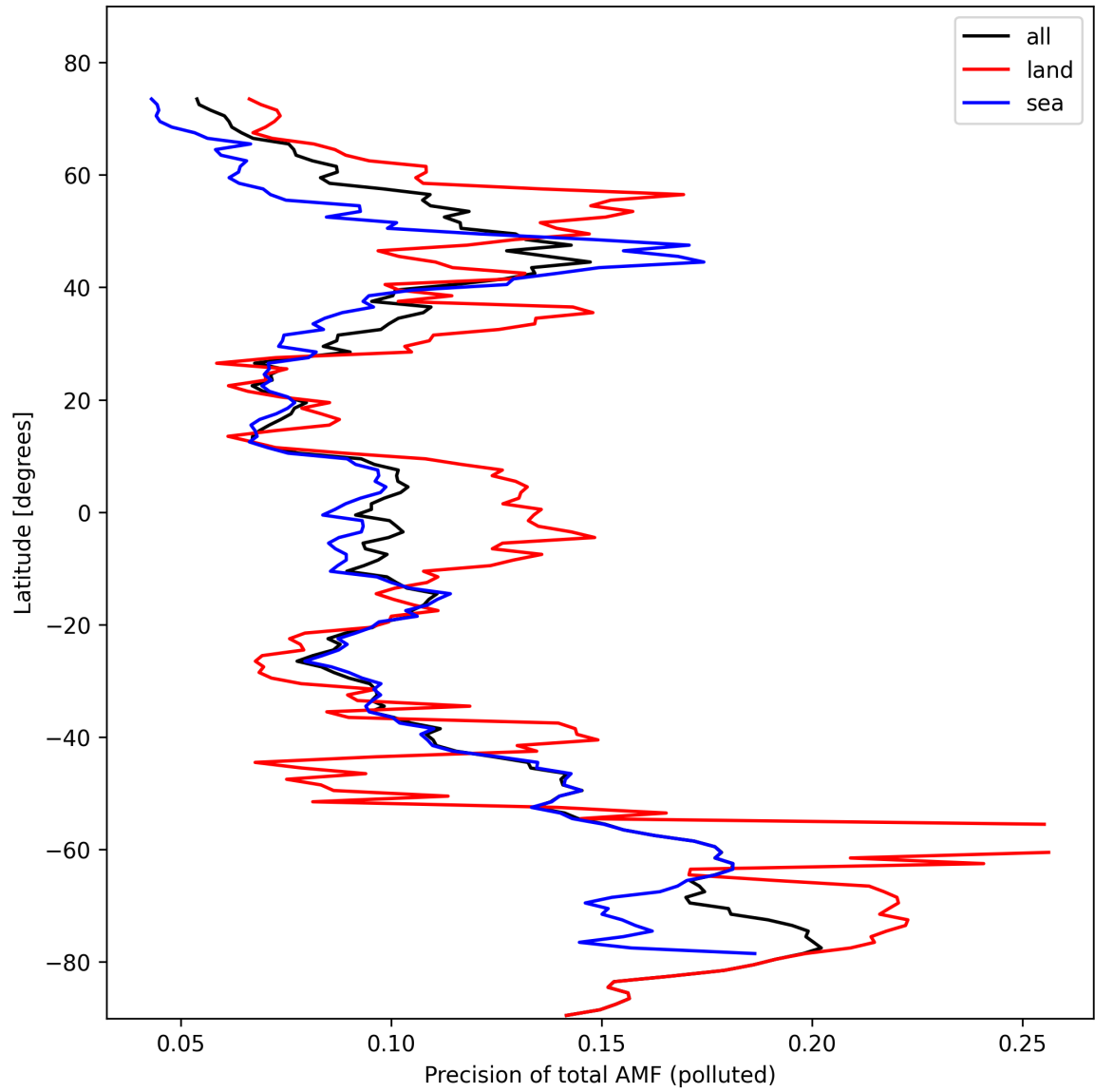
Figure 49: Zonal average of “Precision of total AMF (polluted)” for 2024-10-22 to 2024-10-24.
