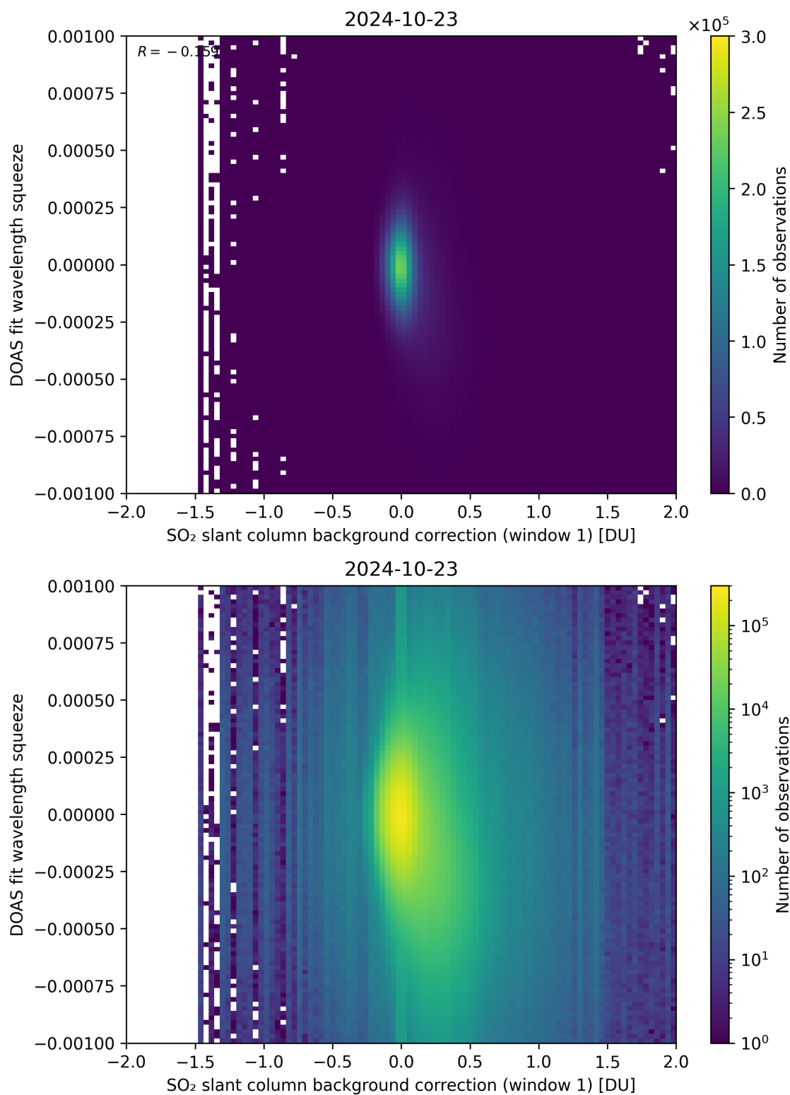
Figure 101: Scatter density plot of “SO 2 slant column background correction (window 1)” against “DOAS fit wavelength squeeze” for 2024-10-22 to 2024-10-24.
