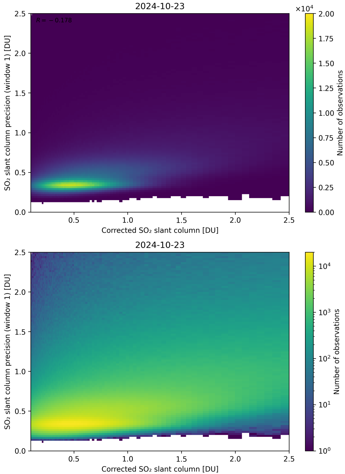
Figure 188: Scatter density plot of “Corrected SO 2 slant column” against “SO 2 slant column precision (window 1)” for 2024-10-22 to 2024-10-24.
