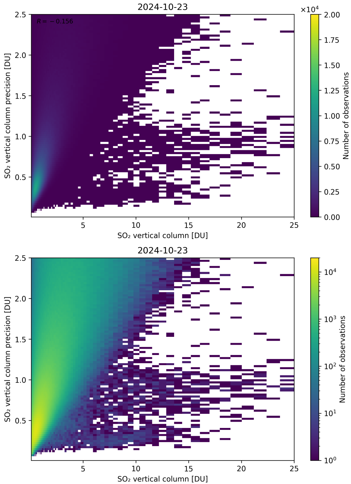
Figure 307: Scatter density plot of “SO 2 vertical column” against “SO 2 vertical column precision” for 2024-10-22 to 2024-10-24.
