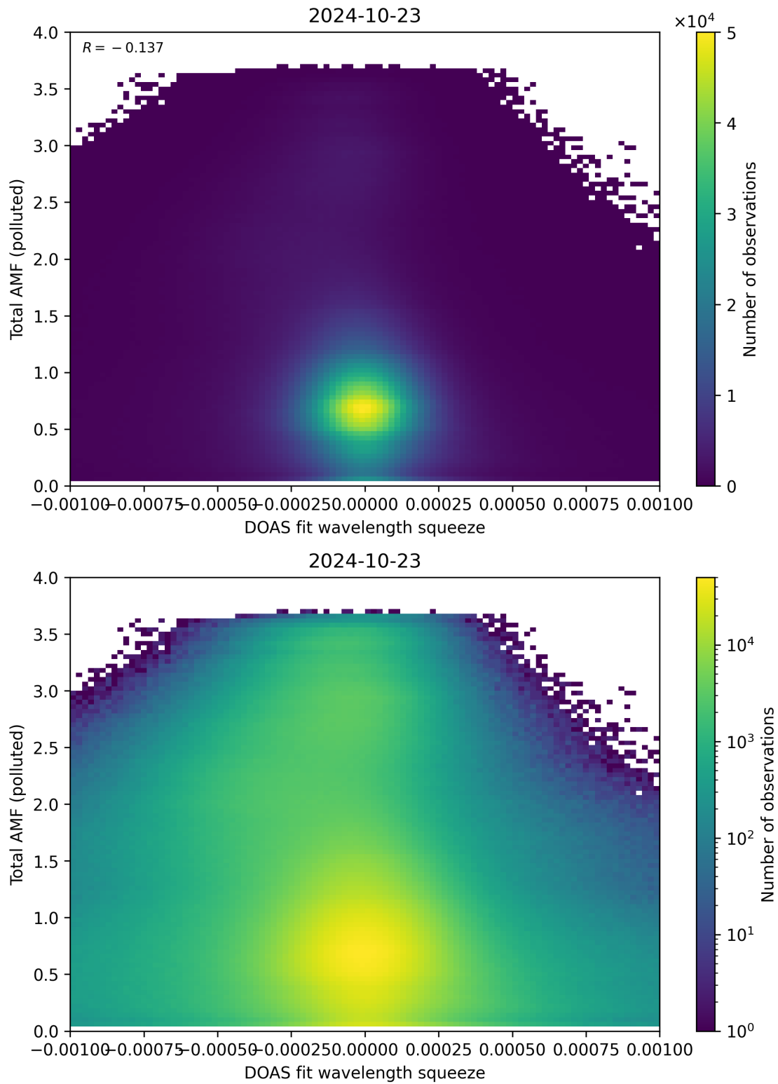
Figure 134: Scatter density plot of “DOAS fit wavelength squeeze” against “Total AMF (polluted)” for 2024-10-22 to 2024-10-24.
