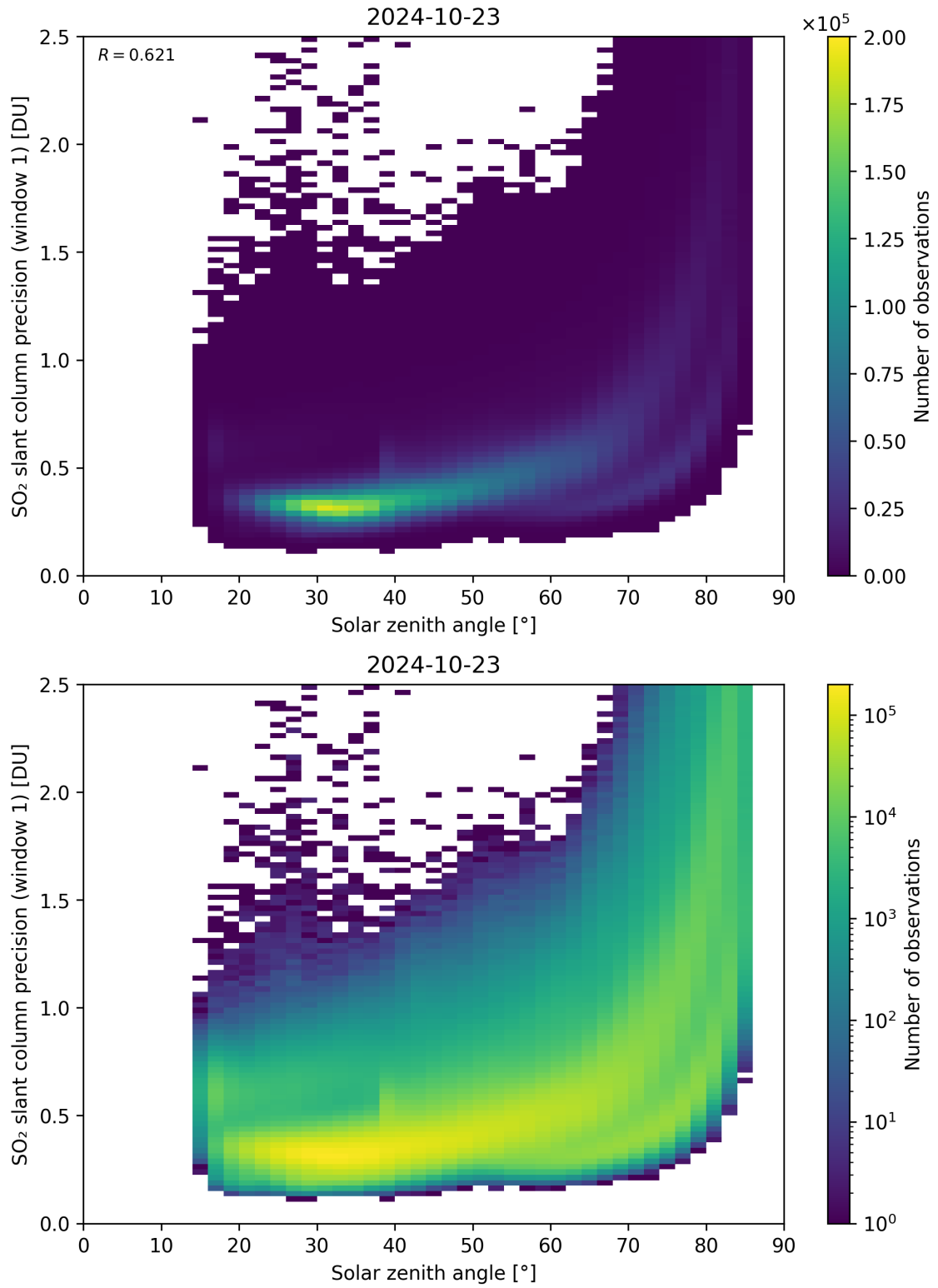
Figure 170: Scatter density plot of “Solar zenith angle” against “SO 2 slant column precision (window 1)” for 2024-10-22 to 2024-10-24.
