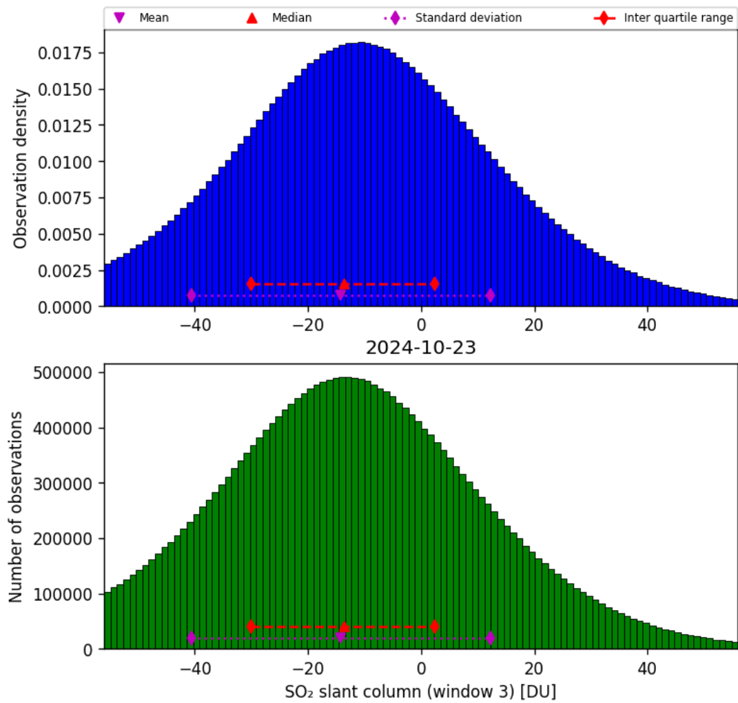
Figure 64: Histogram of “SO 2 slant column (window 3)” for 2024-10-22 to 2024-10-24
