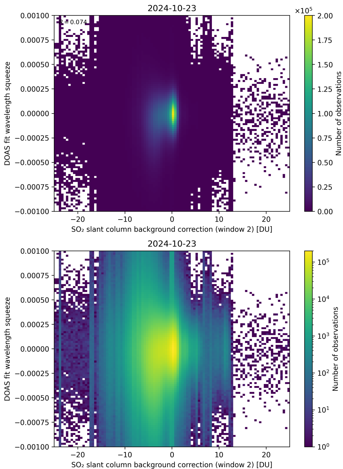
Figure 113: Scatter density plot of “SO 2 slant column background correction (window 2)” against “DOAS fit wavelength squeeze” for 2024-10-22 to 2024-10-24.
