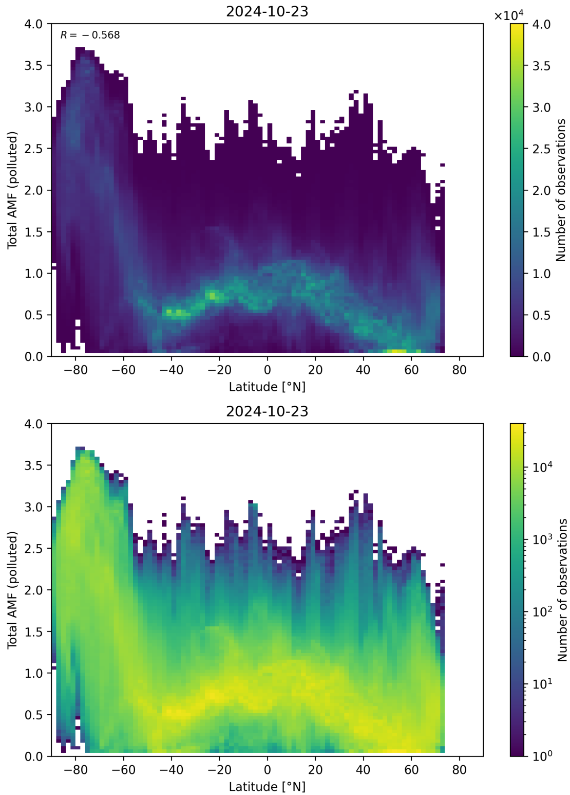
Figure 154: Scatter density plot of “Latitude” against “Total AMF (polluted)” for 2024-10-22 to 2024-10-24.
