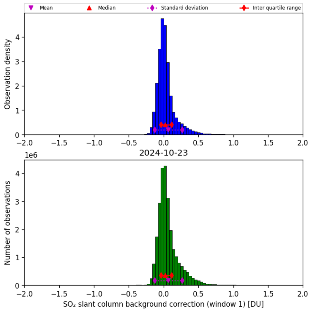
Figure 59: Histogram of “SO 2 slant column background correction (window 1)” for 2024-10-22 to 2024-10-24
