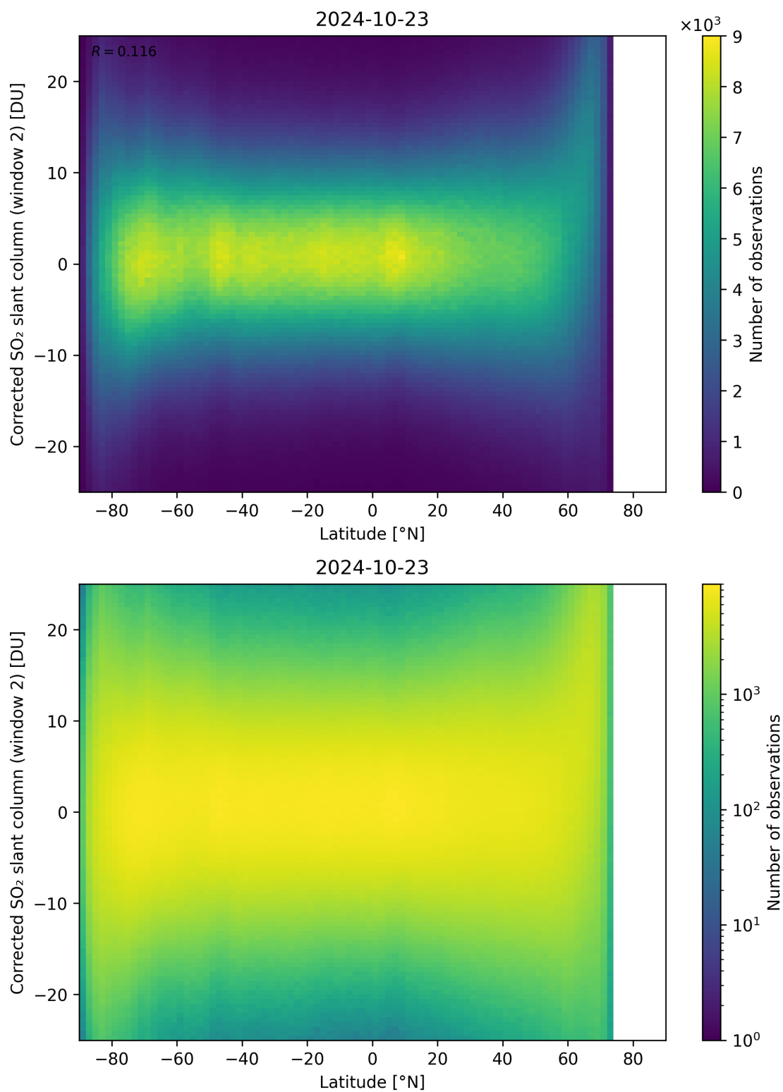
Figure 147: Scatter density plot of “Latitude” against “Corrected SO 2 slant column (window 2)” for 2024-10-22 to 2024-10-24.
