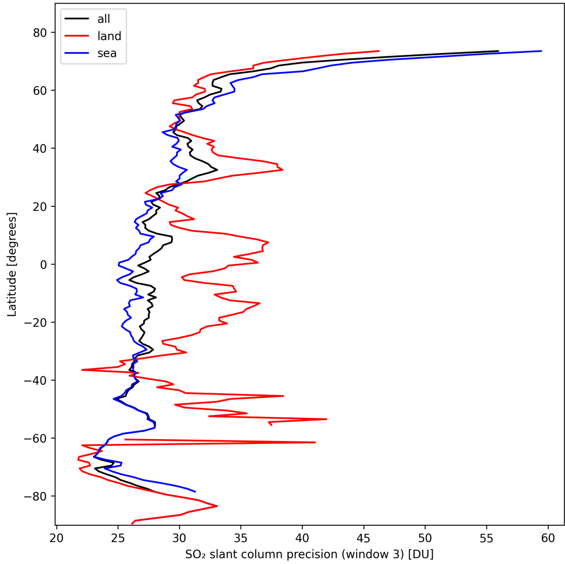
Figure 42: Zonal average of “SO 2 slant column precision (window 3)” for 2024-10-22 to 2024-10-24.
