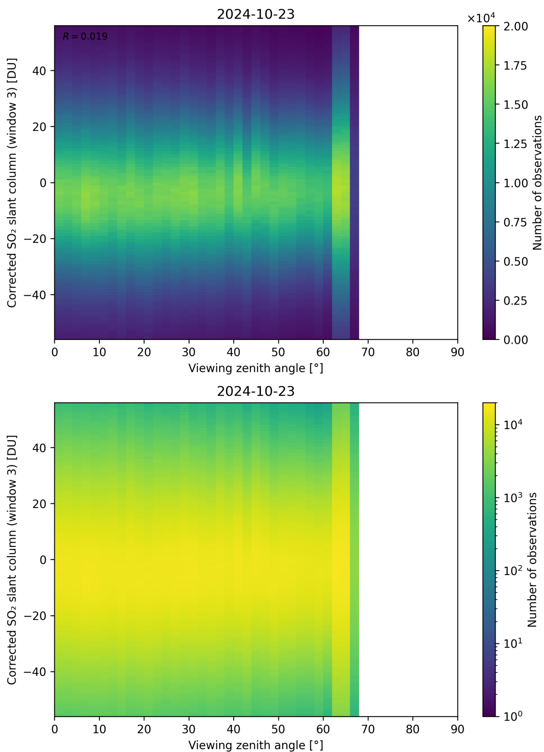
Figure 319: Scatter density plot of “Viewing zenith angle” against “Corrected SO 2 slant column (window 3)” for 2024-10-22 to 2024-10-24.
