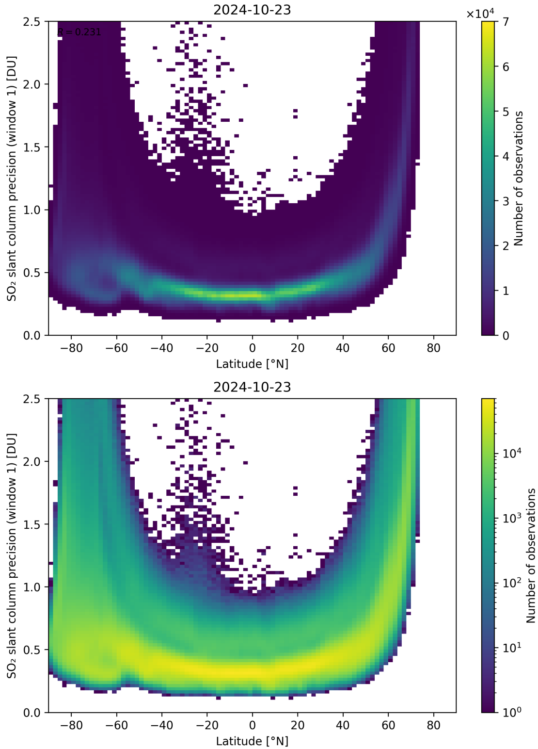
Figure 150: Scatter density plot of “Latitude” against “SO 2 slant column precision (window 1)” for 2024-10-22 to 2024-10-24.
