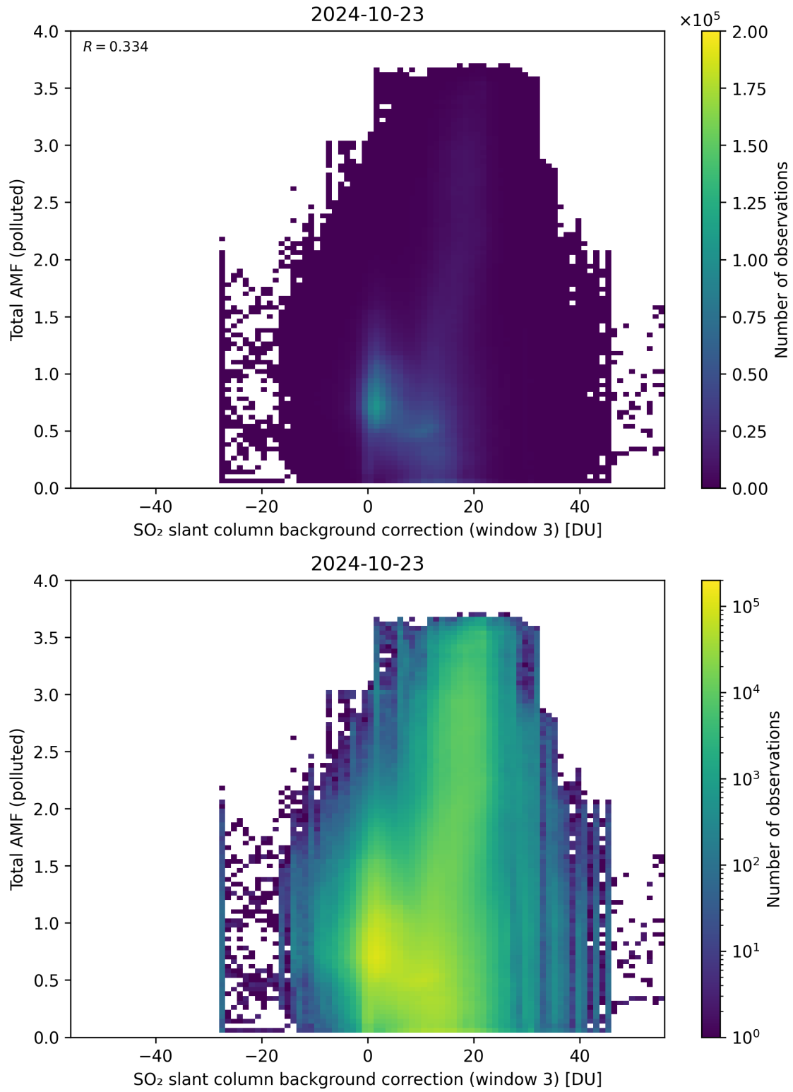
Figure 125: Scatter density plot of “SO 2 slant column background correction (window 3)” against “Total AMF (polluted)” for 2024-10-22 to 2024-10-24.
