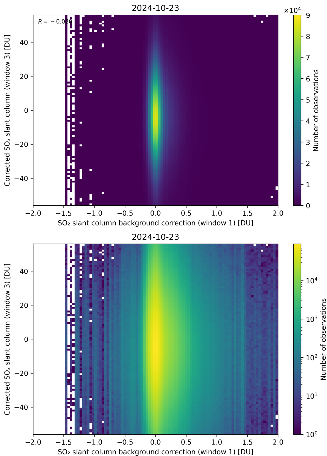
Figure 105: Scatter density plot of “SO 2 slant column background correction (window 1)” against “Corrected SO 2 slant column (window 3)” for 2024-10-22 to 2024-10-24.
