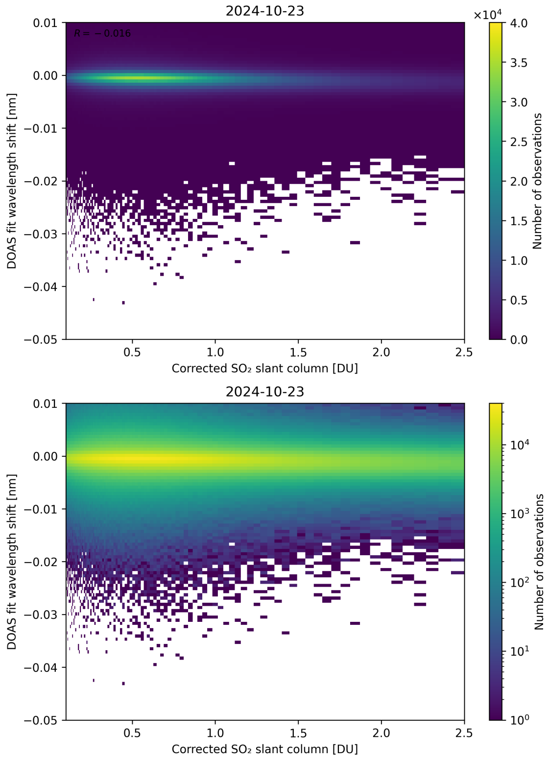
Figure 181: Scatter density plot of “Corrected SO 2 slant column” against “DOAS fit wavelength shift” for 2024-10-22 to 2024-10-24.
