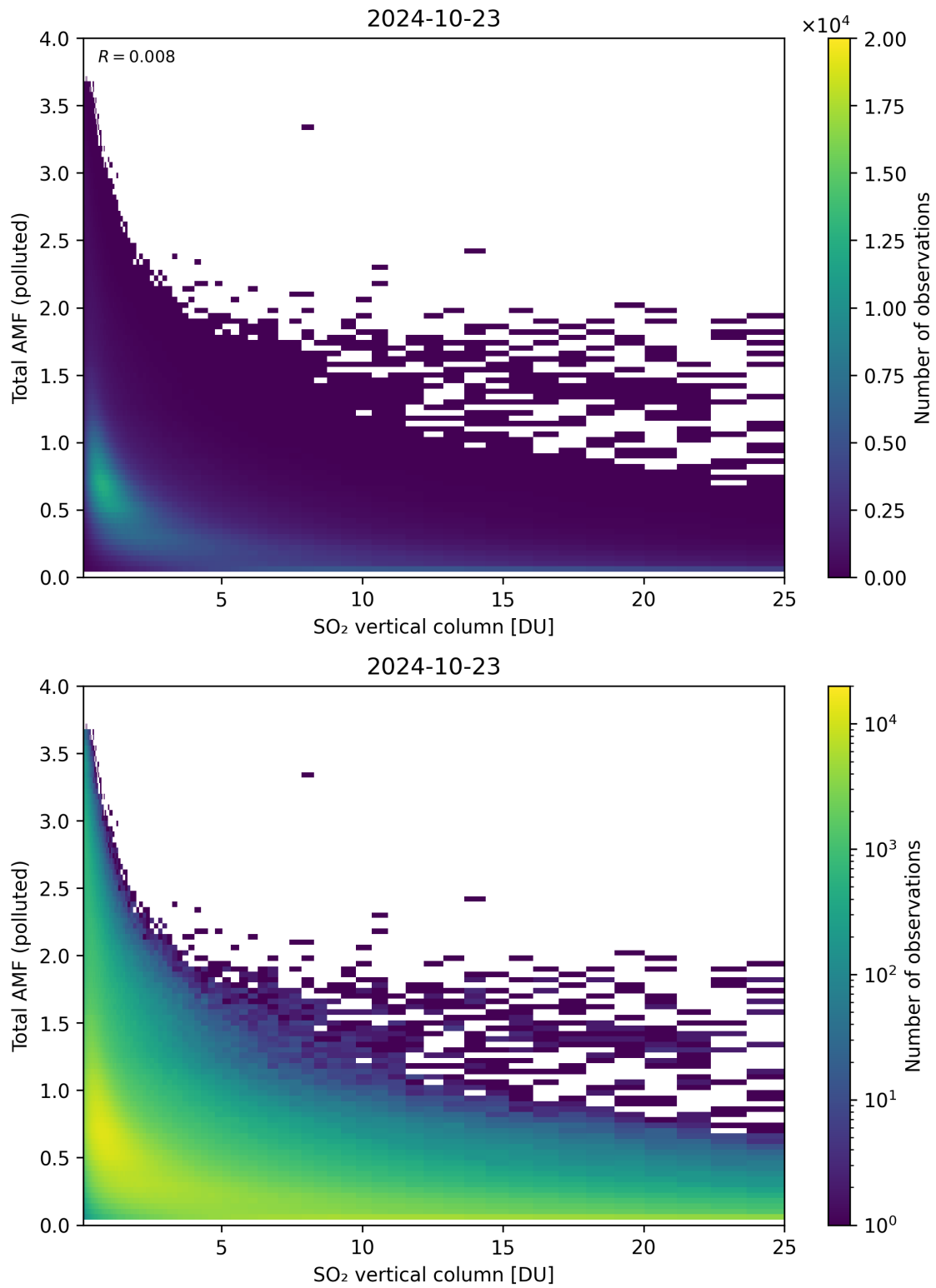
Figure 305: Scatter density plot of “SO 2 vertical column” against “Total AMF (polluted)” for 2024-10-22 to 2024-10-24.
