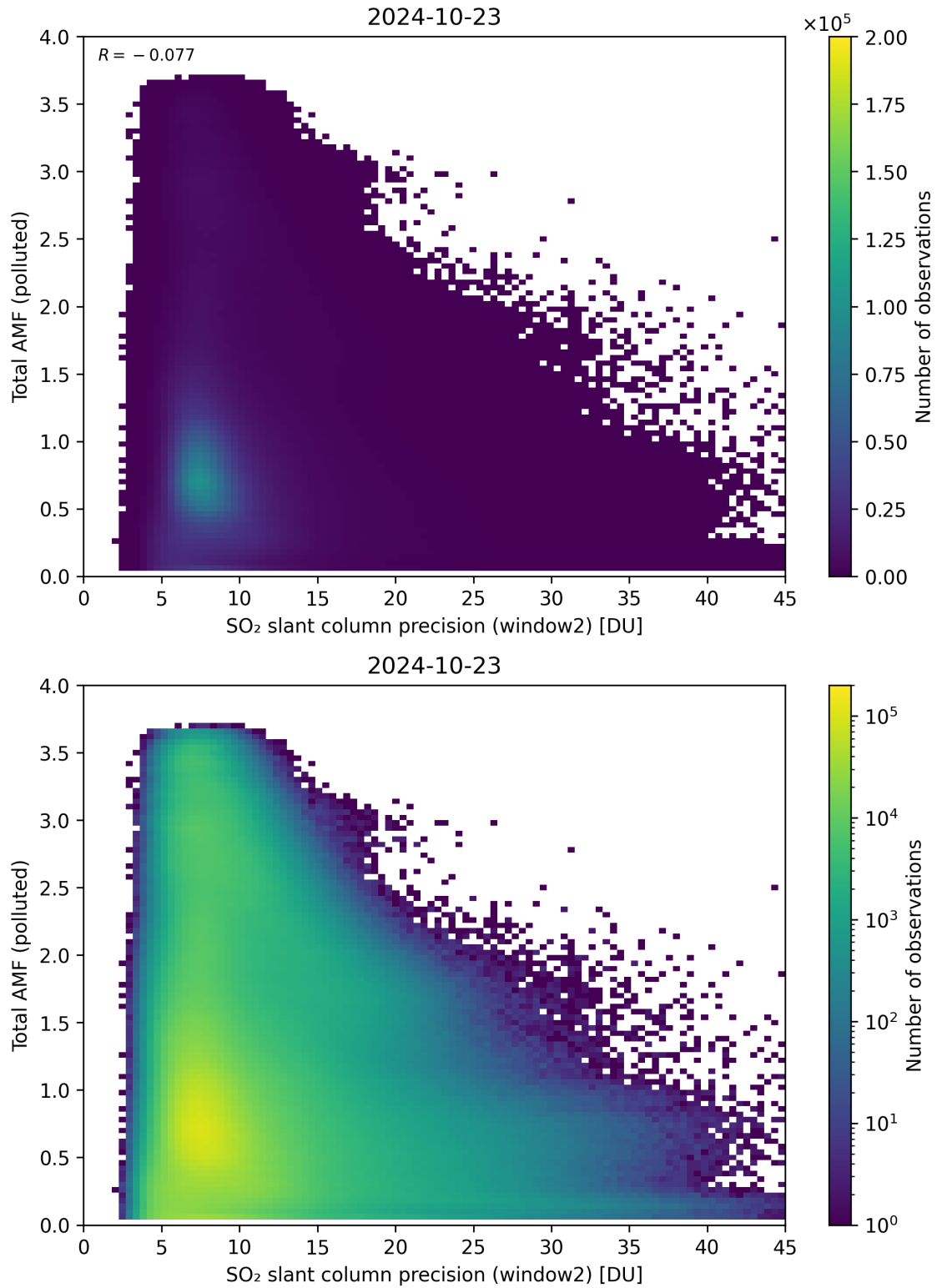
Figure 251: Scatter density plot of “SO 2 slant column precision (window2)” against “Total AMF (polluted)” for 2024-10-22 to 2024-10-24.
