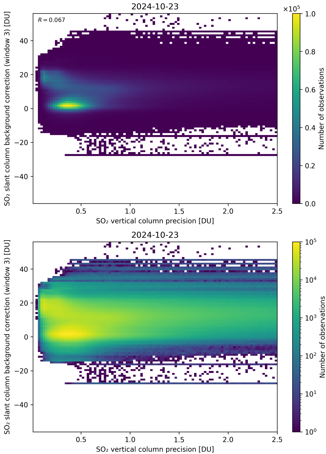
Figure 281: Scatter density plot of “SO 2 vertical column precision” against “SO 2 slant column background correction (window 3)” for 2024-10-22 to 2024-10-24.
