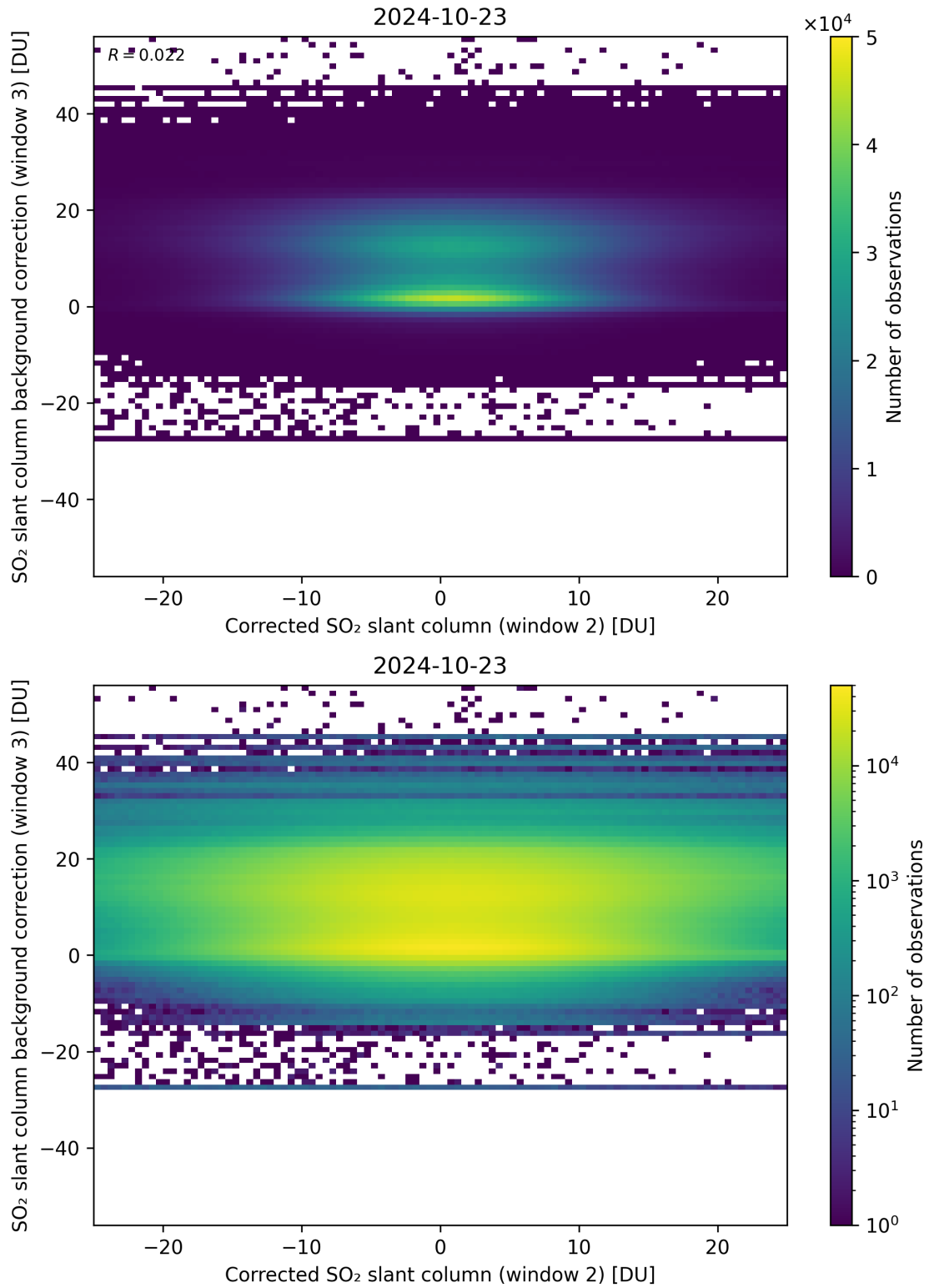
Figure 195: Scatter density plot of “Corrected SO 2 slant column (window 2)” against “SO 2 slant column background correction (window 3)” for 2024-10-22 to 2024-10-24.
