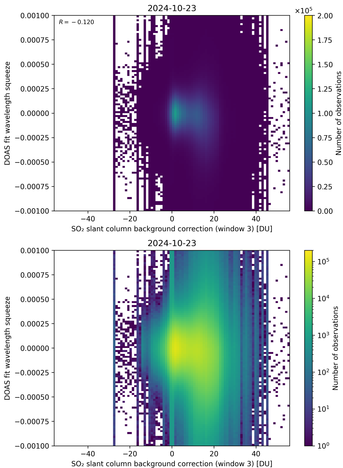
Figure 122: Scatter density plot of “SO 2 slant column background correction (window 3)” against “DOAS fit wavelength squeeze” for 2024-10-22 to 2024-10-24.
