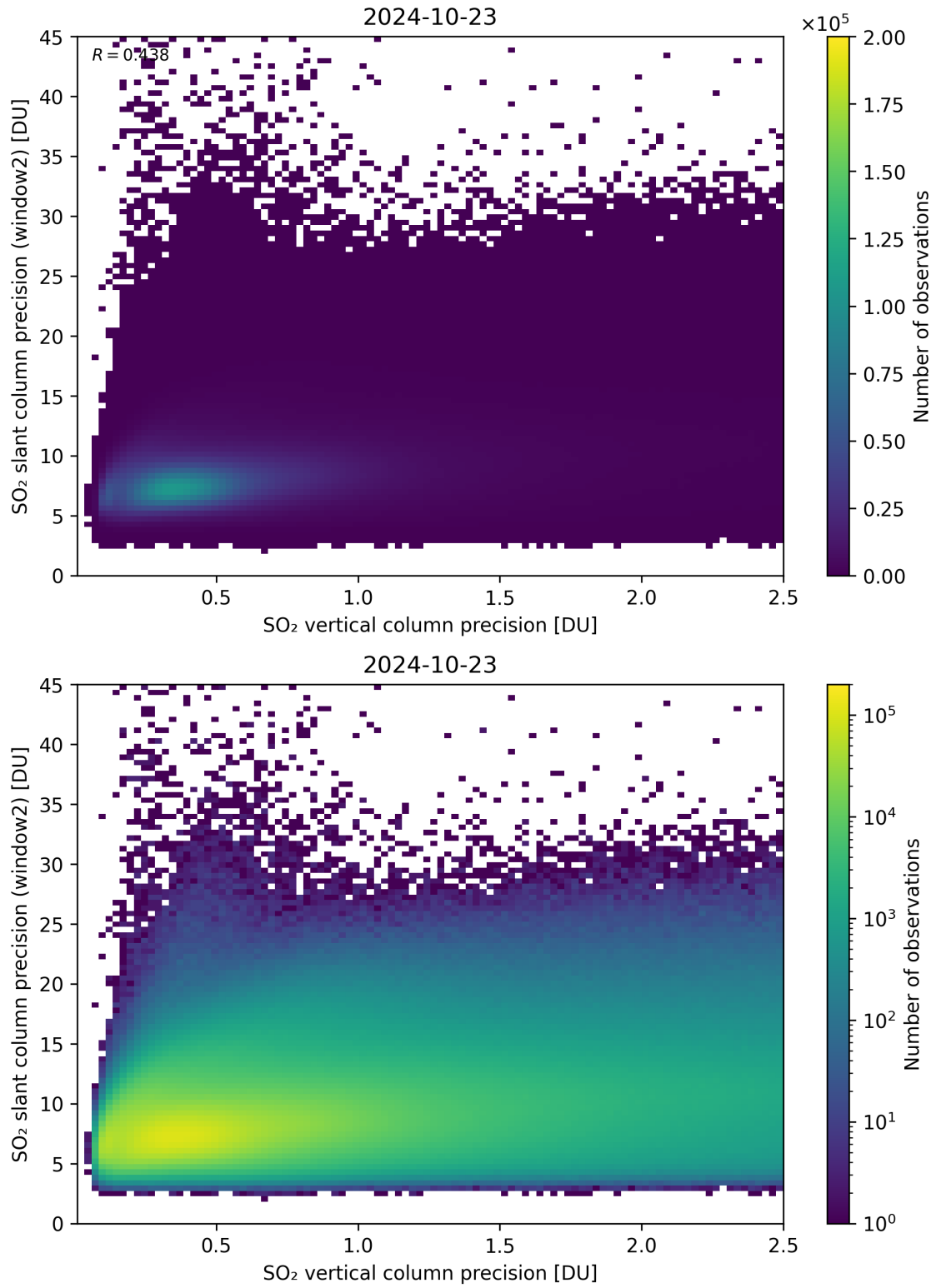
Figure 291: Scatter density plot of “SO 2 vertical column precision” against “SO 2 slant column precision (window2)” for 2024-10-22 to 2024-10-24.
