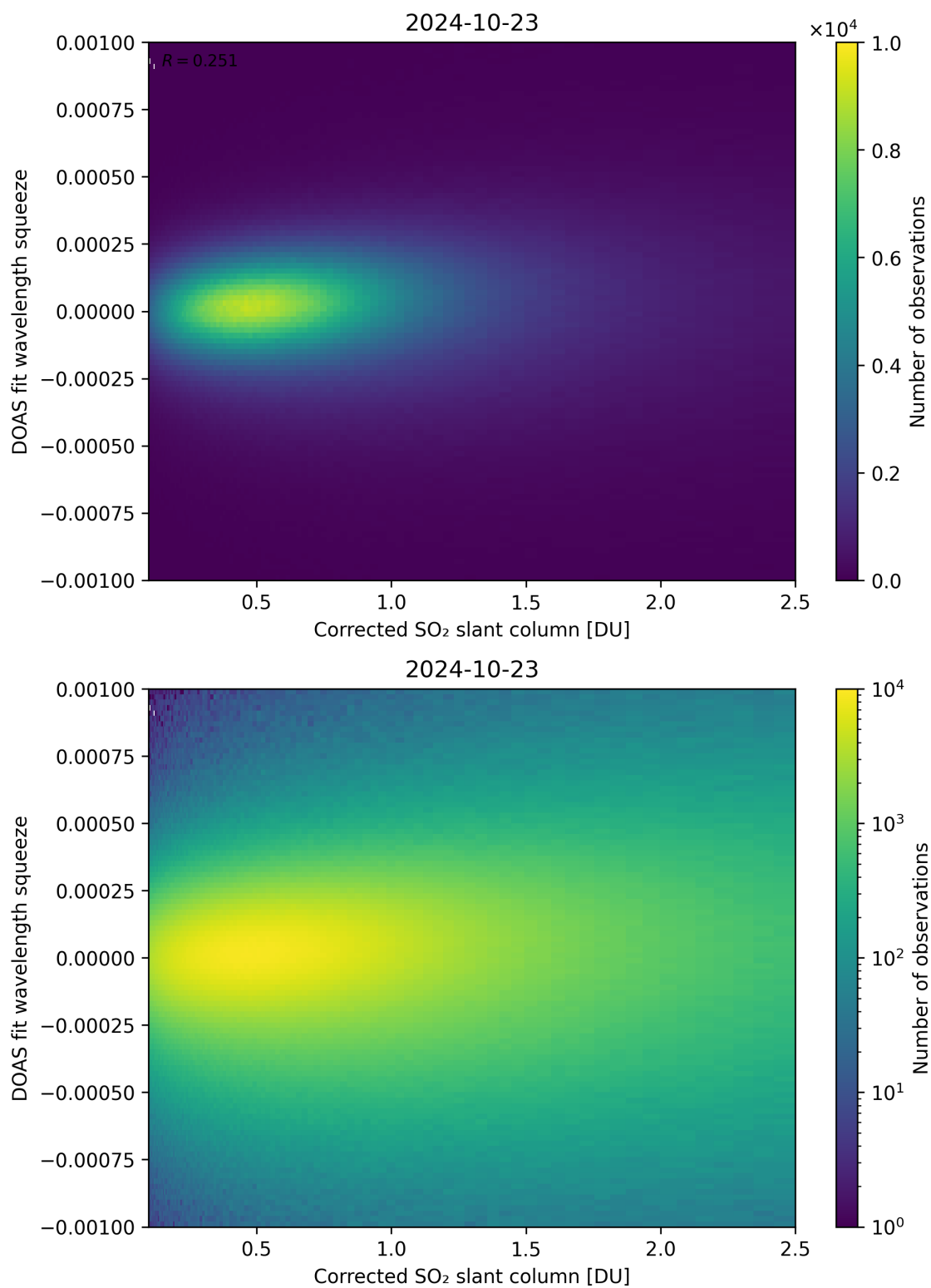
Figure 182: Scatter density plot of “Corrected SO 2 slant column” against “DOAS fit wavelength squeeze” for 2024-10-22 to 2024-10-24.
