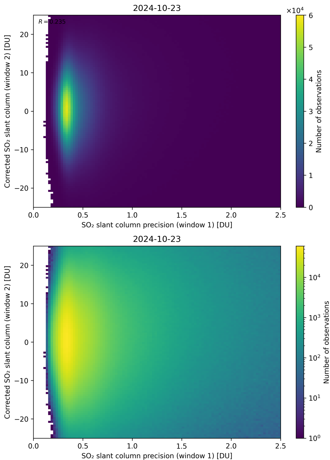
Figure 225: Scatter density plot of “SO 2 slant column precision (window 1)” against “Corrected SO 2 slant column (window 2)” for 2024-10-22 to 2024-10-24.
