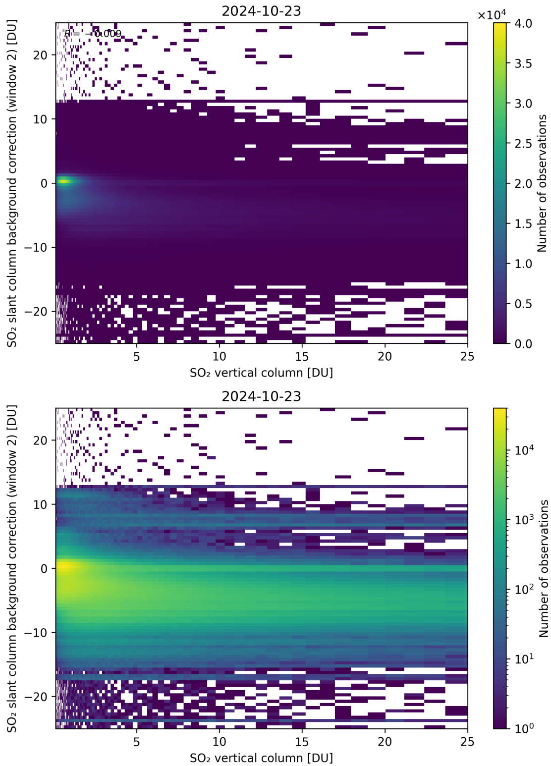
Figure 274: Scatter density plot of “SO 2 vertical column” against “SO 2 slant column background correction (window 2)” for 2024-10-22 to 2024-10-24.
