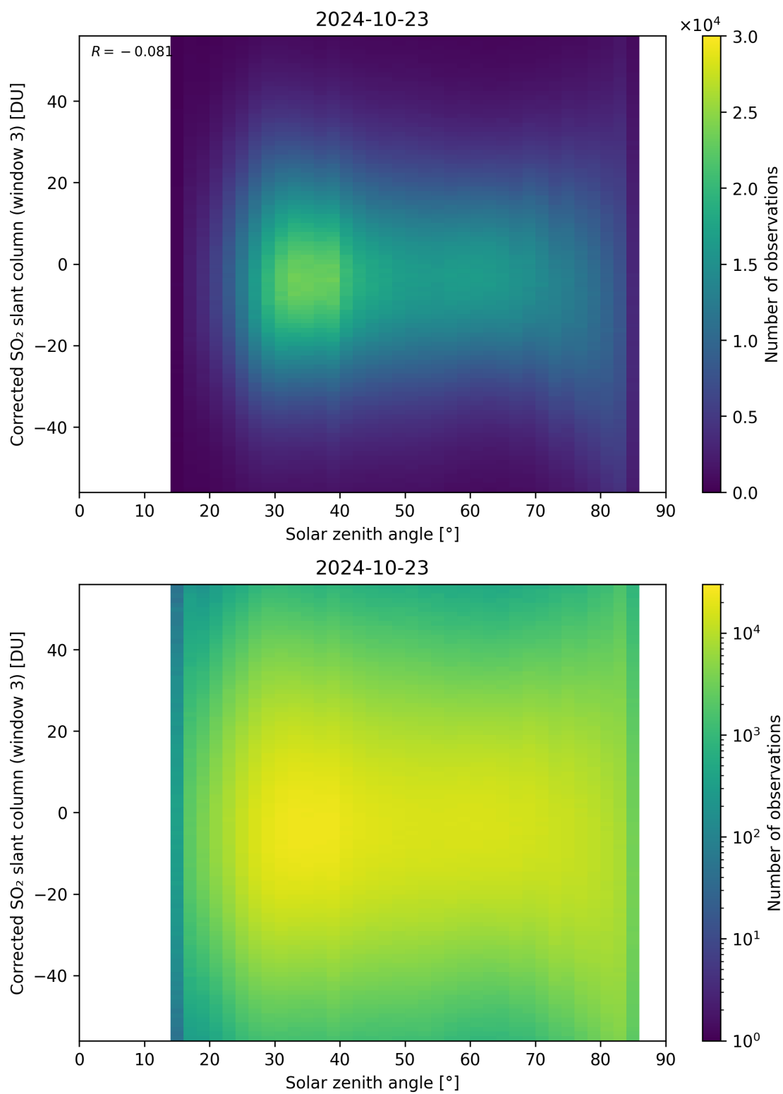
Figure 168: Scatter density plot of “Solar zenith angle” against “Corrected SO 2 slant column (window 3)” for 2024-10-22 to 2024-10-24.
