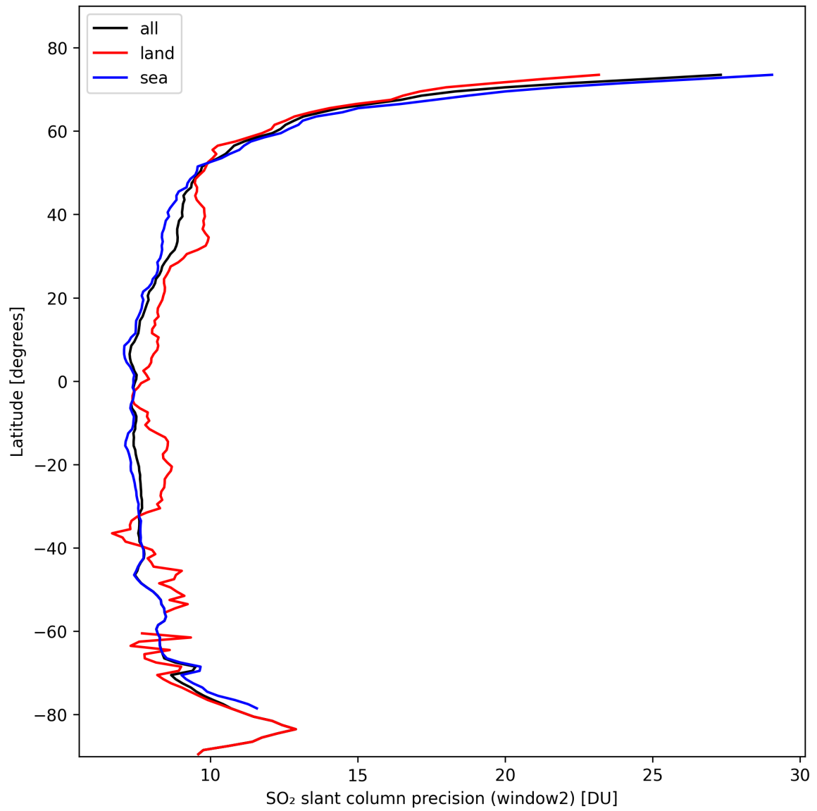
Figure 38: Zonal average of “SO 2 slant column precision (window2)” for 2024-10-22 to 2024-10-24.
