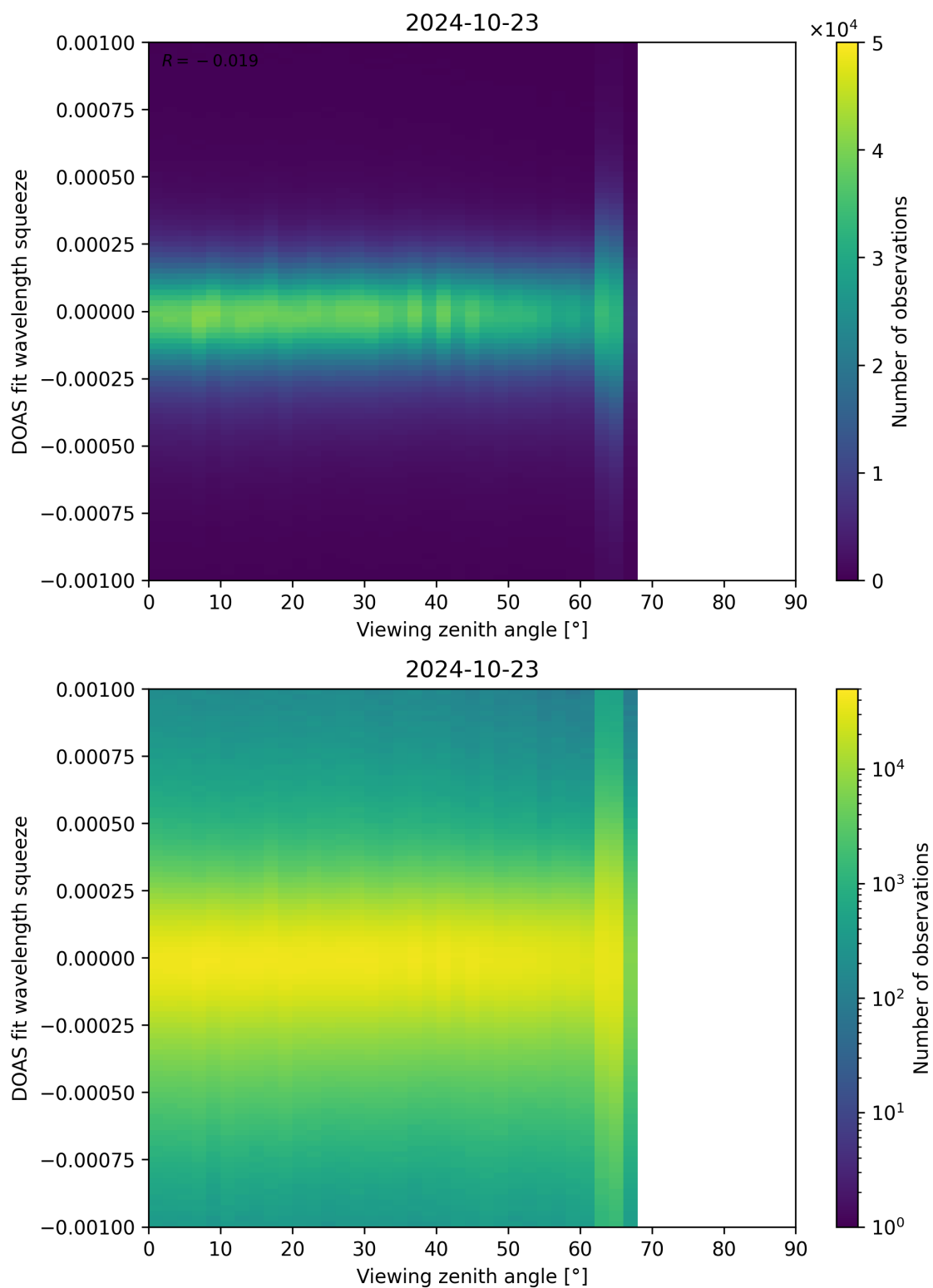
Figure 312: Scatter density plot of “Viewing zenith angle” against “DOAS fit wavelength squeeze” for 2024-10-22 to 2024-10-24.
