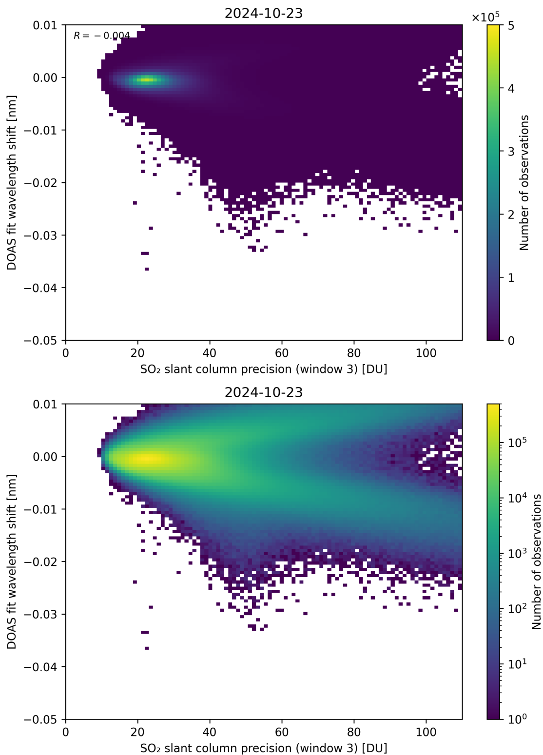
Figure 258: Scatter density plot of “SO 2 slant column precision (window 3)” against “DOAS fit wavelength shift” for 2024-10-22 to 2024-10-24.
