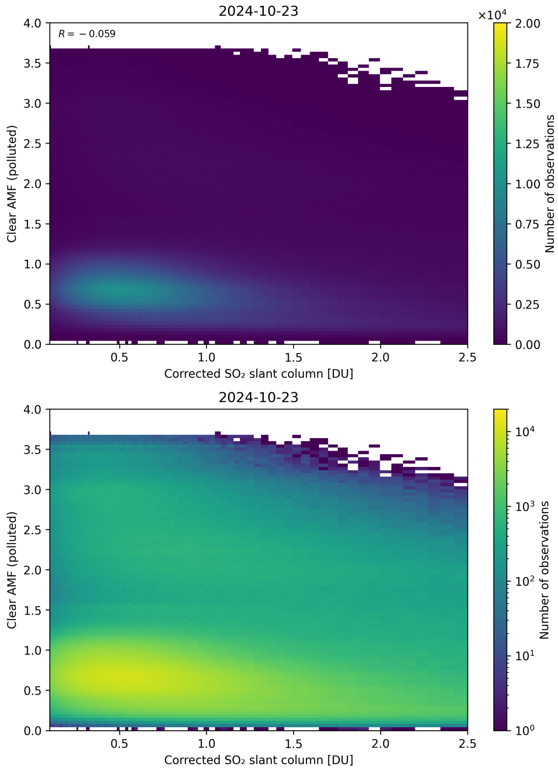
Figure 184: Scatter density plot of “Corrected SO 2 slant column” against “Clear AMF (polluted)” for 2024-10-22 to 2024-10-24.
