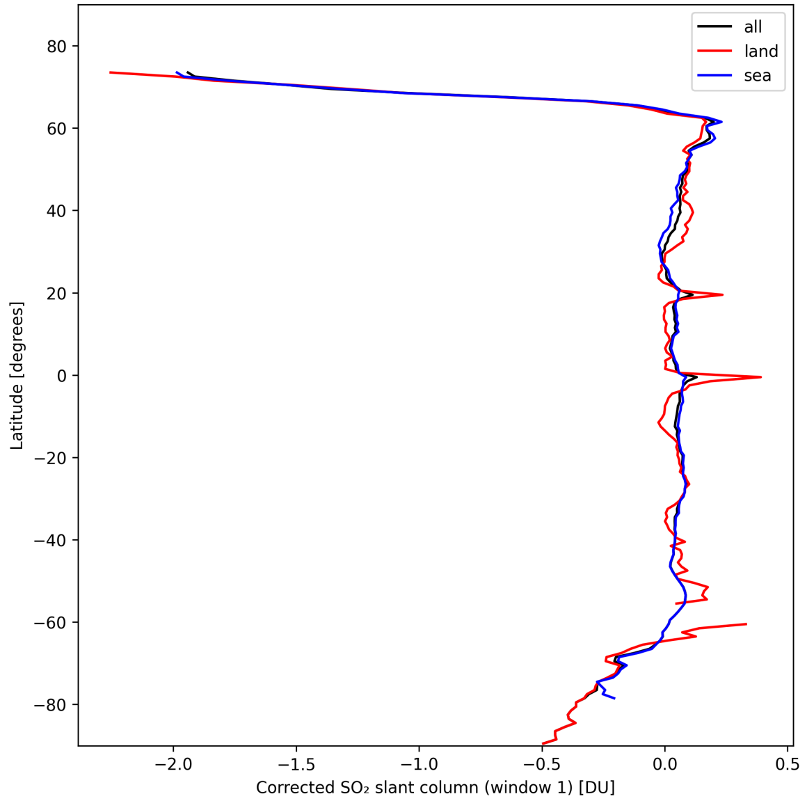
Figure 35: Zonal average of “Corrected SO 2 slant column (window 1)” for 2024-10-22 to 2024-10-24.
