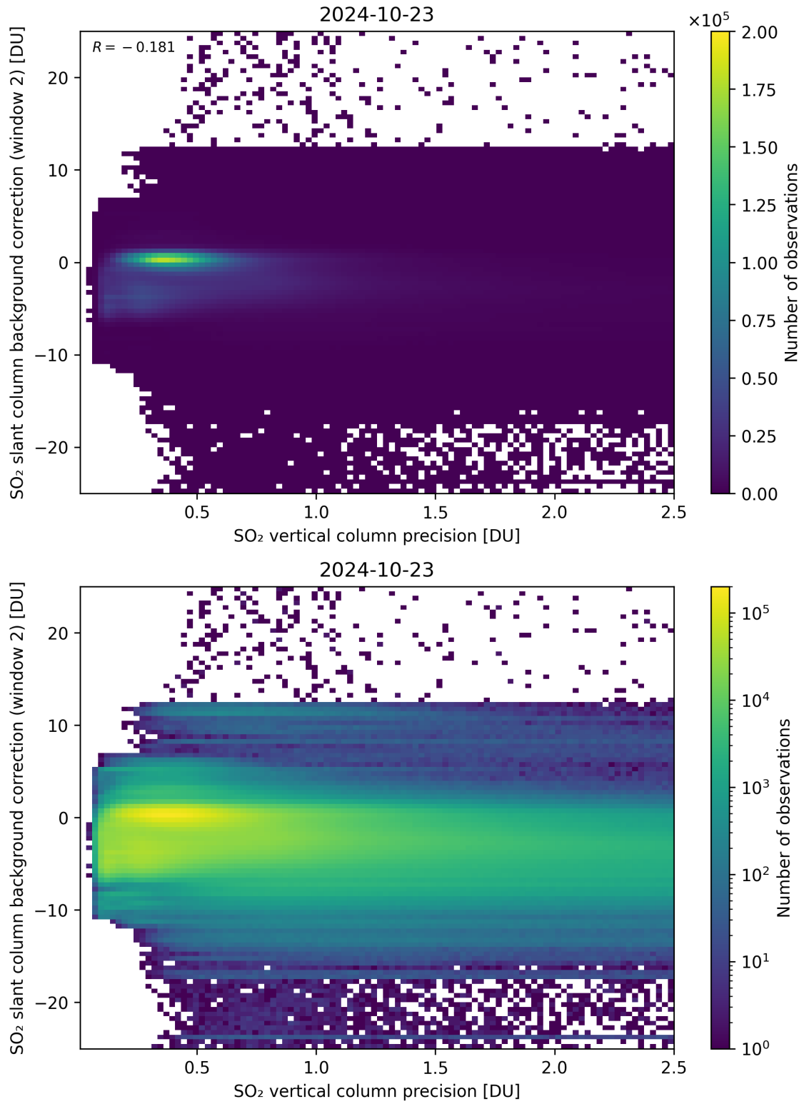
Figure 280: Scatter density plot of “SO 2 vertical column precision” against “SO 2 slant column background correction (window 2)” for 2024-10-22 to 2024-10-24.
