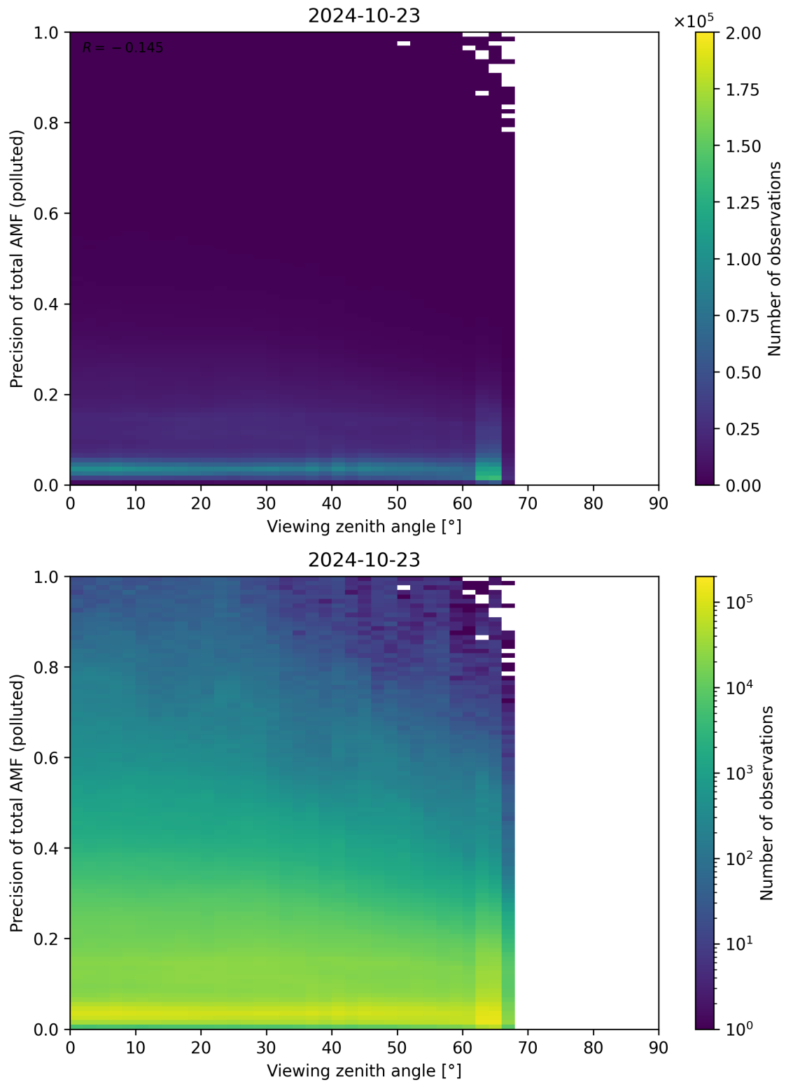
Figure 326: Scatter density plot of “Viewing zenith angle” against “Precision of total AMF (polluted)” for 2024-10-22 to 2024-10-24.
