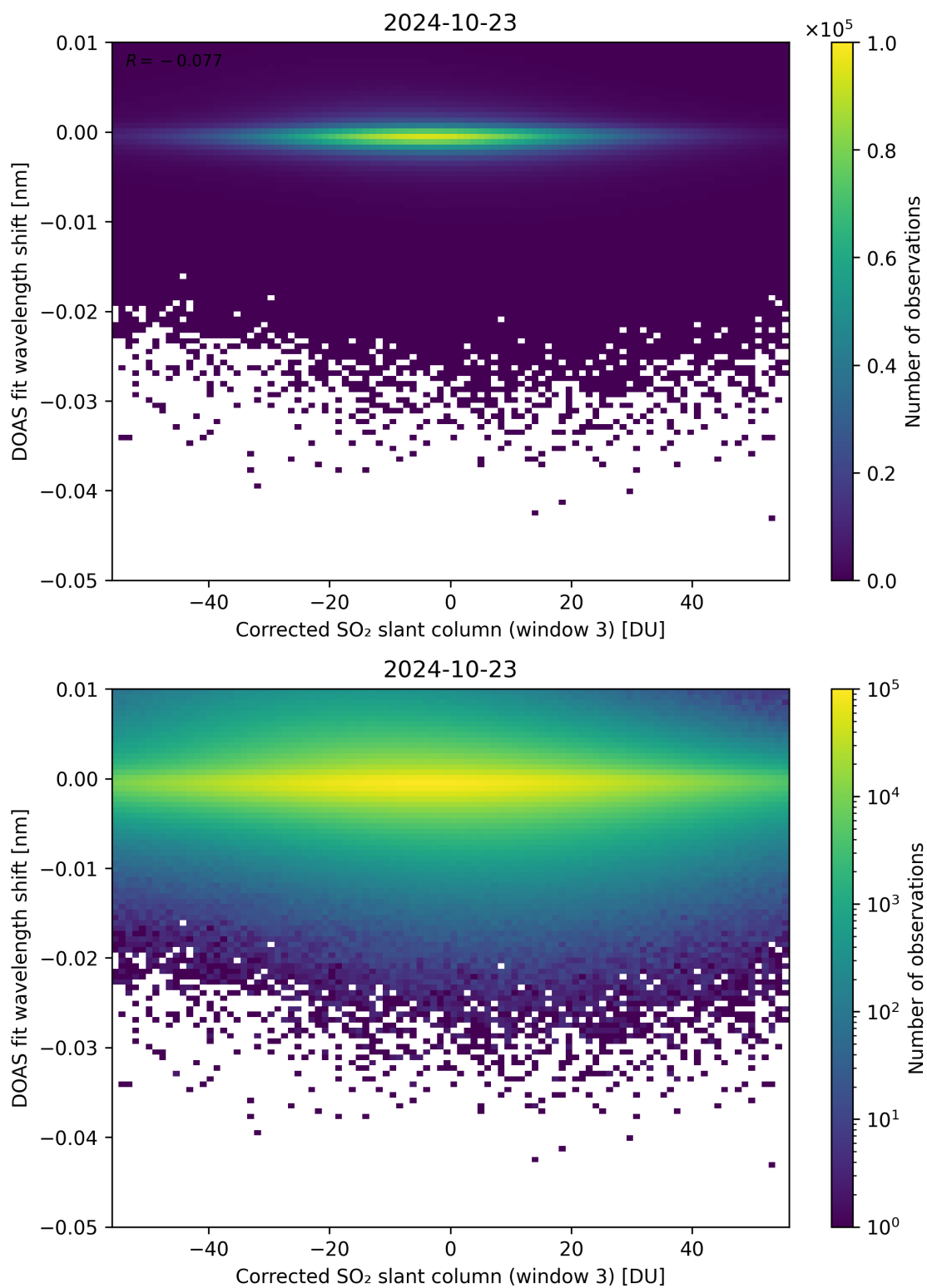
Figure 206: Scatter density plot of “Corrected SO 2 slant column (window 3)” against “DOAS fit wavelength shift” for 2024-10-22 to 2024-10-24.
