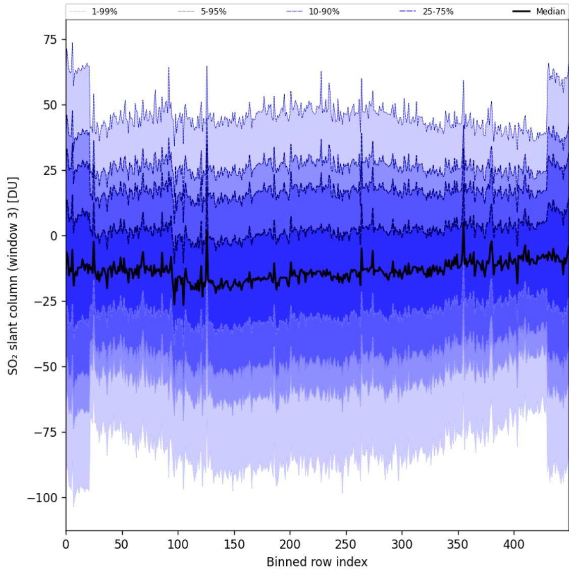
Figure 87: Along track statistics of “SO 2 slant column (window 3)” for 2024-10-22 to 2024-10-24
