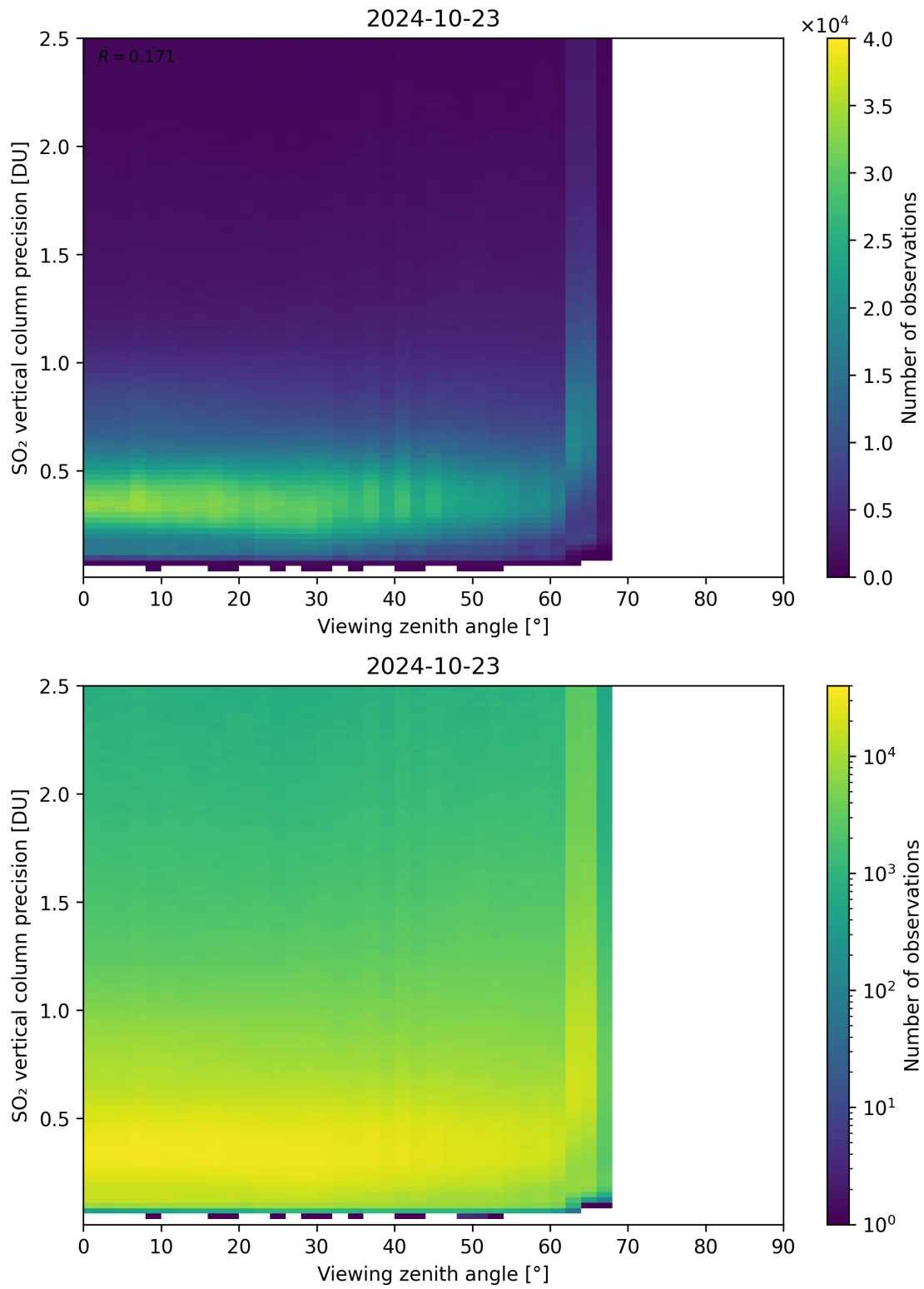
Figure 328: Scatter density plot of “Viewing zenith angle” against “SO 2 vertical column precision” for 2024-10-22 to 2024-10-24.
