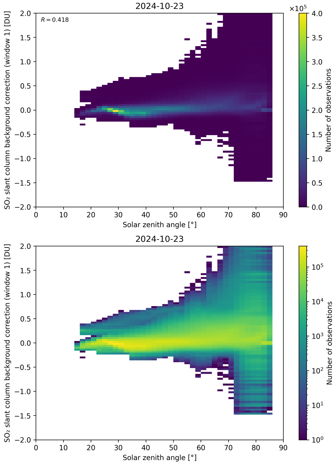
Figure 158: Scatter density plot of “Solar zenith angle” against “SO 2 slant column background correction (window 1)” for 2024-10-22 to 2024-10-24.
