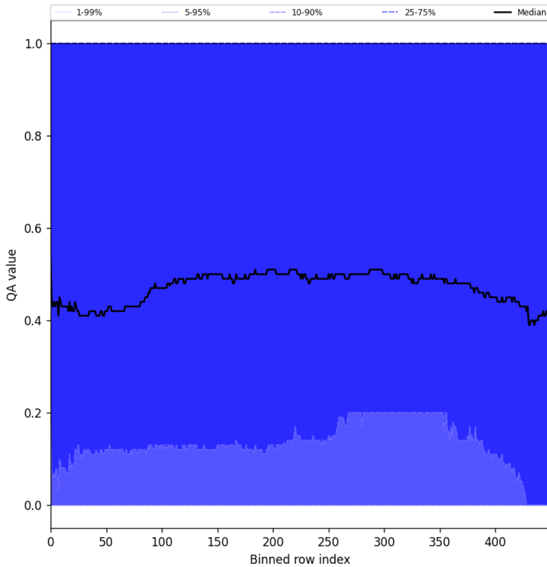
Figure 75: Along track statistics of “QA value” for 2024-10-22 to 2024-10-24
