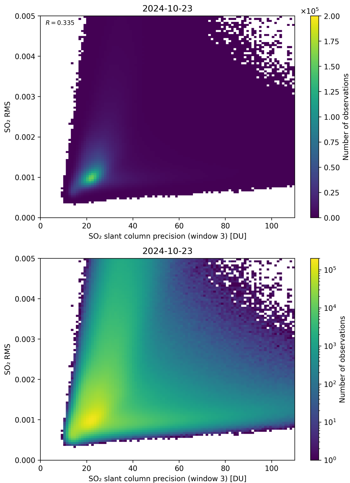
Figure 260: Scatter density plot of “SO 2 slant column precision (window 3)” against “SO 2 RMS” for 2024-10-22 to 2024-10-24.
