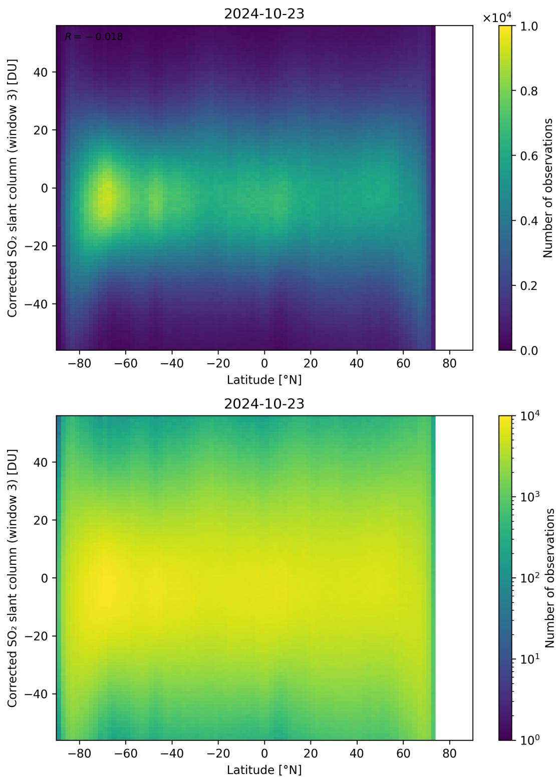
Figure 148: Scatter density plot of “Latitude” against “Corrected SO 2 slant column (window 3)” for 2024-10-22 to 2024-10-24.
