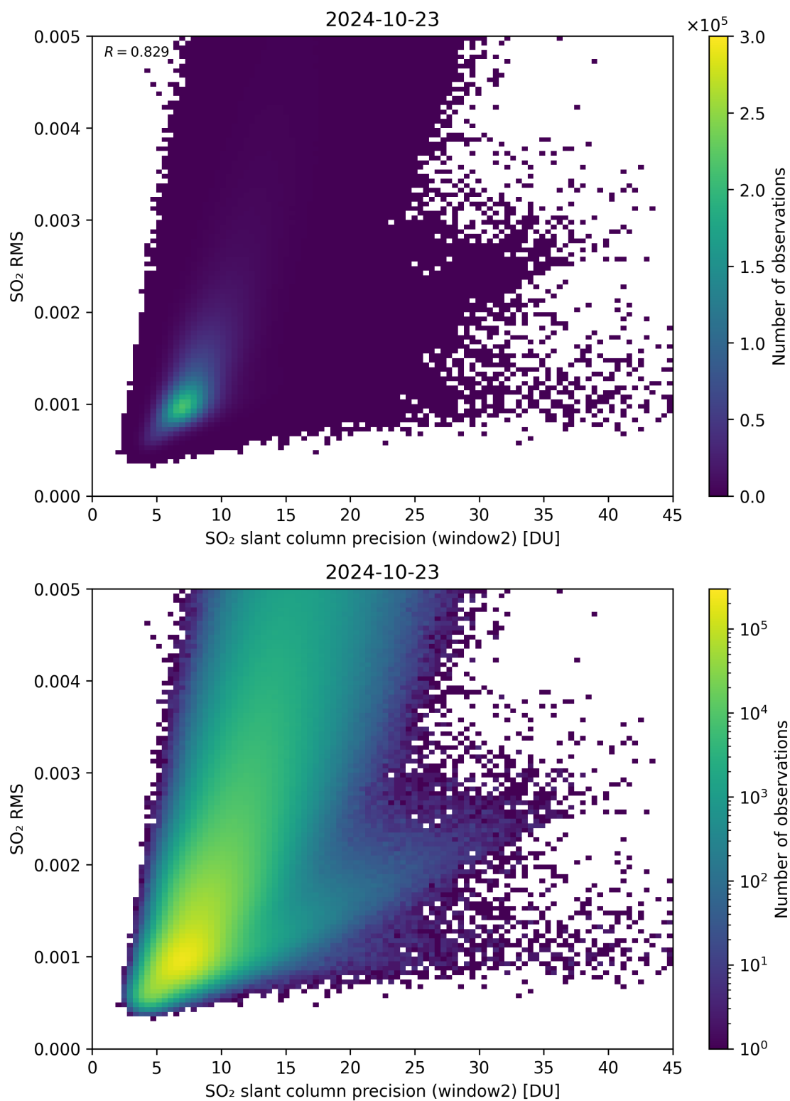
Figure 245: Scatter density plot of “SO 2 slant column precision (window2)” against “SO 2 RMS” for 2024-10-22 to 2024-10-24.
