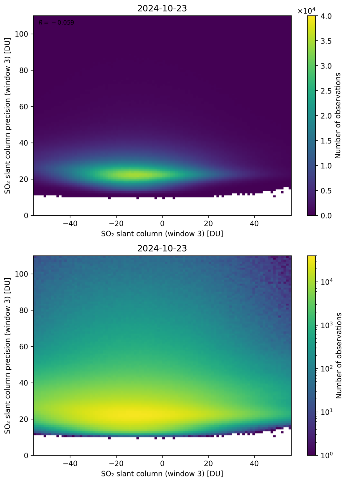
Figure 267: Scatter density plot of “SO 2 slant column (window 3)” against “SO 2 slant column precision (window 3)” for 2024-10-22 to 2024-10-24.
