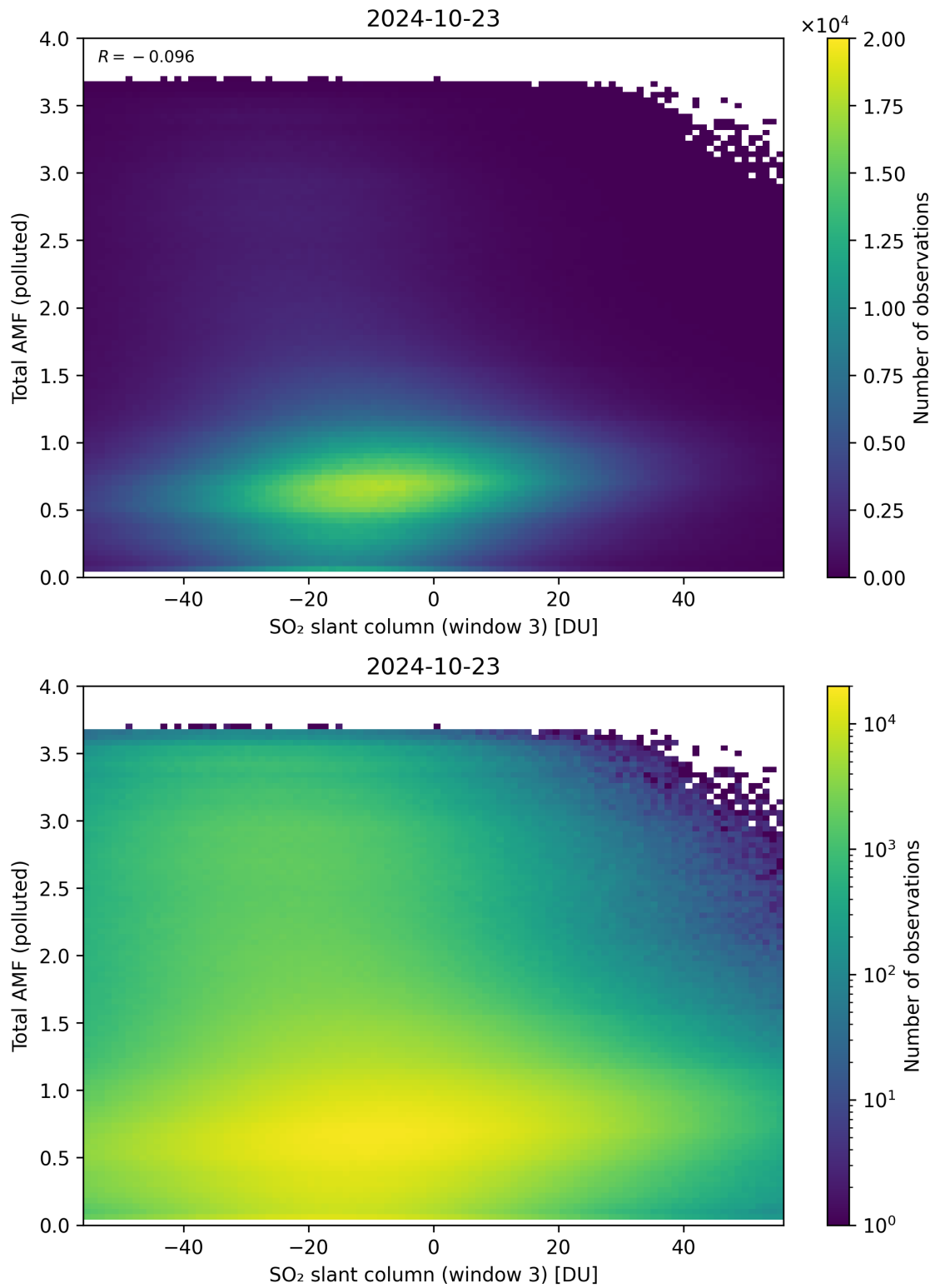
Figure 268: Scatter density plot of “SO 2 slant column (window 3)” against “Total AMF (polluted)” for 2024-10-22 to 2024-10-24.
