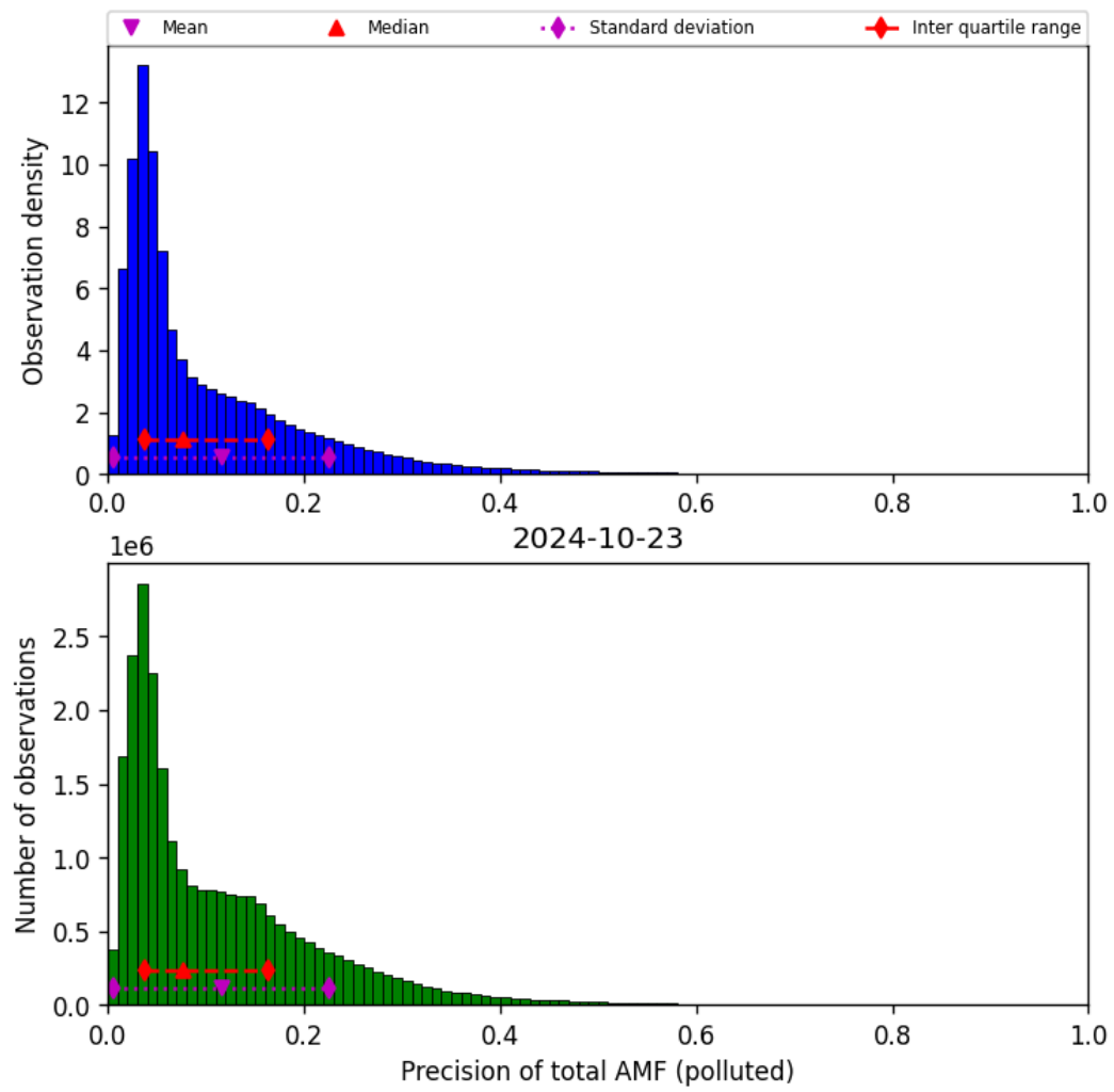
Figure 72: Histogram of “Precision of total AMF (polluted)” for 2024-10-22 to 2024-10-24
