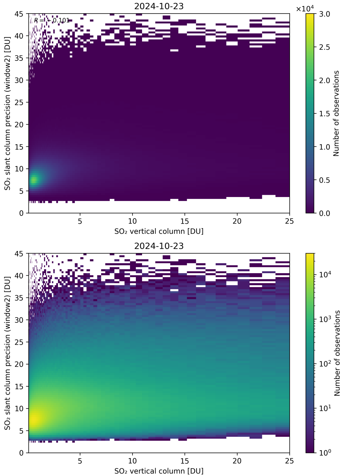
Figure 302: Scatter density plot of “SO 2 vertical column” against “SO 2 slant column precision (window2)” for 2024-10-22 to 2024-10-24.
