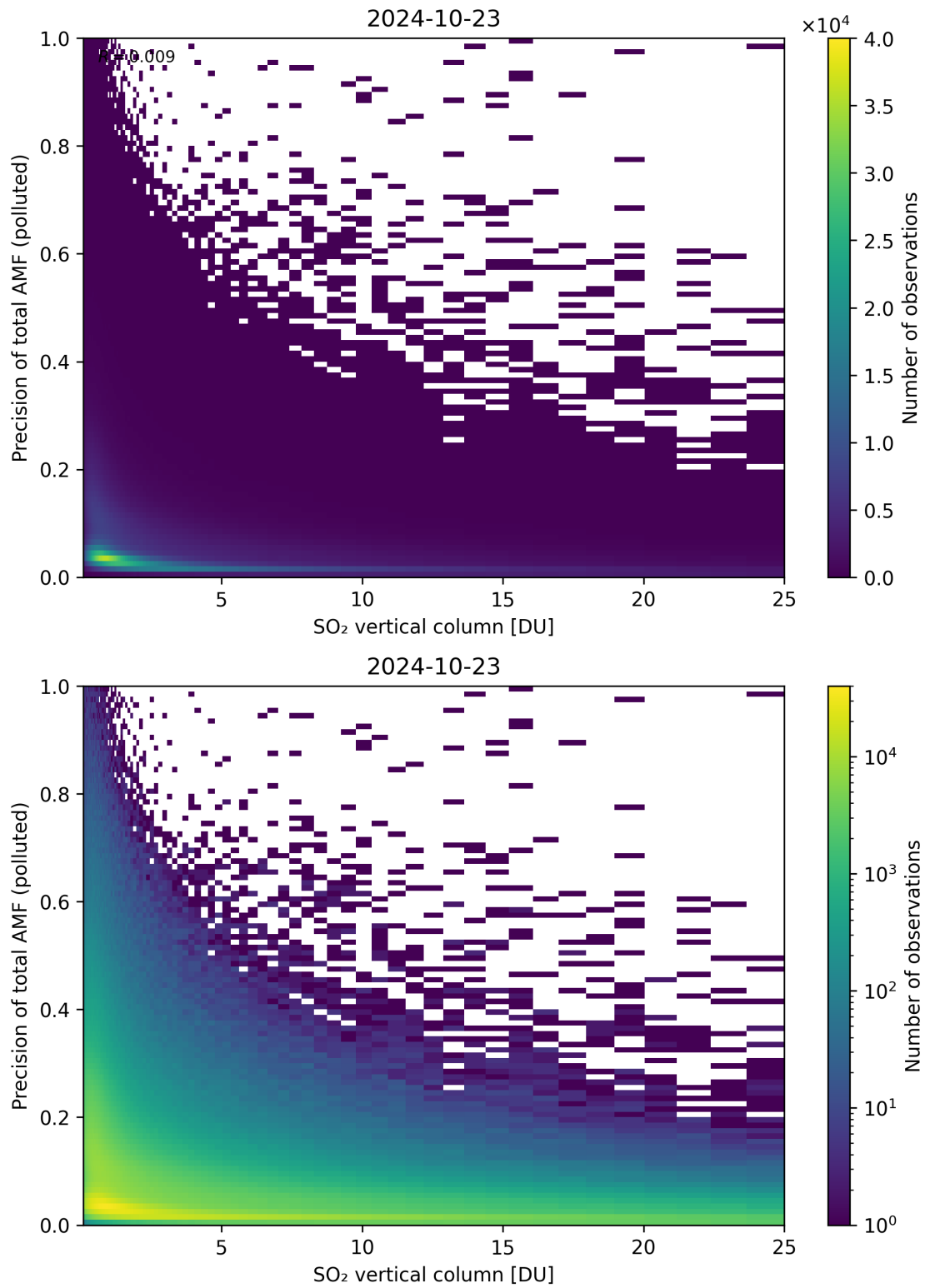
Figure 306: Scatter density plot of “SO 2 vertical column” against “Precision of total AMF (polluted)” for 2024-10-22 to 2024-10-24.
