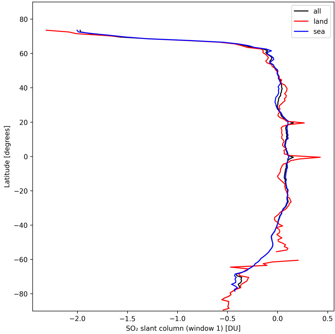
Figure 33: Zonal average of “SO 2 slant column (window 1)” for 2024-10-22 to 2024-10-24.
