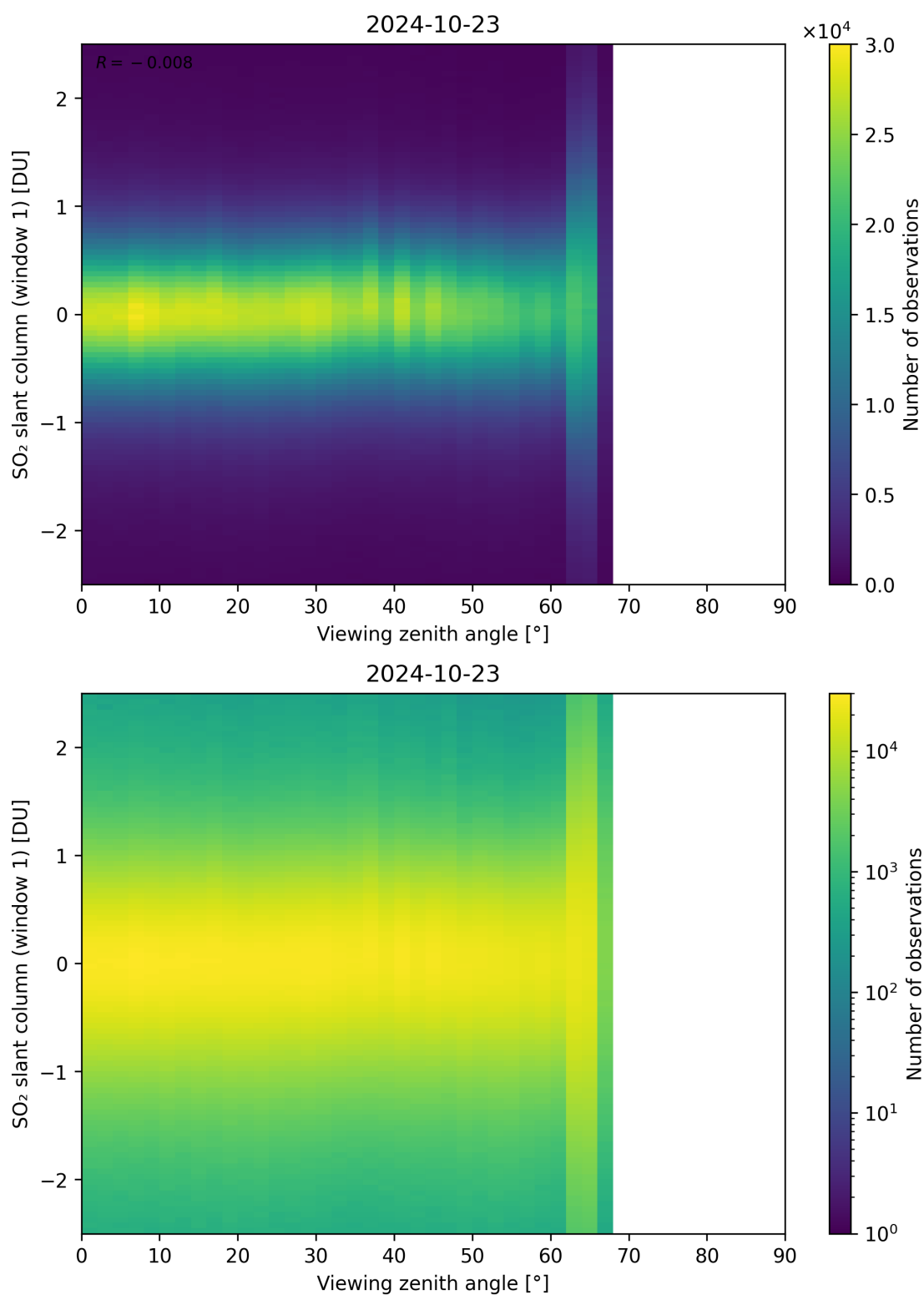
Figure 320: Scatter density plot of “Viewing zenith angle” against “SO 2 slant column (window 1)” for 2024-10-22 to 2024-10-24.
