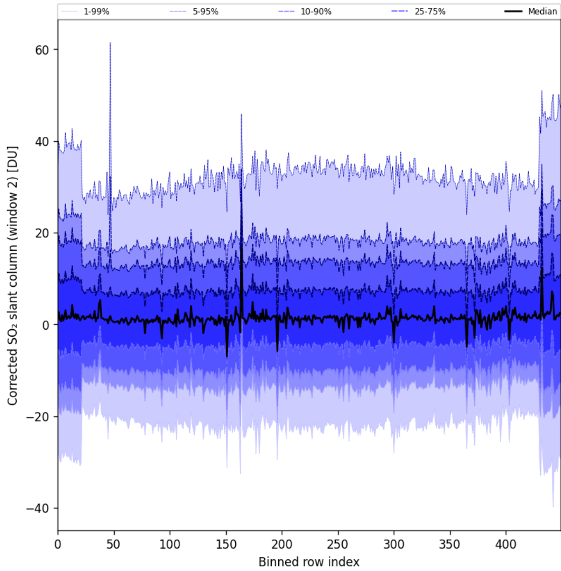
Figure 85: Along track statistics of “Corrected SO 2 slant column (window 2)” for 2024-10-22 to 2024-10-24
