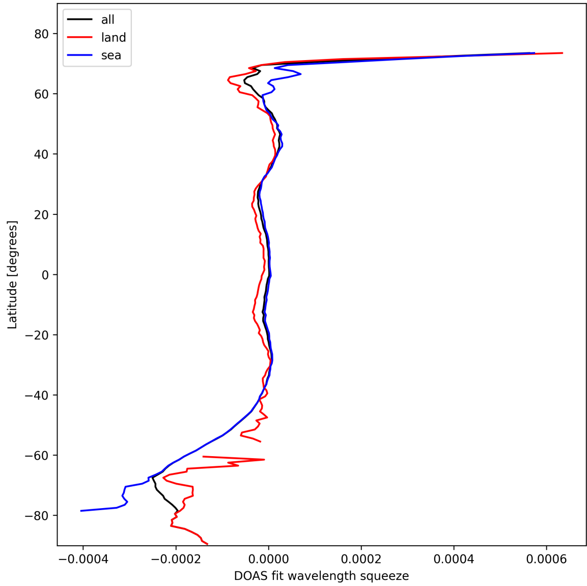
Figure 46: Zonal average of “DOAS fit wavelength squeeze” for 2024-10-22 to 2024-10-24.
