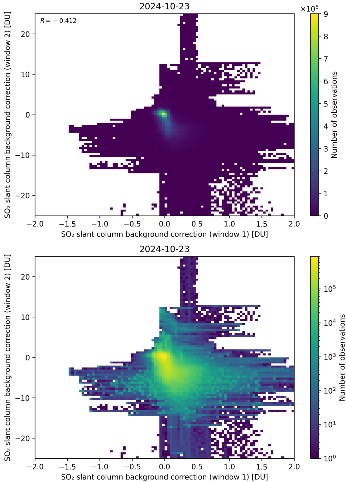
Figure 98: Scatter density plot of “SO 2 slant column background correction (window 1)” against “SO 2 slant column background correction (window 2)” for 2024-10-22 to 2024-10-24.
