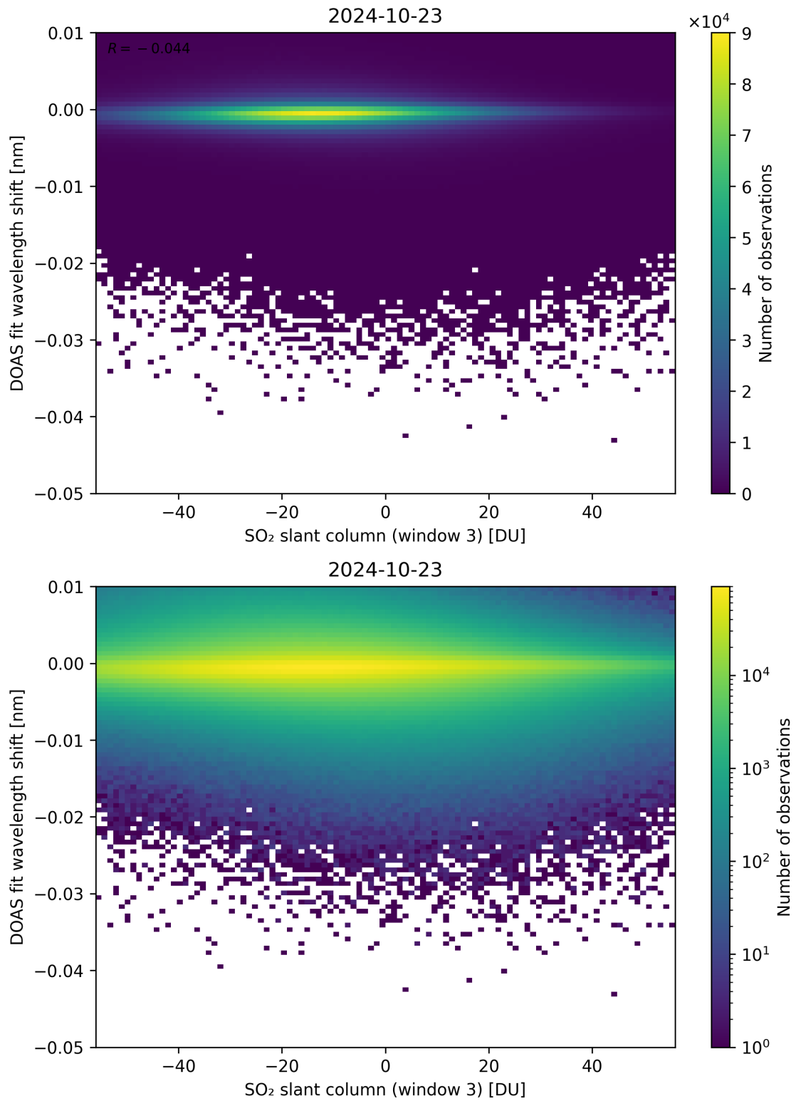
Figure 254: Scatter density plot of “SO 2 slant column (window 3)” against “DOAS fit wavelength shift” for 2024-10-22 to 2024-10-24.
