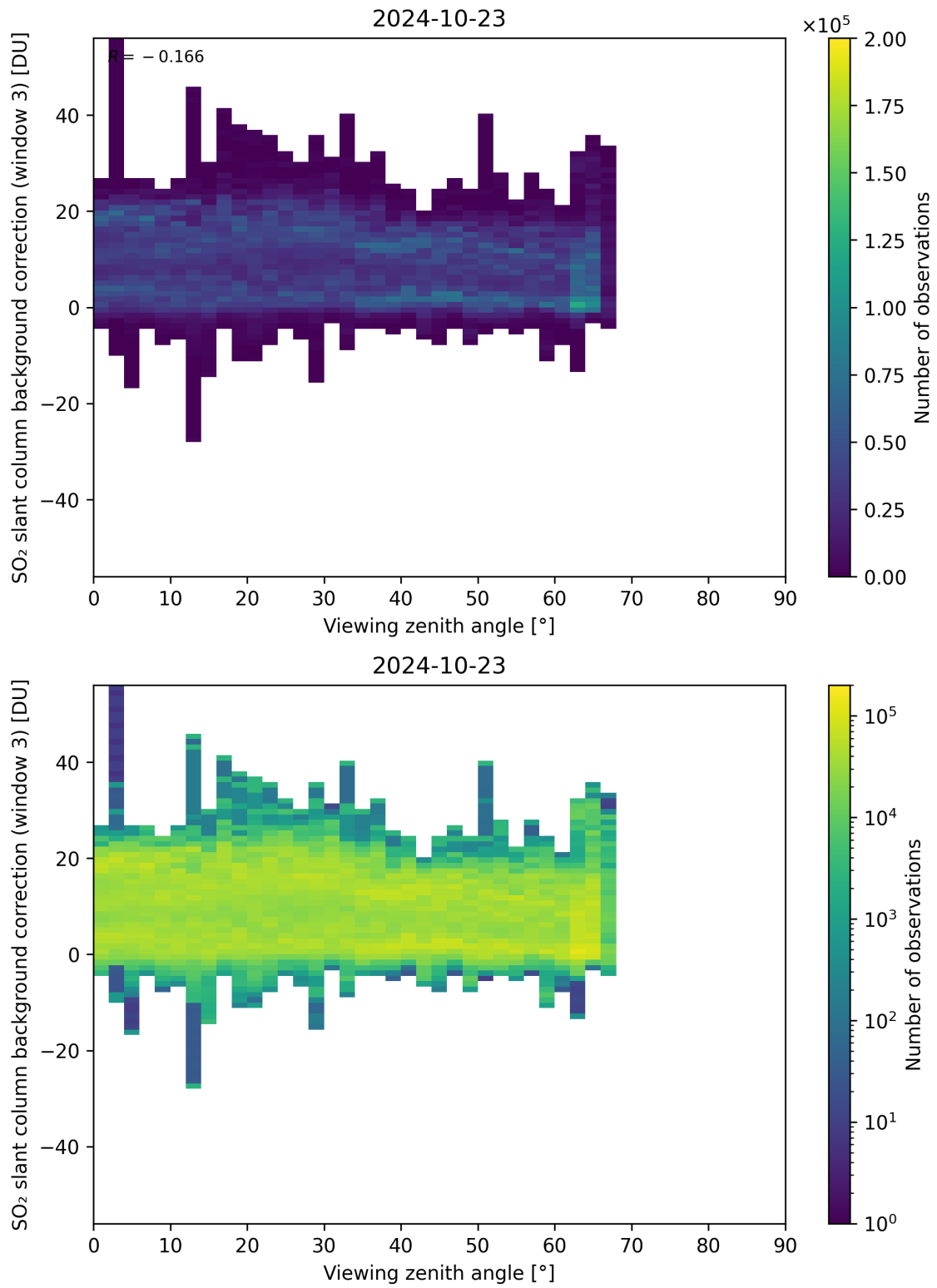
Figure 310: Scatter density plot of “Viewing zenith angle” against “SO 2 slant column background correction (window 3)” for 2024-10-22 to 2024-10-24.
