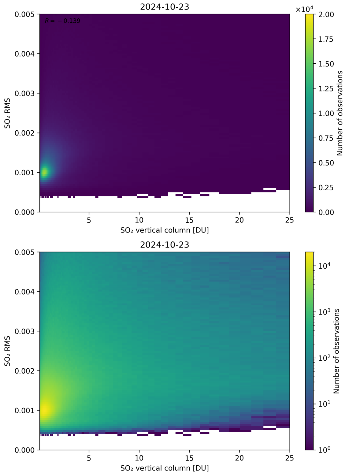
Figure 278: Scatter density plot of “SO 2 vertical column” against “SO 2 RMS” for 2024-10-22 to 2024-10-24.
