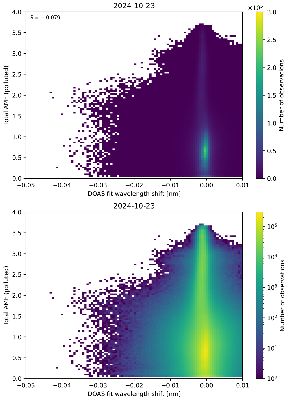
Figure 130: Scatter density plot of “DOAS fit wavelength shift” against “Total AMF (polluted)” for 2024-10-22 to 2024-10-24.
