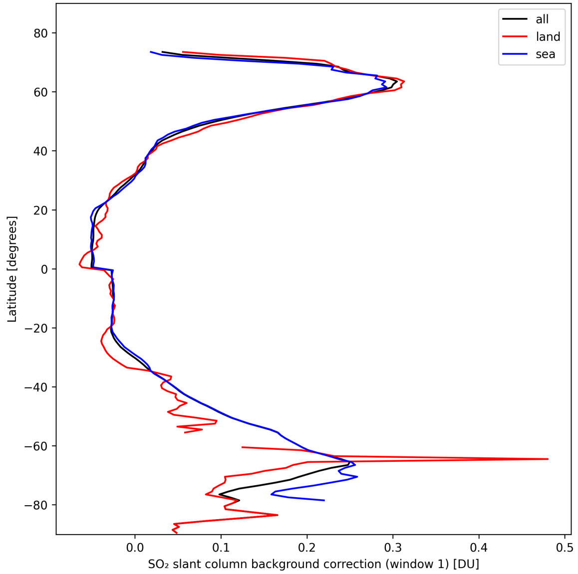
Figure 36: Zonal average of “SO 2 slant column background correction (window 1)” for 2024-10-22 to 2024-10-24.
