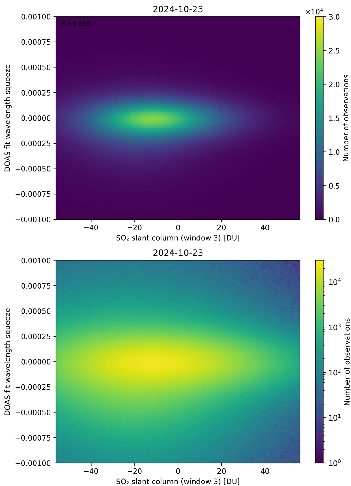
Figure 255: Scatter density plot of “SO 2 slant column (window 3)” against “DOAS fit wavelength squeeze” for 2024-10-22 to 2024-10-24.
