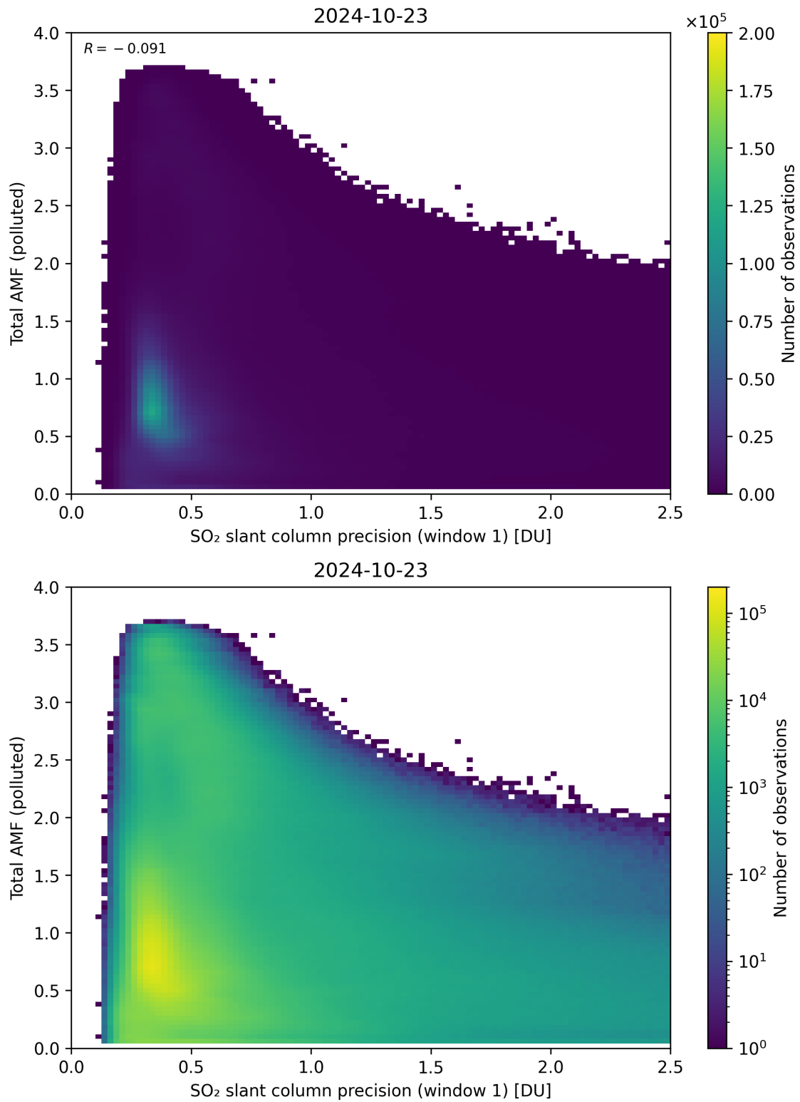
Figure 230: Scatter density plot of “SO 2 slant column precision (window 1)” against “Total AMF (polluted)” for 2024-10-22 to 2024-10-24.
