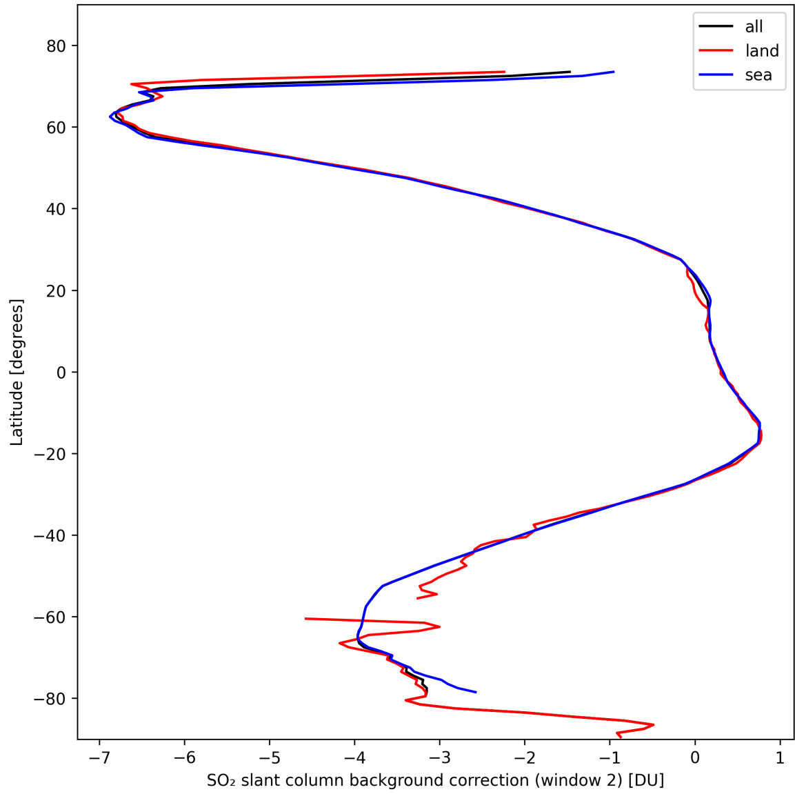
Figure 40: Zonal average of "SO 2 slant column background correction (window 2)" for 2024-10-22 to 2024-10-24.
