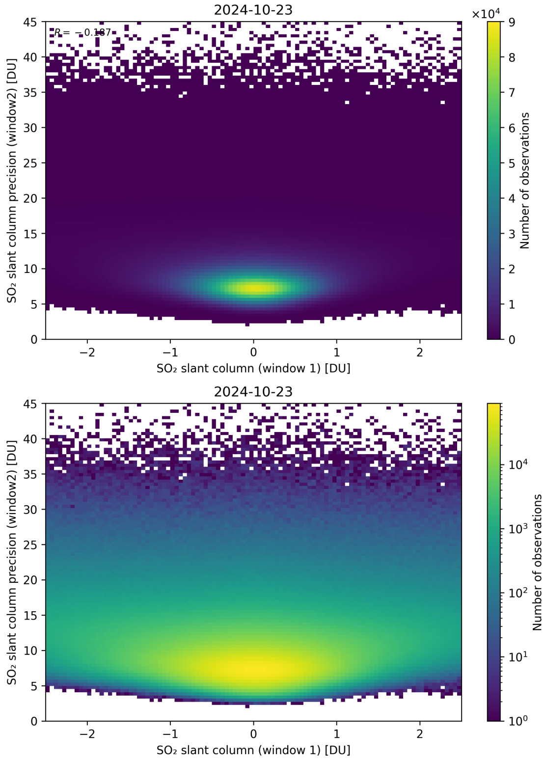
Figure 236: Scatter density plot of “SO 2 slant column (window 1)” against “SO 2 slant column precision (window2)” for 2024-10-22 to 2024-10-24.
