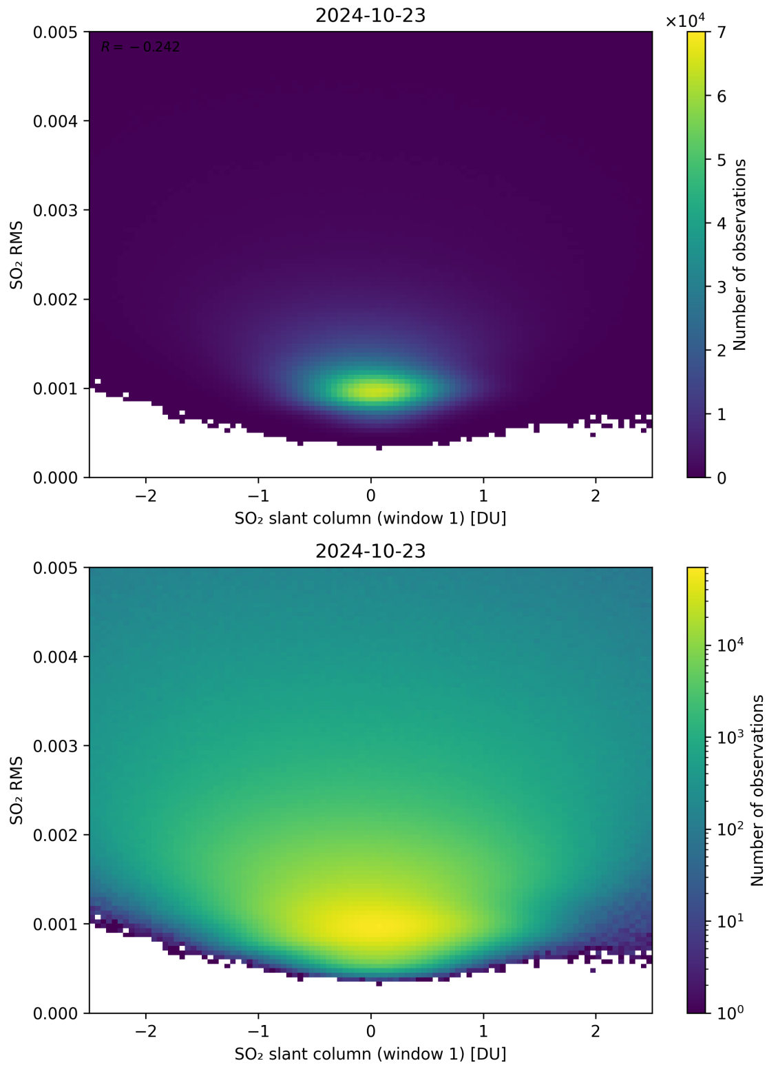
Figure 217: Scatter density plot of “SO 2 slant column (window 1)” against “SO 2 RMS” for 2024-10-22 to 2024-10-24.
