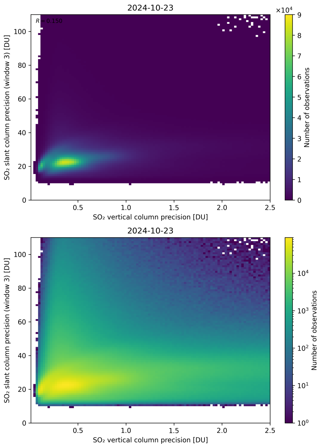
Figure 293: Scatter density plot of “SO 2 vertical column precision” against “SO 2 slant column precision (window 3)” for 2024-10-22 to 2024-10-24.
