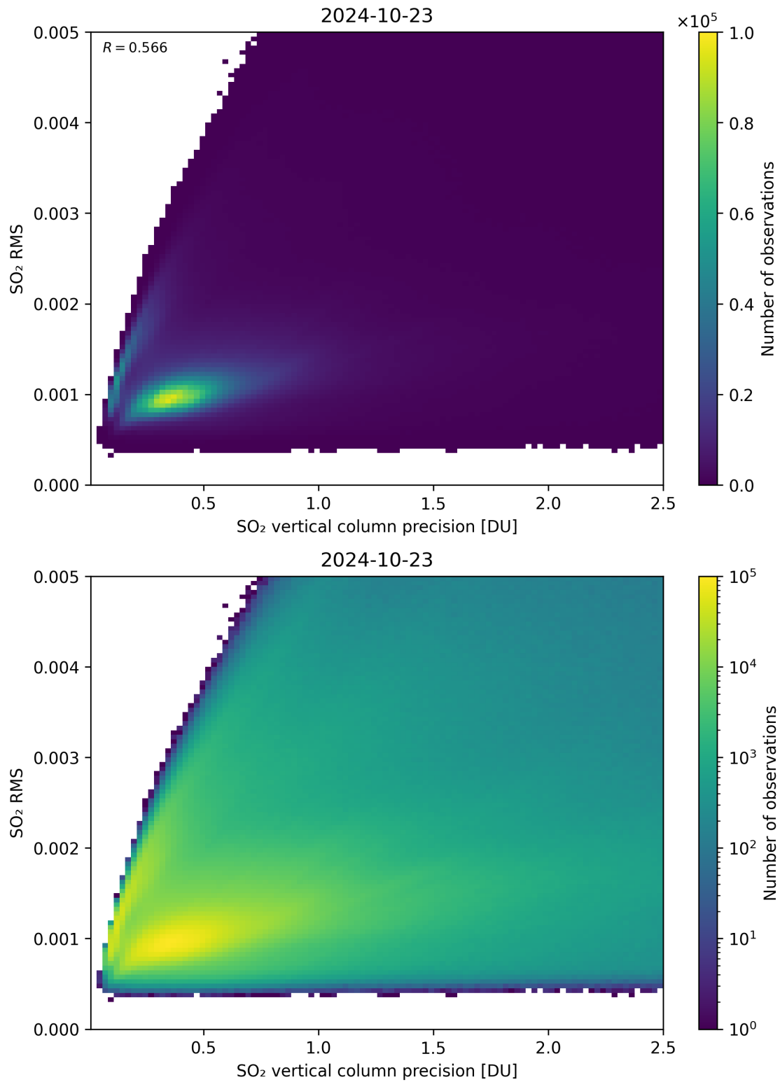
Figure 284: Scatter density plot of “SO 2 vertical column precision” against “SO 2 RMS” for 2024-10-22 to 2024-10-24.
