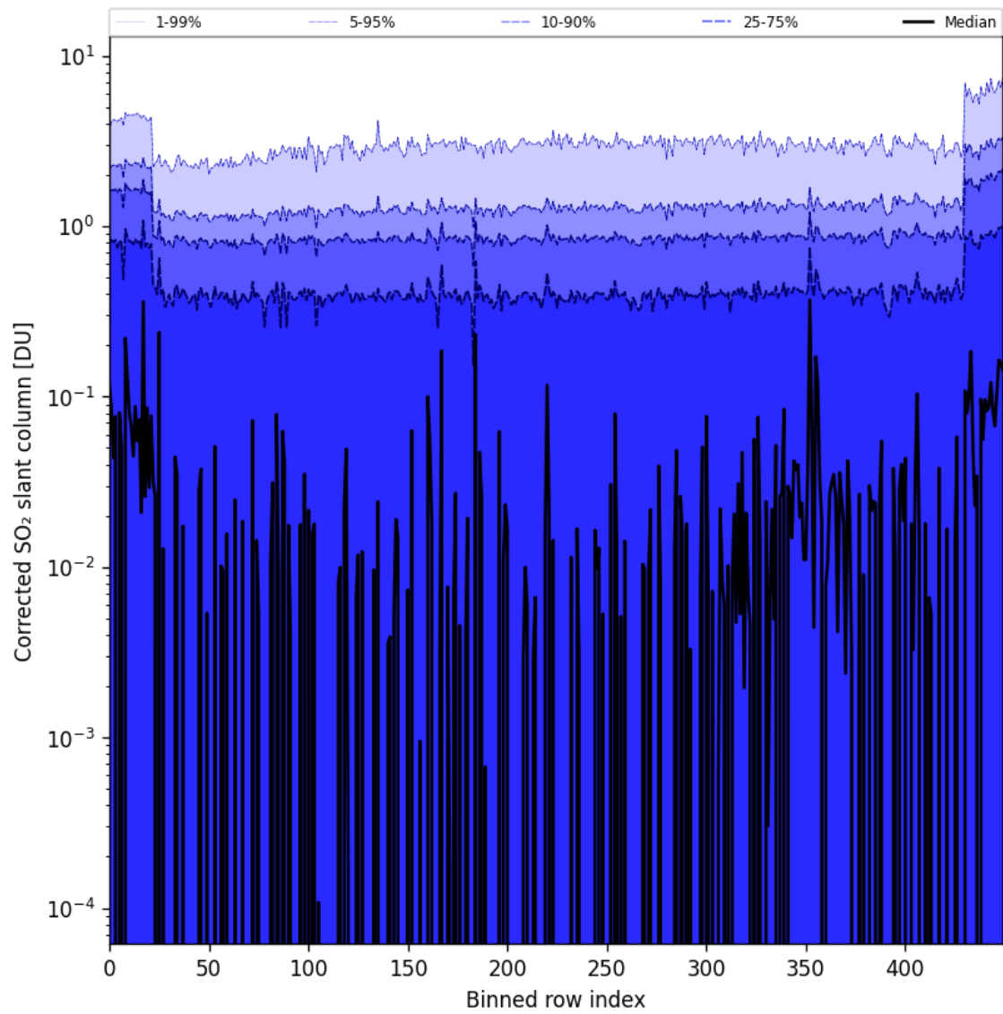
Figure 78: Along track statistics of “Corrected SO 2 slant column” for 2024-10-22 to 2024-10-24
