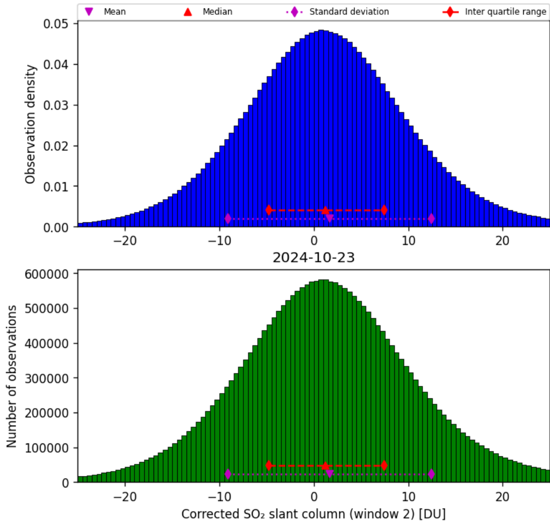
Figure 62: Histogram of “Corrected SO 2 slant column (window 2)” for 2024-10-22 to 2024-10-24
