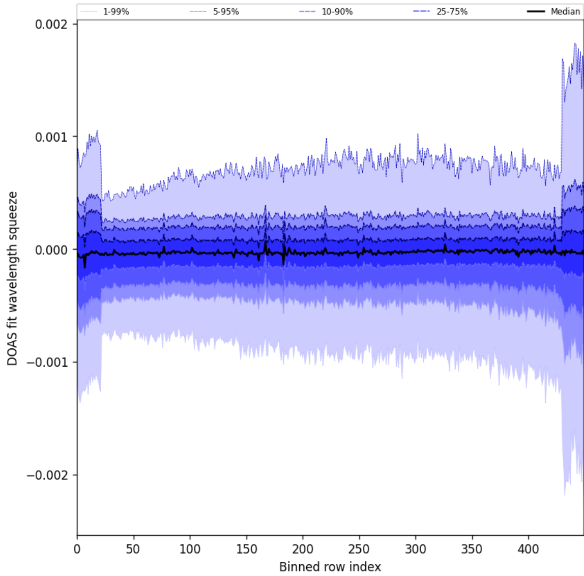
Figure 92: Along track statistics of “DOAS fit wavelength squeeze” for 2024-10-22 to 2024-10-24
