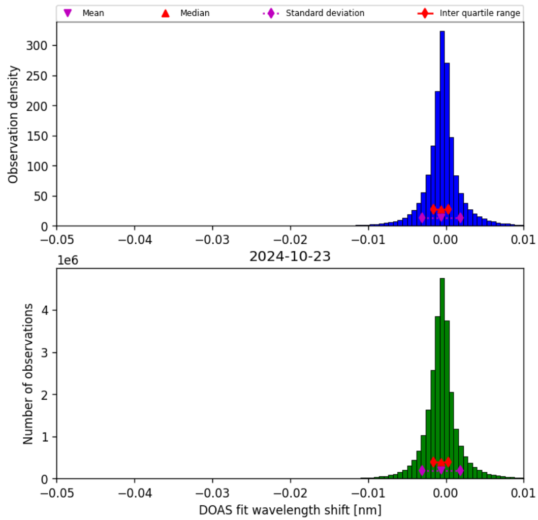
Figure 68: Histogram of “DOAS fit wavelength shift” for 2024-10-22 to 2024-10-24
