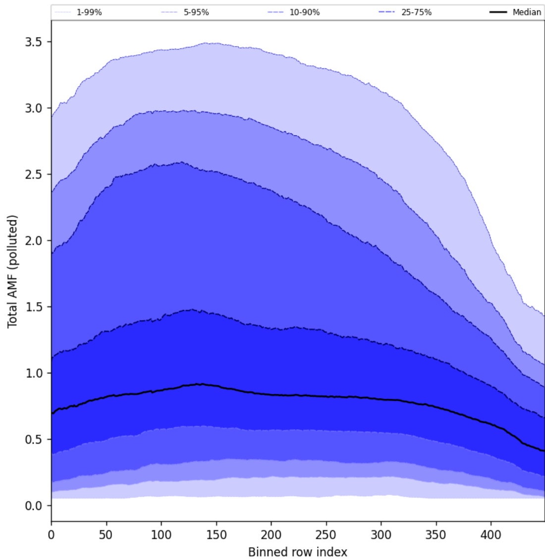
Figure 94: Along track statistics of “Total AMF (polluted)” for 2024-10-22 to 2024-10-24
