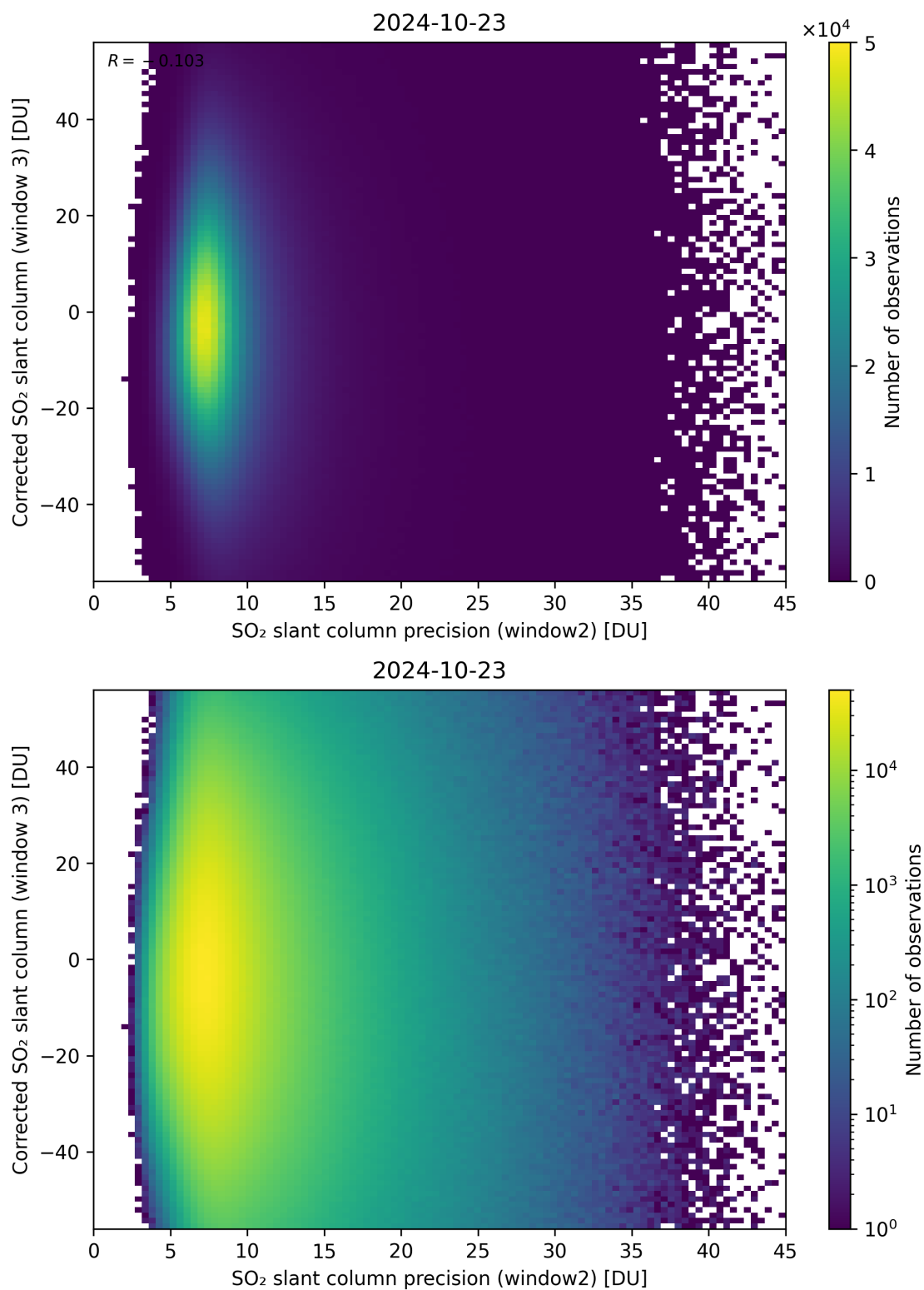
Figure 248: Scatter density plot of “SO 2 slant column precision (window2)” against “Corrected SO 2 slant column (window 3)” for 2024-10-22 to 2024-10-24.
