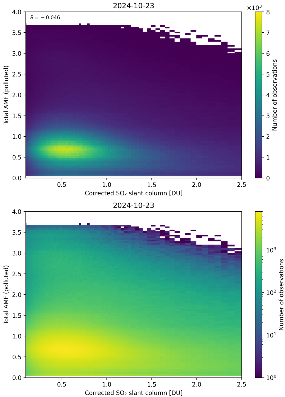
Figure 192: Scatter density plot of “Corrected SO 2 slant column” against “Total AMF (polluted)” for 2024-10-22 to 2024-10-24.
