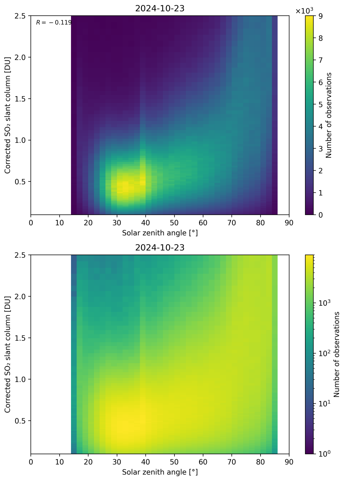
Figure 166: Scatter density plot of “Solar zenith angle” against “Corrected SO 2 slant column” for 2024-10-22 to 2024-10-24.
