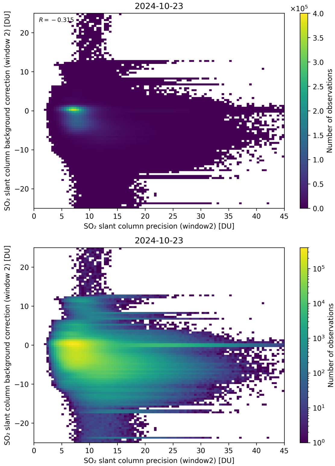
Figure 241: Scatter density plot of “SO 2 slant column precision (window2)” against “SO 2 slant column background correction (window 2)” for 2024-10-22 to 2024-10-24.
