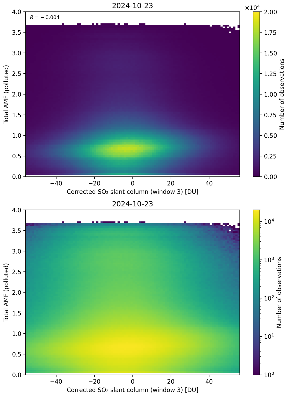
Figure 210: Scatter density plot of “Corrected SO 2 slant column (window 3)” against “Total AMF (polluted)” for 2024-10-22 to 2024-10-24.
