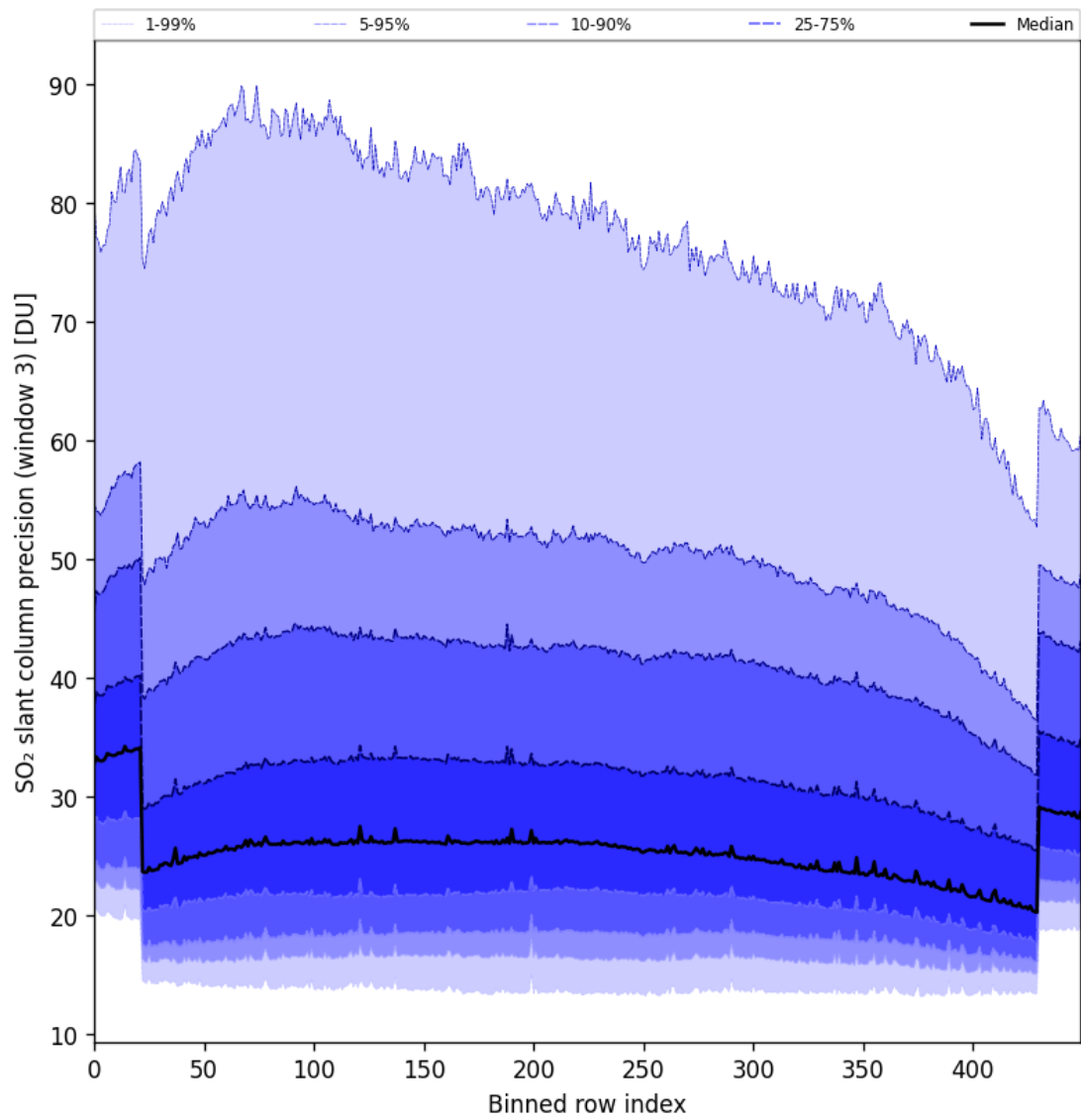
Figure 88: Along track statistics of “SO 2 slant column precision (window 3)” for 2024-10-22 to 2024-10-24
