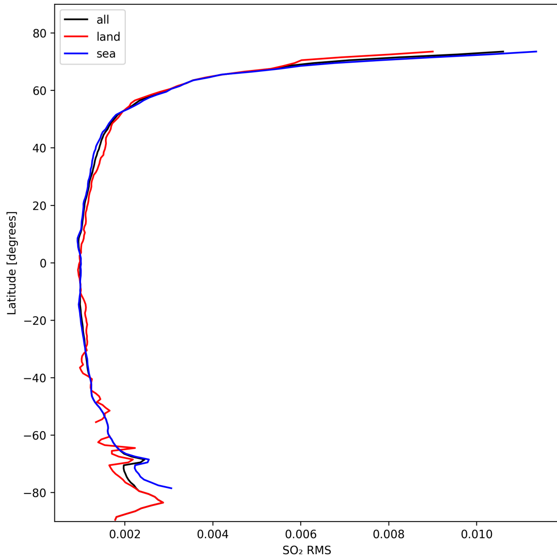
Figure 47: Zonal average of “SO 2 RMS” for 2024-10-22 to 2024-10-24.
