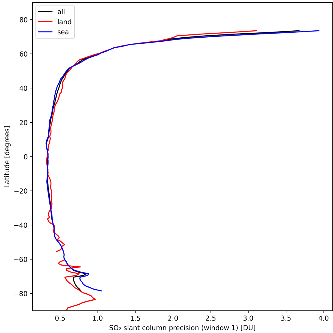
Figure 34: Zonal average of “SO 2 slant column precision (window 1)” for 2024-10-22 to 2024-10-24.
