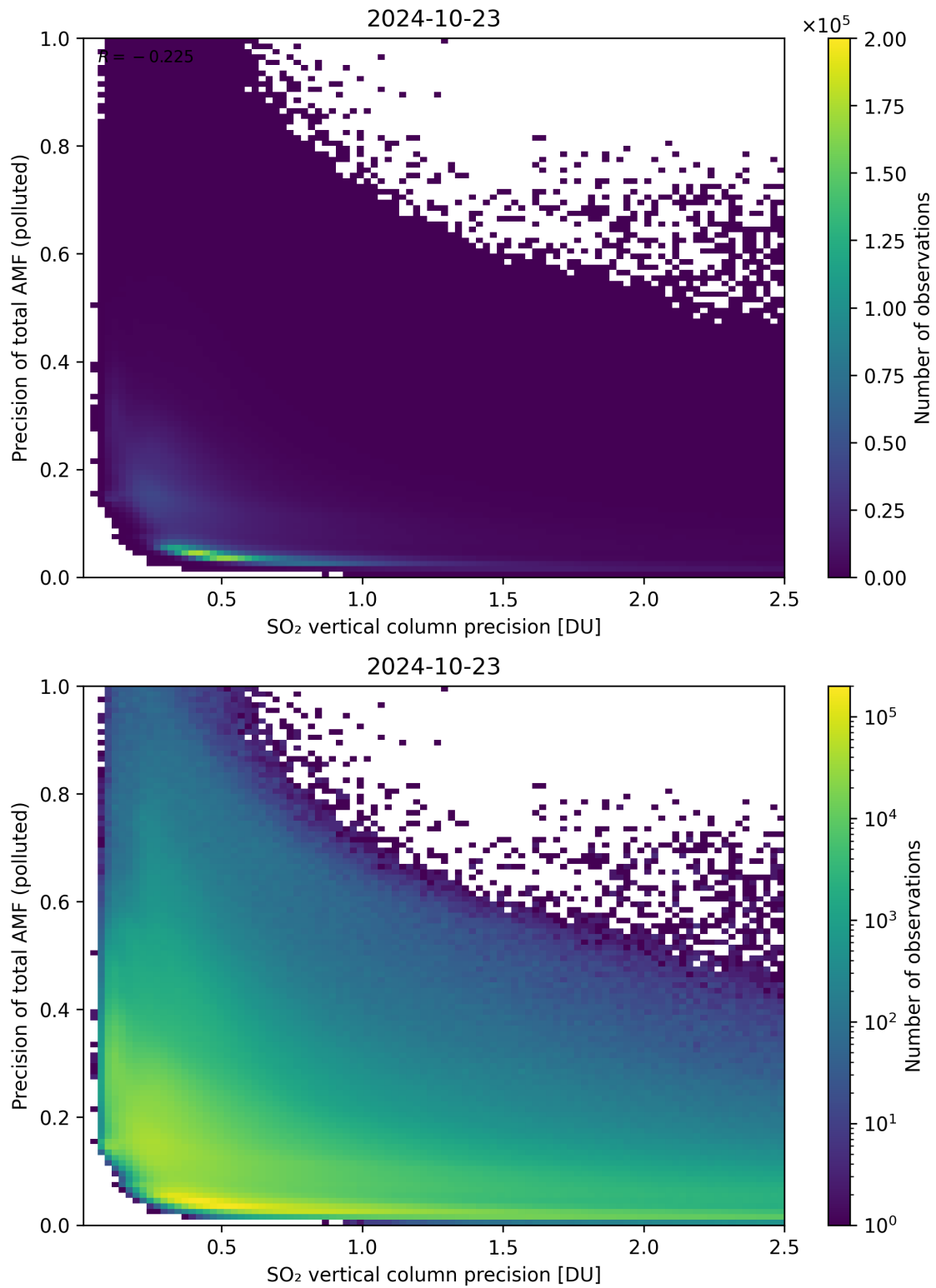
Figure 295: Scatter density plot of “SO 2 vertical column precision” against “Precision of total AMF (polluted)” for 2024-10-22 to 2024-10-24.
