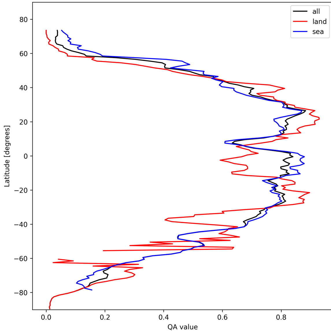
Figure 29: Zonal average of “QA value” for 2024-10-22 to 2024-10-24.
