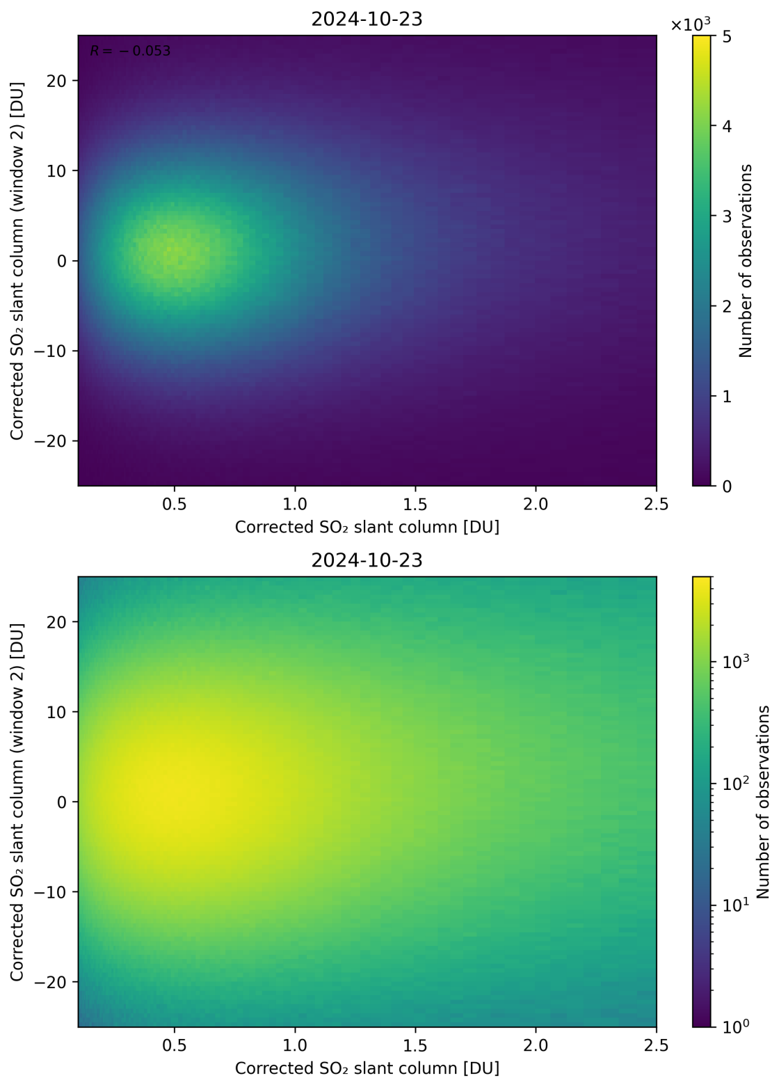
Figure 185: Scatter density plot of “Corrected SO 2 slant column” against “Corrected SO 2 slant column (window 2)” for 2024-10-22 to 2024-10-24.
