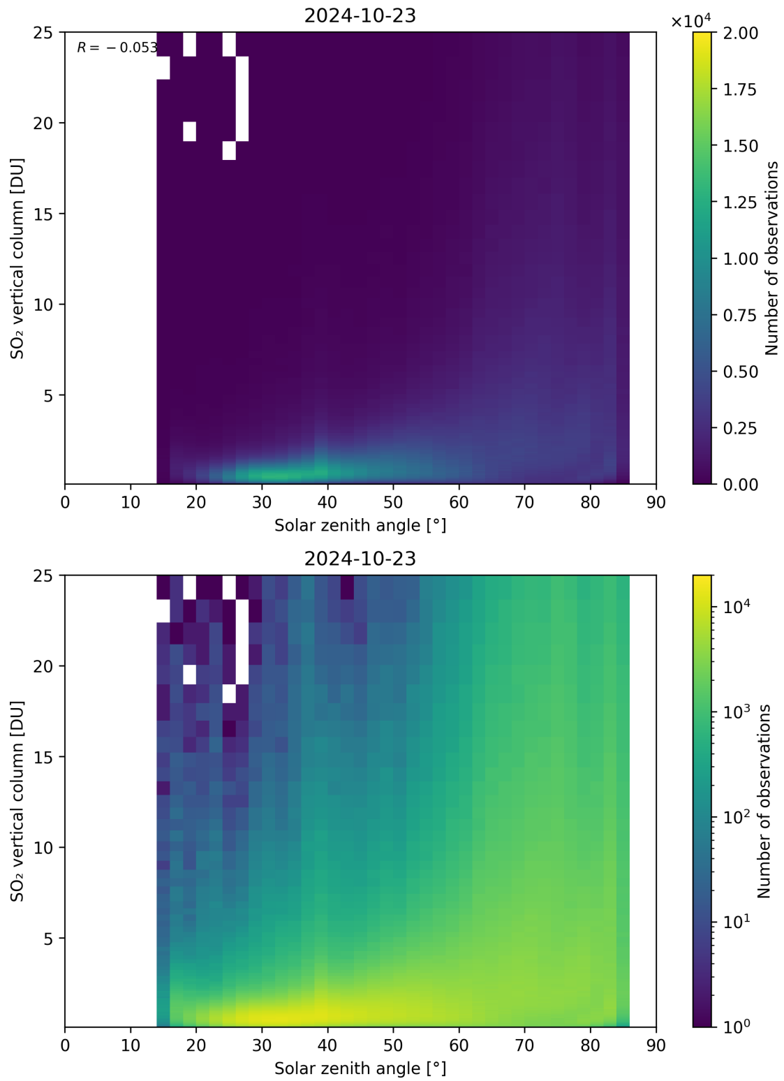
Figure 176: Scatter density plot of “Solar zenith angle” against “SO 2 vertical column” for 2024-10-22 to 2024-10-24.
