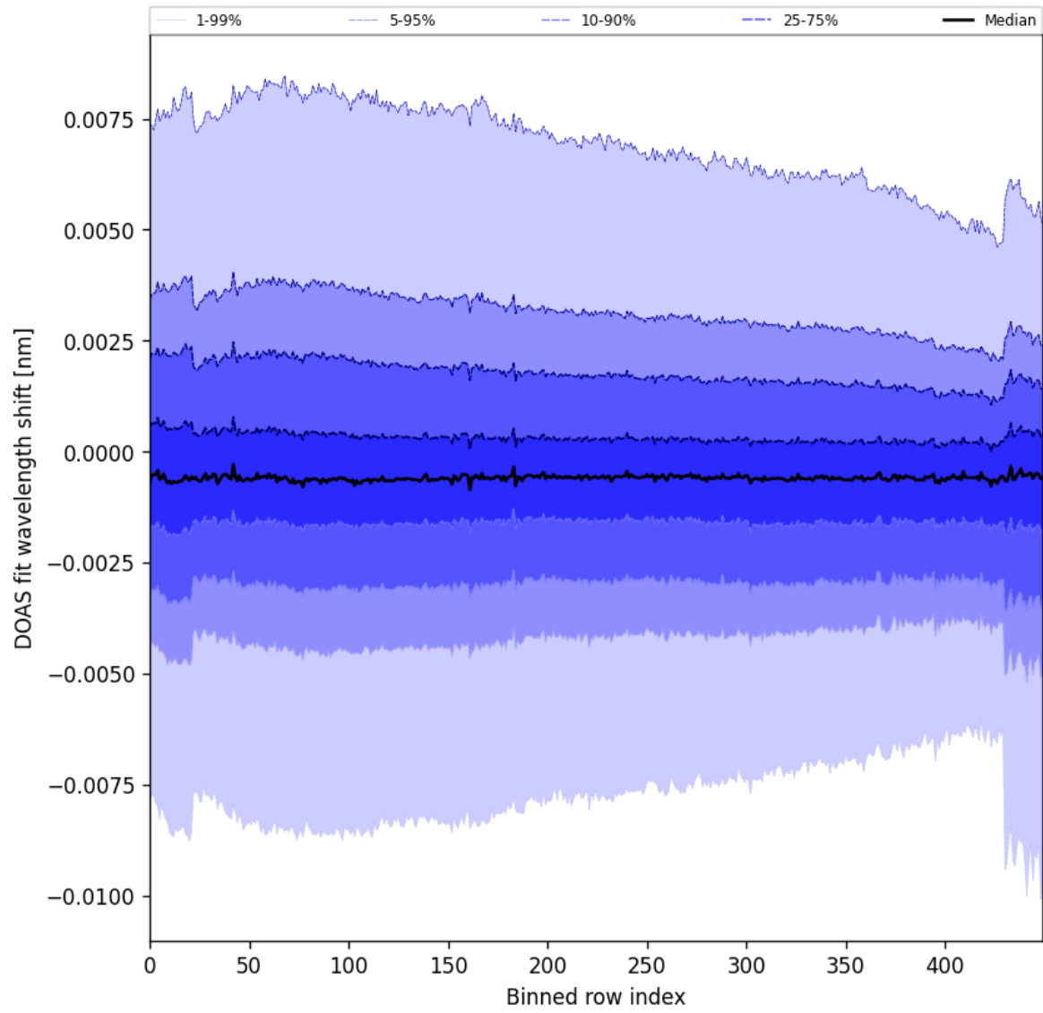
Figure 91: Along track statistics of “DOAS fit wavelength shift” for 2024-10-22 to 2024-10-24
