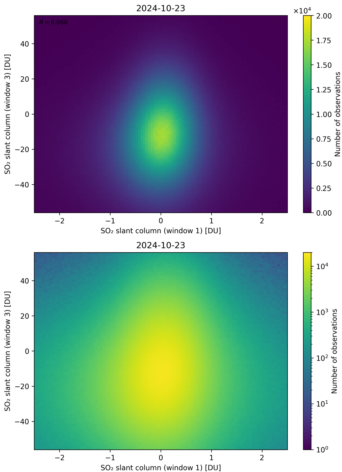
Figure 237: Scatter density plot of “SO 2 slant column (window 1)” against “SO 2 slant column (window 3)” for 2024-10-22 to 2024-10-24.
