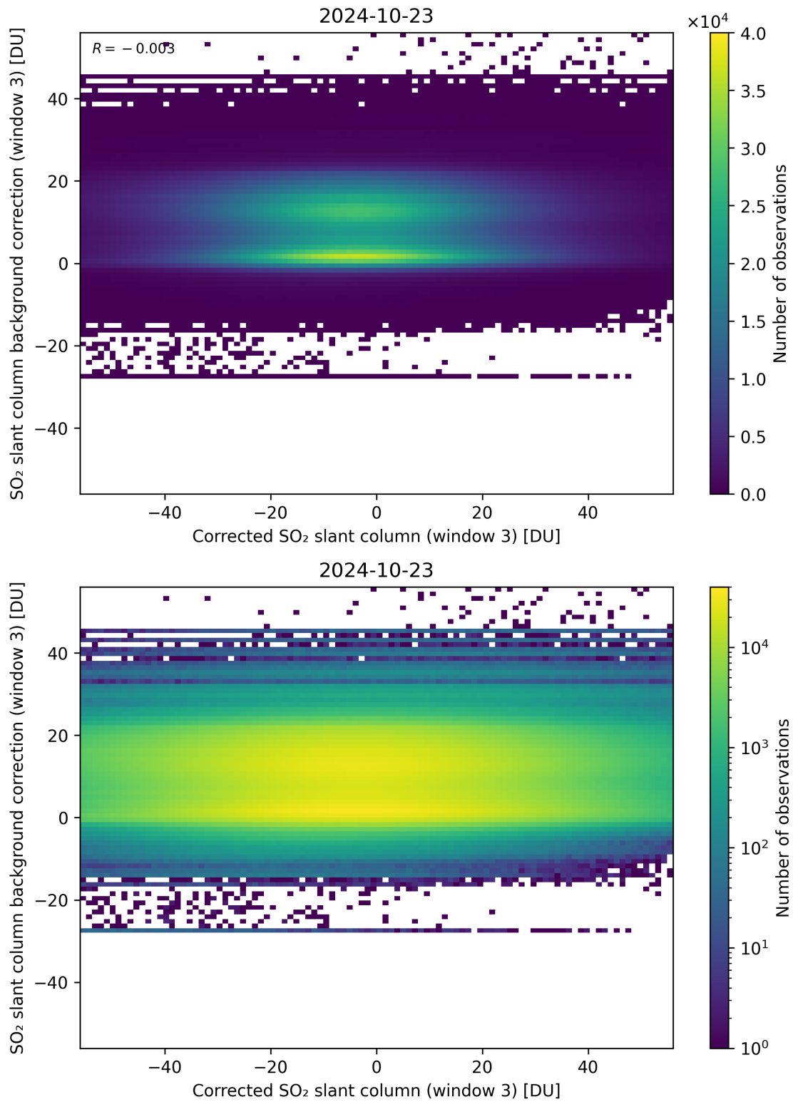
Figure 205: Scatter density plot of “Corrected SO 2 slant column (window 3)” against “SO 2 slant column background correction (window 3)” for 2024-10-22 to 2024-10-24.
