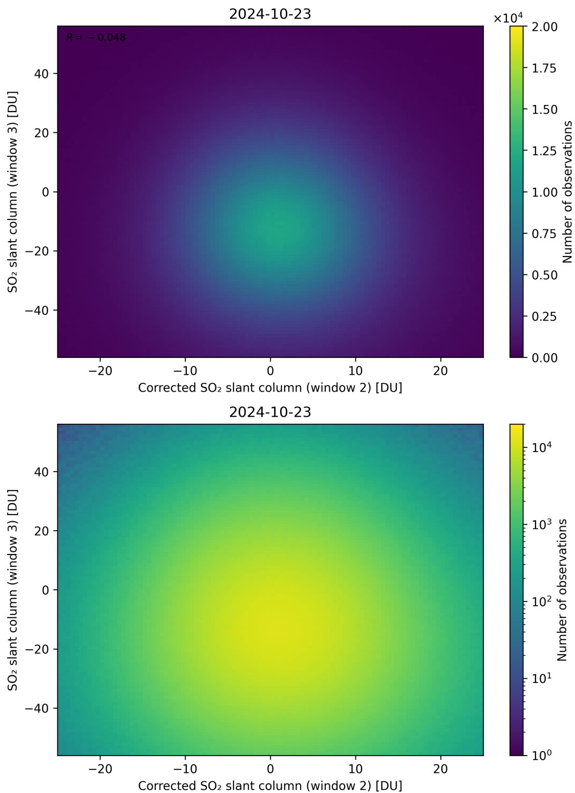
Figure 201: Scatter density plot of “Corrected SO 2 slant column (window 2)” against “SO 2 slant column (window 3)” for 2024-10-22 to 2024-10-24.
