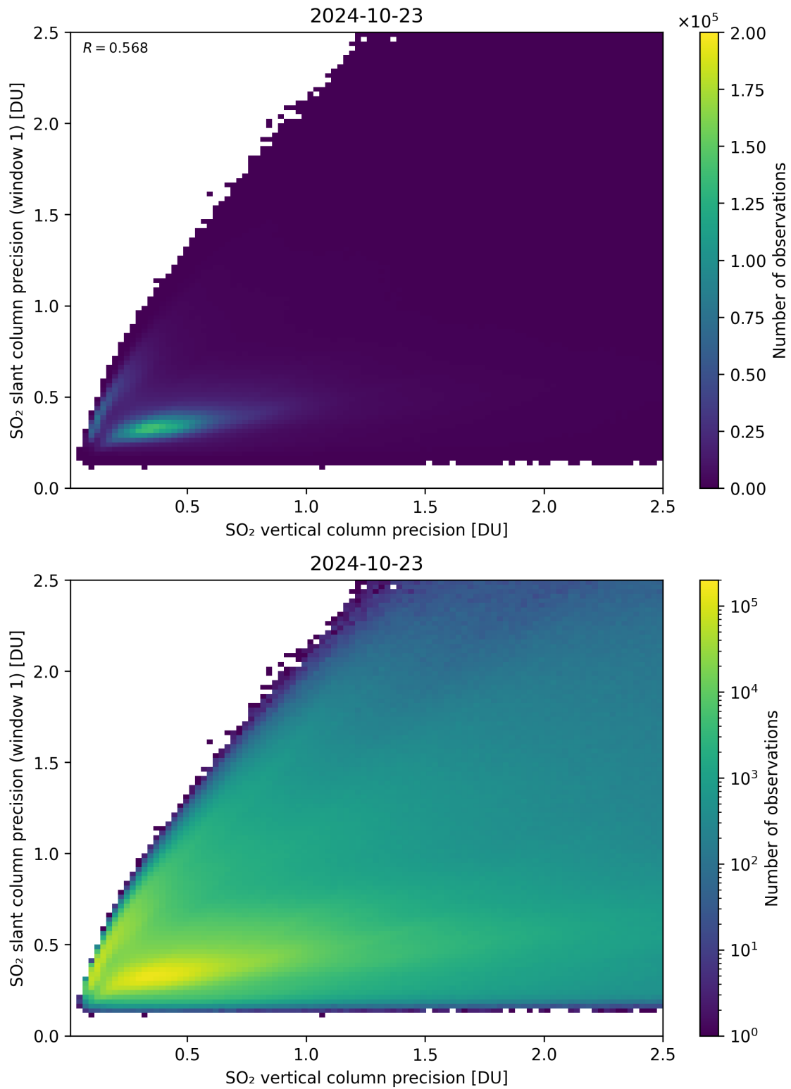
Figure 290: Scatter density plot of “SO 2 vertical column precision” against “SO 2 slant column precision (window 1)” for 2024-10-22 to 2024-10-24.
