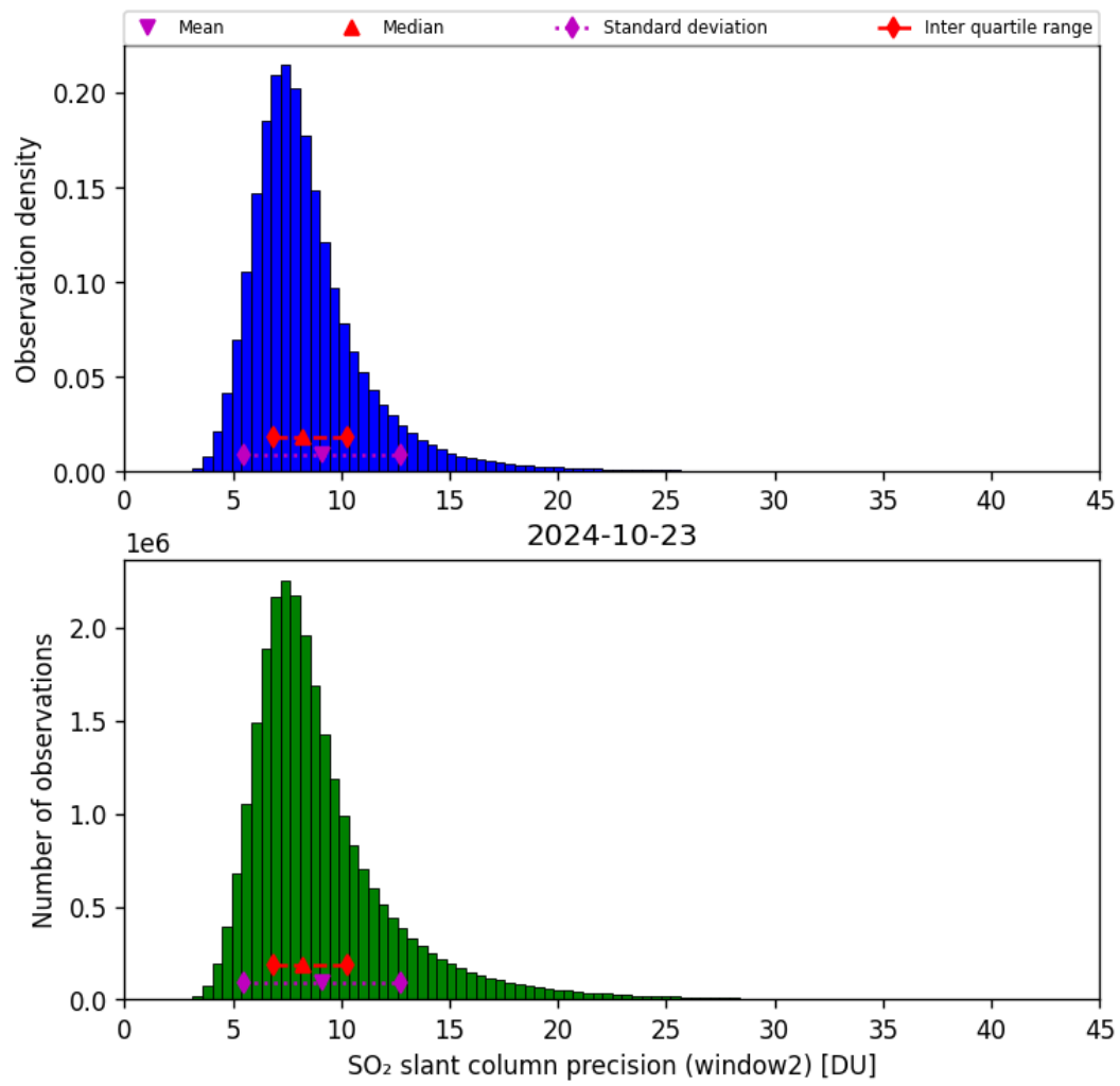
Figure 61: Histogram of “SO 2 slant column precision (window2)” for 2024-10-22 to 2024-10-24
