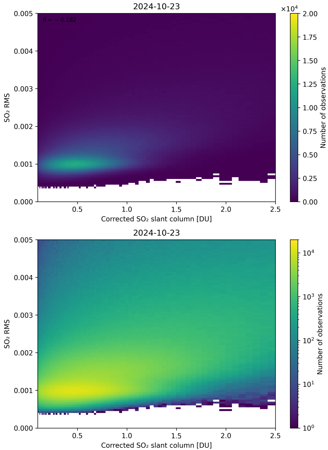
Figure 183: Scatter density plot of “Corrected SO 2 slant column” against “SO 2 RMS” for 2024-10-22 to 2024-10-24.
