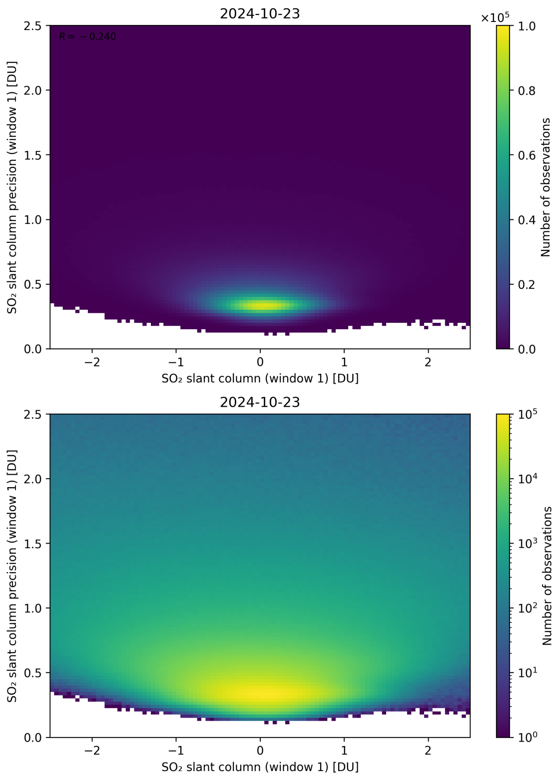
Figure 235: Scatter density plot of “SO 2 slant column (window 1)” against “SO 2 slant column precision (window 1)” for 2024-10-22 to 2024-10-24.
