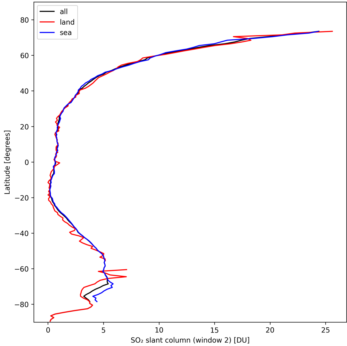
Figure 37: Zonal average of “SO 2 slant column (window 2)” for 2024-10-22 to 2024-10-24.
