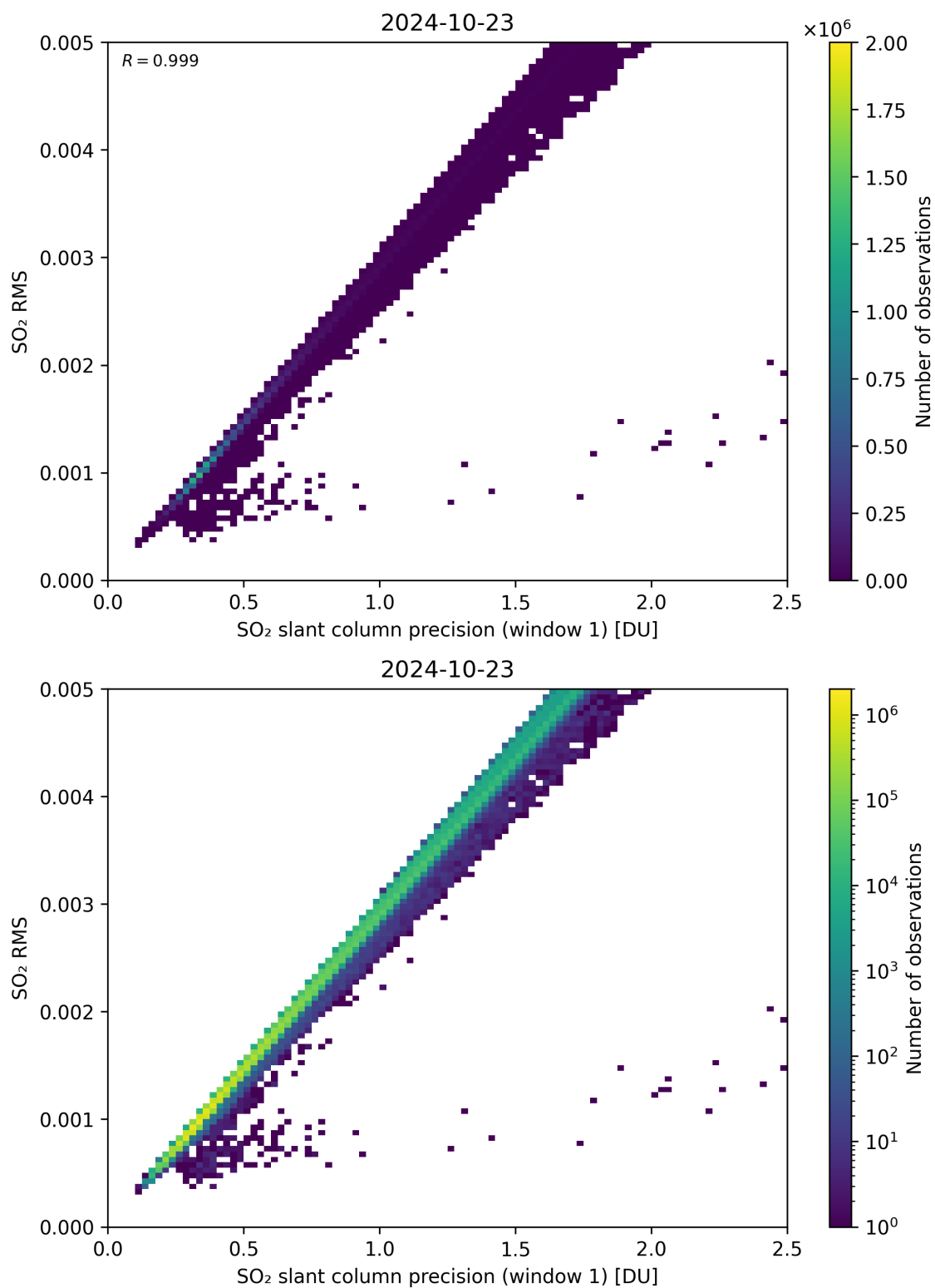
Figure 223: Scatter density plot of “SO 2 slant column precision (window 1)” against “SO 2 RMS” for 2024-10-22 to 2024-10-24.
