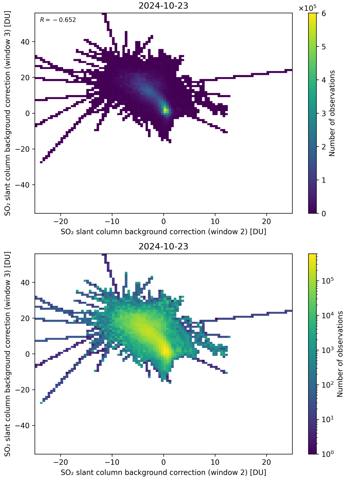
Figure 111: Scatter density plot of “SO 2 slant column background correction (window 2)” against “SO 2 slant column background correction (window 3)” for 2024-10-22 to 2024-10-24.
