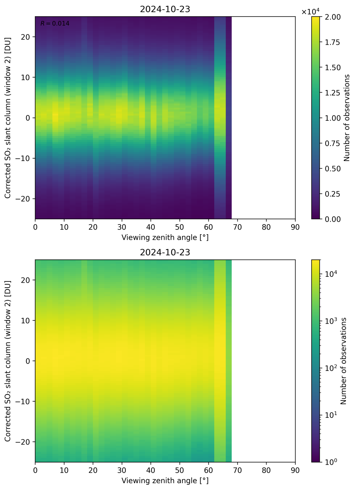
Figure 318: Scatter density plot of “Viewing zenith angle” against “Corrected SO 2 slant column (window 2)” for 2024-10-22 to 2024-10-24.
