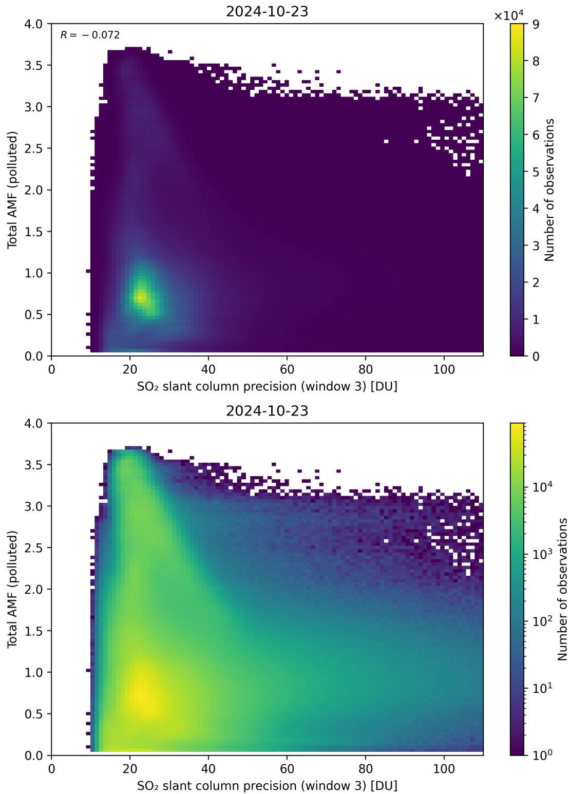
Figure 263: Scatter density plot of “SO 2 slant column precision (window 3)” against “Total AMF (polluted)” for 2024-10-22 to 2024-10-24.
