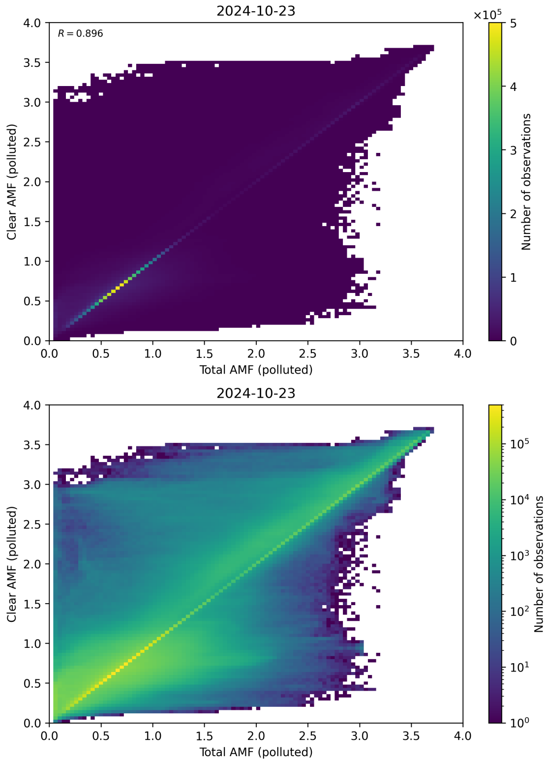
Figure 271: Scatter density plot of “Total AMF (polluted)” against “Clear AMF (polluted)” for 2024-10-22 to 2024-10-24.
