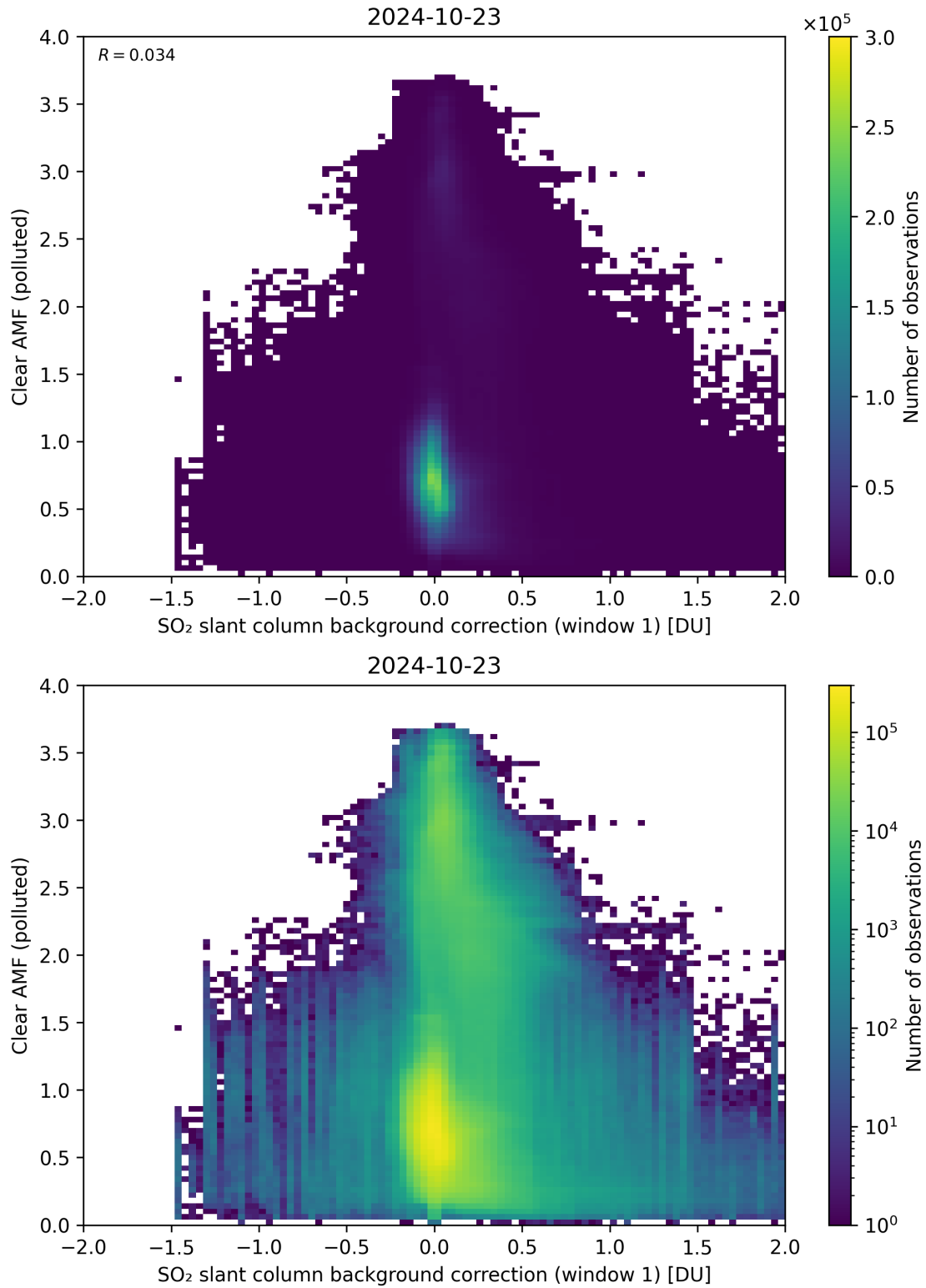
Figure 103: Scatter density plot of “SO 2 slant column background correction (window 1)” against “Clear AMF (polluted)” for 2024-10-22 to 2024-10-24.
