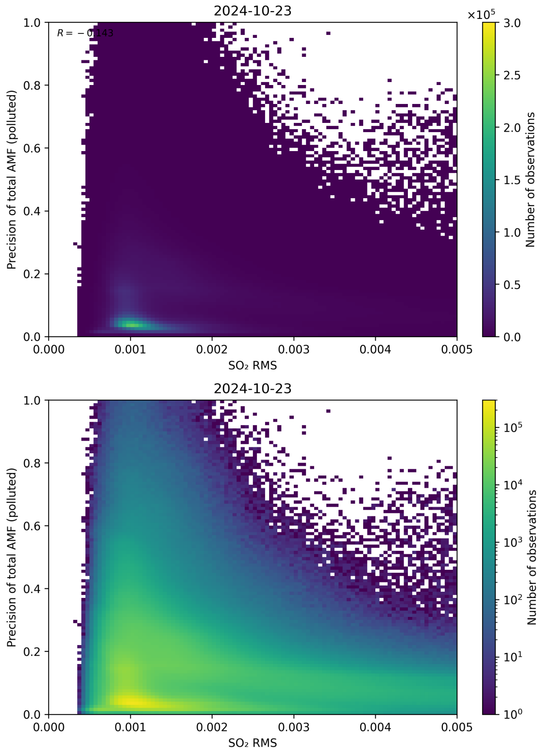
Figure 138: Scatter density plot of “SO 2 RMS” against “Precision of total AMF (polluted)” for 2024-10-22 to 2024-10-24.
