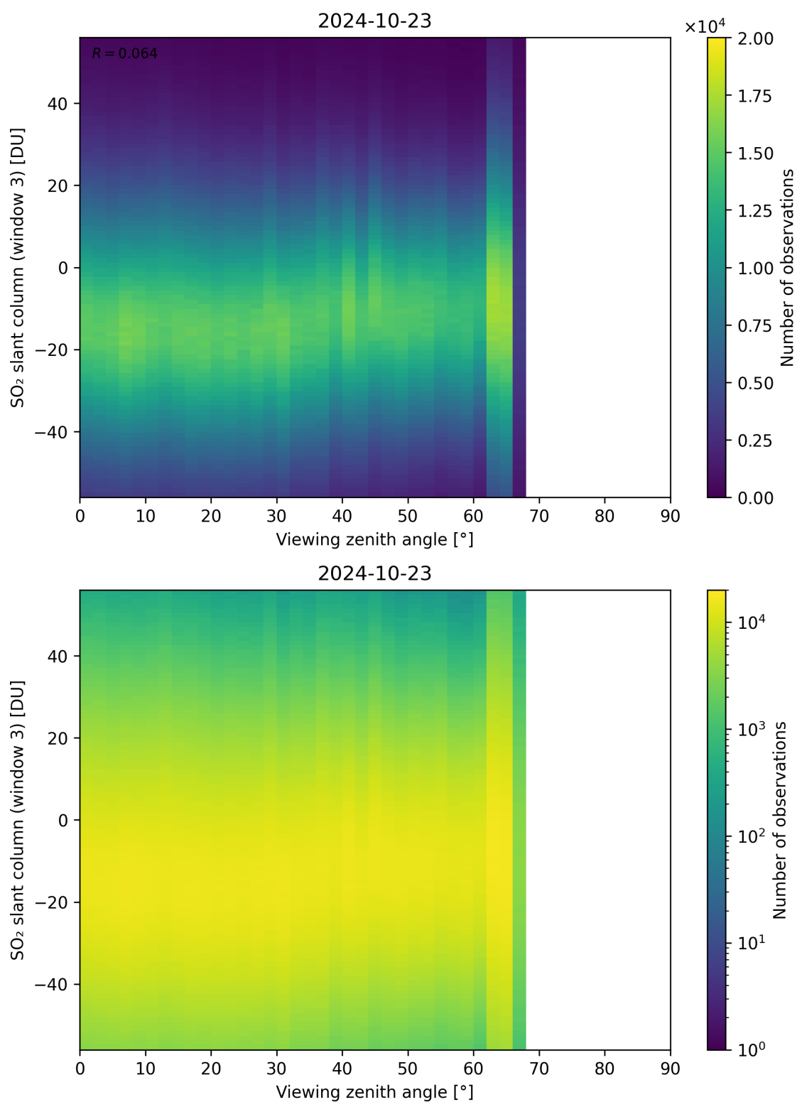
Figure 323: Scatter density plot of “Viewing zenith angle” against “SO 2 slant column (window 3)” for 2024-10-22 to 2024-10-24.
