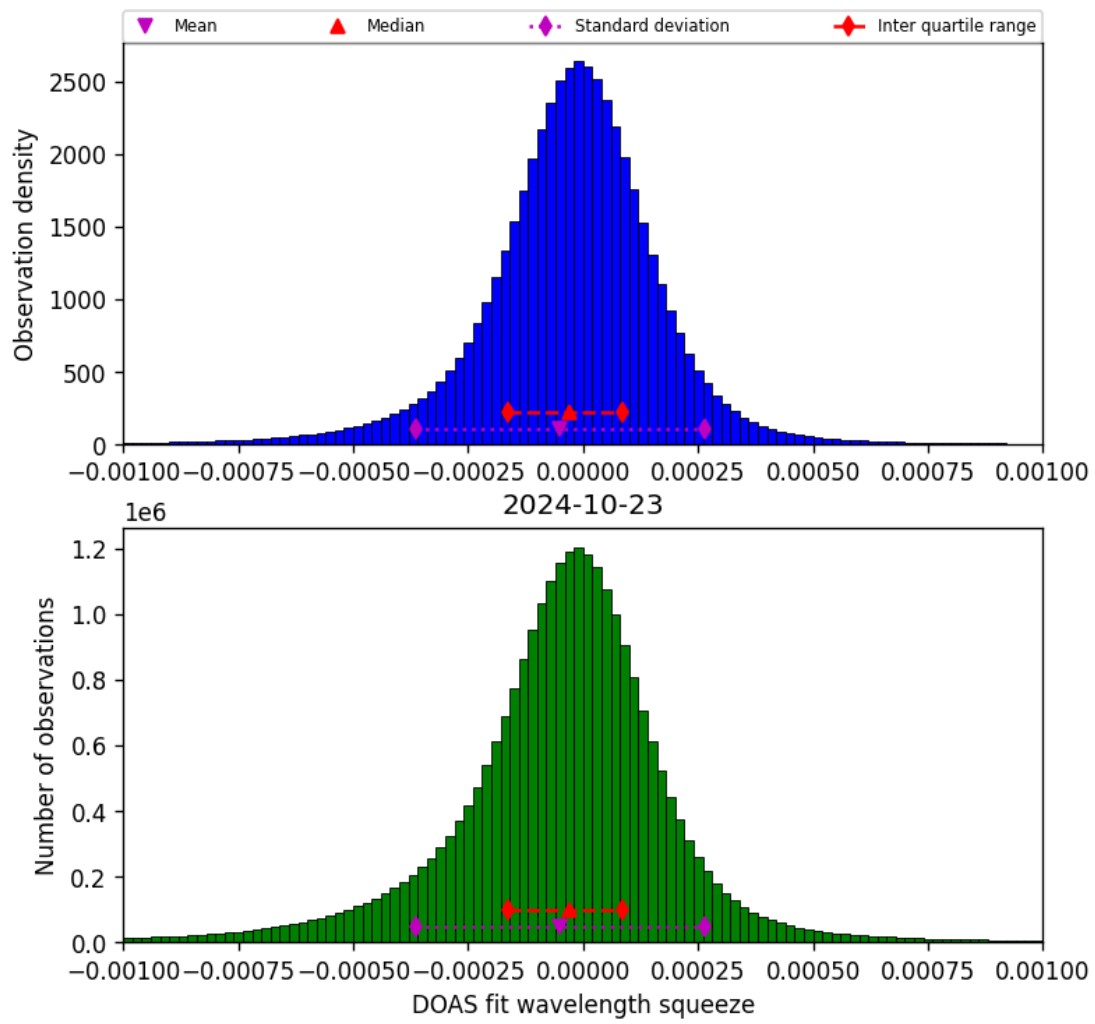
Figure 69: Histogram of “DOAS fit wavelength squeeze” for 2024-10-22 to 2024-10-24
