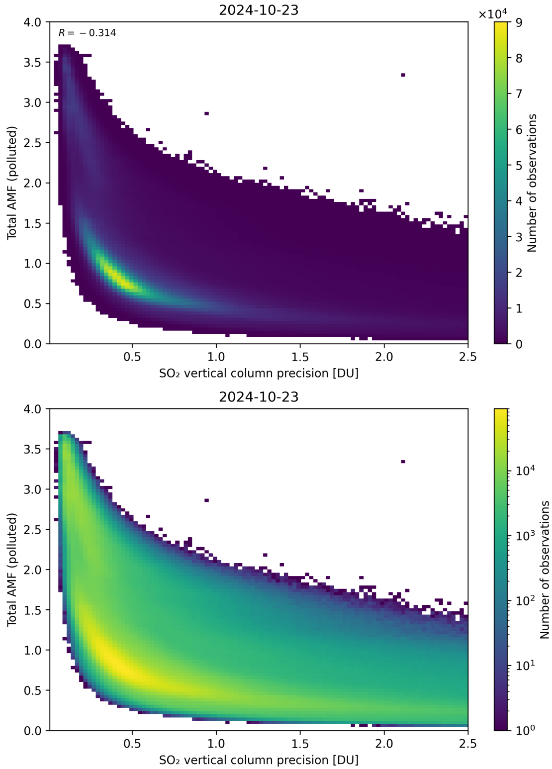
Figure 294: Scatter density plot of “SO 2 vertical column precision” against “Total AMF (polluted)” for 2024-10-22 to 2024-10-24.
