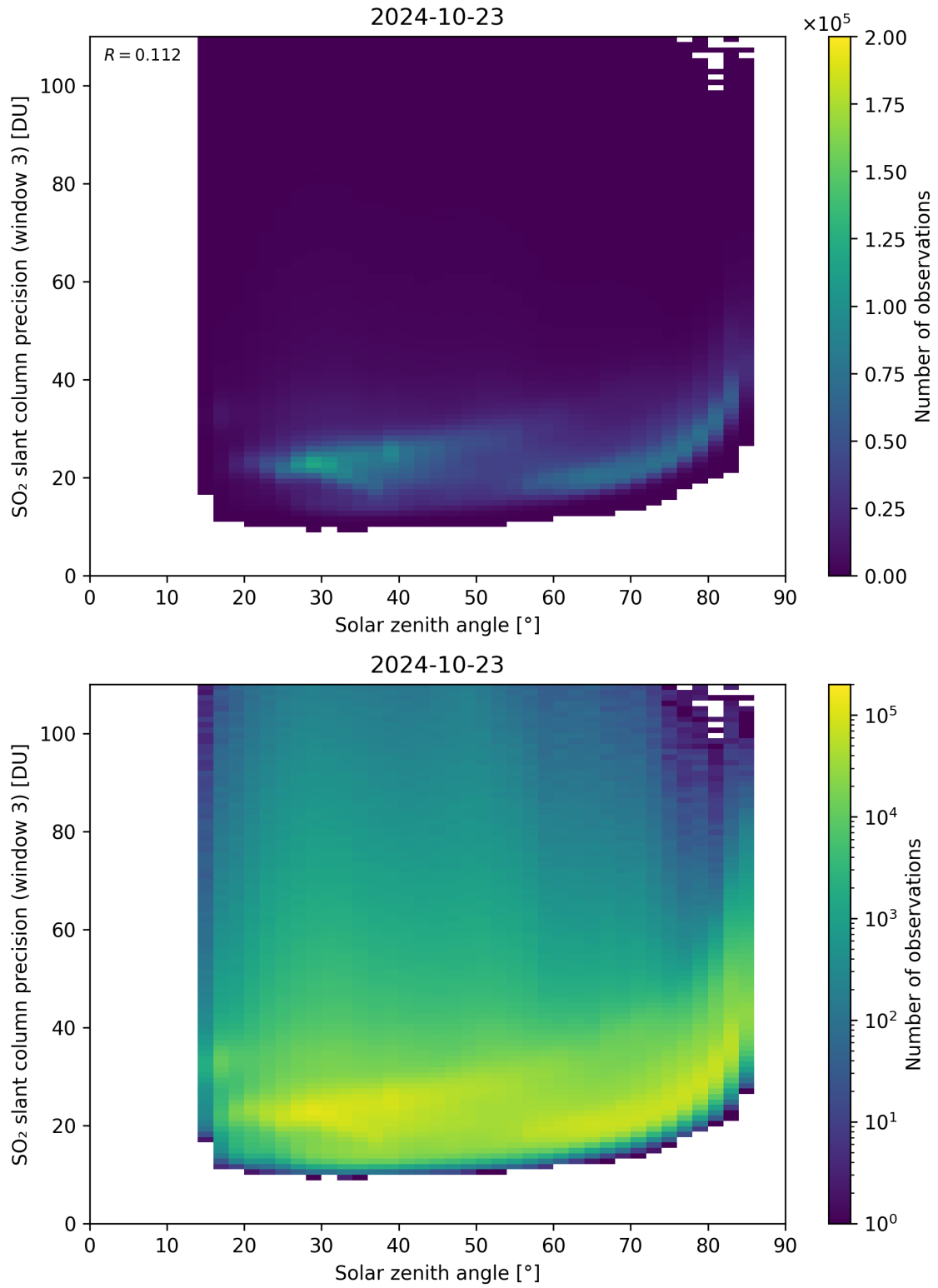
Figure 173: Scatter density plot of “Solar zenith angle” against “SO 2 slant column precision (window 3)” for 2024-10-22 to 2024-10-24.
