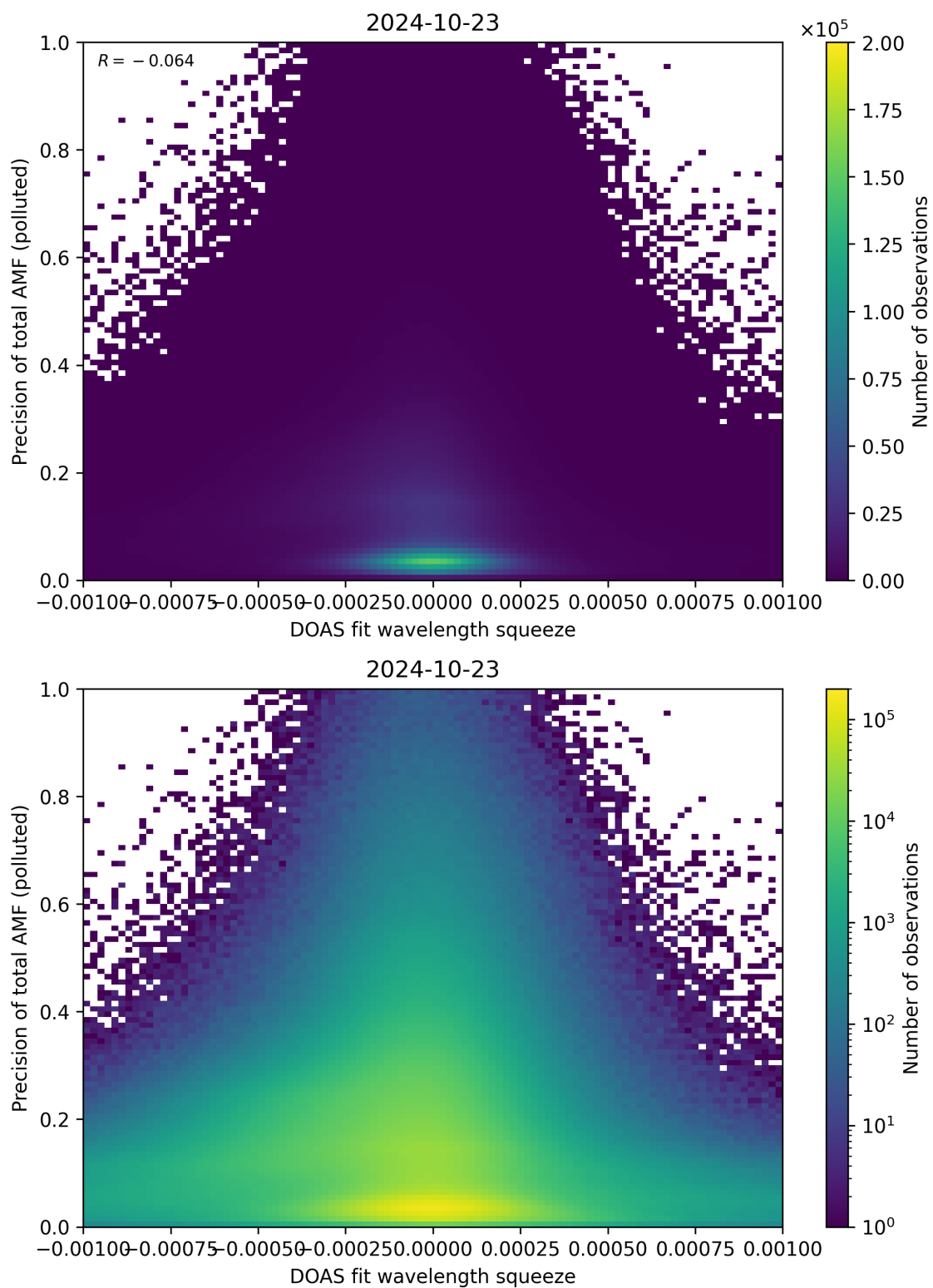
Figure 135: Scatter density plot of “DOAS fit wavelength squeeze” against “Precision of total AMF (polluted)” for 2024-10-22 to 2024-10-24.
