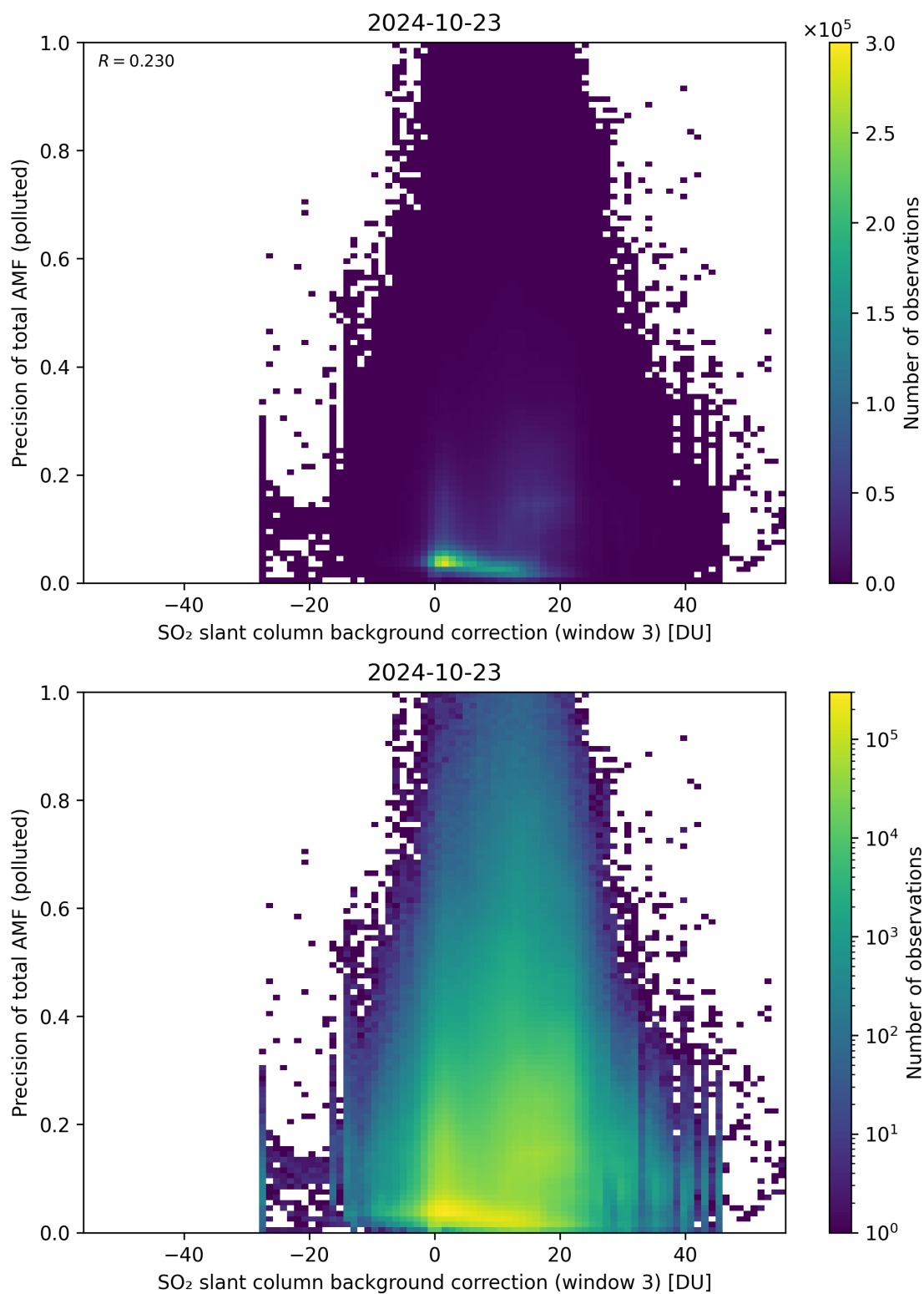
Figure 126: Scatter density plot of “SO 2 slant column background correction (window 3)” against “Precision of total AMF (polluted)” for 2024-10-22 to 2024-10-24.
