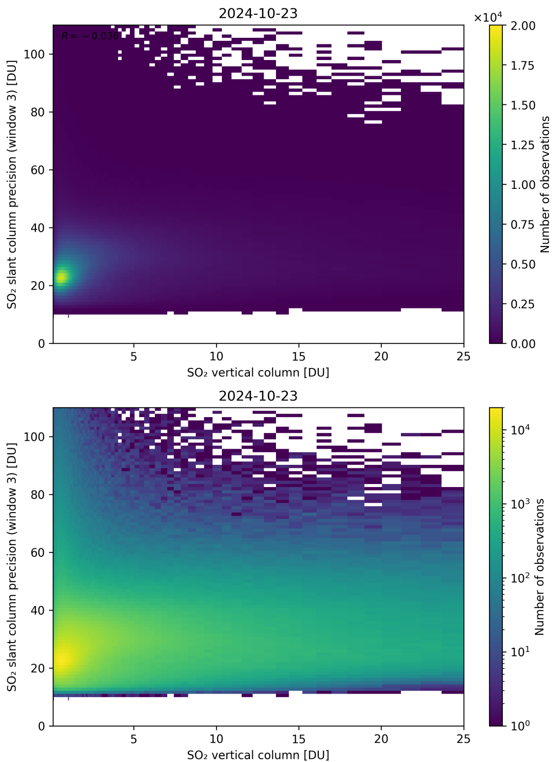
Figure 304: Scatter density plot of “SO 2 vertical column” against “SO 2 slant column precision (window 3)” for 2024-10-22 to 2024-10-24.
