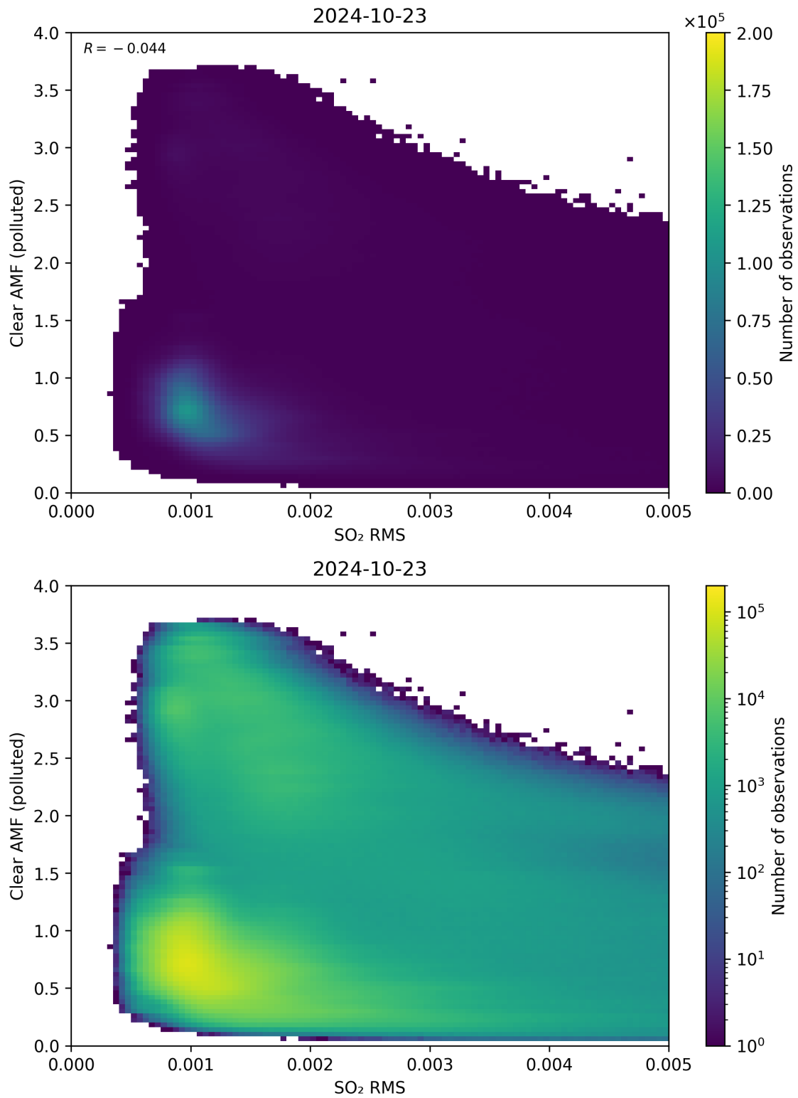
Figure 136: Scatter density plot of “SO 2 RMS” against “Clear AMF (polluted)” for 2024-10-22 to 2024-10-24.
