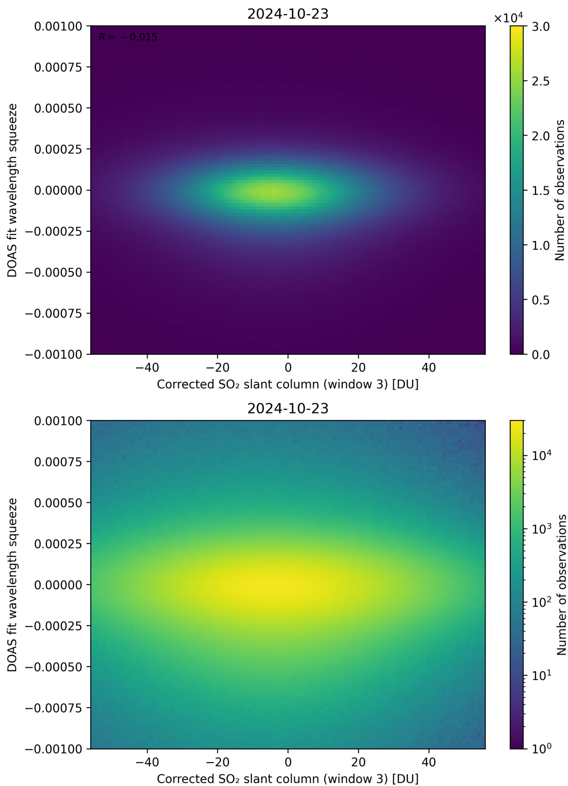
Figure 207: Scatter density plot of “Corrected SO 2 slant column (window 3)” against “DOAS fit wavelength squeeze” for 2024-10-22 to 2024-10-24.
