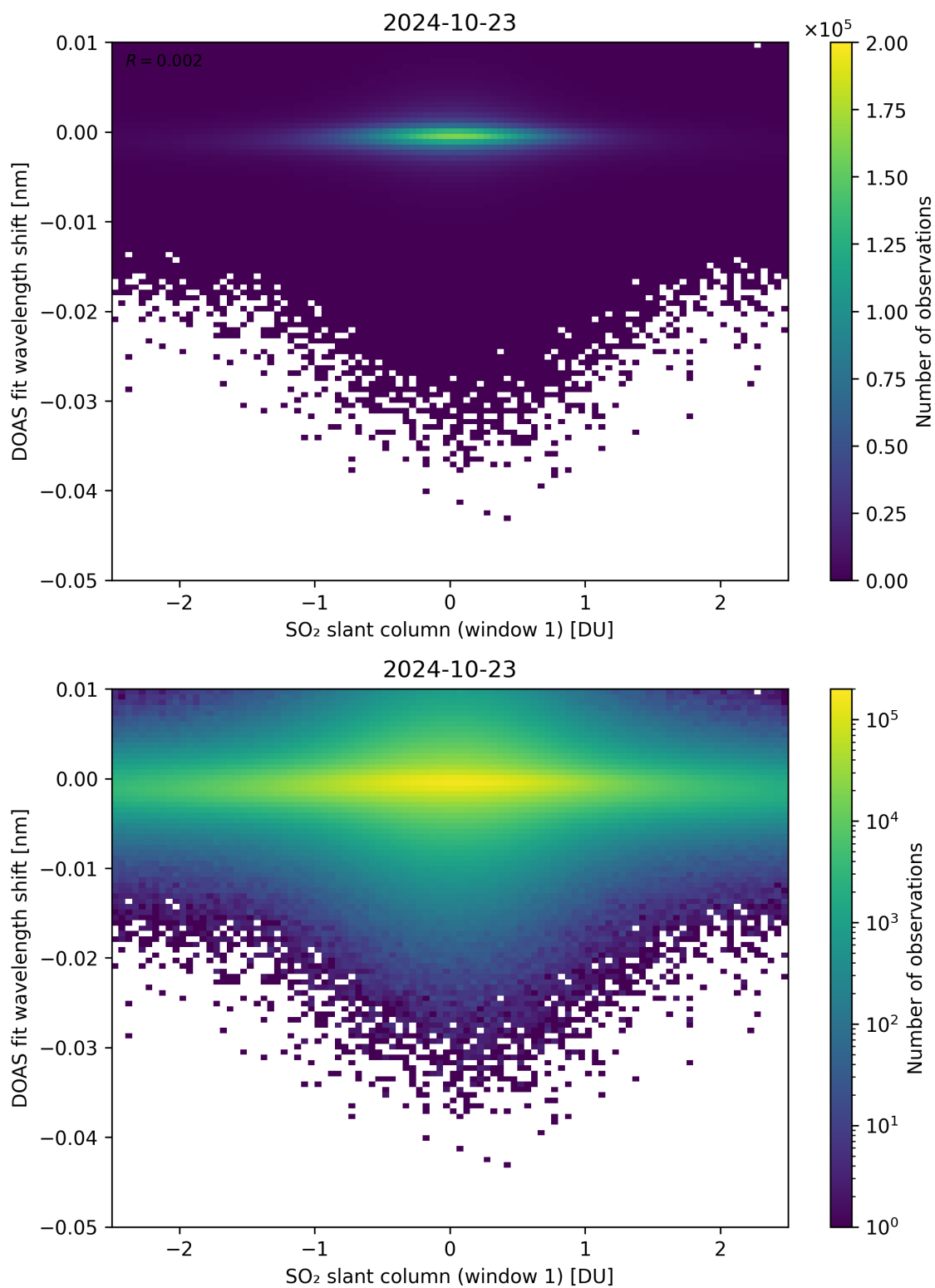
Figure 215: Scatter density plot of “SO 2 slant column (window 1)” against “DOAS fit wavelength shift” for 2024-10-22 to 2024-10-24.
