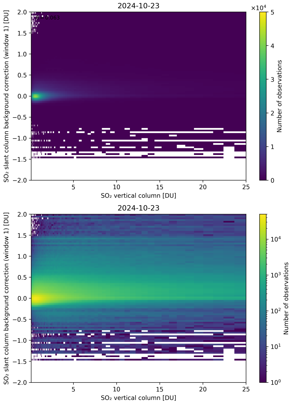
Figure 273: Scatter density plot of “SO 2 vertical column” against “SO 2 slant column background correction (window 1)” for 2024-10-22 to 2024-10-24.
