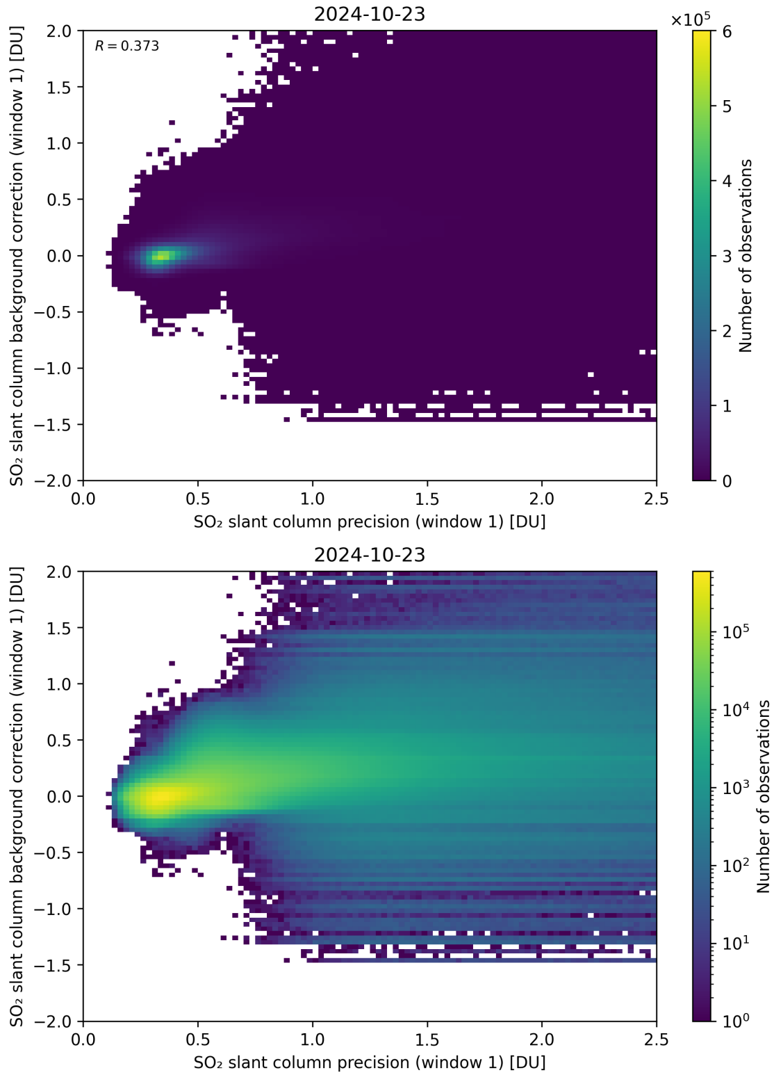
Figure 218: Scatter density plot of “SO 2 slant column precision (window 1)” against “SO 2 slant column background correction (window 1)” for 2024-10-22 to 2024-10-24.
