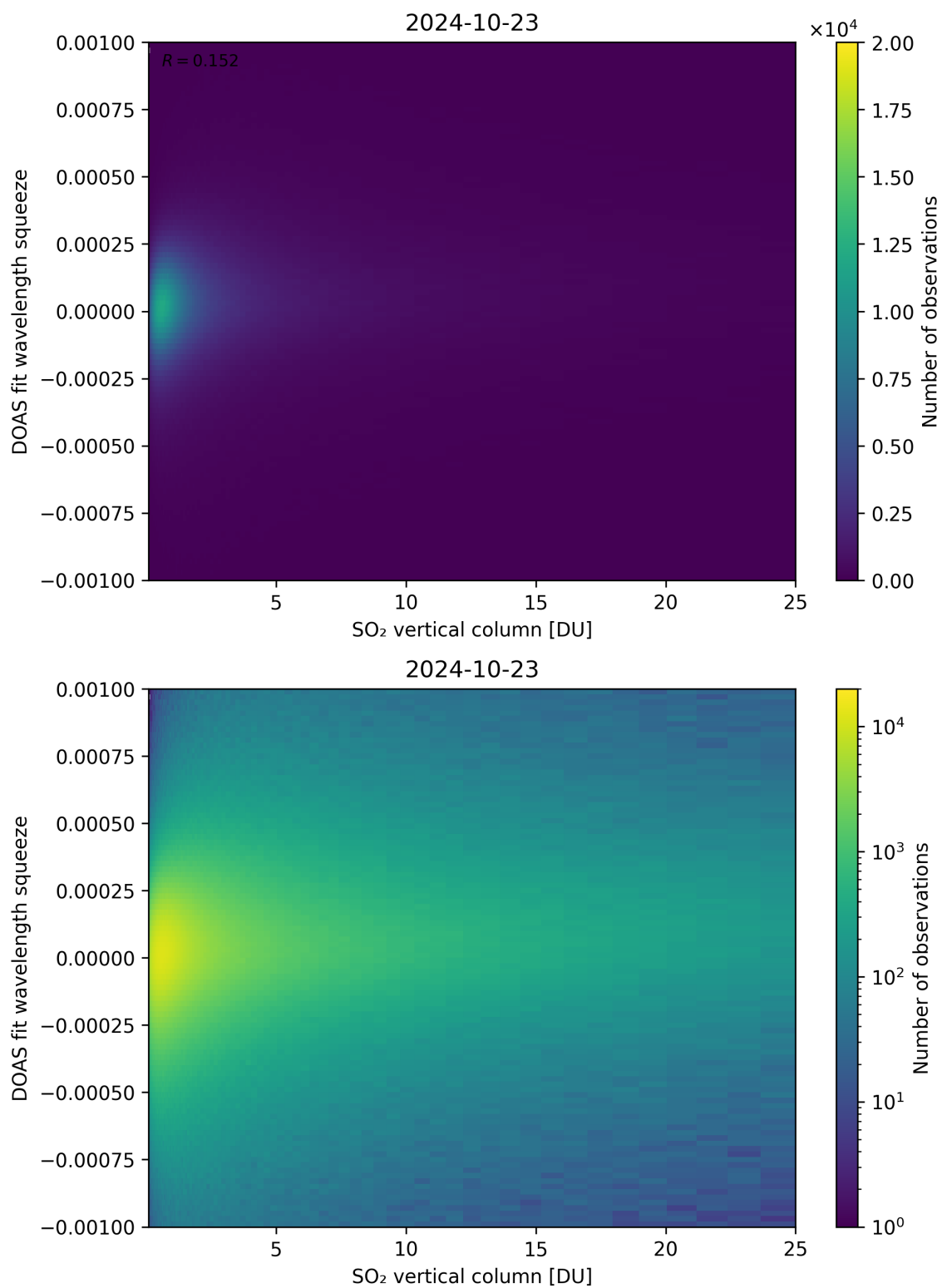
Figure 277: Scatter density plot of “SO 2 vertical column” against “DOAS fit wavelength squeeze” for 2024-10-22 to 2024-10-24.
