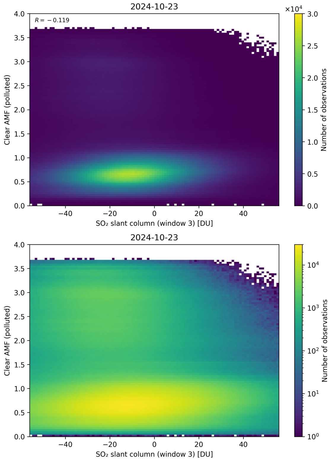
Figure 265: Scatter density plot of “SO 2 slant column (window 3)” against “Clear AMF (polluted)” for 2024-10-22 to 2024-10-24.
