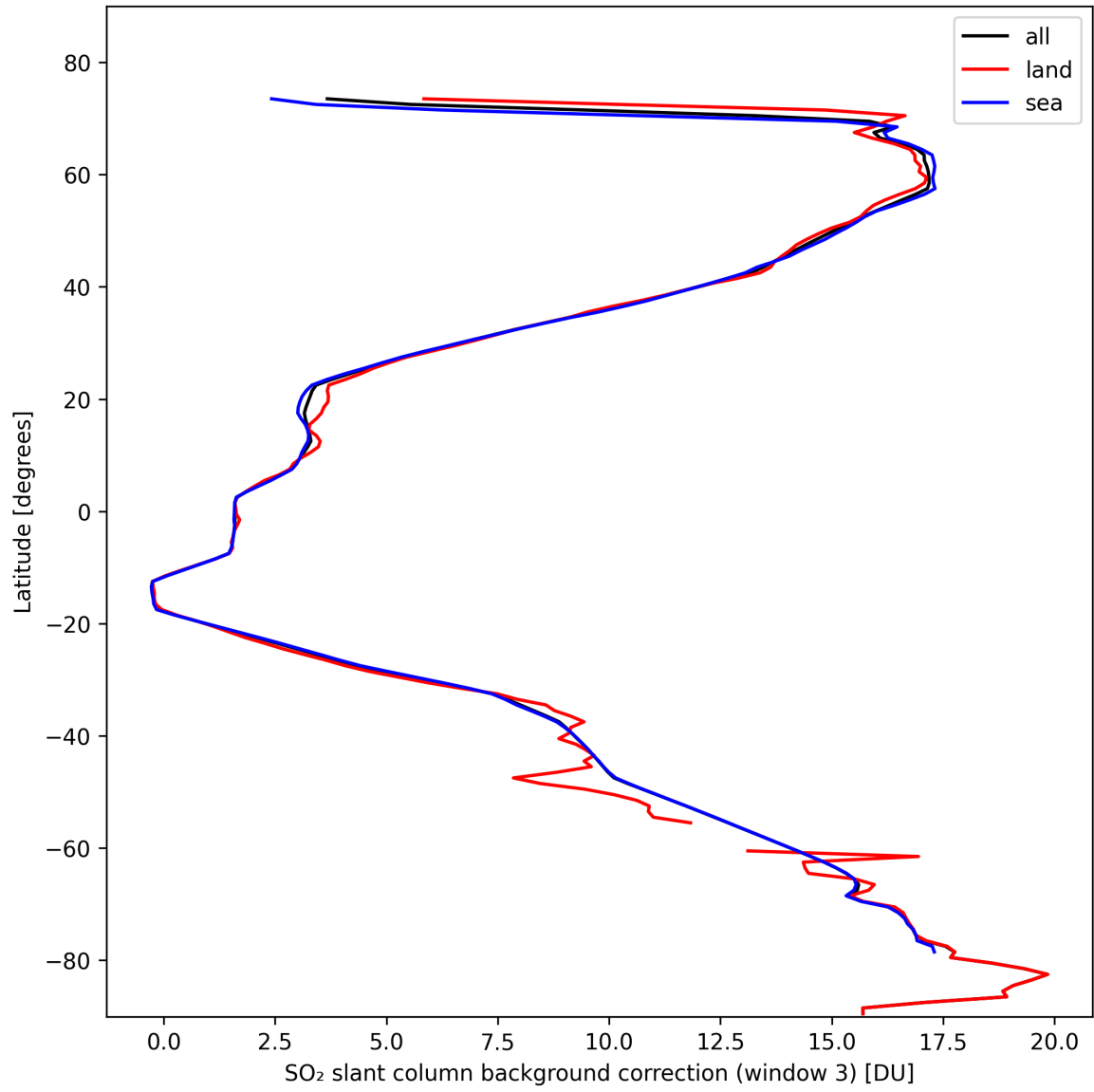
Figure 44: Zonal average of “SO 2 slant column background correction (window 3)” for 2024-10-22 to 2024-10-24.
