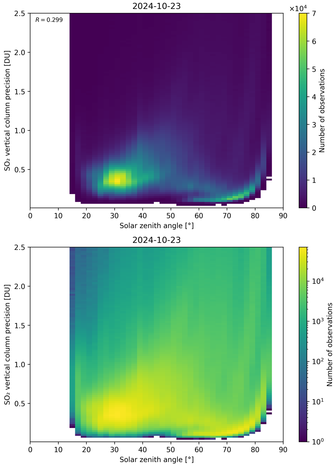
Figure 177: Scatter density plot of “Solar zenith angle” against “SO 2 vertical column precision” for 2024-10-22 to 2024-10-24.
