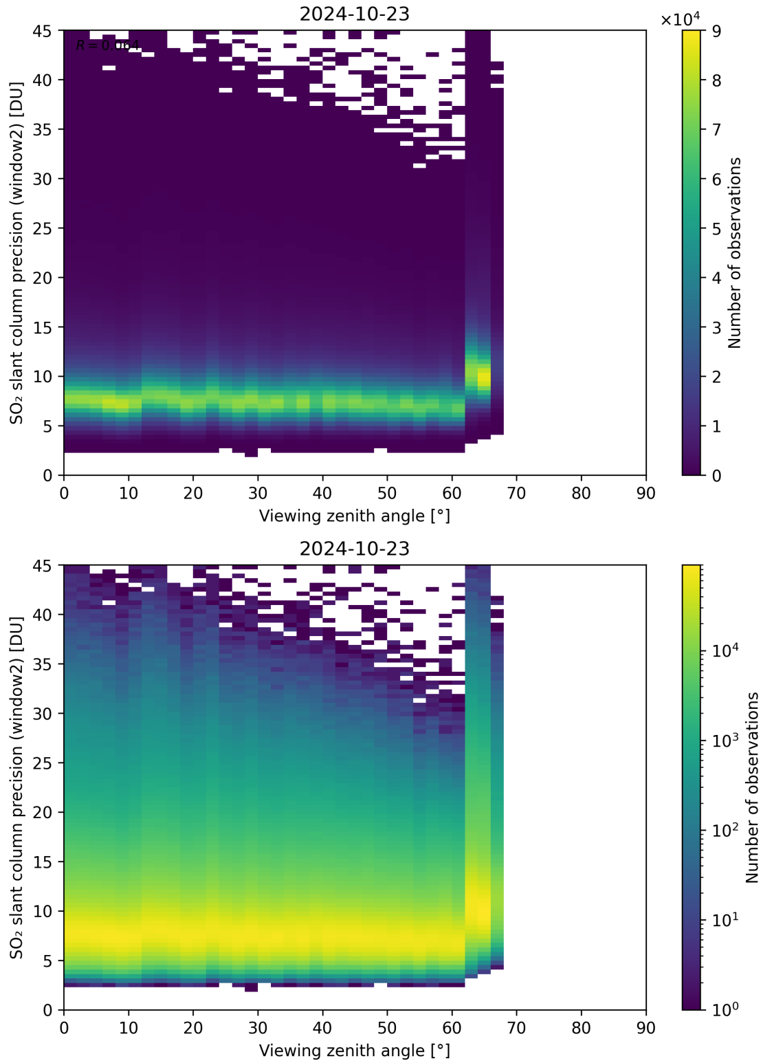
Figure 322: Scatter density plot of “Viewing zenith angle” against “SO 2 slant column precision (window2)” for 2024-10-22 to 2024-10-24.
