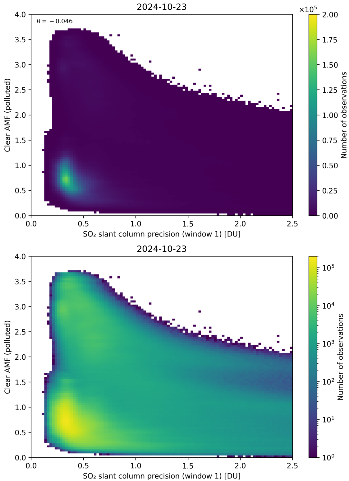
Figure 224: Scatter density plot of “SO 2 slant column precision (window 1)” against “Clear AMF (polluted)” for 2024-10-22 to 2024-10-24.
