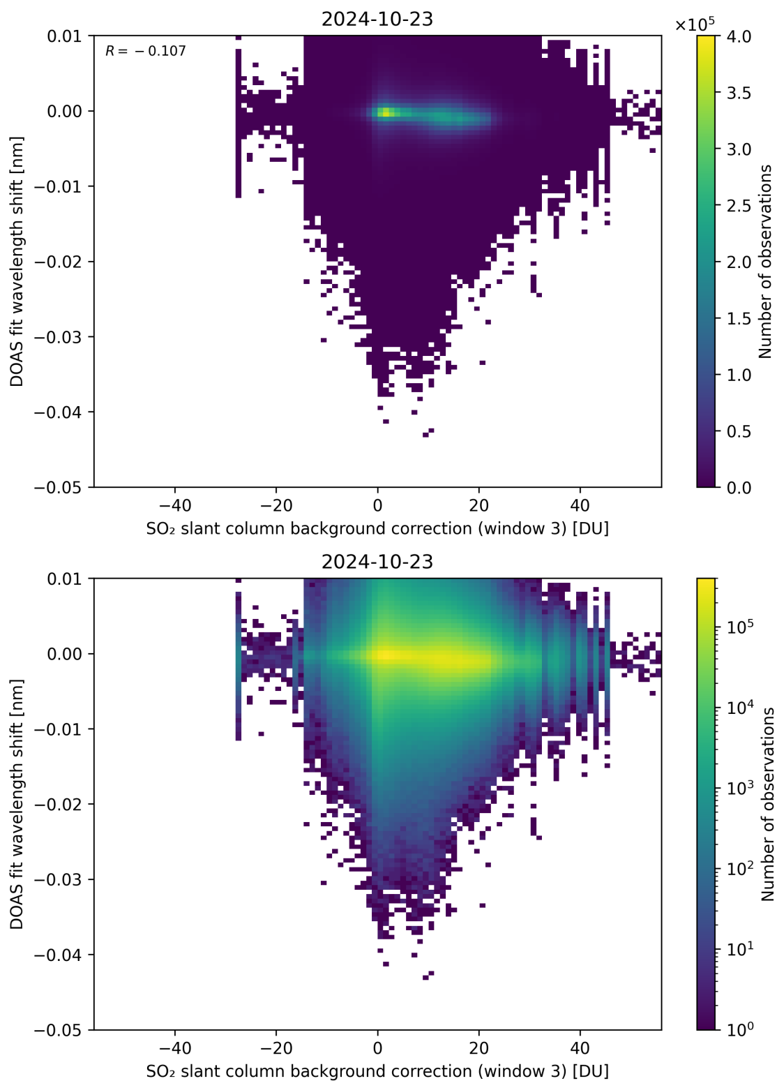
Figure 121: Scatter density plot of “SO 2 slant column background correction (window 3)” against “DOAS fit wavelength shift” for 2024-10-22 to 2024-10-24.
