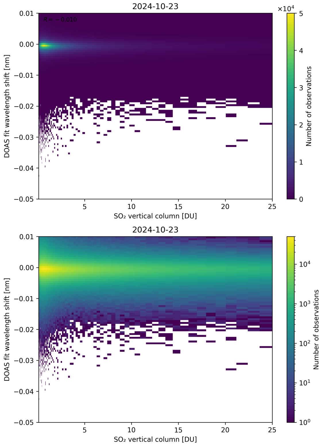
Figure 276: Scatter density plot of “SO 2 vertical column” against “DOAS fit wavelength shift” for 2024-10-22 to 2024-10-24.
