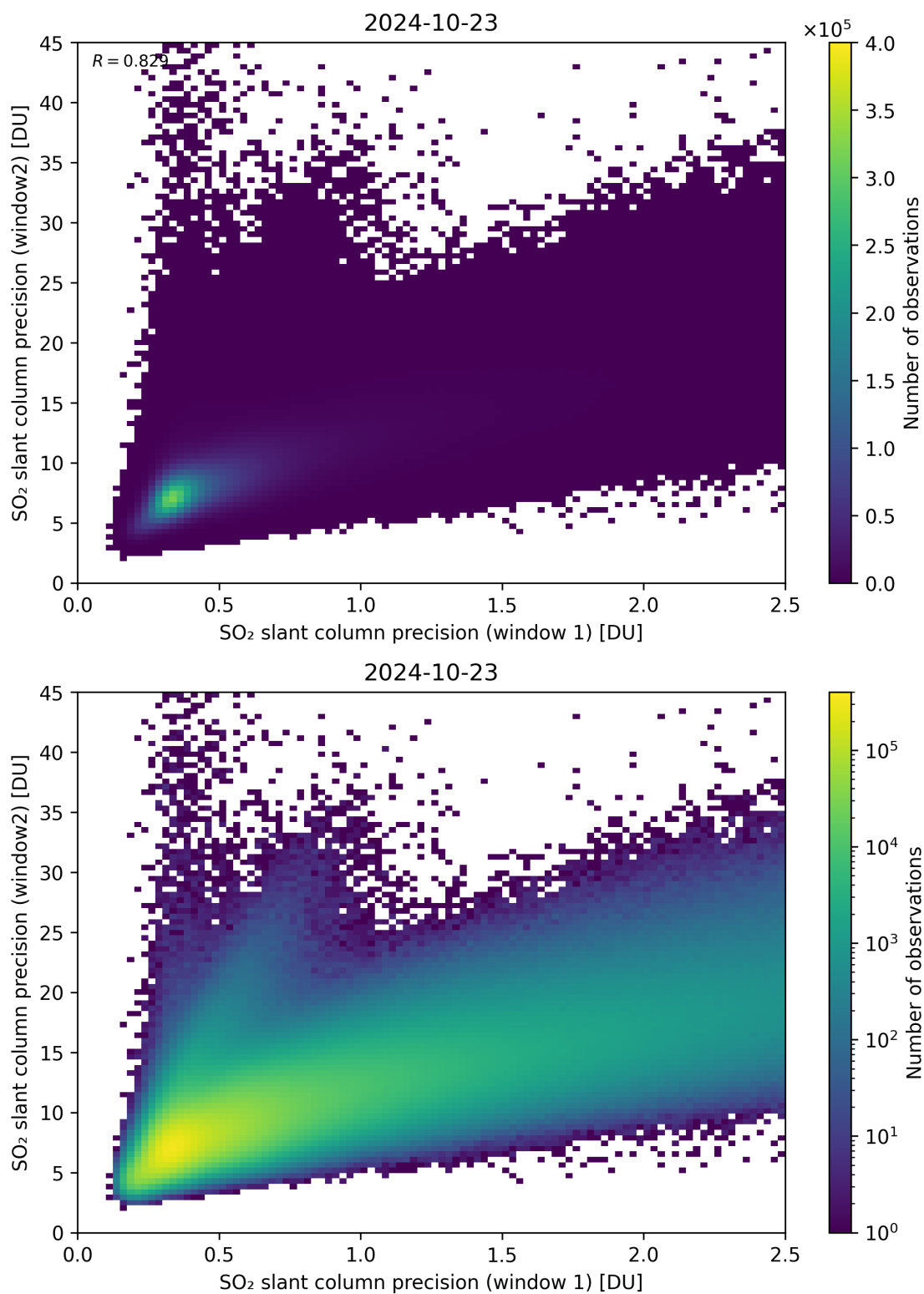
Figure 227: Scatter density plot of “SO 2 slant column precision (window 1)” against “SO 2 slant column precision (window2)” for 2024-10-22 to 2024-10-24.
