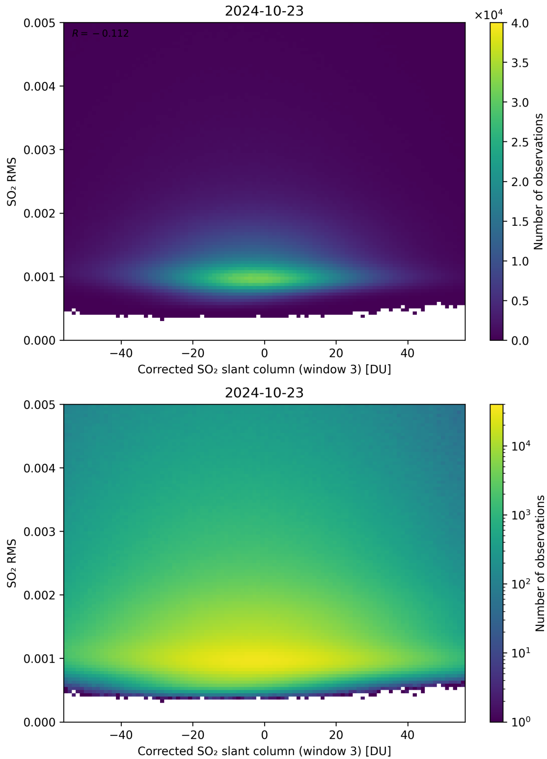
Figure 208: Scatter density plot of “Corrected SO 2 slant column (window 3)” against “SO 2 RMS” for 2024-10-22 to 2024-10-24.
