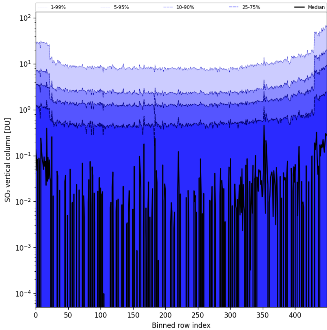
Figure 76: Along track statistics of “SO 2 vertical column” for 2024-10-22 to 2024-10-24
