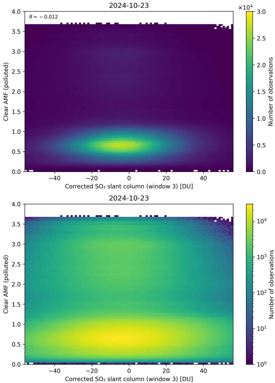
Figure 209: Scatter density plot of “Corrected SO 2 slant column (window 3)” against “Clear AMF (polluted)” for 2024-10-22 to 2024-10-24.
