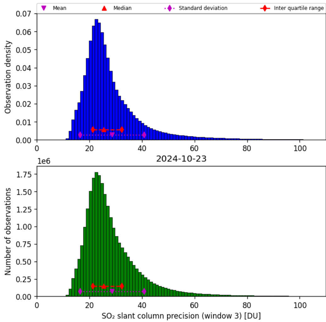
Figure 65: Histogram of “SO 2 slant column precision (window 3)” for 2024-10-22 to 2024-10-24
