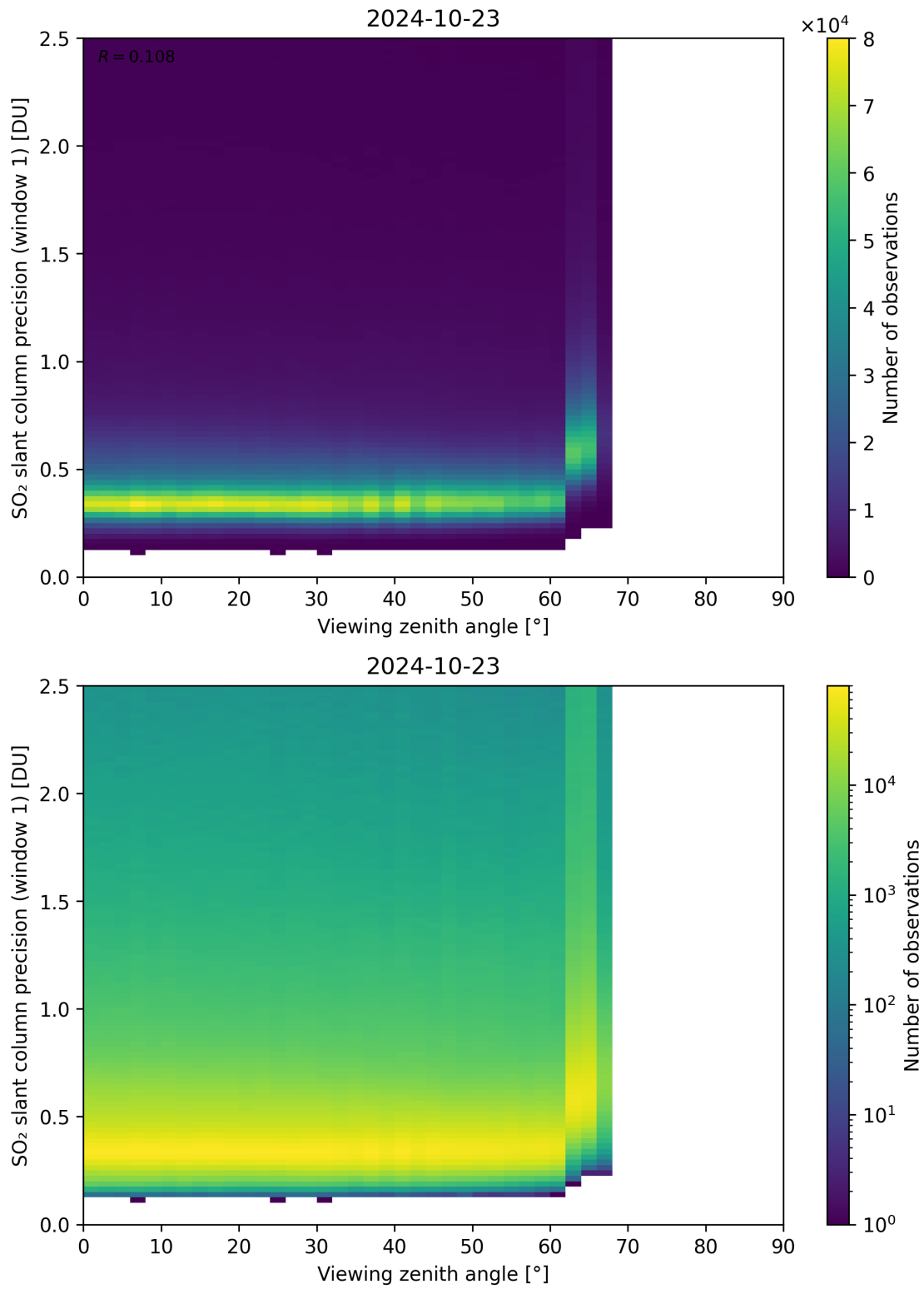
Figure 321: Scatter density plot of “Viewing zenith angle” against “SO 2 slant column precision (window 1)” for 2024-10-22 to 2024-10-24.
