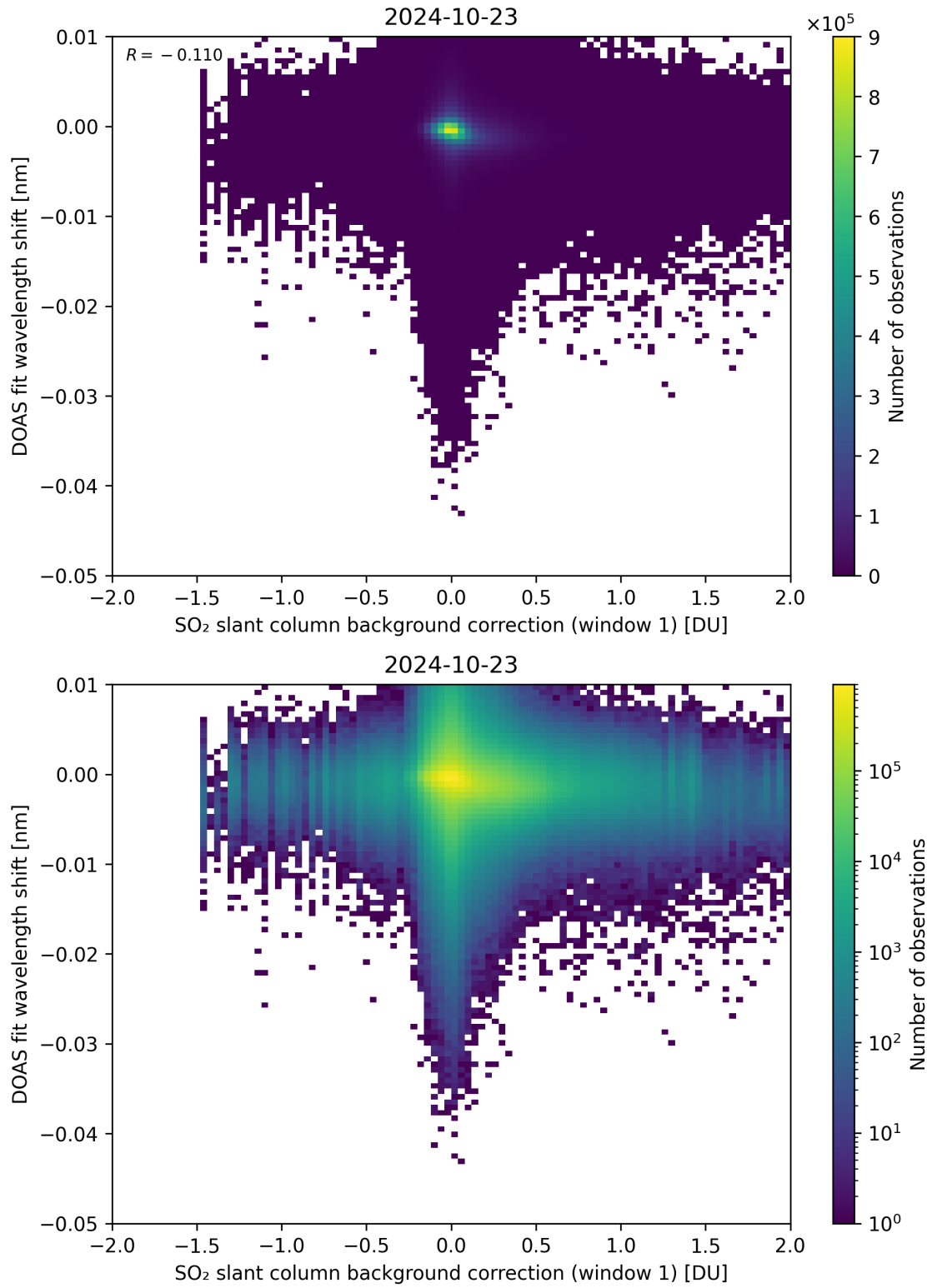
Figure 100: Scatter density plot of “SO 2 slant column background correction (window 1)” against “DOAS fit wavelength shift” for 2024-10-22 to 2024-10-24.
