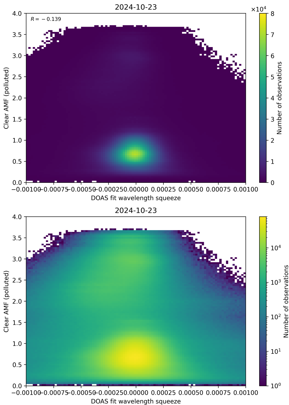
Figure 133: Scatter density plot of “DOAS fit wavelength squeeze” against “Clear AMF (polluted)” for 2024-10-22 to 2024-10-24.
