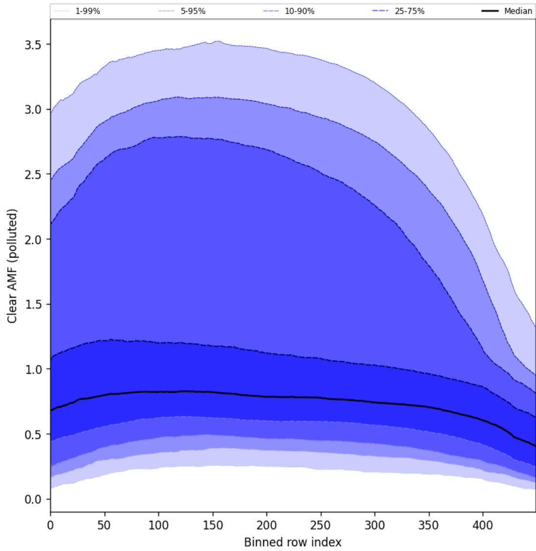
Figure 96: Along track statistics of “Clear AMF (polluted)” for 2024-10-22 to 2024-10-24
