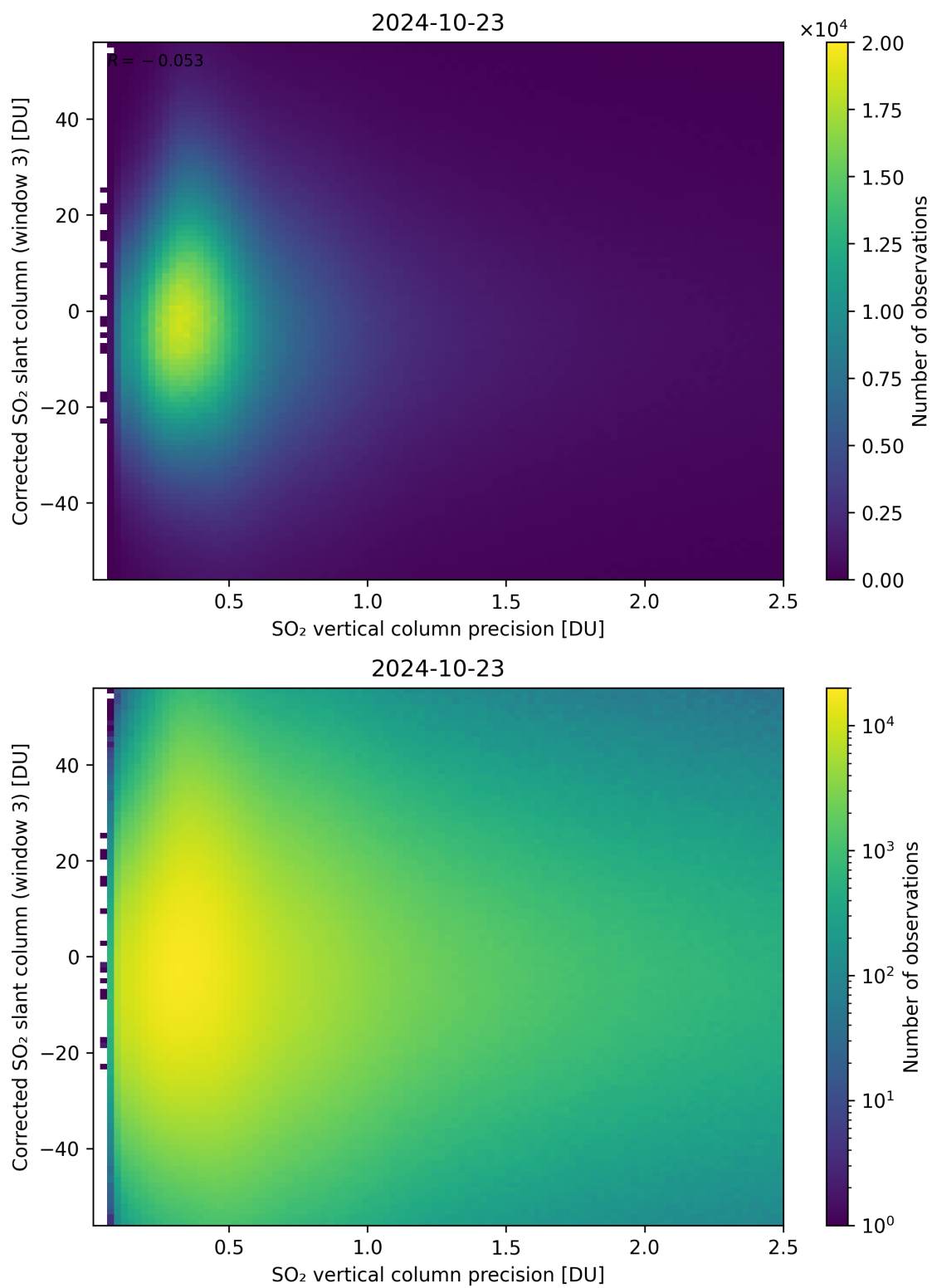
Figure 288: Scatter density plot of “SO 2 vertical column precision” against “Corrected SO 2 slant column (window 3)” for 2024-10-22 to 2024-10-24.
