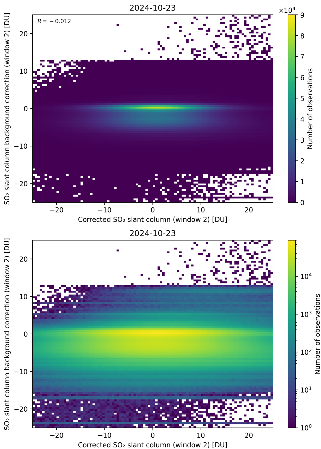
Figure 194: Scatter density plot of “Corrected SO 2 slant column (window 2)” against “SO 2 slant column background correction (window 2)” for 2024-10-22 to 2024-10-24.
