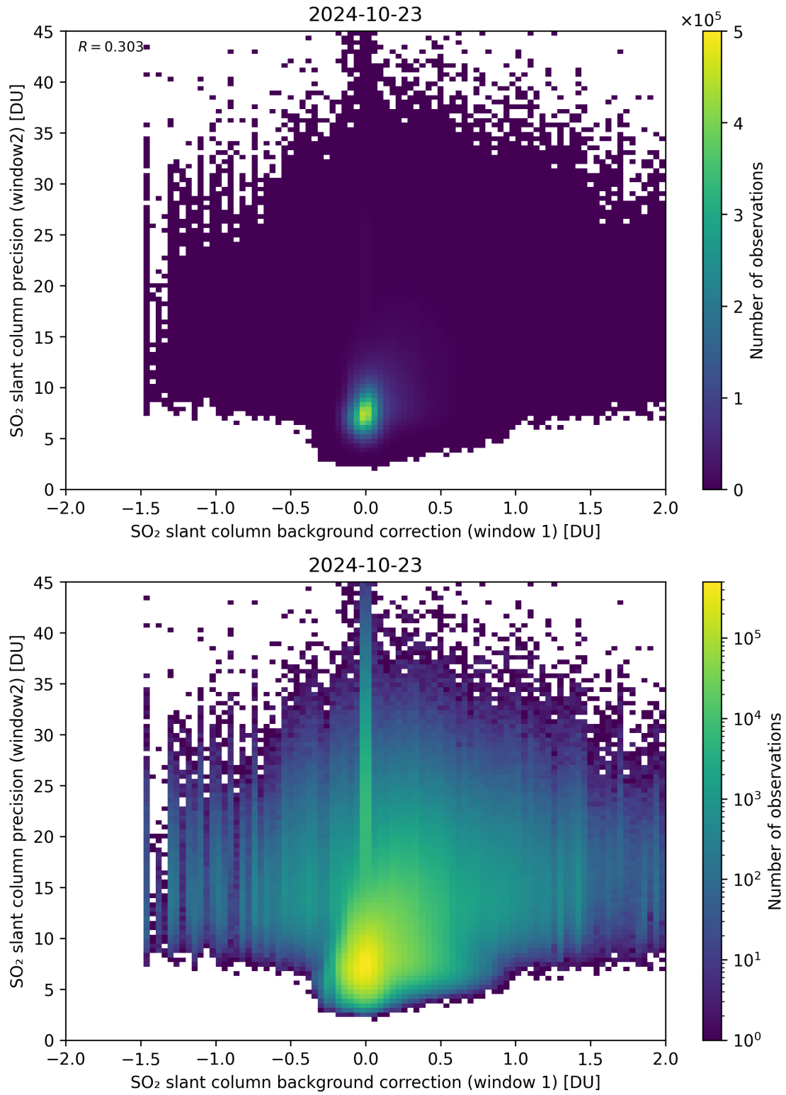
Figure 106: Scatter density plot of “SO 2 slant column background correction (window 1)” against “SO 2 slant column precision (window2)” for 2024-10-22 to 2024-10-24.
