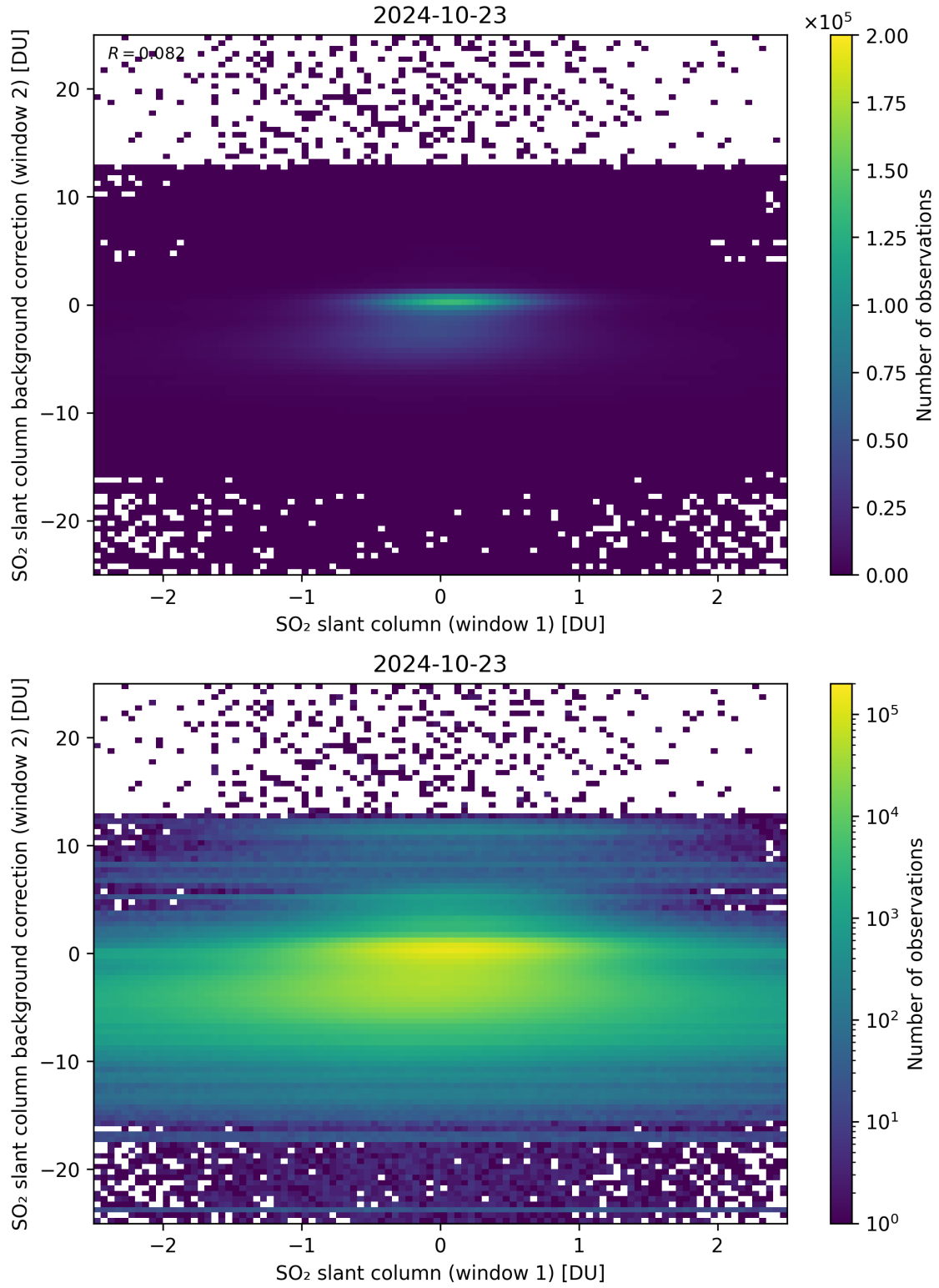
Figure 213: Scatter density plot of “SO 2 slant column (window 1)” against “SO 2 slant column background correction (window 2)” for 2024-10-22 to 2024-10-24.
