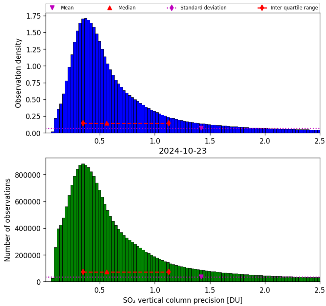
Figure 54: Histogram of “SO 2 vertical column precision” for 2024-10-22 to 2024-10-24
