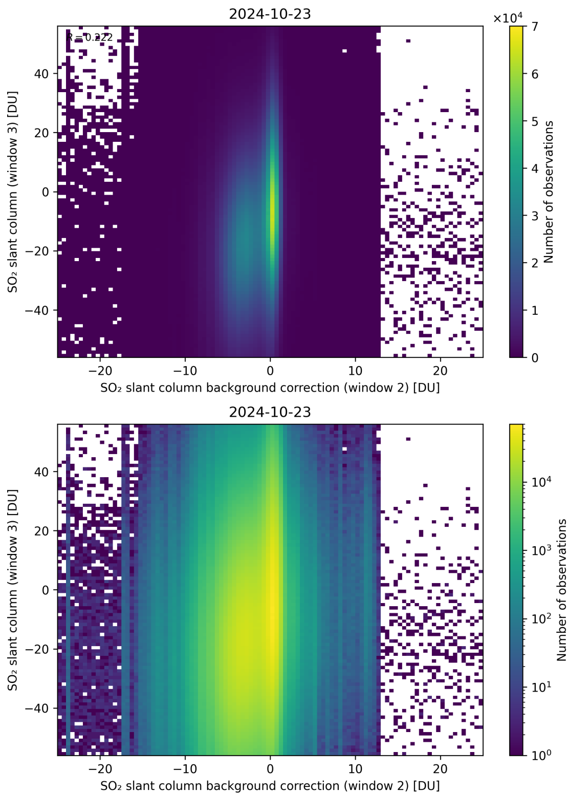
Figure 117: Scatter density plot of “SO 2 slant column background correction (window 2)” against “SO 2 slant column (window 3)” for 2024-10-22 to 2024-10-24.
