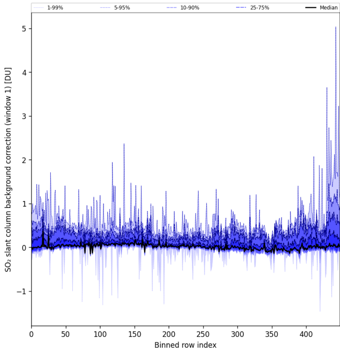
Figure 82: Along track statistics of “SO 2 slant column background correction (window 1)” for 2024-10-22 to 2024-10-24
