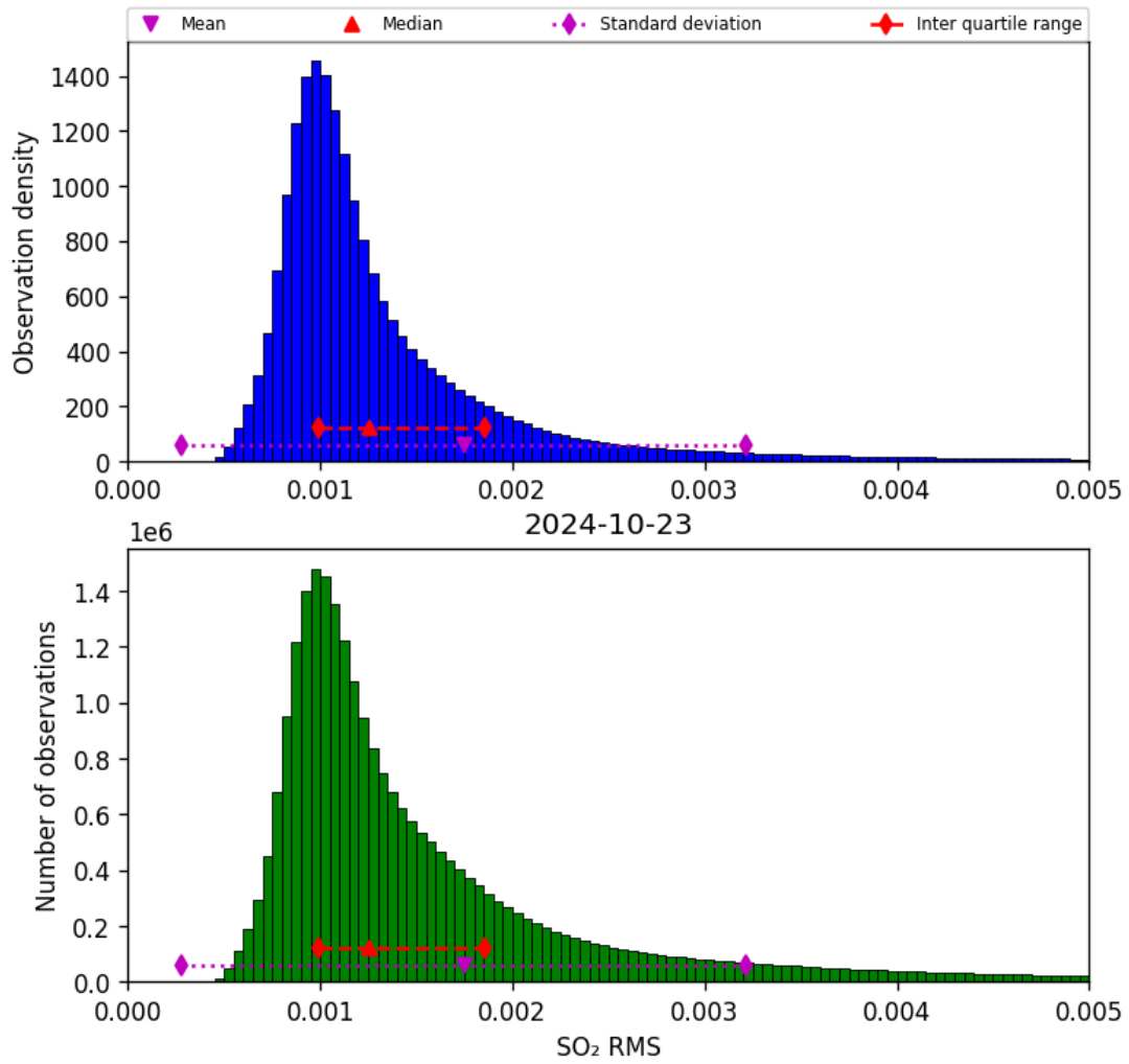
Figure 70: Histogram of “SO 2 RMS” for 2024-10-22 to 2024-10-24
