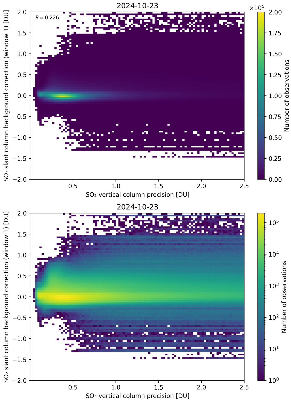
Figure 279: Scatter density plot of “SO 2 vertical column precision” against “SO 2 slant column background correction (window 1)” for 2024-10-22 to 2024-10-24.
