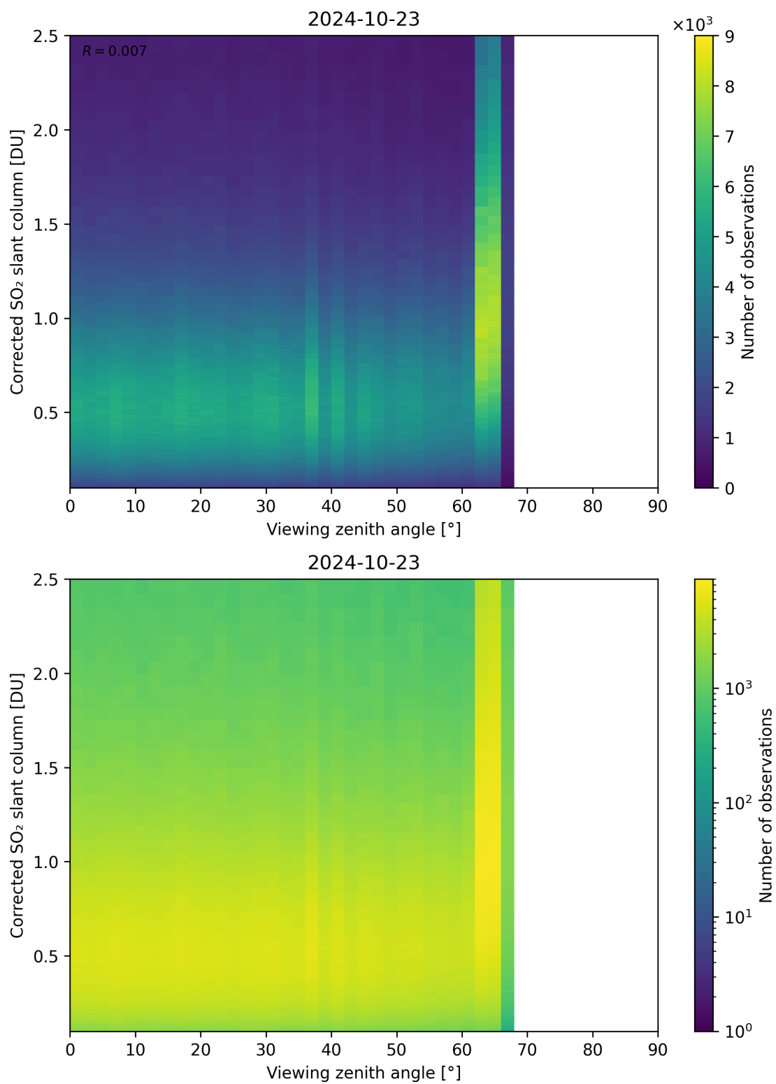
Figure 317: Scatter density plot of “Viewing zenith angle” against “Corrected SO 2 slant column” for 2024-10-22 to 2024-10-24.
