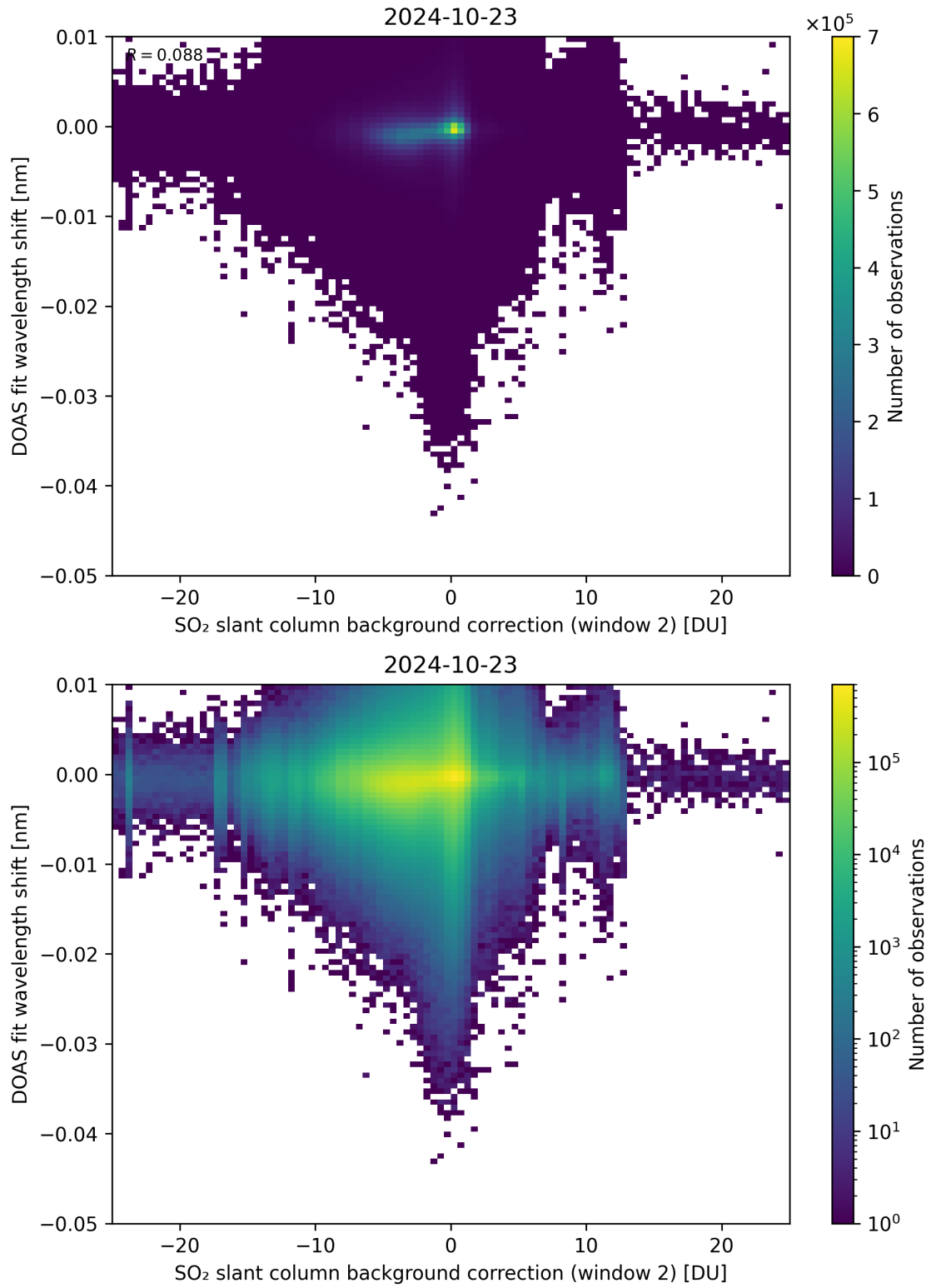
Figure 112: Scatter density plot of “SO 2 slant column background correction (window 2)” against “DOAS fit wavelength shift” for 2024-10-22 to 2024-10-24.
