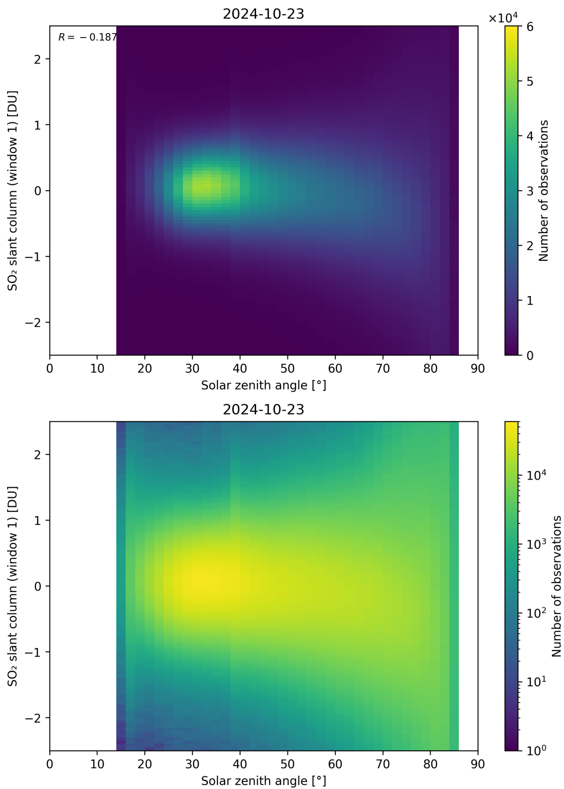
Figure 169: Scatter density plot of “Solar zenith angle” against “SO 2 slant column (window 1)” for 2024-10-22 to 2024-10-24.
