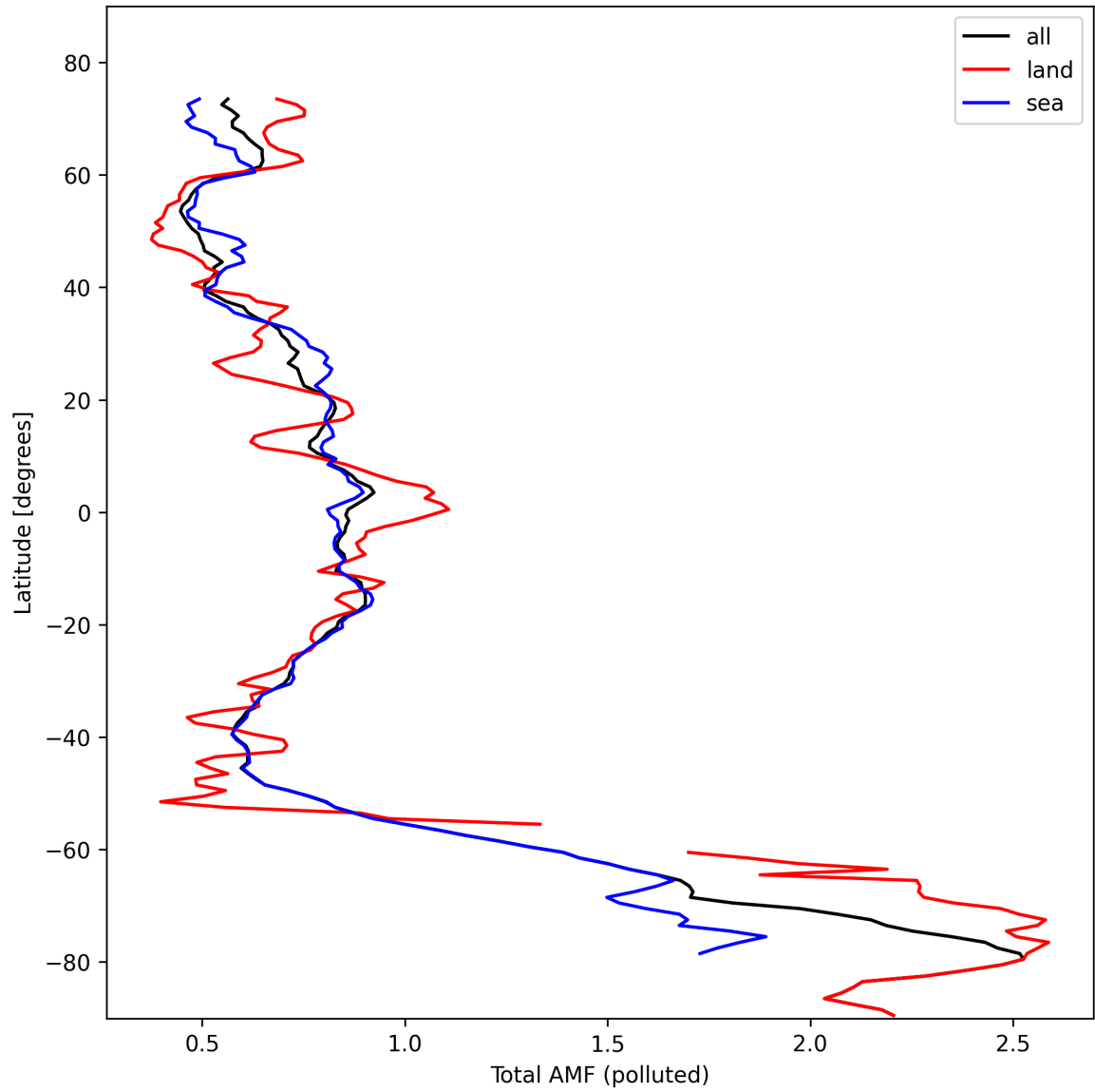
Figure 48: Zonal average of “Total AMF (polluted)” for 2024-10-22 to 2024-10-24.
