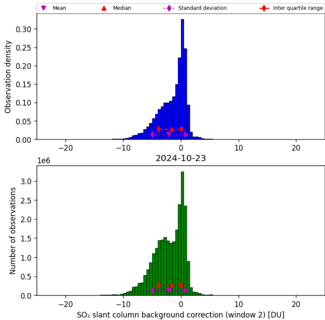
Figure 63: Histogram of “SO 2 slant column background correction (window 2)” for 2024-10-22 to 2024-10-24
