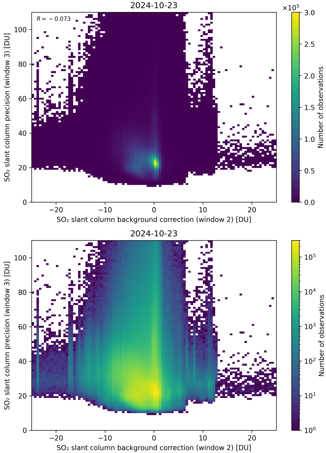
Figure 118: Scatter density plot of “SO 2 slant column background correction (window 2)” against “SO 2 slant column precision (window 3)” for 2024-10-22 to 2024-10-24.
