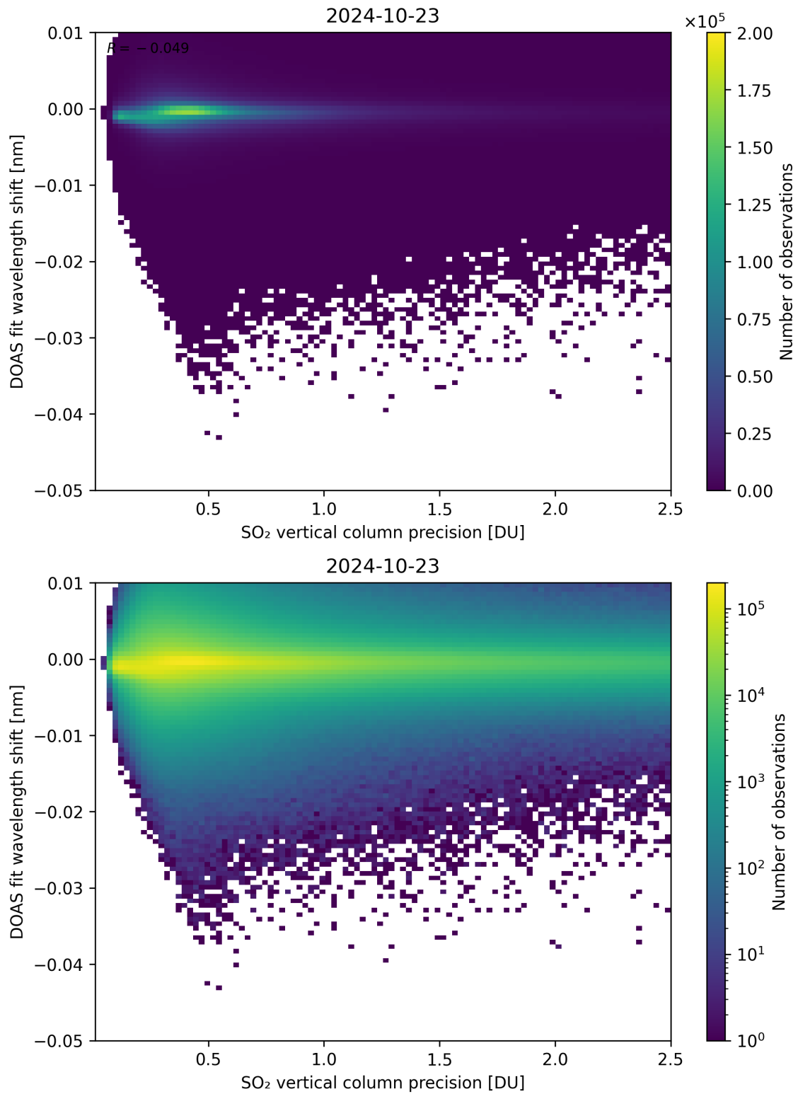
Figure 282: Scatter density plot of “SO 2 vertical column precision” against “DOAS fit wavelength shift” for 2024-10-22 to 2024-10-24.
