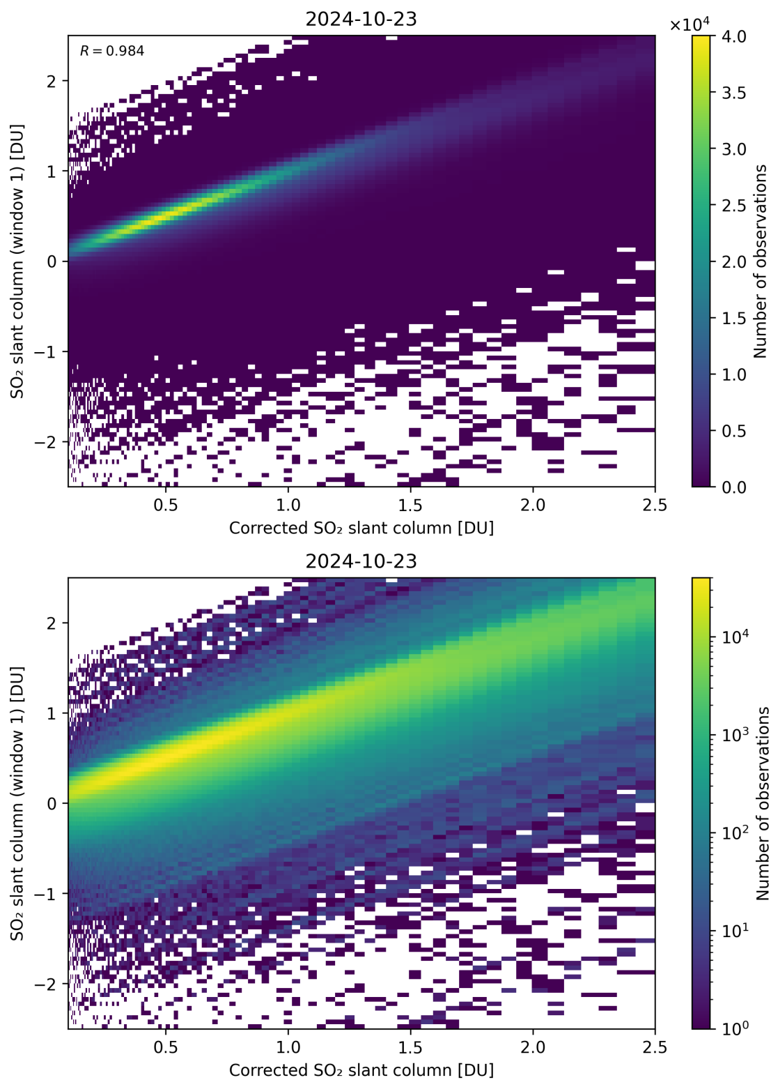
Figure 187: Scatter density plot of “Corrected SO 2 slant column” against “SO 2 slant column (window 1)” for 2024-10-22 to 2024-10-24.
