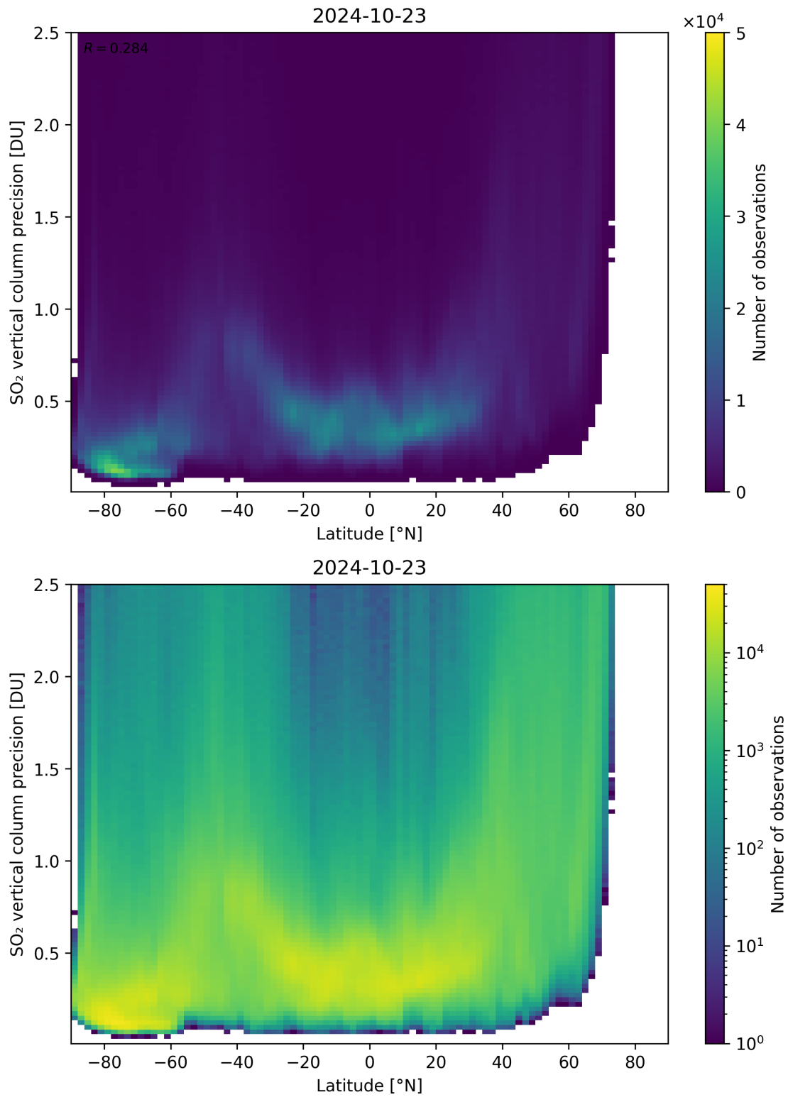
Figure 157: Scatter density plot of “Latitude” against “SO 2 vertical column precision” for 2024-10-22 to 2024-10-24.
