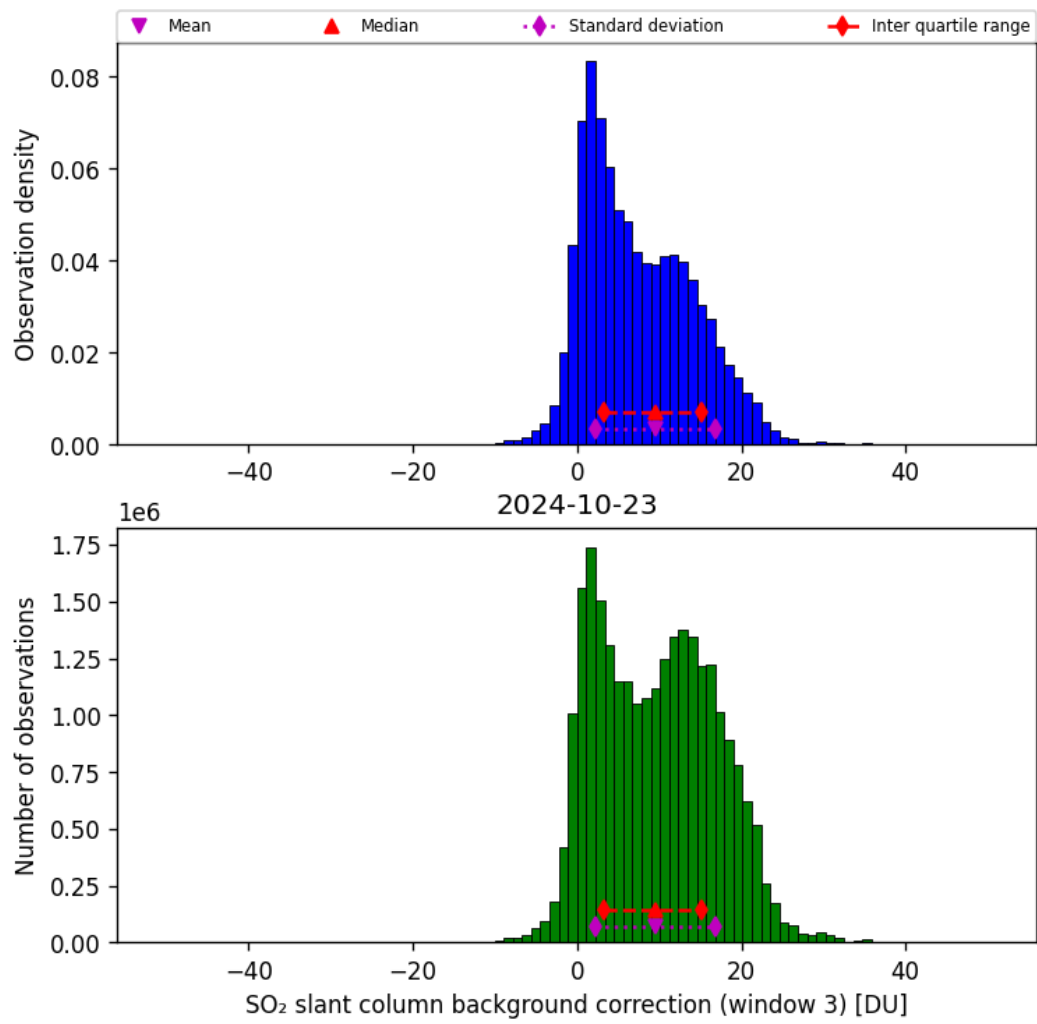
Figure 67: Histogram of “SO 2 slant column background correction (window 3)” for 2024-10-22 to 2024-10-24
