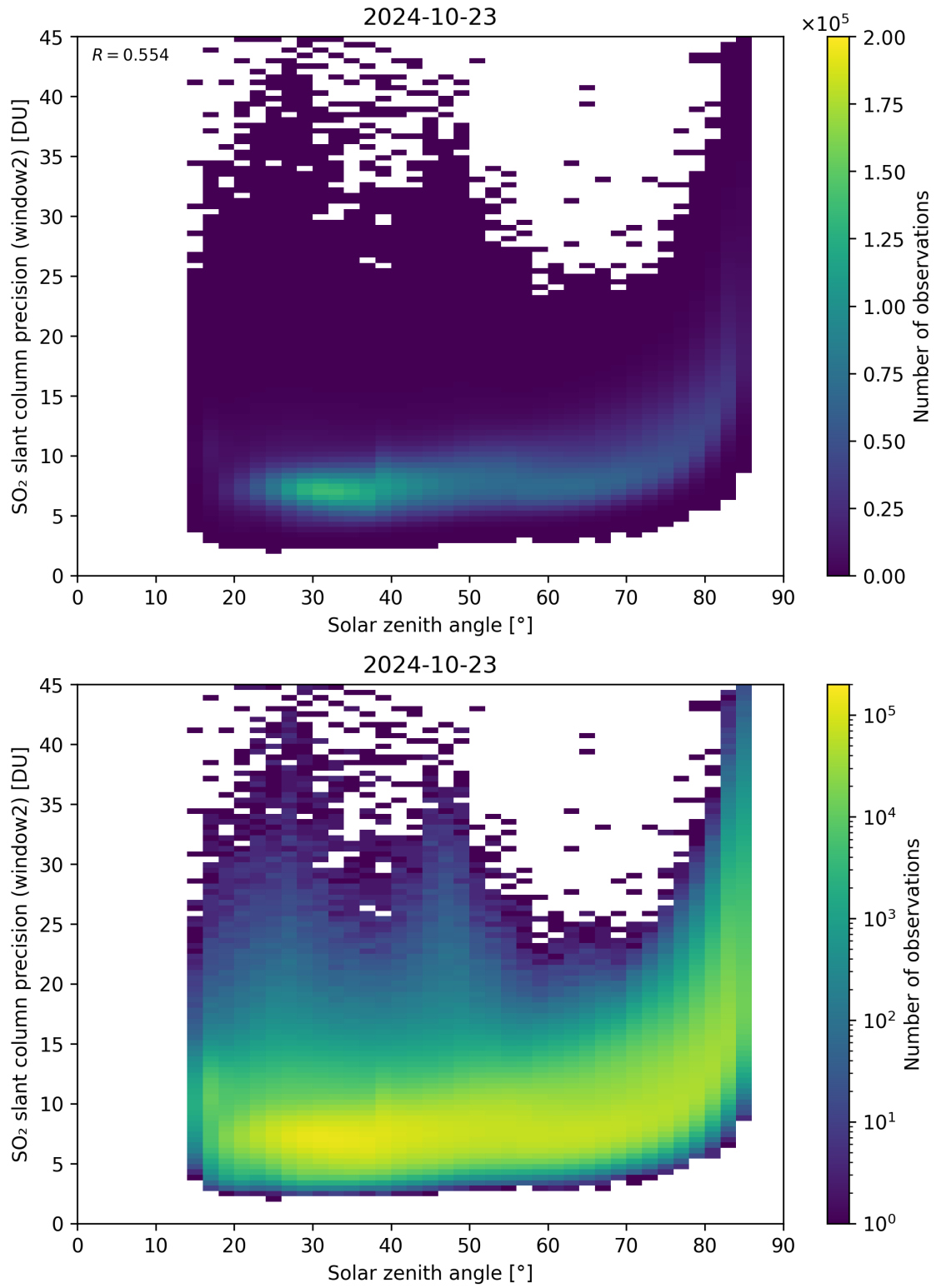
Figure 171: Scatter density plot of “Solar zenith angle” against “SO 2 slant column precision (window2)” for 2024-10-22 to 2024-10-24.
