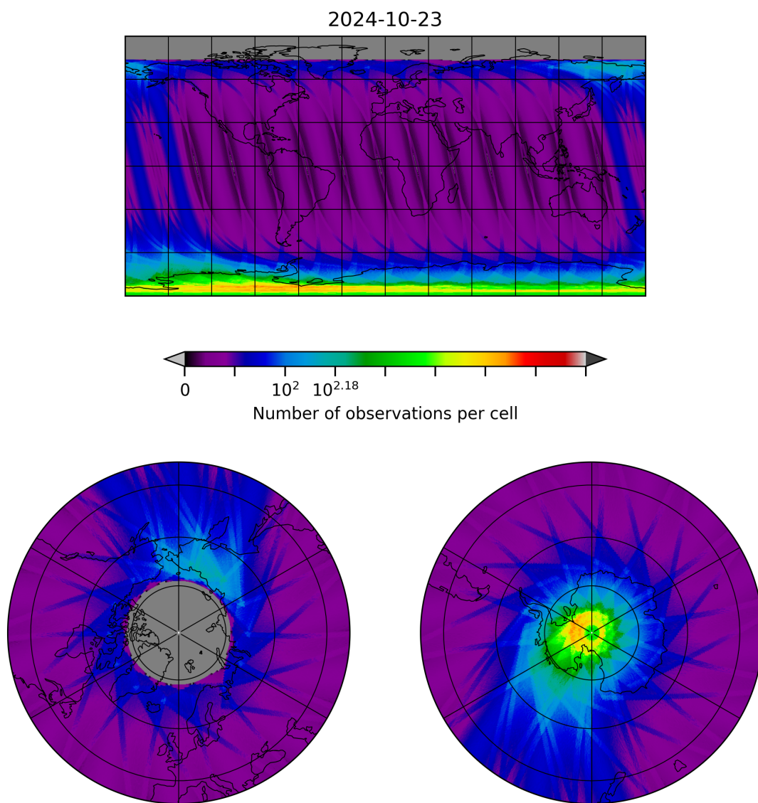
Figure 28: Map of the number of observations for 2024-10-22 to 2024-10-24
