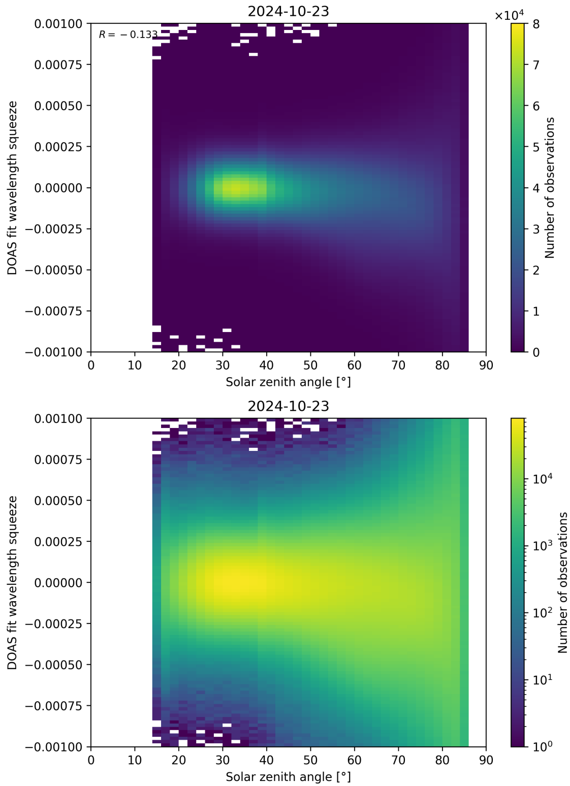
Figure 162: Scatter density plot of “Solar zenith angle” against “DOAS fit wavelength squeeze” for 2024-10-22 to 2024-10-24.
