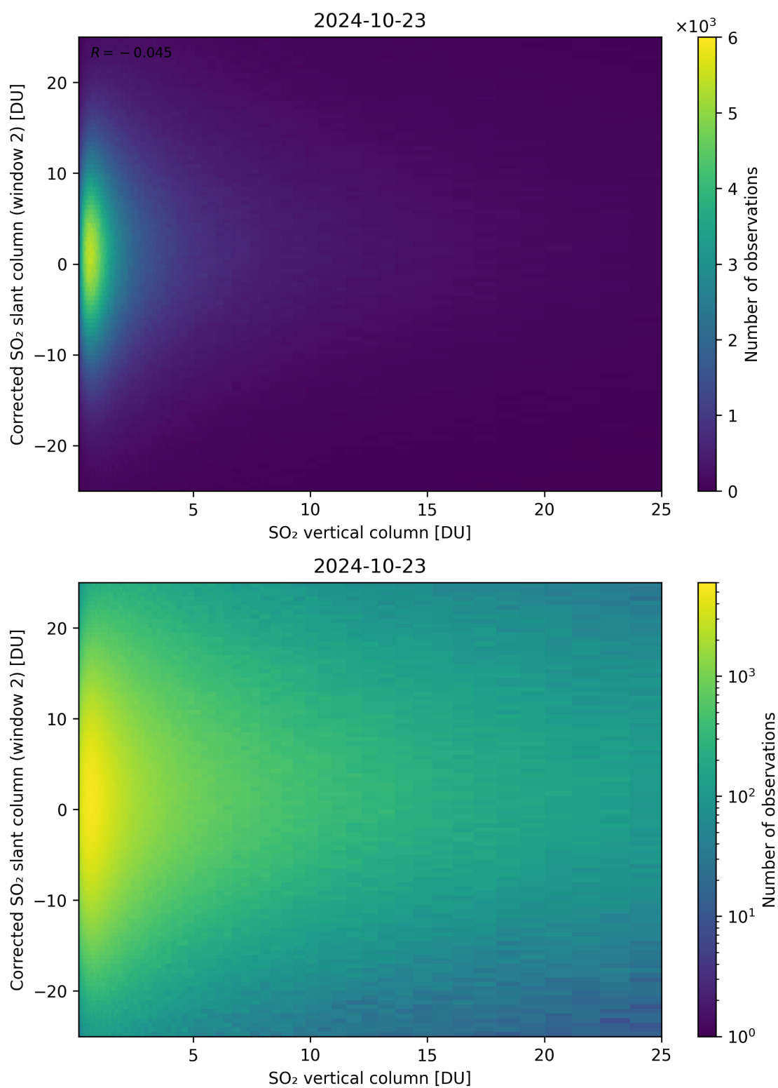
Figure 298: Scatter density plot of “SO 2 vertical column” against “Corrected SO 2 slant column (window 2)” for 2024-10-22 to 2024-10-24.
