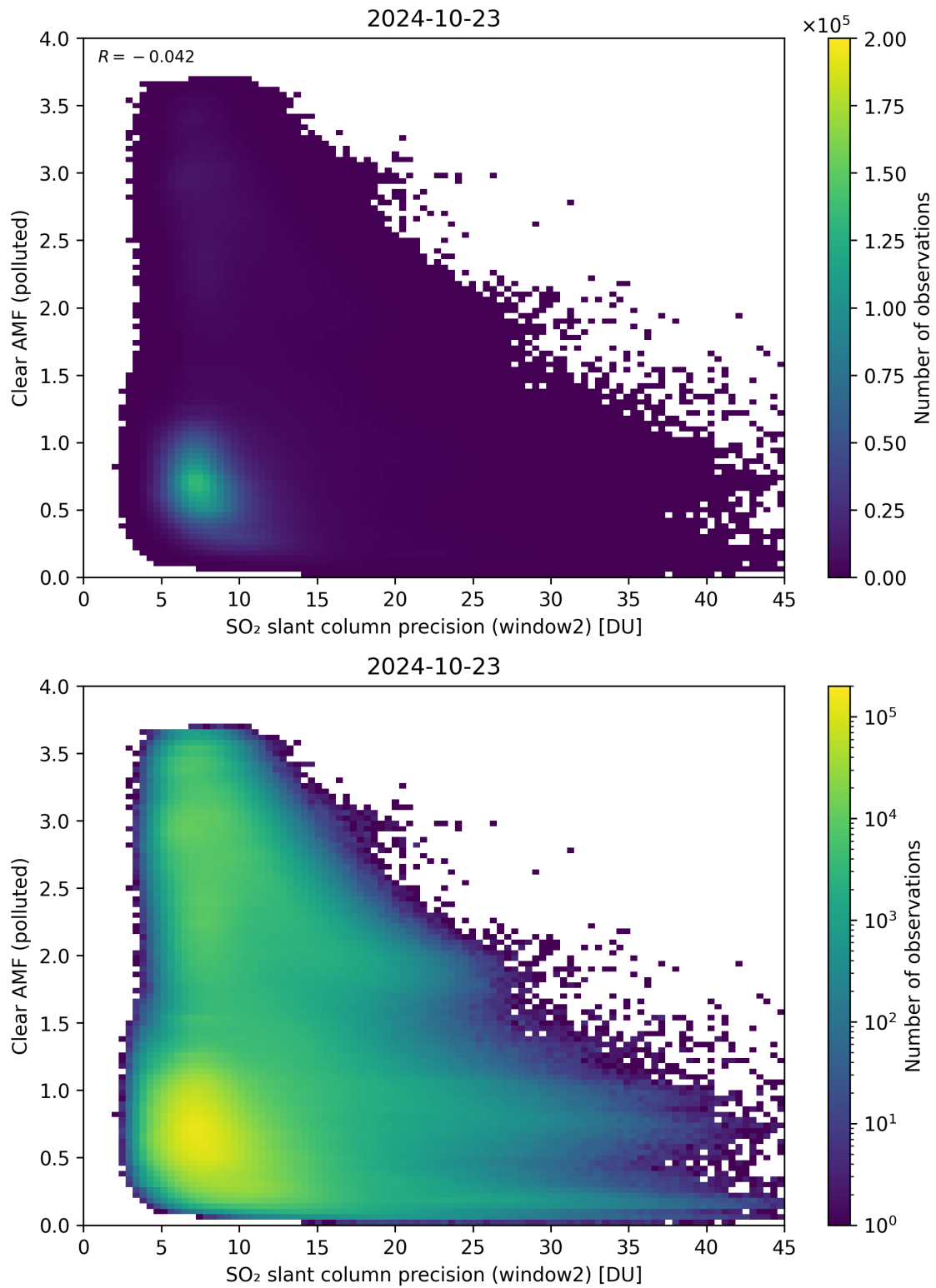
Figure 246: Scatter density plot of “SO 2 slant column precision (window2)” against “Clear AMF (polluted)” for 2024-10-22 to 2024-10-24.
