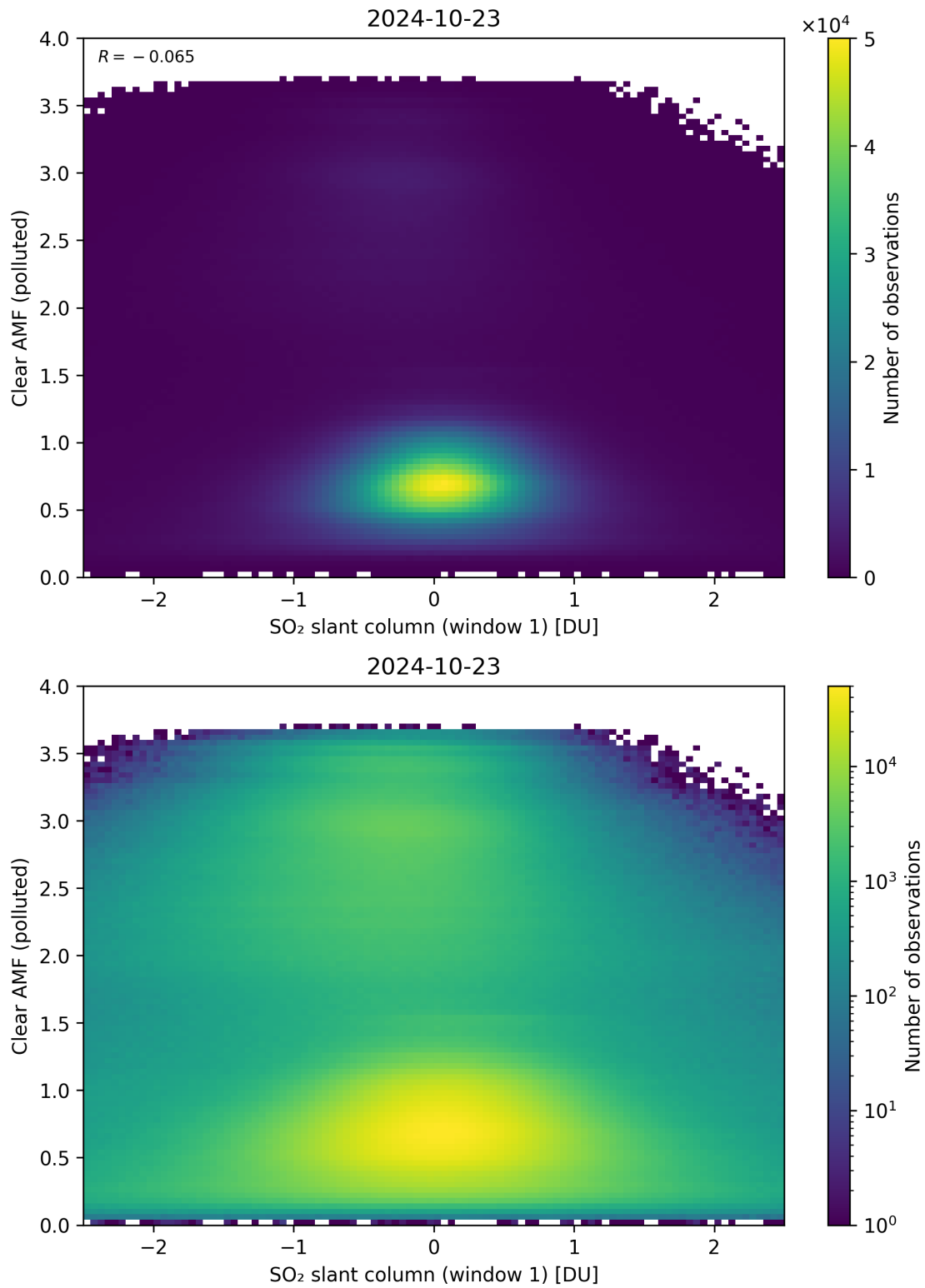
Figure 232: Scatter density plot of “SO 2 slant column (window 1)” against “Clear AMF (polluted)” for 2024-10-22 to 2024-10-24.
