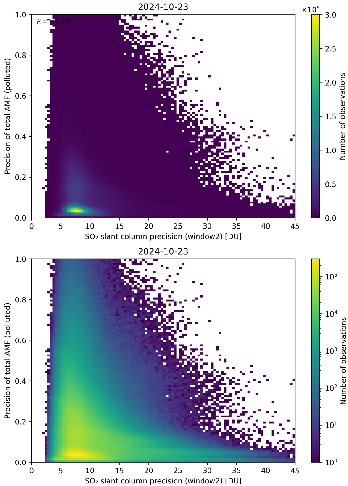
Figure 252: Scatter density plot of “SO 2 slant column precision (window2)” against “Precision of total AMF (polluted)” for 2024-10-22 to 2024-10-24.
