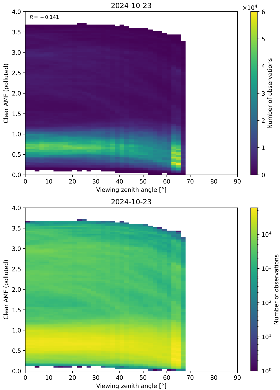
Figure 316: Scatter density plot of “Viewing zenith angle” against “Clear AMF (polluted)” for 2024-10-22 to 2024-10-24.
