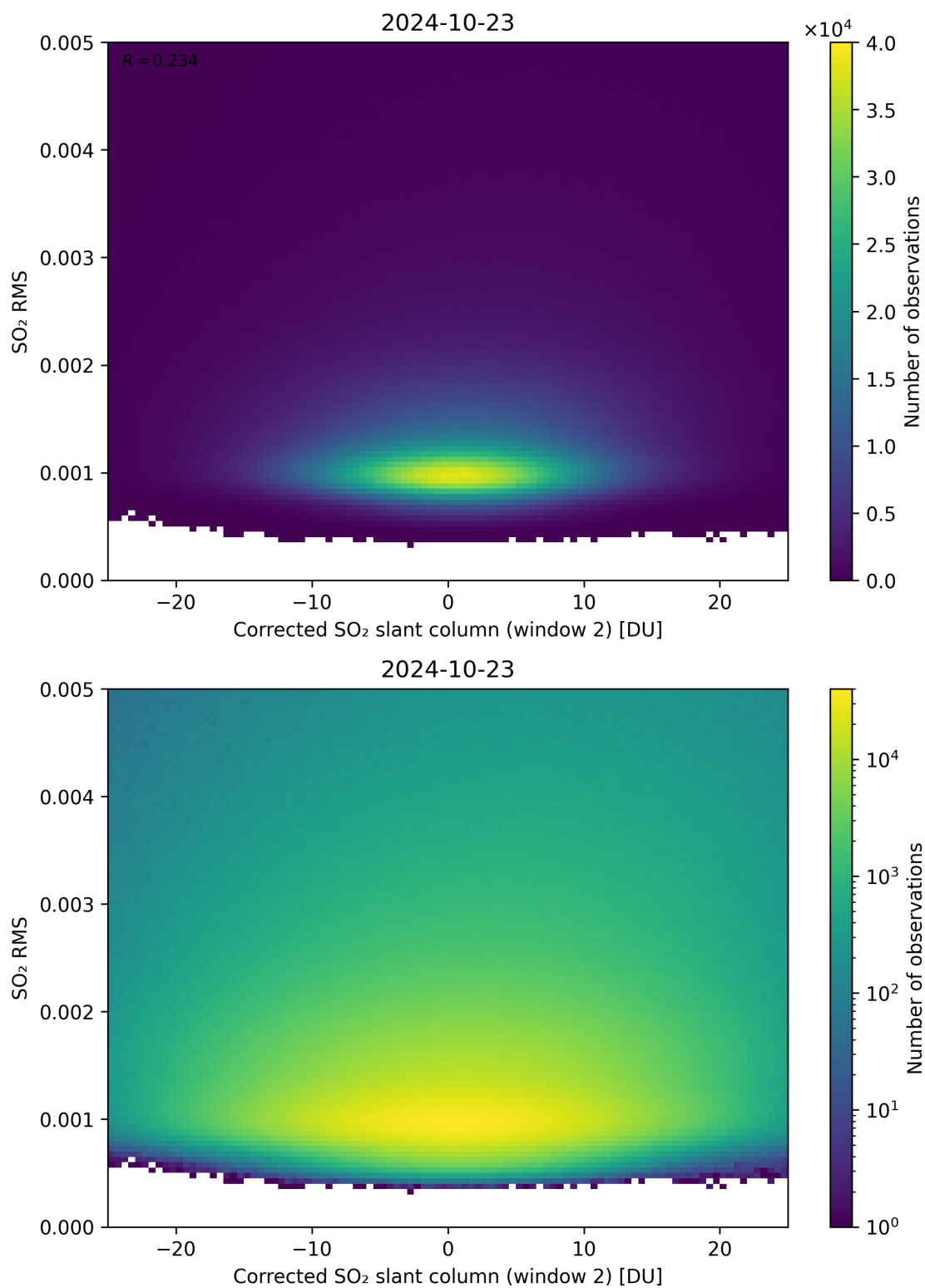
Figure 198: Scatter density plot of “Corrected SO 2 slant column (window 2)” against “SO 2 RMS” for 2024-10-22 to 2024-10-24.
