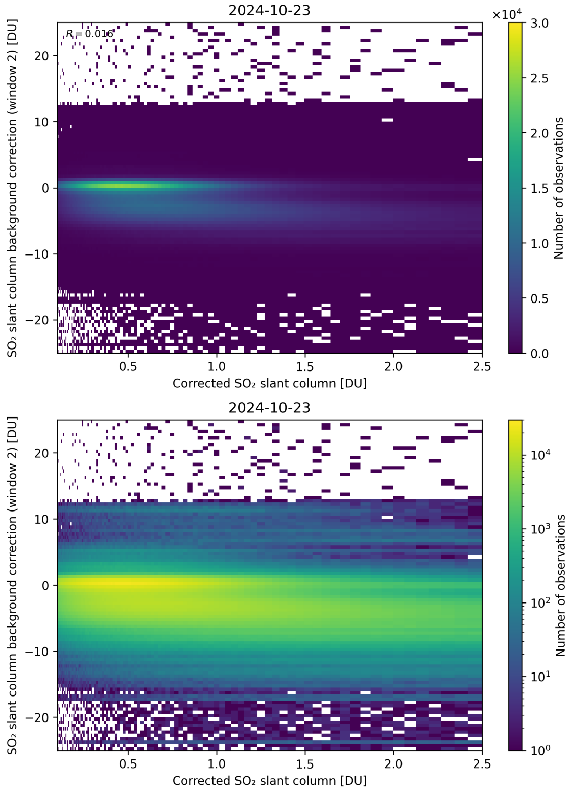
Figure 179: Scatter density plot of “Corrected SO 2 slant column” against “SO 2 slant column background correction (window 2)” for 2024-10-22 to 2024-10-24.
