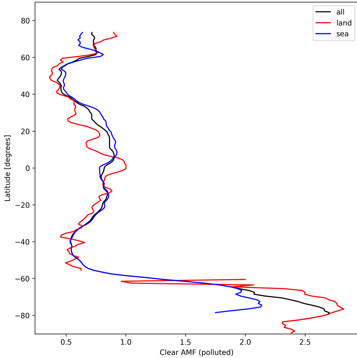
Figure 50: Zonal average of “Clear AMF (polluted)” for 2024-10-22 to 2024-10-24.
