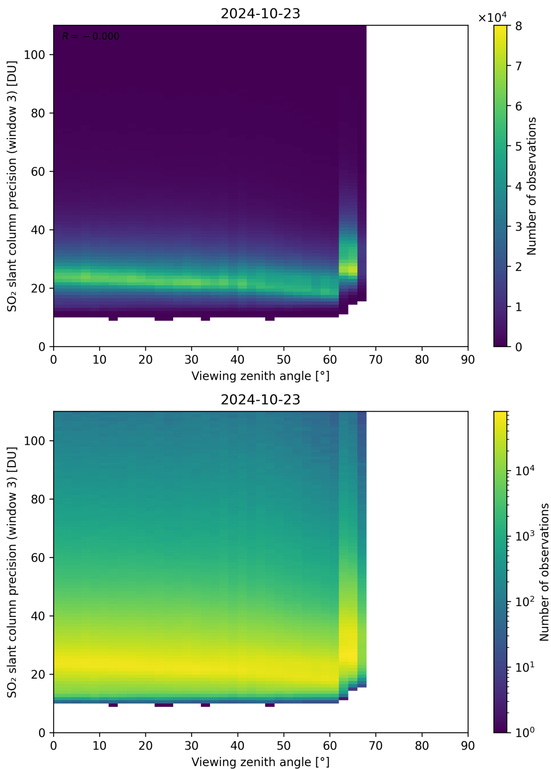
Figure 324: Scatter density plot of “Viewing zenith angle” against “SO 2 slant column precision (window 3)” for 2024-10-22 to 2024-10-24.
