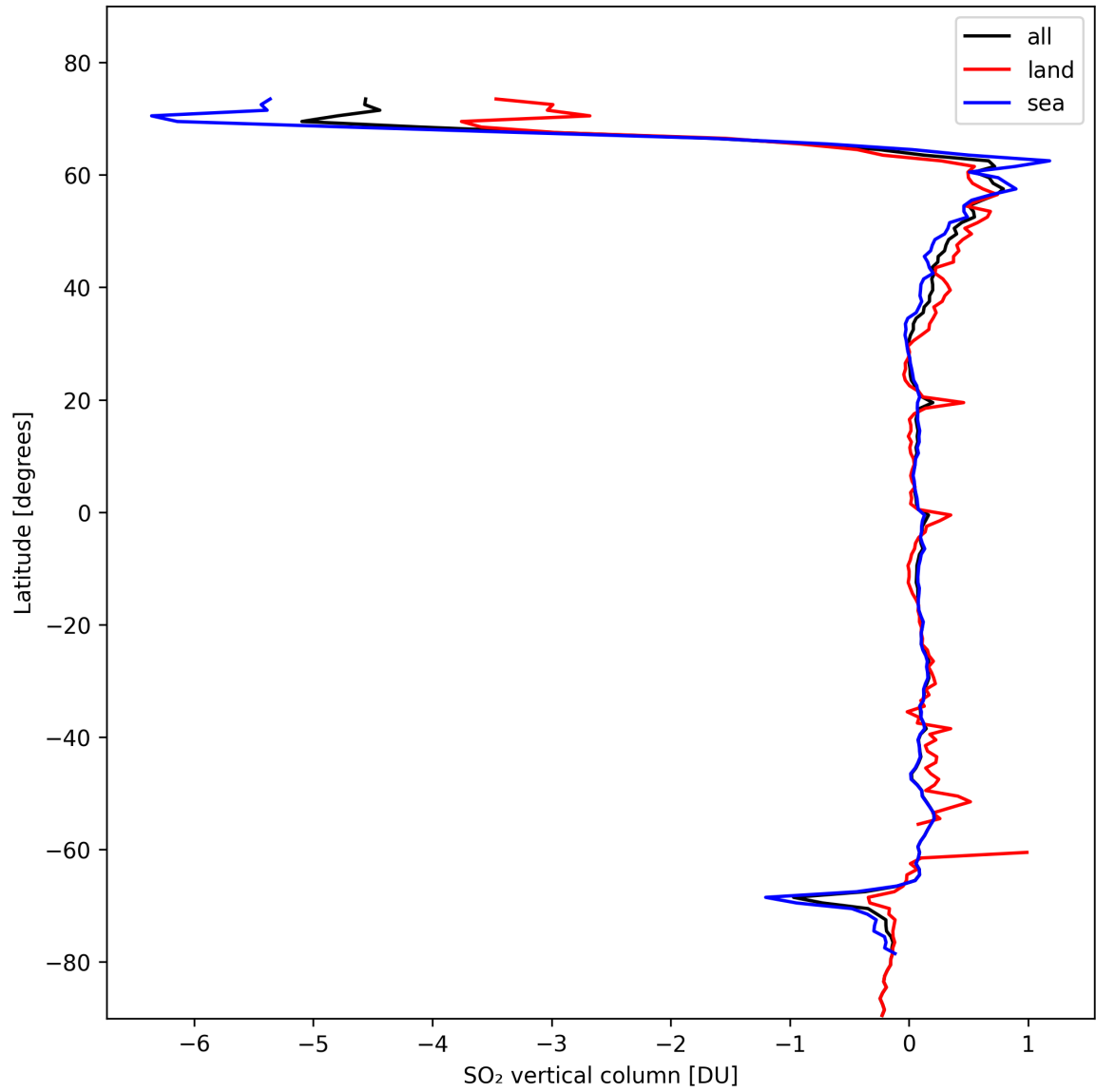
Figure 30: Zonal average of “SO 2 vertical column” for 2024-10-22 to 2024-10-24.
