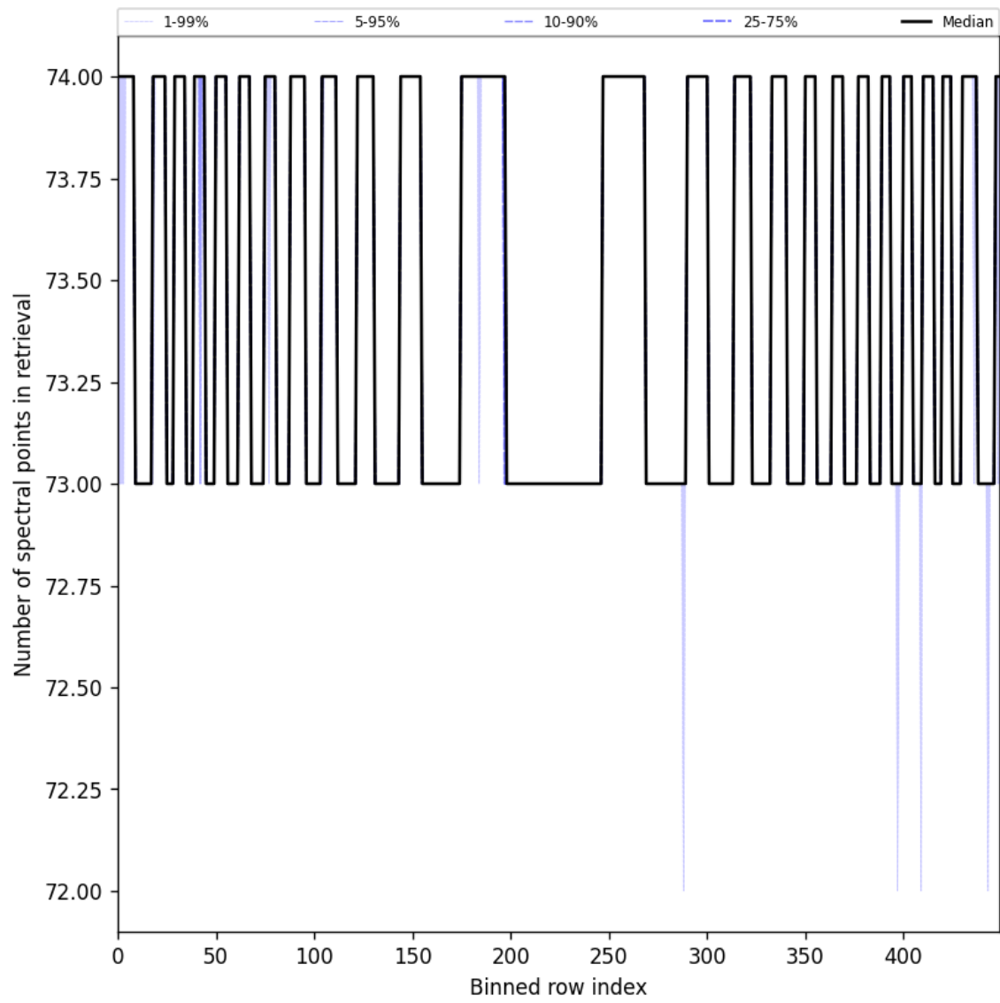
Figure 97: Along track statistics of “Number of spectral points in retrieval” for 2024-10-22 to 2024-10-24
