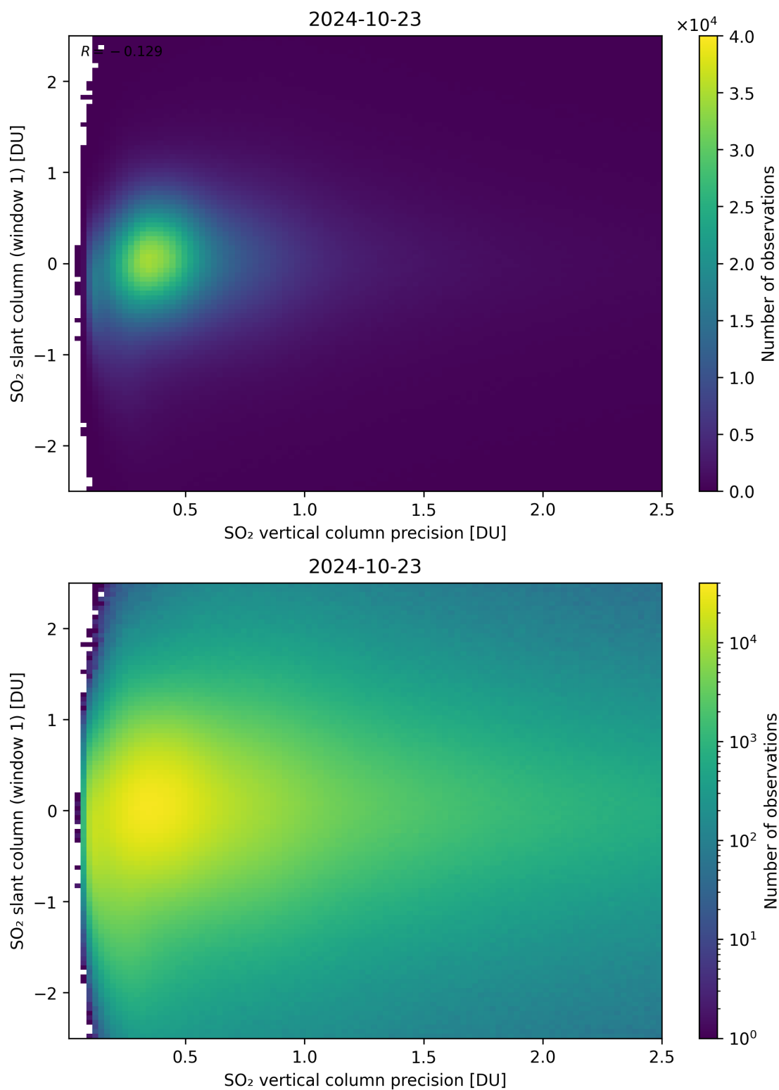
Figure 289: Scatter density plot of “SO 2 vertical column precision” against “SO 2 slant column (window 1)” for 2024-10-22 to 2024-10-24.
