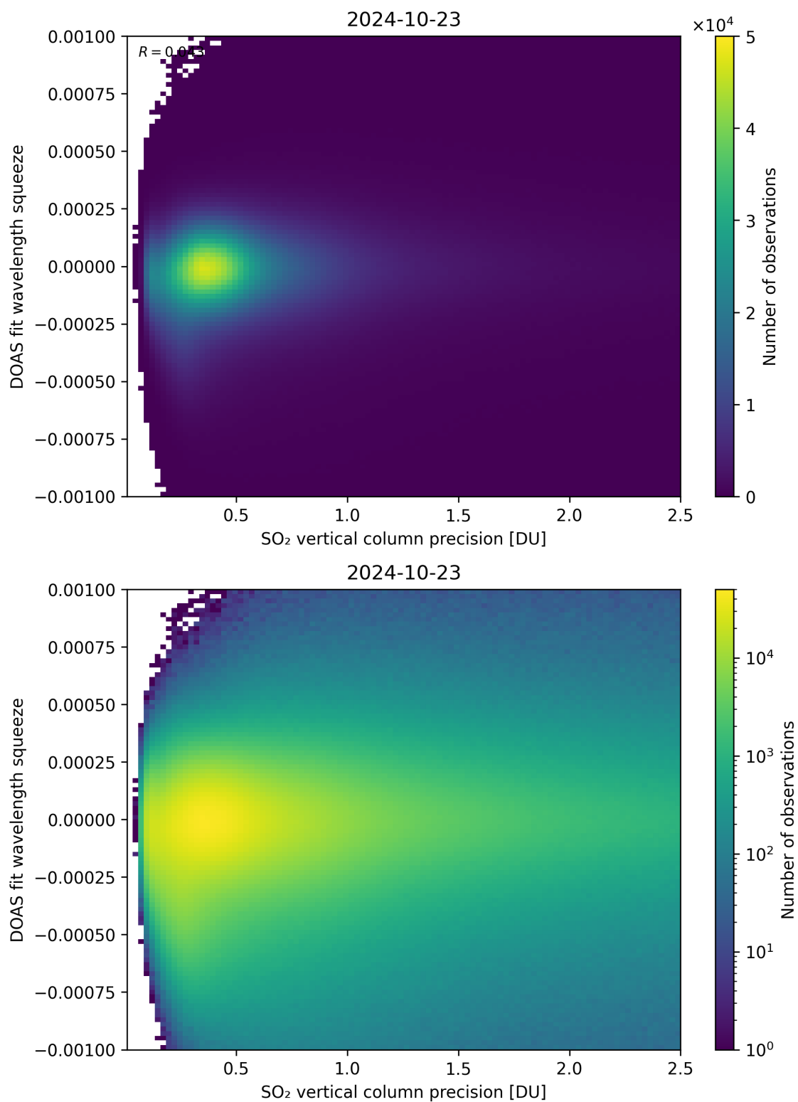
Figure 283: Scatter density plot of “SO 2 vertical column precision” against “DOAS fit wavelength squeeze” for 2024-10-22 to 2024-10-24.
