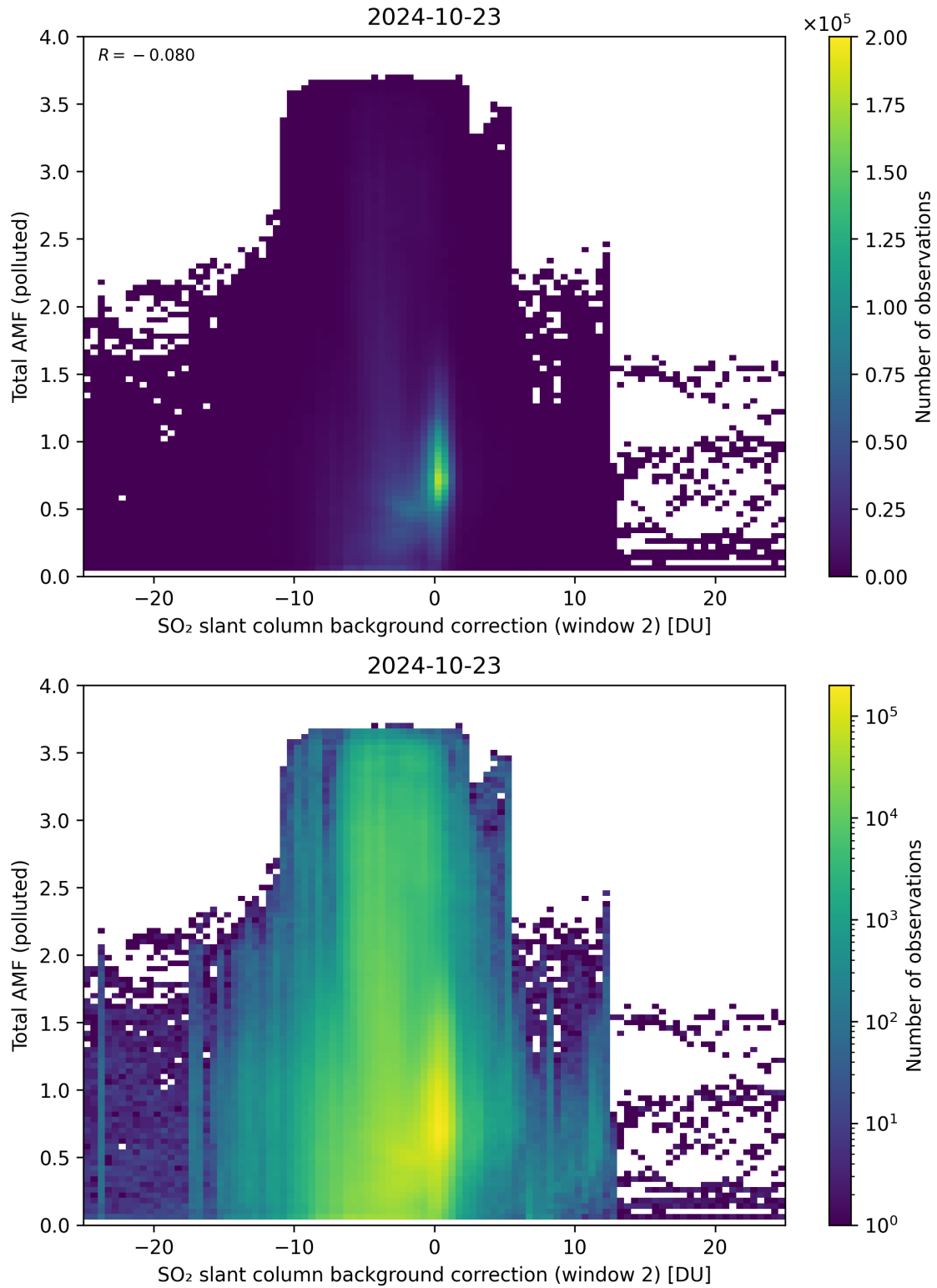
Figure 119: Scatter density plot of “SO 2 slant column background correction (window 2)” against “Total AMF (polluted)” for 2024-10-22 to 2024-10-24.
