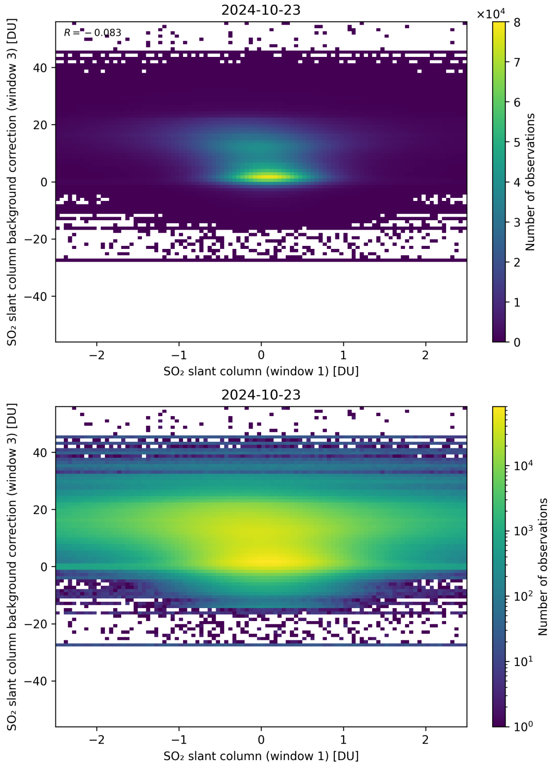
Figure 214: Scatter density plot of “SO 2 slant column (window 1)” against “SO 2 slant column background correction (window 3)” for 2024-10-22 to 2024-10-24.
