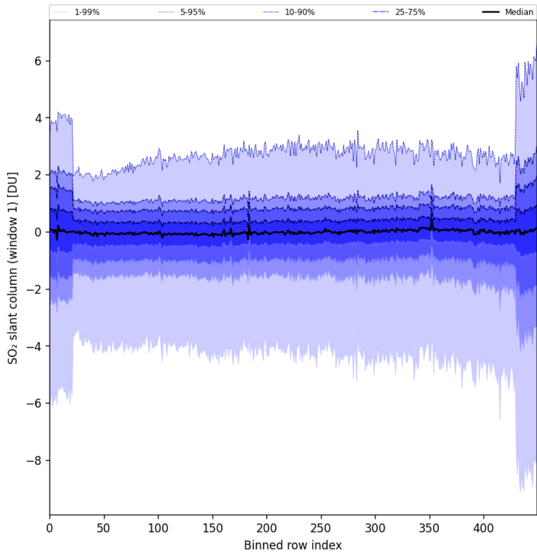
Figure 79: Along track statistics of “SO 2 slant column (window 1)” for 2024-10-22 to 2024-10-24
