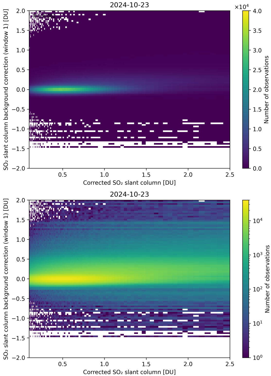
Figure 178: Scatter density plot of “Corrected SO 2 slant column” against “SO 2 slant column background correction (window 1)” for 2024-10-22 to 2024-10-24.
