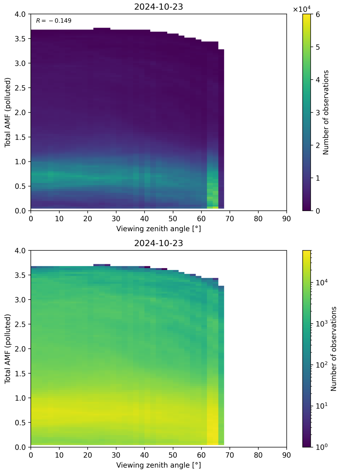
Figure 325: Scatter density plot of “Viewing zenith angle” against “Total AMF (polluted)” for 2024-10-22 to 2024-10-24.
