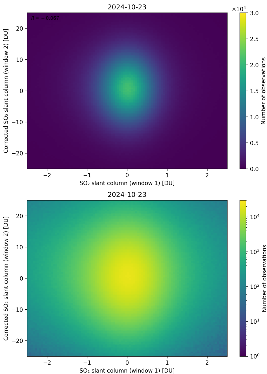
Figure 233: Scatter density plot of “SO 2 slant column (window 1)” against “Corrected SO 2 slant column (window 2)” for 2024-10-22 to 2024-10-24.
