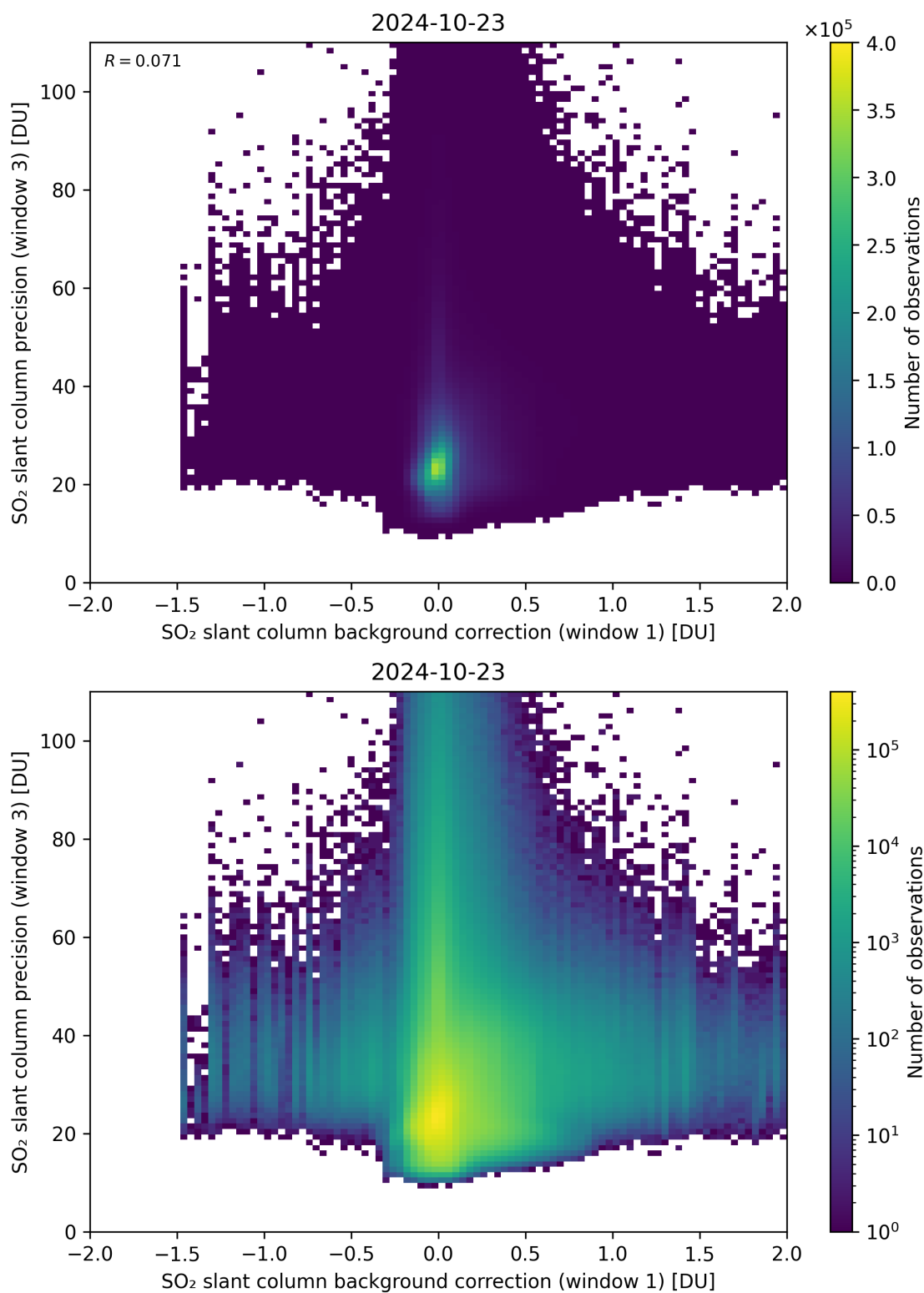
Figure 108: Scatter density plot of “SO 2 slant column background correction (window 1)” against “SO 2 slant column precision (window 3)” for 2024-10-22 to 2024-10-24.
