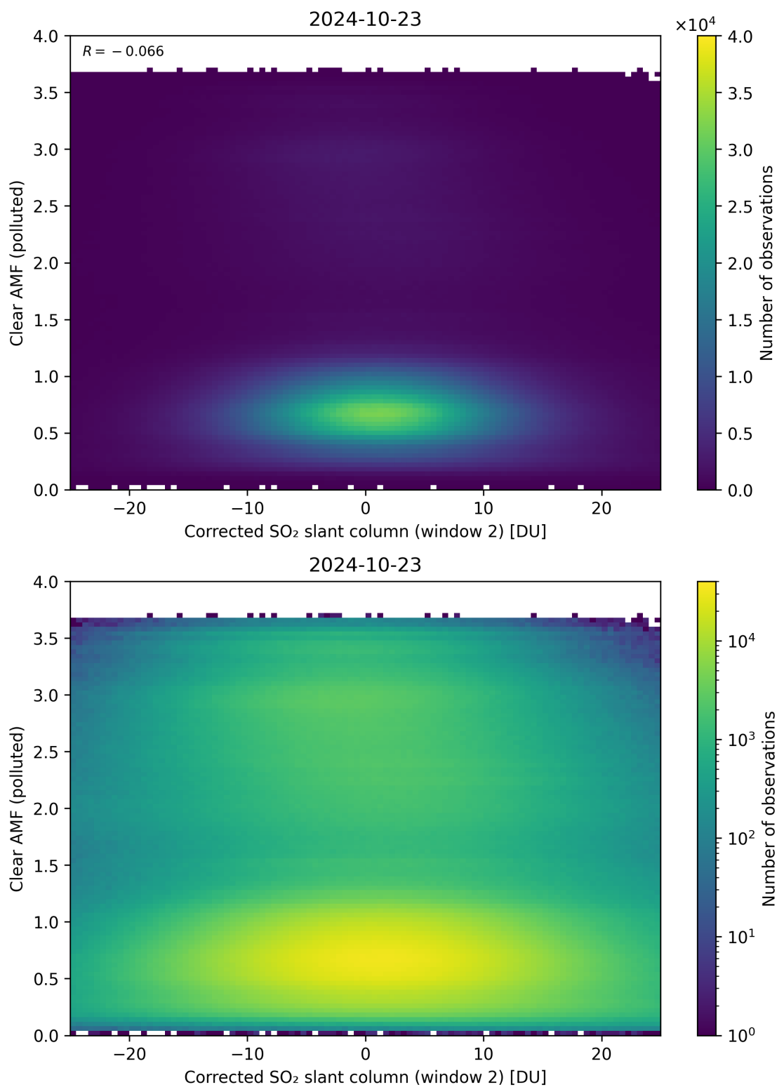
Figure 199: Scatter density plot of “Corrected SO 2 slant column (window 2)” against “Clear AMF (polluted)” for 2024-10-22 to 2024-10-24.
