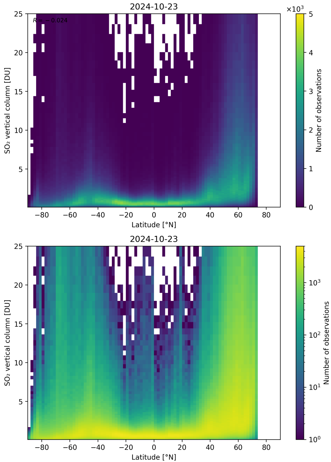
Figure 156: Scatter density plot of “Latitude” against “SO 2 vertical column” for 2024-10-22 to 2024-10-24.
