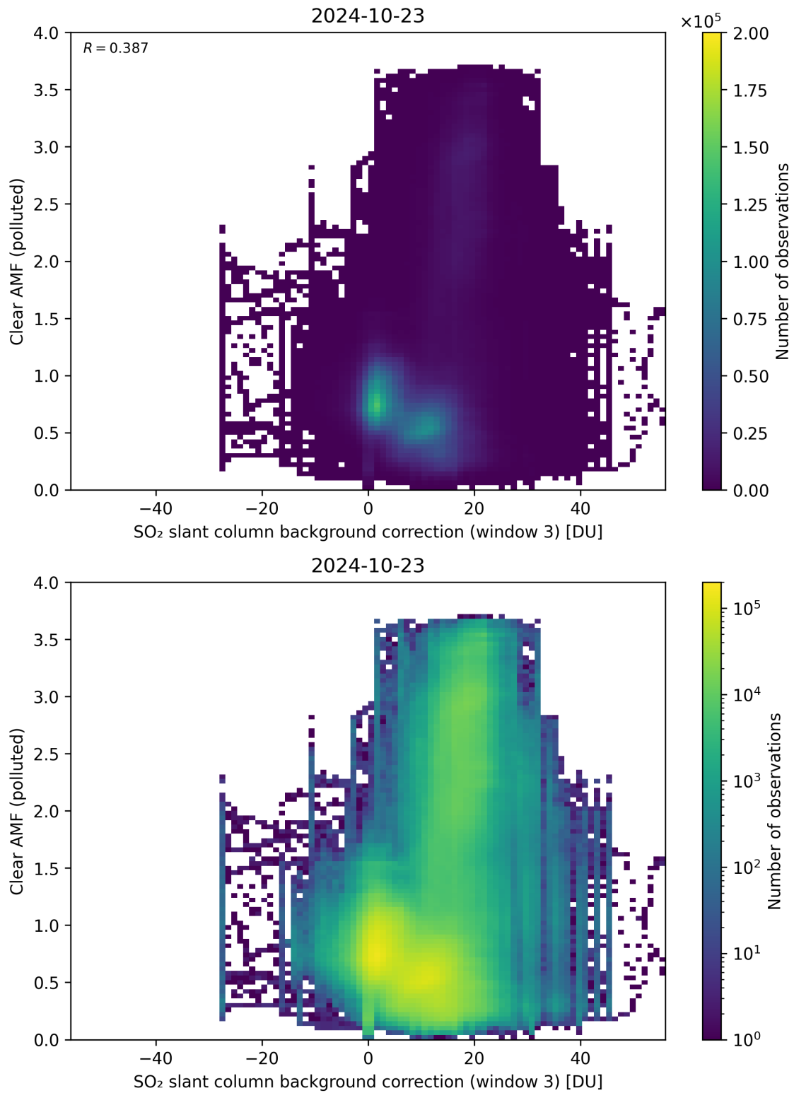
Figure 124: Scatter density plot of “SO 2 slant column background correction (window 3)” against “Clear AMF (polluted)” for 2024-10-22 to 2024-10-24.
