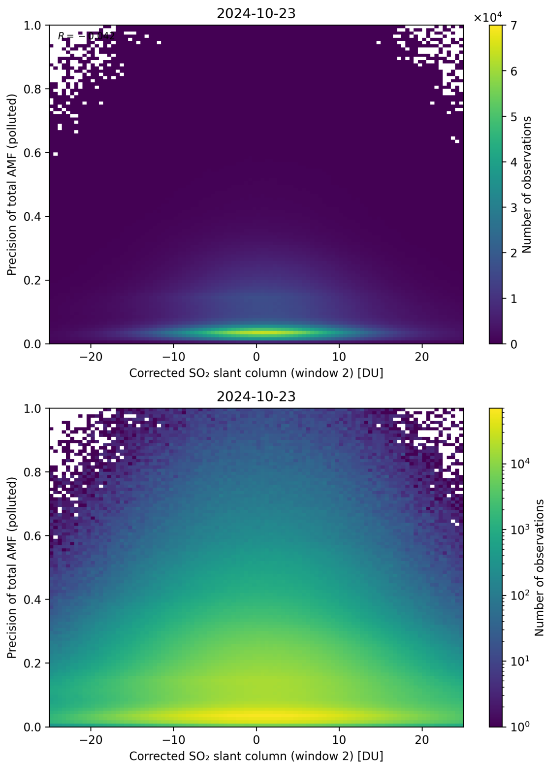
Figure 204: Scatter density plot of “Corrected SO 2 slant column (window 2)” against “Precision of total AMF (polluted)” for 2024-10-22 to 2024-10-24.
