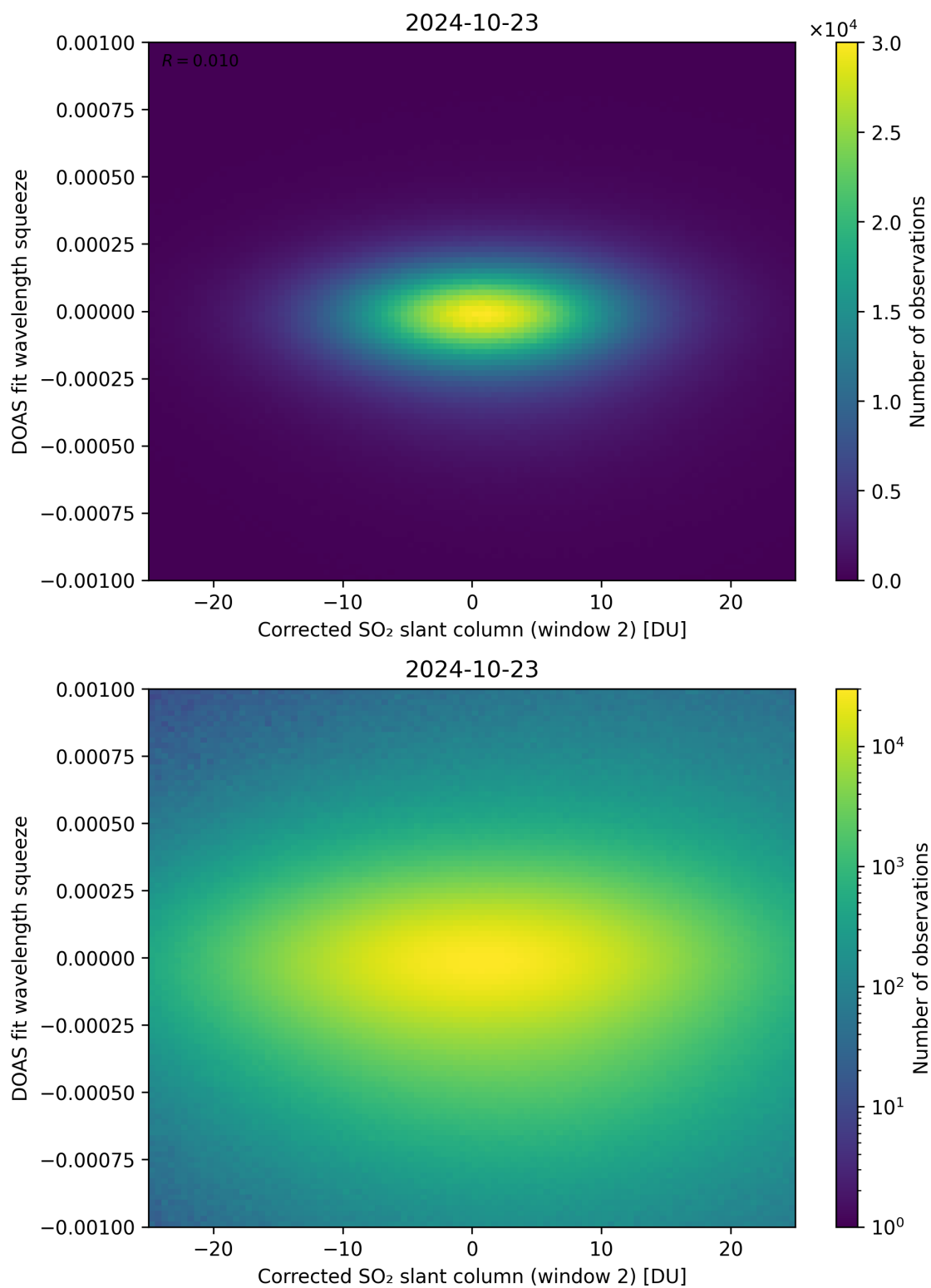
Figure 197: Scatter density plot of “Corrected SO 2 slant column (window 2)” against “DOAS fit wavelength squeeze” for 2024-10-22 to 2024-10-24.
