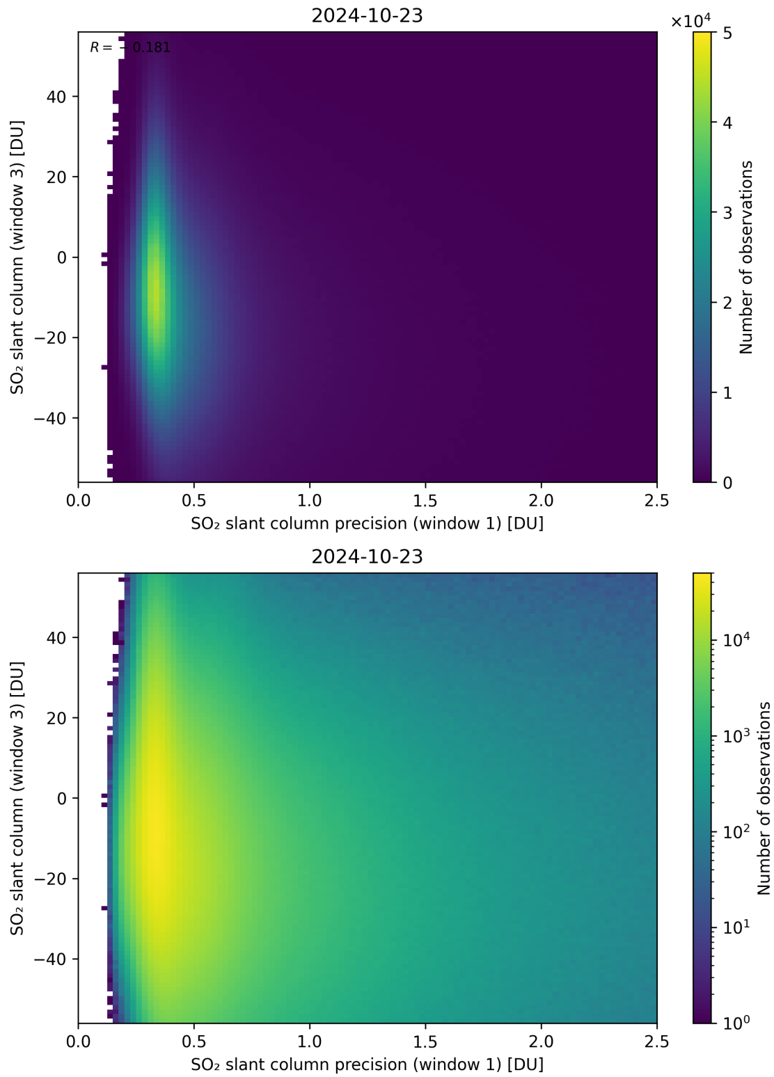
Figure 228: Scatter density plot of “SO 2 slant column precision (window 1)” against “SO 2 slant column (window 3)” for 2024-10-22 to 2024-10-24.
