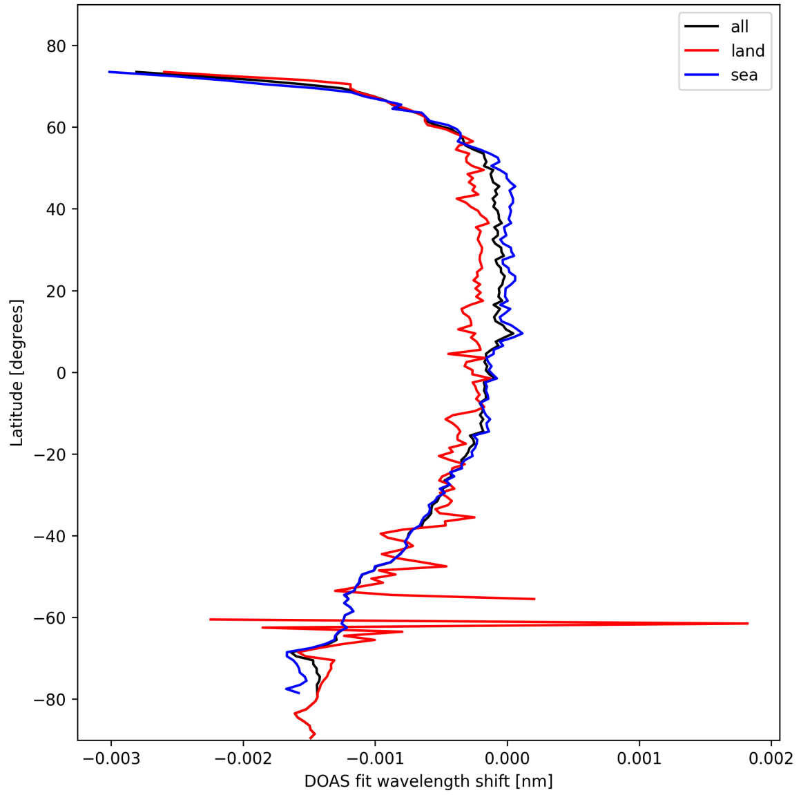
Figure 45: Zonal average of “DOAS fit wavelength shift” for 2024-10-22 to 2024-10-24.
