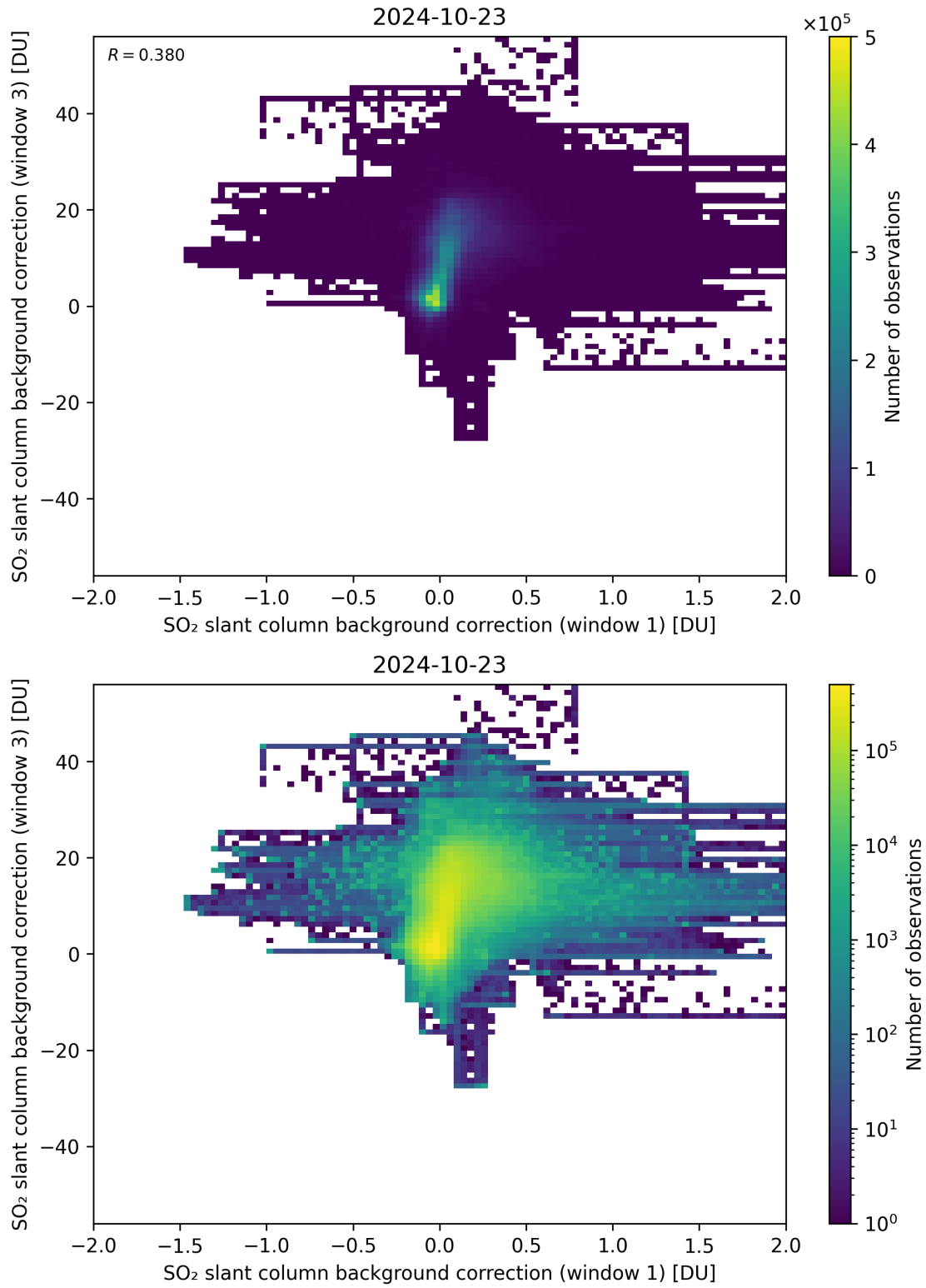
Figure 99: Scatter density plot of “SO 2 slant column background correction (window 1)” against “SO 2 slant column background correction (window 3)” for 2024-10-22 to 2024-10-24.
