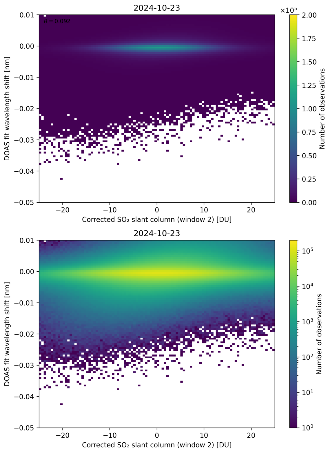
Figure 196: Scatter density plot of “Corrected SO 2 slant column (window 2)” against “DOAS fit wavelength shift” for 2024-10-22 to 2024-10-24.
