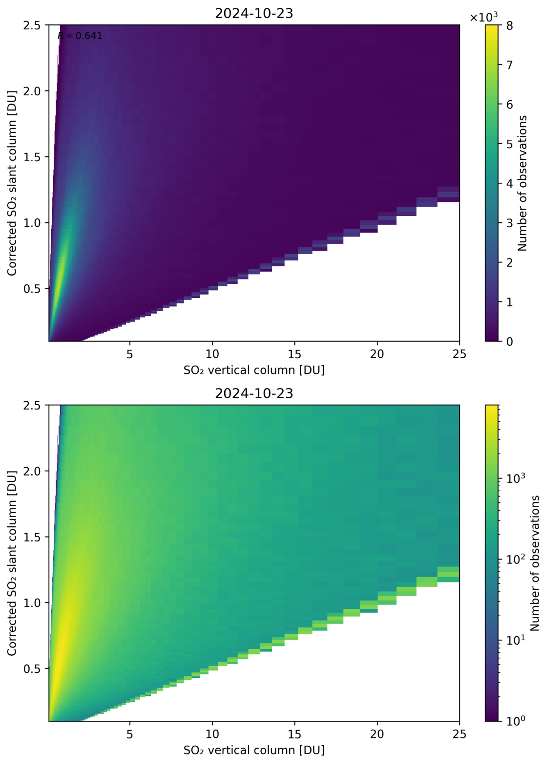
Figure 297: Scatter density plot of “SO 2 vertical column” against “Corrected SO 2 slant column” for 2024-10-22 to 2024-10-24.
