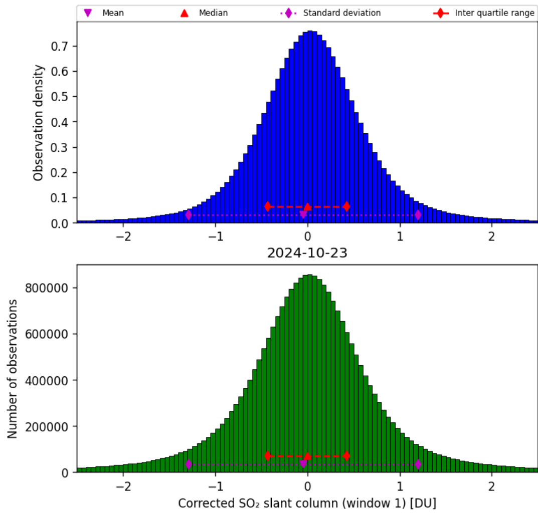
Figure 58: Histogram of “Corrected SO 2 slant column (window 1)” for 2024-10-22 to 2024-10-24
