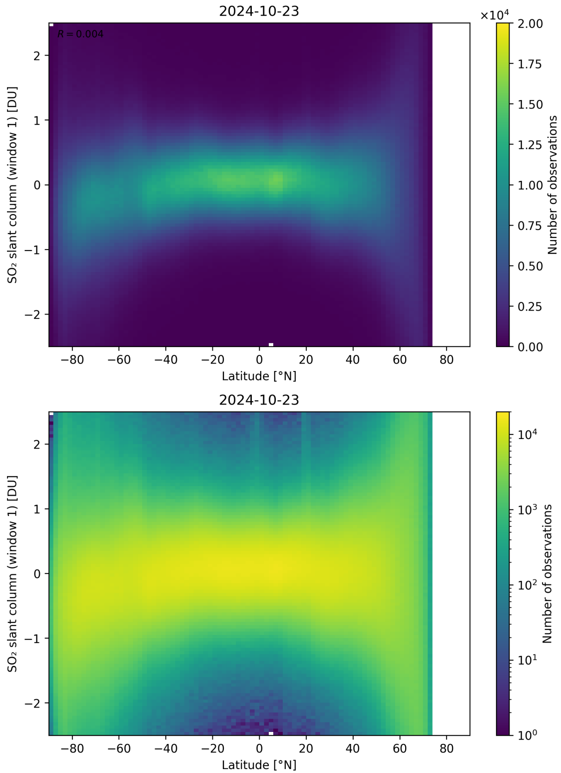
Figure 149: Scatter density plot of “Latitude” against “SO 2 slant column (window 1)” for 2024-10-22 to 2024-10-24.
