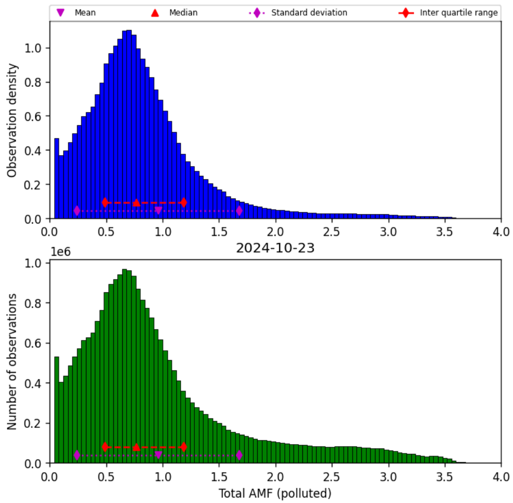
Figure 71: Histogram of “Total AMF (polluted)” for 2024-10-22 to 2024-10-24
