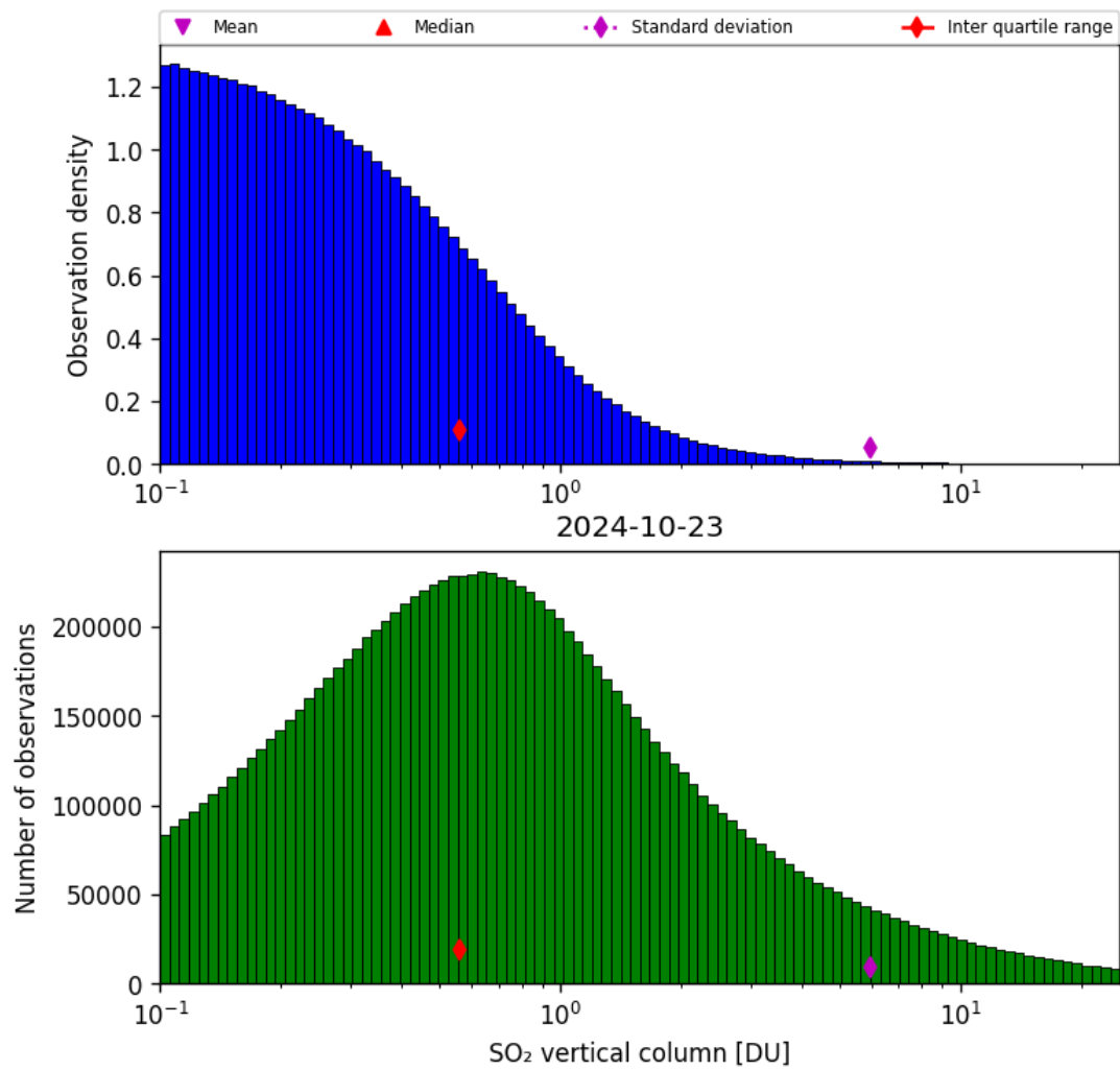
Figure 53: Histogram of “SO 2 vertical column” for 2024-10-22 to 2024-10-24
