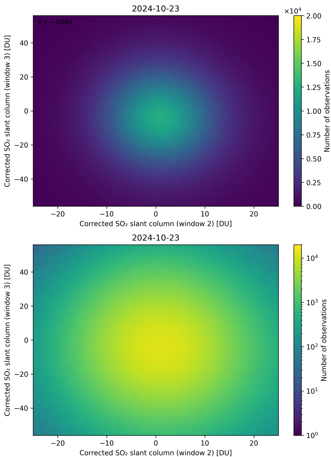
Figure 200: Scatter density plot of “Corrected SO 2 slant column (window 2)” against “Corrected SO 2 slant column (window 3)” for 2024-10-22 to 2024-10-24.
