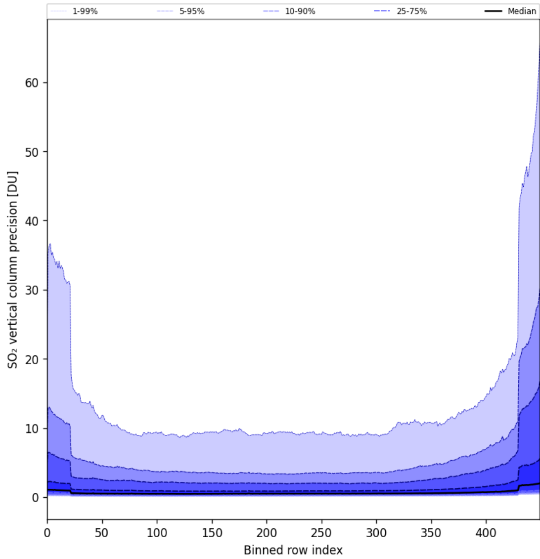
Figure 77: Along track statistics of “SO 2 vertical column precision” for 2024-10-22 to 2024-10-24
