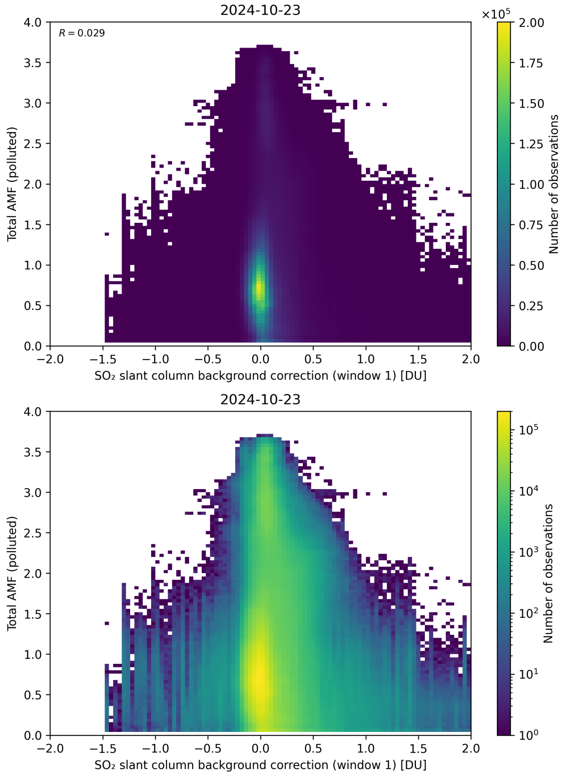
Figure 109: Scatter density plot of “SO 2 slant column background correction (window 1)” against “Total AMF (polluted)” for 2024-10-22 to 2024-10-24.
