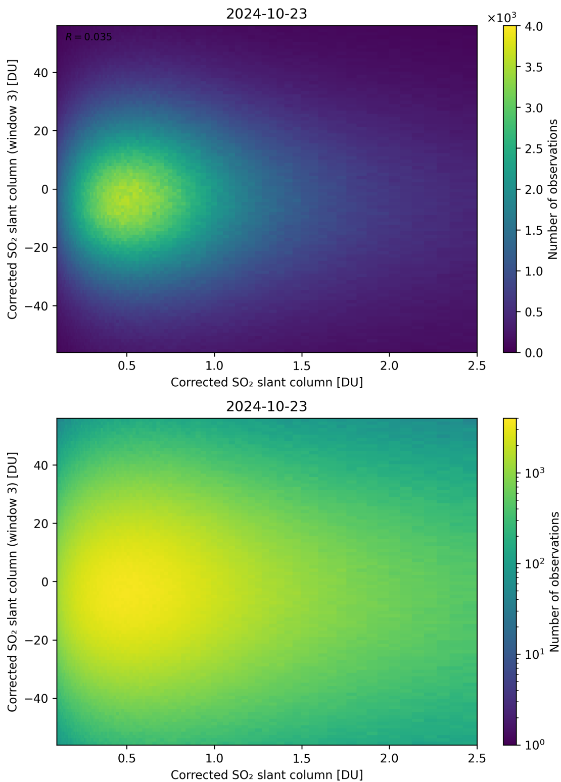
Figure 186: Scatter density plot of “Corrected SO 2 slant column” against “Corrected SO 2 slant column (window 3)” for 2024-10-22 to 2024-10-24.
