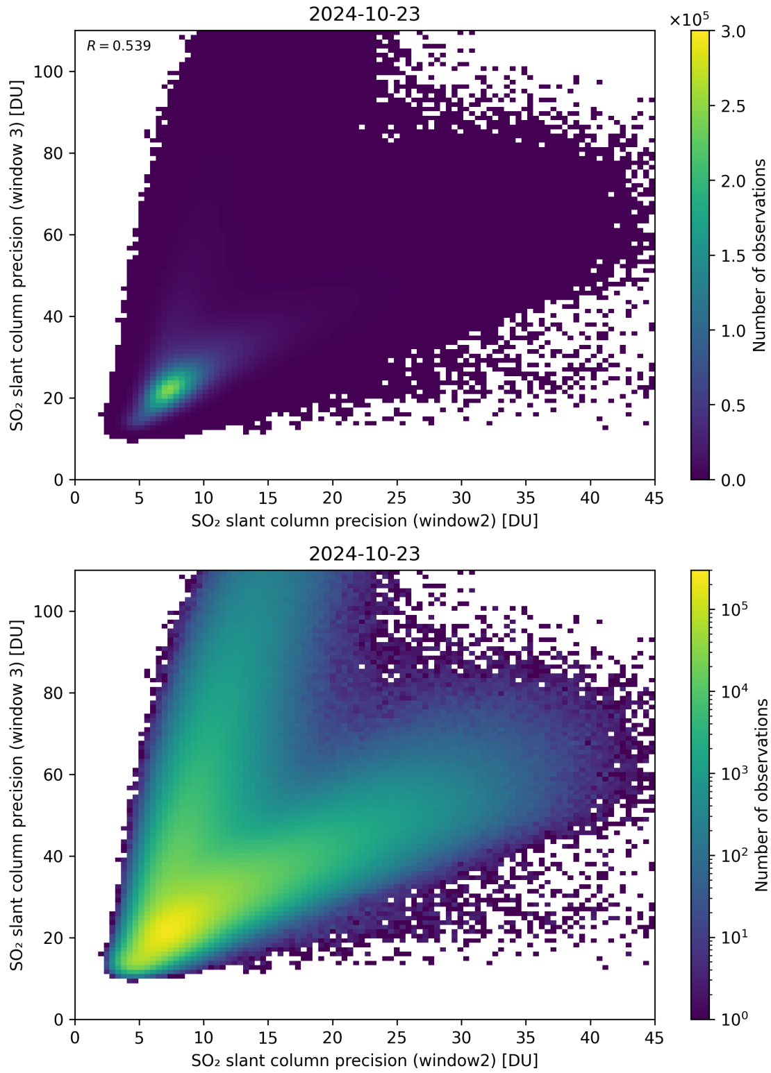
Figure 250: Scatter density plot of “SO 2 slant column precision (window2)” against “SO 2 slant column precision (window 3)” for 2024-10-22 to 2024-10-24.
