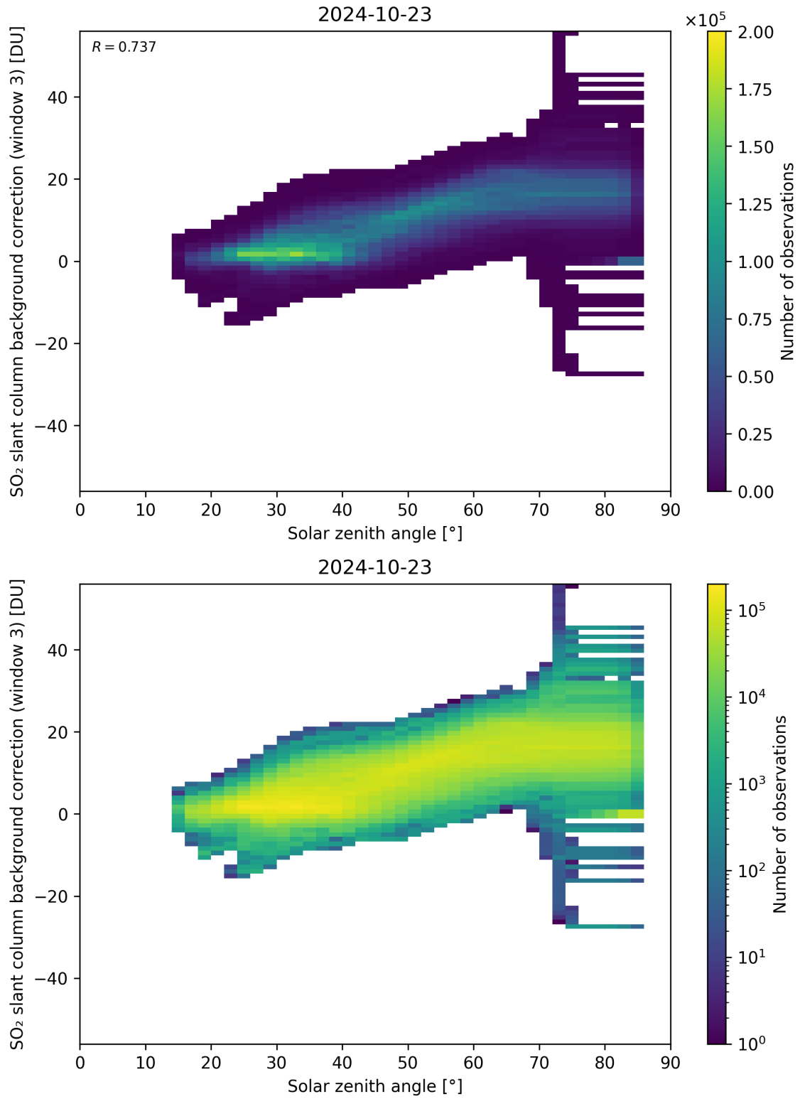
Figure 160: Scatter density plot of “Solar zenith angle” against “SO 2 slant column background correction (window 3)” for 2024-10-22 to 2024-10-24.
