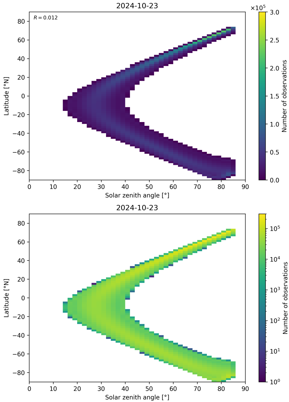
Figure 164: Scatter density plot of “Solar zenith angle” against “Latitude” for 2024-10-22 to 2024-10-24.
