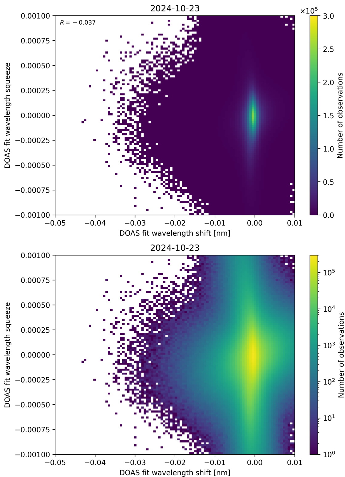
Figure 127: Scatter density plot of “DOAS fit wavelength shift” against “DOAS fit wavelength squeeze” for 2024-10-22 to 2024-10-24.
