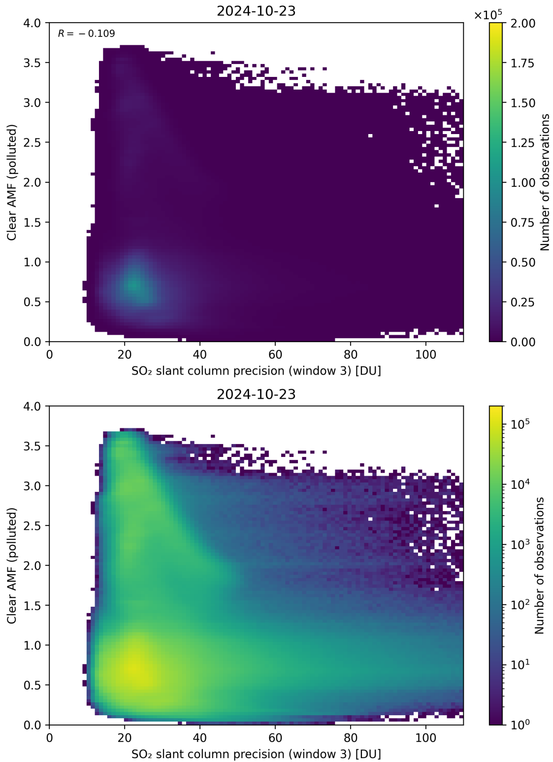
Figure 261: Scatter density plot of “SO 2 slant column precision (window 3)” against “Clear AMF (polluted)” for 2024-10-22 to 2024-10-24.
