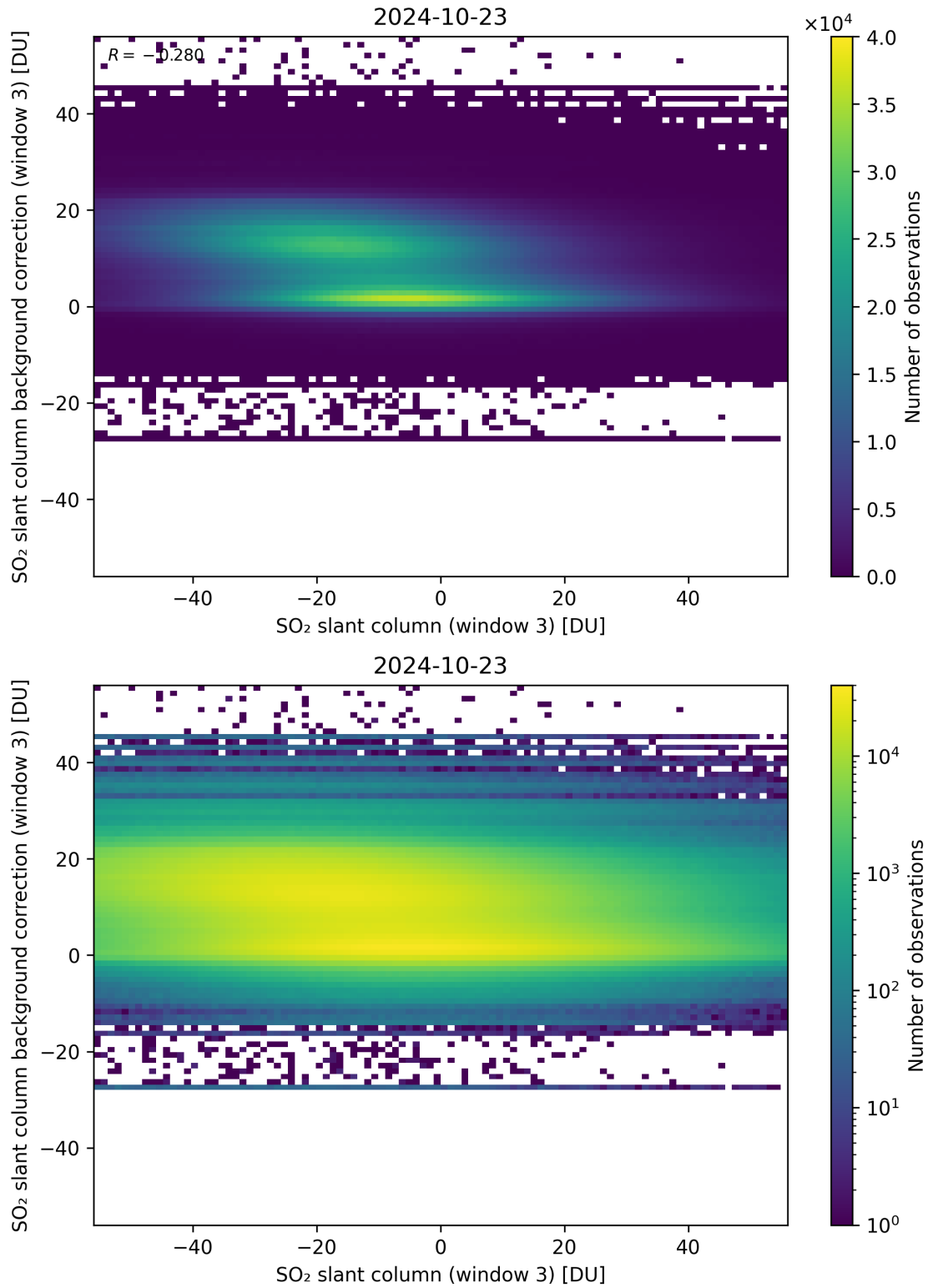
Figure 253: Scatter density plot of “SO 2 slant column (window 3)” against “SO 2 slant column background correction (window 3)” for 2024-10-22 to 2024-10-24.
