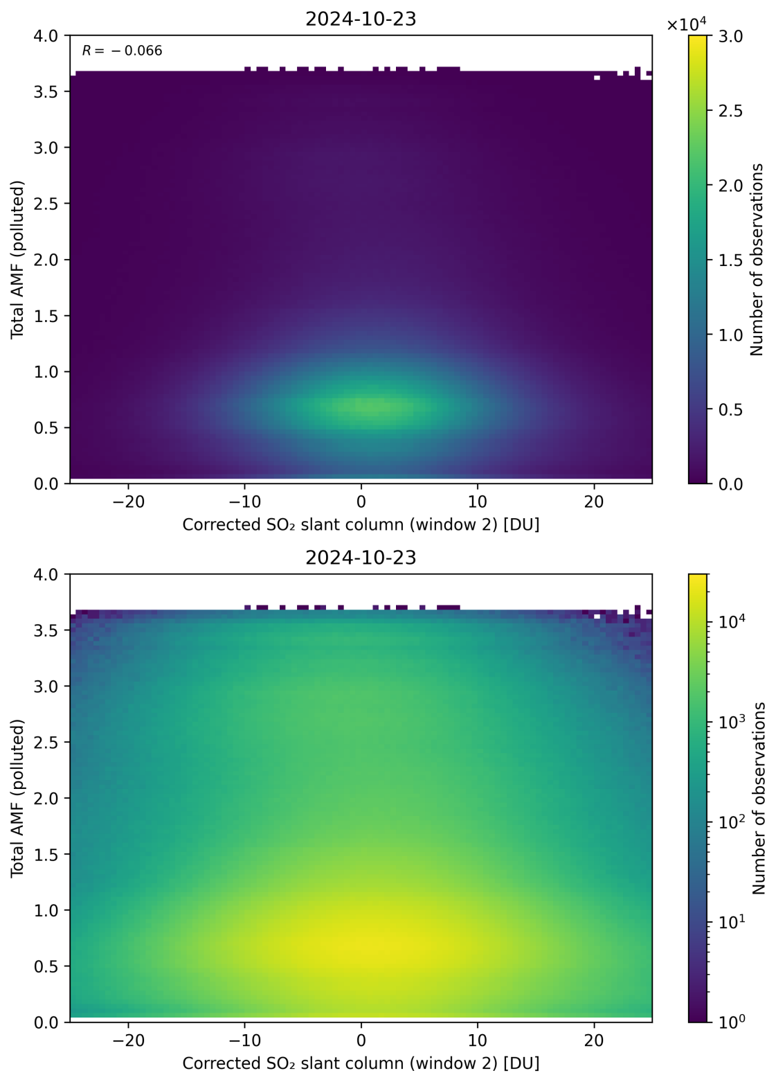
Figure 203: Scatter density plot of “Corrected SO 2 slant column (window 2)” against “Total AMF (polluted)” for 2024-10-22 to 2024-10-24.
