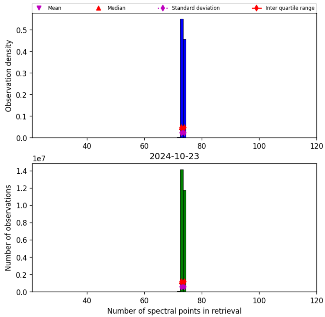
Figure 74: Histogram of “Number of spectral points in retrieval” for 2024-10-22 to 2024-10-24
