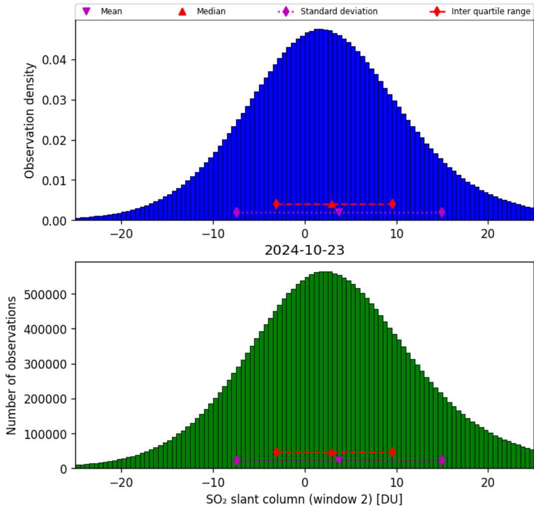
Figure 60: Histogram of “SO 2 slant column (window 2)” for 2024-10-22 to 2024-10-24
