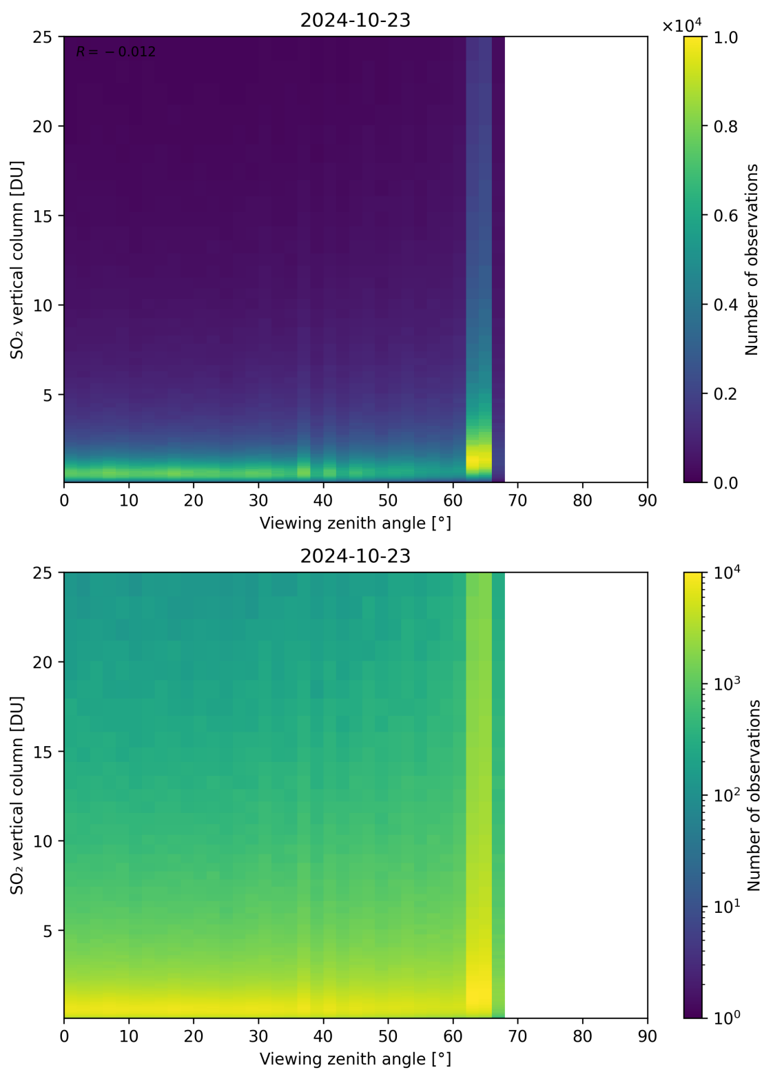
Figure 327: Scatter density plot of “Viewing zenith angle” against “SO 2 vertical column” for 2024-10-22 to 2024-10-24.
