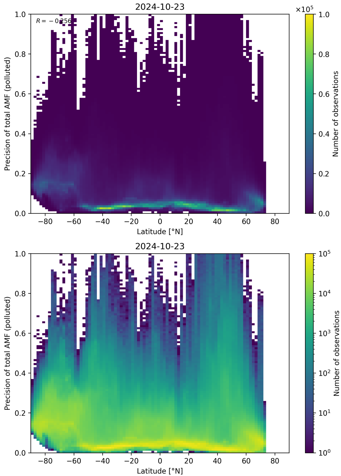
Figure 155: Scatter density plot of “Latitude” against “Precision of total AMF (polluted)” for 2024-10-22 to 2024-10-24.
