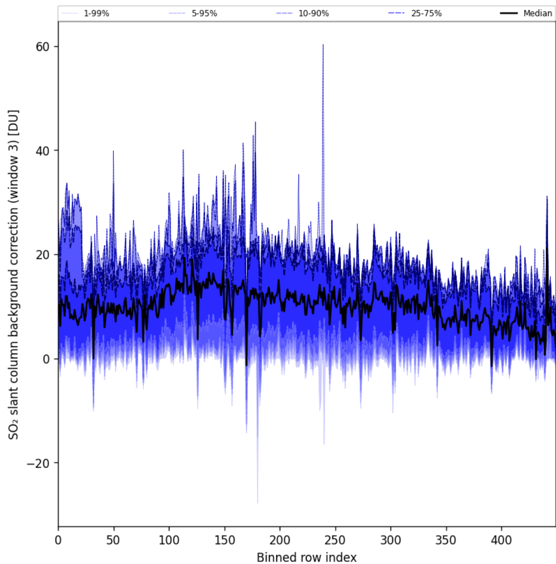
Figure 90: Along track statistics of “SO 2 slant column background correction (window 3)” for 2024-10-22 to 2024-10-24
