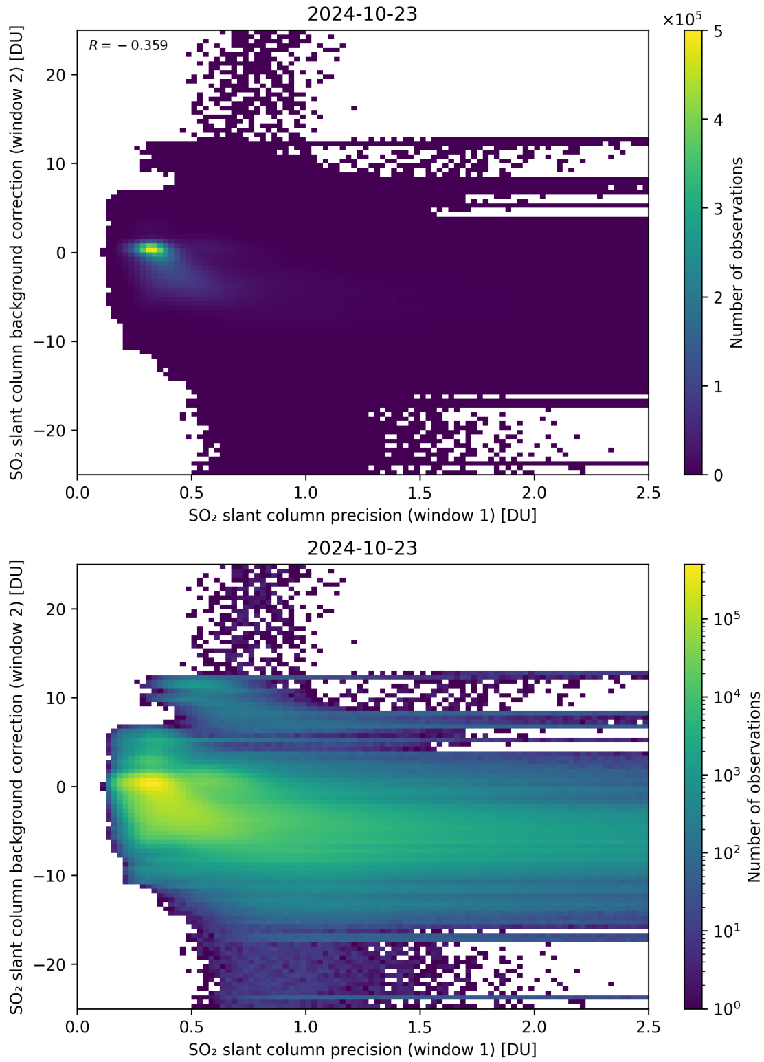
Figure 219: Scatter density plot of “SO 2 slant column precision (window 1)” against “SO 2 slant column background correction (window 2)” for 2024-10-22 to 2024-10-24.
