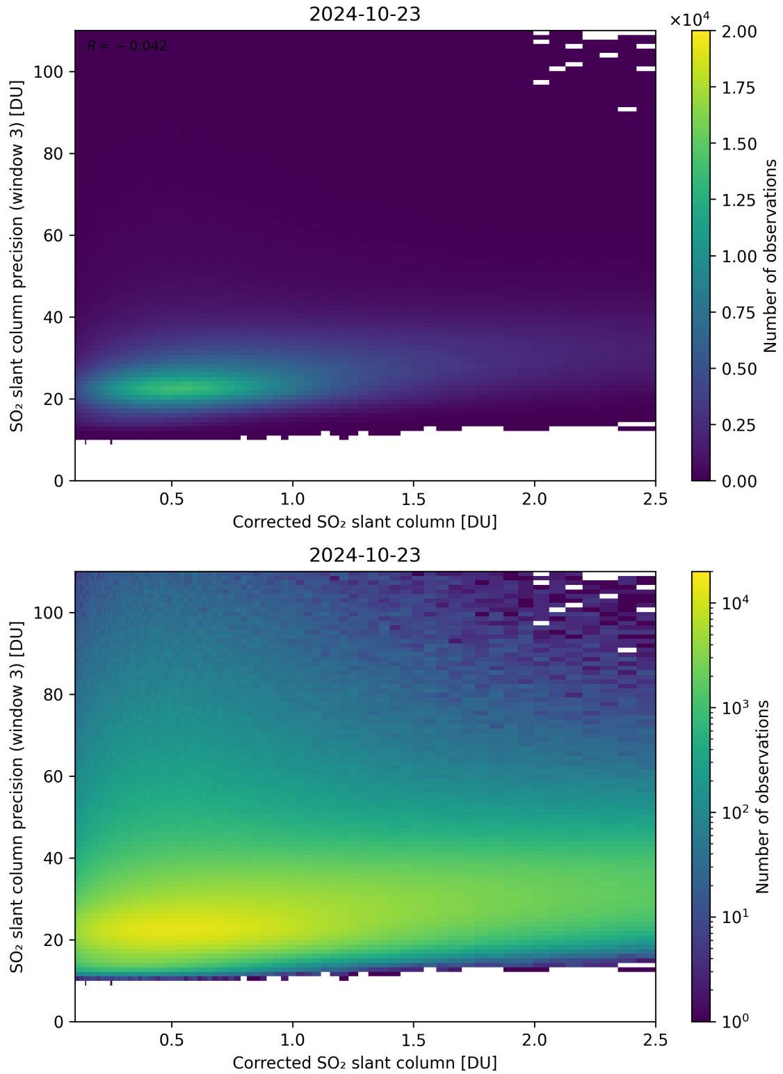
Figure 191: Scatter density plot of “Corrected SO 2 slant column” against “SO 2 slant column precision (window 3)” for 2024-10-22 to 2024-10-24.
