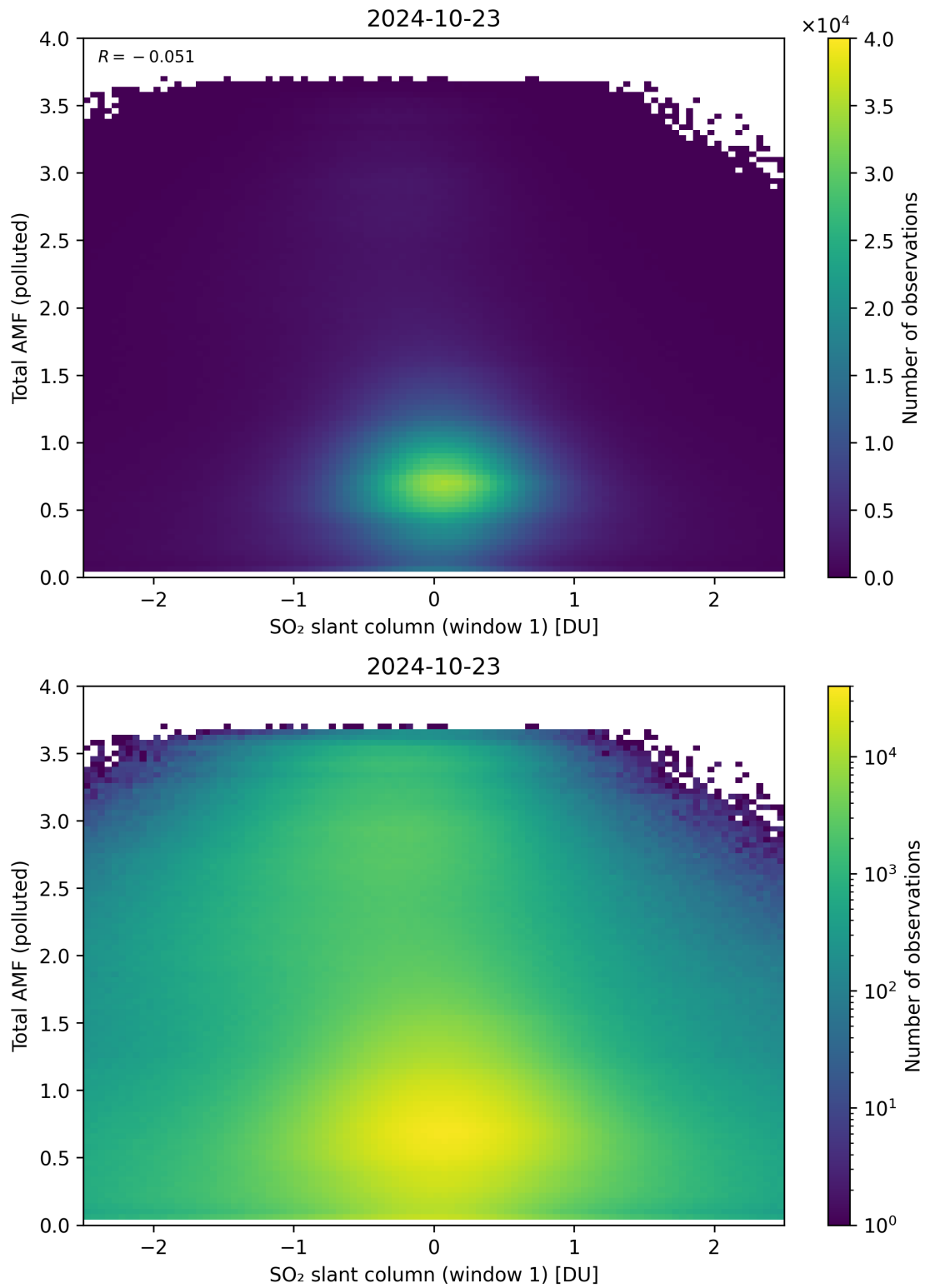
Figure 239: Scatter density plot of “SO 2 slant column (window 1)” against “Total AMF (polluted)” for 2024-10-22 to 2024-10-24.
