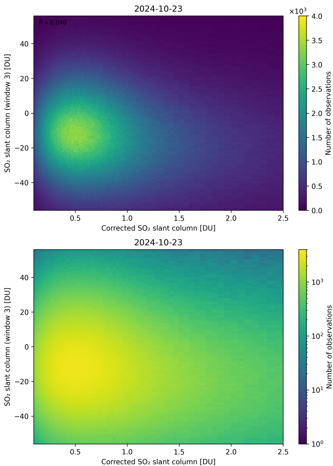
Figure 190: Scatter density plot of “Corrected SO 2 slant column” against “SO 2 slant column (window 3)” for 2024-10-22 to 2024-10-24.
