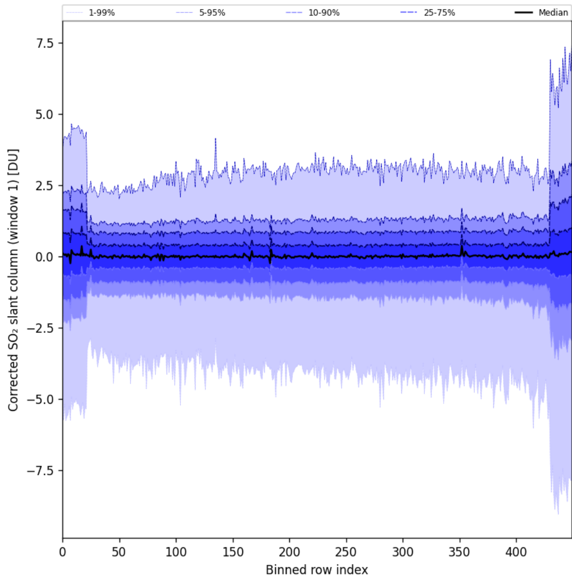
Figure 81: Along track statistics of "Corrected SO 2 slant column (window 1)" for 2024-10-22 to 2024-10-24
