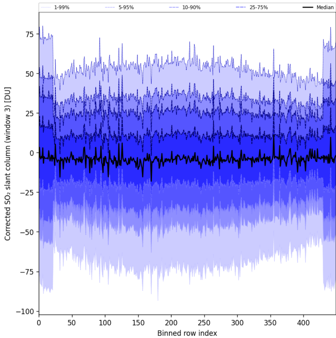
Figure 89: Along track statistics of “Corrected SO 2 slant column (window 3)” for 2024-10-22 to 2024-10-24
