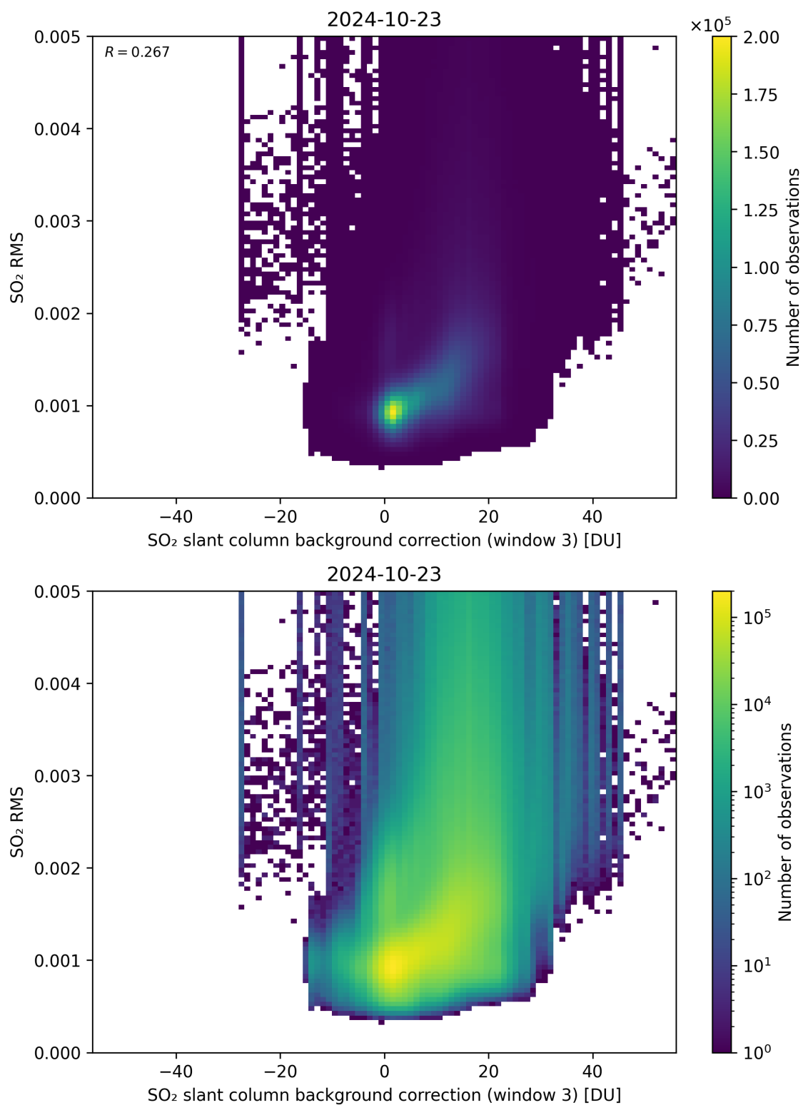
Figure 123: Scatter density plot of “SO 2 slant column background correction (window 3)” against “SO 2 RMS” for 2024-10-22 to 2024-10-24.
