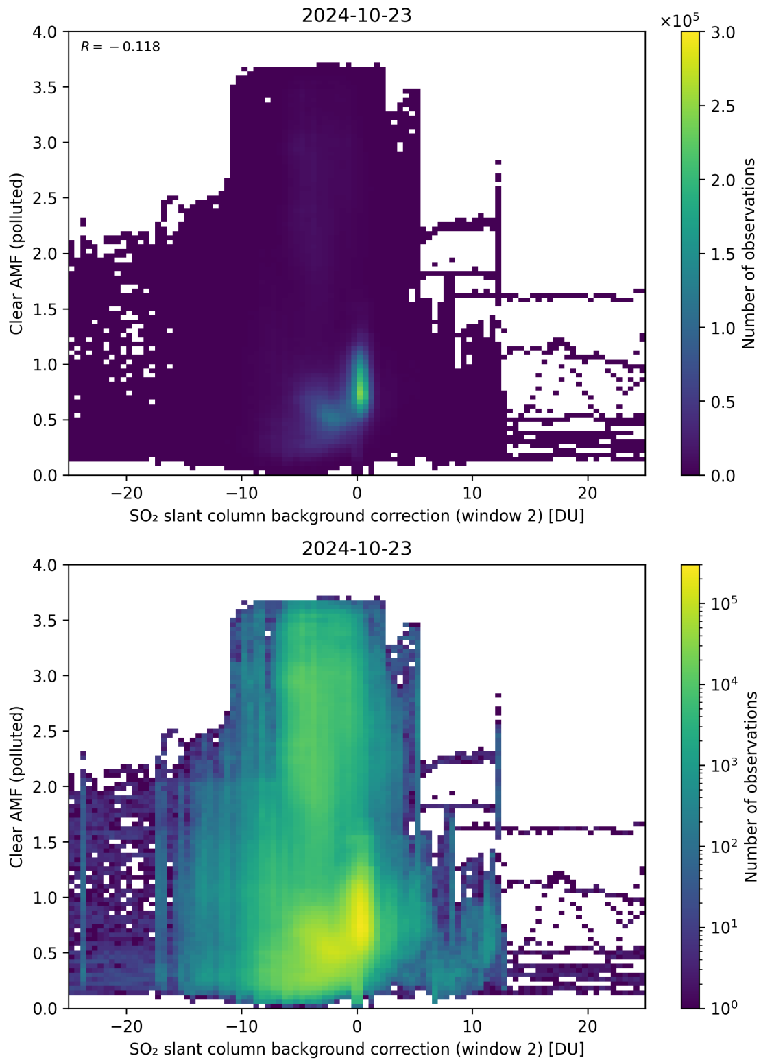
Figure 115: Scatter density plot of “SO 2 slant column background correction (window 2)” against “Clear AMF (polluted)” for 2024-10-22 to 2024-10-24.
