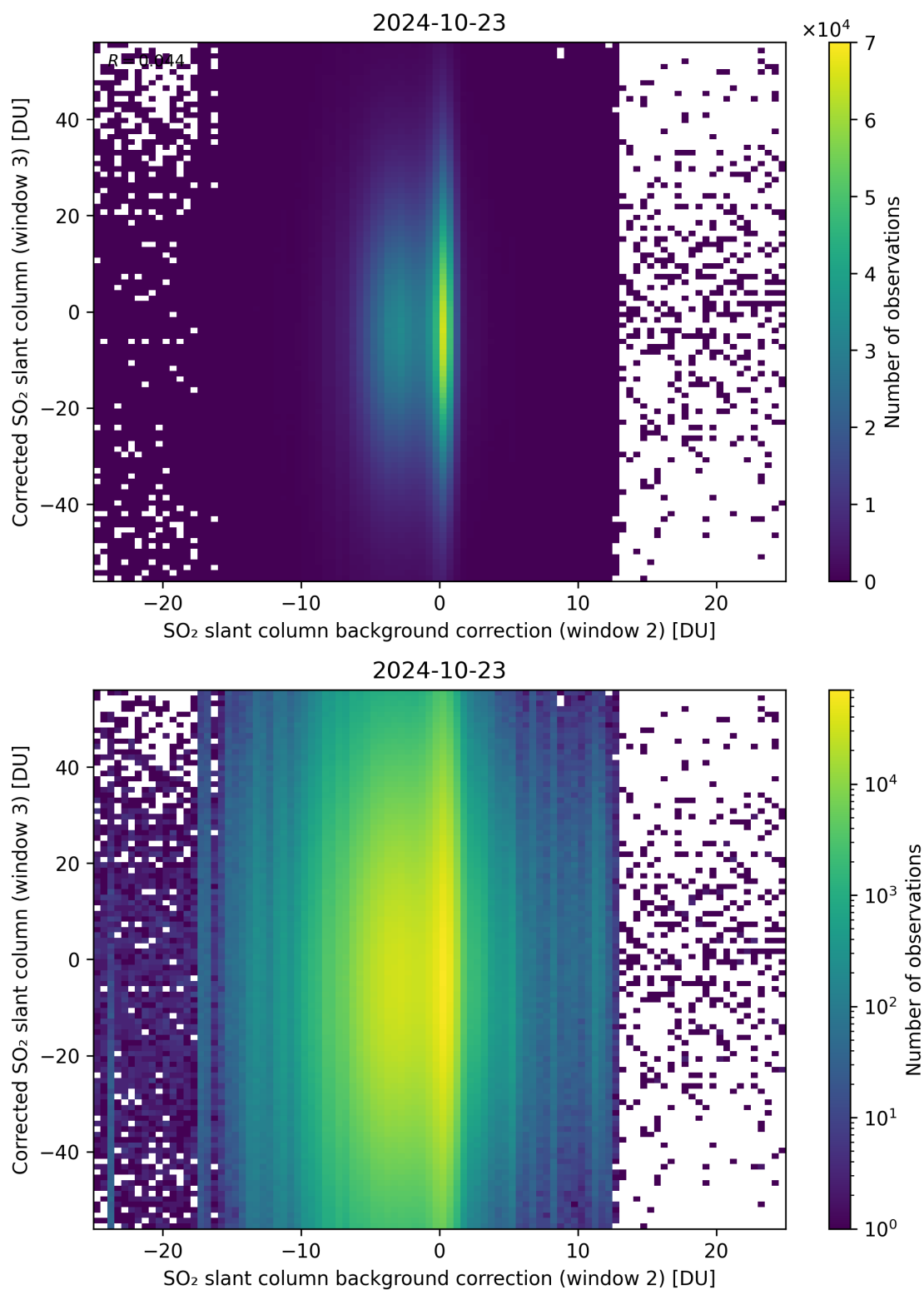
Figure 116: Scatter density plot of “SO 2 slant column background correction (window 2)” against “Corrected SO 2 slant column (window 3)” for 2024-10-22 to 2024-10-24.
