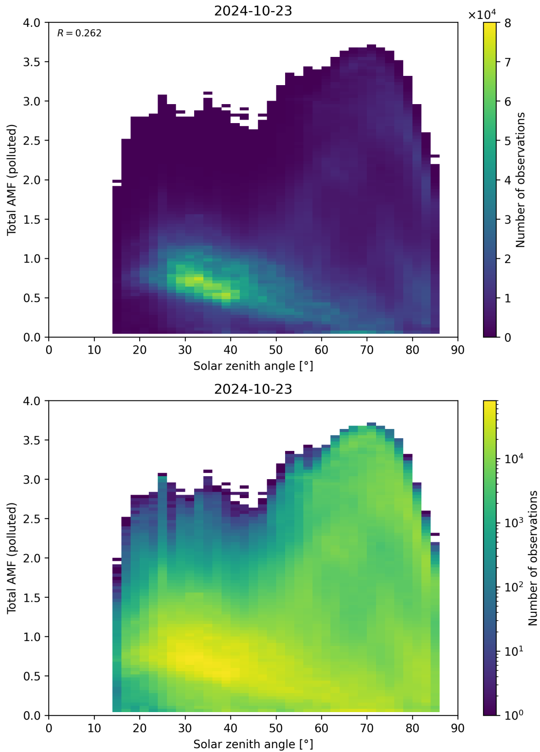
Figure 174: Scatter density plot of “Solar zenith angle” against “Total AMF (polluted)” for 2024-10-22 to 2024-10-24.
