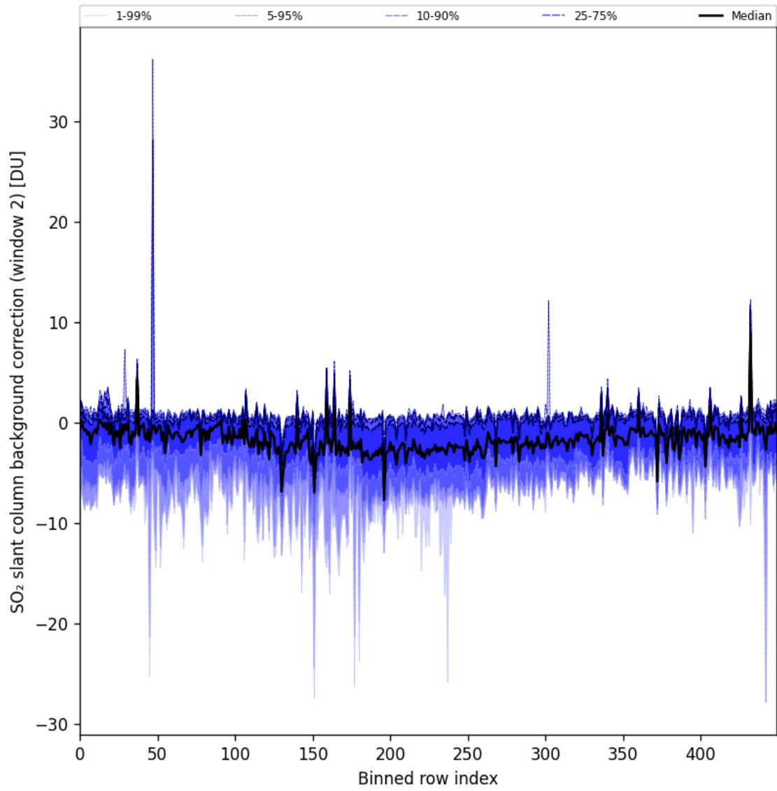
Figure 86: Along track statistics of “SO 2 slant column background correction (window 2)” for 2024-10-22 to 2024-10-24
