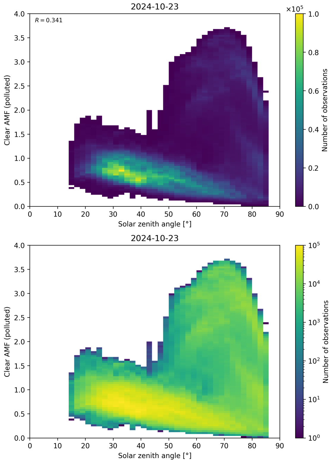
Figure 165: Scatter density plot of “Solar zenith angle” against “Clear AMF (polluted)” for 2024-10-22 to 2024-10-24.
