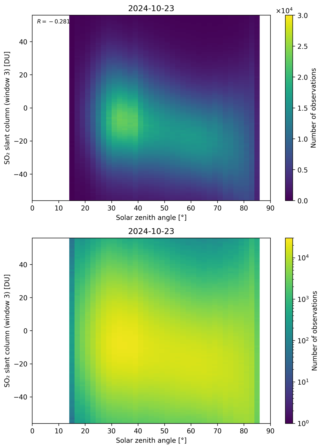
Figure 172: Scatter density plot of “Solar zenith angle” against “SO 2 slant column (window 3)” for 2024-10-22 to 2024-10-24.
