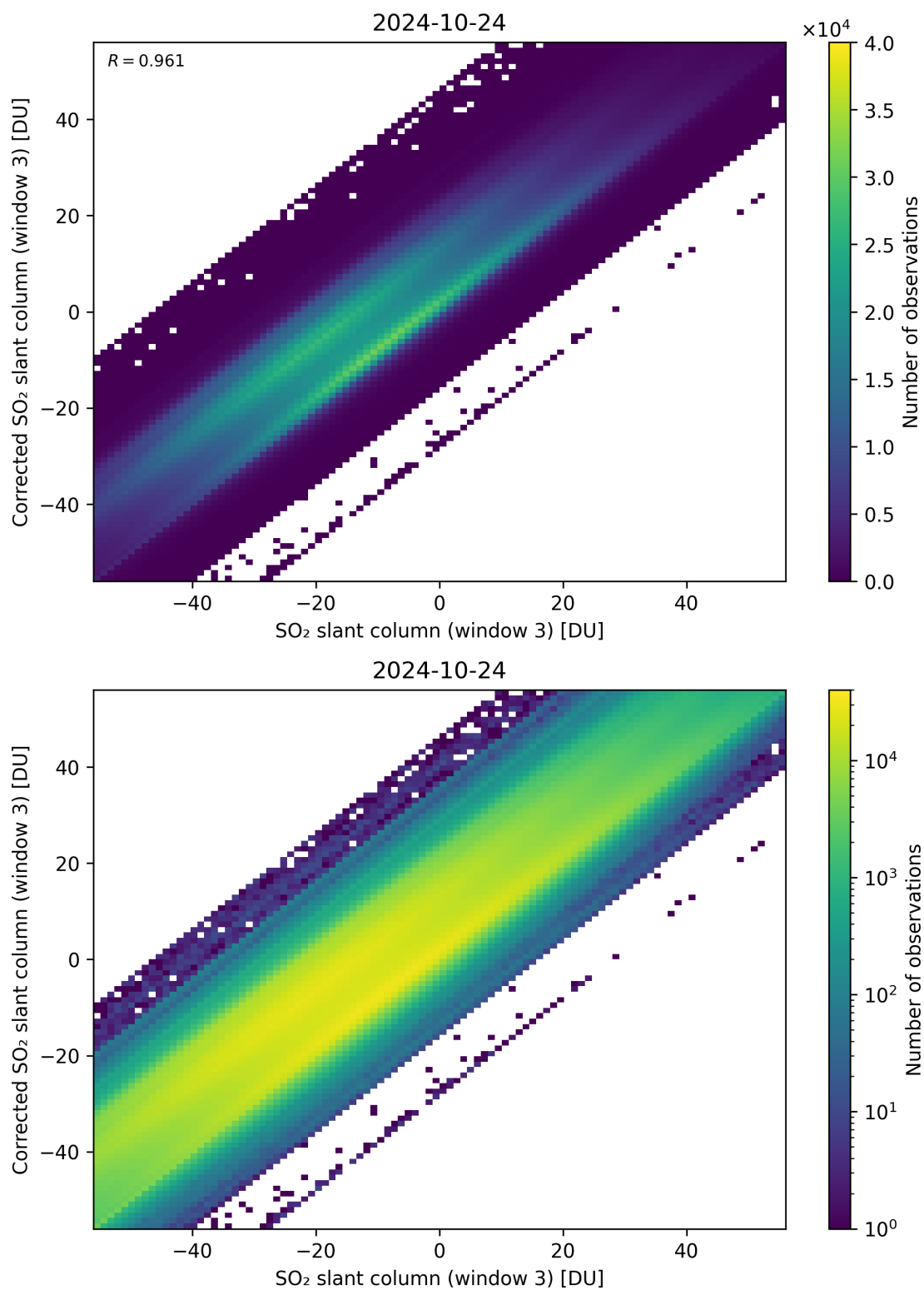
Figure 266: Scatter density plot of “SO 2 slant column (window 3)” against “Corrected SO 2 slant column (window 3)” for 2024-10-24 to 2024-10-25.
