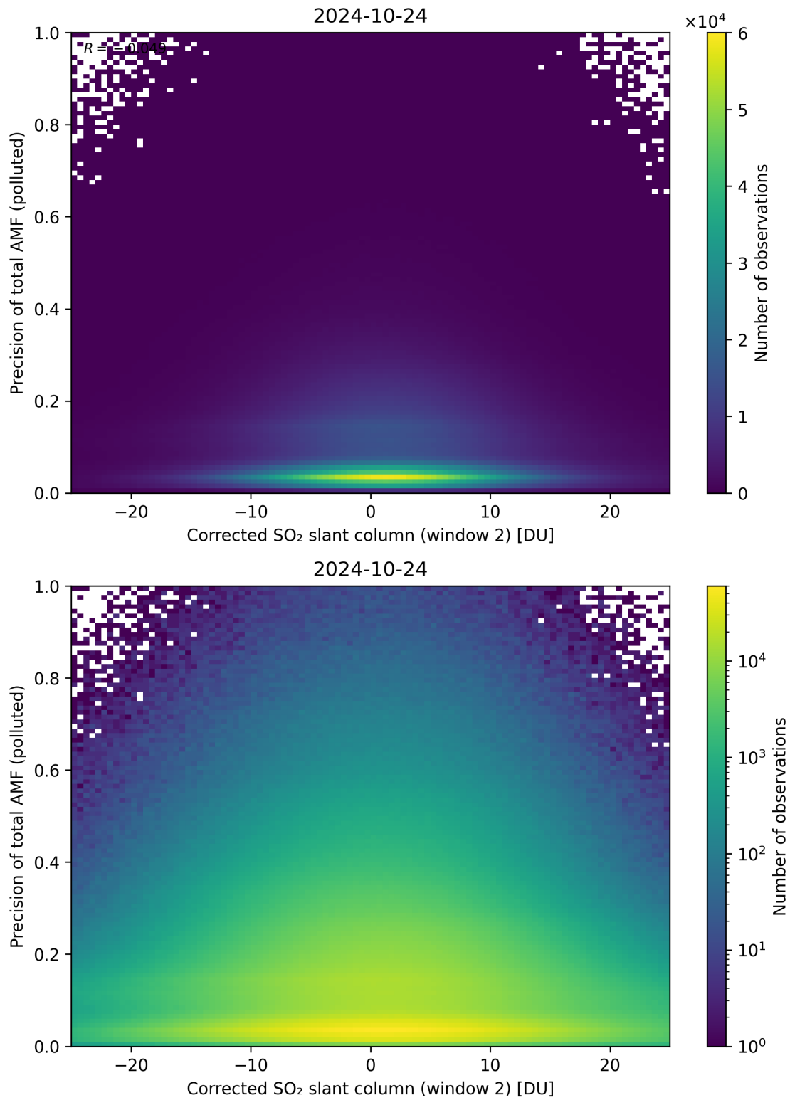
Figure 204: Scatter density plot of “Corrected SO 2 slant column (window 2)” against “Precision of total AMF (polluted)” for 2024-10-24 to 2024-10-25.
