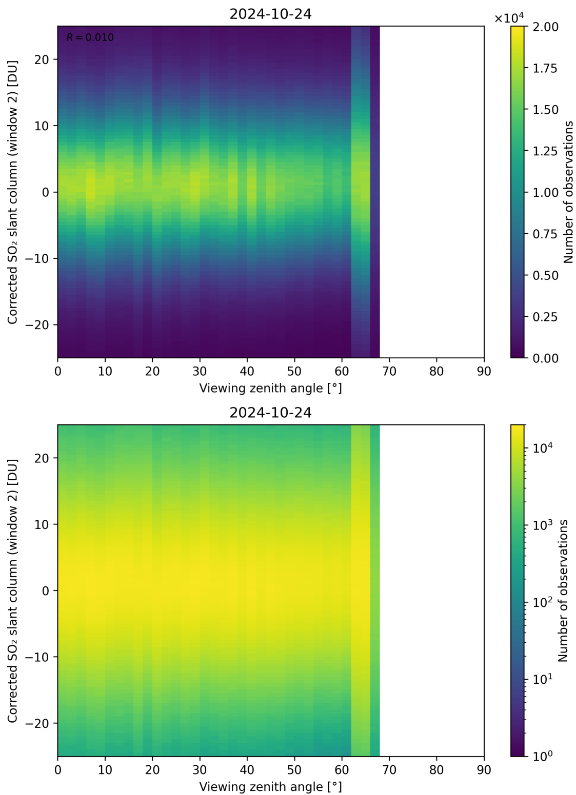
Figure 318: Scatter density plot of “Viewing zenith angle” against “Corrected SO 2 slant column (window 2)” for 2024-10-24 to 2024-10-25.
