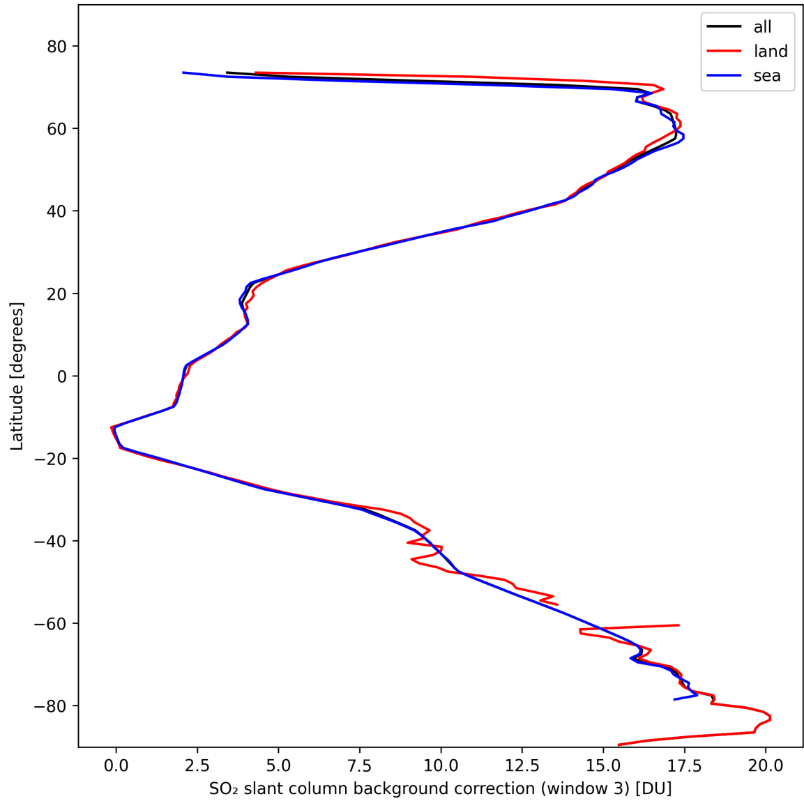
Figure 44: Zonal average of “SO 2 slant column background correction (window 3)” for 2024-10-24 to 2024-10-25.
