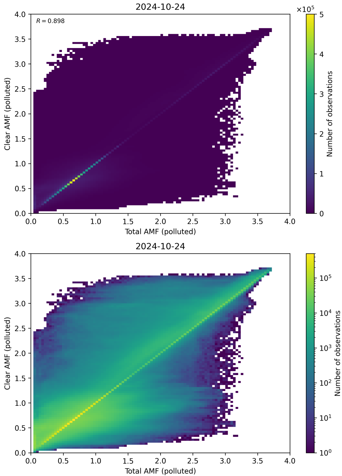
Figure 271: Scatter density plot of “Total AMF (polluted)” against “Clear AMF (polluted)” for 2024-10-24 to 2024-10-25.
