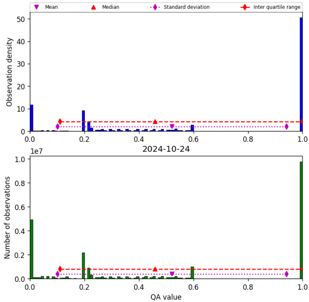
Figure 52: Histogram of “QA value” for 2024-10-24 to 2024-10-25
