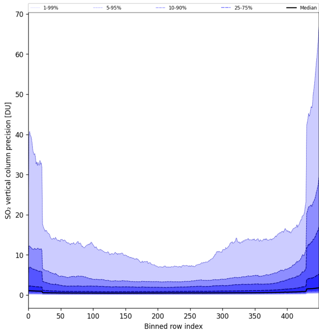
Figure 77: Along track statistics of “SO 2 vertical column precision” for 2024-10-24 to 2024-10-25
