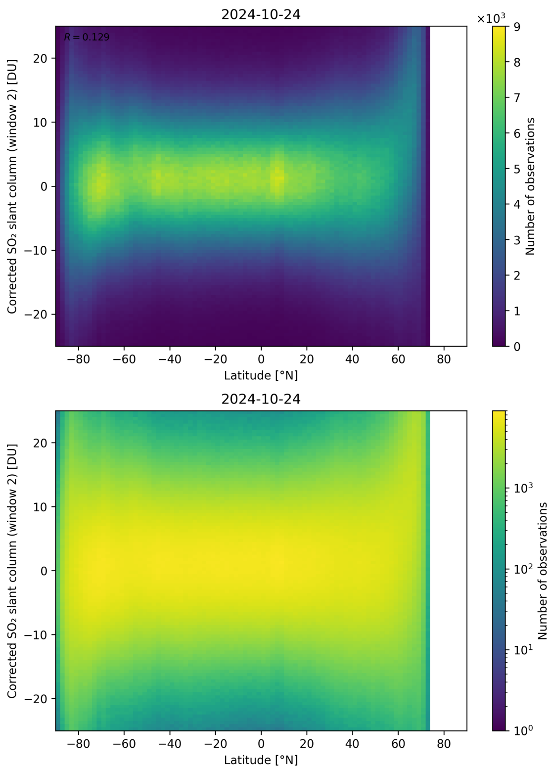
Figure 147: Scatter density plot of “Latitude” against “Corrected SO 2 slant column (window 2)” for 2024-10-24 to 2024-10-25.
