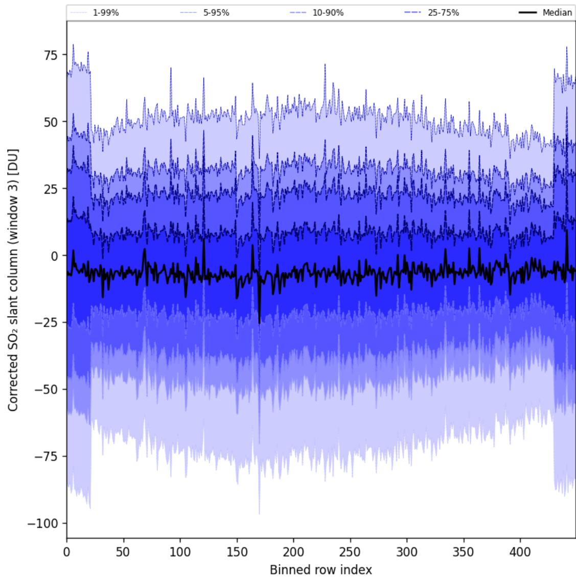
Figure 89: Along track statistics of “Corrected SO 2 slant column (window 3)” for 2024-10-24 to 2024-10-25
