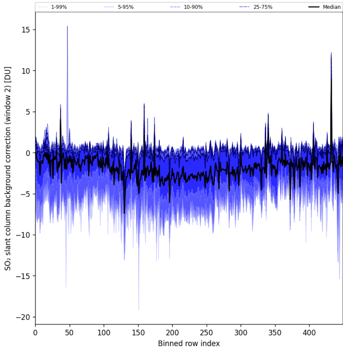
Figure 86: Along track statistics of “SO 2 slant column background correction (window 2)” for 2024-10-24 to 2024-10-25
