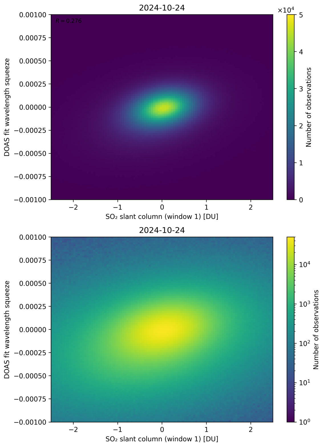
Figure 216: Scatter density plot of “SO 2 slant column (window 1)” against “DOAS fit wavelength squeeze” for 2024-10-24 to 2024-10-25.
