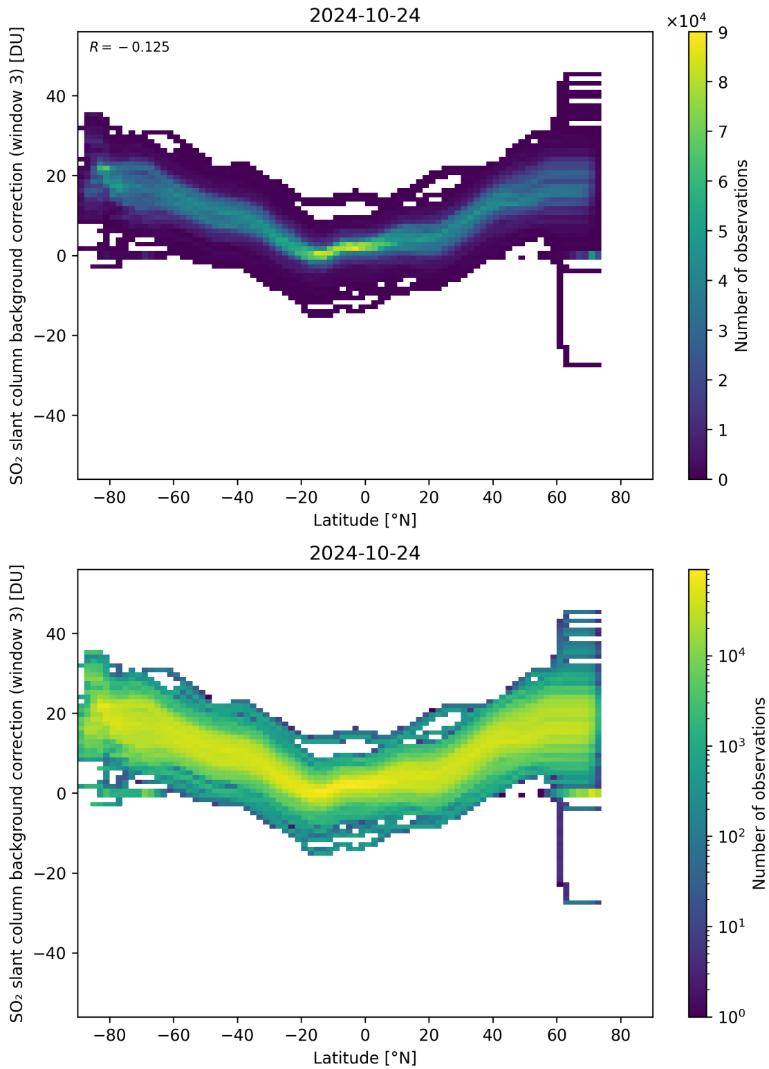
Figure 141: Scatter density plot of “Latitude” against “SO 2 slant column background correction (window 3)” for 2024-10-24 to 2024-10-25.
