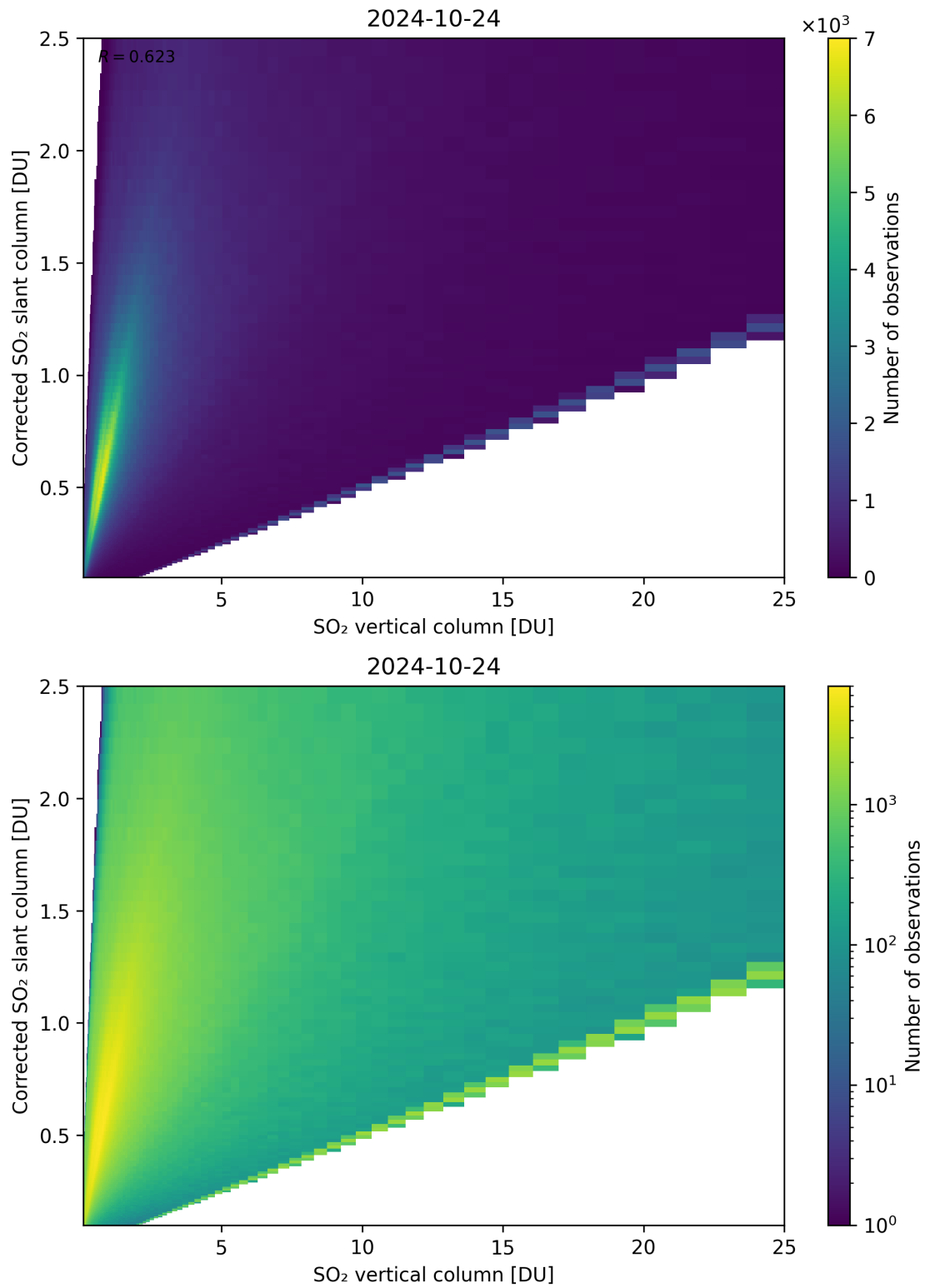
Figure 297: Scatter density plot of “SO 2 vertical column” against “Corrected SO 2 slant column” for 2024-10-24 to 2024-10-25.
