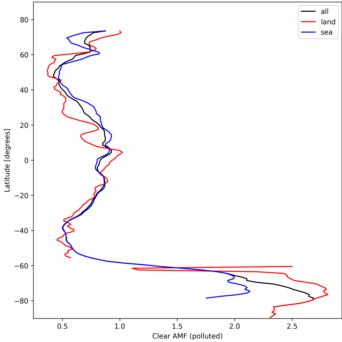
Figure 50: Zonal average of “Clear AMF (polluted)” for 2024-10-24 to 2024-10-25.
