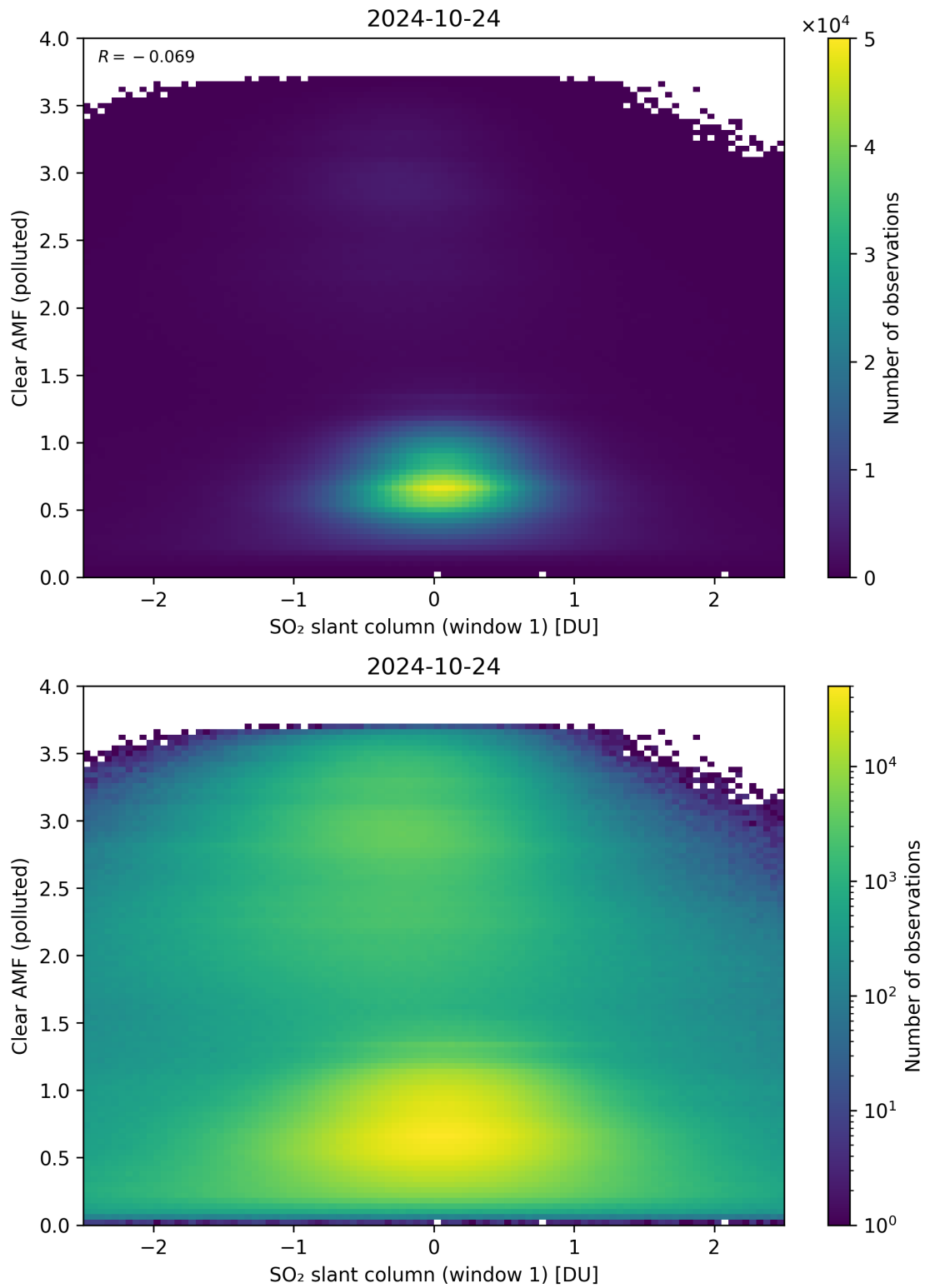
Figure 232: Scatter density plot of “SO 2 slant column (window 1)” against “Clear AMF (polluted)” for 2024-10-24 to 2024-10-25.
