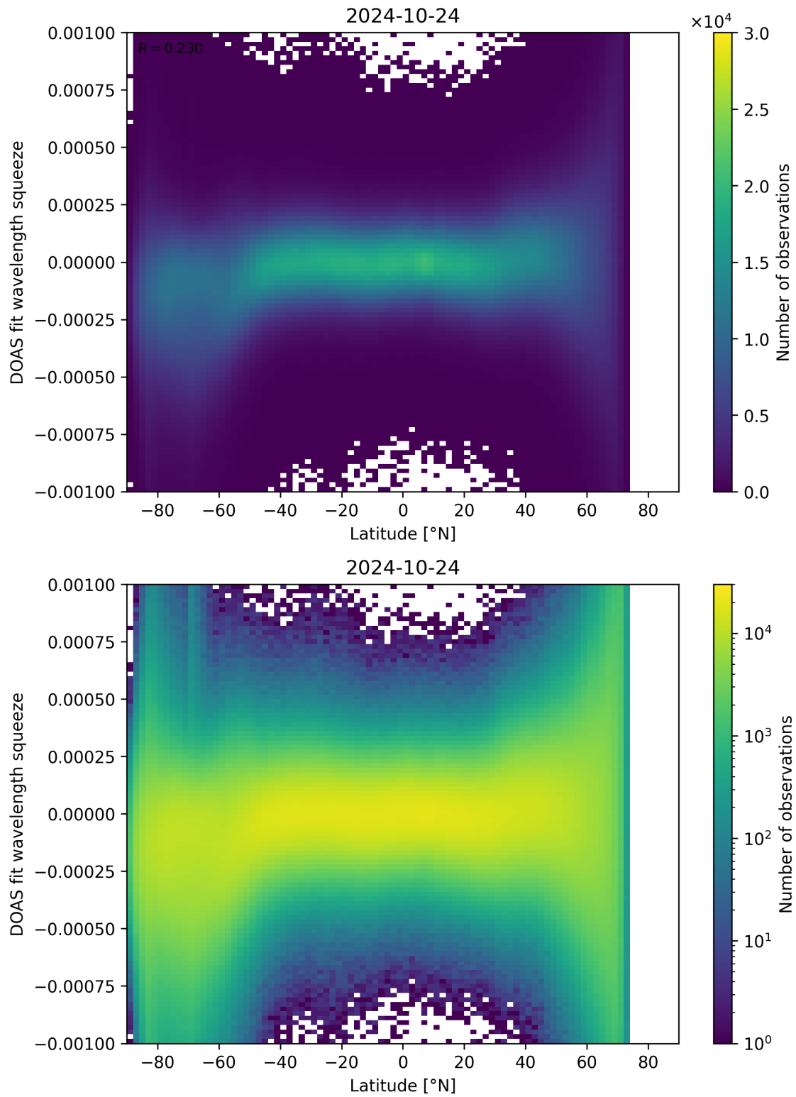
Figure 143: Scatter density plot of “Latitude” against “DOAS fit wavelength squeeze” for 2024-10-24 to 2024-10-25.
