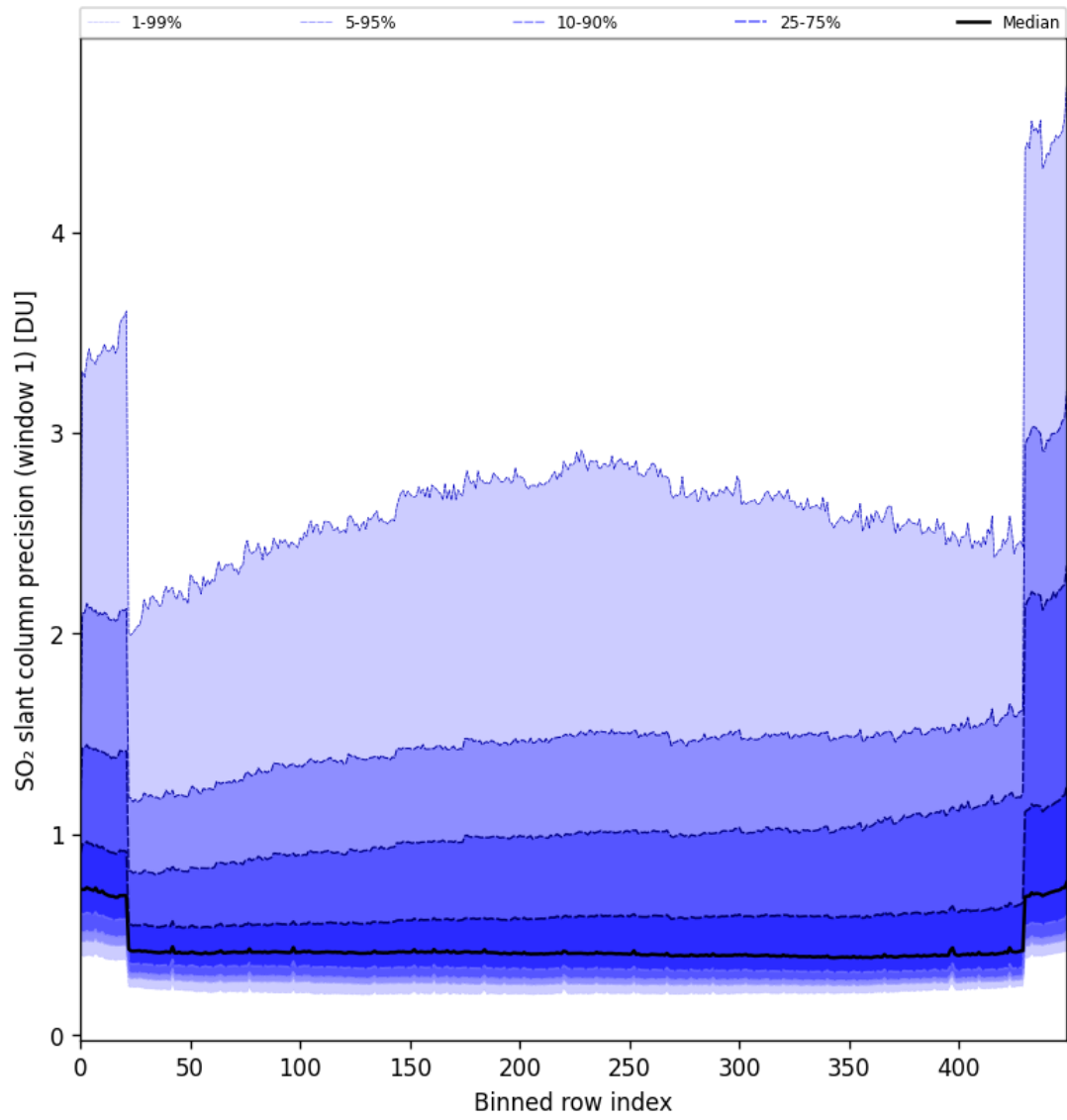
Figure 80: Along track statistics of “SO 2 slant column precision (window 1)” for 2024-10-24 to 2024-10-25
