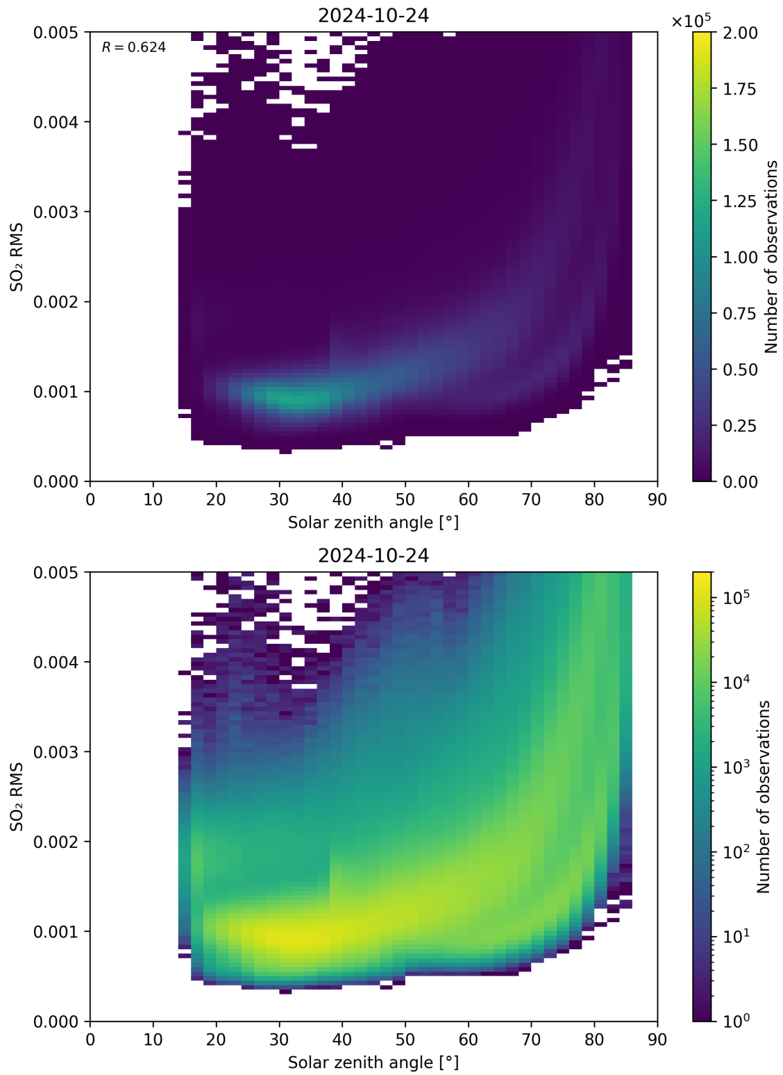
Figure 163: Scatter density plot of “Solar zenith angle” against “SO 2 RMS” for 2024-10-24 to 2024-10-25.
