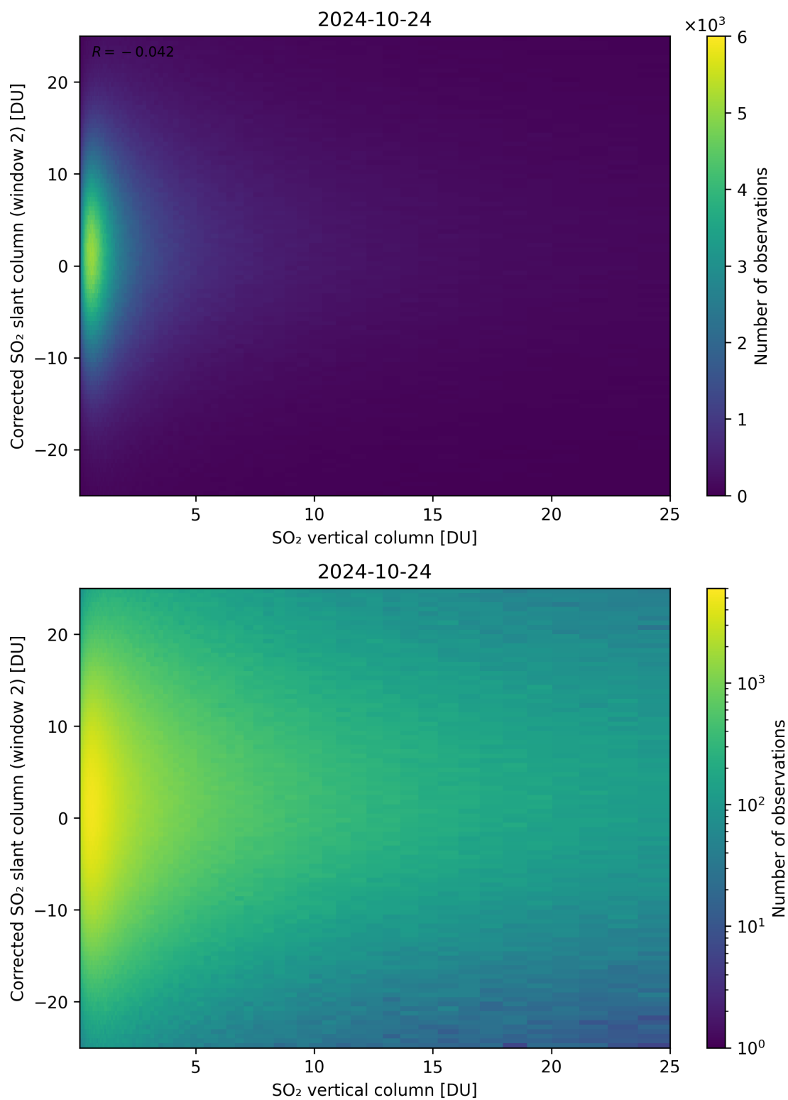
Figure 298: Scatter density plot of “SO 2 vertical column” against “Corrected SO 2 slant column (window 2)” for 2024-10-24 to 2024-10-25.
