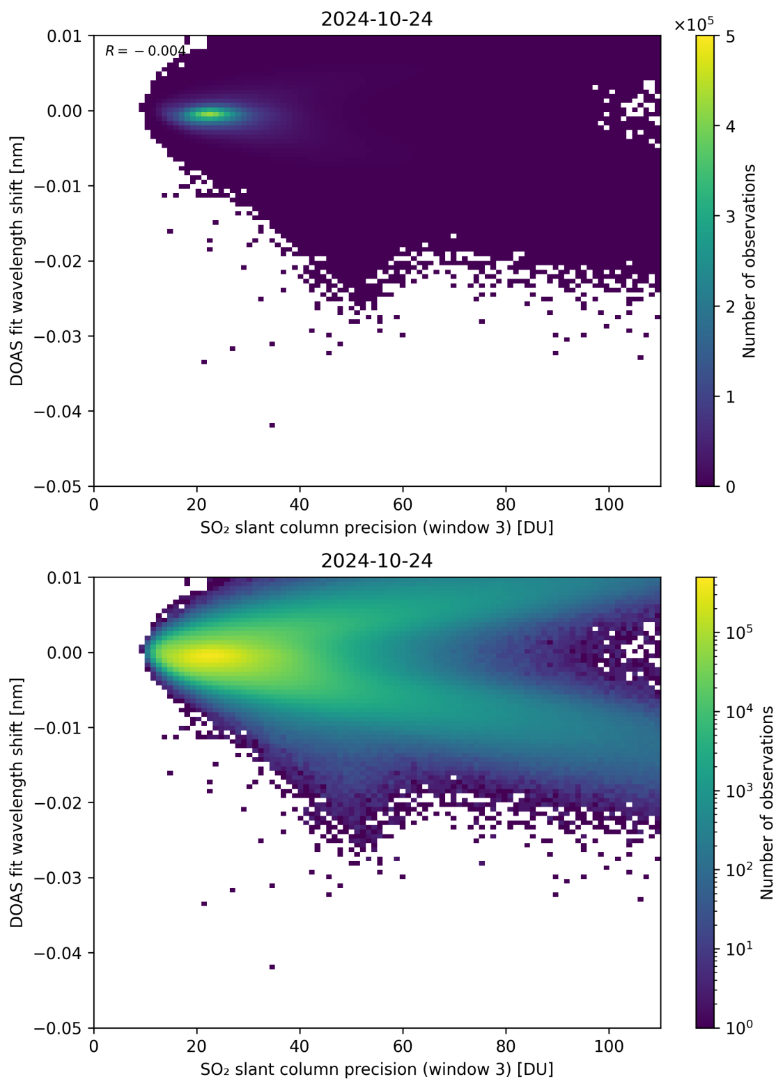
Figure 258: Scatter density plot of “SO 2 slant column precision (window 3)” against “DOAS fit wavelength shift” for 2024-10-24 to 2024-10-25.
