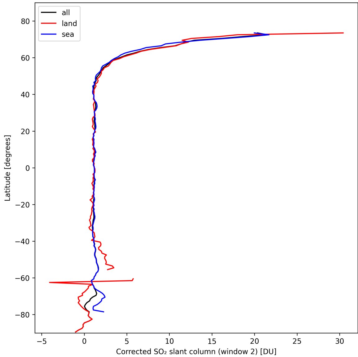
Figure 39: Zonal average of “Corrected SO 2 slant column (window 2)” for 2024-10-24 to 2024-10-25.
