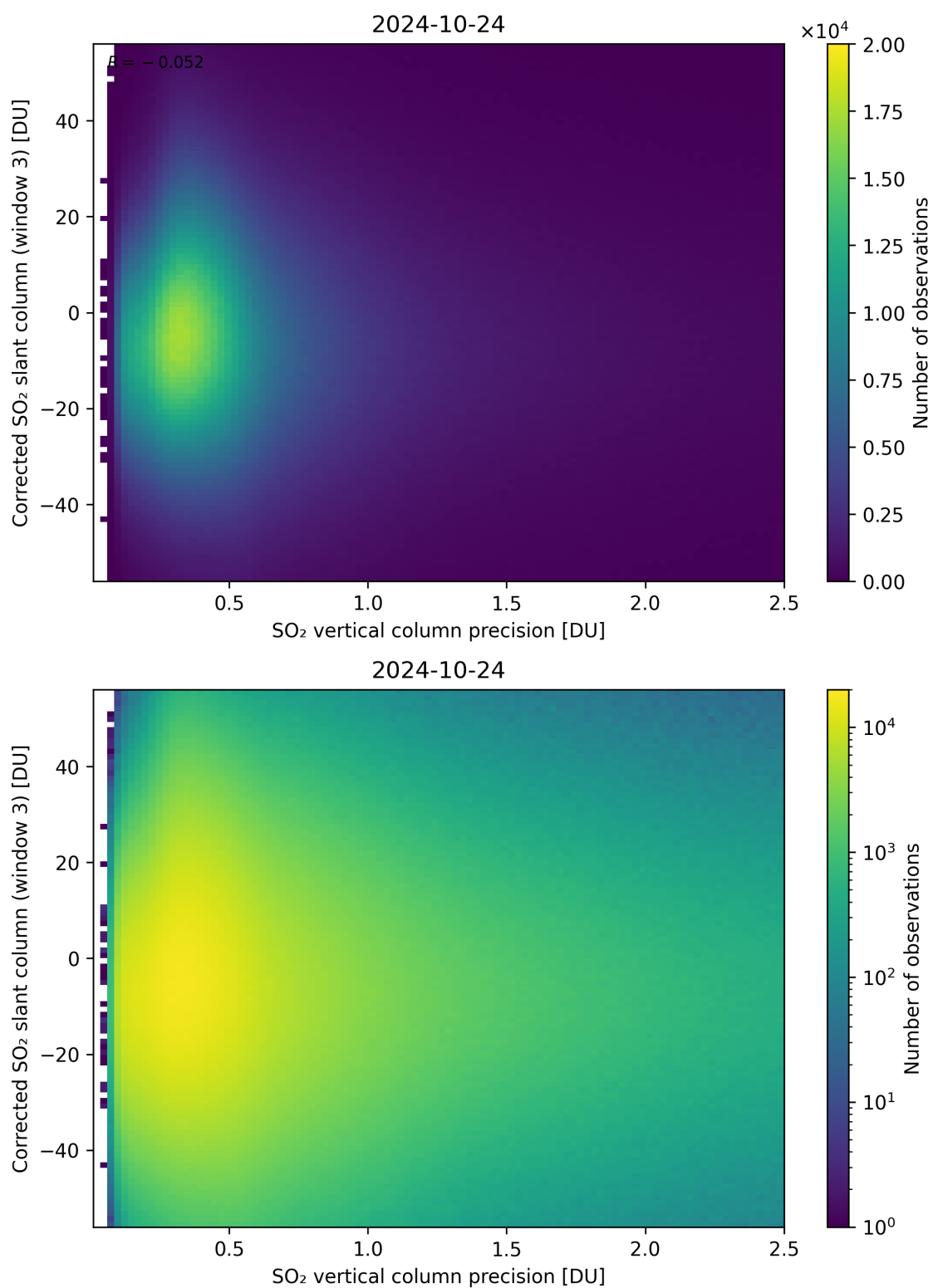
Figure 288: Scatter density plot of “SO 2 vertical column precision” against “Corrected SO 2 slant column (window 3)” for 2024-10-24 to 2024-10-25.
