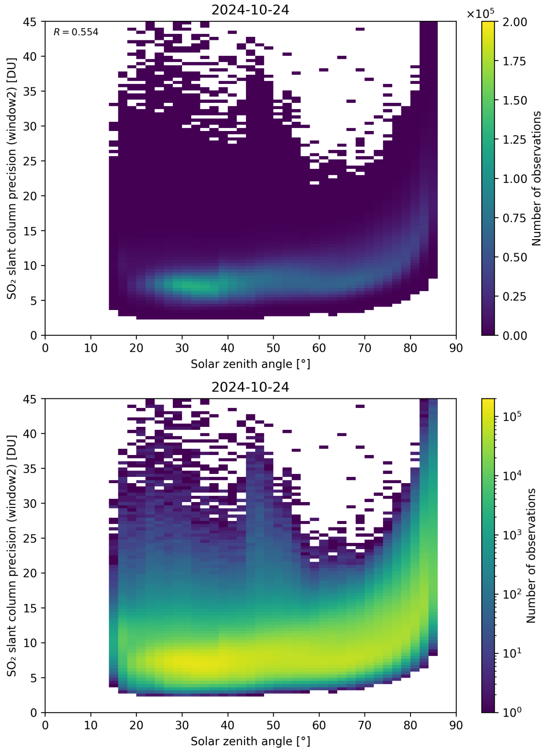
Figure 171: Scatter density plot of “Solar zenith angle” against “SO 2 slant column precision (window2)” for 2024-10-24 to 2024-10-25.
