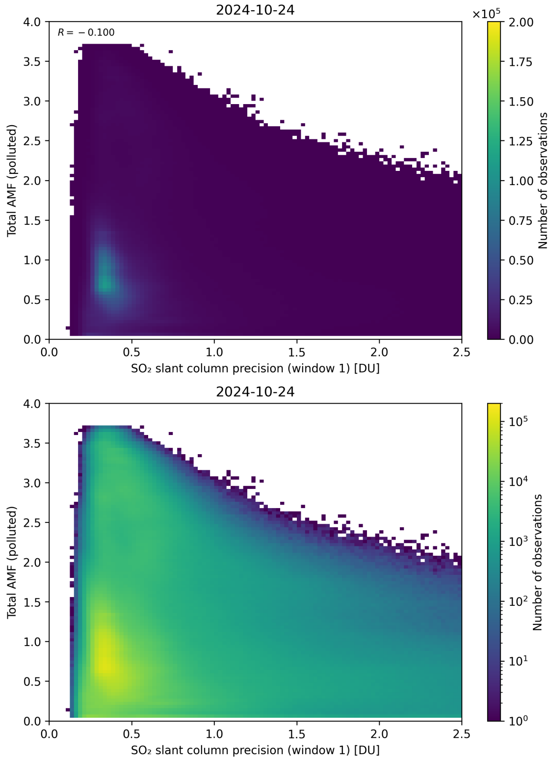
Figure 230: Scatter density plot of “SO 2 slant column precision (window 1)” against “Total AMF (polluted)” for 2024-10-24 to 2024-10-25.
