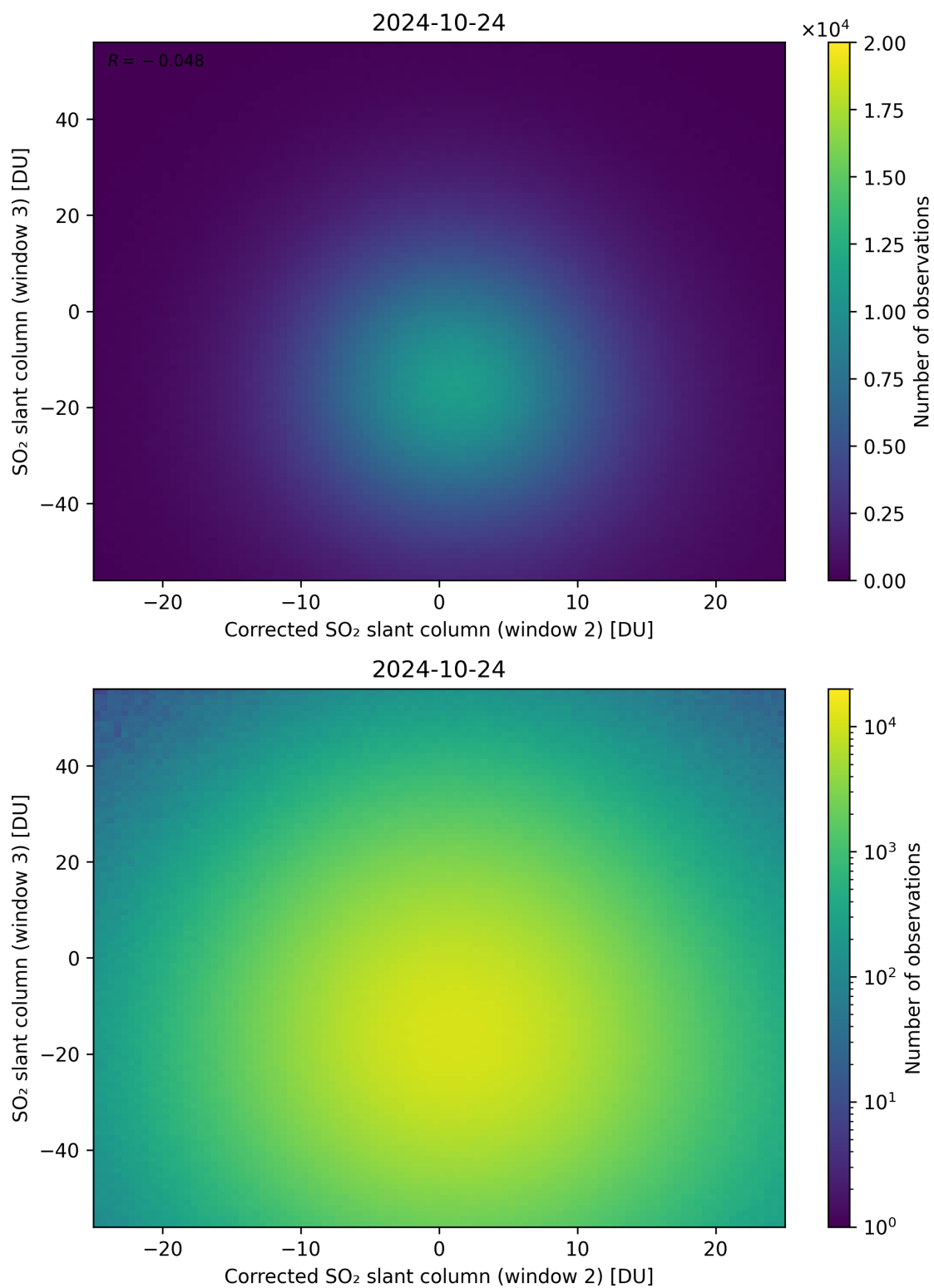
Figure 201: Scatter density plot of “Corrected SO 2 slant column (window 2)” against “SO 2 slant column (window 3)” for 2024-10-24 to 2024-10-25.
