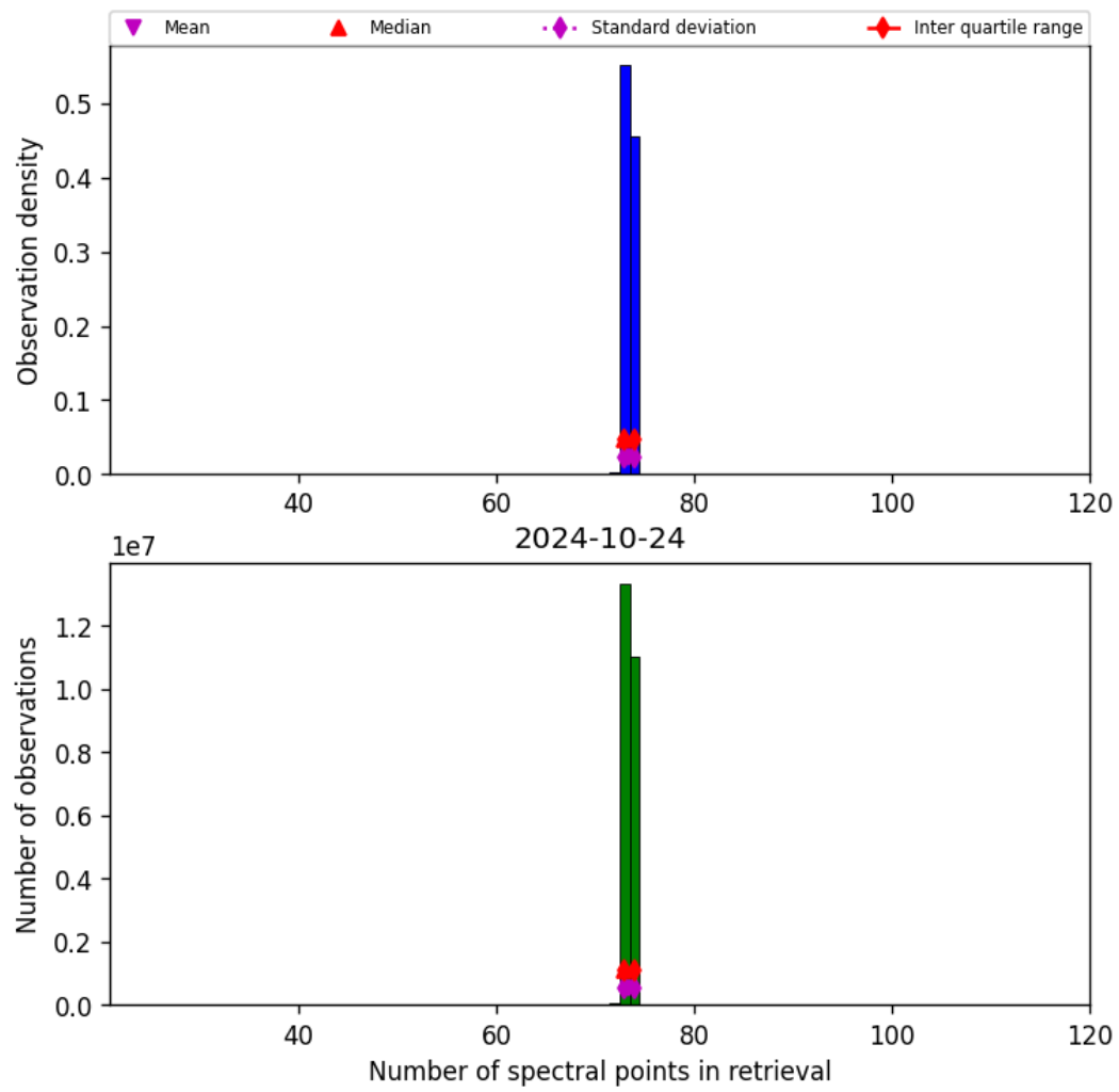
Figure 74: Histogram of “Number of spectral points in retrieval” for 2024-10-24 to 2024-10-25
