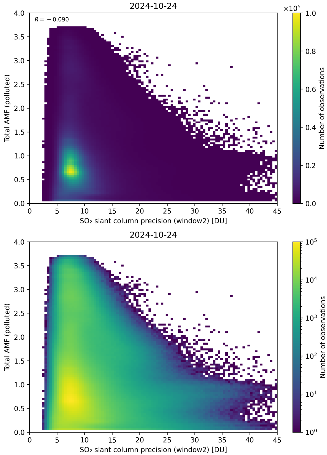
Figure 251: Scatter density plot of “SO 2 slant column precision (window2)” against “Total AMF (polluted)” for 2024-10-24 to 2024-10-25.
