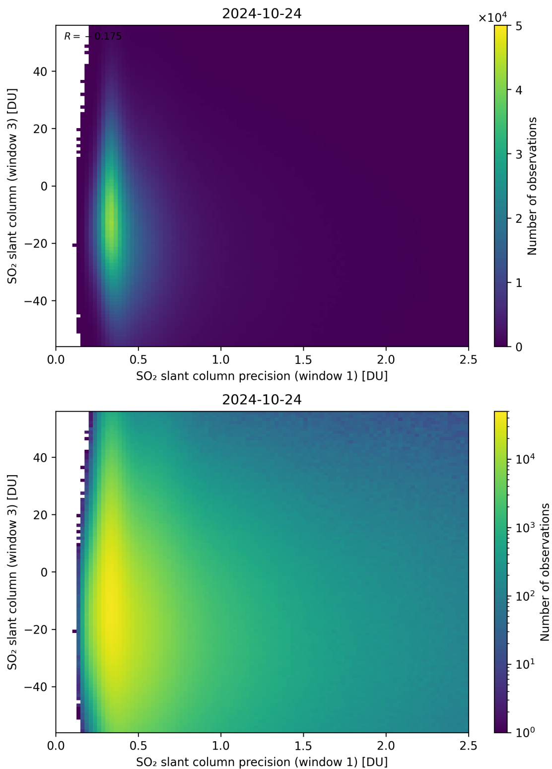
Figure 228: Scatter density plot of “SO 2 slant column precision (window 1)” against “SO 2 slant column (window 3)” for 2024-10-24 to 2024-10-25.
