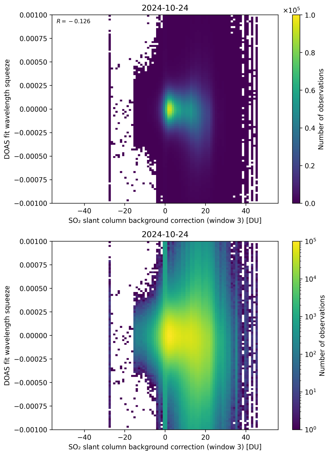
Figure 122: Scatter density plot of “SO 2 slant column background correction (window 3)” against “DOAS fit wavelength squeeze” for 2024-10-24 to 2024-10-25.
