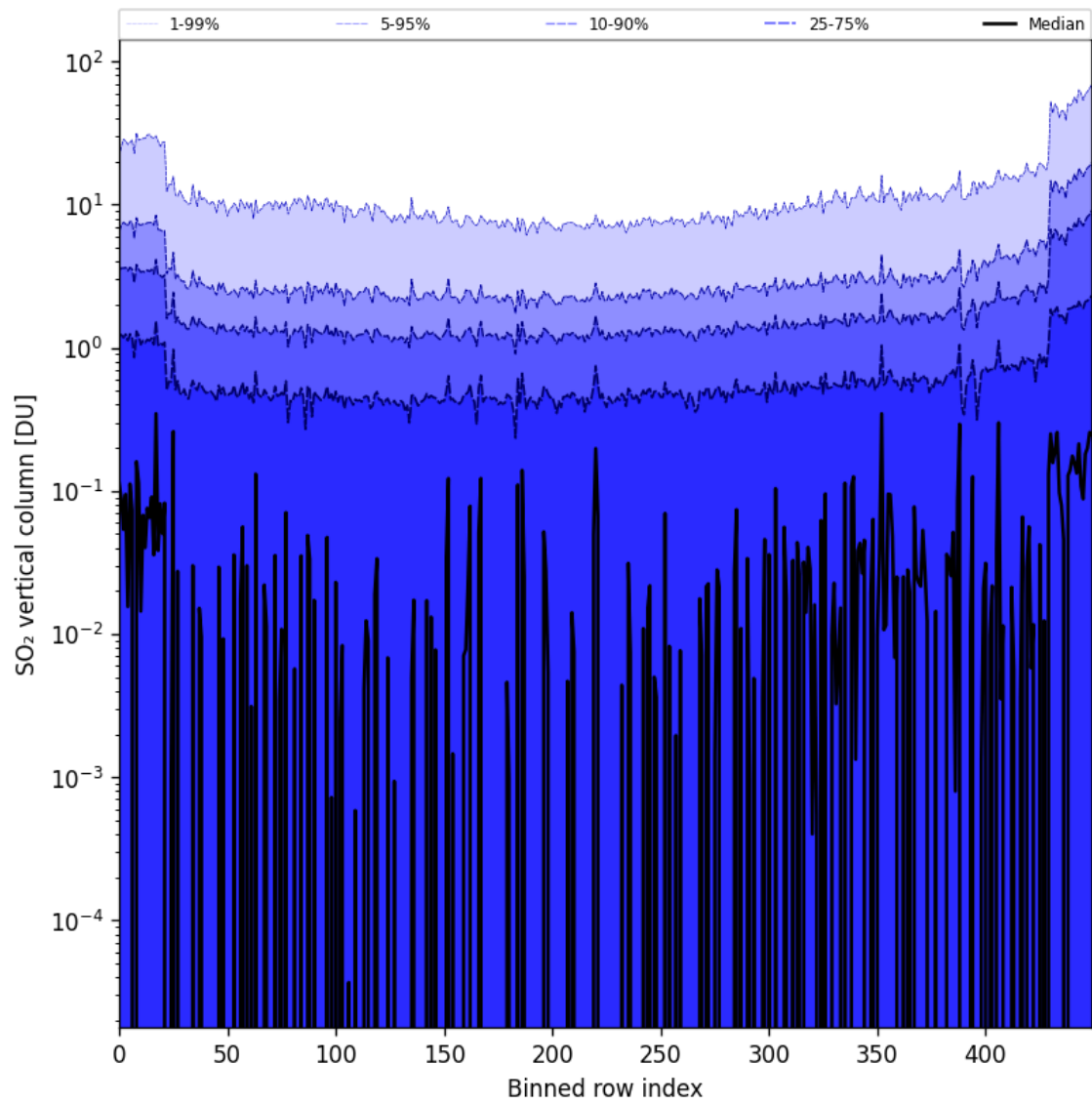
Figure 76: Along track statistics of “SO 2 vertical column” for 2024-10-24 to 2024-10-25
