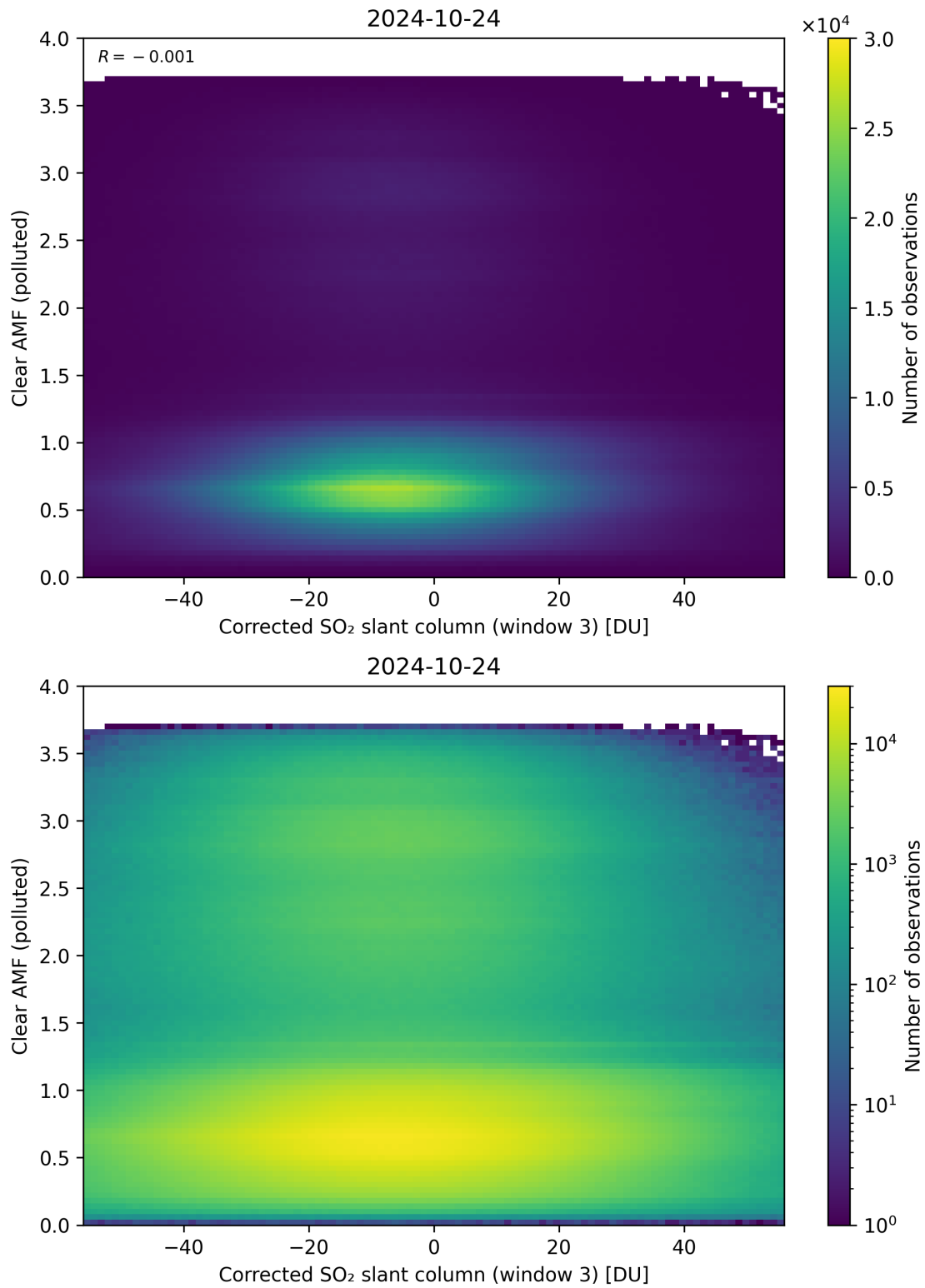
Figure 209: Scatter density plot of “Corrected SO 2 slant column (window 3)” against “Clear AMF (polluted)” for 2024-10-24 to 2024-10-25.
