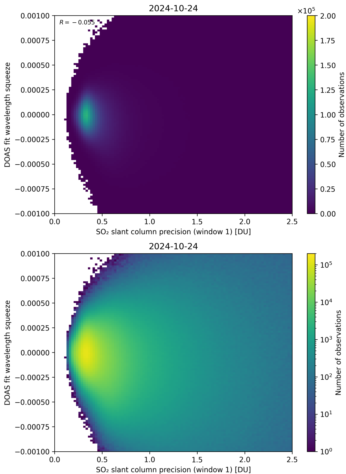
Figure 222: Scatter density plot of “SO 2 slant column precision (window 1)” against “DOAS fit wavelength squeeze” for 2024-10-24 to 2024-10-25.
