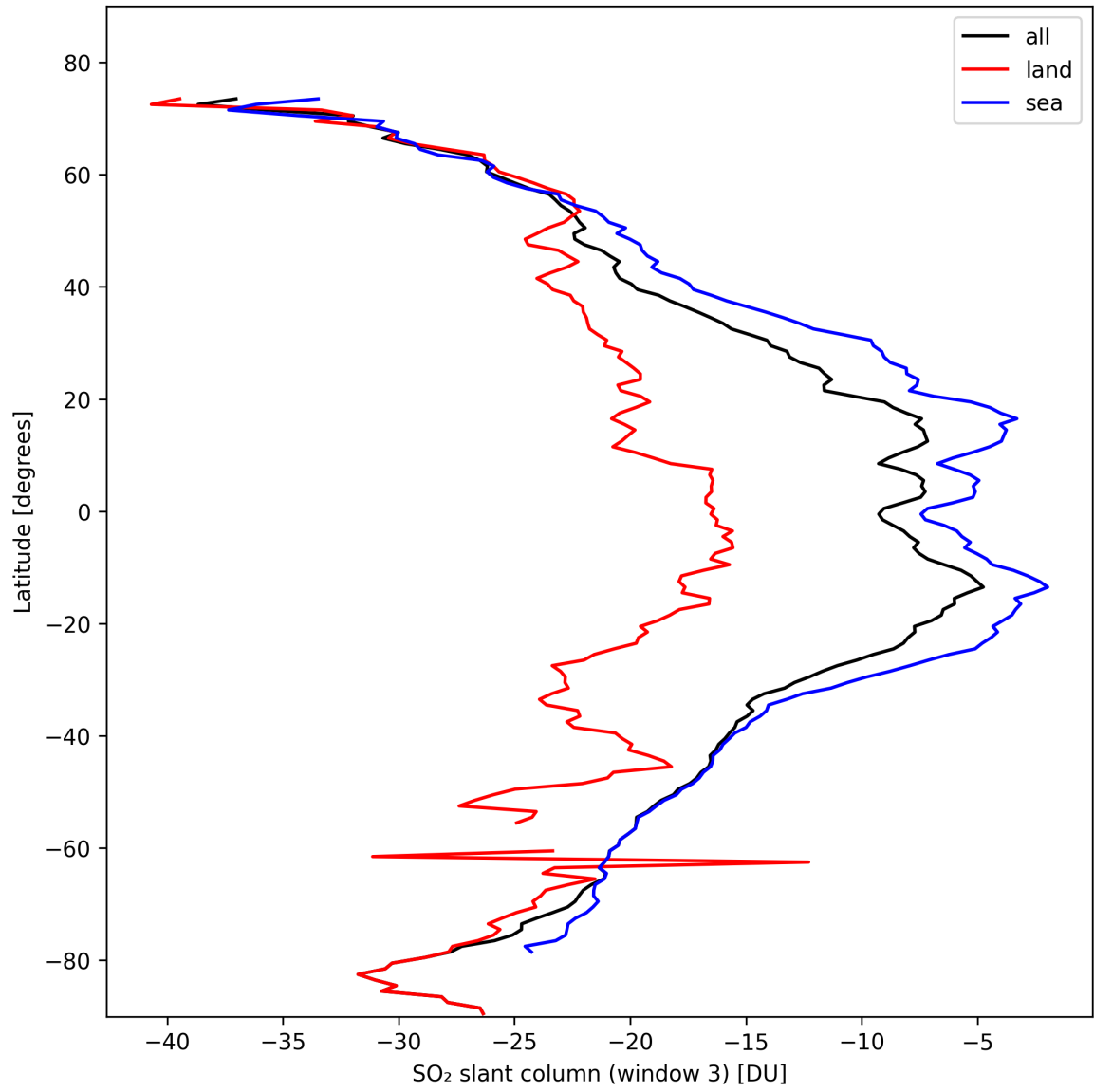
Figure 41: Zonal average of “SO 2 slant column (window 3)” for 2024-10-24 to 2024-10-25.
