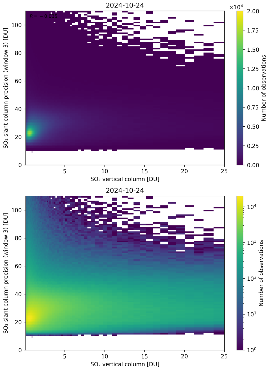
Figure 304: Scatter density plot of “SO 2 vertical column” against “SO 2 slant column precision (window 3)” for 2024-10-24 to 2024-10-25.
