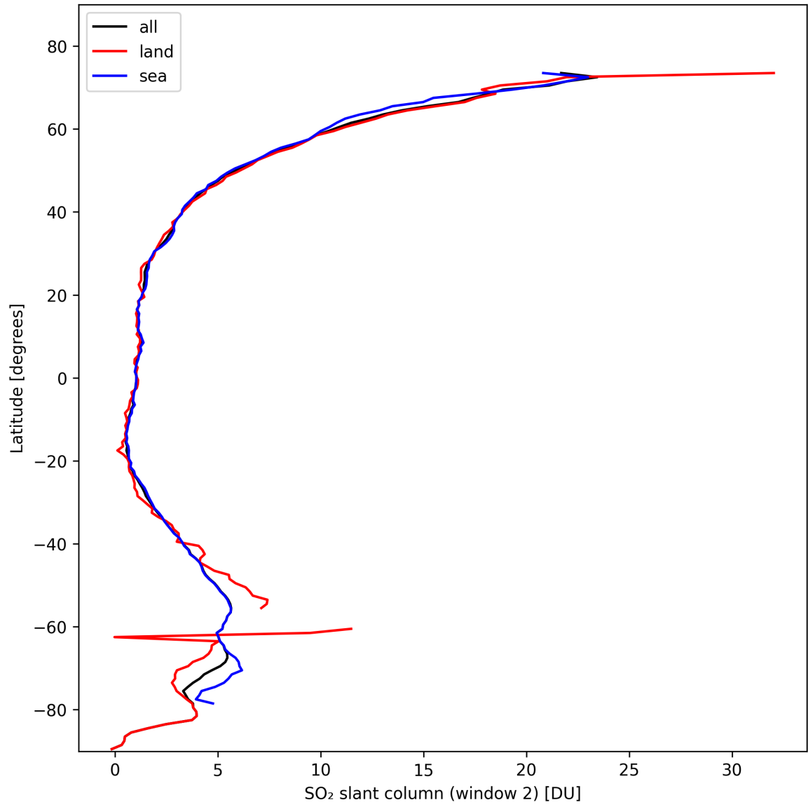
Figure 37: Zonal average of “SO 2 slant column (window 2)” for 2024-10-24 to 2024-10-25.
