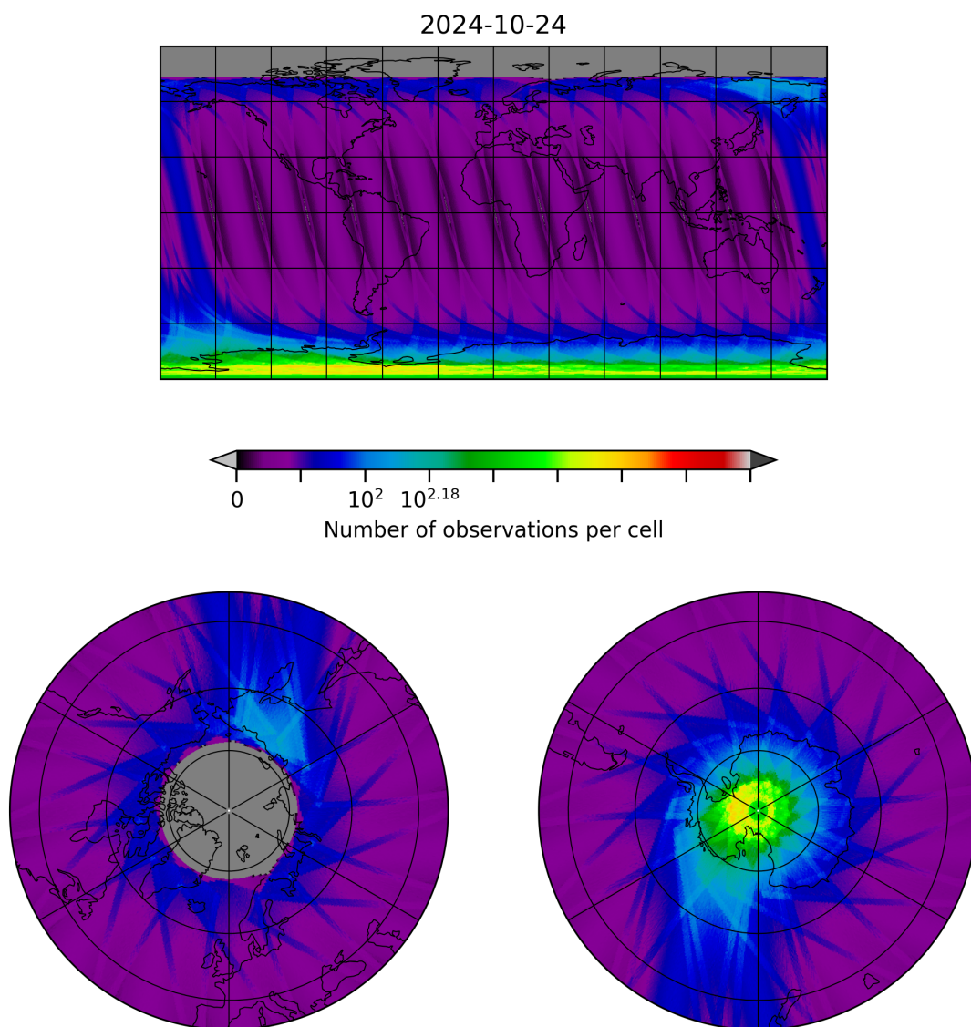
Figure 28: Map of the number of observations for 2024-10-24 to 2024-10-25
