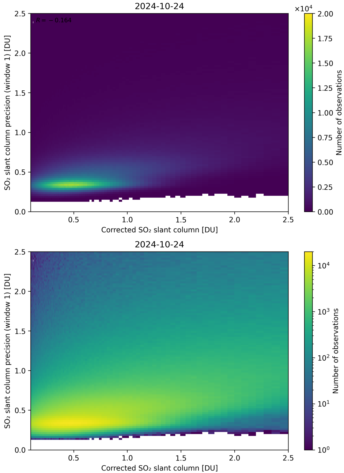
Figure 188: Scatter density plot of “Corrected SO 2 slant column” against “SO 2 slant column precision (window 1)” for 2024-10-24 to 2024-10-25.
