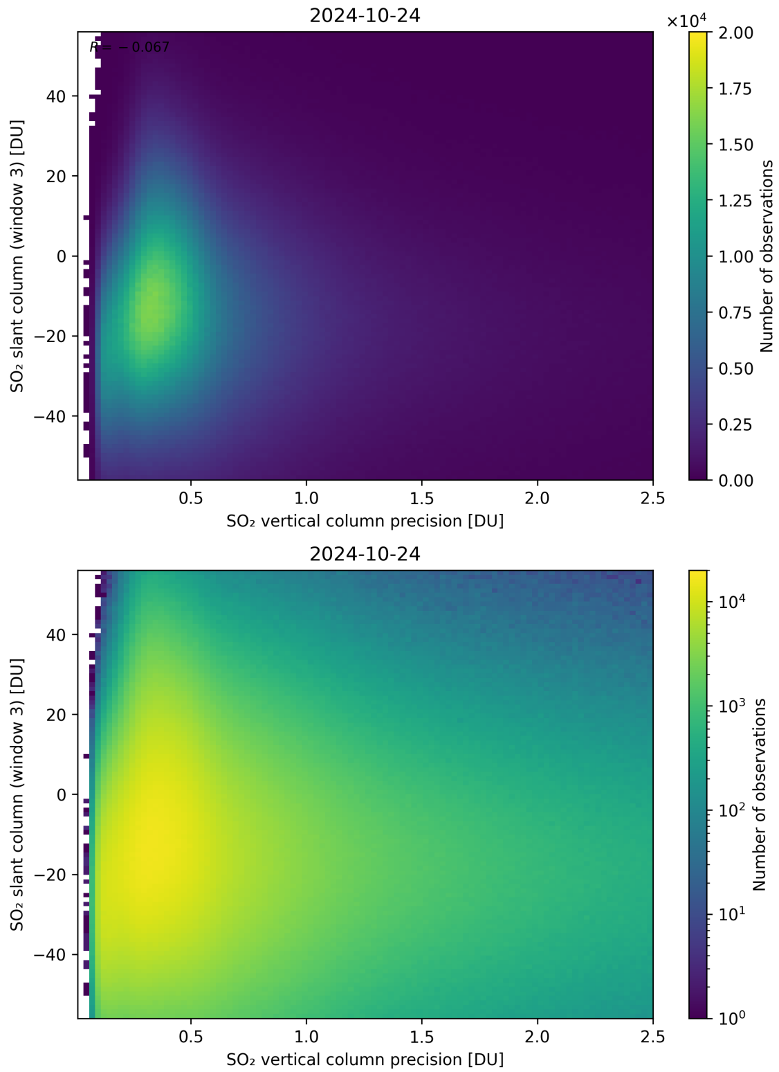
Figure 292: Scatter density plot of “SO 2 vertical column precision” against “SO 2 slant column (window 3)” for 2024-10-24 to 2024-10-25.
