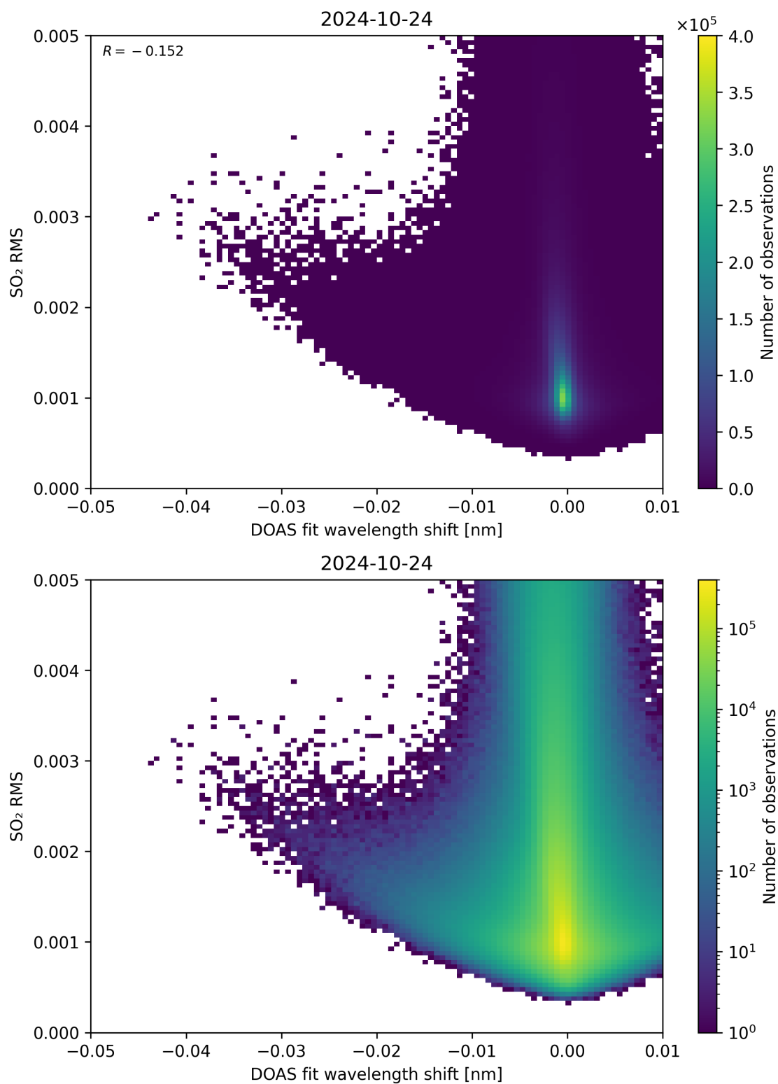
Figure 128: Scatter density plot of “DOAS fit wavelength shift” against “SO 2 RMS” for 2024-10-24 to 2024-10-25.
