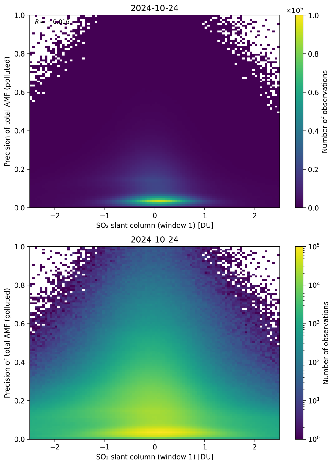
Figure 240: Scatter density plot of “SO 2 slant column (window 1)” against “Precision of total AMF (polluted)” for 2024-10-24 to 2024-10-25.
