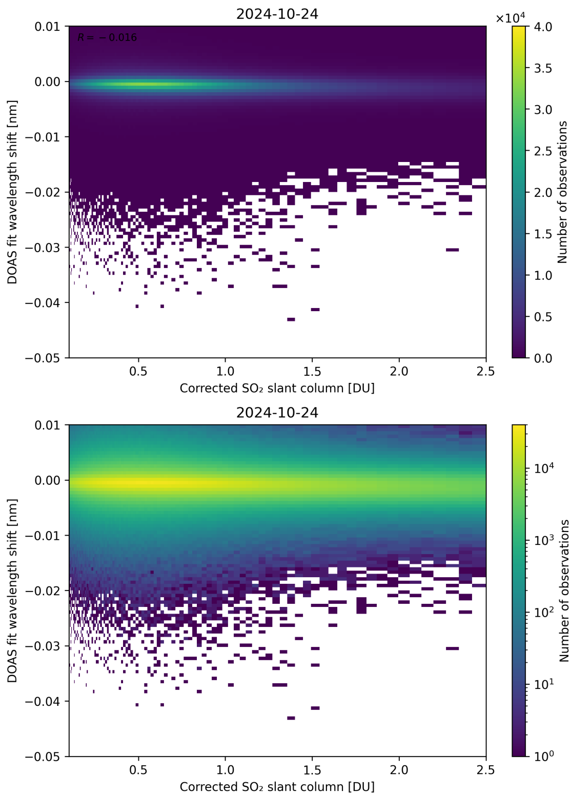
Figure 181: Scatter density plot of “Corrected SO 2 slant column” against “DOAS fit wavelength shift” for 2024-10-24 to 2024-10-25.
