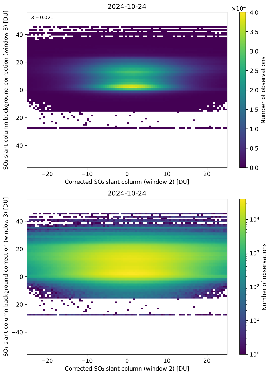
Figure 195: Scatter density plot of “Corrected SO 2 slant column (window 2)” against “SO 2 slant column background correction (window 3)” for 2024-10-24 to 2024-10-25.
