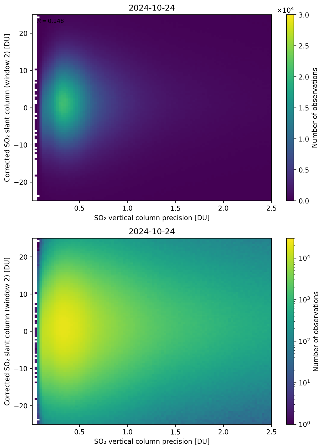
Figure 287: Scatter density plot of “SO 2 vertical column precision” against “Corrected SO 2 slant column (window 2)” for 2024-10-24 to 2024-10-25.
