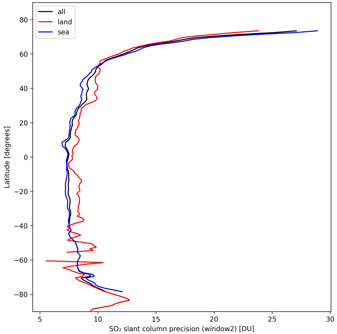
Figure 38: Zonal average of “SO 2 slant column precision (window2)” for 2024-10-24 to 2024-10-25.
