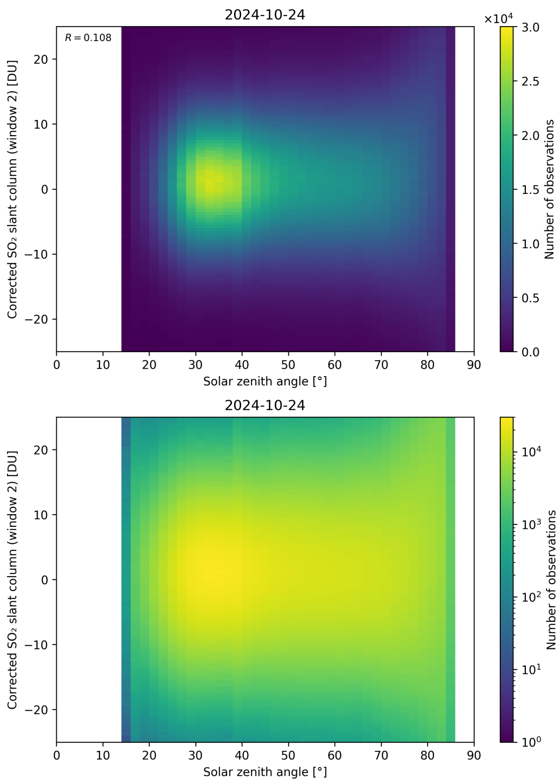
Figure 167: Scatter density plot of “Solar zenith angle” against “Corrected SO 2 slant column (window 2)” for 2024-10-24 to 2024-10-25.
