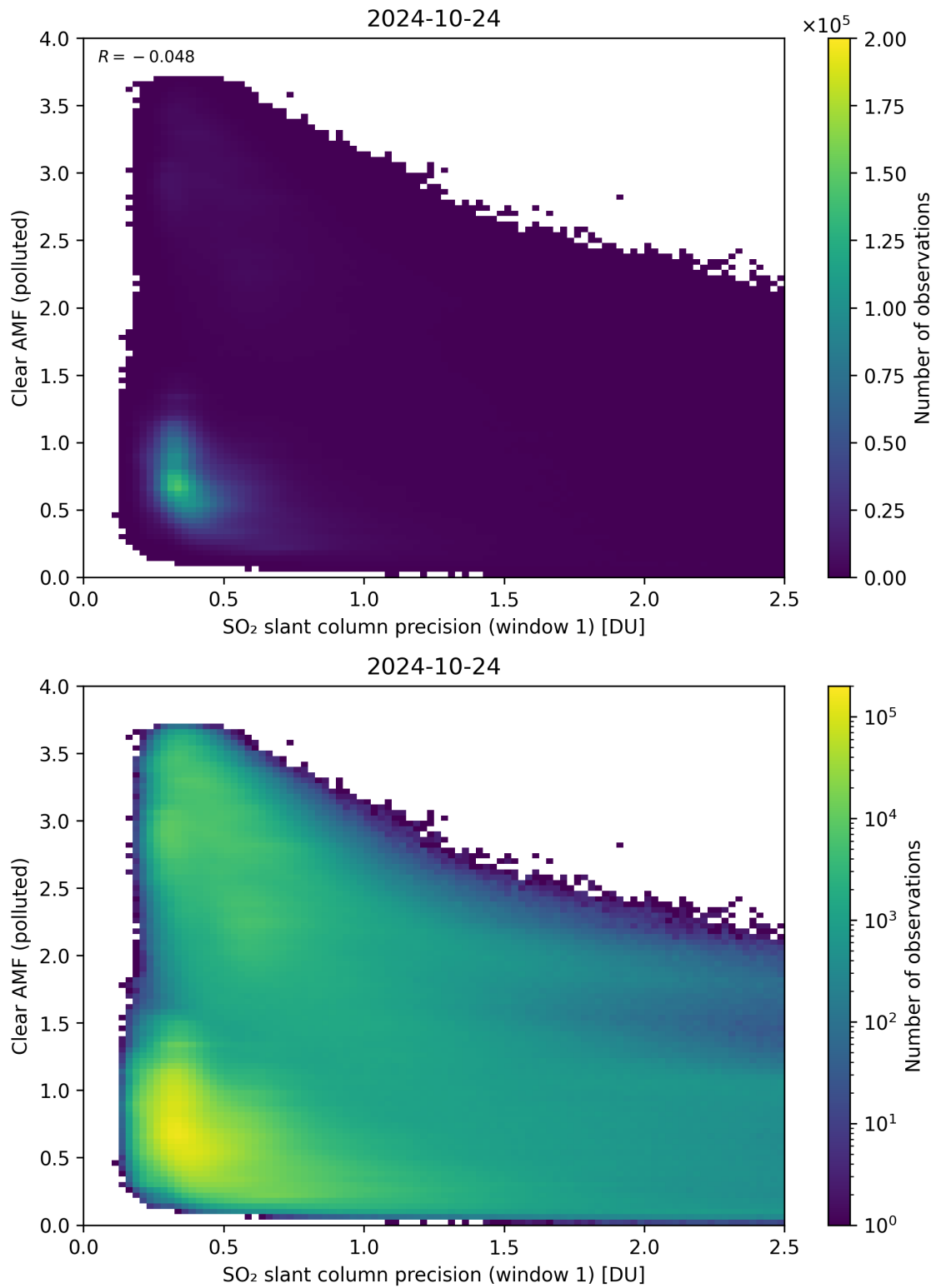
Figure 224: Scatter density plot of “SO 2 slant column precision (window 1)” against “Clear AMF (polluted)” for 2024-10-24 to 2024-10-25.
