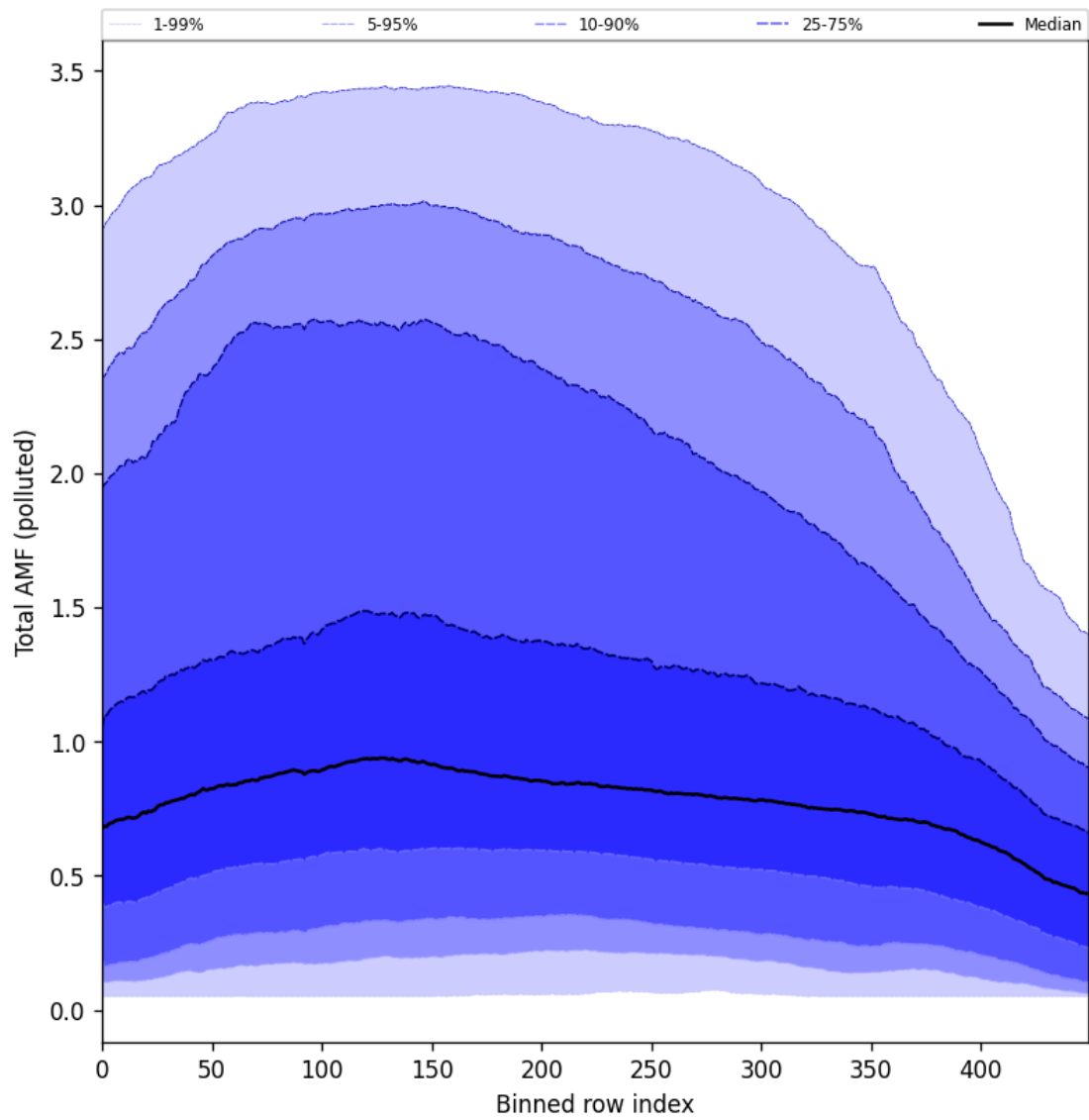
Figure 94: Along track statistics of “Total AMF (polluted)” for 2024-10-24 to 2024-10-25
