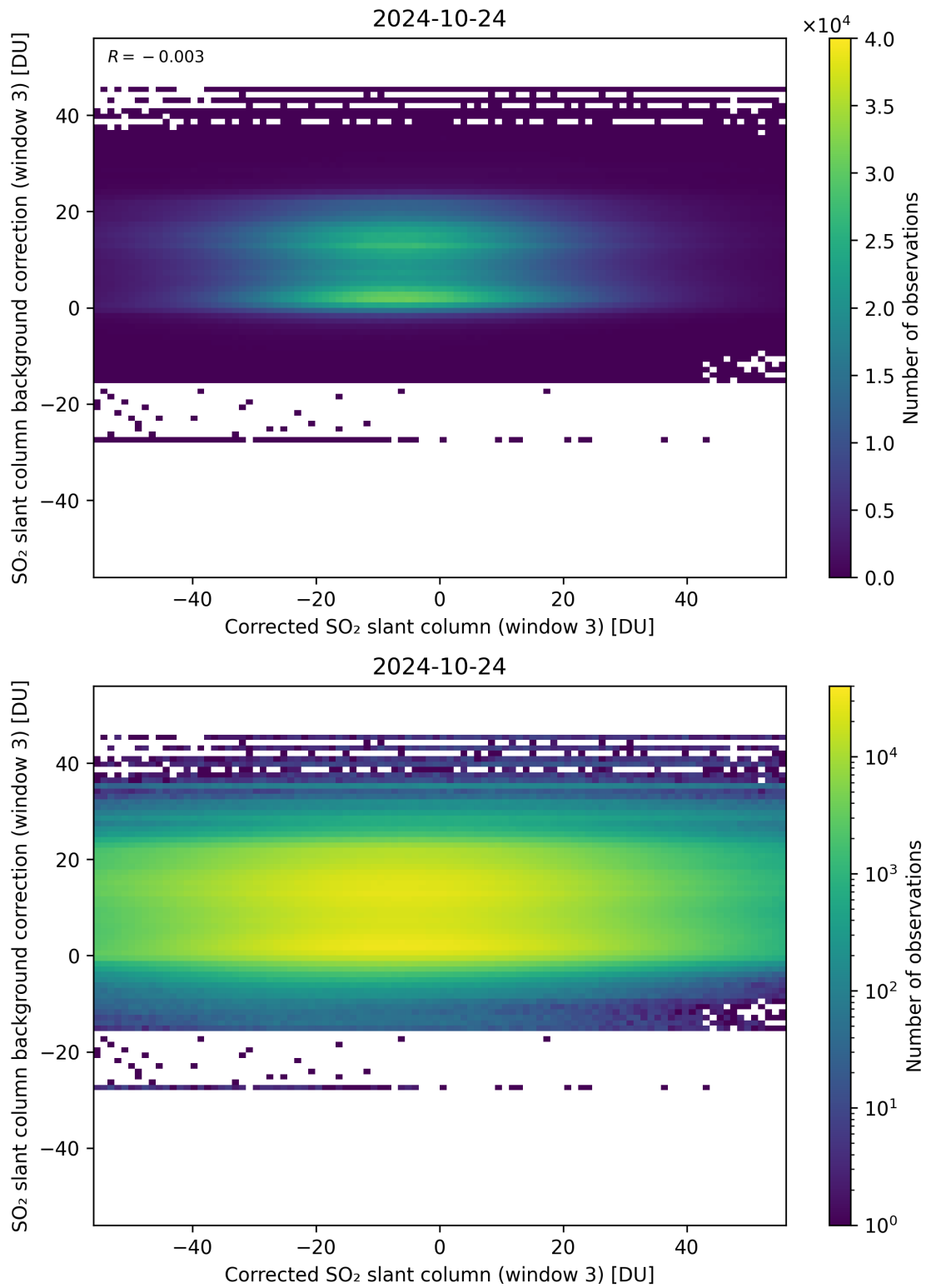
Figure 205: Scatter density plot of “Corrected SO 2 slant column (window 3)” against “SO 2 slant column background correction (window 3)” for 2024-10-24 to 2024-10-25.
