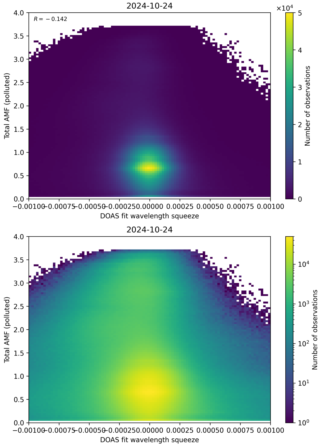
Figure 134: Scatter density plot of “DOAS fit wavelength squeeze” against “Total AMF (polluted)” for 2024-10-24 to 2024-10-25.
