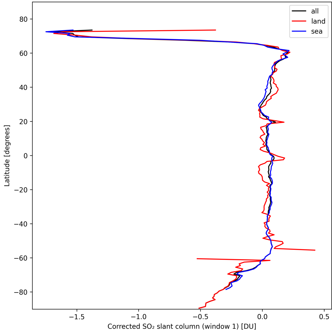
Figure 35: Zonal average of “Corrected SO 2 slant column (window 1)” for 2024-10-24 to 2024-10-25.
