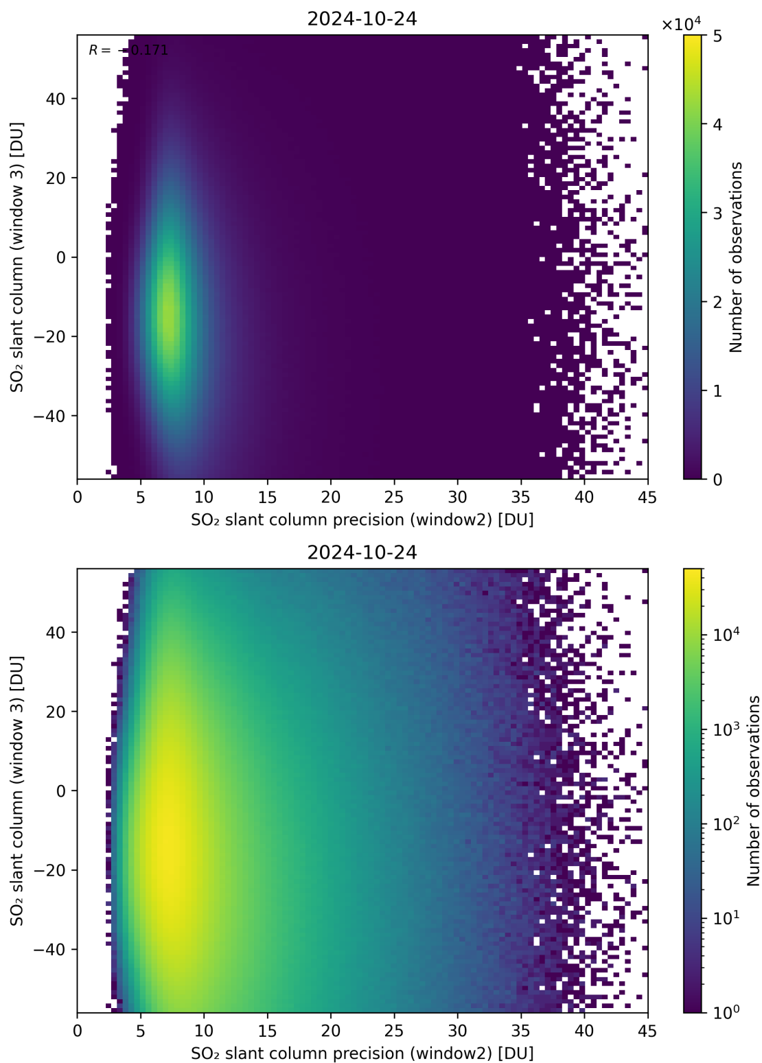
Figure 249: Scatter density plot of “SO 2 slant column precision (window2)” against “SO 2 slant column (window 3)” for 2024-10-24 to 2024-10-25.
