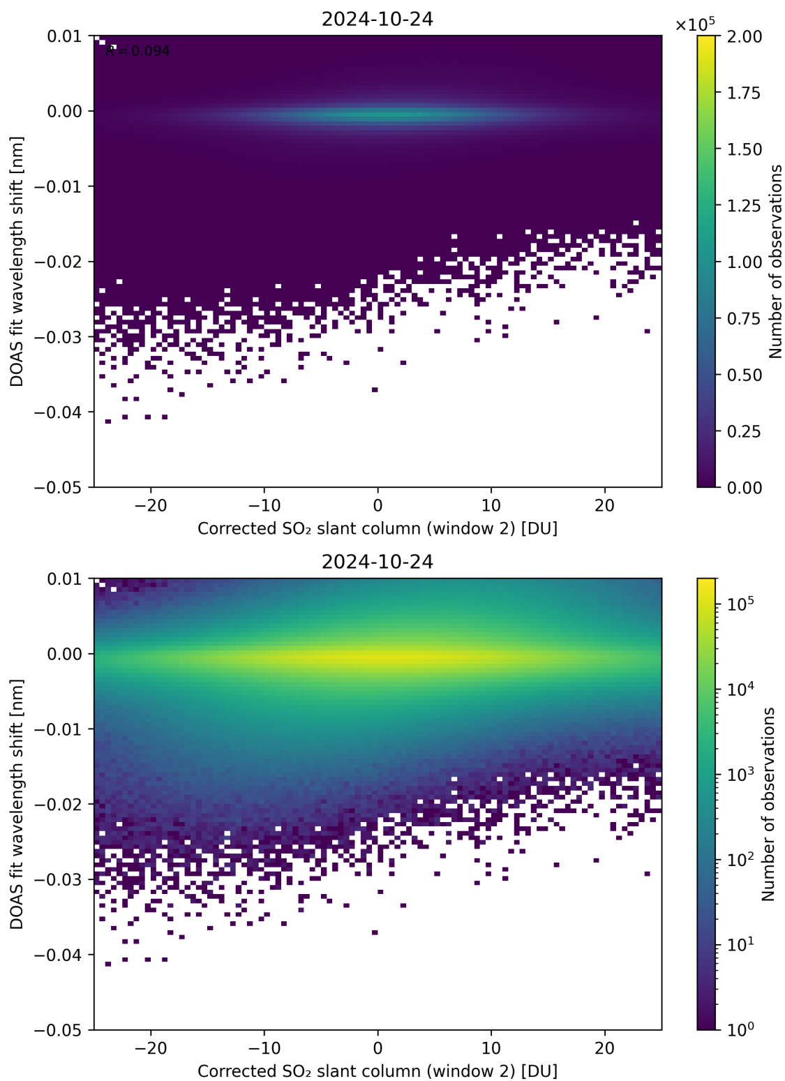
Figure 196: Scatter density plot of “Corrected SO 2 slant column (window 2)” against “DOAS fit wavelength shift” for 2024-10-24 to 2024-10-25.
