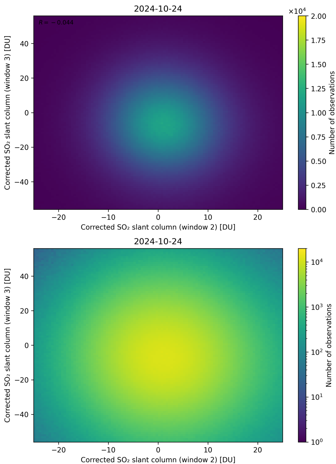
Figure 200: Scatter density plot of “Corrected SO 2 slant column (window 2)” against “Corrected SO 2 slant column (window 3)” for 2024-10-24 to 2024-10-25.
