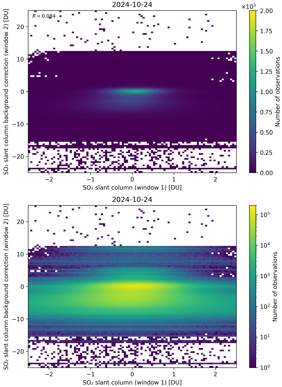
Figure 213: Scatter density plot of “SO 2 slant column (window 1)” against “SO 2 slant column background correction (window 2)” for 2024-10-24 to 2024-10-25.
