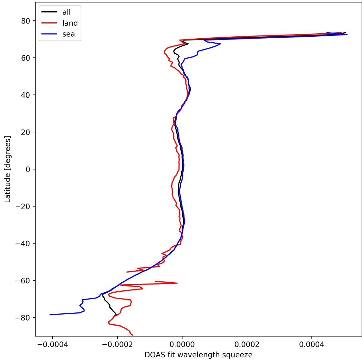
Figure 46: Zonal average of “DOAS fit wavelength squeeze” for 2024-10-24 to 2024-10-25.
