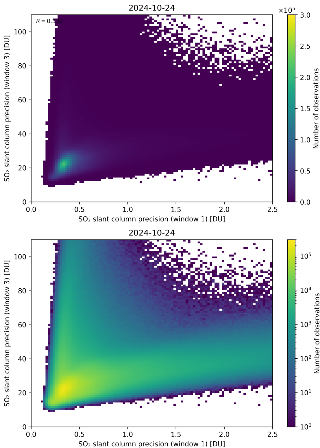
Figure 229: Scatter density plot of “SO 2 slant column precision (window 1)” against “SO 2 slant column precision (window 3)” for 2024-10-24 to 2024-10-25.
