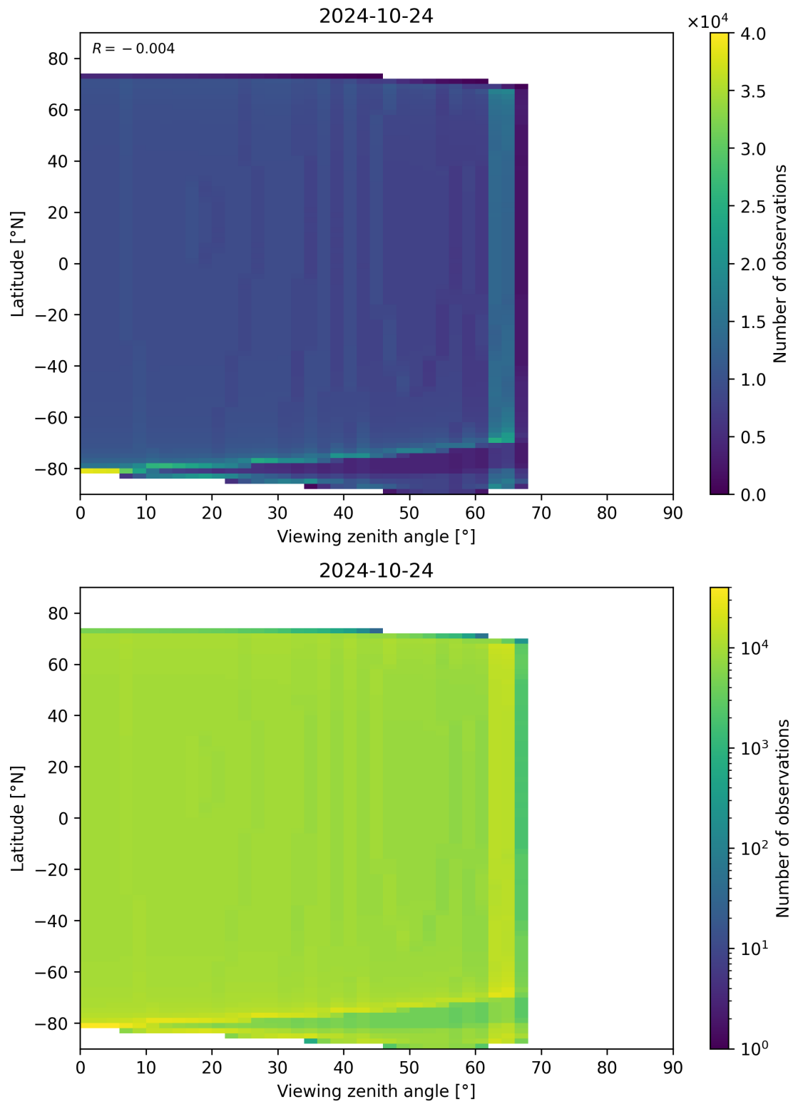
Figure 314: Scatter density plot of “Viewing zenith angle” against “Latitude” for 2024-10-24 to 2024-10-25.
