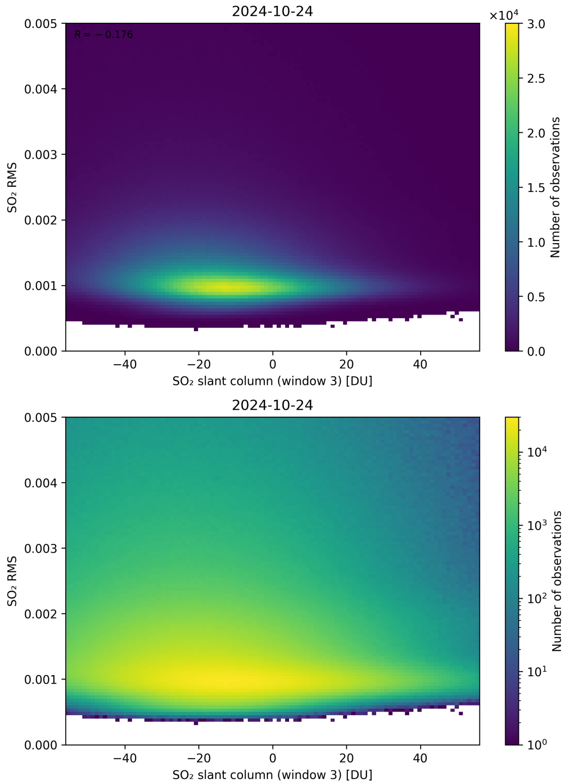
Figure 256: Scatter density plot of “SO 2 slant column (window 3)” against “SO 2 RMS” for 2024-10-24 to 2024-10-25.
