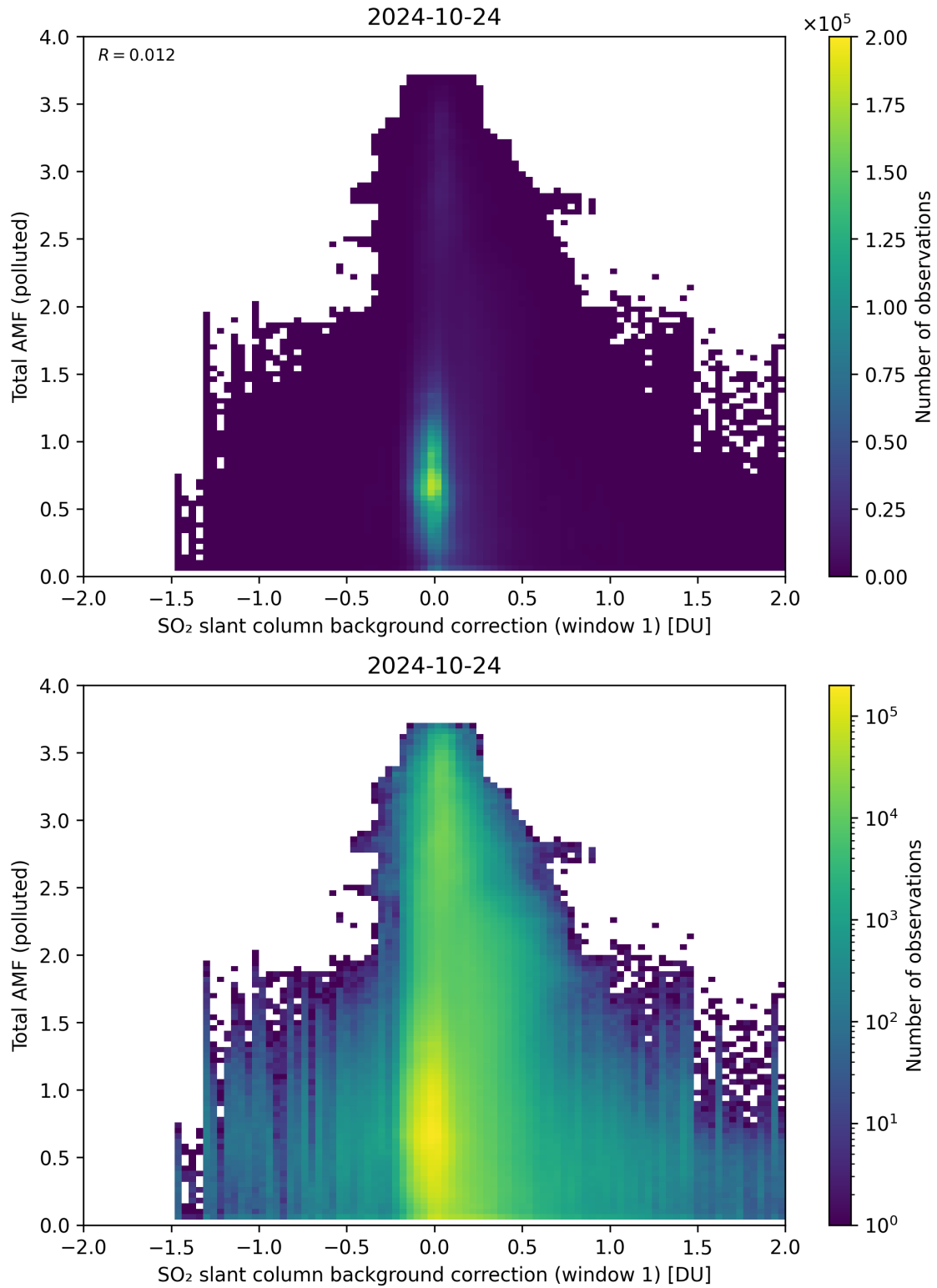
Figure 109: Scatter density plot of “SO 2 slant column background correction (window 1)” against “Total AMF (polluted)” for 2024-10-24 to 2024-10-25.
