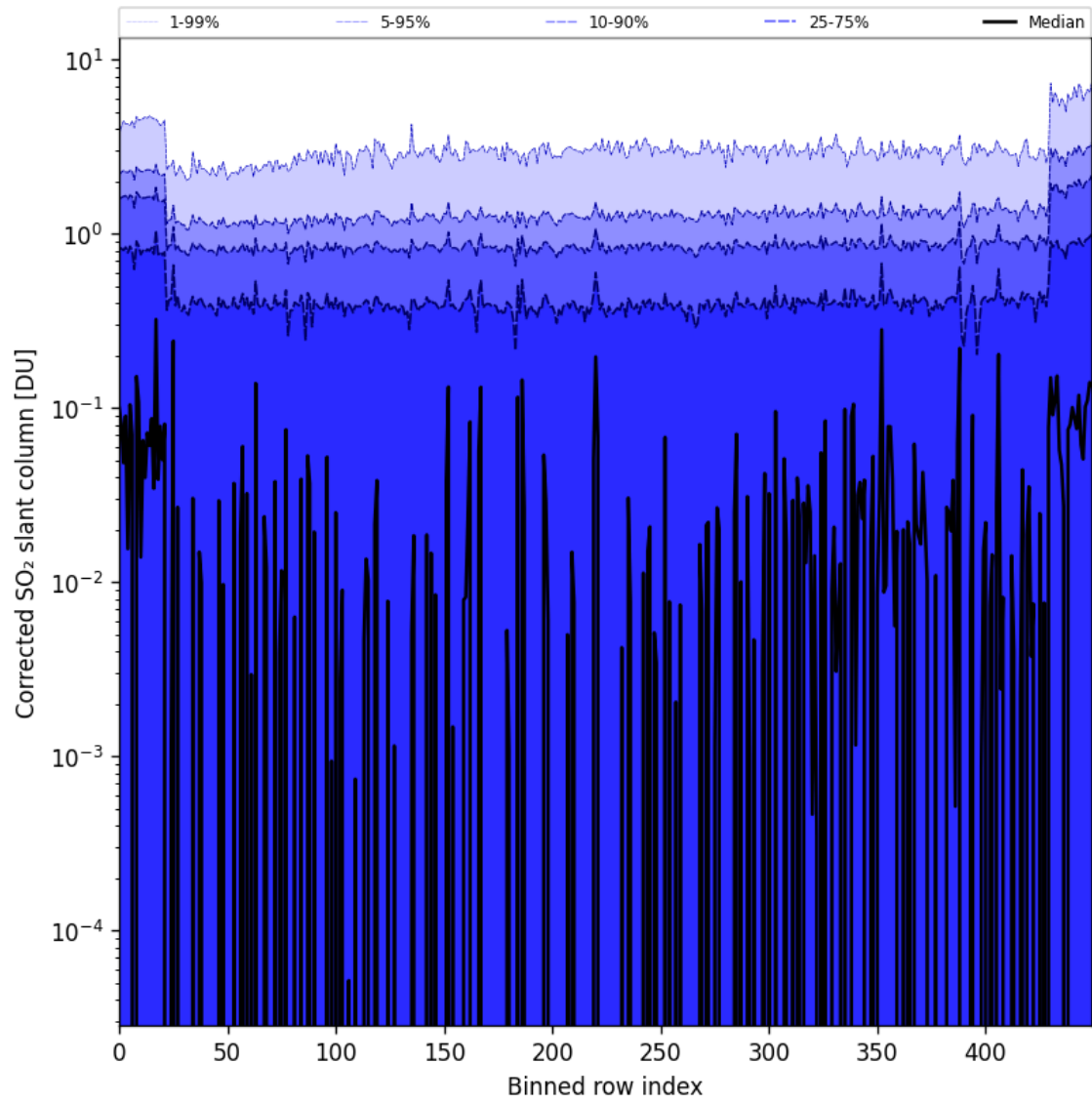
Figure 78: Along track statistics of “Corrected SO 2 slant column” for 2024-10-24 to 2024-10-25
