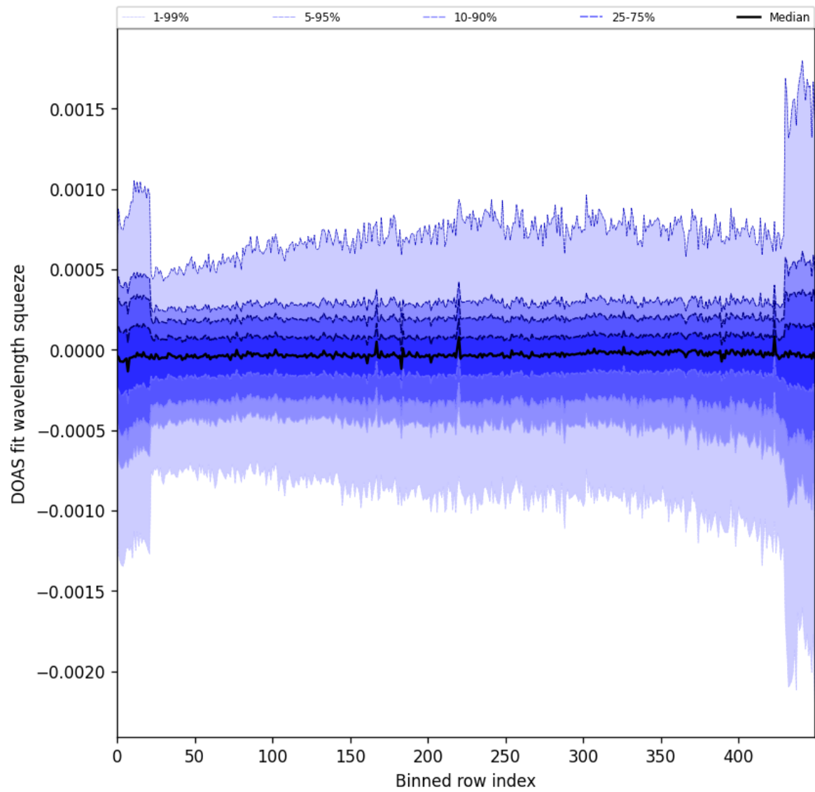
Figure 92: Along track statistics of “DOAS fit wavelength squeeze” for 2024-10-24 to 2024-10-25
