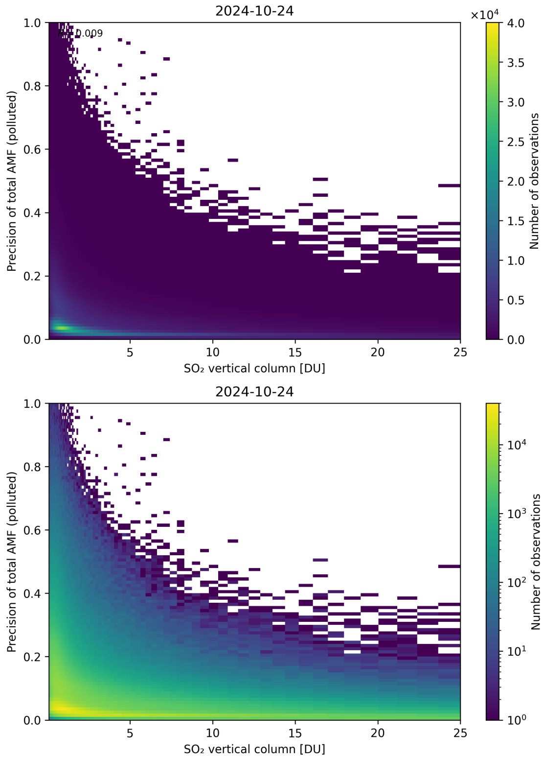
Figure 306: Scatter density plot of “SO 2 vertical column” against “Precision of total AMF (polluted)” for 2024-10-24 to 2024-10-25.
