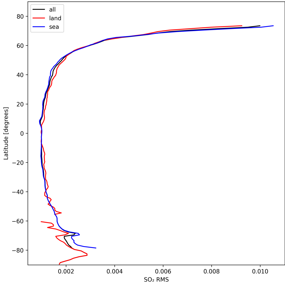
Figure 47: Zonal average of “SO 2 RMS” for 2024-10-24 to 2024-10-25.
