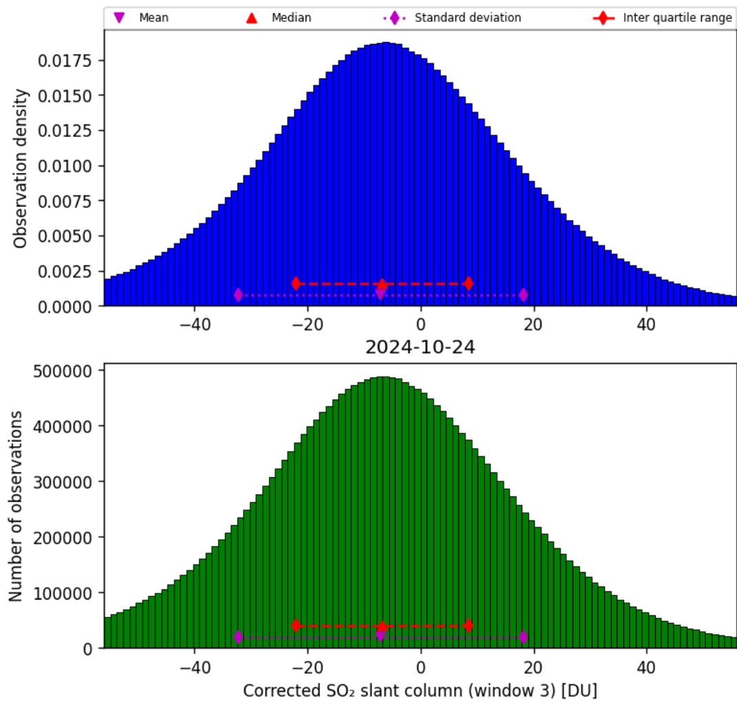
Figure 66: Histogram of “Corrected SO 2 slant column (window 3)” for 2024-10-24 to 2024-10-25
