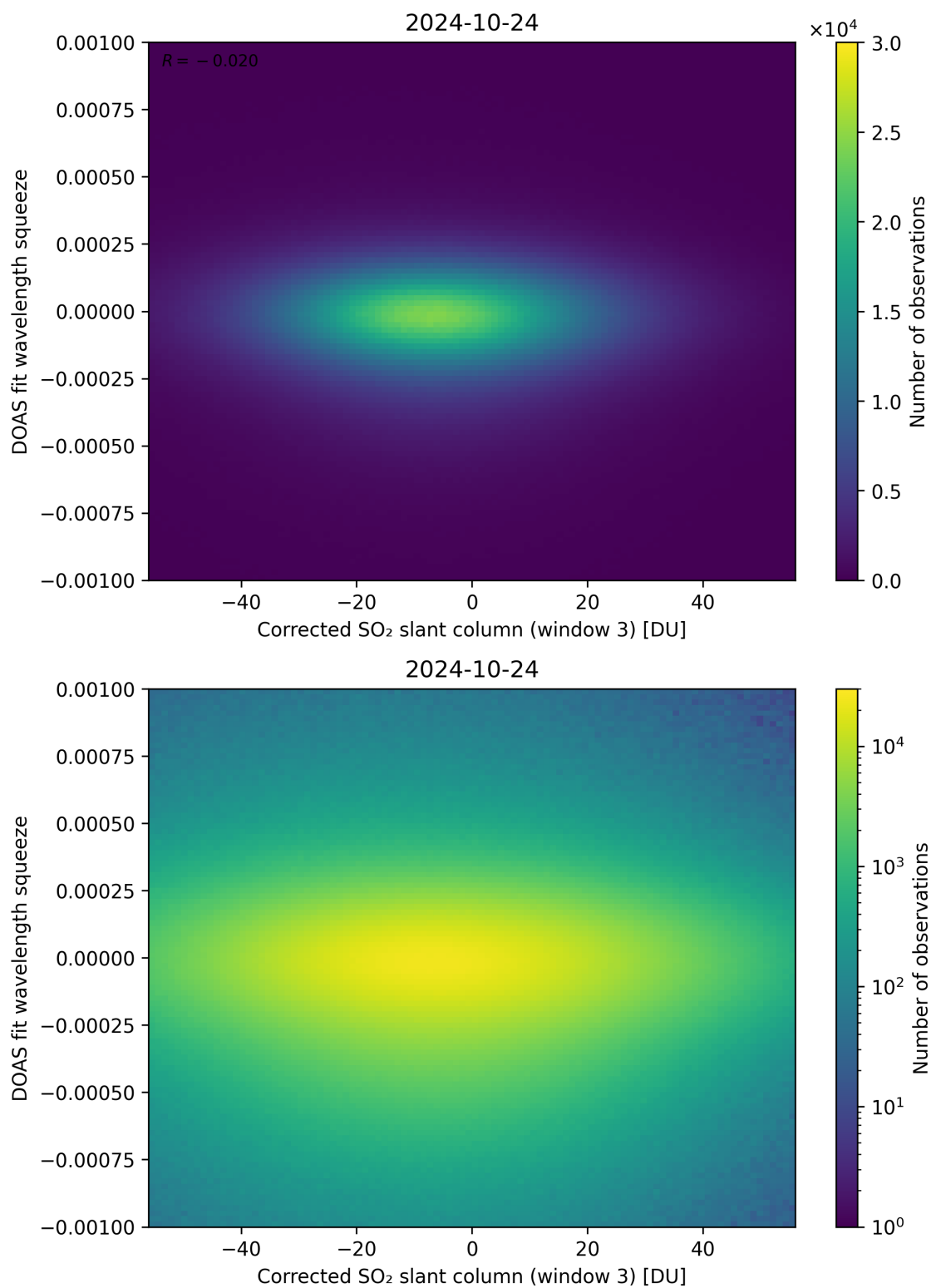
Figure 207: Scatter density plot of “Corrected SO 2 slant column (window 3)” against “DOAS fit wavelength squeeze” for 2024-10-24 to 2024-10-25.
