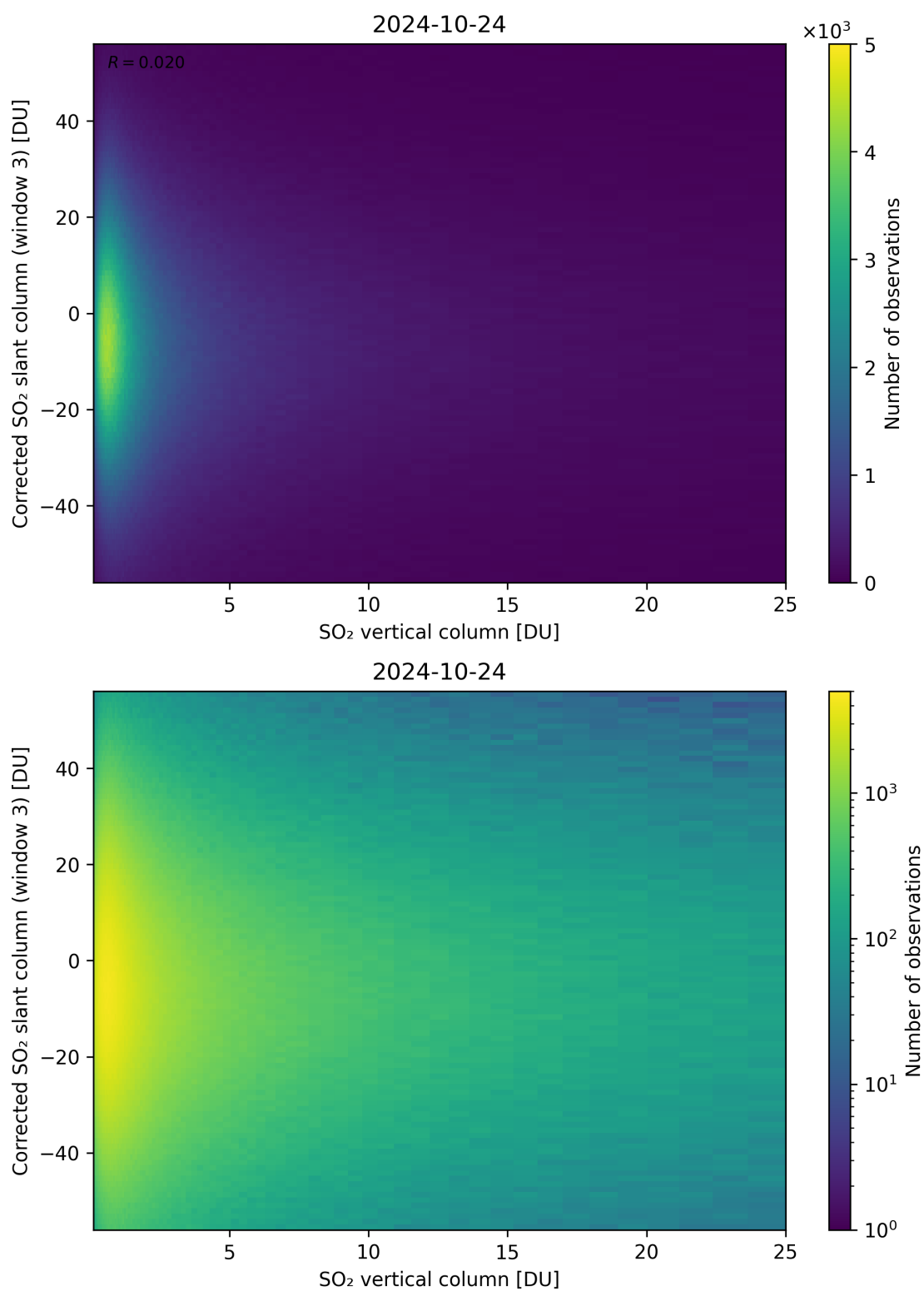
Figure 299: Scatter density plot of “SO 2 vertical column” against “Corrected SO 2 slant column (window 3)” for 2024-10-24 to 2024-10-25.
