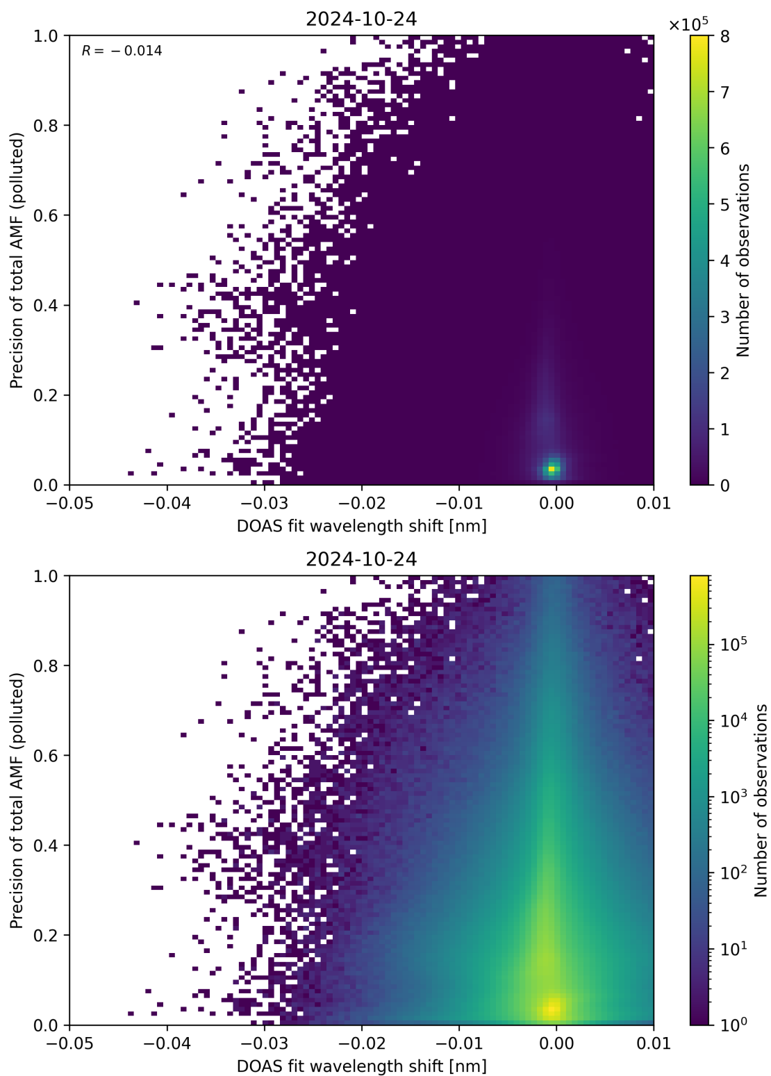
Figure 131: Scatter density plot of “DOAS fit wavelength shift” against “Precision of total AMF (polluted)” for 2024-10-24 to 2024-10-25.
