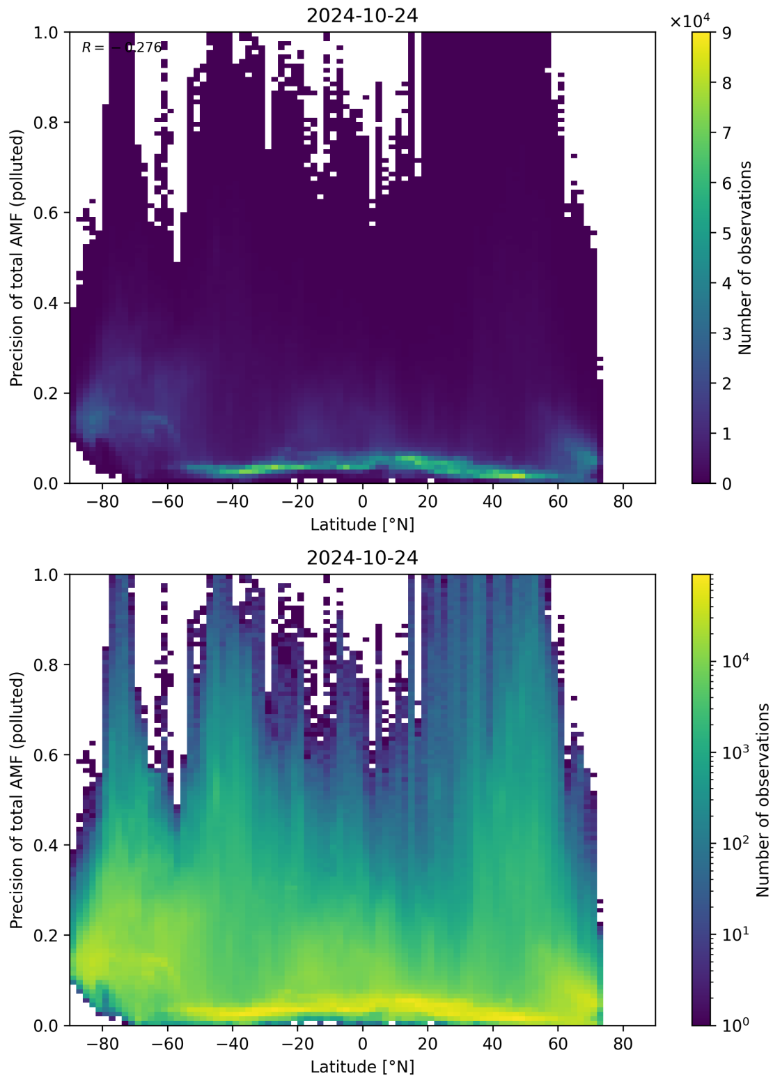
Figure 155: Scatter density plot of “Latitude” against “Precision of total AMF (polluted)” for 2024-10-24 to 2024-10-25.
