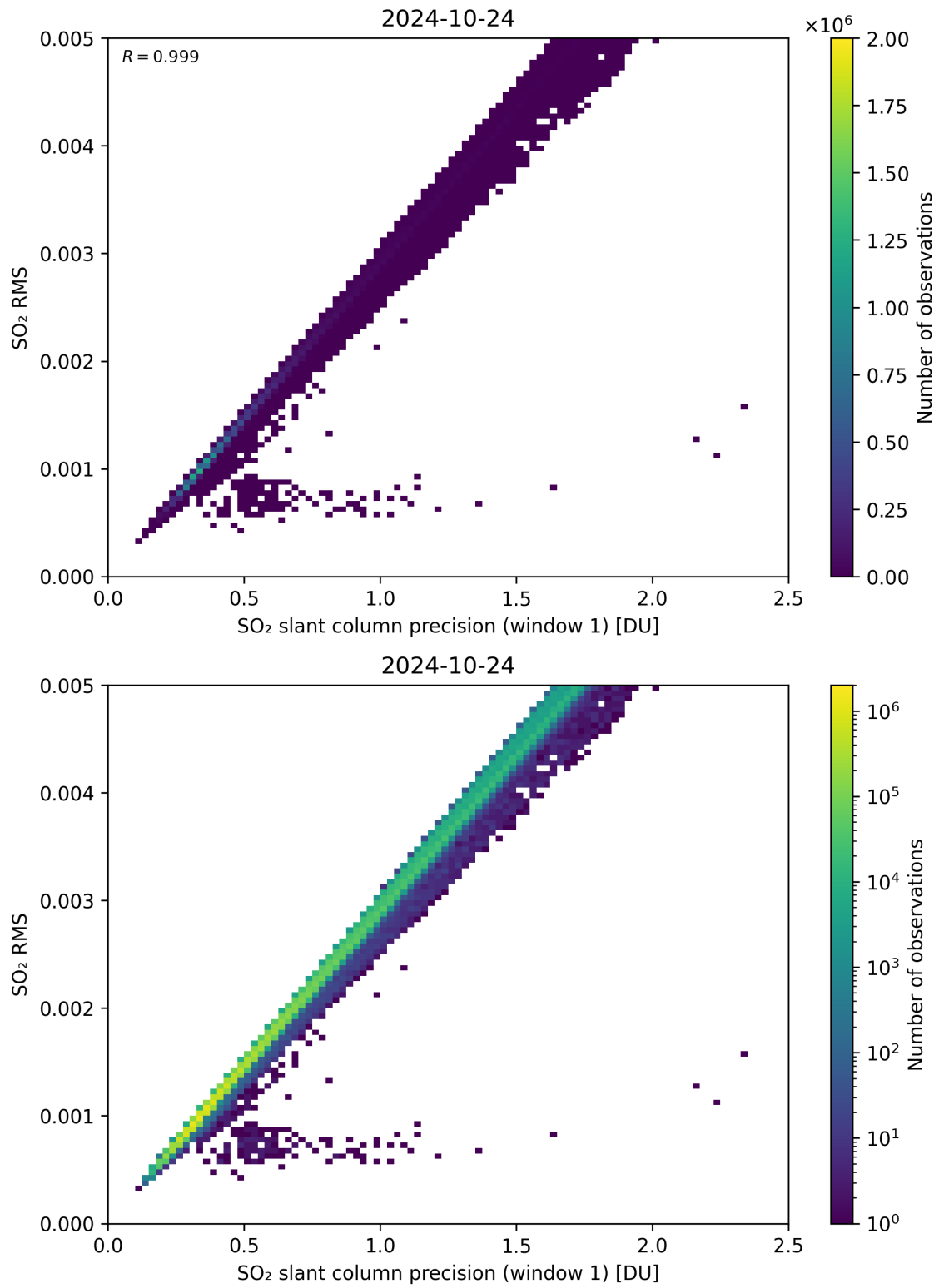
Figure 223: Scatter density plot of “SO 2 slant column precision (window 1)” against “SO 2 RMS” for 2024-10-24 to 2024-10-25.
