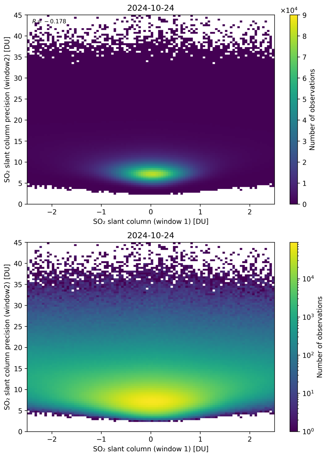
Figure 236: Scatter density plot of “SO 2 slant column (window 1)” against “SO 2 slant column precision (window2)” for 2024-10-24 to 2024-10-25.
