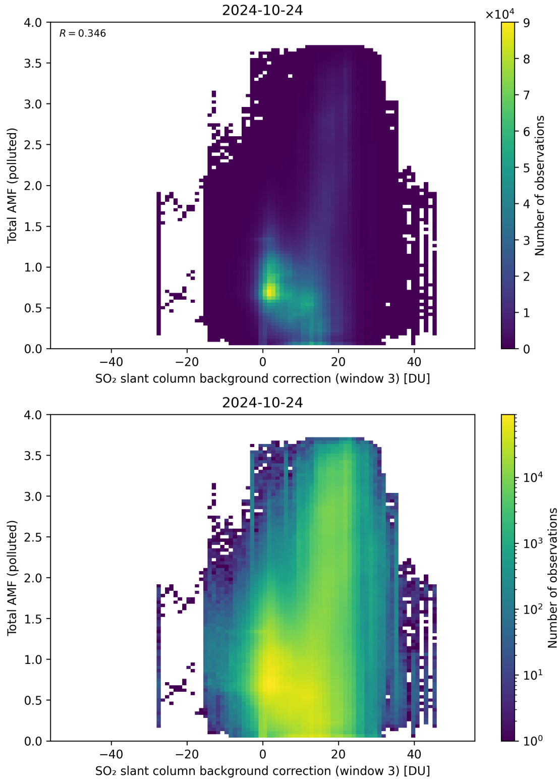
Figure 125: Scatter density plot of “SO 2 slant column background correction (window 3)” against “Total AMF (polluted)” for 2024-10-24 to 2024-10-25.
