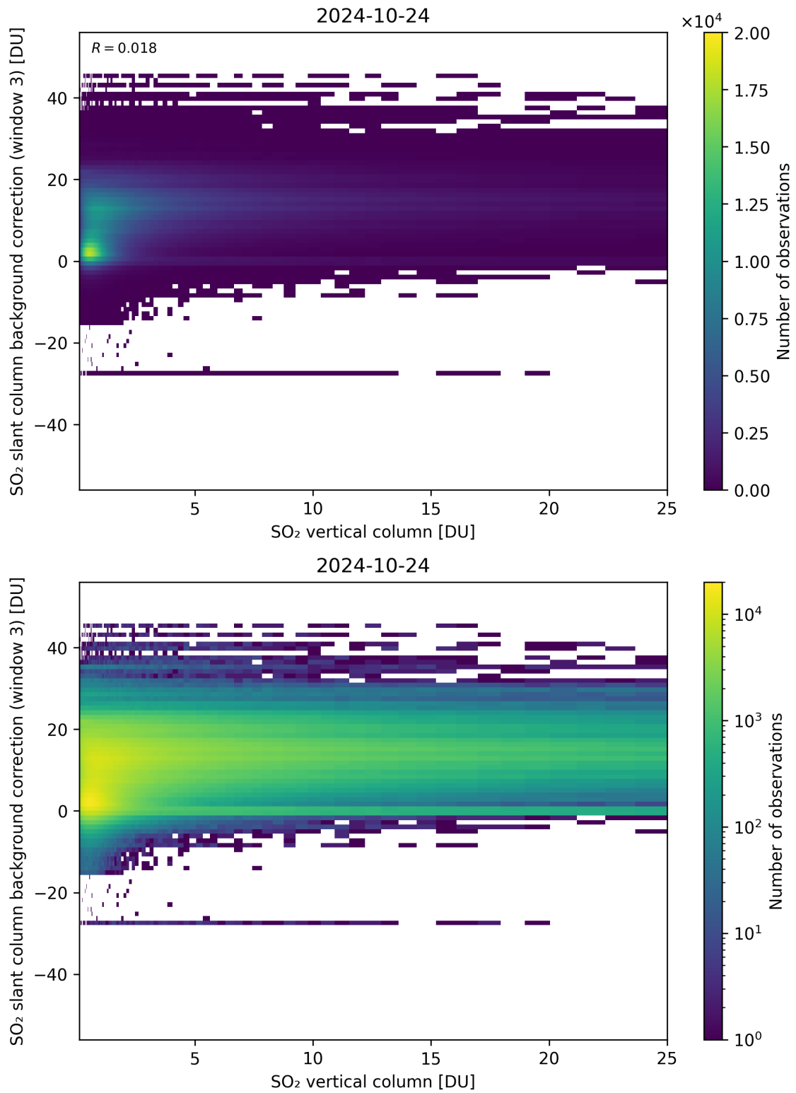
Figure 275: Scatter density plot of “SO 2 vertical column” against “SO 2 slant column background correction (window 3)” for 2024-10-24 to 2024-10-25.
