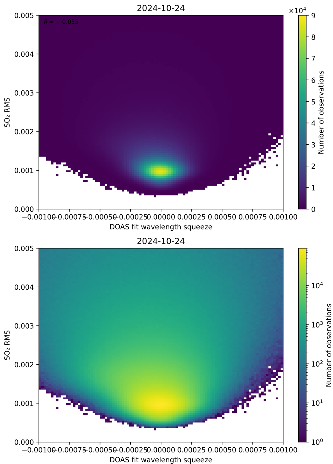
Figure 132: Scatter density plot of “DOAS fit wavelength squeeze” against “SO 2 RMS” for 2024-10-24 to 2024-10-25.
