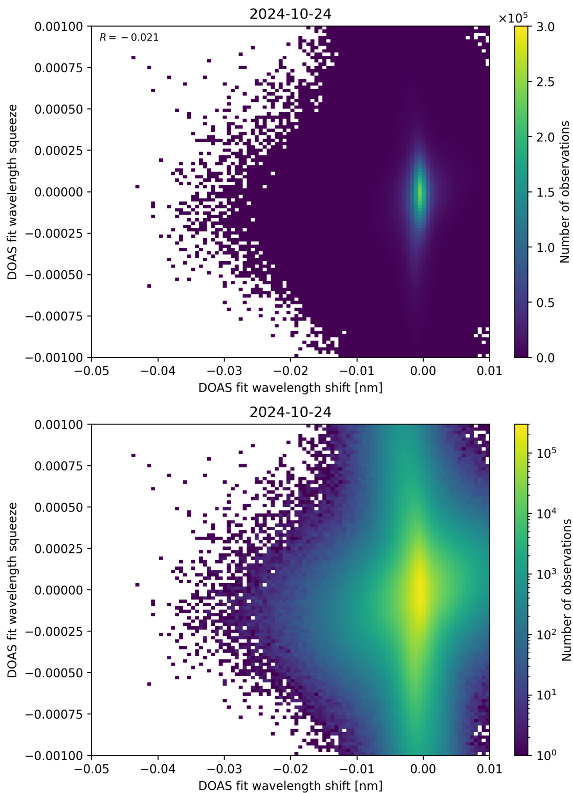
Figure 127: Scatter density plot of “DOAS fit wavelength shift” against “DOAS fit wavelength squeeze” for 2024-10-24 to 2024-10-25.
