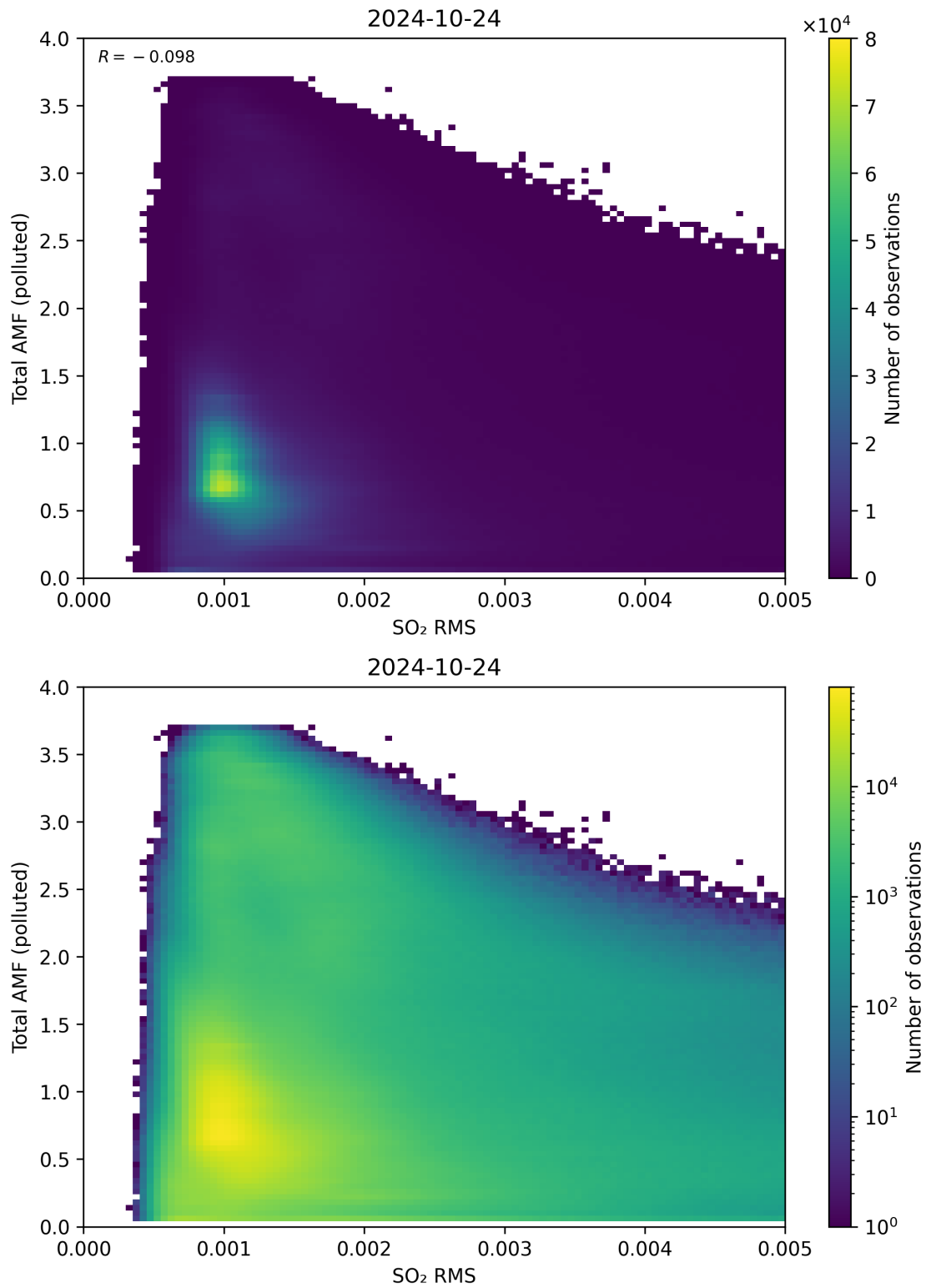
Figure 137: Scatter density plot of “SO 2 RMS” against “Total AMF (polluted)” for 2024-10-24 to 2024-10-25.
