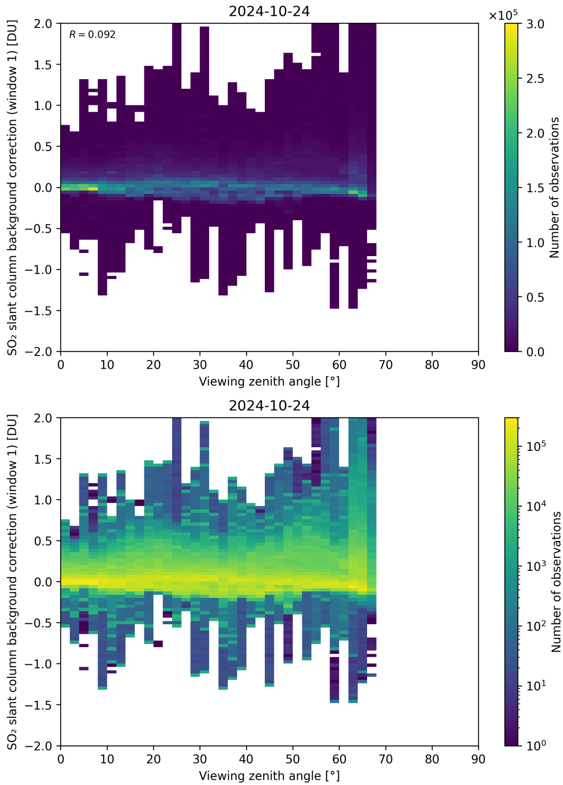
Figure 308: Scatter density plot of “Viewing zenith angle” against “SO 2 slant column background correction (window 1)” for 2024-10-24 to 2024-10-25.
