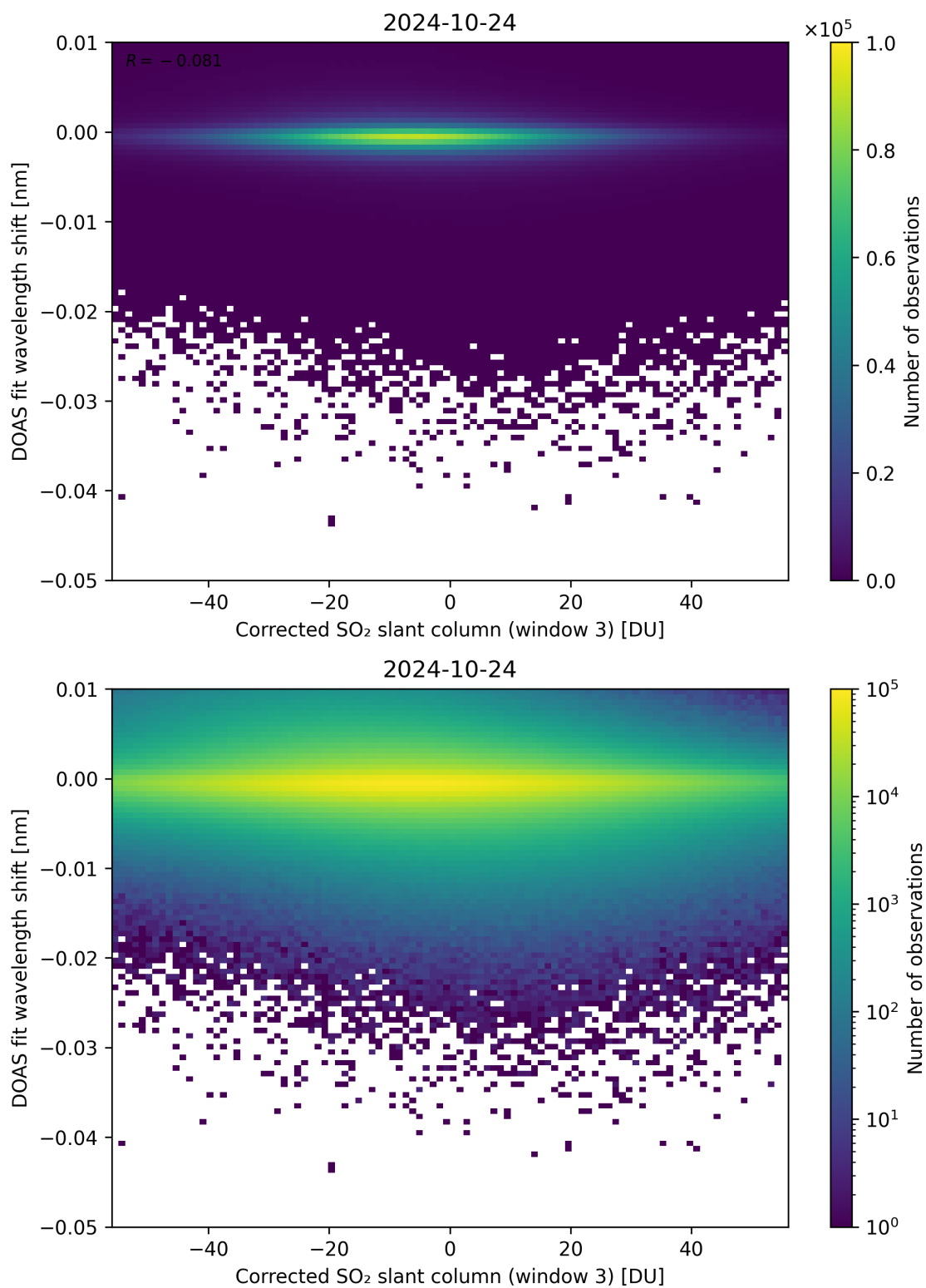
Figure 206: Scatter density plot of “Corrected SO 2 slant column (window 3)” against “DOAS fit wavelength shift” for 2024-10-24 to 2024-10-25.
