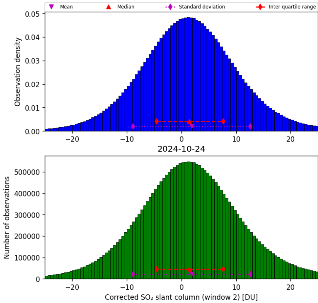
Figure 62: Histogram of “Corrected SO 2 slant column (window 2)” for 2024-10-24 to 2024-10-25
