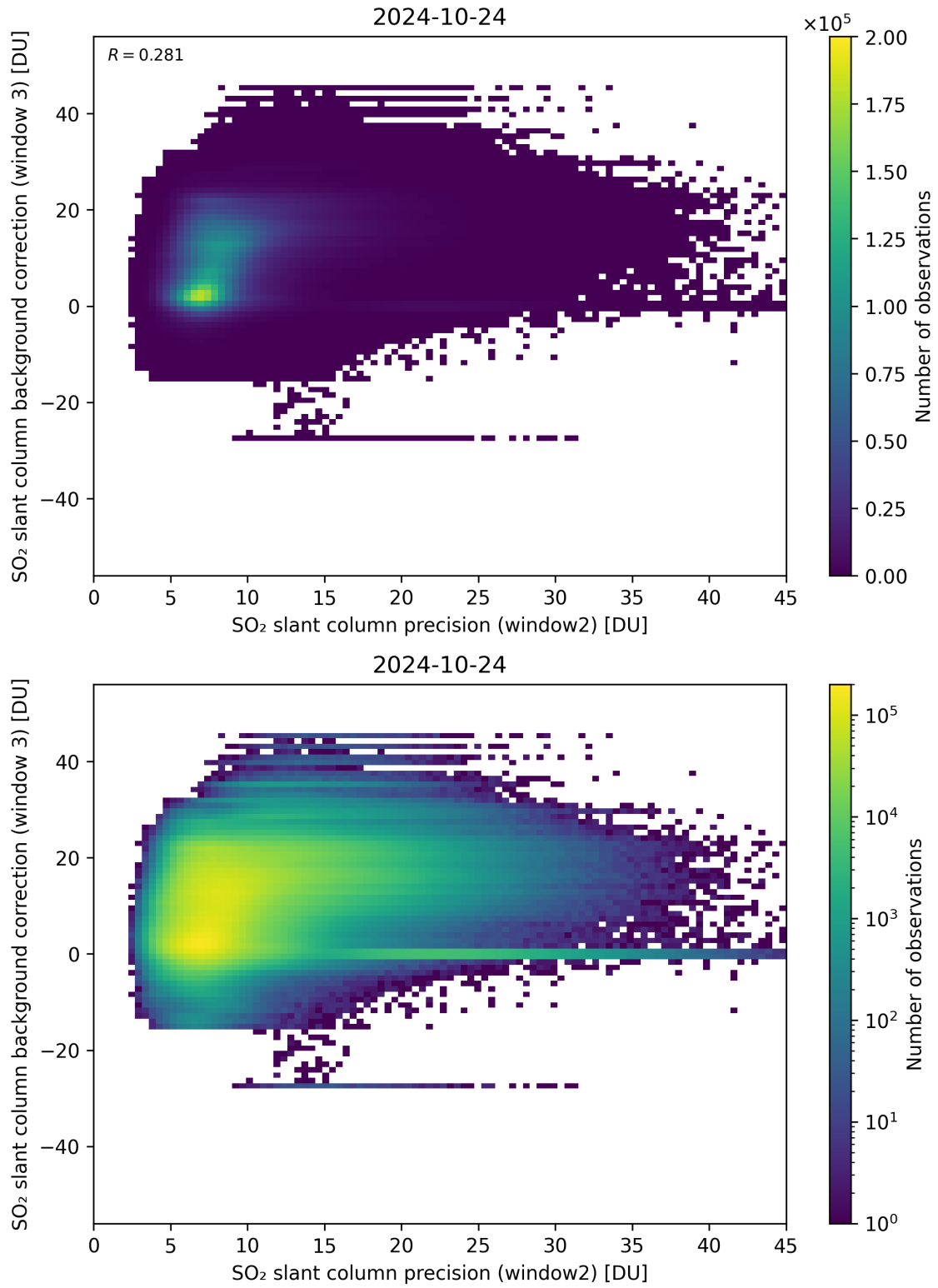
Figure 242: Scatter density plot of “SO 2 slant column precision (window2)” against “SO 2 slant column background correction (window 3)” for 2024-10-24 to 2024-10-25.
