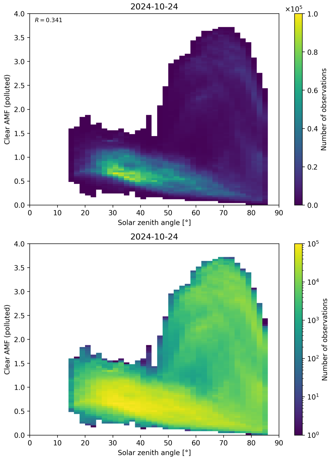
Figure 165: Scatter density plot of “Solar zenith angle” against “Clear AMF (polluted)” for 2024-10-24 to 2024-10-25.
