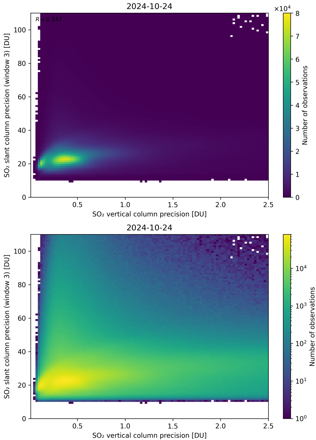
Figure 293: Scatter density plot of “SO 2 vertical column precision” against “SO 2 slant column precision (window 3)” for 2024-10-24 to 2024-10-25.
