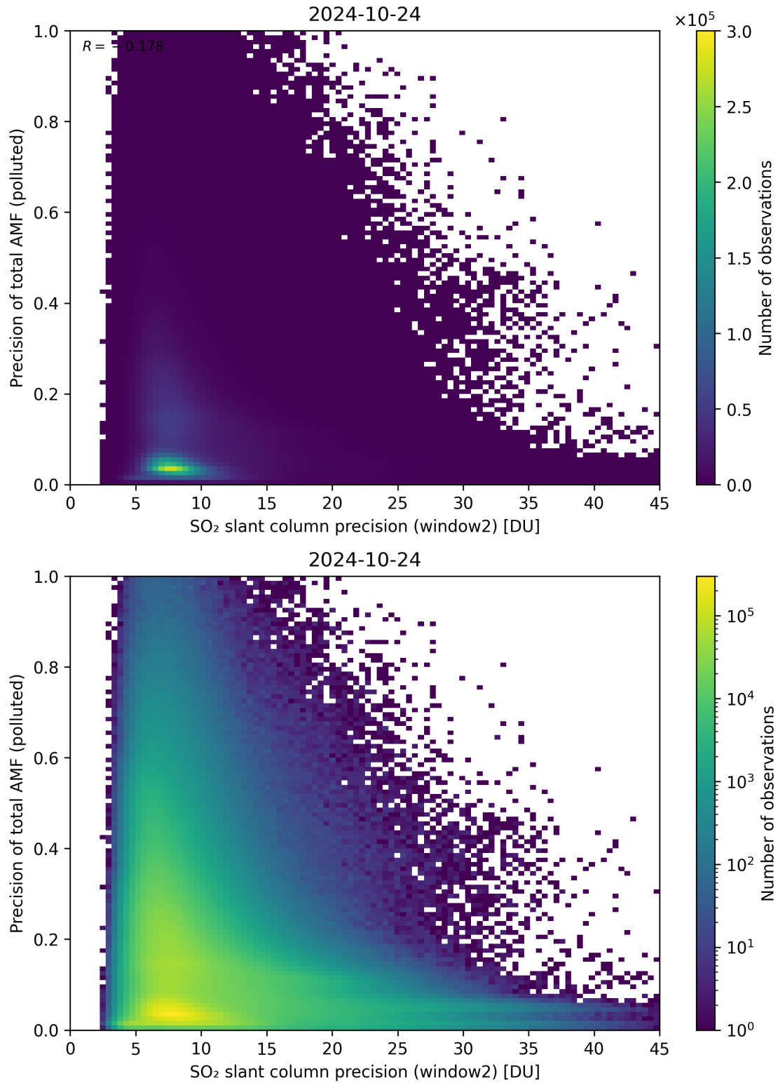
Figure 252: Scatter density plot of “SO 2 slant column precision (window2)” against “Precision of total AMF (polluted)” for 2024-10-24 to 2024-10-25.
