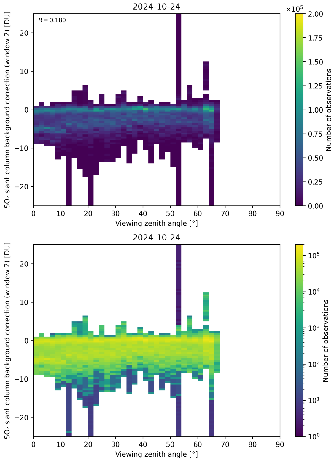
Figure 309: Scatter density plot of “Viewing zenith angle” against “SO 2 slant column background correction (window 2)” for 2024-10-24 to 2024-10-25.
