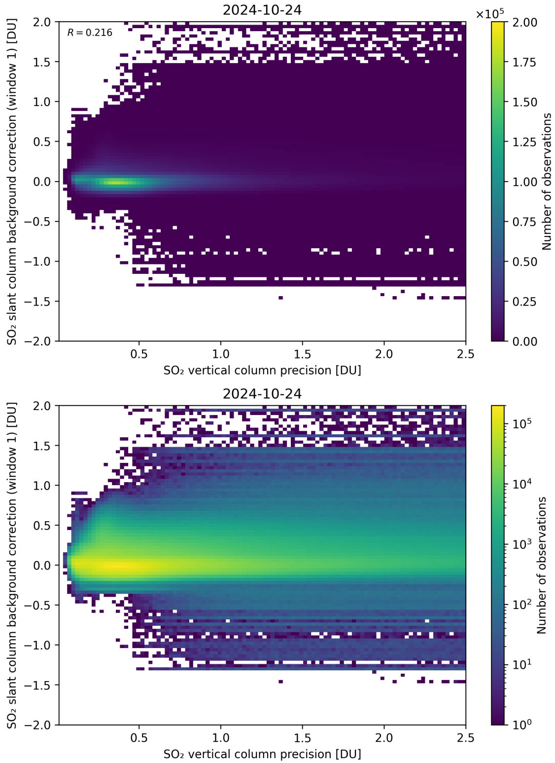
Figure 279: Scatter density plot of “SO 2 vertical column precision” against “SO 2 slant column background correction (window 1)” for 2024-10-24 to 2024-10-25.
