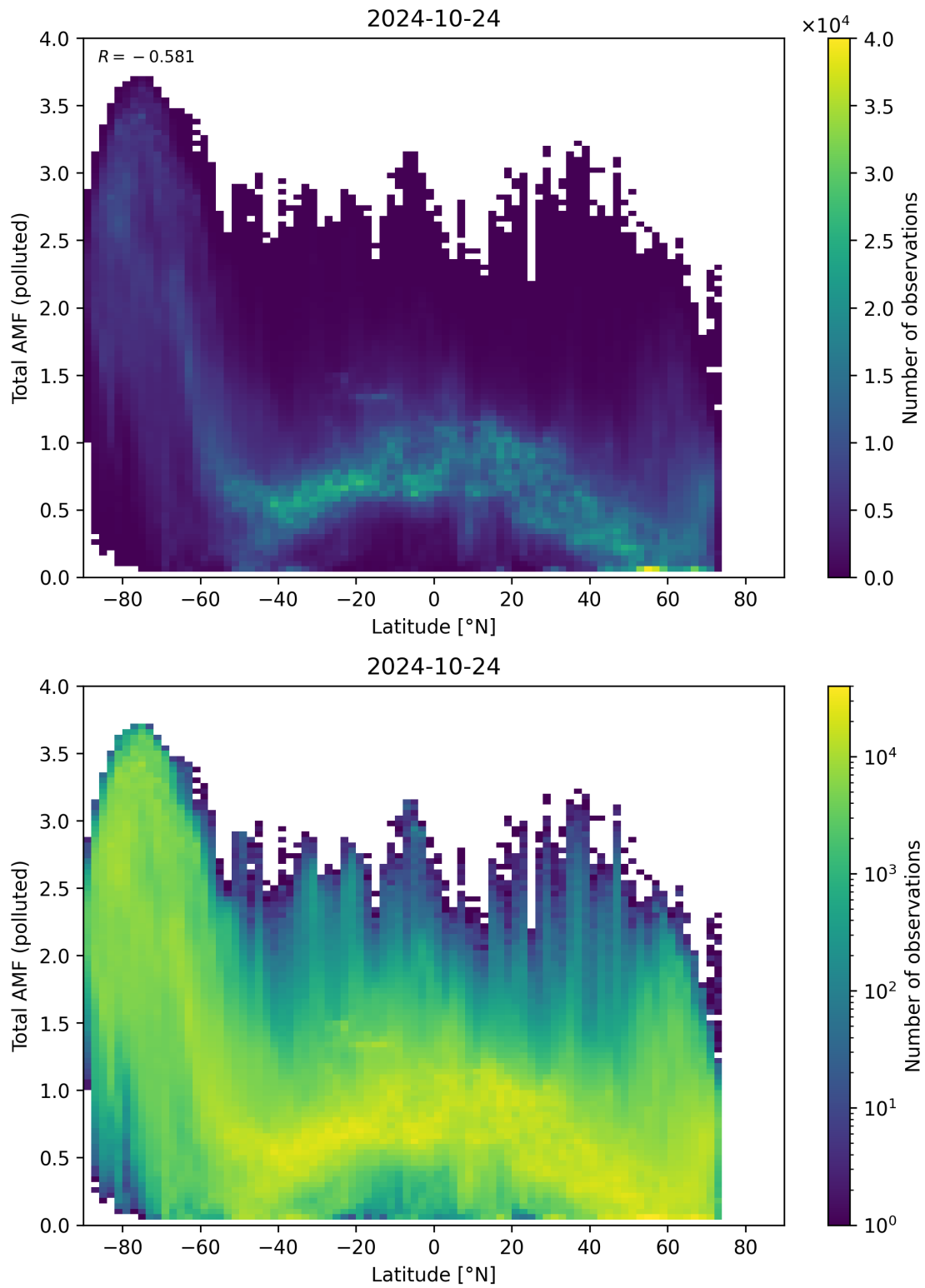
Figure 154: Scatter density plot of “Latitude” against “Total AMF (polluted)” for 2024-10-24 to 2024-10-25.
