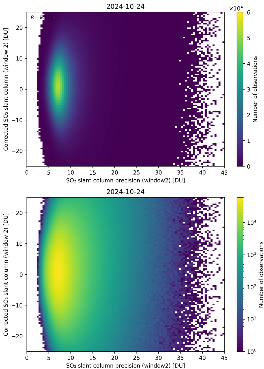
Figure 247: Scatter density plot of “SO 2 slant column precision (window2)” against “Corrected SO 2 slant column (window 2)” for 2024-10-24 to 2024-10-25.
