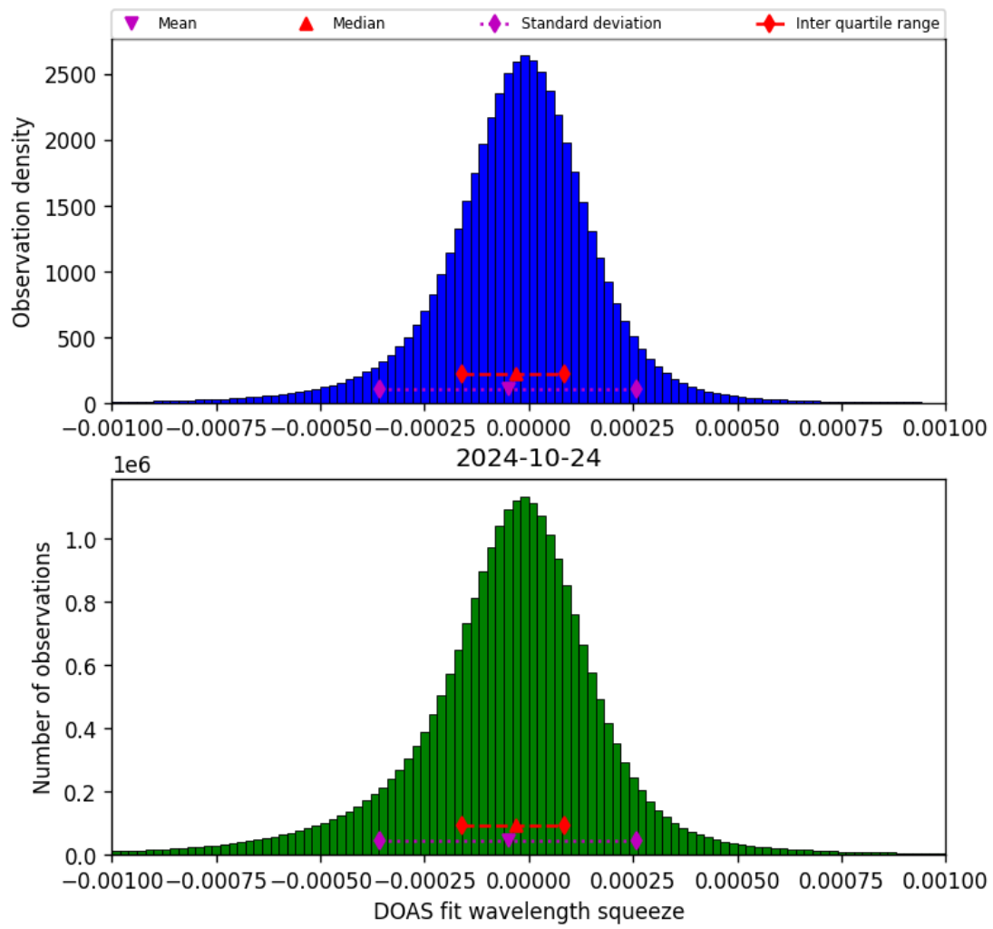
Figure 69: Histogram of "DOAS fit wavelength squeeze" for 2024-10-24 to 2024-10-25
