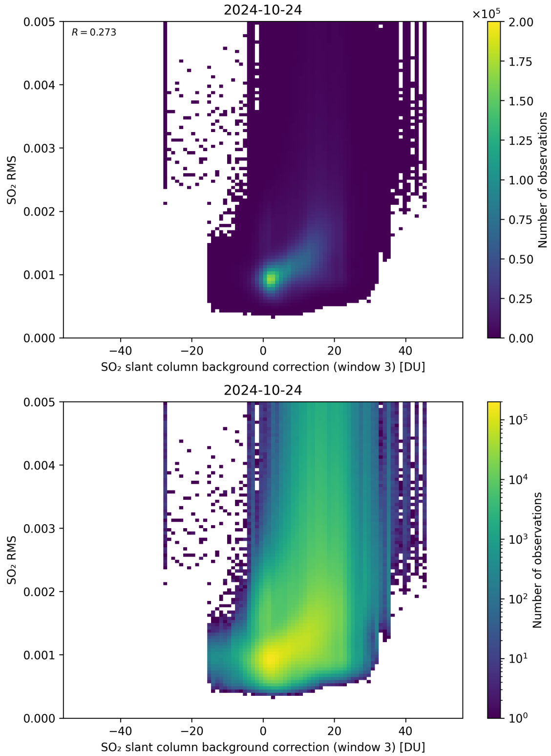
Figure 123: Scatter density plot of “SO 2 slant column background correction (window 3)” against “SO 2 RMS” for 2024-10-24 to 2024-10-25.
