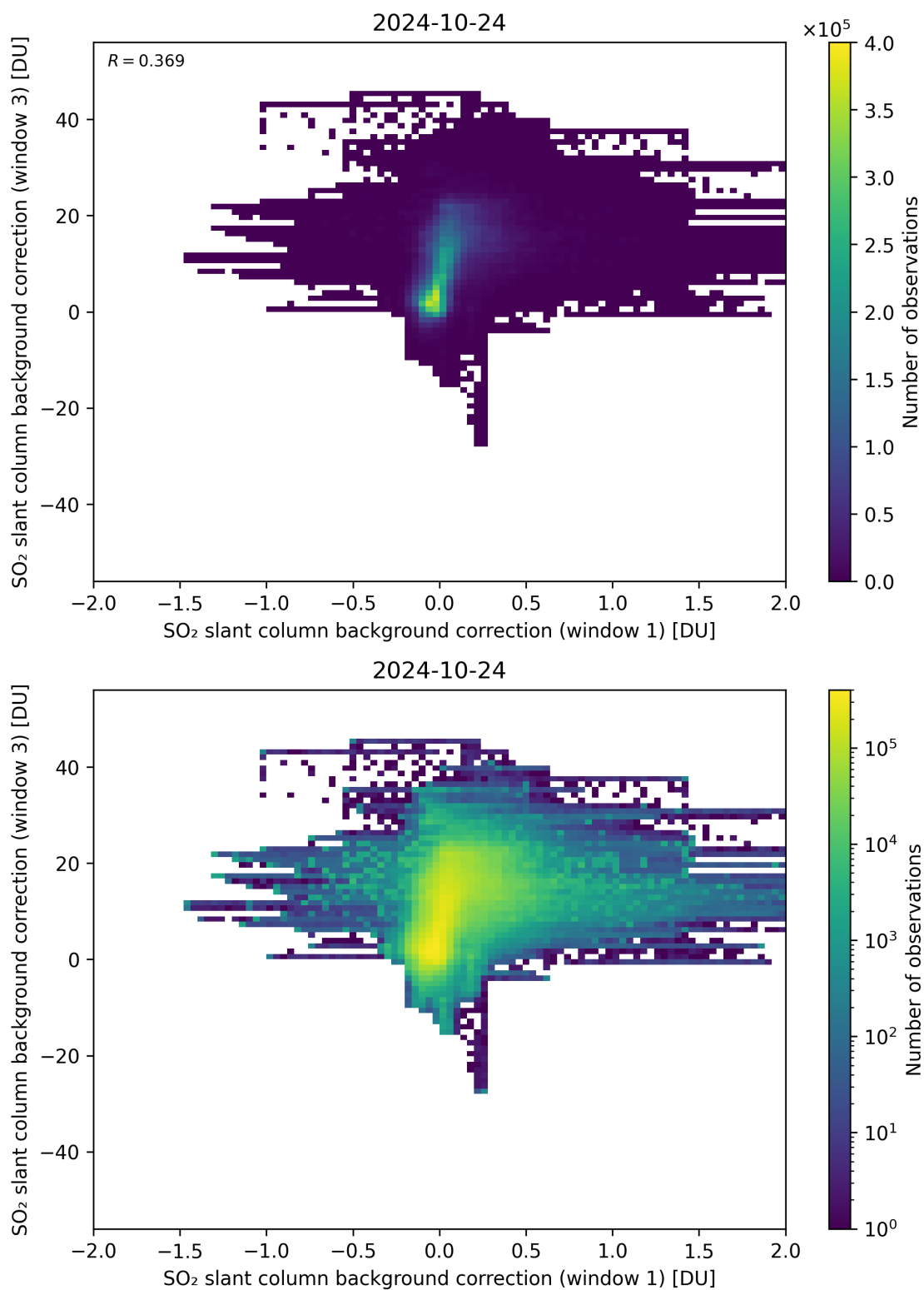
Figure 99: Scatter density plot of “SO 2 slant column background correction (window 1)” against “SO 2 slant column background correction (window 3)” for 2024-10-24 to 2024-10-25.
