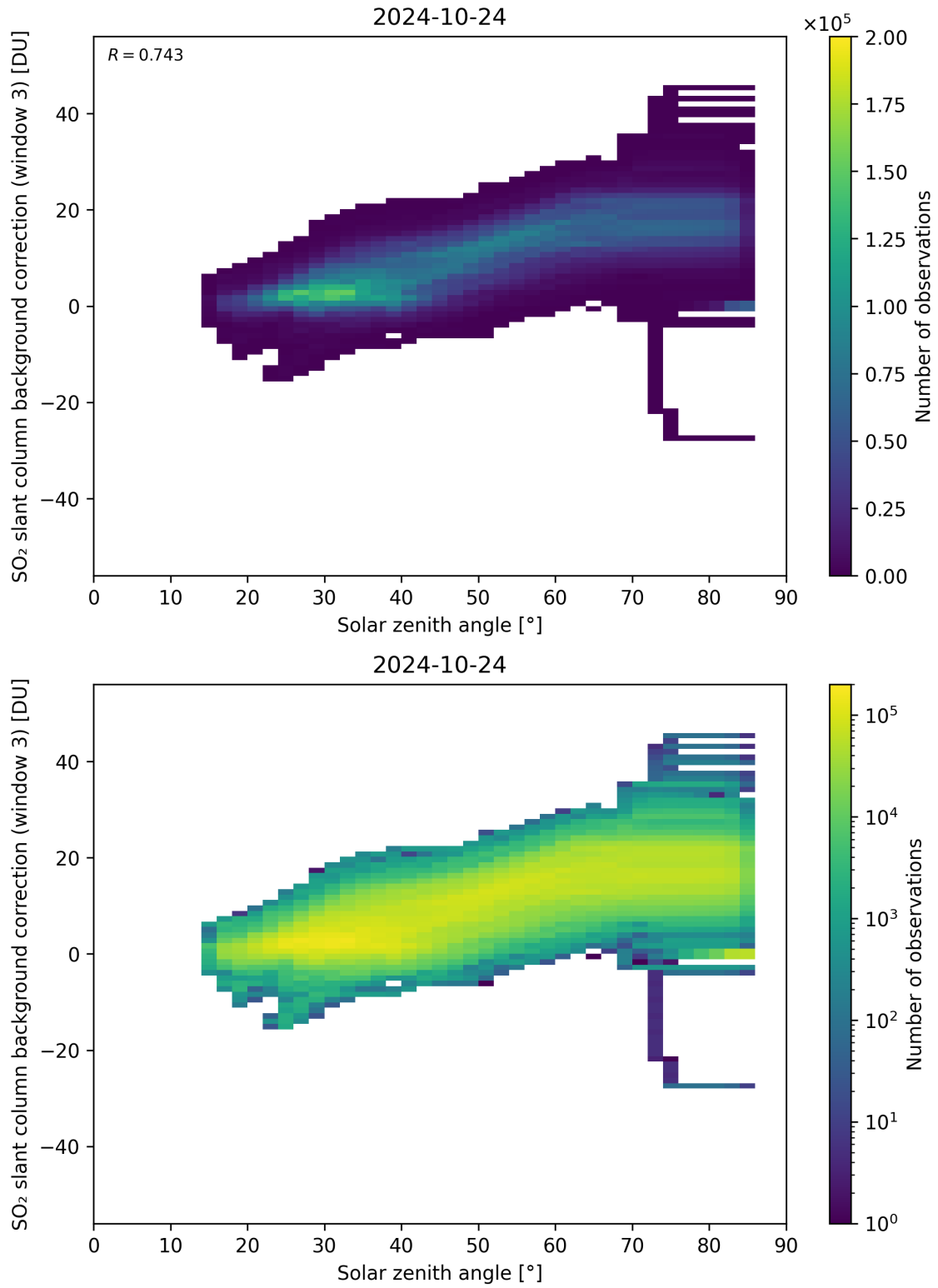
Figure 160: Scatter density plot of “Solar zenith angle” against “SO 2 slant column background correction (window 3)” for 2024-10-24 to 2024-10-25.
