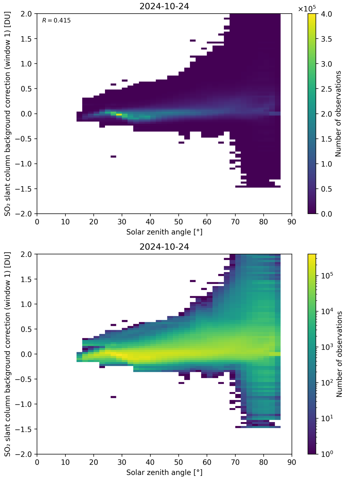
Figure 158: Scatter density plot of “Solar zenith angle” against “SO 2 slant column background correction (window 1)” for 2024-10-24 to 2024-10-25.
