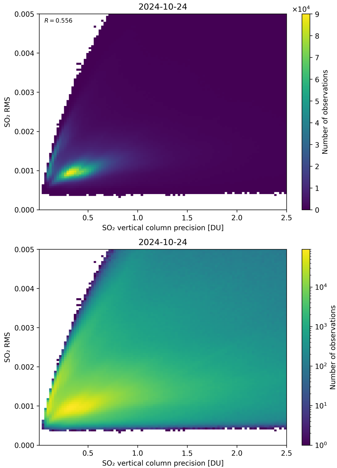
Figure 284: Scatter density plot of “SO 2 vertical column precision” against “SO 2 RMS” for 2024-10-24 to 2024-10-25.
