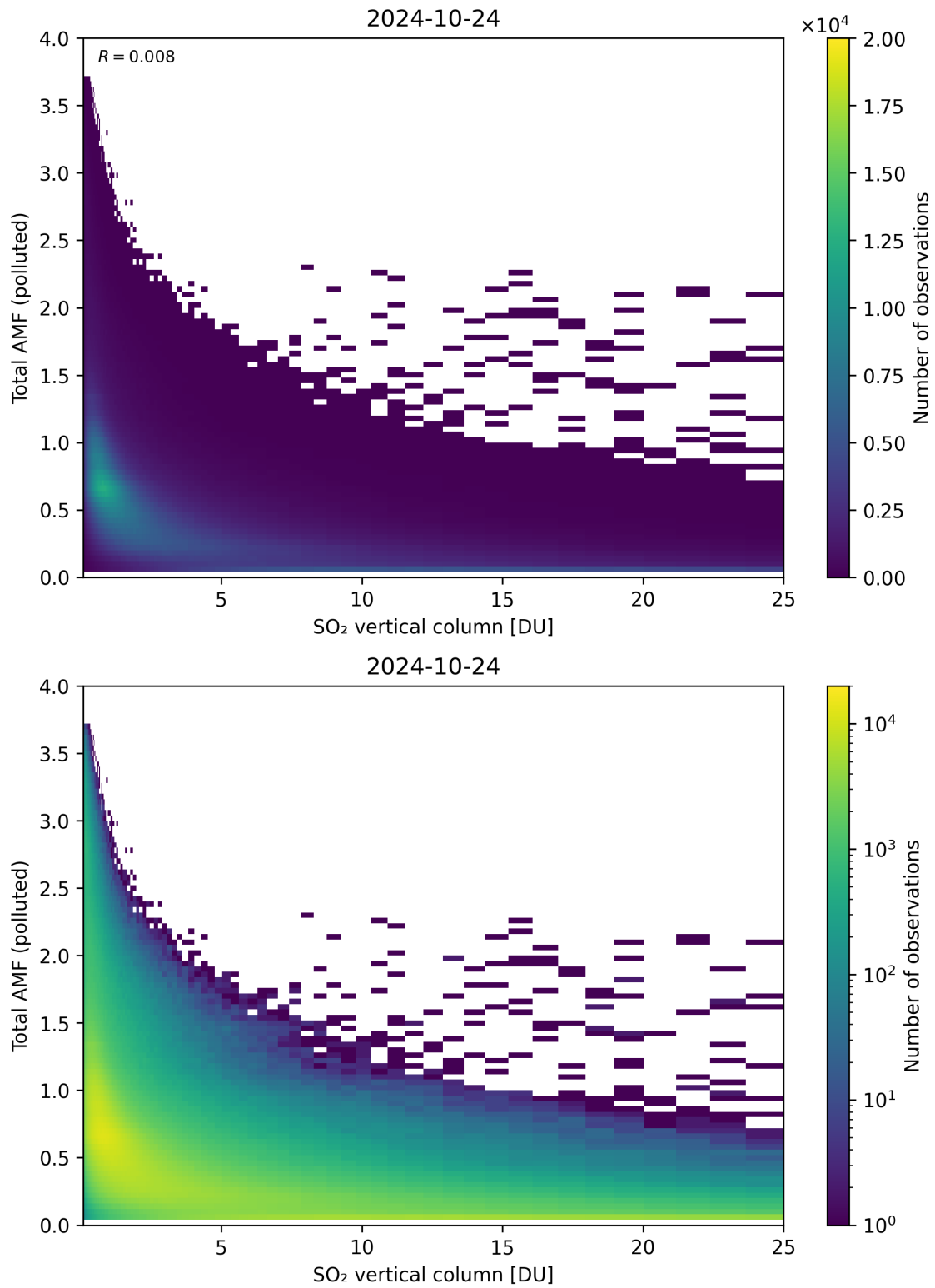
Figure 305: Scatter density plot of “SO 2 vertical column” against “Total AMF (polluted)” for 2024-10-24 to 2024-10-25.
