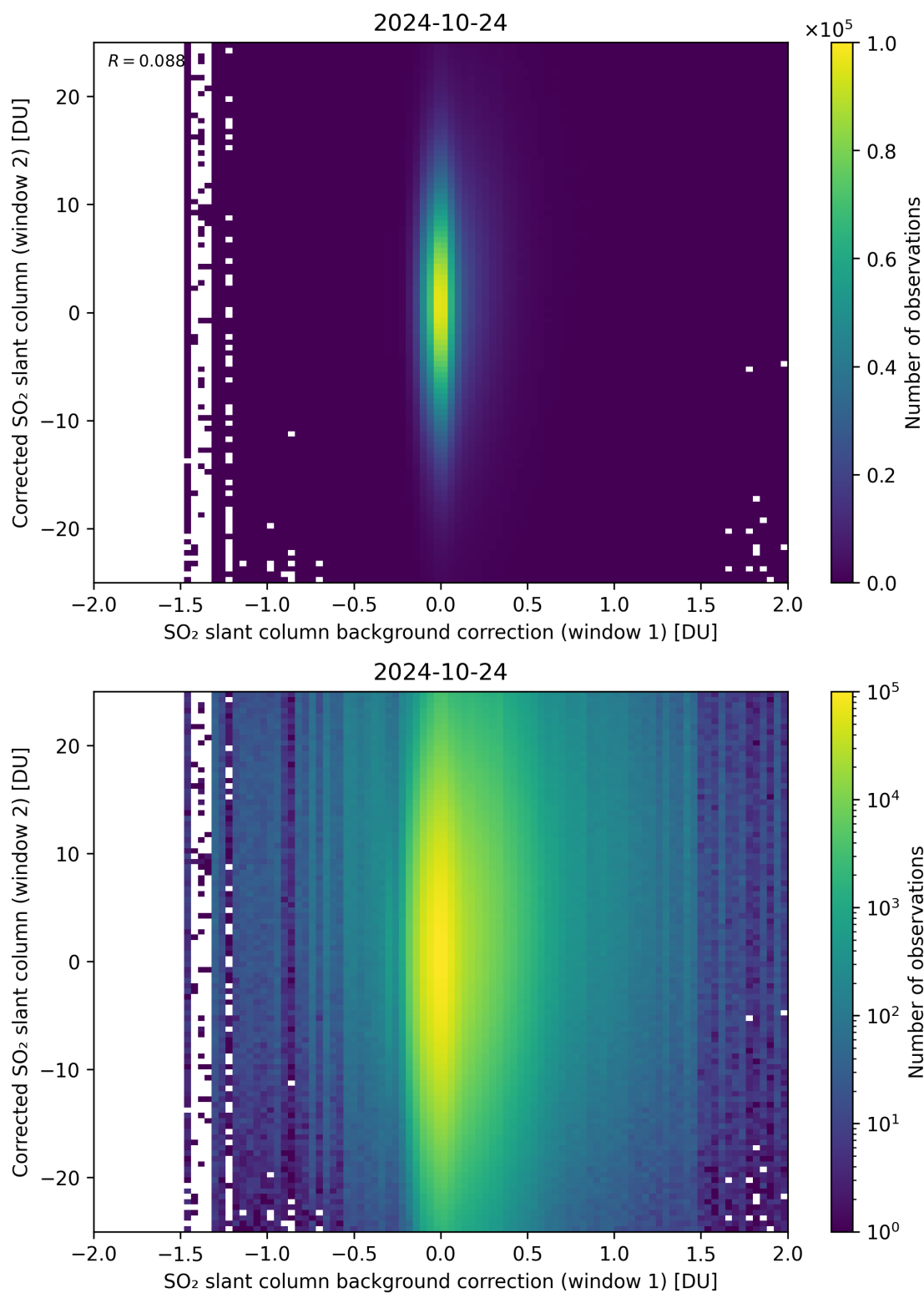
Figure 104: Scatter density plot of “SO 2 slant column background correction (window 1)” against “Corrected SO 2 slant column (window 2)” for 2024-10-24 to 2024-10-25.
