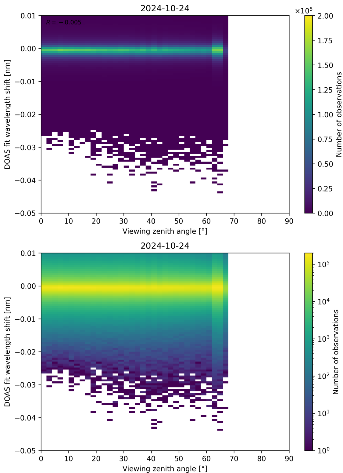
Figure 311: Scatter density plot of “Viewing zenith angle” against “DOAS fit wavelength shift” for 2024-10-24 to 2024-10-25.
