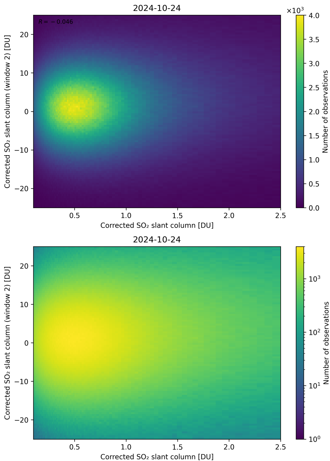
Figure 185: Scatter density plot of “Corrected SO 2 slant column” against “Corrected SO 2 slant column (window 2)” for 2024-10-24 to 2024-10-25.
