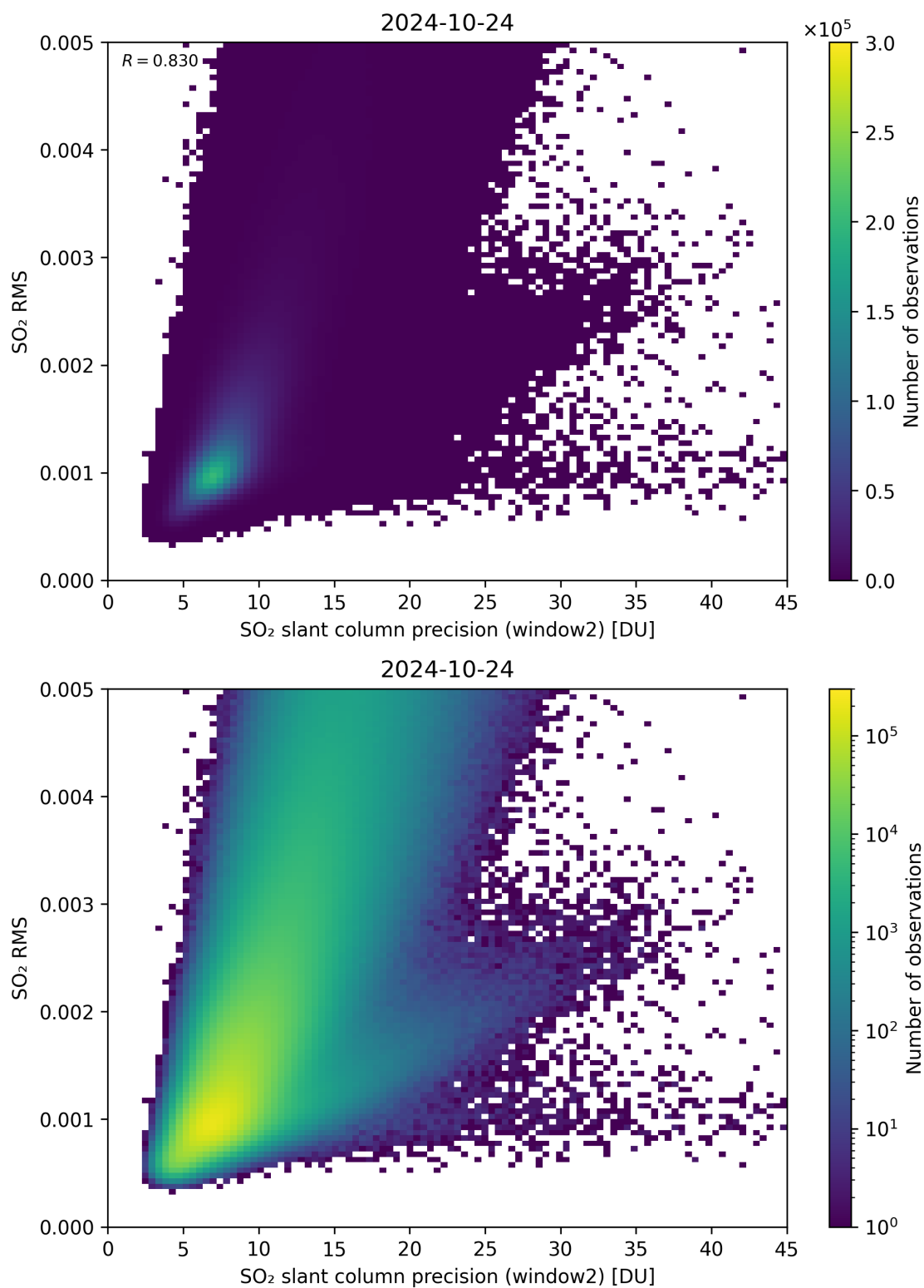
Figure 245: Scatter density plot of “SO 2 slant column precision (window2)” against “SO 2 RMS” for 2024-10-24 to 2024-10-25.
