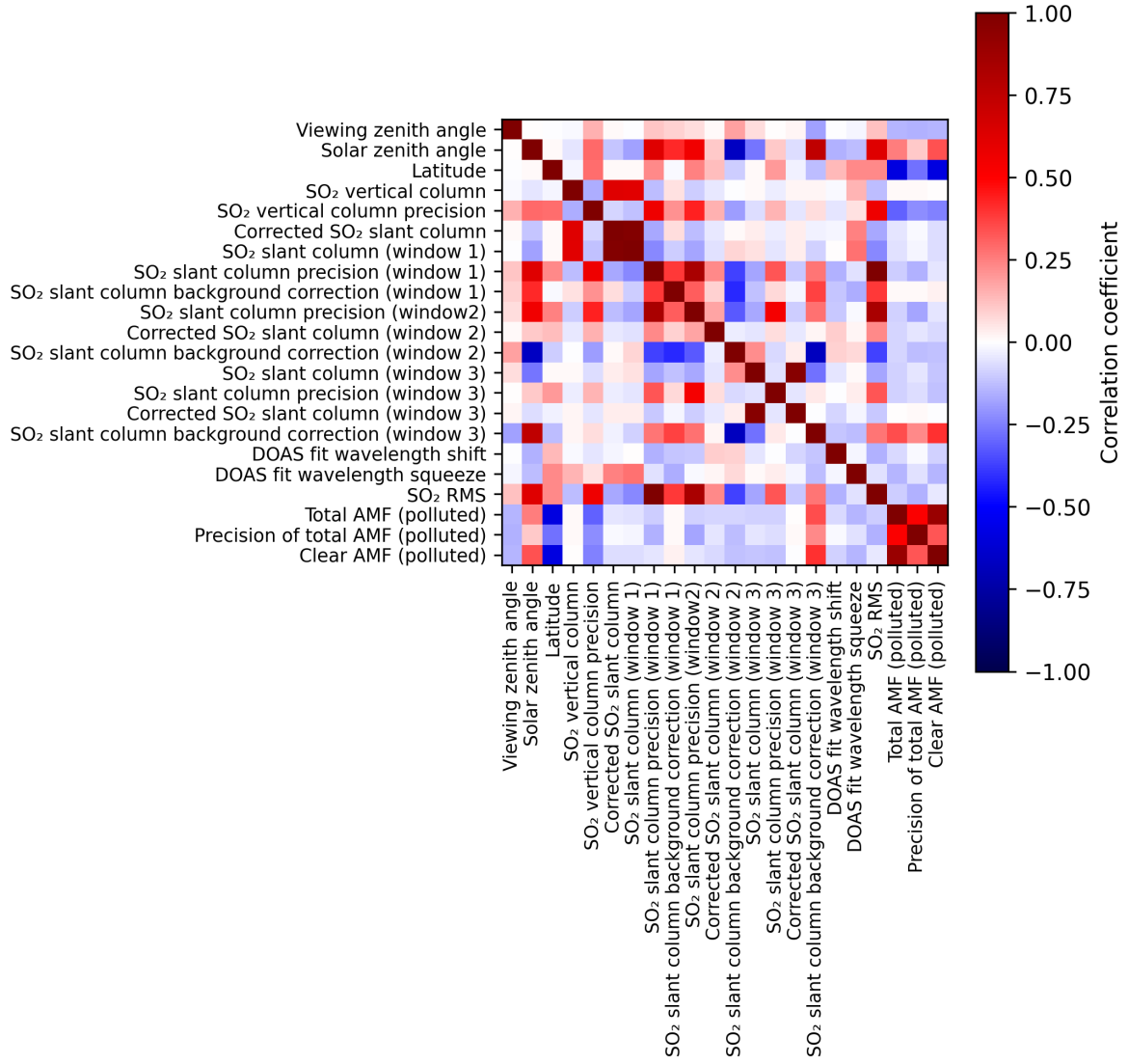
Figure 2: Map of correlation matrix for 2024-10-24 to 2024-10-25.
