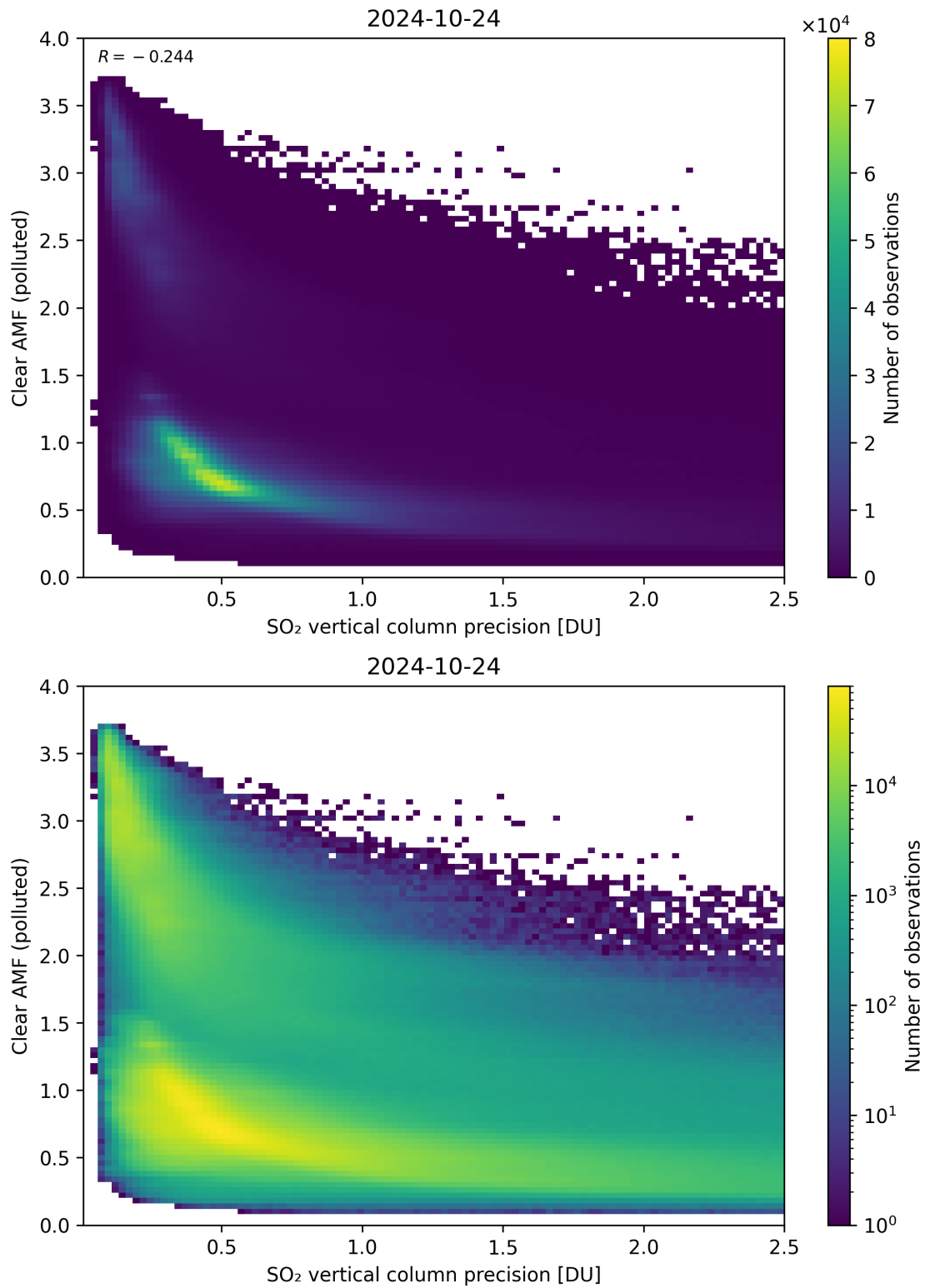
Figure 285: Scatter density plot of “SO 2 vertical column precision” against “Clear AMF (polluted)” for 2024-10-24 to 2024-10-25.
