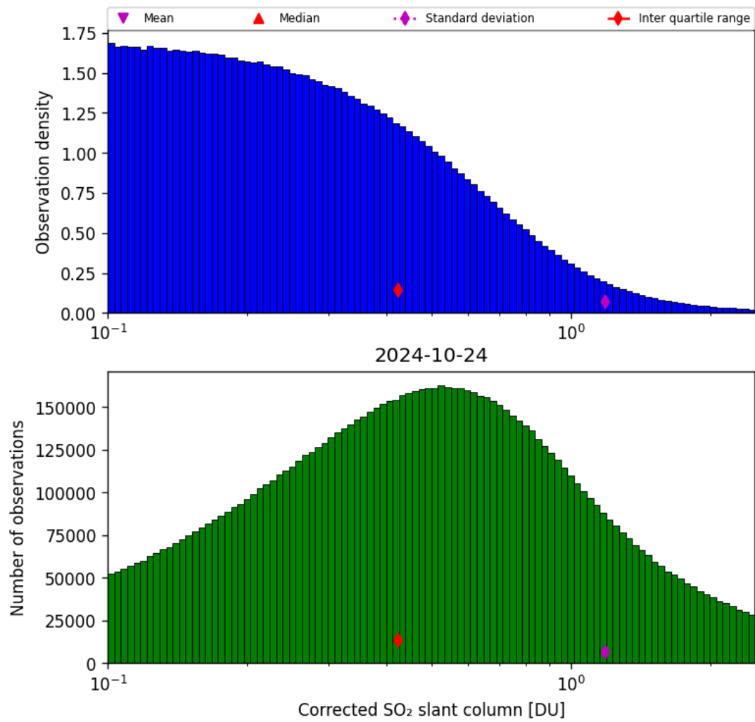
Figure 55: Histogram of “Corrected SO 2 slant column” for 2024-10-24 to 2024-10-25
