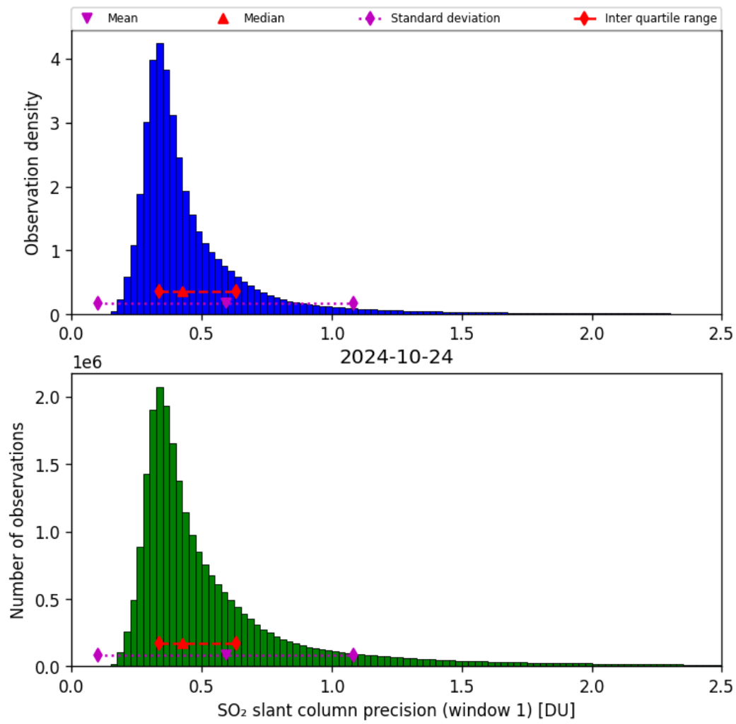
Figure 57: Histogram of “SO 2 slant column precision (window 1)” for 2024-10-24 to 2024-10-25
