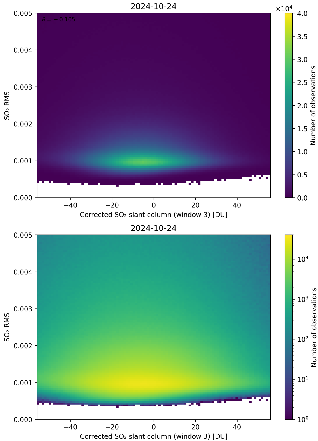
Figure 208: Scatter density plot of “Corrected SO 2 slant column (window 3)” against “SO 2 RMS” for 2024-10-24 to 2024-10-25.
