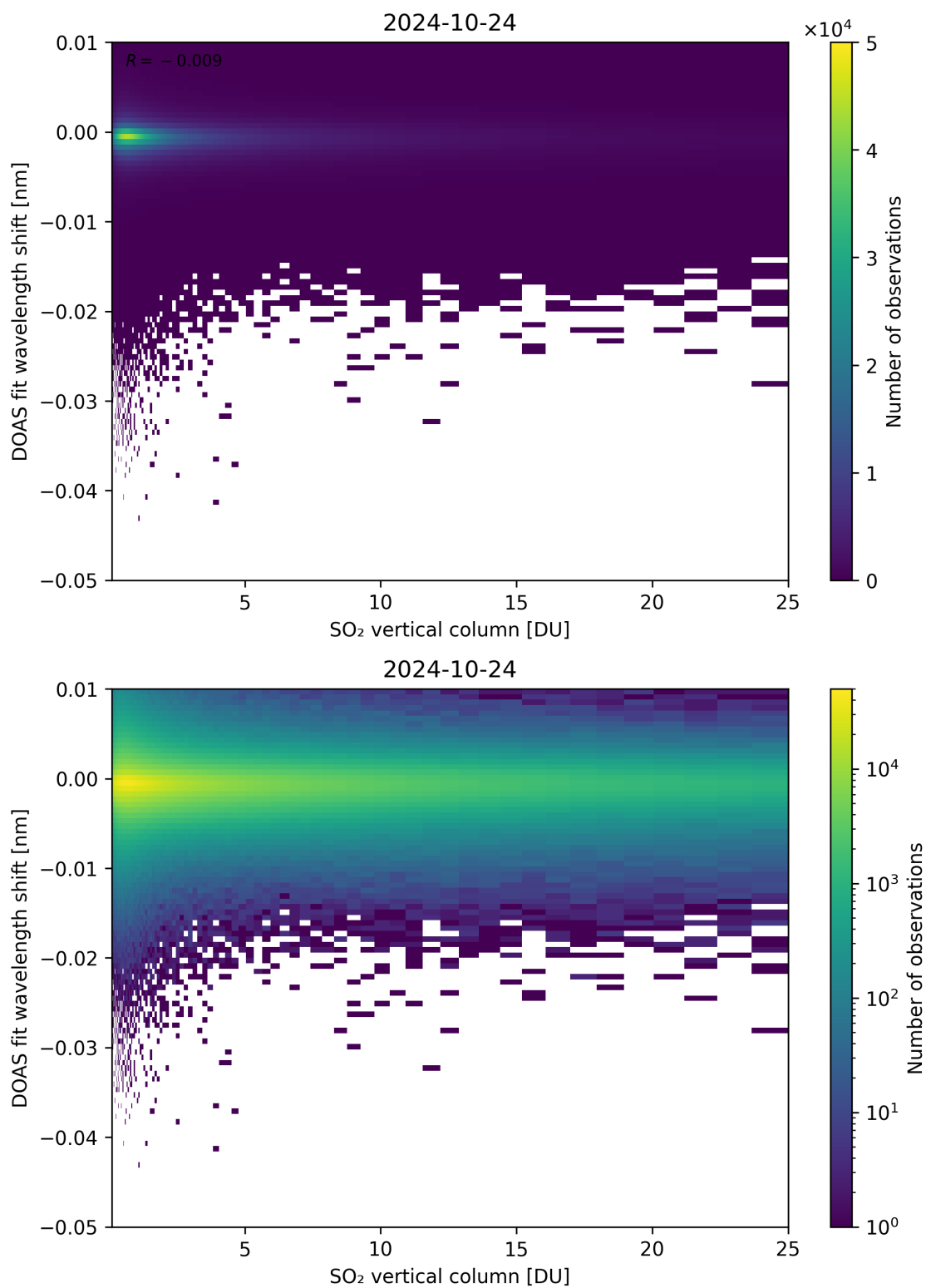
Figure 276: Scatter density plot of “SO 2 vertical column” against “DOAS fit wavelength shift” for 2024-10-24 to 2024-10-25.
