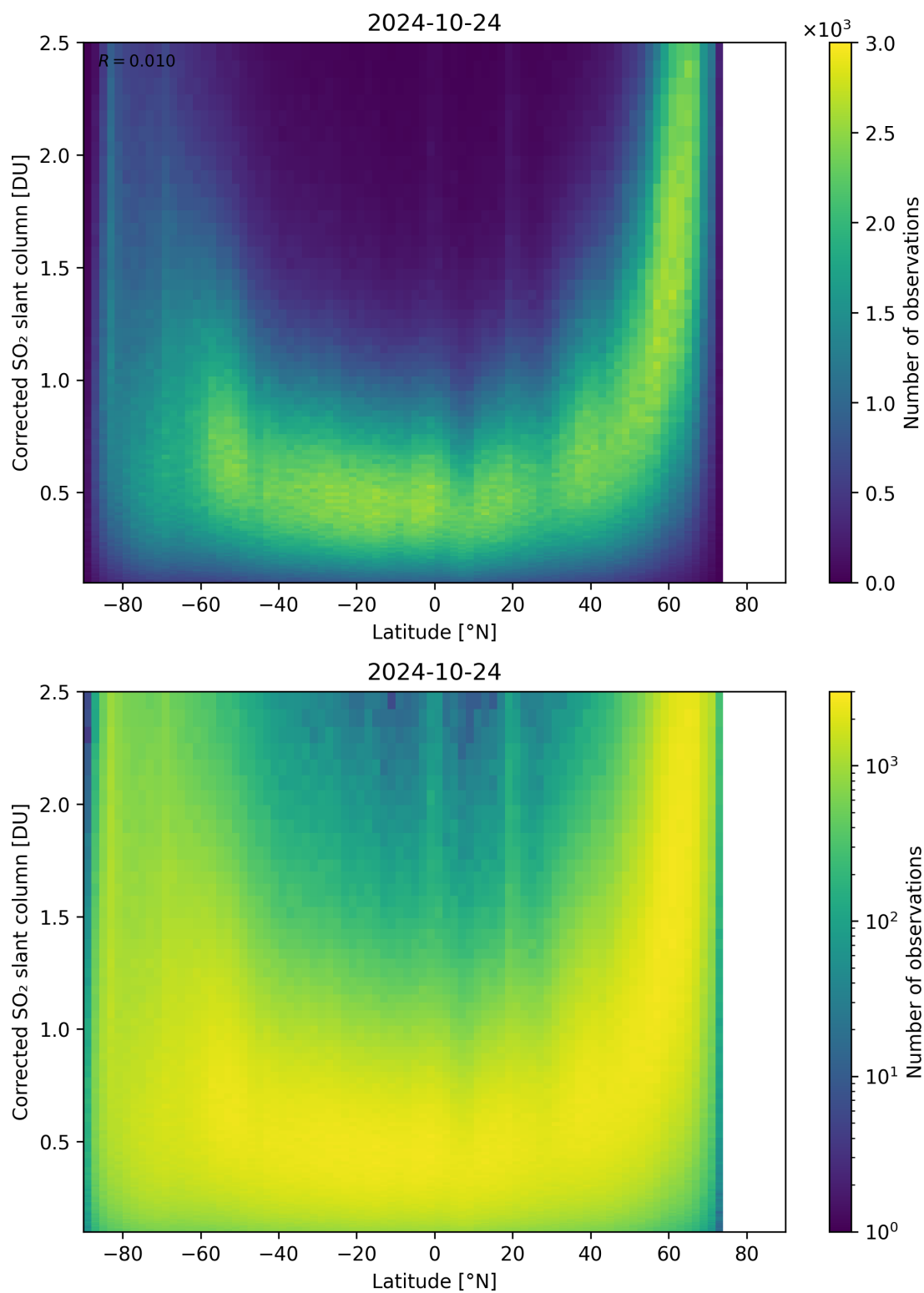
Figure 146: Scatter density plot of “Latitude” against “Corrected SO 2 slant column” for 2024-10-24 to 2024-10-25.
