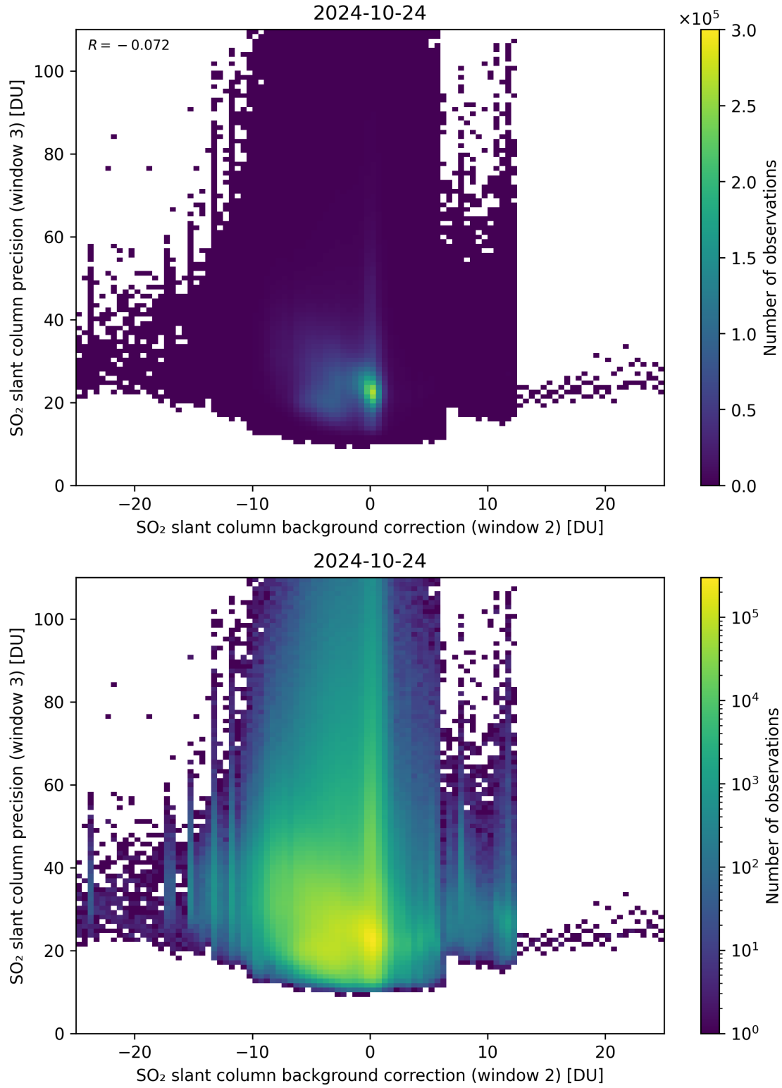
Figure 118: Scatter density plot of “SO 2 slant column background correction (window 2)” against “SO 2 slant column precision (window 3)” for 2024-10-24 to 2024-10-25.
