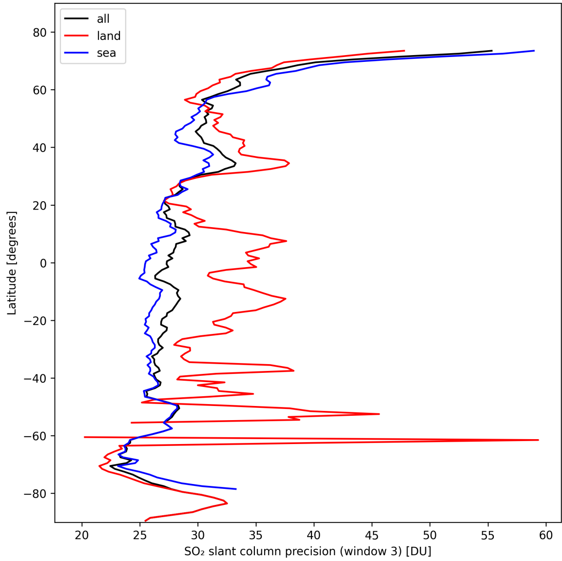
Figure 42: Zonal average of “SO 2 slant column precision (window 3)” for 2024-10-24 to 2024-10-25.
