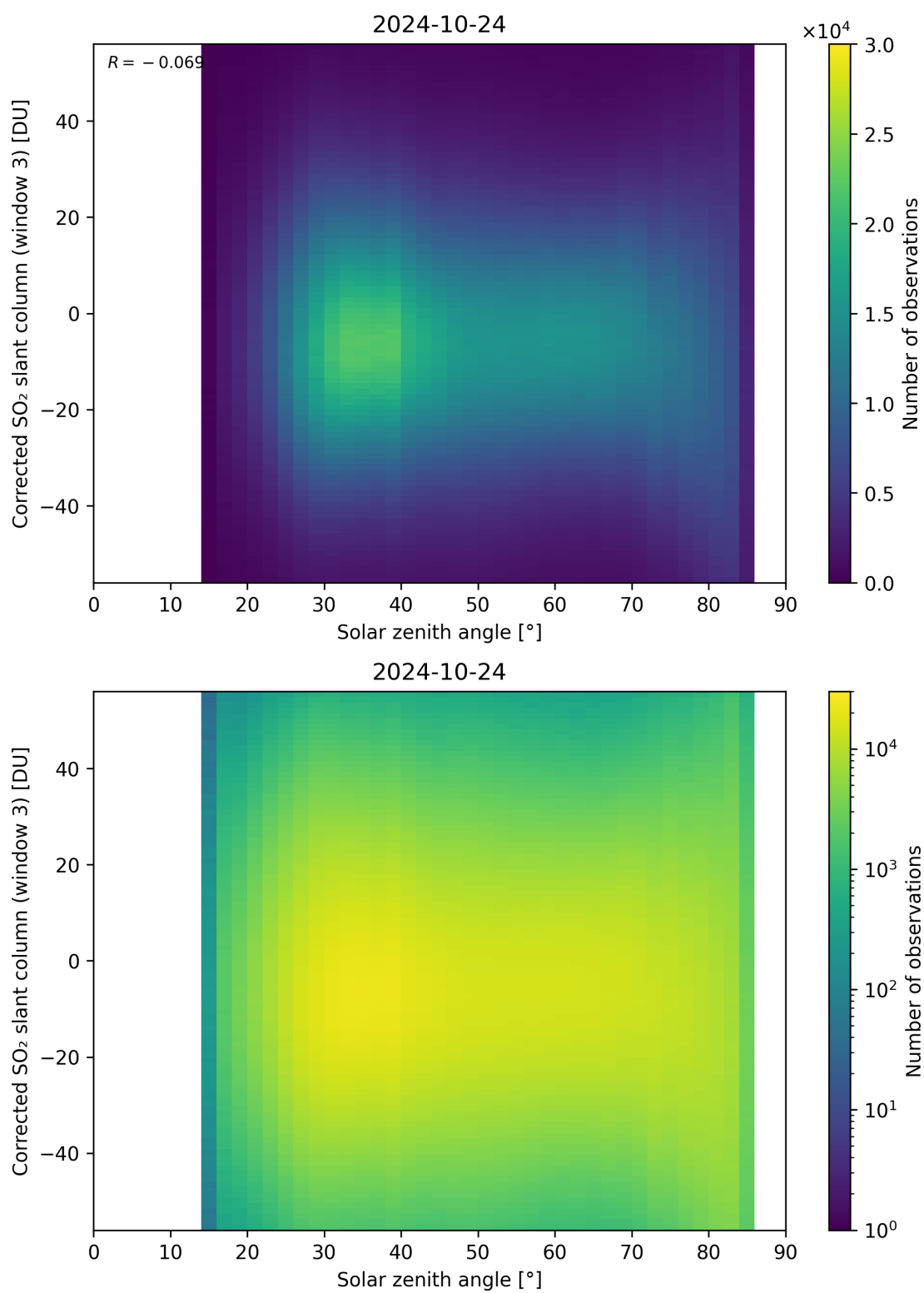
Figure 168: Scatter density plot of “Solar zenith angle” against “Corrected SO 2 slant column (window 3)” for 2024-10-24 to 2024-10-25.
