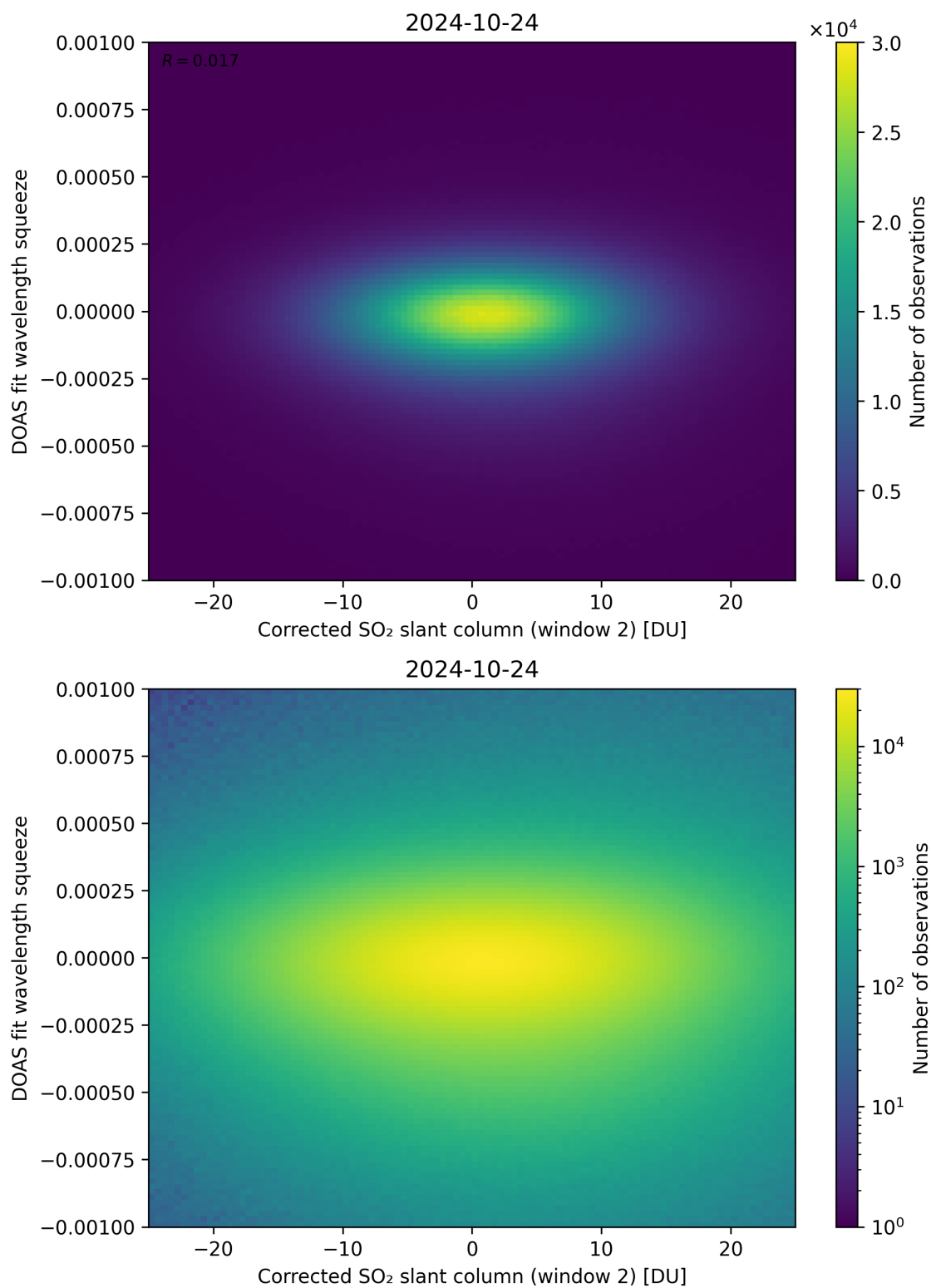
Figure 197: Scatter density plot of “Corrected SO 2 slant column (window 2)” against “DOAS fit wavelength squeeze” for 2024-10-24 to 2024-10-25.
