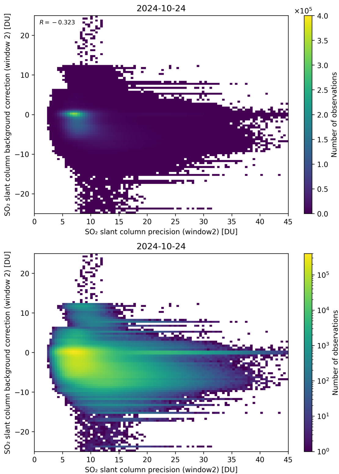
Figure 241: Scatter density plot of “SO 2 slant column precision (window2)” against “SO 2 slant column background correction (window 2)” for 2024-10-24 to 2024-10-25.
