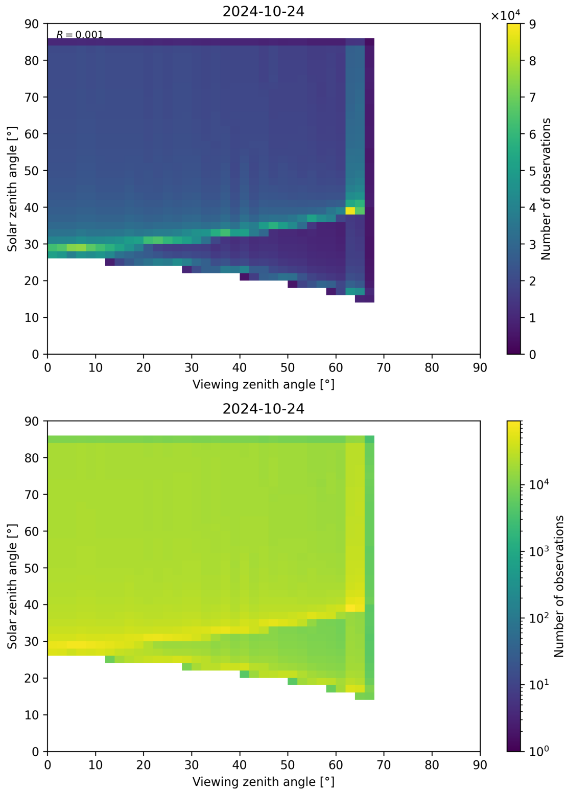
Figure 315: Scatter density plot of “Viewing zenith angle” against “Solar zenith angle” for 2024-10-24 to 2024-10-25.
