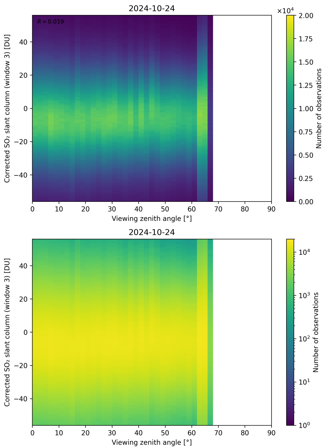
Figure 319: Scatter density plot of “Viewing zenith angle” against “Corrected SO 2 slant column (window 3)” for 2024-10-24 to 2024-10-25.
