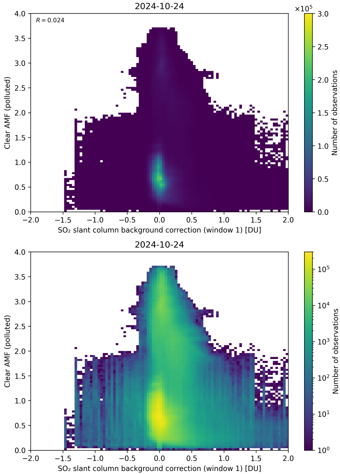
Figure 103: Scatter density plot of “SO 2 slant column background correction (window 1)” against “Clear AMF (polluted)” for 2024-10-24 to 2024-10-25.
