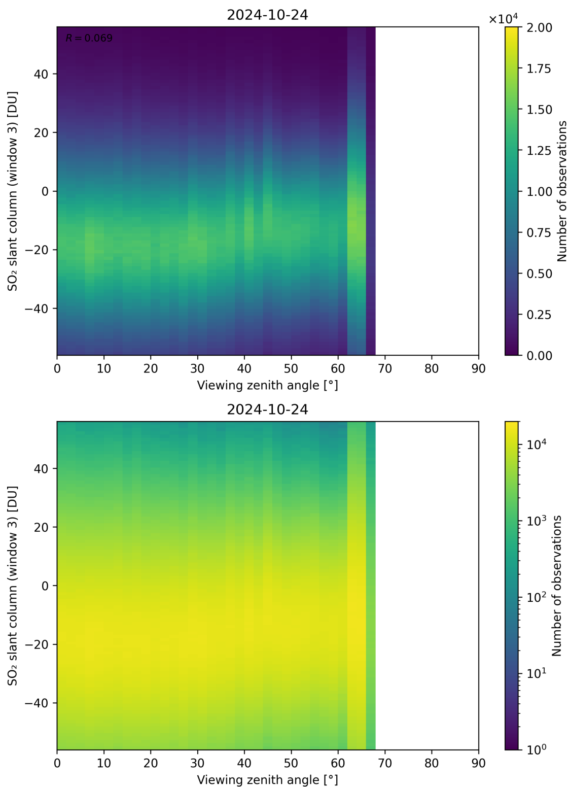
Figure 323: Scatter density plot of “Viewing zenith angle” against “SO 2 slant column (window 3)” for 2024-10-24 to 2024-10-25.
