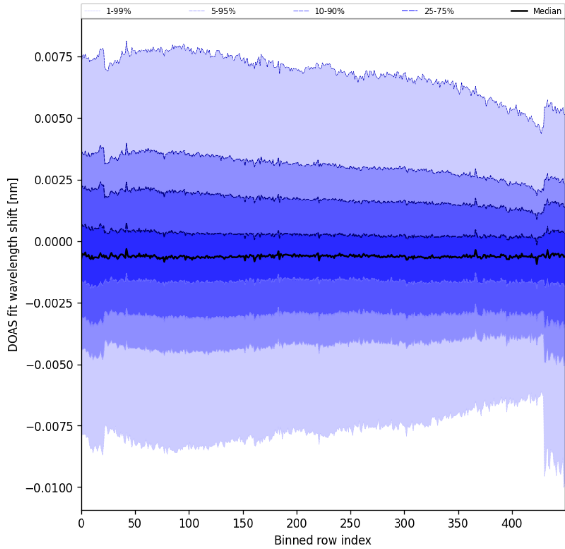
Figure 91: Along track statistics of “DOAS fit wavelength shift” for 2024-10-24 to 2024-10-25
