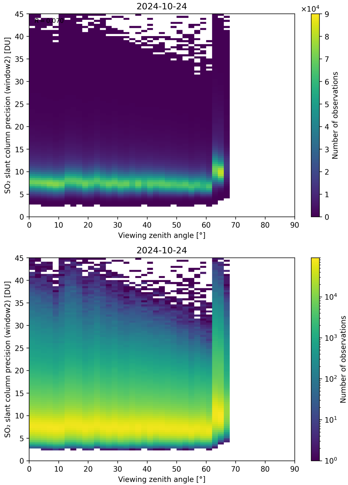
Figure 322: Scatter density plot of “Viewing zenith angle” against “SO 2 slant column precision (window2)” for 2024-10-24 to 2024-10-25.
