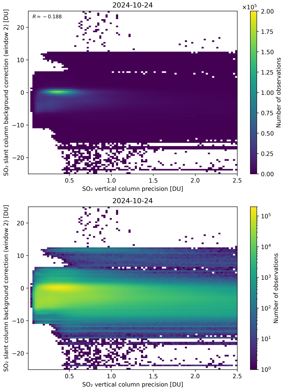
Figure 280: Scatter density plot of “SO 2 vertical column precision” against “SO 2 slant column background correction (window 2)” for 2024-10-24 to 2024-10-25.
