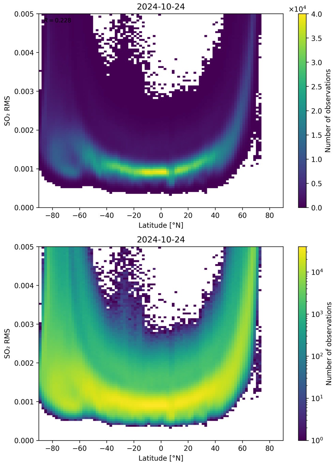
Figure 144: Scatter density plot of “Latitude” against “SO 2 RMS” for 2024-10-24 to 2024-10-25.
