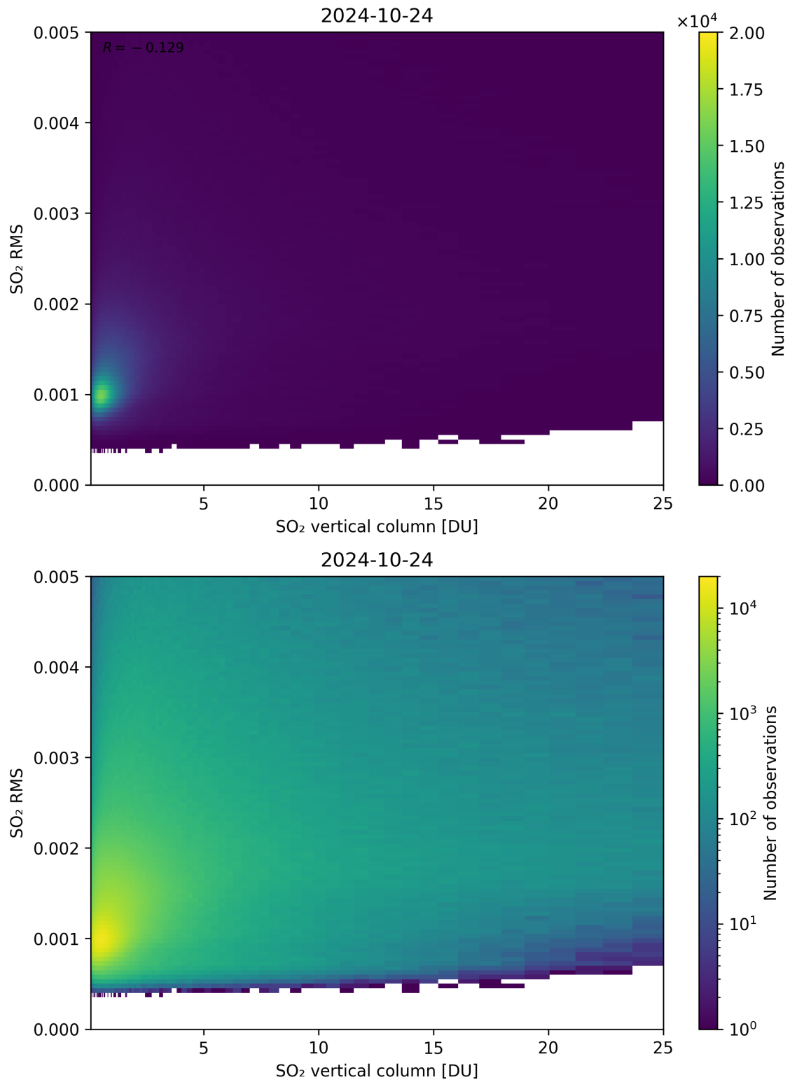
Figure 278: Scatter density plot of “SO 2 vertical column” against “SO 2 RMS” for 2024-10-24 to 2024-10-25.
