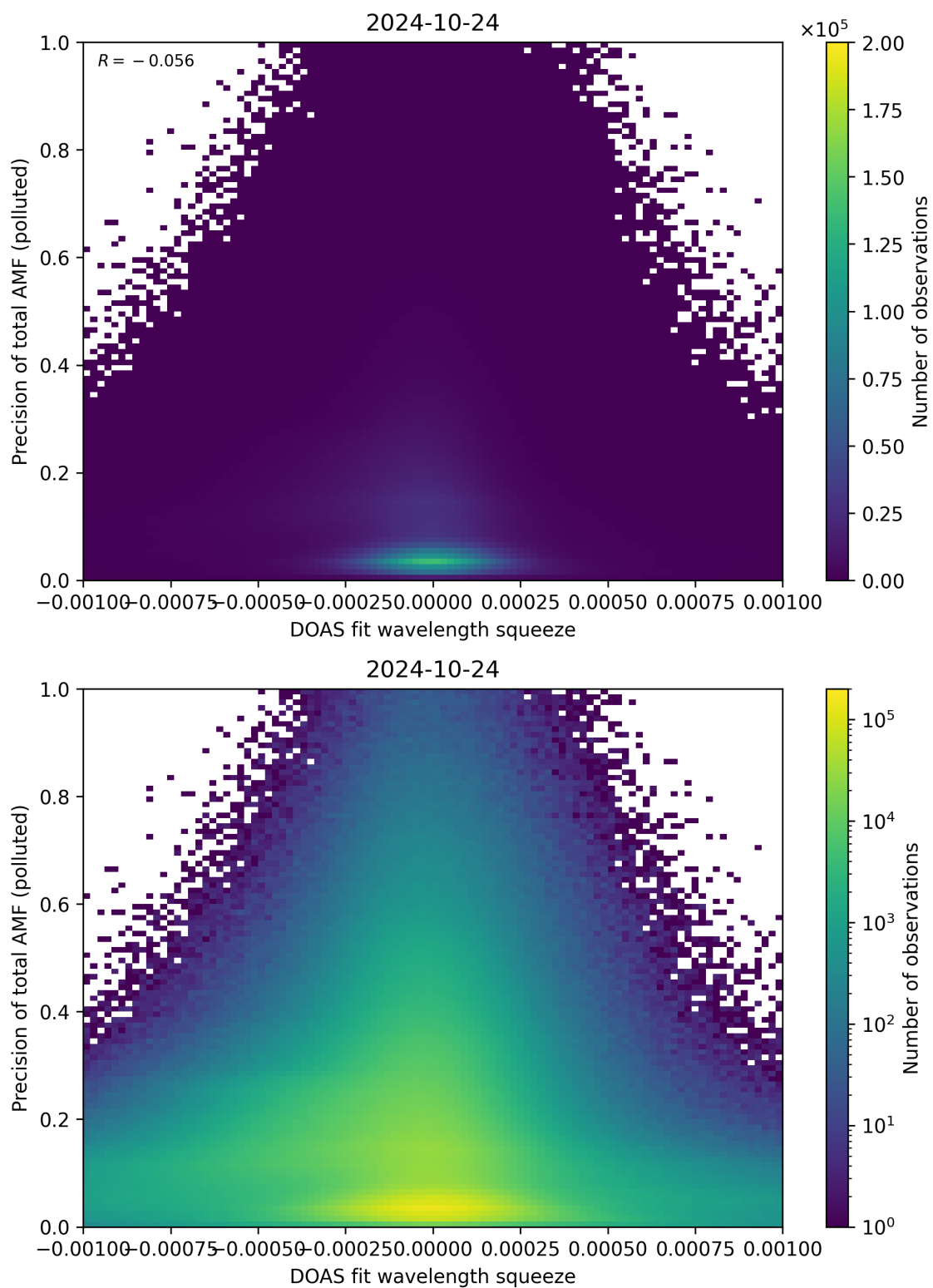
Figure 135: Scatter density plot of “DOAS fit wavelength squeeze” against “Precision of total AMF (polluted)” for 2024-10-24 to 2024-10-25.
