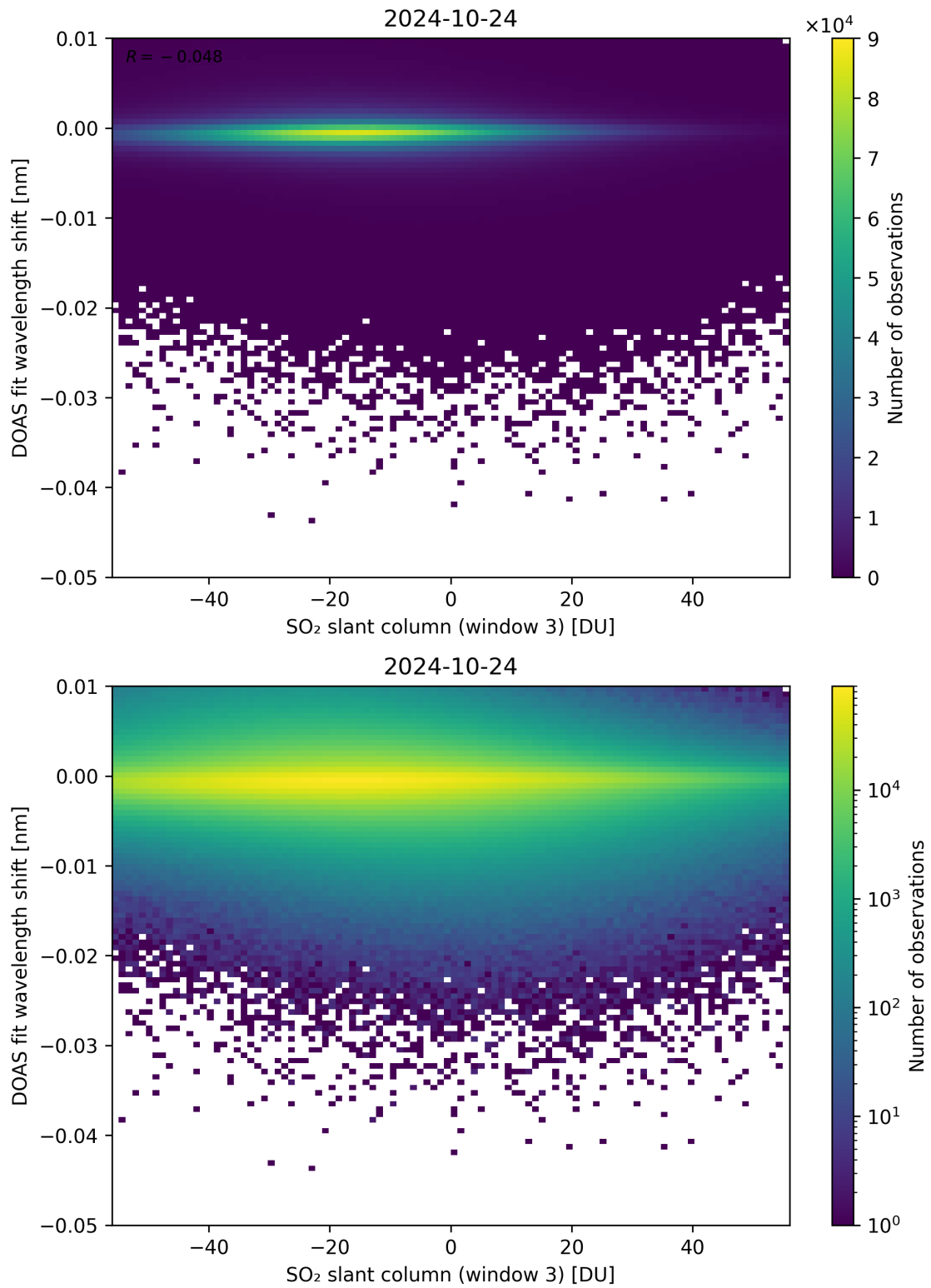
Figure 254: Scatter density plot of “SO 2 slant column (window 3)” against “DOAS fit wavelength shift” for 2024-10-24 to 2024-10-25.
