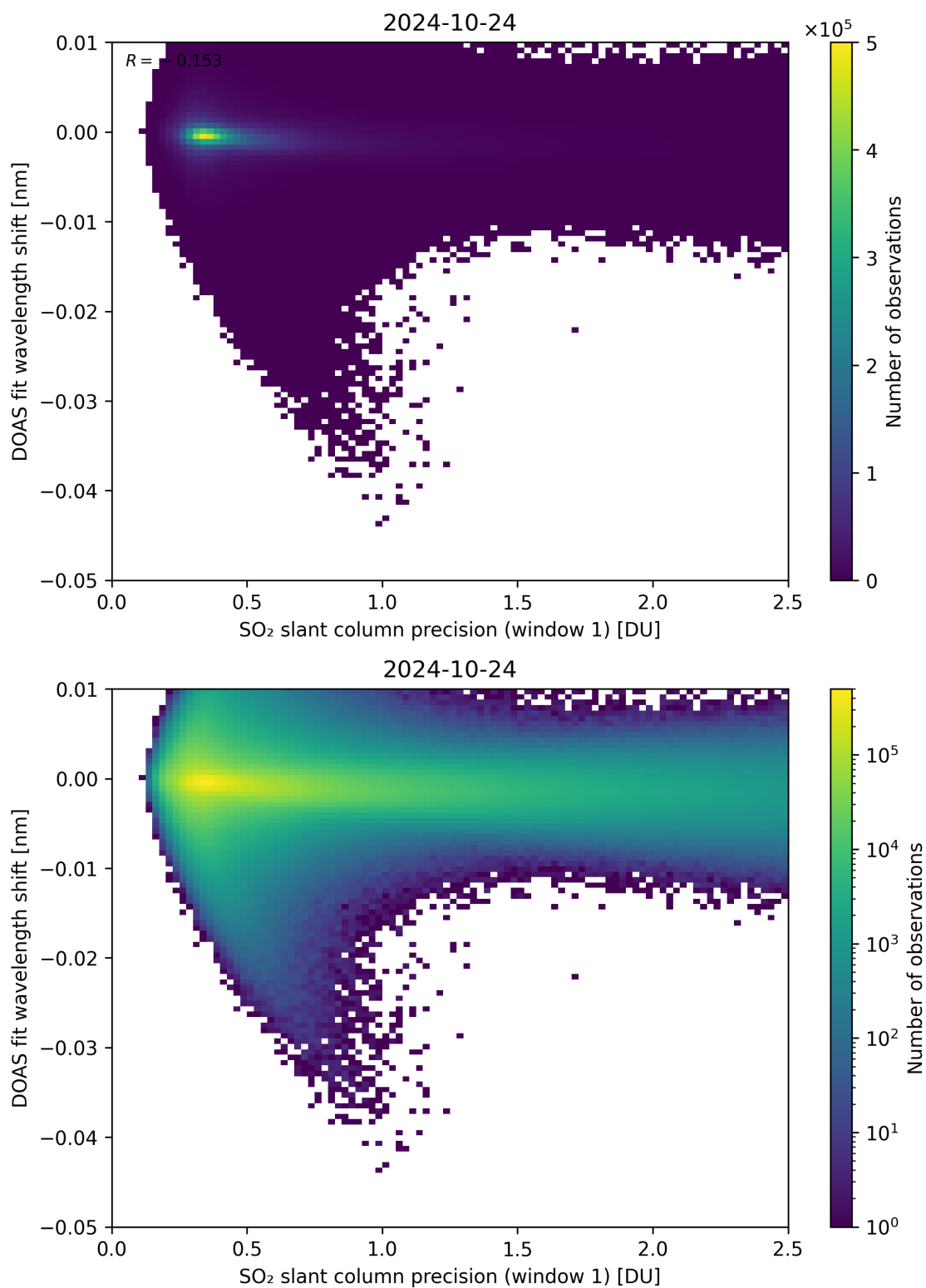
Figure 221: Scatter density plot of “SO 2 slant column precision (window 1)” against “DOAS fit wavelength shift” for 2024-10-24 to 2024-10-25.
