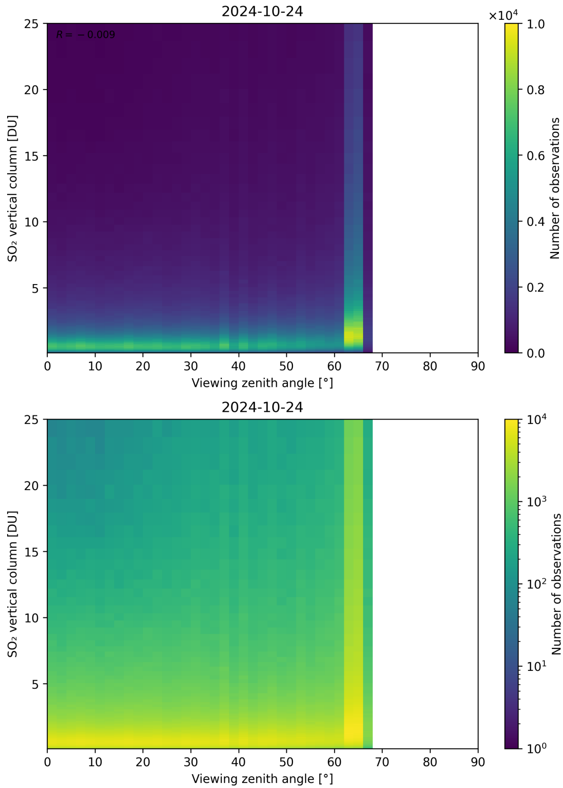
Figure 327: Scatter density plot of “Viewing zenith angle” against “SO 2 vertical column” for 2024-10-24 to 2024-10-25.
