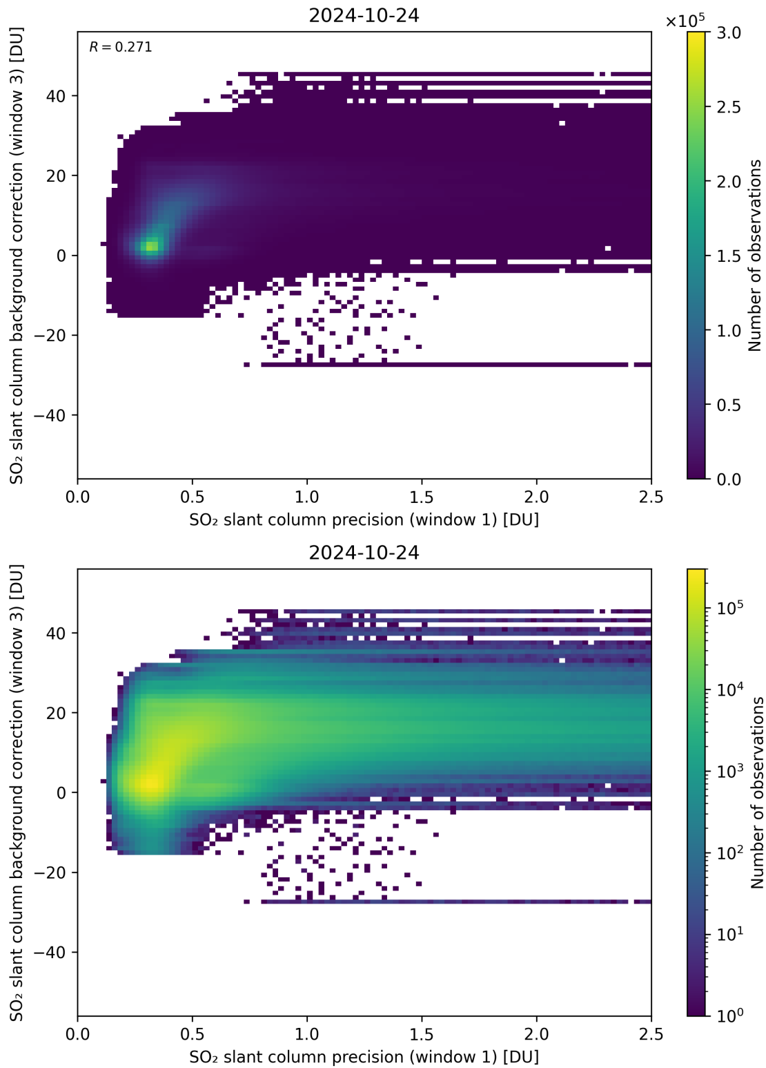
Figure 220: Scatter density plot of “SO 2 slant column precision (window 1)” against “SO 2 slant column background correction (window 3)” for 2024-10-24 to 2024-10-25.
