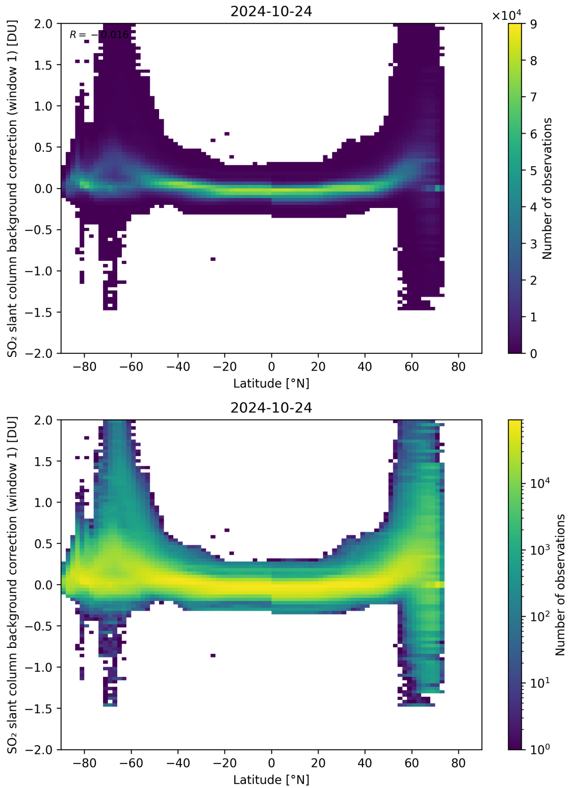
Figure 139: Scatter density plot of “Latitude” against “SO 2 slant column background correction (window 1)” for 2024-10-24 to 2024-10-25.
