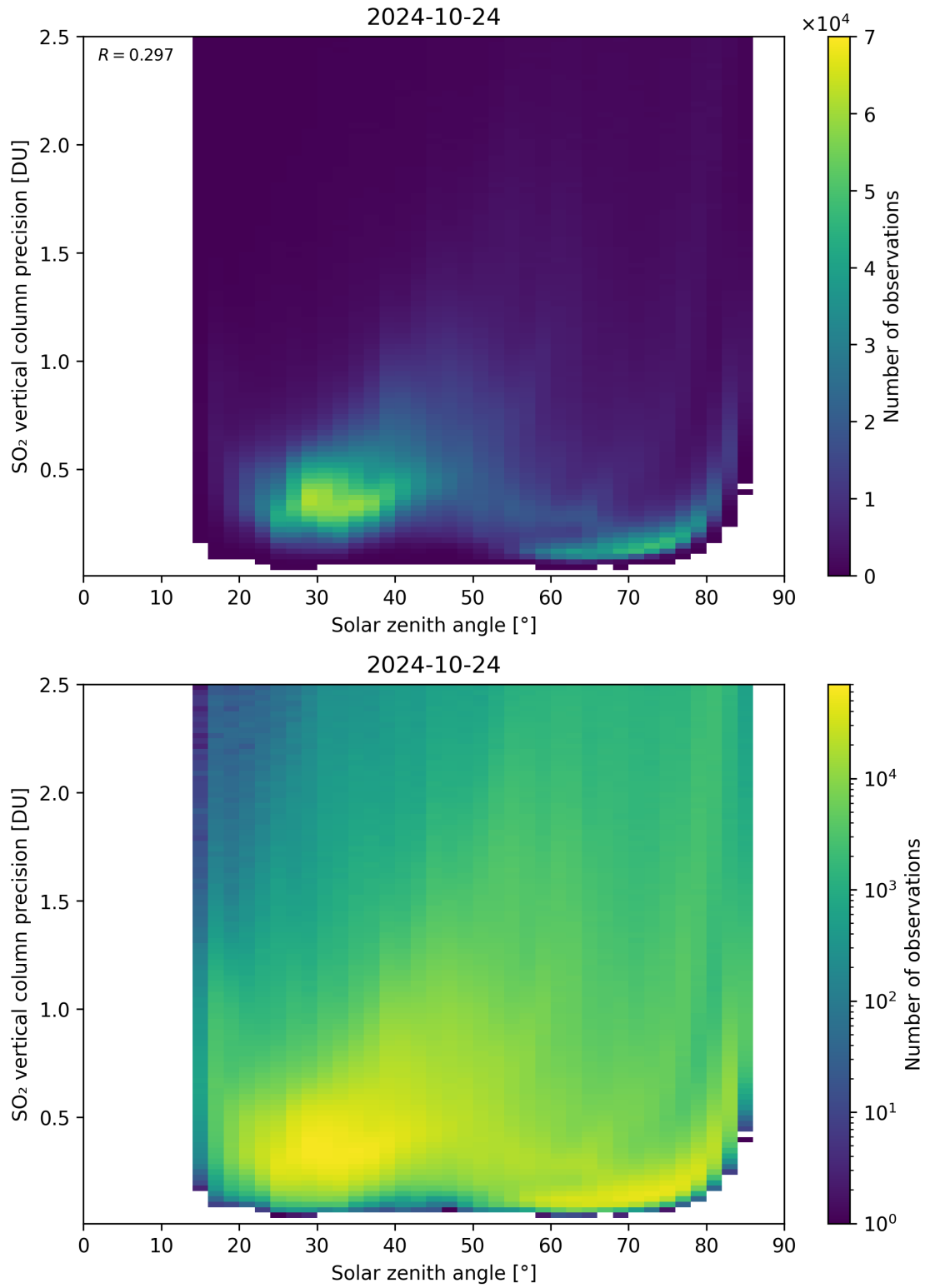
Figure 177: Scatter density plot of “Solar zenith angle” against “SO 2 vertical column precision” for 2024-10-24 to 2024-10-25.
