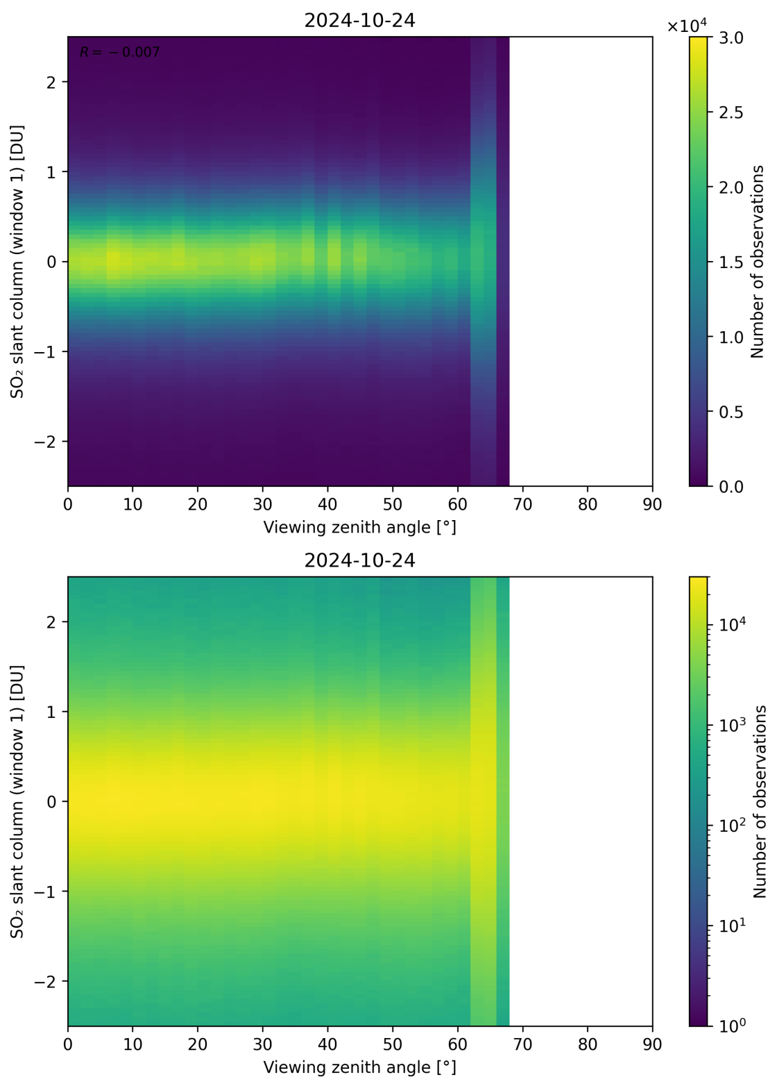
Figure 320: Scatter density plot of “Viewing zenith angle” against “SO 2 slant column (window 1)” for 2024-10-24 to 2024-10-25.
