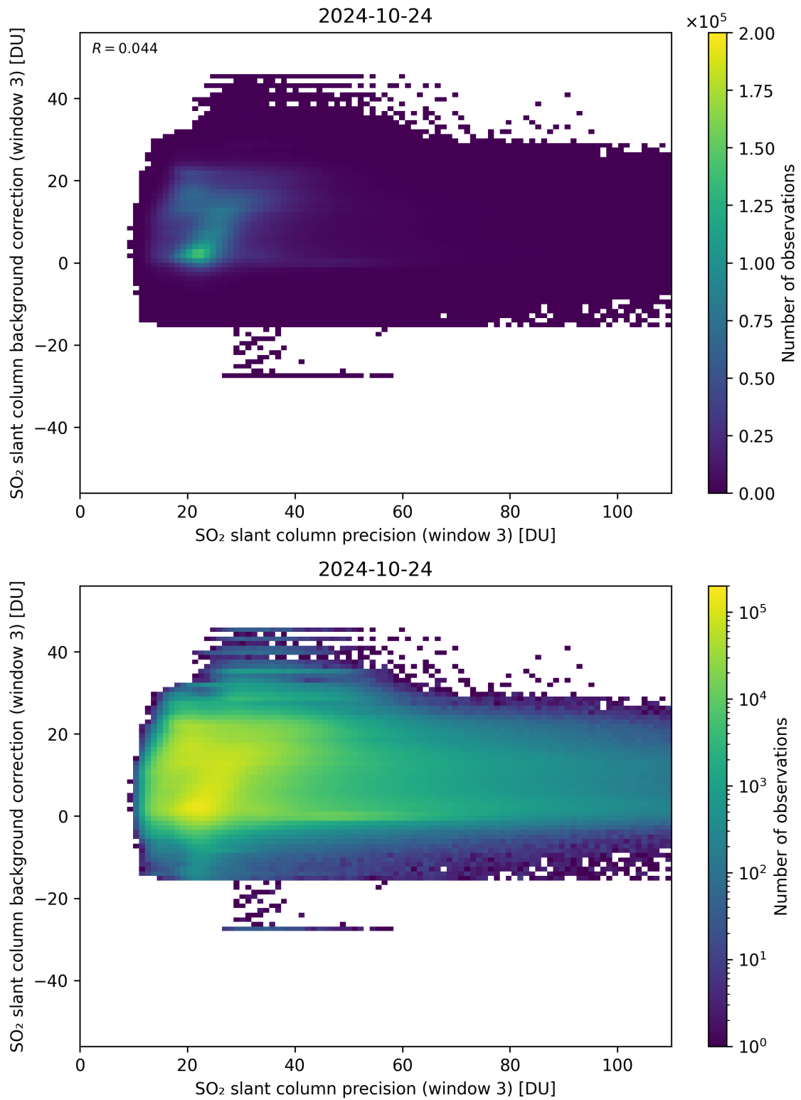
Figure 257: Scatter density plot of “SO 2 slant column precision (window 3)” against “SO 2 slant column background correction (window 3)” for 2024-10-24 to 2024-10-25.
