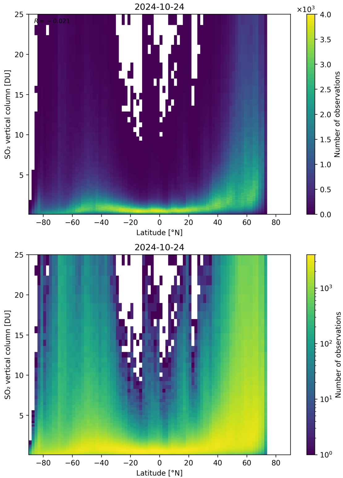
Figure 156: Scatter density plot of “Latitude” against “SO 2 vertical column” for 2024-10-24 to 2024-10-25.
