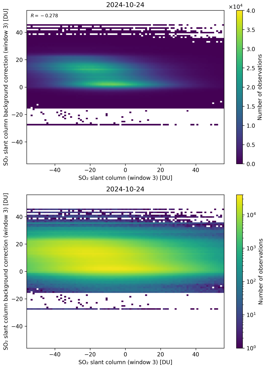
Figure 253: Scatter density plot of “SO 2 slant column (window 3)” against “SO 2 slant column background correction (window 3)” for 2024-10-24 to 2024-10-25.
