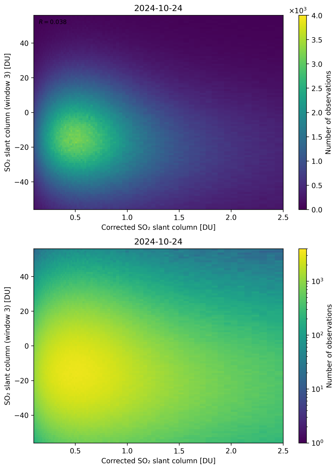
Figure 190: Scatter density plot of “Corrected SO 2 slant column” against “SO 2 slant column (window 3)” for 2024-10-24 to 2024-10-25.
