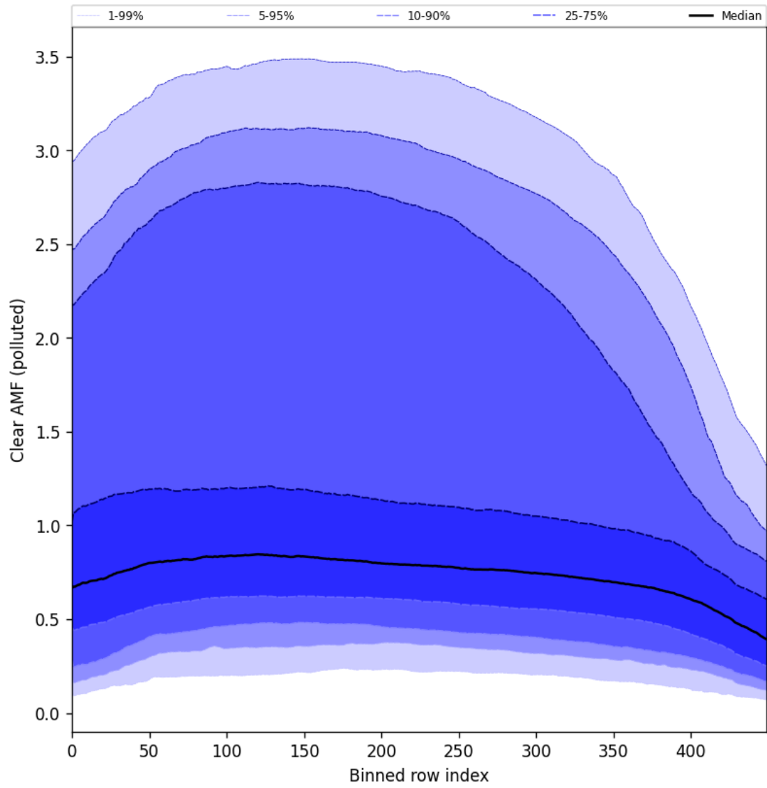
Figure 96: Along track statistics of “Clear AMF (polluted)” for 2024-10-24 to 2024-10-25
