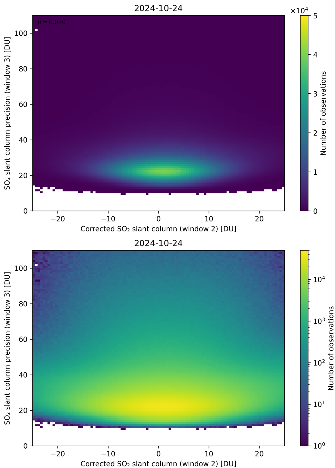
Figure 202: Scatter density plot of “Corrected SO 2 slant column (window 2)” against “SO 2 slant column precision (window 3)” for 2024-10-24 to 2024-10-25.
