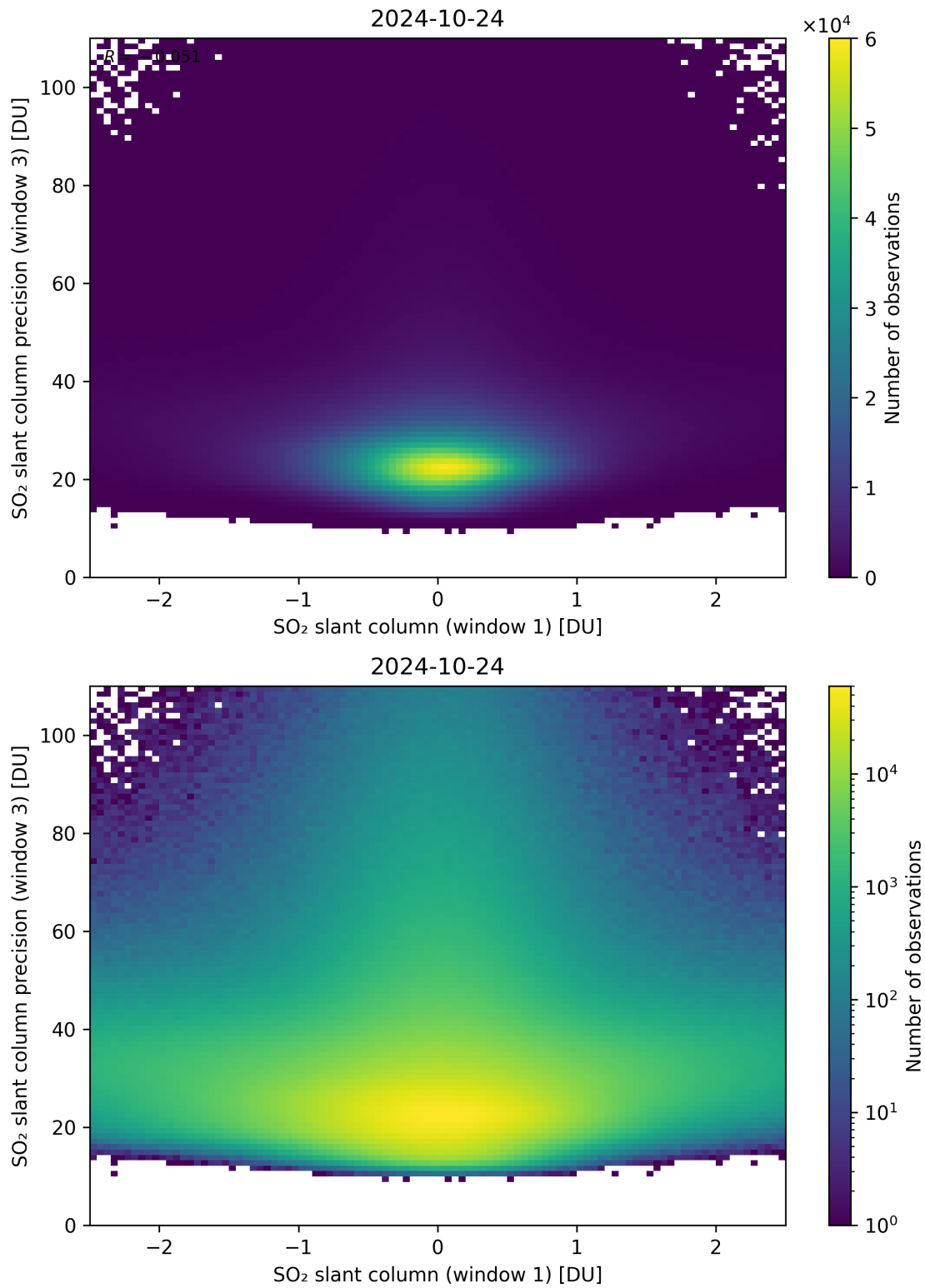
Figure 238: Scatter density plot of “SO 2 slant column (window 1)” against “SO 2 slant column precision (window 3)” for 2024-10-24 to 2024-10-25.
