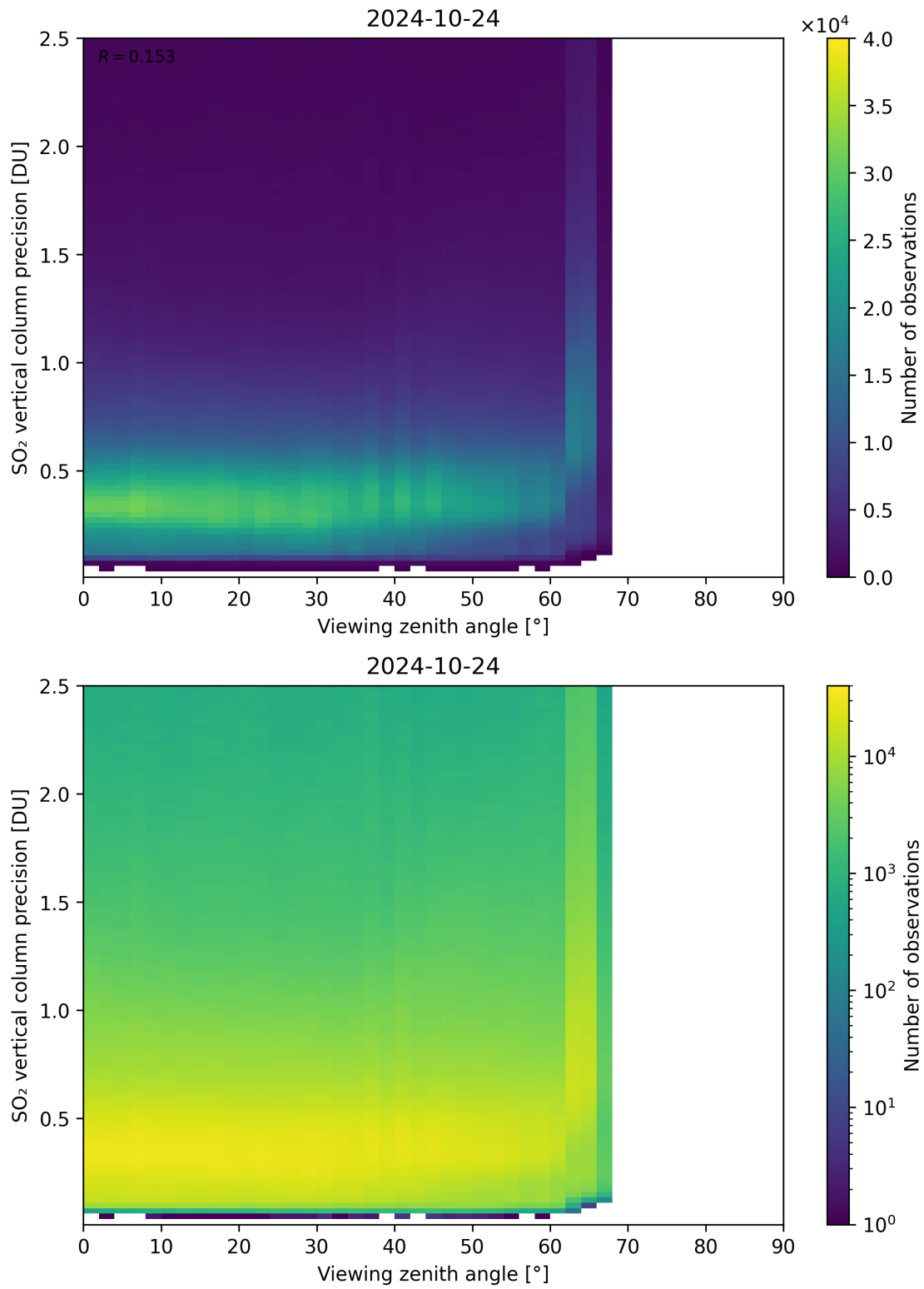
Figure 328: Scatter density plot of “Viewing zenith angle” against “SO 2 vertical column precision” for 2024-10-24 to 2024-10-25.
