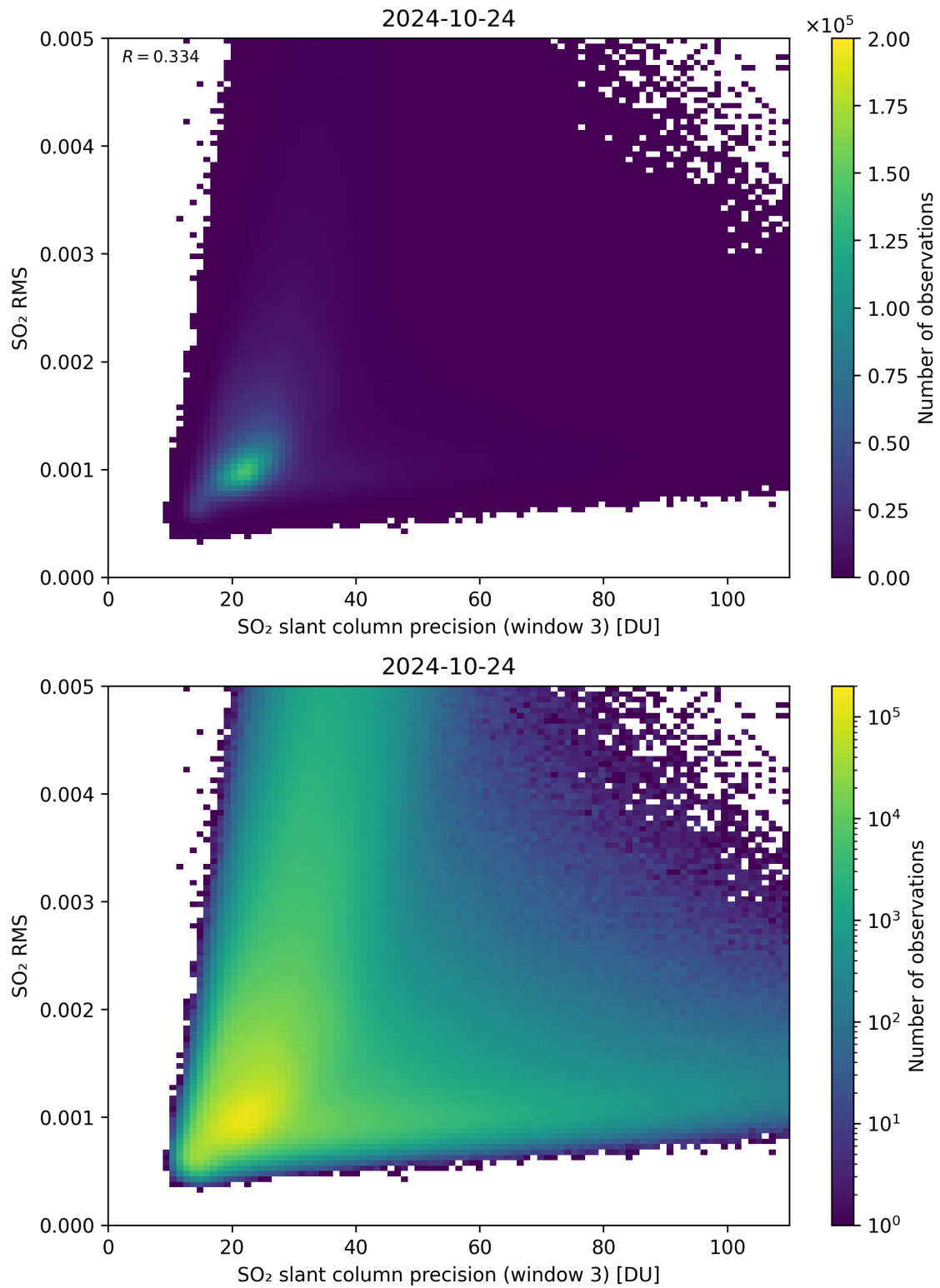
Figure 260: Scatter density plot of “SO 2 slant column precision (window 3)” against “SO 2 RMS” for 2024-10-24 to 2024-10-25.
