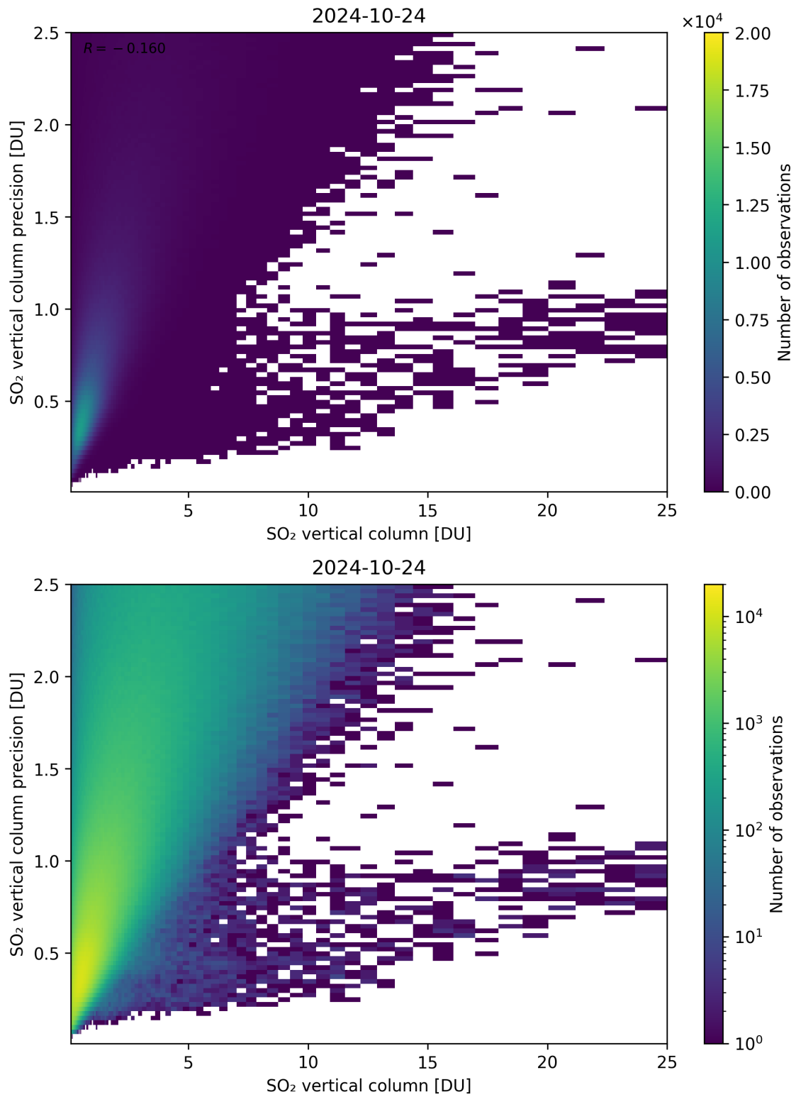
Figure 307: Scatter density plot of “SO 2 vertical column” against “SO 2 vertical column precision” for 2024-10-24 to 2024-10-25.
