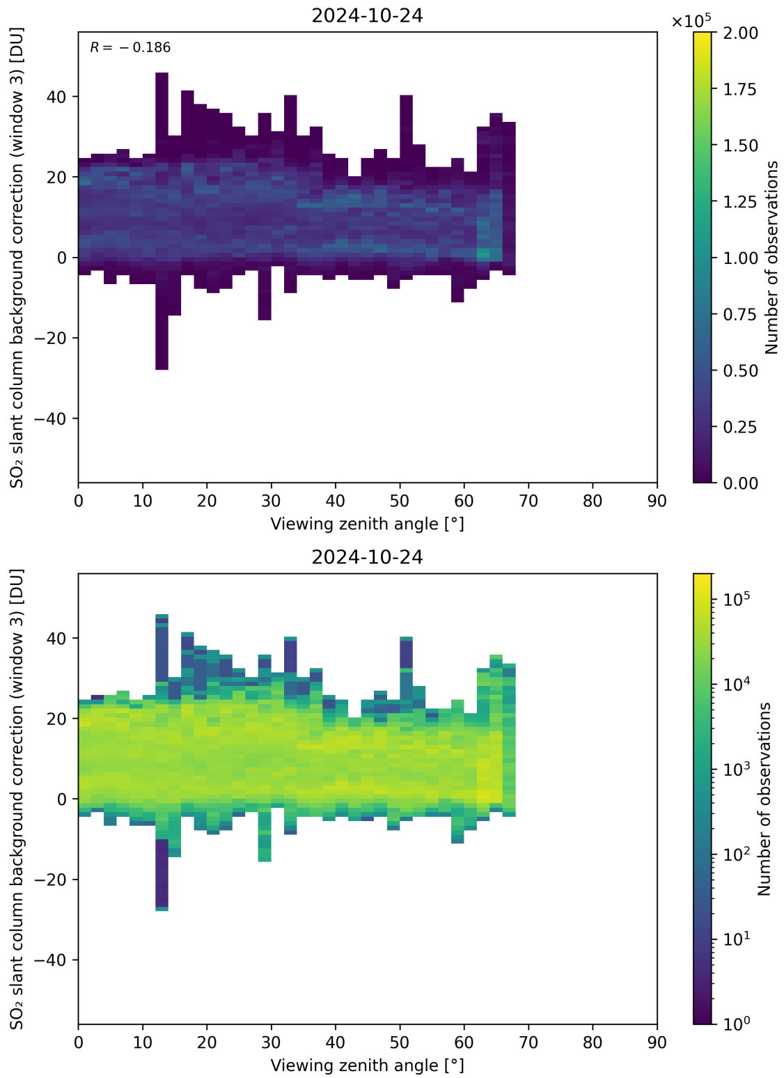
Figure 310: Scatter density plot of “Viewing zenith angle” against “SO 2 slant column background correction (window 3)” for 2024-10-24 to 2024-10-25.
