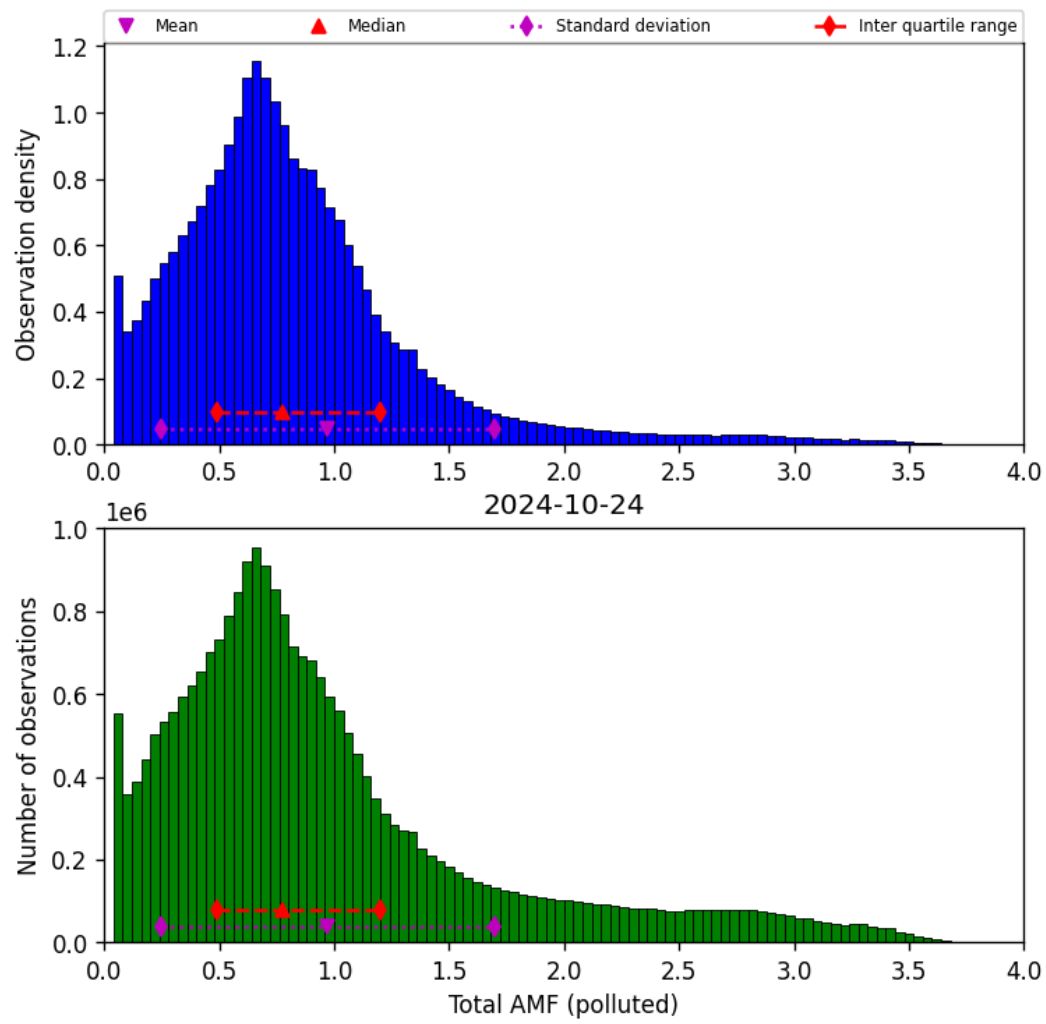
Figure 71: Histogram of “Total AMF (polluted)” for 2024-10-24 to 2024-10-25
