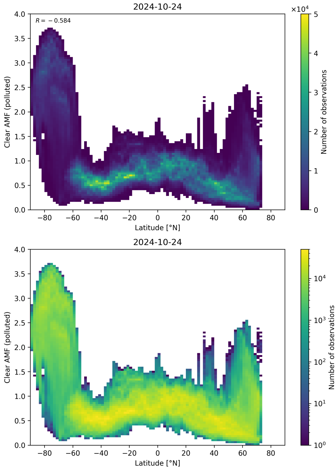
Figure 145: Scatter density plot of “Latitude” against “Clear AMF (polluted)” for 2024-10-24 to 2024-10-25.
