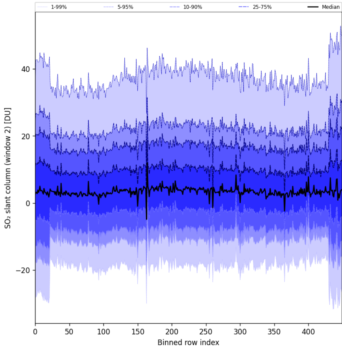
Figure 83: Along track statistics of “SO 2 slant column (window 2)” for 2024-10-24 to 2024-10-25
