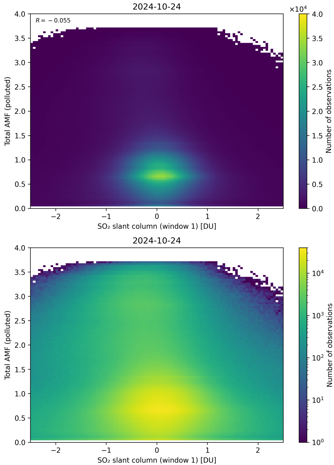
Figure 239: Scatter density plot of “SO 2 slant column (window 1)” against “Total AMF (polluted)” for 2024-10-24 to 2024-10-25.
