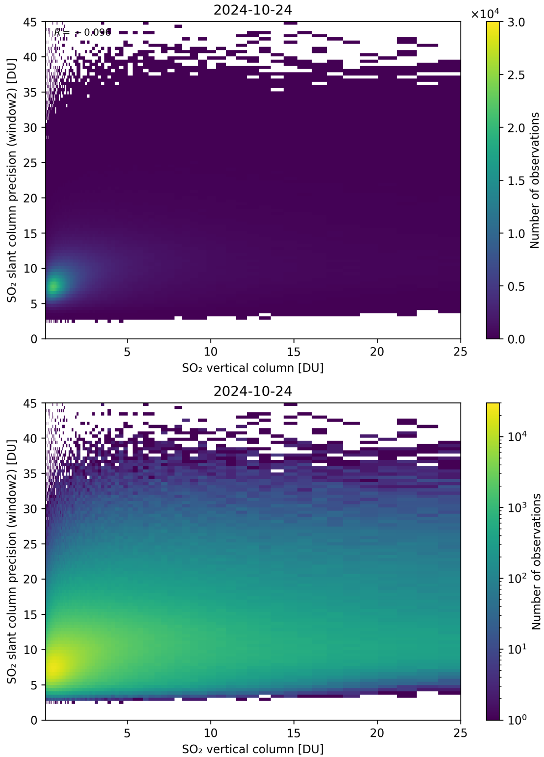
Figure 302: Scatter density plot of “SO 2 vertical column” against “SO 2 slant column precision (window2)” for 2024-10-24 to 2024-10-25.
