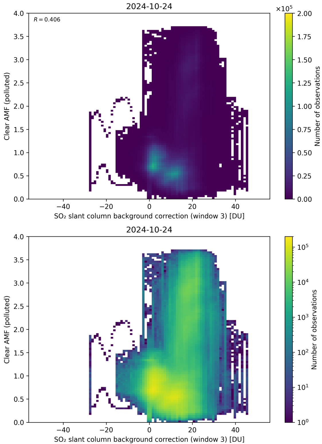
Figure 124: Scatter density plot of “SO 2 slant column background correction (window 3)” against “Clear AMF (polluted)” for 2024-10-24 to 2024-10-25.
