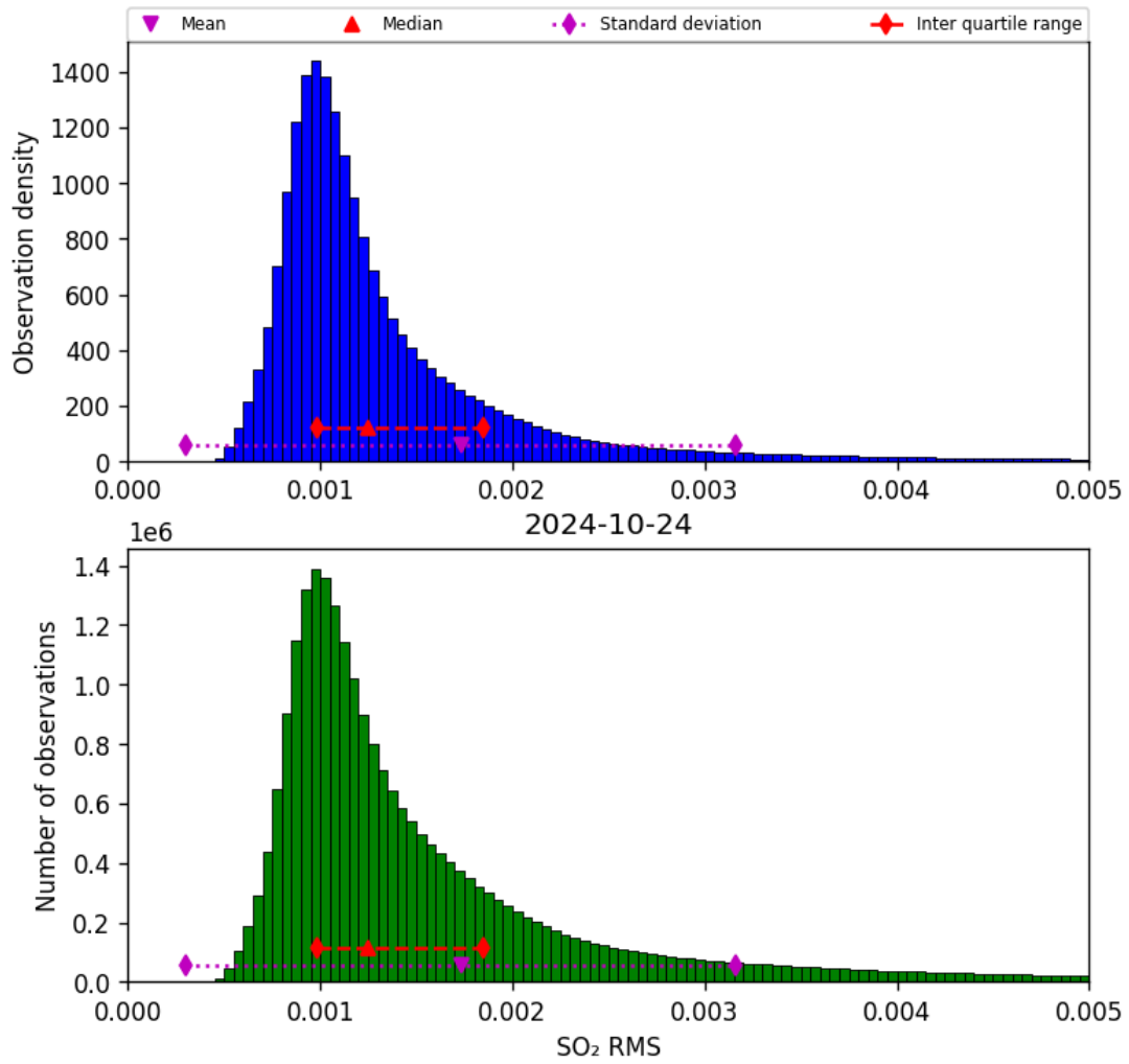
Figure 70: Histogram of “SO 2 RMS” for 2024-10-24 to 2024-10-25
