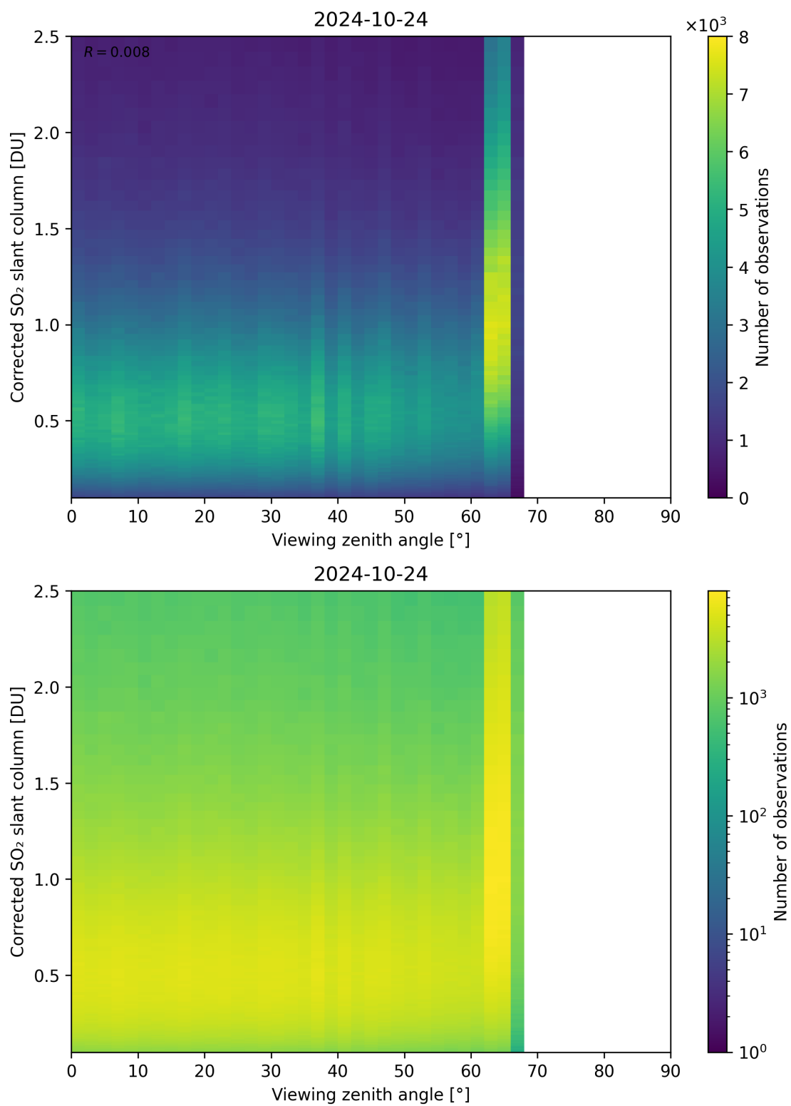
Figure 317: Scatter density plot of “Viewing zenith angle” against “Corrected SO 2 slant column” for 2024-10-24 to 2024-10-25.
