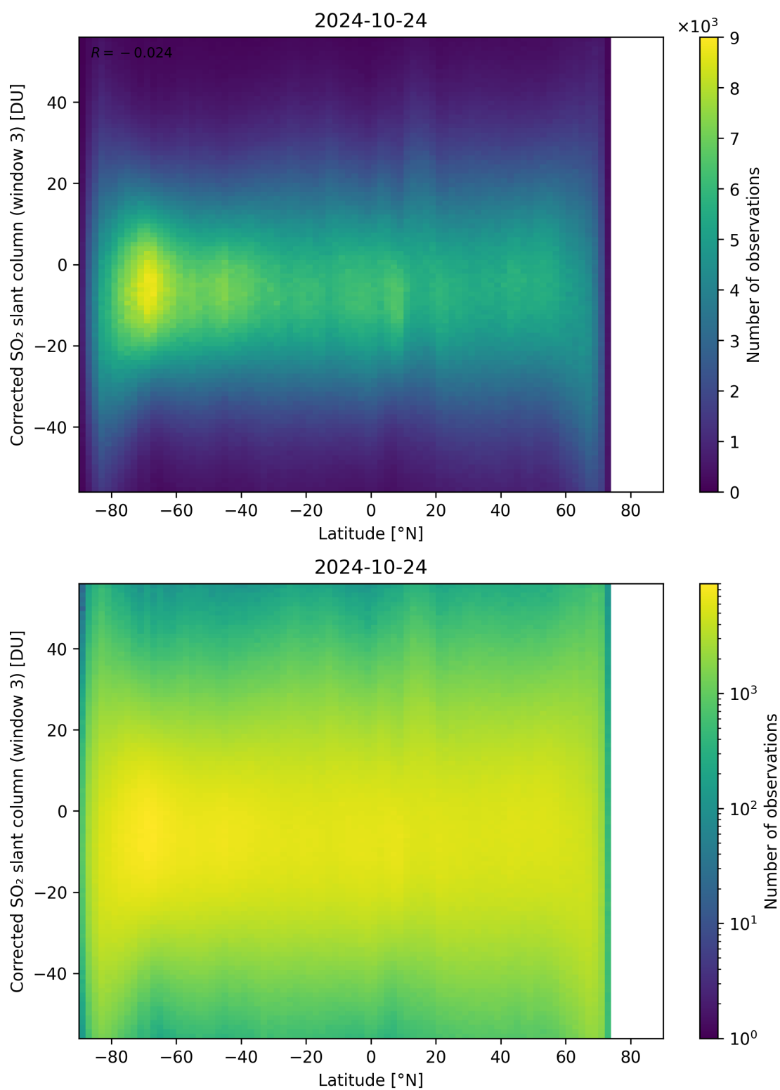
Figure 148: Scatter density plot of “Latitude” against “Corrected SO 2 slant column (window 3)” for 2024-10-24 to 2024-10-25.
