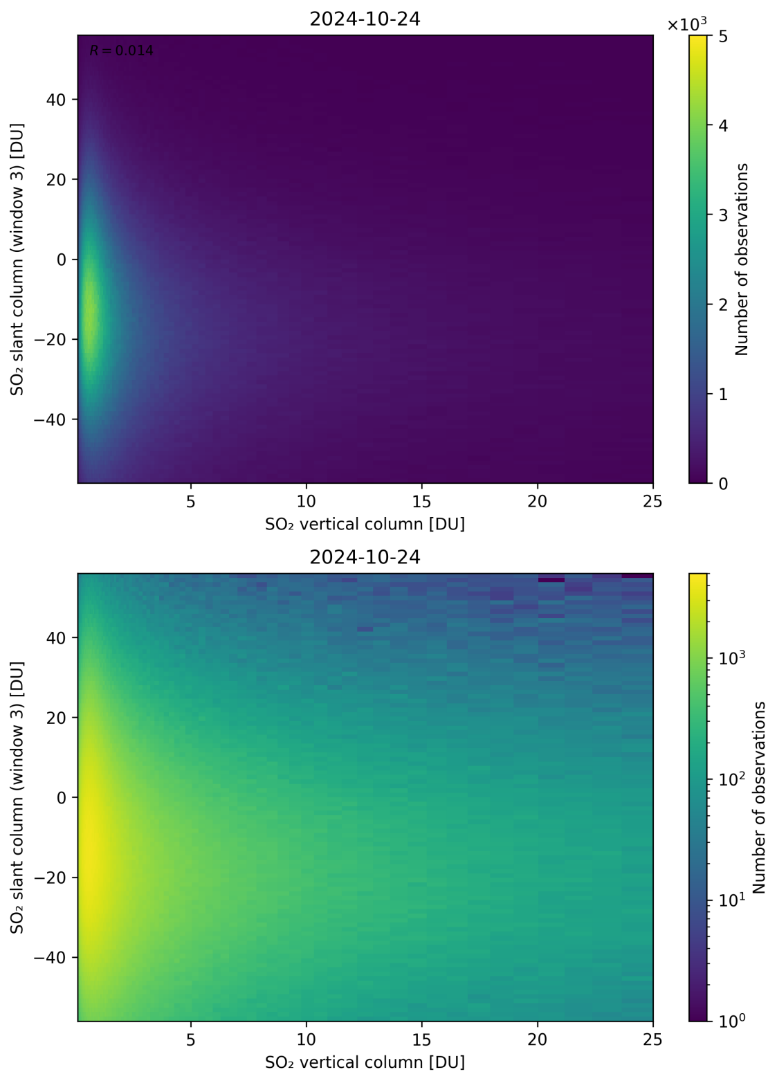
Figure 303: Scatter density plot of “SO 2 vertical column” against “SO 2 slant column (window 3)” for 2024-10-24 to 2024-10-25.
