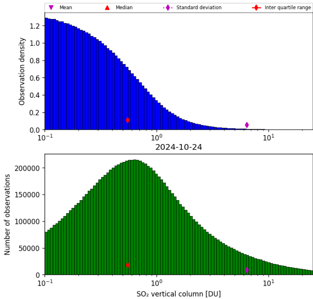
Figure 53: Histogram of “SO 2 vertical column” for 2024-10-24 to 2024-10-25
