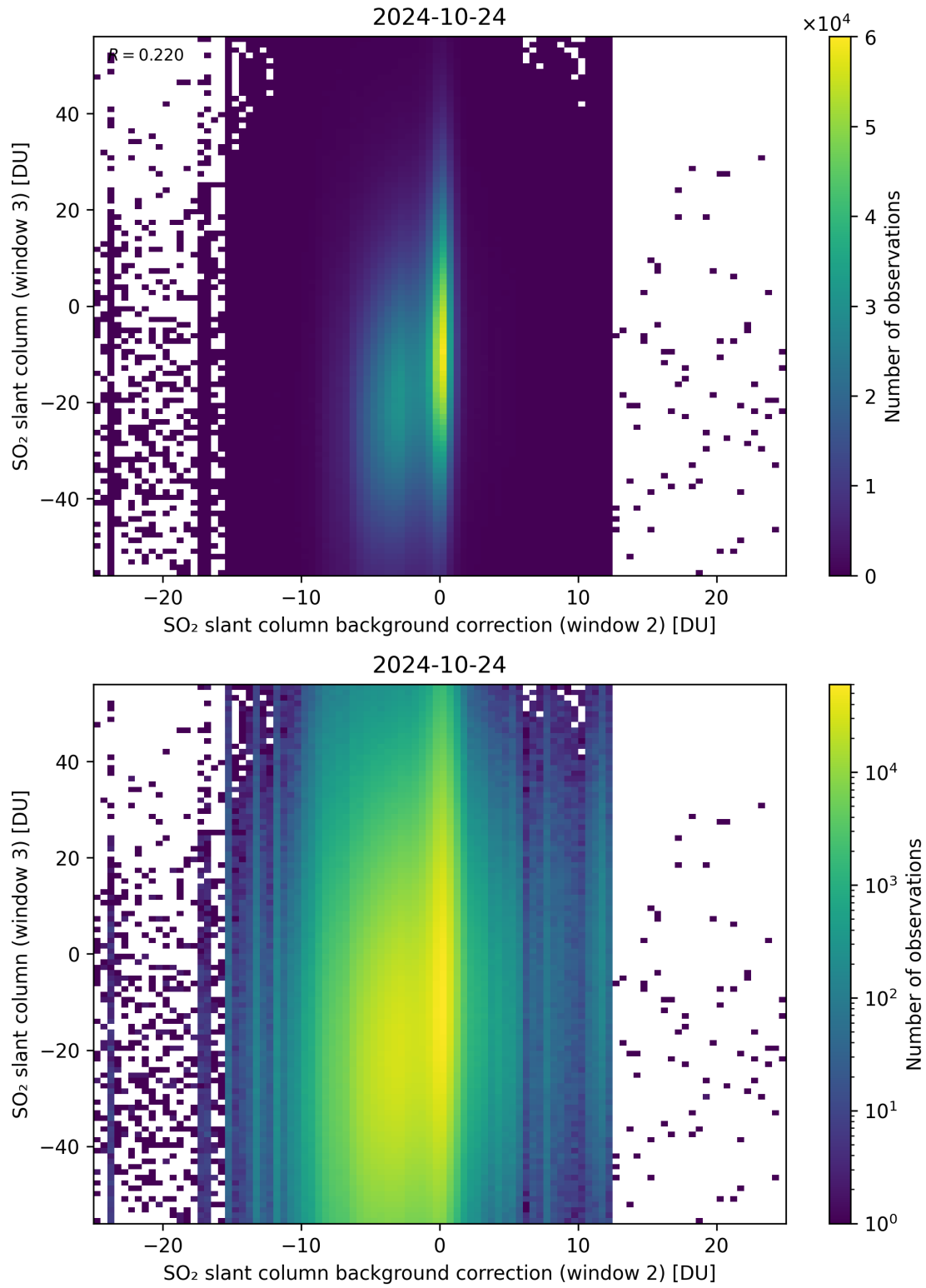
Figure 117: Scatter density plot of “SO 2 slant column background correction (window 2)” against “SO 2 slant column (window 3)” for 2024-10-24 to 2024-10-25.
