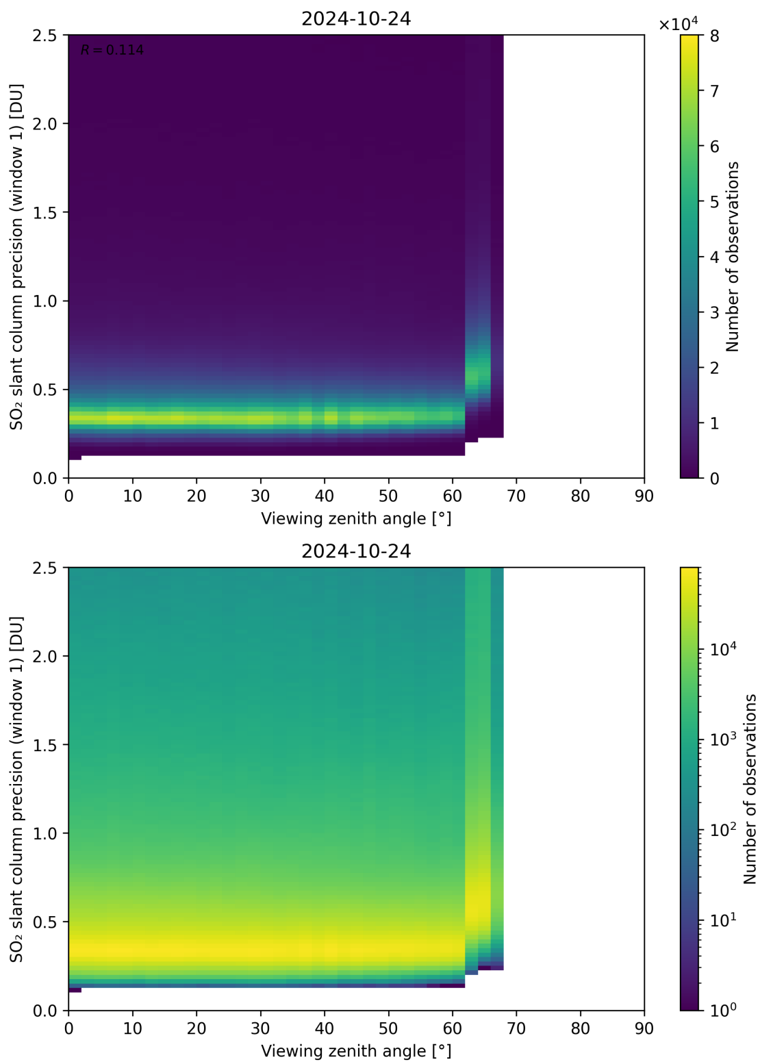
Figure 321: Scatter density plot of “Viewing zenith angle” against “SO 2 slant column precision (window 1)” for 2024-10-24 to 2024-10-25.
