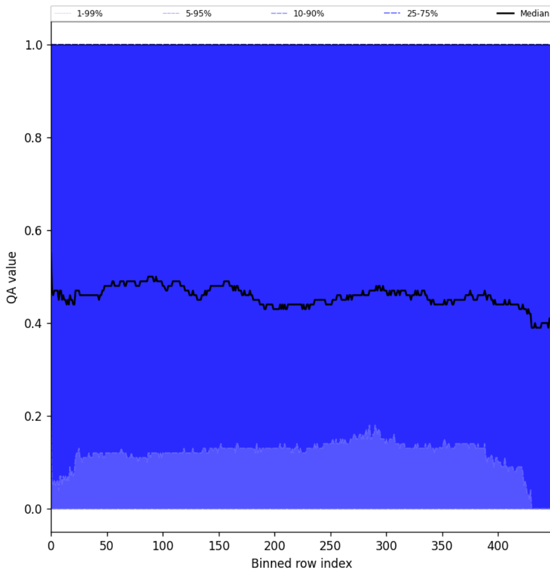
Figure 75: Along track statistics of “QA value” for 2024-10-24 to 2024-10-25
