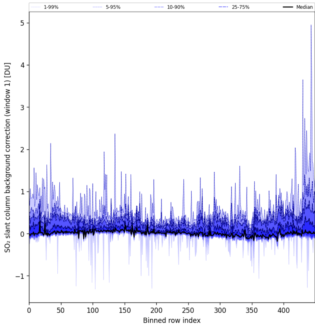
Figure 82: Along track statistics of “SO 2 slant column background correction (window 1)” for 2024-10-24 to 2024-10-25
