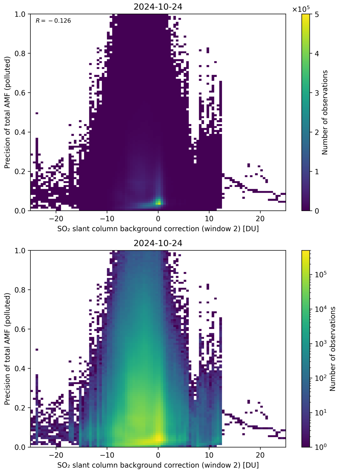
Figure 120: Scatter density plot of “SO 2 slant column background correction (window 2)” against “Precision of total AMF (polluted)” for 2024-10-24 to 2024-10-25.
