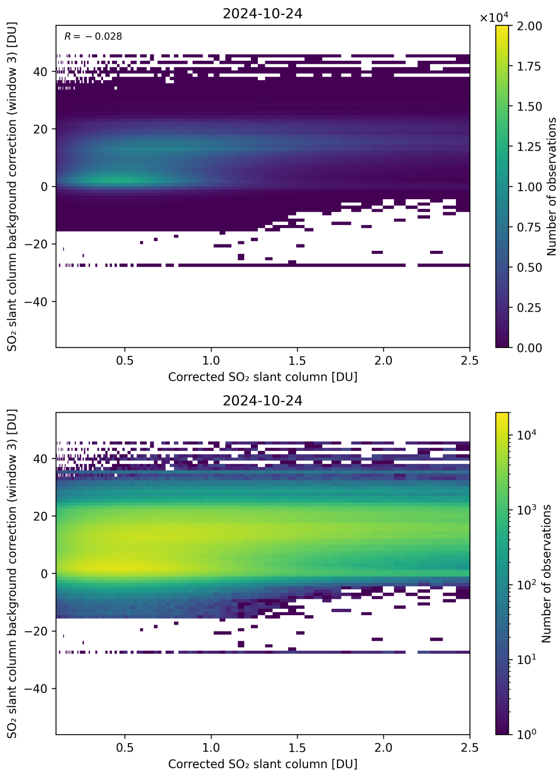
Figure 180: Scatter density plot of “Corrected SO 2 slant column” against “SO 2 slant column background correction (window 3)” for 2024-10-24 to 2024-10-25.
