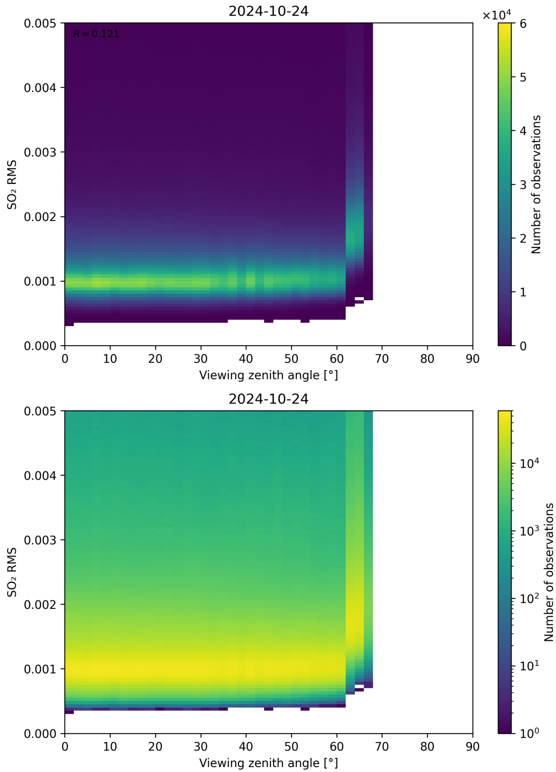
Figure 313: Scatter density plot of “Viewing zenith angle” against “SO 2 RMS” for 2024-10-24 to 2024-10-25.
