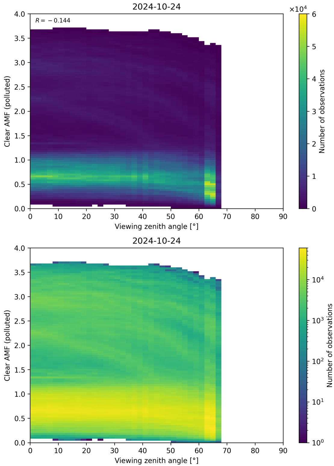
Figure 316: Scatter density plot of “Viewing zenith angle” against “Clear AMF (polluted)” for 2024-10-24 to 2024-10-25.
