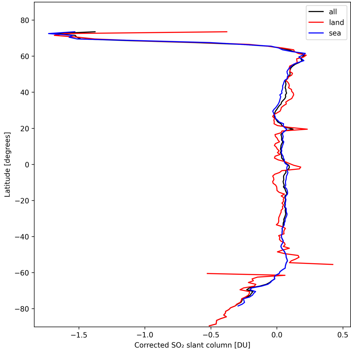
Figure 32: Zonal average of “Corrected SO 2 slant column” for 2024-10-24 to 2024-10-25.
