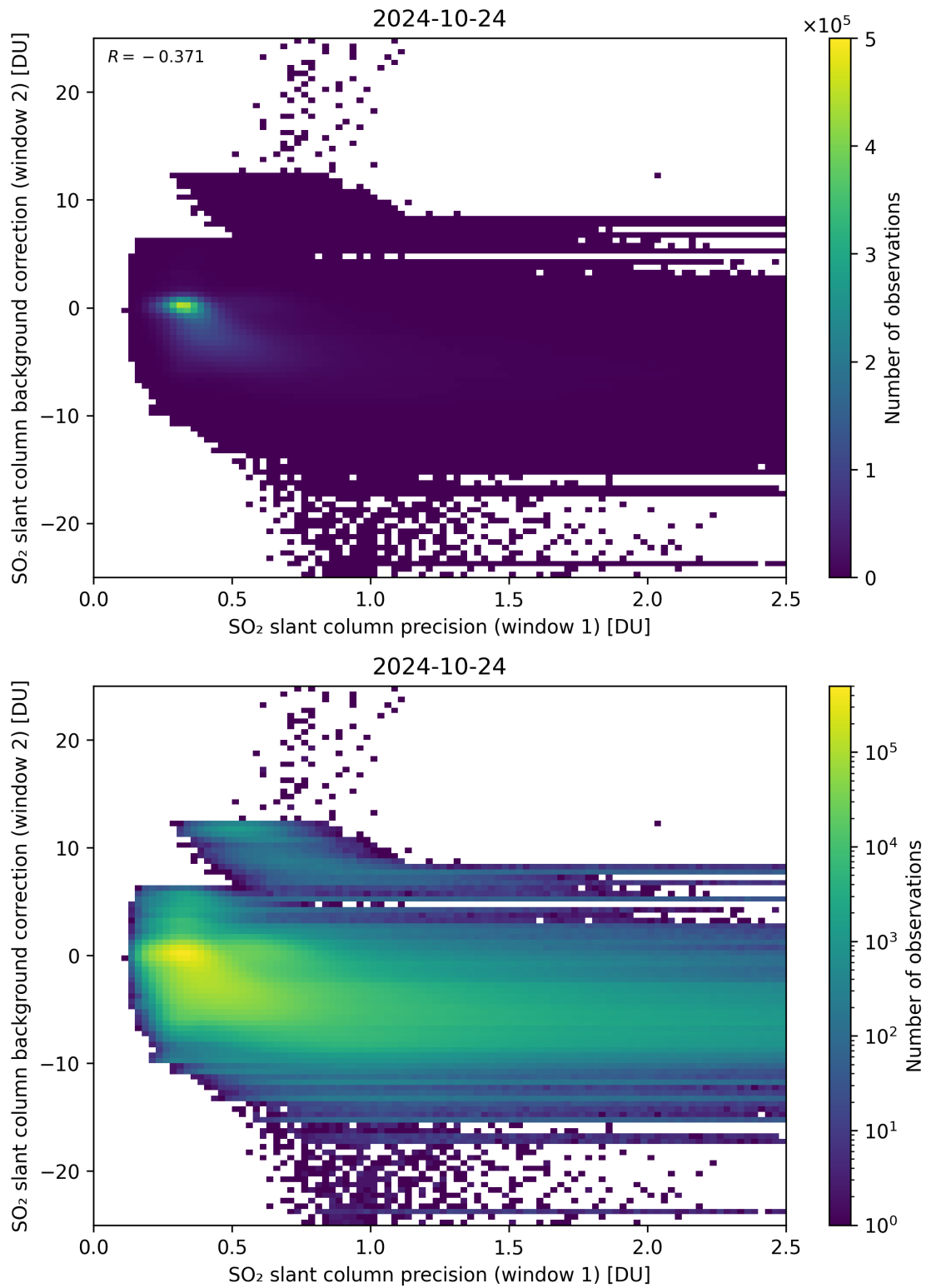
Figure 219: Scatter density plot of “SO 2 slant column precision (window 1)” against “SO 2 slant column background correction (window 2)” for 2024-10-24 to 2024-10-25.
