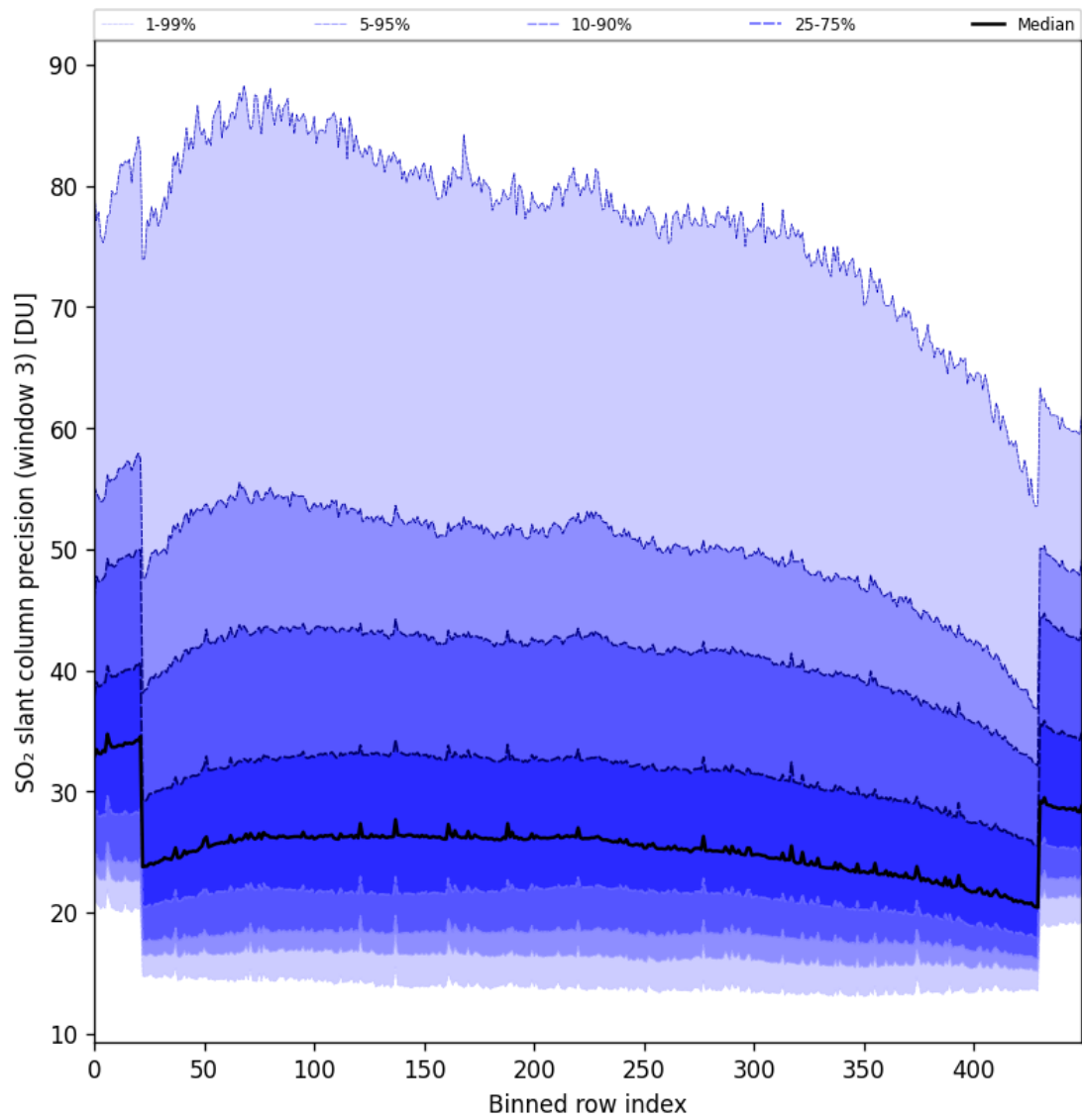
Figure 88: Along track statistics of “SO 2 slant column precision (window 3)” for 2024-10-24 to 2024-10-25
