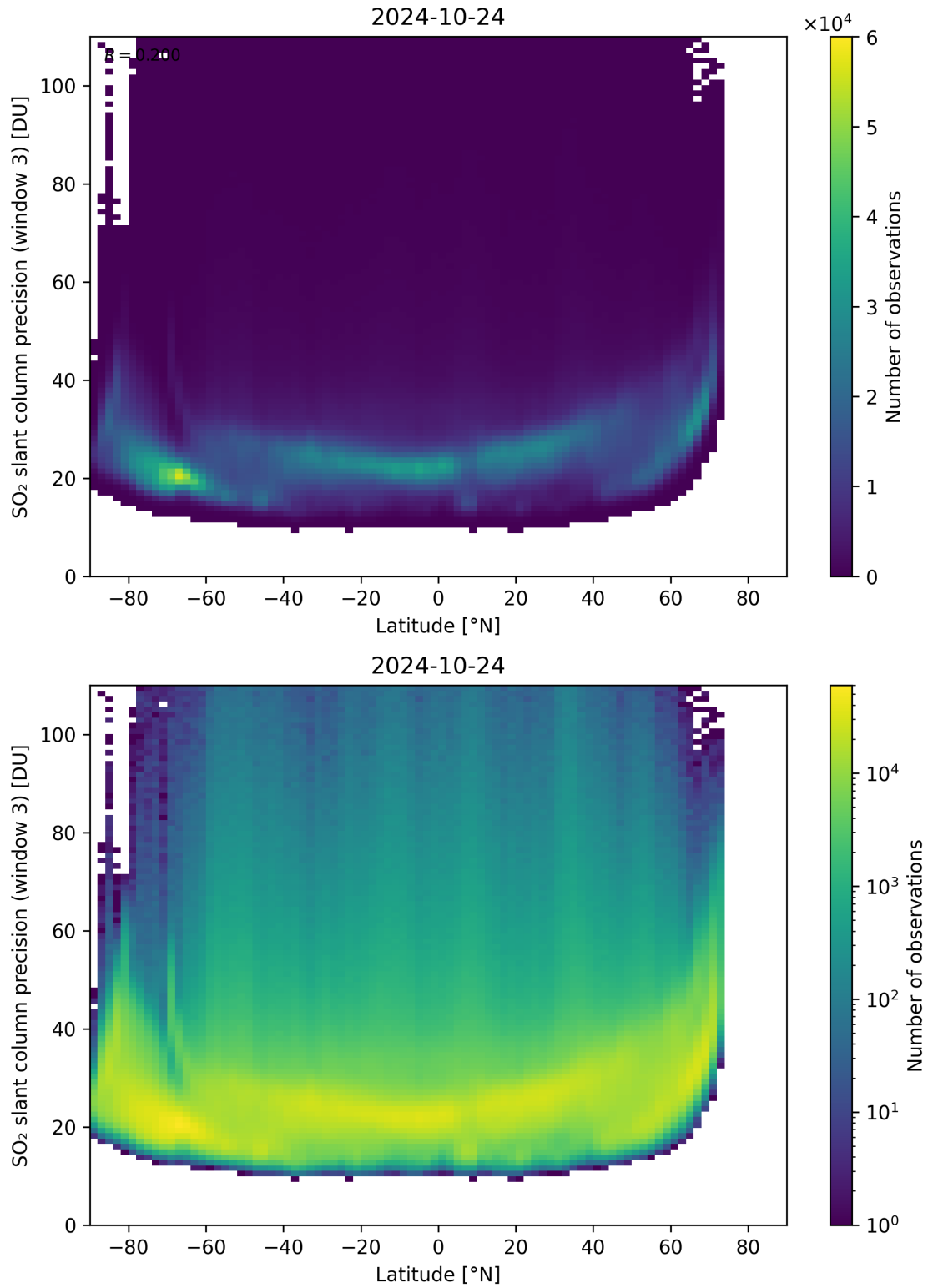
Figure 153: Scatter density plot of “Latitude” against “SO 2 slant column precision (window 3)” for 2024-10-24 to 2024-10-25.
