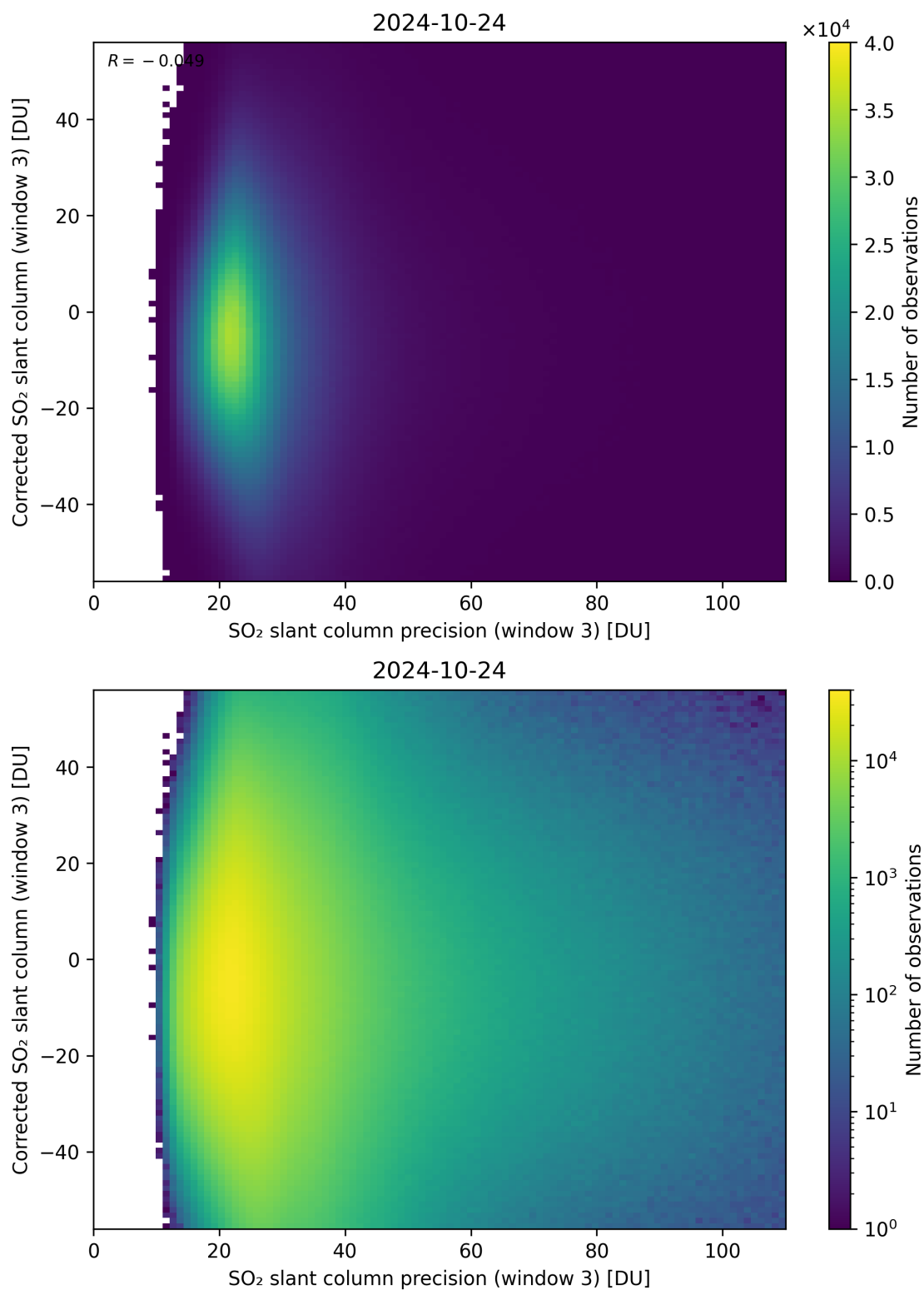
Figure 262: Scatter density plot of “SO 2 slant column precision (window 3)” against “Corrected SO 2 slant column (window 3)” for 2024-10-24 to 2024-10-25.
