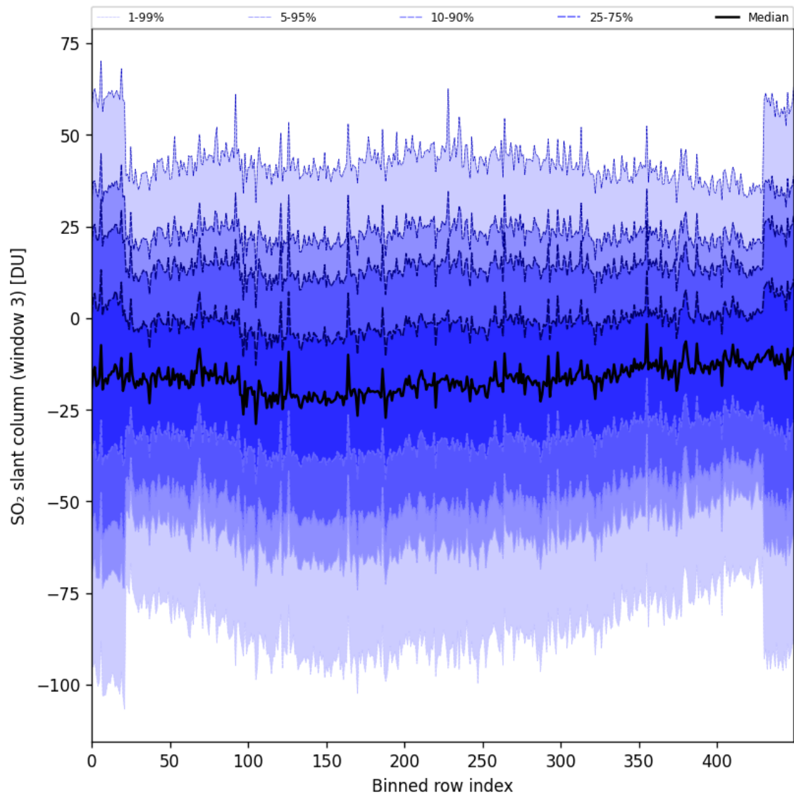
Figure 87: Along track statistics of “SO 2 slant column (window 3)” for 2024-10-24 to 2024-10-25
