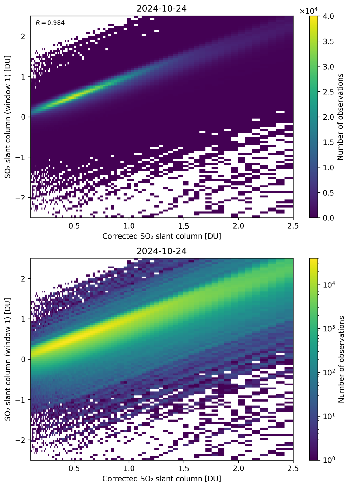
Figure 187: Scatter density plot of “Corrected SO 2 slant column” against “SO 2 slant column (window 1)” for 2024-10-24 to 2024-10-25.
