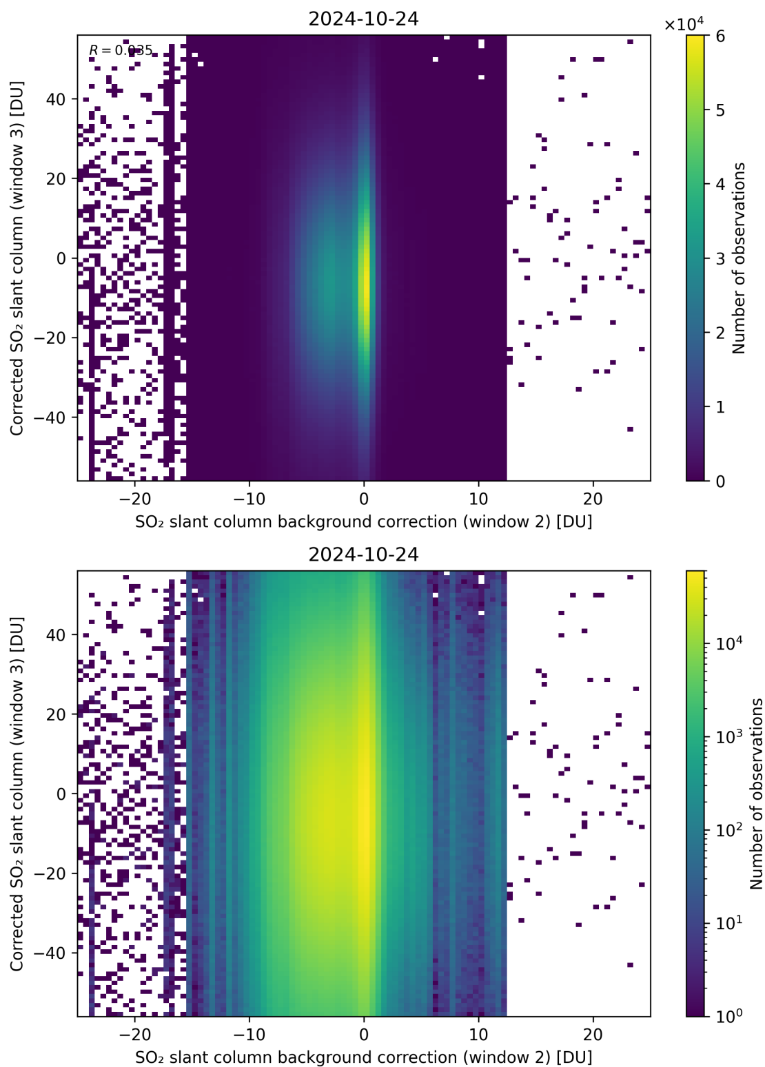
Figure 116: Scatter density plot of “SO 2 slant column background correction (window 2)” against “Corrected SO 2 slant column (window 3)” for 2024-10-24 to 2024-10-25.
