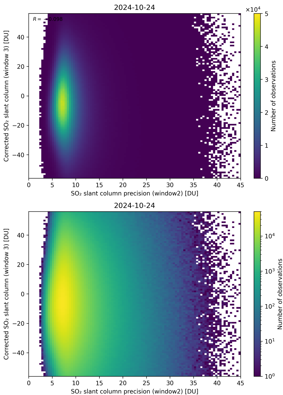
Figure 248: Scatter density plot of “SO 2 slant column precision (window2)” against “Corrected SO 2 slant column (window 3)” for 2024-10-24 to 2024-10-25.
