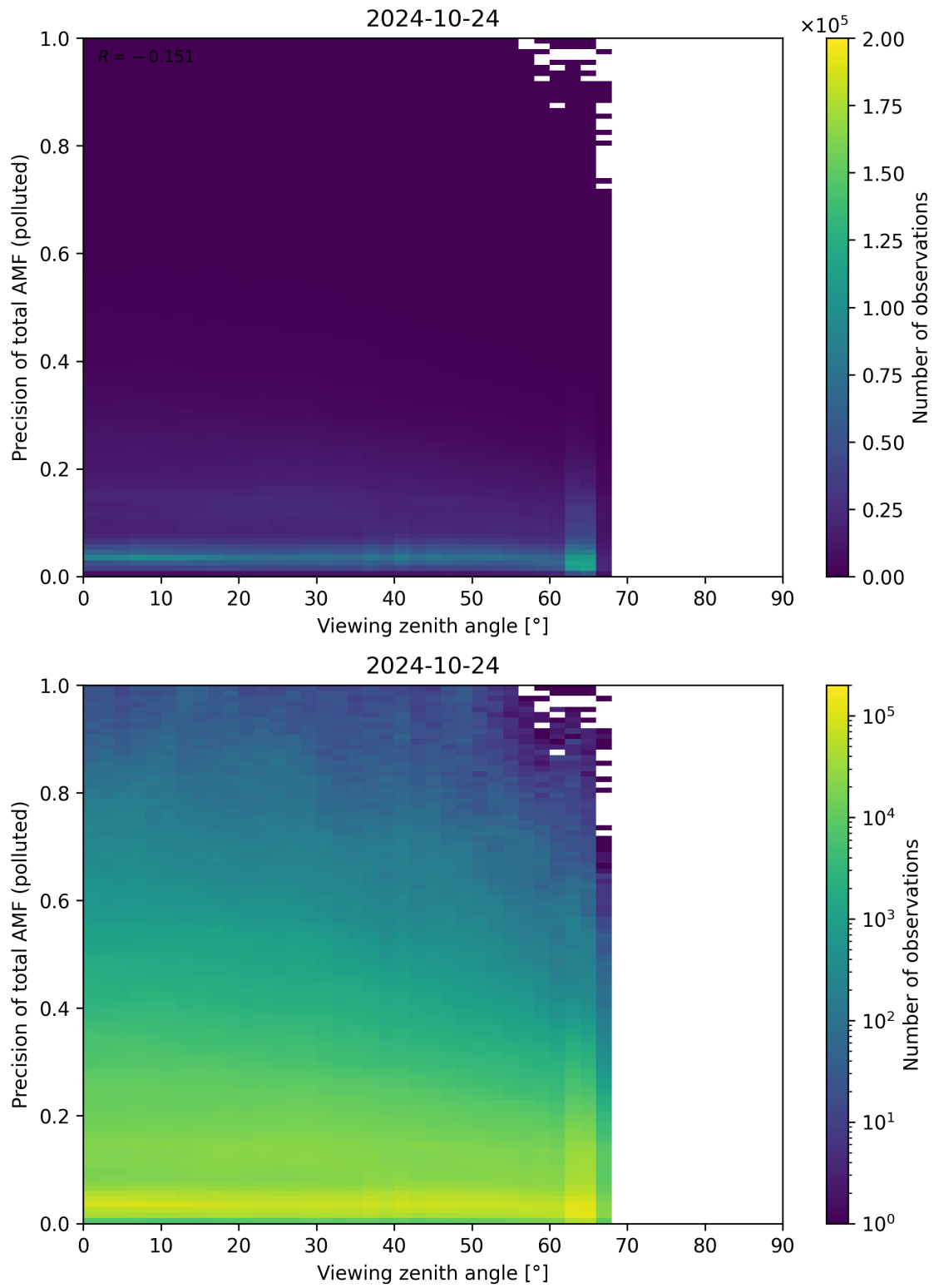
Figure 326: Scatter density plot of “Viewing zenith angle” against “Precision of total AMF (polluted)” for 2024-10-24 to 2024-10-25.
