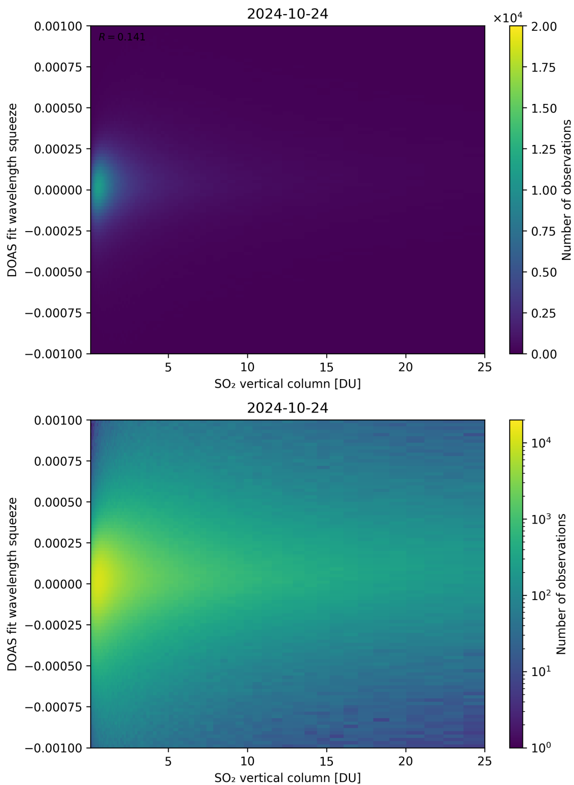
Figure 277: Scatter density plot of “SO 2 vertical column” against “DOAS fit wavelength squeeze” for 2024-10-24 to 2024-10-25.
