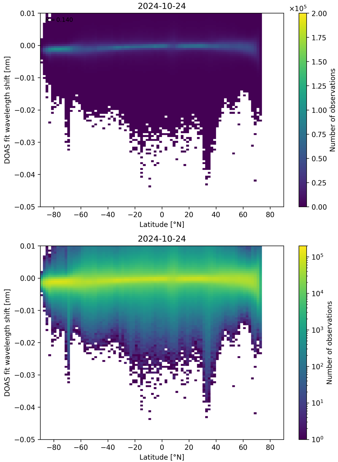
Figure 142: Scatter density plot of “Latitude” against “DOAS fit wavelength shift” for 2024-10-24 to 2024-10-25.
