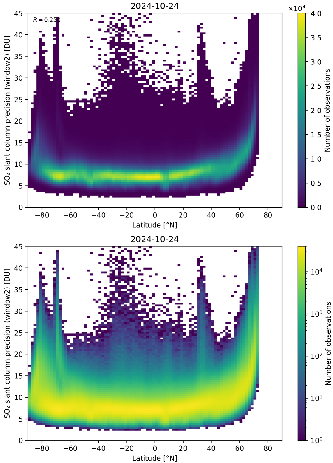
Figure 151: Scatter density plot of “Latitude” against “SO 2 slant column precision (window2)” for 2024-10-24 to 2024-10-25.
