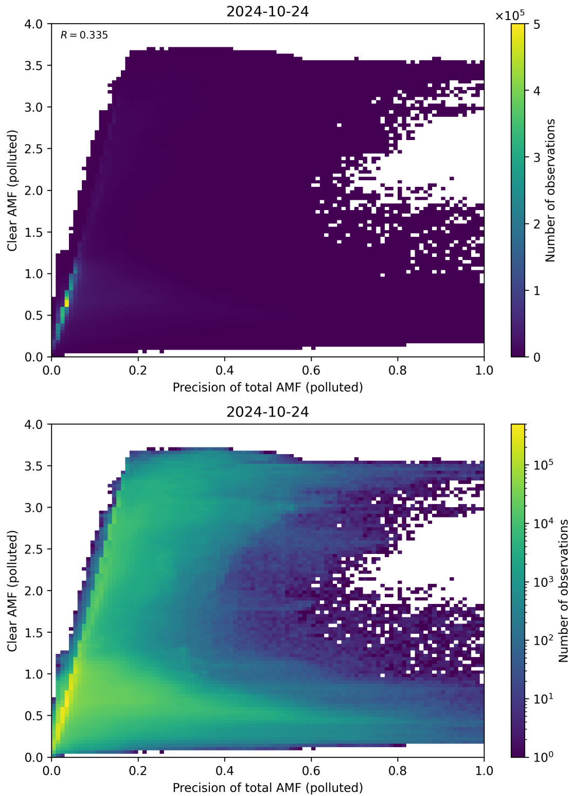
Figure 270: Scatter density plot of “Precision of total AMF (polluted)” against “Clear AMF (polluted)” for 2024-10-24 to 2024-10-25.
