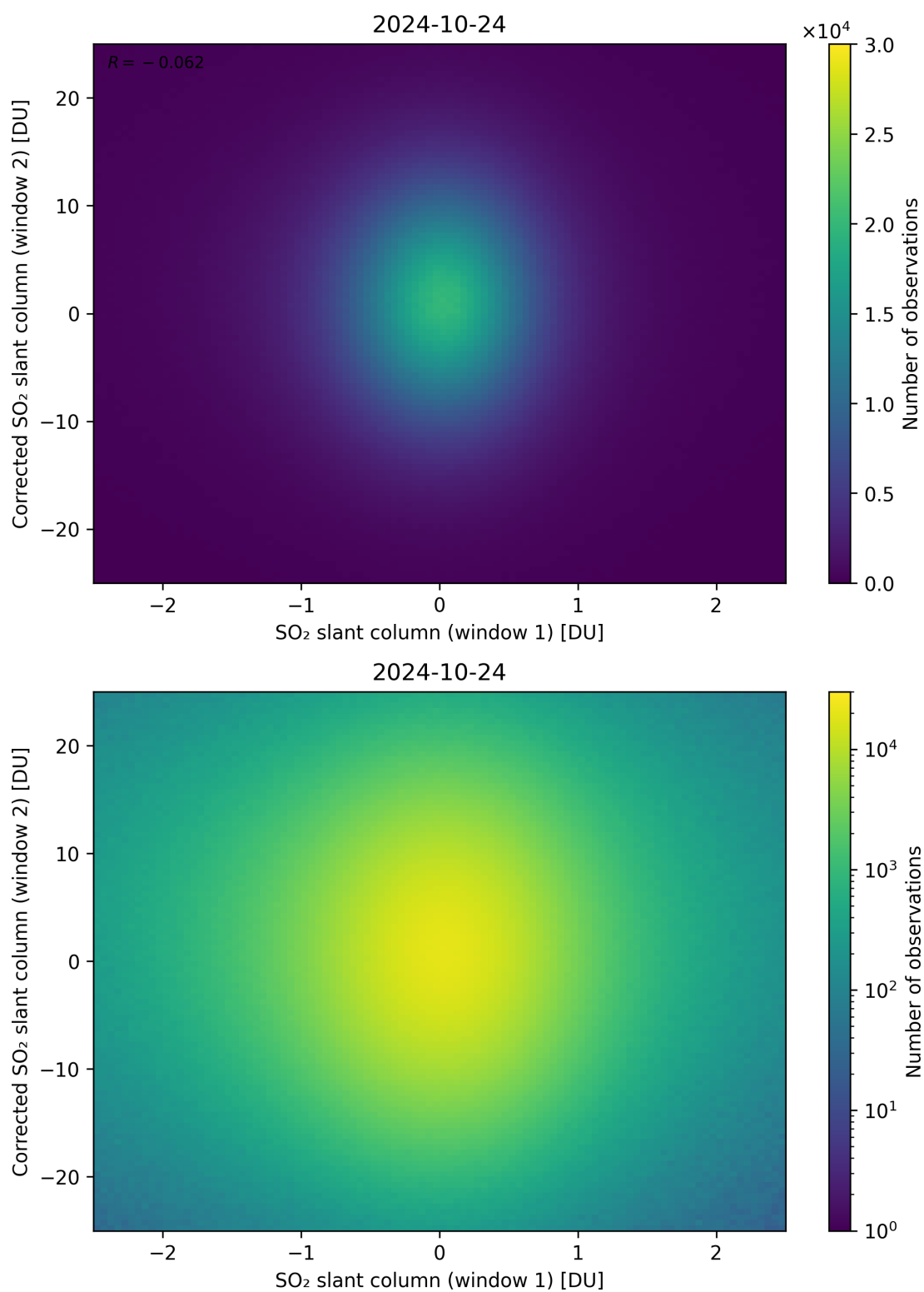
Figure 233: Scatter density plot of “SO 2 slant column (window 1)” against “Corrected SO 2 slant column (window 2)” for 2024-10-24 to 2024-10-25.
