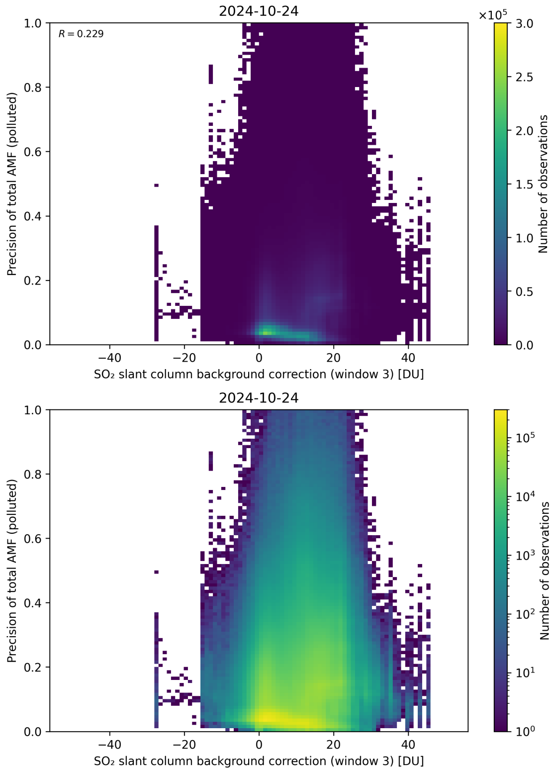
Figure 126: Scatter density plot of “SO 2 slant column background correction (window 3)” against “Precision of total AMF (polluted)” for 2024-10-24 to 2024-10-25.
