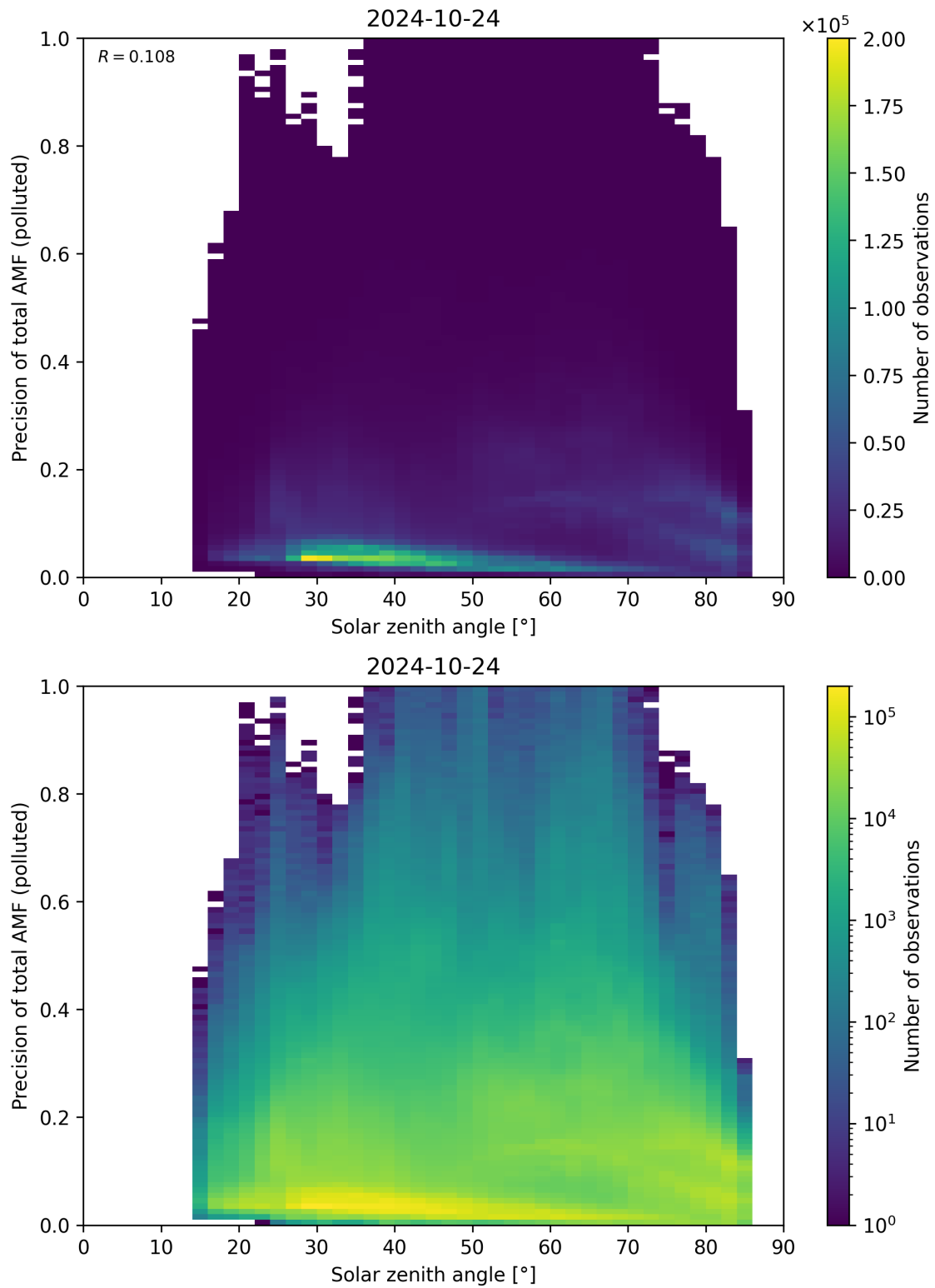
Figure 175: Scatter density plot of “Solar zenith angle” against “Precision of total AMF (polluted)” for 2024-10-24 to 2024-10-25.
