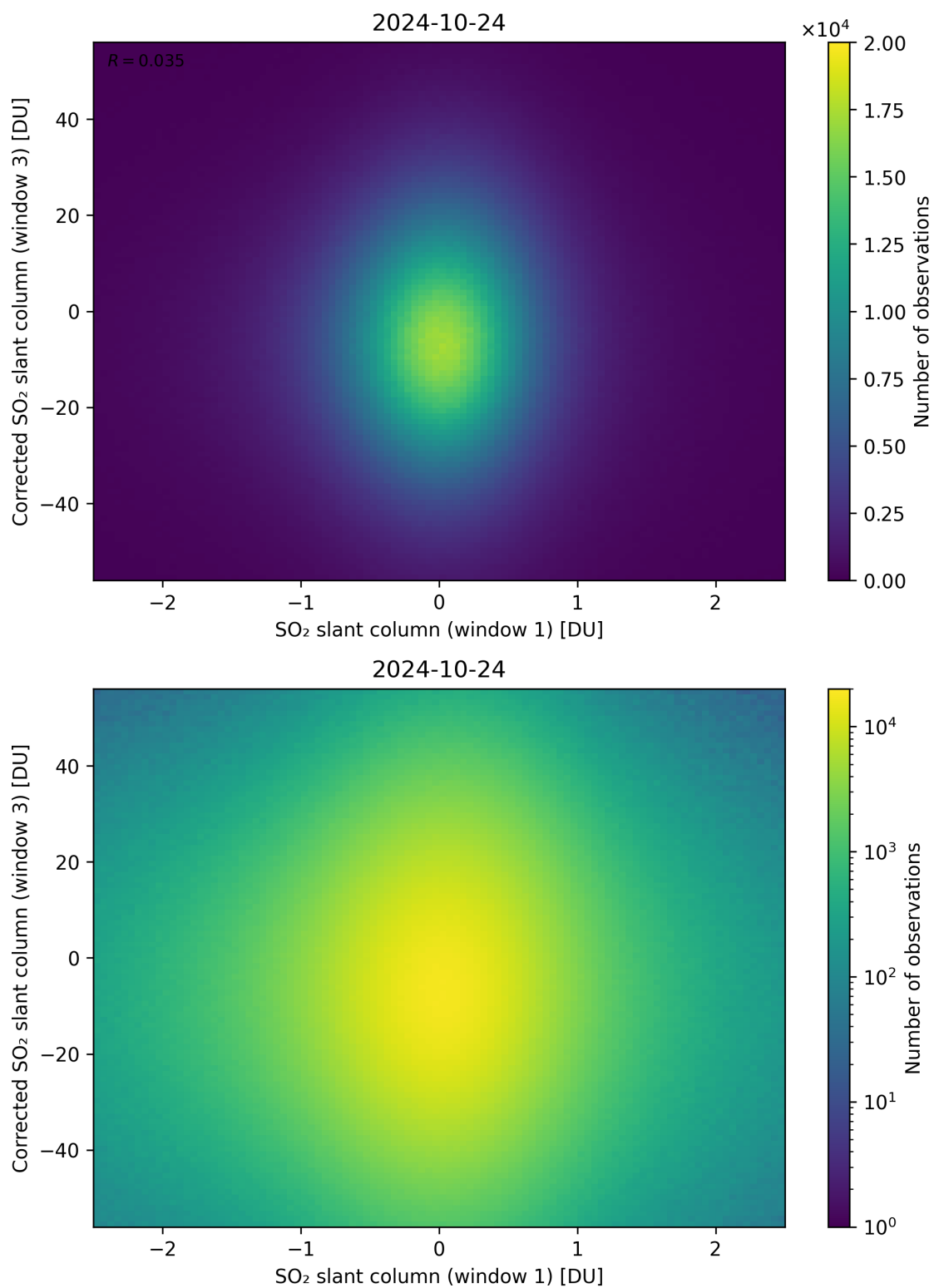
Figure 234: Scatter density plot of “SO 2 slant column (window 1)” against “Corrected SO 2 slant column (window 3)” for 2024-10-24 to 2024-10-25.
