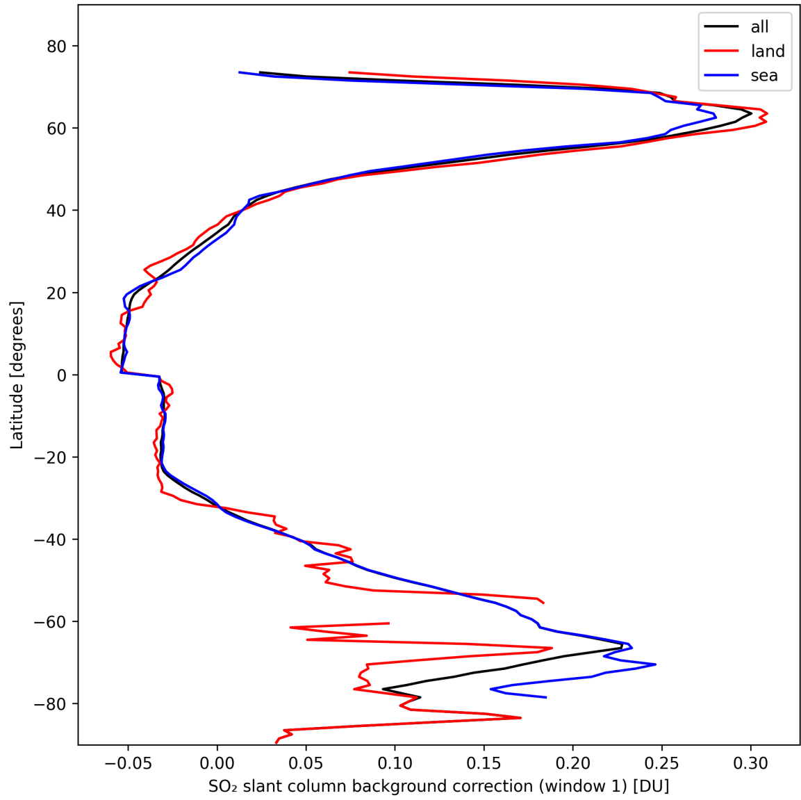
Figure 36: Zonal average of “SO 2 slant column background correction (window 1)” for 2024-10-24 to 2024-10-25.
