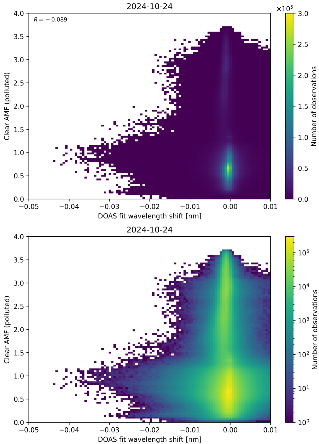
Figure 129: Scatter density plot of “DOAS fit wavelength shift” against “Clear AMF (polluted)” for 2024-10-24 to 2024-10-25.
