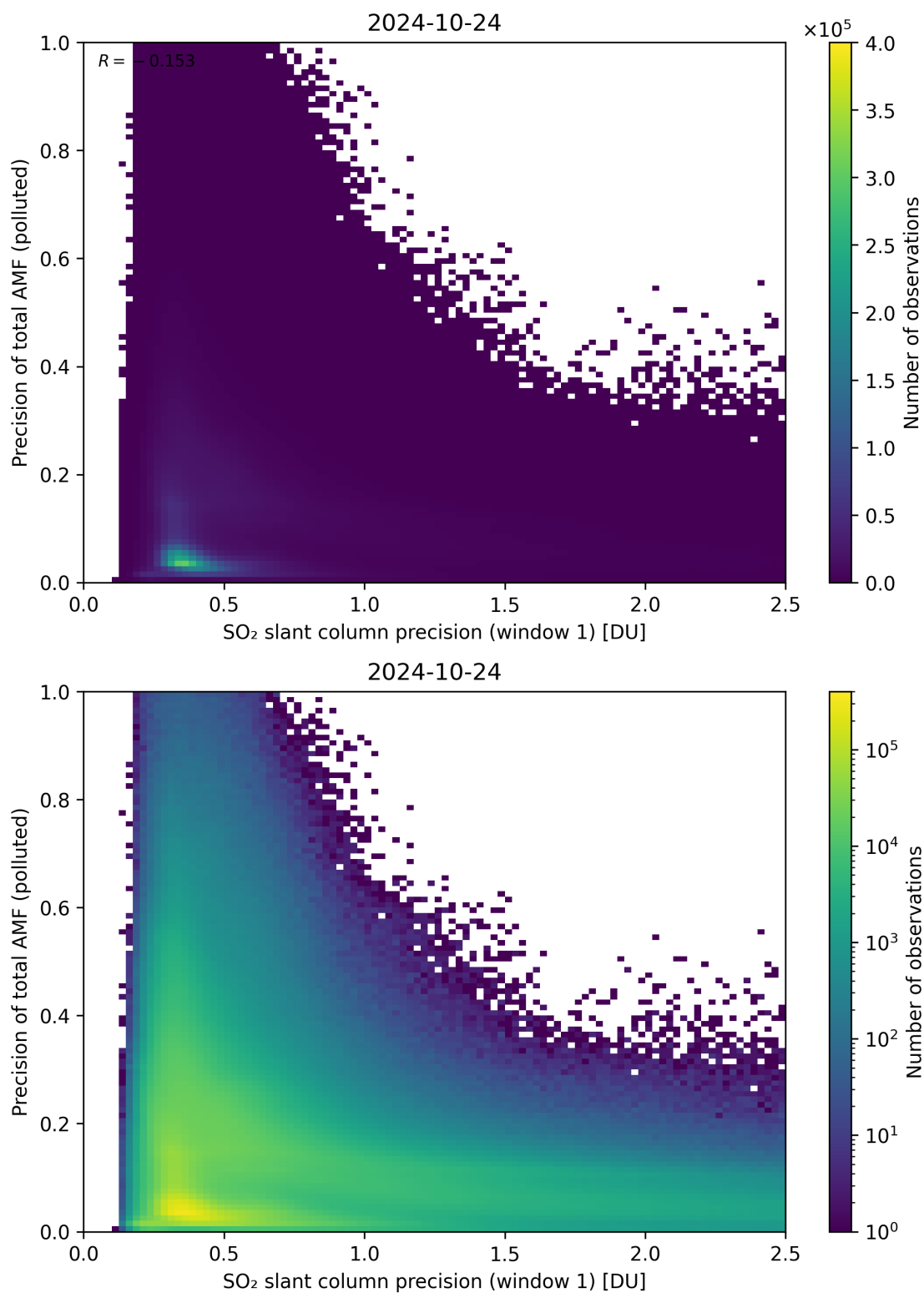
Figure 231: Scatter density plot of “SO 2 slant column precision (window 1)” against “Precision of total AMF (polluted)” for 2024-10-24 to 2024-10-25.
