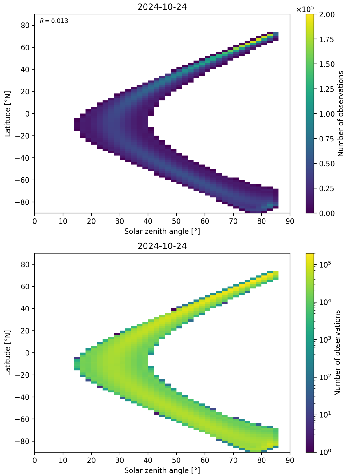
Figure 164: Scatter density plot of “Solar zenith angle” against “Latitude” for 2024-10-24 to 2024-10-25.
