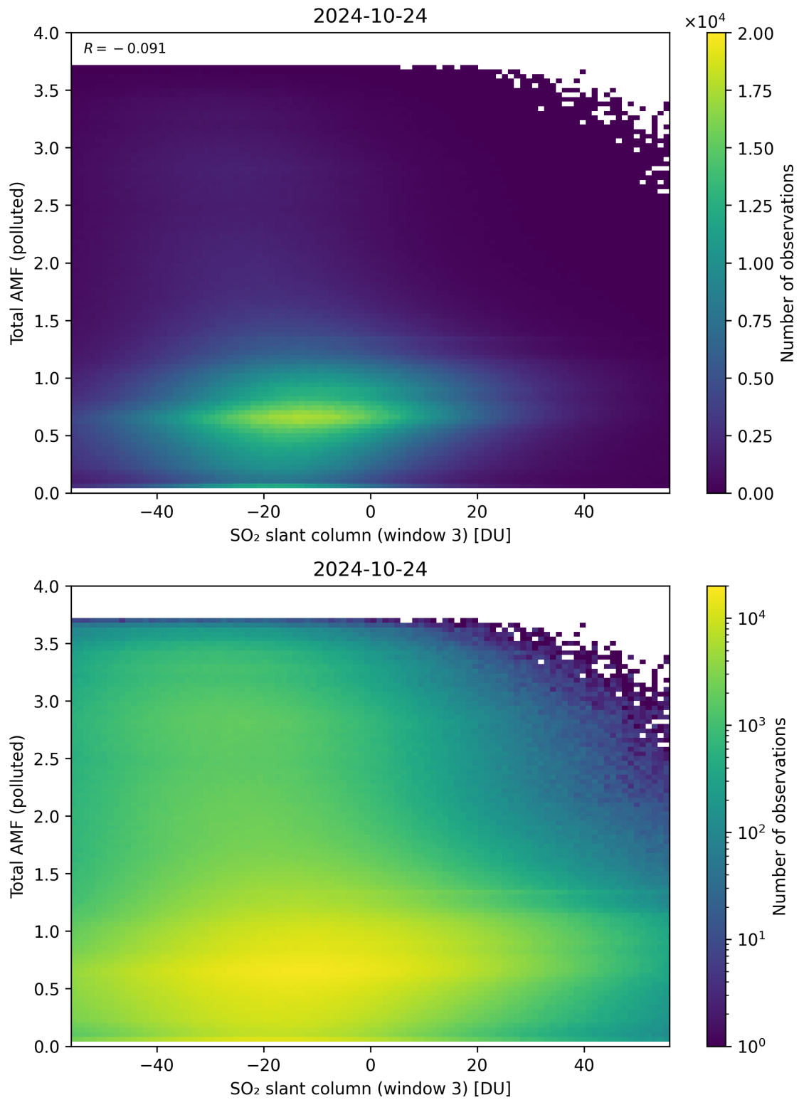
Figure 268: Scatter density plot of “SO 2 slant column (window 3)” against “Total AMF (polluted)” for 2024-10-24 to 2024-10-25.
