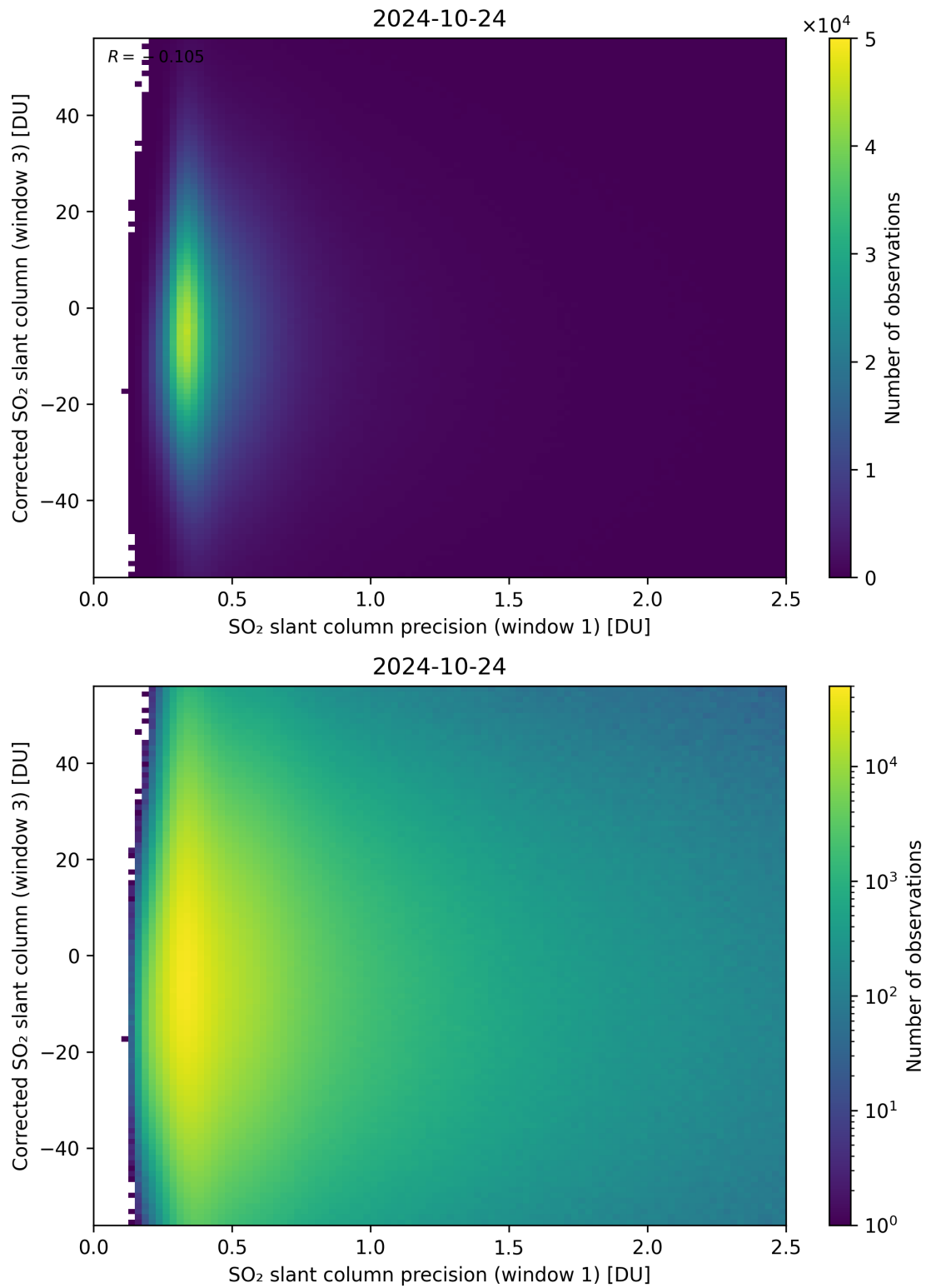
Figure 226: Scatter density plot of “SO 2 slant column precision (window 1)” against “Corrected SO 2 slant column (window 3)” for 2024-10-24 to 2024-10-25.
