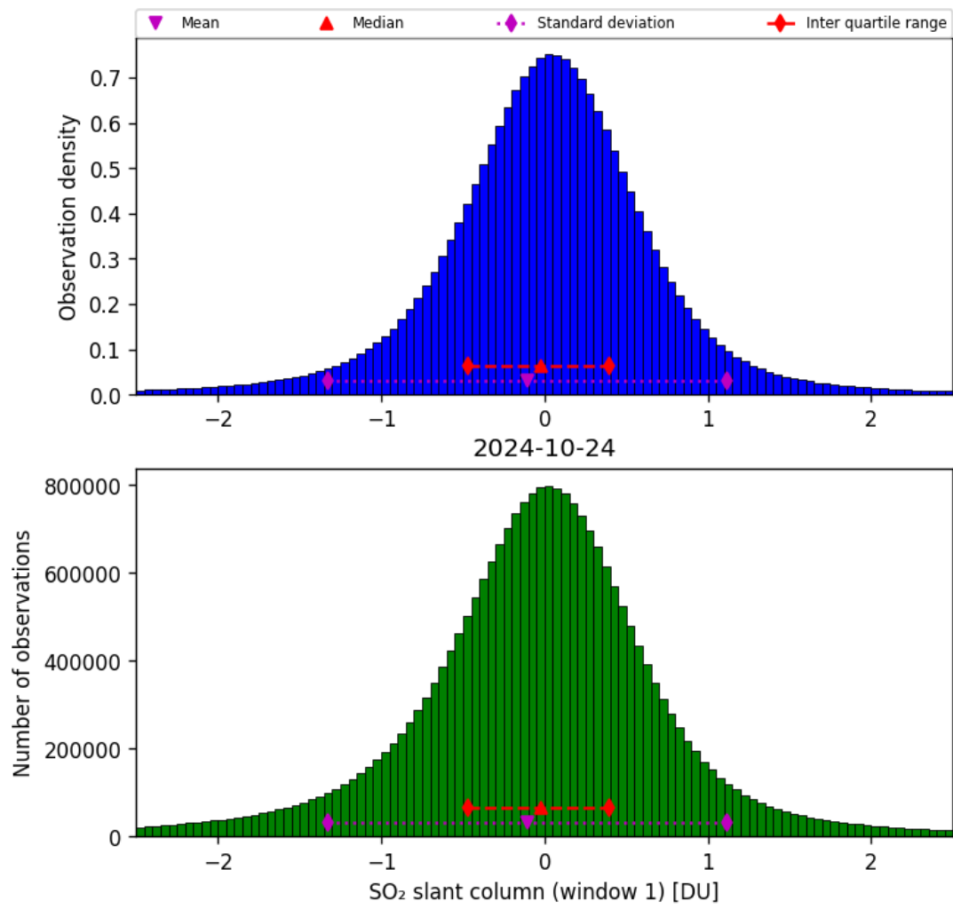
Figure 56: Histogram of “SO 2 slant column (window 1)” for 2024-10-24 to 2024-10-25
