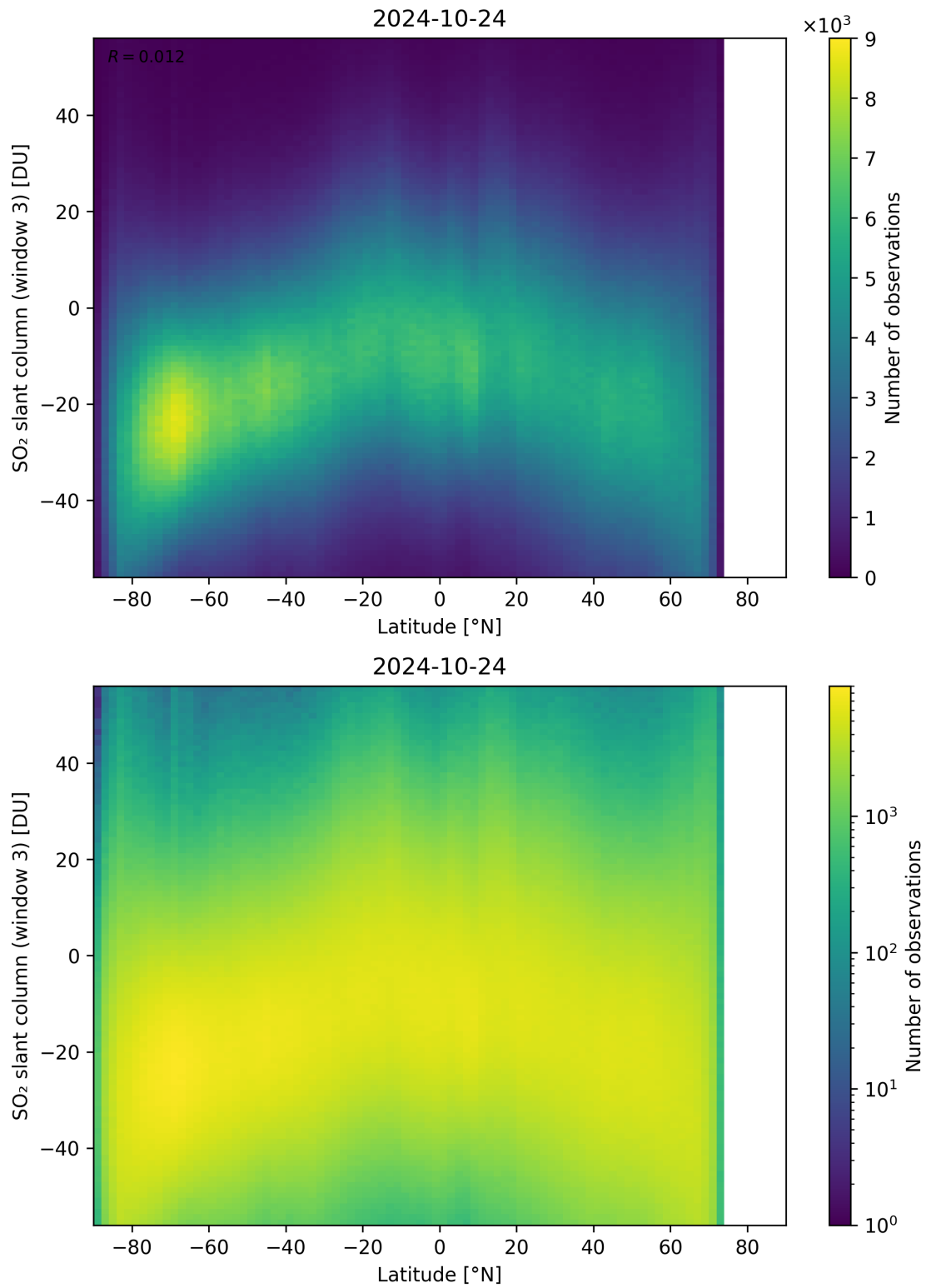
Figure 152: Scatter density plot of “Latitude” against “SO 2 slant column (window 3)” for 2024-10-24 to 2024-10-25.
