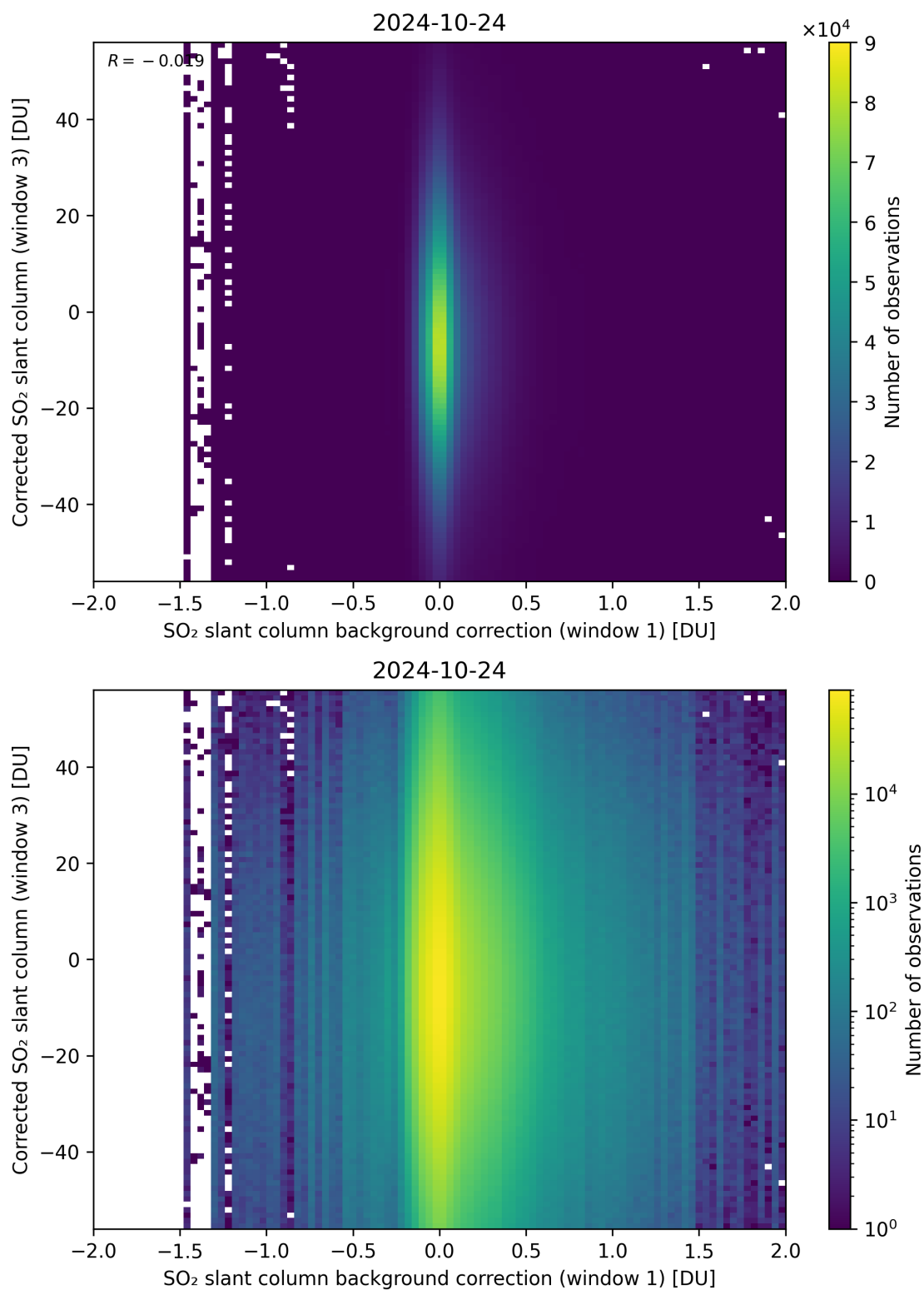
Figure 105: Scatter density plot of “SO 2 slant column background correction (window 1)” against “Corrected SO 2 slant column (window 3)” for 2024-10-24 to 2024-10-25.
