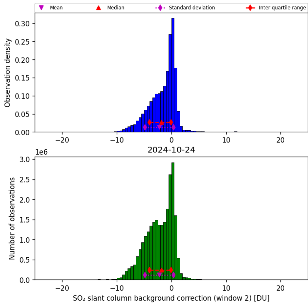
Figure 63: Histogram of “SO 2 slant column background correction (window 2)” for 2024-10-24 to 2024-10-25
