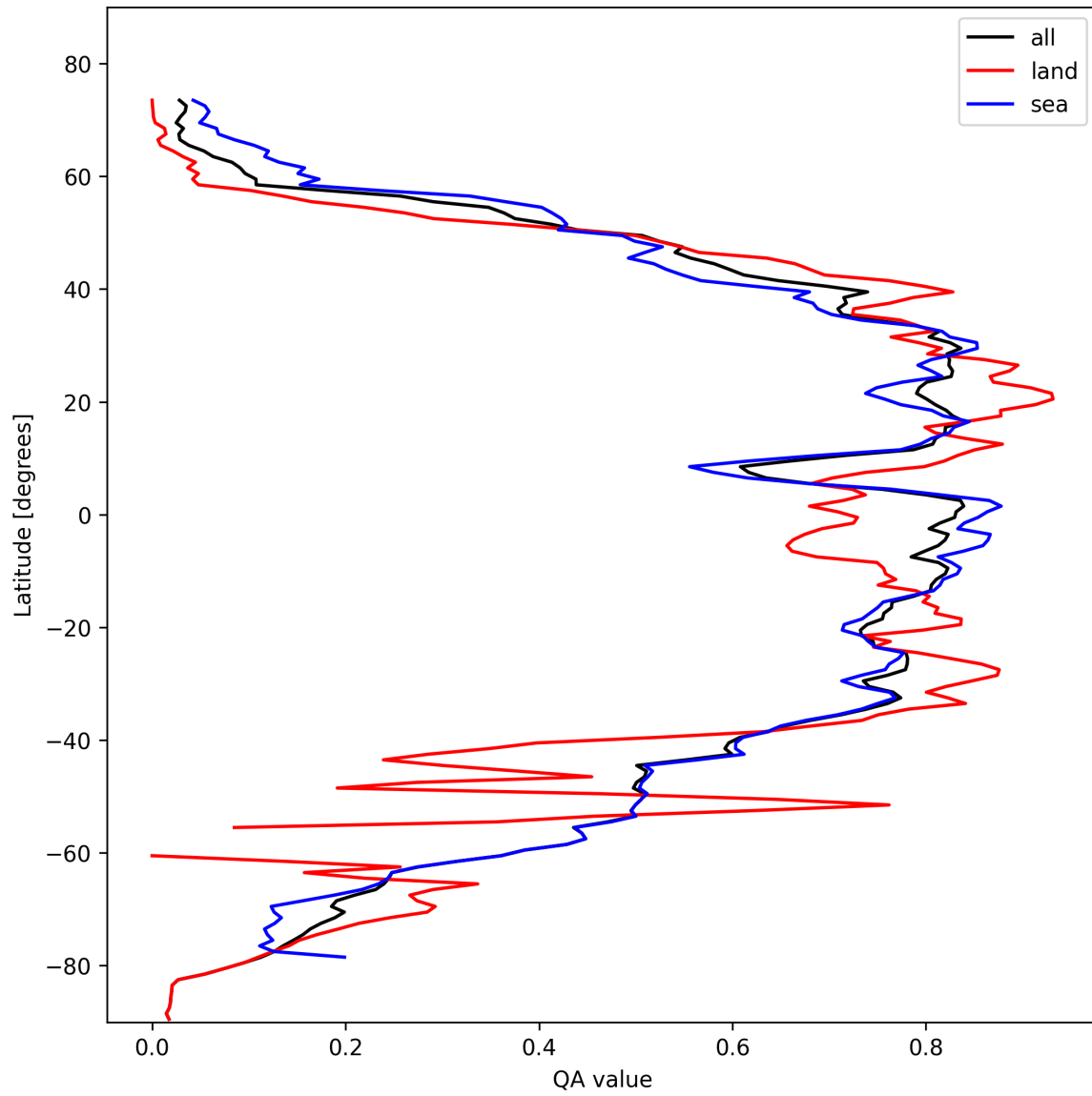
Figure 29: Zonal average of “QA value” for 2024-10-24 to 2024-10-25.
