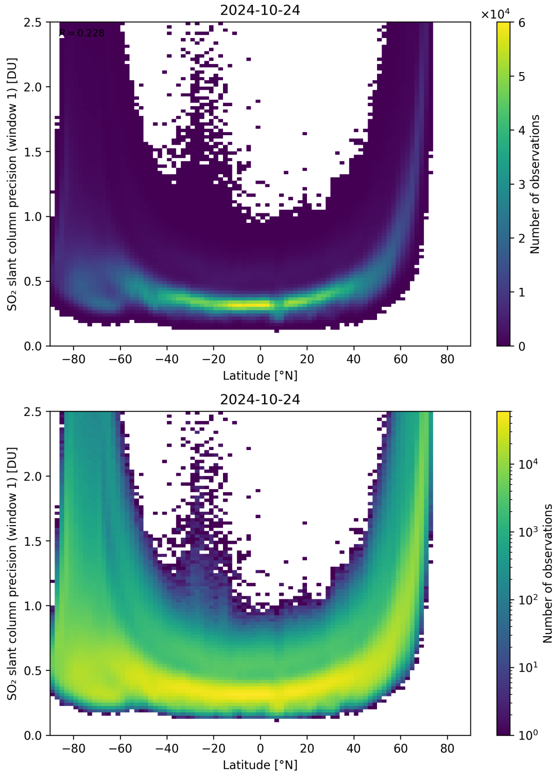
Figure 150: Scatter density plot of “Latitude” against “SO 2 slant column precision (window 1)” for 2024-10-24 to 2024-10-25.
