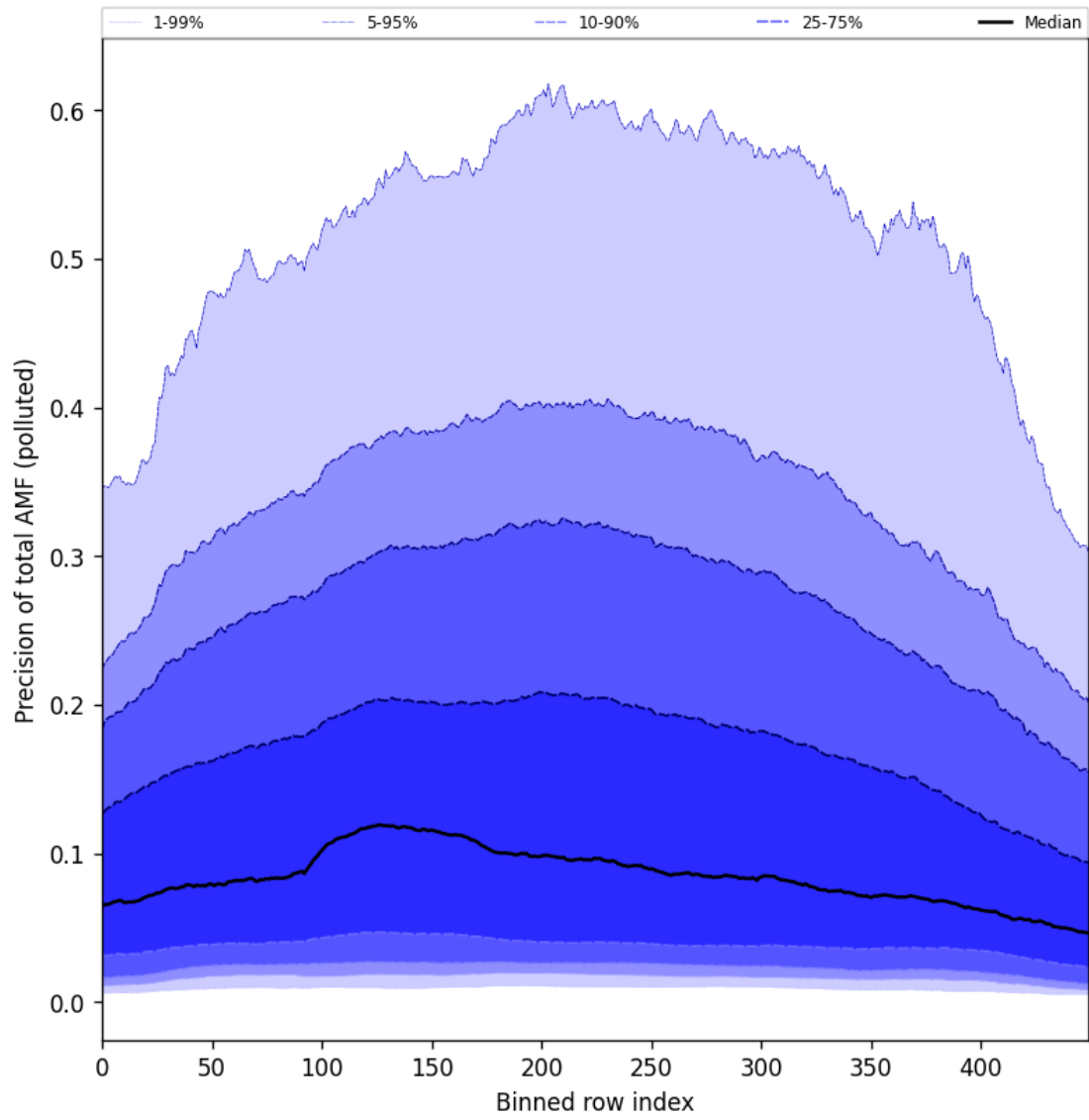
Figure 95: Along track statistics of “Precision of total AMF (polluted)” for 2024-10-24 to 2024-10-25
