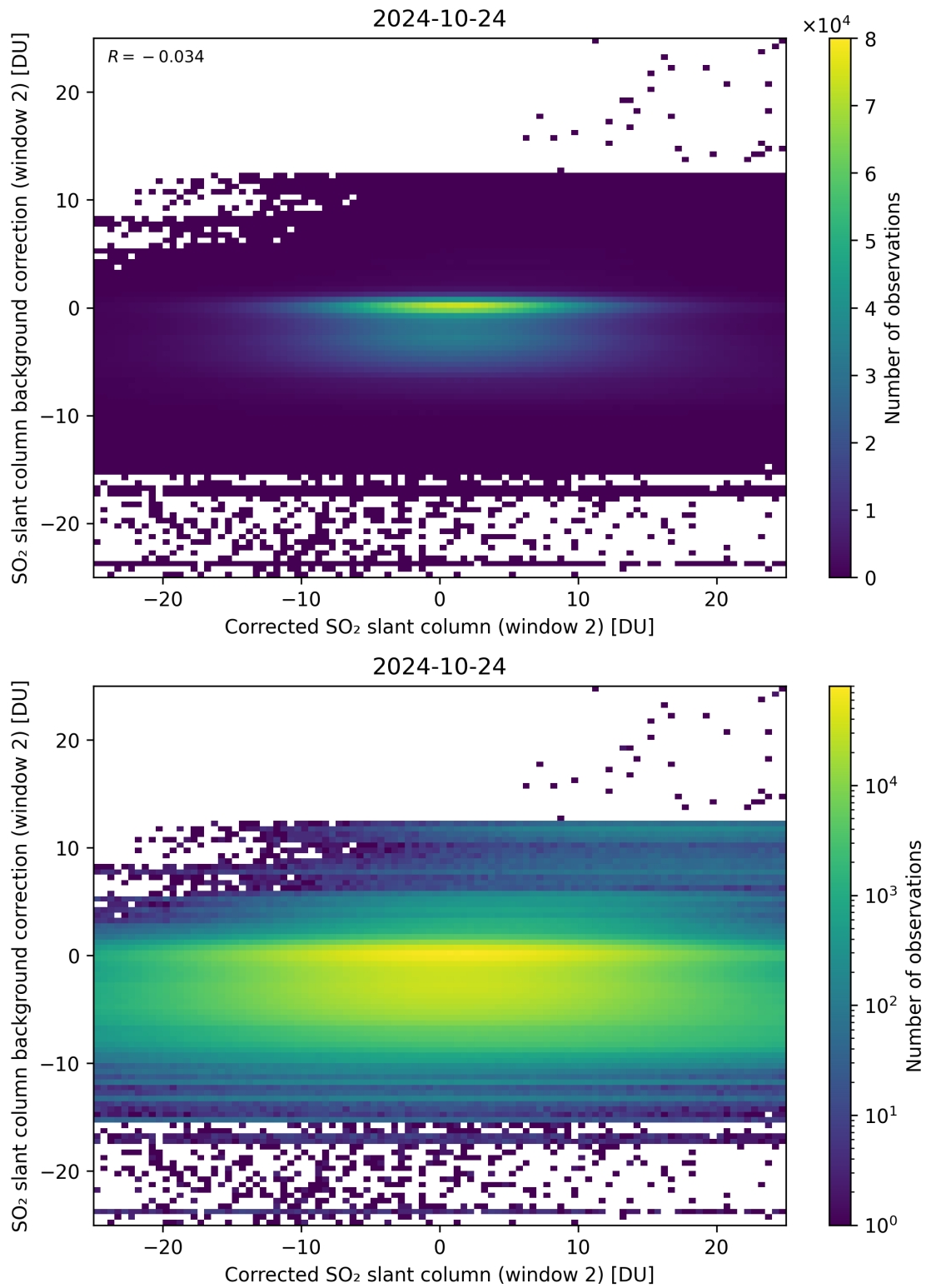
Figure 194: Scatter density plot of “Corrected SO 2 slant column (window 2)” against “SO 2 slant column background correction (window 2)” for 2024-10-24 to 2024-10-25.
