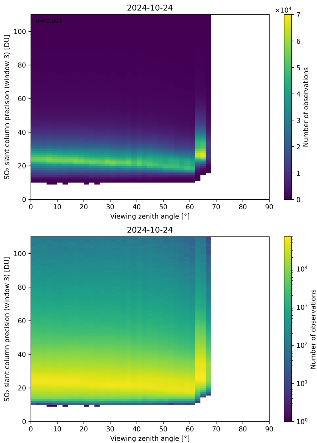
Figure 324: Scatter density plot of “Viewing zenith angle” against “SO 2 slant column precision (window 3)” for 2024-10-24 to 2024-10-25.
