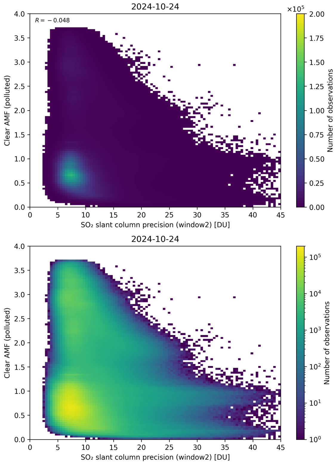
Figure 246: Scatter density plot of “SO 2 slant column precision (window2)” against “Clear AMF (polluted)” for 2024-10-24 to 2024-10-25.
