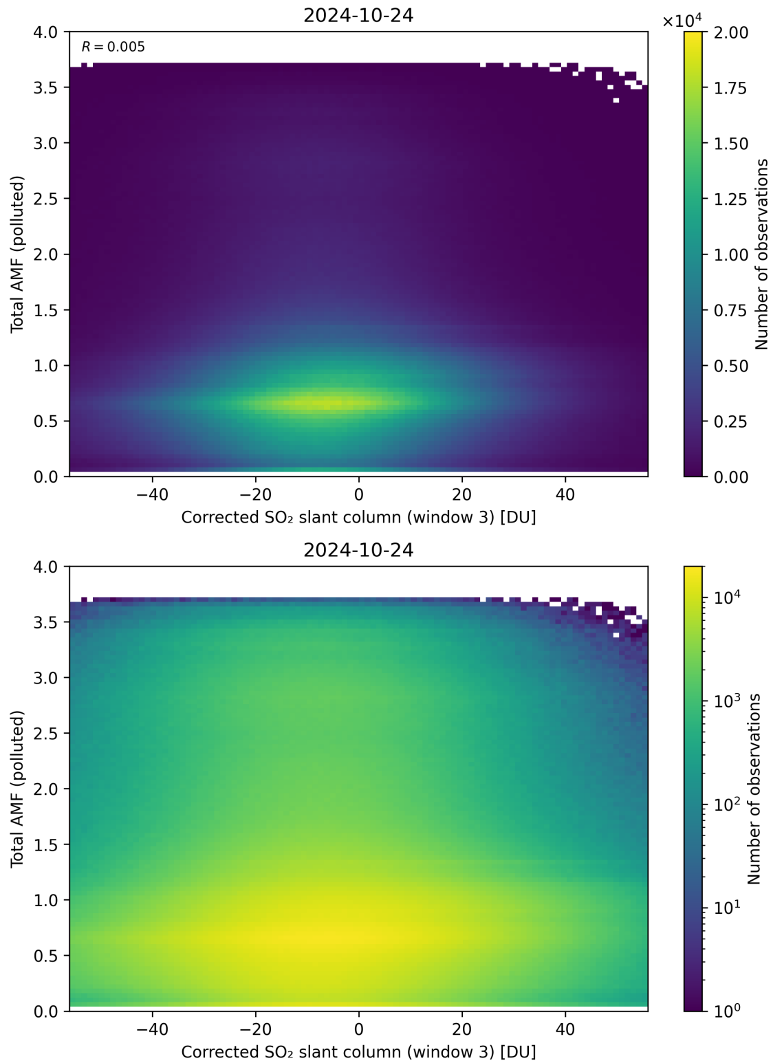
Figure 210: Scatter density plot of “Corrected SO 2 slant column (window 3)” against “Total AMF (polluted)” for 2024-10-24 to 2024-10-25.
