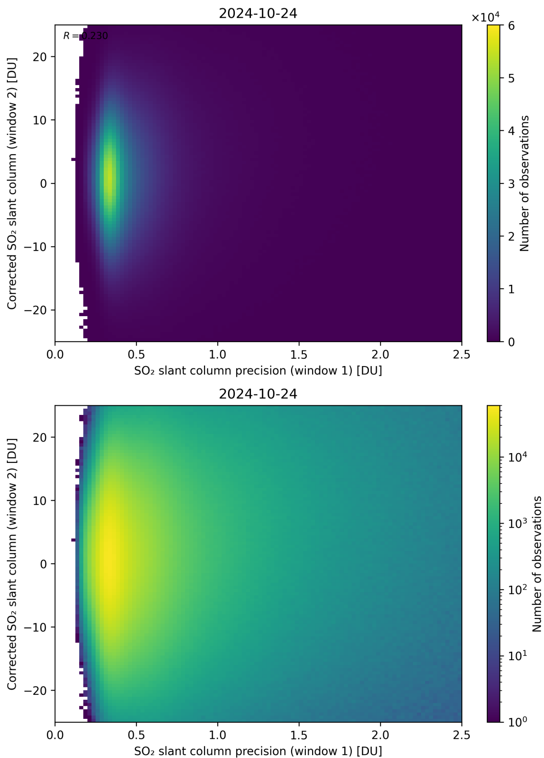
Figure 225: Scatter density plot of “SO 2 slant column precision (window 1)” against “Corrected SO 2 slant column (window 2)” for 2024-10-24 to 2024-10-25.
