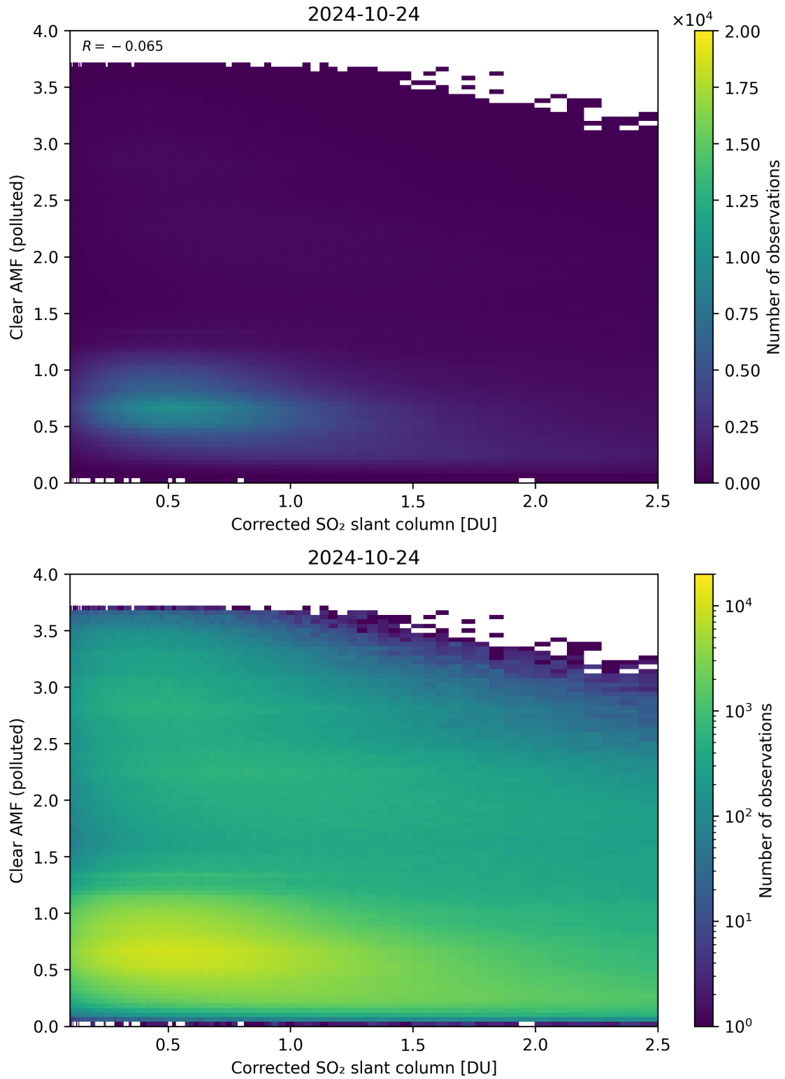
Figure 184: Scatter density plot of “Corrected SO 2 slant column” against “Clear AMF (polluted)” for 2024-10-24 to 2024-10-25.
