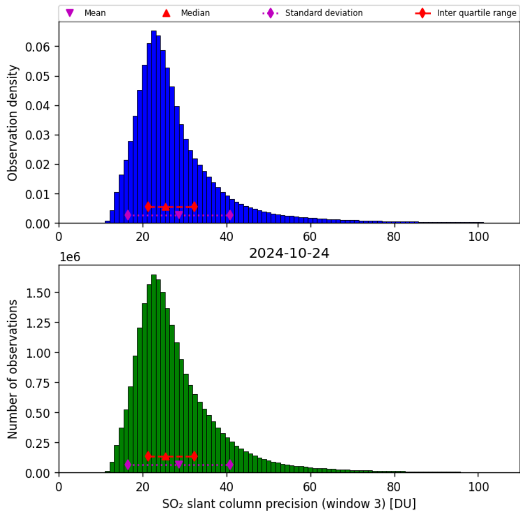
Figure 65: Histogram of “SO 2 slant column precision (window 3)” for 2024-10-24 to 2024-10-25
