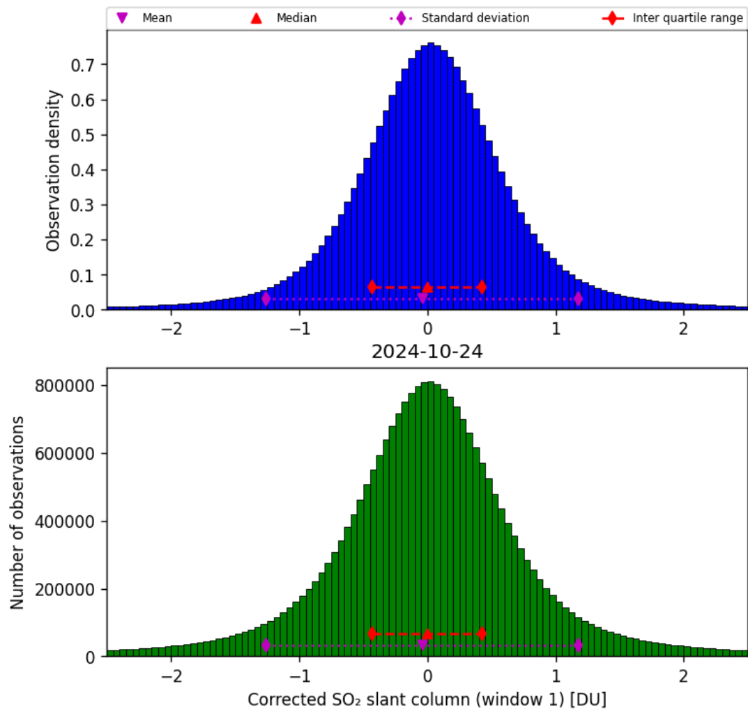
Figure 58: Histogram of “Corrected SO 2 slant column (window 1)” for 2024-10-24 to 2024-10-25
