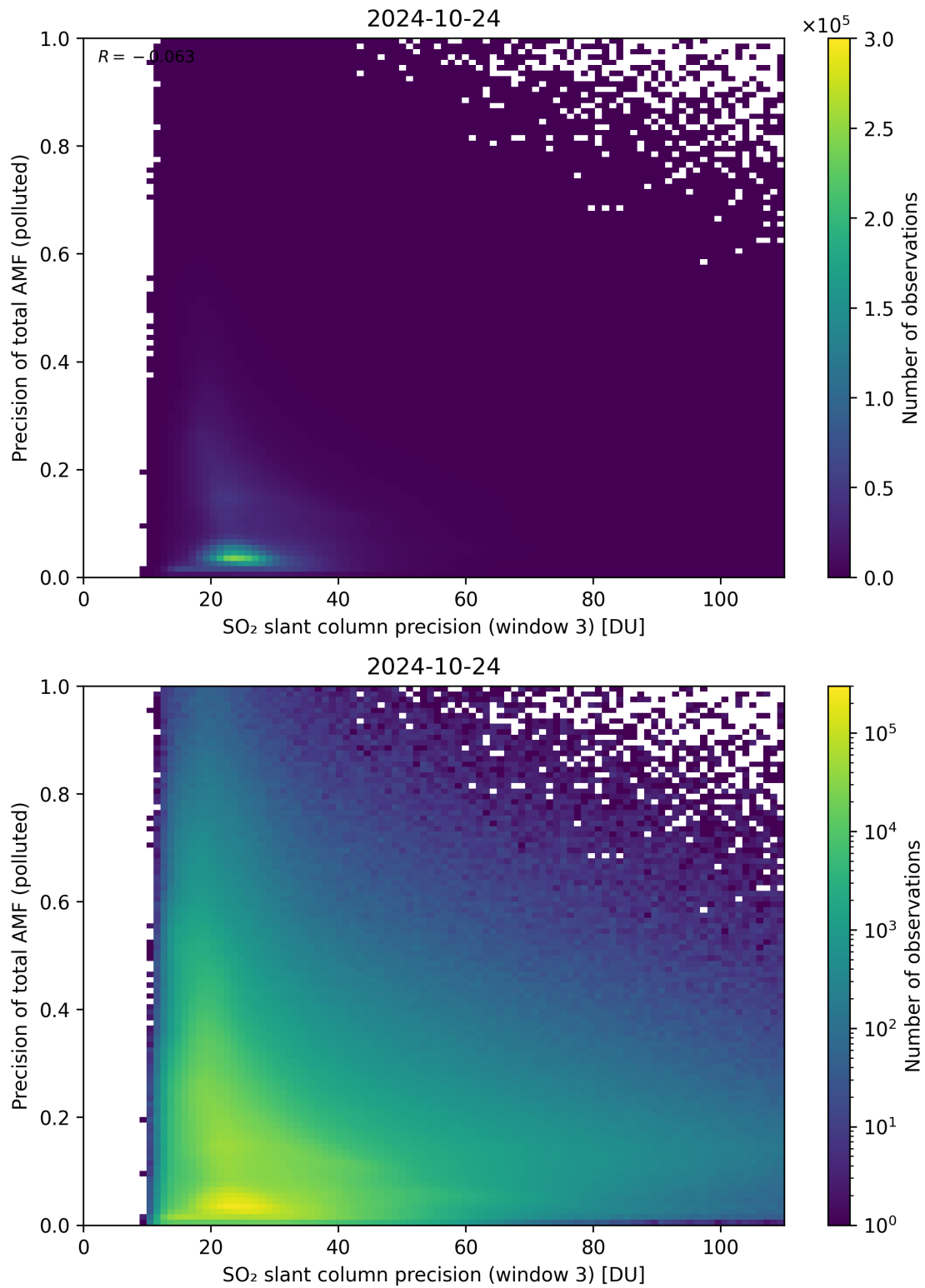
Figure 264: Scatter density plot of “SO 2 slant column precision (window 3)” against “Precision of total AMF (polluted)” for 2024-10-24 to 2024-10-25.
