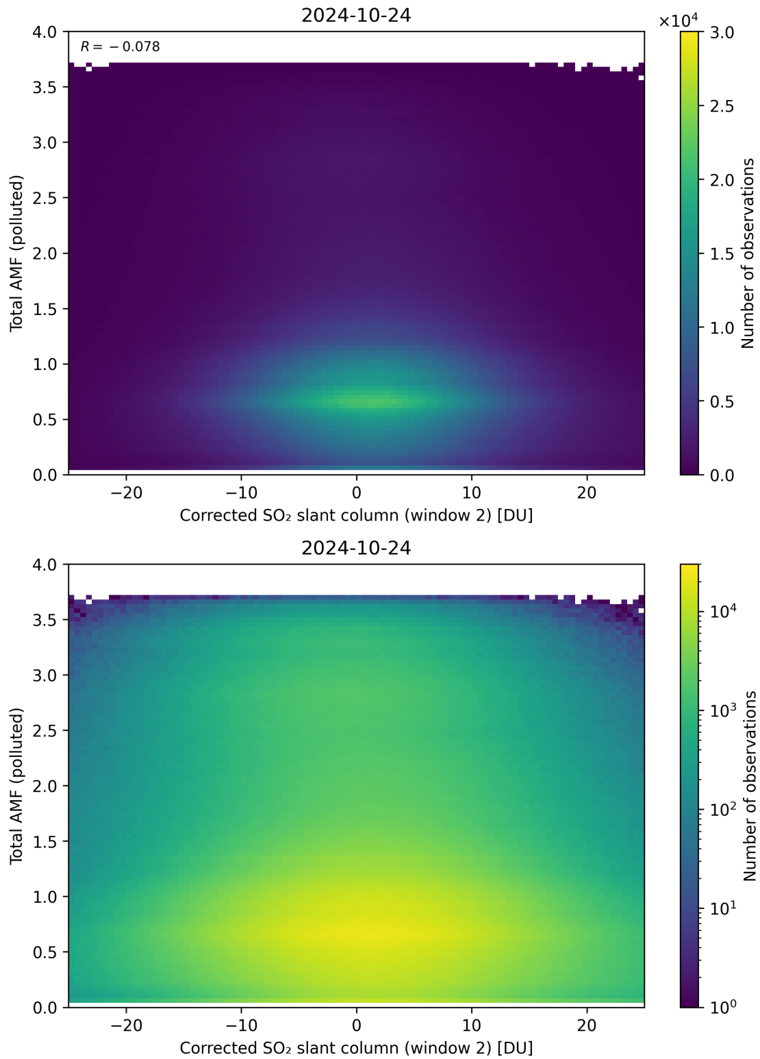
Figure 203: Scatter density plot of “Corrected SO 2 slant column (window 2)” against “Total AMF (polluted)” for 2024-10-24 to 2024-10-25.
