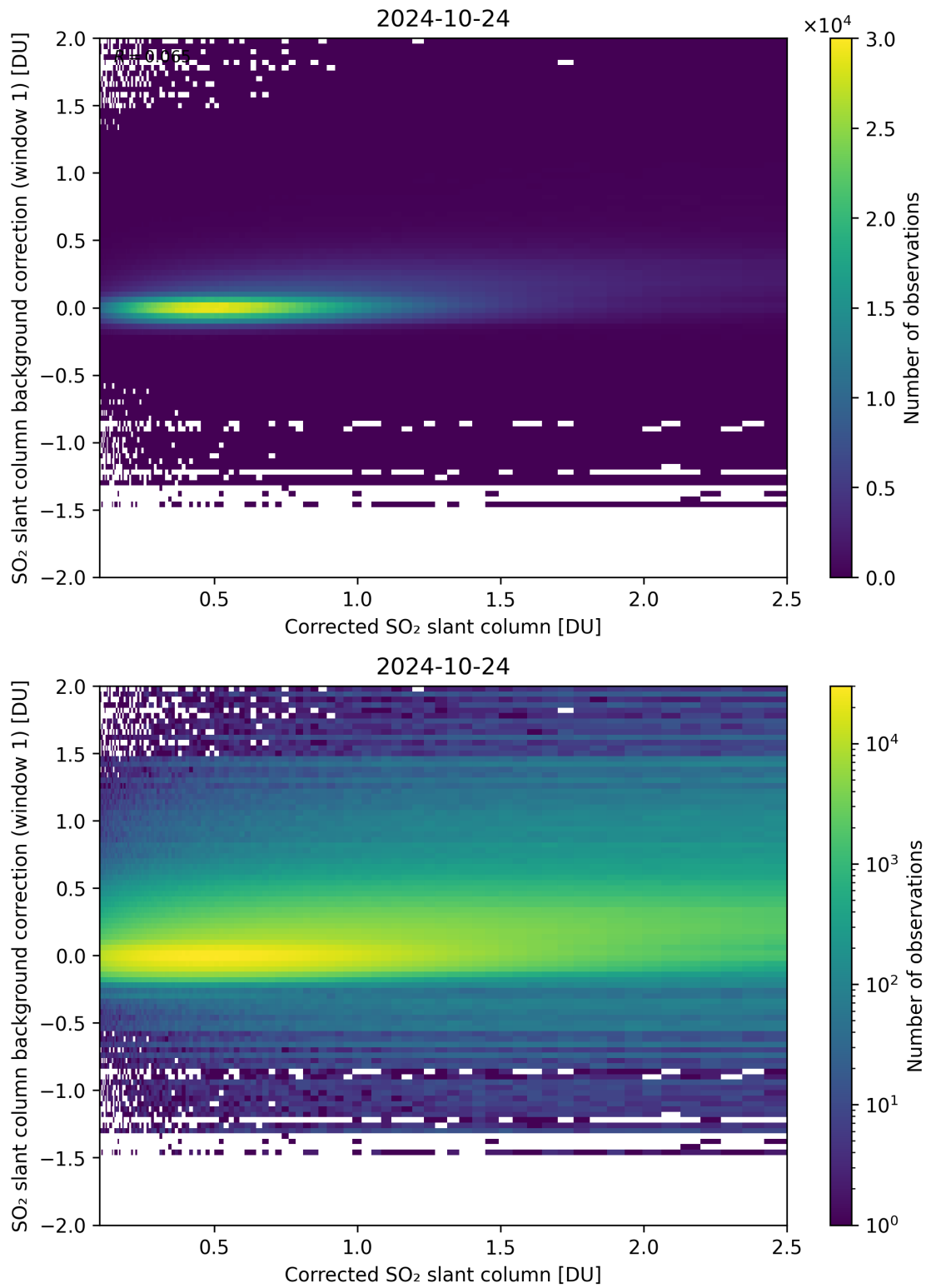
Figure 178: Scatter density plot of “Corrected SO 2 slant column” against “SO 2 slant column background correction (window 1)” for 2024-10-24 to 2024-10-25.
