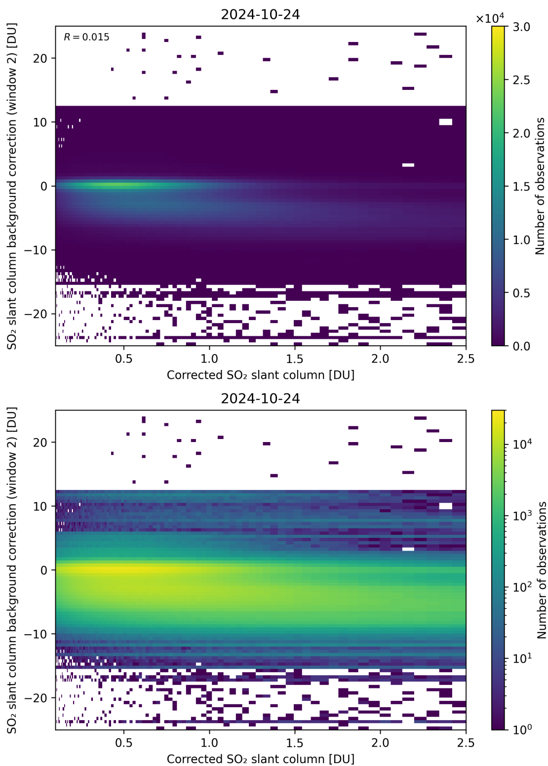
Figure 179: Scatter density plot of “Corrected SO 2 slant column” against “SO 2 slant column background correction (window 2)” for 2024-10-24 to 2024-10-25.
