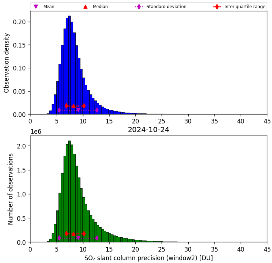
Figure 61: Histogram of “SO 2 slant column precision (window2)” for 2024-10-24 to 2024-10-25
