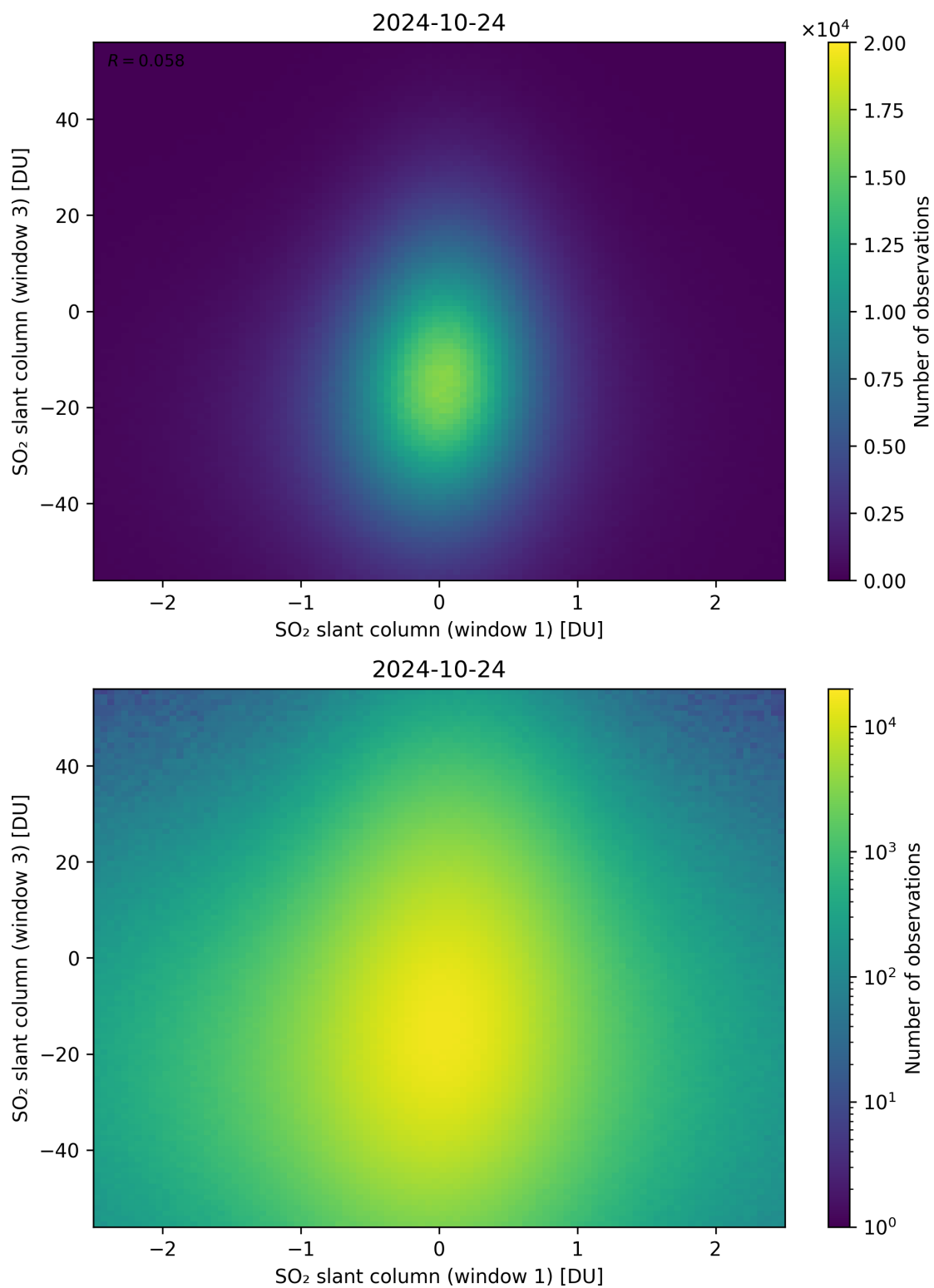
Figure 237: Scatter density plot of “SO 2 slant column (window 1)” against “SO 2 slant column (window 3)” for 2024-10-24 to 2024-10-25.
