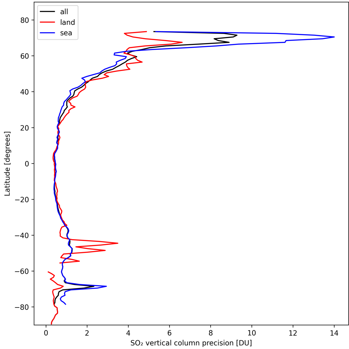
Figure 31: Zonal average of “SO 2 vertical column precision” for 2024-10-24 to 2024-10-25.
