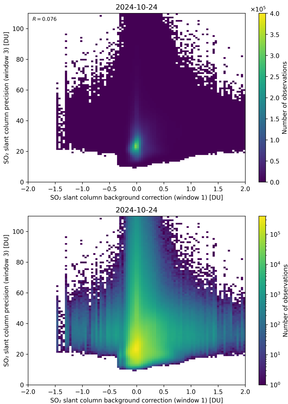
Figure 108: Scatter density plot of “SO 2 slant column background correction (window 1)” against “SO 2 slant column precision (window 3)” for 2024-10-24 to 2024-10-25.
