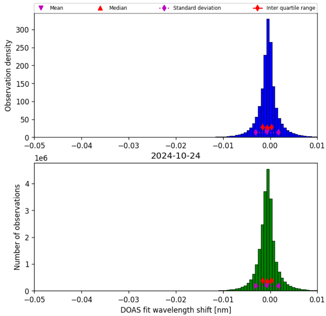
Figure 68: Histogram of “DOAS fit wavelength shift” for 2024-10-24 to 2024-10-25
