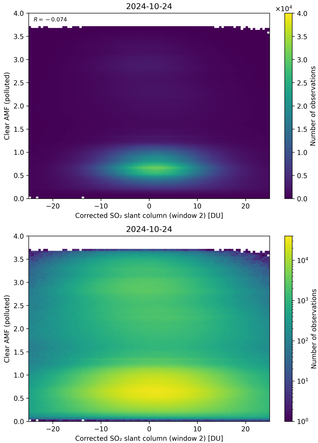
Figure 199: Scatter density plot of “Corrected SO 2 slant column (window 2)” against “Clear AMF (polluted)” for 2024-10-24 to 2024-10-25.
