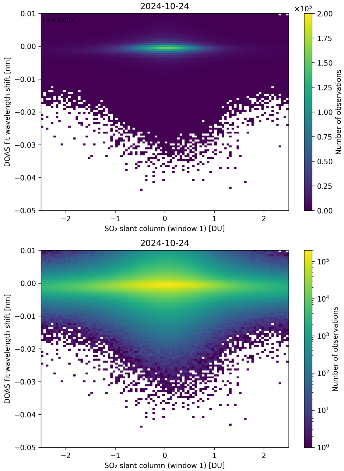
Figure 215: Scatter density plot of “SO 2 slant column (window 1)” against “DOAS fit wavelength shift” for 2024-10-24 to 2024-10-25.
