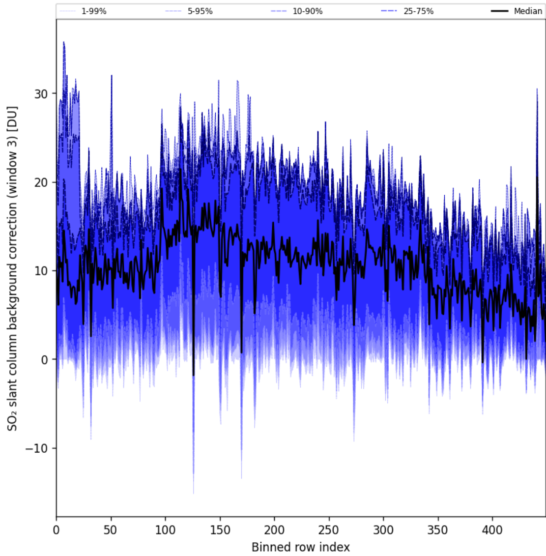
Figure 90: Along track statistics of “SO 2 slant column background correction (window 3)” for 2024-10-24 to 2024-10-25
