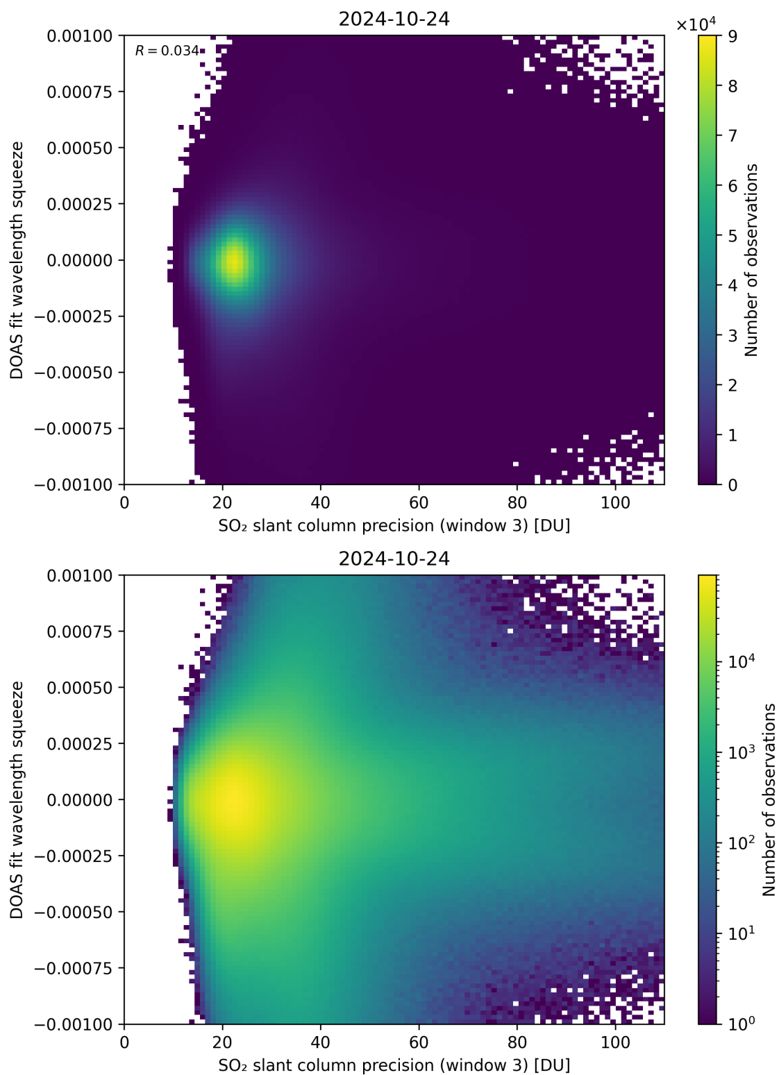
Figure 259: Scatter density plot of “SO 2 slant column precision (window 3)” against “DOAS fit wavelength squeeze” for 2024-10-24 to 2024-10-25.
