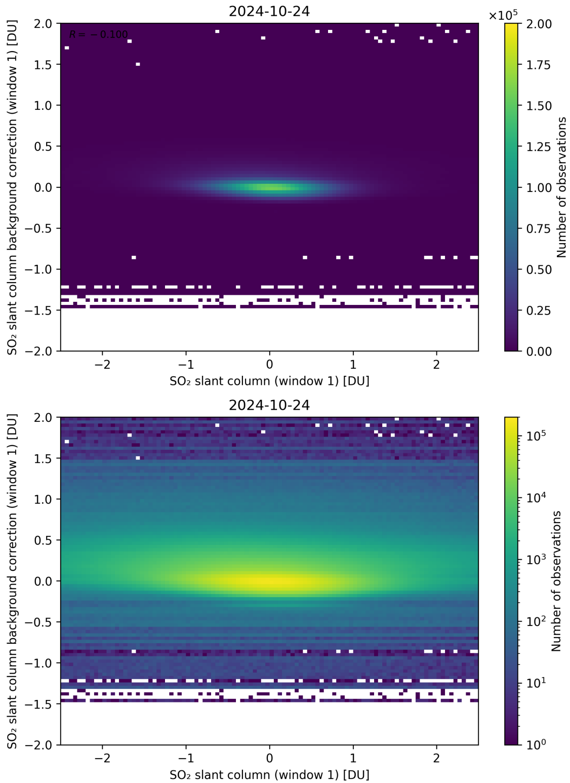
Figure 212: Scatter density plot of “SO 2 slant column (window 1)” against “SO 2 slant column background correction (window 1)” for 2024-10-24 to 2024-10-25.
