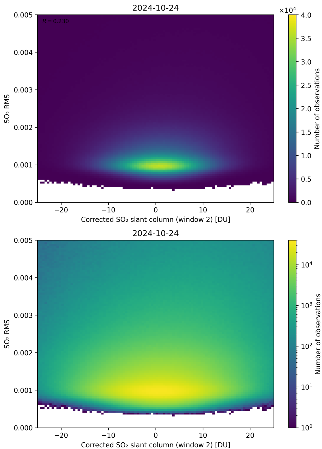
Figure 198: Scatter density plot of “Corrected SO 2 slant column (window 2)” against “SO 2 RMS” for 2024-10-24 to 2024-10-25.
