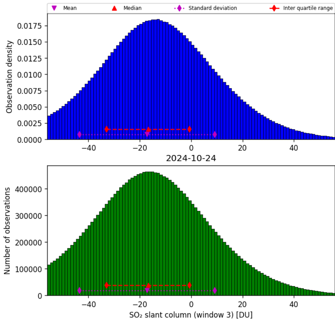
Figure 64: Histogram of “SO 2 slant column (window 3)” for 2024-10-24 to 2024-10-25
