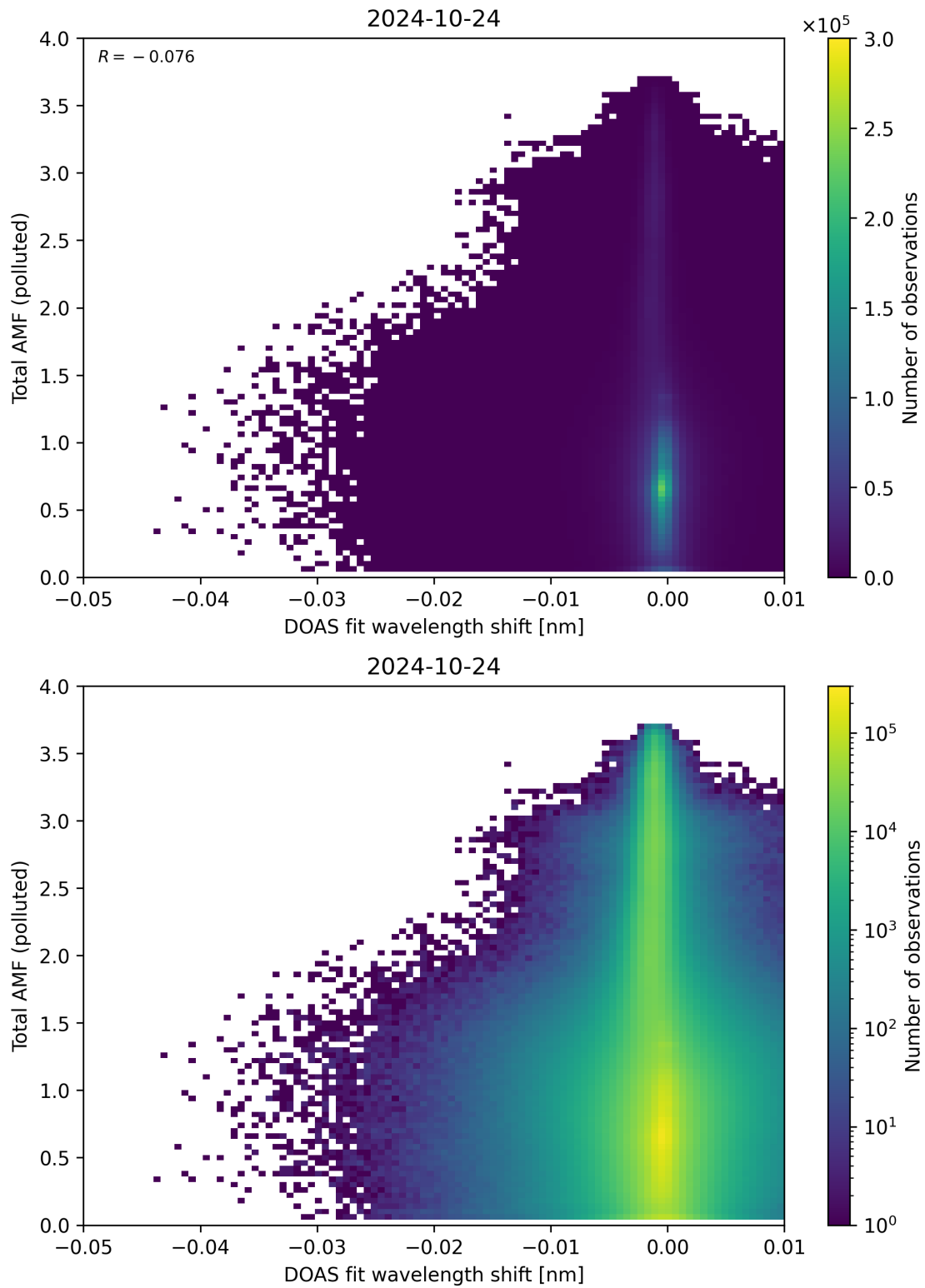
Figure 130: Scatter density plot of “DOAS fit wavelength shift” against “Total AMF (polluted)” for 2024-10-24 to 2024-10-25.
