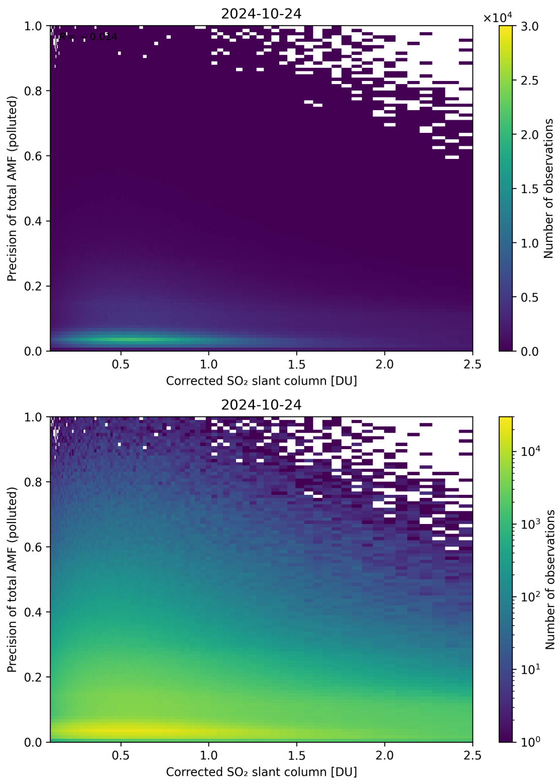
Figure 193: Scatter density plot of “Corrected SO 2 slant column” against “Precision of total AMF (polluted)” for 2024-10-24 to 2024-10-25.
