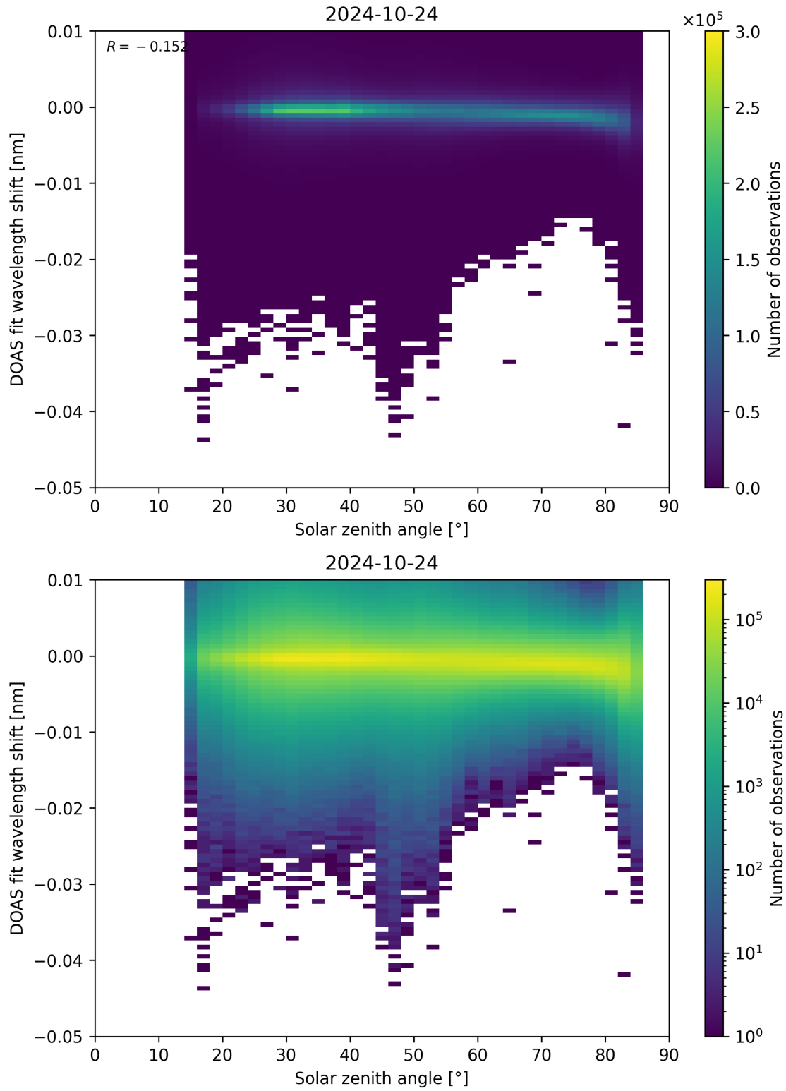
Figure 161: Scatter density plot of “Solar zenith angle” against “DOAS fit wavelength shift” for 2024-10-24 to 2024-10-25.
