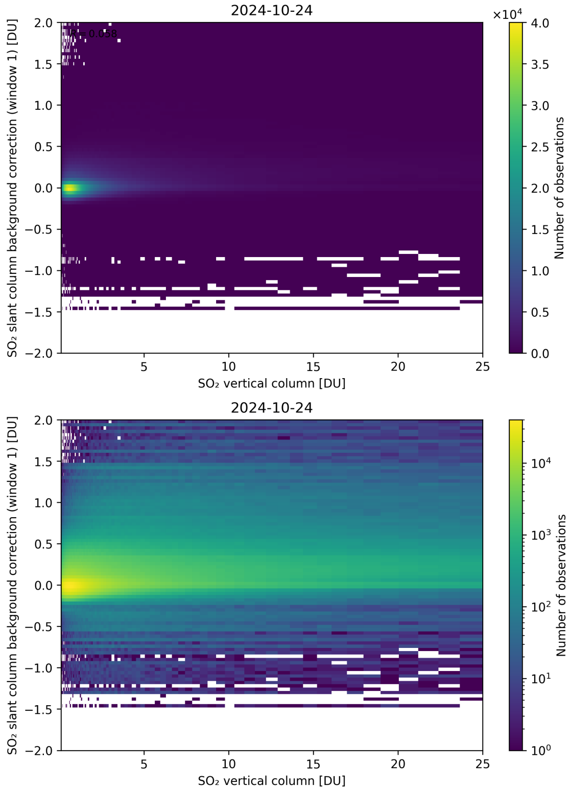
Figure 273: Scatter density plot of “SO 2 vertical column” against “SO 2 slant column background correction (window 1)” for 2024-10-24 to 2024-10-25.
