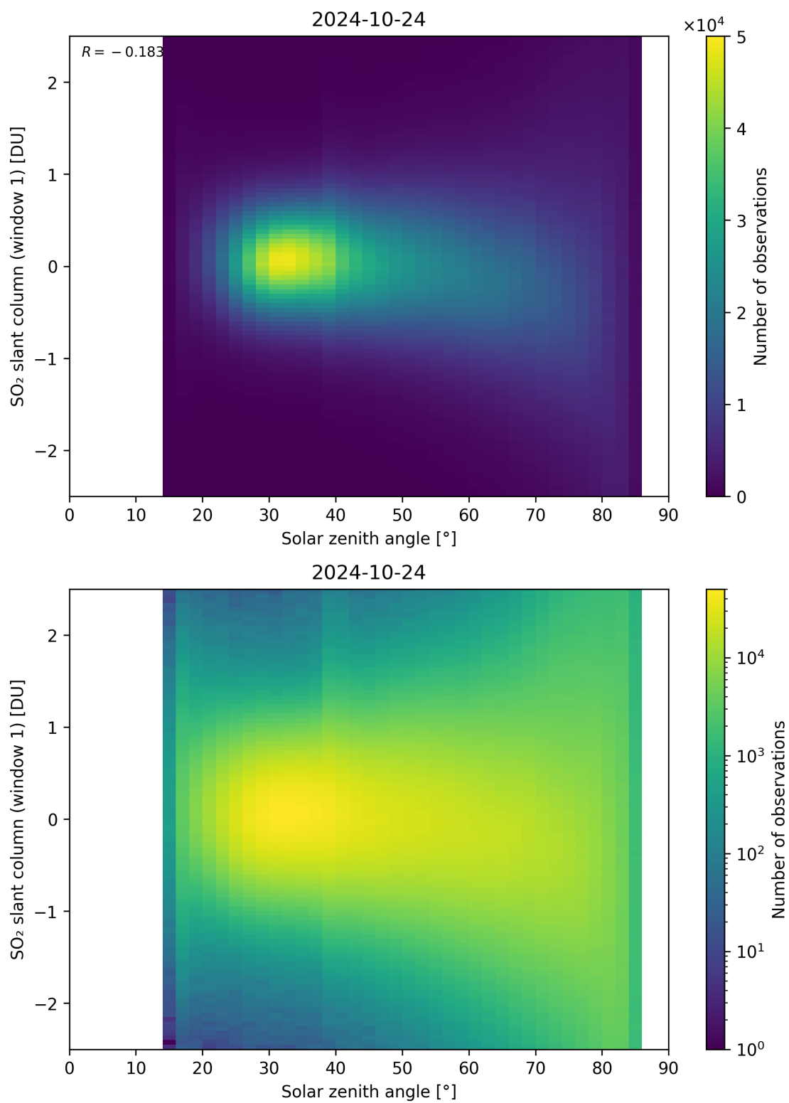
Figure 169: Scatter density plot of “Solar zenith angle” against “SO 2 slant column (window 1)” for 2024-10-24 to 2024-10-25.
