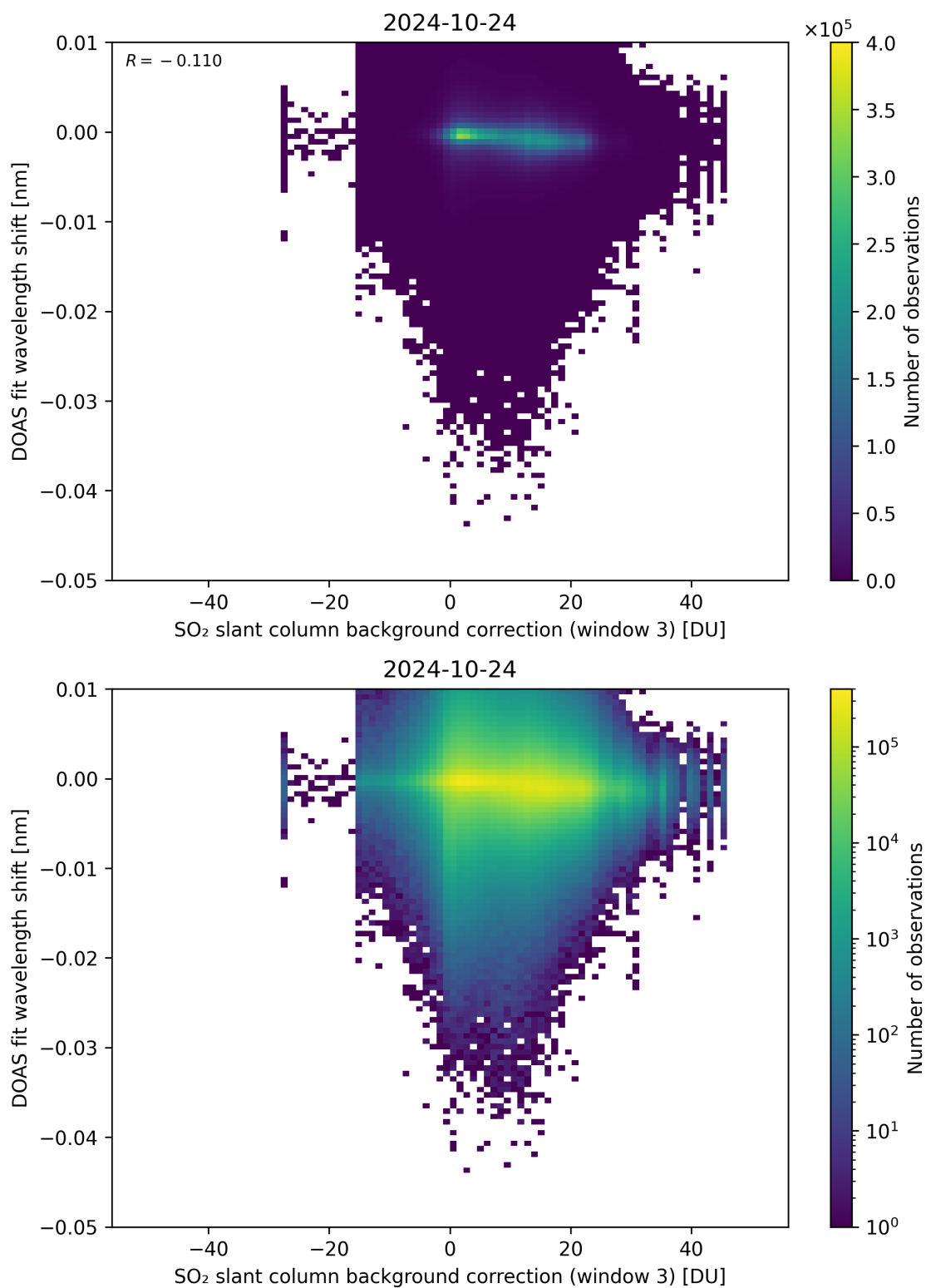
Figure 121: Scatter density plot of “SO 2 slant column background correction (window 3)” against “DOAS fit wavelength shift” for 2024-10-24 to 2024-10-25.
