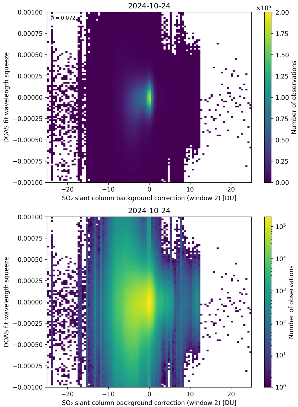
Figure 113: Scatter density plot of “SO 2 slant column background correction (window 2)” against “DOAS fit wavelength squeeze” for 2024-10-24 to 2024-10-25.
