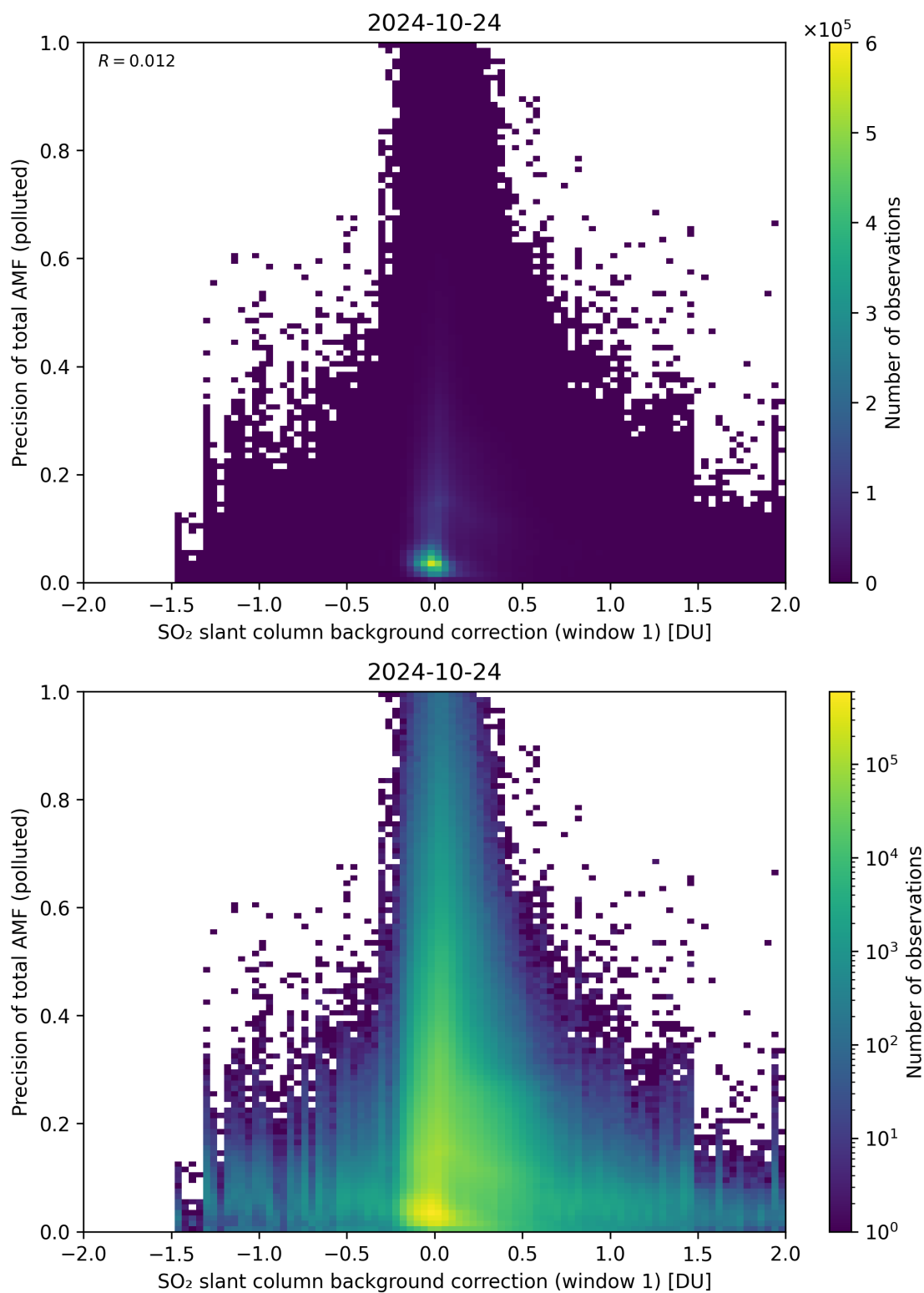
Figure 110: Scatter density plot of “SO 2 slant column background correction (window 1)” against “Precision of total AMF (polluted)” for 2024-10-24 to 2024-10-25.
