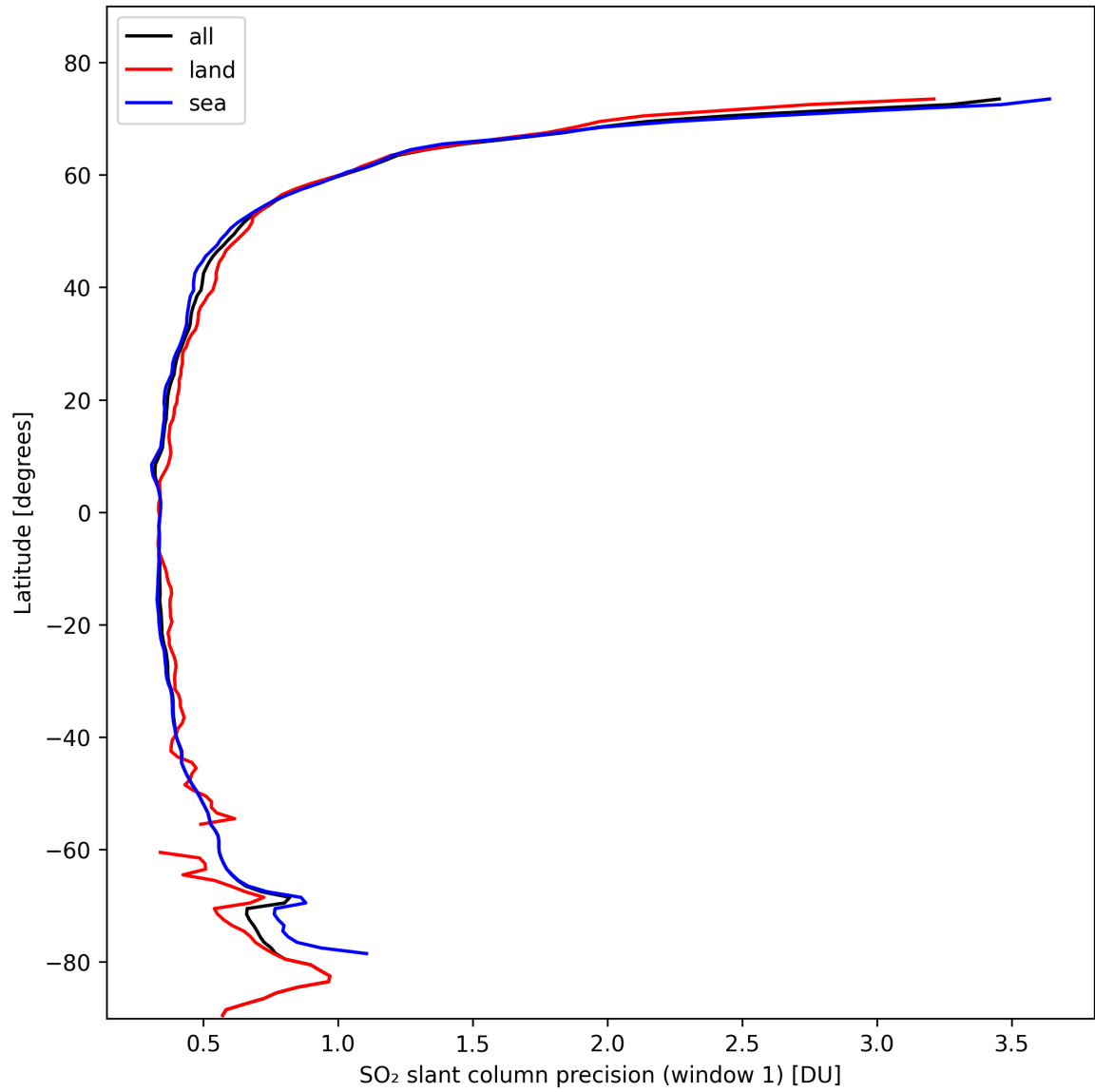
Figure 34: Zonal average of “SO 2 slant column precision (window 1)” for 2024-10-24 to 2024-10-25.
