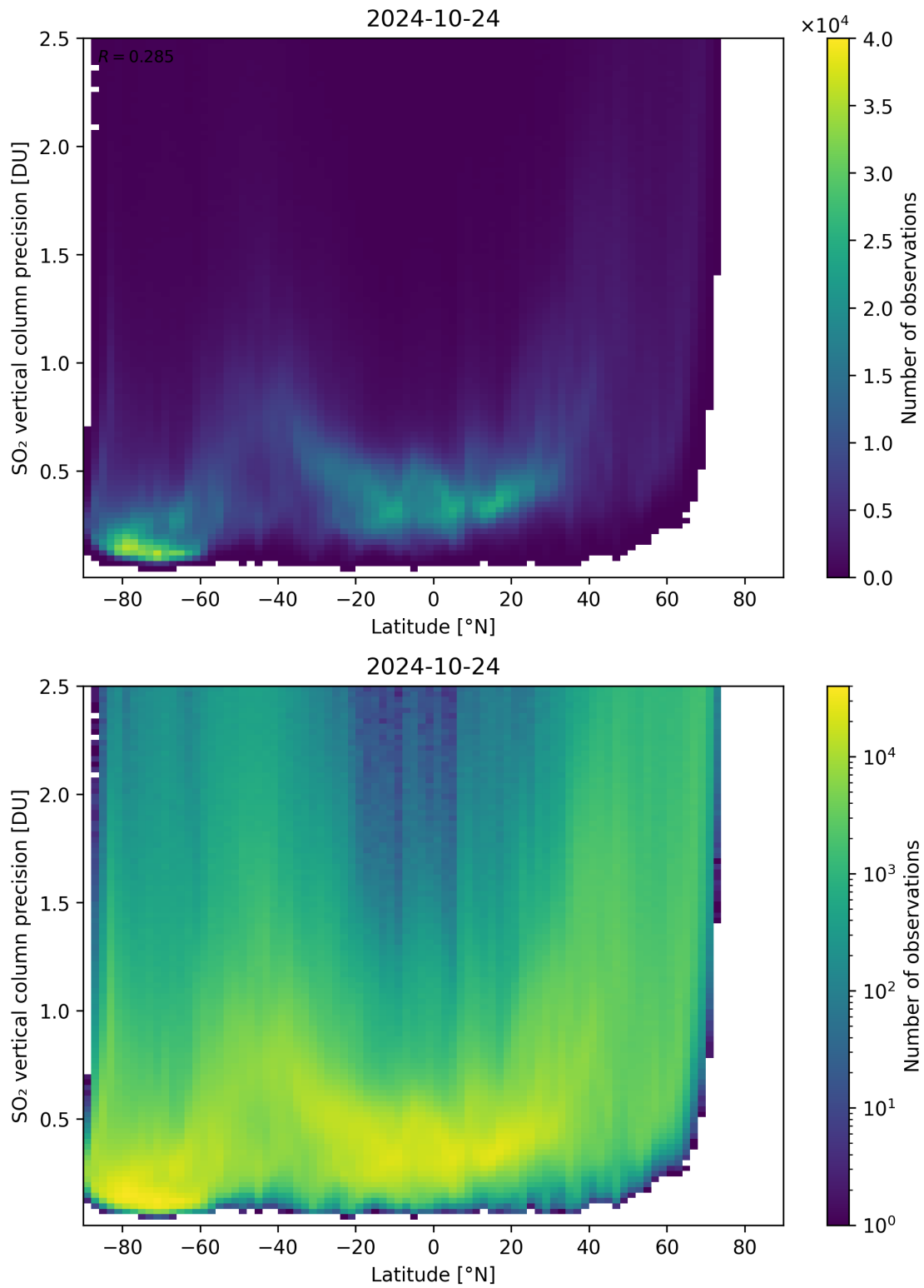
Figure 157: Scatter density plot of “Latitude” against “SO 2 vertical column precision” for 2024-10-24 to 2024-10-25.
