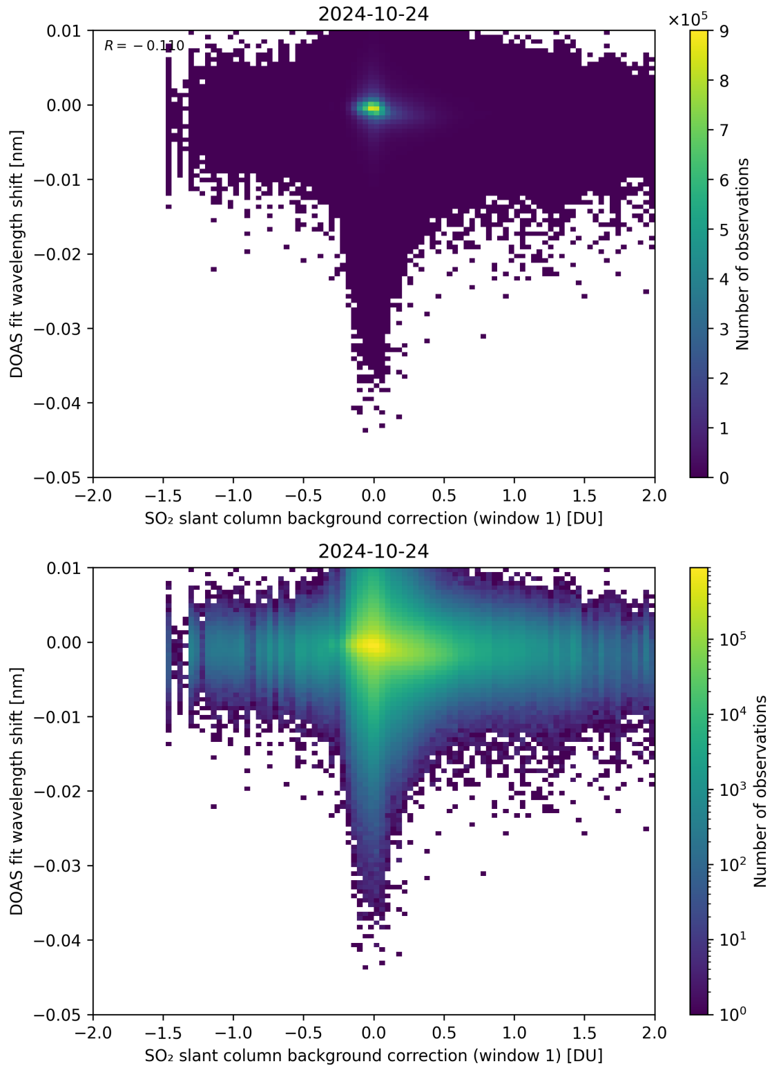
Figure 100: Scatter density plot of “SO 2 slant column background correction (window 1)” against “DOAS fit wavelength shift” for 2024-10-24 to 2024-10-25.
