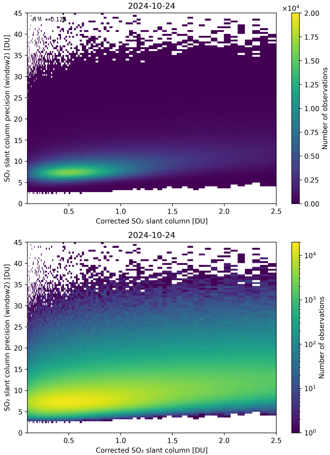
Figure 189: Scatter density plot of “Corrected SO 2 slant column” against “SO 2 slant column precision (window2)” for 2024-10-24 to 2024-10-25.
