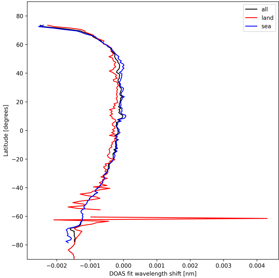
Figure 45: Zonal average of “DOAS fit wavelength shift” for 2024-10-24 to 2024-10-25.
