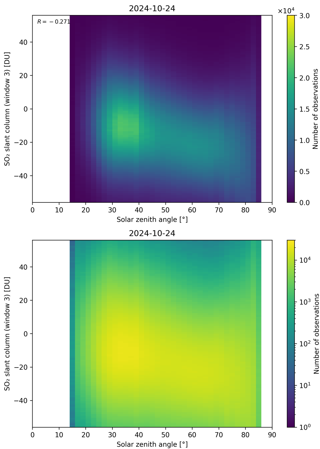
Figure 172: Scatter density plot of “Solar zenith angle” against “SO 2 slant column (window 3)” for 2024-10-24 to 2024-10-25.
