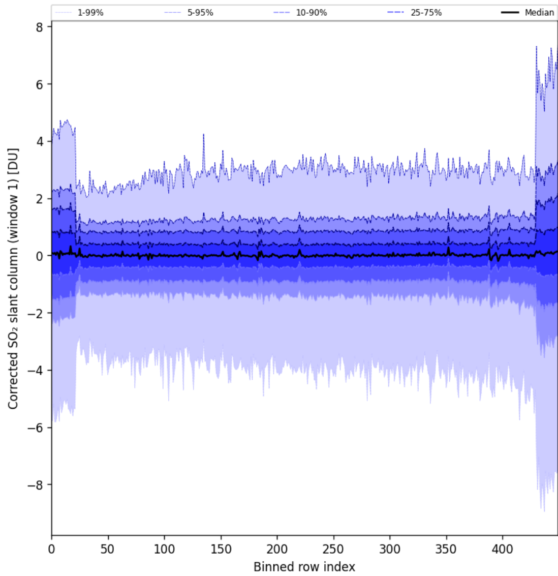
Figure 81: Along track statistics of “Corrected SO 2 slant column (window 1)” for 2024-10-24 to 2024-10-25
