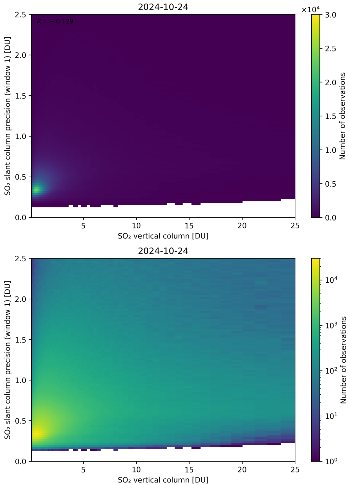
Figure 301: Scatter density plot of “SO 2 vertical column” against “SO 2 slant column precision (window 1)” for 2024-10-24 to 2024-10-25.
