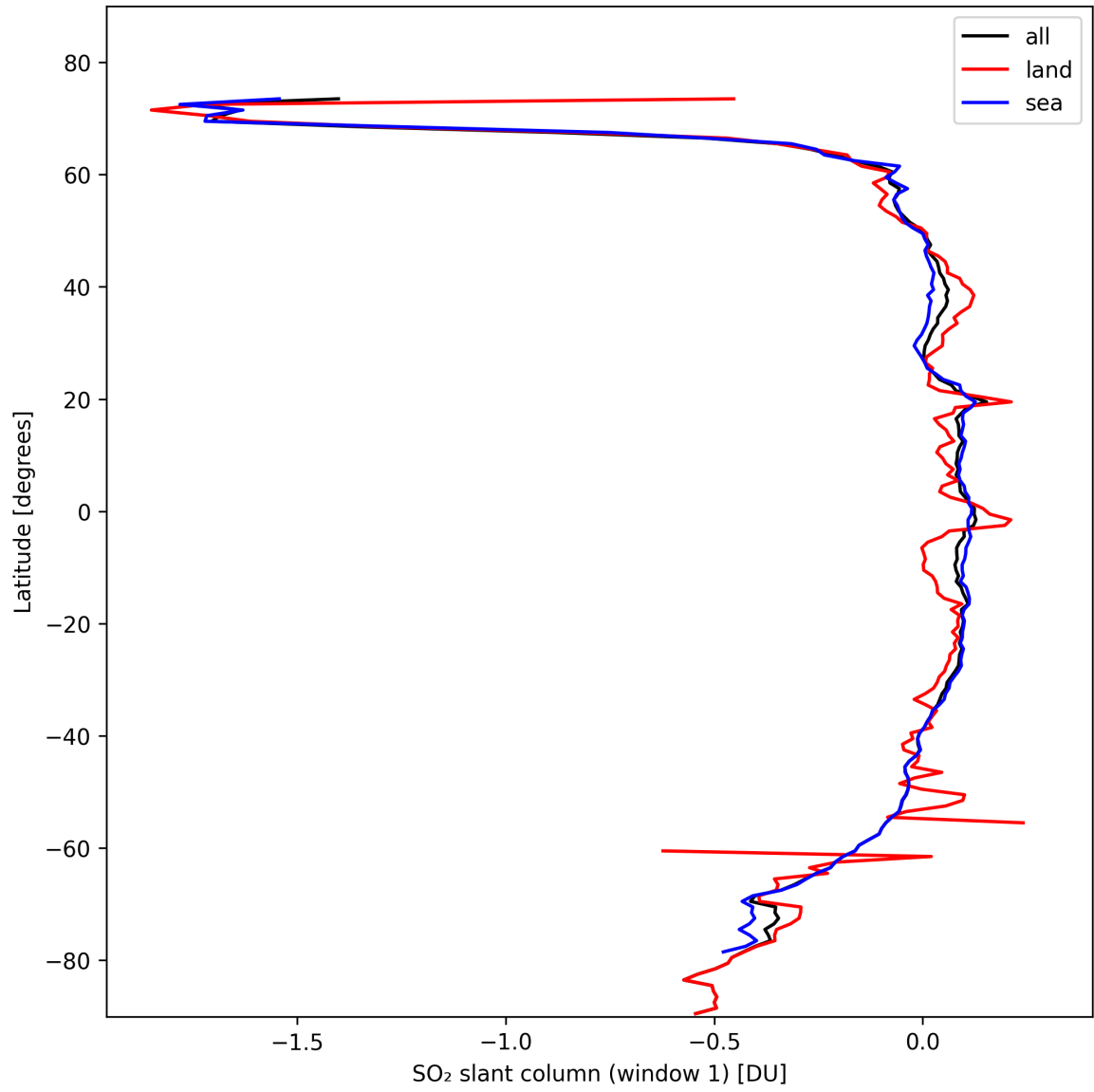
Figure 33: Zonal average of “SO 2 slant column (window 1)” for 2024-10-24 to 2024-10-25.
