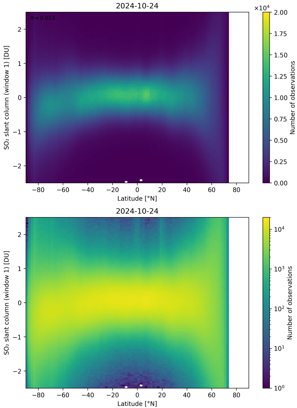
Figure 149: Scatter density plot of “Latitude” against “SO 2 slant column (window 1)” for 2024-10-24 to 2024-10-25.
