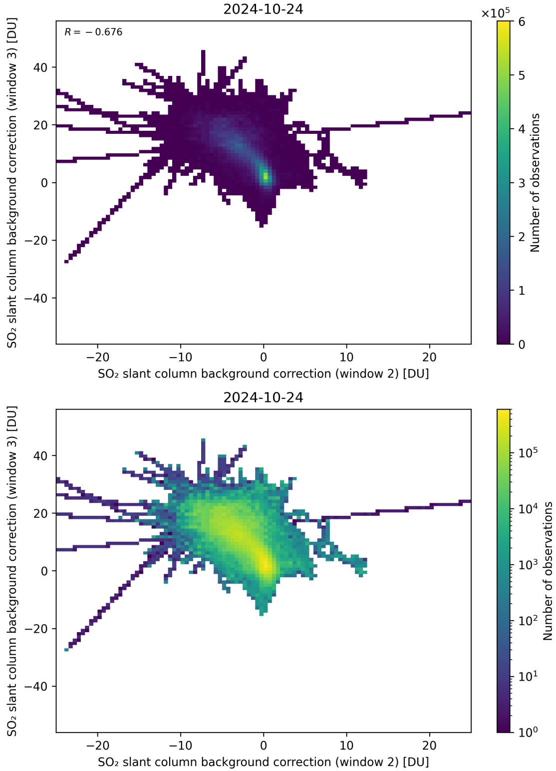
Figure 111: Scatter density plot of “SO 2 slant column background correction (window 2)” against “SO 2 slant column background correction (window 3)” for 2024-10-24 to 2024-10-25.
