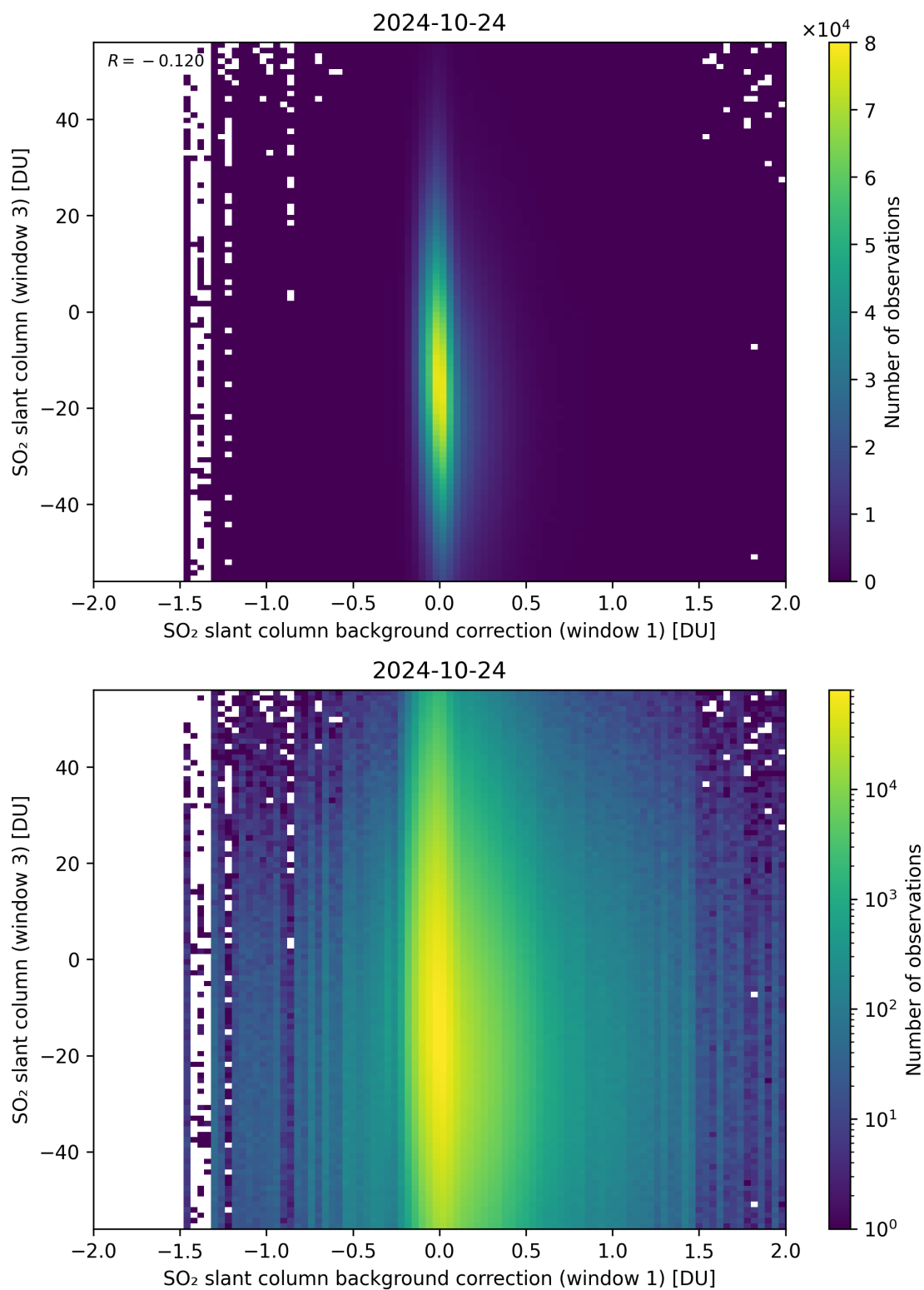
Figure 107: Scatter density plot of “SO 2 slant column background correction (window 1)” against “SO 2 slant column (window 3)” for 2024-10-24 to 2024-10-25.
