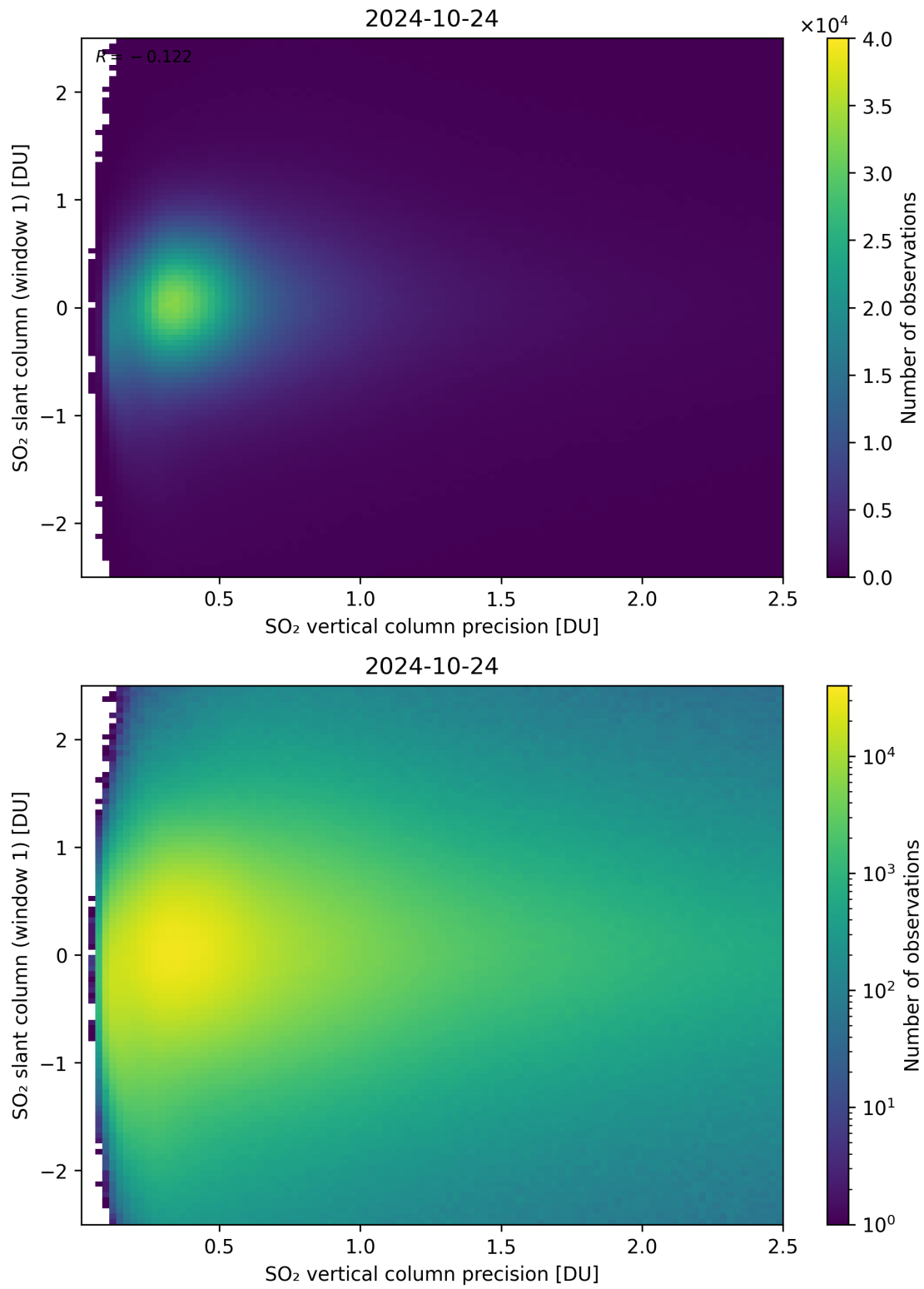
Figure 289: Scatter density plot of “SO 2 vertical column precision” against “SO 2 slant column (window 1)” for 2024-10-24 to 2024-10-25.
