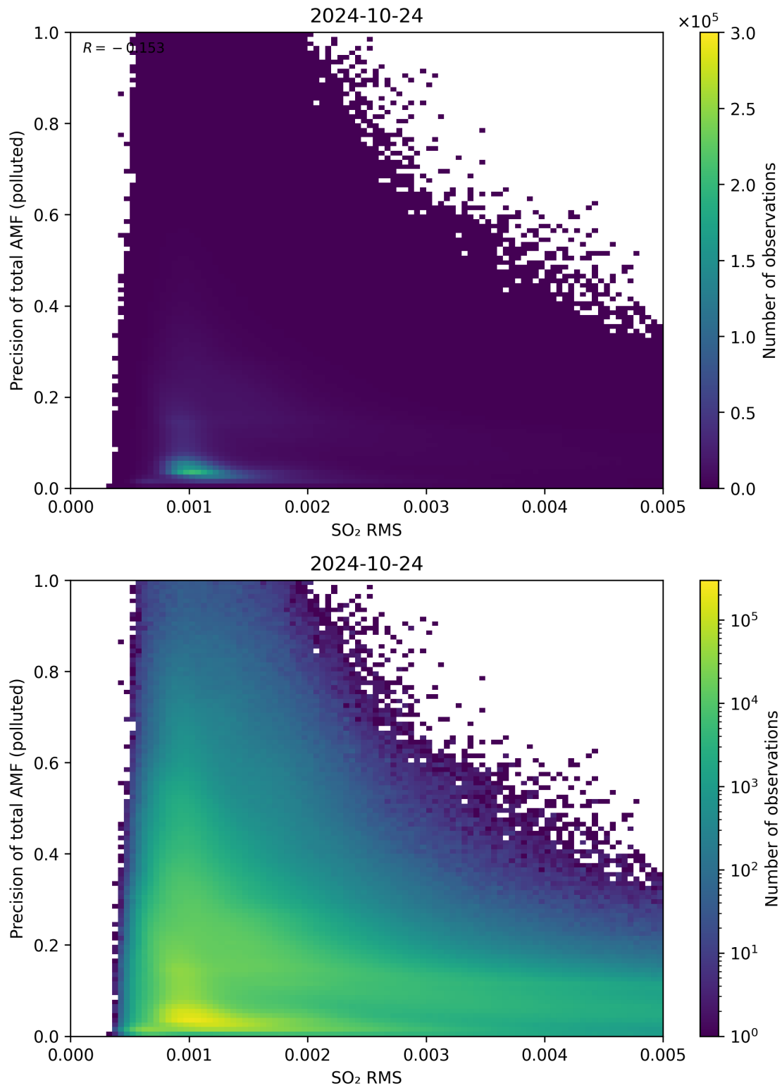
Figure 138: Scatter density plot of “SO 2 RMS” against “Precision of total AMF (polluted)” for 2024-10-24 to 2024-10-25.
