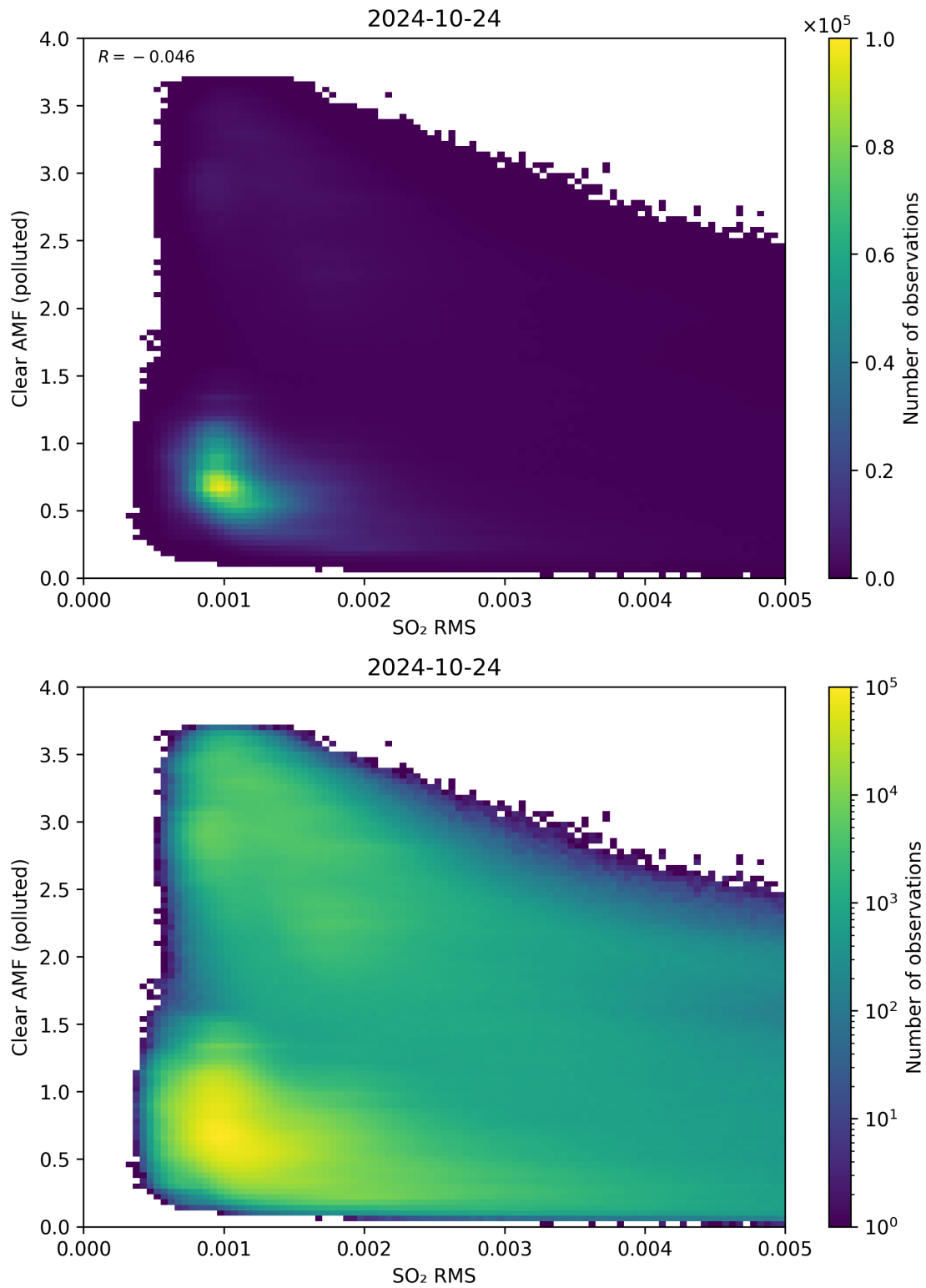
Figure 136: Scatter density plot of “SO 2 RMS” against “Clear AMF (polluted)” for 2024-10-24 to 2024-10-25.
