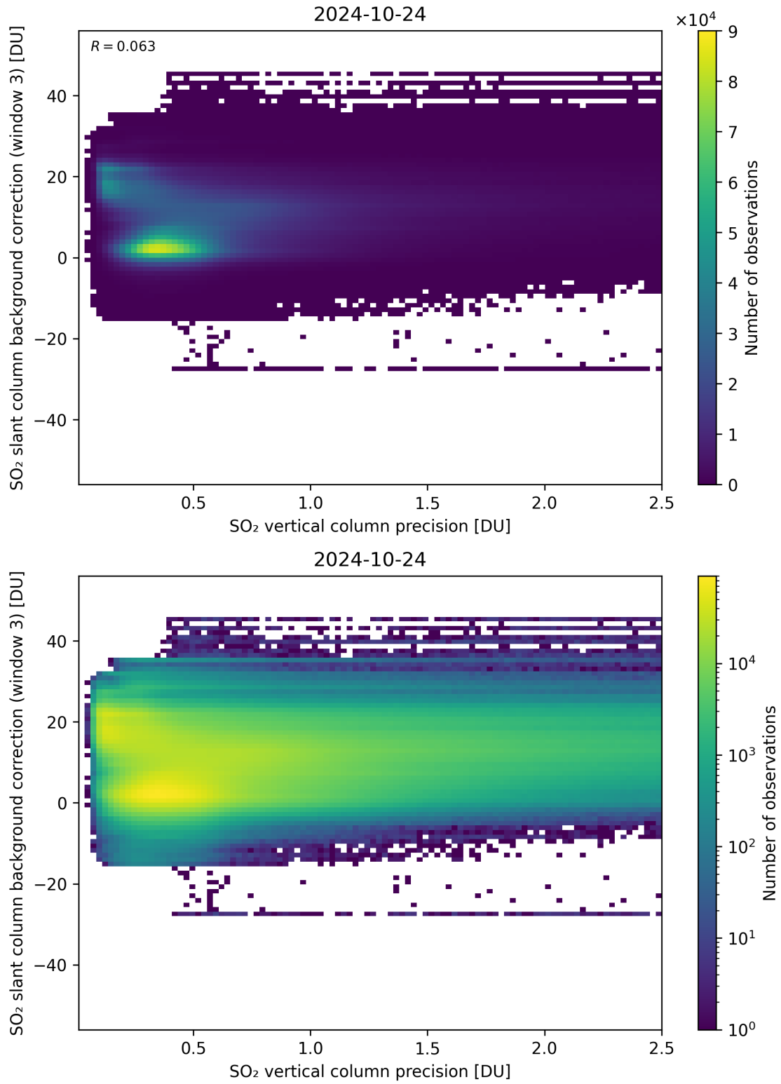
Figure 281: Scatter density plot of “SO 2 vertical column precision” against “SO 2 slant column background correction (window 3)” for 2024-10-24 to 2024-10-25.
