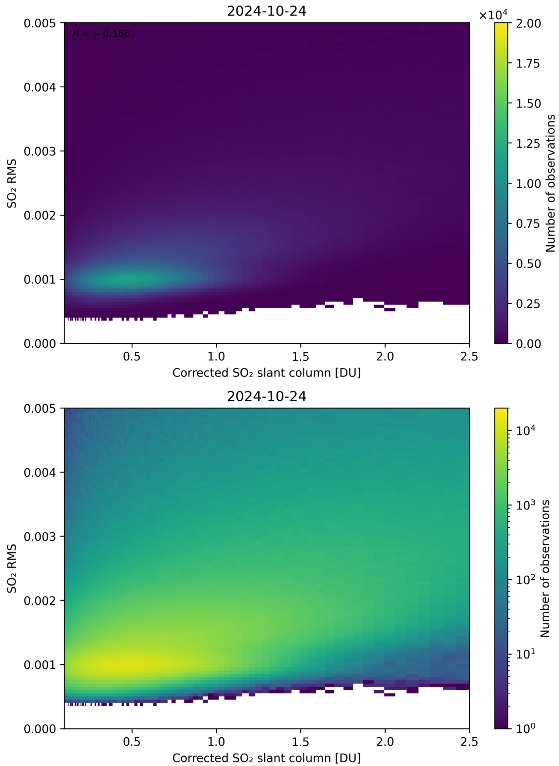
Figure 183: Scatter density plot of “Corrected SO 2 slant column” against “SO 2 RMS” for 2024-10-24 to 2024-10-25.
