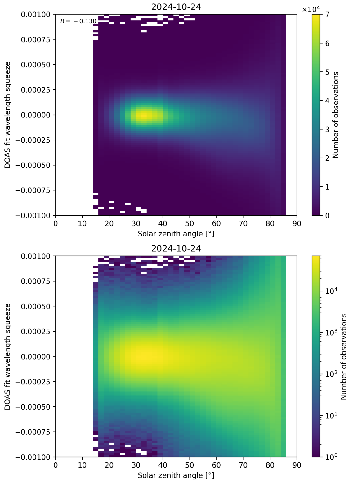
Figure 162: Scatter density plot of “Solar zenith angle” against “DOAS fit wavelength squeeze” for 2024-10-24 to 2024-10-25.
