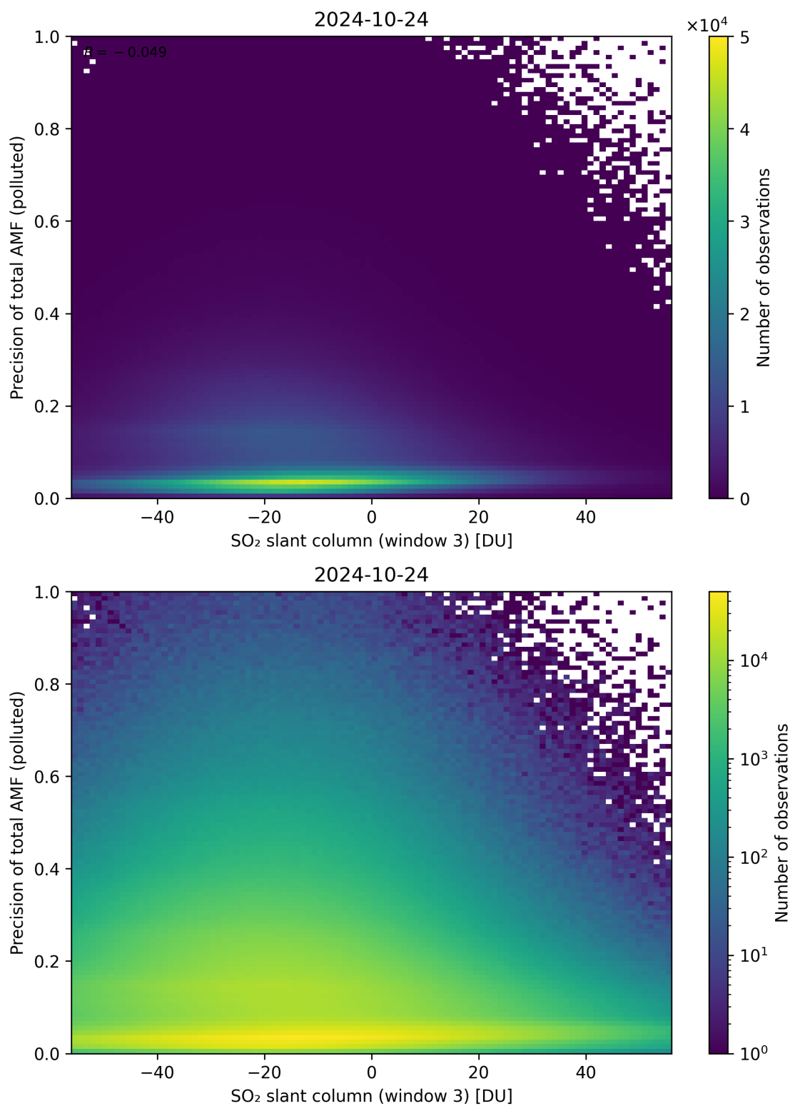
Figure 269: Scatter density plot of “SO 2 slant column (window 3)” against “Precision of total AMF (polluted)” for 2024-10-24 to 2024-10-25.
