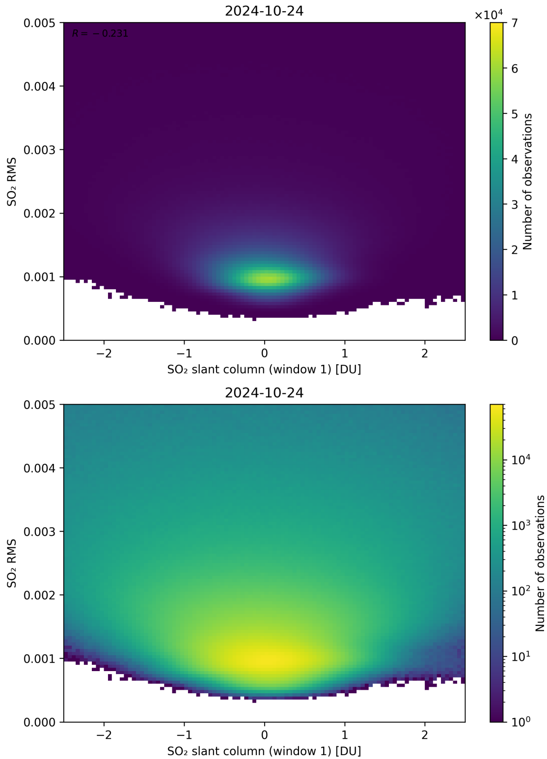
Figure 217: Scatter density plot of “SO 2 slant column (window 1)” against “SO 2 RMS” for 2024-10-24 to 2024-10-25.
