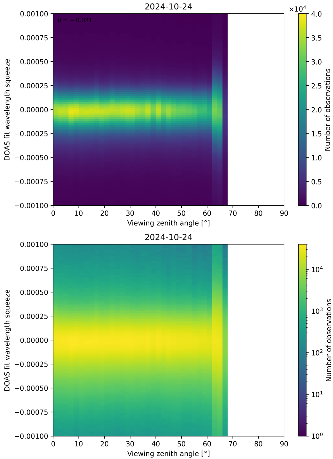
Figure 312: Scatter density plot of “Viewing zenith angle” against “DOAS fit wavelength squeeze” for 2024-10-24 to 2024-10-25.
