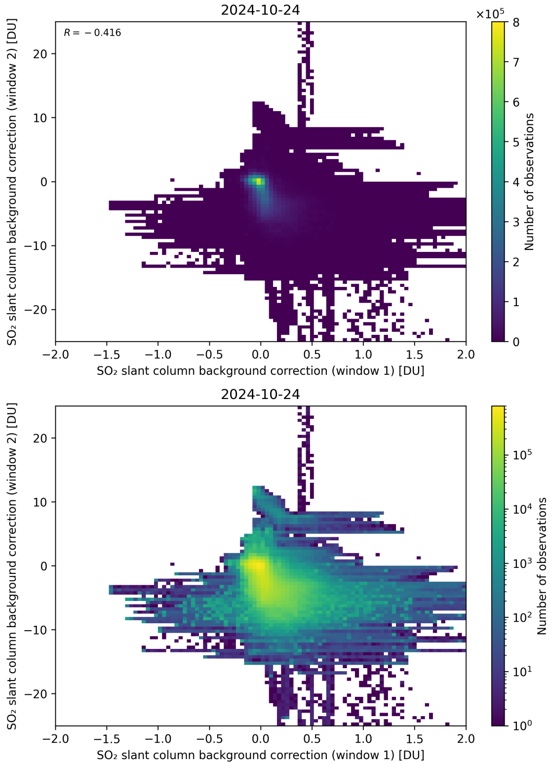
Figure 98: Scatter density plot of “SO 2 slant column background correction (window 1)” against “SO 2 slant column background correction (window 2)” for 2024-10-24 to 2024-10-25.
