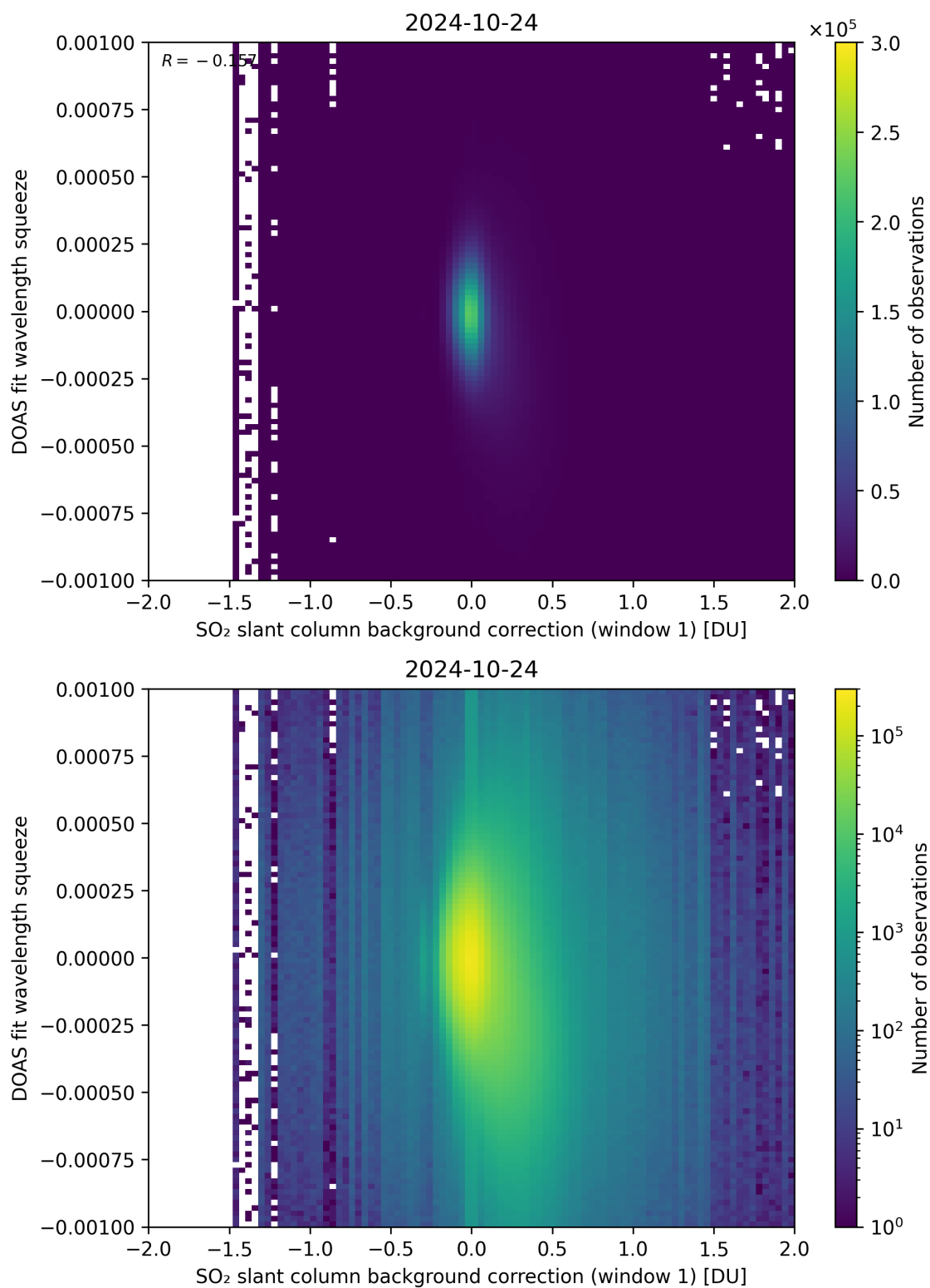
Figure 101: Scatter density plot of “SO 2 slant column background correction (window 1)” against “DOAS fit wavelength squeeze” for 2024-10-24 to 2024-10-25.
