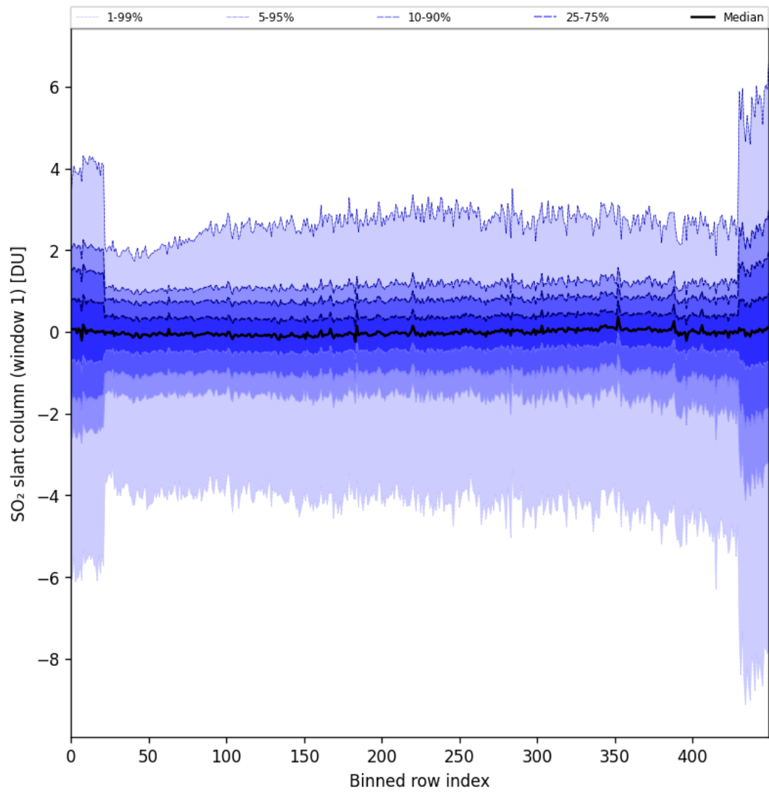
Figure 79: Along track statistics of “SO 2 slant column (window 1)” for 2024-10-24 to 2024-10-25
