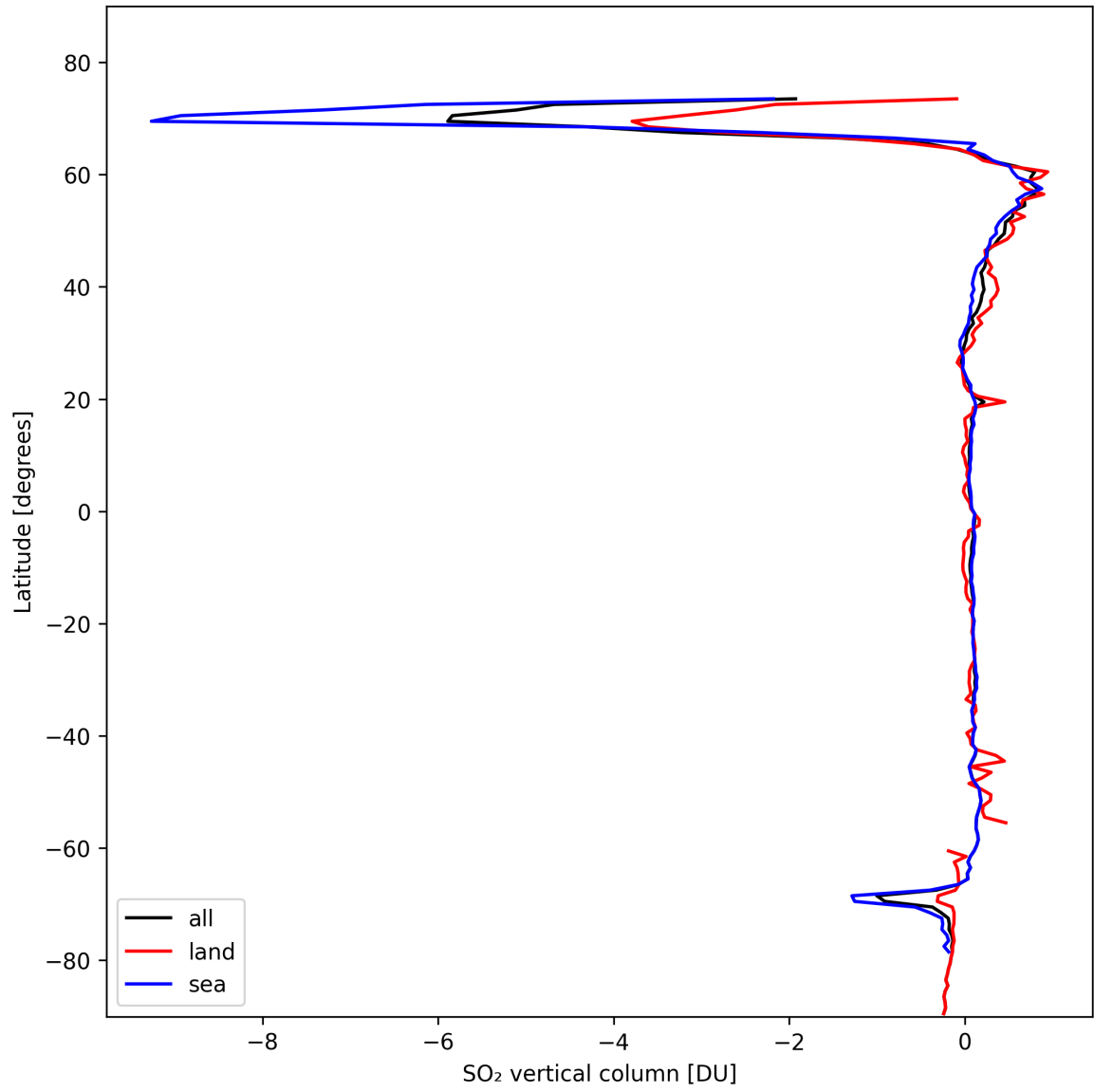
Figure 30: Zonal average of “SO 2 vertical column” for 2024-10-24 to 2024-10-25.
