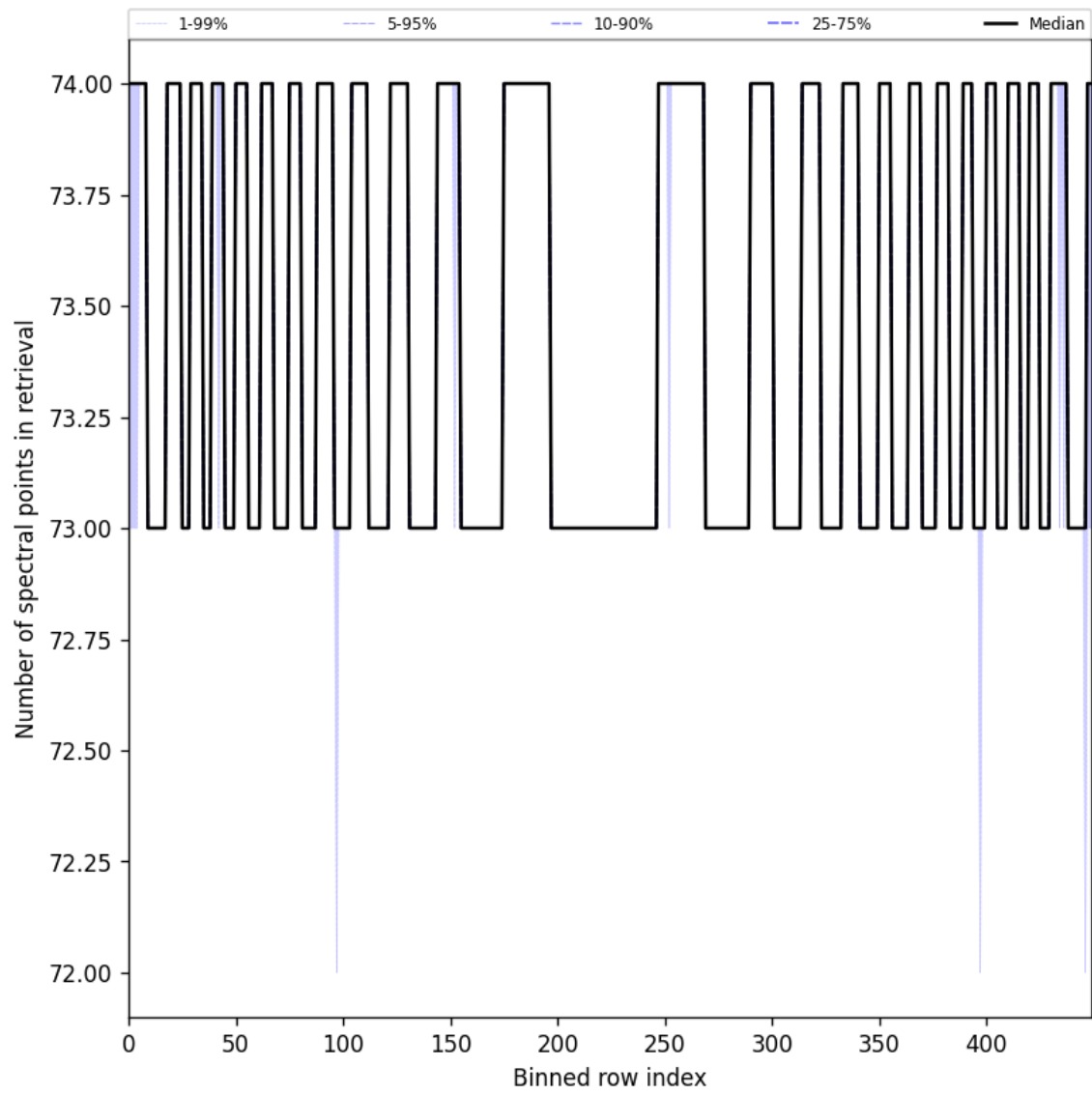
Figure 97: Along track statistics of “Number of spectral points in retrieval” for 2024-10-24 to 2024-10-25
