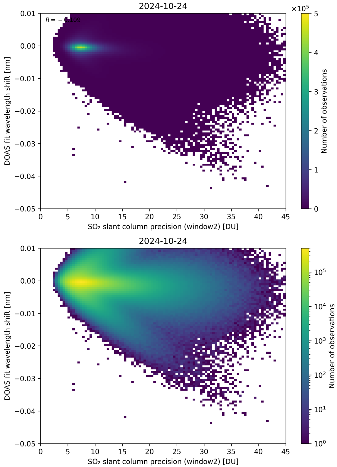
Figure 243: Scatter density plot of “SO 2 slant column precision (window2)” against “DOAS fit wavelength shift” for 2024-10-24 to 2024-10-25.
