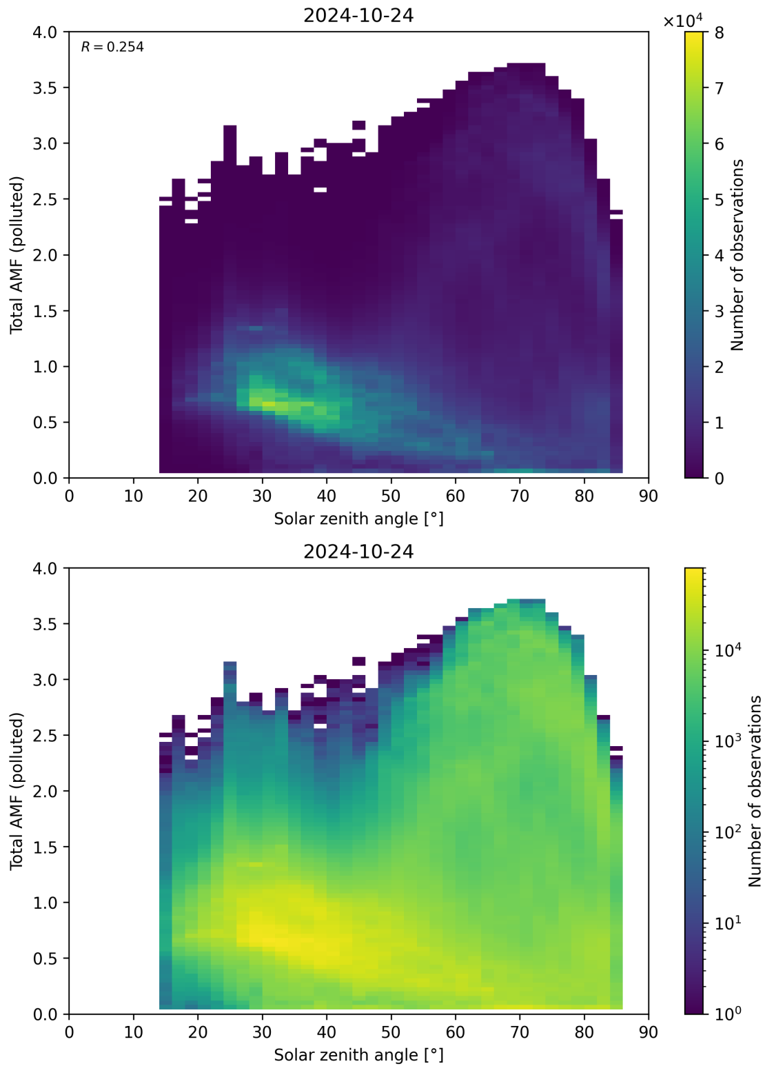
Figure 174: Scatter density plot of “Solar zenith angle” against “Total AMF (polluted)” for 2024-10-24 to 2024-10-25.
