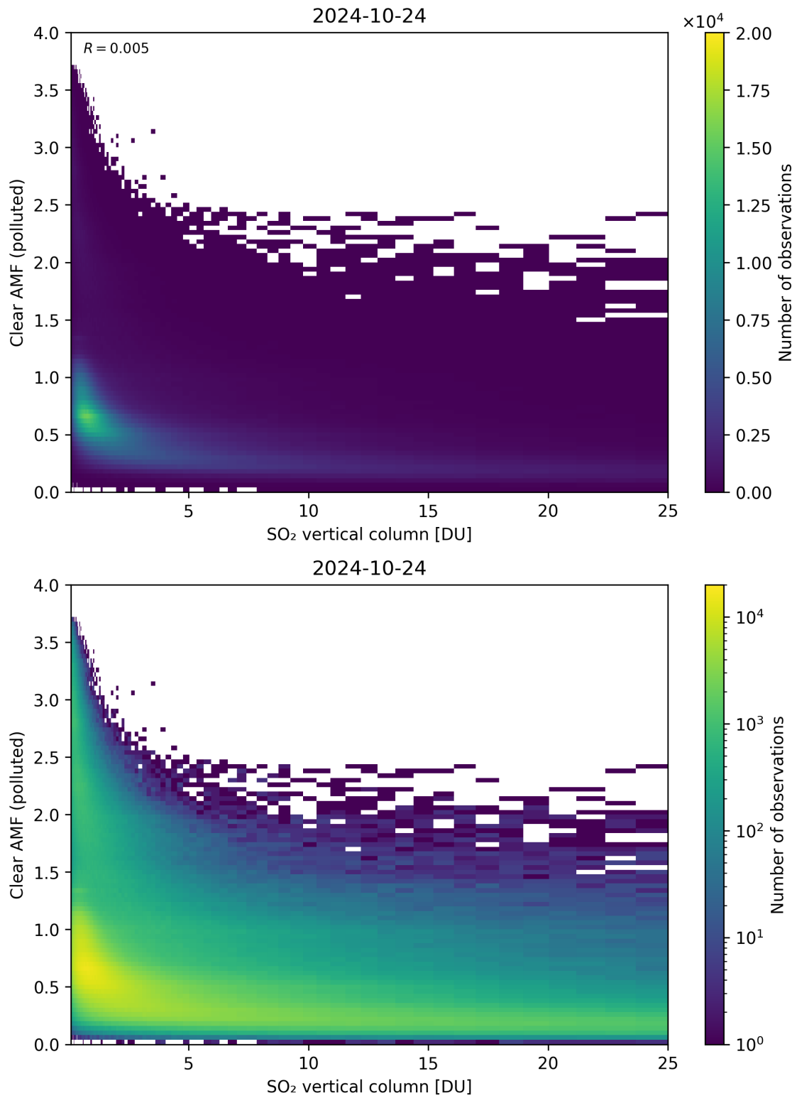
Figure 296: Scatter density plot of “SO 2 vertical column” against “Clear AMF (polluted)” for 2024-10-24 to 2024-10-25.
