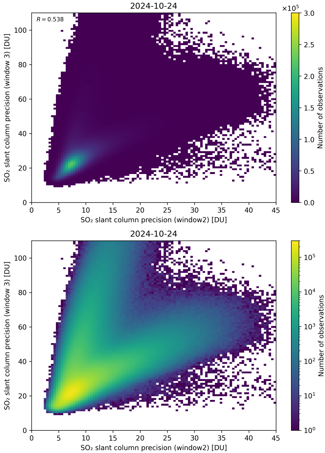
Figure 250: Scatter density plot of “SO 2 slant column precision (window2)” against “SO 2 slant column precision (window 3)” for 2024-10-24 to 2024-10-25.
