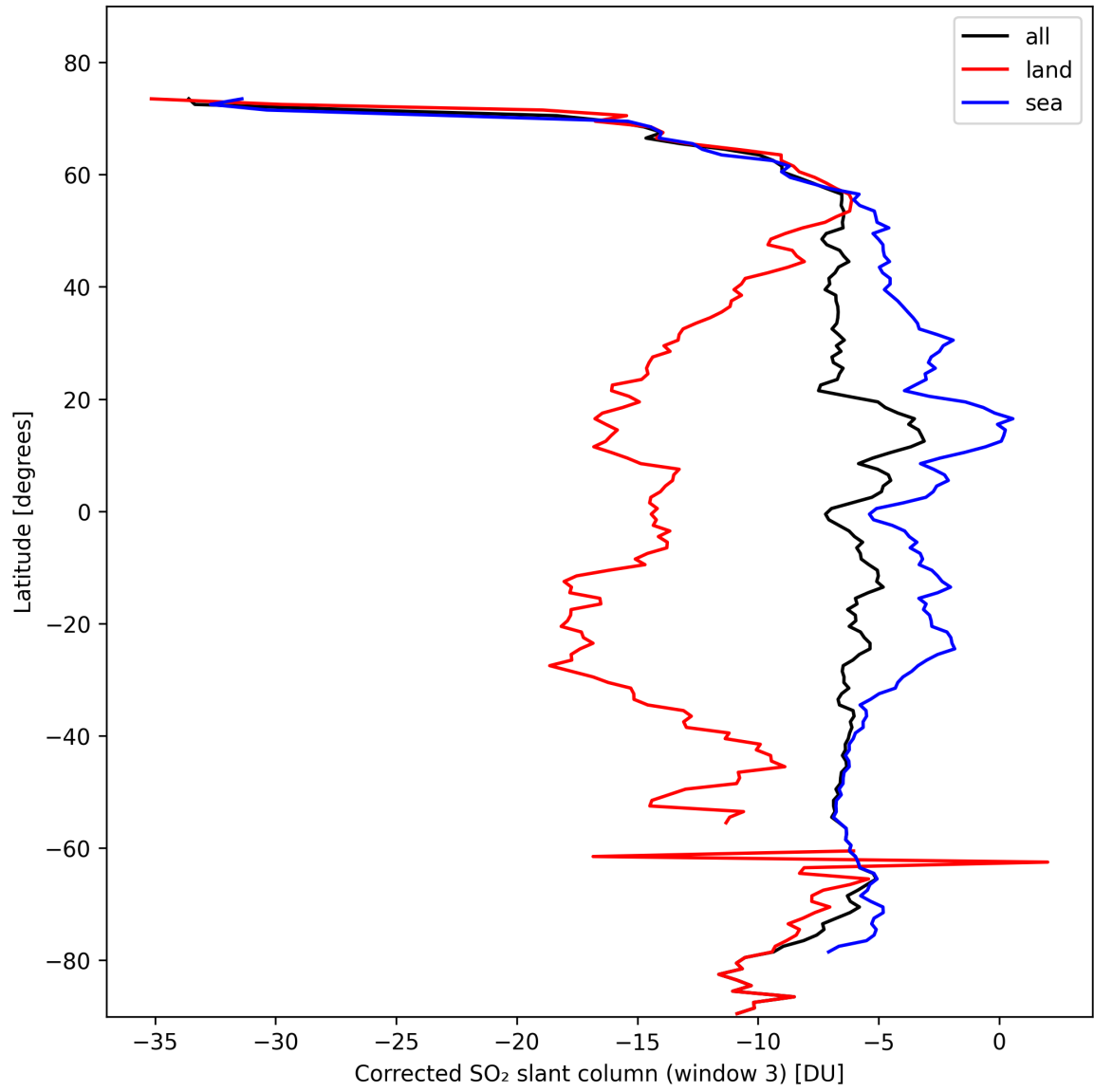
Figure 43: Zonal average of “Corrected SO 2 slant column (window 3)” for 2024-10-24 to 2024-10-25.
