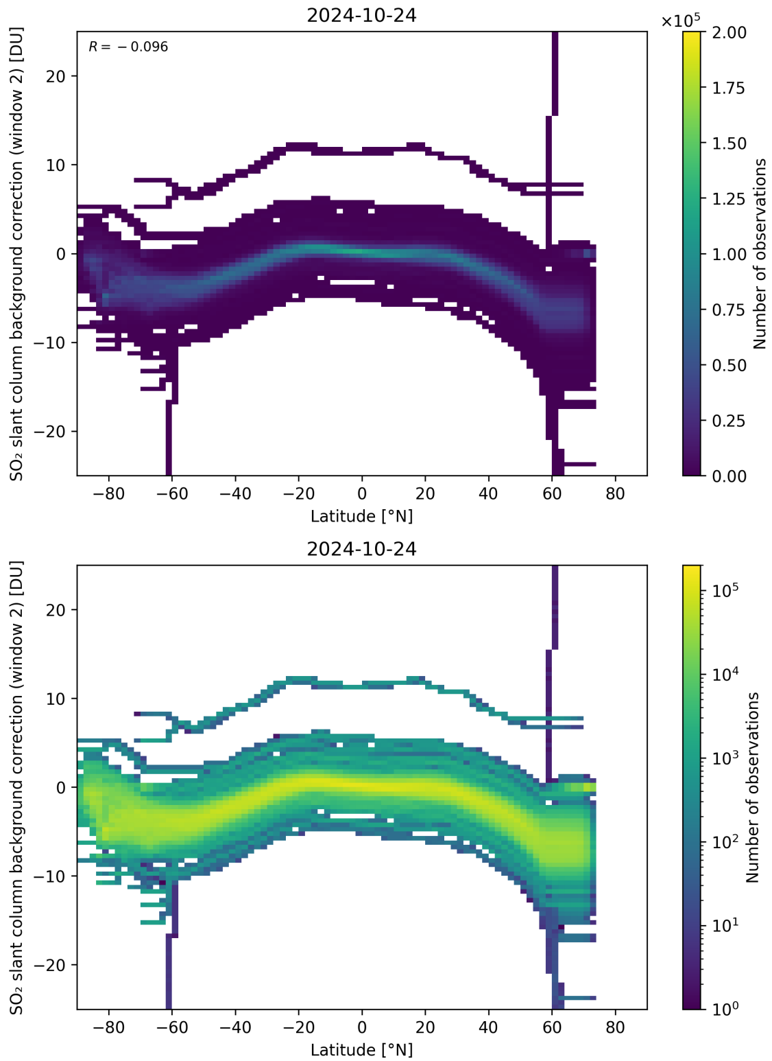
Figure 140: Scatter density plot of “Latitude” against “SO 2 slant column background correction (window 2)” for 2024-10-24 to 2024-10-25.
