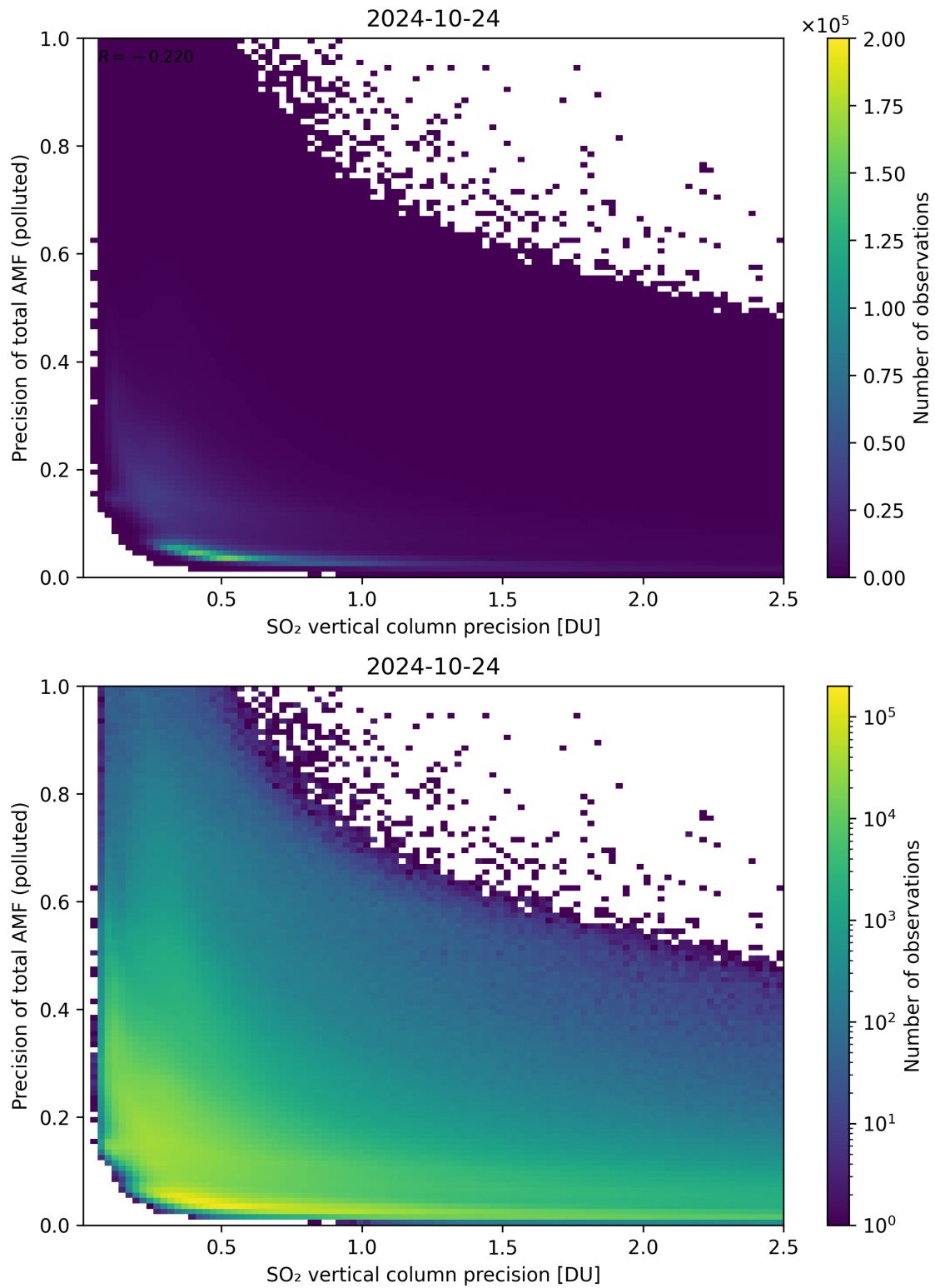
Figure 295: Scatter density plot of “SO 2 vertical column precision” against “Precision of total AMF (polluted)” for 2024-10-24 to 2024-10-25.
