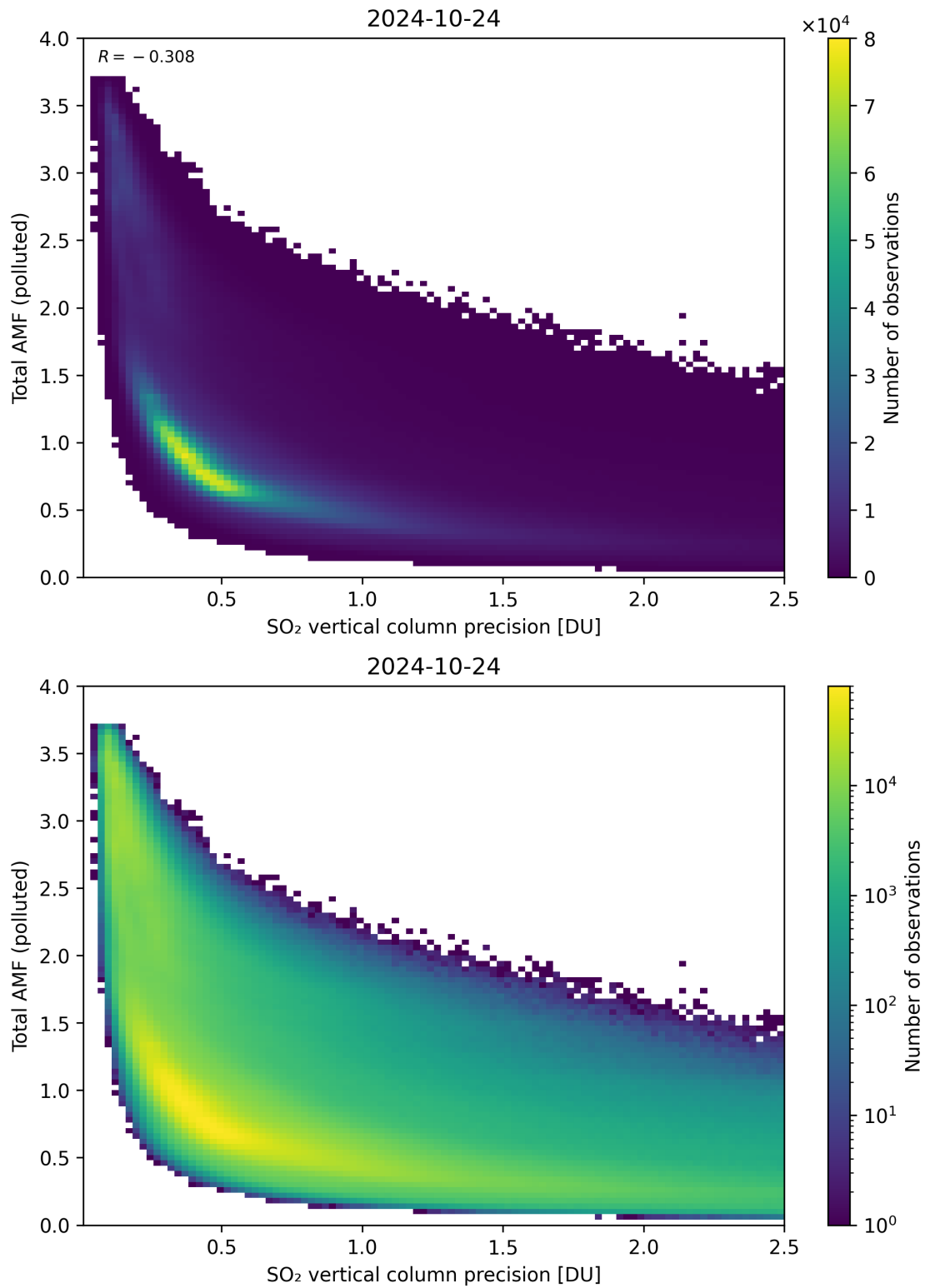
Figure 294: Scatter density plot of “SO 2 vertical column precision” against “Total AMF (polluted)” for 2024-10-24 to 2024-10-25.
