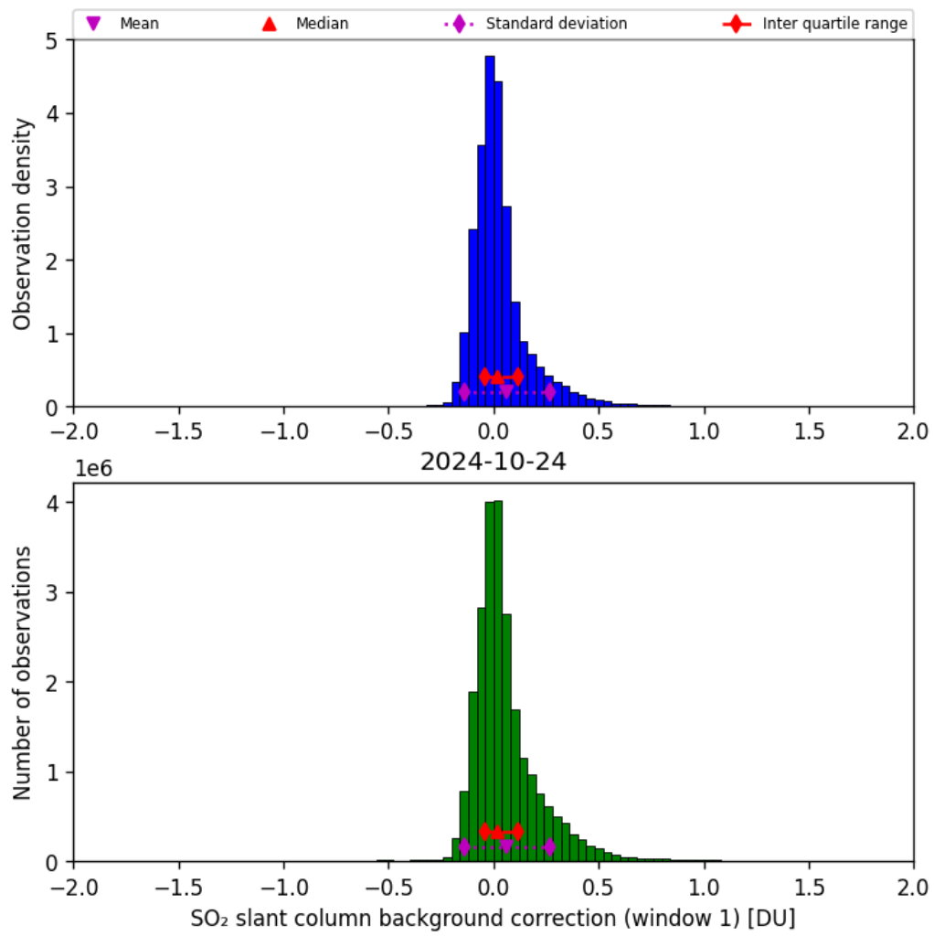
Figure 59: Histogram of “SO 2 slant column background correction (window 1)” for 2024-10-24 to 2024-10-25
