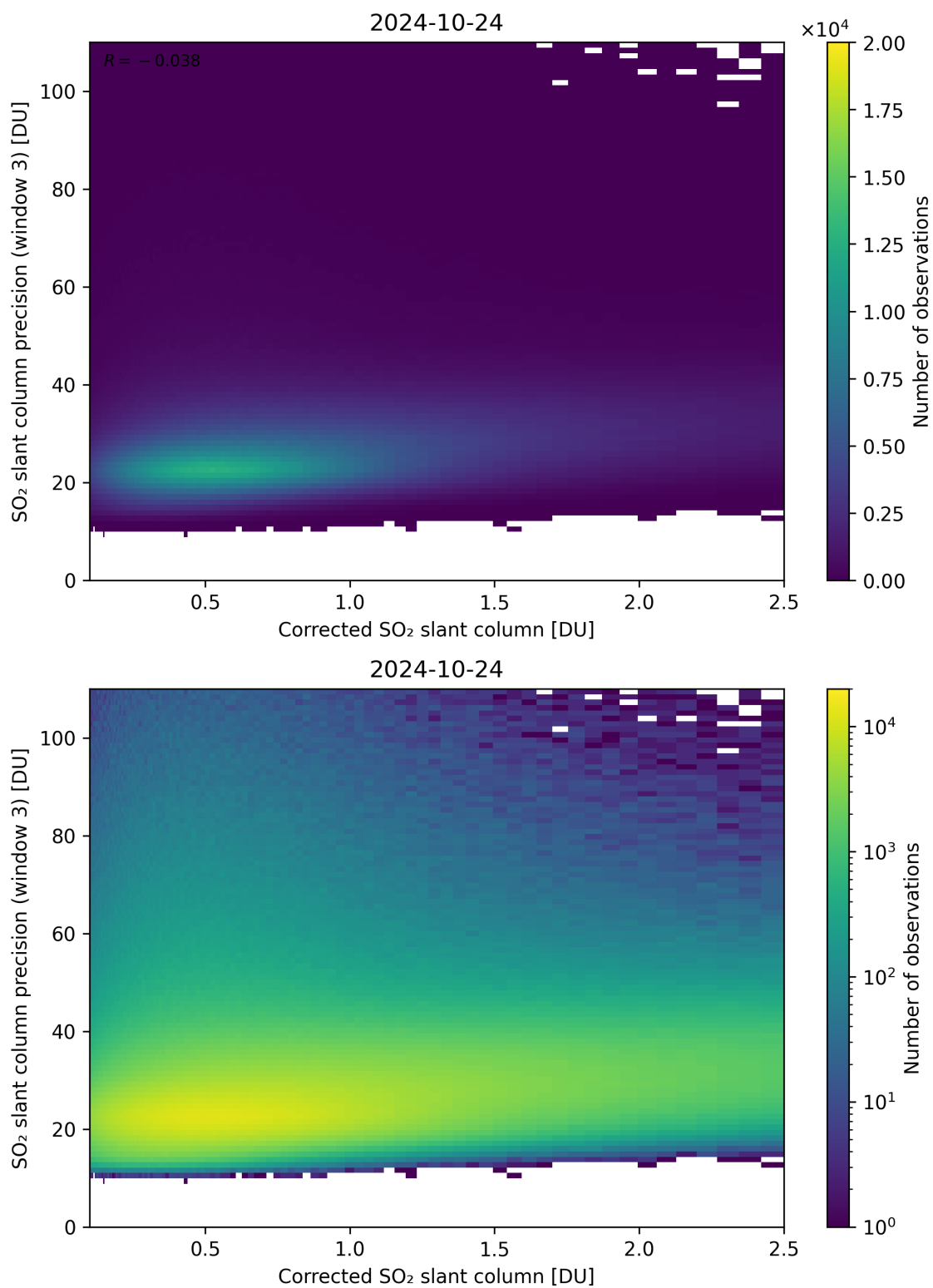
Figure 191: Scatter density plot of “Corrected SO 2 slant column” against “SO 2 slant column precision (window 3)” for 2024-10-24 to 2024-10-25.
