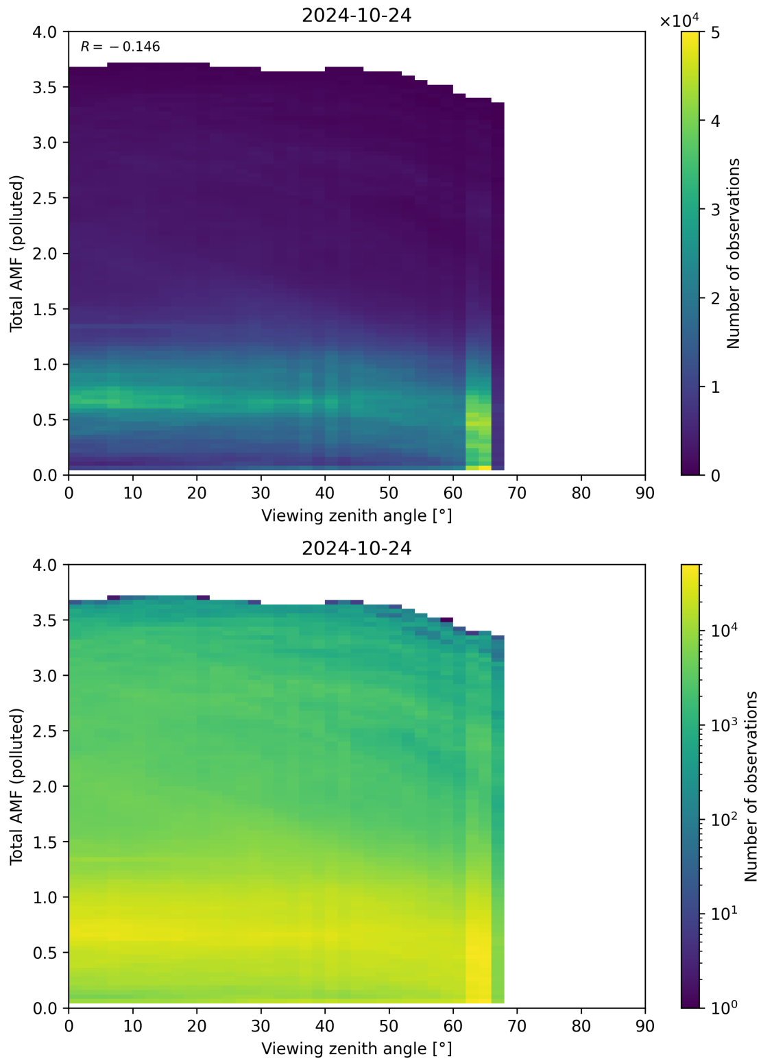
Figure 325: Scatter density plot of “Viewing zenith angle” against “Total AMF (polluted)” for 2024-10-24 to 2024-10-25.
