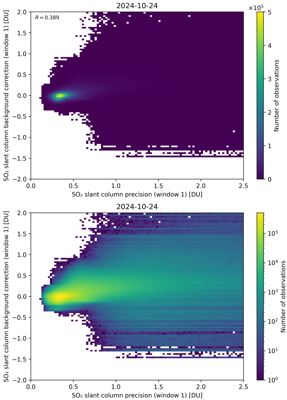
Figure 218: Scatter density plot of “SO 2 slant column precision (window 1)” against “SO 2 slant column background correction (window 1)” for 2024-10-24 to 2024-10-25.
