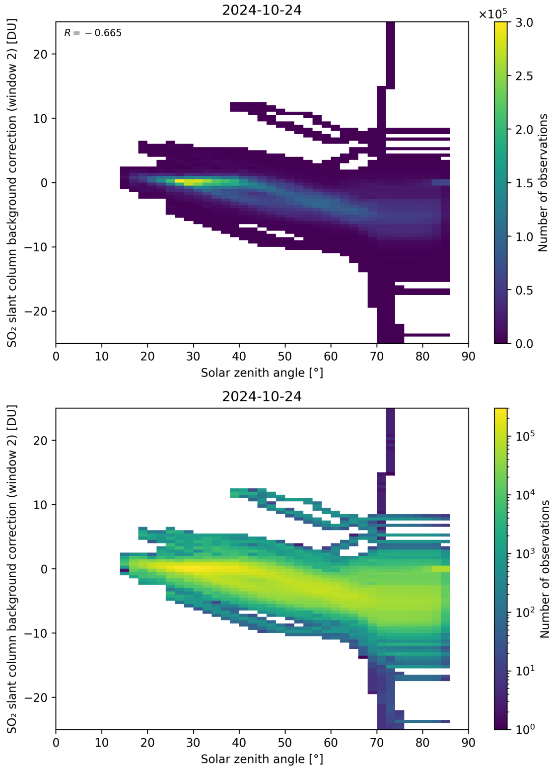
Figure 159: Scatter density plot of “Solar zenith angle” against “SO 2 slant column background correction (window 2)” for 2024-10-24 to 2024-10-25.
