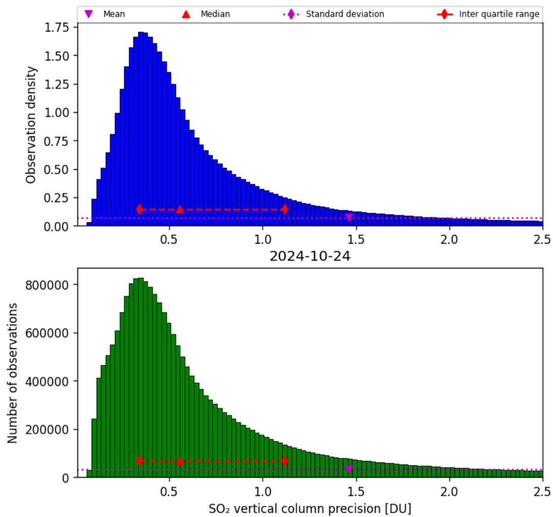
Figure 54: Histogram of “SO 2 vertical column precision” for 2024-10-24 to 2024-10-25
