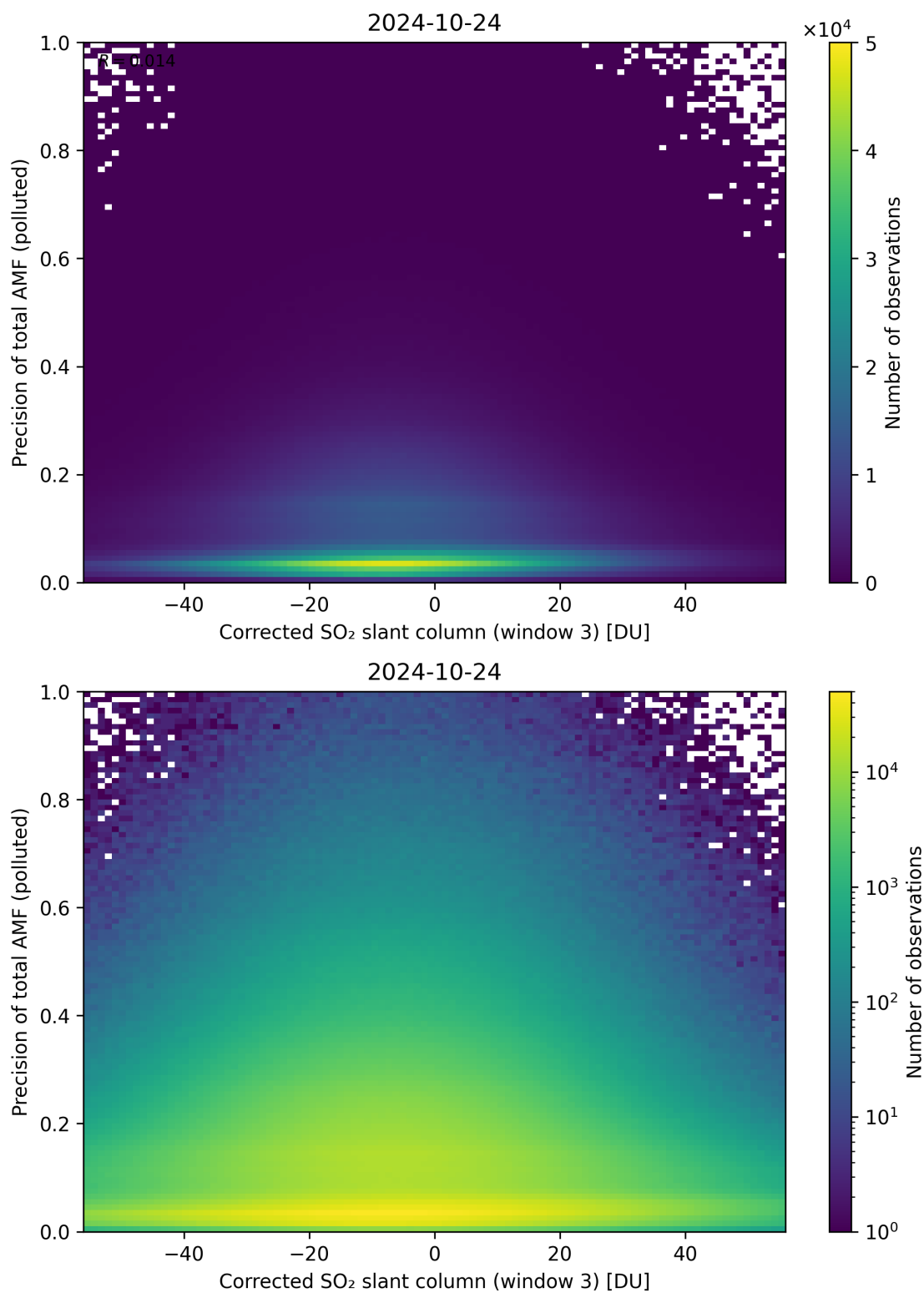
Figure 211: Scatter density plot of “Corrected SO 2 slant column (window 3)” against “Precision of total AMF (polluted)” for 2024-10-24 to 2024-10-25.
