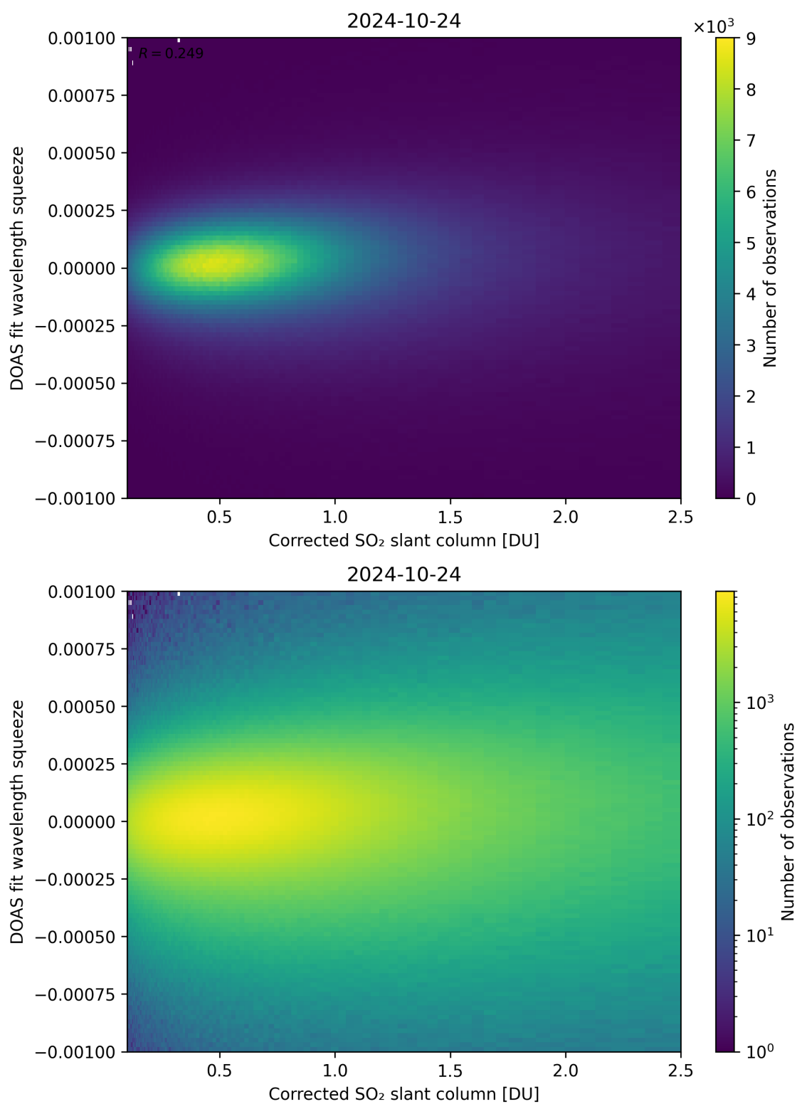
Figure 182: Scatter density plot of “Corrected SO 2 slant column” against “DOAS fit wavelength squeeze” for 2024-10-24 to 2024-10-25.
