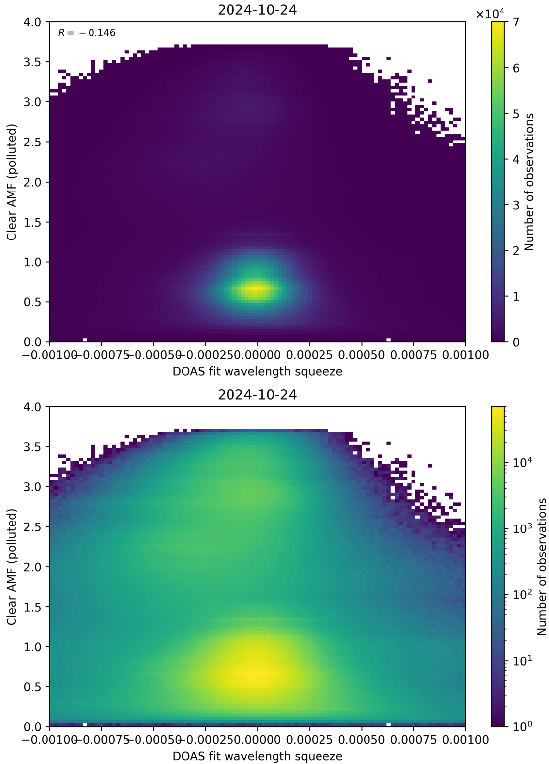
Figure 133: Scatter density plot of “DOAS fit wavelength squeeze” against “Clear AMF (polluted)” for 2024-10-24 to 2024-10-25.
