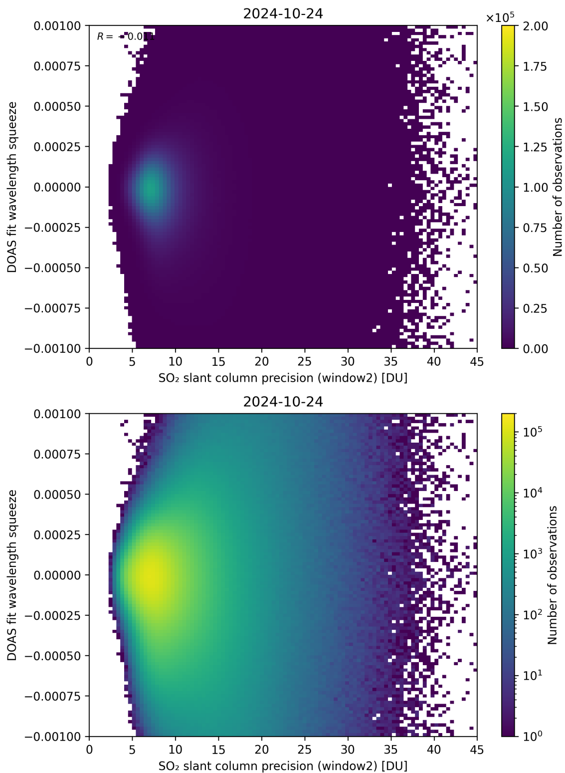
Figure 244: Scatter density plot of “SO 2 slant column precision (window2)” against “DOAS fit wavelength squeeze” for 2024-10-24 to 2024-10-25.
