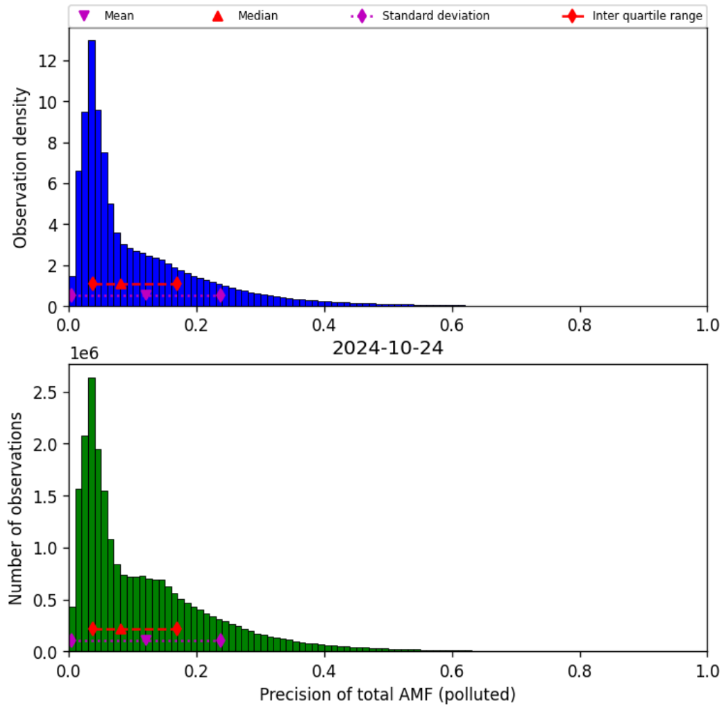
Figure 72: Histogram of “Precision of total AMF (polluted)” for 2024-10-24 to 2024-10-25
