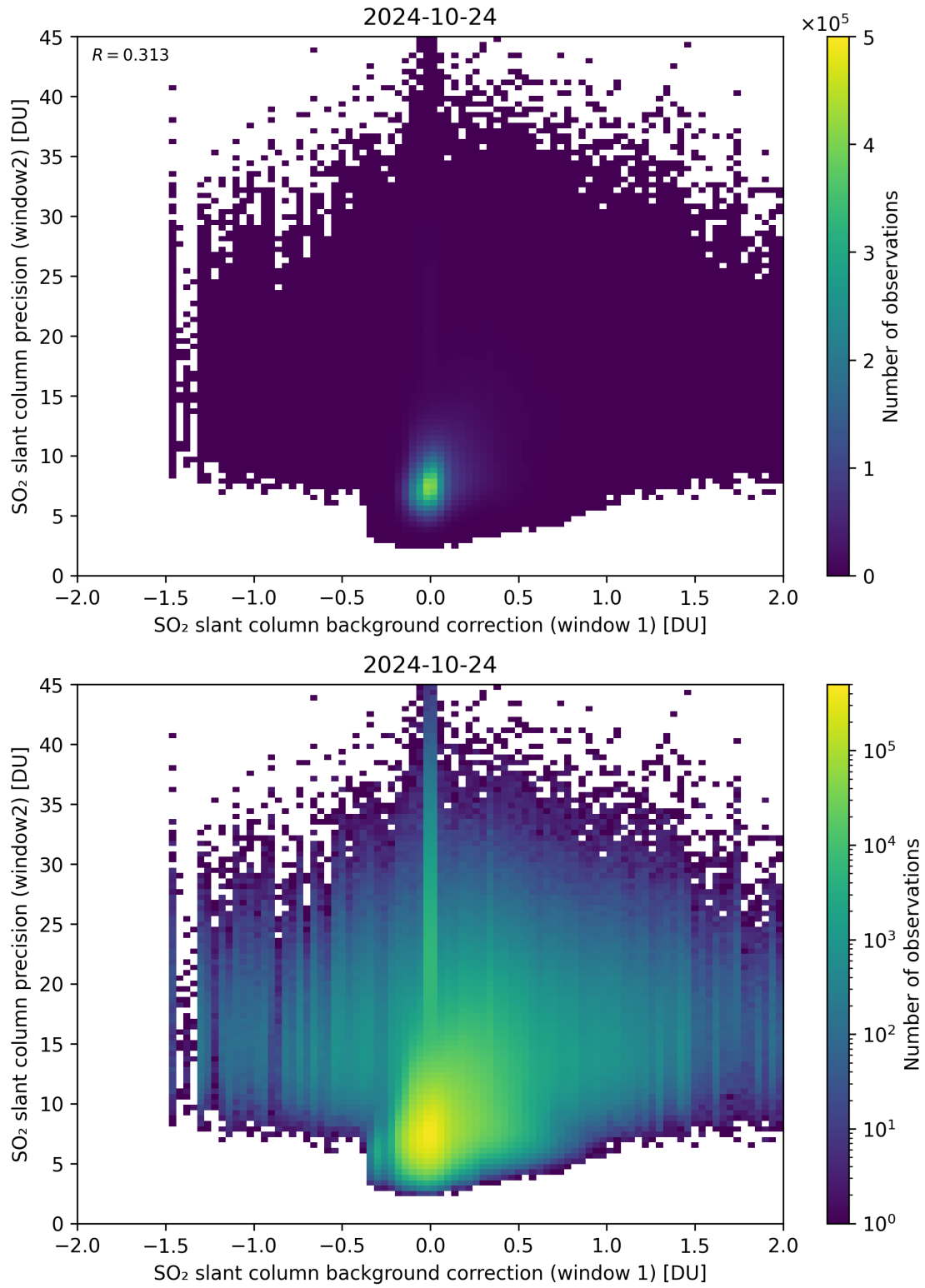
Figure 106: Scatter density plot of “SO 2 slant column background correction (window 1)” against “SO 2 slant column precision (window2)” for 2024-10-24 to 2024-10-25.
