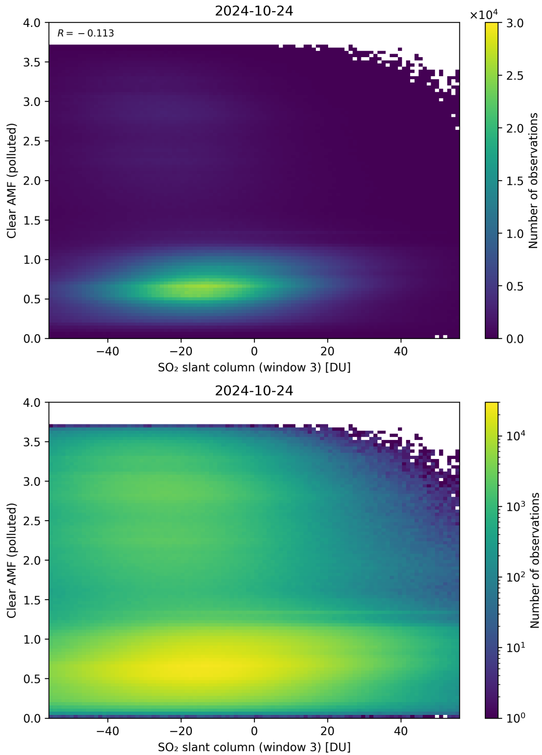
Figure 265: Scatter density plot of “SO 2 slant column (window 3)” against “Clear AMF (polluted)” for 2024-10-24 to 2024-10-25.
