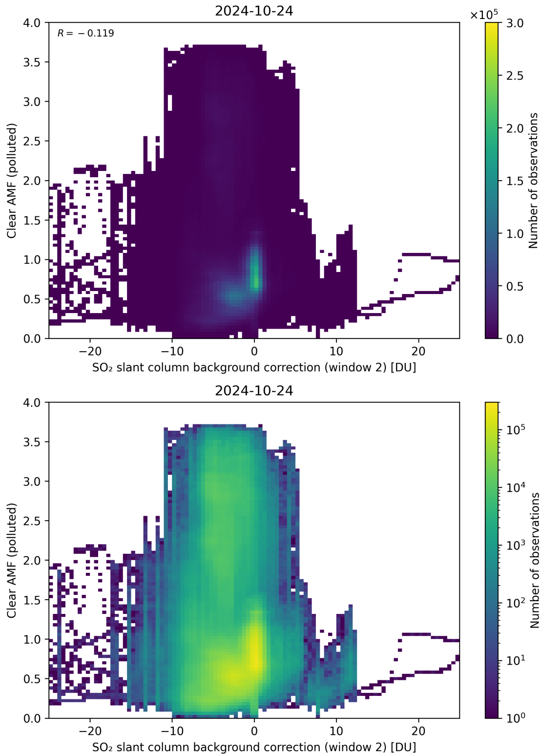
Figure 115: Scatter density plot of “SO 2 slant column background correction (window 2)” against “Clear AMF (polluted)” for 2024-10-24 to 2024-10-25.
