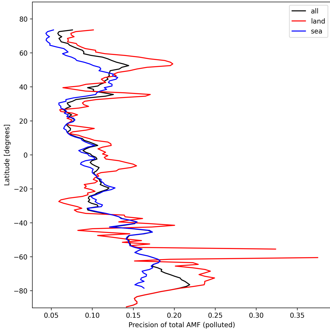
Figure 49: Zonal average of “Precision of total AMF (polluted)” for 2024-10-24 to 2024-10-25.
