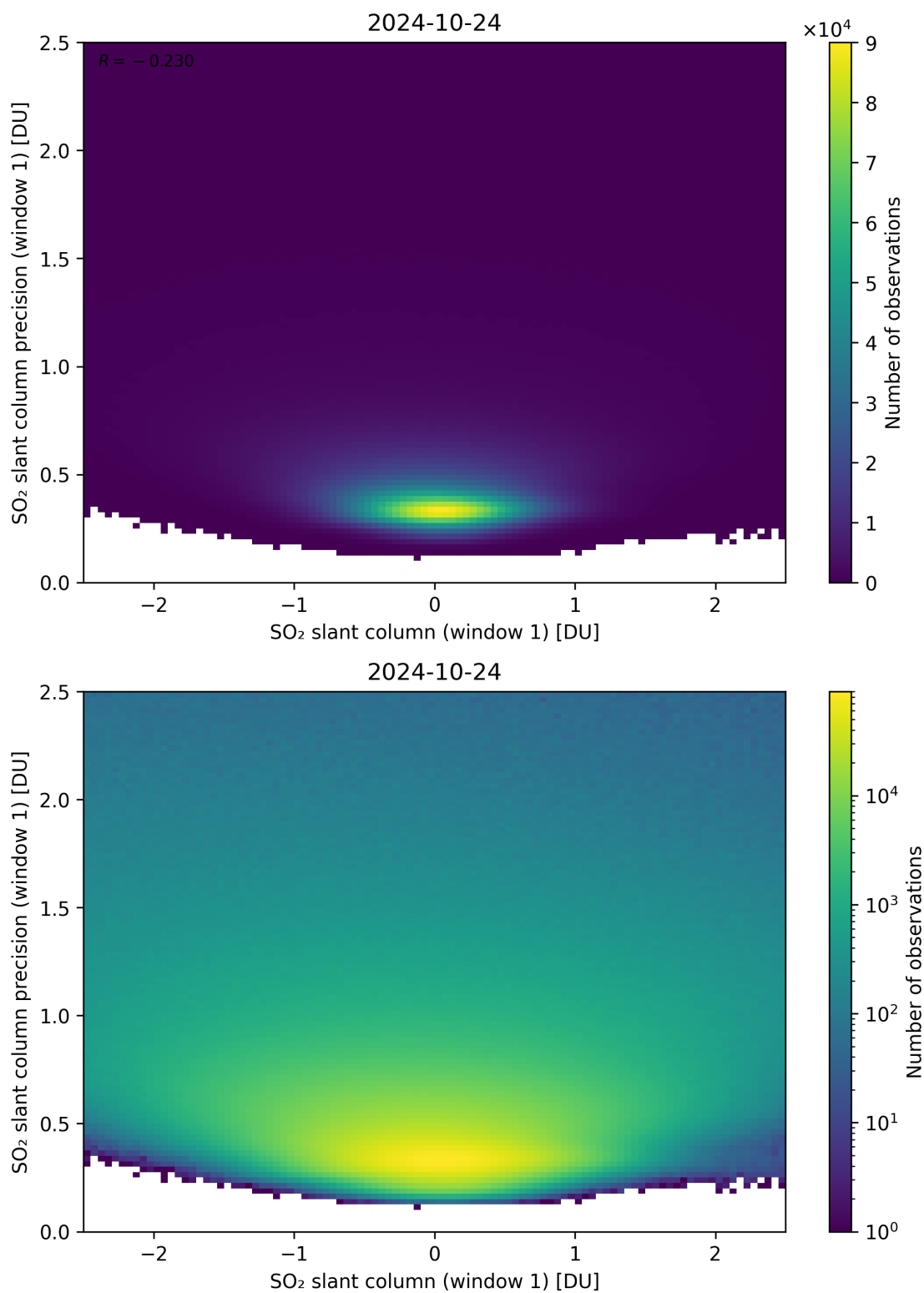
Figure 235: Scatter density plot of “SO 2 slant column (window 1)” against “SO 2 slant column precision (window 1)” for 2024-10-24 to 2024-10-25.
