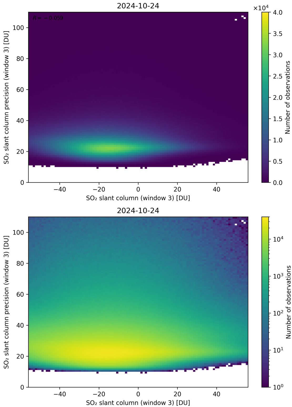
Figure 267: Scatter density plot of “SO 2 slant column (window 3)” against “SO 2 slant column precision (window 3)” for 2024-10-24 to 2024-10-25.
