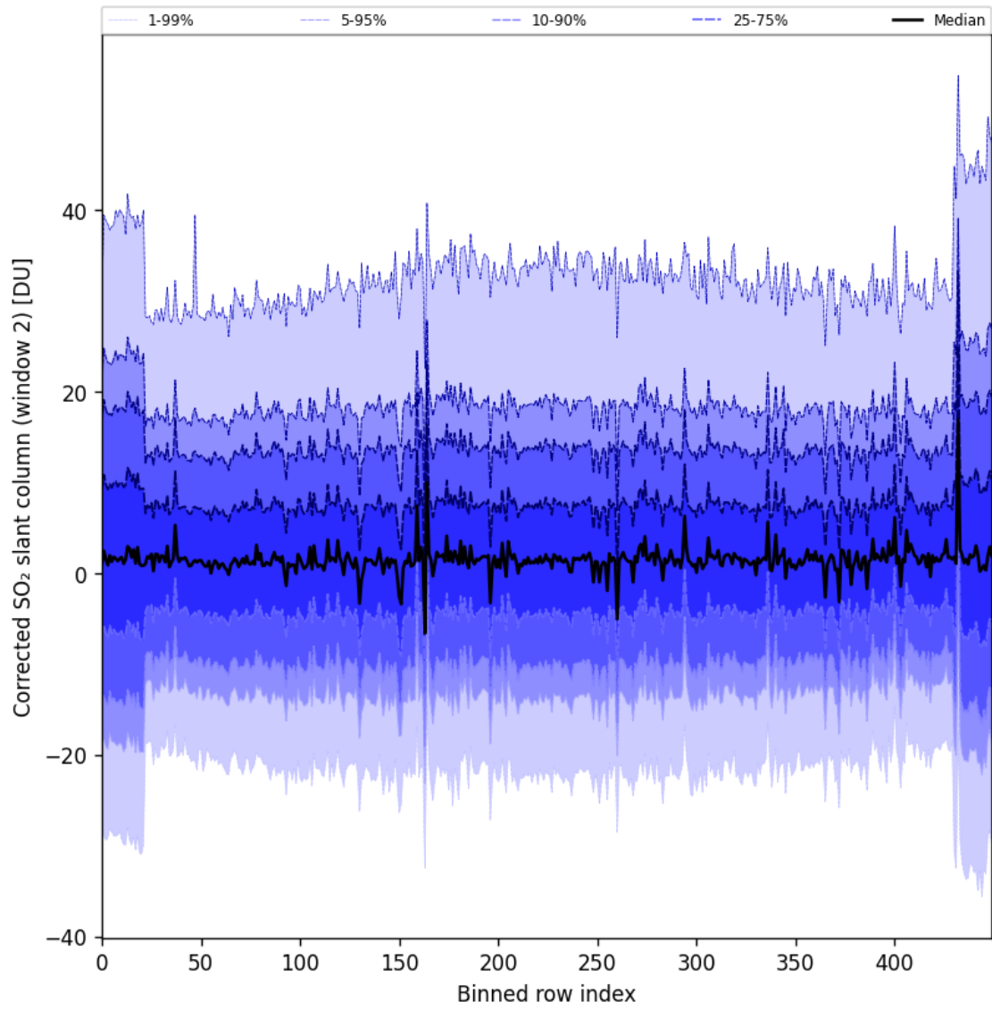
Figure 85: Along track statistics of “Corrected SO 2 slant column (window 2)” for 2024-10-24 to 2024-10-25
