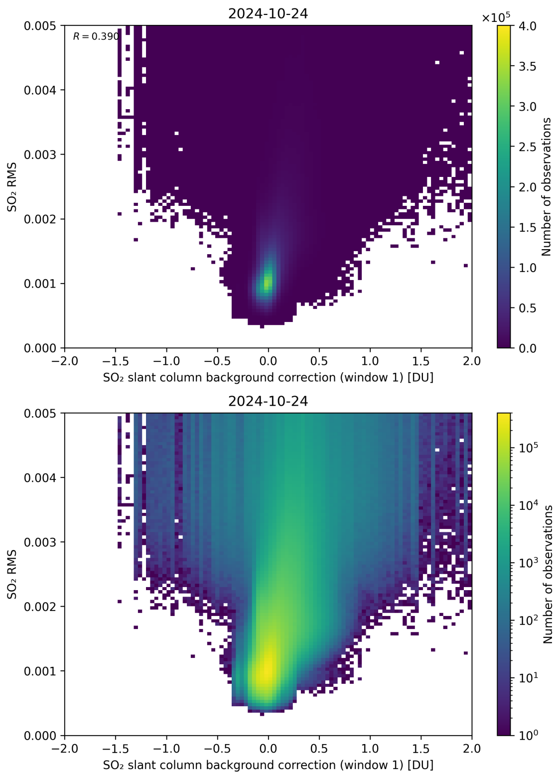
Figure 102: Scatter density plot of “SO 2 slant column background correction (window 1)” against “SO 2 RMS” for 2024-10-24 to 2024-10-25.
