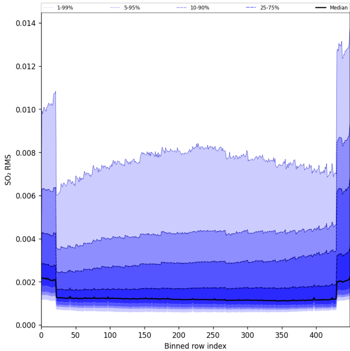
Figure 93: Along track statistics of “SO 2 RMS” for 2024-10-24 to 2024-10-25
