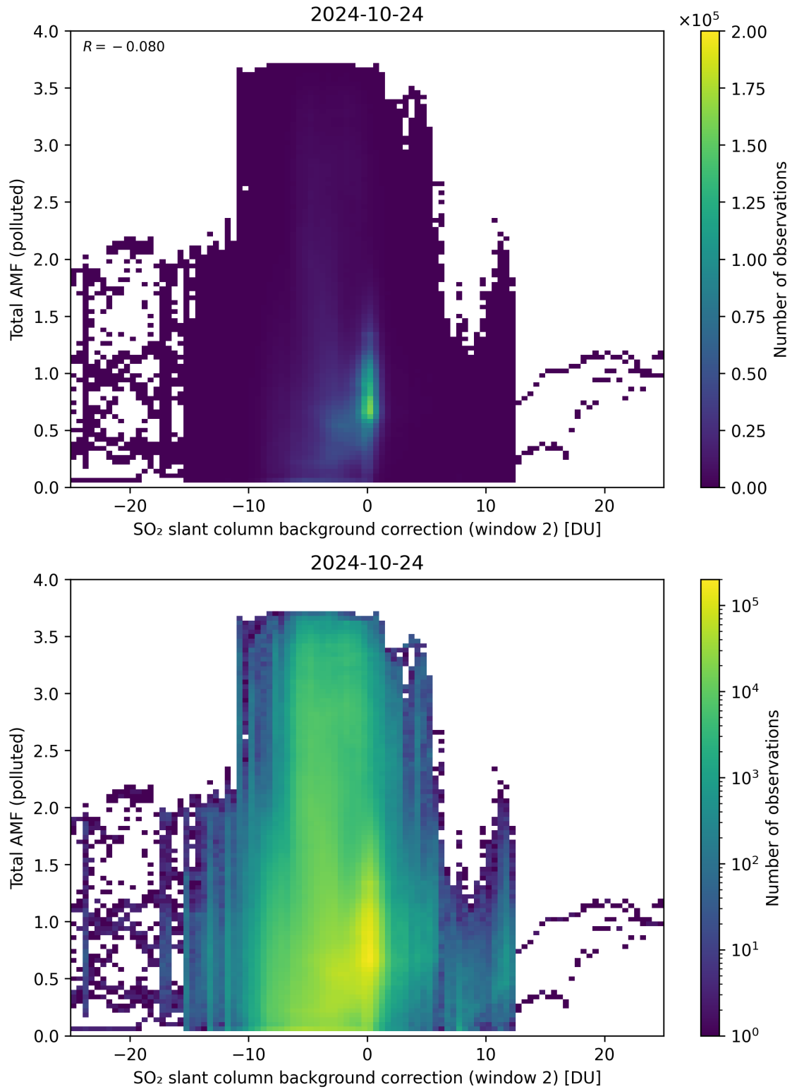
Figure 119: Scatter density plot of “SO 2 slant column background correction (window 2)” against “Total AMF (polluted)” for 2024-10-24 to 2024-10-25.
