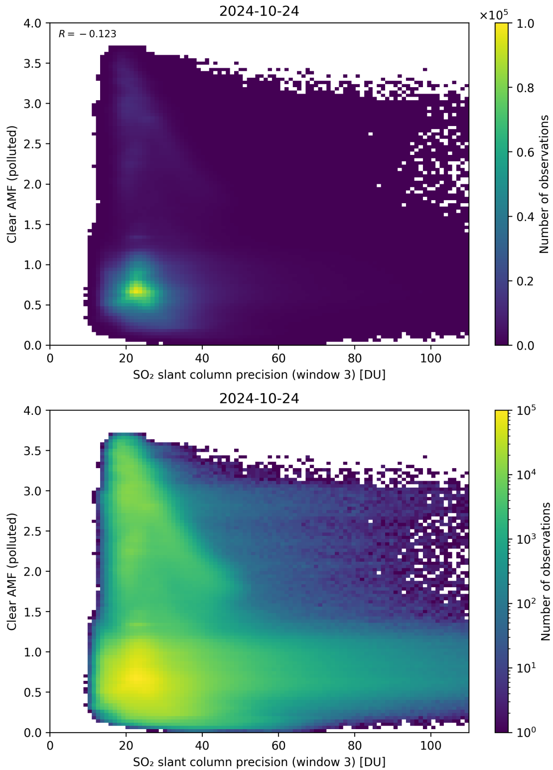
Figure 261: Scatter density plot of “SO 2 slant column precision (window 3)” against “Clear AMF (polluted)” for 2024-10-24 to 2024-10-25.
