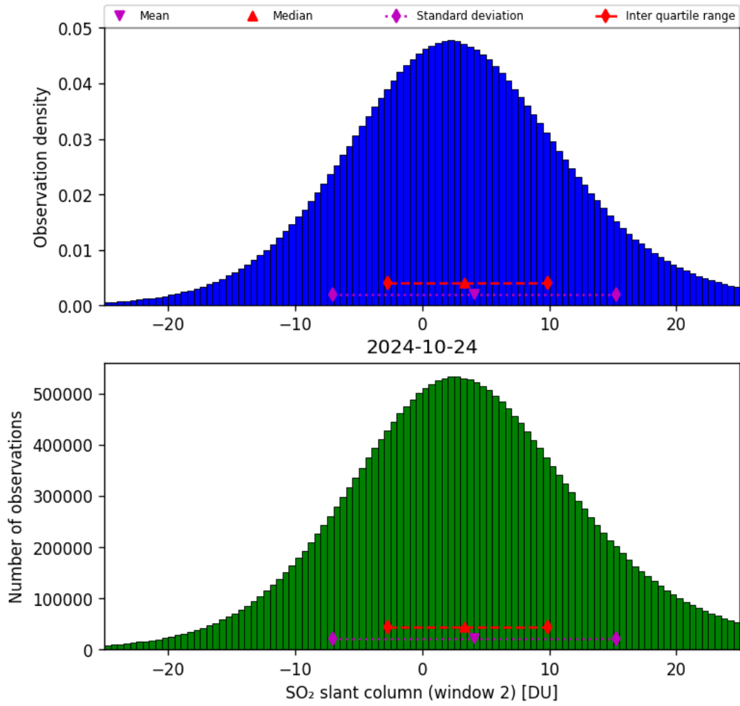
Figure 60: Histogram of “SO 2 slant column (window 2)” for 2024-10-24 to 2024-10-25
