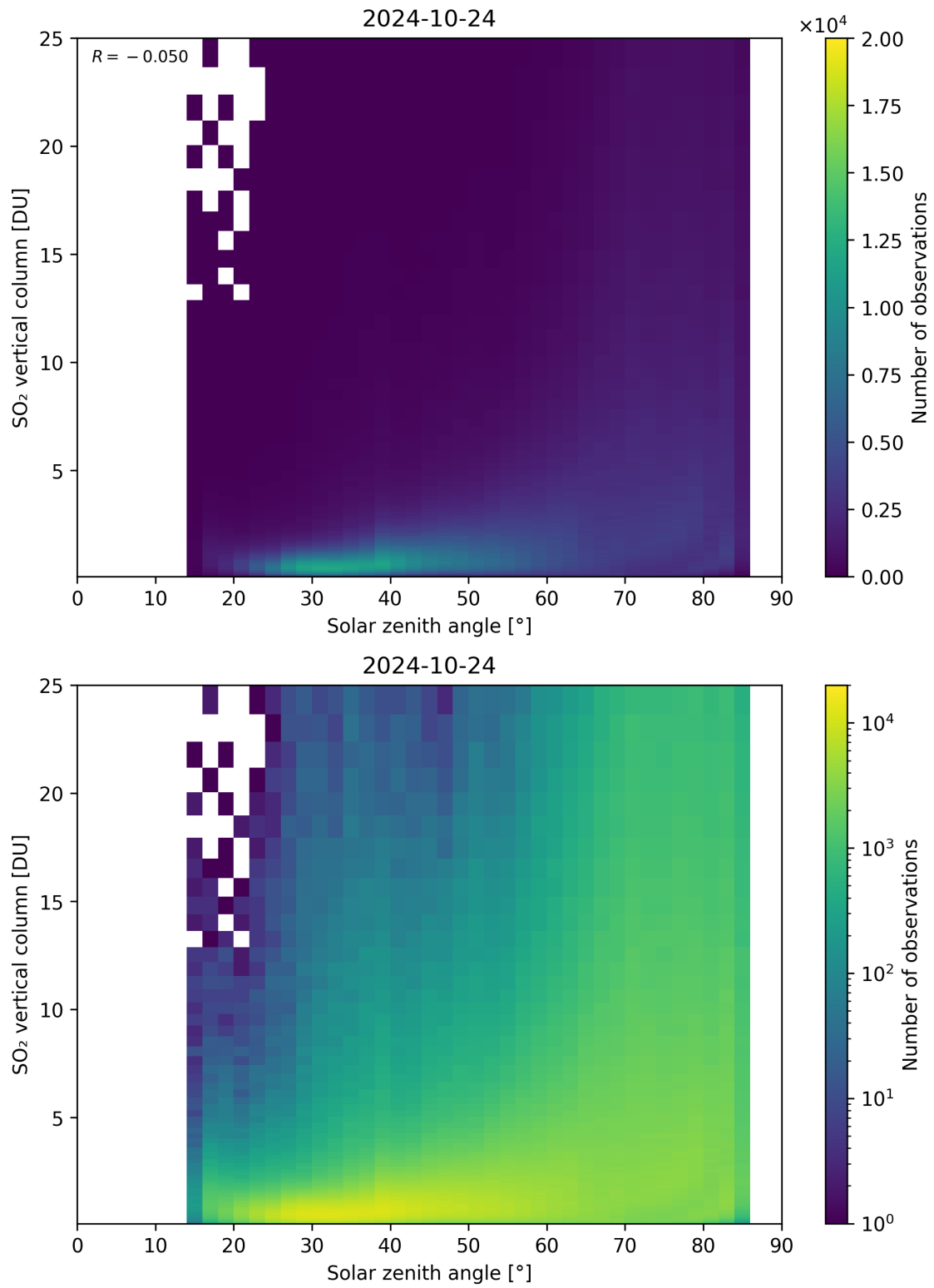
Figure 176: Scatter density plot of “Solar zenith angle” against “SO 2 vertical column” for 2024-10-24 to 2024-10-25.
