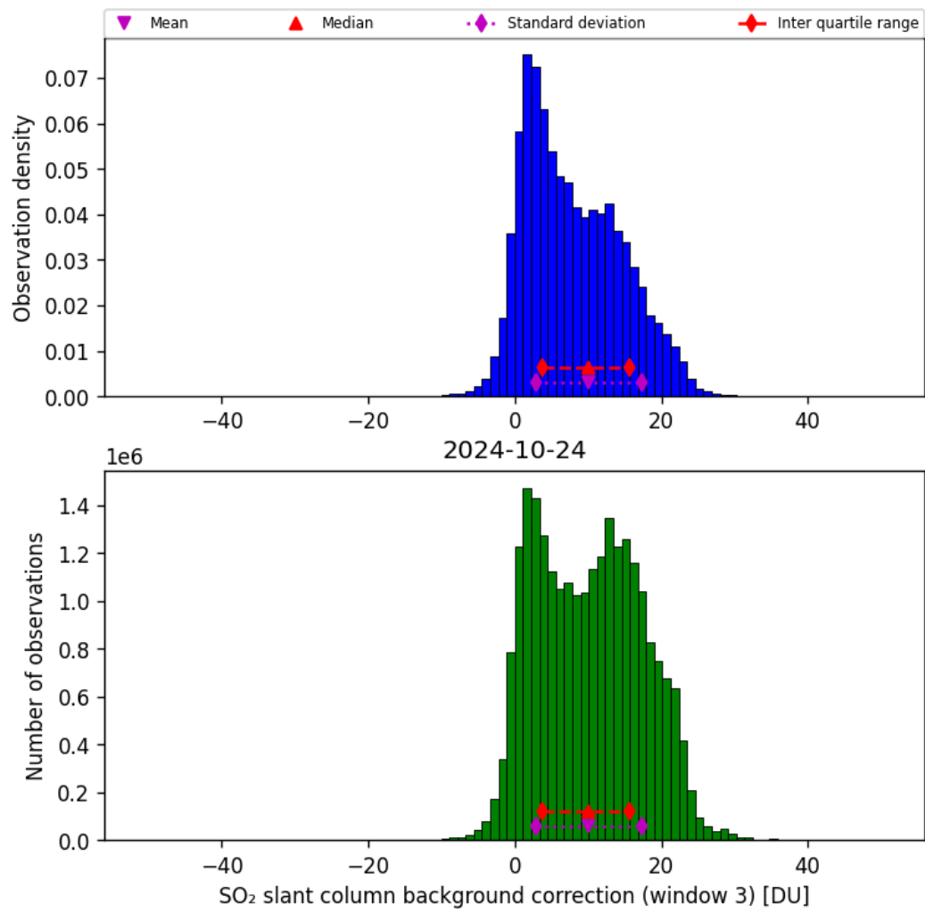
Figure 67: Histogram of “SO 2 slant column background correction (window 3)” for 2024-10-24 to 2024-10-25
