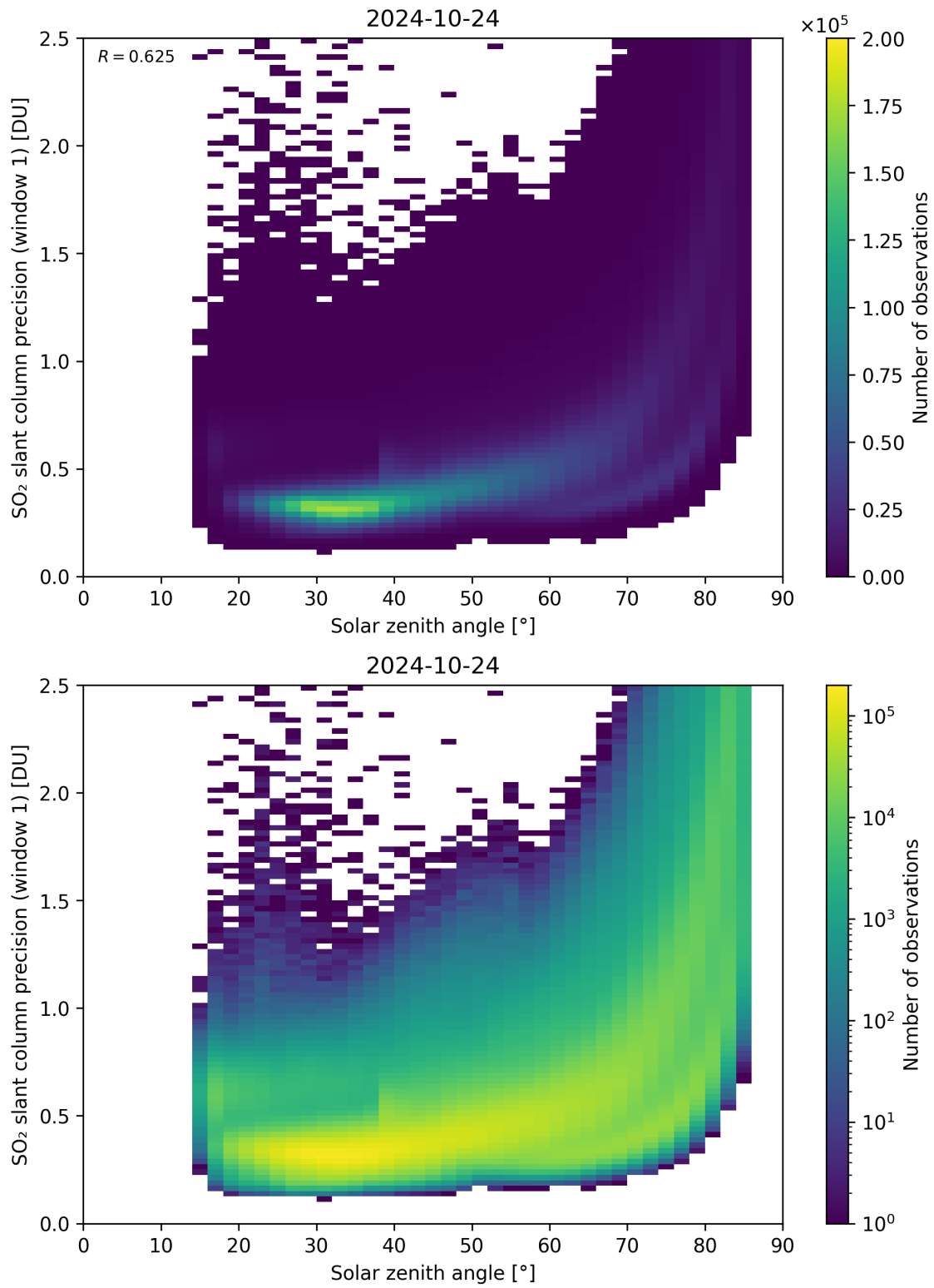
Figure 170: Scatter density plot of “Solar zenith angle” against “SO 2 slant column precision (window 1)” for 2024-10-24 to 2024-10-25.
