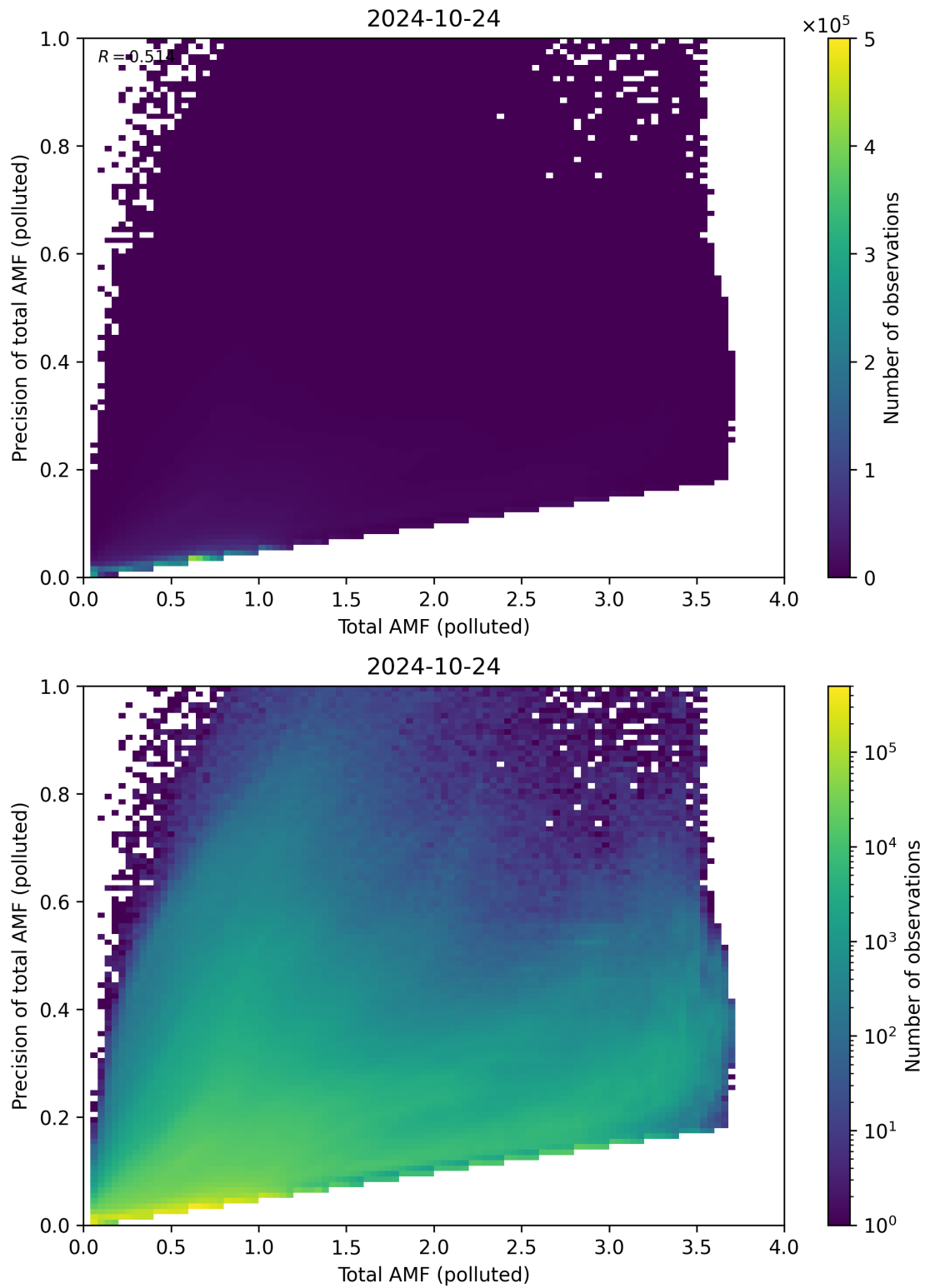
Figure 272: Scatter density plot of “Total AMF (polluted)” against “Precision of total AMF (polluted)” for 2024-10-24 to 2024-10-25.
