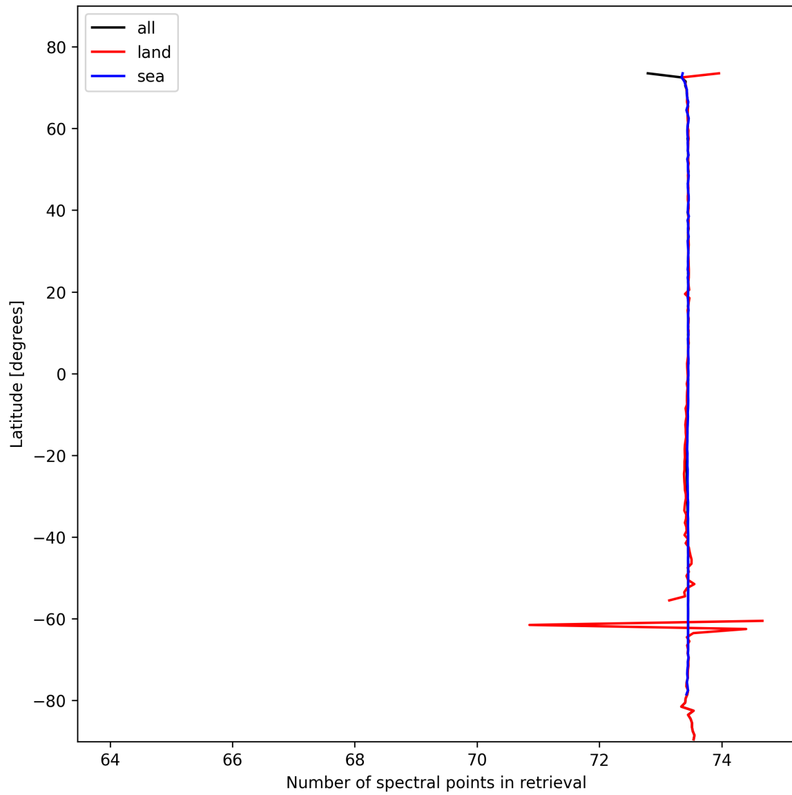
Figure 51: Zonal average of “Number of spectral points in retrieval” for 2024-10-24 to 2024-10-25.
