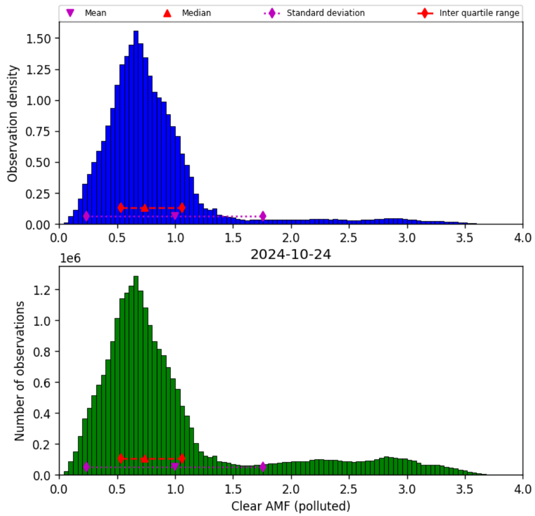
Figure 73: Histogram of "Clear AMF (polluted)" for 2024-10-24 to 2024-10-25
