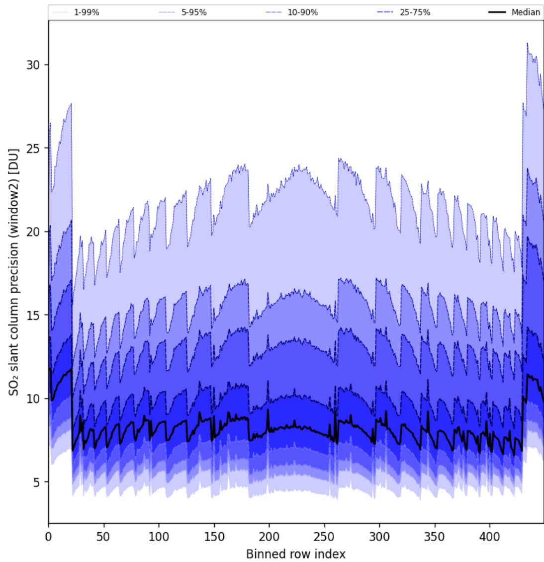
Figure 84: Along track statistics of “SO 2 slant column precision (window2)” for 2024-10-24 to 2024-10-25
