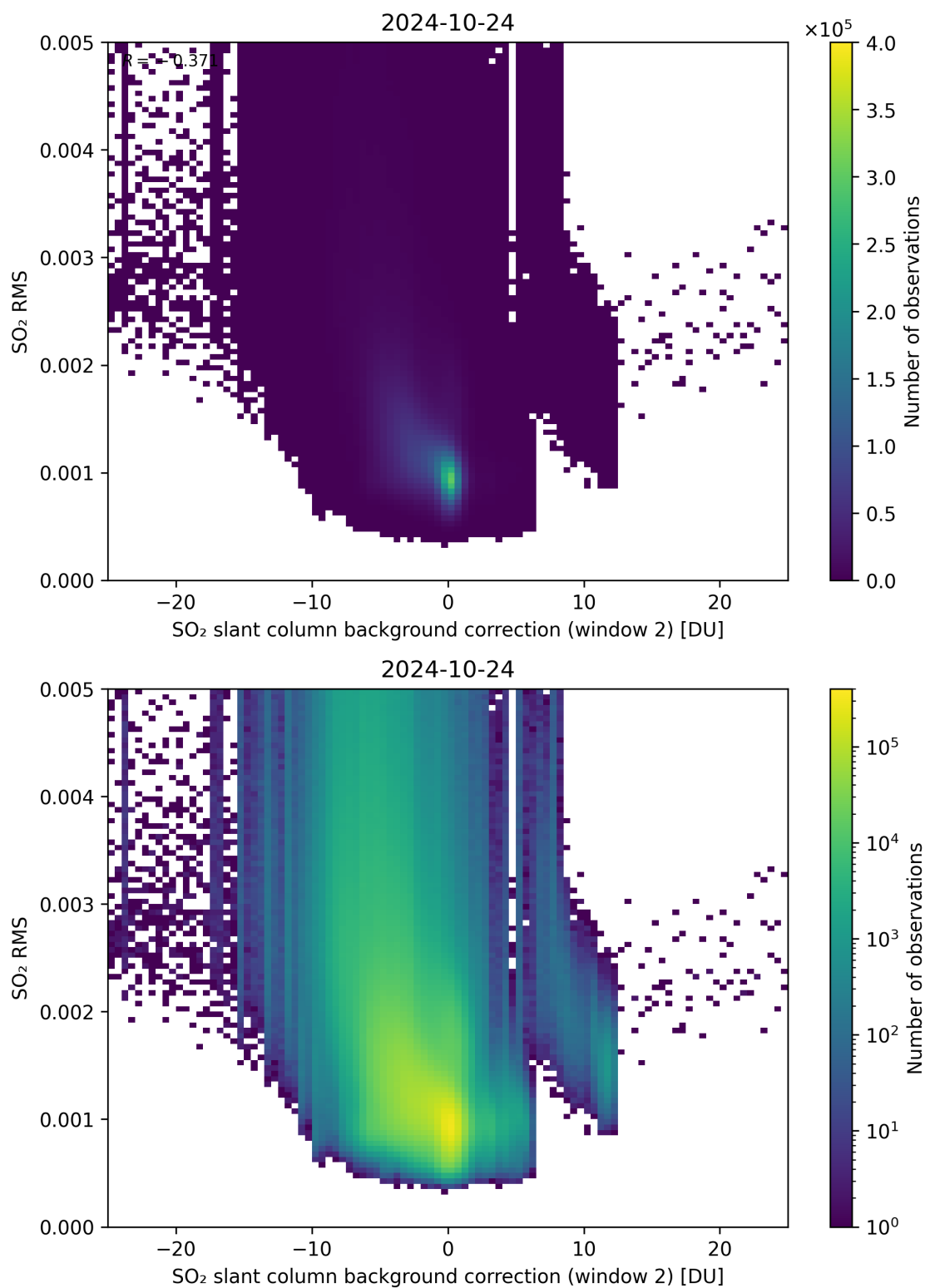
Figure 114: Scatter density plot of “SO 2 slant column background correction (window 2)” against “SO 2 RMS” for 2024-10-24 to 2024-10-25.
