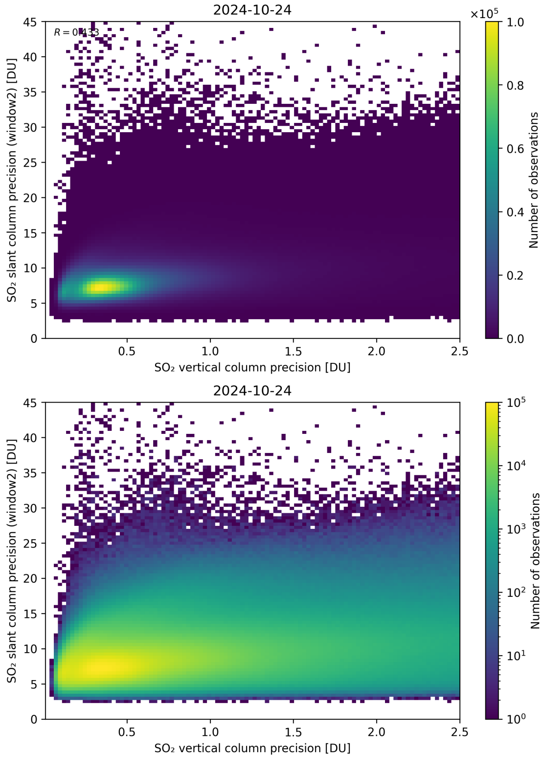
Figure 291: Scatter density plot of “SO 2 vertical column precision” against “SO 2 slant column precision (window2)” for 2024-10-24 to 2024-10-25.
