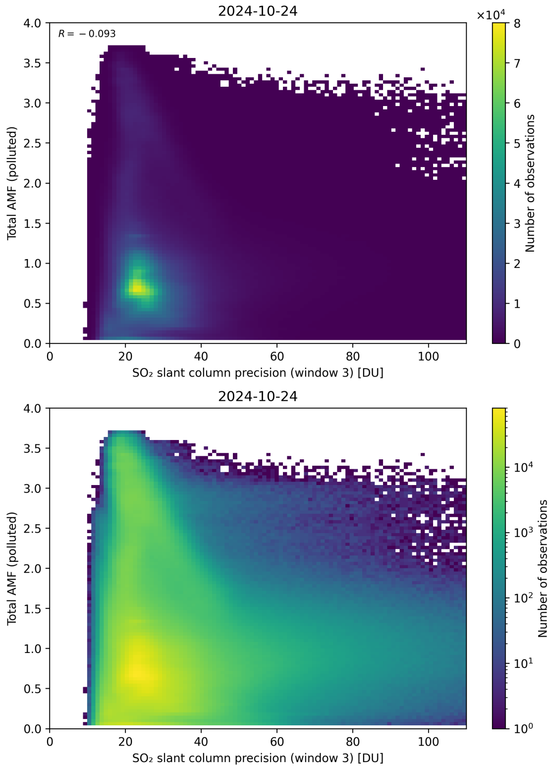
Figure 263: Scatter density plot of “SO 2 slant column precision (window 3)” against “Total AMF (polluted)” for 2024-10-24 to 2024-10-25.
