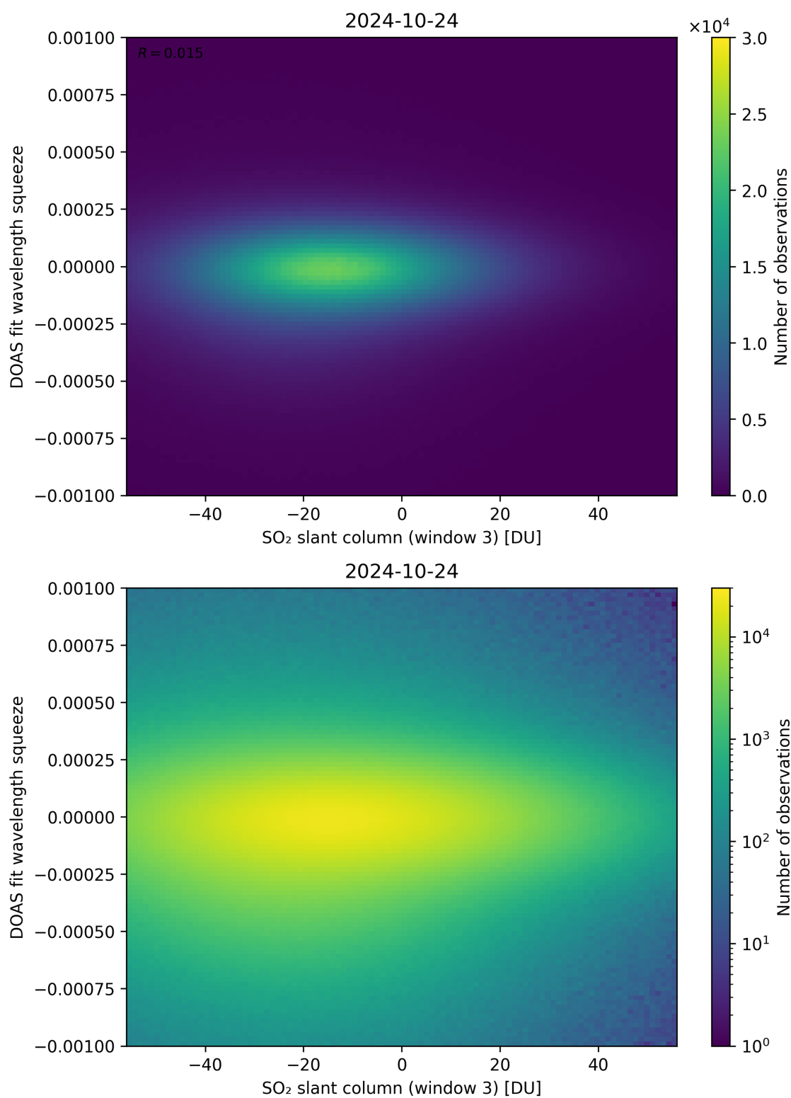
Figure 255: Scatter density plot of “SO 2 slant column (window 3)” against “DOAS fit wavelength squeeze” for 2024-10-24 to 2024-10-25.
