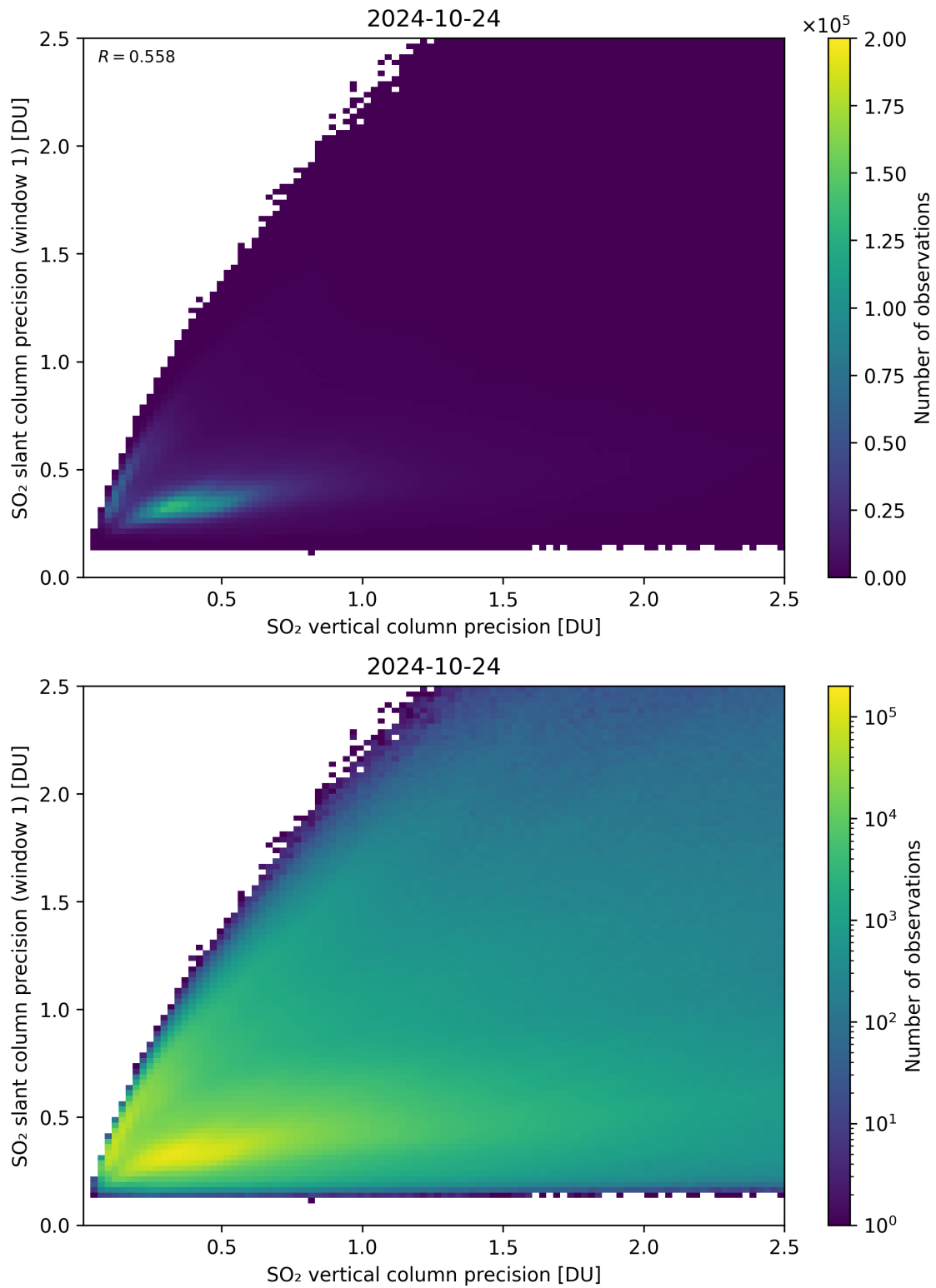
Figure 290: Scatter density plot of “SO 2 vertical column precision” against “SO 2 slant column precision (window 1)” for 2024-10-24 to 2024-10-25.
