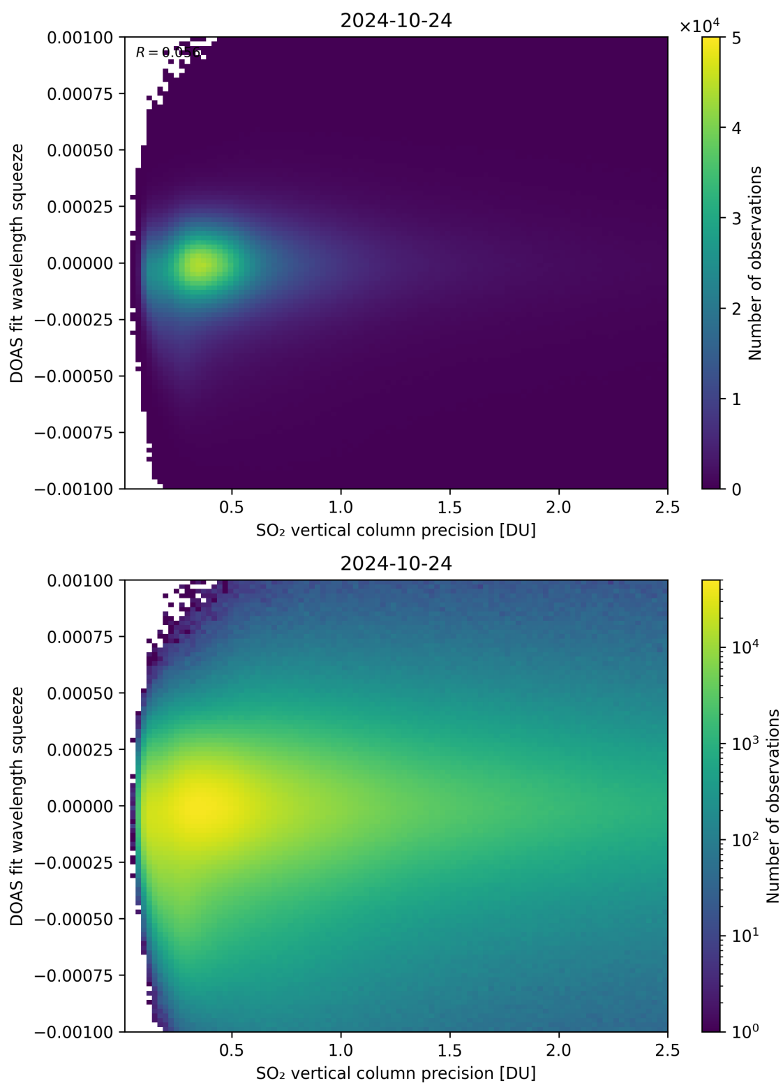
Figure 283: Scatter density plot of “SO 2 vertical column precision” against “DOAS fit wavelength squeeze” for 2024-10-24 to 2024-10-25.
