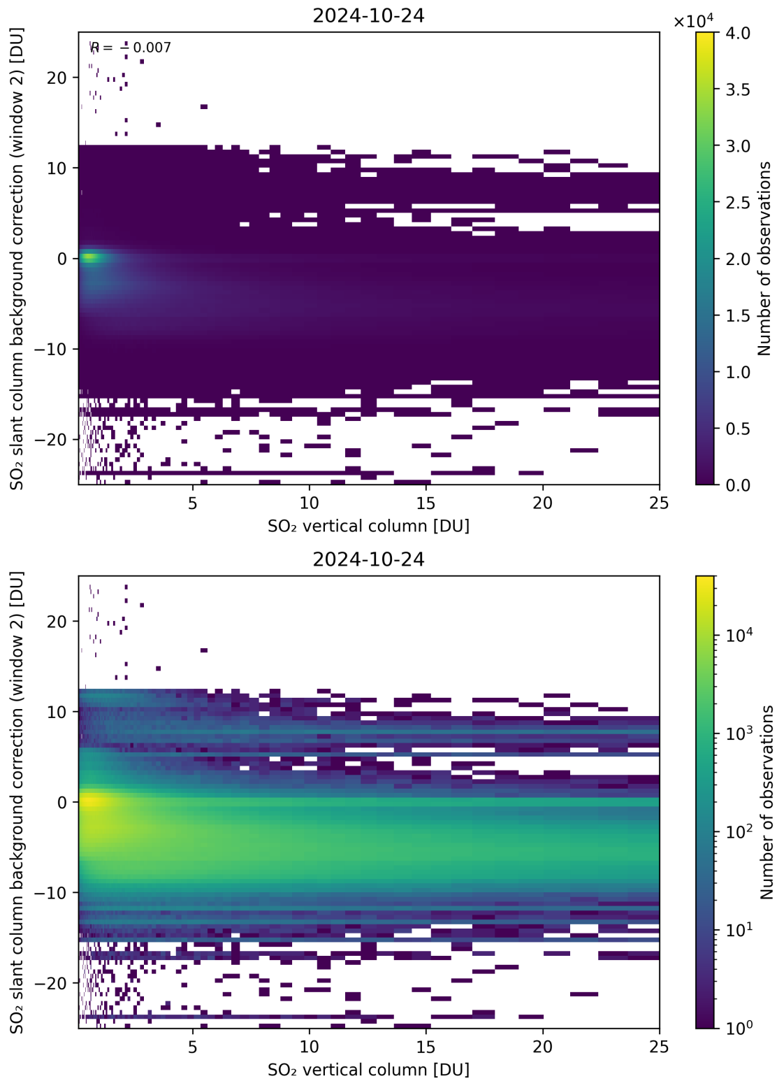
Figure 274: Scatter density plot of “SO 2 vertical column” against “SO 2 slant column background correction (window 2)” for 2024-10-24 to 2024-10-25.
