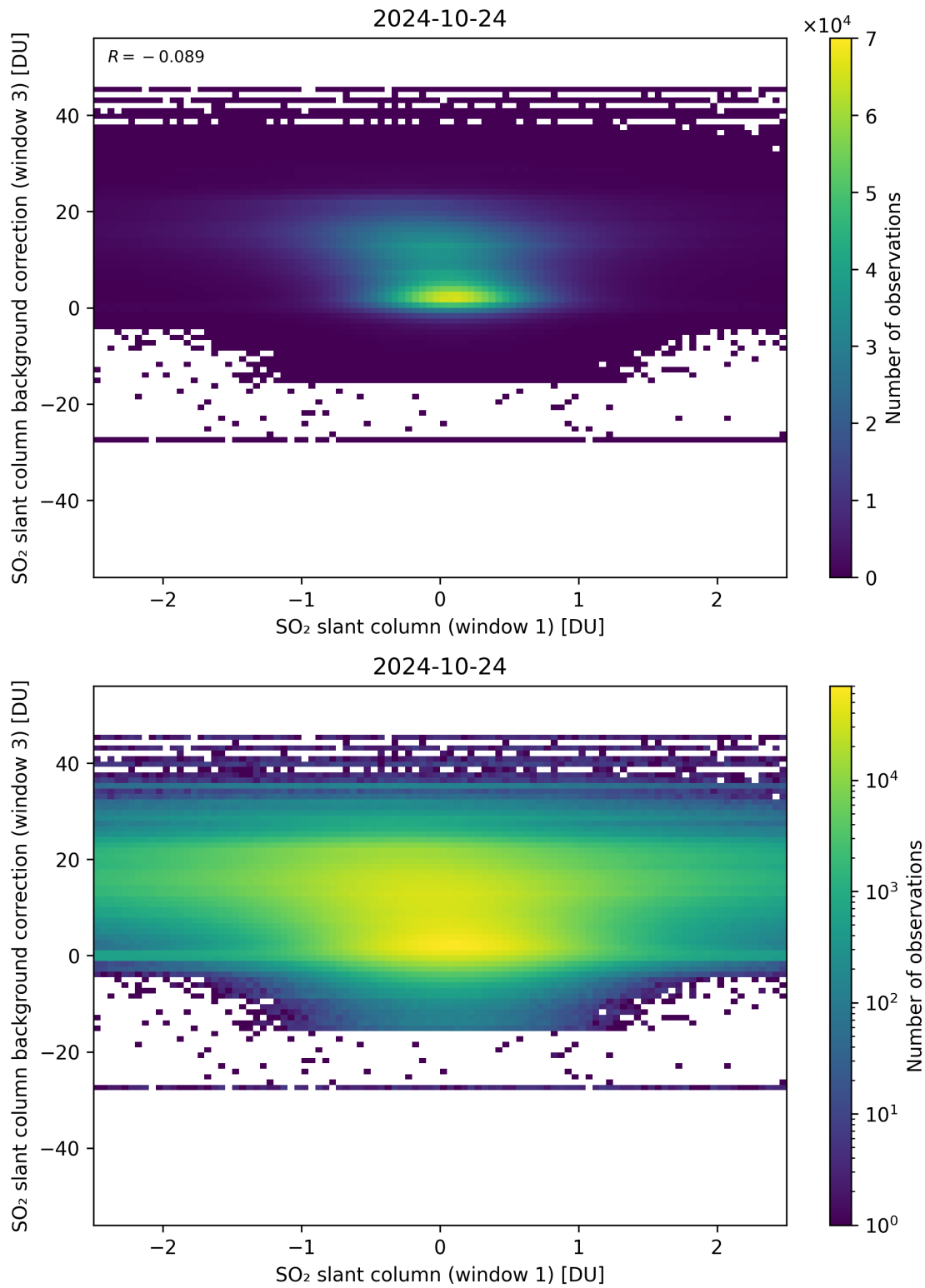
Figure 214: Scatter density plot of “SO 2 slant column (window 1)” against “SO 2 slant column background correction (window 3)” for 2024-10-24 to 2024-10-25.
