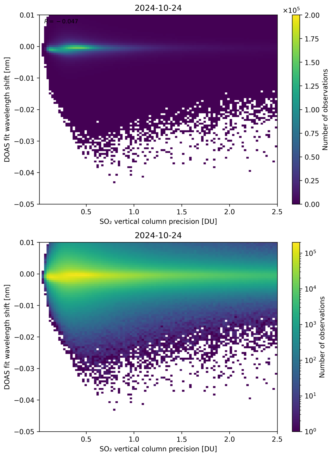
Figure 282: Scatter density plot of “SO 2 vertical column precision” against “DOAS fit wavelength shift” for 2024-10-24 to 2024-10-25.
