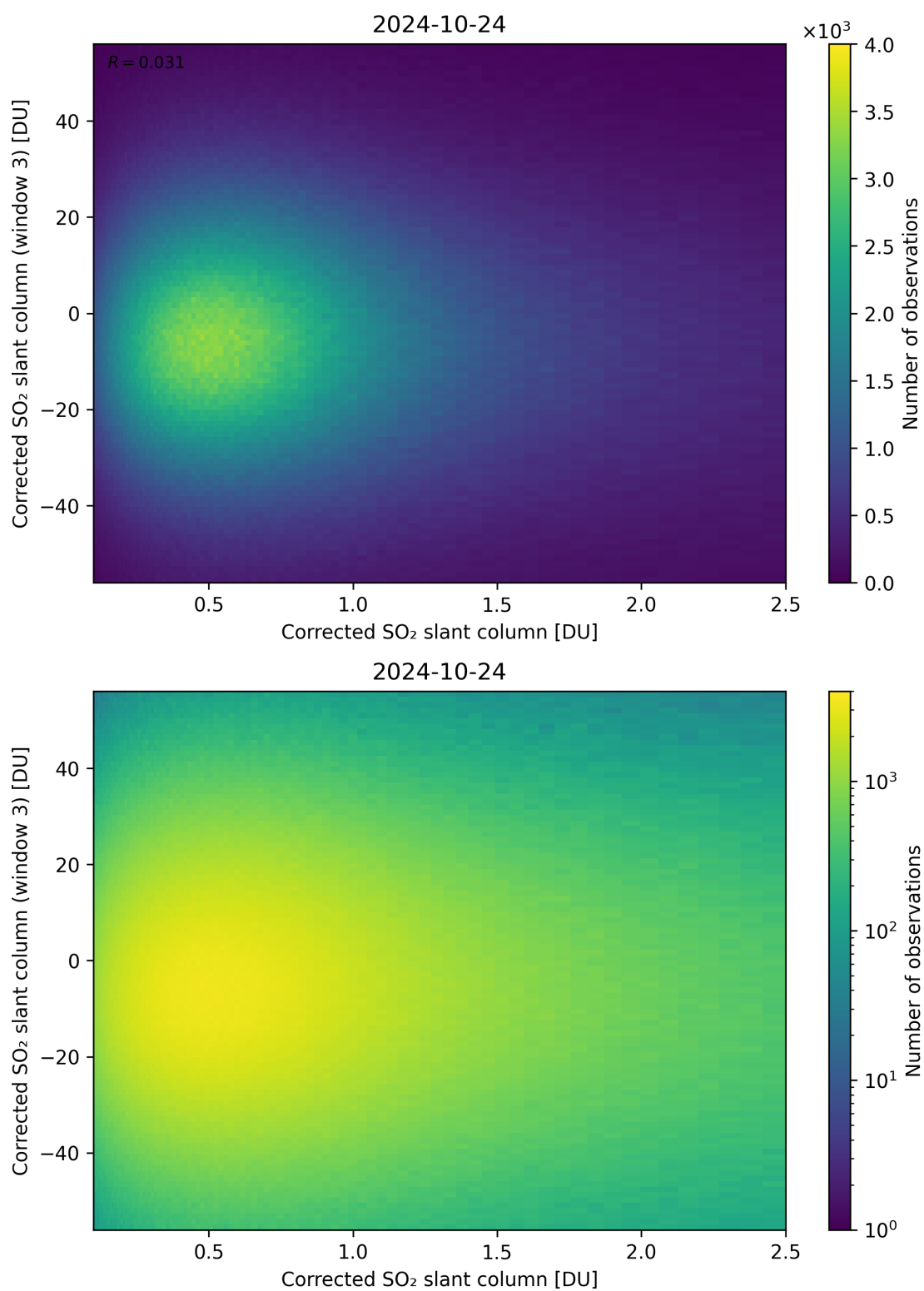
Figure 186: Scatter density plot of “Corrected SO 2 slant column” against “Corrected SO 2 slant column (window 3)” for 2024-10-24 to 2024-10-25.
