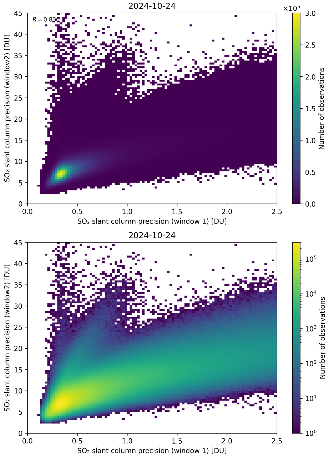
Figure 227: Scatter density plot of “SO 2 slant column precision (window 1)” against “SO 2 slant column precision (window2)” for 2024-10-24 to 2024-10-25.
