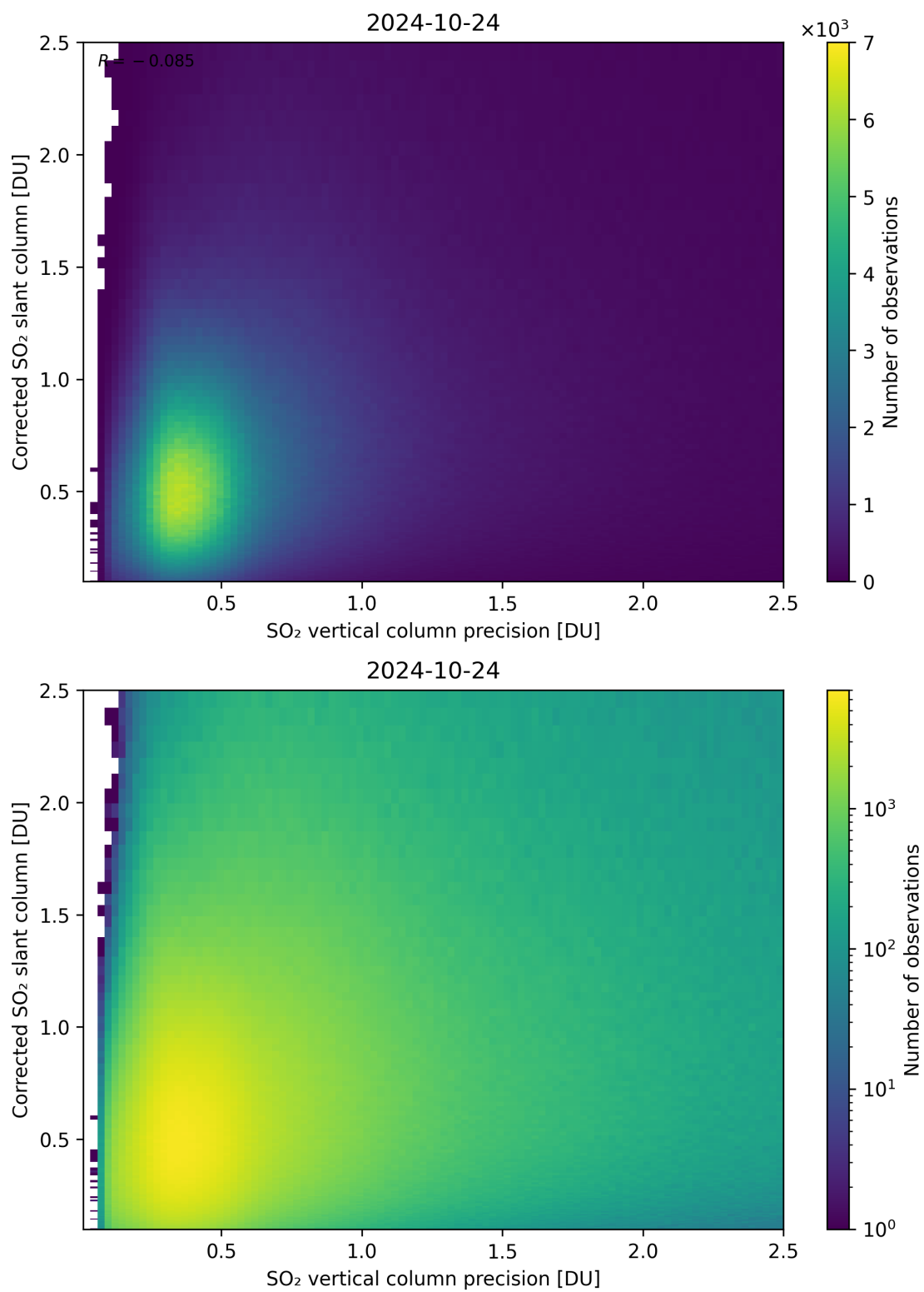
Figure 286: Scatter density plot of “SO 2 vertical column precision” against “Corrected SO 2 slant column” for 2024-10-24 to 2024-10-25.
