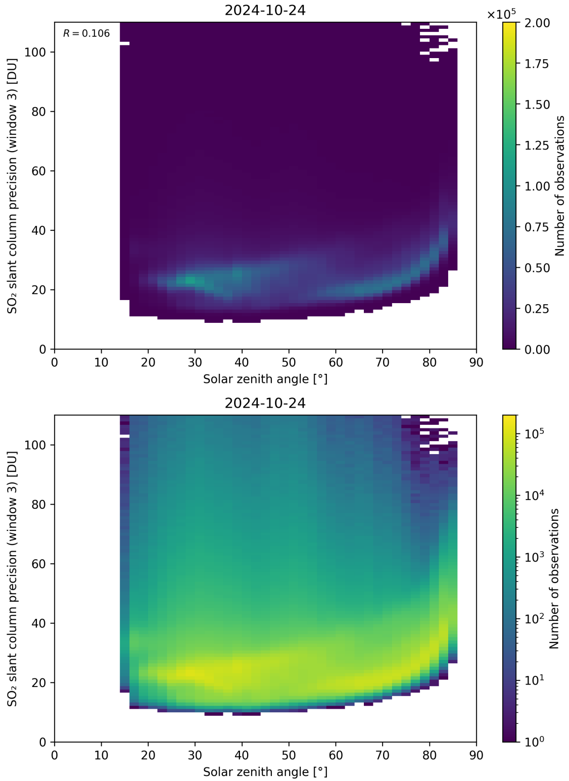
Figure 173: Scatter density plot of “Solar zenith angle” against “SO 2 slant column precision (window 3)” for 2024-10-24 to 2024-10-25.
