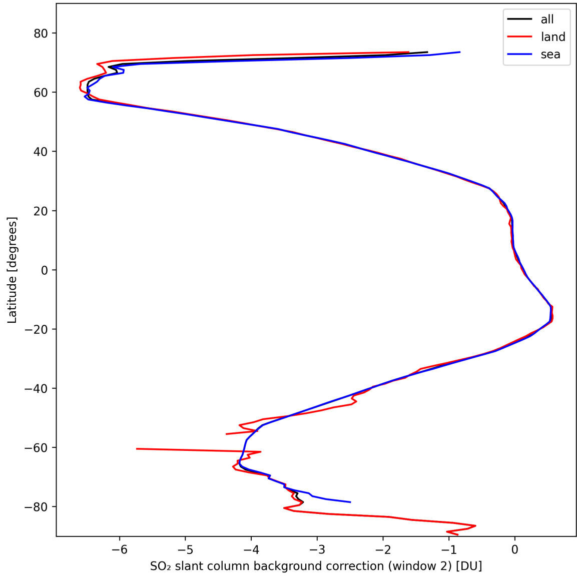
Figure 40: Zonal average of “SO 2 slant column background correction (window 2)” for 2024-10-24 to 2024-10-25.
