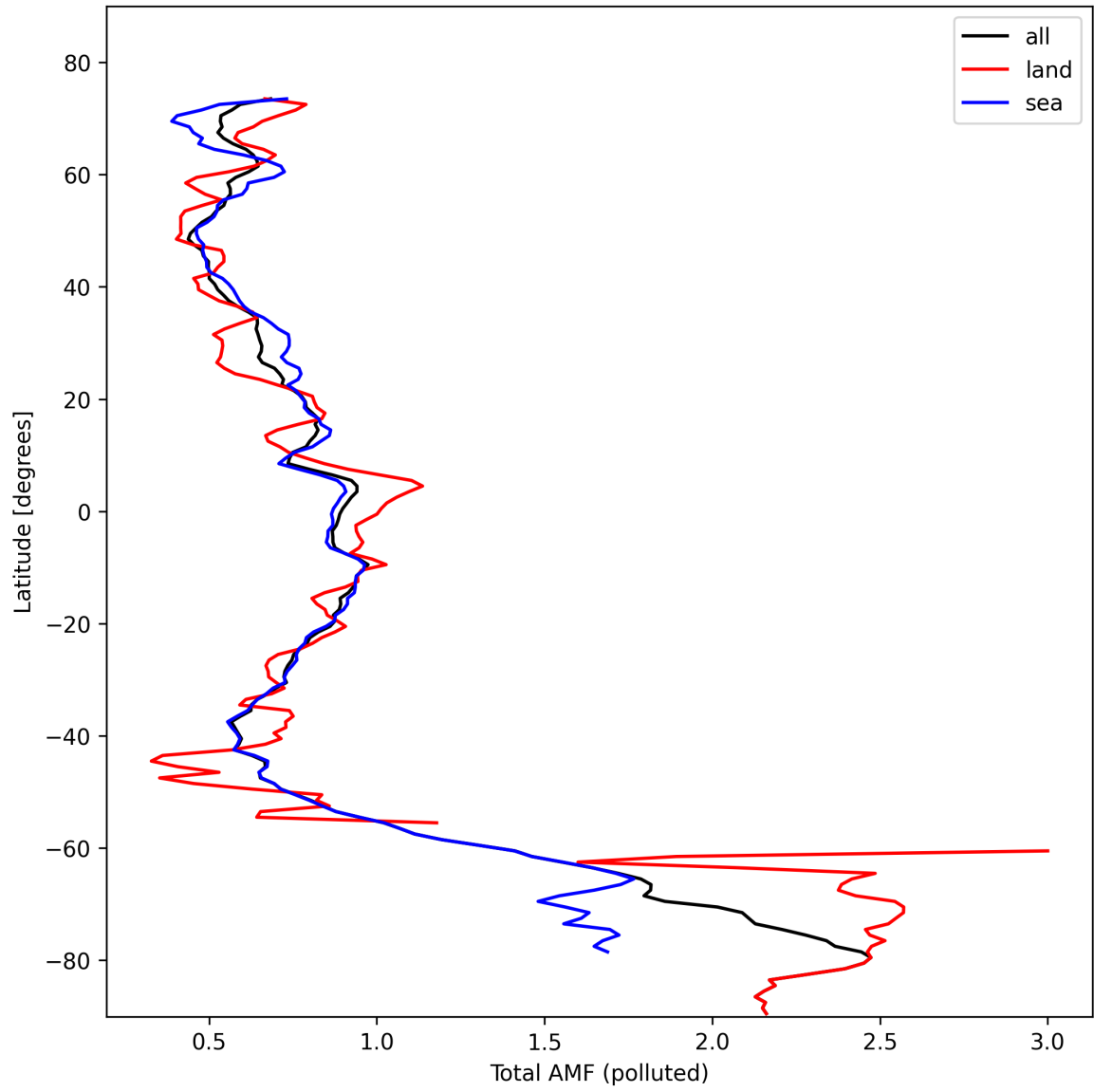
Figure 48: Zonal average of “Total AMF (polluted)” for 2024-10-24 to 2024-10-25.
