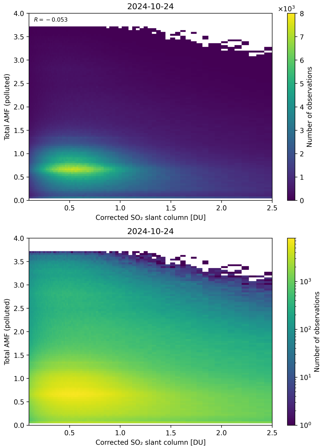
Figure 192: Scatter density plot of “Corrected SO 2 slant column” against “Total AMF (polluted)” for 2024-10-24 to 2024-10-25.
