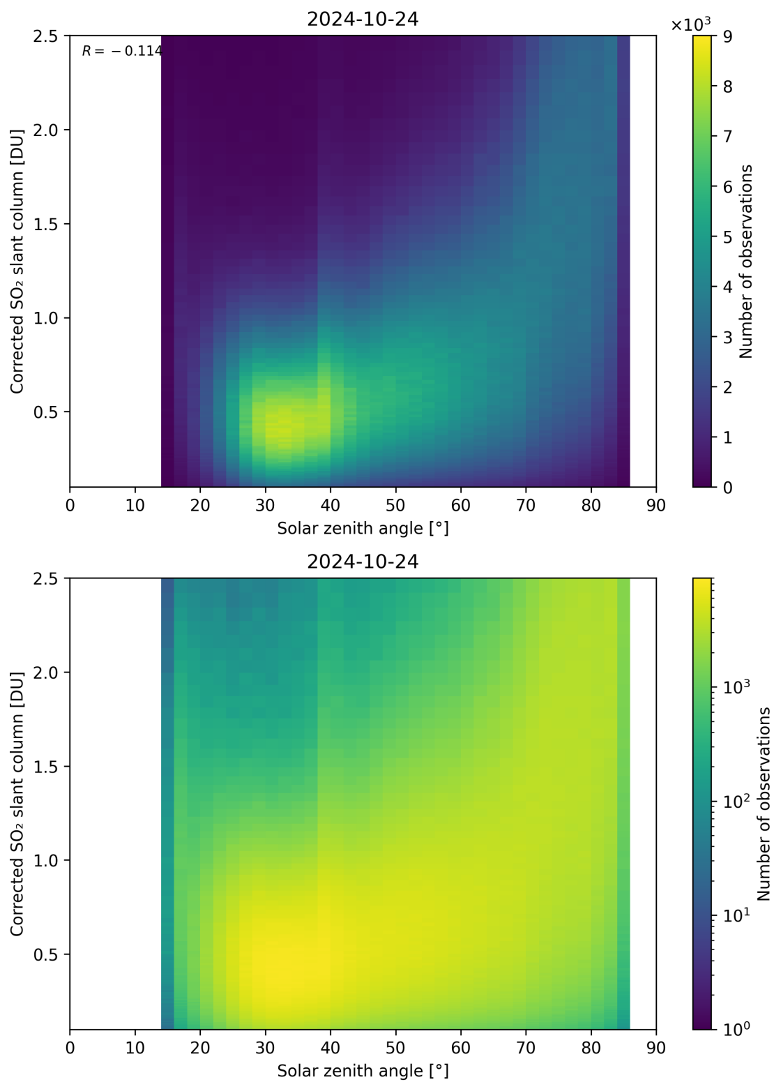
Figure 166: Scatter density plot of “Solar zenith angle” against “Corrected SO 2 slant column” for 2024-10-24 to 2024-10-25.
