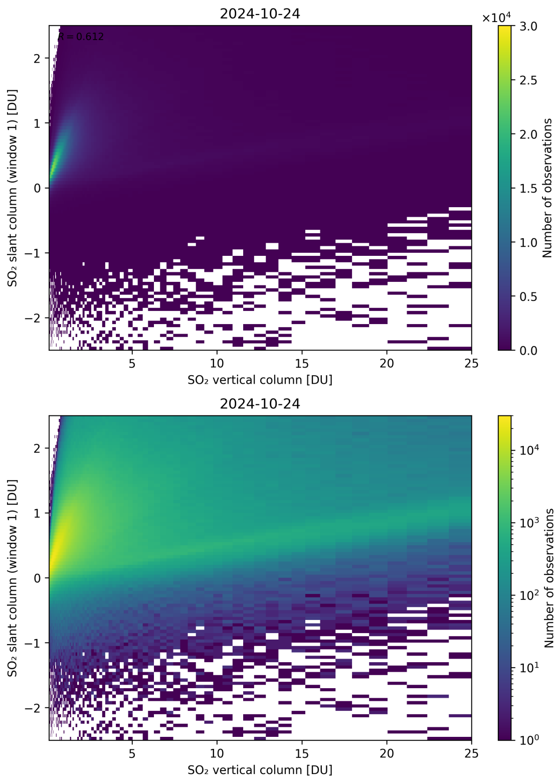
Figure 300: Scatter density plot of “SO 2 vertical column” against “SO 2 slant column (window 1)” for 2024-10-24 to 2024-10-25.
