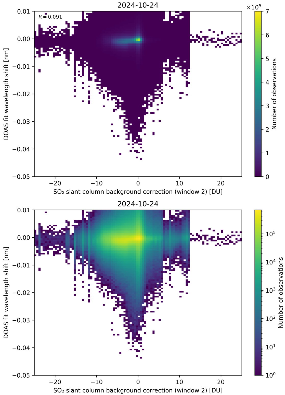
Figure 112: Scatter density plot of “SO 2 slant column background correction (window 2)” against “DOAS fit wavelength shift” for 2024-10-24 to 2024-10-25.
