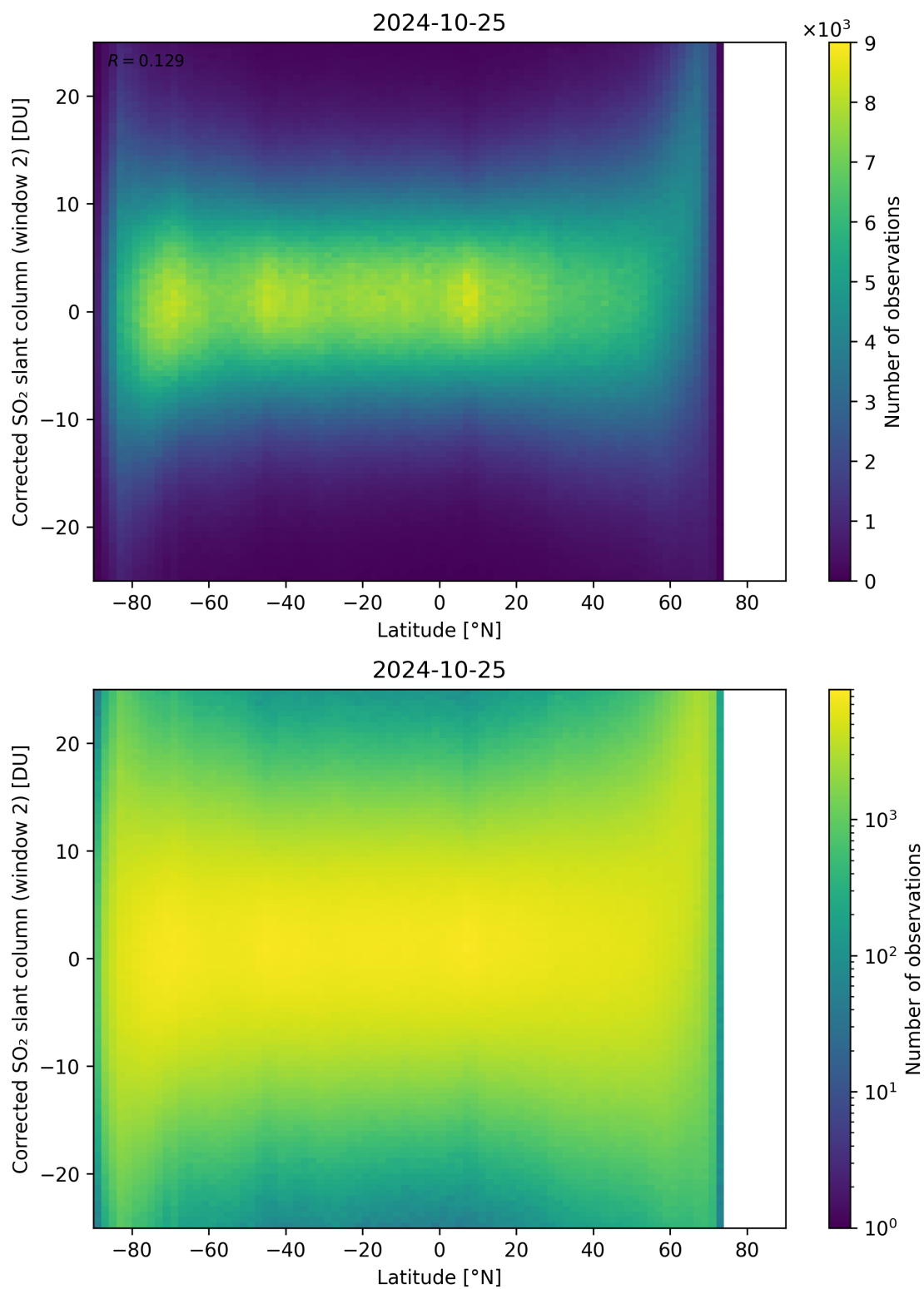
Figure 147: Scatter density plot of “Latitude” against “Corrected SO 2 slant column (window 2)” for 2024-10-24 to 2024-10-26.
