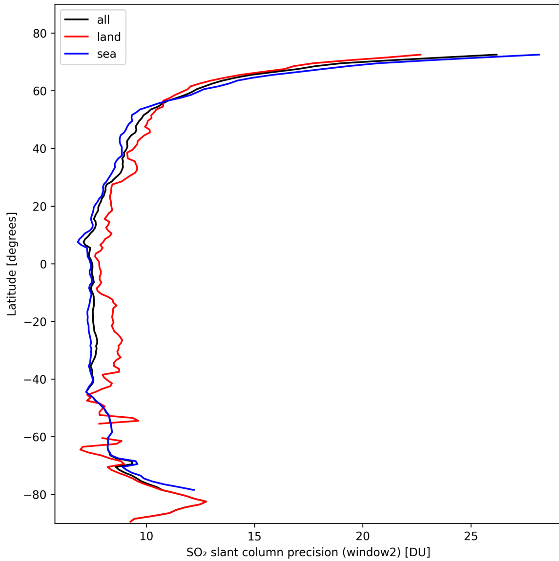
Figure 38: Zonal average of “SO 2 slant column precision (window2)” for 2024-10-24 to 2024-10-26.
