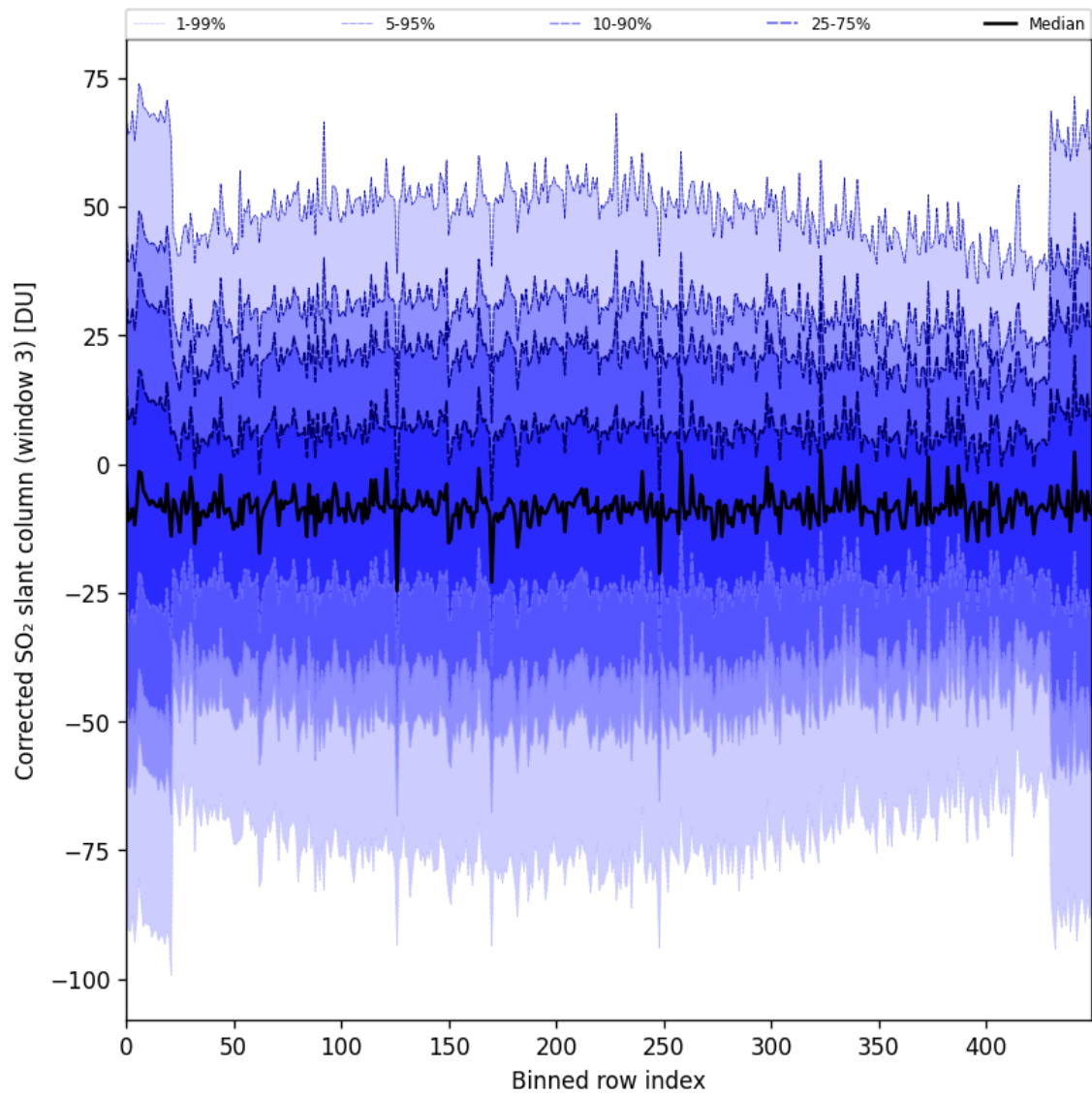
Figure 89: Along track statistics of “Corrected SO 2 slant column (window 3)” for 2024-10-24 to 2024-10-26
