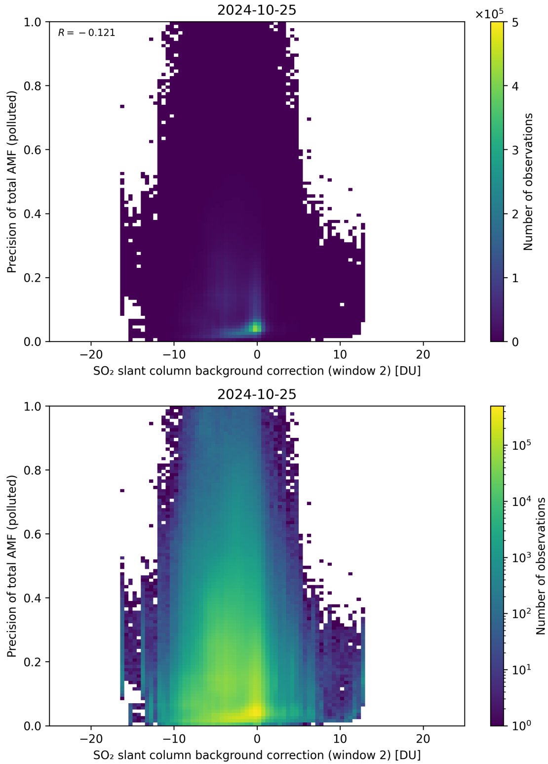
Figure 120: Scatter density plot of “SO 2 slant column background correction (window 2)” against “Precision of total AMF (polluted)” for 2024-10-24 to 2024-10-26.
