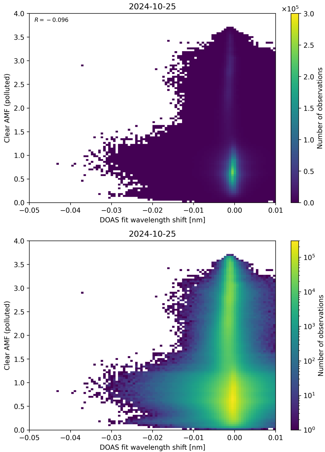
Figure 129: Scatter density plot of “DOAS fit wavelength shift” against “Clear AMF (polluted)” for 2024-10-24 to 2024-10-26.
