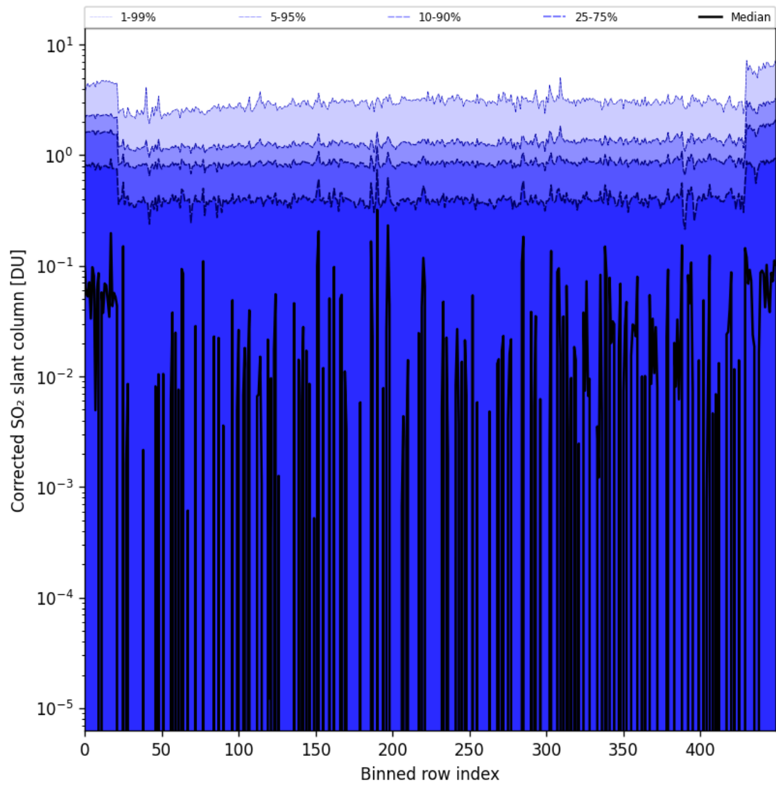
Figure 78: Along track statistics of “Corrected SO 2 slant column” for 2024-10-24 to 2024-10-26
