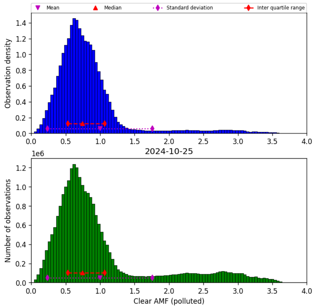
Figure 73: Histogram of “Clear AMF (polluted)” for 2024-10-24 to 2024-10-26
