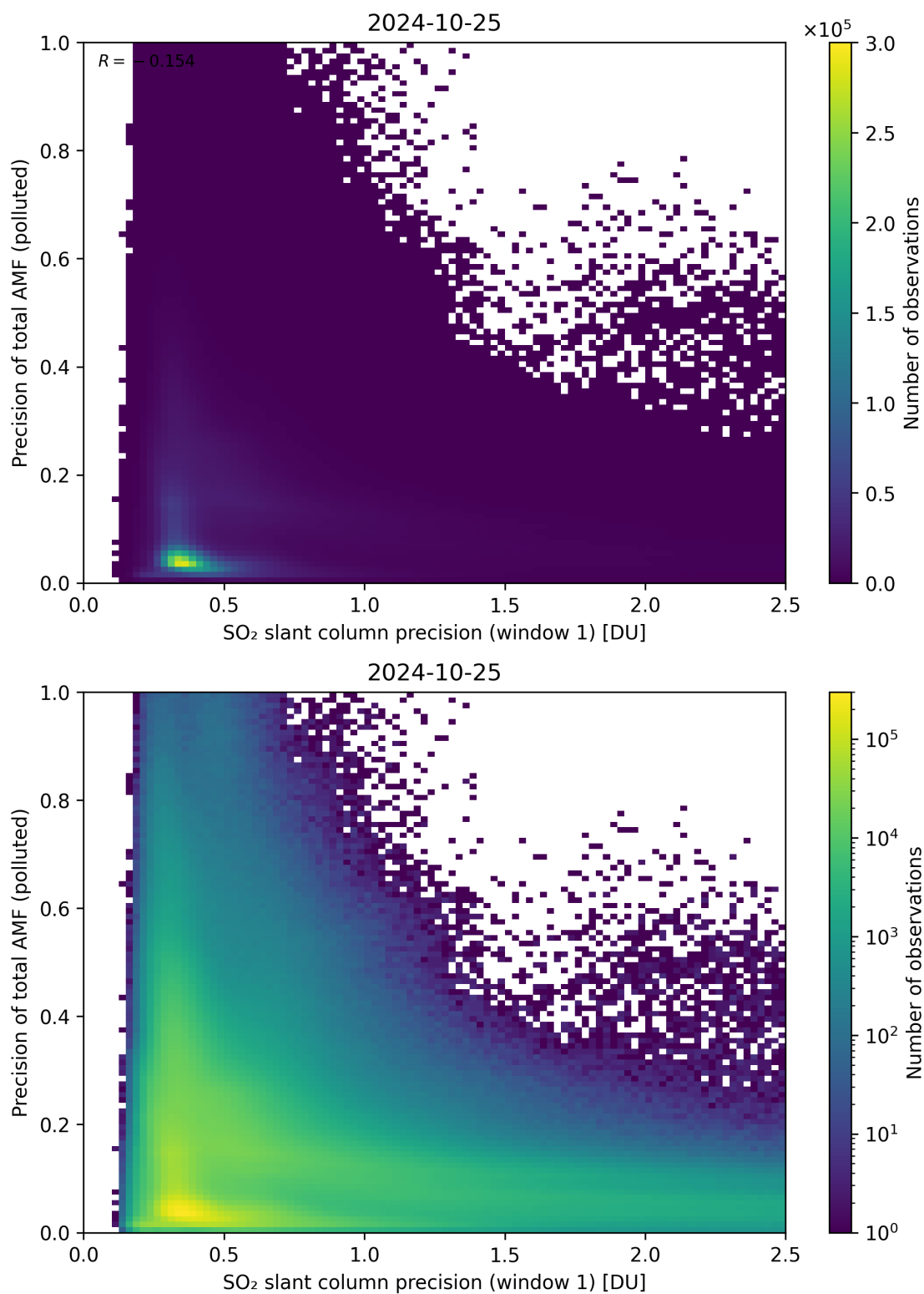
Figure 231: Scatter density plot of “SO 2 slant column precision (window 1)” against “Precision of total AMF (polluted)” for 2024-10-24 to 2024-10-26.
