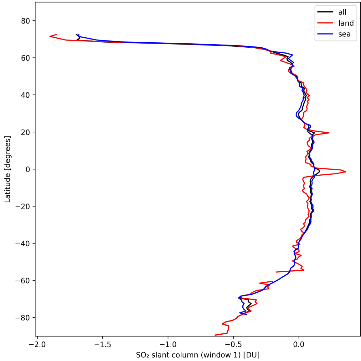
Figure 33: Zonal average of “SO 2 slant column (window 1)” for 2024-10-24 to 2024-10-26.
