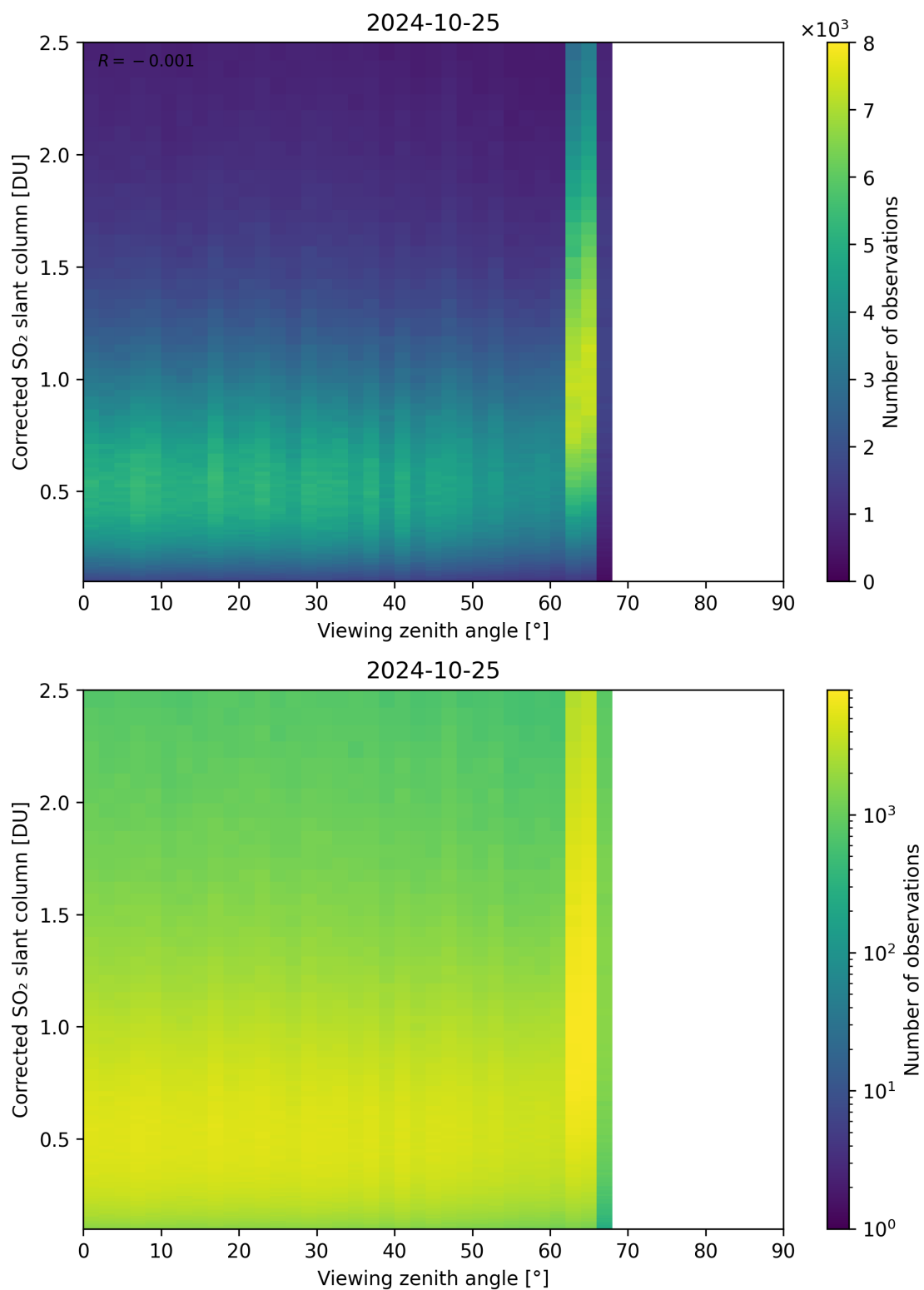
Figure 317: Scatter density plot of “Viewing zenith angle” against “Corrected SO 2 slant column” for 2024-10-24 to 2024-10-26.
