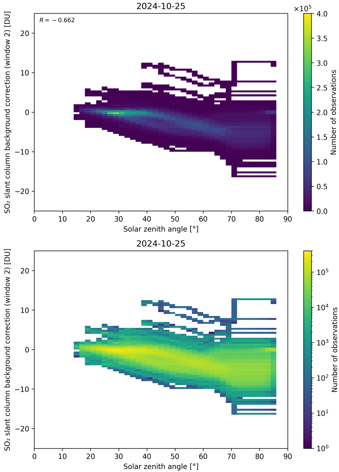
Figure 159: Scatter density plot of “Solar zenith angle” against “SO 2 slant column background correction (window 2)” for 2024-10-24 to 2024-10-26.
