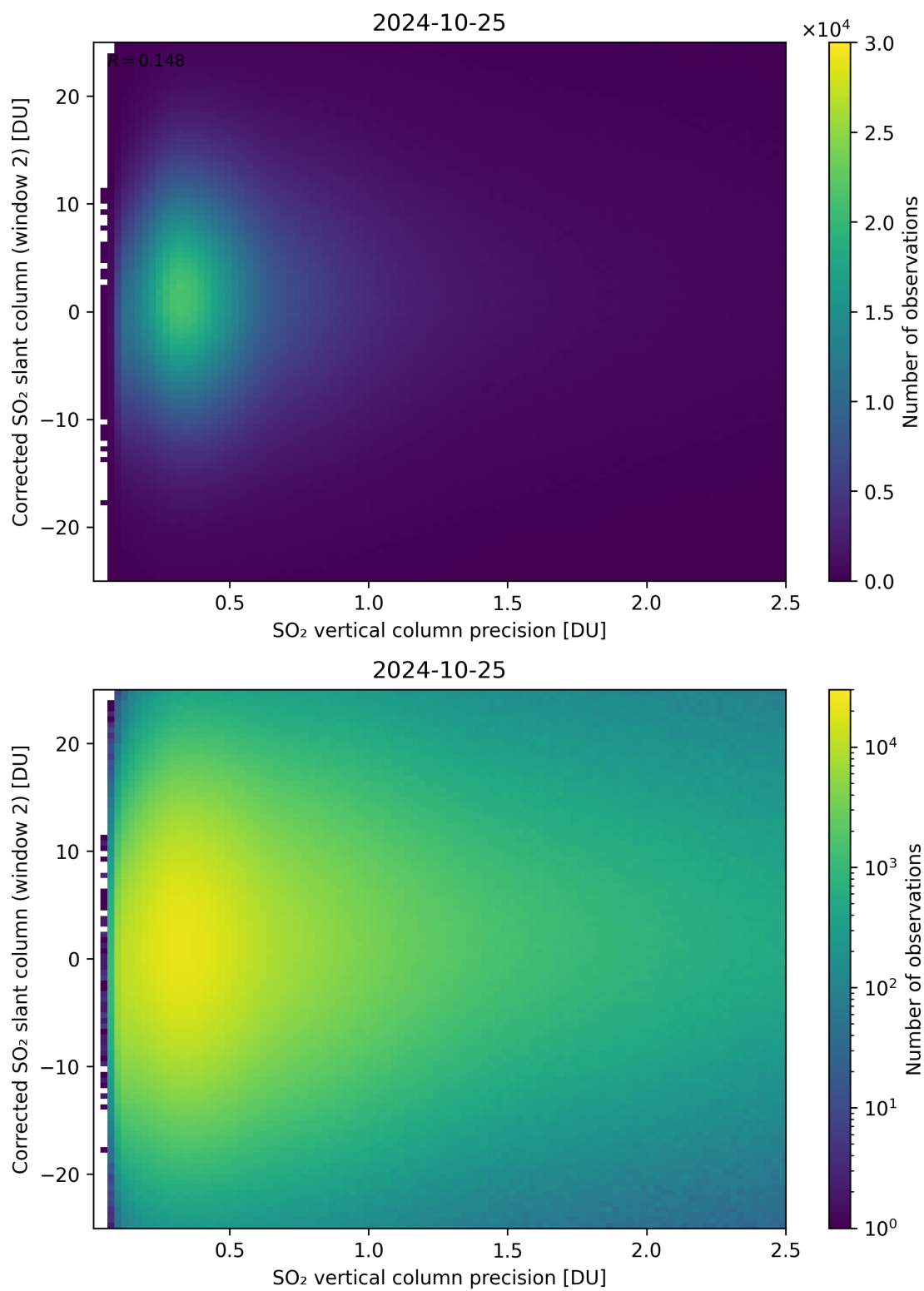
Figure 287: Scatter density plot of “SO 2 vertical column precision” against “Corrected SO 2 slant column (window 2)” for 2024-10-24 to 2024-10-26.
