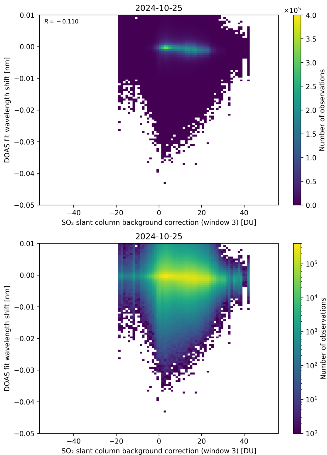
Figure 121: Scatter density plot of “SO 2 slant column background correction (window 3)” against “DOAS fit wavelength shift” for 2024-10-24 to 2024-10-26.
