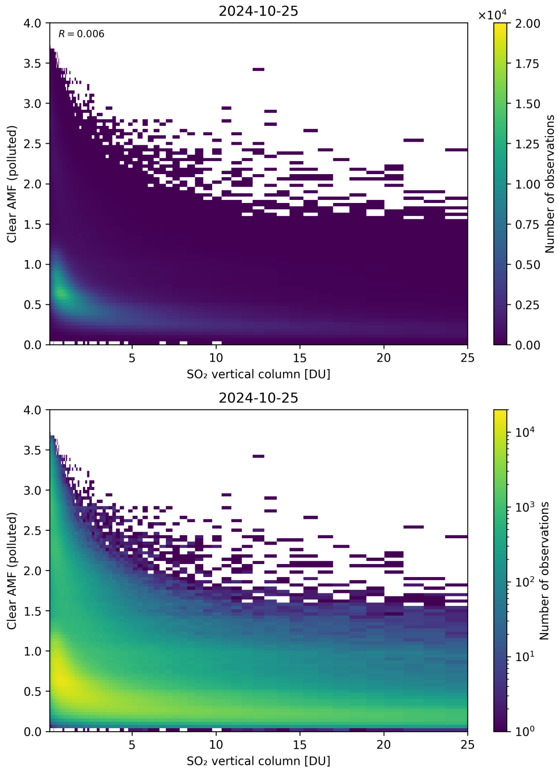
Figure 296: Scatter density plot of “SO 2 vertical column” against “Clear AMF (polluted)” for 2024-10-24 to 2024-10-26.
