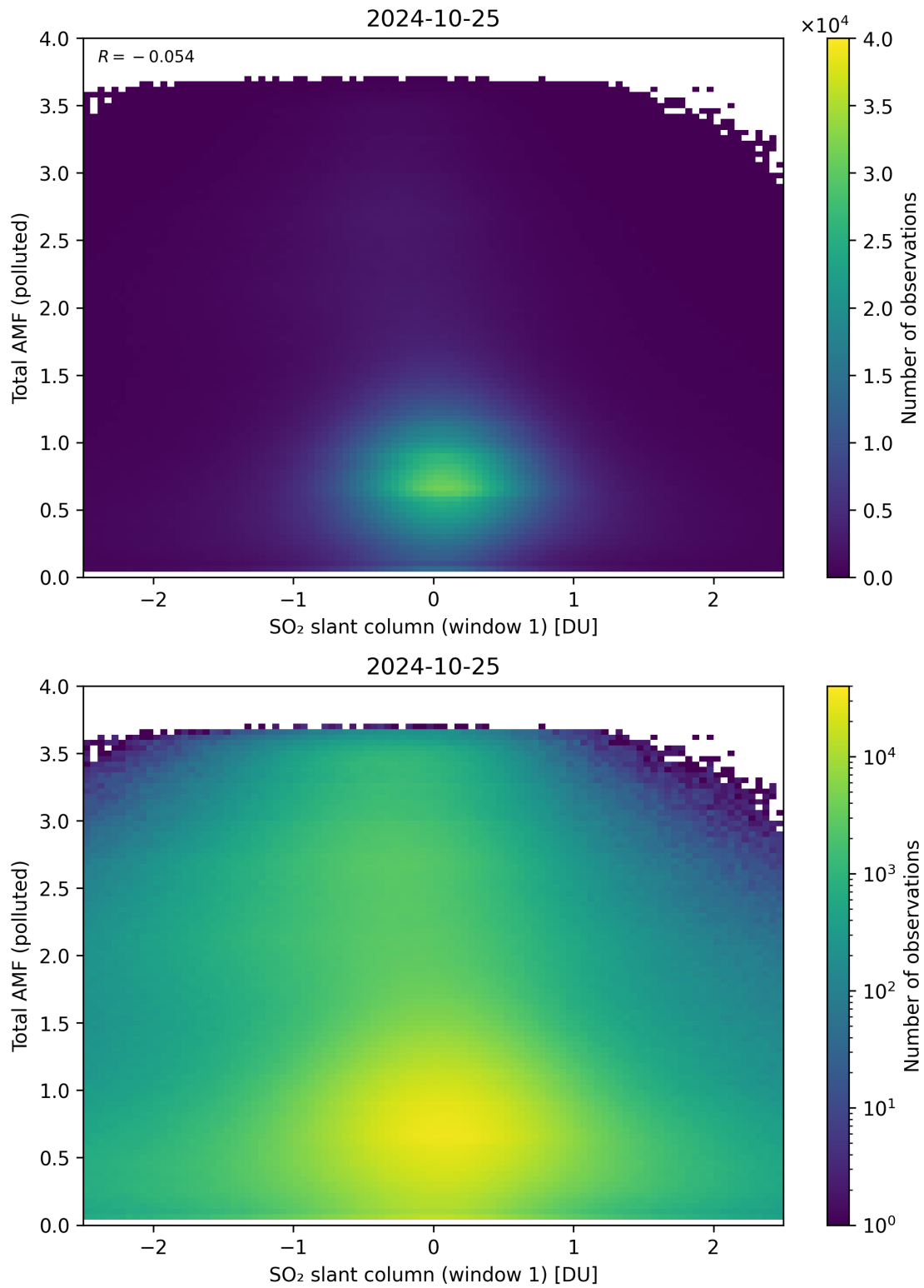
Figure 239: Scatter density plot of “SO 2 slant column (window 1)” against “Total AMF (polluted)” for 2024-10-24 to 2024-10-26.
