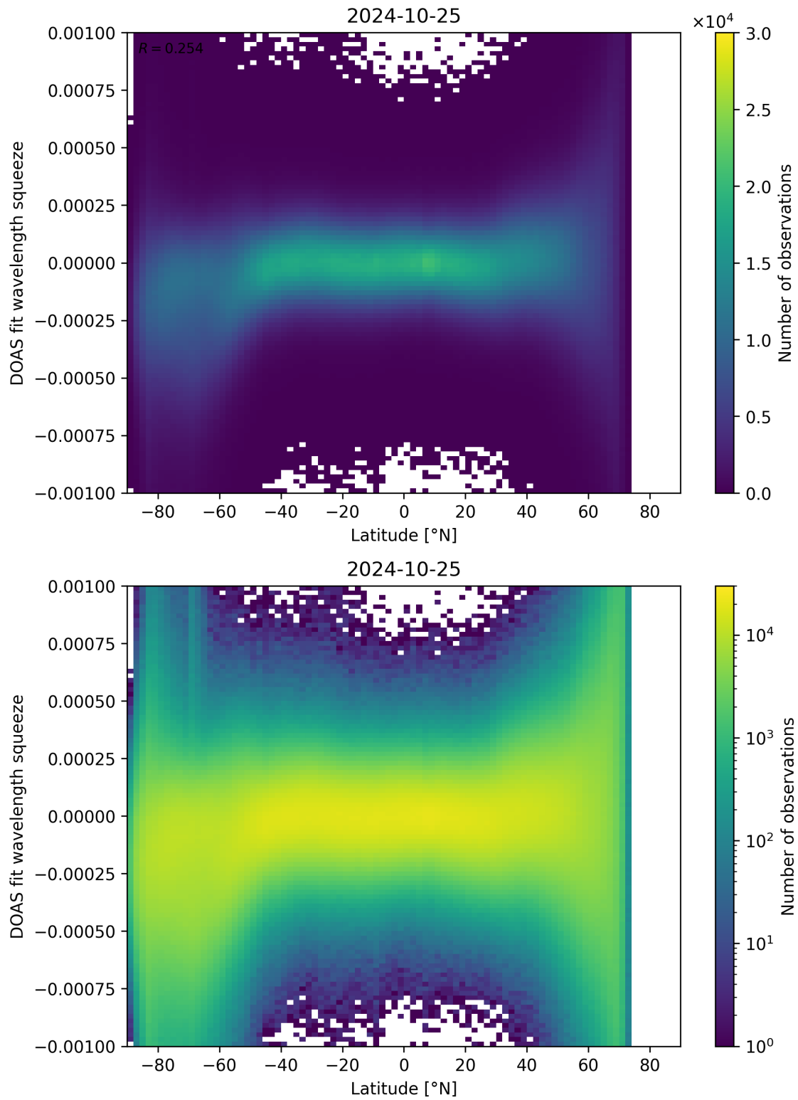
Figure 143: Scatter density plot of “Latitude” against “DOAS fit wavelength squeeze” for 2024-10-24 to 2024-10-26.
