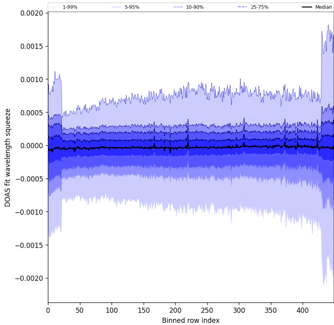
Figure 92: Along track statistics of “DOAS fit wavelength squeeze” for 2024-10-24 to 2024-10-26
