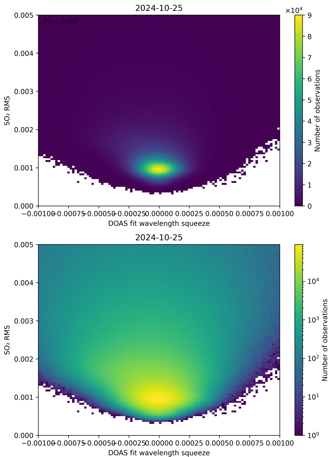
Figure 132: Scatter density plot of “DOAS fit wavelength squeeze” against “SO 2 RMS” for 2024-10-24 to 2024-10-26.
