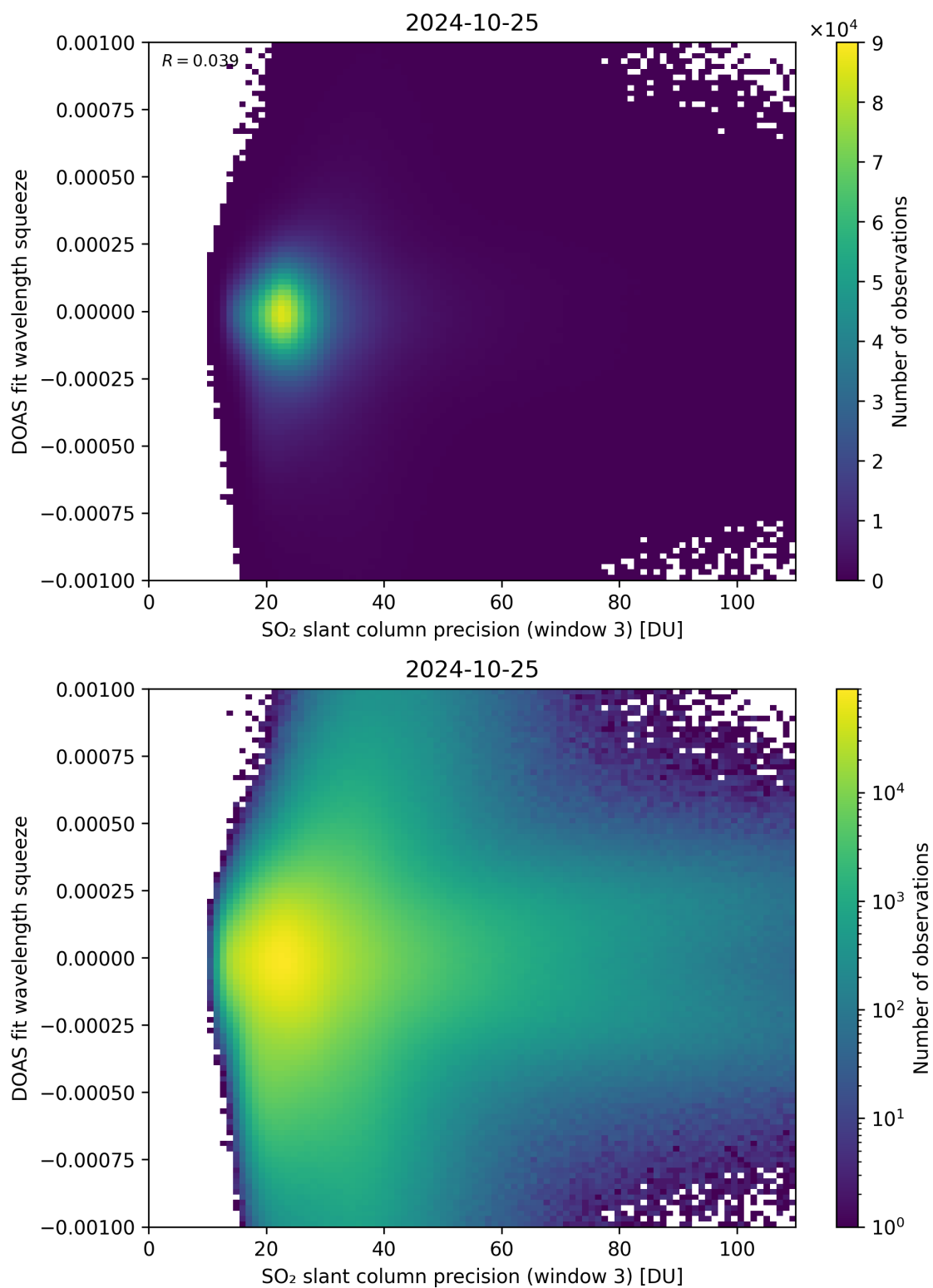
Figure 259: Scatter density plot of “SO 2 slant column precision (window 3)” against “DOAS fit wavelength squeeze” for 2024-10-24 to 2024-10-26.
