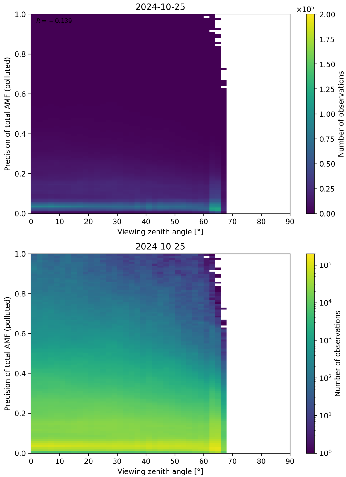
Figure 326: Scatter density plot of “Viewing zenith angle” against “Precision of total AMF (polluted)” for 2024-10-24 to 2024-10-26.
