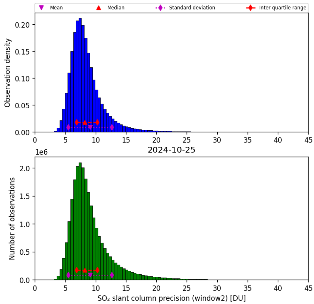
Figure 61: Histogram of “SO 2 slant column precision (window2)” for 2024-10-24 to 2024-10-26
