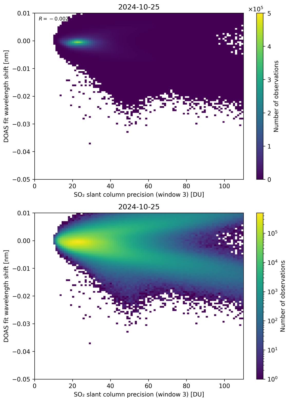
Figure 258: Scatter density plot of “SO 2 slant column precision (window 3)” against “DOAS fit wavelength shift” for 2024-10-24 to 2024-10-26.
