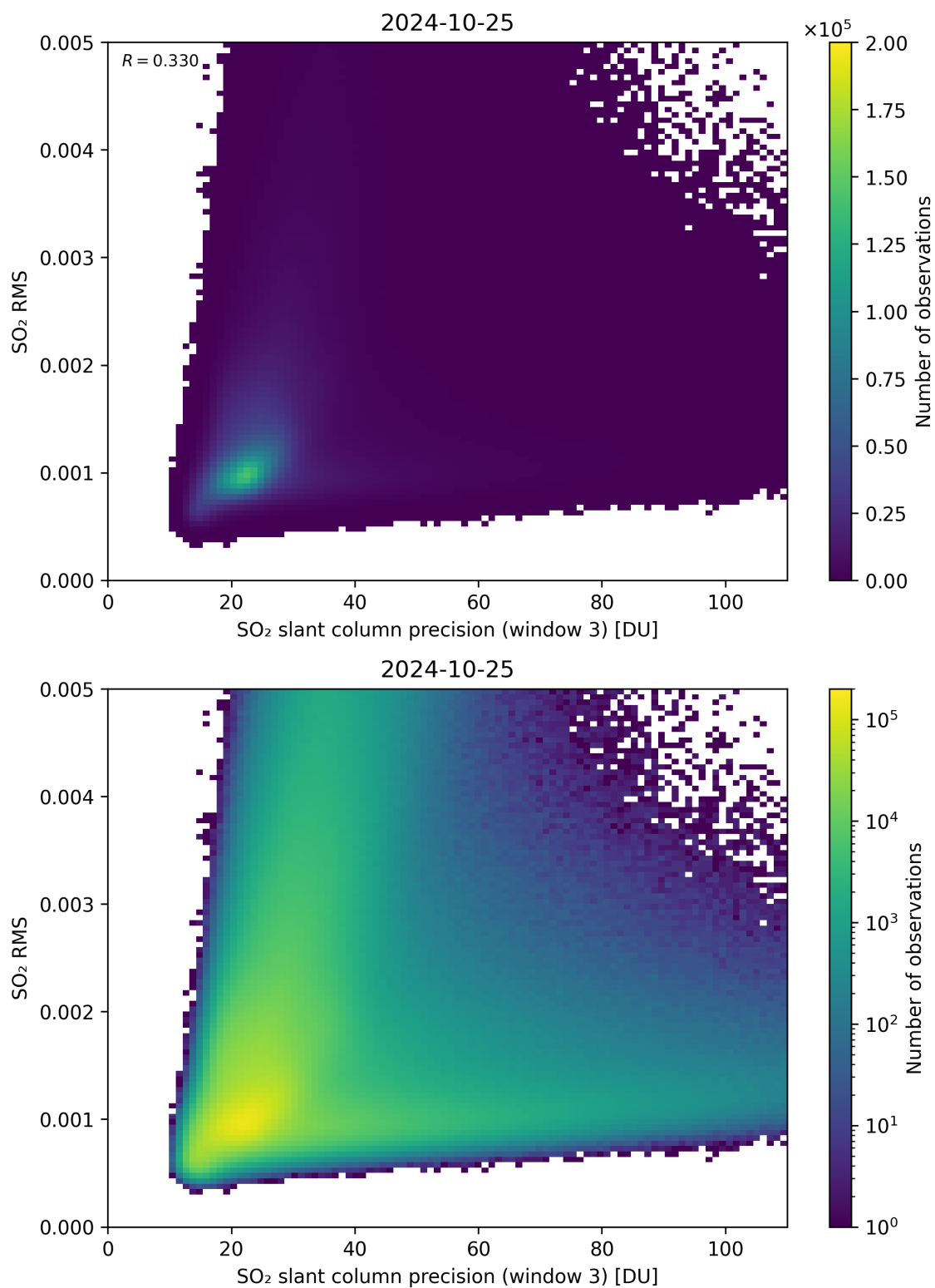
Figure 260: Scatter density plot of “SO 2 slant column precision (window 3)” against “SO 2 RMS” for 2024-10-24 to 2024-10-26.
