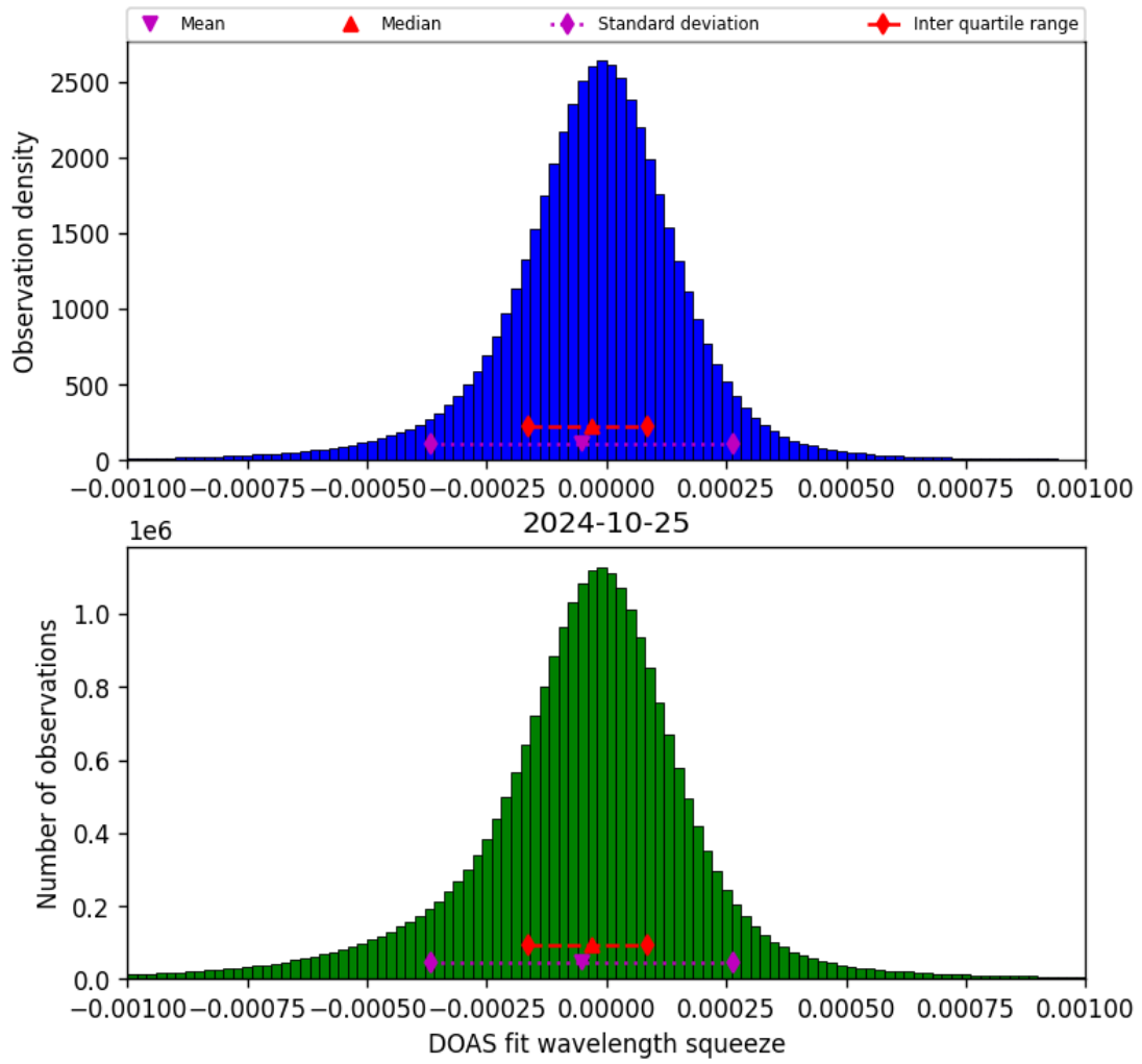
Figure 69: Histogram of “DOAS fit wavelength squeeze” for 2024-10-24 to 2024-10-26
