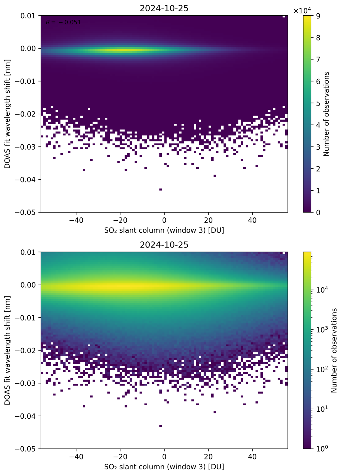
Figure 254: Scatter density plot of “SO 2 slant column (window 3)” against “DOAS fit wavelength shift” for 2024-10-24 to 2024-10-26.
