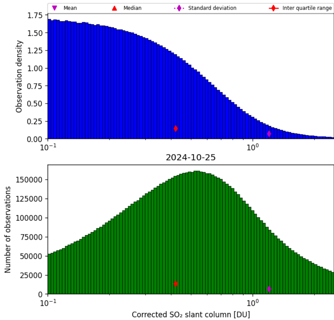
Figure 55: Histogram of “Corrected SO 2 slant column” for 2024-10-24 to 2024-10-26
