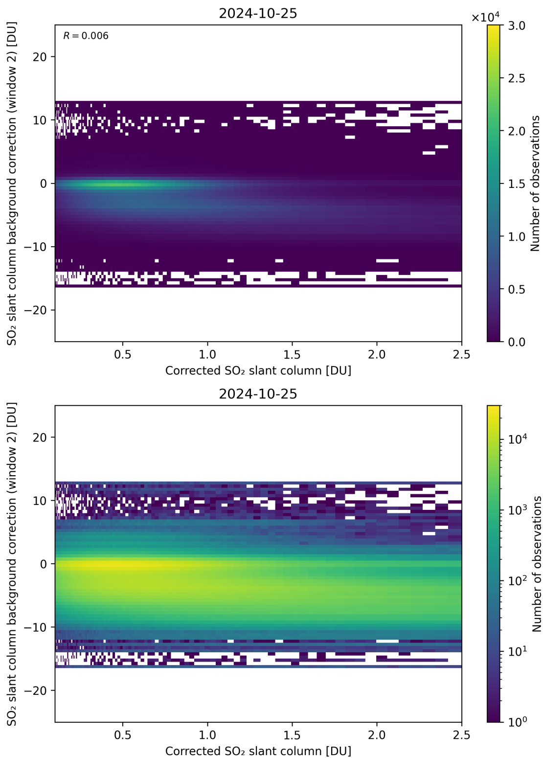
Figure 179: Scatter density plot of “Corrected SO 2 slant column” against “SO 2 slant column background correction (window 2)” for 2024-10-24 to 2024-10-26.
