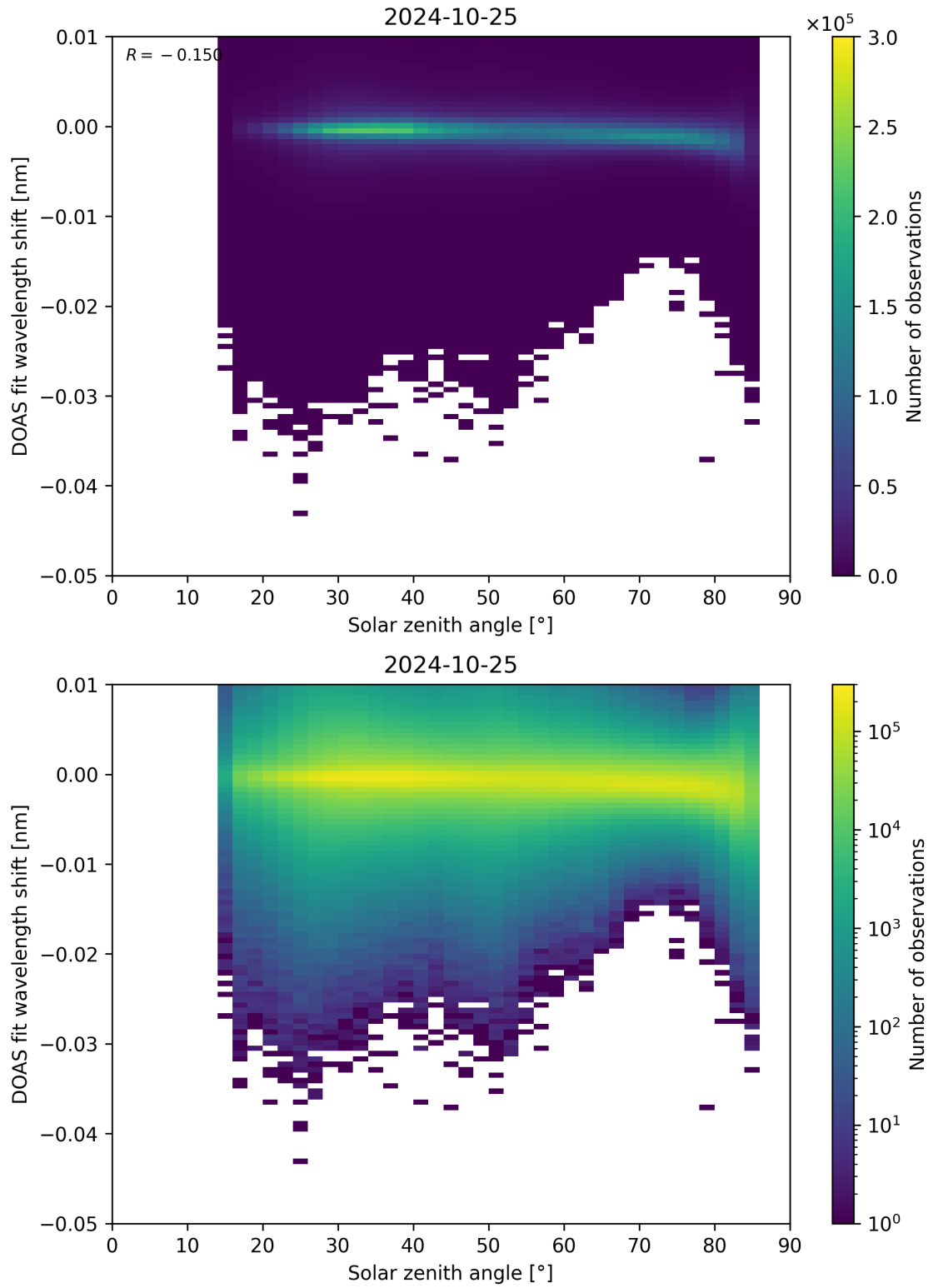
Figure 161: Scatter density plot of “Solar zenith angle” against “DOAS fit wavelength shift” for 2024-10-24 to 2024-10-26.
