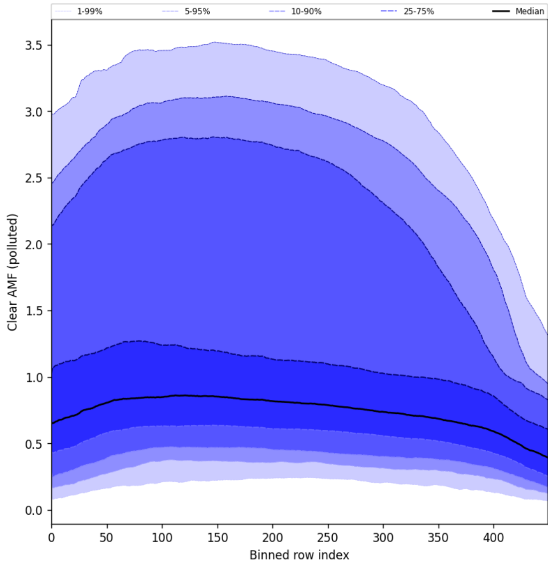
Figure 96: Along track statistics of “Clear AMF (polluted)” for 2024-10-24 to 2024-10-26
