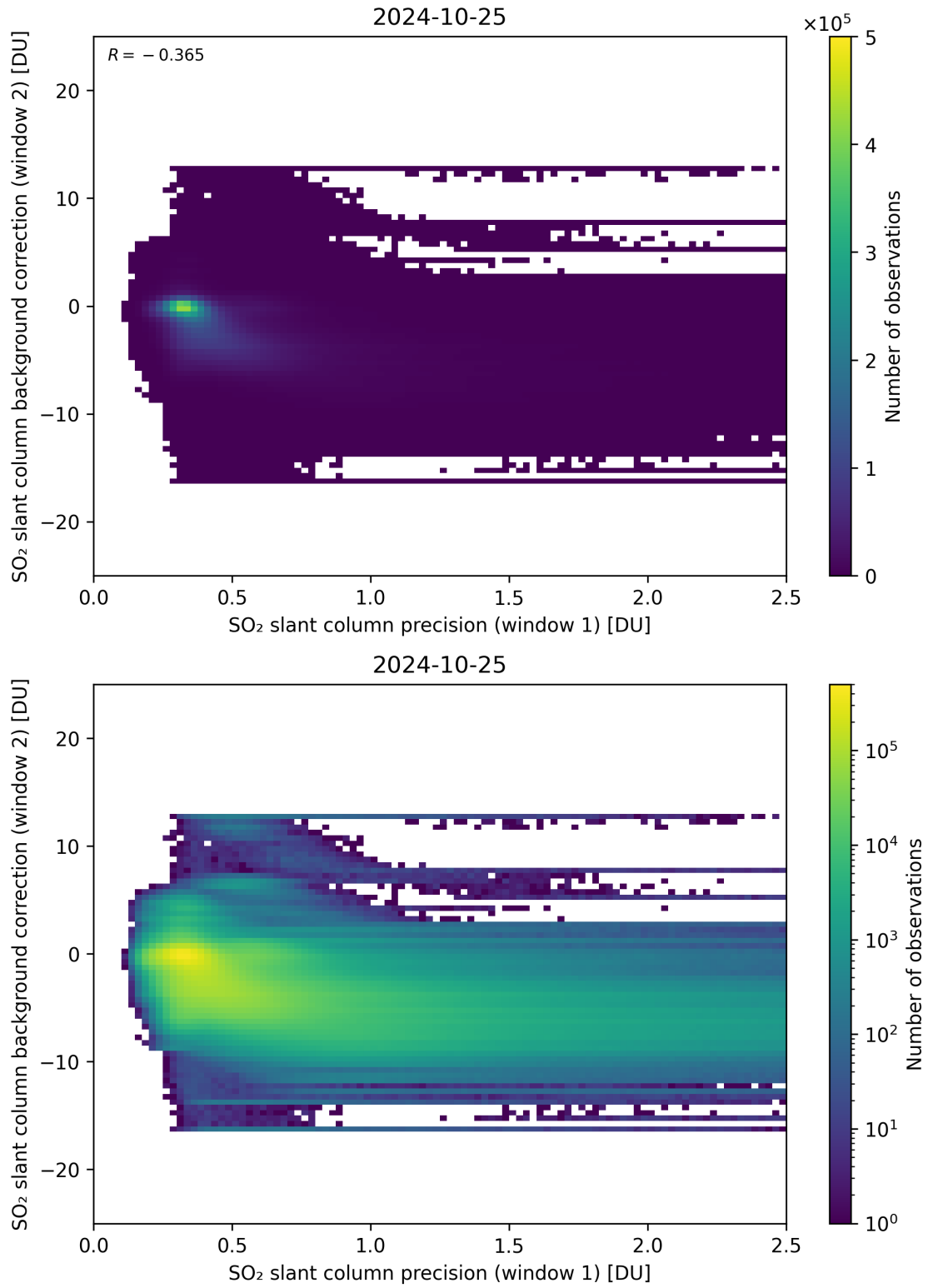
Figure 219: Scatter density plot of “SO 2 slant column precision (window 1)” against “SO 2 slant column background correction (window 2)” for 2024-10-24 to 2024-10-26.
