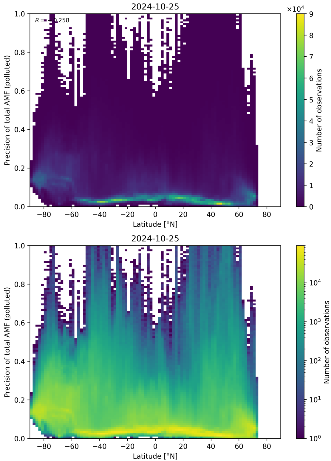
Figure 155: Scatter density plot of “Latitude” against “Precision of total AMF (polluted)” for 2024-10-24 to 2024-10-26.
