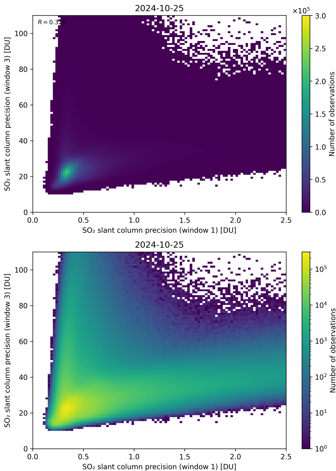
Figure 229: Scatter density plot of “SO 2 slant column precision (window 1)” against “SO 2 slant column precision (window 3)” for 2024-10-24 to 2024-10-26.
