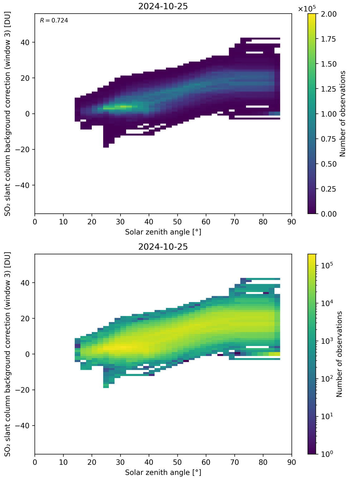
Figure 160: Scatter density plot of “Solar zenith angle” against “SO 2 slant column background correction (window 3)” for 2024-10-24 to 2024-10-26.
