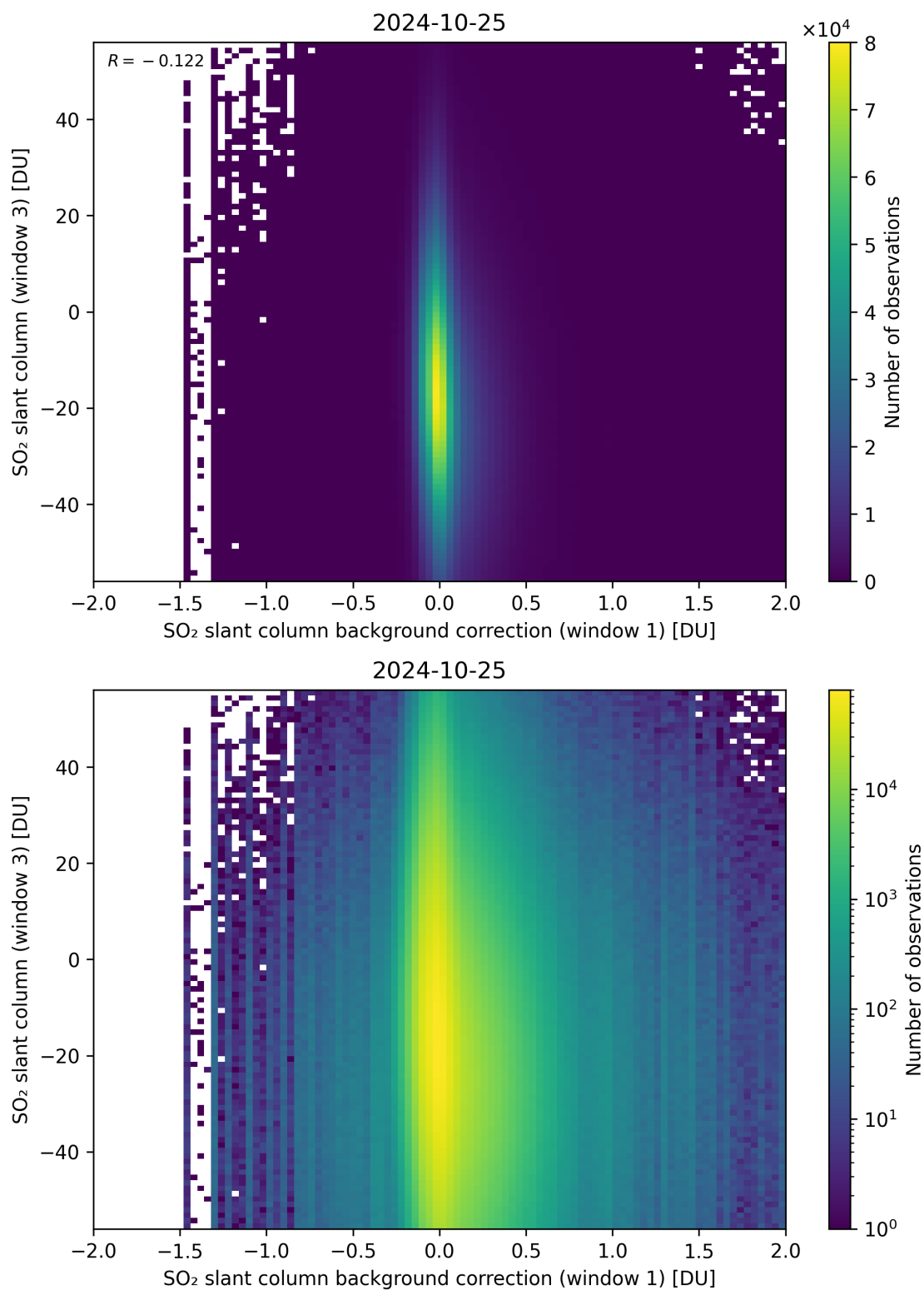
Figure 107: Scatter density plot of “SO 2 slant column background correction (window 1)” against “SO 2 slant column (window 3)” for 2024-10-24 to 2024-10-26.
