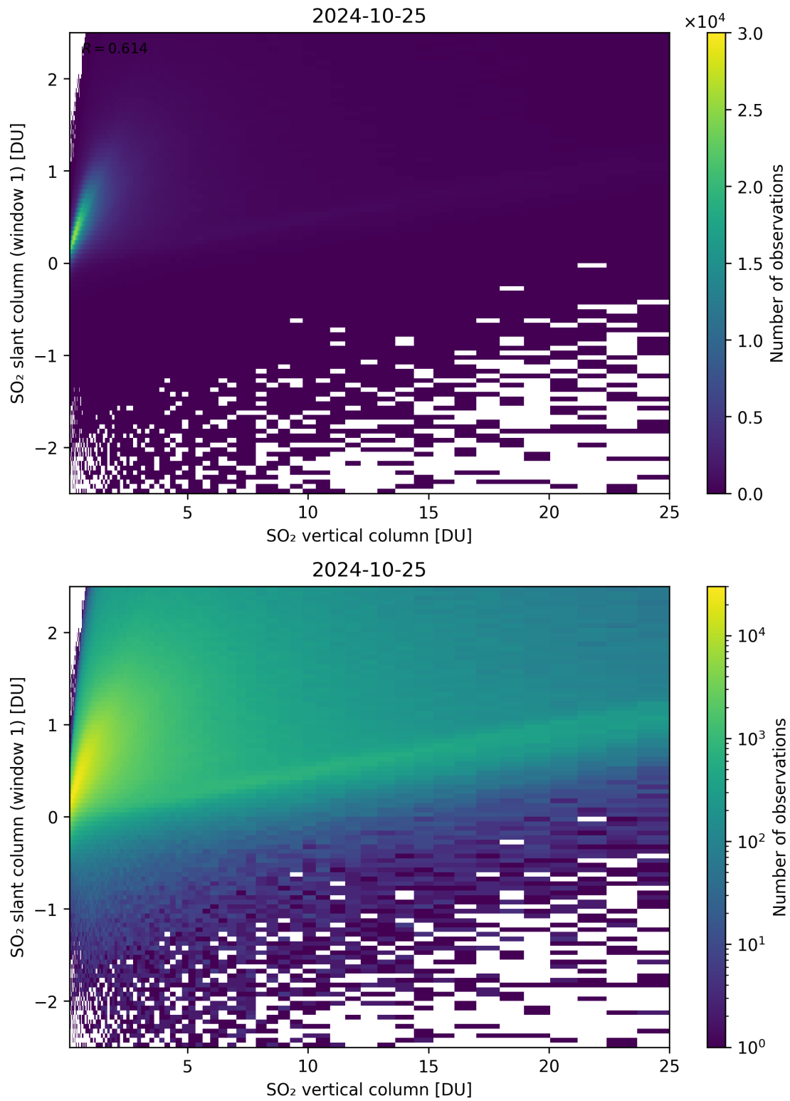
Figure 300: Scatter density plot of “SO 2 vertical column” against “SO 2 slant column (window 1)” for 2024-10-24 to 2024-10-26.
