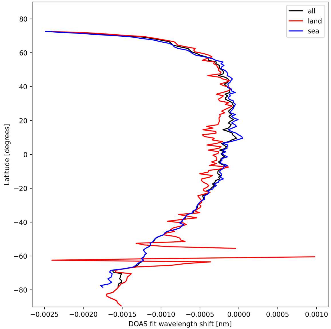
Figure 45: Zonal average of “DOAS fit wavelength shift” for 2024-10-24 to 2024-10-26.
