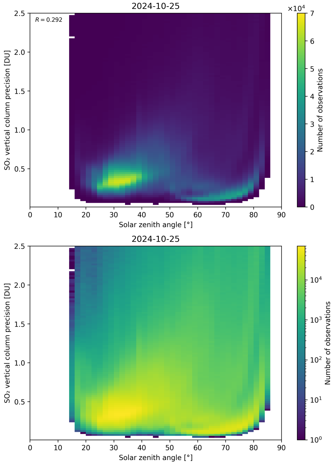
Figure 177: Scatter density plot of “Solar zenith angle” against “SO 2 vertical column precision” for 2024-10-24 to 2024-10-26.
