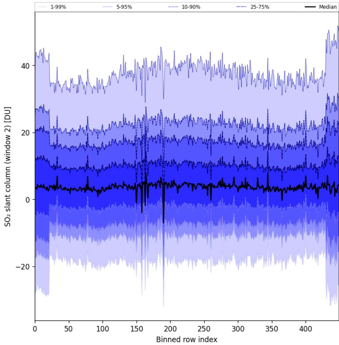
Figure 83: Along track statistics of “SO 2 slant column (window 2)” for 2024-10-24 to 2024-10-26
