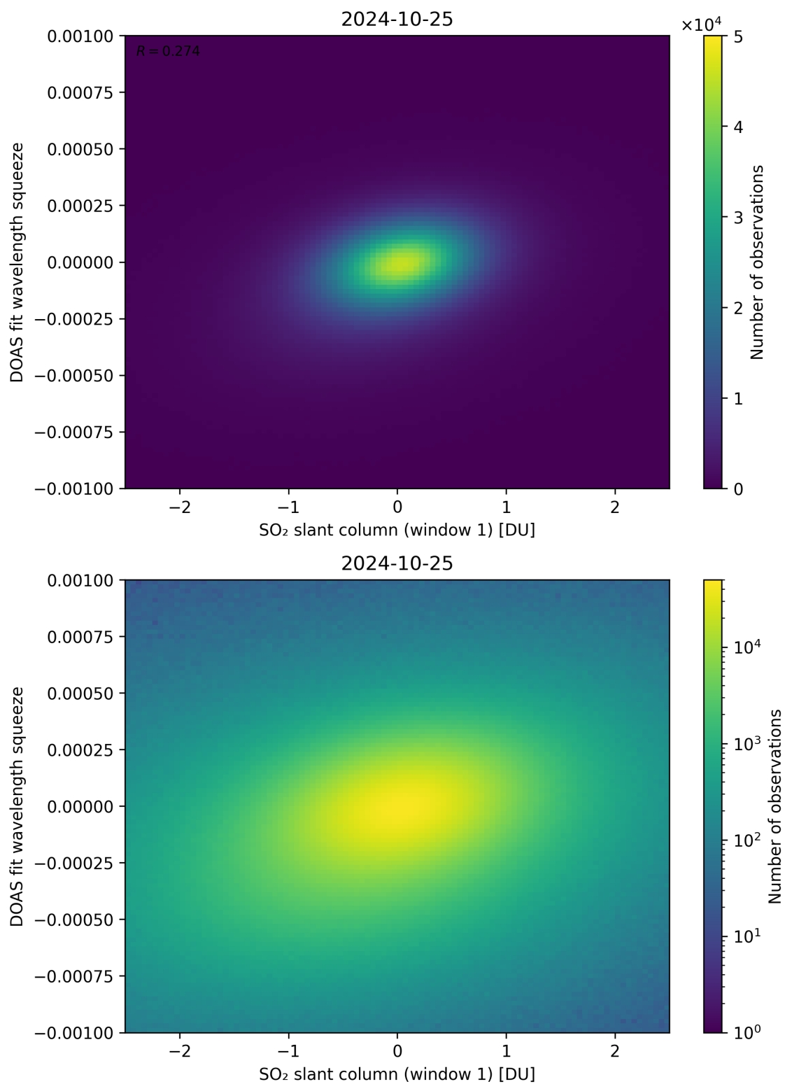
Figure 216: Scatter density plot of “SO 2 slant column (window 1)” against “DOAS fit wavelength squeeze” for 2024-10-24 to 2024-10-26.
