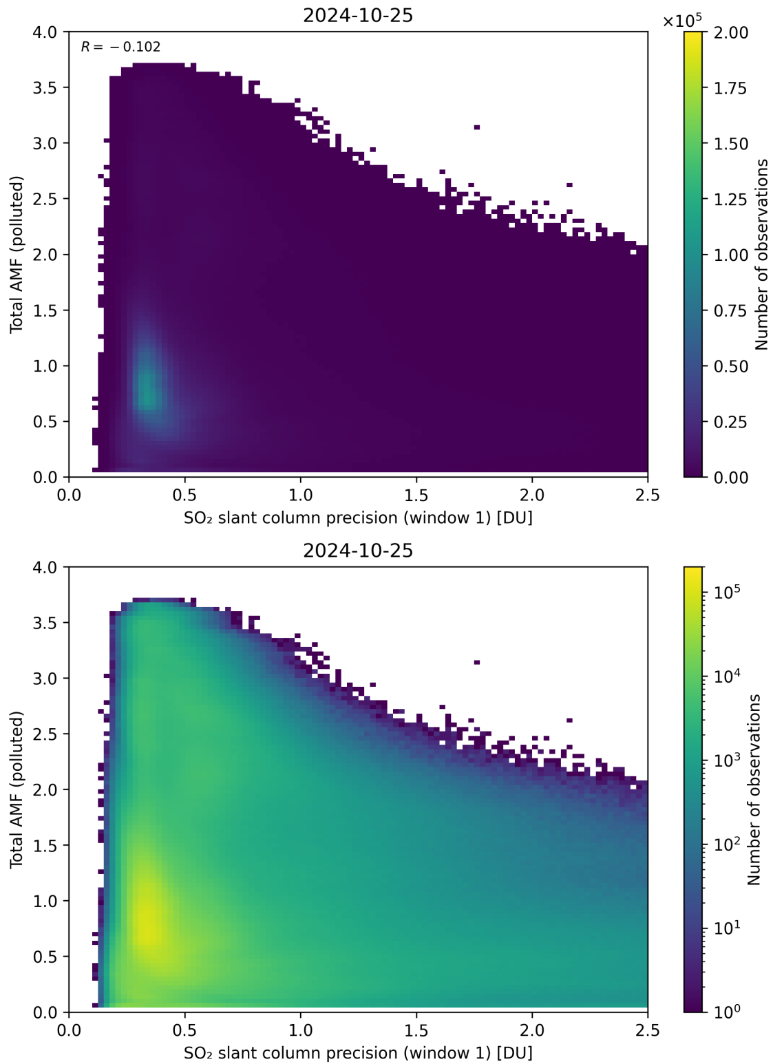
Figure 230: Scatter density plot of “SO 2 slant column precision (window 1)” against “Total AMF (polluted)” for 2024-10-24 to 2024-10-26.
