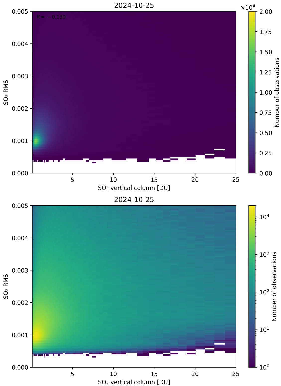
Figure 278: Scatter density plot of “SO 2 vertical column” against “SO 2 RMS” for 2024-10-24 to 2024-10-26.
