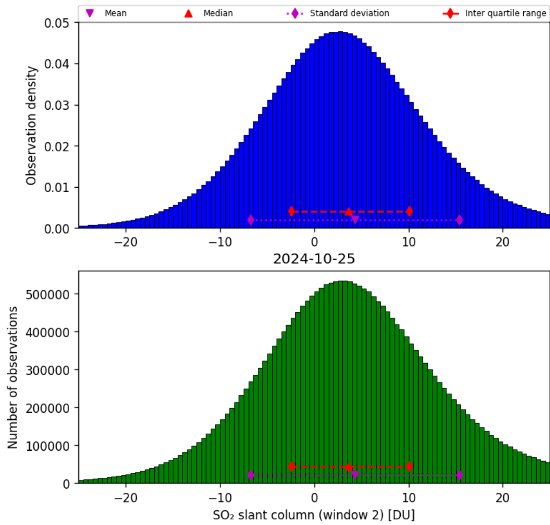
Figure 60: Histogram of “SO 2 slant column (window 2)” for 2024-10-24 to 2024-10-26
