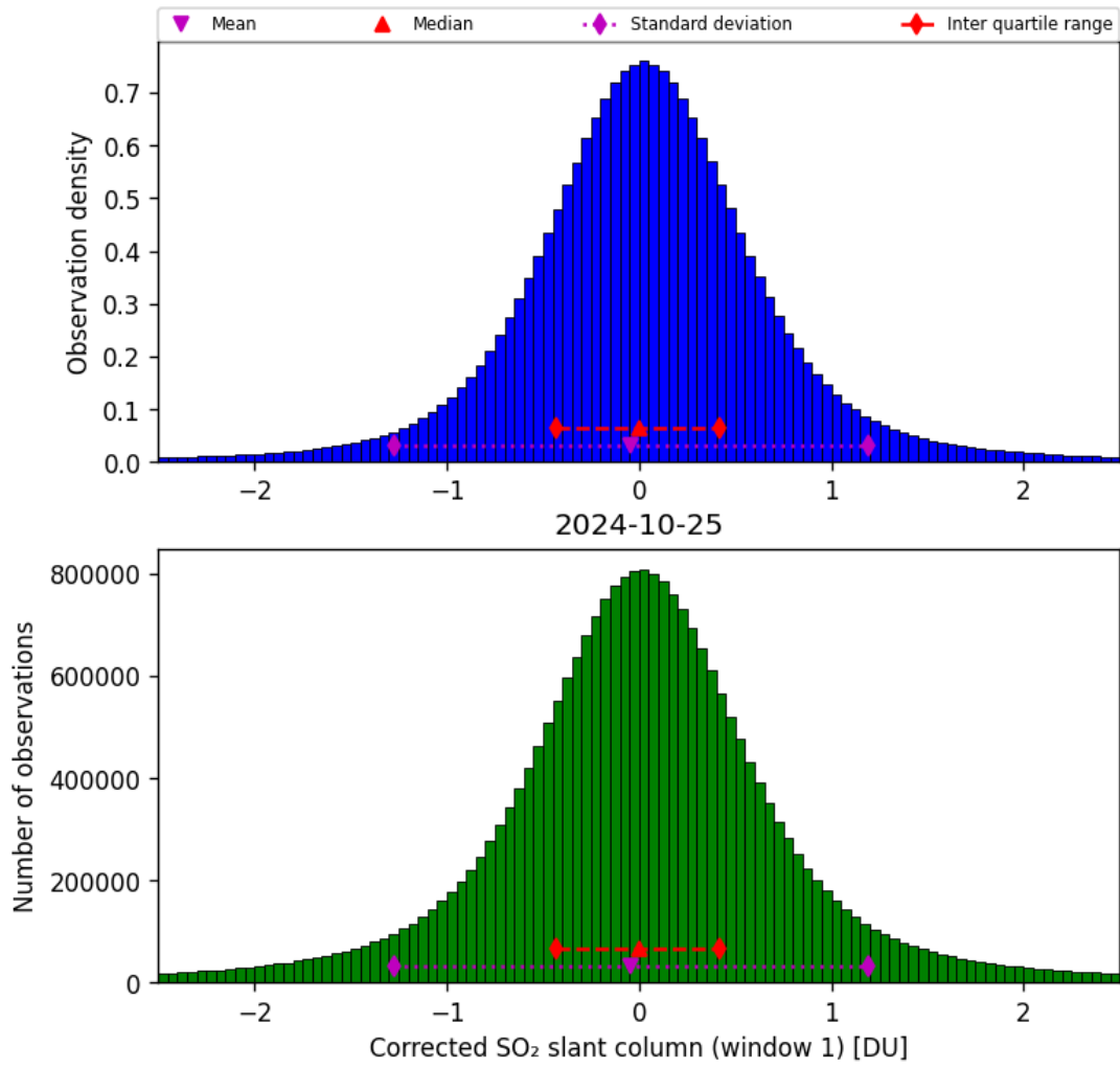
Figure 58: Histogram of “Corrected SO 2 slant column (window 1)” for 2024-10-24 to 2024-10-26
