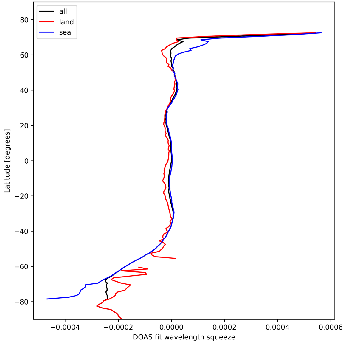
Figure 46: Zonal average of “DOAS fit wavelength squeeze” for 2024-10-24 to 2024-10-26.
