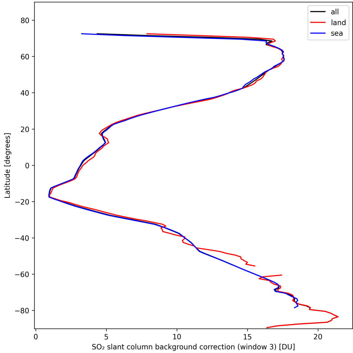
Figure 44: Zonal average of “SO 2 slant column background correction (window 3)” for 2024-10-24 to 2024-10-26.
