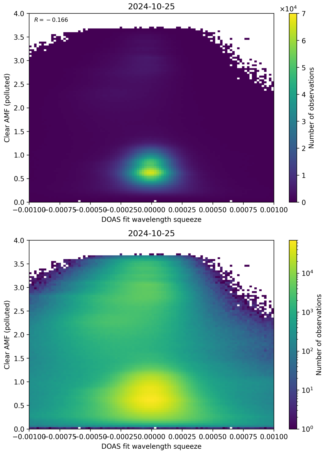
Figure 133: Scatter density plot of “DOAS fit wavelength squeeze” against “Clear AMF (polluted)” for 2024-10-24 to 2024-10-26.
