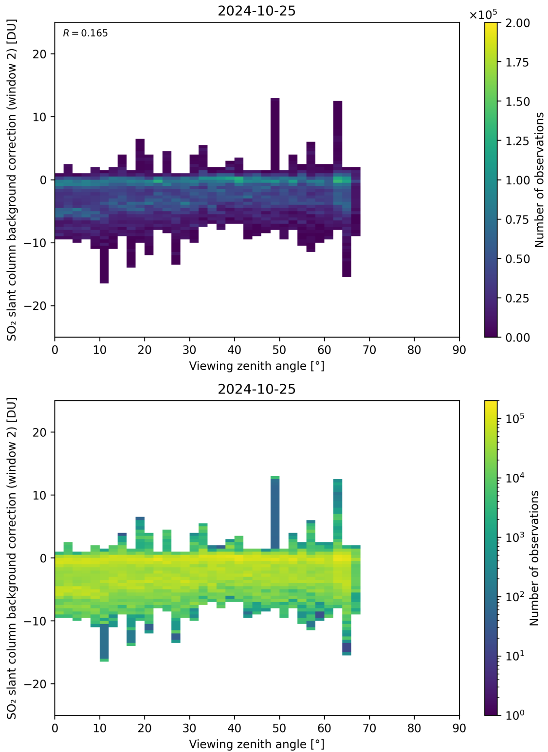
Figure 309: Scatter density plot of “Viewing zenith angle” against “SO 2 slant column background correction (window 2)” for 2024-10-24 to 2024-10-26.
