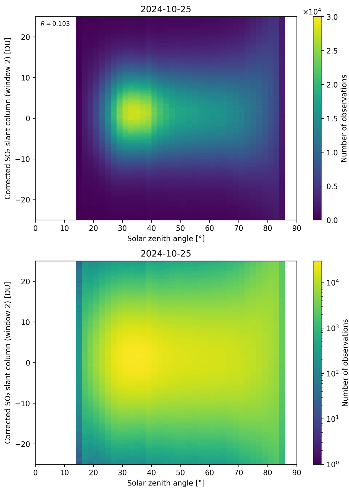
Figure 167: Scatter density plot of “Solar zenith angle” against “Corrected SO 2 slant column (window 2)” for 2024-10-24 to 2024-10-26.
