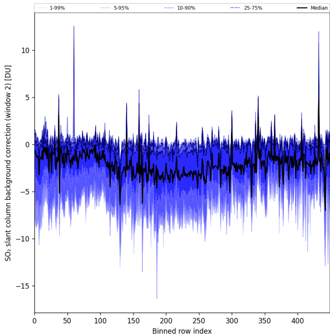
Figure 86: Along track statistics of “SO 2 slant column background correction (window 2)” for 2024-10-24 to 2024-10-26
