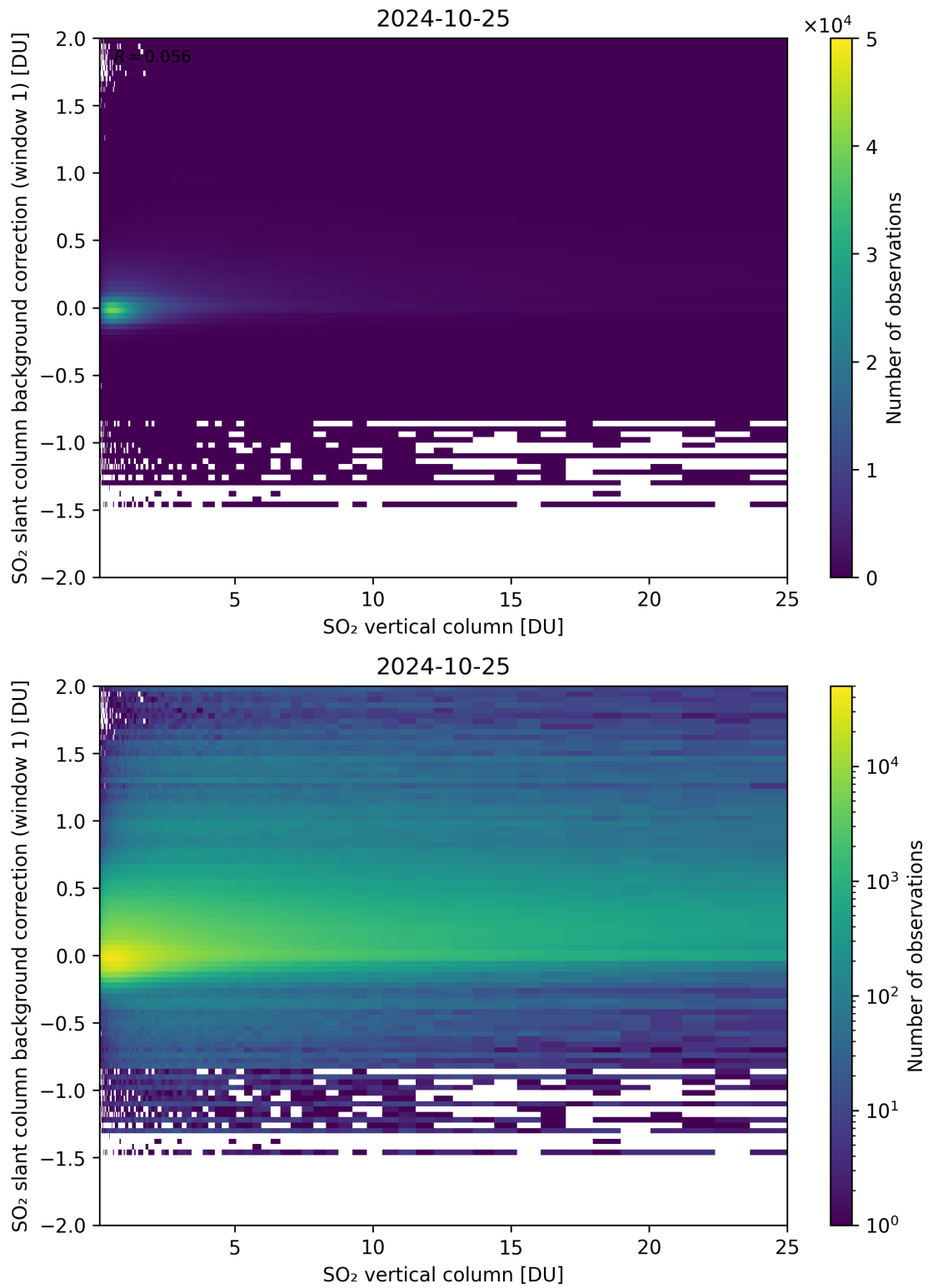
Figure 273: Scatter density plot of “SO 2 vertical column” against “SO 2 slant column background correction (window 1)” for 2024-10-24 to 2024-10-26.
