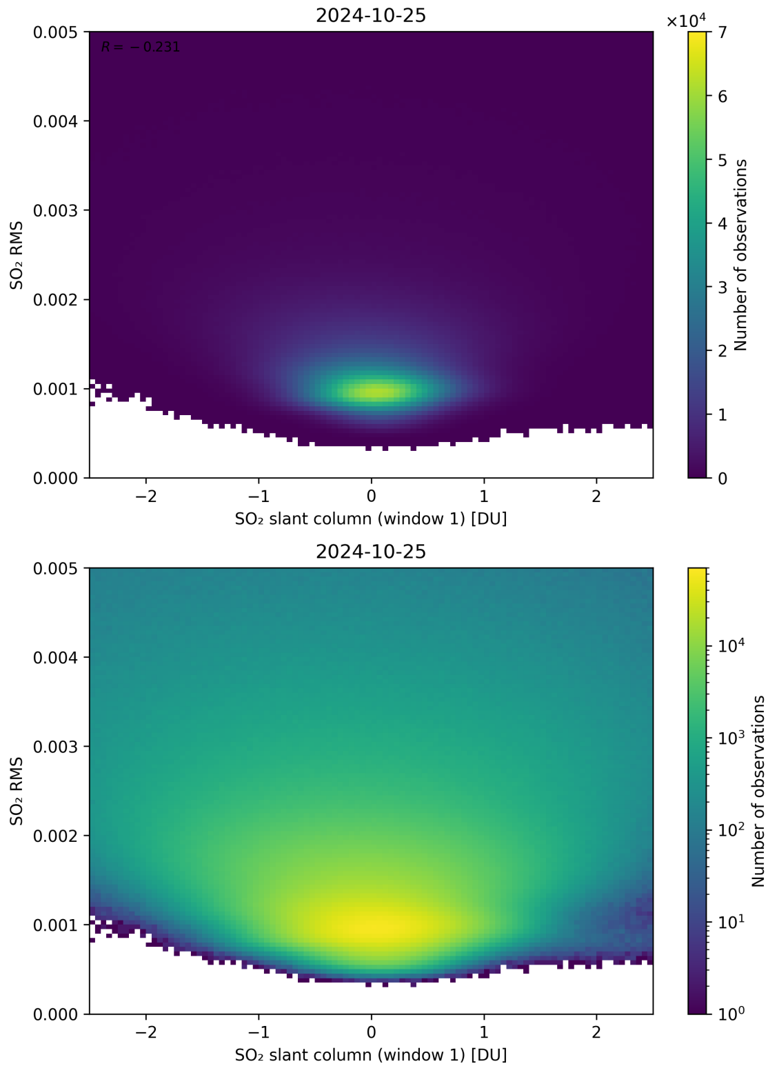
Figure 217: Scatter density plot of “SO 2 slant column (window 1)” against “SO 2 RMS” for 2024-10-24 to 2024-10-26.
