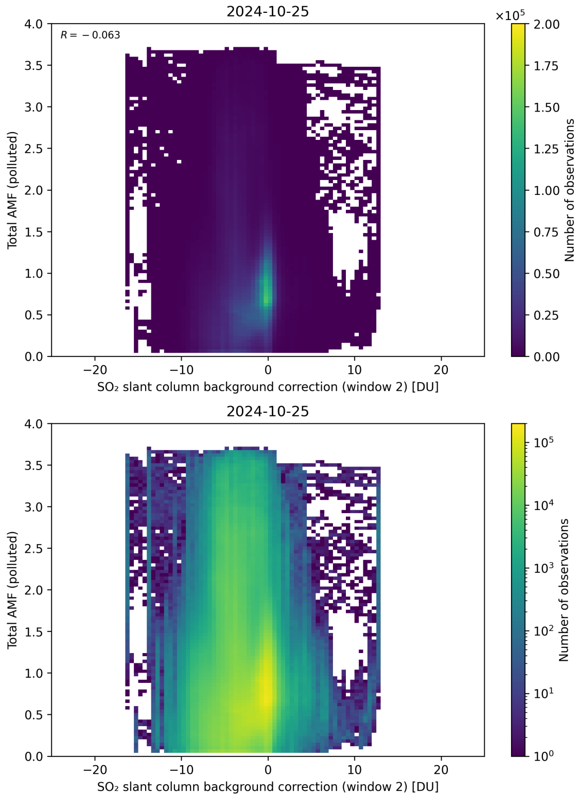
Figure 119: Scatter density plot of “SO 2 slant column background correction (window 2)” against “Total AMF (polluted)” for 2024-10-24 to 2024-10-26.
