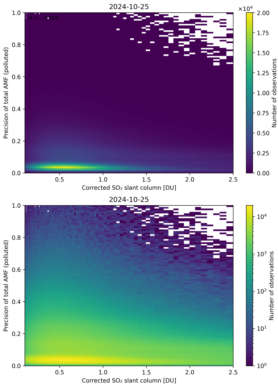
Figure 193: Scatter density plot of “Corrected SO 2 slant column” against “Precision of total AMF (polluted)” for 2024-10-24 to 2024-10-26.
