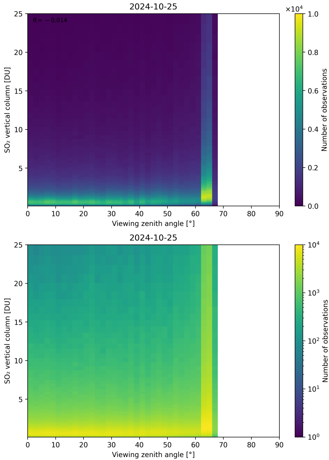
Figure 327: Scatter density plot of “Viewing zenith angle” against “SO 2 vertical column” for 2024-10-24 to 2024-10-26.
