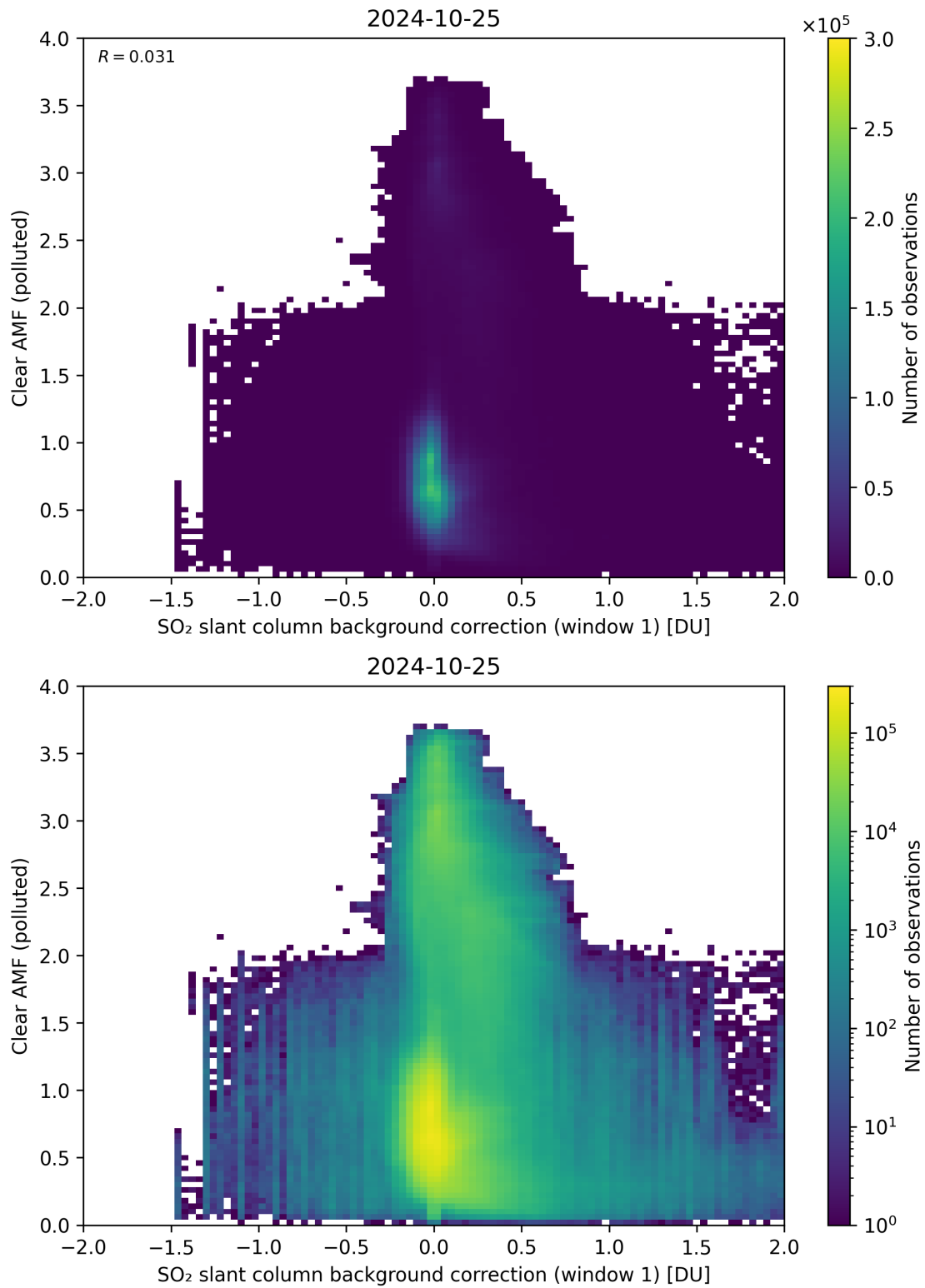
Figure 103: Scatter density plot of “SO 2 slant column background correction (window 1)” against “Clear AMF (polluted)” for 2024-10-24 to 2024-10-26.
