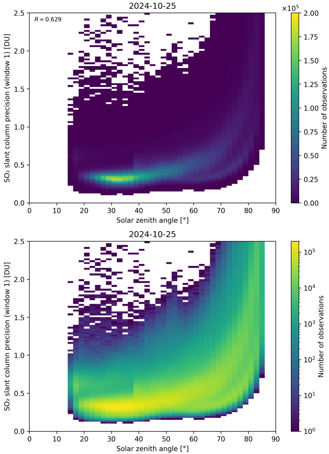
Figure 170: Scatter density plot of “Solar zenith angle” against “SO 2 slant column precision (window 1)” for 2024-10-24 to 2024-10-26.
