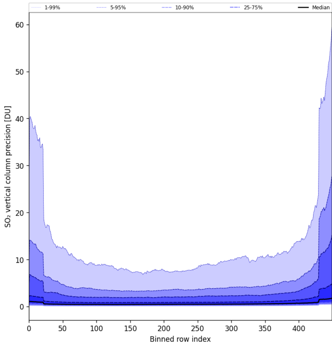
Figure 77: Along track statistics of “SO 2 vertical column precision” for 2024-10-24 to 2024-10-26
