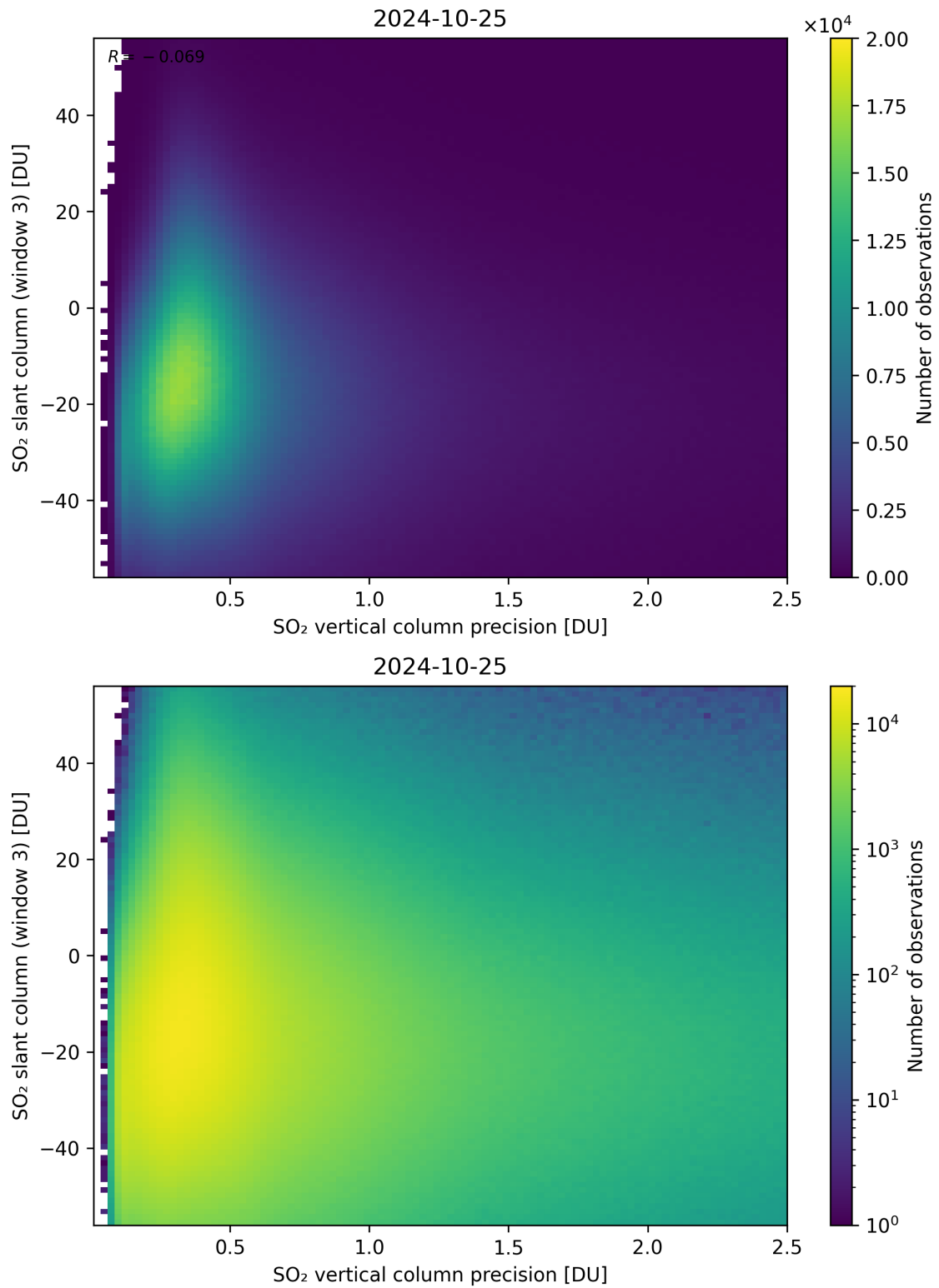
Figure 292: Scatter density plot of “SO 2 vertical column precision” against “SO 2 slant column (window 3)” for 2024-10-24 to 2024-10-26.
