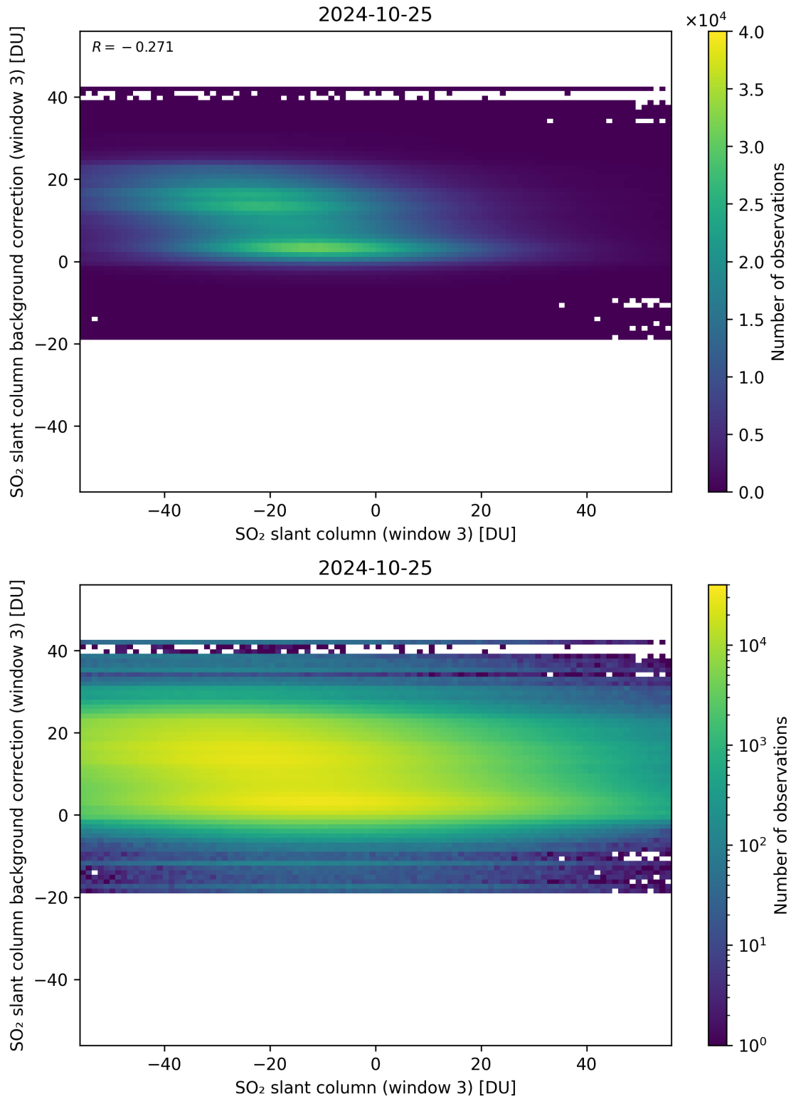
Figure 253: Scatter density plot of “SO 2 slant column (window 3)” against “SO 2 slant column background correction (window 3)” for 2024-10-24 to 2024-10-26.
