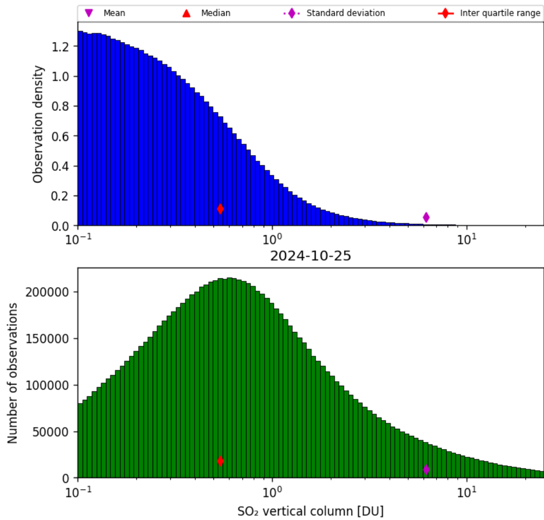
Figure 53: Histogram of “SO 2 vertical column” for 2024-10-24 to 2024-10-26
