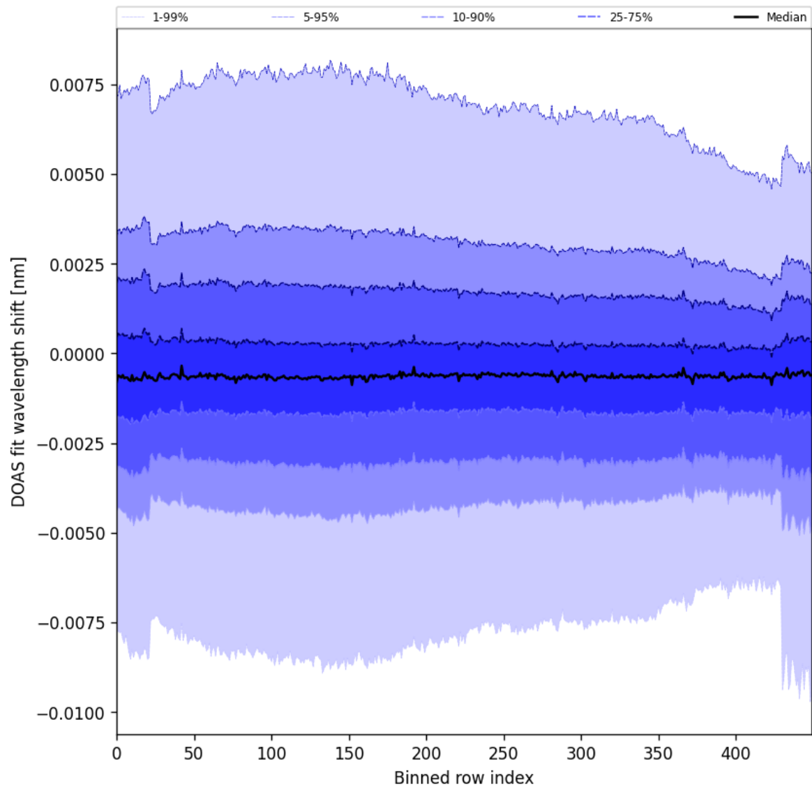
Figure 91: Along track statistics of “DOAS fit wavelength shift” for 2024-10-24 to 2024-10-26
