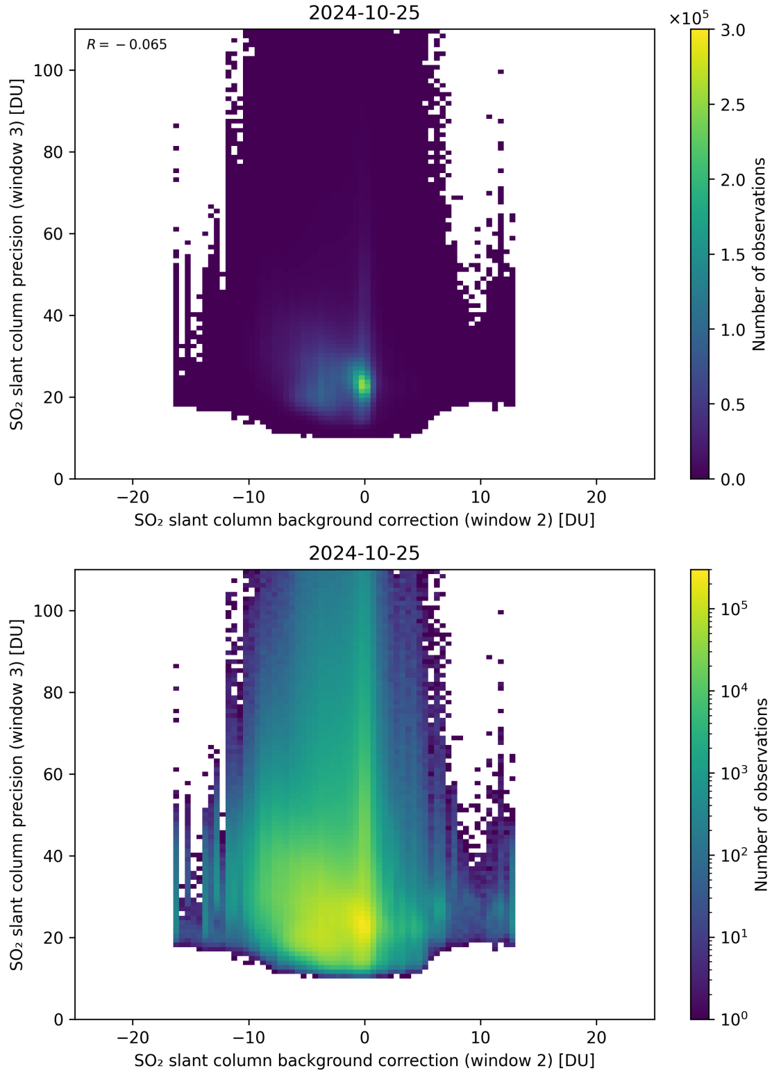
Figure 118: Scatter density plot of “SO 2 slant column background correction (window 2)” against “SO 2 slant column precision (window 3)” for 2024-10-24 to 2024-10-26.
