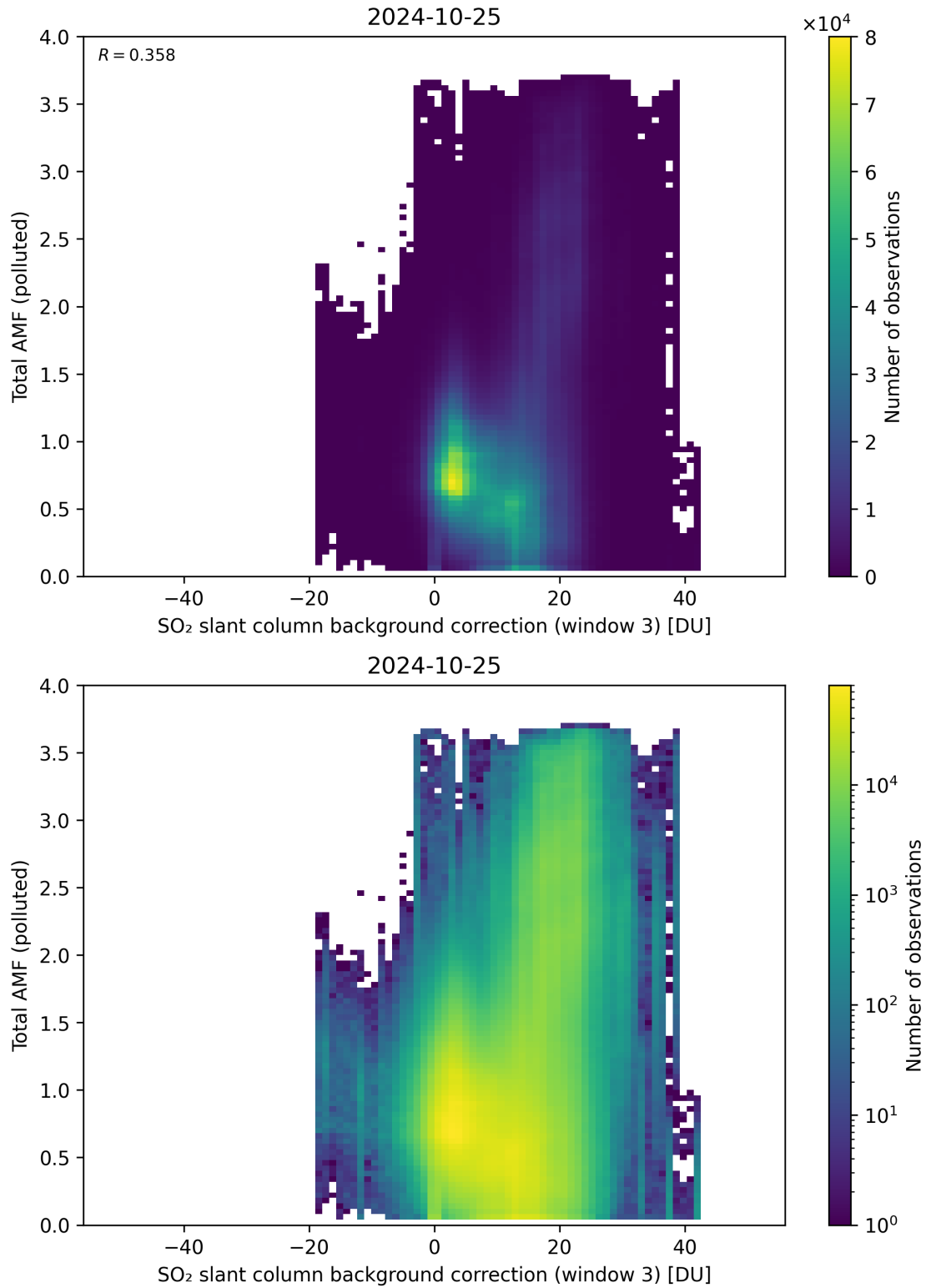
Figure 125: Scatter density plot of “SO 2 slant column background correction (window 3)” against “Total AMF (polluted)” for 2024-10-24 to 2024-10-26.
