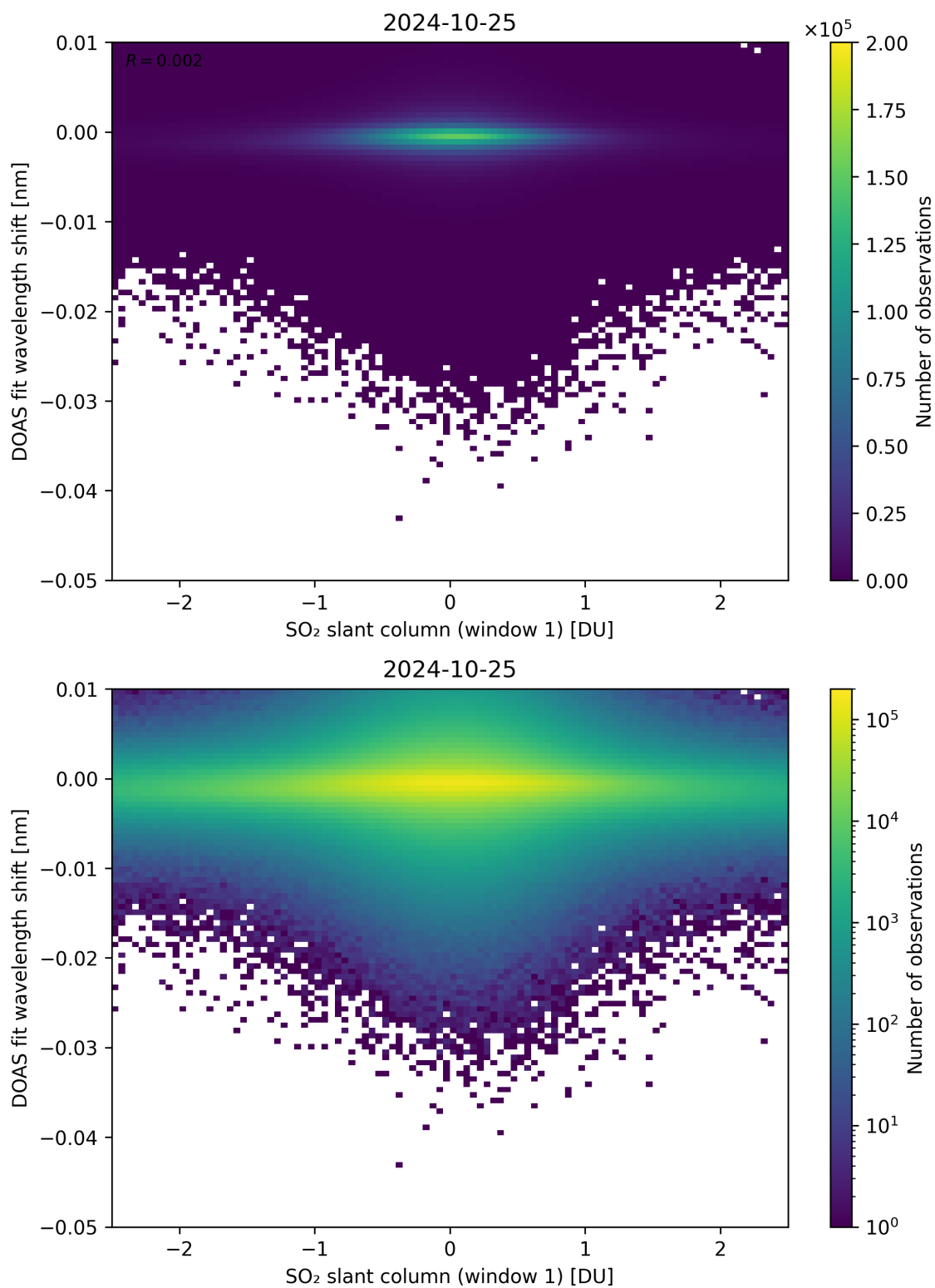
Figure 215: Scatter density plot of “SO 2 slant column (window 1)” against “DOAS fit wavelength shift” for 2024-10-24 to 2024-10-26.
