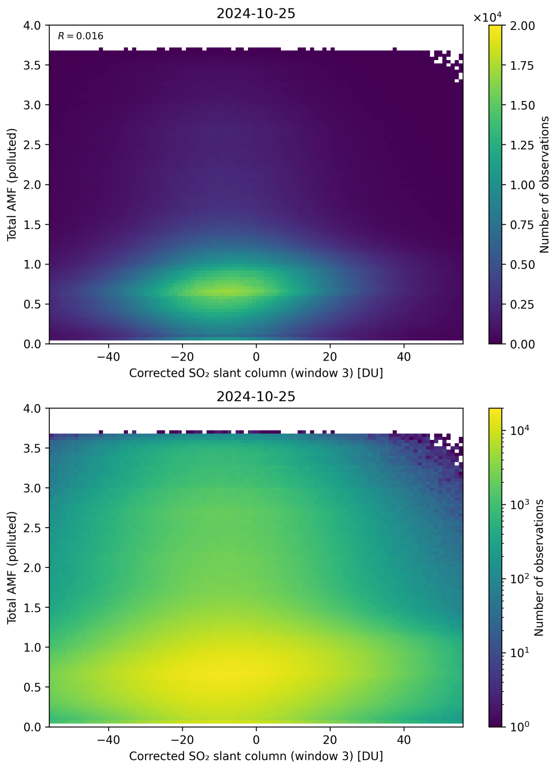
Figure 210: Scatter density plot of “Corrected SO 2 slant column (window 3)” against “Total AMF (polluted)” for 2024-10-24 to 2024-10-26.
