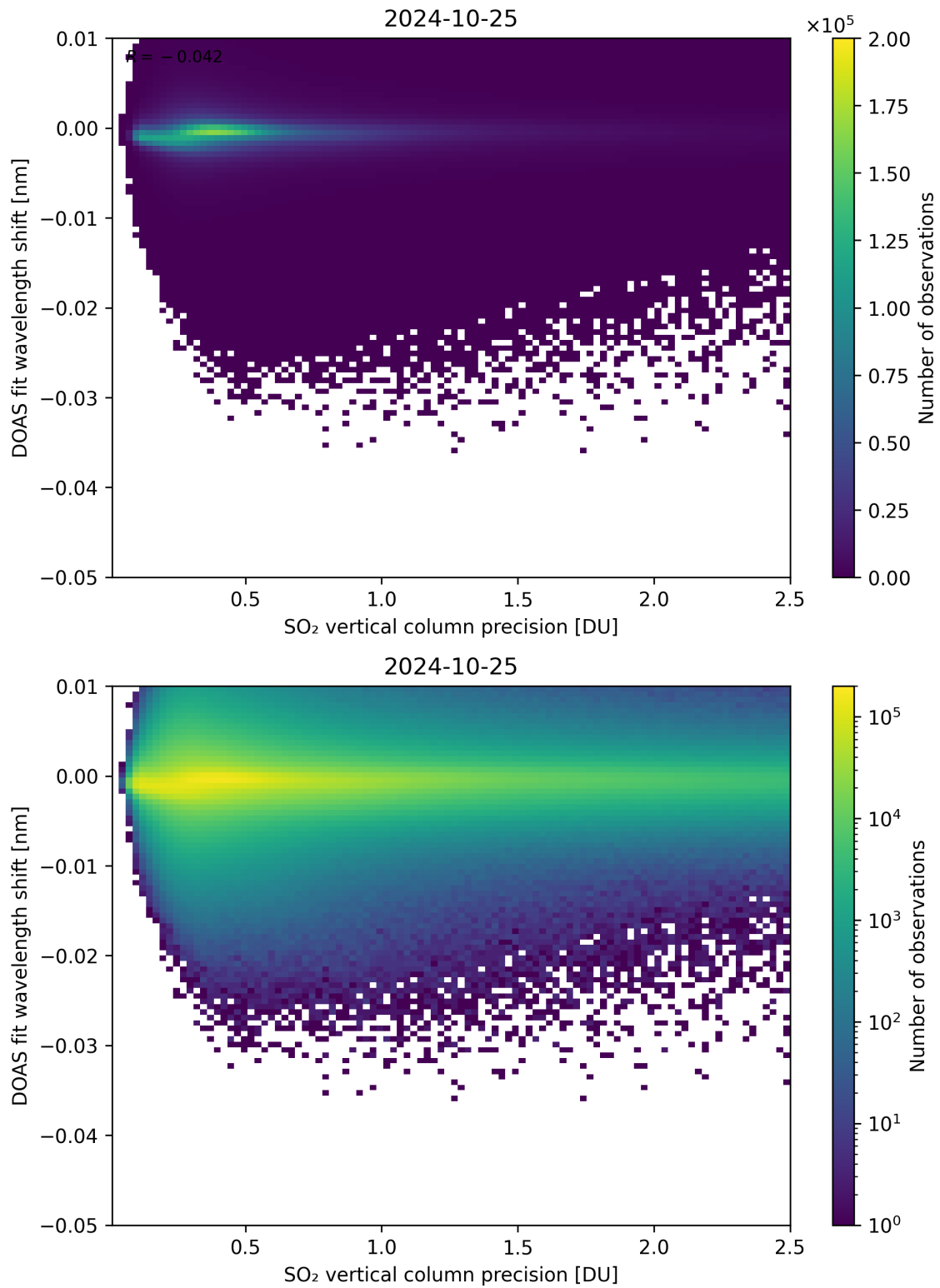
Figure 282: Scatter density plot of “SO 2 vertical column precision” against “DOAS fit wavelength shift” for 2024-10-24 to 2024-10-26.
