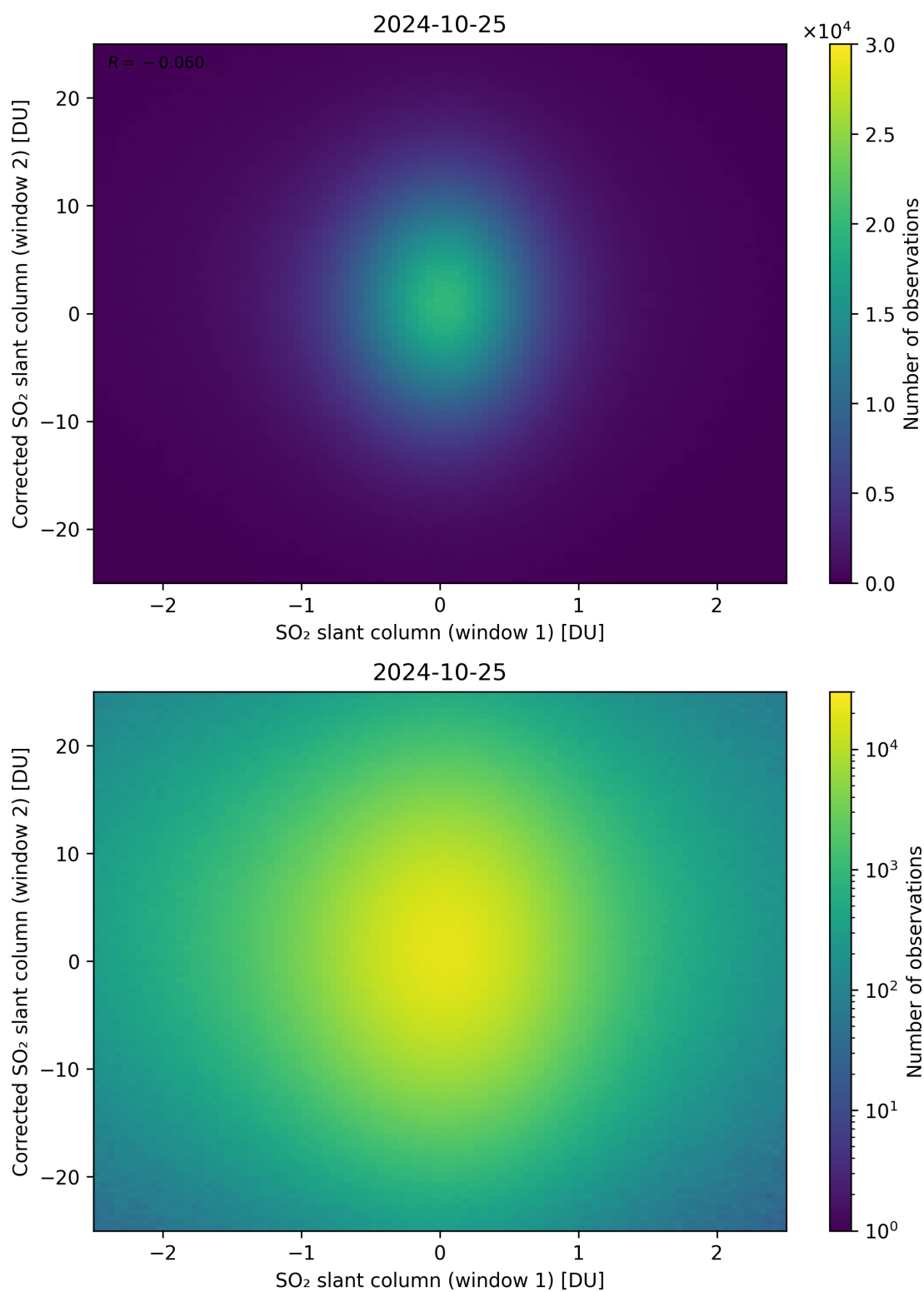
Figure 233: Scatter density plot of “SO 2 slant column (window 1)” against “Corrected SO 2 slant column (window 2)” for 2024-10-24 to 2024-10-26.
