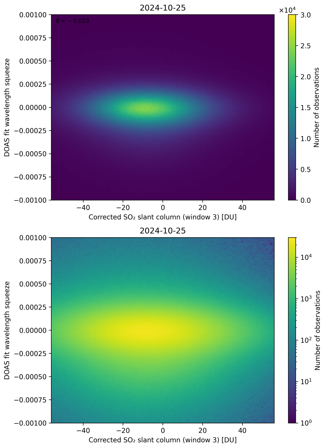
Figure 207: Scatter density plot of “Corrected SO 2 slant column (window 3)” against “DOAS fit wavelength squeeze” for 2024-10-24 to 2024-10-26.
