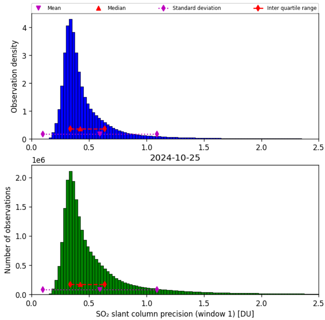
Figure 57: Histogram of “SO 2 slant column precision (window 1)” for 2024-10-24 to 2024-10-26
