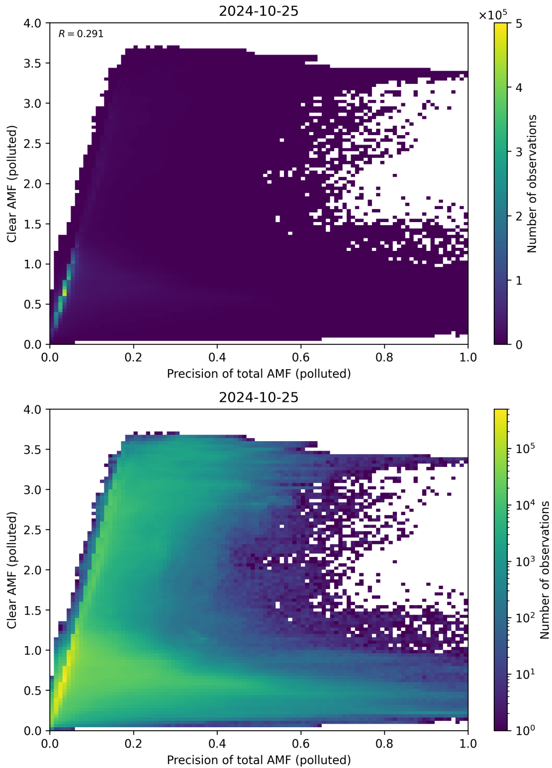
Figure 270: Scatter density plot of “Precision of total AMF (polluted)” against “Clear AMF (polluted)” for 2024-10-24 to 2024-10-26.
