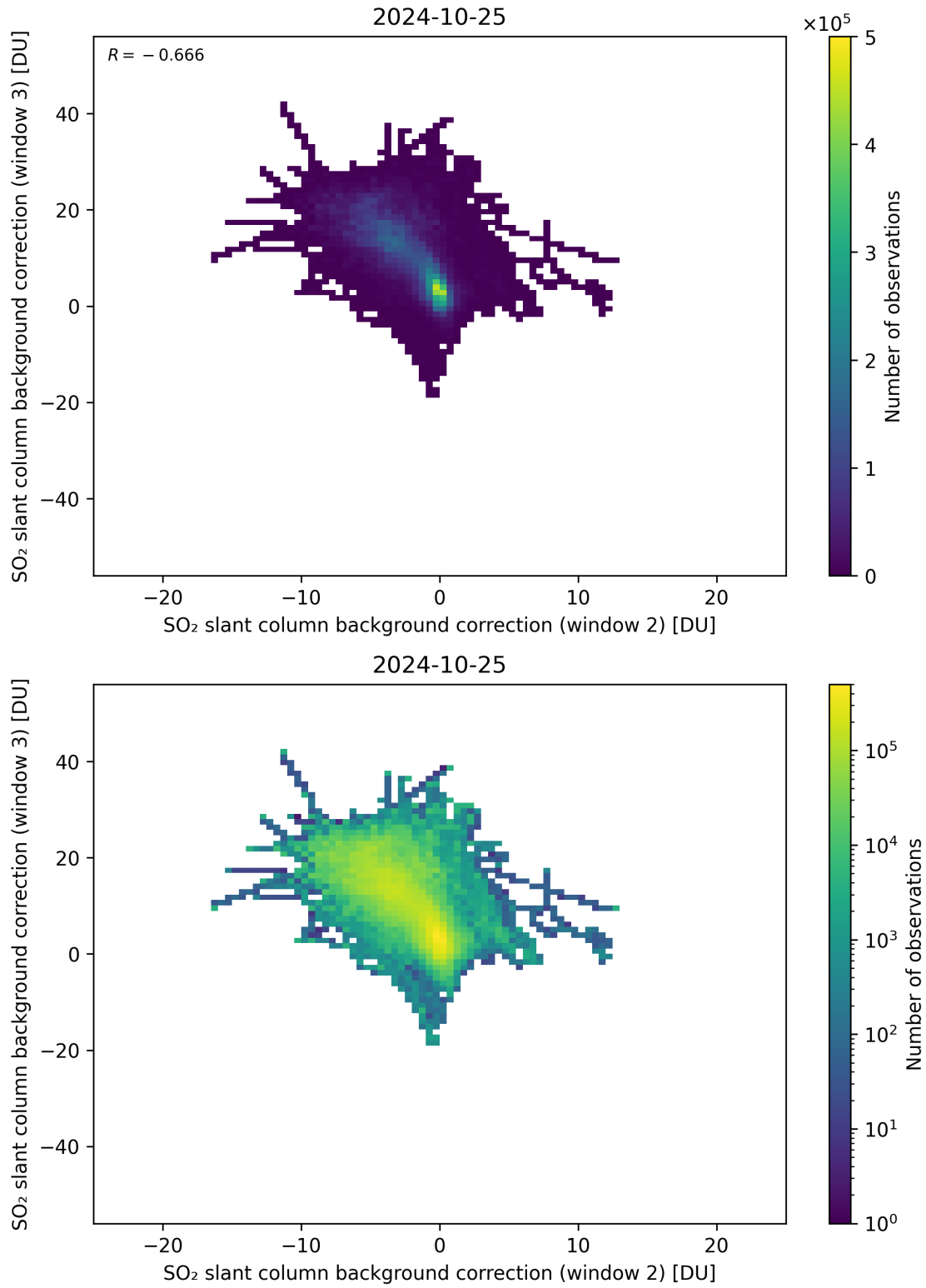
Figure 111: Scatter density plot of “SO 2 slant column background correction (window 2)” against “SO 2 slant column background correction (window 3)” for 2024-10-24 to 2024-10-26.
