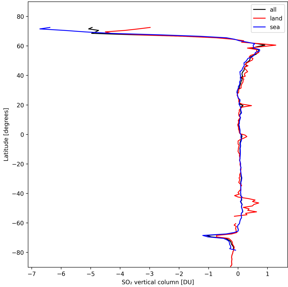
Figure 30: Zonal average of “SO 2 vertical column” for 2024-10-24 to 2024-10-26.
