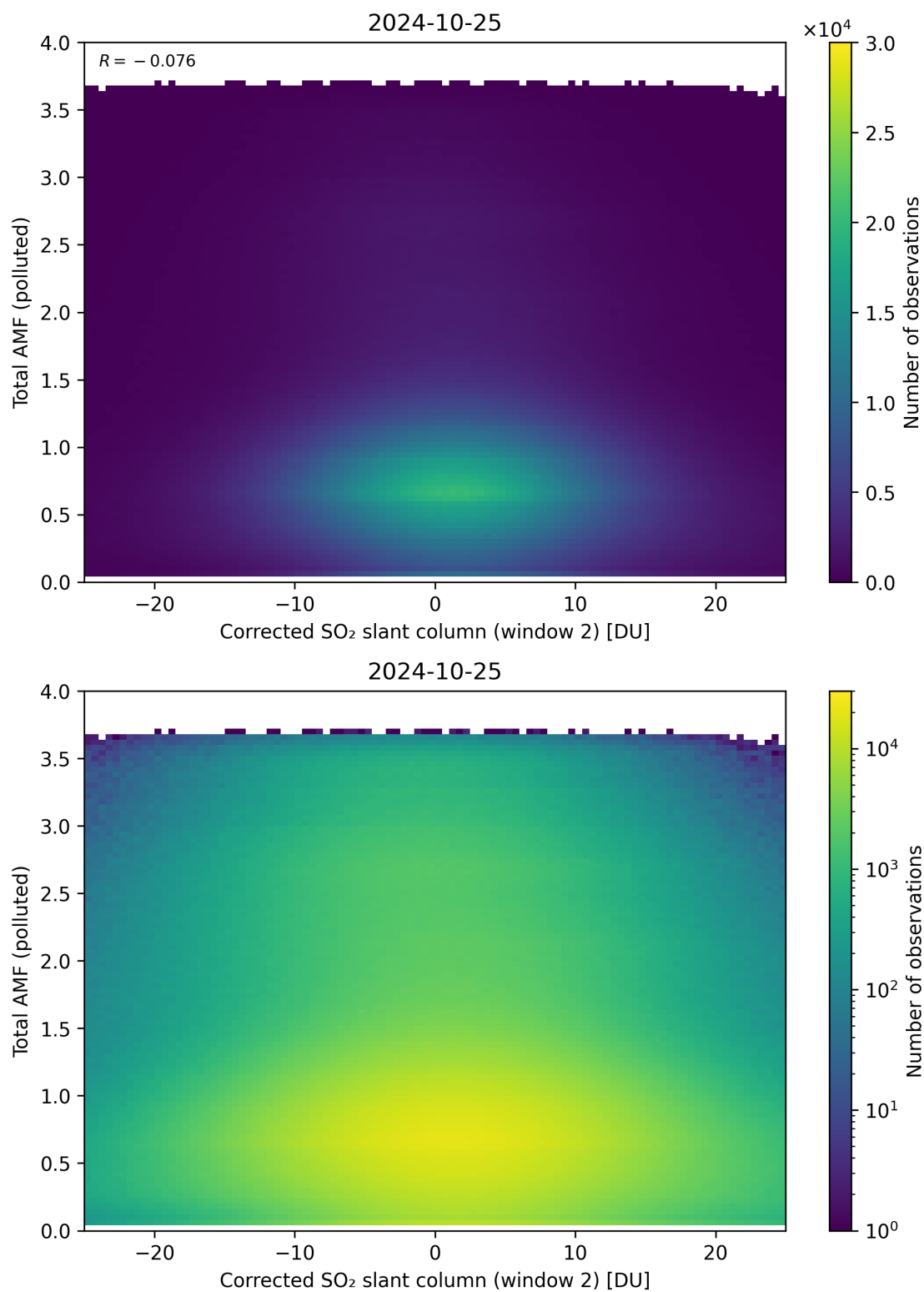
Figure 203: Scatter density plot of “Corrected SO 2 slant column (window 2)” against “Total AMF (polluted)” for 2024-10-24 to 2024-10-26.
