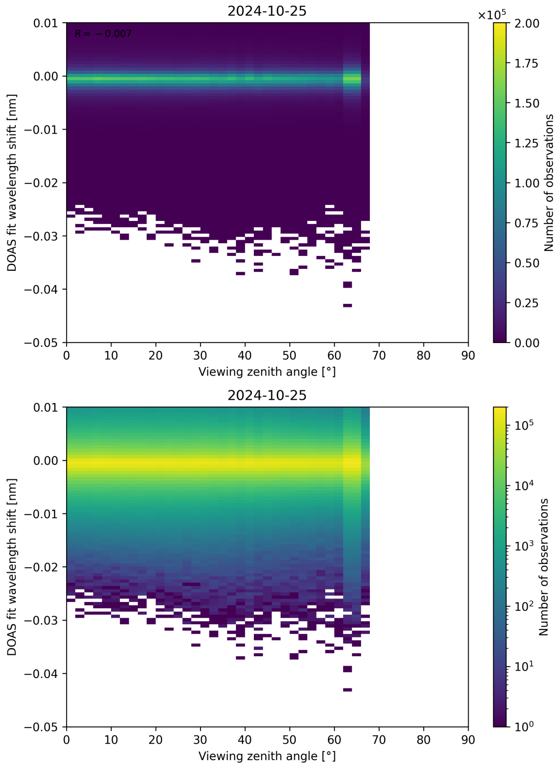
Figure 311: Scatter density plot of “Viewing zenith angle” against “DOAS fit wavelength shift” for 2024-10-24 to 2024-10-26.
