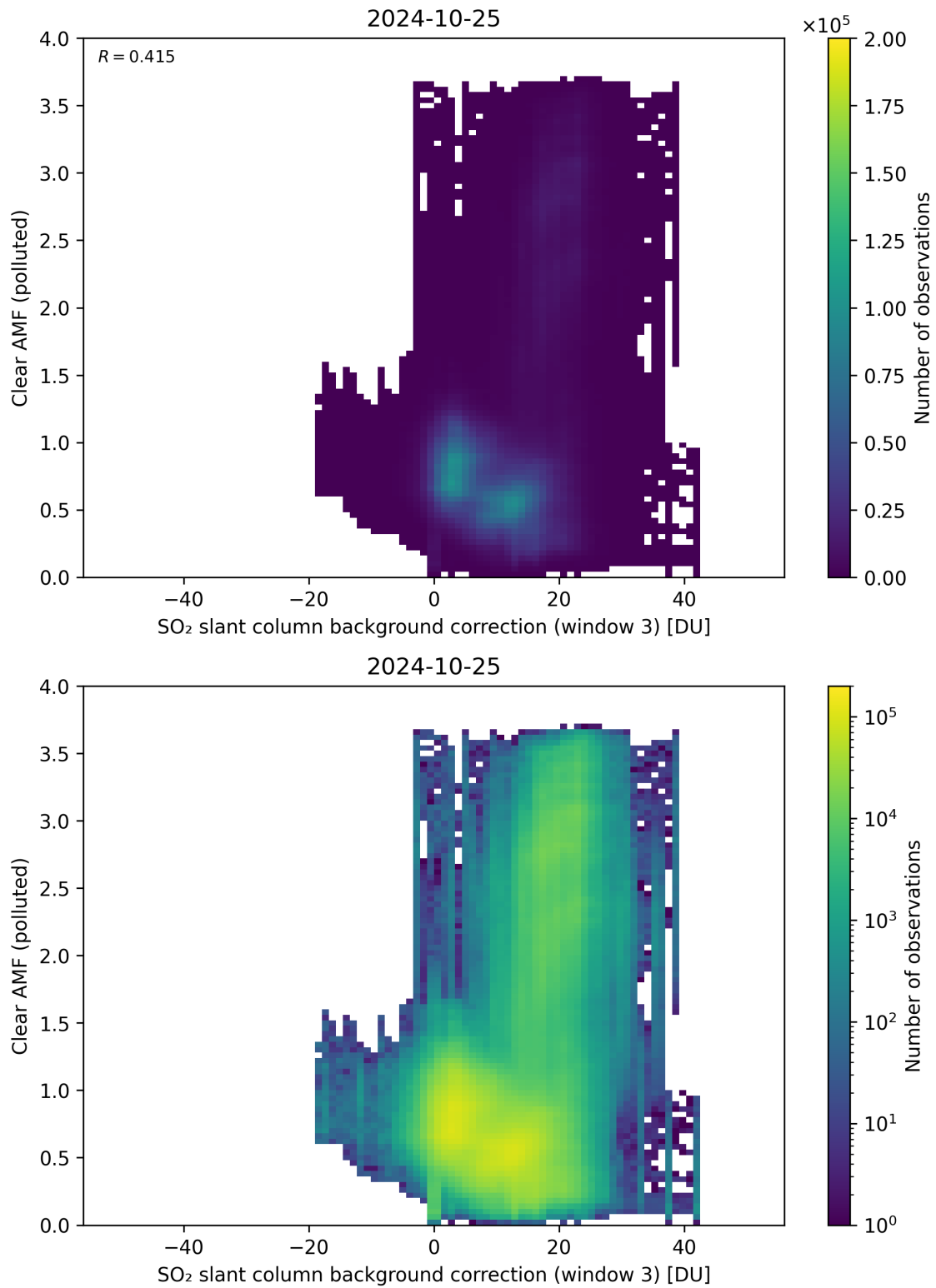
Figure 124: Scatter density plot of “SO 2 slant column background correction (window 3)” against “Clear AMF (polluted)” for 2024-10-24 to 2024-10-26.
