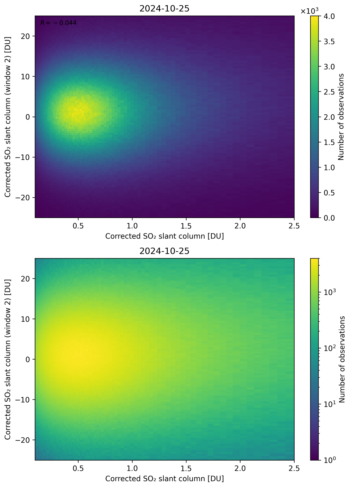
Figure 185: Scatter density plot of “Corrected SO 2 slant column” against “Corrected SO 2 slant column (window 2)” for 2024-10-24 to 2024-10-26.
