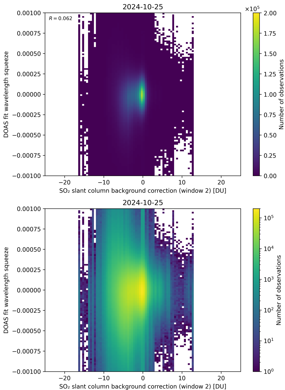
Figure 113: Scatter density plot of “SO 2 slant column background correction (window 2)” against “DOAS fit wavelength squeeze” for 2024-10-24 to 2024-10-26.
