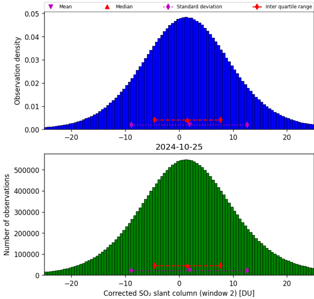
Figure 62: Histogram of “Corrected SO 2 slant column (window 2)” for 2024-10-24 to 2024-10-26
