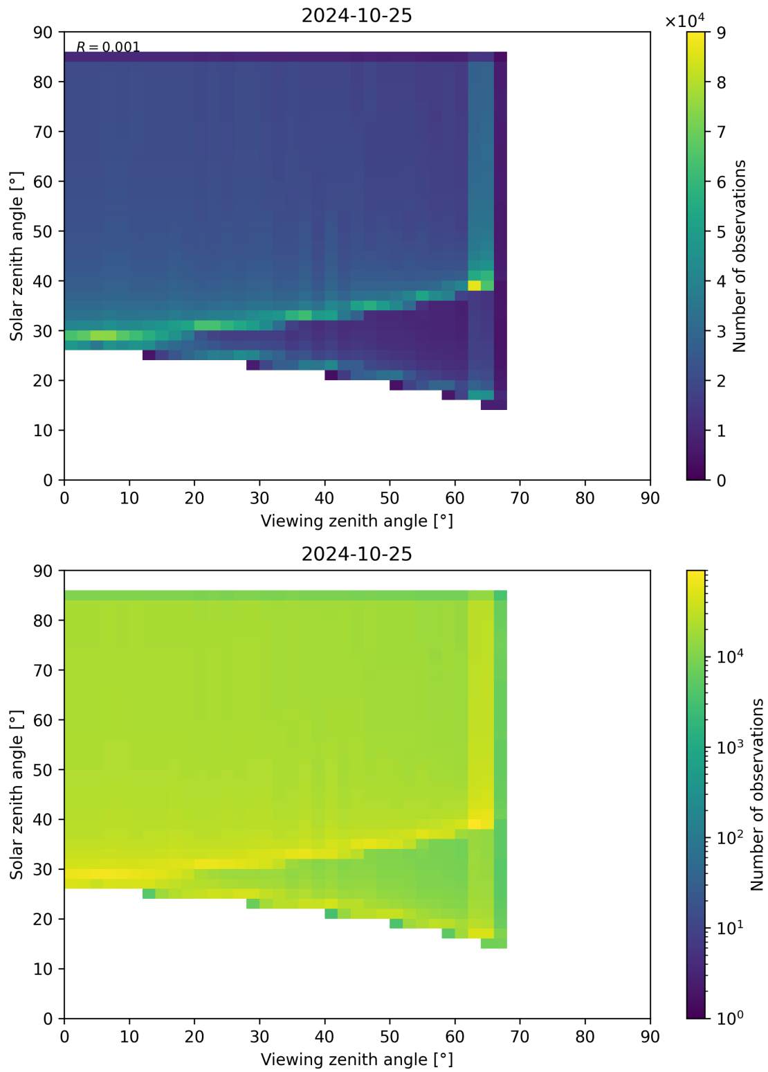
Figure 315: Scatter density plot of “Viewing zenith angle” against “Solar zenith angle” for 2024-10-24 to 2024-10-26.
