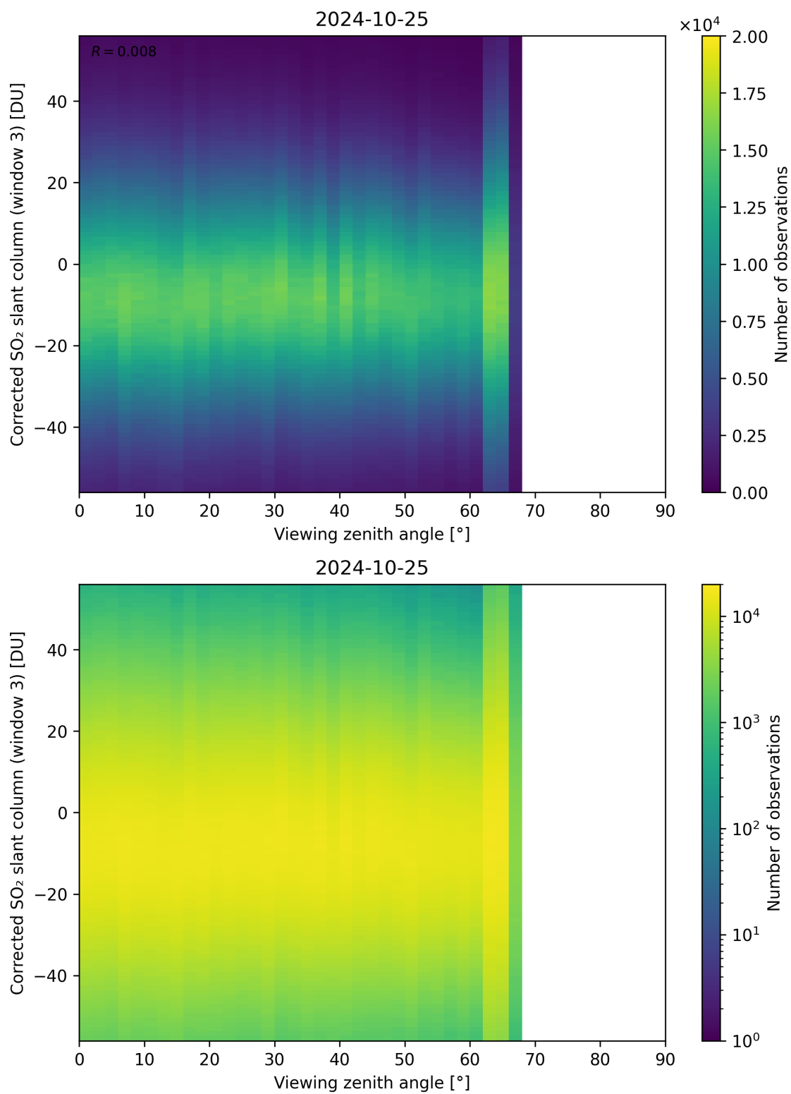
Figure 319: Scatter density plot of “Viewing zenith angle” against “Corrected SO 2 slant column (window 3)” for 2024-10-24 to 2024-10-26.
