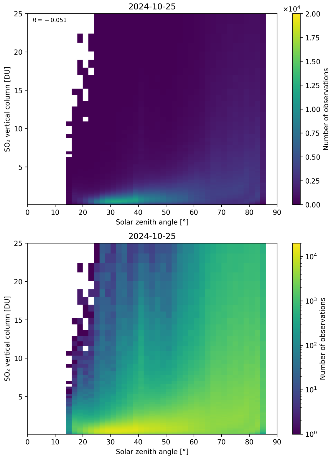
Figure 176: Scatter density plot of “Solar zenith angle” against “SO 2 vertical column” for 2024-10-24 to 2024-10-26.
