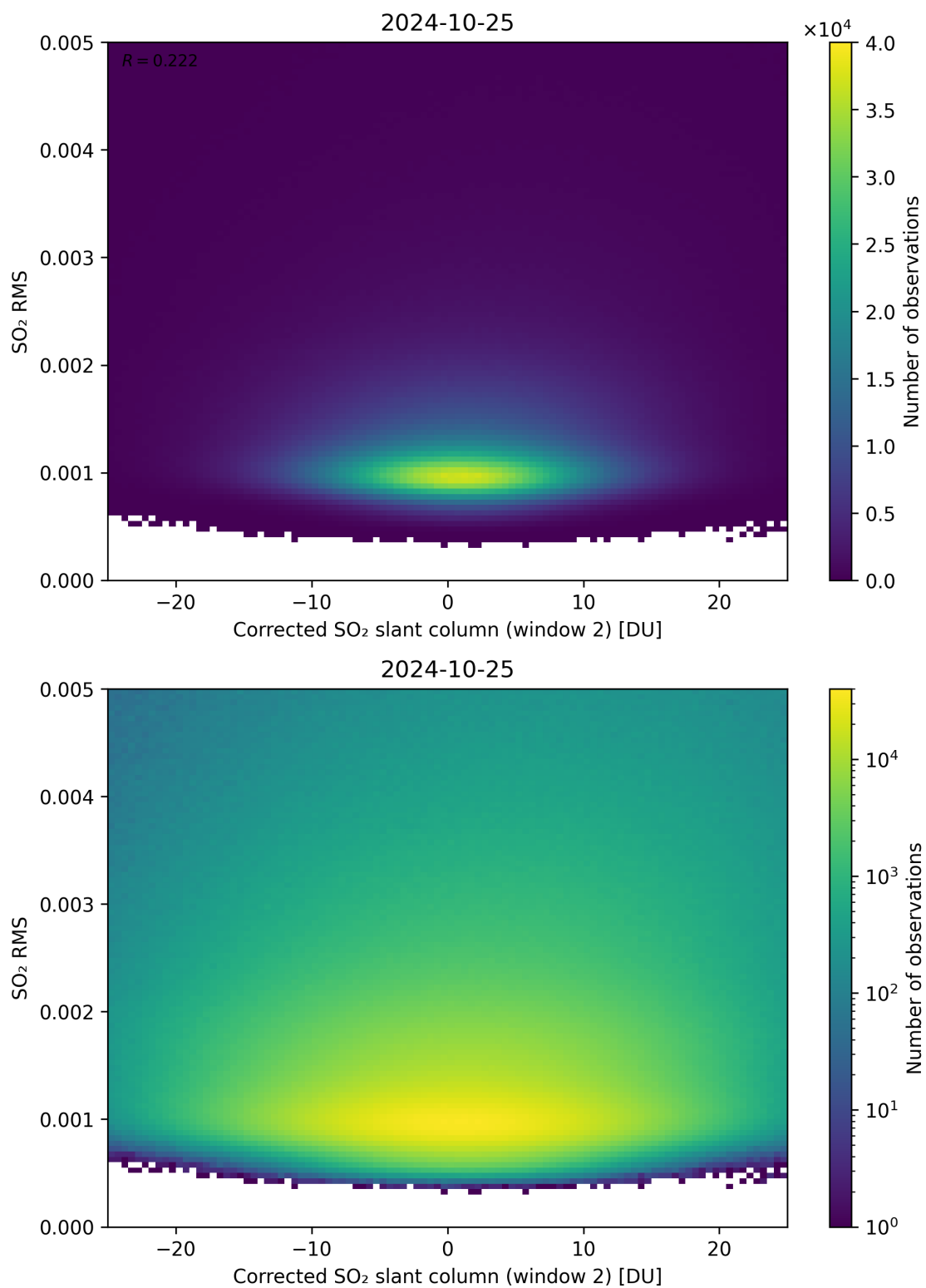
Figure 198: Scatter density plot of “Corrected SO 2 slant column (window 2)” against “SO 2 RMS” for 2024-10-24 to 2024-10-26.
