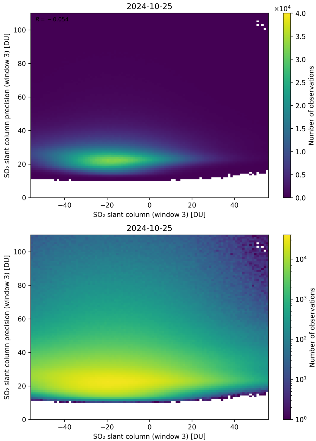
Figure 267: Scatter density plot of “SO 2 slant column (window 3)” against “SO 2 slant column precision (window 3)” for 2024-10-24 to 2024-10-26.
