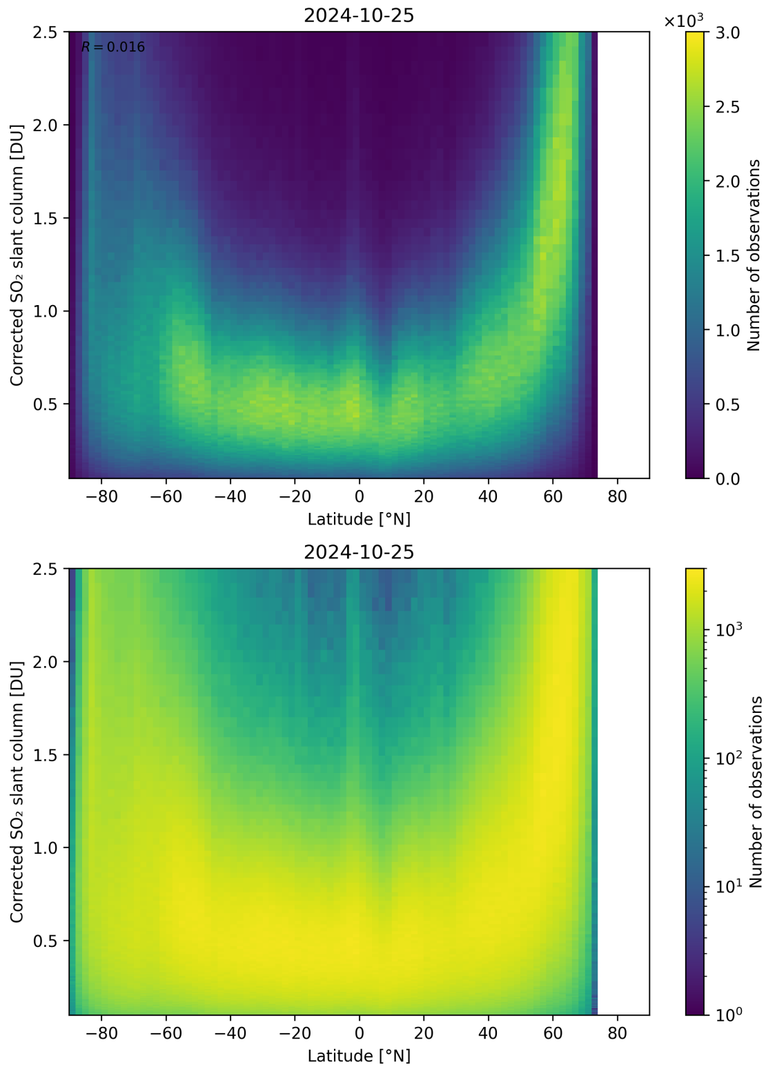
Figure 146: Scatter density plot of “Latitude” against “Corrected SO 2 slant column” for 2024-10-24 to 2024-10-26.
