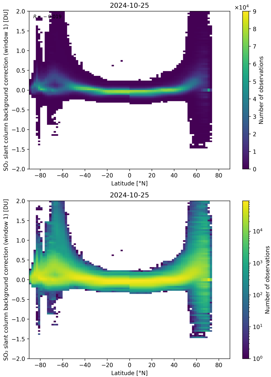
Figure 139: Scatter density plot of “Latitude” against “SO 2 slant column background correction (window 1)” for 2024-10-24 to 2024-10-26.
