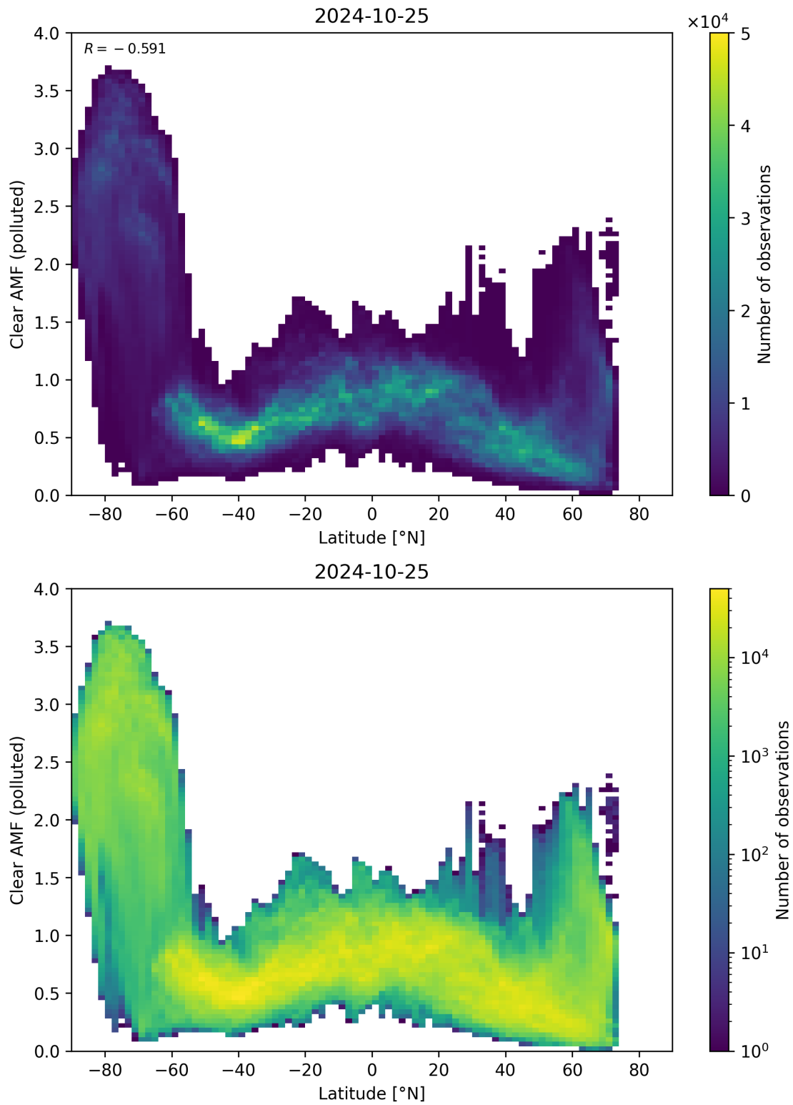
Figure 145: Scatter density plot of “Latitude” against “Clear AMF (polluted)” for 2024-10-24 to 2024-10-26.
