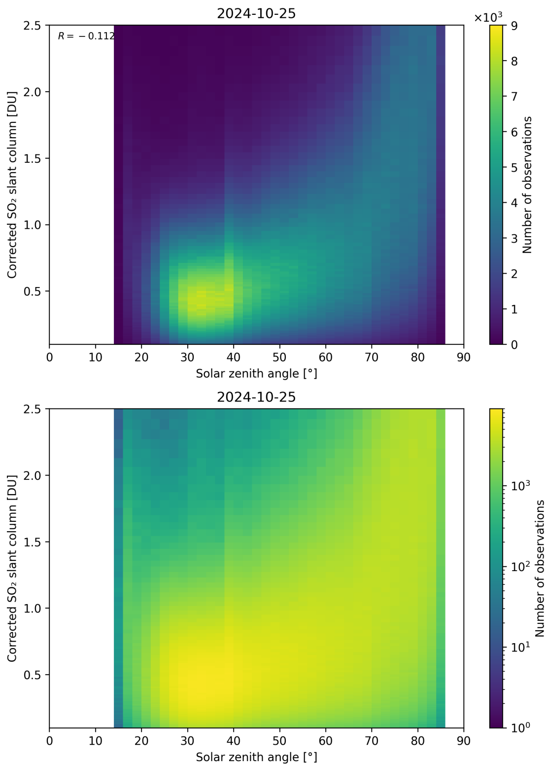
Figure 166: Scatter density plot of “Solar zenith angle” against “Corrected SO 2 slant column” for 2024-10-24 to 2024-10-26.
