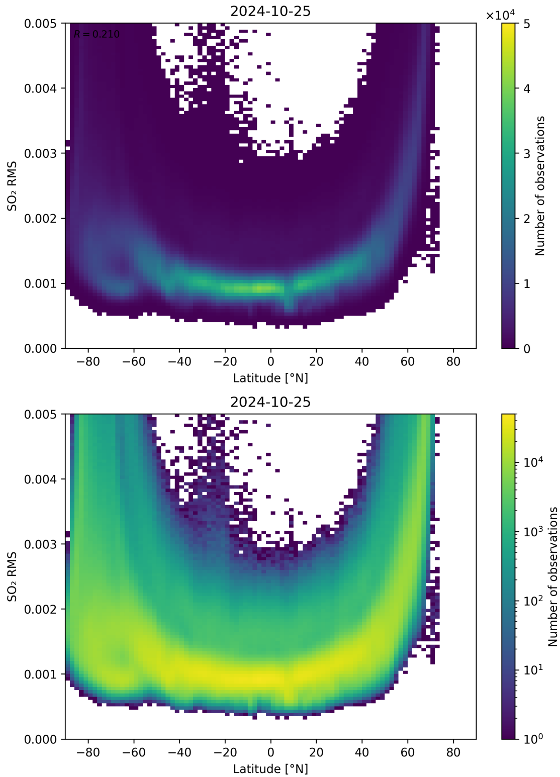
Figure 144: Scatter density plot of “Latitude” against “SO 2 RMS” for 2024-10-24 to 2024-10-26.
