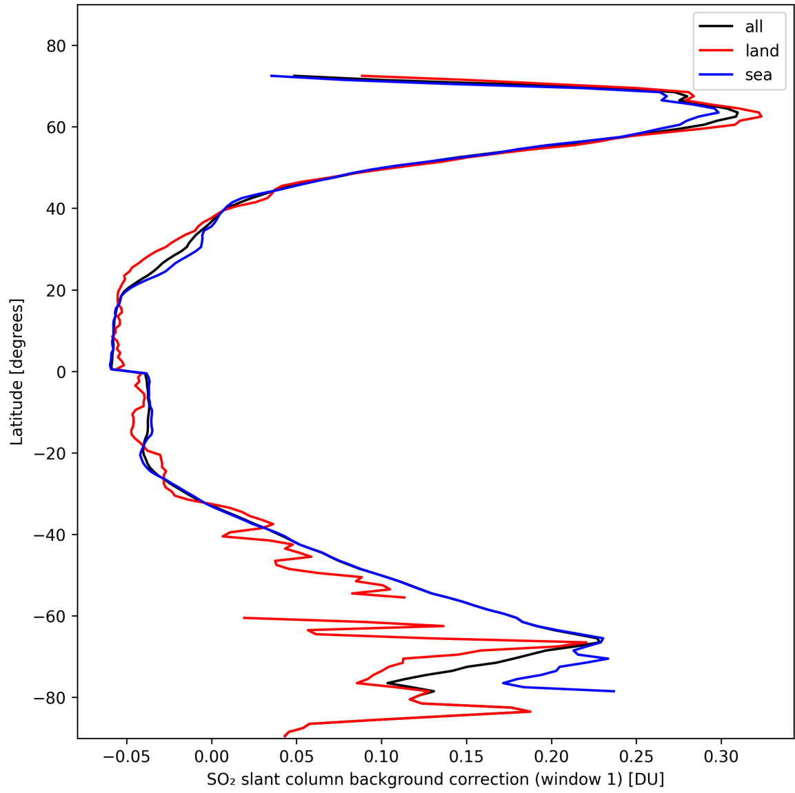
Figure 36: Zonal average of “SO 2 slant column background correction (window 1)” for 2024-10-24 to 2024-10-26.
