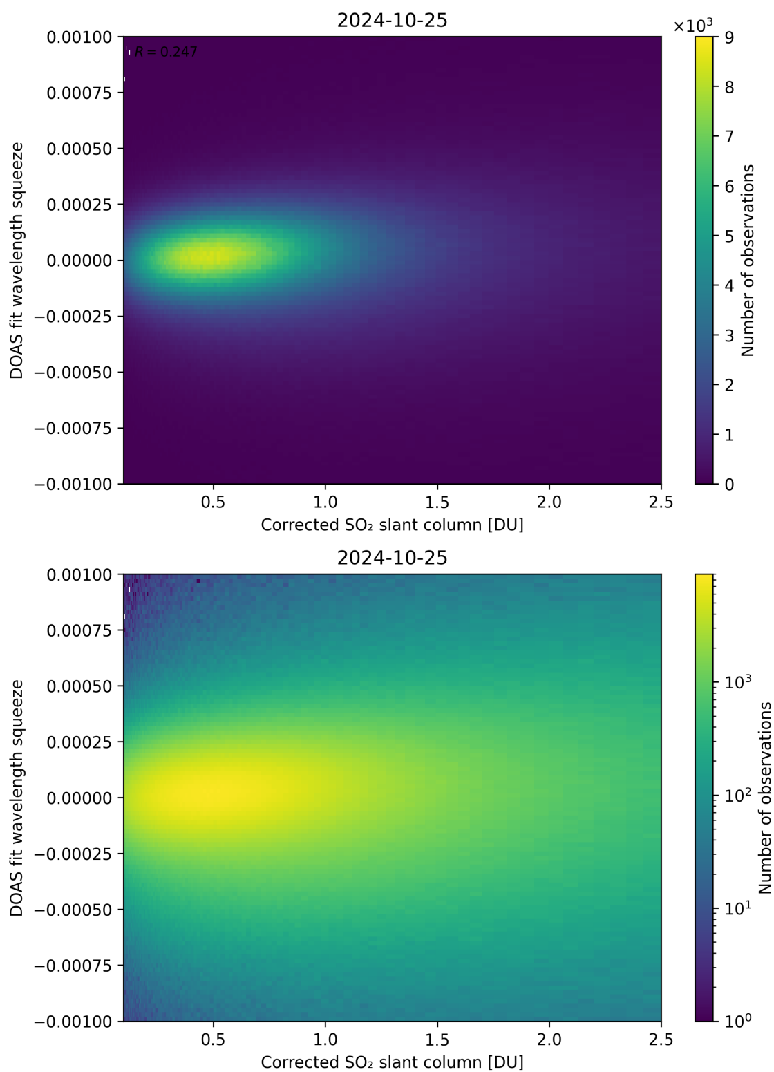
Figure 182: Scatter density plot of “Corrected SO 2 slant column” against “DOAS fit wavelength squeeze” for 2024-10-24 to 2024-10-26.
