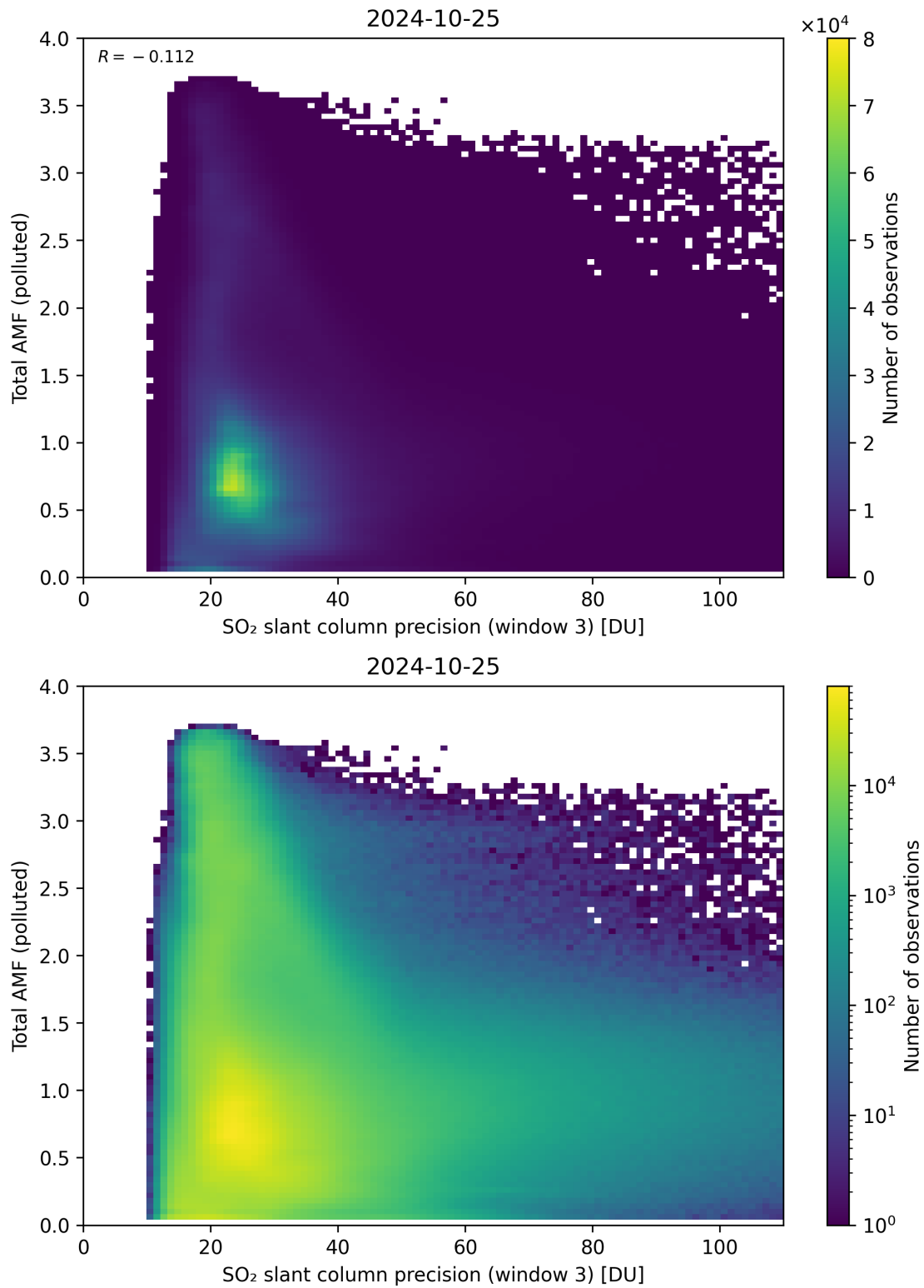
Figure 263: Scatter density plot of “SO 2 slant column precision (window 3)” against “Total AMF (polluted)” for 2024-10-24 to 2024-10-26.
