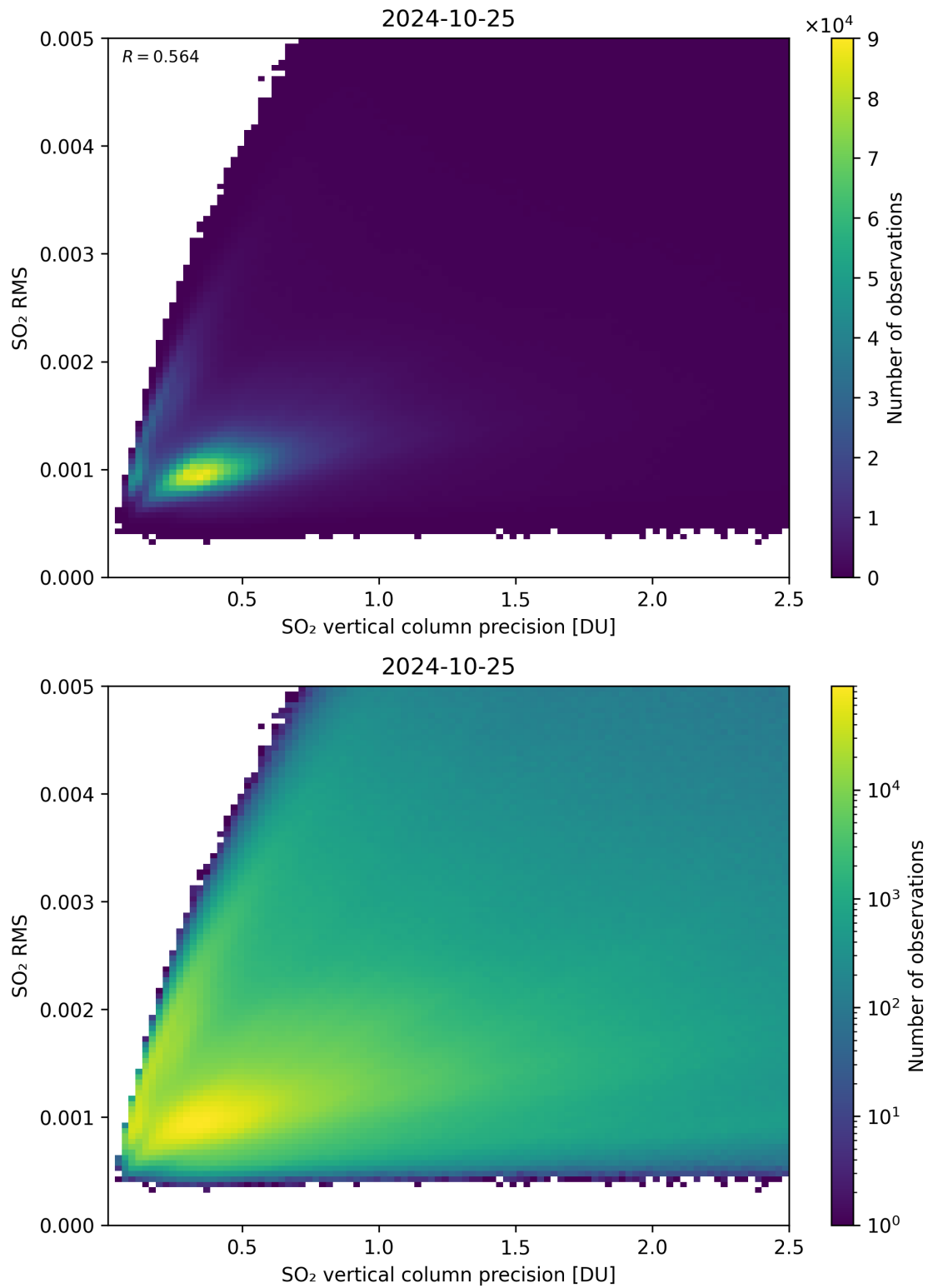
Figure 284: Scatter density plot of “SO 2 vertical column precision” against “SO 2 RMS” for 2024-10-24 to 2024-10-26.
