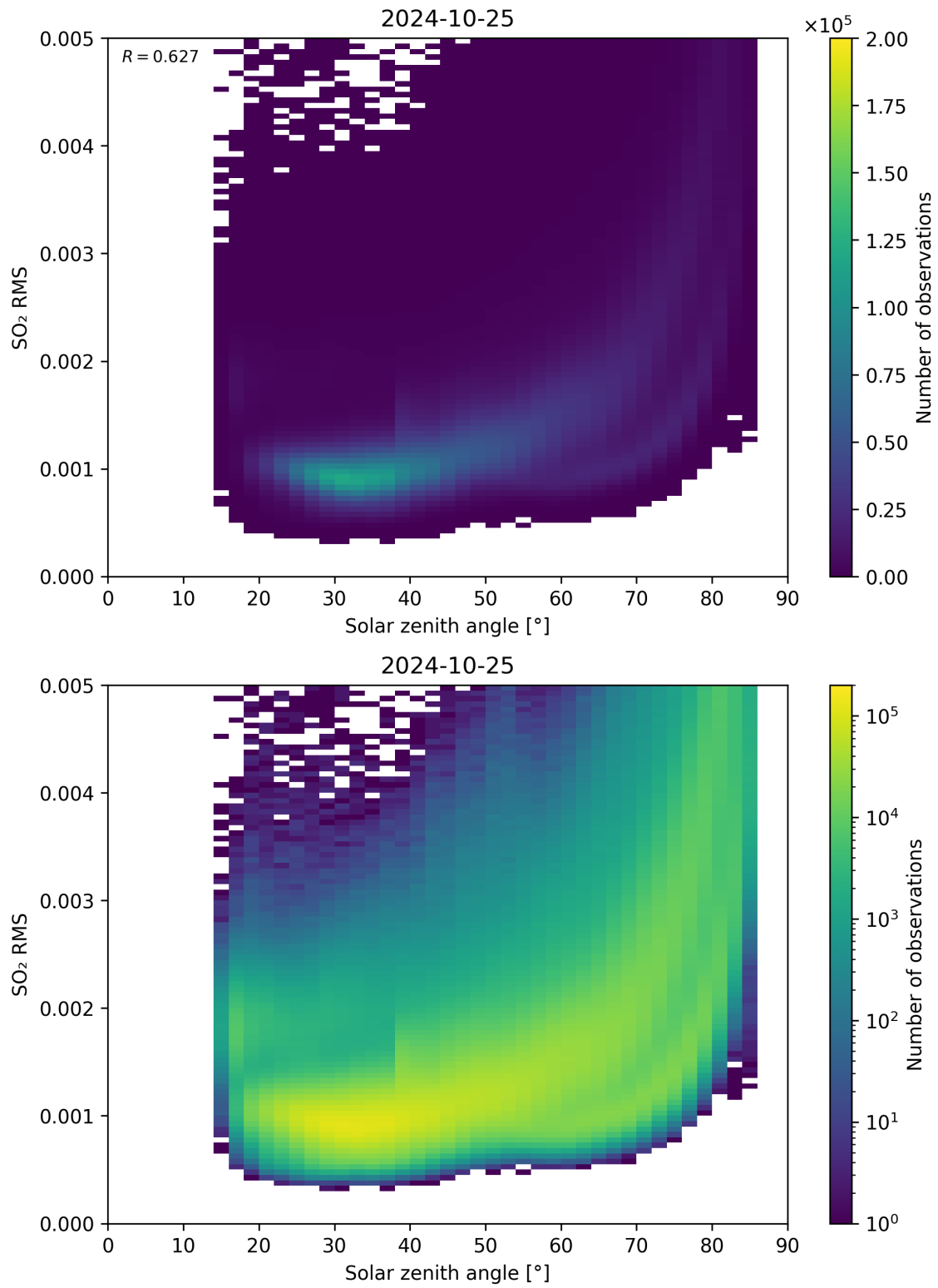
Figure 163: Scatter density plot of “Solar zenith angle” against “SO 2 RMS” for 2024-10-24 to 2024-10-26.
