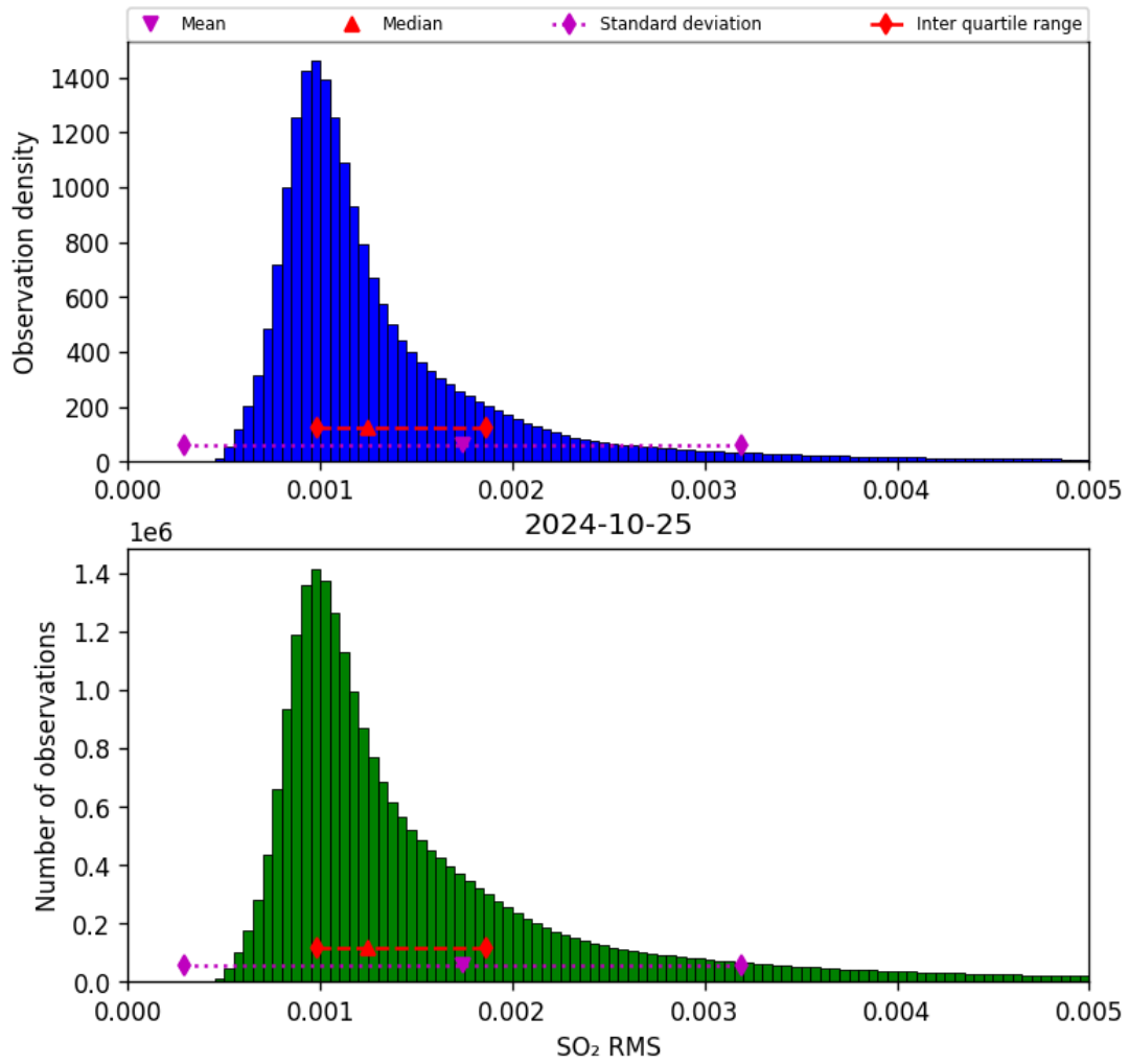
Figure 70: Histogram of “SO 2 RMS” for 2024-10-24 to 2024-10-26
