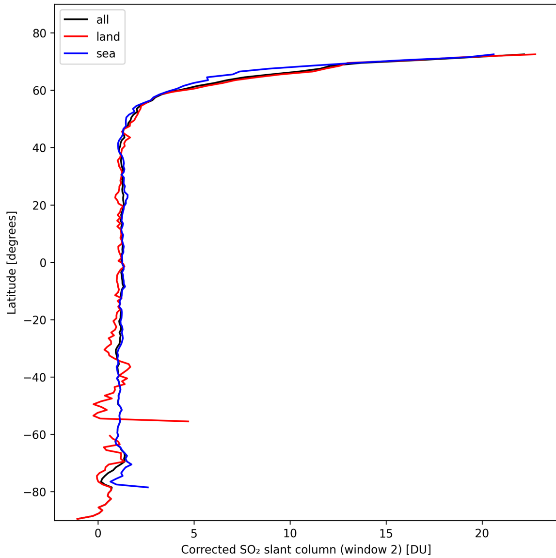
Figure 39: Zonal average of “Corrected SO 2 slant column (window 2)” for 2024-10-24 to 2024-10-26.
