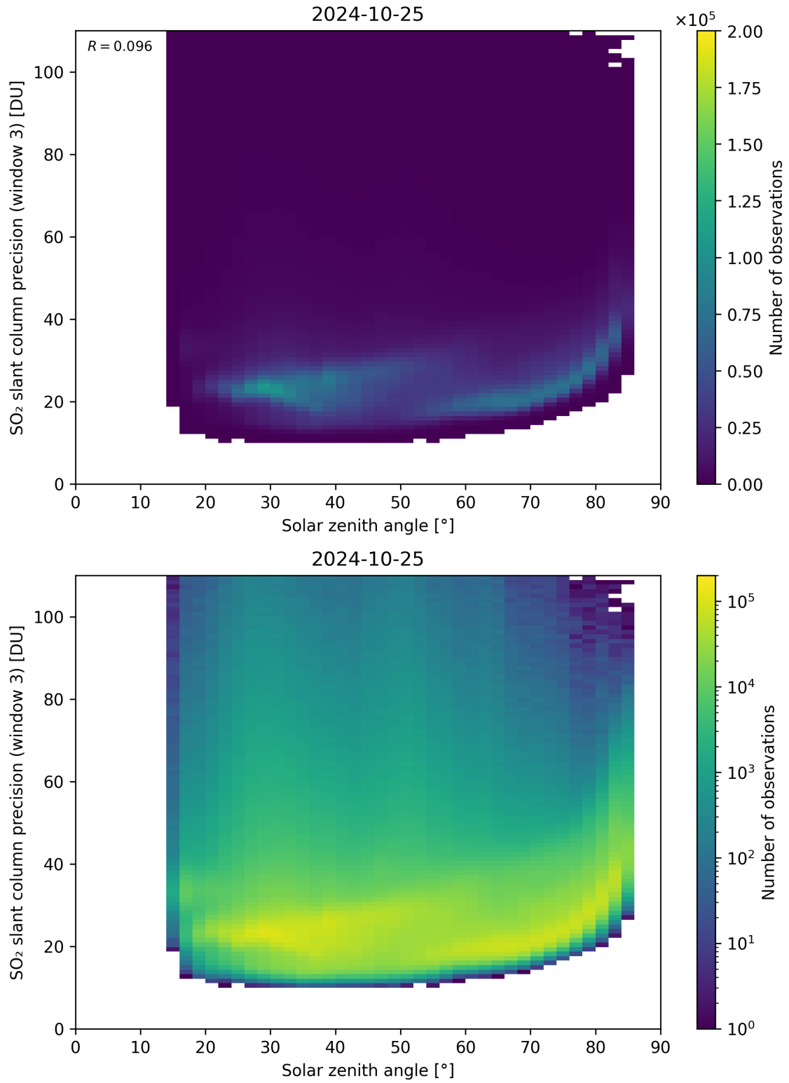
Figure 173: Scatter density plot of “Solar zenith angle” against “SO 2 slant column precision (window 3)” for 2024-10-24 to 2024-10-26.
