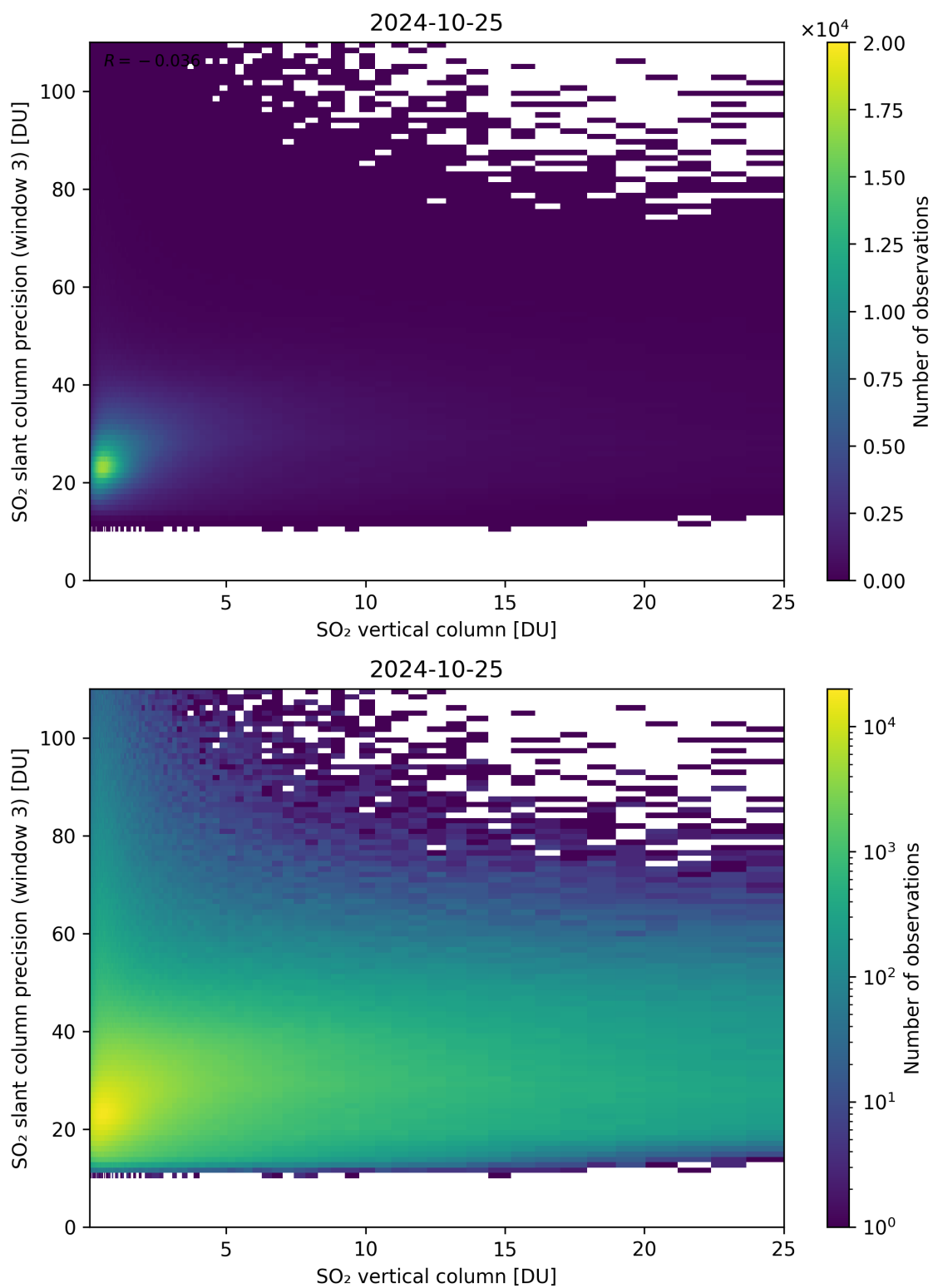
Figure 304: Scatter density plot of “SO 2 vertical column” against “SO 2 slant column precision (window 3)” for 2024-10-24 to 2024-10-26.
