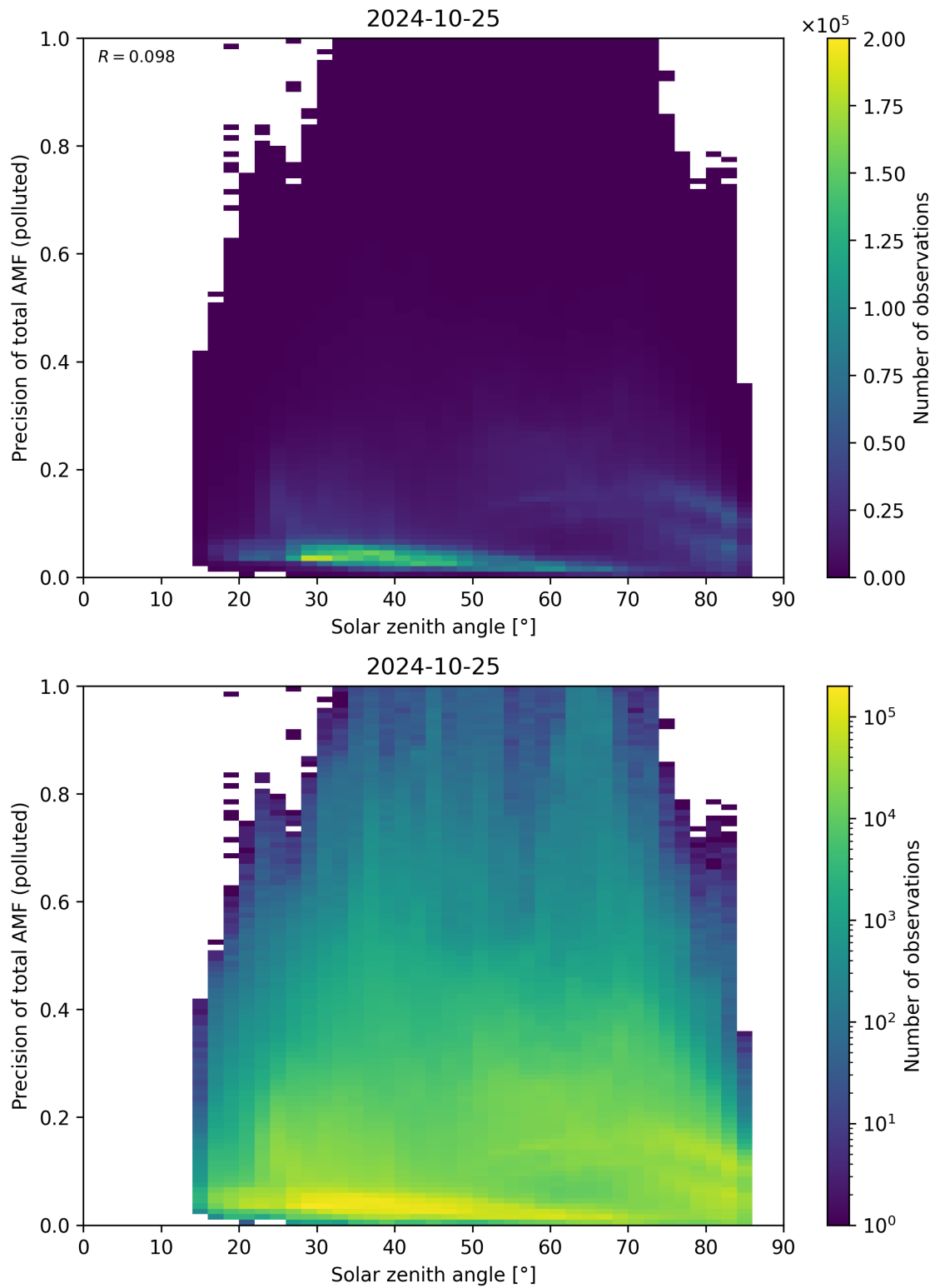
Figure 175: Scatter density plot of “Solar zenith angle” against “Precision of total AMF (polluted)” for 2024-10-24 to 2024-10-26.
