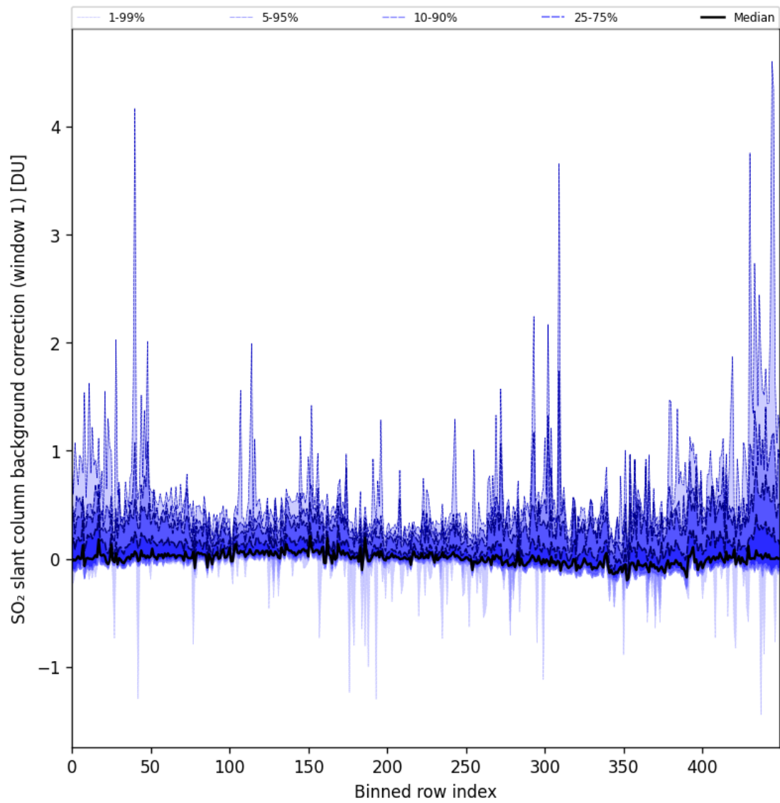
Figure 82: Along track statistics of “SO 2 slant column background correction (window 1)” for 2024-10-24 to 2024-10-26
