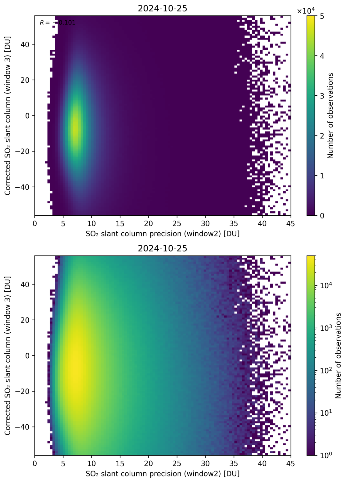
Figure 248: Scatter density plot of “SO 2 slant column precision (window2)” against “Corrected SO 2 slant column (window 3)” for 2024-10-24 to 2024-10-26.
