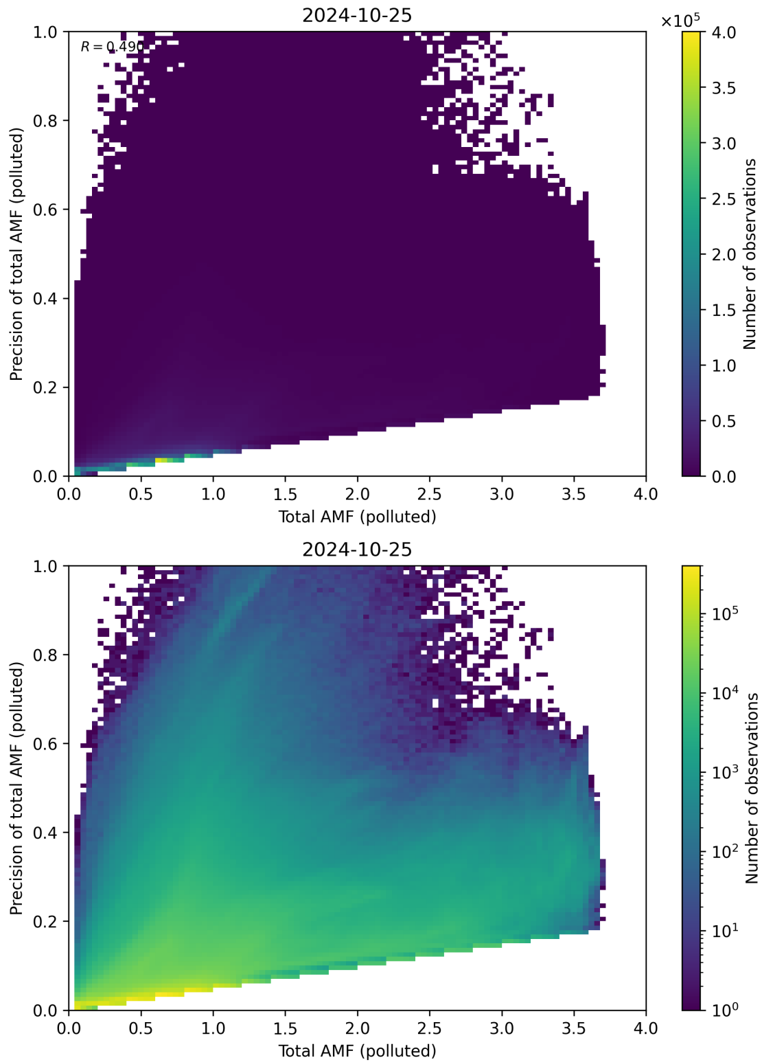
Figure 272: Scatter density plot of “Total AMF (polluted)” against “Precision of total AMF (polluted)” for 2024-10-24 to 2024-10-26.
