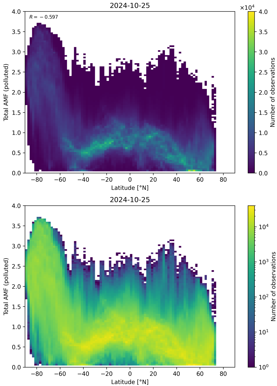
Figure 154: Scatter density plot of “Latitude” against “Total AMF (polluted)” for 2024-10-24 to 2024-10-26.
