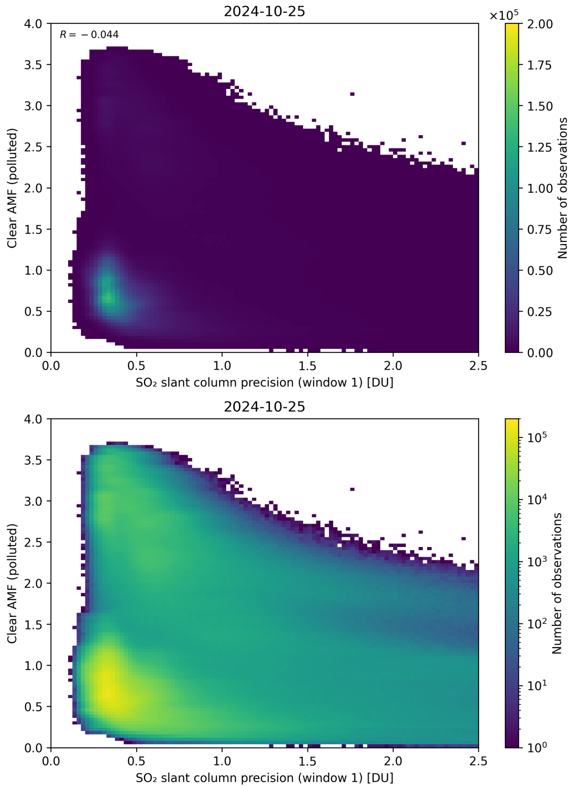
Figure 224: Scatter density plot of “SO 2 slant column precision (window 1)” against “Clear AMF (polluted)” for 2024-10-24 to 2024-10-26.
