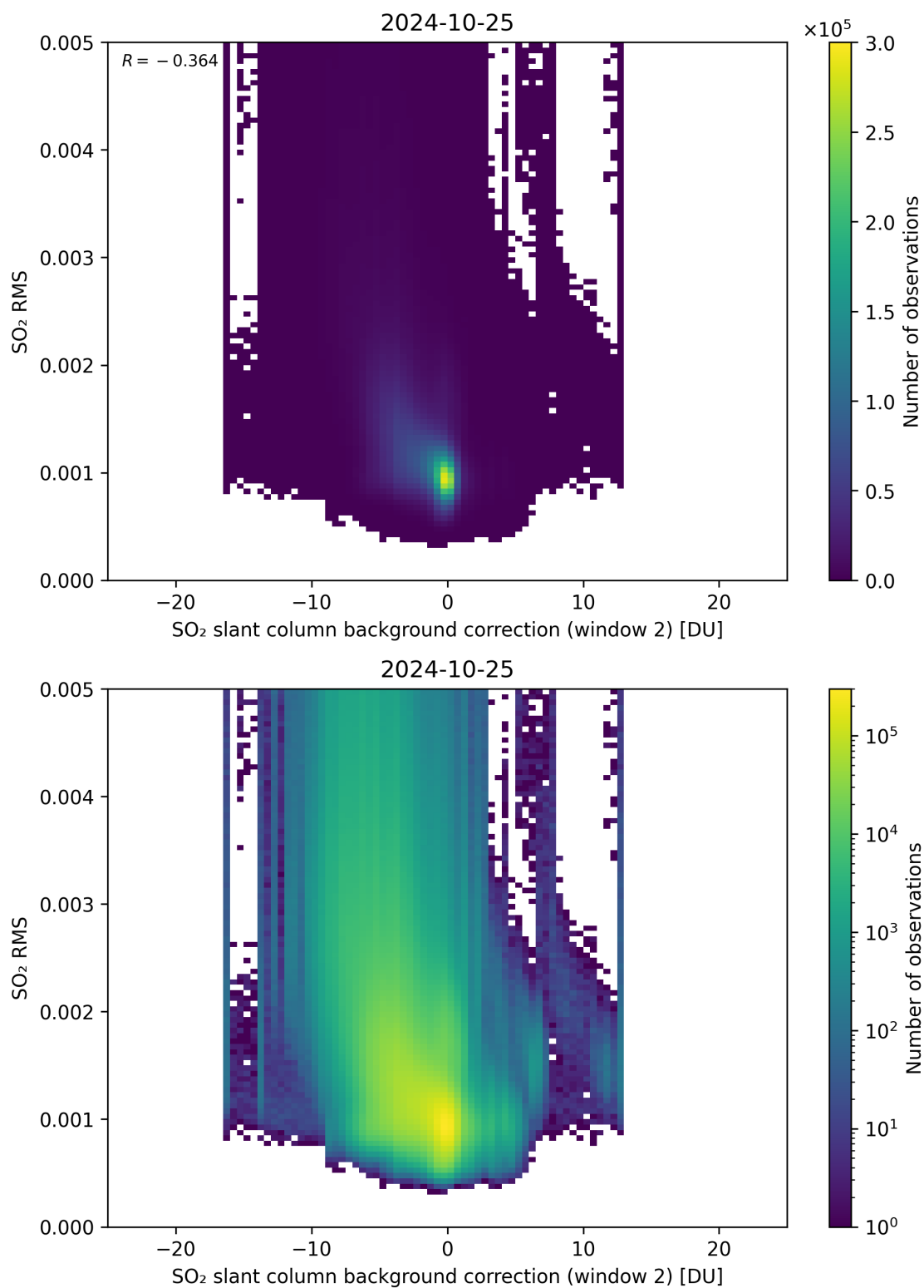
Figure 114: Scatter density plot of “SO 2 slant column background correction (window 2)” against “SO 2 RMS” for 2024-10-24 to 2024-10-26.
