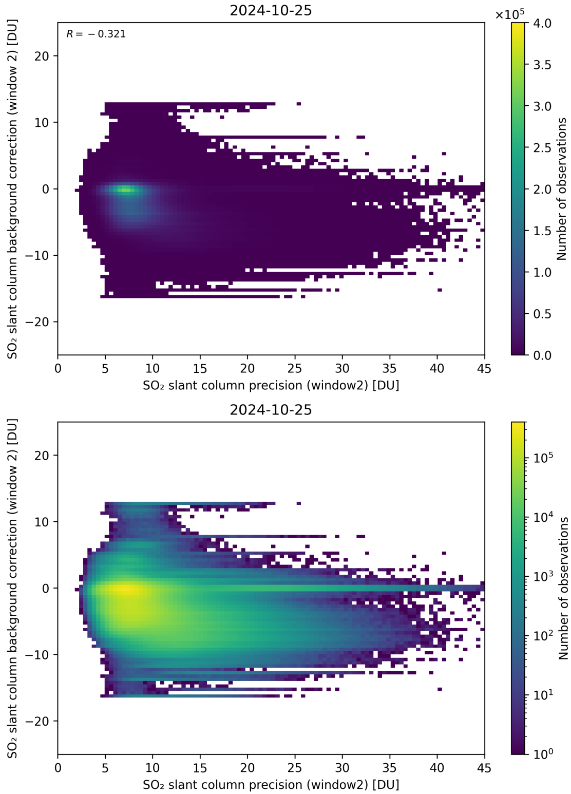
Figure 241: Scatter density plot of “SO 2 slant column precision (window2)” against “SO 2 slant column background correction (window 2)” for 2024-10-24 to 2024-10-26.
