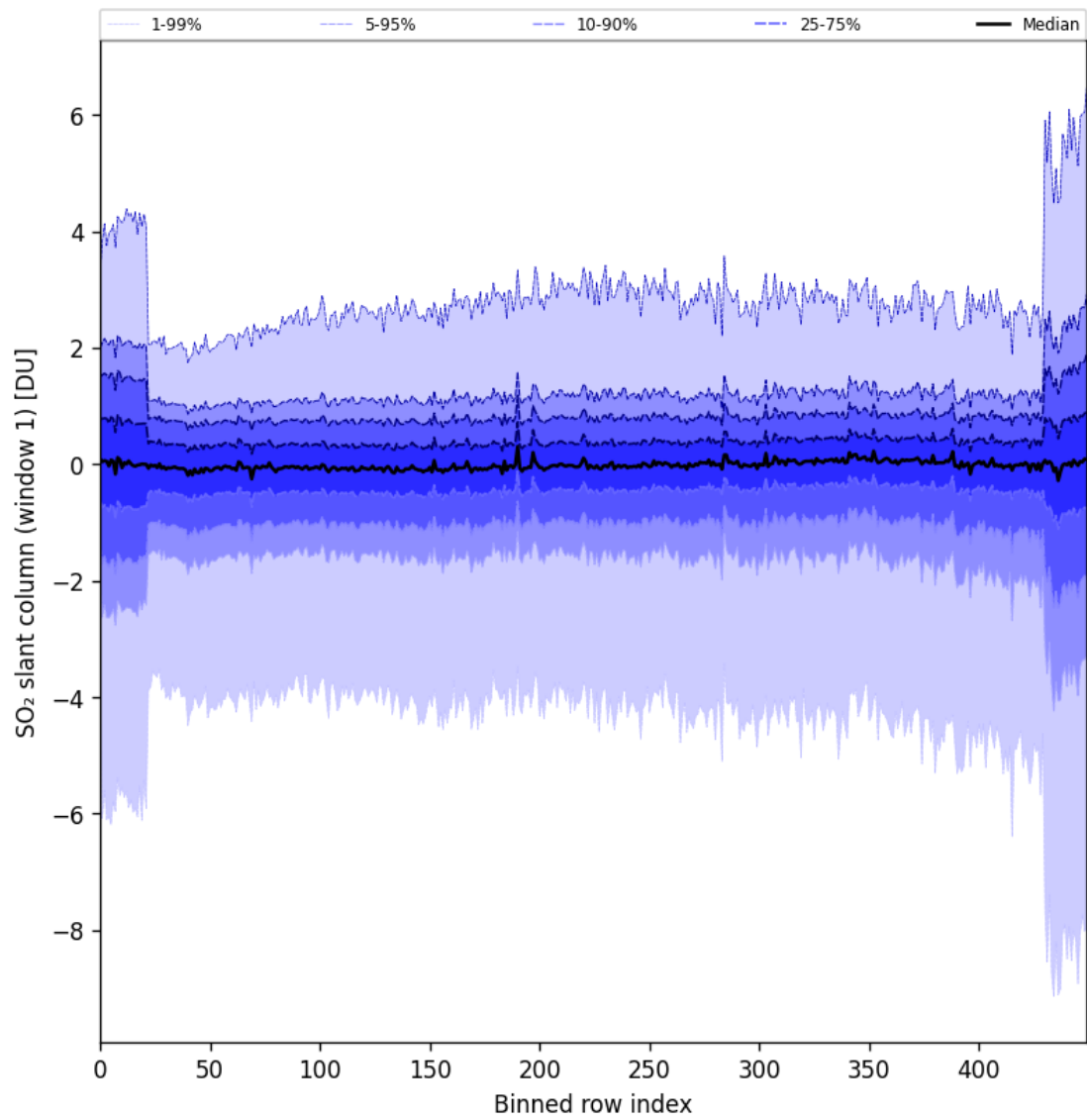
Figure 79: Along track statistics of “SO 2 slant column (window 1)” for 2024-10-24 to 2024-10-26
