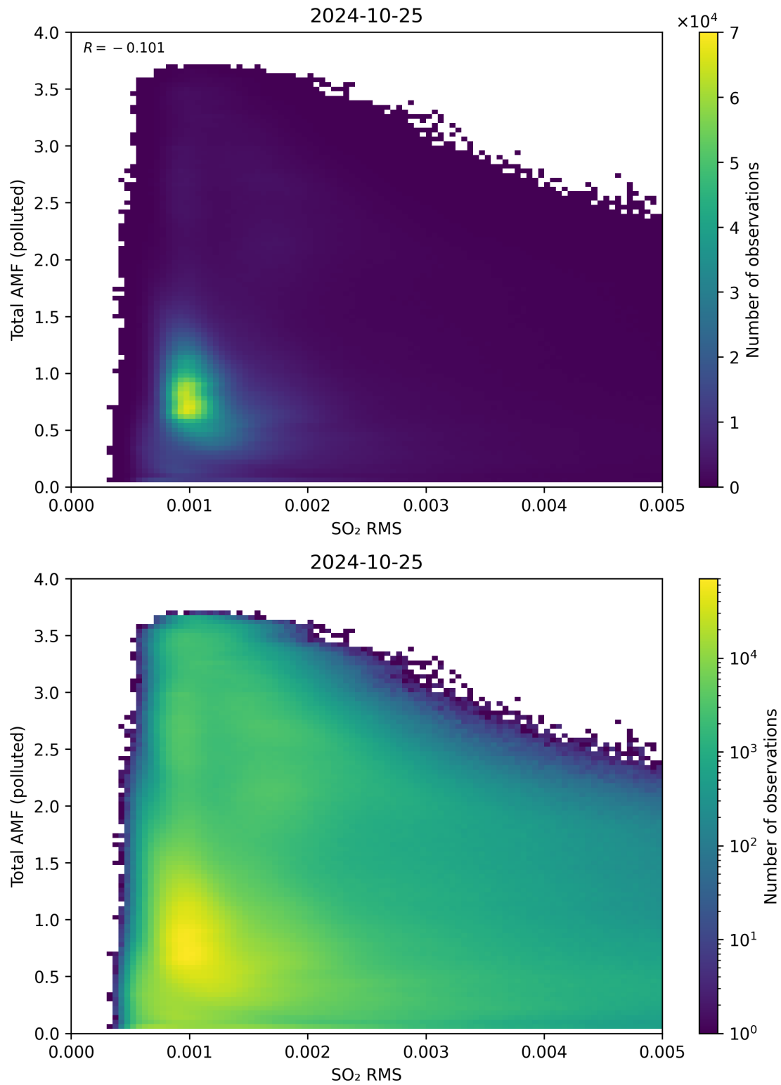
Figure 137: Scatter density plot of “SO 2 RMS” against “Total AMF (polluted)” for 2024-10-24 to 2024-10-26.
