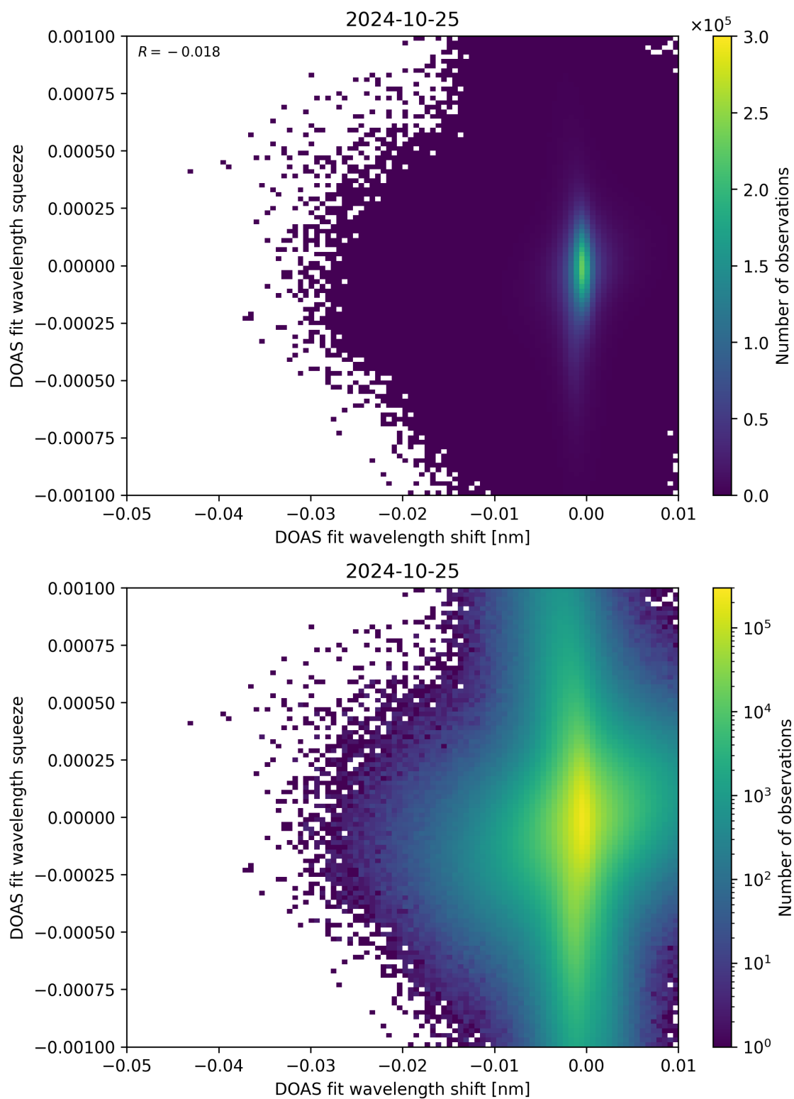
Figure 127: Scatter density plot of “DOAS fit wavelength shift” against “DOAS fit wavelength squeeze” for 2024-10-24 to 2024-10-26.
