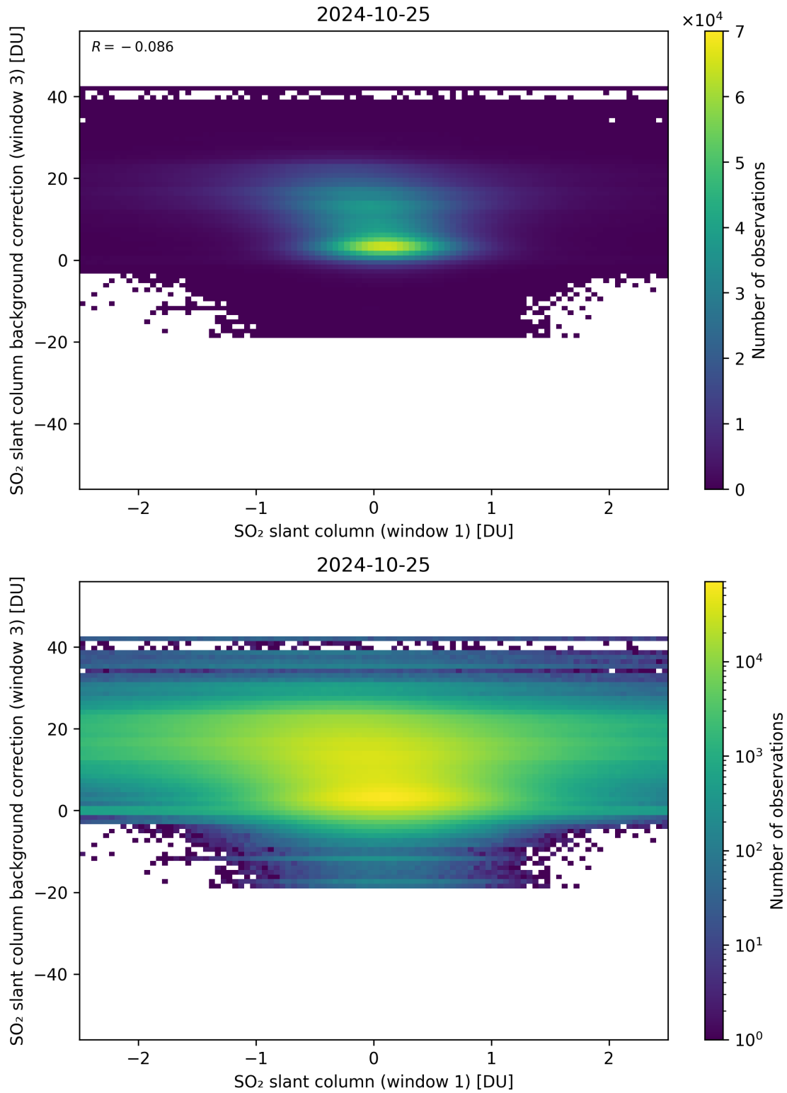
Figure 214: Scatter density plot of “SO 2 slant column (window 1)” against “SO 2 slant column background correction (window 3)” for 2024-10-24 to 2024-10-26.
