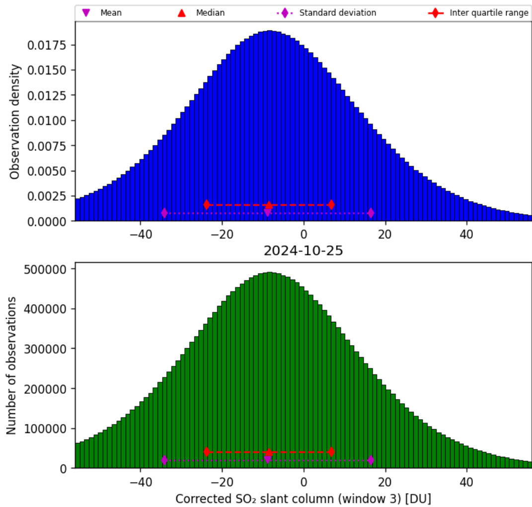
Figure 66: Histogram of “Corrected SO 2 slant column (window 3)” for 2024-10-24 to 2024-10-26
