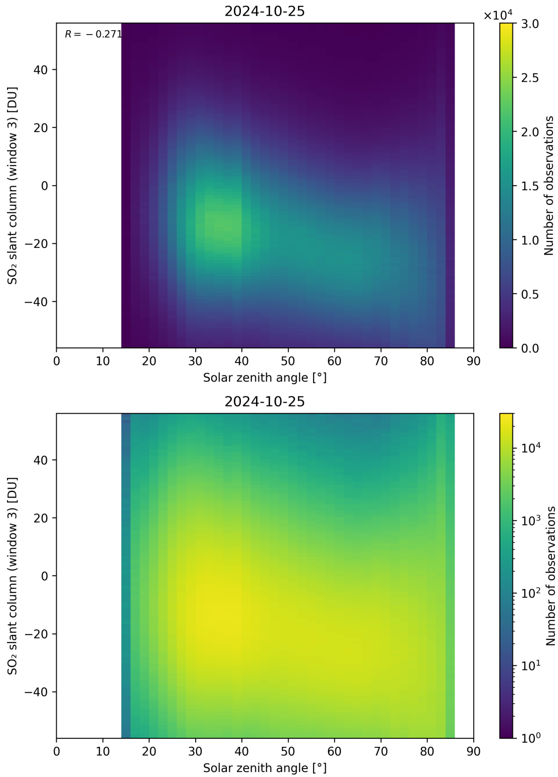
Figure 172: Scatter density plot of “Solar zenith angle” against “SO 2 slant column (window 3)” for 2024-10-24 to 2024-10-26.
