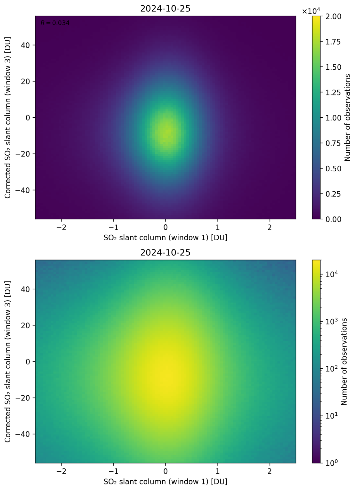
Figure 234: Scatter density plot of “SO 2 slant column (window 1)” against “Corrected SO 2 slant column (window 3)” for 2024-10-24 to 2024-10-26.
