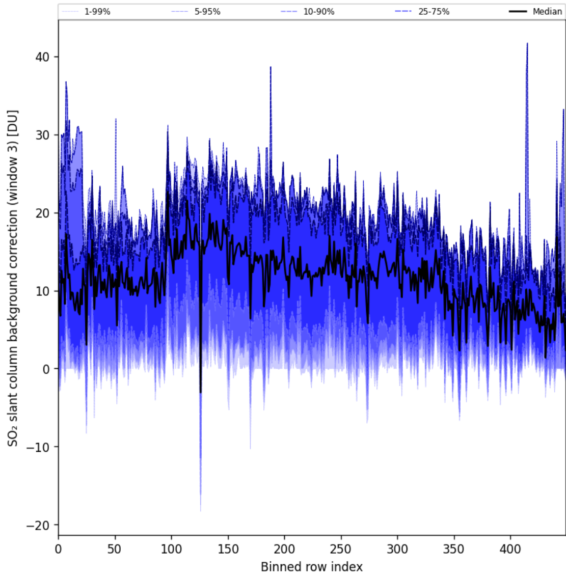
Figure 90: Along track statistics of “SO 2 slant column background correction (window 3)” for 2024-10-24 to 2024-10-26
