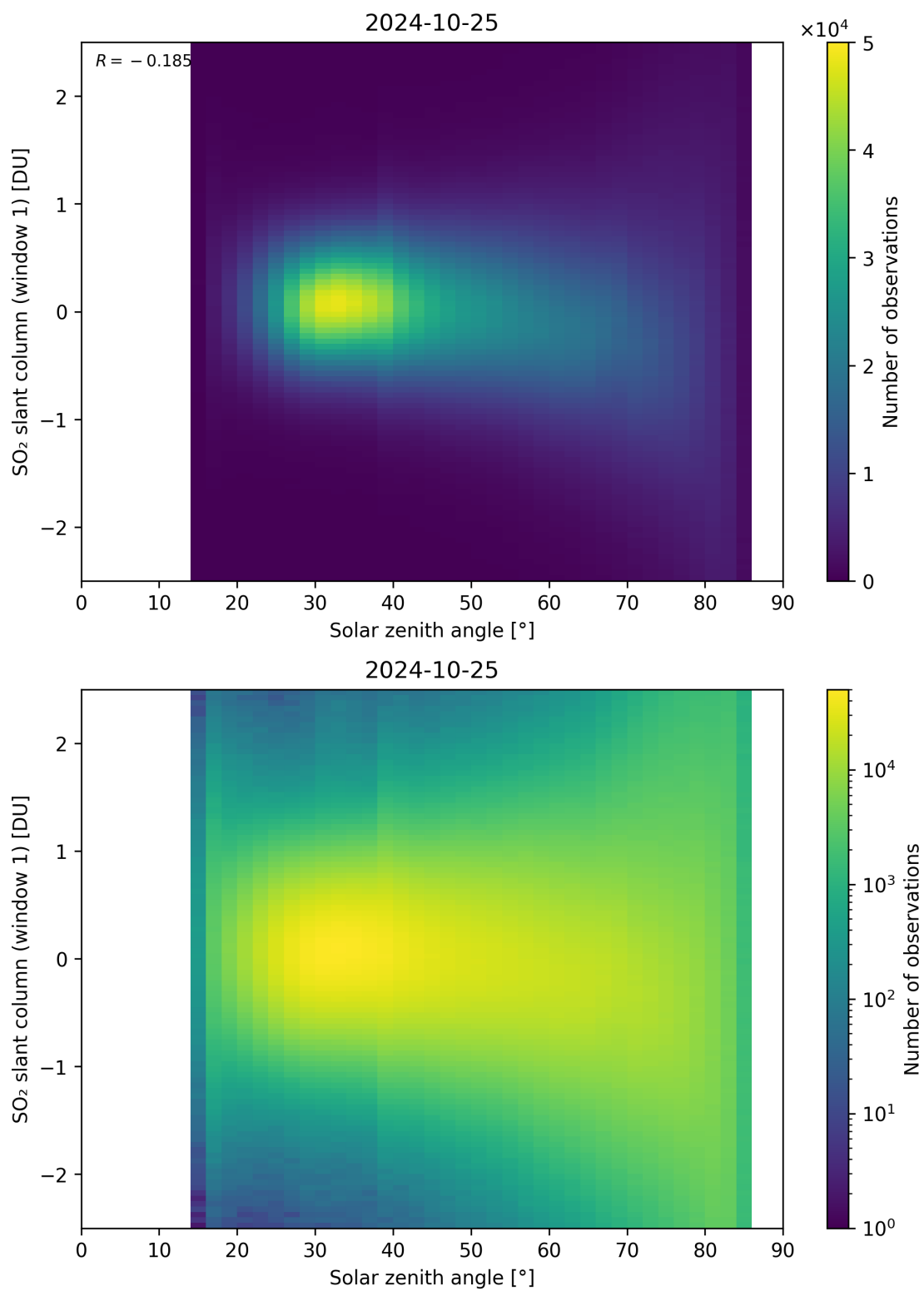
Figure 169: Scatter density plot of “Solar zenith angle” against “SO 2 slant column (window 1)” for 2024-10-24 to 2024-10-26.
