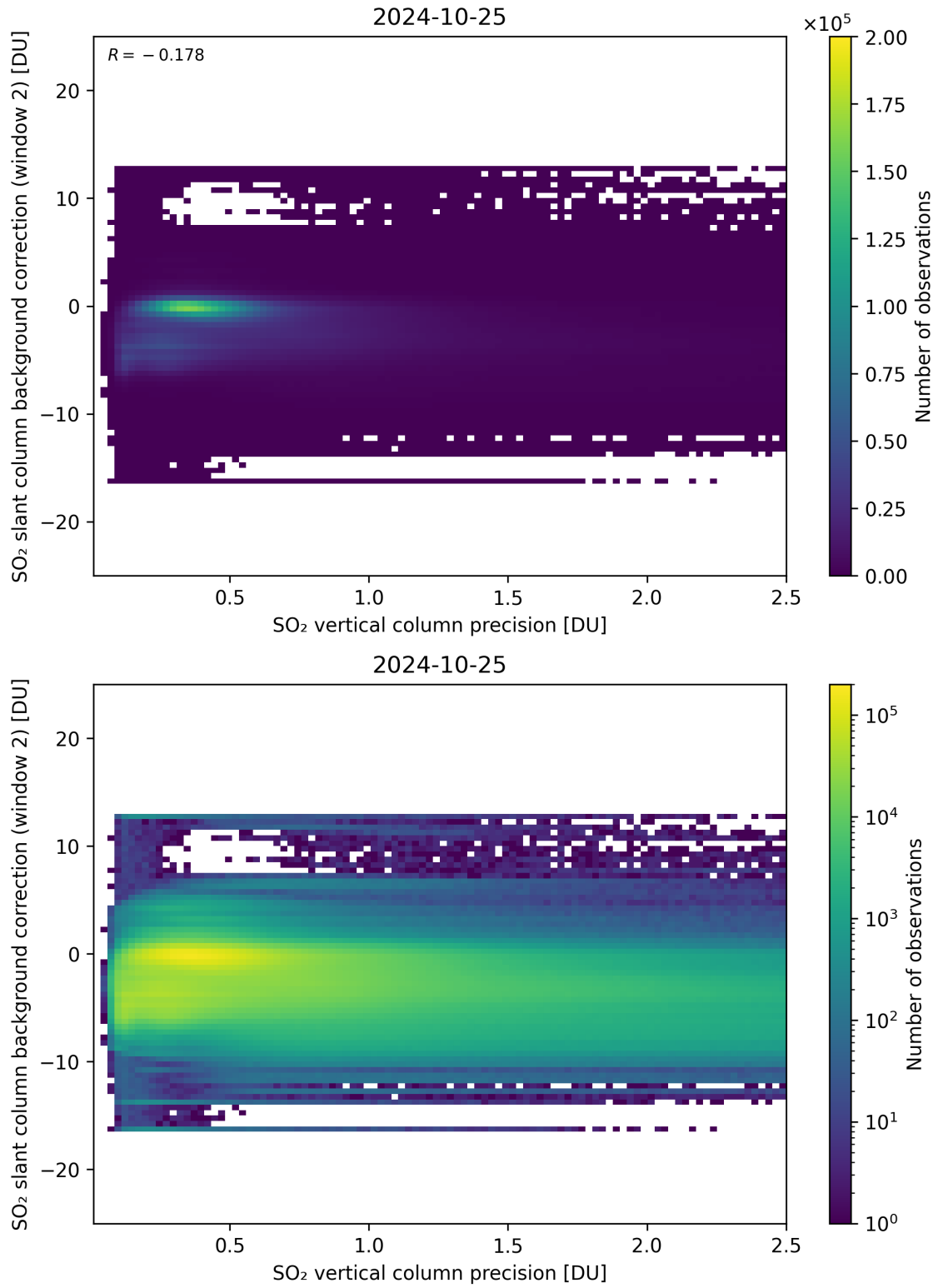
Figure 280: Scatter density plot of “SO 2 vertical column precision” against “SO 2 slant column background correction (window 2)” for 2024-10-24 to 2024-10-26.
