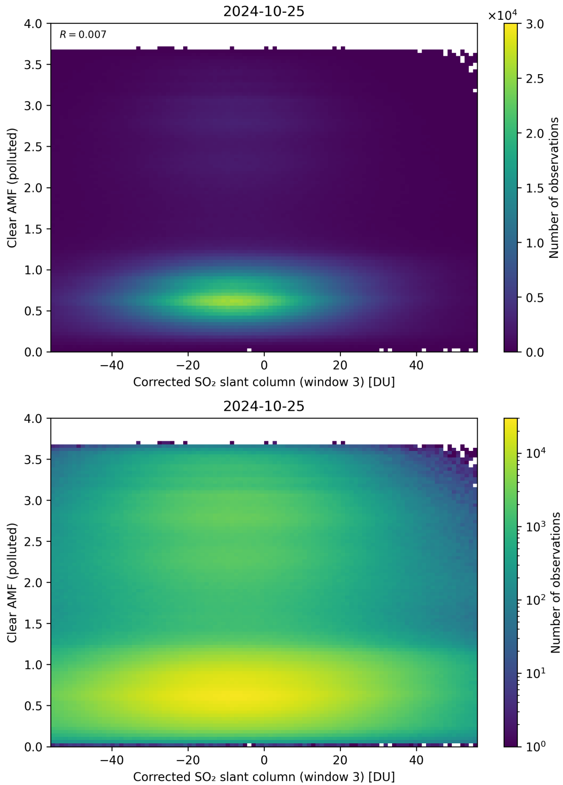
Figure 209: Scatter density plot of “Corrected SO 2 slant column (window 3)” against “Clear AMF (polluted)” for 2024-10-24 to 2024-10-26.
