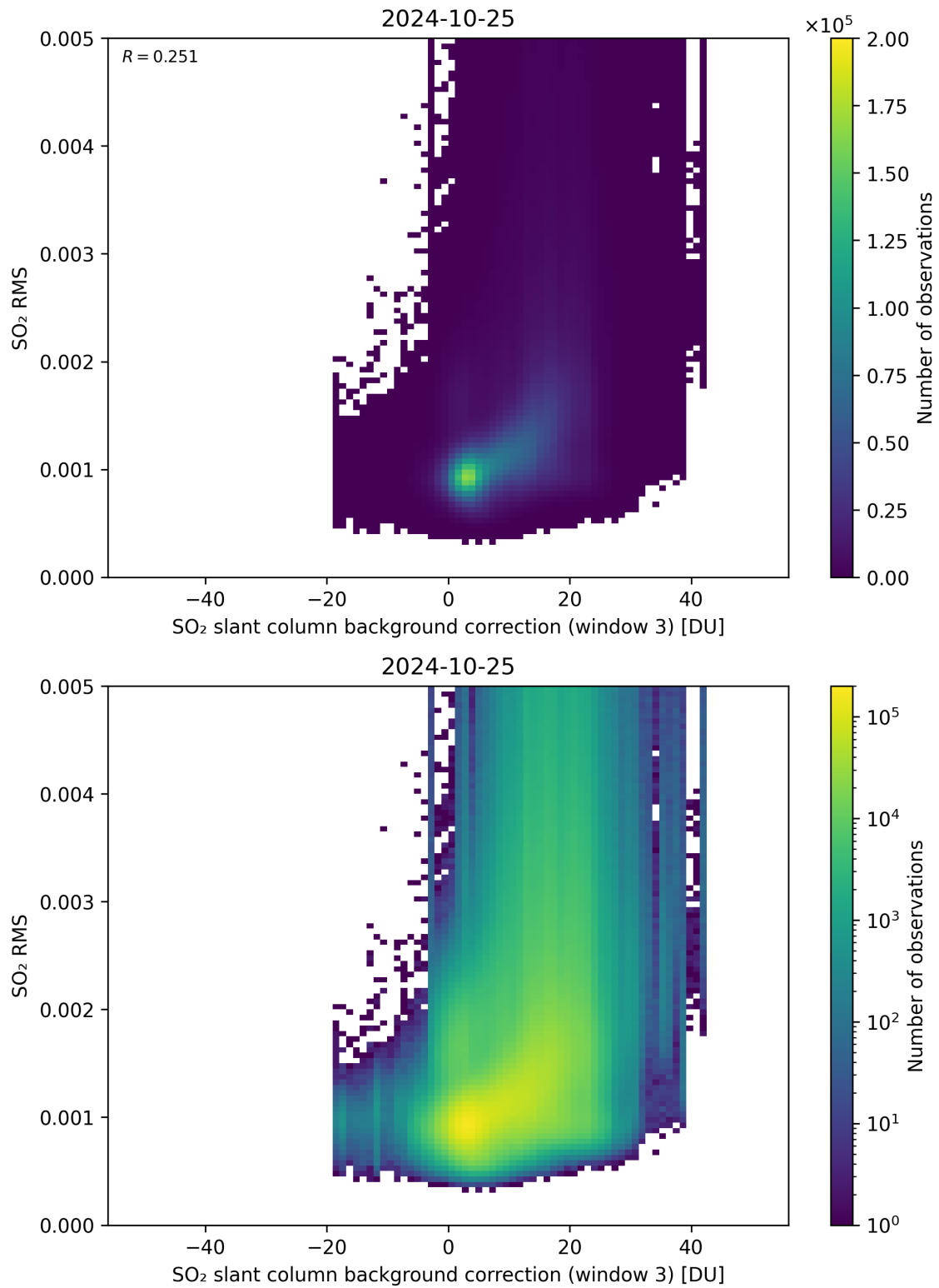
Figure 123: Scatter density plot of “SO 2 slant column background correction (window 3)” against “SO 2 RMS” for 2024-10-24 to 2024-10-26.
