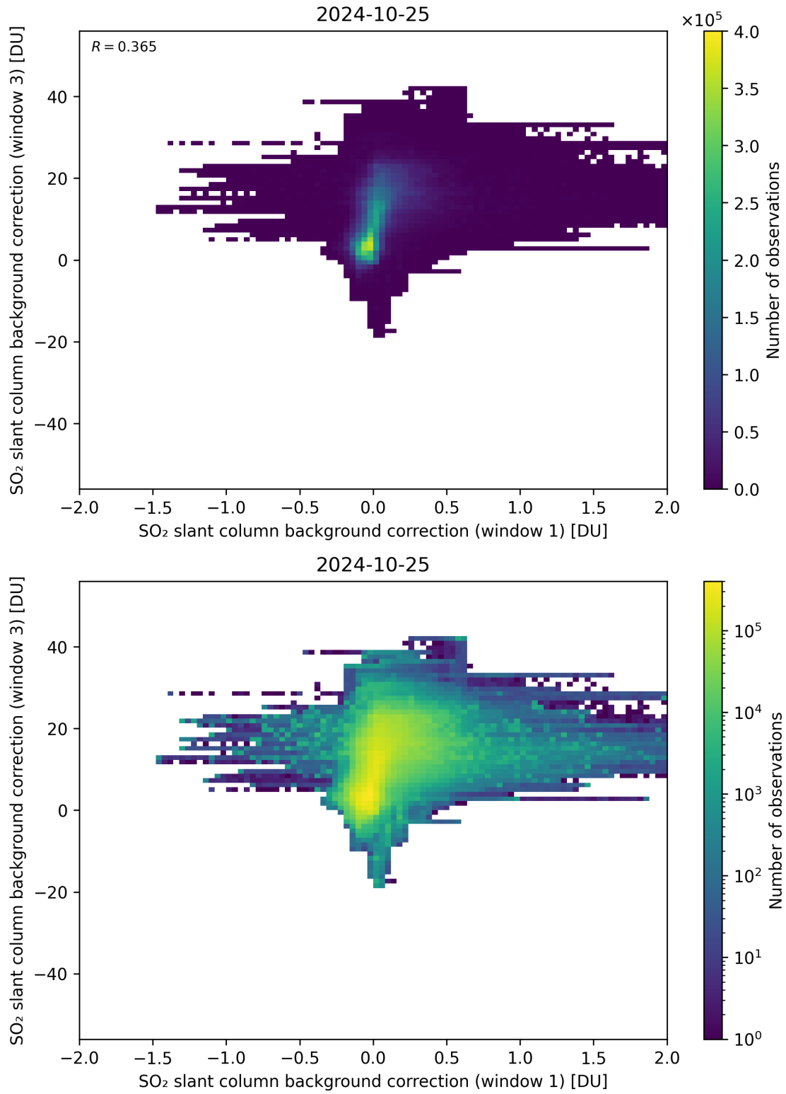
Figure 99: Scatter density plot of “SO 2 slant column background correction (window 1)” against “SO 2 slant column background correction (window 3)” for 2024-10-24 to 2024-10-26.
