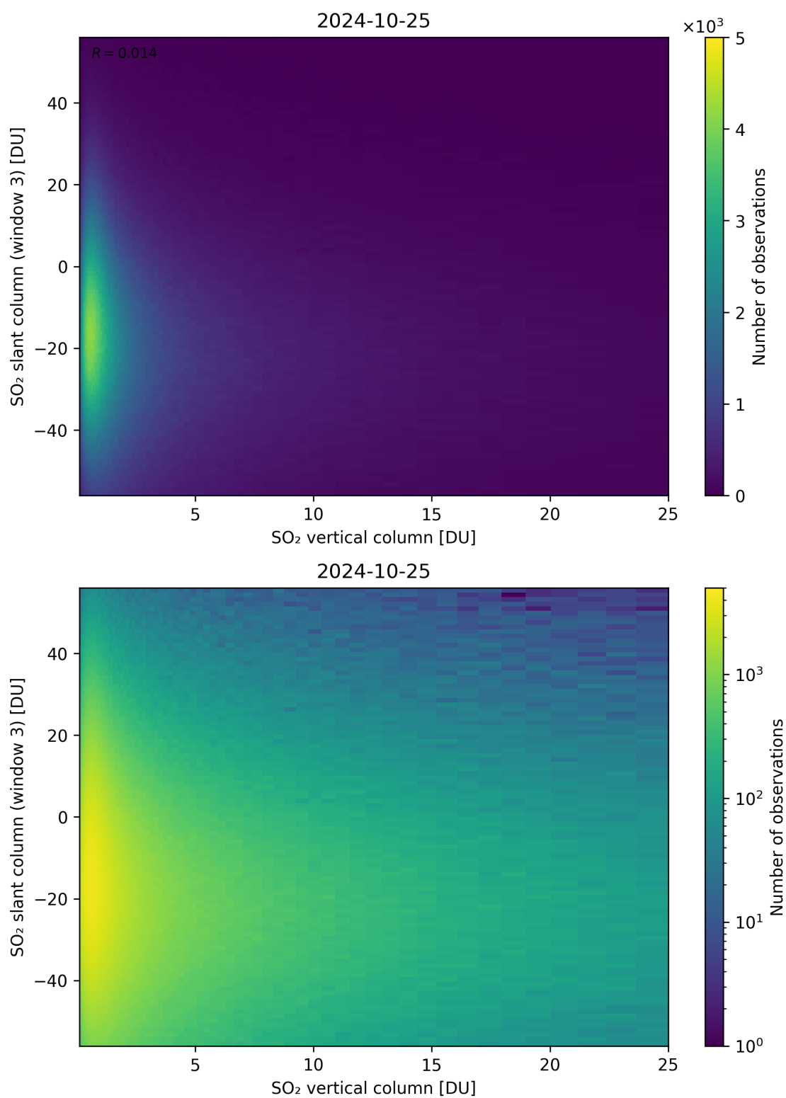
Figure 303: Scatter density plot of “SO 2 vertical column” against “SO 2 slant column (window 3)” for 2024-10-24 to 2024-10-26.
