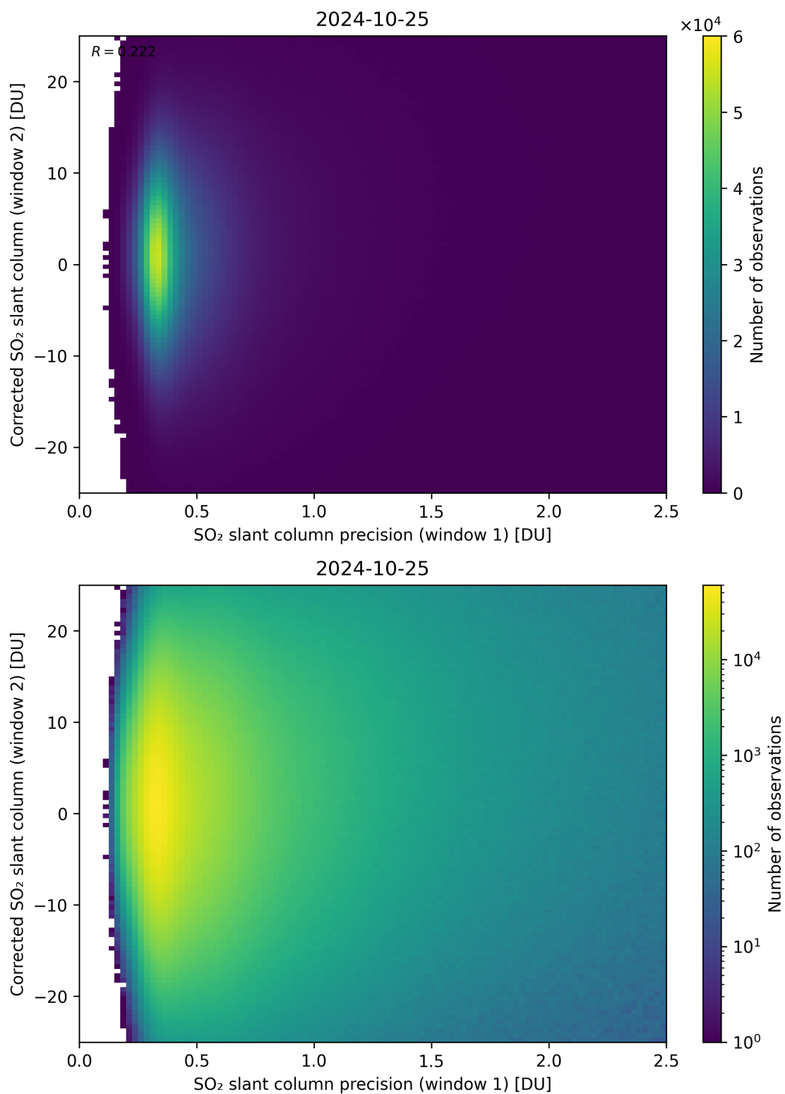
Figure 225: Scatter density plot of “SO 2 slant column precision (window 1)” against “Corrected SO 2 slant column (window 2)” for 2024-10-24 to 2024-10-26.
