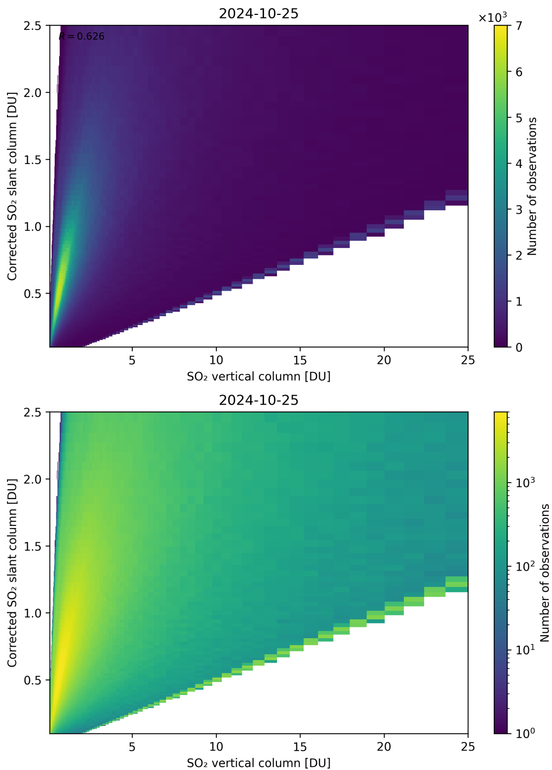
Figure 297: Scatter density plot of “SO 2 vertical column” against “Corrected SO 2 slant column” for 2024-10-24 to 2024-10-26.
