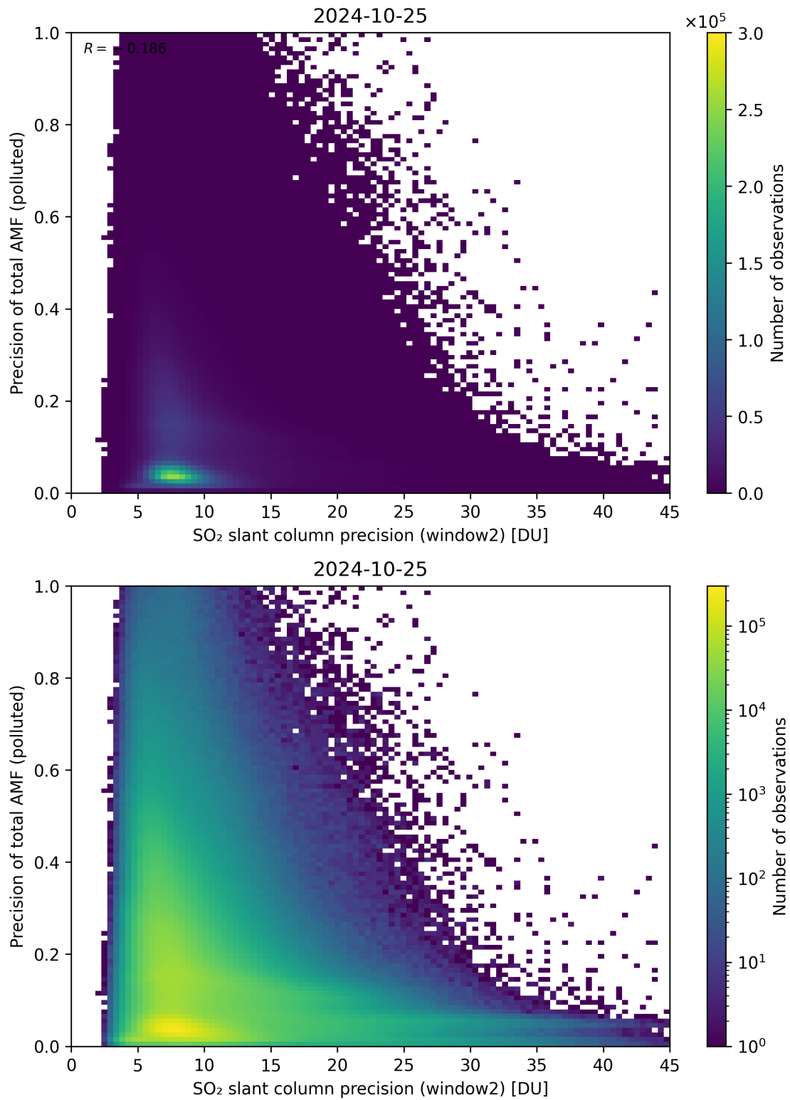
Figure 252: Scatter density plot of “SO 2 slant column precision (window2)” against “Precision of total AMF (polluted)” for 2024-10-24 to 2024-10-26.
