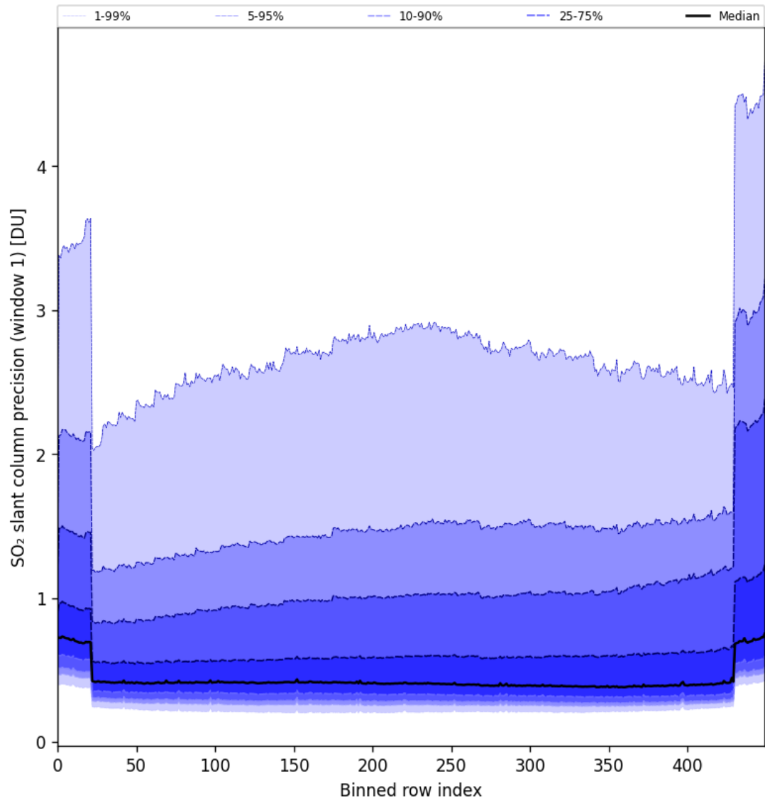
Figure 80: Along track statistics of “SO 2 slant column precision (window 1)” for 2024-10-24 to 2024-10-26
