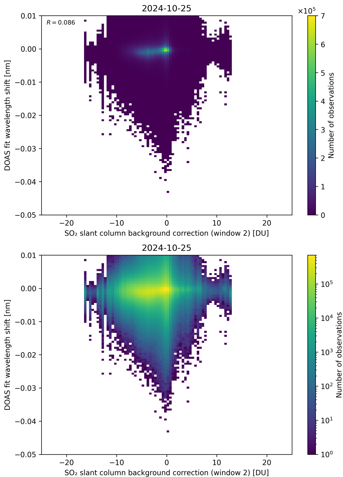
Figure 112: Scatter density plot of “SO 2 slant column background correction (window 2)” against “DOAS fit wavelength shift” for 2024-10-24 to 2024-10-26.
