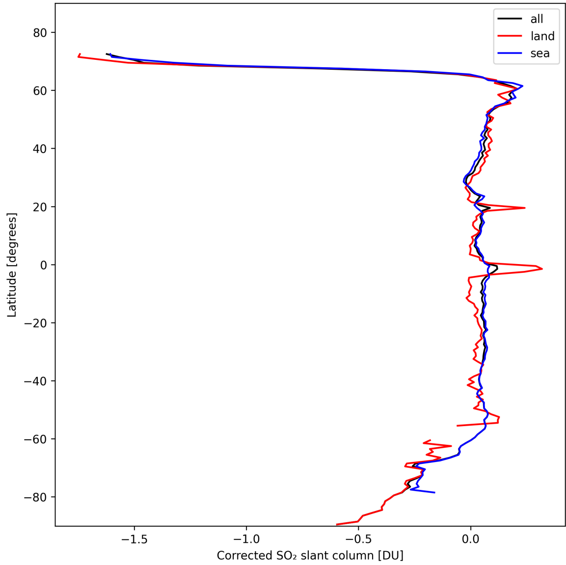
Figure 32: Zonal average of “Corrected SO 2 slant column” for 2024-10-24 to 2024-10-26.
