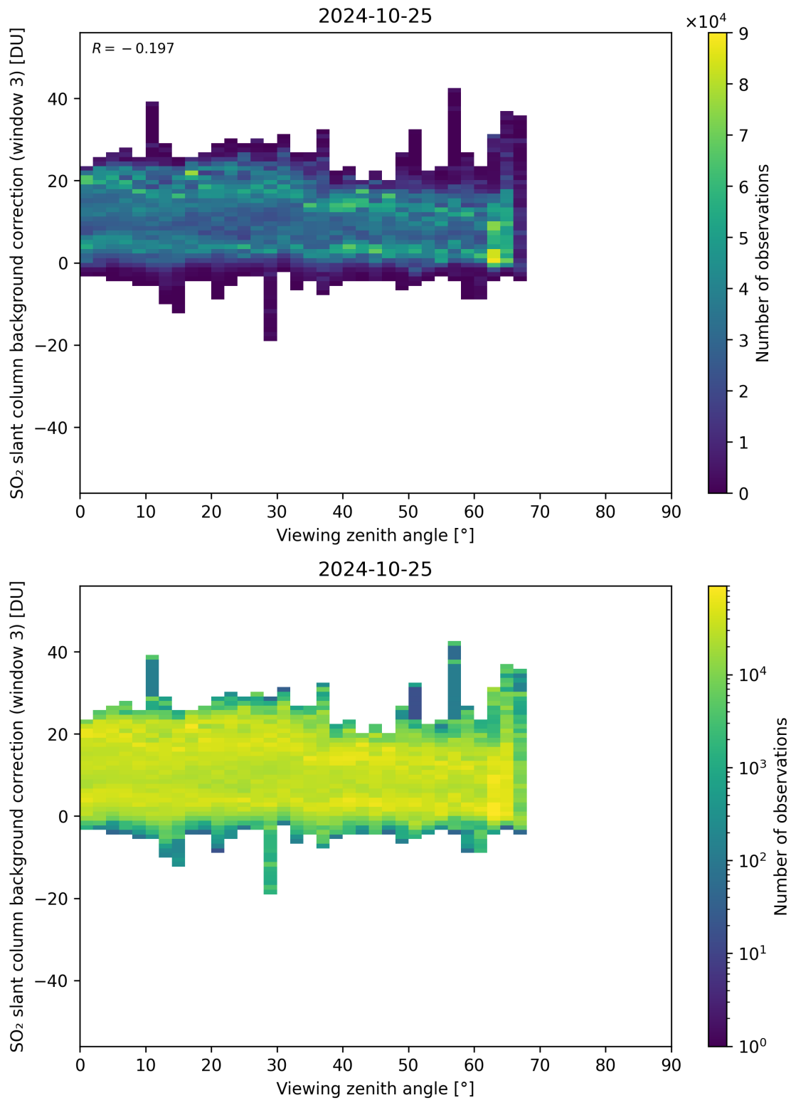
Figure 310: Scatter density plot of “Viewing zenith angle” against “SO 2 slant column background correction (window 3)” for 2024-10-24 to 2024-10-26.
