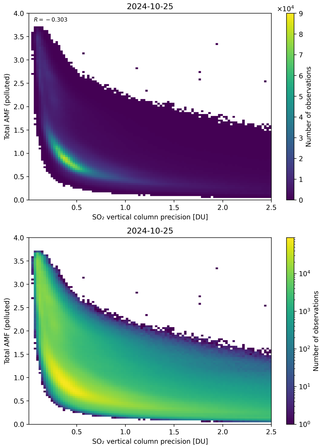
Figure 294: Scatter density plot of “SO 2 vertical column precision” against “Total AMF (polluted)” for 2024-10-24 to 2024-10-26.
