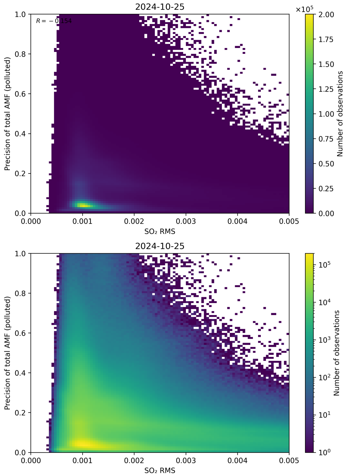
Figure 138: Scatter density plot of “SO 2 RMS” against “Precision of total AMF (polluted)” for 2024-10-24 to 2024-10-26.
