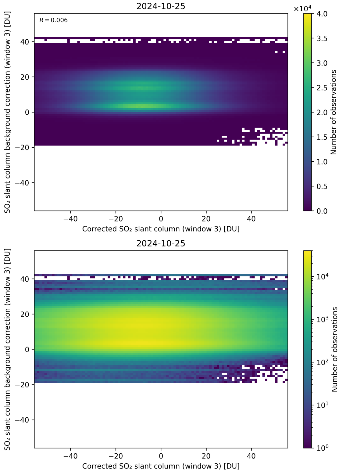
Figure 205: Scatter density plot of “Corrected SO 2 slant column (window 3)” against “SO 2 slant column background correction (window 3)” for 2024-10-24 to 2024-10-26.
