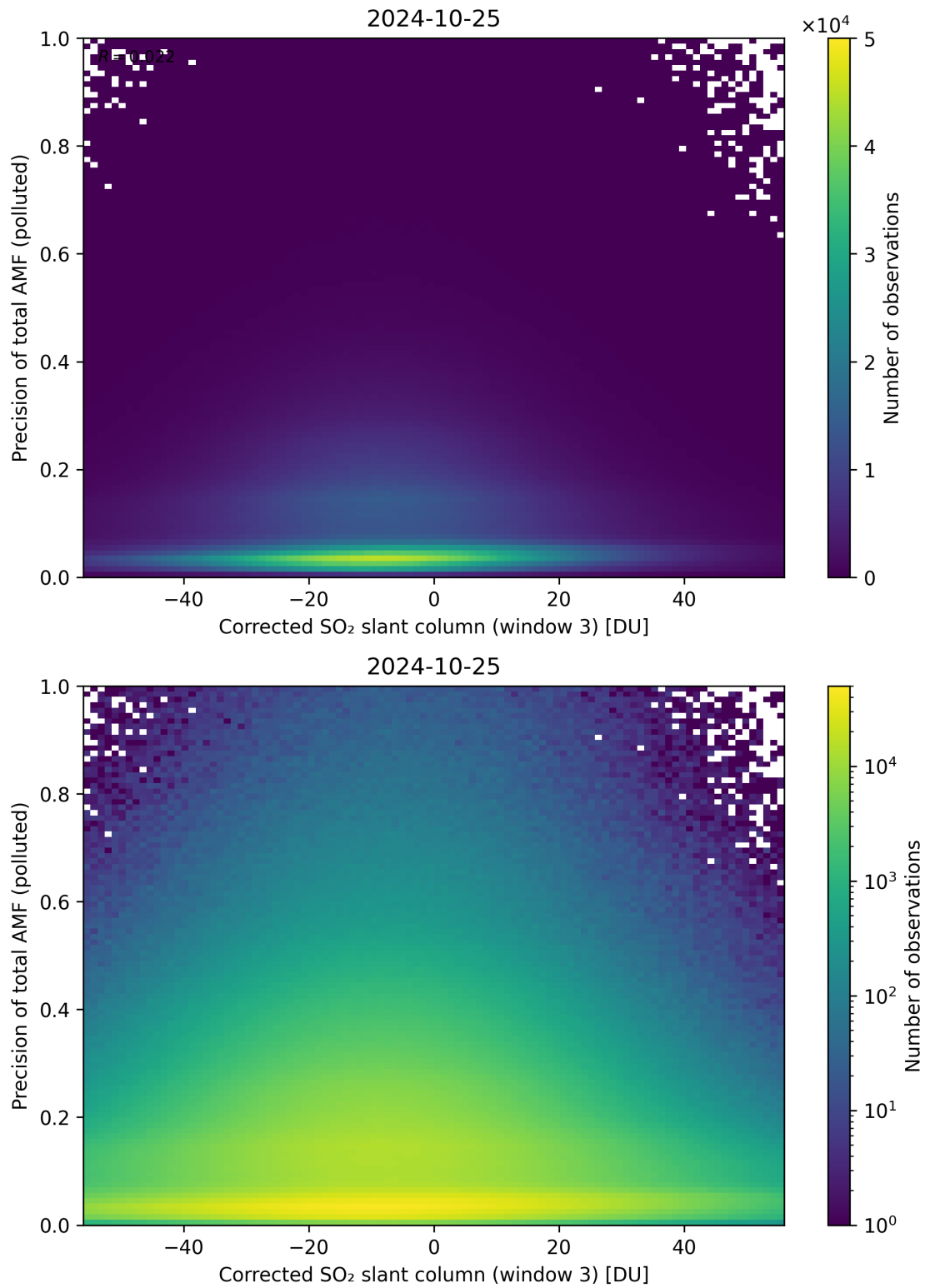
Figure 211: Scatter density plot of “Corrected SO 2 slant column (window 3)” against “Precision of total AMF (polluted)” for 2024-10-24 to 2024-10-26.
