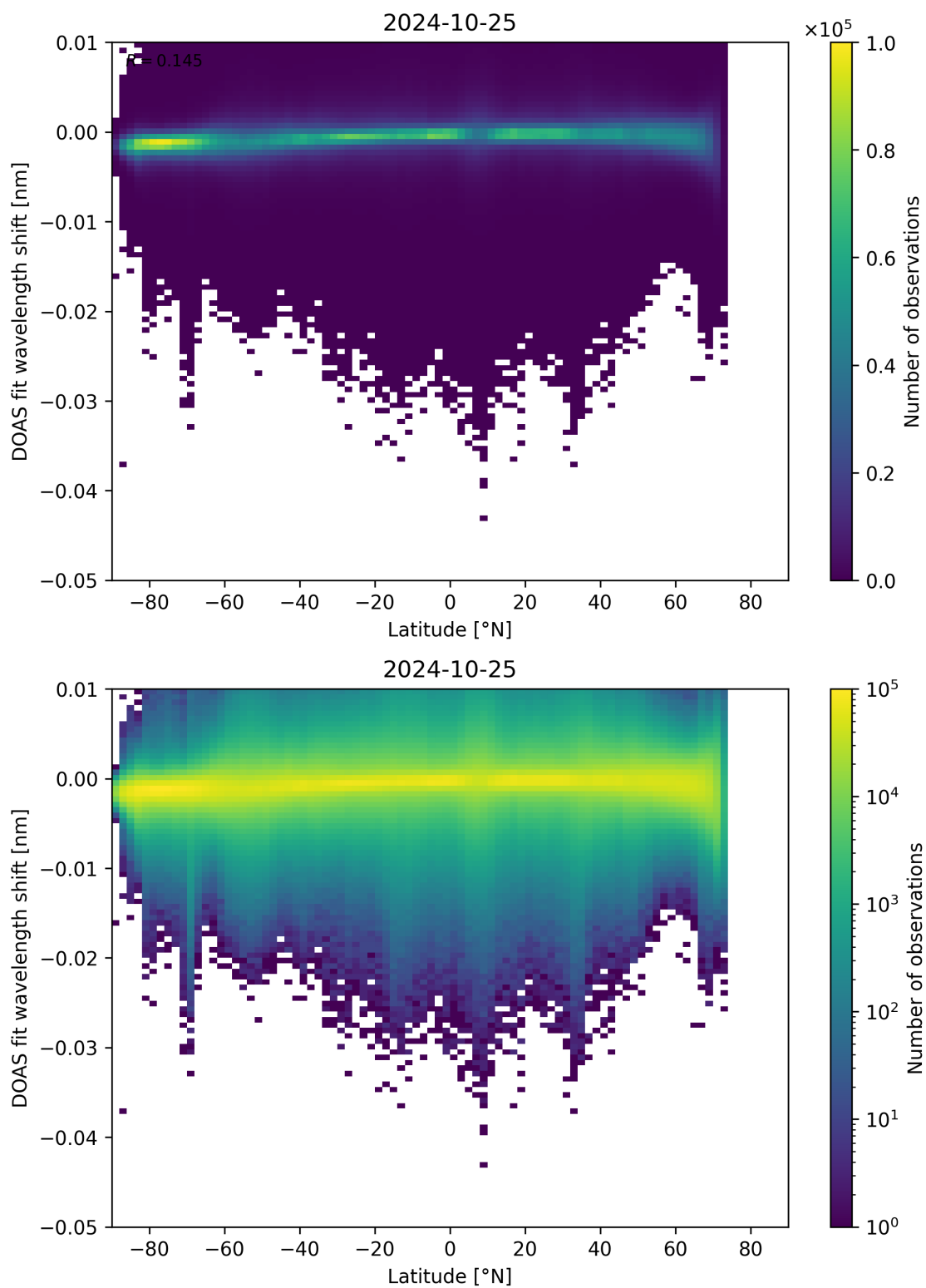
Figure 142: Scatter density plot of “Latitude” against “DOAS fit wavelength shift” for 2024-10-24 to 2024-10-26.
