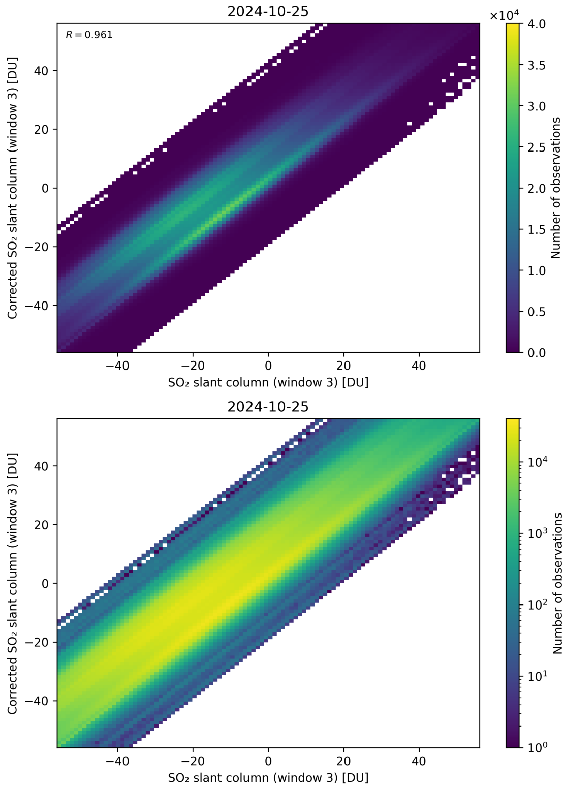
Figure 266: Scatter density plot of “SO 2 slant column (window 3)” against “Corrected SO 2 slant column (window 3)” for 2024-10-24 to 2024-10-26.
