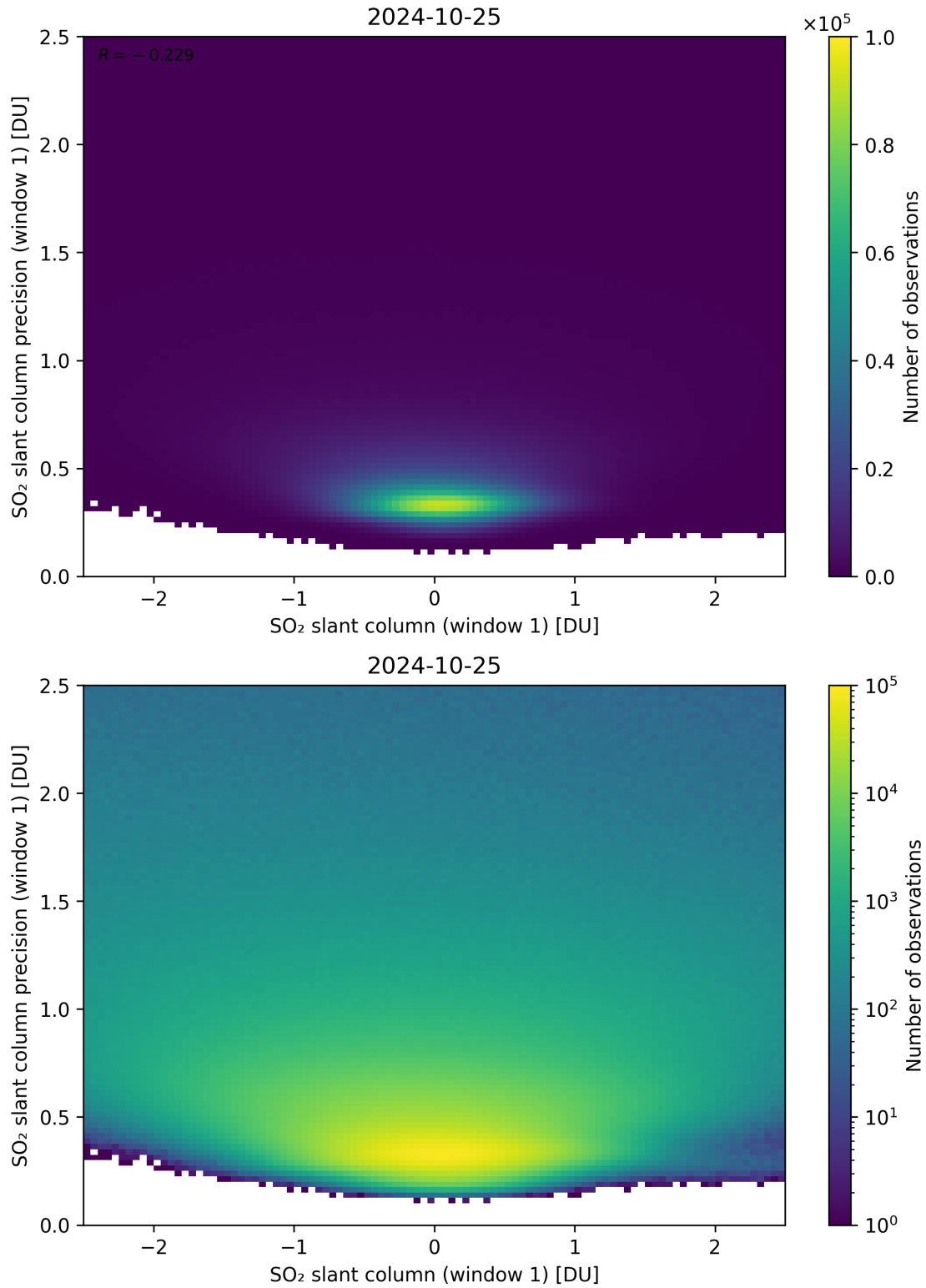
Figure 235: Scatter density plot of “SO 2 slant column (window 1)” against “SO 2 slant column precision (window 1)” for 2024-10-24 to 2024-10-26.
