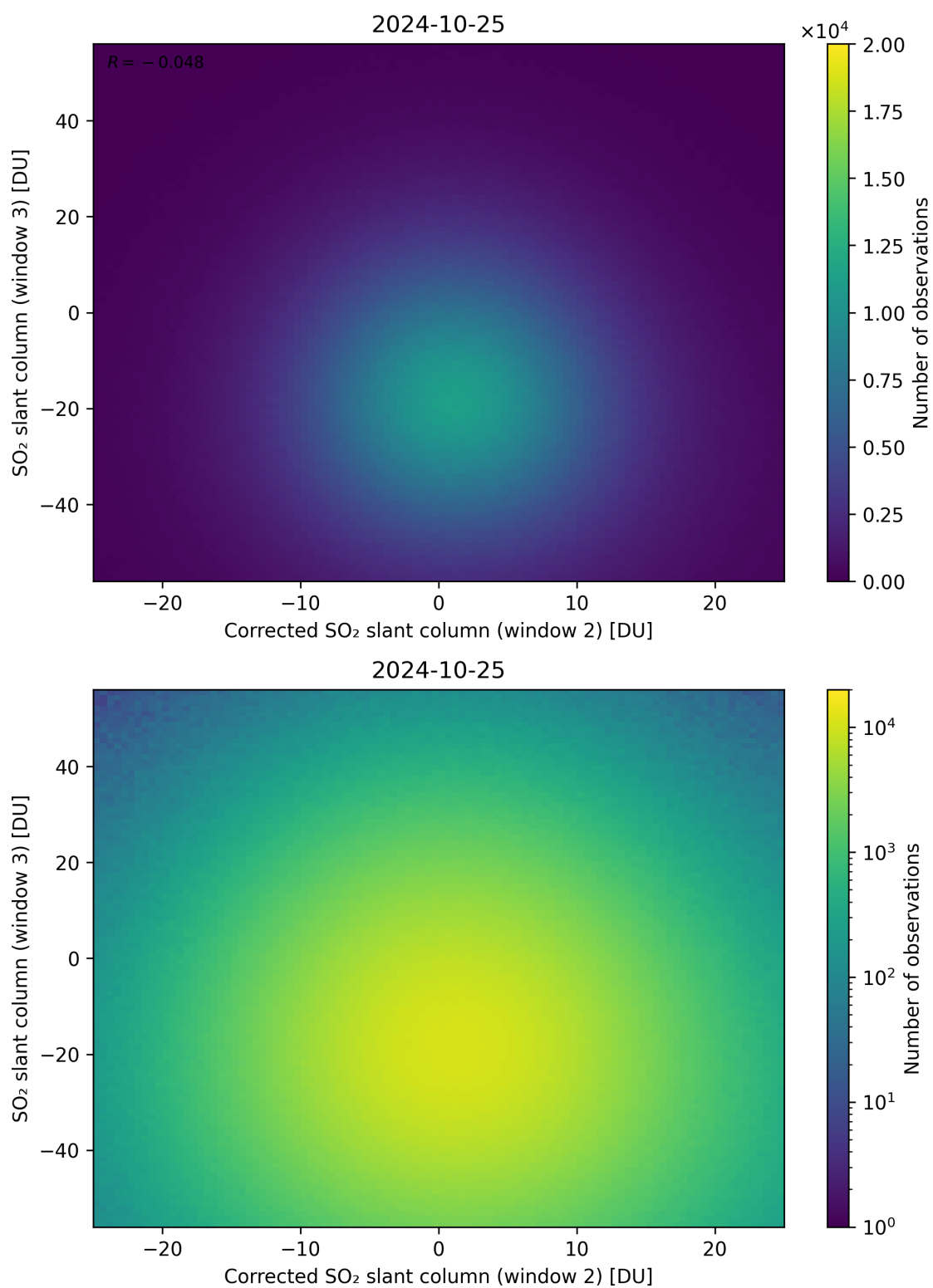
Figure 201: Scatter density plot of “Corrected SO 2 slant column (window 2)” against “SO 2 slant column (window 3)” for 2024-10-24 to 2024-10-26.
