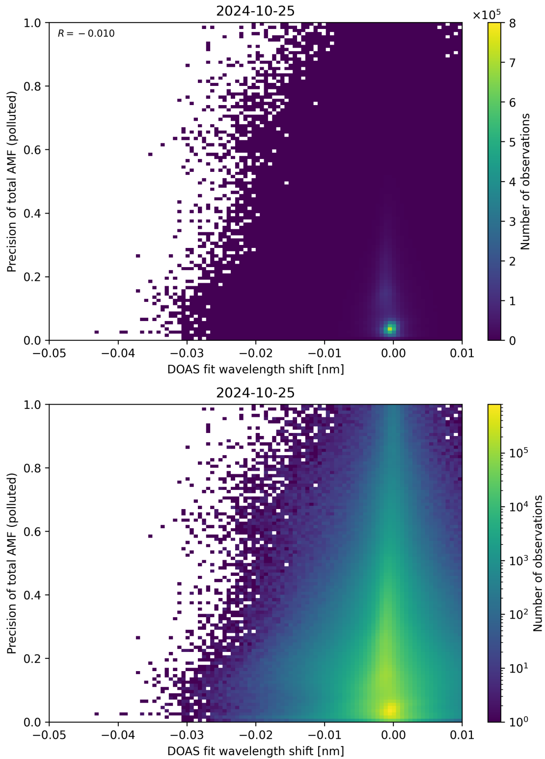
Figure 131: Scatter density plot of “DOAS fit wavelength shift” against “Precision of total AMF (polluted)” for 2024-10-24 to 2024-10-26.
