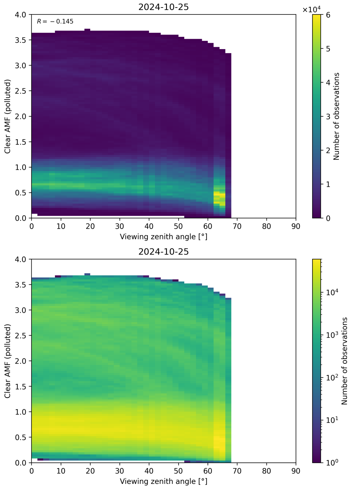
Figure 316: Scatter density plot of “Viewing zenith angle” against “Clear AMF (polluted)” for 2024-10-24 to 2024-10-26.
