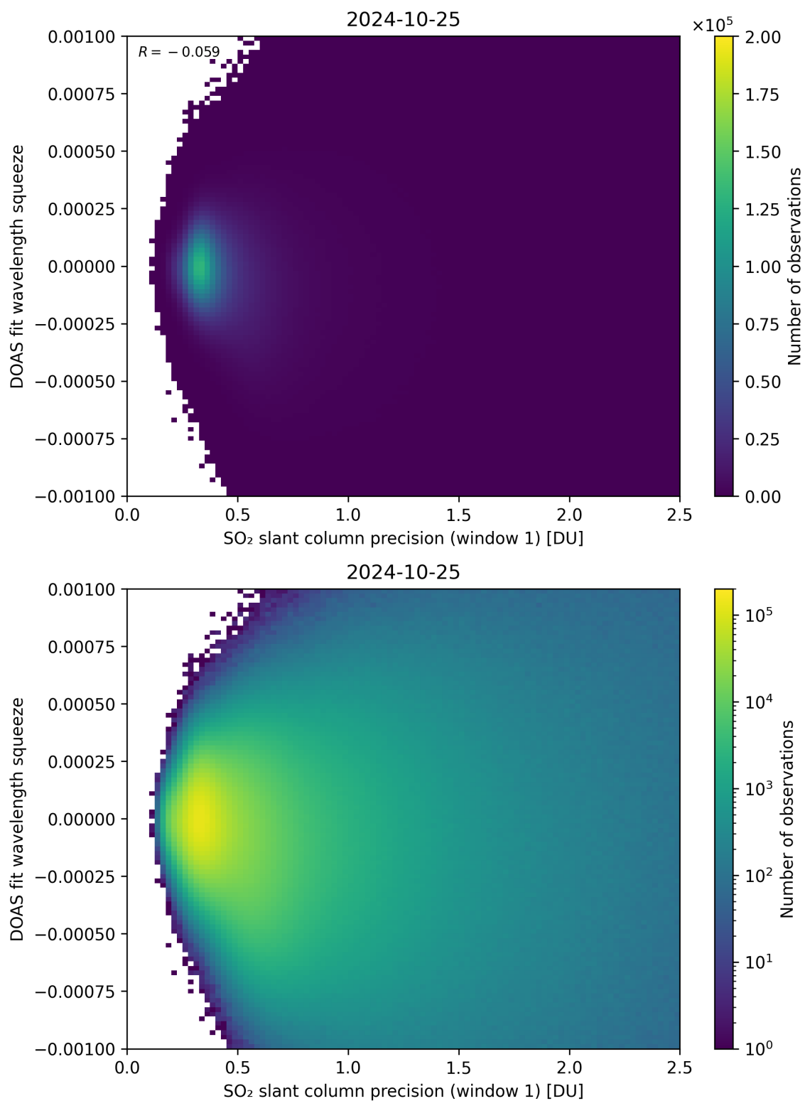
Figure 222: Scatter density plot of “SO 2 slant column precision (window 1)” against “DOAS fit wavelength squeeze” for 2024-10-24 to 2024-10-26.
