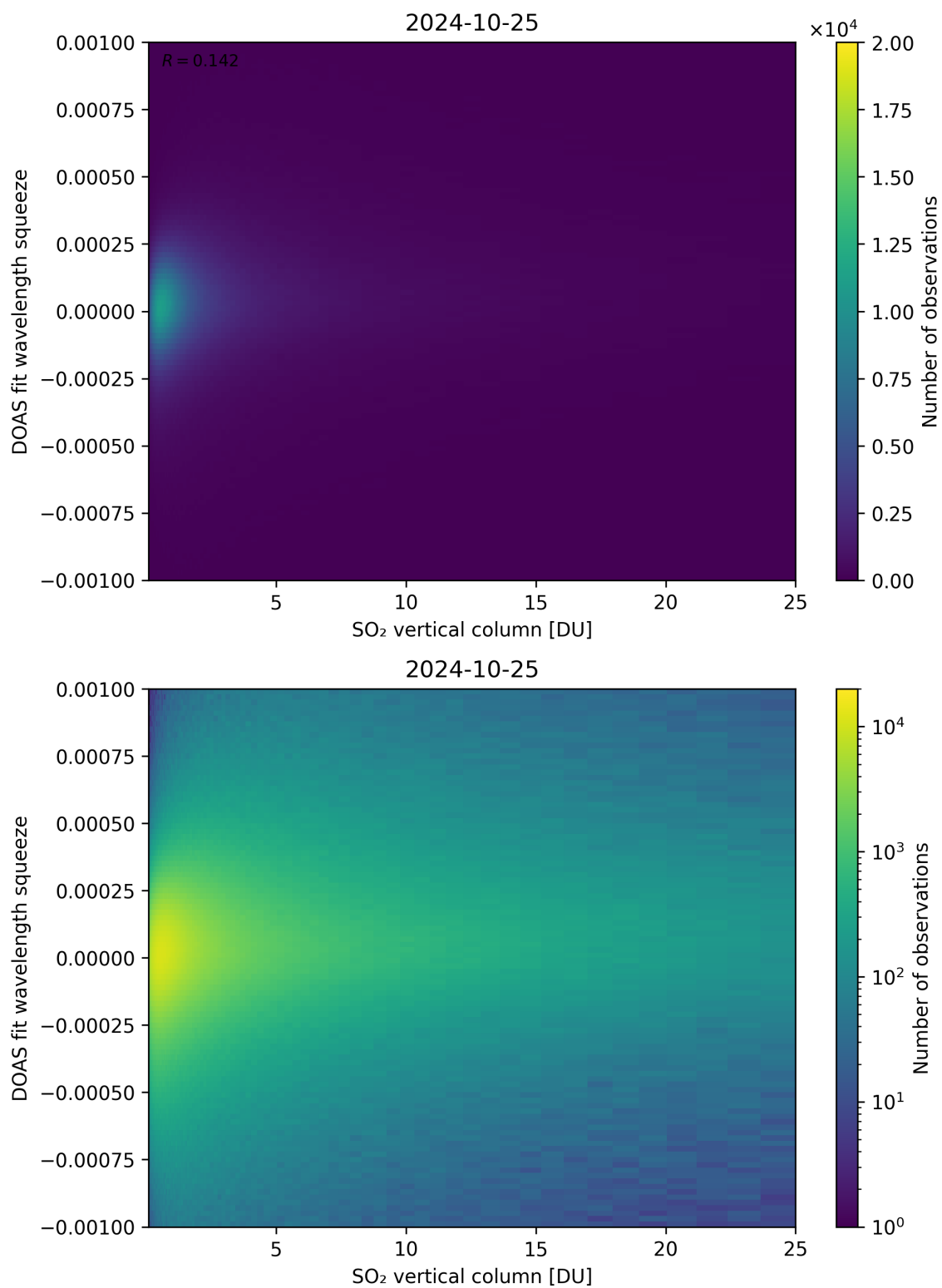
Figure 277: Scatter density plot of “SO 2 vertical column” against “DOAS fit wavelength squeeze” for 2024-10-24 to 2024-10-26.
