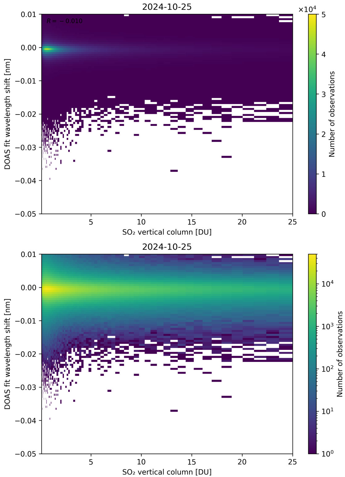
Figure 276: Scatter density plot of “SO 2 vertical column” against “DOAS fit wavelength shift” for 2024-10-24 to 2024-10-26.
