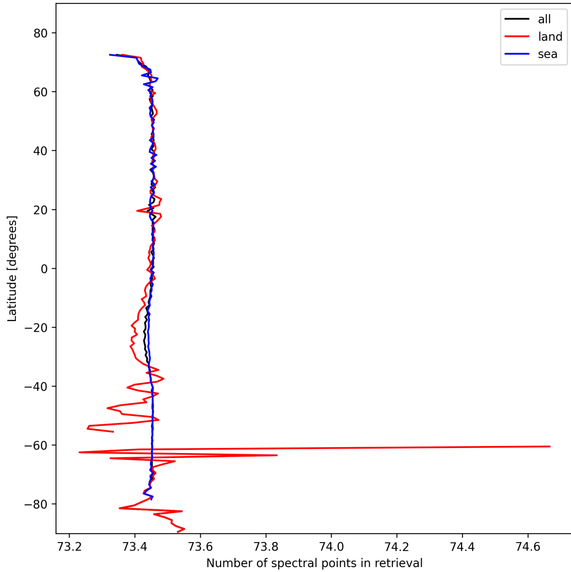
Figure 51: Zonal average of “Number of spectral points in retrieval” for 2024-10-24 to 2024-10-26.
