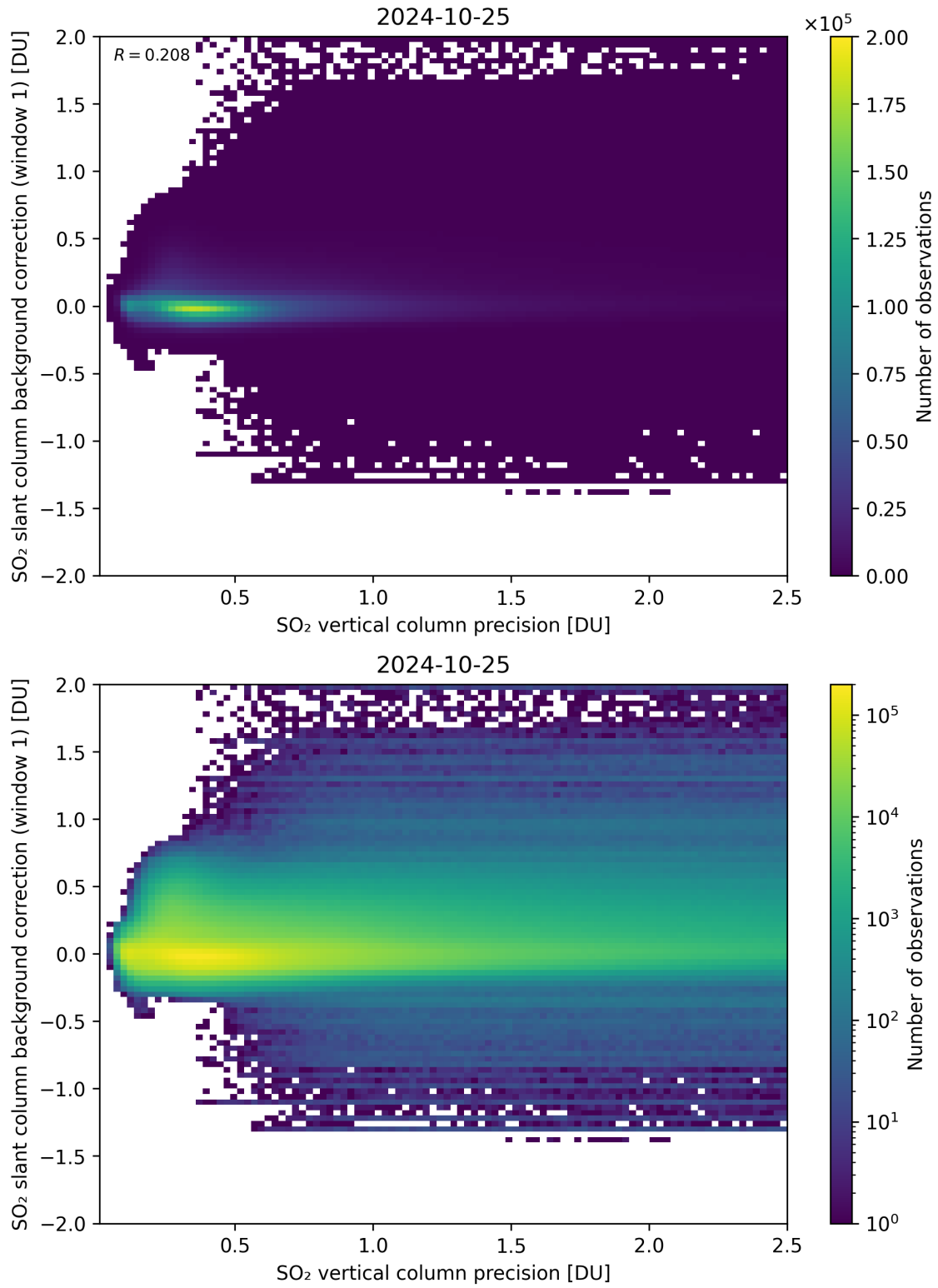
Figure 279: Scatter density plot of “SO 2 vertical column precision” against “SO 2 slant column background correction (window 1)” for 2024-10-24 to 2024-10-26.
