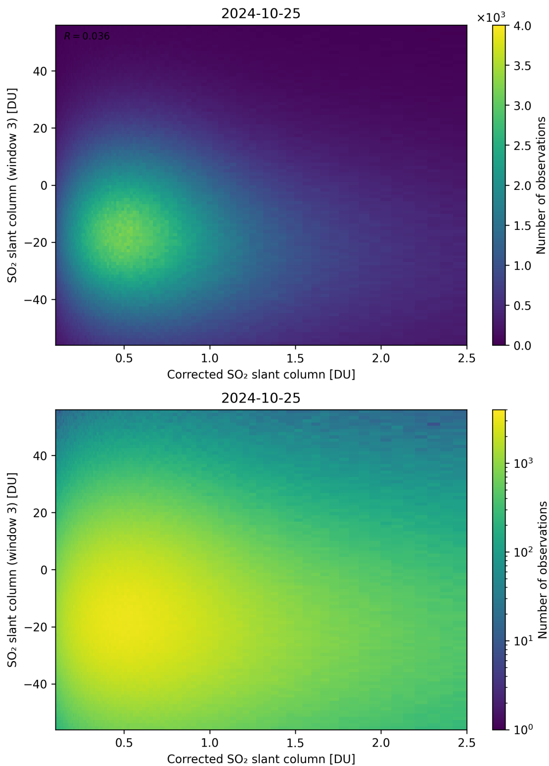
Figure 190: Scatter density plot of “Corrected SO 2 slant column” against “SO 2 slant column (window 3)” for 2024-10-24 to 2024-10-26.
