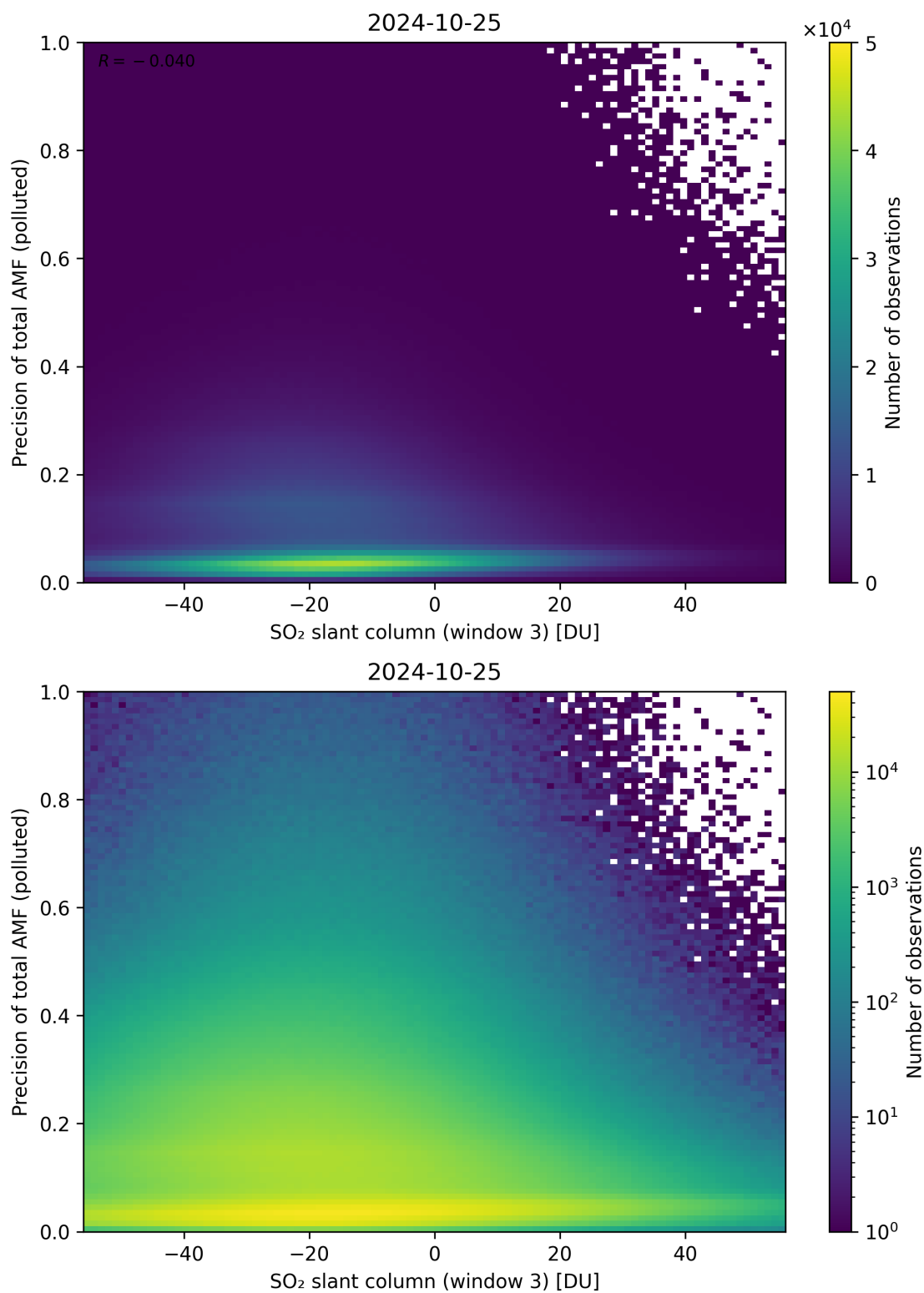
Figure 269: Scatter density plot of “SO 2 slant column (window 3)” against “Precision of total AMF (polluted)” for 2024-10-24 to 2024-10-26.
