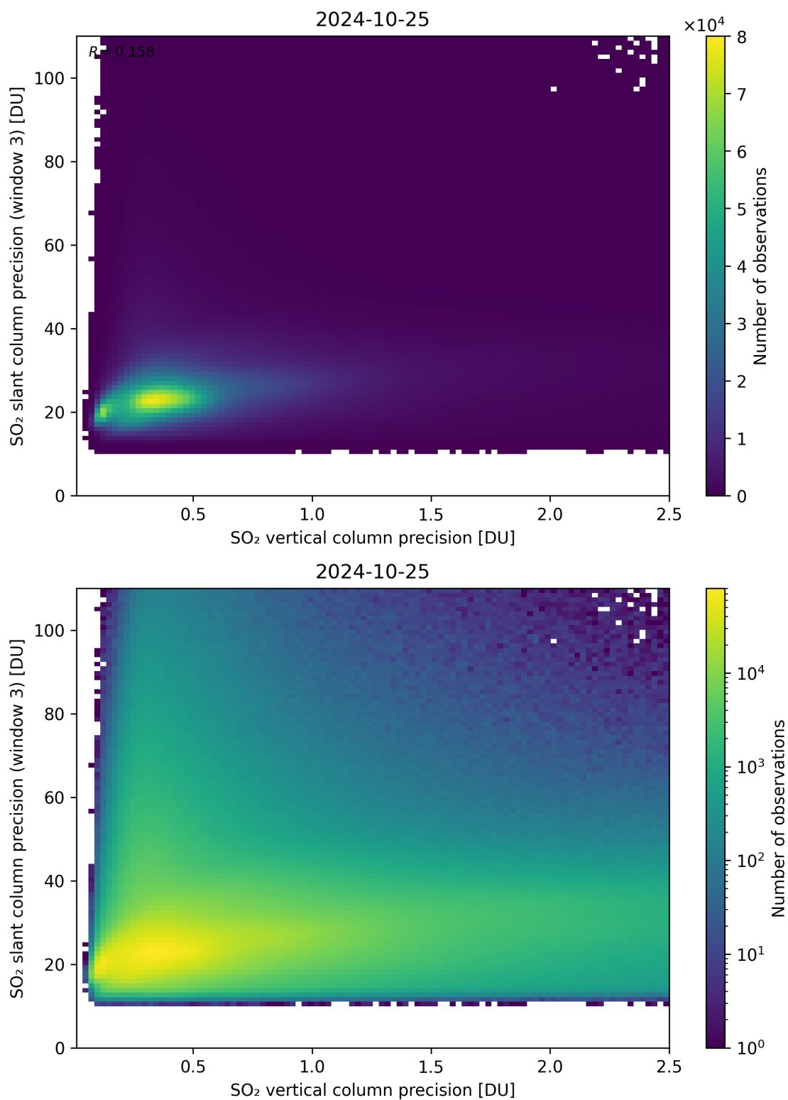
Figure 293: Scatter density plot of “SO 2 vertical column precision” against “SO 2 slant column precision (window 3)” for 2024-10-24 to 2024-10-26.
