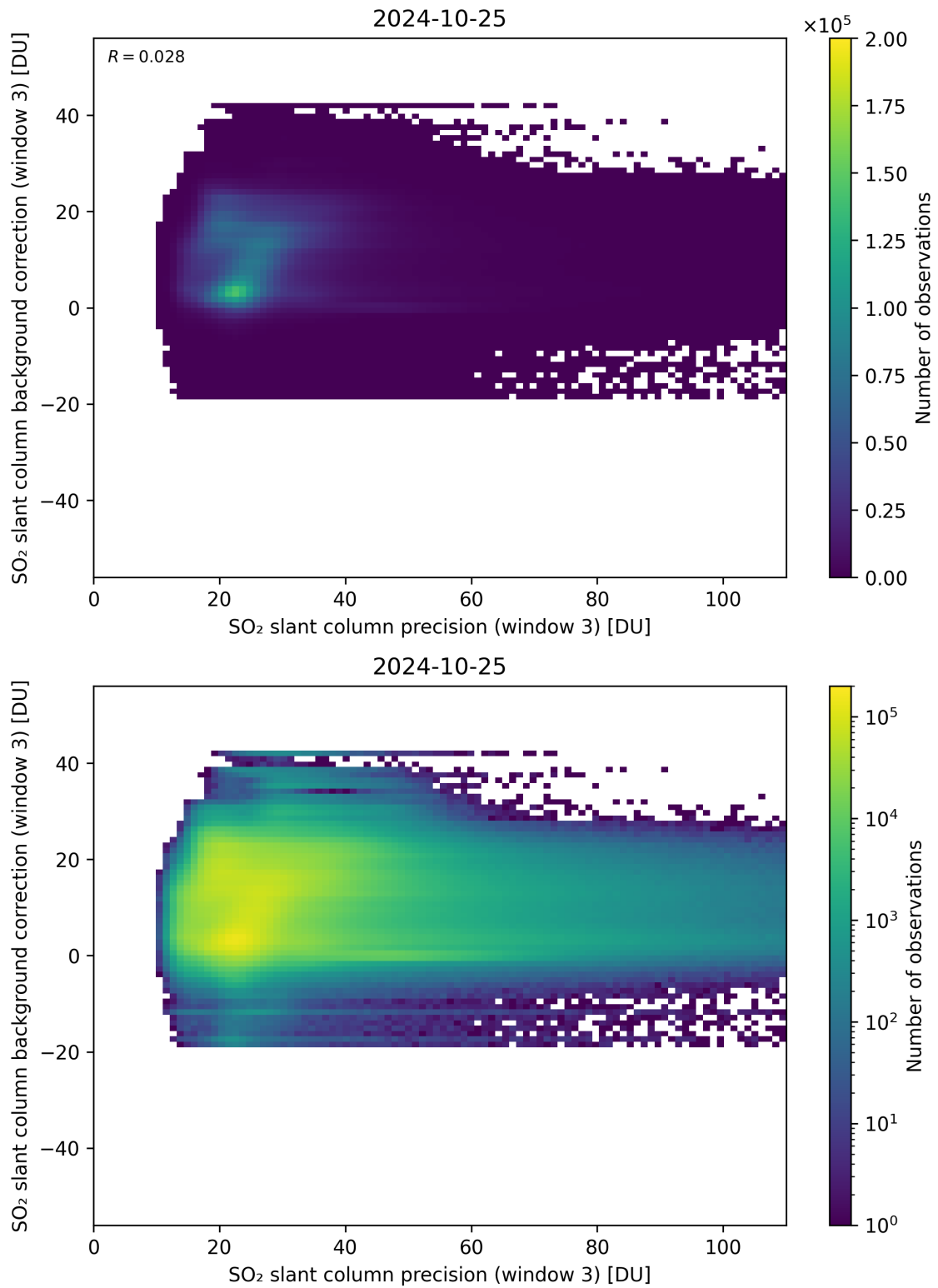
Figure 257: Scatter density plot of “SO 2 slant column precision (window 3)” against “SO 2 slant column background correction (window 3)” for 2024-10-24 to 2024-10-26.
