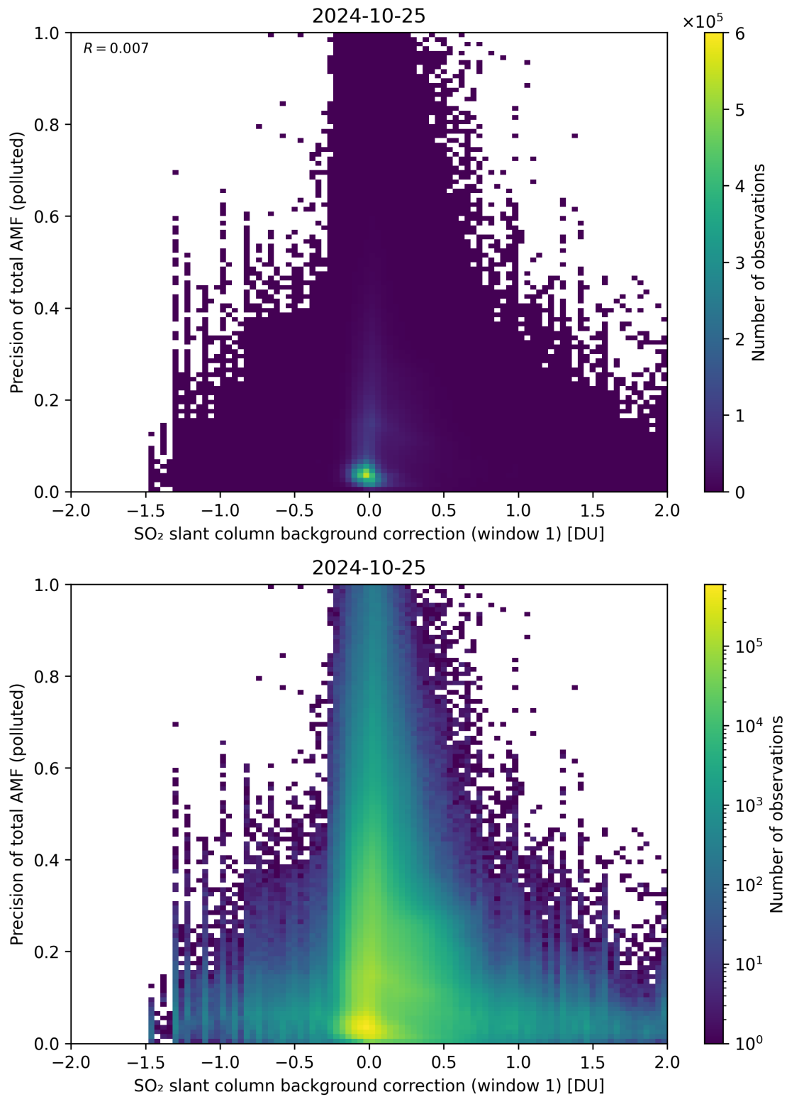
Figure 110: Scatter density plot of “SO 2 slant column background correction (window 1)” against “Precision of total AMF (polluted)” for 2024-10-24 to 2024-10-26.
