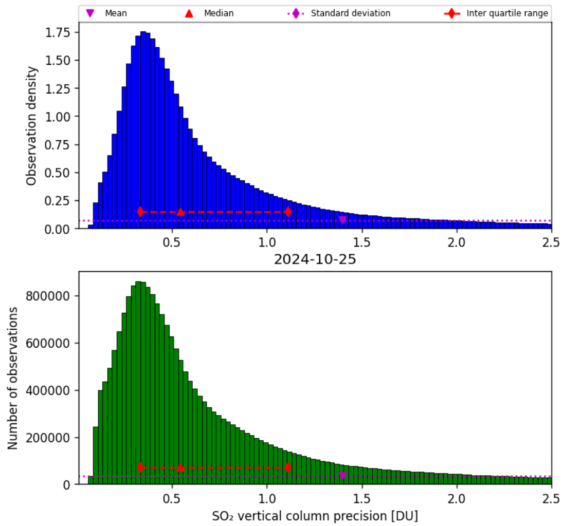
Figure 54: Histogram of “SO 2 vertical column precision” for 2024-10-24 to 2024-10-26
