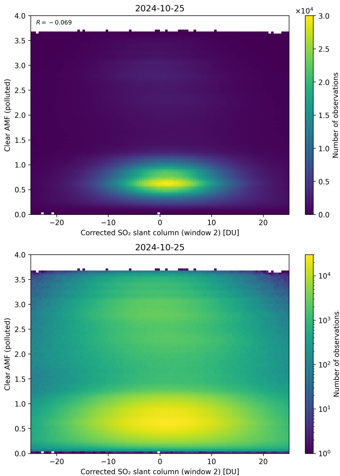
Figure 199: Scatter density plot of “Corrected SO 2 slant column (window 2)” against “Clear AMF (polluted)” for 2024-10-24 to 2024-10-26.
