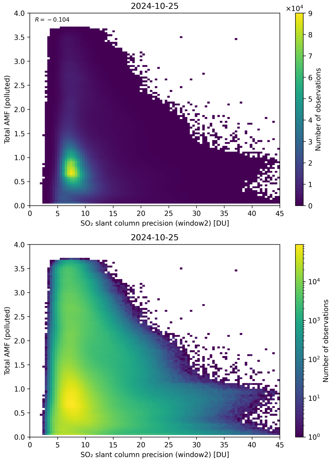
Figure 251: Scatter density plot of “SO 2 slant column precision (window2)” against “Total AMF (polluted)” for 2024-10-24 to 2024-10-26.
