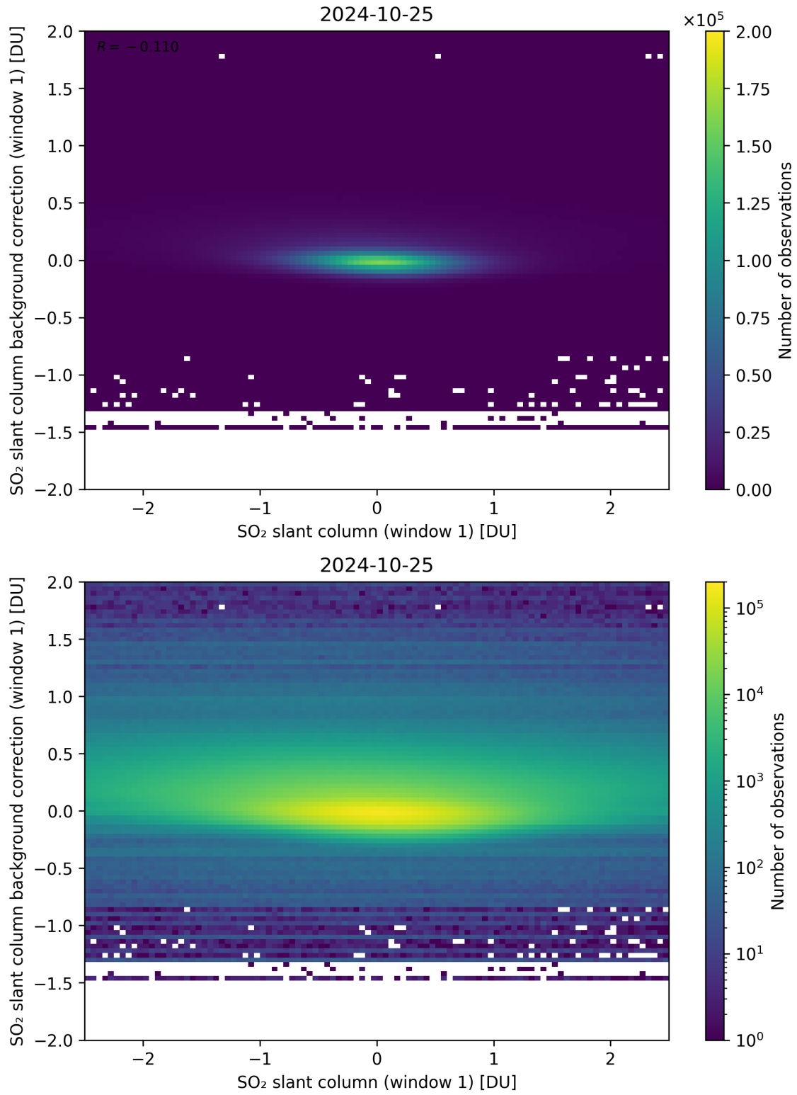
Figure 212: Scatter density plot of “SO 2 slant column (window 1)” against “SO 2 slant column background correction (window 1)” for 2024-10-24 to 2024-10-26.
