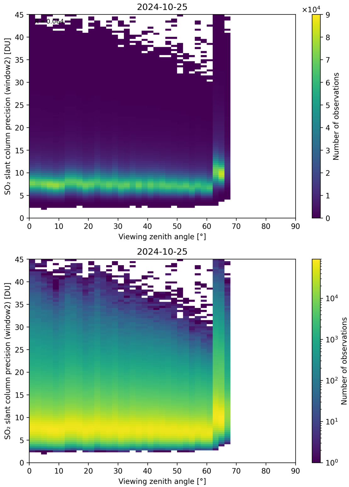
Figure 322: Scatter density plot of “Viewing zenith angle” against “SO 2 slant column precision (window2)” for 2024-10-24 to 2024-10-26.
