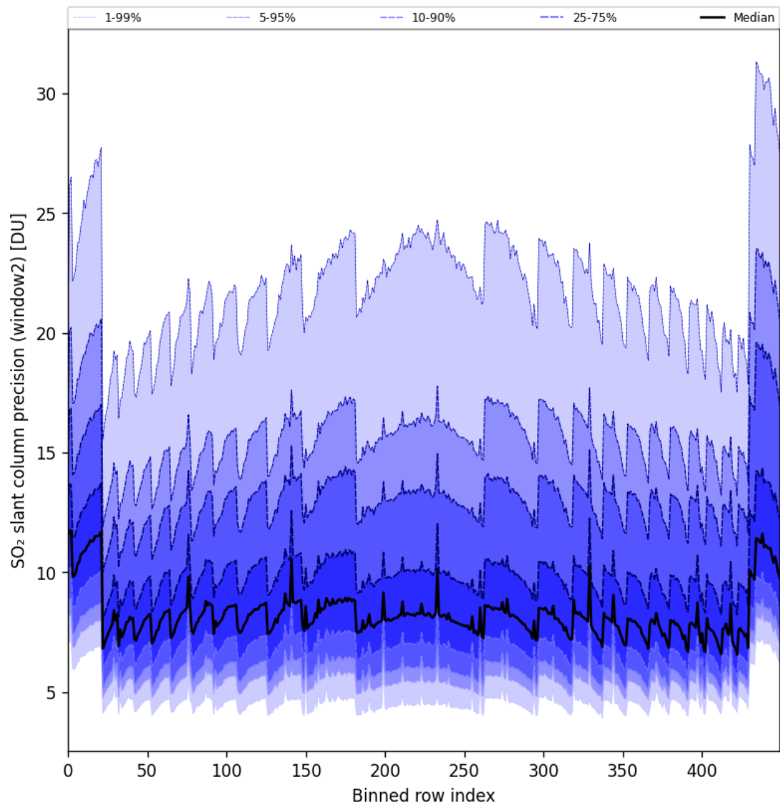
Figure 84: Along track statistics of “SO 2 slant column precision (window2)” for 2024-10-24 to 2024-10-26
