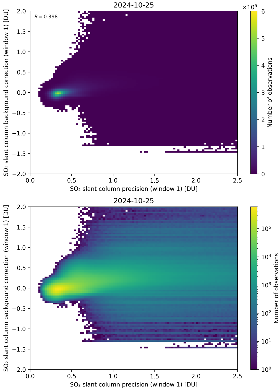
Figure 218: Scatter density plot of “SO 2 slant column precision (window 1)” against “SO 2 slant column background correction (window 1)” for 2024-10-24 to 2024-10-26.
