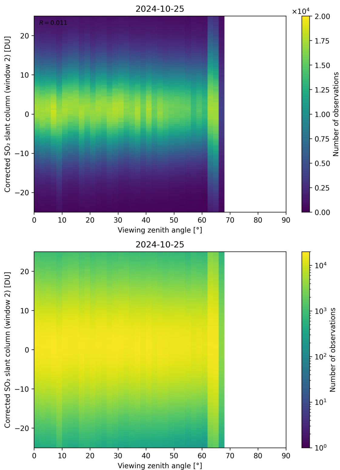
Figure 318: Scatter density plot of “Viewing zenith angle” against “Corrected SO 2 slant column (window 2)” for 2024-10-24 to 2024-10-26.
