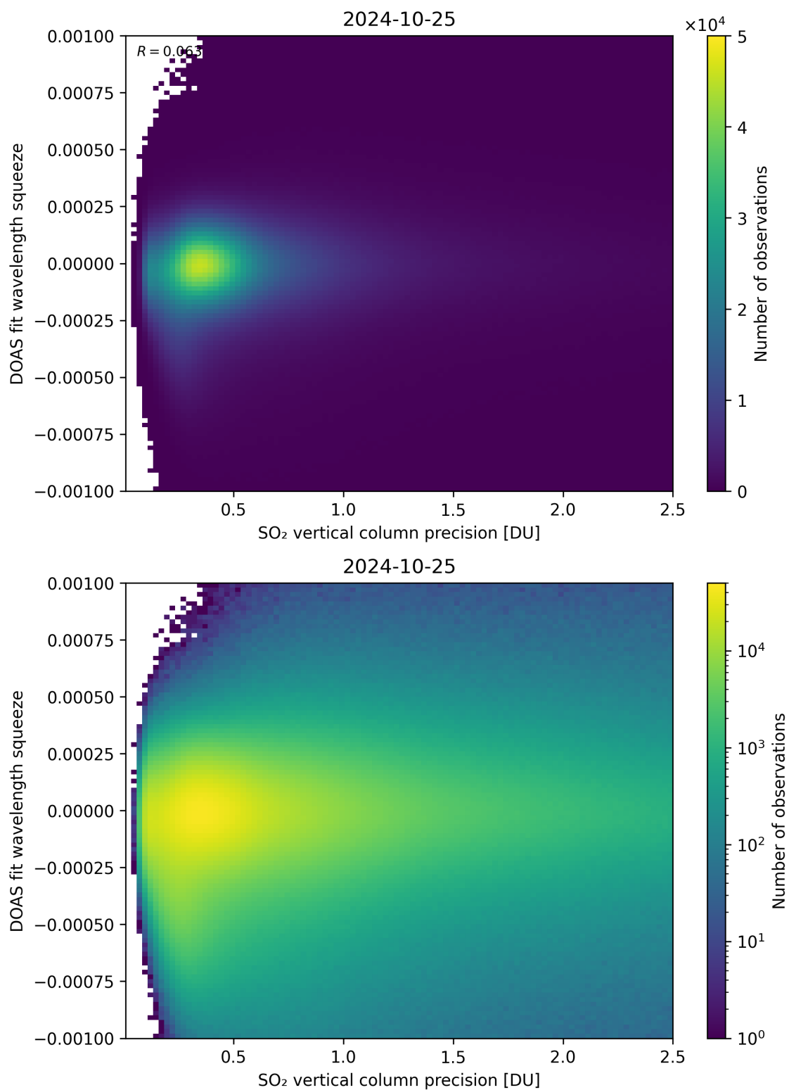
Figure 283: Scatter density plot of “SO 2 vertical column precision” against “DOAS fit wavelength squeeze” for 2024-10-24 to 2024-10-26.
