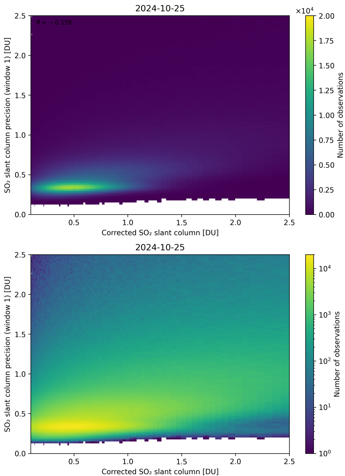
Figure 188: Scatter density plot of “Corrected SO 2 slant column” against “SO 2 slant column precision (window 1)” for 2024-10-24 to 2024-10-26.
