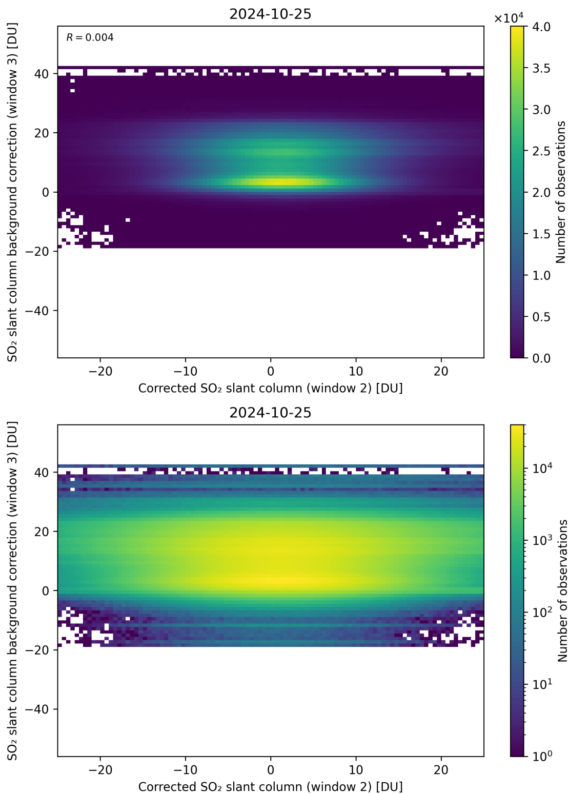
Figure 195: Scatter density plot of “Corrected SO 2 slant column (window 2)” against “SO 2 slant column background correction (window 3)” for 2024-10-24 to 2024-10-26.
