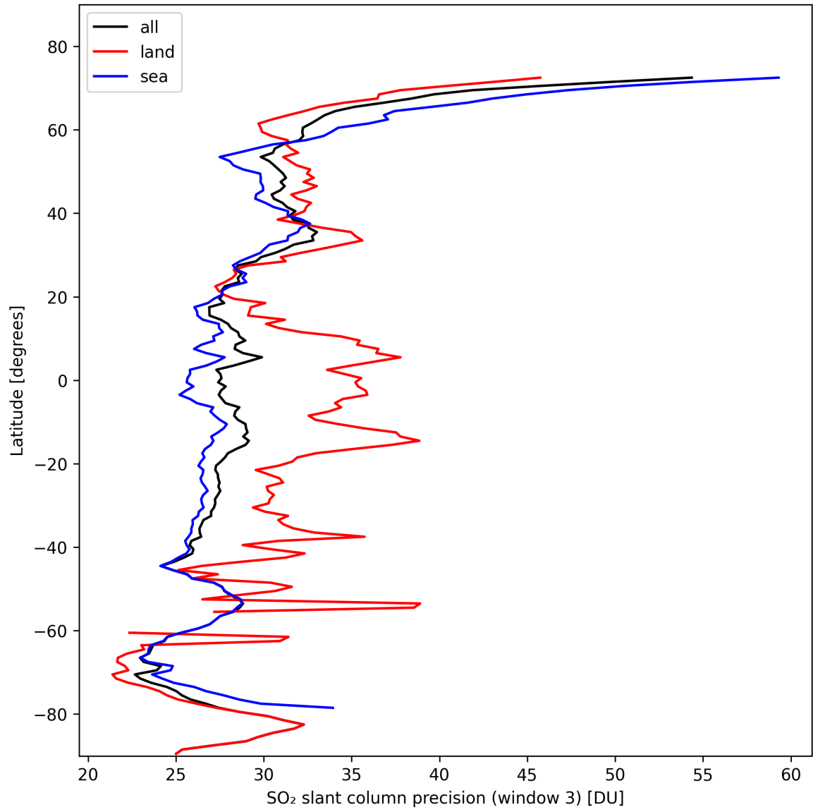
Figure 42: Zonal average of “SO 2 slant column precision (window 3)” for 2024-10-24 to 2024-10-26.
