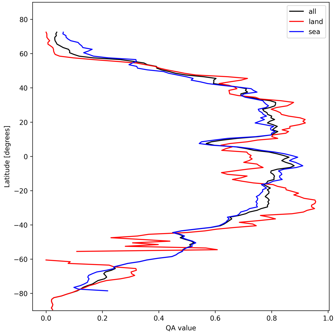
Figure 29: Zonal average of “QA value” for 2024-10-24 to 2024-10-26.
