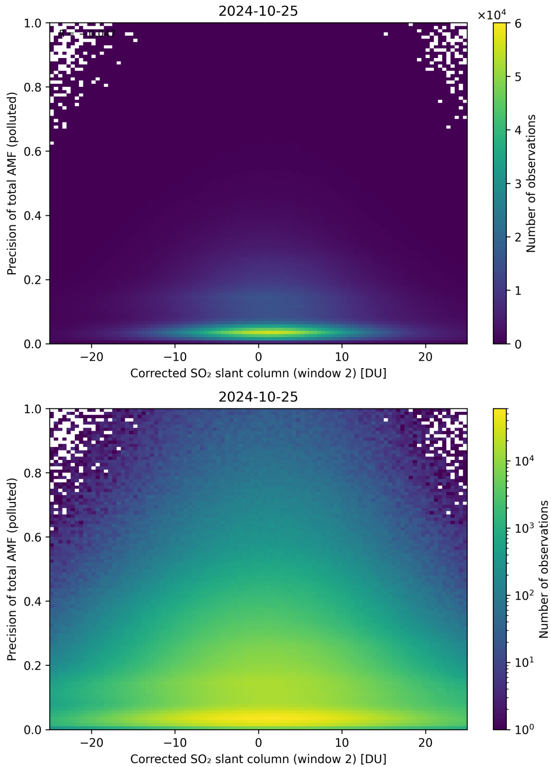
Figure 204: Scatter density plot of “Corrected SO 2 slant column (window 2)” against “Precision of total AMF (polluted)” for 2024-10-24 to 2024-10-26.
