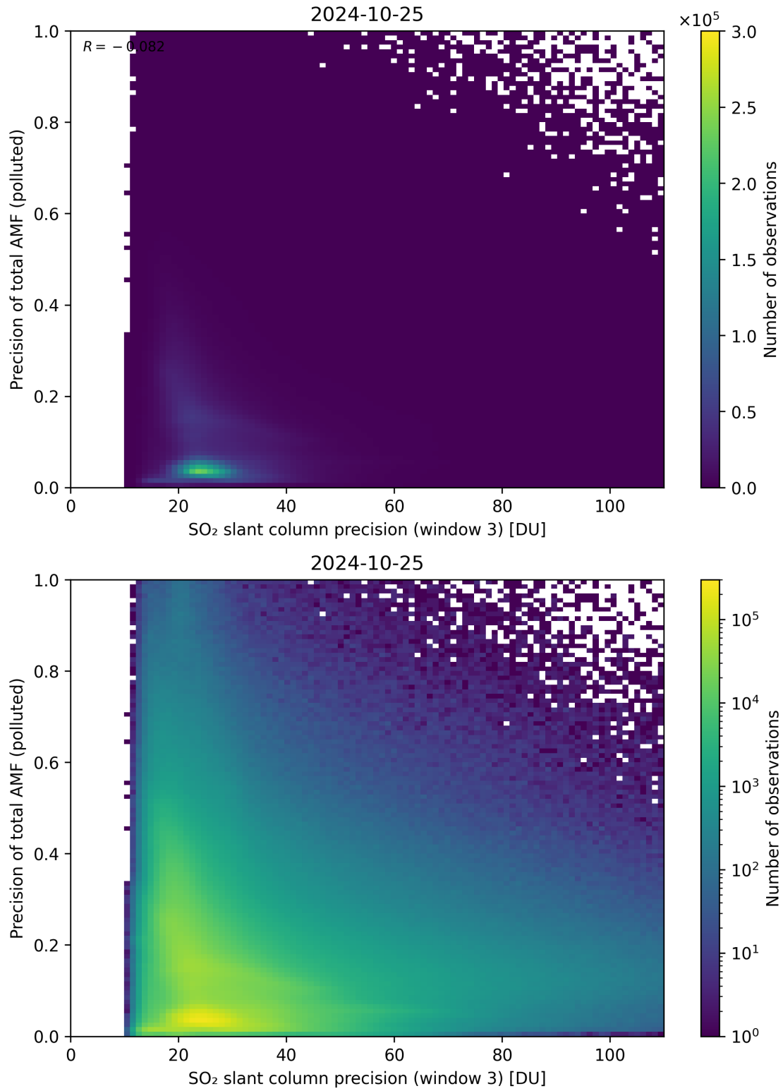
Figure 264: Scatter density plot of “SO 2 slant column precision (window 3)” against “Precision of total AMF (polluted)” for 2024-10-24 to 2024-10-26.
