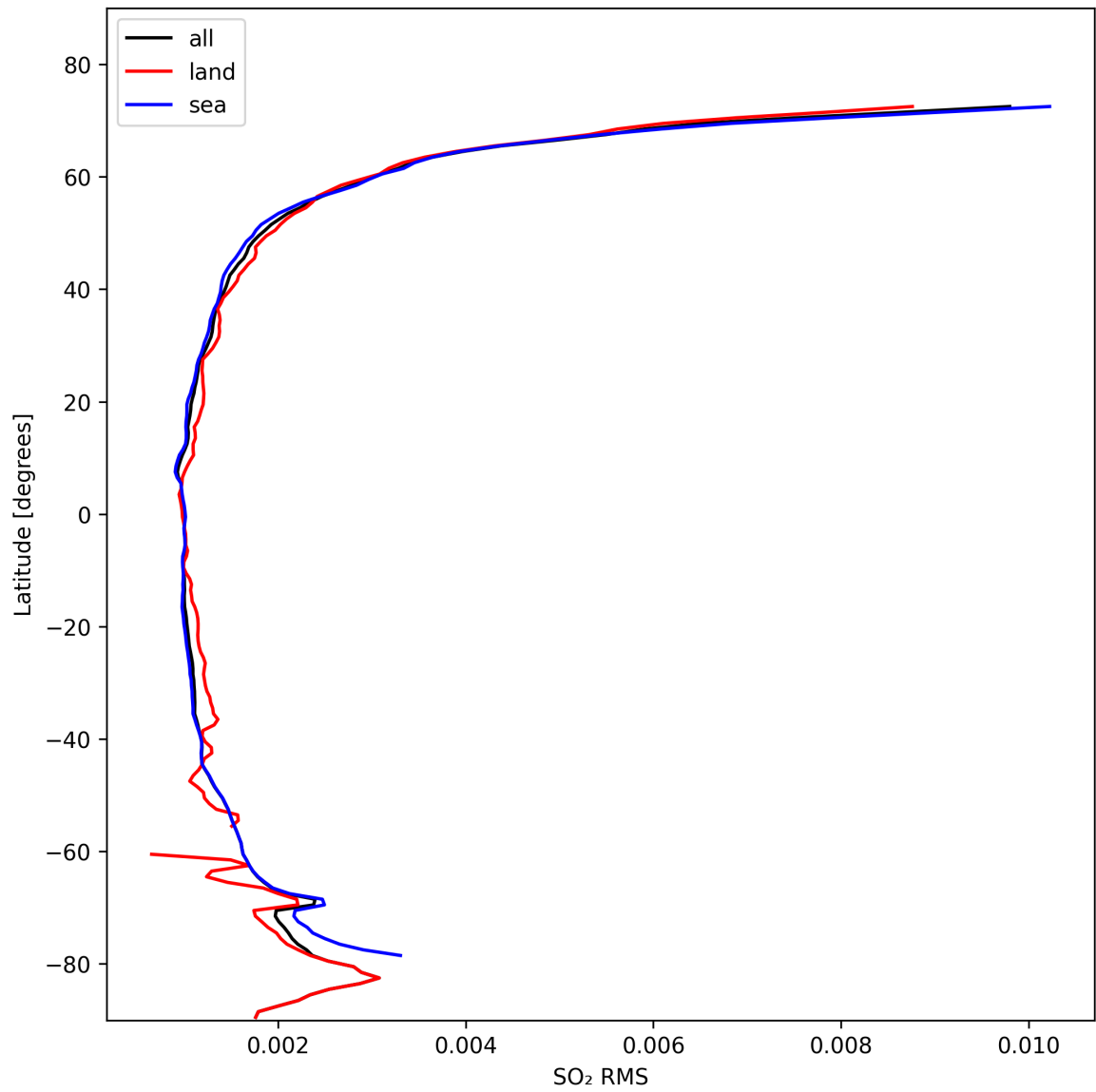
Figure 47: Zonal average of “SO 2 RMS” for 2024-10-24 to 2024-10-26.
