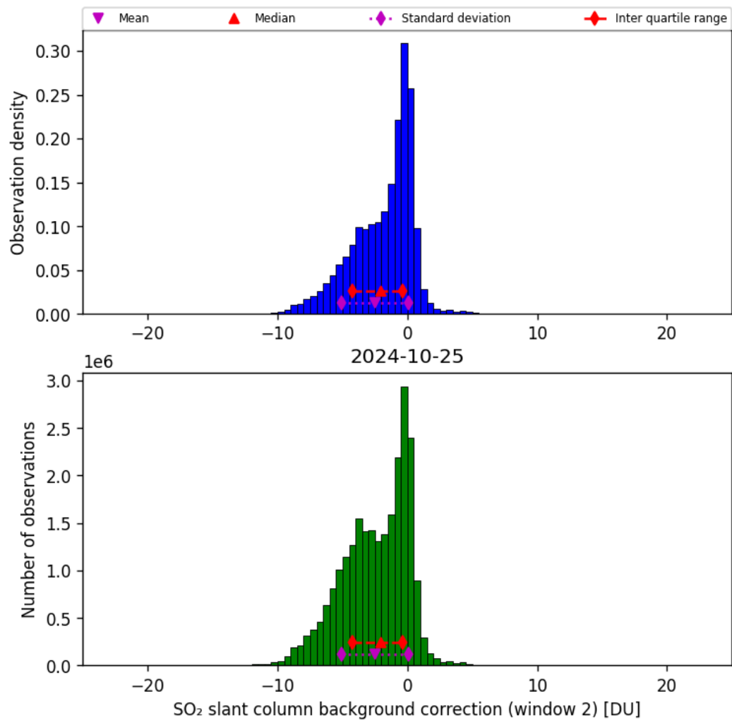
Figure 63: Histogram of “SO 2 slant column background correction (window 2)” for 2024-10-24 to 2024-10-26
