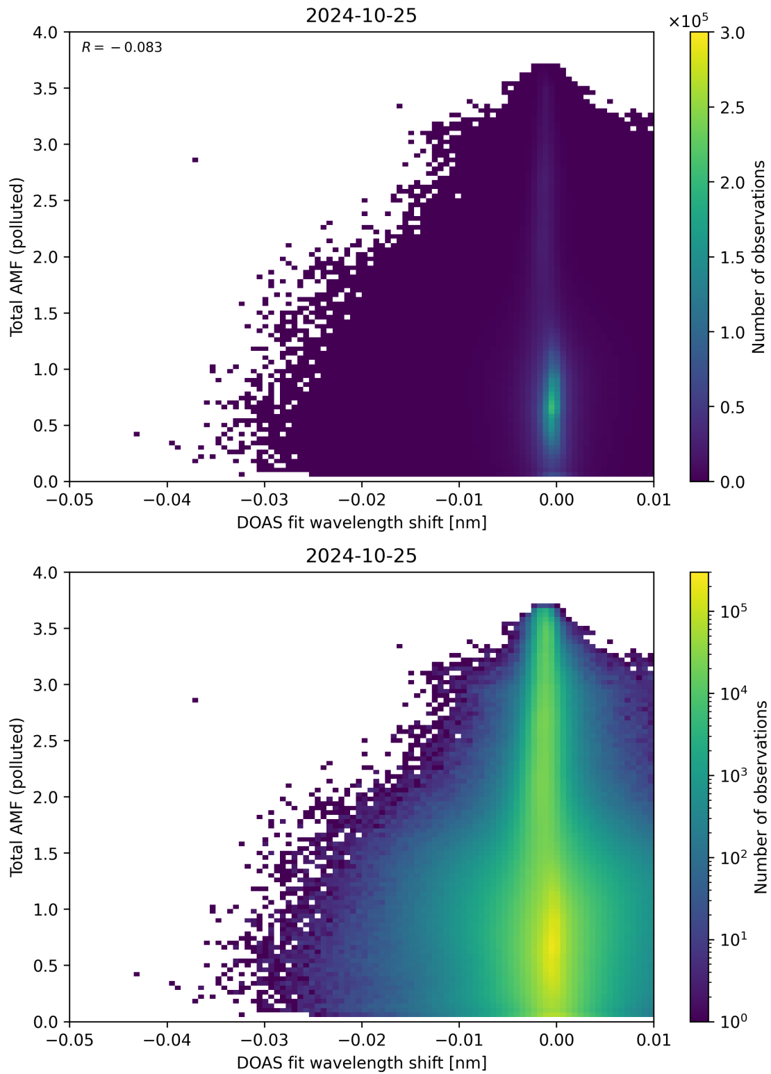
Figure 130: Scatter density plot of “DOAS fit wavelength shift” against “Total AMF (polluted)” for 2024-10-24 to 2024-10-26.
