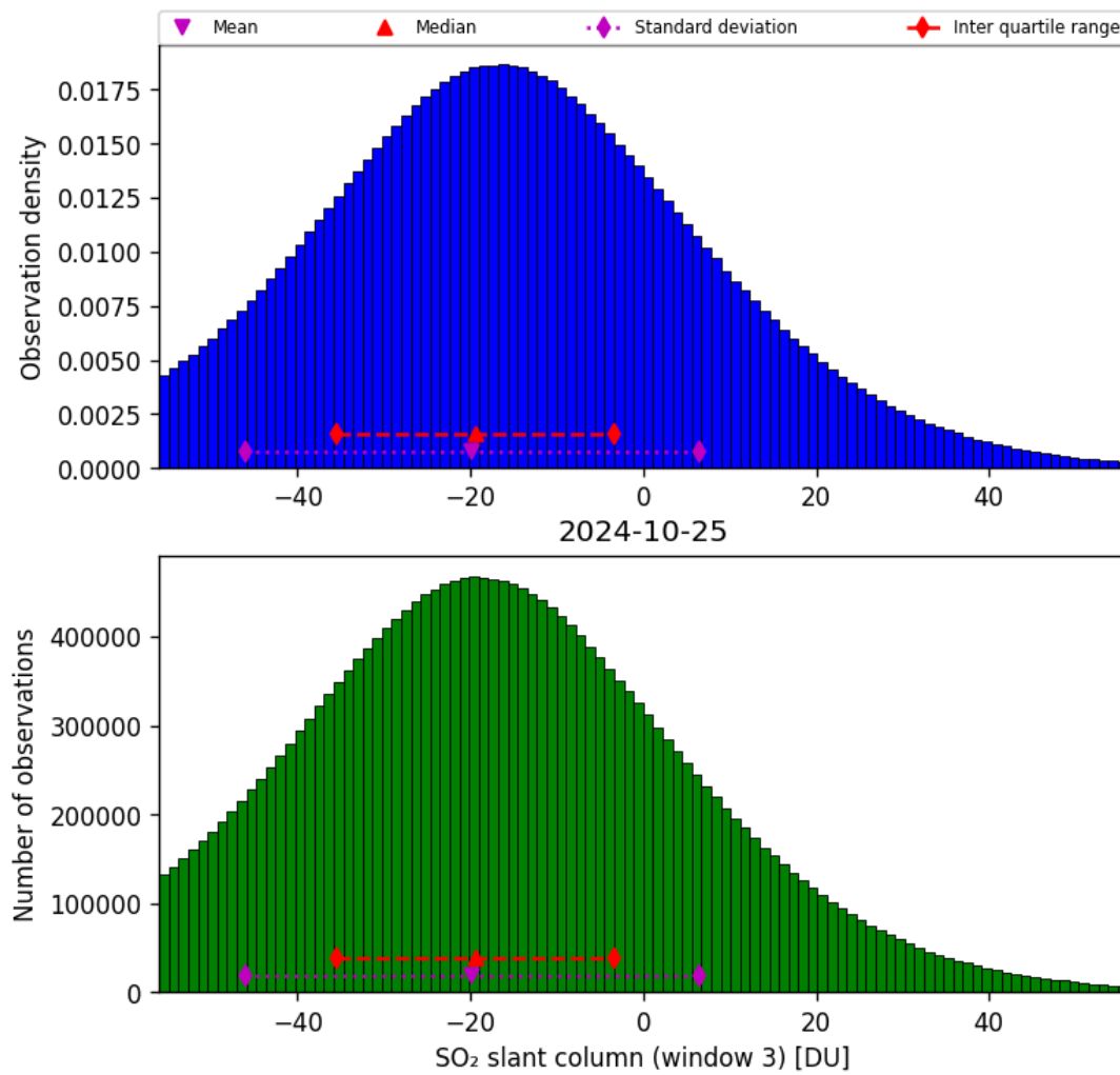
Figure 64: Histogram of “SO 2 slant column (window 3)” for 2024-10-24 to 2024-10-26
