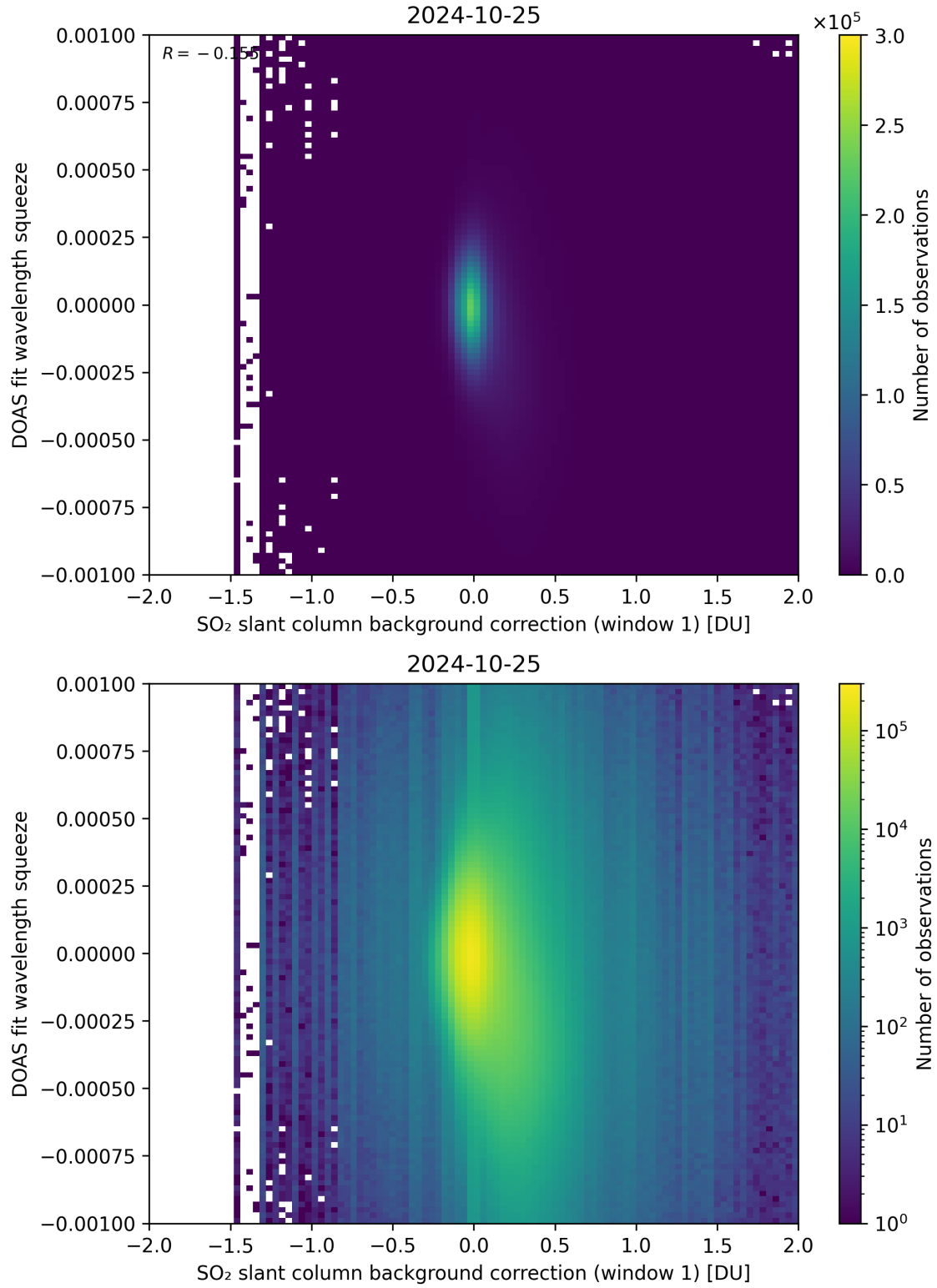
Figure 101: Scatter density plot of “SO 2 slant column background correction (window 1)” against “DOAS fit wavelength squeeze” for 2024-10-24 to 2024-10-26.
