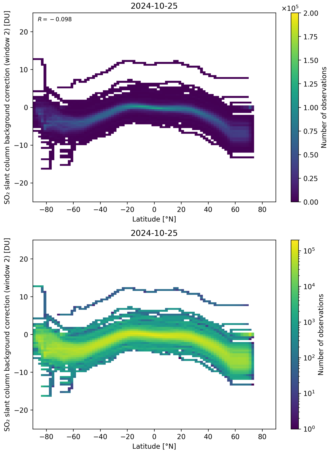
Figure 140: Scatter density plot of “Latitude” against “SO 2 slant column background correction (window 2)” for 2024-10-24 to 2024-10-26.
