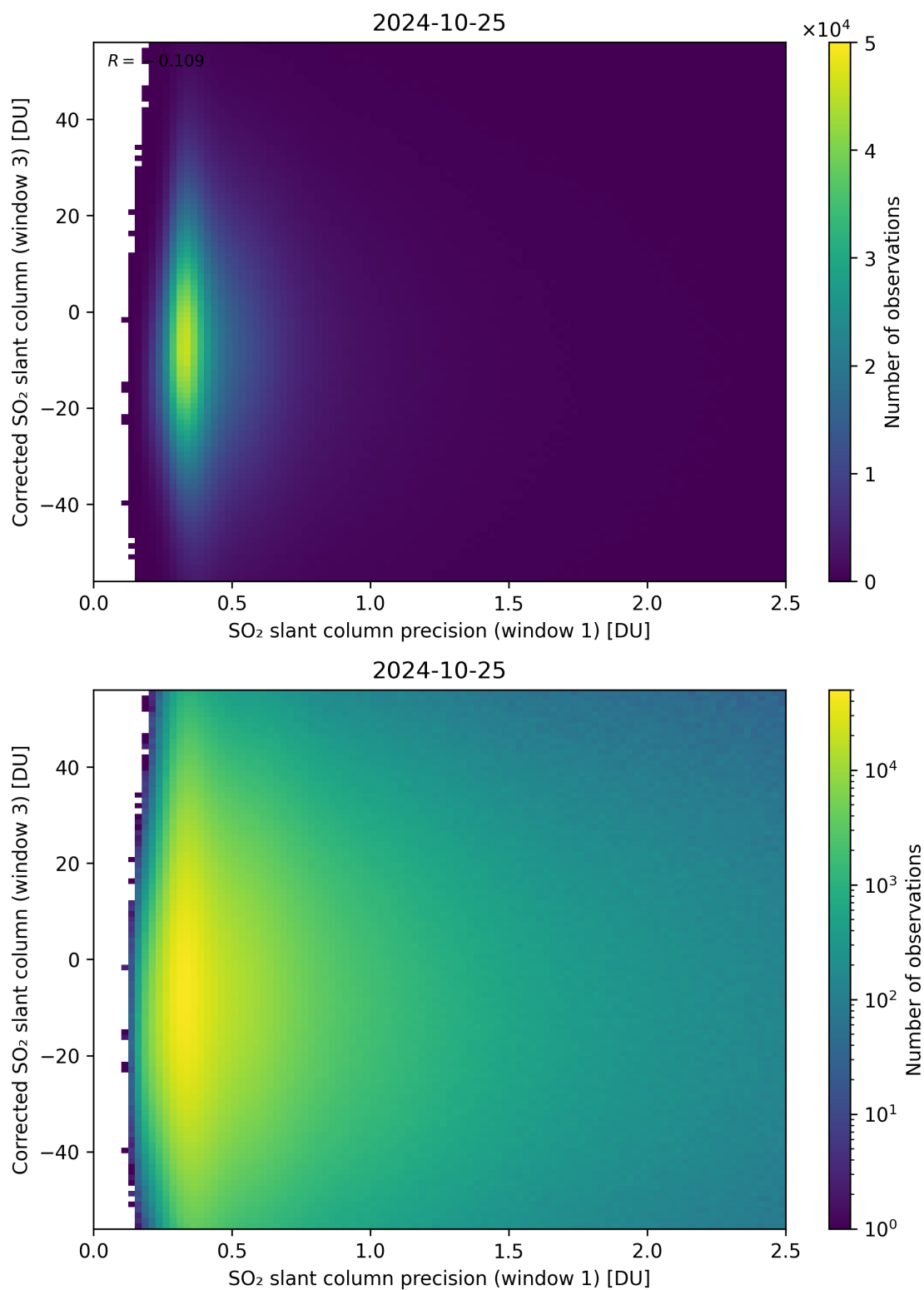
Figure 226: Scatter density plot of “SO 2 slant column precision (window 1)” against “Corrected SO 2 slant column (window 3)” for 2024-10-24 to 2024-10-26.
