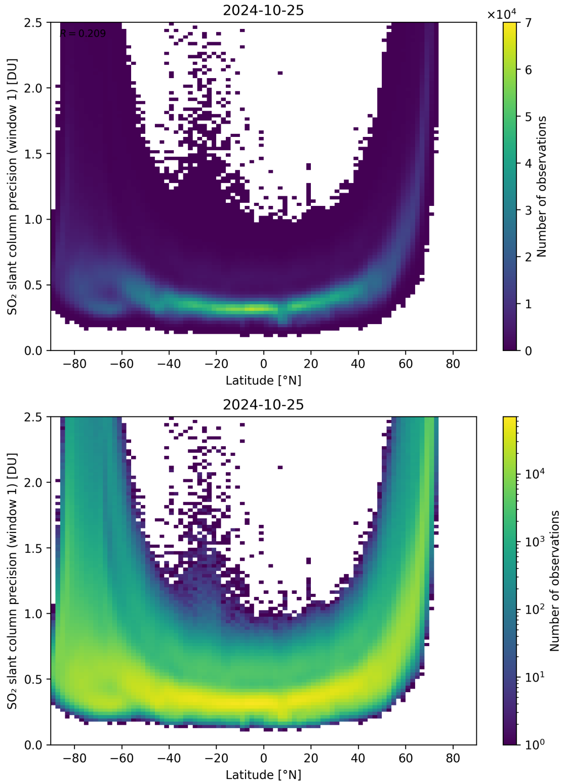
Figure 150: Scatter density plot of “Latitude” against “SO 2 slant column precision (window 1)” for 2024-10-24 to 2024-10-26.
