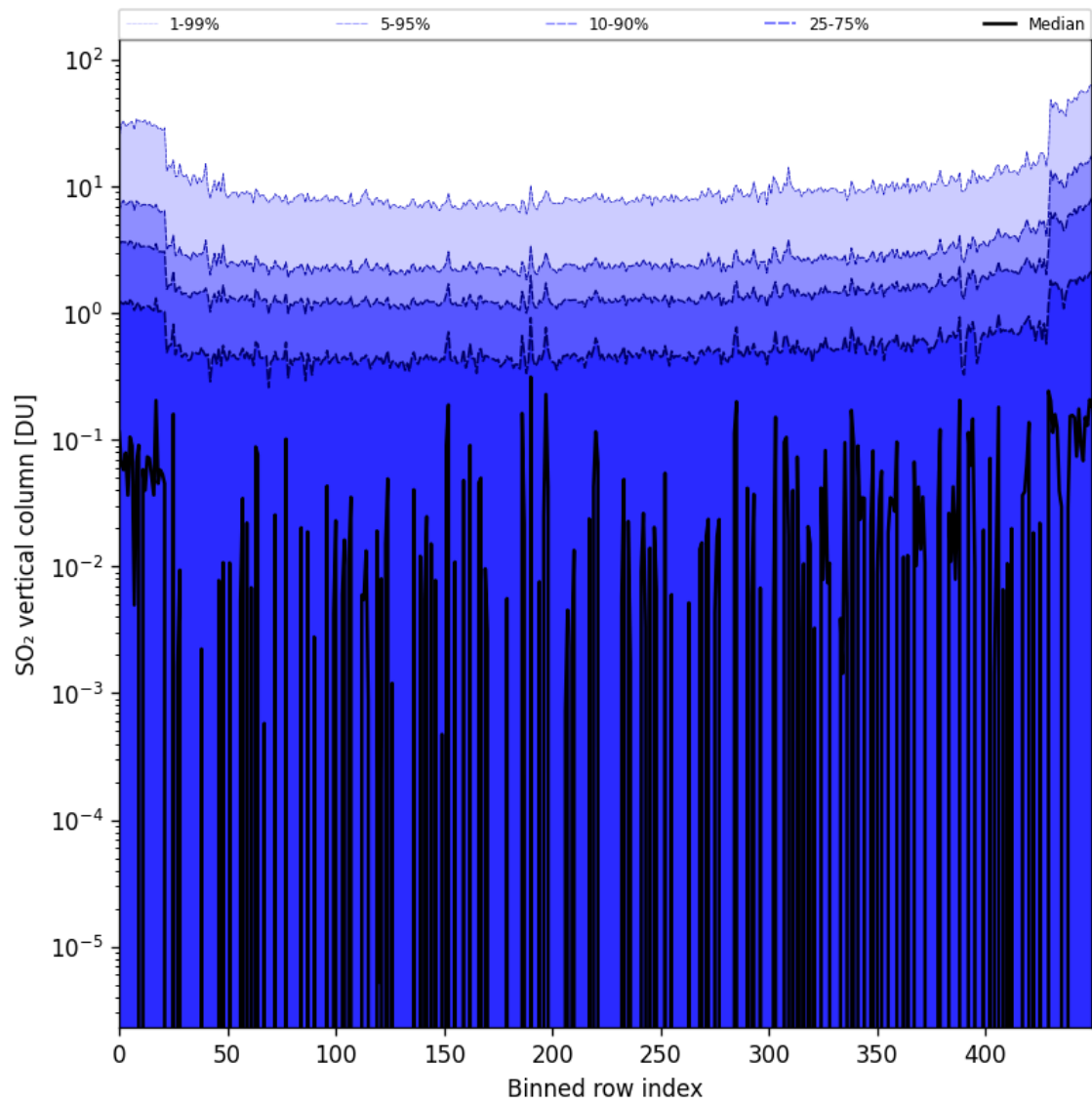
Figure 76: Along track statistics of “SO 2 vertical column” for 2024-10-24 to 2024-10-26
