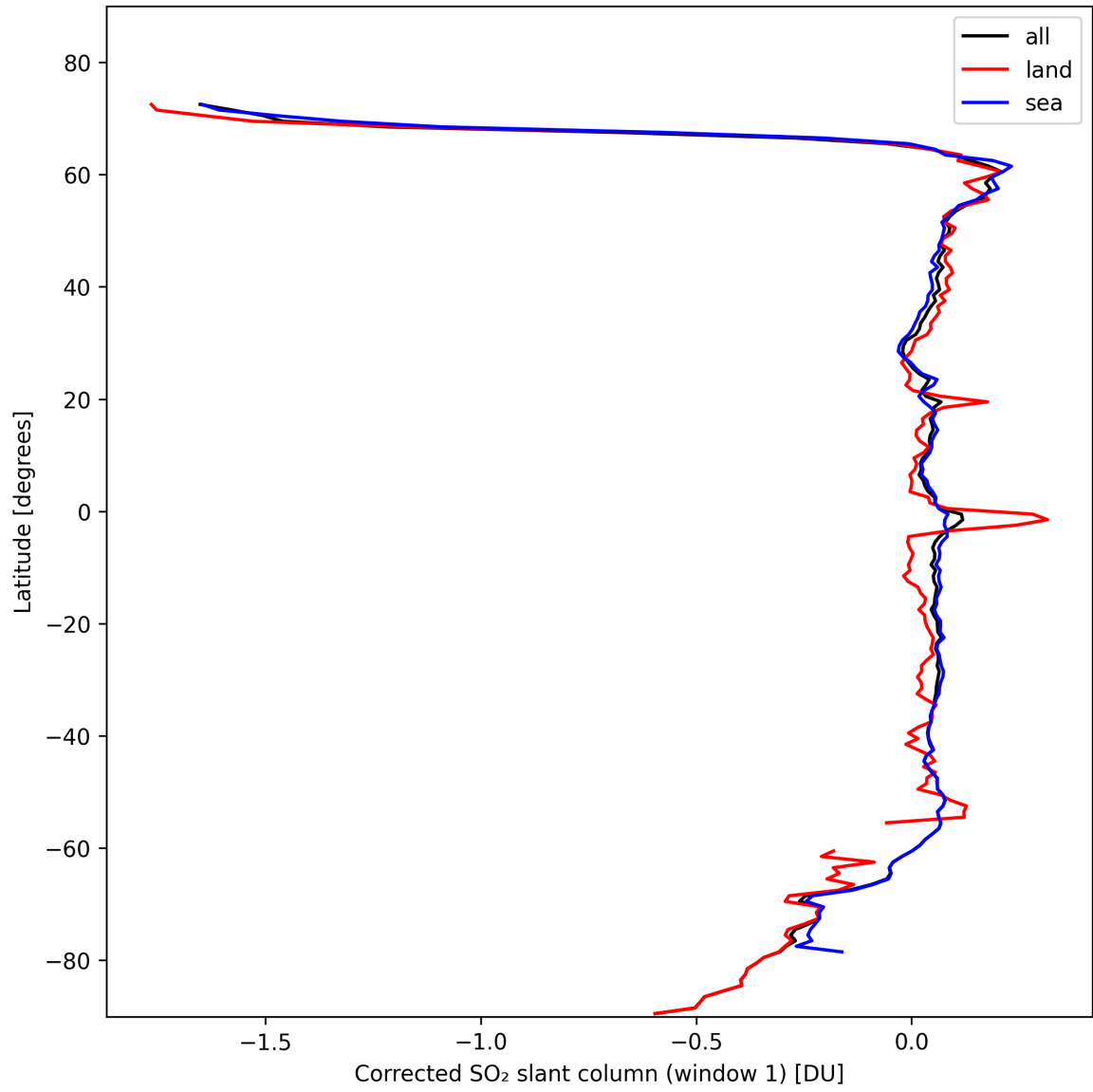
Figure 35: Zonal average of “Corrected SO 2 slant column (window 1)” for 2024-10-24 to 2024-10-26.
