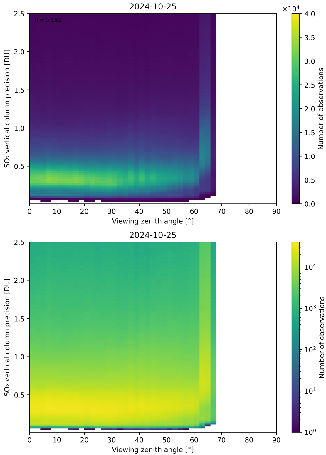
Figure 328: Scatter density plot of “Viewing zenith angle” against “SO 2 vertical column precision” for 2024-10-24 to 2024-10-26.
