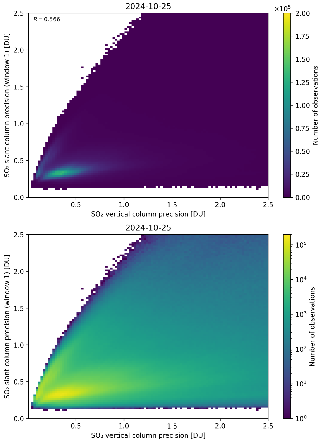
Figure 290: Scatter density plot of “SO 2 vertical column precision” against “SO 2 slant column precision (window 1)” for 2024-10-24 to 2024-10-26.
