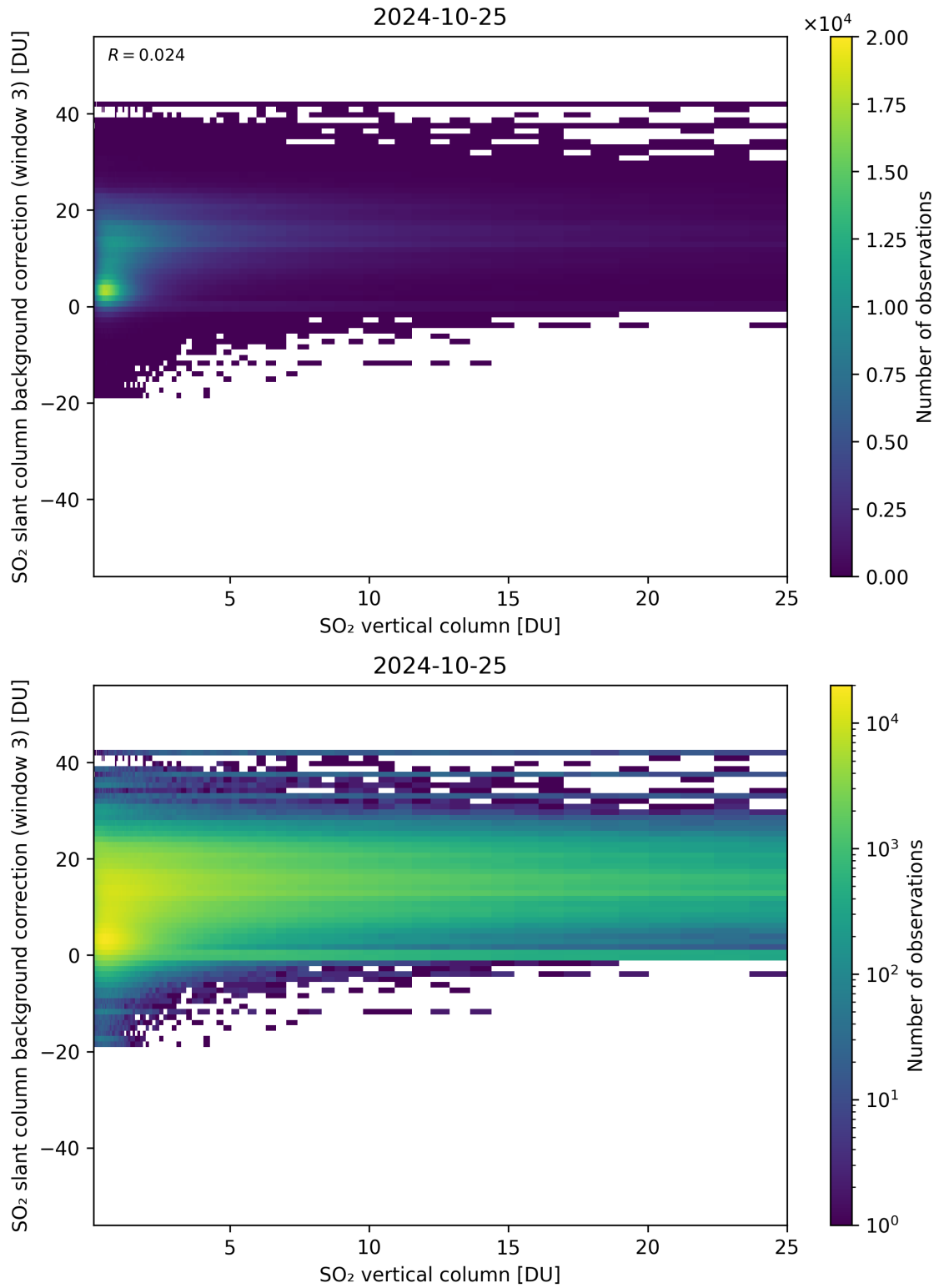
Figure 275: Scatter density plot of “SO 2 vertical column” against “SO 2 slant column background correction (window 3)” for 2024-10-24 to 2024-10-26.
