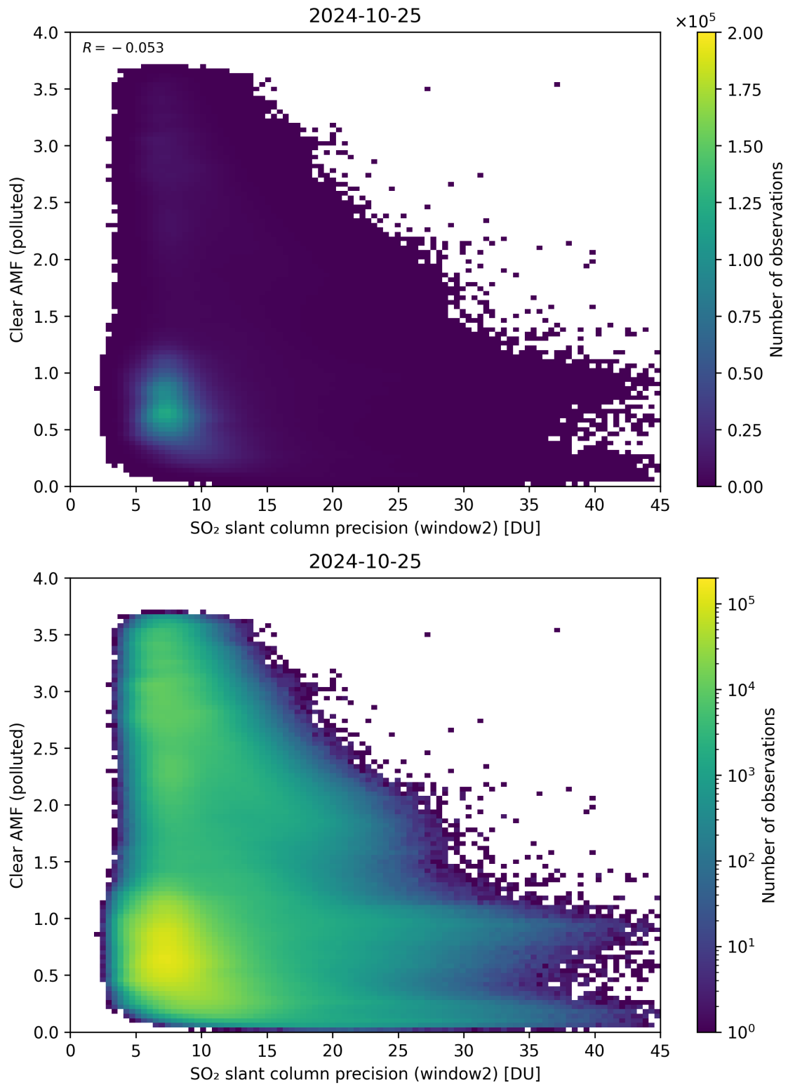
Figure 246: Scatter density plot of “SO 2 slant column precision (window2)” against “Clear AMF (polluted)” for 2024-10-24 to 2024-10-26.
