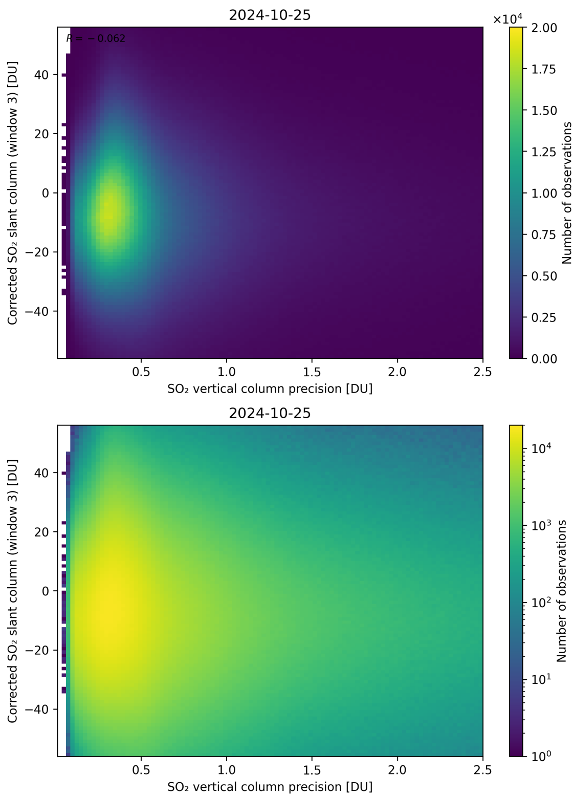
Figure 288: Scatter density plot of “SO 2 vertical column precision” against “Corrected SO 2 slant column (window 3)” for 2024-10-24 to 2024-10-26.
