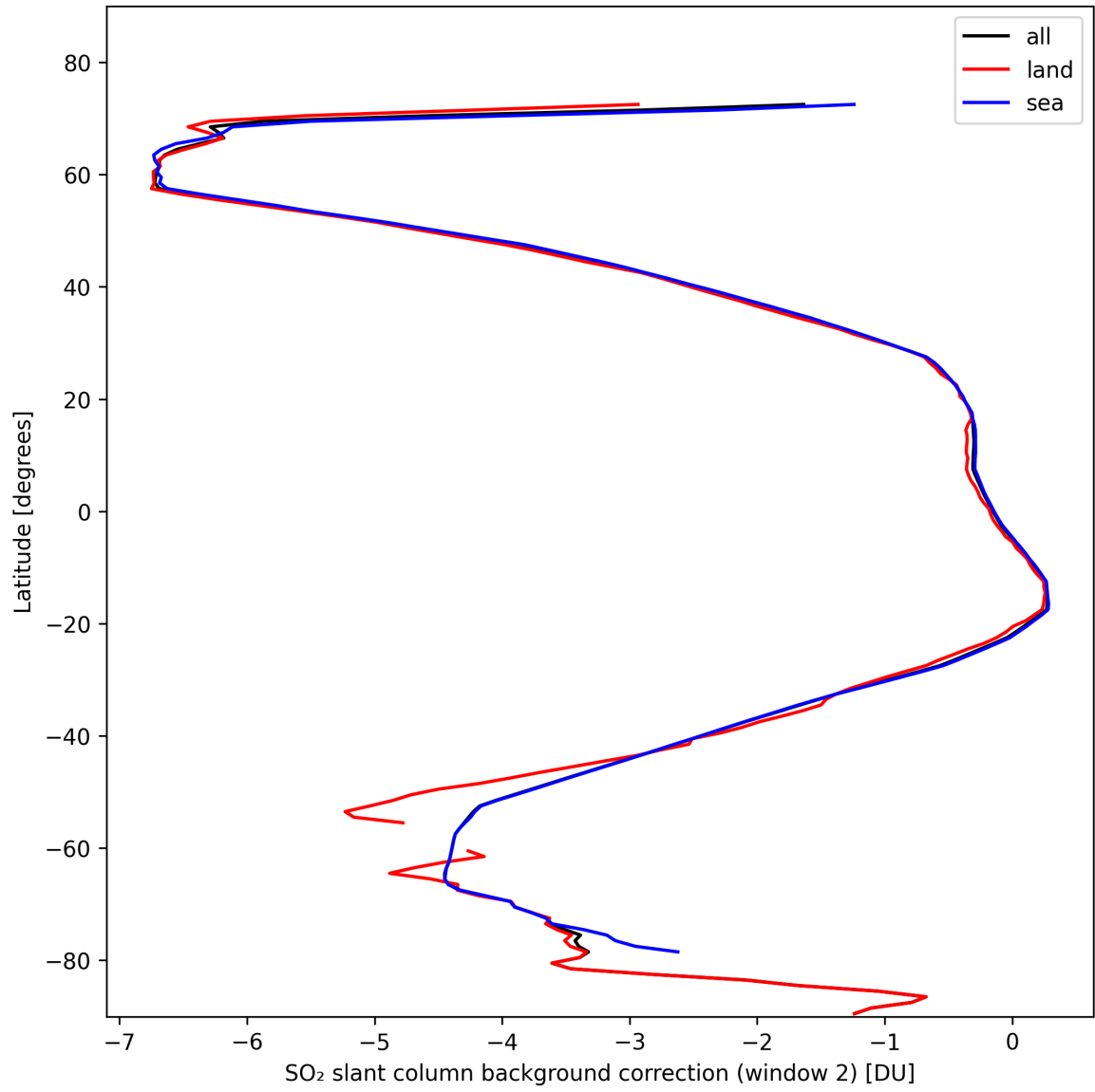
Figure 40: Zonal average of “SO 2 slant column background correction (window 2)” for 2024-10-24 to 2024-10-26.
