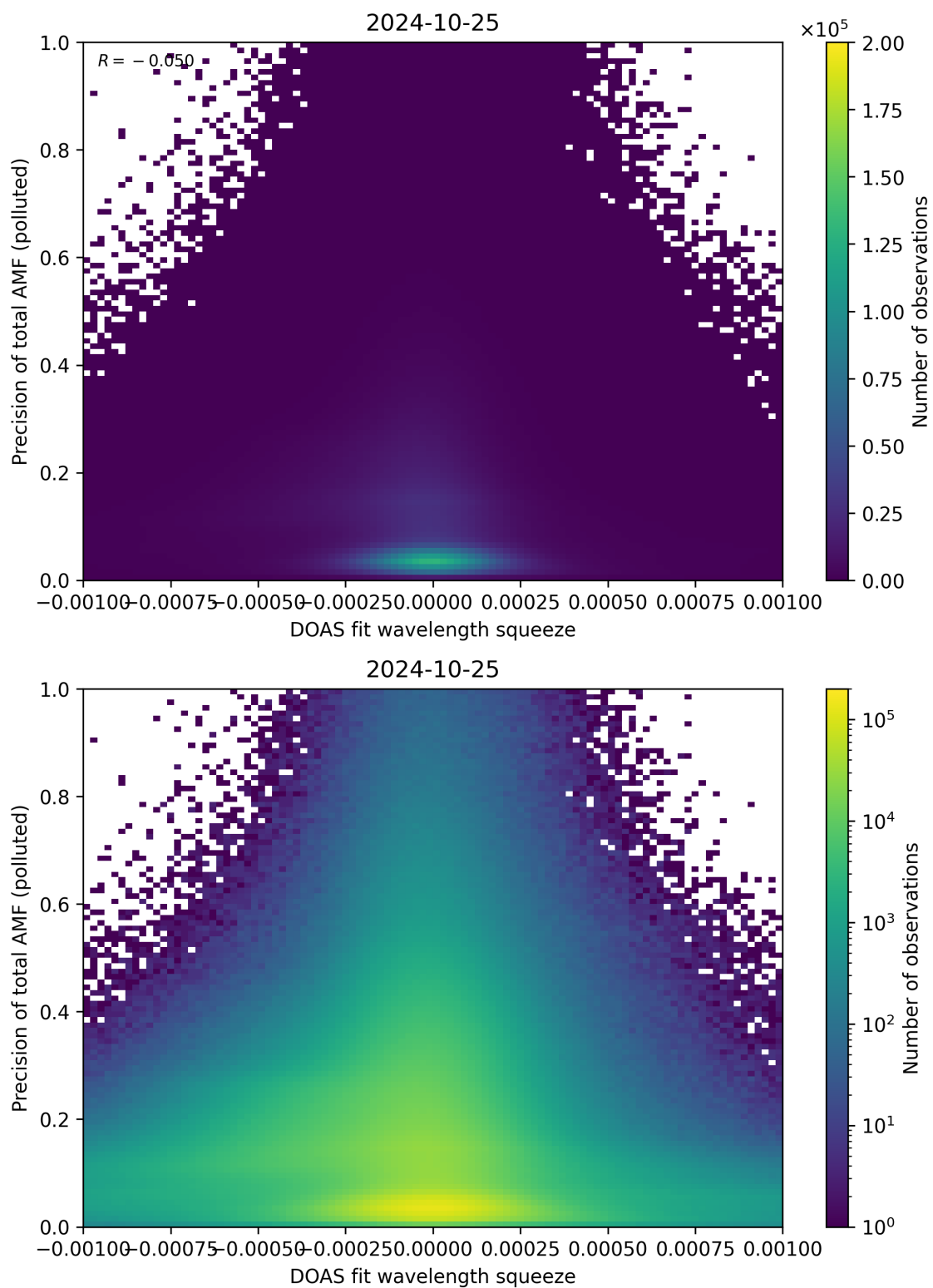
Figure 135: Scatter density plot of “DOAS fit wavelength squeeze” against “Precision of total AMF (polluted)” for 2024-10-24 to 2024-10-26.
