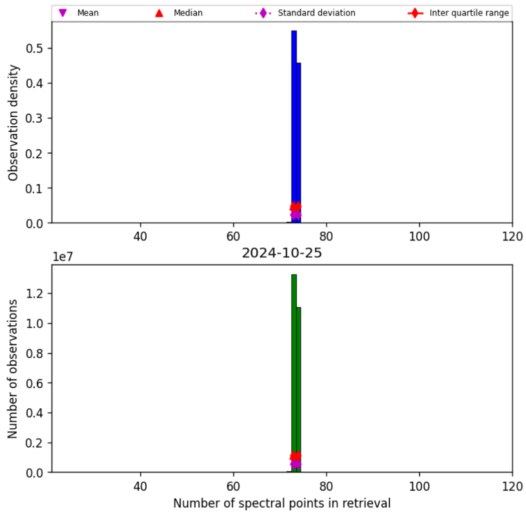
Figure 74: Histogram of “Number of spectral points in retrieval” for 2024-10-24 to 2024-10-26
