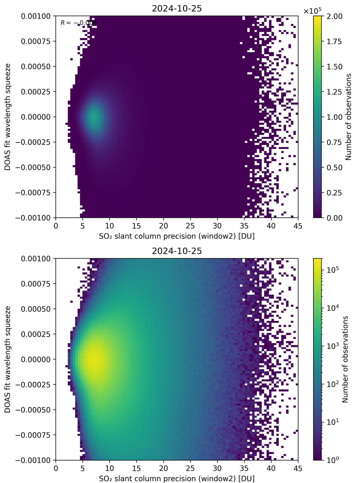
Figure 244: Scatter density plot of “SO 2 slant column precision (window2)” against “DOAS fit wavelength squeeze” for 2024-10-24 to 2024-10-26.
