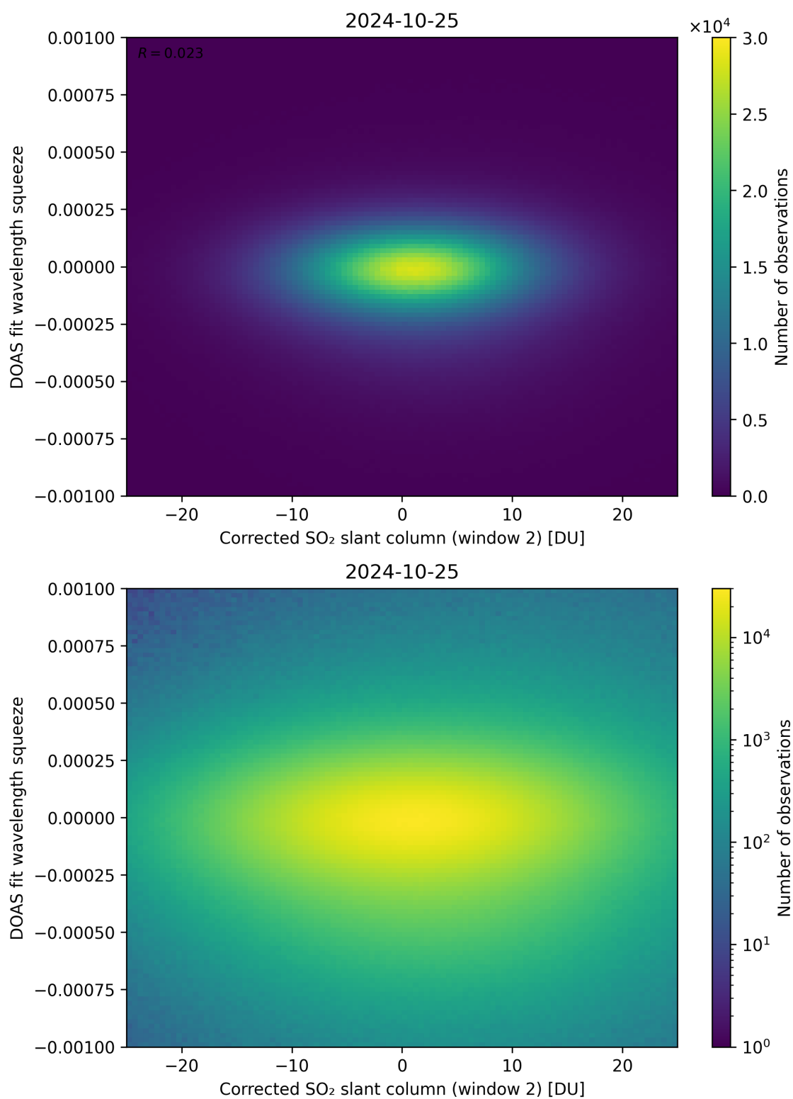
Figure 197: Scatter density plot of “Corrected SO 2 slant column (window 2)” against “DOAS fit wavelength squeeze” for 2024-10-24 to 2024-10-26.
