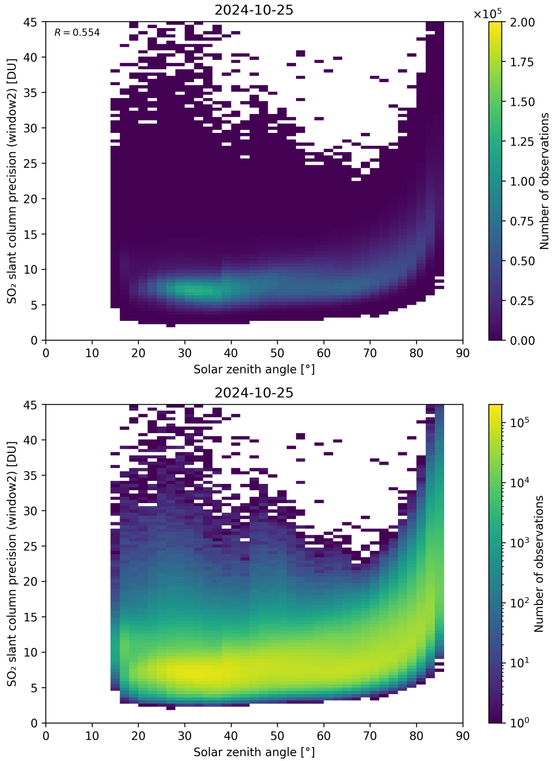
Figure 171: Scatter density plot of “Solar zenith angle” against “SO 2 slant column precision (window2)” for 2024-10-24 to 2024-10-26.
