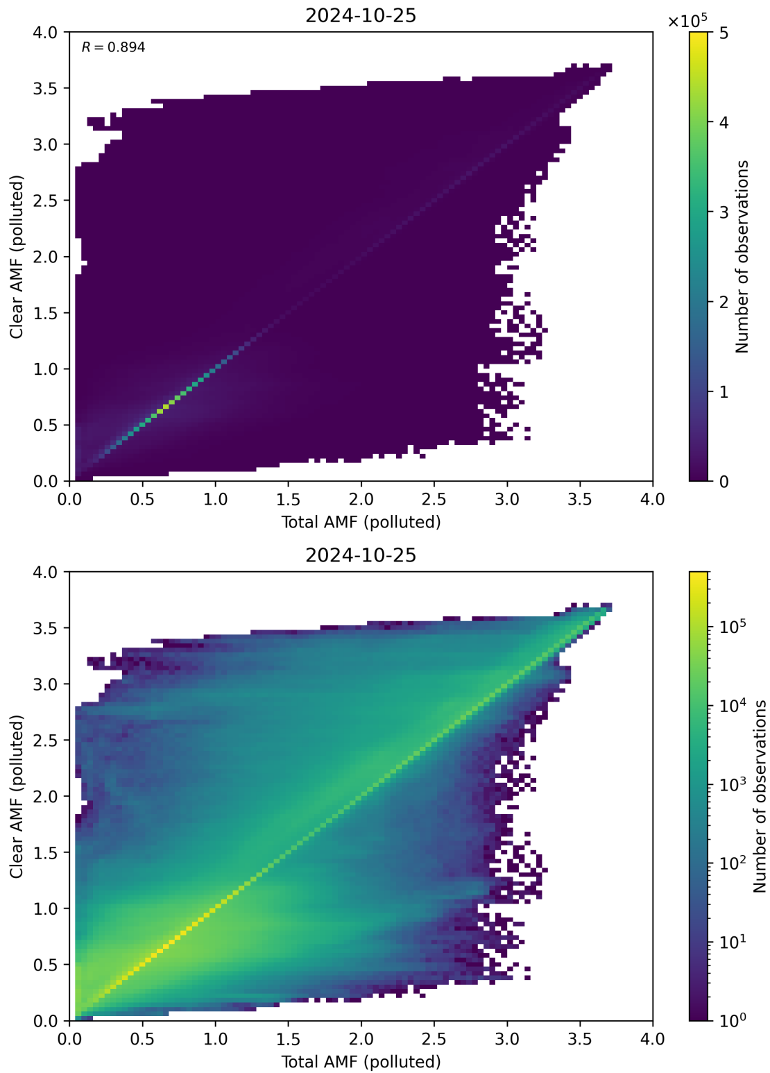
Figure 271: Scatter density plot of “Total AMF (polluted)” against “Clear AMF (polluted)” for 2024-10-24 to 2024-10-26.
