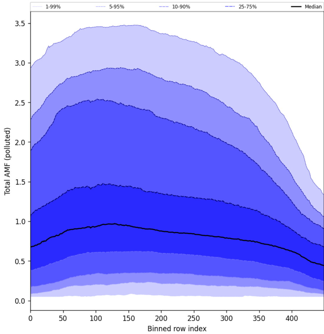
Figure 94: Along track statistics of “Total AMF (polluted)” for 2024-10-24 to 2024-10-26
