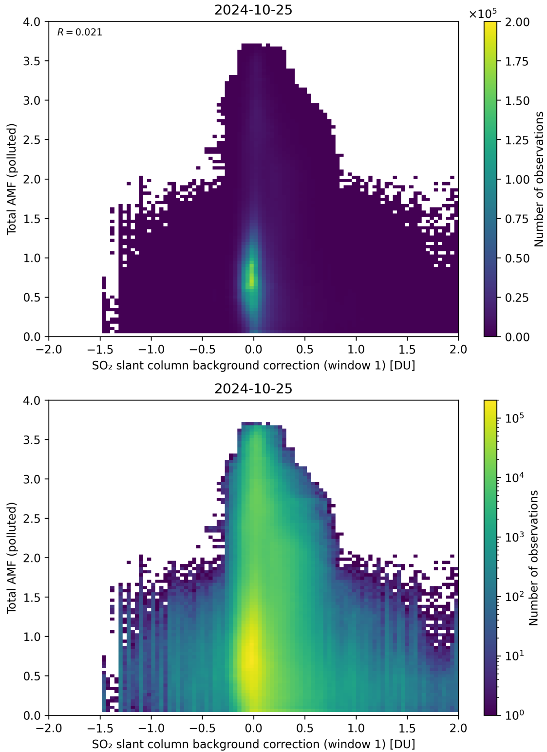
Figure 109: Scatter density plot of “SO 2 slant column background correction (window 1)” against “Total AMF (polluted)” for 2024-10-24 to 2024-10-26.
