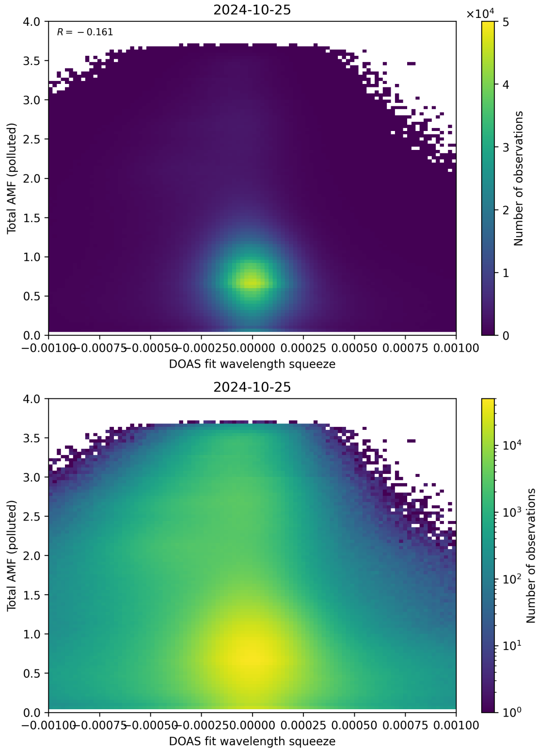
Figure 134: Scatter density plot of “DOAS fit wavelength squeeze” against “Total AMF (polluted)” for 2024-10-24 to 2024-10-26.
