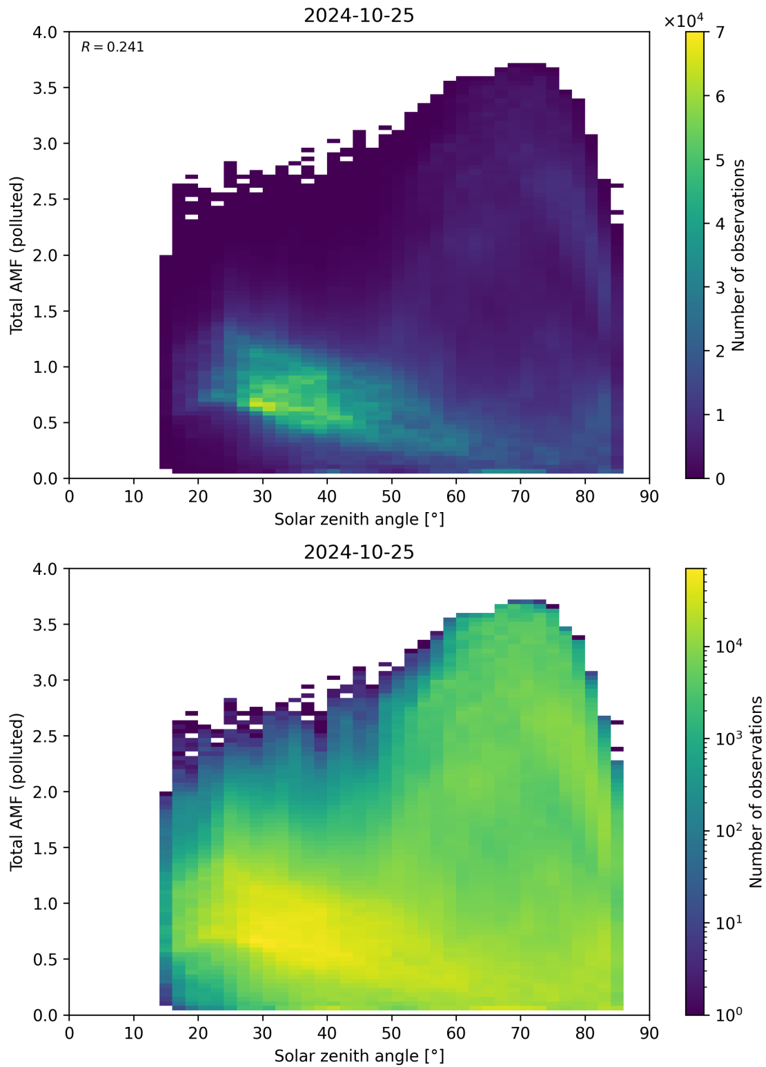
Figure 174: Scatter density plot of “Solar zenith angle” against “Total AMF (polluted)” for 2024-10-24 to 2024-10-26.
