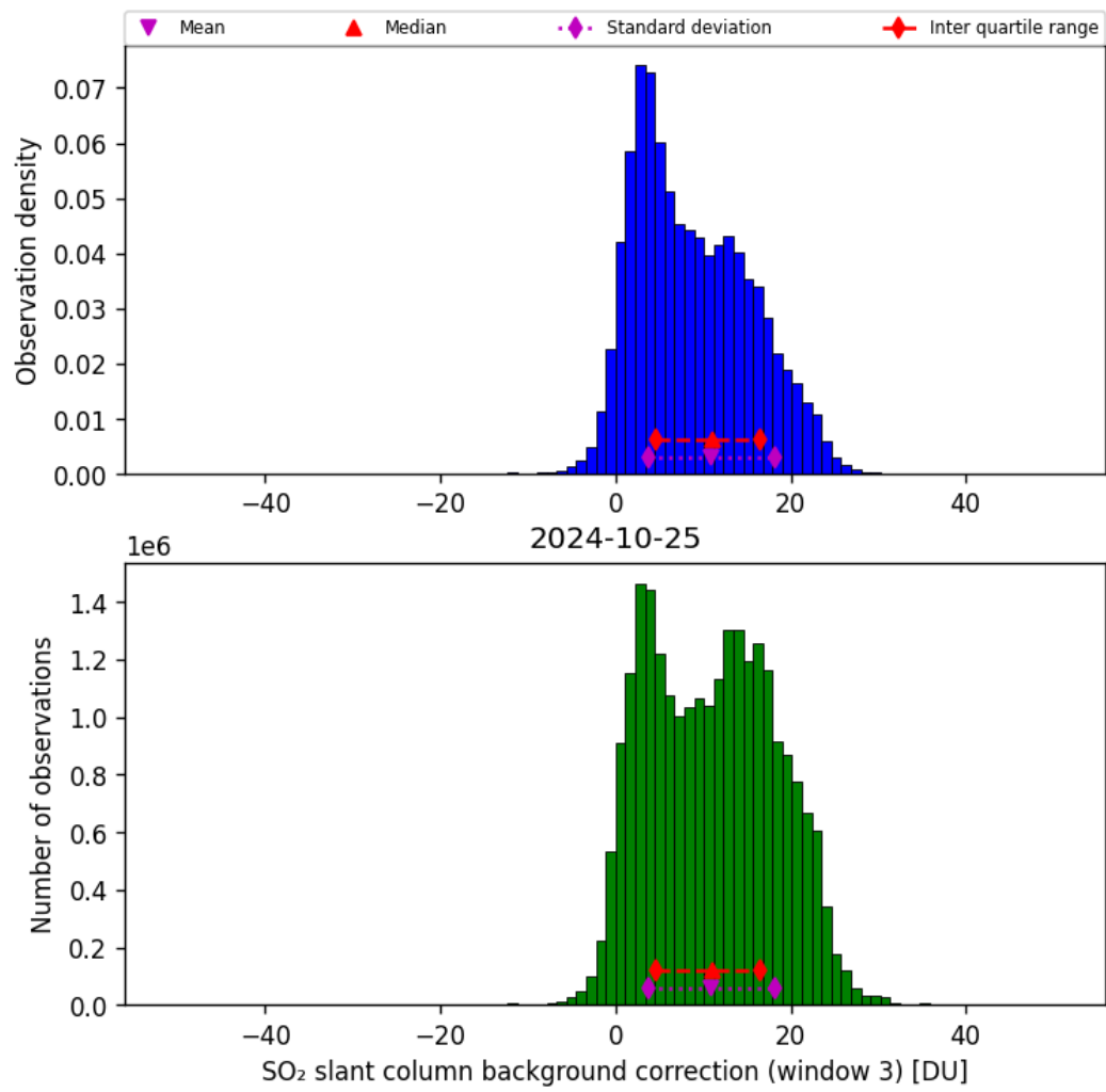
Figure 67: Histogram of “SO 2 slant column background correction (window 3)” for 2024-10-24 to 2024-10-26
