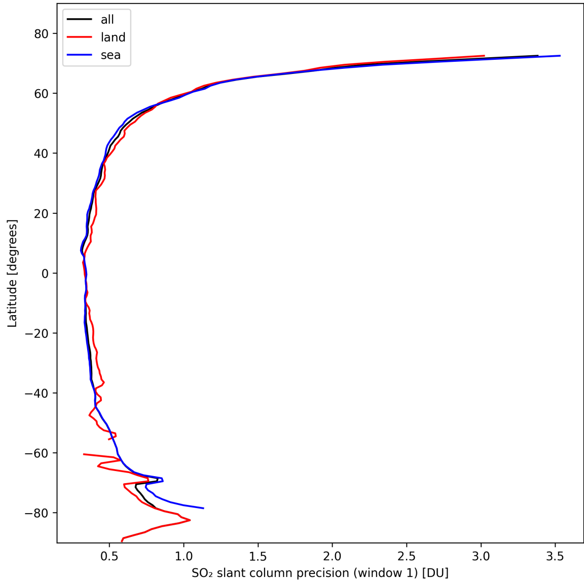
Figure 34: Zonal average of “SO 2 slant column precision (window 1)” for 2024-10-24 to 2024-10-26.
