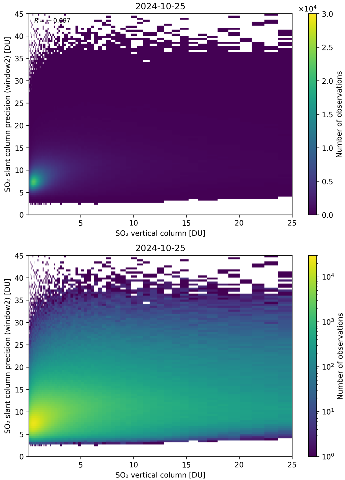
Figure 302: Scatter density plot of “SO 2 vertical column” against “SO 2 slant column precision (window2)” for 2024-10-24 to 2024-10-26.
