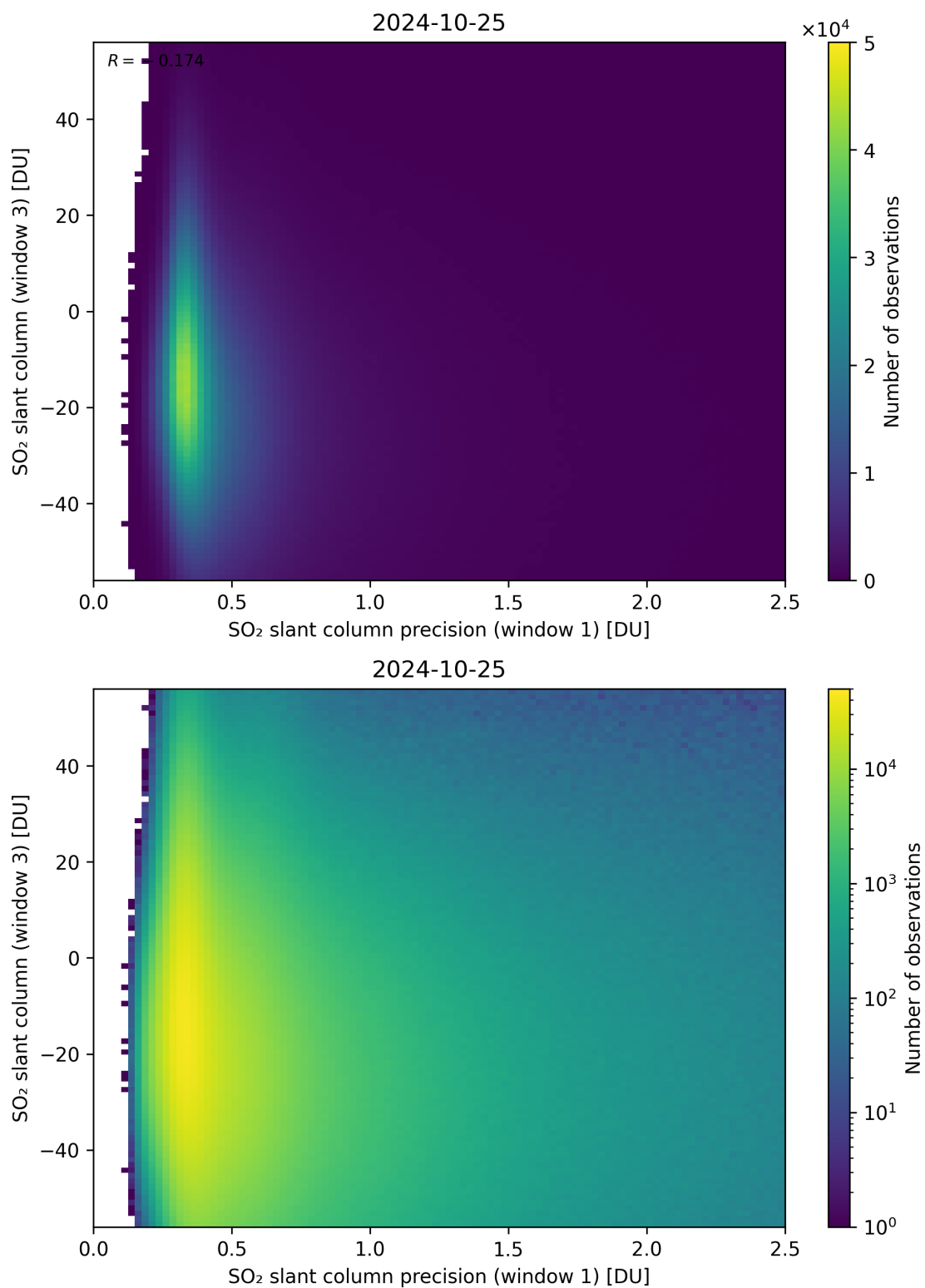
Figure 228: Scatter density plot of “SO 2 slant column precision (window 1)” against “SO 2 slant column (window 3)” for 2024-10-24 to 2024-10-26.
