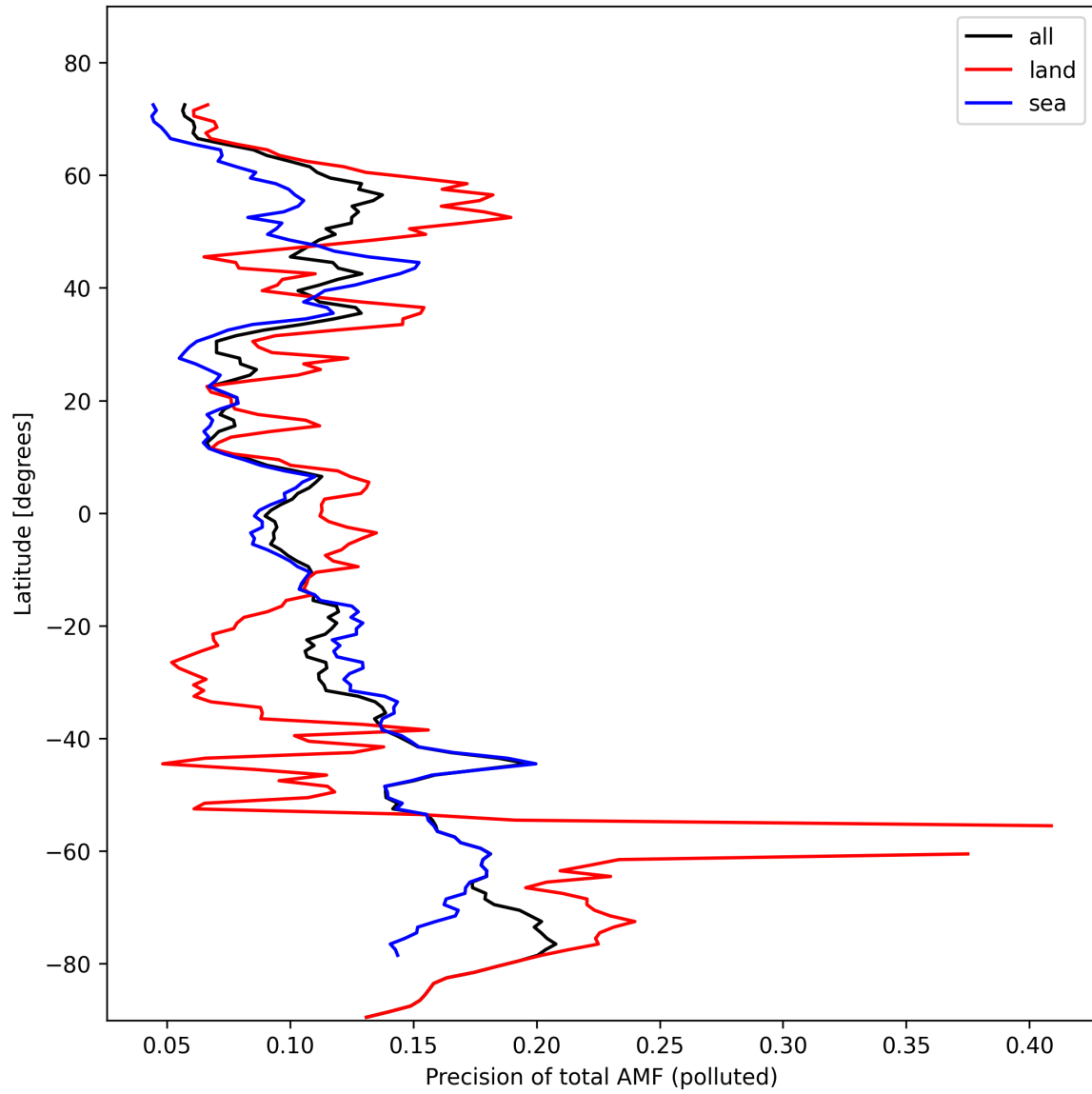
Figure 49: Zonal average of “Precision of total AMF (polluted)” for 2024-10-24 to 2024-10-26.
