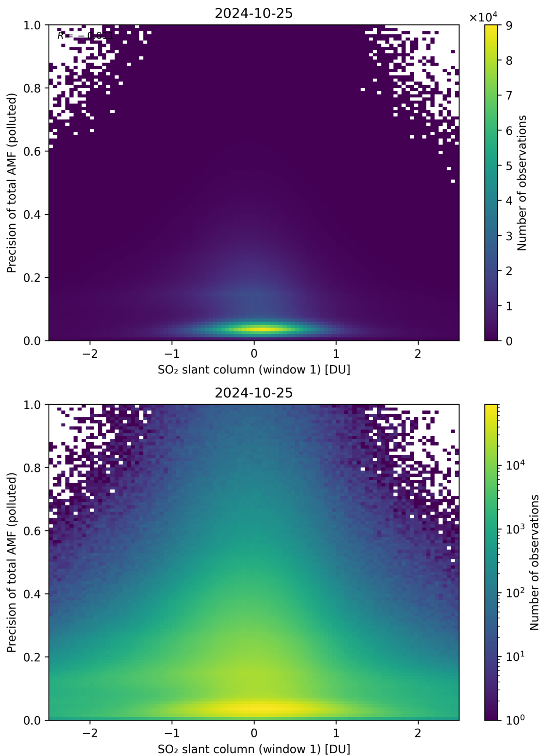
Figure 240: Scatter density plot of “SO 2 slant column (window 1)” against “Precision of total AMF (polluted)” for 2024-10-24 to 2024-10-26.
