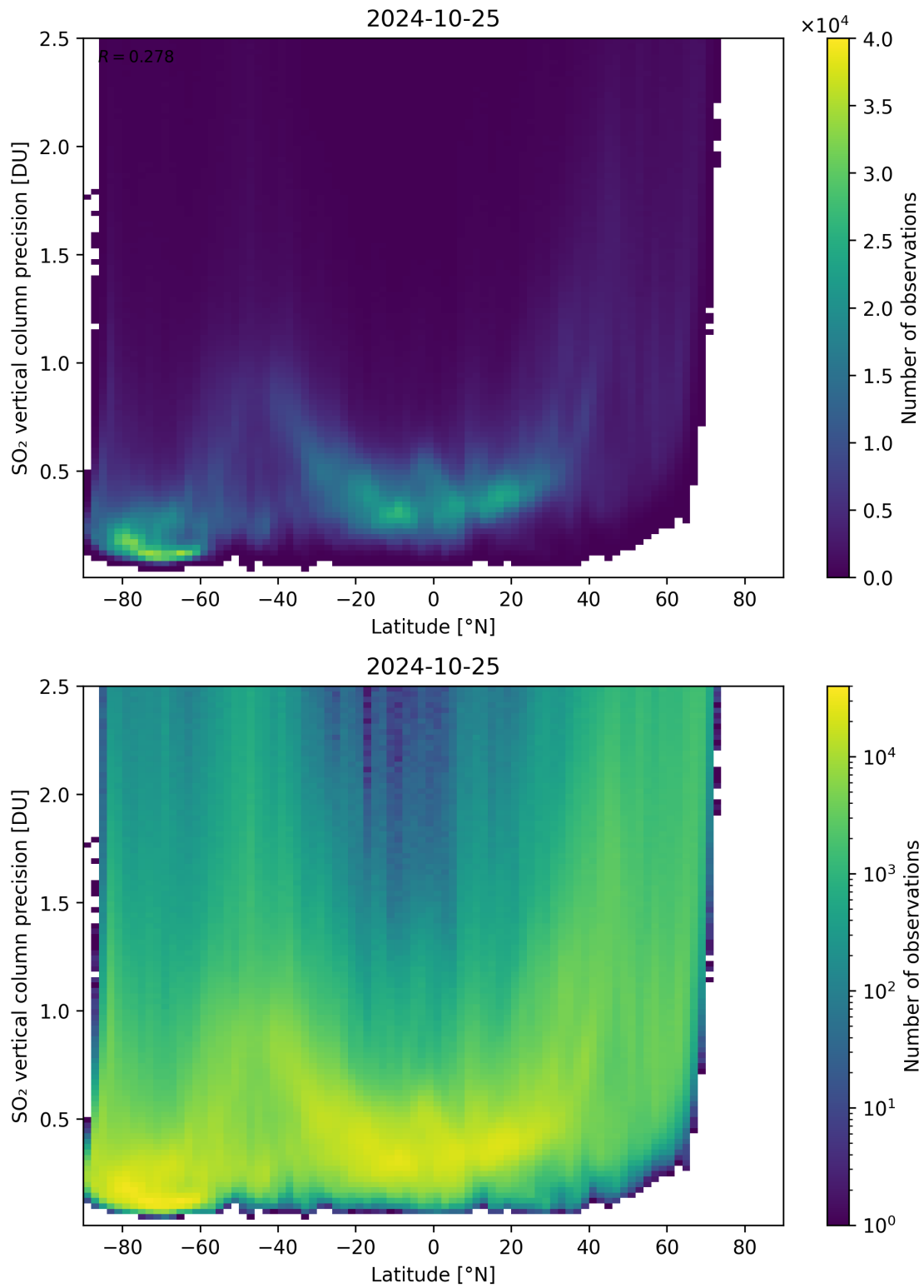
Figure 157: Scatter density plot of “Latitude” against “SO 2 vertical column precision” for 2024-10-24 to 2024-10-26.
