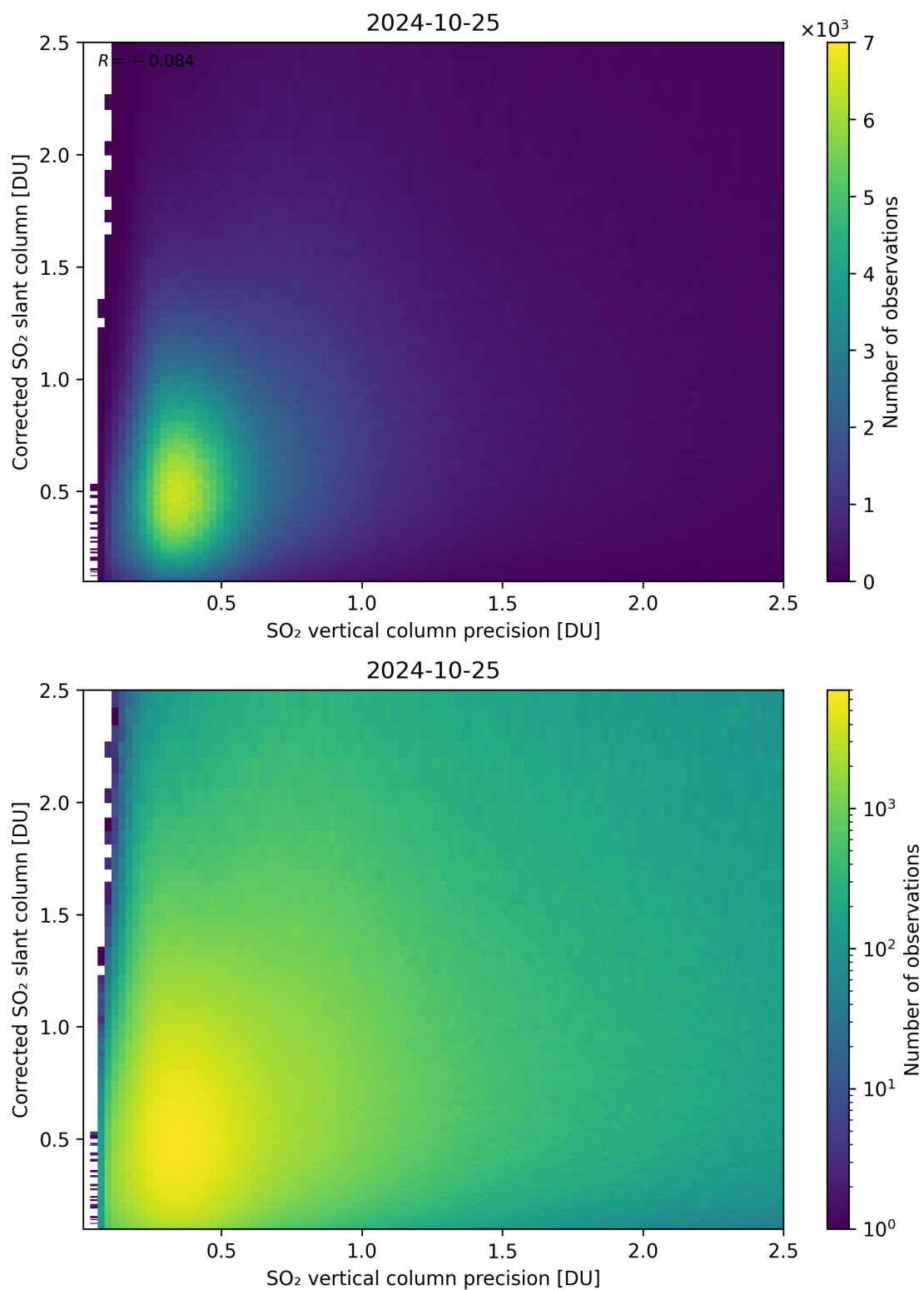
Figure 286: Scatter density plot of “SO 2 vertical column precision” against “Corrected SO 2 slant column” for 2024-10-24 to 2024-10-26.
