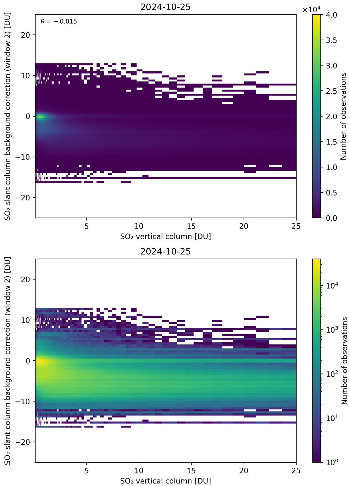
Figure 274: Scatter density plot of “SO 2 vertical column” against “SO 2 slant column background correction (window 2)” for 2024-10-24 to 2024-10-26.
