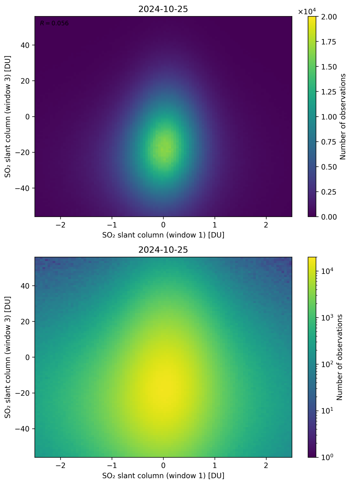
Figure 237: Scatter density plot of “SO 2 slant column (window 1)” against “SO 2 slant column (window 3)” for 2024-10-24 to 2024-10-26.
