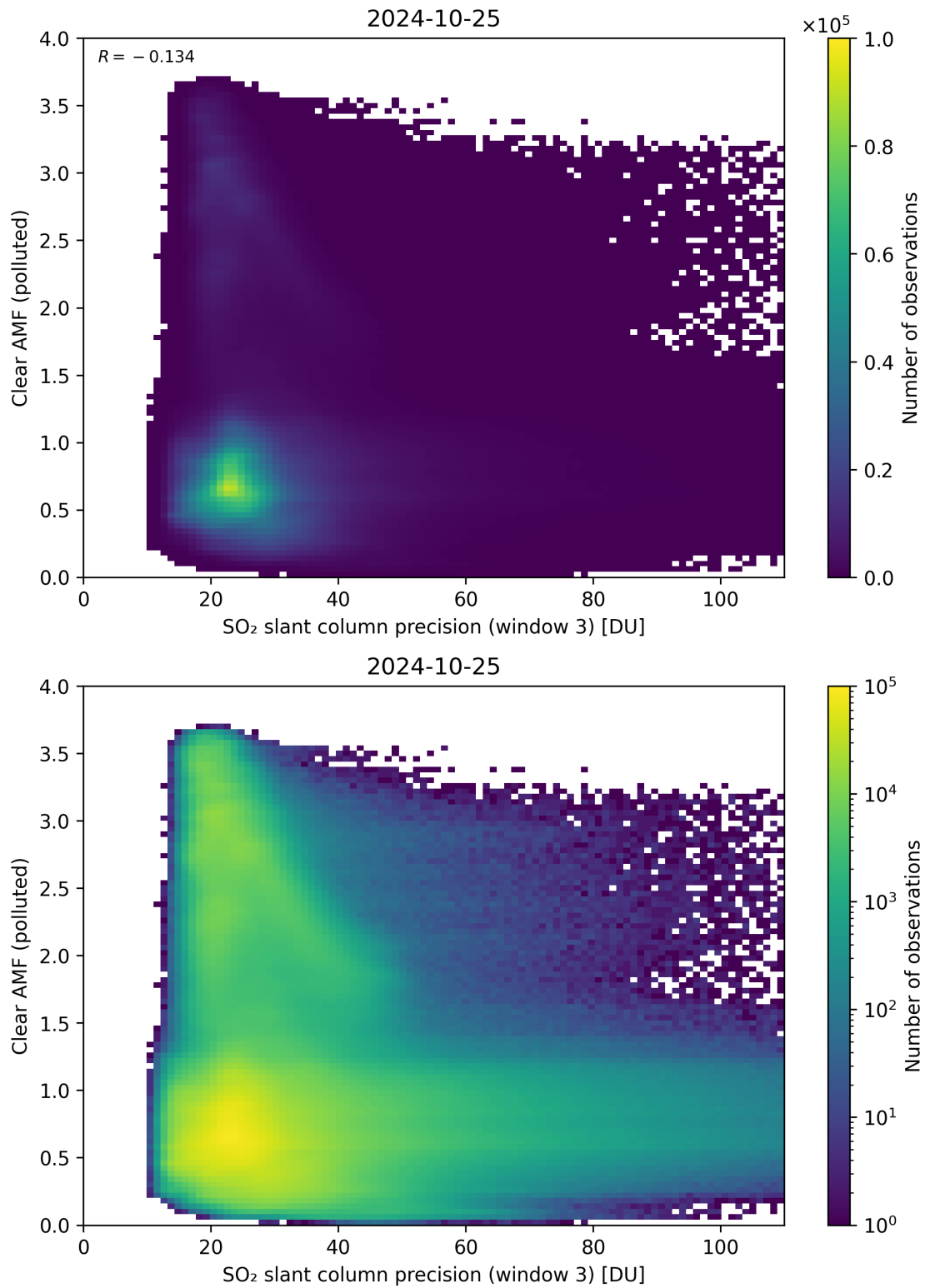
Figure 261: Scatter density plot of “SO 2 slant column precision (window 3)” against “Clear AMF (polluted)” for 2024-10-24 to 2024-10-26.
