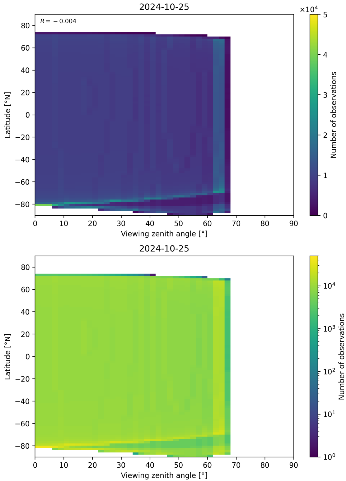
Figure 314: Scatter density plot of “Viewing zenith angle” against “Latitude” for 2024-10-24 to 2024-10-26.
