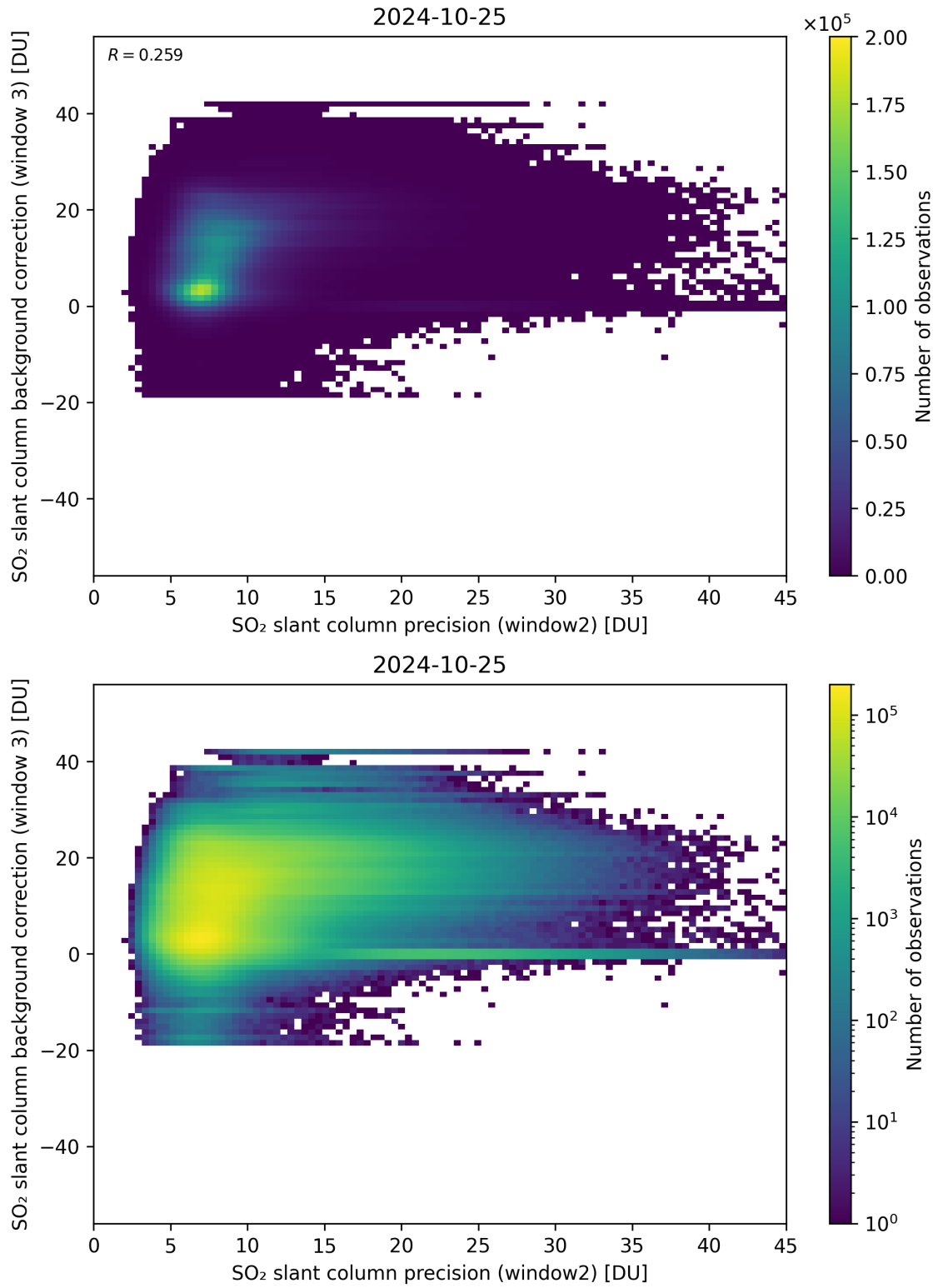
Figure 242: Scatter density plot of “SO 2 slant column precision (window2)” against “SO 2 slant column background correction (window 3)” for 2024-10-24 to 2024-10-26.
