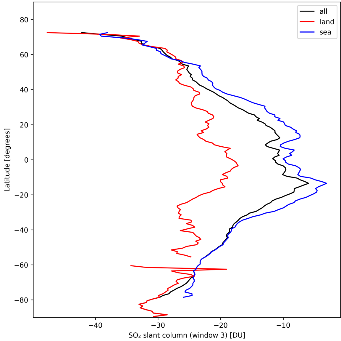
Figure 41: Zonal average of “SO 2 slant column (window 3)” for 2024-10-24 to 2024-10-26.
