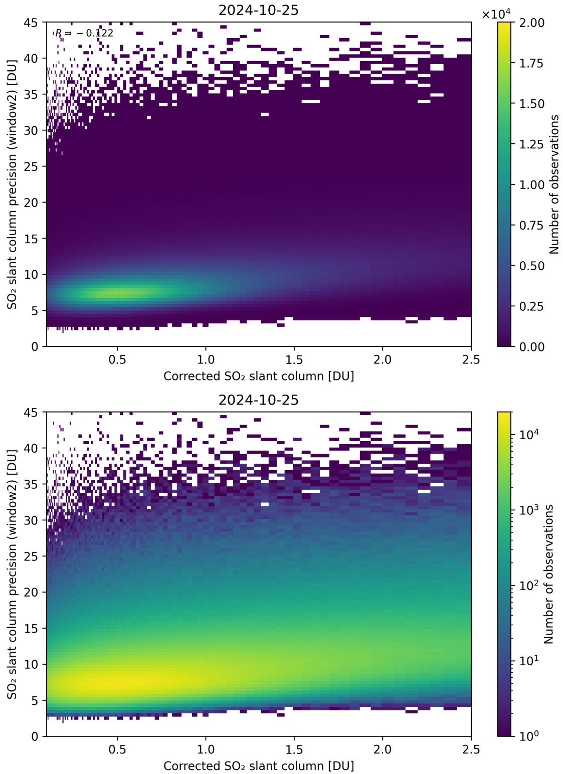
Figure 189: Scatter density plot of “Corrected SO 2 slant column” against “SO 2 slant column precision (window2)” for 2024-10-24 to 2024-10-26.
