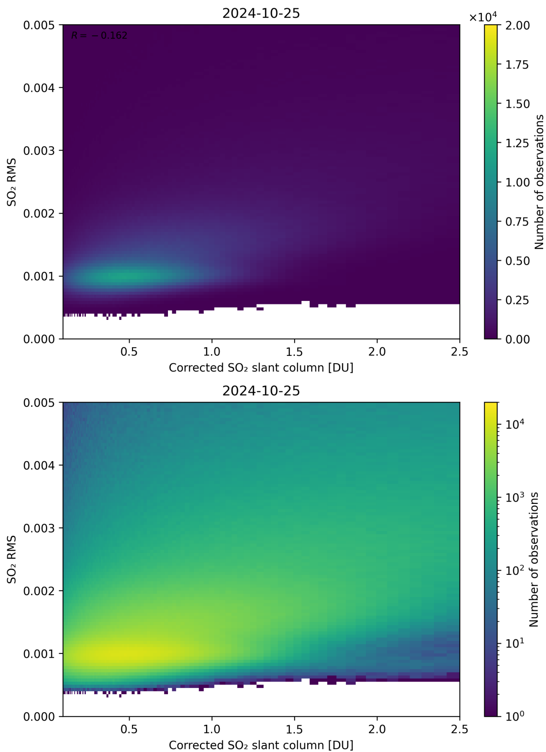
Figure 183: Scatter density plot of “Corrected SO 2 slant column” against “SO 2 RMS” for 2024-10-24 to 2024-10-26.
