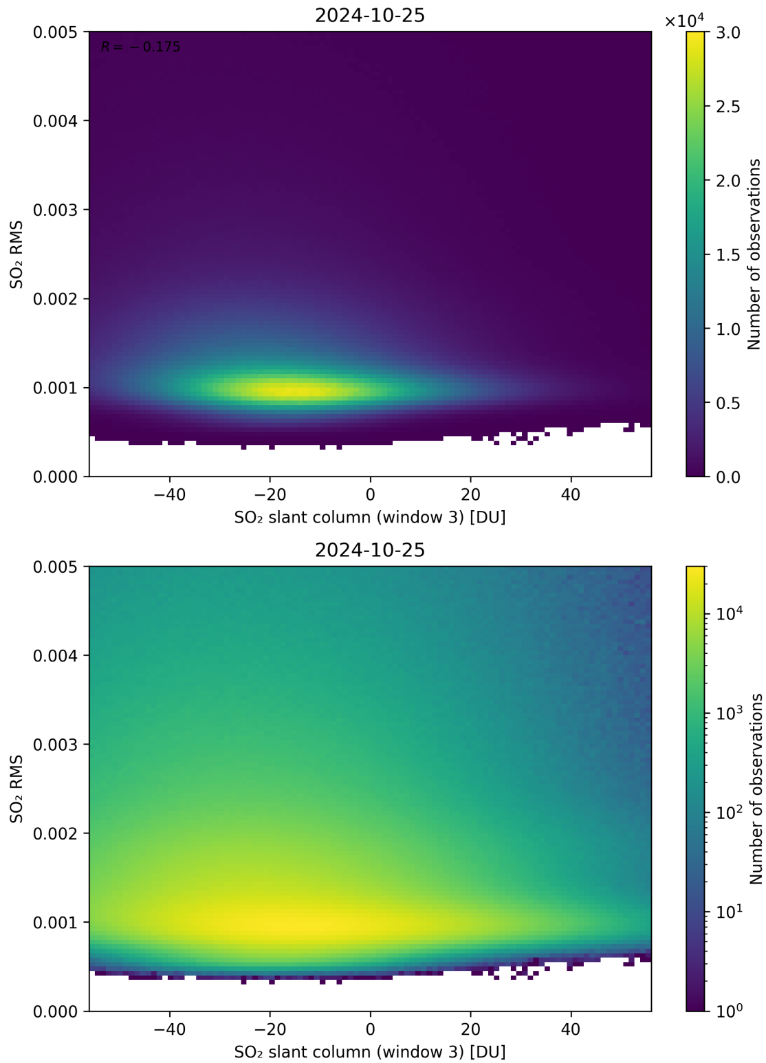
Figure 256: Scatter density plot of “SO 2 slant column (window 3)” against “SO 2 RMS” for 2024-10-24 to 2024-10-26.
