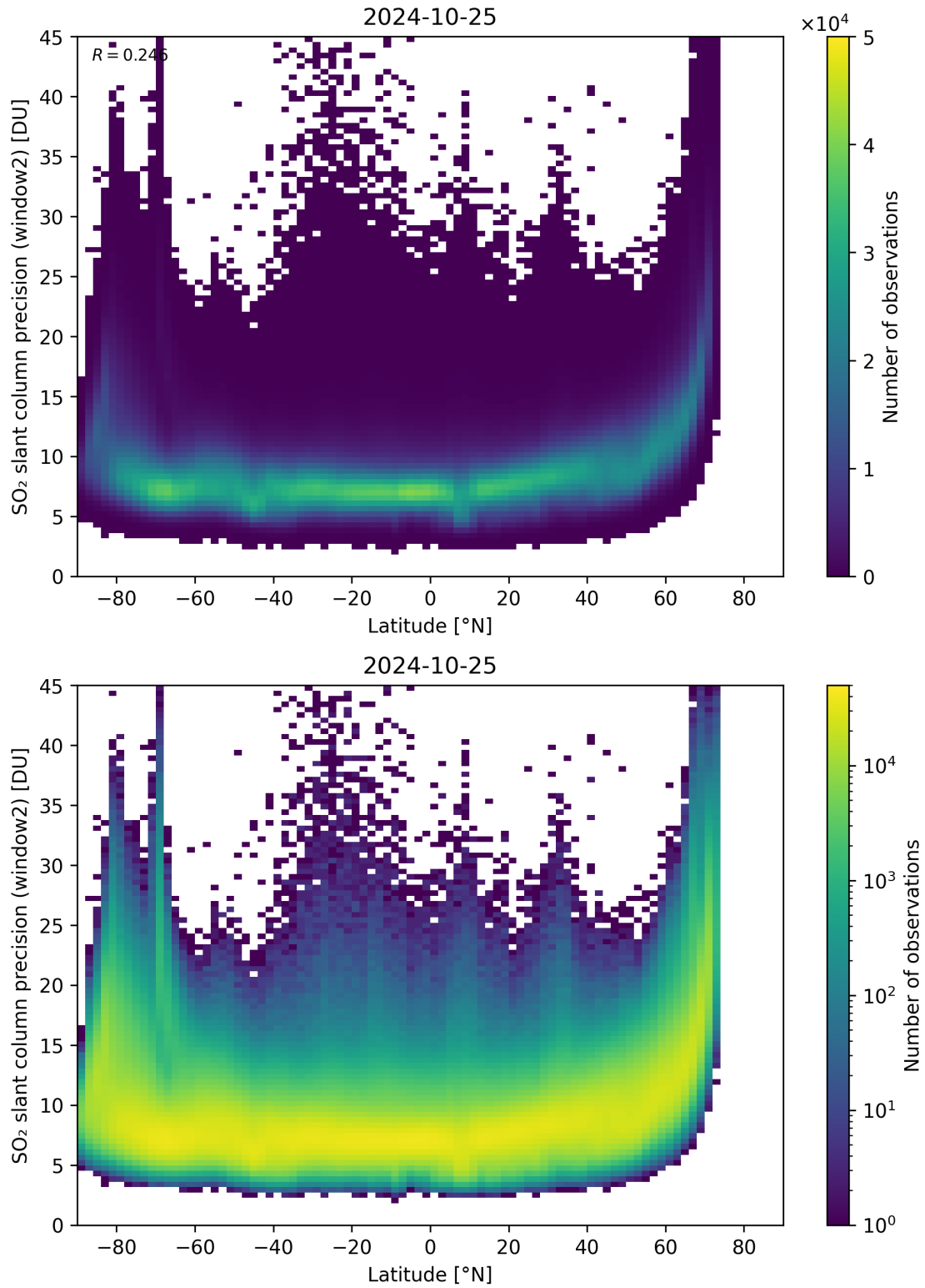
Figure 151: Scatter density plot of “Latitude” against “SO 2 slant column precision (window2)” for 2024-10-24 to 2024-10-26.
