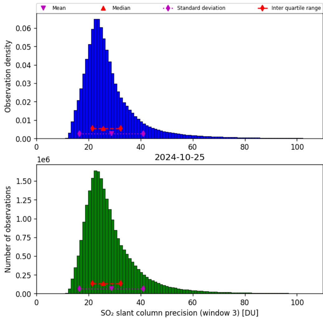
Figure 65: Histogram of “SO 2 slant column precision (window 3)” for 2024-10-24 to 2024-10-26
