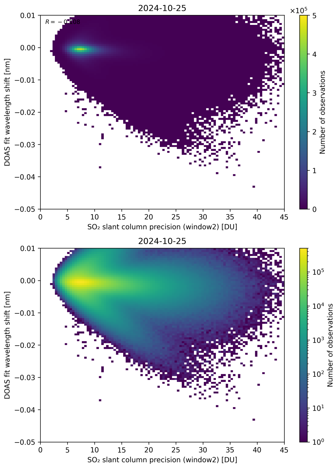
Figure 243: Scatter density plot of “SO 2 slant column precision (window2)” against “DOAS fit wavelength shift” for 2024-10-24 to 2024-10-26.
