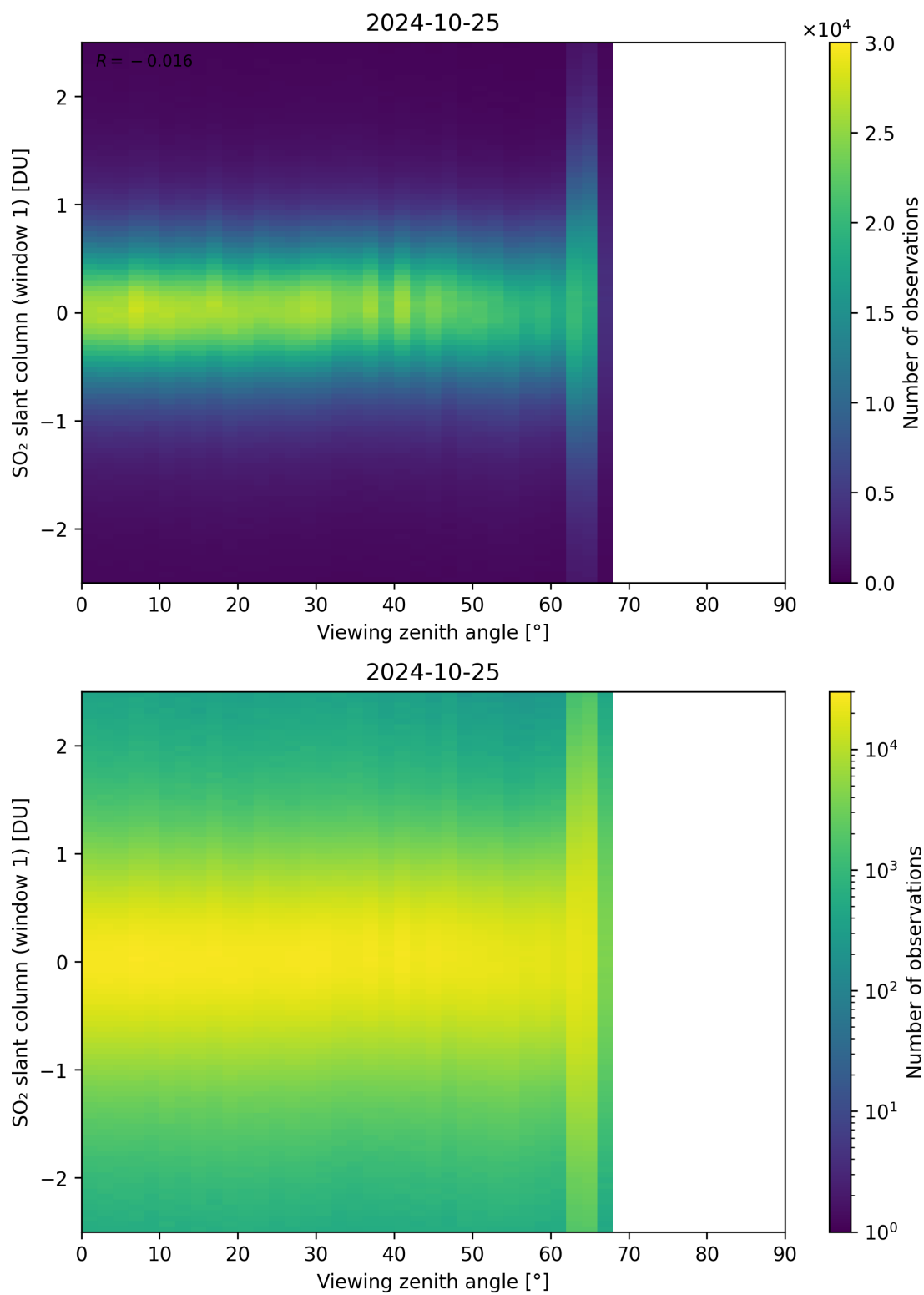
Figure 320: Scatter density plot of “Viewing zenith angle” against “SO 2 slant column (window 1)” for 2024-10-24 to 2024-10-26.
