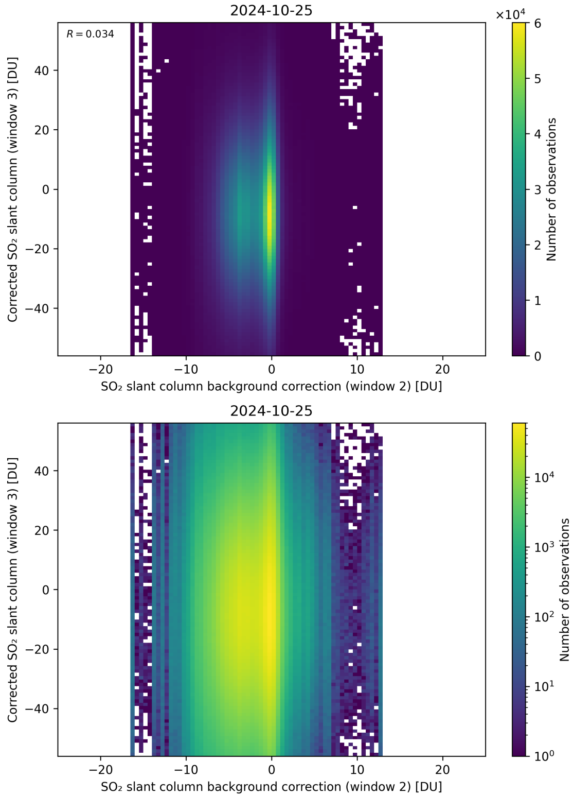
Figure 116: Scatter density plot of “SO 2 slant column background correction (window 2)” against “Corrected SO 2 slant column (window 3)” for 2024-10-24 to 2024-10-26.
