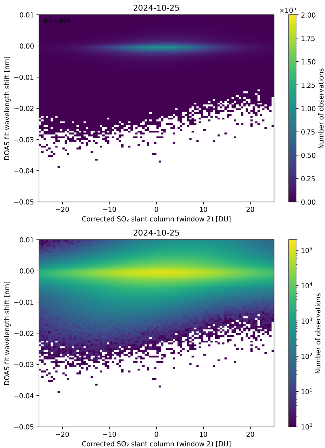
Figure 196: Scatter density plot of “Corrected SO 2 slant column (window 2)” against “DOAS fit wavelength shift” for 2024-10-24 to 2024-10-26.
