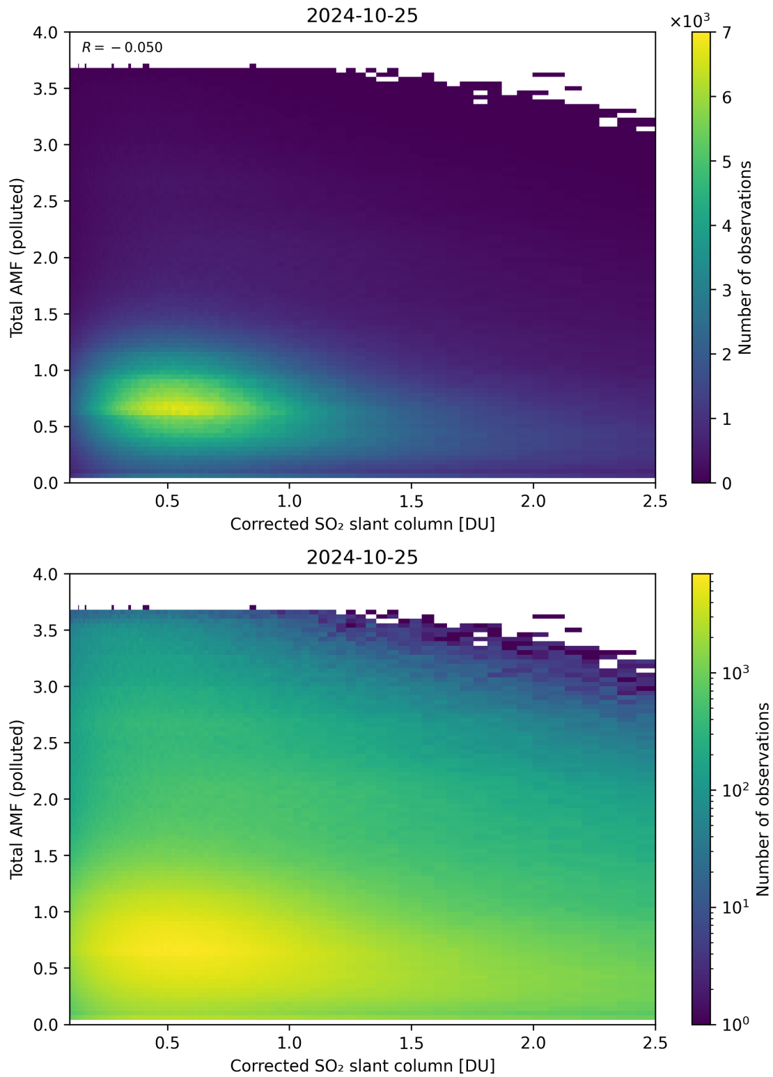
Figure 192: Scatter density plot of “Corrected SO 2 slant column” against “Total AMF (polluted)” for 2024-10-24 to 2024-10-26.
