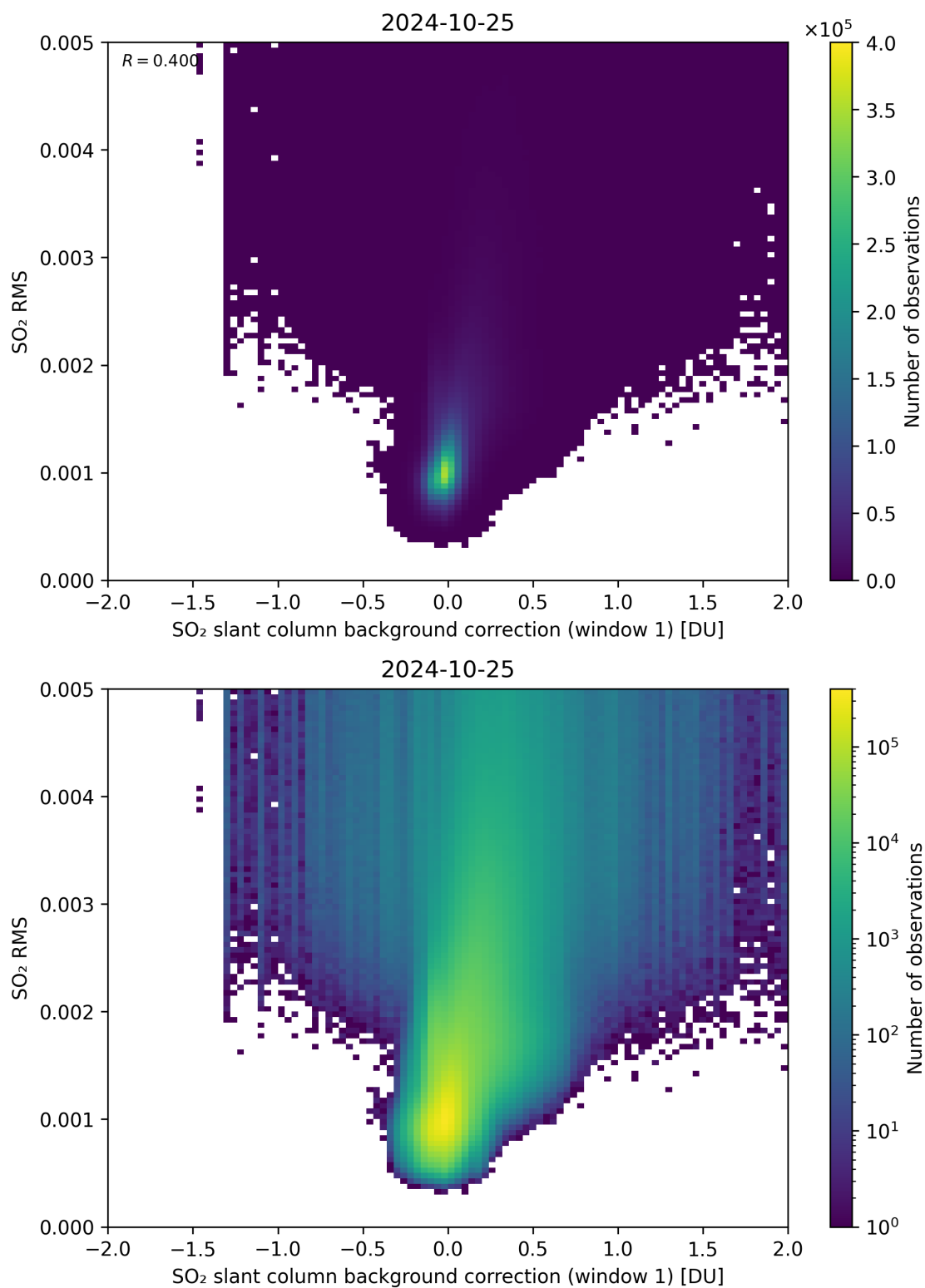
Figure 102: Scatter density plot of “SO 2 slant column background correction (window 1)” against “SO 2 RMS” for 2024-10-24 to 2024-10-26.
