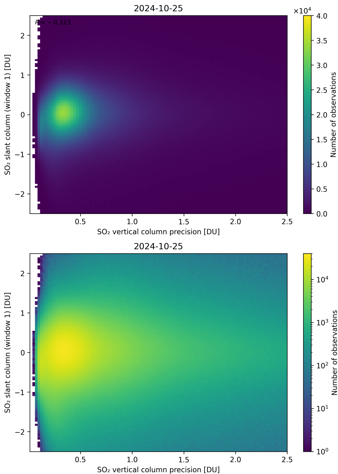
Figure 289: Scatter density plot of “SO 2 vertical column precision” against “SO 2 slant column (window 1)” for 2024-10-24 to 2024-10-26.
