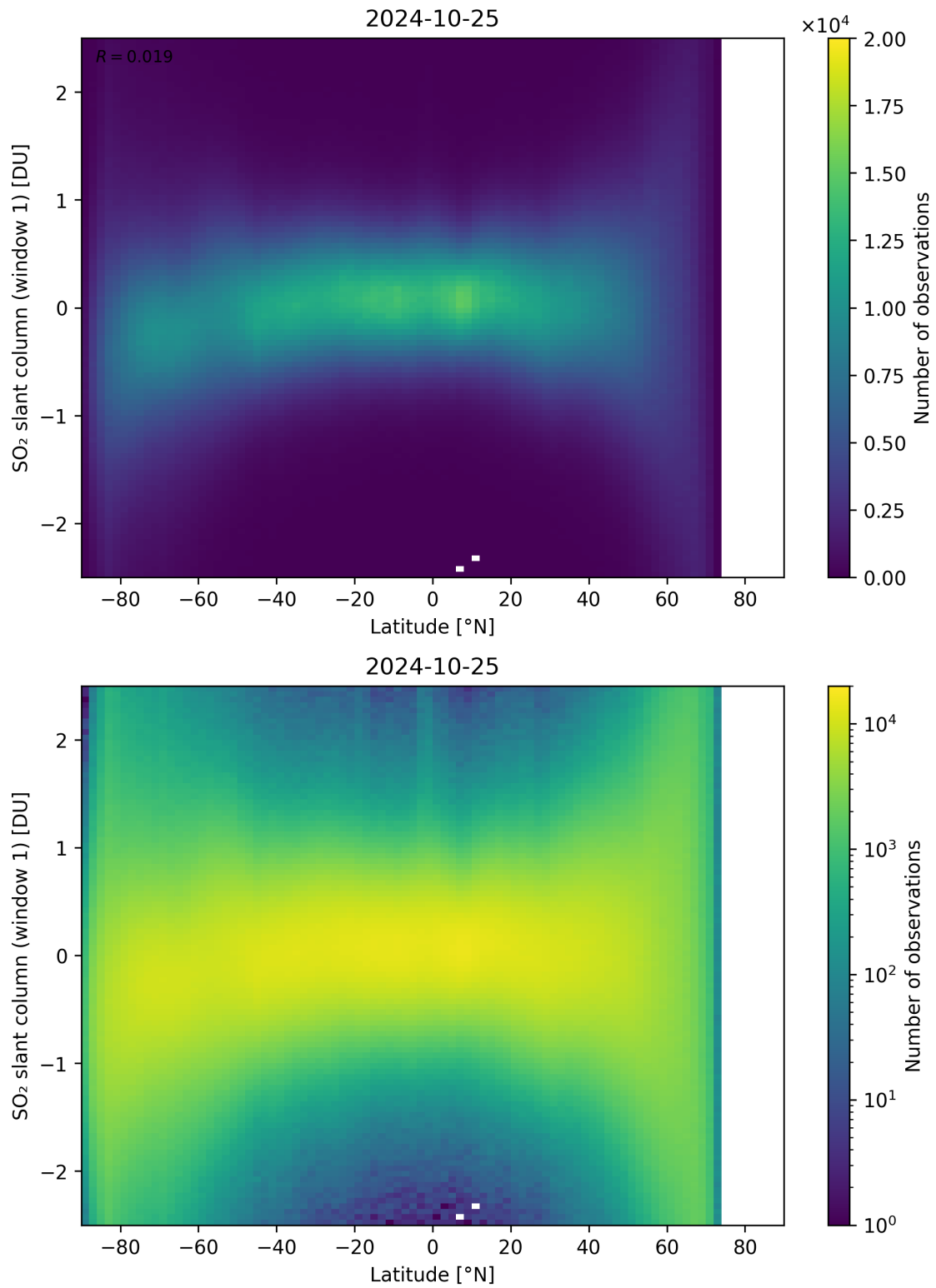
Figure 149: Scatter density plot of “Latitude” against “SO 2 slant column (window 1)” for 2024-10-24 to 2024-10-26.
