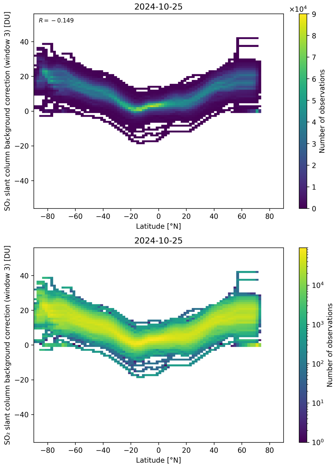
Figure 141: Scatter density plot of “Latitude” against “SO 2 slant column background correction (window 3)” for 2024-10-24 to 2024-10-26.
