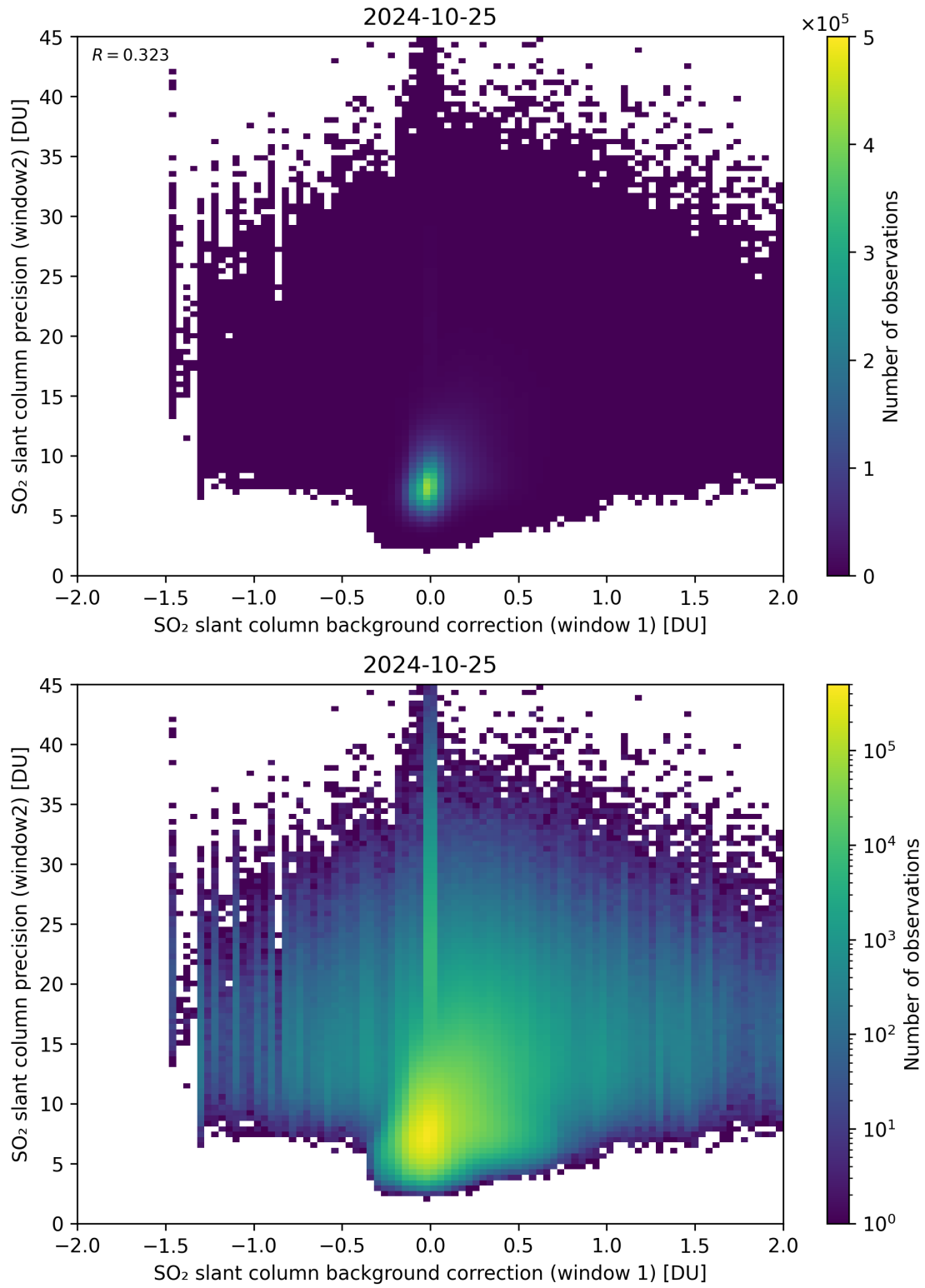
Figure 106: Scatter density plot of “SO 2 slant column background correction (window 1)” against “SO 2 slant column precision (window2)” for 2024-10-24 to 2024-10-26.
