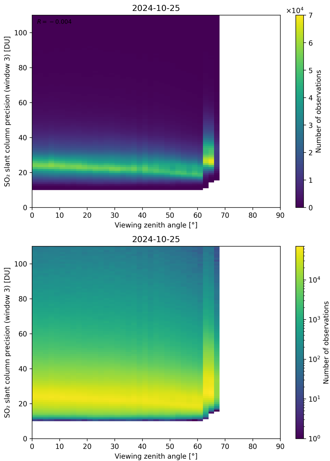
Figure 324: Scatter density plot of “Viewing zenith angle” against “SO 2 slant column precision (window 3)” for 2024-10-24 to 2024-10-26.
