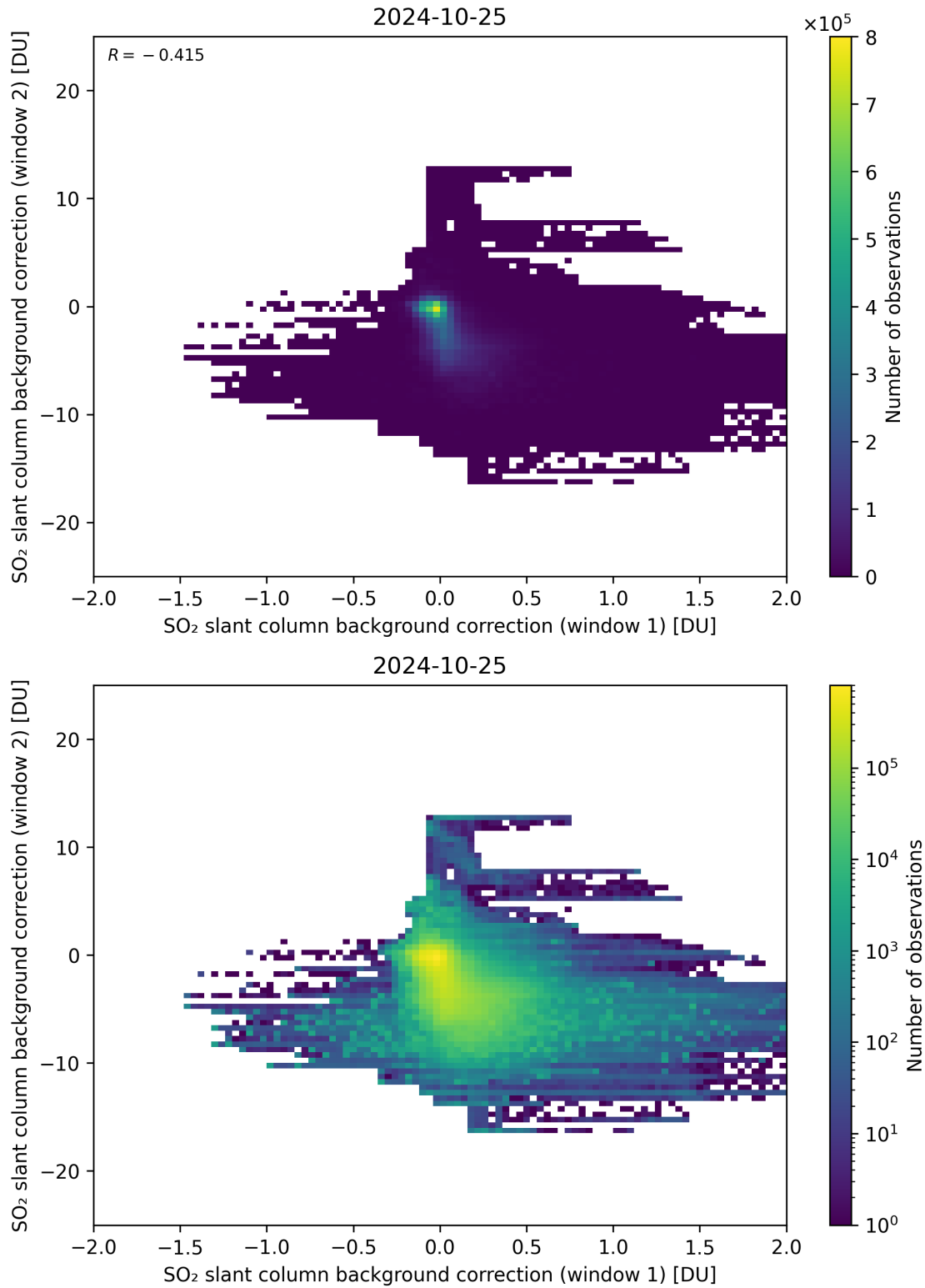
Figure 98: Scatter density plot of “SO 2 slant column background correction (window 1)” against “SO 2 slant column background correction (window 2)” for 2024-10-24 to 2024-10-26.
