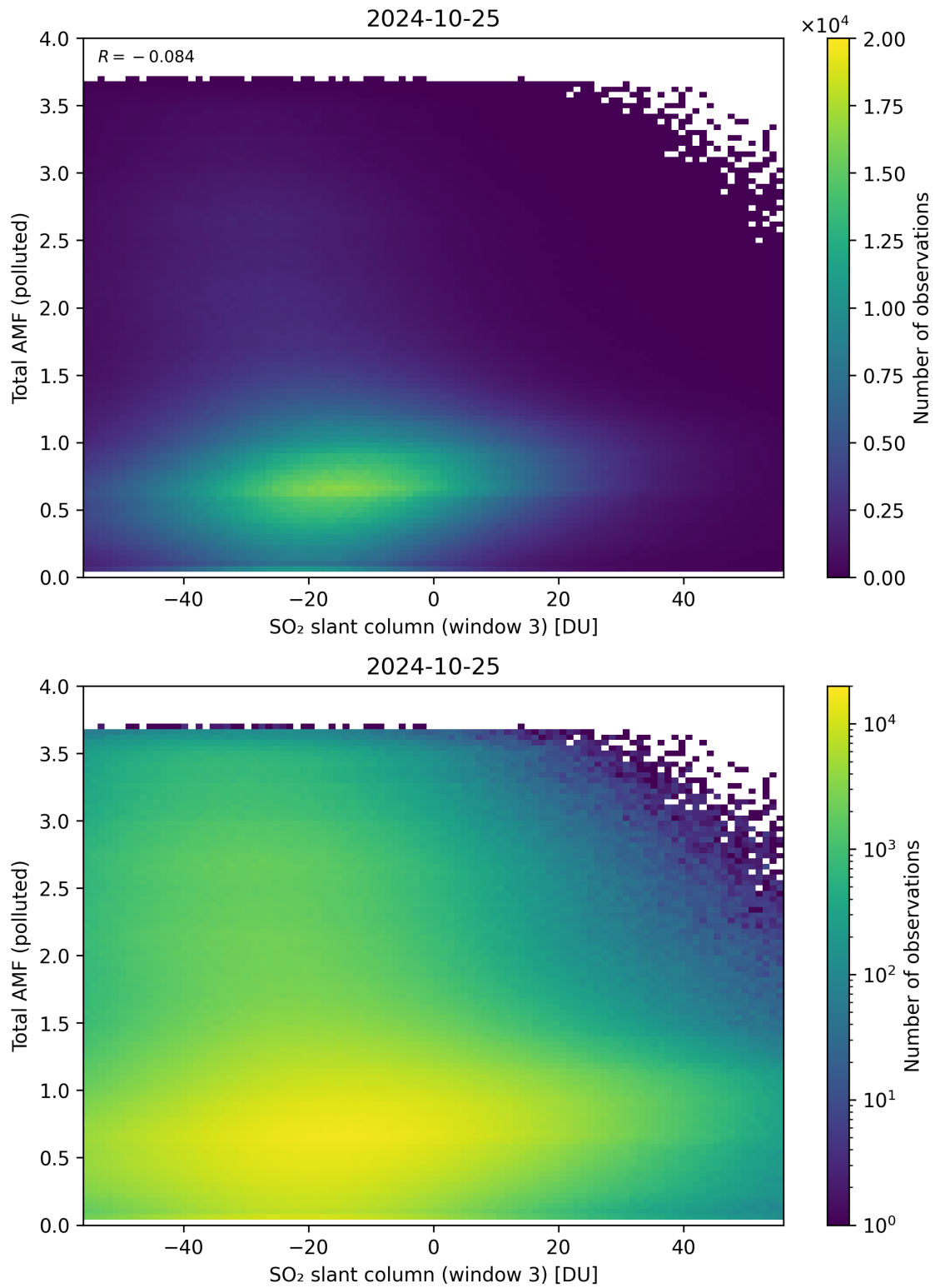
Figure 268: Scatter density plot of “SO 2 slant column (window 3)” against “Total AMF (polluted)” for 2024-10-24 to 2024-10-26.
