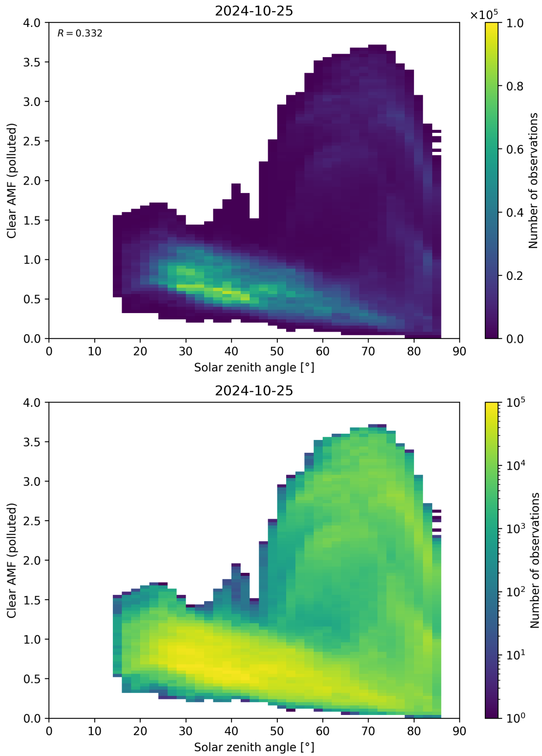
Figure 165: Scatter density plot of “Solar zenith angle” against “Clear AMF (polluted)” for 2024-10-24 to 2024-10-26.
