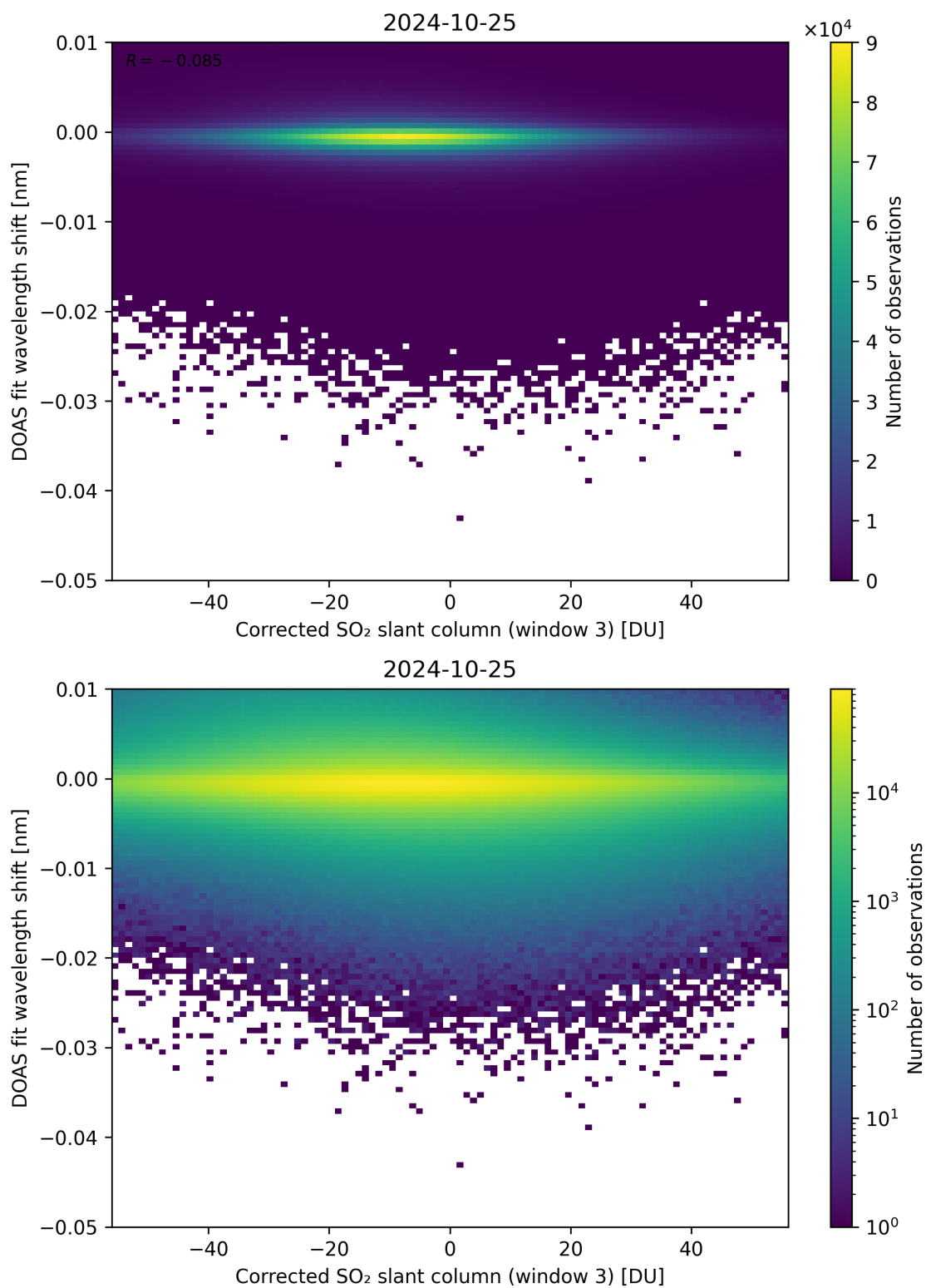
Figure 206: Scatter density plot of “Corrected SO 2 slant column (window 3)” against “DOAS fit wavelength shift” for 2024-10-24 to 2024-10-26.
