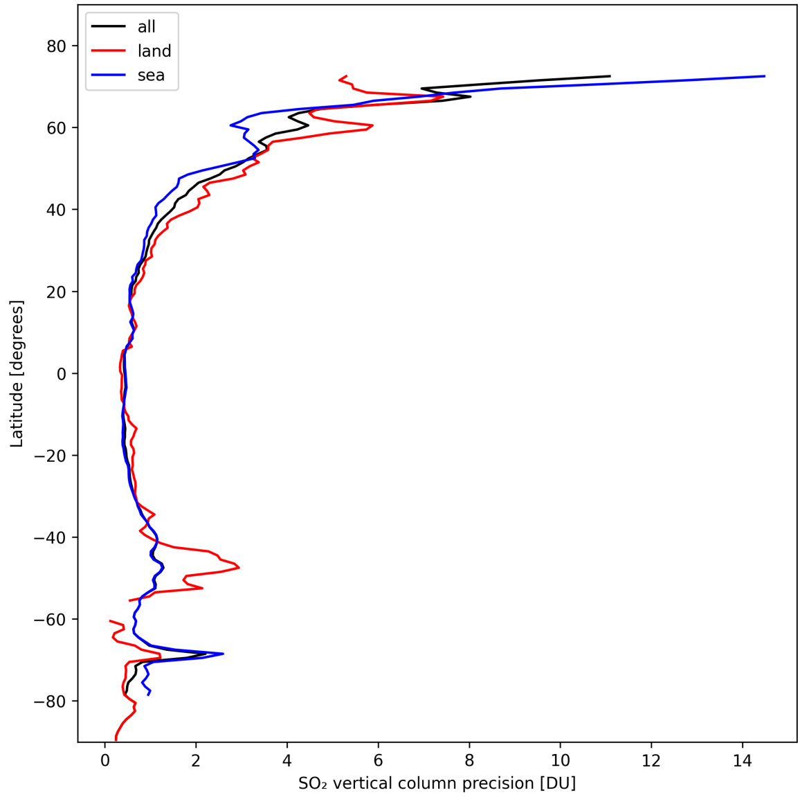
Figure 31: Zonal average of “SO 2 vertical column precision” for 2024-10-24 to 2024-10-26.
