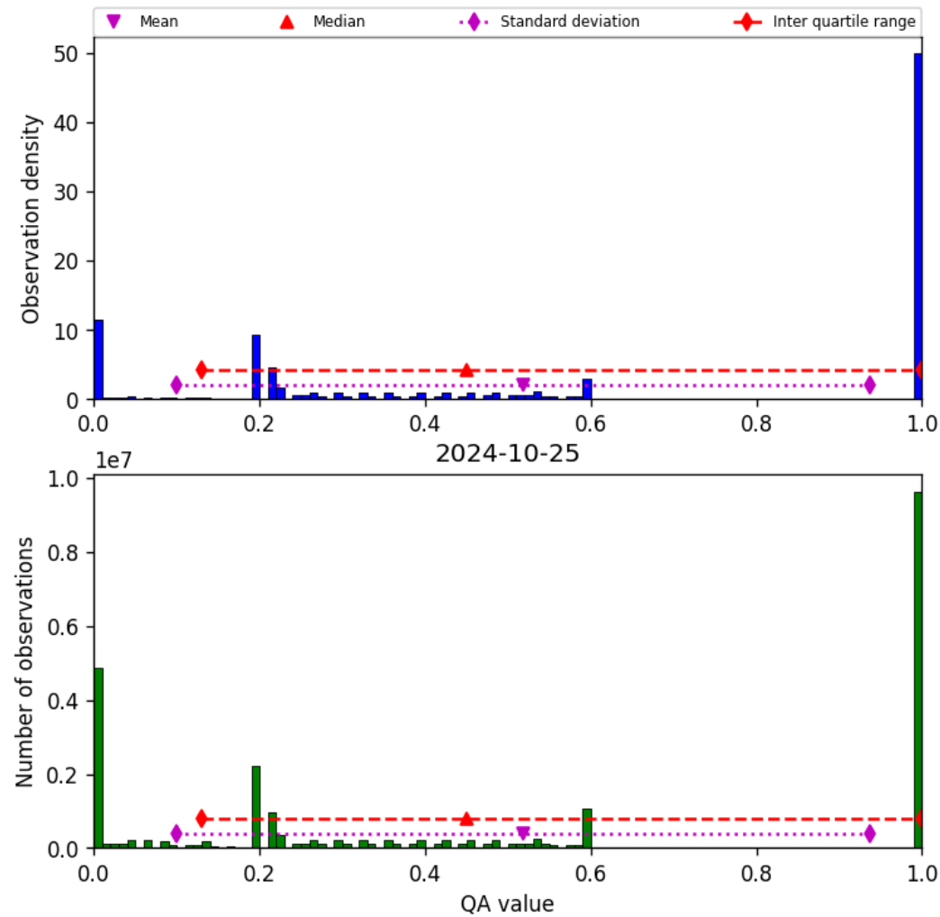
Figure 52: Histogram of “QA value” for 2024-10-24 to 2024-10-26
