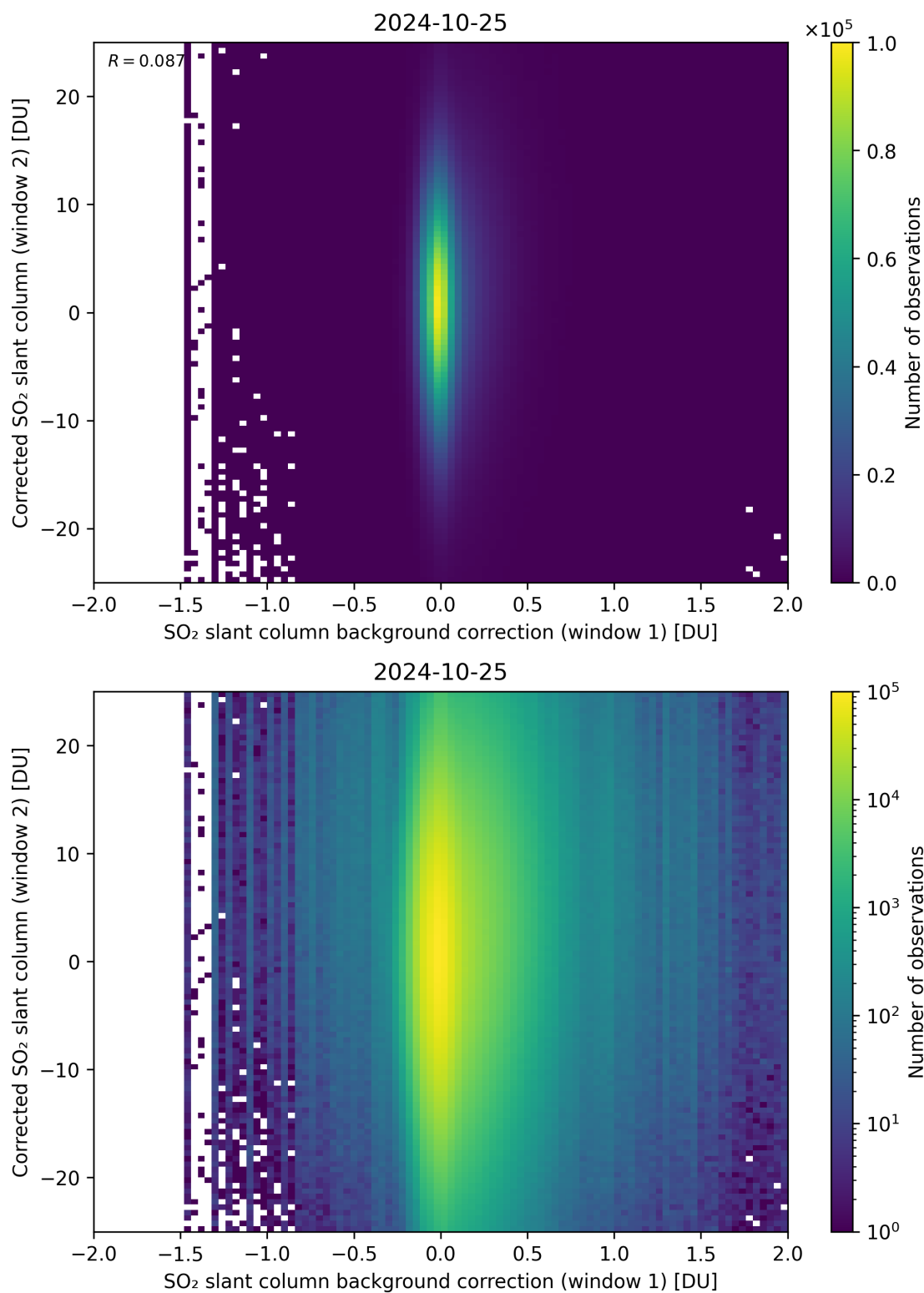
Figure 104: Scatter density plot of “SO 2 slant column background correction (window 1)” against “Corrected SO 2 slant column (window 2)” for 2024-10-24 to 2024-10-26.
