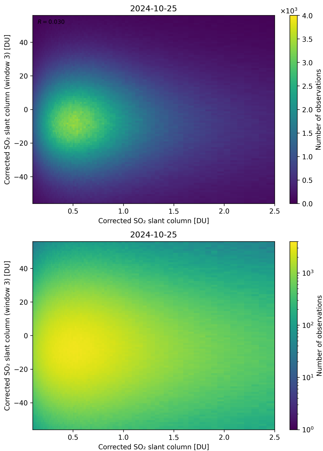
Figure 186: Scatter density plot of “Corrected SO 2 slant column” against “Corrected SO 2 slant column (window 3)” for 2024-10-24 to 2024-10-26.
