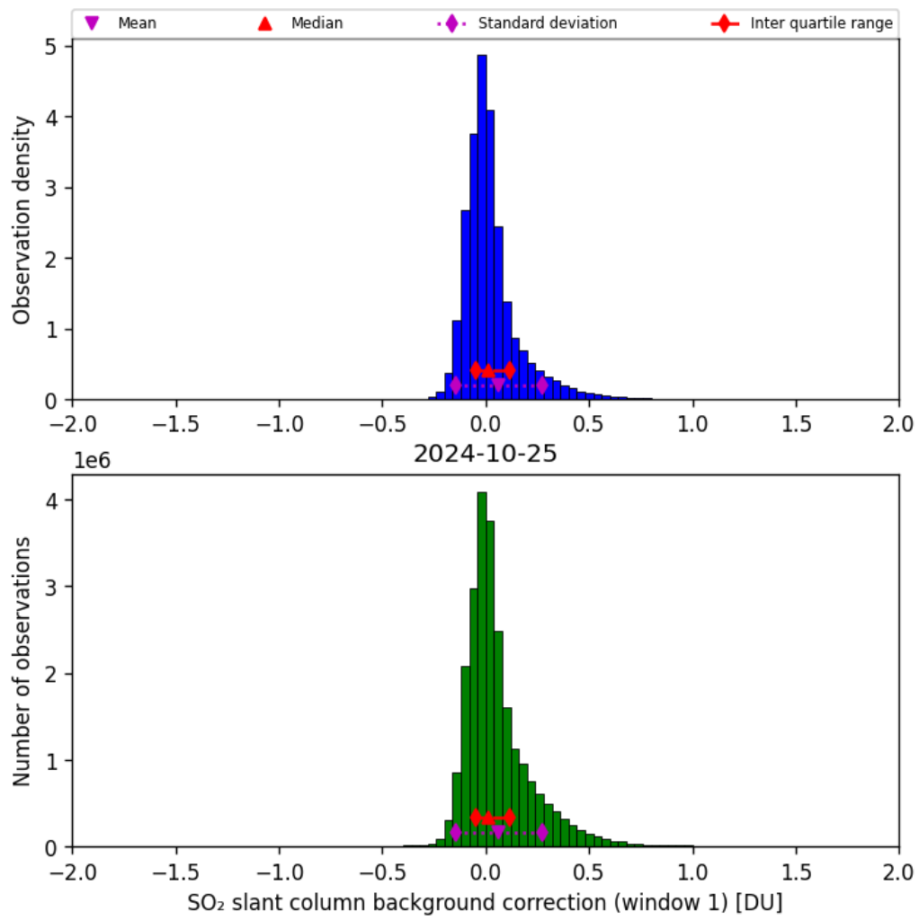
Figure 59: Histogram of “SO 2 slant column background correction (window 1)” for 2024-10-24 to 2024-10-26
