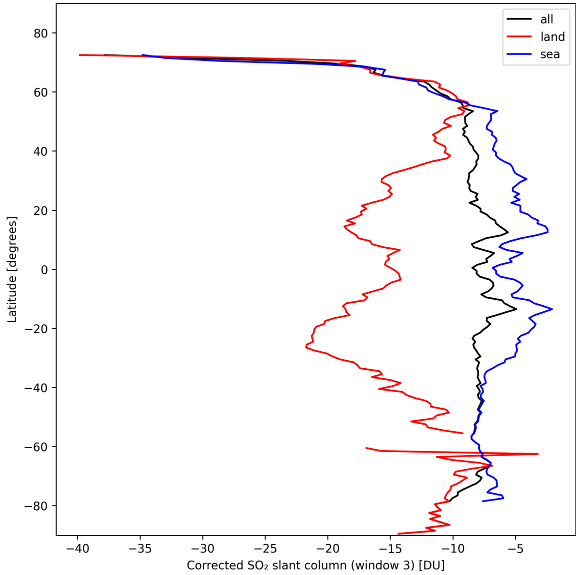
Figure 43: Zonal average of “Corrected SO 2 slant column (window 3)” for 2024-10-24 to 2024-10-26.
