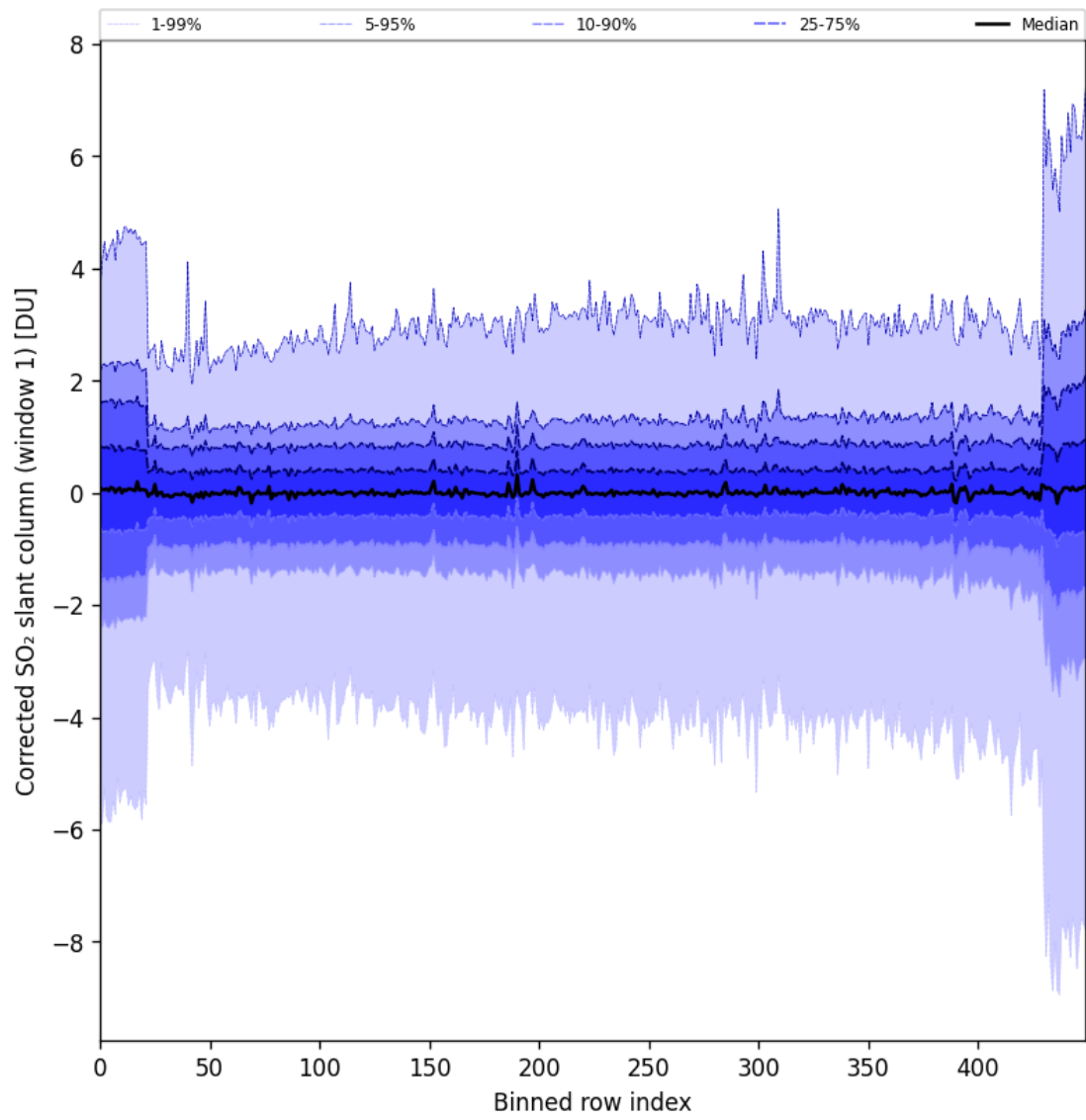
Figure 81: Along track statistics of “Corrected SO 2 slant column (window 1)” for 2024-10-24 to 2024-10-26
