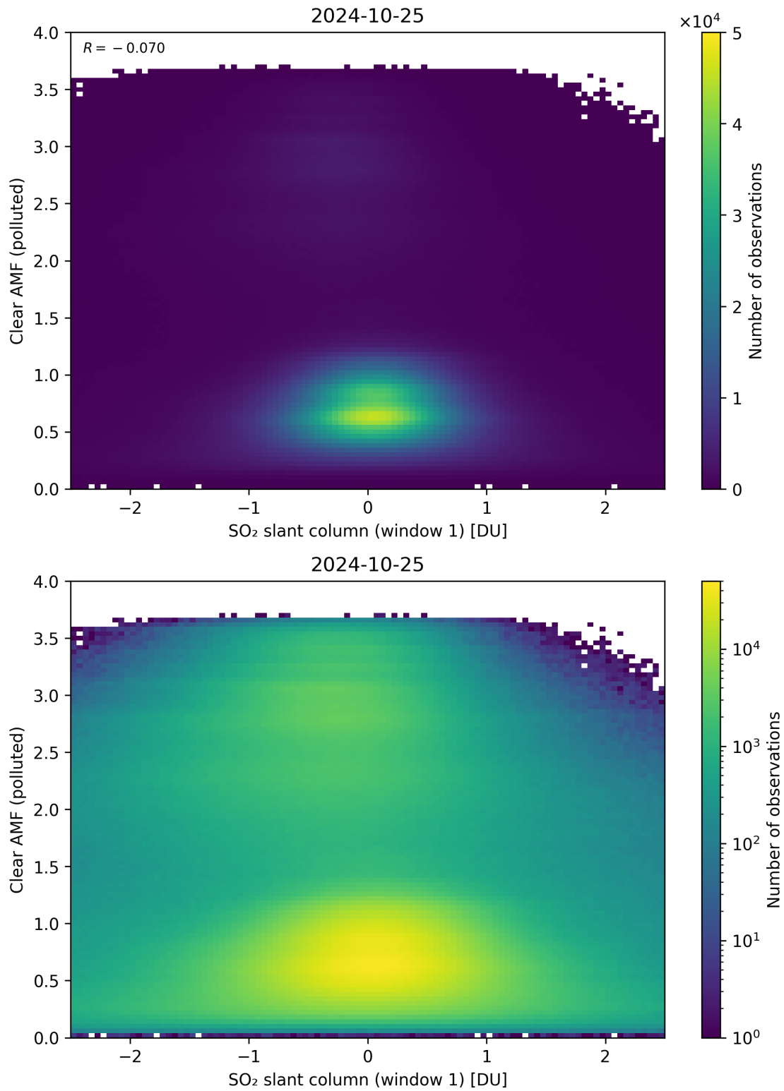
Figure 232: Scatter density plot of “SO 2 slant column (window 1)” against “Clear AMF (polluted)” for 2024-10-24 to 2024-10-26.
