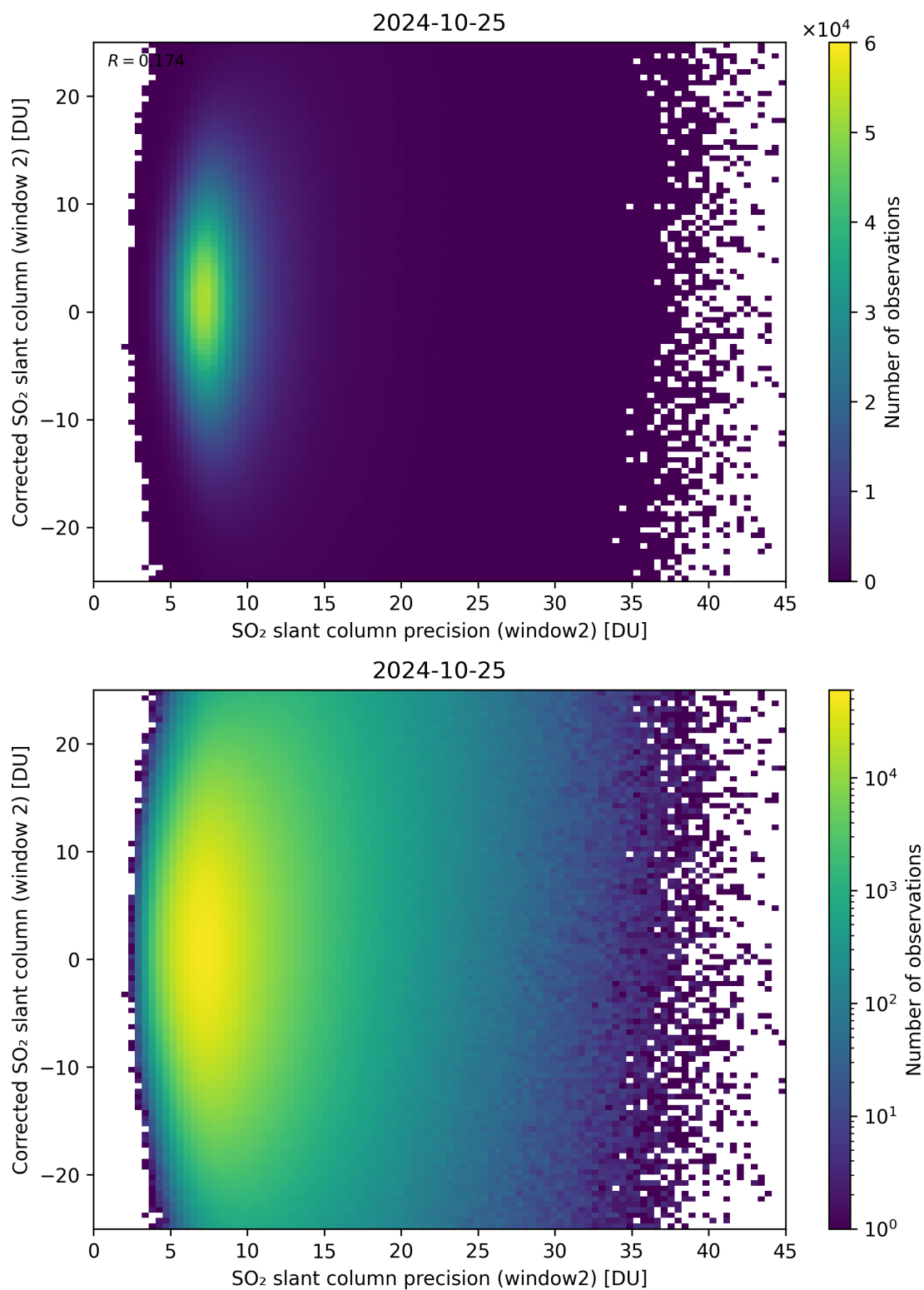
Figure 247: Scatter density plot of “SO 2 slant column precision (window2)” against “Corrected SO 2 slant column (window 2)” for 2024-10-24 to 2024-10-26.
