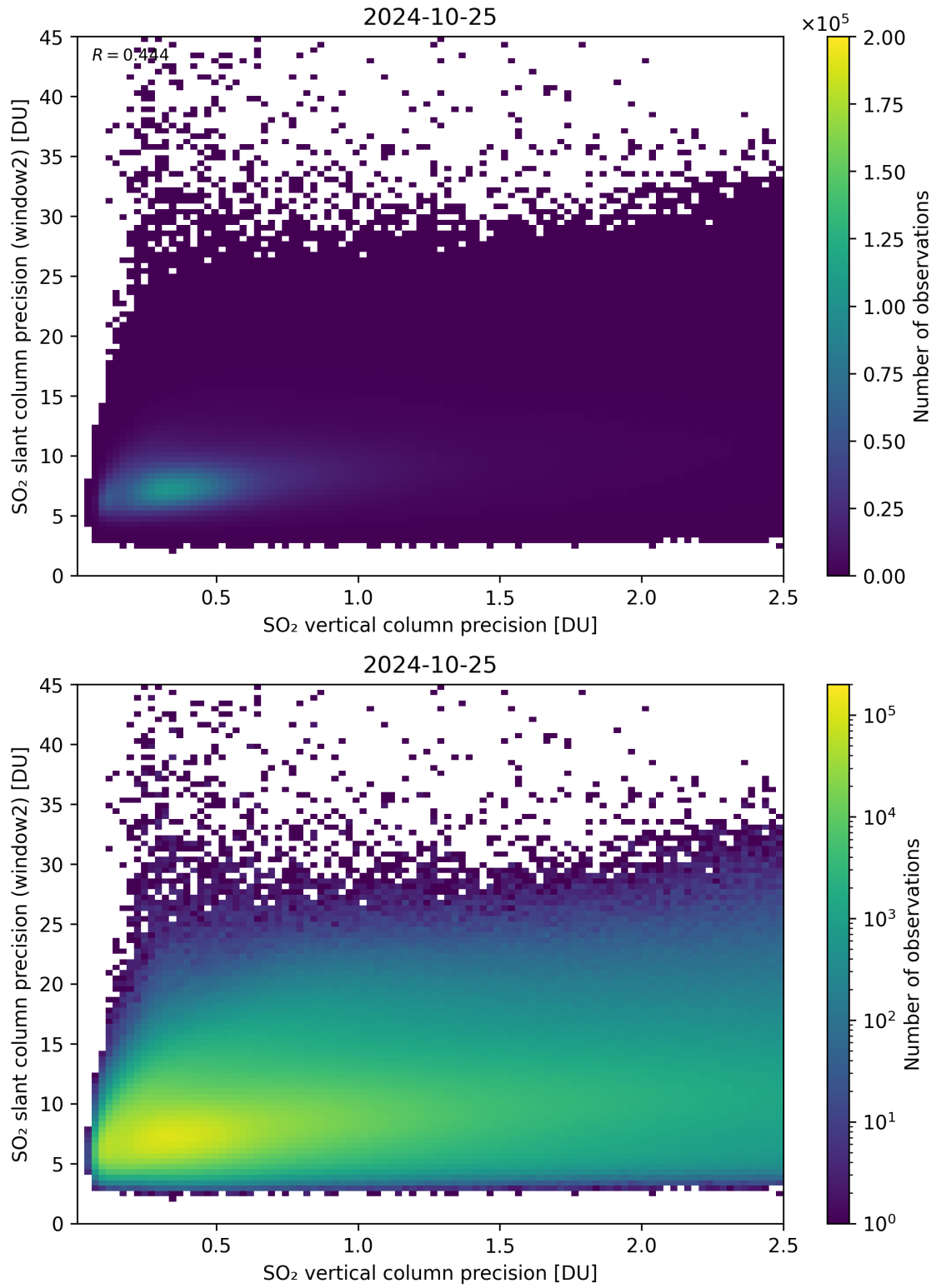
Figure 291: Scatter density plot of “SO 2 vertical column precision” against “SO 2 slant column precision (window2)” for 2024-10-24 to 2024-10-26.
