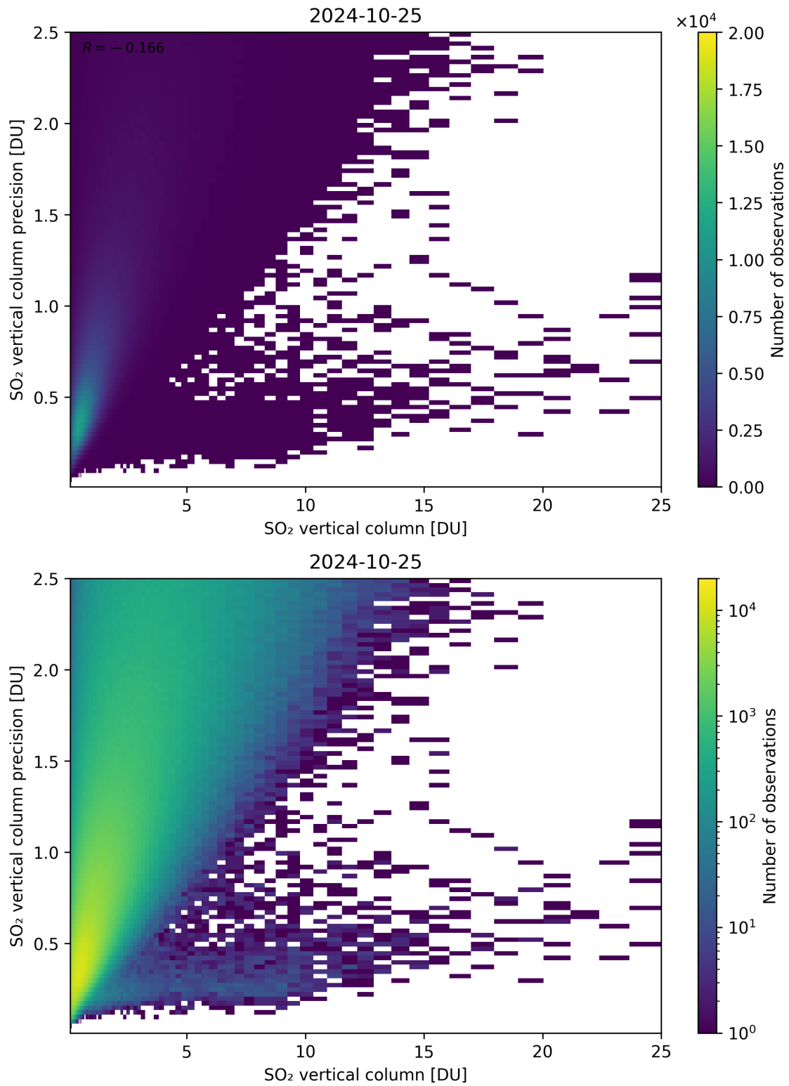
Figure 307: Scatter density plot of “SO 2 vertical column” against “SO 2 vertical column precision” for 2024-10-24 to 2024-10-26.
