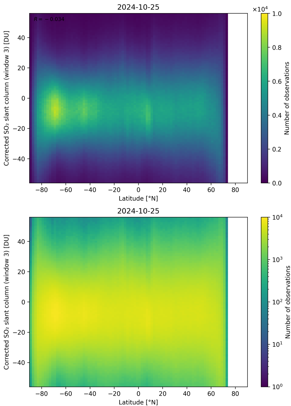
Figure 148: Scatter density plot of “Latitude” against “Corrected SO 2 slant column (window 3)” for 2024-10-24 to 2024-10-26.
