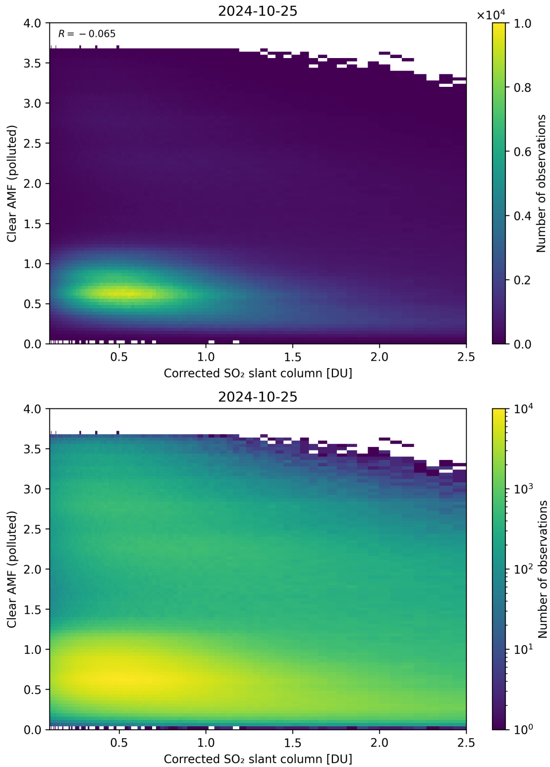
Figure 184: Scatter density plot of “Corrected SO 2 slant column” against “Clear AMF (polluted)” for 2024-10-24 to 2024-10-26.
