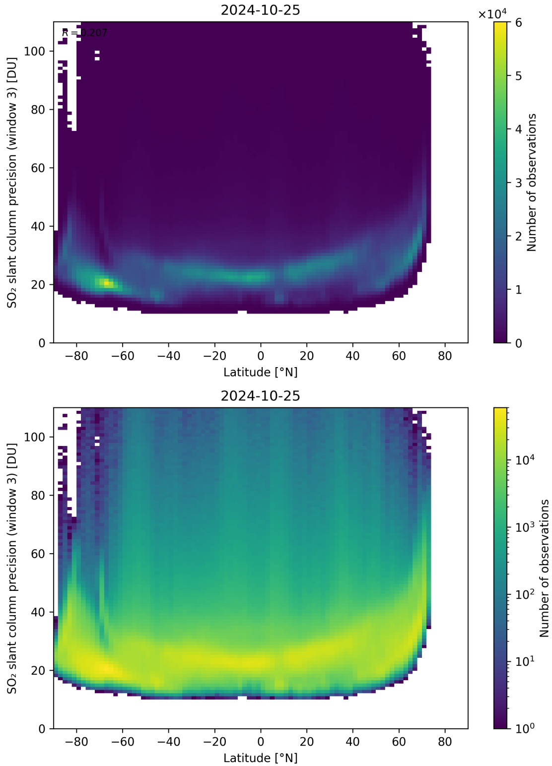
Figure 153: Scatter density plot of “Latitude” against “SO 2 slant column precision (window 3)” for 2024-10-24 to 2024-10-26.
