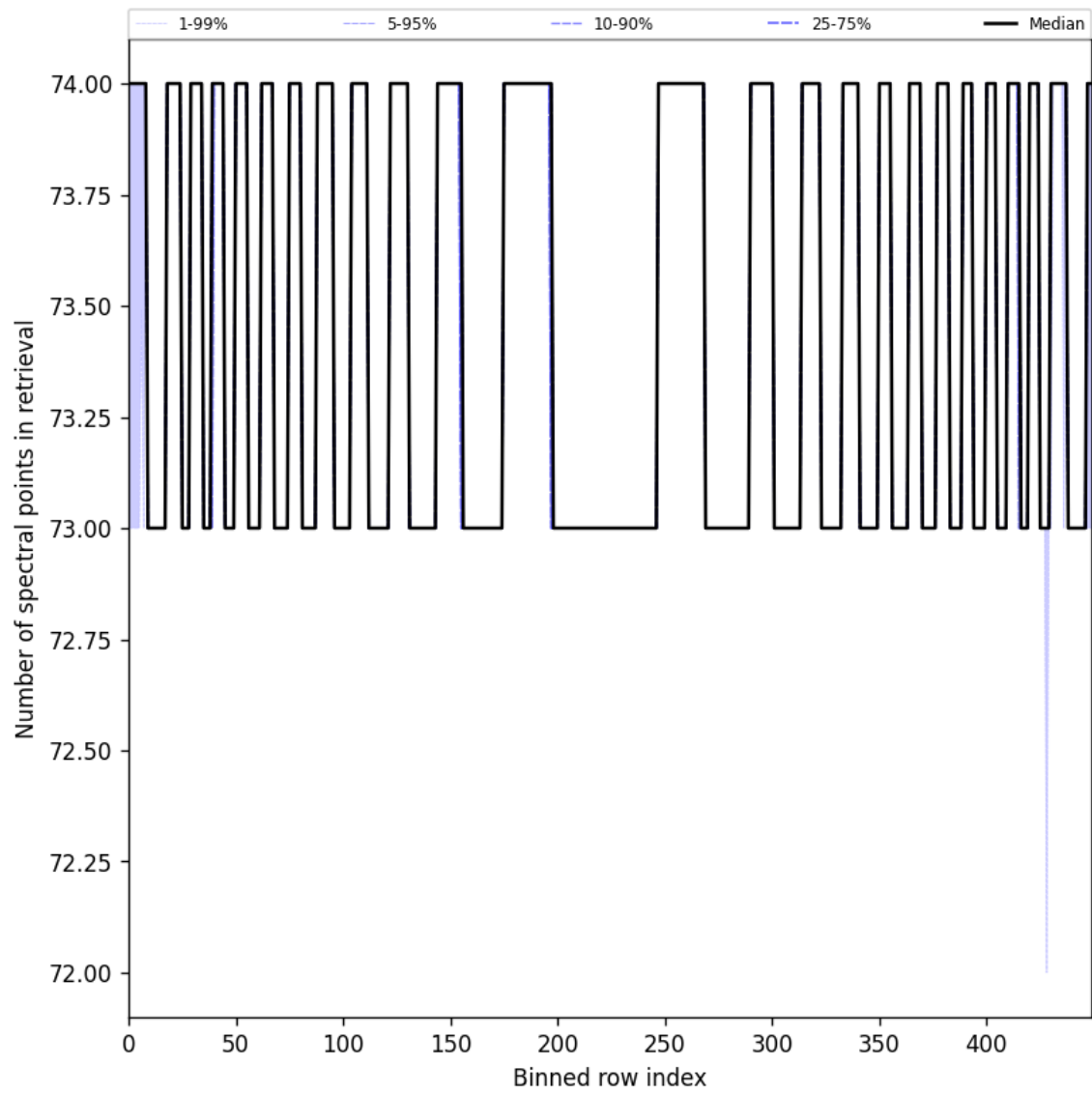
Figure 97: Along track statistics of “Number of spectral points in retrieval” for 2024-10-24 to 2024-10-26
