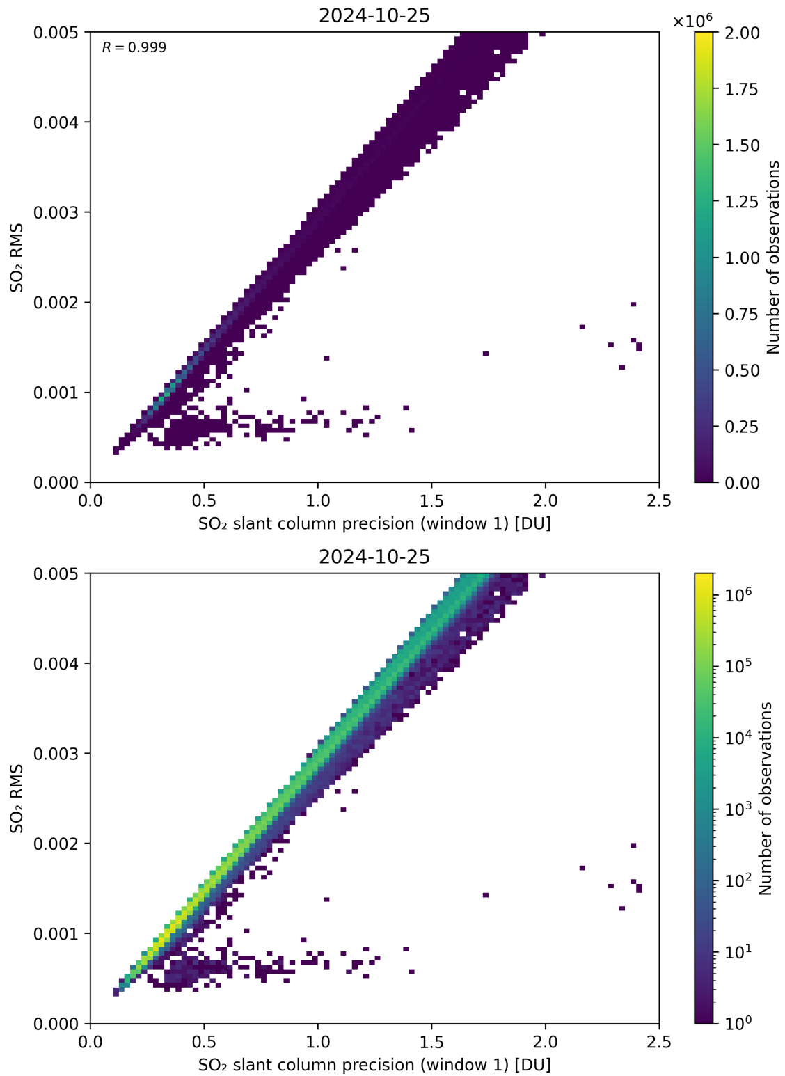
Figure 223: Scatter density plot of “SO 2 slant column precision (window 1)” against “SO 2 RMS” for 2024-10-24 to 2024-10-26.
