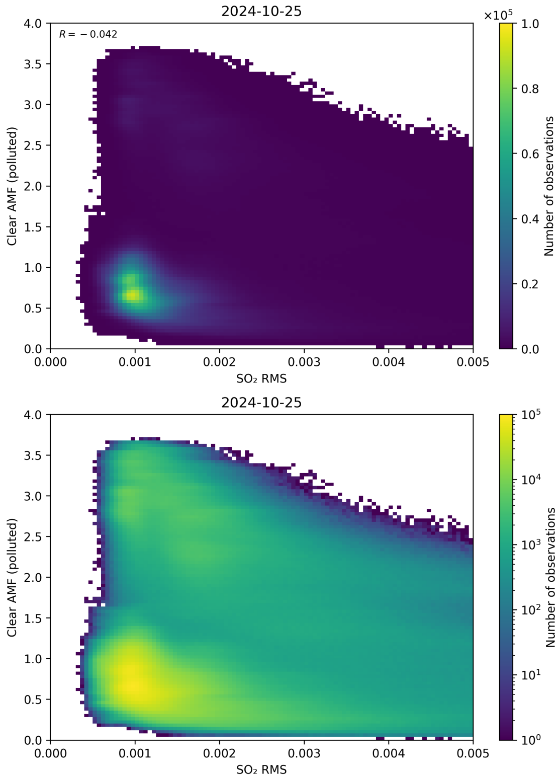
Figure 136: Scatter density plot of “SO 2 RMS” against “Clear AMF (polluted)” for 2024-10-24 to 2024-10-26.
