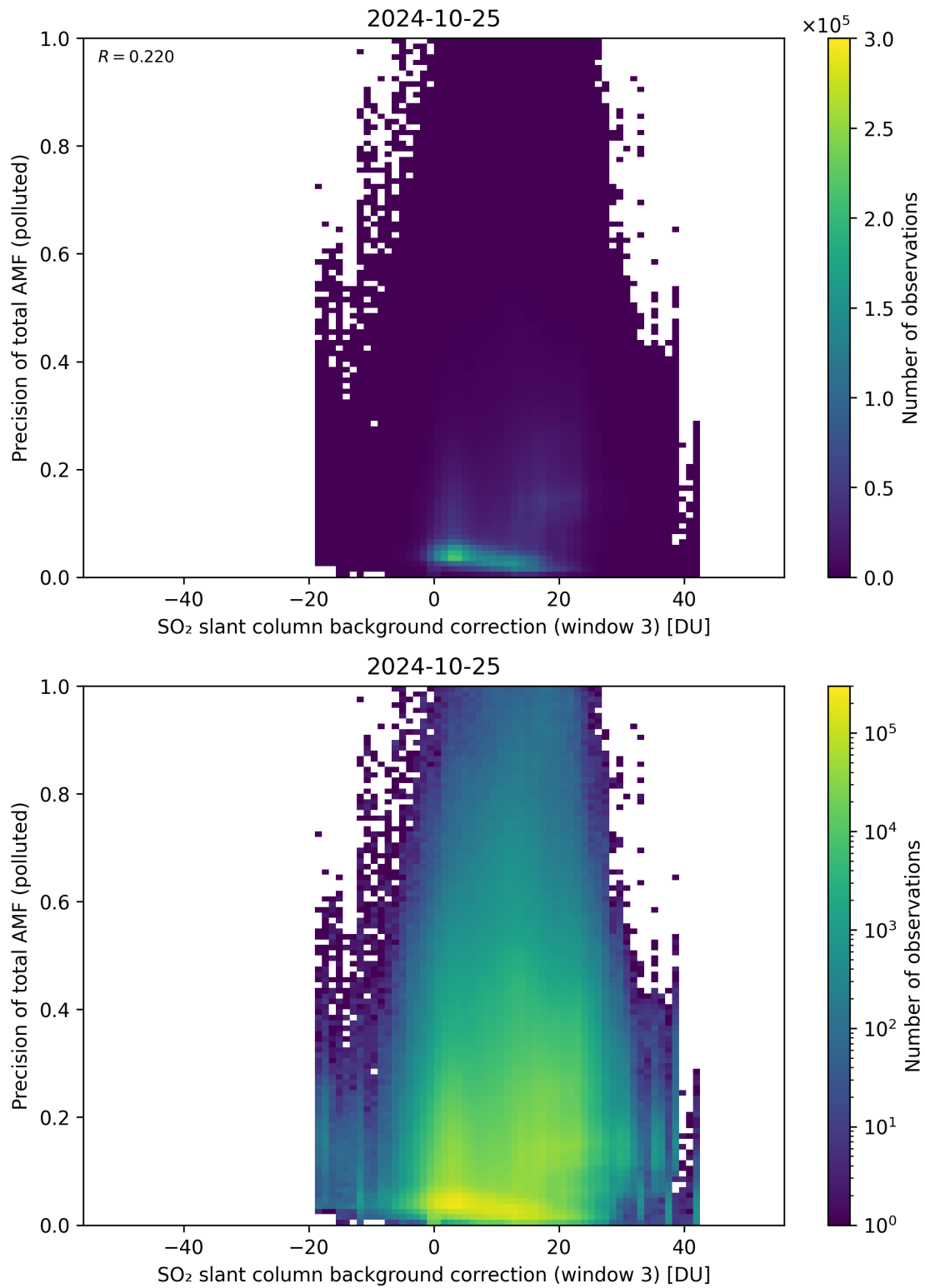
Figure 126: Scatter density plot of “SO 2 slant column background correction (window 3)” against “Precision of total AMF (polluted)” for 2024-10-24 to 2024-10-26.
