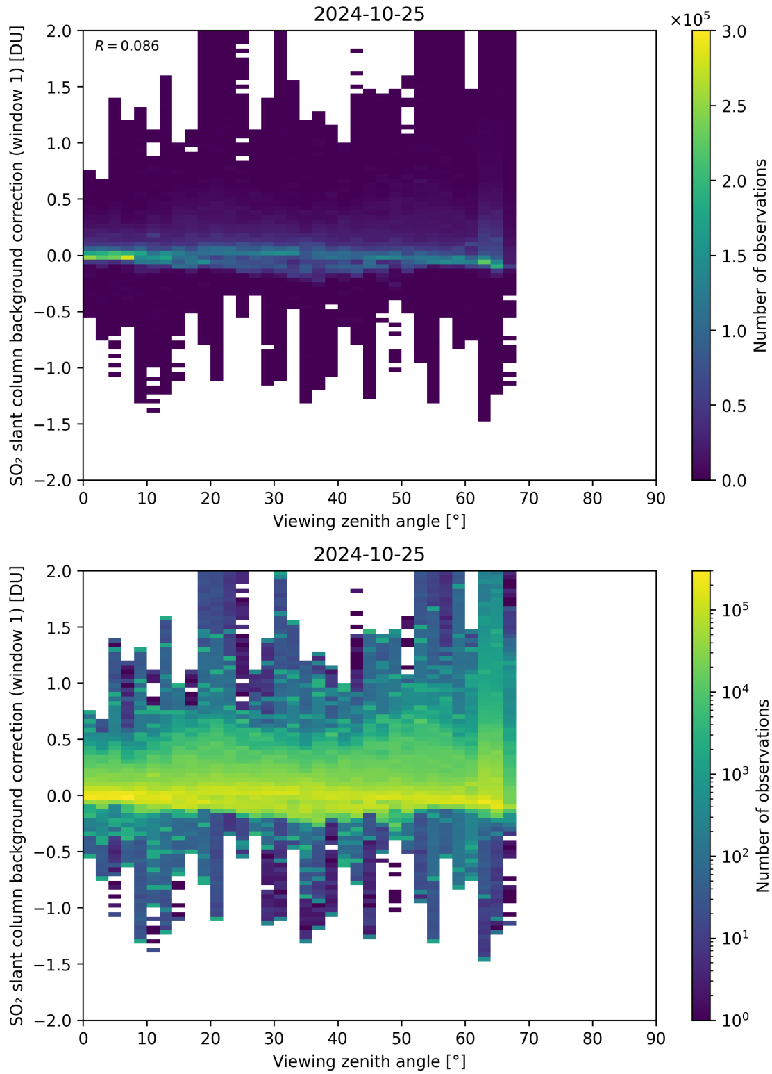
Figure 308: Scatter density plot of “Viewing zenith angle” against “SO 2 slant column background correction (window 1)” for 2024-10-24 to 2024-10-26.
