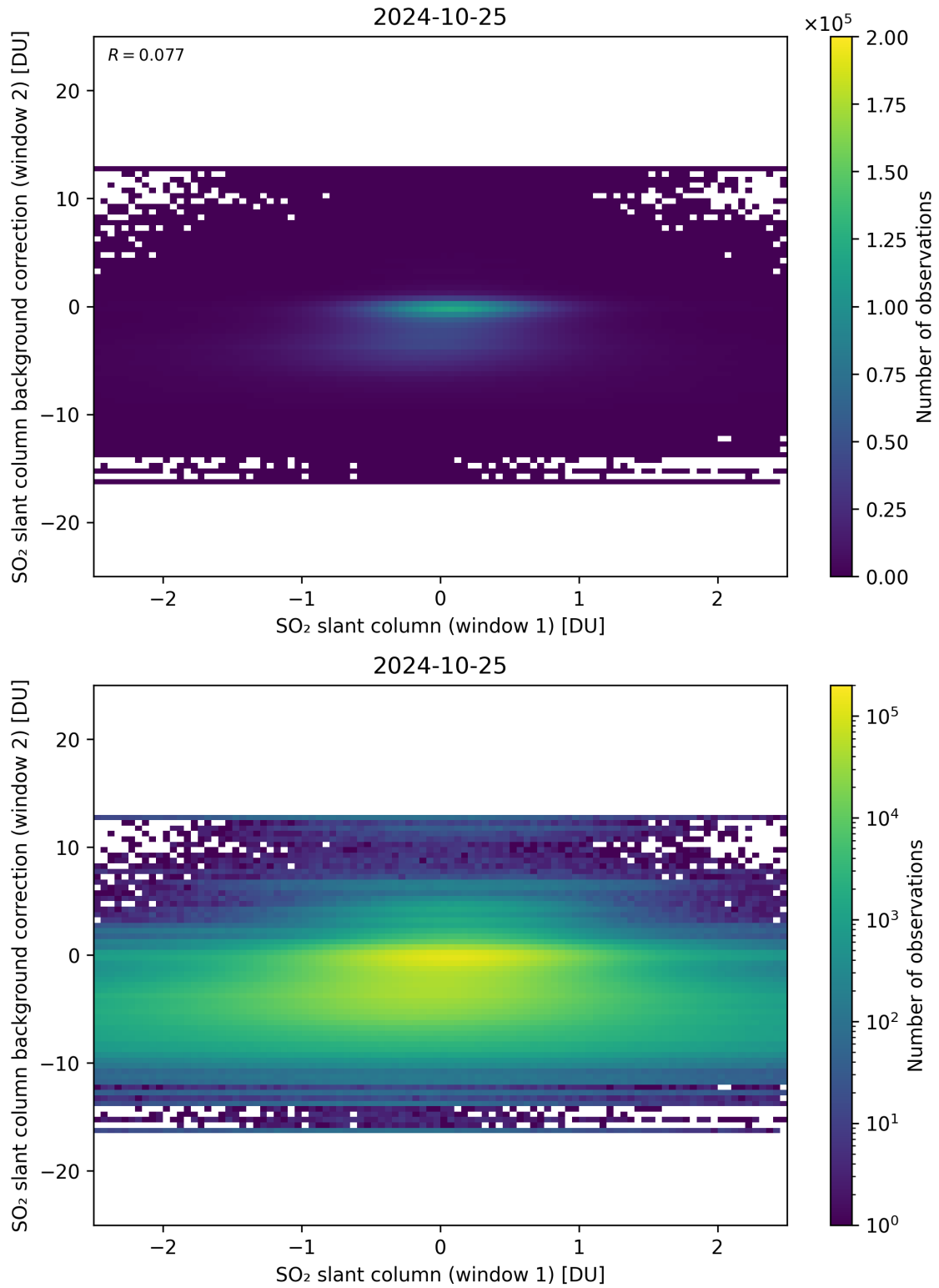
Figure 213: Scatter density plot of “SO 2 slant column (window 1)” against “SO 2 slant column background correction (window 2)” for 2024-10-24 to 2024-10-26.
