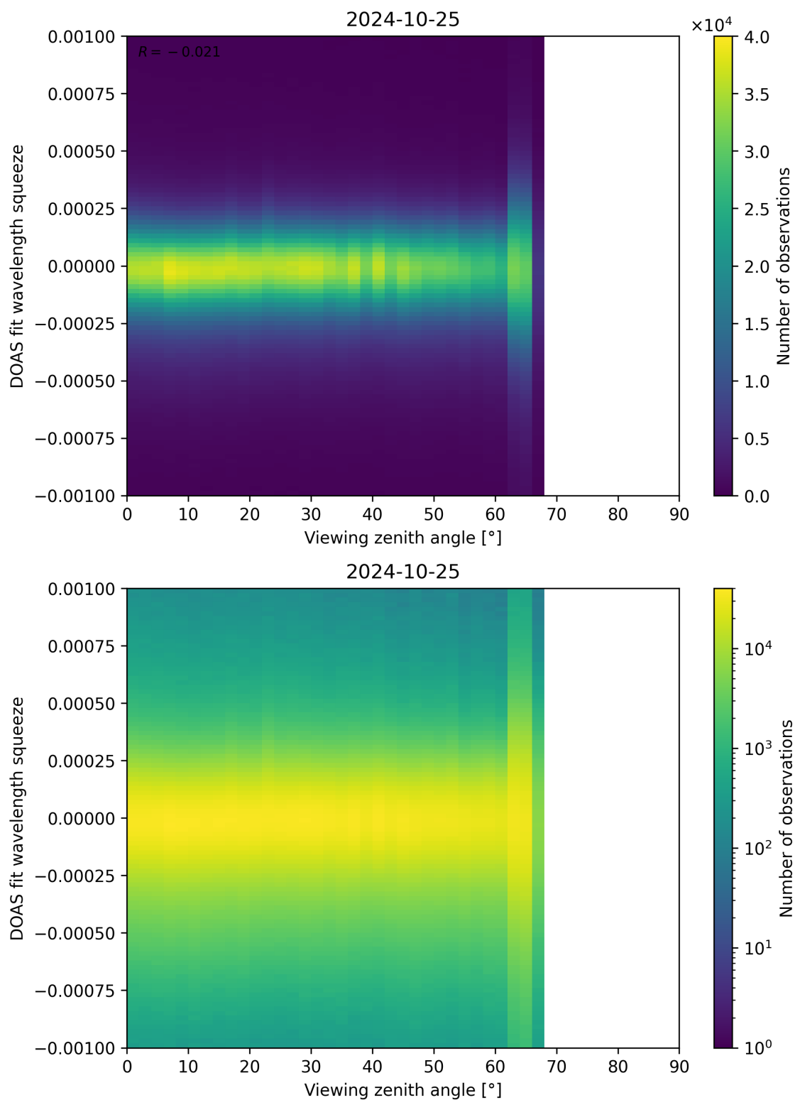
Figure 312: Scatter density plot of “Viewing zenith angle” against “DOAS fit wavelength squeeze” for 2024-10-24 to 2024-10-26.
