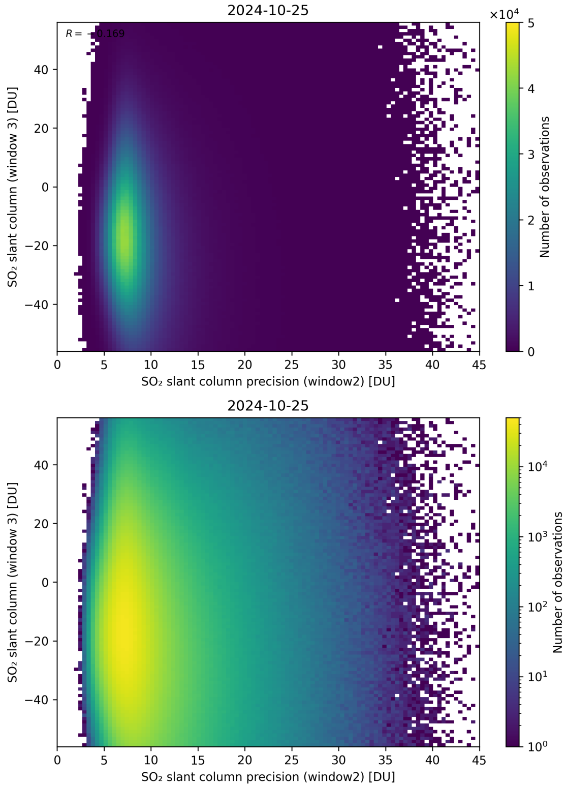
Figure 249: Scatter density plot of “SO 2 slant column precision (window2)” against “SO 2 slant column (window 3)” for 2024-10-24 to 2024-10-26.
