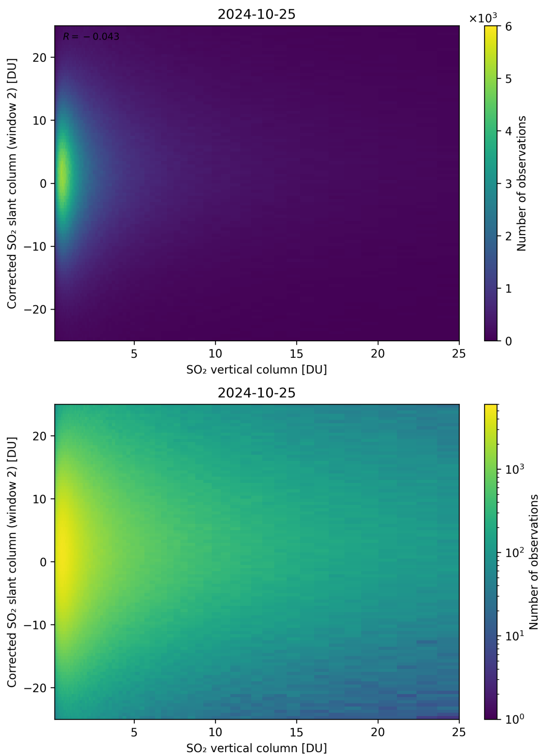
Figure 298: Scatter density plot of “SO 2 vertical column” against “Corrected SO 2 slant column (window 2)” for 2024-10-24 to 2024-10-26.
