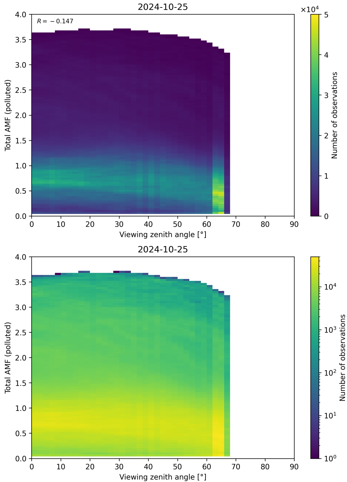
Figure 325: Scatter density plot of “Viewing zenith angle” against “Total AMF (polluted)” for 2024-10-24 to 2024-10-26.
