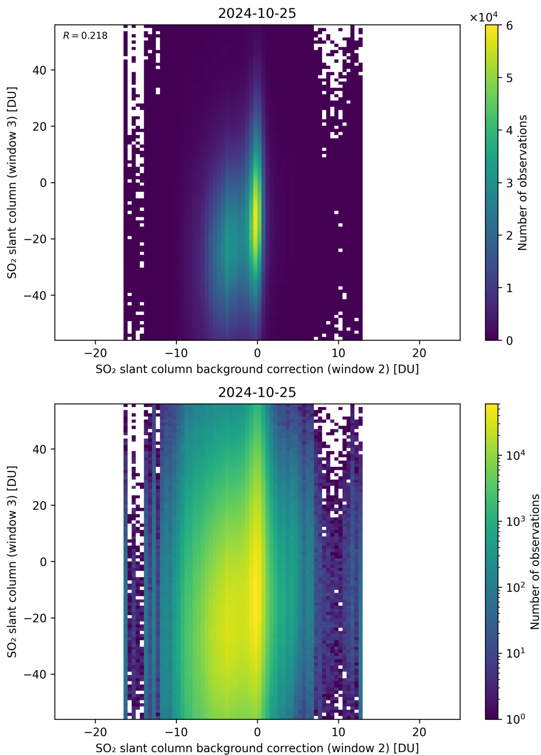
Figure 117: Scatter density plot of “SO 2 slant column background correction (window 2)” against “SO 2 slant column (window 3)” for 2024-10-24 to 2024-10-26.
