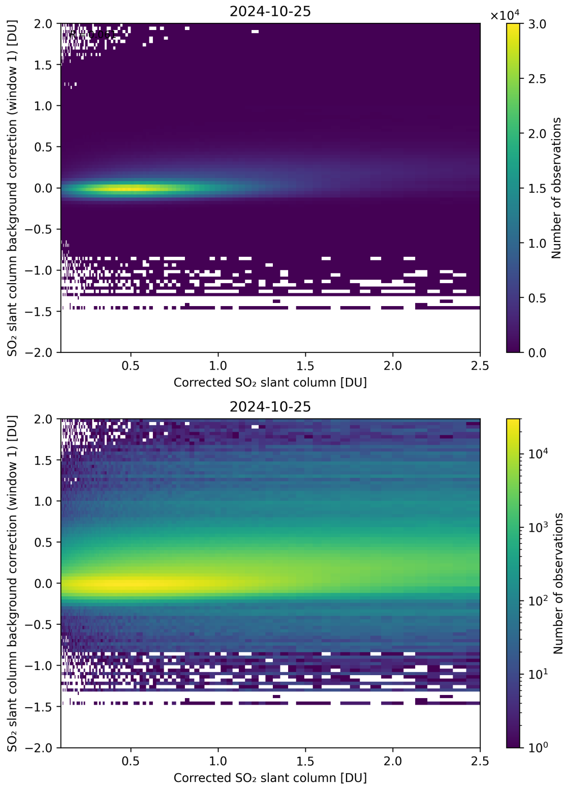
Figure 178: Scatter density plot of “Corrected SO 2 slant column” against “SO 2 slant column background correction (window 1)” for 2024-10-24 to 2024-10-26.
