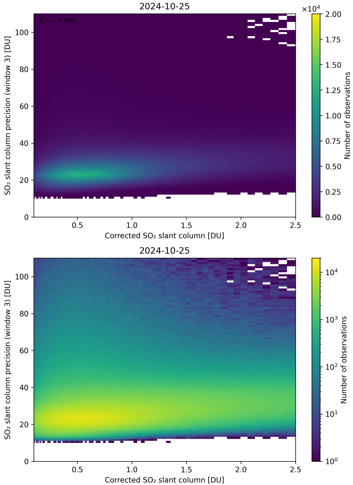
Figure 191: Scatter density plot of “Corrected SO 2 slant column” against “SO 2 slant column precision (window 3)” for 2024-10-24 to 2024-10-26.
