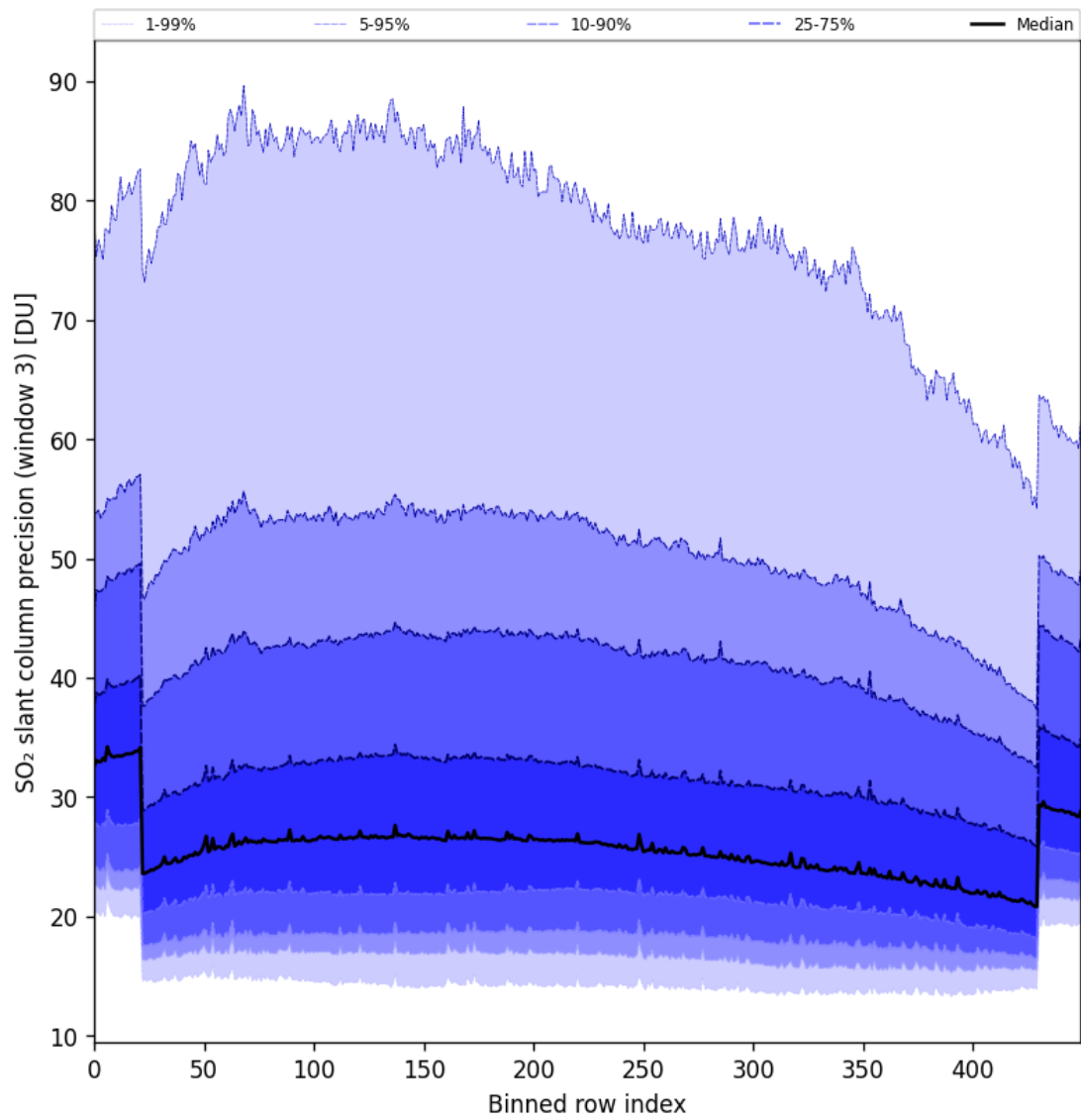
Figure 88: Along track statistics of “SO 2 slant column precision (window 3)” for 2024-10-24 to 2024-10-26
