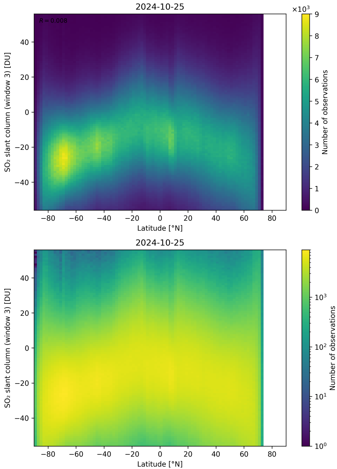
Figure 152: Scatter density plot of “Latitude” against “SO 2 slant column (window 3)” for 2024-10-24 to 2024-10-26.
