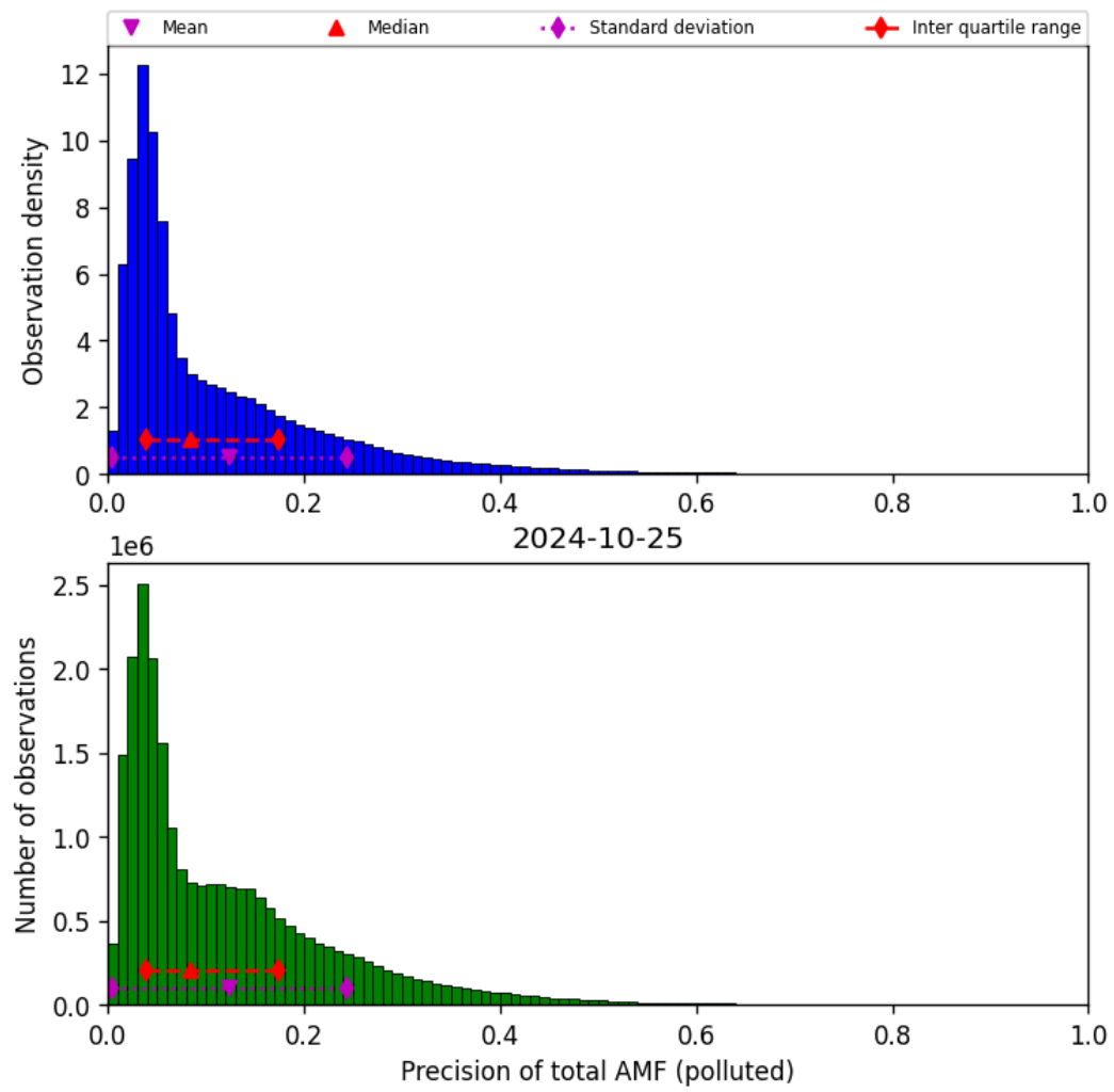
Figure 72: Histogram of “Precision of total AMF (polluted)” for 2024-10-24 to 2024-10-26
