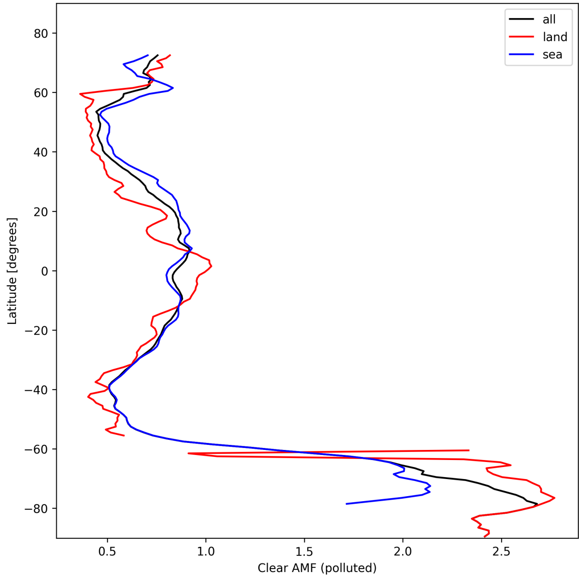
Figure 50: Zonal average of “Clear AMF (polluted)” for 2024-10-24 to 2024-10-26.
