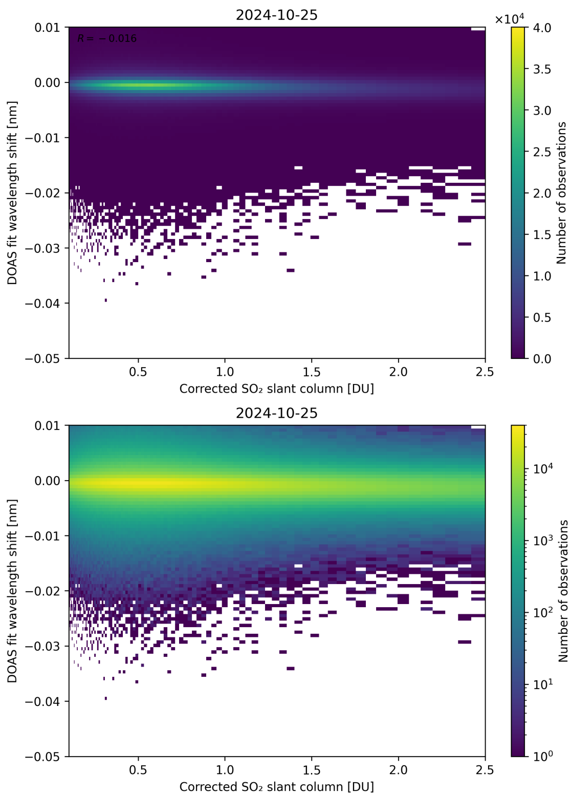
Figure 181: Scatter density plot of “Corrected SO 2 slant column” against “DOAS fit wavelength shift” for 2024-10-24 to 2024-10-26.
