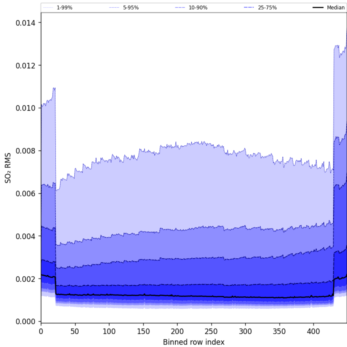
Figure 93: Along track statistics of “SO 2 RMS” for 2024-10-24 to 2024-10-26
