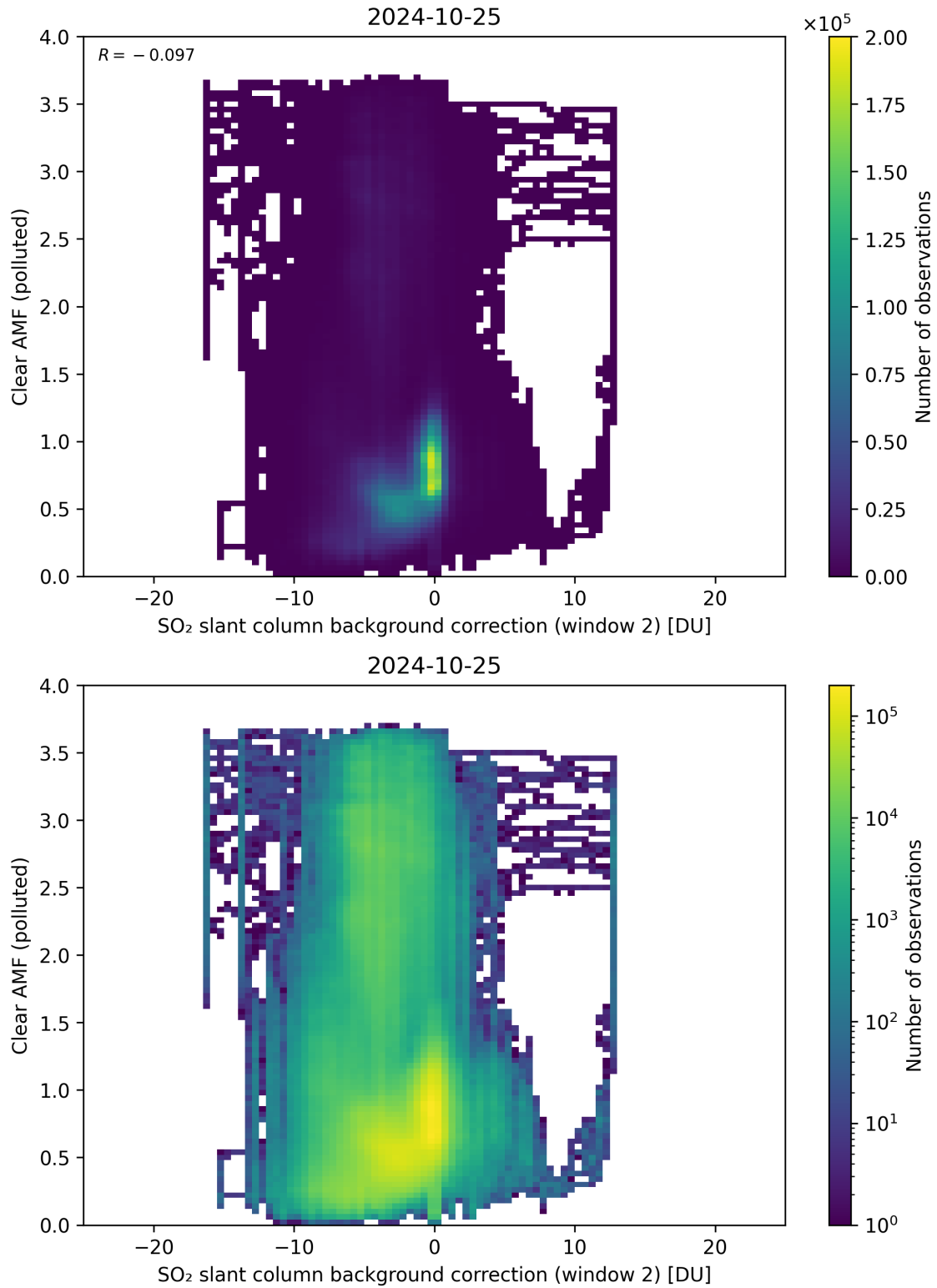
Figure 115: Scatter density plot of “SO 2 slant column background correction (window 2)” against “Clear AMF (polluted)” for 2024-10-24 to 2024-10-26.
