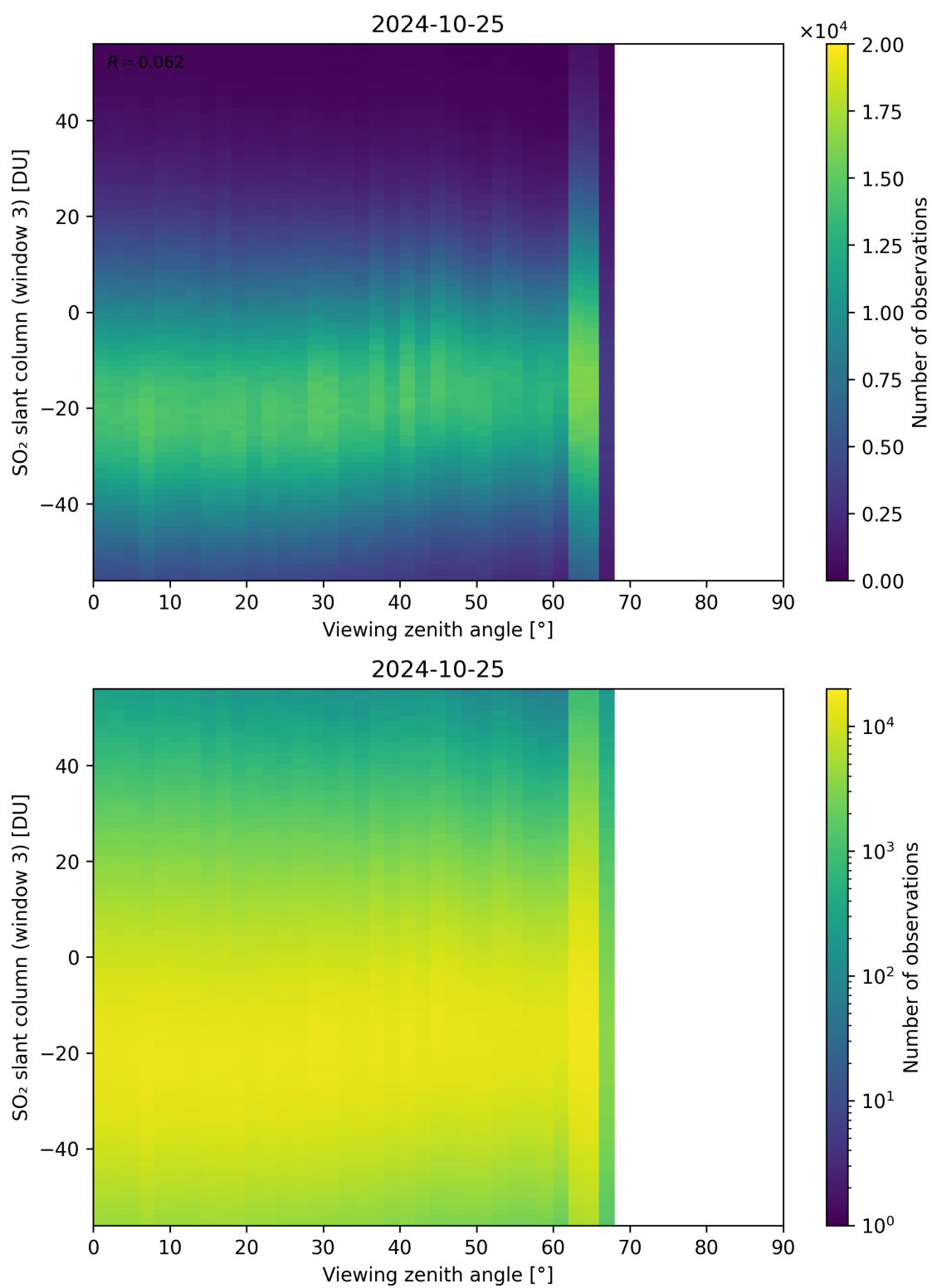
Figure 323: Scatter density plot of “Viewing zenith angle” against “SO 2 slant column (window 3)” for 2024-10-24 to 2024-10-26.
