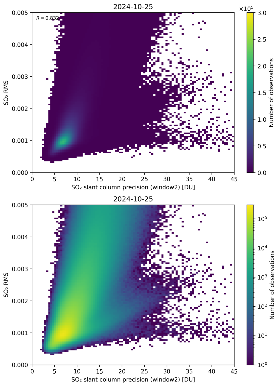
Figure 245: Scatter density plot of “SO 2 slant column precision (window2)” against “SO 2 RMS” for 2024-10-24 to 2024-10-26.
