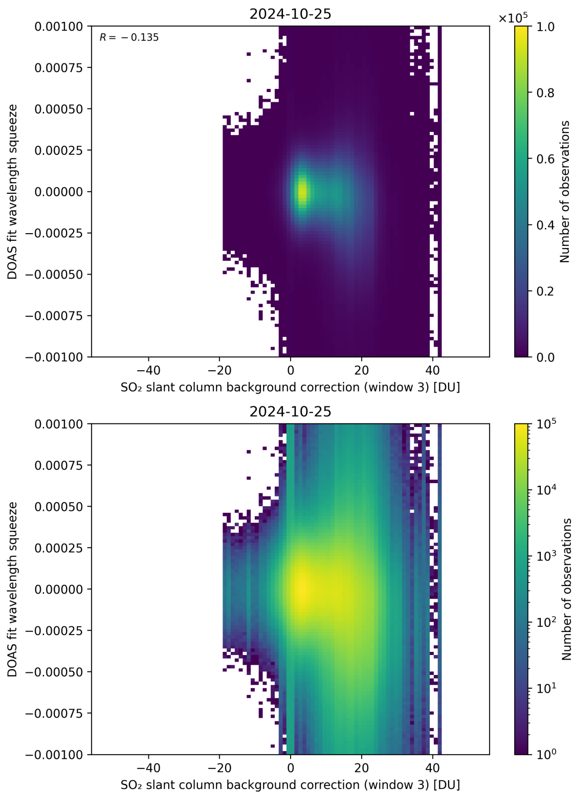
Figure 122: Scatter density plot of “SO 2 slant column background correction (window 3)” against “DOAS fit wavelength squeeze” for 2024-10-24 to 2024-10-26.
