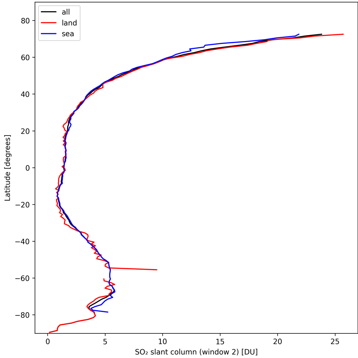
Figure 37: Zonal average of “SO 2 slant column (window 2)” for 2024-10-24 to 2024-10-26.
