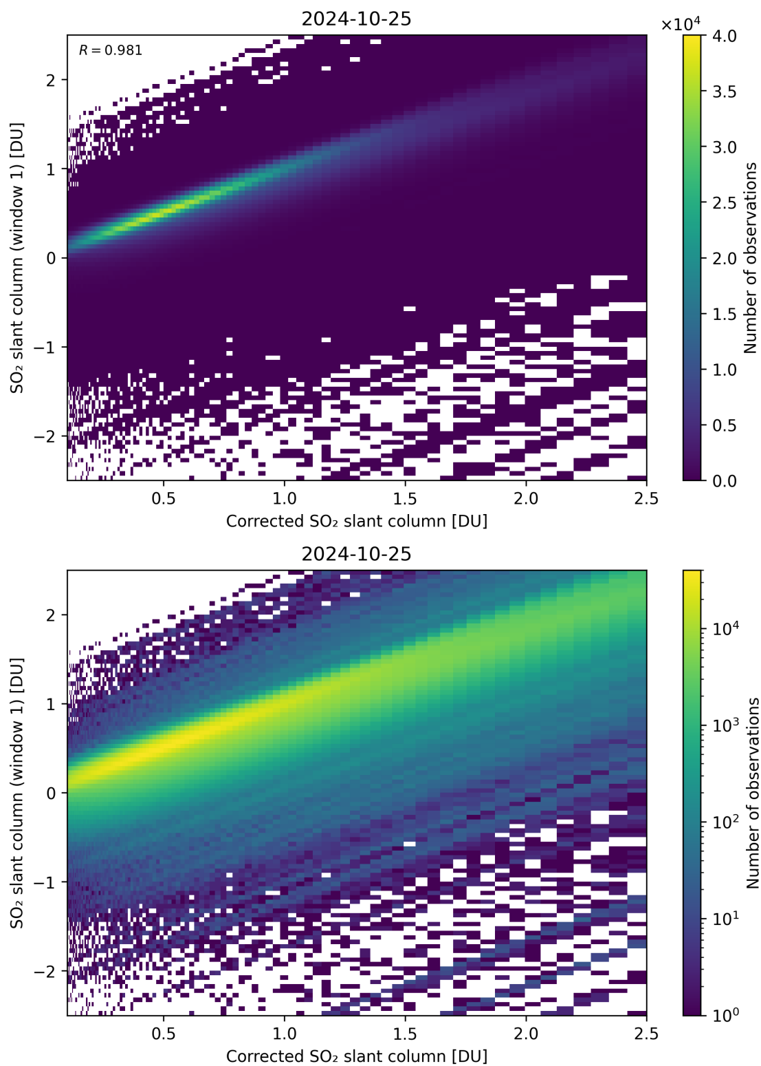
Figure 187: Scatter density plot of “Corrected SO 2 slant column” against “SO 2 slant column (window 1)” for 2024-10-24 to 2024-10-26.
