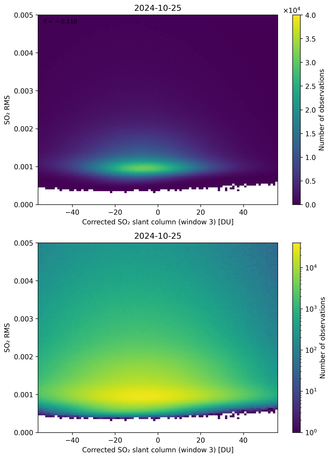
Figure 208: Scatter density plot of “Corrected SO 2 slant column (window 3)” against “SO 2 RMS” for 2024-10-24 to 2024-10-26.
