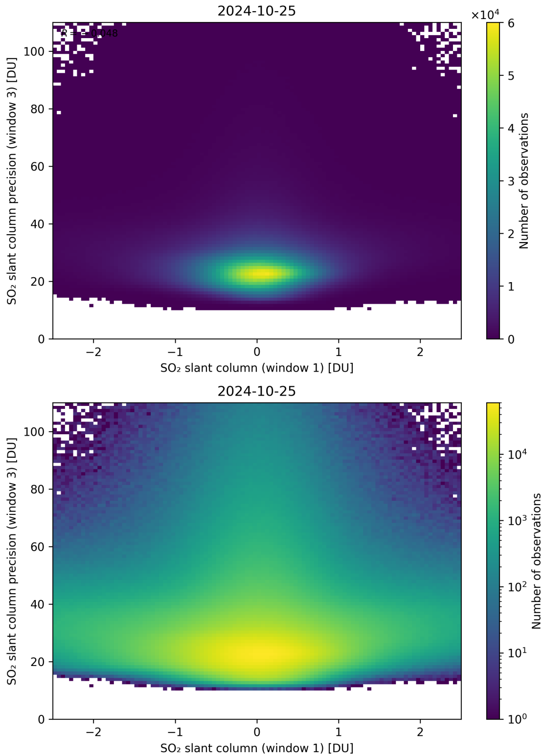
Figure 238: Scatter density plot of “SO 2 slant column (window 1)” against “SO 2 slant column precision (window 3)” for 2024-10-24 to 2024-10-26.
