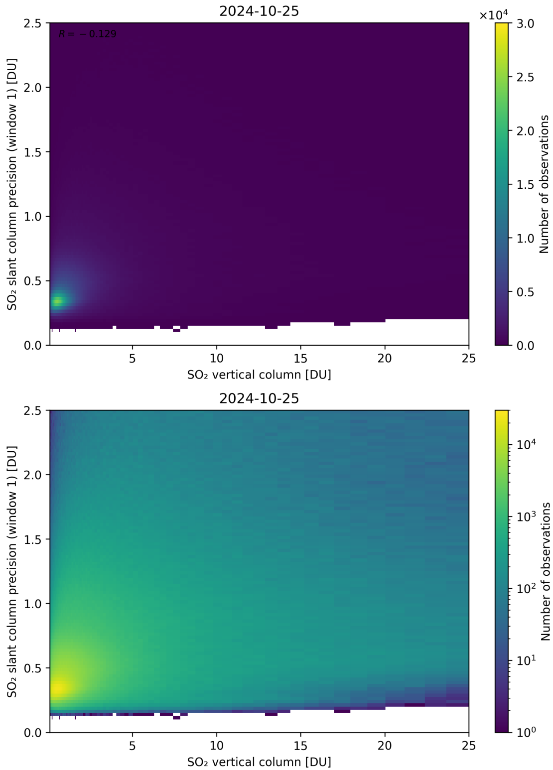
Figure 301: Scatter density plot of “SO 2 vertical column” against “SO 2 slant column precision (window 1)” for 2024-10-24 to 2024-10-26.
