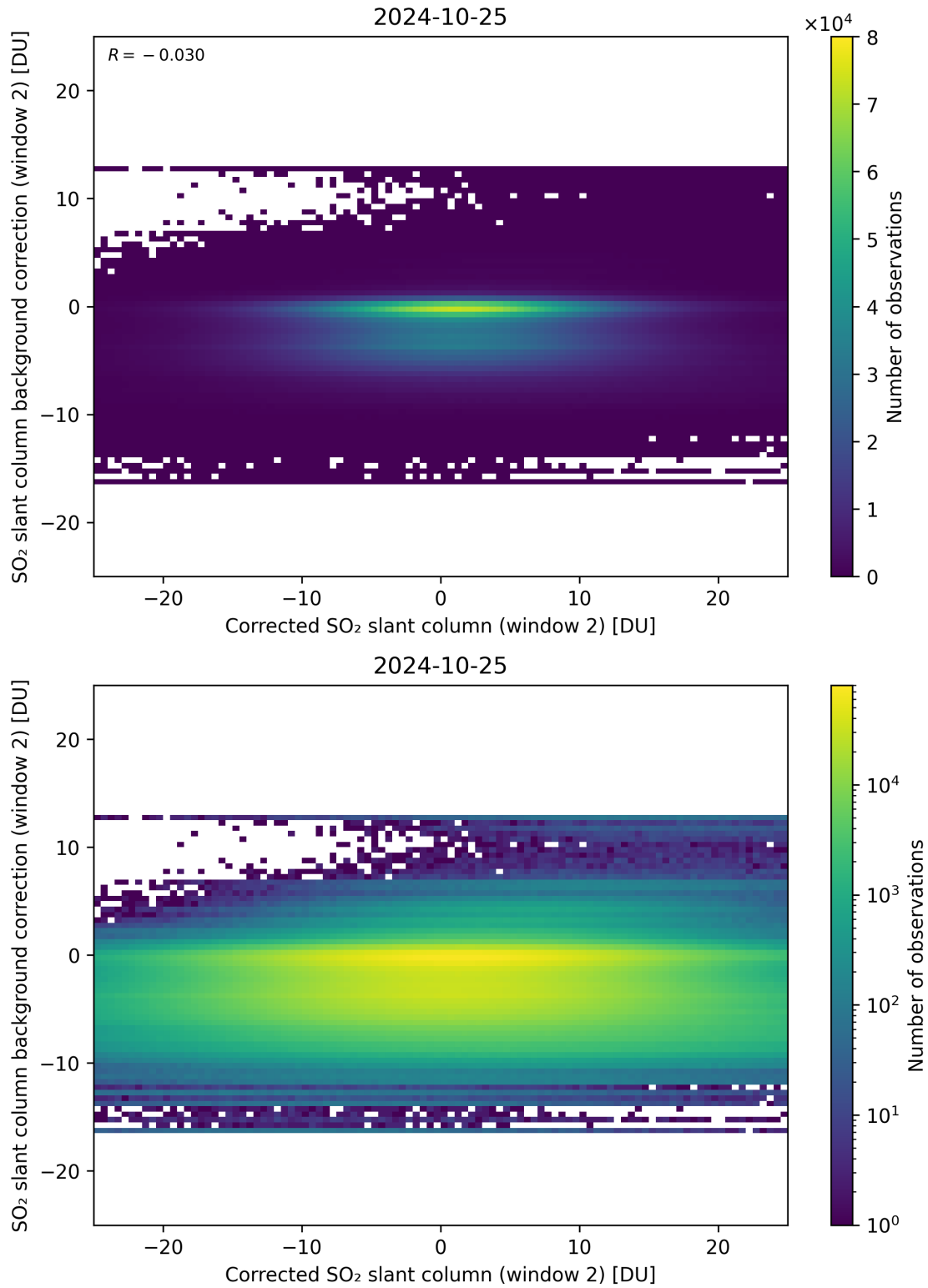
Figure 194: Scatter density plot of “Corrected SO 2 slant column (window 2)” against “SO 2 slant column background correction (window 2)” for 2024-10-24 to 2024-10-26.
