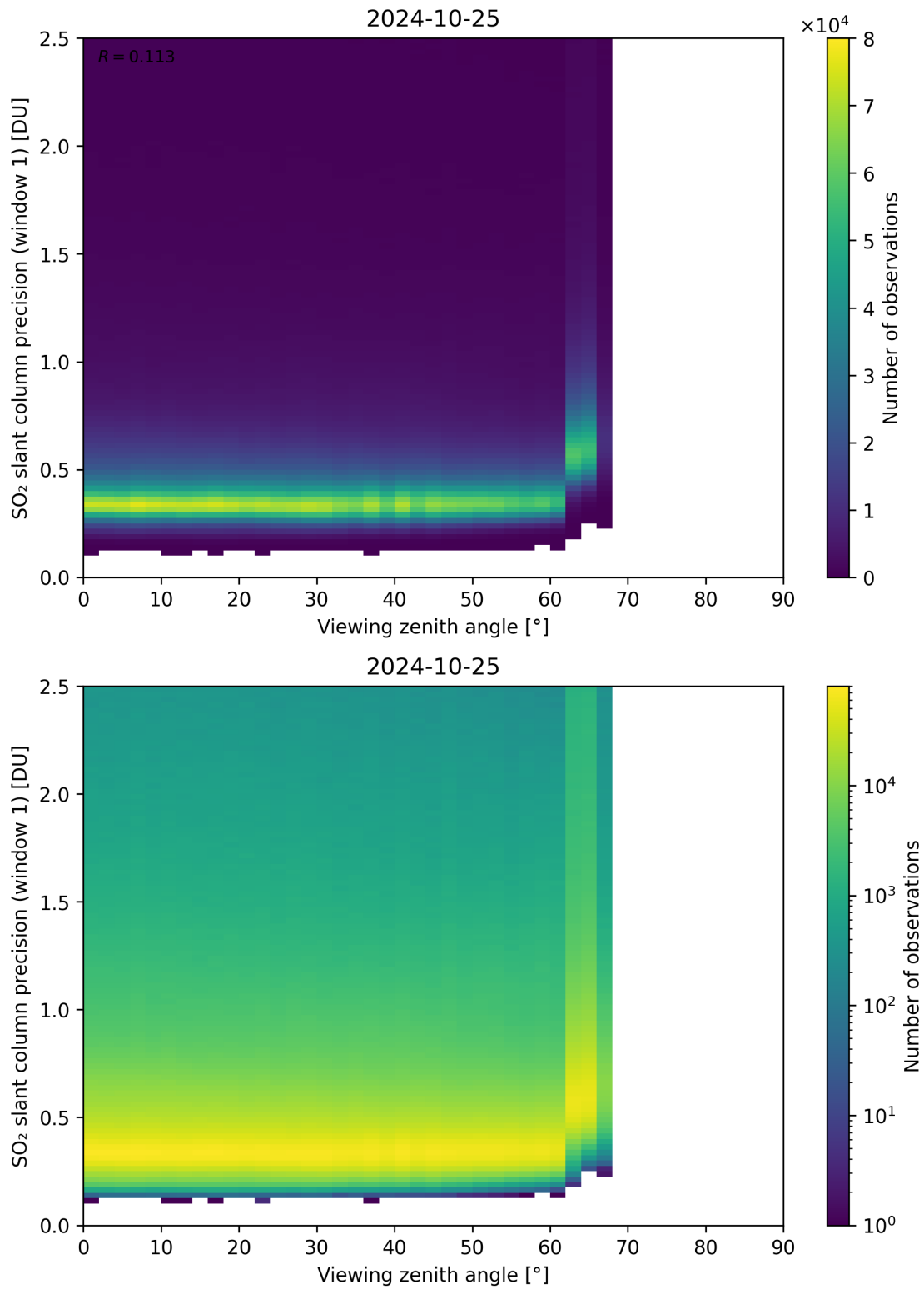
Figure 321: Scatter density plot of “Viewing zenith angle” against “SO 2 slant column precision (window 1)” for 2024-10-24 to 2024-10-26.
