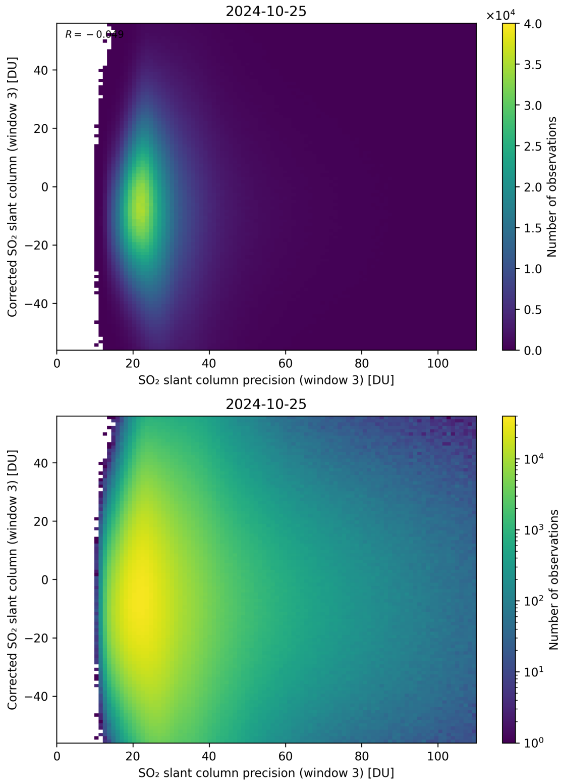
Figure 262: Scatter density plot of “SO 2 slant column precision (window 3)” against “Corrected SO 2 slant column (window 3)” for 2024-10-24 to 2024-10-26.
