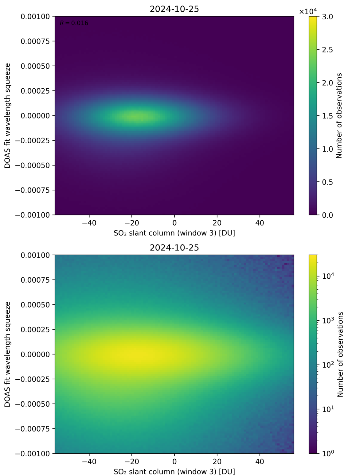
Figure 255: Scatter density plot of “SO 2 slant column (window 3)” against “DOAS fit wavelength squeeze” for 2024-10-24 to 2024-10-26.
