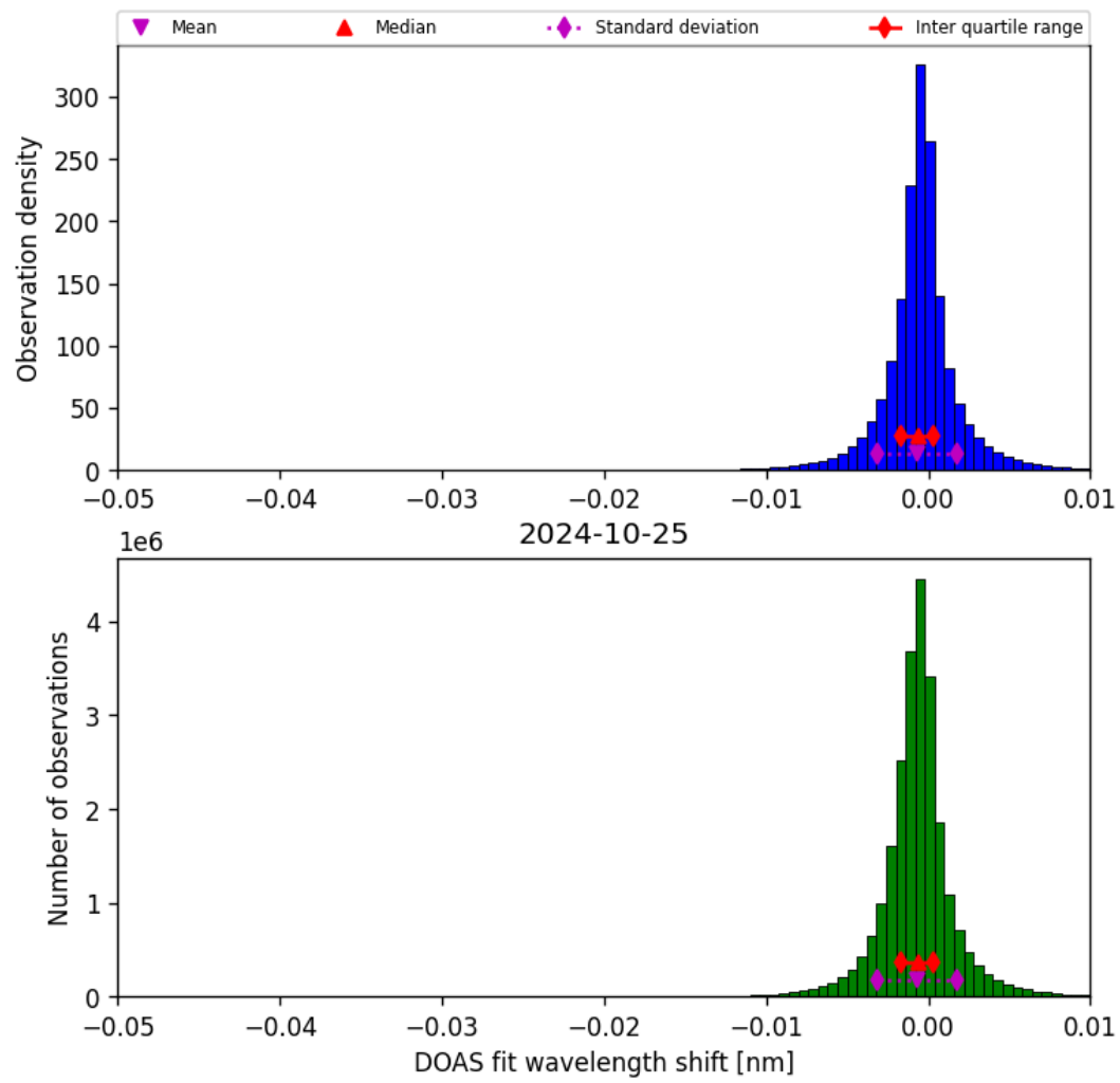
Figure 68: Histogram of “DOAS fit wavelength shift” for 2024-10-24 to 2024-10-26
