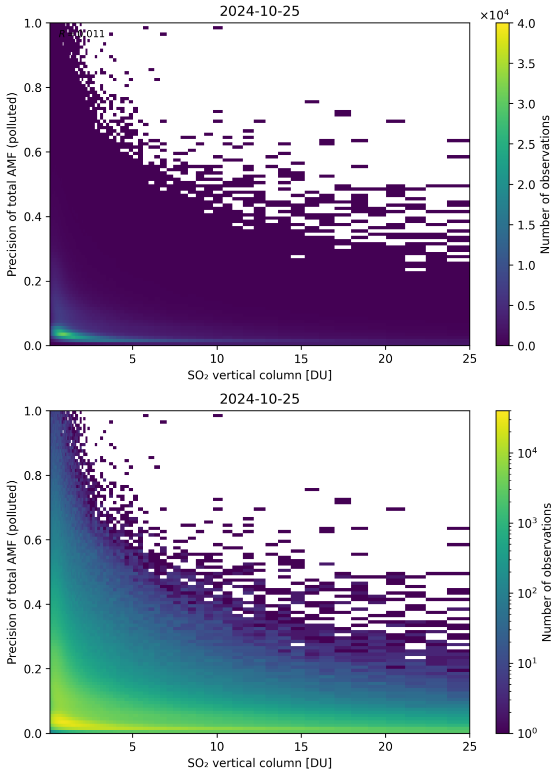
Figure 306: Scatter density plot of “SO 2 vertical column” against “Precision of total AMF (polluted)” for 2024-10-24 to 2024-10-26.
