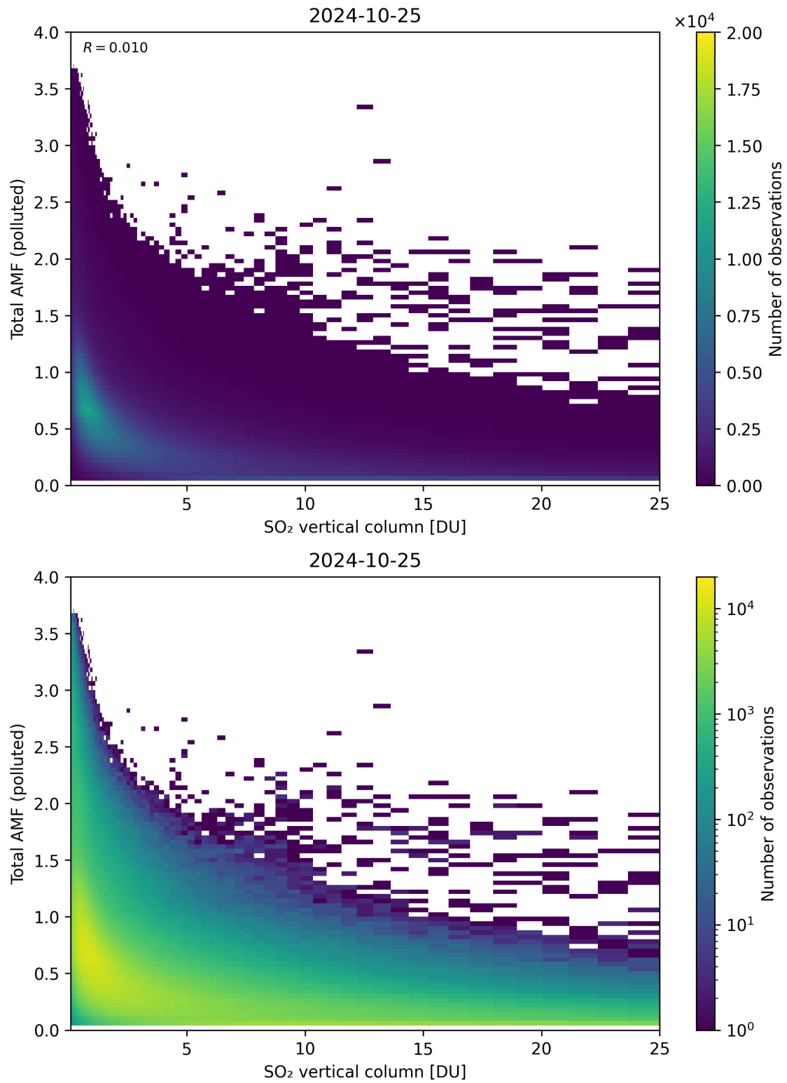
Figure 305: Scatter density plot of “SO 2 vertical column” against “Total AMF (polluted)” for 2024-10-24 to 2024-10-26.
