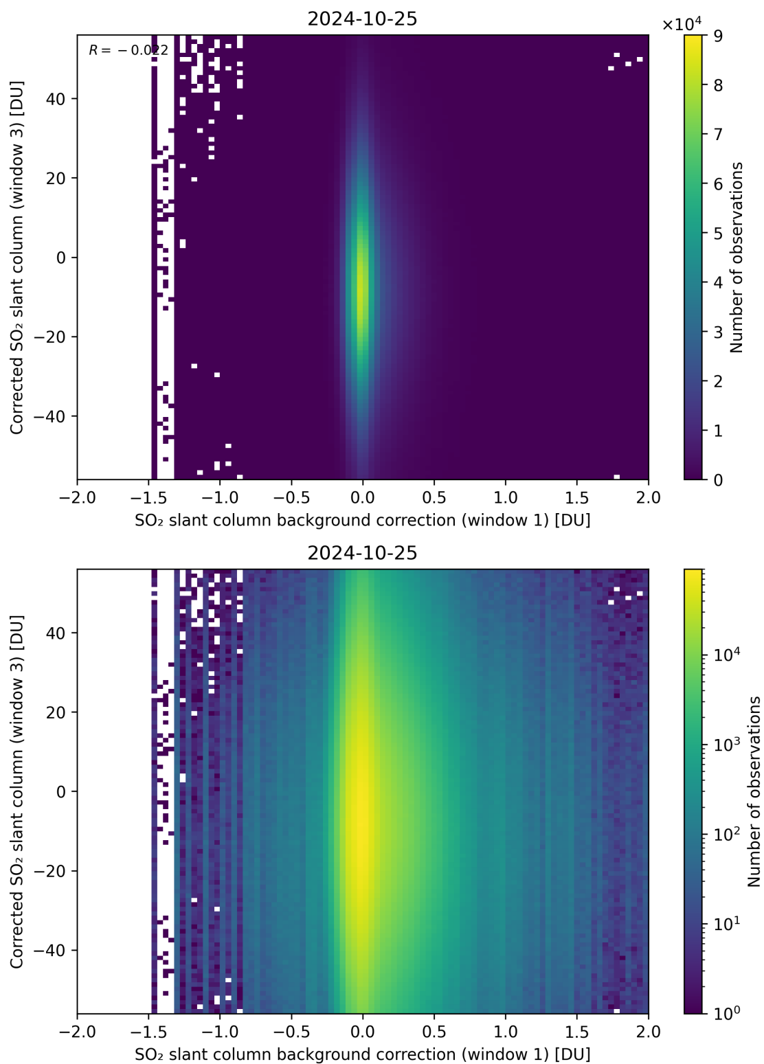
Figure 105: Scatter density plot of “SO 2 slant column background correction (window 1)” against “Corrected SO 2 slant column (window 3)” for 2024-10-24 to 2024-10-26.
