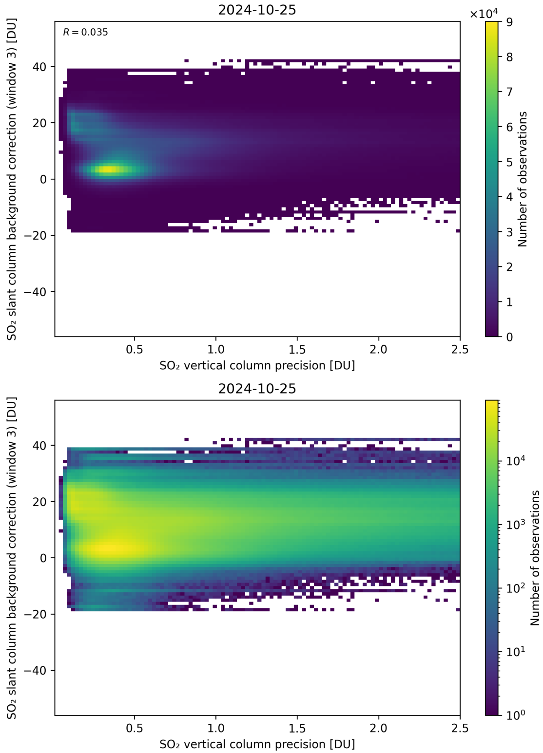
Figure 281: Scatter density plot of “SO 2 vertical column precision” against “SO 2 slant column background correction (window 3)” for 2024-10-24 to 2024-10-26.
