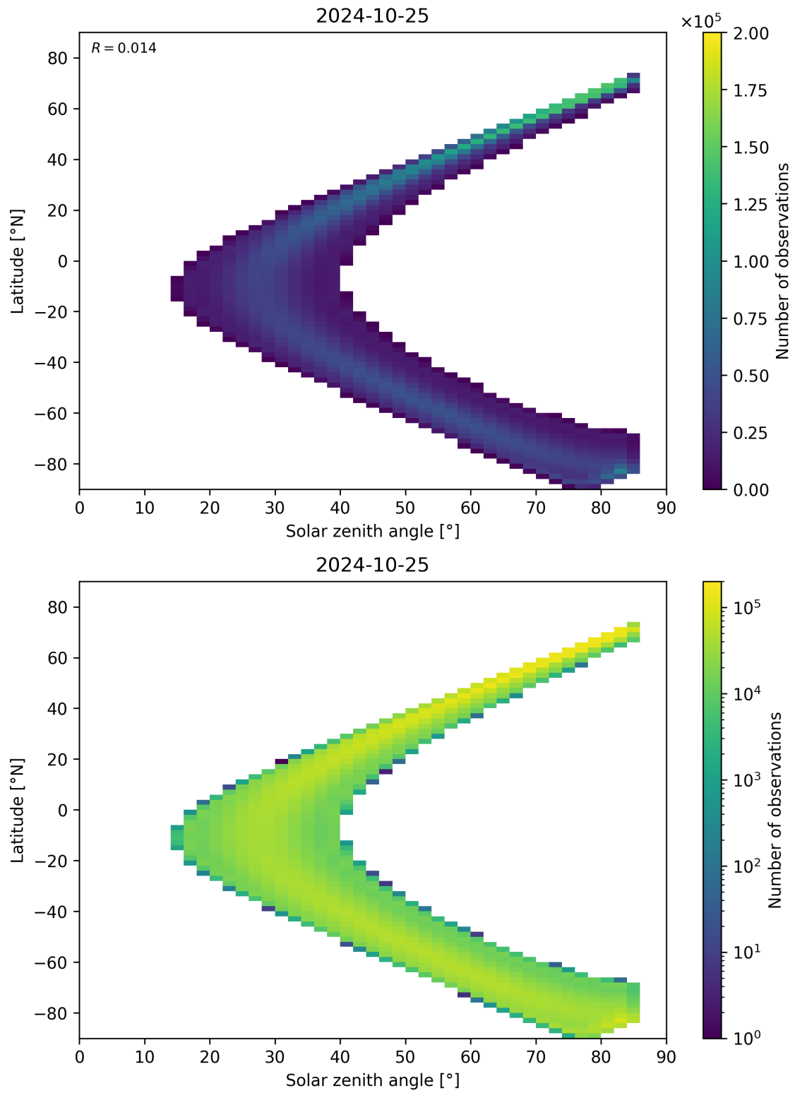
Figure 164: Scatter density plot of “Solar zenith angle” against “Latitude” for 2024-10-24 to 2024-10-26.
