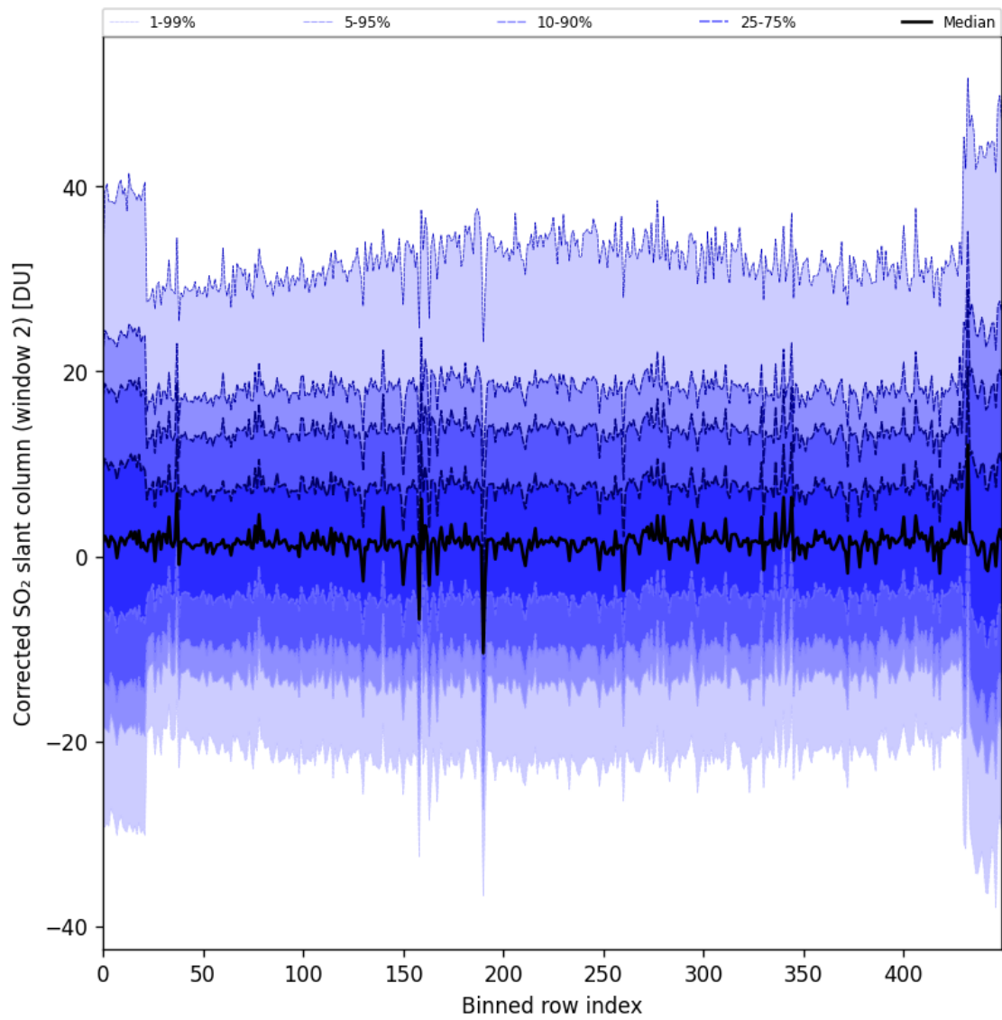
Figure 85: Along track statistics of “Corrected SO 2 slant column (window 2)” for 2024-10-24 to 2024-10-26
