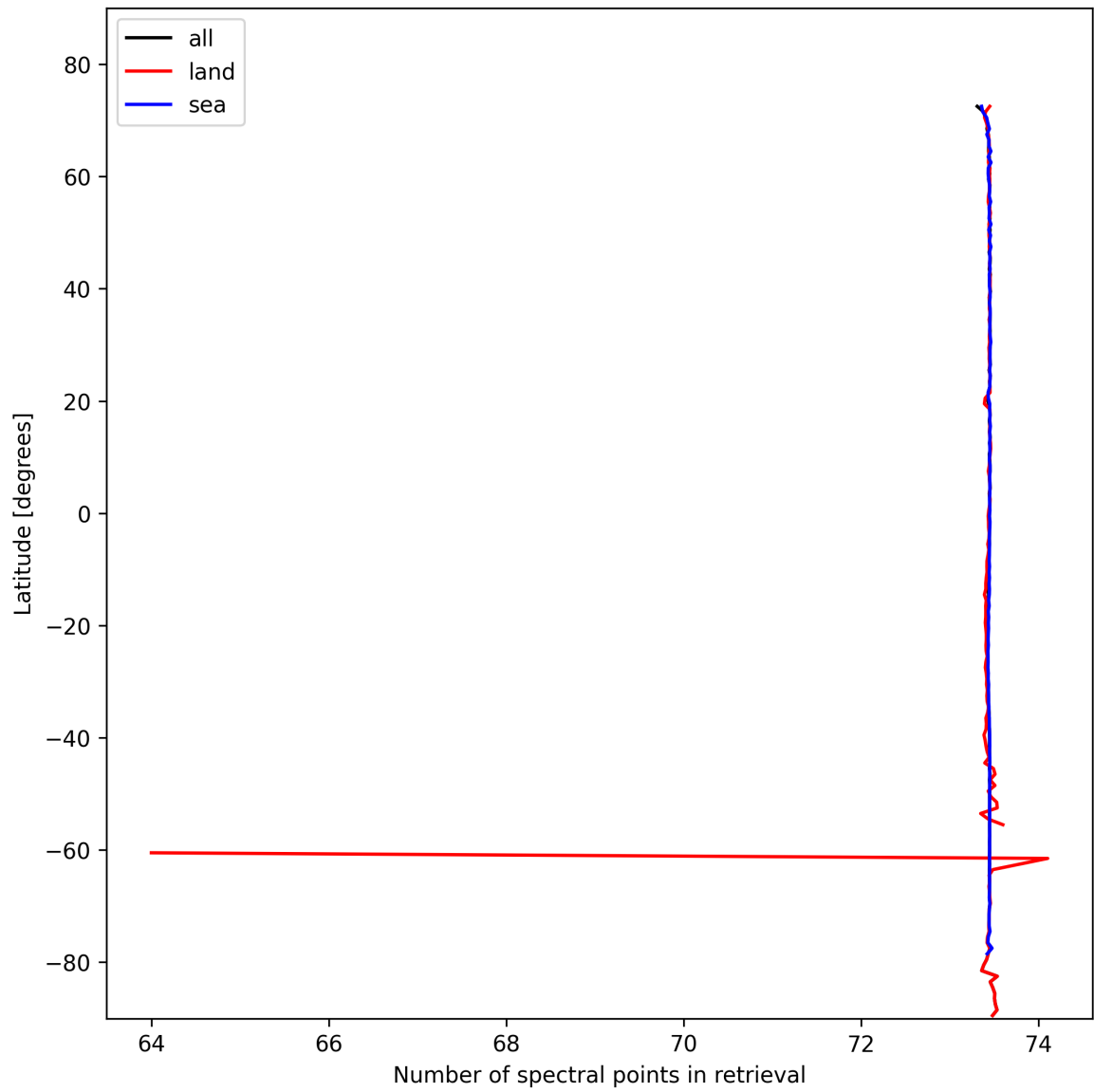
Figure 51: Zonal average of “Number of spectral points in retrieval” for 2024-10-25 to 2024-10-27.
