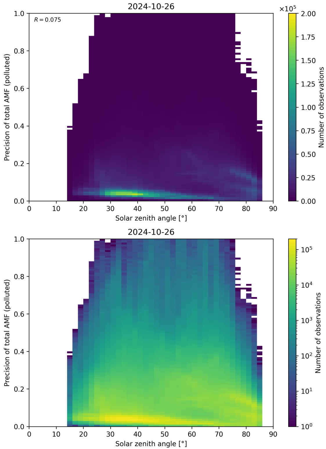
Figure 175: Scatter density plot of “Solar zenith angle” against “Precision of total AMF (polluted)” for 2024-10-25 to 2024-10-27.
