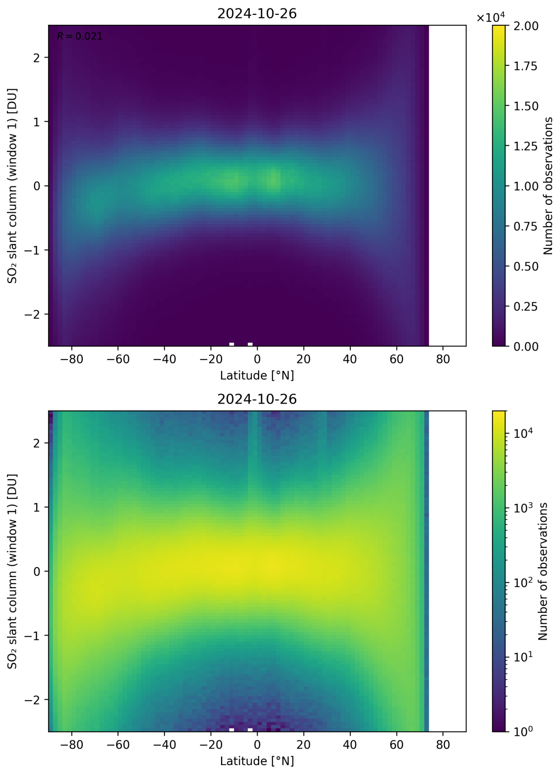
Figure 149: Scatter density plot of “Latitude” against “SO 2 slant column (window 1)” for 2024-10-25 to 2024-10-27.
