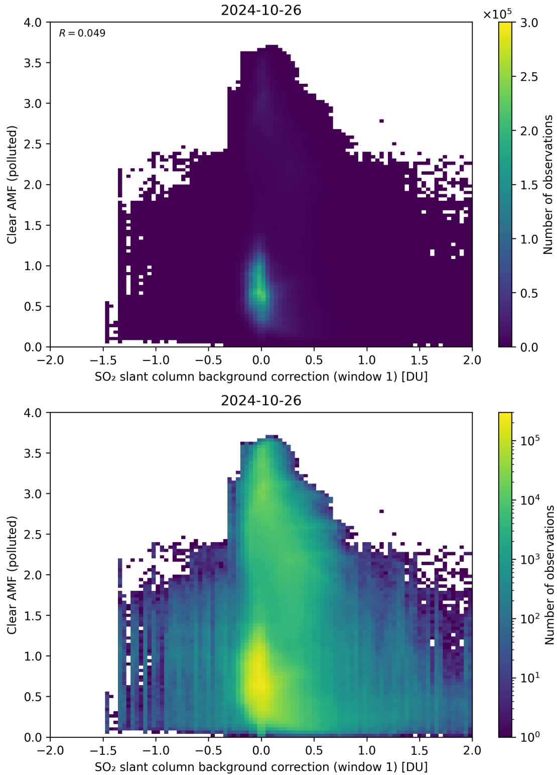
Figure 103: Scatter density plot of “SO 2 slant column background correction (window 1)” against “Clear AMF (polluted)” for 2024-10-25 to 2024-10-27.
