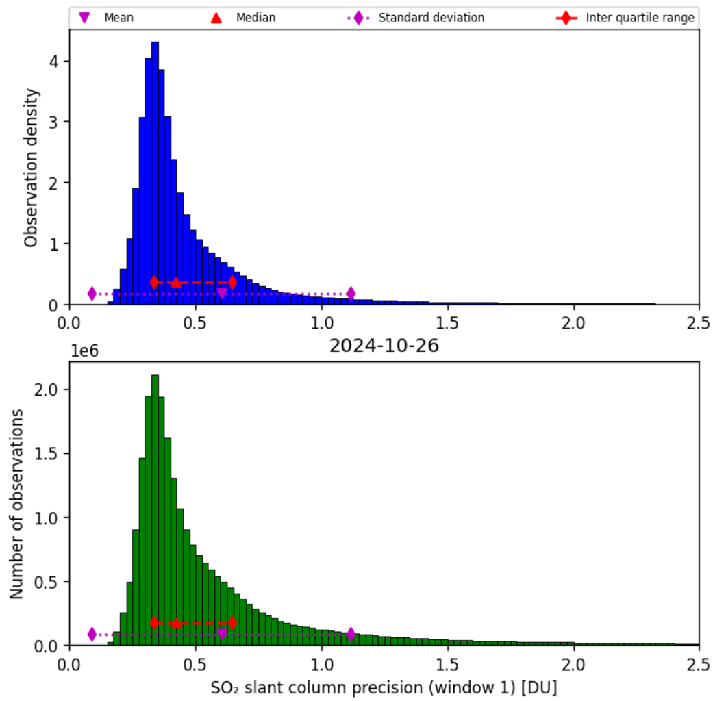
Figure 57: Histogram of “SO 2 slant column precision (window 1)” for 2024-10-25 to 2024-10-27
