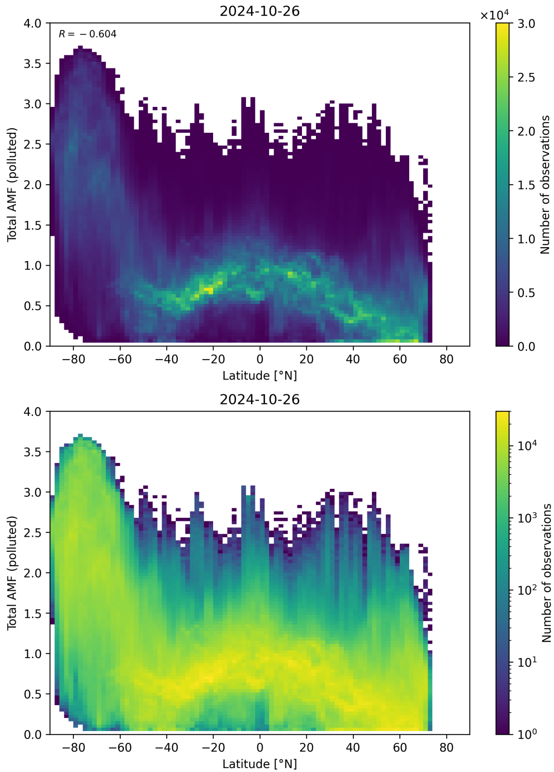
Figure 154: Scatter density plot of “Latitude” against “Total AMF (polluted)” for 2024-10-25 to 2024-10-27.
