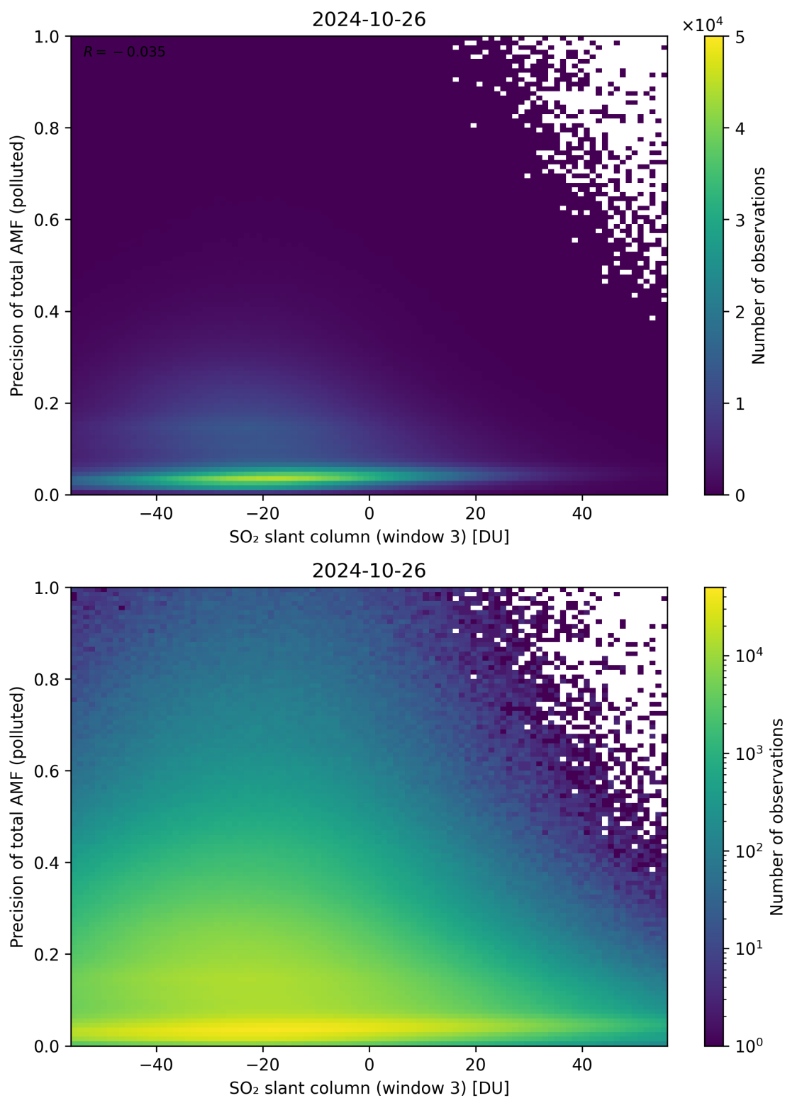
Figure 269: Scatter density plot of “SO 2 slant column (window 3)” against “Precision of total AMF (polluted)” for 2024-10-25 to 2024-10-27.
