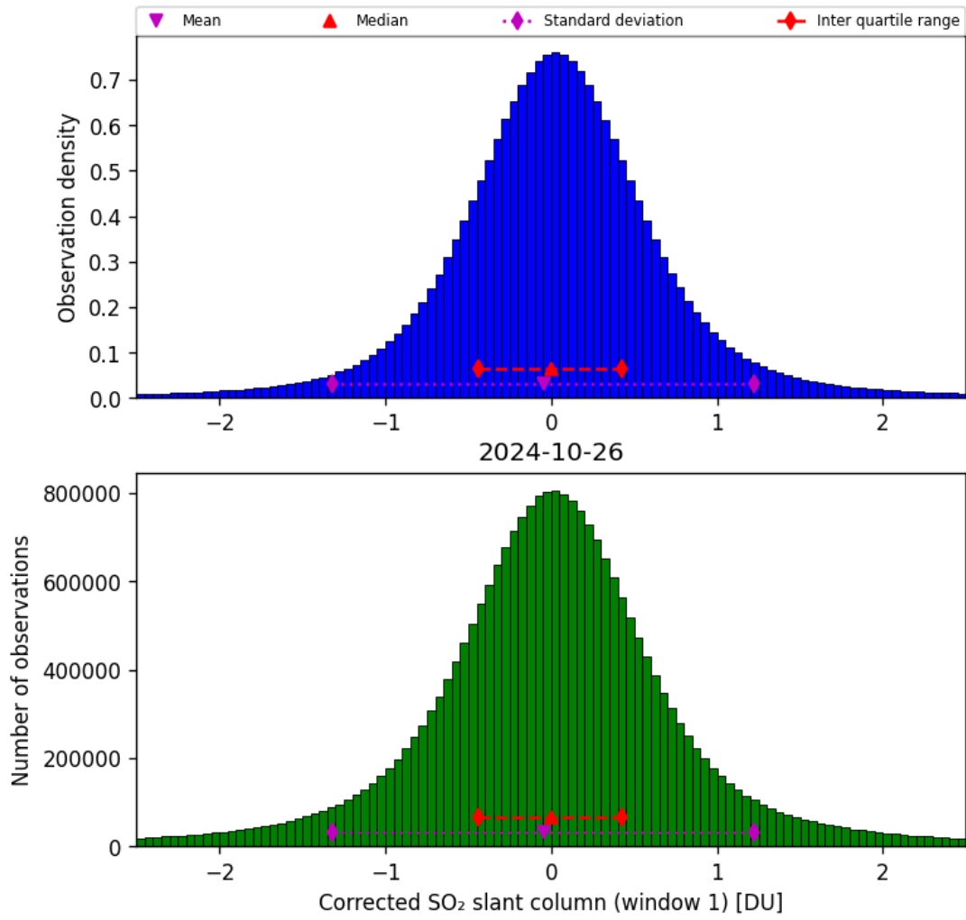
Figure 58: Histogram of “Corrected SO 2 slant column (window 1)” for 2024-10-25 to 2024-10-27
