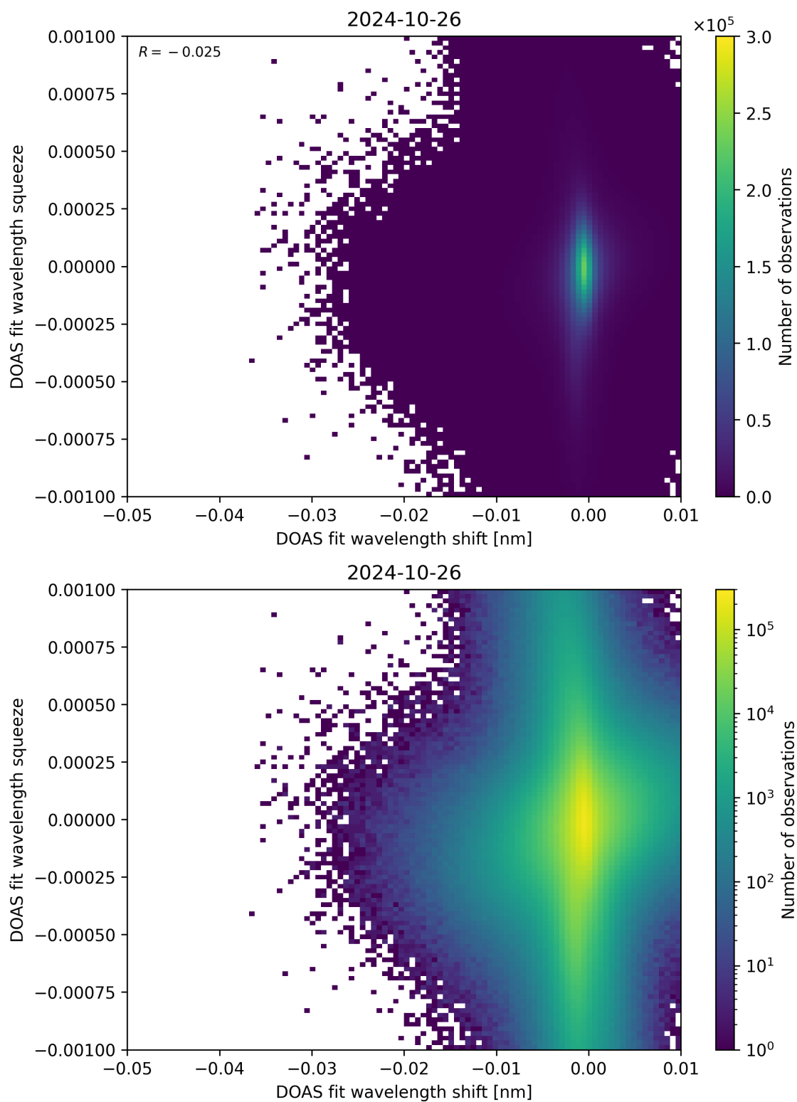
Figure 127: Scatter density plot of “DOAS fit wavelength shift” against “DOAS fit wavelength squeeze” for 2024-10-25 to 2024-10-27.
