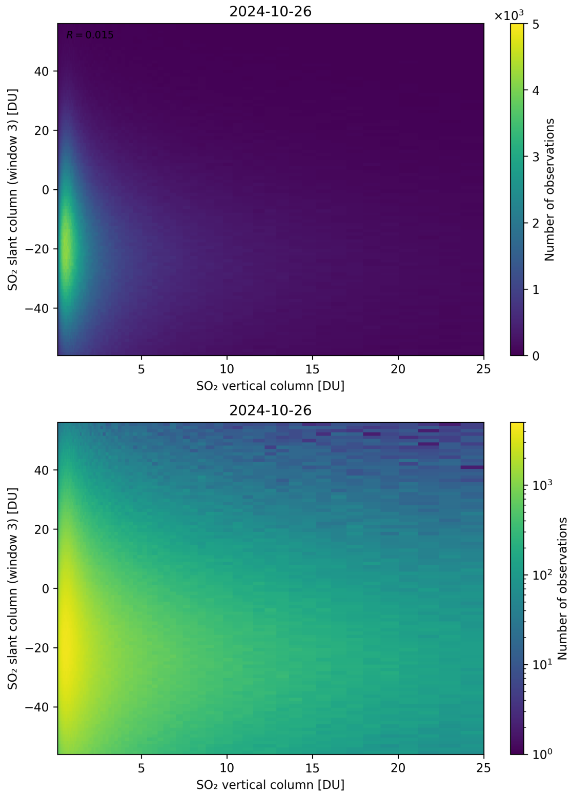
Figure 303: Scatter density plot of “SO 2 vertical column” against “SO 2 slant column (window 3)” for 2024-10-25 to 2024-10-27.
