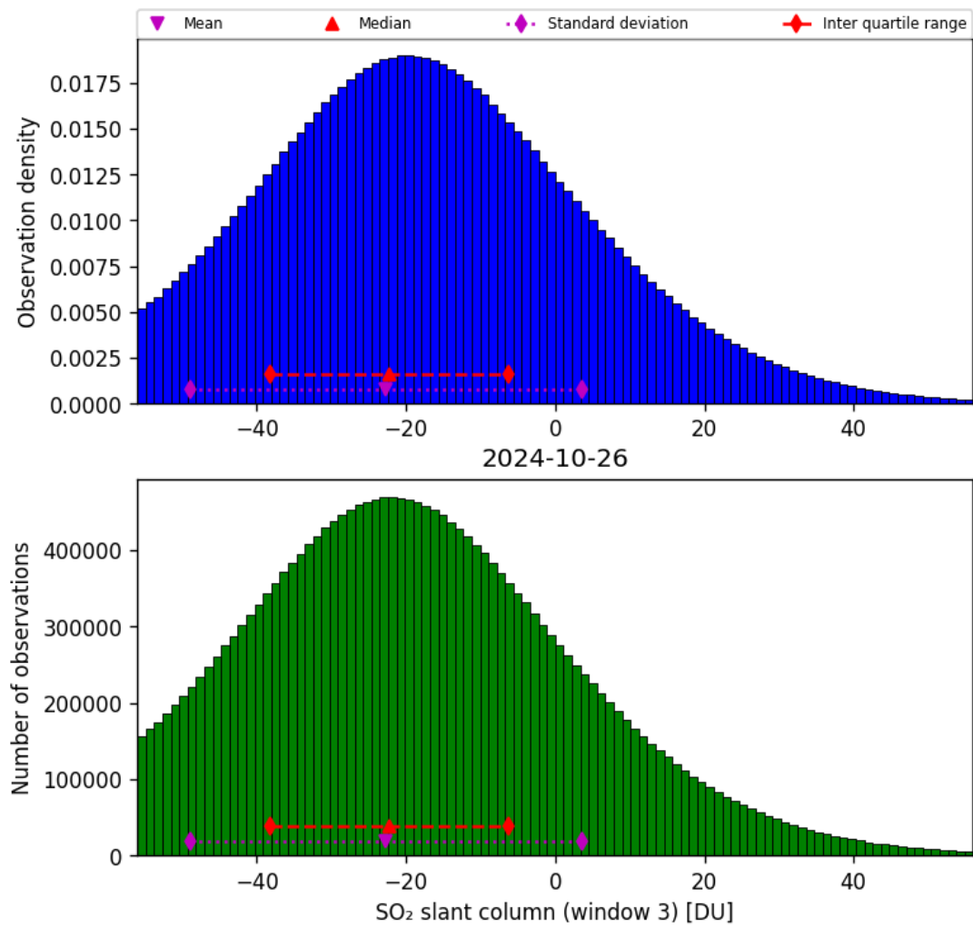
Figure 64: Histogram of “SO 2 slant column (window 3)” for 2024-10-25 to 2024-10-27
