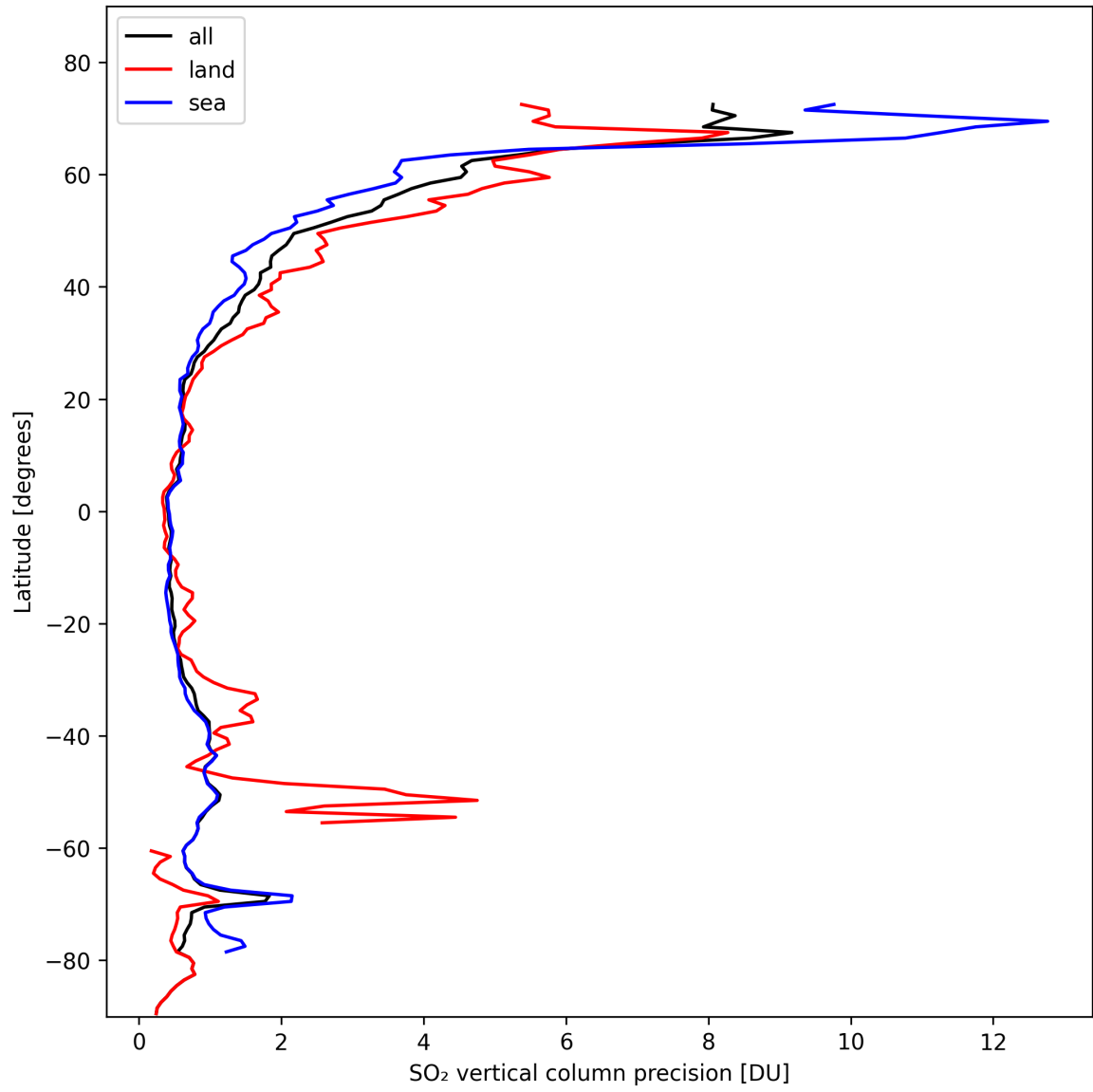
Figure 31: Zonal average of “SO 2 vertical column precision” for 2024-10-25 to 2024-10-27.
