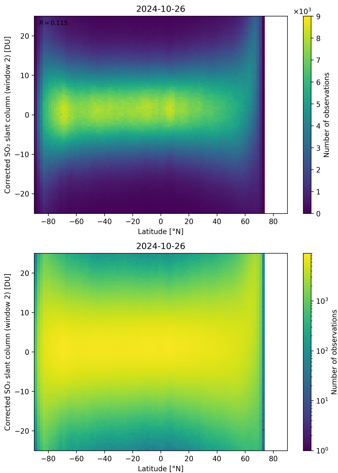
Figure 147: Scatter density plot of “Latitude” against “Corrected SO 2 slant column (window 2)” for 2024-10-25 to 2024-10-27.
