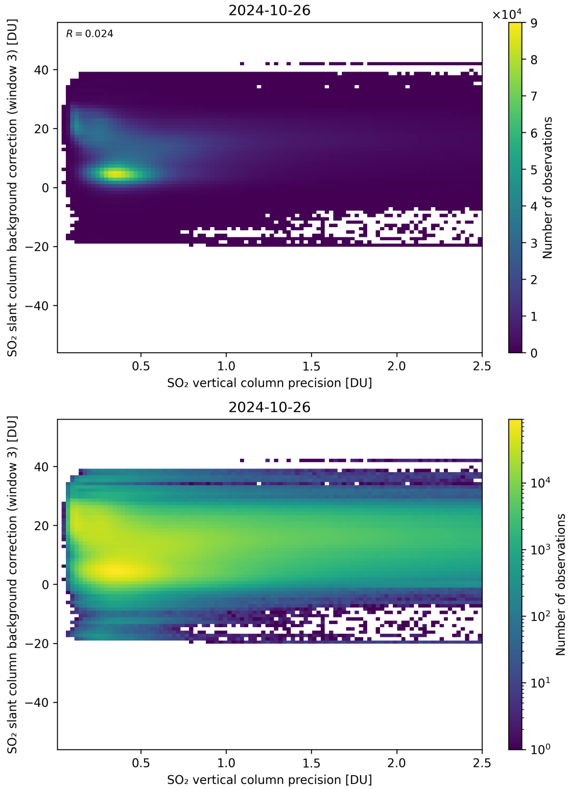
Figure 281: Scatter density plot of “SO 2 vertical column precision” against “SO 2 slant column background correction (window 3)” for 2024-10-25 to 2024-10-27.
