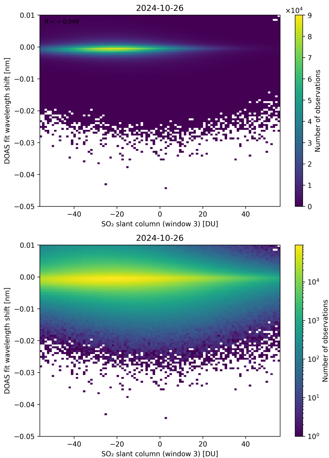
Figure 254: Scatter density plot of “SO 2 slant column (window 3)” against “DOAS fit wavelength shift” for 2024-10-25 to 2024-10-27.
