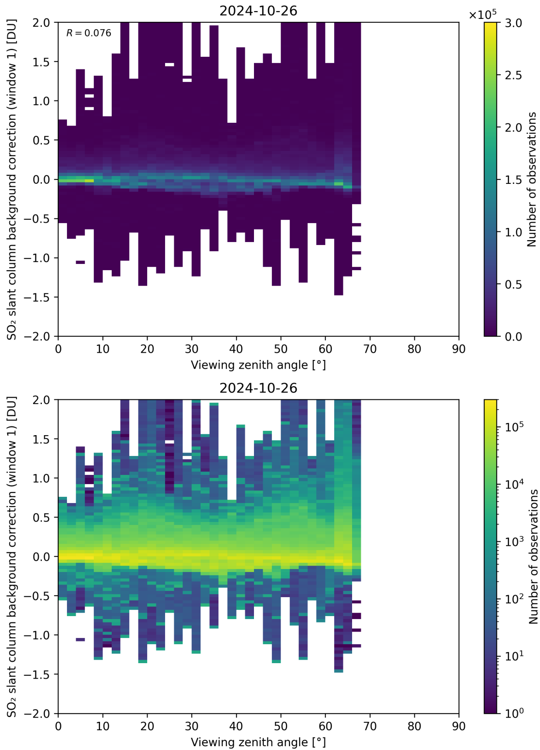
Figure 308: Scatter density plot of “Viewing zenith angle” against “SO 2 slant column background correction (window 1)” for 2024-10-25 to 2024-10-27.
