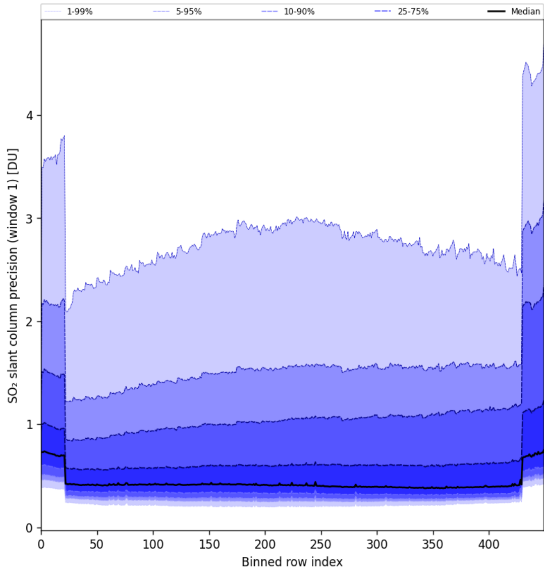
Figure 80: Along track statistics of “SO 2 slant column precision (window 1)” for 2024-10-25 to 2024-10-27
