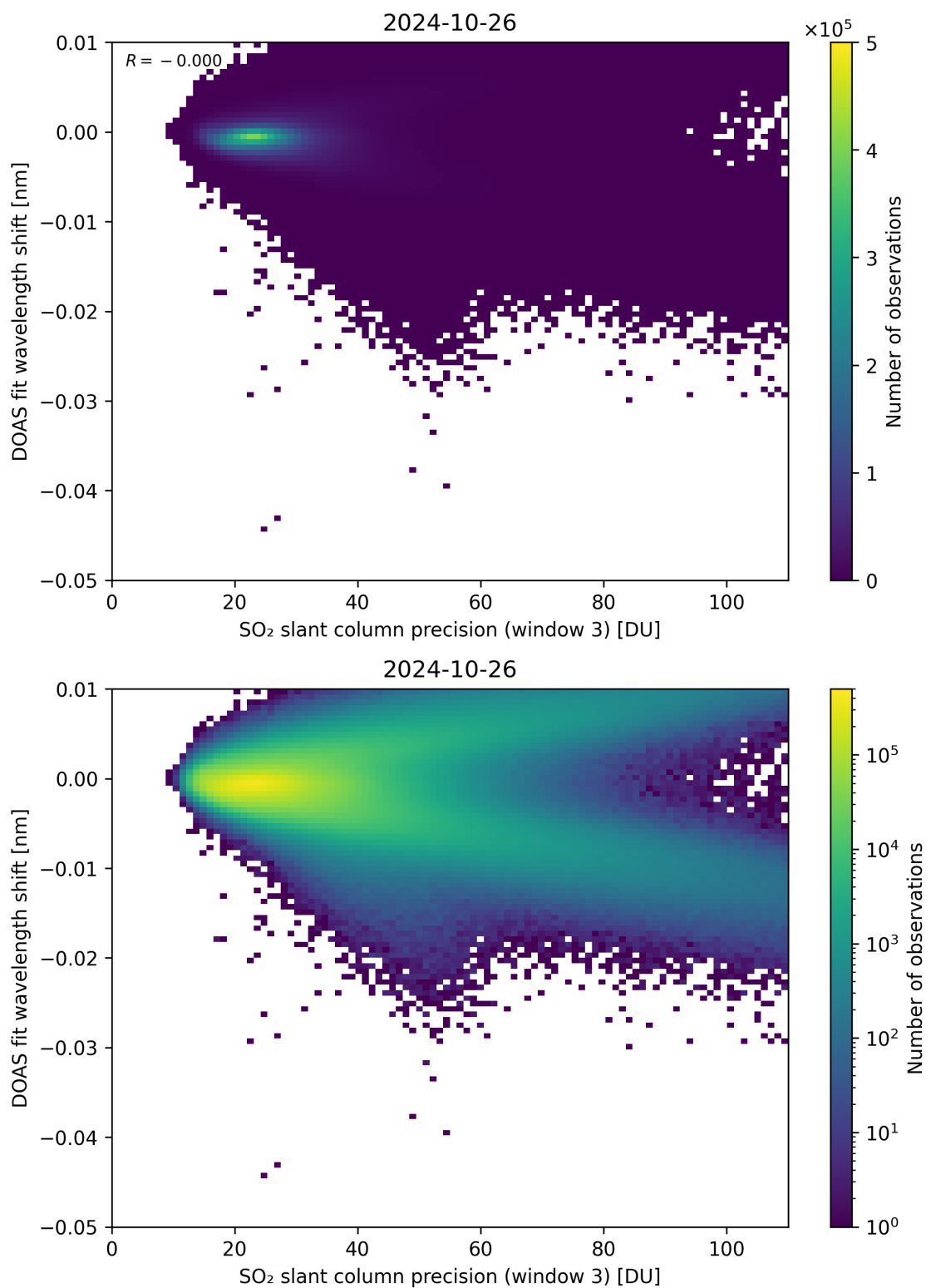
Figure 258: Scatter density plot of “SO 2 slant column precision (window 3)” against “DOAS fit wavelength shift” for 2024-10-25 to 2024-10-27.
