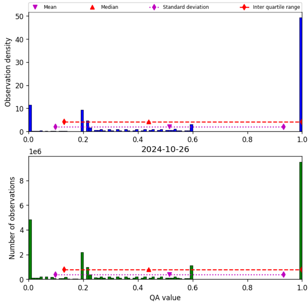
Figure 52: Histogram of “QA value” for 2024-10-25 to 2024-10-27
