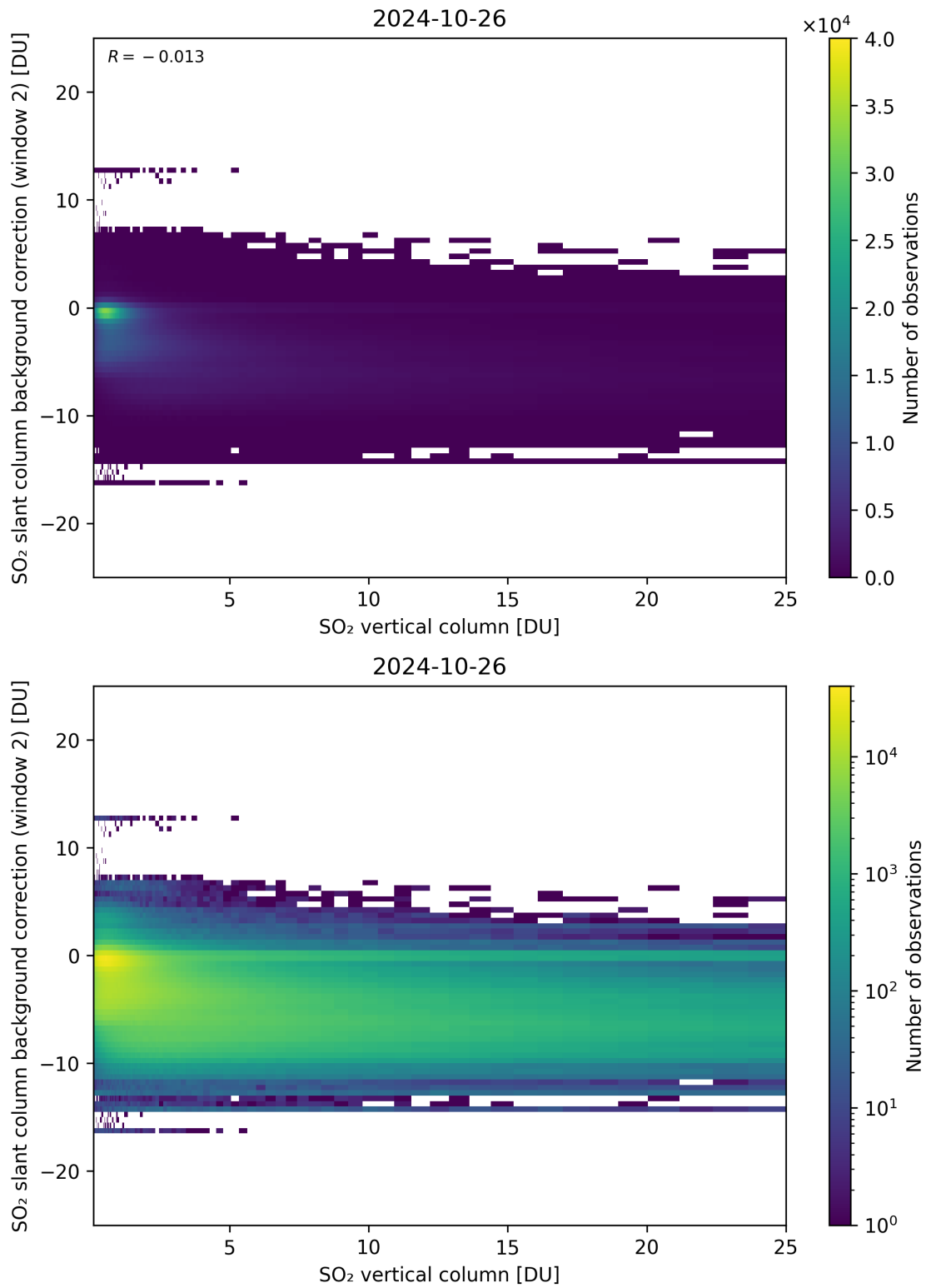
Figure 274: Scatter density plot of “SO 2 vertical column” against “SO 2 slant column background correction (window 2)” for 2024-10-25 to 2024-10-27.
