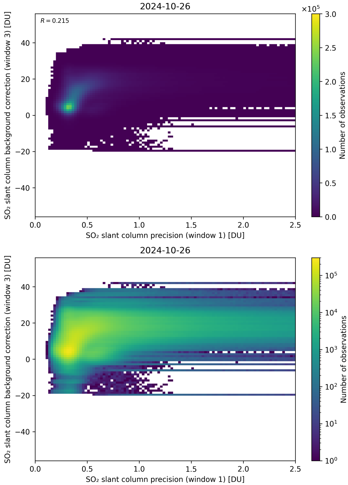
Figure 220: Scatter density plot of “SO 2 slant column precision (window 1)” against “SO 2 slant column background correction (window 3)” for 2024-10-25 to 2024-10-27.
