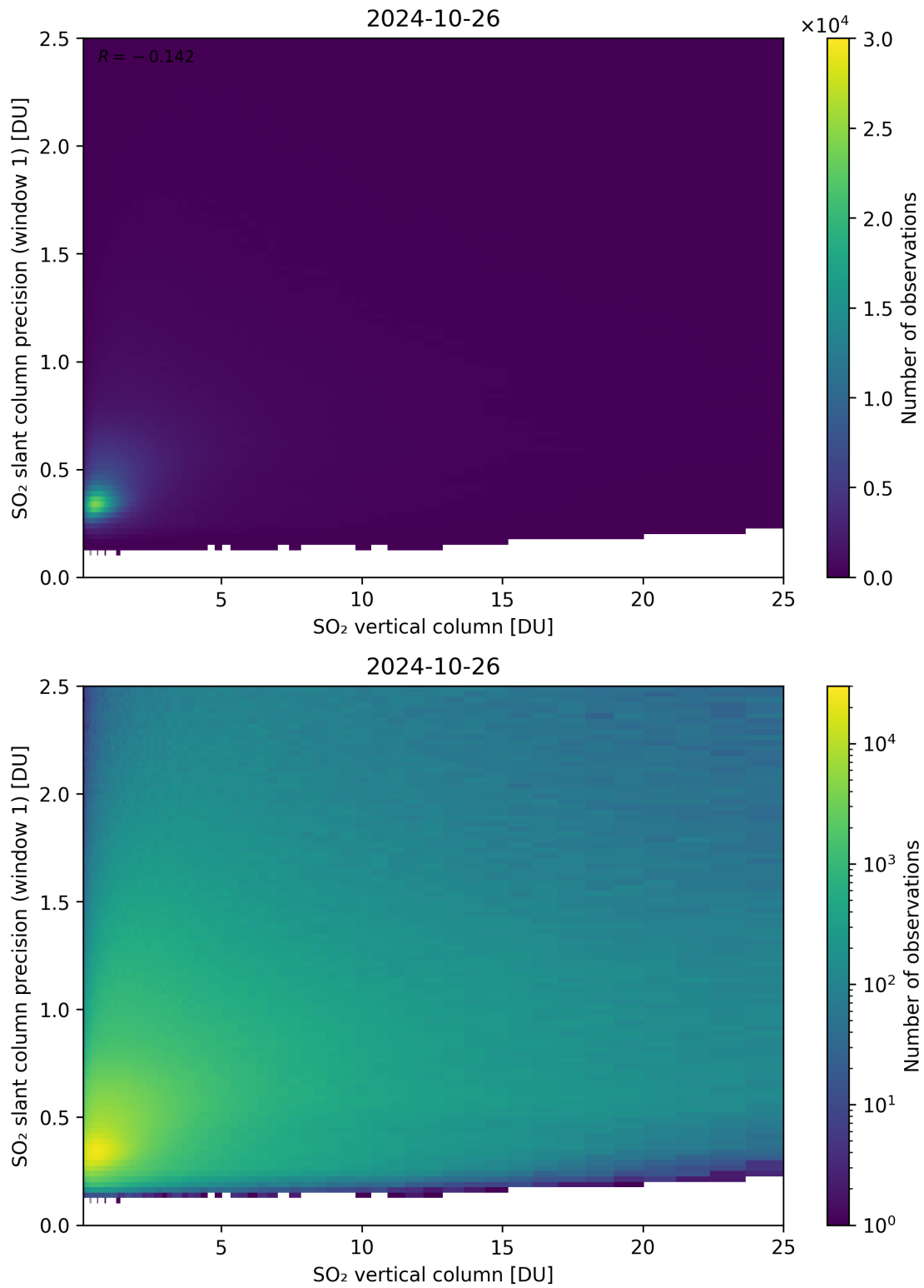
Figure 301: Scatter density plot of “SO 2 vertical column” against “SO 2 slant column precision (window 1)” for 2024-10-25 to 2024-10-27.
