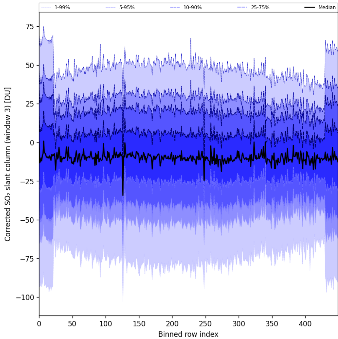
Figure 89: Along track statistics of “Corrected SO 2 slant column (window 3)” for 2024-10-25 to 2024-10-27
