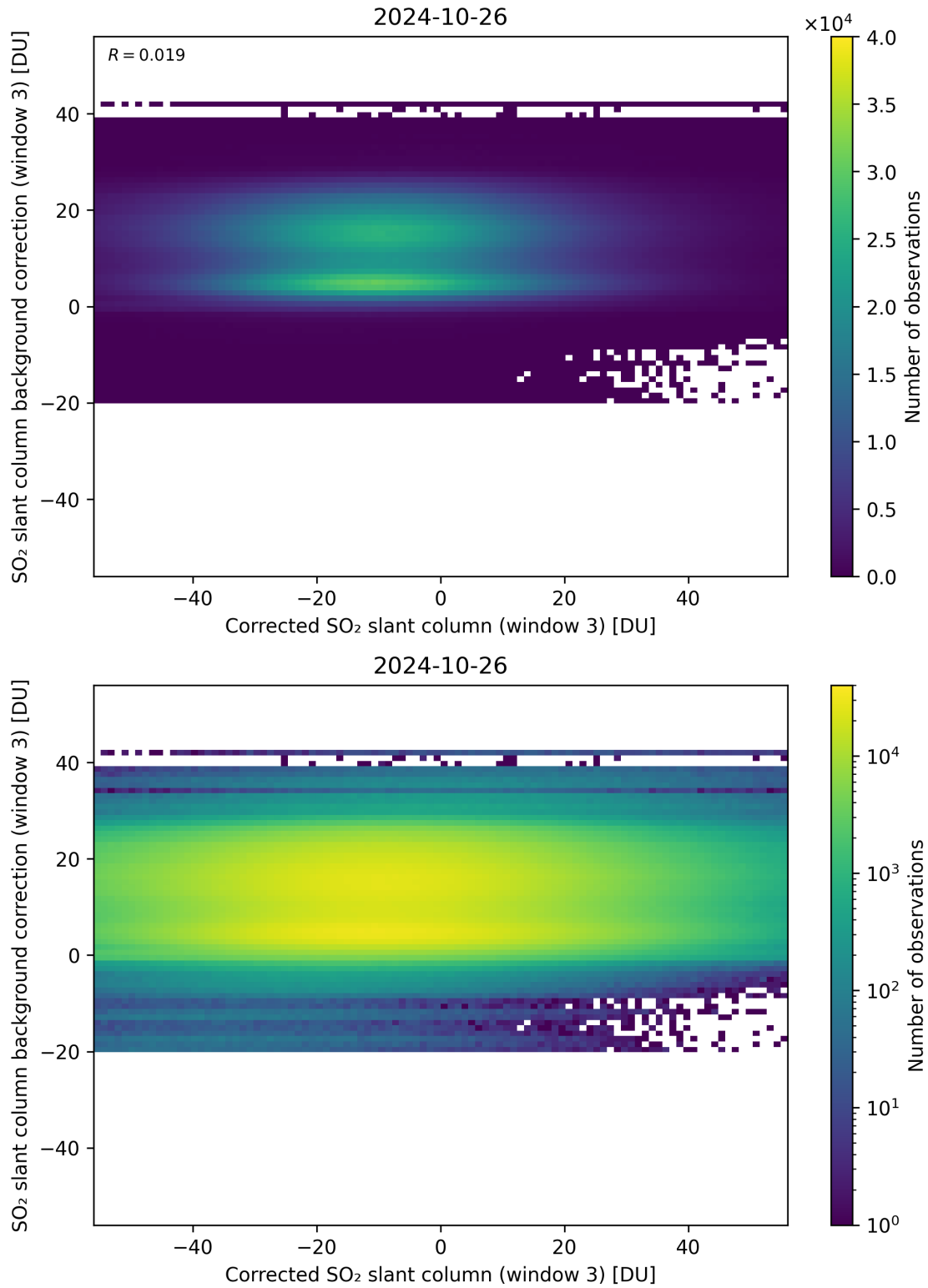
Figure 205: Scatter density plot of “Corrected SO 2 slant column (window 3)” against “SO 2 slant column background correction (window 3)” for 2024-10-25 to 2024-10-27.
