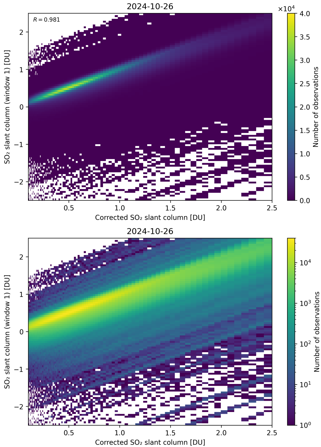
Figure 187: Scatter density plot of “Corrected SO 2 slant column” against “SO 2 slant column (window 1)” for 2024-10-25 to 2024-10-27.
