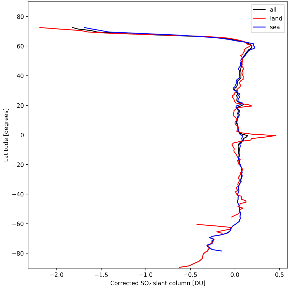
Figure 32: Zonal average of “Corrected SO 2 slant column” for 2024-10-25 to 2024-10-27.
