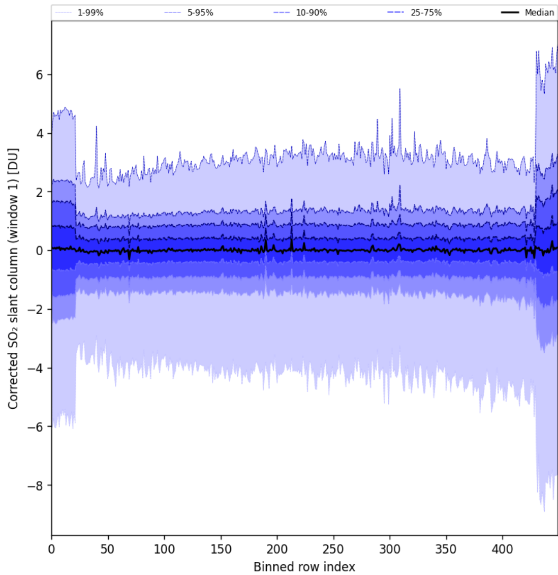
Figure 81: Along track statistics of “Corrected SO 2 slant column (window 1)” for 2024-10-25 to 2024-10-27
