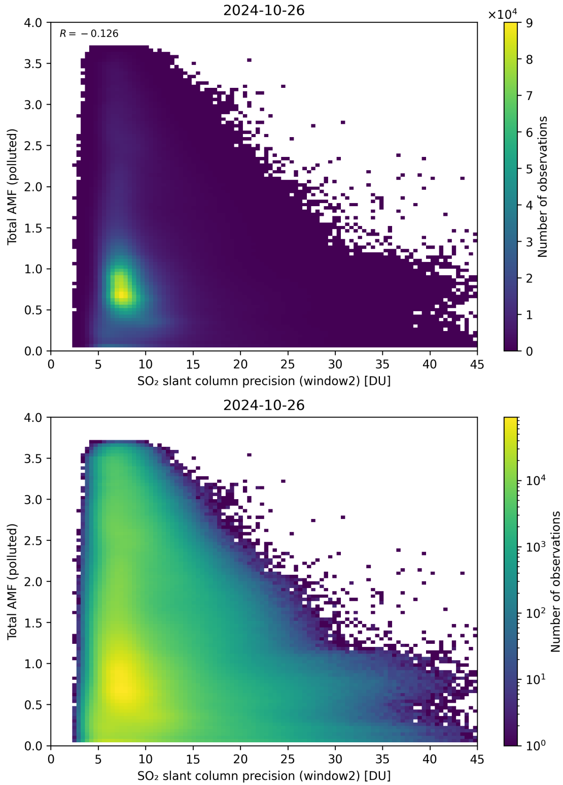
Figure 251: Scatter density plot of “SO 2 slant column precision (window2)” against “Total AMF (polluted)” for 2024-10-25 to 2024-10-27.
