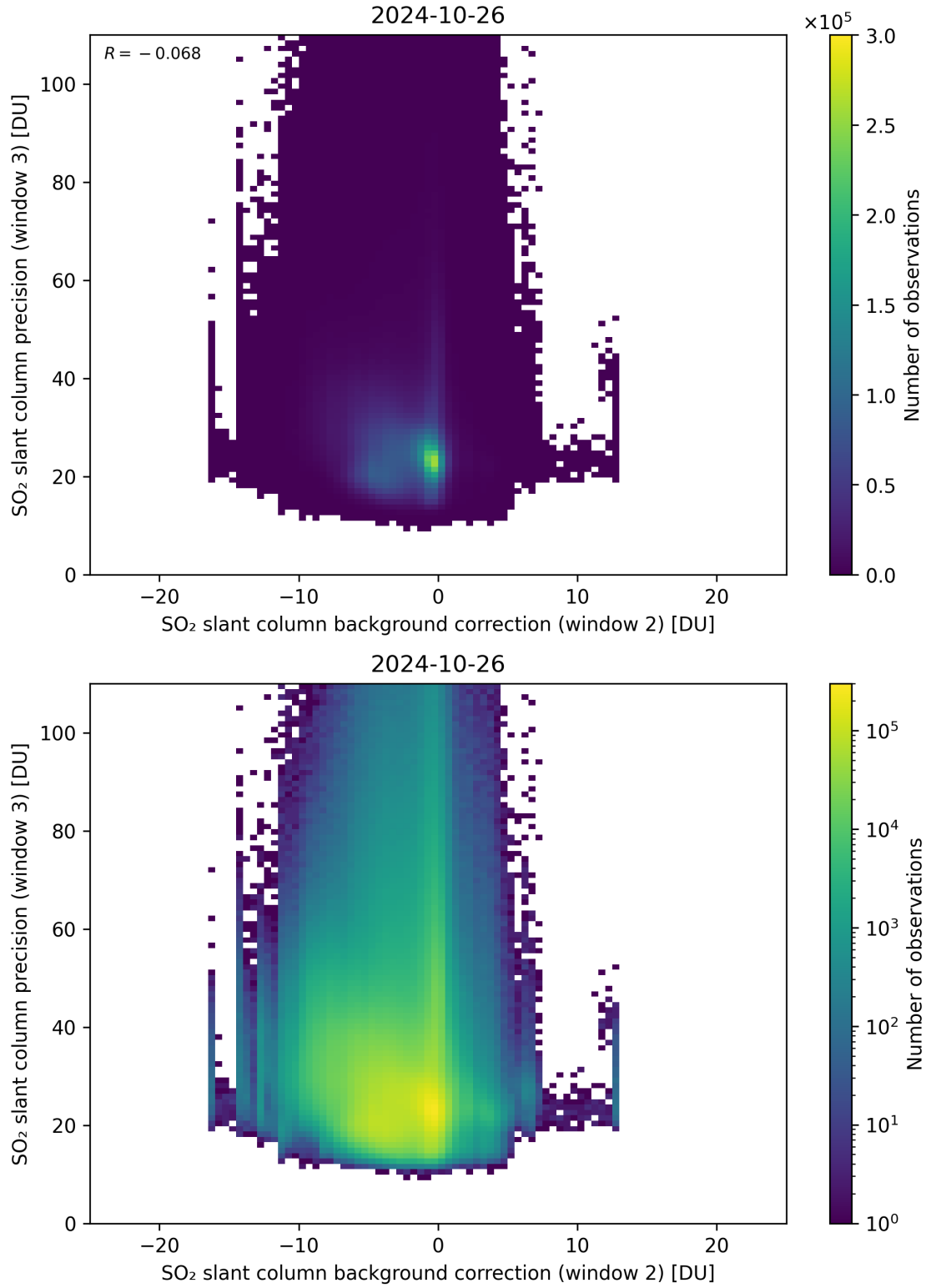
Figure 118: Scatter density plot of “SO 2 slant column background correction (window 2)” against “SO 2 slant column precision (window 3)” for 2024-10-25 to 2024-10-27.
