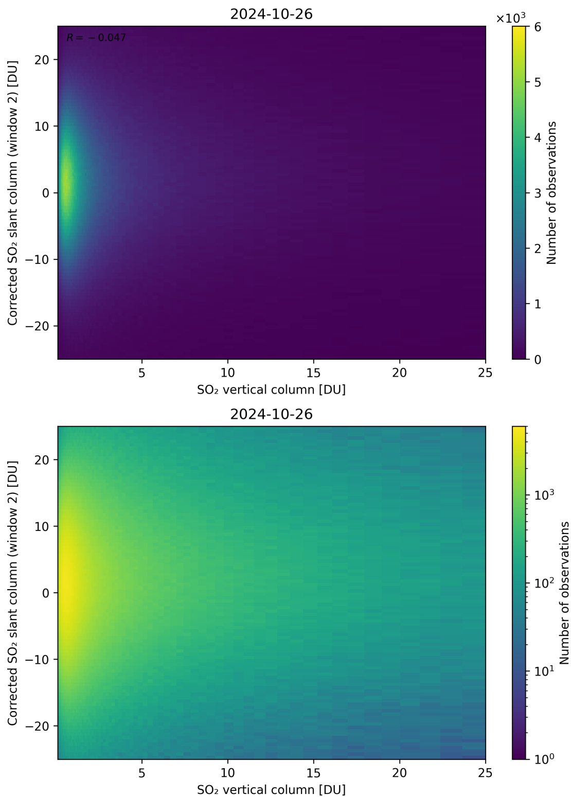
Figure 298: Scatter density plot of “SO 2 vertical column” against “Corrected SO 2 slant column (window 2)” for 2024-10-25 to 2024-10-27.
