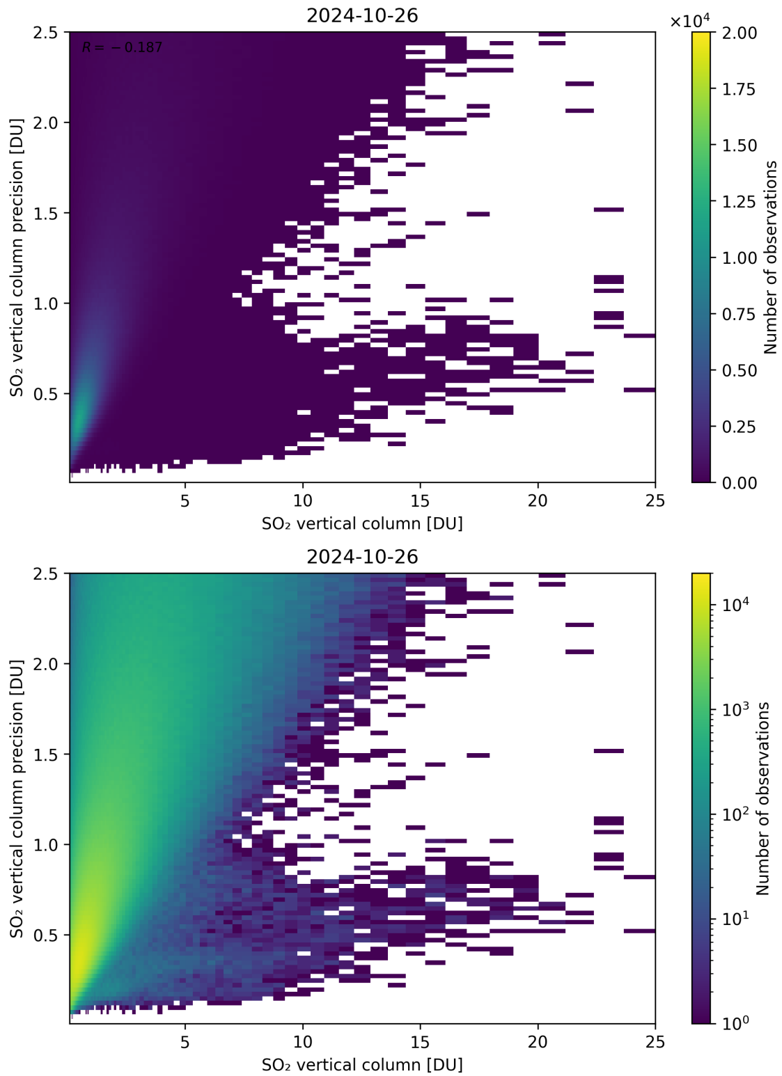
Figure 307: Scatter density plot of “SO 2 vertical column” against “SO 2 vertical column precision” for 2024-10-25 to 2024-10-27.
