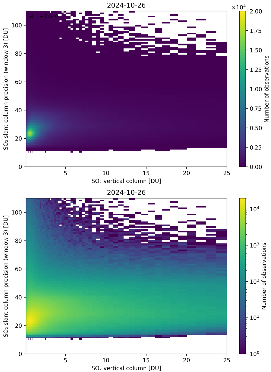
Figure 304: Scatter density plot of “SO 2 vertical column” against “SO 2 slant column precision (window 3)” for 2024-10-25 to 2024-10-27.
