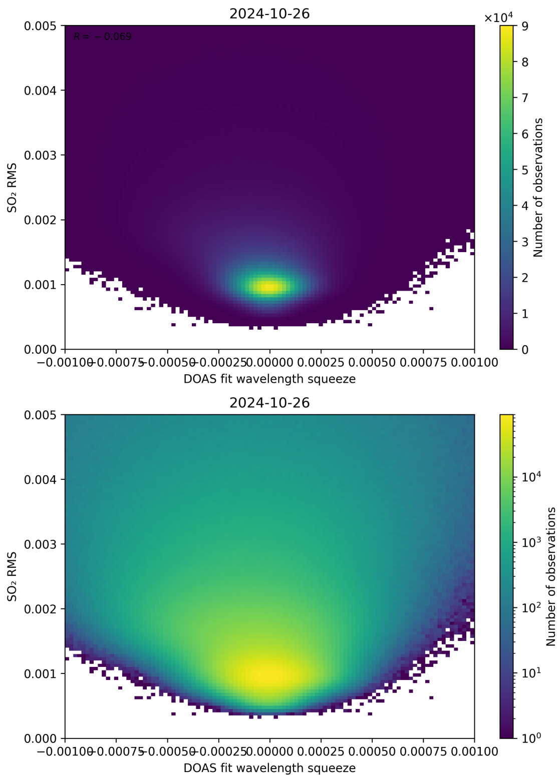
Figure 132: Scatter density plot of “DOAS fit wavelength squeeze” against “SO 2 RMS” for 2024-10-25 to 2024-10-27.
