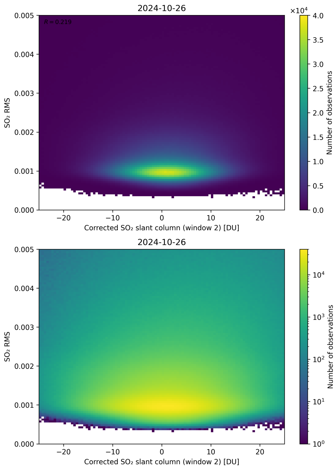
Figure 198: Scatter density plot of “Corrected SO 2 slant column (window 2)” against “SO 2 RMS” for 2024-10-25 to 2024-10-27.
