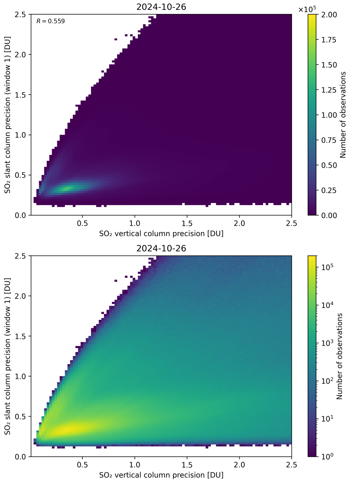
Figure 290: Scatter density plot of “SO 2 vertical column precision” against “SO 2 slant column precision (window 1)” for 2024-10-25 to 2024-10-27.
