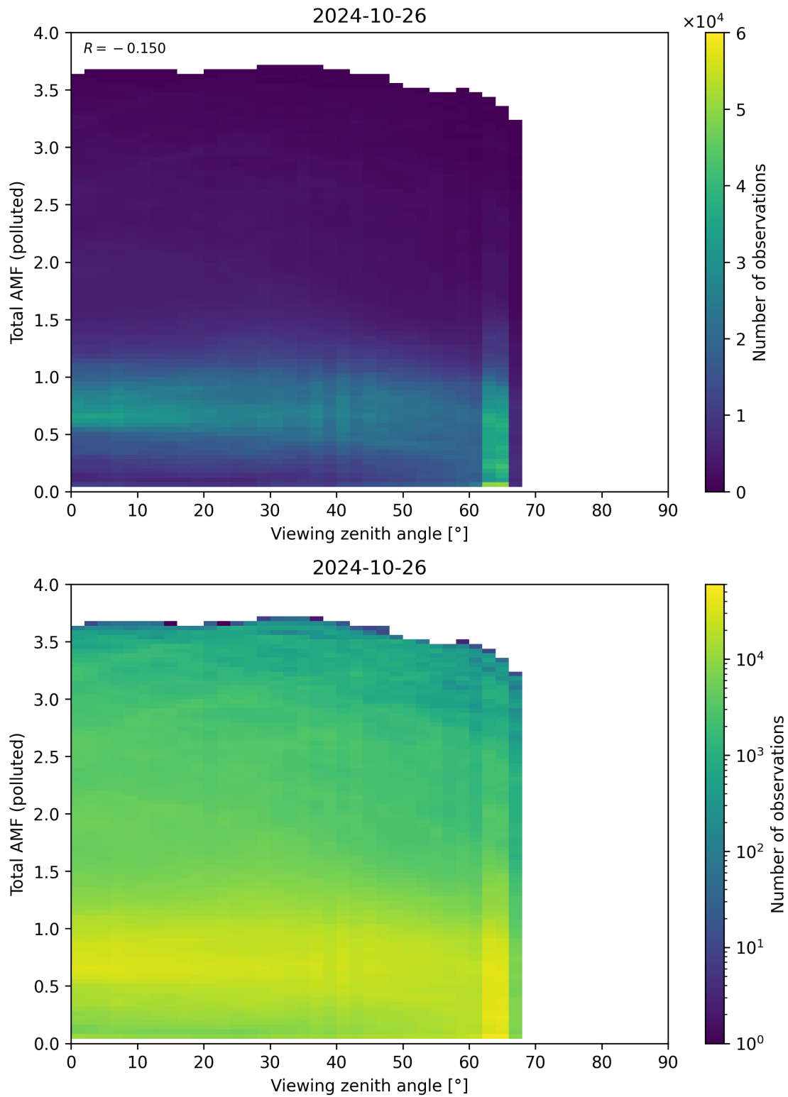
Figure 325: Scatter density plot of “Viewing zenith angle” against “Total AMF (polluted)” for 2024-10-25 to 2024-10-27.
