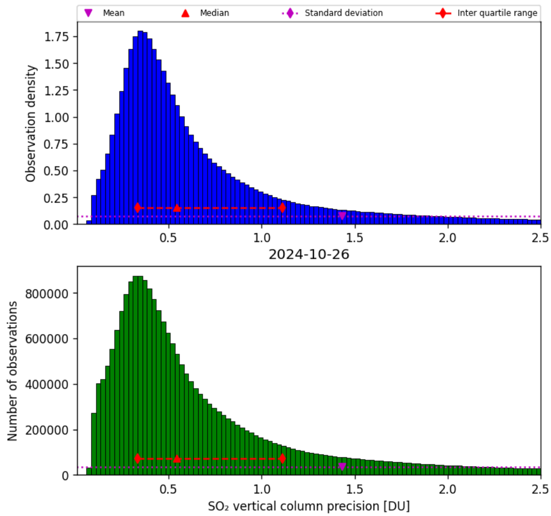
Figure 54: Histogram of “SO 2 vertical column precision” for 2024-10-25 to 2024-10-27
