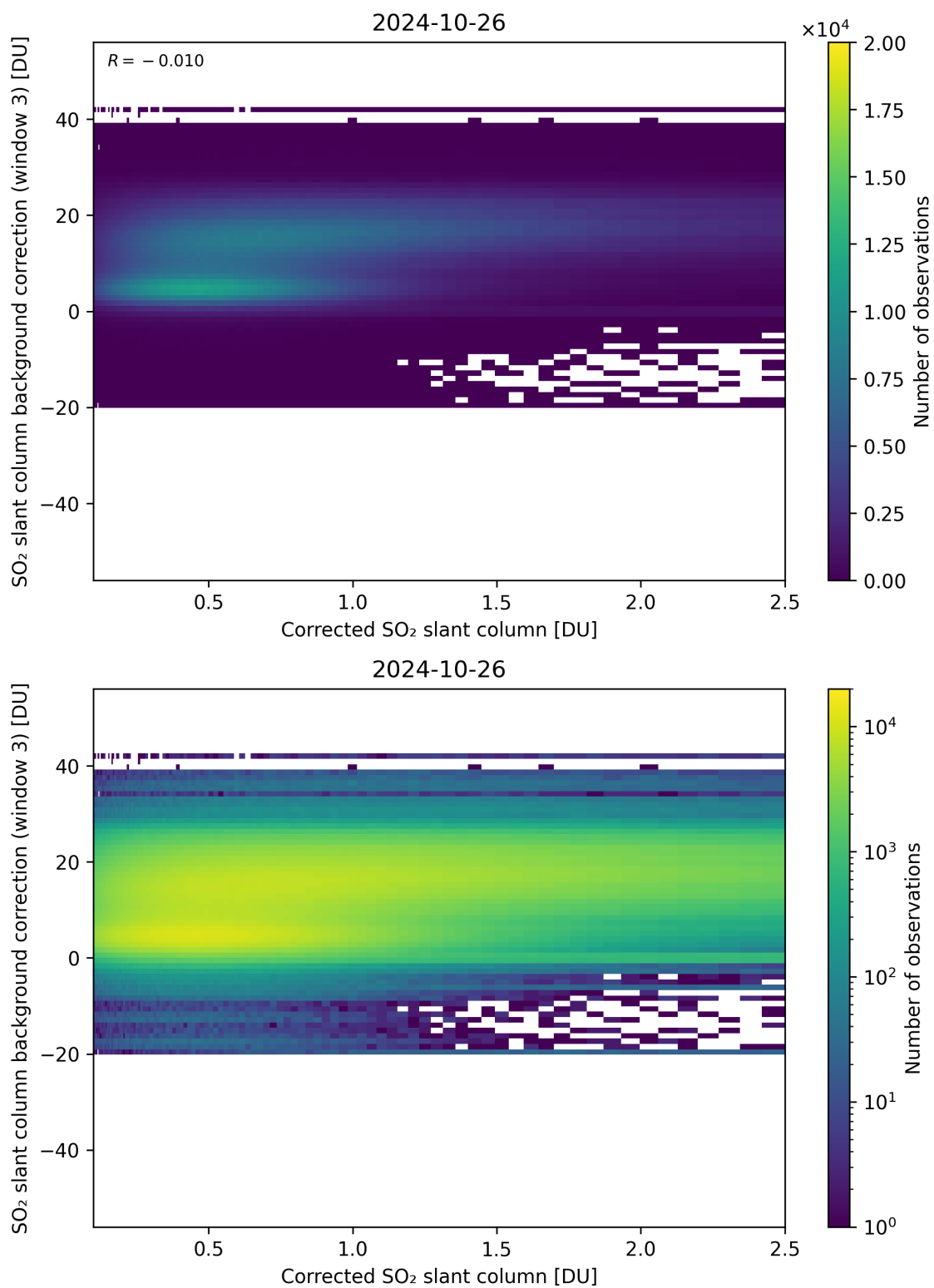
Figure 180: Scatter density plot of “Corrected SO 2 slant column” against “SO 2 slant column background correction (window 3)” for 2024-10-25 to 2024-10-27.
