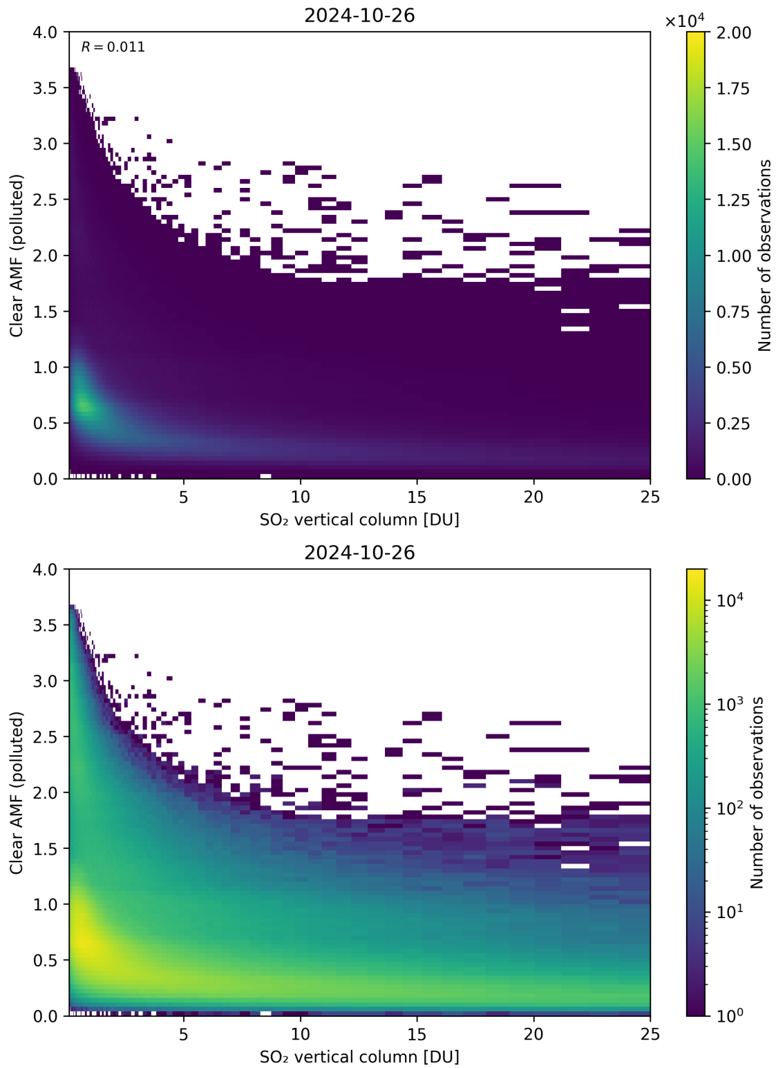
Figure 296: Scatter density plot of “SO 2 vertical column” against “Clear AMF (polluted)” for 2024-10-25 to 2024-10-27.
