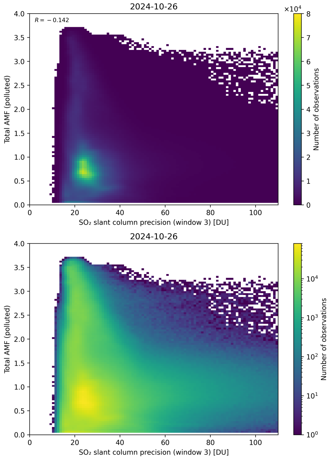
Figure 263: Scatter density plot of “SO 2 slant column precision (window 3)” against “Total AMF (polluted)” for 2024-10-25 to 2024-10-27.
