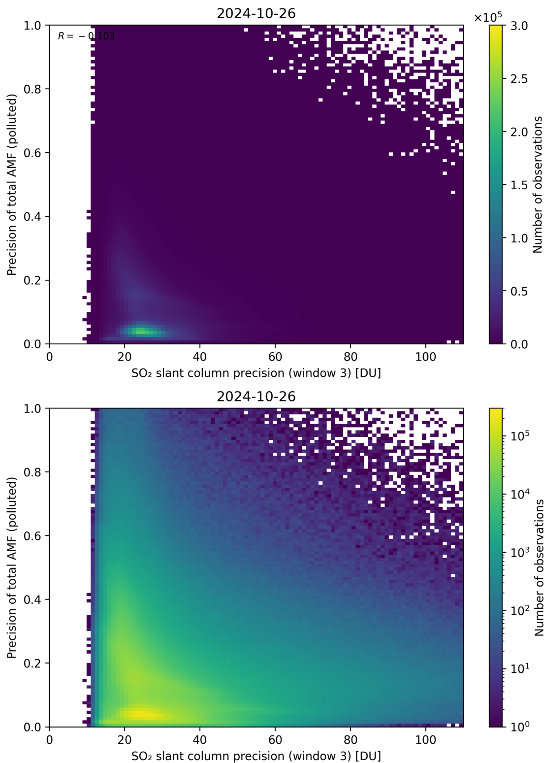
Figure 264: Scatter density plot of “SO 2 slant column precision (window 3)” against “Precision of total AMF (polluted)” for 2024-10-25 to 2024-10-27.
