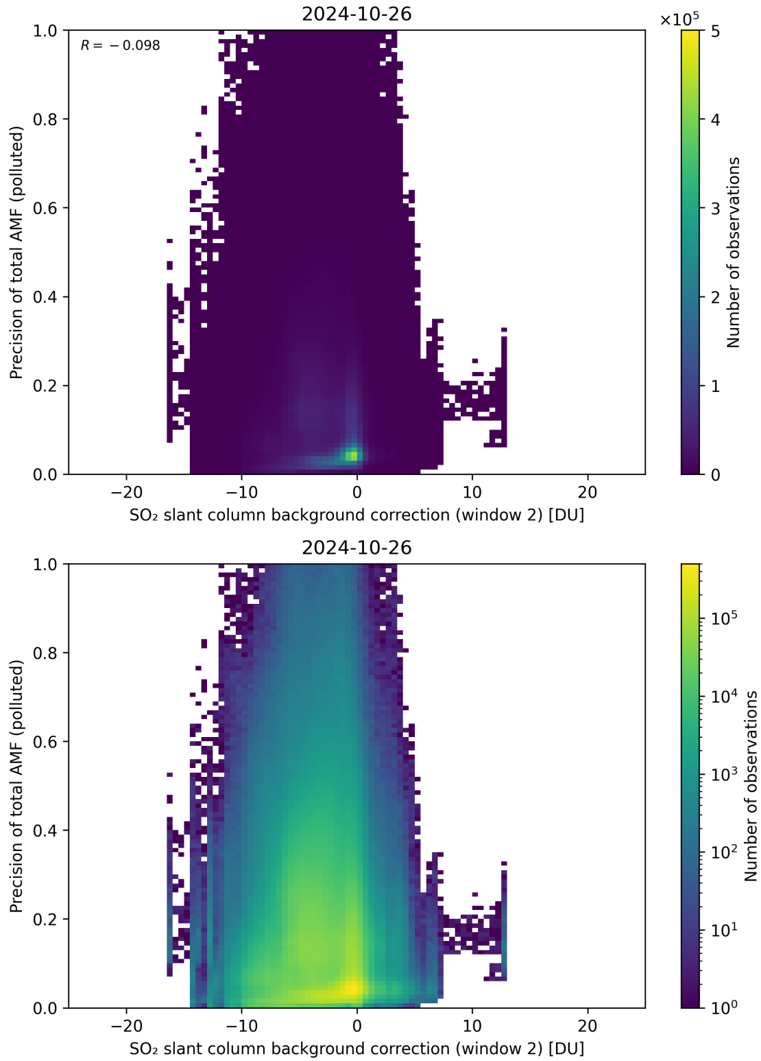
Figure 120: Scatter density plot of “SO 2 slant column background correction (window 2)” against “Precision of total AMF (polluted)” for 2024-10-25 to 2024-10-27.
