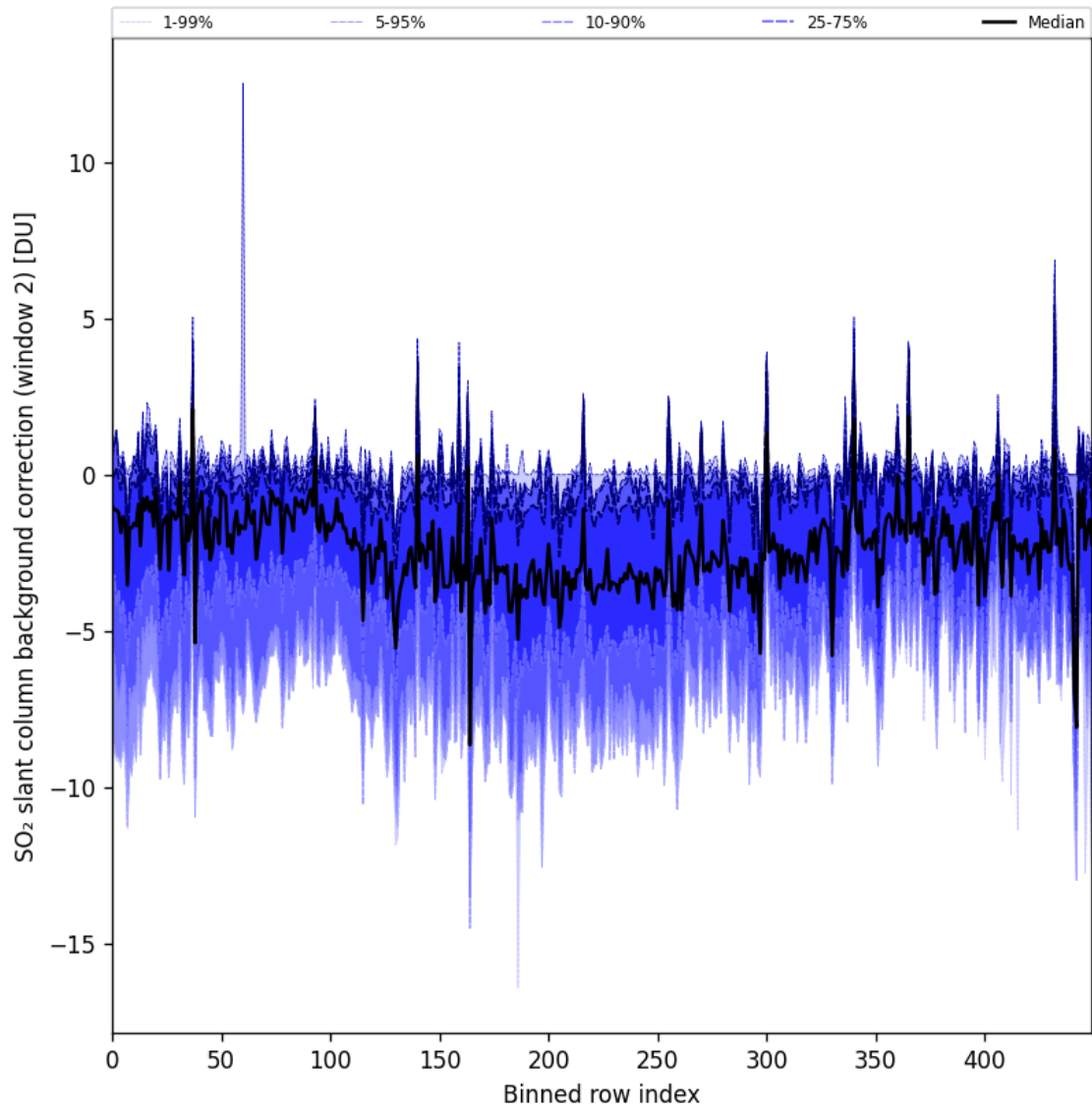
Figure 86: Along track statistics of “SO 2 slant column background correction (window 2)” for 2024-10-25 to 2024-10-27
