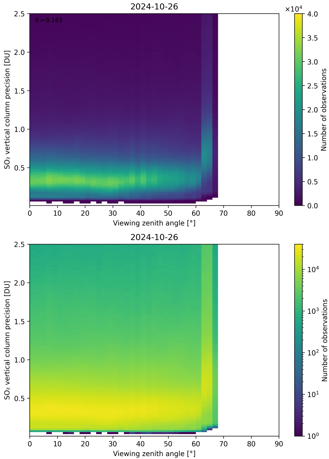
Figure 328: Scatter density plot of “Viewing zenith angle” against “SO 2 vertical column precision” for 2024-10-25 to 2024-10-27.
