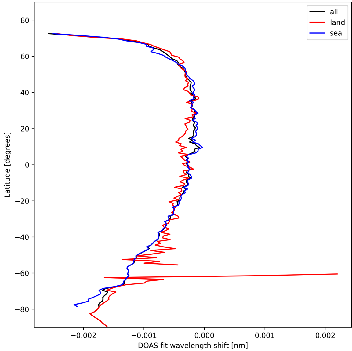
Figure 45: Zonal average of “DOAS fit wavelength shift” for 2024-10-25 to 2024-10-27.
