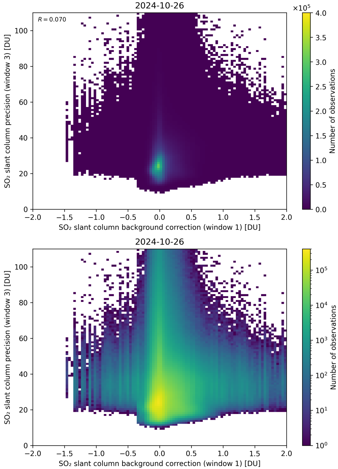
Figure 108: Scatter density plot of “SO 2 slant column background correction (window 1)” against “SO 2 slant column precision (window 3)” for 2024-10-25 to 2024-10-27.
