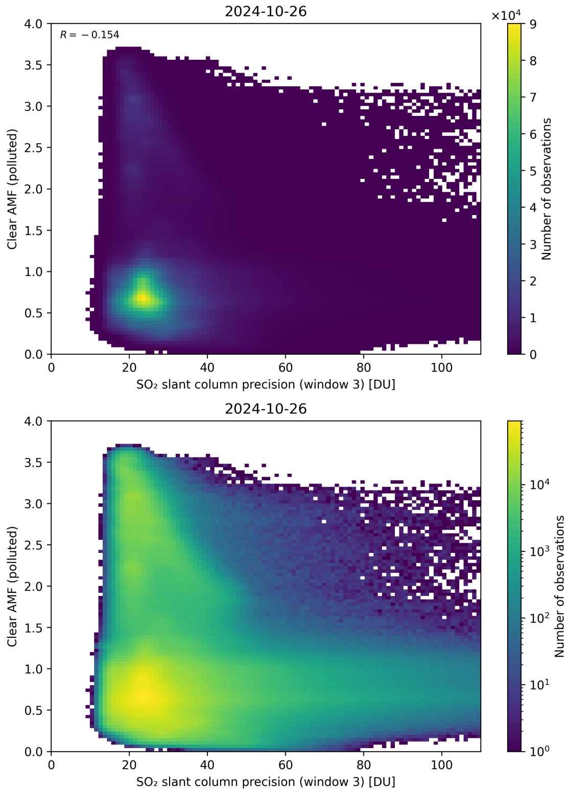
Figure 261: Scatter density plot of “SO 2 slant column precision (window 3)” against “Clear AMF (polluted)” for 2024-10-25 to 2024-10-27.
