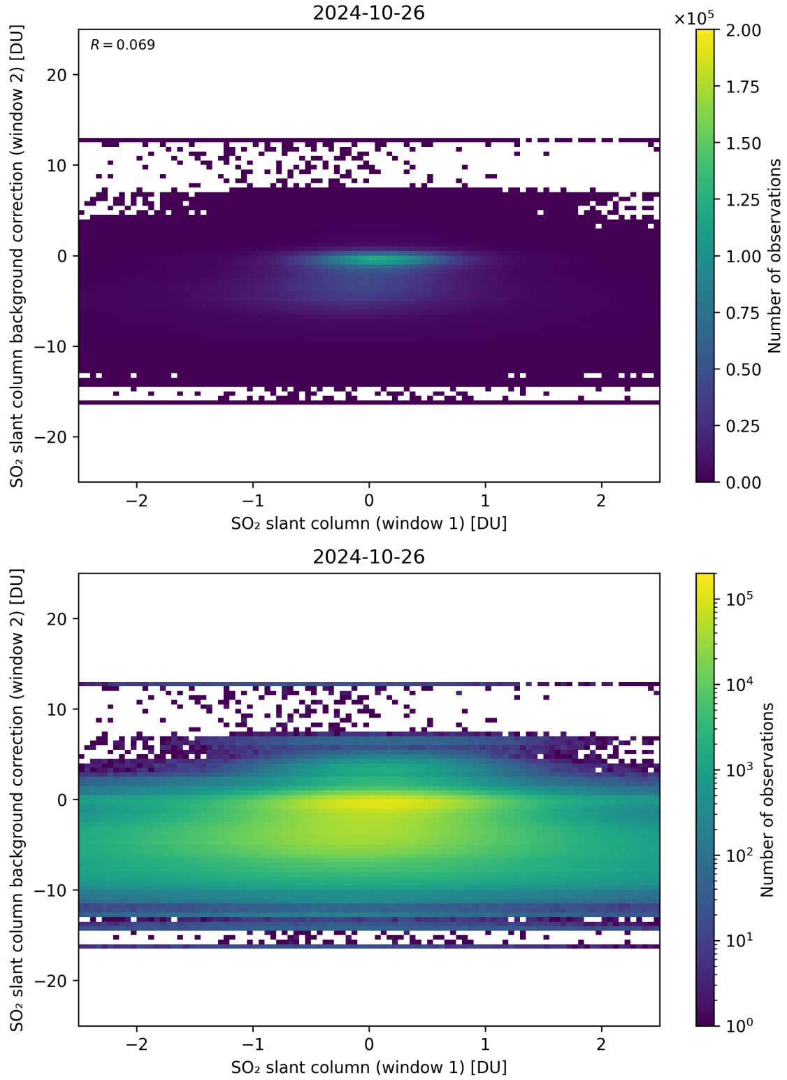
Figure 213: Scatter density plot of “SO 2 slant column (window 1)” against “SO 2 slant column background correction (window 2)” for 2024-10-25 to 2024-10-27.
