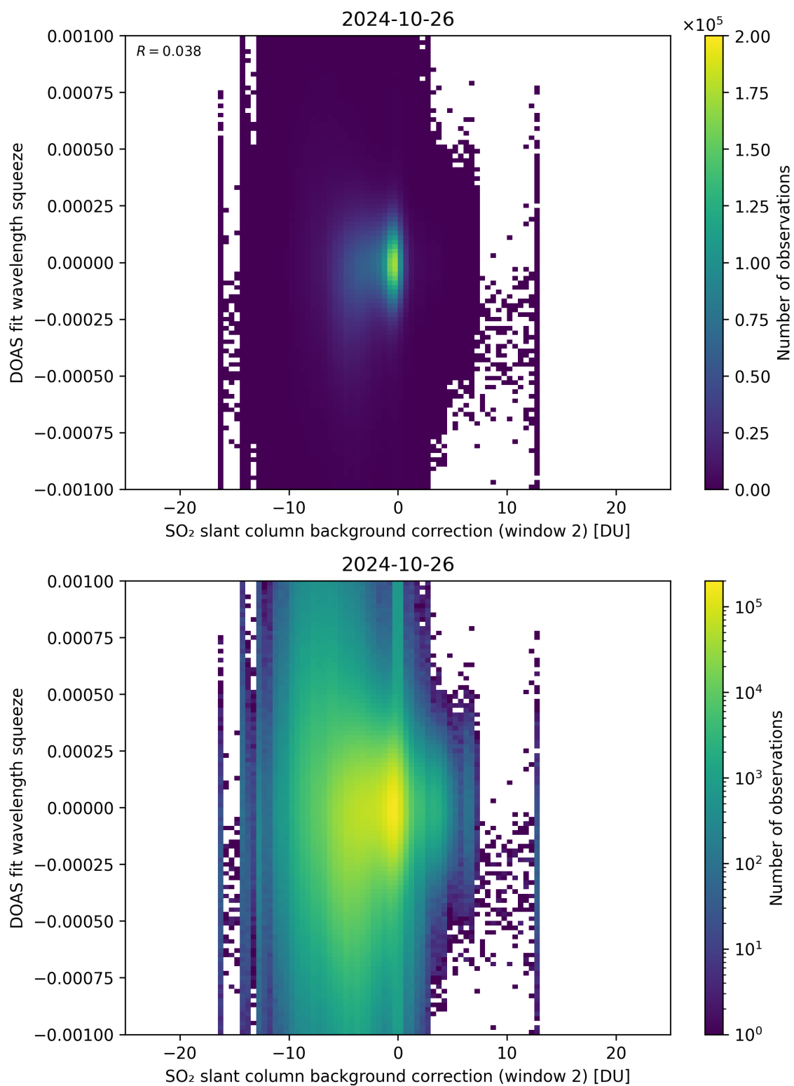
Figure 113: Scatter density plot of “SO 2 slant column background correction (window 2)” against “DOAS fit wavelength squeeze” for 2024-10-25 to 2024-10-27.
