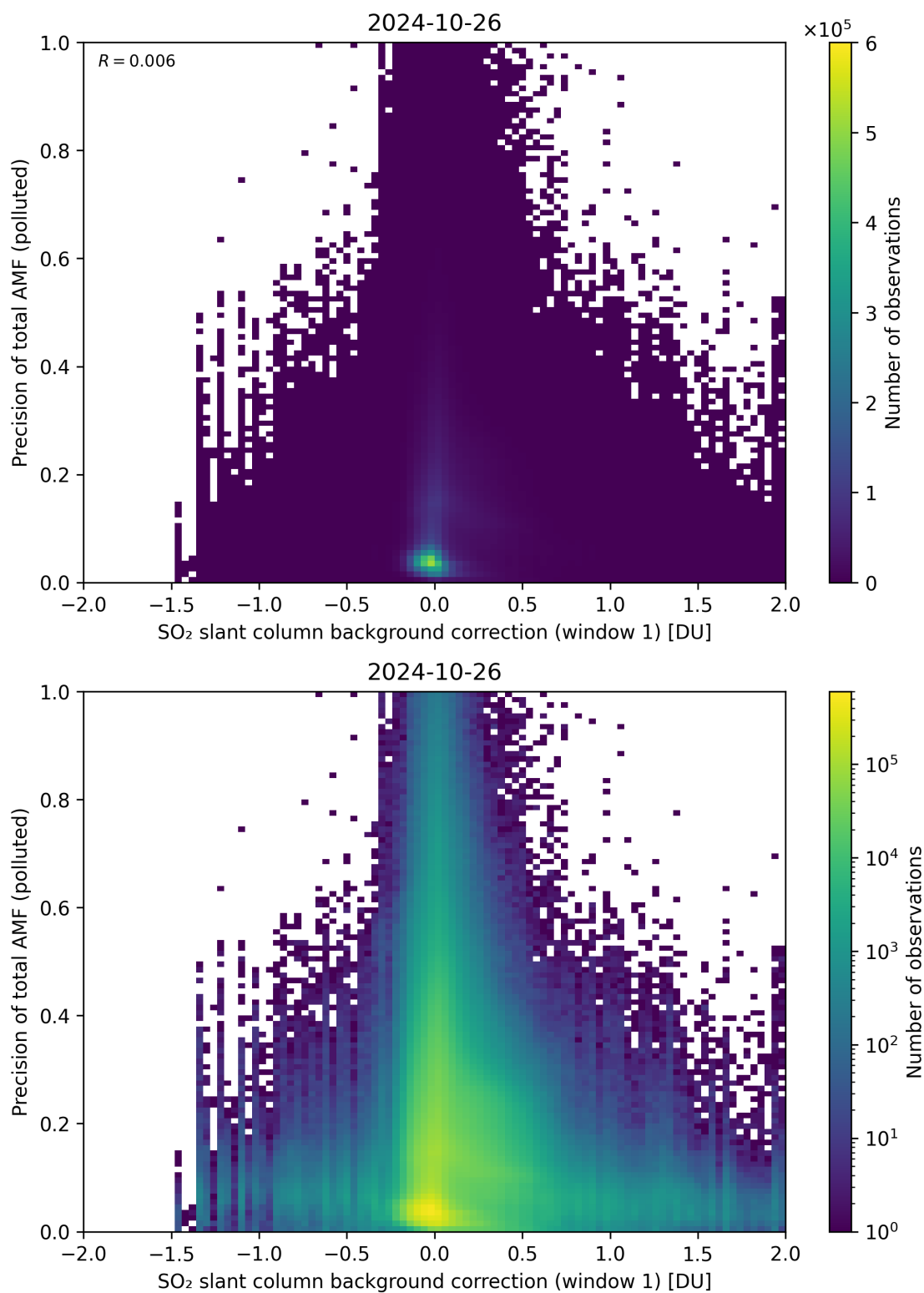
Figure 110: Scatter density plot of “SO 2 slant column background correction (window 1)” against “Precision of total AMF (polluted)” for 2024-10-25 to 2024-10-27.
