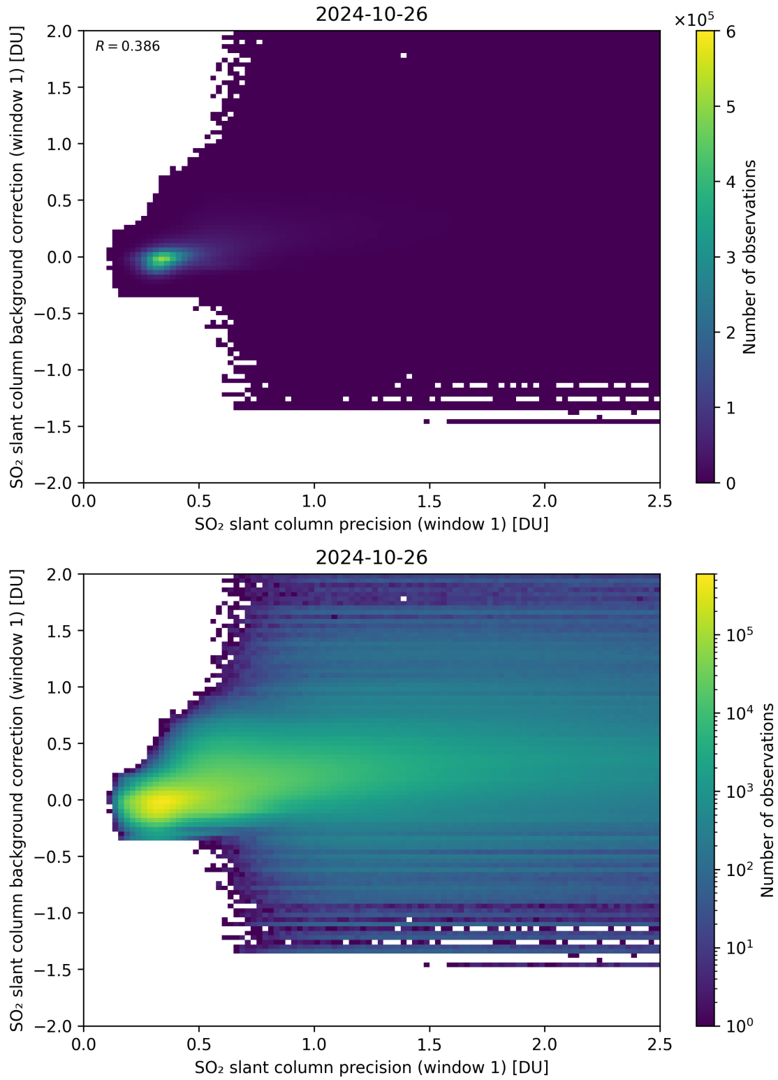
Figure 218: Scatter density plot of “SO 2 slant column precision (window 1)” against “SO 2 slant column background correction (window 1)” for 2024-10-25 to 2024-10-27.
