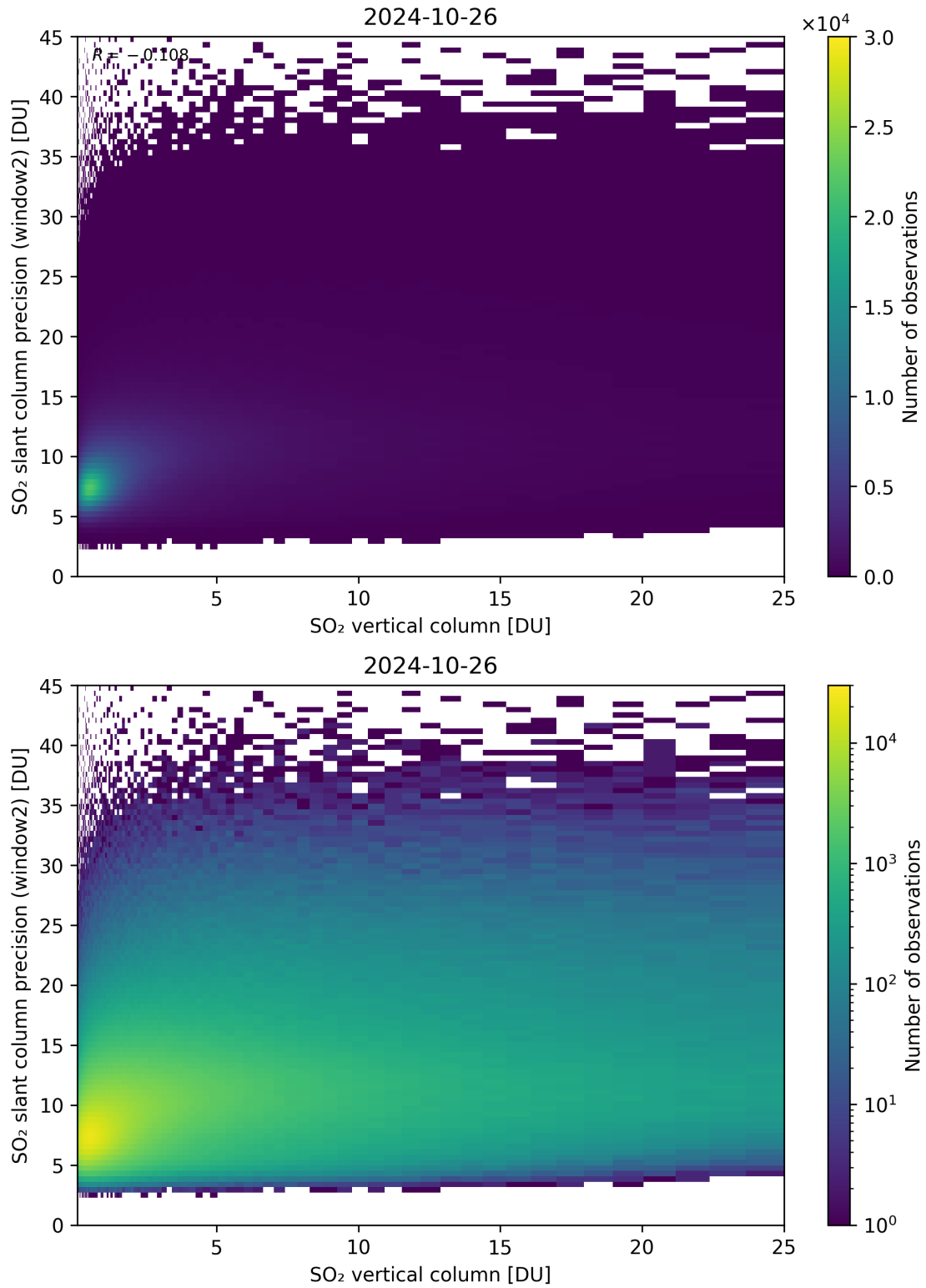
Figure 302: Scatter density plot of “SO 2 vertical column” against “SO 2 slant column precision (window2)” for 2024-10-25 to 2024-10-27.
