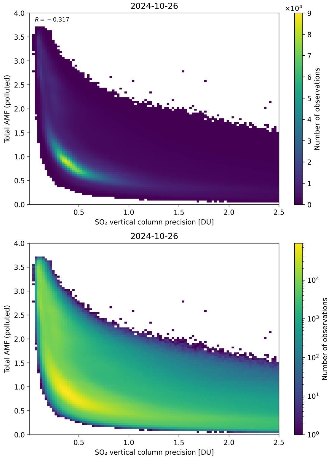
Figure 294: Scatter density plot of “SO 2 vertical column precision” against “Total AMF (polluted)” for 2024-10-25 to 2024-10-27.
