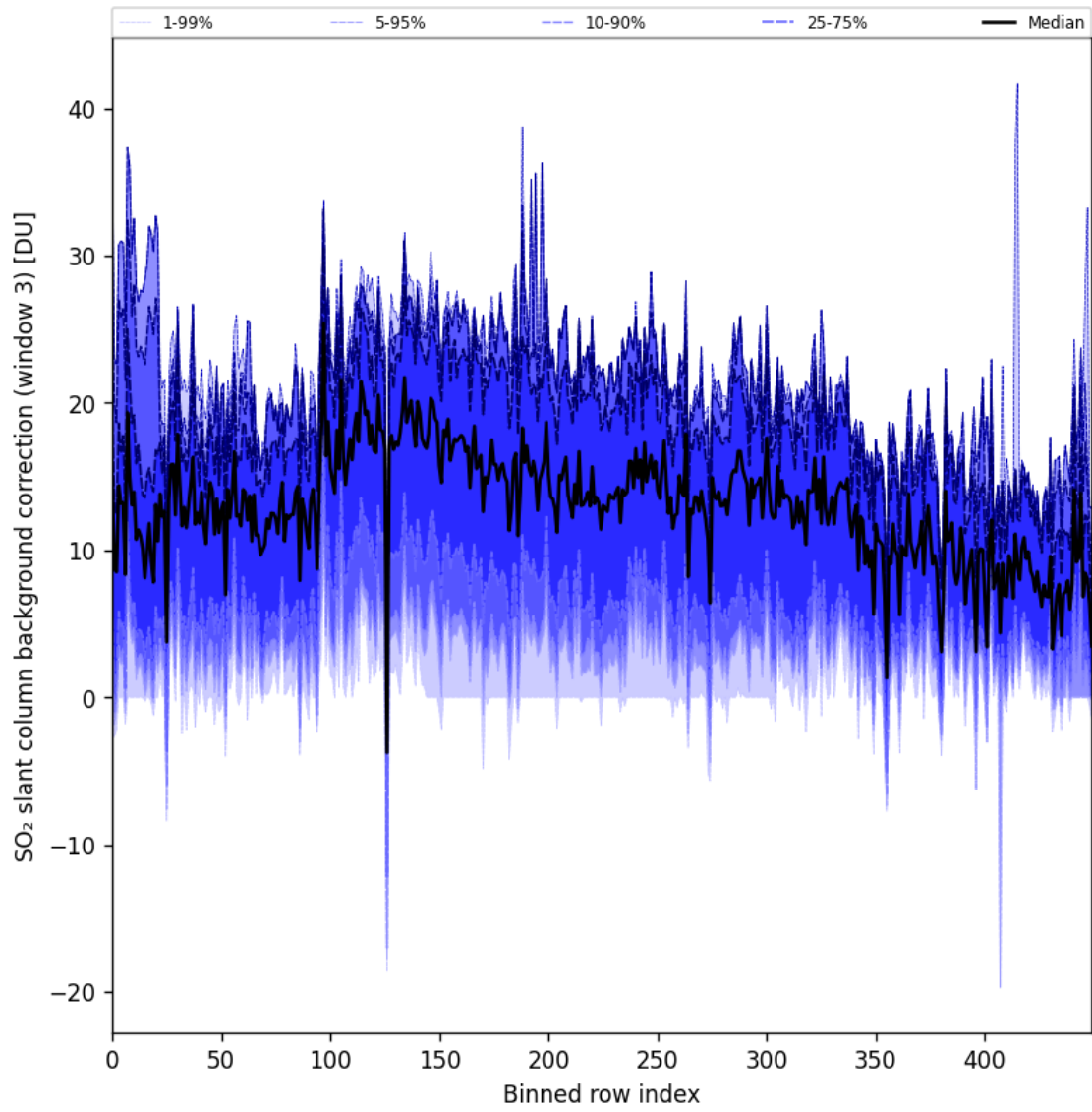
Figure 90: Along track statistics of “SO 2 slant column background correction (window 3)” for 2024-10-25 to 2024-10-27
