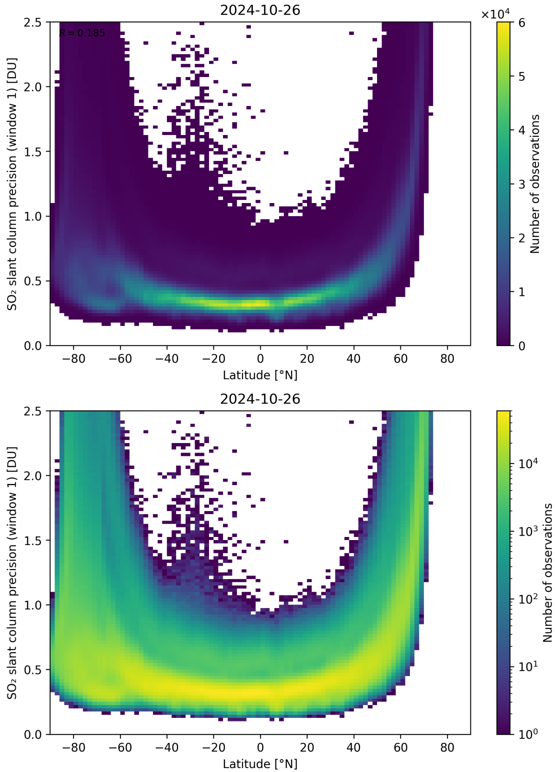
Figure 150: Scatter density plot of “Latitude” against “SO 2 slant column precision (window 1)” for 2024-10-25 to 2024-10-27.
