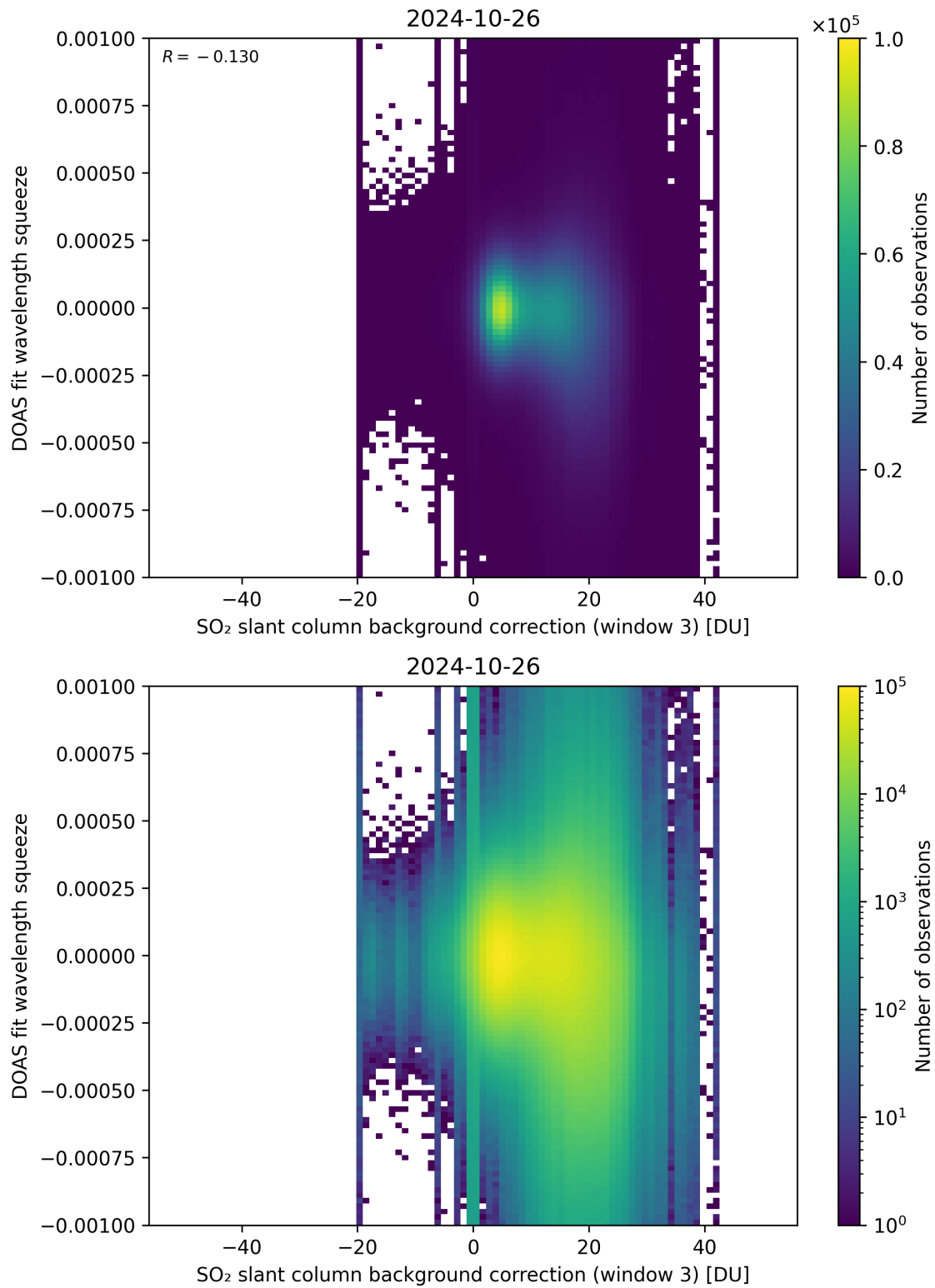
Figure 122: Scatter density plot of “SO 2 slant column background correction (window 3)” against “DOAS fit wavelength squeeze” for 2024-10-25 to 2024-10-27.
