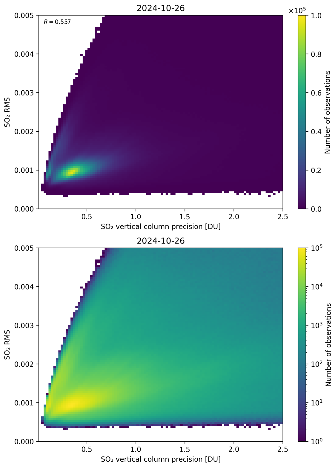
Figure 284: Scatter density plot of “SO 2 vertical column precision” against “SO 2 RMS” for 2024-10-25 to 2024-10-27.
