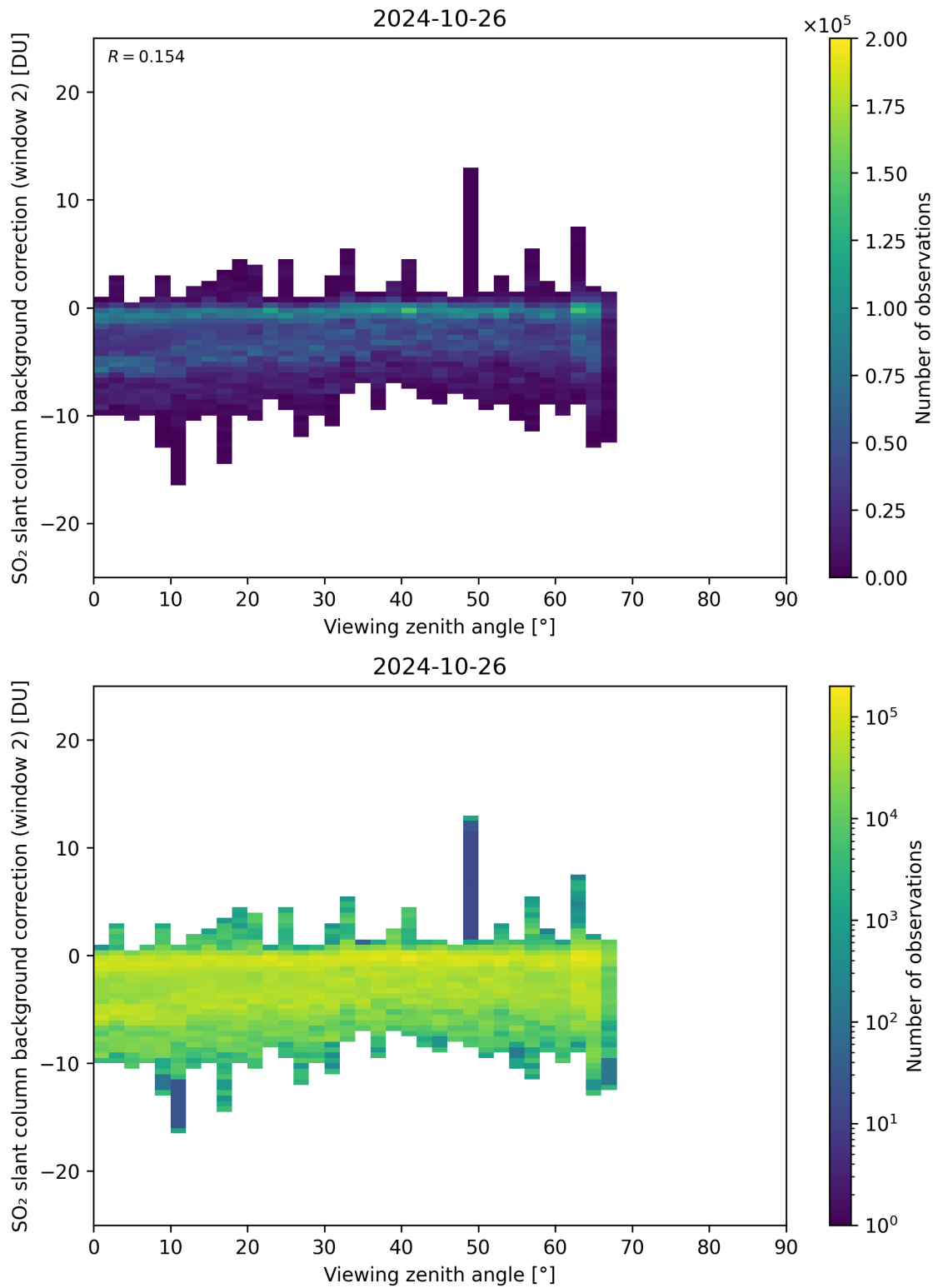
Figure 309: Scatter density plot of “Viewing zenith angle” against “SO 2 slant column background correction (window 2)” for 2024-10-25 to 2024-10-27.
