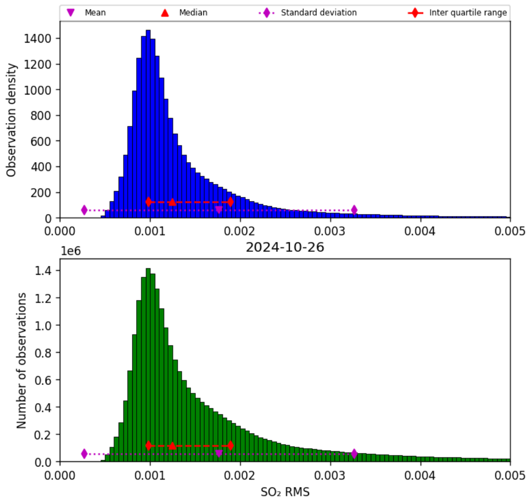
Figure 70: Histogram of “SO 2 RMS” for 2024-10-25 to 2024-10-27
