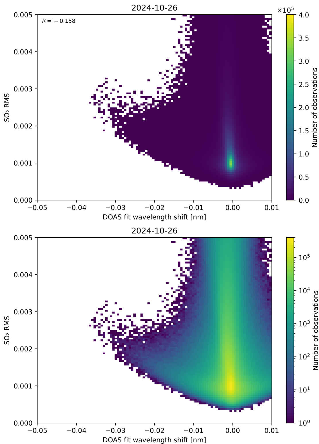
Figure 128: Scatter density plot of “DOAS fit wavelength shift” against “SO 2 RMS” for 2024-10-25 to 2024-10-27.
