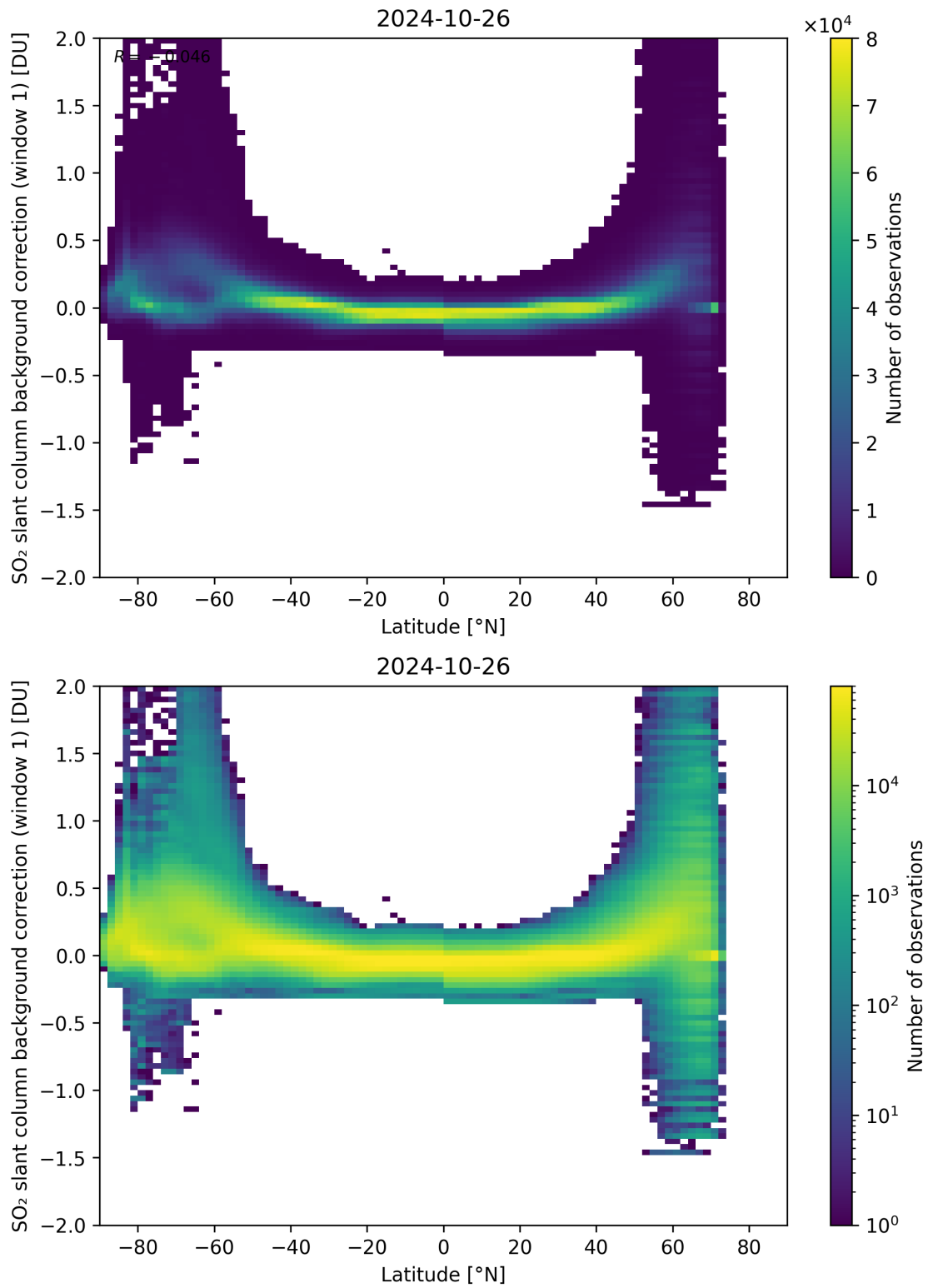
Figure 139: Scatter density plot of “Latitude” against “SO 2 slant column background correction (window 1)” for 2024-10-25 to 2024-10-27.
