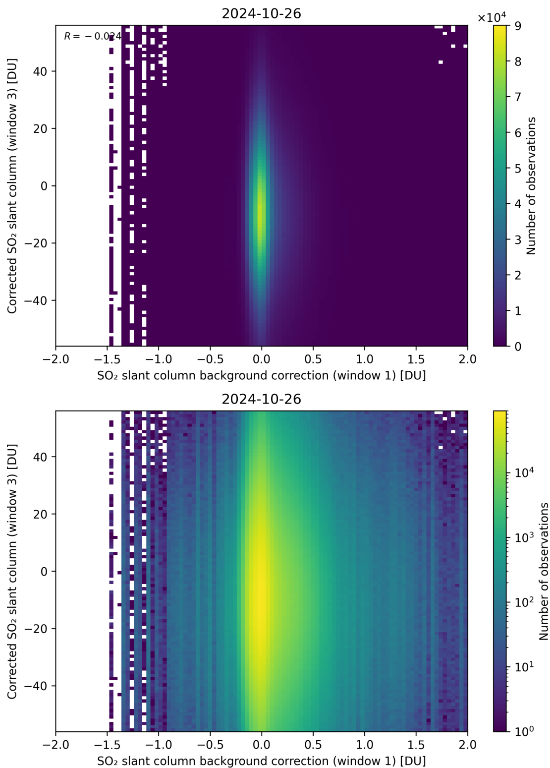
Figure 105: Scatter density plot of “SO 2 slant column background correction (window 1)” against “Corrected SO 2 slant column (window 3)” for 2024-10-25 to 2024-10-27.
