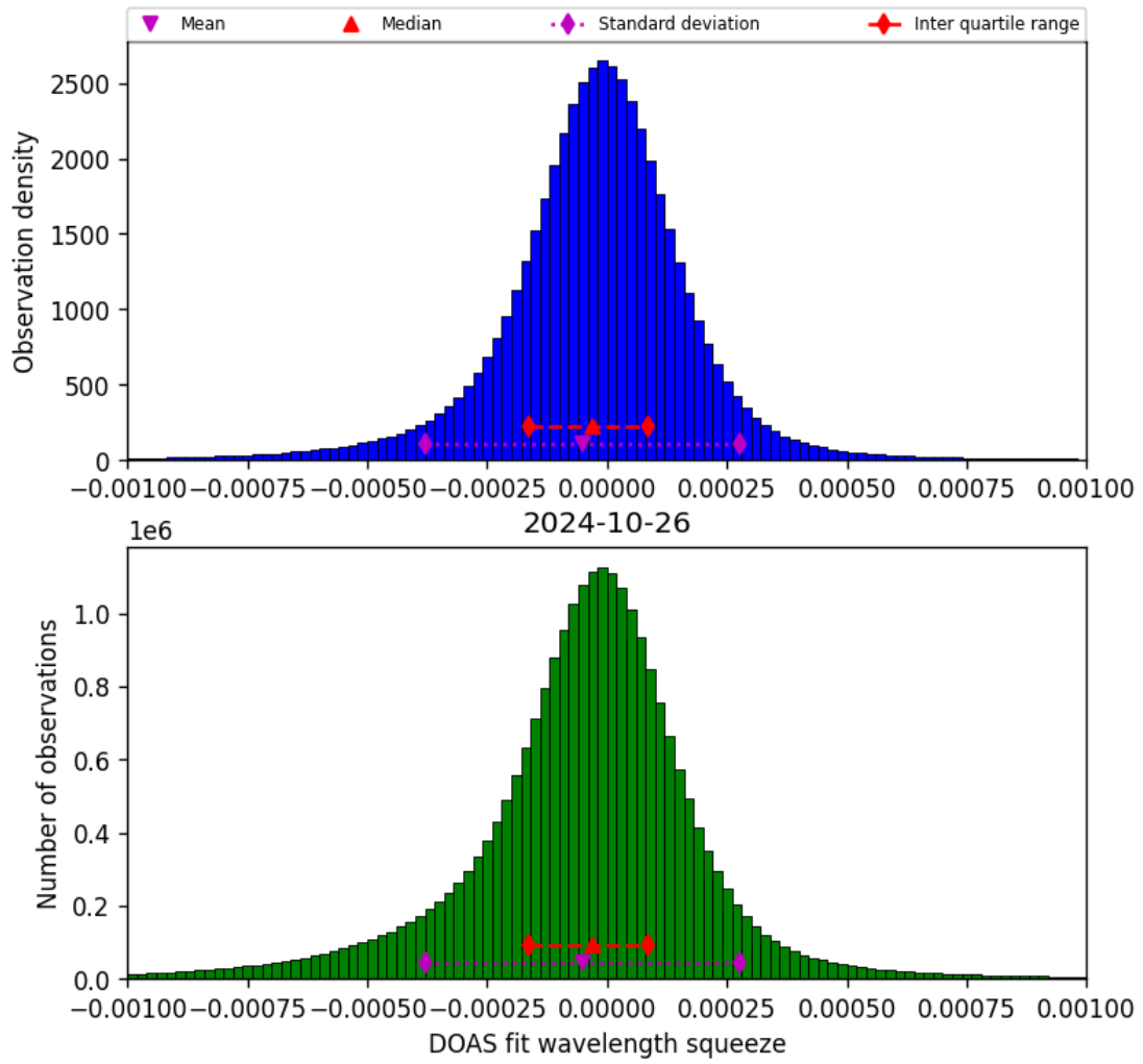
Figure 69: Histogram of “DOAS fit wavelength squeeze” for 2024-10-25 to 2024-10-27
