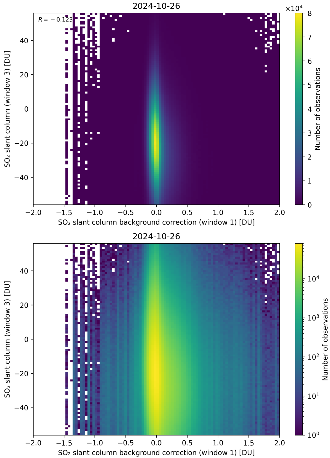
Figure 107: Scatter density plot of “SO 2 slant column background correction (window 1)” against “SO 2 slant column (window 3)” for 2024-10-25 to 2024-10-27.
