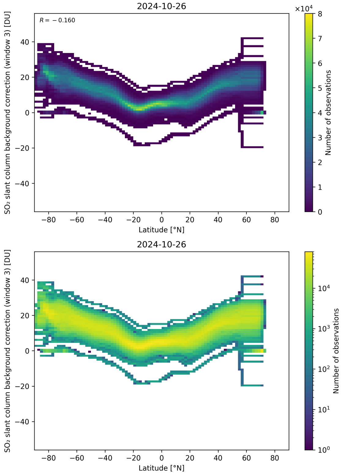
Figure 141: Scatter density plot of “Latitude” against “SO 2 slant column background correction (window 3)” for 2024-10-25 to 2024-10-27.
