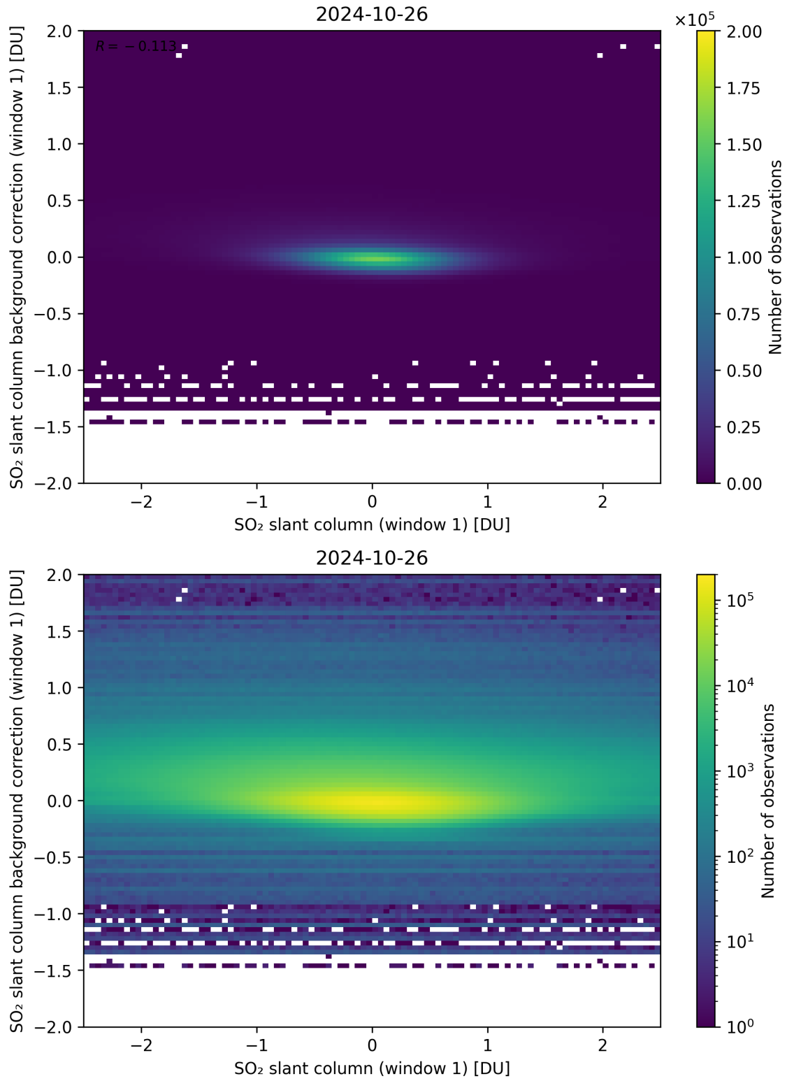
Figure 212: Scatter density plot of “SO 2 slant column (window 1)” against “SO 2 slant column background correction (window 1)” for 2024-10-25 to 2024-10-27.
