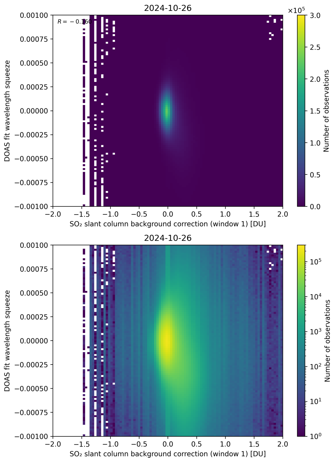
Figure 101: Scatter density plot of “SO 2 slant column background correction (window 1)” against “DOAS fit wavelength squeeze” for 2024-10-25 to 2024-10-27.
