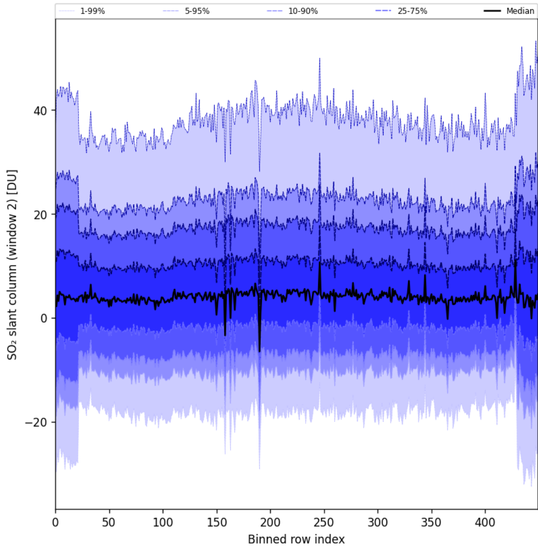
Figure 83: Along track statistics of “SO 2 slant column (window 2)” for 2024-10-25 to 2024-10-27
