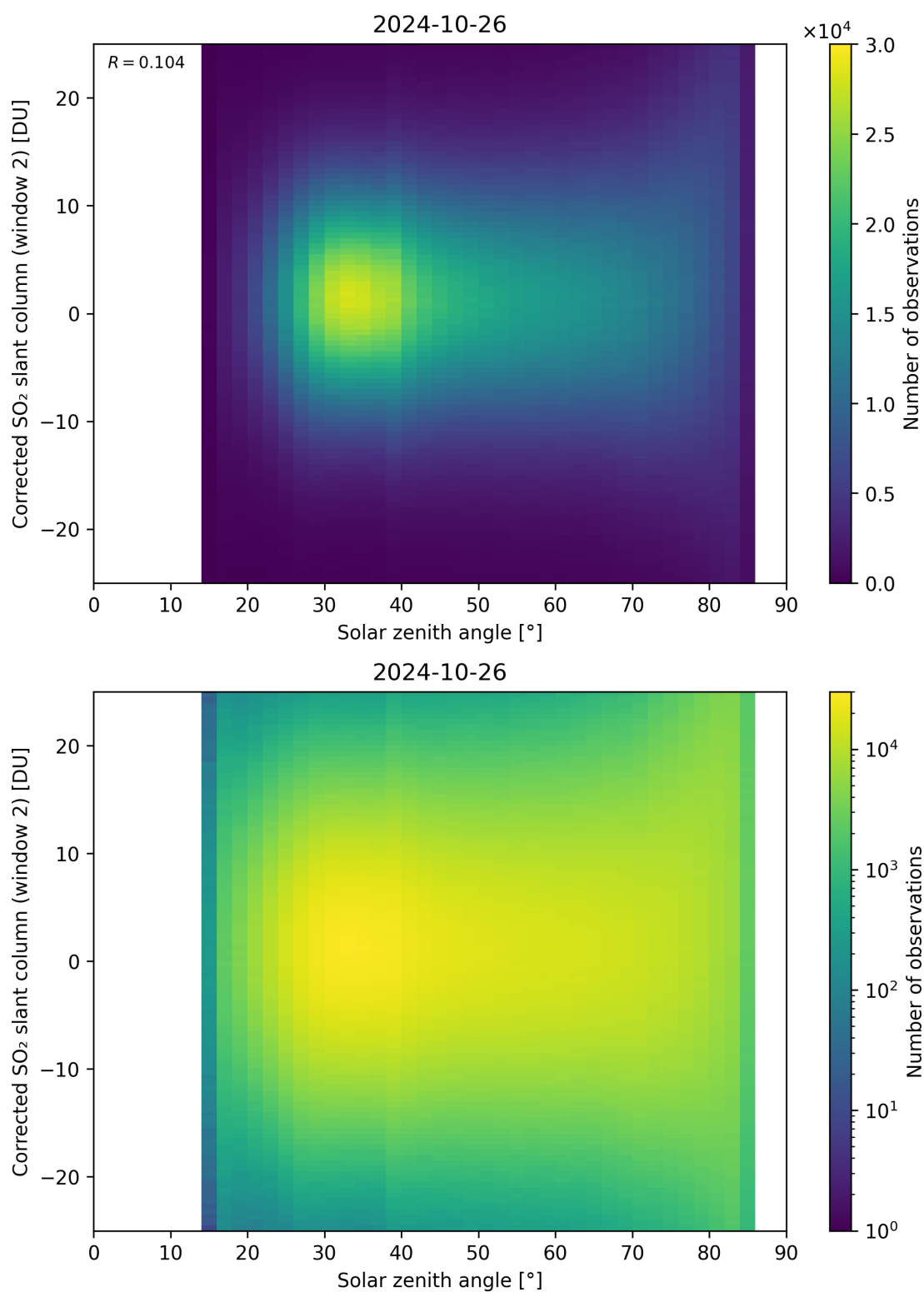
Figure 167: Scatter density plot of “Solar zenith angle” against “Corrected SO 2 slant column (window 2)” for 2024-10-25 to 2024-10-27.
