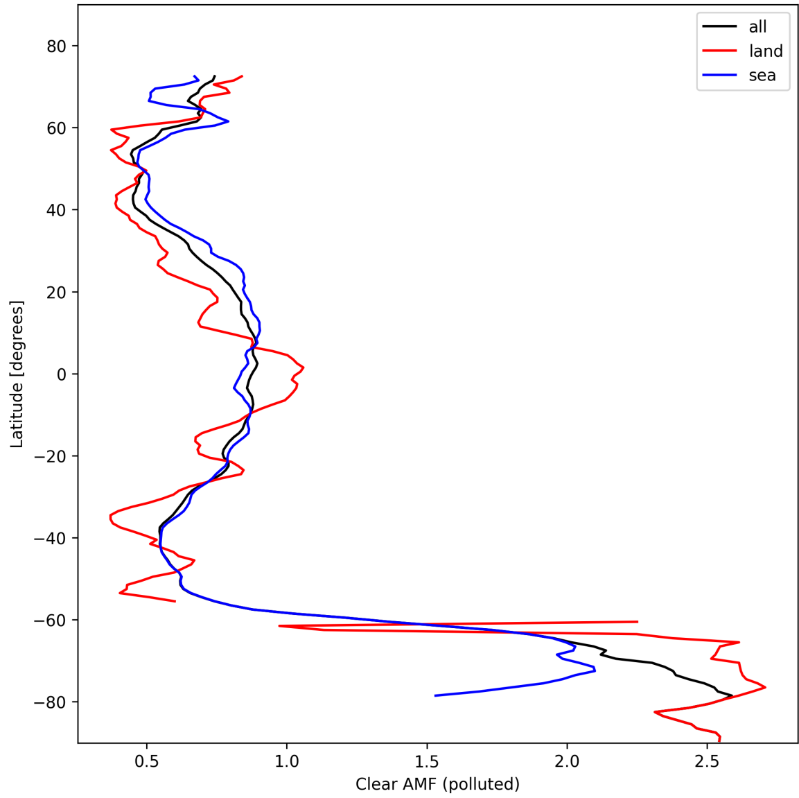
Figure 50: Zonal average of “Clear AMF (polluted)” for 2024-10-25 to 2024-10-27.
