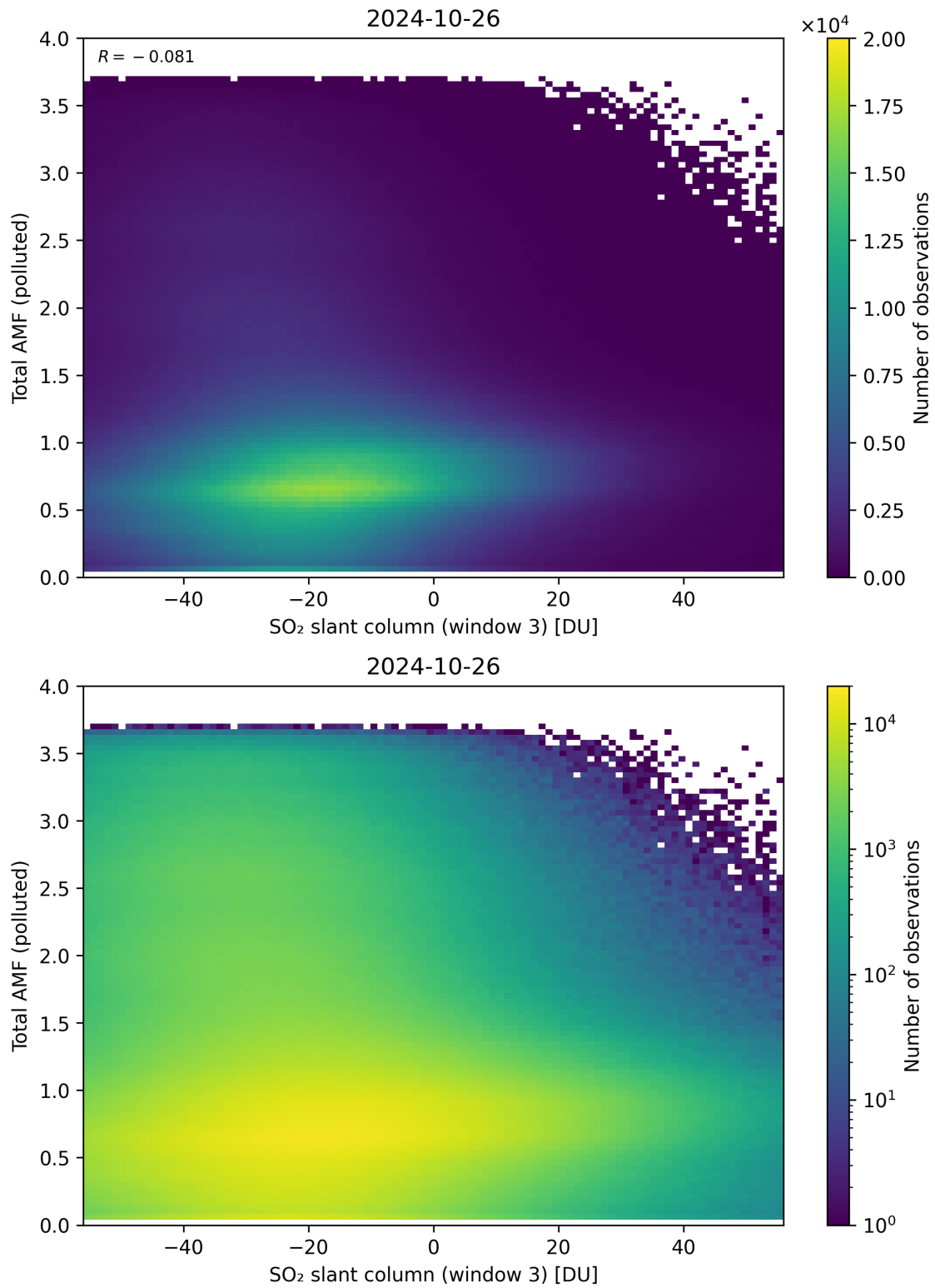
Figure 268: Scatter density plot of “SO 2 slant column (window 3)” against “Total AMF (polluted)” for 2024-10-25 to 2024-10-27.
