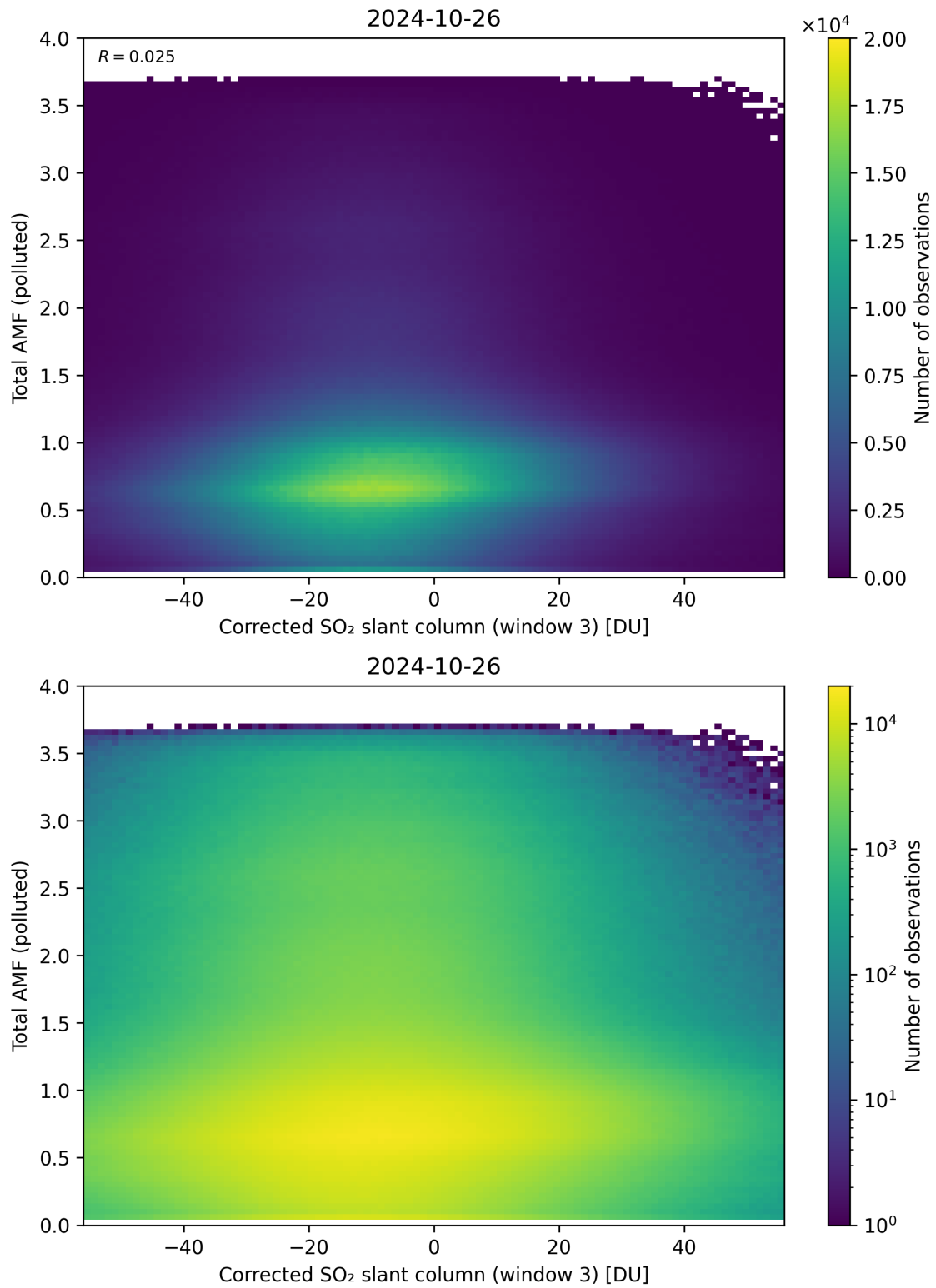
Figure 210: Scatter density plot of “Corrected SO 2 slant column (window 3)” against “Total AMF (polluted)” for 2024-10-25 to 2024-10-27.
