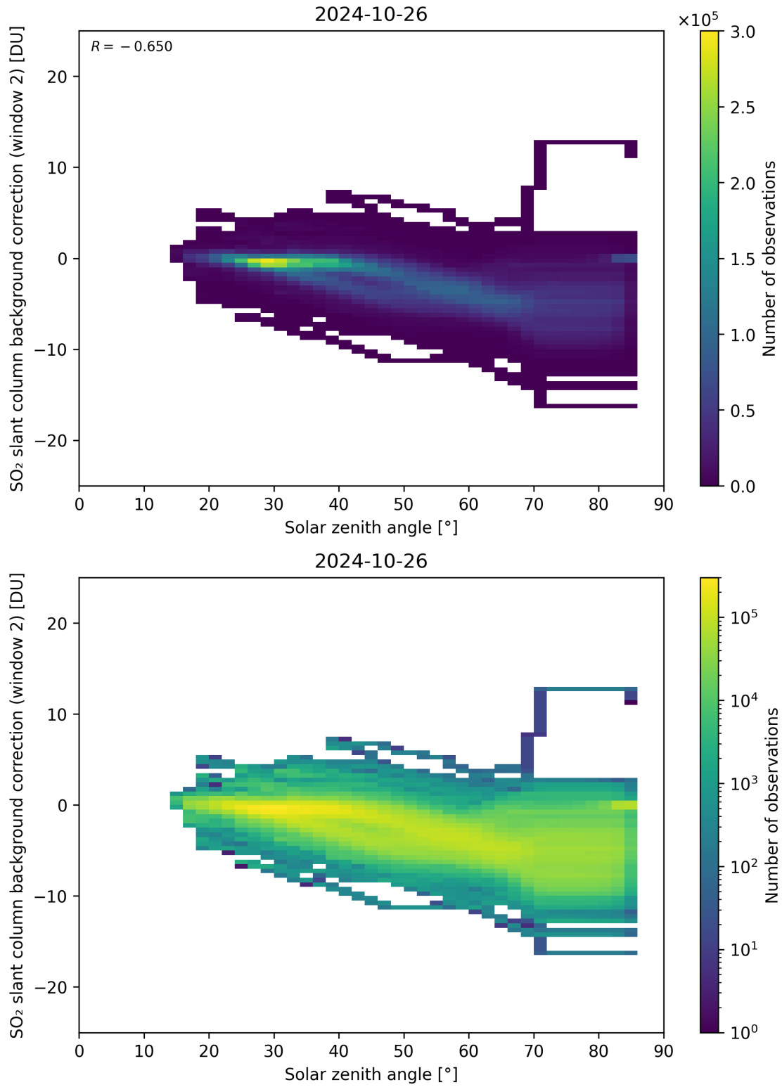
Figure 159: Scatter density plot of “Solar zenith angle” against “SO 2 slant column background correction (window 2)” for 2024-10-25 to 2024-10-27.
