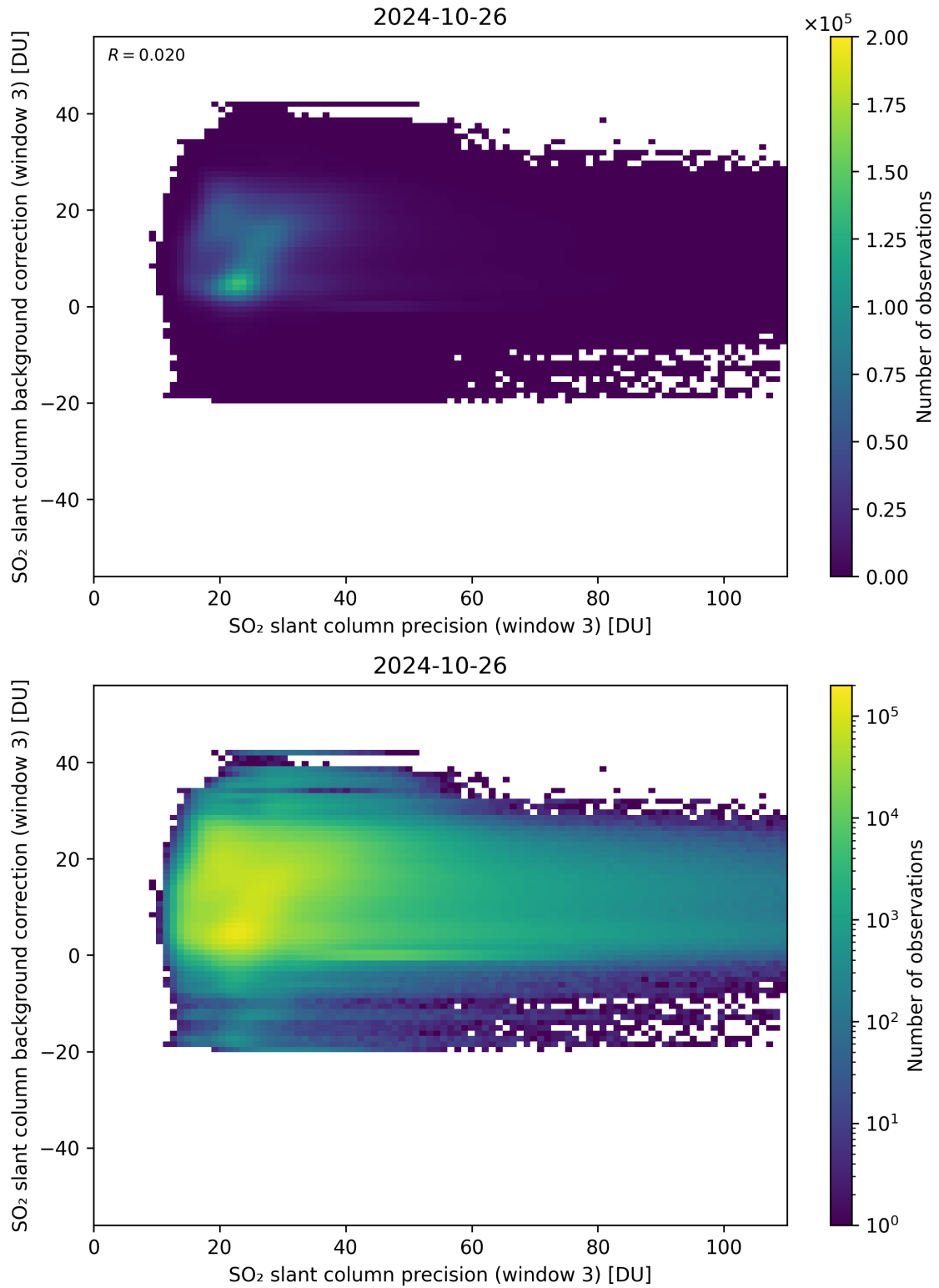
Figure 257: Scatter density plot of “SO 2 slant column precision (window 3)” against “SO 2 slant column background correction (window 3)” for 2024-10-25 to 2024-10-27.
