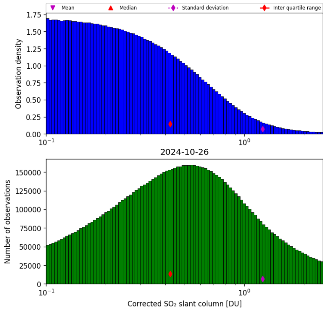
Figure 55: Histogram of “Corrected SO 2 slant column” for 2024-10-25 to 2024-10-27
