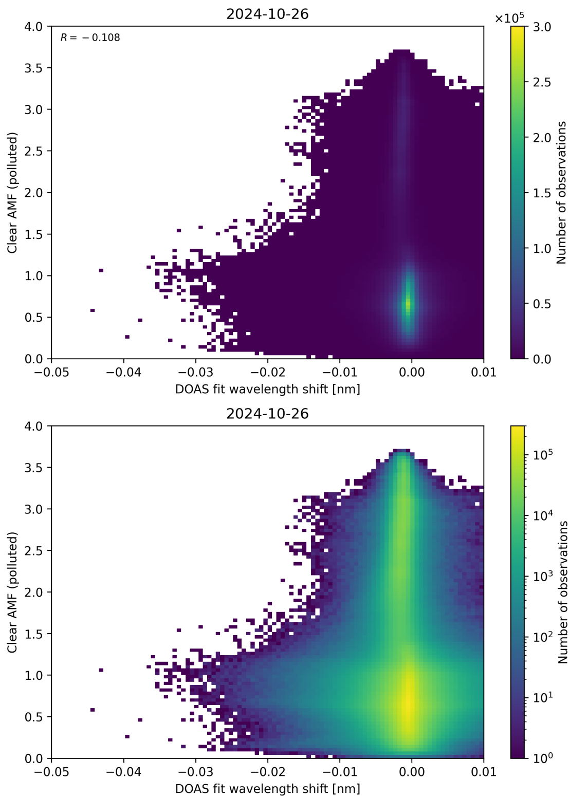
Figure 129: Scatter density plot of “DOAS fit wavelength shift” against “Clear AMF (polluted)” for 2024-10-25 to 2024-10-27.
