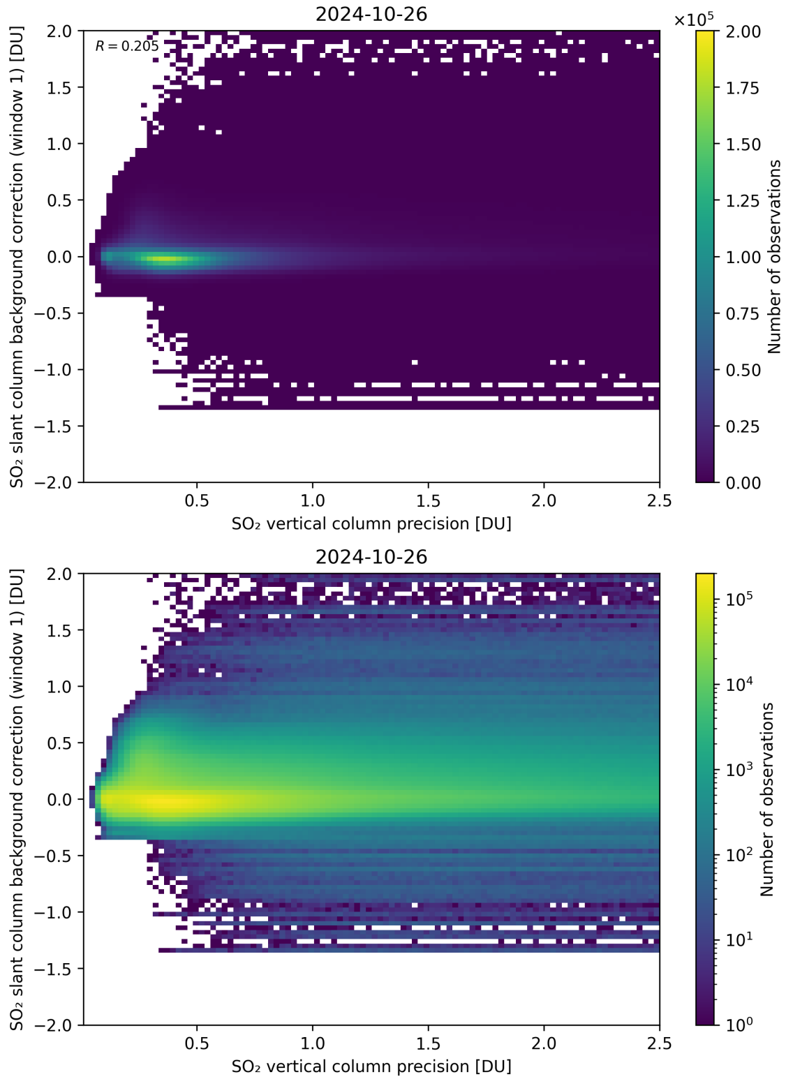
Figure 279: Scatter density plot of “SO 2 vertical column precision” against “SO 2 slant column background correction (window 1)” for 2024-10-25 to 2024-10-27.
