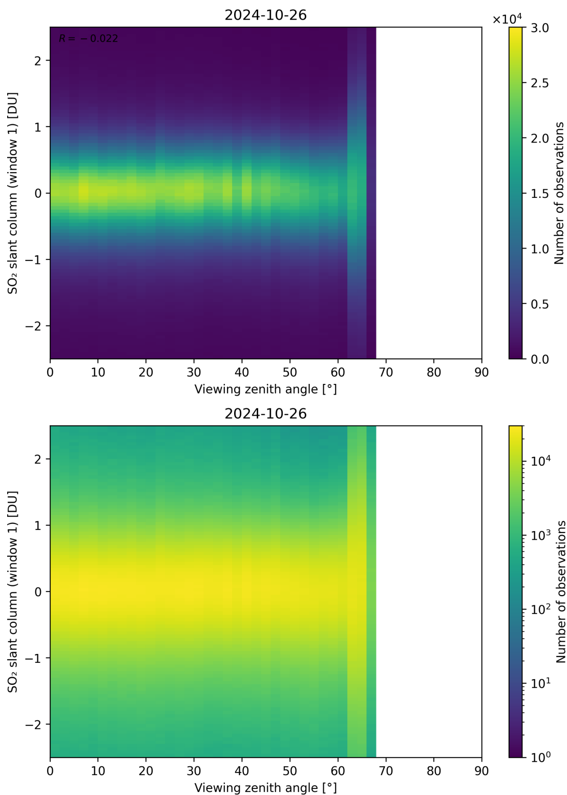
Figure 320: Scatter density plot of “Viewing zenith angle” against “SO 2 slant column (window 1)” for 2024-10-25 to 2024-10-27.
