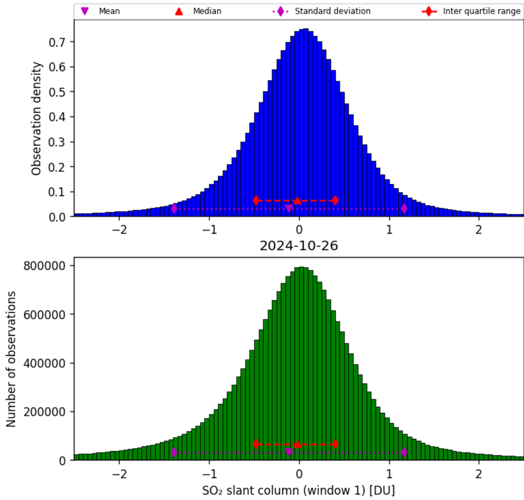
Figure 56: Histogram of “SO 2 slant column (window 1)” for 2024-10-25 to 2024-10-27
