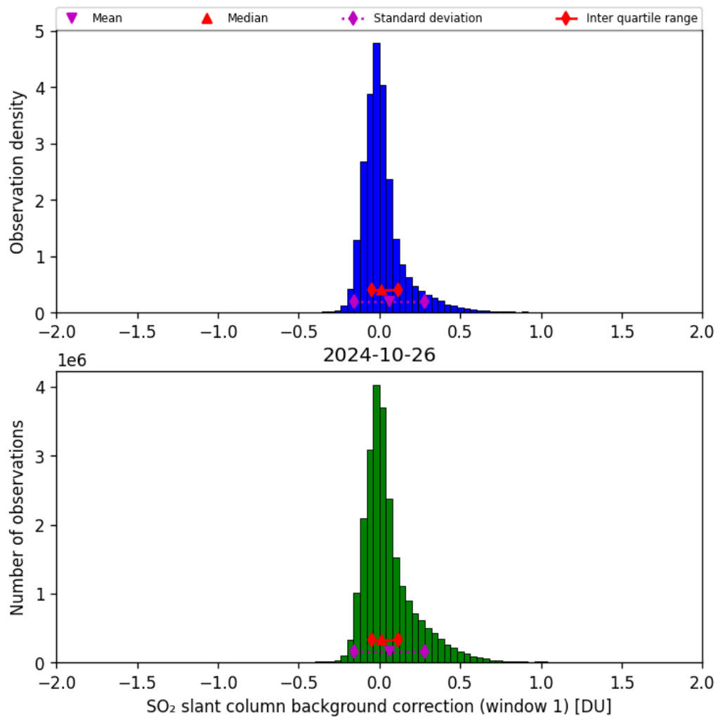
Figure 59: Histogram of “SO 2 slant column background correction (window 1)” for 2024-10-25 to 2024-10-27
