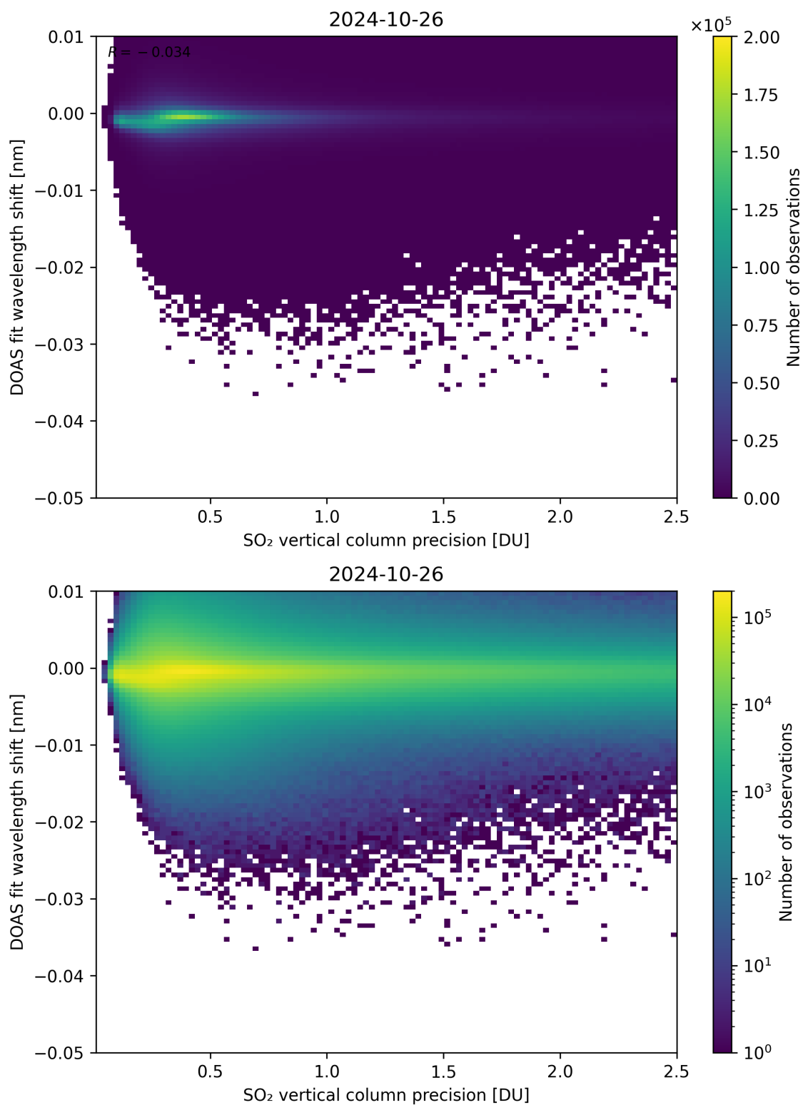
Figure 282: Scatter density plot of “SO 2 vertical column precision” against “DOAS fit wavelength shift” for 2024-10-25 to 2024-10-27.
