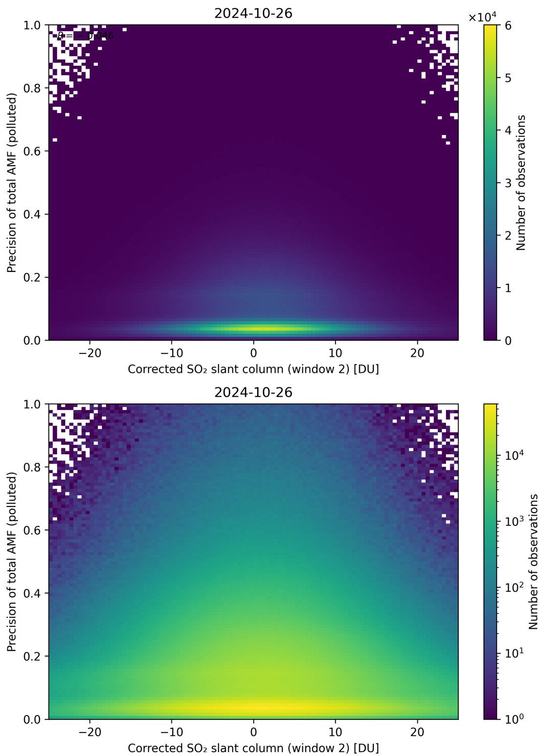
Figure 204: Scatter density plot of “Corrected SO 2 slant column (window 2)” against “Precision of total AMF (polluted)” for 2024-10-25 to 2024-10-27.
