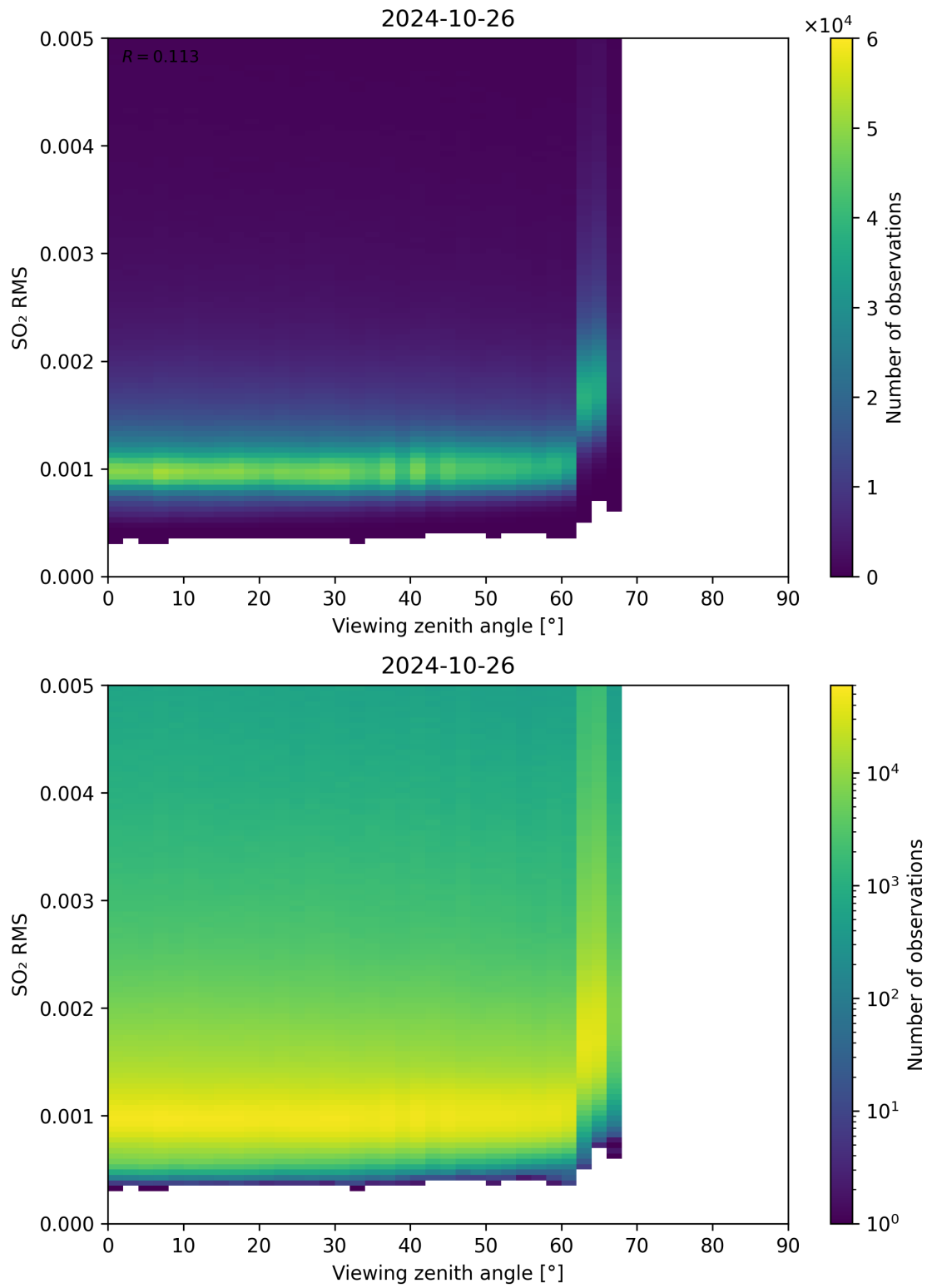
Figure 313: Scatter density plot of “Viewing zenith angle” against “SO 2 RMS” for 2024-10-25 to 2024-10-27.
