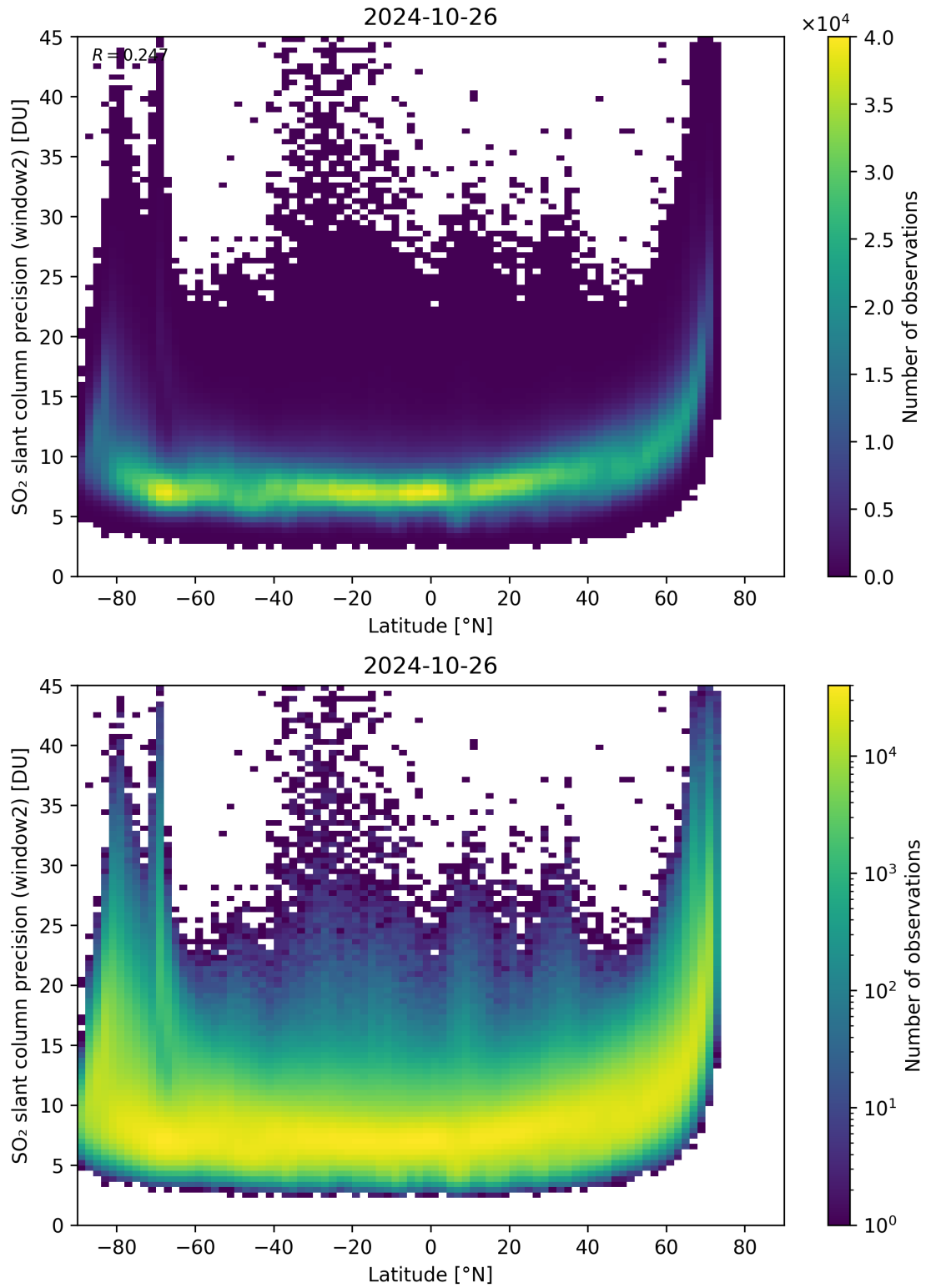
Figure 151: Scatter density plot of “Latitude” against “SO 2 slant column precision (window2)” for 2024-10-25 to 2024-10-27.
