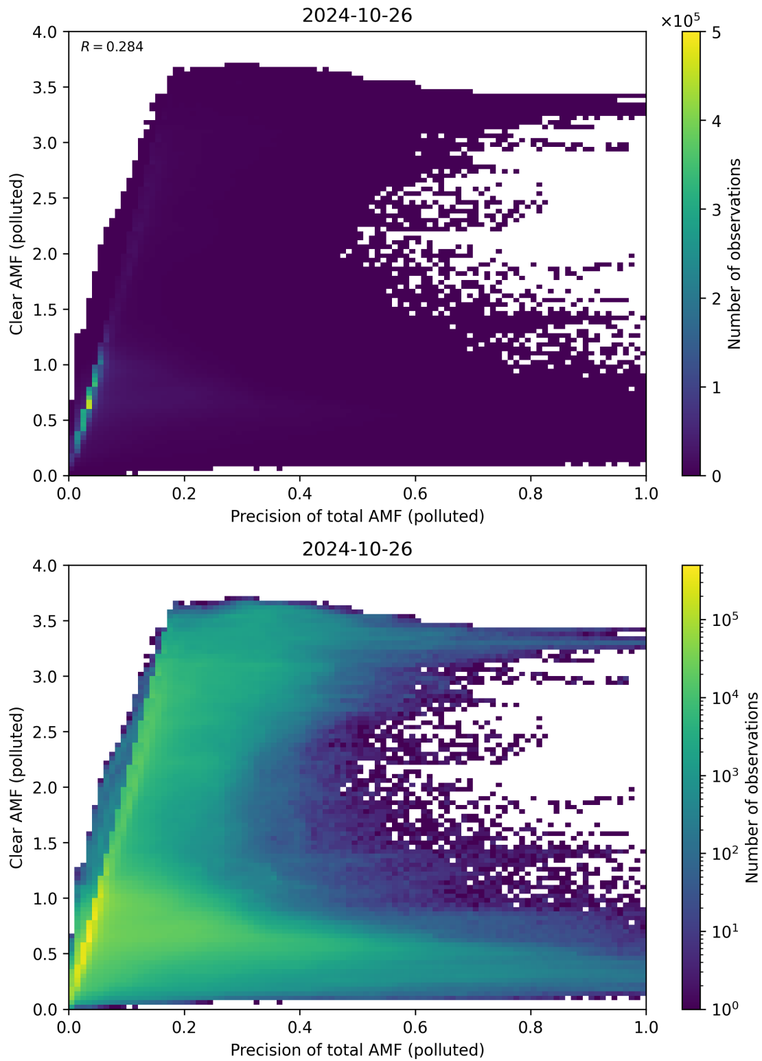
Figure 270: Scatter density plot of “Precision of total AMF (polluted)” against “Clear AMF (polluted)” for 2024-10-25 to 2024-10-27.
