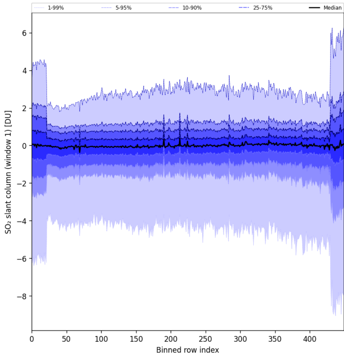
Figure 79: Along track statistics of “SO 2 slant column (window 1)” for 2024-10-25 to 2024-10-27
