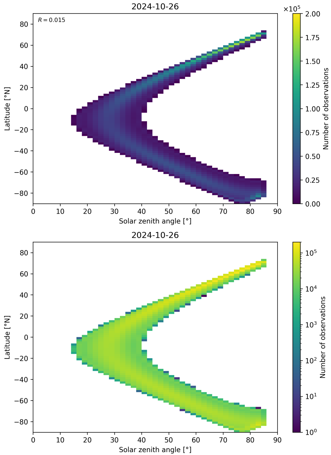
Figure 164: Scatter density plot of “Solar zenith angle” against “Latitude” for 2024-10-25 to 2024-10-27.
