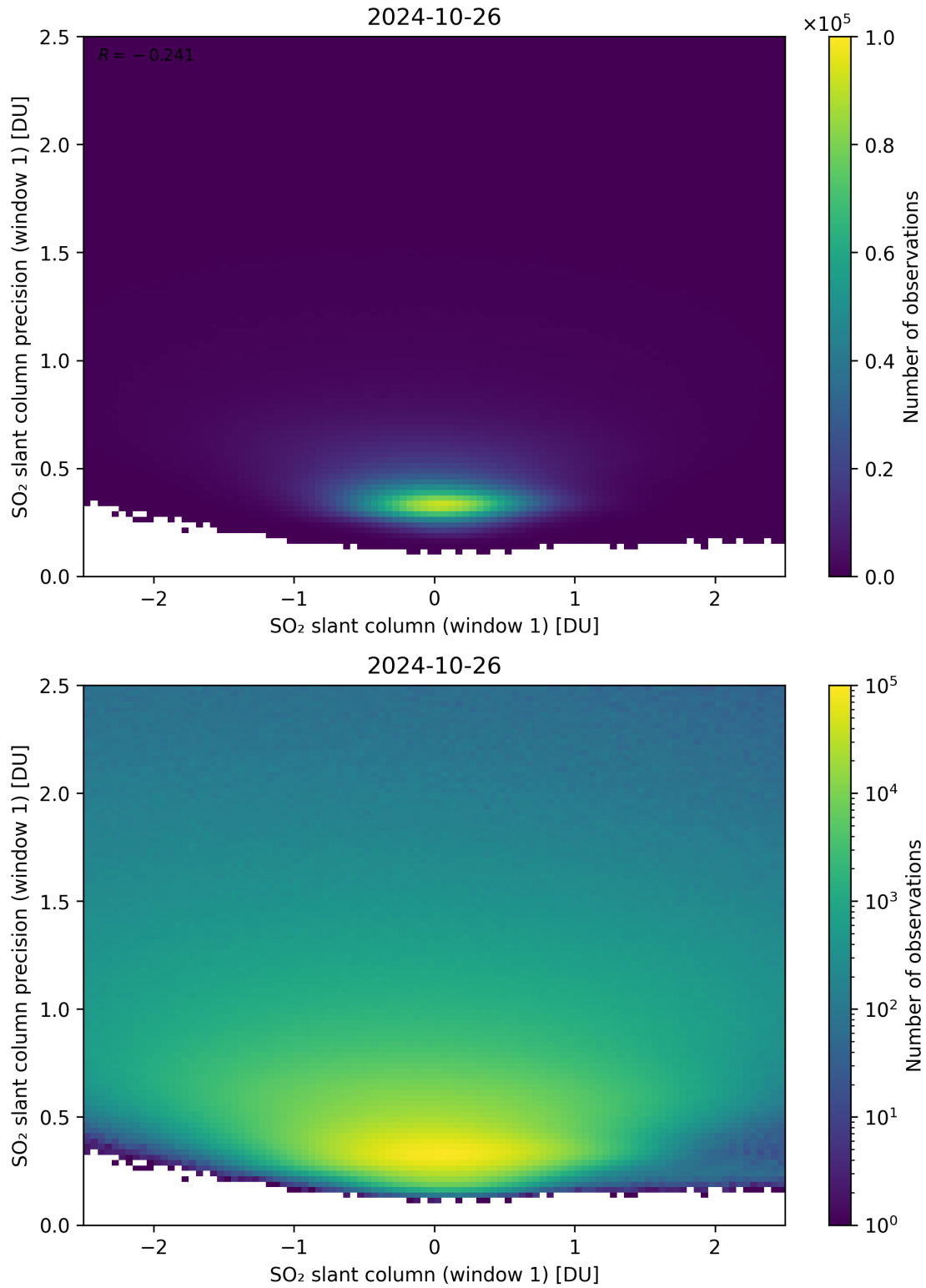
Figure 235: Scatter density plot of “SO 2 slant column (window 1)” against “SO 2 slant column precision (window 1)” for 2024-10-25 to 2024-10-27.
