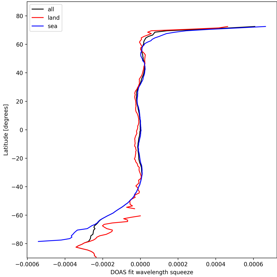
Figure 46: Zonal average of “DOAS fit wavelength squeeze” for 2024-10-25 to 2024-10-27.
