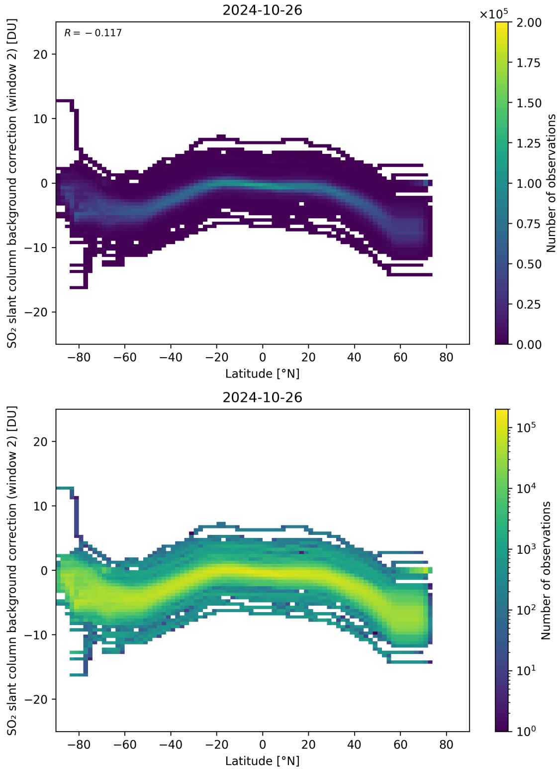
Figure 140: Scatter density plot of “Latitude” against “SO 2 slant column background correction (window 2)” for 2024-10-25 to 2024-10-27.
