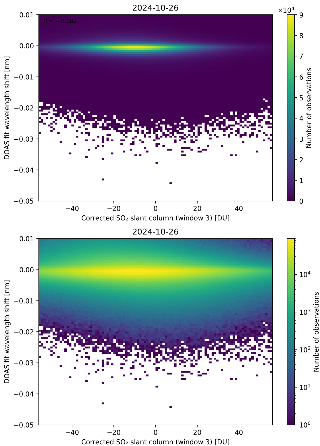
Figure 206: Scatter density plot of “Corrected SO 2 slant column (window 3)” against “DOAS fit wavelength shift” for 2024-10-25 to 2024-10-27.
