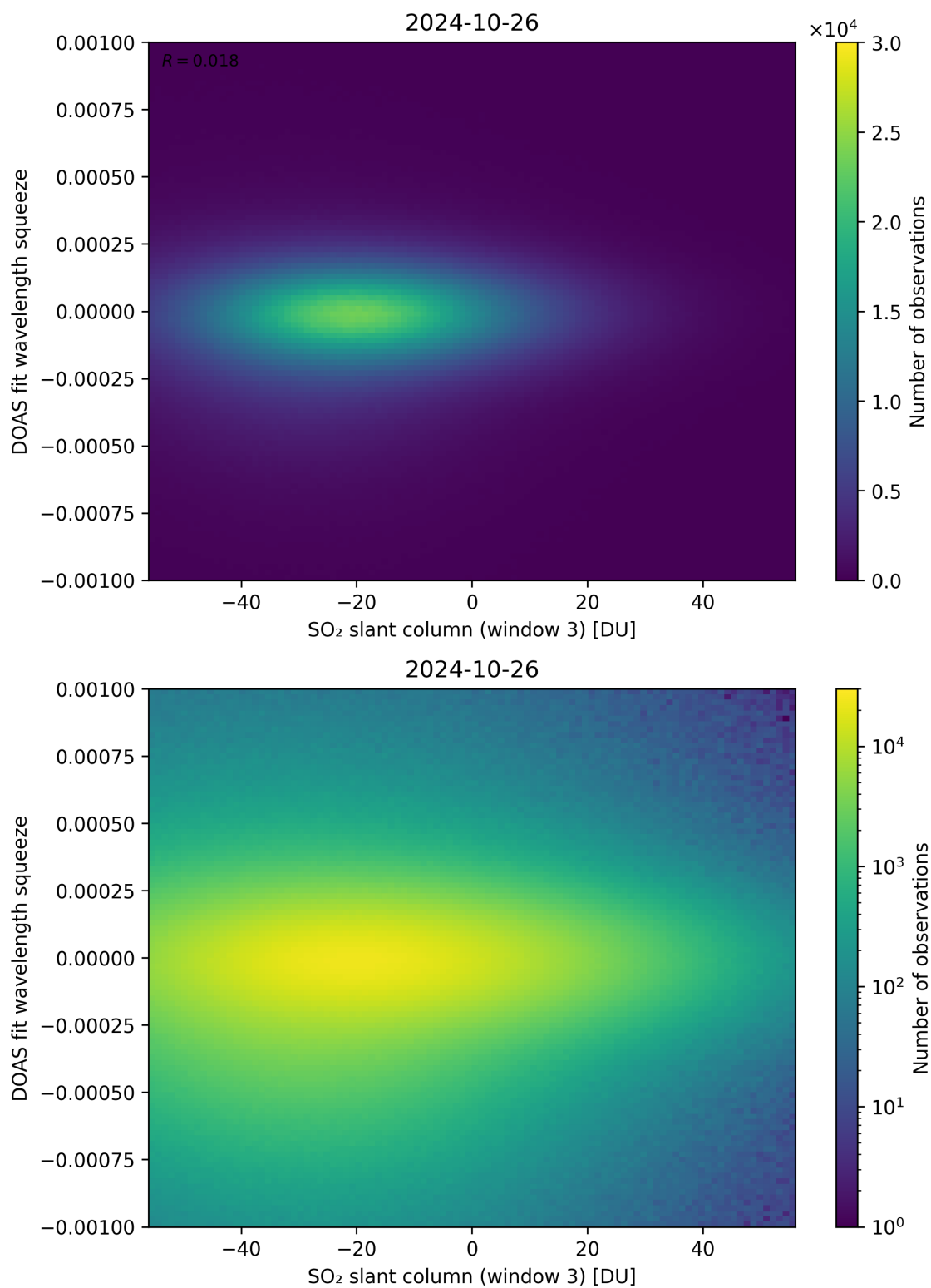
Figure 255: Scatter density plot of “SO 2 slant column (window 3)” against “DOAS fit wavelength squeeze” for 2024-10-25 to 2024-10-27.
