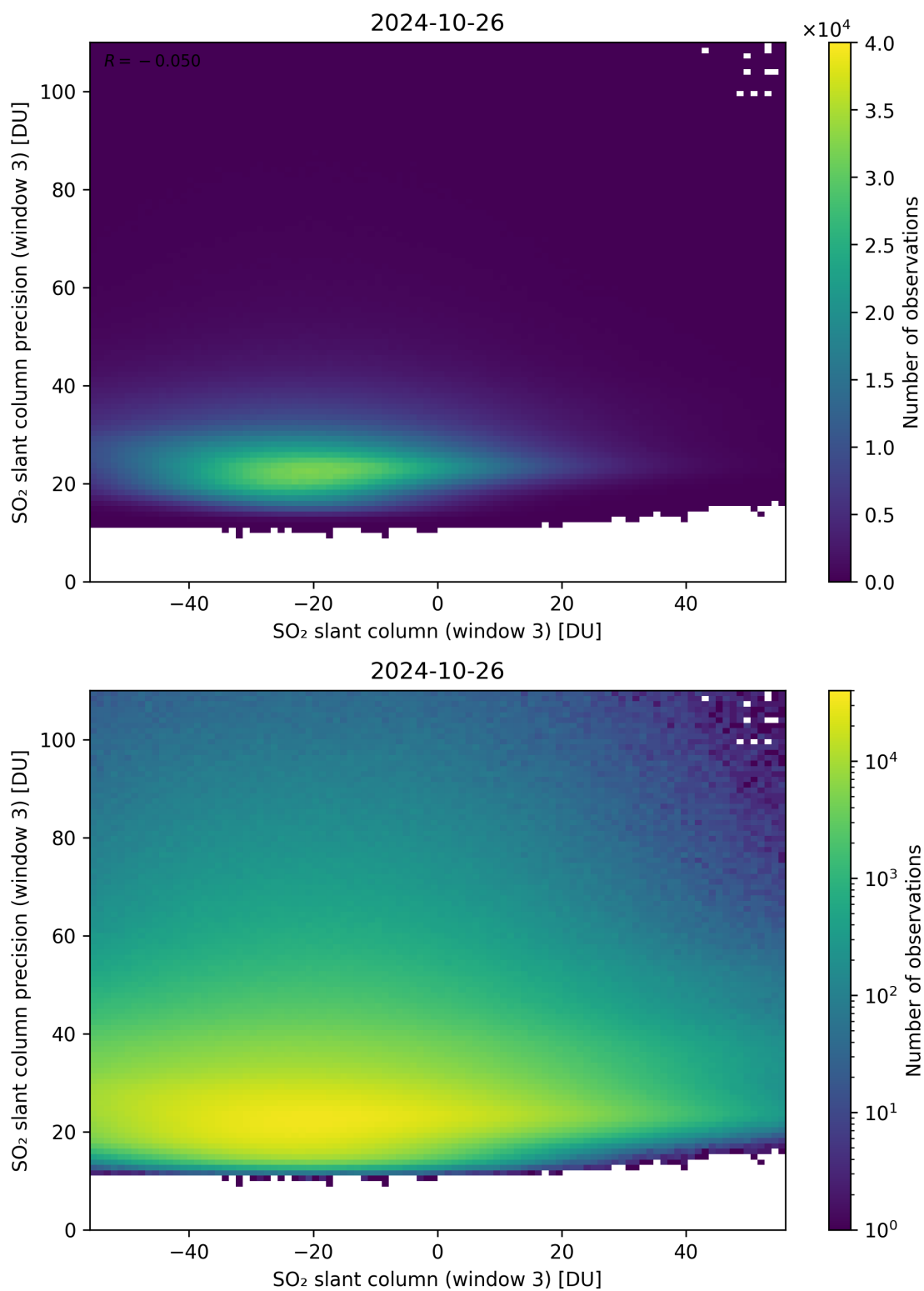
Figure 267: Scatter density plot of “SO 2 slant column (window 3)” against “SO 2 slant column precision (window 3)” for 2024-10-25 to 2024-10-27.
