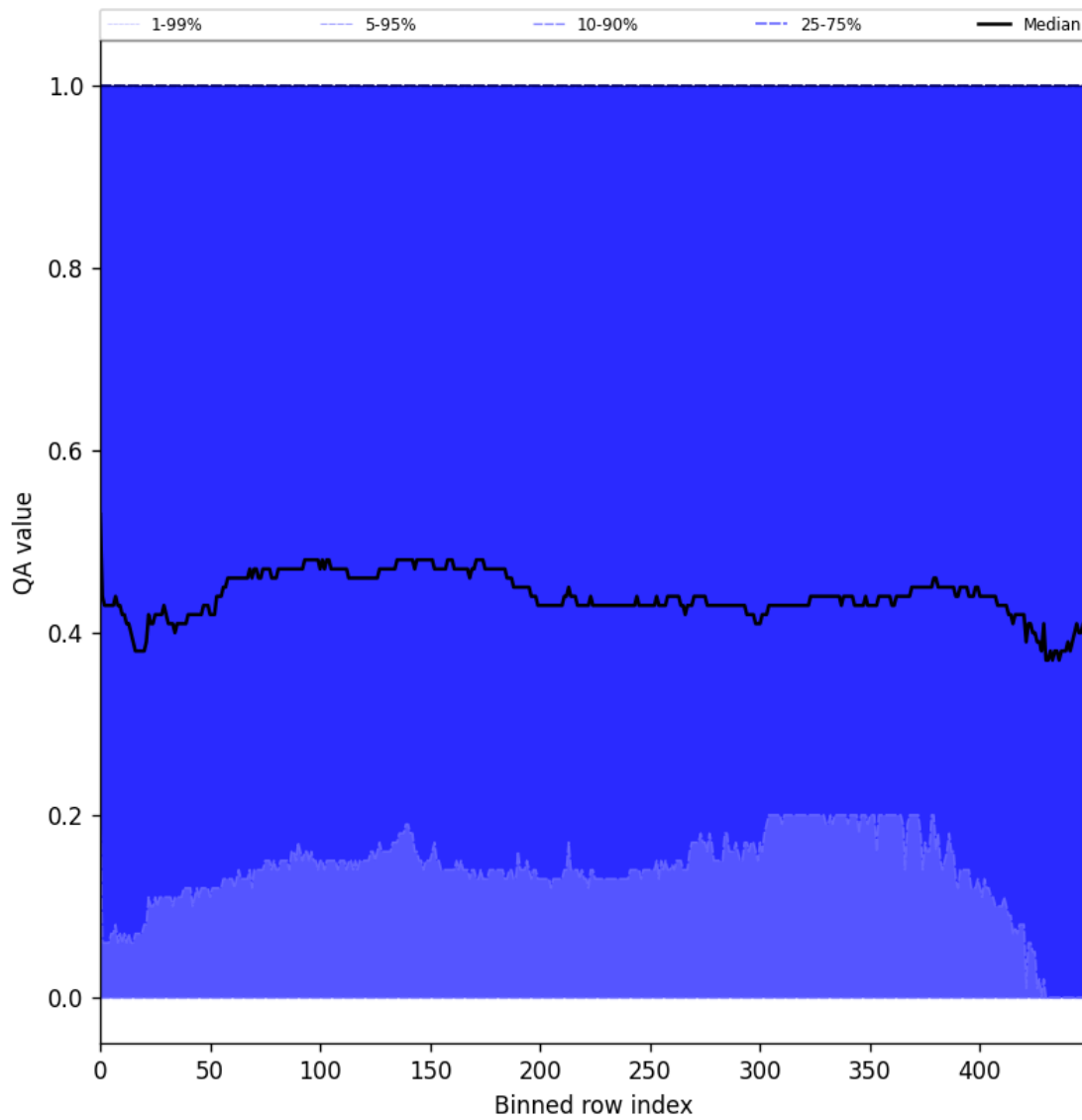
Figure 75: Along track statistics of “QA value” for 2024-10-25 to 2024-10-27
