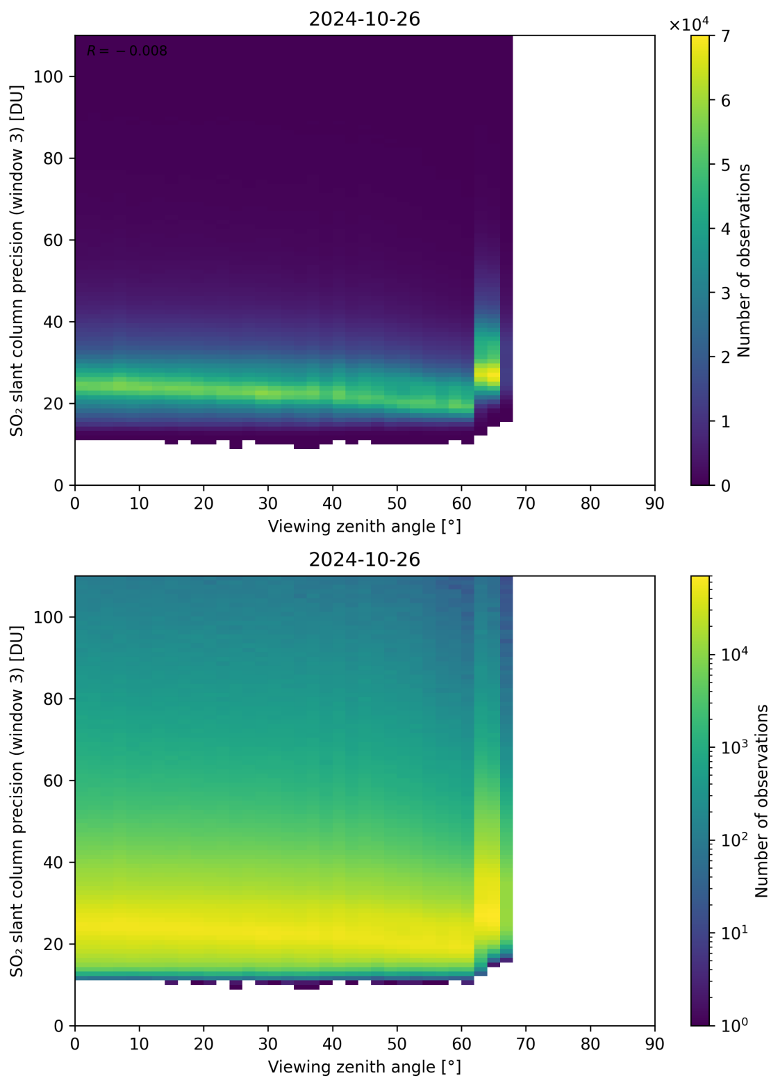
Figure 324: Scatter density plot of “Viewing zenith angle” against “SO 2 slant column precision (window 3)” for 2024-10-25 to 2024-10-27.
