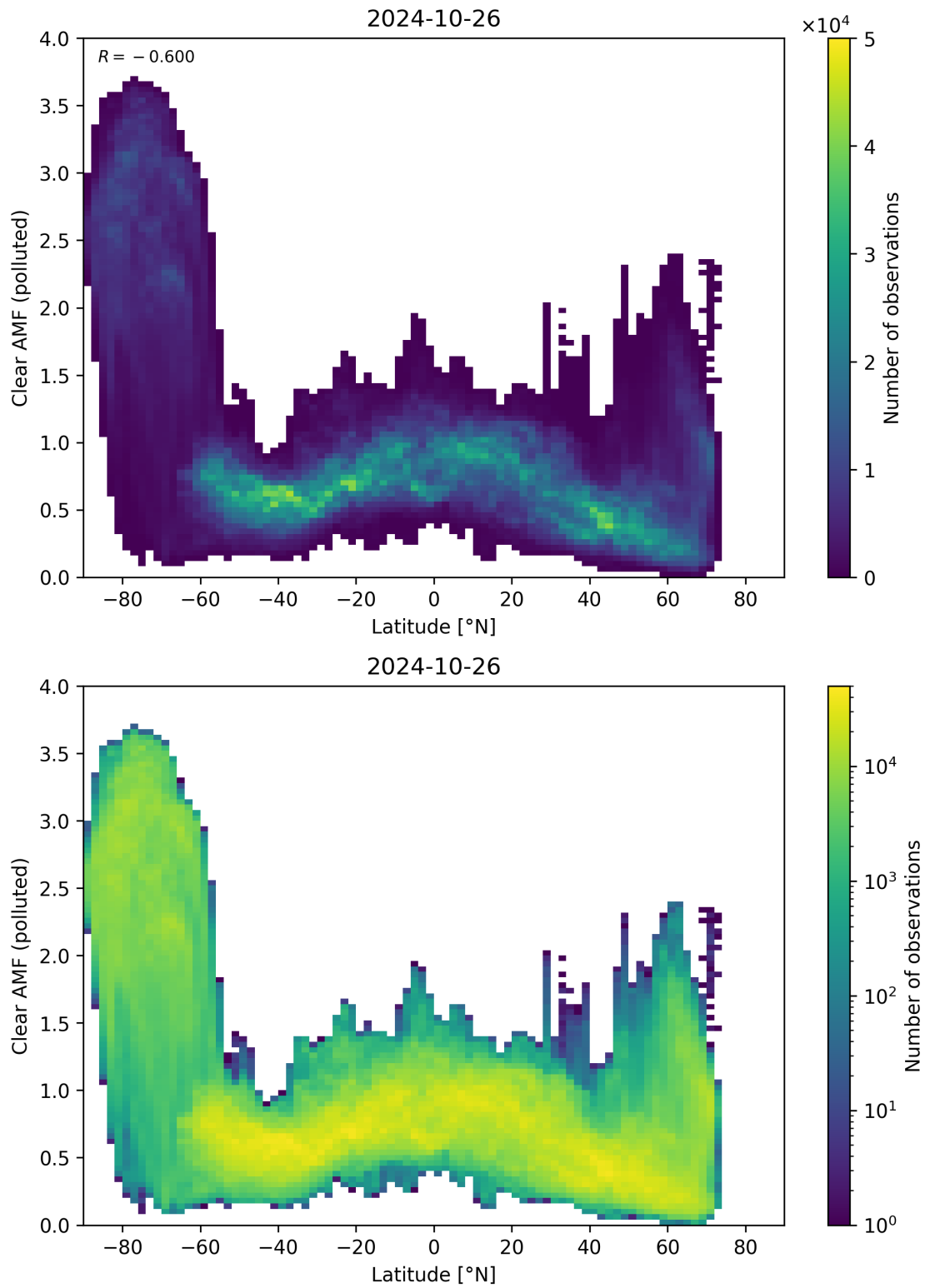
Figure 145: Scatter density plot of “Latitude” against “Clear AMF (polluted)” for 2024-10-25 to 2024-10-27.
