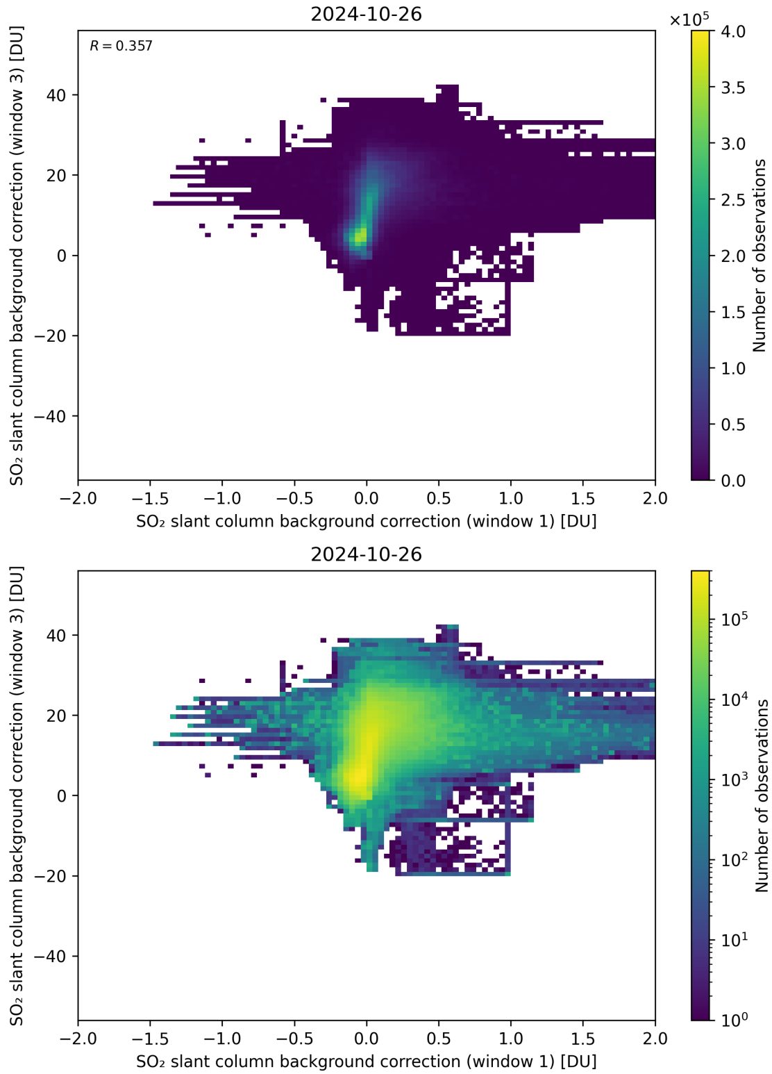
Figure 99: Scatter density plot of “SO 2 slant column background correction (window 1)” against “SO 2 slant column background correction (window 3)” for 2024-10-25 to 2024-10-27.
