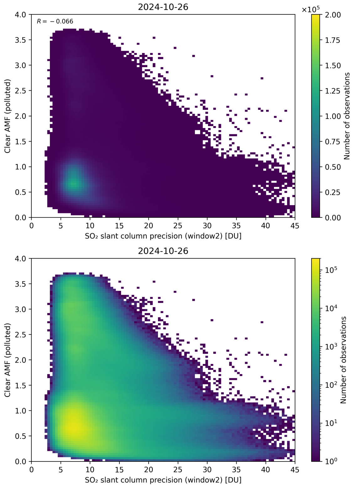
Figure 246: Scatter density plot of “SO 2 slant column precision (window2)” against “Clear AMF (polluted)” for 2024-10-25 to 2024-10-27.
