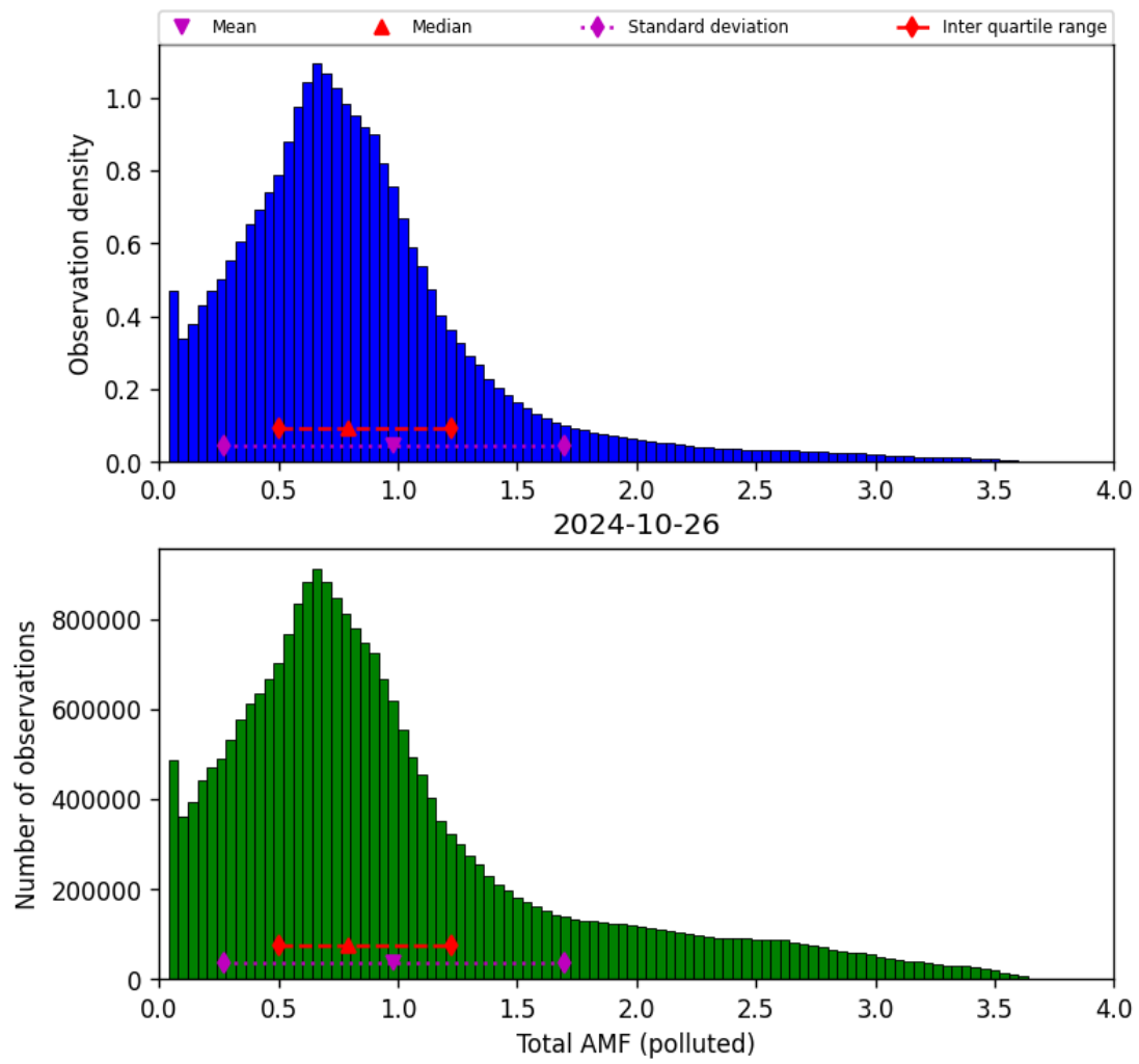
Figure 71: Histogram of “Total AMF (polluted)” for 2024-10-25 to 2024-10-27
