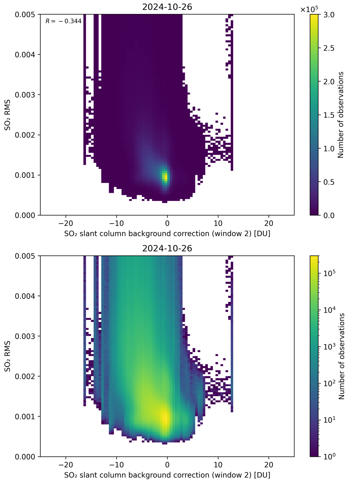
Figure 114: Scatter density plot of “SO 2 slant column background correction (window 2)” against “SO 2 RMS” for 2024-10-25 to 2024-10-27.
