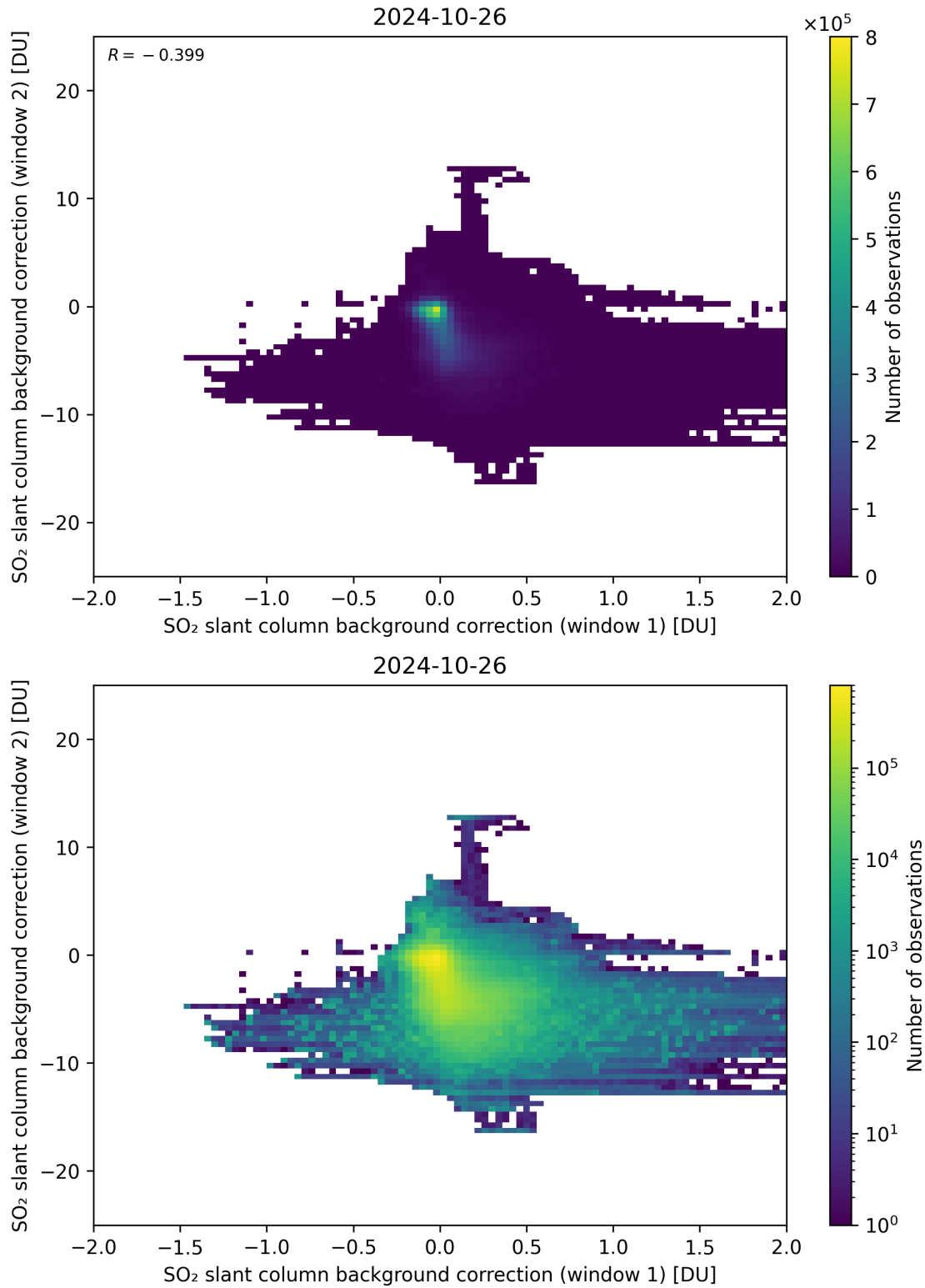
Figure 98: Scatter density plot of “SO 2 slant column background correction (window 1)” against “SO 2 slant column background correction (window 2)” for 2024-10-25 to 2024-10-27.
