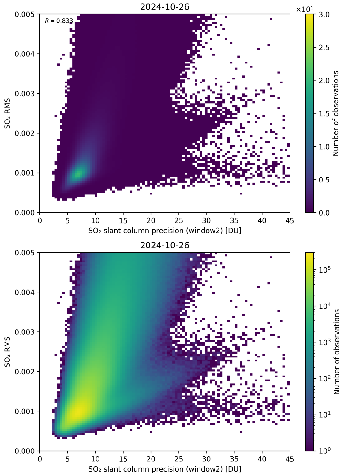
Figure 245: Scatter density plot of “SO 2 slant column precision (window2)” against “SO 2 RMS” for 2024-10-25 to 2024-10-27.
