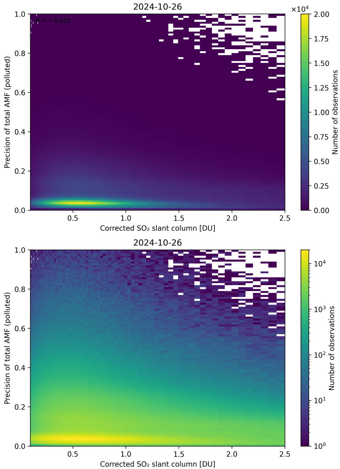
Figure 193: Scatter density plot of “Corrected SO 2 slant column” against “Precision of total AMF (polluted)” for 2024-10-25 to 2024-10-27.
