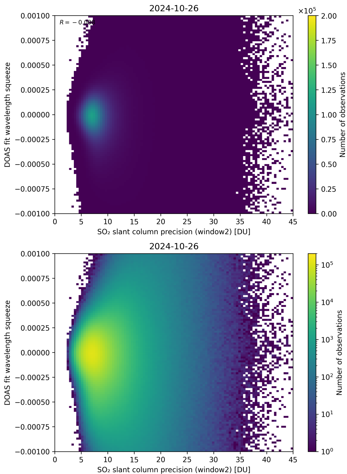
Figure 244: Scatter density plot of “SO 2 slant column precision (window2)” against “DOAS fit wavelength squeeze” for 2024-10-25 to 2024-10-27.
