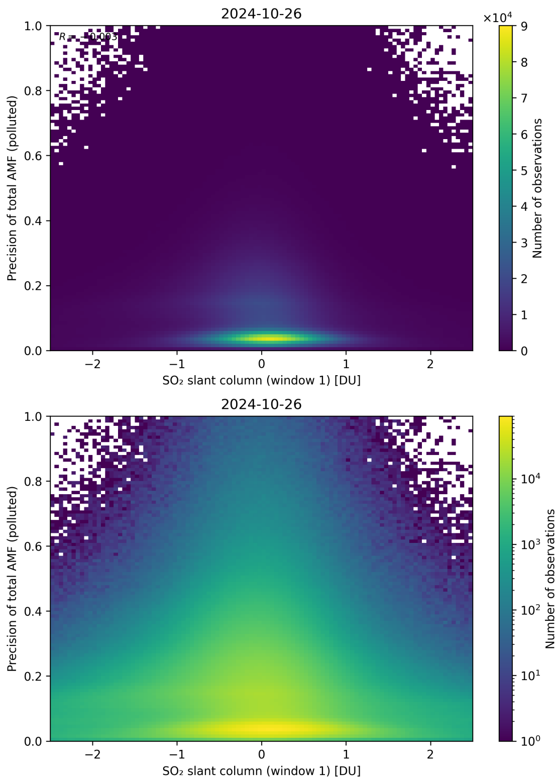
Figure 240: Scatter density plot of “SO 2 slant column (window 1)” against “Precision of total AMF (polluted)” for 2024-10-25 to 2024-10-27.
