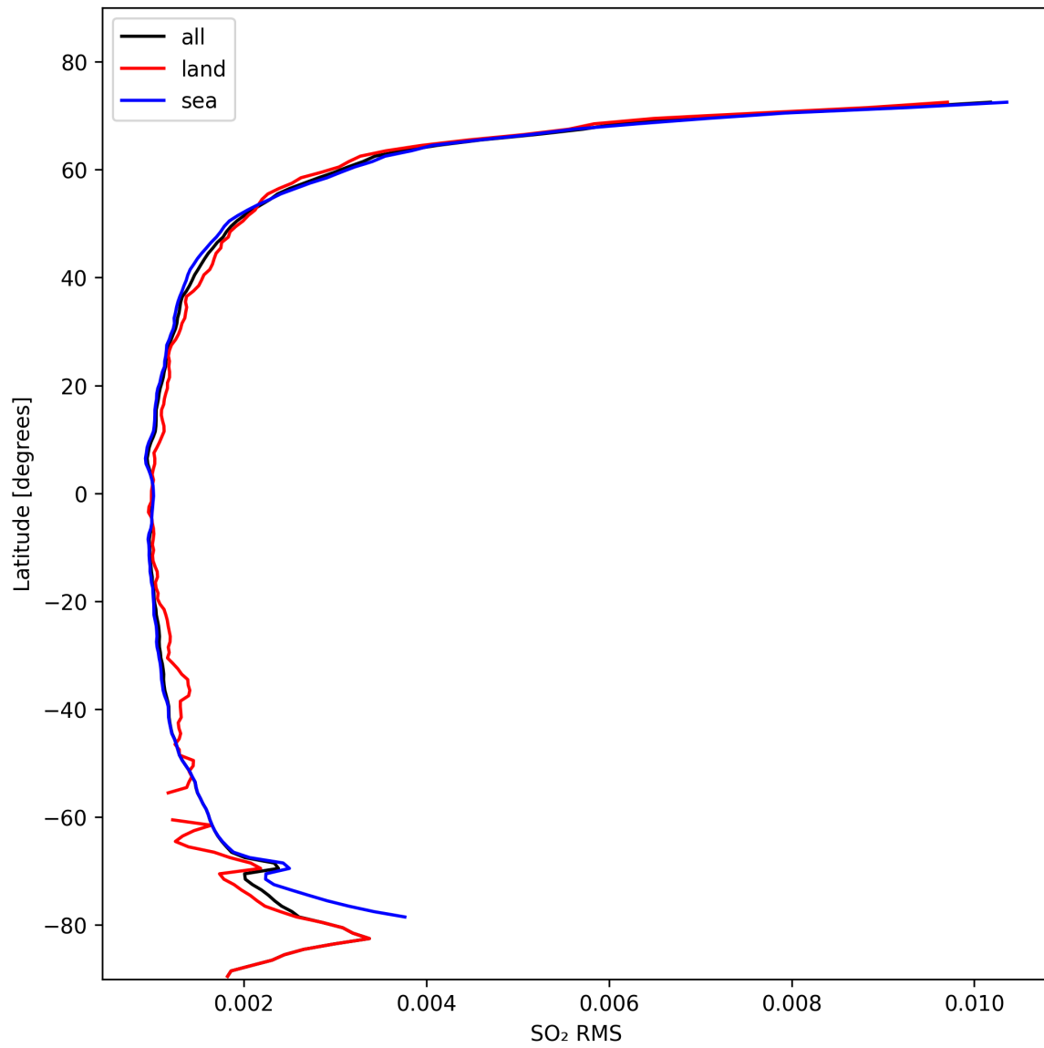
Figure 47: Zonal average of “SO 2 RMS” for 2024-10-25 to 2024-10-27.
