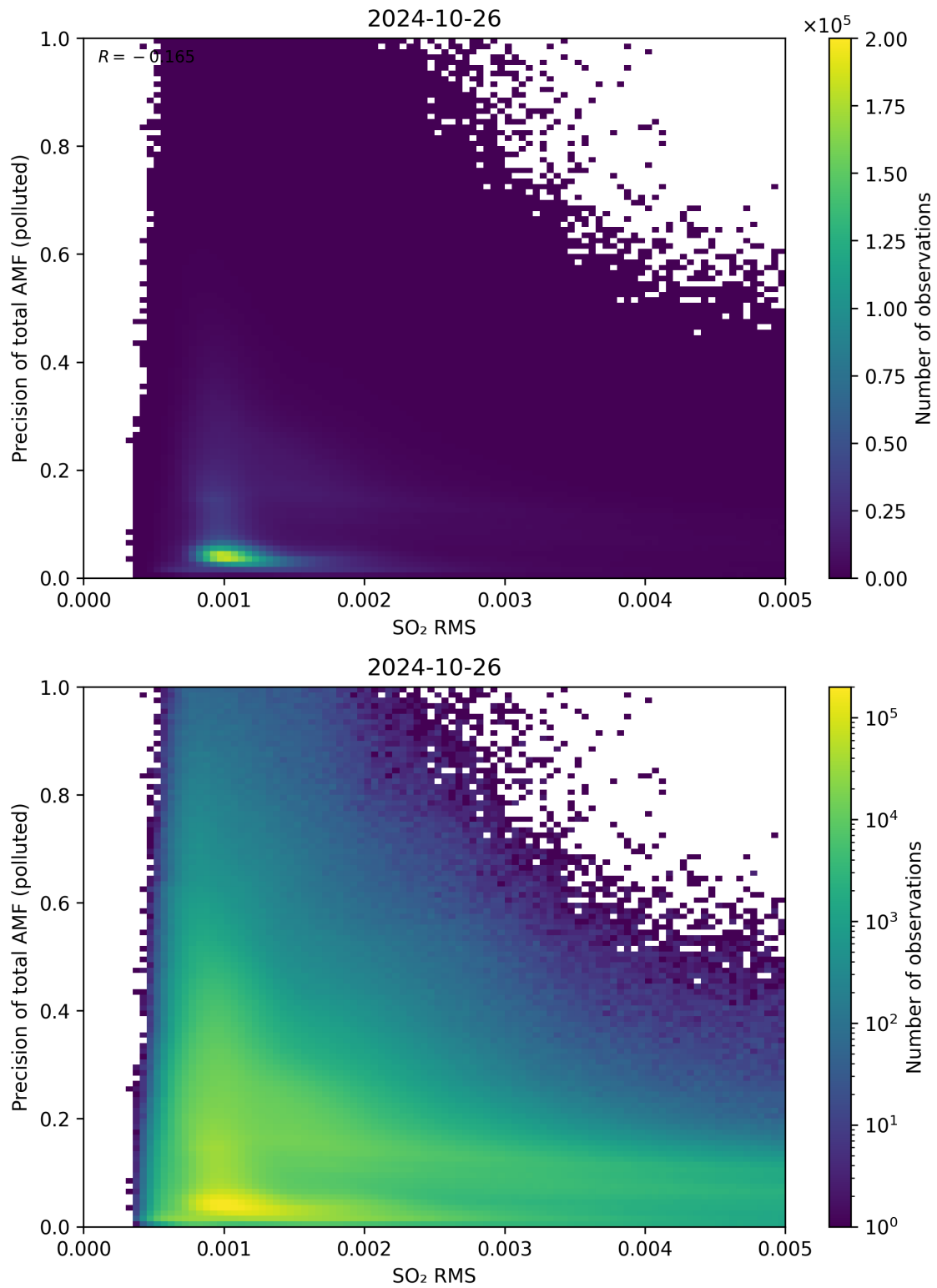
Figure 138: Scatter density plot of “SO 2 RMS” against “Precision of total AMF (polluted)” for 2024-10-25 to 2024-10-27.
