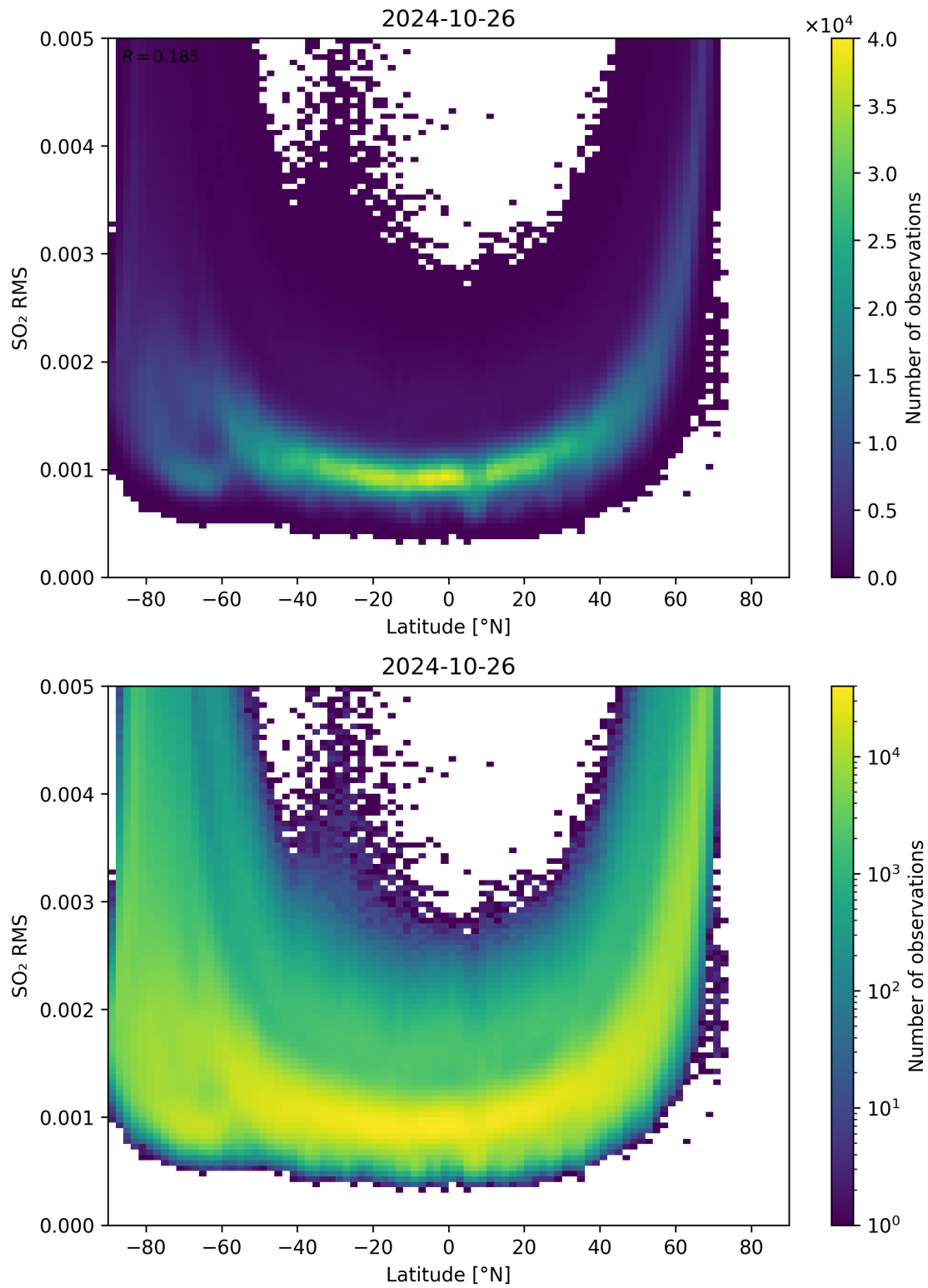
Figure 144: Scatter density plot of “Latitude” against “SO 2 RMS” for 2024-10-25 to 2024-10-27.
