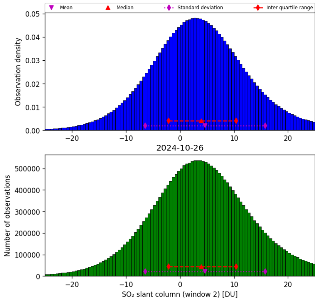
Figure 60: Histogram of “SO 2 slant column (window 2)” for 2024-10-25 to 2024-10-27
