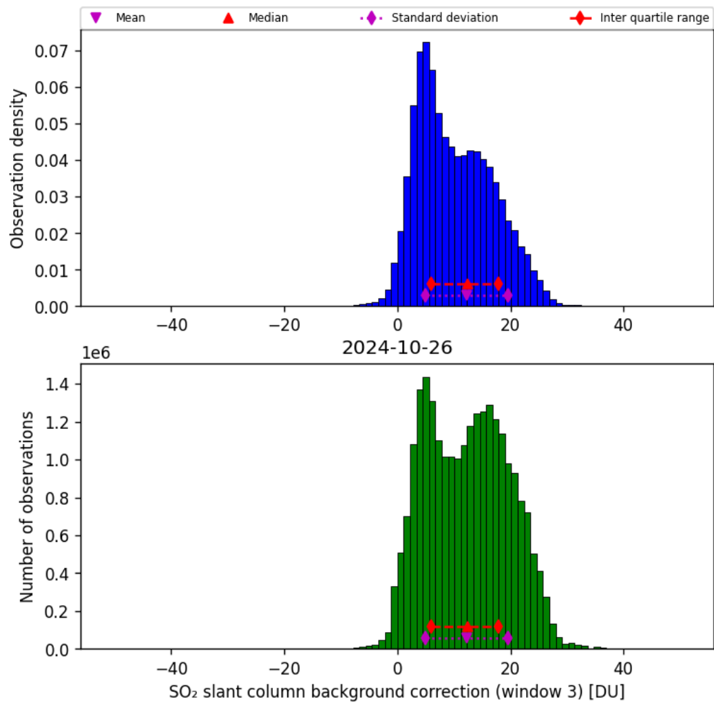
Figure 67: Histogram of “SO 2 slant column background correction (window 3)” for 2024-10-25 to 2024-10-27
