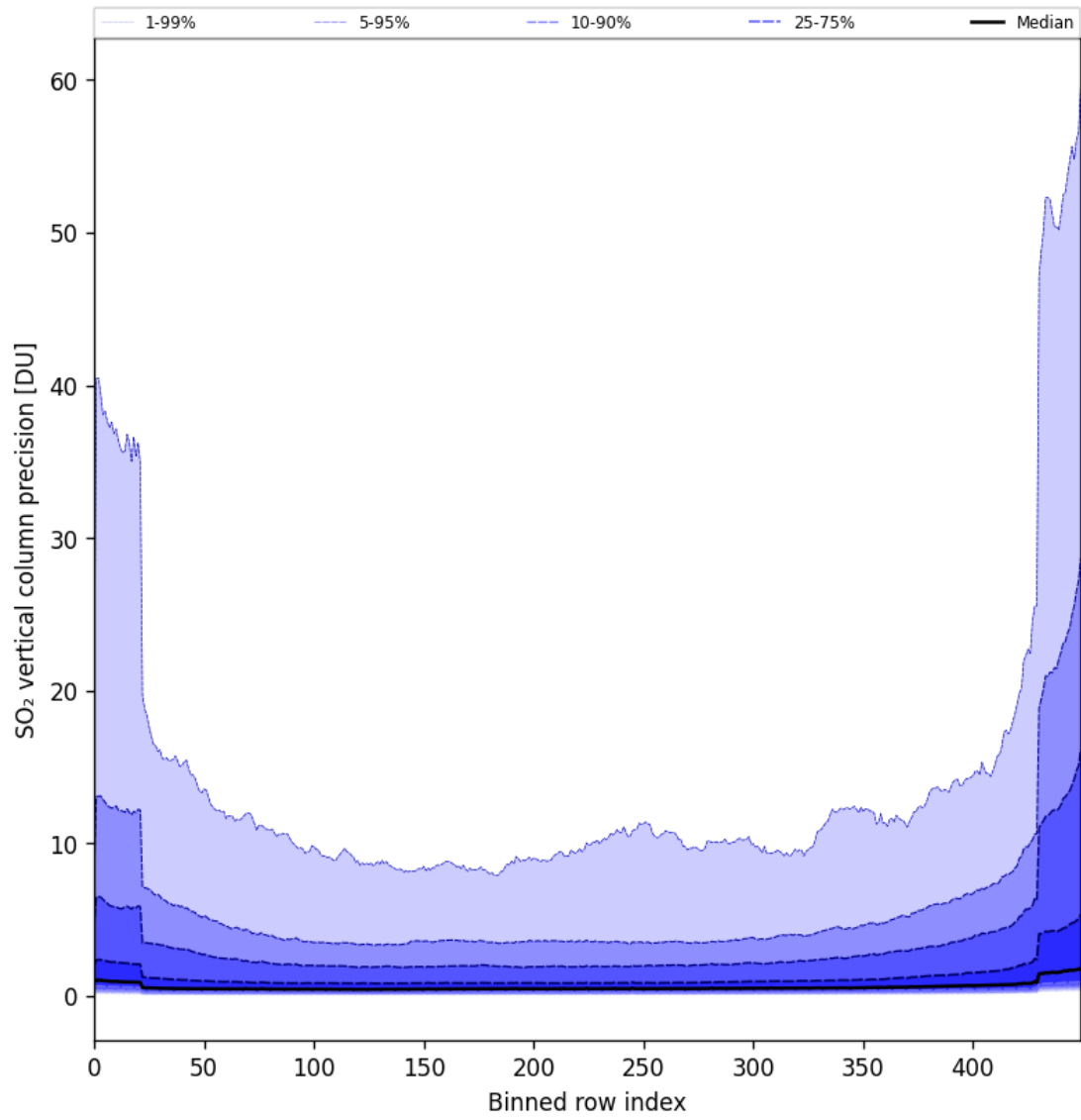
Figure 77: Along track statistics of “SO 2 vertical column precision” for 2024-10-25 to 2024-10-27
