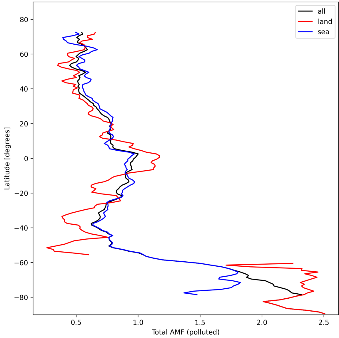
Figure 48: Zonal average of “Total AMF (polluted)” for 2024-10-25 to 2024-10-27.
