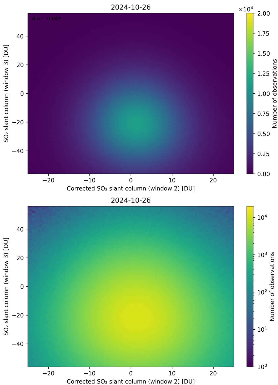
Figure 201: Scatter density plot of “Corrected SO 2 slant column (window 2)” against “SO 2 slant column (window 3)” for 2024-10-25 to 2024-10-27.
