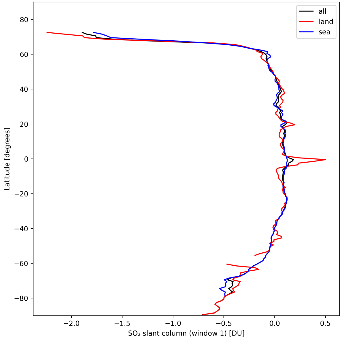
Figure 33: Zonal average of “SO 2 slant column (window 1)” for 2024-10-25 to 2024-10-27.
