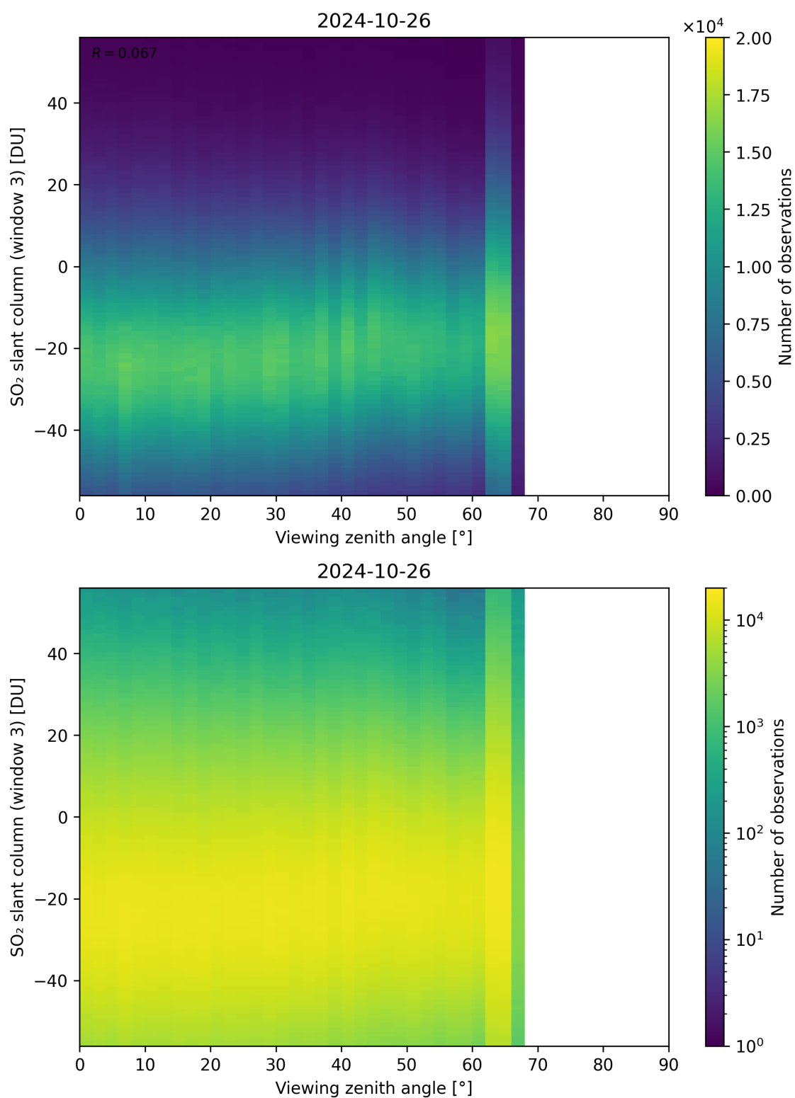
Figure 323: Scatter density plot of “Viewing zenith angle” against “SO 2 slant column (window 3)” for 2024-10-25 to 2024-10-27.
