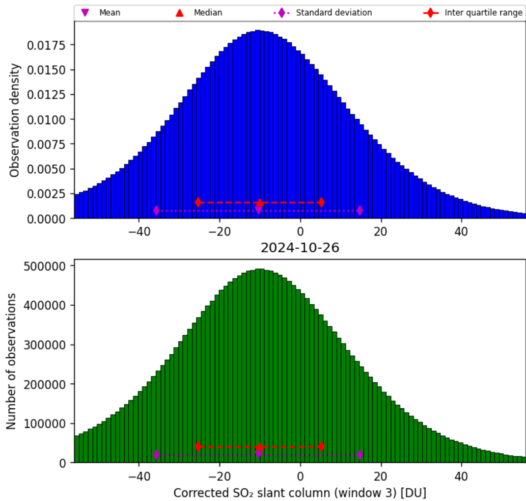
Figure 66: Histogram of “Corrected SO 2 slant column (window 3)” for 2024-10-25 to 2024-10-27
