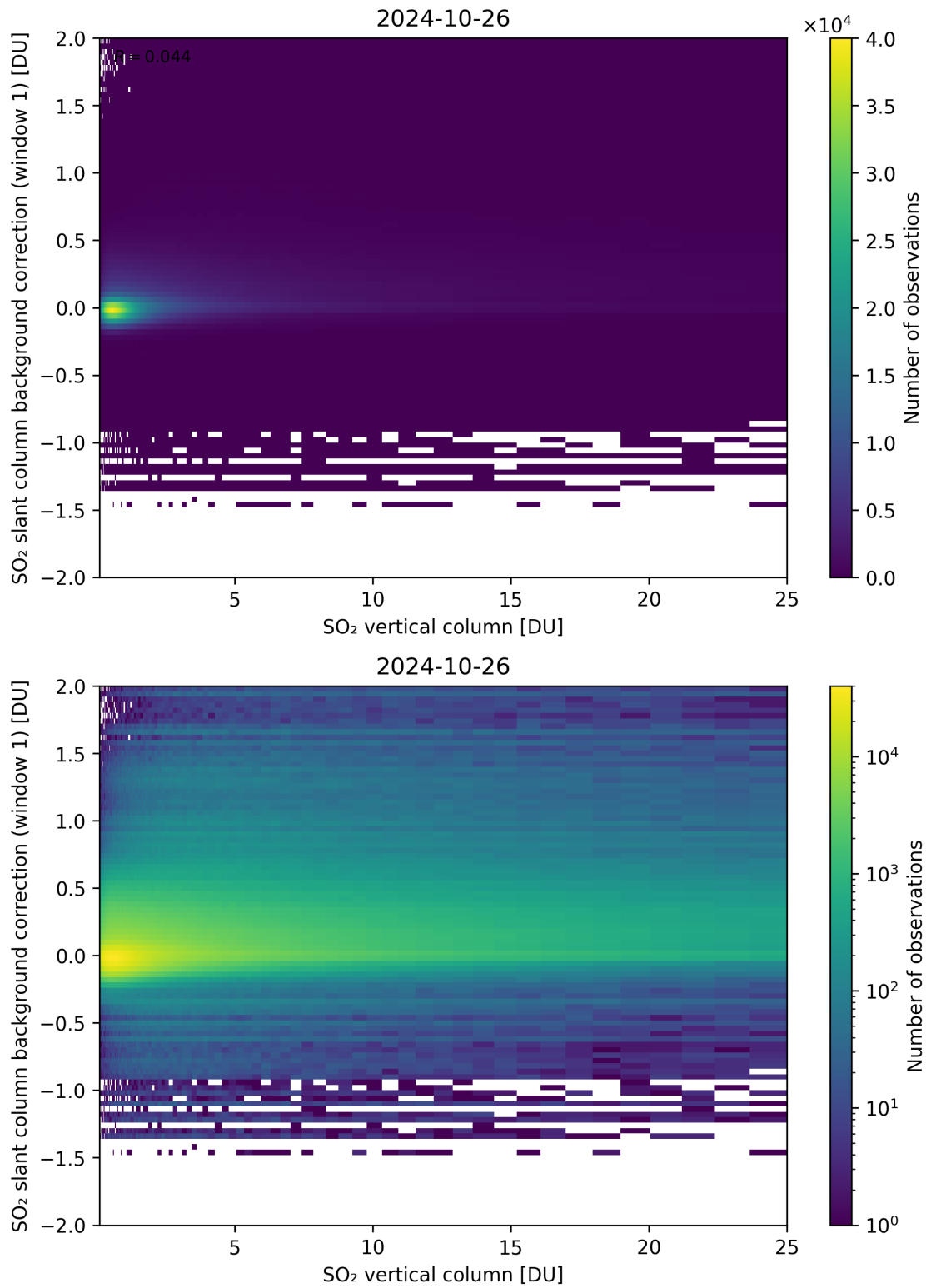
Figure 273: Scatter density plot of “SO 2 vertical column” against “SO 2 slant column background correction (window 1)” for 2024-10-25 to 2024-10-27.
