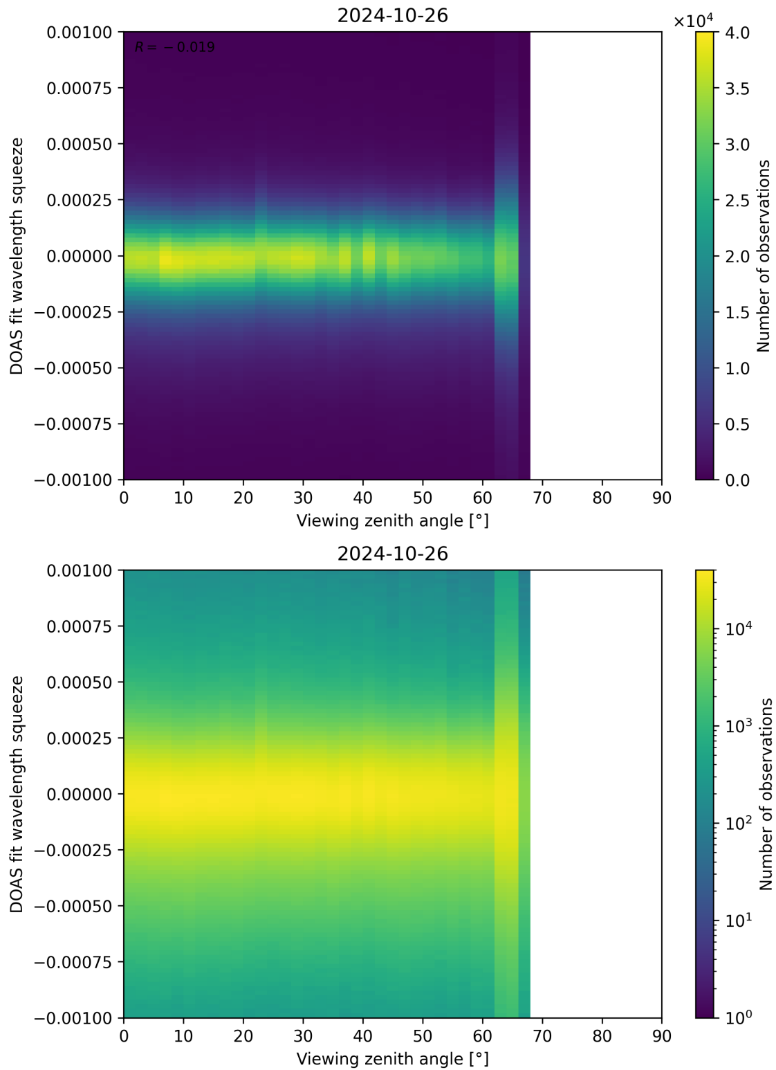
Figure 312: Scatter density plot of “Viewing zenith angle” against “DOAS fit wavelength squeeze” for 2024-10-25 to 2024-10-27.
