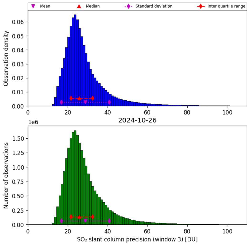
Figure 65: Histogram of “SO 2 slant column precision (window 3)” for 2024-10-25 to 2024-10-27
