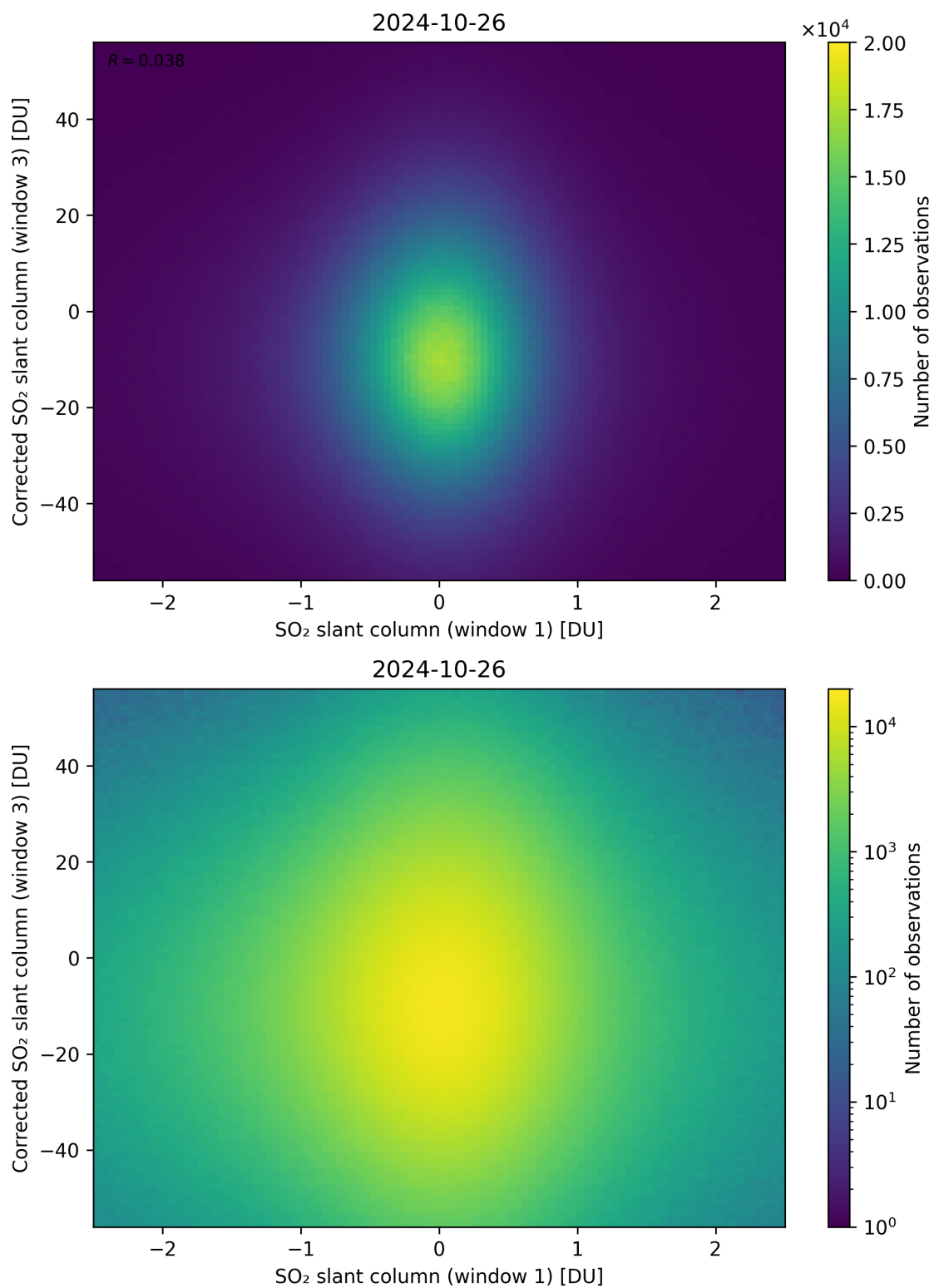
Figure 234: Scatter density plot of “SO 2 slant column (window 1)” against “Corrected SO 2 slant column (window 3)” for 2024-10-25 to 2024-10-27.
