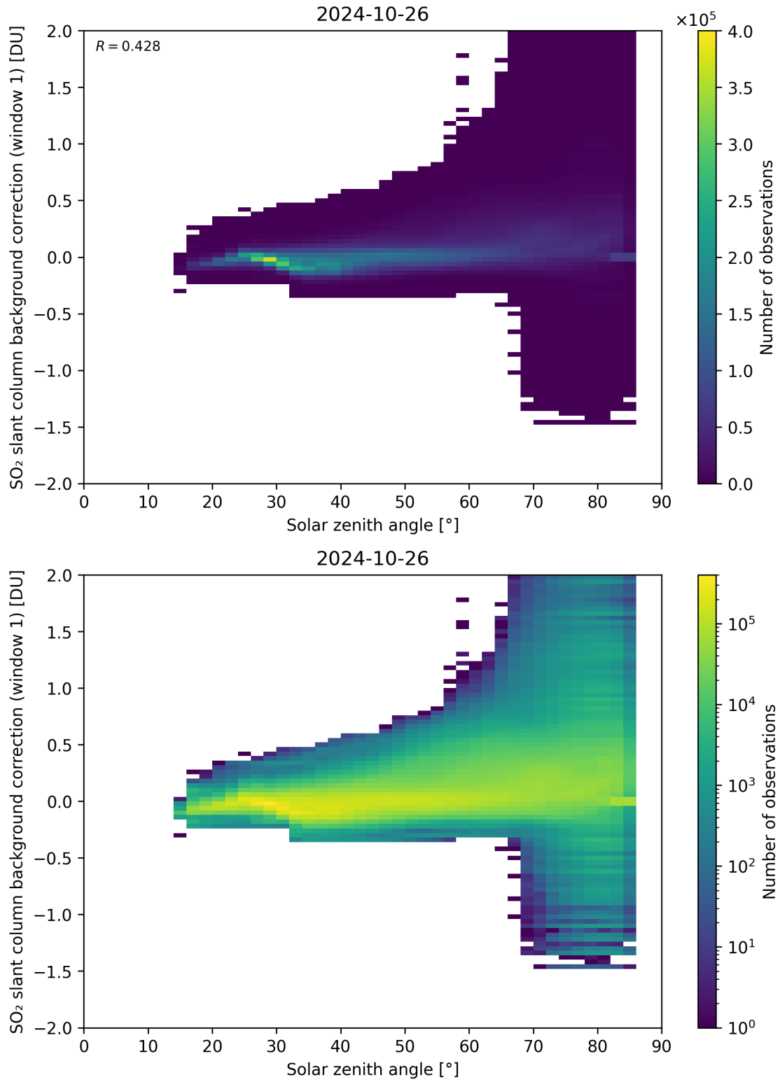
Figure 158: Scatter density plot of “Solar zenith angle” against “SO 2 slant column background correction (window 1)” for 2024-10-25 to 2024-10-27.
