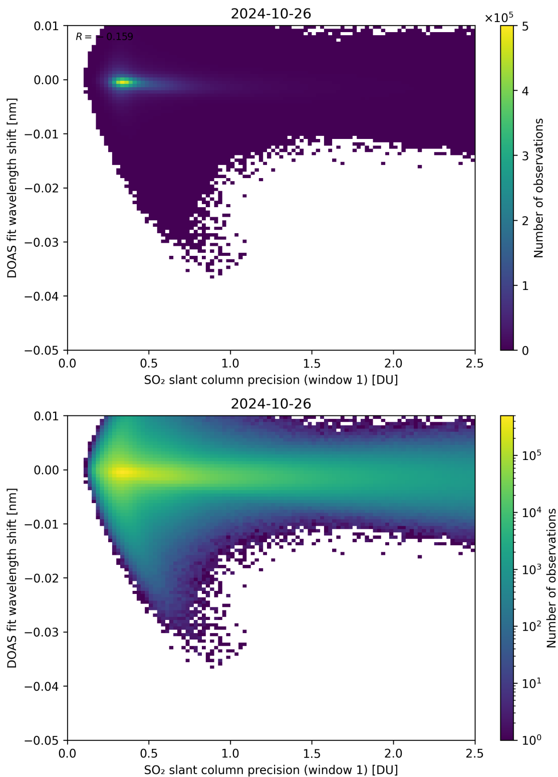
Figure 221: Scatter density plot of “SO 2 slant column precision (window 1)” against “DOAS fit wavelength shift” for 2024-10-25 to 2024-10-27.
