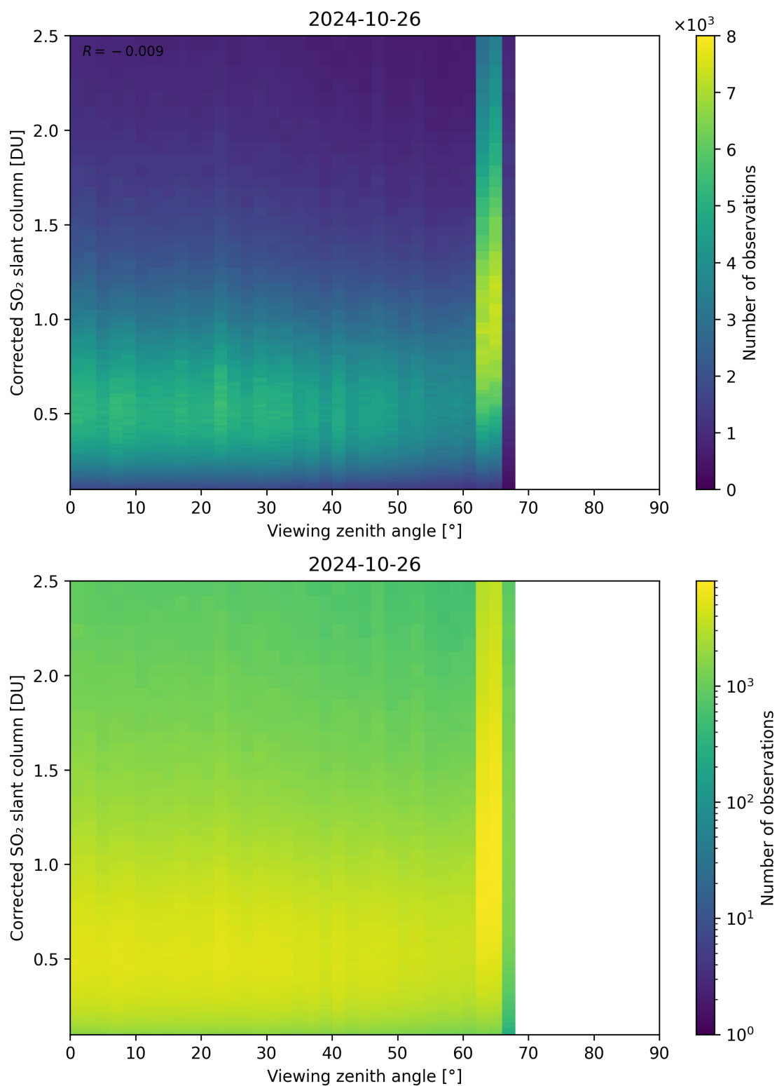
Figure 317: Scatter density plot of “Viewing zenith angle” against “Corrected SO 2 slant column” for 2024-10-25 to 2024-10-27.
