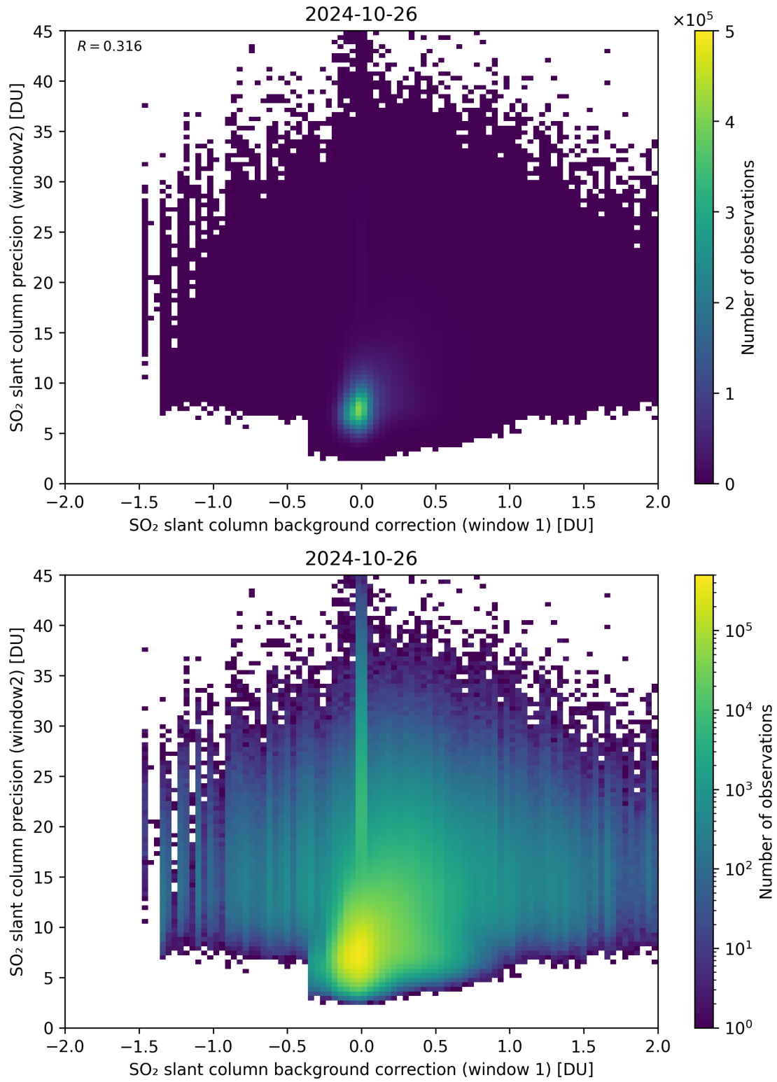
Figure 106: Scatter density plot of “SO 2 slant column background correction (window 1)” against “SO 2 slant column precision (window2)” for 2024-10-25 to 2024-10-27.
