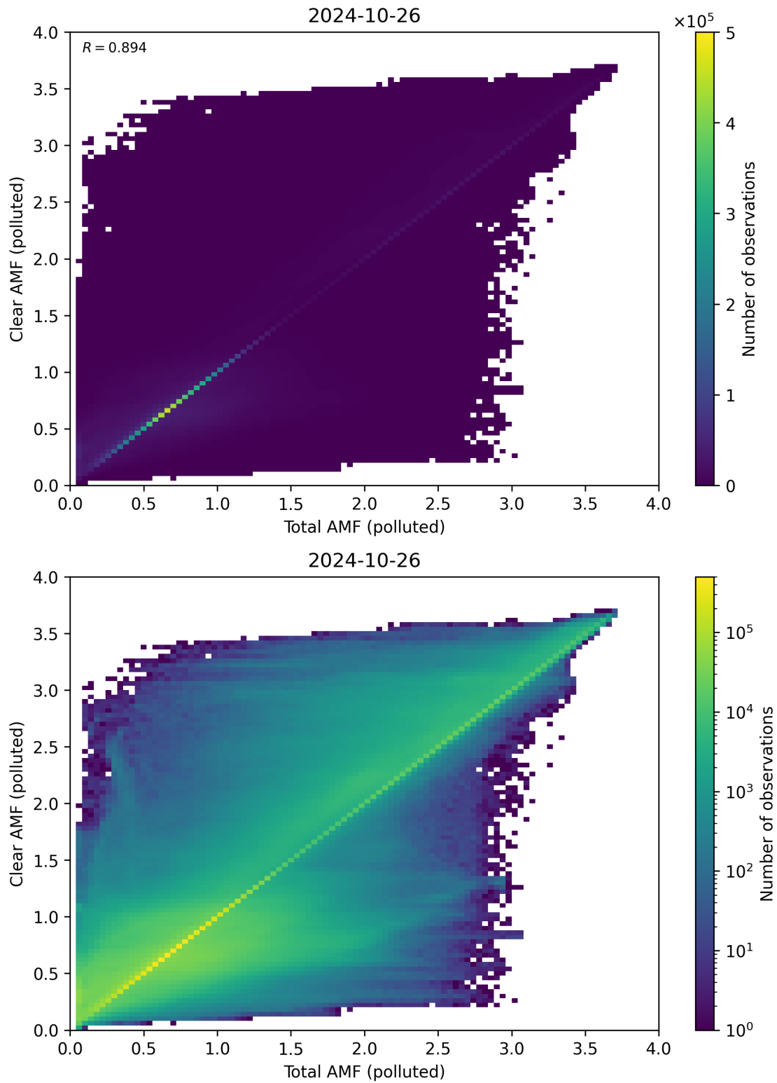
Figure 271: Scatter density plot of “Total AMF (polluted)” against “Clear AMF (polluted)” for 2024-10-25 to 2024-10-27.
