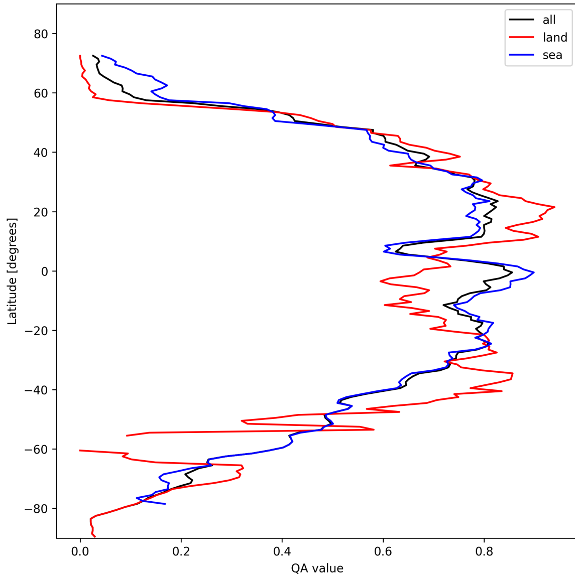
Figure 29: Zonal average of “QA value” for 2024-10-25 to 2024-10-27.
