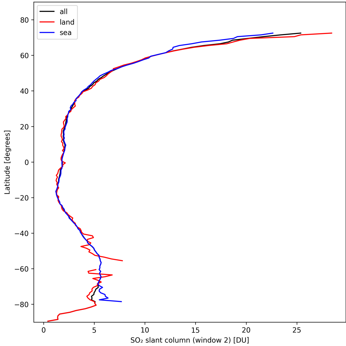
Figure 37: Zonal average of “SO 2 slant column (window 2)” for 2024-10-25 to 2024-10-27.
