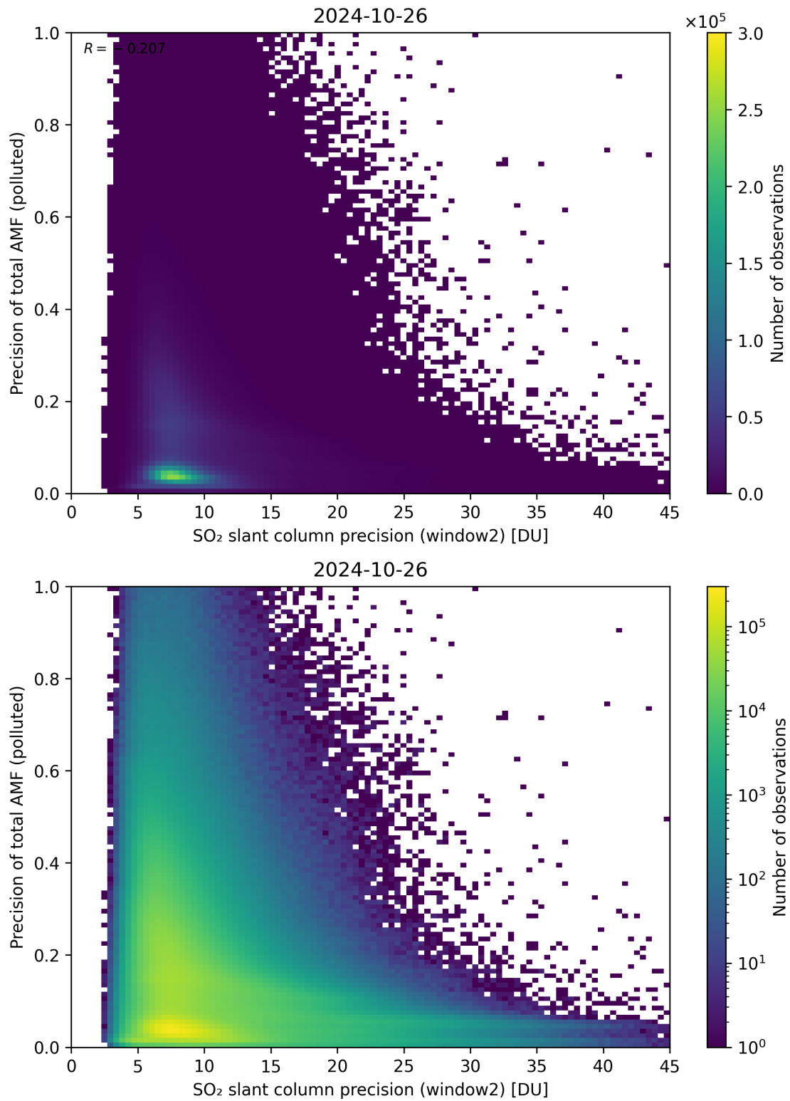
Figure 252: Scatter density plot of “SO 2 slant column precision (window2)” against “Precision of total AMF (polluted)” for 2024-10-25 to 2024-10-27.
