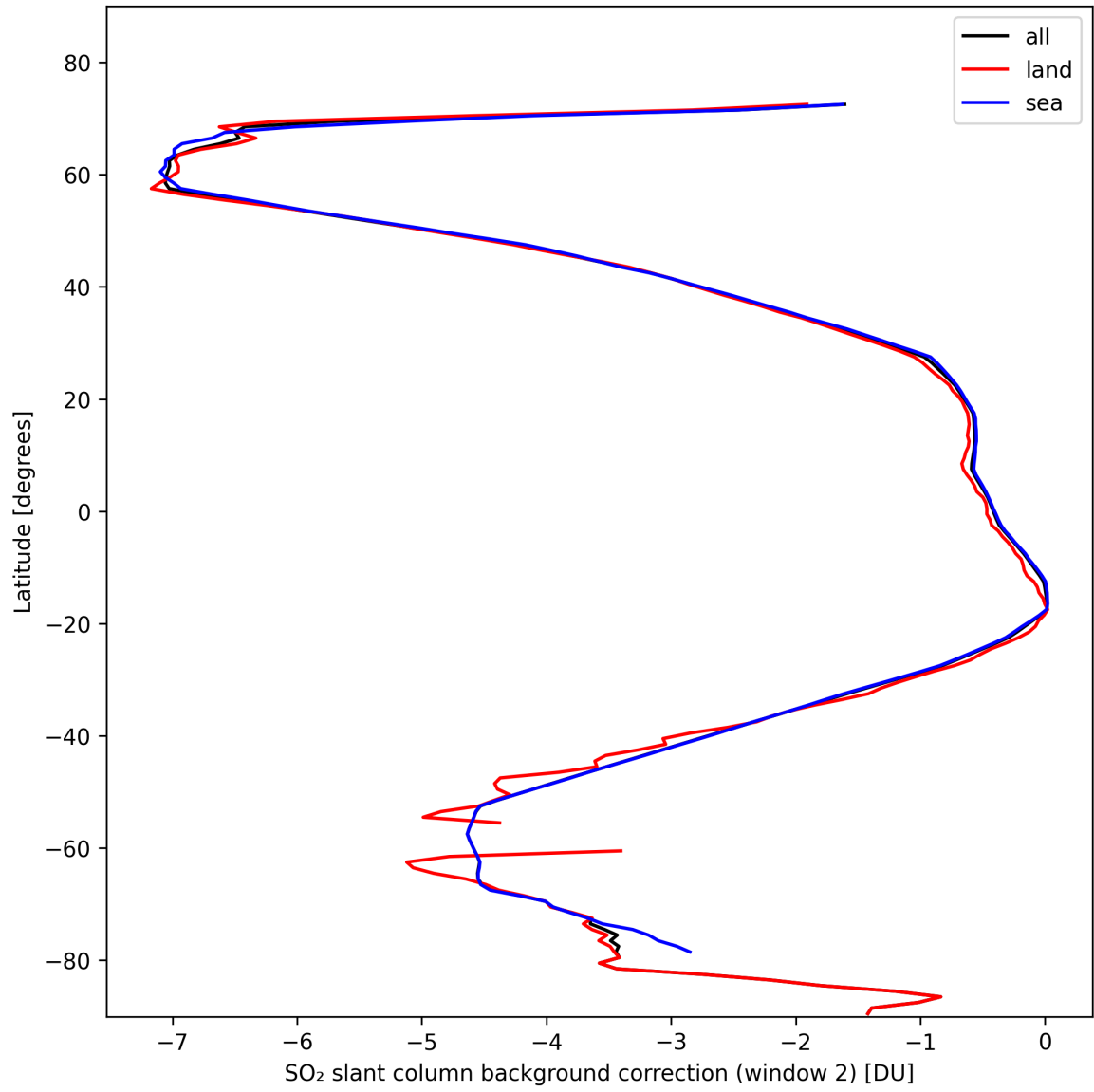
Figure 40: Zonal average of “SO 2 slant column background correction (window 2)” for 2024-10-25 to 2024-10-27.
