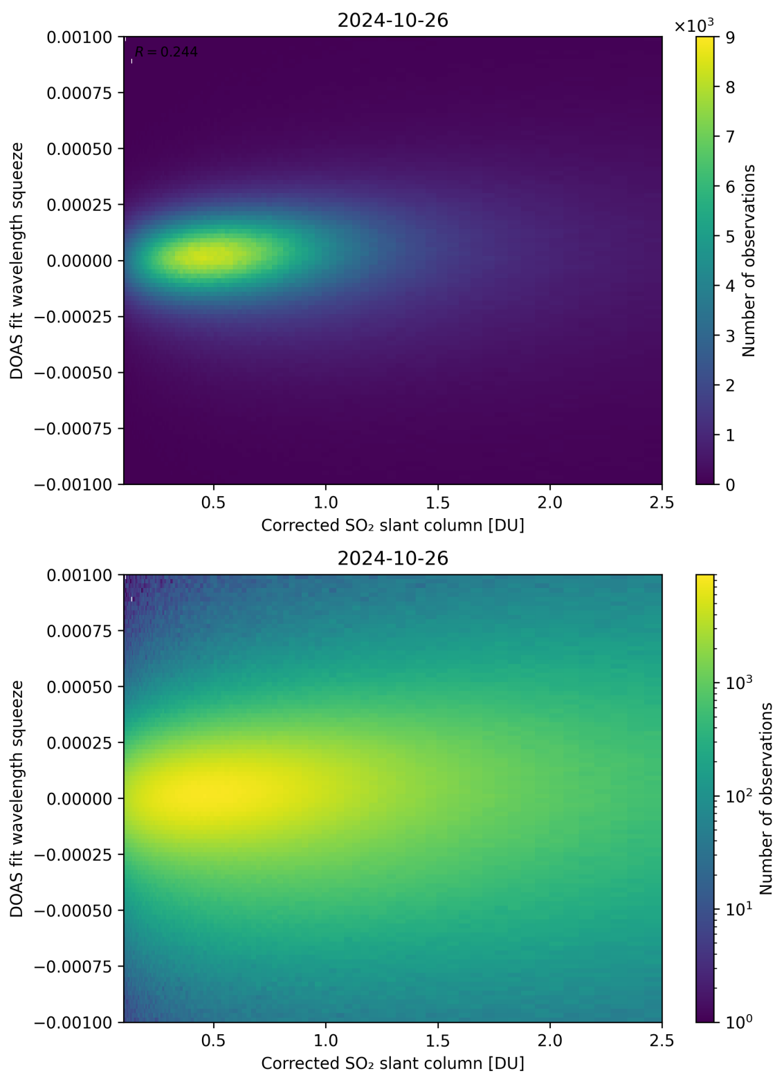
Figure 182: Scatter density plot of “Corrected SO 2 slant column” against “DOAS fit wavelength squeeze” for 2024-10-25 to 2024-10-27.
