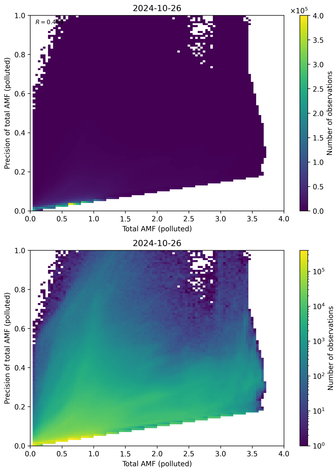
Figure 272: Scatter density plot of “Total AMF (polluted)” against “Precision of total AMF (polluted)” for 2024-10-25 to 2024-10-27.
