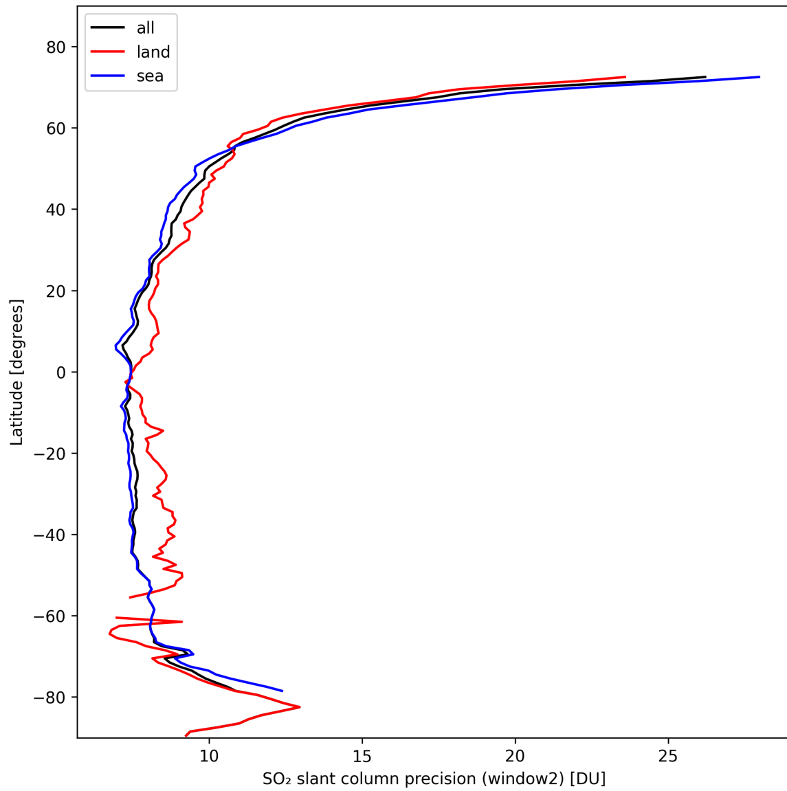
Figure 38: Zonal average of “SO 2 slant column precision (window2)” for 2024-10-25 to 2024-10-27.
