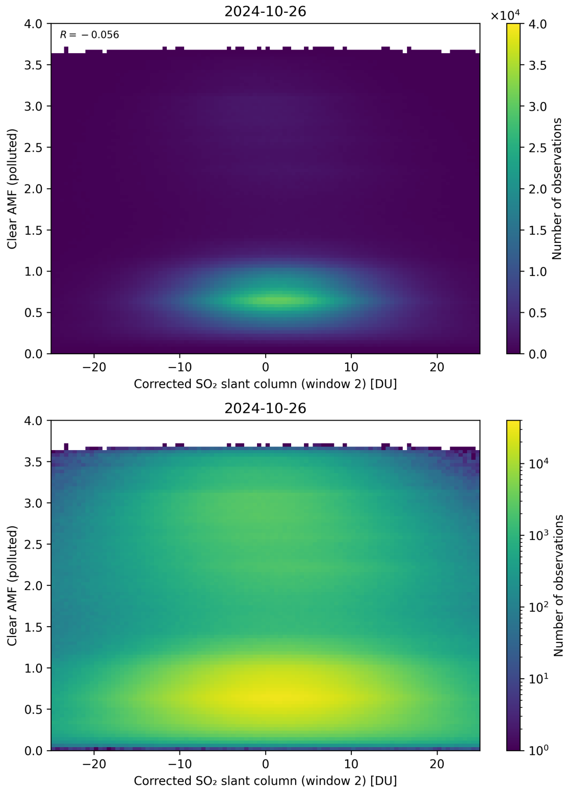
Figure 199: Scatter density plot of “Corrected SO 2 slant column (window 2)” against “Clear AMF (polluted)” for 2024-10-25 to 2024-10-27.
