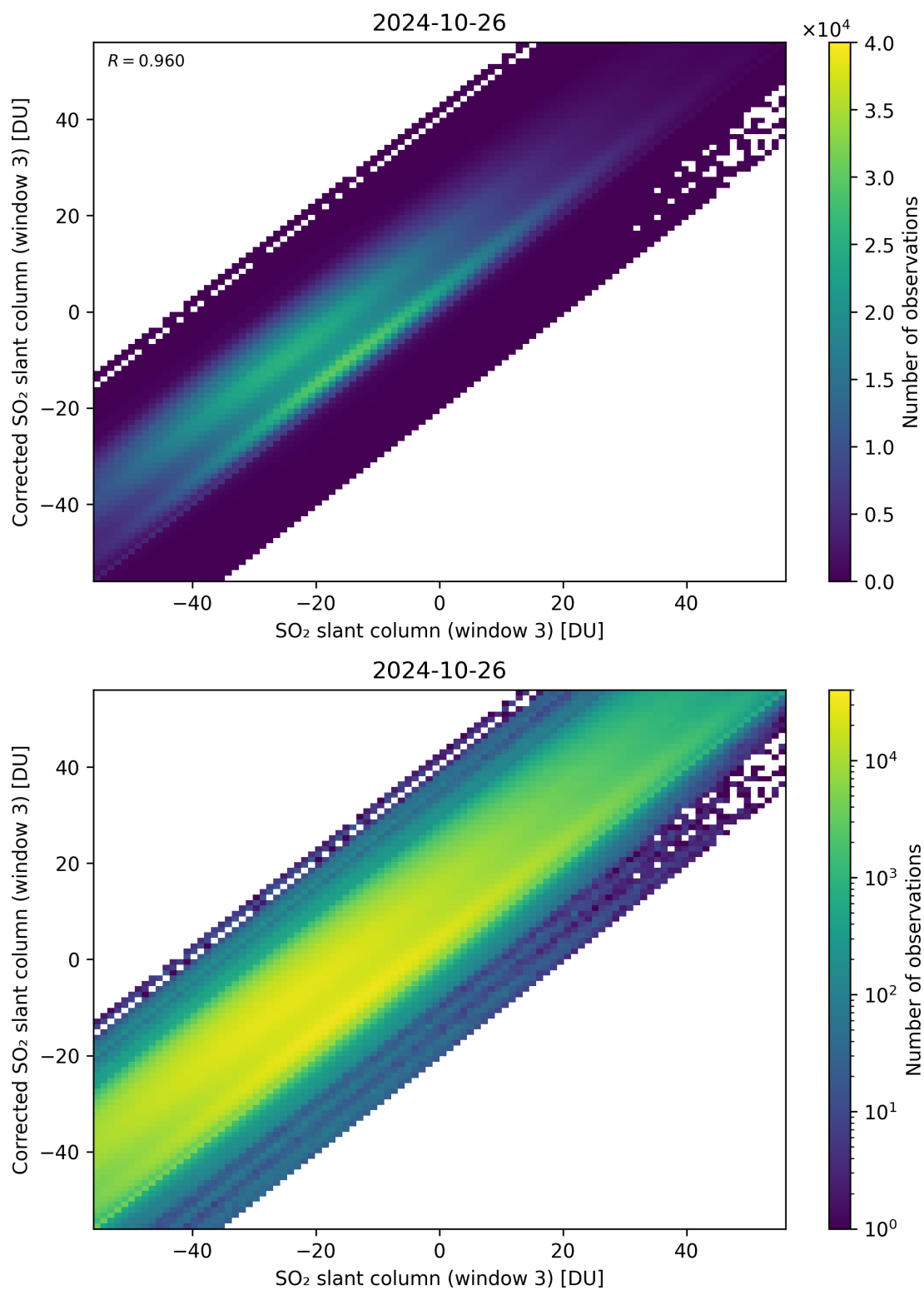
Figure 266: Scatter density plot of “SO 2 slant column (window 3)” against “Corrected SO 2 slant column (window 3)” for 2024-10-25 to 2024-10-27.
