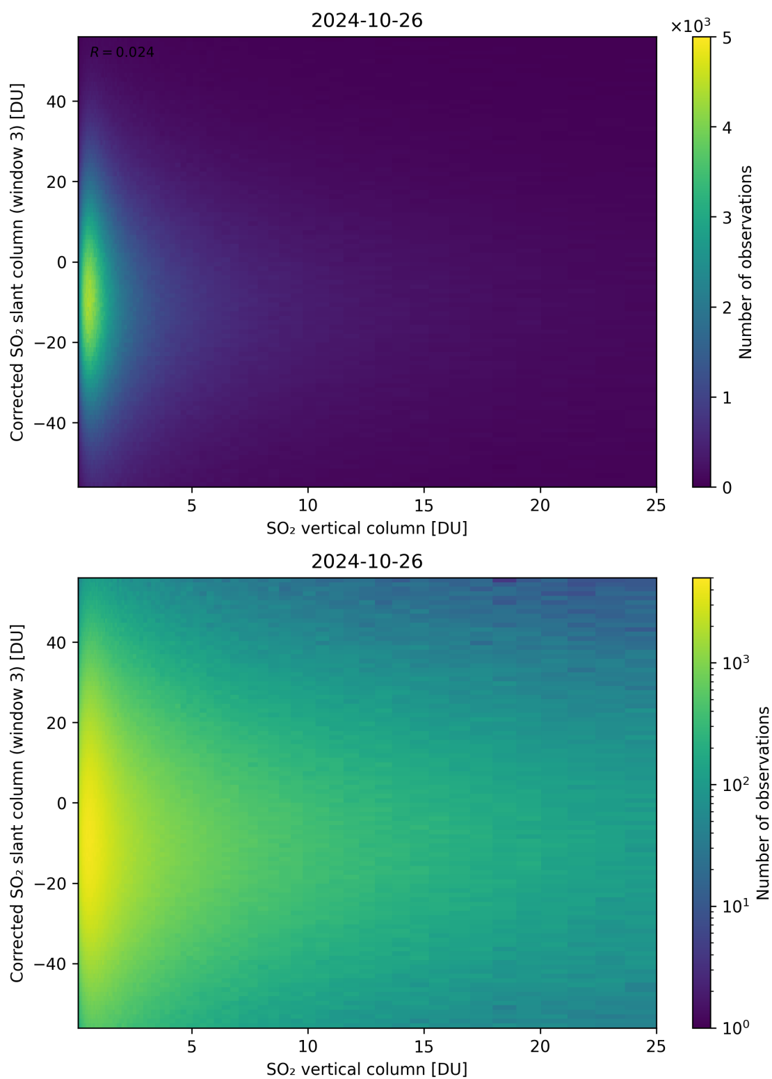
Figure 299: Scatter density plot of “SO 2 vertical column” against “Corrected SO 2 slant column (window 3)” for 2024-10-25 to 2024-10-27.
