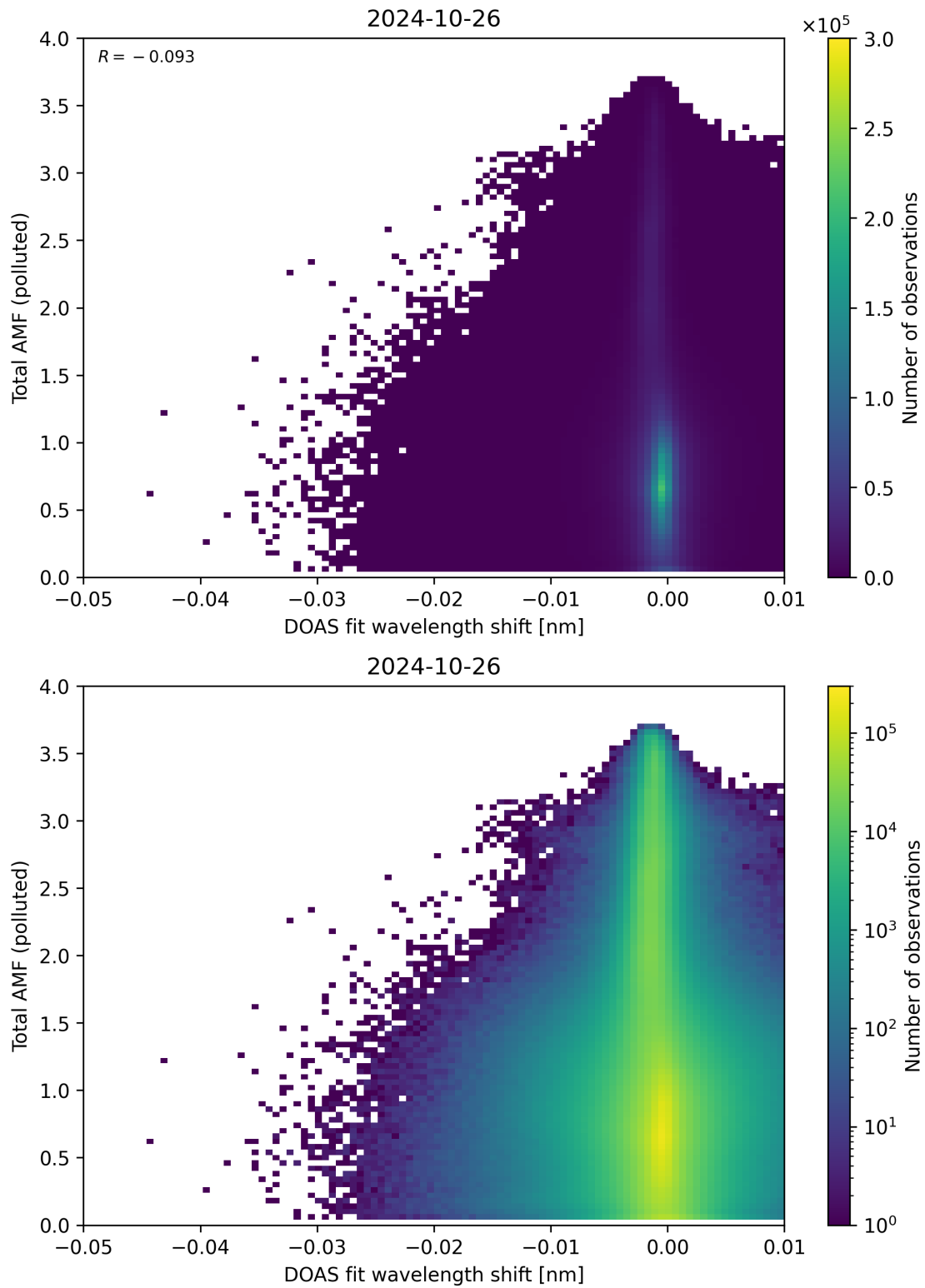
Figure 130: Scatter density plot of “DOAS fit wavelength shift” against “Total AMF (polluted)” for 2024-10-25 to 2024-10-27.
