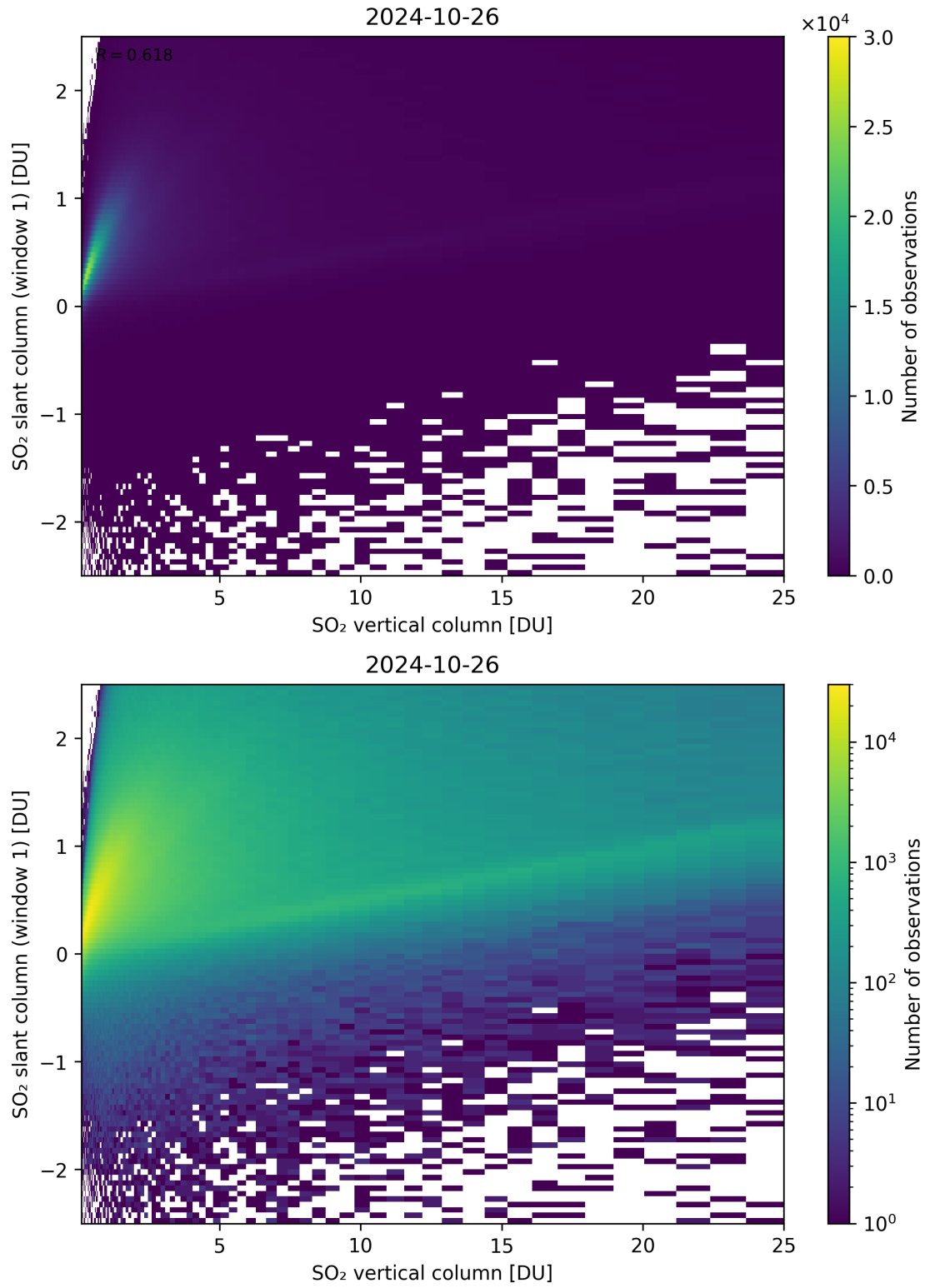
Figure 300: Scatter density plot of “SO 2 vertical column” against “SO 2 slant column (window 1)” for 2024-10-25 to 2024-10-27.
