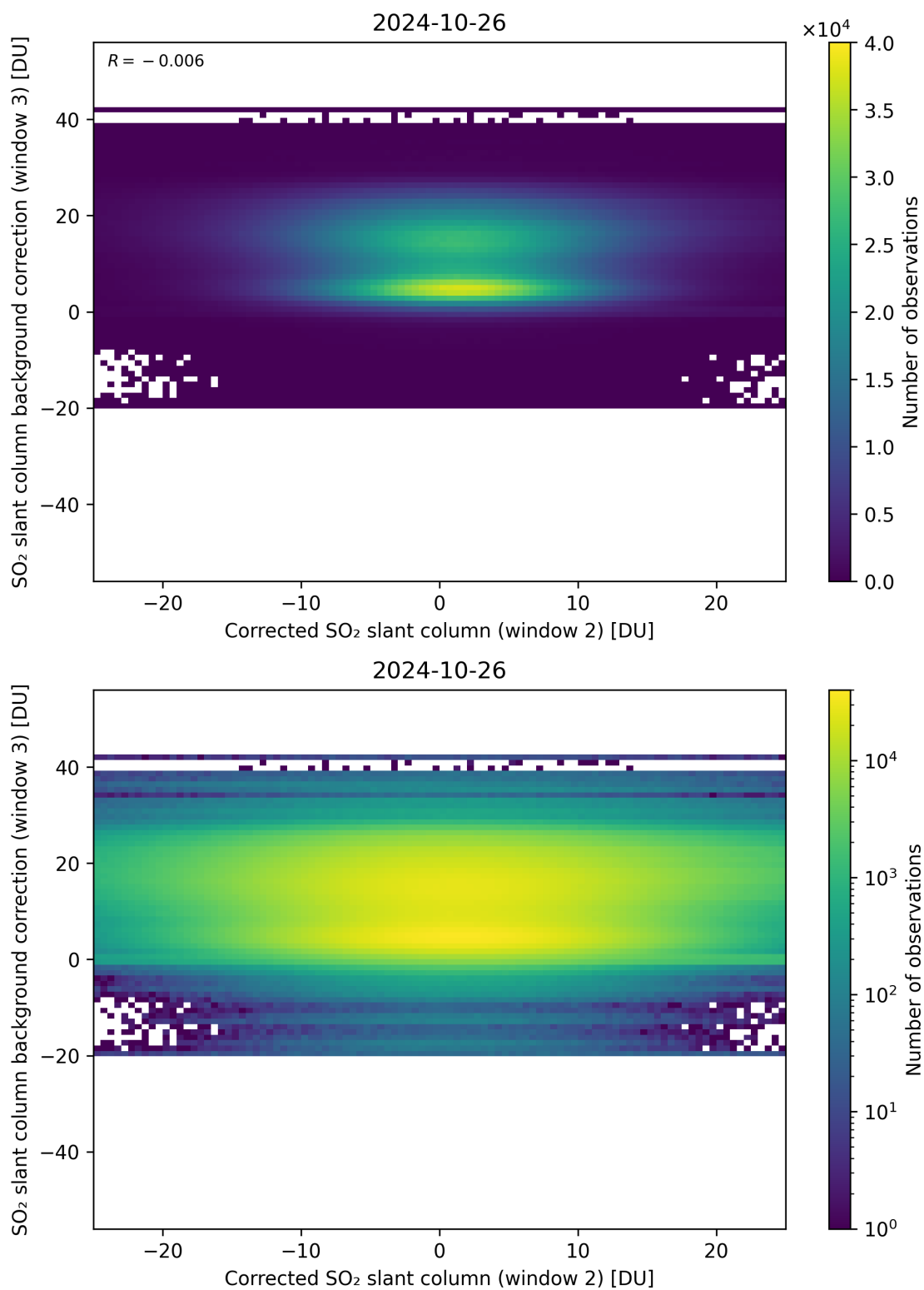
Figure 195: Scatter density plot of “Corrected SO 2 slant column (window 2)” against “SO 2 slant column background correction (window 3)” for 2024-10-25 to 2024-10-27.
