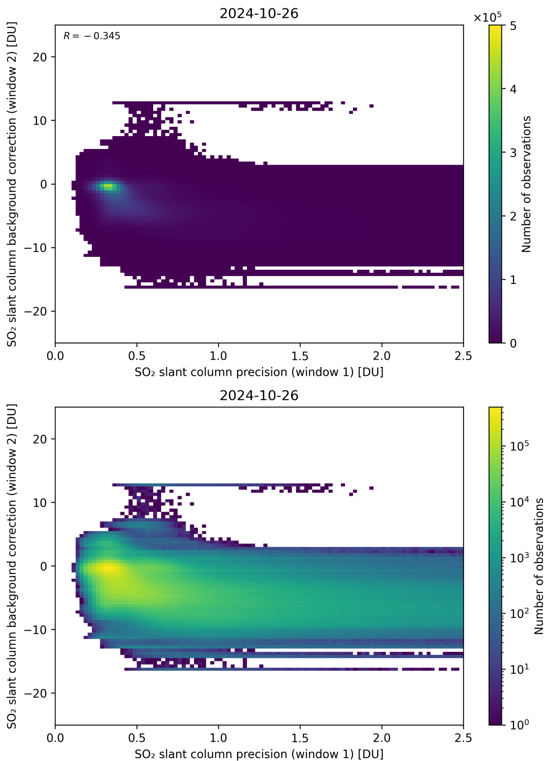
Figure 219: Scatter density plot of “SO 2 slant column precision (window 1)” against “SO 2 slant column background correction (window 2)” for 2024-10-25 to 2024-10-27.
