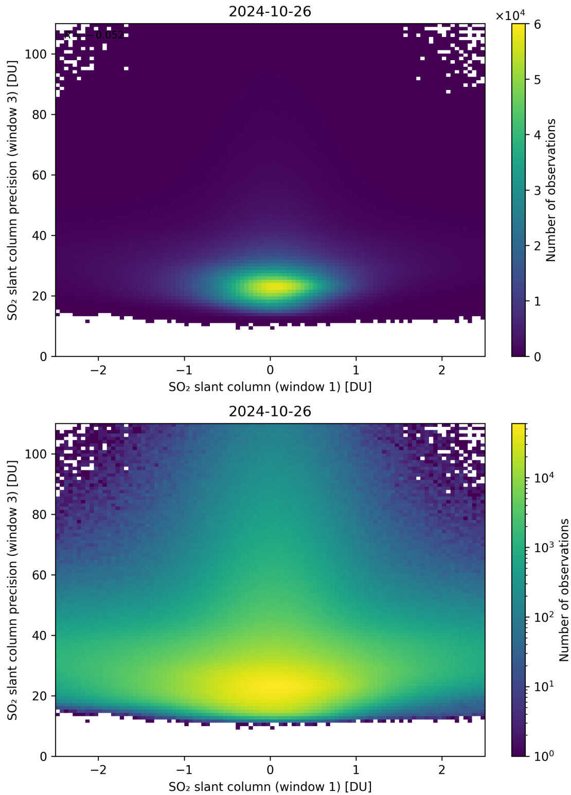
Figure 238: Scatter density plot of “SO 2 slant column (window 1)” against “SO 2 slant column precision (window 3)” for 2024-10-25 to 2024-10-27.
