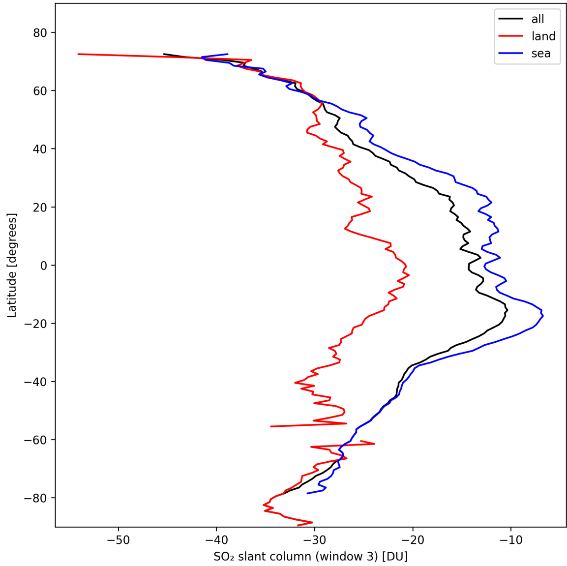
Figure 41: Zonal average of “SO 2 slant column (window 3)” for 2024-10-25 to 2024-10-27.
