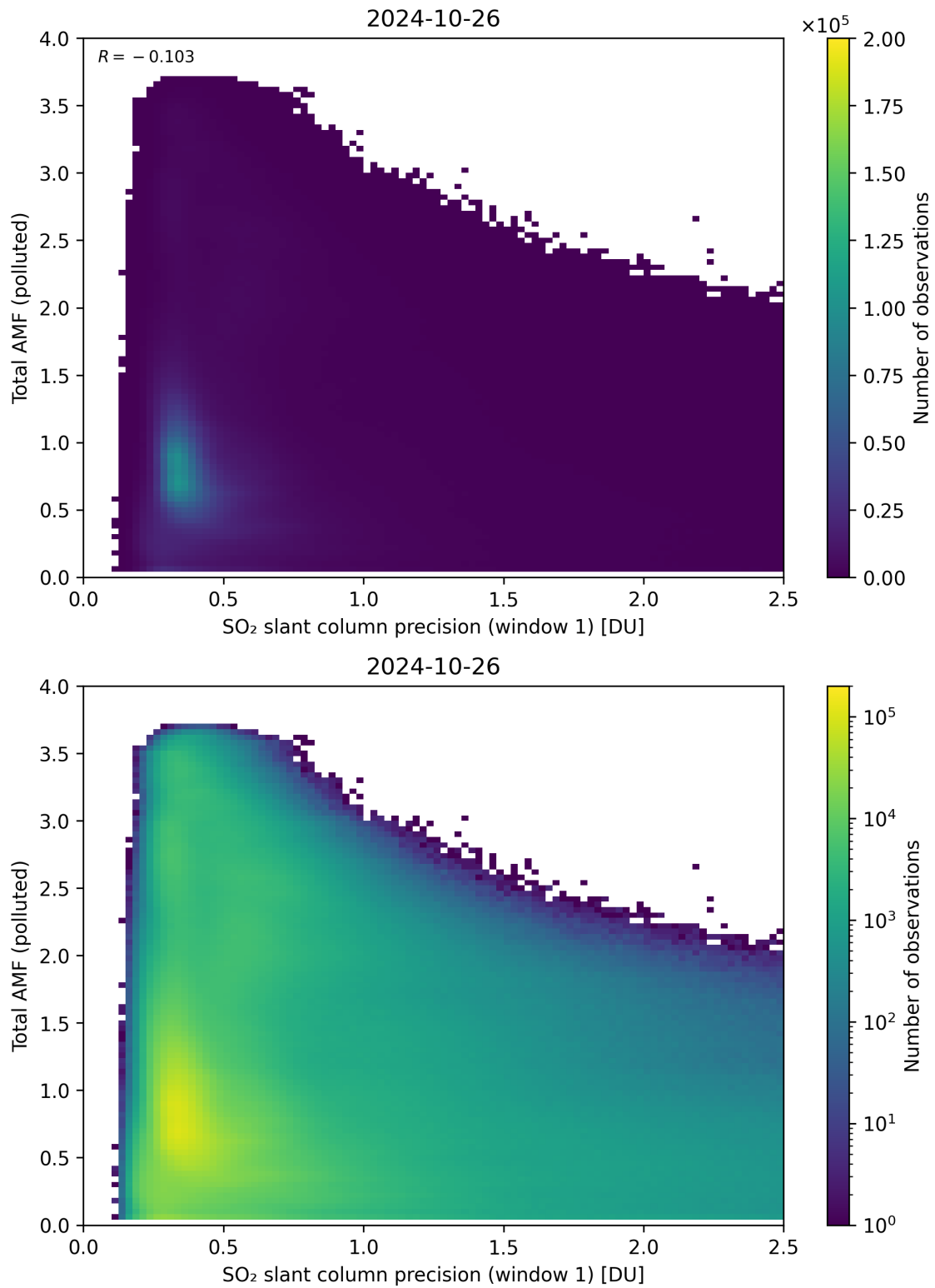
Figure 230: Scatter density plot of “SO 2 slant column precision (window 1)” against “Total AMF (polluted)” for 2024-10-25 to 2024-10-27.
