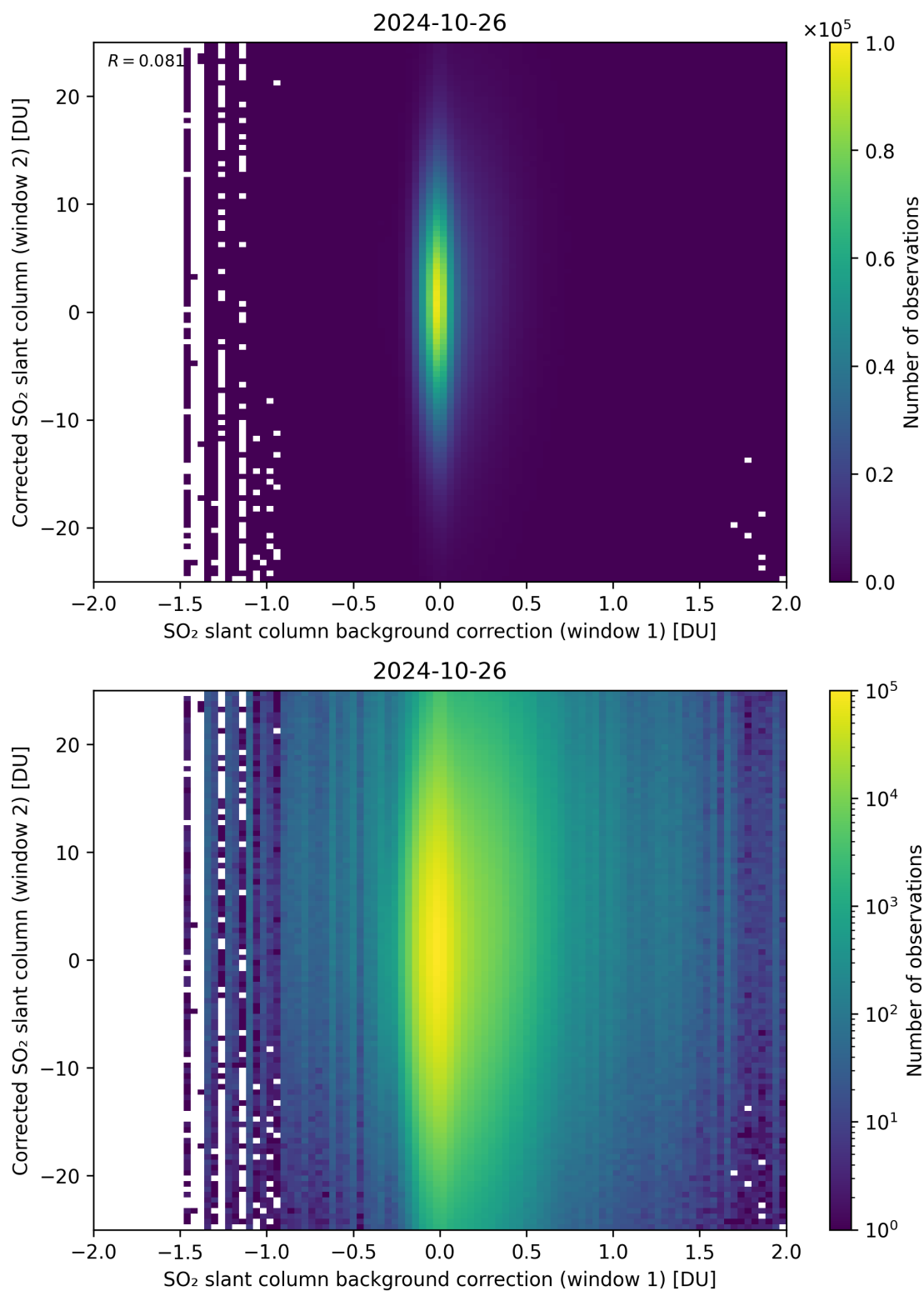
Figure 104: Scatter density plot of “SO 2 slant column background correction (window 1)” against “Corrected SO 2 slant column (window 2)” for 2024-10-25 to 2024-10-27.
