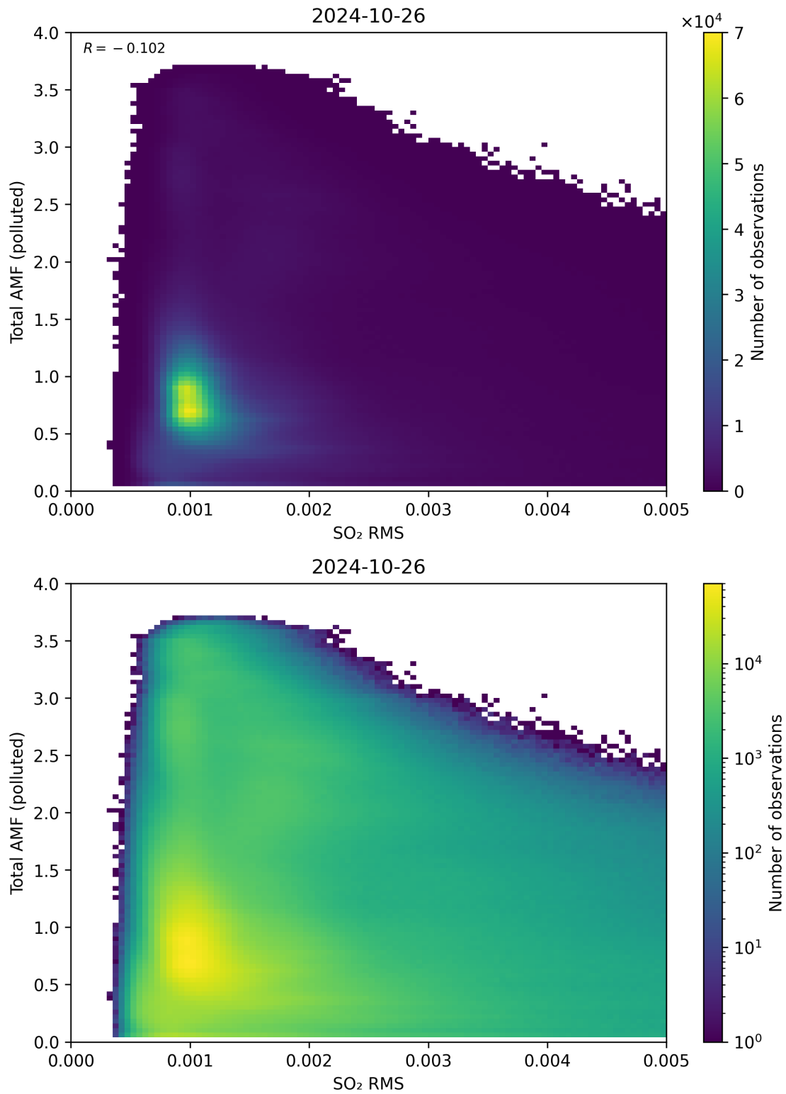
Figure 137: Scatter density plot of “SO 2 RMS” against “Total AMF (polluted)” for 2024-10-25 to 2024-10-27.
