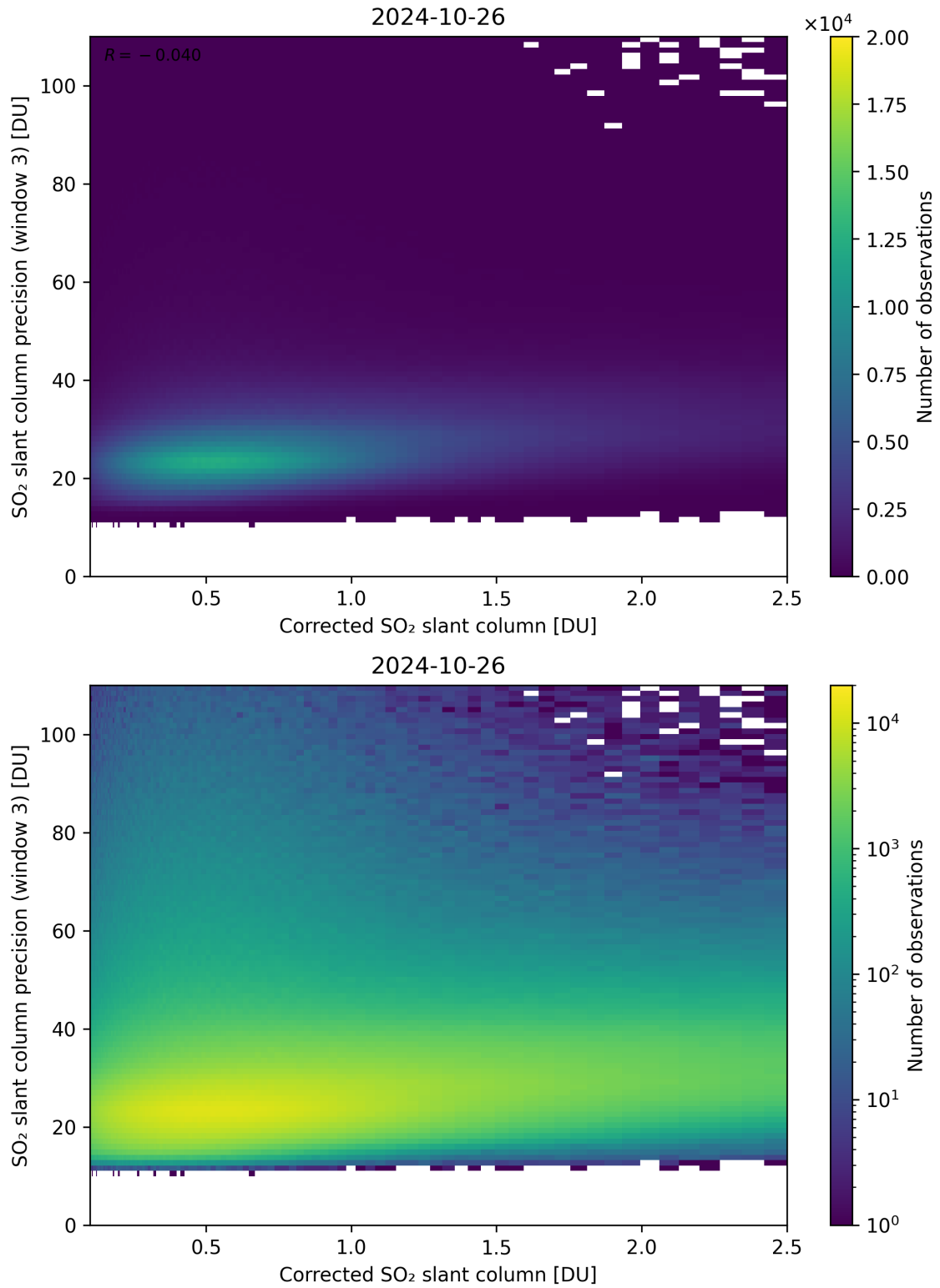
Figure 191: Scatter density plot of “Corrected SO 2 slant column” against “SO 2 slant column precision (window 3)” for 2024-10-25 to 2024-10-27.
