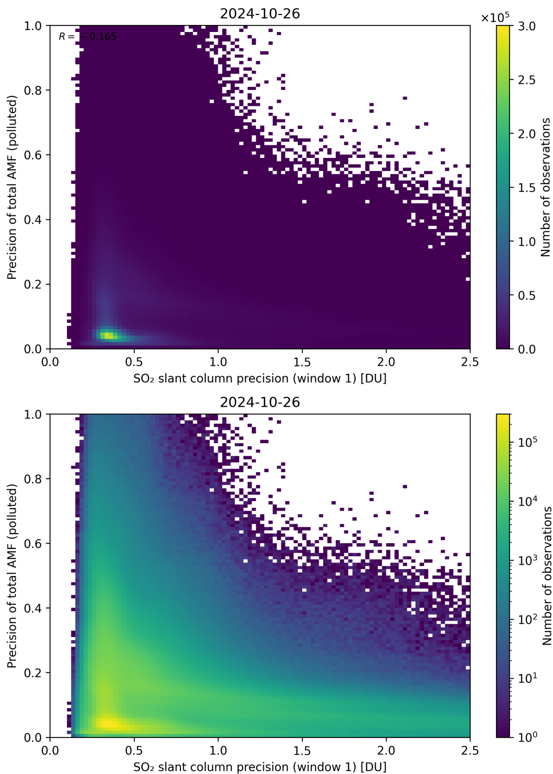
Figure 231: Scatter density plot of “SO 2 slant column precision (window 1)” against “Precision of total AMF (polluted)” for 2024-10-25 to 2024-10-27.
