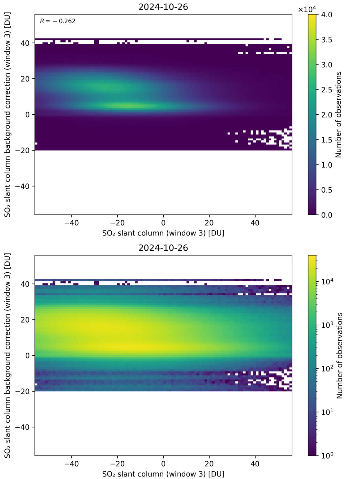
Figure 253: Scatter density plot of “SO 2 slant column (window 3)” against “SO 2 slant column background correction (window 3)” for 2024-10-25 to 2024-10-27.
