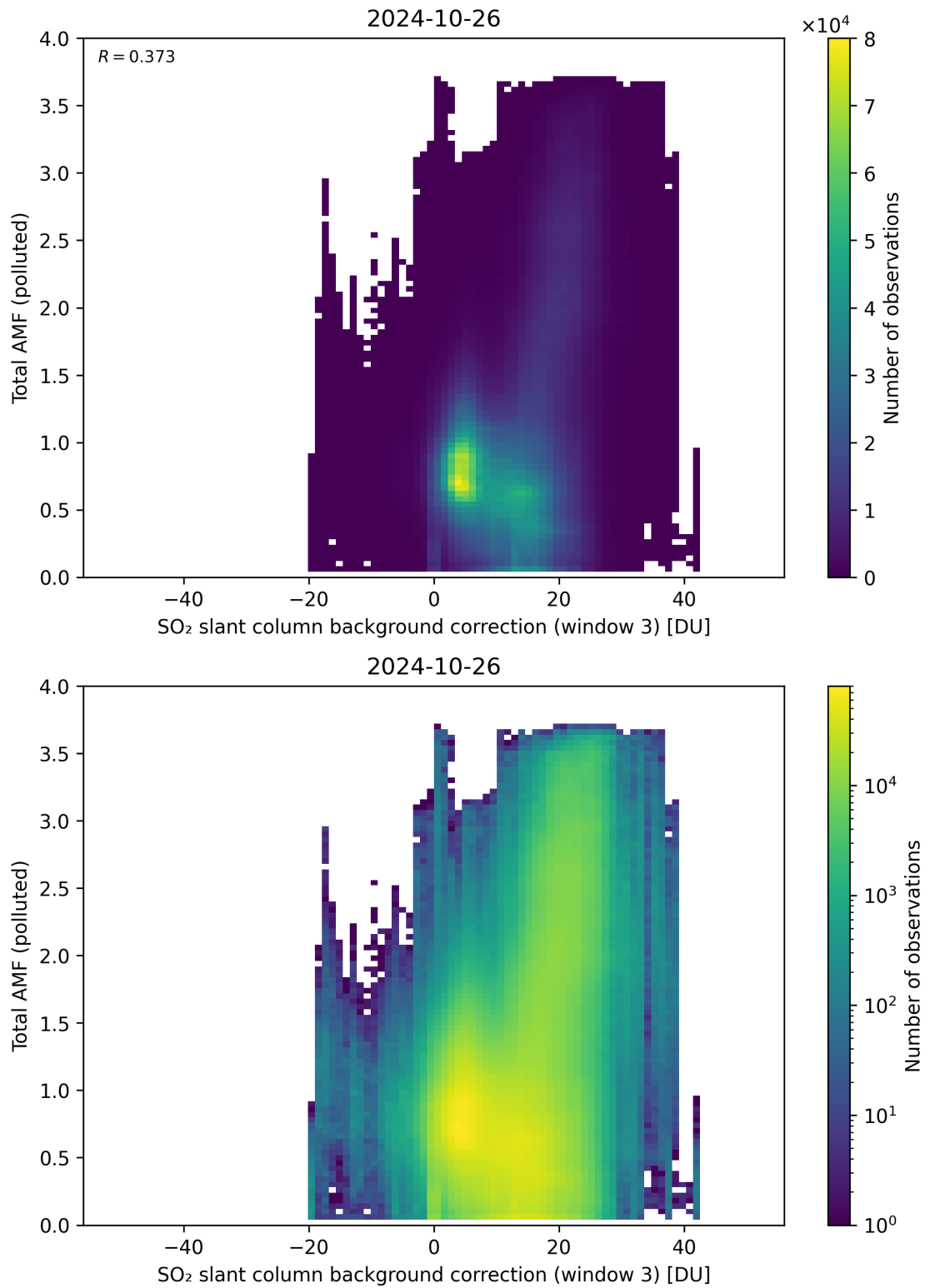
Figure 125: Scatter density plot of “SO 2 slant column background correction (window 3)” against “Total AMF (polluted)” for 2024-10-25 to 2024-10-27.
