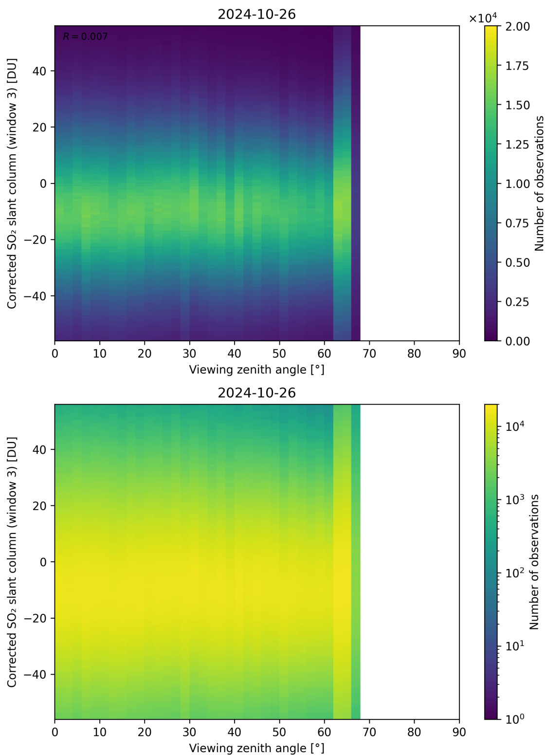
Figure 319: Scatter density plot of “Viewing zenith angle” against “Corrected SO 2 slant column (window 3)” for 2024-10-25 to 2024-10-27.
