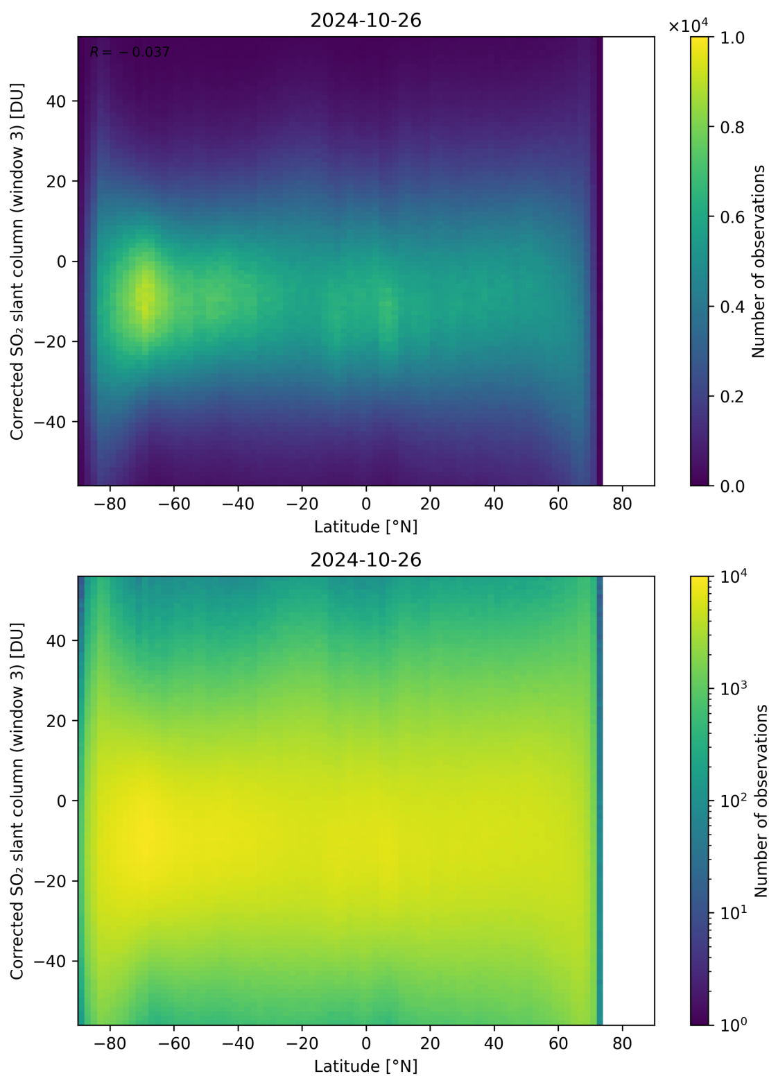
Figure 148: Scatter density plot of “Latitude” against “Corrected SO 2 slant column (window 3)” for 2024-10-25 to 2024-10-27.
