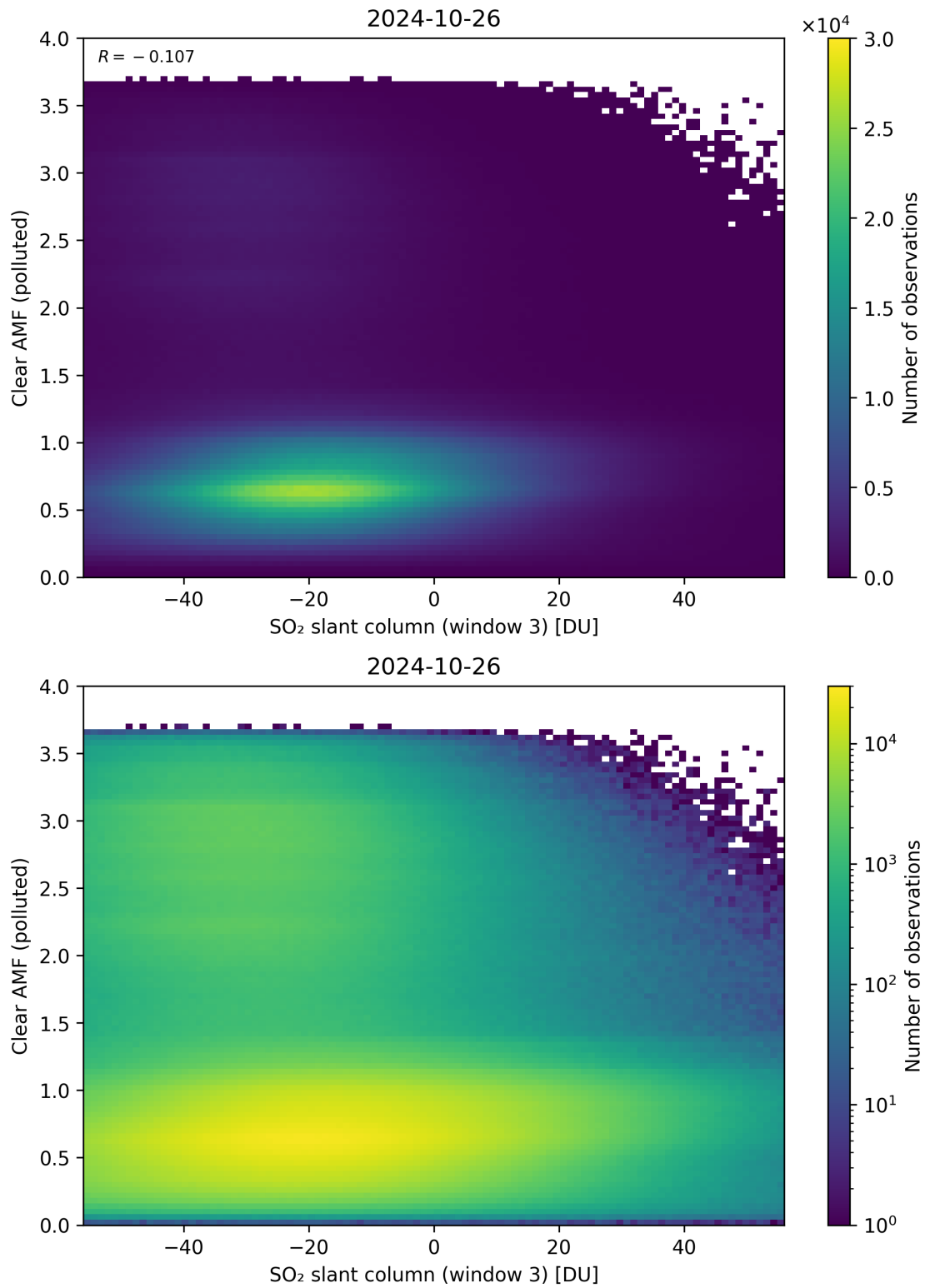
Figure 265: Scatter density plot of “SO 2 slant column (window 3)” against “Clear AMF (polluted)” for 2024-10-25 to 2024-10-27.
