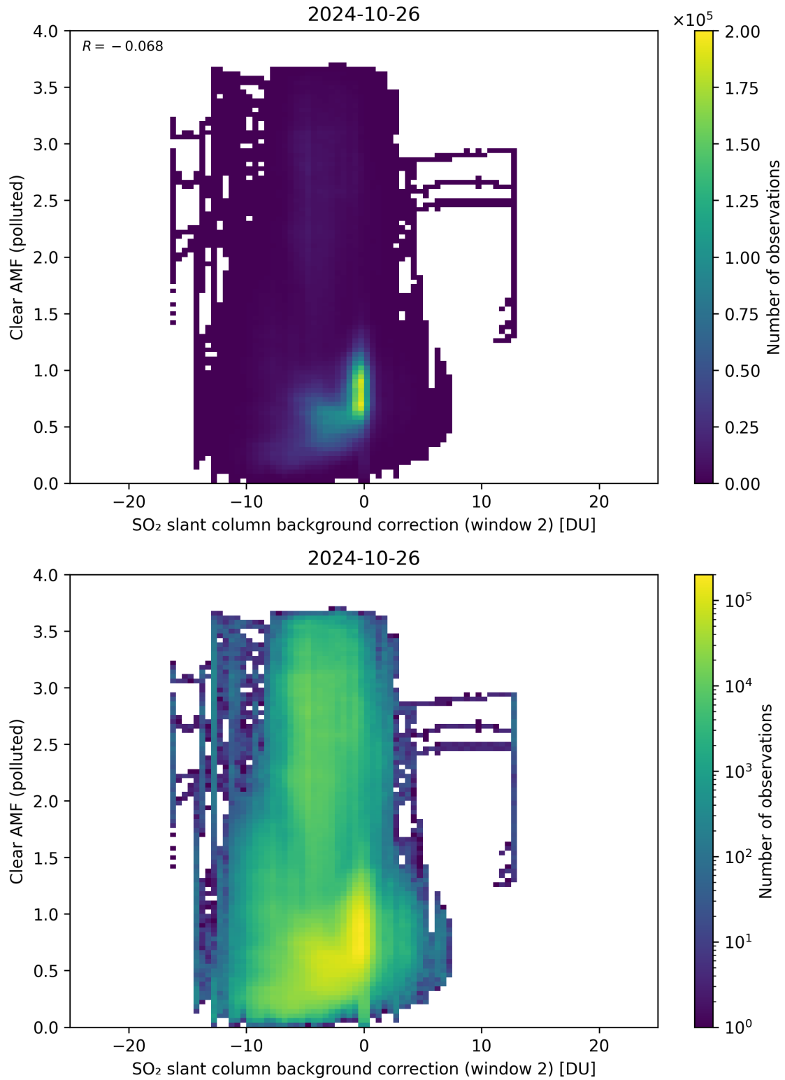
Figure 115: Scatter density plot of “SO 2 slant column background correction (window 2)” against “Clear AMF (polluted)” for 2024-10-25 to 2024-10-27.
