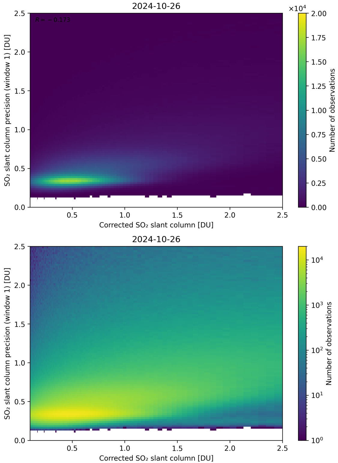
Figure 188: Scatter density plot of “Corrected SO 2 slant column” against “SO 2 slant column precision (window 1)” for 2024-10-25 to 2024-10-27.
