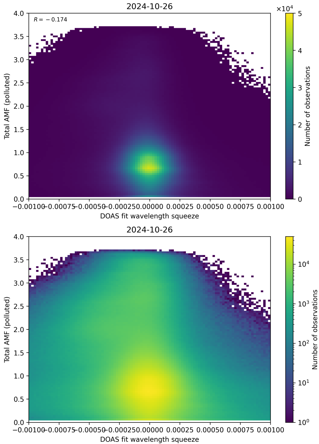
Figure 134: Scatter density plot of “DOAS fit wavelength squeeze” against “Total AMF (polluted)” for 2024-10-25 to 2024-10-27.
