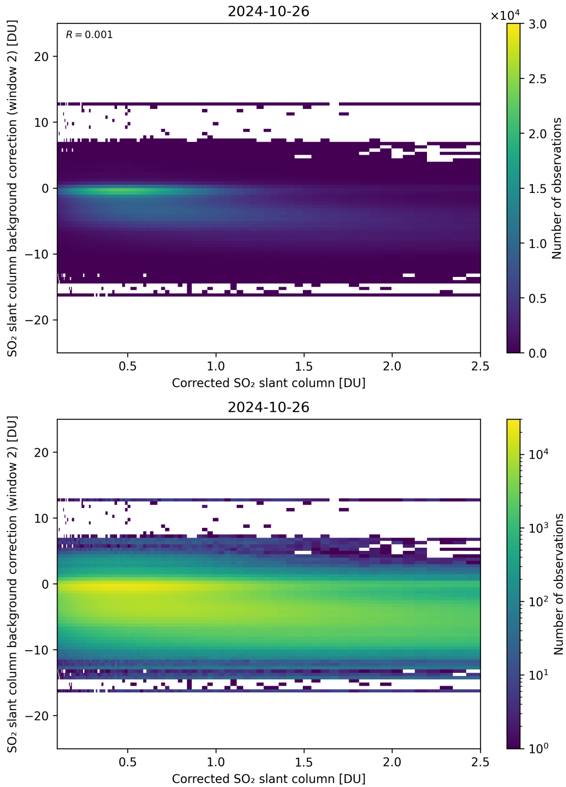
Figure 179: Scatter density plot of “Corrected SO 2 slant column” against “SO 2 slant column background correction (window 2)” for 2024-10-25 to 2024-10-27.
