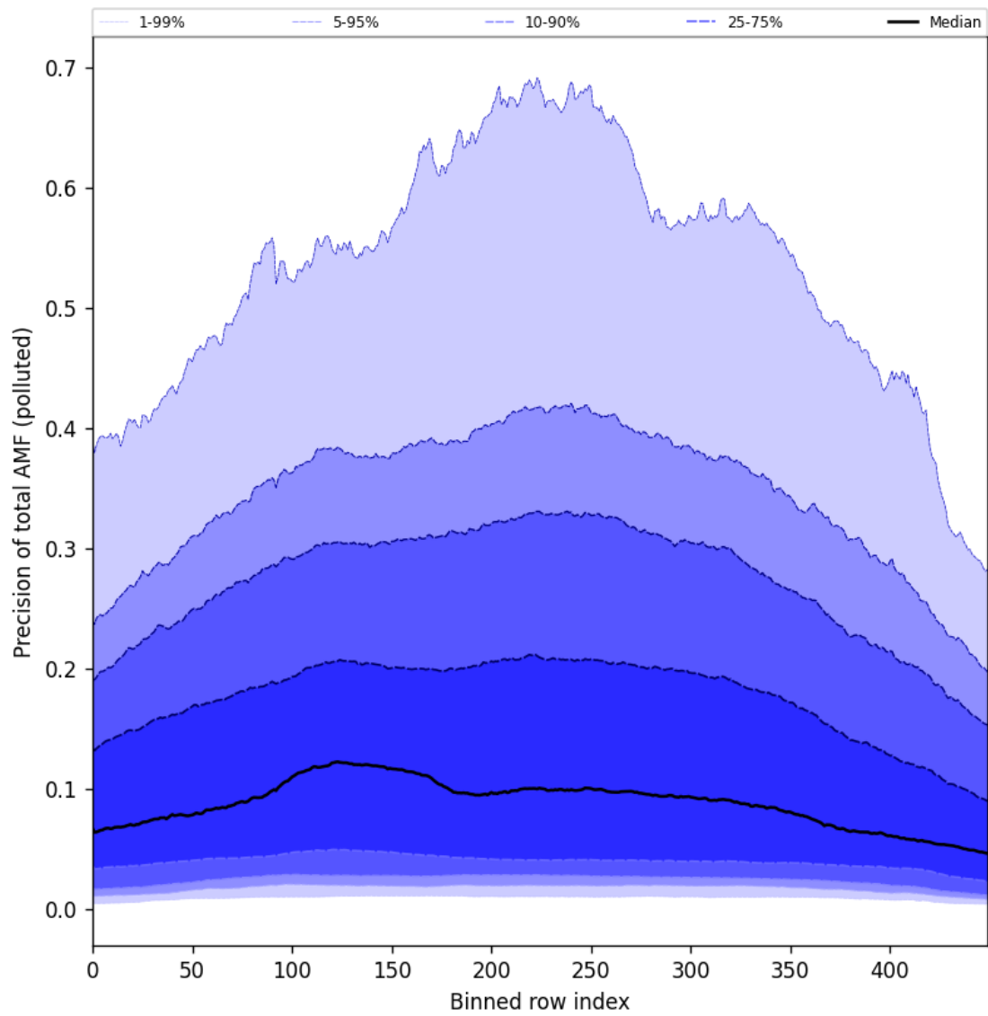
Figure 95: Along track statistics of “Precision of total AMF (polluted)” for 2024-10-25 to 2024-10-27
