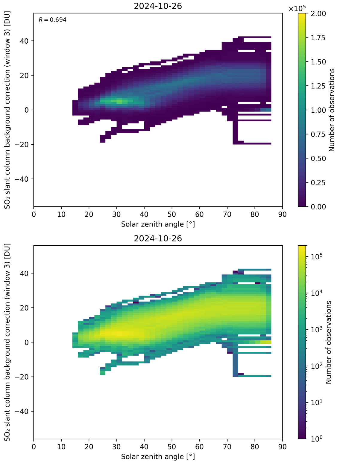
Figure 160: Scatter density plot of “Solar zenith angle” against “SO 2 slant column background correction (window 3)” for 2024-10-25 to 2024-10-27.
