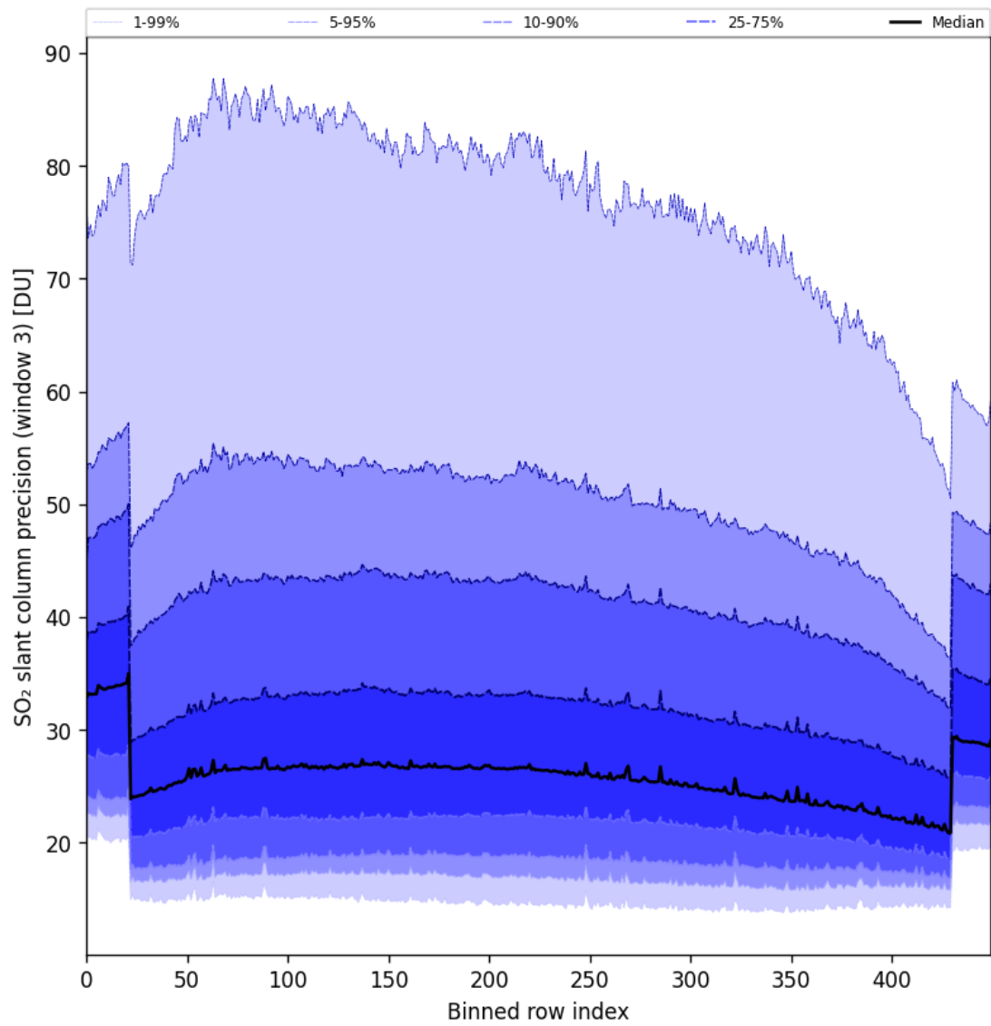
Figure 88: Along track statistics of “SO 2 slant column precision (window 3)” for 2024-10-25 to 2024-10-27
