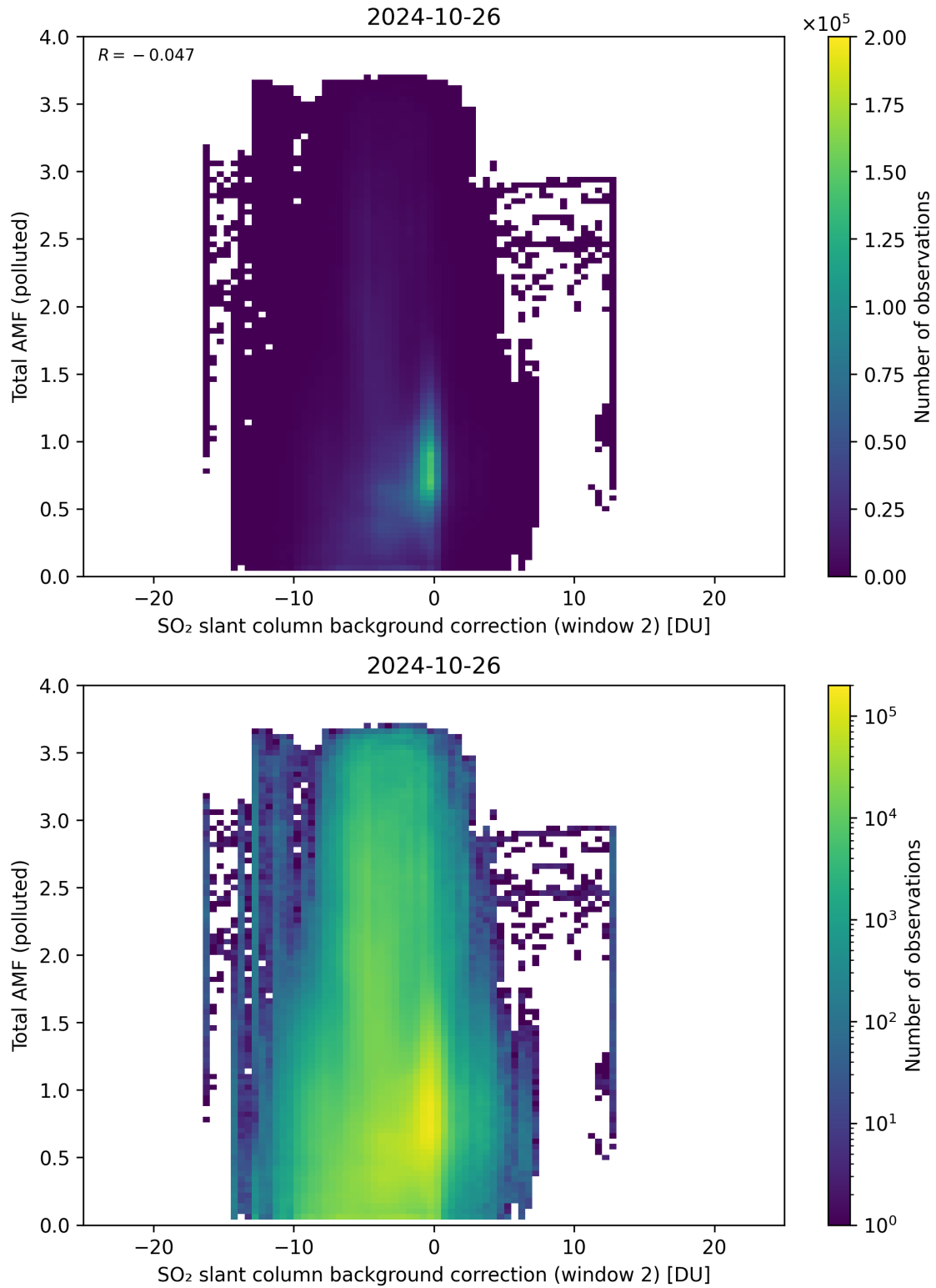
Figure 119: Scatter density plot of “SO 2 slant column background correction (window 2)” against “Total AMF (polluted)” for 2024-10-25 to 2024-10-27.
