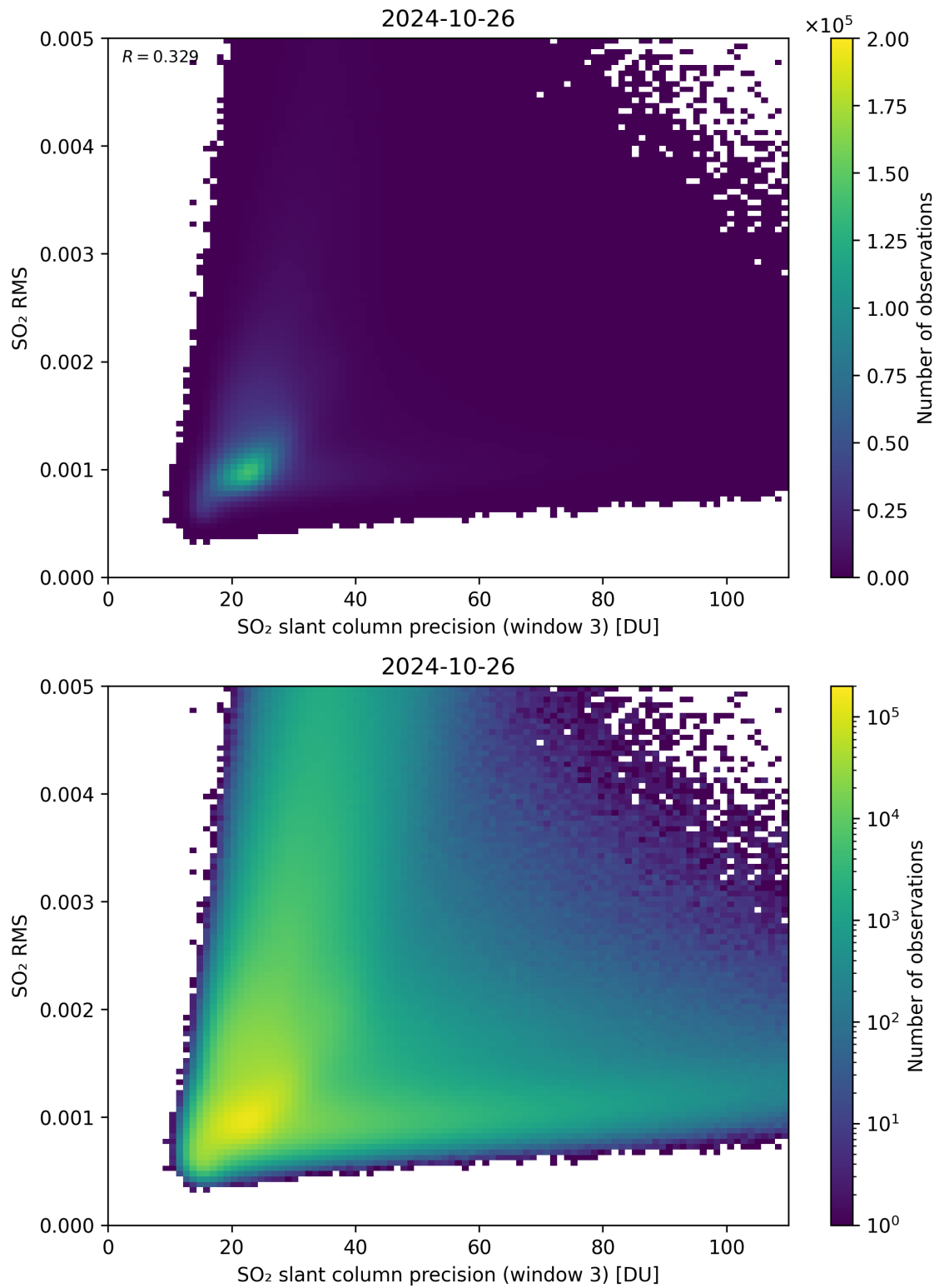
Figure 260: Scatter density plot of “SO 2 slant column precision (window 3)” against “SO 2 RMS” for 2024-10-25 to 2024-10-27.
