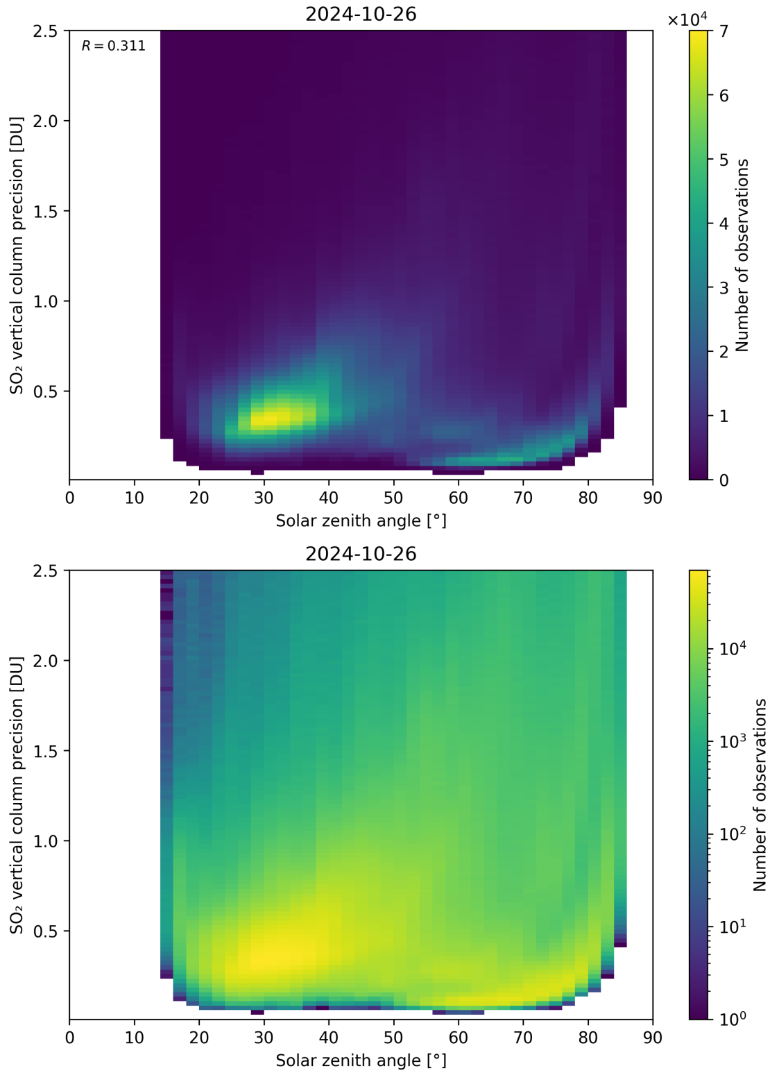
Figure 177: Scatter density plot of “Solar zenith angle” against “SO 2 vertical column precision” for 2024-10-25 to 2024-10-27.
