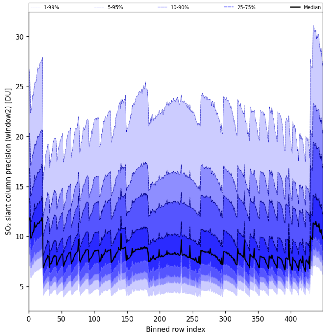
Figure 84: Along track statistics of “SO 2 slant column precision (window2)” for 2024-10-25 to 2024-10-27
