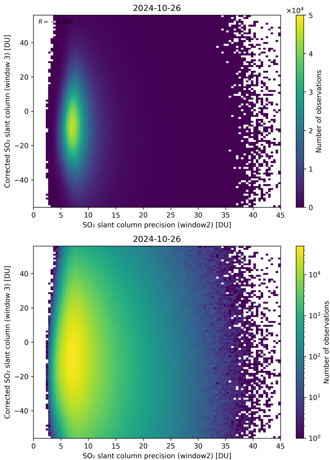
Figure 248: Scatter density plot of “SO 2 slant column precision (window2)” against “Corrected SO 2 slant column (window 3)” for 2024-10-25 to 2024-10-27.
