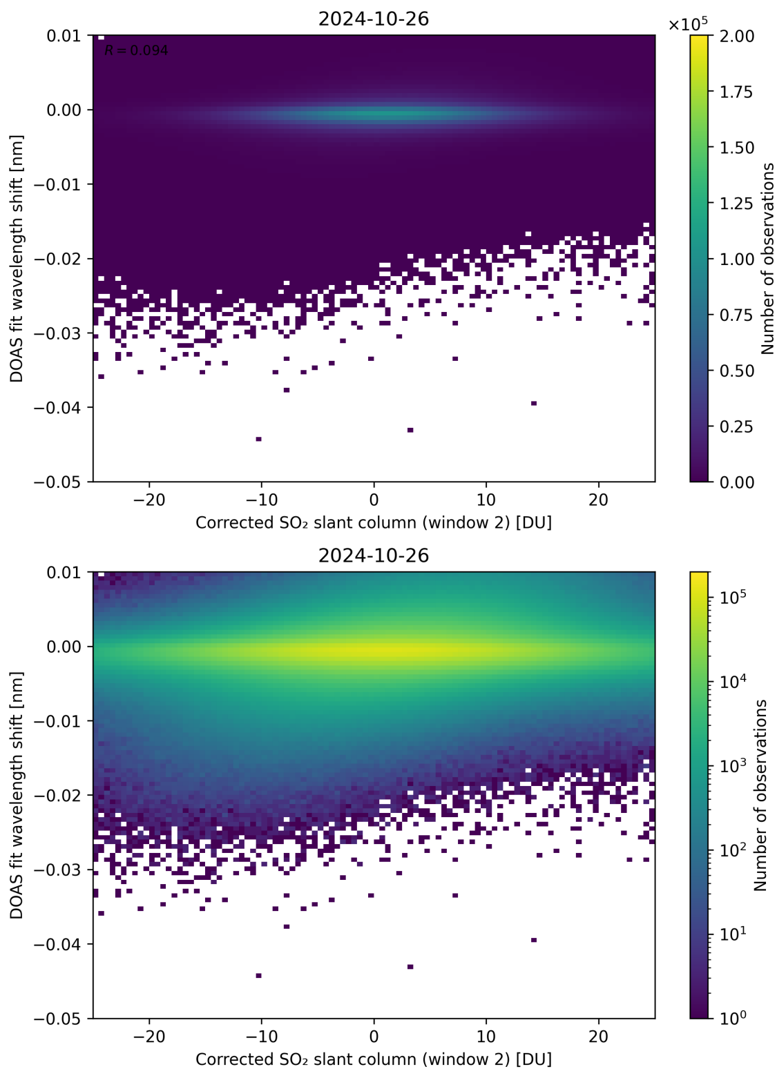
Figure 196: Scatter density plot of “Corrected SO 2 slant column (window 2)” against “DOAS fit wavelength shift” for 2024-10-25 to 2024-10-27.
