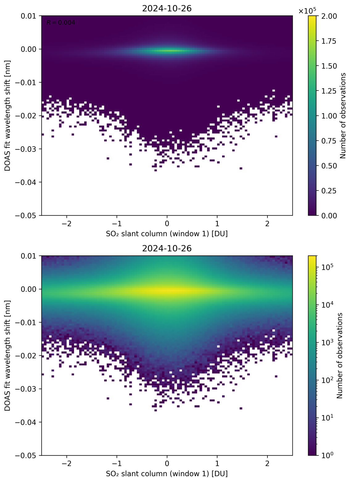
Figure 215: Scatter density plot of “SO 2 slant column (window 1)” against “DOAS fit wavelength shift” for 2024-10-25 to 2024-10-27.
