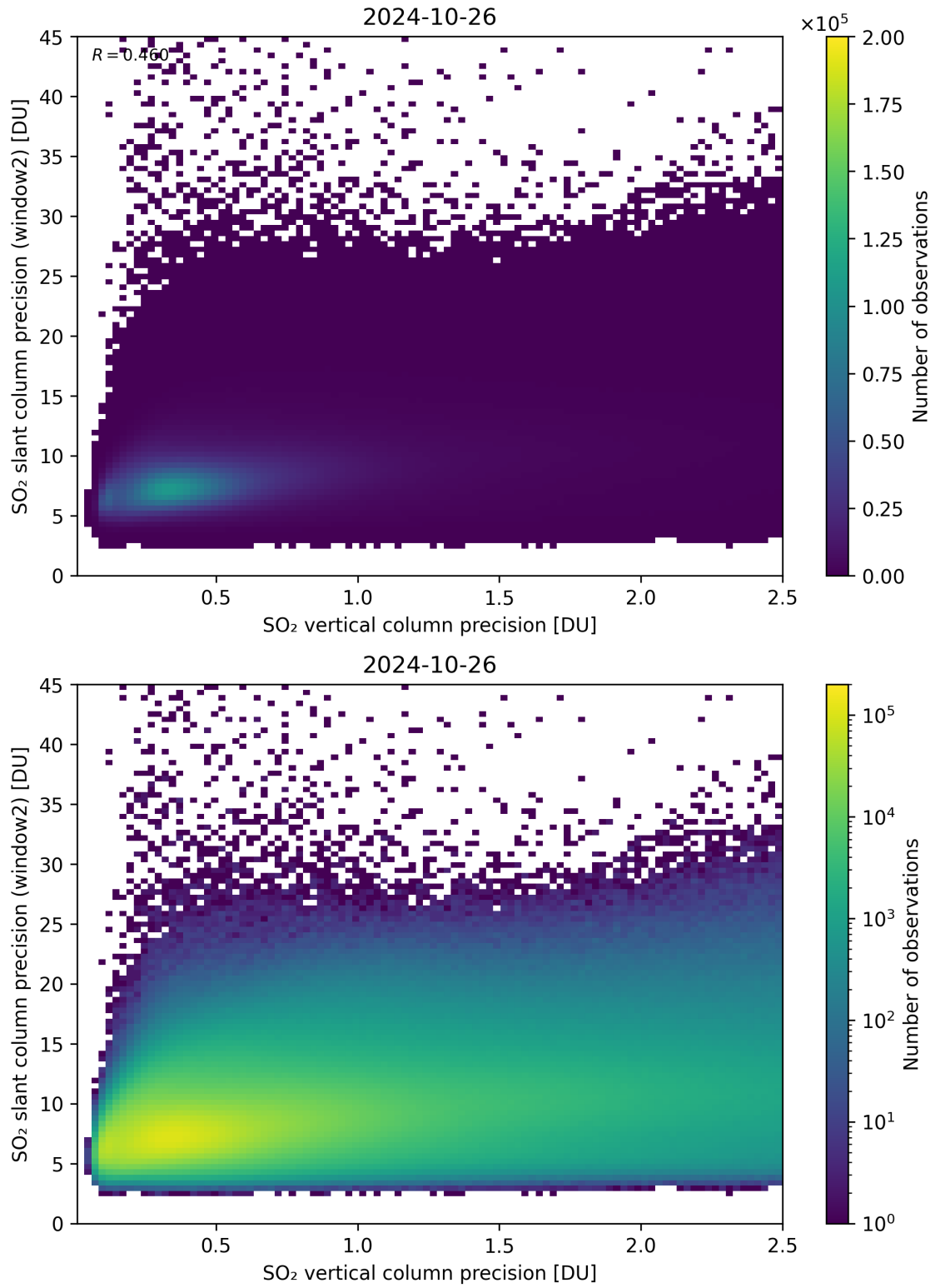
Figure 291: Scatter density plot of “SO 2 vertical column precision” against “SO 2 slant column precision (window2)” for 2024-10-25 to 2024-10-27.
