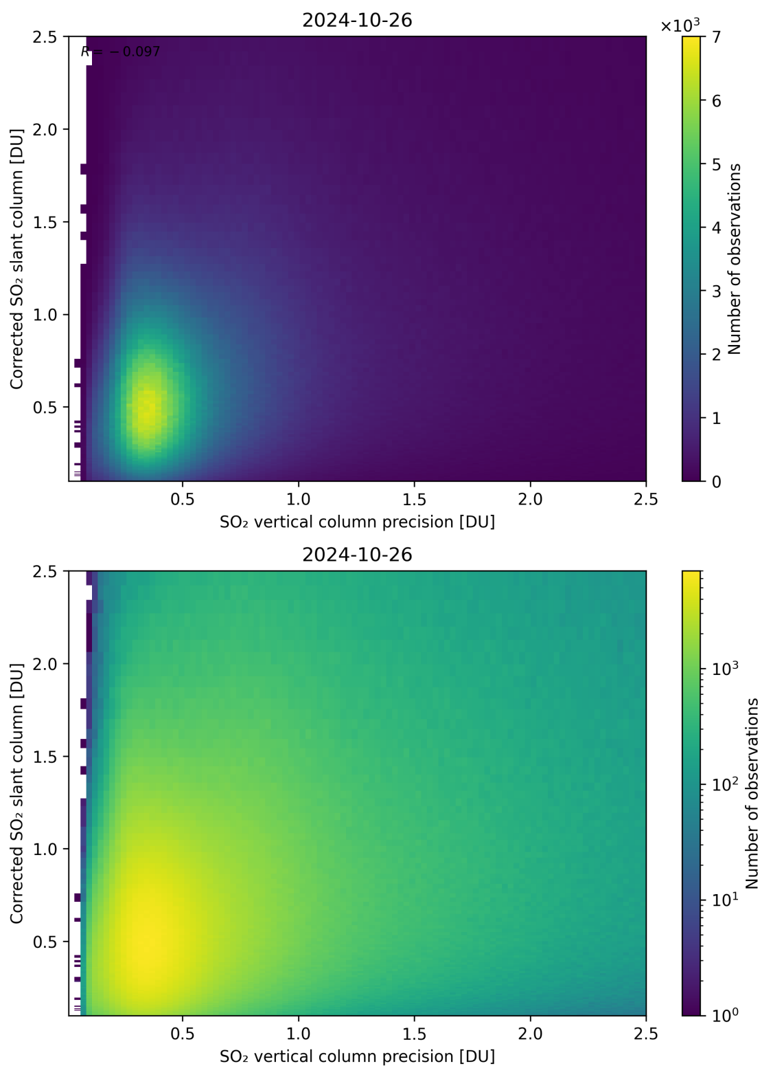
Figure 286: Scatter density plot of “SO 2 vertical column precision” against “Corrected SO 2 slant column” for 2024-10-25 to 2024-10-27.
