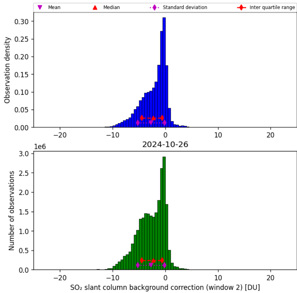
Figure 63: Histogram of “SO 2 slant column background correction (window 2)” for 2024-10-25 to 2024-10-27
