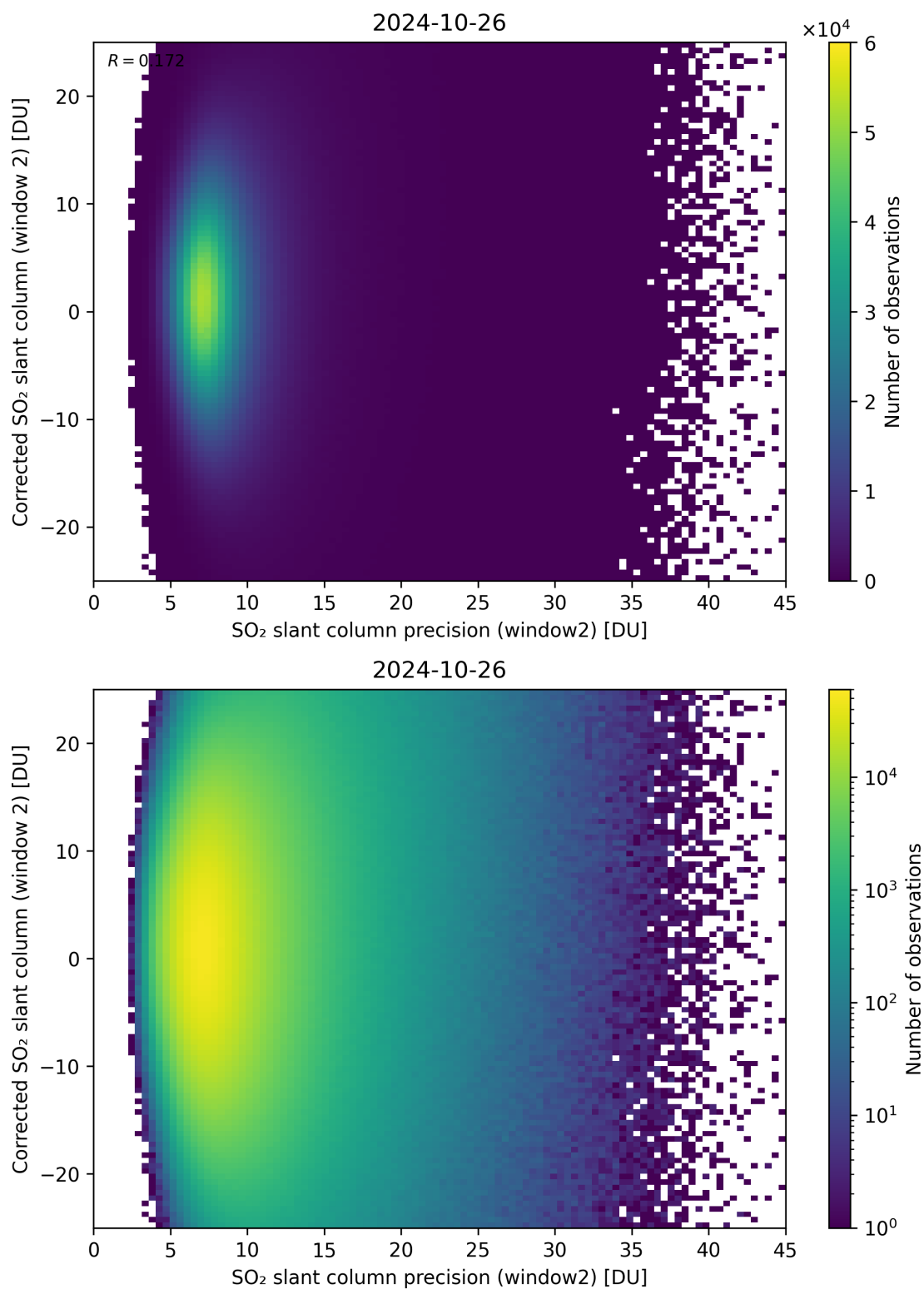
Figure 247: Scatter density plot of “SO 2 slant column precision (window2)” against “Corrected SO 2 slant column (window 2)” for 2024-10-25 to 2024-10-27.
