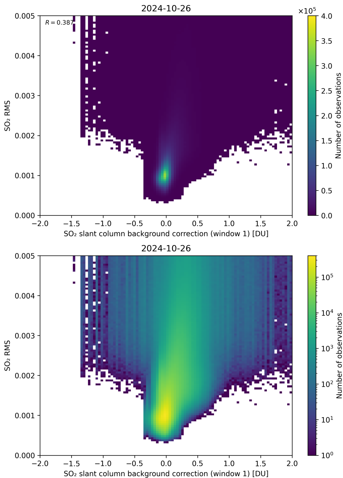
Figure 102: Scatter density plot of “SO 2 slant column background correction (window 1)” against “SO 2 RMS” for 2024-10-25 to 2024-10-27.
