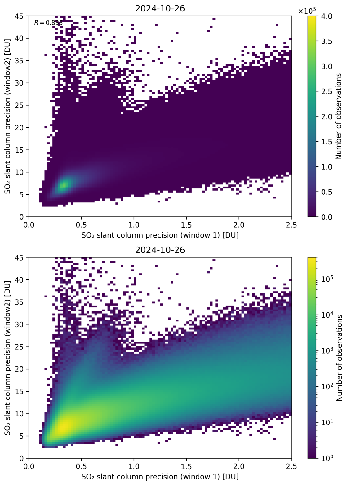
Figure 227: Scatter density plot of “SO 2 slant column precision (window 1)” against “SO 2 slant column precision (window 2)” for 2024-10-25 to 2024-10-27.
