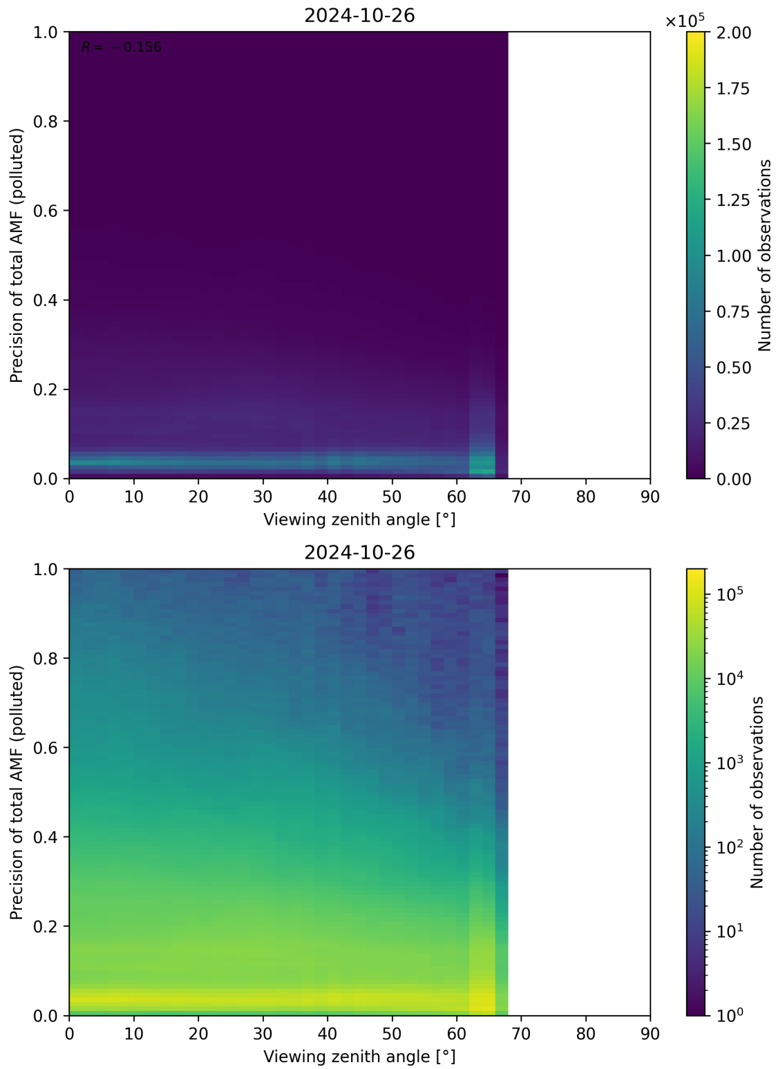
Figure 326: Scatter density plot of “Viewing zenith angle” against “Precision of total AMF (polluted)” for 2024-10-25 to 2024-10-27.
