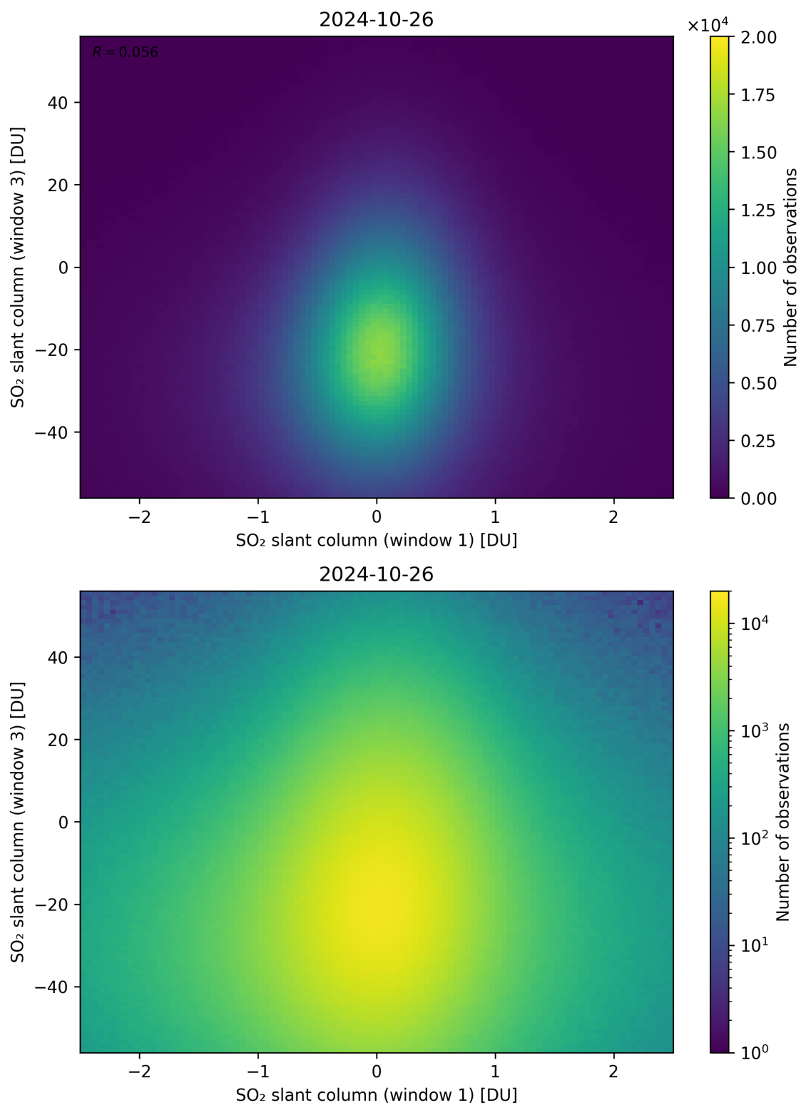
Figure 237: Scatter density plot of “SO 2 slant column (window 1)” against “SO 2 slant column (window 3)” for 2024-10-25 to 2024-10-27.
