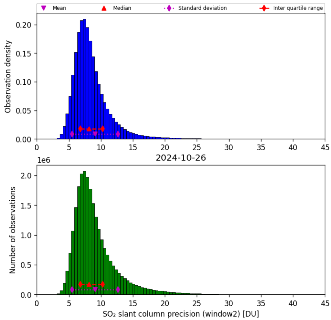
Figure 61: Histogram of “SO 2 slant column precision (window2)” for 2024-10-25 to 2024-10-27
