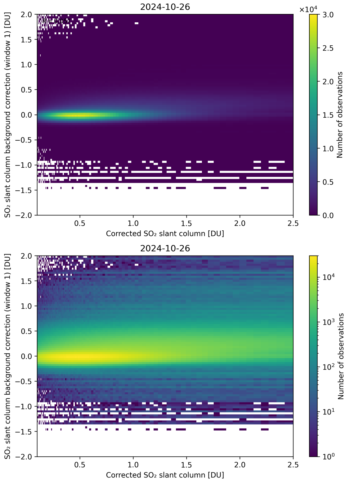
Figure 178: Scatter density plot of “Corrected SO 2 slant column” against “SO 2 slant column background correction (window 1)” for 2024-10-25 to 2024-10-27.
