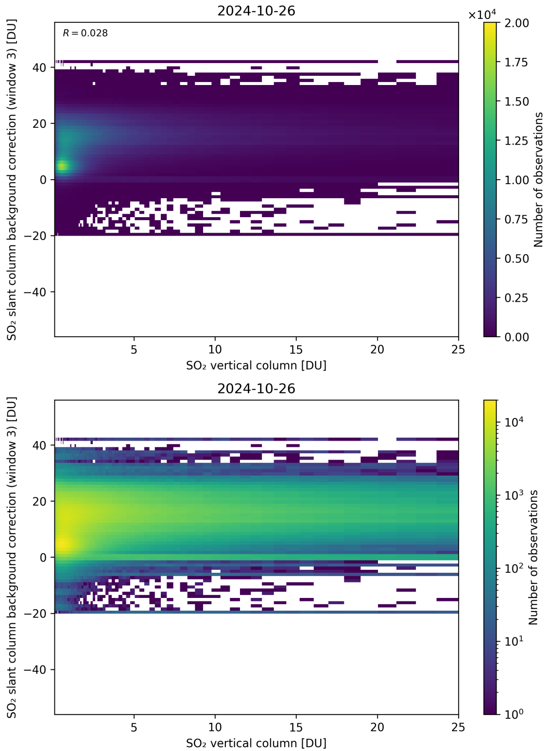
Figure 275: Scatter density plot of “SO 2 vertical column” against “SO 2 slant column background correction (window 3)” for 2024-10-25 to 2024-10-27.
