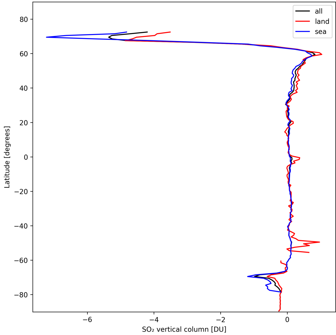
Figure 30: Zonal average of “SO 2 vertical column” for 2024-10-25 to 2024-10-27.
