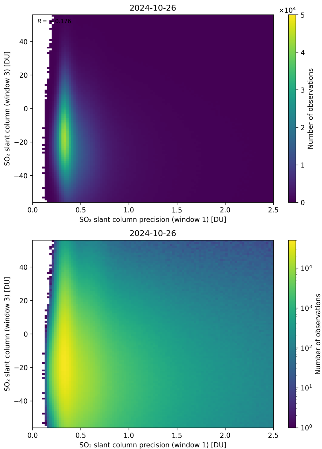
Figure 228: Scatter density plot of “SO 2 slant column precision (window 1)” against “SO 2 slant column (window 3)” for 2024-10-25 to 2024-10-27.
