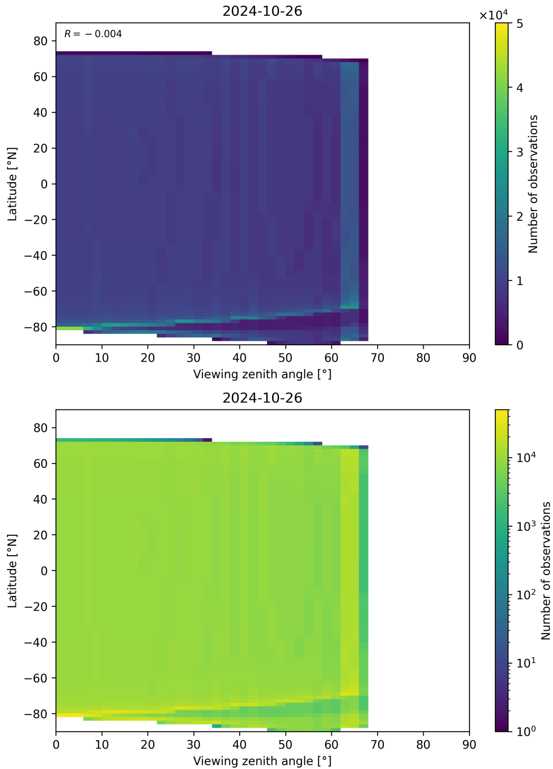
Figure 314: Scatter density plot of “Viewing zenith angle” against “Latitude” for 2024-10-25 to 2024-10-27.
