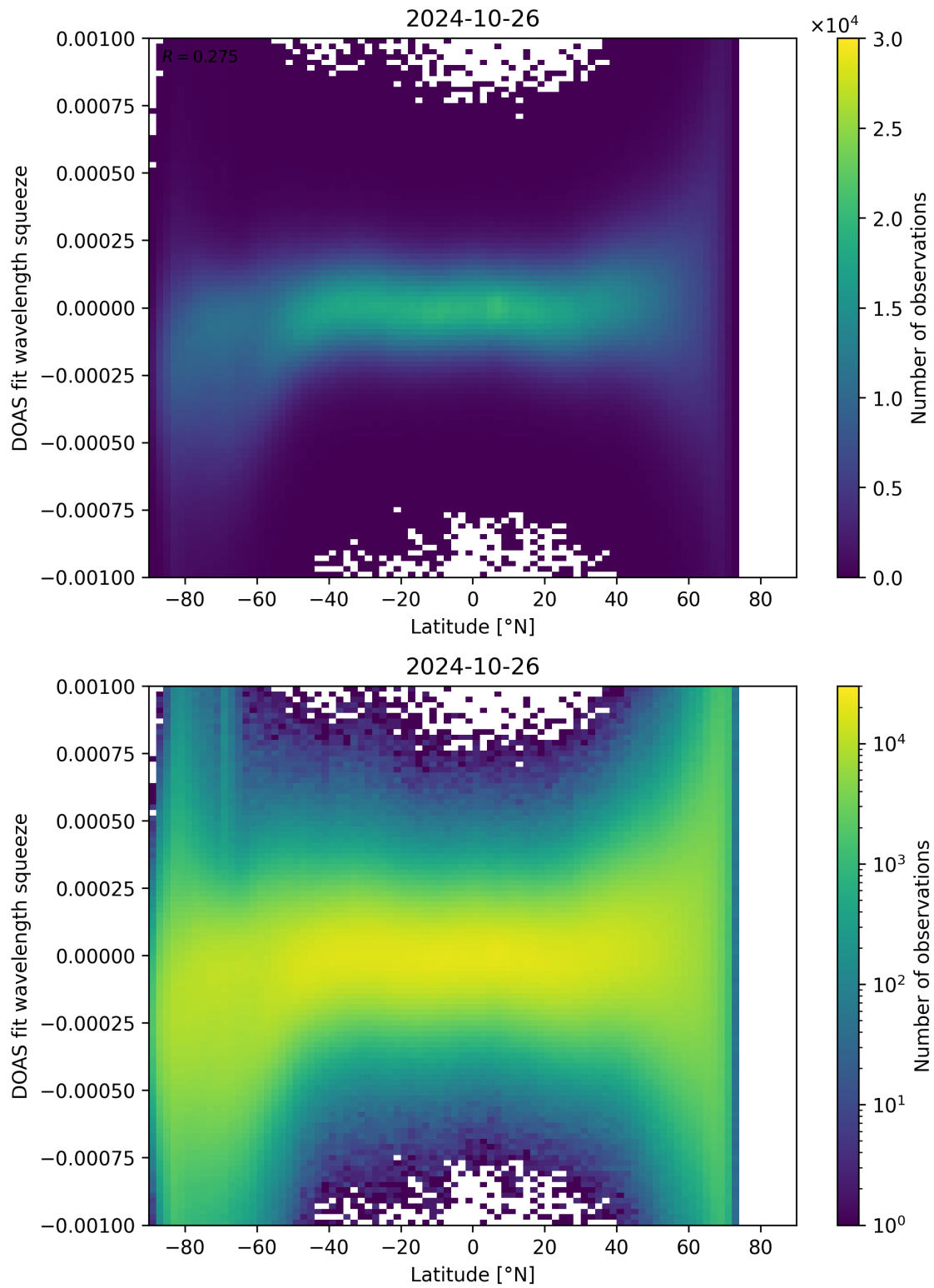
Figure 143: Scatter density plot of “Latitude” against “DOAS fit wavelength squeeze” for 2024-10-25 to 2024-10-27.
