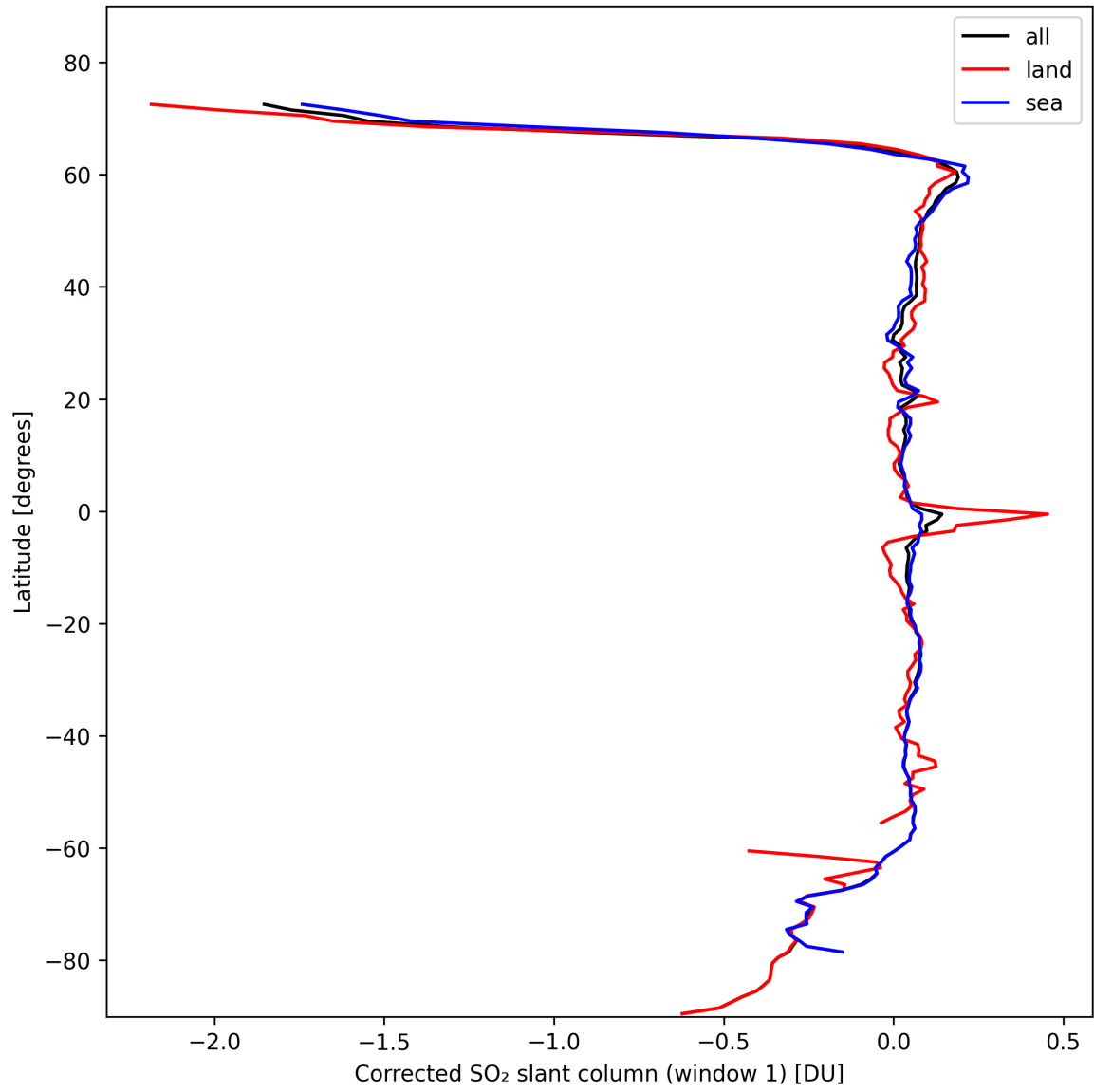
Figure 35: Zonal average of “Corrected SO 2 slant column (window 1)” for 2024-10-25 to 2024-10-27.
