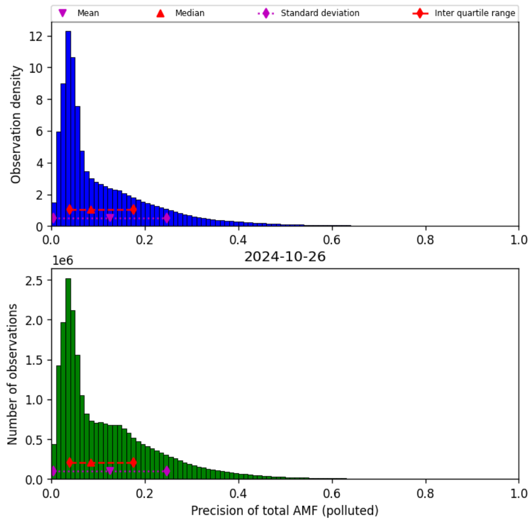
Figure 72: Histogram of “Precision of total AMF (polluted)” for 2024-10-25 to 2024-10-27
