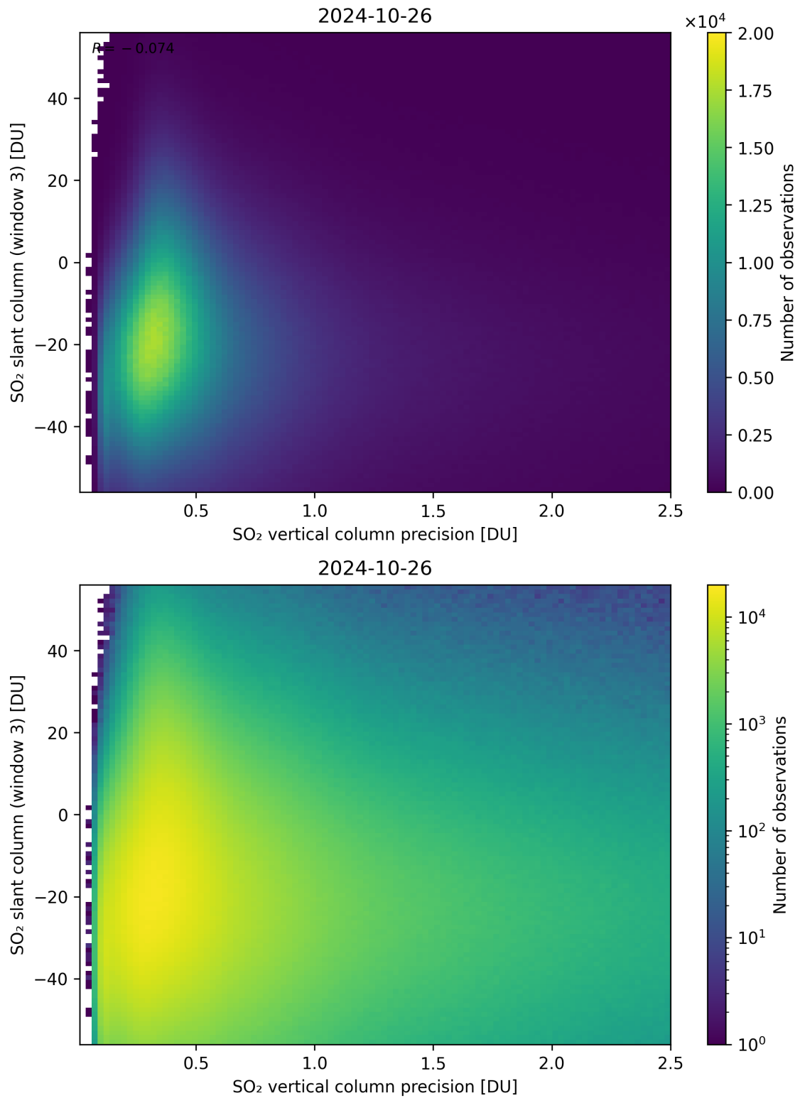
Figure 292: Scatter density plot of “SO 2 vertical column precision” against “SO 2 slant column (window 3)” for 2024-10-25 to 2024-10-27.
