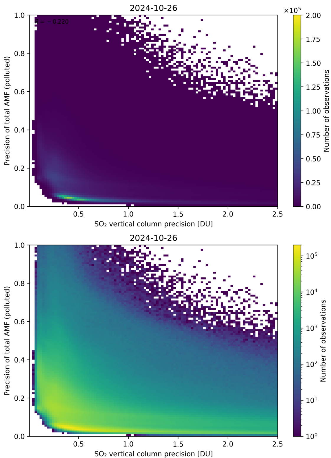
Figure 295: Scatter density plot of “SO 2 vertical column precision” against “Precision of total AMF (polluted)” for 2024-10-25 to 2024-10-27.
