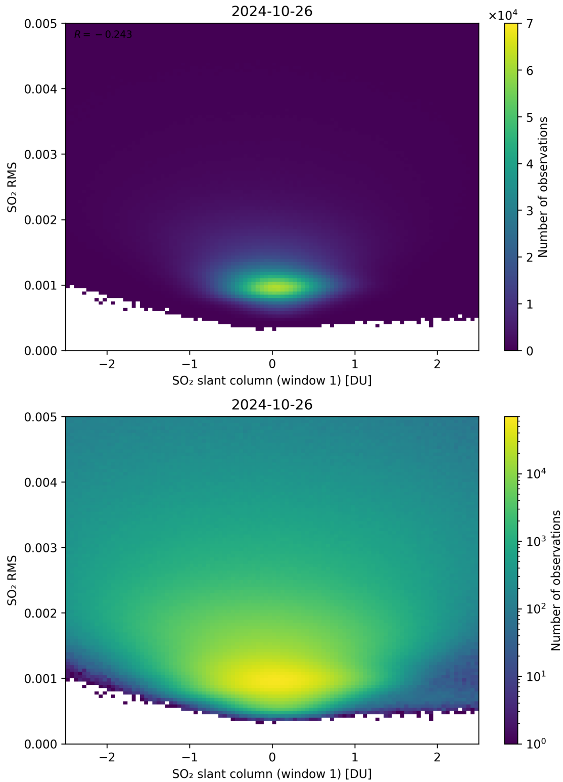
Figure 217: Scatter density plot of “SO 2 slant column (window 1)” against “SO 2 RMS” for 2024-10-25 to 2024-10-27.
