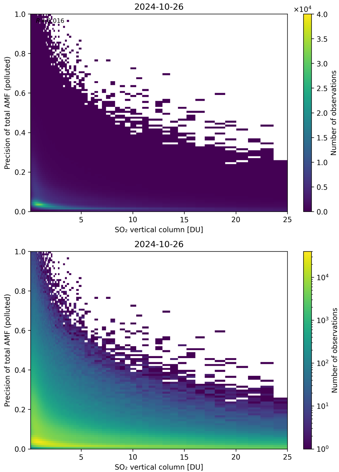
Figure 306: Scatter density plot of “SO 2 vertical column” against “Precision of total AMF (polluted)” for 2024-10-25 to 2024-10-27.
