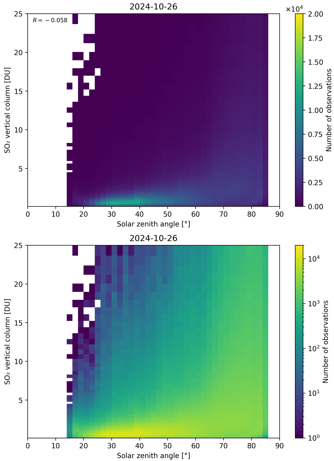
Figure 176: Scatter density plot of “Solar zenith angle” against “SO 2 vertical column” for 2024-10-25 to 2024-10-27.
