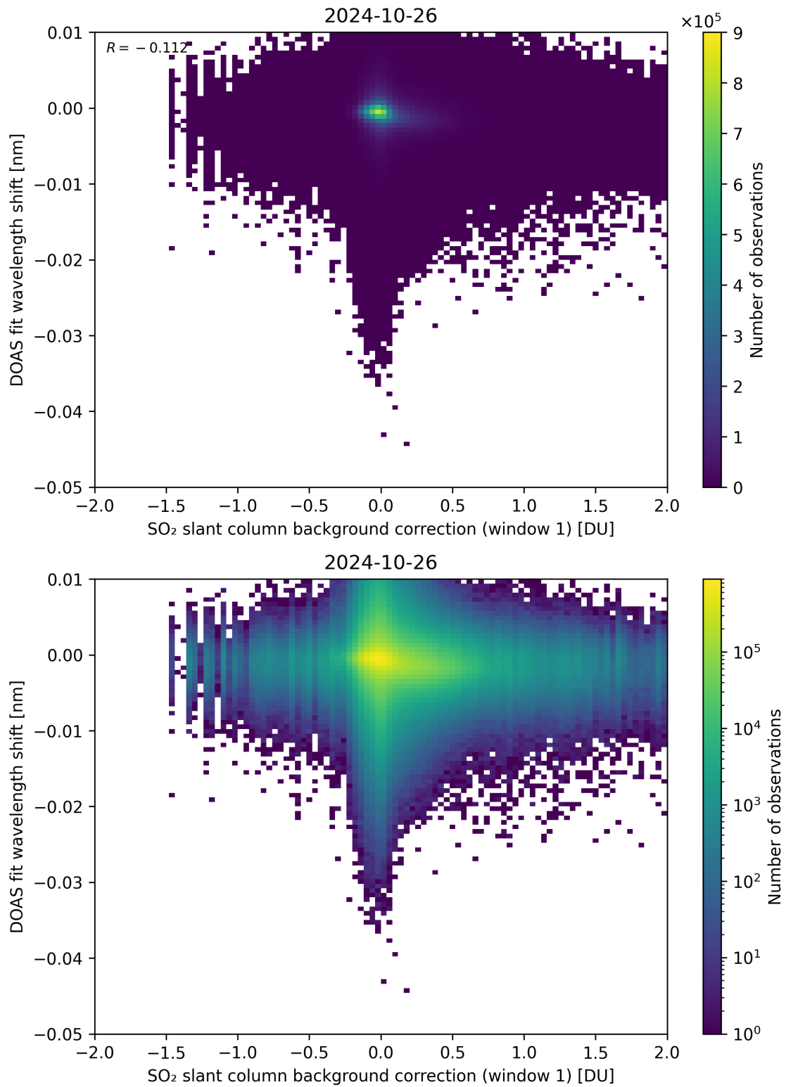
Figure 100: Scatter density plot of “SO 2 slant column background correction (window 1)” against “DOAS fit wavelength shift” for 2024-10-25 to 2024-10-27.
