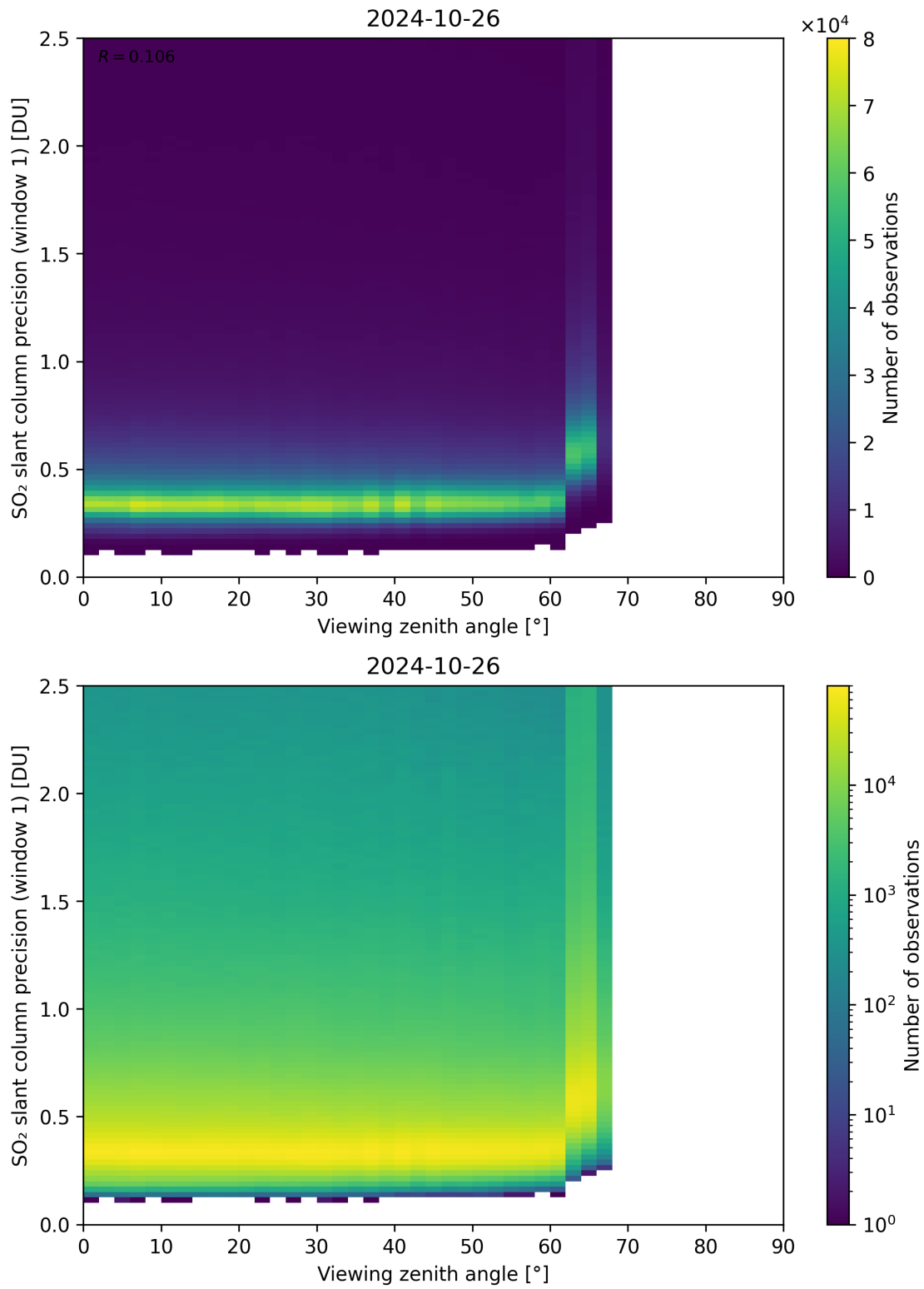
Figure 321: Scatter density plot of “Viewing zenith angle” against “SO 2 slant column precision (window 1)” for 2024-10-25 to 2024-10-27.
