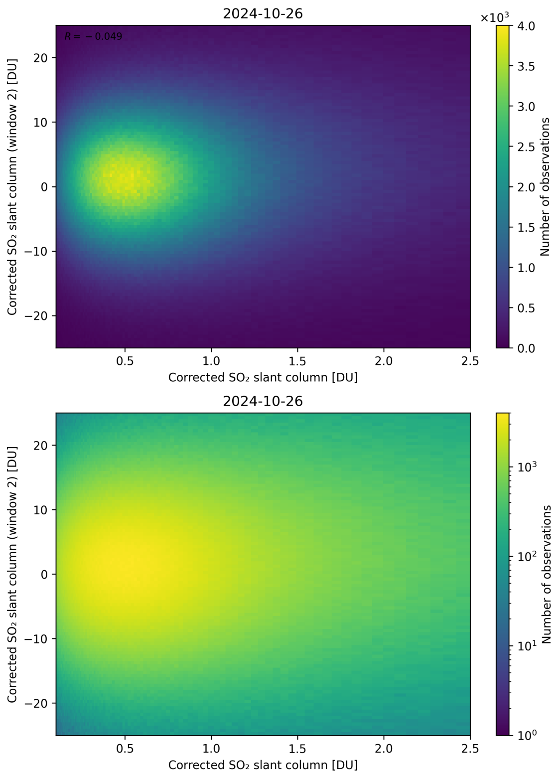
Figure 185: Scatter density plot of “Corrected SO 2 slant column” against “Corrected SO 2 slant column (window 2)” for 2024-10-25 to 2024-10-27.
