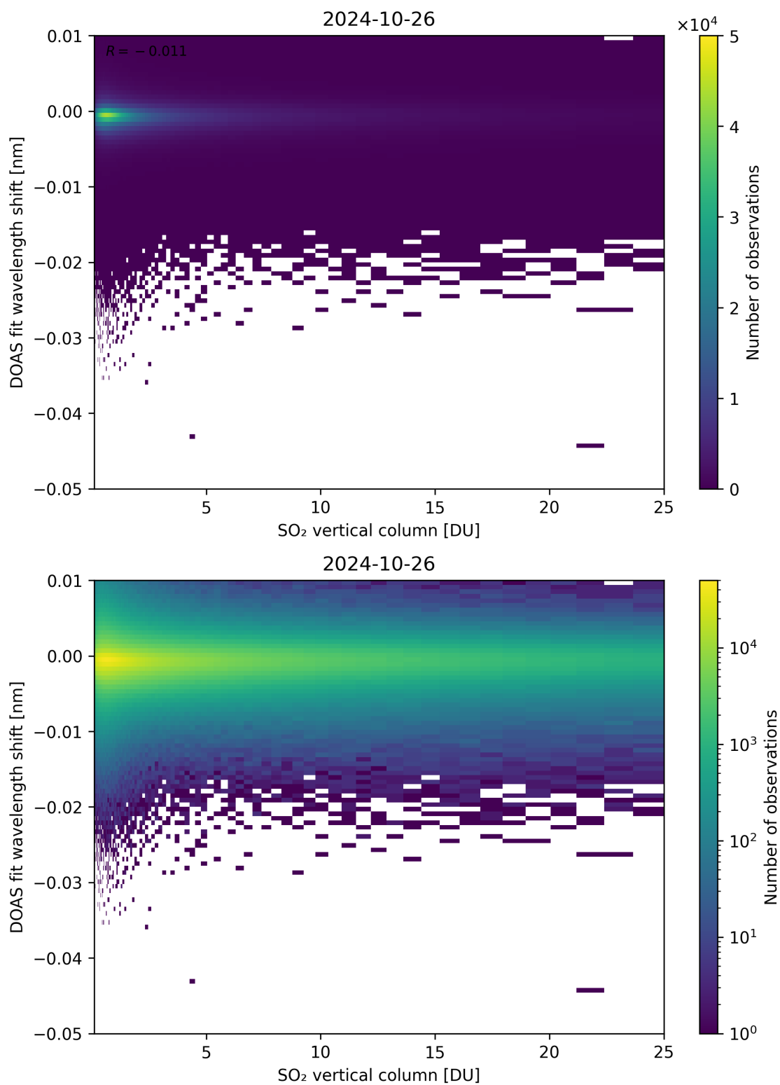
Figure 276: Scatter density plot of “SO 2 vertical column” against “DOAS fit wavelength shift” for 2024-10-25 to 2024-10-27.
