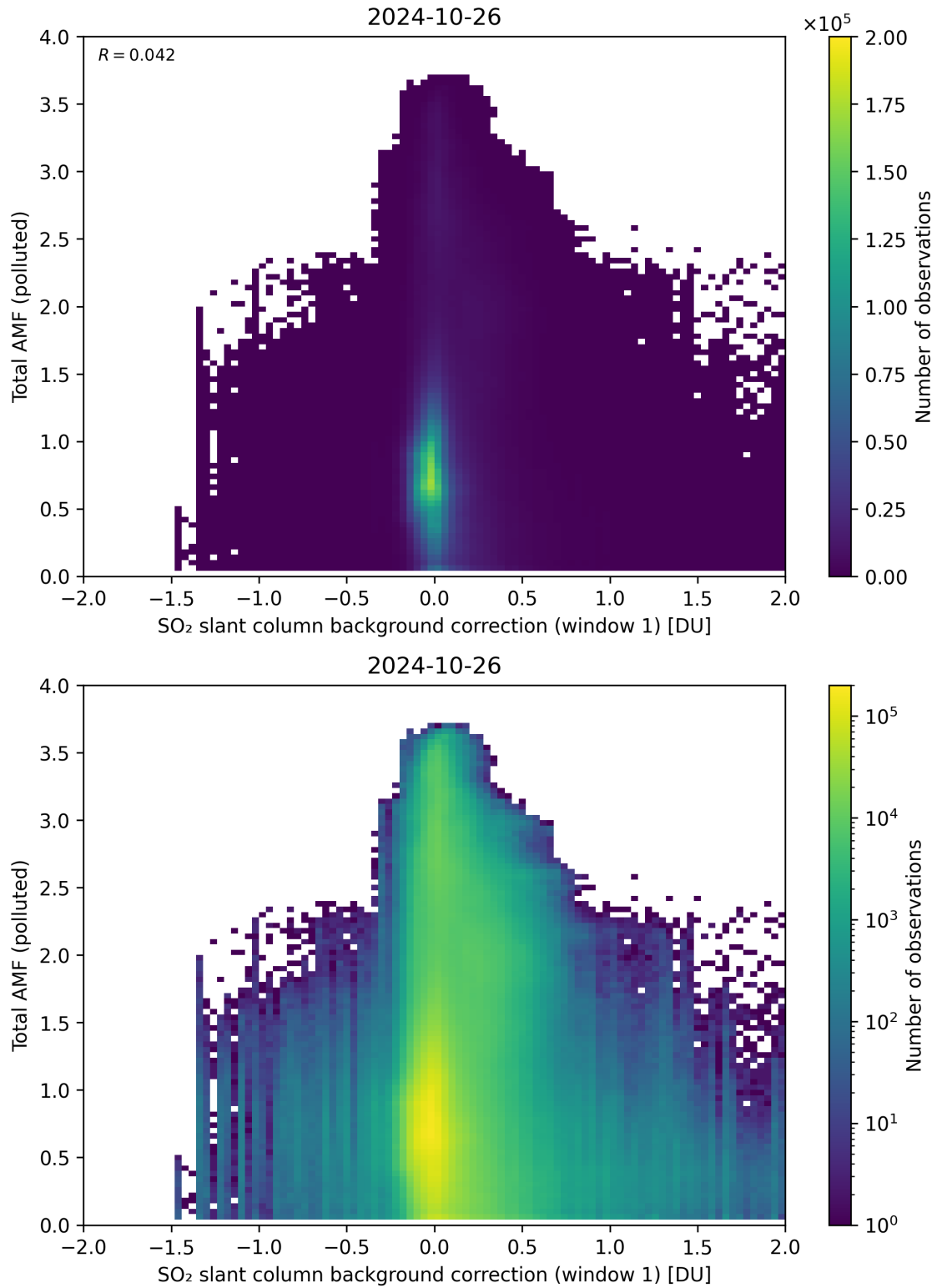
Figure 109: Scatter density plot of “SO 2 slant column background correction (window 1)” against “Total AMF (polluted)” for 2024-10-25 to 2024-10-27.
