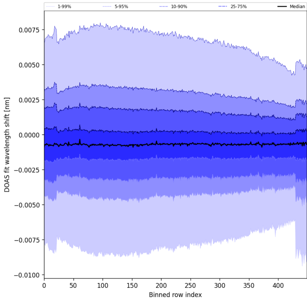
Figure 91: Along track statistics of “DOAS fit wavelength shift” for 2024-10-25 to 2024-10-27
