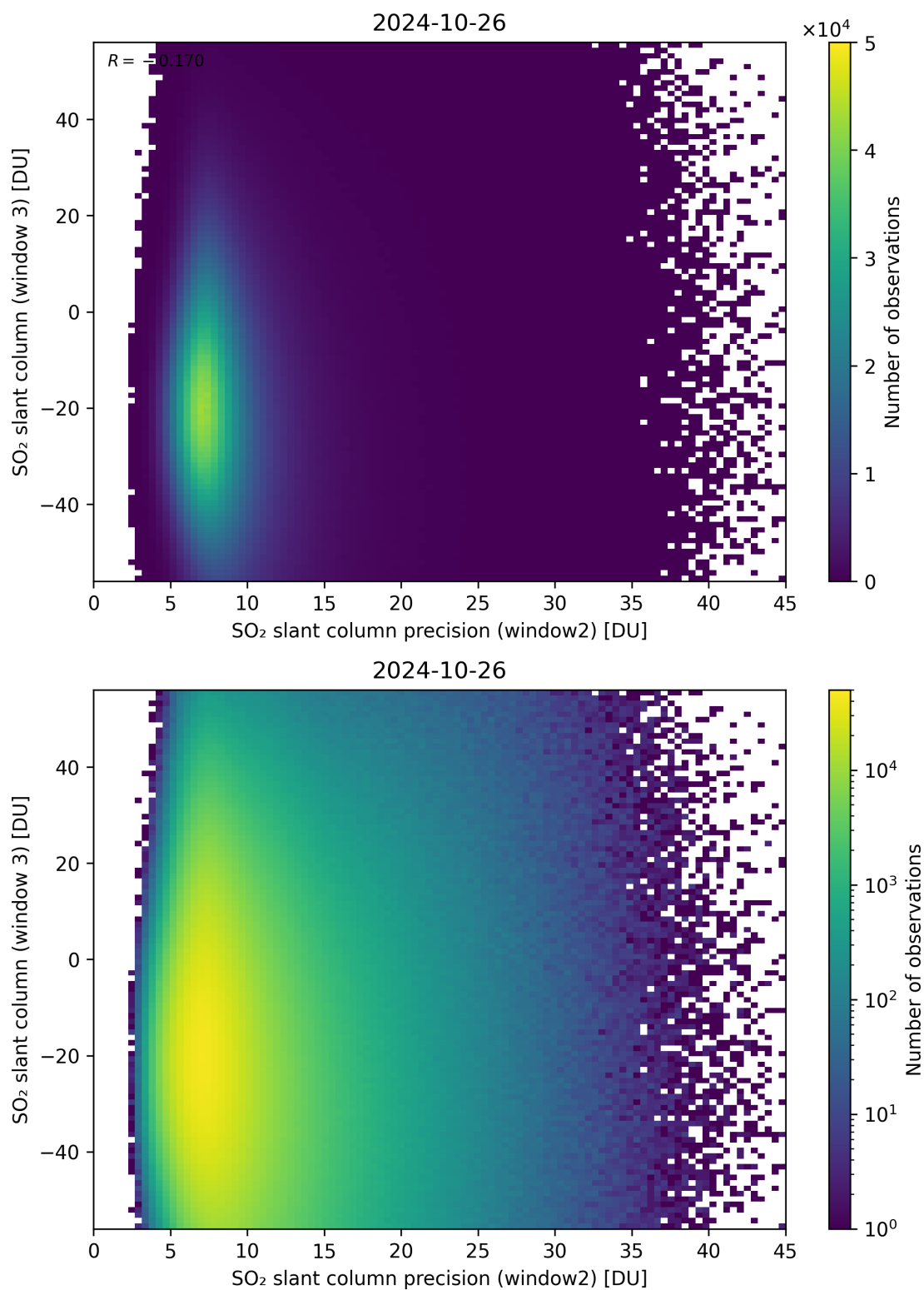
Figure 249: Scatter density plot of “SO 2 slant column precision (window2)” against “SO 2 slant column (window 3)” for 2024-10-25 to 2024-10-27.
