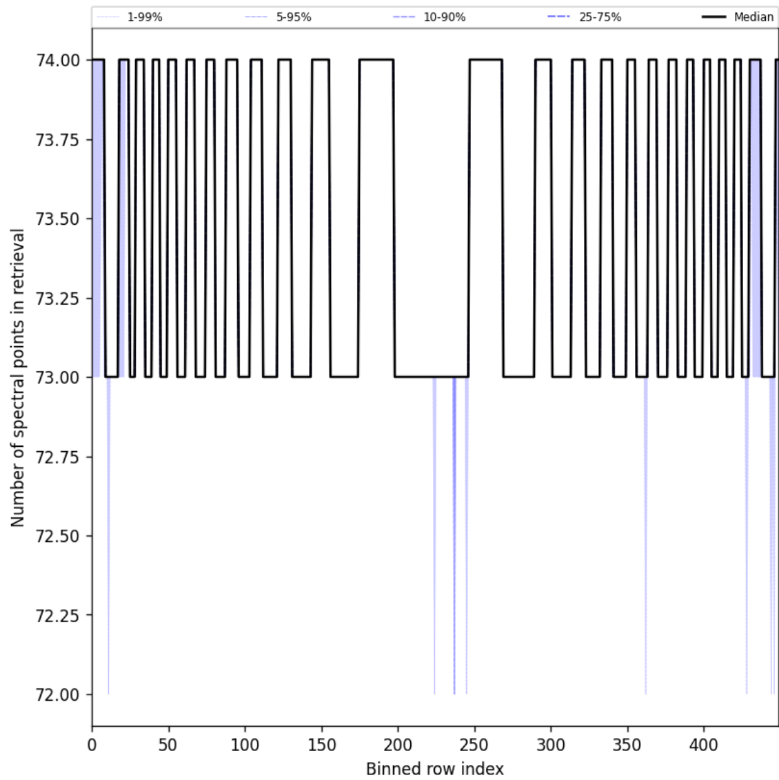
Figure 97: Along track statistics of “Number of spectral points in retrieval” for 2024-10-25 to 2024-10-27
