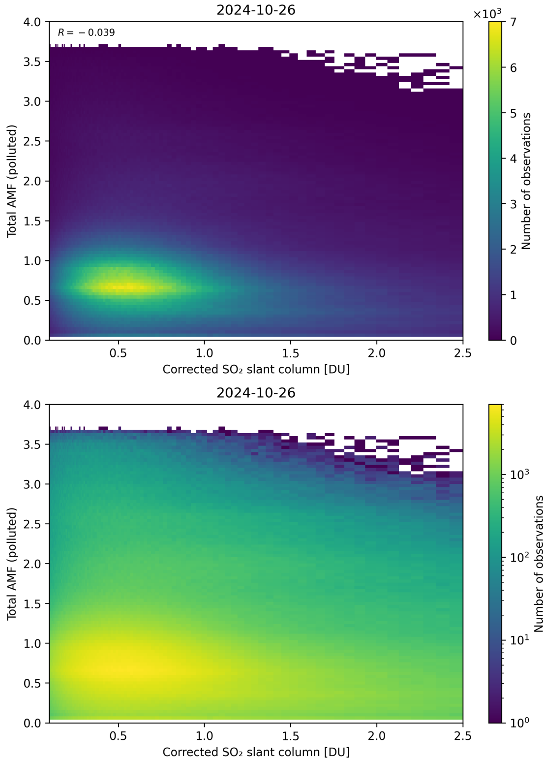
Figure 192: Scatter density plot of “Corrected SO 2 slant column” against “Total AMF (polluted)” for 2024-10-25 to 2024-10-27.
