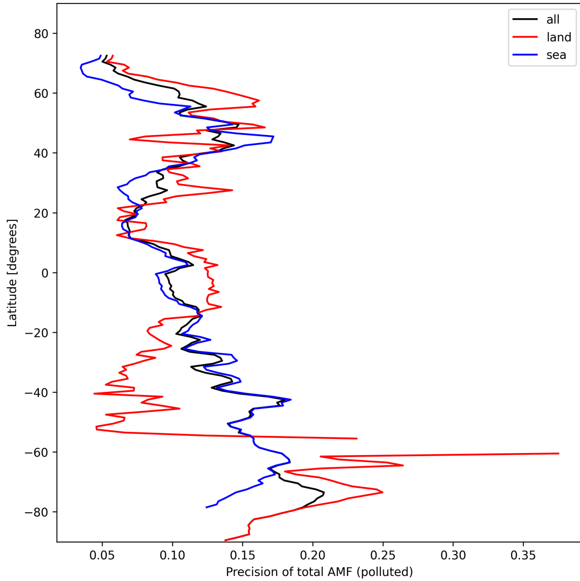
Figure 49: Zonal average of “Precision of total AMF (polluted)” for 2024-10-25 to 2024-10-27.
