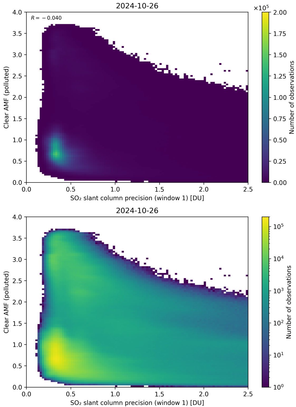
Figure 224: Scatter density plot of “SO 2 slant column precision (window 1)” against “Clear AMF (polluted)” for 2024-10-25 to 2024-10-27.
