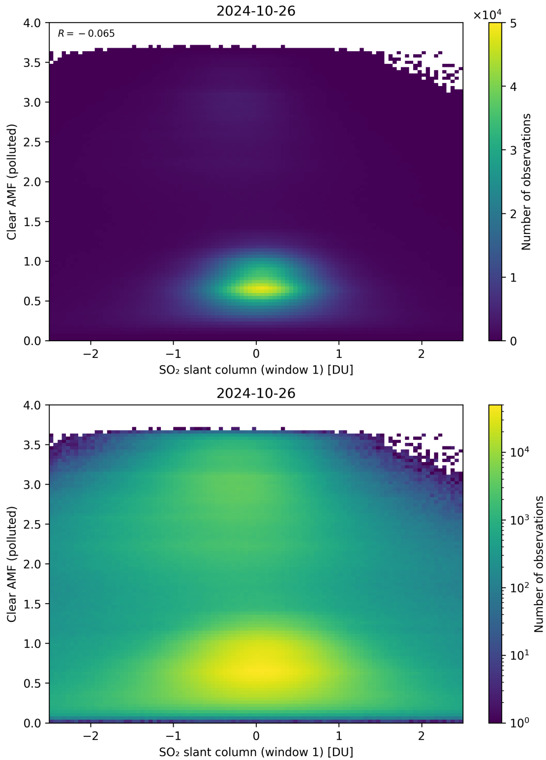
Figure 232: Scatter density plot of “SO 2 slant column (window 1)” against “Clear AMF (polluted)” for 2024-10-25 to 2024-10-27.
