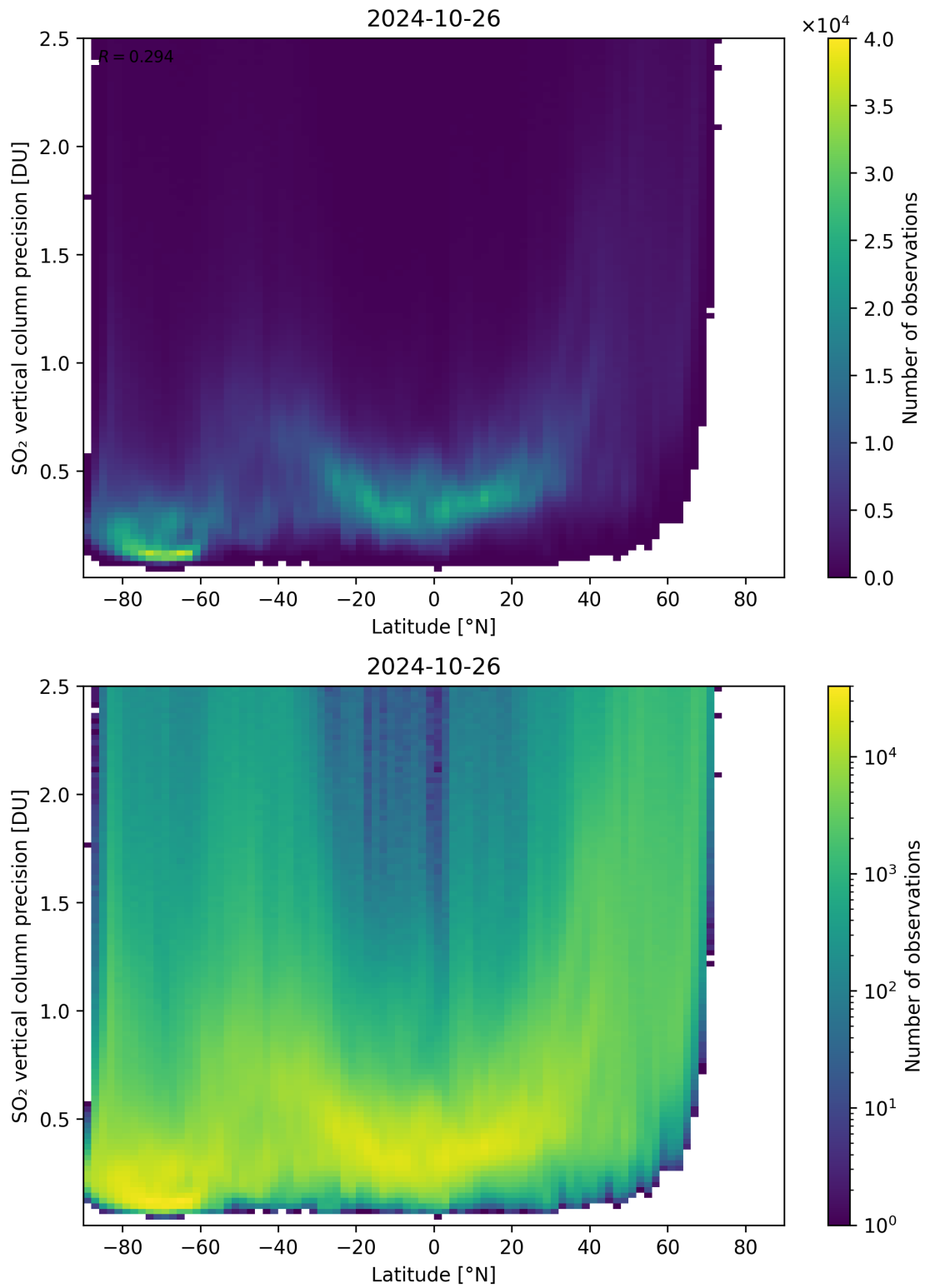
Figure 157: Scatter density plot of “Latitude” against “SO 2 vertical column precision” for 2024-10-25 to 2024-10-27.
