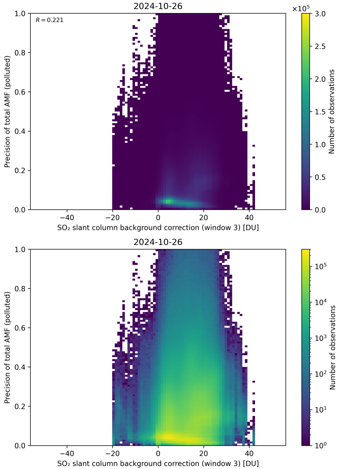
Figure 126: Scatter density plot of “SO 2 slant column background correction (window 3)” against “Precision of total AMF (polluted)” for 2024-10-25 to 2024-10-27.
