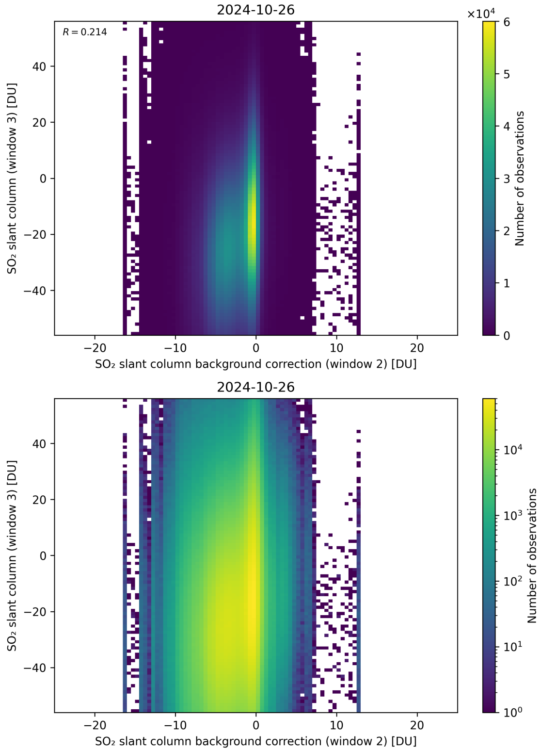
Figure 117: Scatter density plot of “SO 2 slant column background correction (window 2)” against “SO 2 slant column (window 3)” for 2024-10-25 to 2024-10-27.
