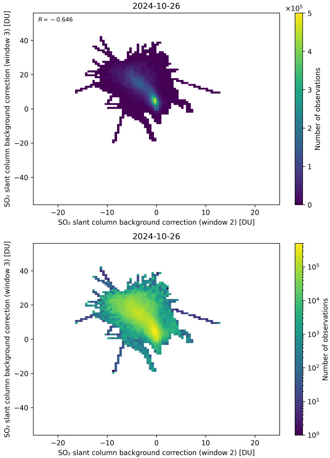
Figure 111: Scatter density plot of “SO 2 slant column background correction (window 2)” against “SO 2 slant column background correction (window 3)” for 2024-10-25 to 2024-10-27.
