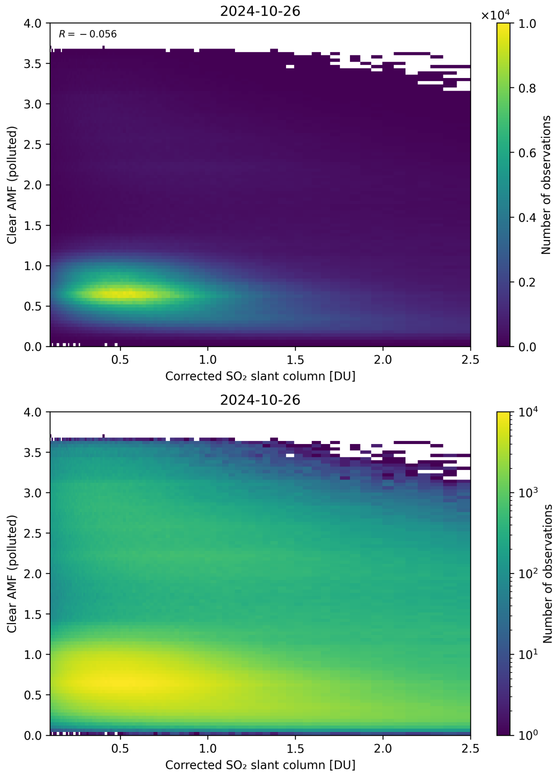
Figure 184: Scatter density plot of “Corrected SO 2 slant column” against “Clear AMF (polluted)” for 2024-10-25 to 2024-10-27.
