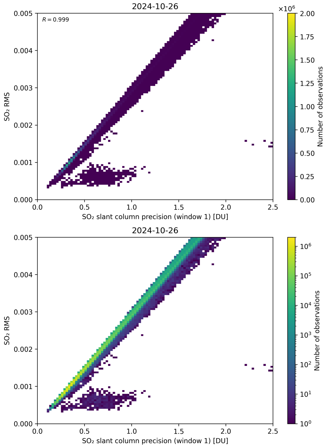
Figure 223: Scatter density plot of “SO 2 slant column precision (window 1)” against “SO 2 RMS” for 2024-10-25 to 2024-10-27.
