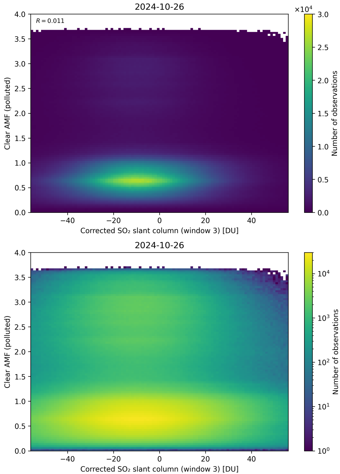
Figure 209: Scatter density plot of “Corrected SO 2 slant column (window 3)” against “Clear AMF (polluted)” for 2024-10-25 to 2024-10-27.
