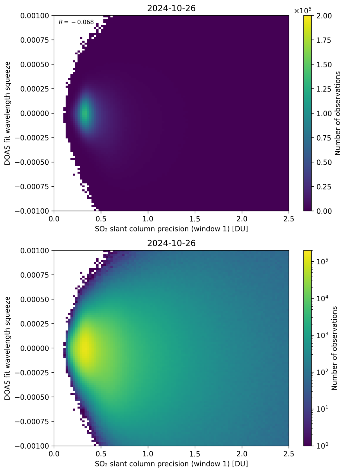
Figure 222: Scatter density plot of “SO 2 slant column precision (window 1)” against “DOAS fit wavelength squeeze” for 2024-10-25 to 2024-10-27.
