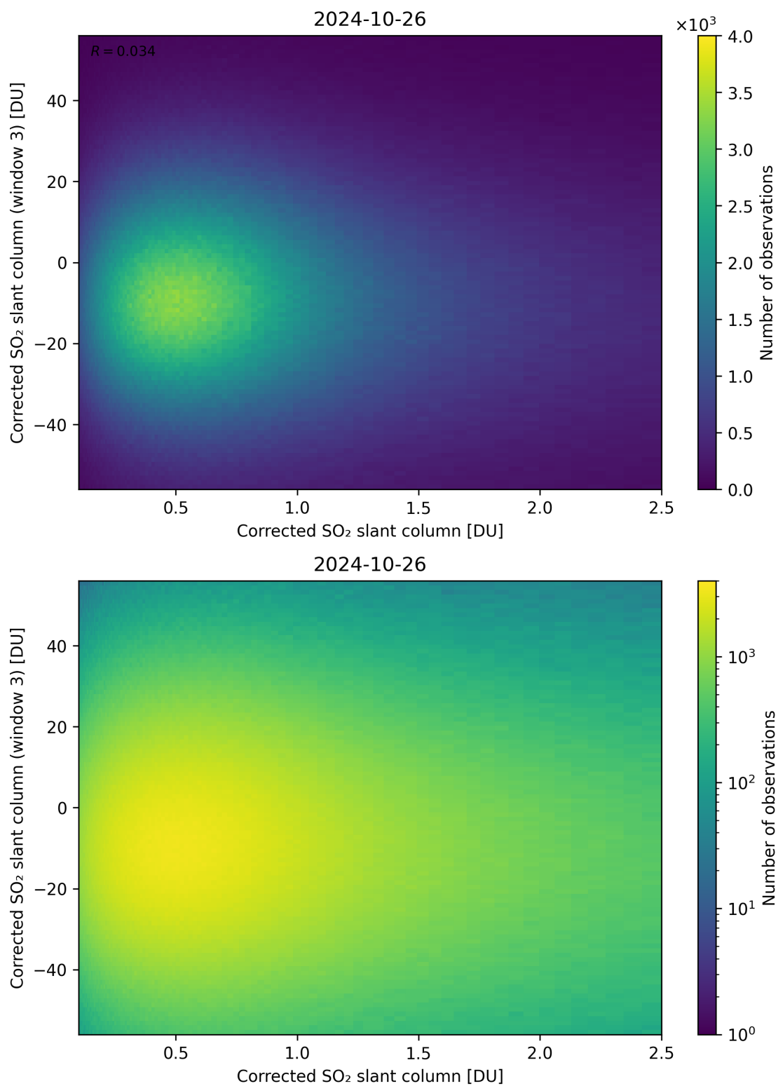
Figure 186: Scatter density plot of “Corrected SO 2 slant column” against “Corrected SO 2 slant column (window 3)” for 2024-10-25 to 2024-10-27.
