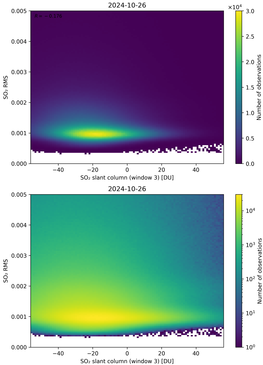
Figure 256: Scatter density plot of “SO 2 slant column (window 3)” against “SO 2 RMS” for 2024-10-25 to 2024-10-27.
