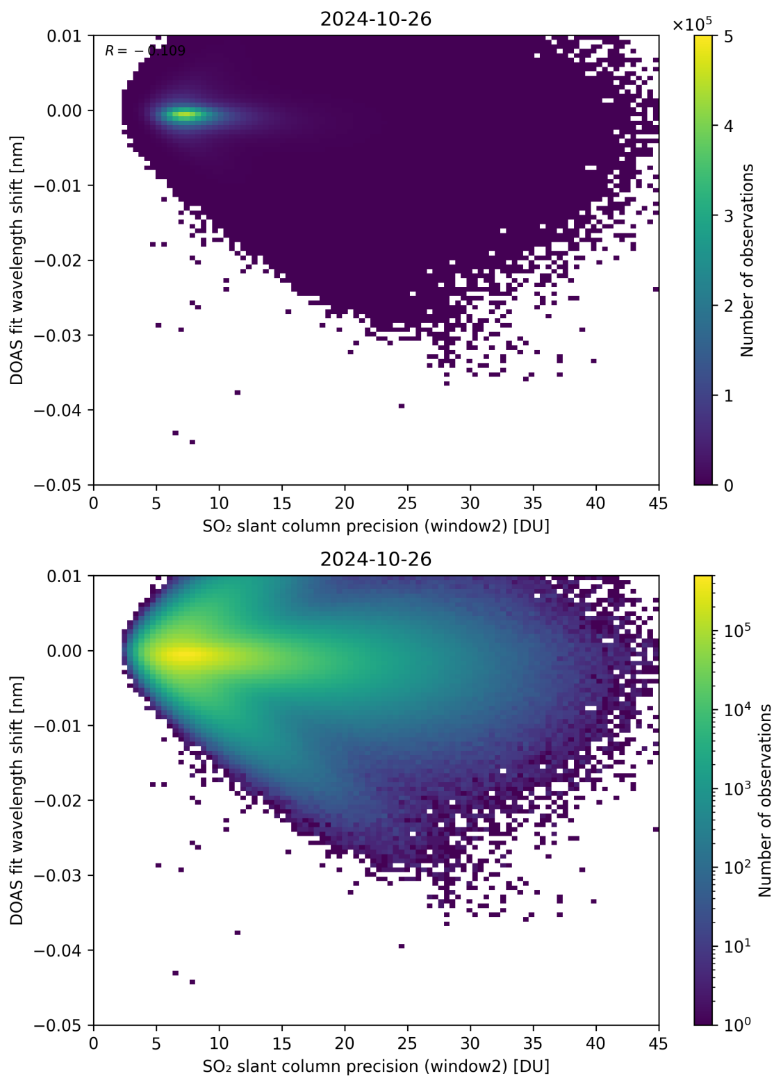
Figure 243: Scatter density plot of “SO 2 slant column precision (window2)” against “DOAS fit wavelength shift” for 2024-10-25 to 2024-10-27.
