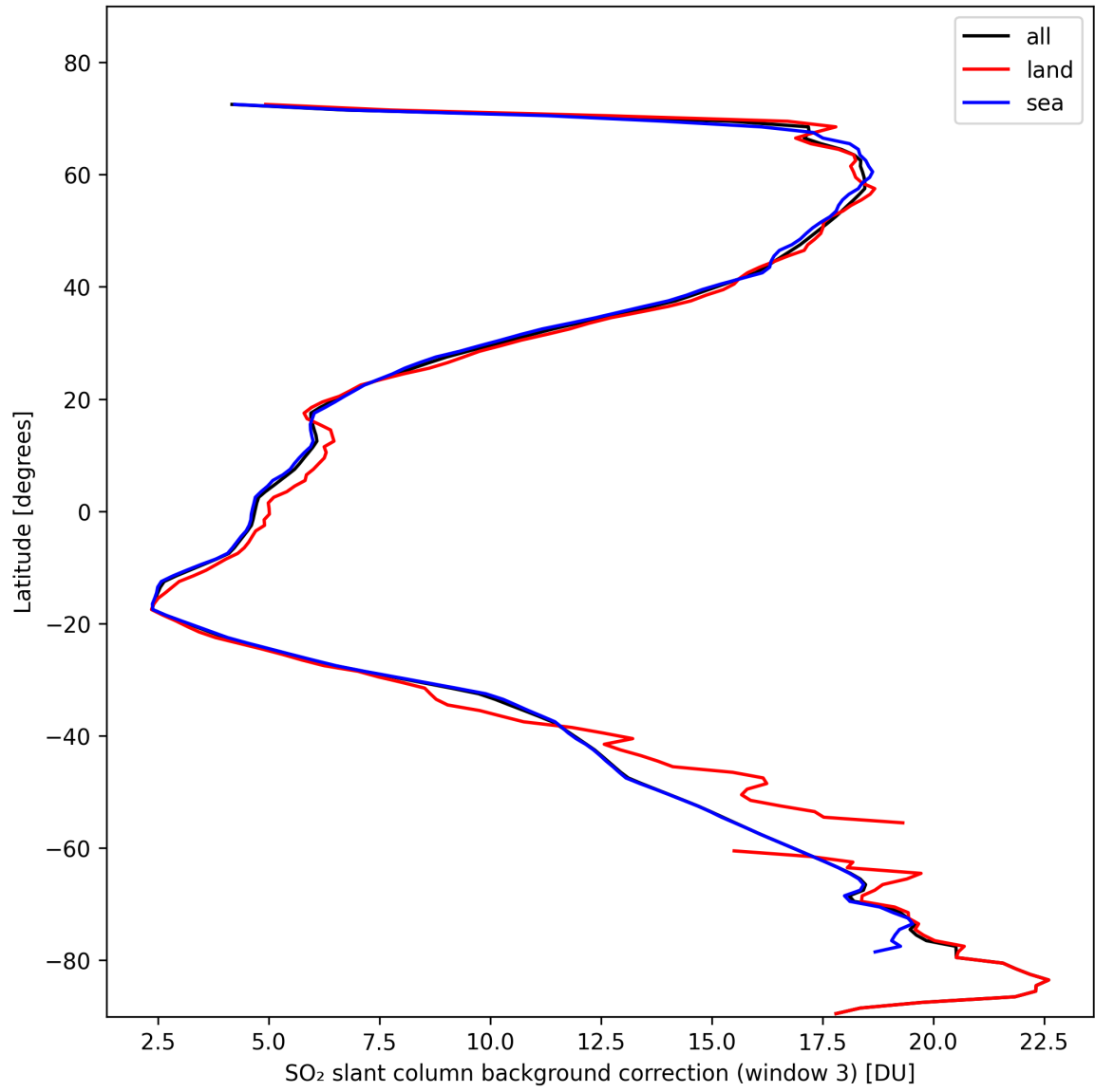
Figure 44: Zonal average of “SO 2 slant column background correction (window 3)” for 2024-10-25 to 2024-10-27.
