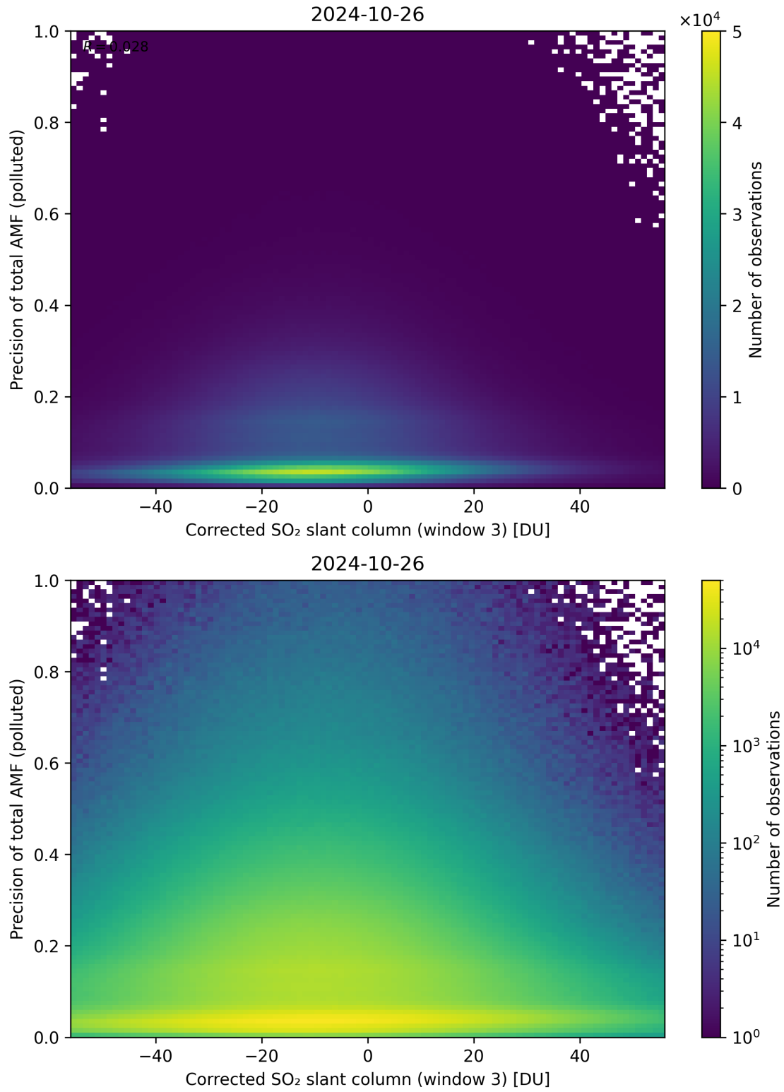
Figure 211: Scatter density plot of “Corrected SO 2 slant column (window 3)” against “Precision of total AMF (polluted)” for 2024-10-25 to 2024-10-27.
