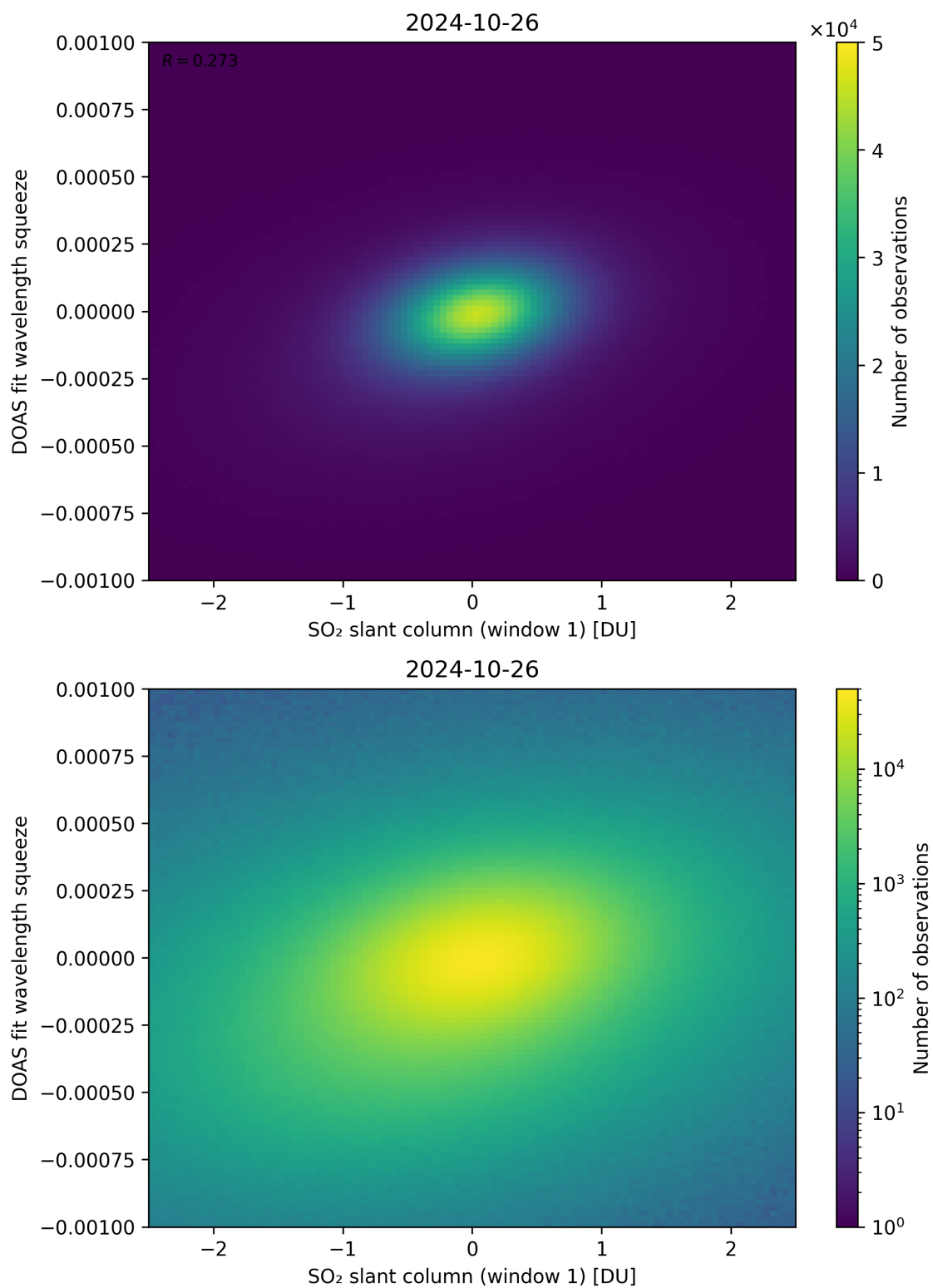
Figure 216: Scatter density plot of “SO 2 slant column (window 1)” against “DOAS fit wavelength squeeze” for 2024-10-25 to 2024-10-27.
