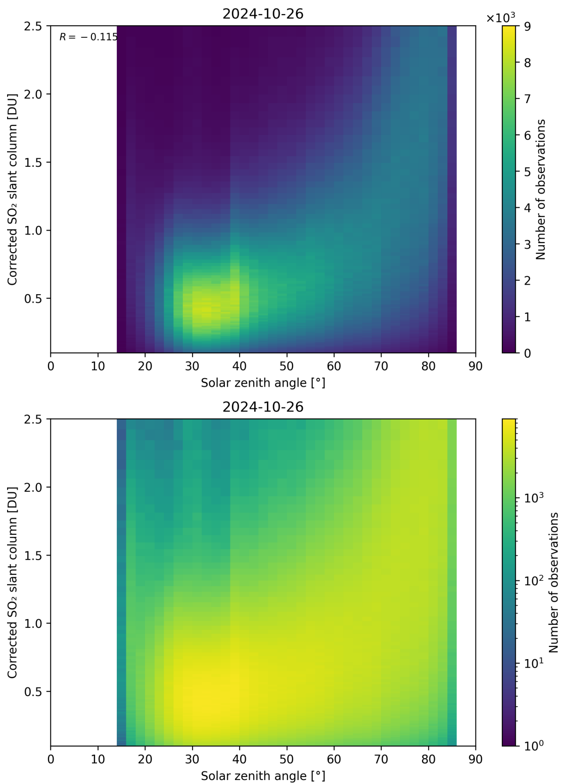
Figure 166: Scatter density plot of “Solar zenith angle” against “Corrected SO 2 slant column” for 2024-10-25 to 2024-10-27.
