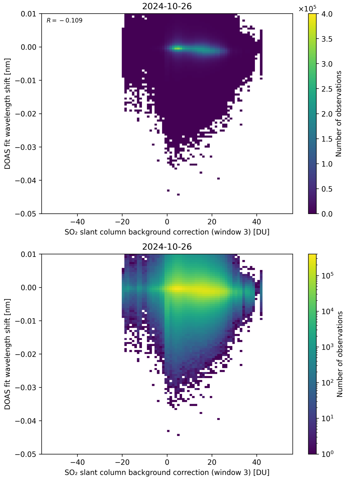
Figure 121: Scatter density plot of “SO 2 slant column background correction (window 3)” against “DOAS fit wavelength shift” for 2024-10-25 to 2024-10-27.
