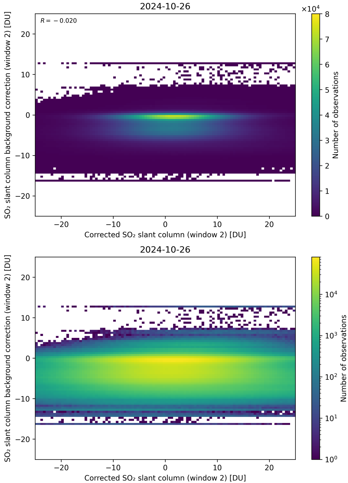
Figure 194: Scatter density plot of “Corrected SO 2 slant column (window 2)” against “SO 2 slant column background correction (window 2)” for 2024-10-25 to 2024-10-27.
