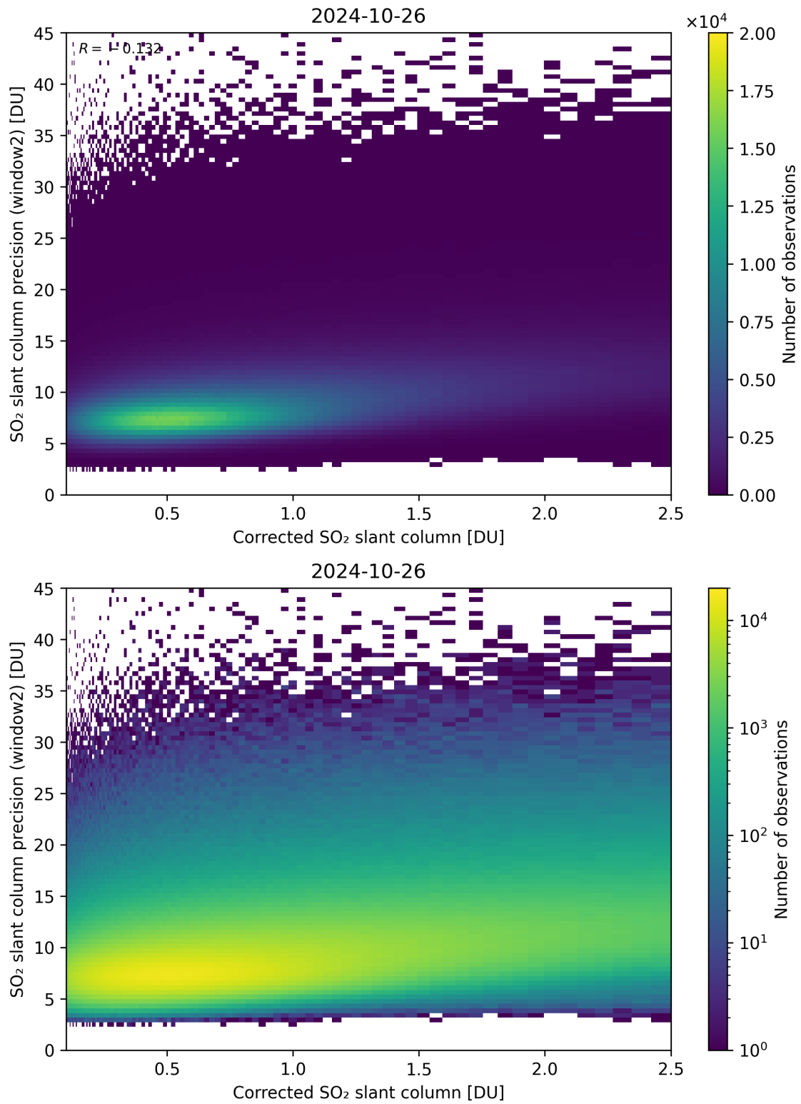
Figure 189: Scatter density plot of “Corrected SO 2 slant column” against “SO 2 slant column precision (window2)” for 2024-10-25 to 2024-10-27.
