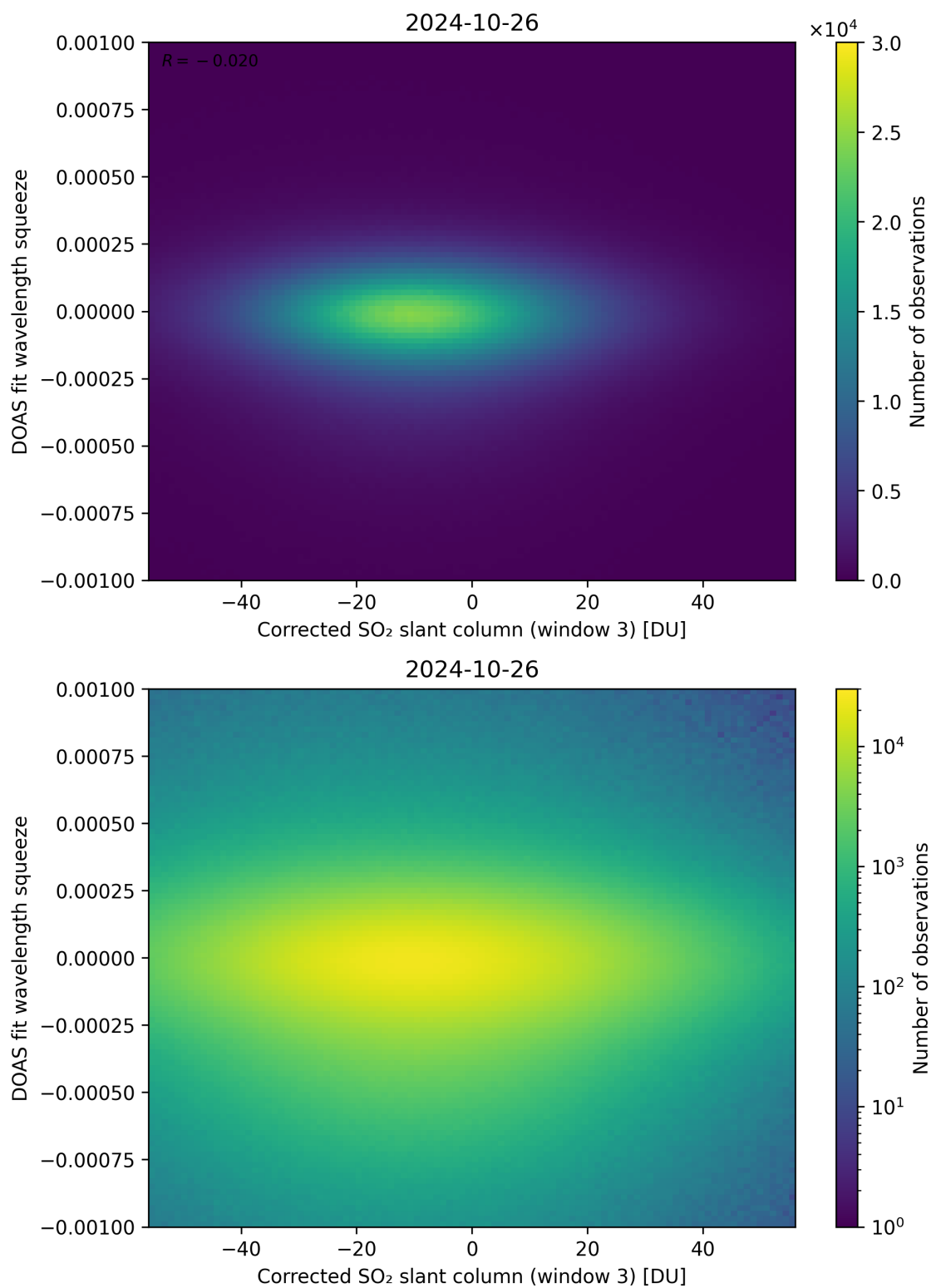
Figure 207: Scatter density plot of “Corrected SO 2 slant column (window 3)” against “DOAS fit wavelength squeeze” for 2024-10-25 to 2024-10-27.
