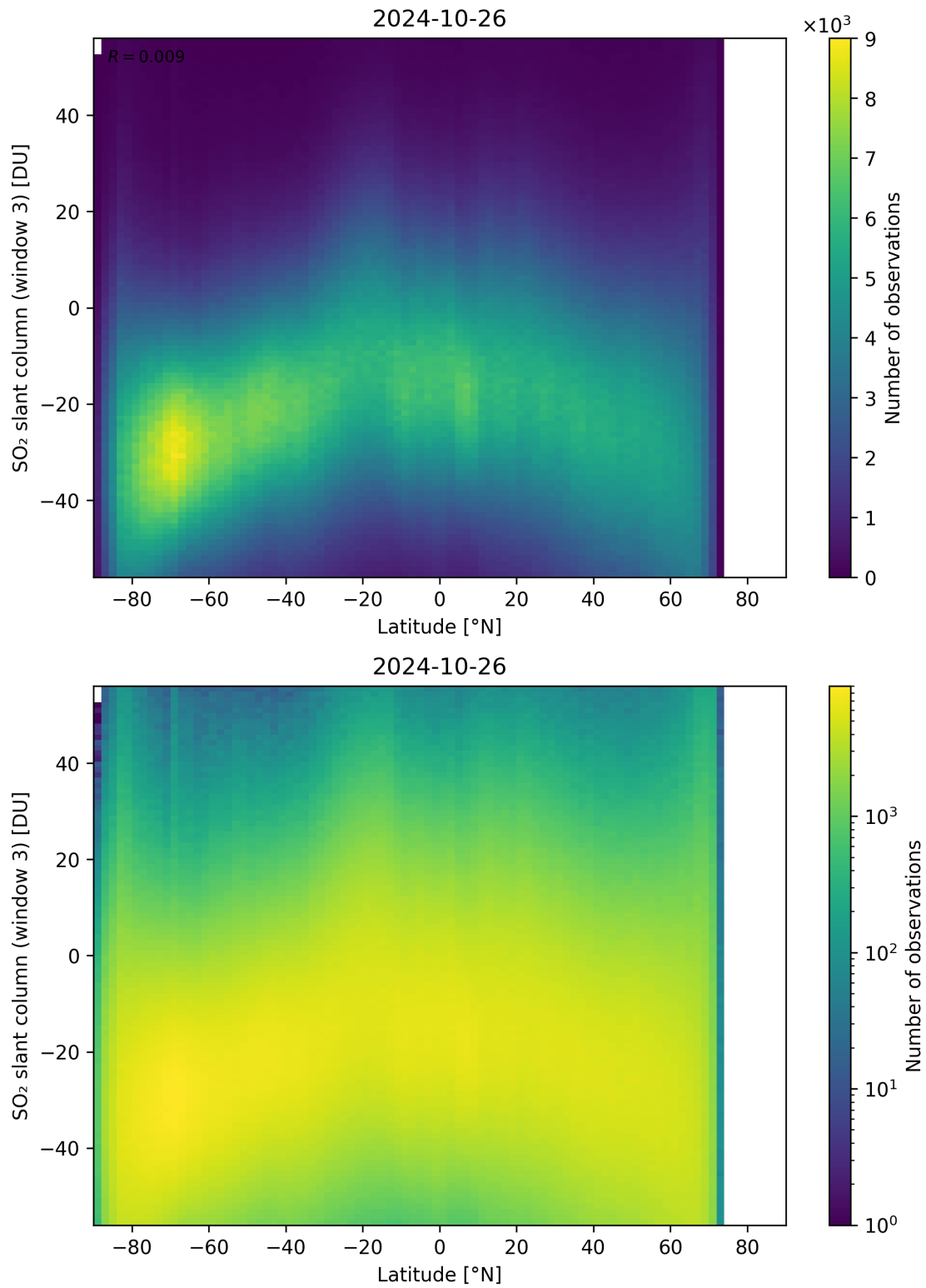
Figure 152: Scatter density plot of “Latitude” against “SO 2 slant column (window 3)” for 2024-10-25 to 2024-10-27.
