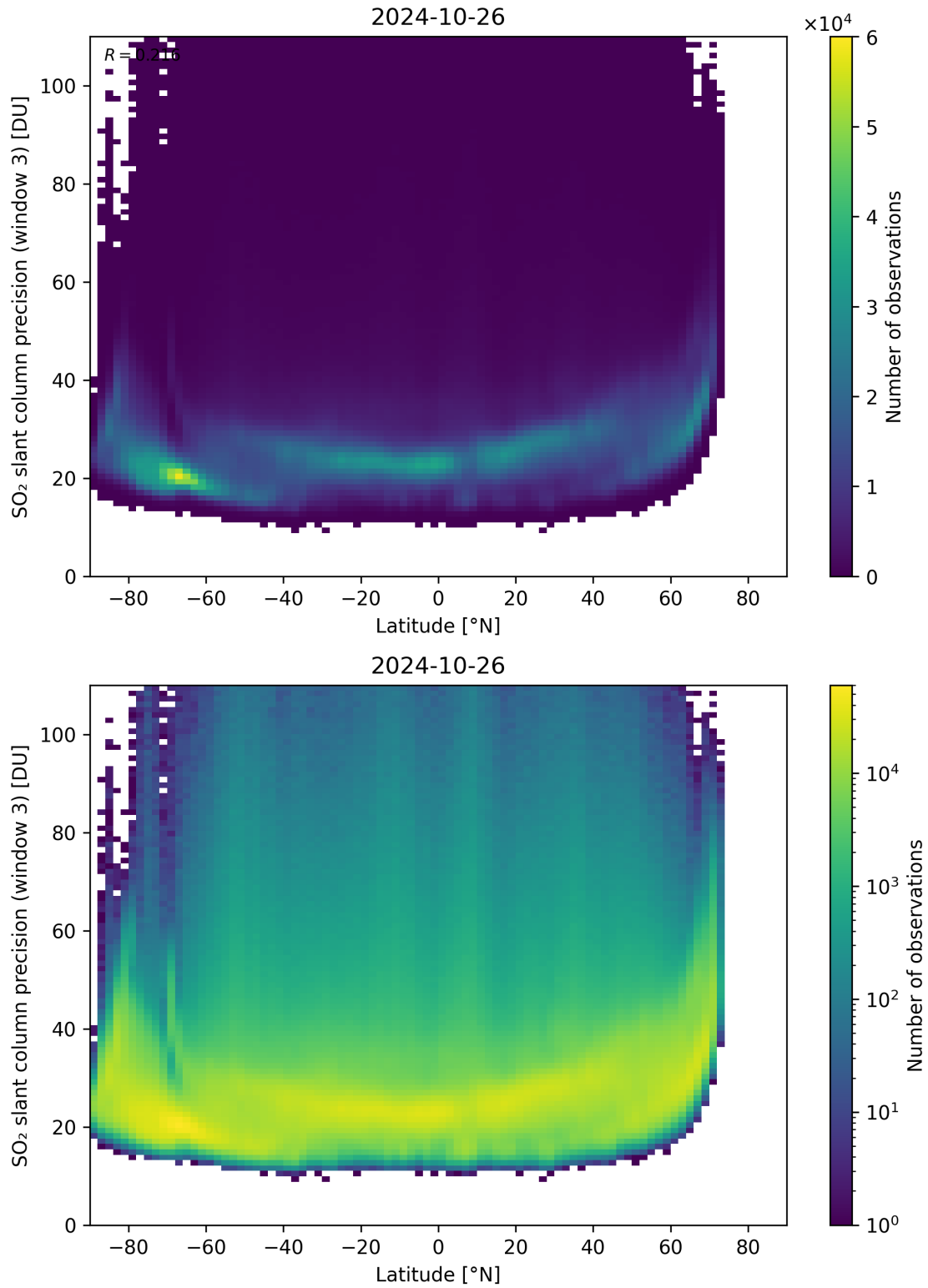
Figure 153: Scatter density plot of “Latitude” against “SO 2 slant column precision (window 3)” for 2024-10-25 to 2024-10-27.
