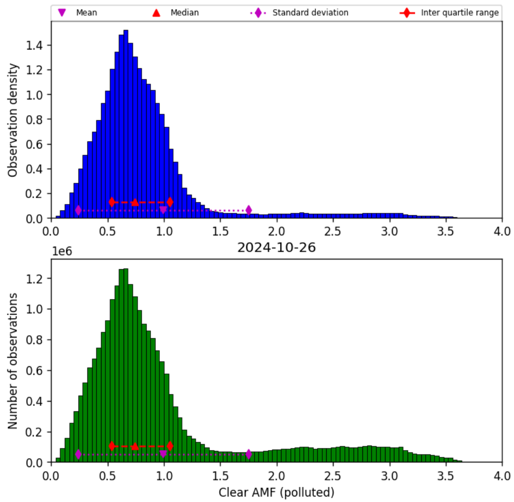
Figure 73: Histogram of “Clear AMF (polluted)” for 2024-10-25 to 2024-10-27
