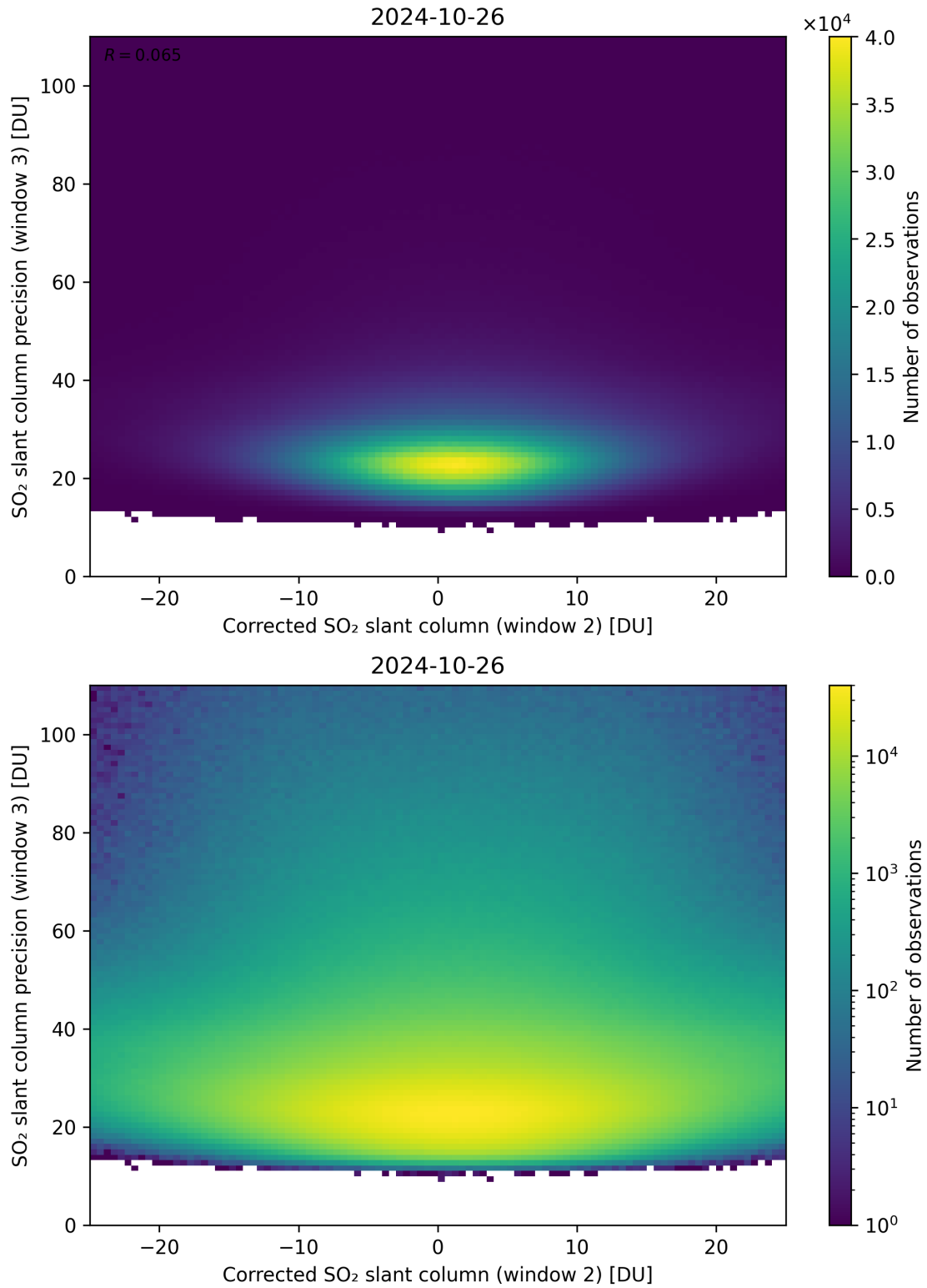
Figure 202: Scatter density plot of “Corrected SO 2 slant column (window 2)” against “SO 2 slant column precision (window 3)” for 2024-10-25 to 2024-10-27.
