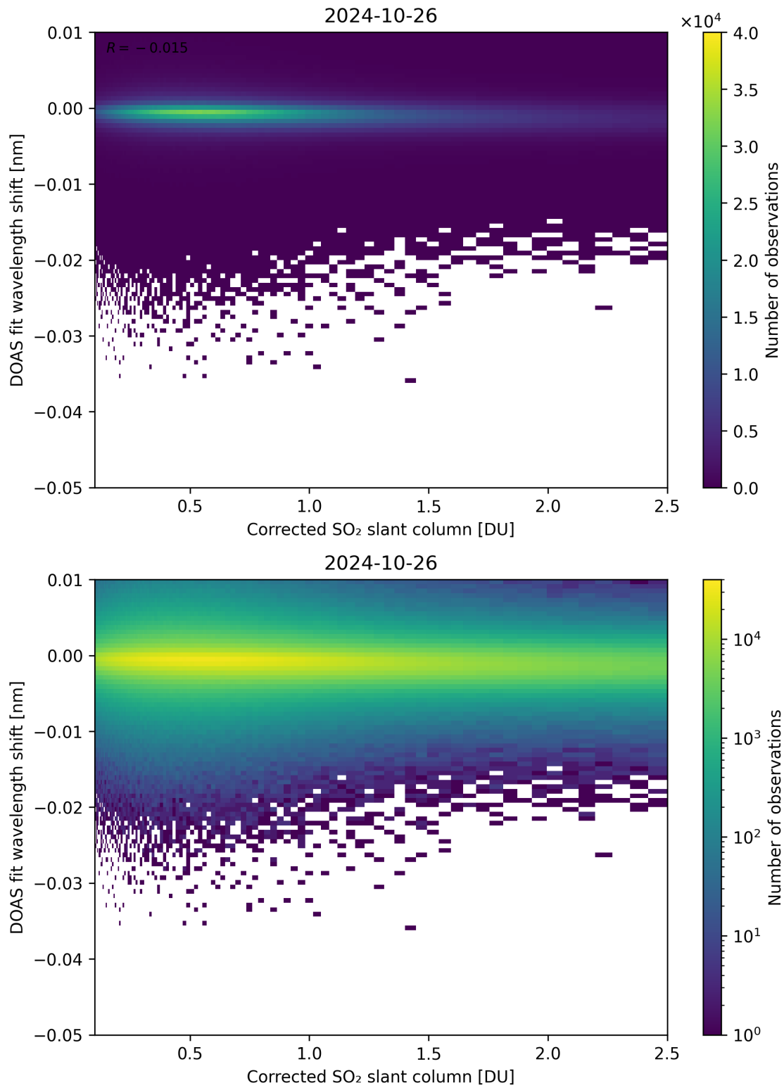
Figure 181: Scatter density plot of “Corrected SO 2 slant column” against “DOAS fit wavelength shift” for 2024-10-25 to 2024-10-27.
