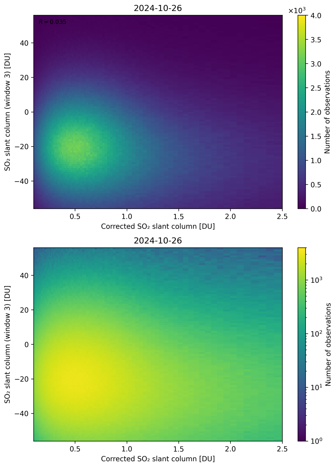
Figure 190: Scatter density plot of “Corrected SO 2 slant column” against “SO 2 slant column (window 3)” for 2024-10-25 to 2024-10-27.
