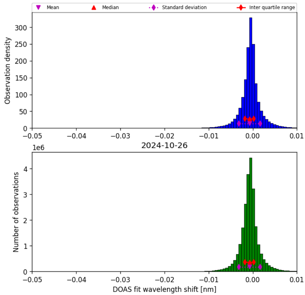
Figure 68: Histogram of “DOAS fit wavelength shift” for 2024-10-25 to 2024-10-27
