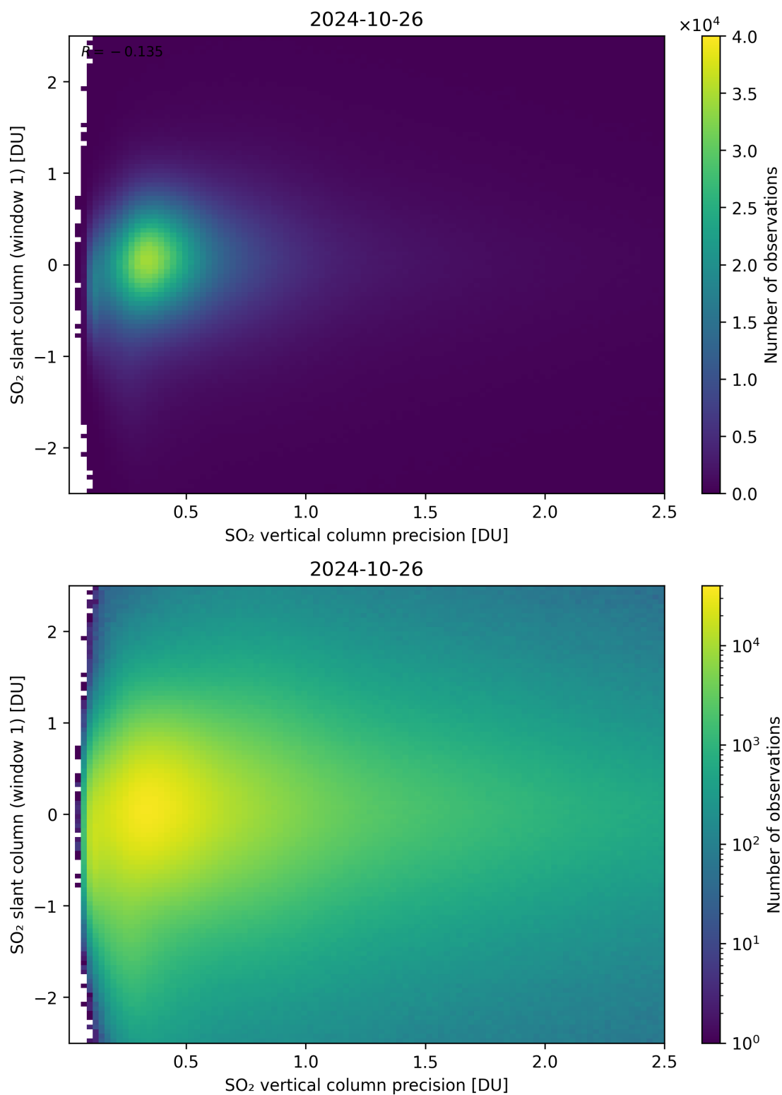
Figure 289: Scatter density plot of “SO 2 vertical column precision” against “SO 2 slant column (window 1)” for 2024-10-25 to 2024-10-27.
