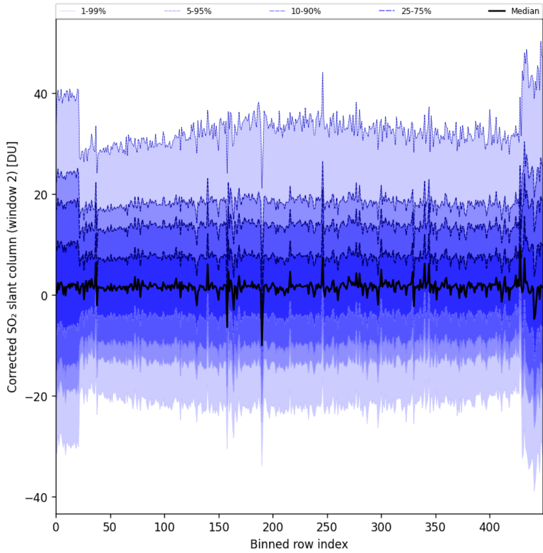
Figure 85: Along track statistics of “Corrected SO 2 slant column (window 2)” for 2024-10-25 to 2024-10-27
