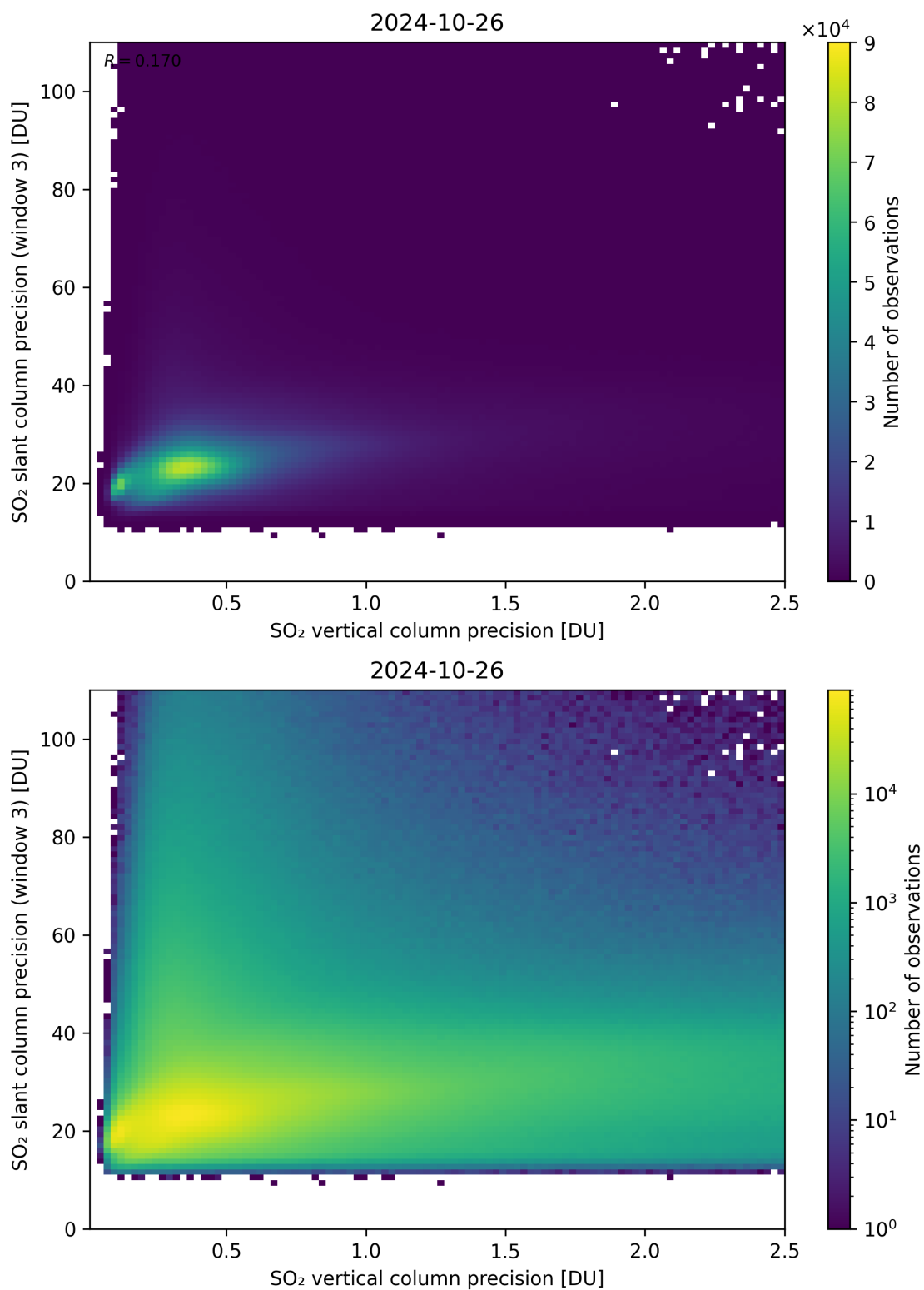
Figure 293: Scatter density plot of “SO 2 vertical column precision” against “SO 2 slant column precision (window 3)” for 2024-10-25 to 2024-10-27.
