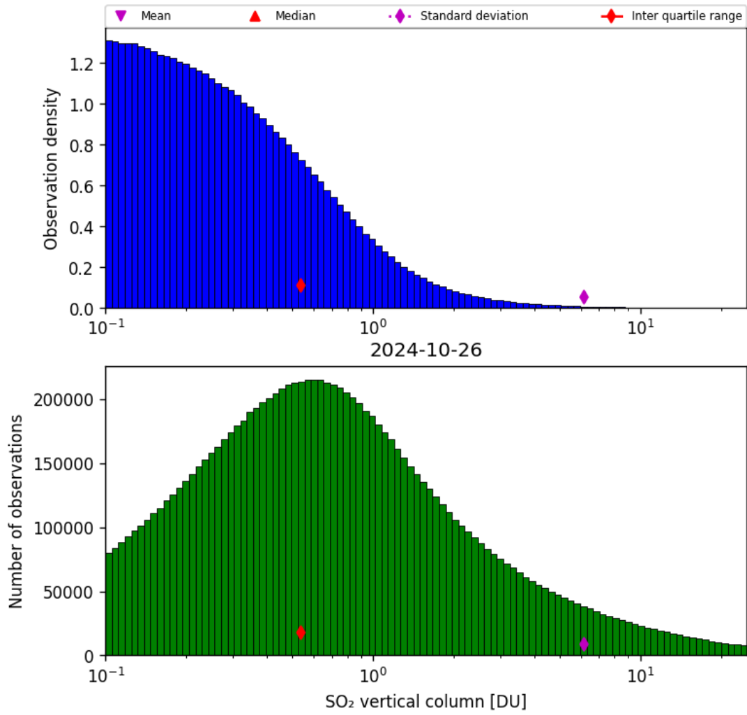
Figure 53: Histogram of “SO 2 vertical column” for 2024-10-25 to 2024-10-27
