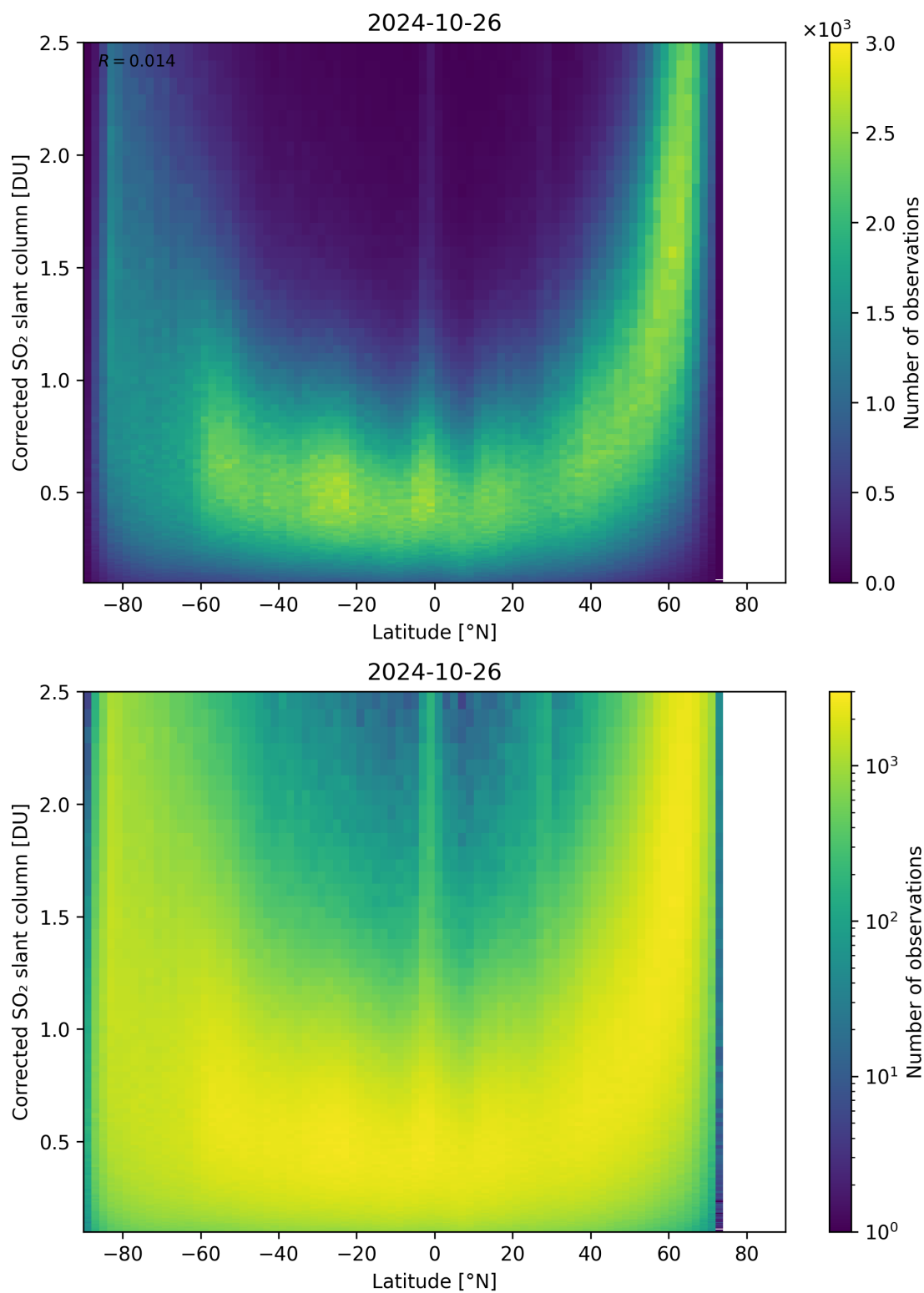
Figure 146: Scatter density plot of “Latitude” against “Corrected SO 2 slant column” for 2024-10-25 to 2024-10-27.
