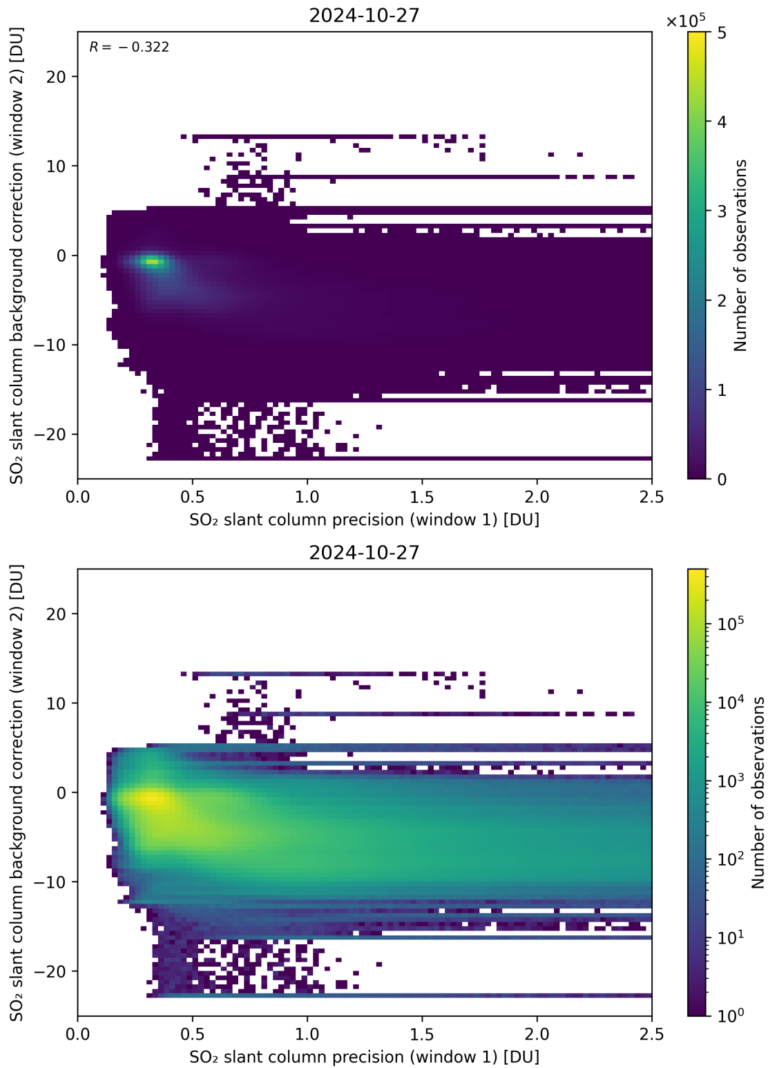
Figure 219: Scatter density plot of “SO 2 slant column precision (window 1)” against “SO 2 slant column background correction (window 2)” for 2024-10-26 to 2024-10-28.
