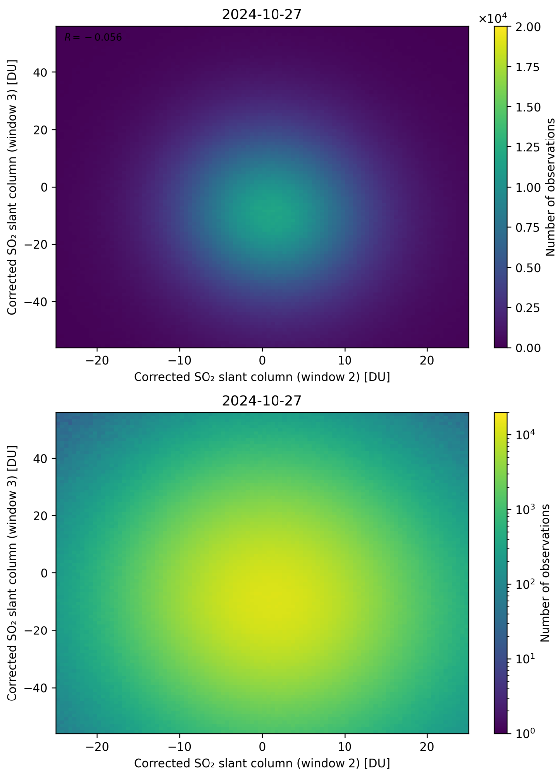
Figure 200: Scatter density plot of “Corrected SO 2 slant column (window 2)” against “Corrected SO 2 slant column (window 3)” for 2024-10-26 to 2024-10-28.
