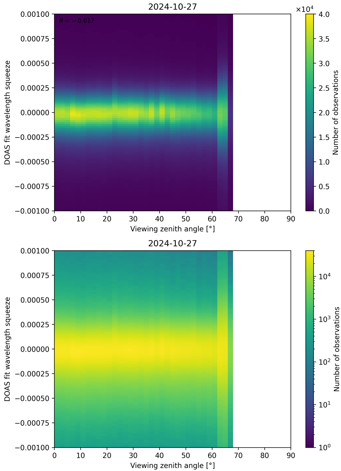
Figure 312: Scatter density plot of “Viewing zenith angle” against “DOAS fit wavelength squeeze” for 2024-10-26 to 2024-10-28.
