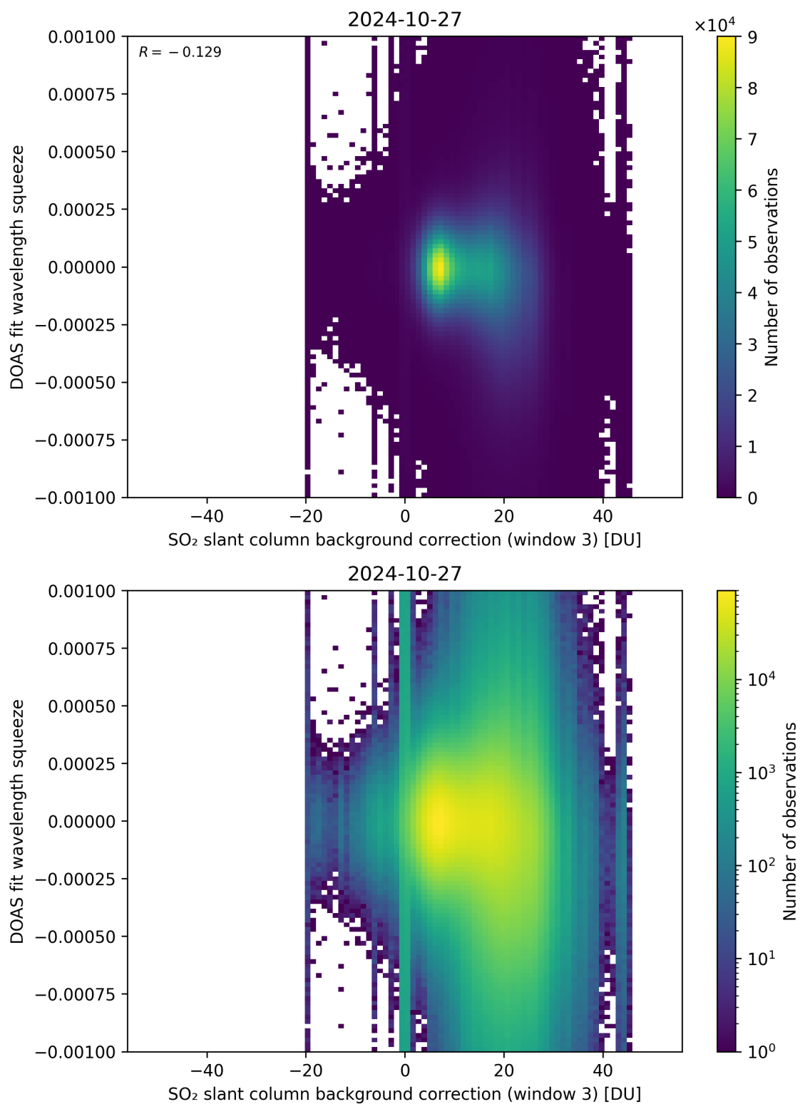
Figure 122: Scatter density plot of “SO 2 slant column background correction (window 3)” against “DOAS fit wavelength squeeze” for 2024-10-26 to 2024-10-28.
