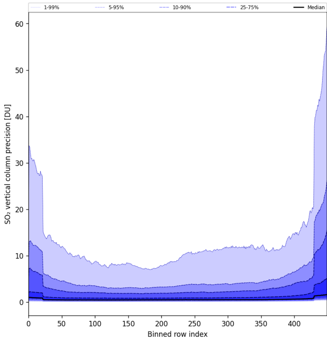
Figure 77: Along track statistics of “SO 2 vertical column precision” for 2024-10-26 to 2024-10-28
