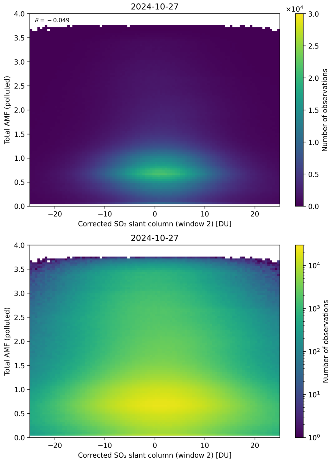
Figure 203: Scatter density plot of “Corrected SO 2 slant column (window 2)” against “Total AMF (polluted)” for 2024-10-26 to 2024-10-28.
