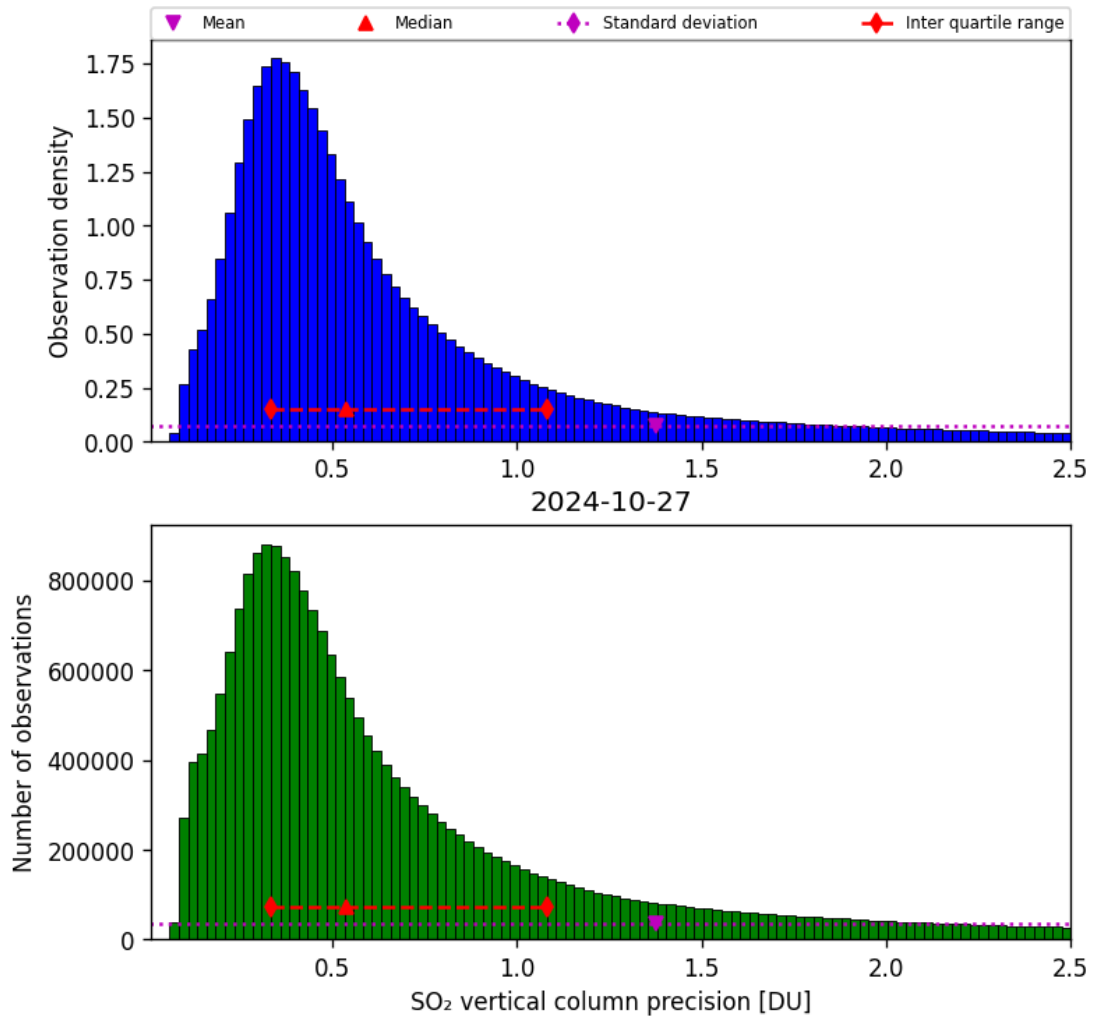
Figure 54: Histogram of “SO 2 vertical column precision” for 2024-10-26 to 2024-10-28
