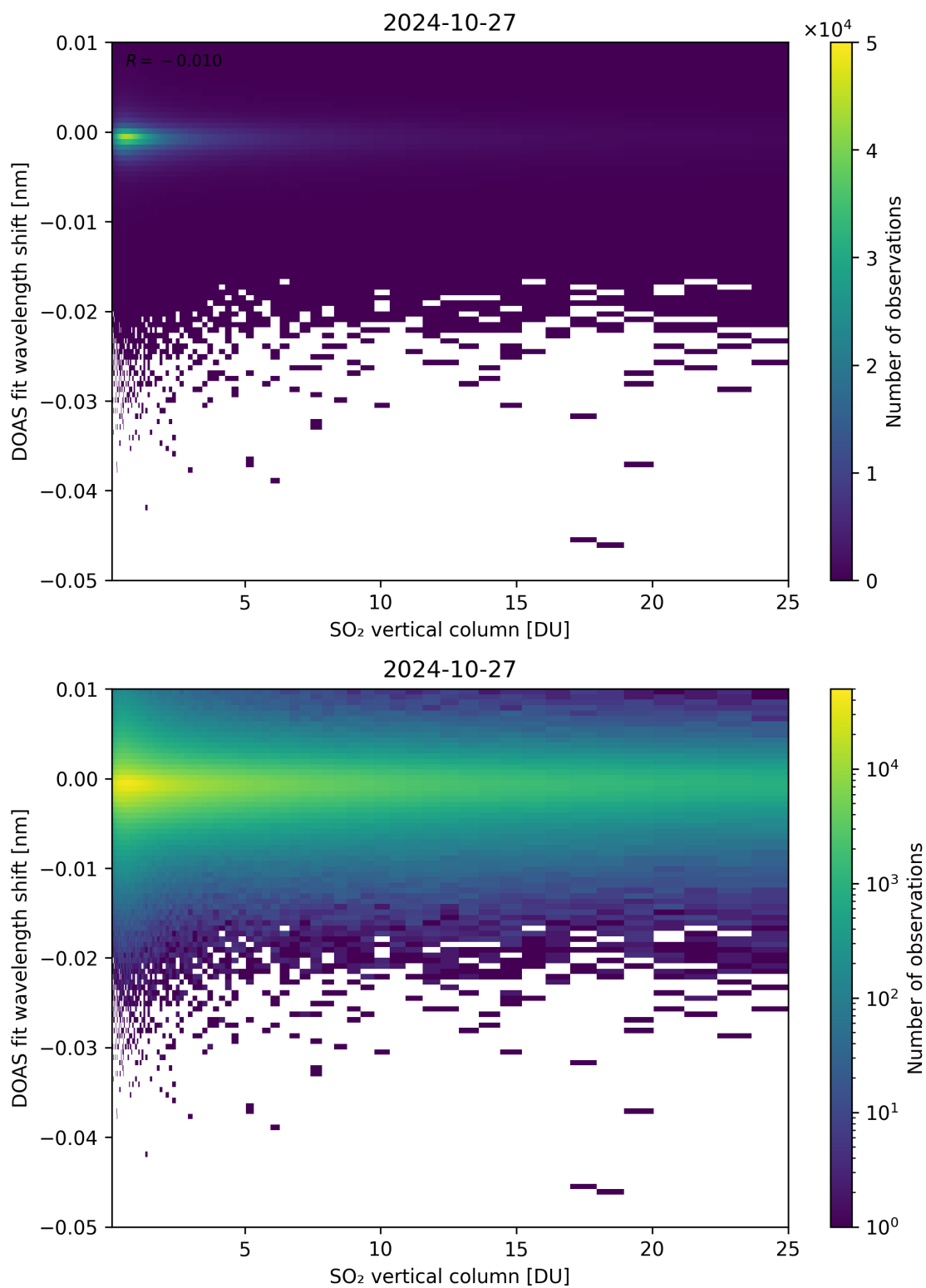
Figure 276: Scatter density plot of “SO 2 vertical column” against “DOAS fit wavelength shift” for 2024-10-26 to 2024-10-28.
