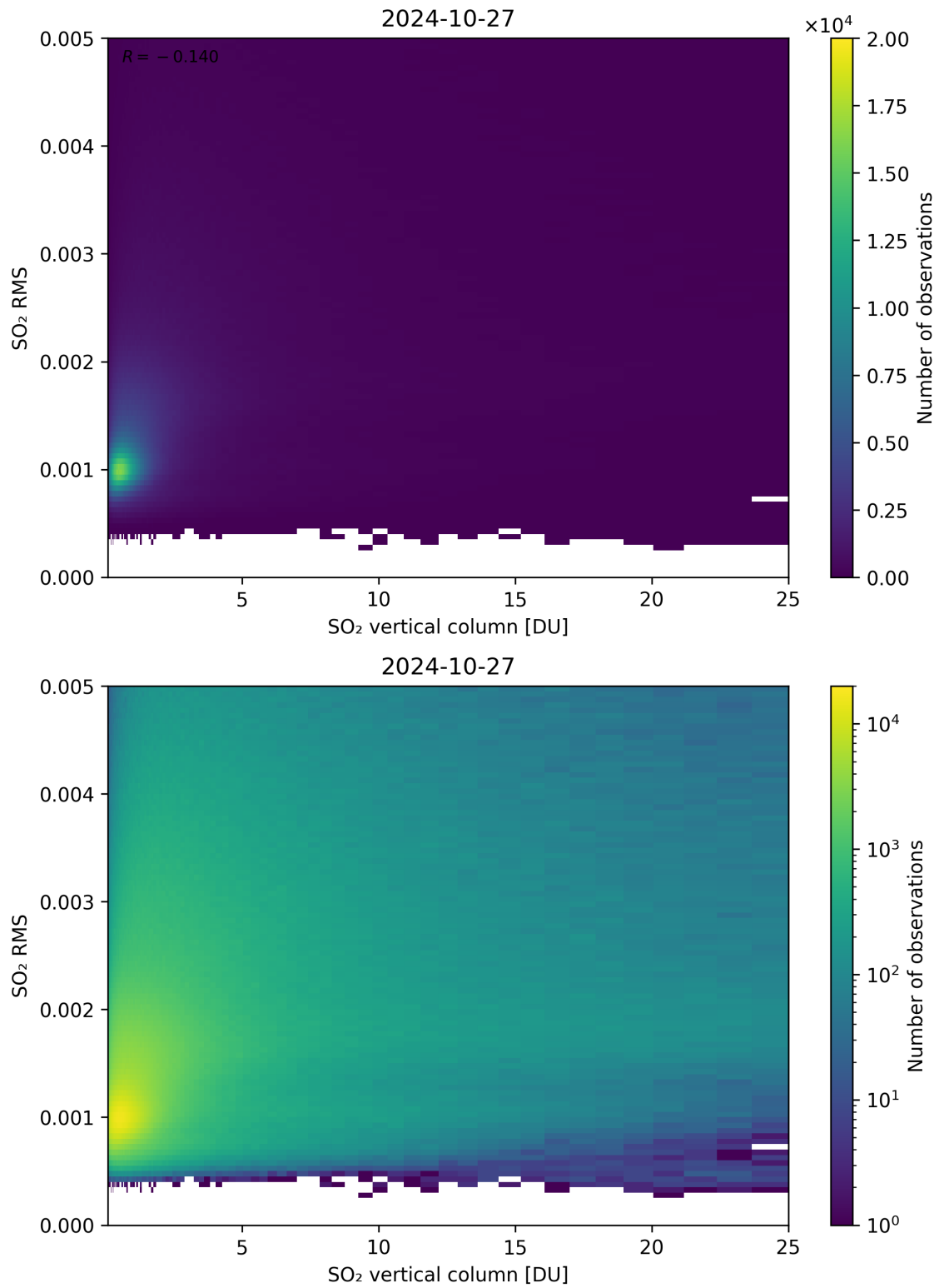
Figure 278: Scatter density plot of “SO 2 vertical column” against “SO 2 RMS” for 2024-10-26 to 2024-10-28.
