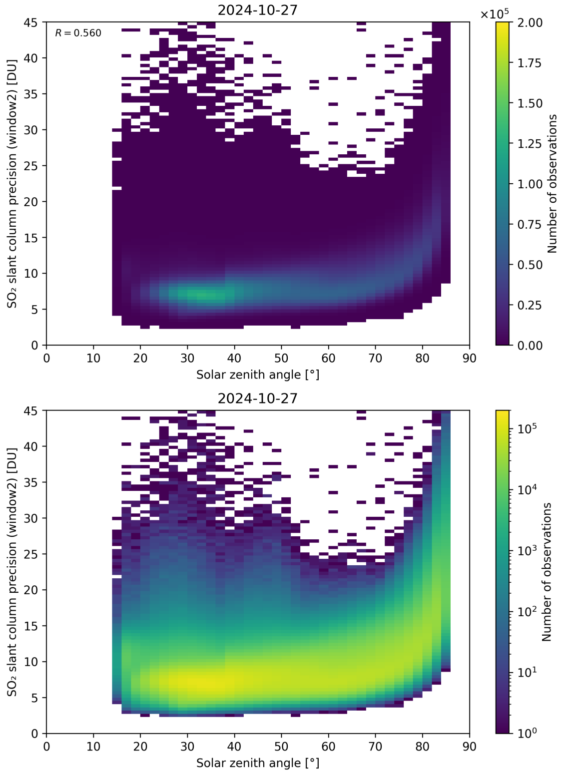
Figure 171: Scatter density plot of “Solar zenith angle” against “SO 2 slant column precision (window2)” for 2024-10-26 to 2024-10-28.
