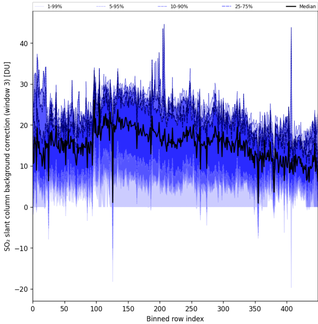
Figure 90: Along track statistics of “SO 2 slant column background correction (window 3)” for 2024-10-26 to 2024-10-28
