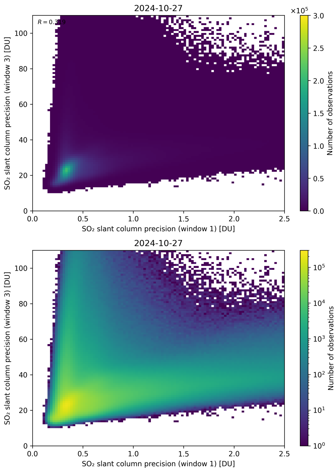
Figure 229: Scatter density plot of “SO 2 slant column precision (window 1)” against “SO 2 slant column precision (window 3)” for 2024-10-26 to 2024-10-28.
