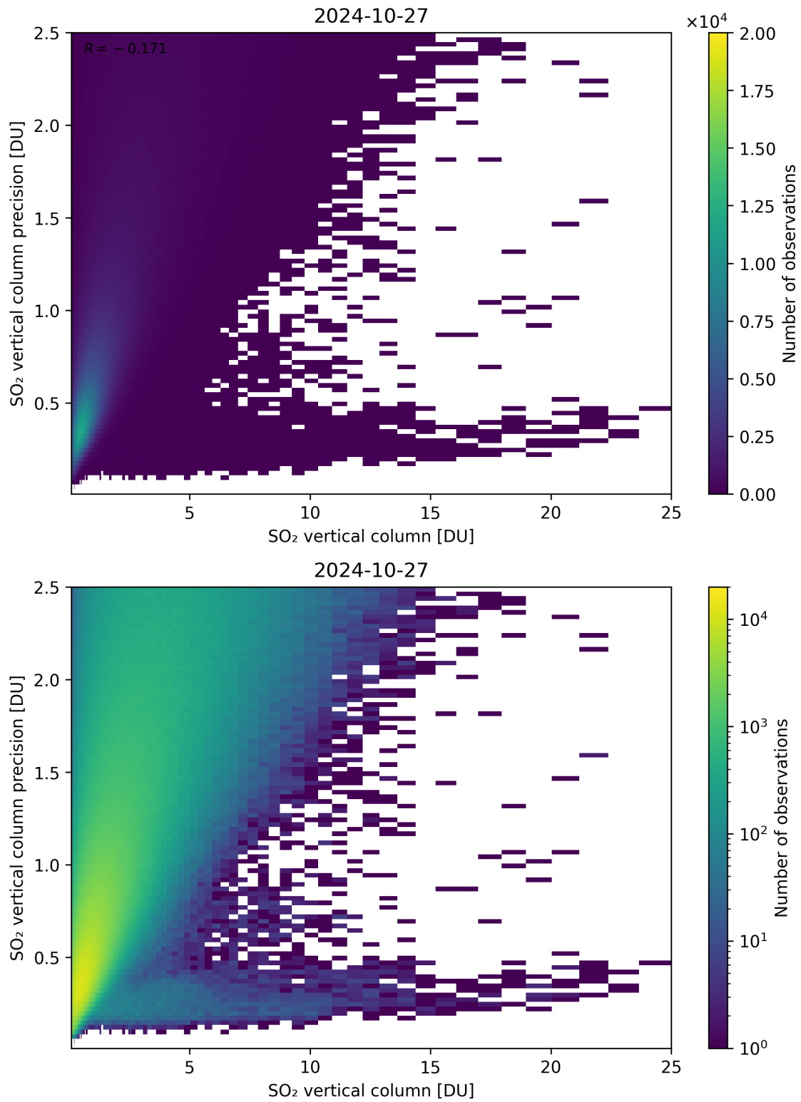
Figure 307: Scatter density plot of “SO 2 vertical column” against “SO 2 vertical column precision” for 2024-10-26 to 2024-10-28.
