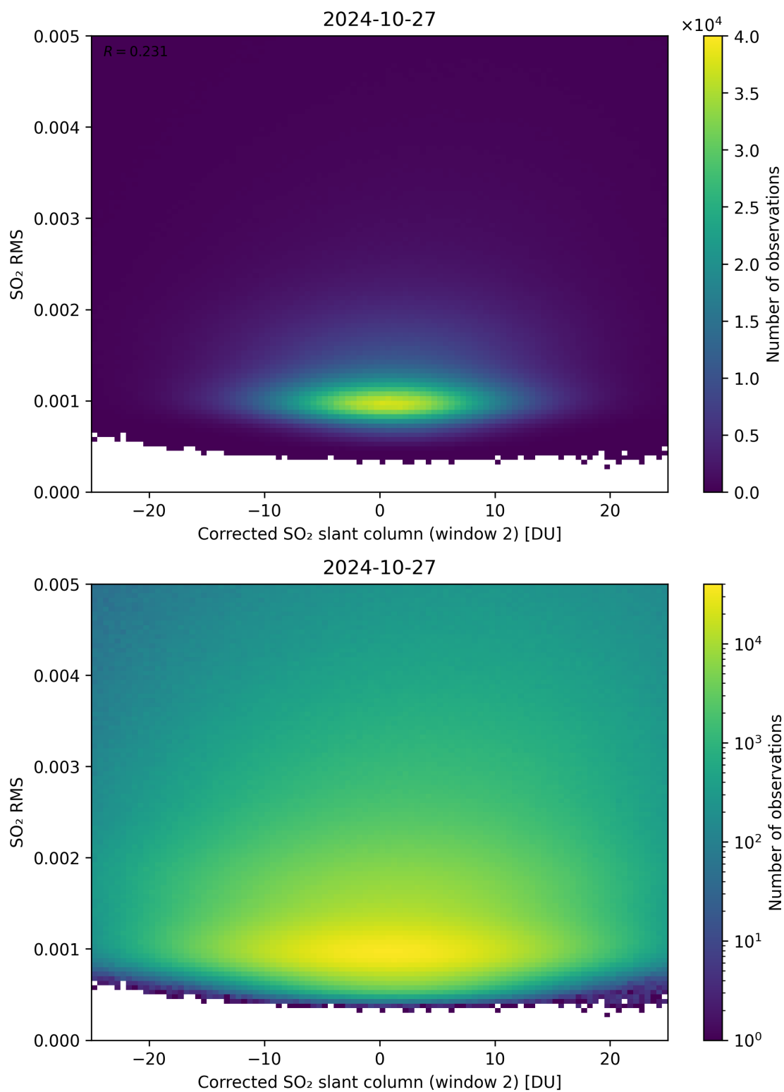
Figure 198: Scatter density plot of “Corrected SO 2 slant column (window 2)” against “SO 2 RMS” for 2024-10-26 to 2024-10-28.
