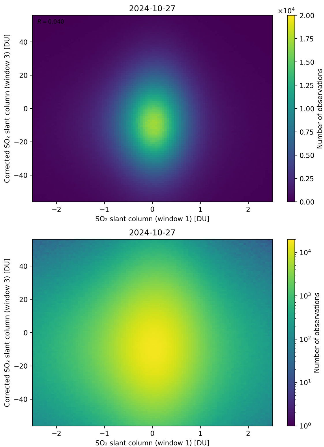
Figure 234: Scatter density plot of “SO 2 slant column (window 1)” against “Corrected SO 2 slant column (window 3)” for 2024-10-26 to 2024-10-28.
