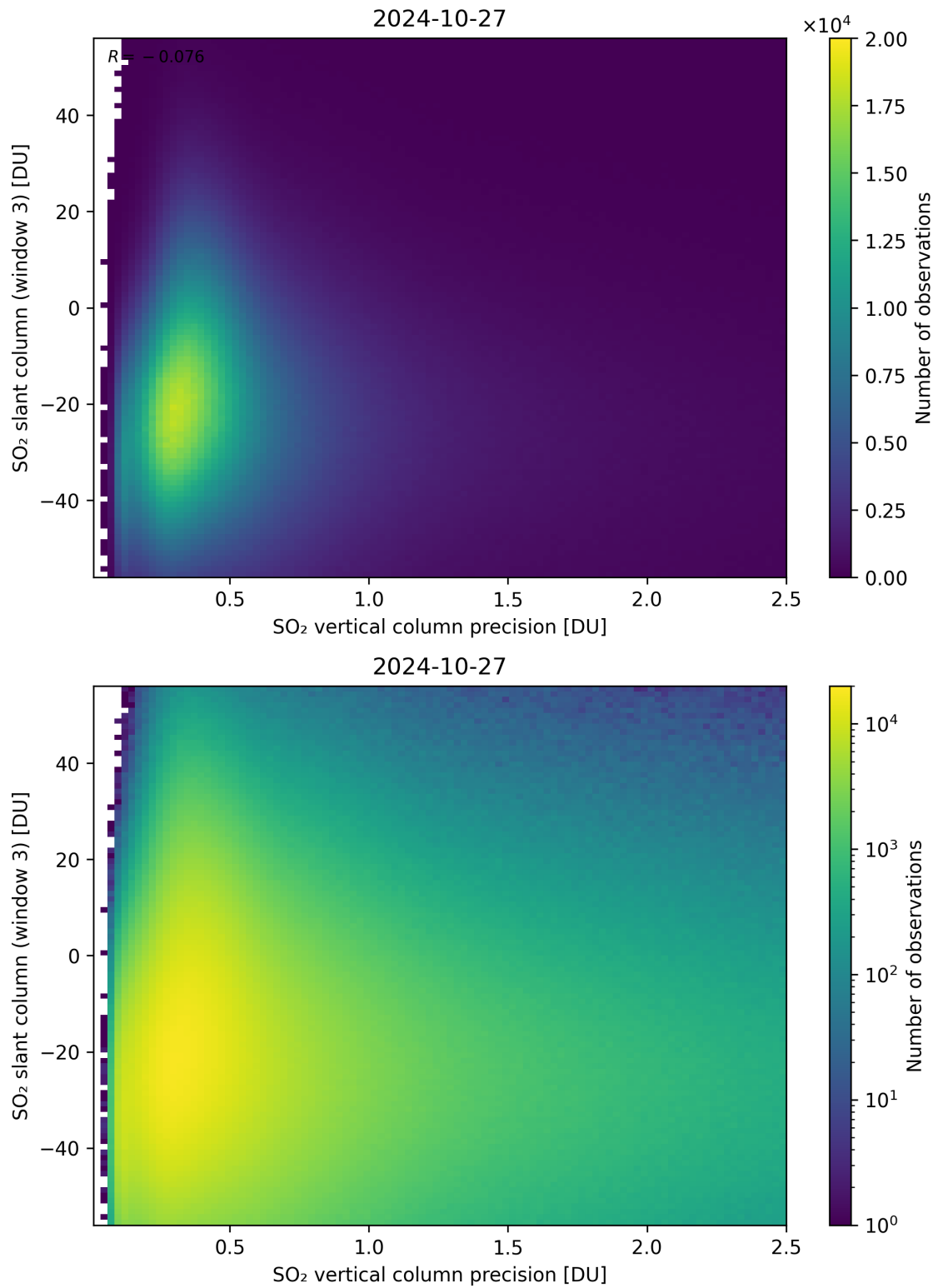
Figure 292: Scatter density plot of “SO 2 vertical column precision” against “SO 2 slant column (window 3)” for 2024-10-26 to 2024-10-28.
