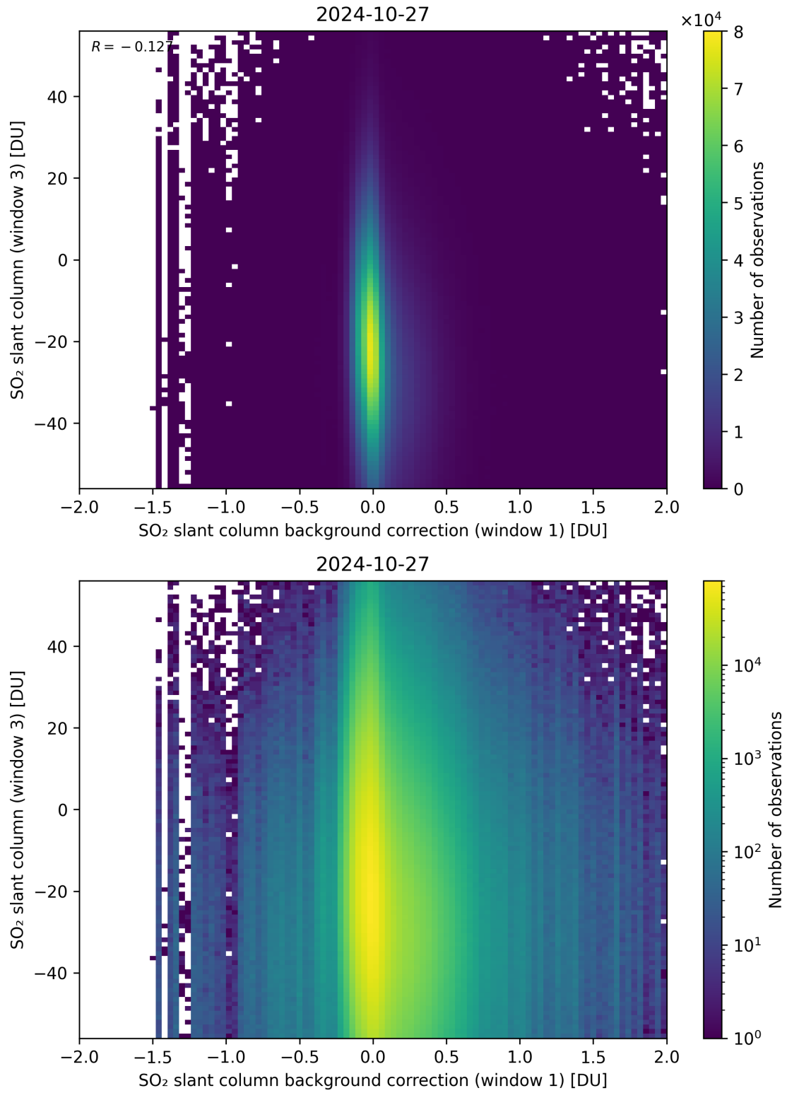
Figure 107: Scatter density plot of “SO 2 slant column background correction (window 1)” against “SO 2 slant column (window 3)” for 2024-10-26 to 2024-10-28.
