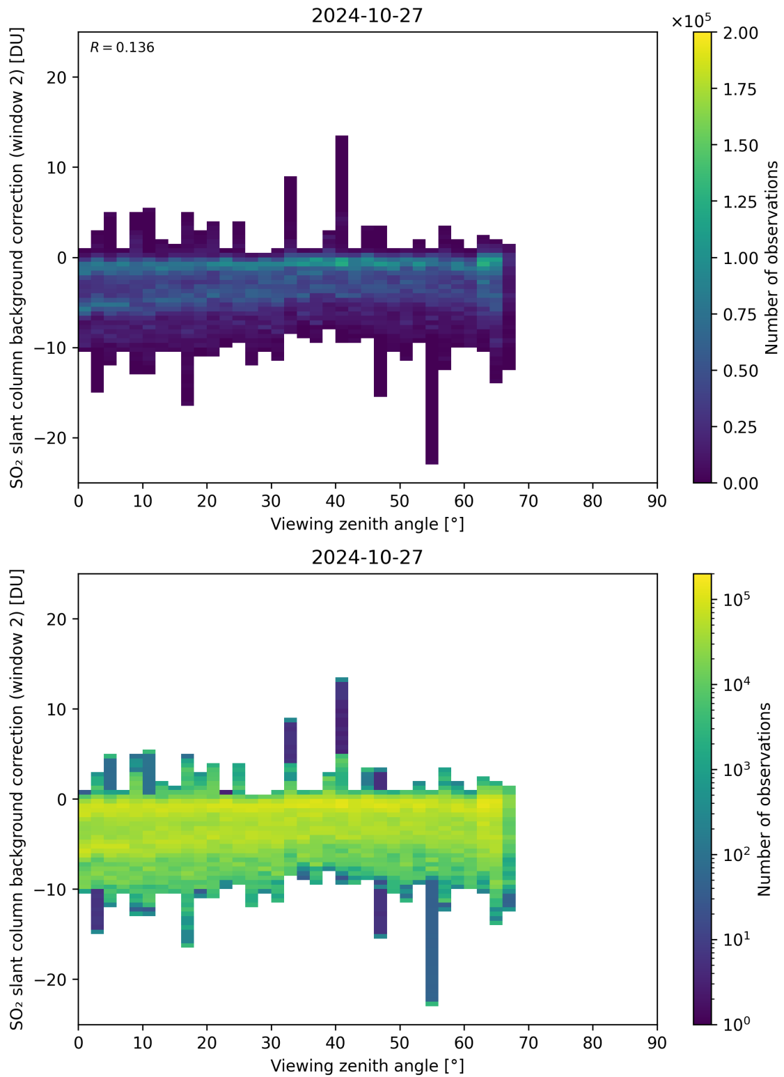
Figure 309: Scatter density plot of “Viewing zenith angle” against “SO 2 slant column background correction (window 2)” for 2024-10-26 to 2024-10-28.
