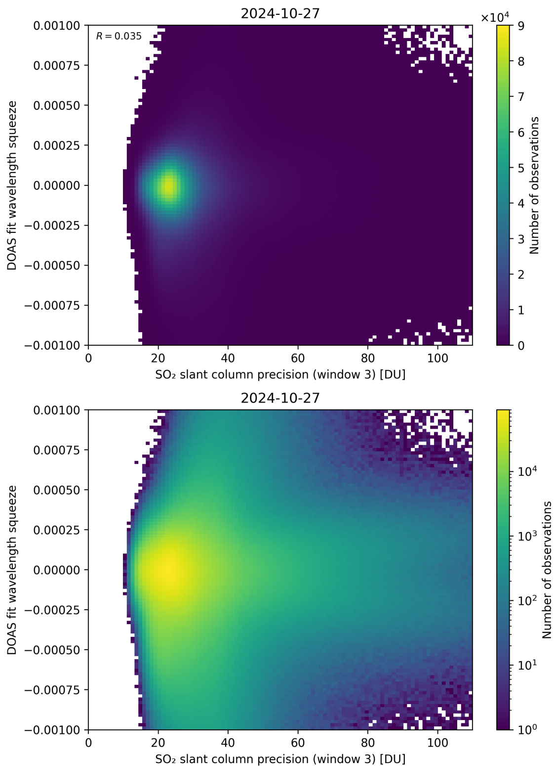
Figure 259: Scatter density plot of “SO 2 slant column precision (window 3)” against “DOAS fit wavelength squeeze” for 2024-10-26 to 2024-10-28.
