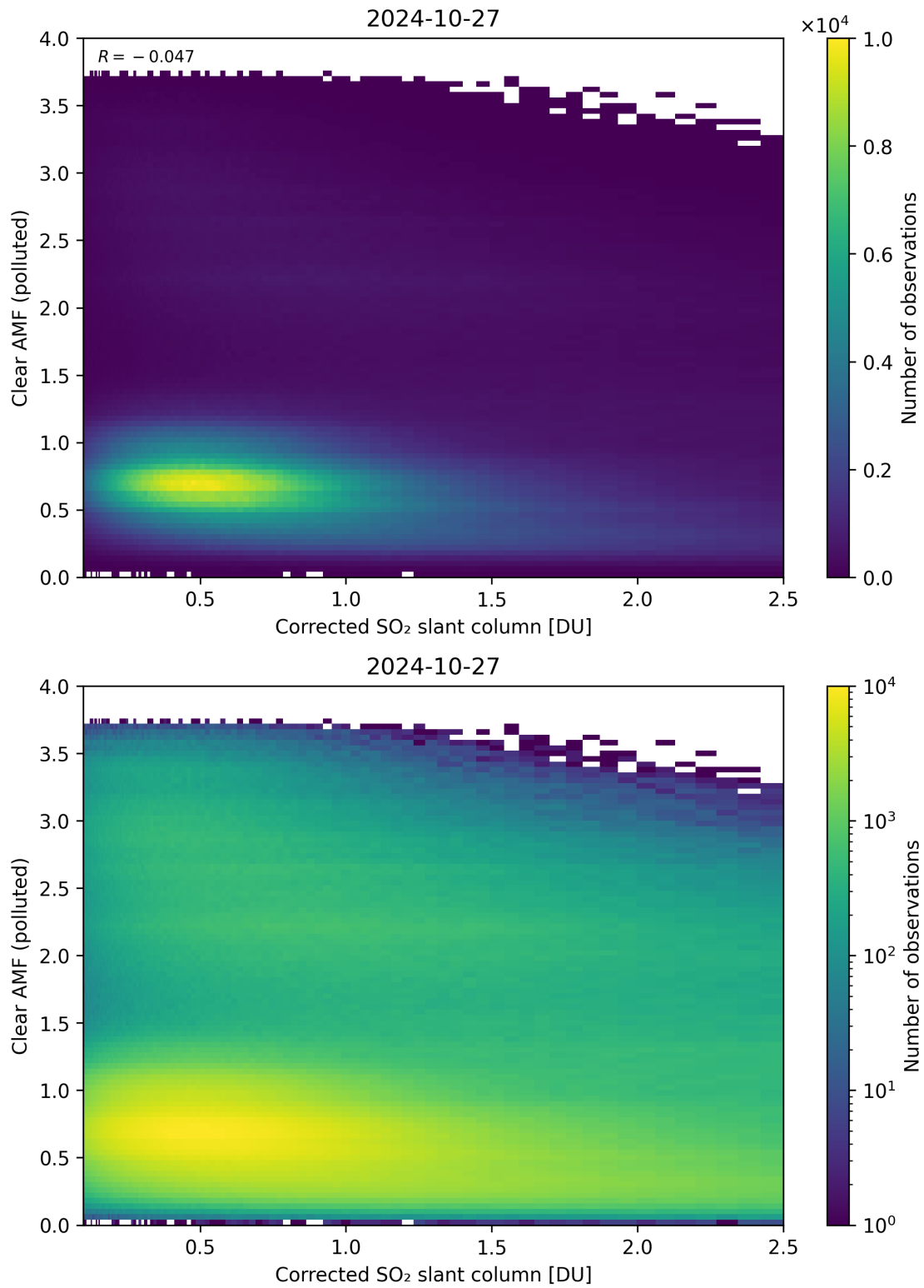
Figure 184: Scatter density plot of “Corrected SO 2 slant column” against “Clear AMF (polluted)” for 2024-10-26 to 2024-10-28.
