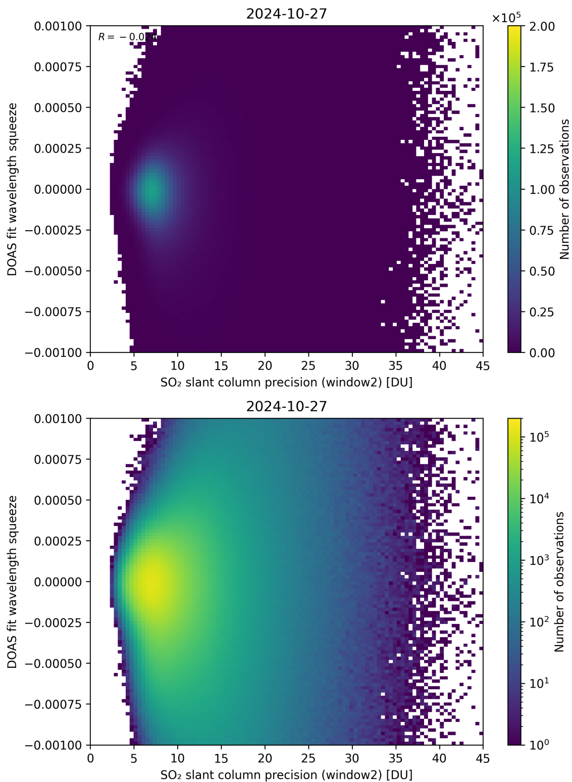
Figure 244: Scatter density plot of “SO 2 slant column precision (window2)” against “DOAS fit wavelength squeeze” for 2024-10-26 to 2024-10-28.
