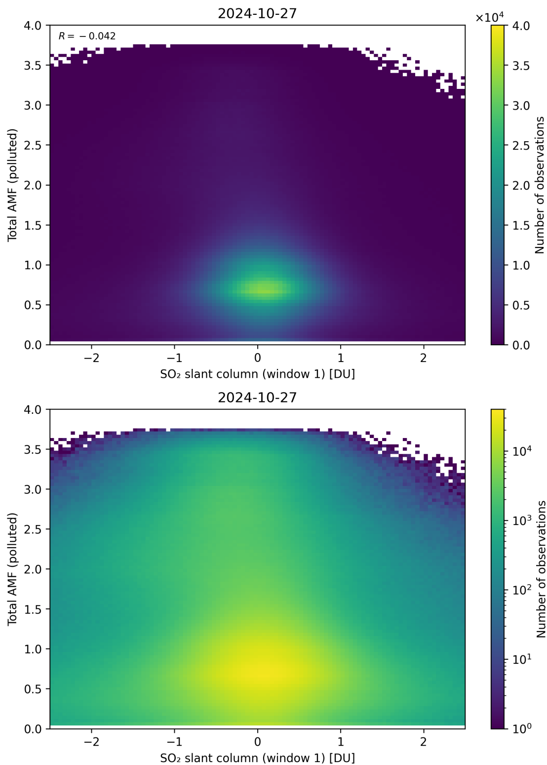
Figure 239: Scatter density plot of “SO 2 slant column (window 1)” against “Total AMF (polluted)” for 2024-10-26 to 2024-10-28.
