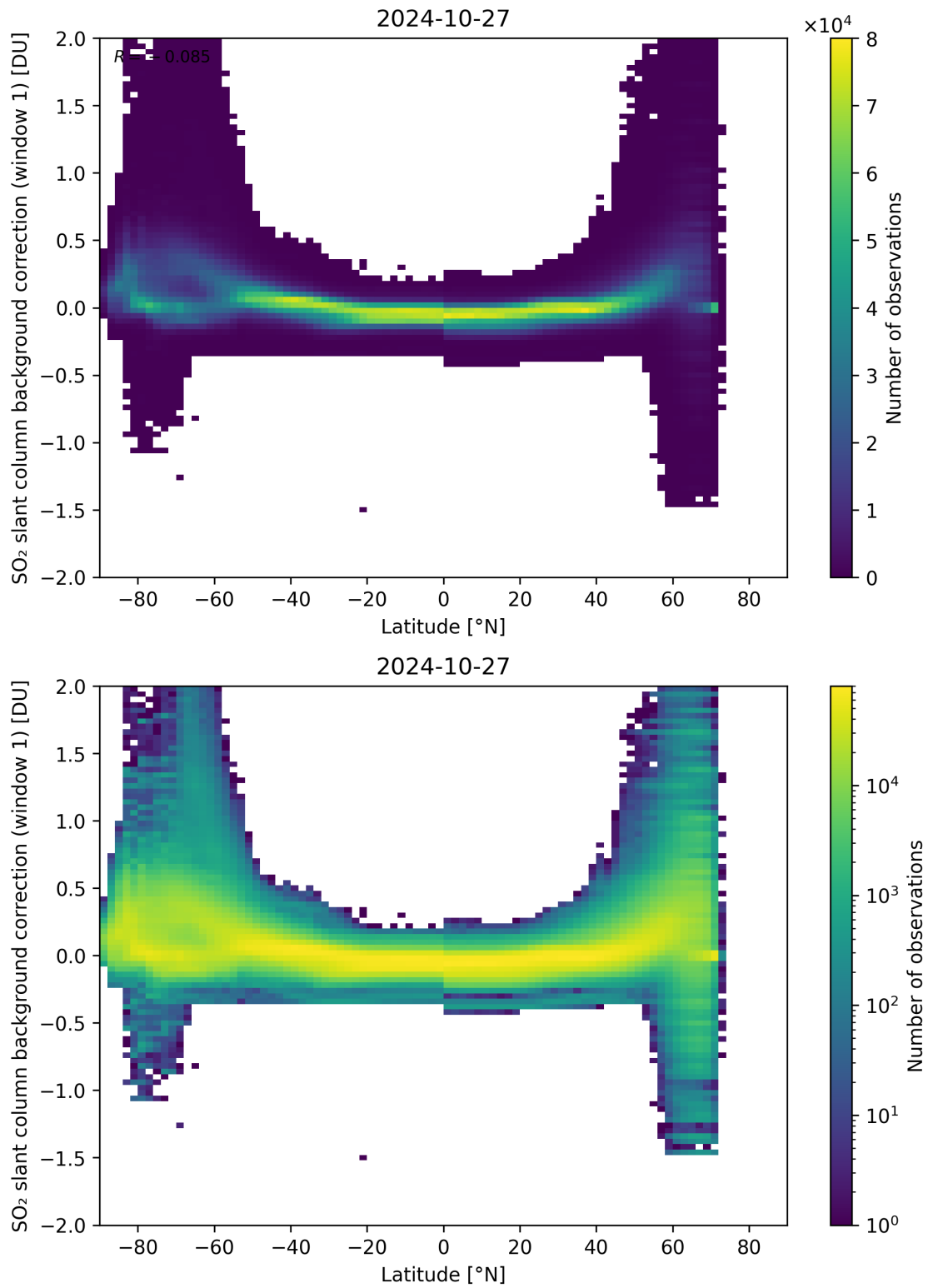
Figure 139: Scatter density plot of “Latitude” against “SO 2 slant column background correction (window 1)” for 2024-10-26 to 2024-10-28.
