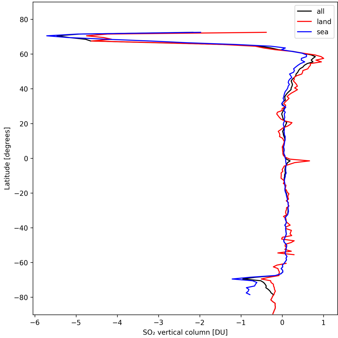
Figure 30: Zonal average of “SO 2 vertical column” for 2024-10-26 to 2024-10-28.
