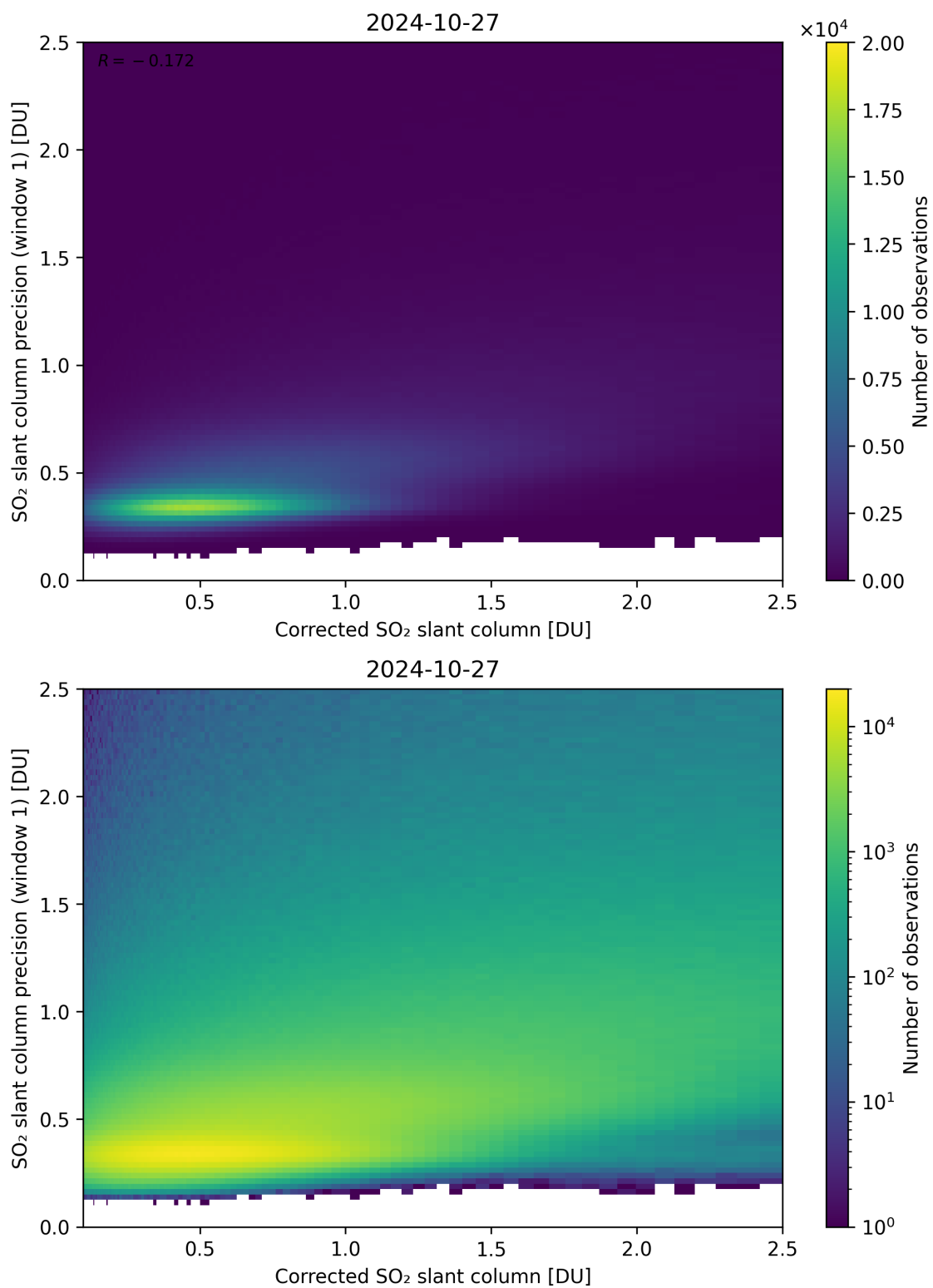
Figure 188: Scatter density plot of “Corrected SO 2 slant column” against “SO 2 slant column precision (window 1)” for 2024-10-26 to 2024-10-28.
