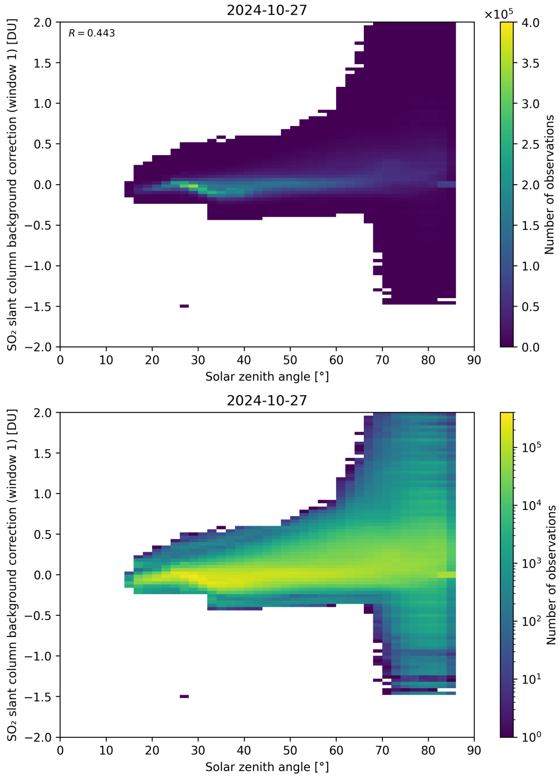
Figure 158: Scatter density plot of “Solar zenith angle” against “SO 2 slant column background correction (window 1)” for 2024-10-26 to 2024-10-28.
