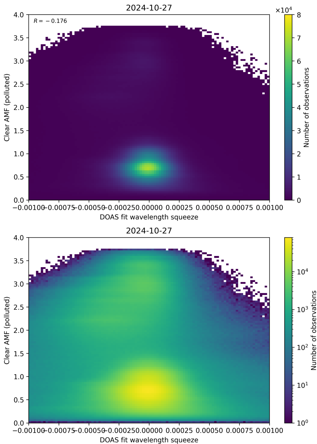
Figure 133: Scatter density plot of “DOAS fit wavelength squeeze” against “Clear AMF (polluted)” for 2024-10-26 to 2024-10-28.
