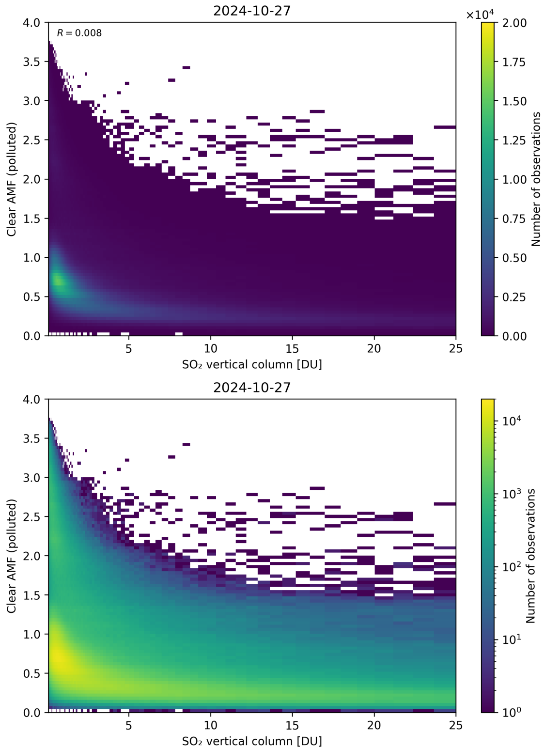
Figure 296: Scatter density plot of “SO 2 vertical column” against “Clear AMF (polluted)” for 2024-10-26 to 2024-10-28.
