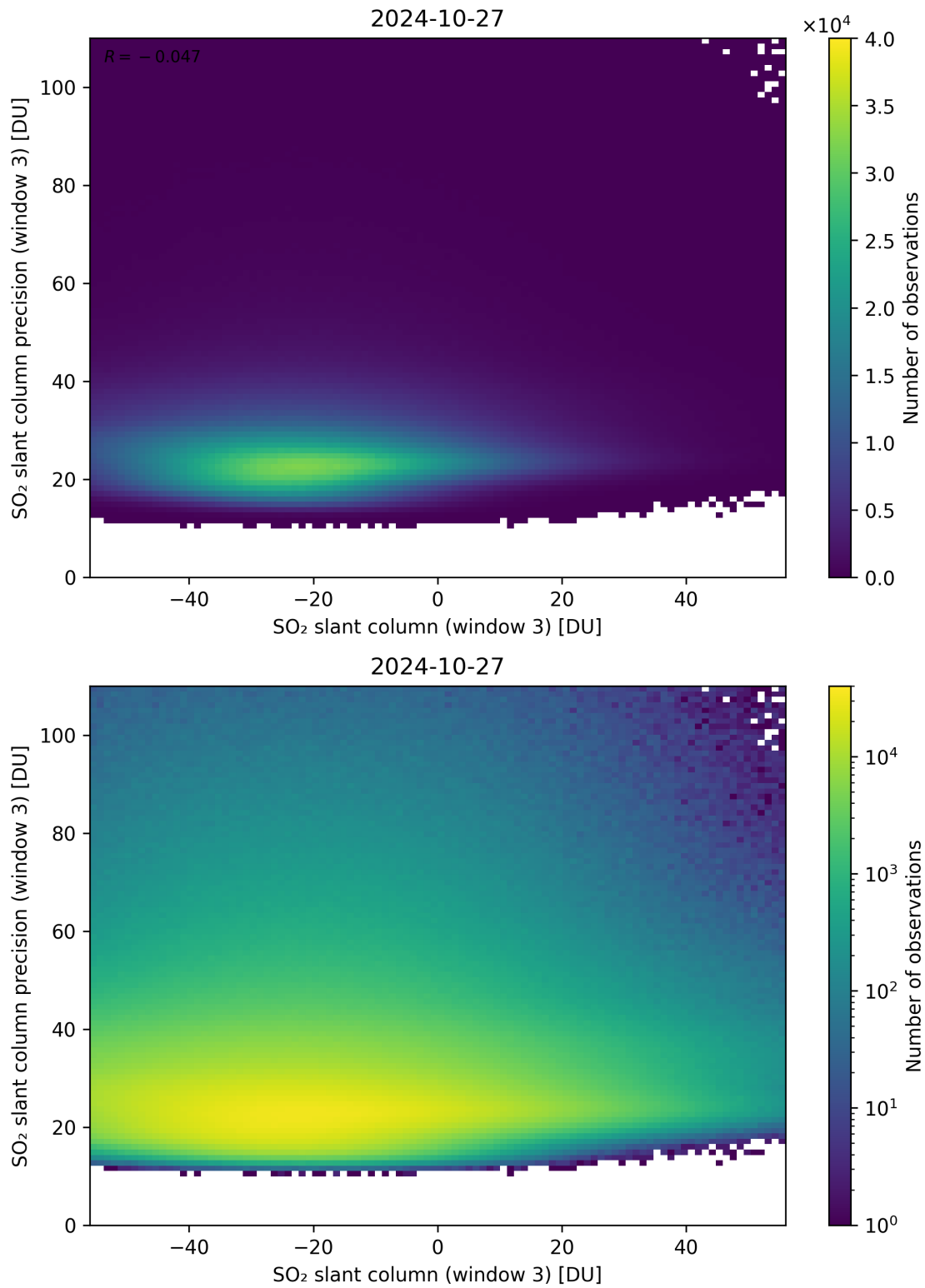
Figure 267: Scatter density plot of “SO 2 slant column (window 3)” against “SO 2 slant column precision (window 3)” for 2024-10-26 to 2024-10-28.
