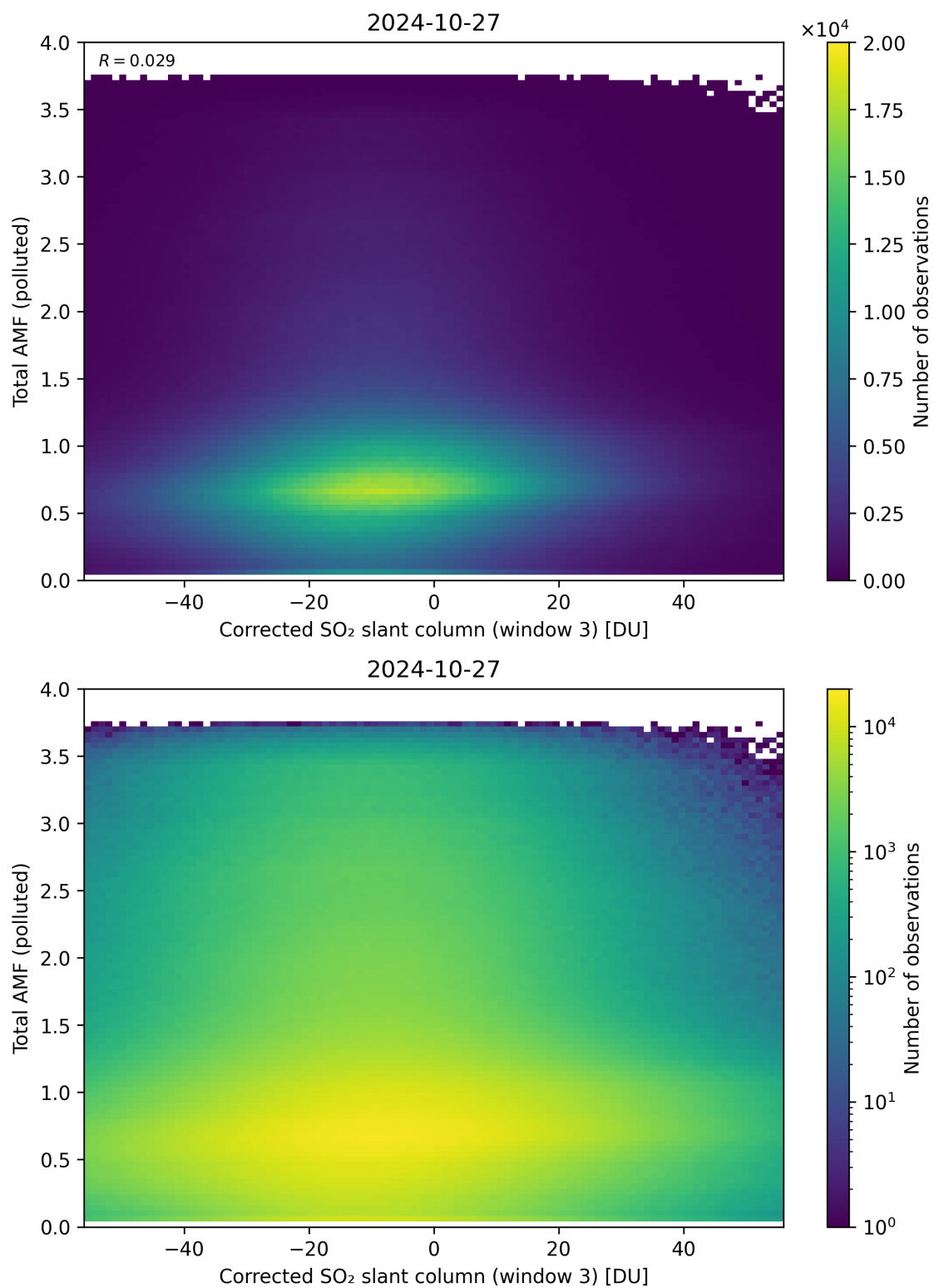
Figure 210: Scatter density plot of “Corrected SO 2 slant column (window 3)” against “Total AMF (polluted)” for 2024-10-26 to 2024-10-28.
