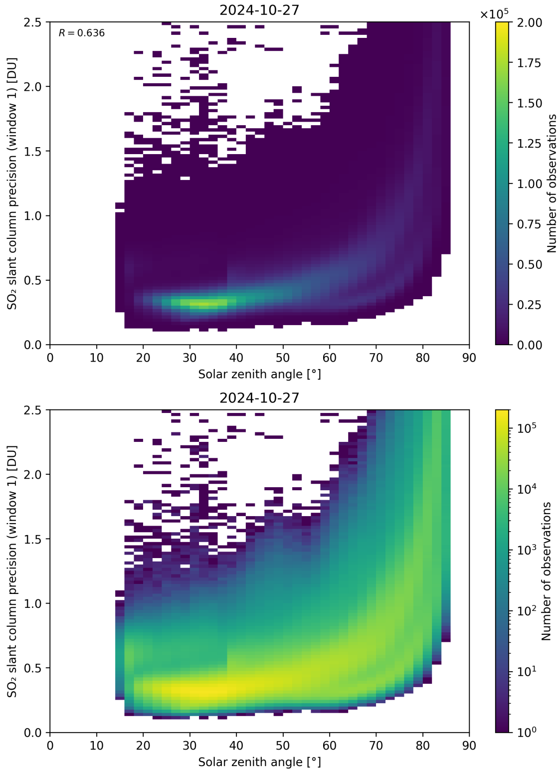
Figure 170: Scatter density plot of “Solar zenith angle” against “SO 2 slant column precision (window 1)” for 2024-10-26 to 2024-10-28.
