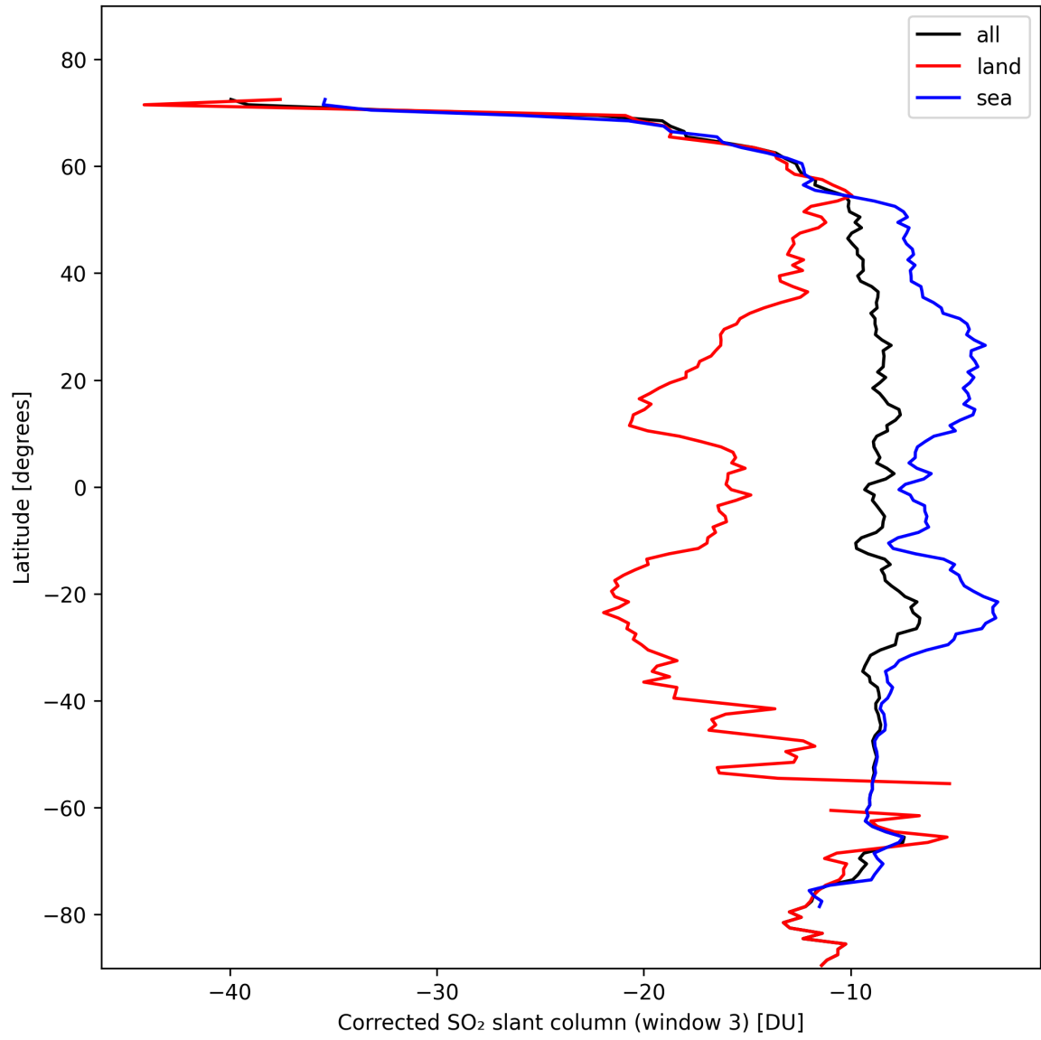
Figure 43: Zonal average of “Corrected SO 2 slant column (window 3)” for 2024-10-26 to 2024-10-28.
