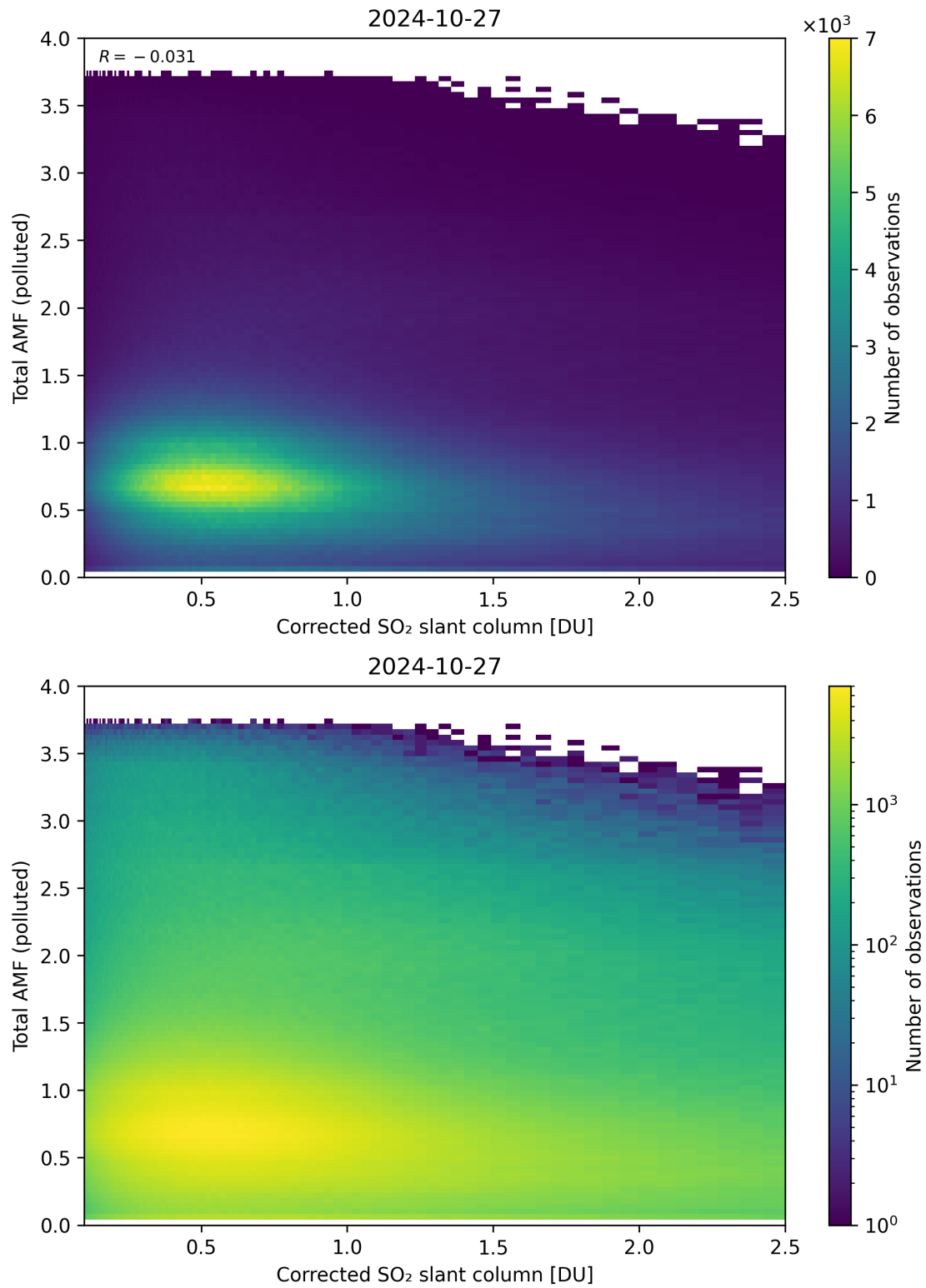
Figure 192: Scatter density plot of “Corrected SO 2 slant column” against “Total AMF (polluted)” for 2024-10-26 to 2024-10-28.
