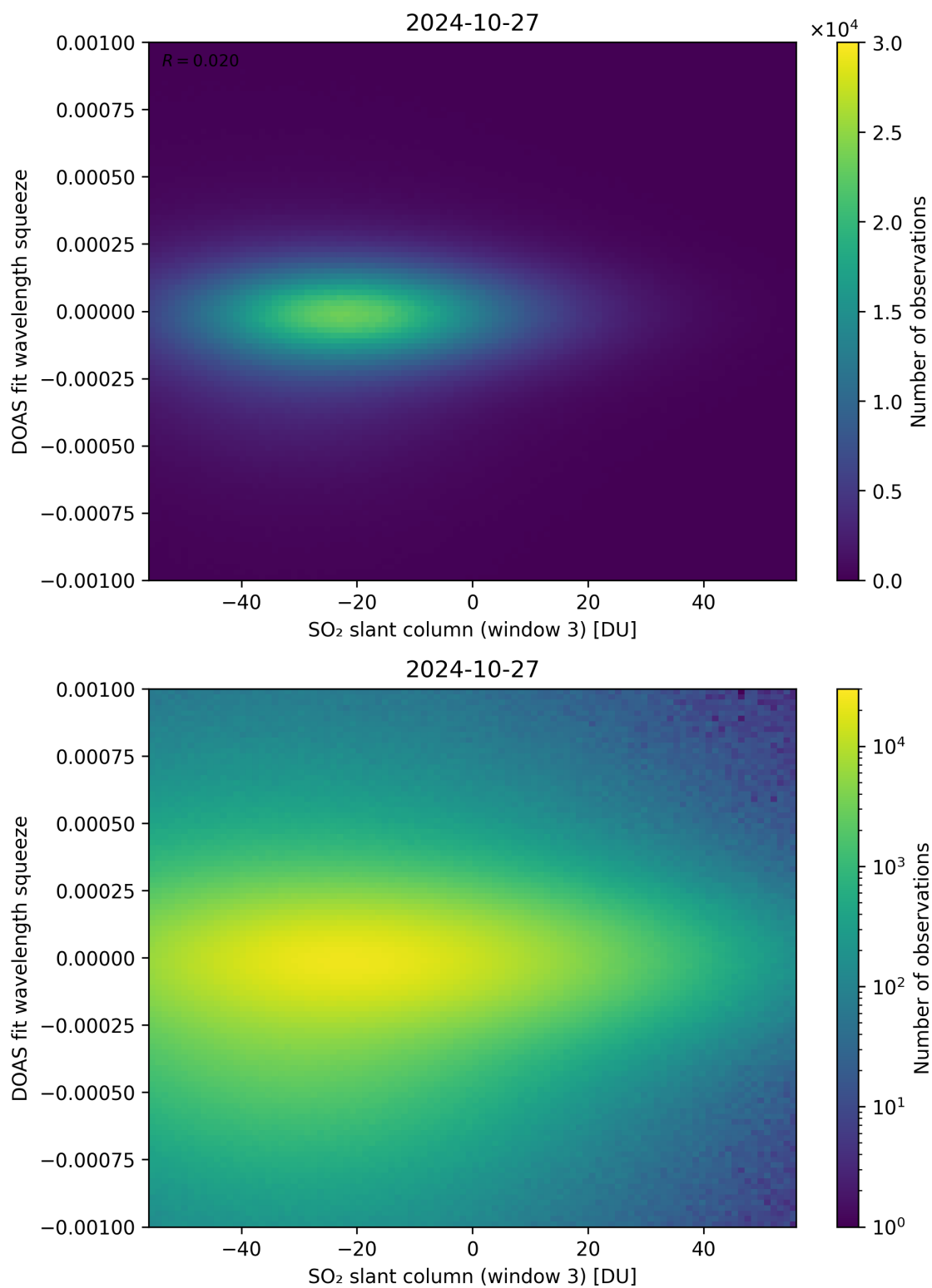
Figure 255: Scatter density plot of “SO 2 slant column (window 3)” against “DOAS fit wavelength squeeze” for 2024-10-26 to 2024-10-28.
