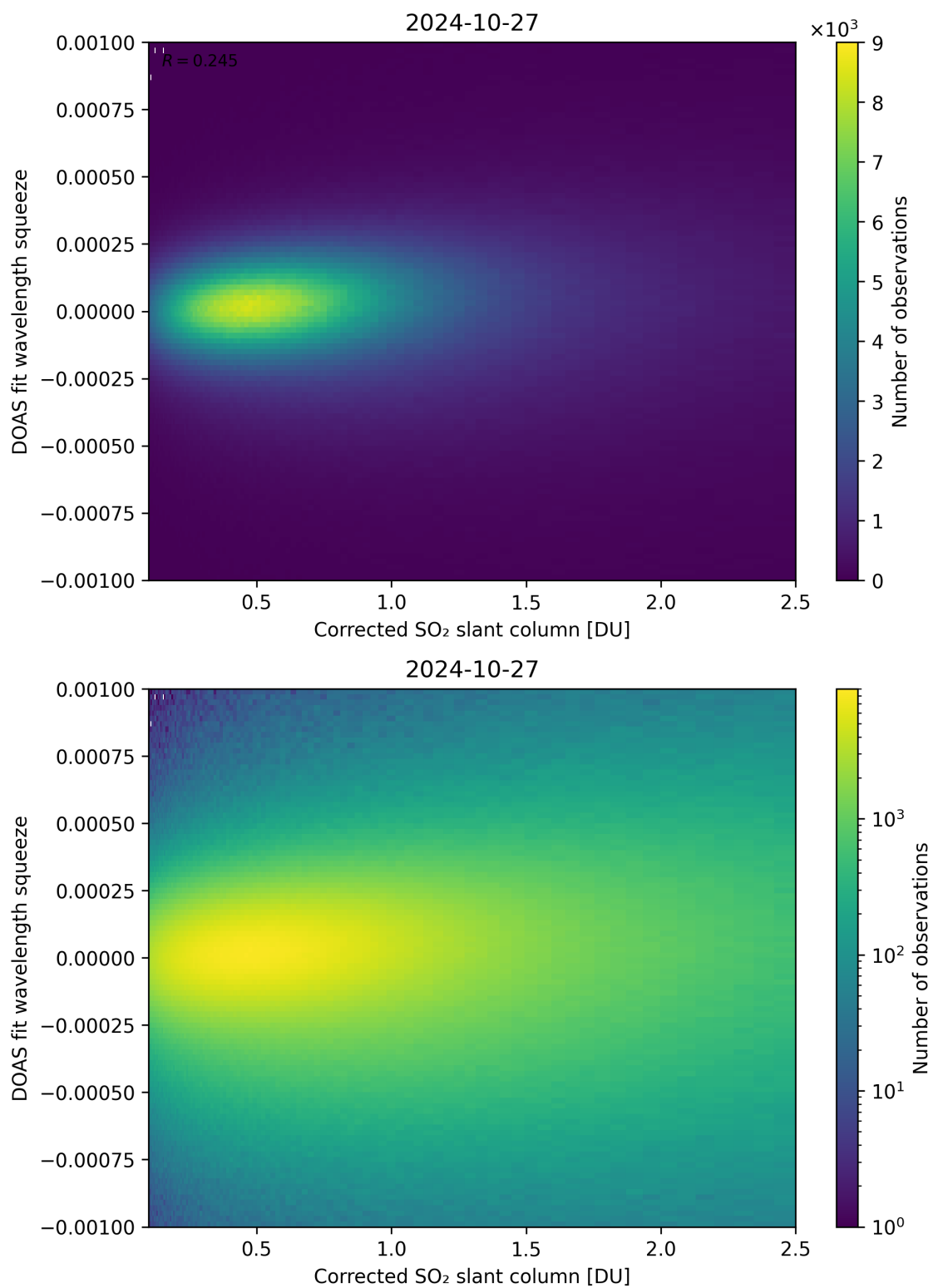
Figure 182: Scatter density plot of “Corrected SO 2 slant column” against “DOAS fit wavelength squeeze” for 2024-10-26 to 2024-10-28.
