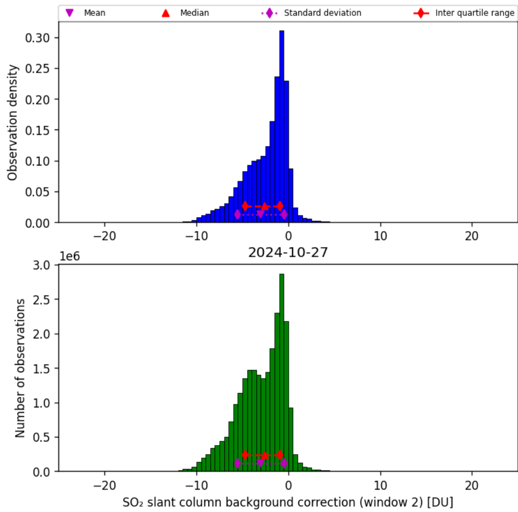
Figure 63: Histogram of “SO 2 slant column background correction (window 2)” for 2024-10-26 to 2024-10-28
