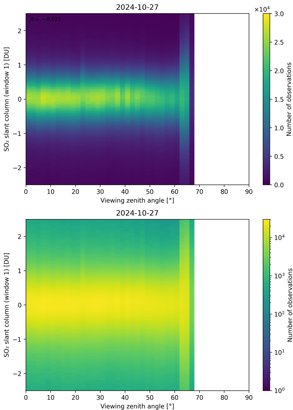
Figure 320: Scatter density plot of “Viewing zenith angle” against “SO 2 slant column (window 1)” for 2024-10-26 to 2024-10-28.
