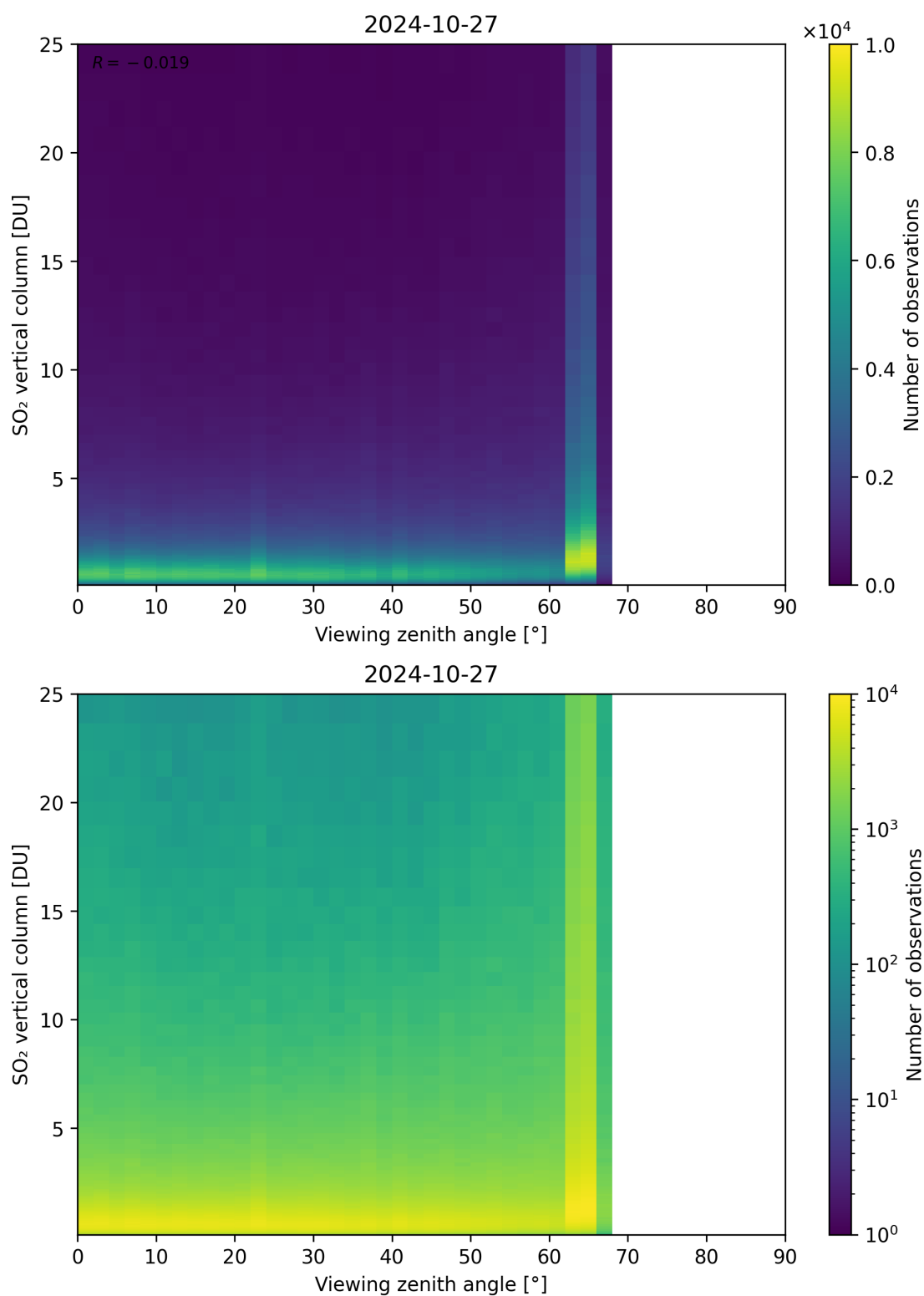
Figure 327: Scatter density plot of “Viewing zenith angle” against “SO 2 vertical column” for 2024-10-26 to 2024-10-28.
