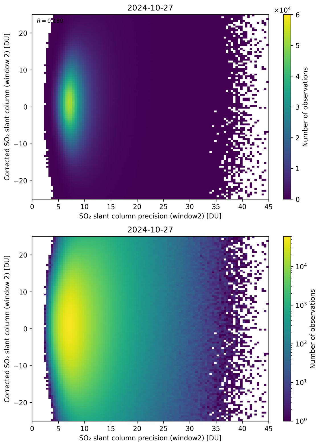
Figure 247: Scatter density plot of “SO 2 slant column precision (window2)” against “Corrected SO 2 slant column (window 2)” for 2024-10-26 to 2024-10-28.
