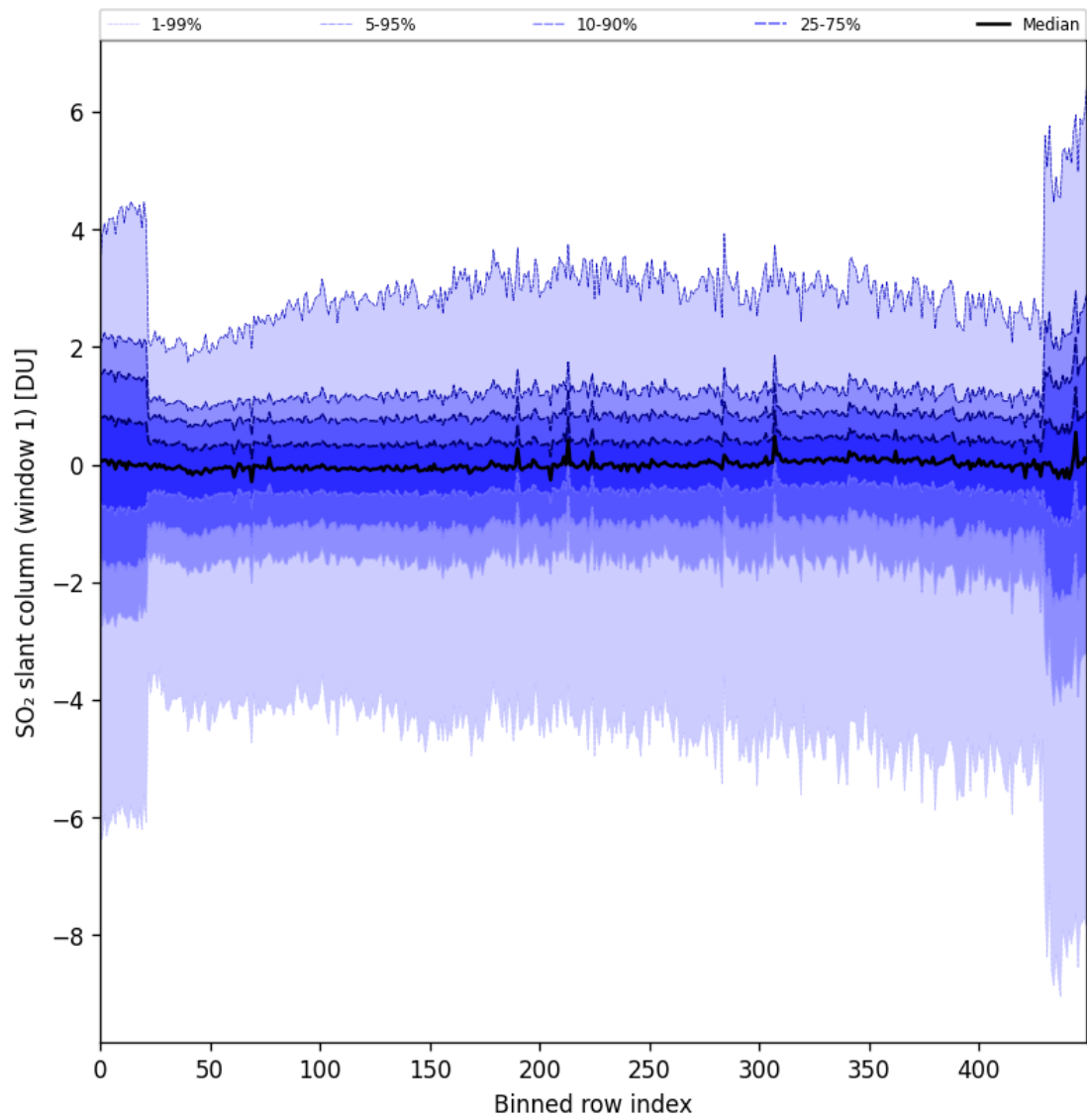
Figure 79: Along track statistics of “SO 2 slant column (window 1)” for 2024-10-26 to 2024-10-28
