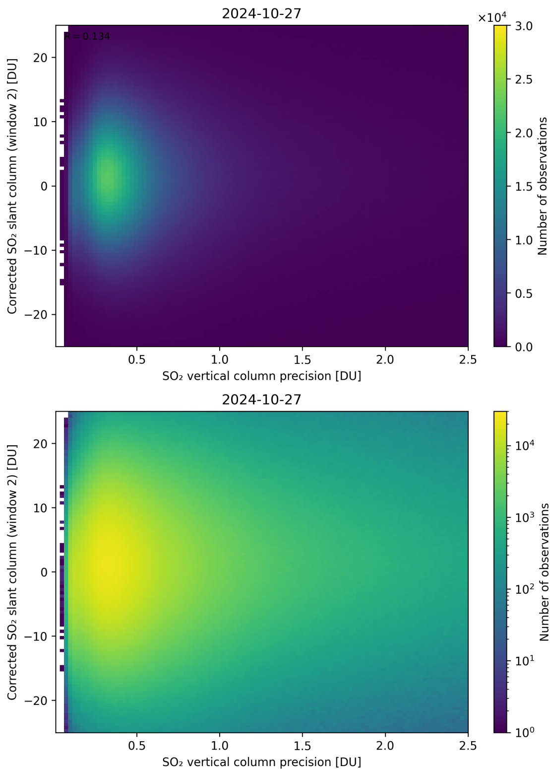
Figure 287: Scatter density plot of “SO 2 vertical column precision” against “Corrected SO 2 slant column (window 2)” for 2024-10-26 to 2024-10-28.
