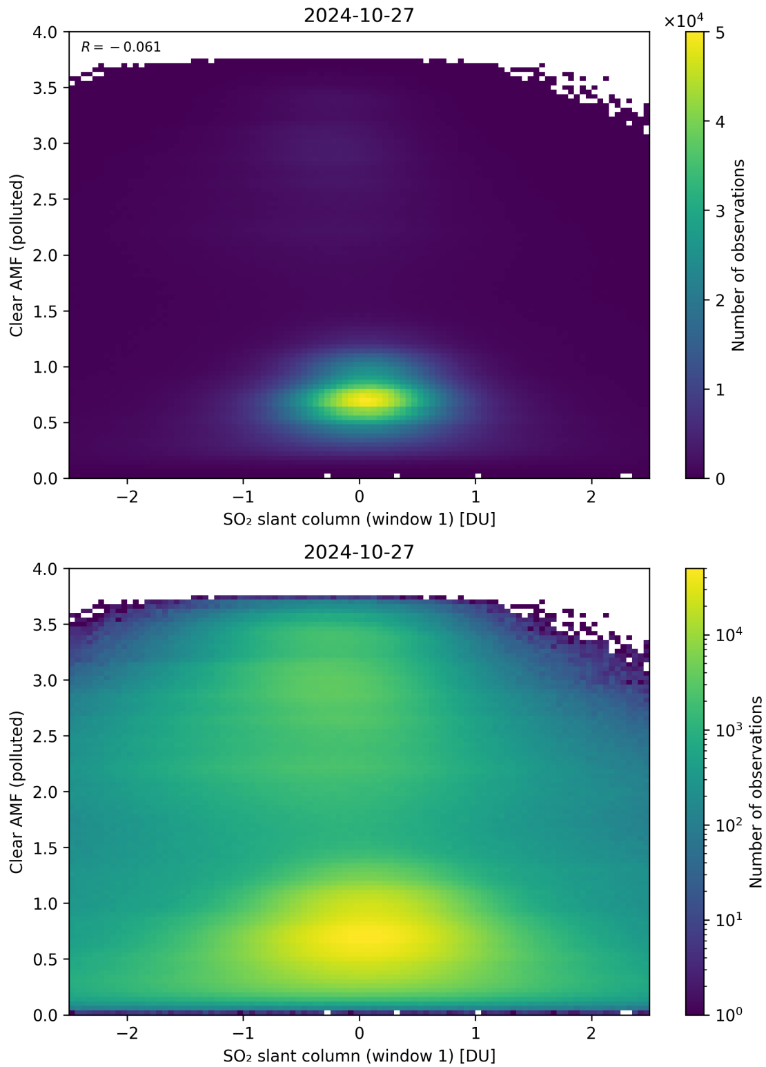
Figure 232: Scatter density plot of “SO 2 slant column (window 1)” against “Clear AMF (polluted)” for 2024-10-26 to 2024-10-28.
