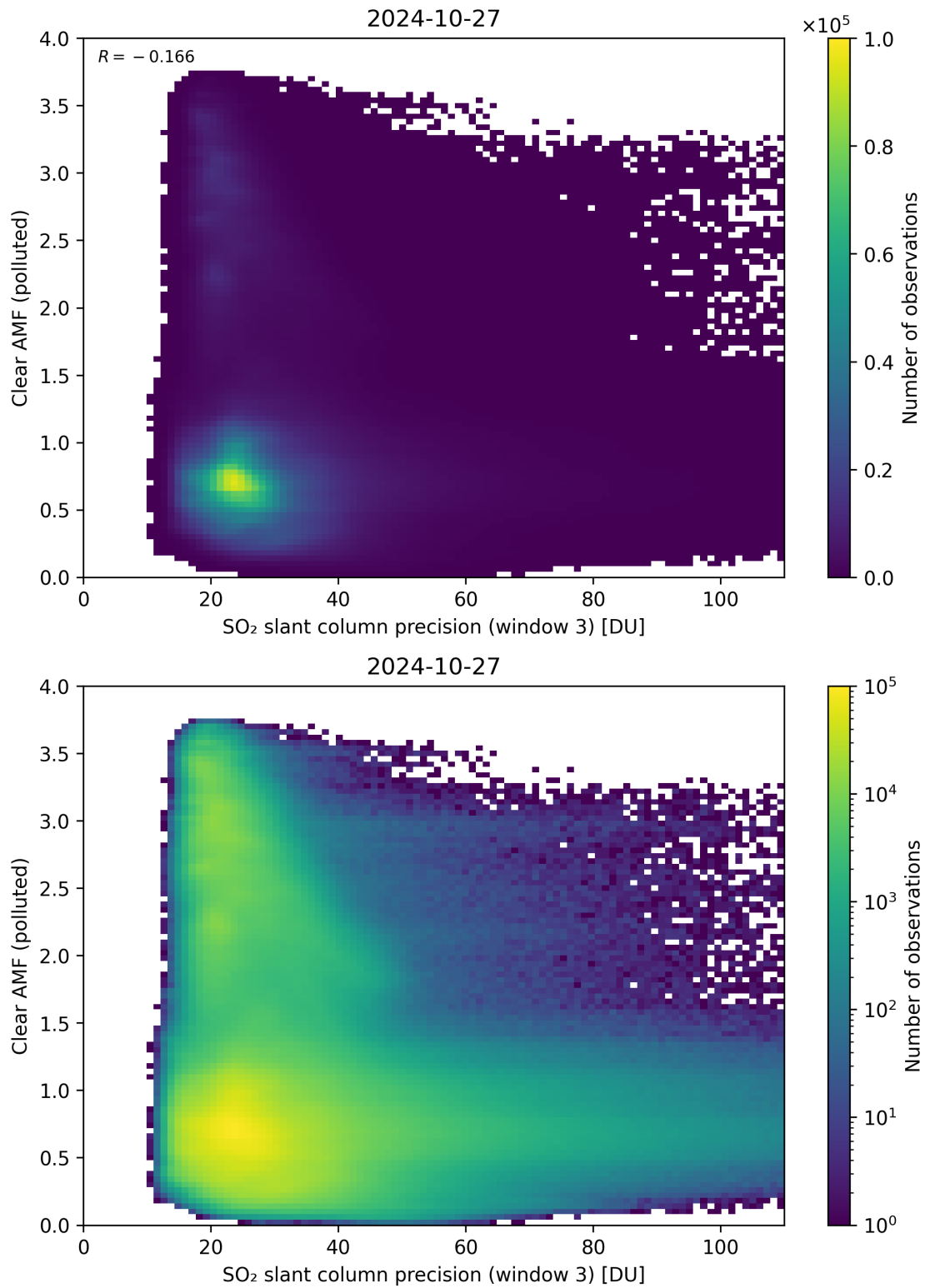
Figure 261: Scatter density plot of “SO 2 slant column precision (window 3)” against “Clear AMF (polluted)” for 2024-10-26 to 2024-10-28.
