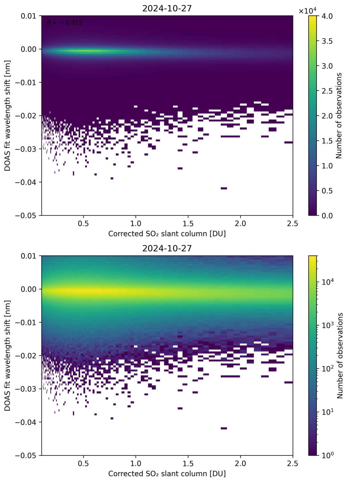
Figure 181: Scatter density plot of “Corrected SO 2 slant column” against “DOAS fit wavelength shift” for 2024-10-26 to 2024-10-28.
