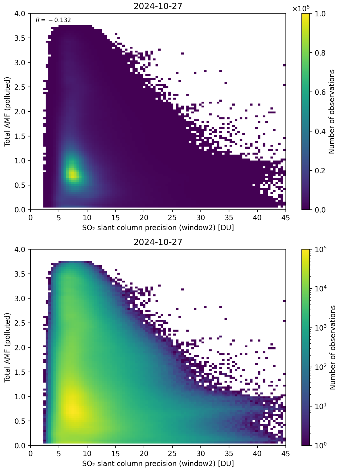
Figure 251: Scatter density plot of “SO 2 slant column precision (window2)” against “Total AMF (polluted)” for 2024-10-26 to 2024-10-28.
