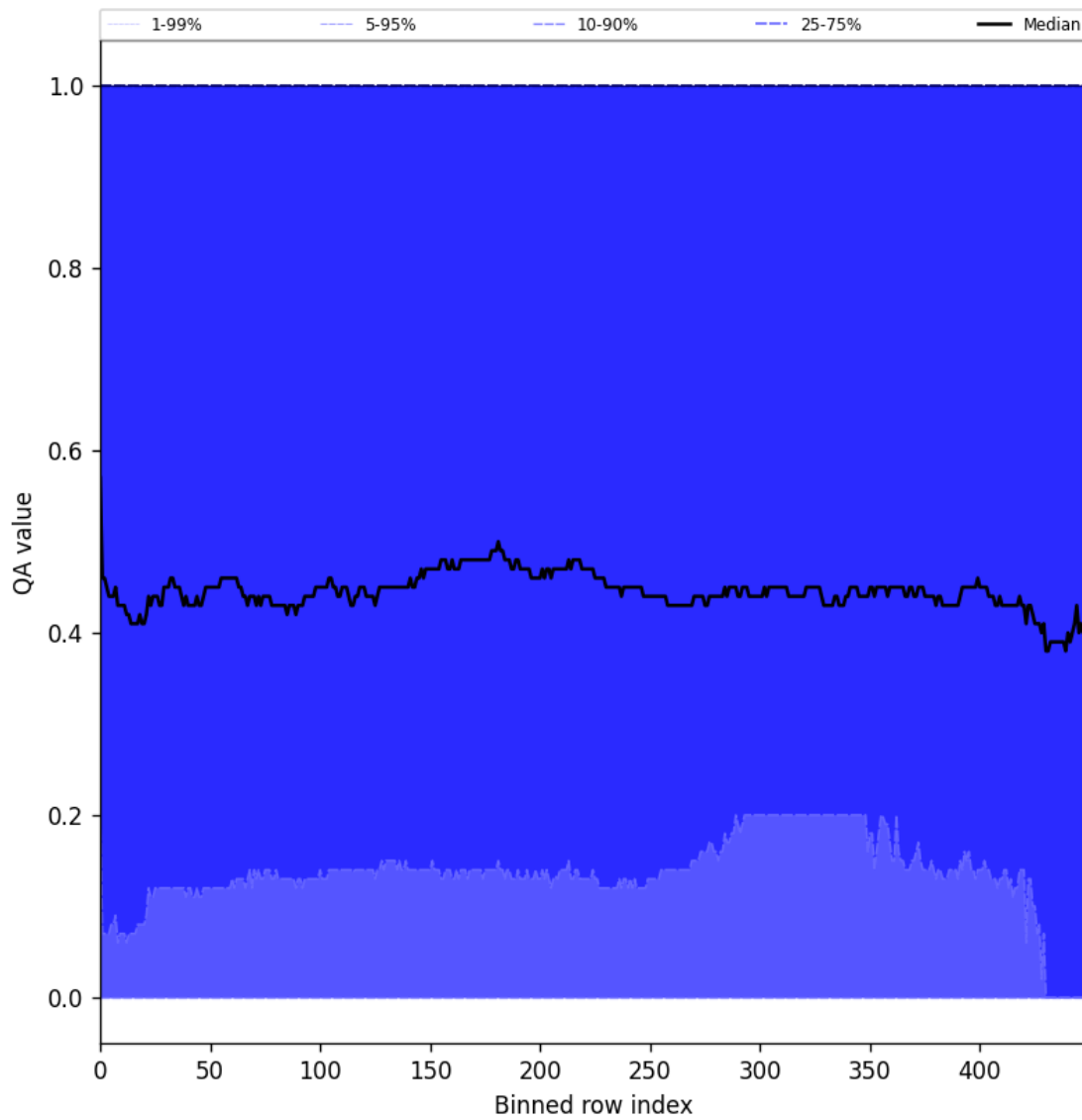
Figure 75: Along track statistics of “QA value” for 2024-10-26 to 2024-10-28
