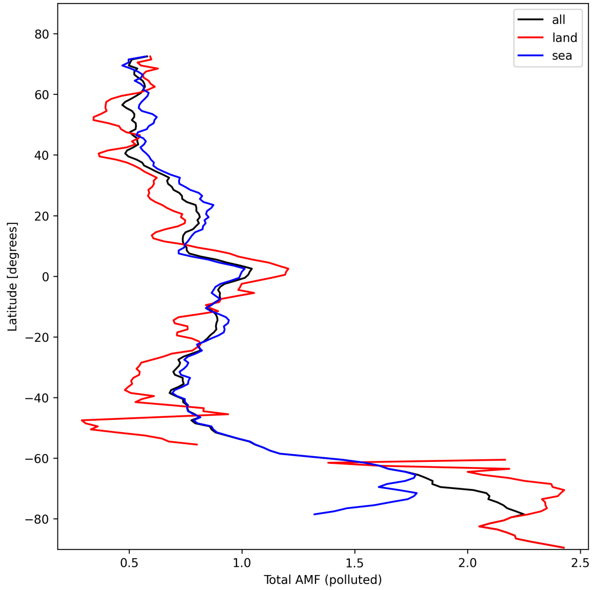
Figure 48: Zonal average of “Total AMF (polluted)” for 2024-10-26 to 2024-10-28.
