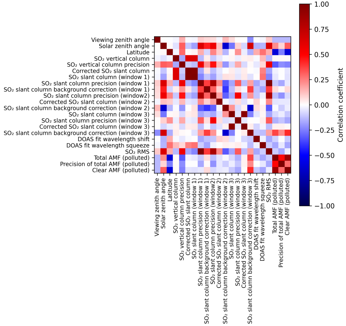
Figure 2: Map of correlation matrix for 2024-10-26 to 2024-10-28.
