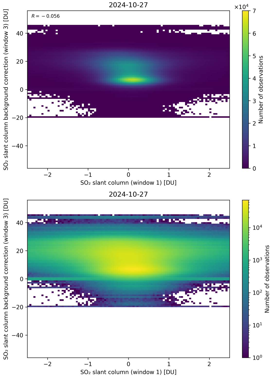
Figure 214: Scatter density plot of “SO 2 slant column (window 1)” against “SO 2 slant column background correction (window 3)” for 2024-10-26 to 2024-10-28.
