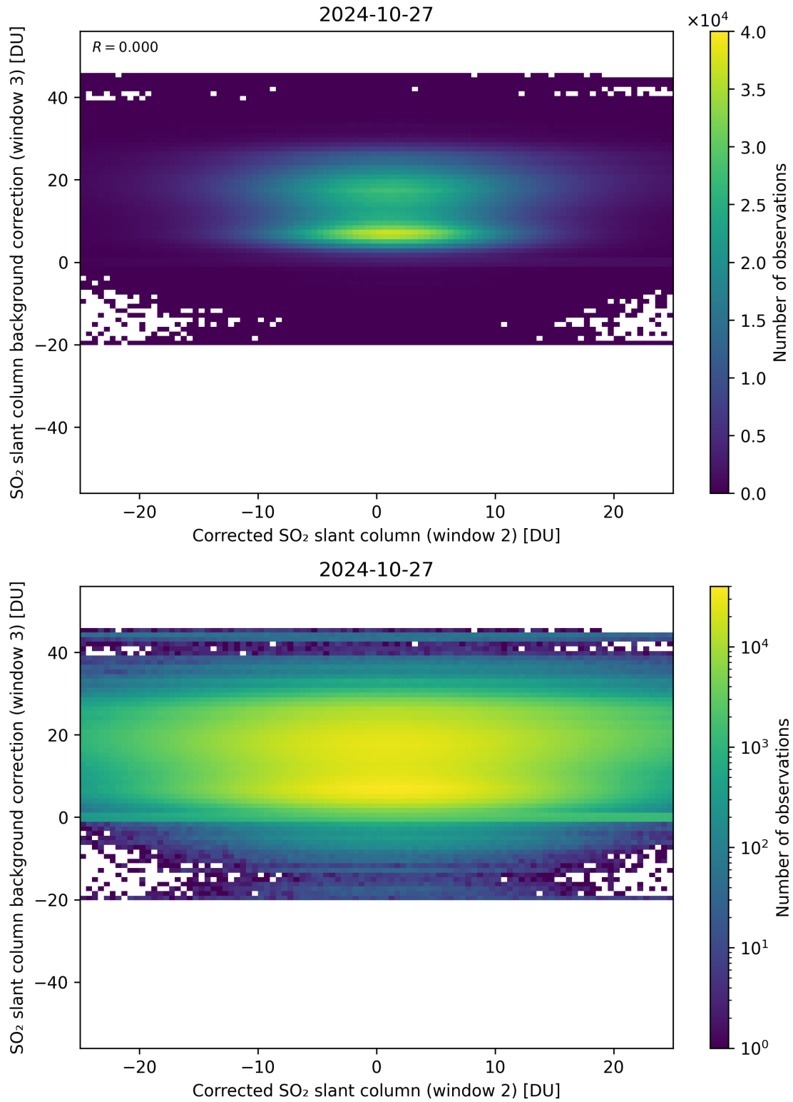
Figure 195: Scatter density plot of “Corrected SO 2 slant column (window 2)” against “SO 2 slant column background correction (window 3)” for 2024-10-26 to 2024-10-28.
