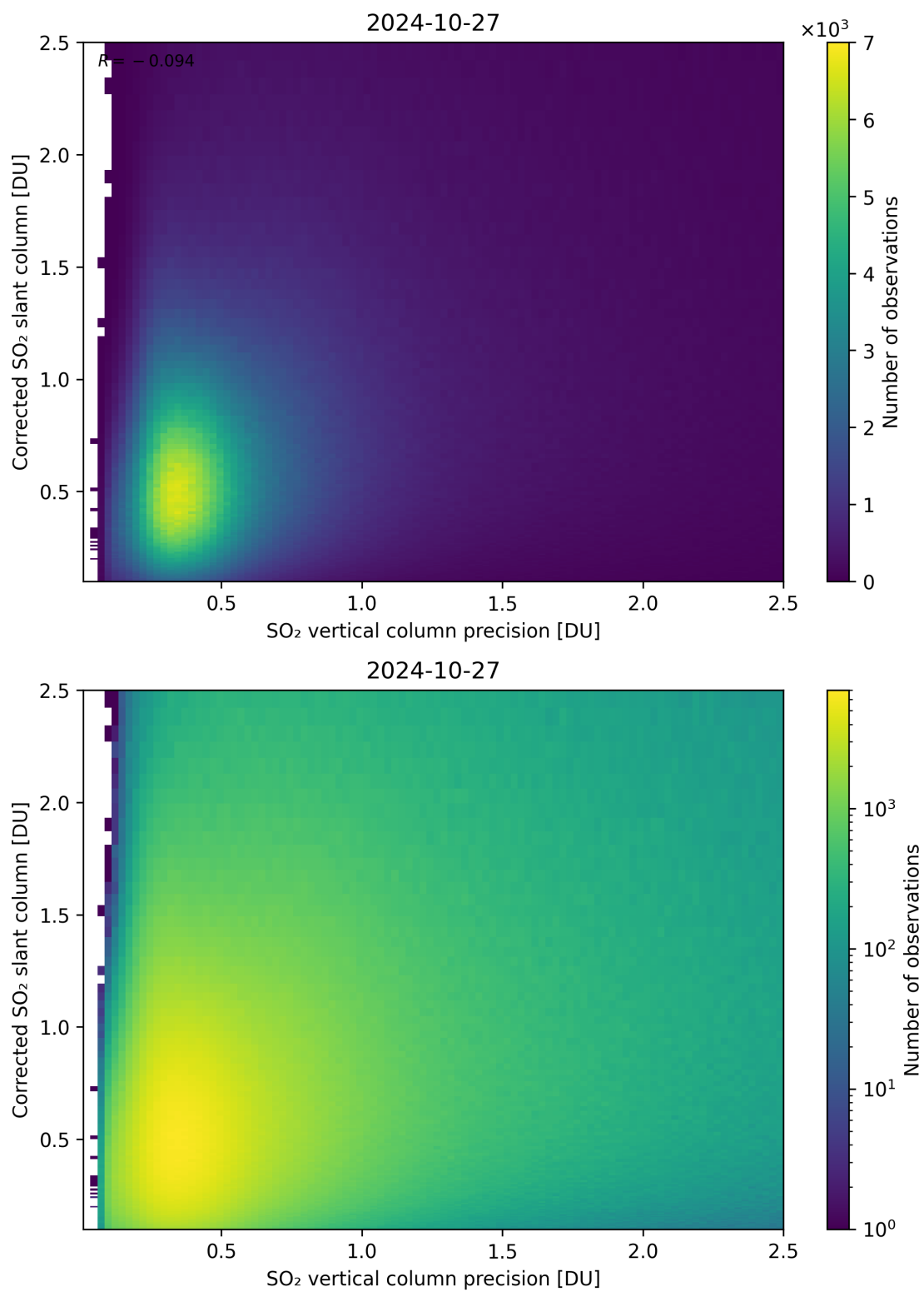
Figure 286: Scatter density plot of “SO 2 vertical column precision” against “Corrected SO 2 slant column” for 2024-10-26 to 2024-10-28.
