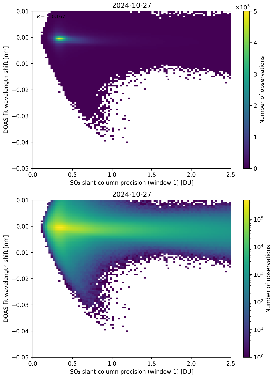
Figure 221: Scatter density plot of “SO 2 slant column precision (window 1)” against “DOAS fit wavelength shift” for 2024-10-26 to 2024-10-28.
