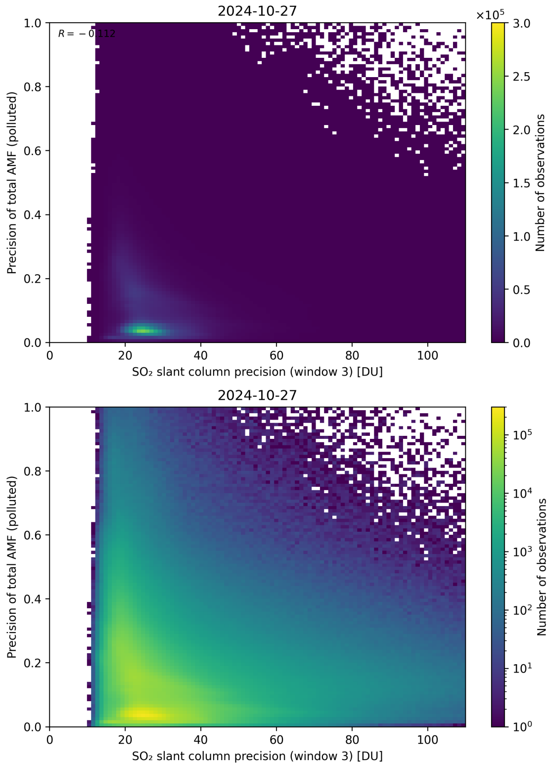
Figure 264: Scatter density plot of “SO 2 slant column precision (window 3)” against “Precision of total AMF (polluted)” for 2024-10-26 to 2024-10-28.
