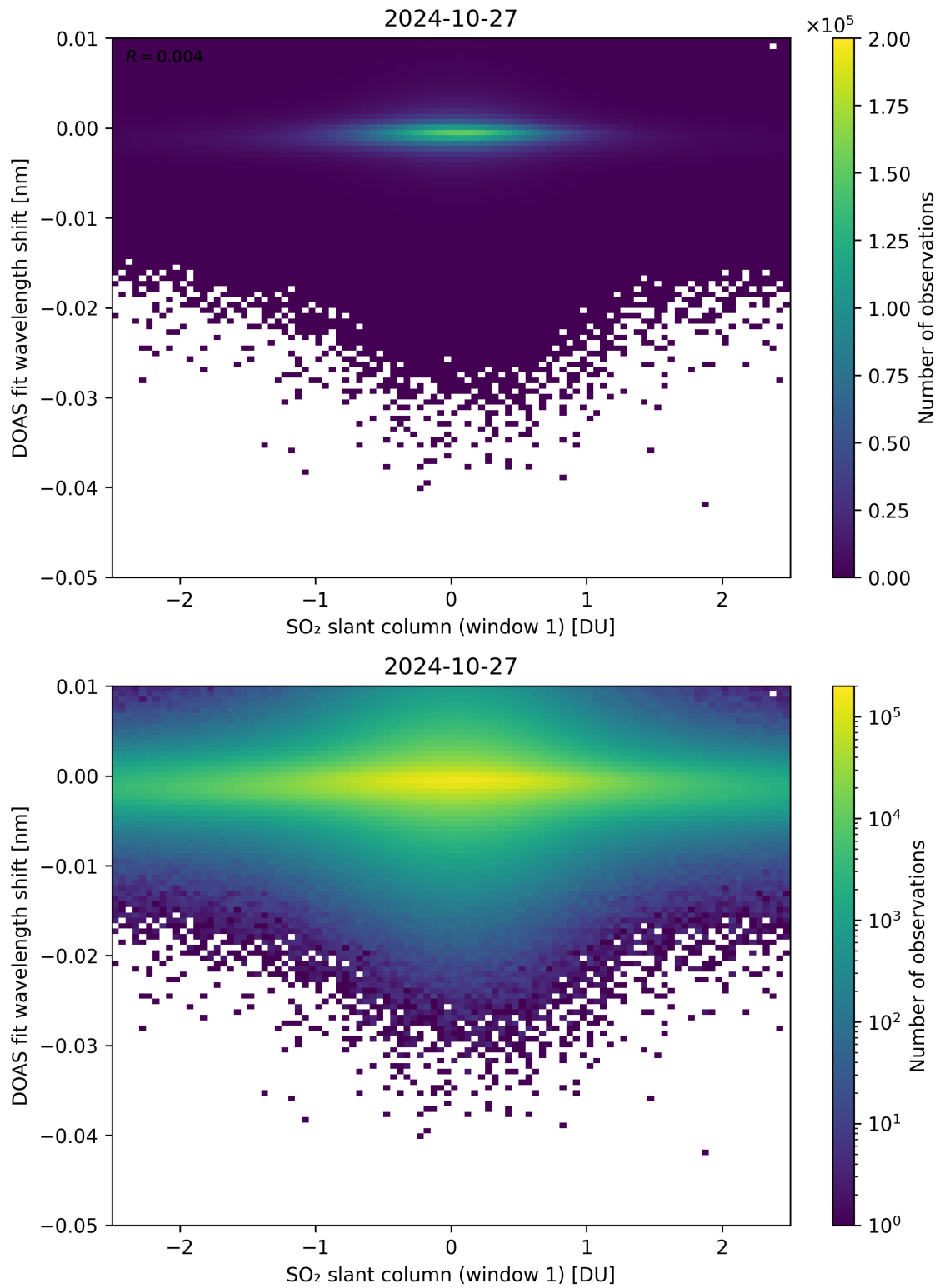
Figure 215: Scatter density plot of “SO 2 slant column (window 1)” against “DOAS fit wavelength shift” for 2024-10-26 to 2024-10-28.
