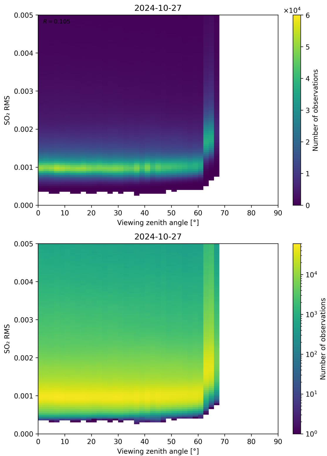
Figure 313: Scatter density plot of “Viewing zenith angle” against “SO 2 RMS” for 2024-10-26 to 2024-10-28.
