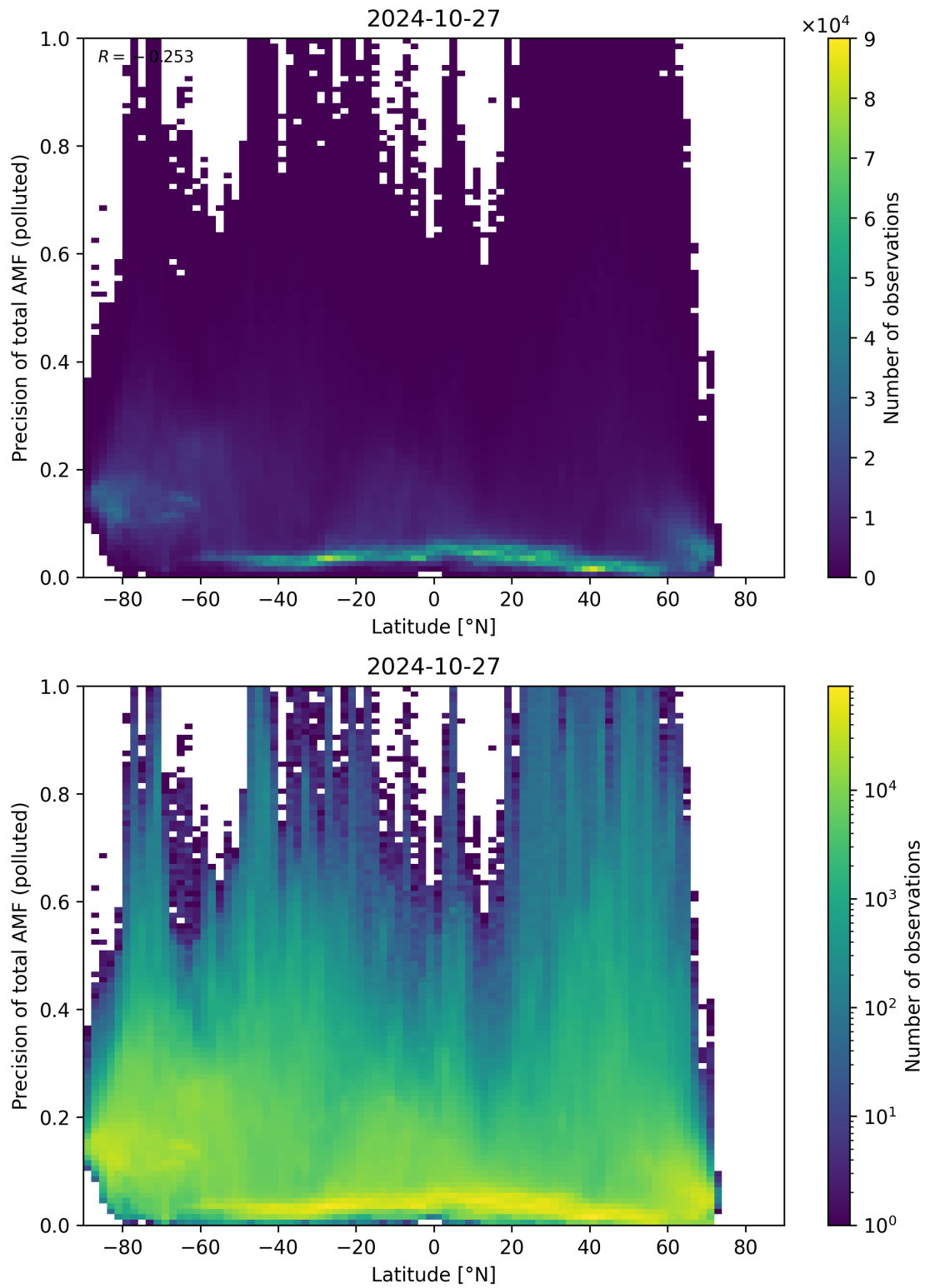
Figure 155: Scatter density plot of “Latitude” against “Precision of total AMF (polluted)” for 2024-10-26 to 2024-10-28.
