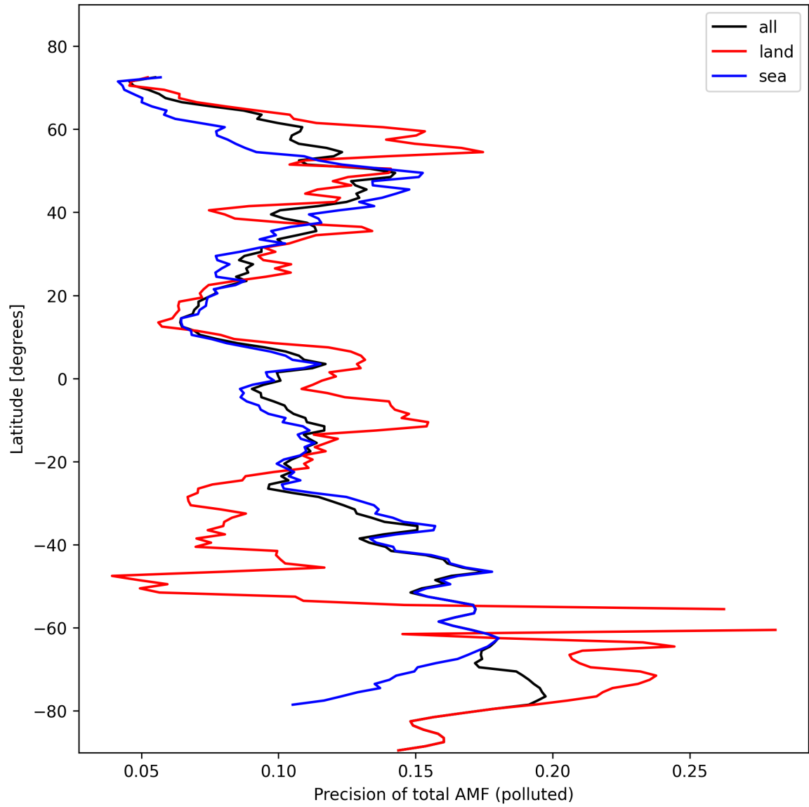
Figure 49: Zonal average of “Precision of total AMF (polluted)” for 2024-10-26 to 2024-10-28.
