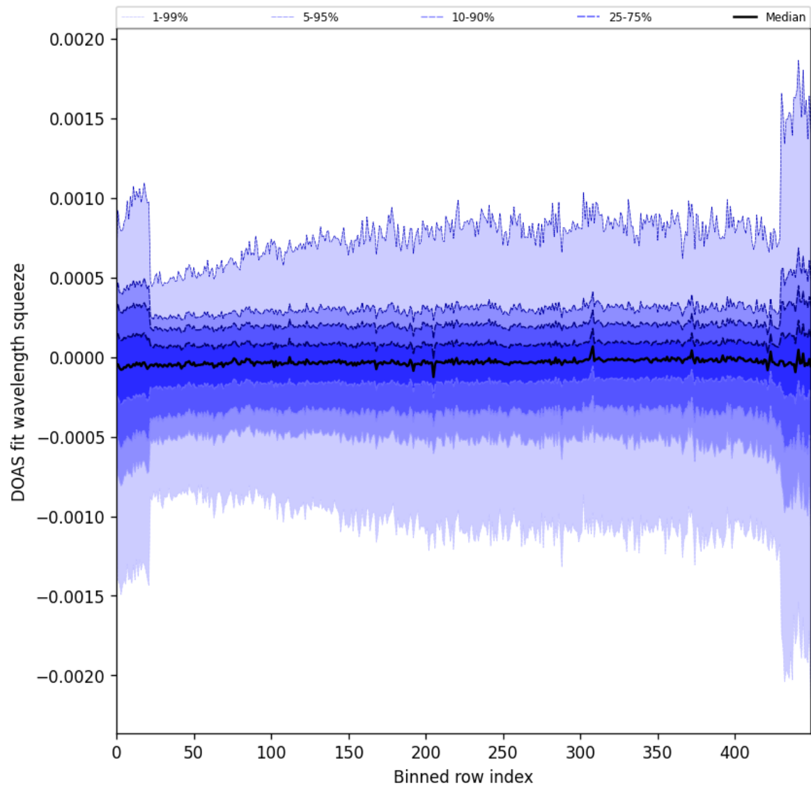
Figure 92: Along track statistics of “DOAS fit wavelength squeeze” for 2024-10-26 to 2024-10-28
