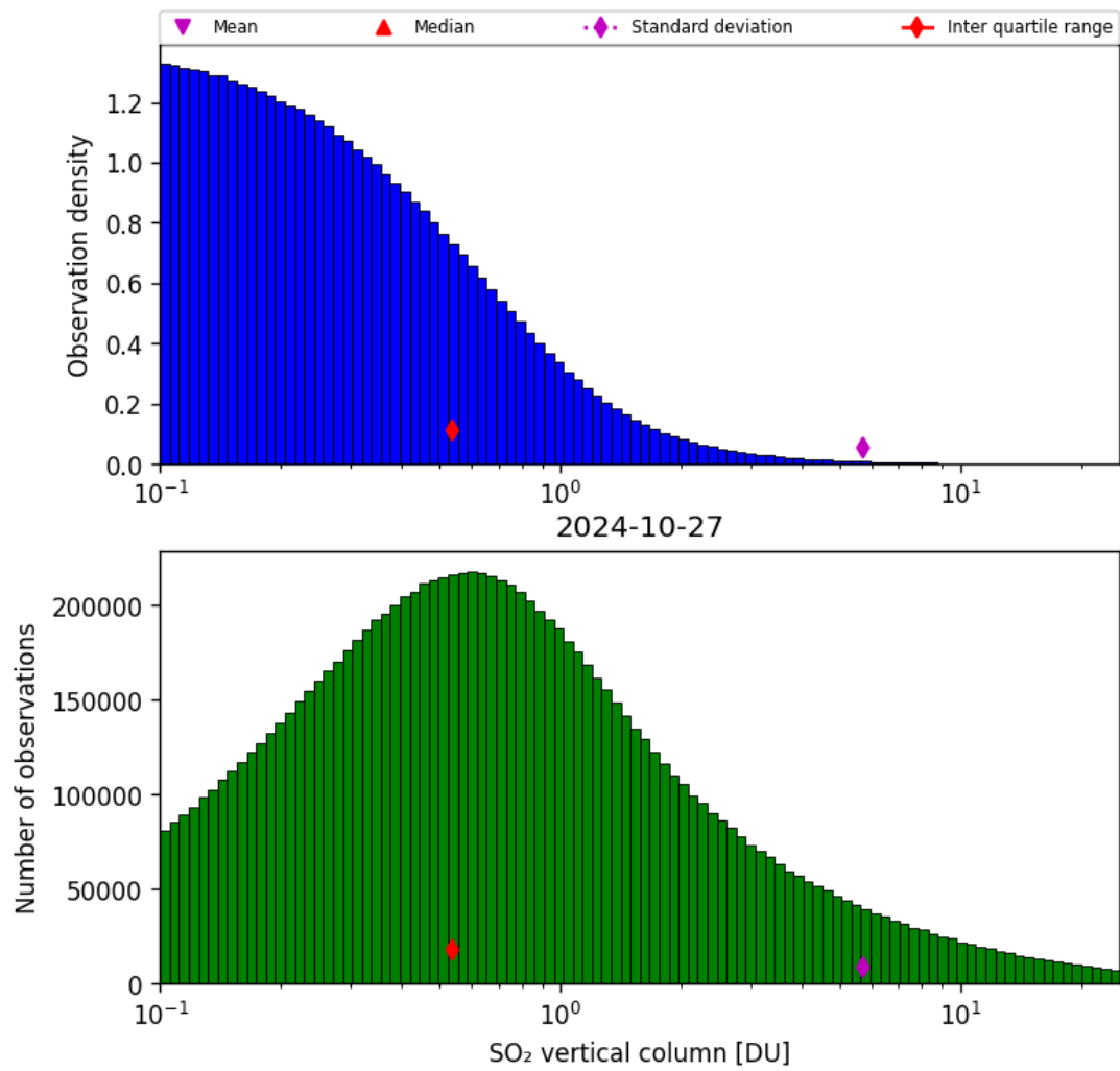
Figure 53: Histogram of “SO 2 vertical column” for 2024-10-26 to 2024-10-28
