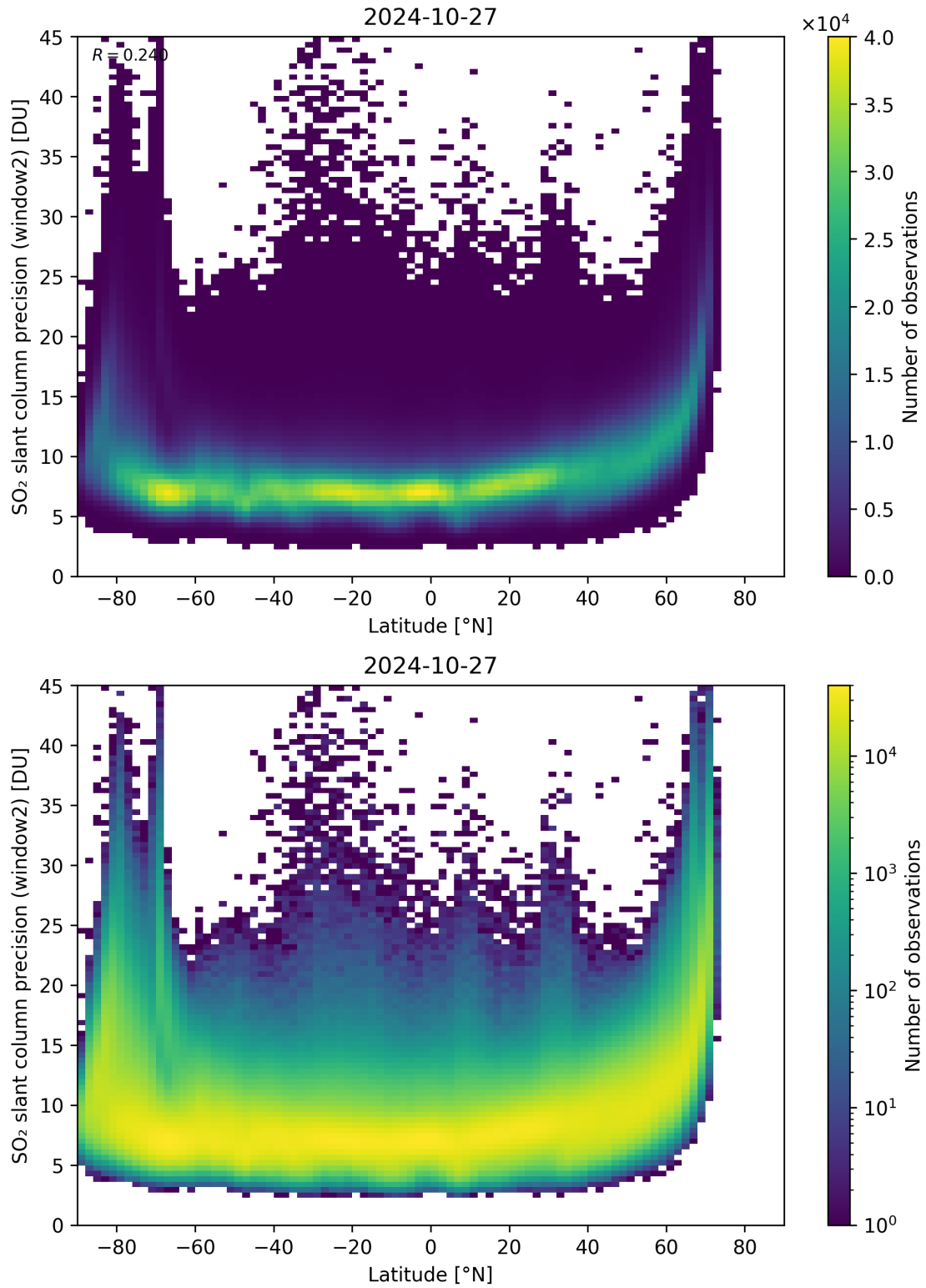
Figure 151: Scatter density plot of “Latitude” against “SO 2 slant column precision (window2)” for 2024-10-26 to 2024-10-28.
