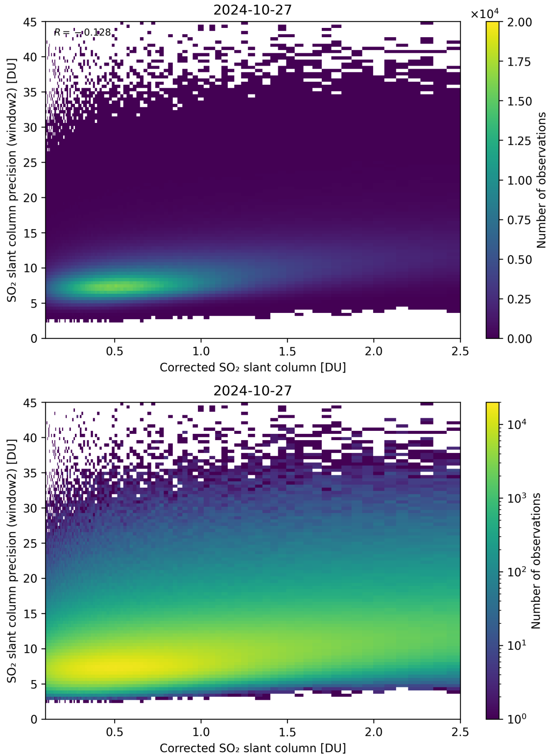
Figure 189: Scatter density plot of “Corrected SO 2 slant column” against “SO 2 slant column precision (window2)” for 2024-10-26 to 2024-10-28.
