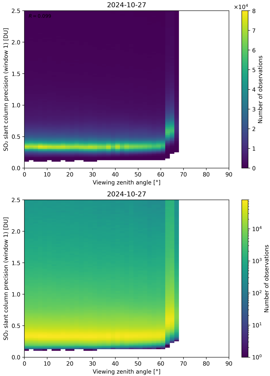
Figure 321: Scatter density plot of “Viewing zenith angle” against “SO 2 slant column precision (window 1)” for 2024-10-26 to 2024-10-28.
