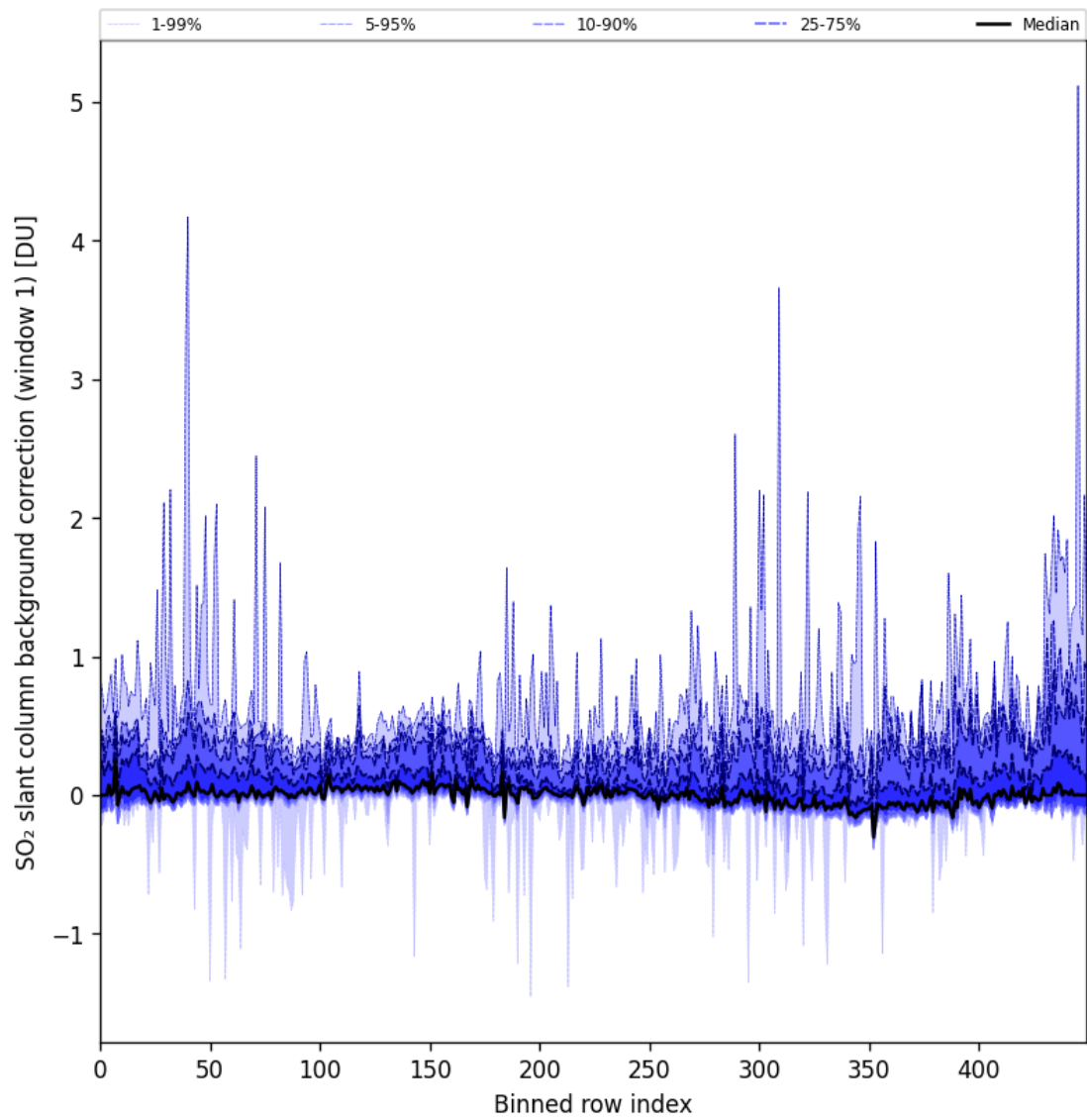
Figure 82: Along track statistics of “SO 2 slant column background correction (window 1)” for 2024-10-26 to 2024-10-28
