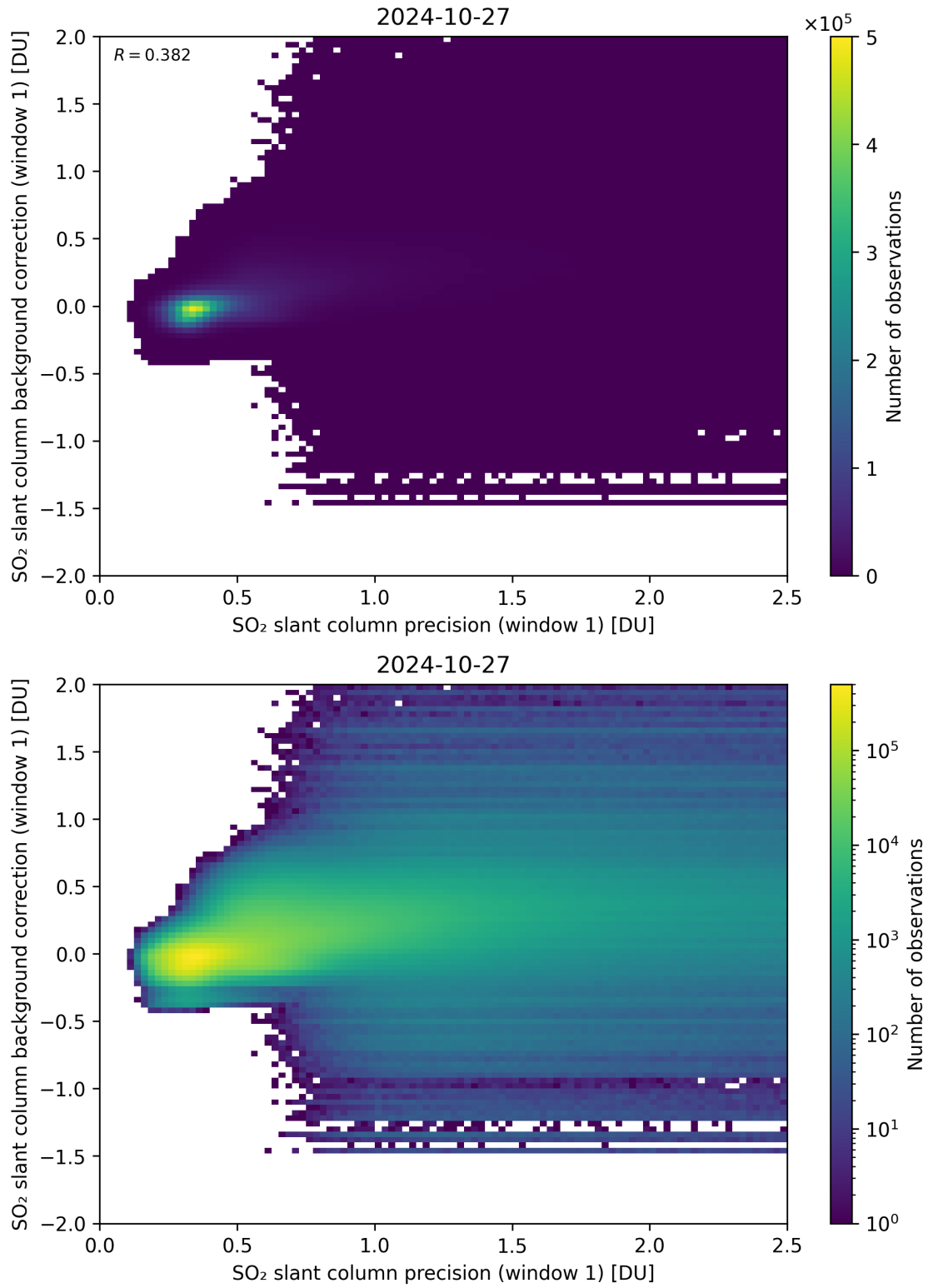
Figure 218: Scatter density plot of “SO 2 slant column precision (window 1)” against “SO 2 slant column background correction (window 1)” for 2024-10-26 to 2024-10-28.
