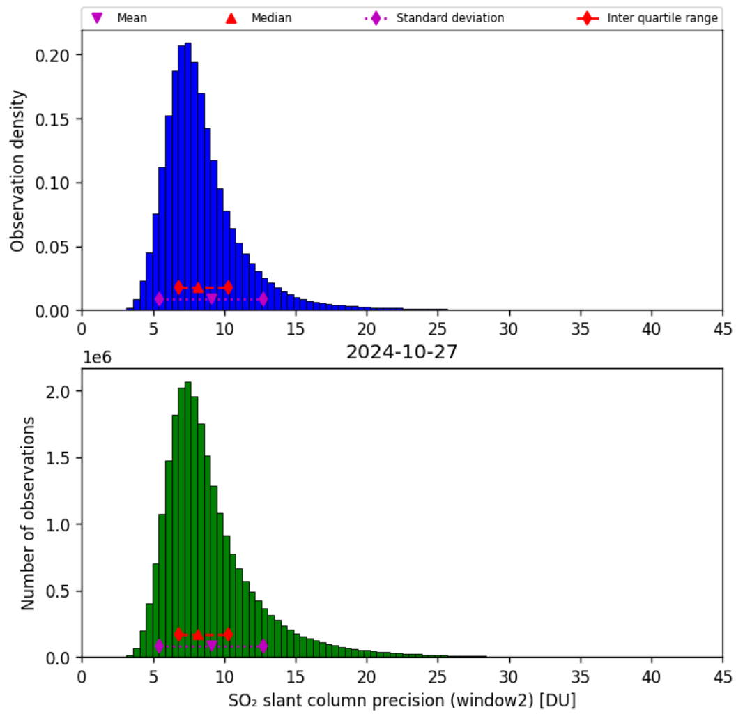
Figure 61: Histogram of “SO 2 slant column precision (window2)” for 2024-10-26 to 2024-10-28
