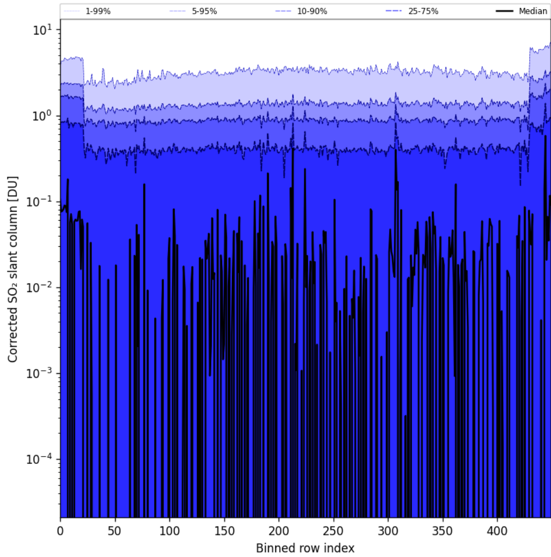
Figure 78: Along track statistics of “Corrected SO 2 slant column” for 2024-10-26 to 2024-10-28
