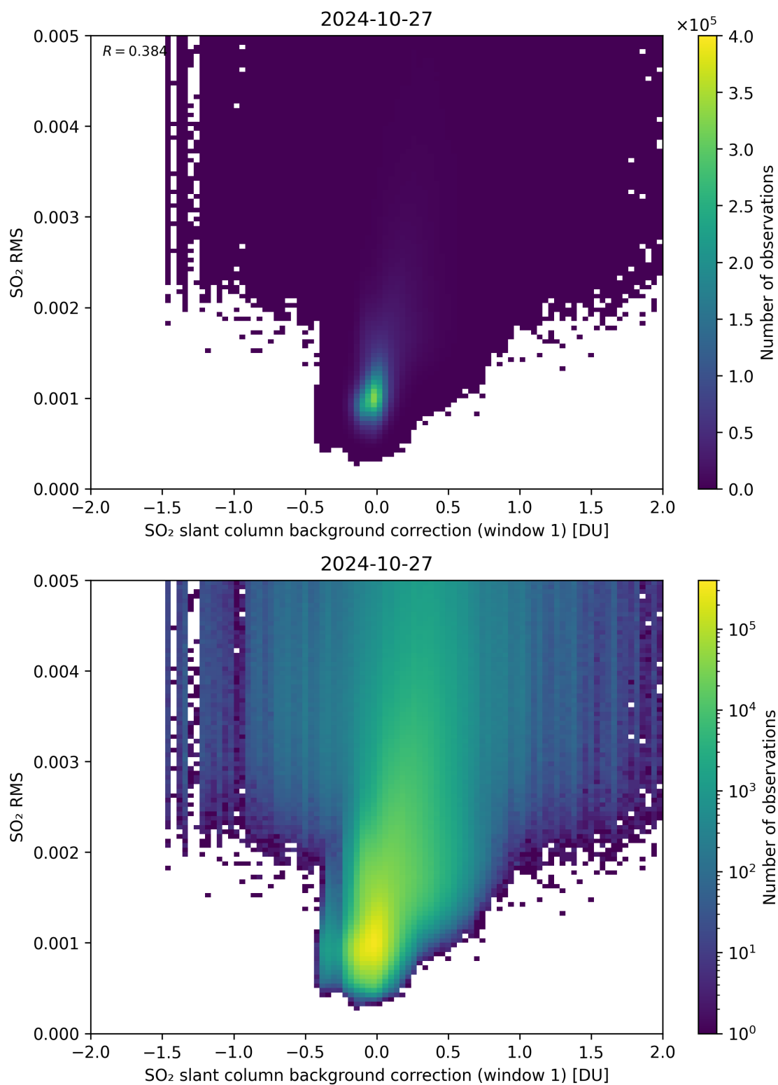
Figure 102: Scatter density plot of “SO 2 slant column background correction (window 1)” against “SO 2 RMS” for 2024-10-26 to 2024-10-28.
