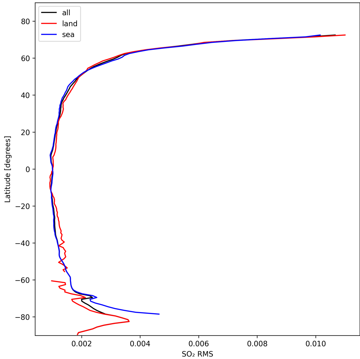
Figure 47: Zonal average of “SO 2 RMS” for 2024-10-26 to 2024-10-28.
