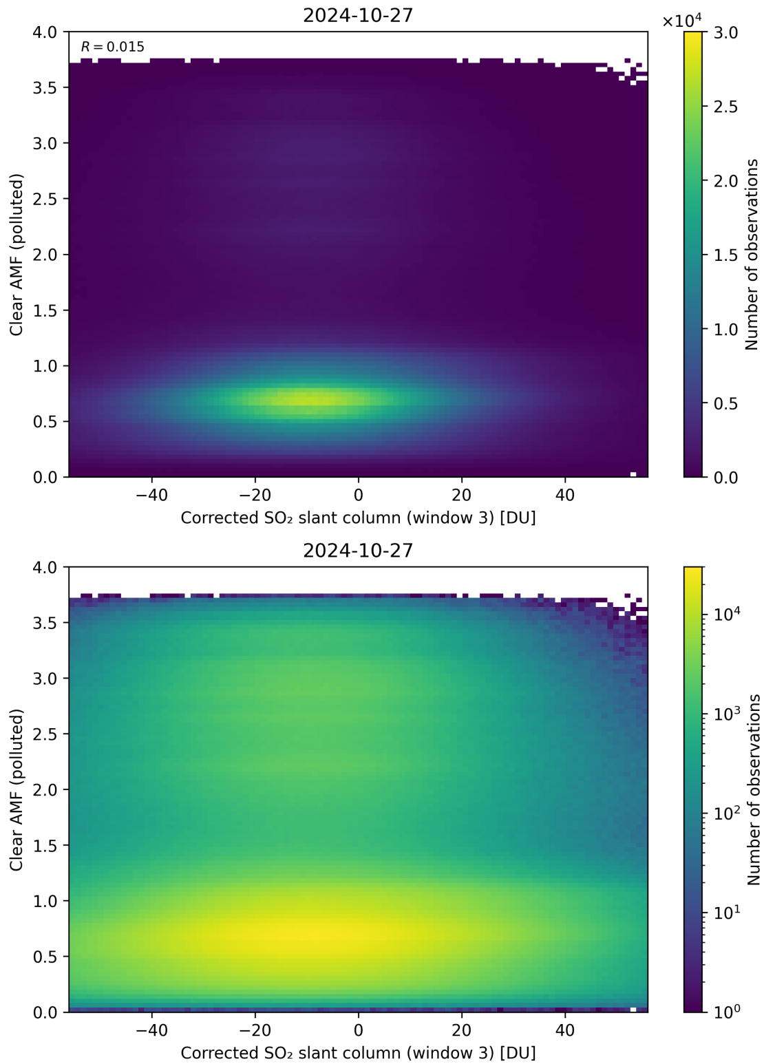
Figure 209: Scatter density plot of “Corrected SO 2 slant column (window 3)” against “Clear AMF (polluted)” for 2024-10-26 to 2024-10-28.
