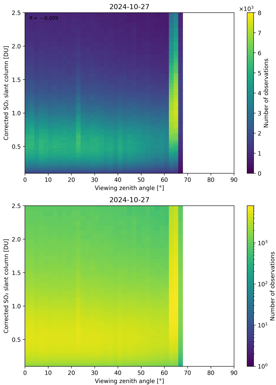
Figure 317: Scatter density plot of “Viewing zenith angle” against “Corrected SO 2 slant column” for 2024-10-26 to 2024-10-28.
