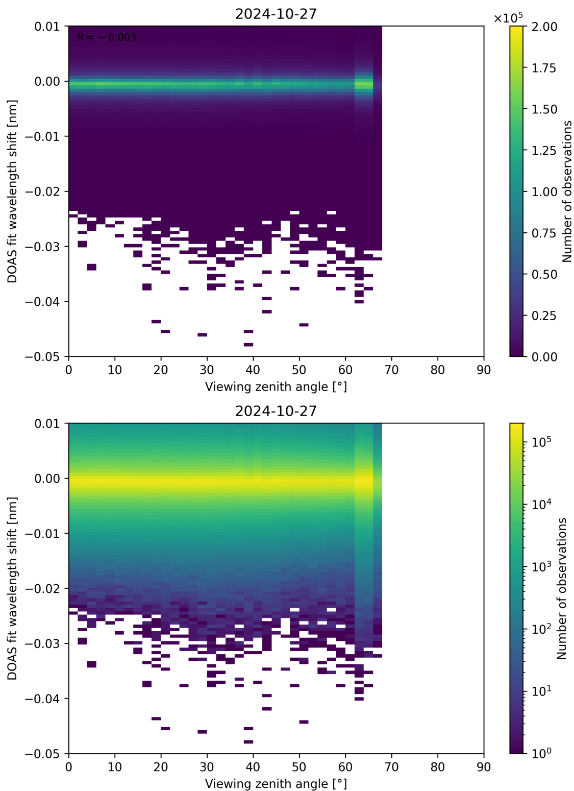
Figure 311: Scatter density plot of “Viewing zenith angle” against “DOAS fit wavelength shift” for 2024-10-26 to 2024-10-28.
