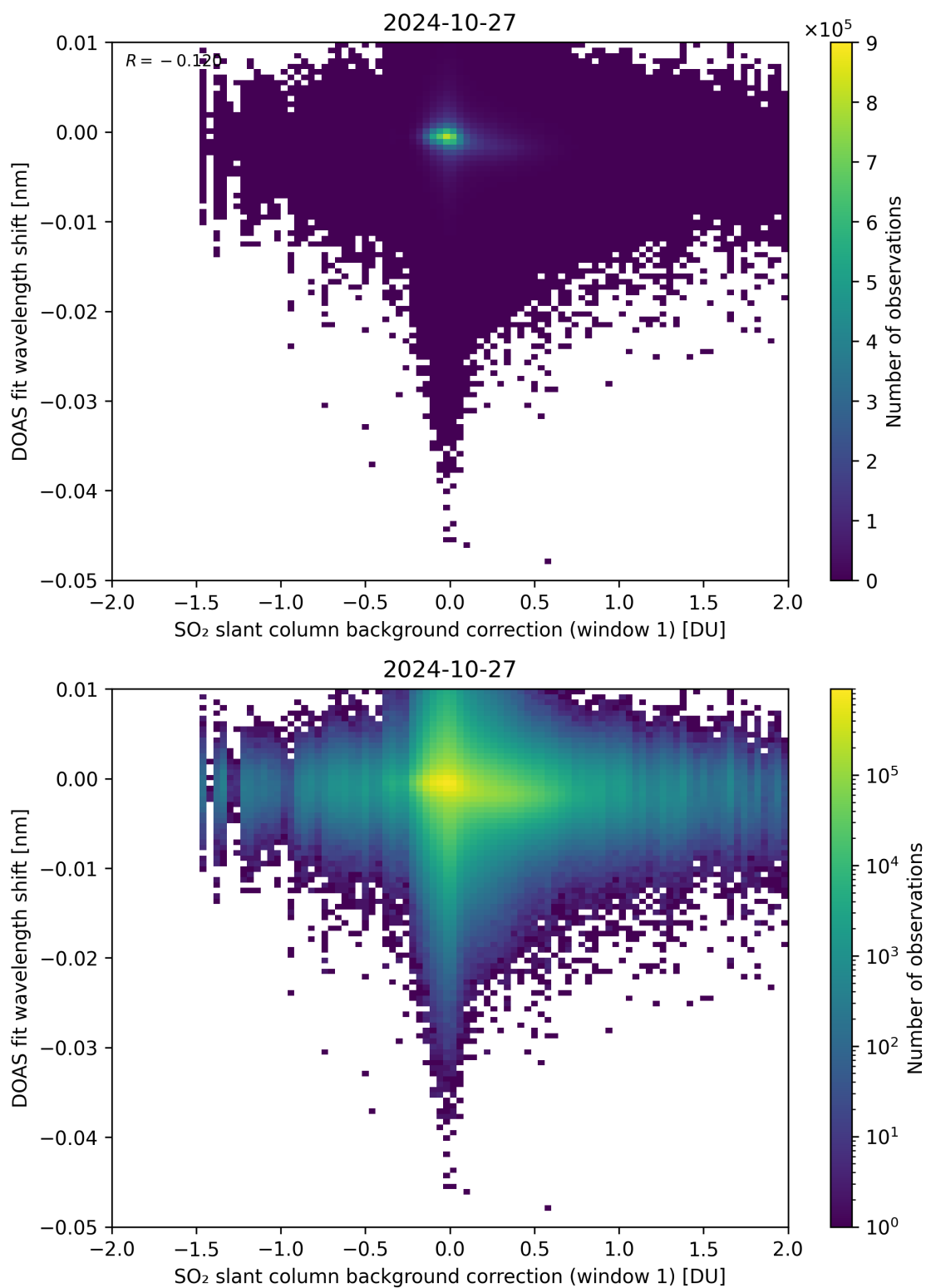
Figure 100: Scatter density plot of “SO 2 slant column background correction (window 1)” against “DOAS fit wavelength shift” for 2024-10-26 to 2024-10-28.
