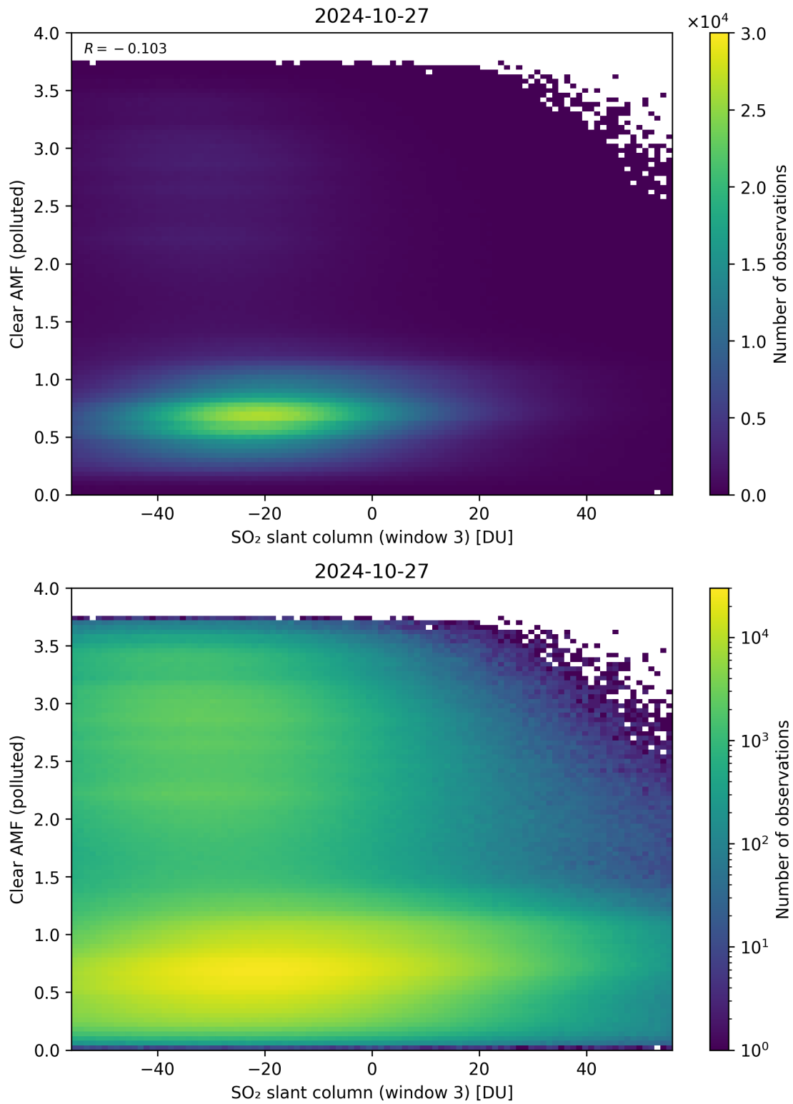
Figure 265: Scatter density plot of “SO 2 slant column (window 3)” against “Clear AMF (polluted)” for 2024-10-26 to 2024-10-28.
