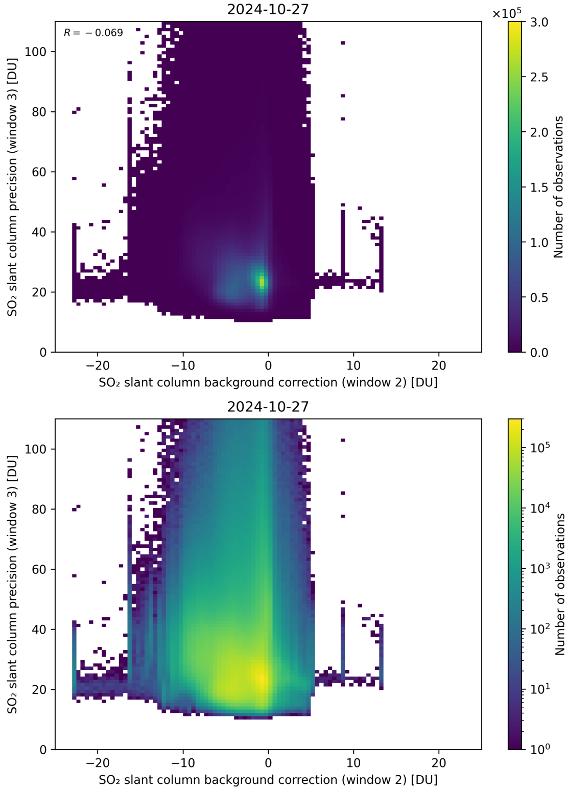
Figure 118: Scatter density plot of “SO 2 slant column background correction (window 2)” against “SO 2 slant column precision (window 3)” for 2024-10-26 to 2024-10-28.
