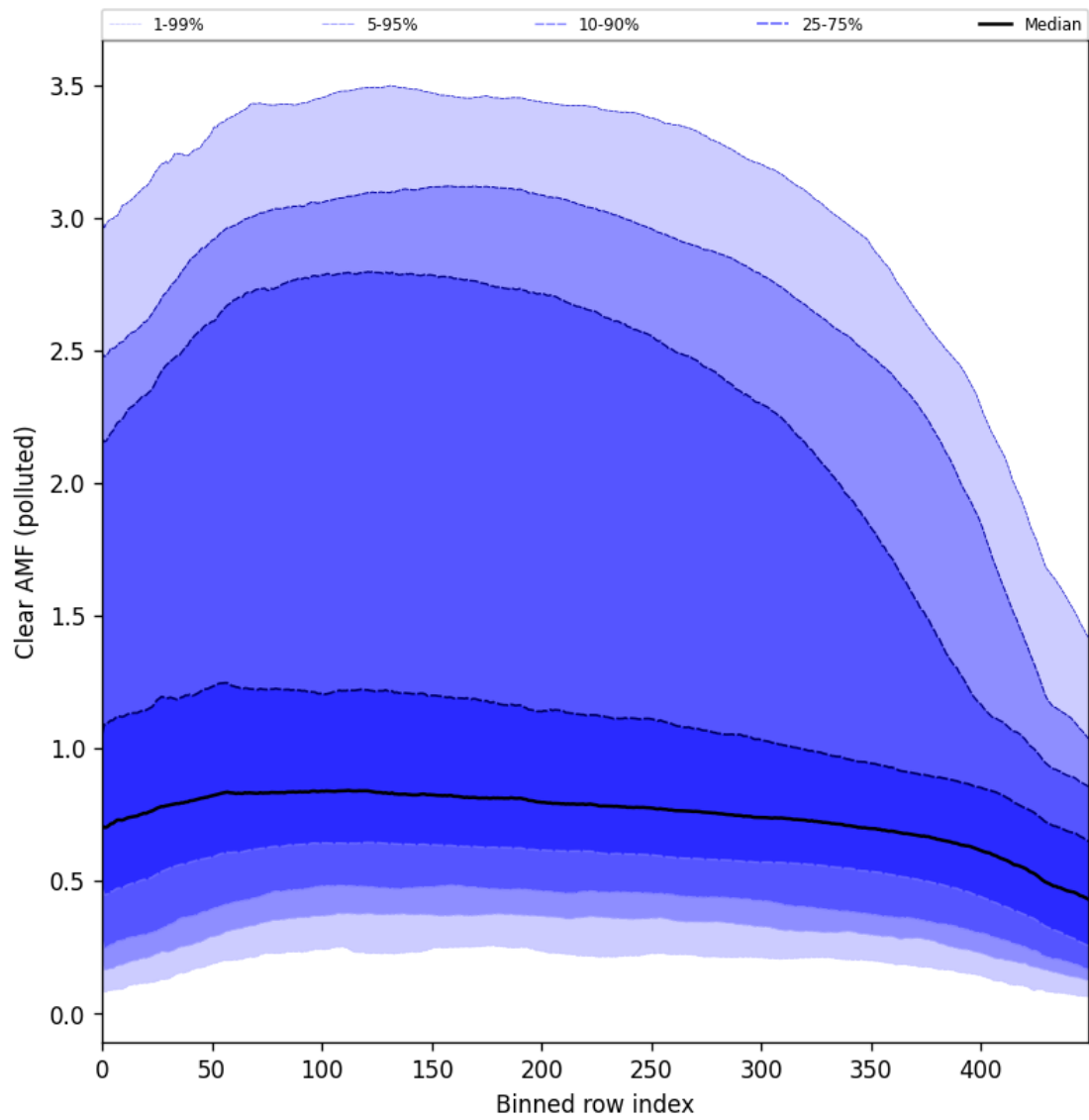
Figure 96: Along track statistics of “Clear AMF (polluted)” for 2024-10-26 to 2024-10-28
