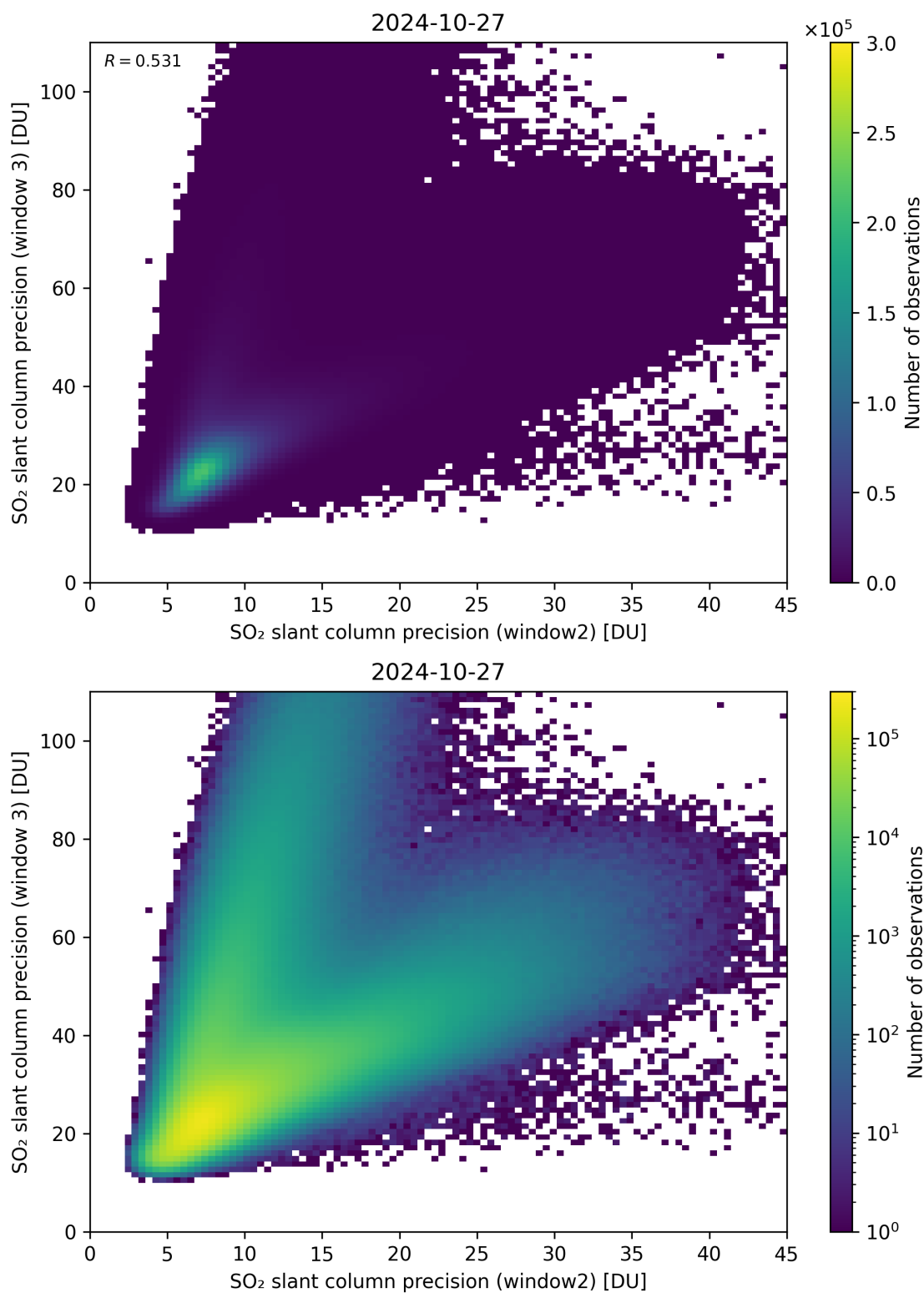
Figure 250: Scatter density plot of “SO 2 slant column precision (window2)” against “SO 2 slant column precision (window 3)” for 2024-10-26 to 2024-10-28.
