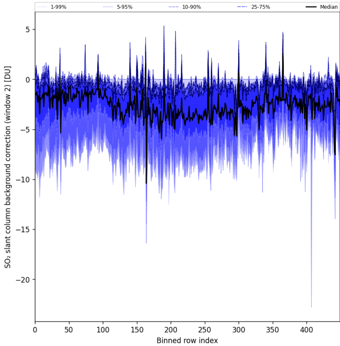
Figure 86: Along track statistics of “SO 2 slant column background correction (window 2)” for 2024-10-26 to 2024-10-28
