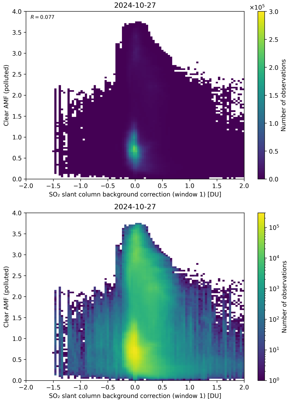
Figure 103: Scatter density plot of “SO 2 slant column background correction (window 1)” against “Clear AMF (polluted)” for 2024-10-26 to 2024-10-28.
