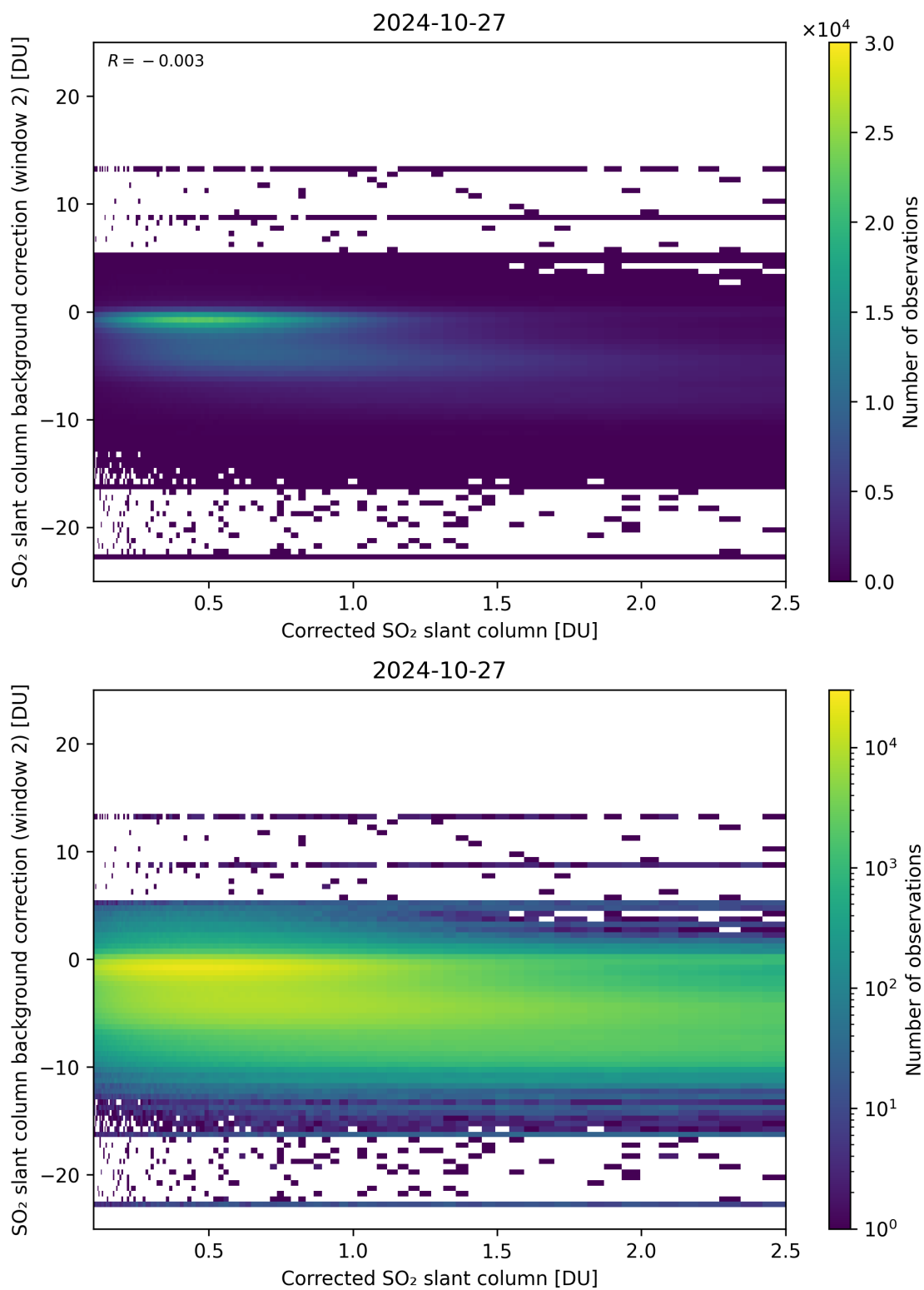
Figure 179: Scatter density plot of “Corrected SO 2 slant column” against “SO 2 slant column background correction (window 2)” for 2024-10-26 to 2024-10-28.
