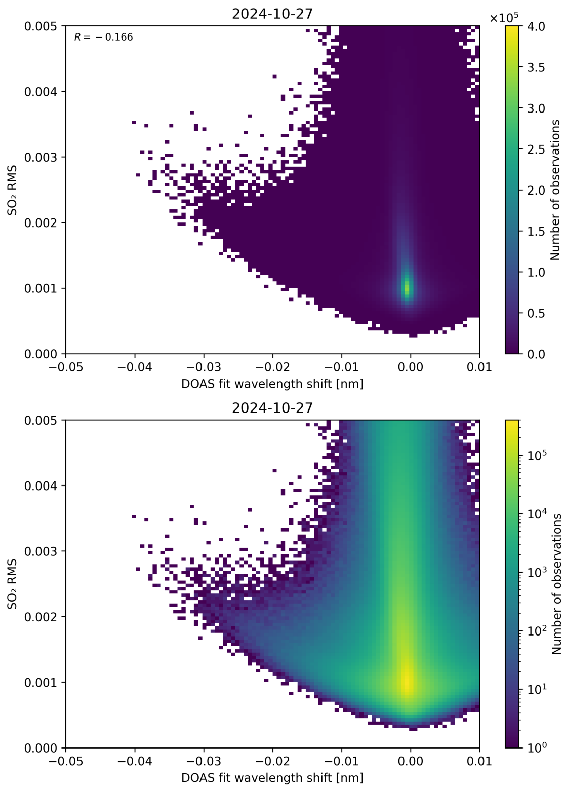
Figure 128: Scatter density plot of “DOAS fit wavelength shift” against “SO 2 RMS” for 2024-10-26 to 2024-10-28.
