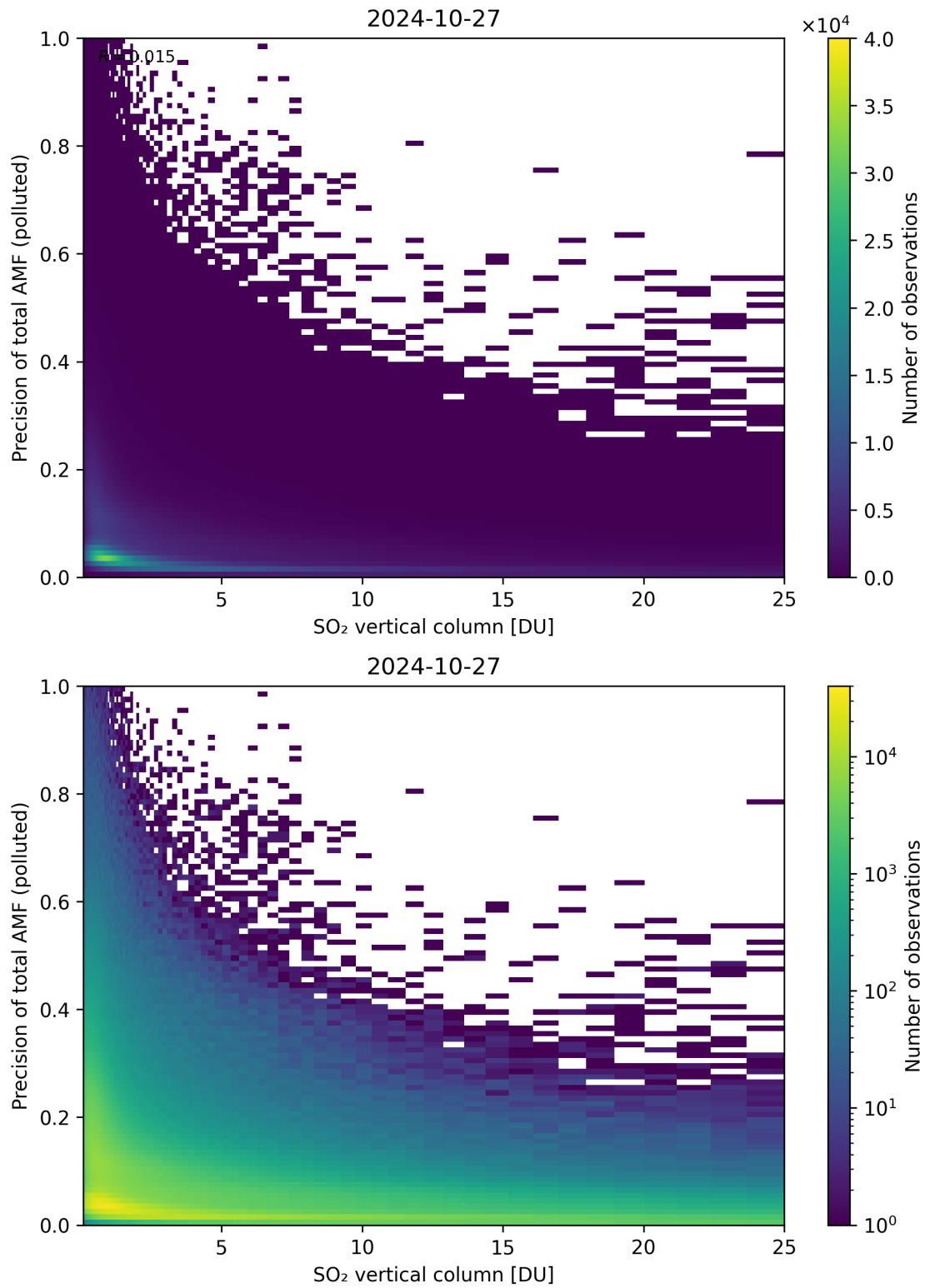
Figure 306: Scatter density plot of “SO 2 vertical column” against “Precision of total AMF (polluted)” for 2024-10-26 to 2024-10-28.
