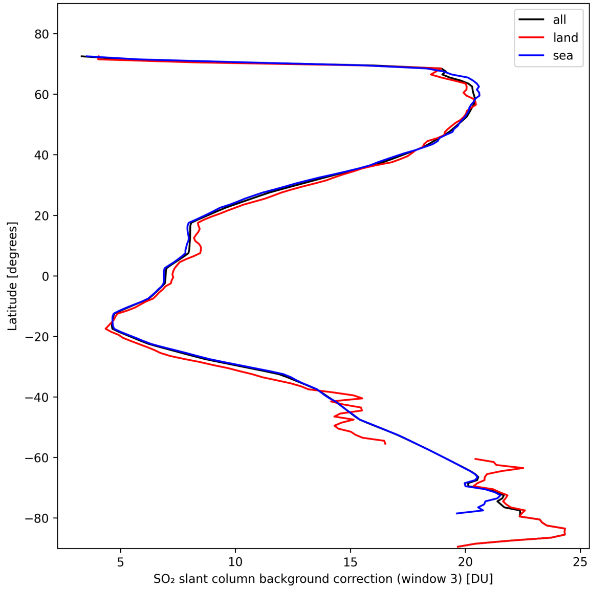
Figure 44: Zonal average of “SO 2 slant column background correction (window 3)” for 2024-10-26 to 2024-10-28.
