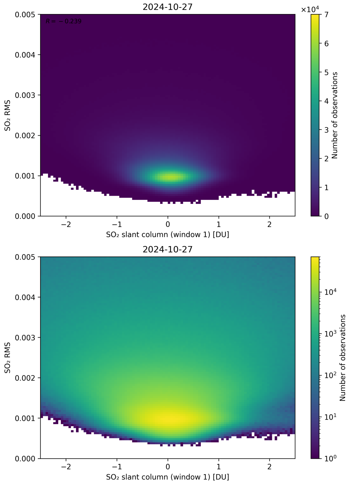
Figure 217: Scatter density plot of “SO 2 slant column (window 1)” against “SO 2 RMS” for 2024-10-26 to 2024-10-28.
