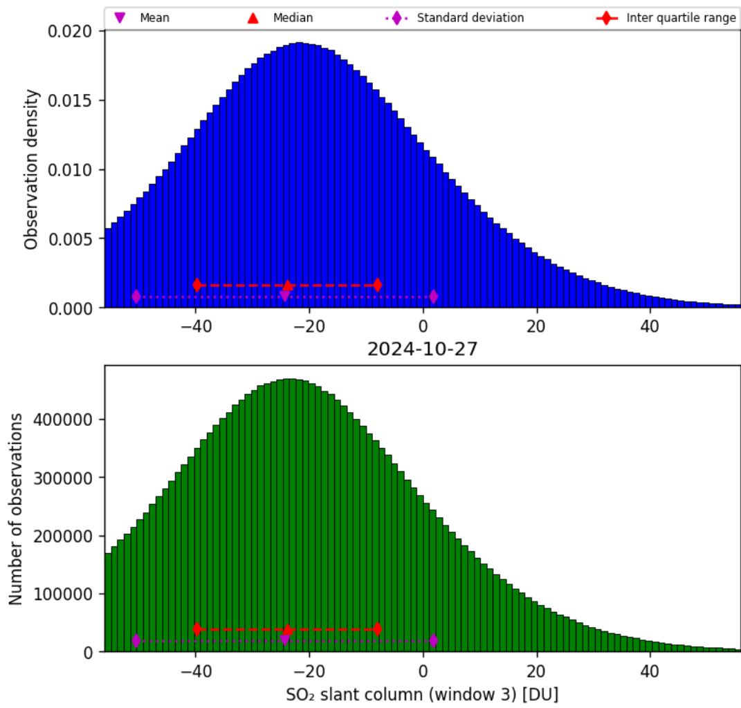
Figure 64: Histogram of “SO 2 slant column (window 3)” for 2024-10-26 to 2024-10-28
