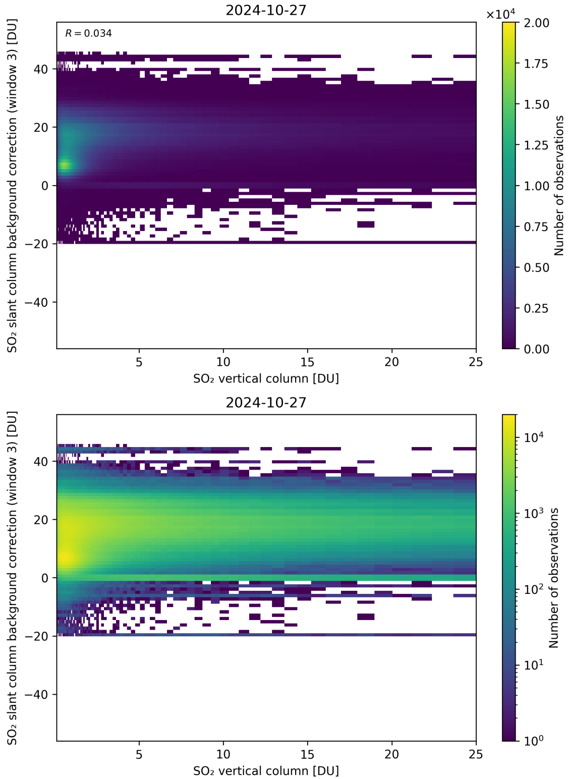
Figure 275: Scatter density plot of “SO 2 vertical column” against “SO 2 slant column background correction (window 3)” for 2024-10-26 to 2024-10-28.
