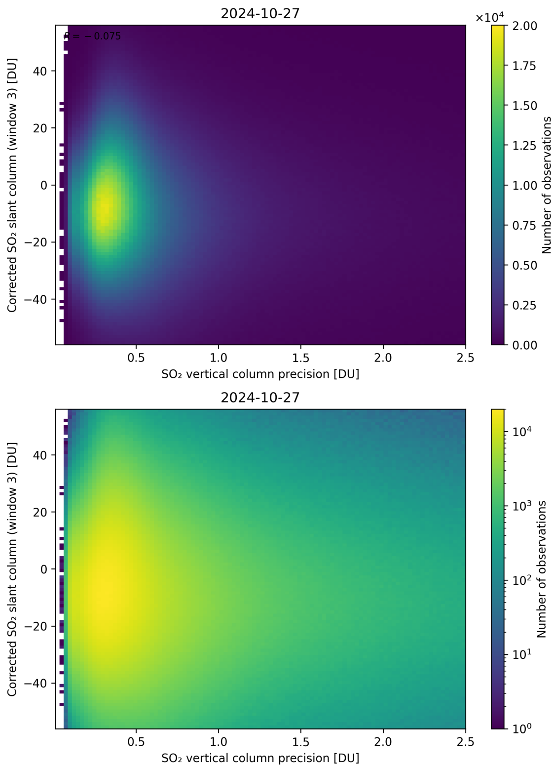
Figure 288: Scatter density plot of “SO 2 vertical column precision” against “Corrected SO 2 slant column (window 3)” for 2024-10-26 to 2024-10-28.
