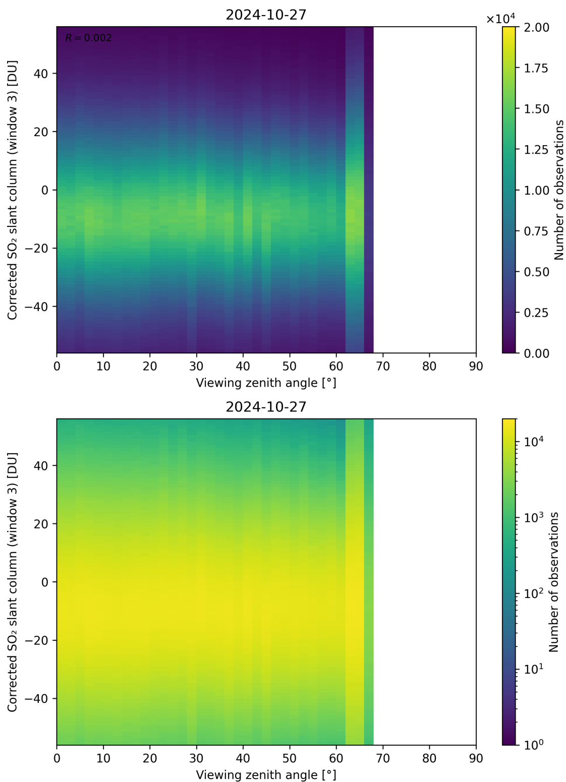
Figure 319: Scatter density plot of “Viewing zenith angle” against “Corrected SO 2 slant column (window 3)” for 2024-10-26 to 2024-10-28.
