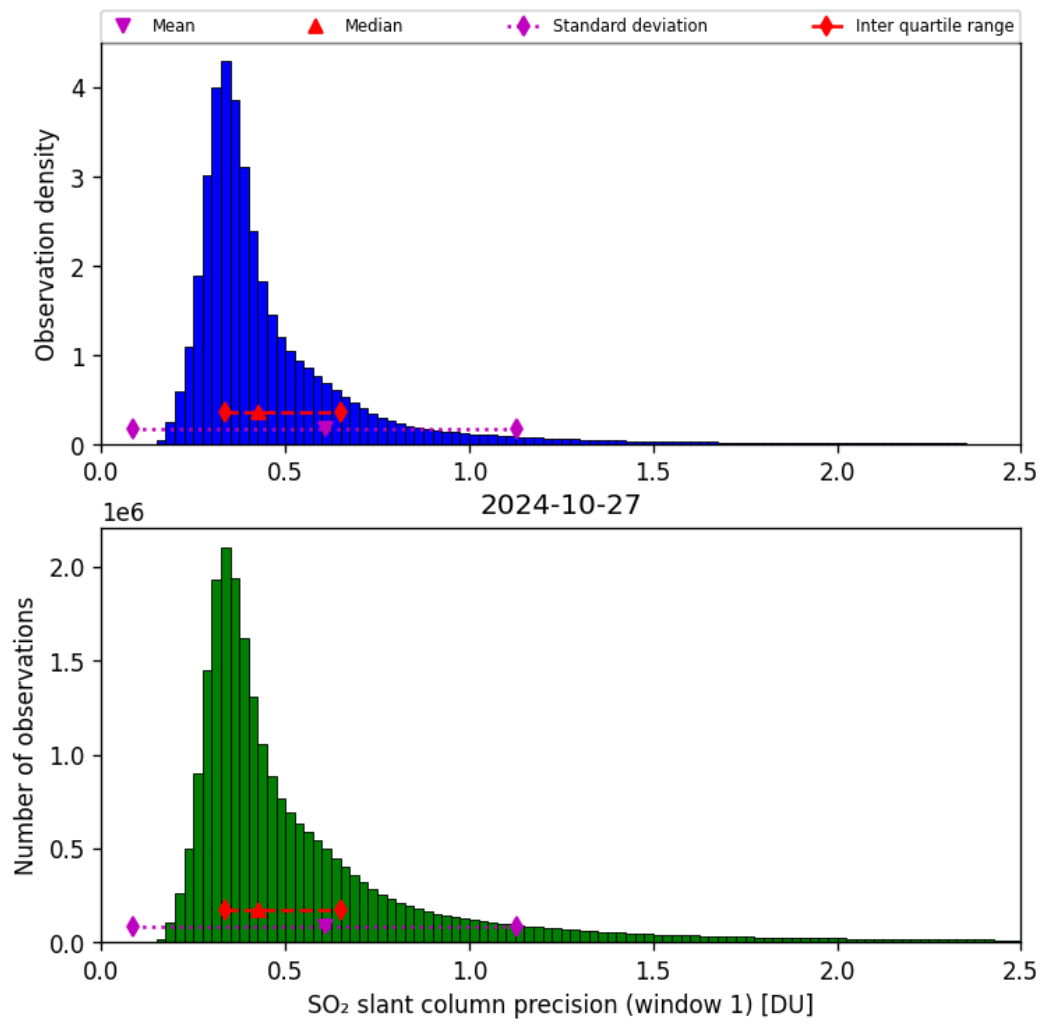
Figure 57: Histogram of “SO 2 slant column precision (window 1)” for 2024-10-26 to 2024-10-28
