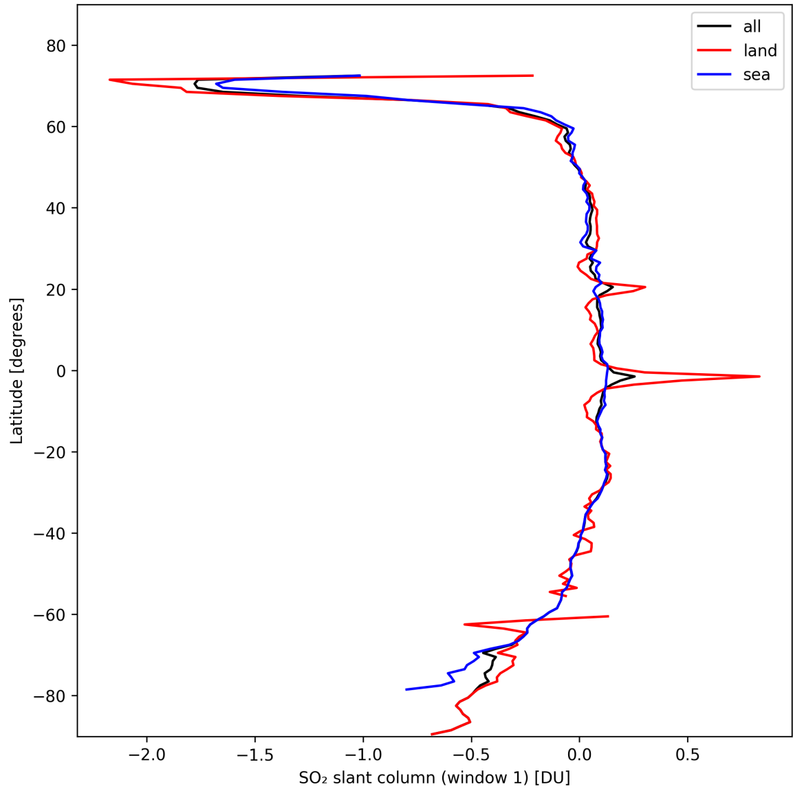
Figure 33: Zonal average of “SO 2 slant column (window 1)” for 2024-10-26 to 2024-10-28.
