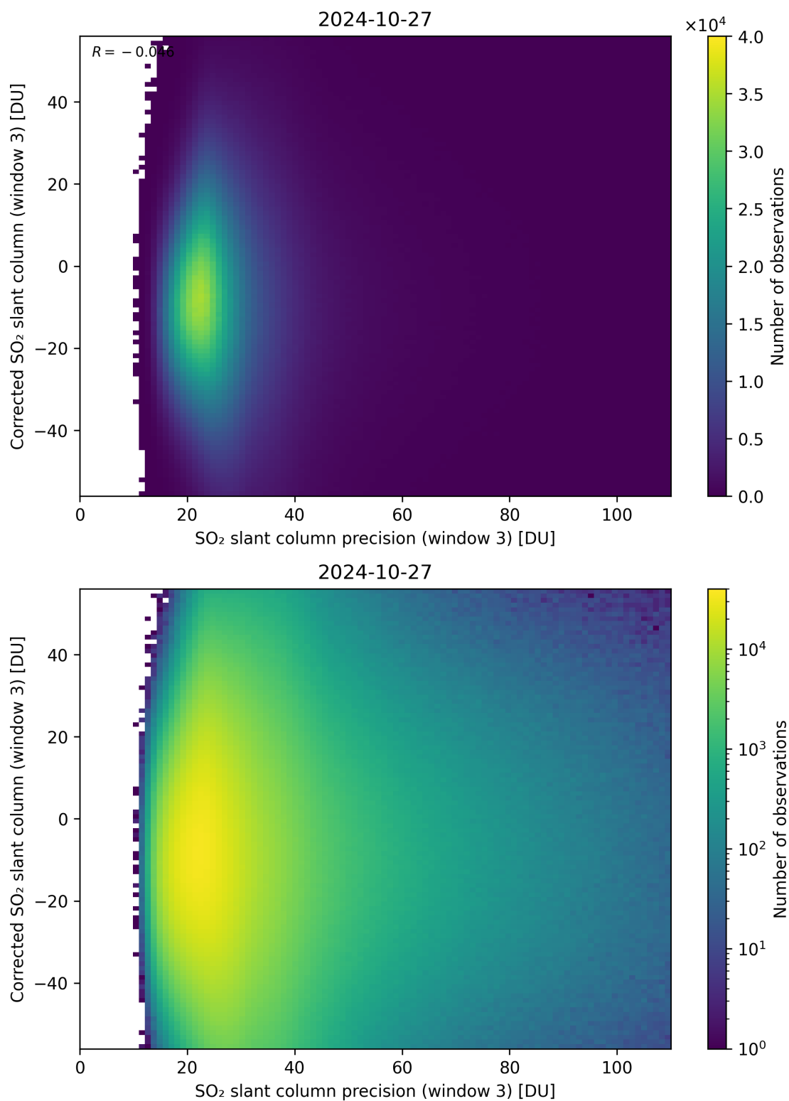
Figure 262: Scatter density plot of “SO 2 slant column precision (window 3)” against “Corrected SO 2 slant column (window 3)” for 2024-10-26 to 2024-10-28.
