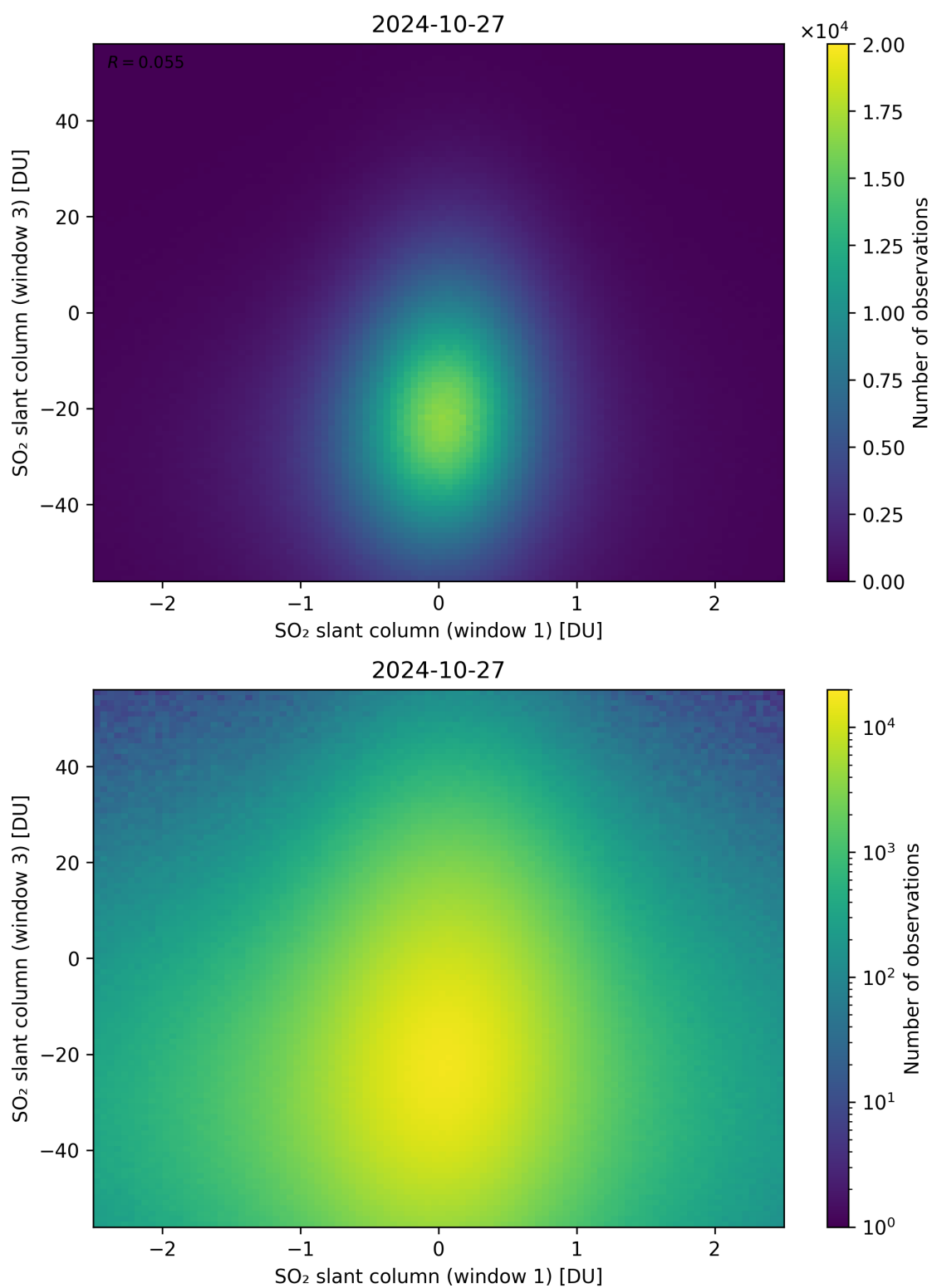
Figure 237: Scatter density plot of “SO 2 slant column (window 1)” against “SO 2 slant column (window 3)” for 2024-10-26 to 2024-10-28.
