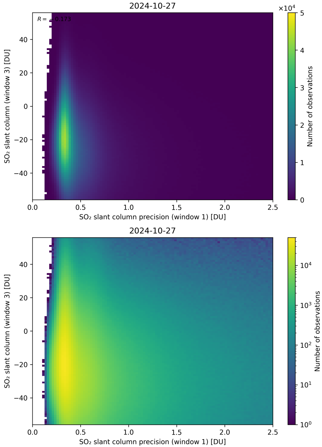
Figure 228: Scatter density plot of “SO 2 slant column precision (window 1)” against “SO 2 slant column (window 3)” for 2024-10-26 to 2024-10-28.
