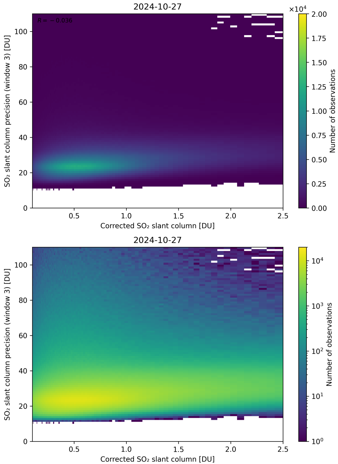
Figure 191: Scatter density plot of “Corrected SO 2 slant column” against “SO 2 slant column precision (window 3)” for 2024-10-26 to 2024-10-28.
