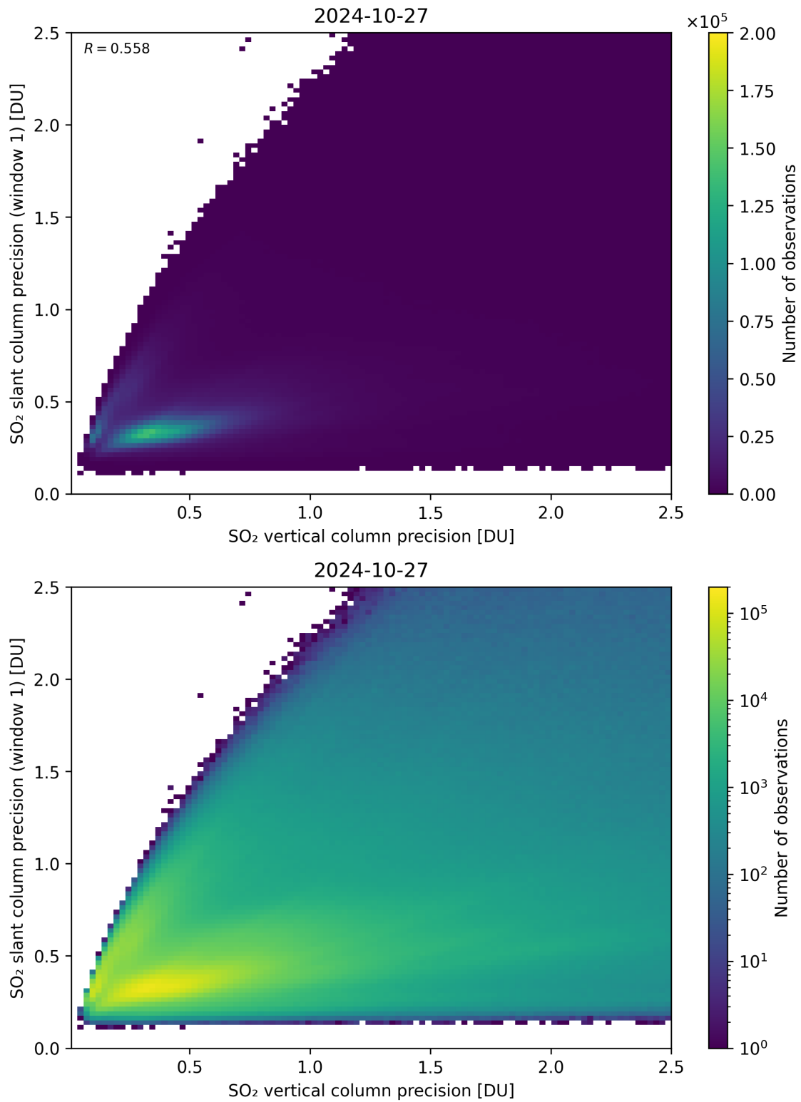
Figure 290: Scatter density plot of “SO 2 vertical column precision” against “SO 2 slant column precision (window 1)” for 2024-10-26 to 2024-10-28.
