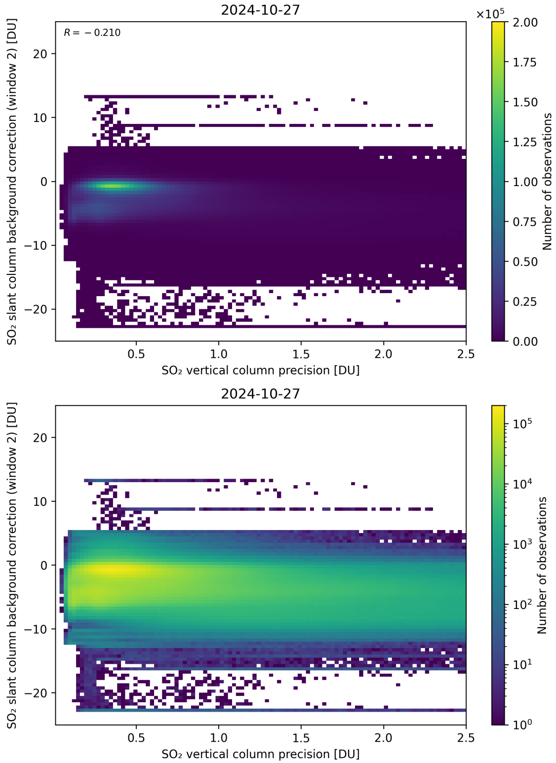
Figure 280: Scatter density plot of “SO 2 vertical column precision” against “SO 2 slant column background correction (window 2)” for 2024-10-26 to 2024-10-28.
