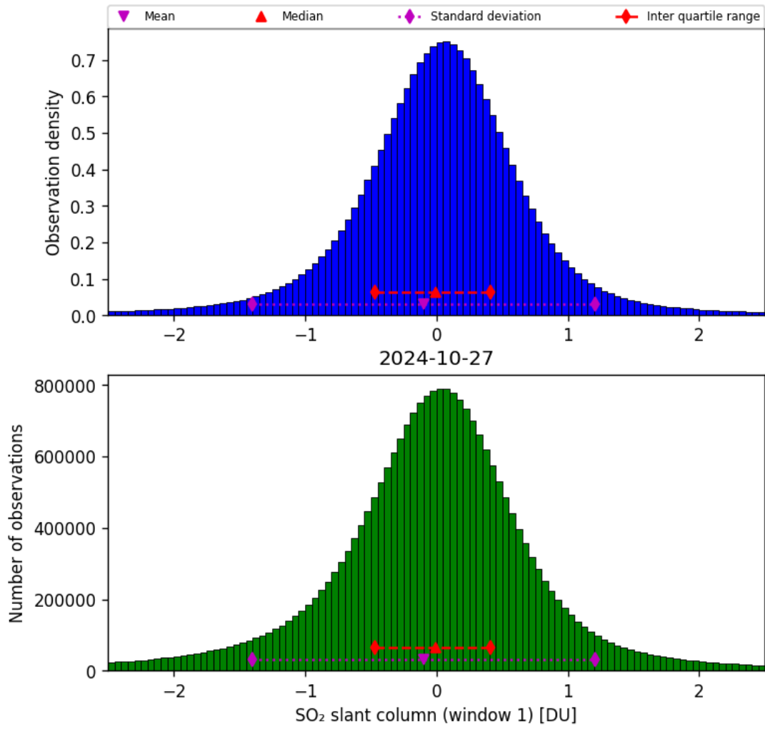
Figure 56: Histogram of “SO 2 slant column (window 1)” for 2024-10-26 to 2024-10-28
