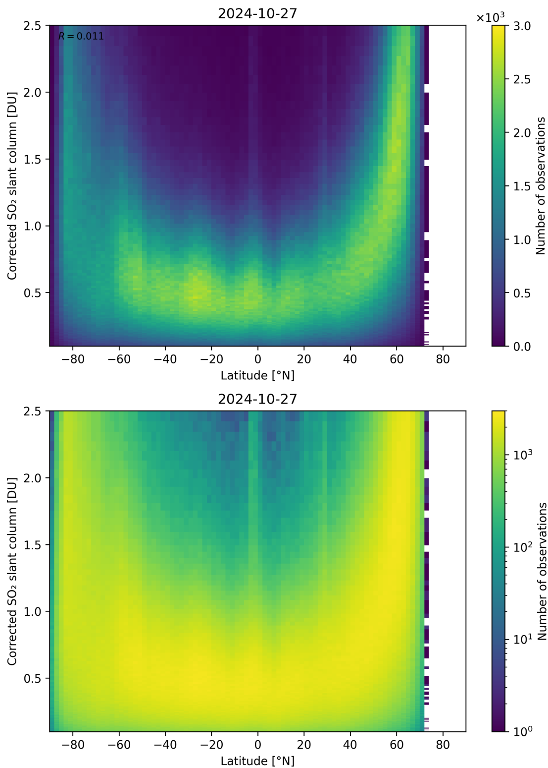
Figure 146: Scatter density plot of “Latitude” against “Corrected SO 2 slant column” for 2024-10-26 to 2024-10-28.
