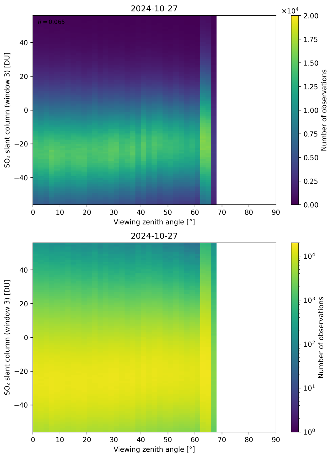
Figure 323: Scatter density plot of “Viewing zenith angle” against “SO 2 slant column (window 3)” for 2024-10-26 to 2024-10-28.
