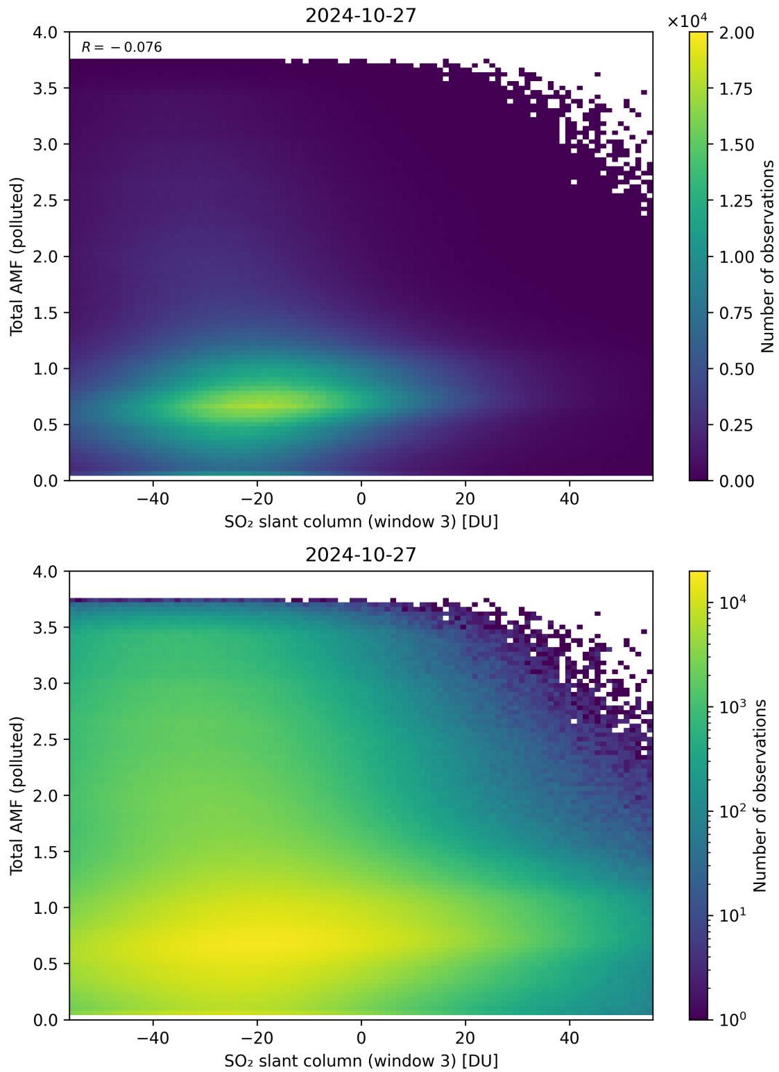
Figure 268: Scatter density plot of “SO 2 slant column (window 3)” against “Total AMF (polluted)” for 2024-10-26 to 2024-10-28.
