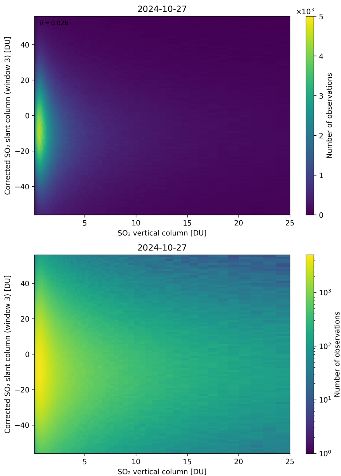
Figure 299: Scatter density plot of “SO 2 vertical column” against “Corrected SO 2 slant column (window 3)” for 2024-10-26 to 2024-10-28.
