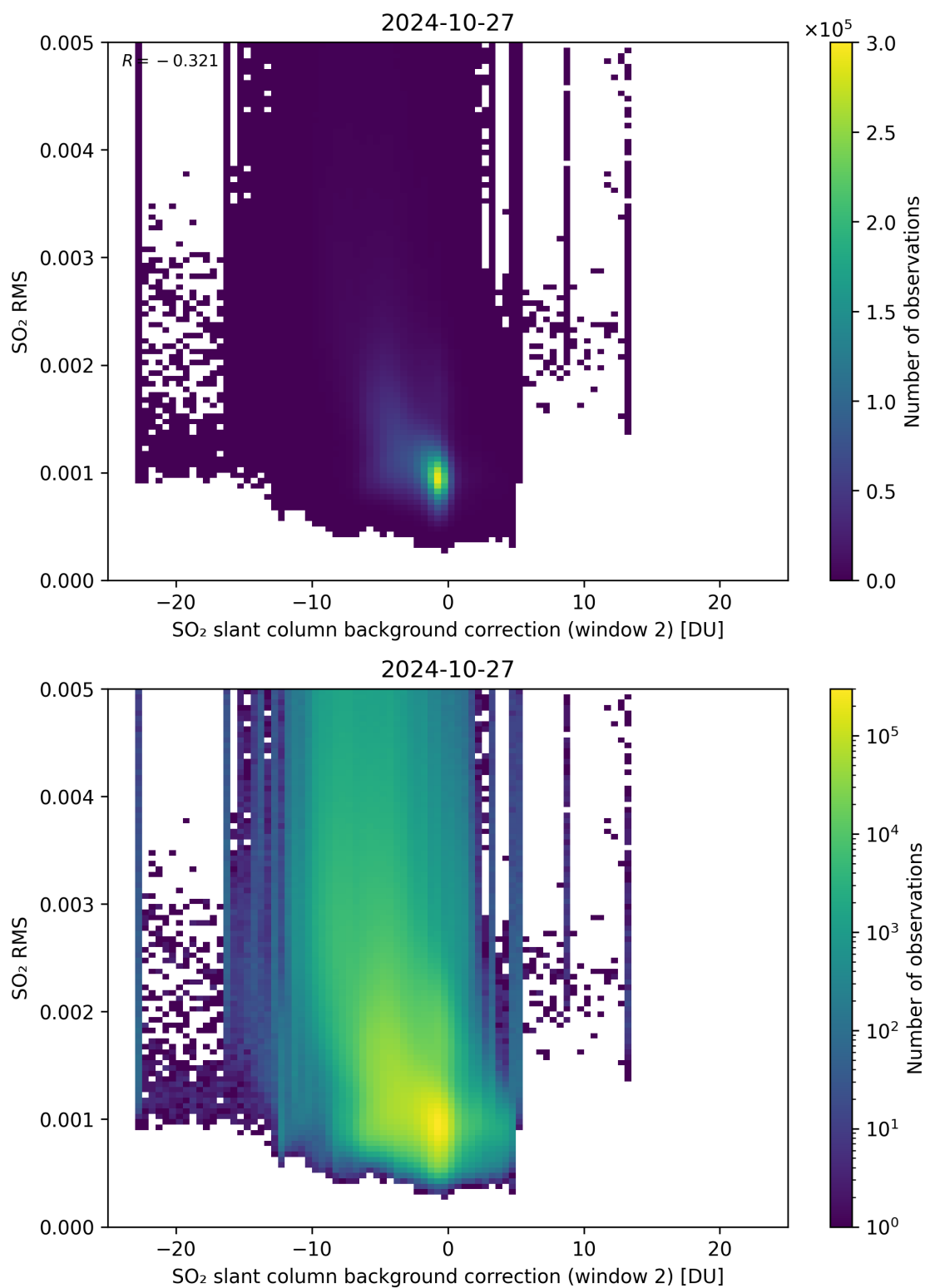
Figure 114: Scatter density plot of “SO 2 slant column background correction (window 2)” against “SO 2 RMS” for 2024-10-26 to 2024-10-28.
