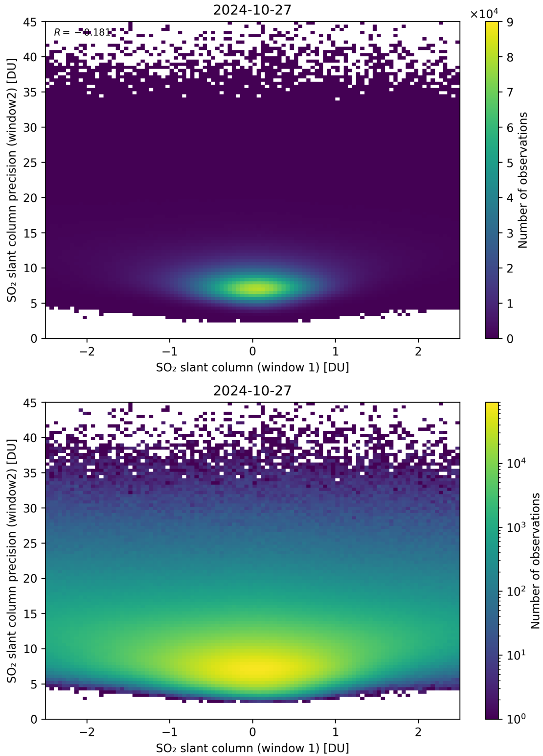
Figure 236: Scatter density plot of “SO 2 slant column (window 1)” against “SO 2 slant column precision (window2)” for 2024-10-26 to 2024-10-28.
