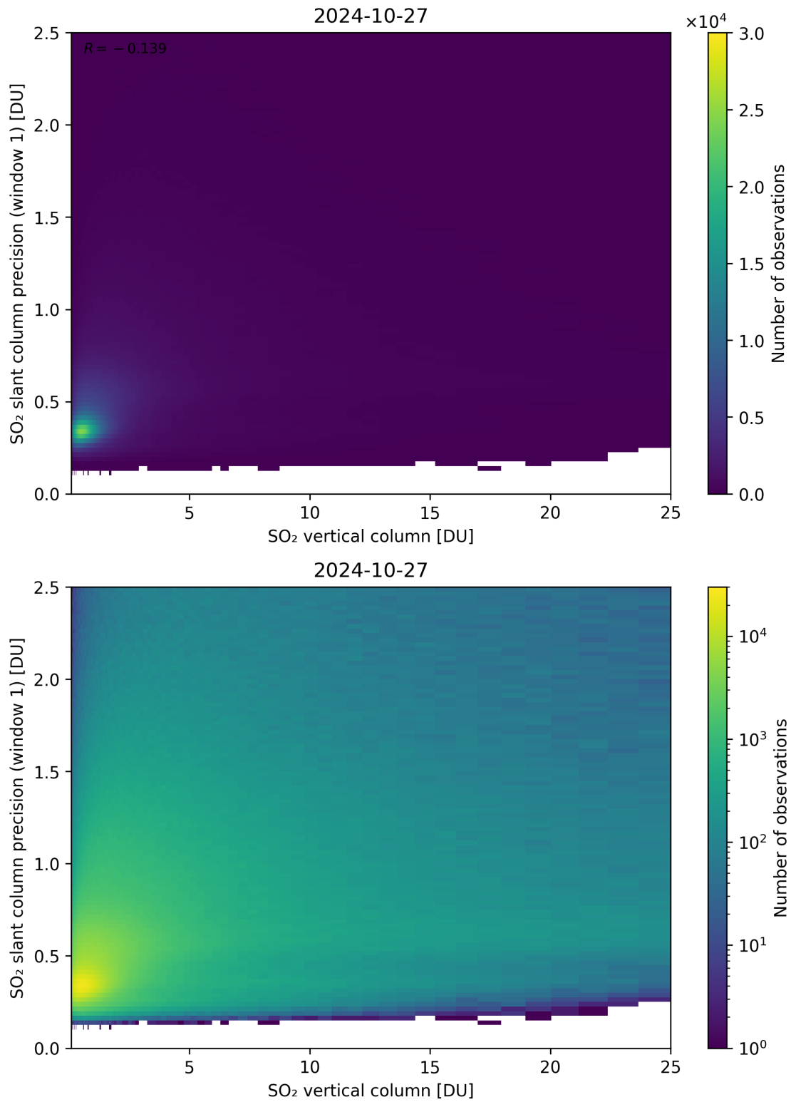
Figure 301: Scatter density plot of “SO 2 vertical column” against “SO 2 slant column precision (window 1)” for 2024-10-26 to 2024-10-28.
