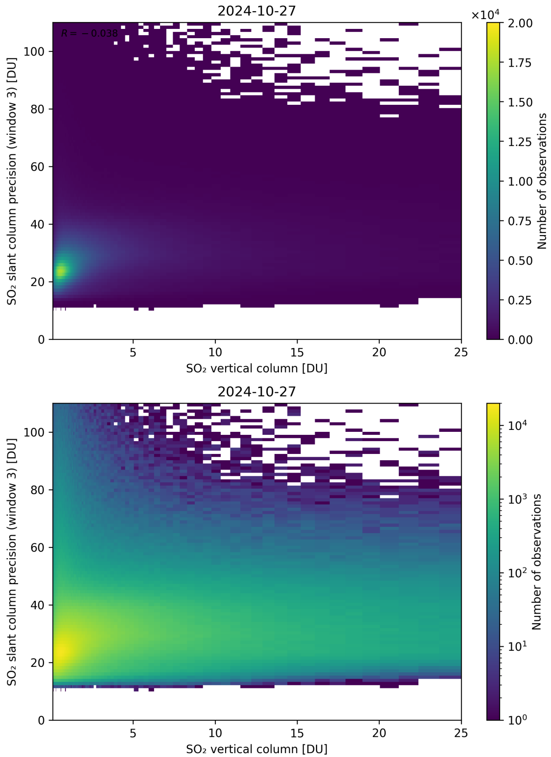
Figure 304: Scatter density plot of “SO 2 vertical column” against “SO 2 slant column precision (window 3)” for 2024-10-26 to 2024-10-28.
