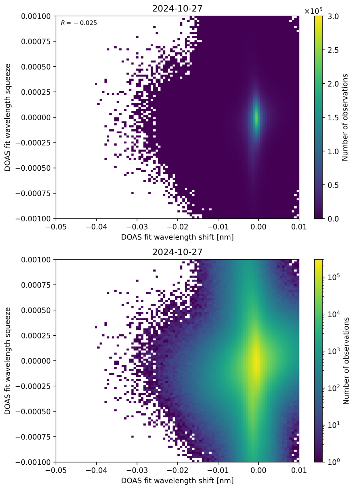
Figure 127: Scatter density plot of “DOAS fit wavelength shift” against “DOAS fit wavelength squeeze” for 2024-10-26 to 2024-10-28.
