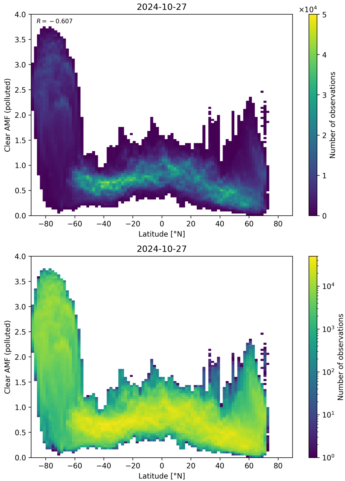
Figure 145: Scatter density plot of “Latitude” against “Clear AMF (polluted)” for 2024-10-26 to 2024-10-28.
