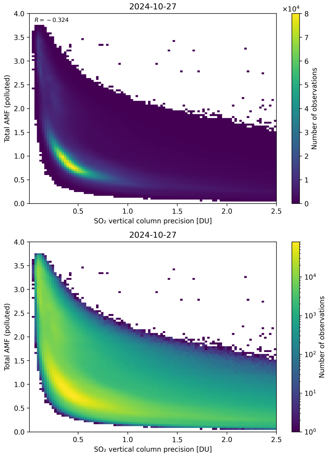
Figure 294: Scatter density plot of “SO 2 vertical column precision” against “Total AMF (polluted)” for 2024-10-26 to 2024-10-28.
