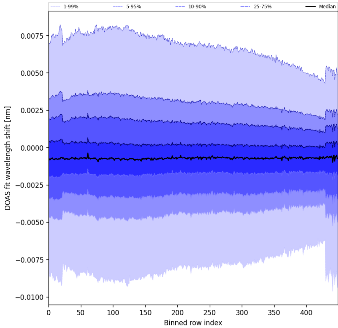
Figure 91: Along track statistics of “DOAS fit wavelength shift” for 2024-10-26 to 2024-10-28
