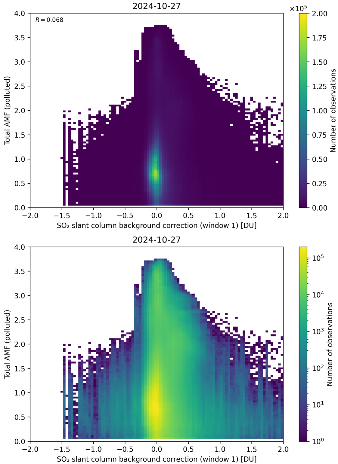
Figure 109: Scatter density plot of “SO 2 slant column background correction (window 1)” against “Total AMF (polluted)” for 2024-10-26 to 2024-10-28.
