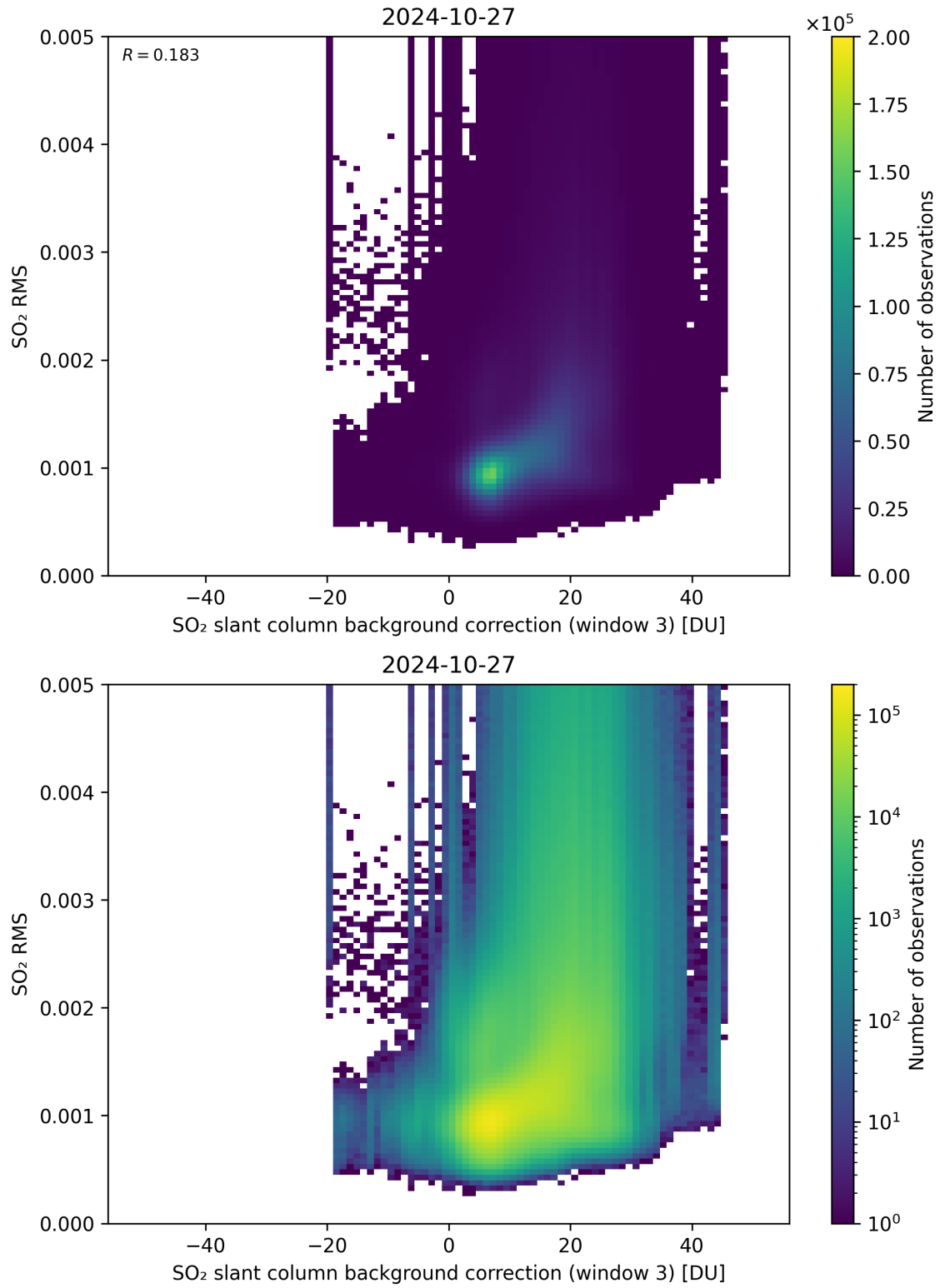
Figure 123: Scatter density plot of “SO 2 slant column background correction (window 3)” against “SO 2 RMS” for 2024-10-26 to 2024-10-28.
