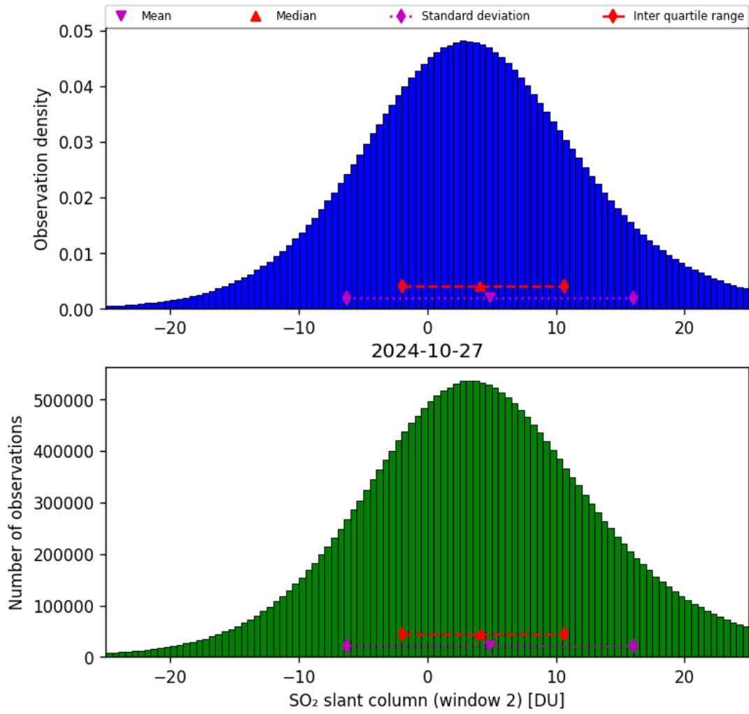
Figure 60: Histogram of “SO 2 slant column (window 2)” for 2024-10-26 to 2024-10-28
