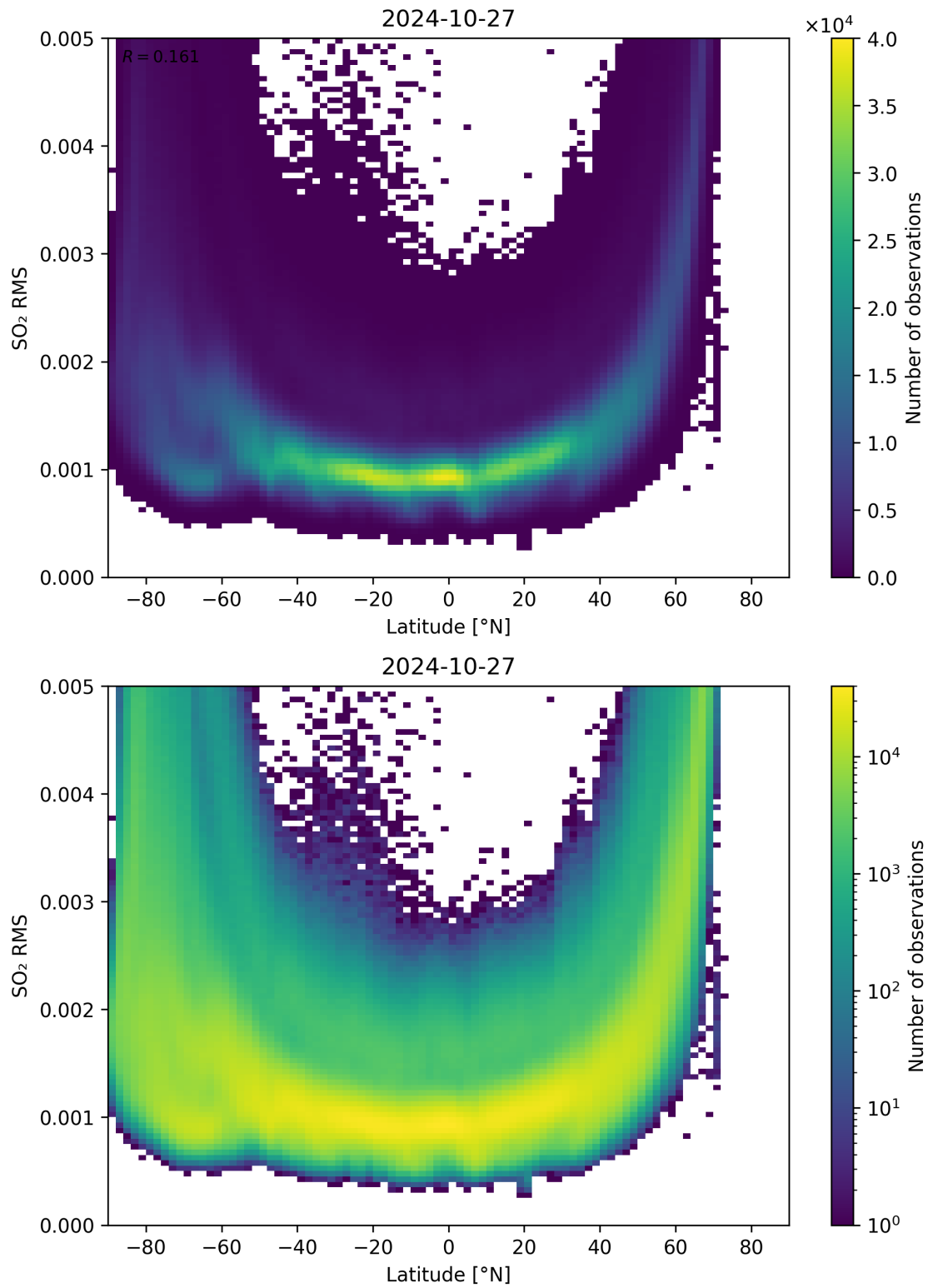
Figure 144: Scatter density plot of “Latitude” against “SO 2 RMS” for 2024-10-26 to 2024-10-28.
