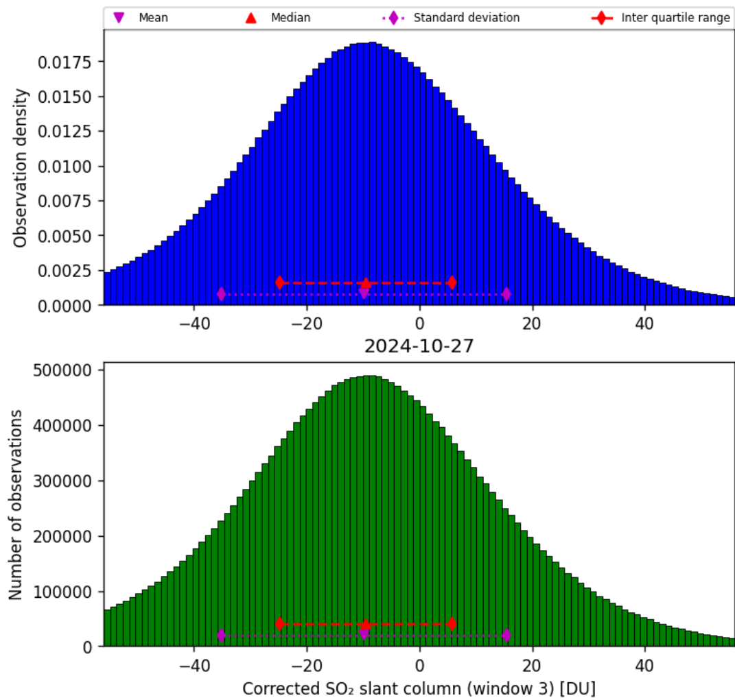
Figure 66: Histogram of “Corrected SO 2 slant column (window 3)” for 2024-10-26 to 2024-10-28
