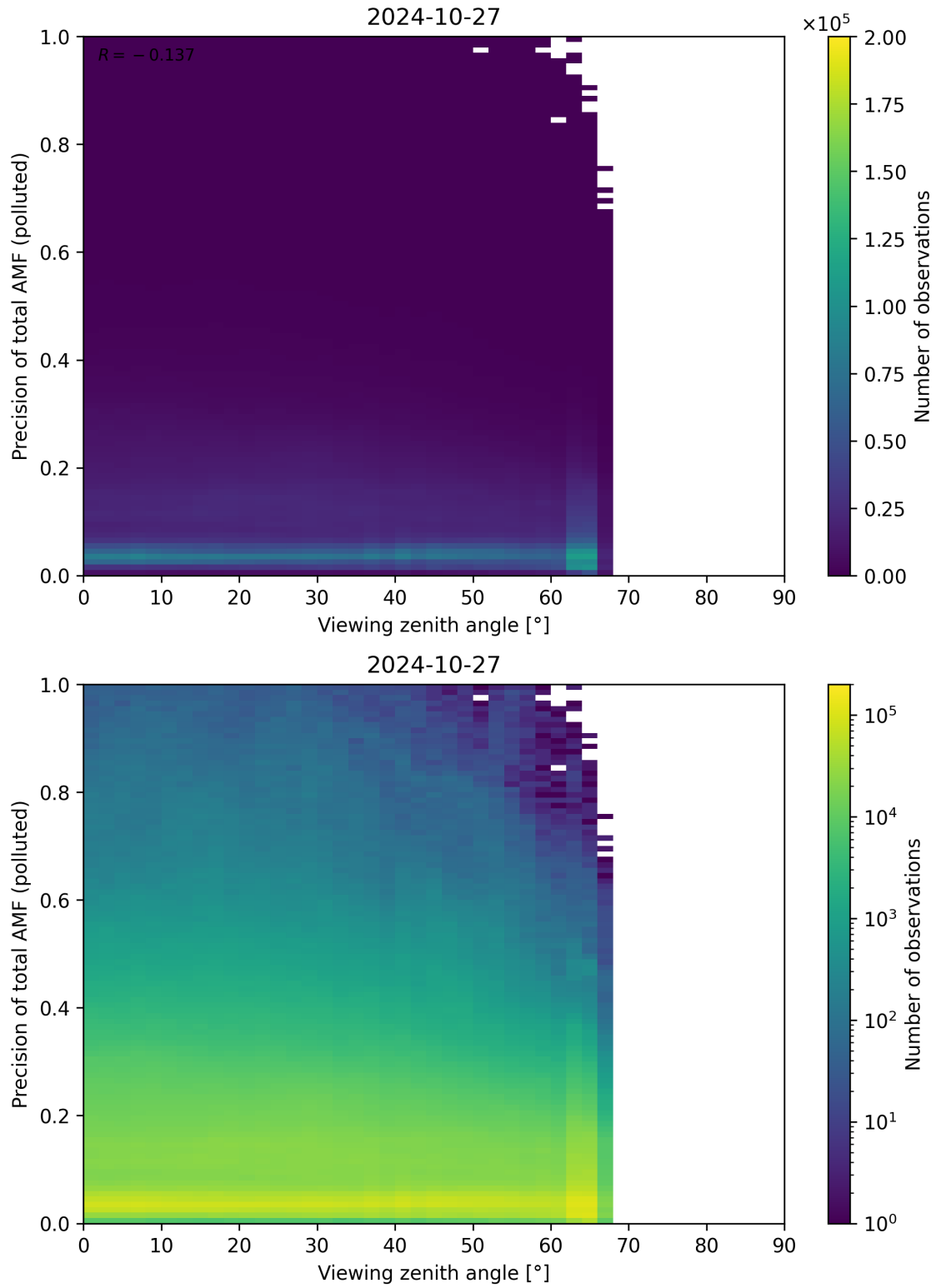
Figure 326: Scatter density plot of “Viewing zenith angle” against “Precision of total AMF (polluted)” for 2024-10-26 to 2024-10-28.
