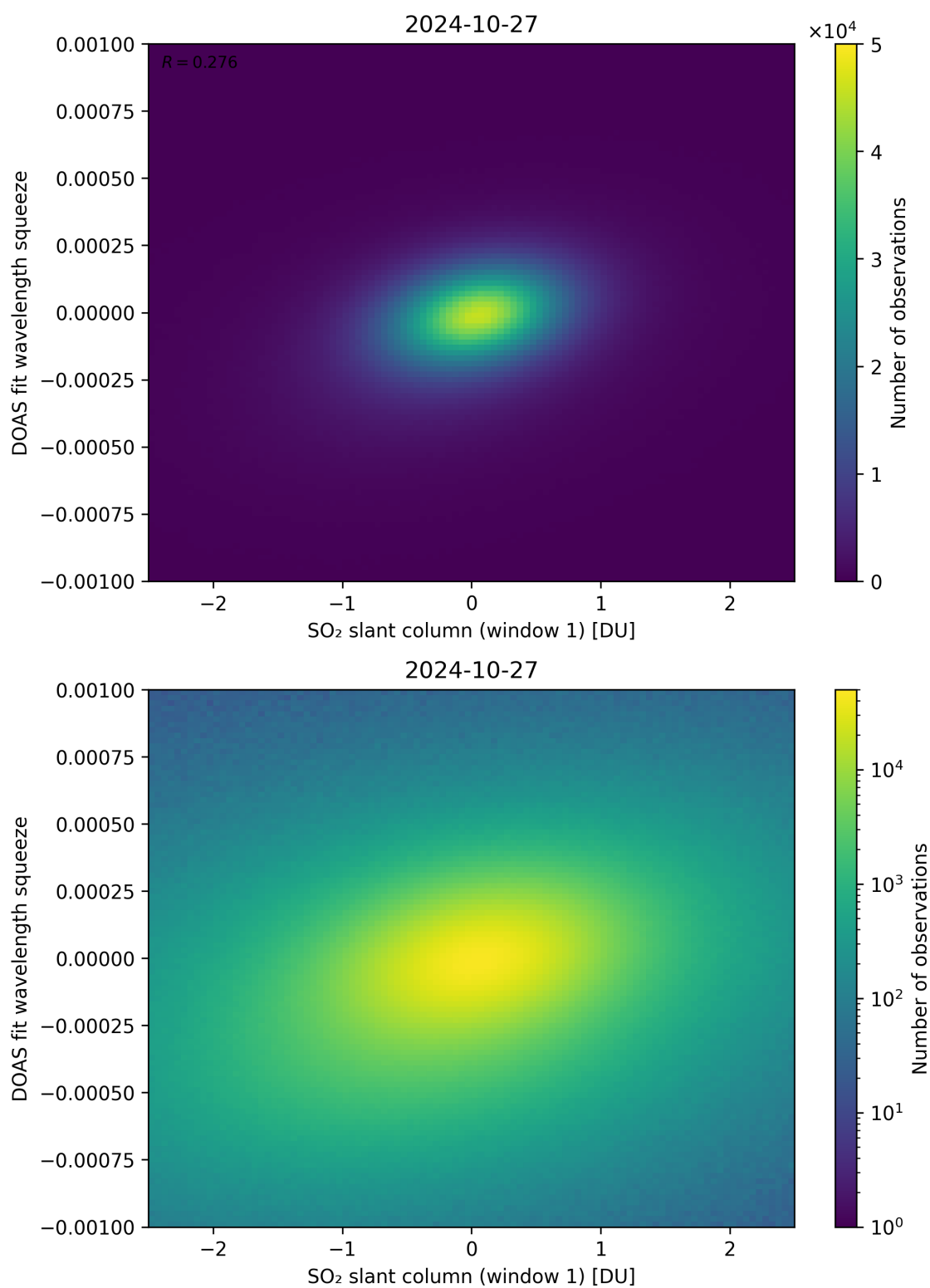
Figure 216: Scatter density plot of “SO 2 slant column (window 1)” against “DOAS fit wavelength squeeze” for 2024-10-26 to 2024-10-28.
