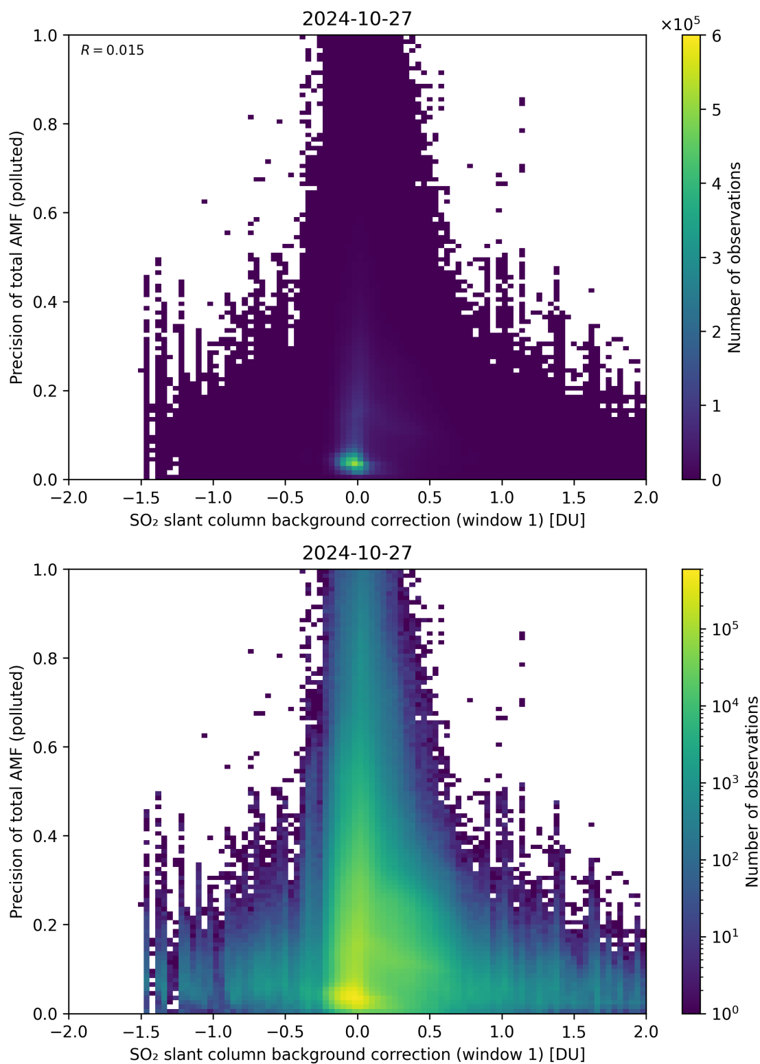
Figure 110: Scatter density plot of “SO 2 slant column background correction (window 1)” against “Precision of total AMF (polluted)” for 2024-10-26 to 2024-10-28.
