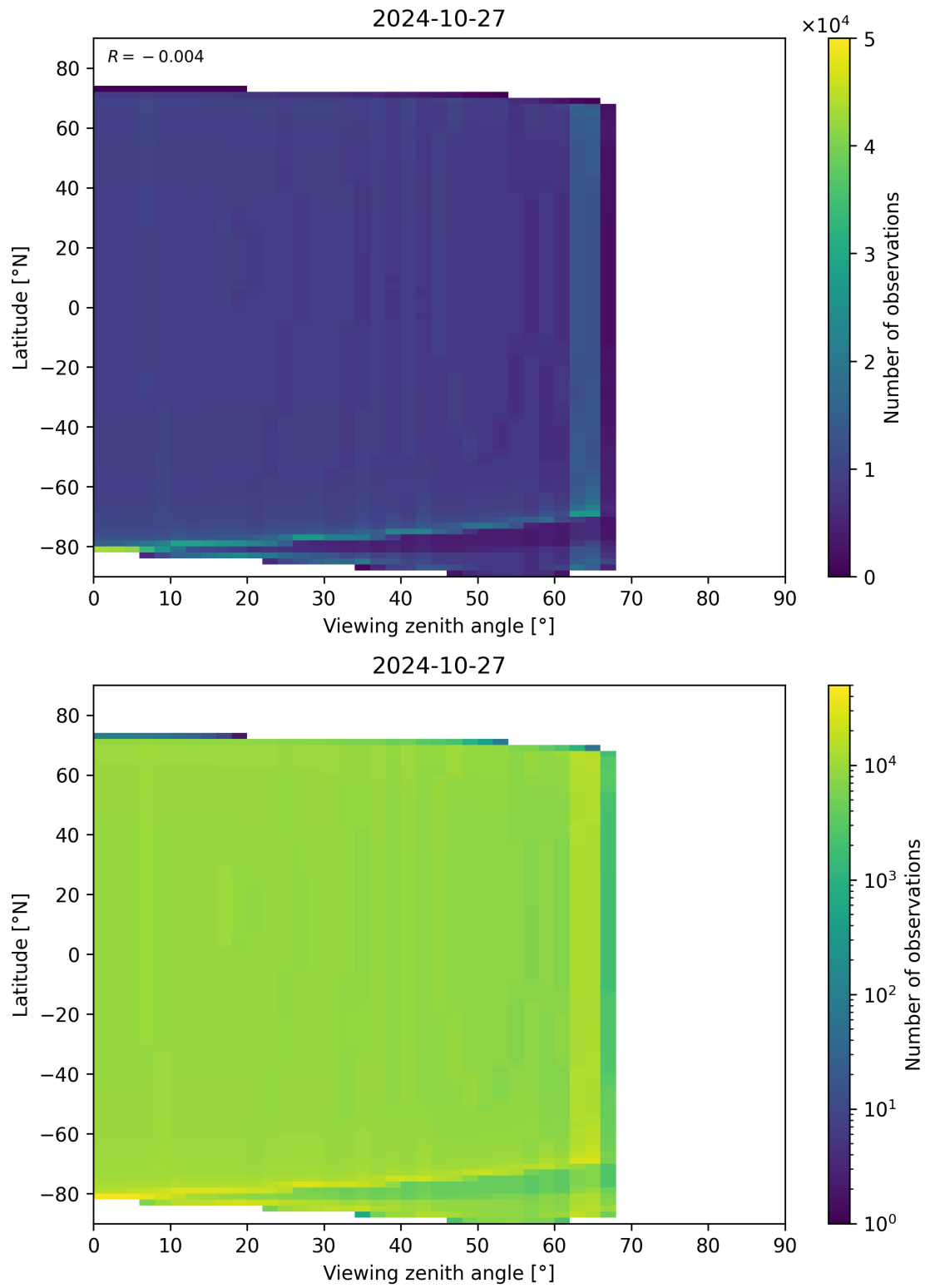
Figure 314: Scatter density plot of “Viewing zenith angle” against “Latitude” for 2024-10-26 to 2024-10-28.
