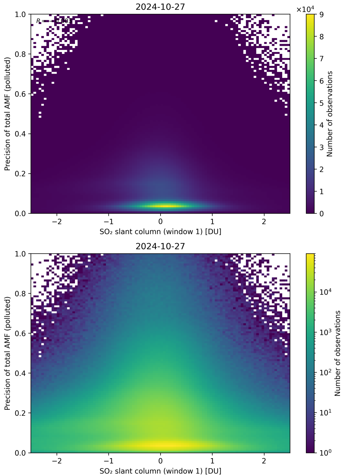
Figure 240: Scatter density plot of “SO 2 slant column (window 1)” against “Precision of total AMF (polluted)” for 2024-10-26 to 2024-10-28.
