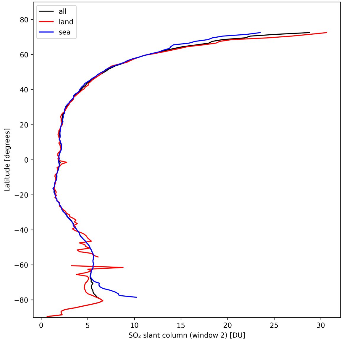
Figure 37: Zonal average of “SO 2 slant column (window 2)” for 2024-10-26 to 2024-10-28.
