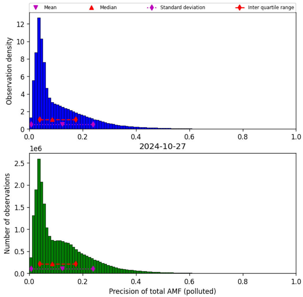
Figure 72: Histogram of “Precision of total AMF (polluted)” for 2024-10-26 to 2024-10-28
