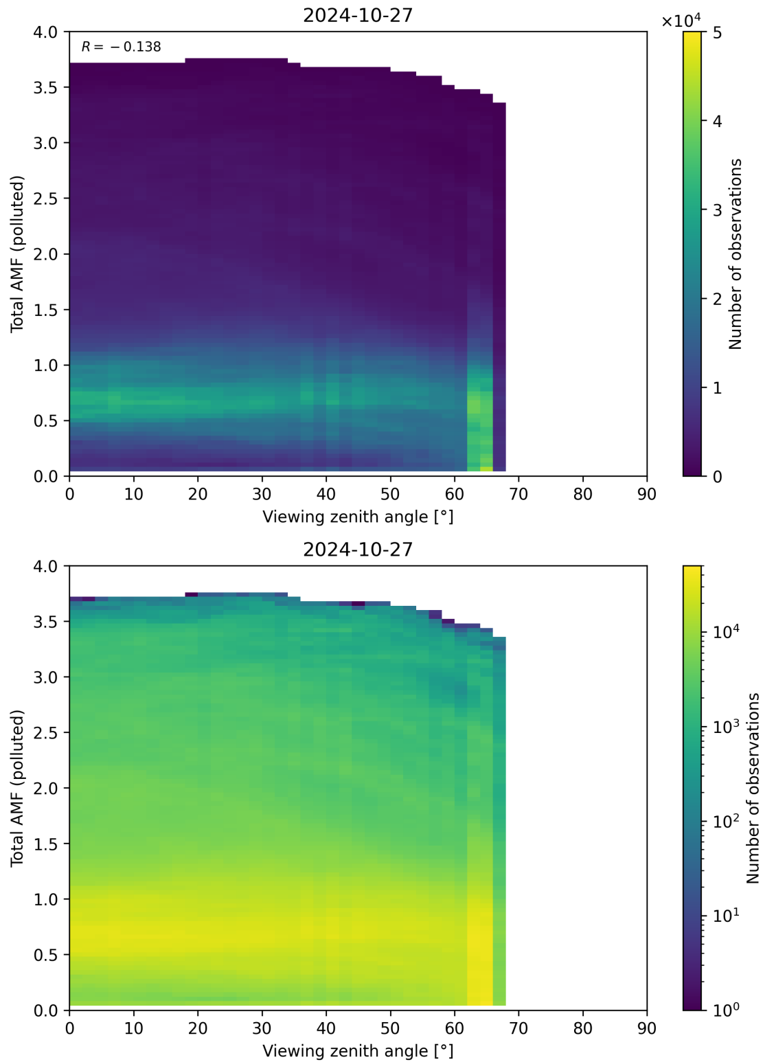
Figure 325: Scatter density plot of “Viewing zenith angle” against “Total AMF (polluted)” for 2024-10-26 to 2024-10-28.
