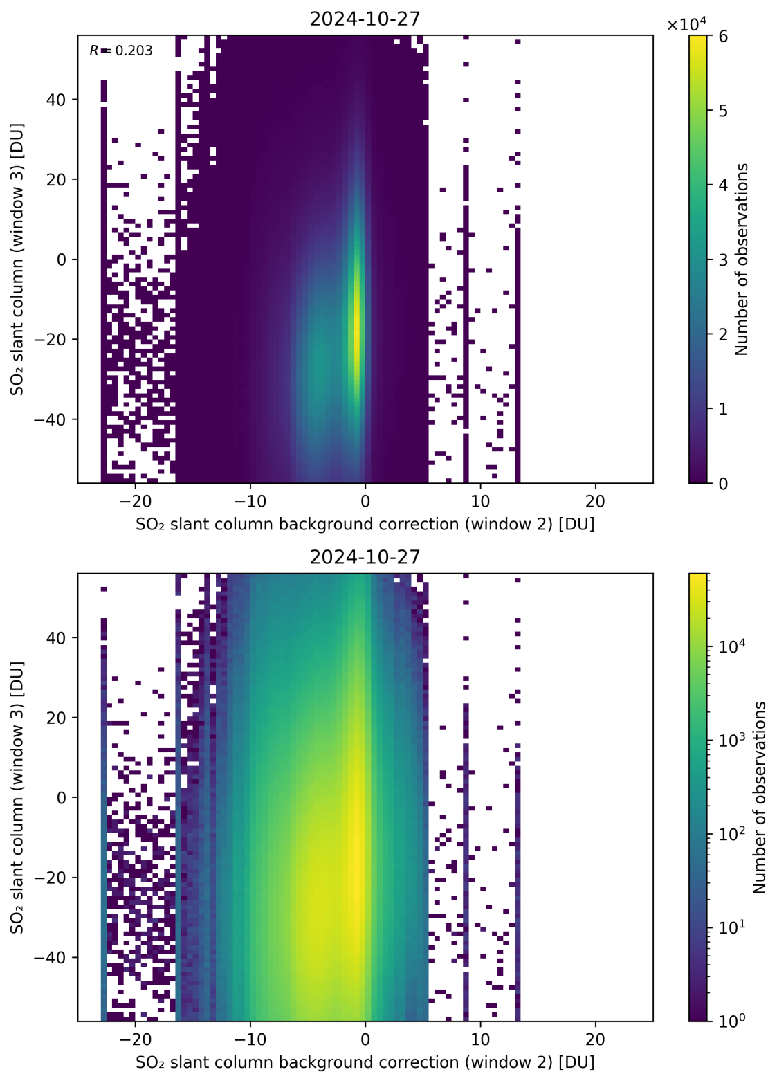
Figure 117: Scatter density plot of “SO 2 slant column background correction (window 2)” against “SO 2 slant column (window 3)” for 2024-10-26 to 2024-10-28.
