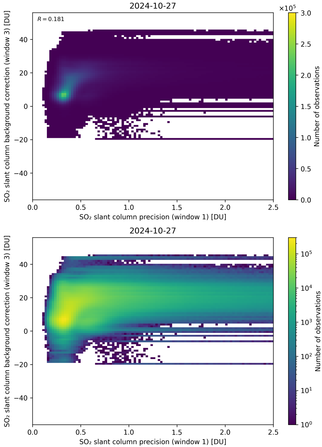
Figure 220: Scatter density plot of “SO 2 slant column precision (window 1)” against “SO 2 slant column background correction (window 3)” for 2024-10-26 to 2024-10-28.
