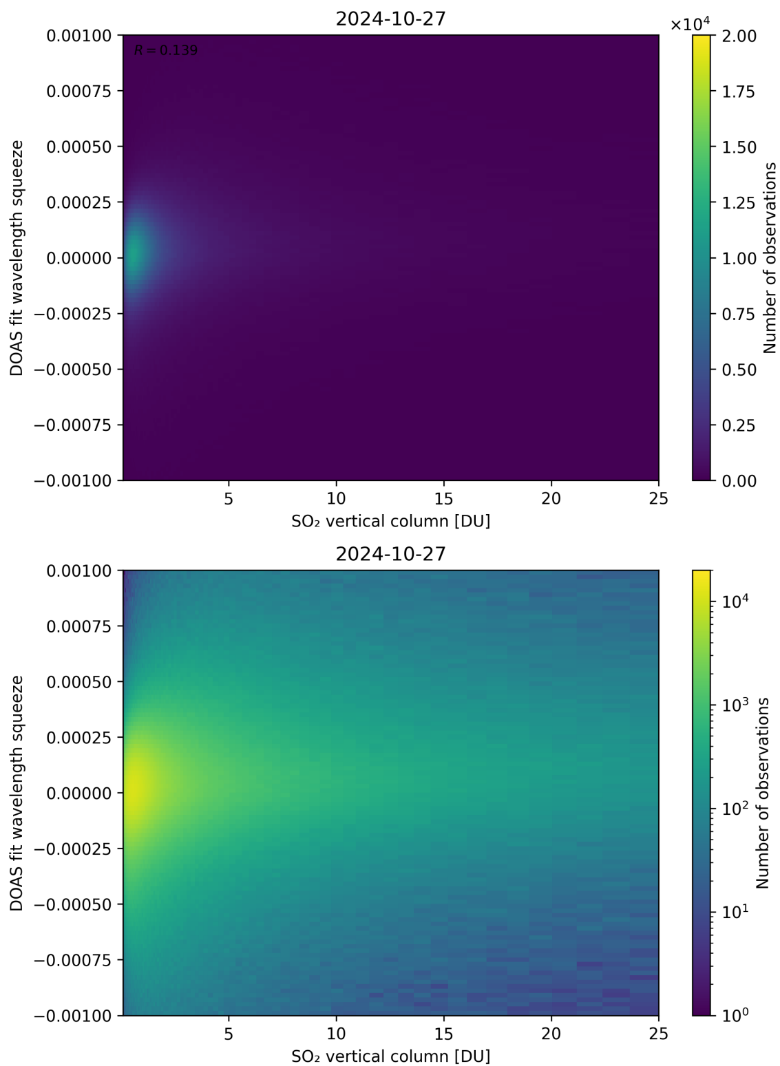
Figure 277: Scatter density plot of “SO 2 vertical column” against “DOAS fit wavelength squeeze” for 2024-10-26 to 2024-10-28.
