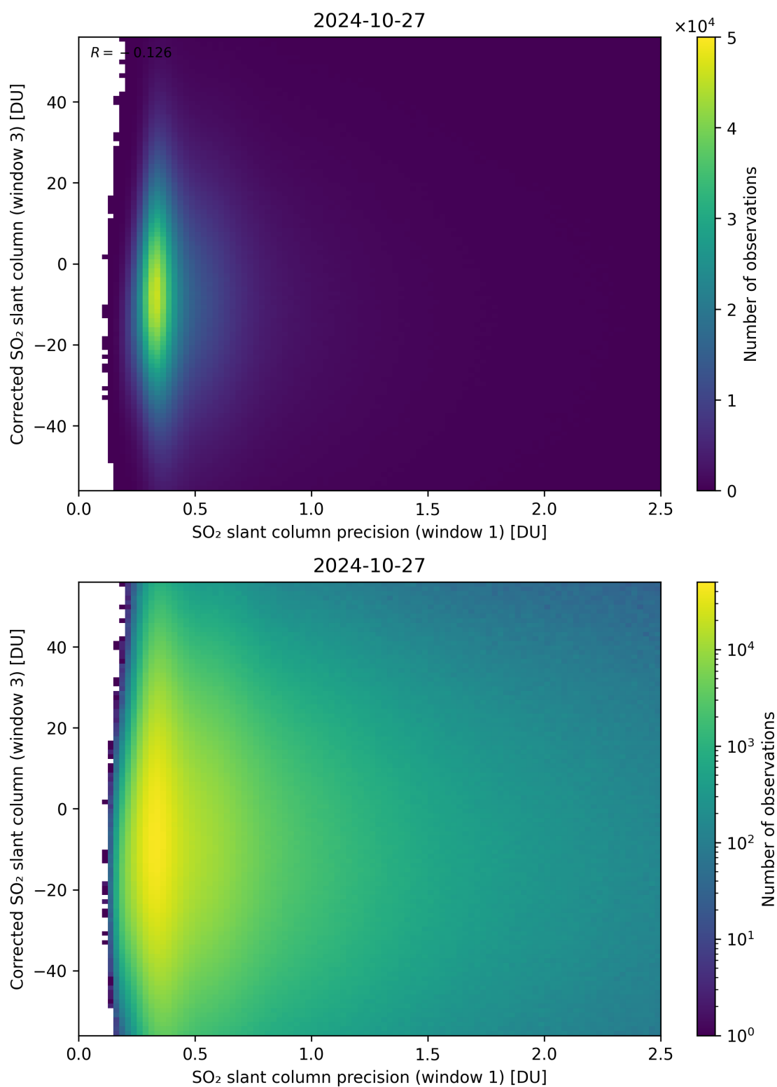
Figure 226: Scatter density plot of “SO 2 slant column precision (window 1)” against “Corrected SO 2 slant column (window 3)” for 2024-10-26 to 2024-10-28.
