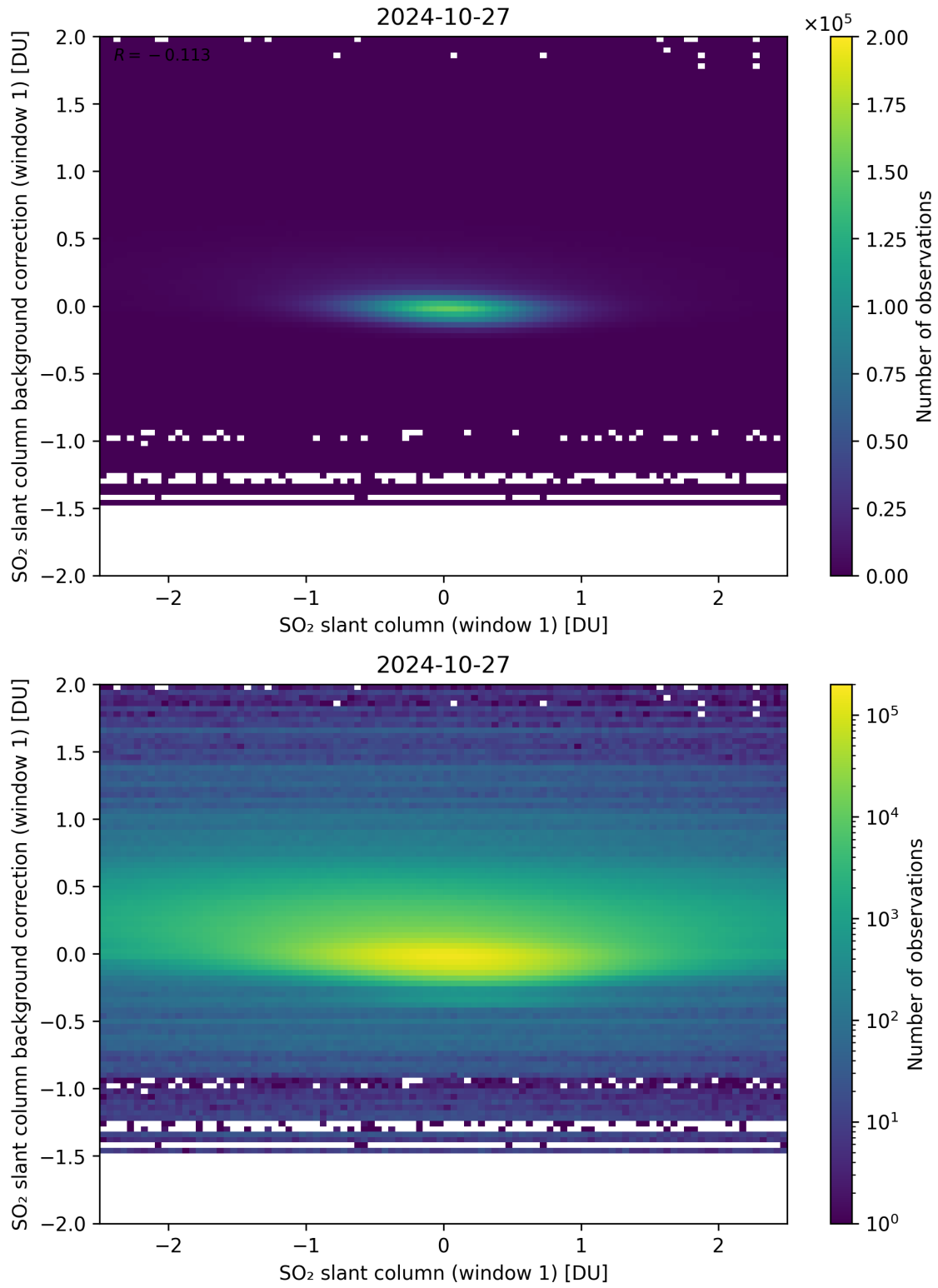
Figure 212: Scatter density plot of “SO 2 slant column (window 1)” against “SO 2 slant column background correction (window 1)” for 2024-10-26 to 2024-10-28.
