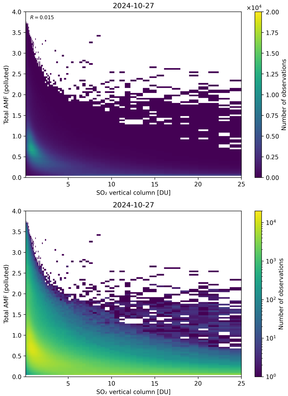
Figure 305: Scatter density plot of “SO 2 vertical column” against “Total AMF (polluted)” for 2024-10-26 to 2024-10-28.
