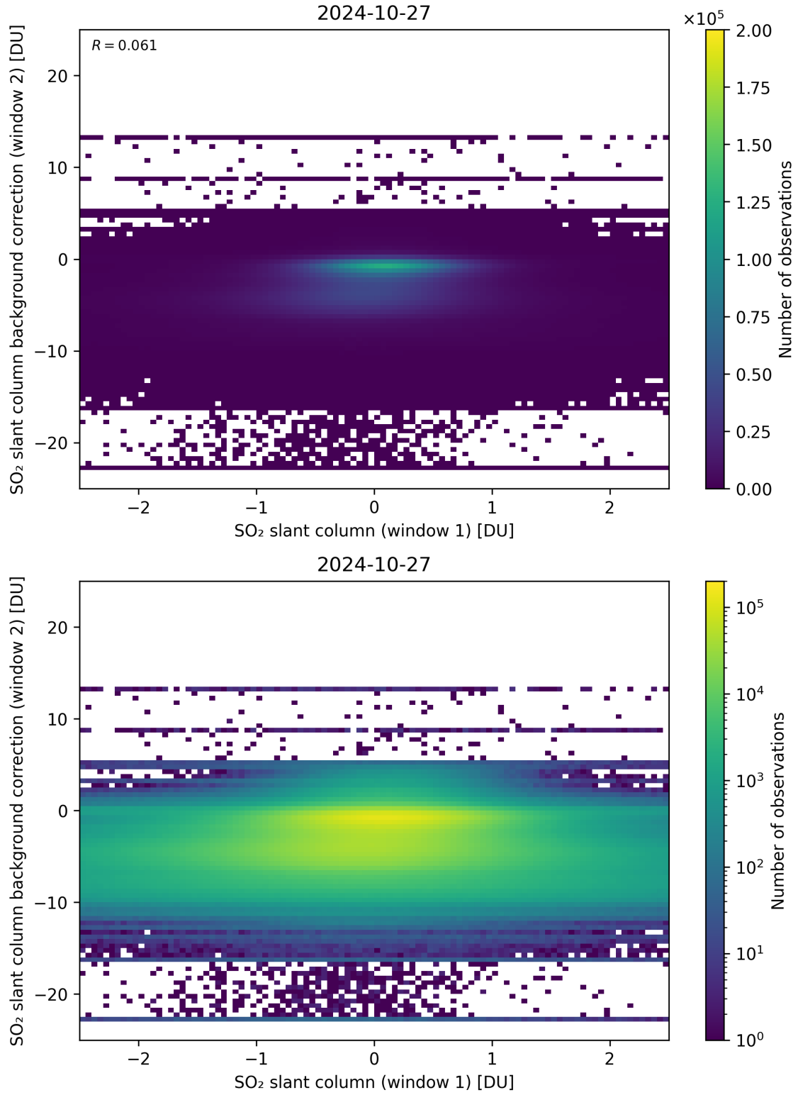
Figure 213: Scatter density plot of “SO 2 slant column (window 1)” against “SO 2 slant column background correction (window 2)” for 2024-10-26 to 2024-10-28.
