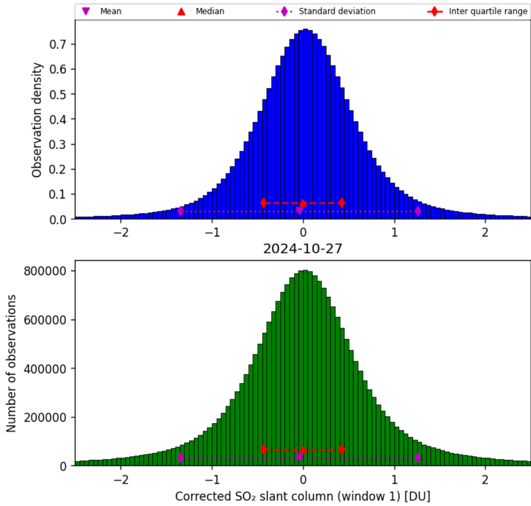
Figure 58: Histogram of “Corrected SO 2 slant column (window 1)” for 2024-10-26 to 2024-10-28
