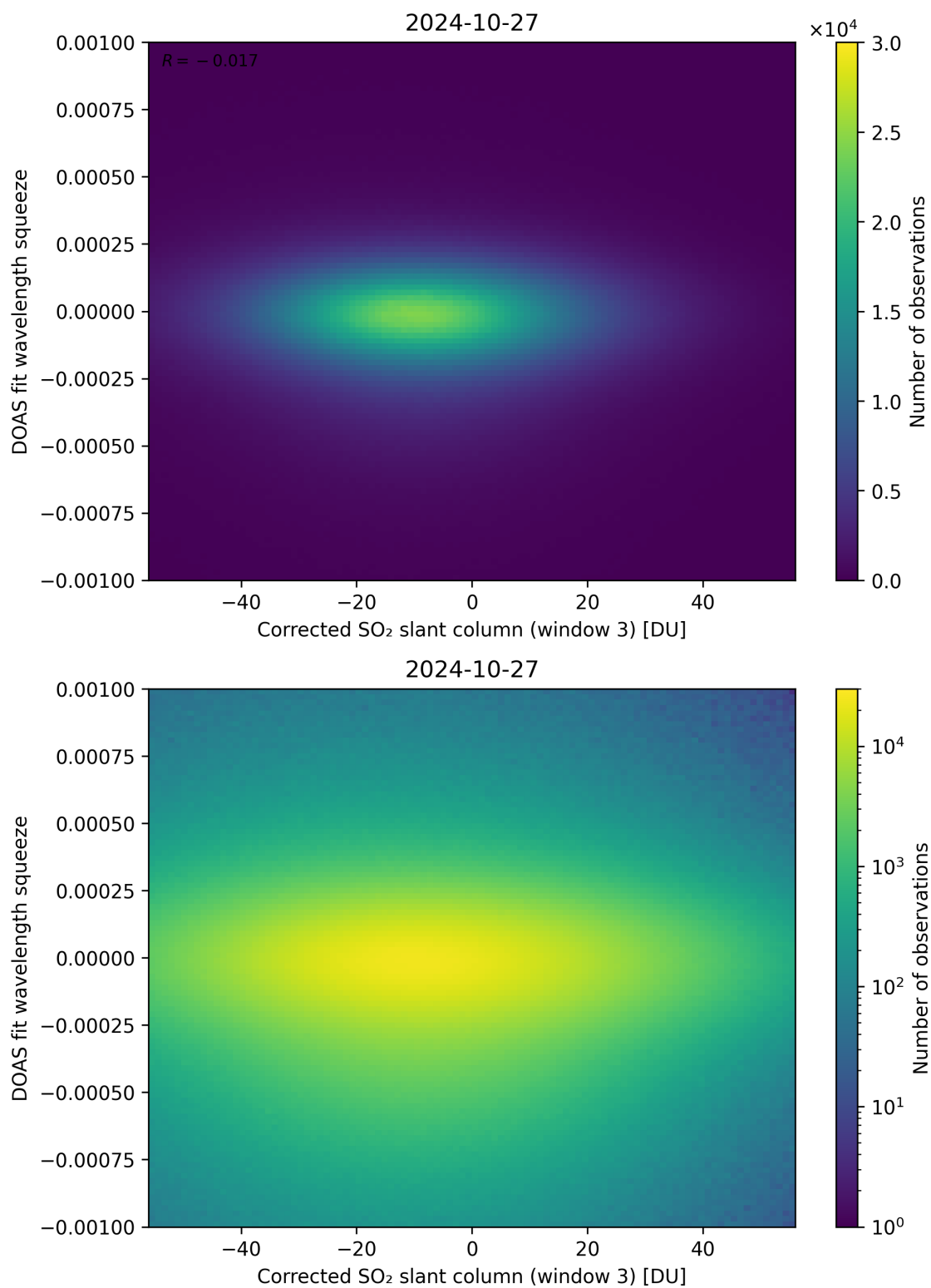
Figure 207: Scatter density plot of “Corrected SO 2 slant column (window 3)” against “DOAS fit wavelength squeeze” for 2024-10-26 to 2024-10-28.
