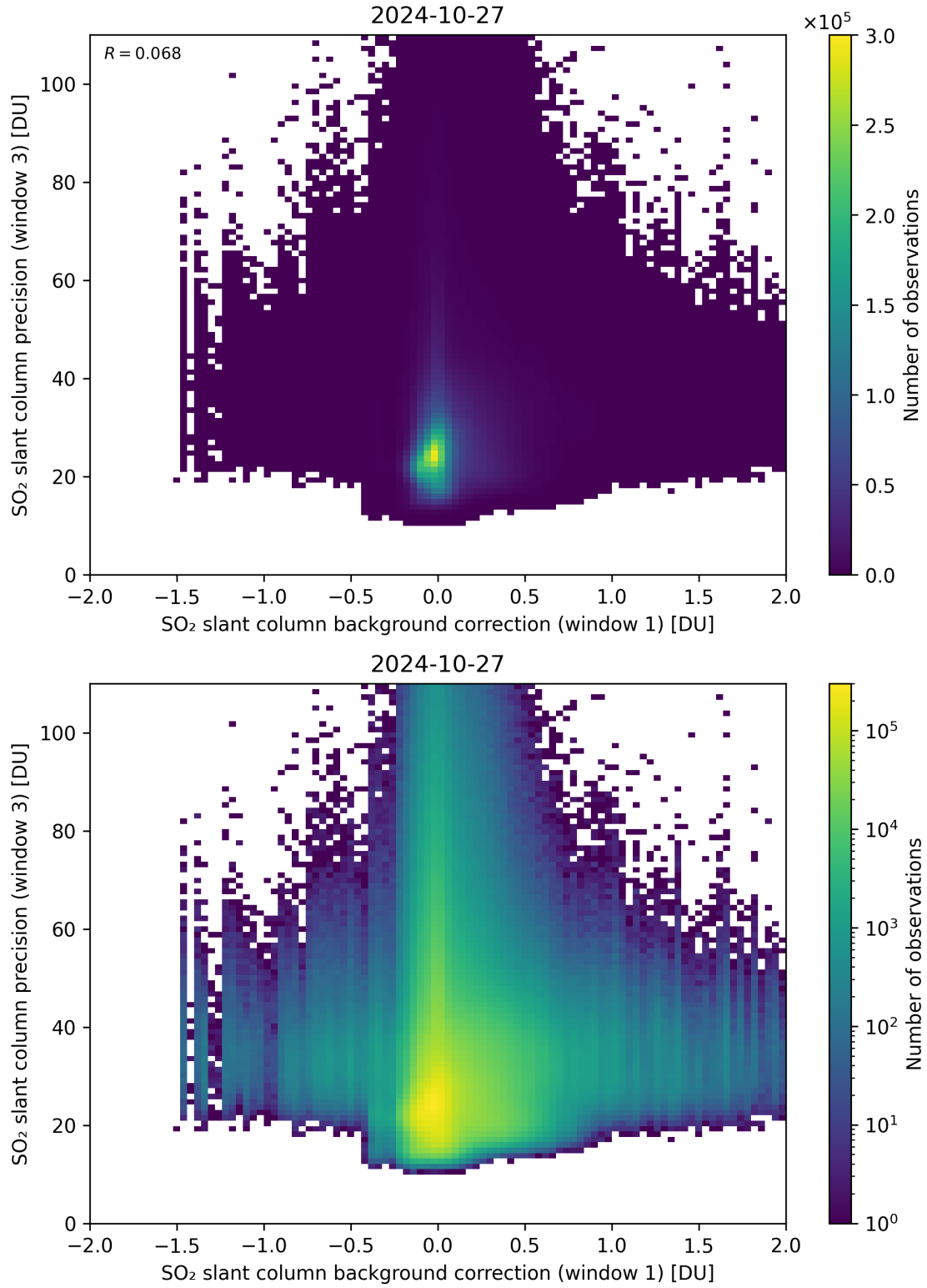
Figure 108: Scatter density plot of “SO 2 slant column background correction (window 1)” against “SO 2 slant column precision (window 3)” for 2024-10-26 to 2024-10-28.
