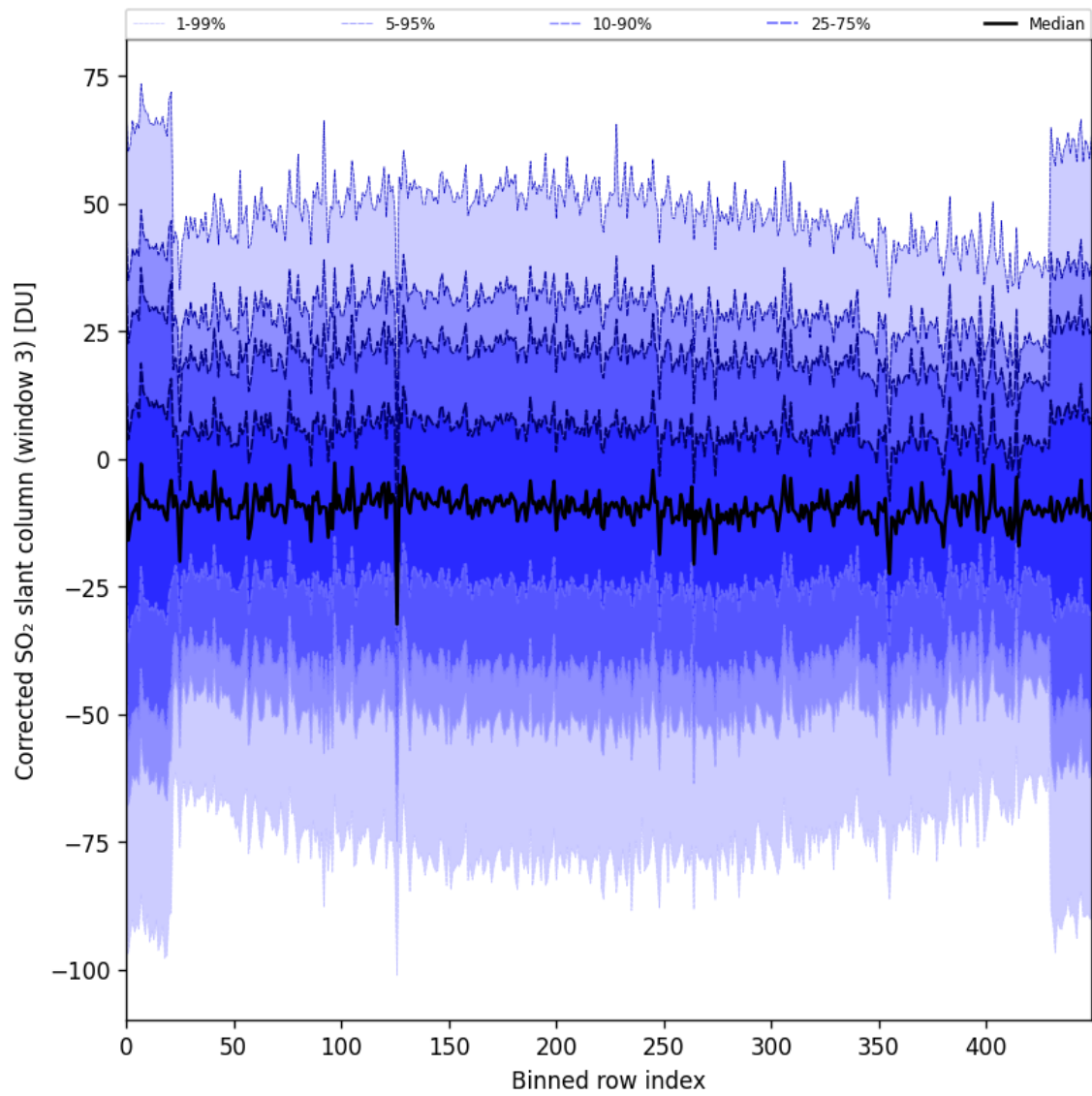
Figure 89: Along track statistics of “Corrected SO 2 slant column (window 3)” for 2024-10-26 to 2024-10-28
