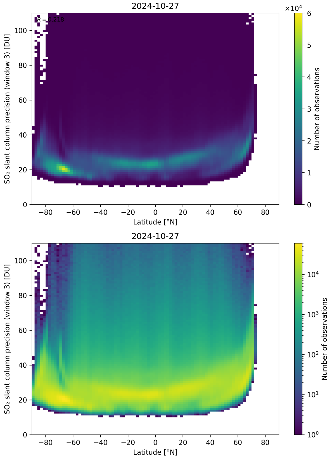
Figure 153: Scatter density plot of “Latitude” against “SO 2 slant column precision (window 3)” for 2024-10-26 to 2024-10-28.
