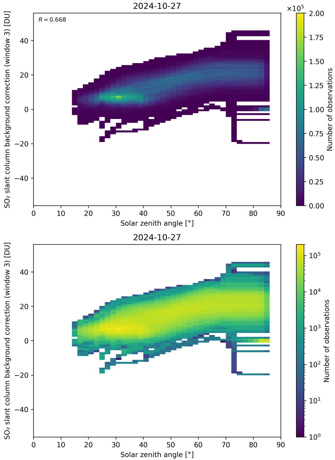
Figure 160: Scatter density plot of “Solar zenith angle” against “SO 2 slant column background correction (window 3)” for 2024-10-26 to 2024-10-28.
