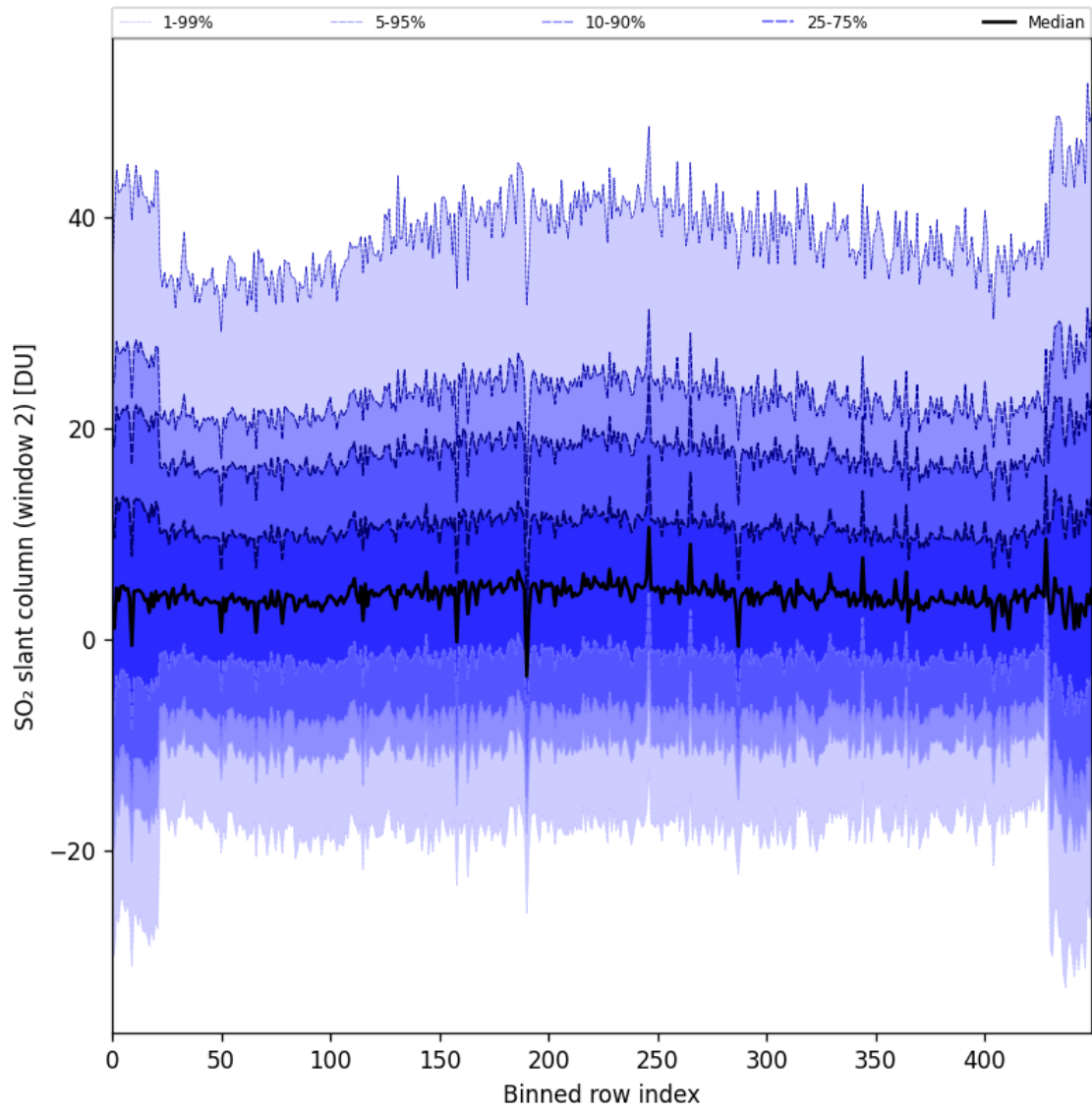
Figure 83: Along track statistics of “SO 2 slant column (window 2)” for 2024-10-26 to 2024-10-28
