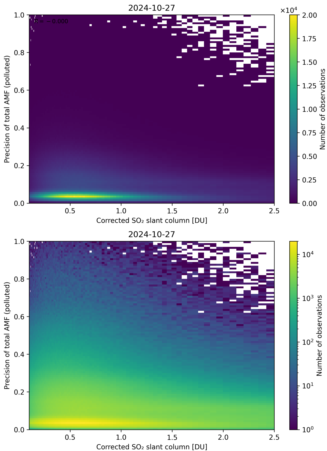
Figure 193: Scatter density plot of “Corrected SO 2 slant column” against “Precision of total AMF (polluted)” for 2024-10-26 to 2024-10-28.
