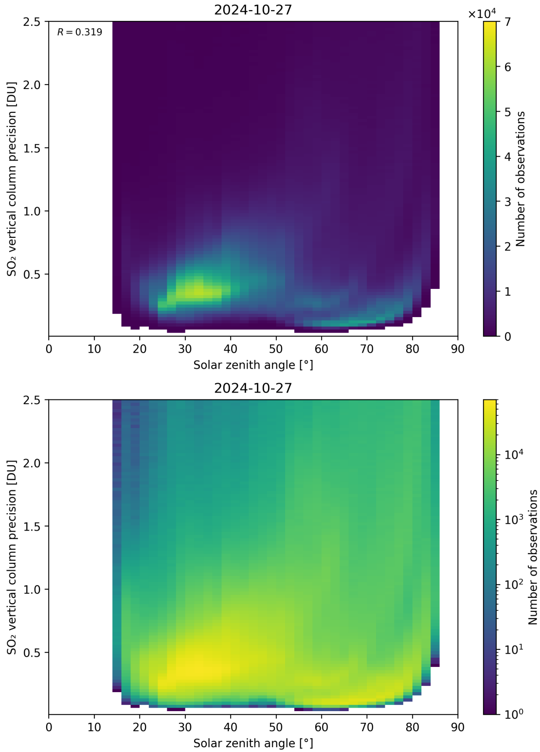
Figure 177: Scatter density plot of “Solar zenith angle” against “SO 2 vertical column precision” for 2024-10-26 to 2024-10-28.
