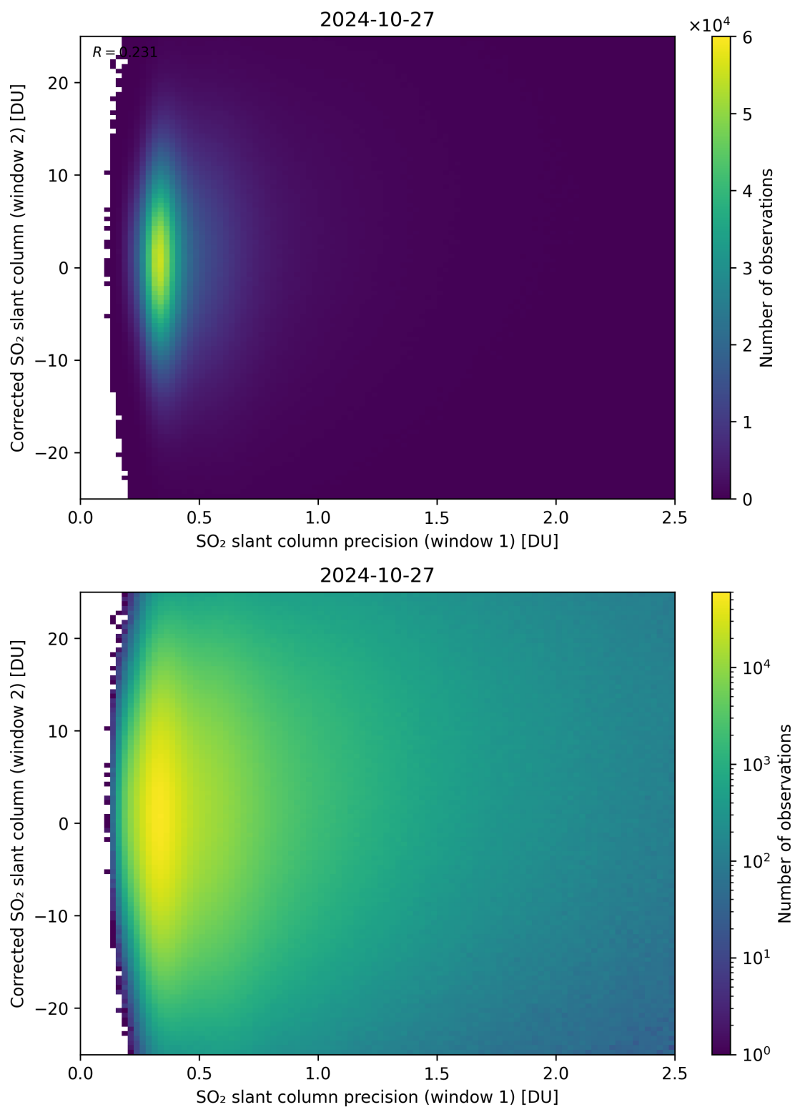
Figure 225: Scatter density plot of “SO 2 slant column precision (window 1)” against “Corrected SO 2 slant column (window 2)” for 2024-10-26 to 2024-10-28.
