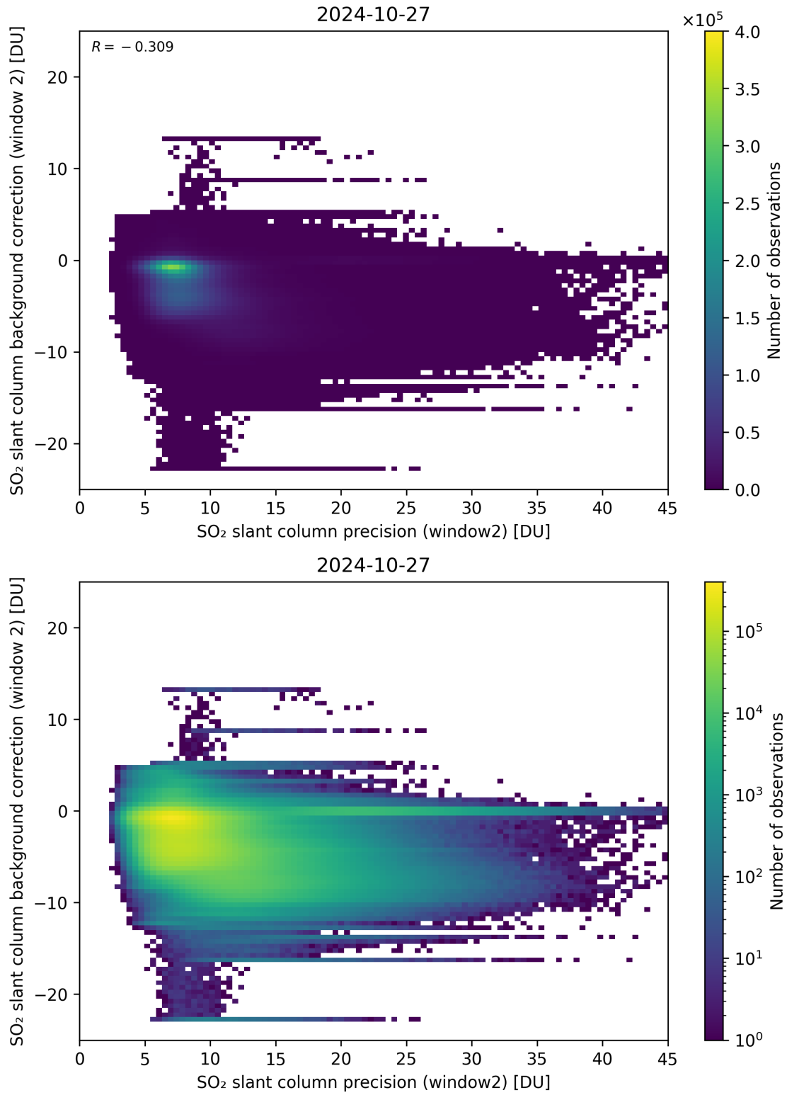
Figure 241: Scatter density plot of “SO 2 slant column precision (window2)” against “SO 2 slant column background correction (window 2)” for 2024-10-26 to 2024-10-28.
