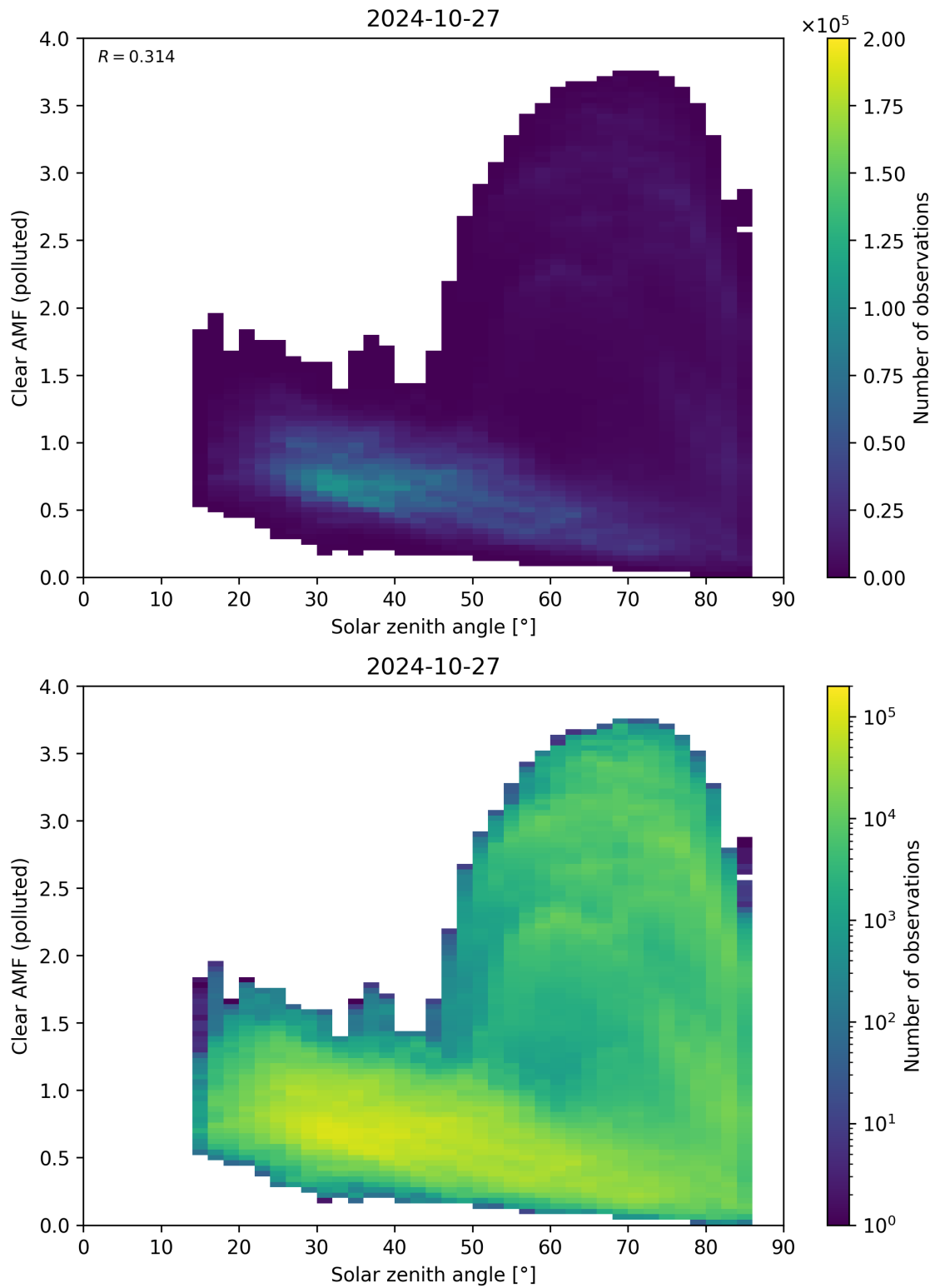
Figure 165: Scatter density plot of “Solar zenith angle” against “Clear AMF (polluted)” for 2024-10-26 to 2024-10-28.
