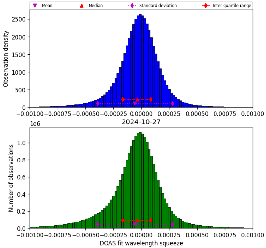
Figure 69: Histogram of “DOAS fit wavelength squeeze” for 2024-10-26 to 2024-10-28
