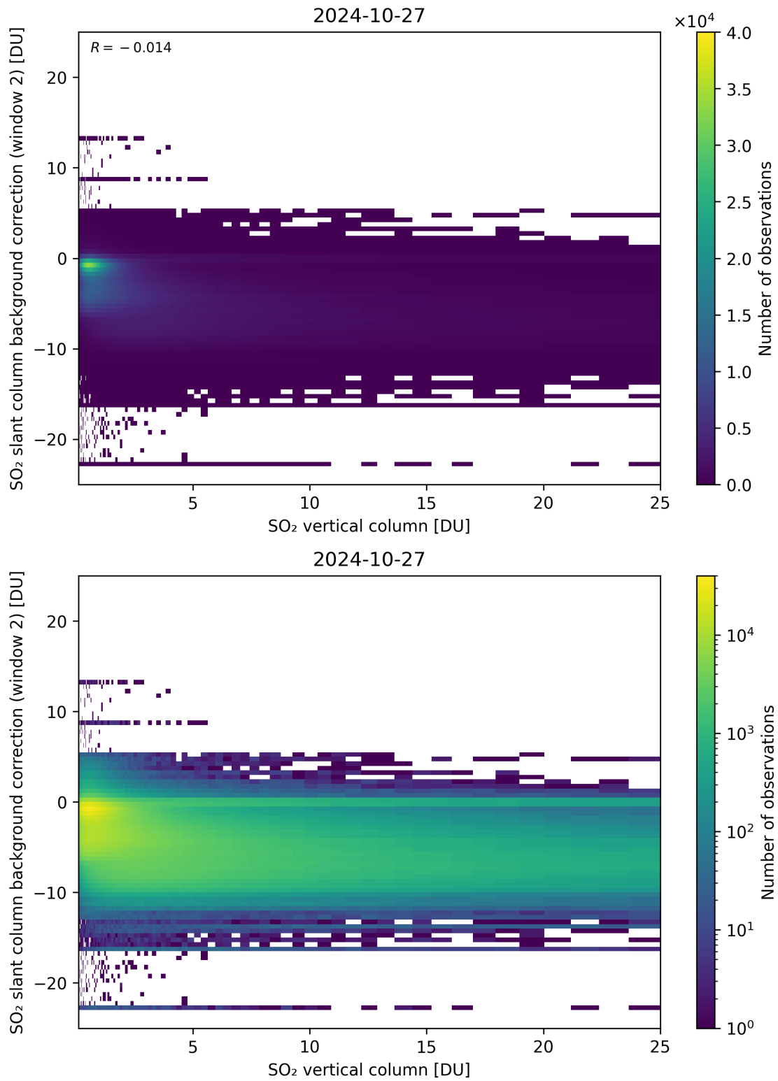
Figure 274: Scatter density plot of “SO 2 vertical column” against “SO 2 slant column background correction (window 2)” for 2024-10-26 to 2024-10-28.
