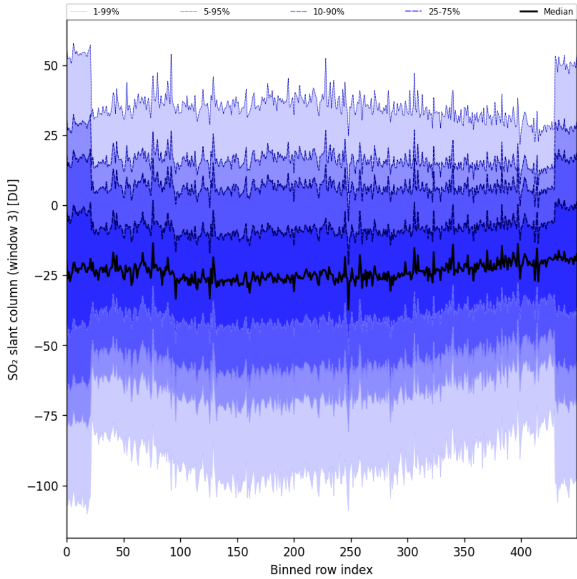
Figure 87: Along track statistics of “SO 2 slant column (window 3)” for 2024-10-26 to 2024-10-28
