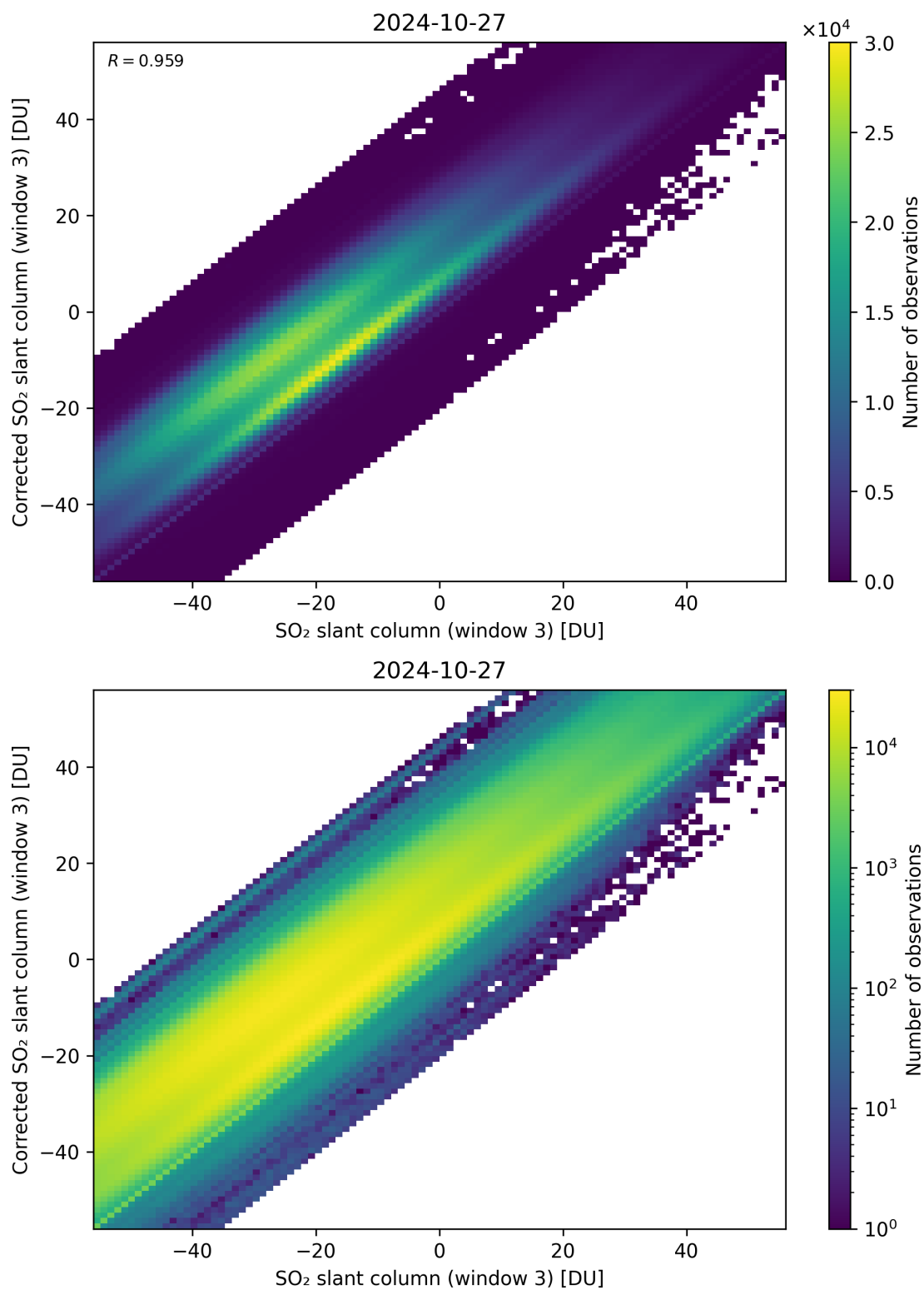
Figure 266: Scatter density plot of “SO 2 slant column (window 3)” against “Corrected SO 2 slant column (window 3)” for 2024-10-26 to 2024-10-28.
