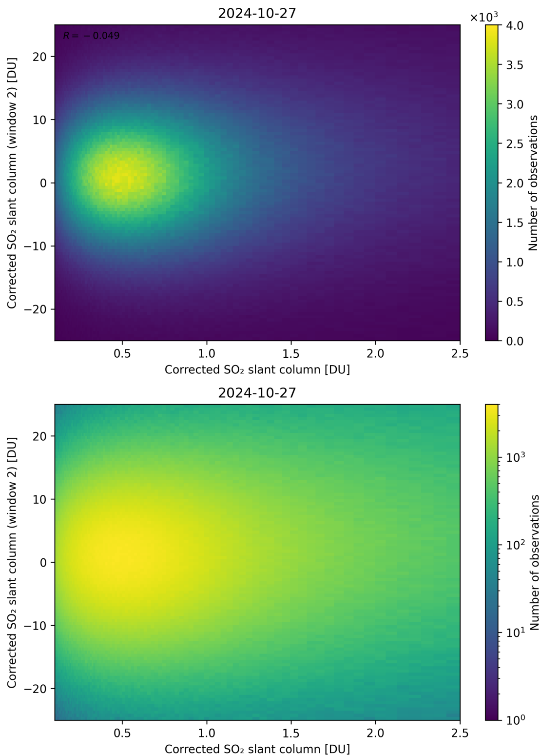
Figure 185: Scatter density plot of “Corrected SO 2 slant column” against “Corrected SO 2 slant column (window 2)” for 2024-10-26 to 2024-10-28.
