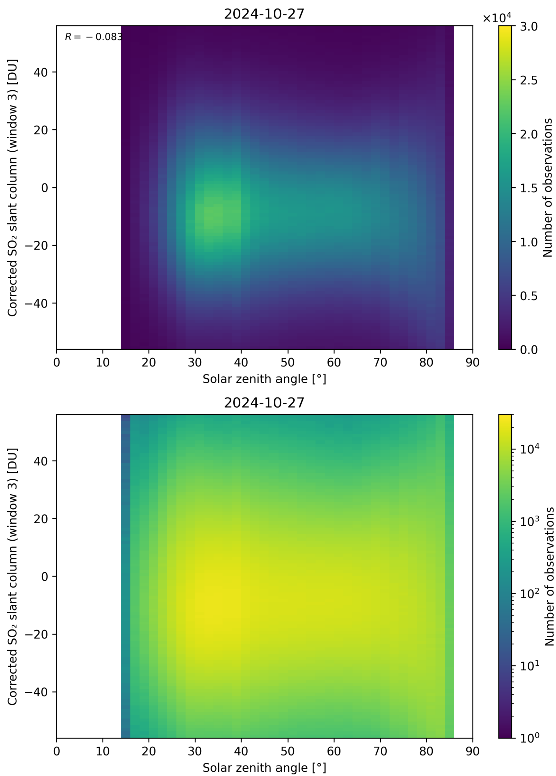
Figure 168: Scatter density plot of “Solar zenith angle” against “Corrected SO 2 slant column (window 3)” for 2024-10-26 to 2024-10-28.
