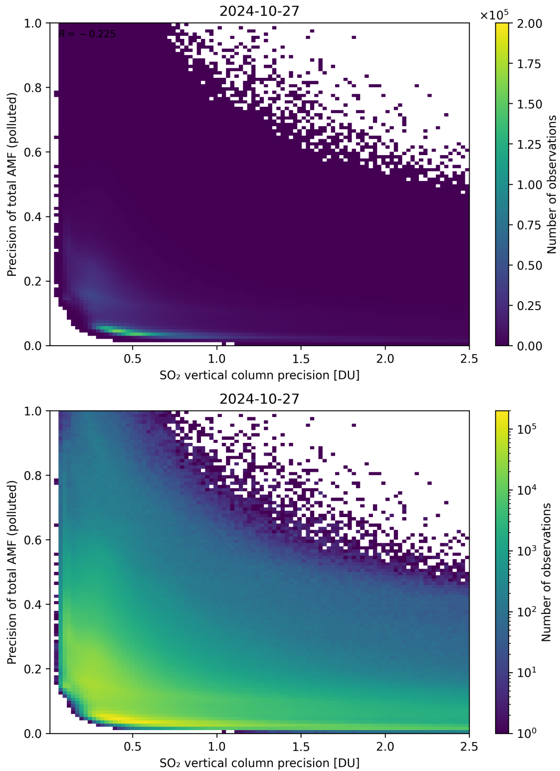
Figure 295: Scatter density plot of “SO 2 vertical column precision” against “Precision of total AMF (polluted)” for 2024-10-26 to 2024-10-28.
