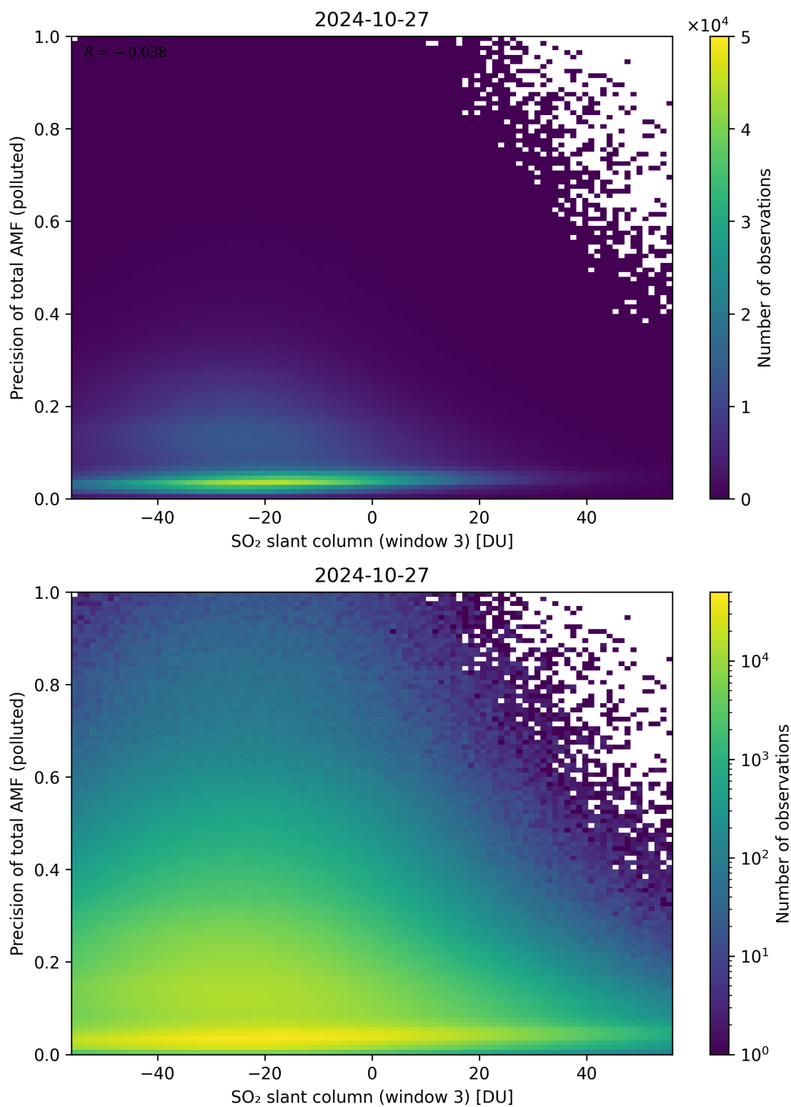
Figure 269: Scatter density plot of “SO 2 slant column (window 3)” against “Precision of total AMF (polluted)” for 2024-10-26 to 2024-10-28.
