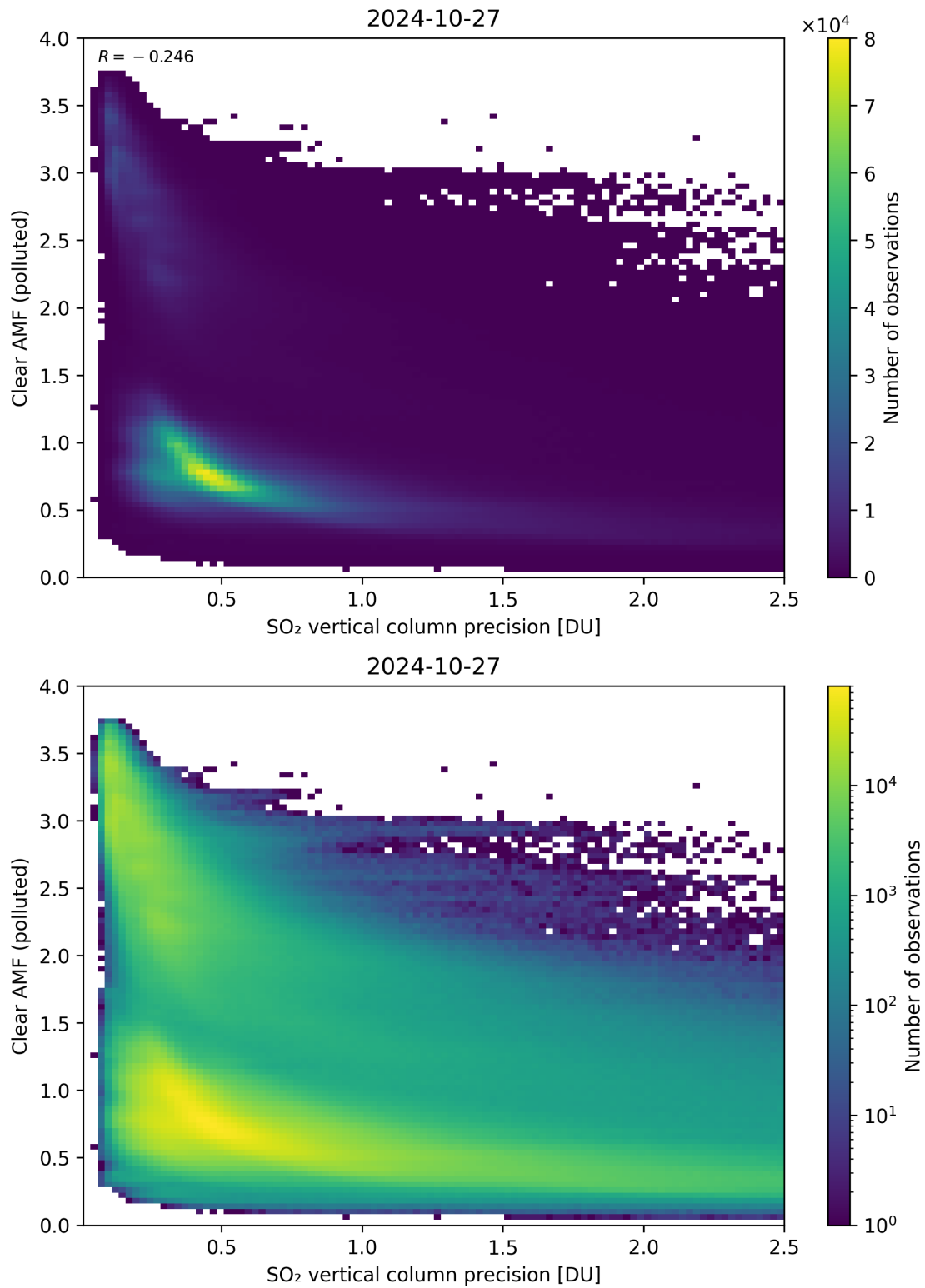
Figure 285: Scatter density plot of “SO 2 vertical column precision” against “Clear AMF (polluted)” for 2024-10-26 to 2024-10-28.
