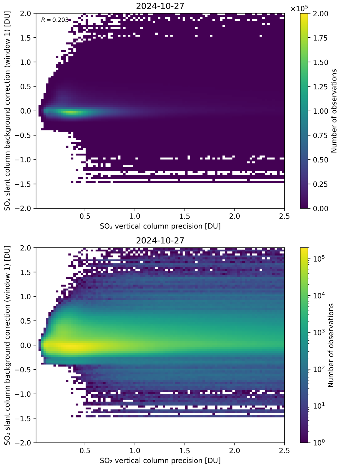
Figure 279: Scatter density plot of “SO 2 vertical column precision” against “SO 2 slant column background correction (window 1)” for 2024-10-26 to 2024-10-28.
