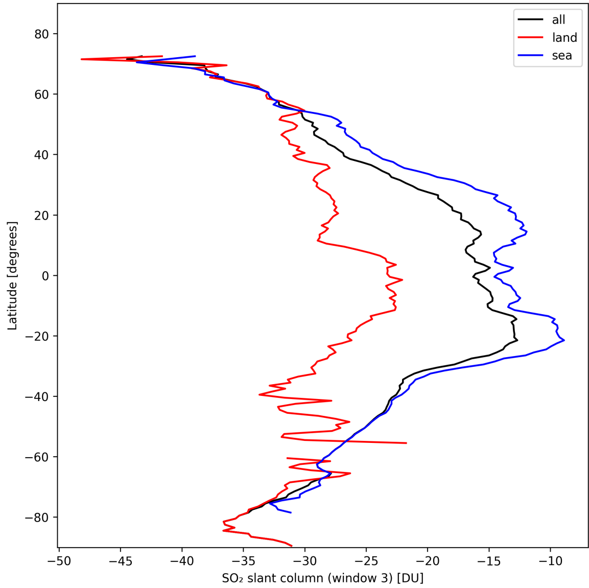
Figure 41: Zonal average of “SO 2 slant column (window 3)” for 2024-10-26 to 2024-10-28.
