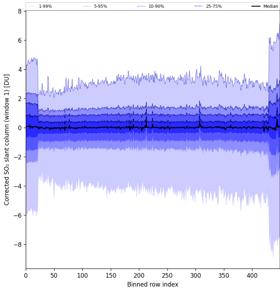
Figure 81: Along track statistics of “Corrected SO 2 slant column (window 1)” for 2024-10-26 to 2024-10-28
