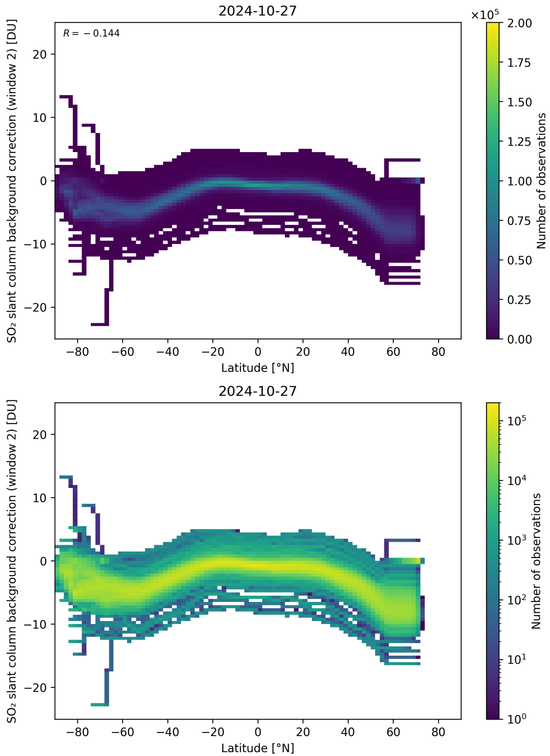
Figure 140: Scatter density plot of “Latitude” against “SO 2 slant column background correction (window 2)” for 2024-10-26 to 2024-10-28.
