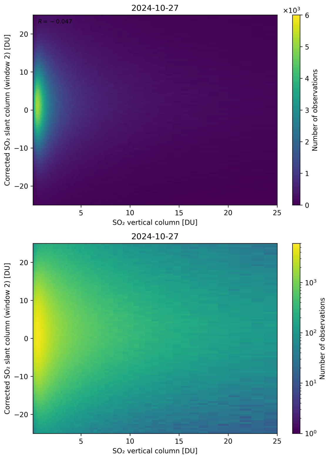
Figure 298: Scatter density plot of “SO 2 vertical column” against “Corrected SO 2 slant column (window 2)” for 2024-10-26 to 2024-10-28.
