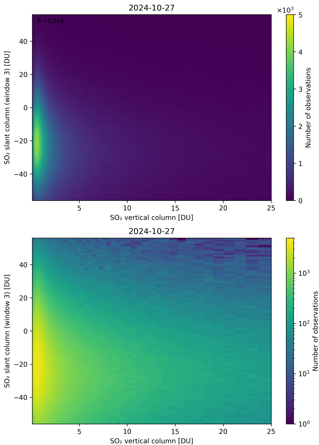
Figure 303: Scatter density plot of “SO 2 vertical column” against “SO 2 slant column (window 3)” for 2024-10-26 to 2024-10-28.
