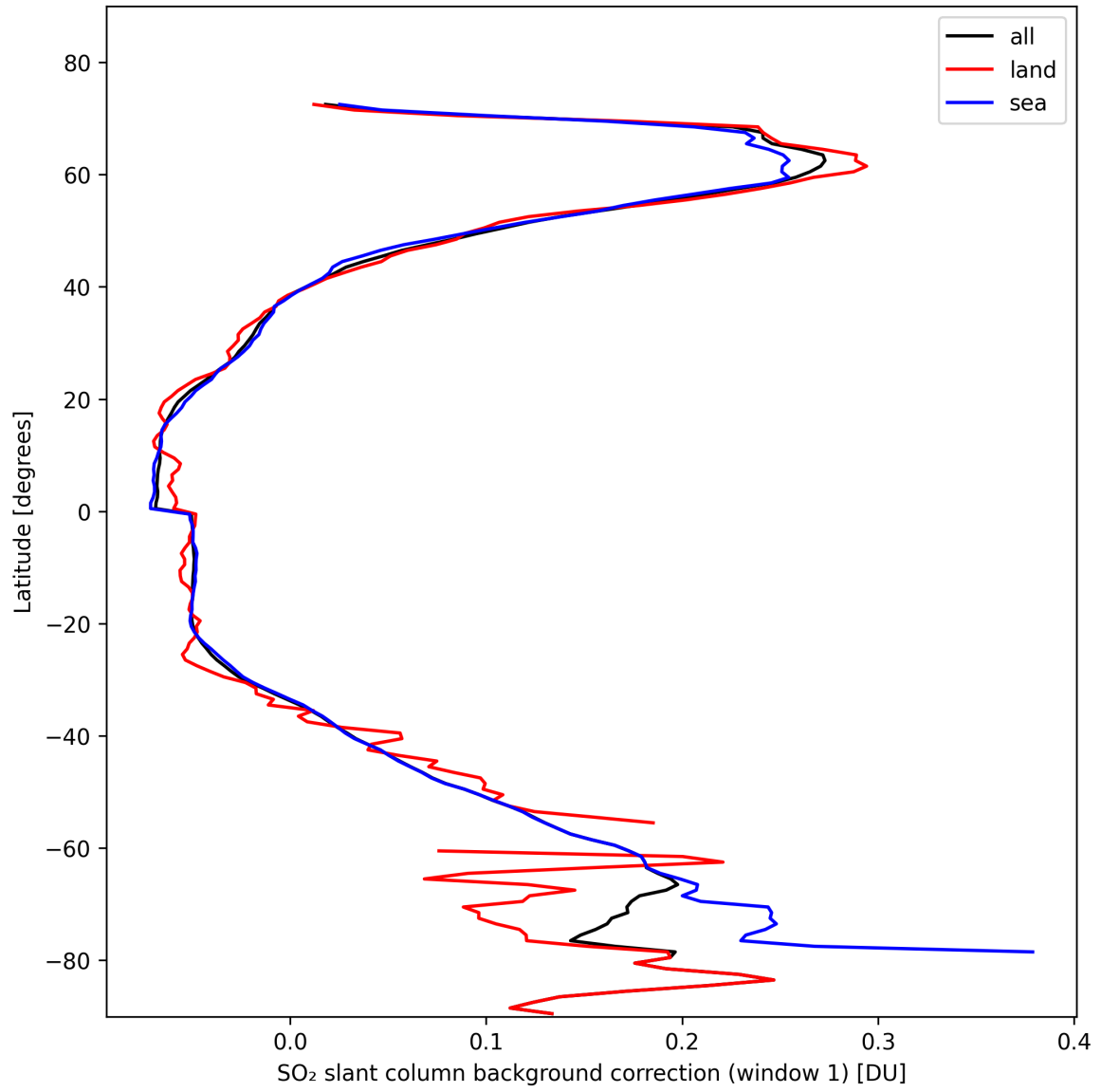
Figure 36: Zonal average of “SO 2 slant column background correction (window 1)” for 2024-10-26 to 2024-10-28.
