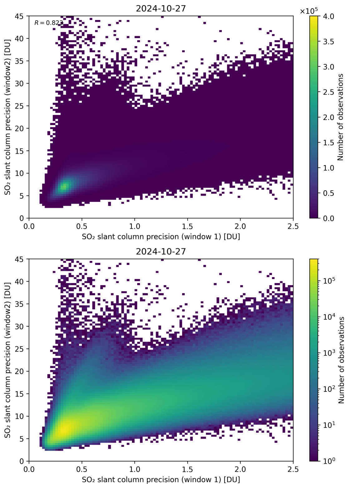
Figure 227: Scatter density plot of “SO 2 slant column precision (window 1)” against “SO 2 slant column precision (window 2)” for 2024-10-26 to 2024-10-28.
