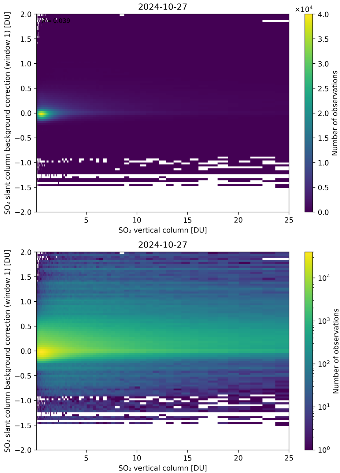
Figure 273: Scatter density plot of “SO 2 vertical column” against “SO 2 slant column background correction (window 1)” for 2024-10-26 to 2024-10-28.
