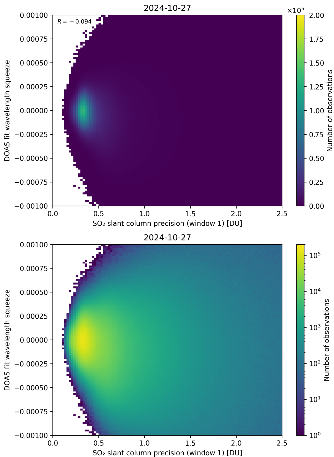
Figure 222: Scatter density plot of “SO 2 slant column precision (window 1)” against “DOAS fit wavelength squeeze” for 2024-10-26 to 2024-10-28.
