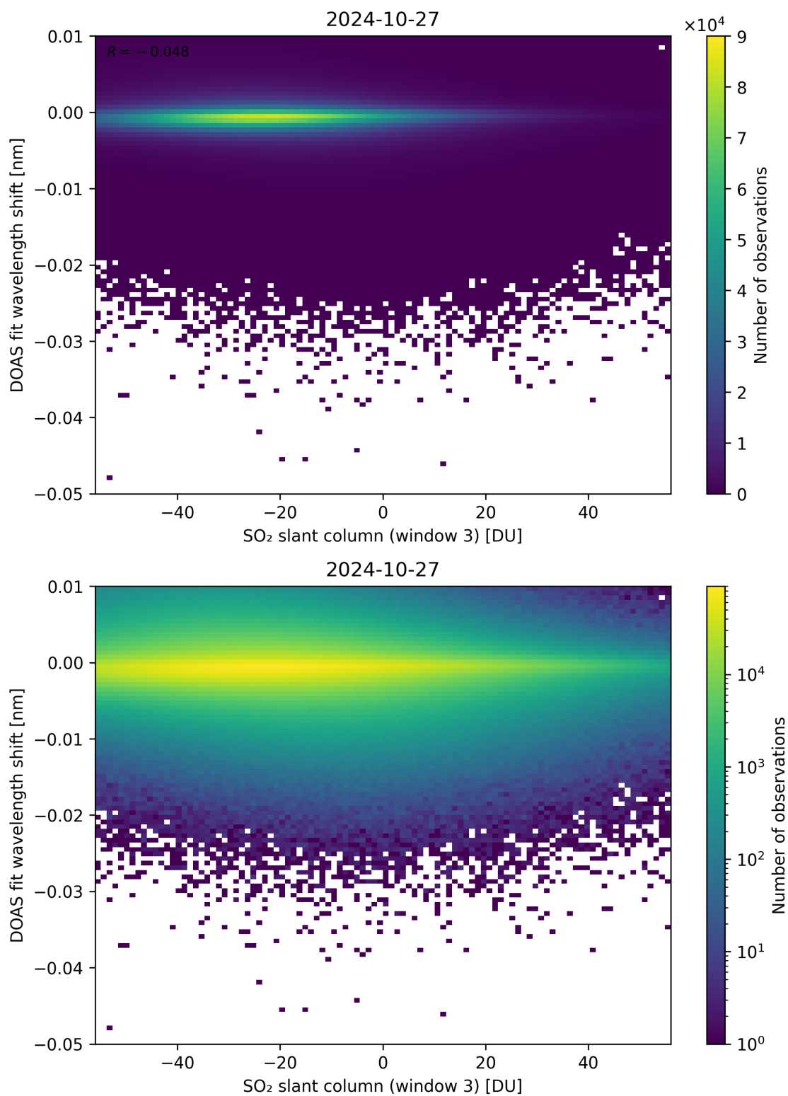
Figure 254: Scatter density plot of “SO 2 slant column (window 3)” against “DOAS fit wavelength shift” for 2024-10-26 to 2024-10-28.
