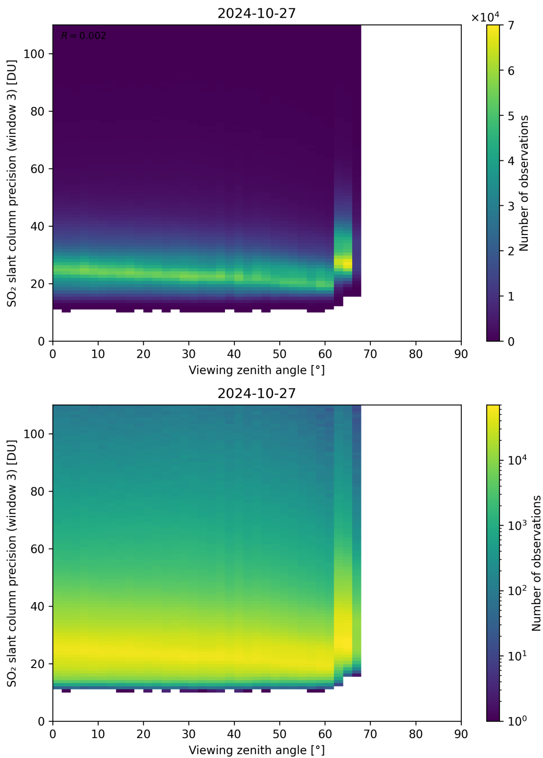
Figure 324: Scatter density plot of “Viewing zenith angle” against “SO 2 slant column precision (window 3)” for 2024-10-26 to 2024-10-28.
