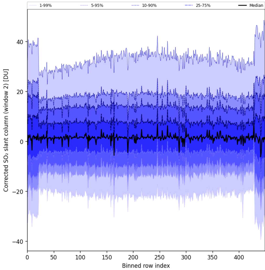
Figure 85: Along track statistics of “Corrected SO 2 slant column (window 2)” for 2024-10-26 to 2024-10-28
