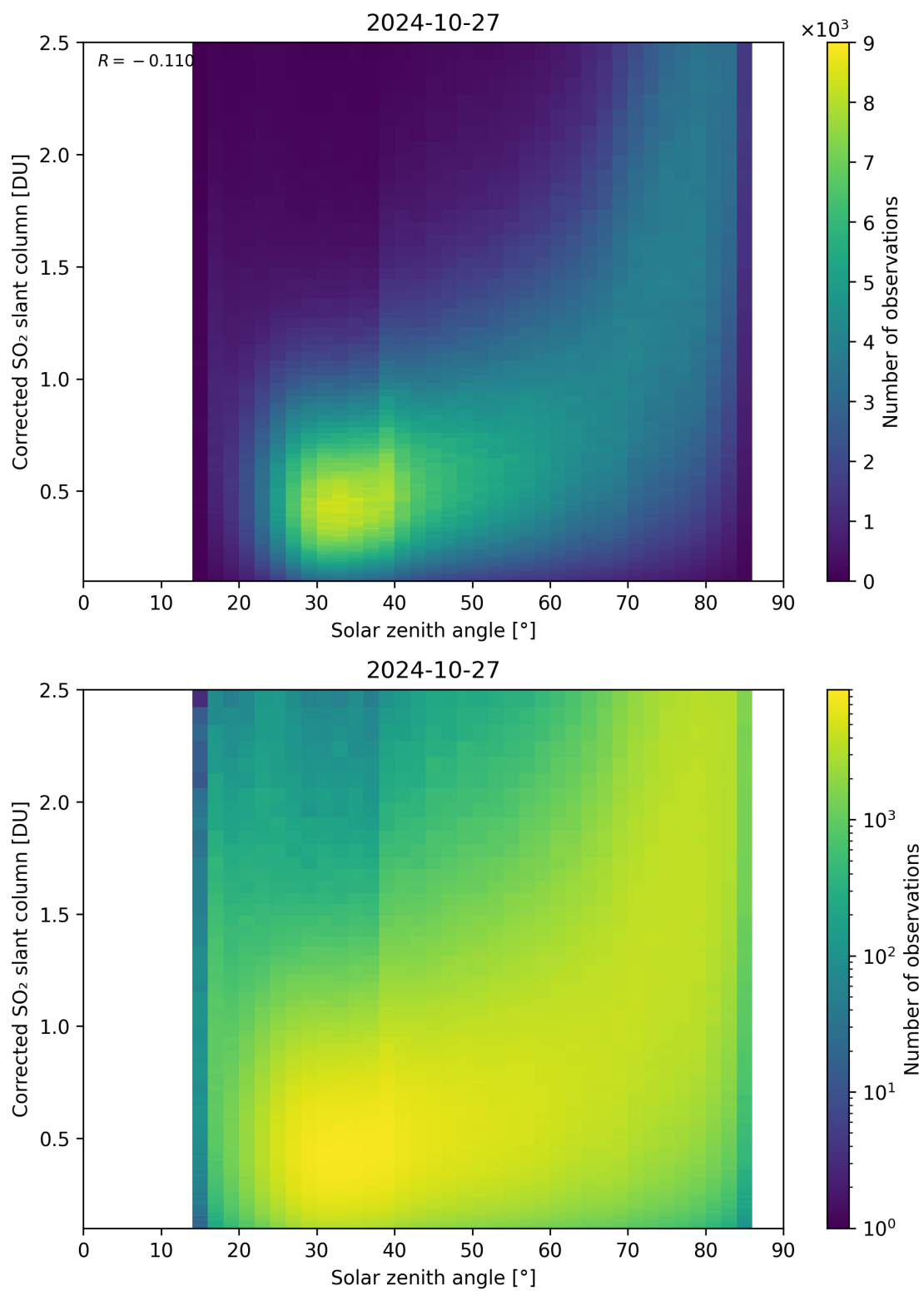
Figure 166: Scatter density plot of “Solar zenith angle” against “Corrected SO 2 slant column” for 2024-10-26 to 2024-10-28.
