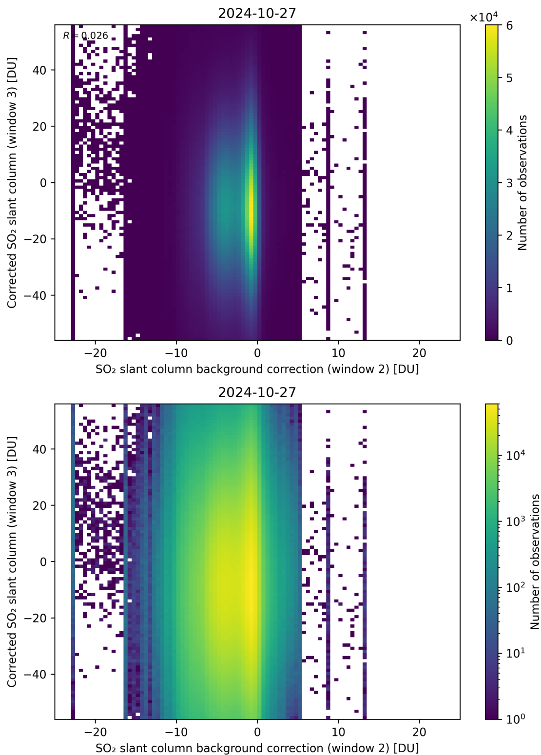
Figure 116: Scatter density plot of “SO 2 slant column background correction (window 2)” against “Corrected SO 2 slant column (window 3)” for 2024-10-26 to 2024-10-28.
