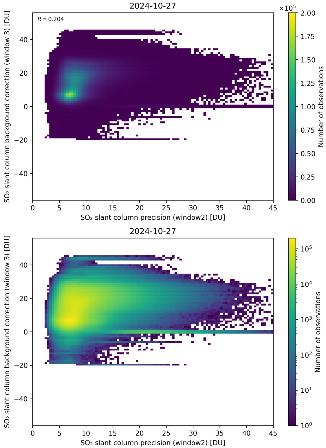
Figure 242: Scatter density plot of “SO 2 slant column precision (window2)” against “SO 2 slant column background correction (window 3)” for 2024-10-26 to 2024-10-28.
