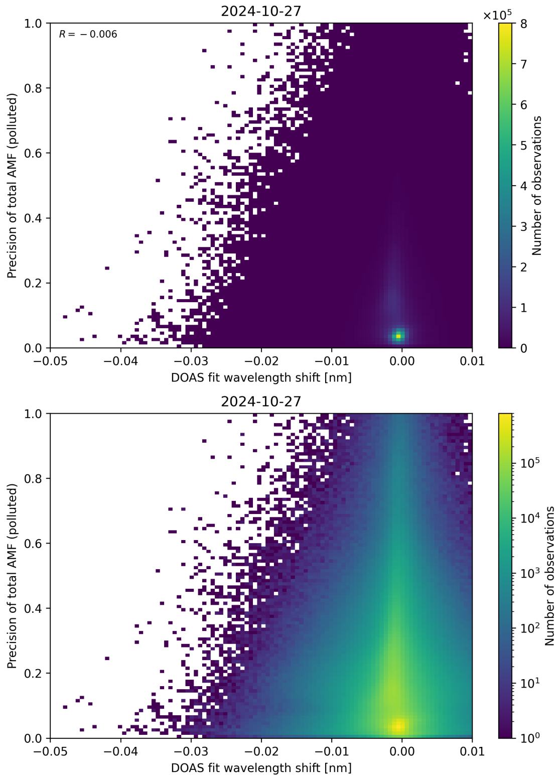
Figure 131: Scatter density plot of “DOAS fit wavelength shift” against “Precision of total AMF (polluted)” for 2024-10-26 to 2024-10-28.
