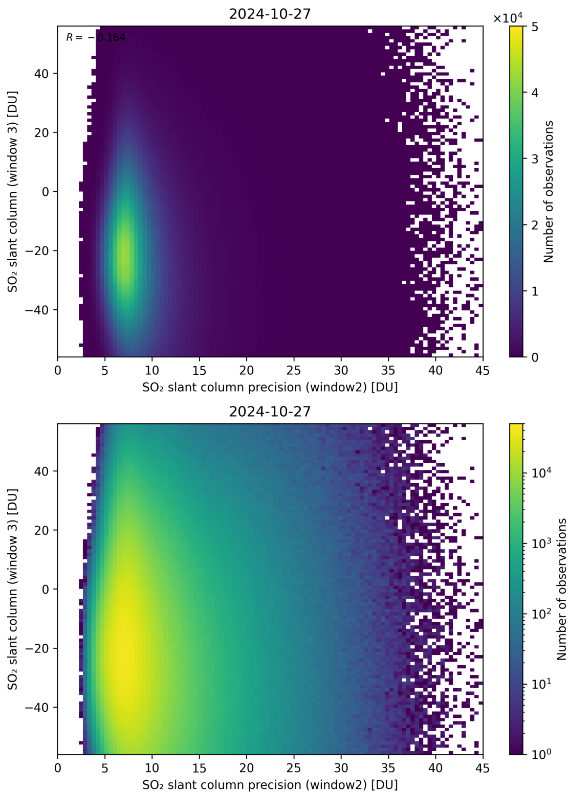
Figure 249: Scatter density plot of “SO 2 slant column precision (window2)” against “SO 2 slant column (window 3)” for 2024-10-26 to 2024-10-28.
