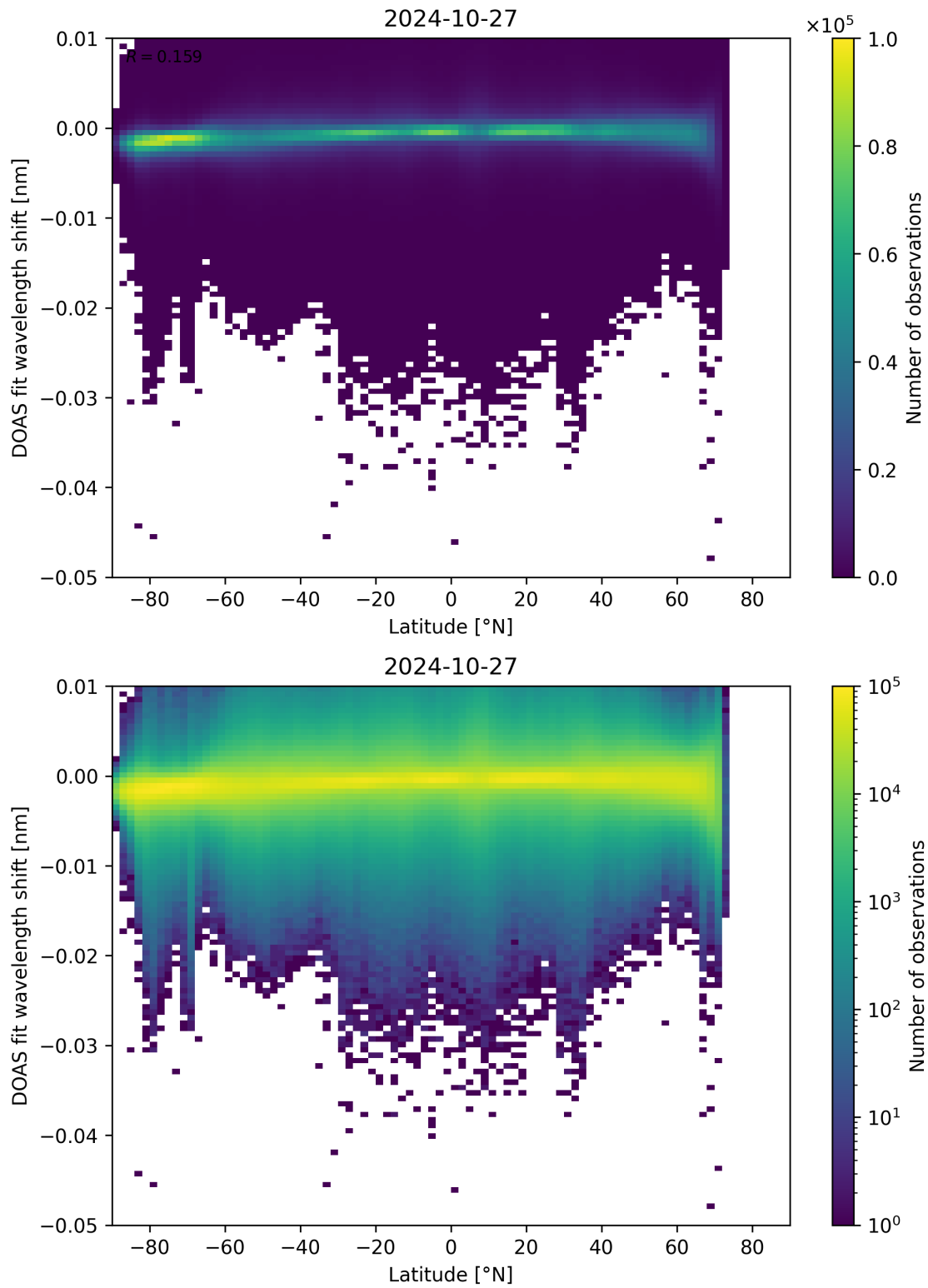
Figure 142: Scatter density plot of “Latitude” against “DOAS fit wavelength shift” for 2024-10-26 to 2024-10-28.
