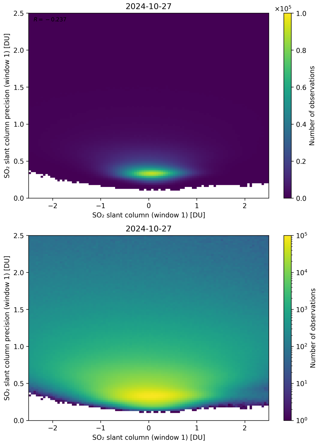
Figure 235: Scatter density plot of “SO 2 slant column (window 1)” against “SO 2 slant column precision (window 1)” for 2024-10-26 to 2024-10-28.
