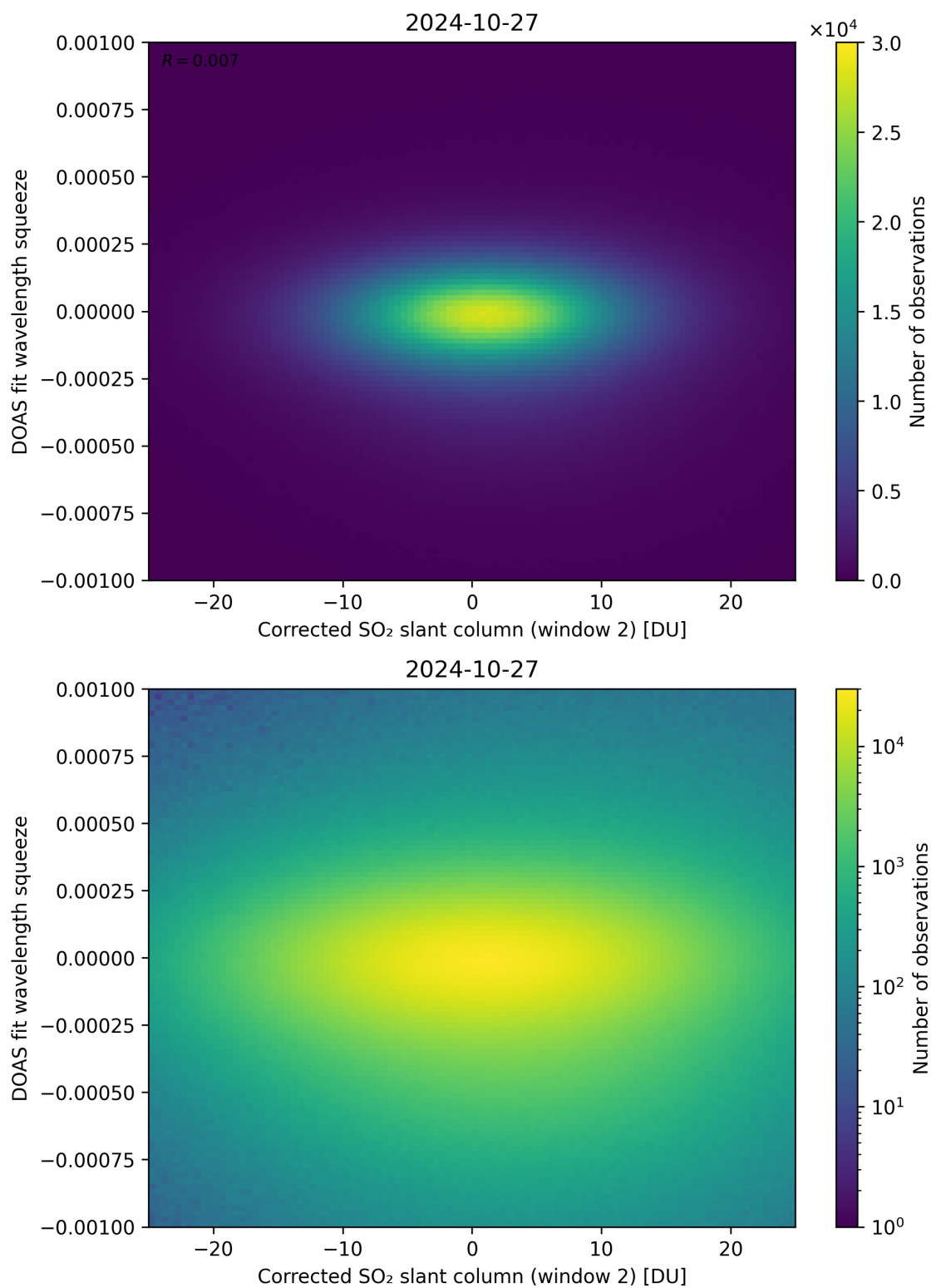
Figure 197: Scatter density plot of “Corrected SO 2 slant column (window 2)” against “DOAS fit wavelength squeeze” for 2024-10-26 to 2024-10-28.
