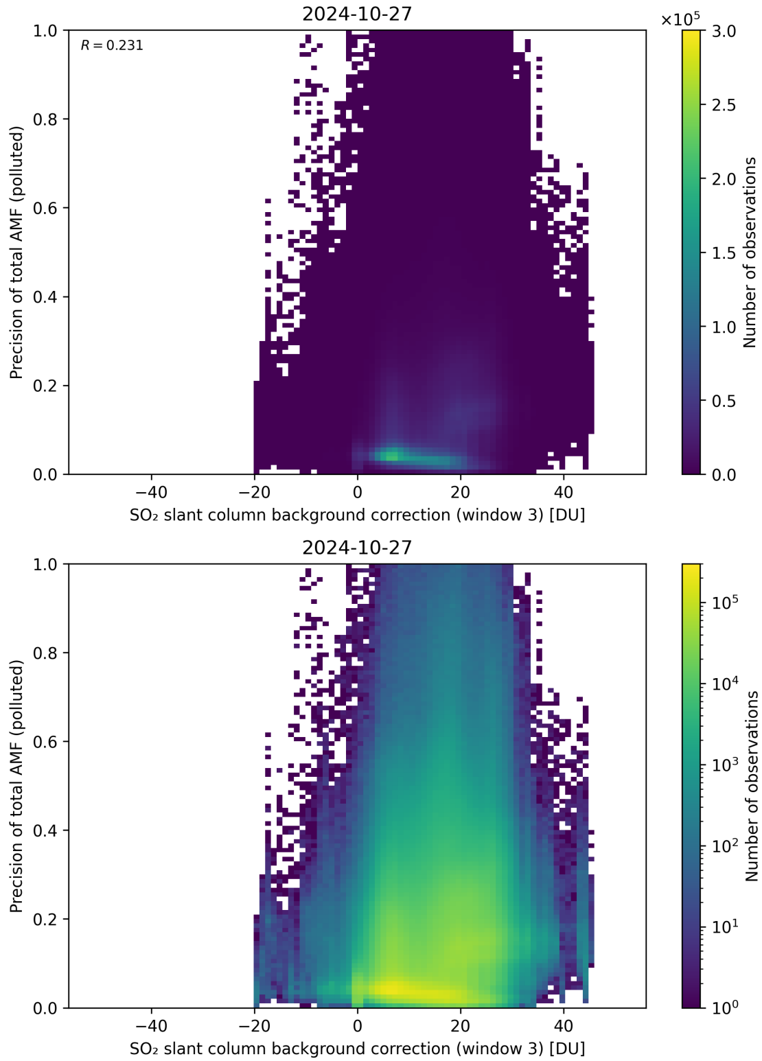
Figure 126: Scatter density plot of “SO 2 slant column background correction (window 3)” against “Precision of total AMF (polluted)” for 2024-10-26 to 2024-10-28.
