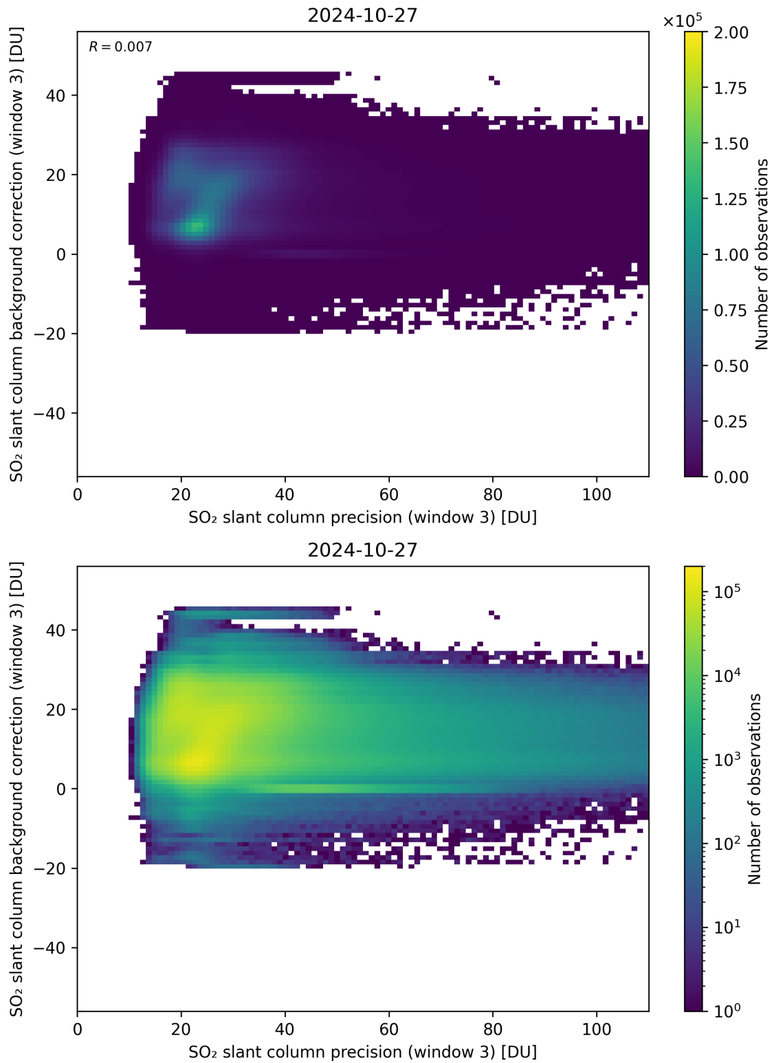
Figure 257: Scatter density plot of “SO 2 slant column precision (window 3)” against “SO 2 slant column background correction (window 3)” for 2024-10-26 to 2024-10-28.
