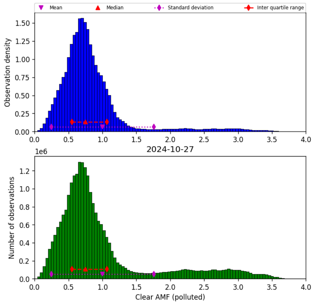
Figure 73: Histogram of “Clear AMF (polluted)” for 2024-10-26 to 2024-10-28
