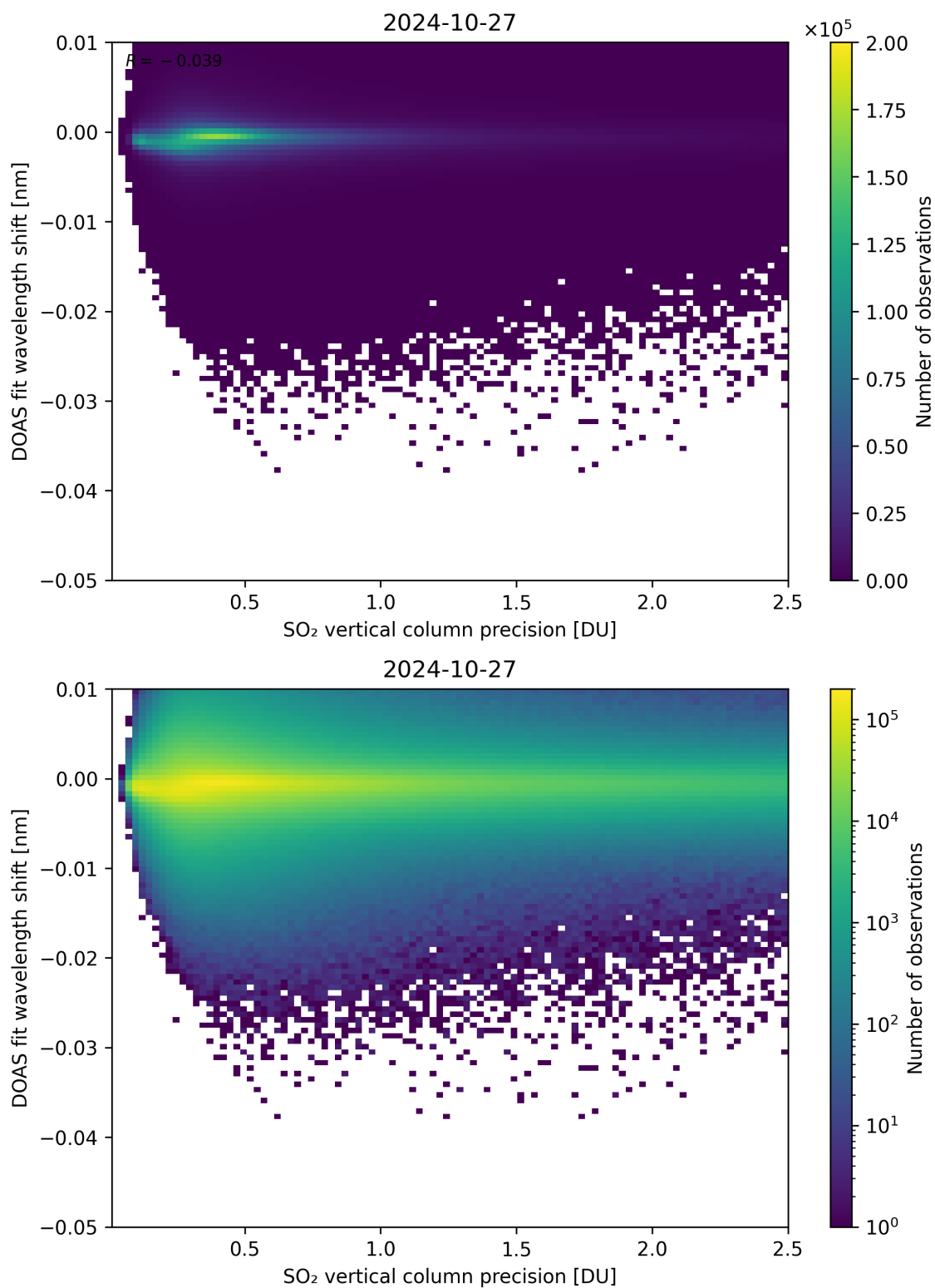
Figure 282: Scatter density plot of “SO 2 vertical column precision” against “DOAS fit wavelength shift” for 2024-10-26 to 2024-10-28.
