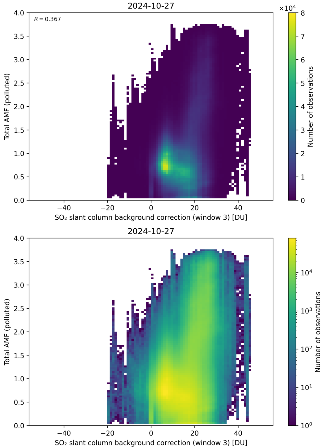
Figure 125: Scatter density plot of “SO 2 slant column background correction (window 3)” against “Total AMF (polluted)” for 2024-10-26 to 2024-10-28.
