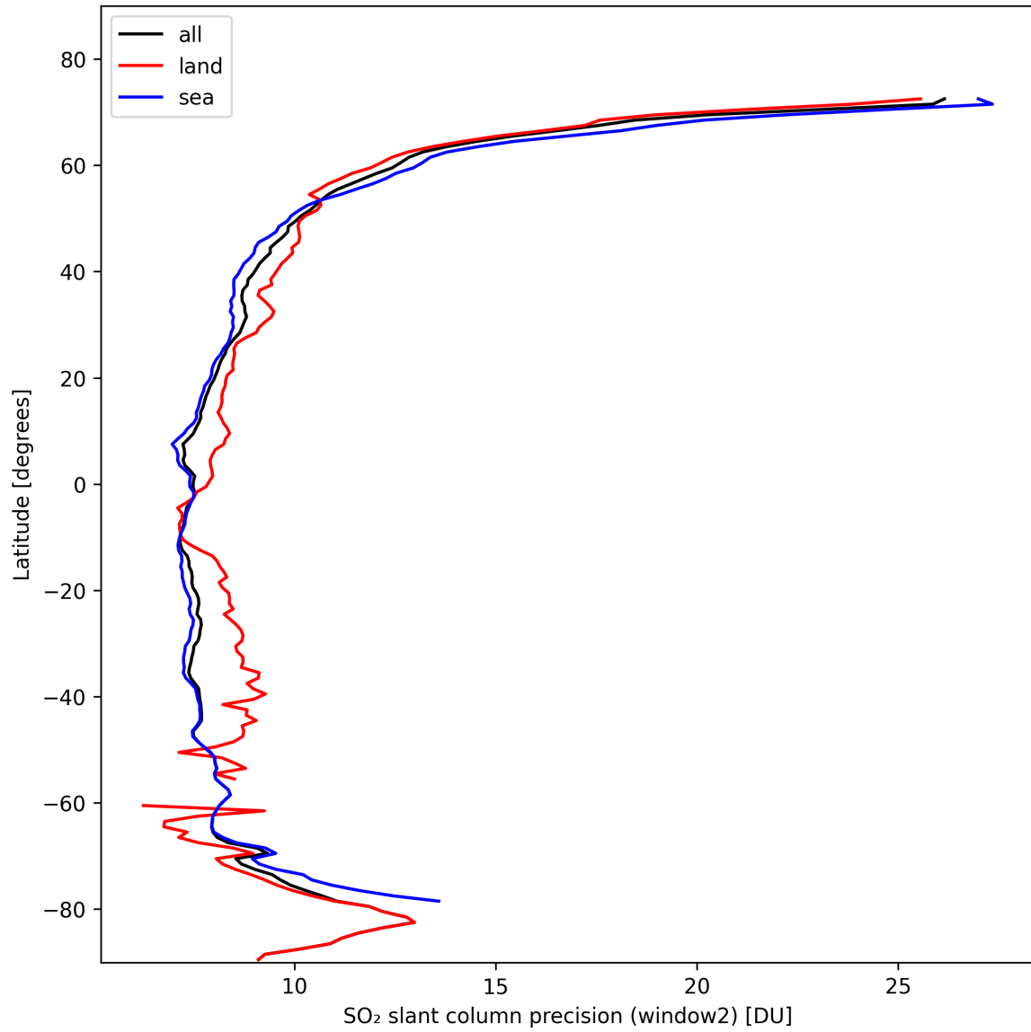
Figure 38: Zonal average of “SO 2 slant column precision (window2)” for 2024-10-26 to 2024-10-28.
