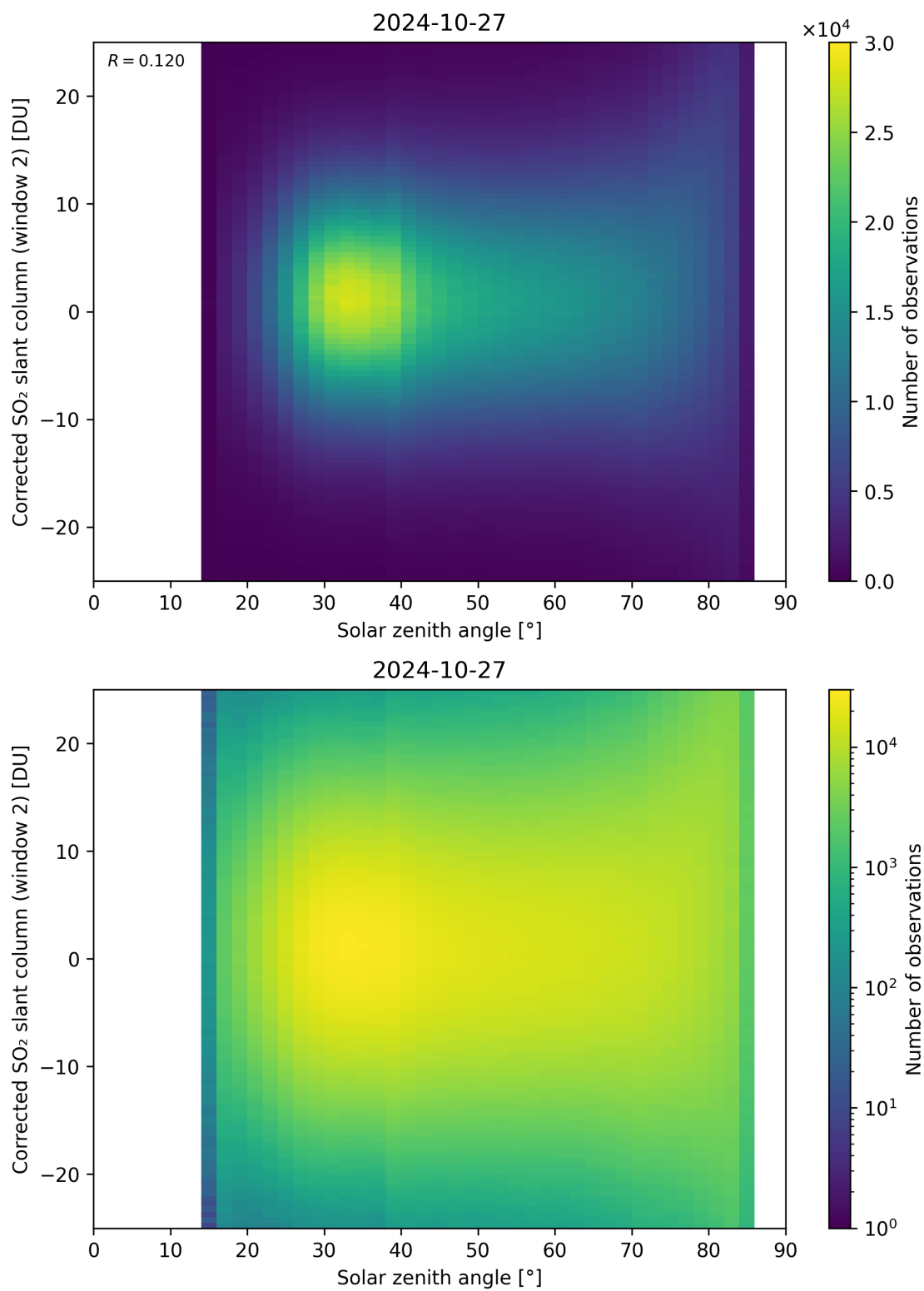
Figure 167: Scatter density plot of “Solar zenith angle” against “Corrected SO 2 slant column (window 2)” for 2024-10-26 to 2024-10-28.
