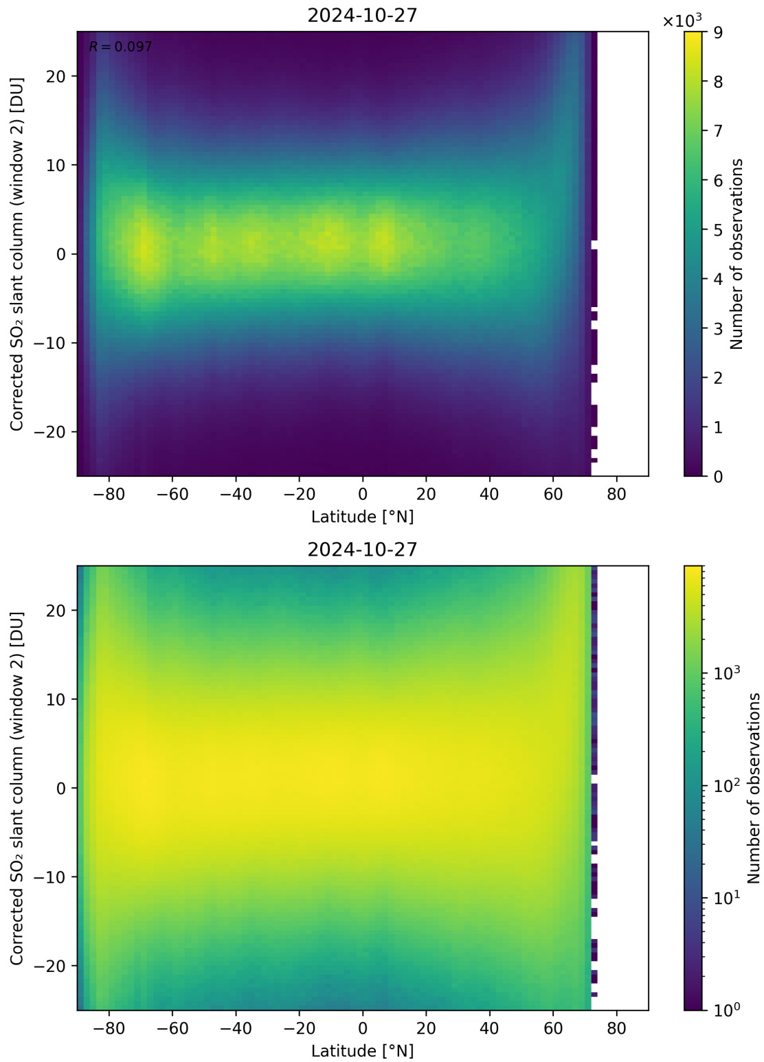
Figure 147: Scatter density plot of “Latitude” against “Corrected SO 2 slant column (window 2)” for 2024-10-26 to 2024-10-28.
