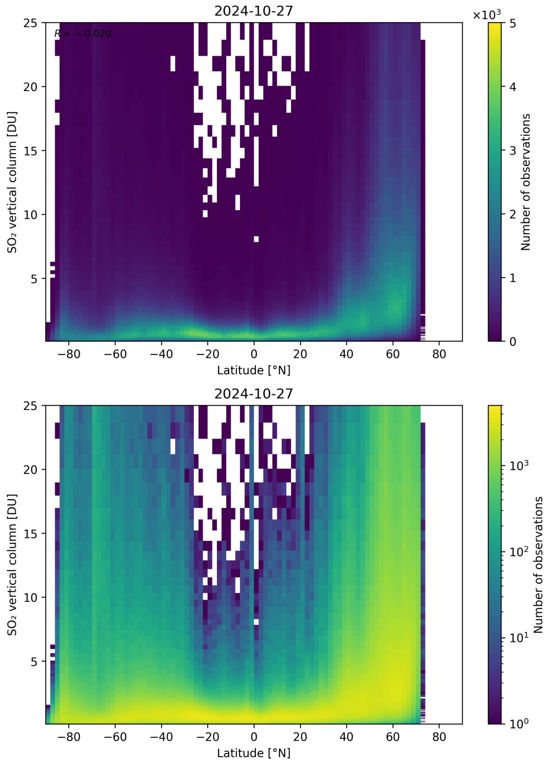
Figure 156: Scatter density plot of “Latitude” against “SO 2 vertical column” for 2024-10-26 to 2024-10-28.
