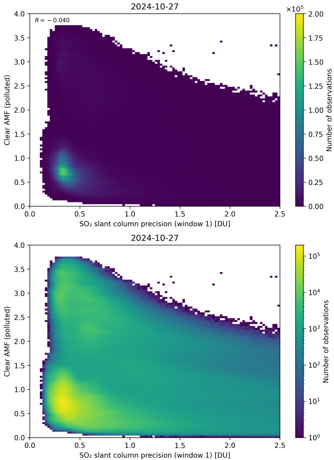
Figure 224: Scatter density plot of “SO 2 slant column precision (window 1)” against “Clear AMF (polluted)” for 2024-10-26 to 2024-10-28.
