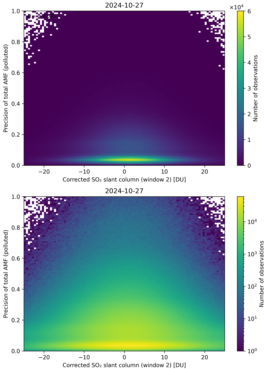
Figure 204: Scatter density plot of “Corrected SO 2 slant column (window 2)” against “Precision of total AMF (polluted)” for 2024-10-26 to 2024-10-28.
