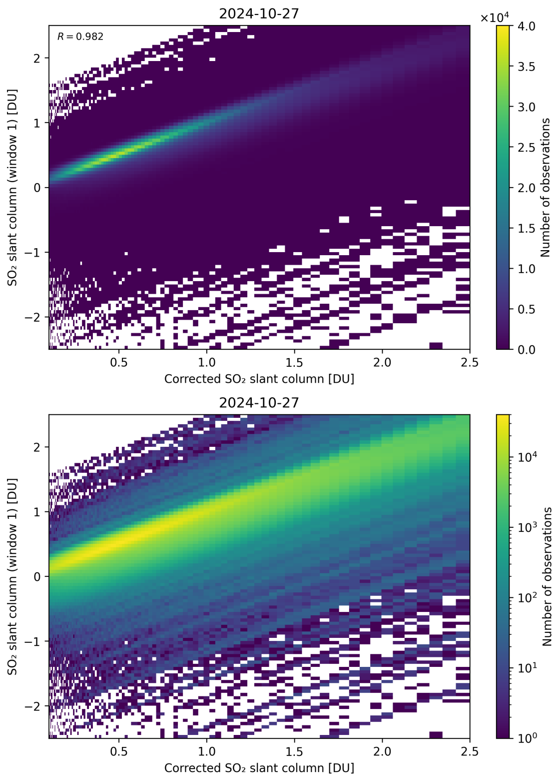
Figure 187: Scatter density plot of “Corrected SO 2 slant column” against “SO 2 slant column (window 1)” for 2024-10-26 to 2024-10-28.
