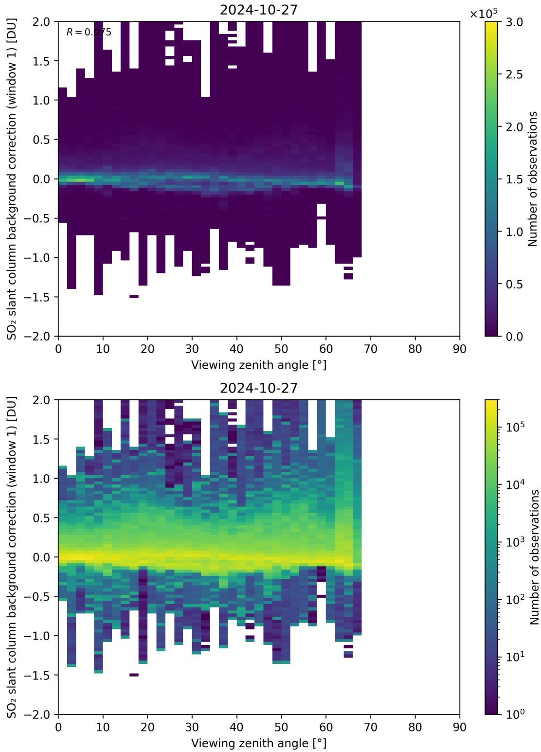
Figure 308: Scatter density plot of “Viewing zenith angle” against “SO 2 slant column background correction (window 1)” for 2024-10-26 to 2024-10-28.
