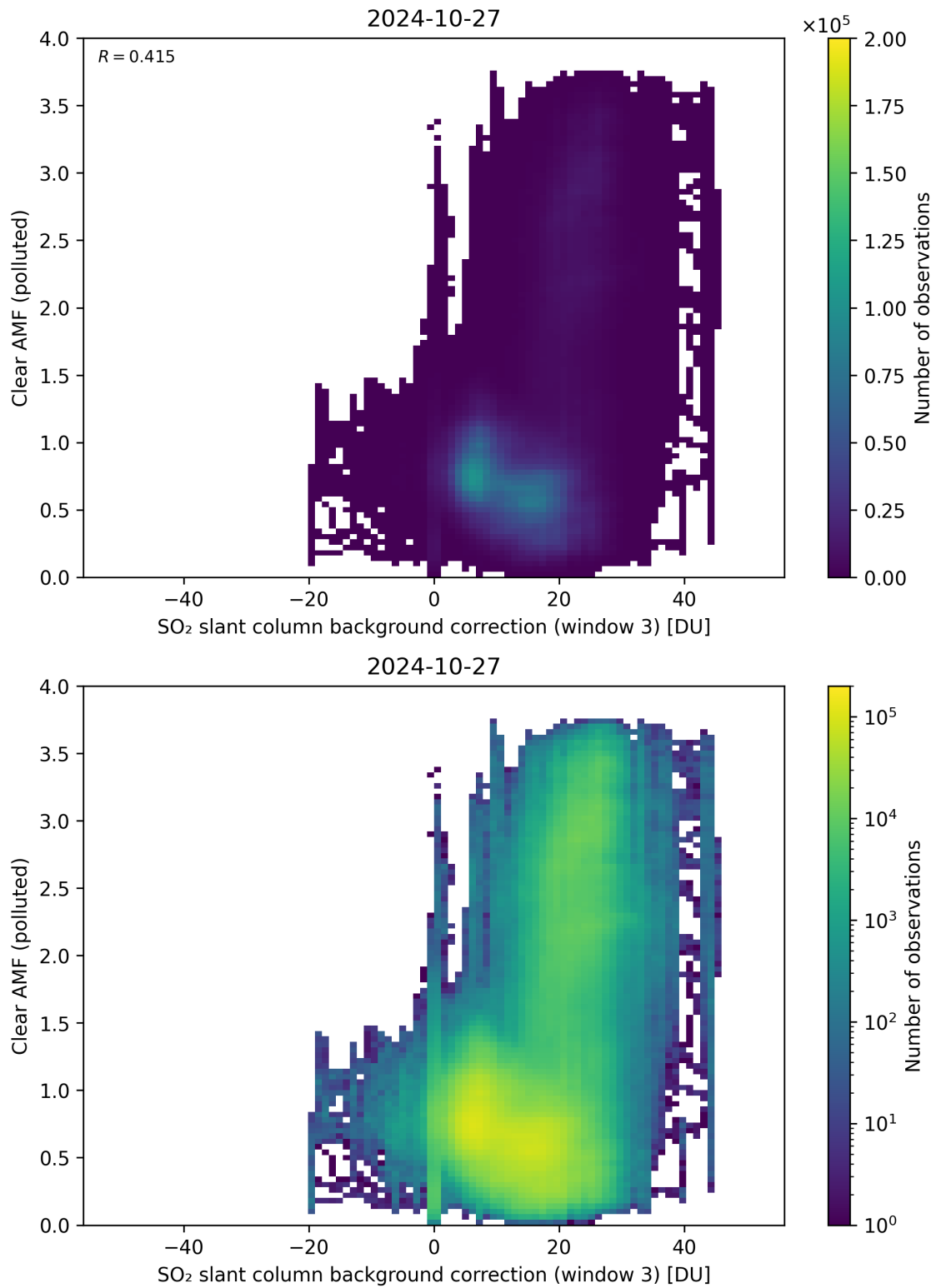
Figure 124: Scatter density plot of “SO 2 slant column background correction (window 3)” against “Clear AMF (polluted)” for 2024-10-26 to 2024-10-28.
