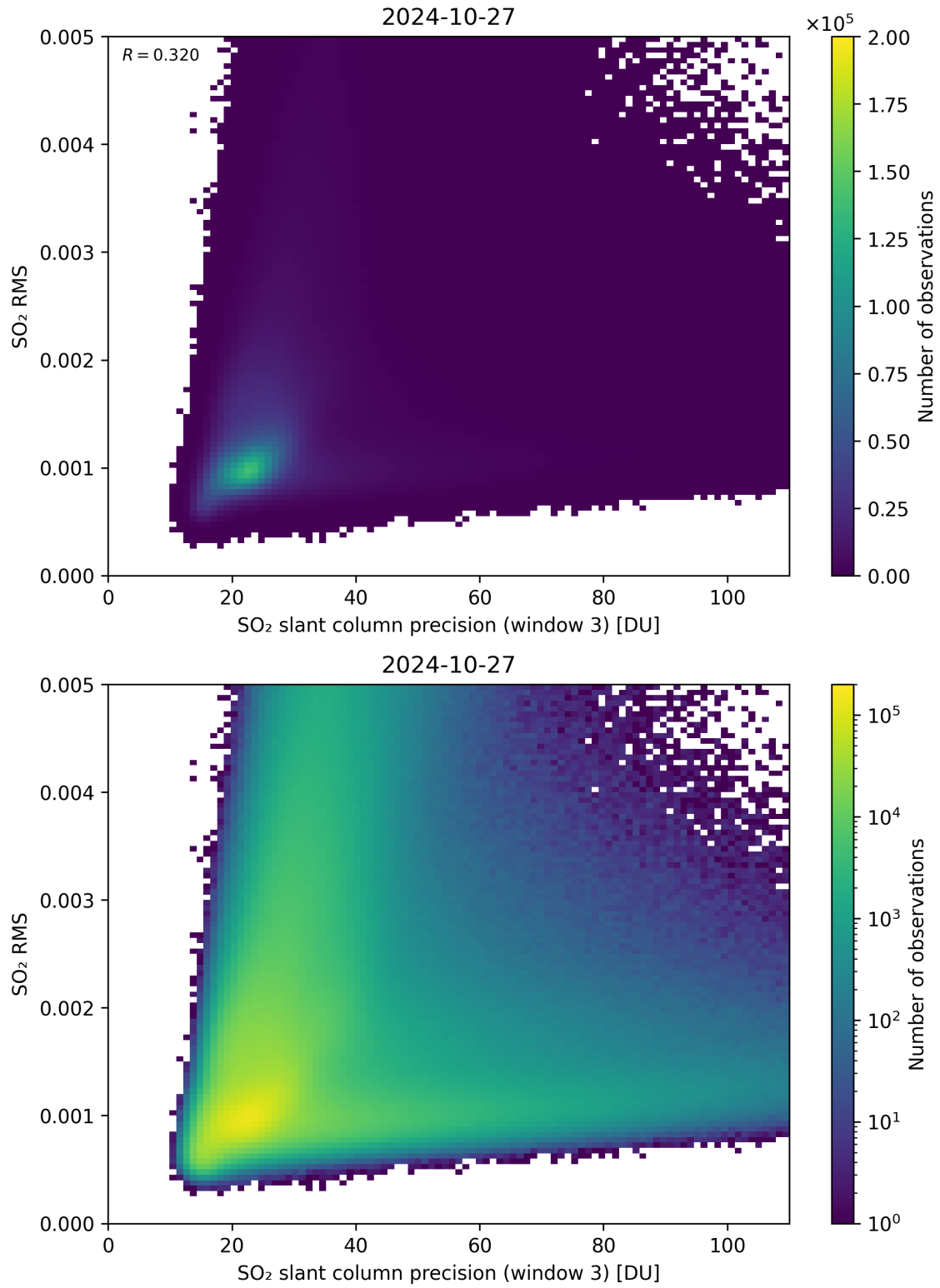
Figure 260: Scatter density plot of “SO 2 slant column precision (window 3)” against “SO 2 RMS” for 2024-10-26 to 2024-10-28.
