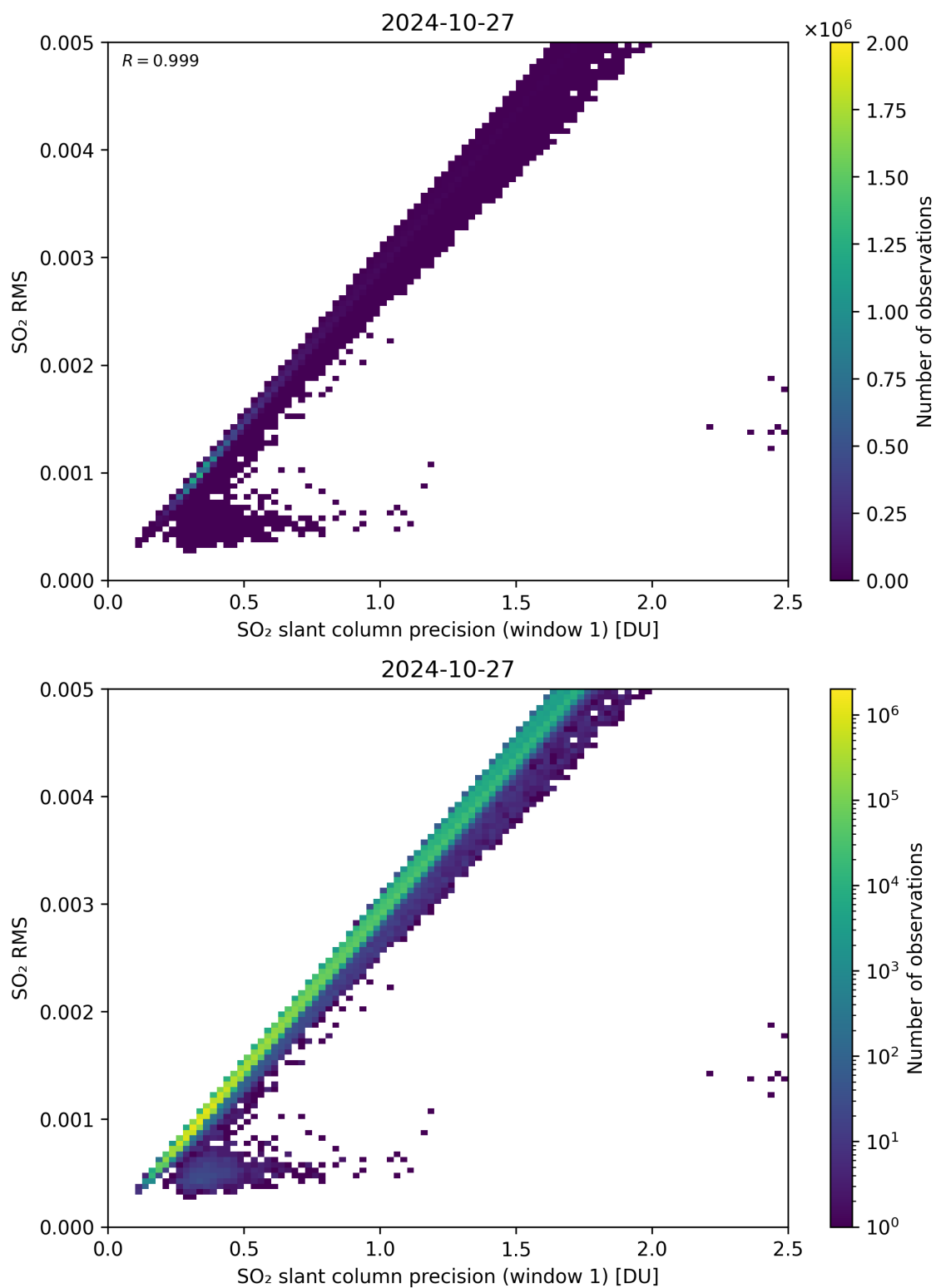
Figure 223: Scatter density plot of “SO 2 slant column precision (window 1)” against “SO 2 RMS” for 2024-10-26 to 2024-10-28.
