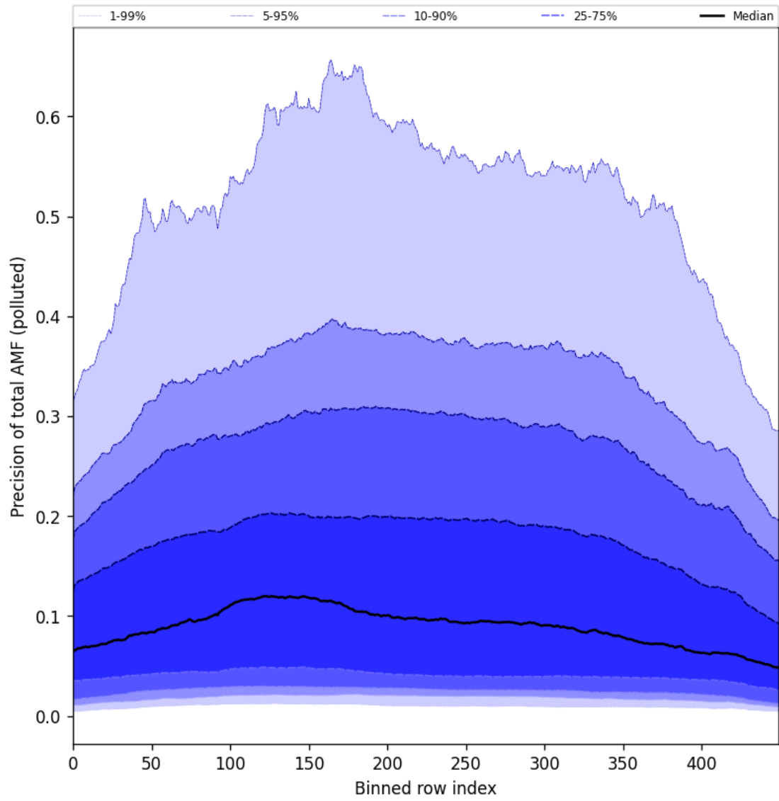
Figure 95: Along track statistics of “Precision of total AMF (polluted)” for 2024-10-26 to 2024-10-28
