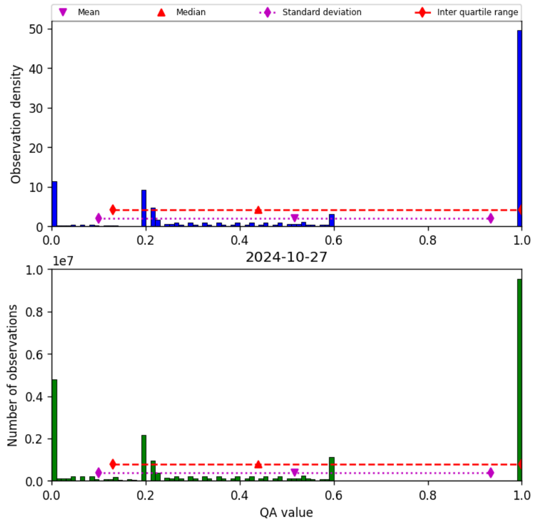
Figure 52: Histogram of “QA value” for 2024-10-26 to 2024-10-28
