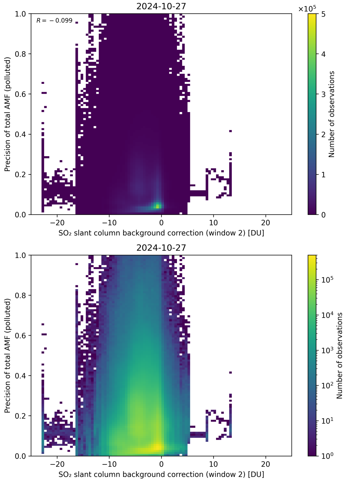
Figure 120: Scatter density plot of “SO 2 slant column background correction (window 2)” against “Precision of total AMF (polluted)” for 2024-10-26 to 2024-10-28.
