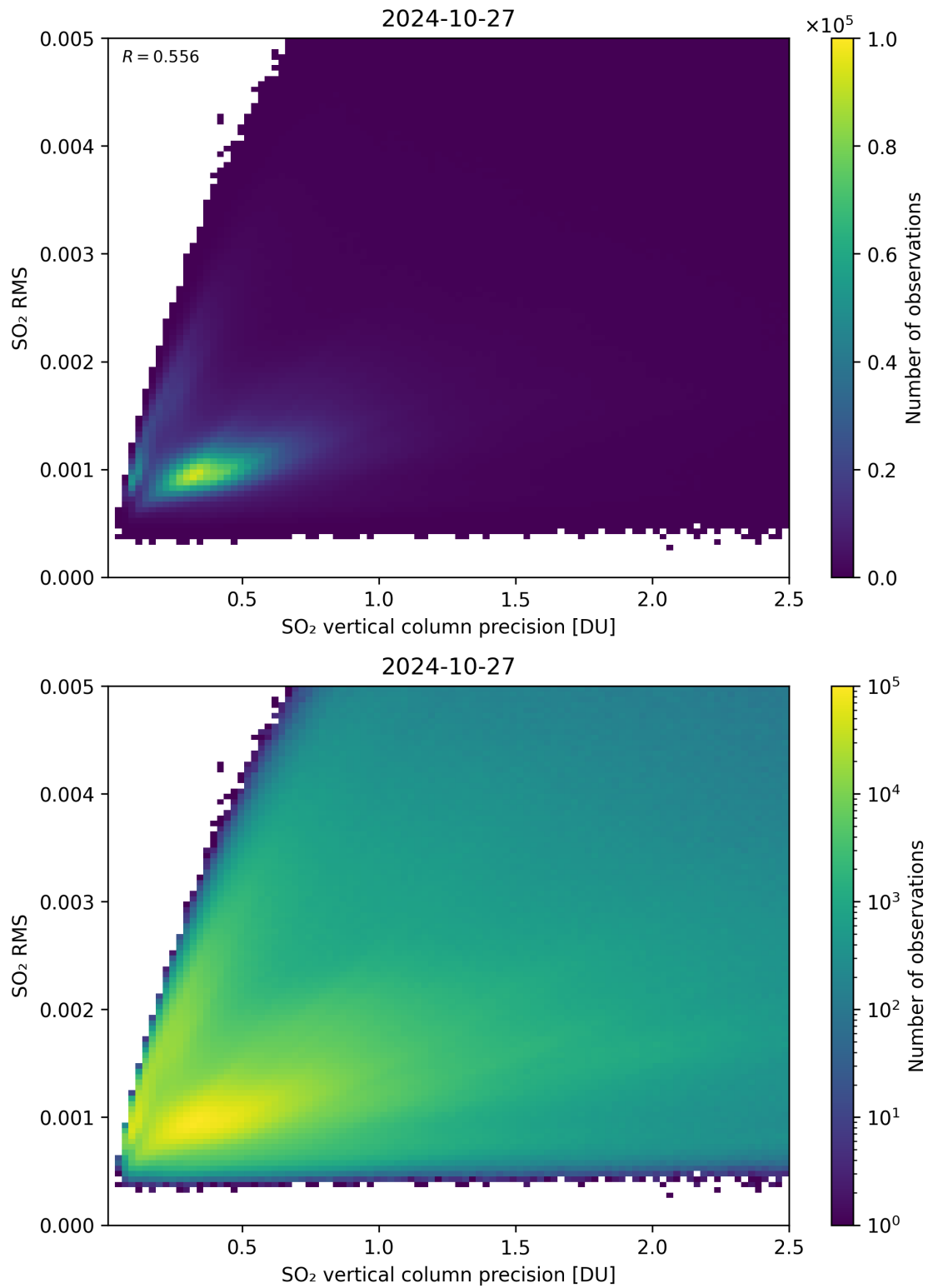
Figure 284: Scatter density plot of “SO 2 vertical column precision” against “SO 2 RMS” for 2024-10-26 to 2024-10-28.
