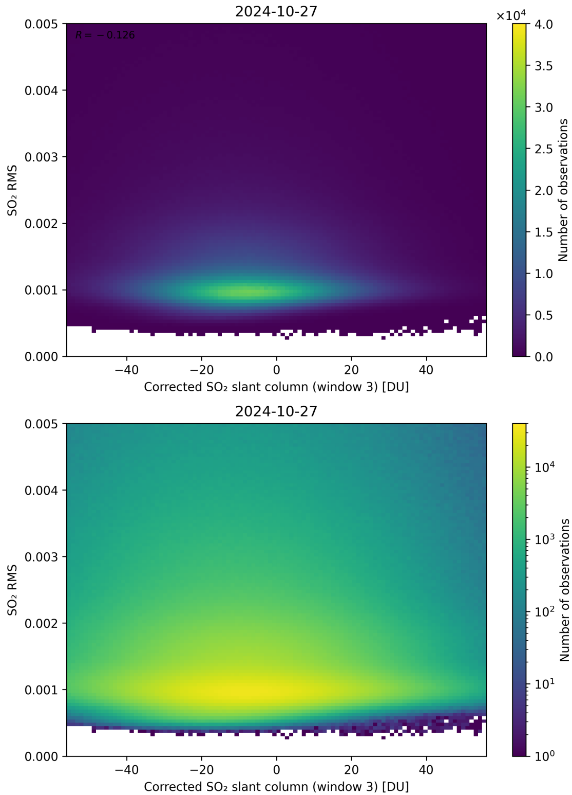
Figure 208: Scatter density plot of “Corrected SO 2 slant column (window 3)” against “SO 2 RMS” for 2024-10-26 to 2024-10-28.
