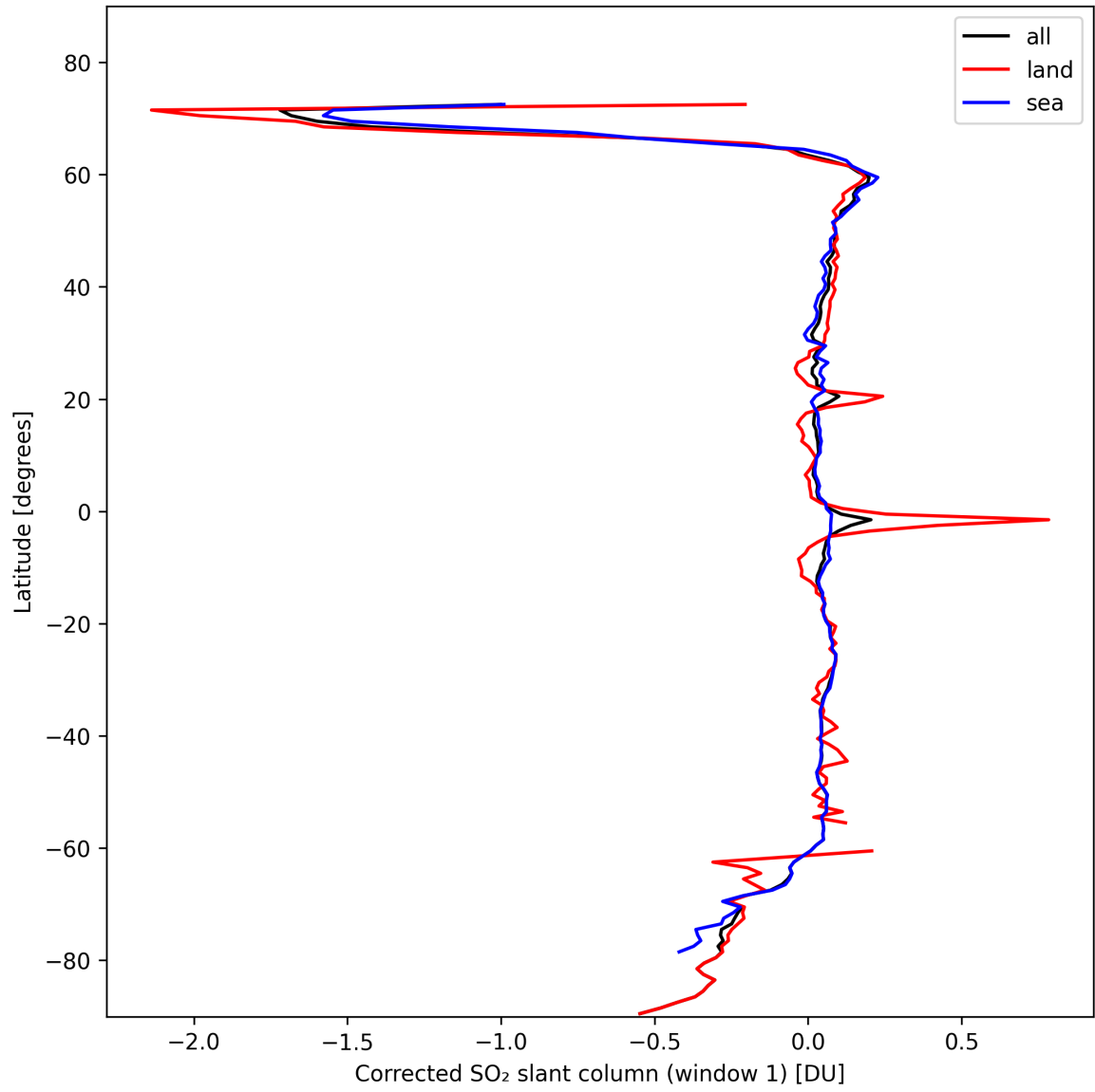
Figure 35: Zonal average of “Corrected SO 2 slant column (window 1)” for 2024-10-26 to 2024-10-28.
