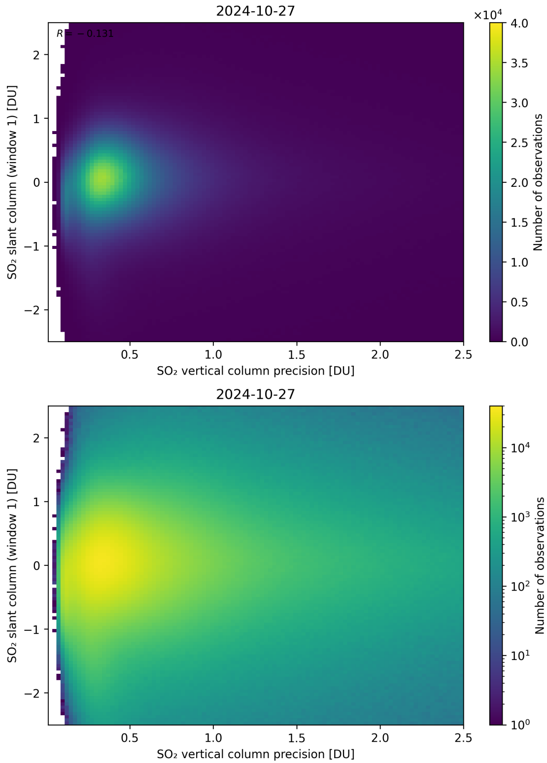
Figure 289: Scatter density plot of “SO 2 vertical column precision” against “SO 2 slant column (window 1)” for 2024-10-26 to 2024-10-28.
