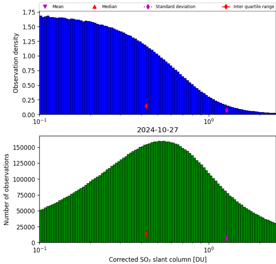
Figure 55: Histogram of “Corrected SO 2 slant column” for 2024-10-26 to 2024-10-28
