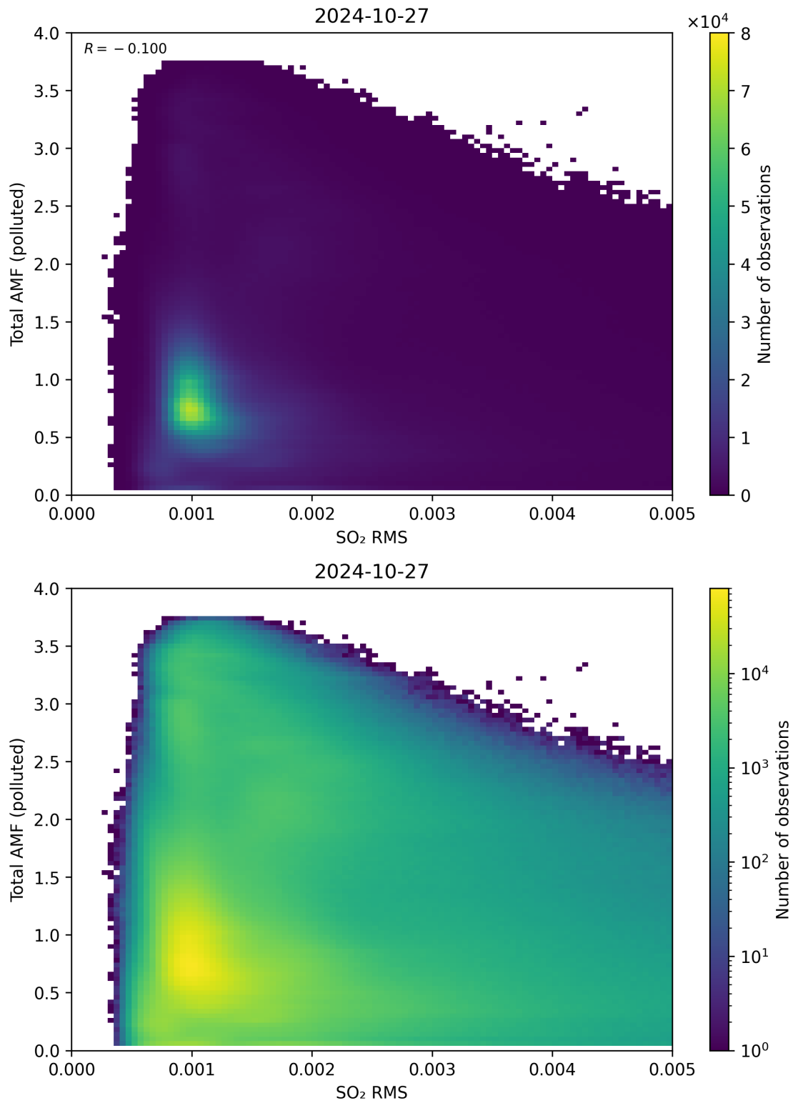
Figure 137: Scatter density plot of “SO 2 RMS” against “Total AMF (polluted)” for 2024-10-26 to 2024-10-28.
