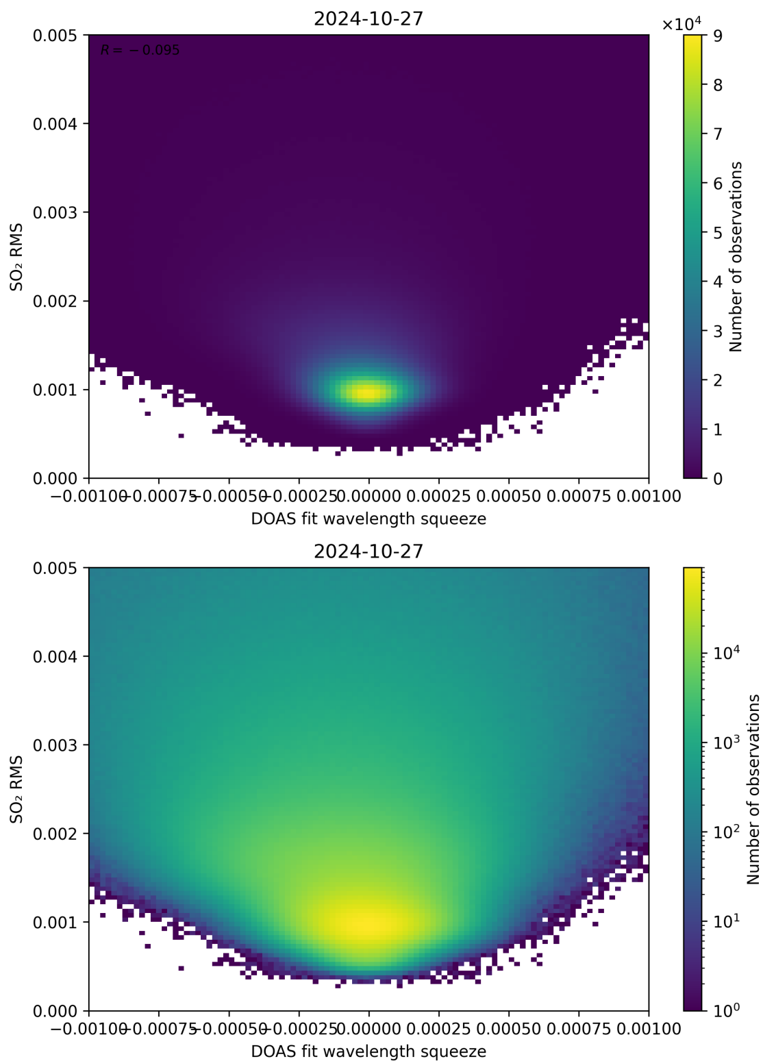
Figure 132: Scatter density plot of “DOAS fit wavelength squeeze” against “SO 2 RMS” for 2024-10-26 to 2024-10-28.
