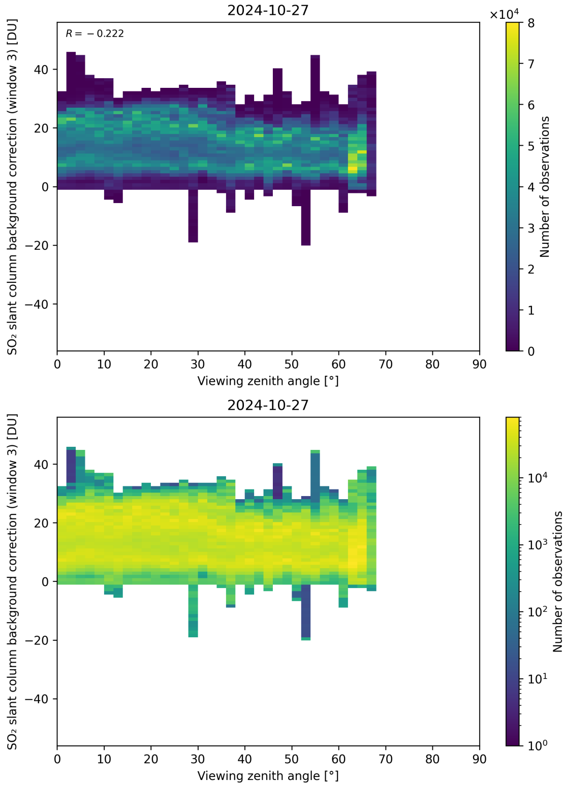
Figure 310: Scatter density plot of “Viewing zenith angle” against “SO 2 slant column background correction (window 3)” for 2024-10-26 to 2024-10-28.
