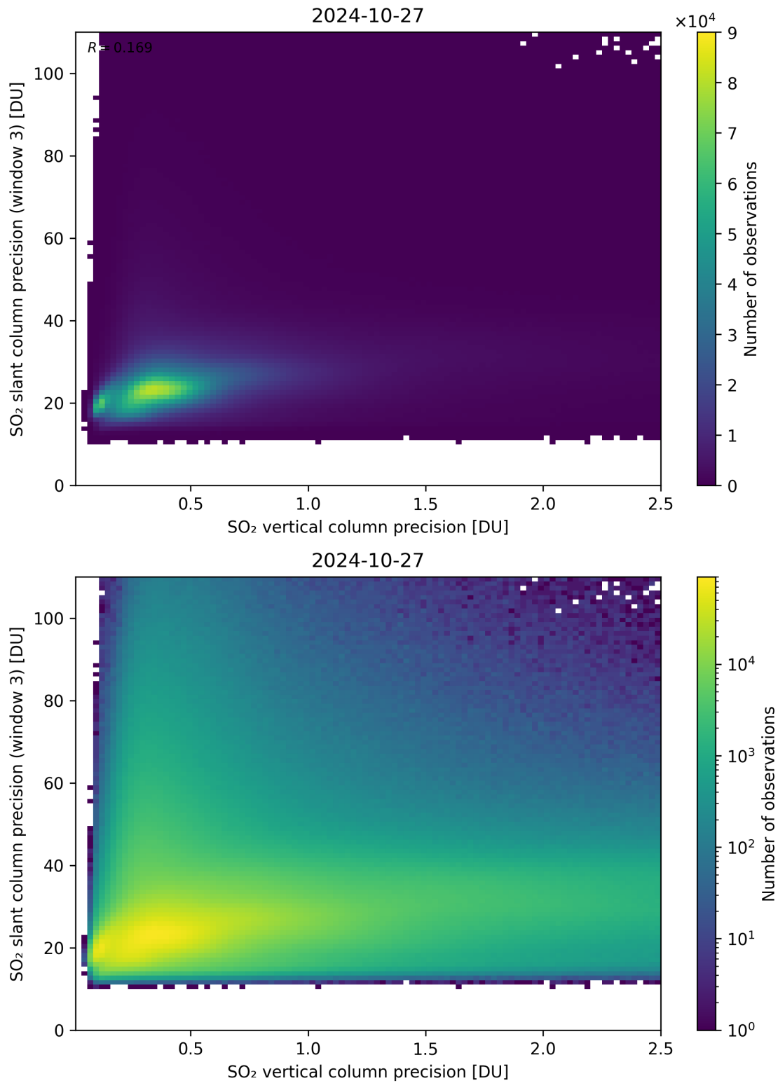
Figure 293: Scatter density plot of “SO 2 vertical column precision” against “SO 2 slant column precision (window 3)” for 2024-10-26 to 2024-10-28.
