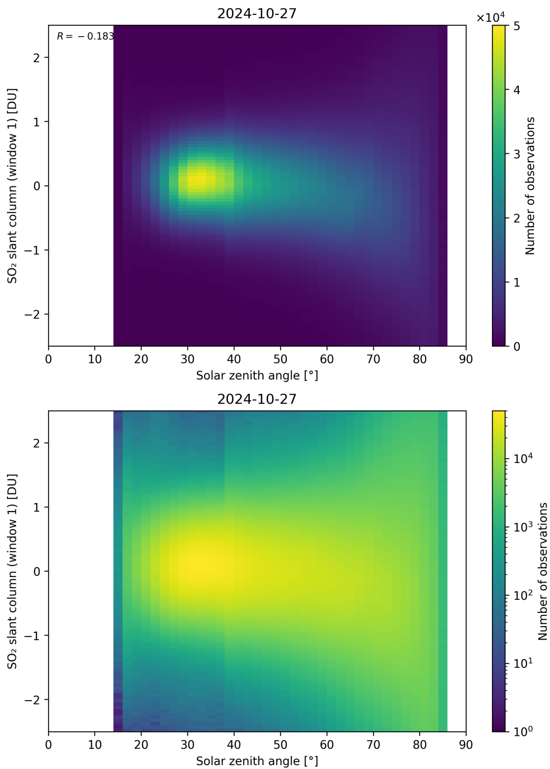
Figure 169: Scatter density plot of “Solar zenith angle” against “SO 2 slant column (window 1)” for 2024-10-26 to 2024-10-28.
