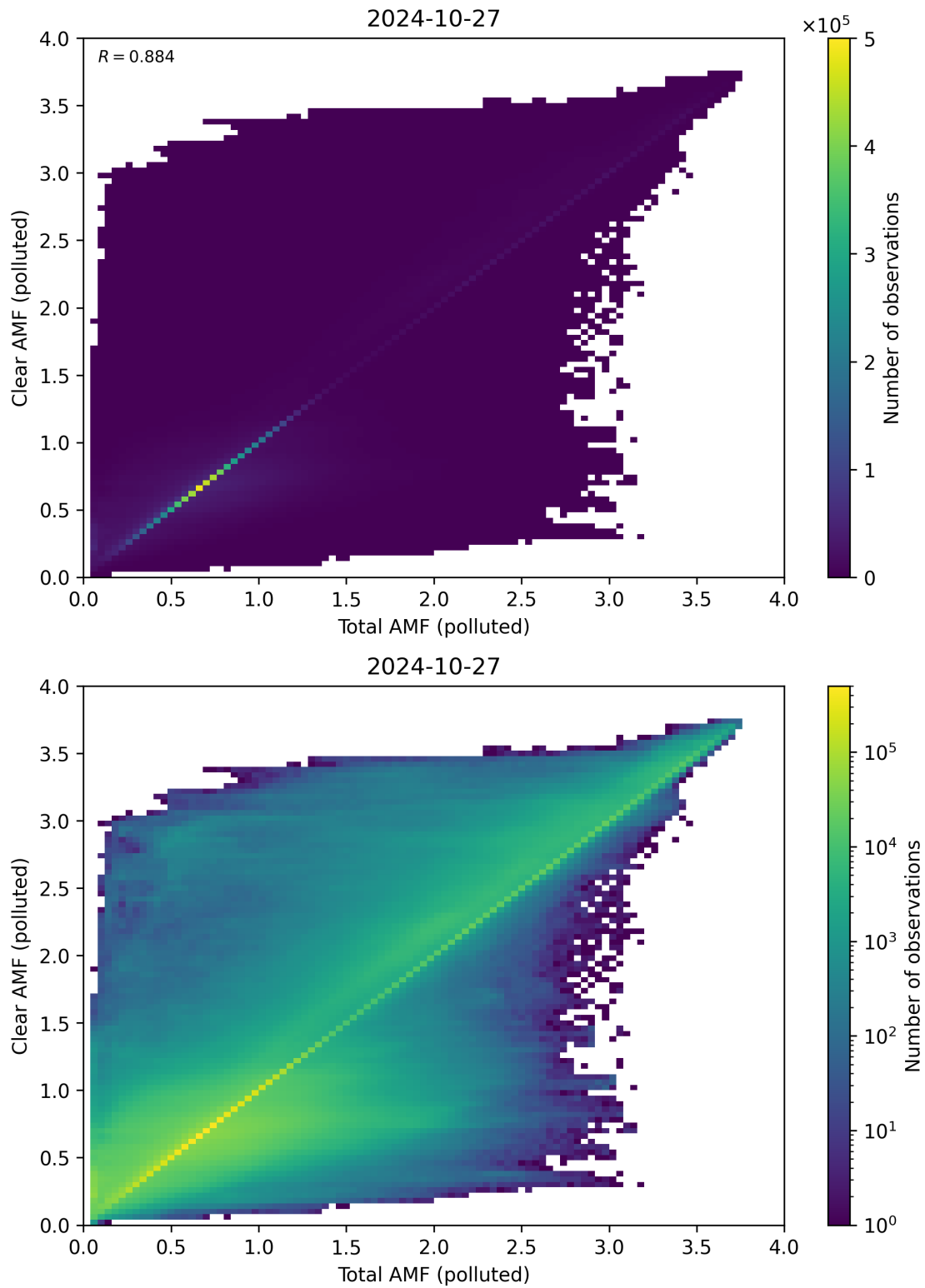
Figure 271: Scatter density plot of “Total AMF (polluted)” against “Clear AMF (polluted)” for 2024-10-26 to 2024-10-28.
