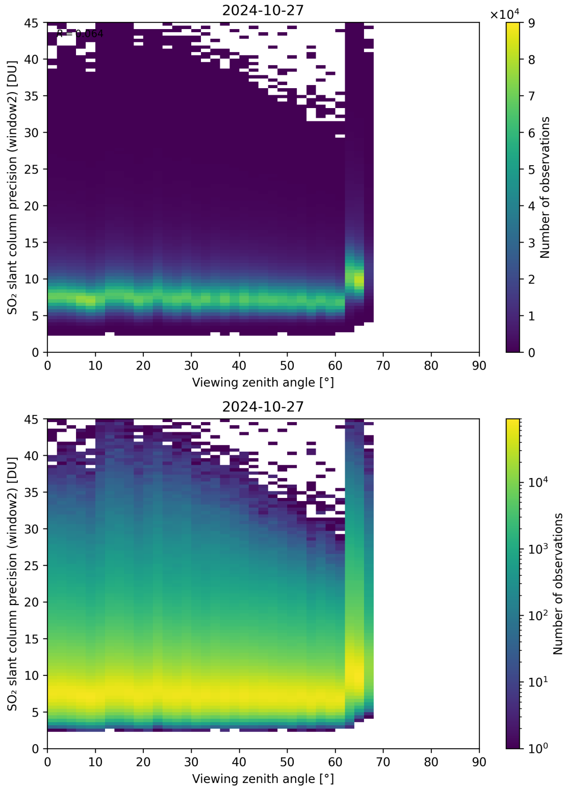
Figure 322: Scatter density plot of “Viewing zenith angle” against “SO 2 slant column precision (window2)” for 2024-10-26 to 2024-10-28.
