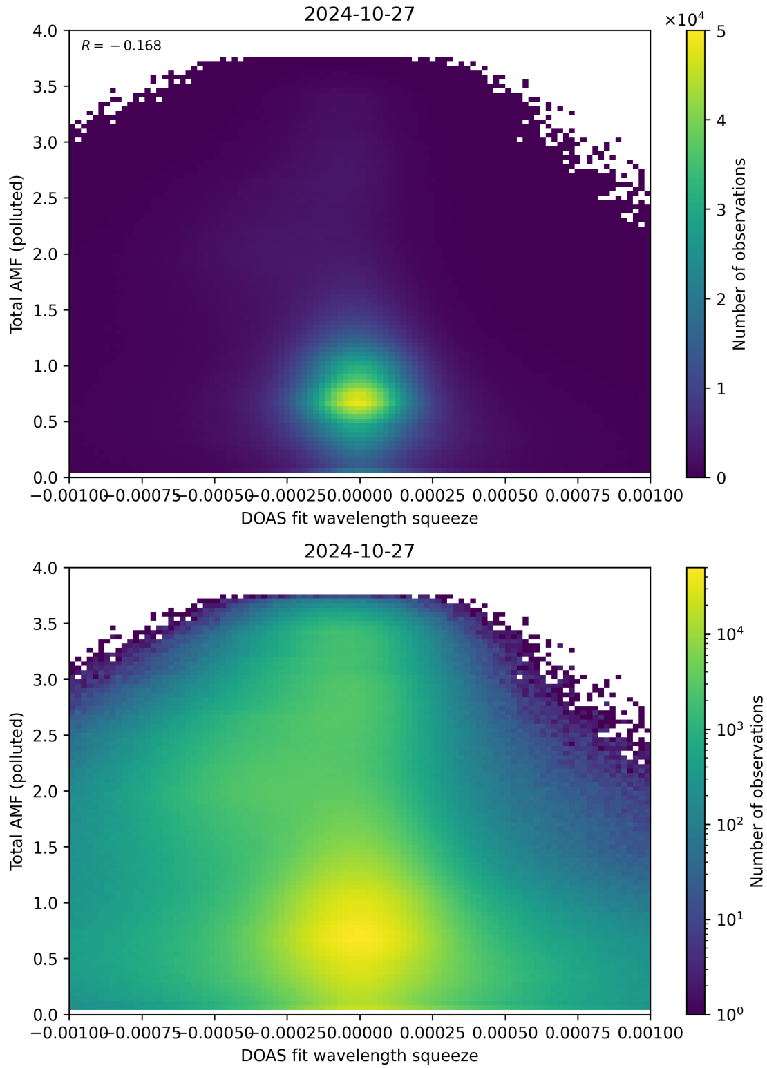
Figure 134: Scatter density plot of “DOAS fit wavelength squeeze” against “Total AMF (polluted)” for 2024-10-26 to 2024-10-28.
