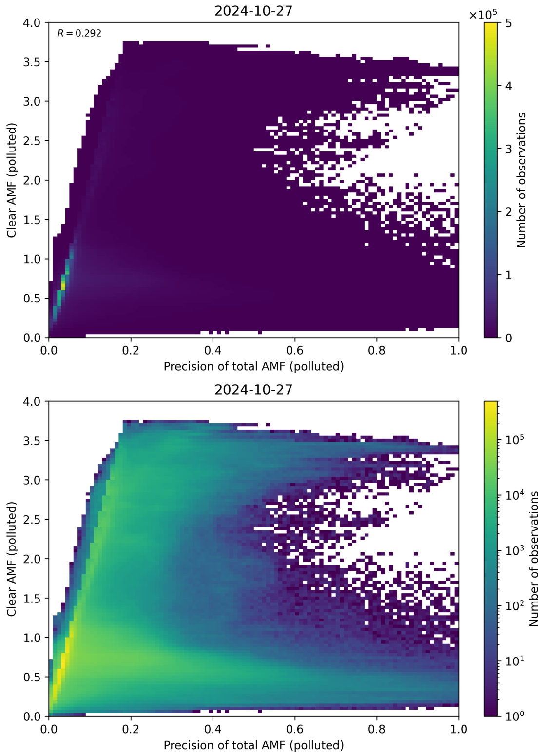
Figure 270: Scatter density plot of “Precision of total AMF (polluted)” against “Clear AMF (polluted)” for 2024-10-26 to 2024-10-28.
