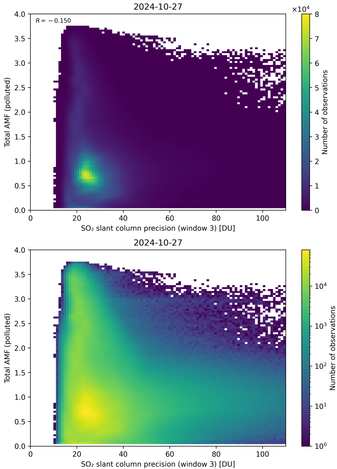
Figure 263: Scatter density plot of “SO 2 slant column precision (window 3)” against “Total AMF (polluted)” for 2024-10-26 to 2024-10-28.
