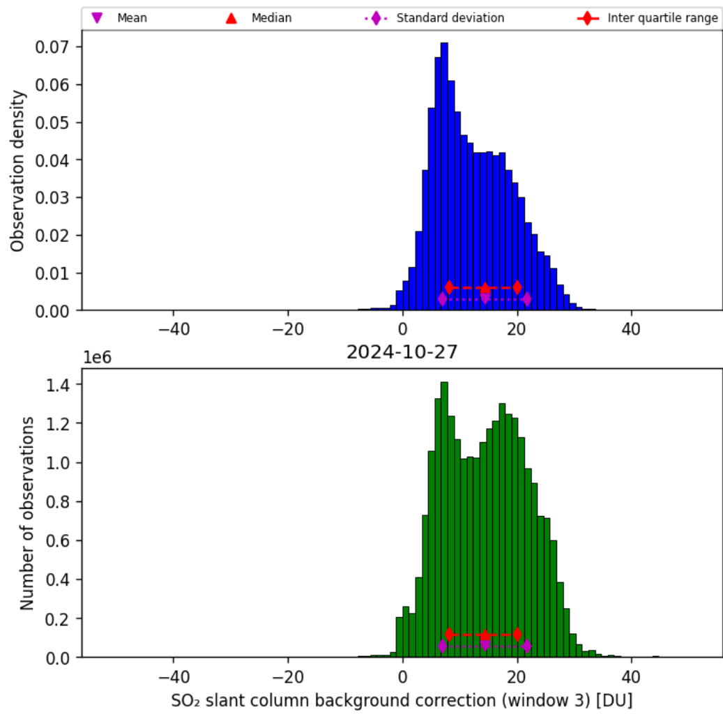
Figure 67: Histogram of “SO 2 slant column background correction (window 3)” for 2024-10-26 to 2024-10-28
