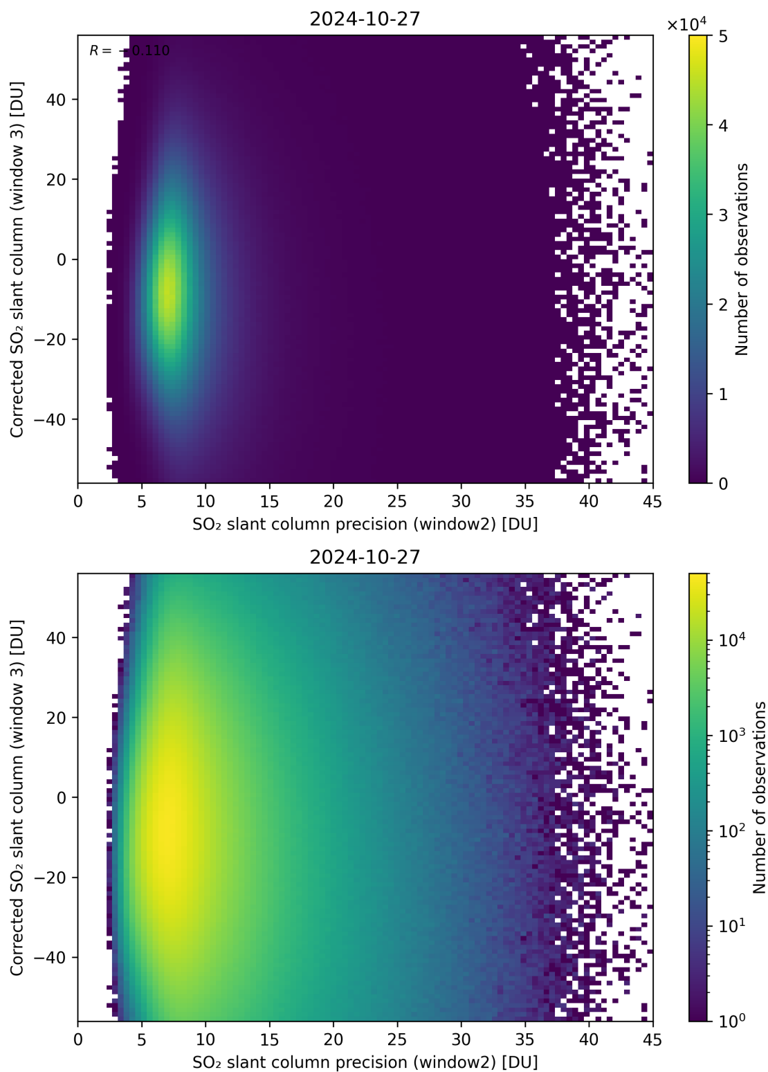
Figure 248: Scatter density plot of “SO 2 slant column precision (window2)” against “Corrected SO 2 slant column (window 3)” for 2024-10-26 to 2024-10-28.
