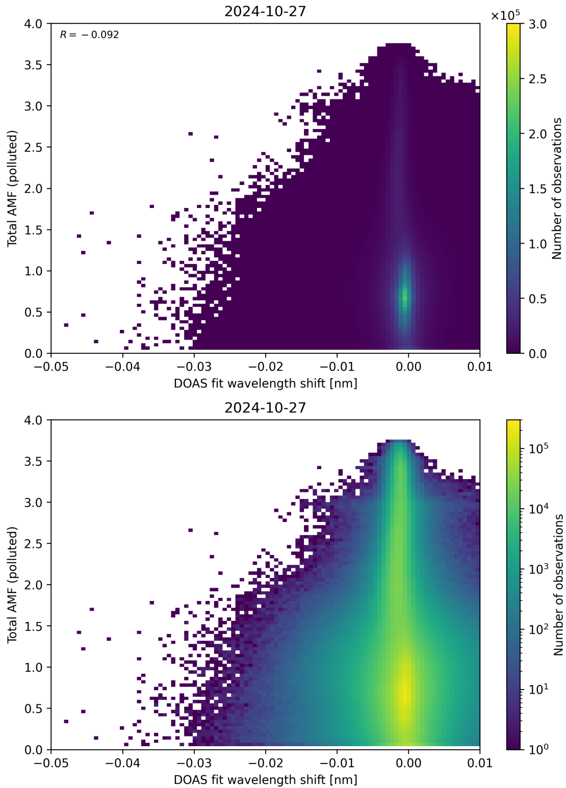
Figure 130: Scatter density plot of “DOAS fit wavelength shift” against “Total AMF (polluted)” for 2024-10-26 to 2024-10-28.
