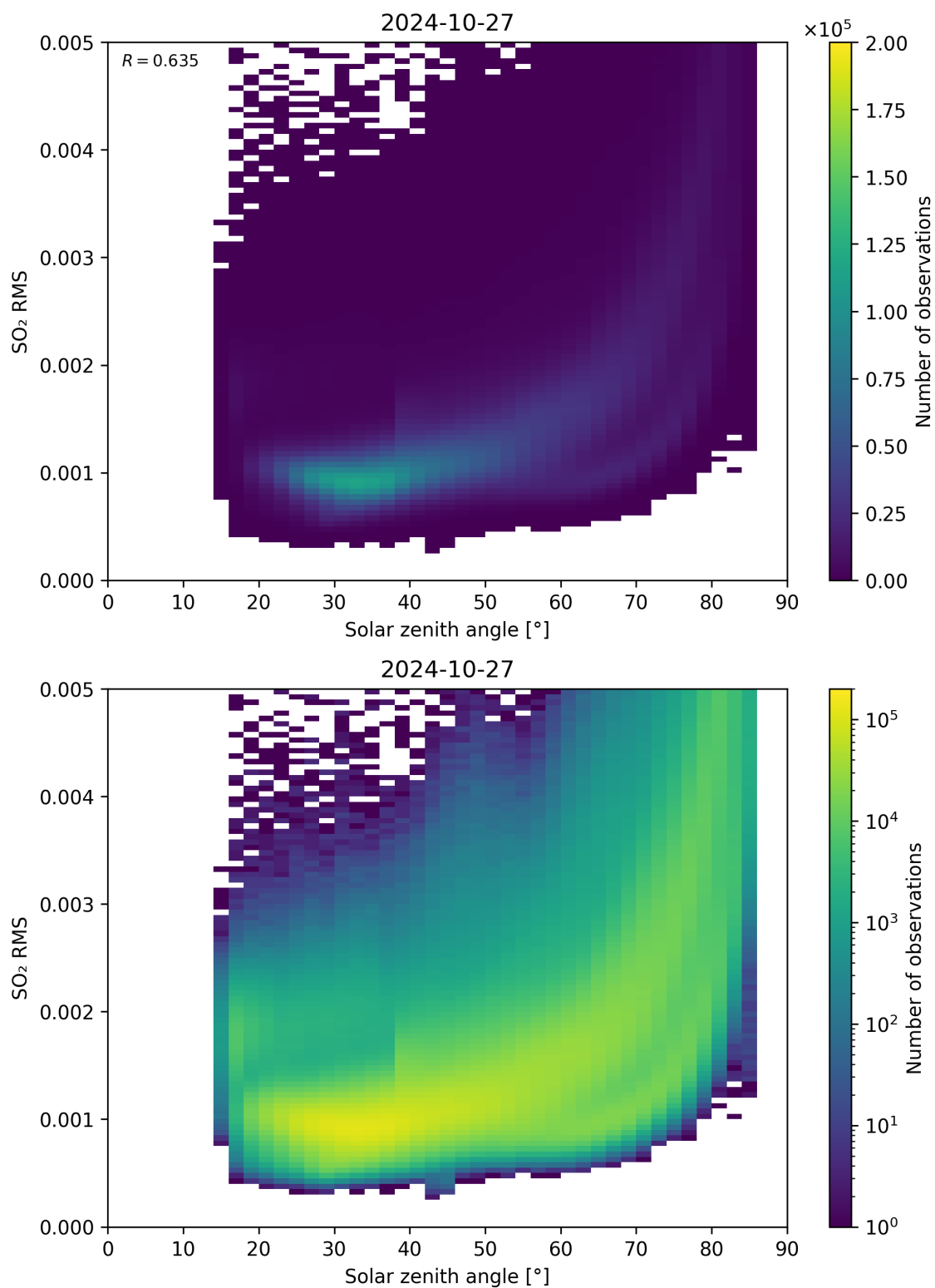
Figure 163: Scatter density plot of “Solar zenith angle” against “SO 2 RMS” for 2024-10-26 to 2024-10-28.
