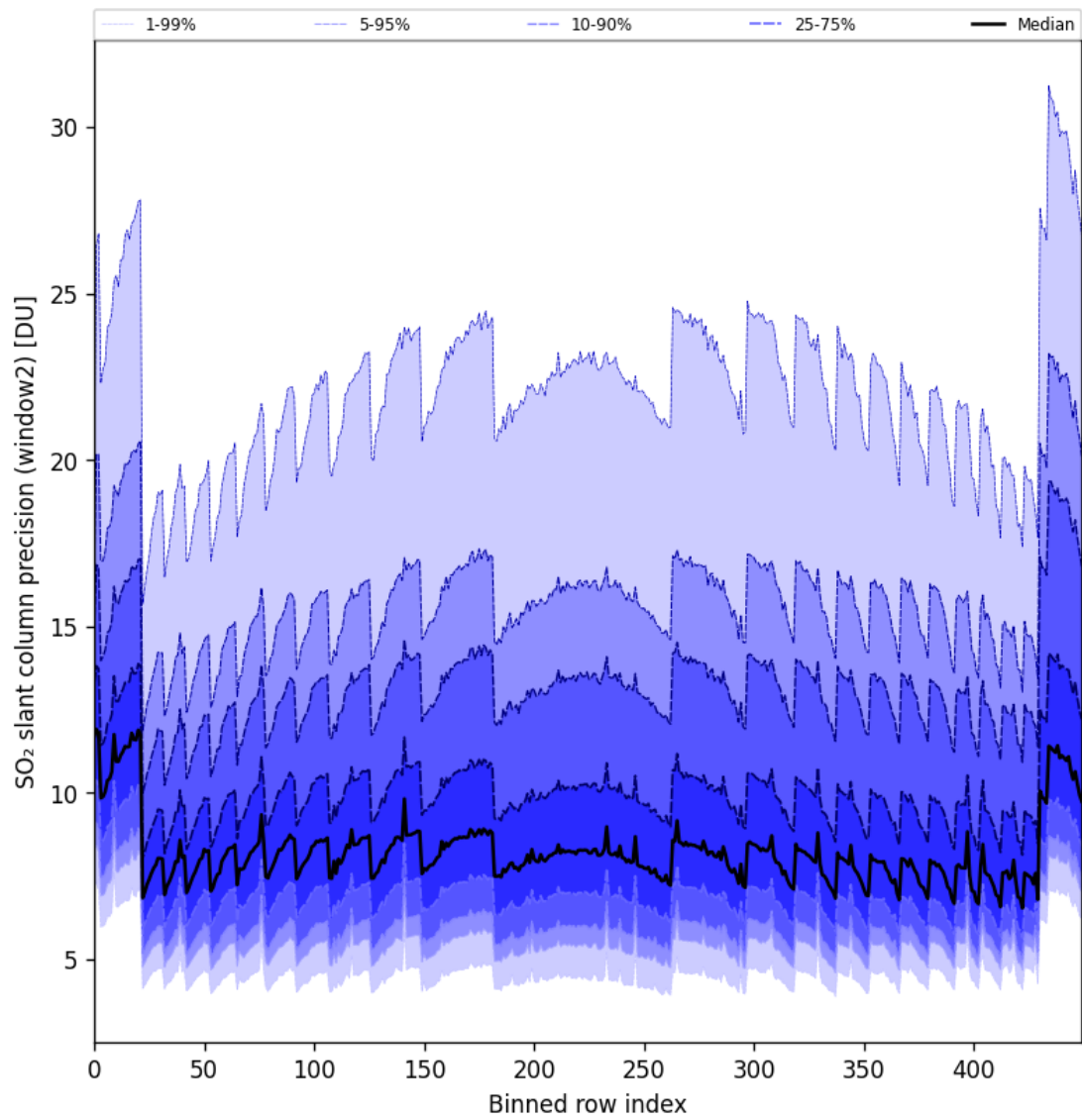
Figure 84: Along track statistics of “SO 2 slant column precision (window2)” for 2024-10-26 to 2024-10-28
