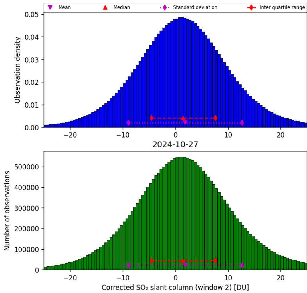
Figure 62: Histogram of “Corrected SO 2 slant column (window 2)” for 2024-10-26 to 2024-10-28
