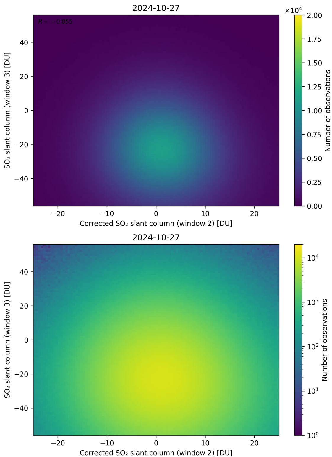
Figure 201: Scatter density plot of “Corrected SO 2 slant column (window 2)” against “SO 2 slant column (window 3)” for 2024-10-26 to 2024-10-28.
