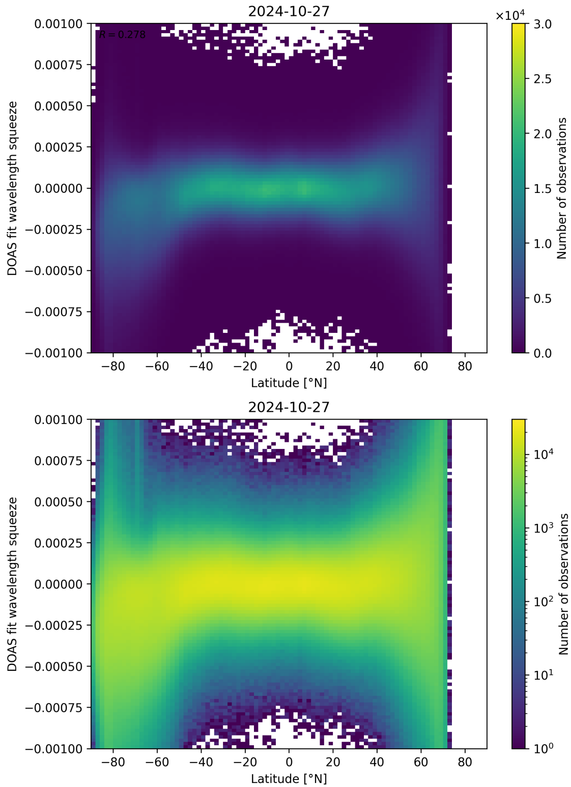
Figure 143: Scatter density plot of “Latitude” against “DOAS fit wavelength squeeze” for 2024-10-26 to 2024-10-28.
