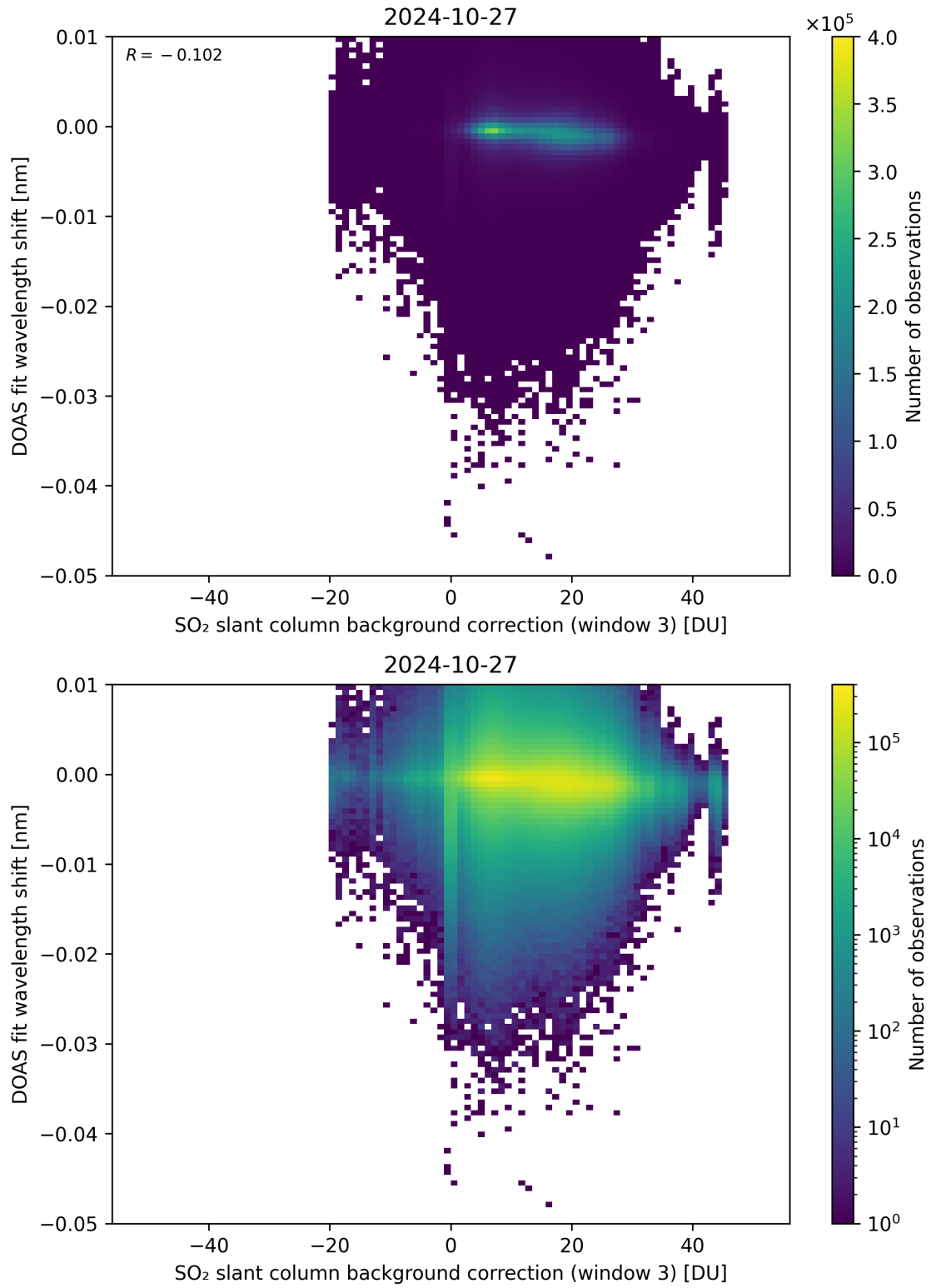
Figure 121: Scatter density plot of “SO 2 slant column background correction (window 3)” against “DOAS fit wavelength shift” for 2024-10-26 to 2024-10-28.
