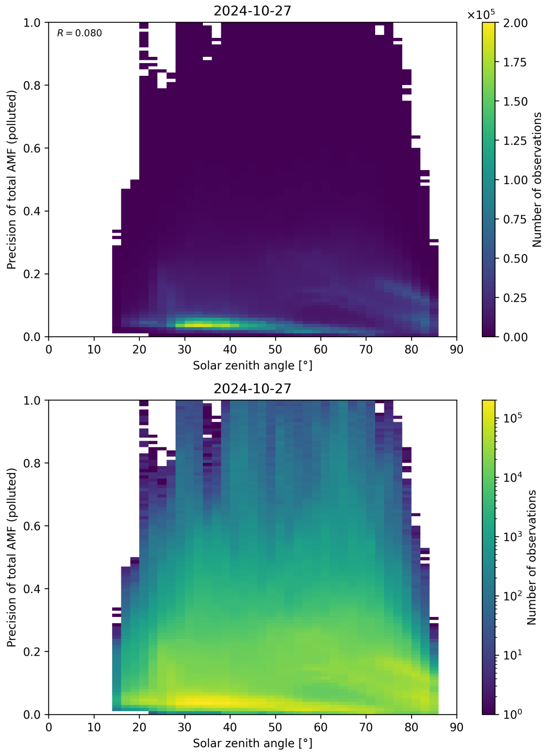
Figure 175: Scatter density plot of “Solar zenith angle” against “Precision of total AMF (polluted)” for 2024-10-26 to 2024-10-28.
