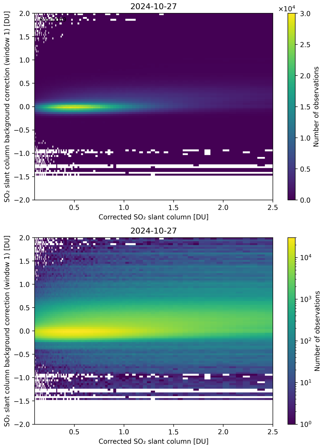
Figure 178: Scatter density plot of “Corrected SO 2 slant column” against “SO 2 slant column background correction (window 1)” for 2024-10-26 to 2024-10-28.
