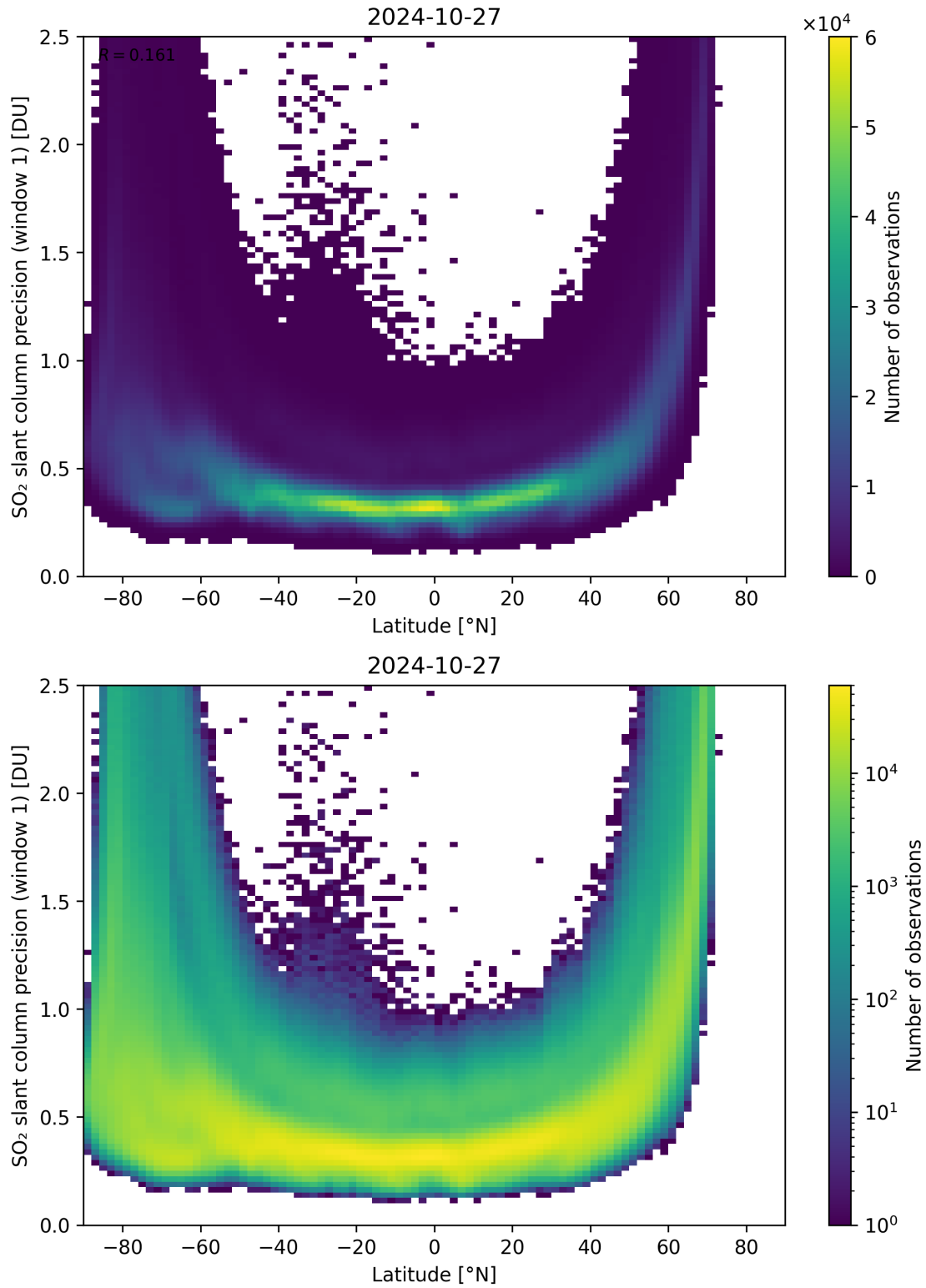
Figure 150: Scatter density plot of “Latitude” against “SO 2 slant column precision (window 1)” for 2024-10-26 to 2024-10-28.
