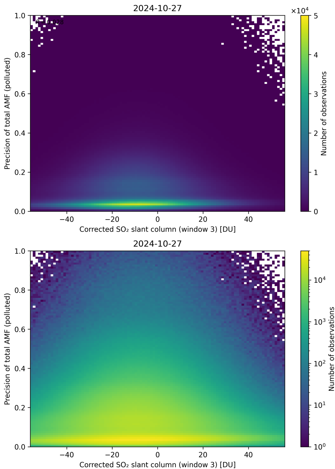
Figure 211: Scatter density plot of “Corrected SO 2 slant column (window 3)” against “Precision of total AMF (polluted)” for 2024-10-26 to 2024-10-28.
