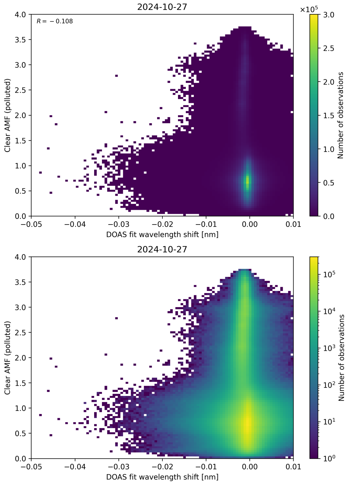
Figure 129: Scatter density plot of “DOAS fit wavelength shift” against “Clear AMF (polluted)” for 2024-10-26 to 2024-10-28.
