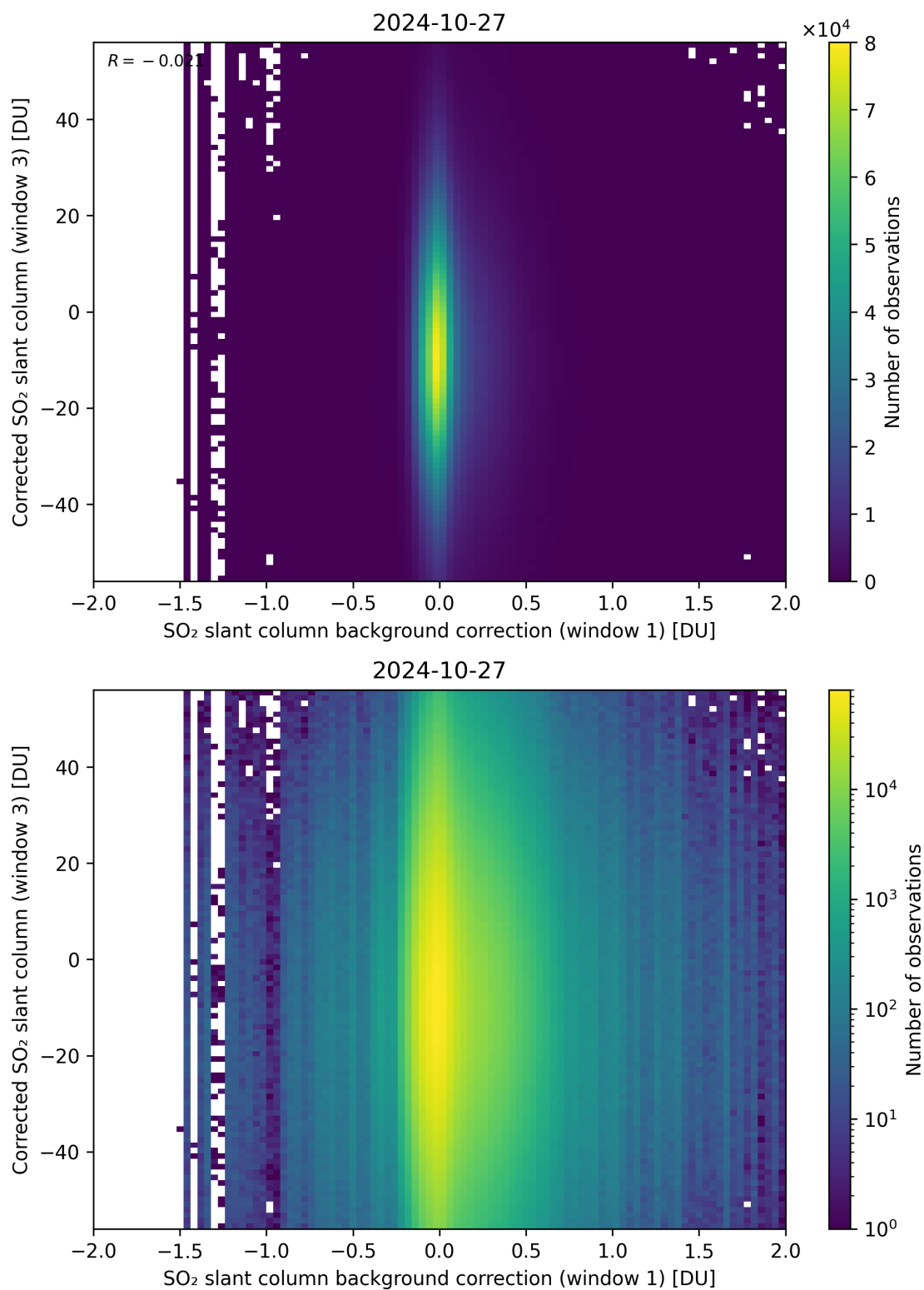
Figure 105: Scatter density plot of “SO 2 slant column background correction (window 1)” against “Corrected SO 2 slant column (window 3)” for 2024-10-26 to 2024-10-28.
