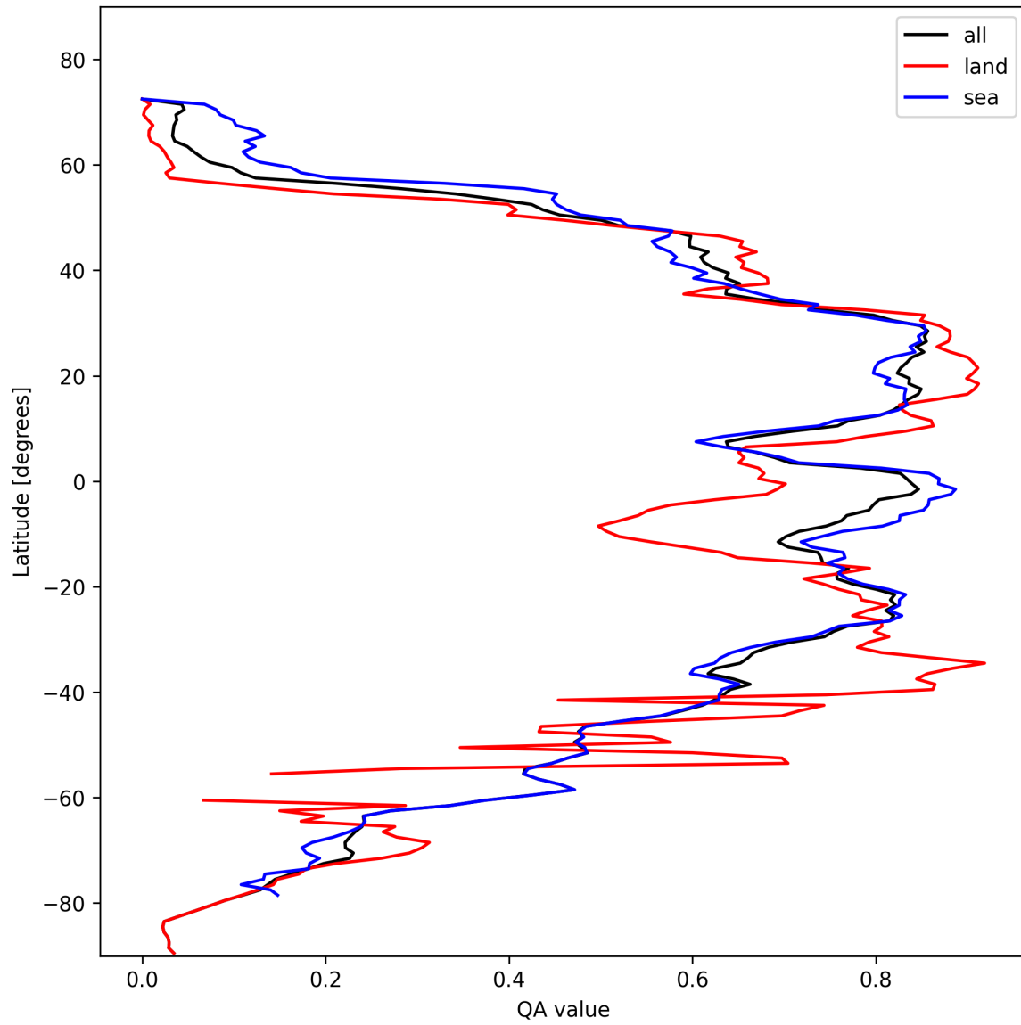
Figure 29: Zonal average of “QA value” for 2024-10-26 to 2024-10-28.
