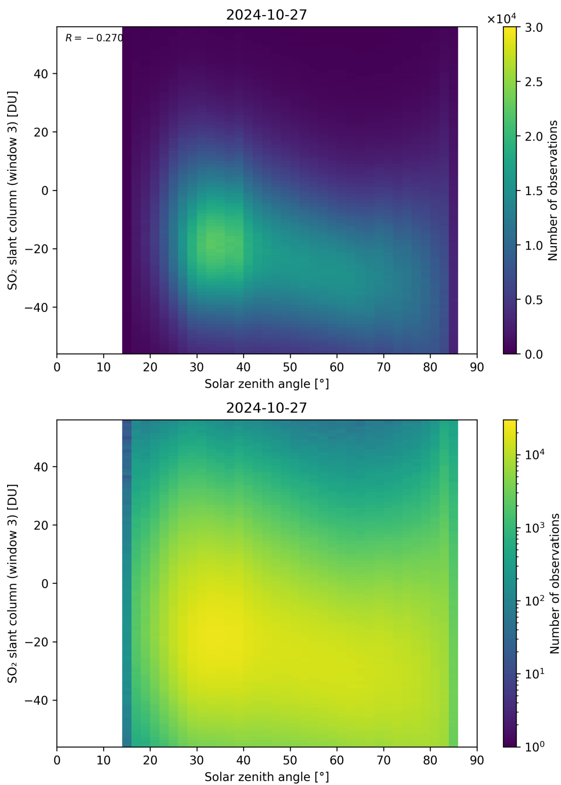
Figure 172: Scatter density plot of “Solar zenith angle” against “SO 2 slant column (window 3)” for 2024-10-26 to 2024-10-28.
