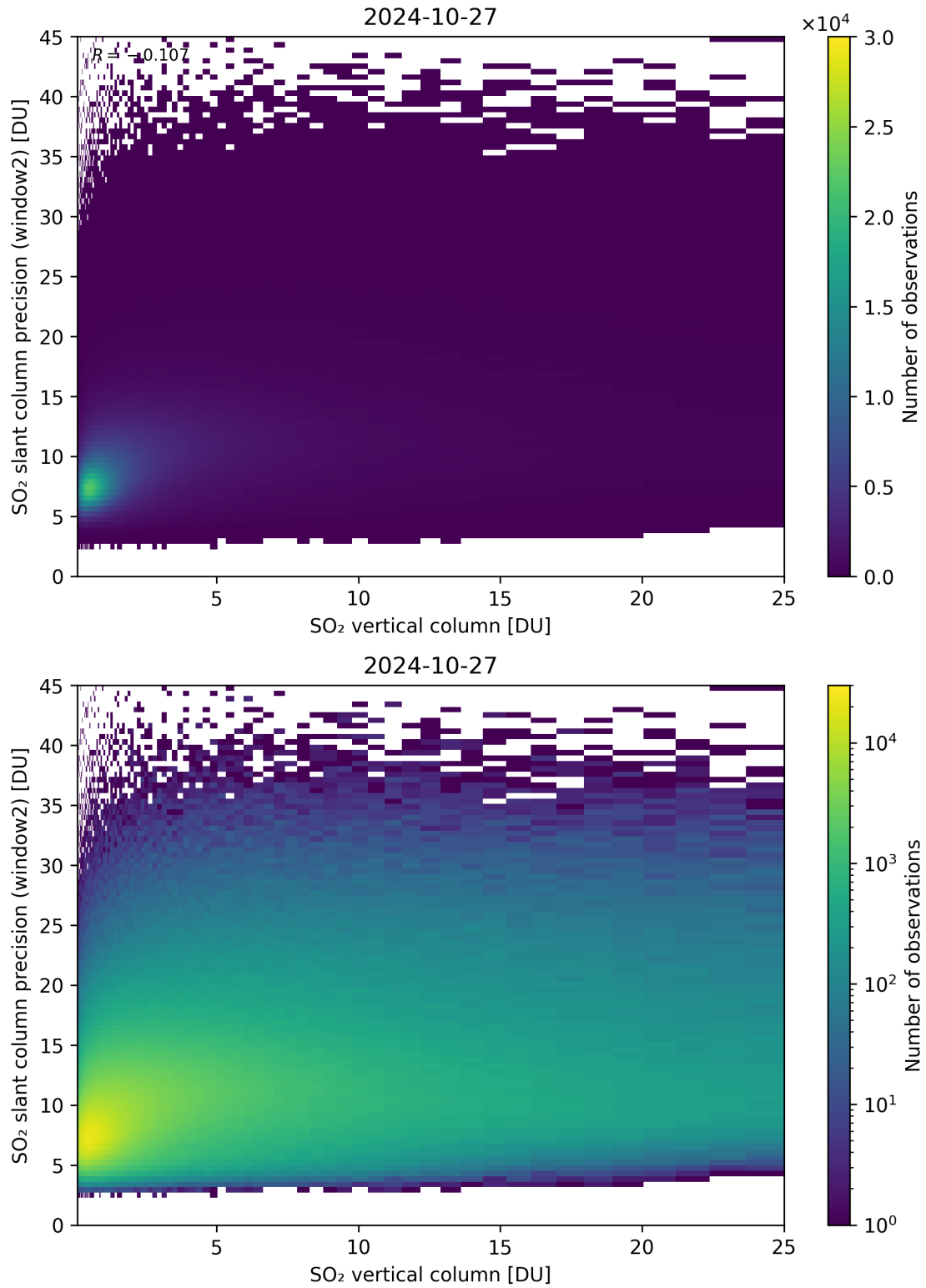
Figure 302: Scatter density plot of “SO 2 vertical column” against “SO 2 slant column precision (window2)” for 2024-10-26 to 2024-10-28.
