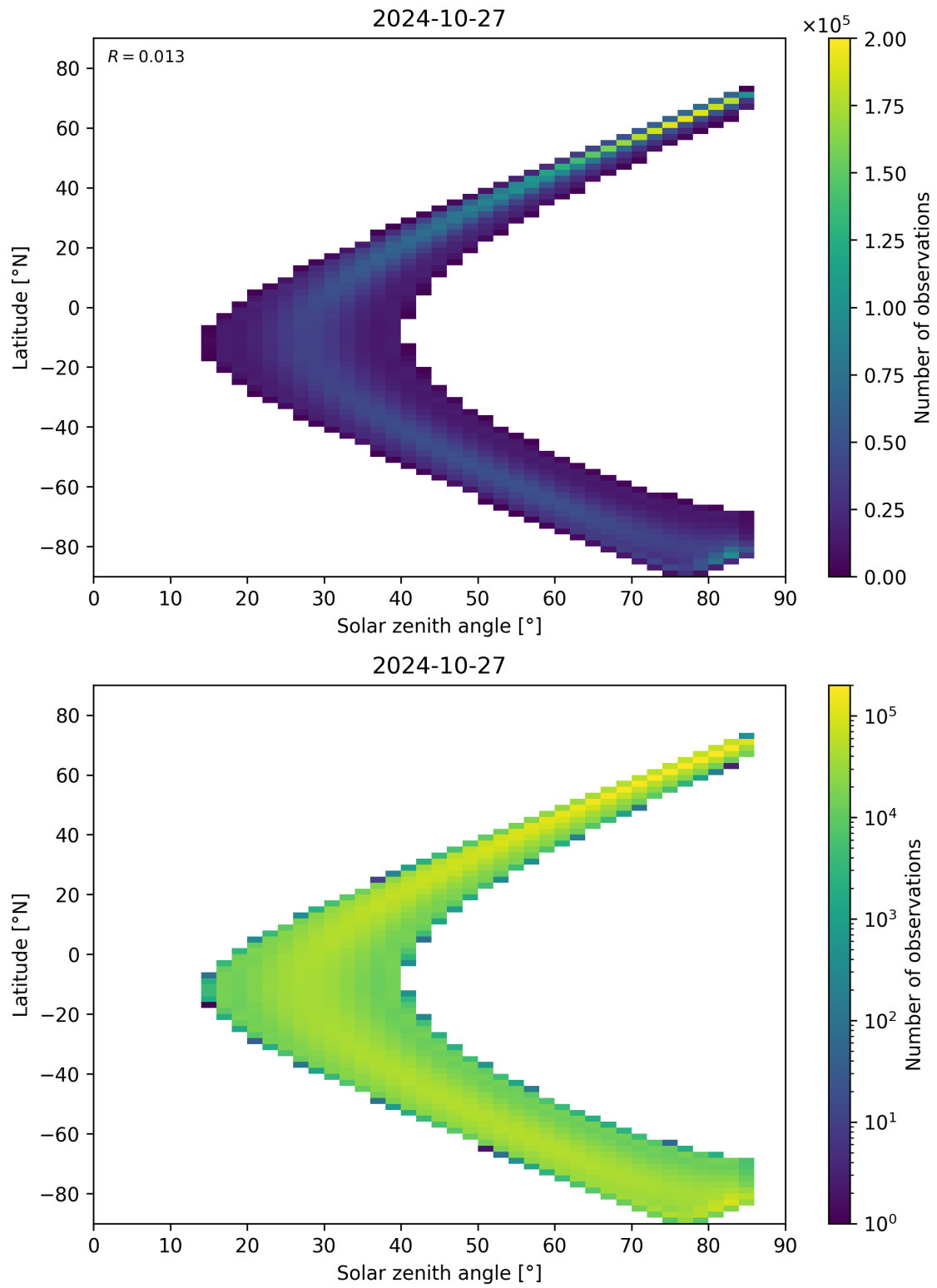
Figure 164: Scatter density plot of “Solar zenith angle” against “Latitude” for 2024-10-26 to 2024-10-28.
