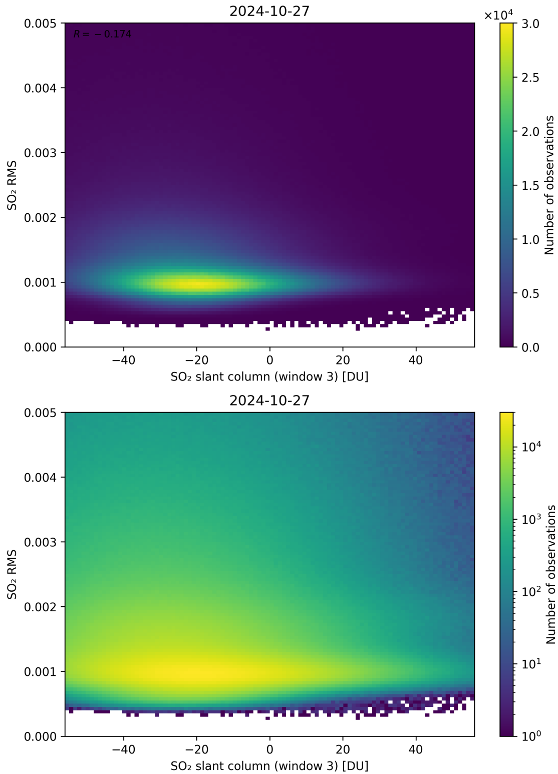
Figure 256: Scatter density plot of “SO 2 slant column (window 3)” against “SO 2 RMS” for 2024-10-26 to 2024-10-28.
