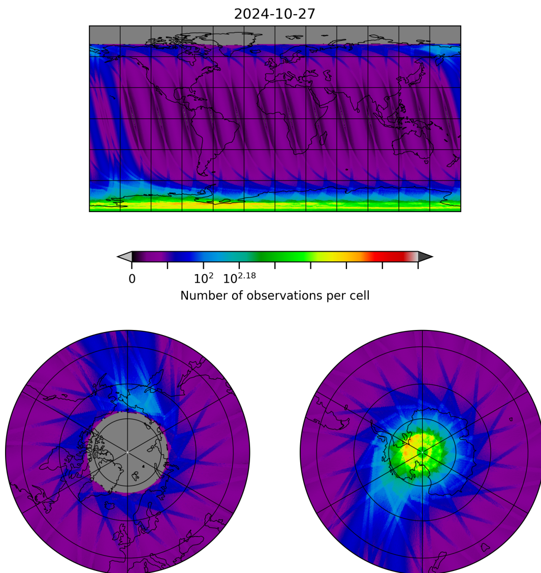
Figure 28: Map of the number of observations for 2024-10-26 to 2024-10-28
