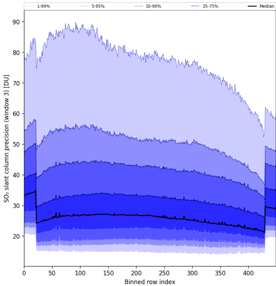
Figure 88: Along track statistics of “SO 2 slant column precision (window 3)” for 2024-10-26 to 2024-10-28
