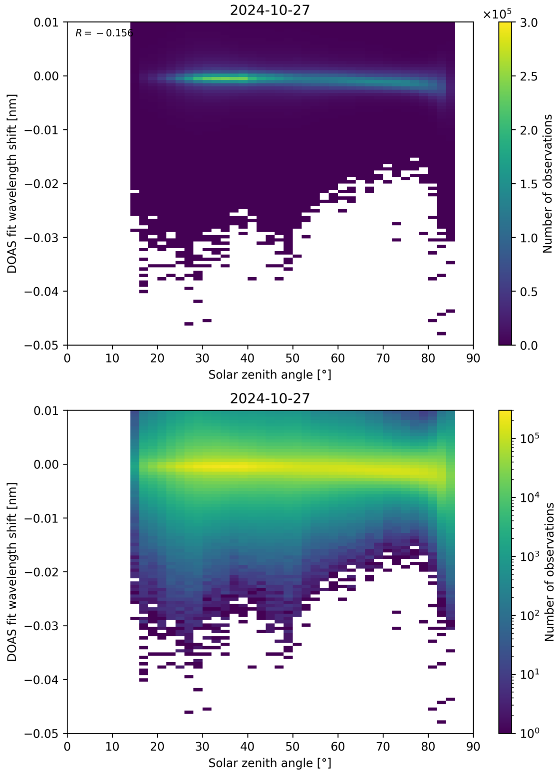
Figure 161: Scatter density plot of “Solar zenith angle” against “DOAS fit wavelength shift” for 2024-10-26 to 2024-10-28.
