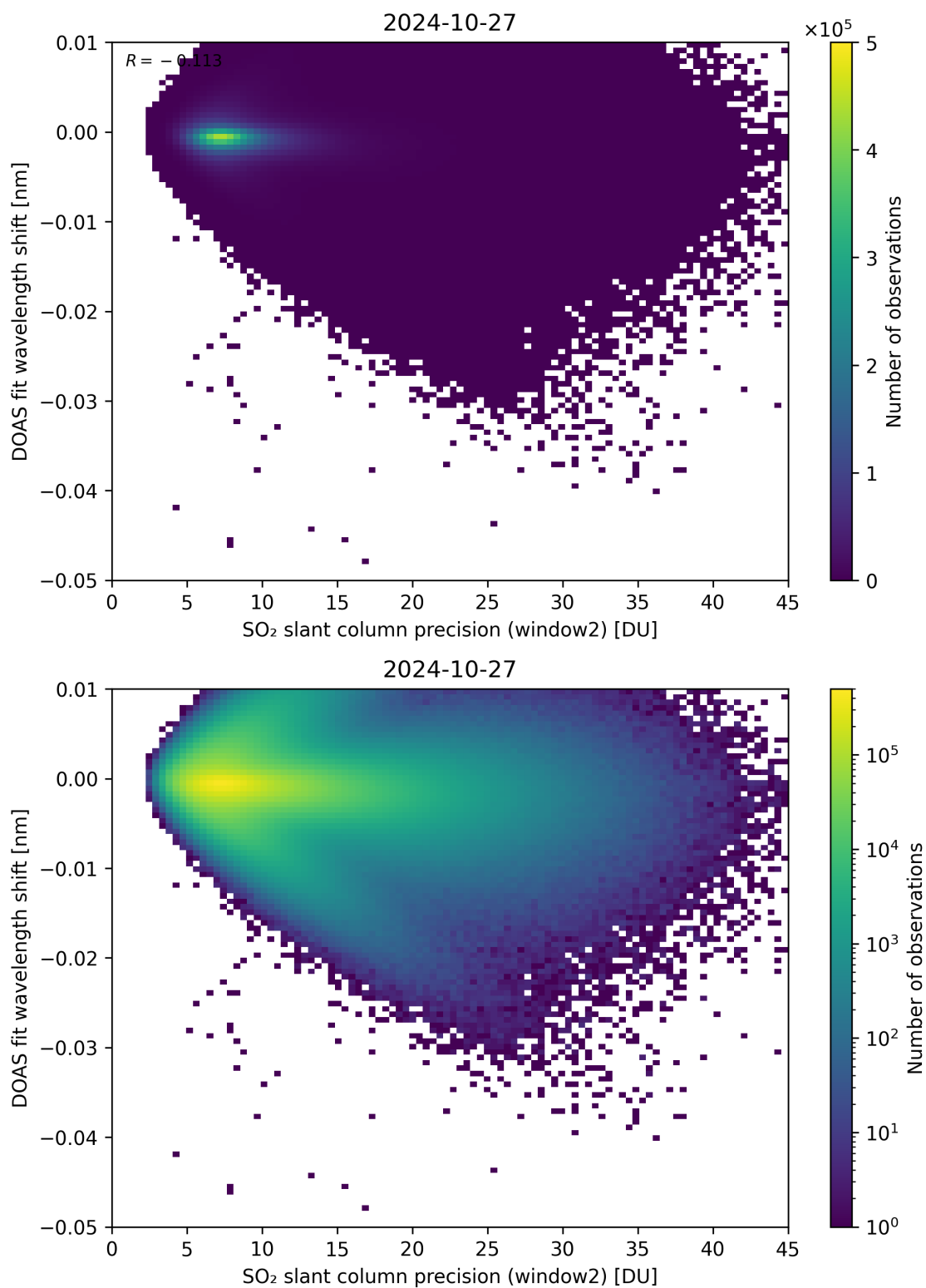
Figure 243: Scatter density plot of “SO 2 slant column precision (window2)” against “DOAS fit wavelength shift” for 2024-10-26 to 2024-10-28.
