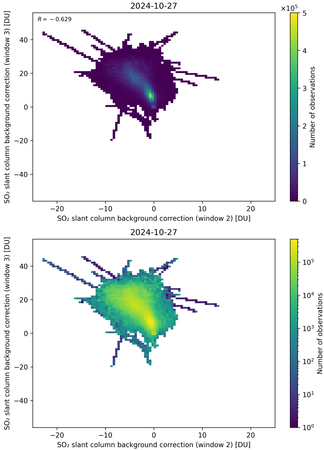
Figure 111: Scatter density plot of “SO 2 slant column background correction (window 2)” against “SO 2 slant column background correction (window 3)” for 2024-10-26 to 2024-10-28.
