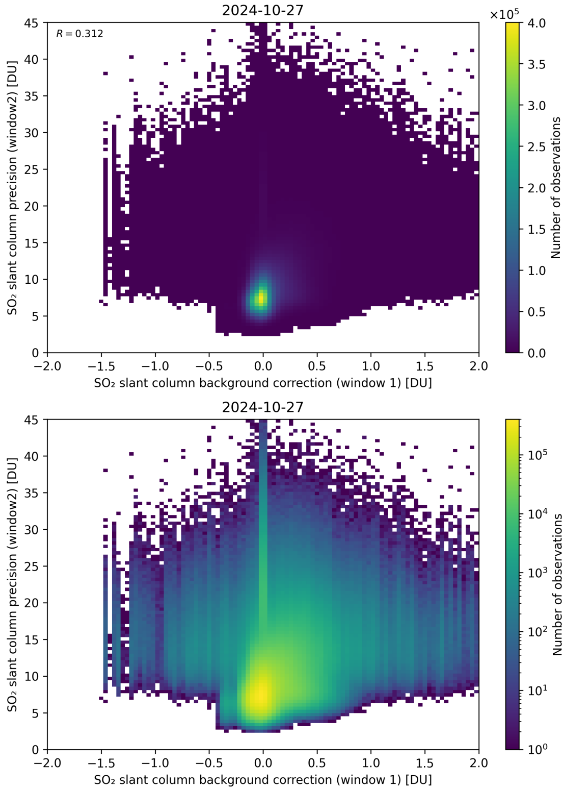
Figure 106: Scatter density plot of “SO 2 slant column background correction (window 1)” against “SO 2 slant column precision (window2)” for 2024-10-26 to 2024-10-28.
