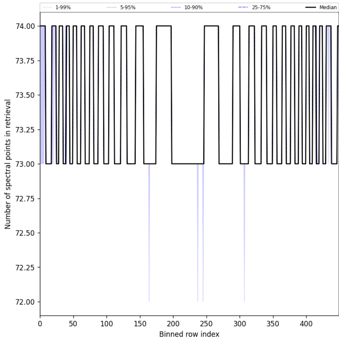
Figure 97: Along track statistics of “Number of spectral points in retrieval” for 2024-10-26 to 2024-10-28
