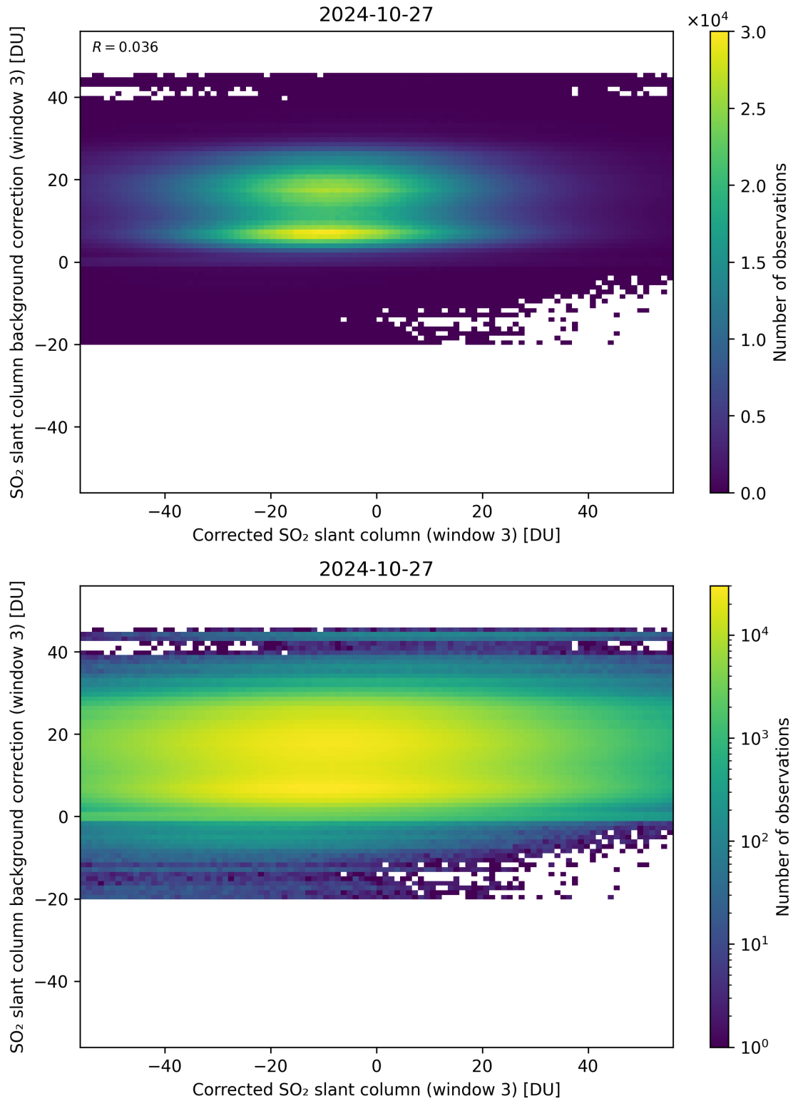
Figure 205: Scatter density plot of “Corrected SO 2 slant column (window 3)” against “SO 2 slant column background correction (window 3)” for 2024-10-26 to 2024-10-28.
