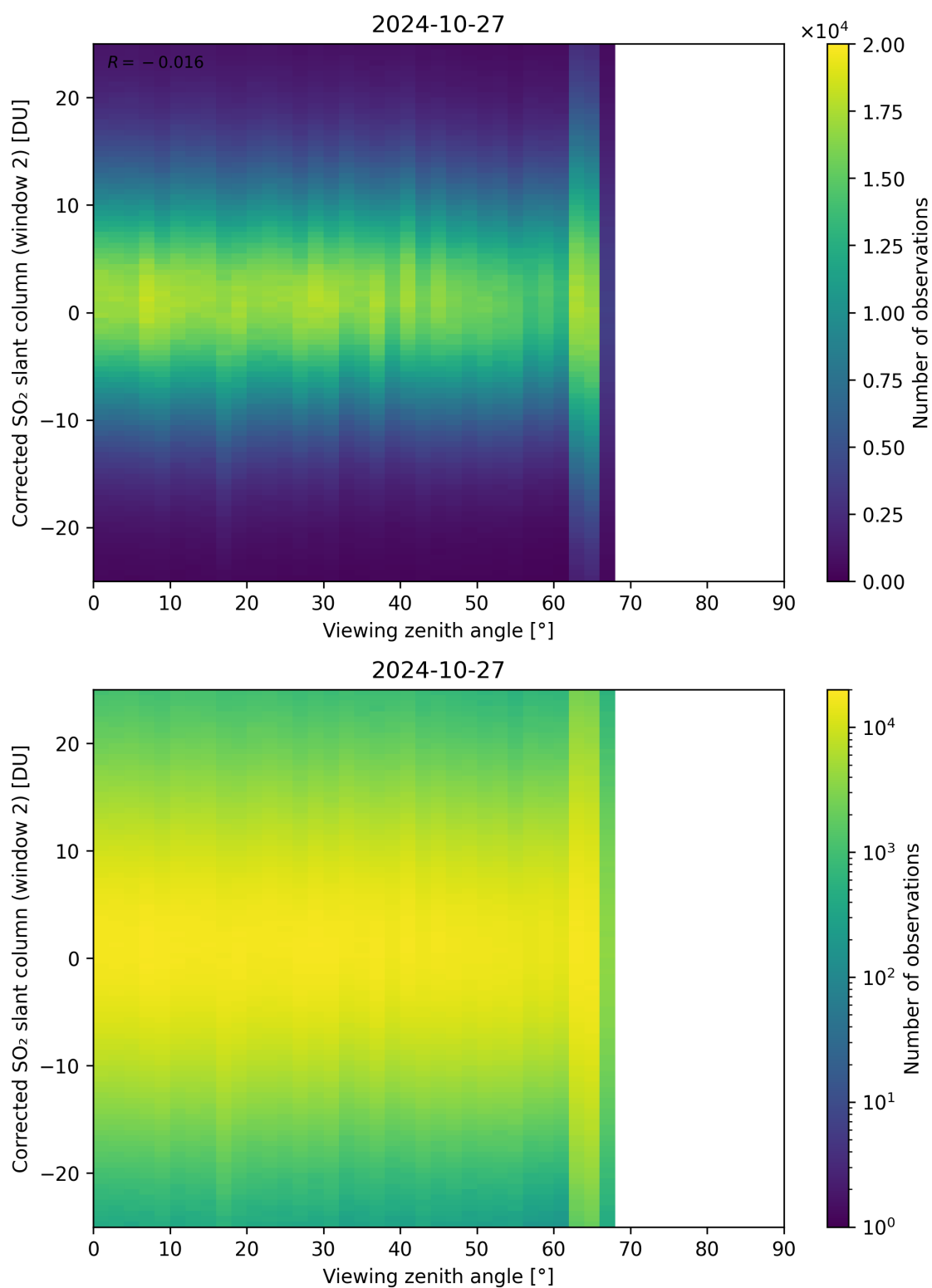
Figure 318: Scatter density plot of “Viewing zenith angle” against “Corrected SO 2 slant column (window 2)” for 2024-10-26 to 2024-10-28.
