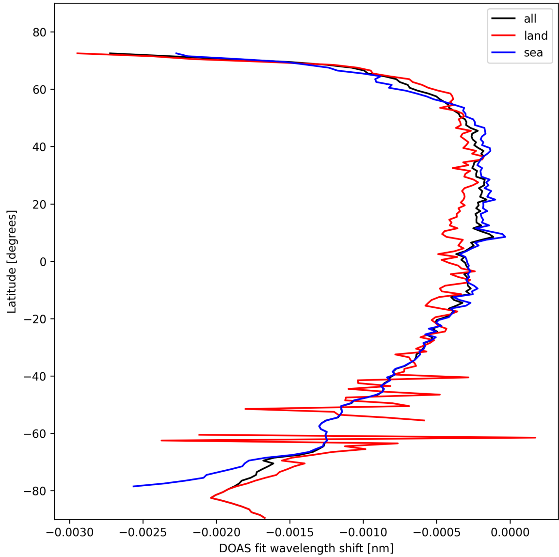
Figure 45: Zonal average of “DOAS fit wavelength shift” for 2024-10-26 to 2024-10-28.
