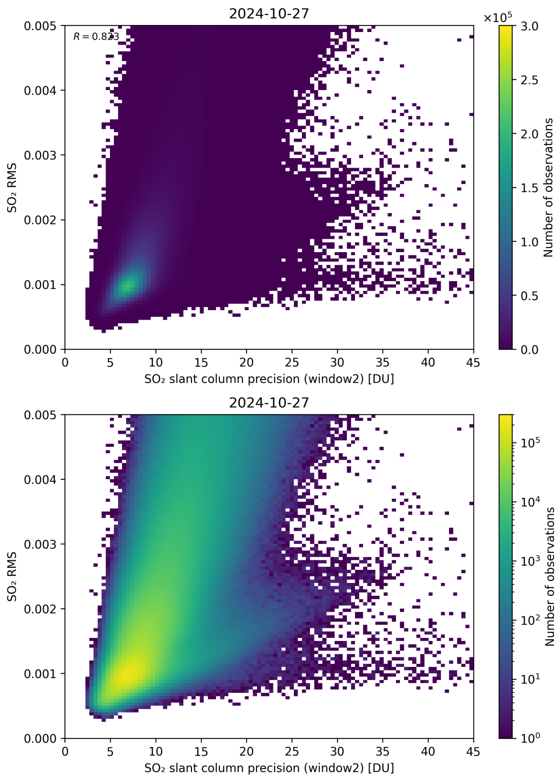
Figure 245: Scatter density plot of “SO 2 slant column precision (window2)” against “SO 2 RMS” for 2024-10-26 to 2024-10-28.
