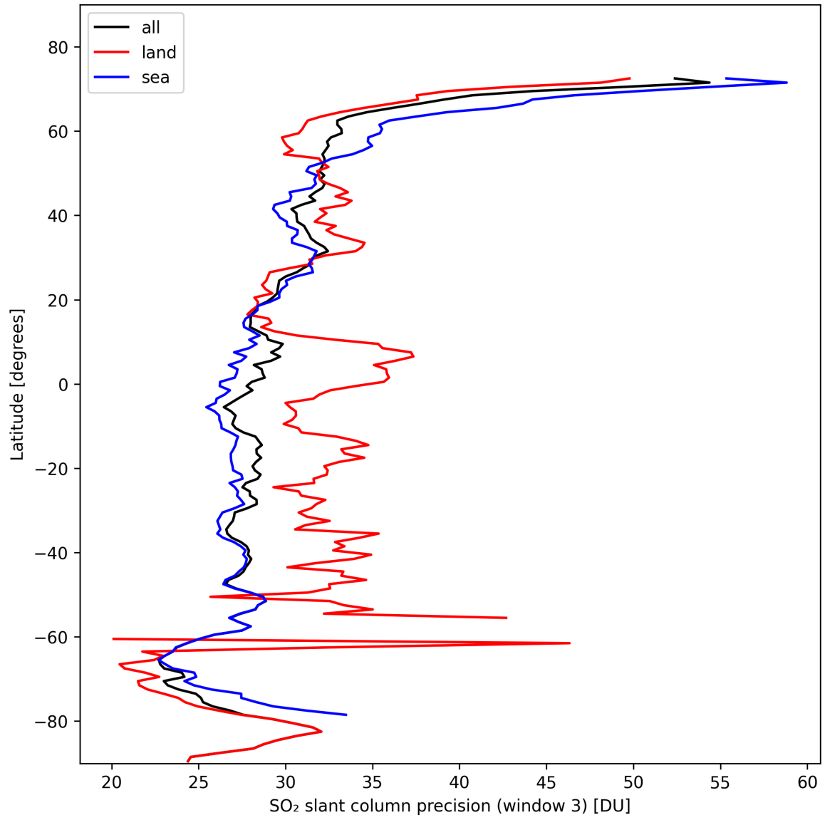
Figure 42: Zonal average of “SO 2 slant column precision (window 3)” for 2024-10-26 to 2024-10-28.
