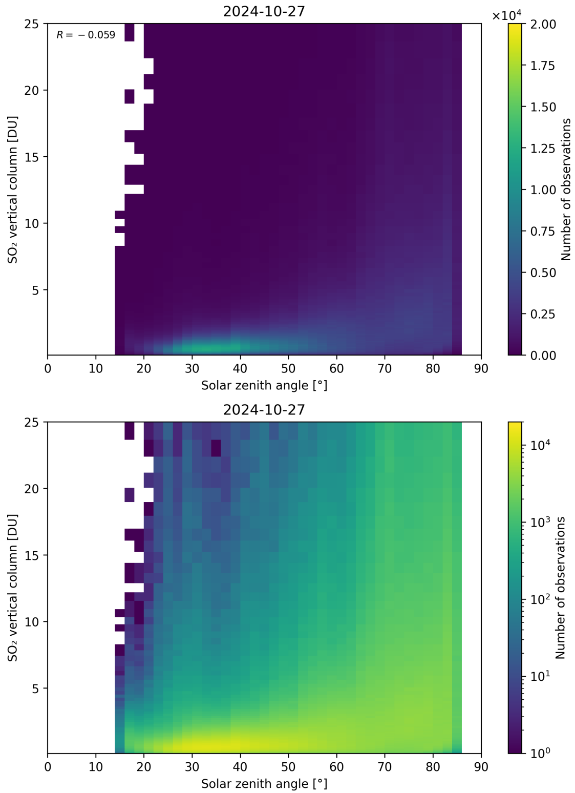
Figure 176: Scatter density plot of “Solar zenith angle” against “SO 2 vertical column” for 2024-10-26 to 2024-10-28.
