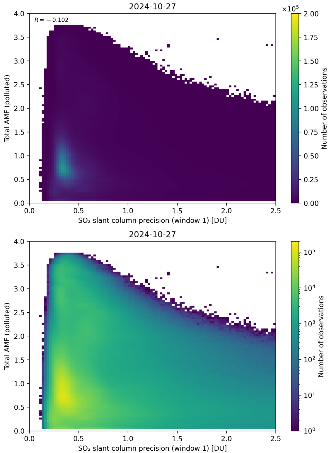
Figure 230: Scatter density plot of “SO 2 slant column precision (window 1)” against “Total AMF (polluted)” for 2024-10-26 to 2024-10-28.
