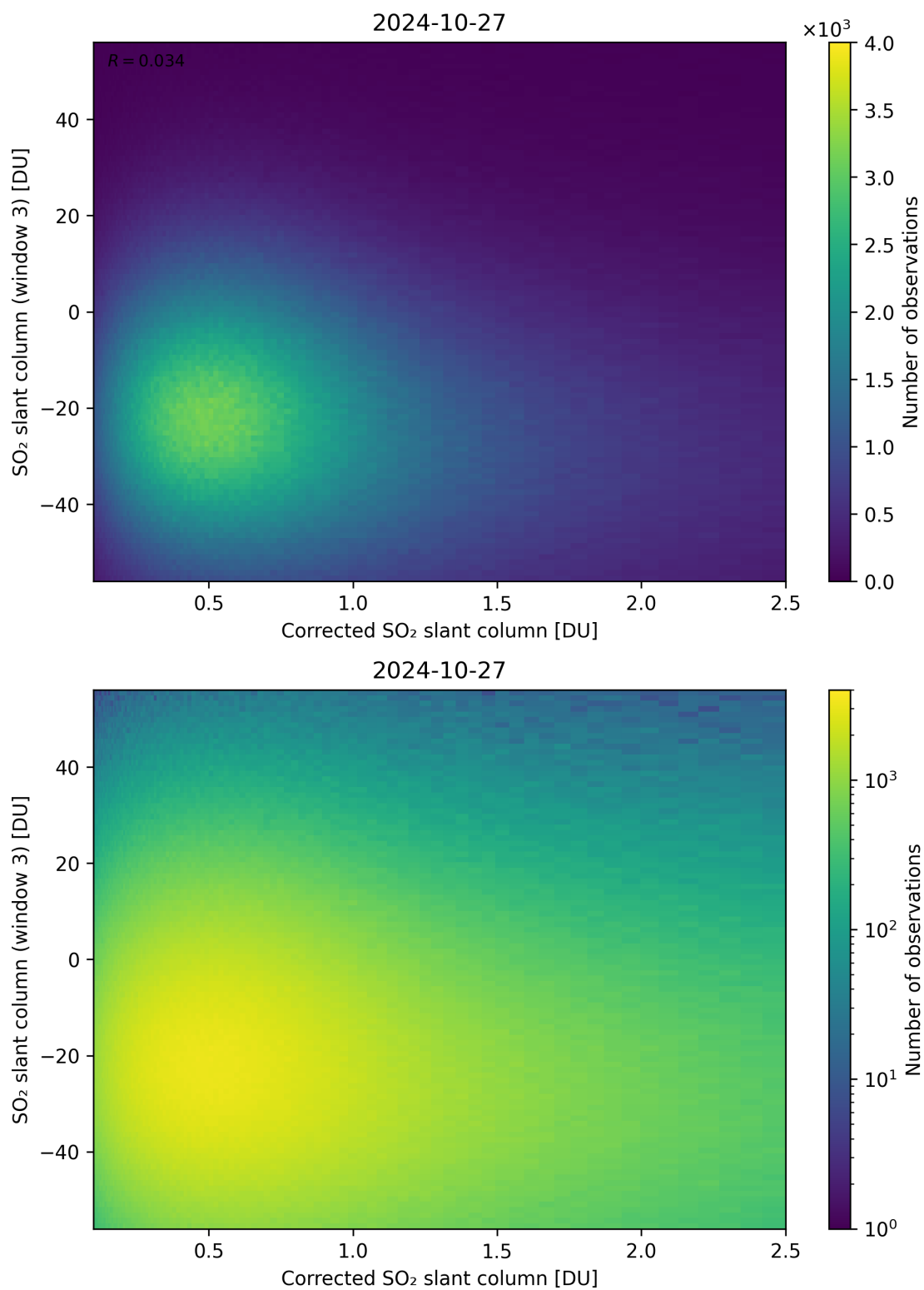
Figure 190: Scatter density plot of “Corrected SO 2 slant column” against “SO 2 slant column (window 3)” for 2024-10-26 to 2024-10-28.
