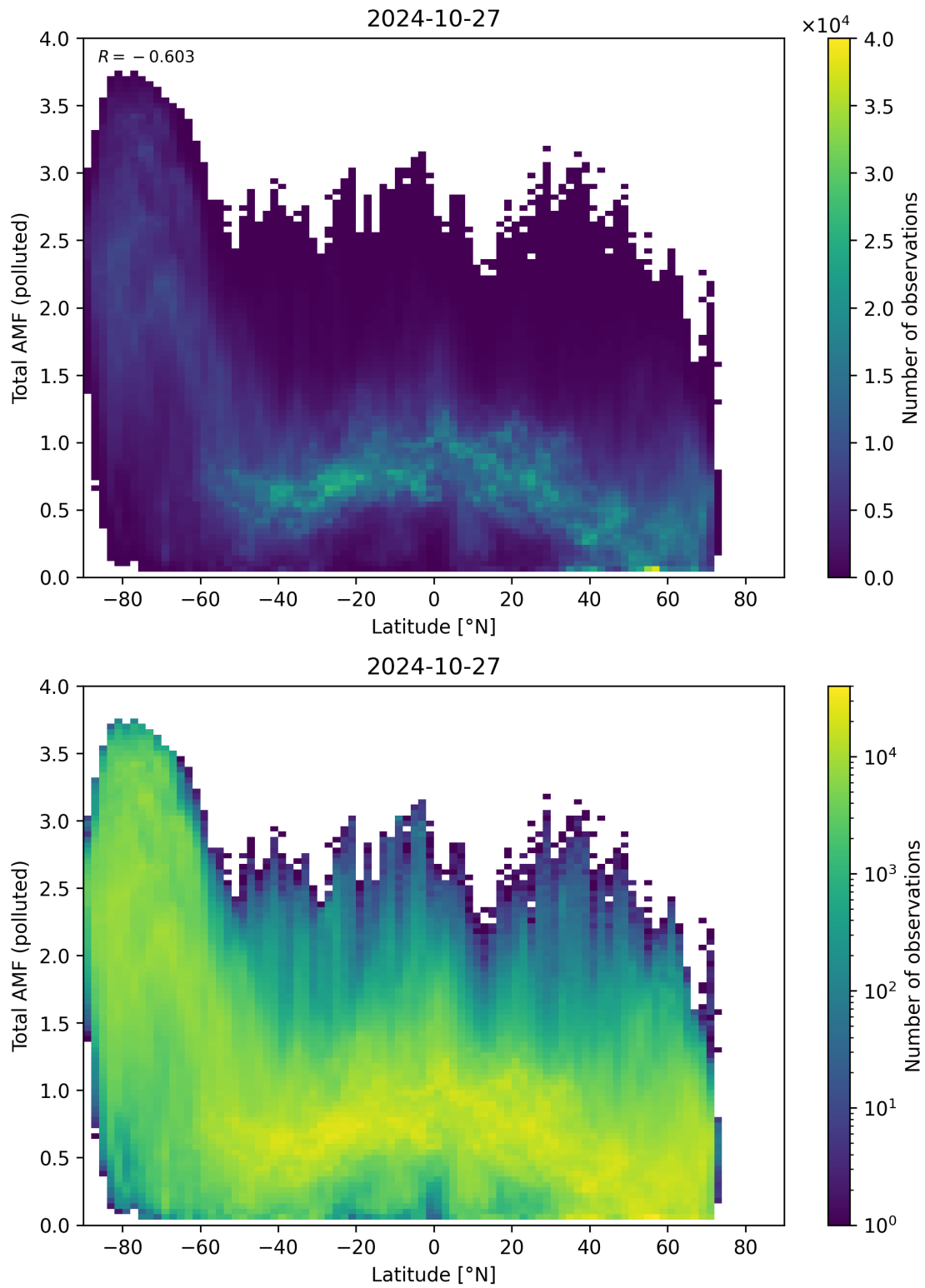
Figure 154: Scatter density plot of “Latitude” against “Total AMF (polluted)” for 2024-10-26 to 2024-10-28.
