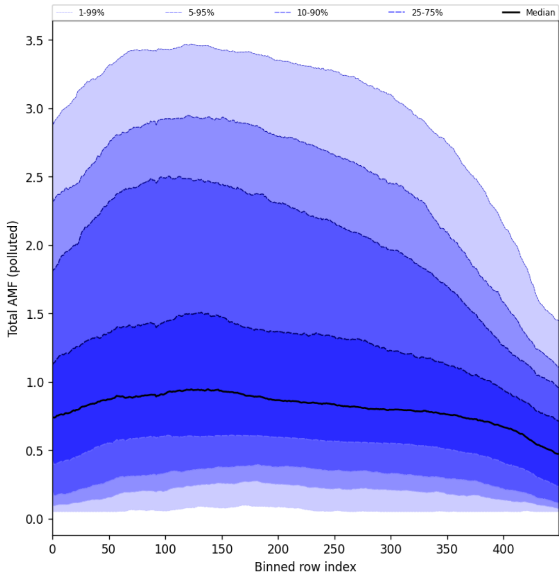
Figure 94: Along track statistics of “Total AMF (polluted)” for 2024-10-26 to 2024-10-28
