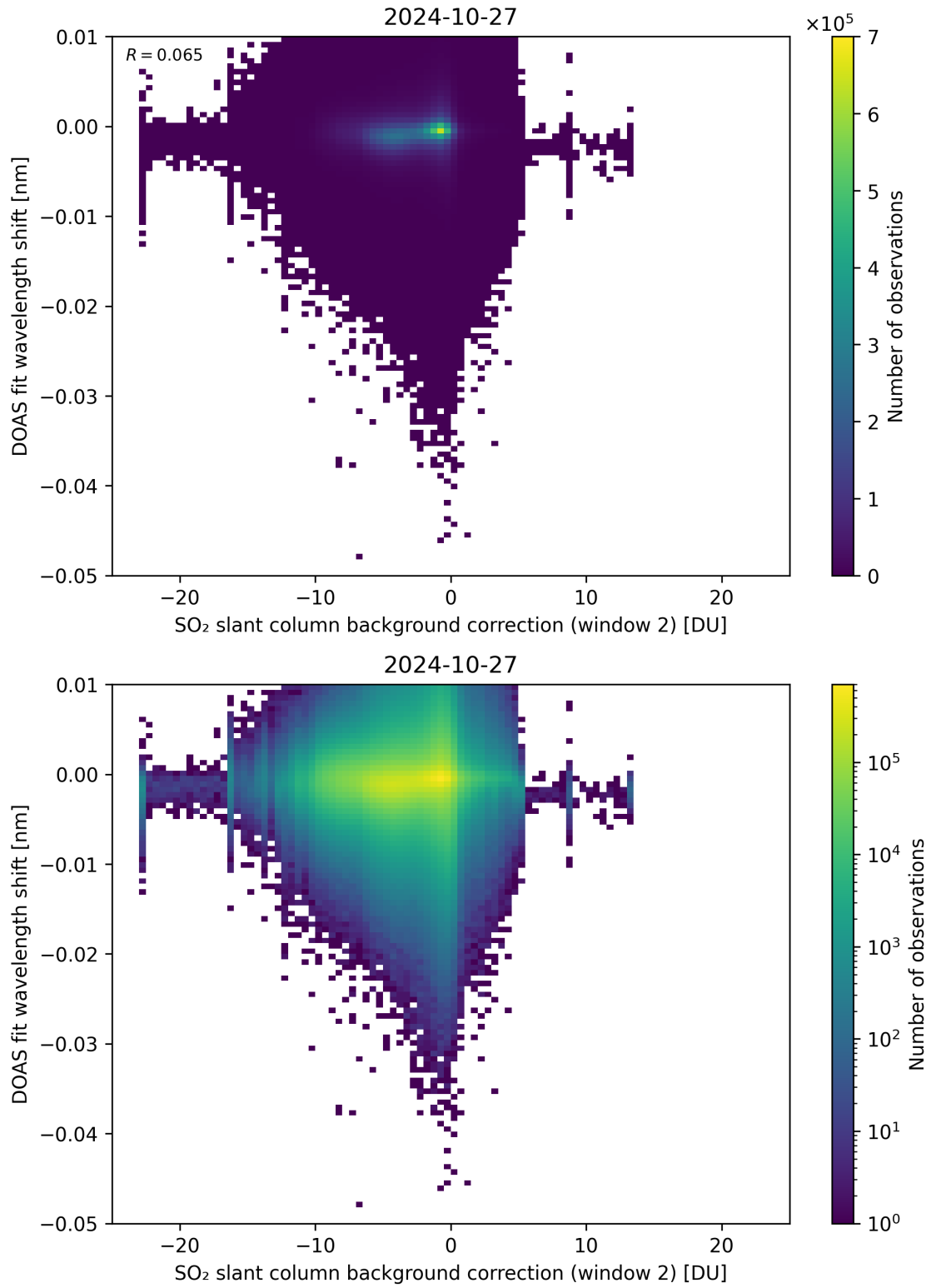
Figure 112: Scatter density plot of “SO 2 slant column background correction (window 2)” against “DOAS fit wavelength shift” for 2024-10-26 to 2024-10-28.
