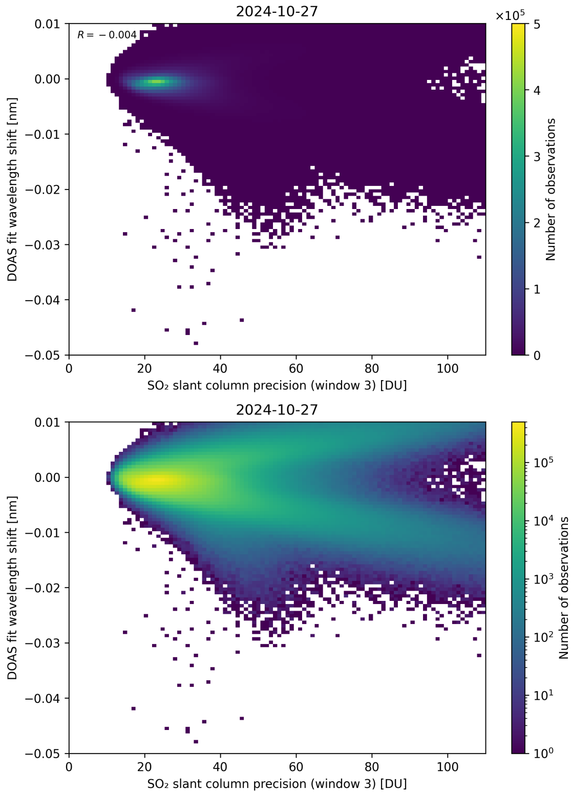
Figure 258: Scatter density plot of “SO 2 slant column precision (window 3)” against “DOAS fit wavelength shift” for 2024-10-26 to 2024-10-28.
