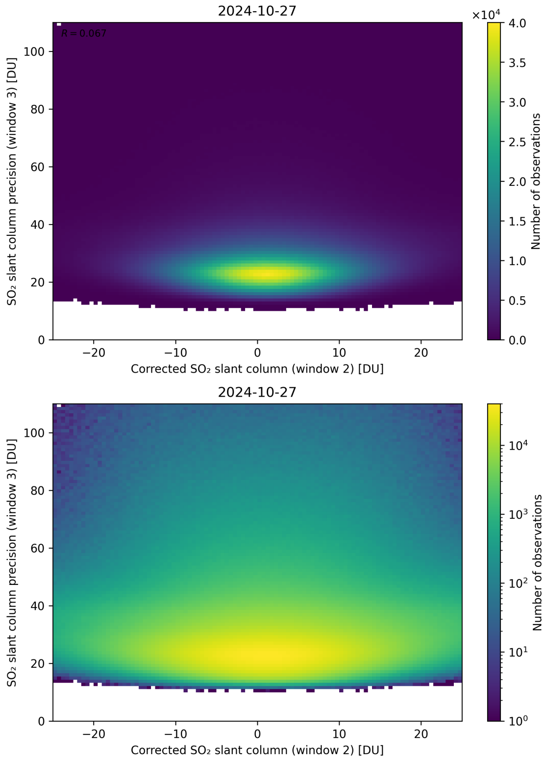
Figure 202: Scatter density plot of “Corrected SO 2 slant column (window 2)” against “SO 2 slant column precision (window 3)” for 2024-10-26 to 2024-10-28.
