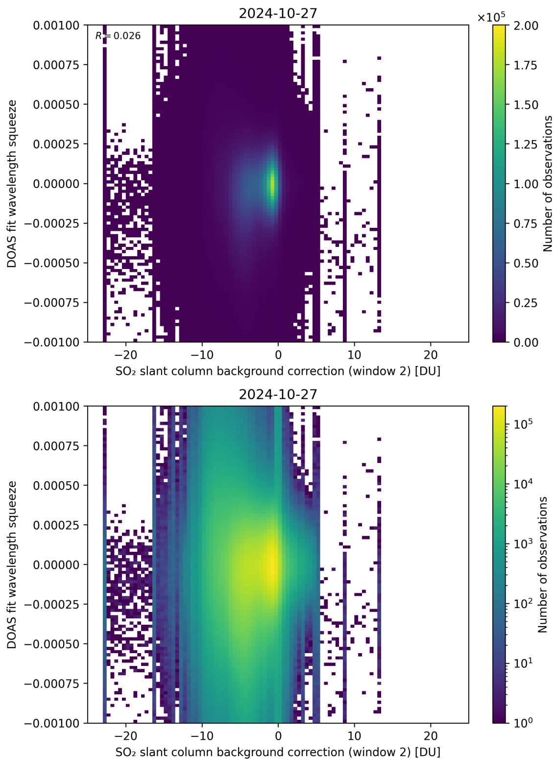
Figure 113: Scatter density plot of “SO 2 slant column background correction (window 2)” against “DOAS fit wavelength squeeze” for 2024-10-26 to 2024-10-28.
