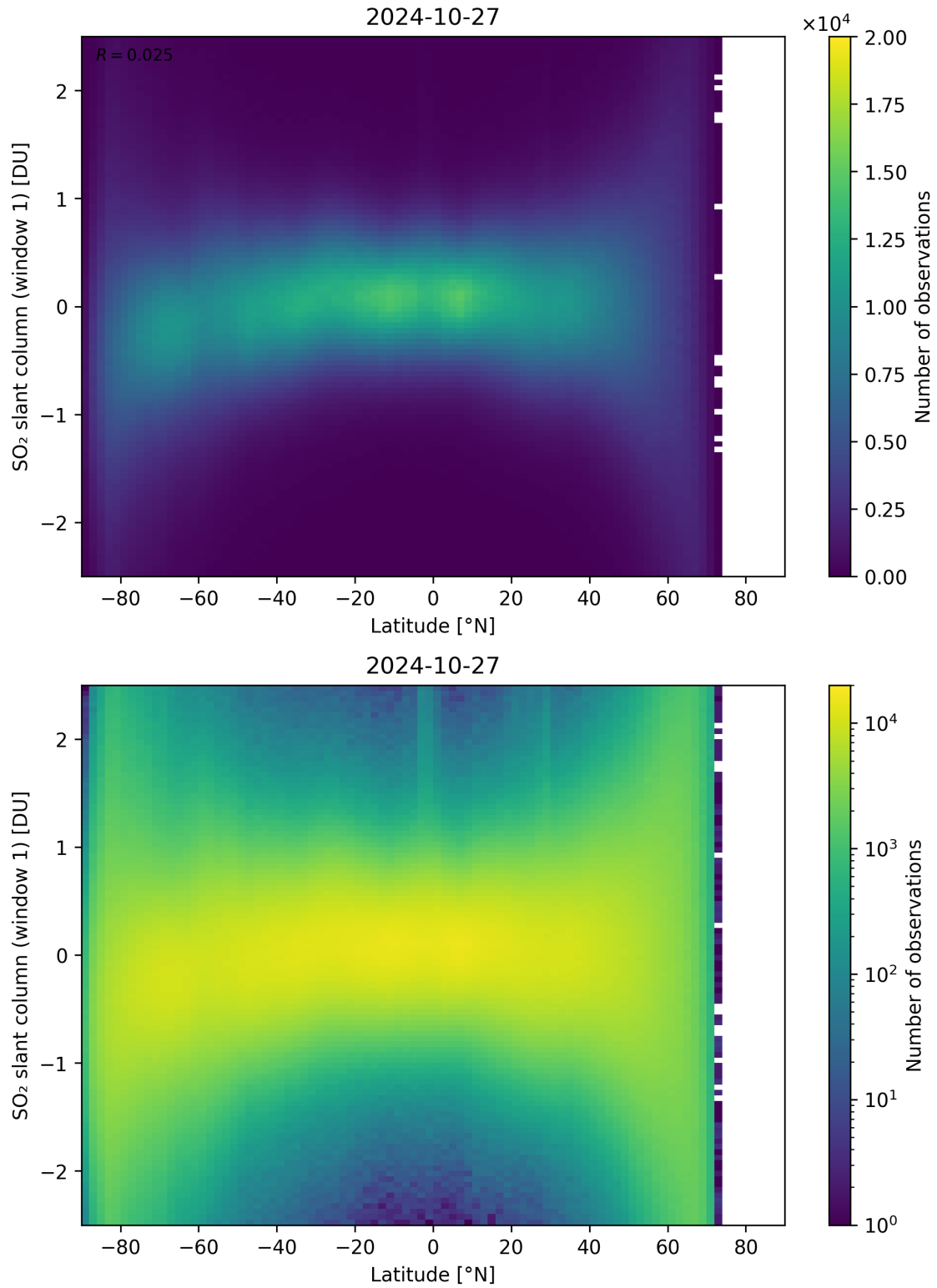
Figure 149: Scatter density plot of “Latitude” against “SO 2 slant column (window 1)” for 2024-10-26 to 2024-10-28.
