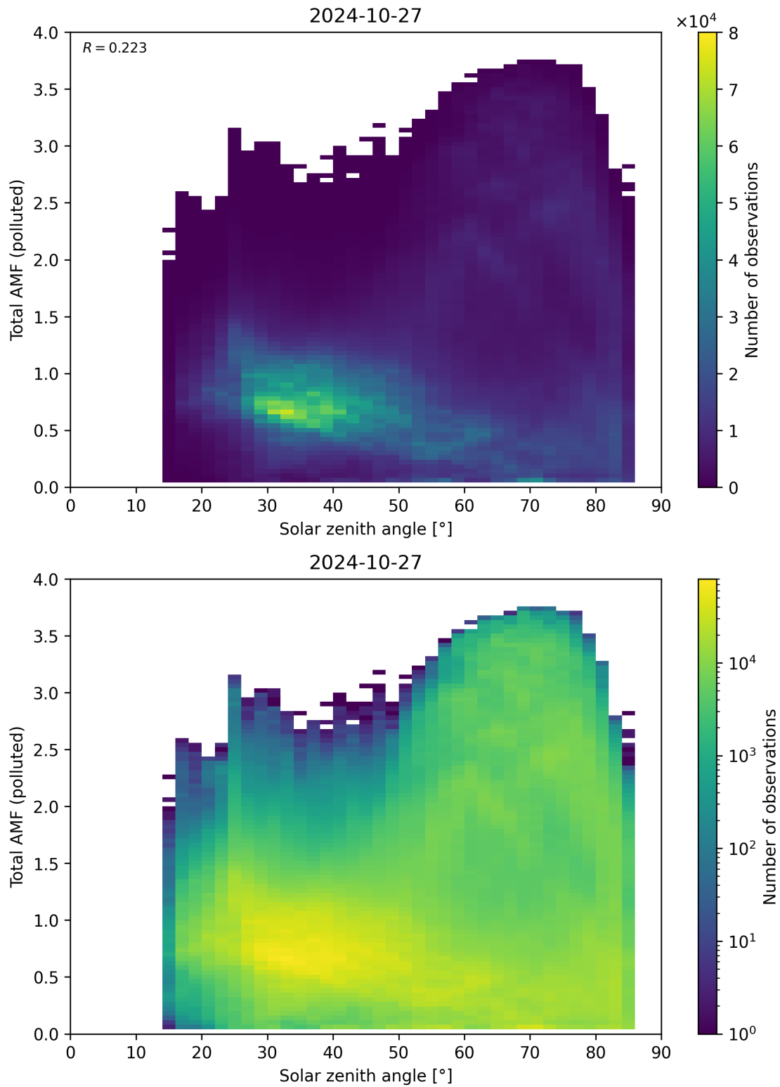
Figure 174: Scatter density plot of “Solar zenith angle” against “Total AMF (polluted)” for 2024-10-26 to 2024-10-28.
