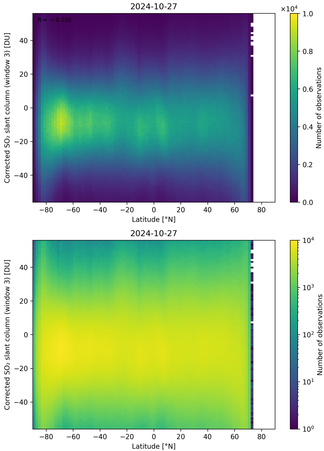
Figure 148: Scatter density plot of “Latitude” against “Corrected SO 2 slant column (window 3)” for 2024-10-26 to 2024-10-28.
