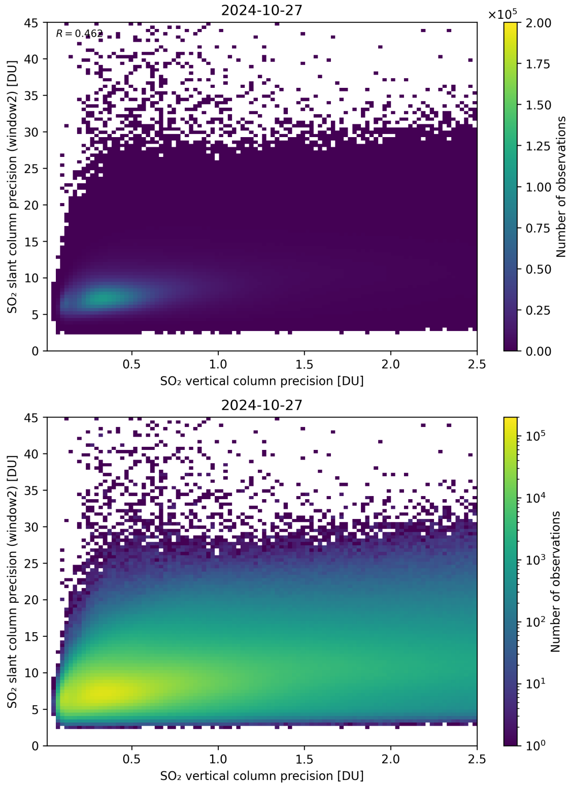
Figure 291: Scatter density plot of “SO 2 vertical column precision” against “SO 2 slant column precision (window2)” for 2024-10-26 to 2024-10-28.
