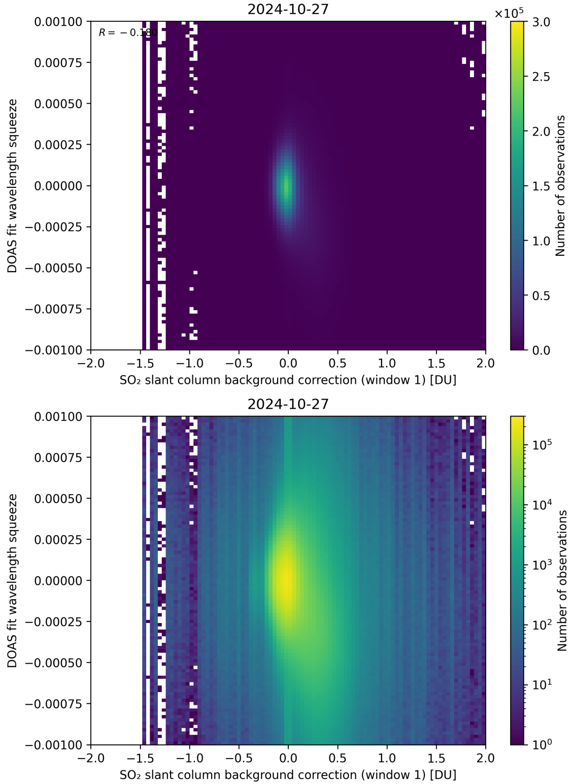
Figure 101: Scatter density plot of “SO 2 slant column background correction (window 1)” against “DOAS fit wavelength squeeze” for 2024-10-26 to 2024-10-28.
