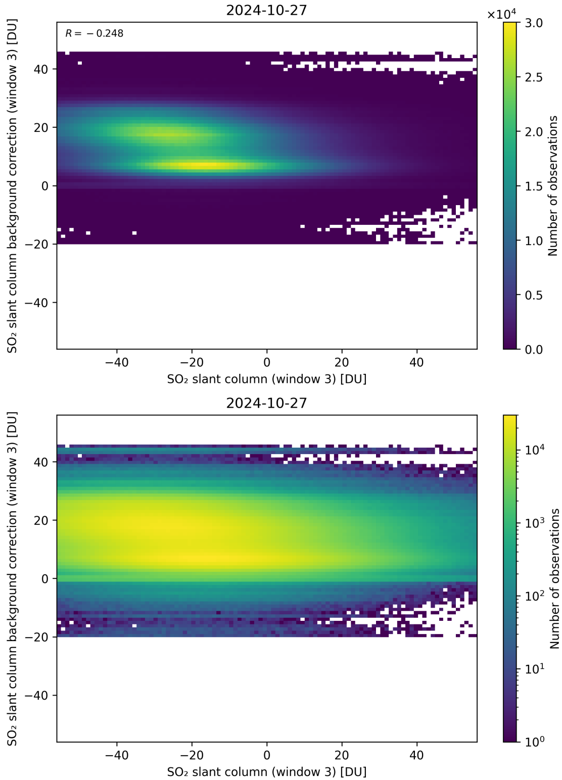
Figure 253: Scatter density plot of “SO 2 slant column (window 3)” against “SO 2 slant column background correction (window 3)” for 2024-10-26 to 2024-10-28.
