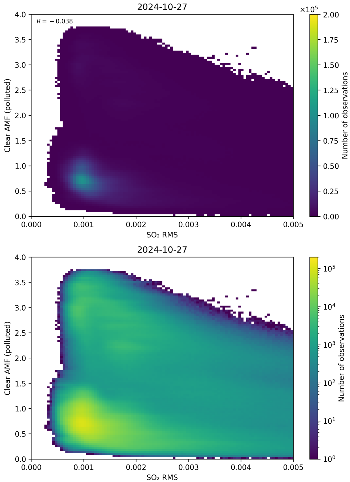
Figure 136: Scatter density plot of “SO 2 RMS” against “Clear AMF (polluted)” for 2024-10-26 to 2024-10-28.
