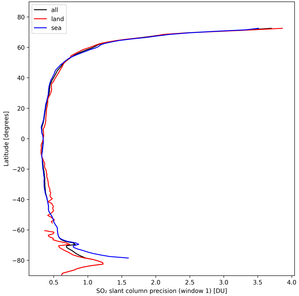
Figure 34: Zonal average of “SO 2 slant column precision (window 1)” for 2024-10-26 to 2024-10-28.
