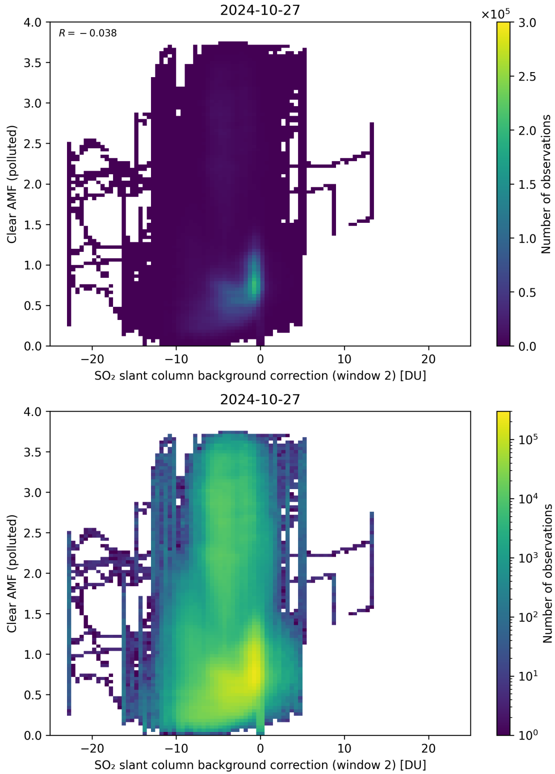
Figure 115: Scatter density plot of “SO 2 slant column background correction (window 2)” against “Clear AMF (polluted)” for 2024-10-26 to 2024-10-28.
