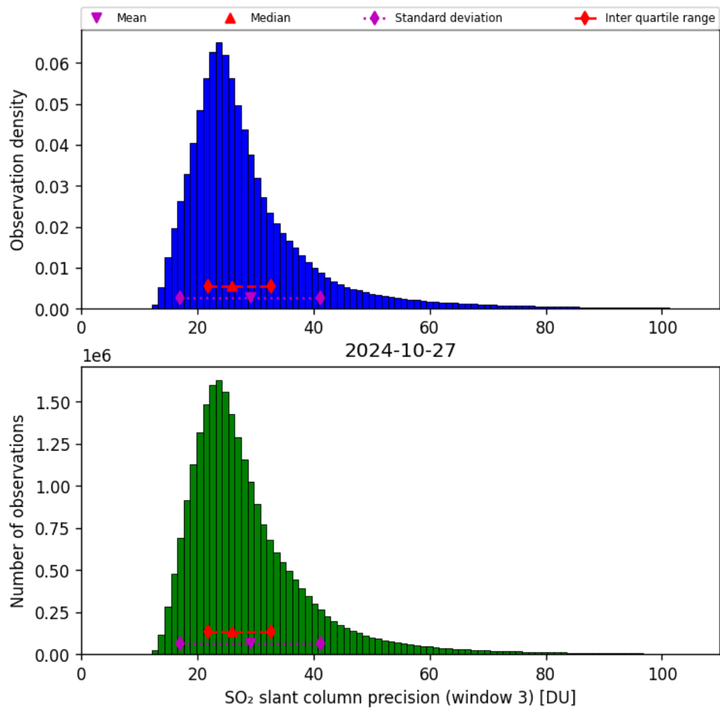
Figure 65: Histogram of “SO 2 slant column precision (window 3)” for 2024-10-26 to 2024-10-28
