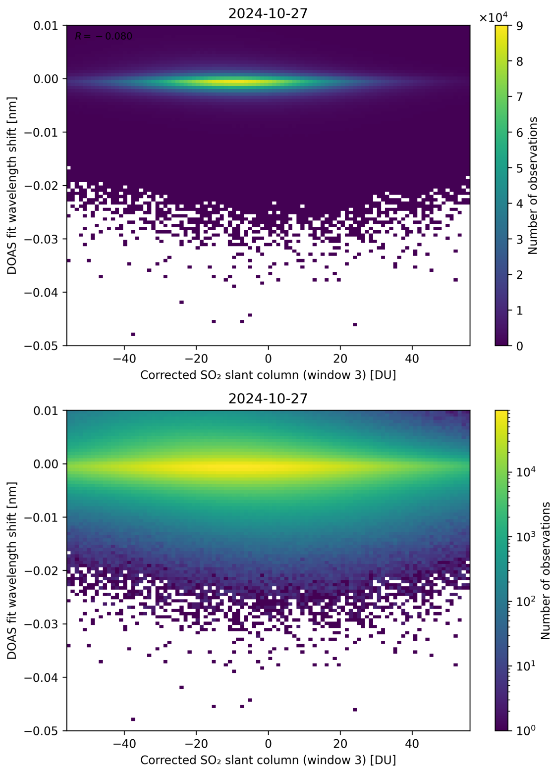
Figure 206: Scatter density plot of “Corrected SO 2 slant column (window 3)” against “DOAS fit wavelength shift” for 2024-10-26 to 2024-10-28.
