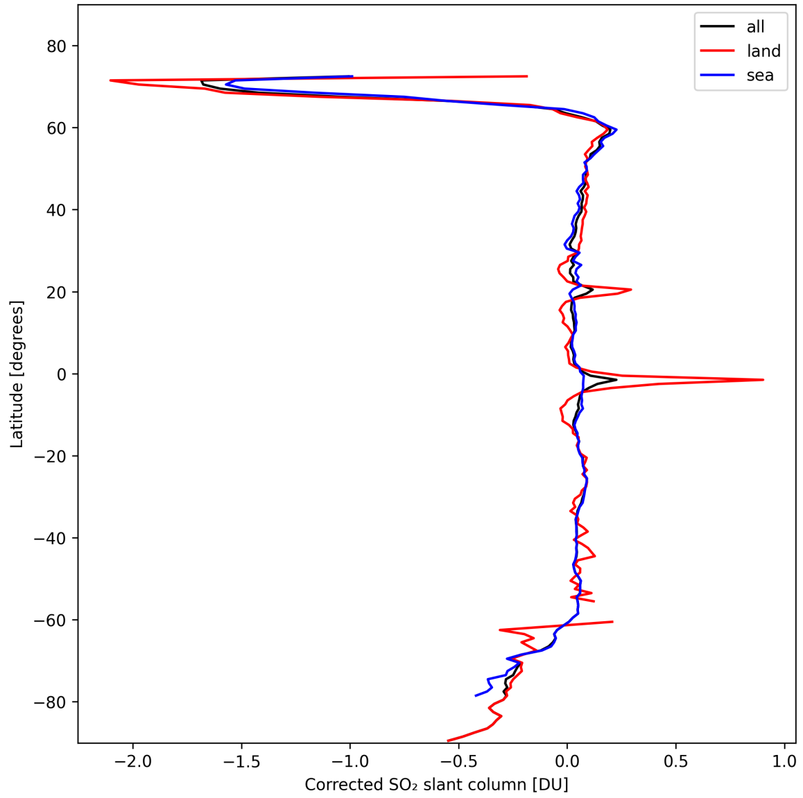
Figure 32: Zonal average of “Corrected SO 2 slant column” for 2024-10-26 to 2024-10-28.
