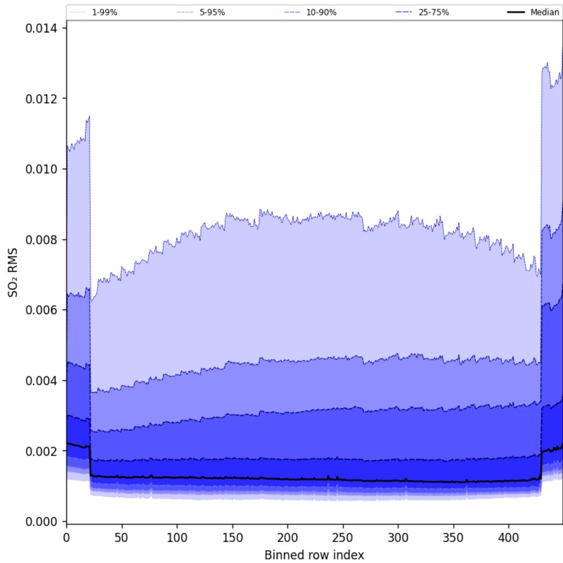
Figure 93: Along track statistics of “SO 2 RMS” for 2024-10-26 to 2024-10-28
