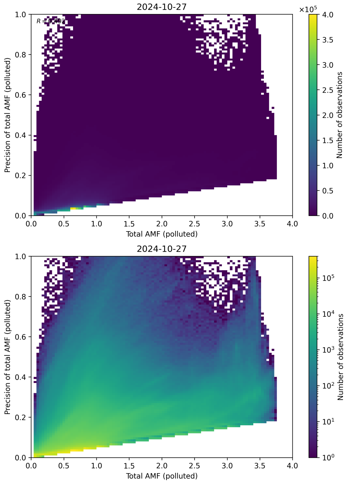
Figure 272: Scatter density plot of “Total AMF (polluted)” against “Precision of total AMF (polluted)” for 2024-10-26 to 2024-10-28.
