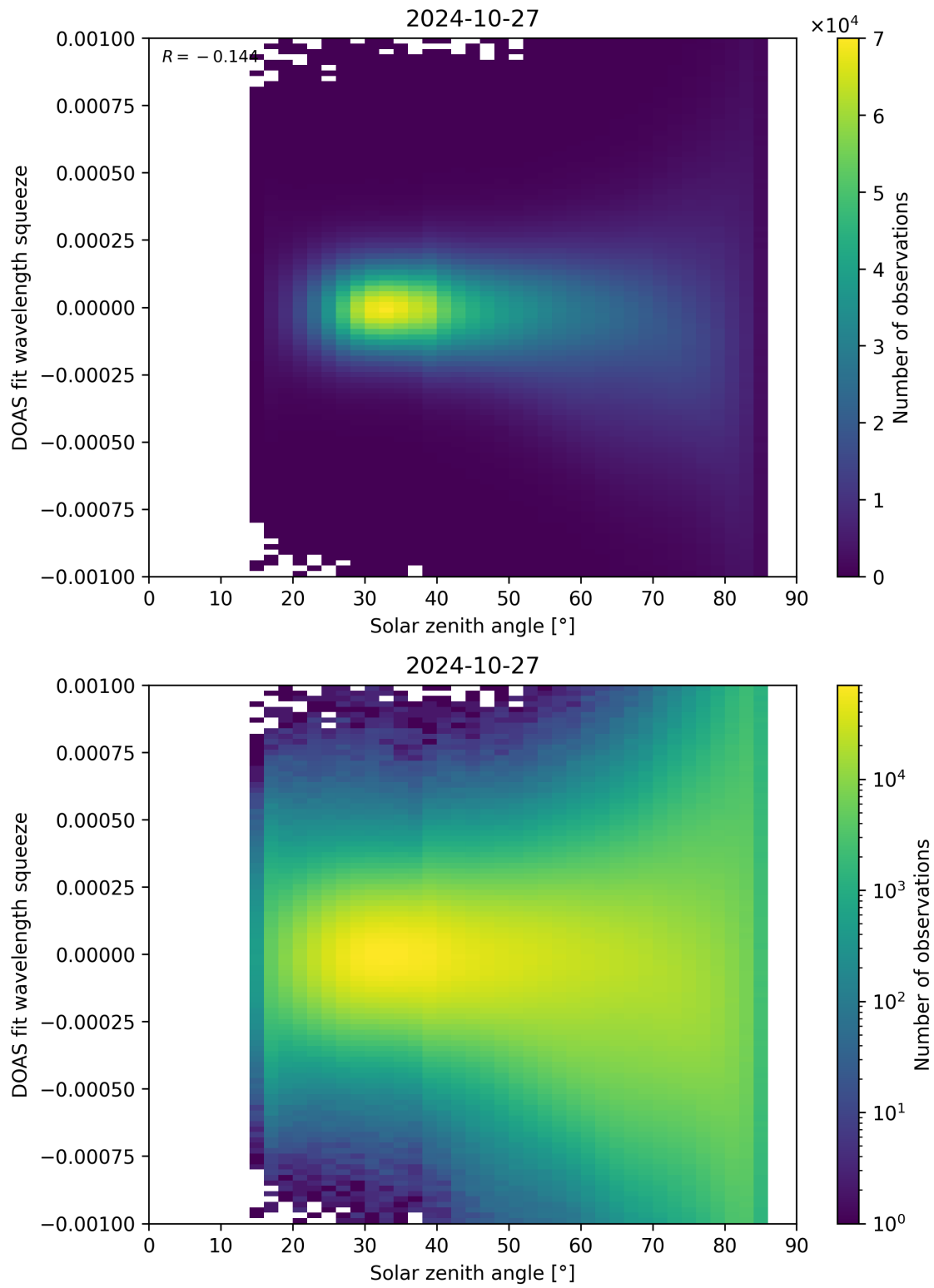
Figure 162: Scatter density plot of “Solar zenith angle” against “DOAS fit wavelength squeeze” for 2024-10-26 to 2024-10-28.
