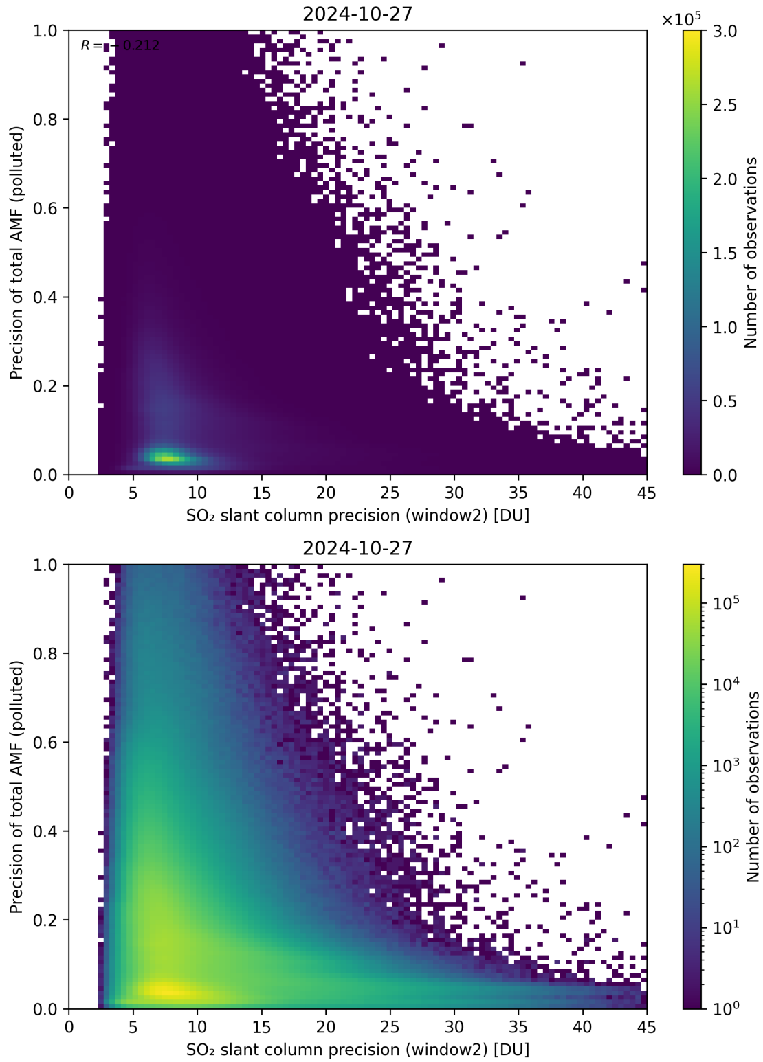
Figure 252: Scatter density plot of “SO 2 slant column precision (window2)” against “Precision of total AMF (polluted)” for 2024-10-26 to 2024-10-28.
