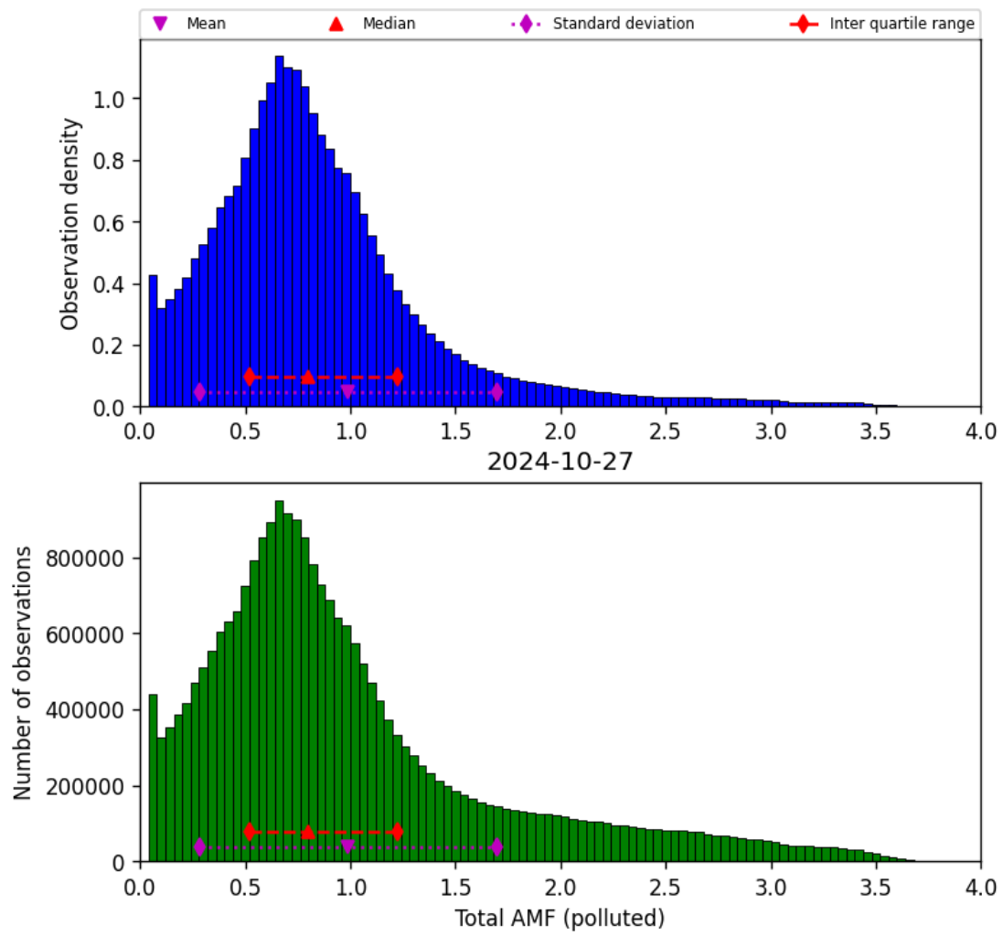
Figure 71: Histogram of “Total AMF (polluted)” for 2024-10-26 to 2024-10-28
