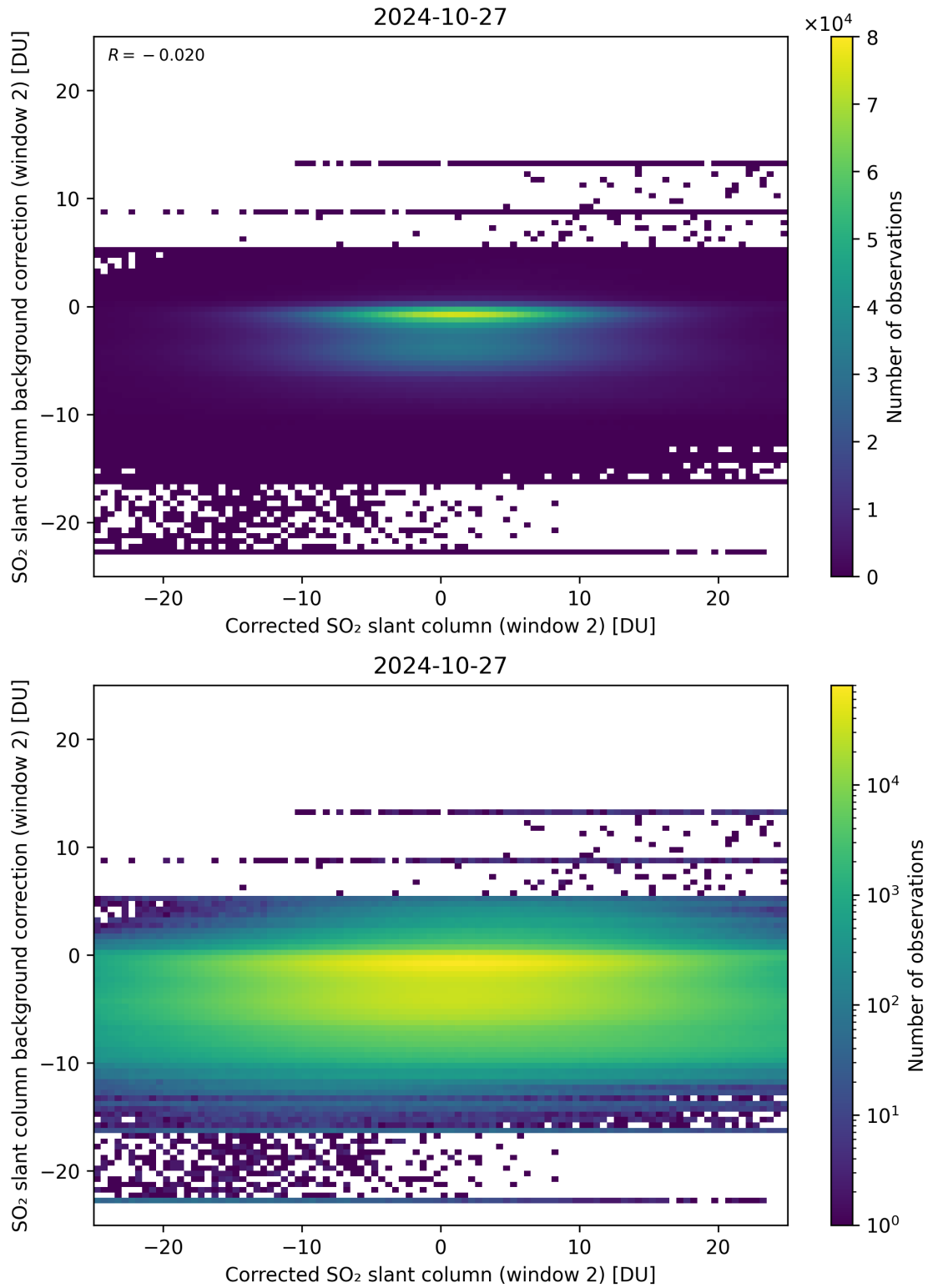
Figure 194: Scatter density plot of “Corrected SO 2 slant column (window 2)” against “SO 2 slant column background correction (window 2)” for 2024-10-26 to 2024-10-28.
