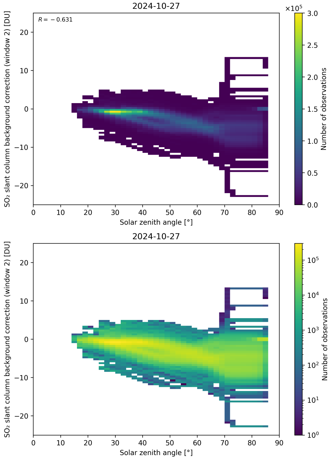
Figure 159: Scatter density plot of “Solar zenith angle” against “SO 2 slant column background correction (window 2)” for 2024-10-26 to 2024-10-28.
