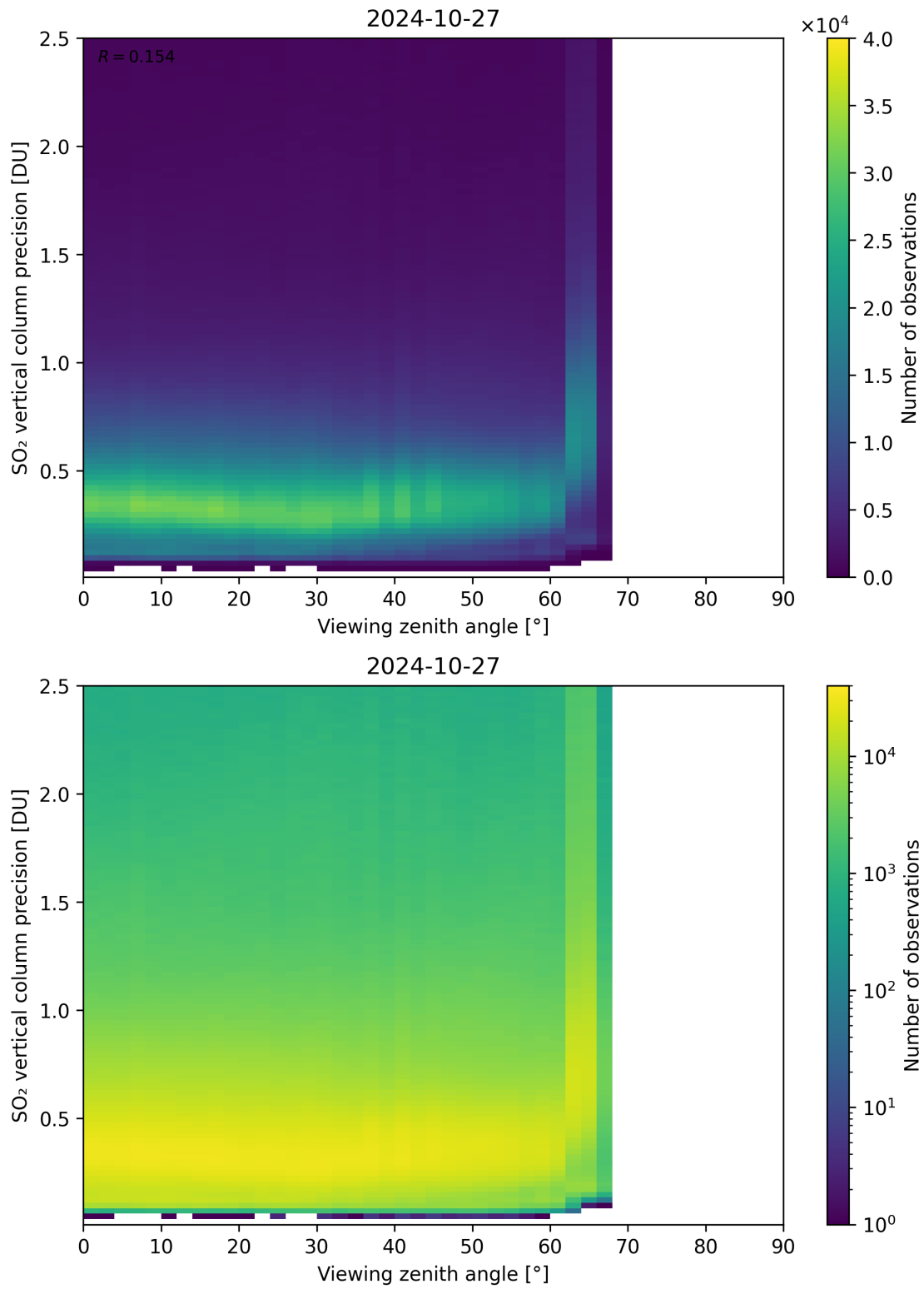
Figure 328: Scatter density plot of “Viewing zenith angle” against “SO 2 vertical column precision” for 2024-10-26 to 2024-10-28.
