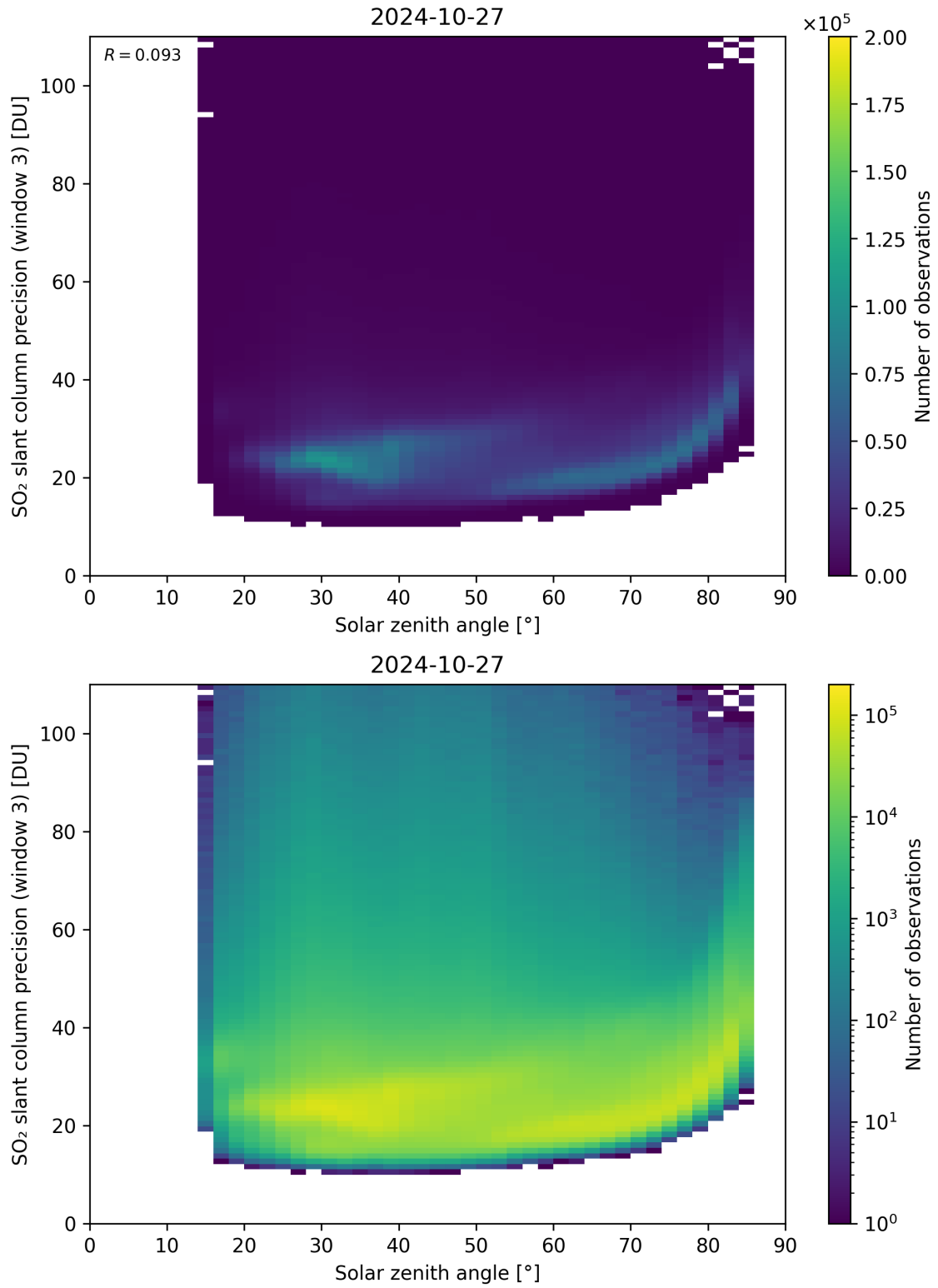
Figure 173: Scatter density plot of “Solar zenith angle” against “SO 2 slant column precision (window 3)” for 2024-10-26 to 2024-10-28.
