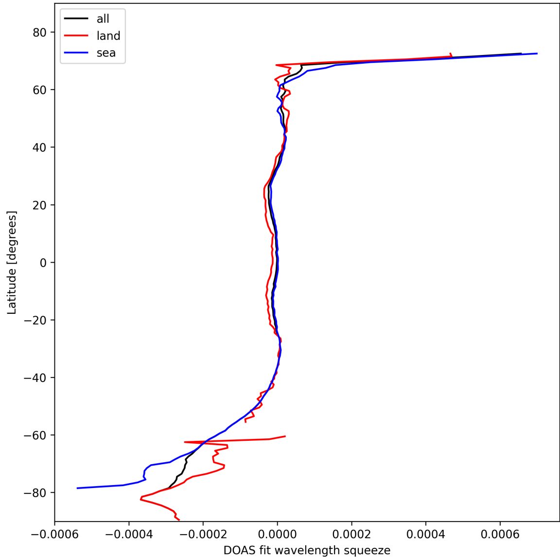
Figure 46: Zonal average of “DOAS fit wavelength squeeze” for 2024-10-26 to 2024-10-28.
