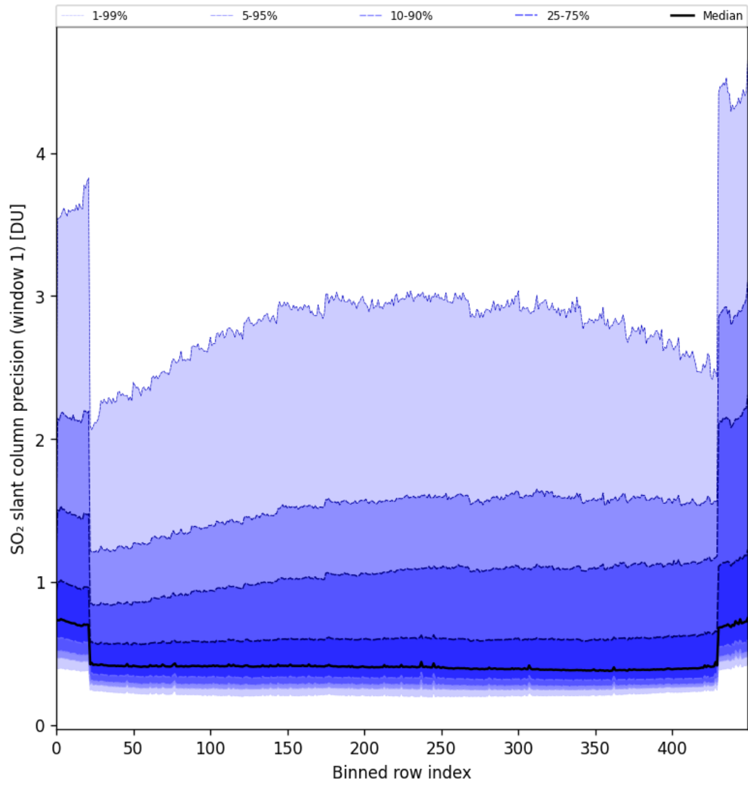
Figure 80: Along track statistics of “SO 2 slant column precision (window 1)” for 2024-10-26 to 2024-10-28
