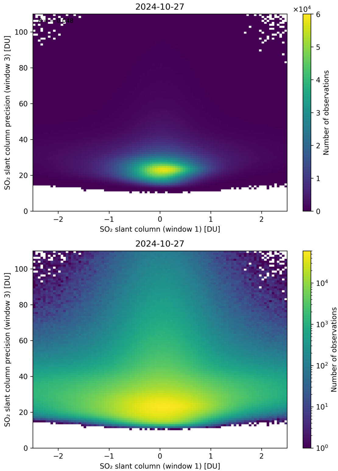
Figure 238: Scatter density plot of “SO 2 slant column (window 1)” against “SO 2 slant column precision (window 3)” for 2024-10-26 to 2024-10-28.
