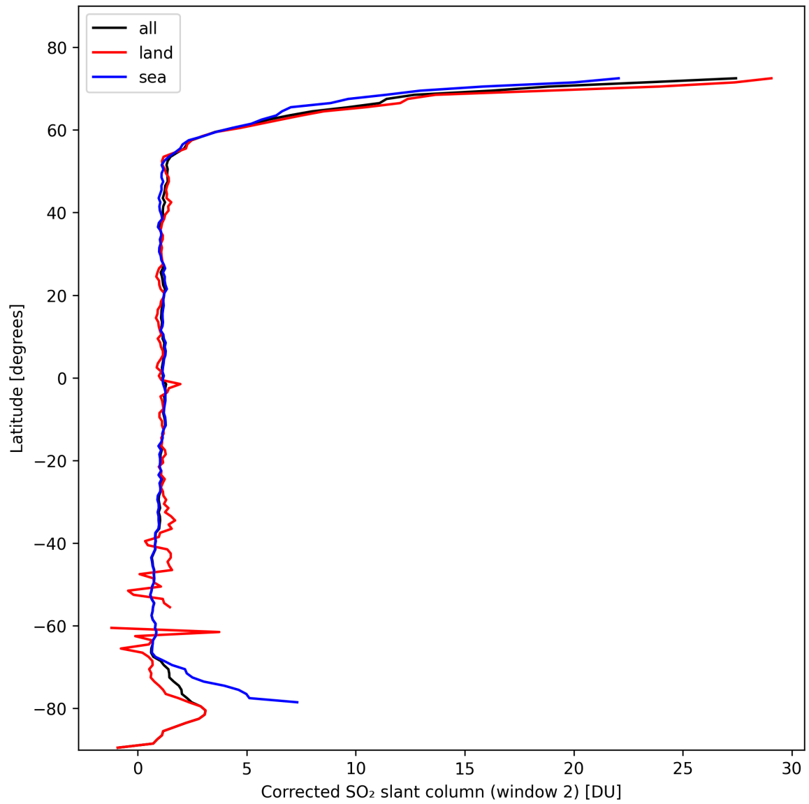
Figure 39: Zonal average of “Corrected SO 2 slant column (window 2)” for 2024-10-26 to 2024-10-28.
