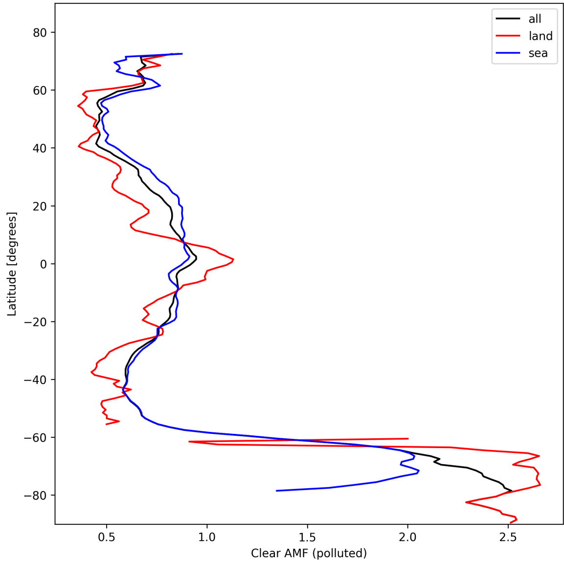
Figure 50: Zonal average of “Clear AMF (polluted)” for 2024-10-26 to 2024-10-28.
