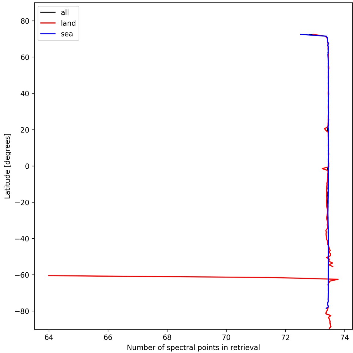
Figure 51: Zonal average of “Number of spectral points in retrieval” for 2024-10-26 to 2024-10-28.
