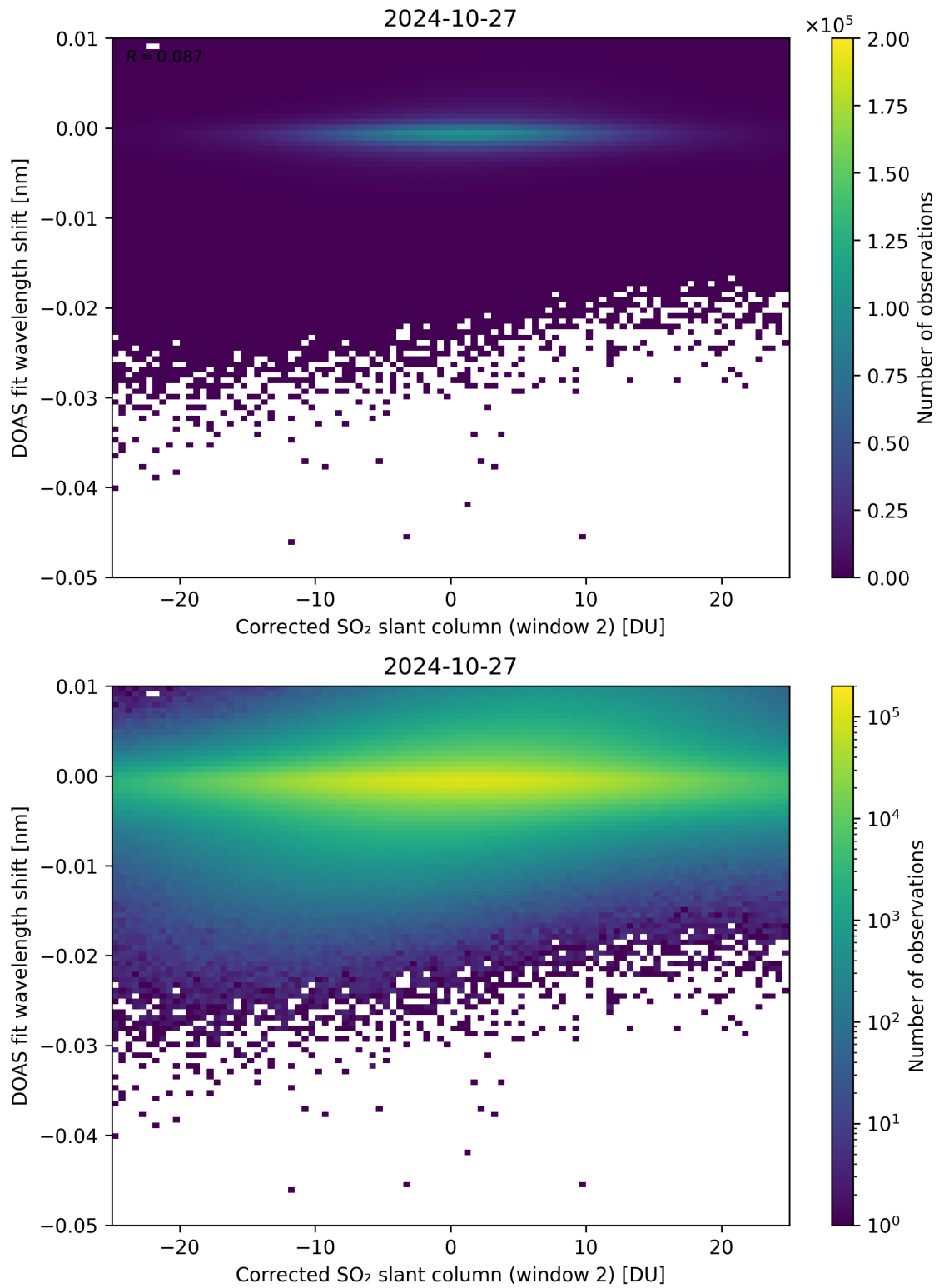
Figure 196: Scatter density plot of “Corrected SO 2 slant column (window 2)” against “DOAS fit wavelength shift” for 2024-10-26 to 2024-10-28.
