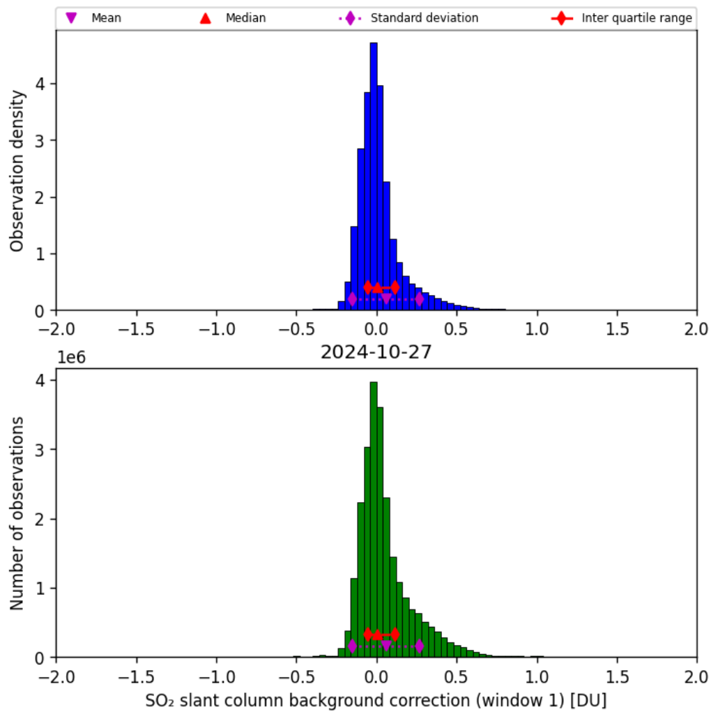
Figure 59: Histogram of “SO 2 slant column background correction (window 1)” for 2024-10-26 to 2024-10-28
