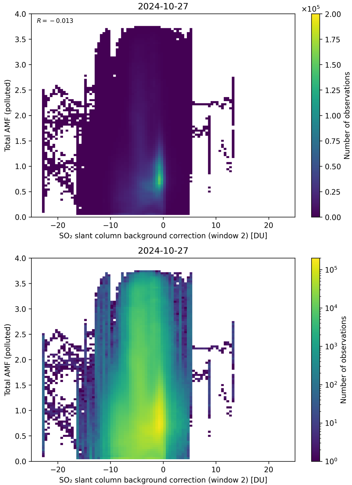
Figure 119: Scatter density plot of “SO 2 slant column background correction (window 2)” against “Total AMF (polluted)” for 2024-10-26 to 2024-10-28.
