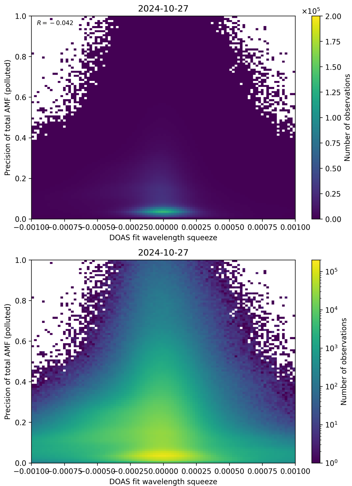
Figure 135: Scatter density plot of “DOAS fit wavelength squeeze” against “Precision of total AMF (polluted)” for 2024-10-26 to 2024-10-28.
