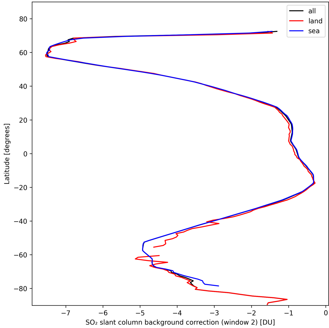
Figure 40: Zonal average of “SO 2 slant column background correction (window 2)” for 2024-10-26 to 2024-10-28.
