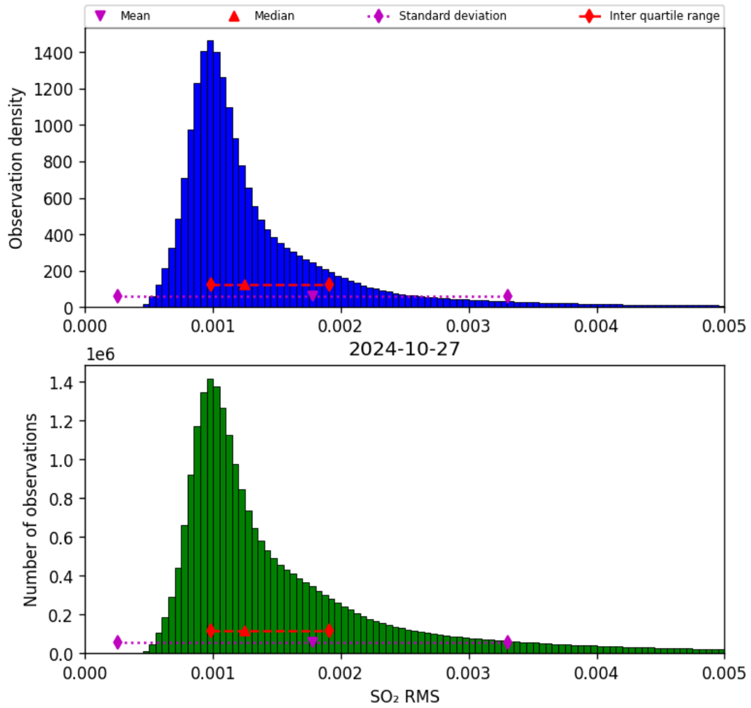
Figure 70: Histogram of “SO 2 RMS” for 2024-10-26 to 2024-10-28
