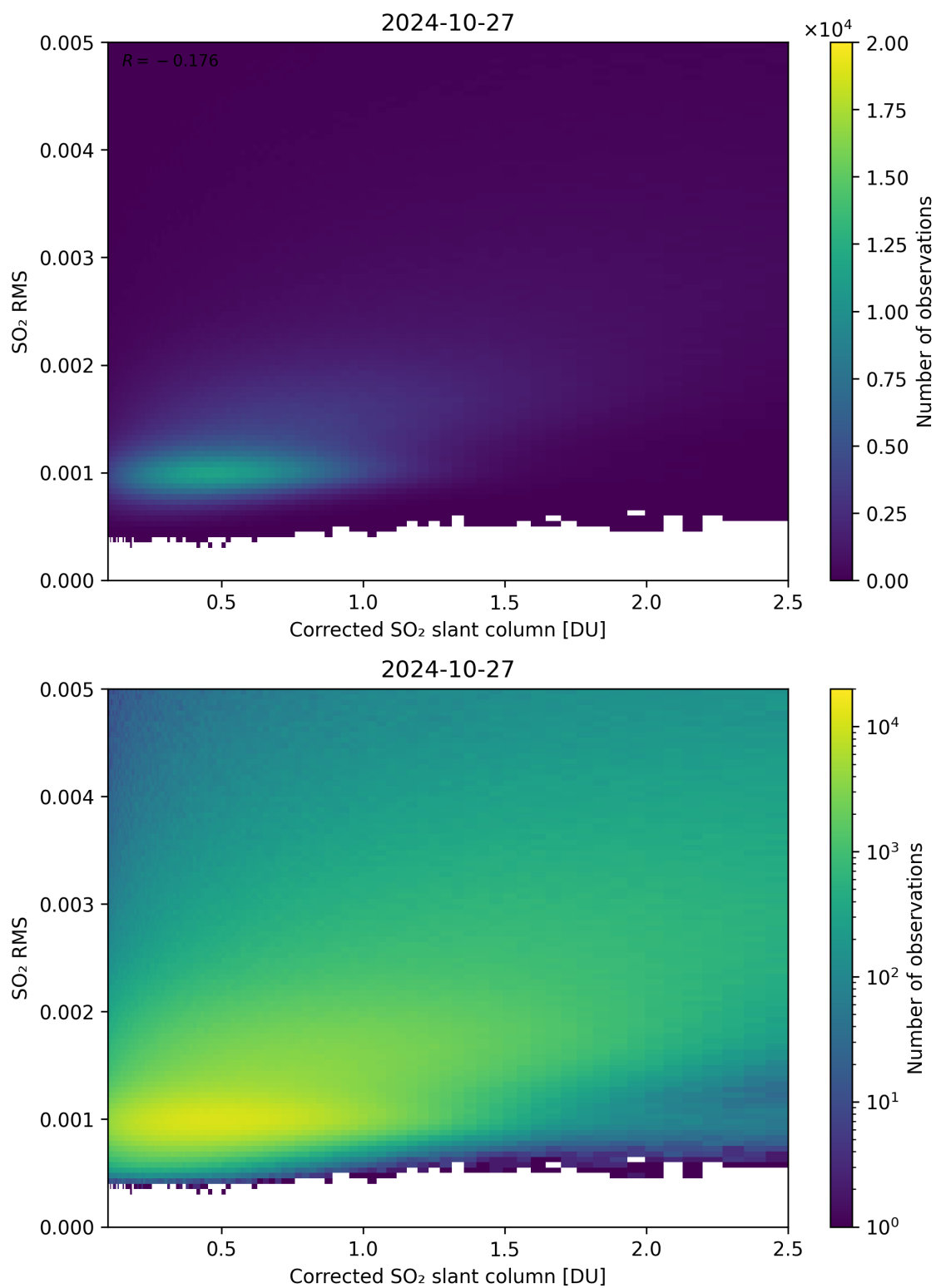
Figure 183: Scatter density plot of “Corrected SO 2 slant column” against “SO 2 RMS” for 2024-10-26 to 2024-10-28.
