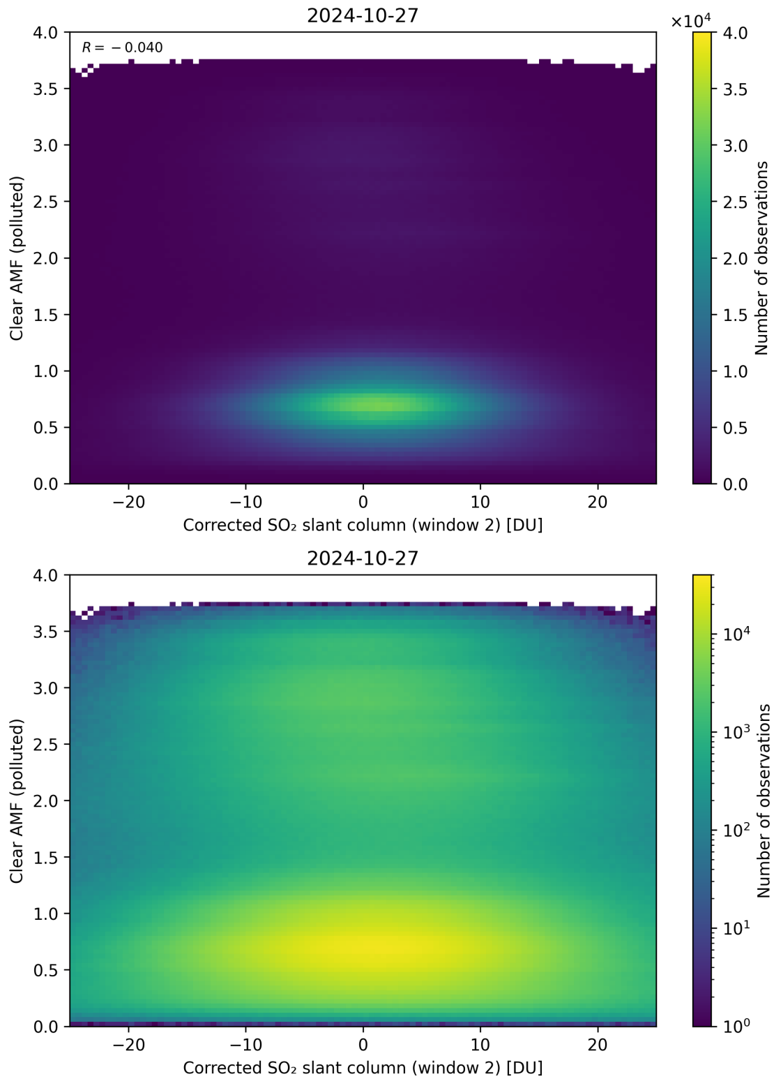
Figure 199: Scatter density plot of “Corrected SO 2 slant column (window 2)” against “Clear AMF (polluted)” for 2024-10-26 to 2024-10-28.
