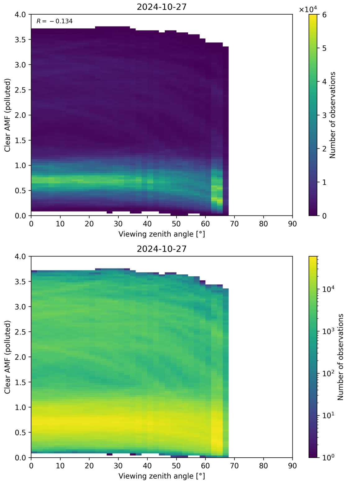
Figure 316: Scatter density plot of “Viewing zenith angle” against “Clear AMF (polluted)” for 2024-10-26 to 2024-10-28.
