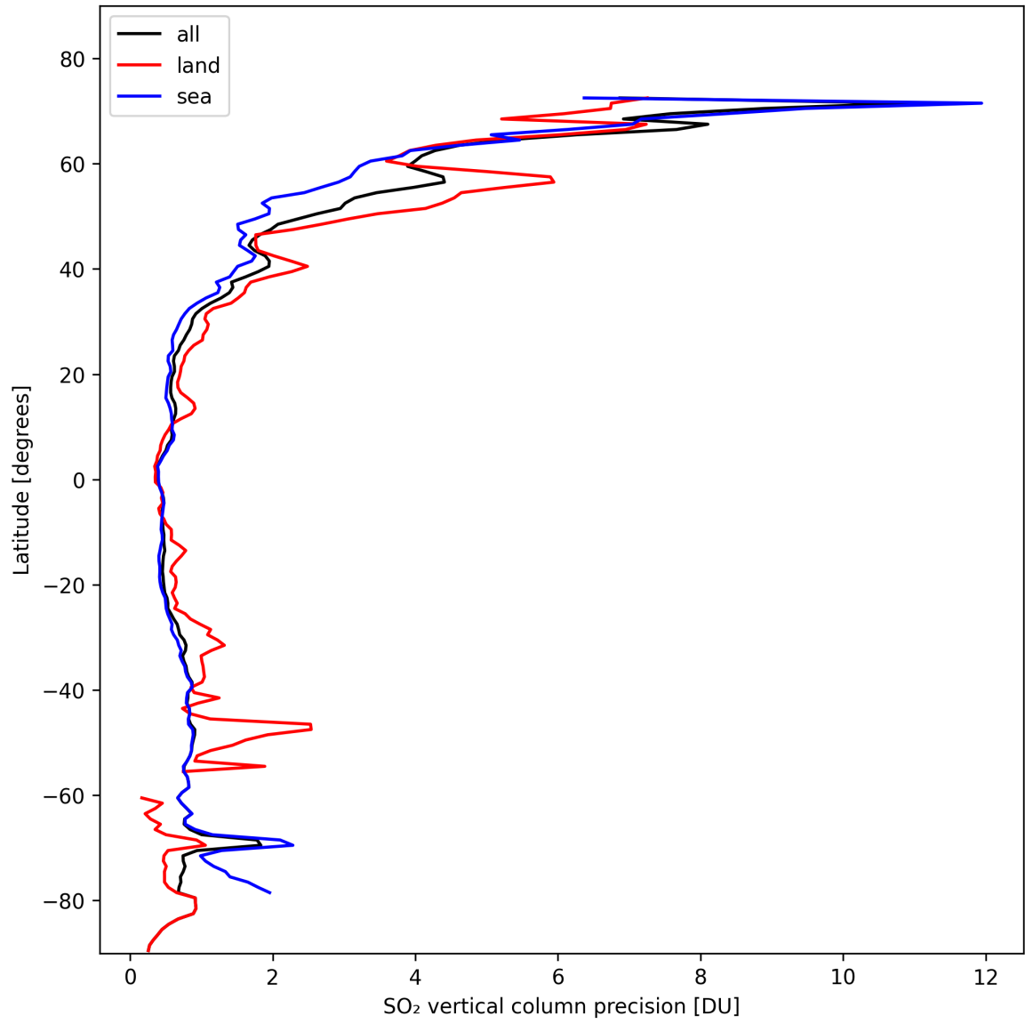
Figure 31: Zonal average of “SO 2 vertical column precision” for 2024-10-26 to 2024-10-28.
