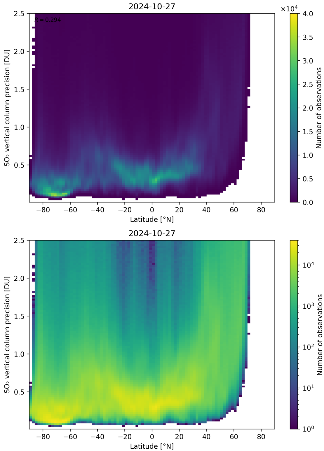
Figure 157: Scatter density plot of “Latitude” against “SO 2 vertical column precision” for 2024-10-26 to 2024-10-28.
