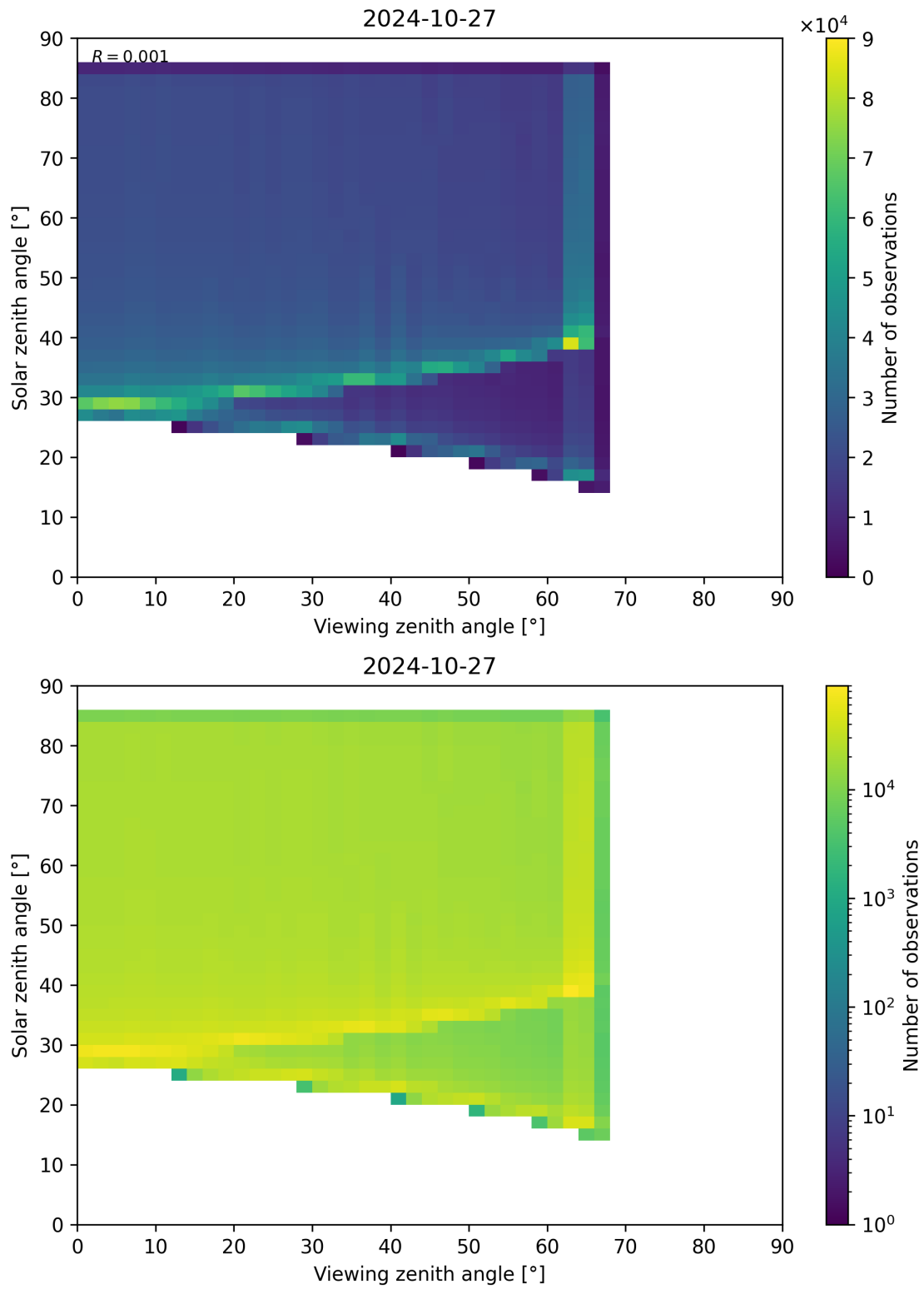
Figure 315: Scatter density plot of “Viewing zenith angle” against “Solar zenith angle” for 2024-10-26 to 2024-10-28.
