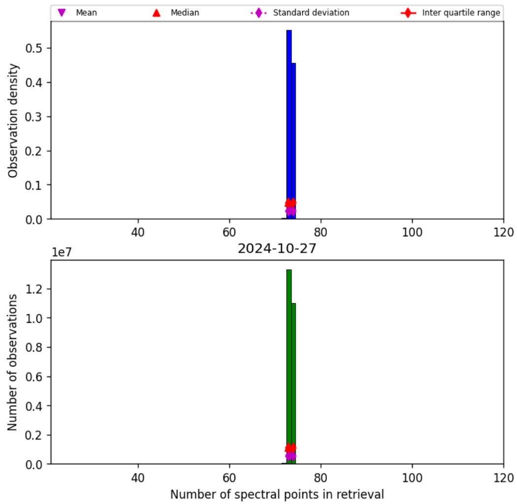
Figure 74: Histogram of “Number of spectral points in retrieval” for 2024-10-26 to 2024-10-28
