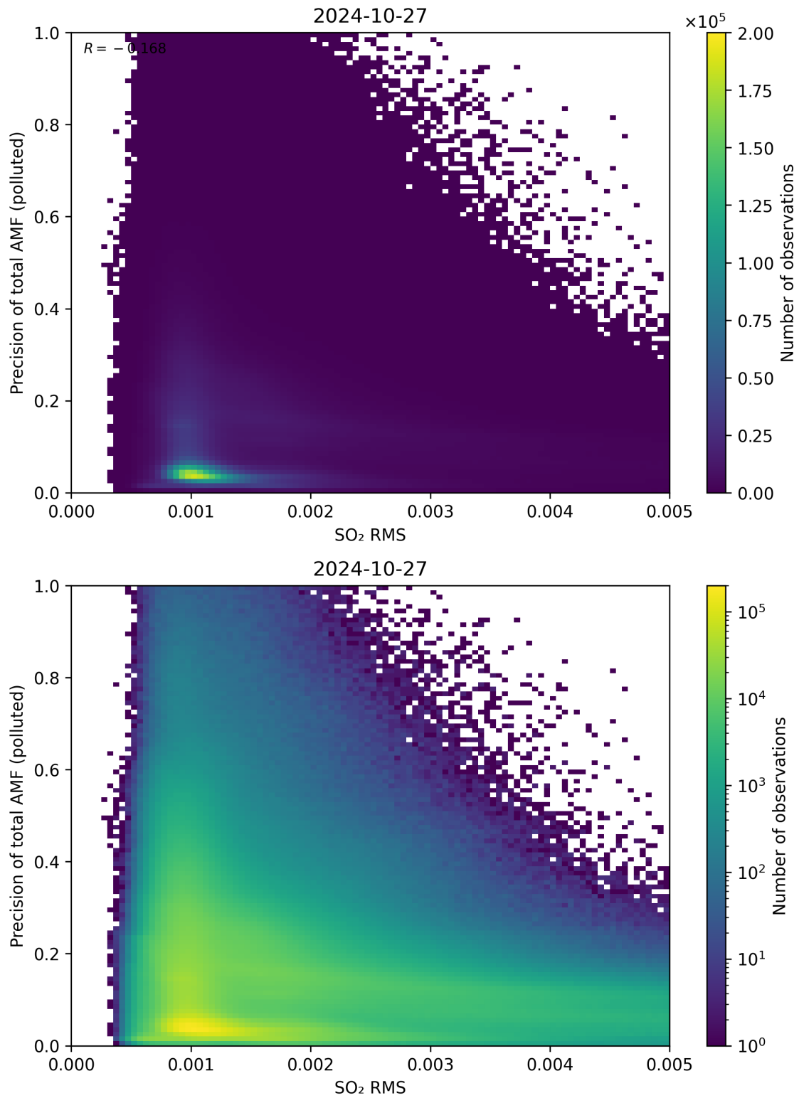
Figure 138: Scatter density plot of “SO 2 RMS” against “Precision of total AMF (polluted)” for 2024-10-26 to 2024-10-28.
