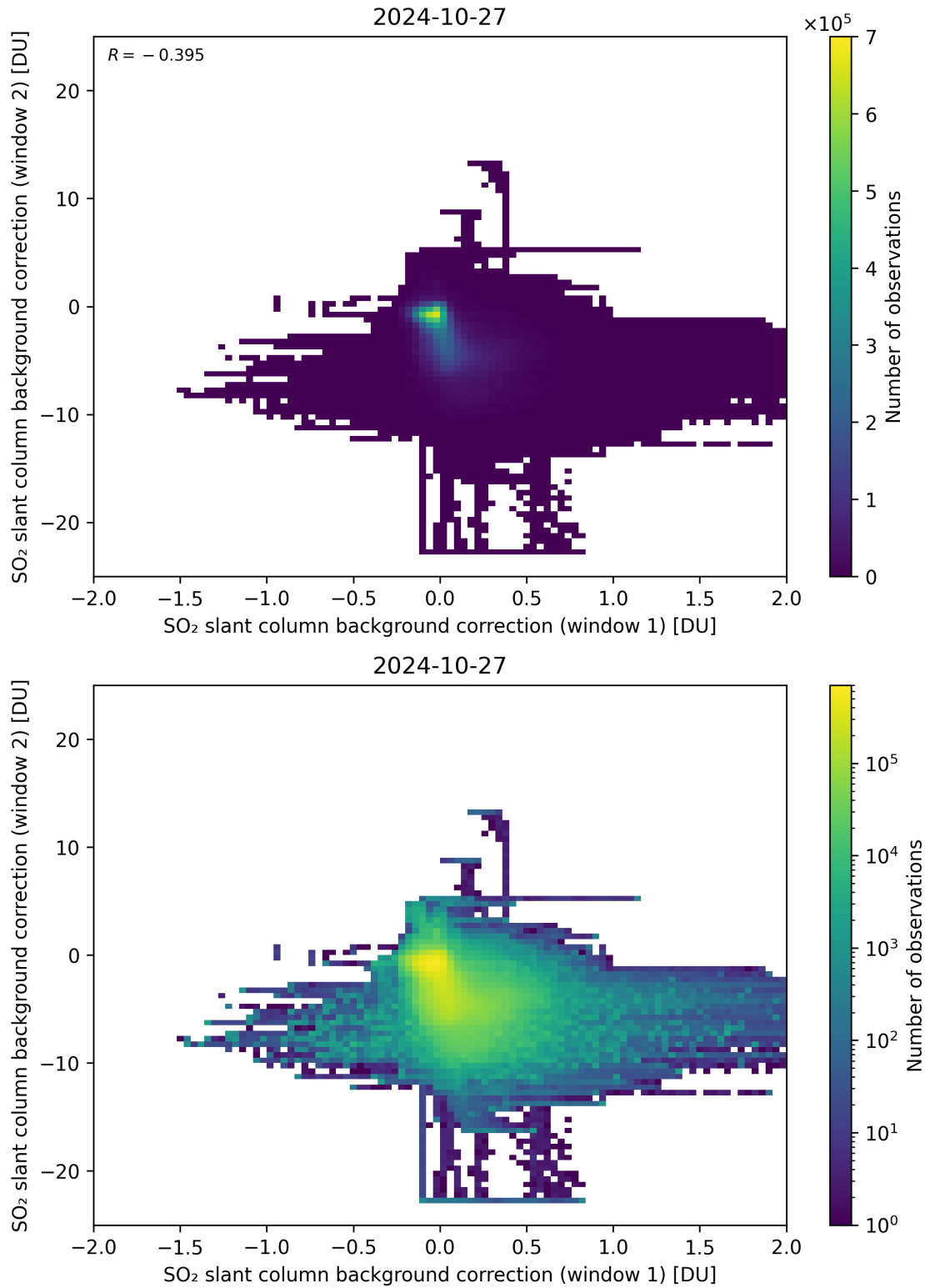
Figure 98: Scatter density plot of “SO 2 slant column background correction (window 1)” against “SO 2 slant column background correction (window 2)” for 2024-10-26 to 2024-10-28.
