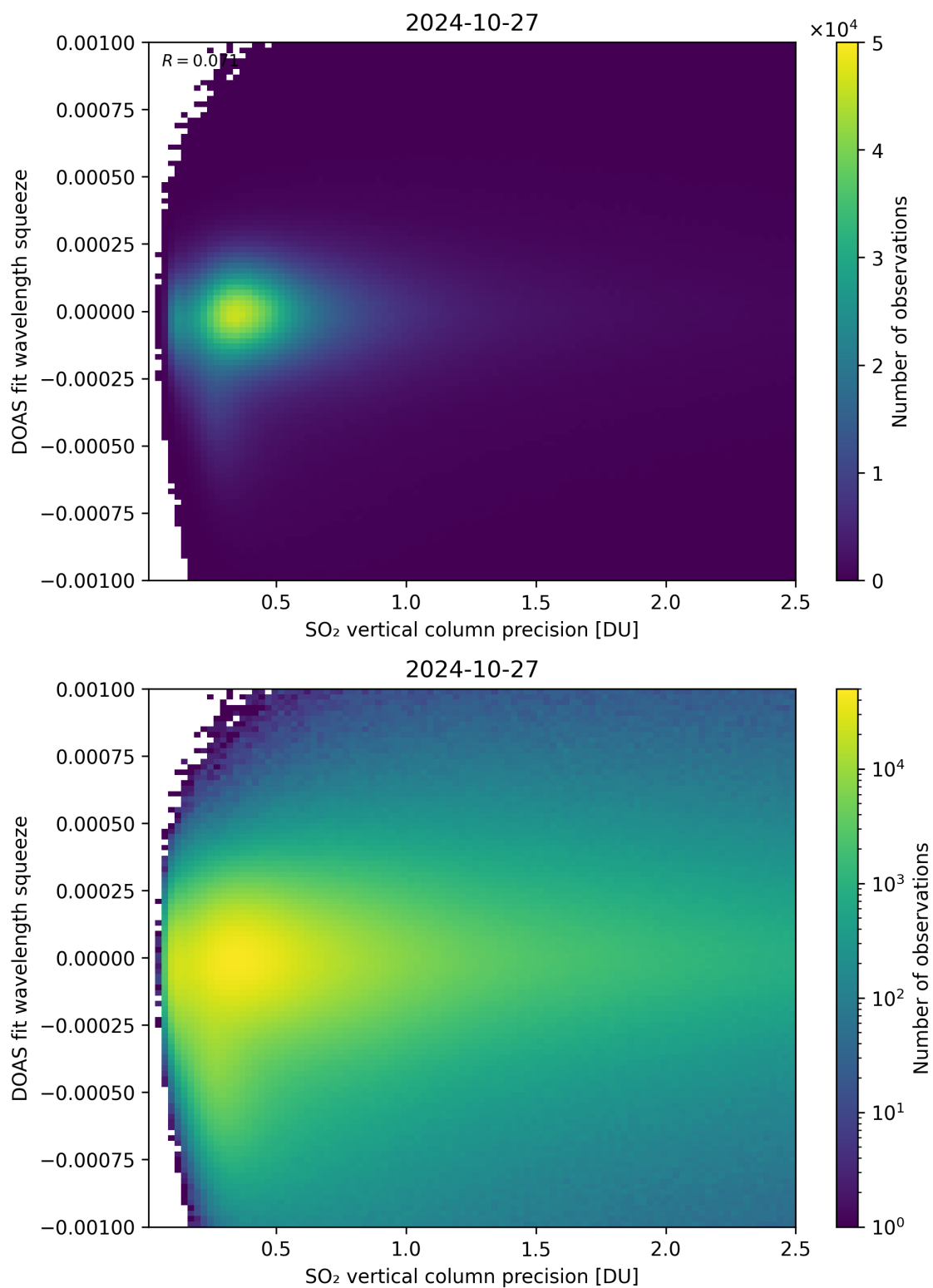
Figure 283: Scatter density plot of “SO 2 vertical column precision” against “DOAS fit wavelength squeeze” for 2024-10-26 to 2024-10-28.
