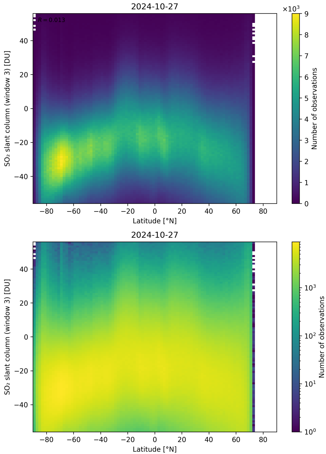
Figure 152: Scatter density plot of “Latitude” against “SO 2 slant column (window 3)” for 2024-10-26 to 2024-10-28.
