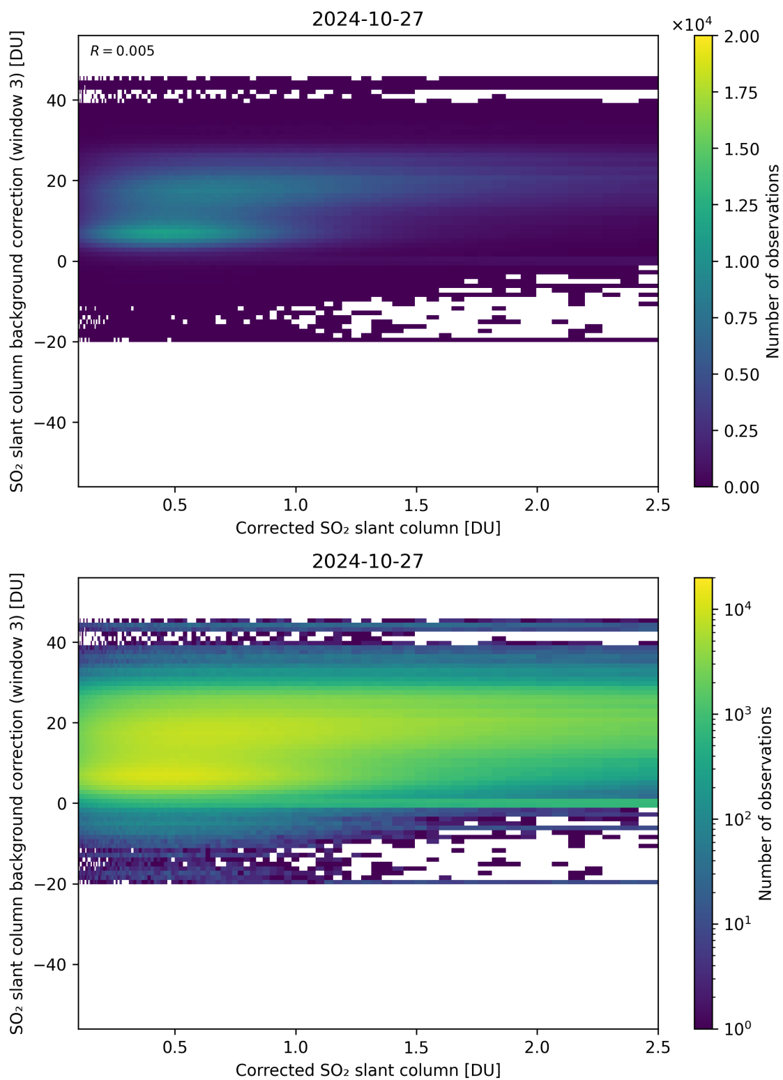
Figure 180: Scatter density plot of “Corrected SO 2 slant column” against “SO 2 slant column background correction (window 3)” for 2024-10-26 to 2024-10-28.
