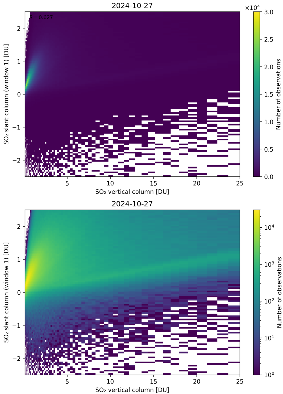
Figure 300: Scatter density plot of “SO 2 vertical column” against “SO 2 slant column (window 1)” for 2024-10-26 to 2024-10-28.
