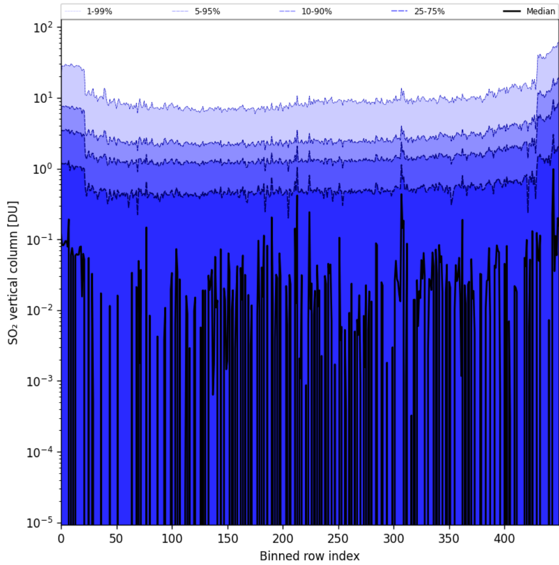
Figure 76: Along track statistics of “SO 2 vertical column” for 2024-10-26 to 2024-10-28
