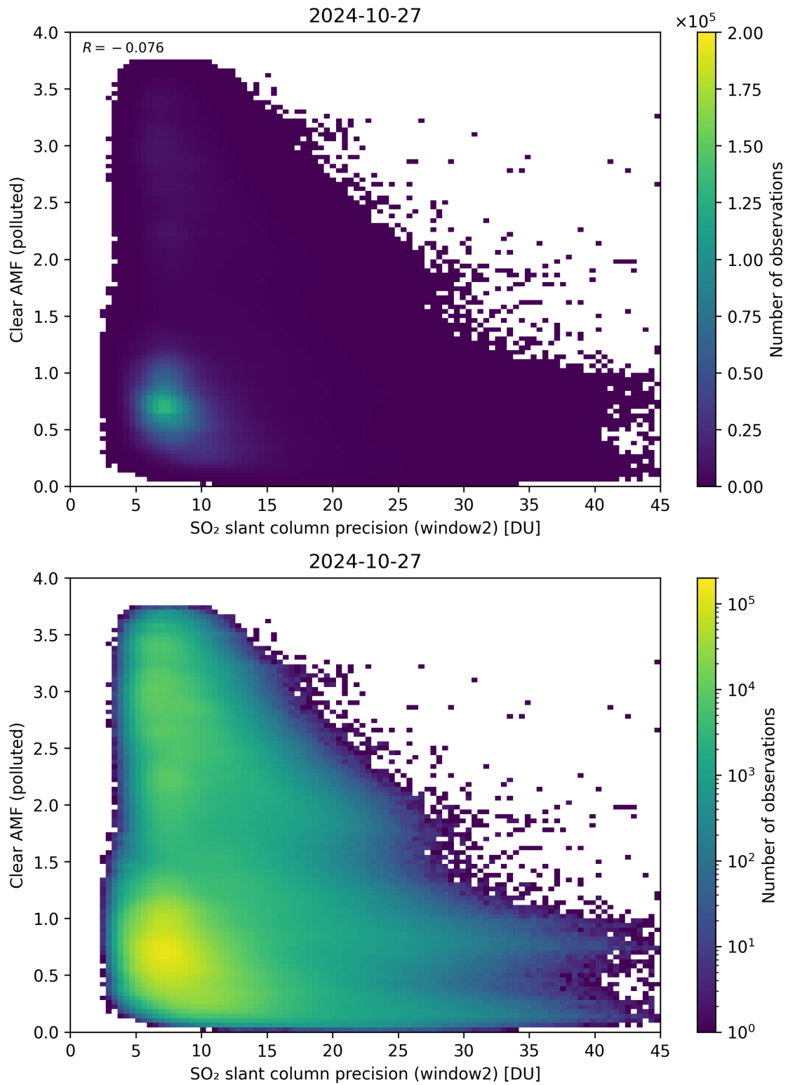
Figure 246: Scatter density plot of “SO 2 slant column precision (window2)” against “Clear AMF (polluted)” for 2024-10-26 to 2024-10-28.
