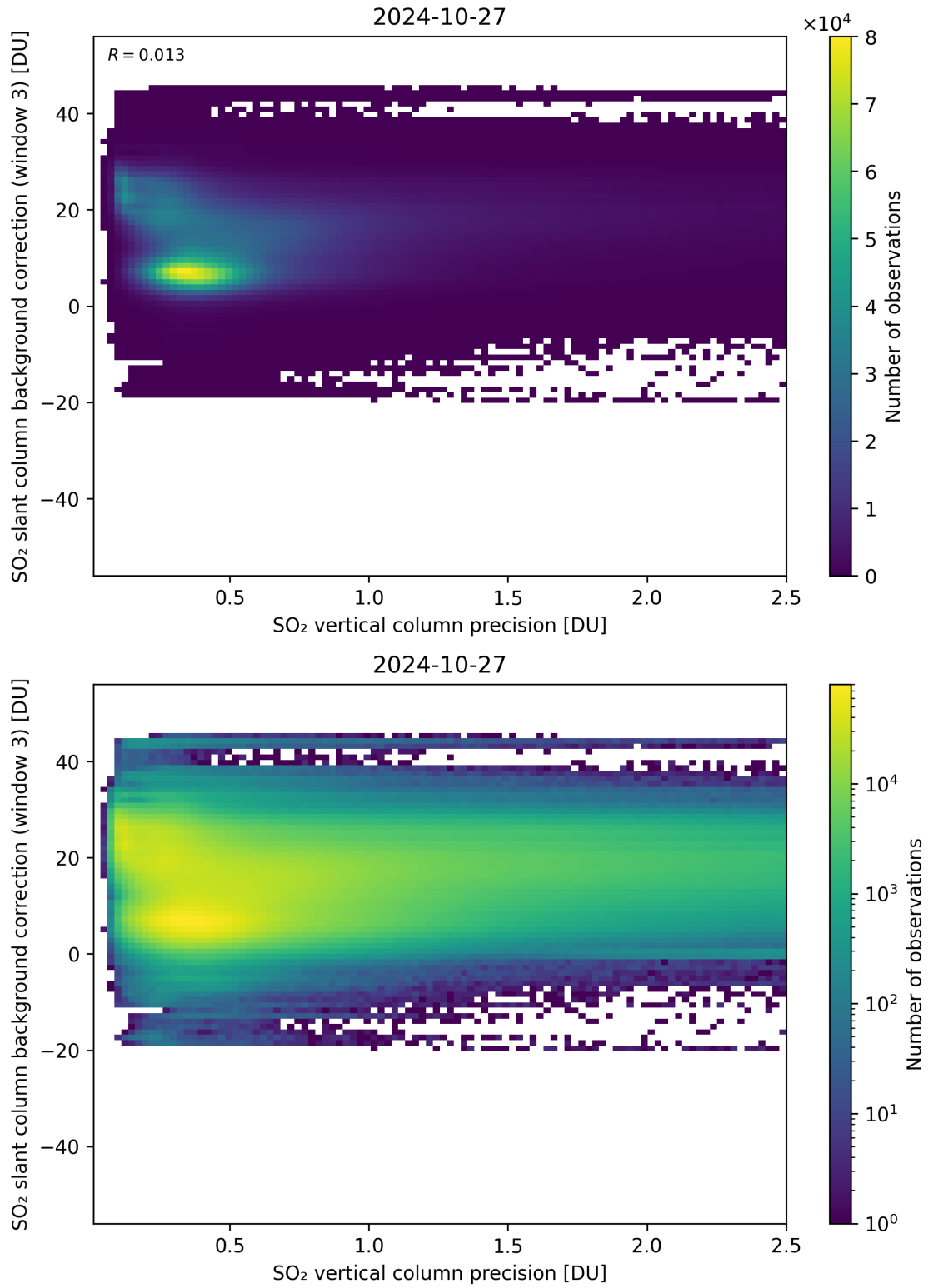
Figure 281: Scatter density plot of “SO 2 vertical column precision” against “SO 2 slant column background correction (window 3)” for 2024-10-26 to 2024-10-28.
