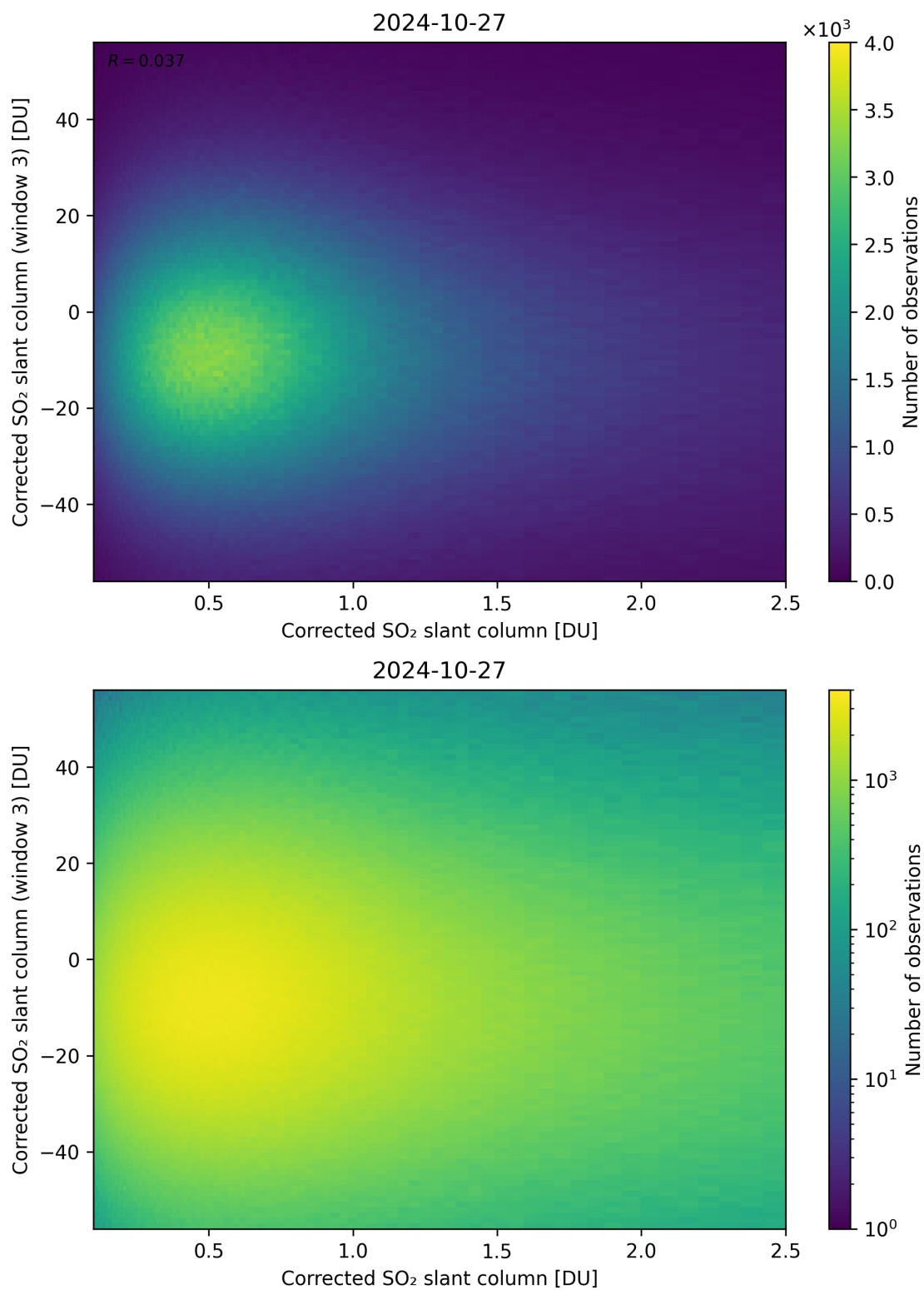
Figure 186: Scatter density plot of “Corrected SO 2 slant column” against “Corrected SO 2 slant column (window 3)” for 2024-10-26 to 2024-10-28.
