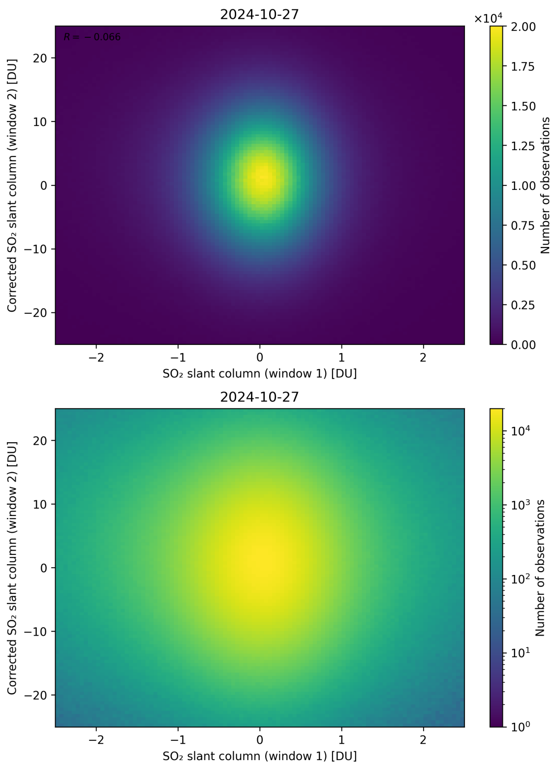
Figure 233: Scatter density plot of “SO 2 slant column (window 1)” against “Corrected SO 2 slant column (window 2)” for 2024-10-26 to 2024-10-28.
