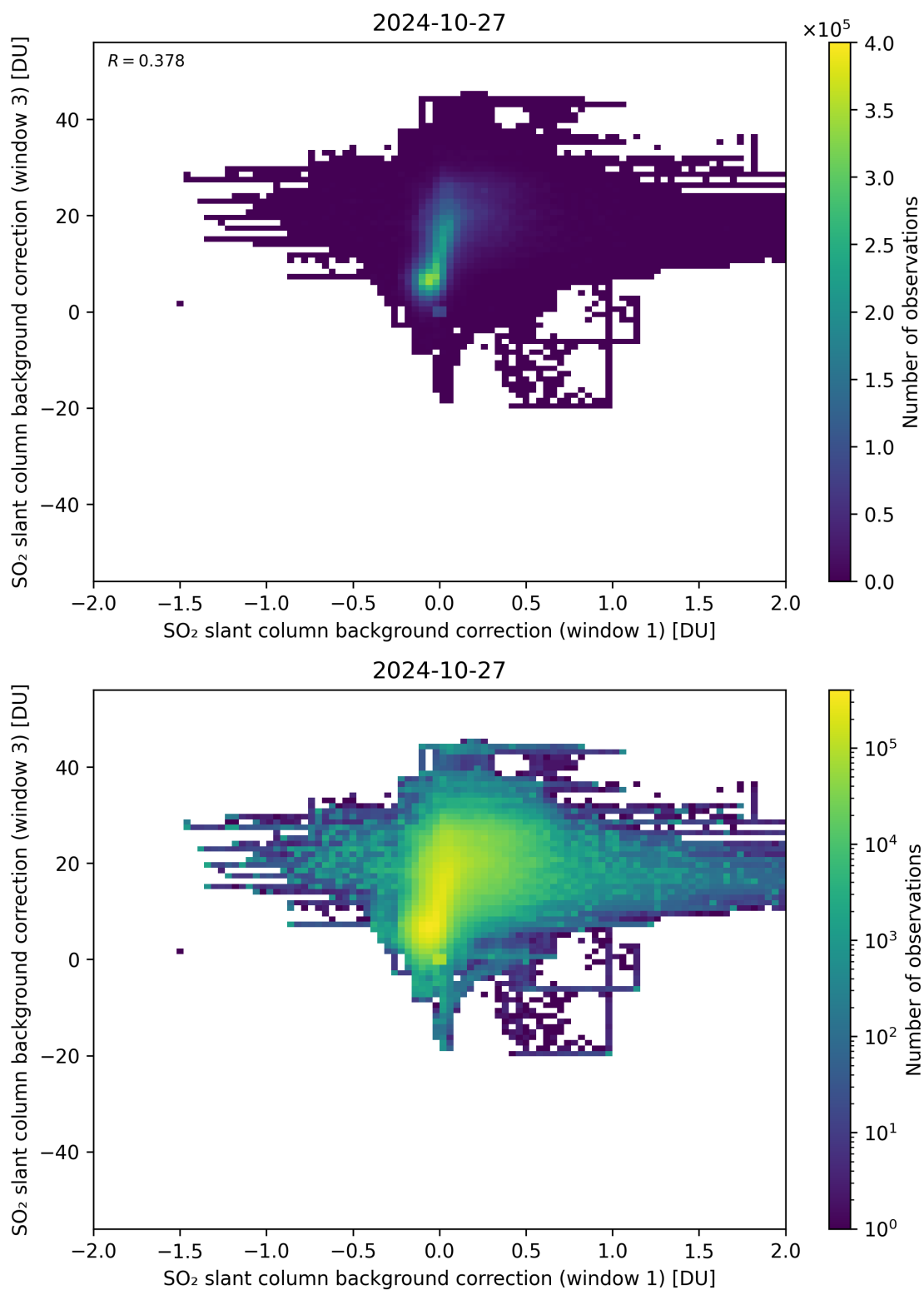
Figure 99: Scatter density plot of “SO 2 slant column background correction (window 1)” against “SO 2 slant column background correction (window 3)” for 2024-10-26 to 2024-10-28.
