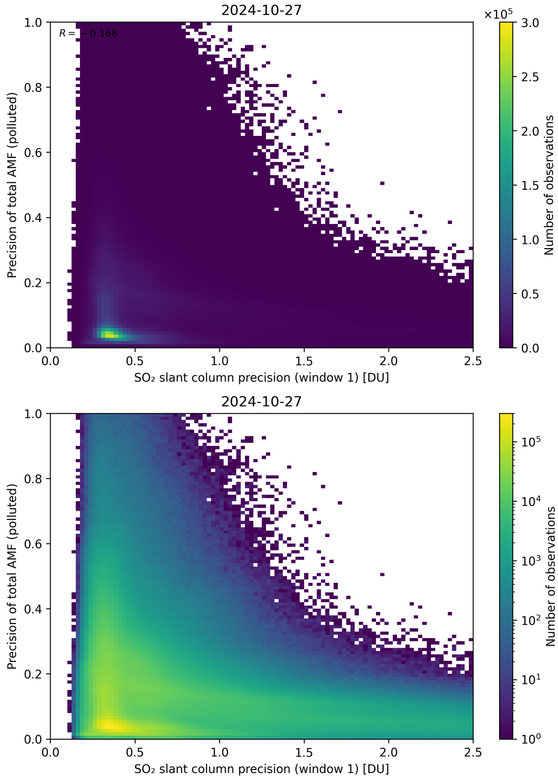
Figure 231: Scatter density plot of “SO 2 slant column precision (window 1)” against “Precision of total AMF (polluted)” for 2024-10-26 to 2024-10-28.
