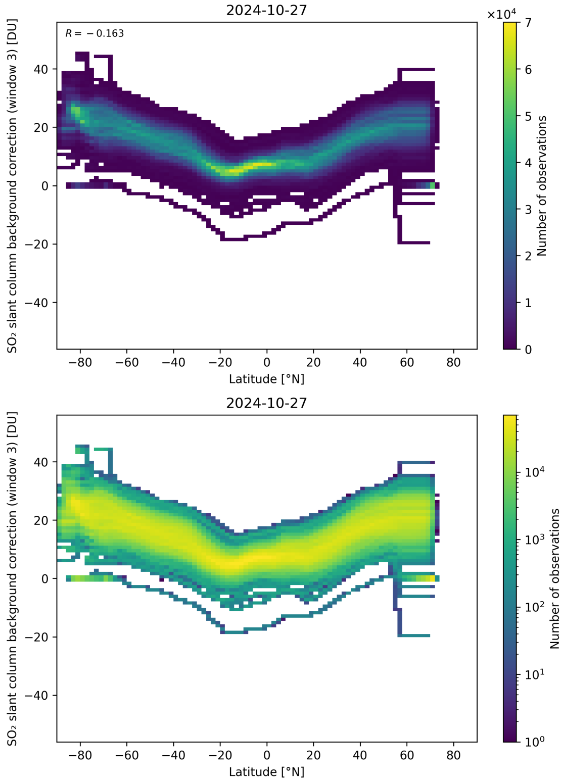
Figure 141: Scatter density plot of “Latitude” against “SO 2 slant column background correction (window 3)” for 2024-10-26 to 2024-10-28.
