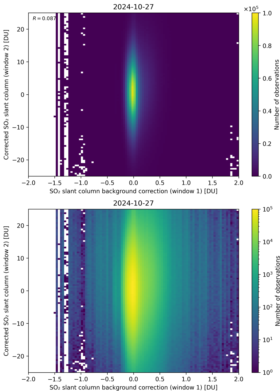
Figure 104: Scatter density plot of “SO 2 slant column background correction (window 1)” against “Corrected SO 2 slant column (window 2)” for 2024-10-26 to 2024-10-28.
