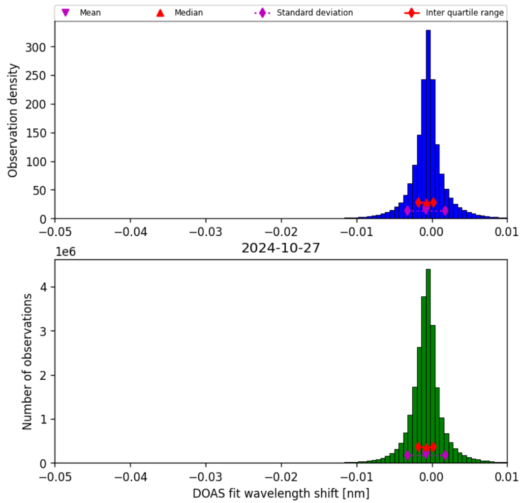
Figure 68: Histogram of “DOAS fit wavelength shift” for 2024-10-26 to 2024-10-28
