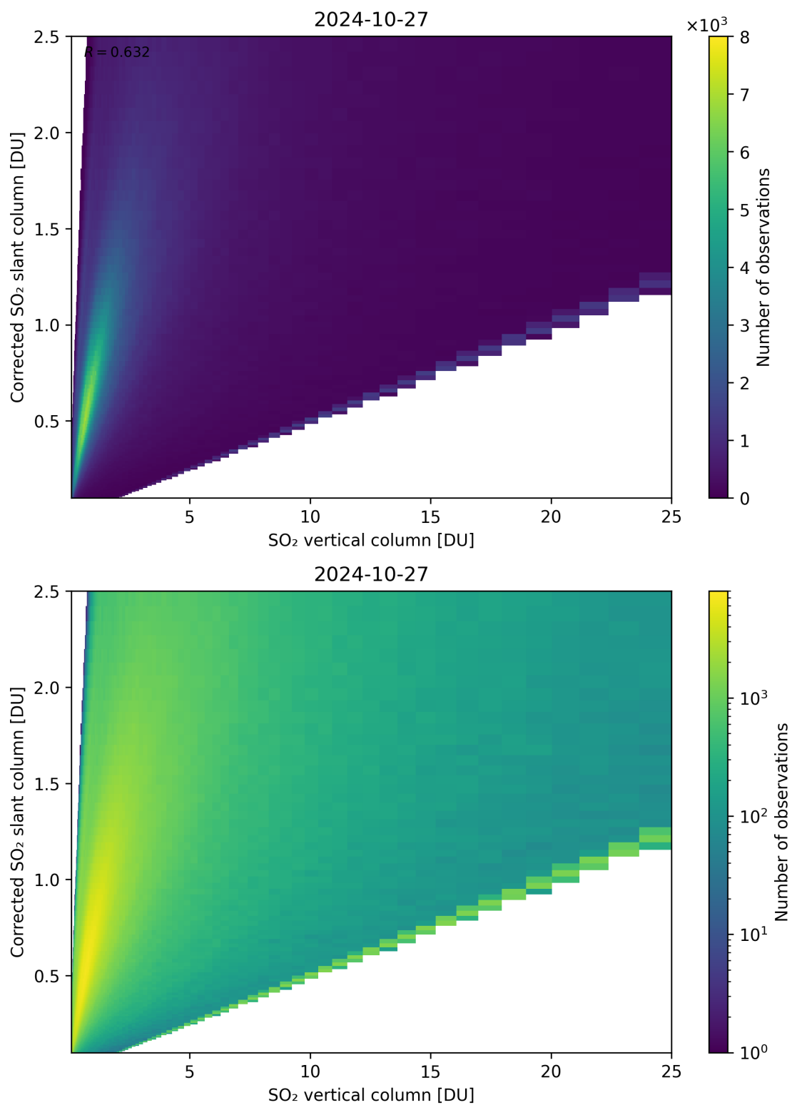
Figure 297: Scatter density plot of “SO 2 vertical column” against “Corrected SO 2 slant column” for 2024-10-26 to 2024-10-28.
