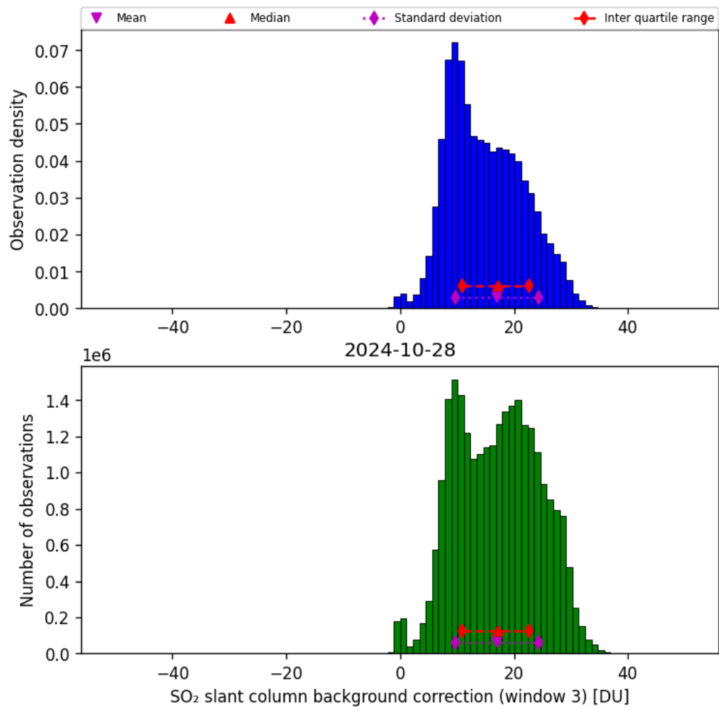
Figure 67: Histogram of “SO 2 slant column background correction (window 3)” for 2024-10-27 to 2024-10-29
