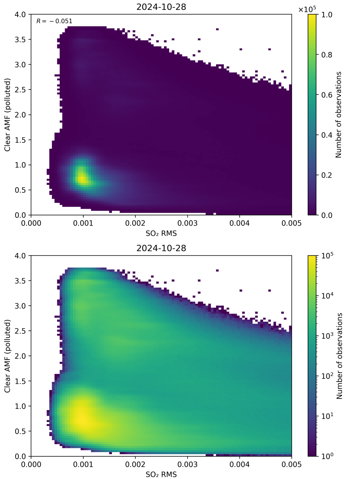
Figure 136: Scatter density plot of “SO 2 RMS” against “Clear AMF (polluted)” for 2024-10-27 to 2024-10-29.
