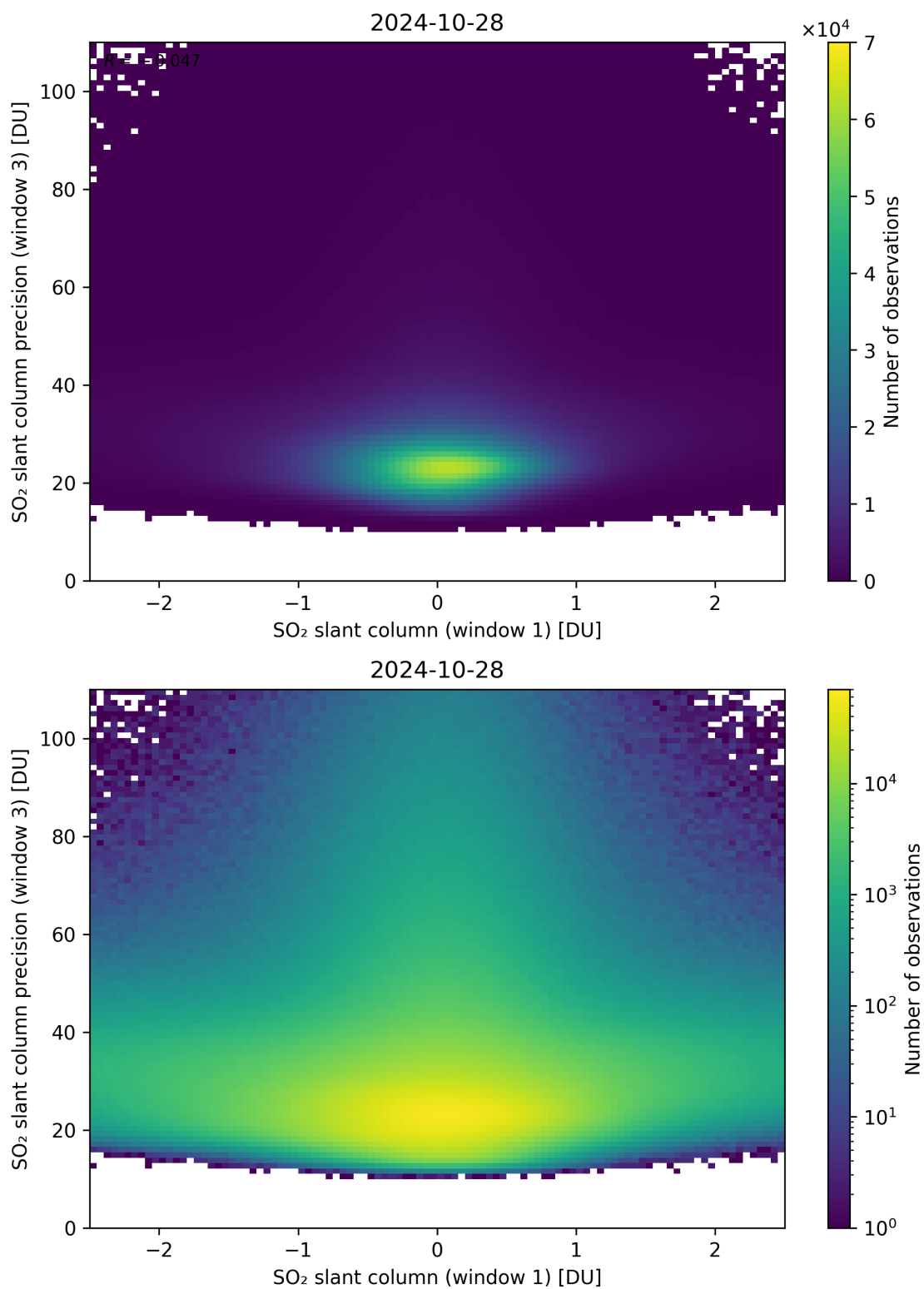
Figure 238: Scatter density plot of “SO 2 slant column (window 1)” against “SO 2 slant column precision (window 3)” for 2024-10-27 to 2024-10-29.
