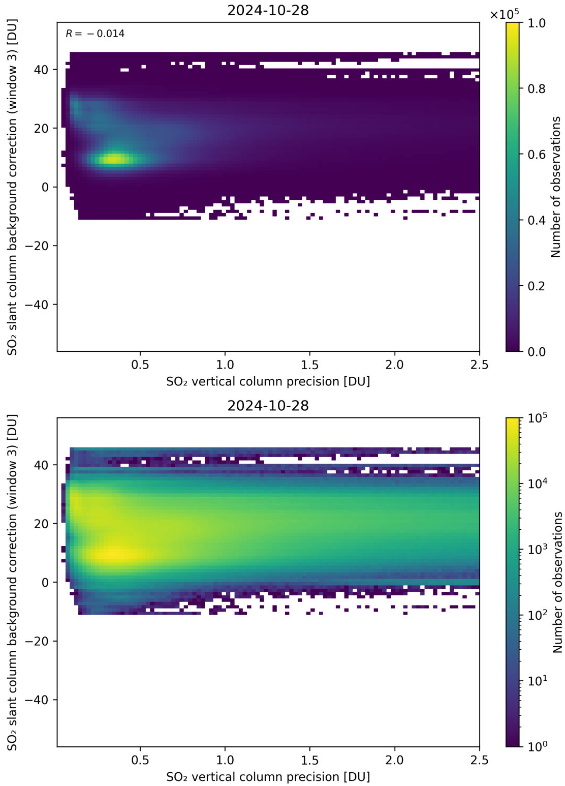
Figure 281: Scatter density plot of “SO 2 vertical column precision” against “SO 2 slant column background correction (window 3)” for 2024-10-27 to 2024-10-29.
