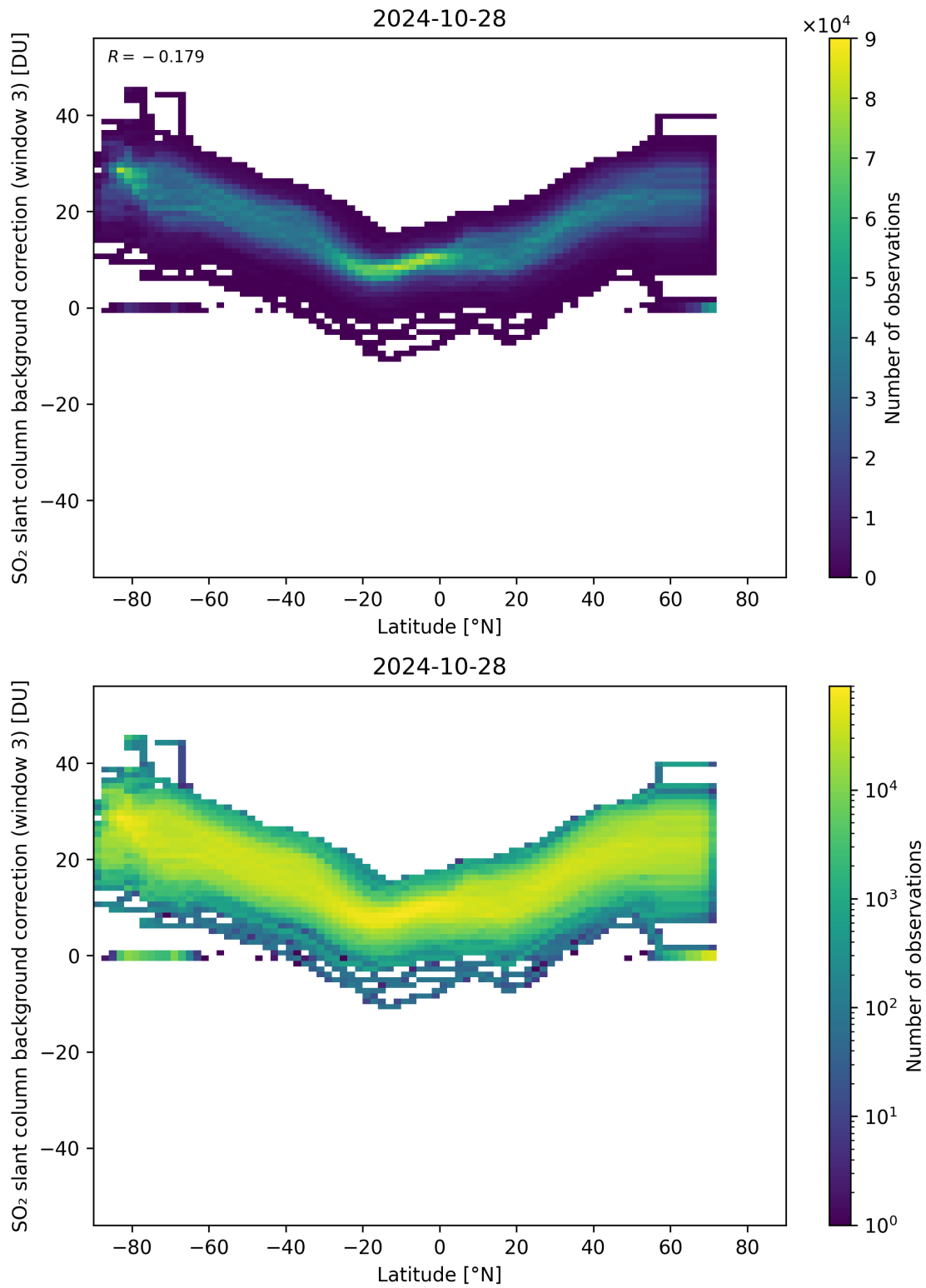
Figure 141: Scatter density plot of “Latitude” against “SO 2 slant column background correction (window 3)” for 2024-10-27 to 2024-10-29.
