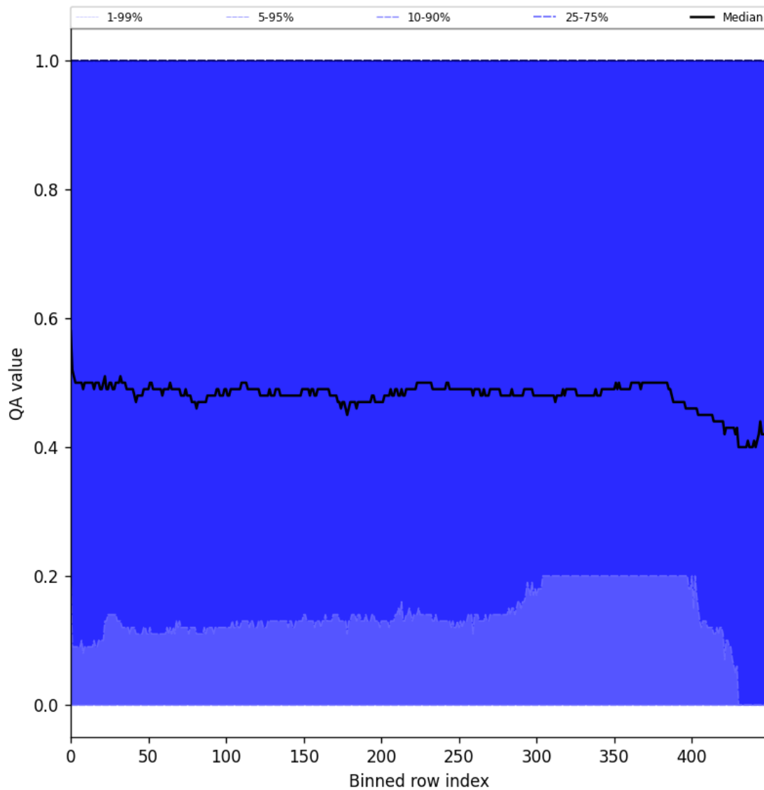
Figure 75: Along track statistics of “QA value” for 2024-10-27 to 2024-10-29
