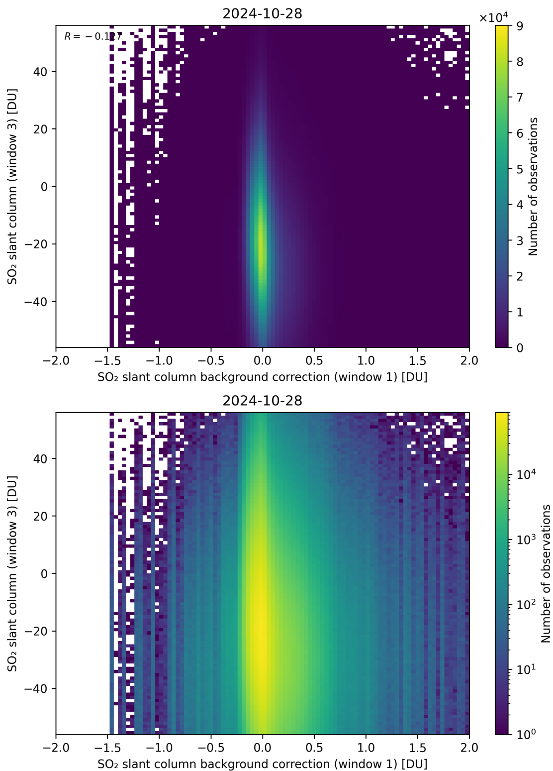
Figure 107: Scatter density plot of “SO 2 slant column background correction (window 1)” against “SO 2 slant column (window 3)” for 2024-10-27 to 2024-10-29.
