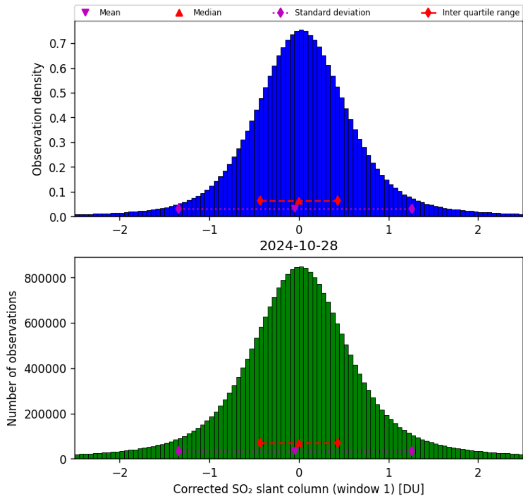
Figure 58: Histogram of “Corrected SO 2 slant column (window 1)” for 2024-10-27 to 2024-10-29
