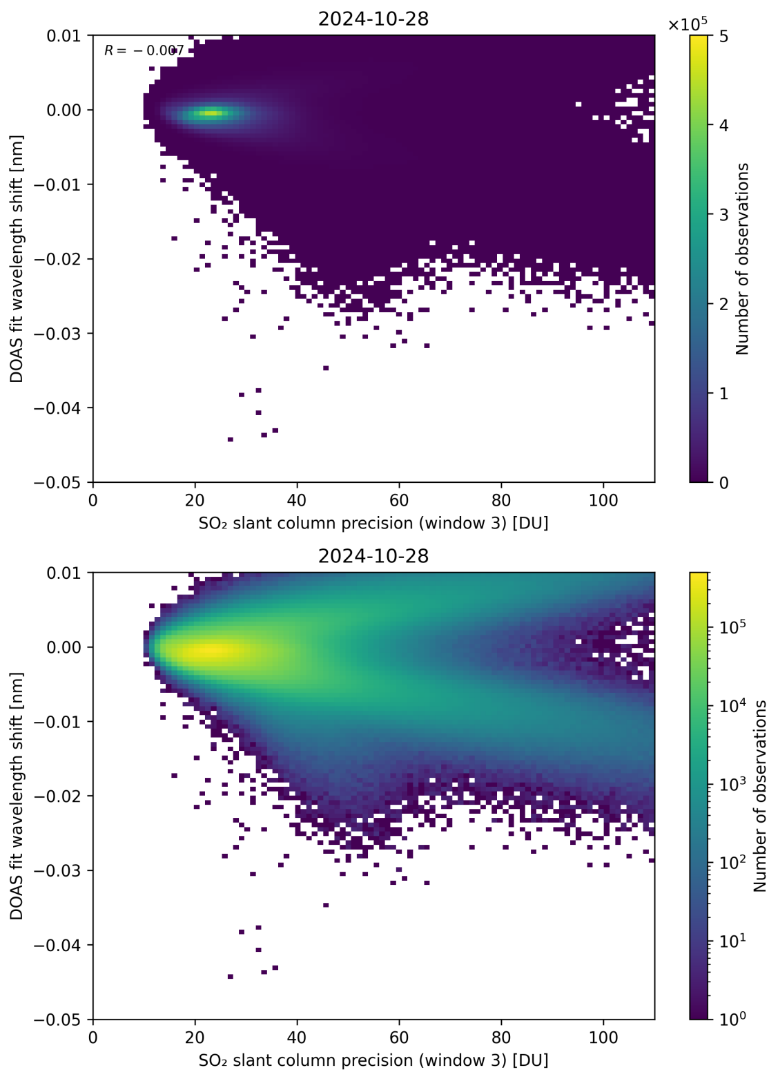
Figure 258: Scatter density plot of “SO 2 slant column precision (window 3)” against “DOAS fit wavelength shift” for 2024-10-27 to 2024-10-29.
