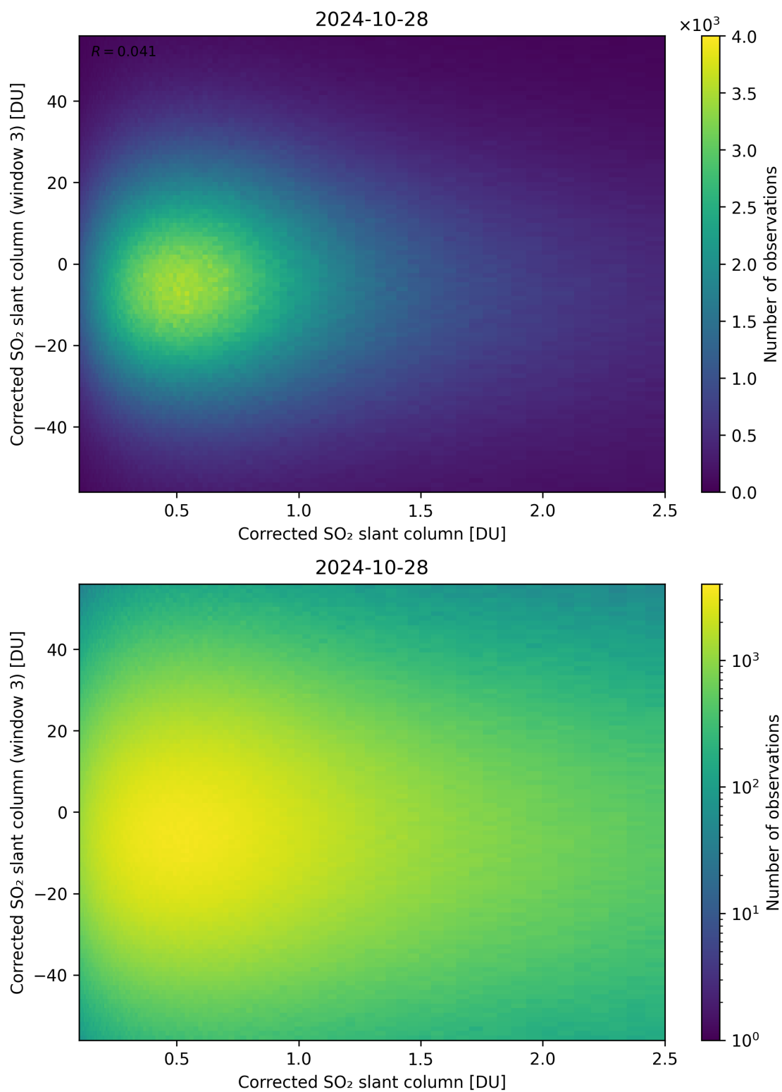
Figure 186: Scatter density plot of “Corrected SO 2 slant column” against “Corrected SO 2 slant column (window 3)” for 2024-10-27 to 2024-10-29.
