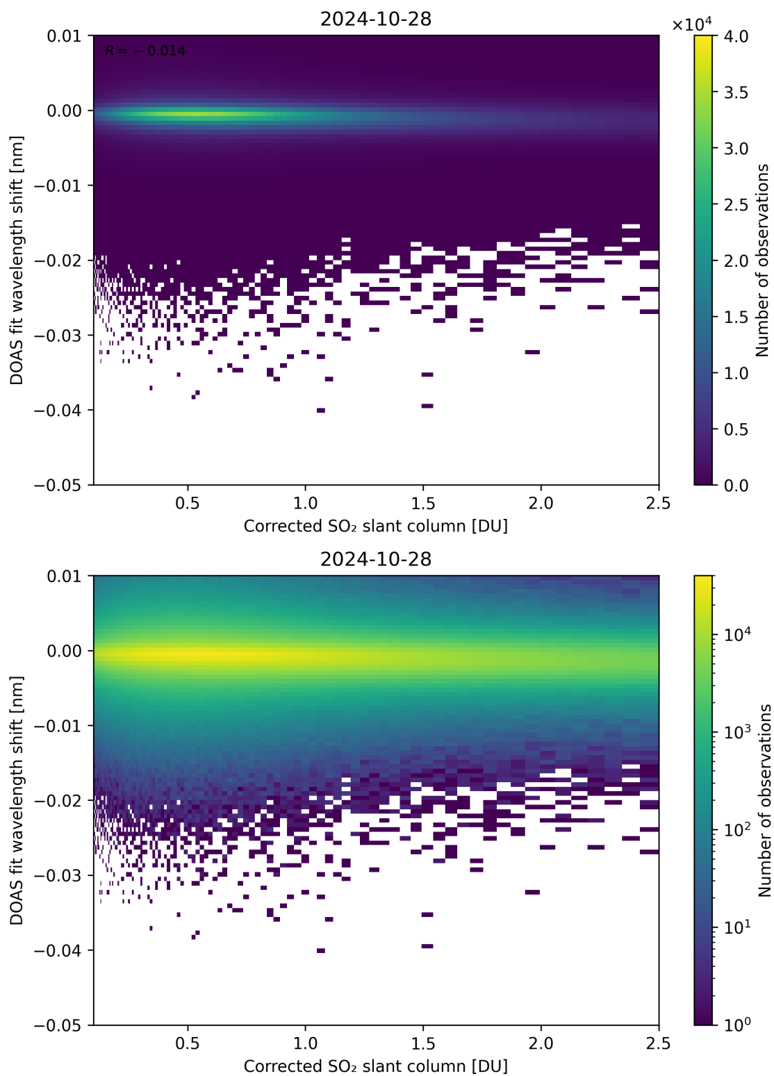
Figure 181: Scatter density plot of “Corrected SO 2 slant column” against “DOAS fit wavelength shift” for 2024-10-27 to 2024-10-29.
