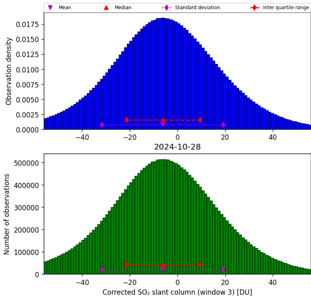
Figure 66: Histogram of “Corrected SO 2 slant column (window 3)” for 2024-10-27 to 2024-10-29
