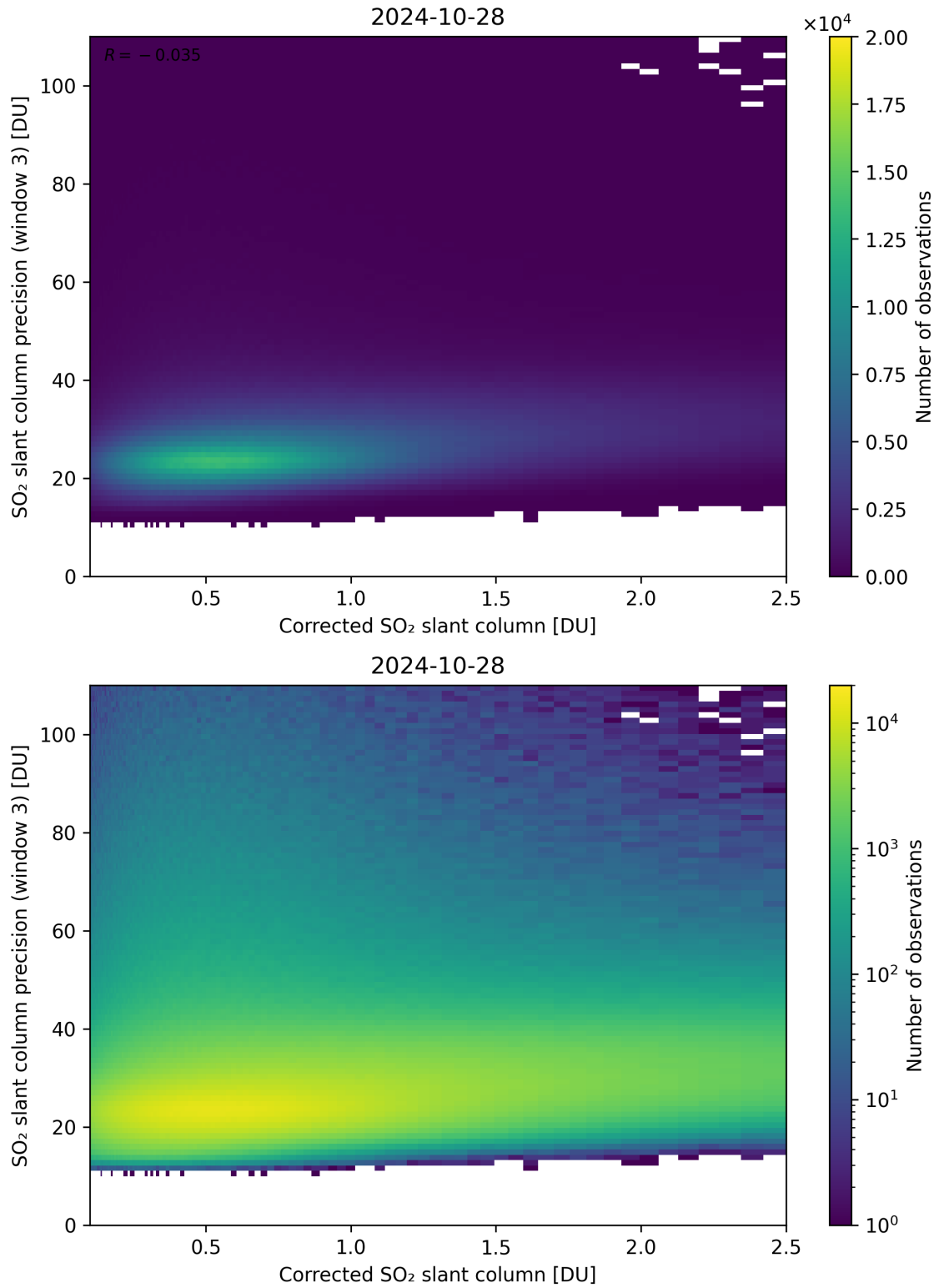
Figure 191: Scatter density plot of “Corrected SO 2 slant column” against “SO 2 slant column precision (window 3)” for 2024-10-27 to 2024-10-29.
