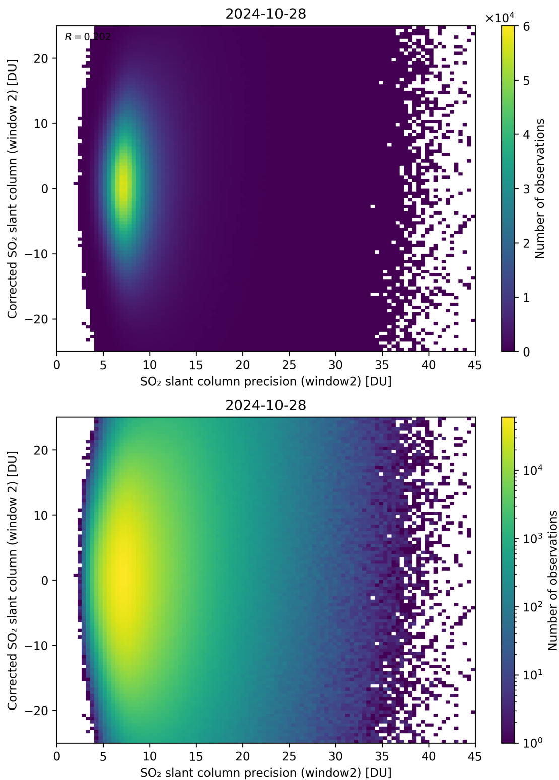
Figure 247: Scatter density plot of “SO 2 slant column precision (window2)” against “Corrected SO 2 slant column (window 2)” for 2024-10-27 to 2024-10-29.
