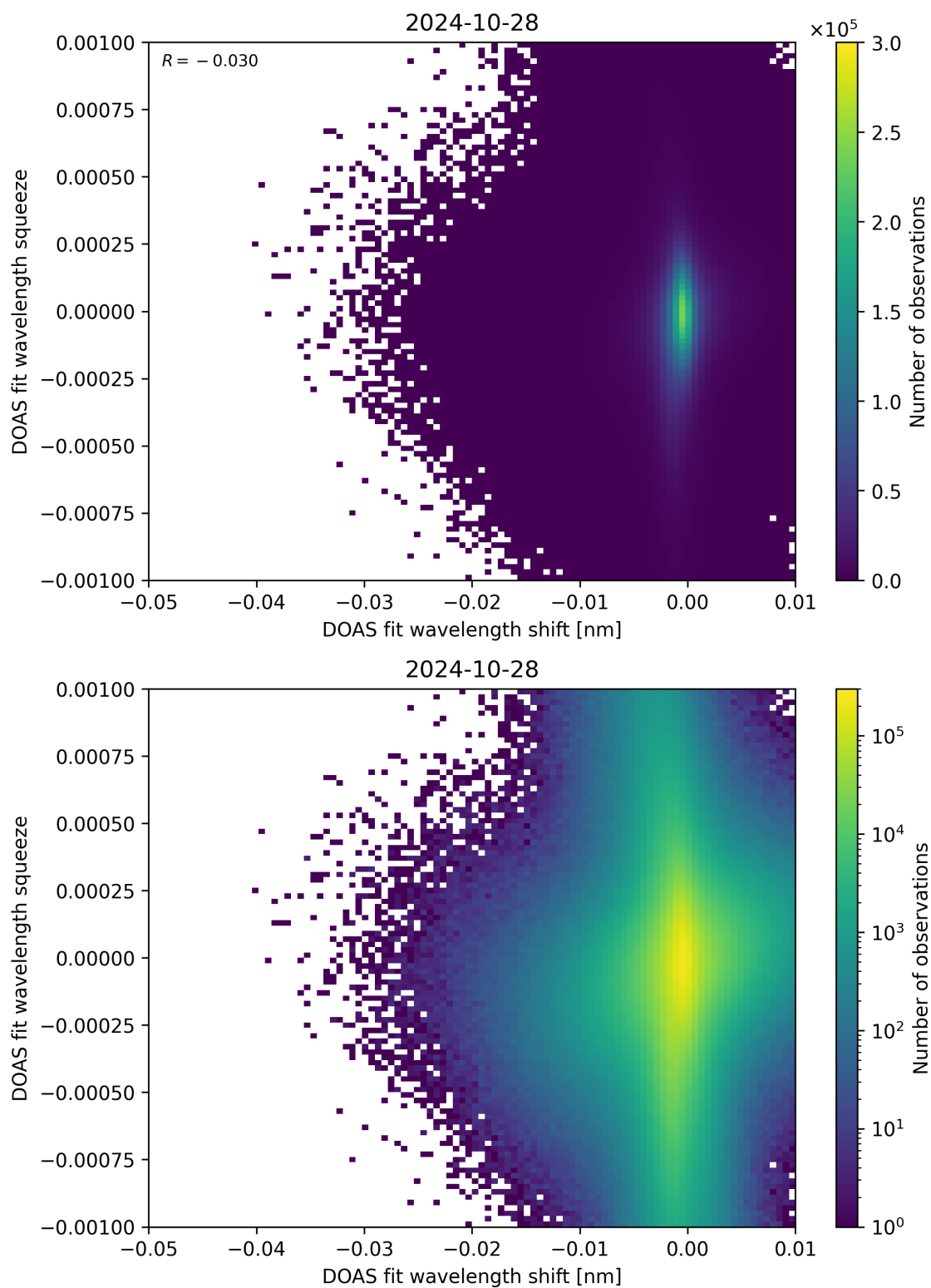
Figure 127: Scatter density plot of “DOAS fit wavelength shift” against “DOAS fit wavelength squeeze” for 2024-10-27 to 2024-10-29.
