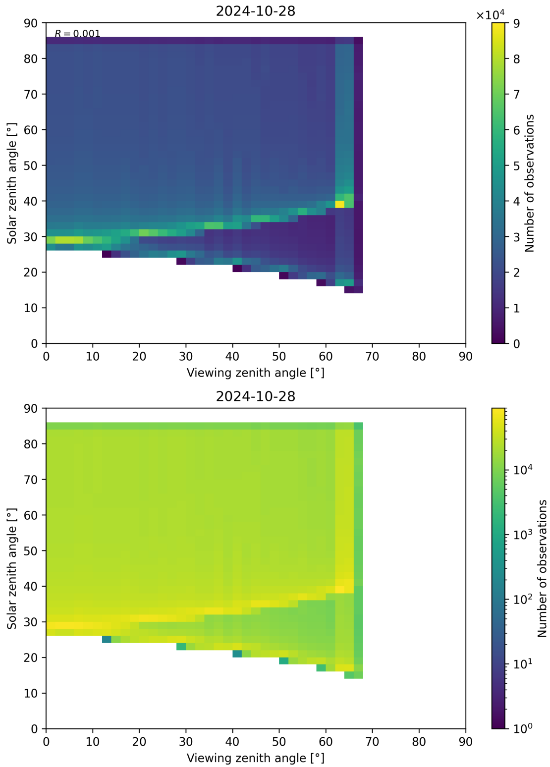
Figure 315: Scatter density plot of “Viewing zenith angle” against “Solar zenith angle” for 2024-10-27 to 2024-10-29.
