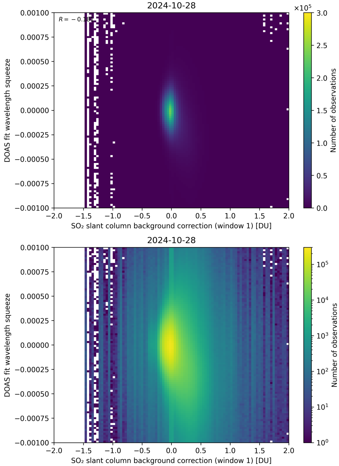
Figure 101: Scatter density plot of “SO 2 slant column background correction (window 1)” against “DOAS fit wavelength squeeze” for 2024-10-27 to 2024-10-29.
