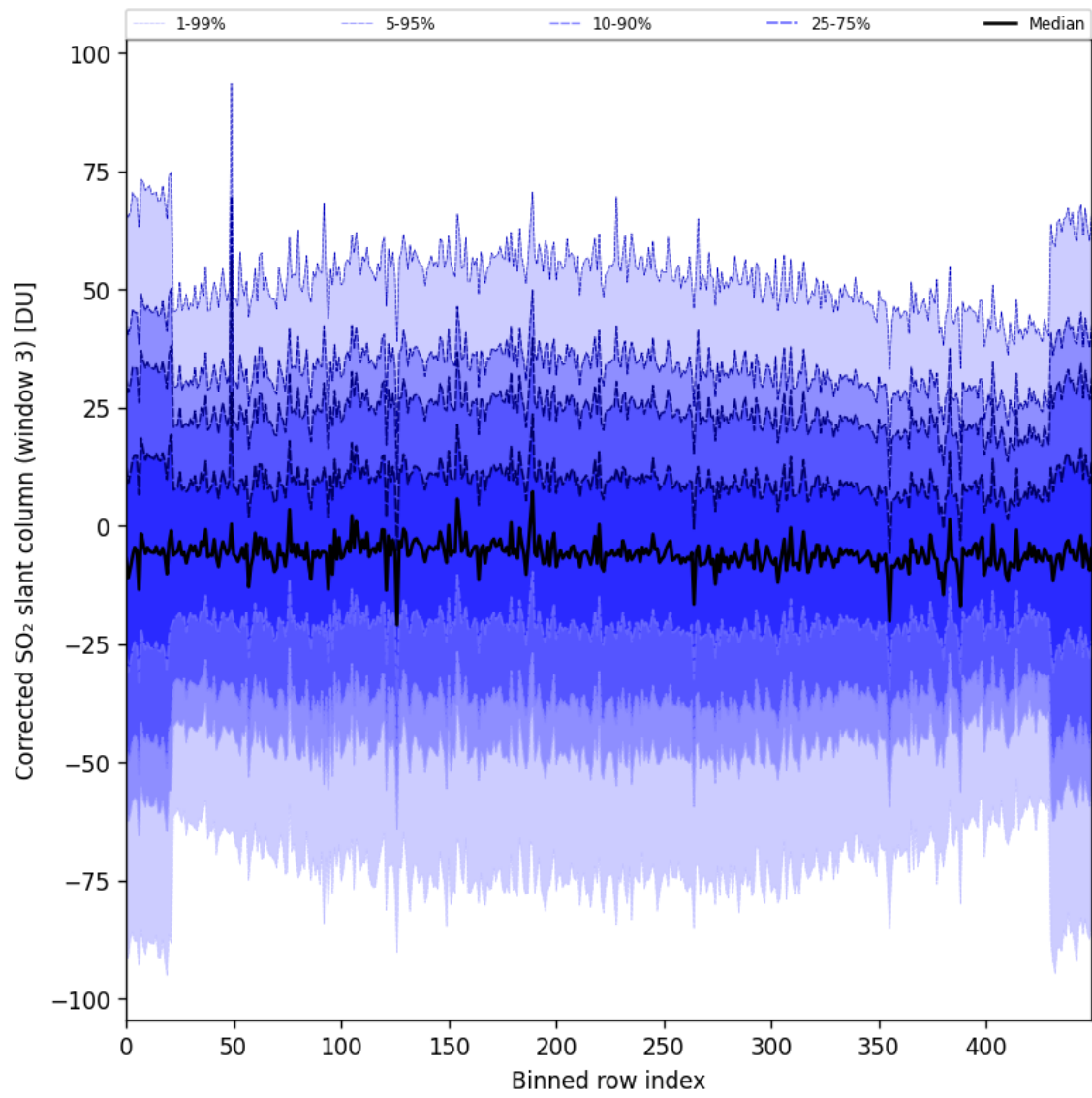
Figure 89: Along track statistics of “Corrected SO 2 slant column (window 3)” for 2024-10-27 to 2024-10-29
