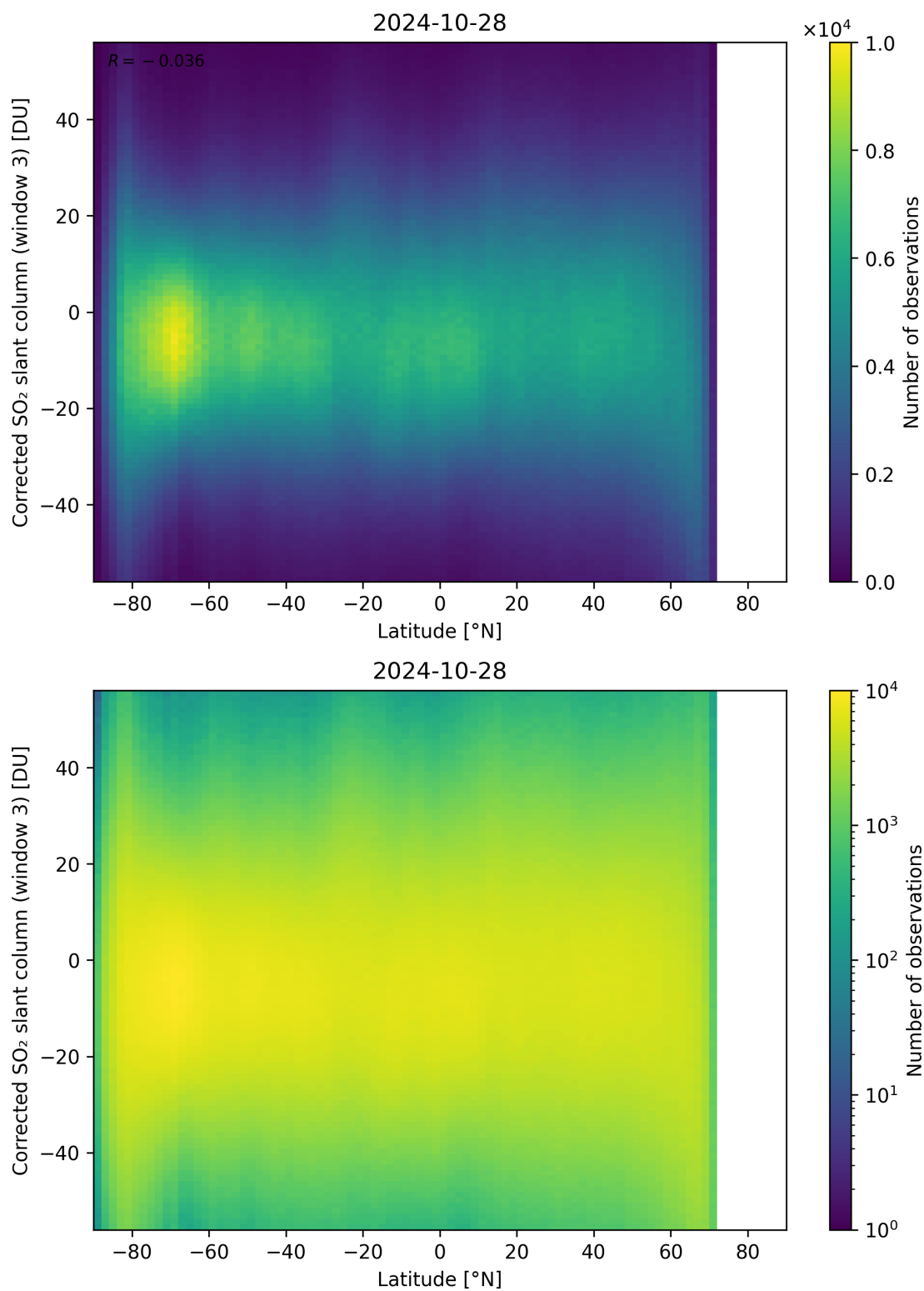
Figure 148: Scatter density plot of “Latitude” against “Corrected SO 2 slant column (window 3)” for 2024-10-27 to 2024-10-29.
