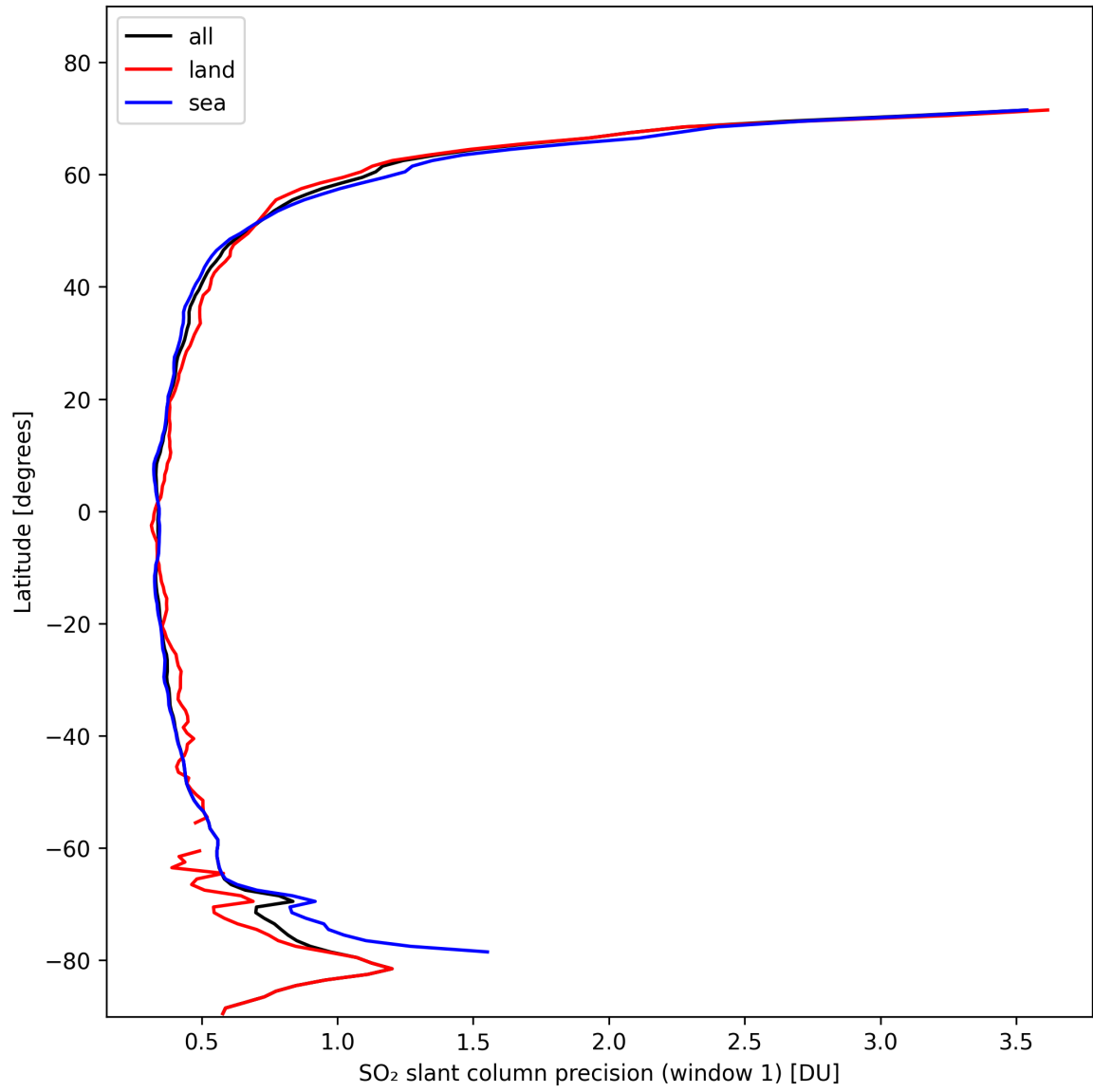
Figure 34: Zonal average of “SO 2 slant column precision (window 1)” for 2024-10-27 to 2024-10-29.
