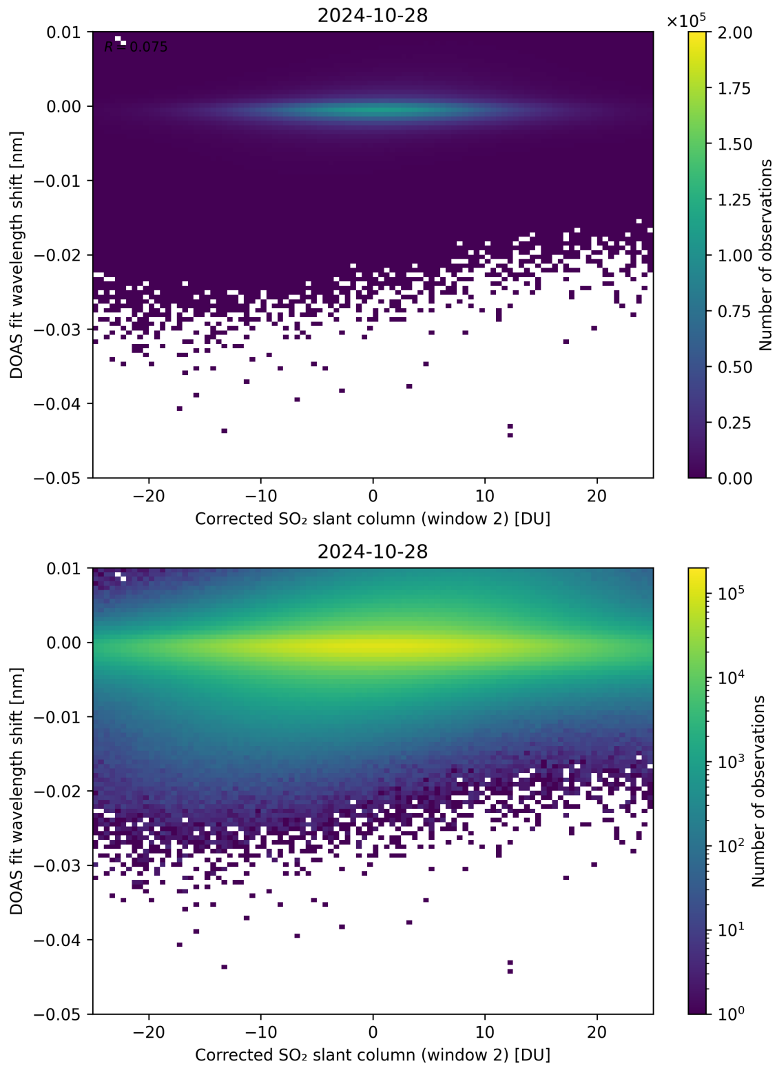
Figure 196: Scatter density plot of “Corrected SO 2 slant column (window 2)” against “DOAS fit wavelength shift” for 2024-10-27 to 2024-10-29.
