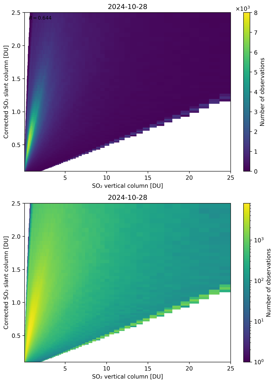
Figure 297: Scatter density plot of “SO 2 vertical column” against “Corrected SO 2 slant column” for 2024-10-27 to 2024-10-29.
