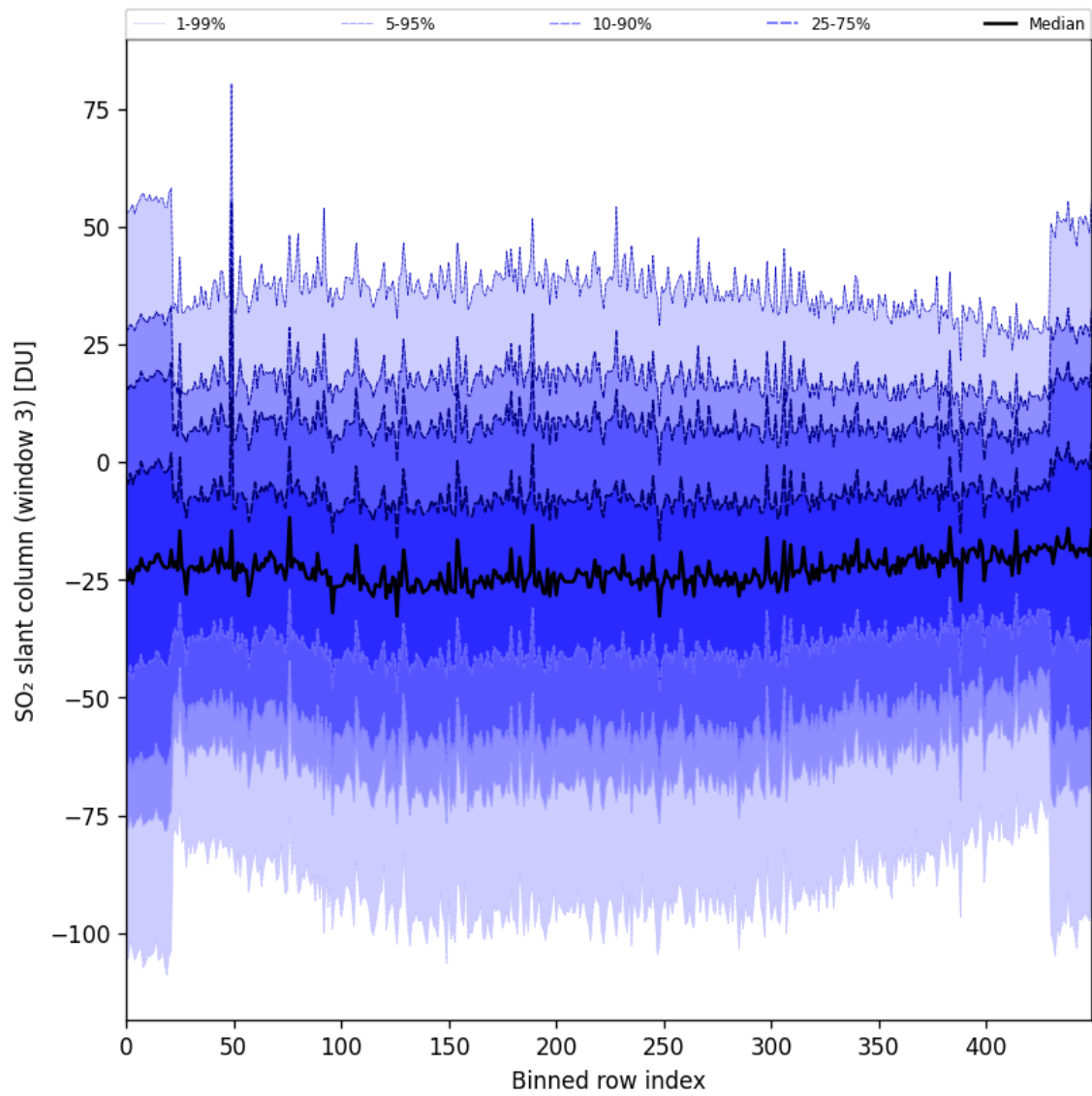
Figure 87: Along track statistics of “SO 2 slant column (window 3)” for 2024-10-27 to 2024-10-29
