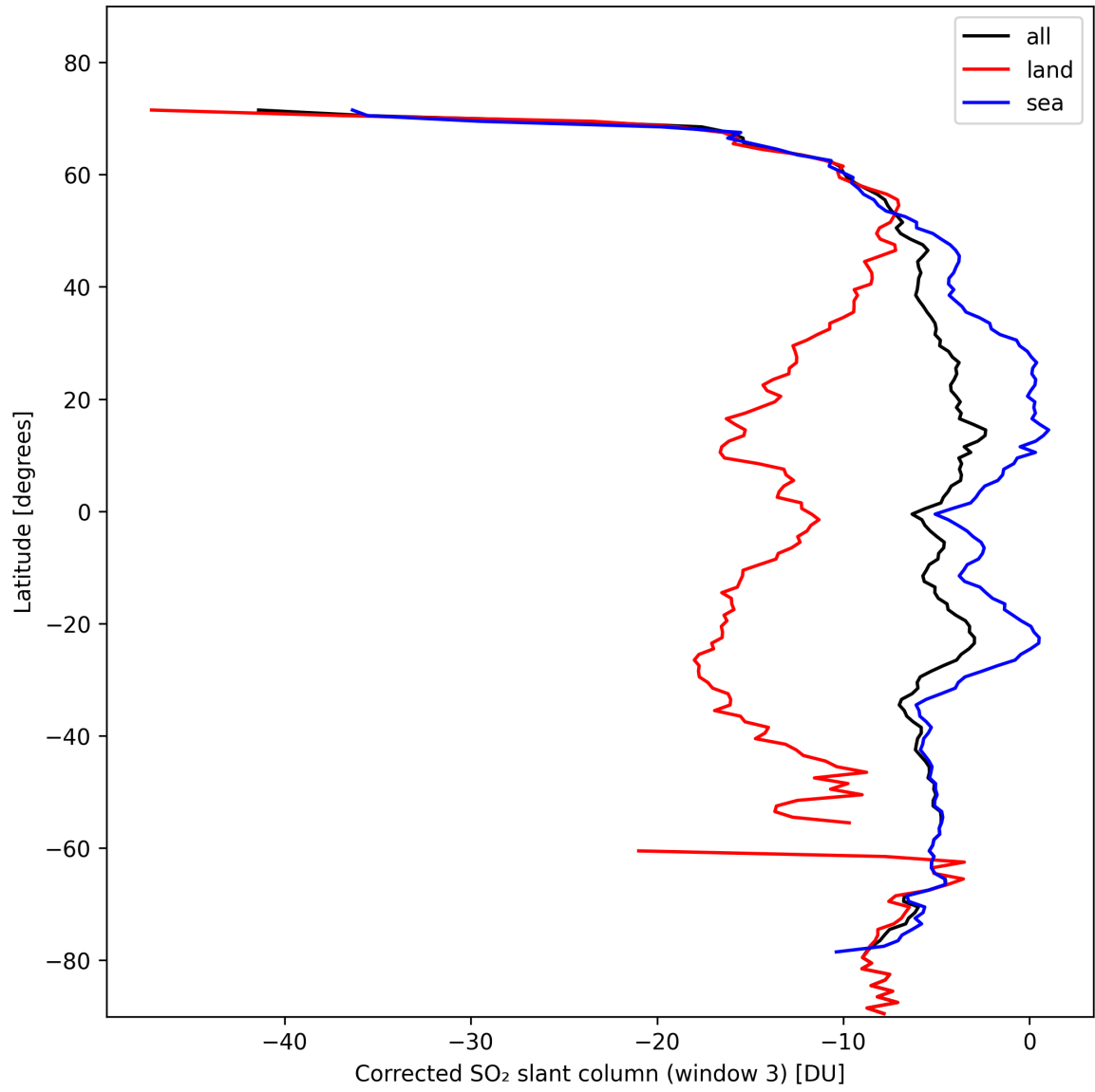
Figure 43: Zonal average of “Corrected SO 2 slant column (window 3)” for 2024-10-27 to 2024-10-29.
