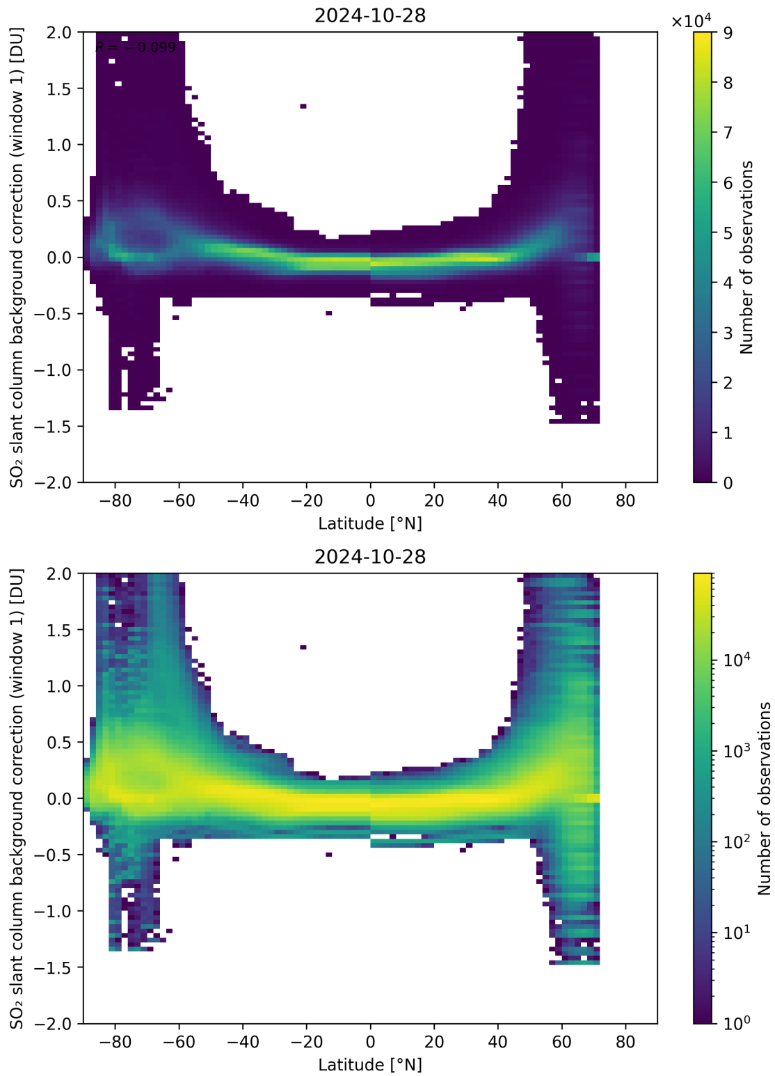
Figure 139: Scatter density plot of “Latitude” against “SO 2 slant column background correction (window 1)” for 2024-10-27 to 2024-10-29.
