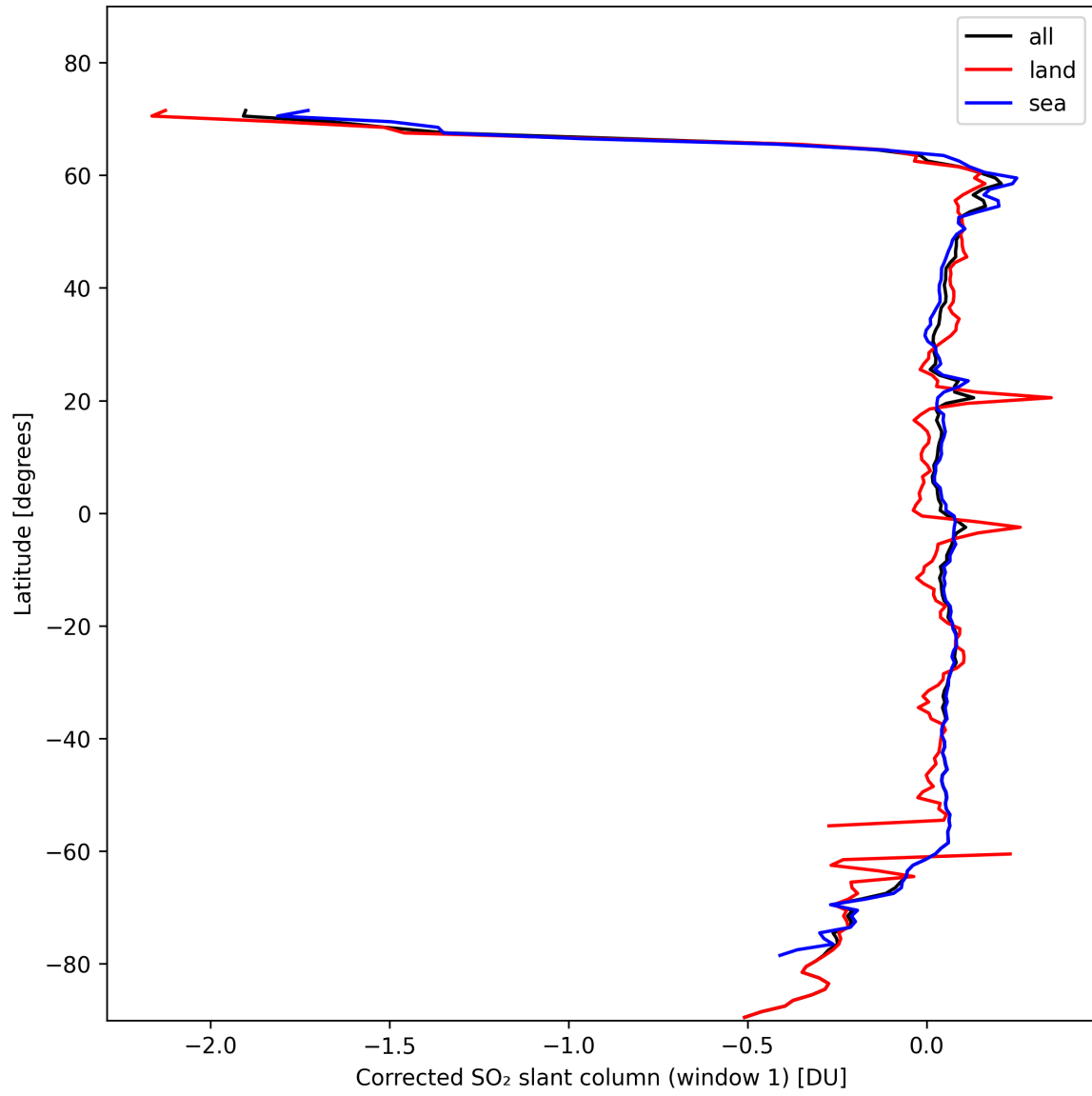
Figure 35: Zonal average of “Corrected SO 2 slant column (window 1)” for 2024-10-27 to 2024-10-29.
