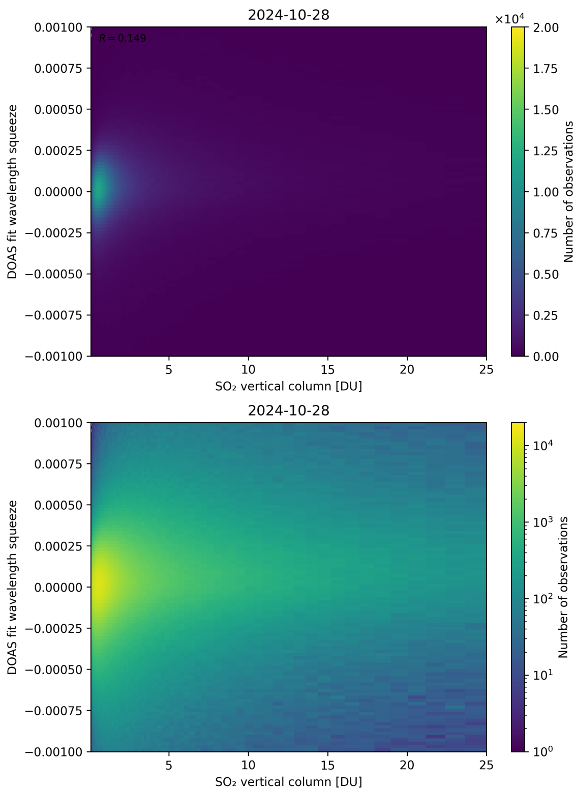
Figure 277: Scatter density plot of “SO 2 vertical column” against “DOAS fit wavelength squeeze” for 2024-10-27 to 2024-10-29.
