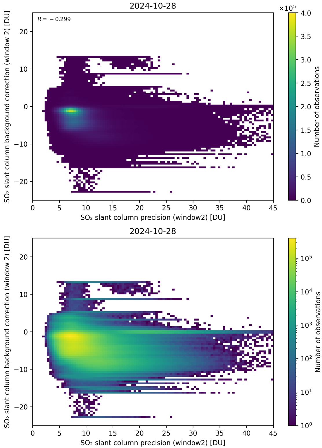
Figure 241: Scatter density plot of “SO 2 slant column precision (window2)” against “SO 2 slant column background correction (window 2)” for 2024-10-27 to 2024-10-29.
