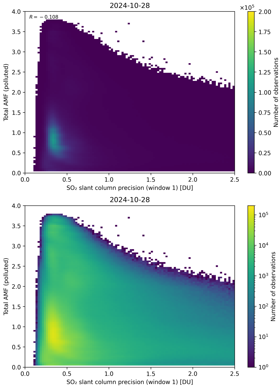
Figure 230: Scatter density plot of “SO 2 slant column precision (window 1)” against “Total AMF (polluted)” for 2024-10-27 to 2024-10-29.
