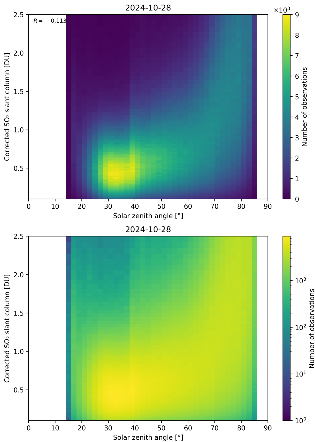
Figure 166: Scatter density plot of “Solar zenith angle” against “Corrected SO 2 slant column” for 2024-10-27 to 2024-10-29.
