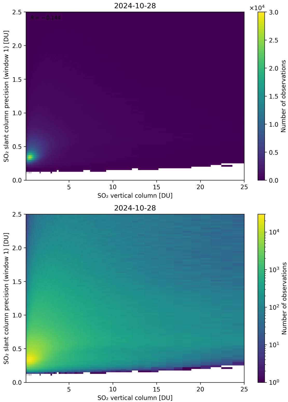
Figure 301: Scatter density plot of “SO 2 vertical column” against “SO 2 slant column precision (window 1)” for 2024-10-27 to 2024-10-29.
