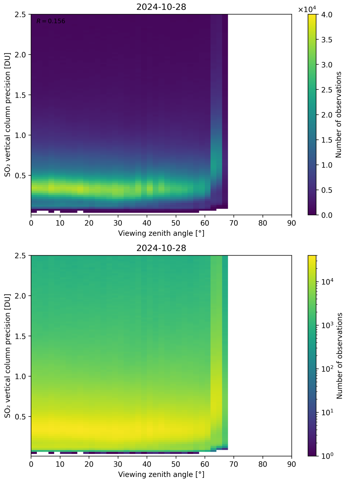
Figure 328: Scatter density plot of “Viewing zenith angle” against “SO 2 vertical column precision” for 2024-10-27 to 2024-10-29.
