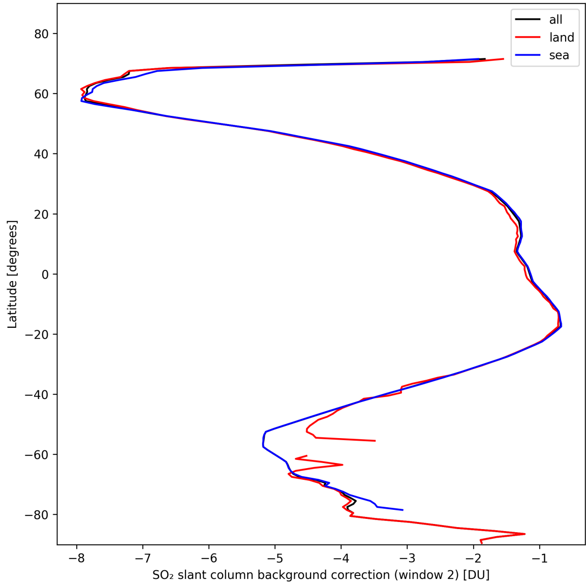
Figure 40: Zonal average of “SO 2 slant column background correction (window 2)” for 2024-10-27 to 2024-10-29.
