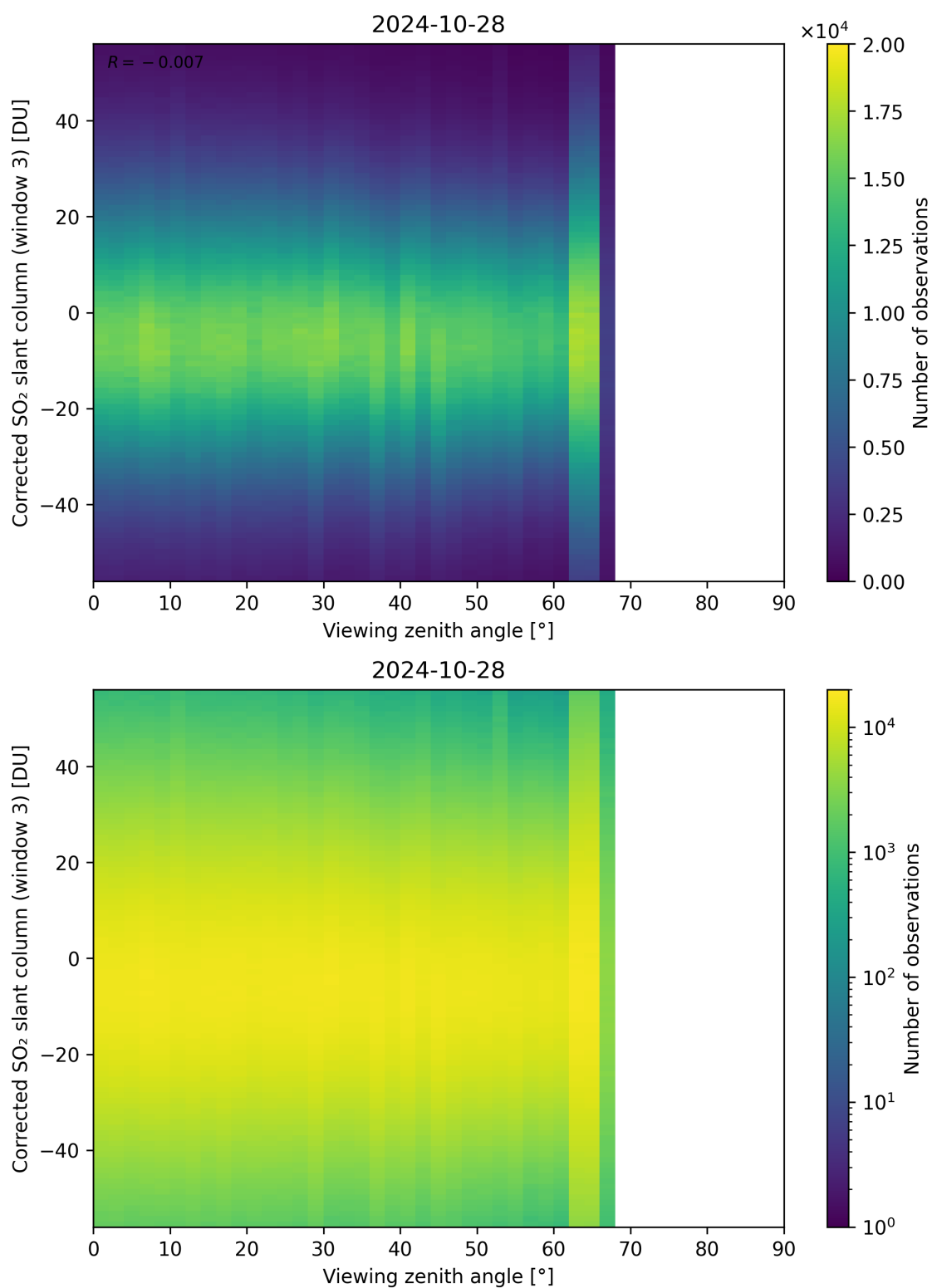
Figure 319: Scatter density plot of “Viewing zenith angle” against “Corrected SO 2 slant column (window 3)” for 2024-10-27 to 2024-10-29.
