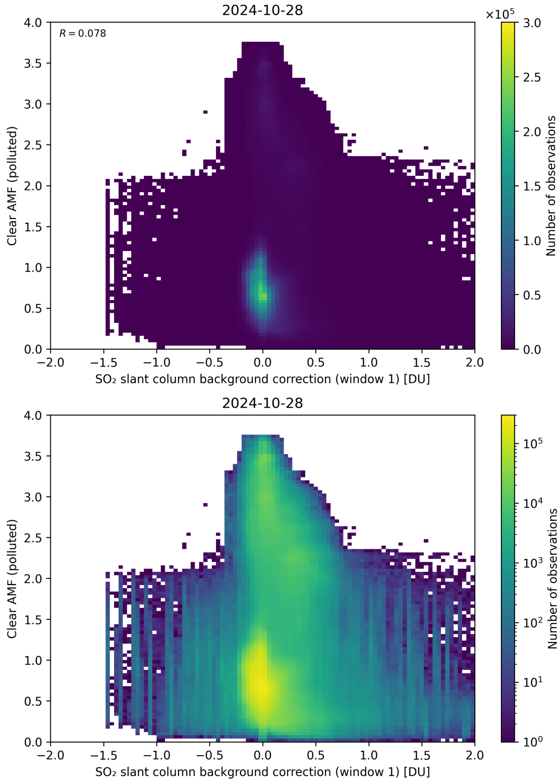
Figure 103: Scatter density plot of “SO 2 slant column background correction (window 1)” against “Clear AMF (polluted)” for 2024-10-27 to 2024-10-29.
