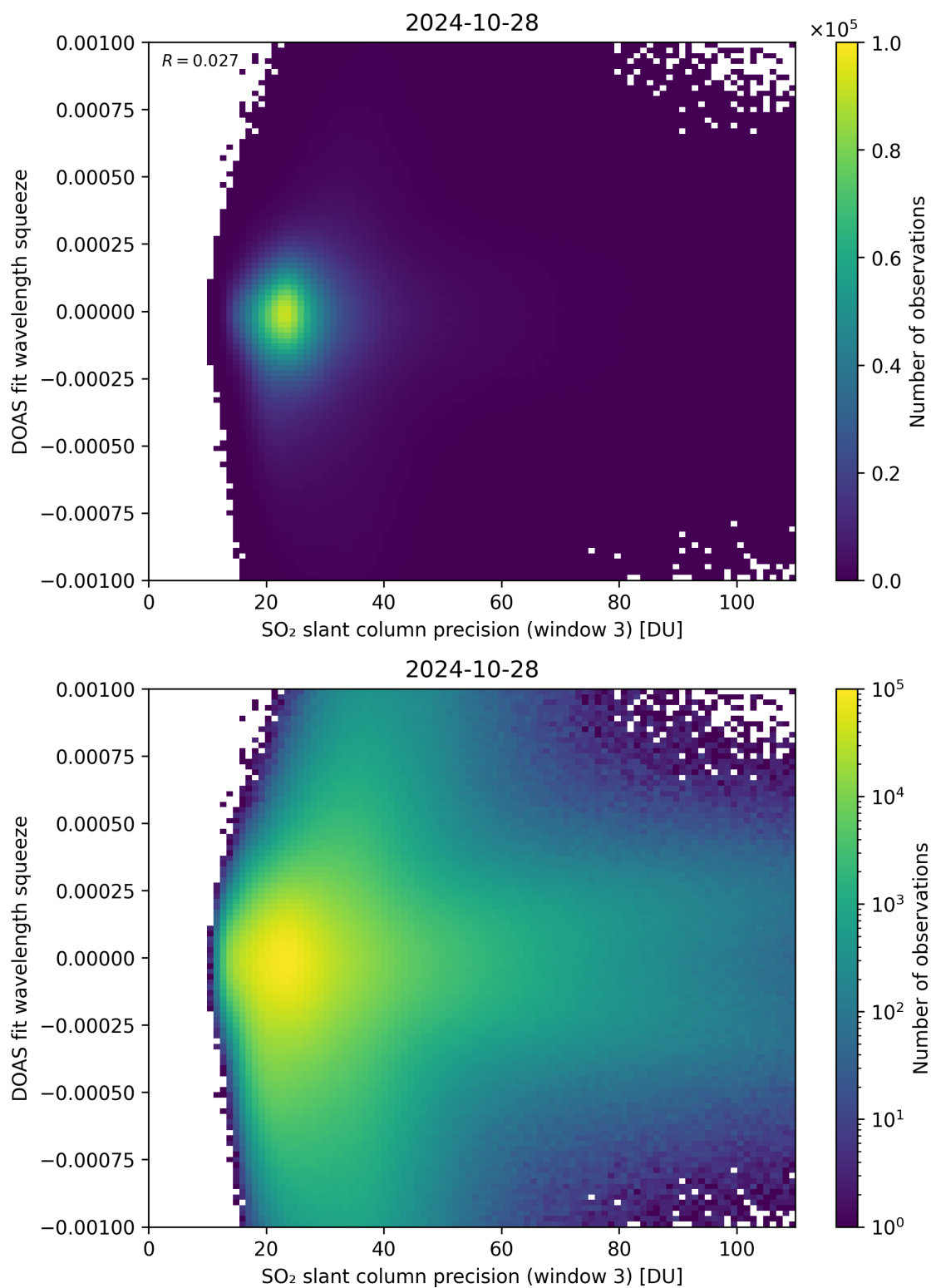
Figure 259: Scatter density plot of “SO 2 slant column precision (window 3)” against “DOAS fit wavelength squeeze” for 2024-10-27 to 2024-10-29.
