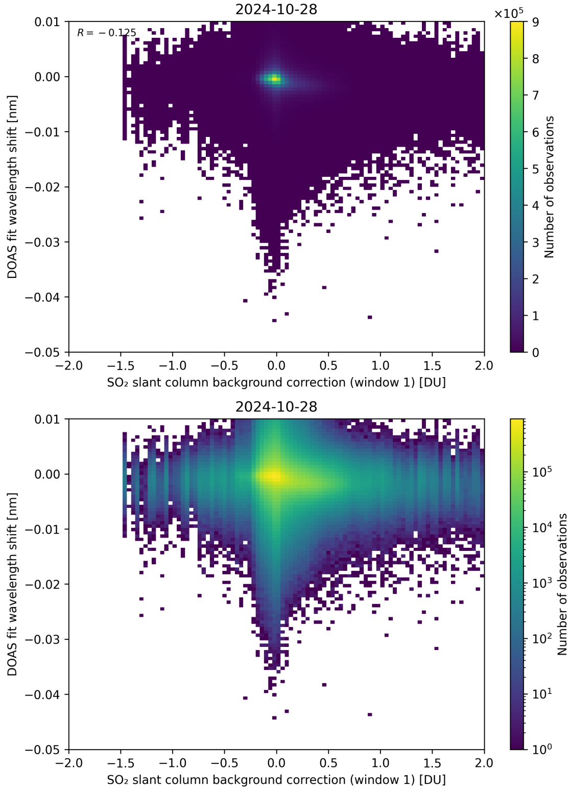
Figure 100: Scatter density plot of “SO 2 slant column background correction (window 1)” against “DOAS fit wavelength shift” for 2024-10-27 to 2024-10-29.
