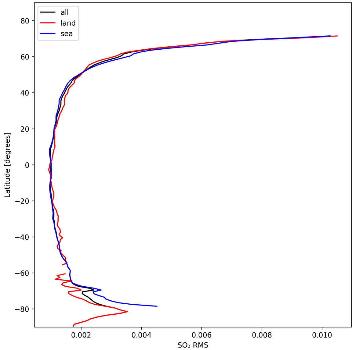
Figure 47: Zonal average of “SO 2 RMS” for 2024-10-27 to 2024-10-29.
