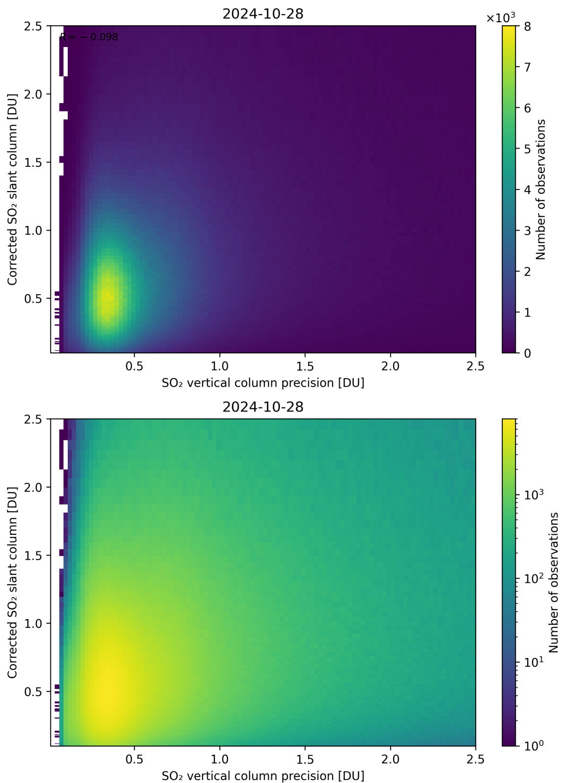
Figure 286: Scatter density plot of “SO 2 vertical column precision” against “Corrected SO 2 slant column” for 2024-10-27 to 2024-10-29.
