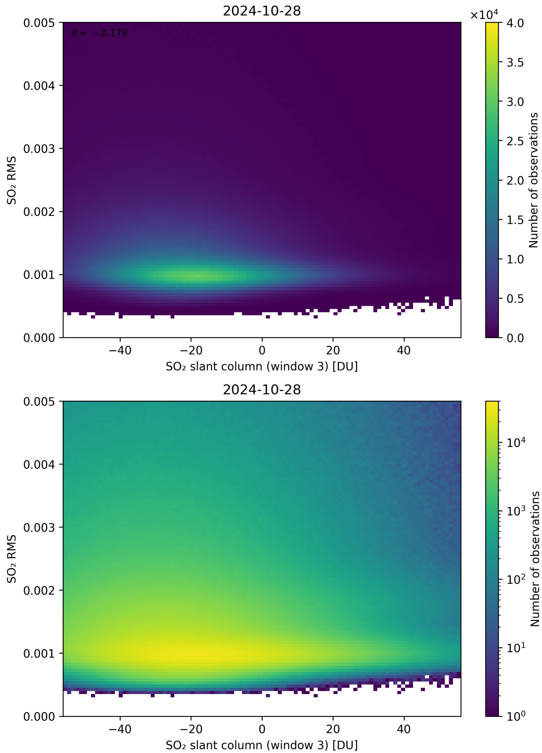
Figure 256: Scatter density plot of “SO 2 slant column (window 3)” against “SO 2 RMS” for 2024-10-27 to 2024-10-29.
