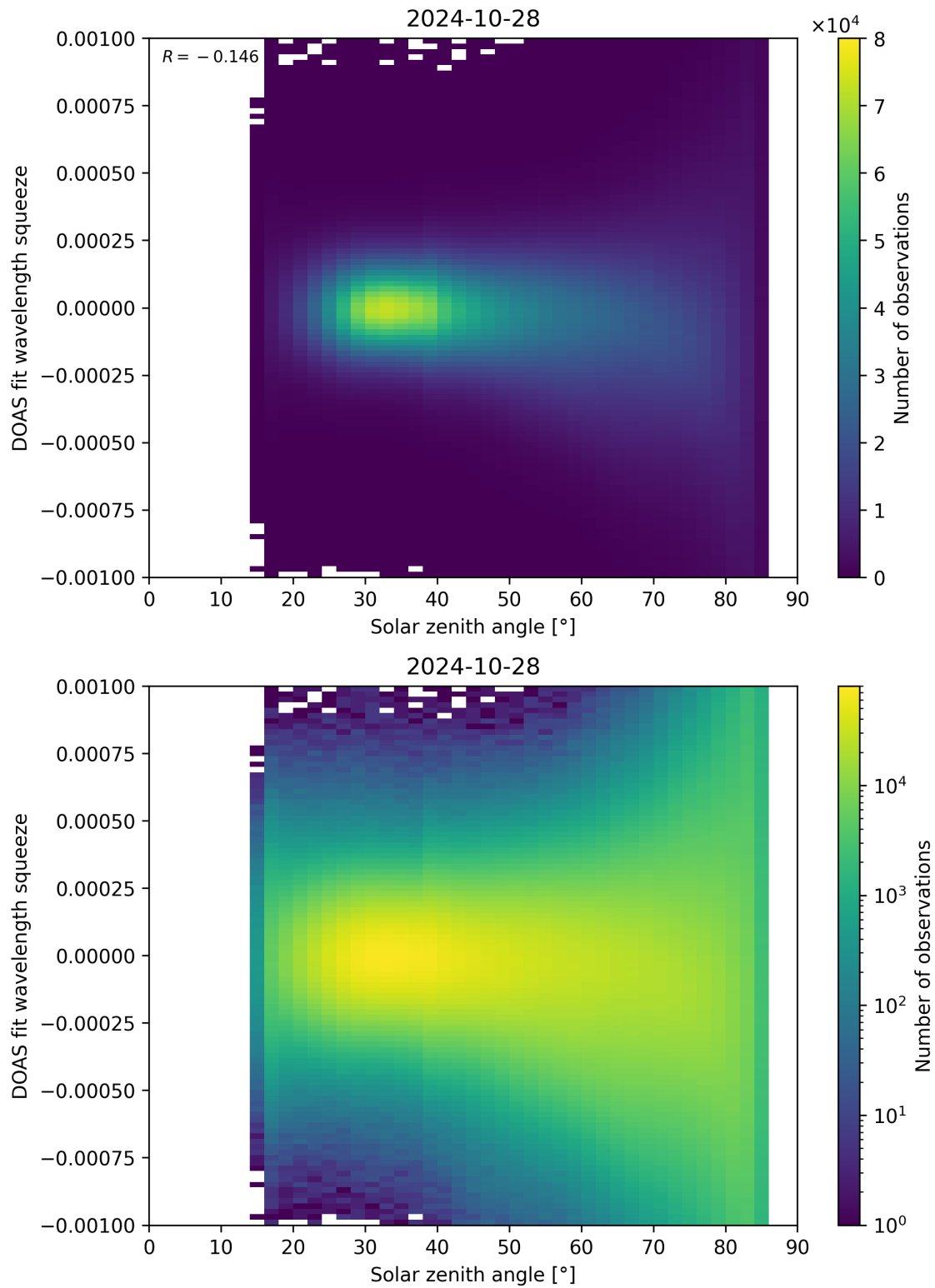
Figure 162: Scatter density plot of “Solar zenith angle” against “DOAS fit wavelength squeeze” for 2024-10-27 to 2024-10-29.
