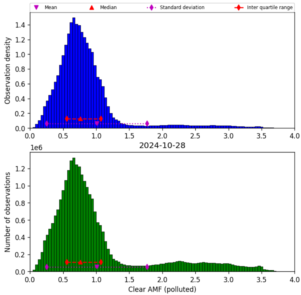
Figure 73: Histogram of “Clear AMF (polluted)” for 2024-10-27 to 2024-10-29
