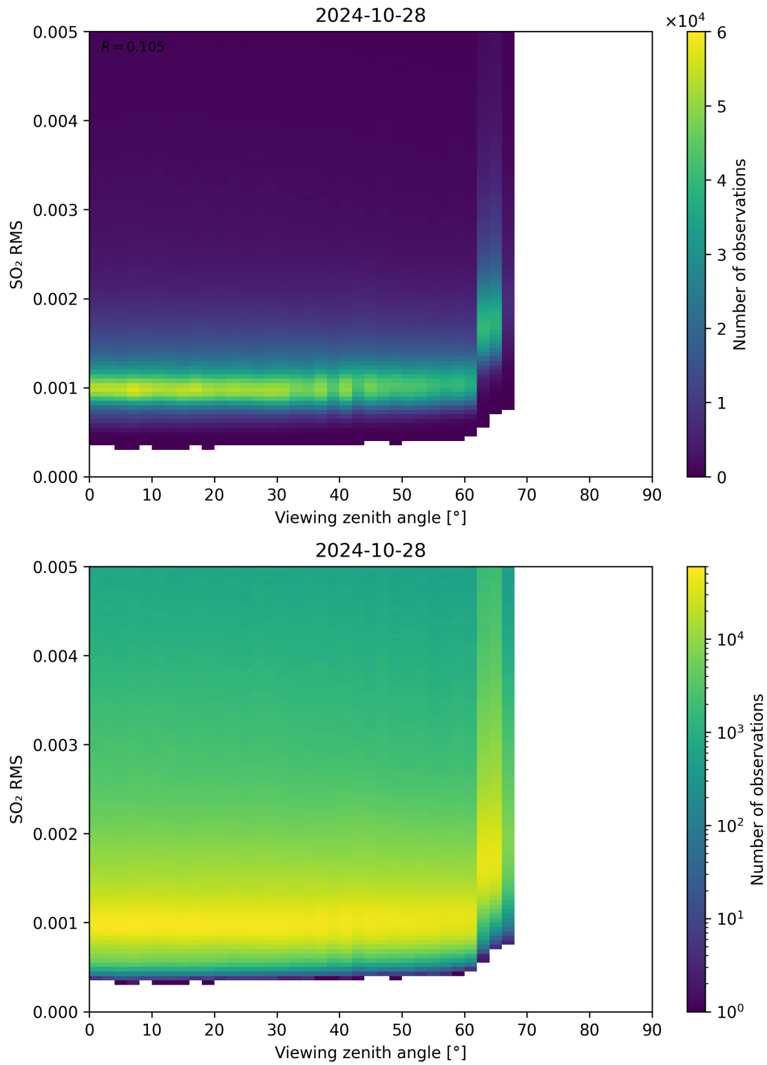
Figure 313: Scatter density plot of “Viewing zenith angle” against “SO 2 RMS” for 2024-10-27 to 2024-10-29.
