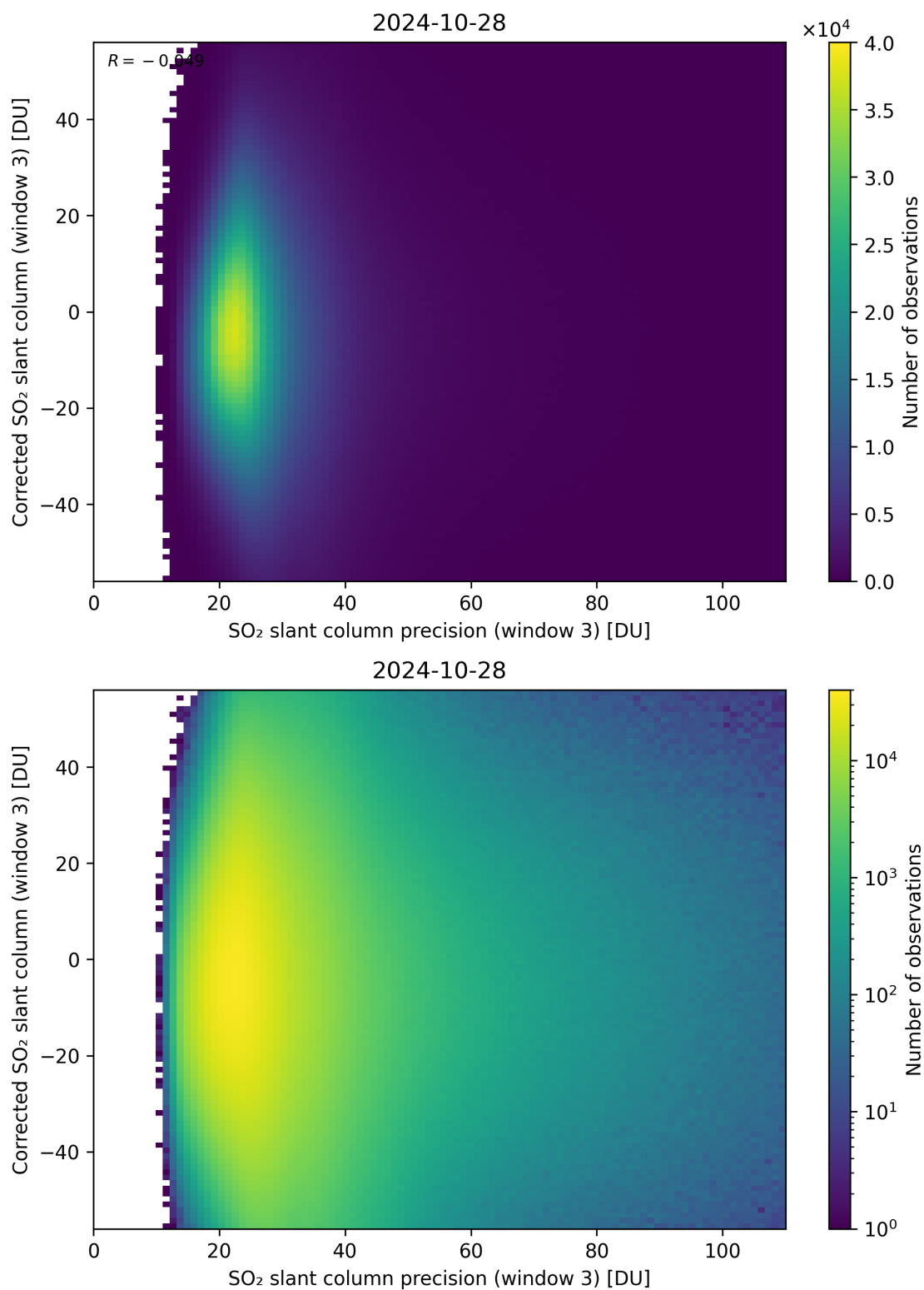
Figure 262: Scatter density plot of “SO 2 slant column precision (window 3)” against “Corrected SO 2 slant column (window 3)” for 2024-10-27 to 2024-10-29.
