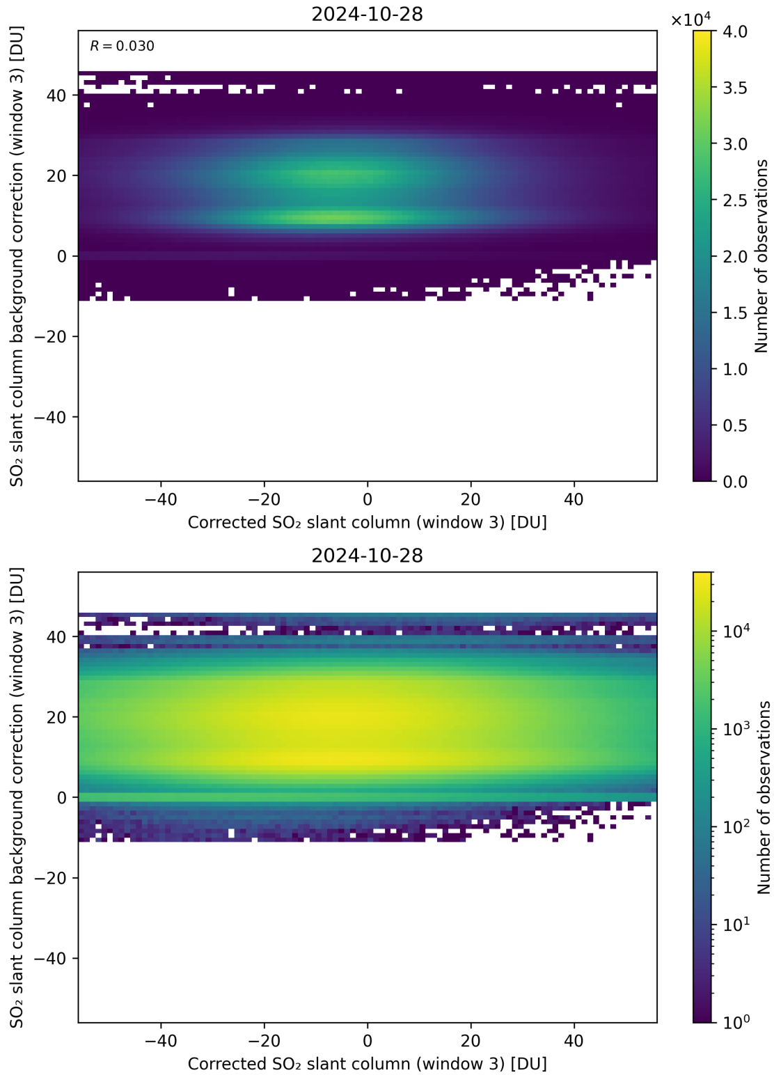
Figure 205: Scatter density plot of “Corrected SO 2 slant column (window 3)” against “SO 2 slant column background correction (window 3)” for 2024-10-27 to 2024-10-29.
