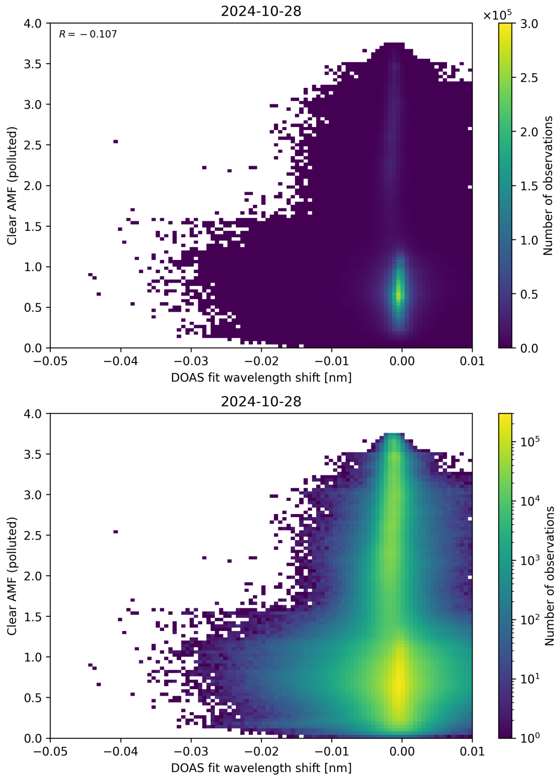
Figure 129: Scatter density plot of “DOAS fit wavelength shift” against “Clear AMF (polluted)” for 2024-10-27 to 2024-10-29.
