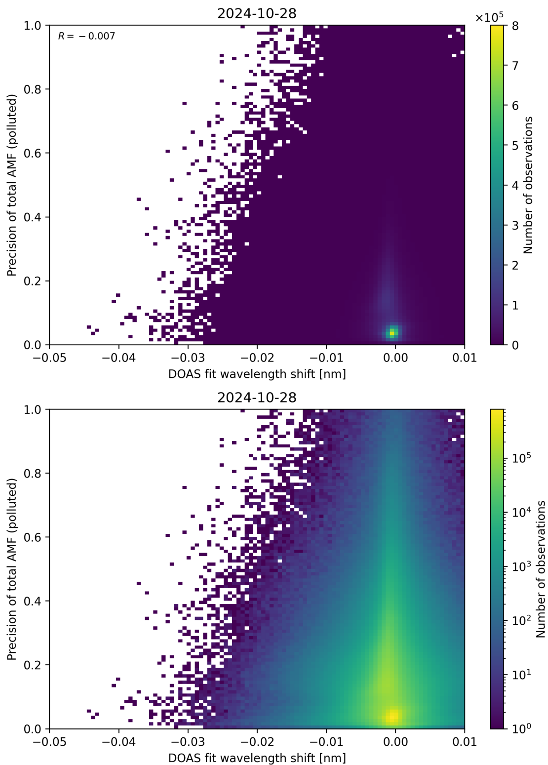
Figure 131: Scatter density plot of “DOAS fit wavelength shift” against “Precision of total AMF (polluted)” for 2024-10-27 to 2024-10-29.
