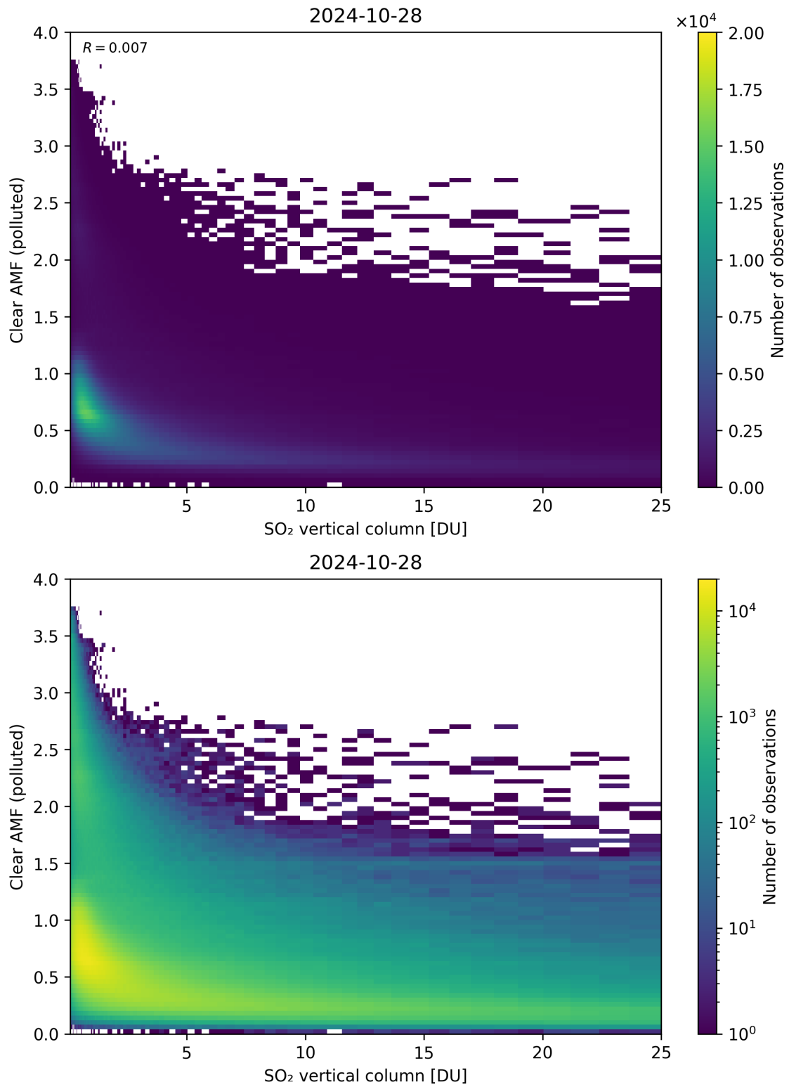
Figure 296: Scatter density plot of “SO 2 vertical column” against “Clear AMF (polluted)” for 2024-10-27 to 2024-10-29.
