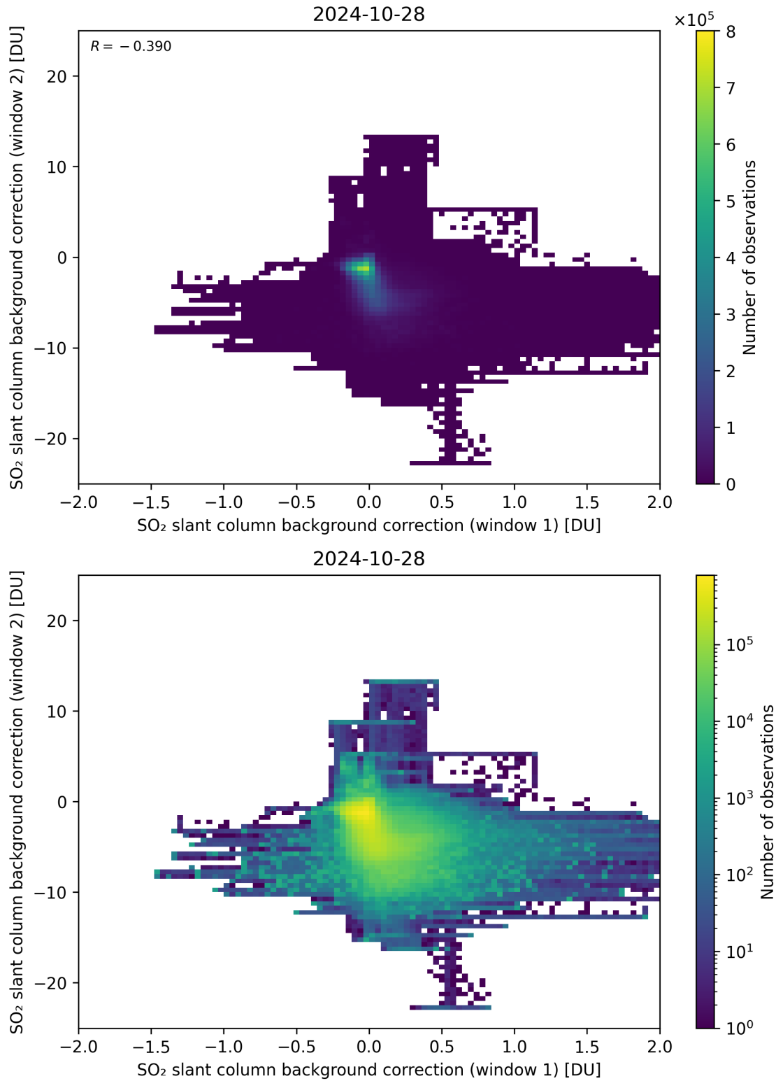
Figure 98: Scatter density plot of “SO 2 slant column background correction (window 1)” against “SO 2 slant column background correction (window 2)” for 2024-10-27 to 2024-10-29.
