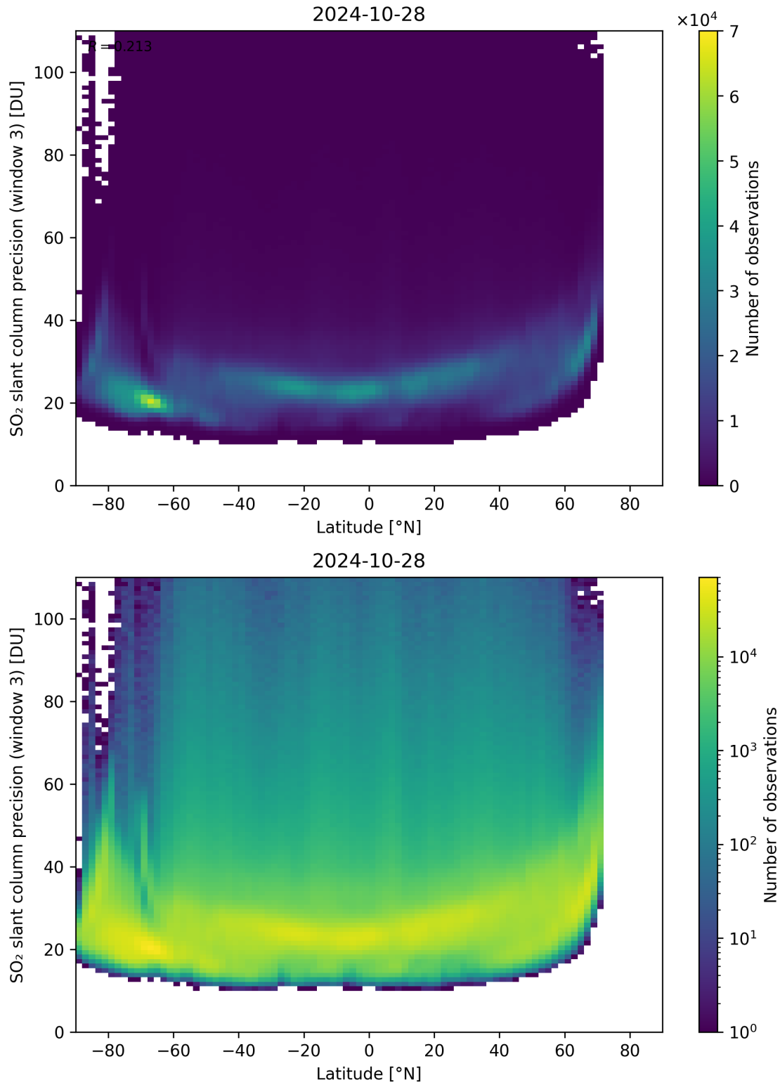
Figure 153: Scatter density plot of “Latitude” against “SO 2 slant column precision (window 3)” for 2024-10-27 to 2024-10-29.
