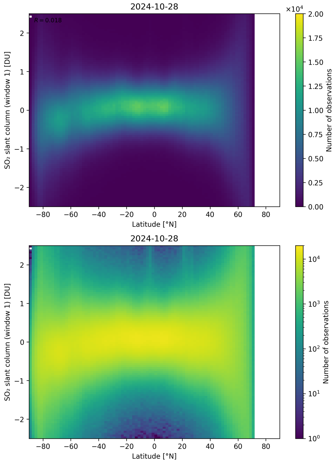
Figure 149: Scatter density plot of “Latitude” against “SO 2 slant column (window 1)” for 2024-10-27 to 2024-10-29.
