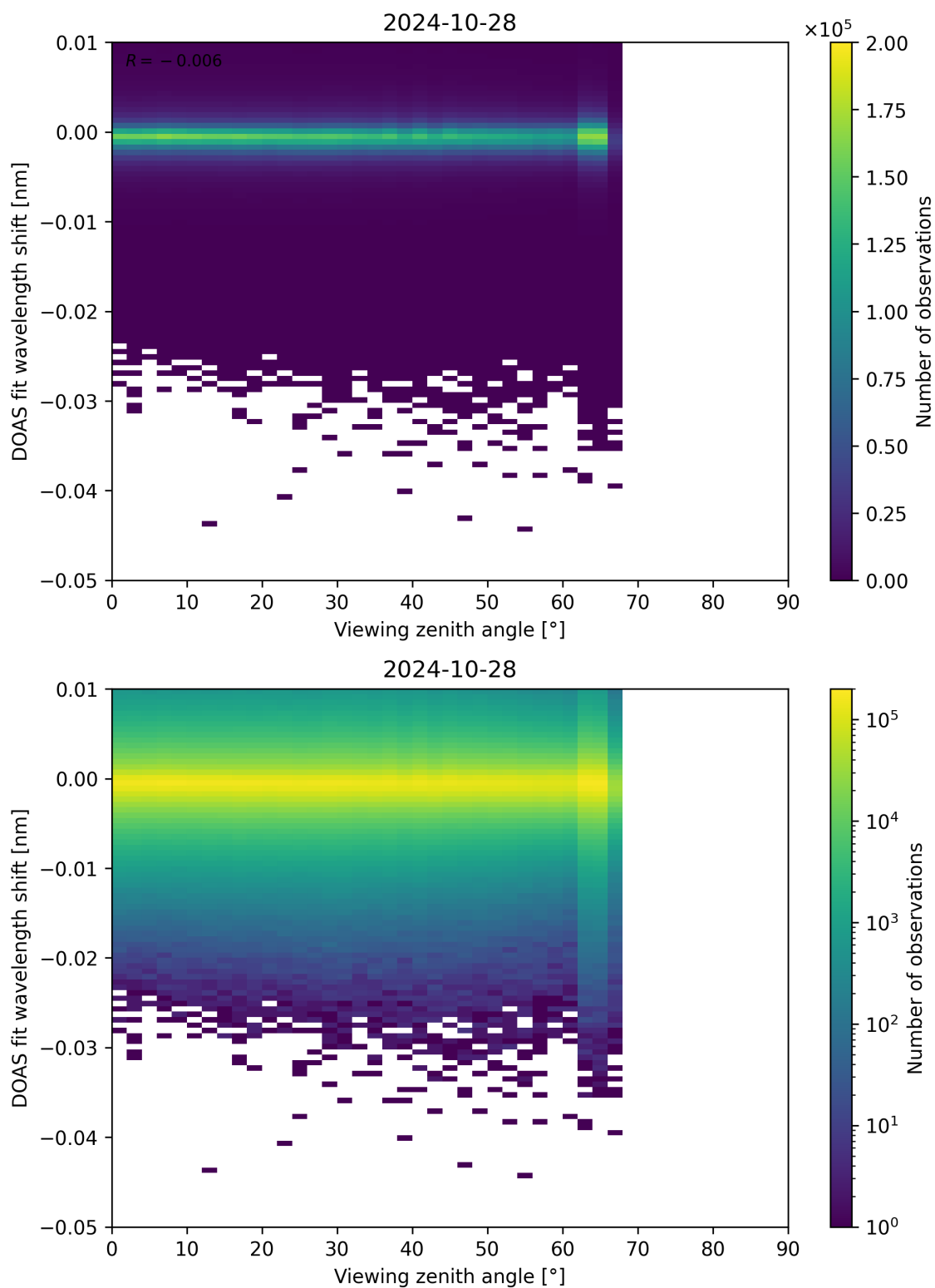
Figure 311: Scatter density plot of “Viewing zenith angle” against “DOAS fit wavelength shift” for 2024-10-27 to 2024-10-29.
