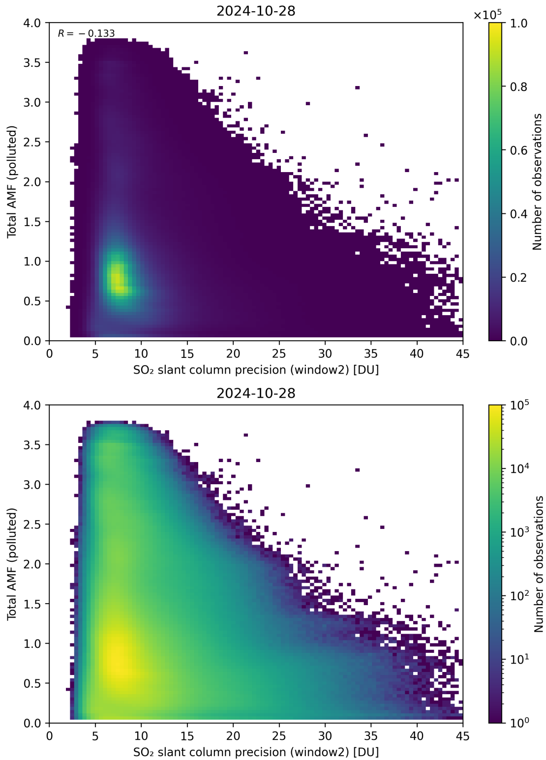
Figure 251: Scatter density plot of “SO 2 slant column precision (window2)” against “Total AMF (polluted)” for 2024-10-27 to 2024-10-29.
