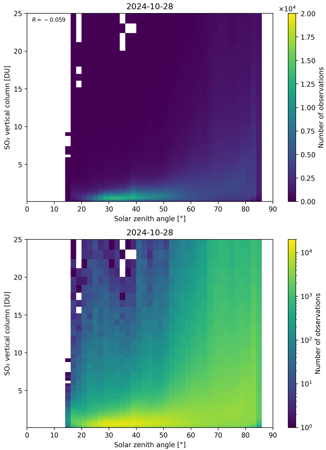
Figure 176: Scatter density plot of “Solar zenith angle” against “SO 2 vertical column” for 2024-10-27 to 2024-10-29.
