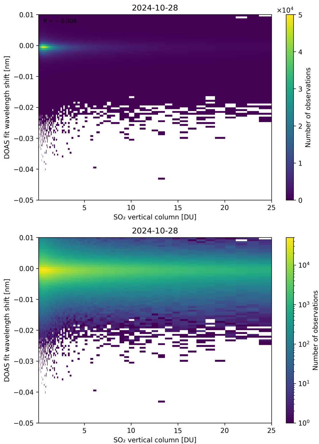
Figure 276: Scatter density plot of “SO 2 vertical column” against “DOAS fit wavelength shift” for 2024-10-27 to 2024-10-29.
