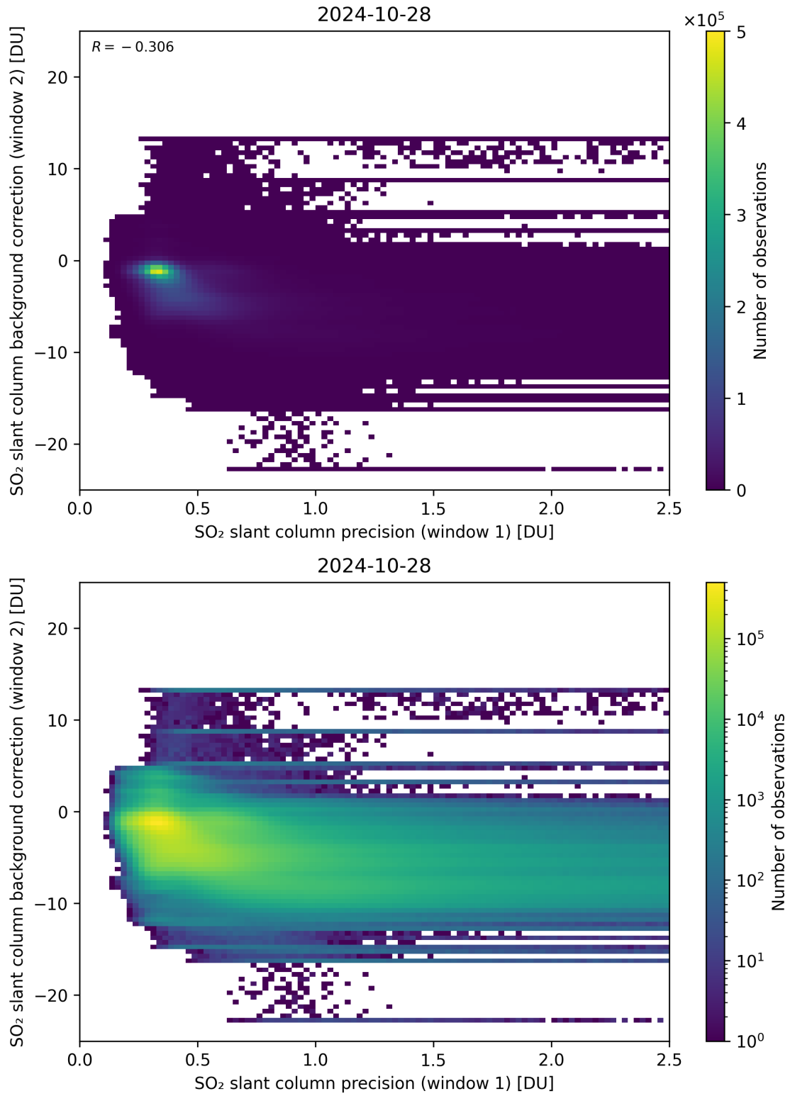
Figure 219: Scatter density plot of “SO 2 slant column precision (window 1)” against “SO 2 slant column background correction (window 2)” for 2024-10-27 to 2024-10-29.
