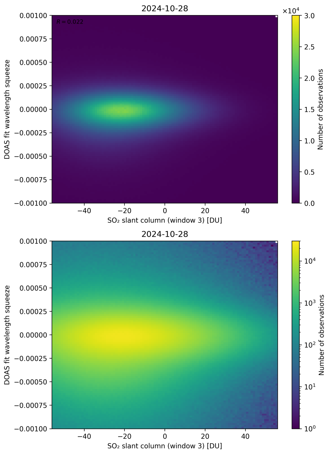
Figure 255: Scatter density plot of “SO 2 slant column (window 3)” against “DOAS fit wavelength squeeze” for 2024-10-27 to 2024-10-29.
