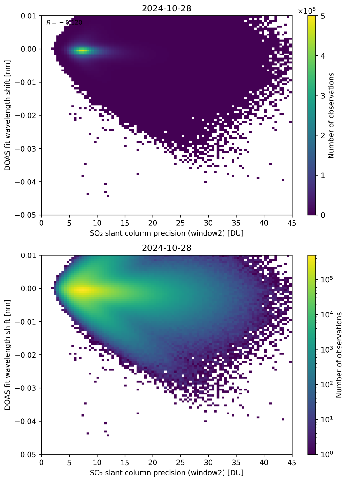
Figure 243: Scatter density plot of “SO 2 slant column precision (window2)” against “DOAS fit wavelength shift” for 2024-10-27 to 2024-10-29.
