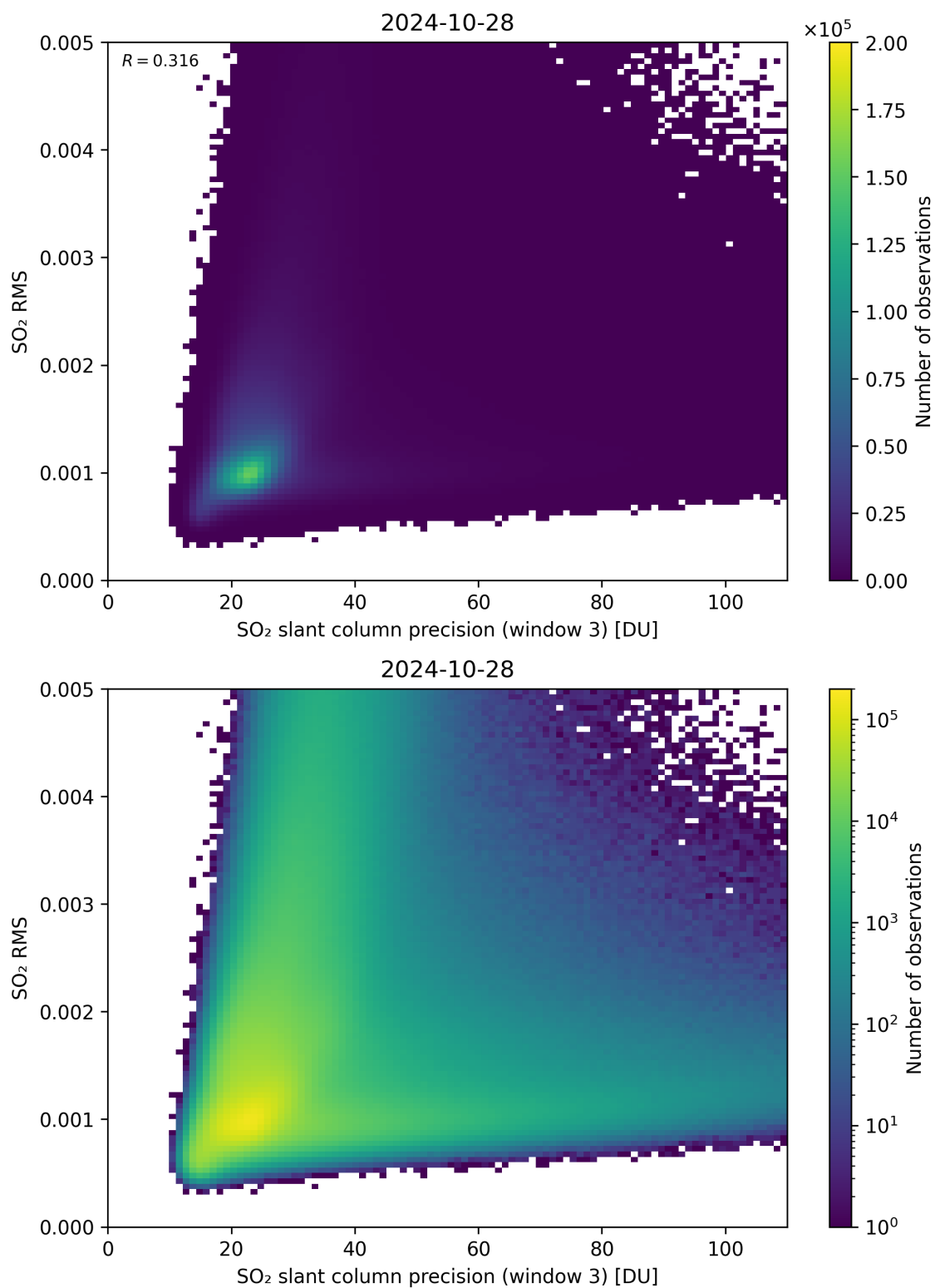
Figure 260: Scatter density plot of “SO 2 slant column precision (window 3)” against “SO 2 RMS” for 2024-10-27 to 2024-10-29.
