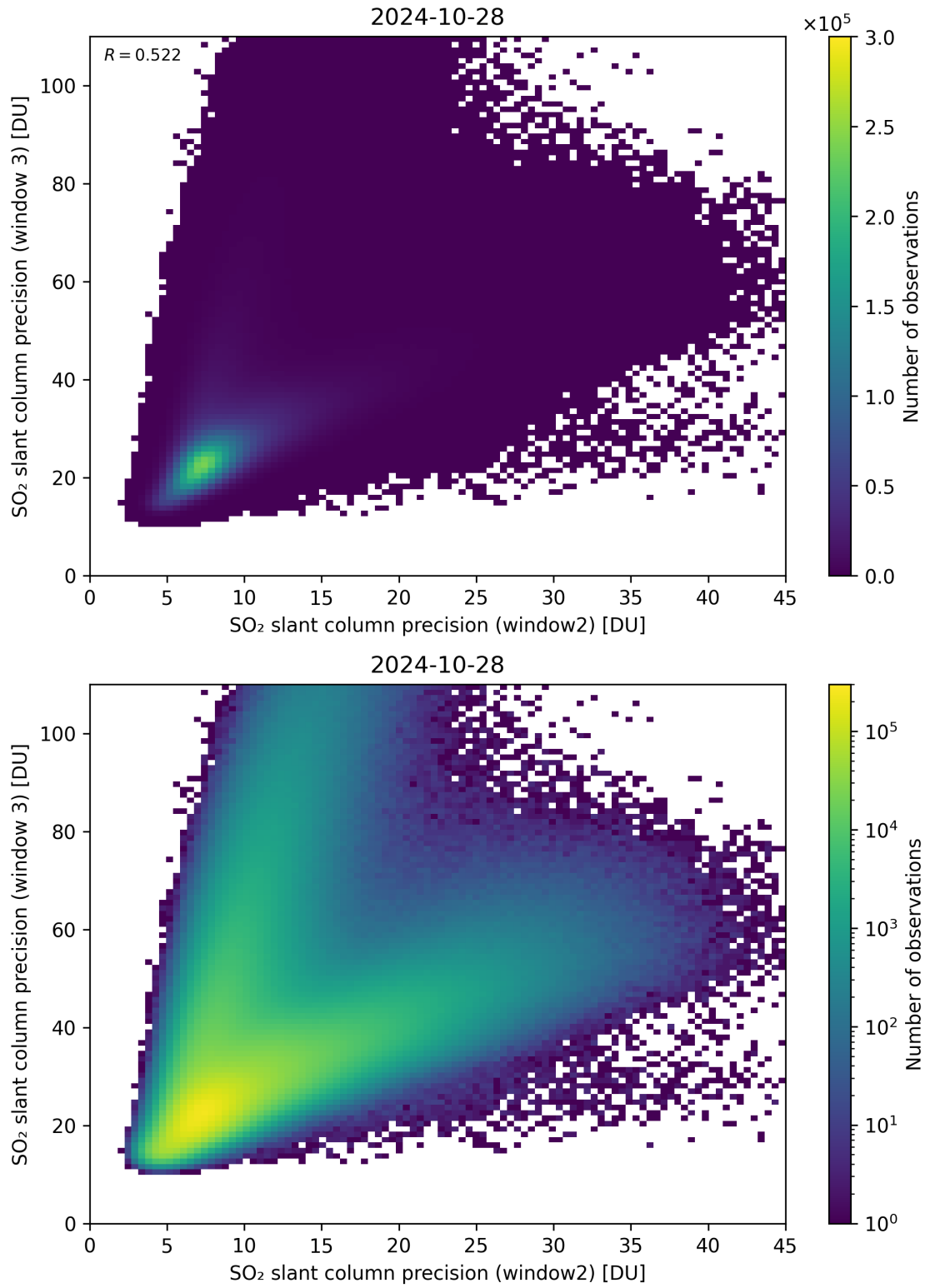
Figure 250: Scatter density plot of “SO 2 slant column precision (window2)” against “SO 2 slant column precision (window 3)” for 2024-10-27 to 2024-10-29.
