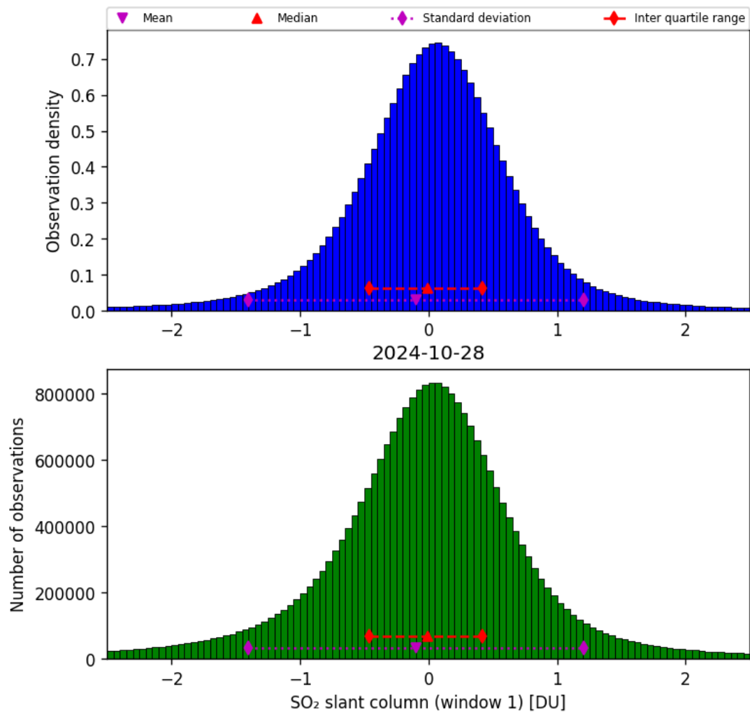
Figure 56: Histogram of “SO 2 slant column (window 1)” for 2024-10-27 to 2024-10-29
