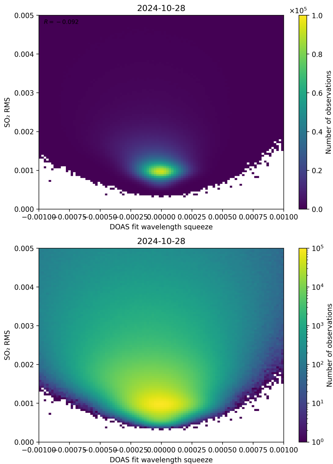
Figure 132: Scatter density plot of “DOAS fit wavelength squeeze” against “SO 2 RMS” for 2024-10-27 to 2024-10-29.
