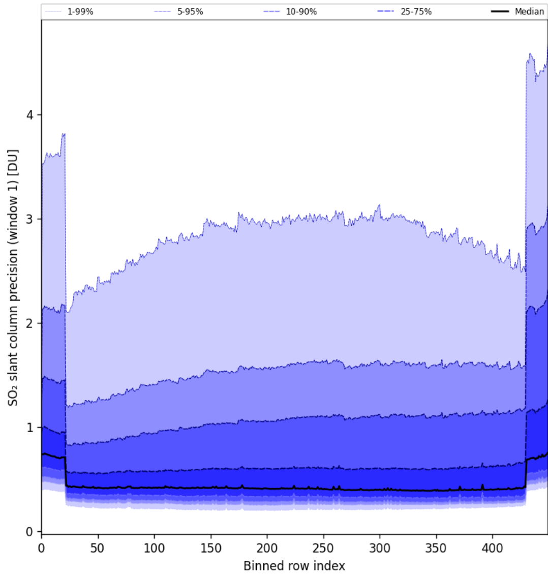
Figure 80: Along track statistics of “SO 2 slant column precision (window 1)” for 2024-10-27 to 2024-10-29
