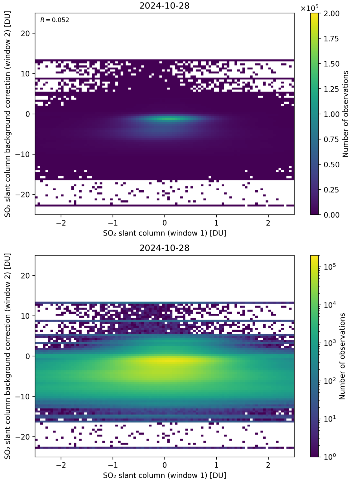
Figure 213: Scatter density plot of “SO 2 slant column (window 1)” against “SO 2 slant column background correction (window 2)” for 2024-10-27 to 2024-10-29.
