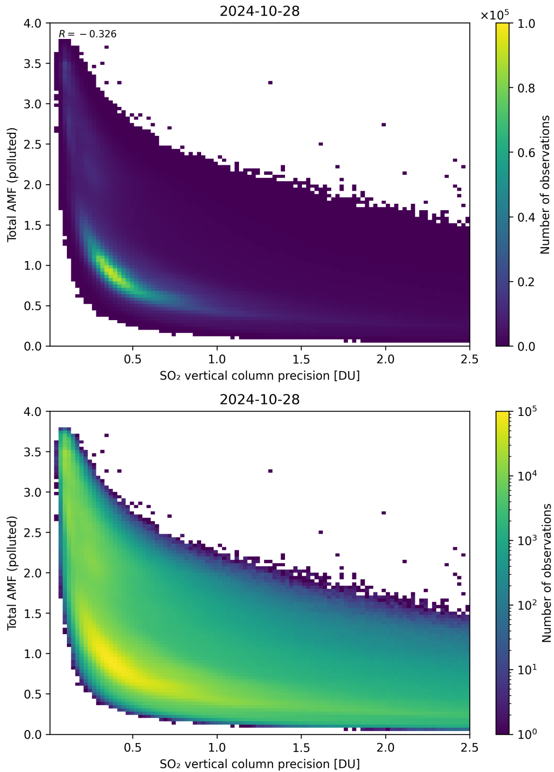
Figure 294: Scatter density plot of “SO 2 vertical column precision” against “Total AMF (polluted)” for 2024-10-27 to 2024-10-29.
