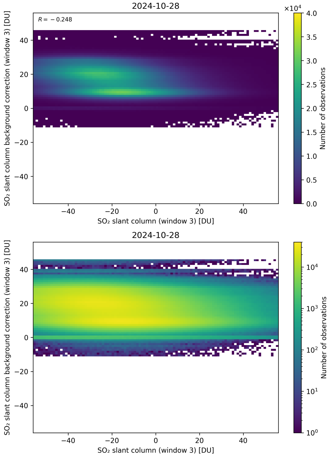
Figure 253: Scatter density plot of “SO 2 slant column (window 3)” against “SO 2 slant column background correction (window 3)” for 2024-10-27 to 2024-10-29.
