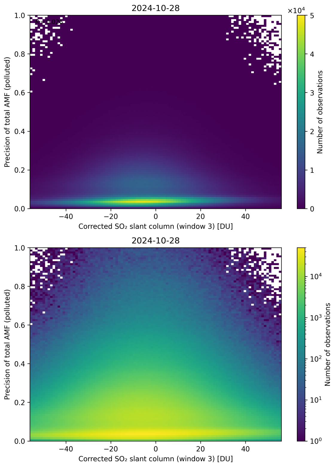
Figure 211: Scatter density plot of “Corrected SO 2 slant column (window 3)” against “Precision of total AMF (polluted)” for 2024-10-27 to 2024-10-29.
