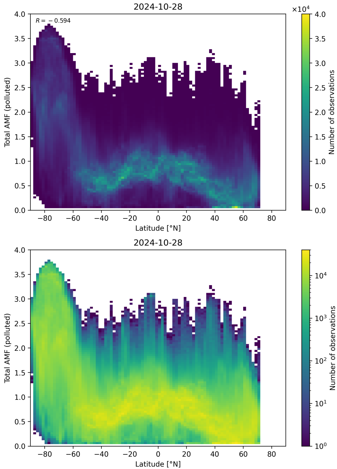
Figure 154: Scatter density plot of “Latitude” against “Total AMF (polluted)” for 2024-10-27 to 2024-10-29.
