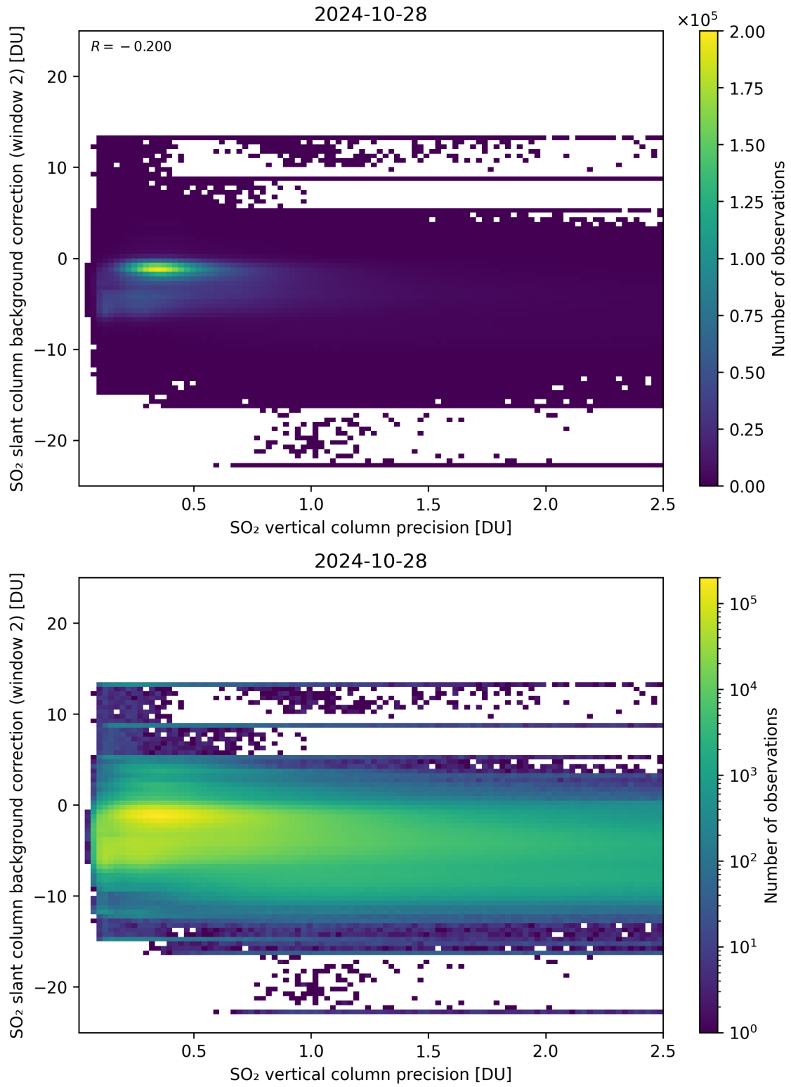
Figure 280: Scatter density plot of “SO 2 vertical column precision” against “SO 2 slant column background correction (window 2)” for 2024-10-27 to 2024-10-29.
