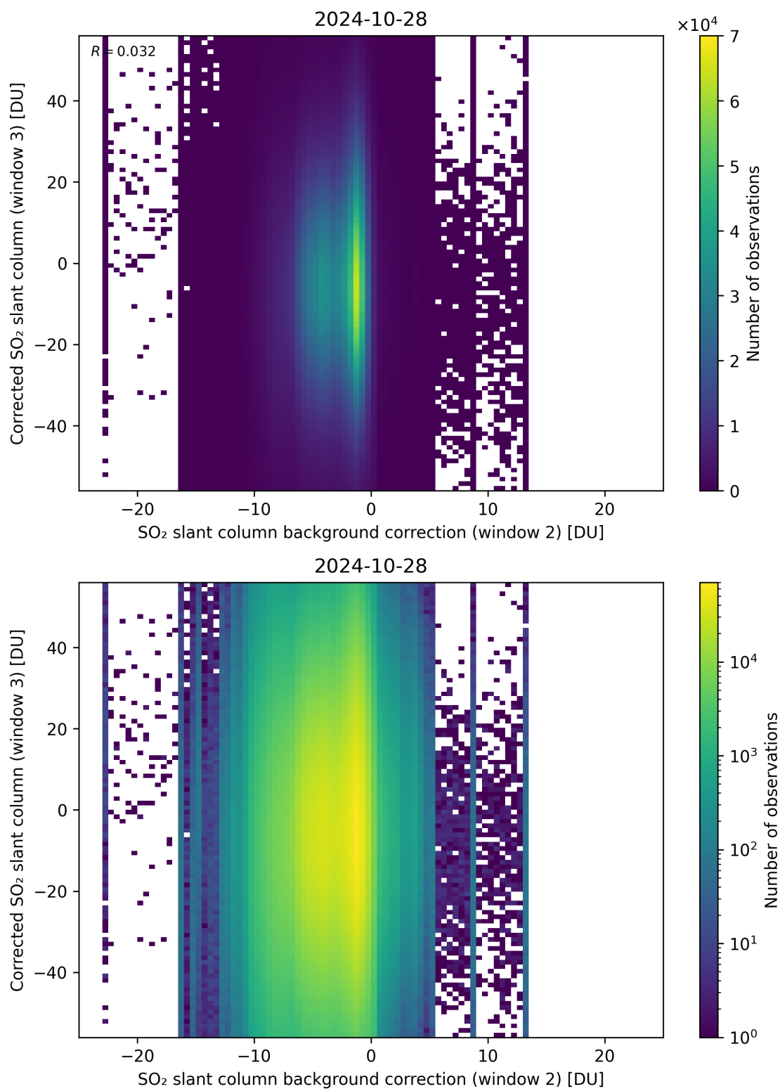
Figure 116: Scatter density plot of “SO 2 slant column background correction (window 2)” against “Corrected SO 2 slant column (window 3)” for 2024-10-27 to 2024-10-29.
