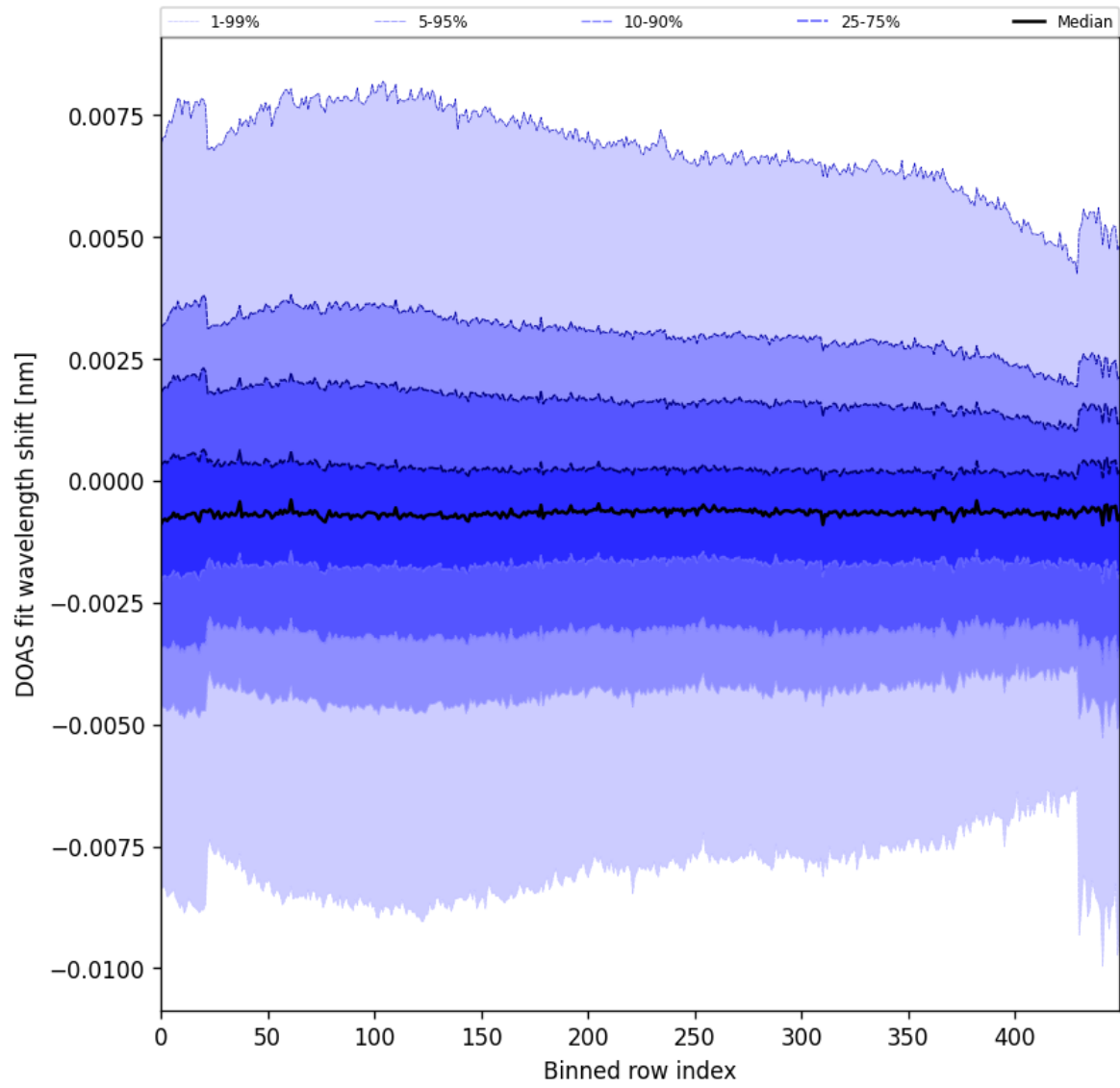
Figure 91: Along track statistics of “DOAS fit wavelength shift” for 2024-10-27 to 2024-10-29
