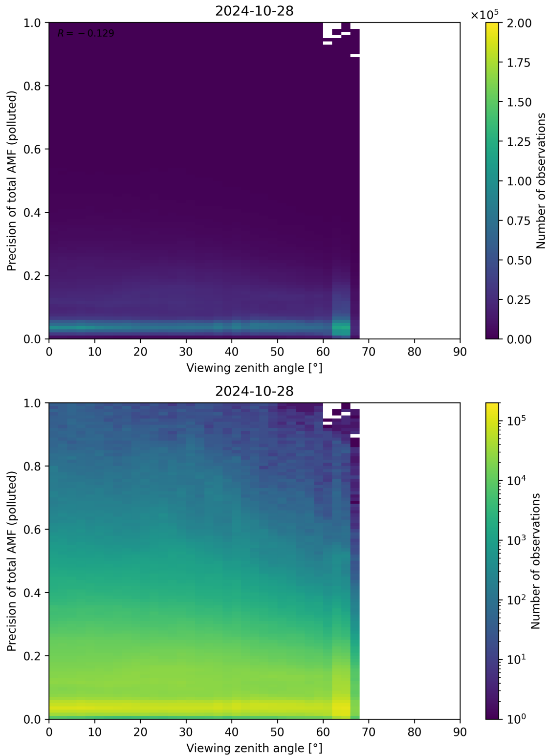
Figure 326: Scatter density plot of “Viewing zenith angle” against “Precision of total AMF (polluted)” for 2024-10-27 to 2024-10-29.
