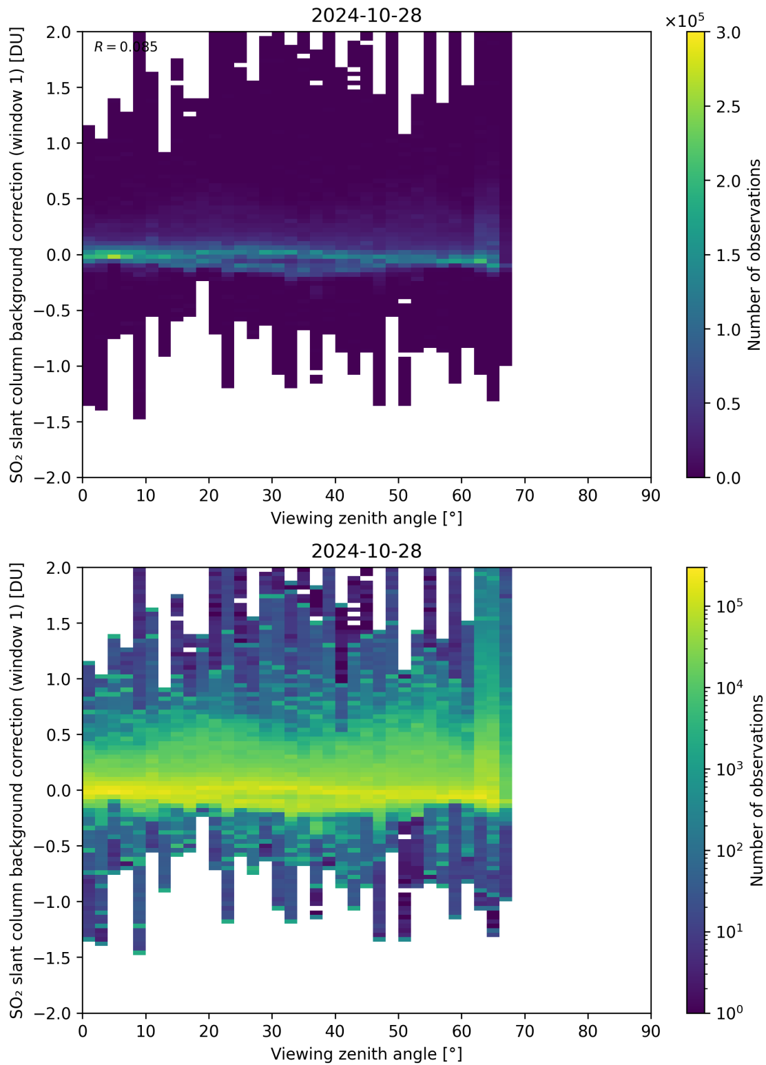
Figure 308: Scatter density plot of “Viewing zenith angle” against “SO 2 slant column background correction (window 1)” for 2024-10-27 to 2024-10-29.
