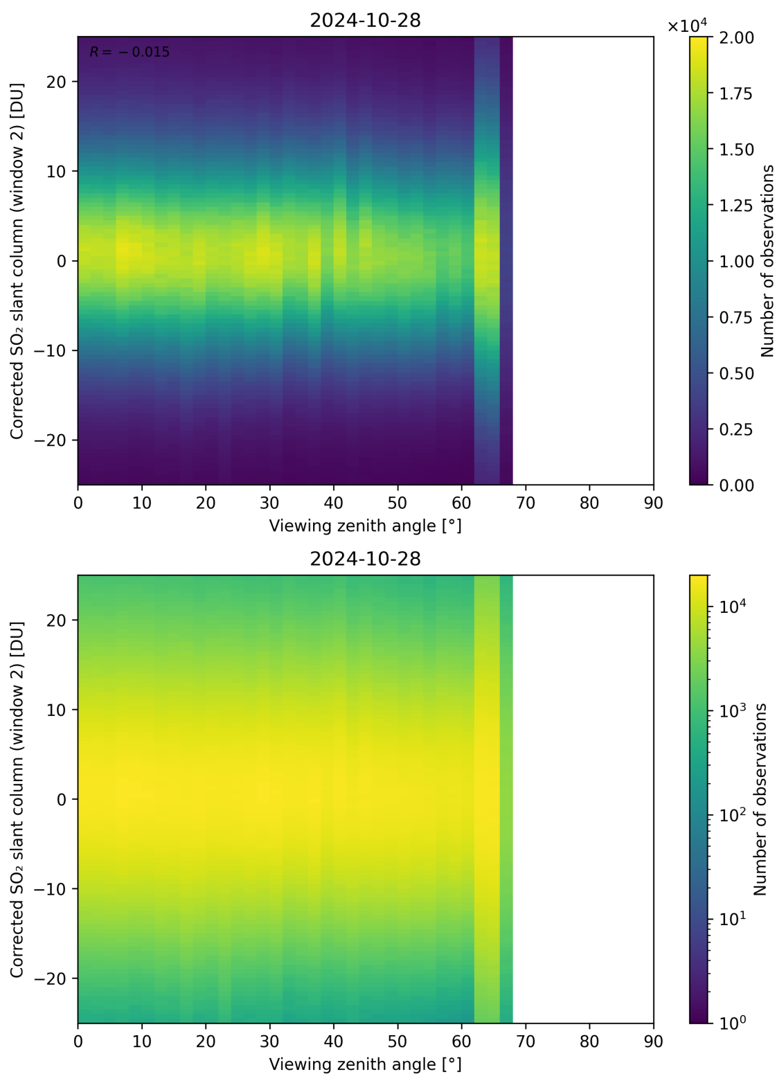
Figure 318: Scatter density plot of “Viewing zenith angle” against “Corrected SO 2 slant column (window 2)” for 2024-10-27 to 2024-10-29.
