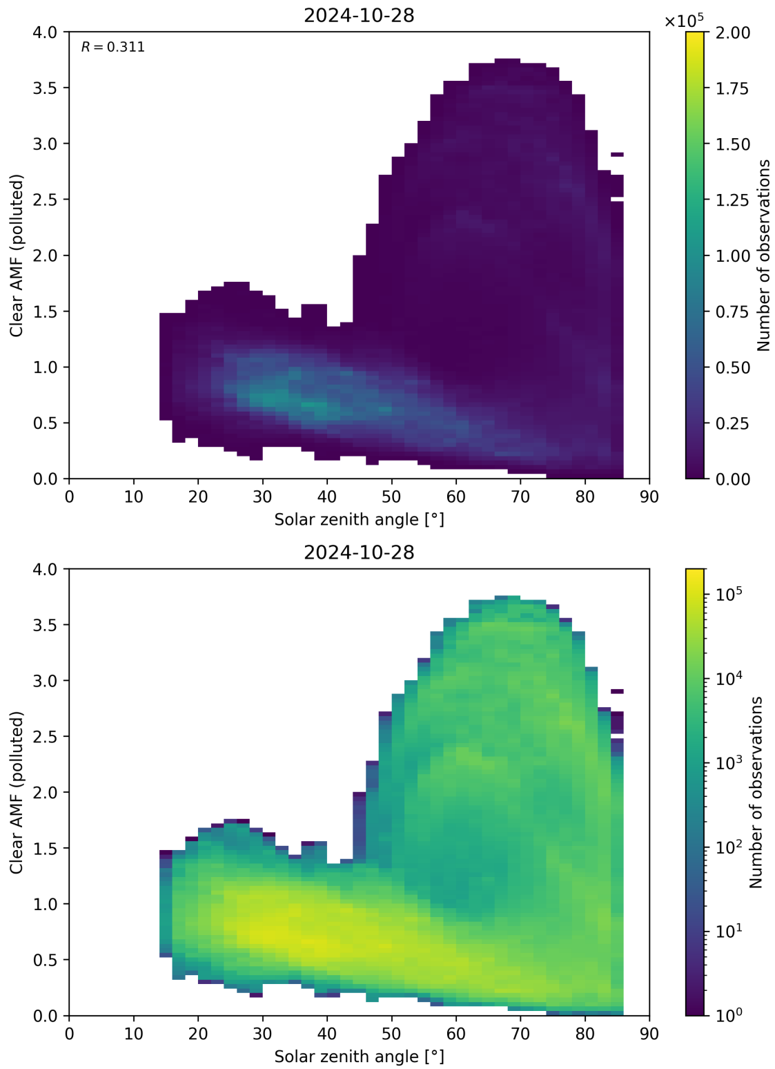
Figure 165: Scatter density plot of “Solar zenith angle” against “Clear AMF (polluted)” for 2024-10-27 to 2024-10-29.
