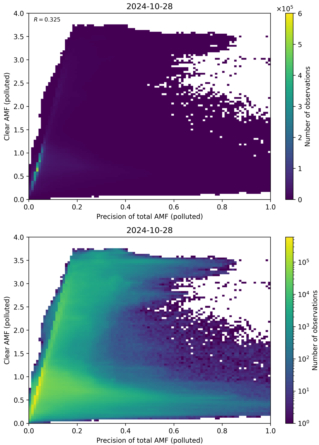
Figure 270: Scatter density plot of “Precision of total AMF (polluted)” against “Clear AMF (polluted)” for 2024-10-27 to 2024-10-29.
