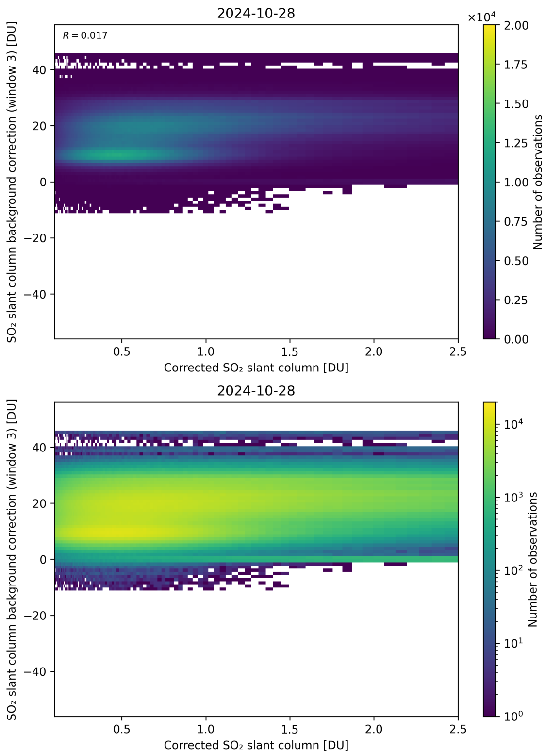
Figure 180: Scatter density plot of “Corrected SO 2 slant column” against “SO 2 slant column background correction (window 3)” for 2024-10-27 to 2024-10-29.
