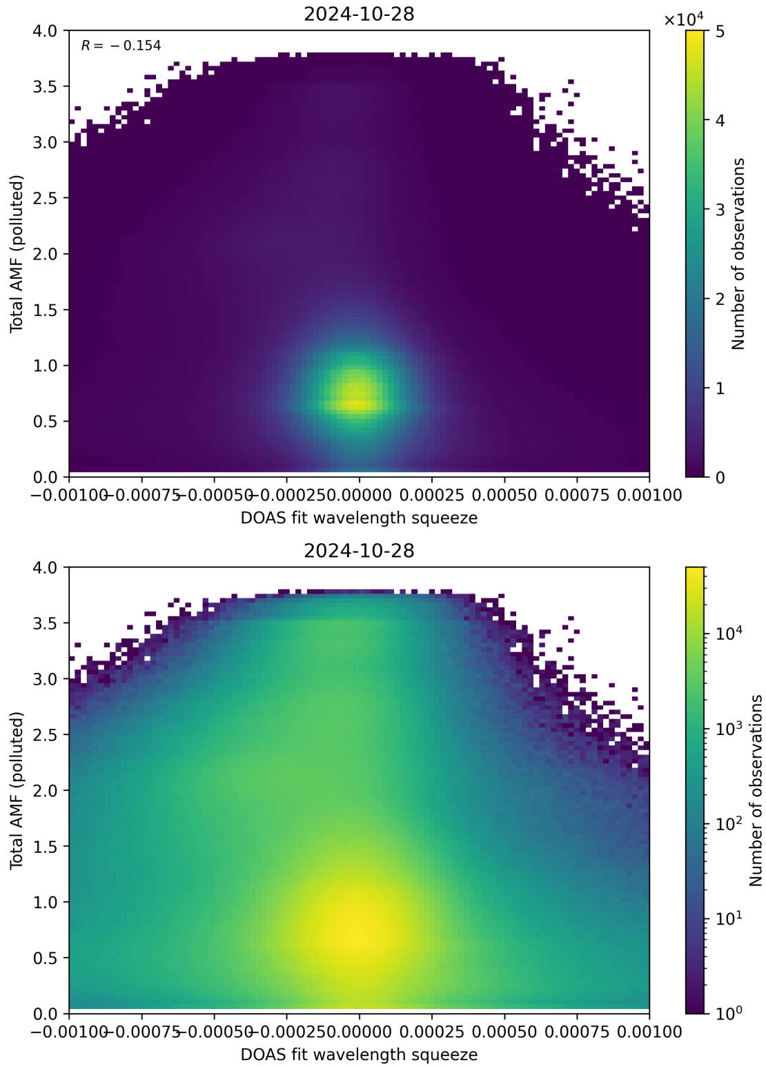
Figure 134: Scatter density plot of “DOAS fit wavelength squeeze” against “Total AMF (polluted)” for 2024-10-27 to 2024-10-29.
