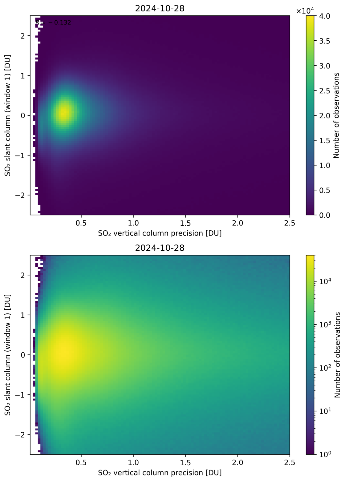
Figure 289: Scatter density plot of “SO 2 vertical column precision” against “SO 2 slant column (window 1)” for 2024-10-27 to 2024-10-29.
