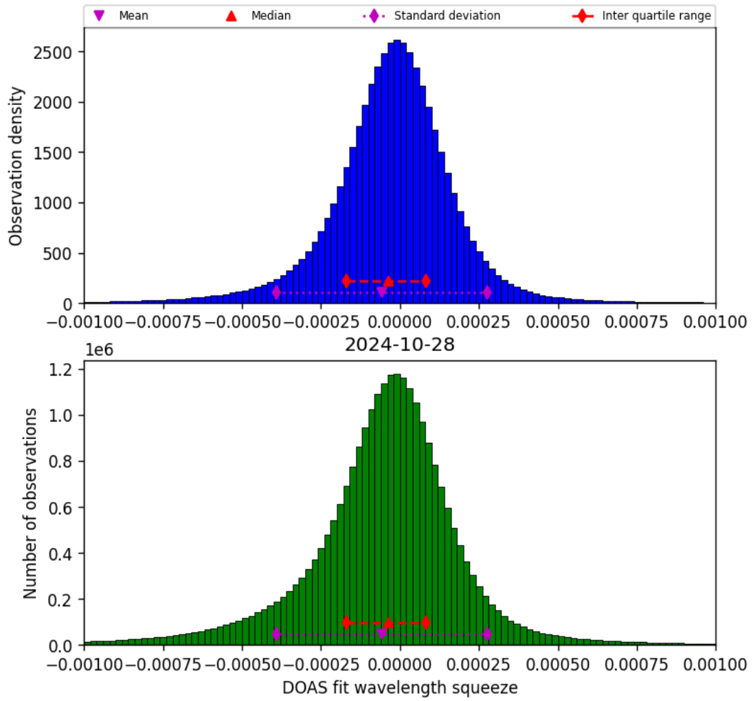
Figure 69: Histogram of “DOAS fit wavelength squeeze” for 2024-10-27 to 2024-10-29
