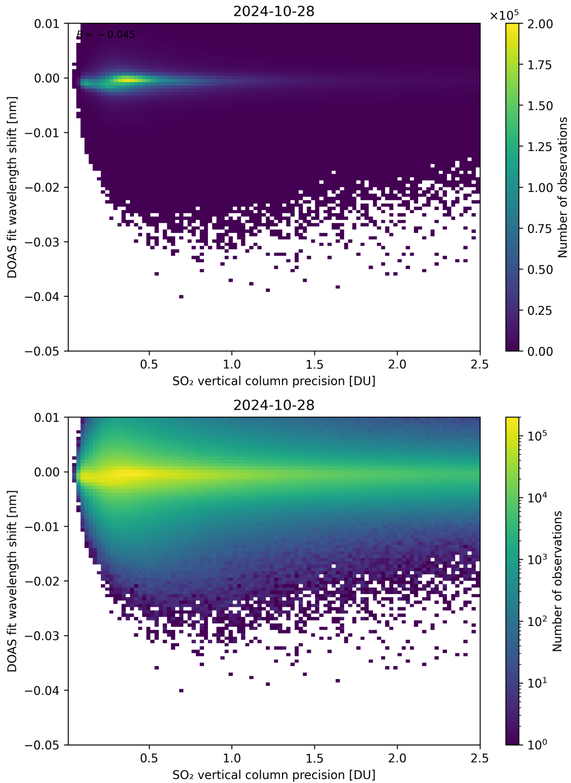
Figure 282: Scatter density plot of “SO 2 vertical column precision” against “DOAS fit wavelength shift” for 2024-10-27 to 2024-10-29.
