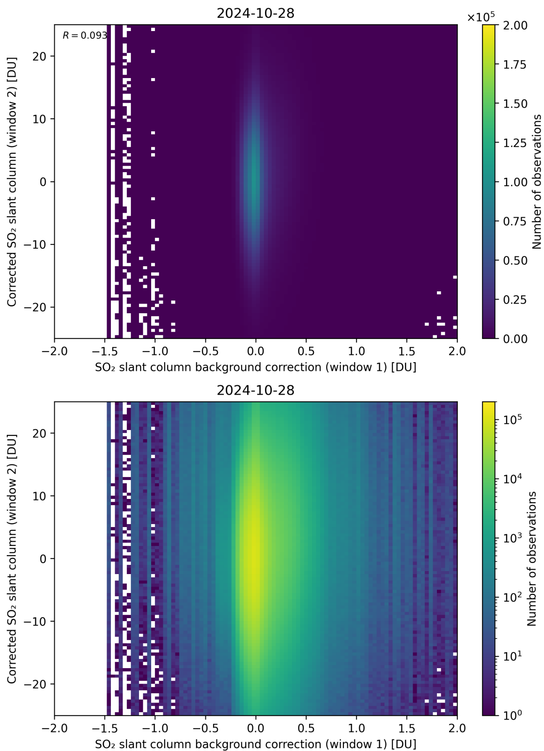
Figure 104: Scatter density plot of “SO 2 slant column background correction (window 1)” against “Corrected SO 2 slant column (window 2)” for 2024-10-27 to 2024-10-29.
