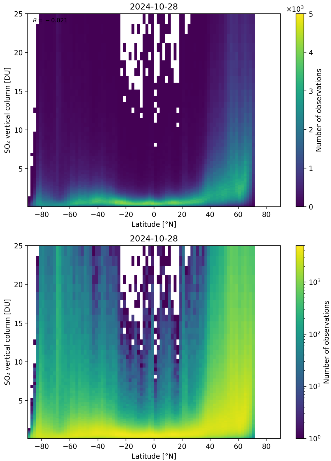
Figure 156: Scatter density plot of “Latitude” against “SO 2 vertical column” for 2024-10-27 to 2024-10-29.
