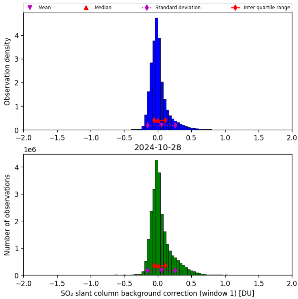
Figure 59: Histogram of “SO 2 slant column background correction (window 1)” for 2024-10-27 to 2024-10-29
