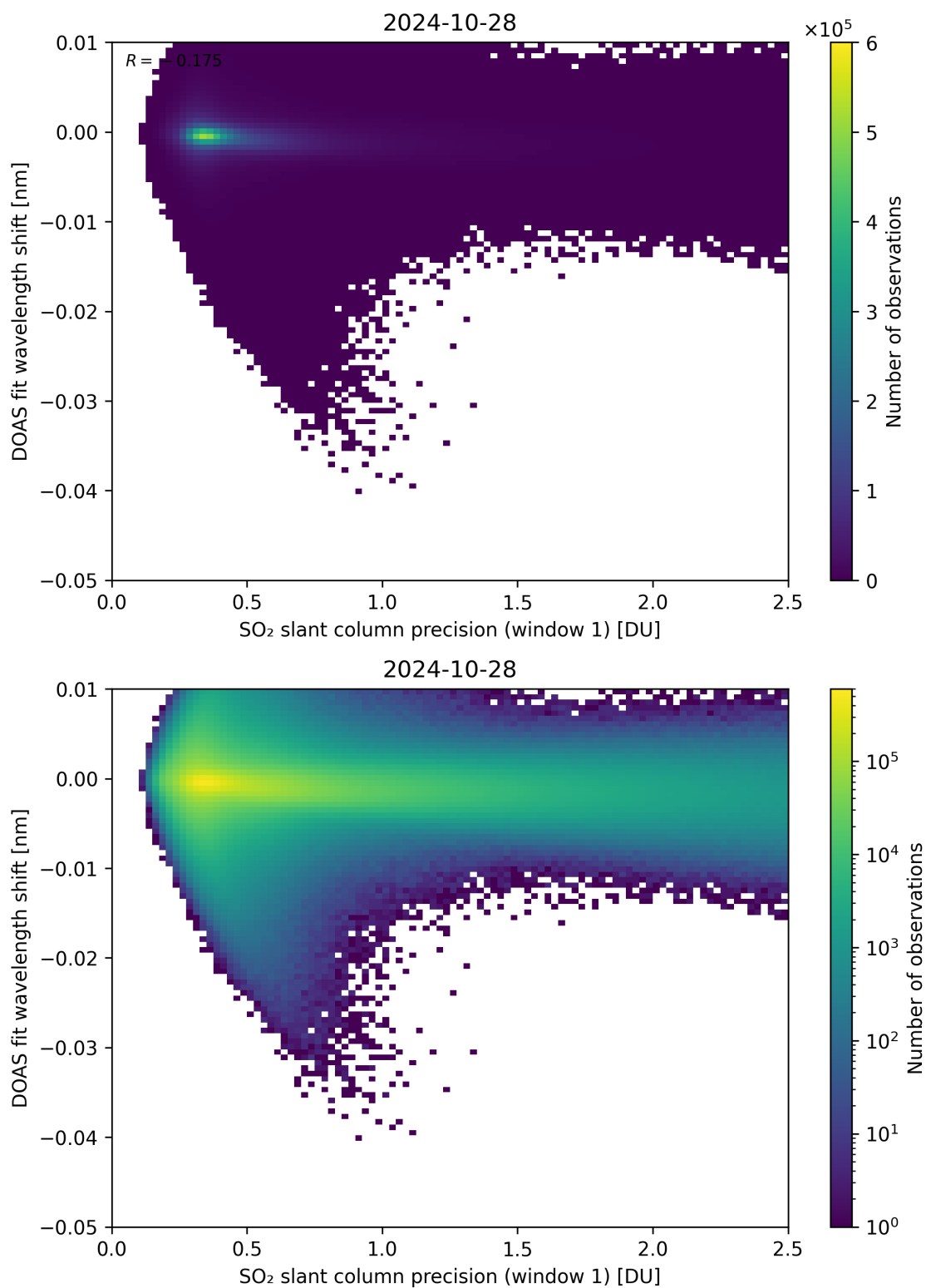
Figure 221: Scatter density plot of “SO 2 slant column precision (window 1)” against “DOAS fit wavelength shift” for 2024-10-27 to 2024-10-29.
