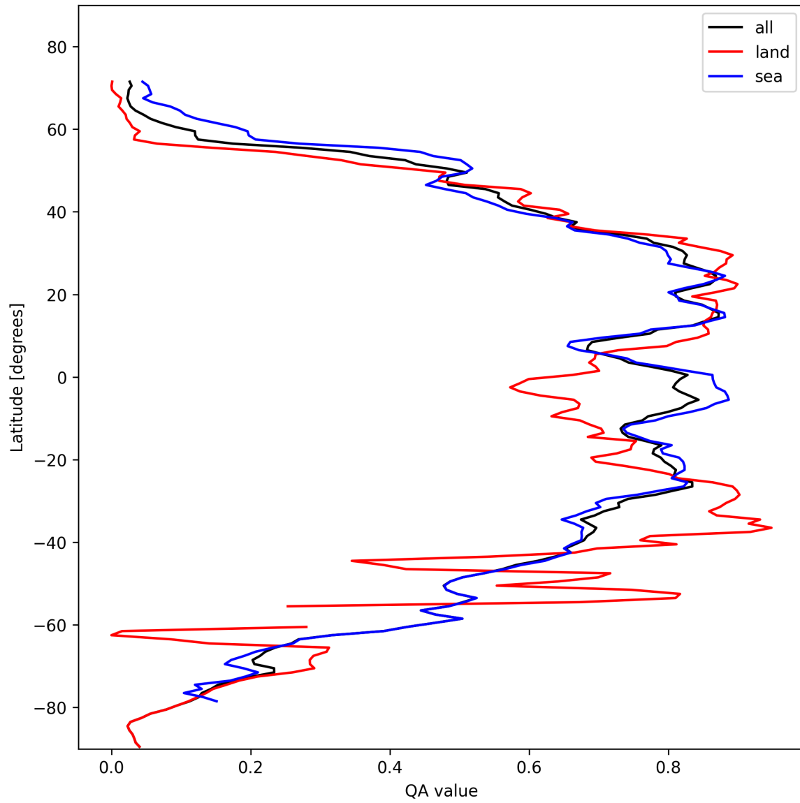
Figure 29: Zonal average of “QA value” for 2024-10-27 to 2024-10-29.
