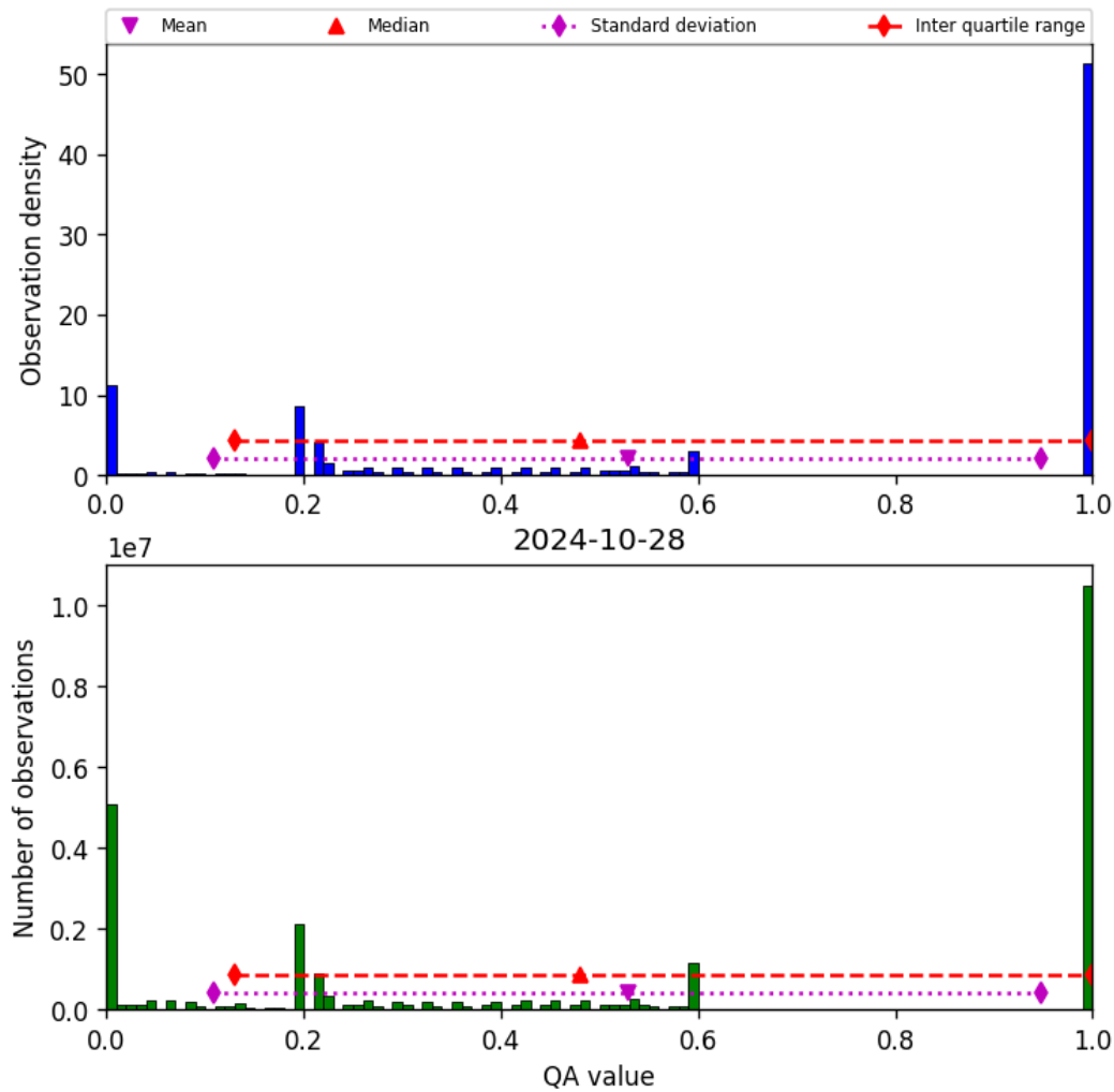
Figure 52: Histogram of “QA value” for 2024-10-27 to 2024-10-29
