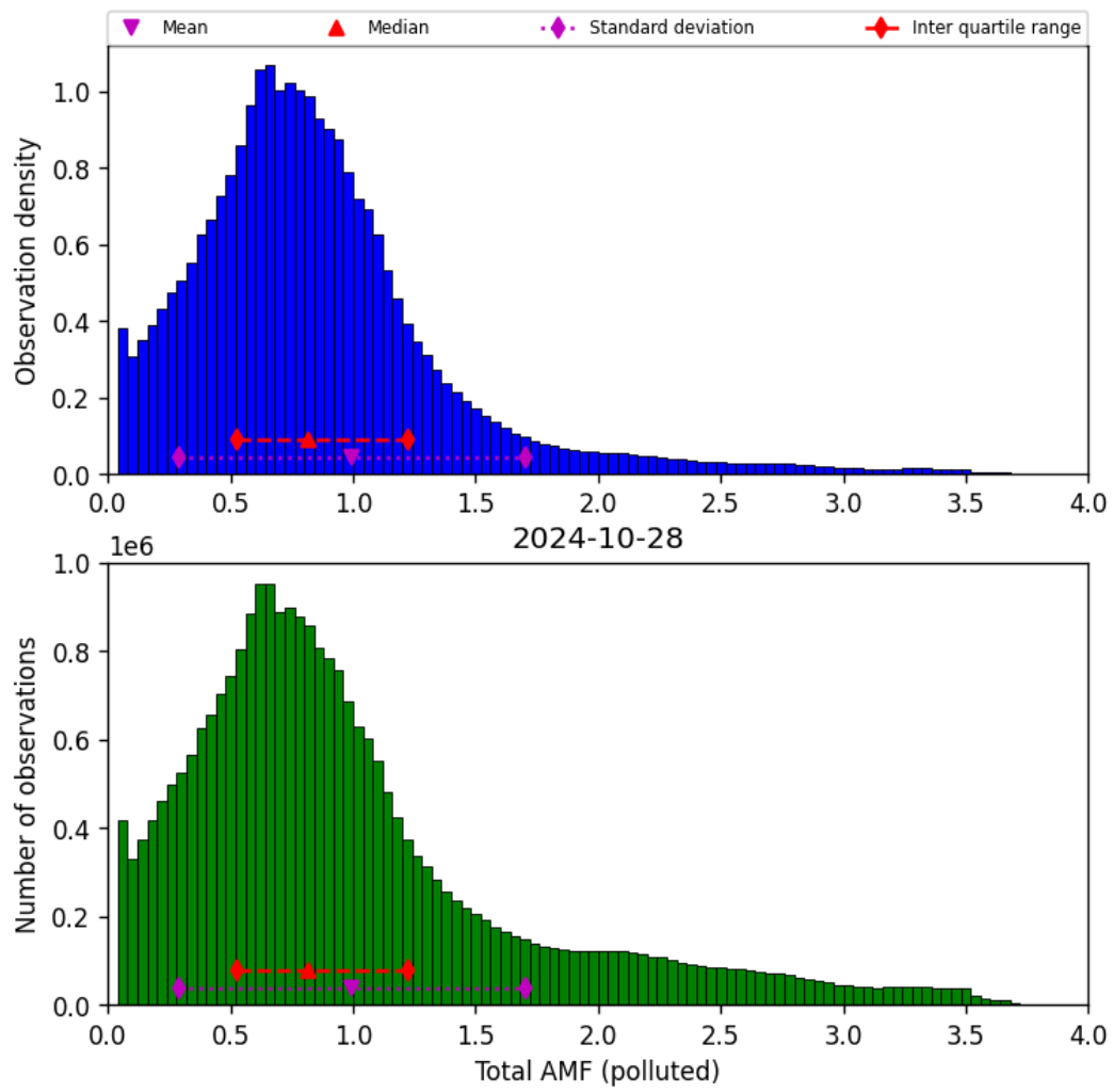
Figure 71: Histogram of “Total AMF (polluted)” for 2024-10-27 to 2024-10-29
