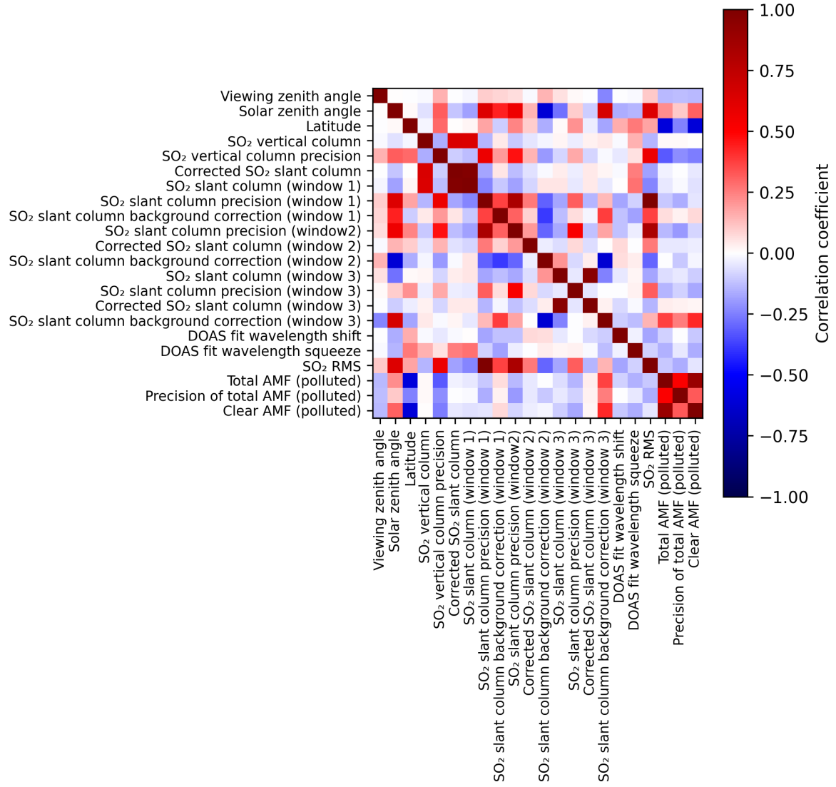
Figure 2: Map of correlation matrix for 2024-10-27 to 2024-10-29.
