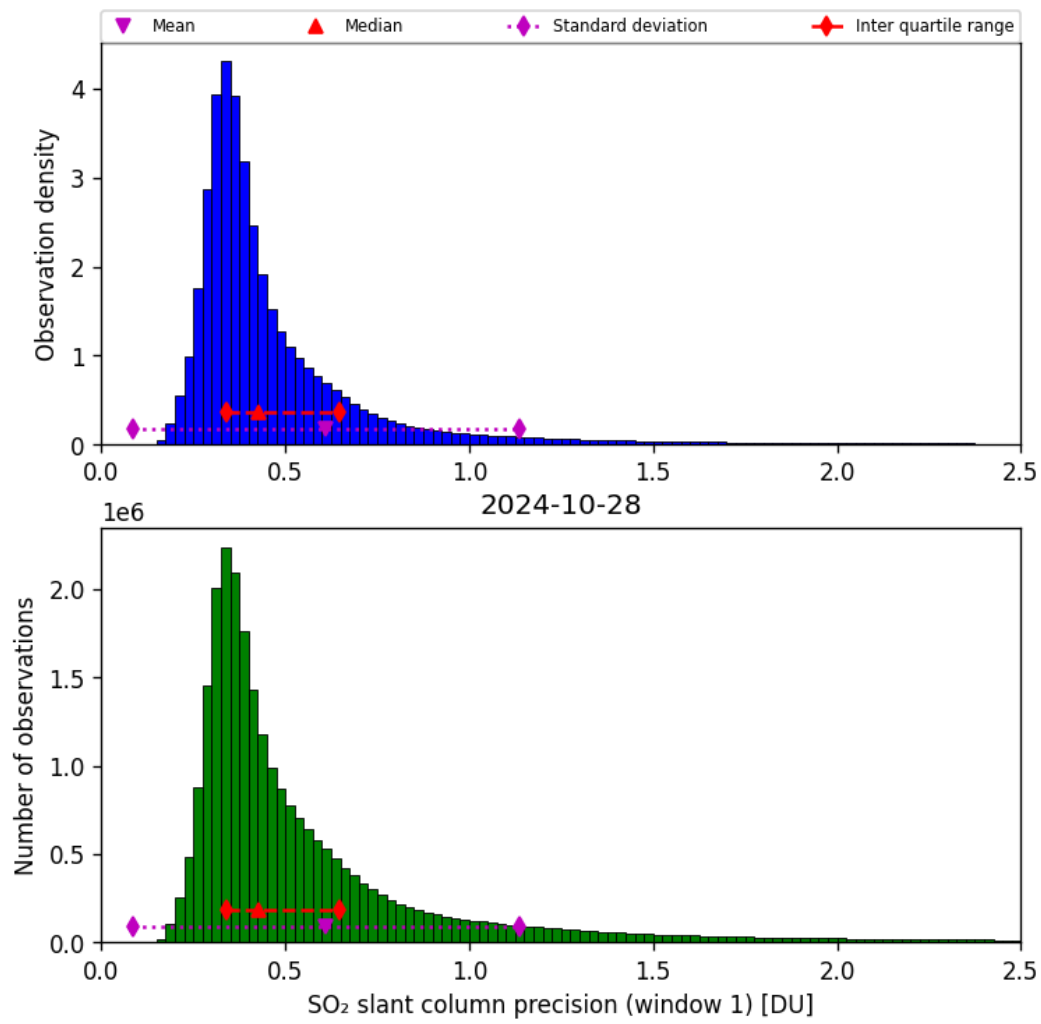
Figure 57: Histogram of “SO 2 slant column precision (window 1)” for 2024-10-27 to 2024-10-29
