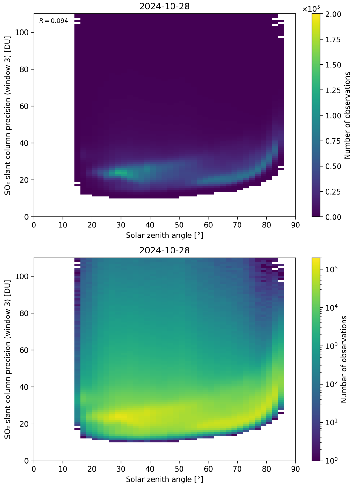
Figure 173: Scatter density plot of “Solar zenith angle” against “SO 2 slant column precision (window 3)” for 2024-10-27 to 2024-10-29.
