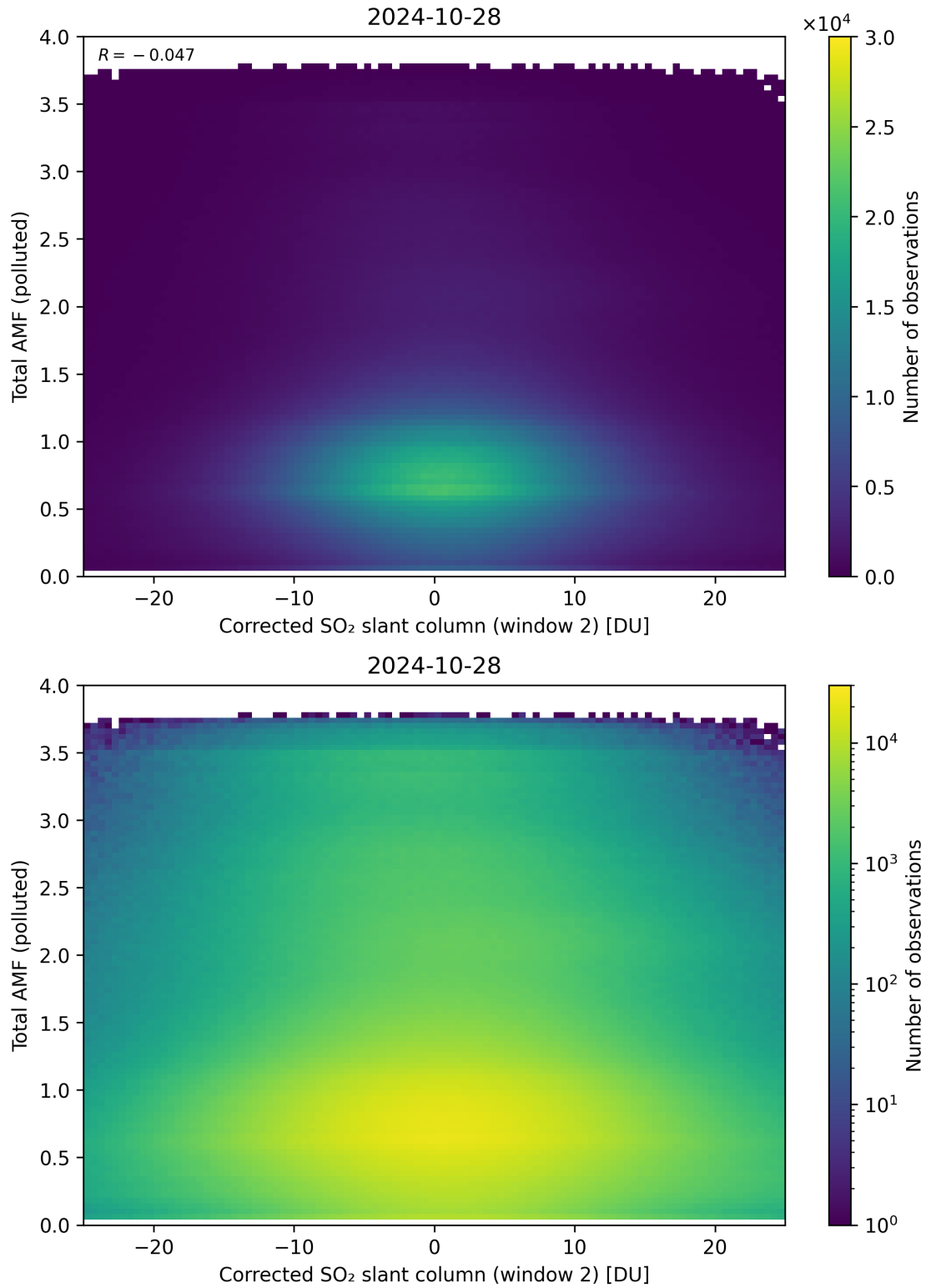
Figure 203: Scatter density plot of “Corrected SO 2 slant column (window 2)” against “Total AMF (polluted)” for 2024-10-27 to 2024-10-29.
