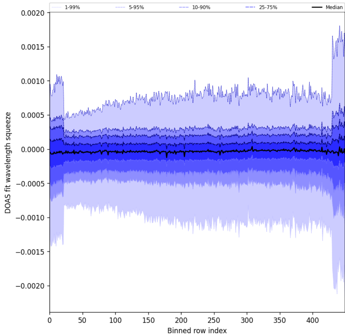
Figure 92: Along track statistics of “DOAS fit wavelength squeeze” for 2024-10-27 to 2024-10-29
