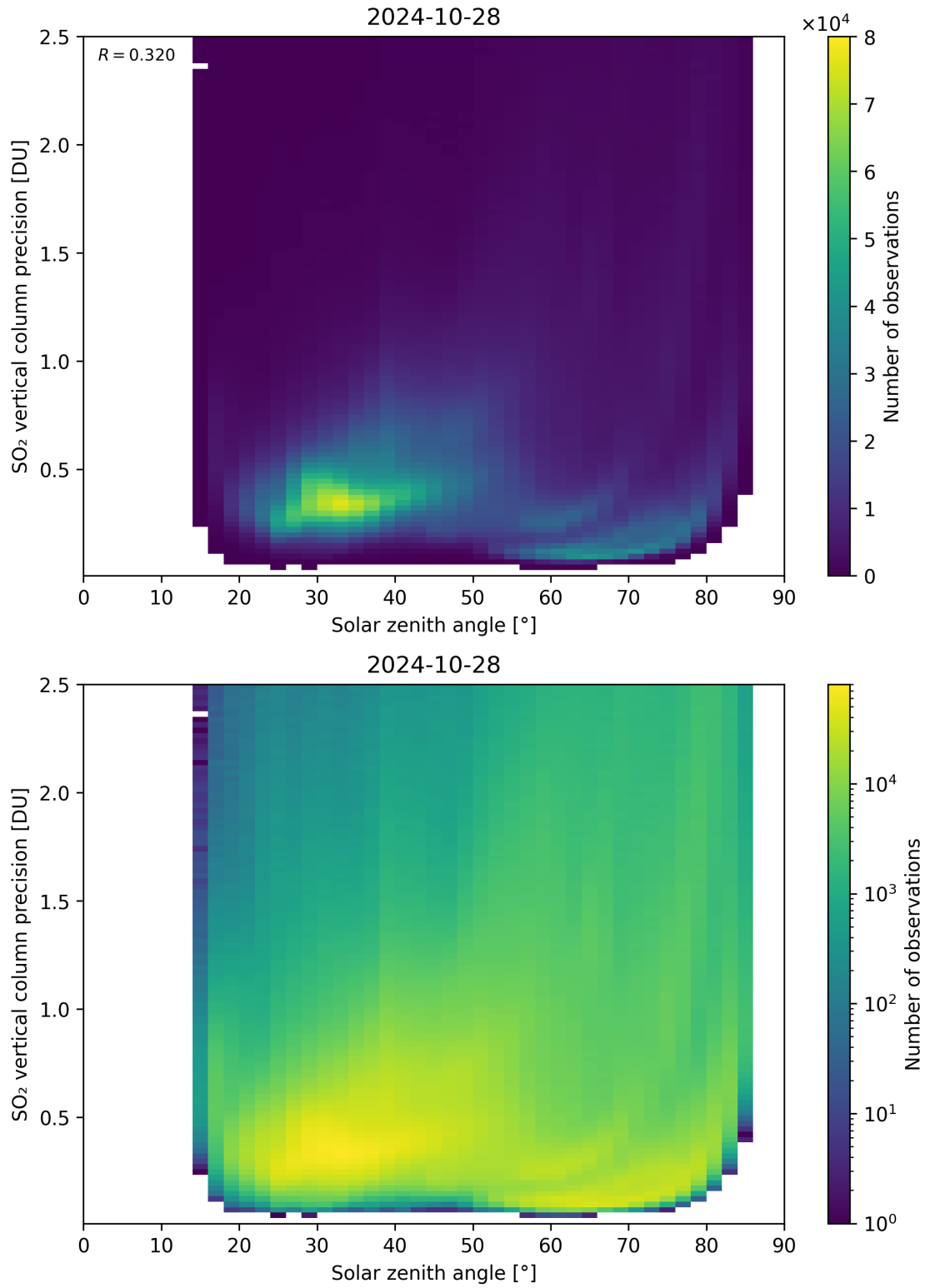
Figure 177: Scatter density plot of “Solar zenith angle” against “SO 2 vertical column precision” for 2024-10-27 to 2024-10-29.
