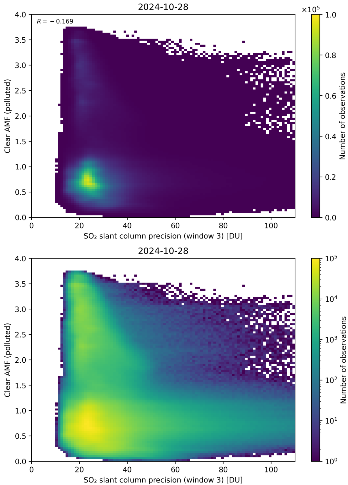
Figure 261: Scatter density plot of “SO 2 slant column precision (window 3)” against “Clear AMF (polluted)” for 2024-10-27 to 2024-10-29.
