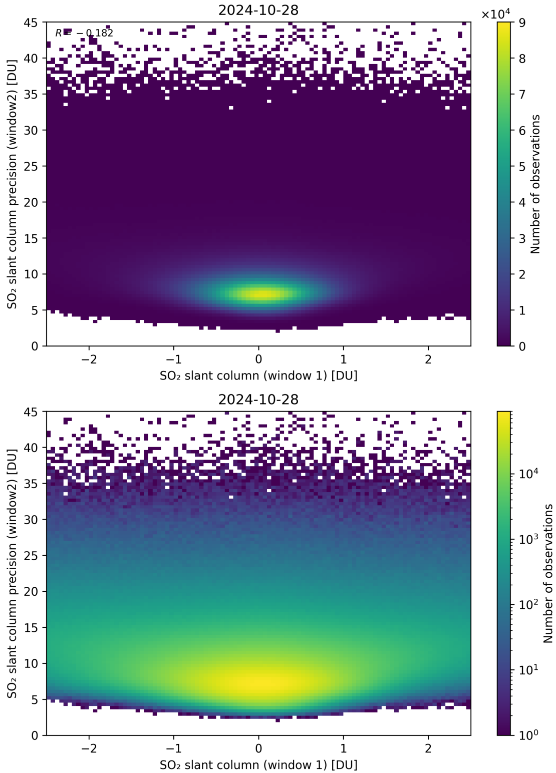
Figure 236: Scatter density plot of “SO 2 slant column (window 1)” against “SO 2 slant column precision (window2)” for 2024-10-27 to 2024-10-29.
