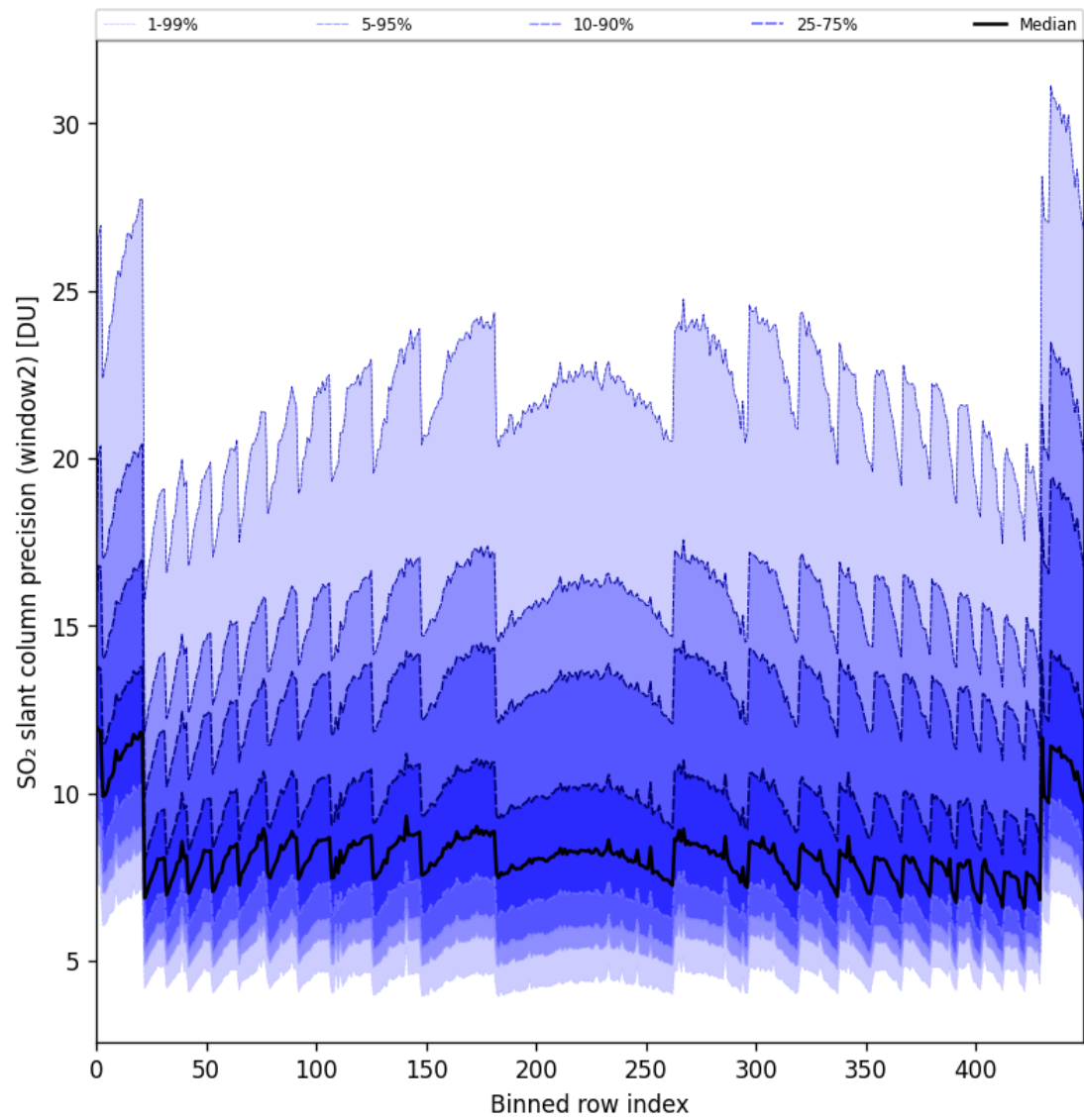
Figure 84: Along track statistics of “SO 2 slant column precision (window2)” for 2024-10-27 to 2024-10-29
