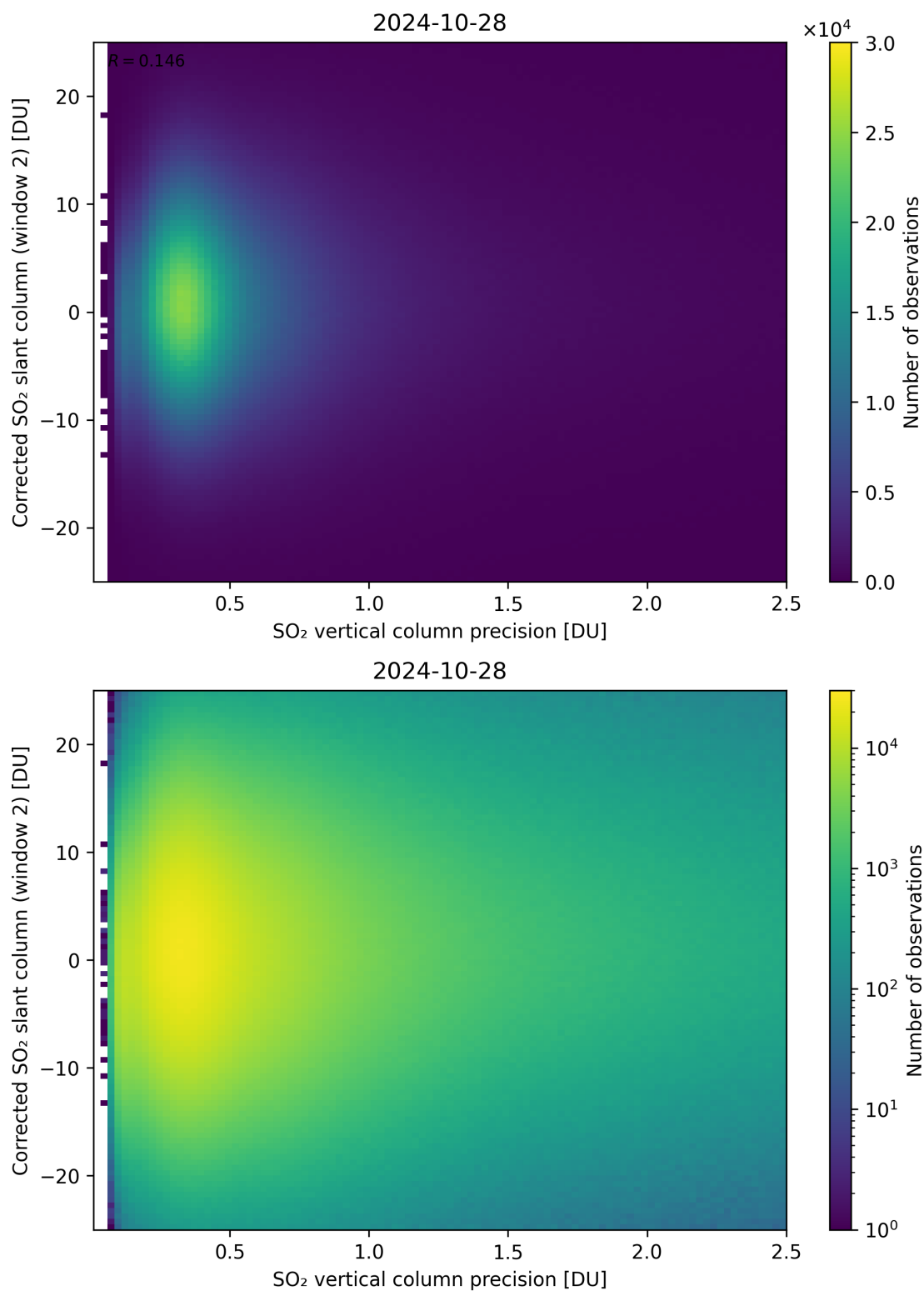
Figure 287: Scatter density plot of “SO 2 vertical column precision” against “Corrected SO 2 slant column (window 2)” for 2024-10-27 to 2024-10-29.
