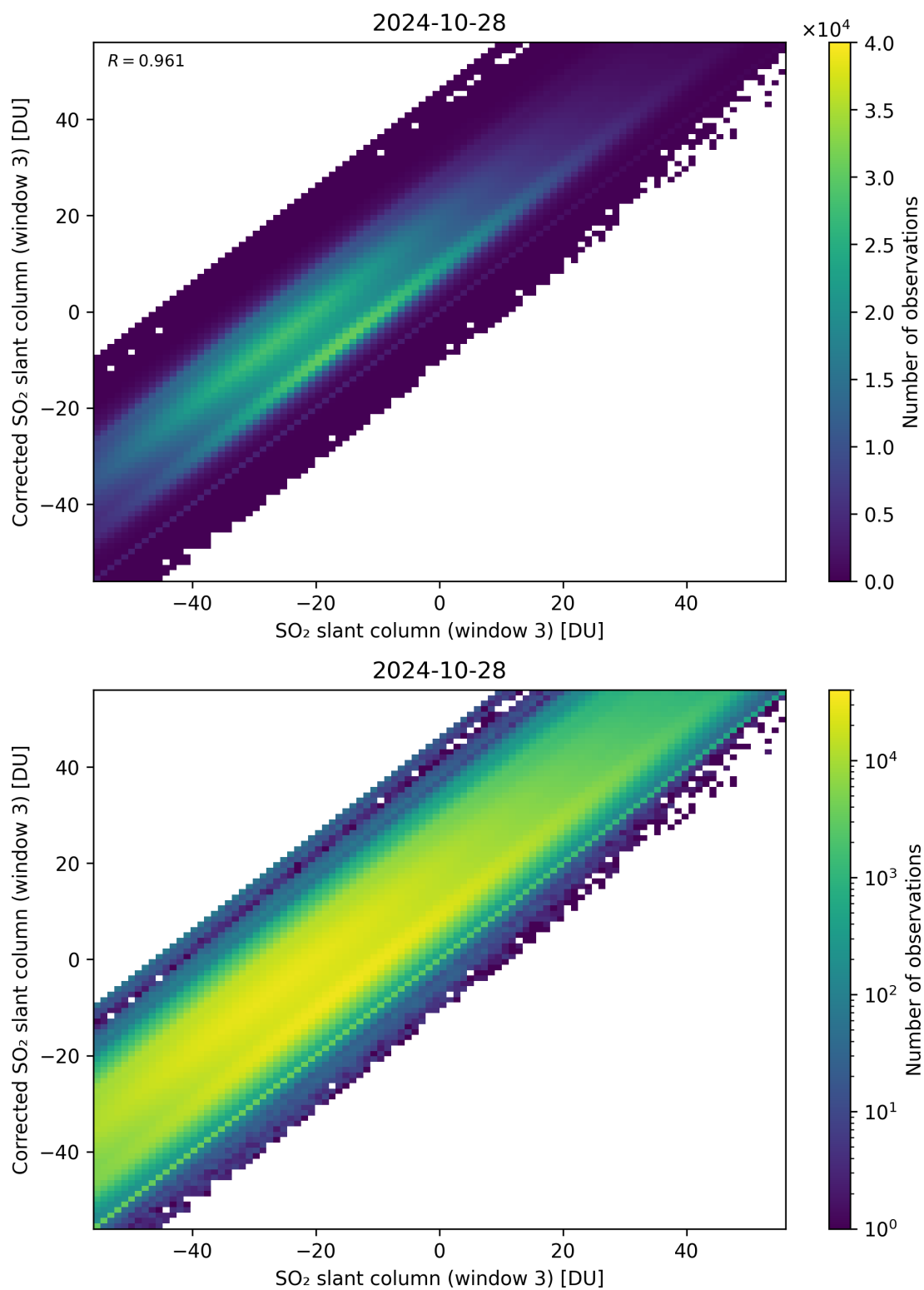
Figure 266: Scatter density plot of “SO 2 slant column (window 3)” against “Corrected SO 2 slant column (window 3)” for 2024-10-27 to 2024-10-29.
