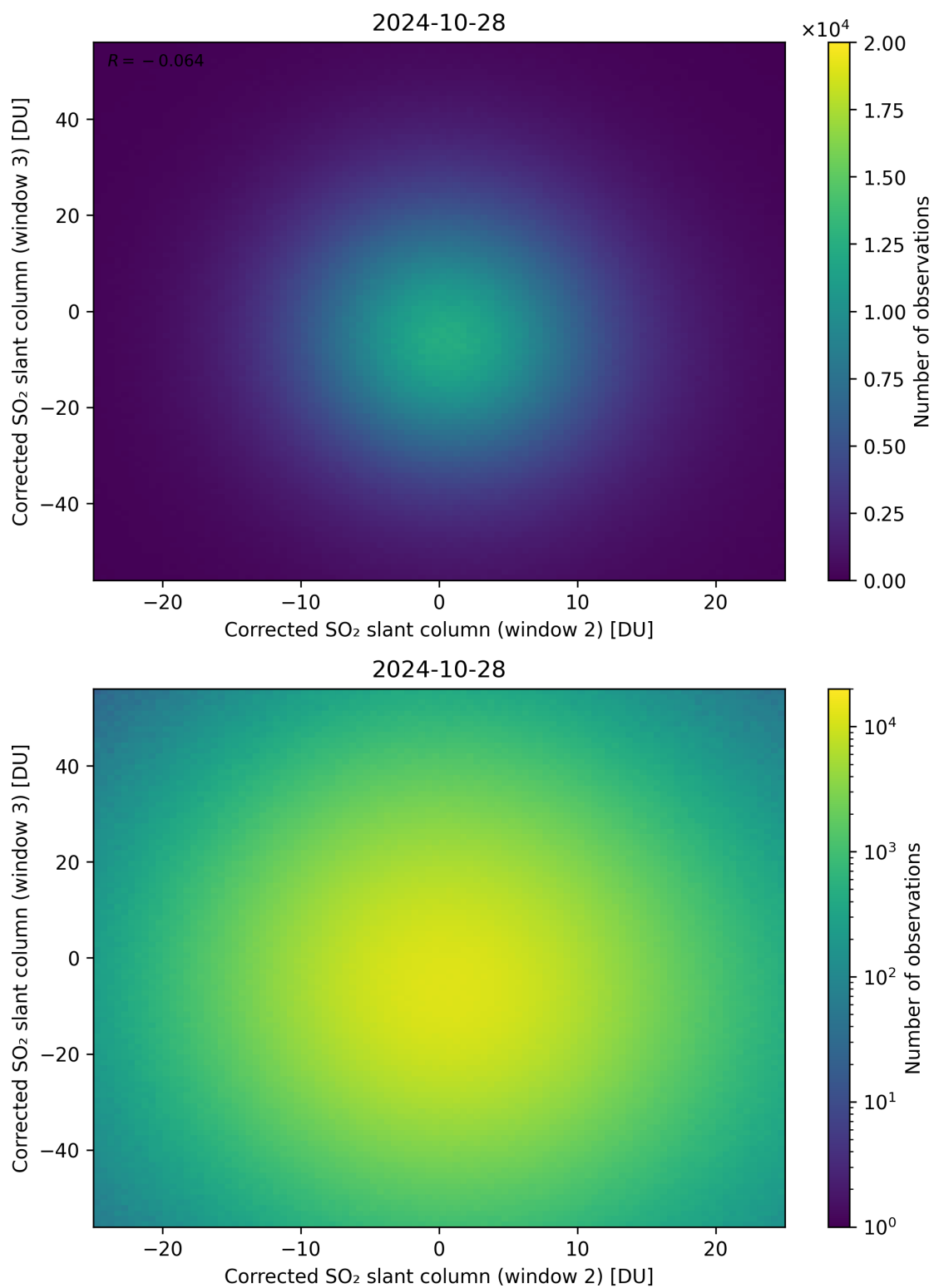
Figure 200: Scatter density plot of “Corrected SO 2 slant column (window 2)” against “Corrected SO 2 slant column (window 3)” for 2024-10-27 to 2024-10-29.
