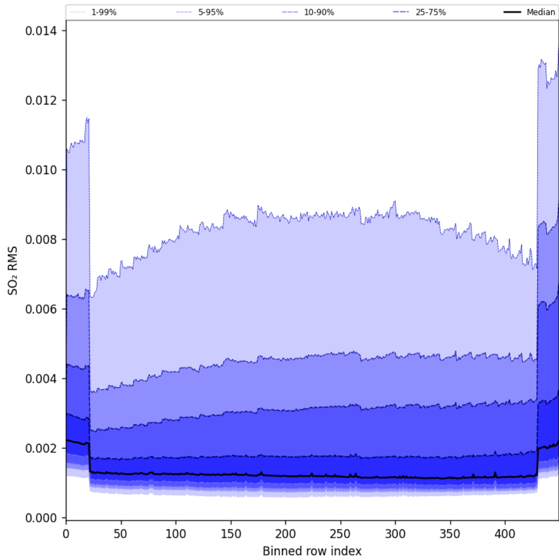
Figure 93: Along track statistics of “SO 2 RMS” for 2024-10-27 to 2024-10-29
