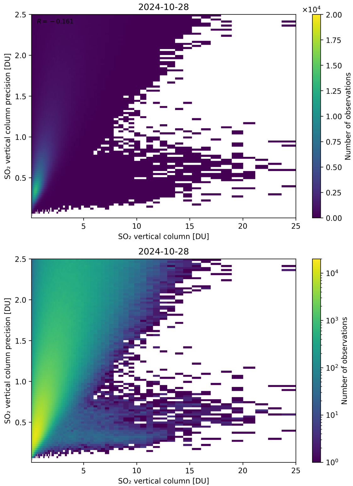
Figure 307: Scatter density plot of “SO 2 vertical column” against “SO 2 vertical column precision” for 2024-10-27 to 2024-10-29.
