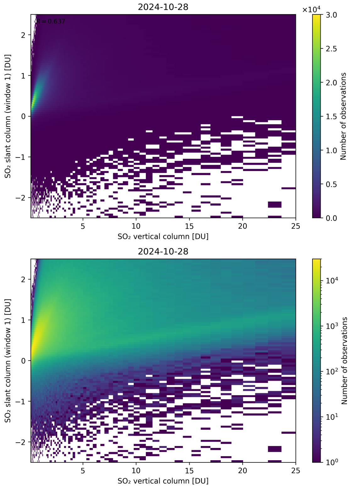
Figure 300: Scatter density plot of “SO 2 vertical column” against “SO 2 slant column (window 1)” for 2024-10-27 to 2024-10-29.
