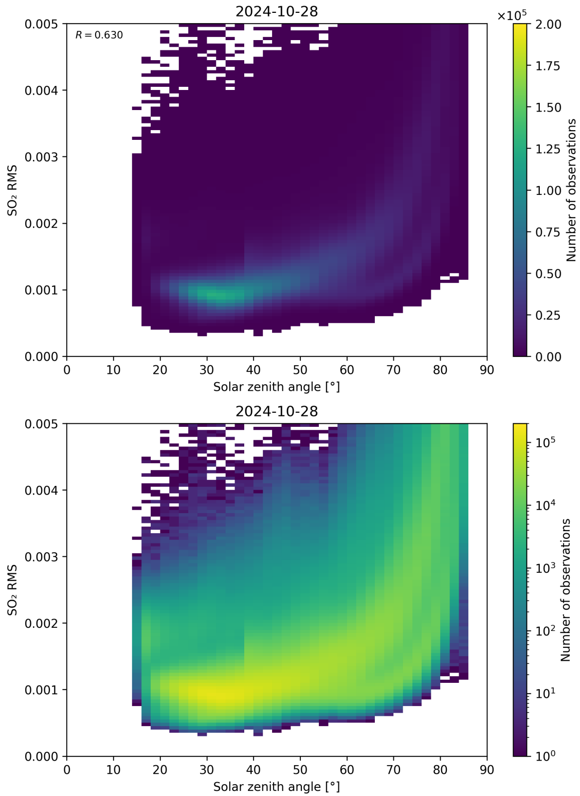
Figure 163: Scatter density plot of “Solar zenith angle” against “SO 2 RMS” for 2024-10-27 to 2024-10-29.
