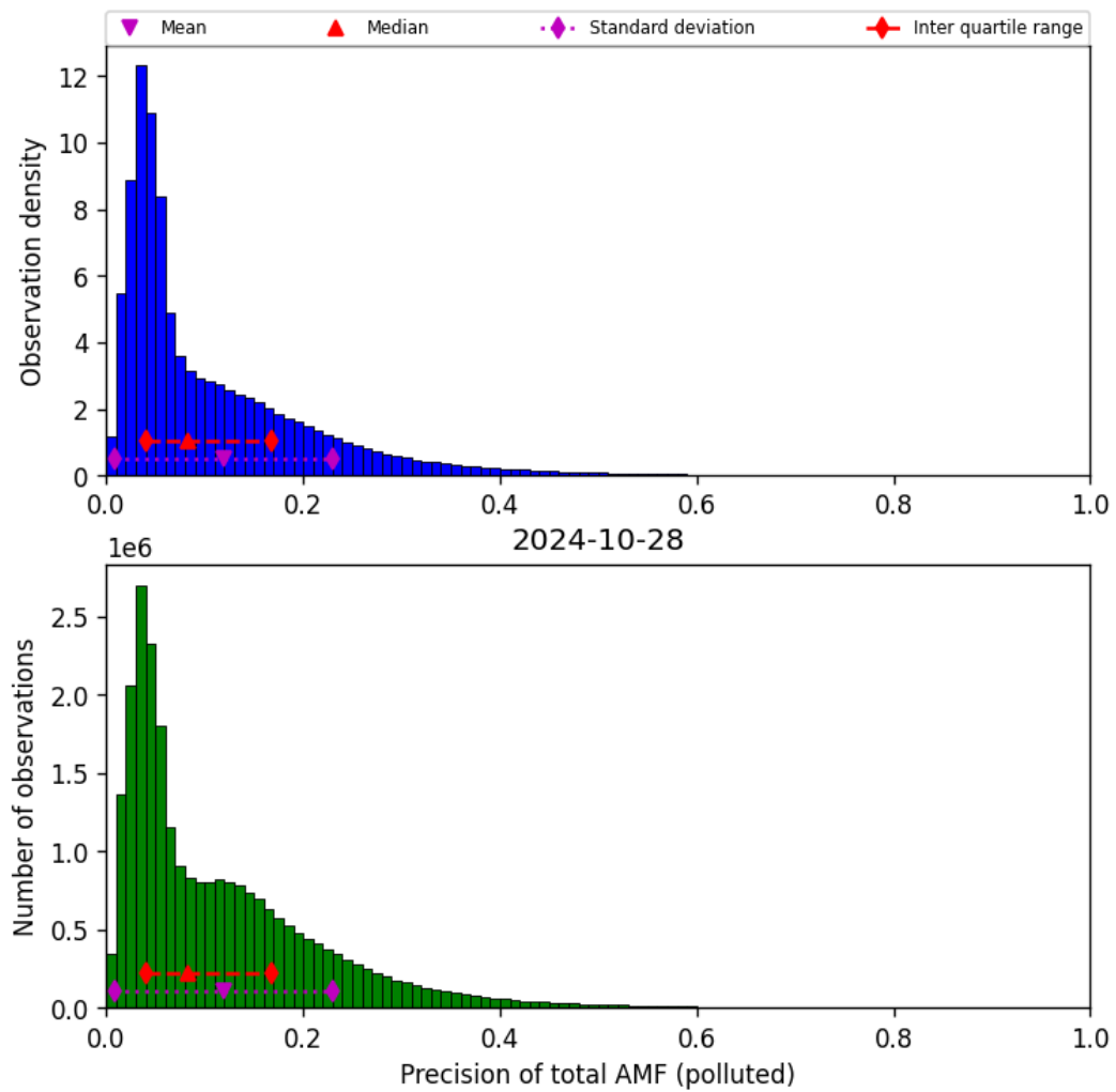
Figure 72: Histogram of “Precision of total AMF (polluted)” for 2024-10-27 to 2024-10-29
