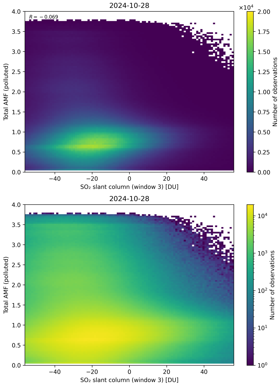
Figure 268: Scatter density plot of “SO 2 slant column (window 3)” against “Total AMF (polluted)” for 2024-10-27 to 2024-10-29.
