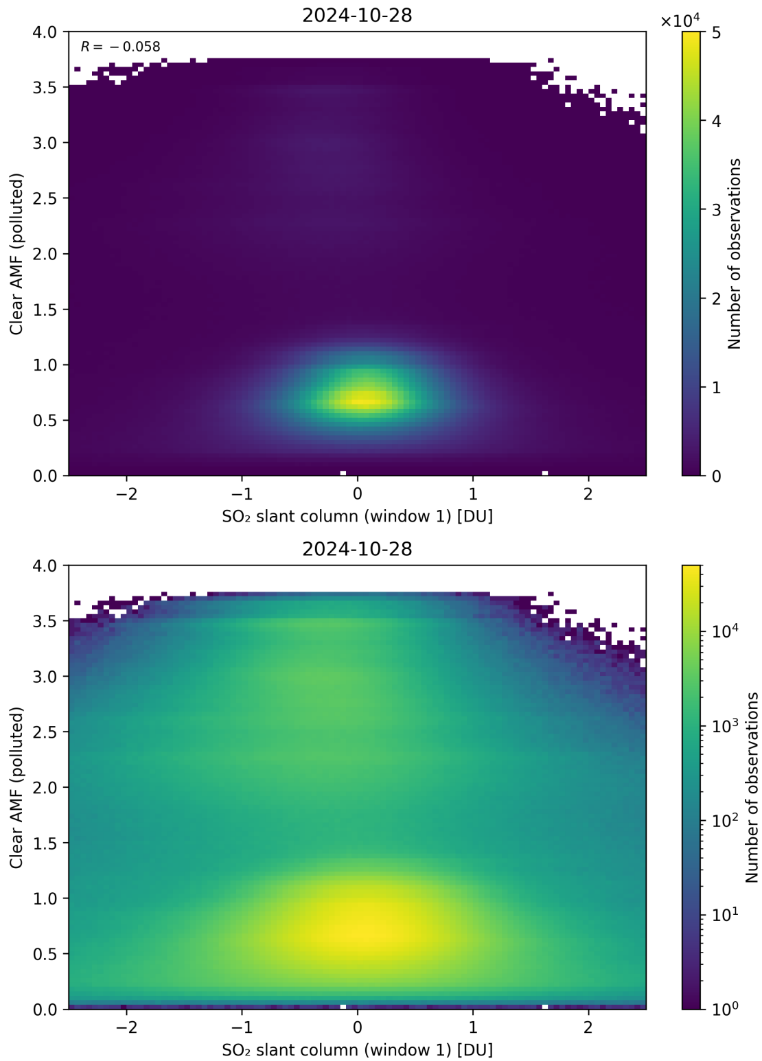
Figure 232: Scatter density plot of “SO 2 slant column (window 1)” against “Clear AMF (polluted)” for 2024-10-27 to 2024-10-29.
