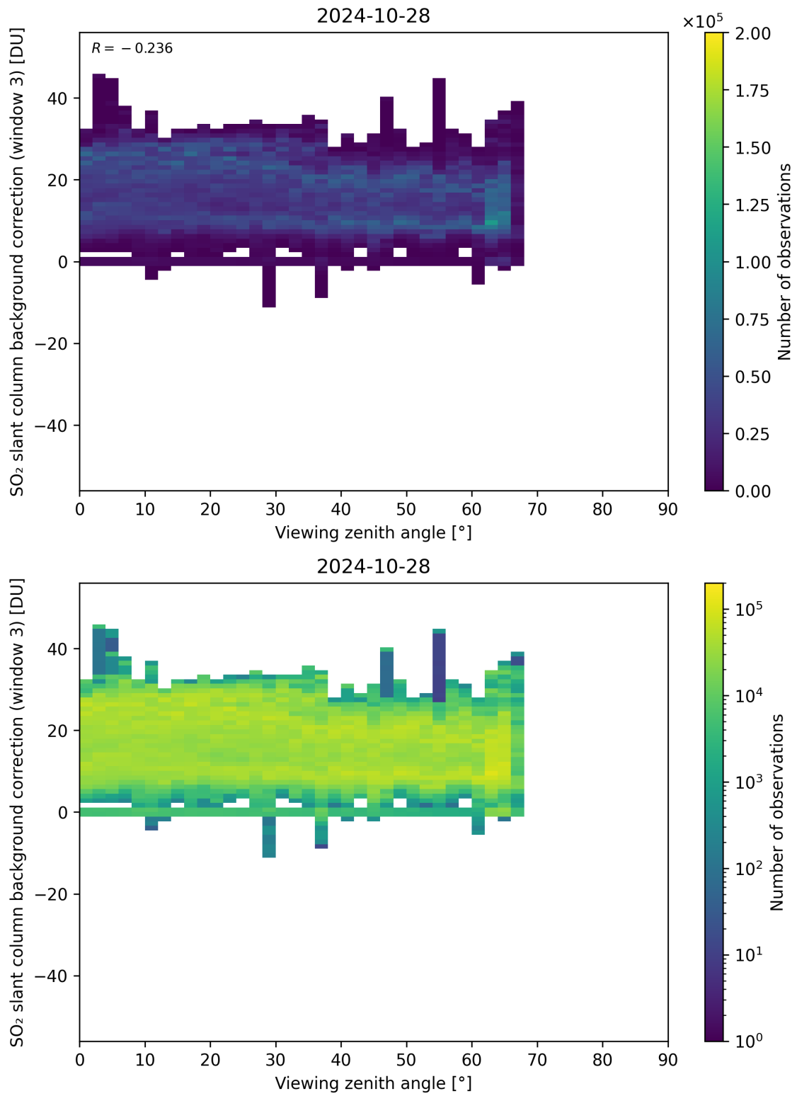
Figure 310: Scatter density plot of “Viewing zenith angle” against “SO 2 slant column background correction (window 3)” for 2024-10-27 to 2024-10-29.
