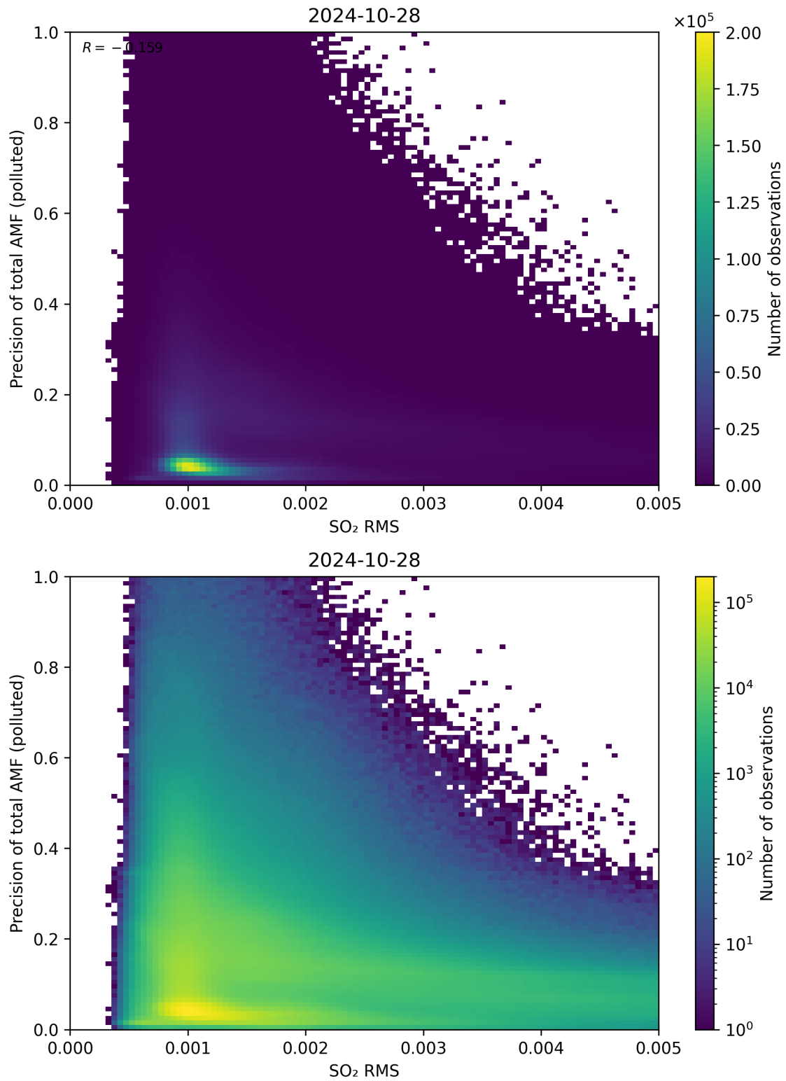
Figure 138: Scatter density plot of “SO 2 RMS” against “Precision of total AMF (polluted)” for 2024-10-27 to 2024-10-29.
