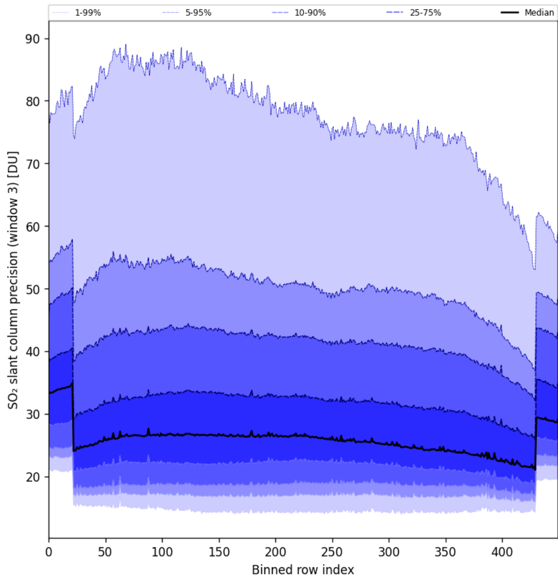
Figure 88: Along track statistics of “SO 2 slant column precision (window 3)” for 2024-10-27 to 2024-10-29
