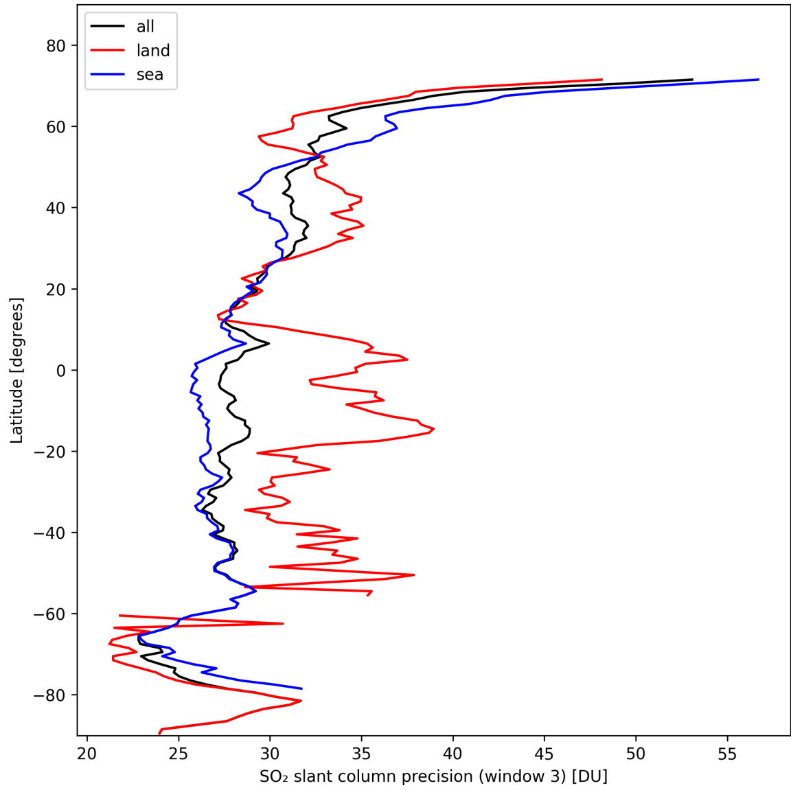
Figure 42: Zonal average of “SO 2 slant column precision (window 3)” for 2024-10-27 to 2024-10-29.
