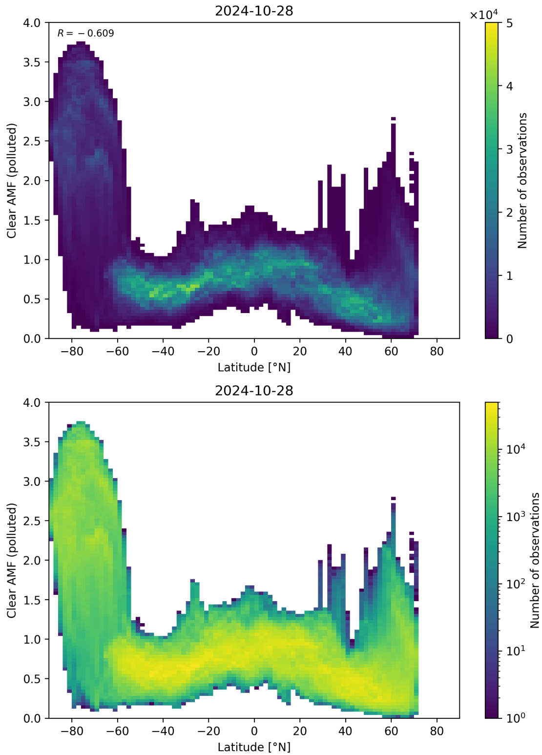
Figure 145: Scatter density plot of “Latitude” against “Clear AMF (polluted)” for 2024-10-27 to 2024-10-29.
