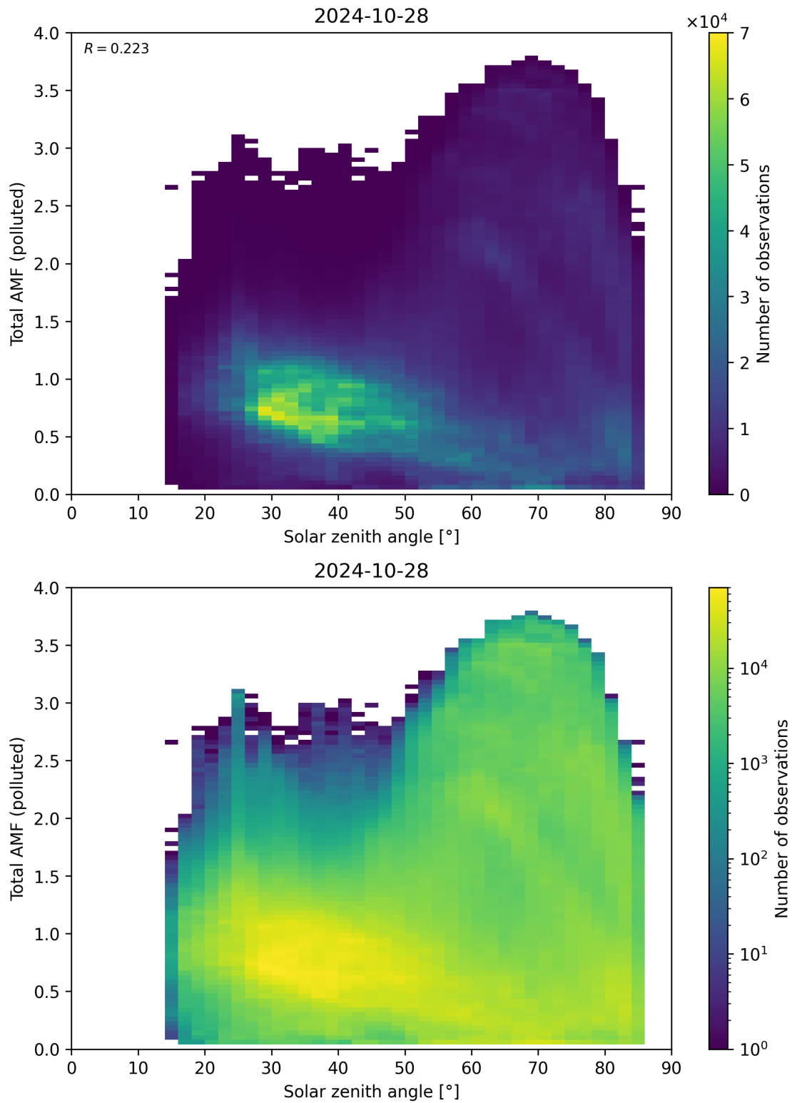
Figure 174: Scatter density plot of “Solar zenith angle” against “Total AMF (polluted)” for 2024-10-27 to 2024-10-29.
