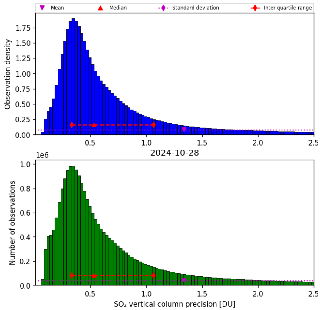
Figure 54: Histogram of “SO 2 vertical column precision” for 2024-10-27 to 2024-10-29
