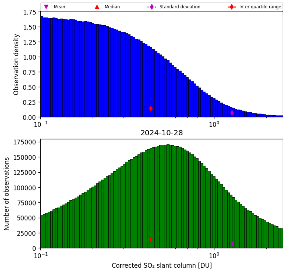
Figure 55: Histogram of “Corrected SO 2 slant column” for 2024-10-27 to 2024-10-29
