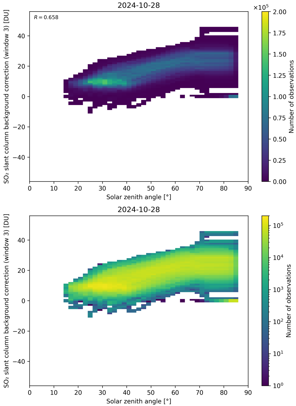
Figure 160: Scatter density plot of “Solar zenith angle” against “SO 2 slant column background correction (window 3)” for 2024-10-27 to 2024-10-29.
