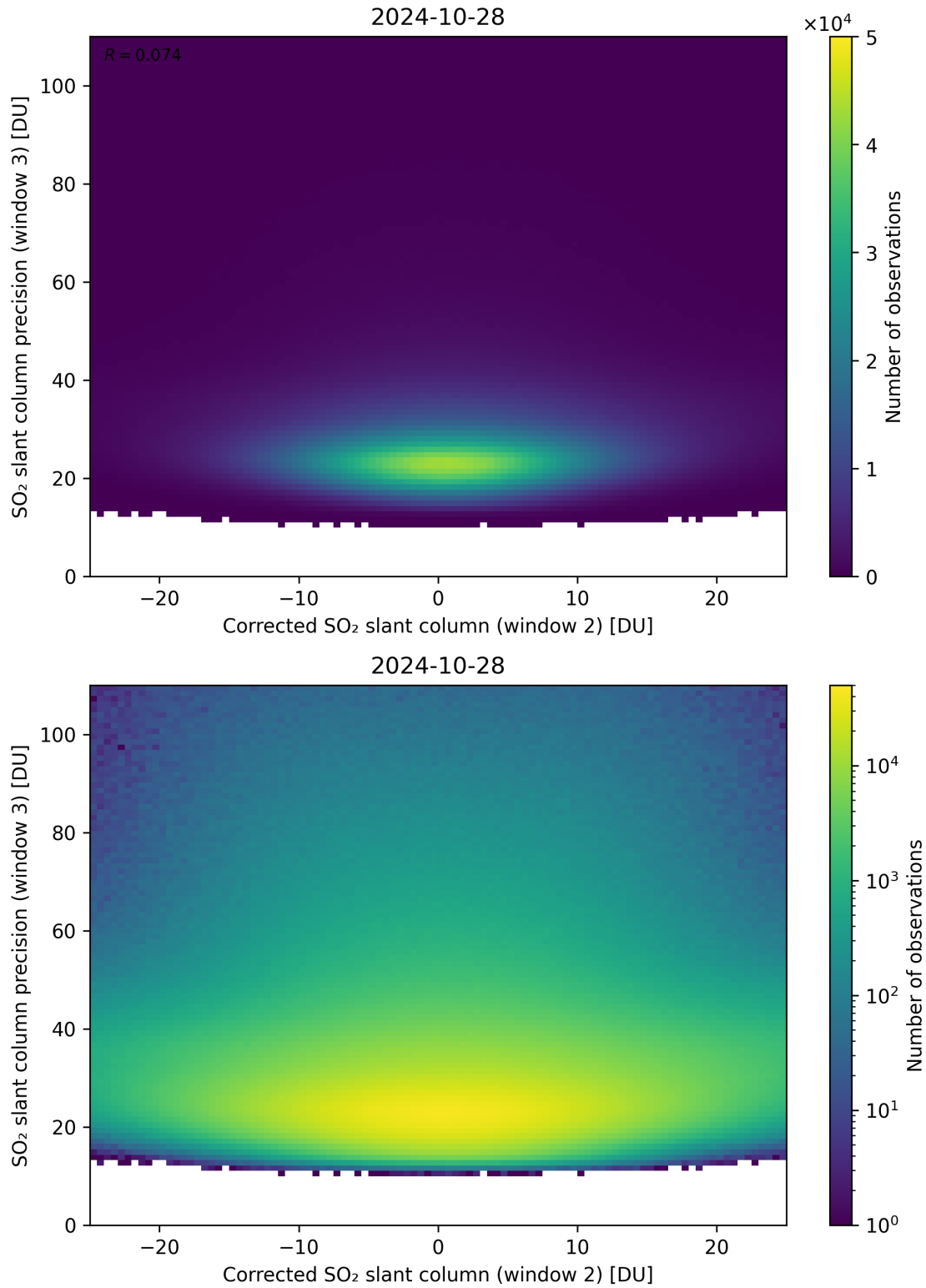
Figure 202: Scatter density plot of “Corrected SO 2 slant column (window 2)” against “SO 2 slant column precision (window 3)” for 2024-10-27 to 2024-10-29.
