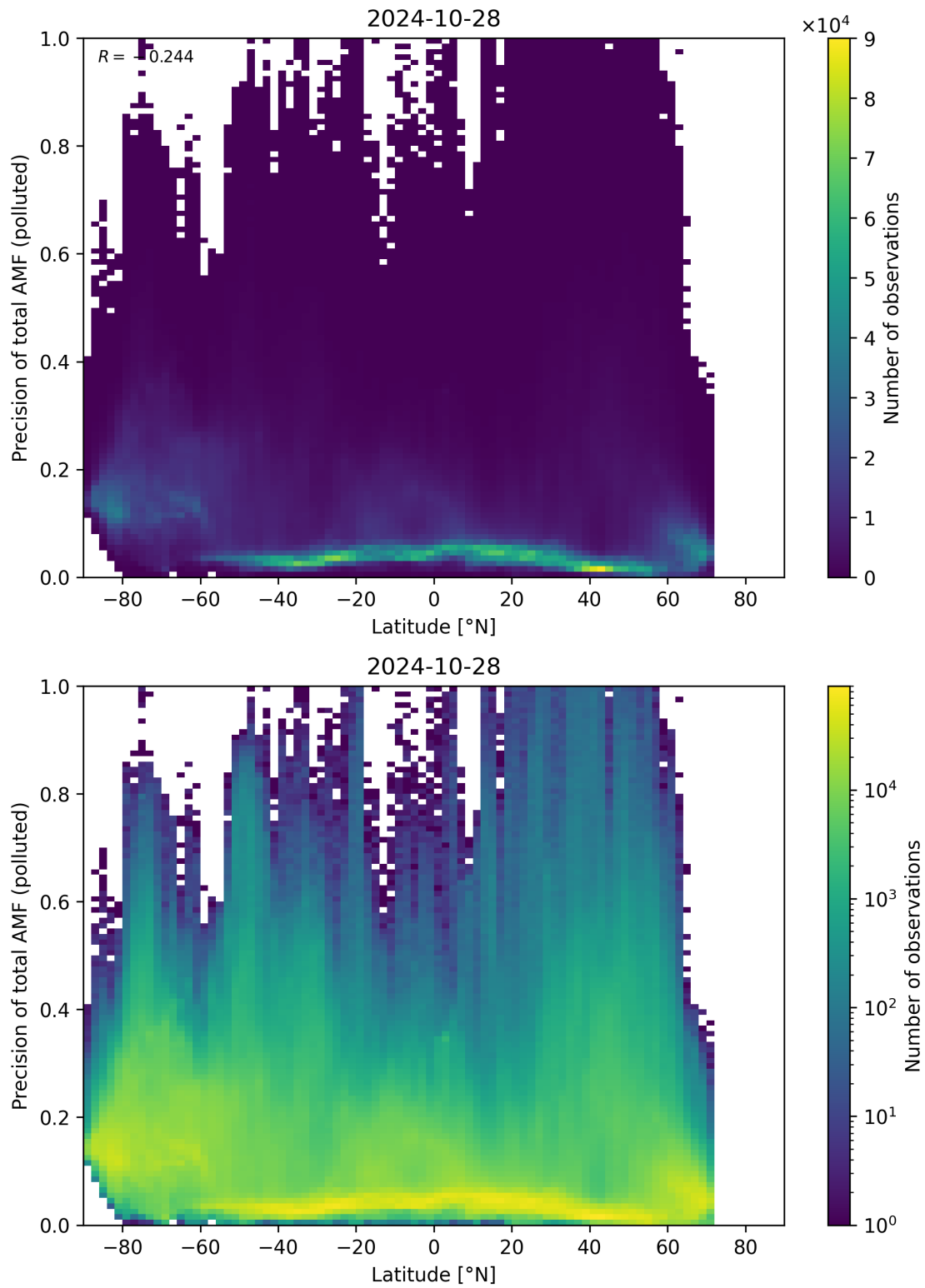
Figure 155: Scatter density plot of “Latitude” against “Precision of total AMF (polluted)” for 2024-10-27 to 2024-10-29.
