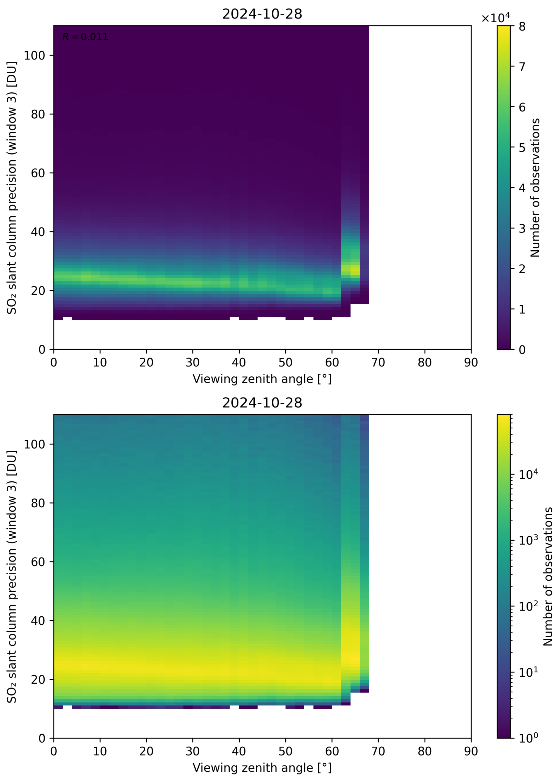
Figure 324: Scatter density plot of “Viewing zenith angle” against “SO 2 slant column precision (window 3)” for 2024-10-27 to 2024-10-29.
