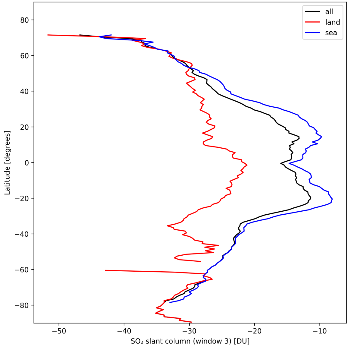
Figure 41: Zonal average of “SO 2 slant column (window 3)” for 2024-10-27 to 2024-10-29.
