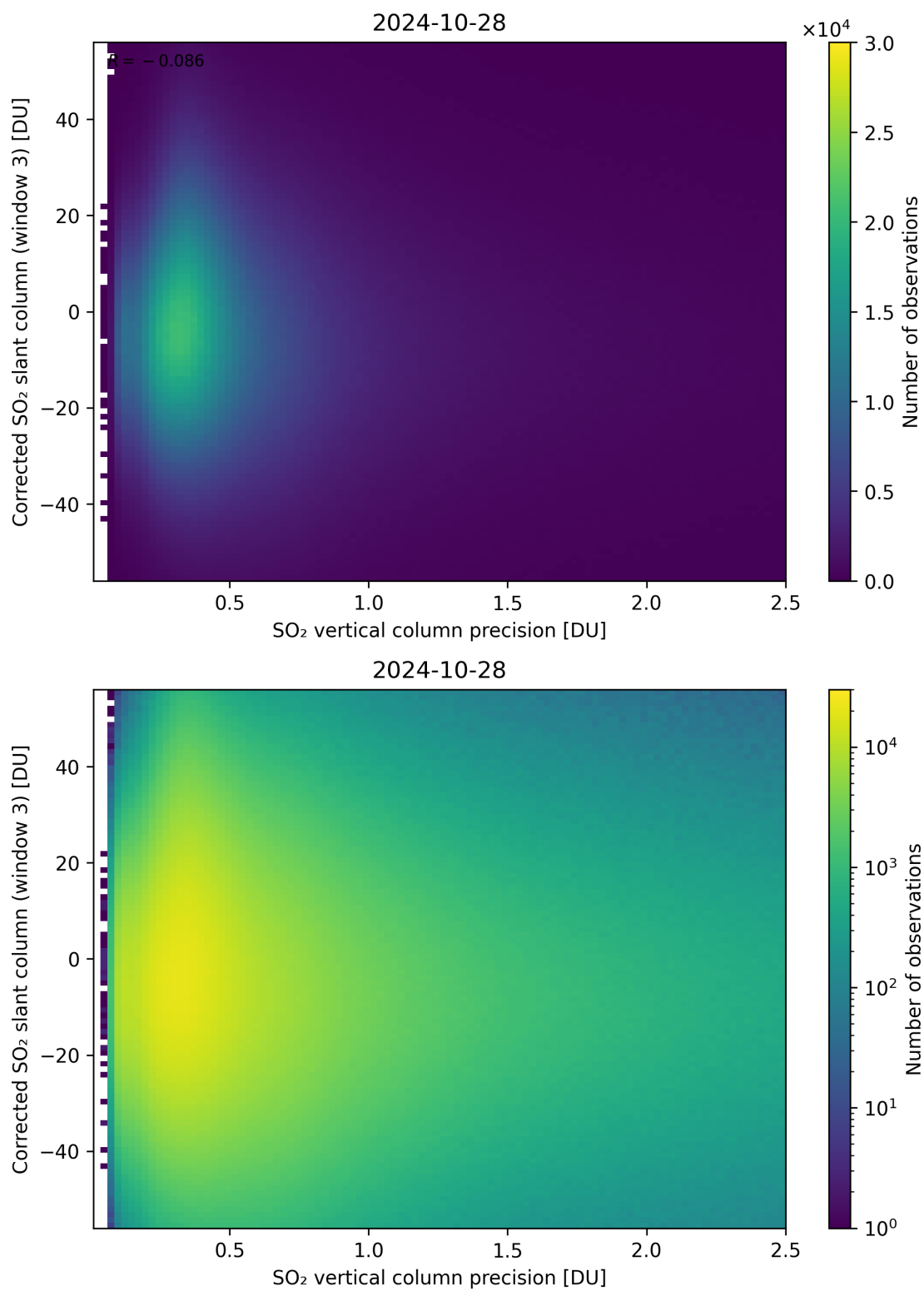
Figure 288: Scatter density plot of “SO 2 vertical column precision” against “Corrected SO 2 slant column (window 3)” for 2024-10-27 to 2024-10-29.
