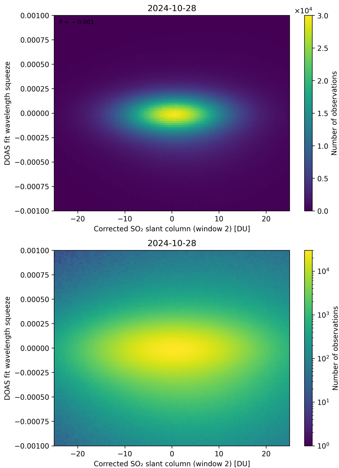
Figure 197: Scatter density plot of “Corrected SO 2 slant column (window 2)” against “DOAS fit wavelength squeeze” for 2024-10-27 to 2024-10-29.
