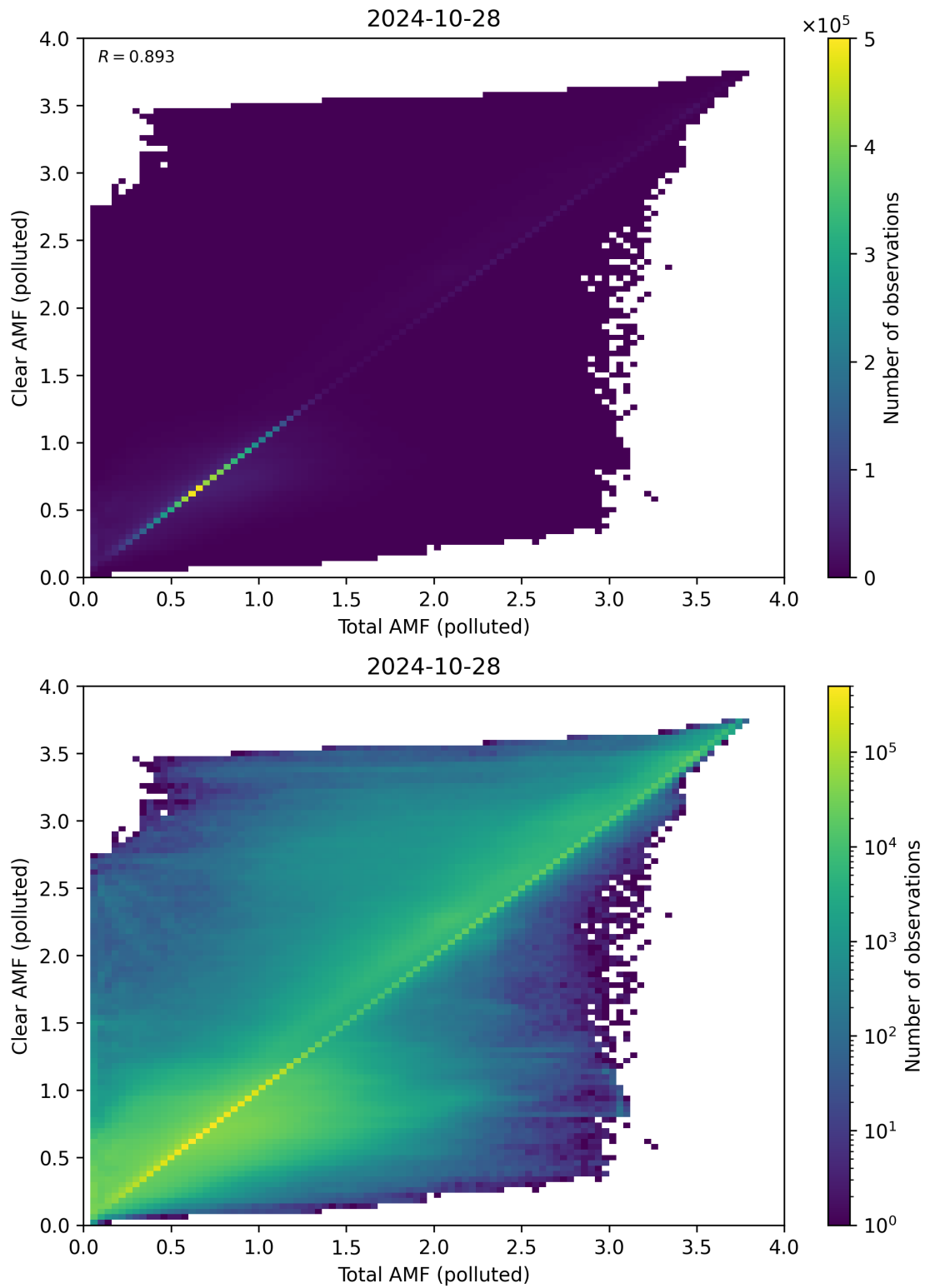
Figure 271: Scatter density plot of “Total AMF (polluted)” against “Clear AMF (polluted)” for 2024-10-27 to 2024-10-29.
