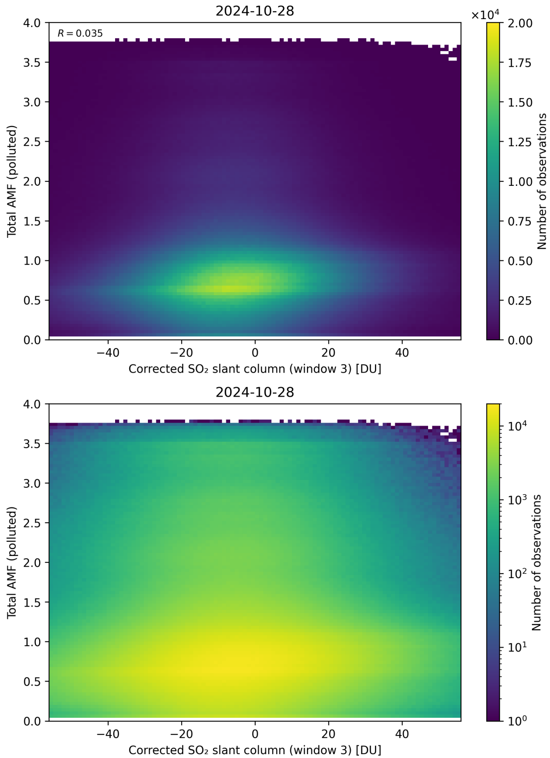
Figure 210: Scatter density plot of “Corrected SO 2 slant column (window 3)” against “Total AMF (polluted)” for 2024-10-27 to 2024-10-29.
