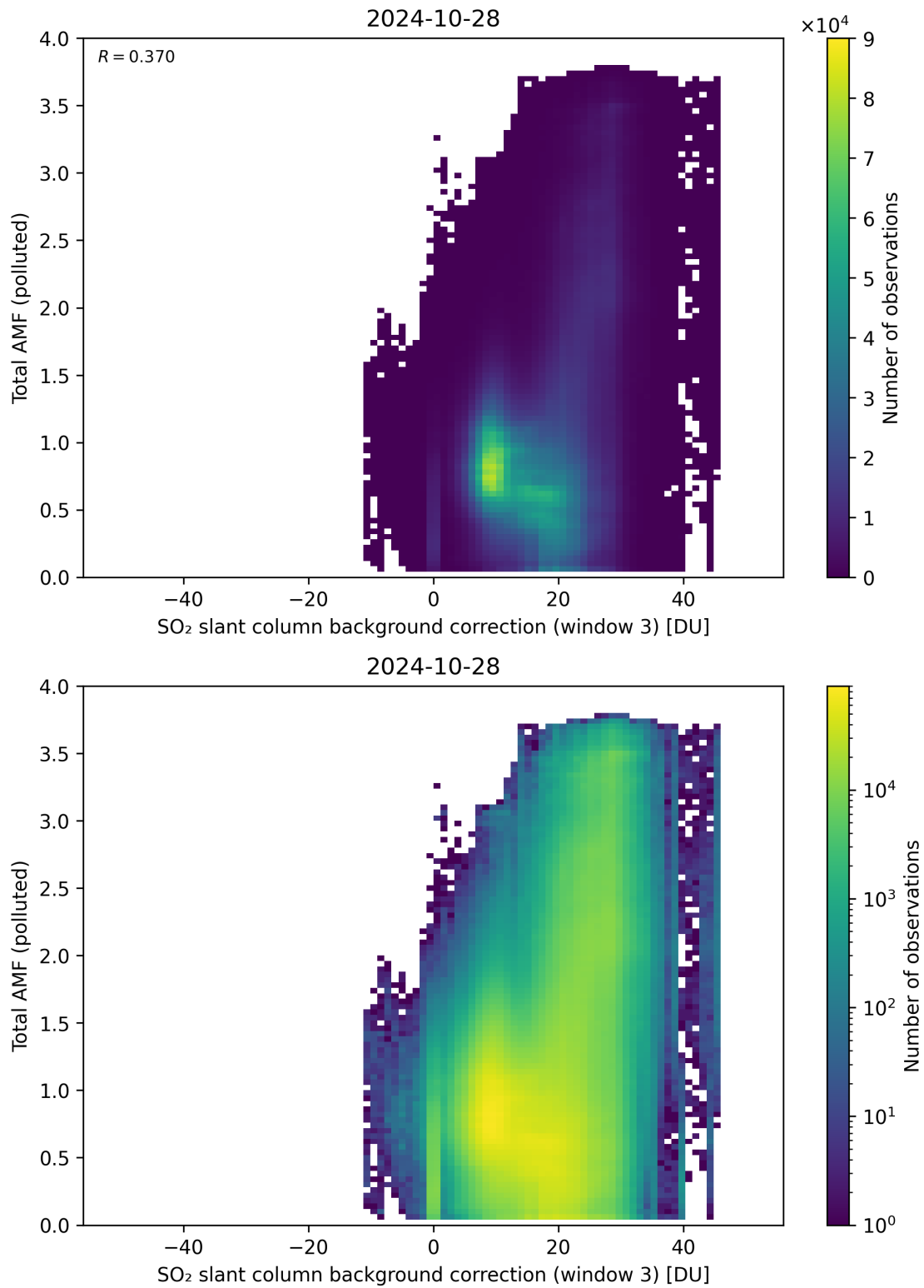
Figure 125: Scatter density plot of “SO 2 slant column background correction (window 3)” against “Total AMF (polluted)” for 2024-10-27 to 2024-10-29.
