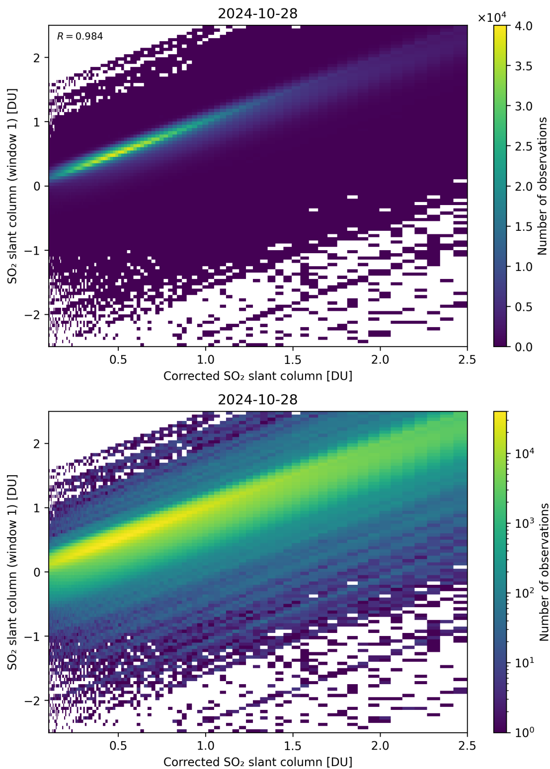
Figure 187: Scatter density plot of “Corrected SO 2 slant column” against “SO 2 slant column (window 1)” for 2024-10-27 to 2024-10-29.
