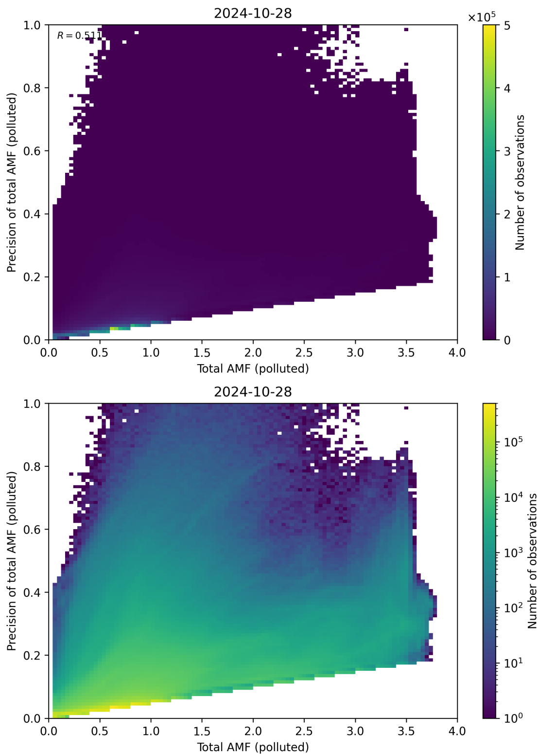
Figure 272: Scatter density plot of “Total AMF (polluted)” against “Precision of total AMF (polluted)” for 2024-10-27 to 2024-10-29.
