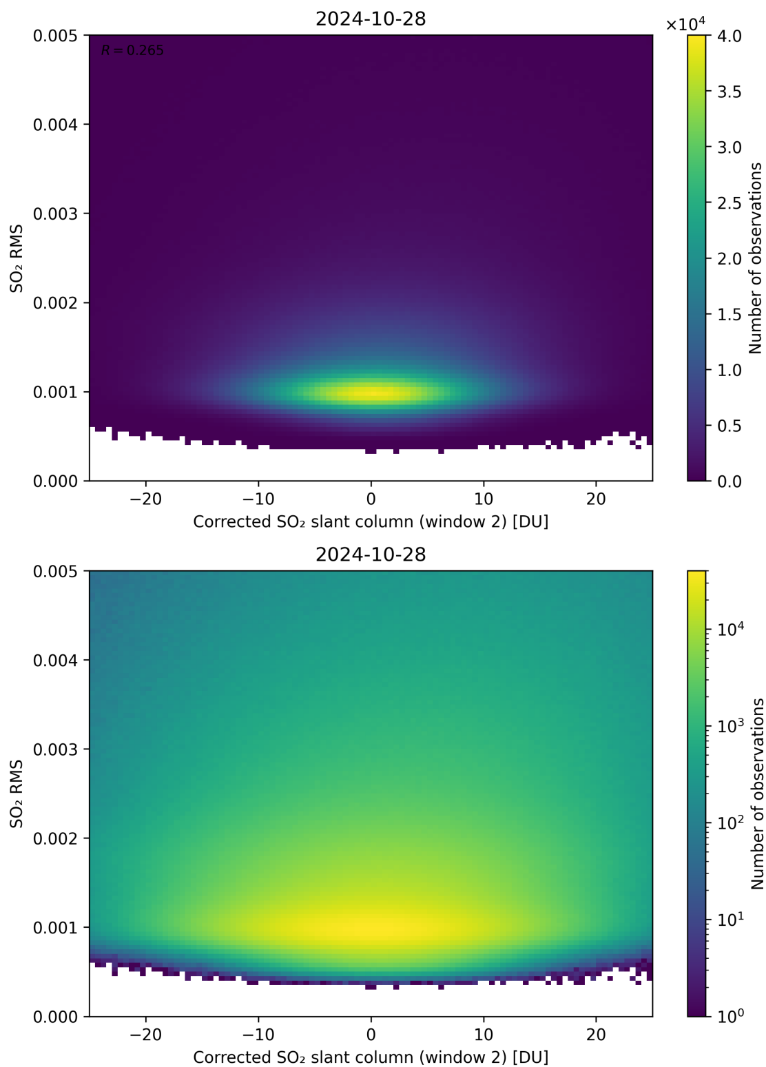
Figure 198: Scatter density plot of “Corrected SO 2 slant column (window 2)” against “SO 2 RMS” for 2024-10-27 to 2024-10-29.
