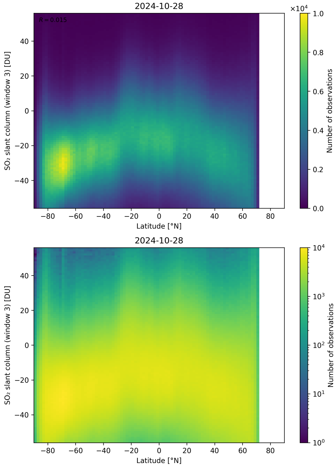
Figure 152: Scatter density plot of “Latitude” against “SO 2 slant column (window 3)” for 2024-10-27 to 2024-10-29.
