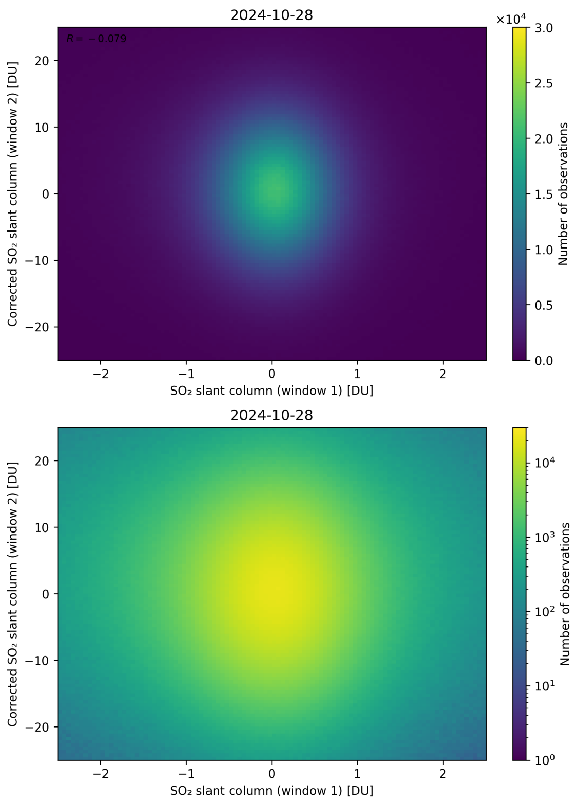
Figure 233: Scatter density plot of “SO 2 slant column (window 1)” against “Corrected SO 2 slant column (window 2)” for 2024-10-27 to 2024-10-29.
