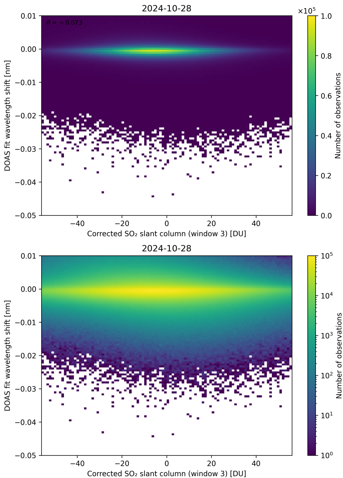
Figure 206: Scatter density plot of “Corrected SO 2 slant column (window 3)” against “DOAS fit wavelength shift” for 2024-10-27 to 2024-10-29.
