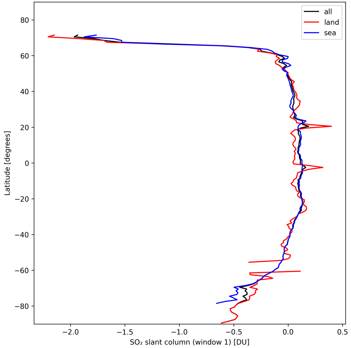
Figure 33: Zonal average of “SO 2 slant column (window 1)” for 2024-10-27 to 2024-10-29.
