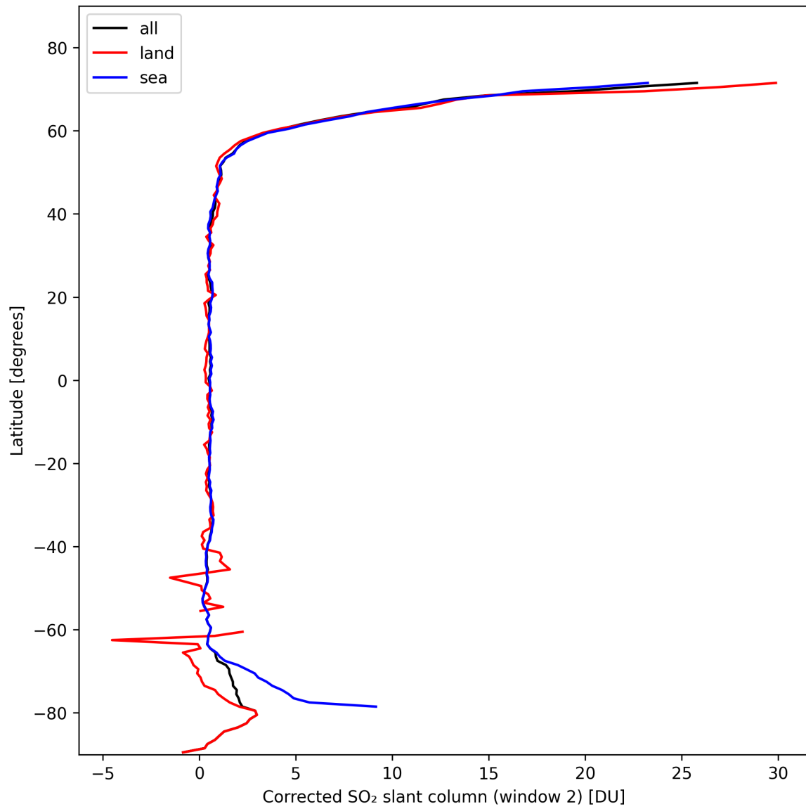
Figure 39: Zonal average of “Corrected SO 2 slant column (window 2)” for 2024-10-27 to 2024-10-29.
