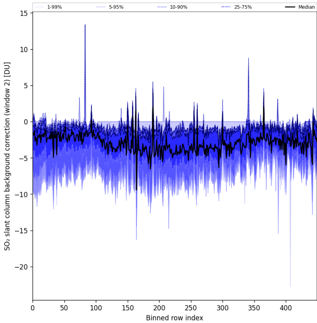
Figure 86: Along track statistics of “SO 2 slant column background correction (window 2)” for 2024-10-27 to 2024-10-29
