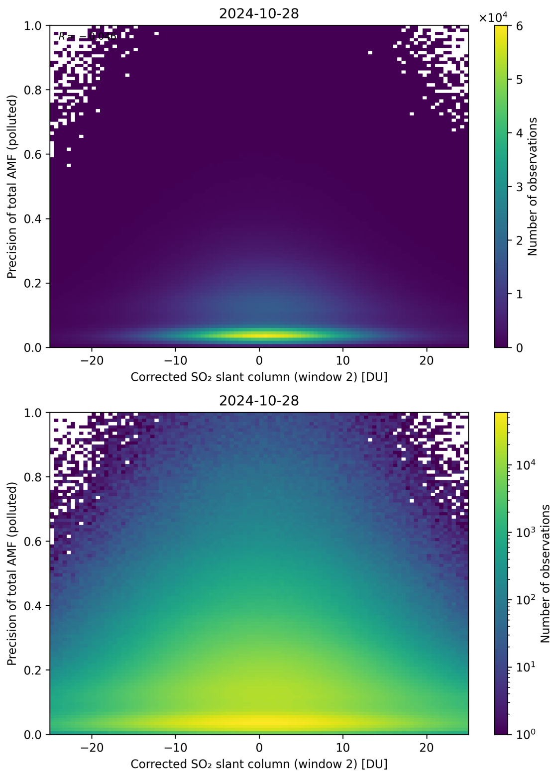
Figure 204: Scatter density plot of “Corrected SO 2 slant column (window 2)” against “Precision of total AMF (polluted)” for 2024-10-27 to 2024-10-29.
