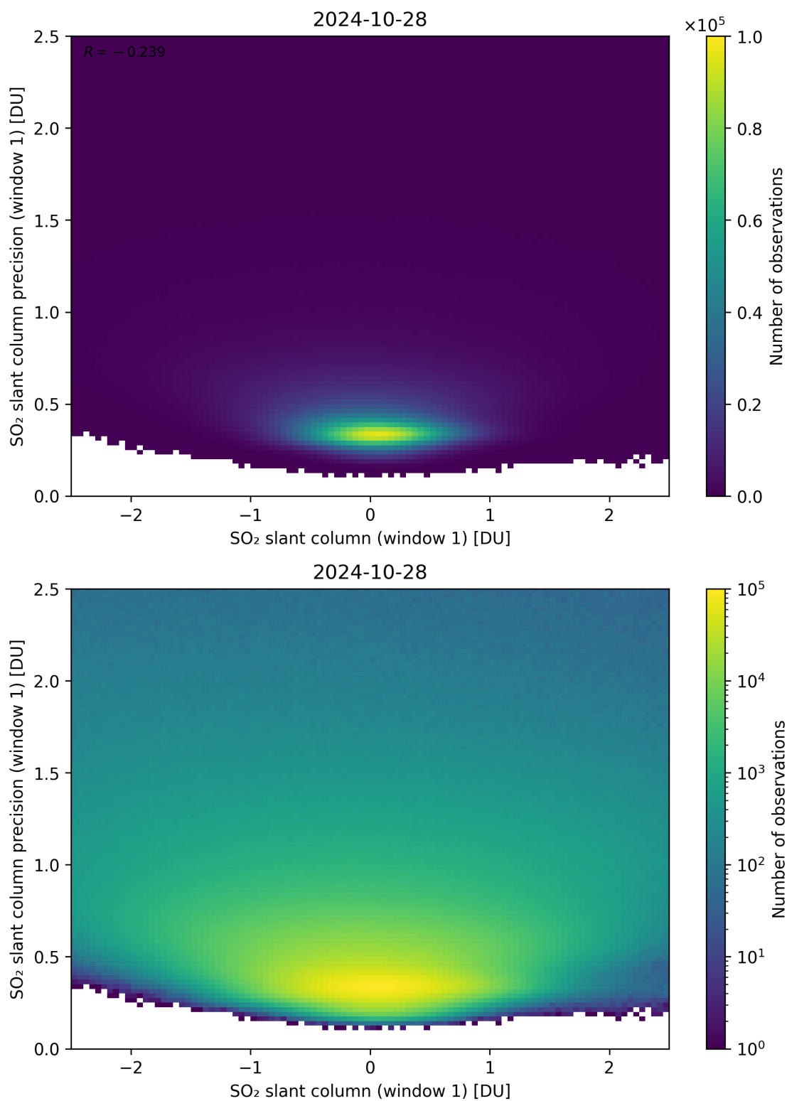
Figure 235: Scatter density plot of “SO 2 slant column (window 1)” against “SO 2 slant column precision (window 1)” for 2024-10-27 to 2024-10-29.
