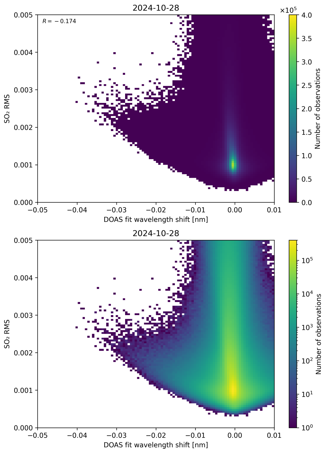
Figure 128: Scatter density plot of “DOAS fit wavelength shift” against “SO 2 RMS” for 2024-10-27 to 2024-10-29.
