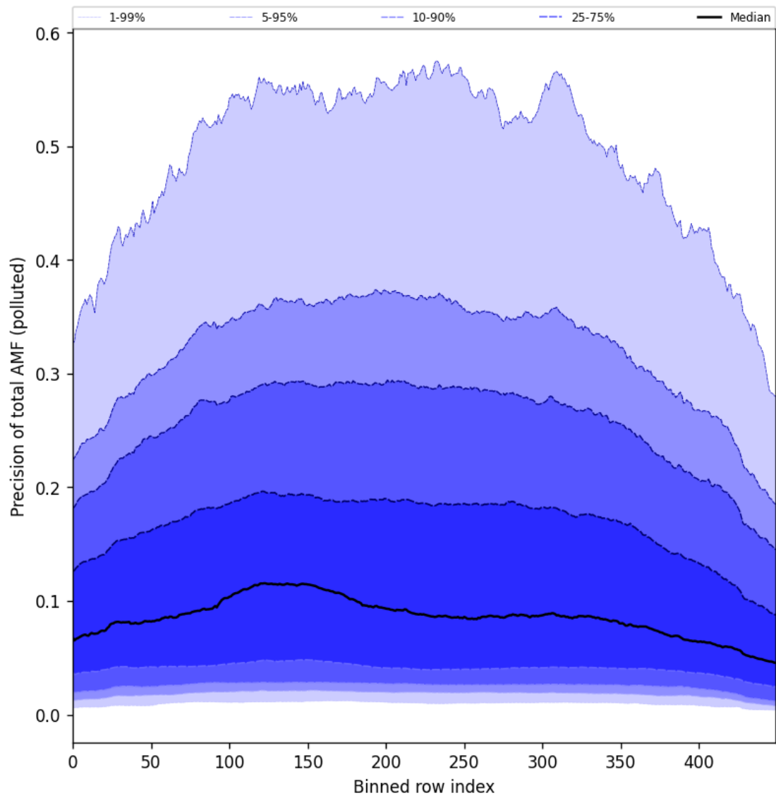
Figure 95: Along track statistics of “Precision of total AMF (polluted)” for 2024-10-27 to 2024-10-29
