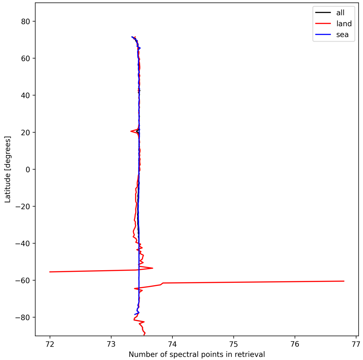
Figure 51: Zonal average of “Number of spectral points in retrieval” for 2024-10-27 to 2024-10-29.
