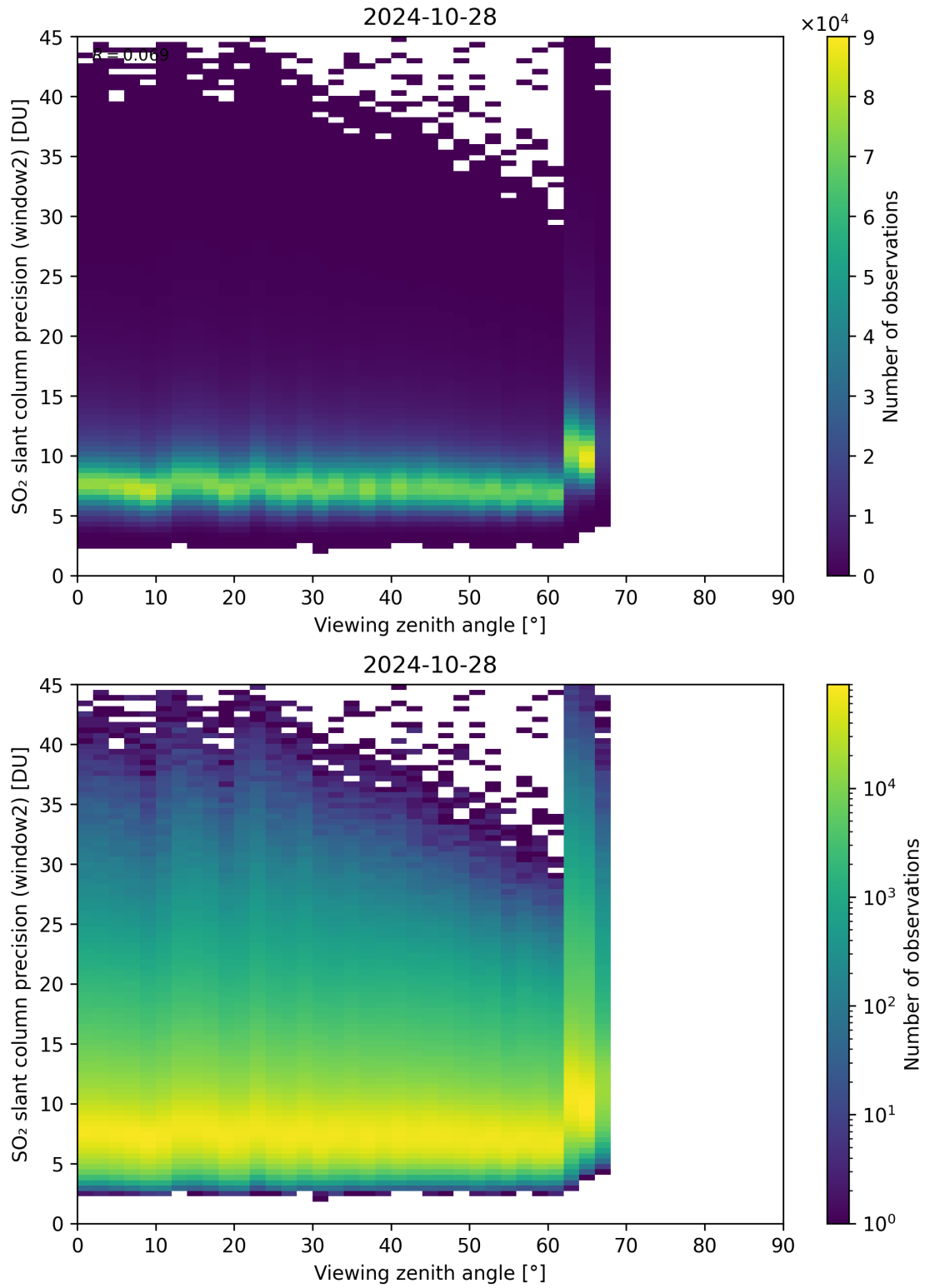
Figure 322: Scatter density plot of “Viewing zenith angle” against “SO 2 slant column precision (window2)” for 2024-10-27 to 2024-10-29.
