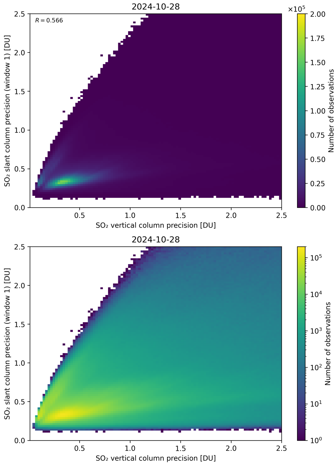
Figure 290: Scatter density plot of “SO 2 vertical column precision” against “SO 2 slant column precision (window 1)” for 2024-10-27 to 2024-10-29.
