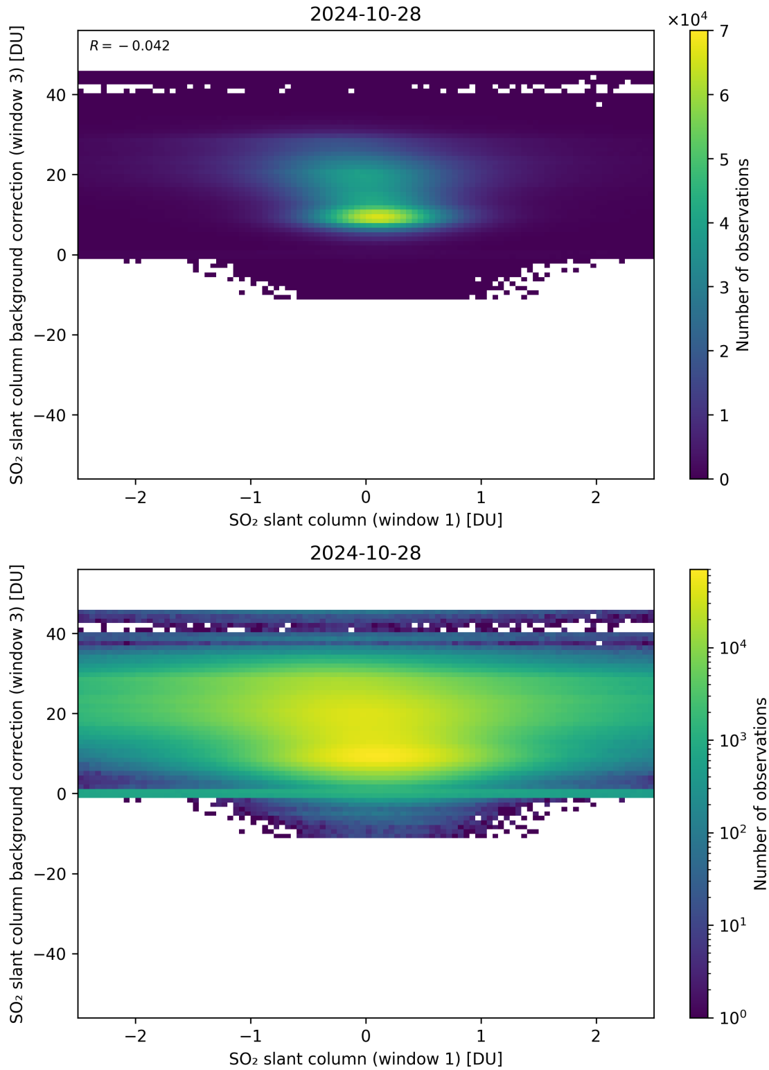
Figure 214: Scatter density plot of “SO 2 slant column (window 1)” against “SO 2 slant column background correction (window 3)” for 2024-10-27 to 2024-10-29.
