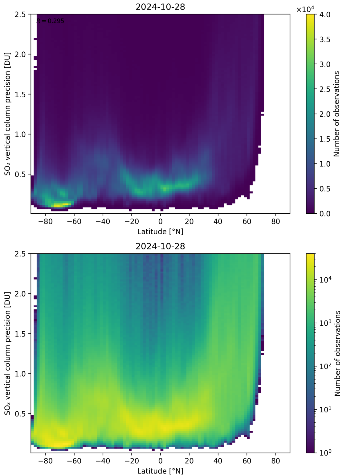
Figure 157: Scatter density plot of “Latitude” against “SO 2 vertical column precision” for 2024-10-27 to 2024-10-29.
