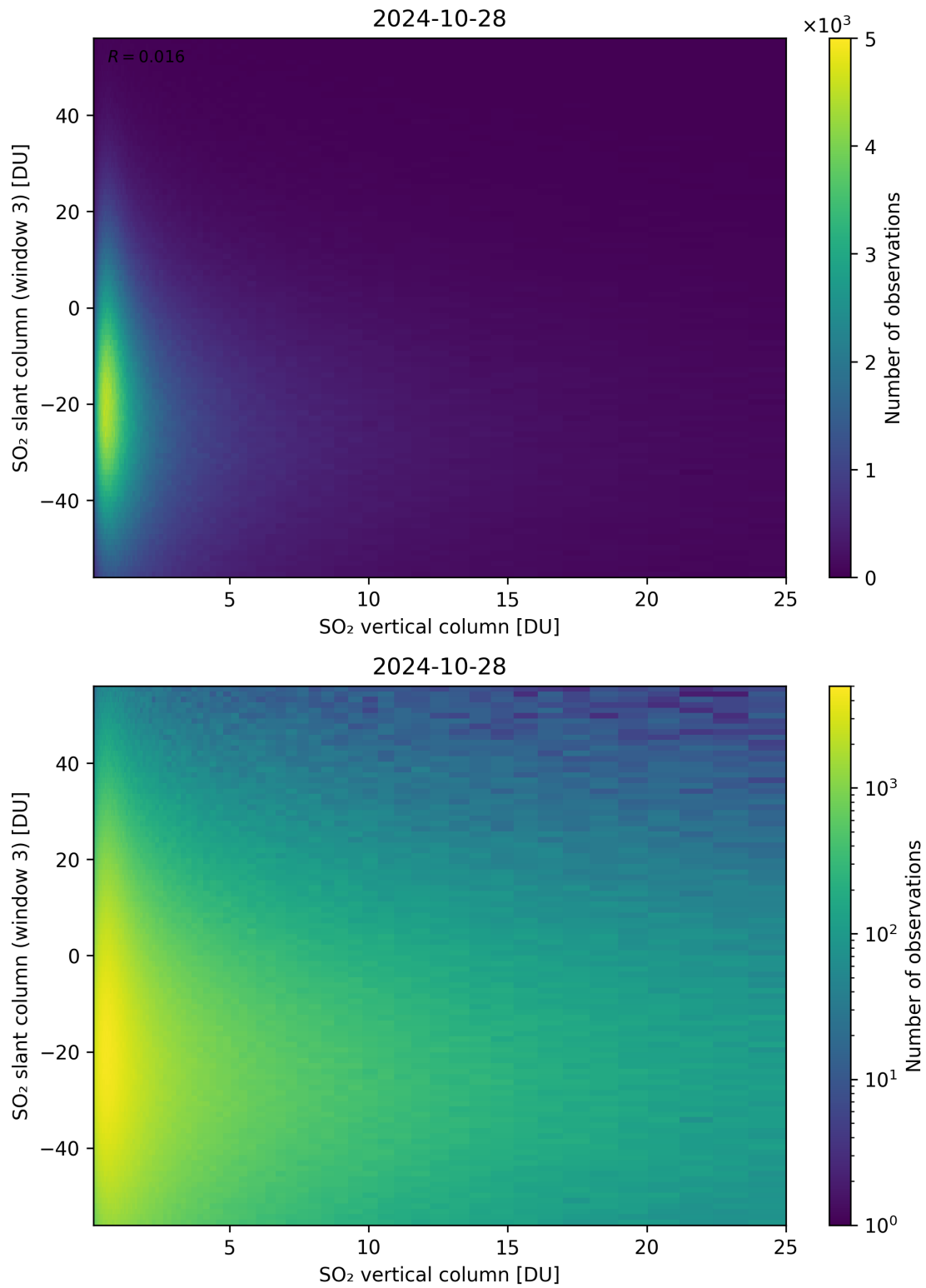
Figure 303: Scatter density plot of “SO 2 vertical column” against “SO 2 slant column (window 3)” for 2024-10-27 to 2024-10-29.
