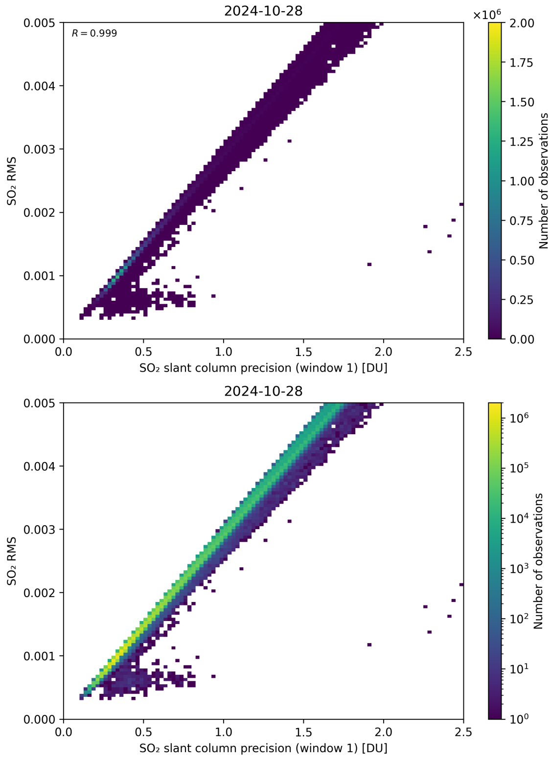
Figure 223: Scatter density plot of “SO 2 slant column precision (window 1)” against “SO 2 RMS” for 2024-10-27 to 2024-10-29.
