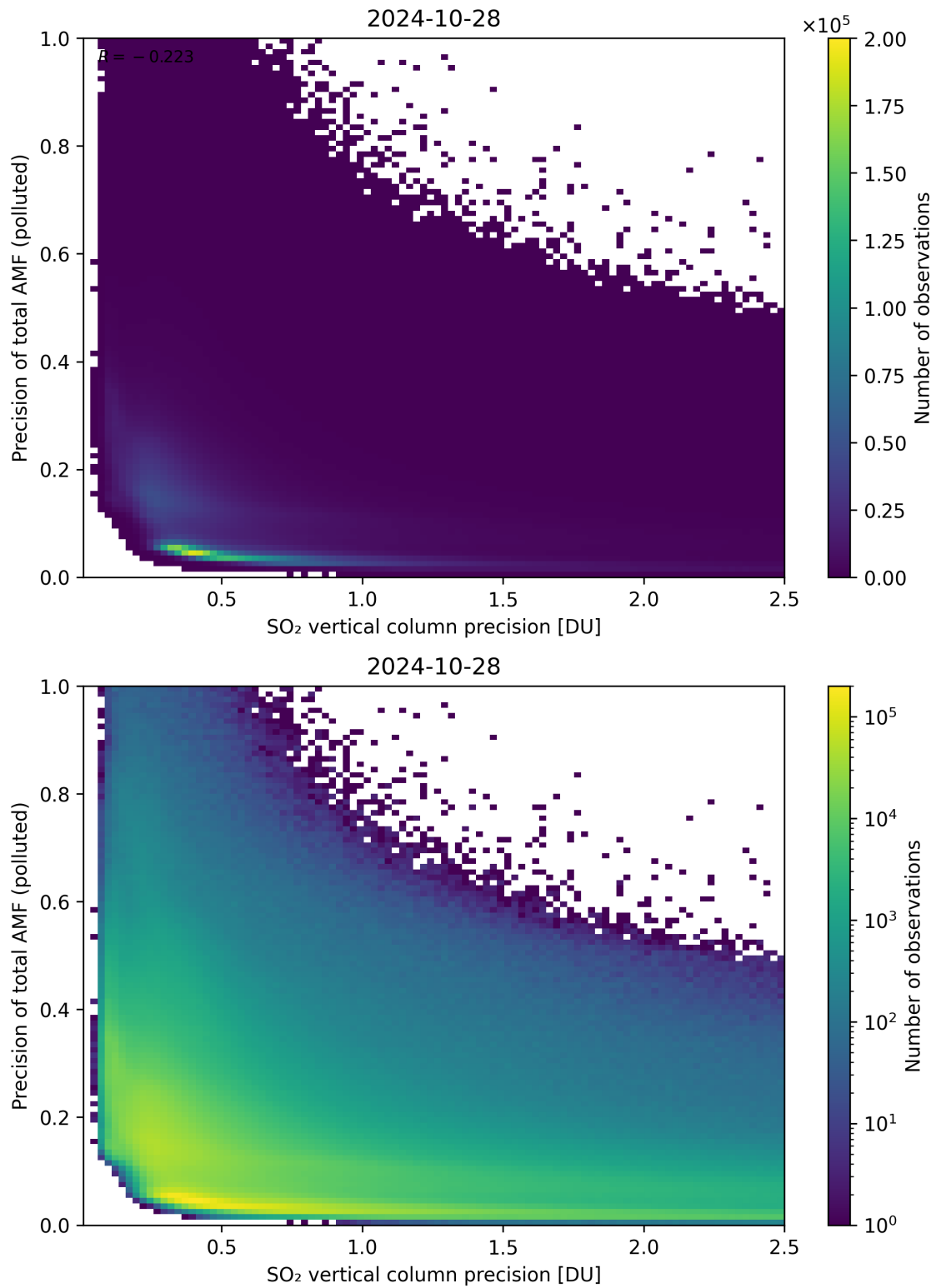
Figure 295: Scatter density plot of “SO 2 vertical column precision” against “Precision of total AMF (polluted)” for 2024-10-27 to 2024-10-29.
