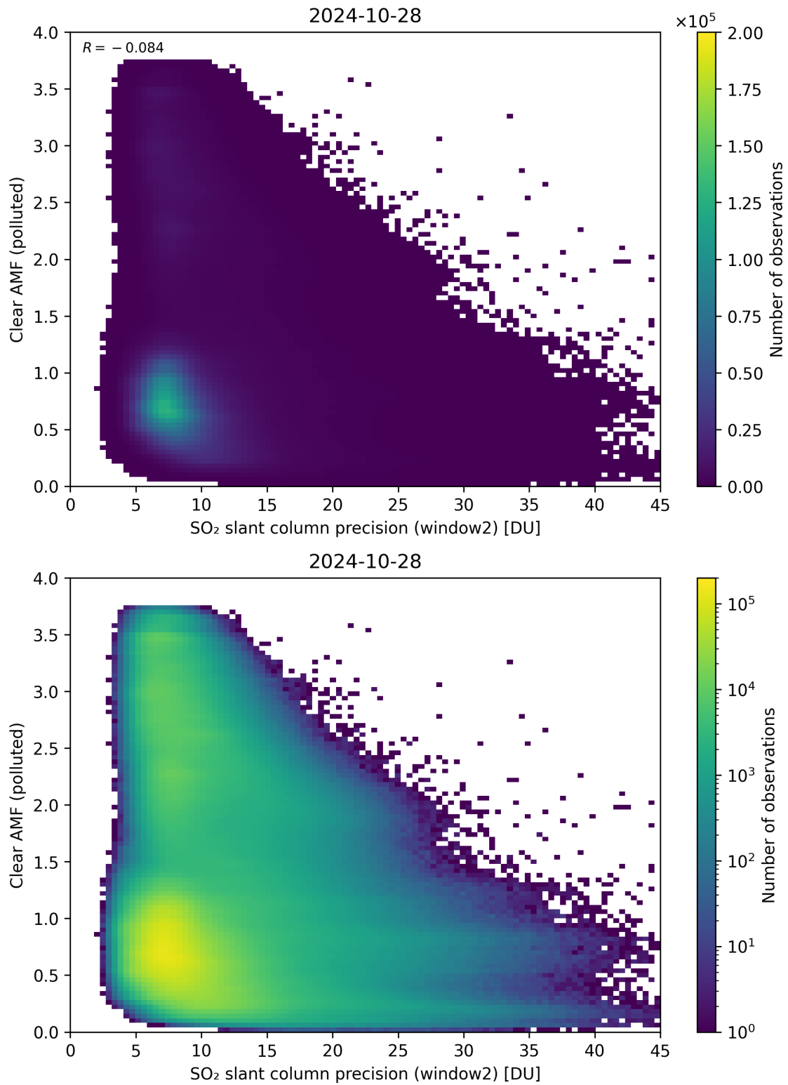
Figure 246: Scatter density plot of “SO 2 slant column precision (window2)” against “Clear AMF (polluted)” for 2024-10-27 to 2024-10-29.
