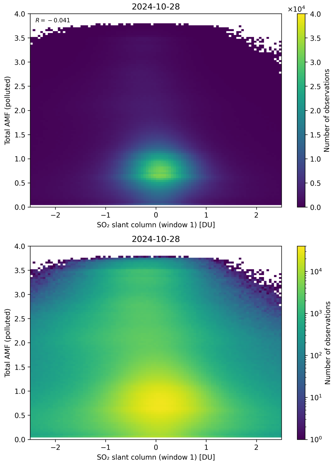
Figure 239: Scatter density plot of “SO 2 slant column (window 1)” against “Total AMF (polluted)” for 2024-10-27 to 2024-10-29.
