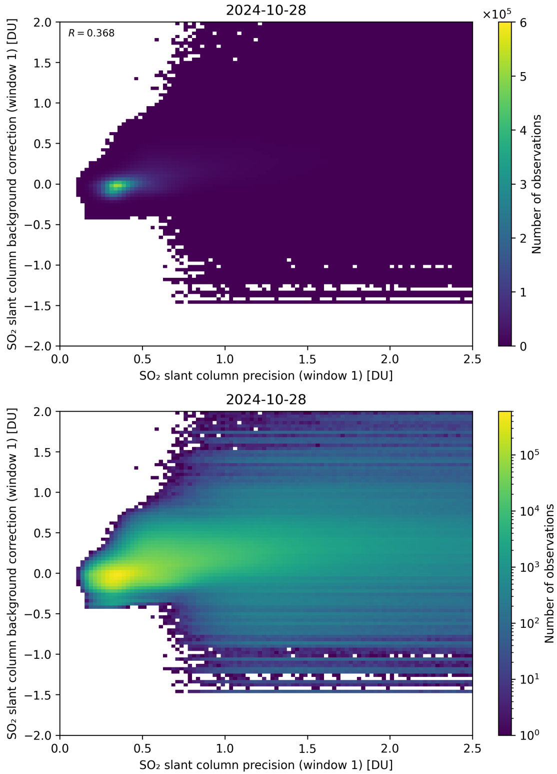
Figure 218: Scatter density plot of “SO 2 slant column precision (window 1)” against “SO 2 slant column background correction (window 1)” for 2024-10-27 to 2024-10-29.
