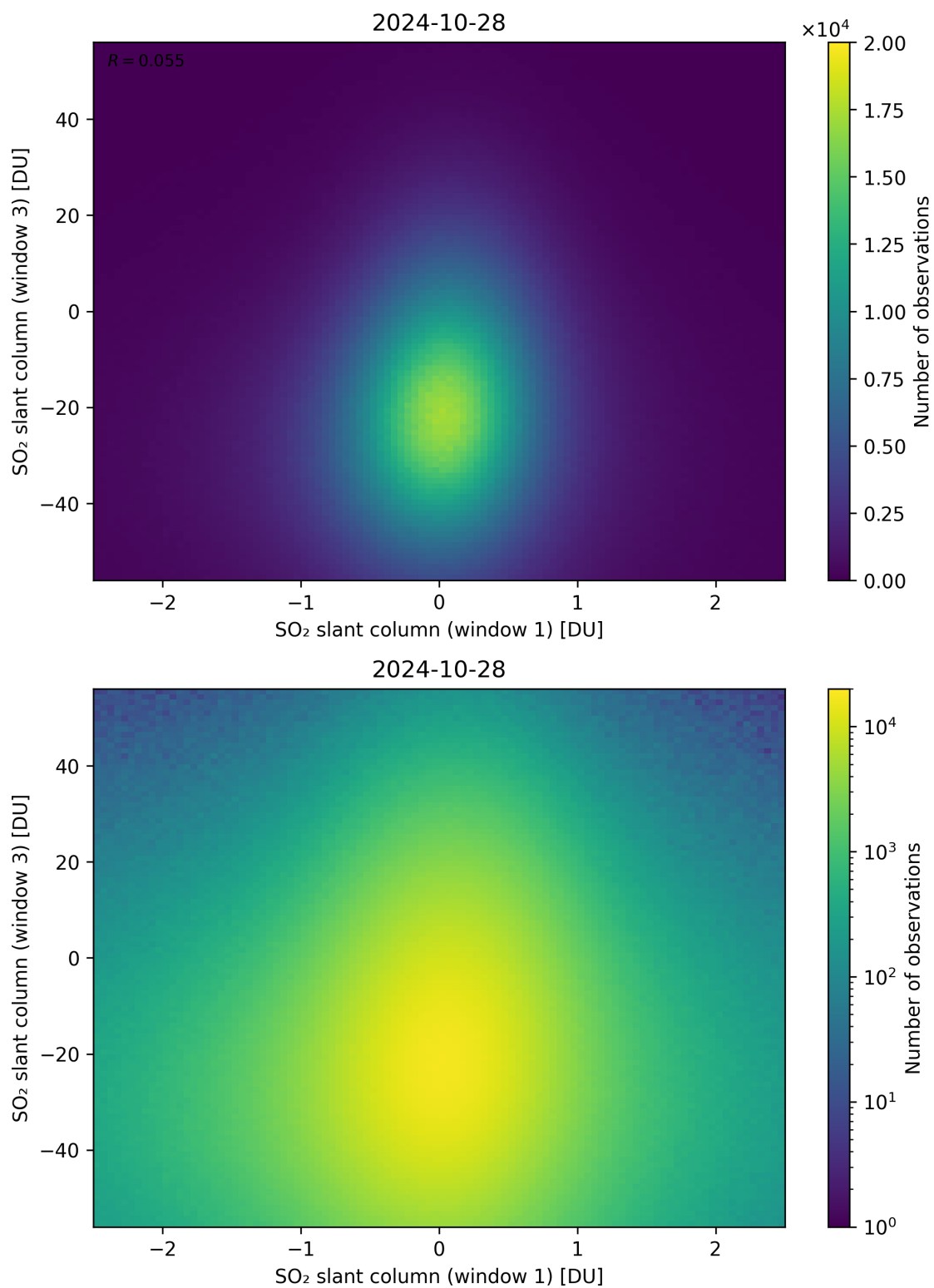
Figure 237: Scatter density plot of “SO 2 slant column (window 1)” against “SO 2 slant column (window 3)” for 2024-10-27 to 2024-10-29.
