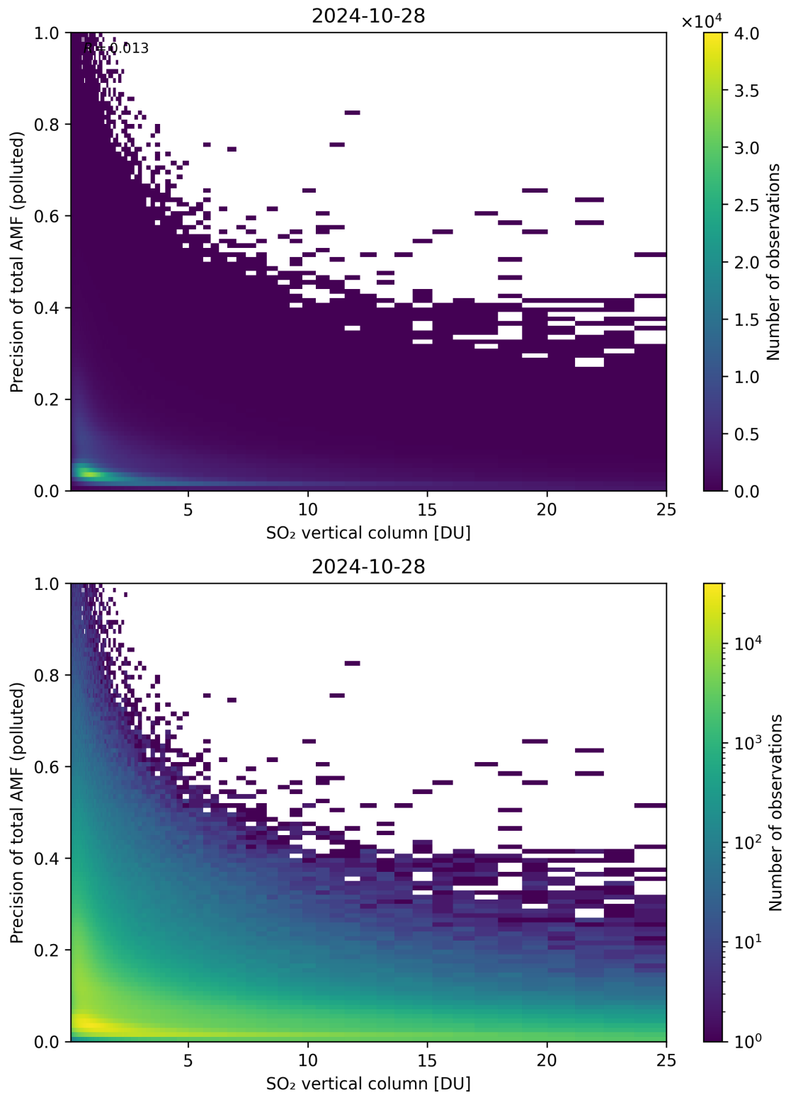
Figure 306: Scatter density plot of “SO 2 vertical column” against “Precision of total AMF (polluted)” for 2024-10-27 to 2024-10-29.
