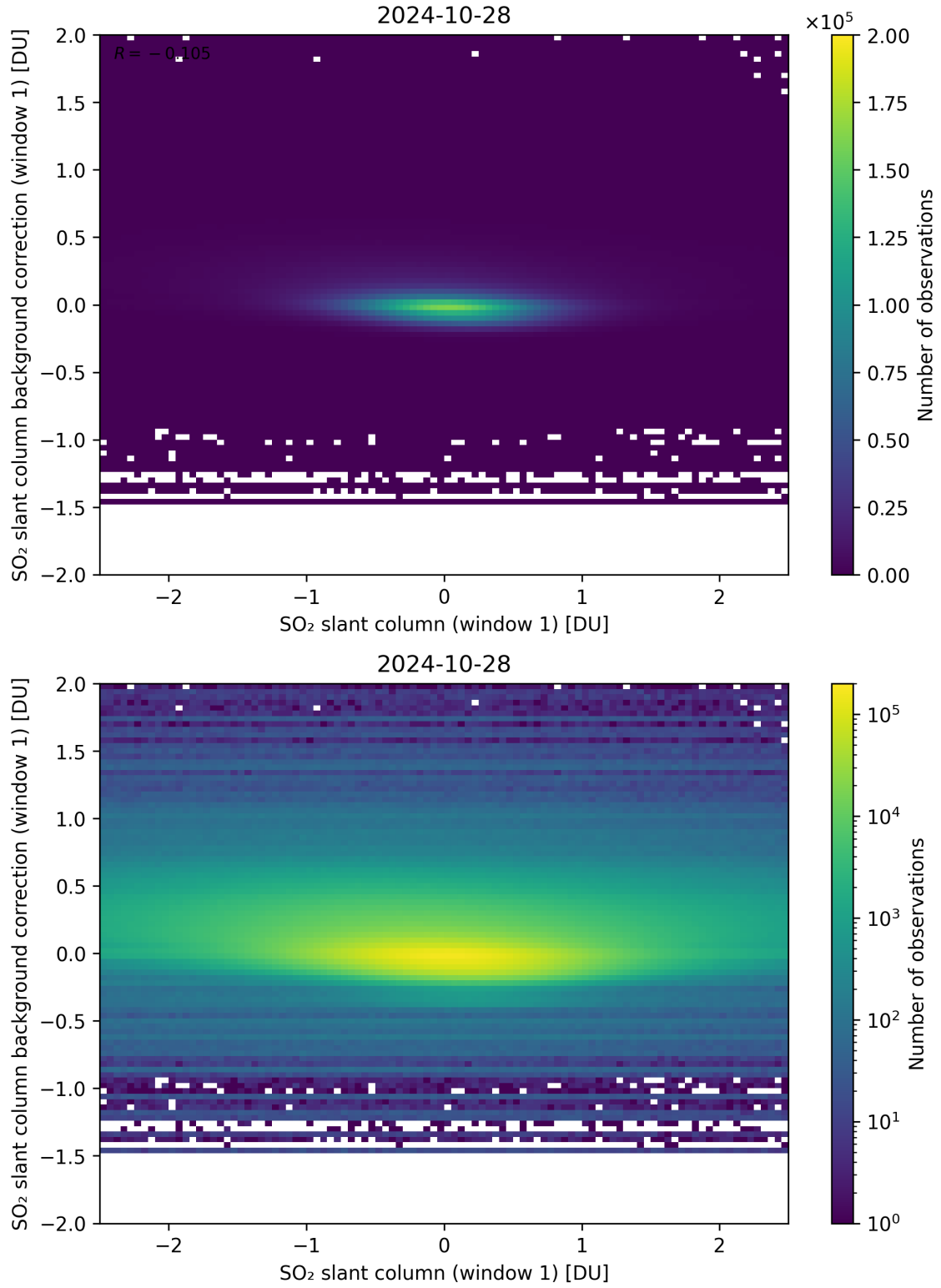
Figure 212: Scatter density plot of “SO 2 slant column (window 1)” against “SO 2 slant column background correction (window 1)” for 2024-10-27 to 2024-10-29.
