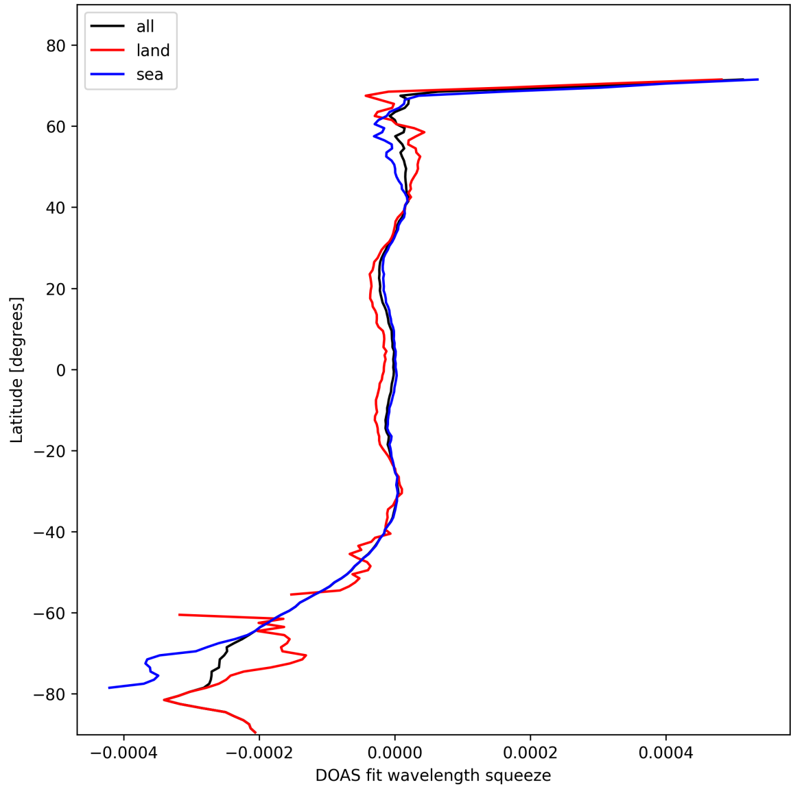
Figure 46: Zonal average of “DOAS fit wavelength squeeze” for 2024-10-27 to 2024-10-29.
