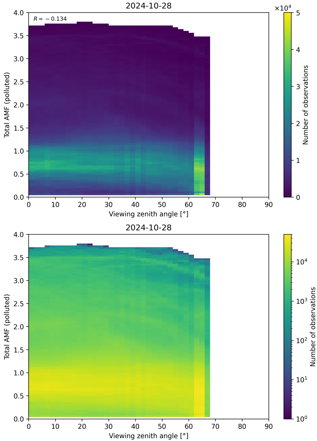
Figure 325: Scatter density plot of “Viewing zenith angle” against “Total AMF (polluted)” for 2024-10-27 to 2024-10-29.
