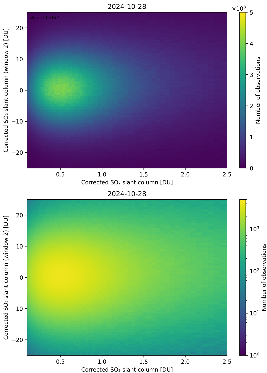
Figure 185: Scatter density plot of “Corrected SO 2 slant column” against “Corrected SO 2 slant column (window 2)” for 2024-10-27 to 2024-10-29.
