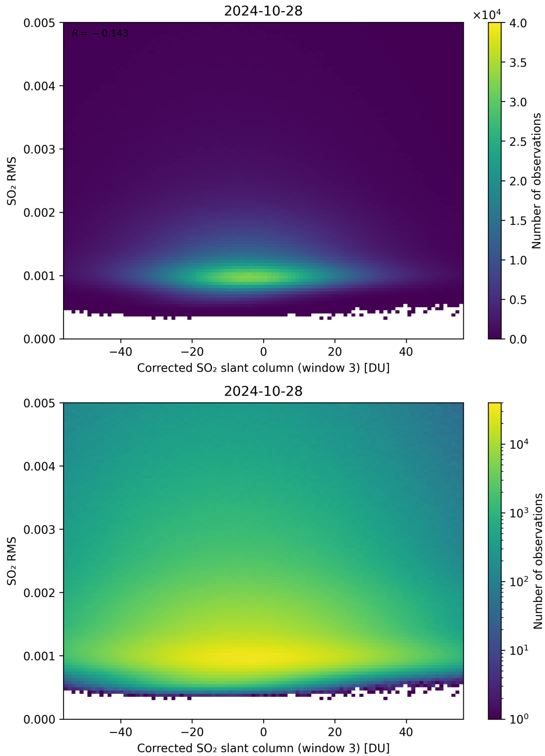
Figure 208: Scatter density plot of “Corrected SO 2 slant column (window 3)” against “SO 2 RMS” for 2024-10-27 to 2024-10-29.
