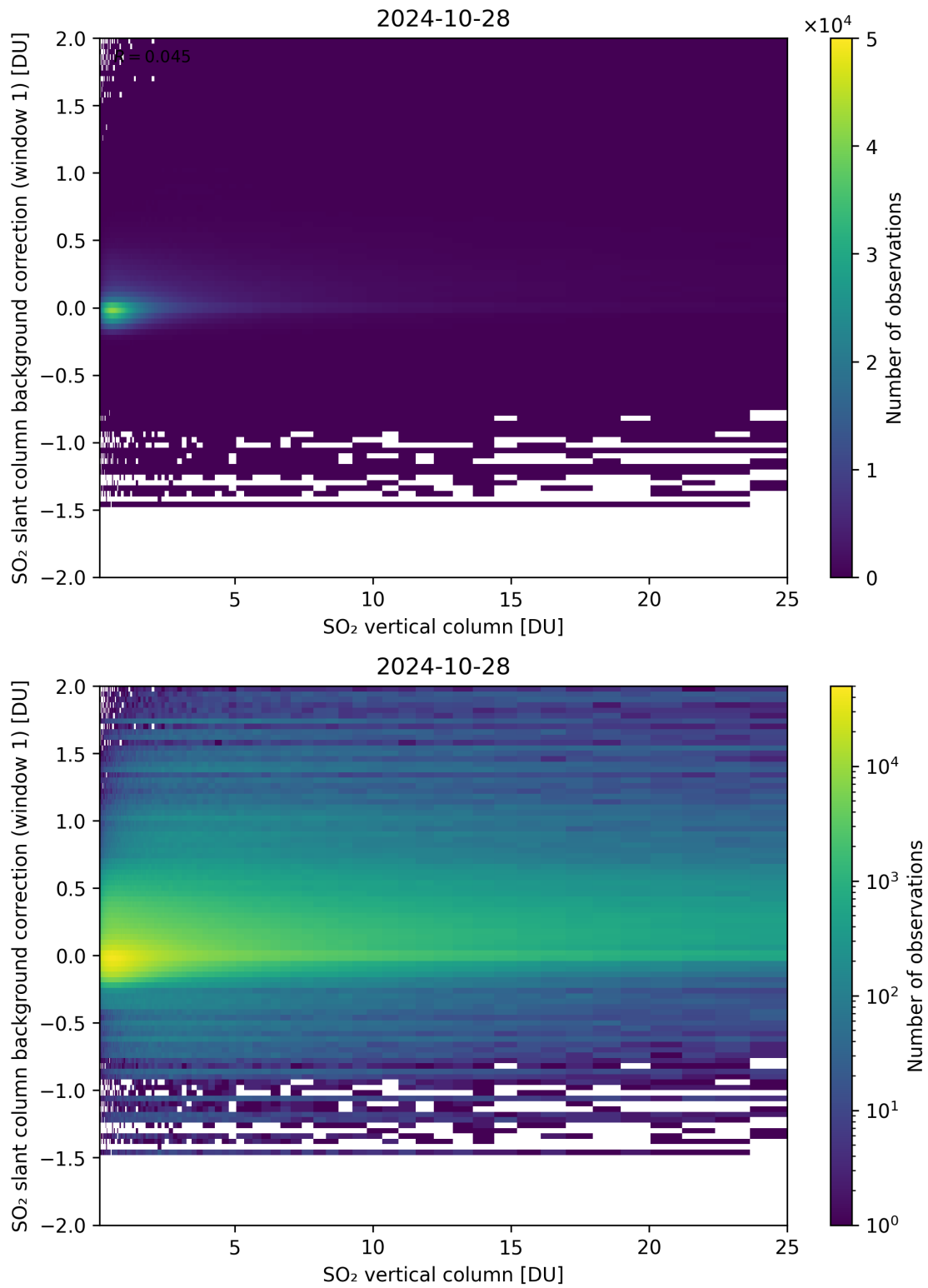
Figure 273: Scatter density plot of “SO 2 vertical column” against “SO 2 slant column background correction (window 1)” for 2024-10-27 to 2024-10-29.
