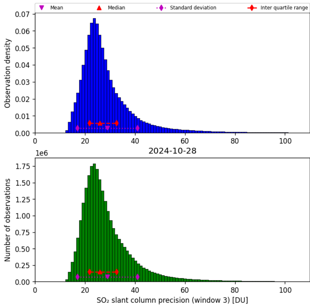
Figure 65: Histogram of “SO 2 slant column precision (window 3)” for 2024-10-27 to 2024-10-29
