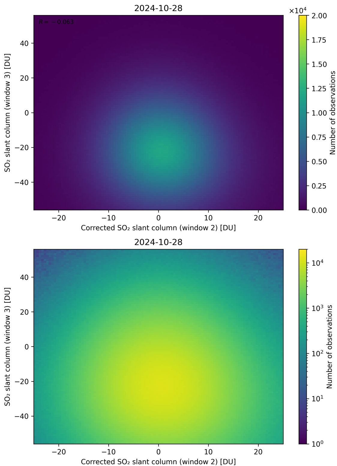
Figure 201: Scatter density plot of “Corrected SO 2 slant column (window 2)” against “SO 2 slant column (window 3)” for 2024-10-27 to 2024-10-29.
