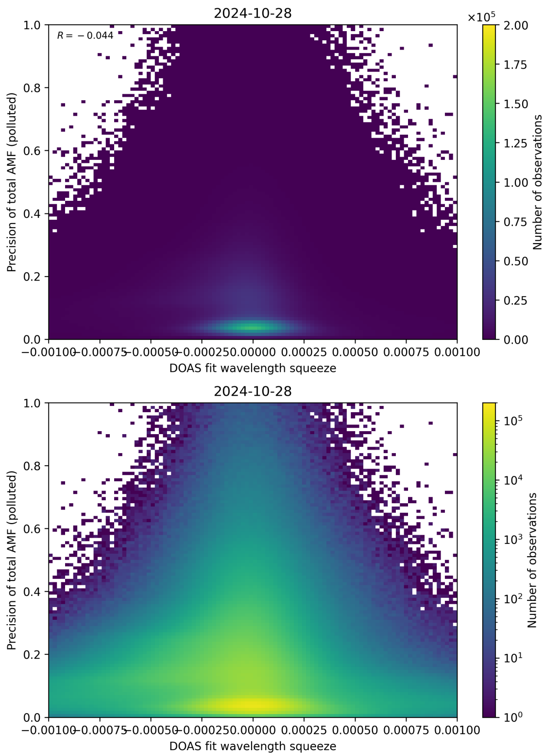
Figure 135: Scatter density plot of “DOAS fit wavelength squeeze” against “Precision of total AMF (polluted)” for 2024-10-27 to 2024-10-29.
