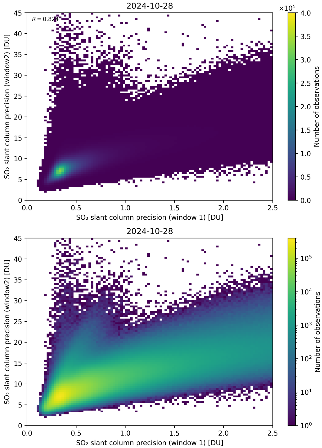
Figure 227: Scatter density plot of “SO 2 slant column precision (window 1)” against “SO 2 slant column precision (window2)” for 2024-10-27 to 2024-10-29.
