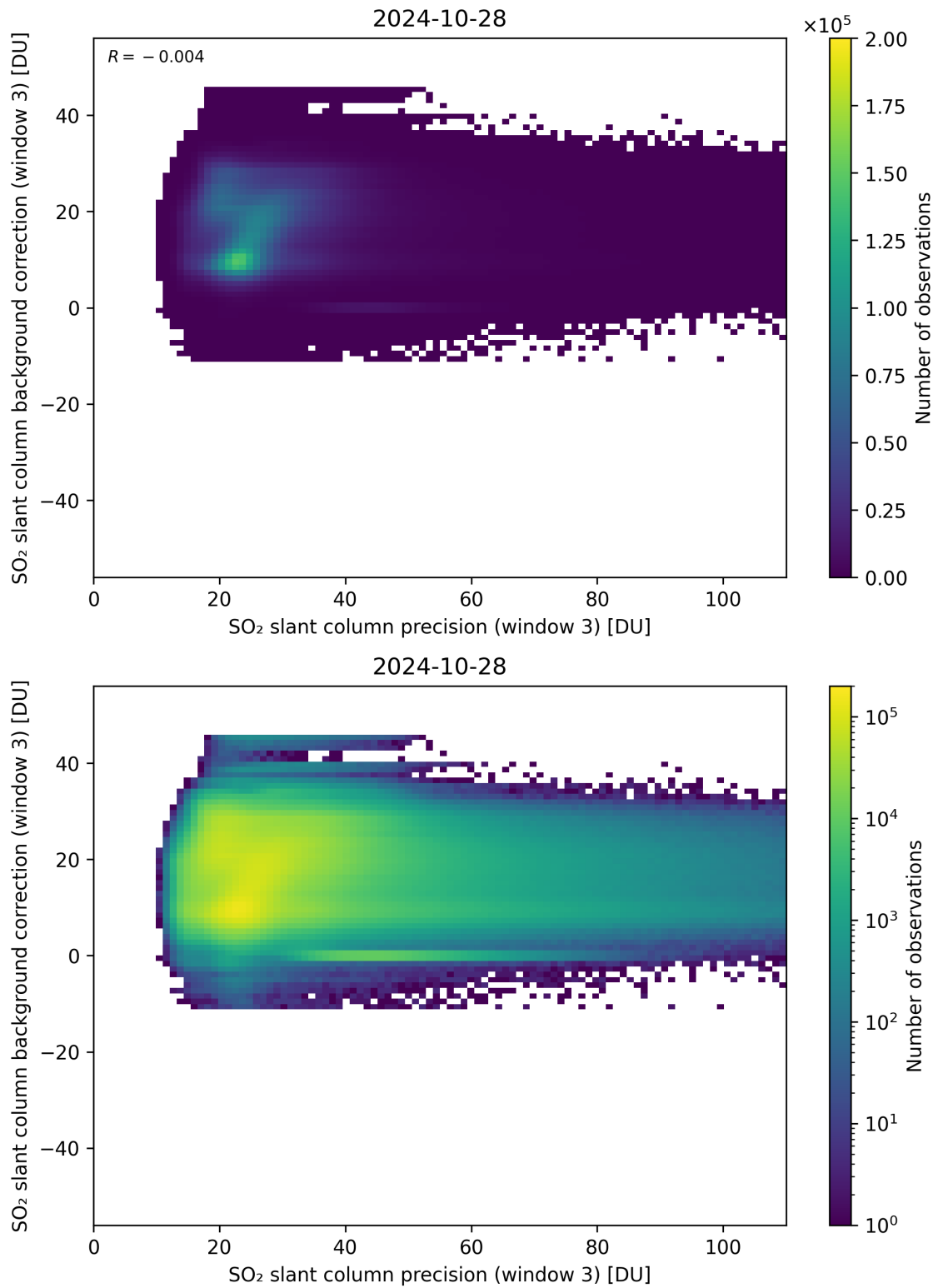
Figure 257: Scatter density plot of “SO 2 slant column precision (window 3)” against “SO 2 slant column background correction (window 3)” for 2024-10-27 to 2024-10-29.
