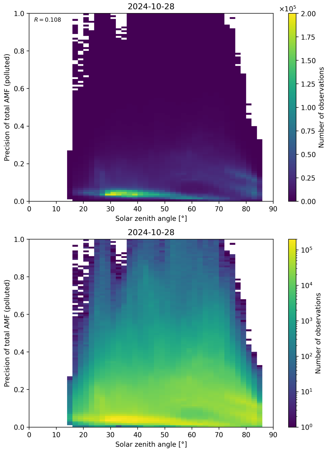
Figure 175: Scatter density plot of “Solar zenith angle” against “Precision of total AMF (polluted)” for 2024-10-27 to 2024-10-29.
