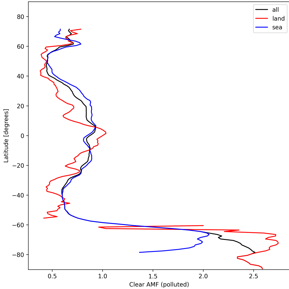
Figure 50: Zonal average of “Clear AMF (polluted)” for 2024-10-27 to 2024-10-29.
