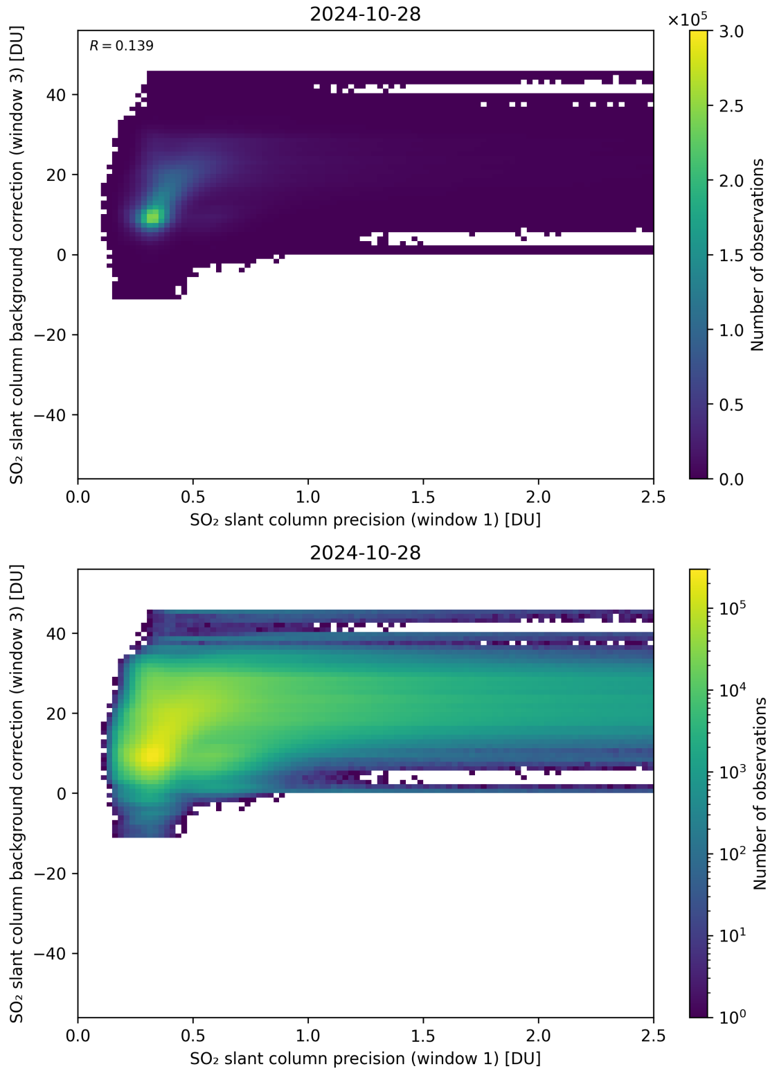
Figure 220: Scatter density plot of “SO 2 slant column precision (window 1)” against “SO 2 slant column background correction (window 3)” for 2024-10-27 to 2024-10-29.
