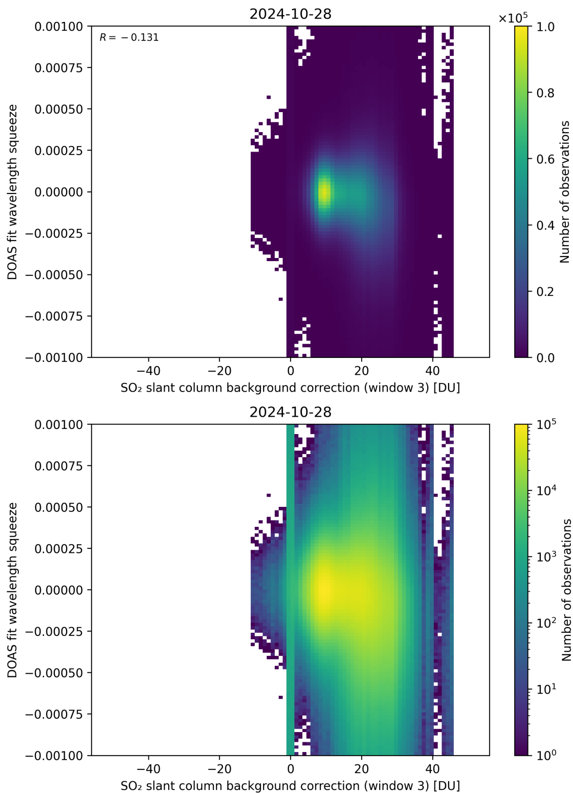
Figure 122: Scatter density plot of “SO 2 slant column background correction (window 3)” against “DOAS fit wavelength squeeze” for 2024-10-27 to 2024-10-29.
