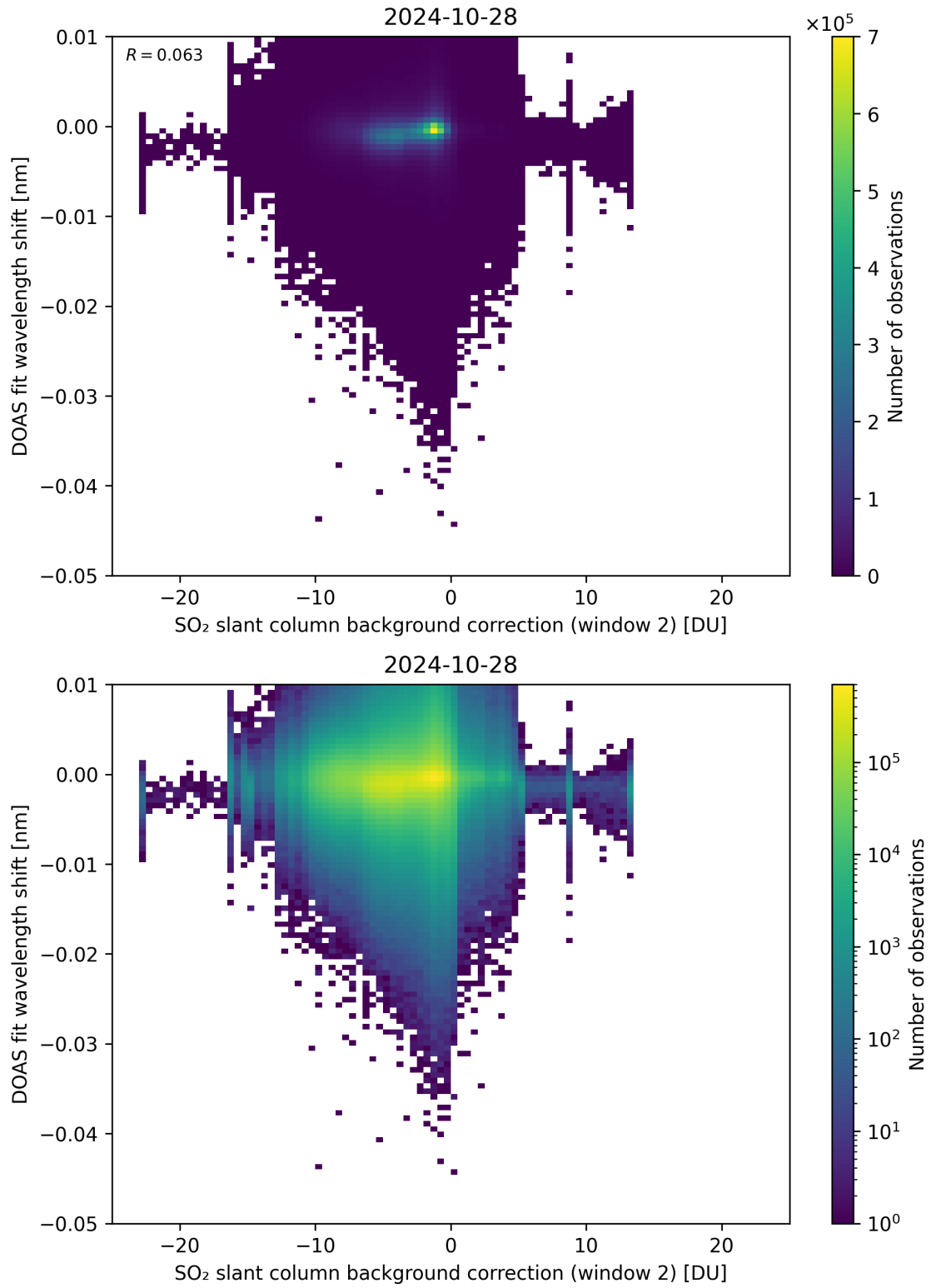
Figure 112: Scatter density plot of “SO 2 slant column background correction (window 2)” against “DOAS fit wavelength shift” for 2024-10-27 to 2024-10-29.
