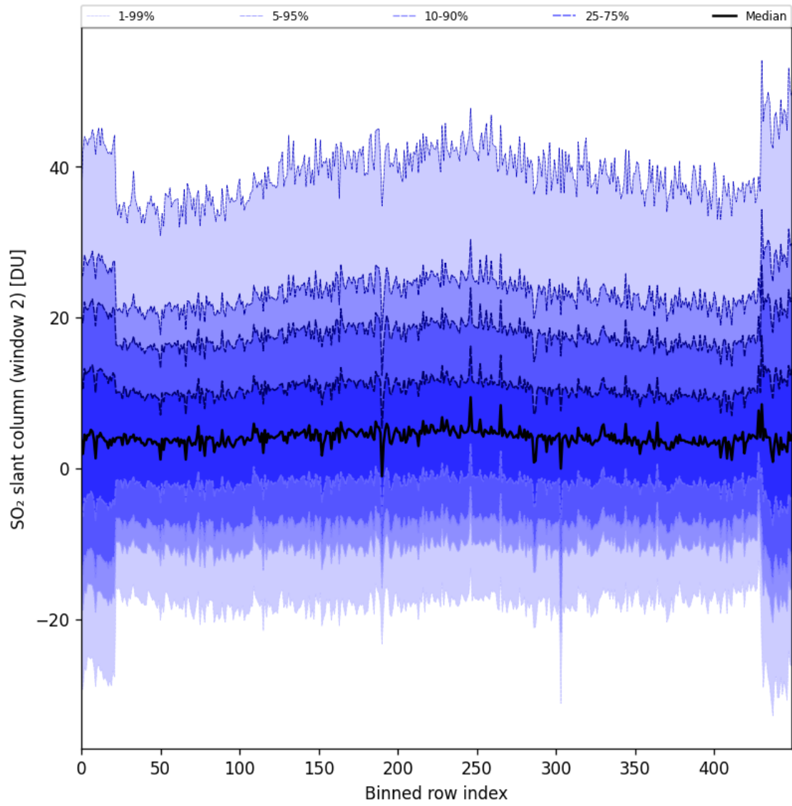
Figure 83: Along track statistics of “SO 2 slant column (window 2)” for 2024-10-27 to 2024-10-29
