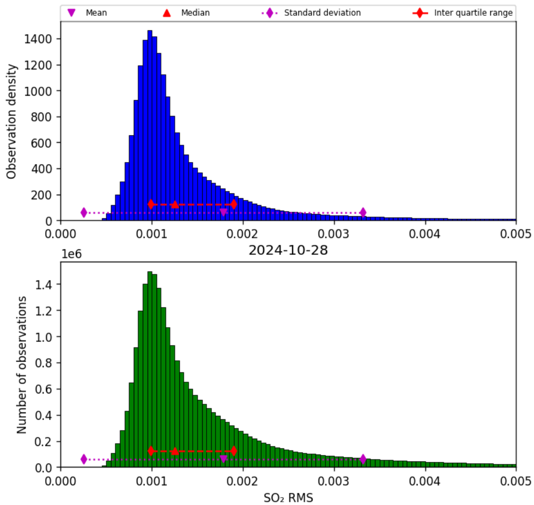
Figure 70: Histogram of “SO 2 RMS” for 2024-10-27 to 2024-10-29
