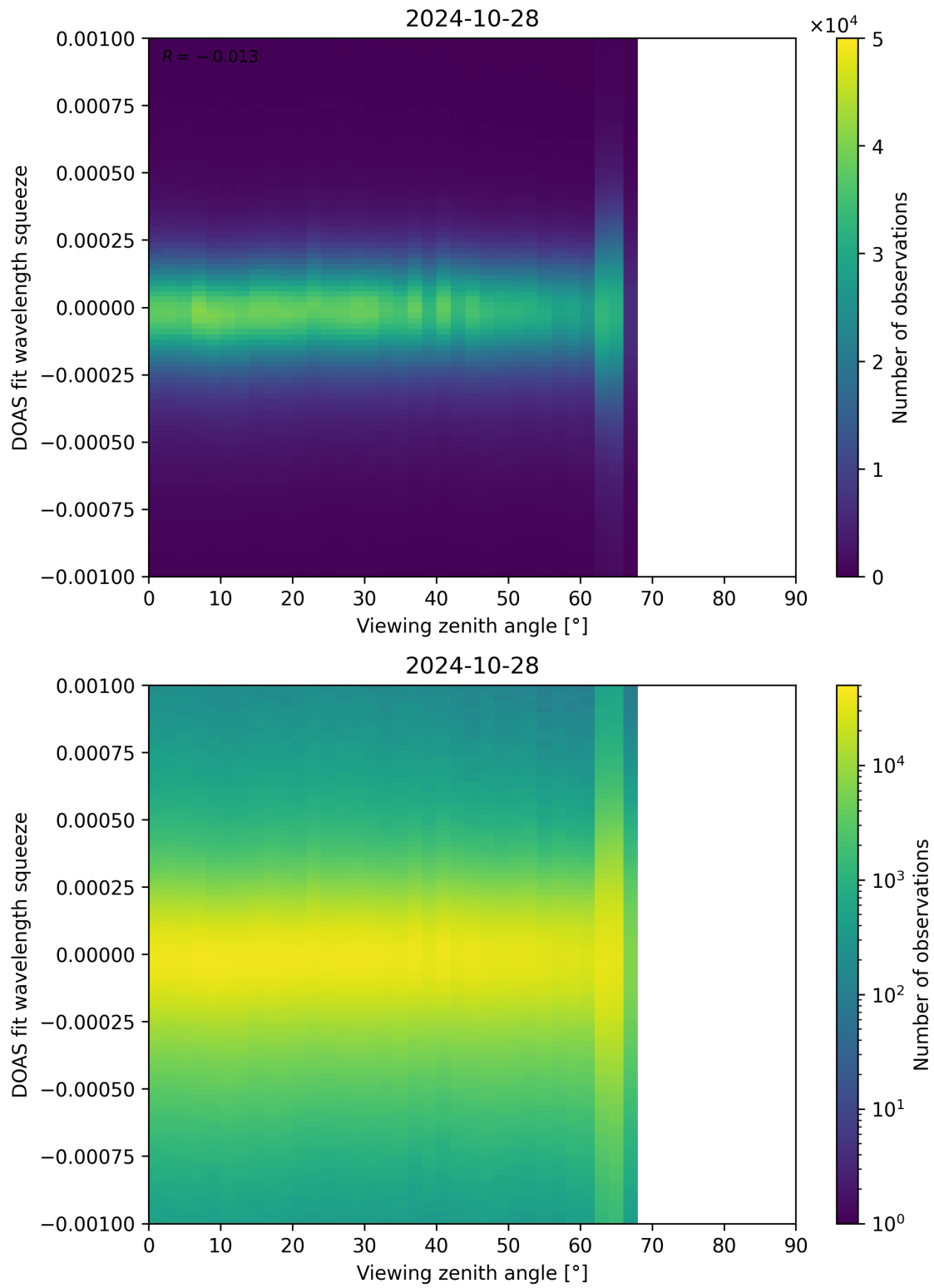
Figure 312: Scatter density plot of “Viewing zenith angle” against “DOAS fit wavelength squeeze” for 2024-10-27 to 2024-10-29.
