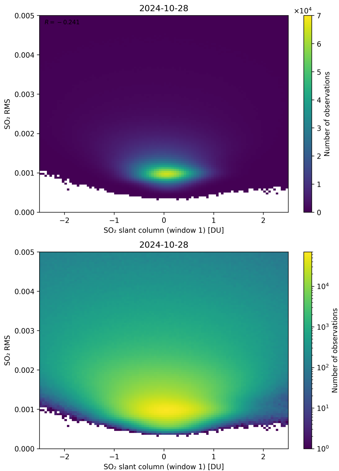
Figure 217: Scatter density plot of “SO 2 slant column (window 1)” against “SO 2 RMS” for 2024-10-27 to 2024-10-29.
