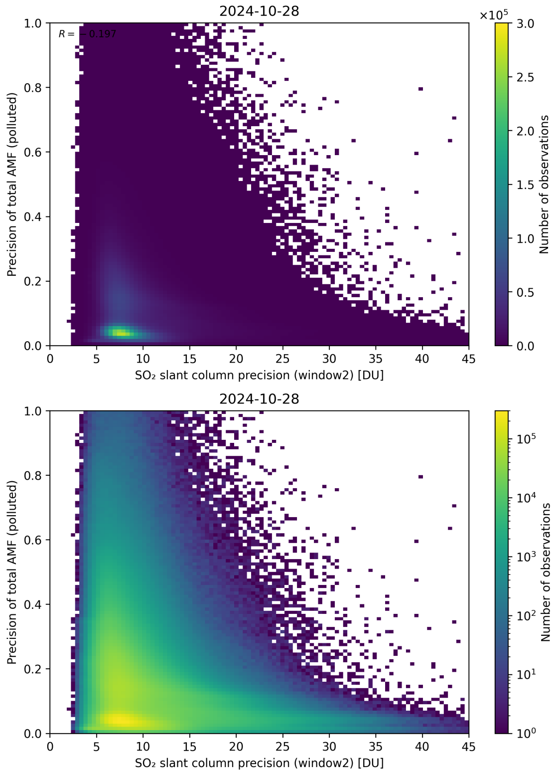
Figure 252: Scatter density plot of “SO 2 slant column precision (window2)” against “Precision of total AMF (polluted)” for 2024-10-27 to 2024-10-29.
