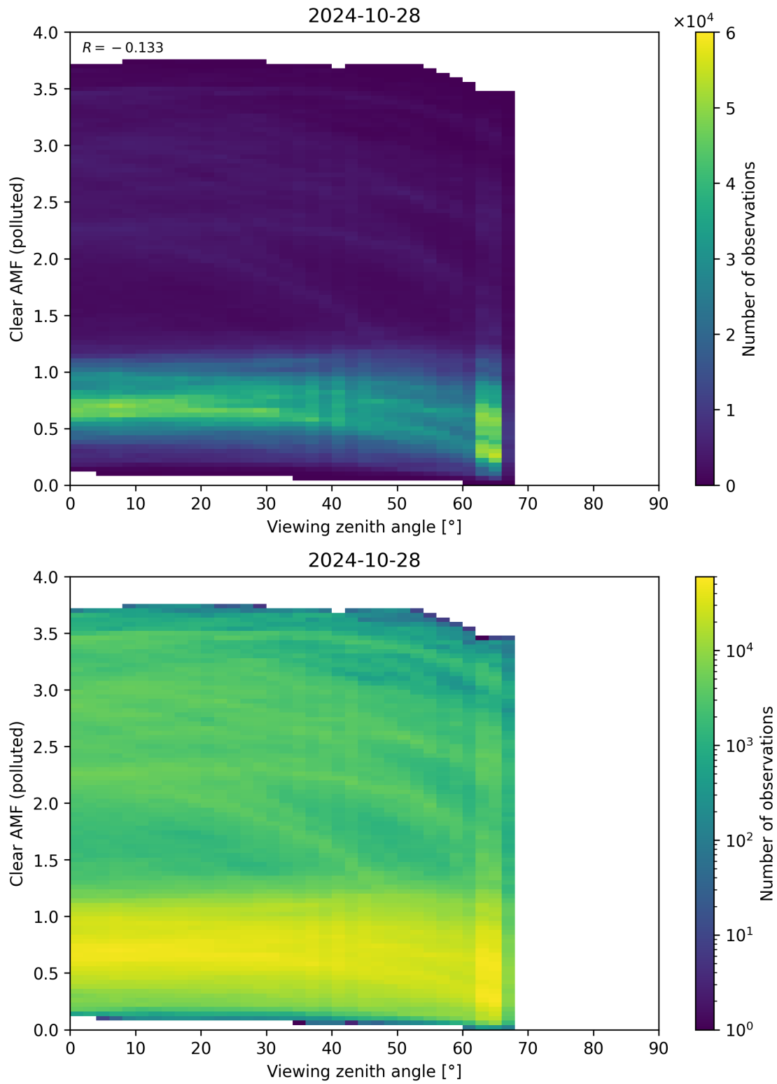
Figure 316: Scatter density plot of “Viewing zenith angle” against “Clear AMF (polluted)” for 2024-10-27 to 2024-10-29.
