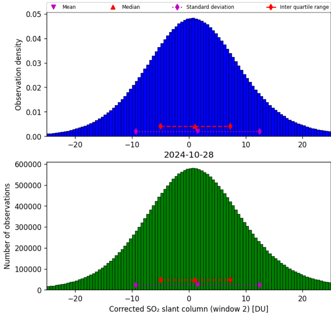
Figure 62: Histogram of “Corrected SO 2 slant column (window 2)” for 2024-10-27 to 2024-10-29
