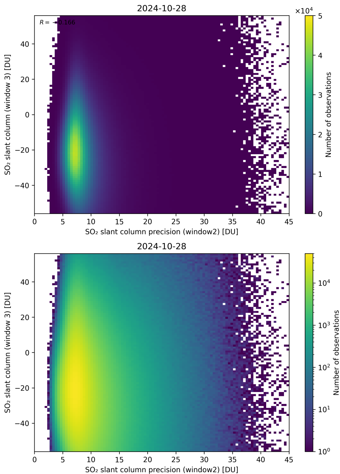
Figure 249: Scatter density plot of “SO 2 slant column precision (window2)” against “SO 2 slant column (window 3)” for 2024-10-27 to 2024-10-29.
