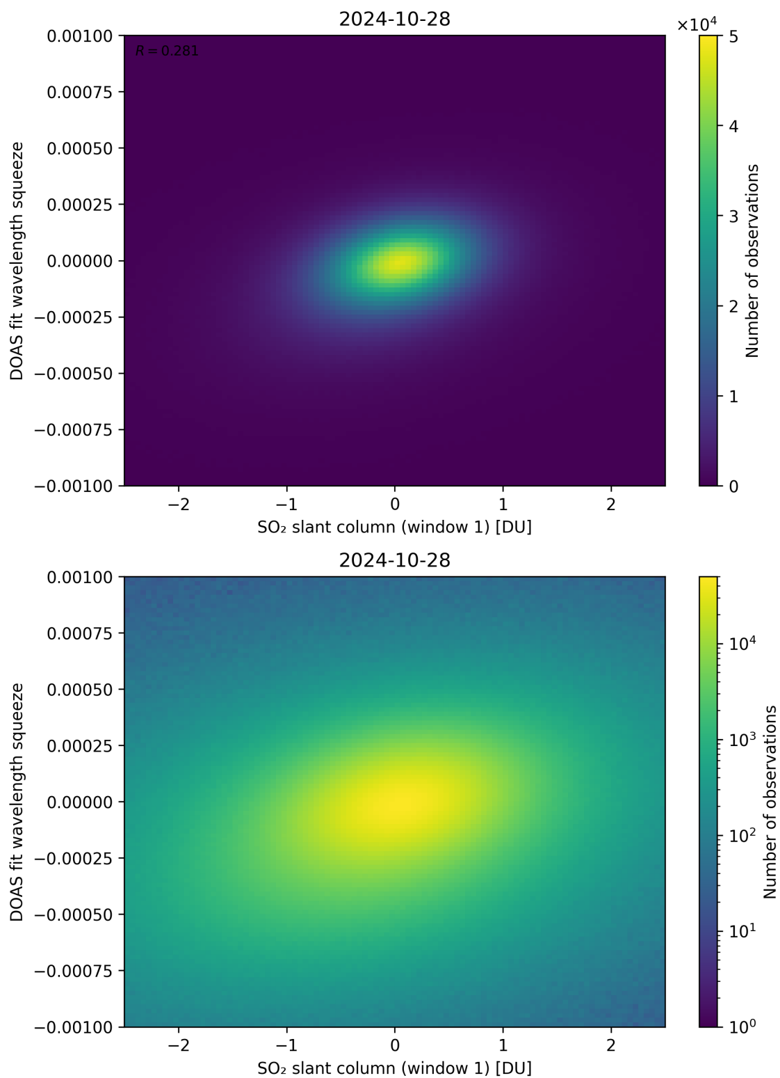
Figure 216: Scatter density plot of “SO 2 slant column (window 1)” against “DOAS fit wavelength squeeze” for 2024-10-27 to 2024-10-29.
