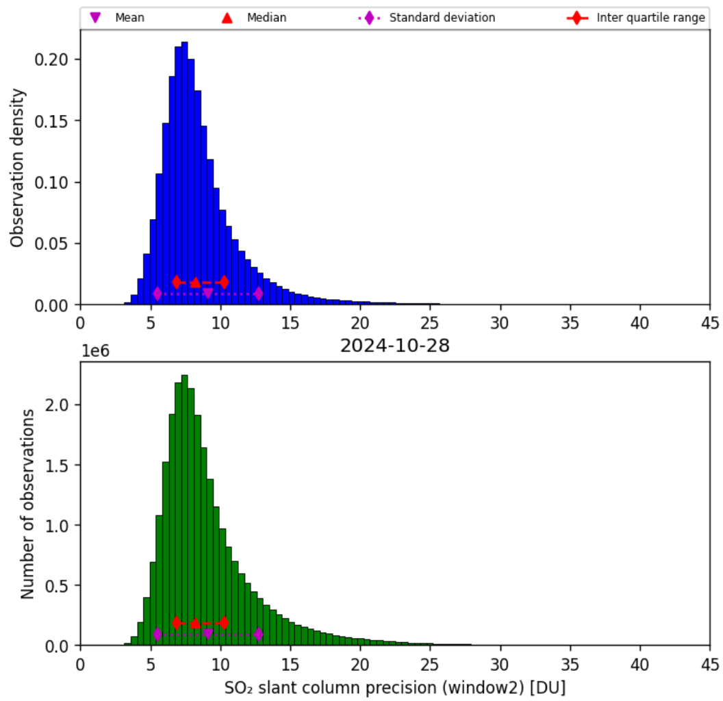
Figure 61: Histogram of “SO 2 slant column precision (window2)” for 2024-10-27 to 2024-10-29
