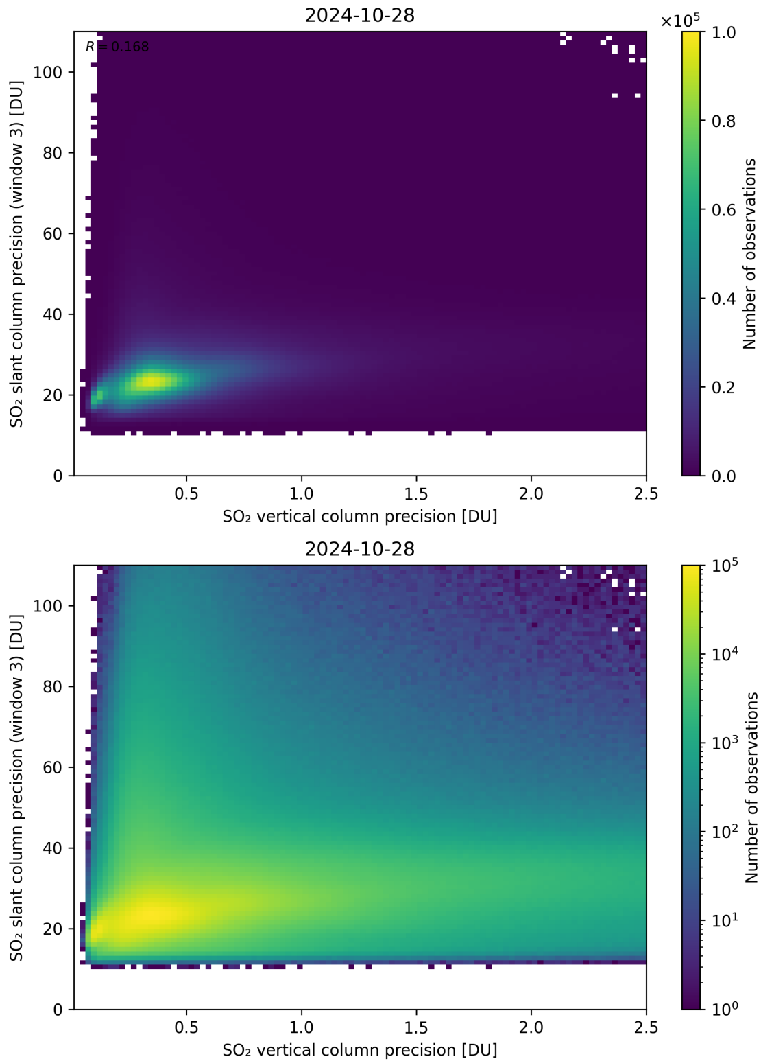
Figure 293: Scatter density plot of “SO 2 vertical column precision” against “SO 2 slant column precision (window 3)” for 2024-10-27 to 2024-10-29.
