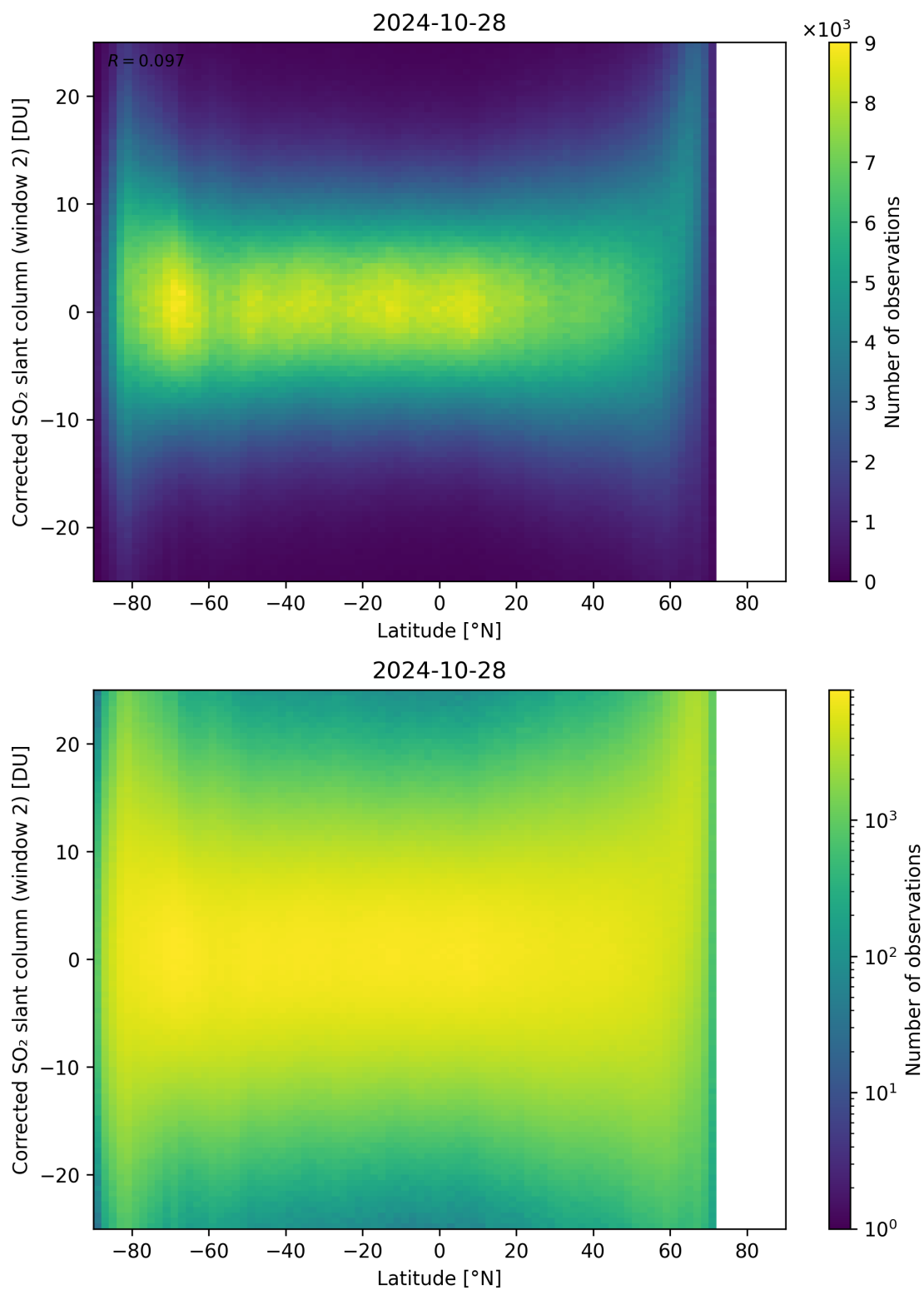
Figure 147: Scatter density plot of “Latitude” against “Corrected SO 2 slant column (window 2)” for 2024-10-27 to 2024-10-29.
