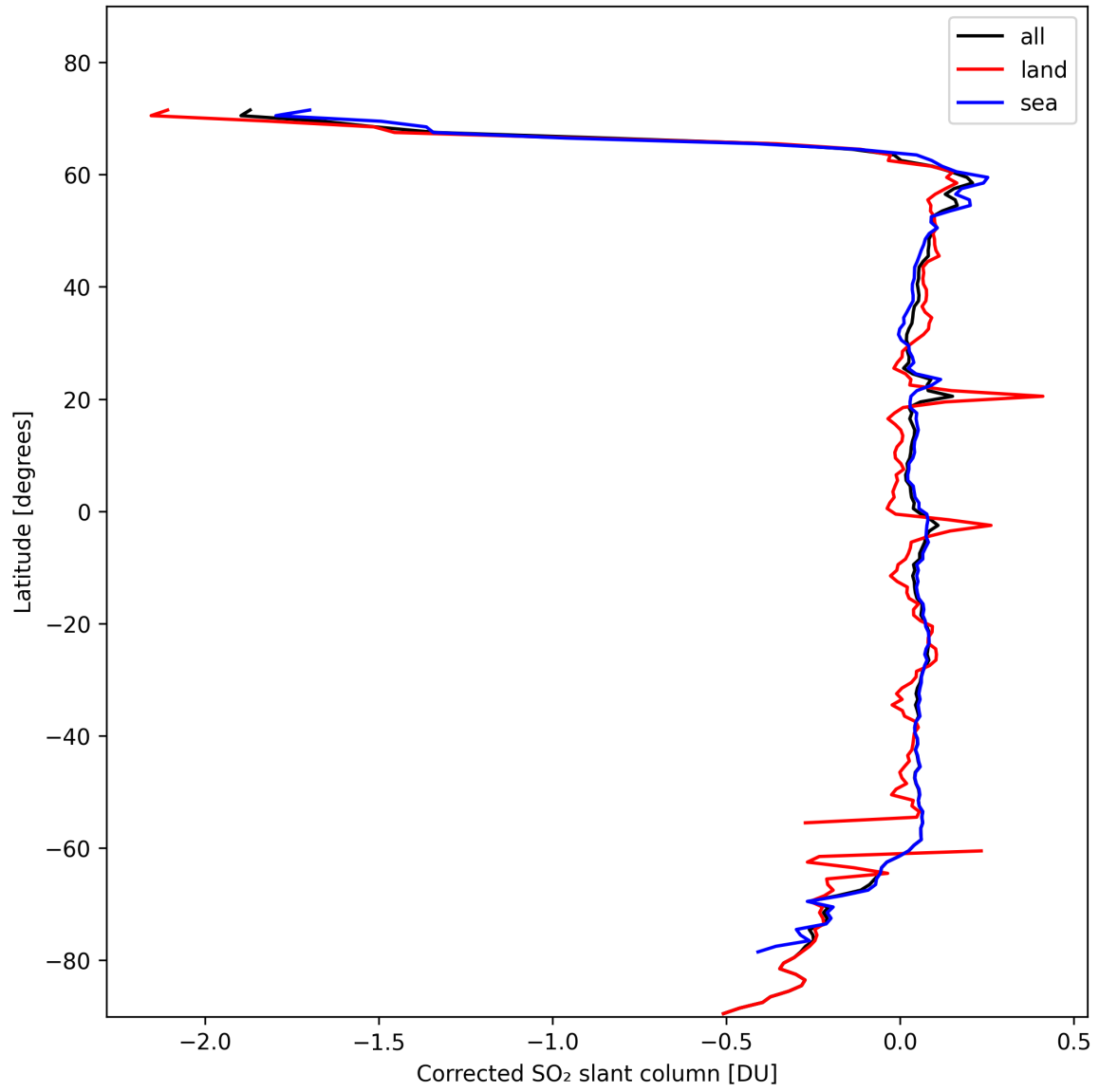
Figure 32: Zonal average of “Corrected SO 2 slant column” for 2024-10-27 to 2024-10-29.
