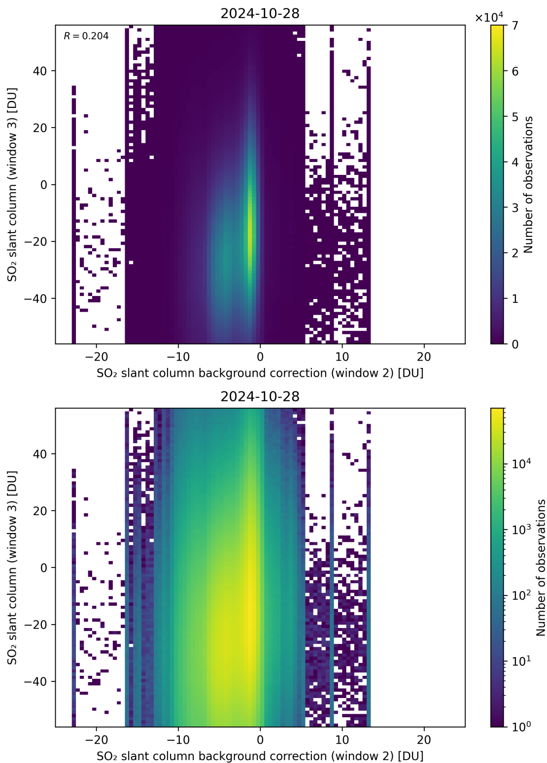
Figure 117: Scatter density plot of “SO 2 slant column background correction (window 2)” against “SO 2 slant column (window 3)” for 2024-10-27 to 2024-10-29.
