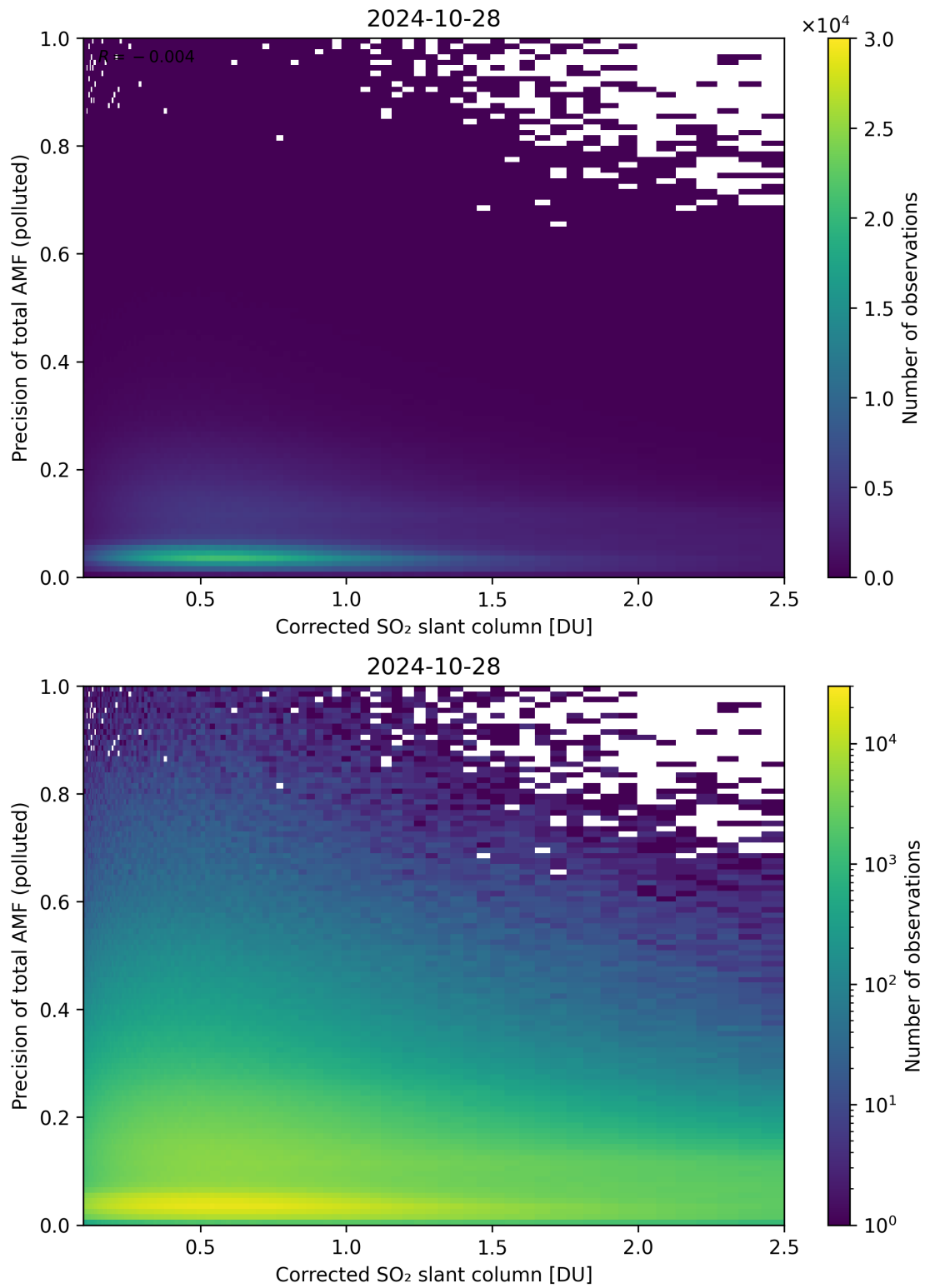
Figure 193: Scatter density plot of “Corrected SO 2 slant column” against “Precision of total AMF (polluted)” for 2024-10-27 to 2024-10-29.
