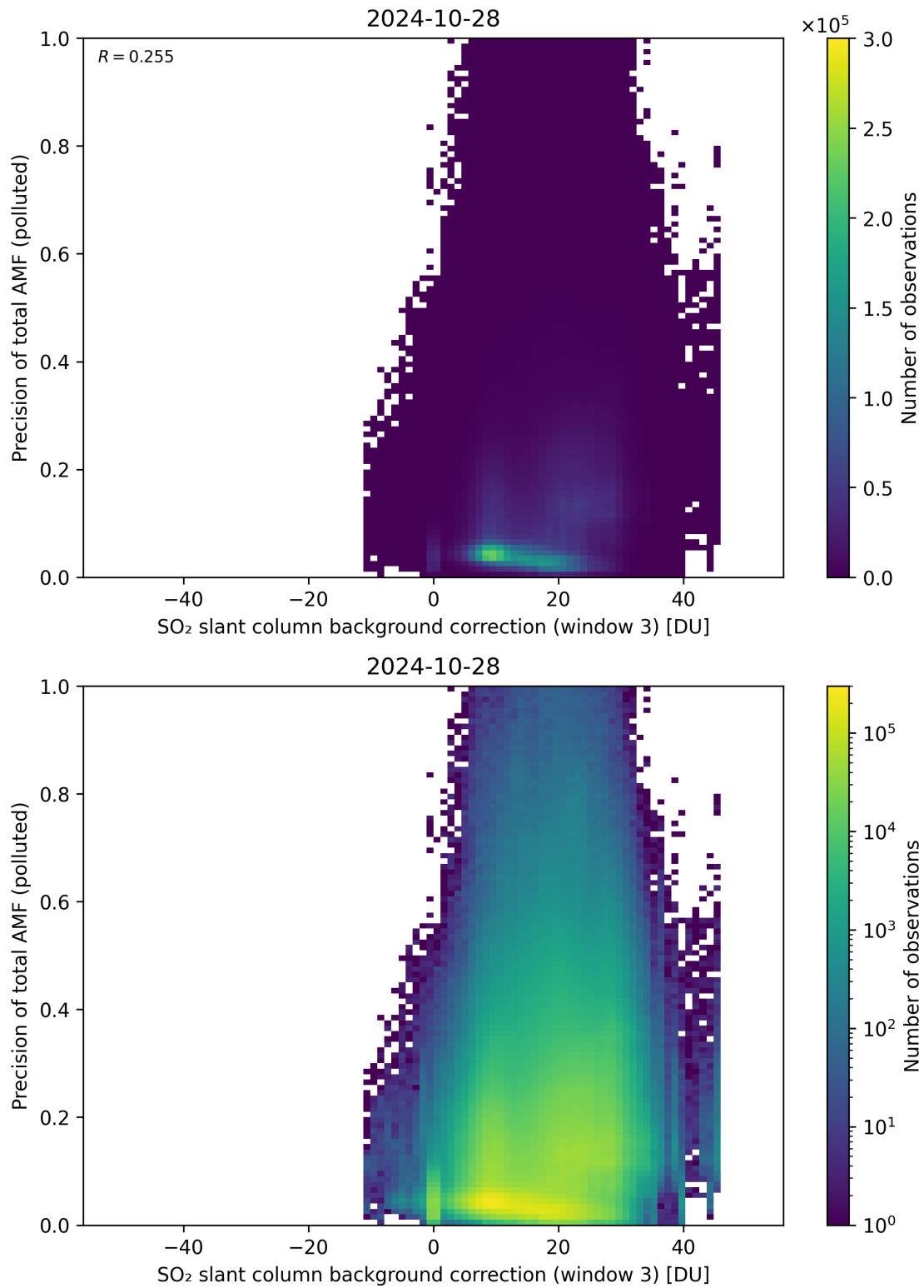
Figure 126: Scatter density plot of “SO 2 slant column background correction (window 3)” against “Precision of total AMF (polluted)” for 2024-10-27 to 2024-10-29.
