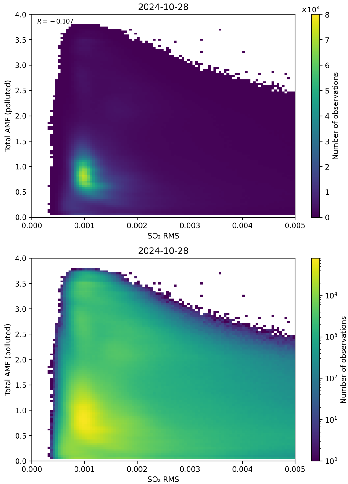
Figure 137: Scatter density plot of “SO 2 RMS” against “Total AMF (polluted)” for 2024-10-27 to 2024-10-29.
