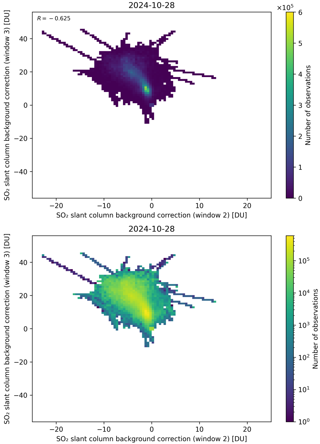
Figure 111: Scatter density plot of “SO 2 slant column background correction (window 2)” against “SO 2 slant column background correction (window 3)” for 2024-10-27 to 2024-10-29.
