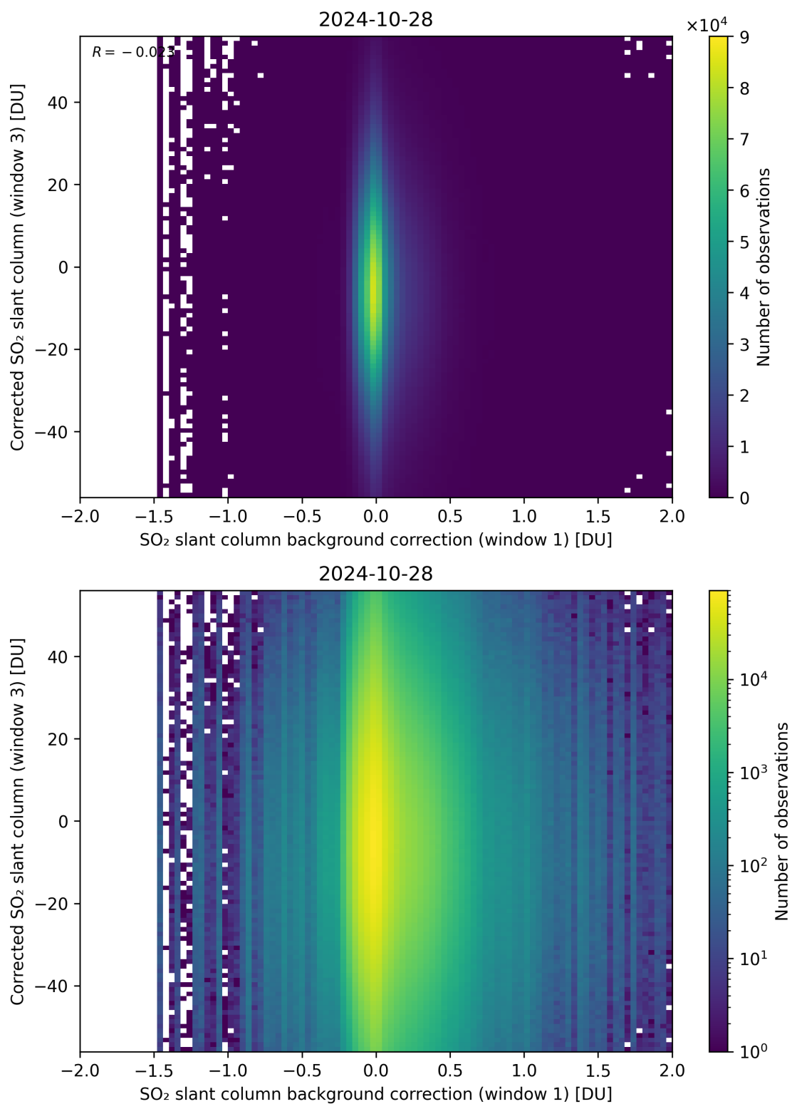
Figure 105: Scatter density plot of “SO 2 slant column background correction (window 1)” against “Corrected SO 2 slant column (window 3)” for 2024-10-27 to 2024-10-29.
