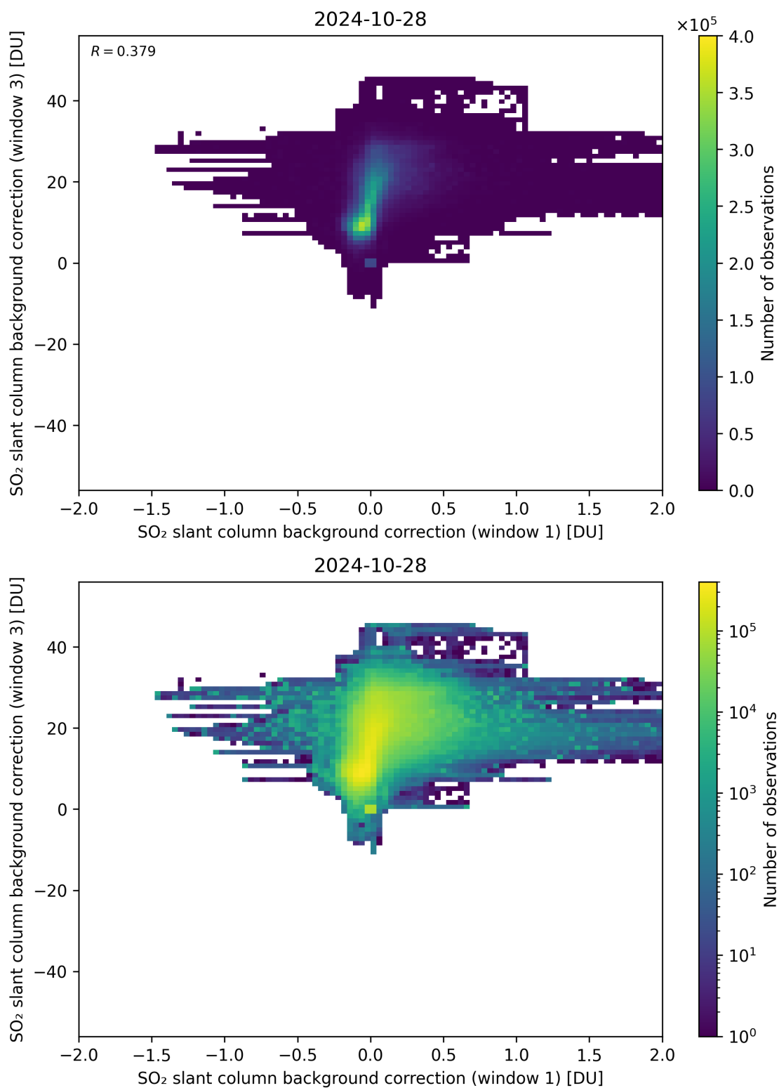
Figure 99: Scatter density plot of “SO 2 slant column background correction (window 1)” against “SO 2 slant column background correction (window 3)” for 2024-10-27 to 2024-10-29.
