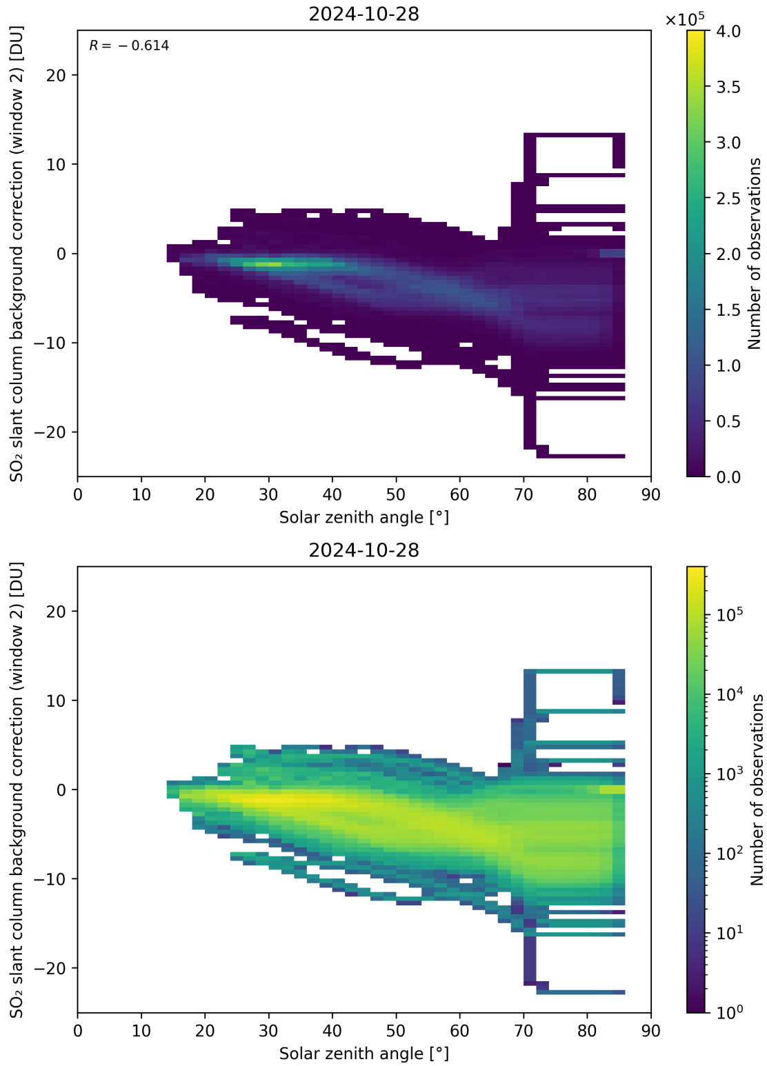
Figure 159: Scatter density plot of “Solar zenith angle” against “SO 2 slant column background correction (window 2)” for 2024-10-27 to 2024-10-29.
