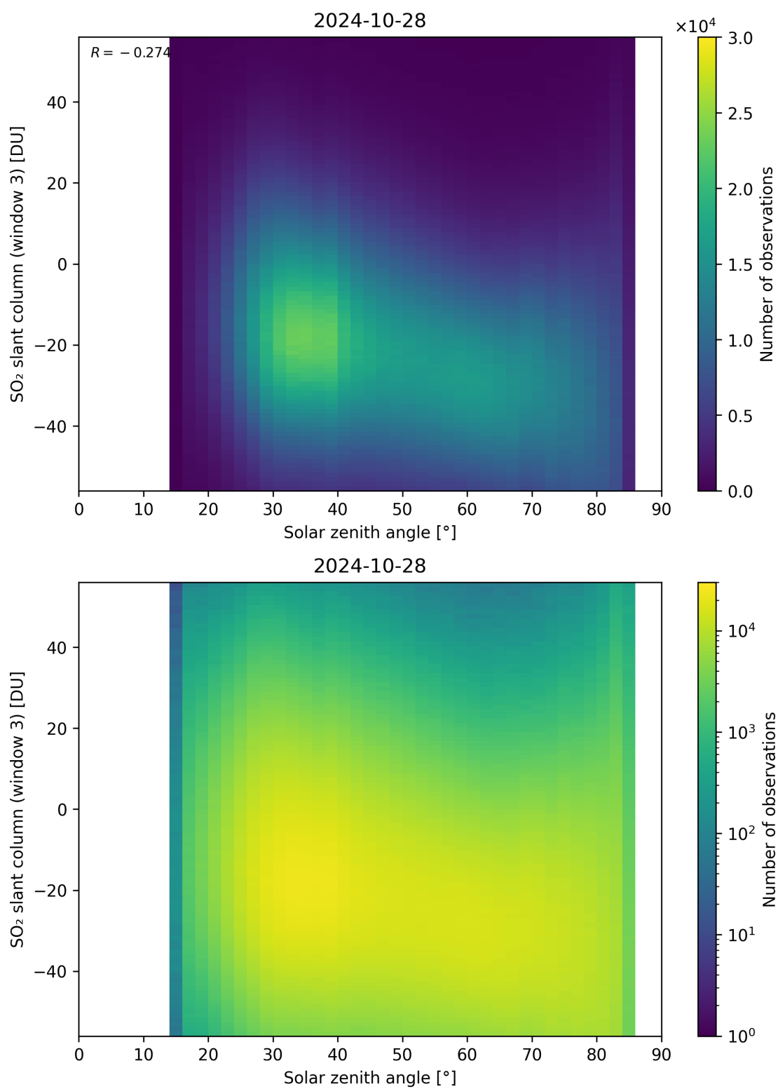
Figure 172: Scatter density plot of “Solar zenith angle” against “SO 2 slant column (window 3)” for 2024-10-27 to 2024-10-29.
