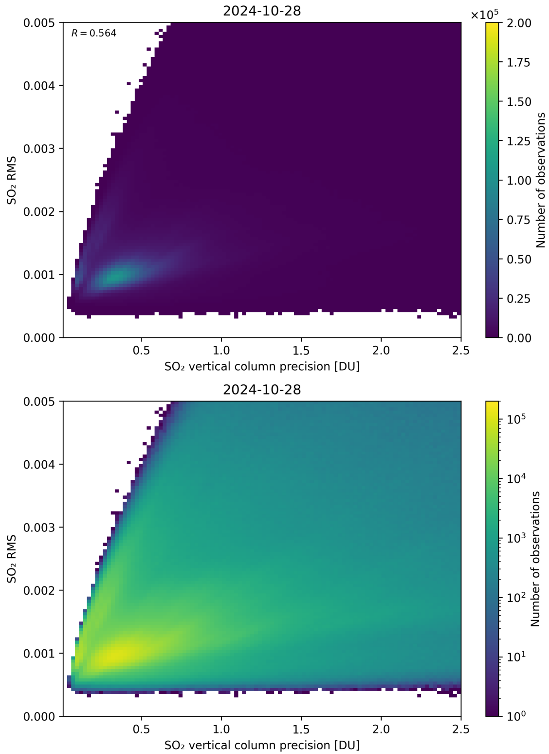
Figure 284: Scatter density plot of “SO 2 vertical column precision” against “SO 2 RMS” for 2024-10-27 to 2024-10-29.
