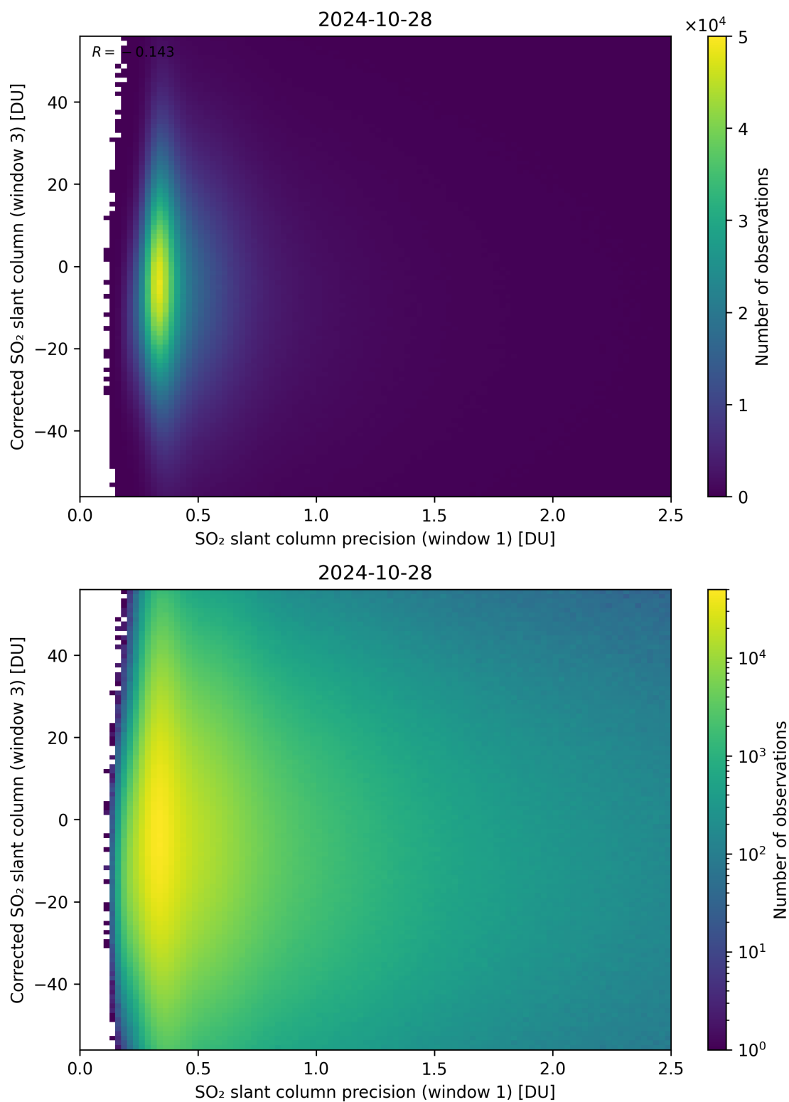
Figure 226: Scatter density plot of “SO 2 slant column precision (window 1)” against “Corrected SO 2 slant column (window 3)” for 2024-10-27 to 2024-10-29.
