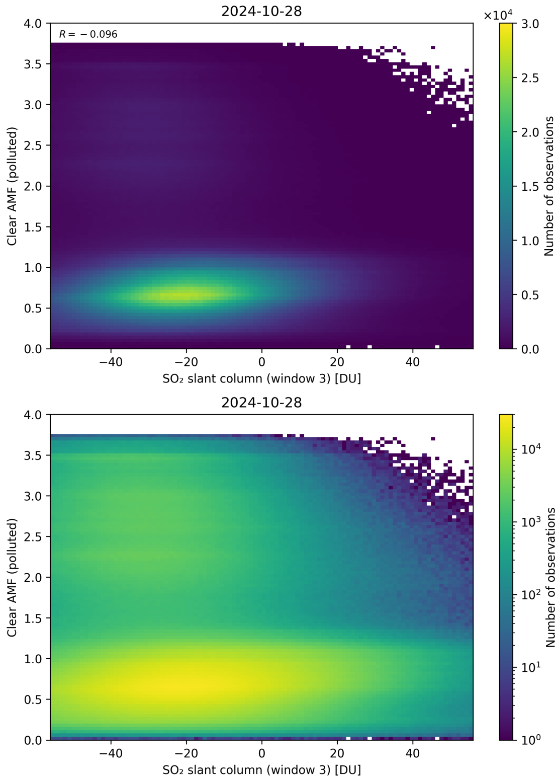
Figure 265: Scatter density plot of “SO 2 slant column (window 3)” against “Clear AMF (polluted)” for 2024-10-27 to 2024-10-29.
