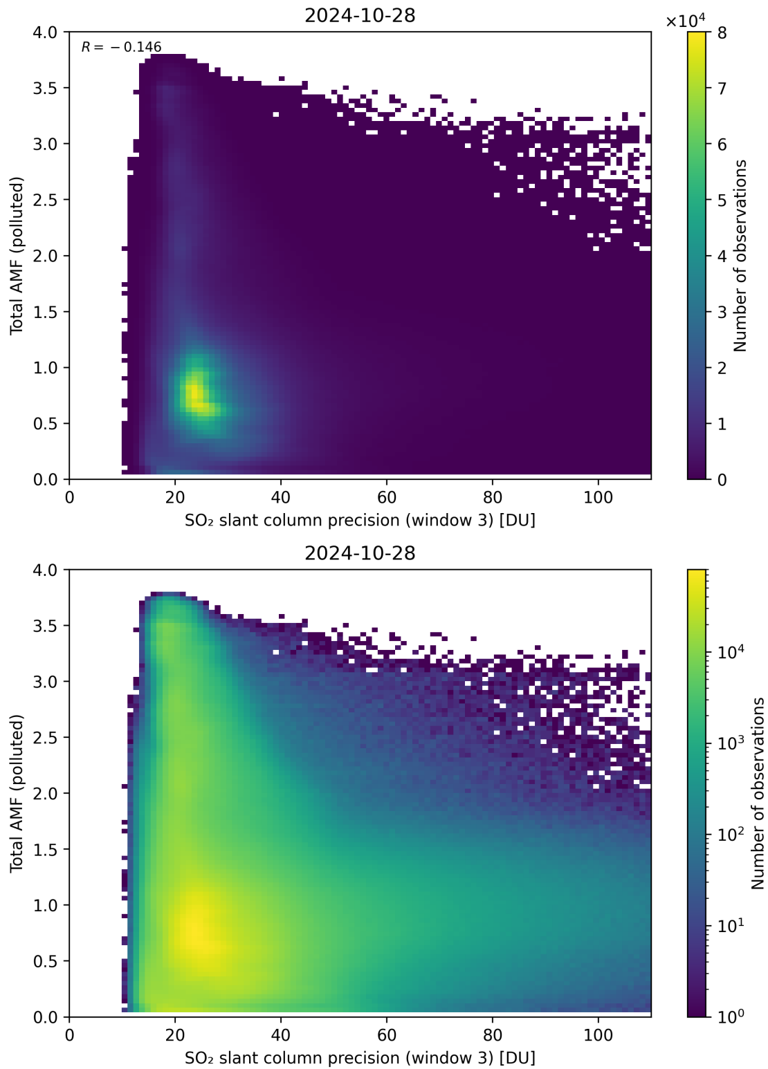
Figure 263: Scatter density plot of “SO 2 slant column precision (window 3)” against “Total AMF (polluted)” for 2024-10-27 to 2024-10-29.
