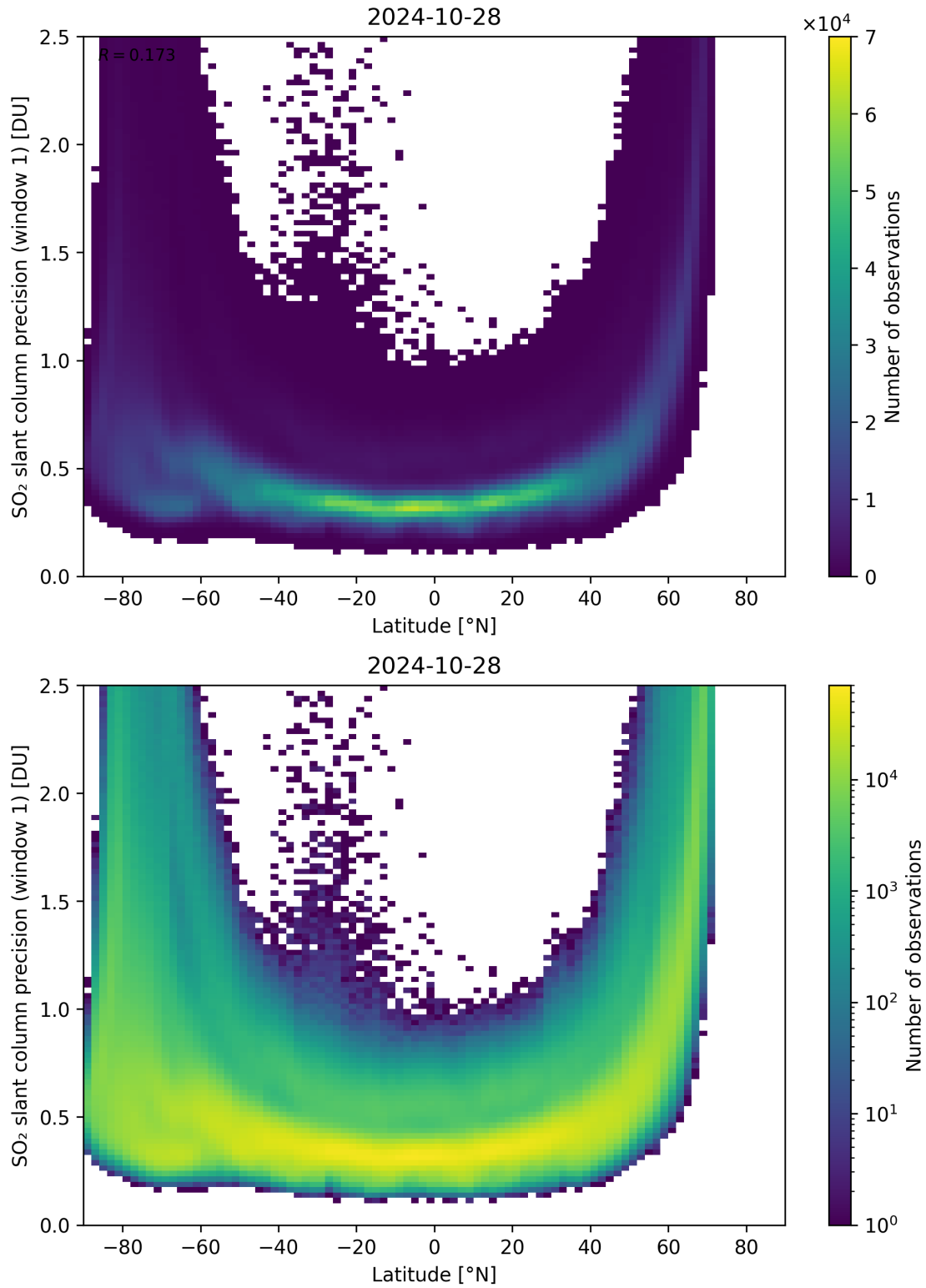
Figure 150: Scatter density plot of “Latitude” against “SO 2 slant column precision (window 1)” for 2024-10-27 to 2024-10-29.
