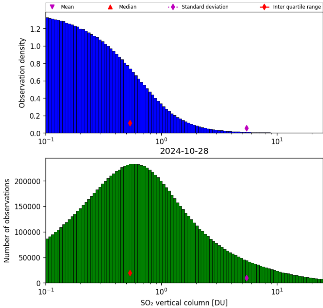
Figure 53: Histogram of “SO 2 vertical column” for 2024-10-27 to 2024-10-29
