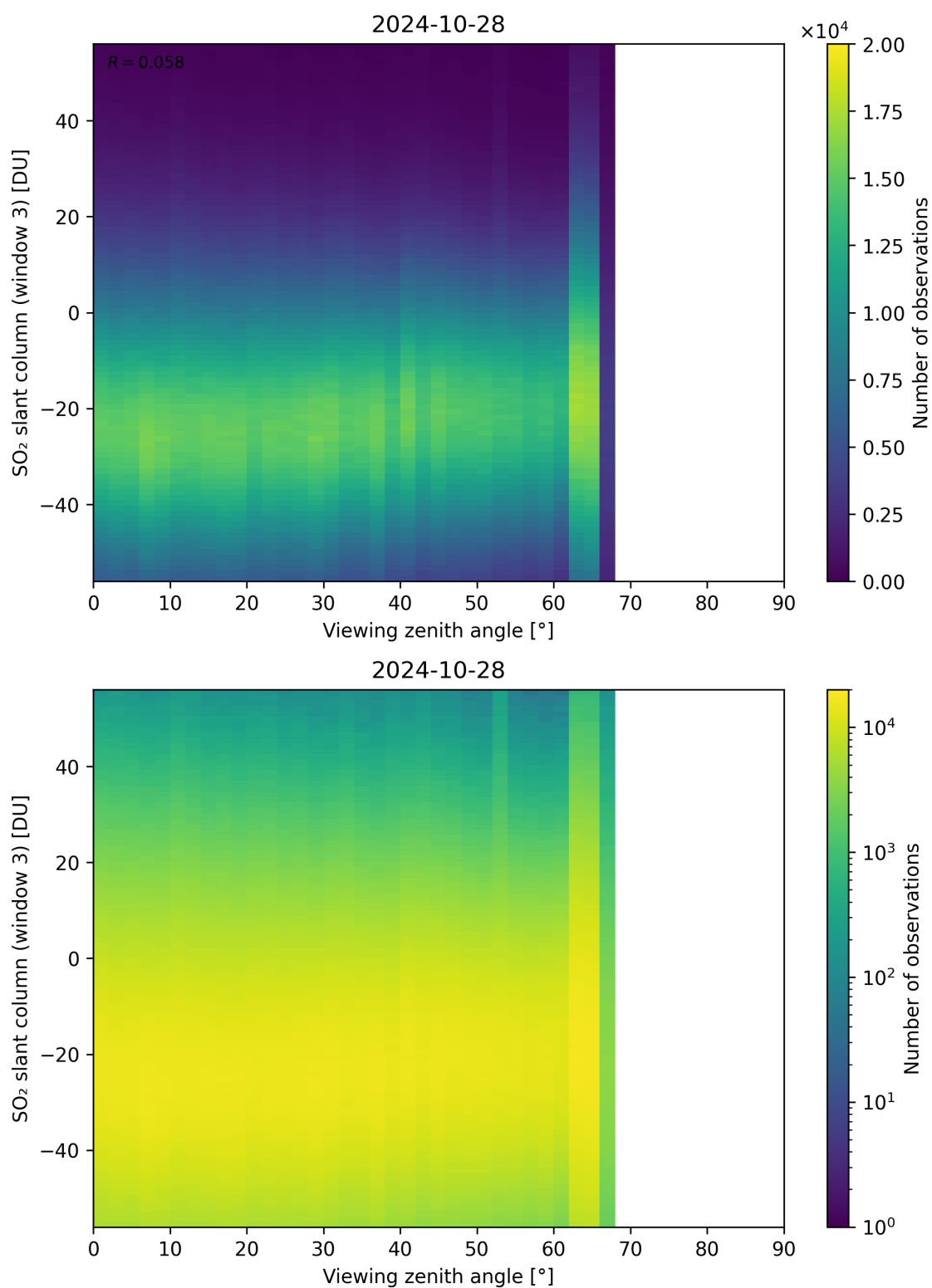
Figure 323: Scatter density plot of “Viewing zenith angle” against “SO 2 slant column (window 3)” for 2024-10-27 to 2024-10-29.
