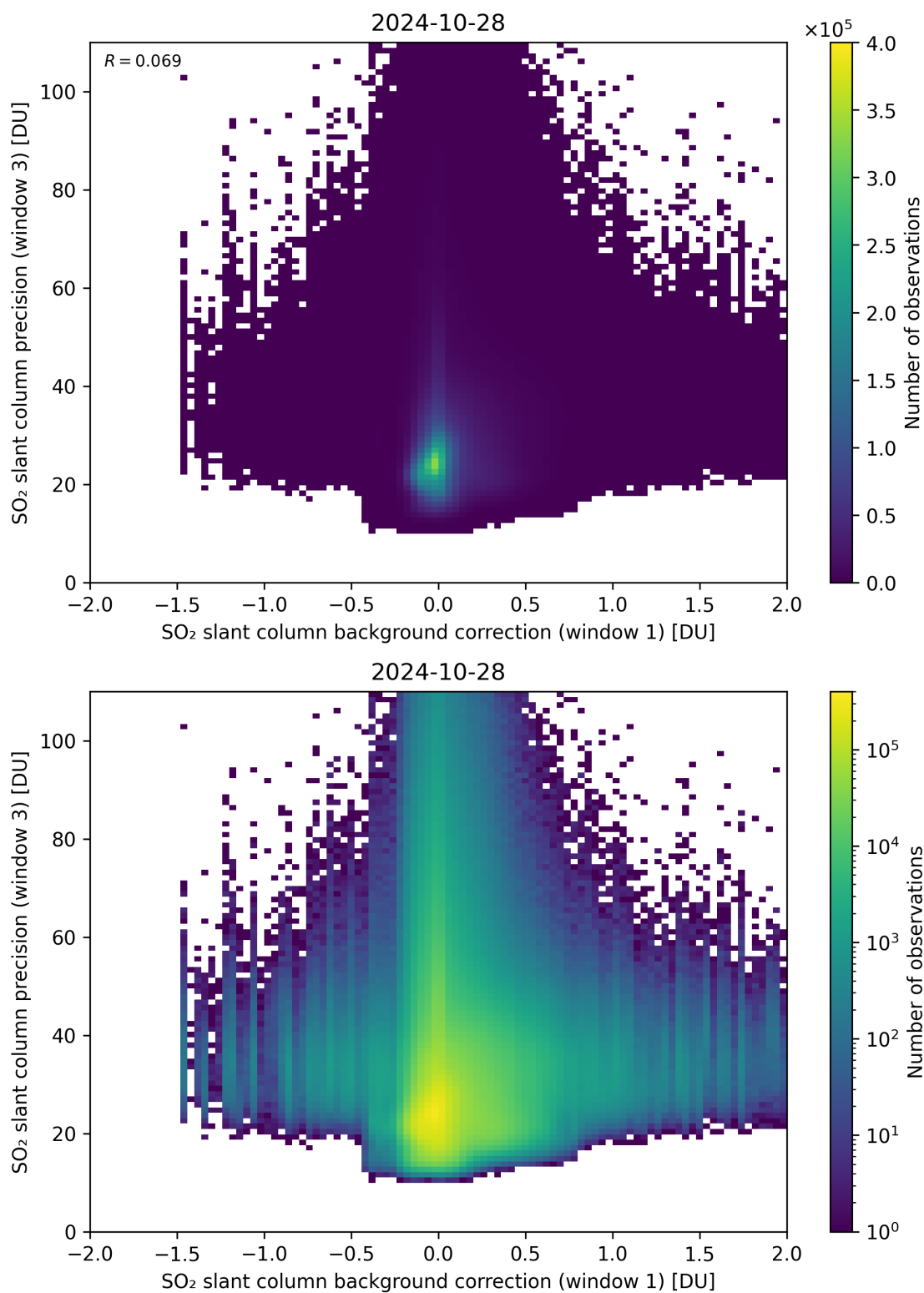
Figure 108: Scatter density plot of “SO 2 slant column background correction (window 1)” against “SO 2 slant column precision (window 3)” for 2024-10-27 to 2024-10-29.
