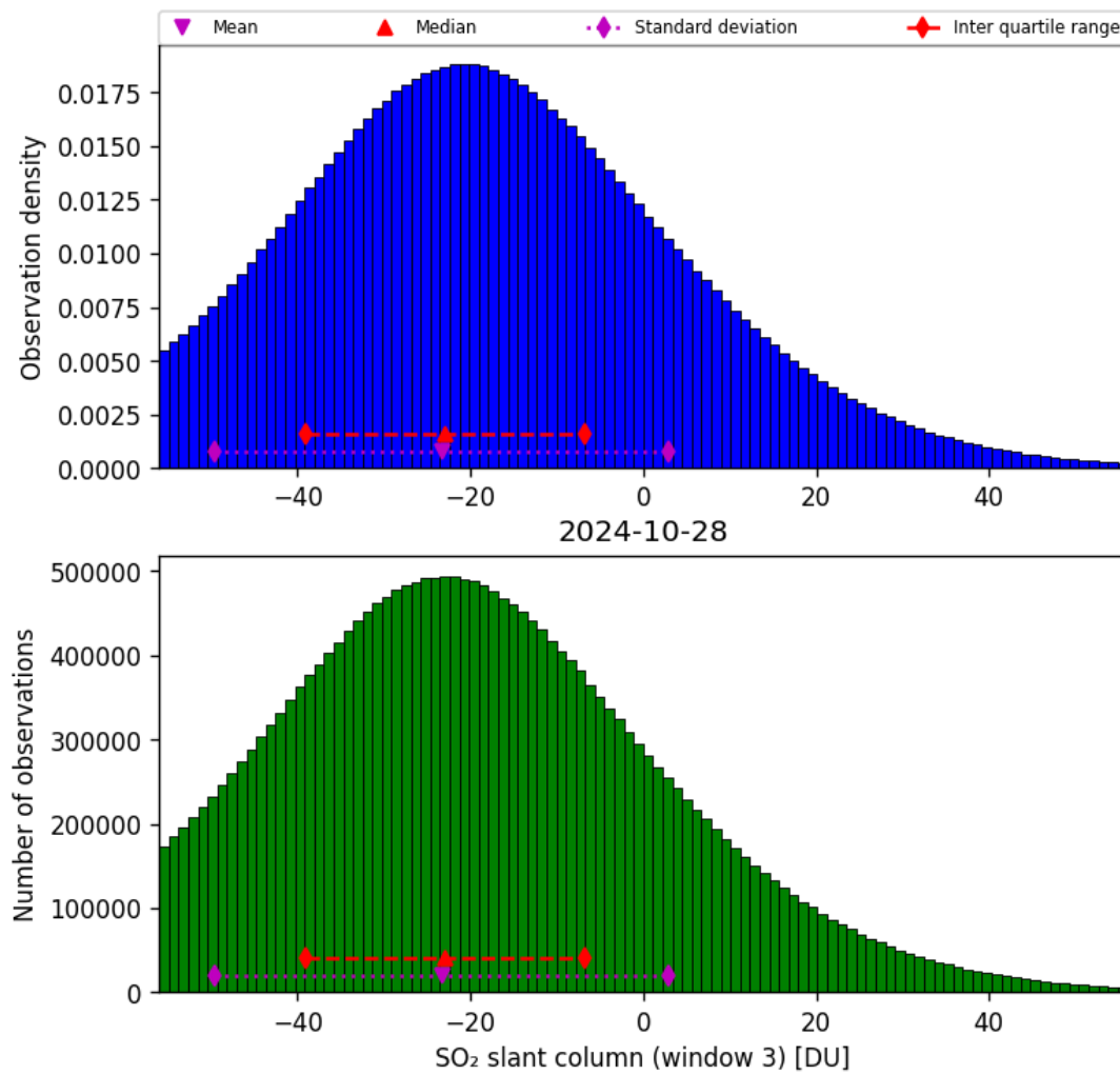
Figure 64: Histogram of “SO 2 slant column (window 3)” for 2024-10-27 to 2024-10-29
