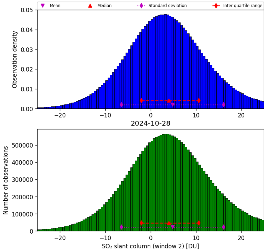
Figure 60: Histogram of “SO 2 slant column (window 2)” for 2024-10-27 to 2024-10-29
