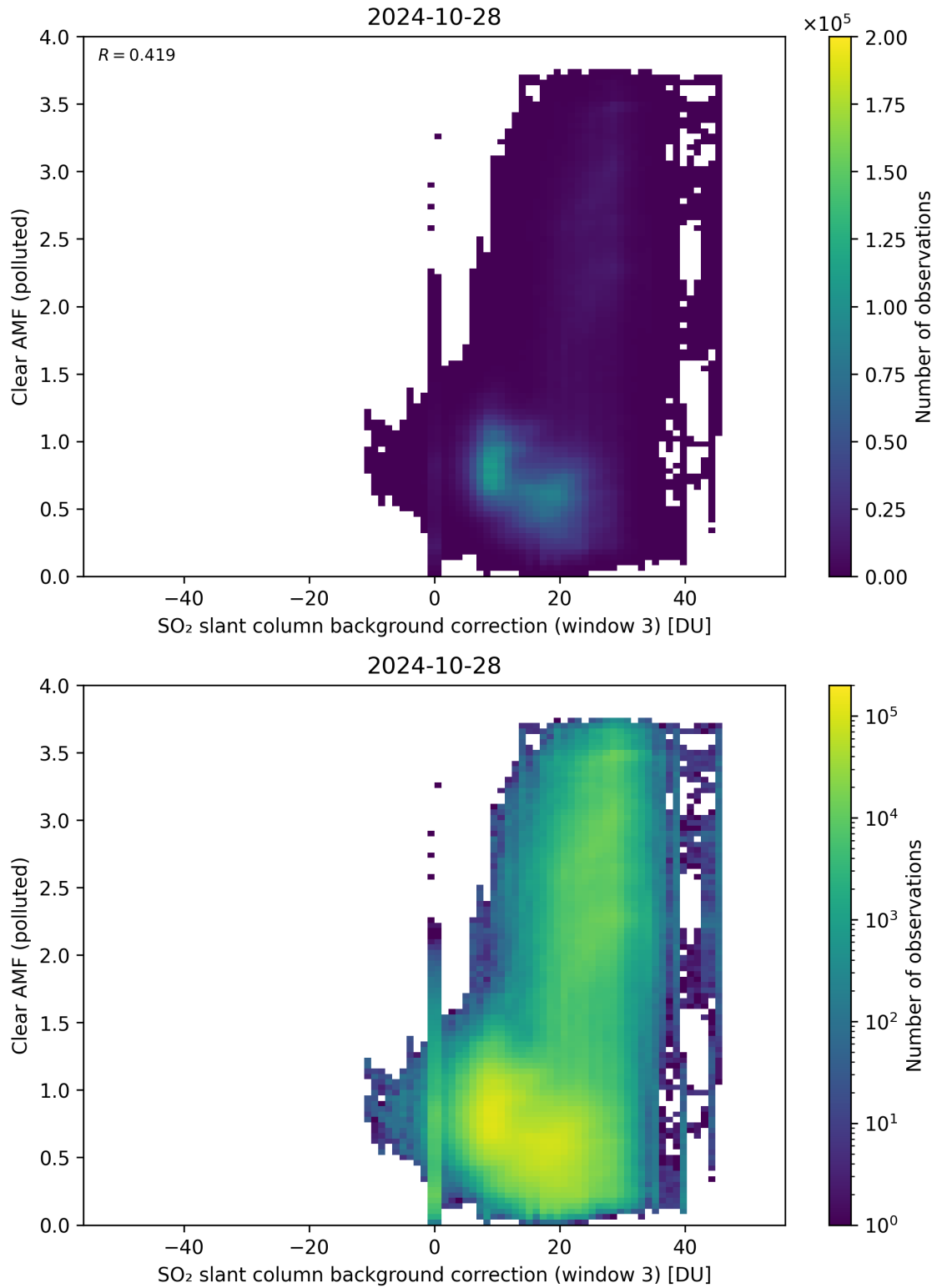
Figure 124: Scatter density plot of “SO 2 slant column background correction (window 3)” against “Clear AMF (polluted)” for 2024-10-27 to 2024-10-29.
