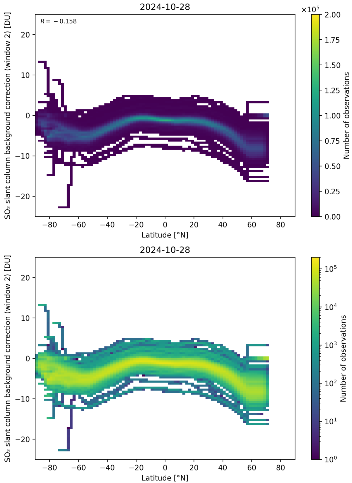
Figure 140: Scatter density plot of “Latitude” against “SO 2 slant column background correction (window 2)” for 2024-10-27 to 2024-10-29.
