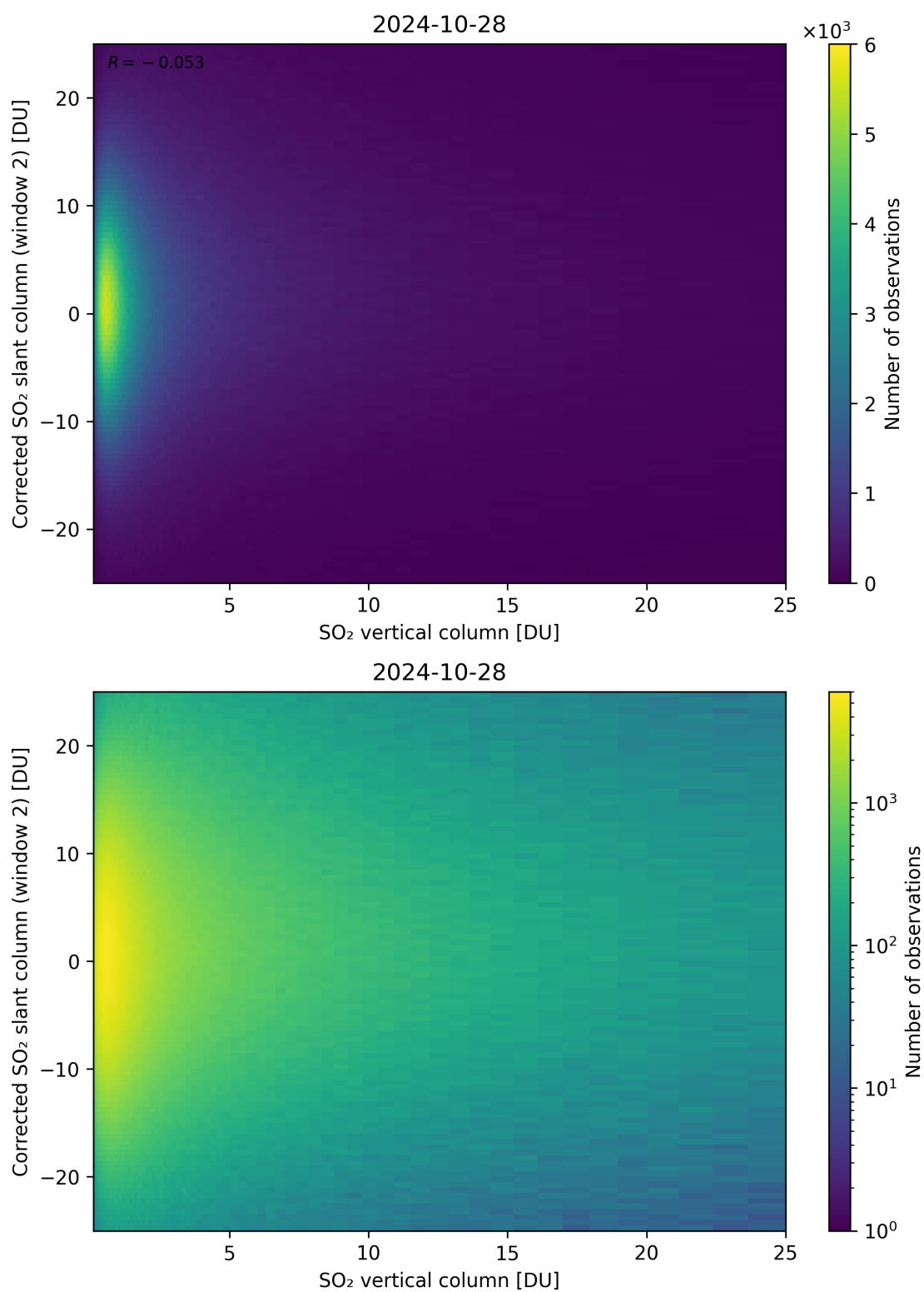
Figure 298: Scatter density plot of “SO 2 vertical column” against “Corrected SO 2 slant column (window 2)” for 2024-10-27 to 2024-10-29.
