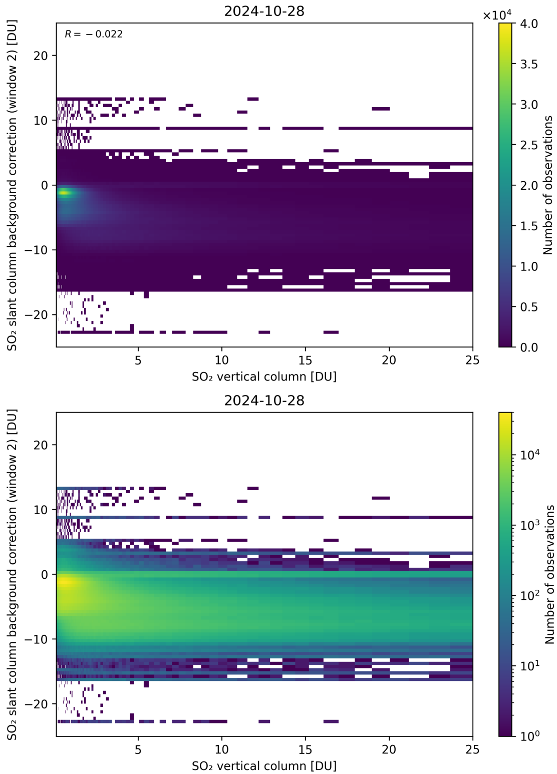
Figure 274: Scatter density plot of “SO 2 vertical column” against “SO 2 slant column background correction (window 2)” for 2024-10-27 to 2024-10-29.
