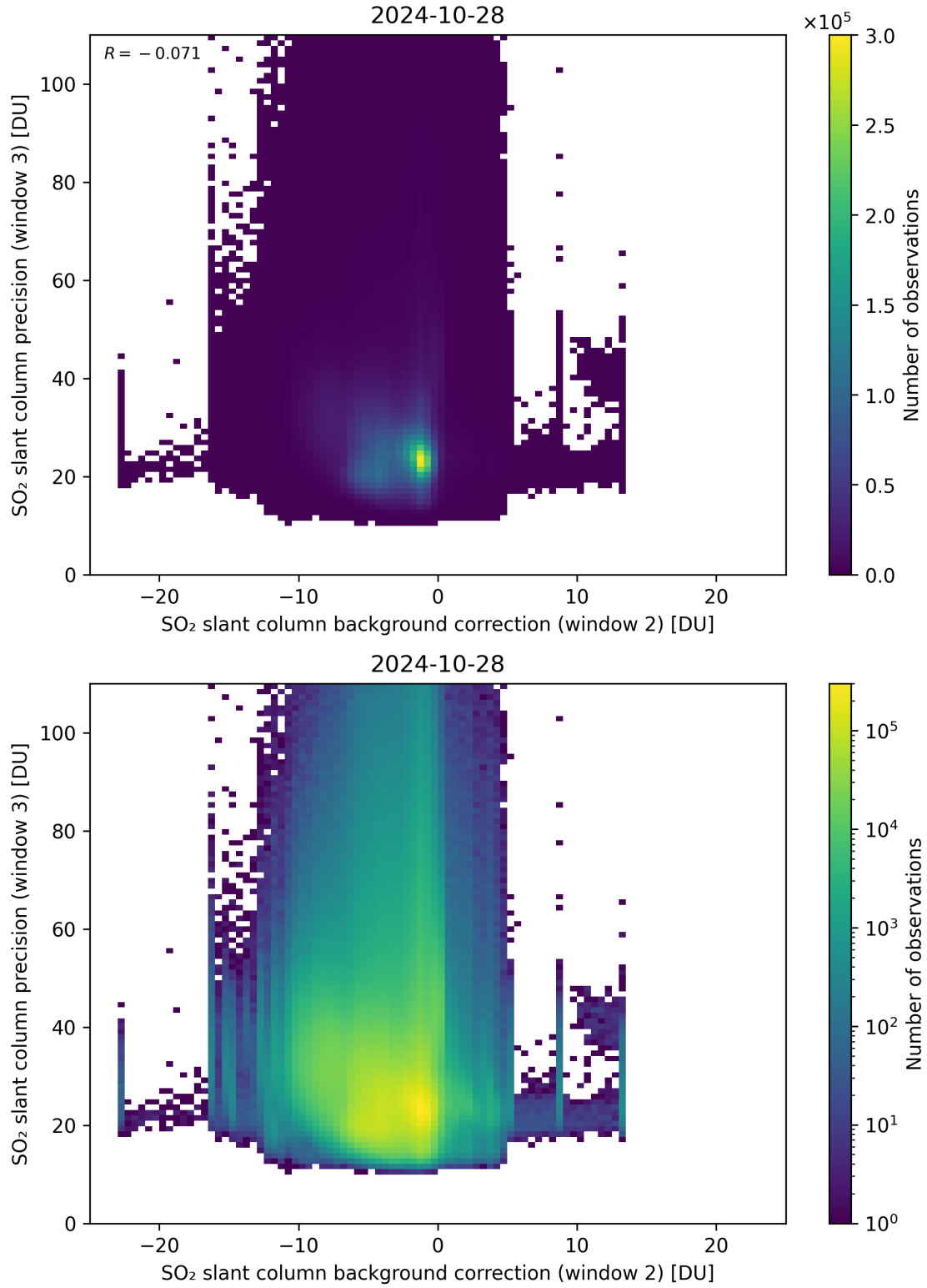
Figure 118: Scatter density plot of “SO 2 slant column background correction (window 2)” against “SO 2 slant column precision (window 3)” for 2024-10-27 to 2024-10-29.
