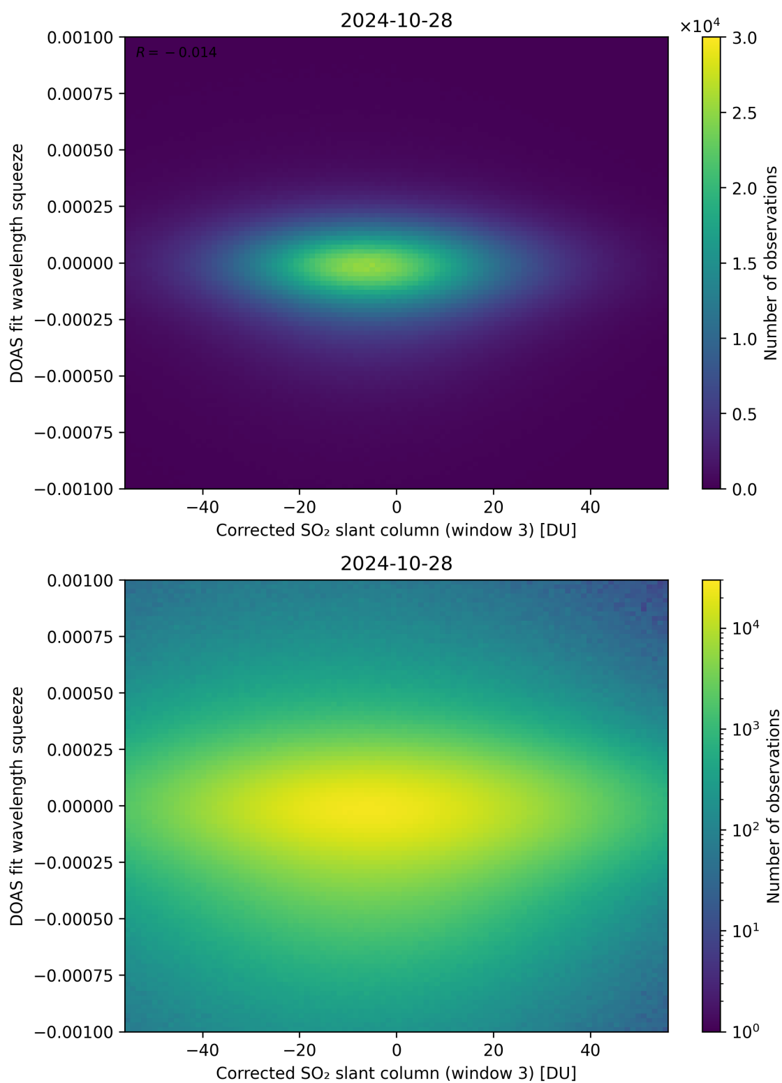
Figure 207: Scatter density plot of “Corrected SO 2 slant column (window 3)” against “DOAS fit wavelength squeeze” for 2024-10-27 to 2024-10-29.
