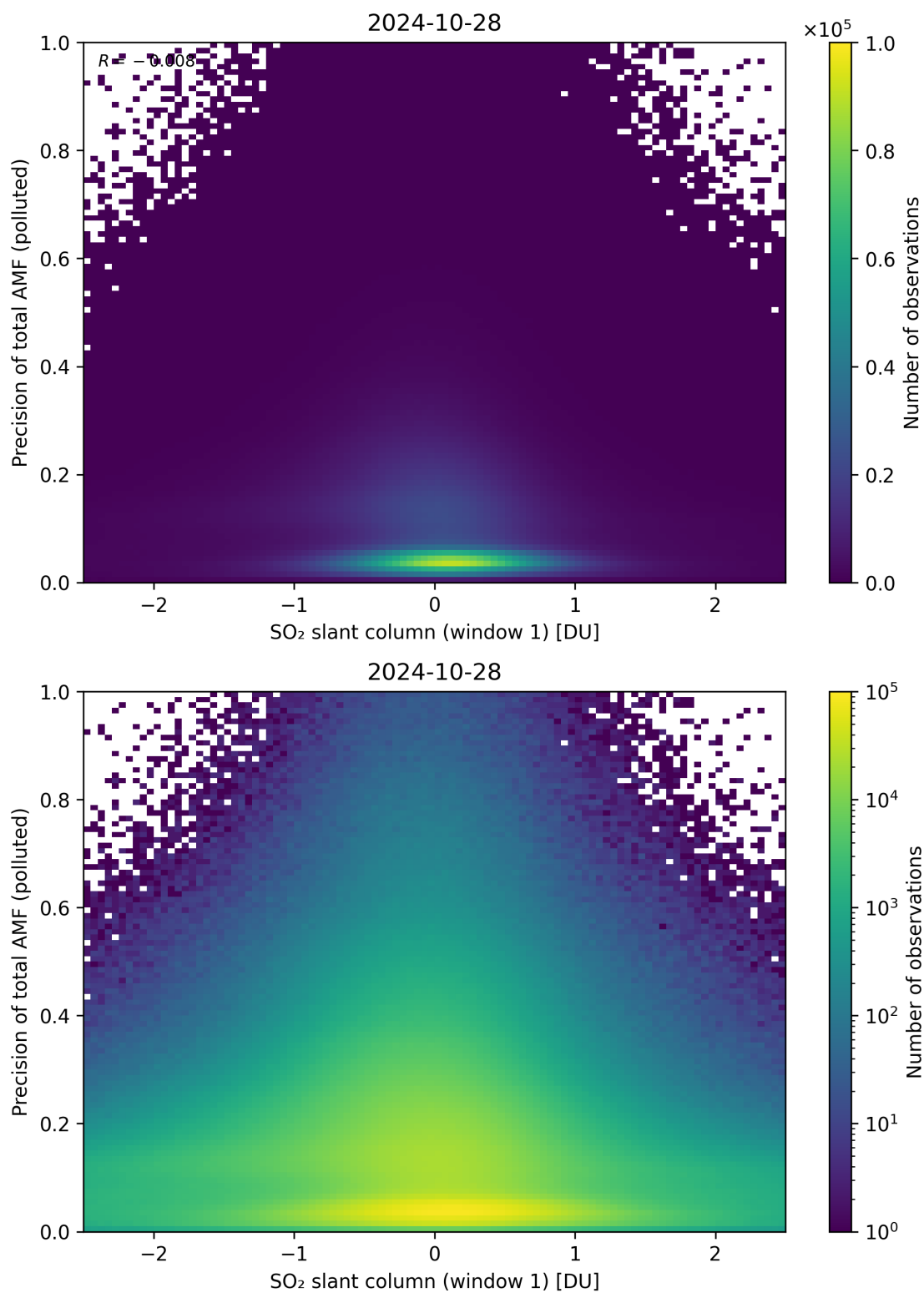
Figure 240: Scatter density plot of “SO 2 slant column (window 1)” against “Precision of total AMF (polluted)” for 2024-10-27 to 2024-10-29.
