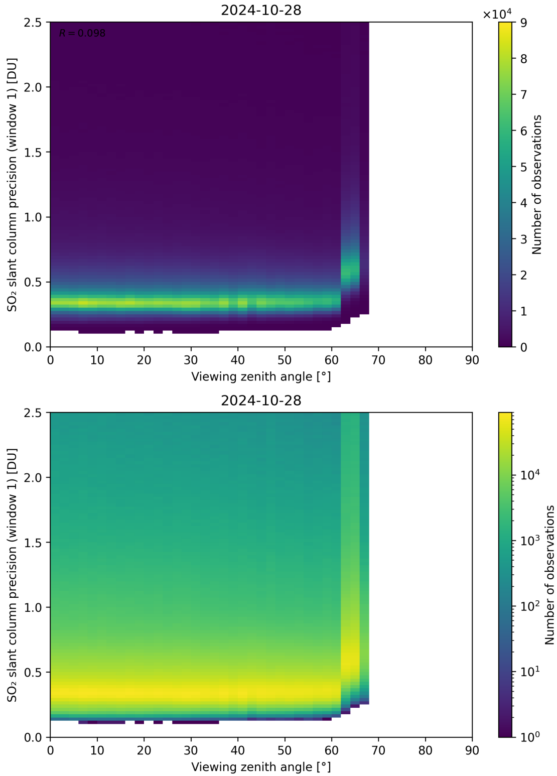
Figure 321: Scatter density plot of “Viewing zenith angle” against “SO 2 slant column precision (window 1)” for 2024-10-27 to 2024-10-29.
