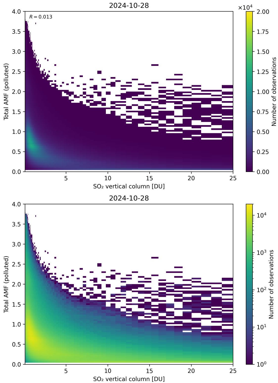
Figure 305: Scatter density plot of “SO 2 vertical column” against “Total AMF (polluted)” for 2024-10-27 to 2024-10-29.
