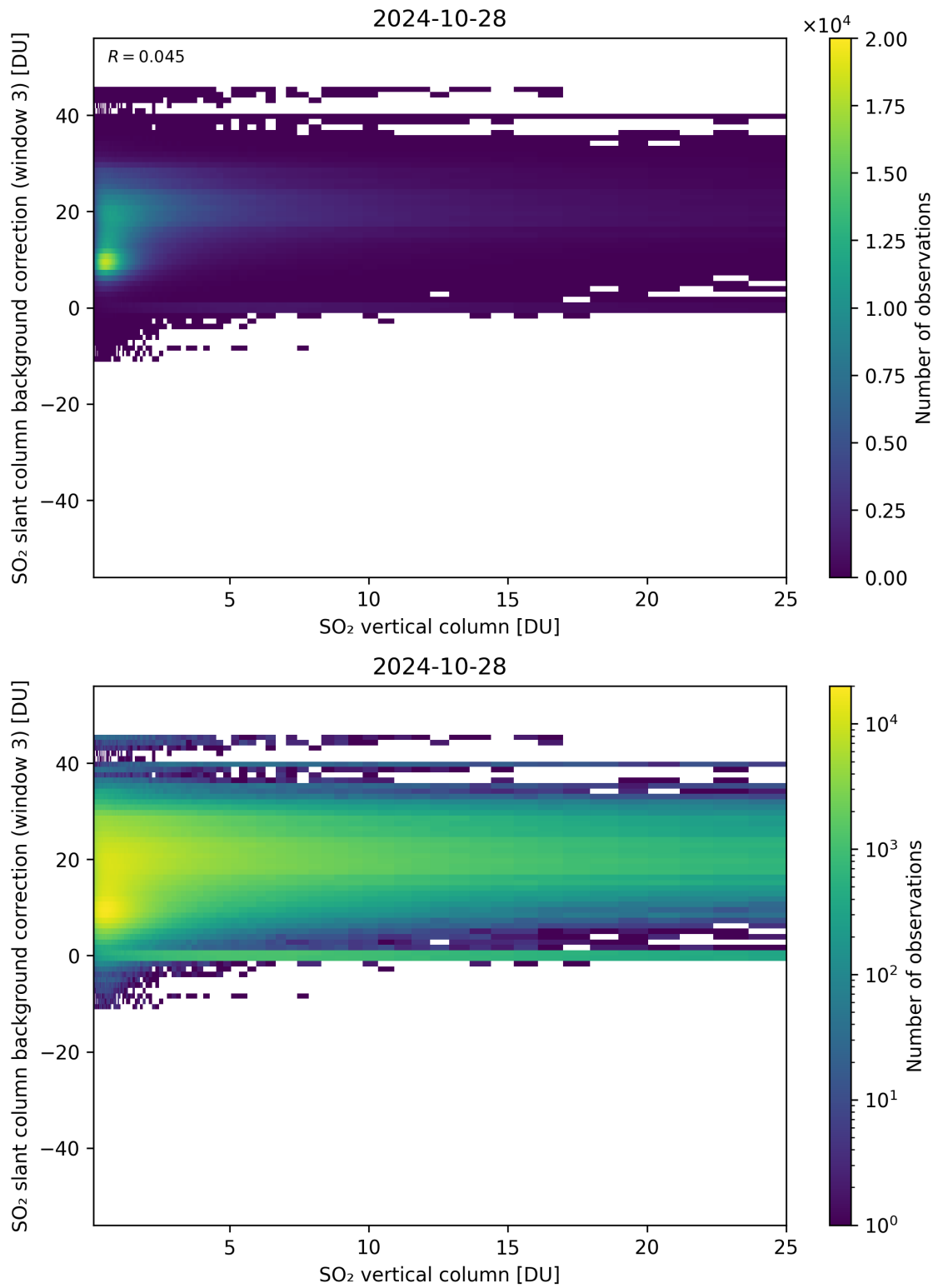
Figure 275: Scatter density plot of “SO 2 vertical column” against “SO 2 slant column background correction (window 3)” for 2024-10-27 to 2024-10-29.
