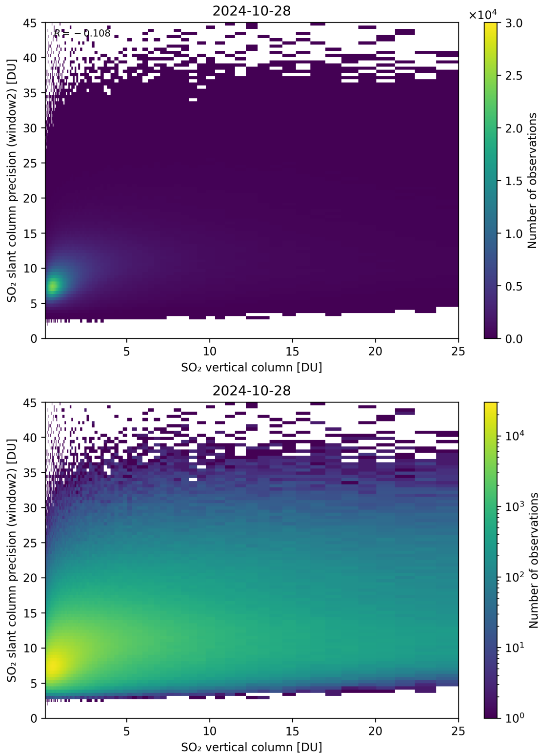
Figure 302: Scatter density plot of “SO 2 vertical column” against “SO 2 slant column precision (window2)” for 2024-10-27 to 2024-10-29.
