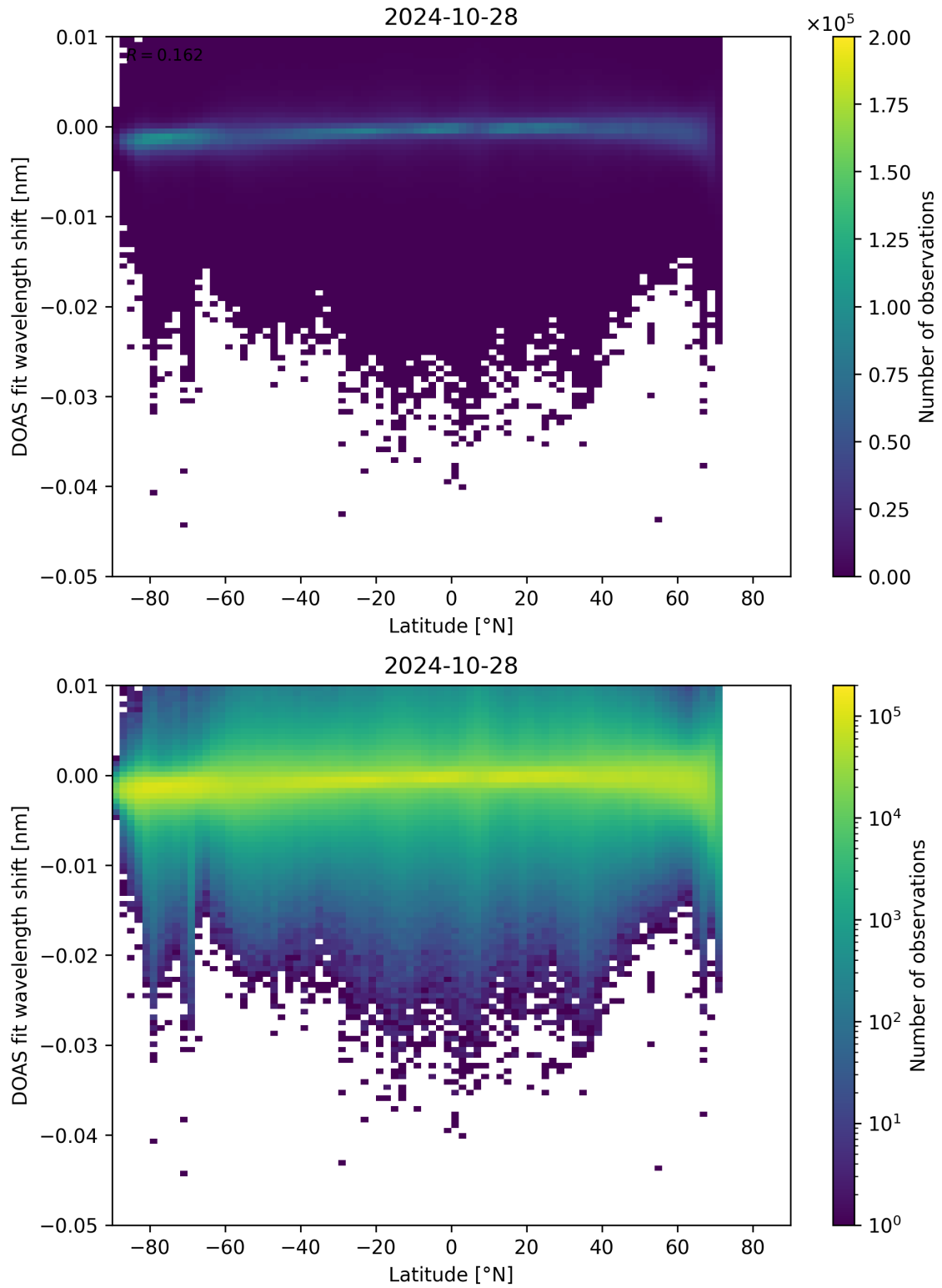
Figure 142: Scatter density plot of “Latitude” against “DOAS fit wavelength shift” for 2024-10-27 to 2024-10-29.
