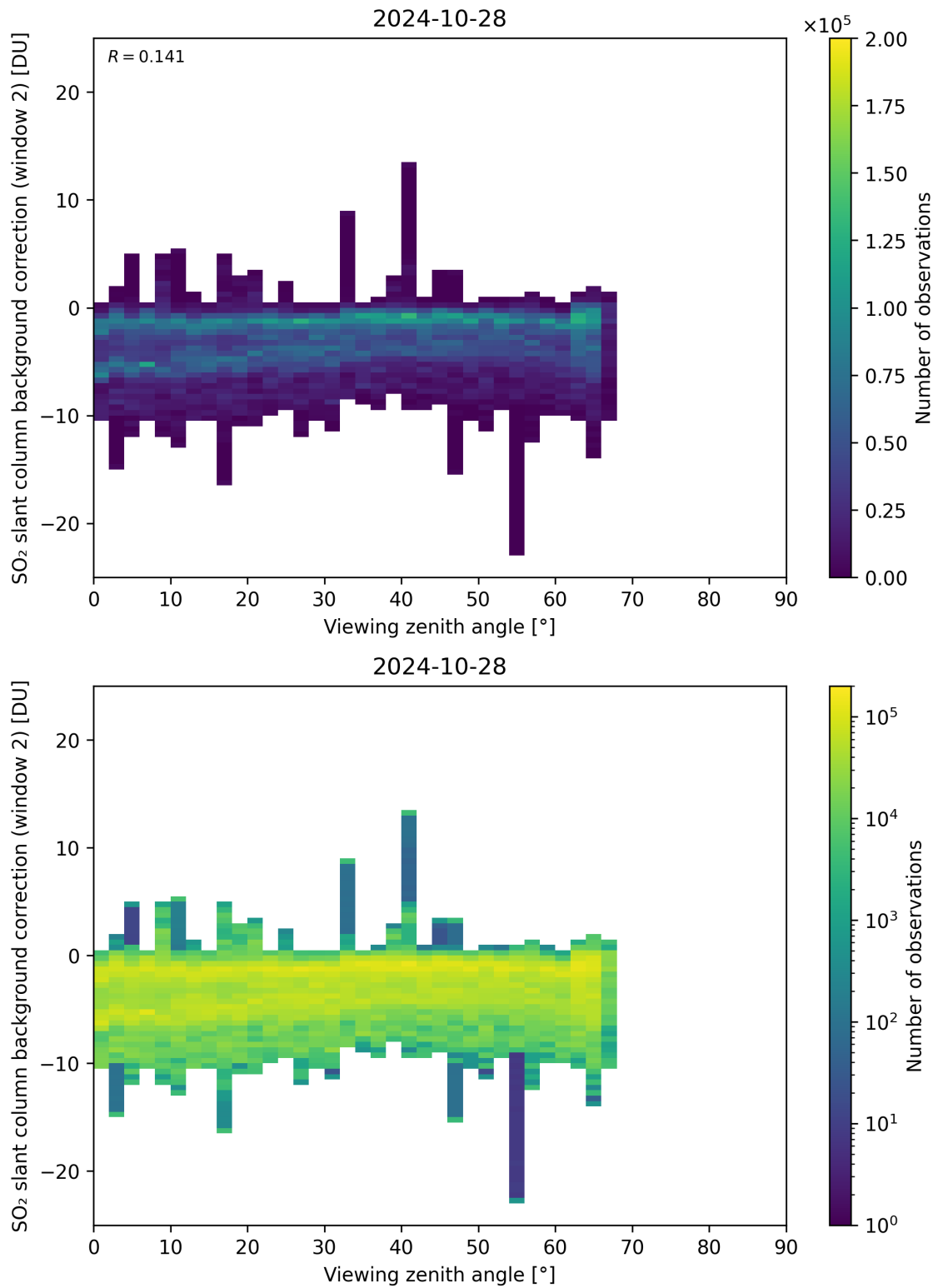
Figure 309: Scatter density plot of “Viewing zenith angle” against “SO 2 slant column background correction (window 2)” for 2024-10-27 to 2024-10-29.
