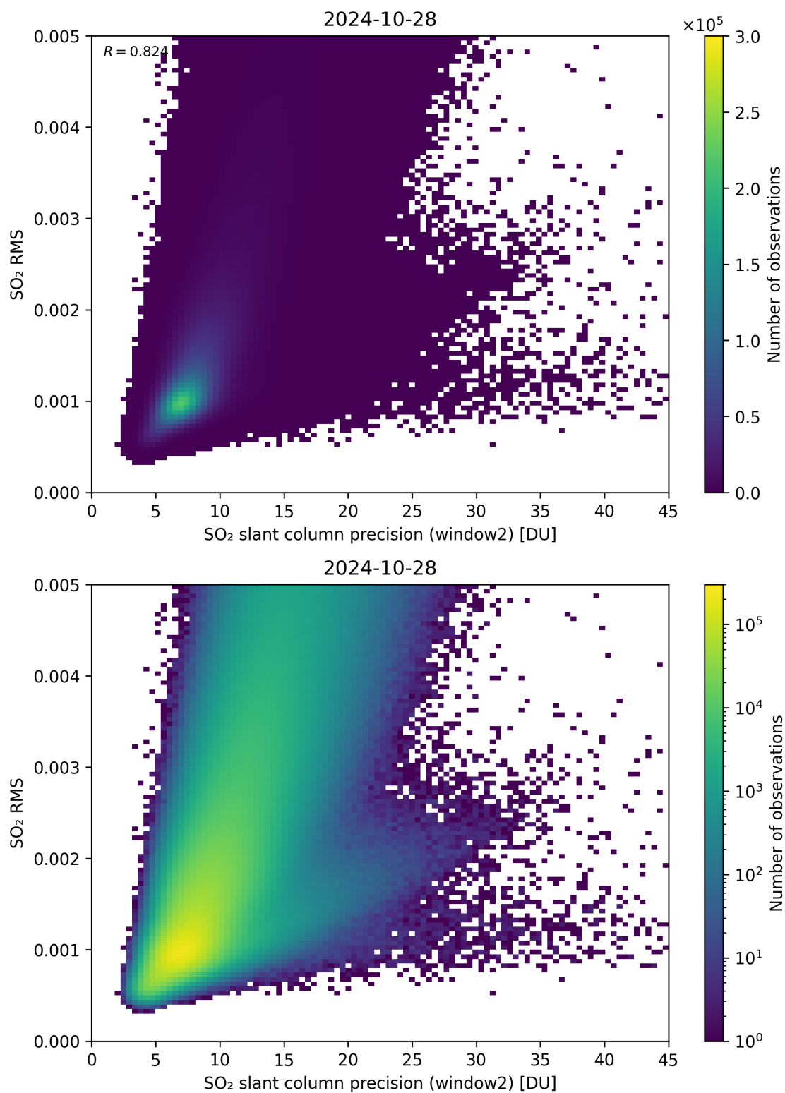
Figure 245: Scatter density plot of “SO 2 slant column precision (window2)” against “SO 2 RMS” for 2024-10-27 to 2024-10-29.
