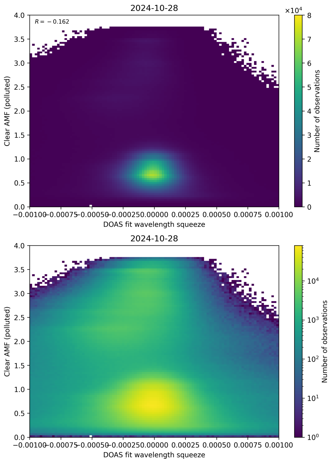
Figure 133: Scatter density plot of “DOAS fit wavelength squeeze” against “Clear AMF (polluted)” for 2024-10-27 to 2024-10-29.
