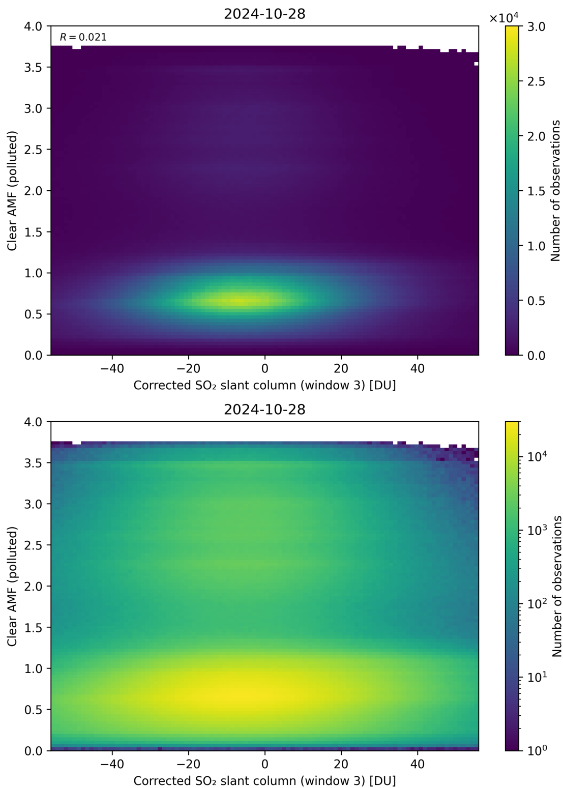
Figure 209: Scatter density plot of “Corrected SO 2 slant column (window 3)” against “Clear AMF (polluted)” for 2024-10-27 to 2024-10-29.
