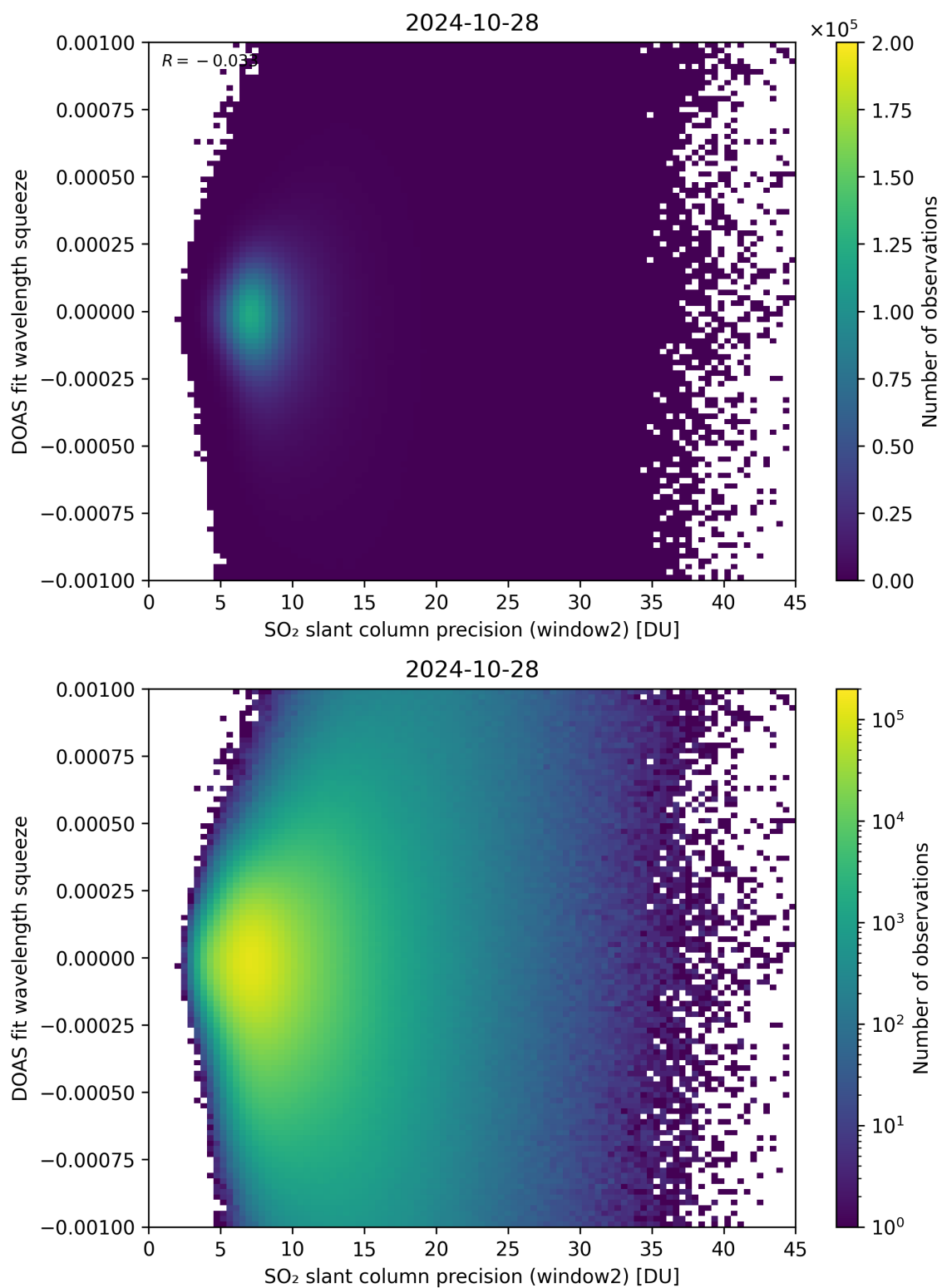
Figure 244: Scatter density plot of “SO 2 slant column precision (window2)” against “DOAS fit wavelength squeeze” for 2024-10-27 to 2024-10-29.
