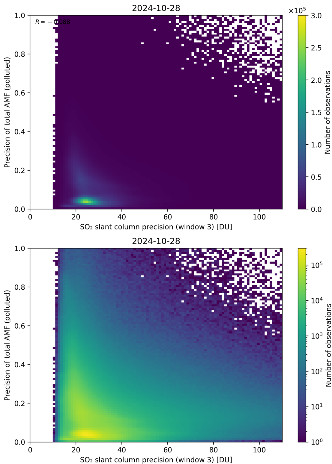
Figure 264: Scatter density plot of “SO 2 slant column precision (window 3)” against “Precision of total AMF (polluted)” for 2024-10-27 to 2024-10-29.
