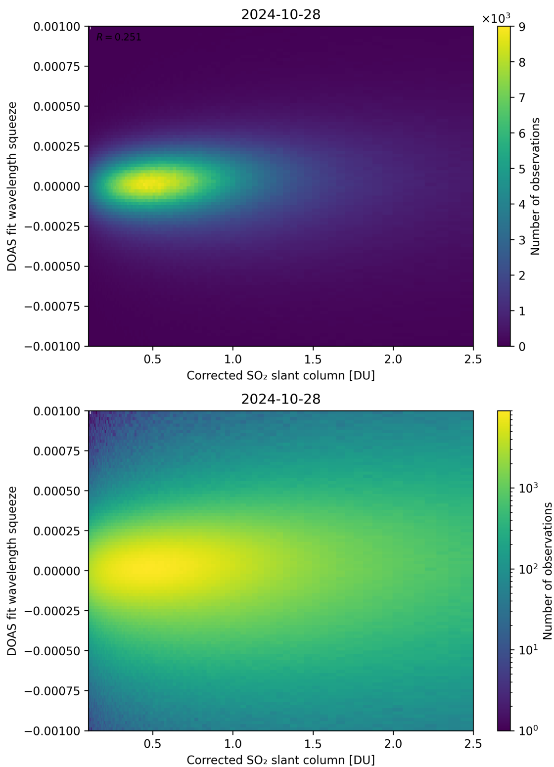
Figure 182: Scatter density plot of “Corrected SO 2 slant column” against “DOAS fit wavelength squeeze” for 2024-10-27 to 2024-10-29.
