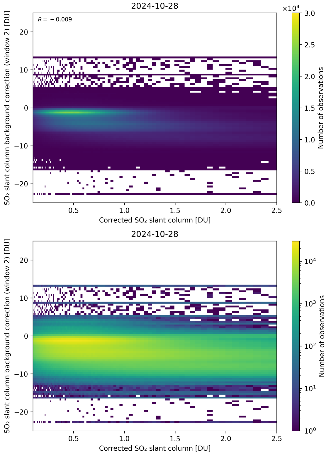
Figure 179: Scatter density plot of “Corrected SO 2 slant column” against “SO 2 slant column background correction (window 2)” for 2024-10-27 to 2024-10-29.
