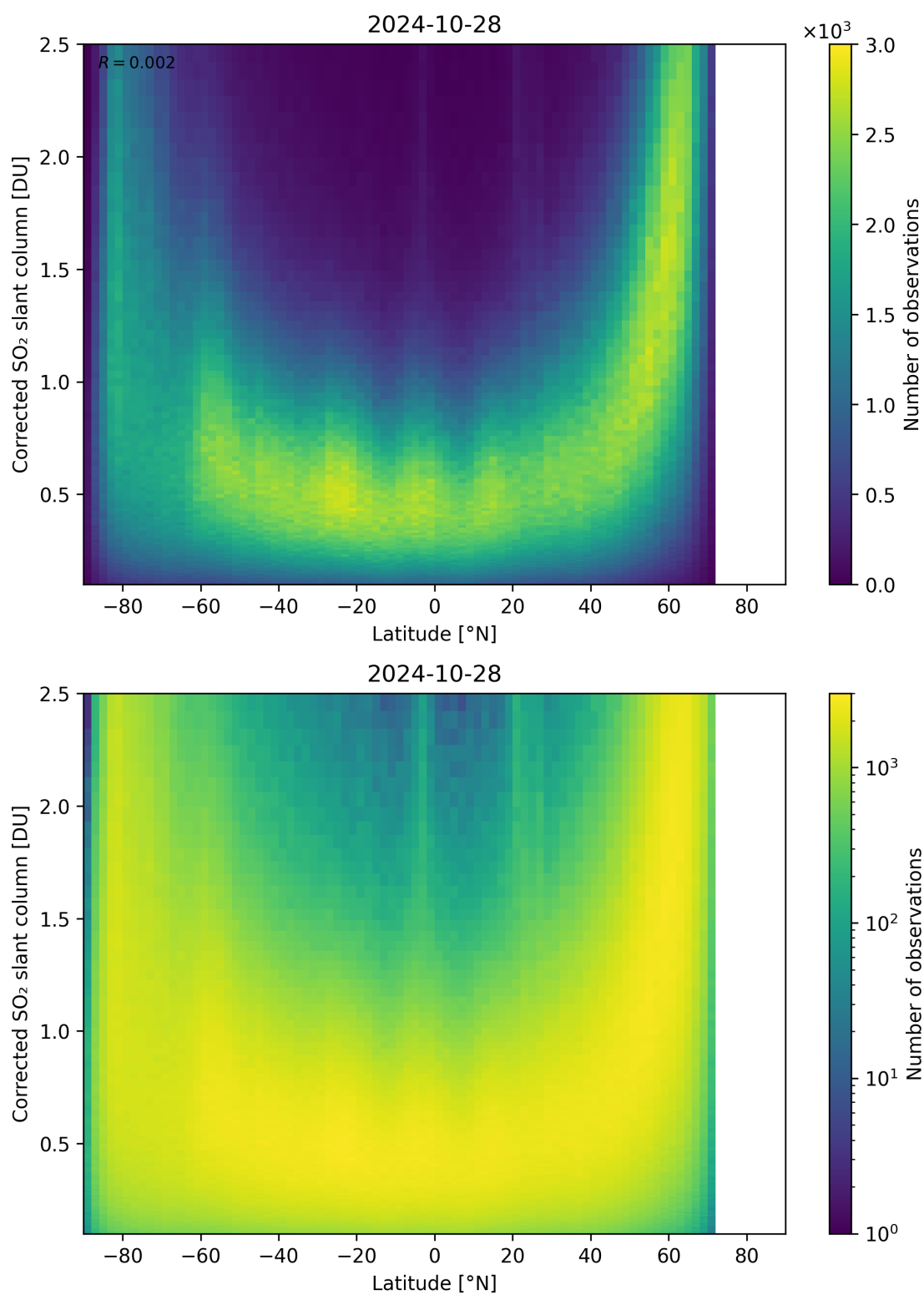
Figure 146: Scatter density plot of “Latitude” against “Corrected SO 2 slant column” for 2024-10-27 to 2024-10-29.
