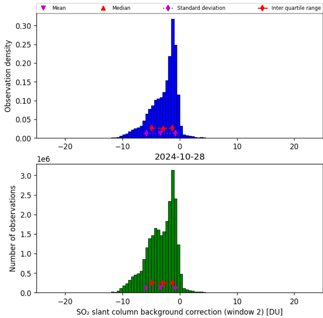
Figure 63: Histogram of “SO 2 slant column background correction (window 2)” for 2024-10-27 to 2024-10-29
