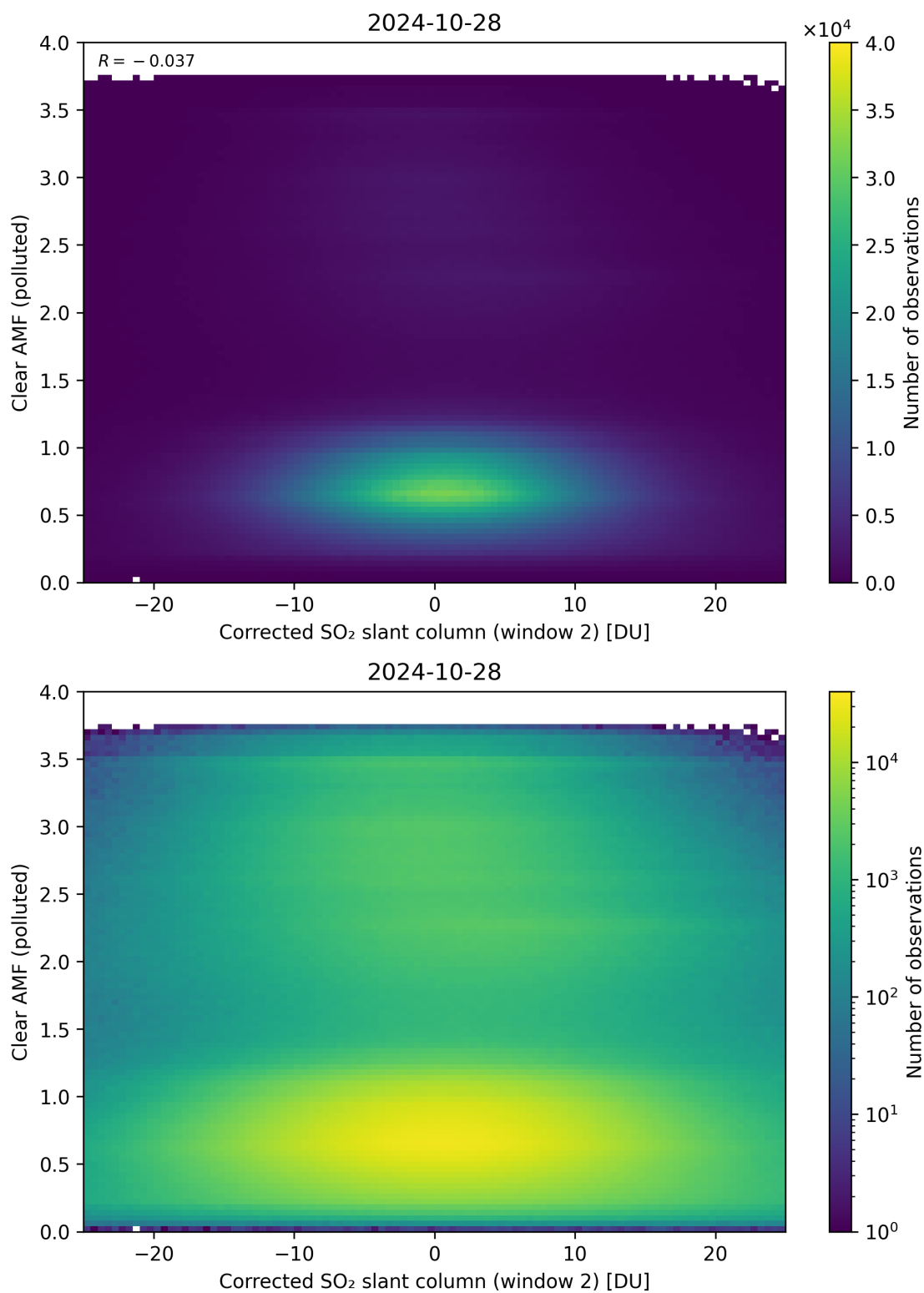
Figure 199: Scatter density plot of “Corrected SO 2 slant column (window 2)” against “Clear AMF (polluted)” for 2024-10-27 to 2024-10-29.
