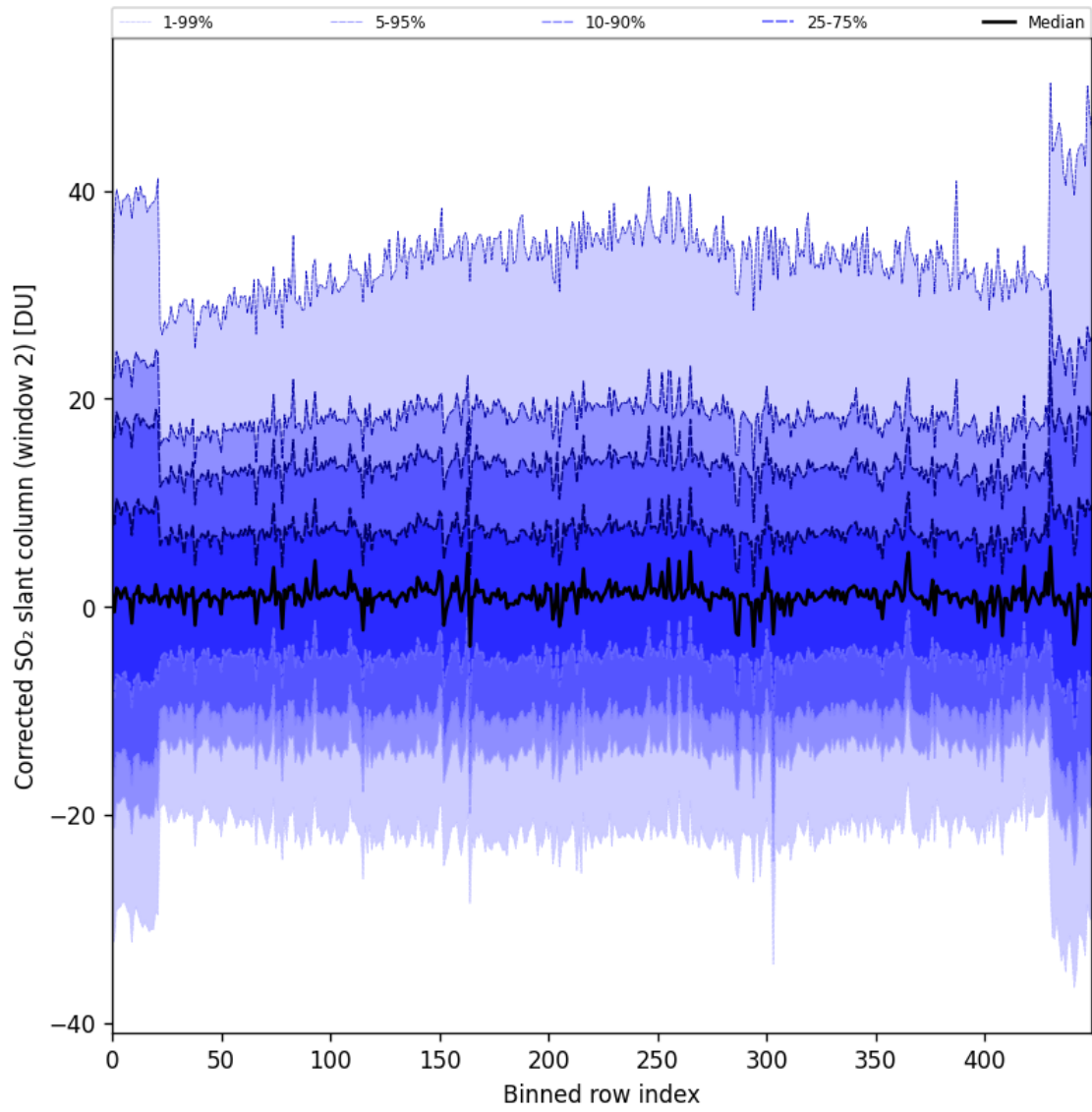
Figure 85: Along track statistics of “Corrected SO 2 slant column (window 2)” for 2024-10-27 to 2024-10-29
