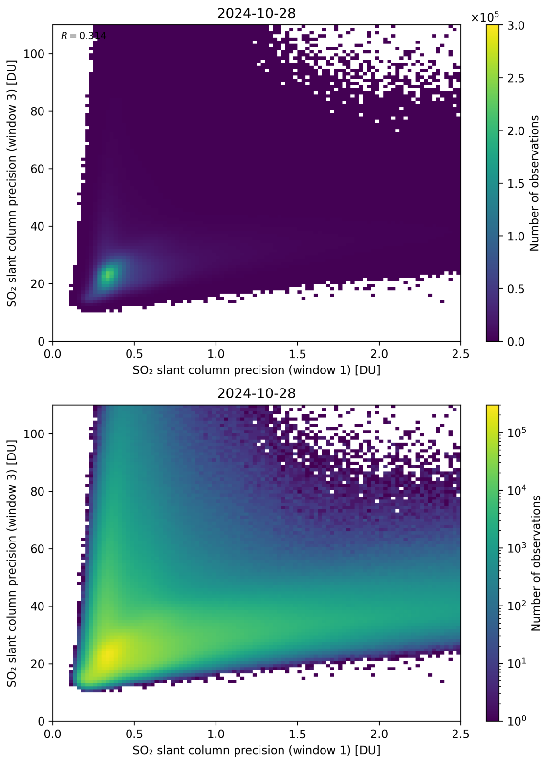
Figure 229: Scatter density plot of “SO 2 slant column precision (window 1)” against “SO 2 slant column precision (window 3)” for 2024-10-27 to 2024-10-29.
