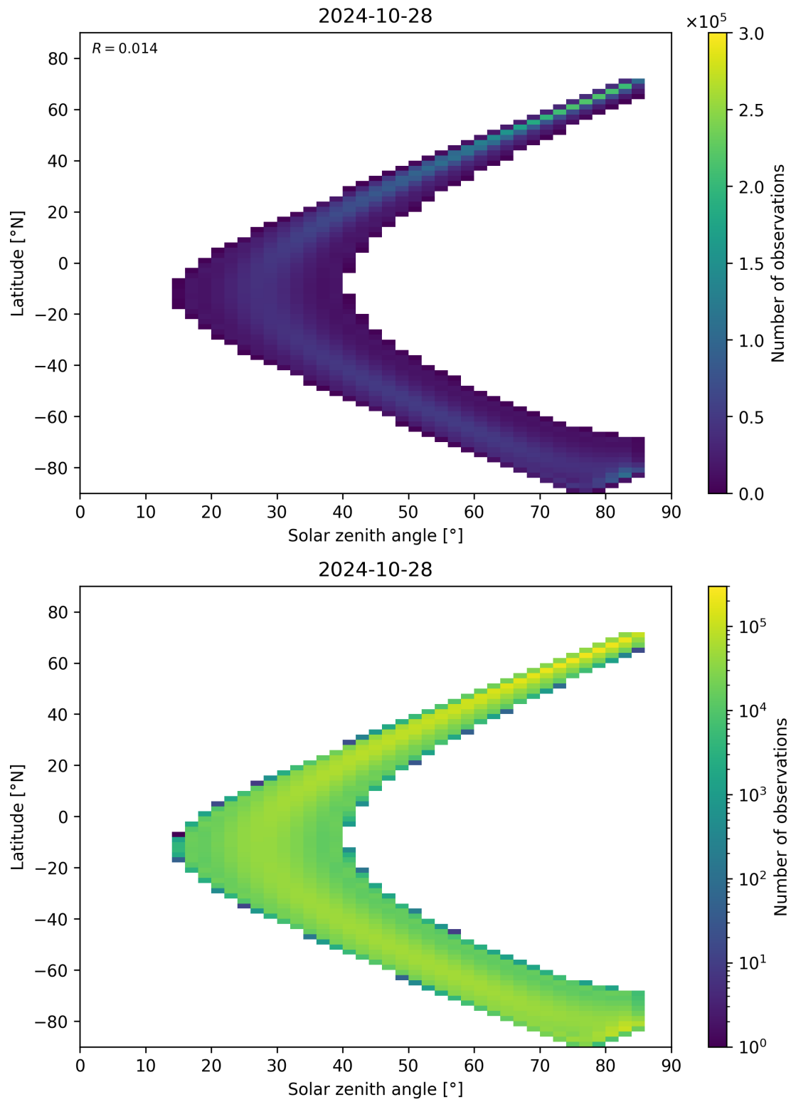
Figure 164: Scatter density plot of “Solar zenith angle” against “Latitude” for 2024-10-27 to 2024-10-29.
