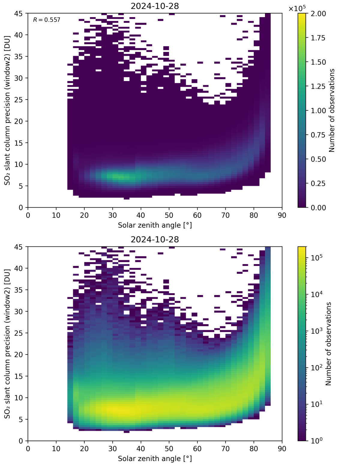
Figure 171: Scatter density plot of “Solar zenith angle” against “SO 2 slant column precision (window2)” for 2024-10-27 to 2024-10-29.
