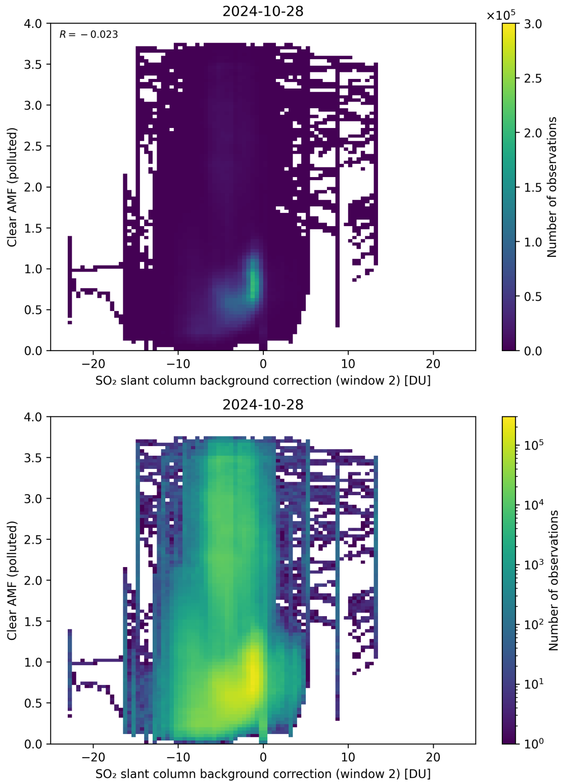
Figure 115: Scatter density plot of “SO 2 slant column background correction (window 2)” against “Clear AMF (polluted)” for 2024-10-27 to 2024-10-29.
