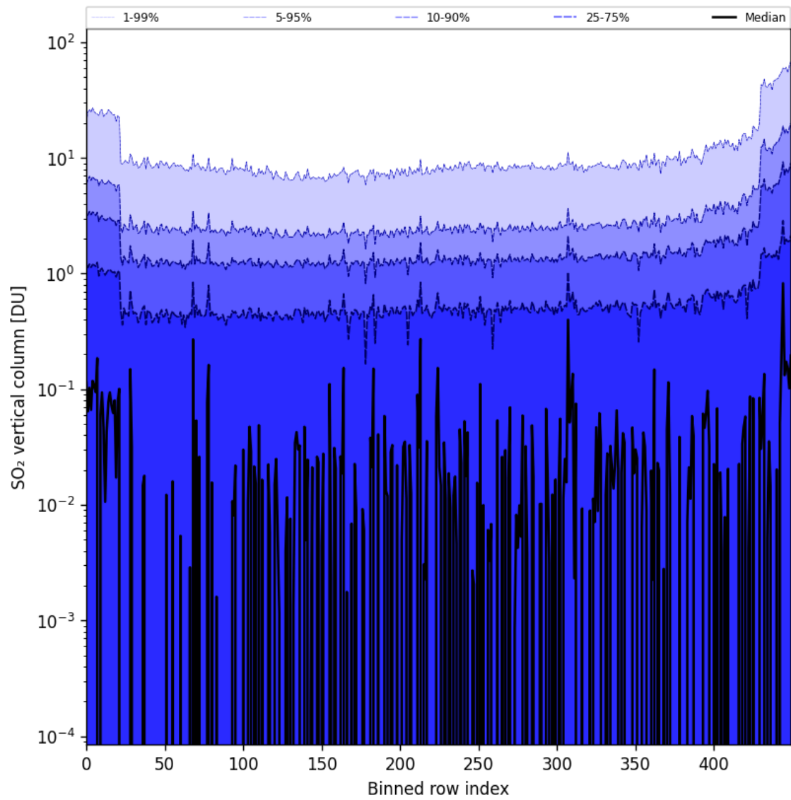
Figure 76: Along track statistics of “SO 2 vertical column” for 2024-10-27 to 2024-10-29
