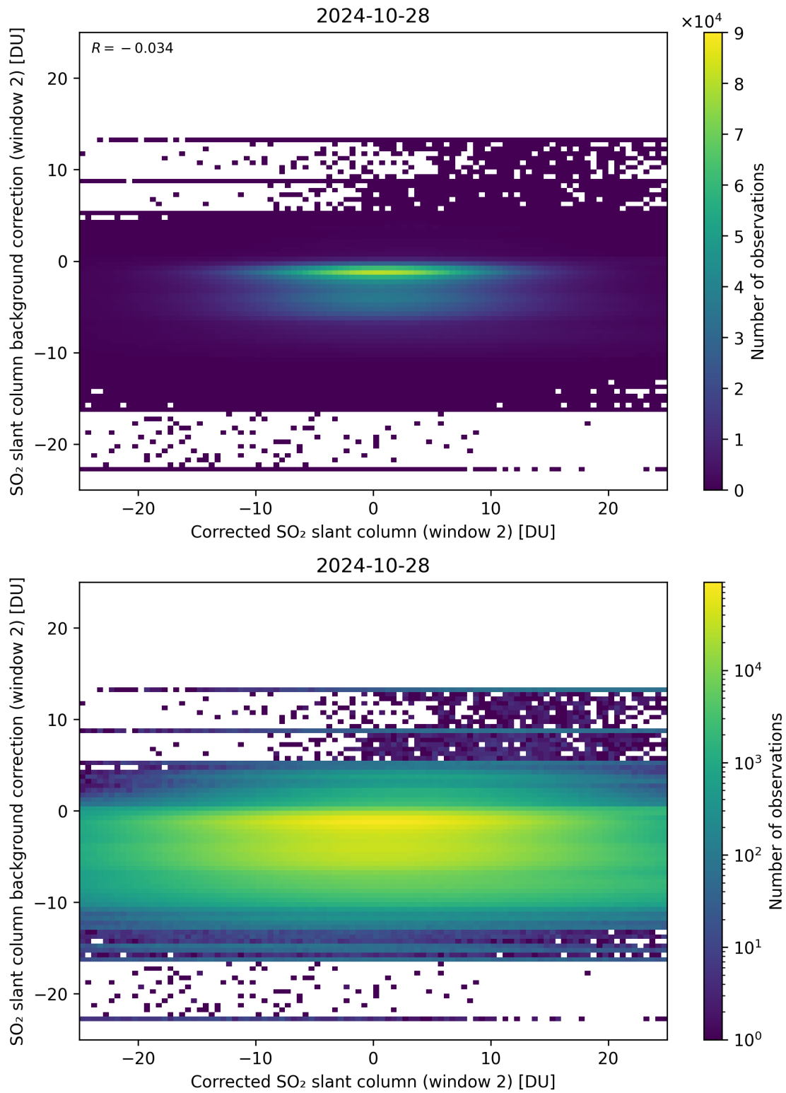
Figure 194: Scatter density plot of “Corrected SO 2 slant column (window 2)” against “SO 2 slant column background correction (window 2)” for 2024-10-27 to 2024-10-29.
