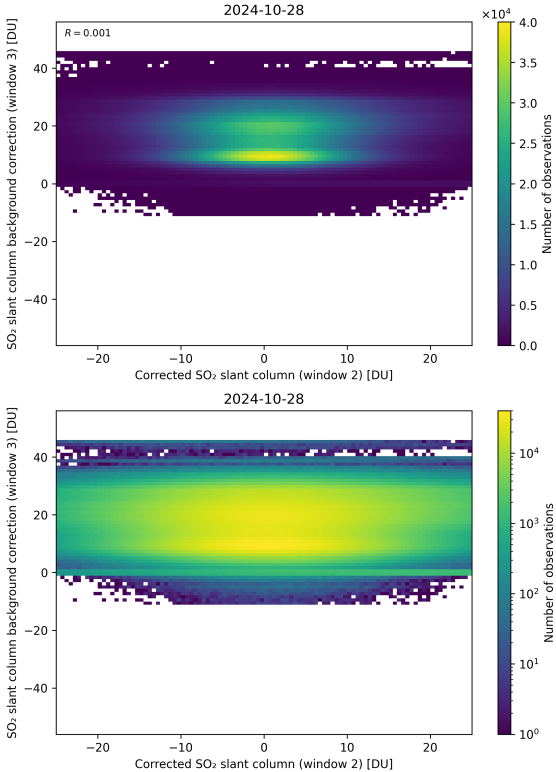
Figure 195: Scatter density plot of “Corrected SO 2 slant column (window 2)” against “SO 2 slant column background correction (window 3)” for 2024-10-27 to 2024-10-29.
