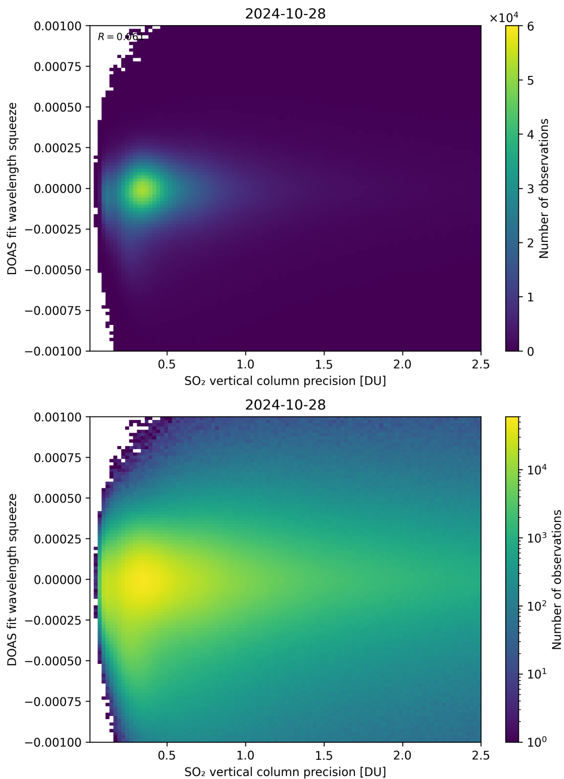
Figure 283: Scatter density plot of “SO 2 vertical column precision” against “DOAS fit wavelength squeeze” for 2024-10-27 to 2024-10-29.
