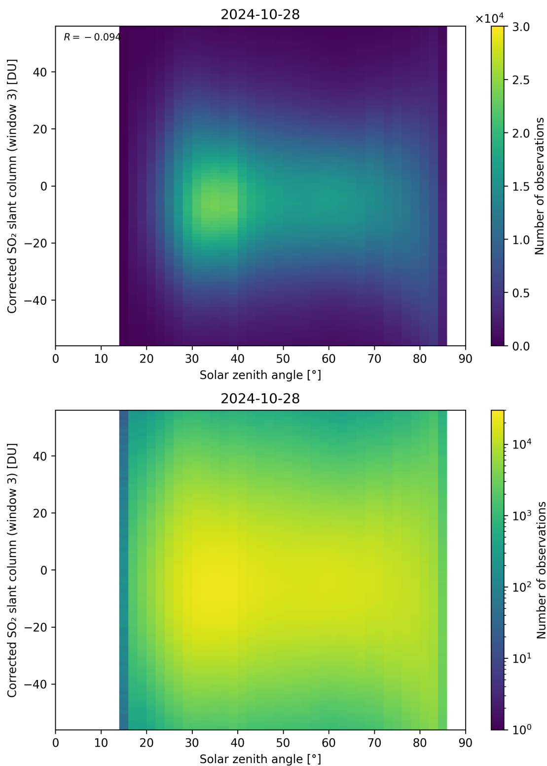
Figure 168: Scatter density plot of “Solar zenith angle” against “Corrected SO 2 slant column (window 3)” for 2024-10-27 to 2024-10-29.
