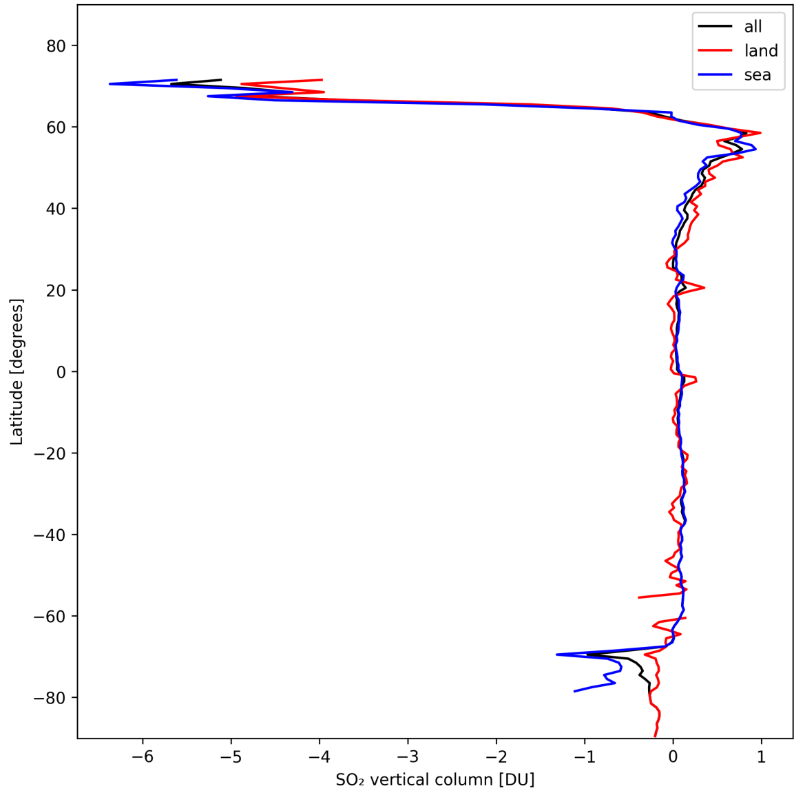
Figure 30: Zonal average of “SO 2 vertical column” for 2024-10-27 to 2024-10-29.
