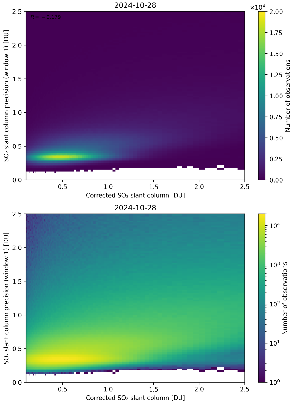
Figure 188: Scatter density plot of “Corrected SO 2 slant column” against “SO 2 slant column precision (window 1)” for 2024-10-27 to 2024-10-29.
