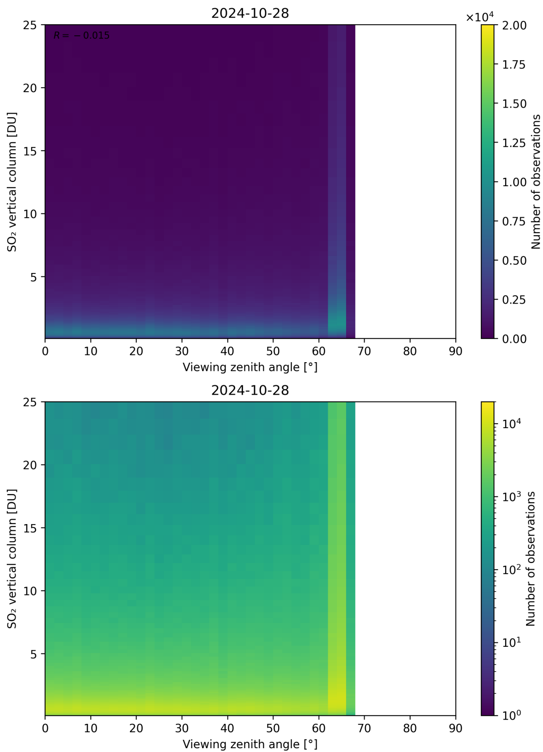
Figure 327: Scatter density plot of “Viewing zenith angle” against “SO 2 vertical column” for 2024-10-27 to 2024-10-29.
