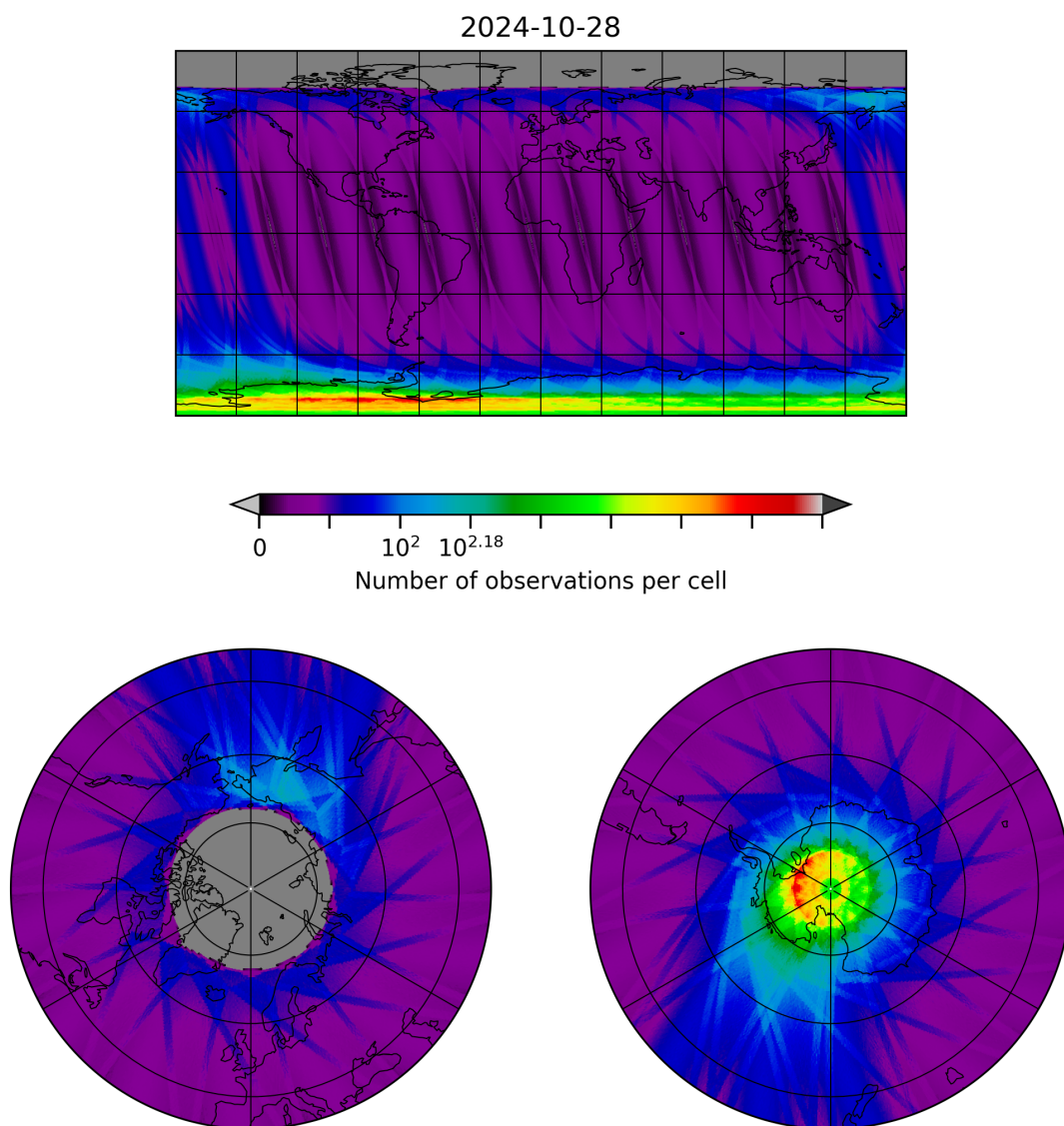
Figure 28: Map of the number of observations for 2024-10-27 to 2024-10-29
