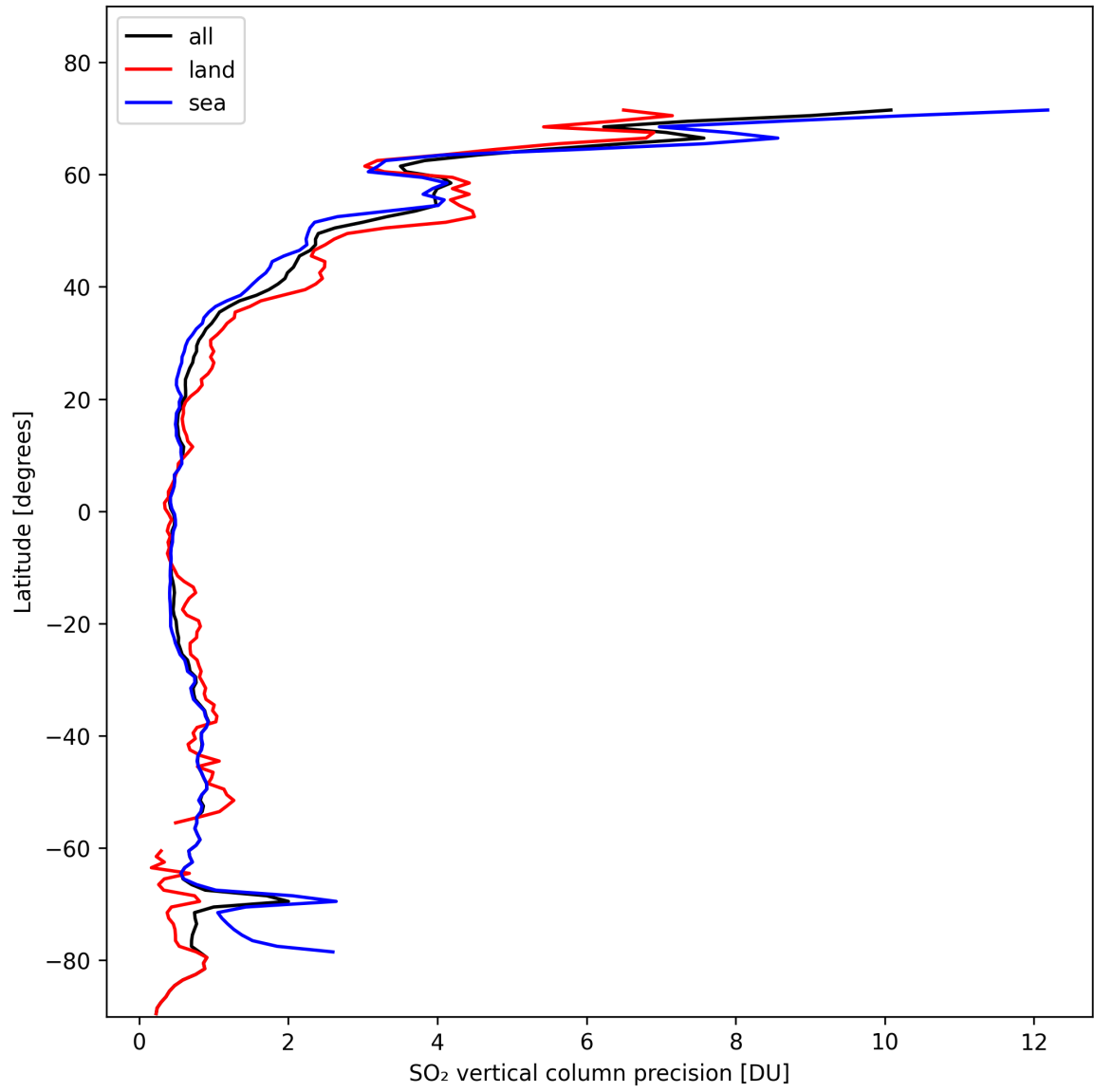
Figure 31: Zonal average of “SO 2 vertical column precision” for 2024-10-27 to 2024-10-29.
