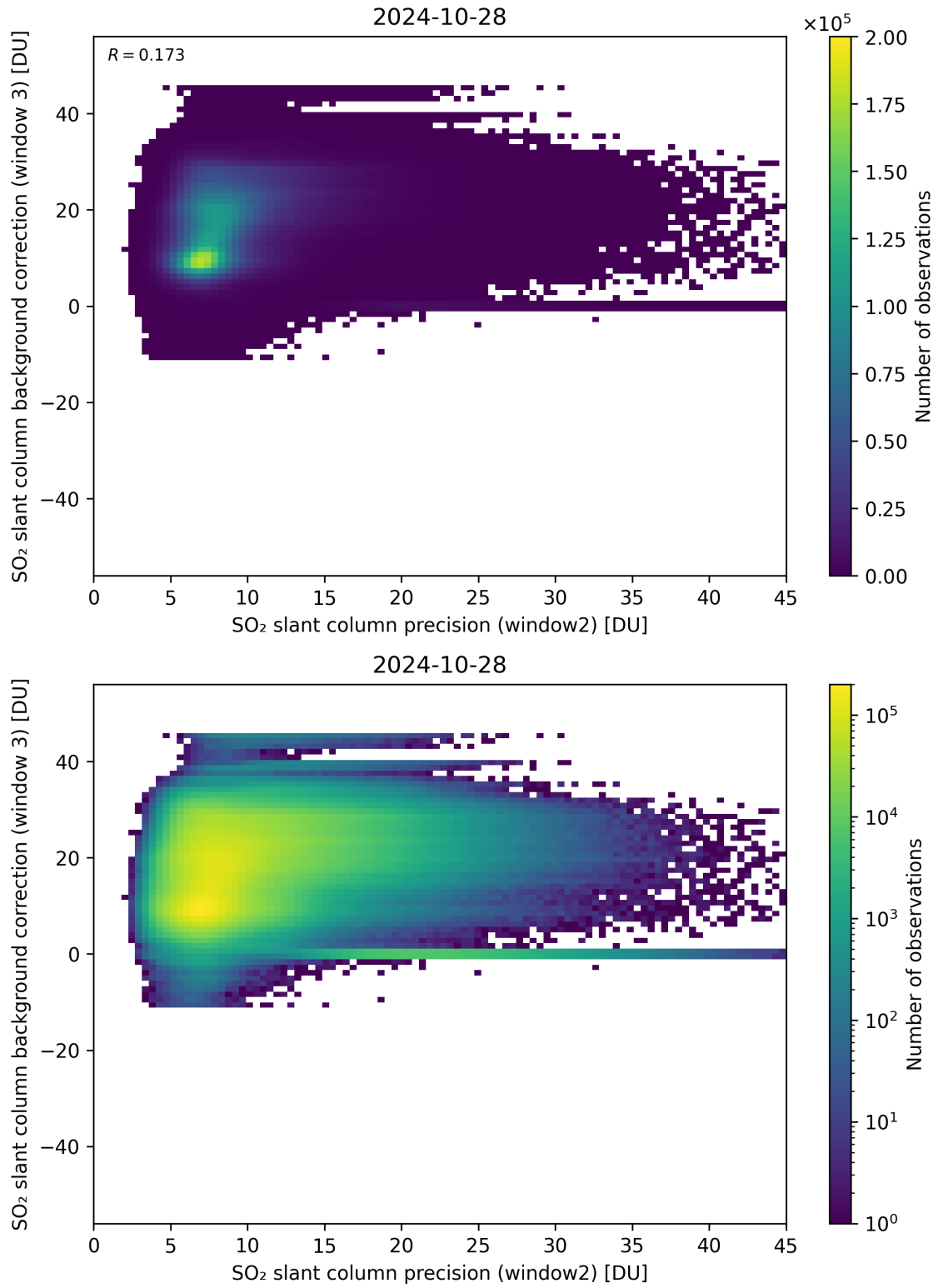
Figure 242: Scatter density plot of “SO 2 slant column precision (window2)” against “SO 2 slant column background correction (window 3)” for 2024-10-27 to 2024-10-29.
