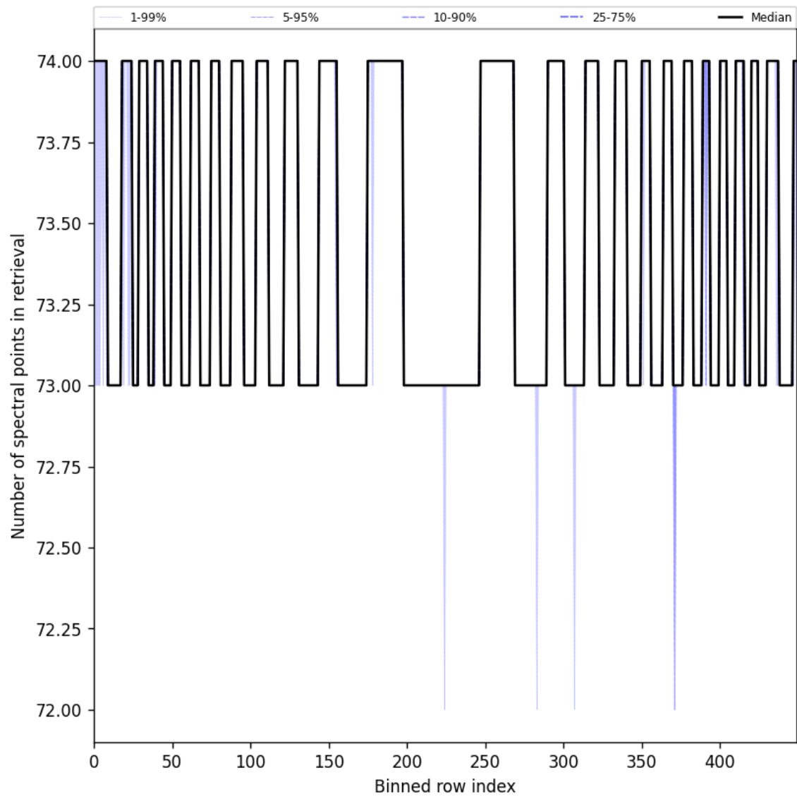
Figure 97: Along track statistics of “Number of spectral points in retrieval” for 2024-10-27 to 2024-10-29
