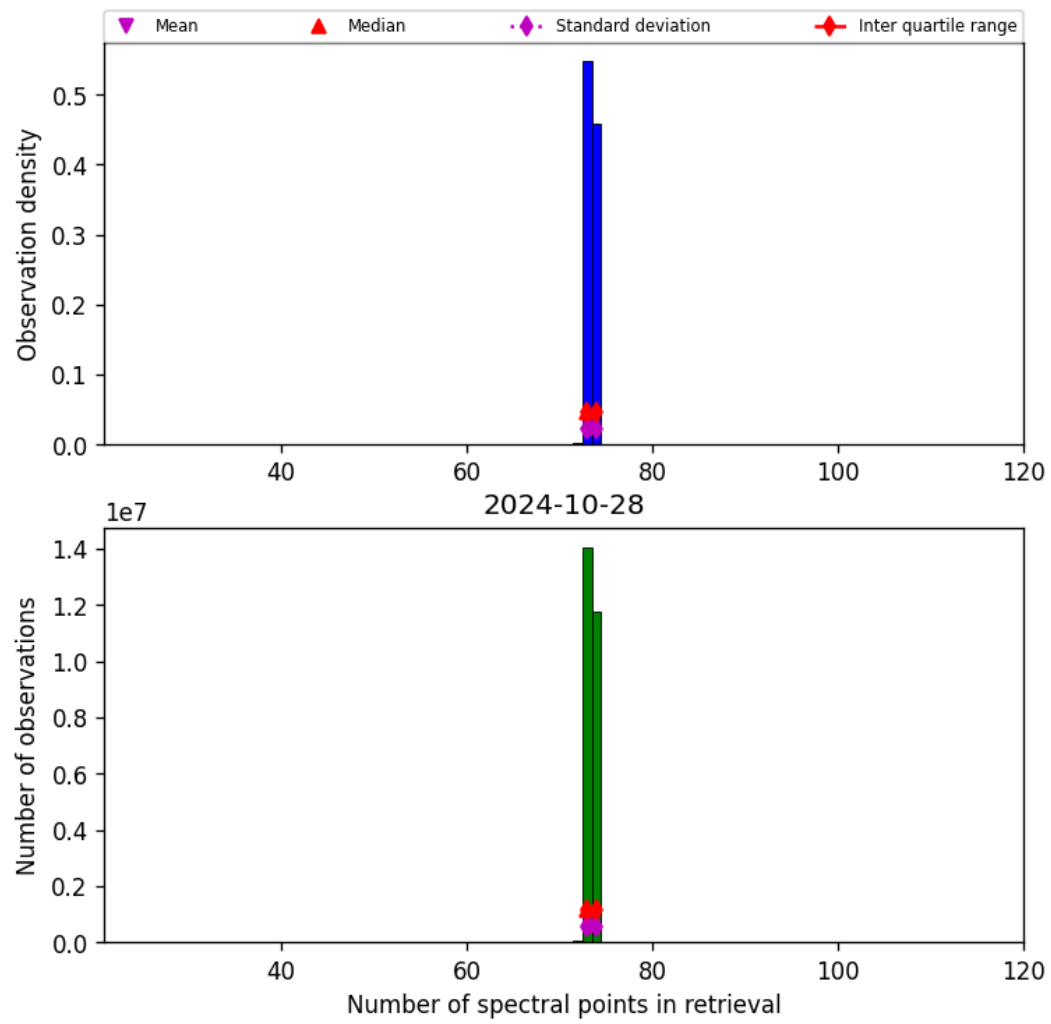
Figure 74: Histogram of “Number of spectral points in retrieval” for 2024-10-27 to 2024-10-29
