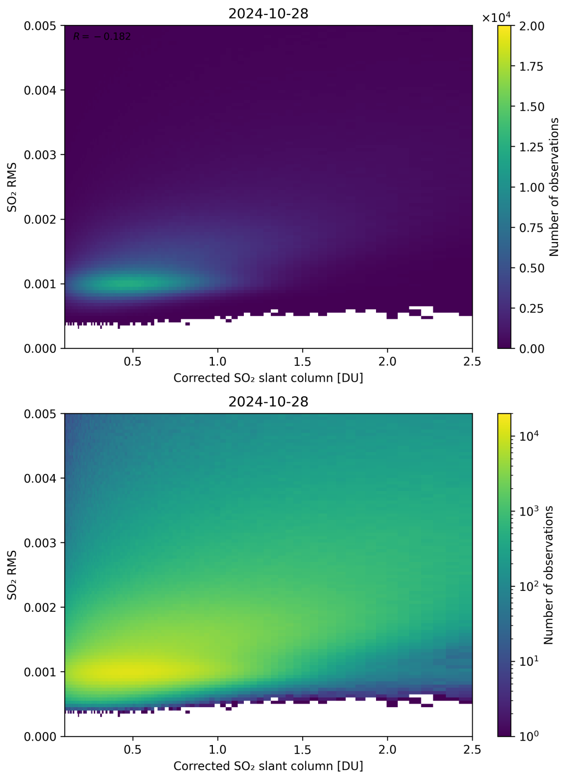
Figure 183: Scatter density plot of “Corrected SO 2 slant column” against “SO 2 RMS” for 2024-10-27 to 2024-10-29.
