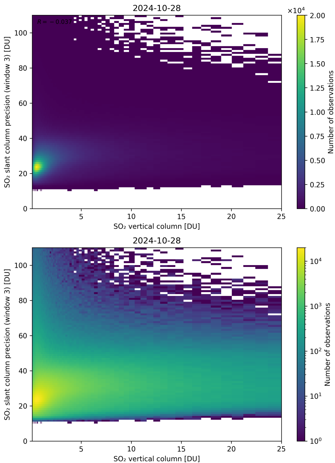
Figure 304: Scatter density plot of “SO 2 vertical column” against “SO 2 slant column precision (window 3)” for 2024-10-27 to 2024-10-29.
