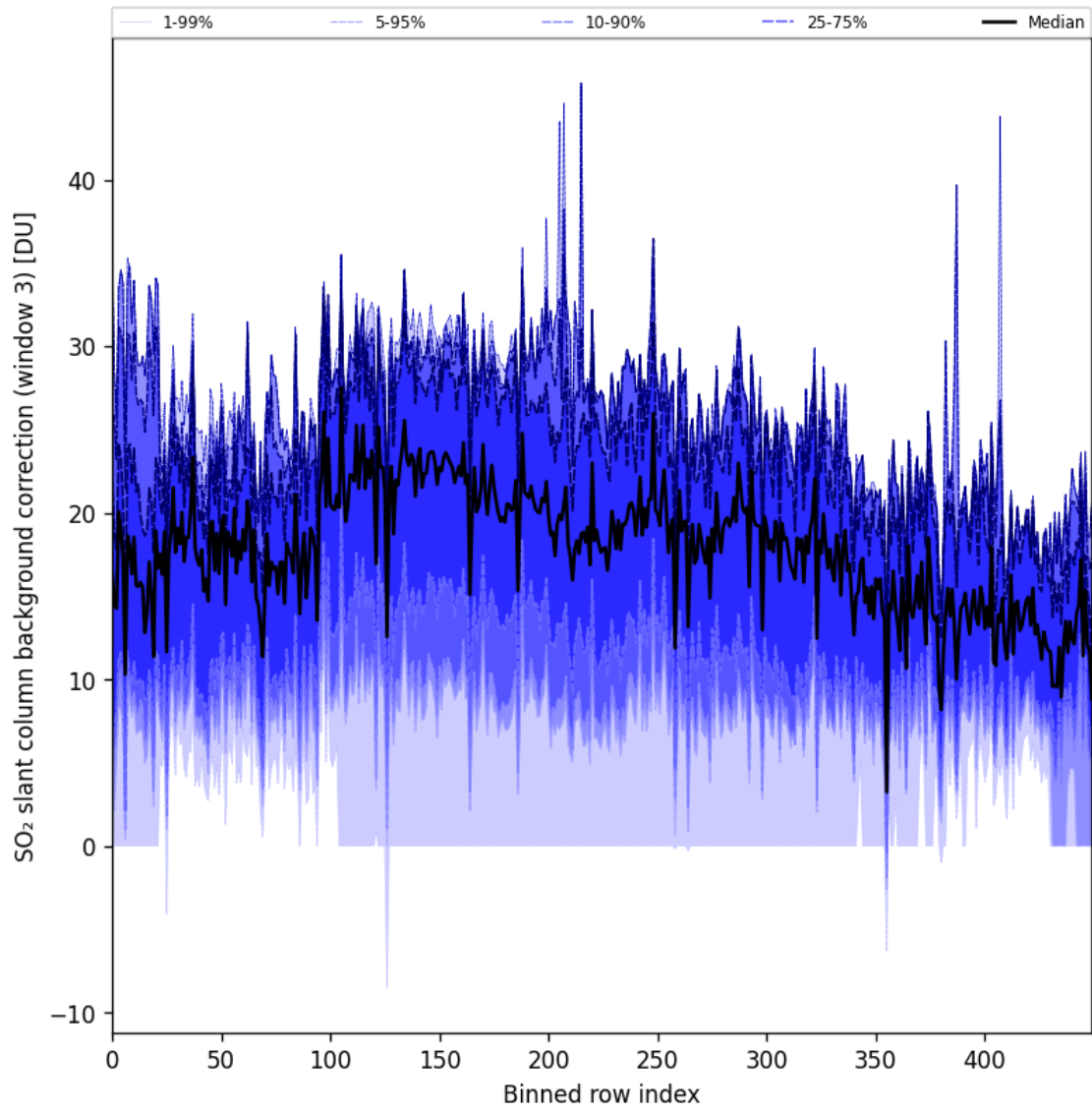
Figure 90: Along track statistics of “SO 2 slant column background correction (window 3)” for 2024-10-27 to 2024-10-29
