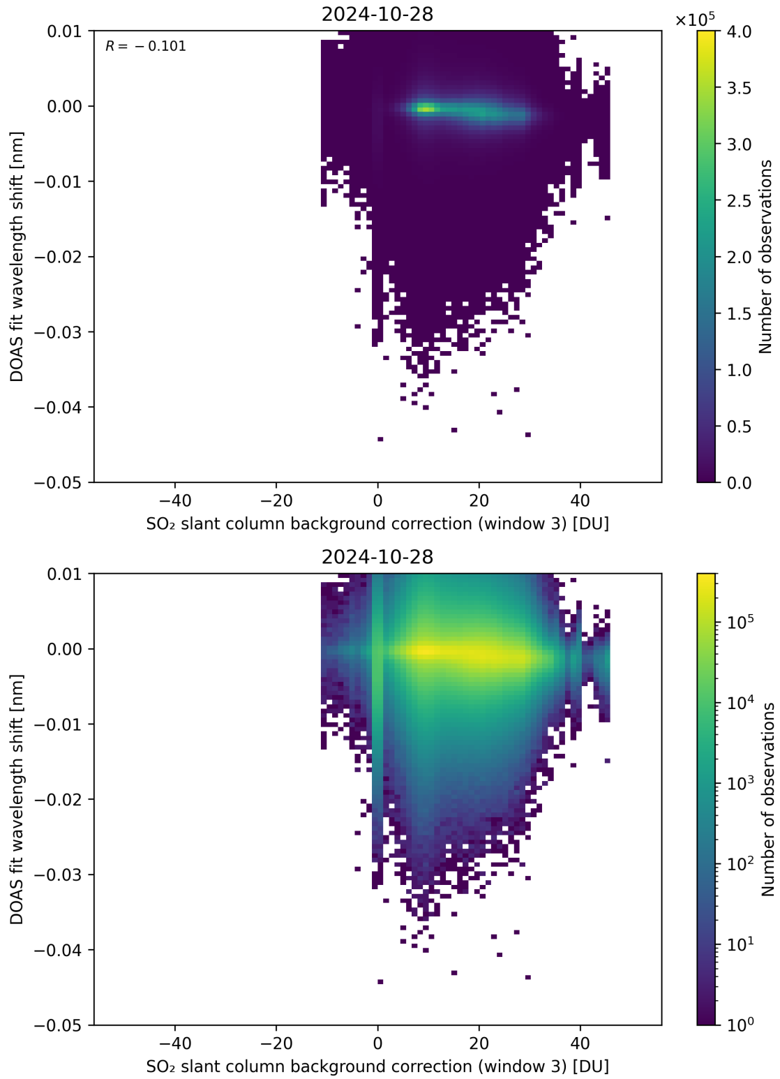
Figure 121: Scatter density plot of “SO 2 slant column background correction (window 3)” against “DOAS fit wavelength shift” for 2024-10-27 to 2024-10-29.
