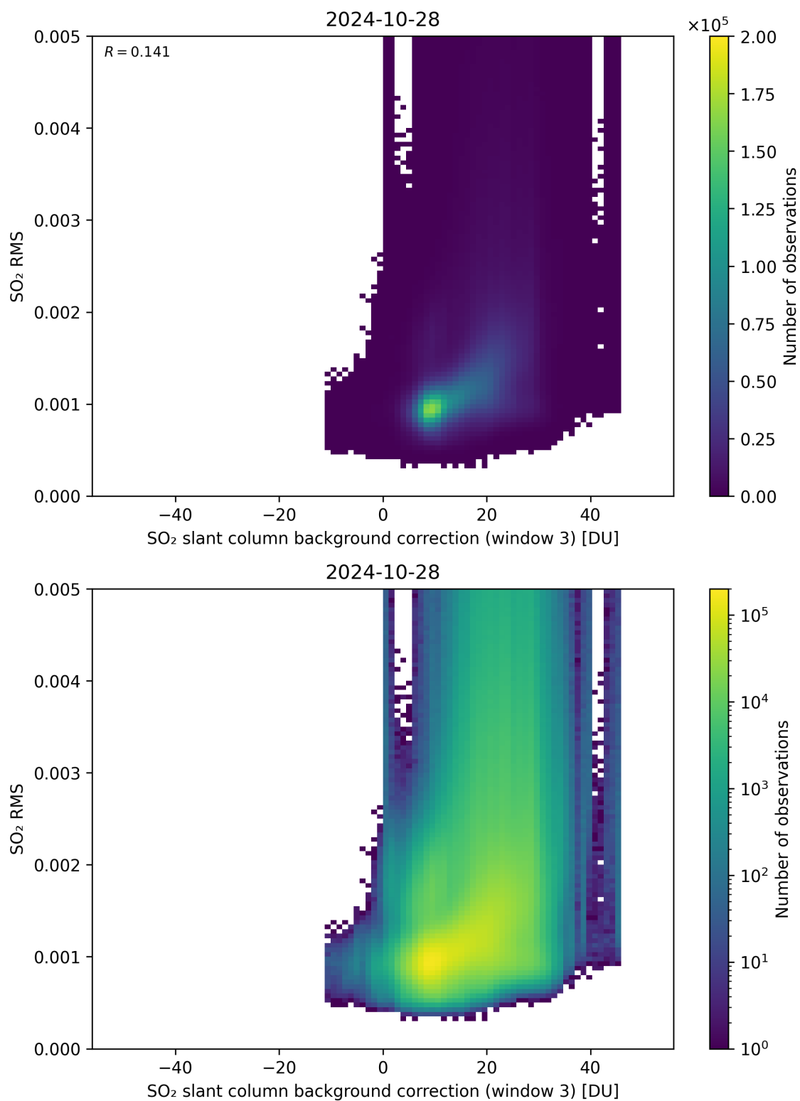
Figure 123: Scatter density plot of “SO 2 slant column background correction (window 3)” against “SO 2 RMS” for 2024-10-27 to 2024-10-29.
