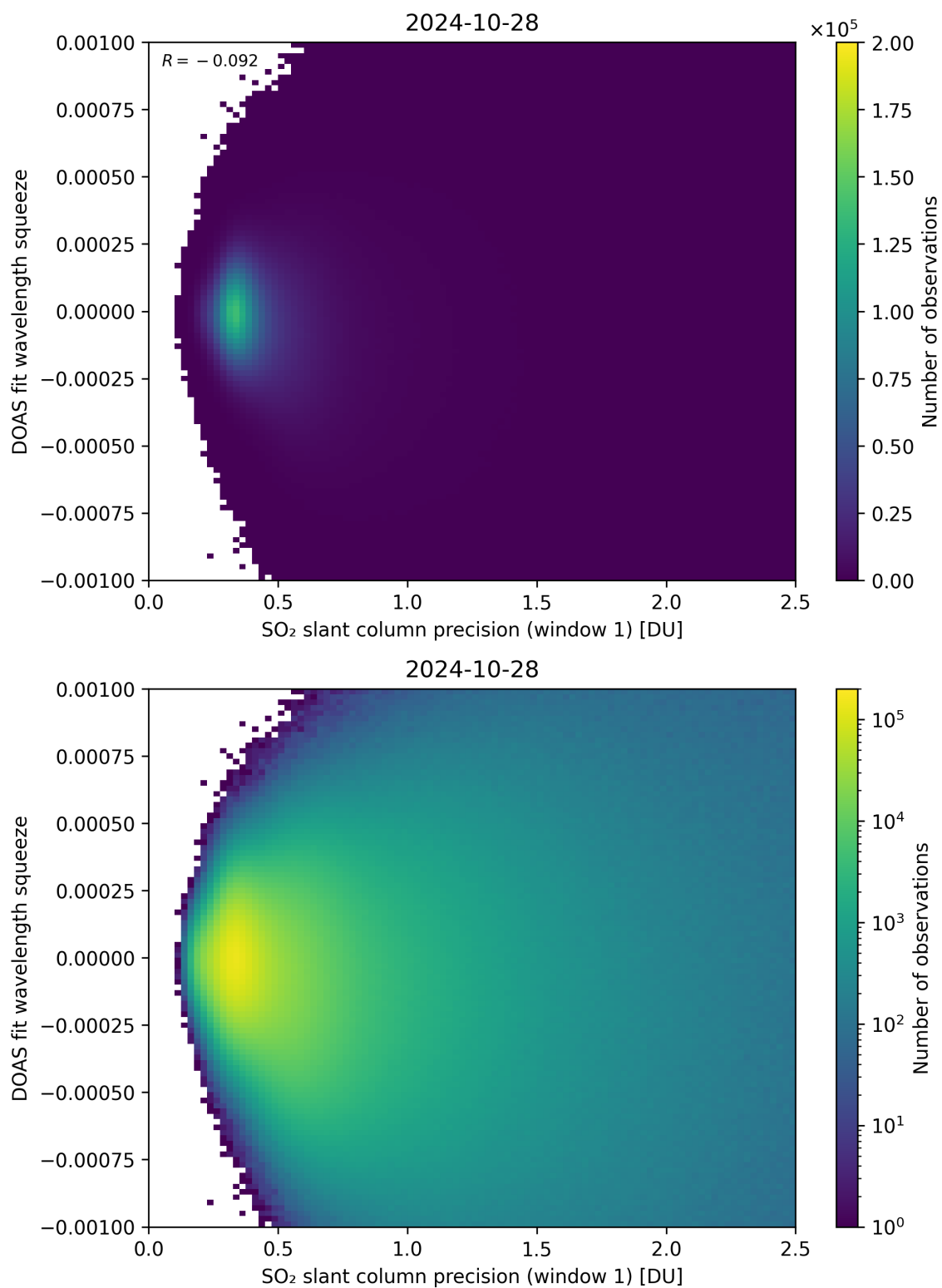
Figure 222: Scatter density plot of “SO 2 slant column precision (window 1)” against “DOAS fit wavelength squeeze” for 2024-10-27 to 2024-10-29.
