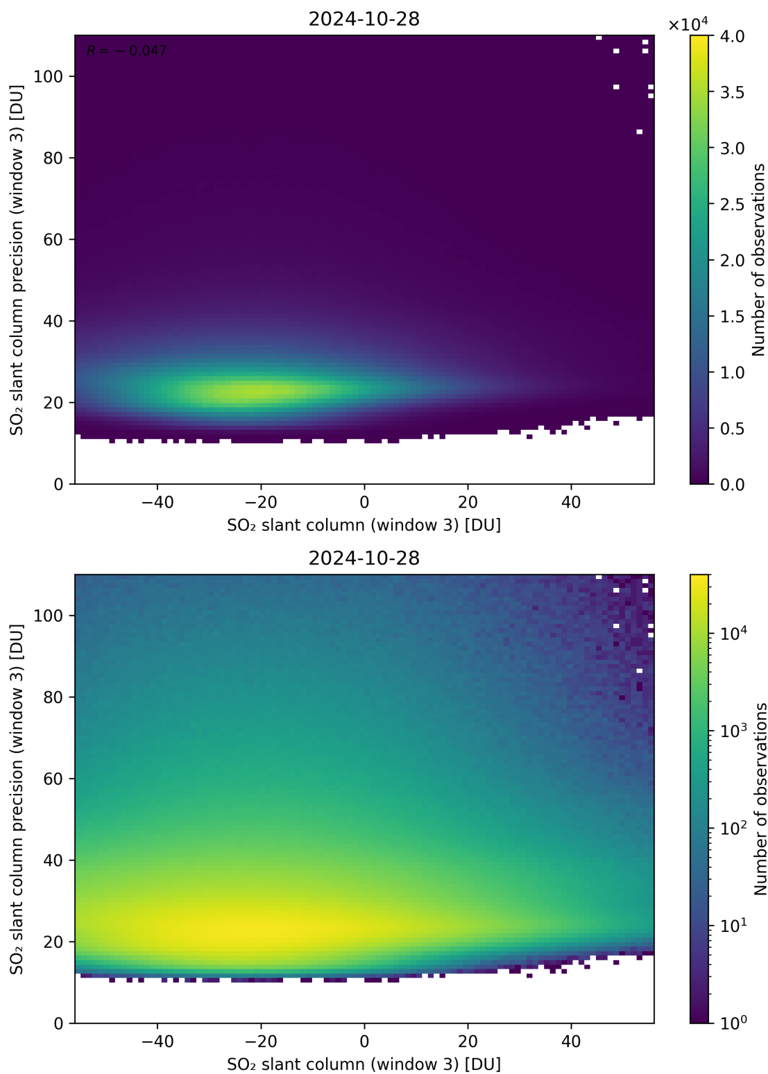
Figure 267: Scatter density plot of “SO 2 slant column (window 3)” against “SO 2 slant column precision (window 3)” for 2024-10-27 to 2024-10-29.
