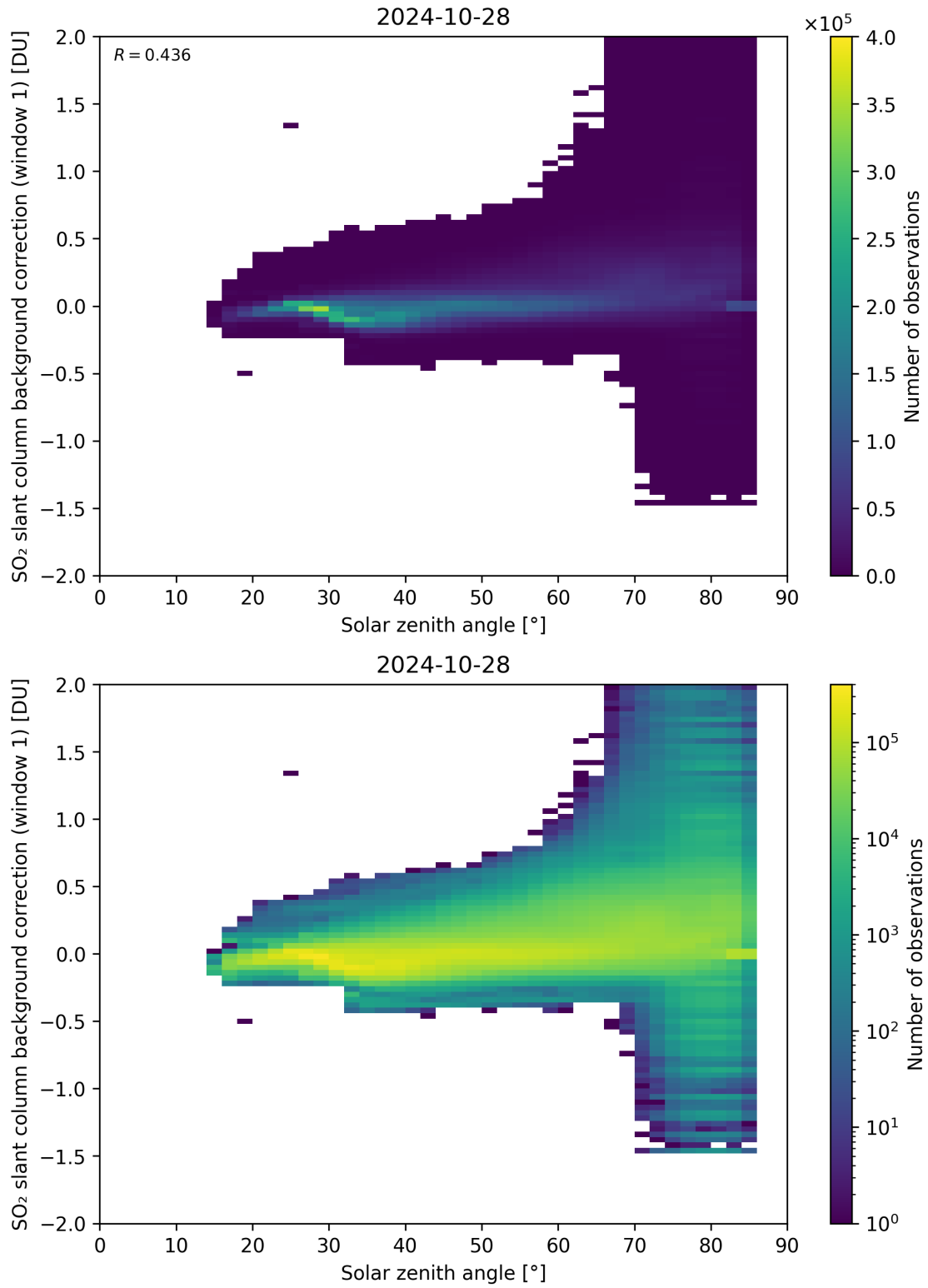
Figure 158: Scatter density plot of “Solar zenith angle” against “SO 2 slant column background correction (window 1)” for 2024-10-27 to 2024-10-29.
