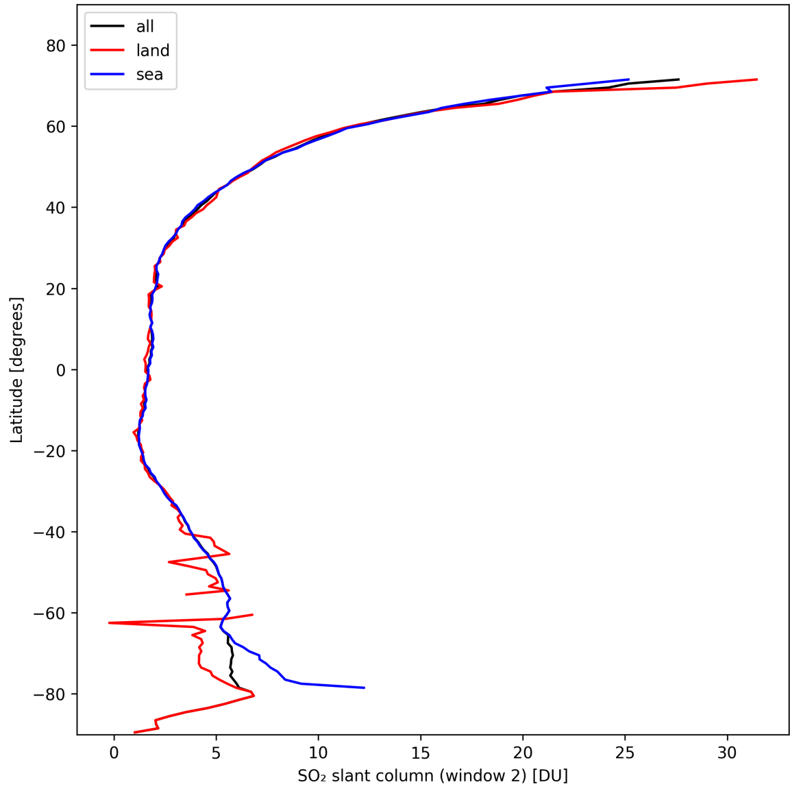
Figure 37: Zonal average of “SO 2 slant column (window 2)” for 2024-10-27 to 2024-10-29.
