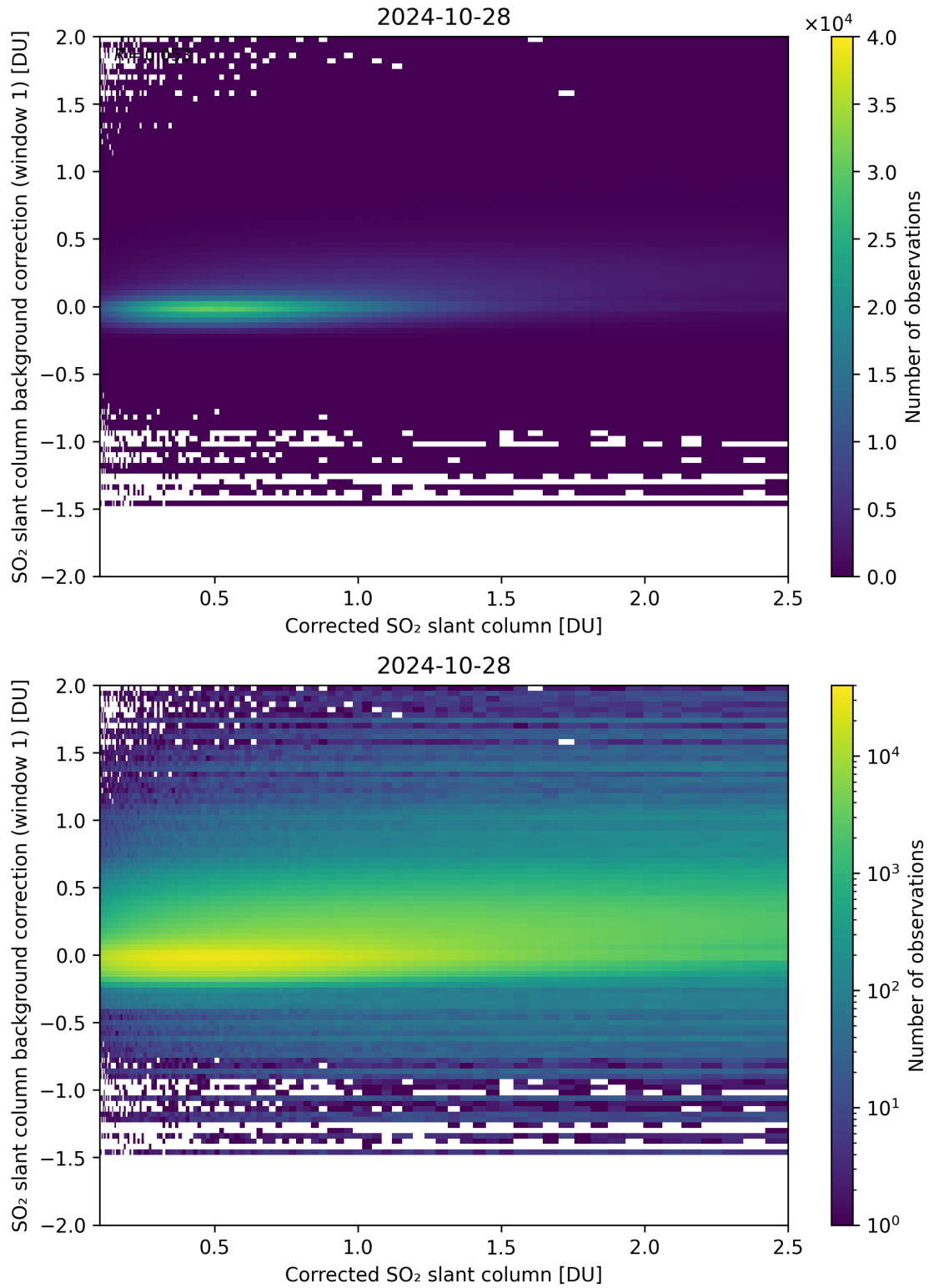
Figure 178: Scatter density plot of “Corrected SO 2 slant column” against “SO 2 slant column background correction (window 1)” for 2024-10-27 to 2024-10-29.
