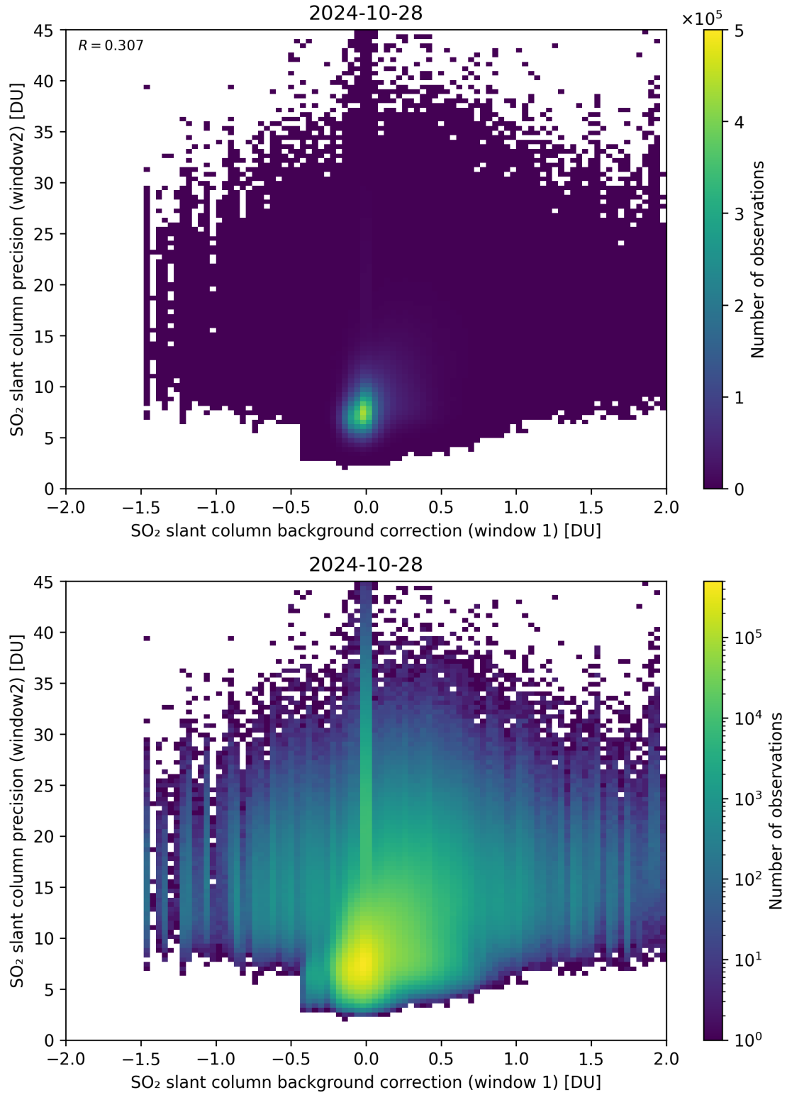
Figure 106: Scatter density plot of “SO 2 slant column background correction (window 1)” against “SO 2 slant column precision (window2)” for 2024-10-27 to 2024-10-29.
