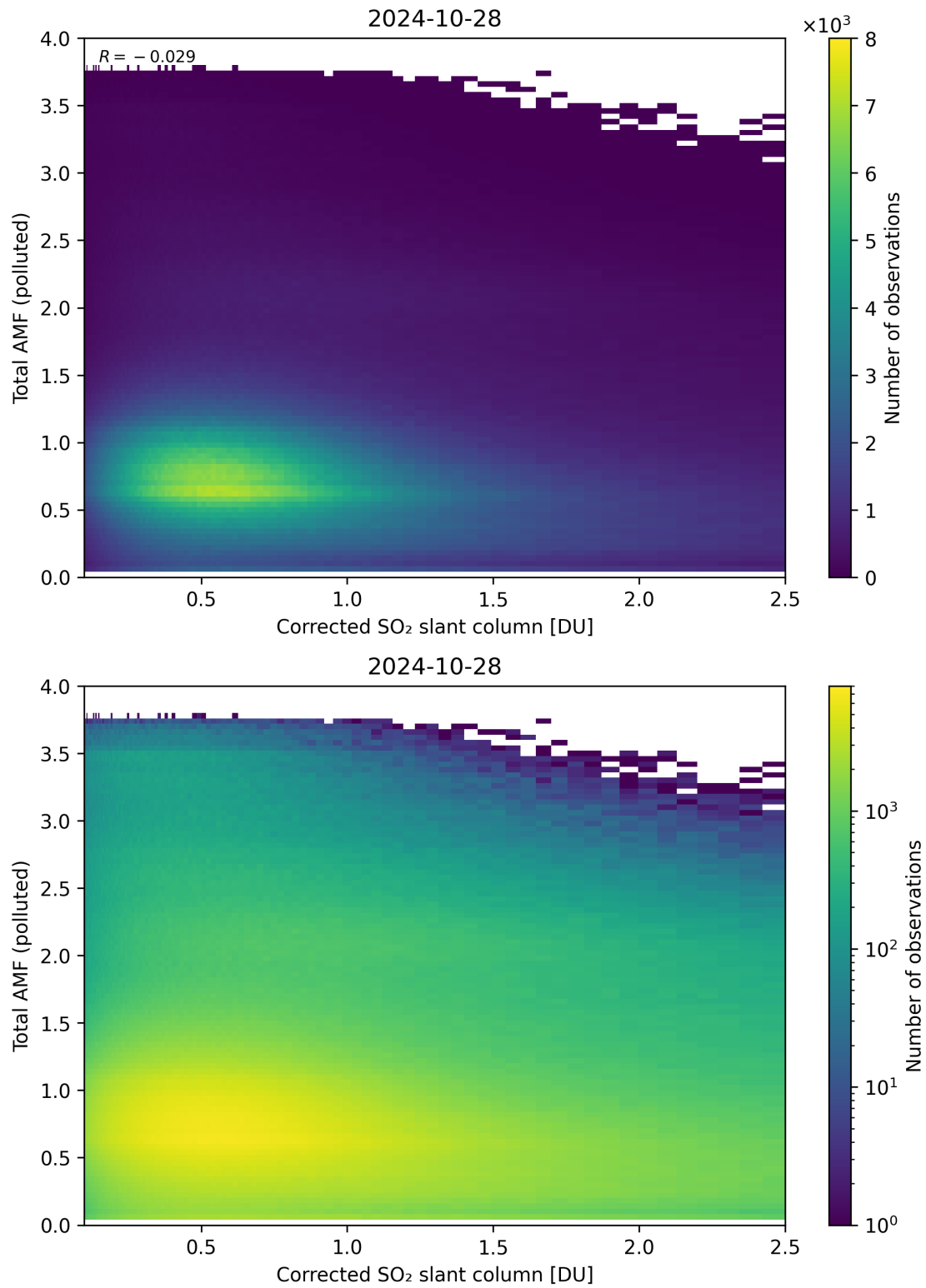
Figure 192: Scatter density plot of “Corrected SO 2 slant column” against “Total AMF (polluted)” for 2024-10-27 to 2024-10-29.
