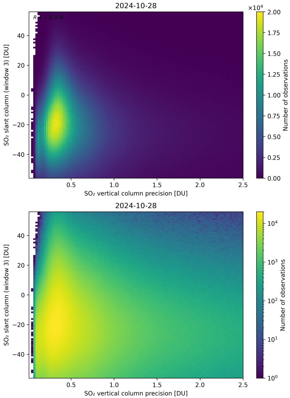
Figure 292: Scatter density plot of “SO 2 vertical column precision” against “SO 2 slant column (window 3)” for 2024-10-27 to 2024-10-29.
