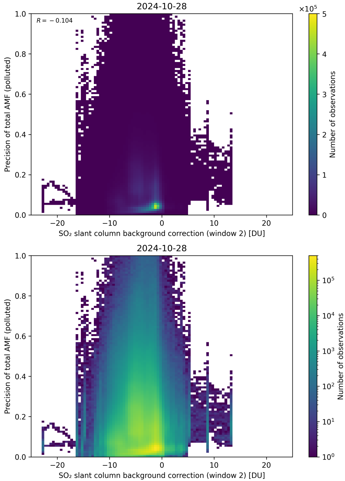
Figure 120: Scatter density plot of “SO 2 slant column background correction (window 2)” against “Precision of total AMF (polluted)” for 2024-10-27 to 2024-10-29.
