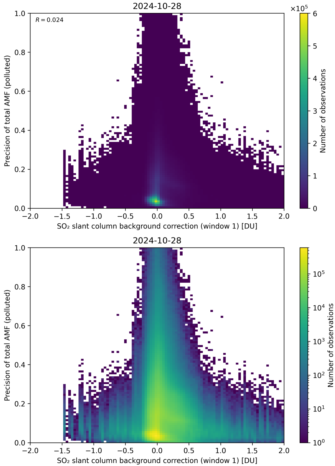
Figure 110: Scatter density plot of “SO 2 slant column background correction (window 1)” against “Precision of total AMF (polluted)” for 2024-10-27 to 2024-10-29.
