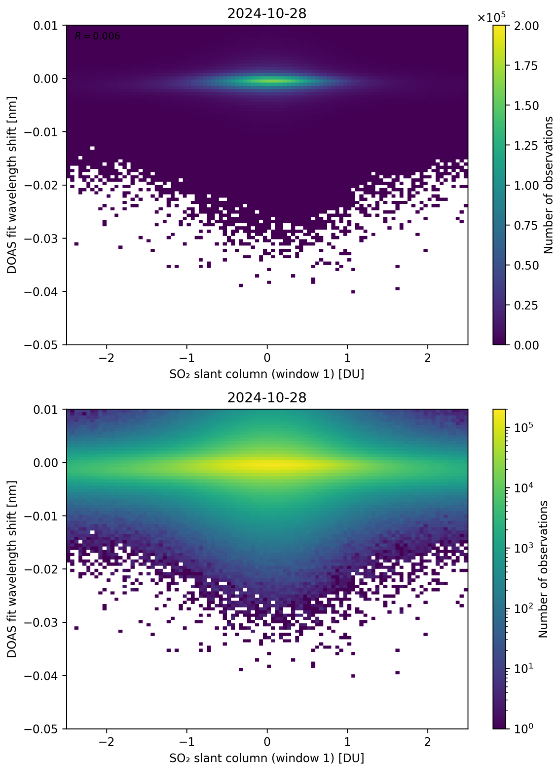
Figure 215: Scatter density plot of “SO 2 slant column (window 1)” against “DOAS fit wavelength shift” for 2024-10-27 to 2024-10-29.
