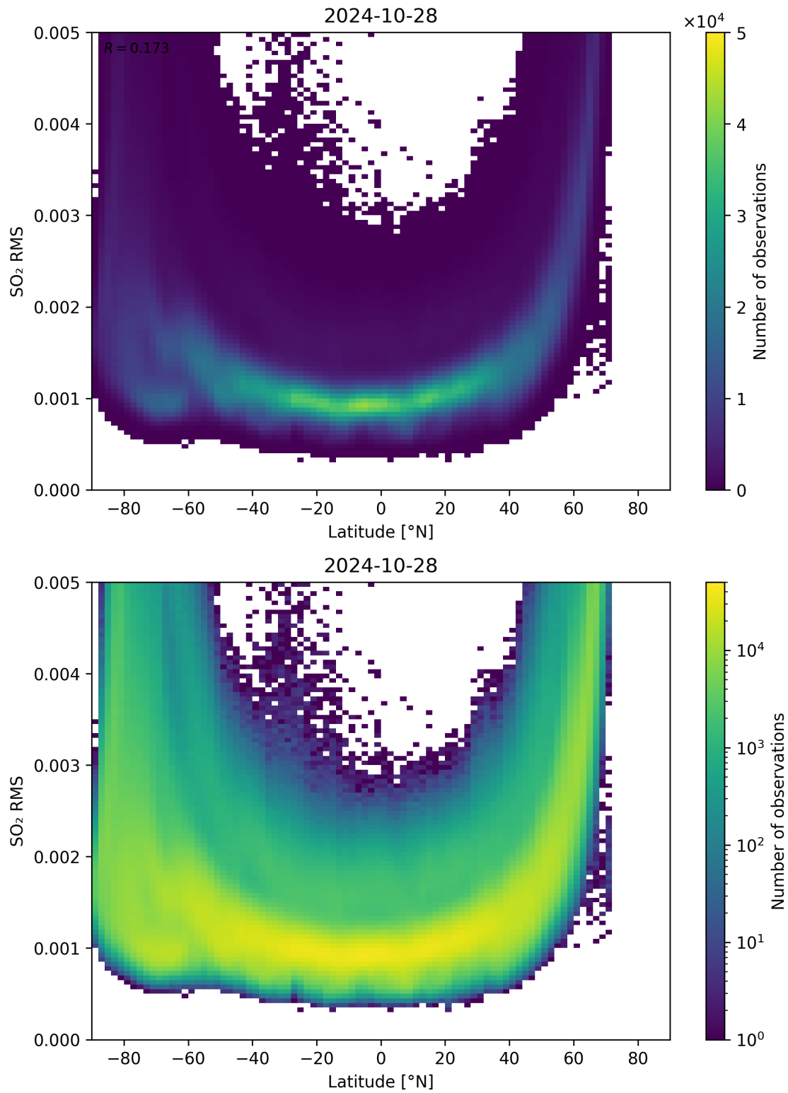
Figure 144: Scatter density plot of “Latitude” against “SO 2 RMS” for 2024-10-27 to 2024-10-29.
