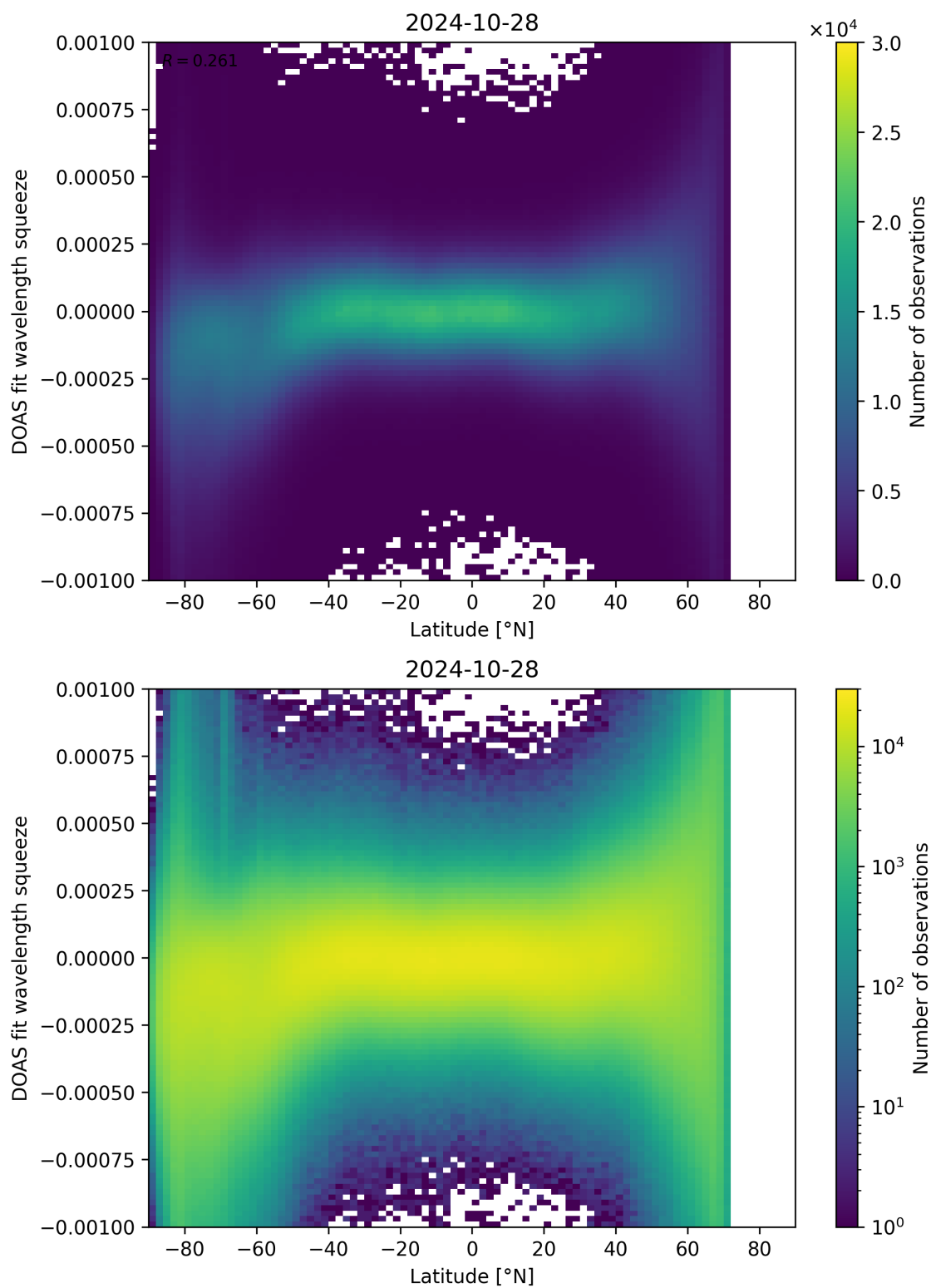
Figure 143: Scatter density plot of “Latitude” against “DOAS fit wavelength squeeze” for 2024-10-27 to 2024-10-29.
