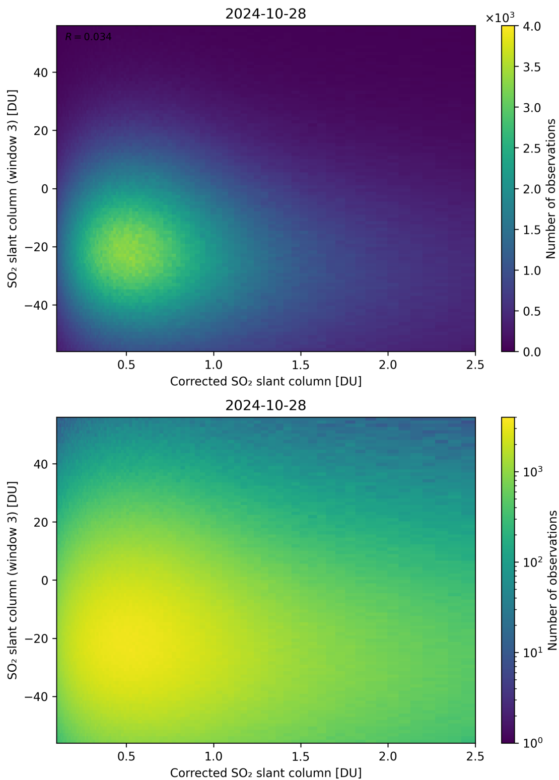
Figure 190: Scatter density plot of “Corrected SO 2 slant column” against “SO 2 slant column (window 3)” for 2024-10-27 to 2024-10-29.
