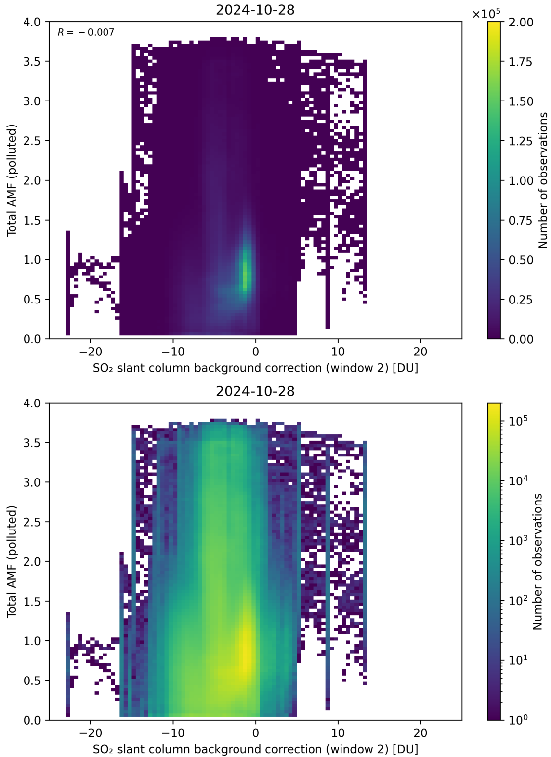
Figure 119: Scatter density plot of “SO 2 slant column background correction (window 2)” against “Total AMF (polluted)” for 2024-10-27 to 2024-10-29.
