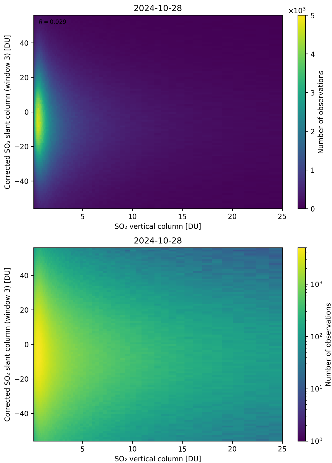
Figure 299: Scatter density plot of “SO 2 vertical column” against “Corrected SO 2 slant column (window 3)” for 2024-10-27 to 2024-10-29.
