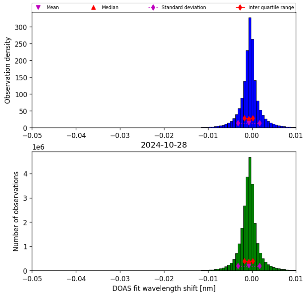
Figure 68: Histogram of “DOAS fit wavelength shift” for 2024-10-27 to 2024-10-29
