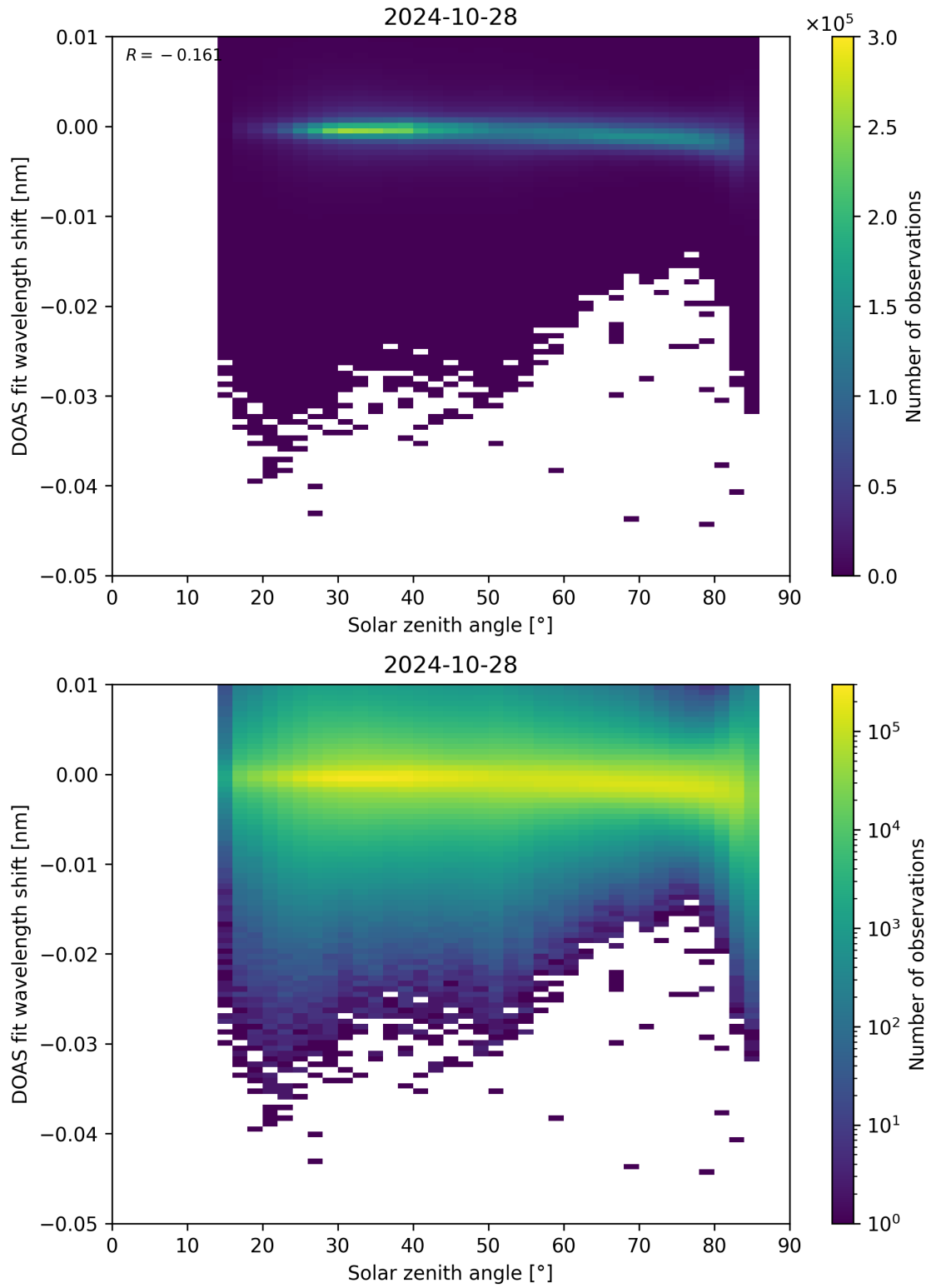
Figure 161: Scatter density plot of “Solar zenith angle” against “DOAS fit wavelength shift” for 2024-10-27 to 2024-10-29.
