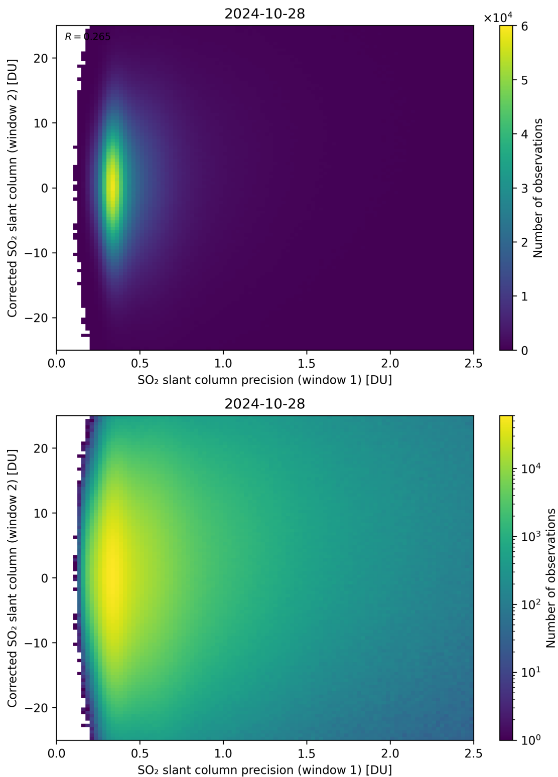
Figure 225: Scatter density plot of “SO 2 slant column precision (window 1)” against “Corrected SO 2 slant column (window 2)” for 2024-10-27 to 2024-10-29.
