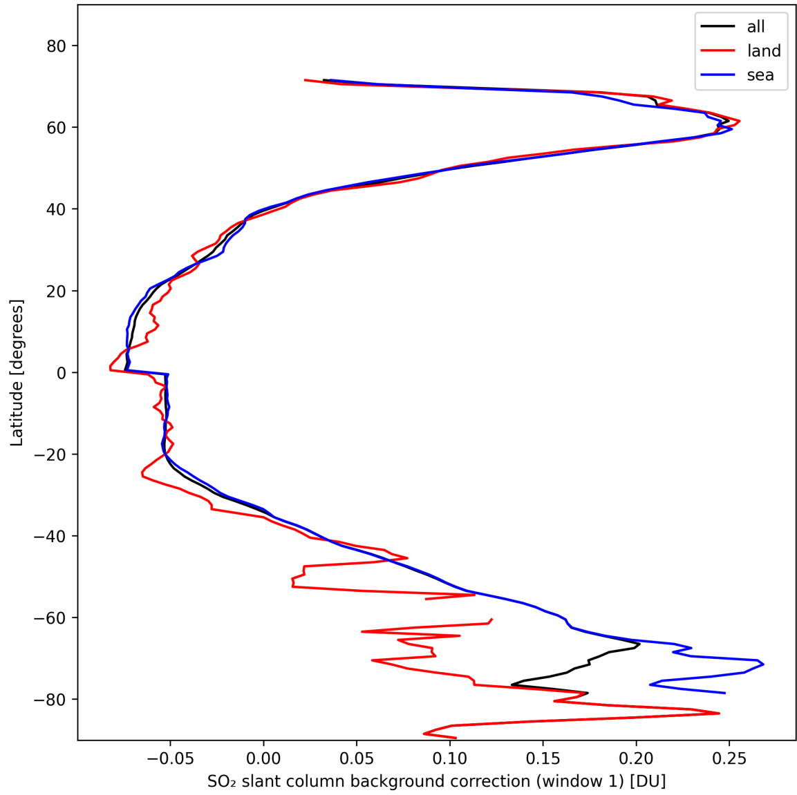
Figure 36: Zonal average of “SO 2 slant column background correction (window 1)” for 2024-10-27 to 2024-10-29.
