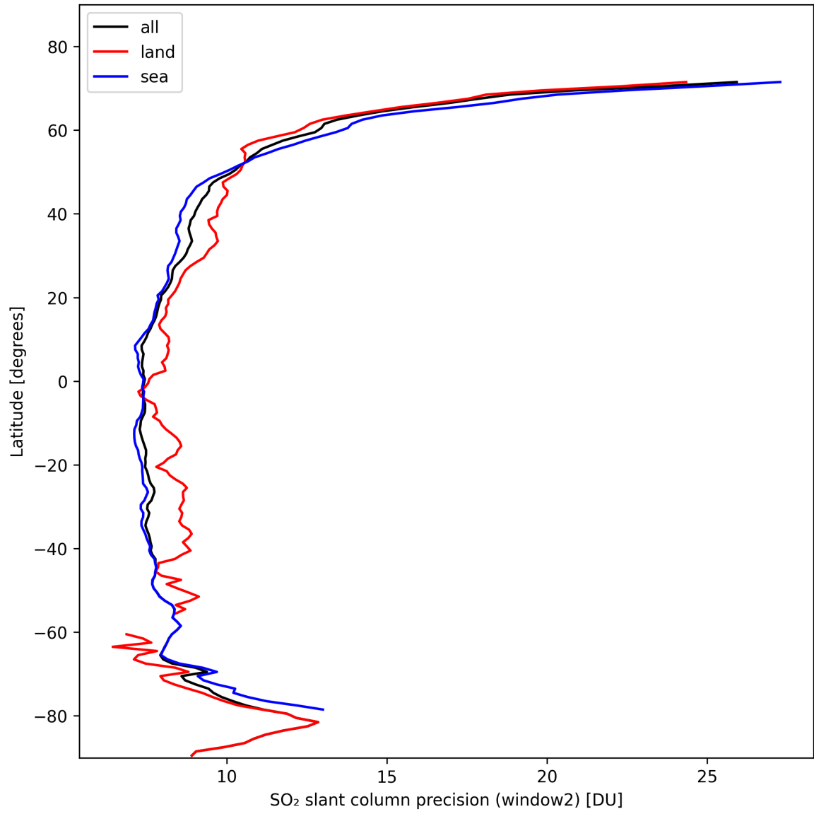
Figure 38: Zonal average of “SO 2 slant column precision (window2)” for 2024-10-27 to 2024-10-29.
