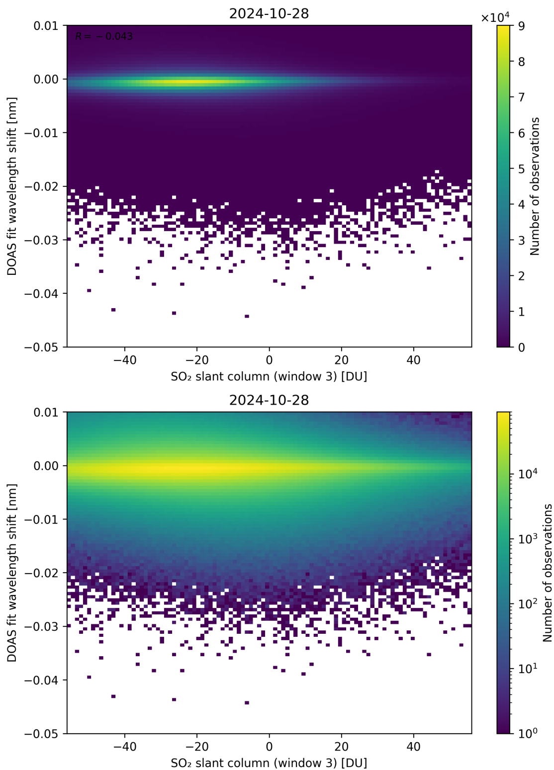
Figure 254: Scatter density plot of “SO 2 slant column (window 3)” against “DOAS fit wavelength shift” for 2024-10-27 to 2024-10-29.
