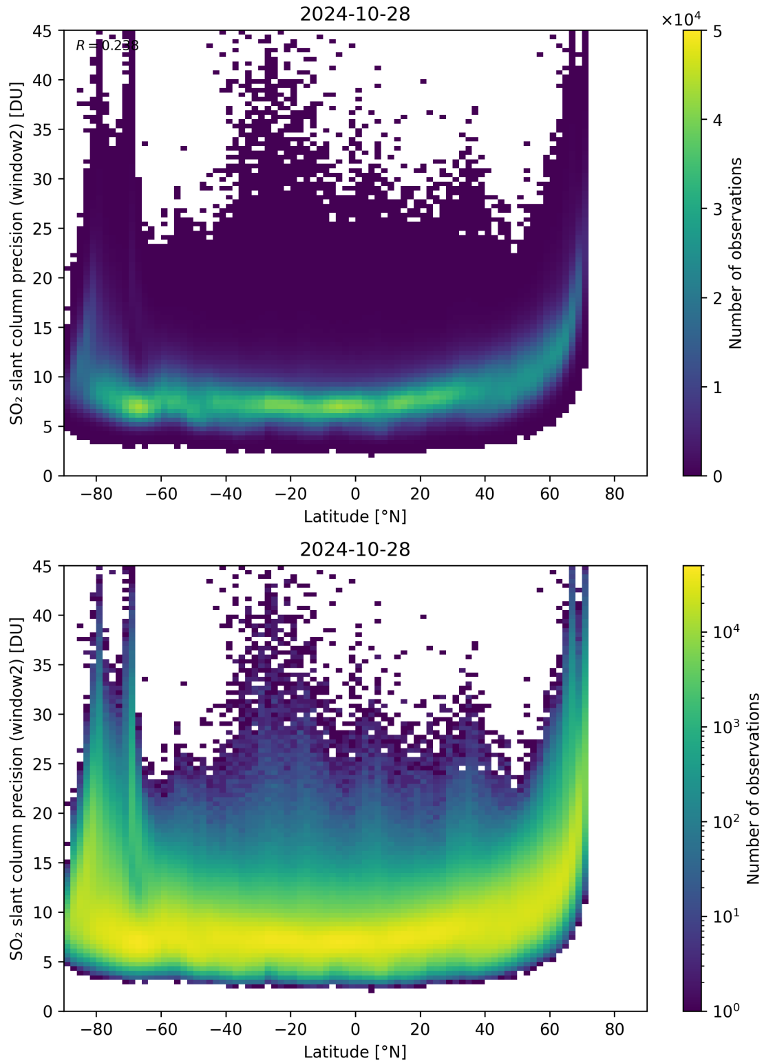
Figure 151: Scatter density plot of “Latitude” against “SO 2 slant column precision (window2)” for 2024-10-27 to 2024-10-29.
