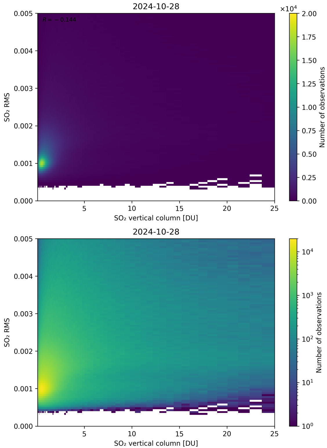
Figure 278: Scatter density plot of “SO 2 vertical column” against “SO 2 RMS” for 2024-10-27 to 2024-10-29.
