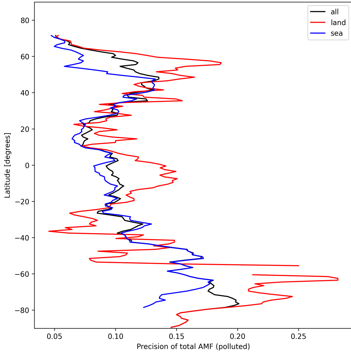
Figure 49: Zonal average of “Precision of total AMF (polluted)” for 2024-10-27 to 2024-10-29.
