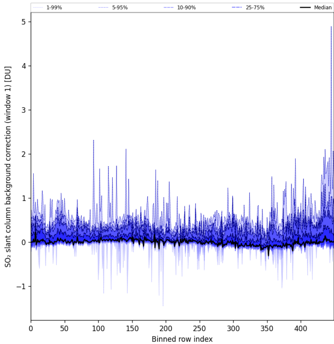
Figure 82: Along track statistics of “SO 2 slant column background correction (window 1)” for 2024-10-27 to 2024-10-29
