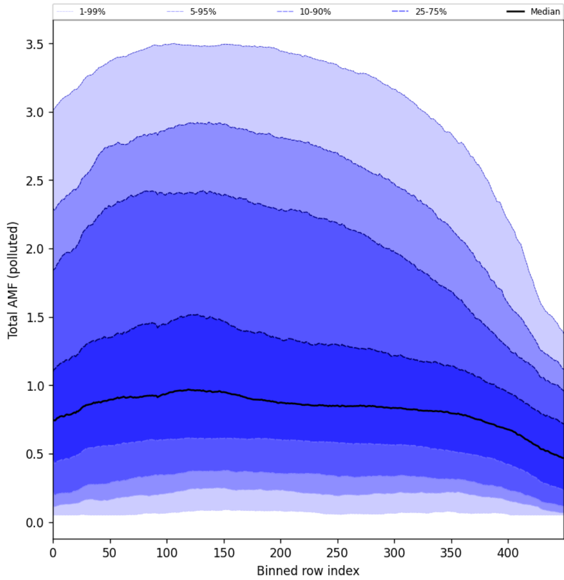
Figure 94: Along track statistics of “Total AMF (polluted)” for 2024-10-27 to 2024-10-29
