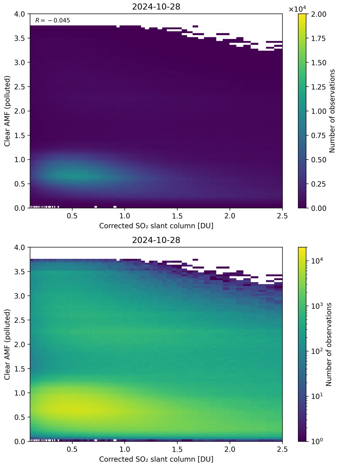
Figure 184: Scatter density plot of “Corrected SO 2 slant column” against “Clear AMF (polluted)” for 2024-10-27 to 2024-10-29.
