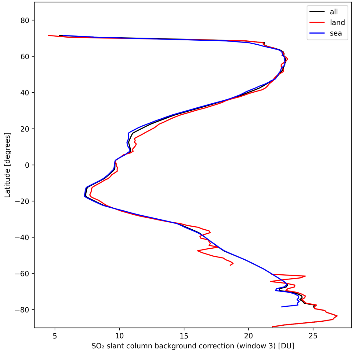
Figure 44: Zonal average of “SO 2 slant column background correction (window 3)” for 2024-10-27 to 2024-10-29.
