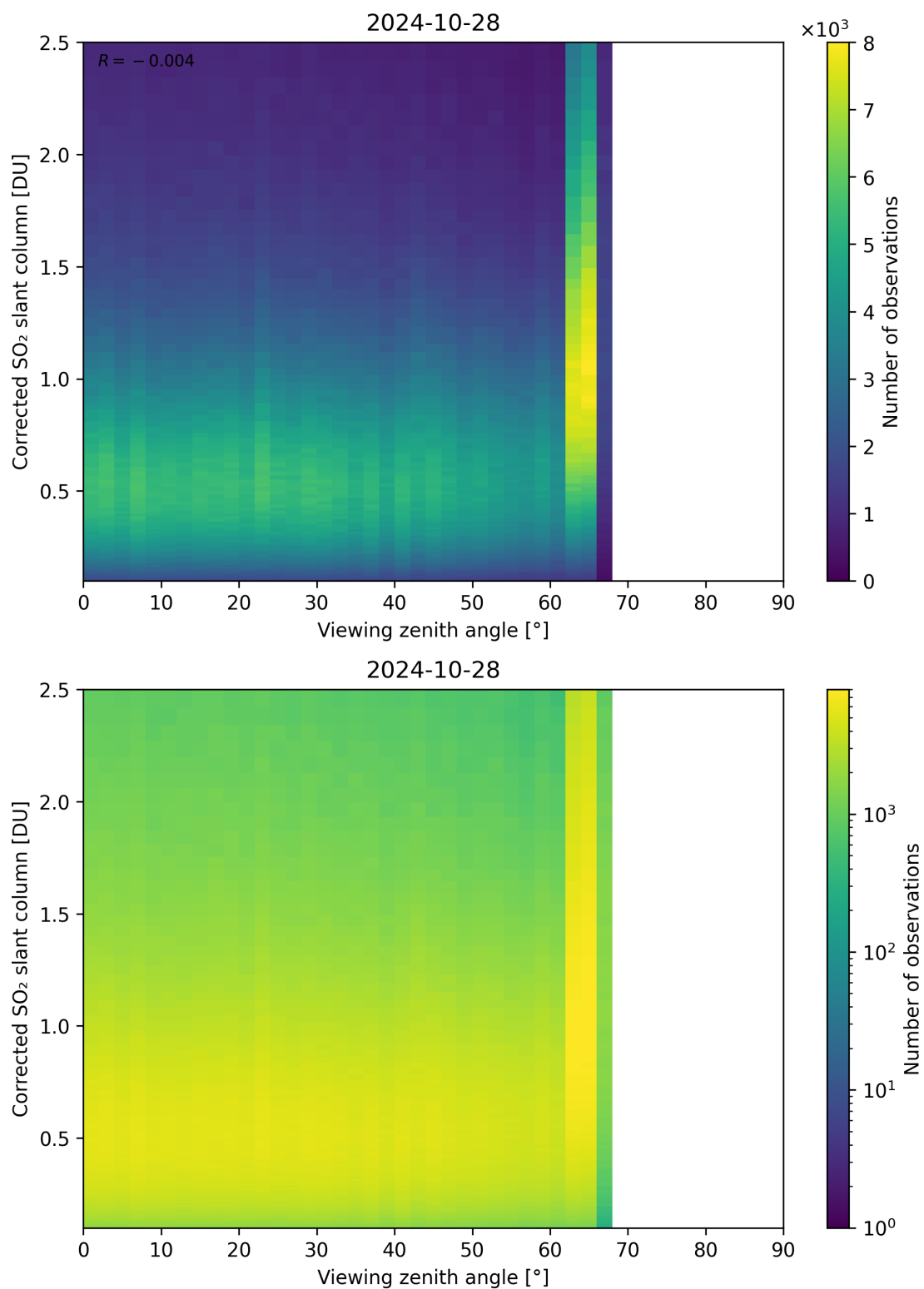
Figure 317: Scatter density plot of “Viewing zenith angle” against “Corrected SO 2 slant column” for 2024-10-27 to 2024-10-29.
