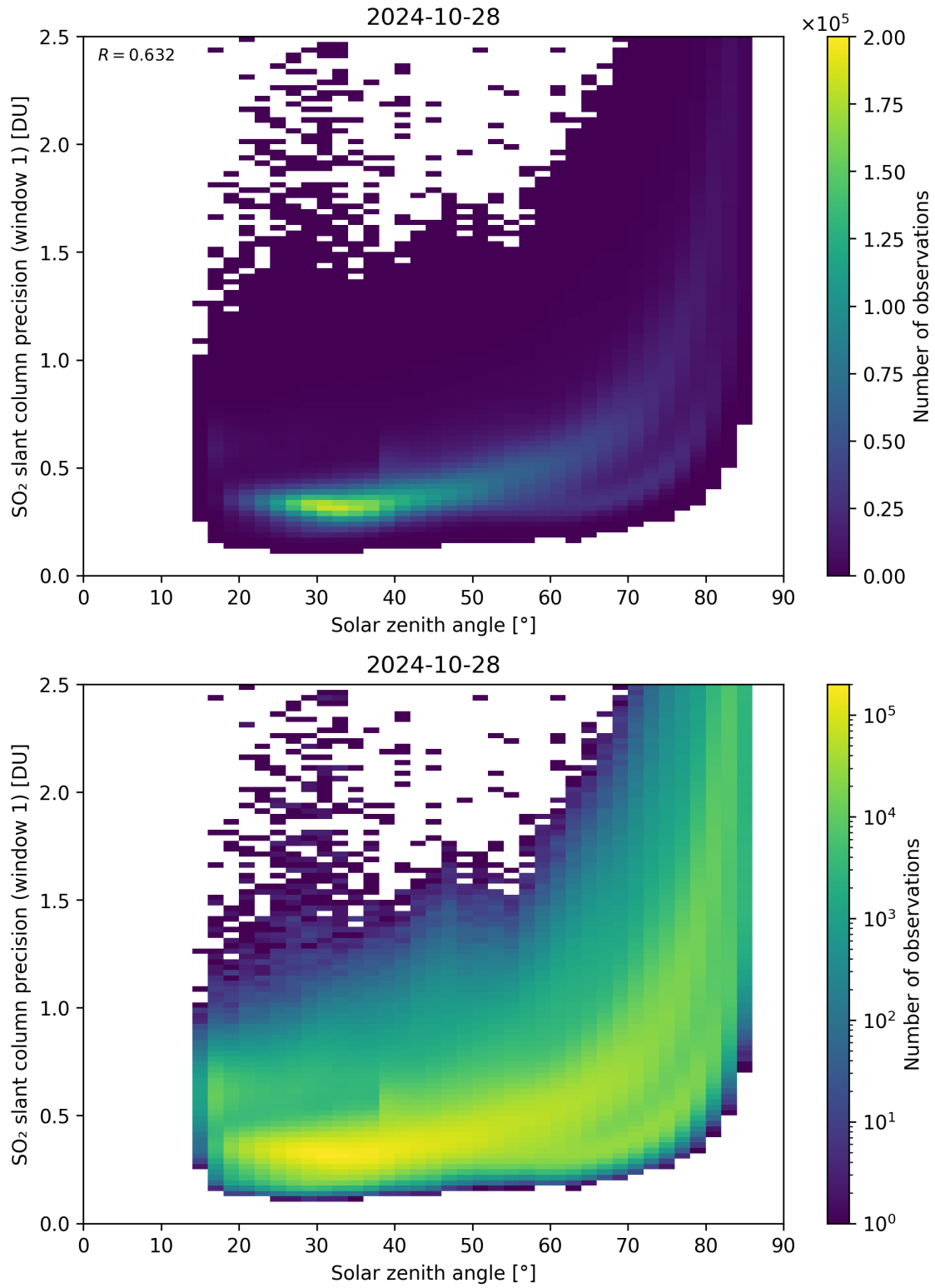
Figure 170: Scatter density plot of “Solar zenith angle” against “SO 2 slant column precision (window 1)” for 2024-10-27 to 2024-10-29.
