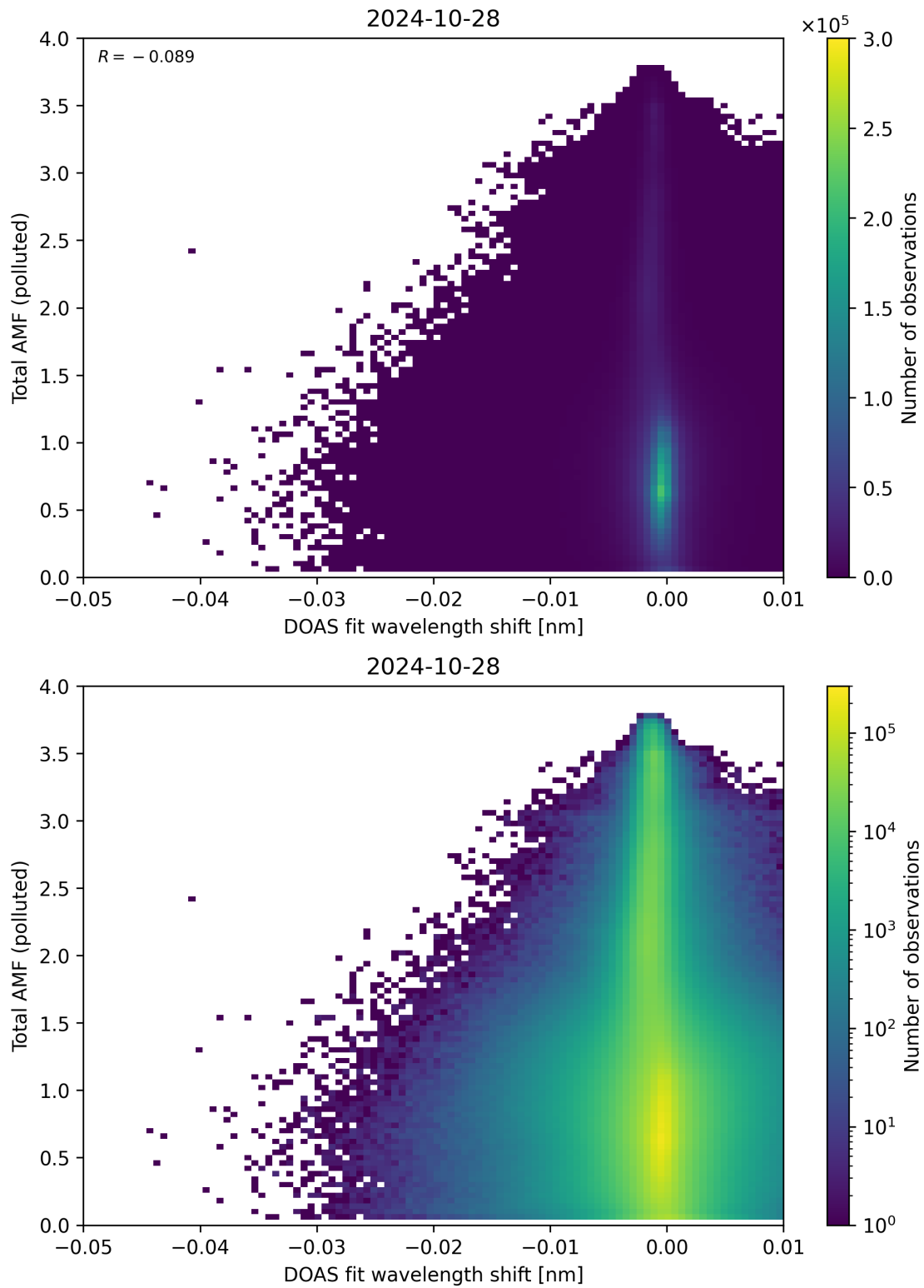
Figure 130: Scatter density plot of “DOAS fit wavelength shift” against “Total AMF (polluted)” for 2024-10-27 to 2024-10-29.
