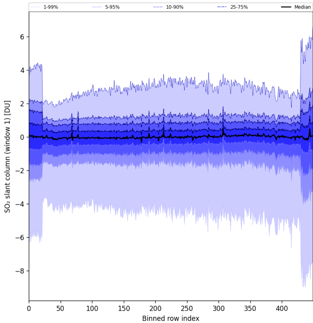
Figure 79: Along track statistics of “SO 2 slant column (window 1)” for 2024-10-27 to 2024-10-29
