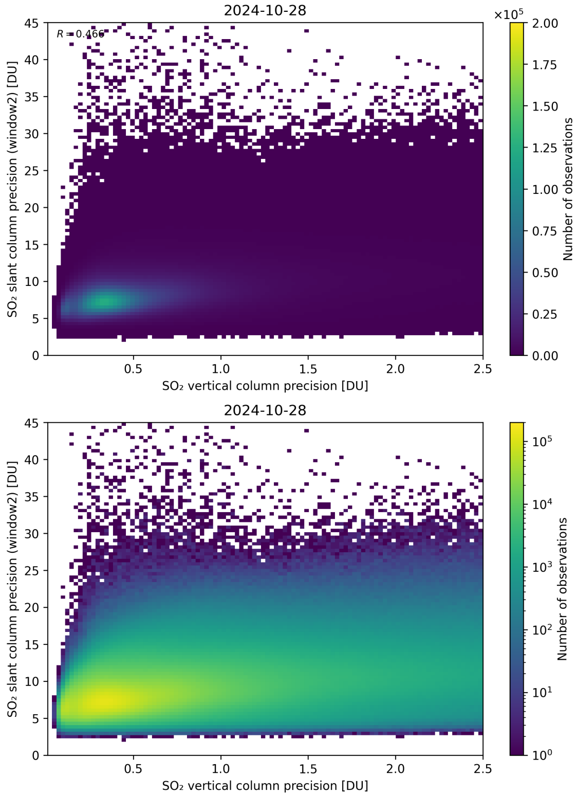
Figure 291: Scatter density plot of “SO 2 vertical column precision” against “SO 2 slant column precision (window2)” for 2024-10-27 to 2024-10-29.
