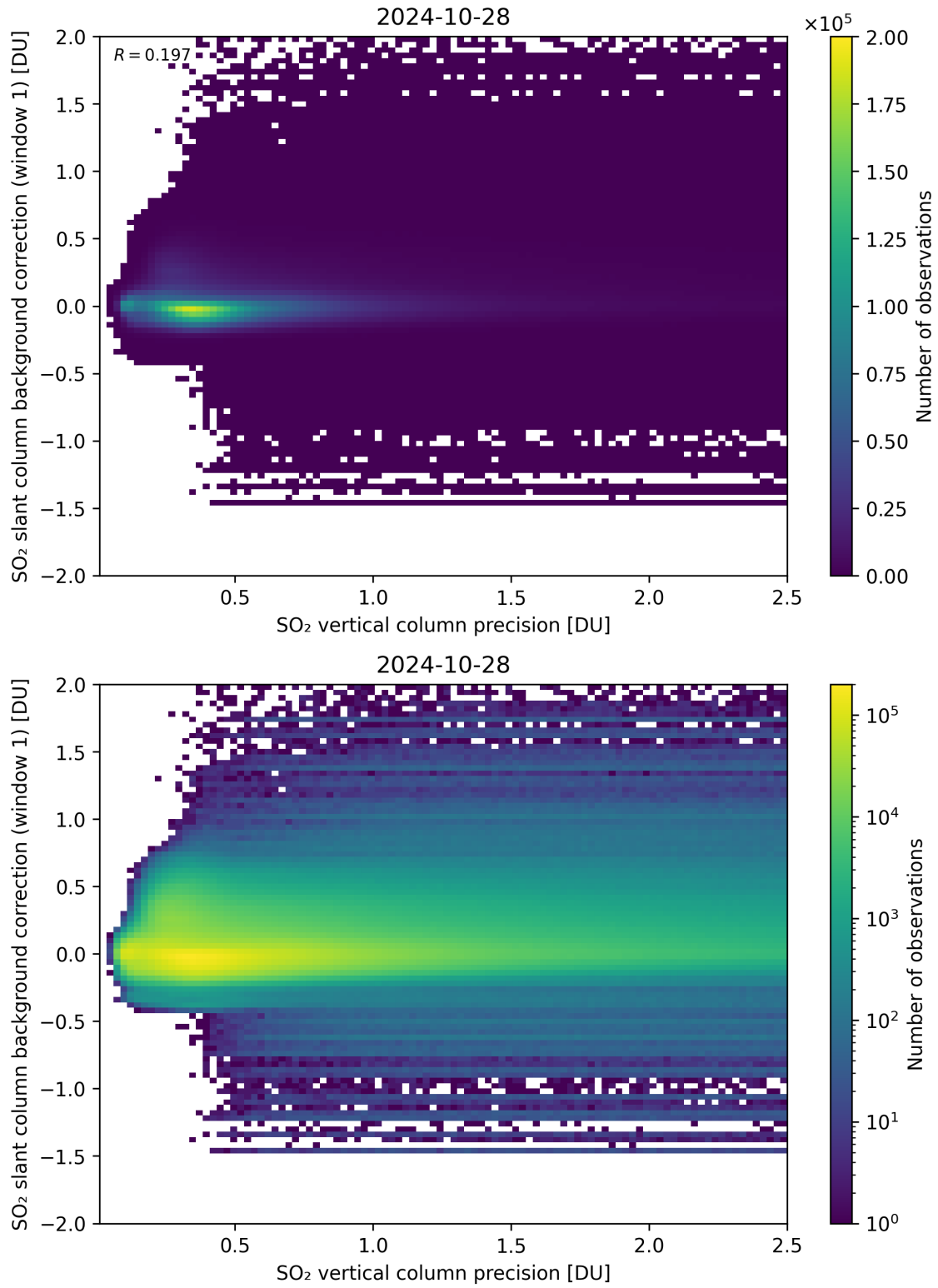
Figure 279: Scatter density plot of “SO 2 vertical column precision” against “SO 2 slant column background correction (window 1)” for 2024-10-27 to 2024-10-29.
