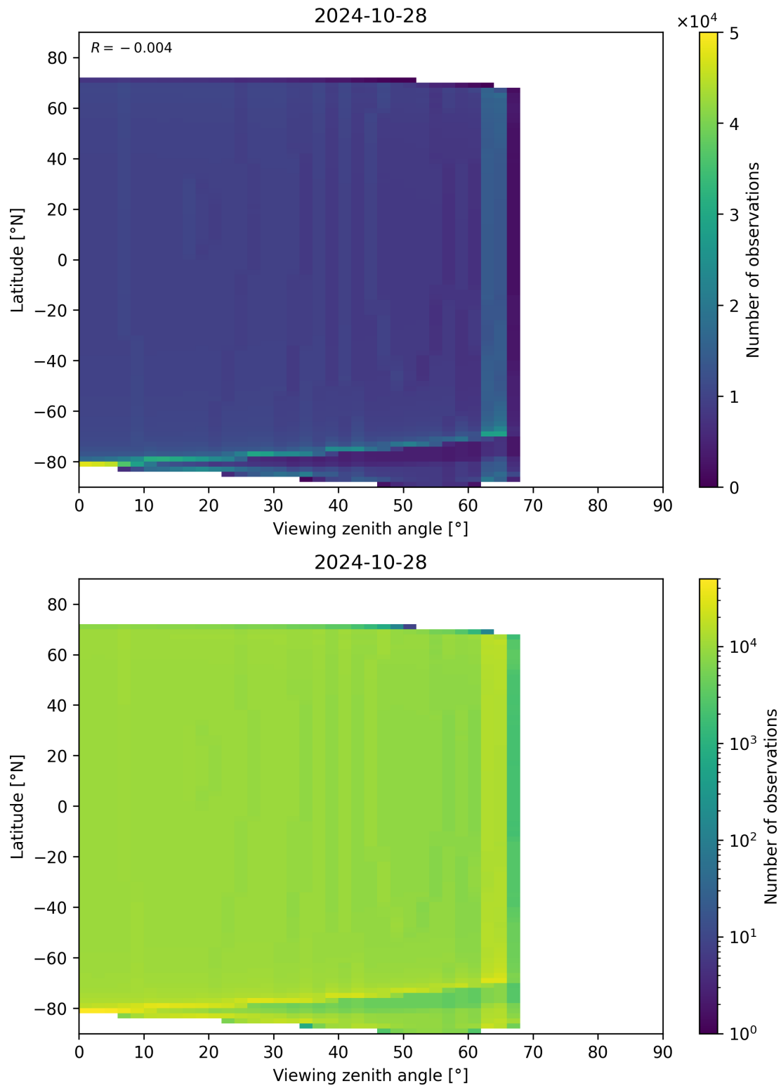
Figure 314: Scatter density plot of “Viewing zenith angle” against “Latitude” for 2024-10-27 to 2024-10-29.
