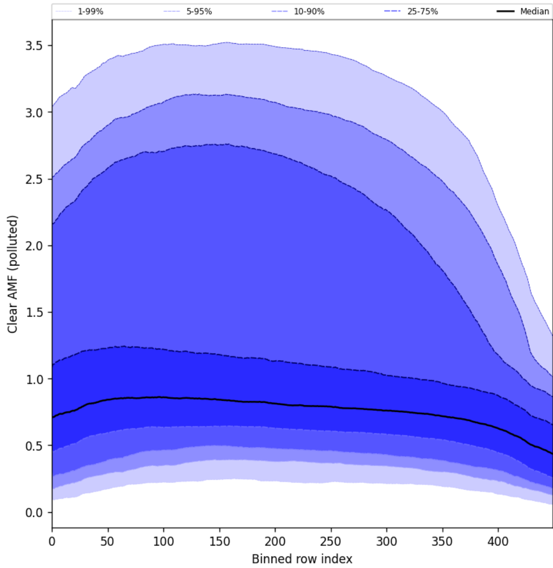
Figure 96: Along track statistics of “Clear AMF (polluted)” for 2024-10-27 to 2024-10-29
