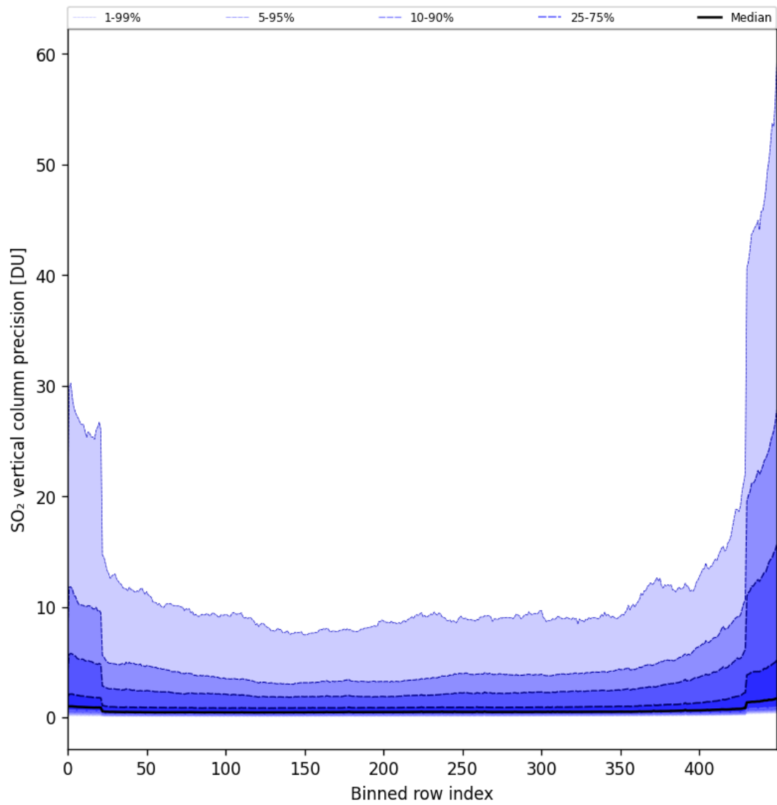
Figure 77: Along track statistics of “SO 2 vertical column precision” for 2024-10-27 to 2024-10-29
