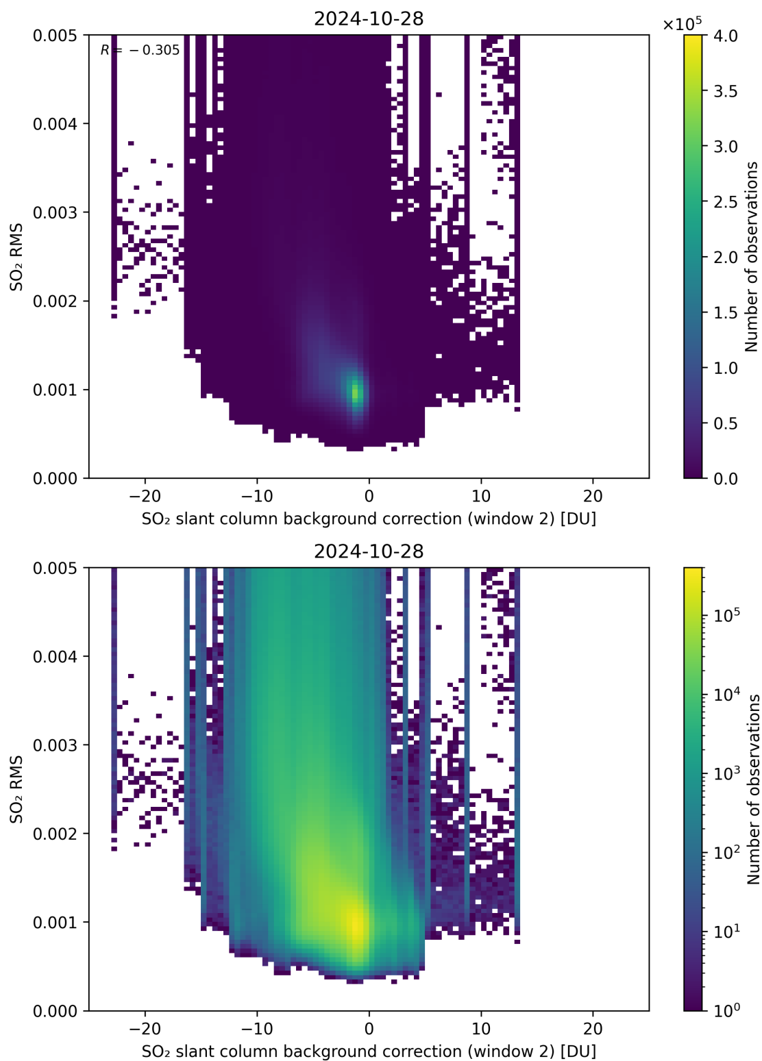
Figure 114: Scatter density plot of “SO 2 slant column background correction (window 2)” against “SO 2 RMS” for 2024-10-27 to 2024-10-29.
