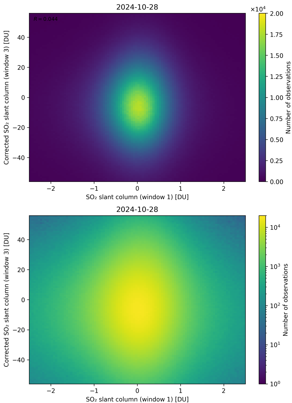
Figure 234: Scatter density plot of “SO 2 slant column (window 1)” against “Corrected SO 2 slant column (window 3)” for 2024-10-27 to 2024-10-29.
