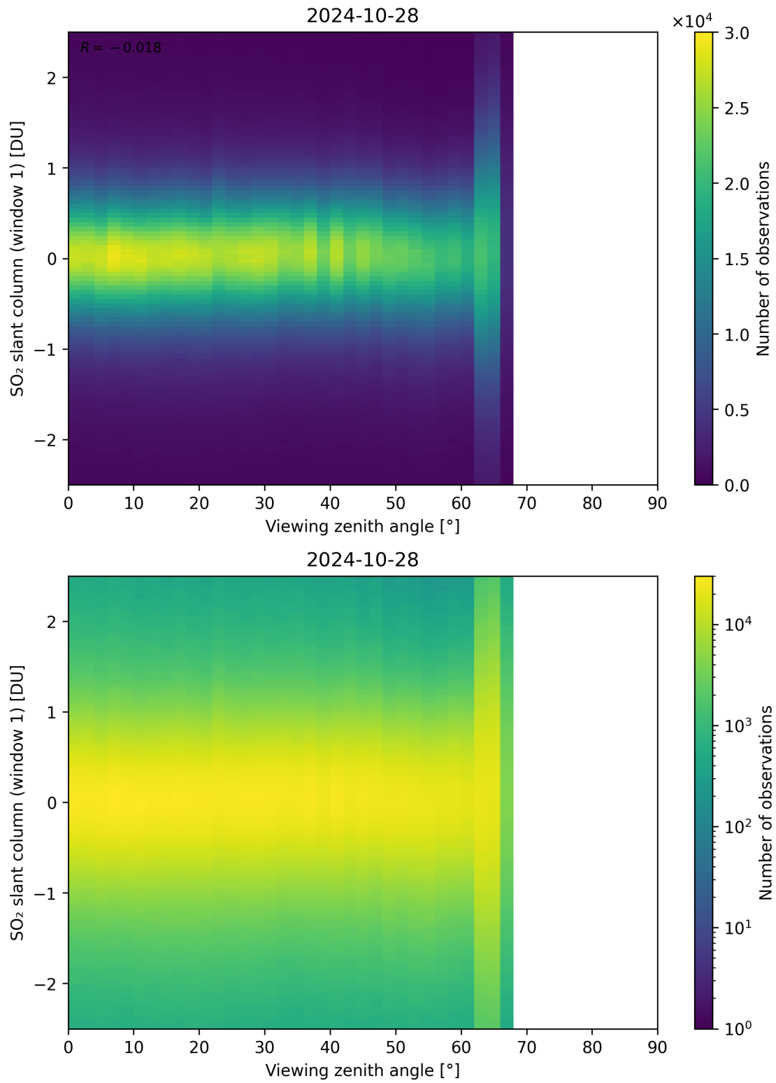
Figure 320: Scatter density plot of “Viewing zenith angle” against “SO 2 slant column (window 1)” for 2024-10-27 to 2024-10-29.
