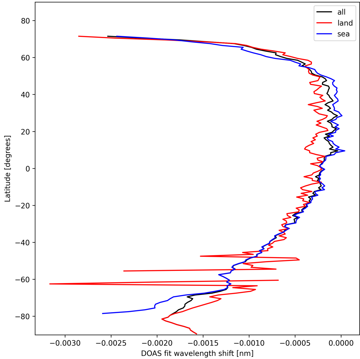
Figure 45: Zonal average of “DOAS fit wavelength shift” for 2024-10-27 to 2024-10-29.
