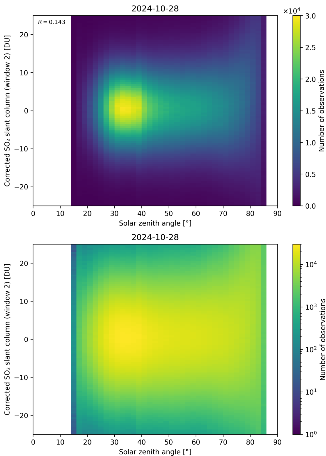
Figure 167: Scatter density plot of “Solar zenith angle” against “Corrected SO 2 slant column (window 2)” for 2024-10-27 to 2024-10-29.
