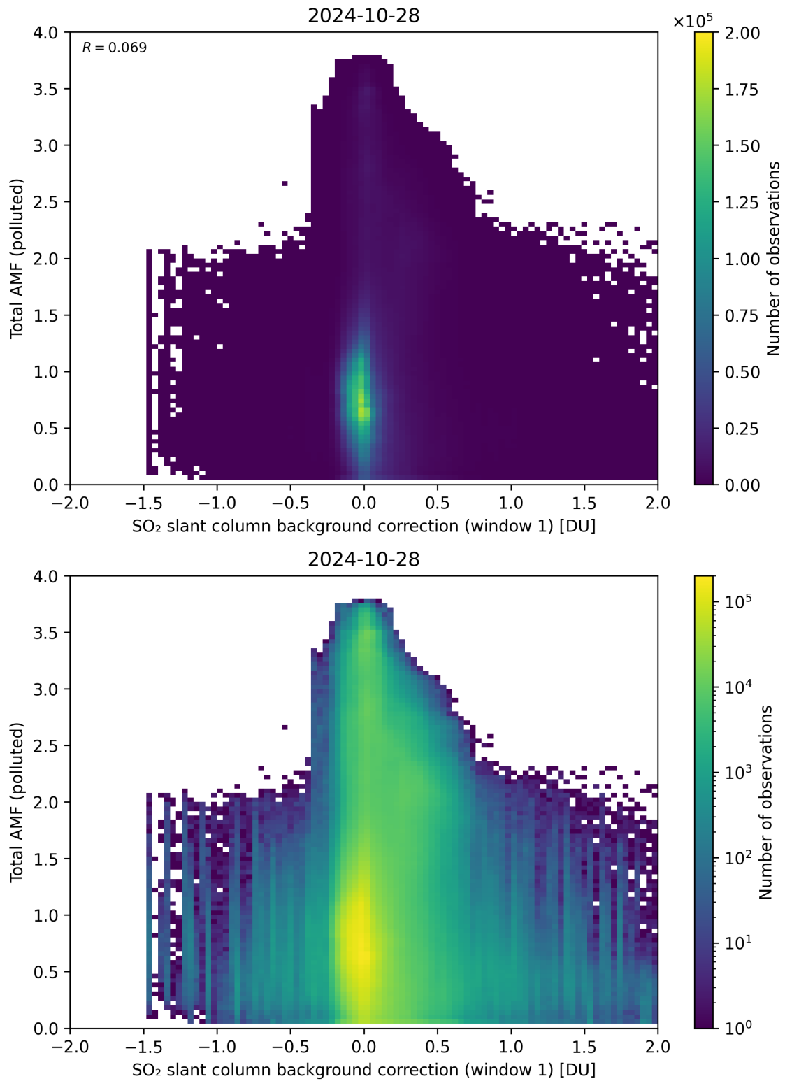
Figure 109: Scatter density plot of “SO 2 slant column background correction (window 1)” against “Total AMF (polluted)” for 2024-10-27 to 2024-10-29.
