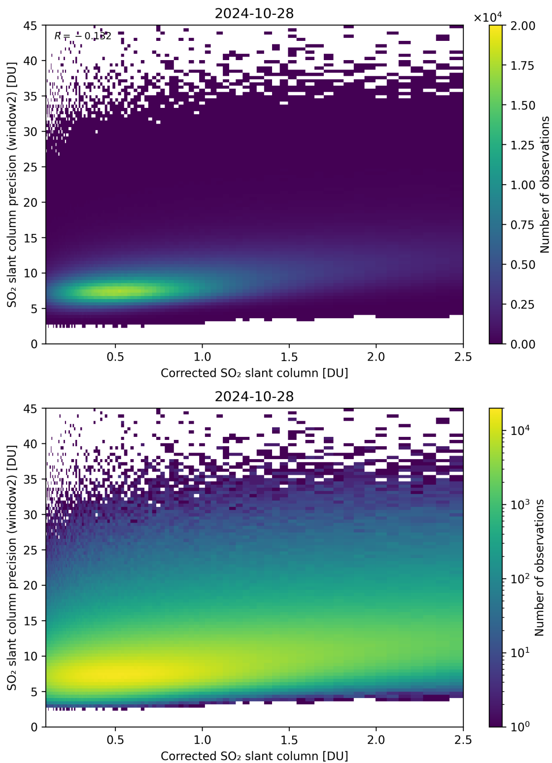
Figure 189: Scatter density plot of “Corrected SO 2 slant column” against “SO 2 slant column precision (window2)” for 2024-10-27 to 2024-10-29.
