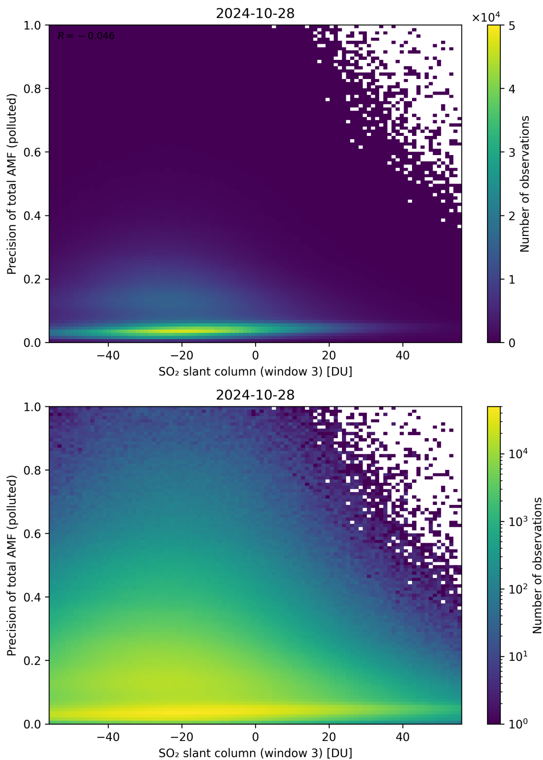
Figure 269: Scatter density plot of “SO 2 slant column (window 3)” against “Precision of total AMF (polluted)” for 2024-10-27 to 2024-10-29.
