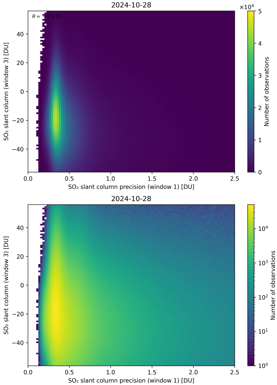
Figure 228: Scatter density plot of “SO 2 slant column precision (window 1)” against “SO 2 slant column (window 3)” for 2024-10-27 to 2024-10-29.
