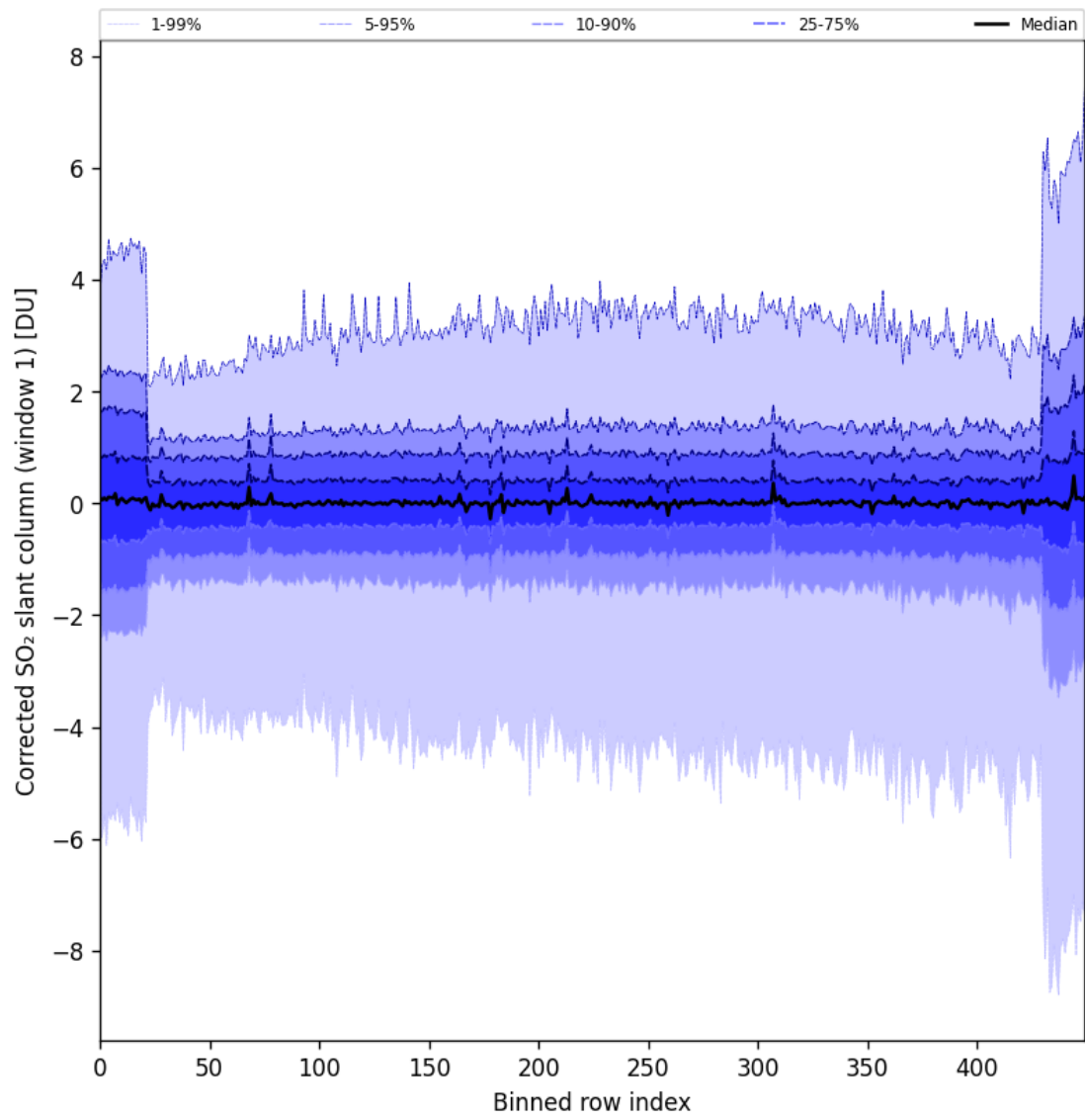
Figure 81: Along track statistics of “Corrected SO 2 slant column (window 1)” for 2024-10-27 to 2024-10-29
