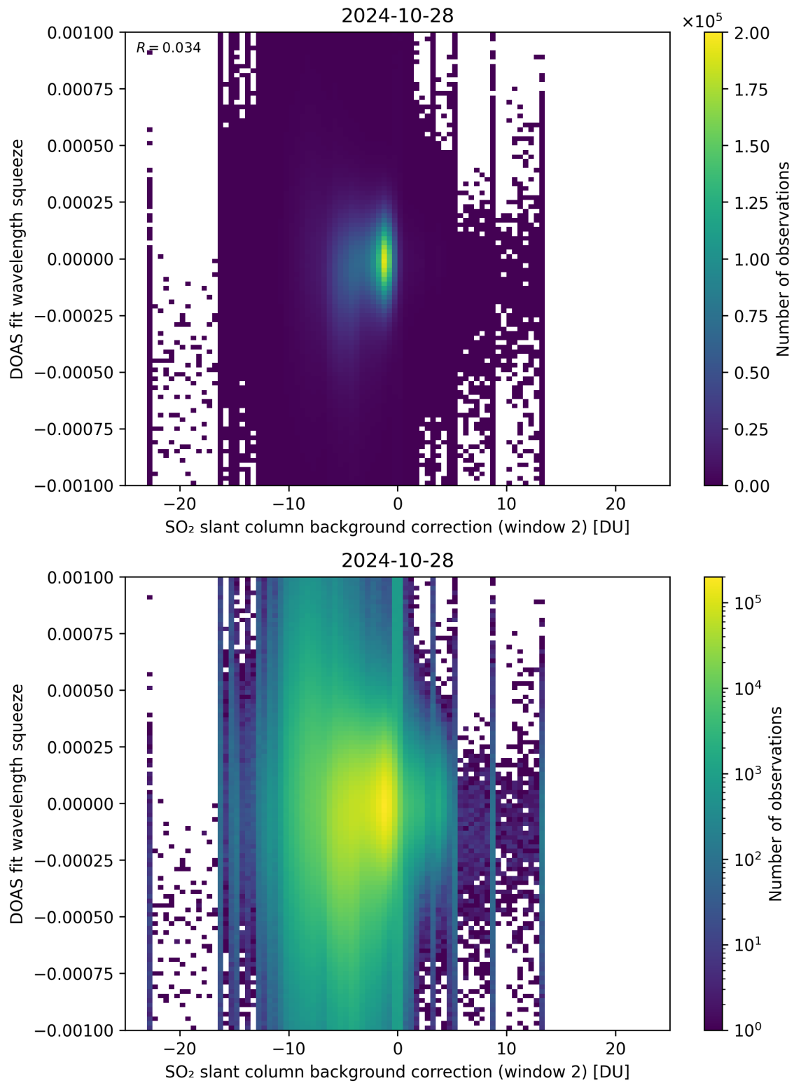
Figure 113: Scatter density plot of “SO 2 slant column background correction (window 2)” against “DOAS fit wavelength squeeze” for 2024-10-27 to 2024-10-29.
