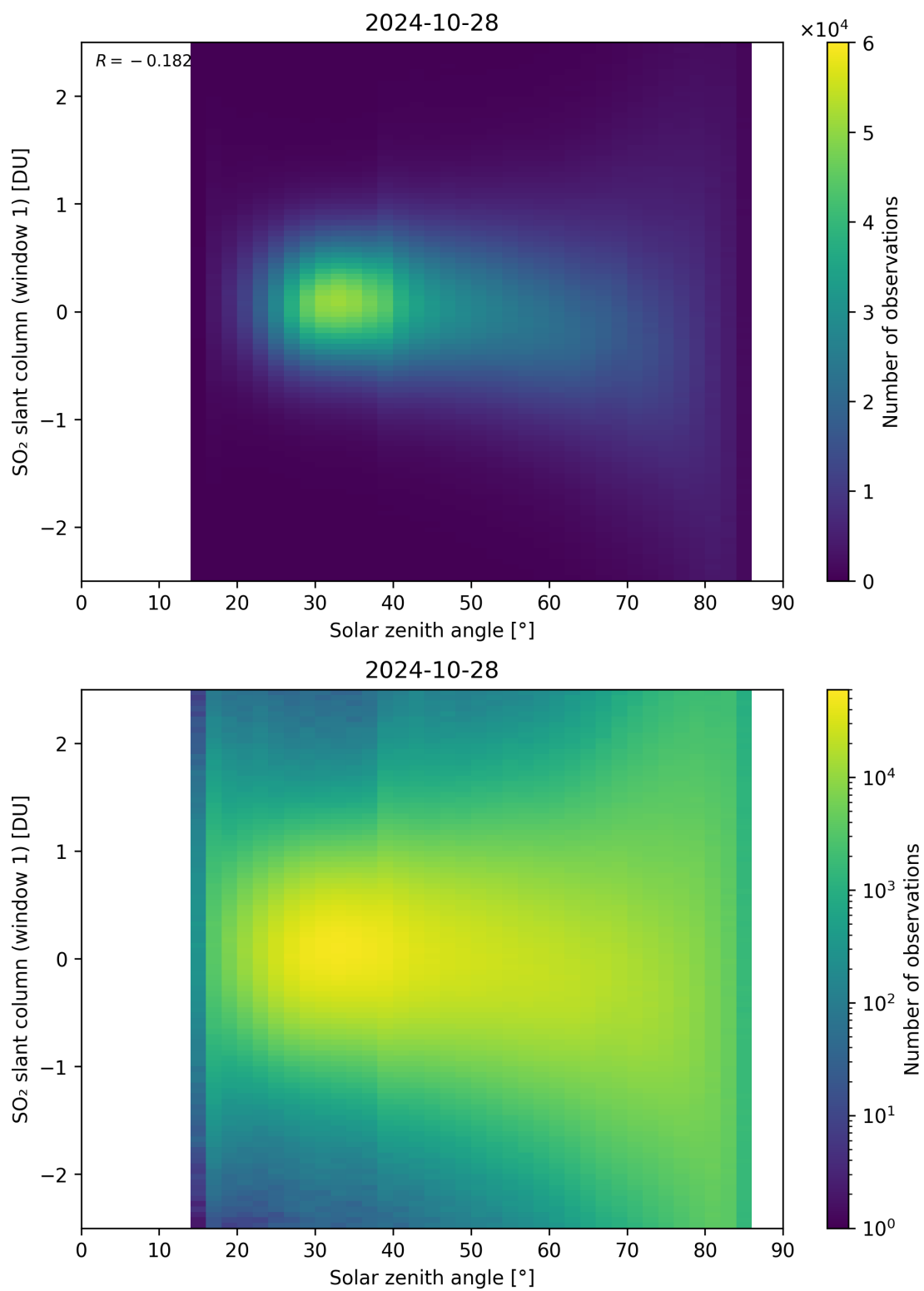
Figure 169: Scatter density plot of “Solar zenith angle” against “SO 2 slant column (window 1)” for 2024-10-27 to 2024-10-29.
