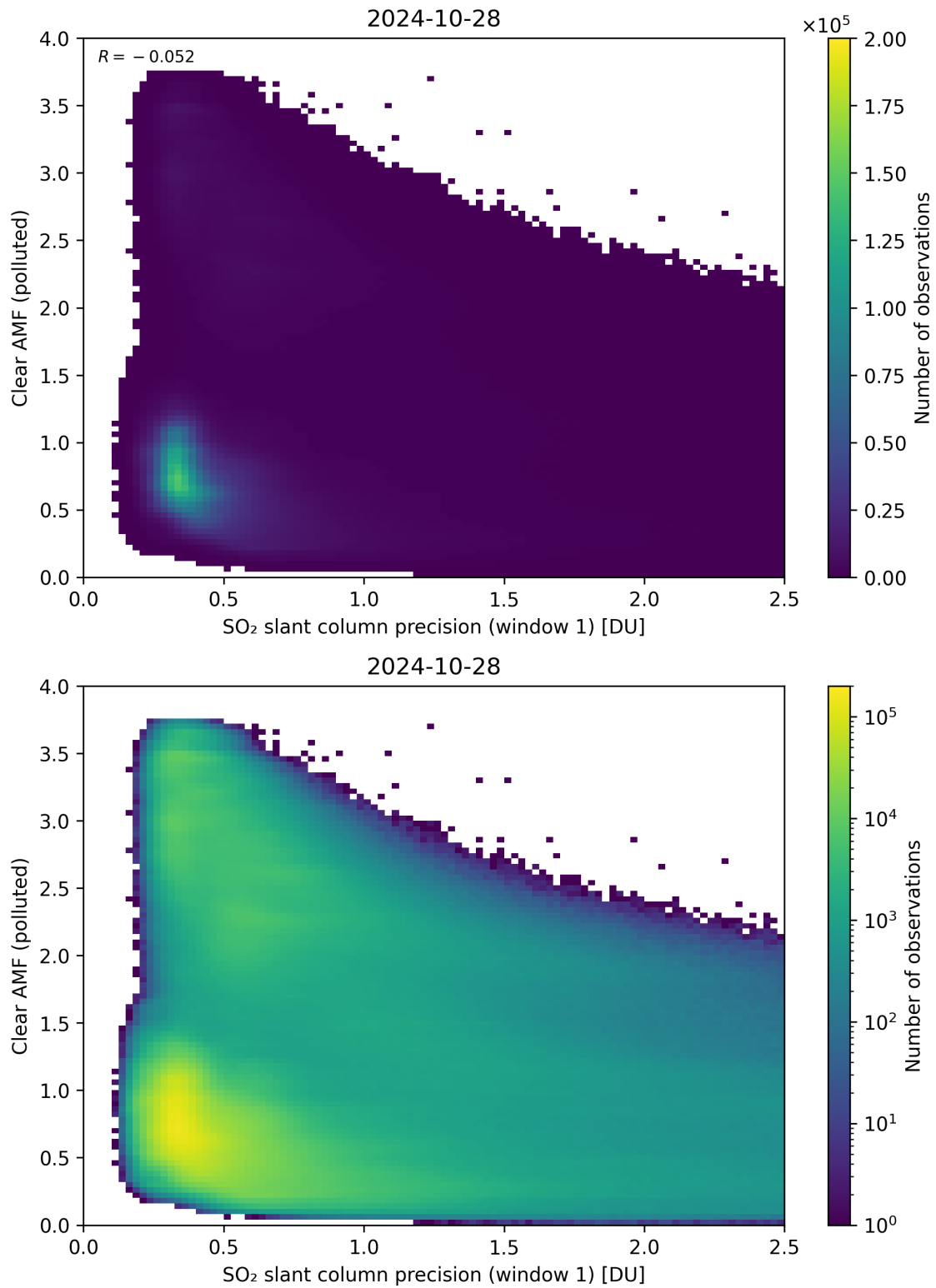
Figure 224: Scatter density plot of “SO 2 slant column precision (window 1)” against “Clear AMF (polluted)” for 2024-10-27 to 2024-10-29.
