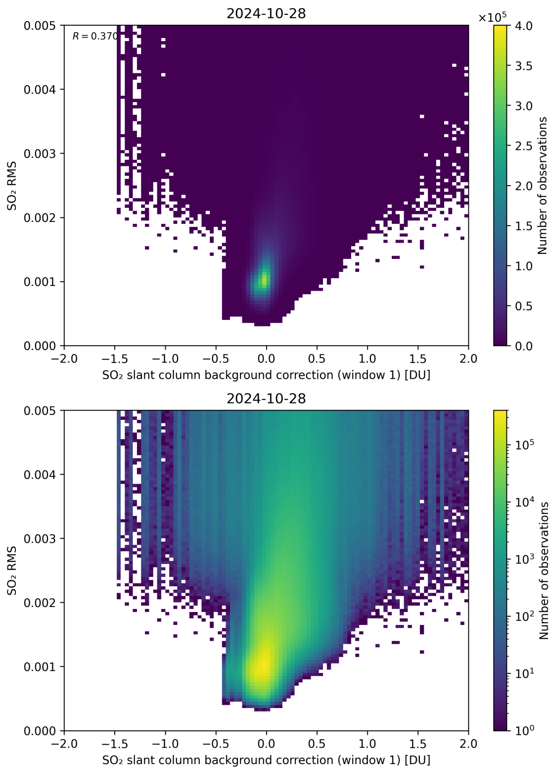
Figure 102: Scatter density plot of “SO 2 slant column background correction (window 1)” against “SO 2 RMS” for 2024-10-27 to 2024-10-29.
