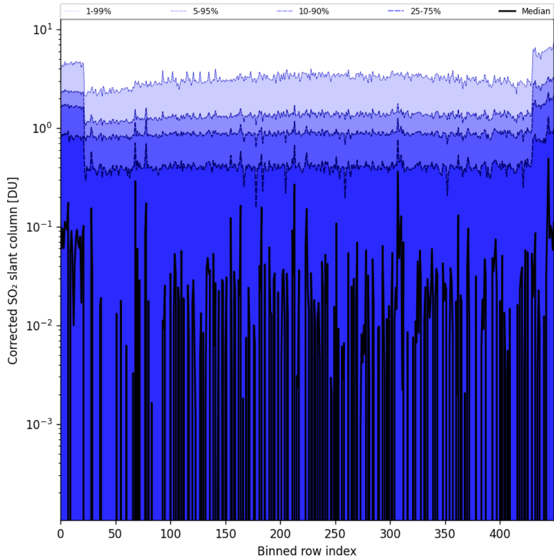
Figure 78: Along track statistics of "Corrected SO 2 slant column" for 2024-10-27 to 2024-10-29
