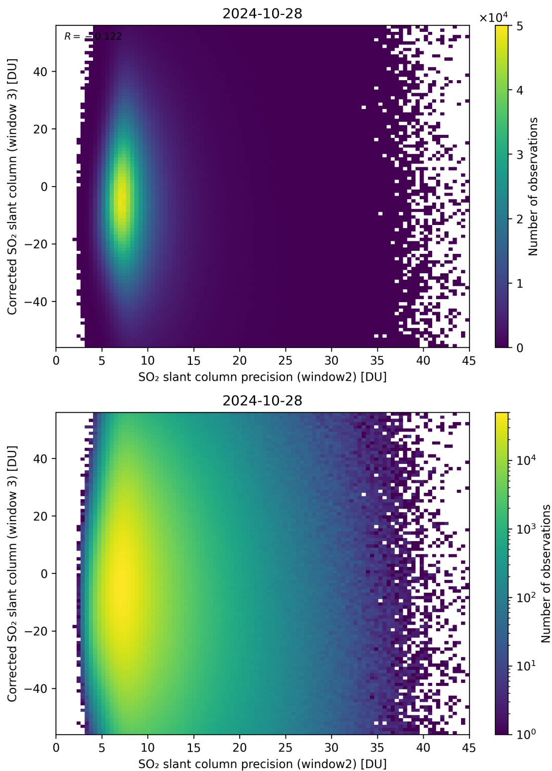
Figure 248: Scatter density plot of “SO 2 slant column precision (window2)” against “Corrected SO 2 slant column (window 3)” for 2024-10-27 to 2024-10-29.
