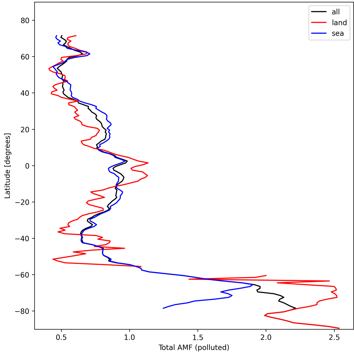
Figure 48: Zonal average of “Total AMF (polluted)” for 2024-10-27 to 2024-10-29.
