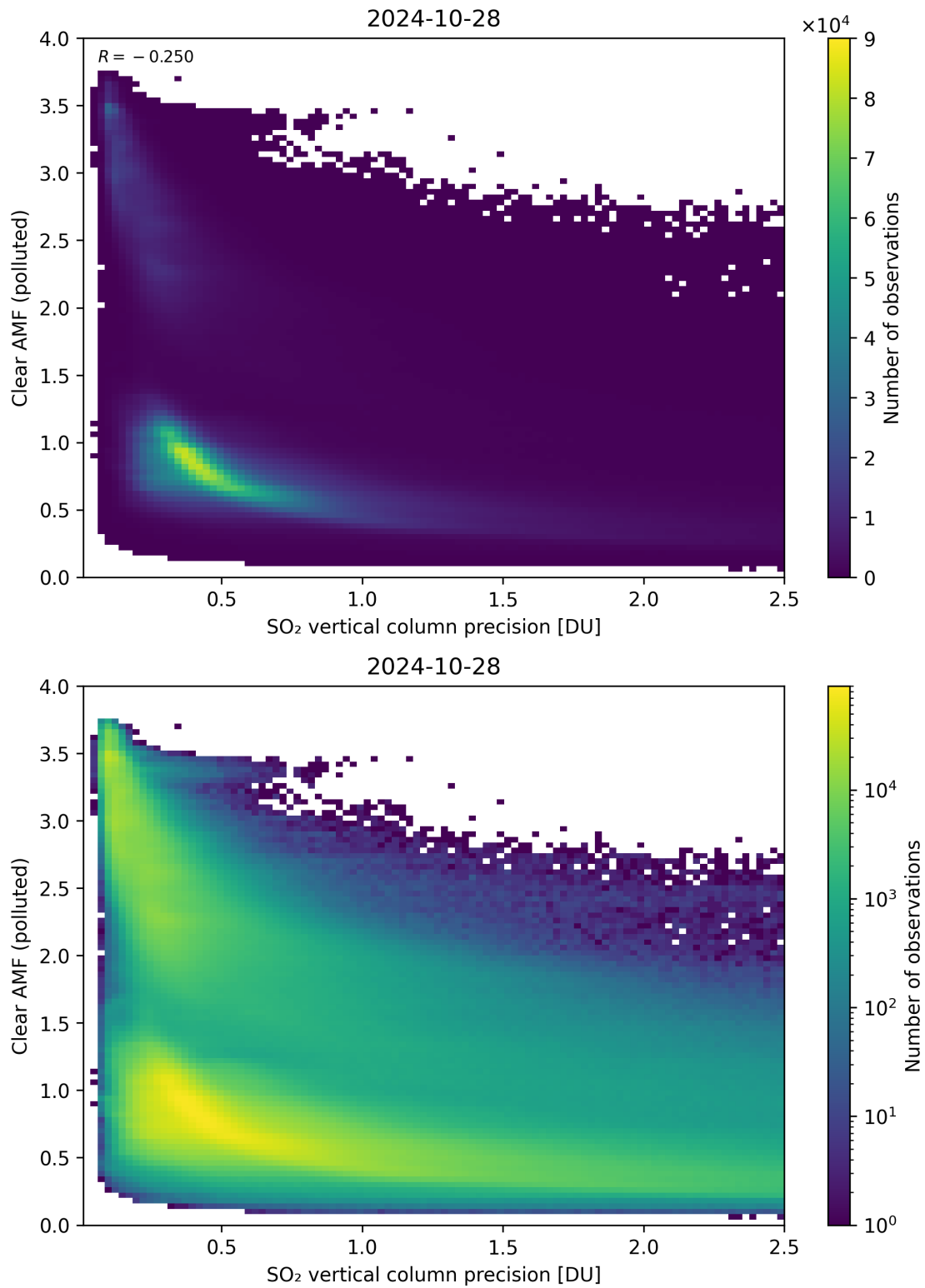
Figure 285: Scatter density plot of “SO 2 vertical column precision” against “Clear AMF (polluted)” for 2024-10-27 to 2024-10-29.
