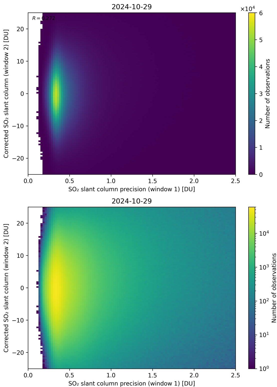
Figure 225: Scatter density plot of “SO 2 slant column precision (window 1)” against “Corrected SO 2 slant column (window 2)” for 2024-10-29 to 2024-10-30.
