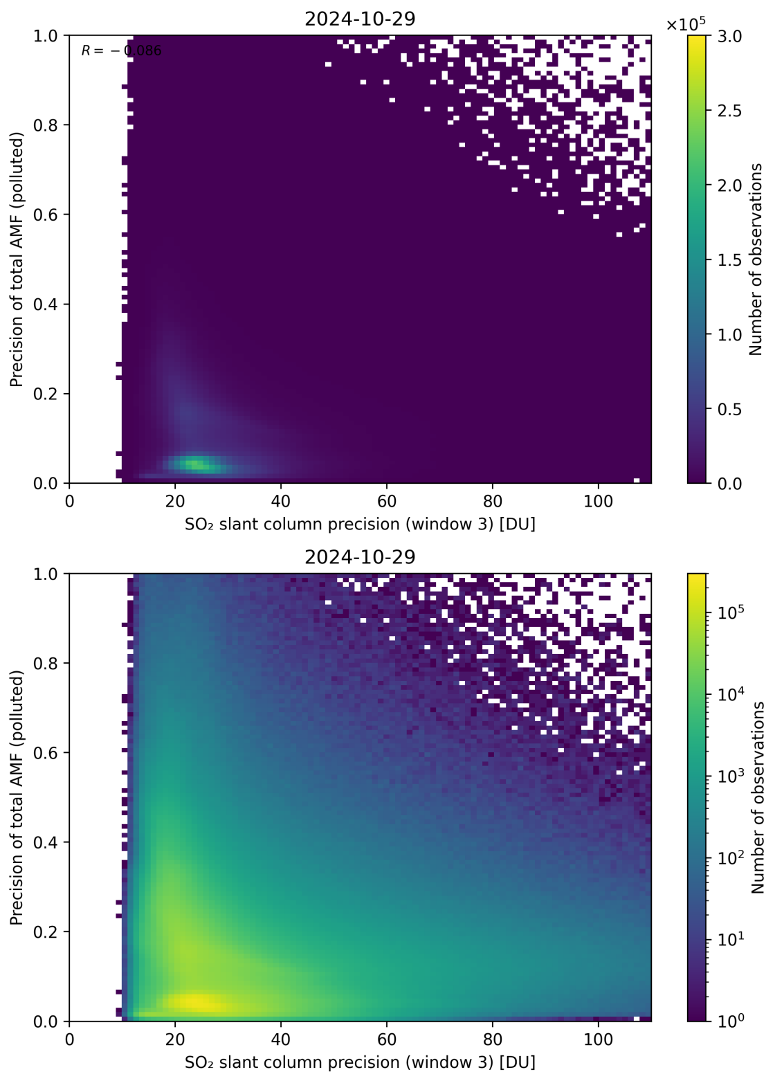
Figure 264: Scatter density plot of “SO 2 slant column precision (window 3)” against “Precision of total AMF (polluted)” for 2024-10-29 to 2024-10-30.
