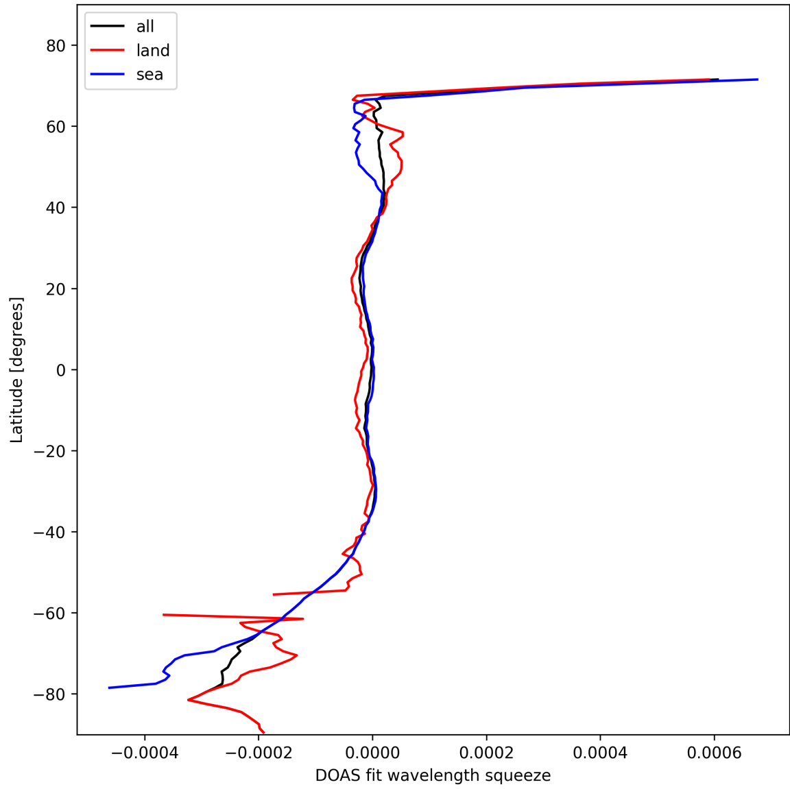
Figure 46: Zonal average of “DOAS fit wavelength squeeze” for 2024-10-29 to 2024-10-30.
