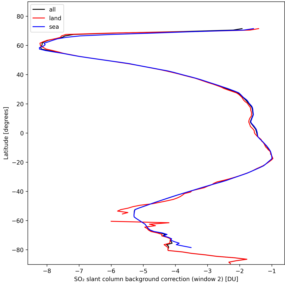
Figure 40: Zonal average of “SO 2 slant column background correction (window 2)” for 2024-10-29 to 2024-10-30.
