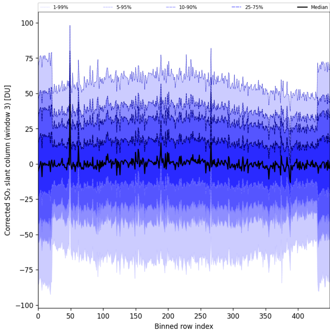
Figure 89: Along track statistics of “Corrected SO 2 slant column (window 3)” for 2024-10-29 to 2024-10-30
