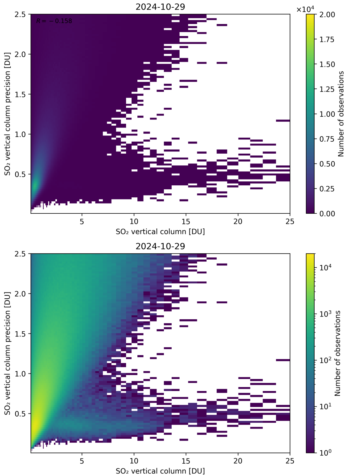
Figure 307: Scatter density plot of “SO 2 vertical column” against “SO 2 vertical column precision” for 2024-10-29 to 2024-10-30.
