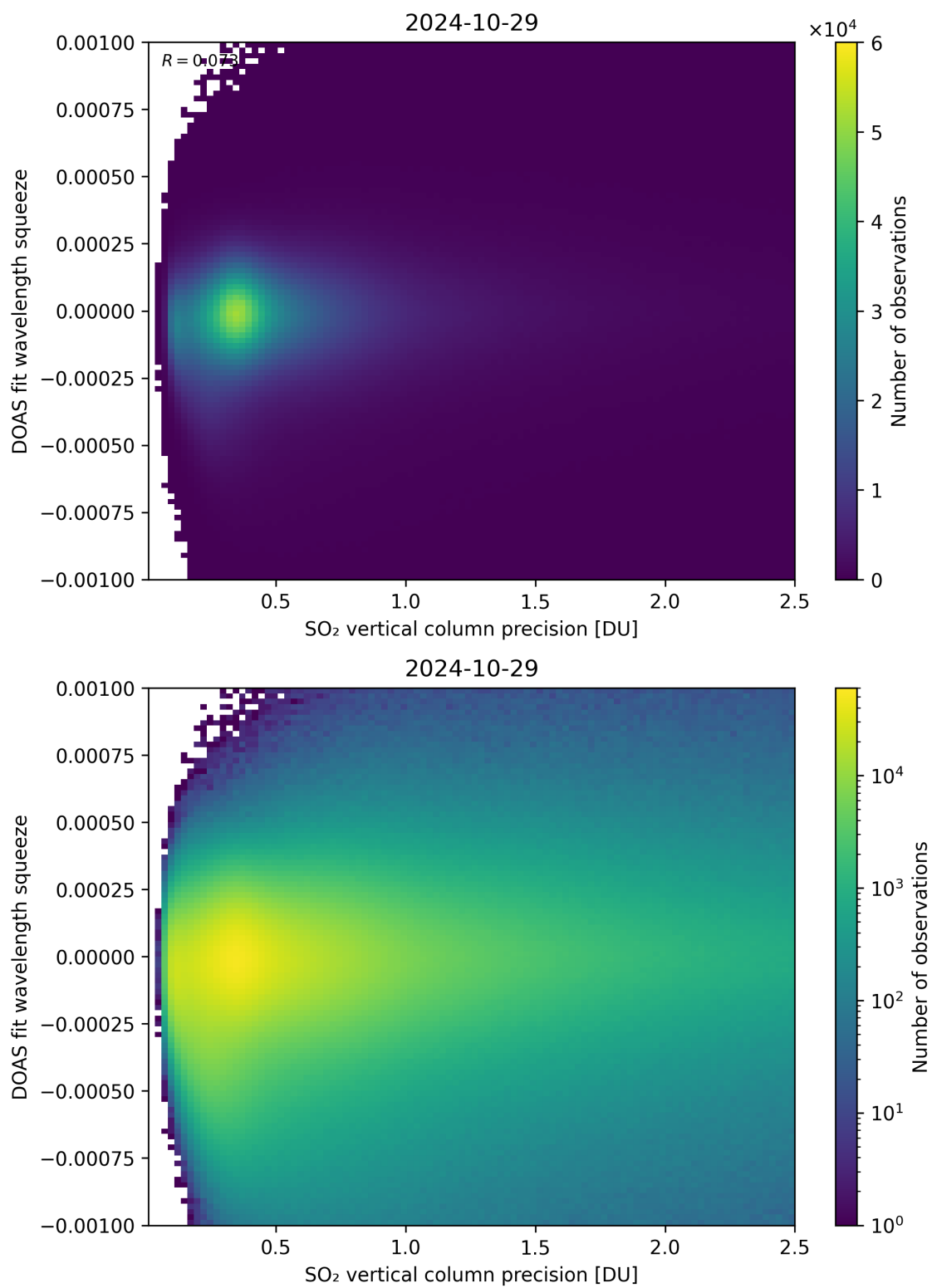
Figure 283: Scatter density plot of “SO 2 vertical column precision” against “DOAS fit wavelength squeeze” for 2024-10-29 to 2024-10-30.
