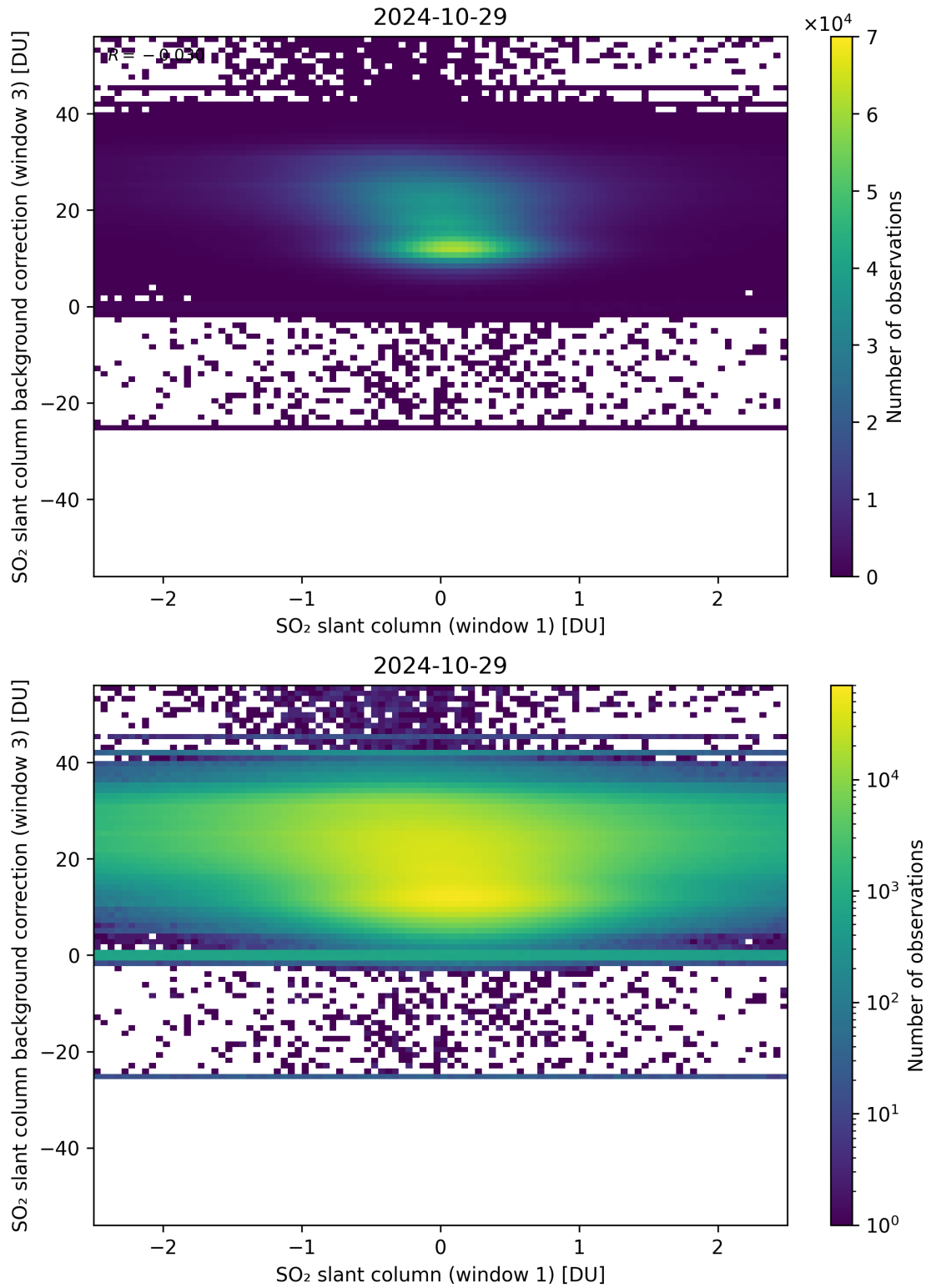
Figure 214: Scatter density plot of “SO 2 slant column (window 1)” against “SO 2 slant column background correction (window 3)” for 2024-10-29 to 2024-10-30.
