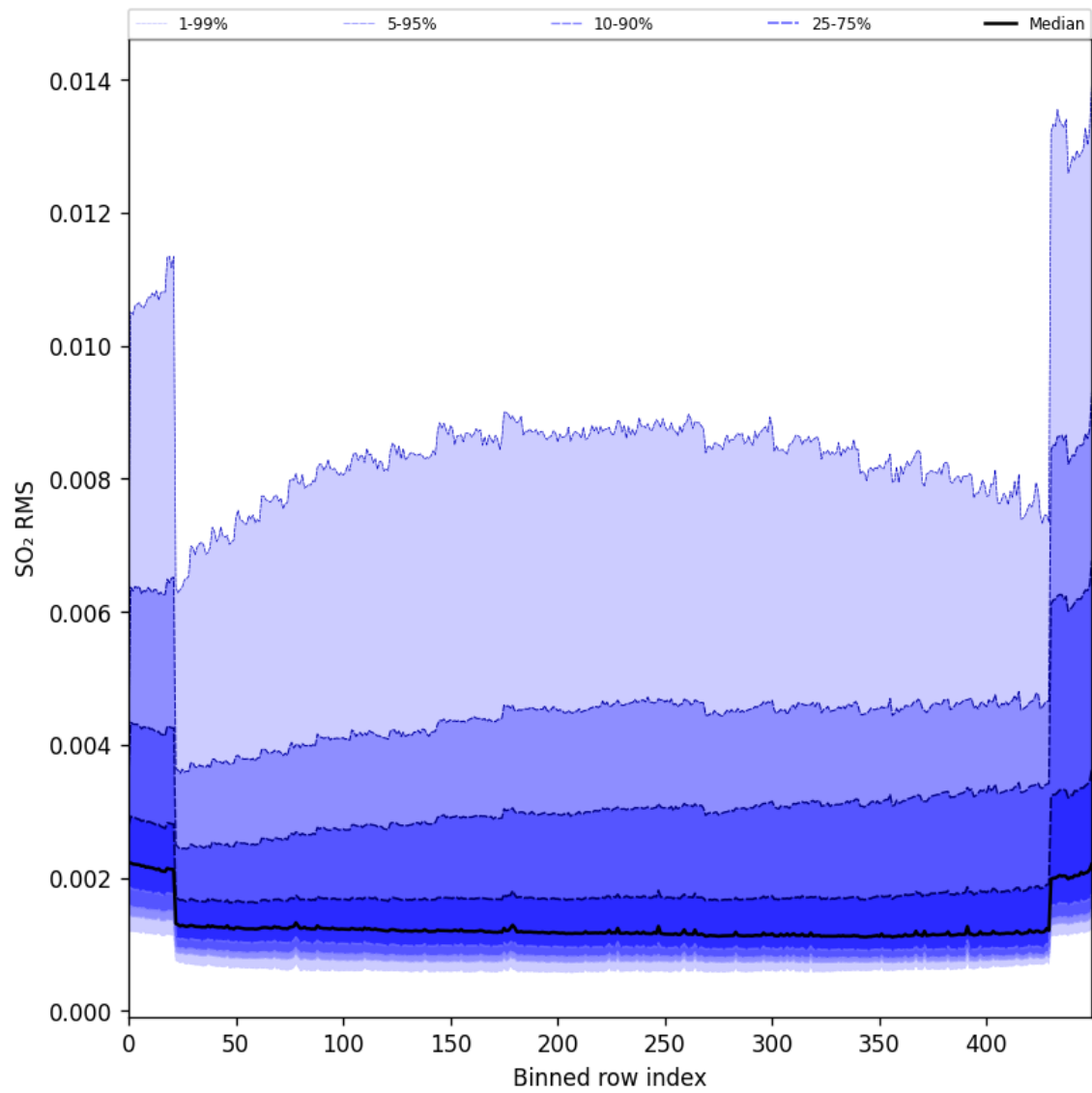
Figure 93: Along track statistics of “SO 2 RMS” for 2024-10-29 to 2024-10-30
