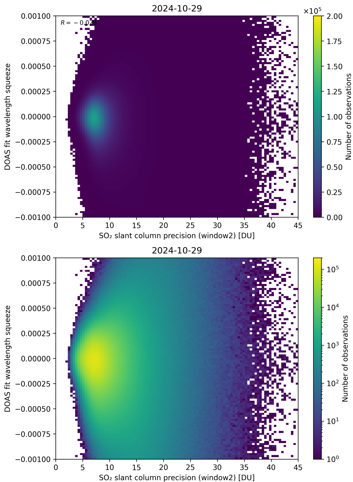
Figure 244: Scatter density plot of “SO 2 slant column precision (window2)” against “DOAS fit wavelength squeeze” for 2024-10-29 to 2024-10-30.
