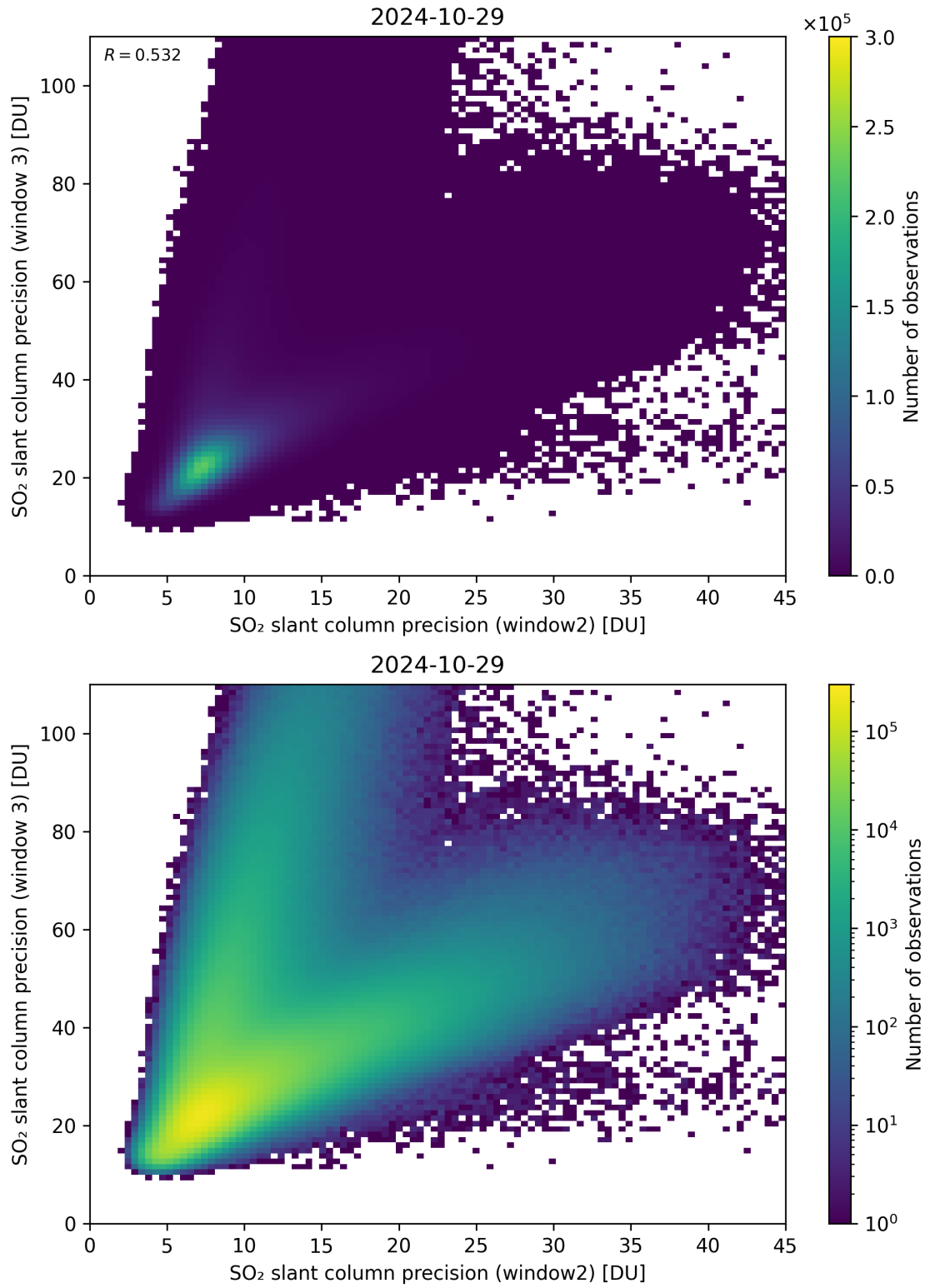
Figure 250: Scatter density plot of “SO 2 slant column precision (window2)” against “SO 2 slant column precision (window 3)” for 2024-10-29 to 2024-10-30.
