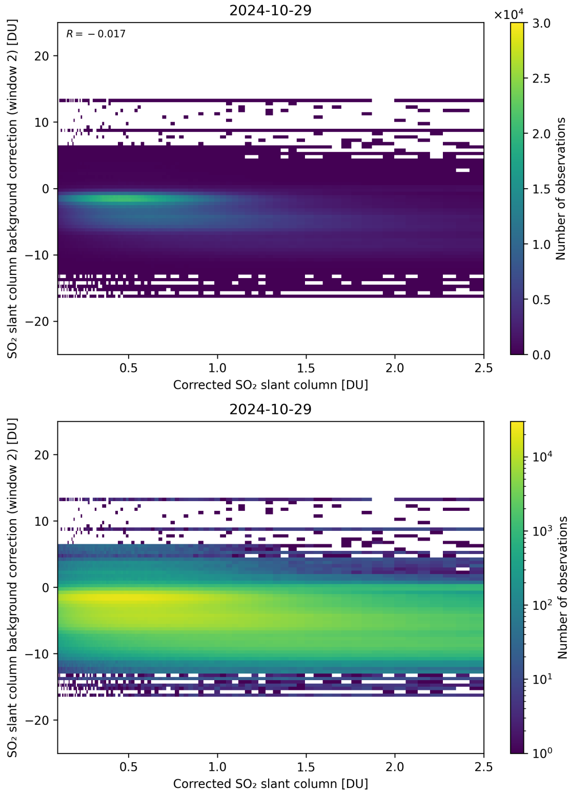
Figure 179: Scatter density plot of “Corrected SO 2 slant column” against “SO 2 slant column background correction (window 2)” for 2024-10-29 to 2024-10-30.
