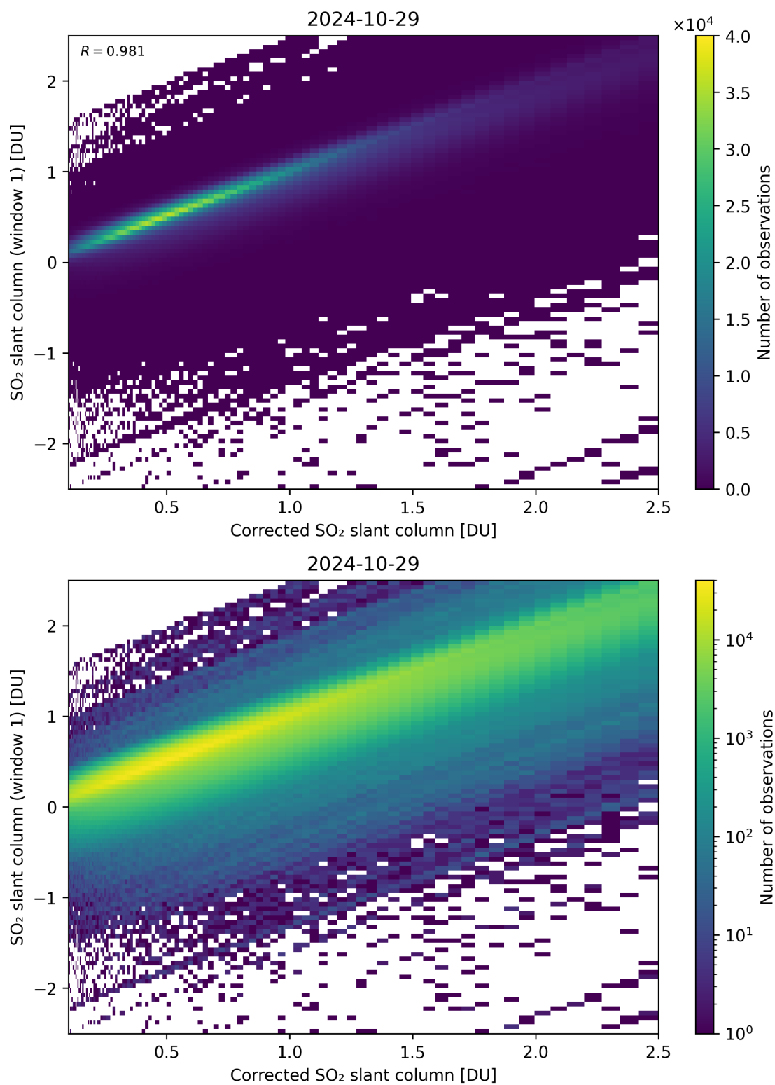
Figure 187: Scatter density plot of “Corrected SO 2 slant column” against “SO 2 slant column (window 1)” for 2024-10-29 to 2024-10-30.
