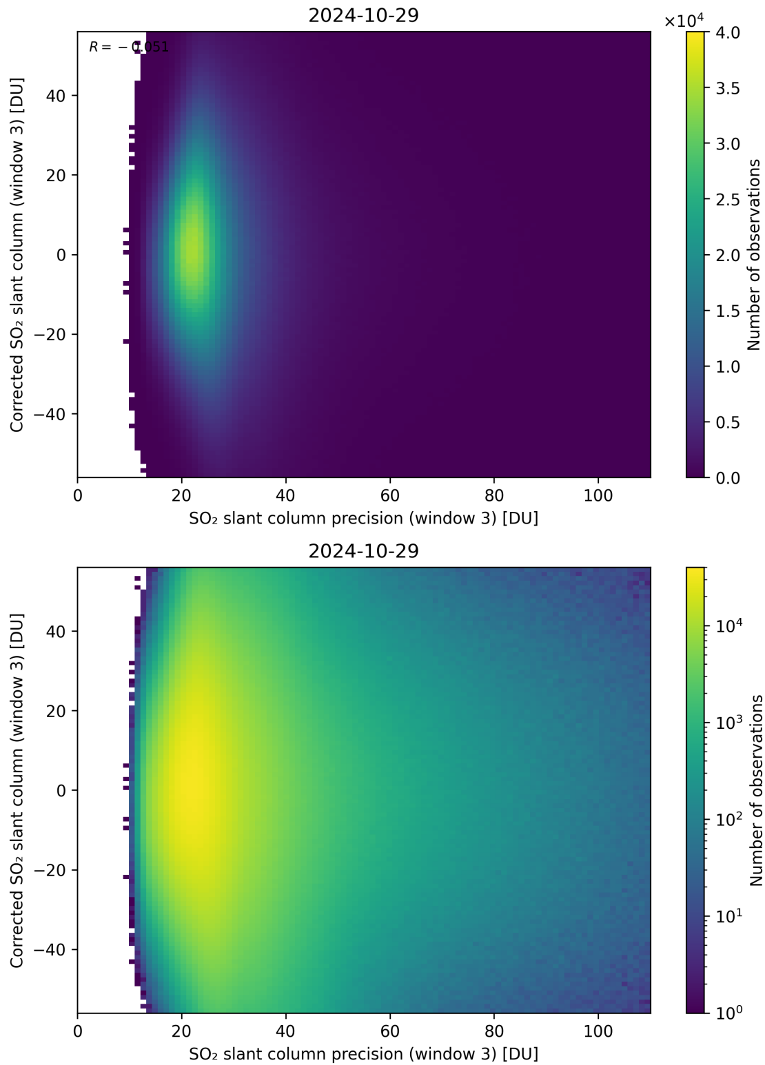
Figure 262: Scatter density plot of “SO 2 slant column precision (window 3)” against “Corrected SO 2 slant column (window 3)” for 2024-10-29 to 2024-10-30.
