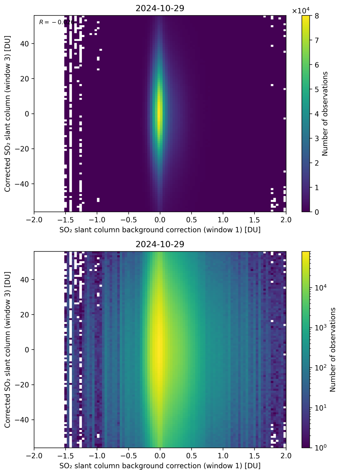
Figure 105: Scatter density plot of “SO 2 slant column background correction (window 1)” against “Corrected SO 2 slant column (window 3)” for 2024-10-29 to 2024-10-30.
