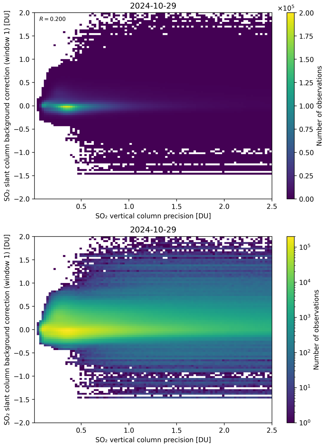
Figure 279: Scatter density plot of “SO 2 vertical column precision” against “SO 2 slant column background correction (window 1)” for 2024-10-29 to 2024-10-30.
