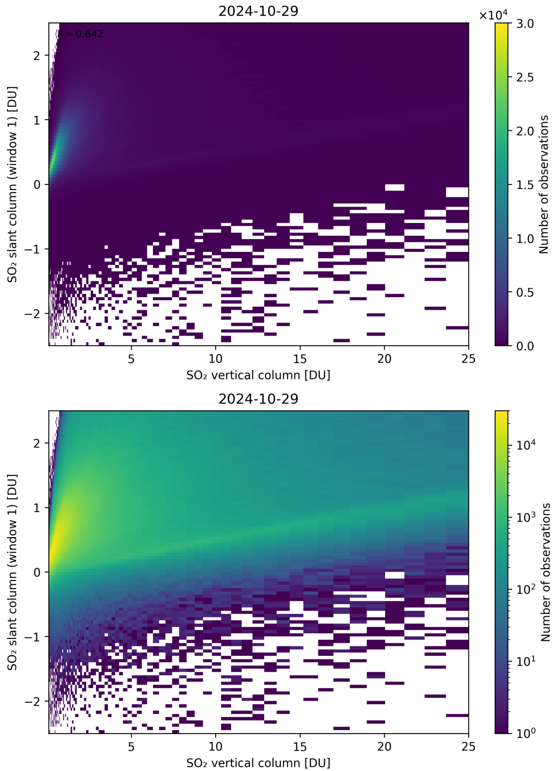
Figure 300: Scatter density plot of “SO 2 vertical column” against “SO 2 slant column (window 1)” for 2024-10-29 to 2024-10-30.
