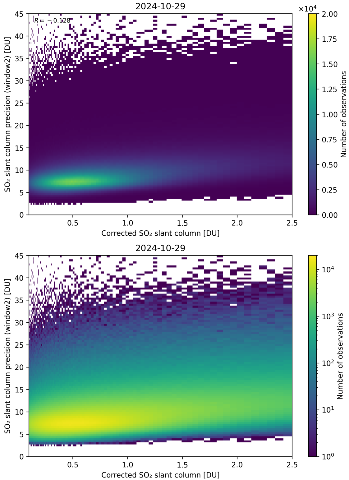
Figure 189: Scatter density plot of “Corrected SO 2 slant column” against “SO 2 slant column precision (window2)” for 2024-10-29 to 2024-10-30.
