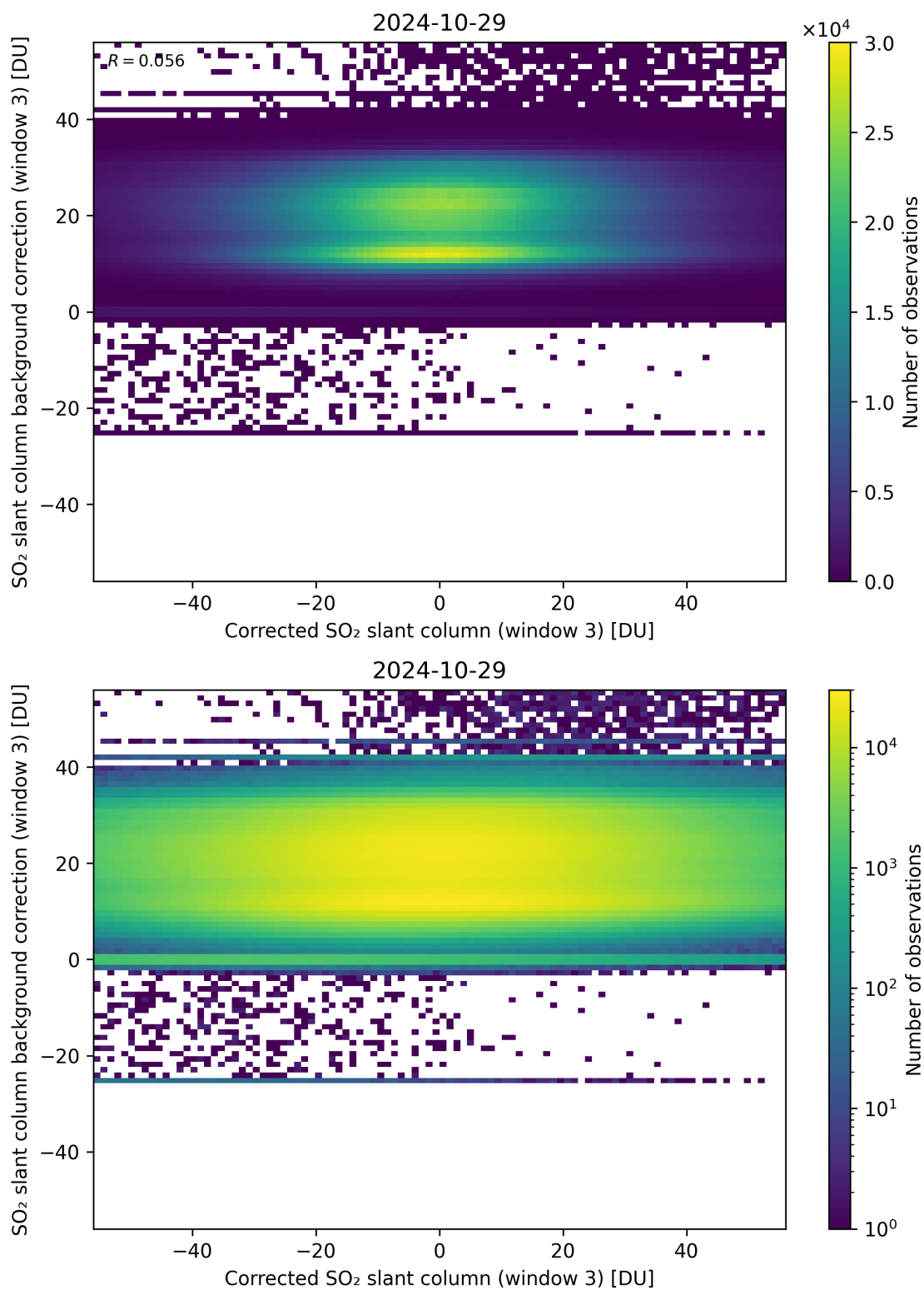
Figure 205: Scatter density plot of “Corrected SO 2 slant column (window 3)” against “SO 2 slant column background correction (window 3)” for 2024-10-29 to 2024-10-30.
