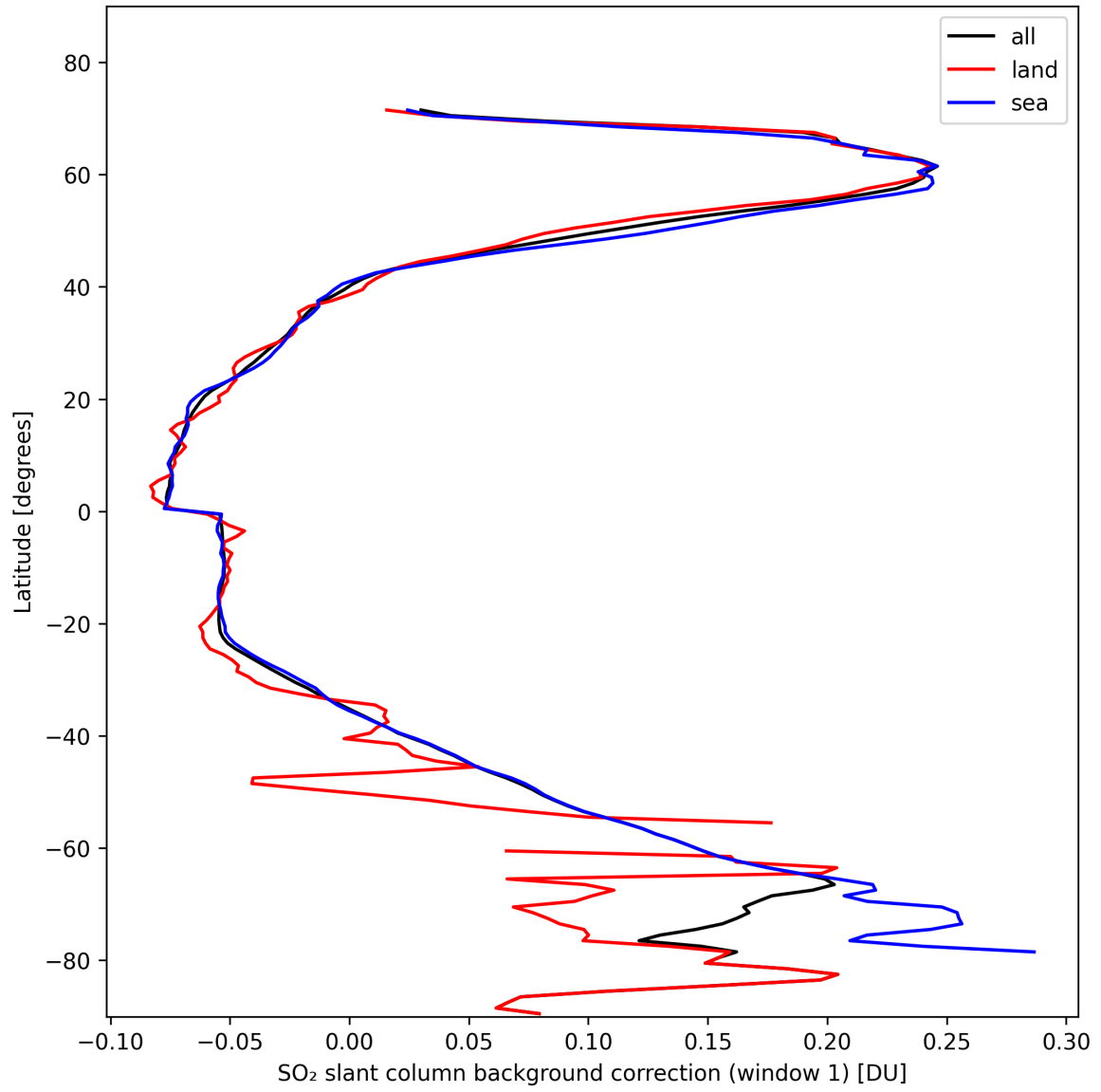
Figure 36: Zonal average of “SO 2 slant column background correction (window 1)” for 2024-10-29 to 2024-10-30.
