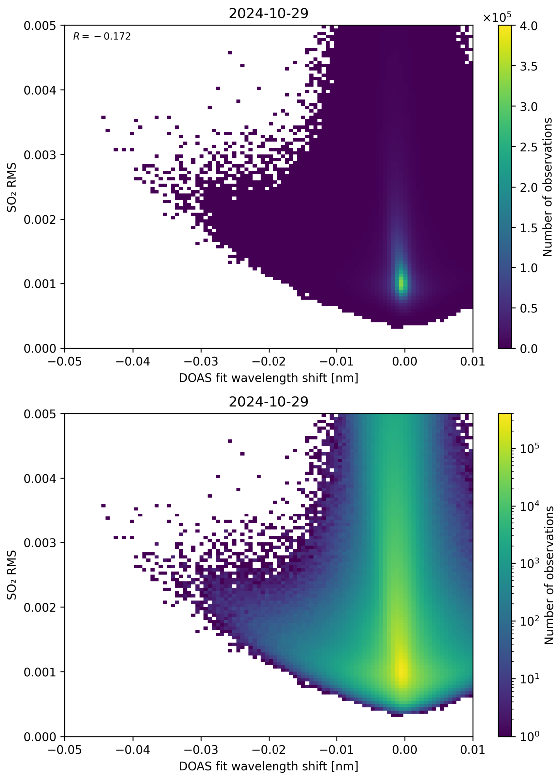
Figure 128: Scatter density plot of “DOAS fit wavelength shift” against “SO 2 RMS” for 2024-10-29 to 2024-10-30.
