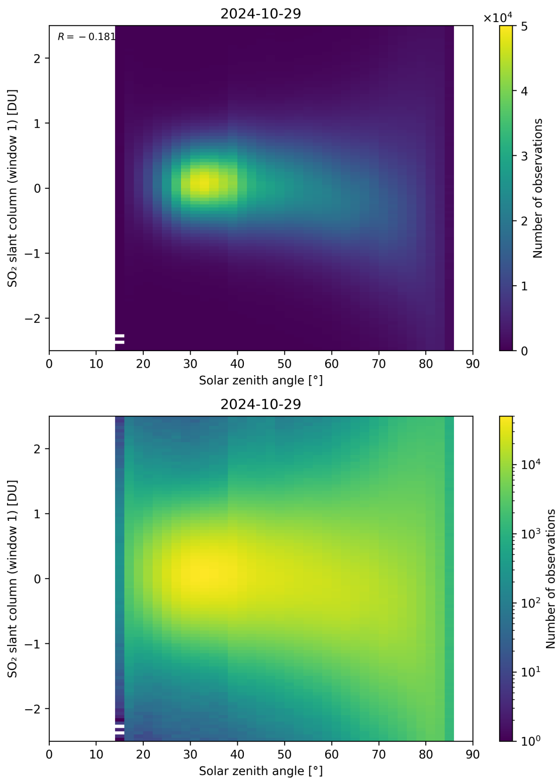
Figure 169: Scatter density plot of “Solar zenith angle” against “SO 2 slant column (window 1)” for 2024-10-29 to 2024-10-30.
