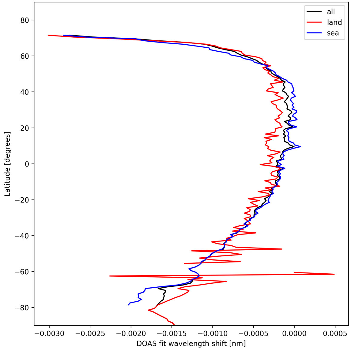
Figure 45: Zonal average of “DOAS fit wavelength shift” for 2024-10-29 to 2024-10-30.
