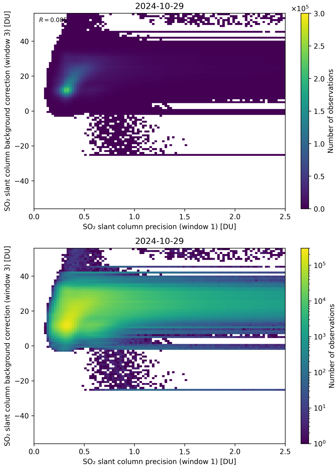
Figure 220: Scatter density plot of “SO 2 slant column precision (window 1)” against “SO 2 slant column background correction (window 3)” for 2024-10-29 to 2024-10-30.
