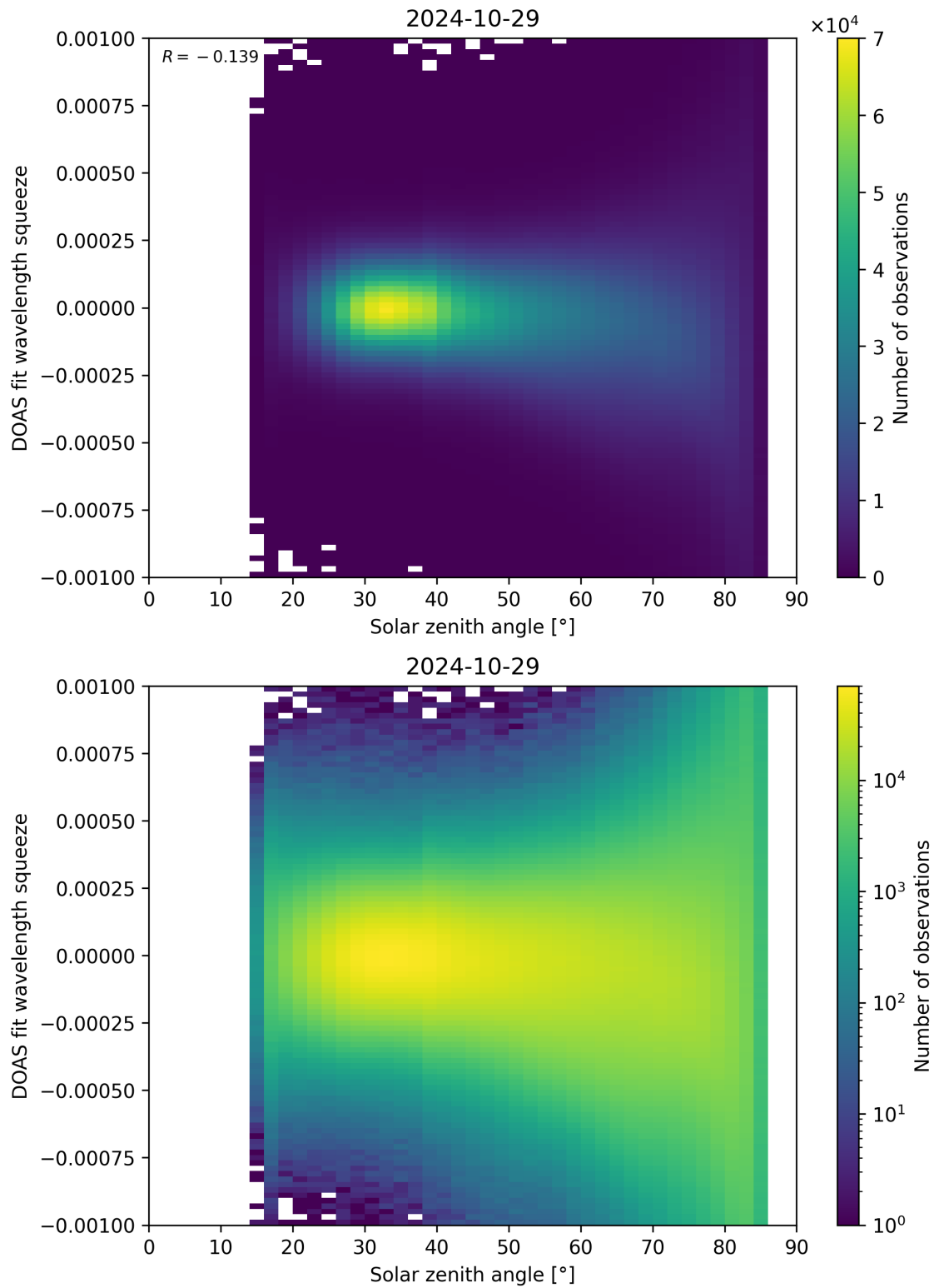
Figure 162: Scatter density plot of “Solar zenith angle” against “DOAS fit wavelength squeeze” for 2024-10-29 to 2024-10-30.
