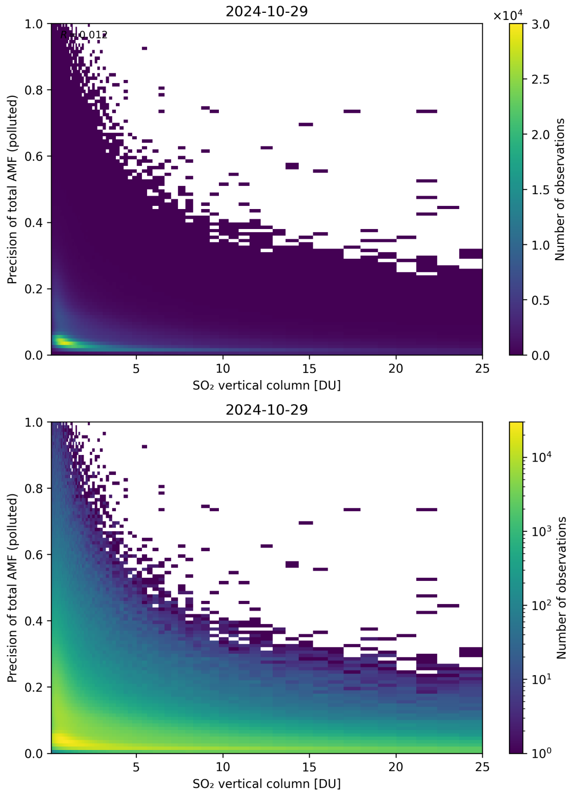
Figure 306: Scatter density plot of “SO 2 vertical column” against “Precision of total AMF (polluted)” for 2024-10-29 to 2024-10-30.
