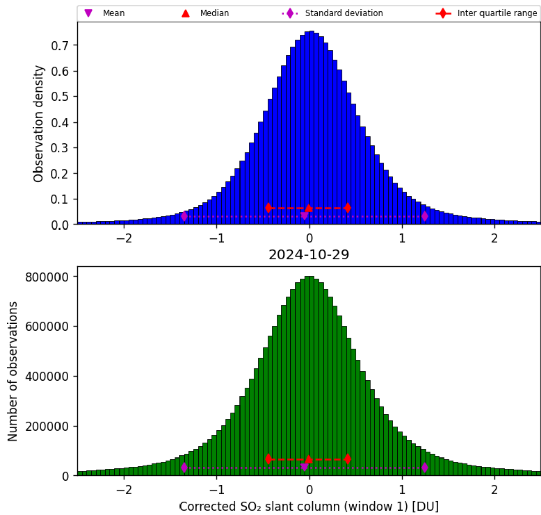
Figure 58: Histogram of “Corrected SO 2 slant column (window 1)” for 2024-10-29 to 2024-10-30
