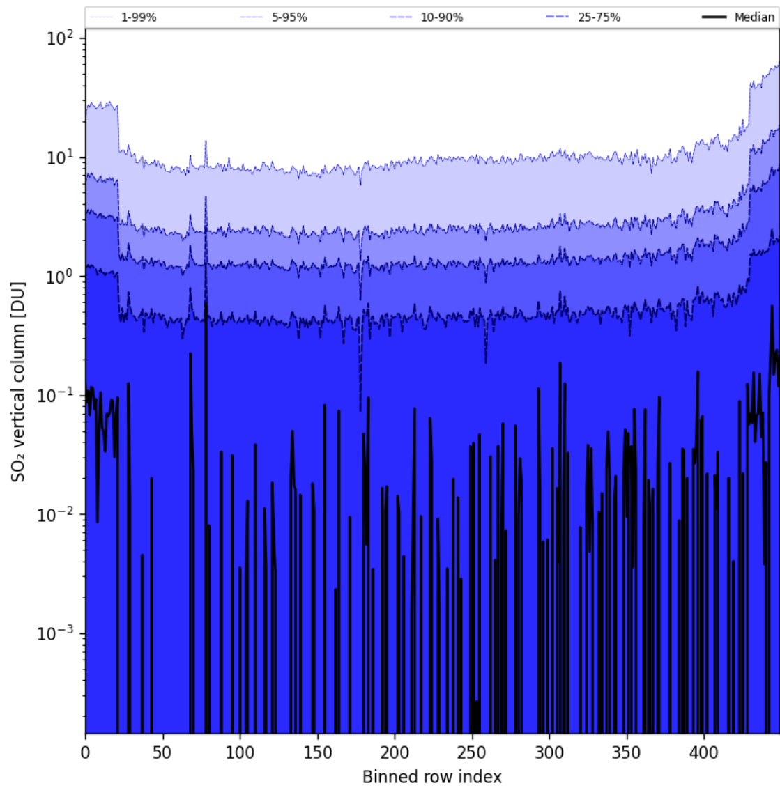
Figure 76: Along track statistics of “SO 2 vertical column” for 2024-10-29 to 2024-10-30
