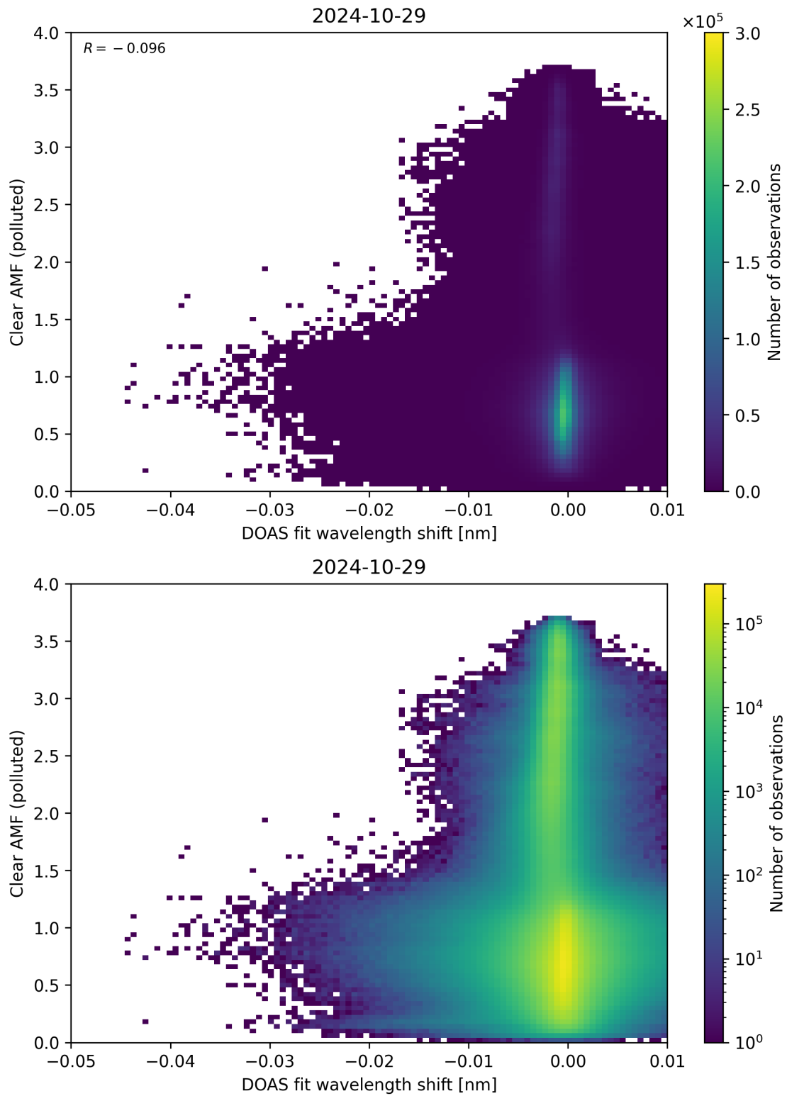
Figure 129: Scatter density plot of “DOAS fit wavelength shift” against “Clear AMF (polluted)” for 2024-10-29 to 2024-10-30.
