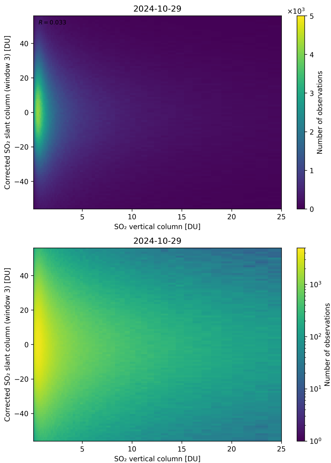
Figure 299: Scatter density plot of “SO 2 vertical column” against “Corrected SO 2 slant column (window 3)” for 2024-10-29 to 2024-10-30.
