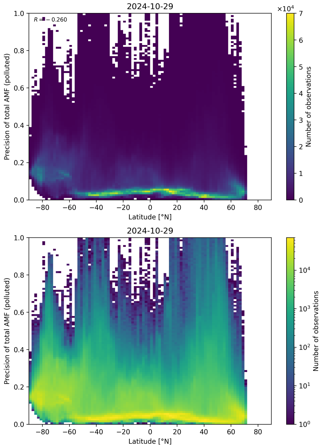
Figure 155: Scatter density plot of “Latitude” against “Precision of total AMF (polluted)” for 2024-10-29 to 2024-10-30.
