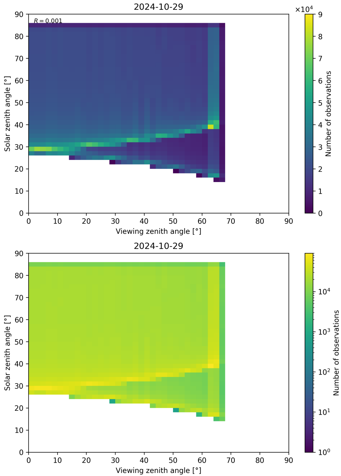
Figure 315: Scatter density plot of “Viewing zenith angle” against “Solar zenith angle” for 2024-10-29 to 2024-10-30.
