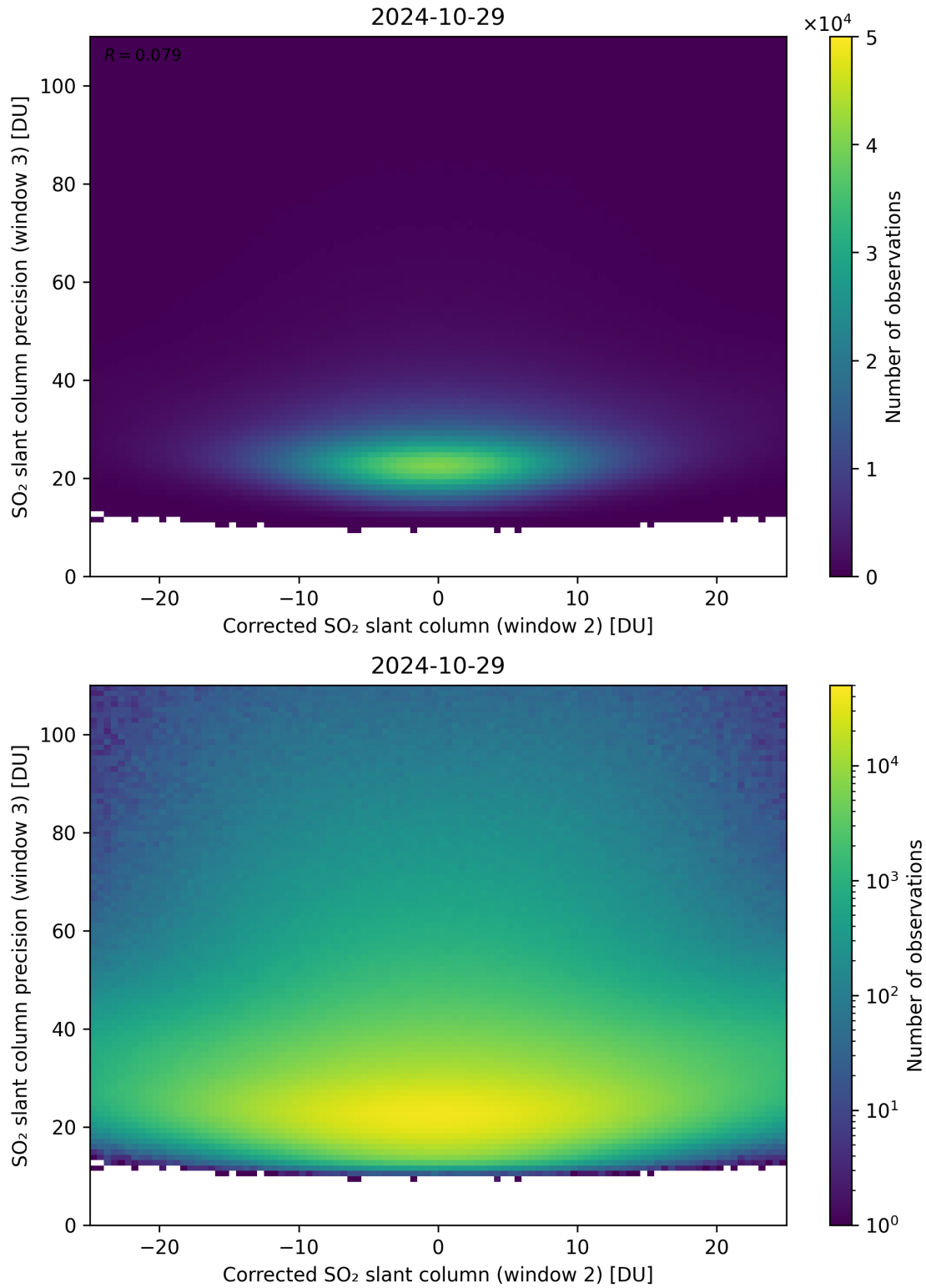
Figure 202: Scatter density plot of “Corrected SO 2 slant column (window 2)” against “SO 2 slant column precision (window 3)” for 2024-10-29 to 2024-10-30.
