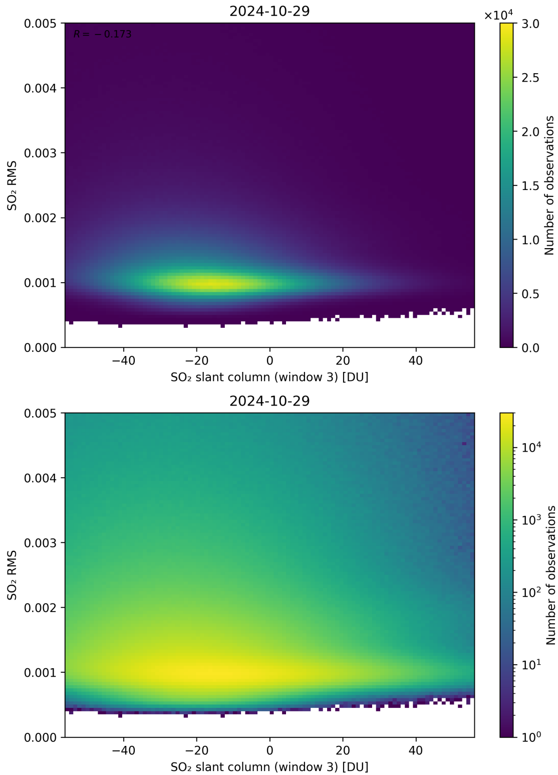
Figure 256: Scatter density plot of “SO 2 slant column (window 3)” against “SO 2 RMS” for 2024-10-29 to 2024-10-30.
