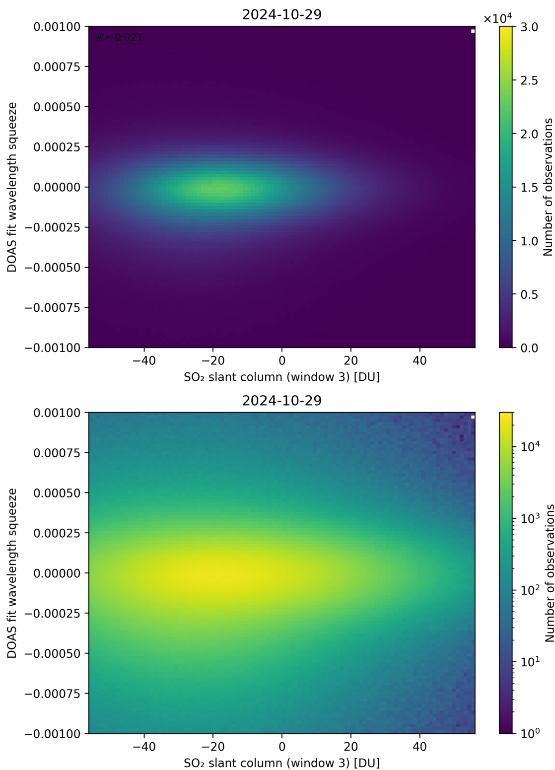
Figure 255: Scatter density plot of “SO 2 slant column (window 3)” against “DOAS fit wavelength squeeze” for 2024-10-29 to 2024-10-30.
