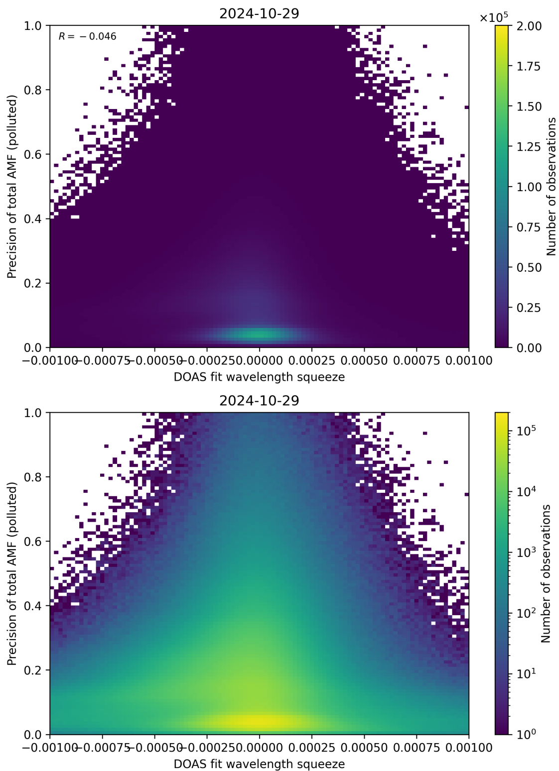
Figure 135: Scatter density plot of “DOAS fit wavelength squeeze” against “Precision of total AMF (polluted)” for 2024-10-29 to 2024-10-30.
