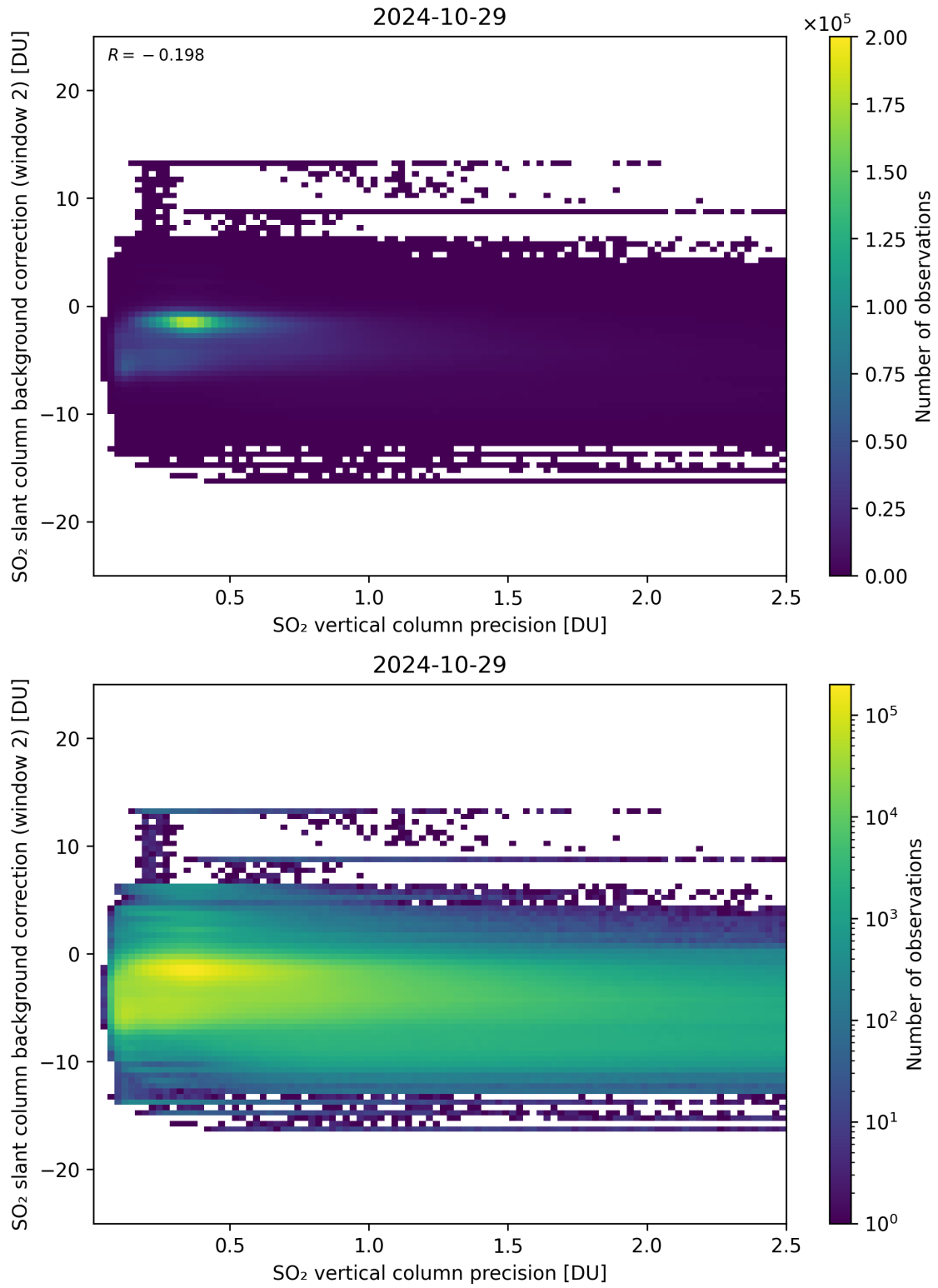
Figure 280: Scatter density plot of “SO 2 vertical column precision” against “SO 2 slant column background correction (window 2)” for 2024-10-29 to 2024-10-30.
