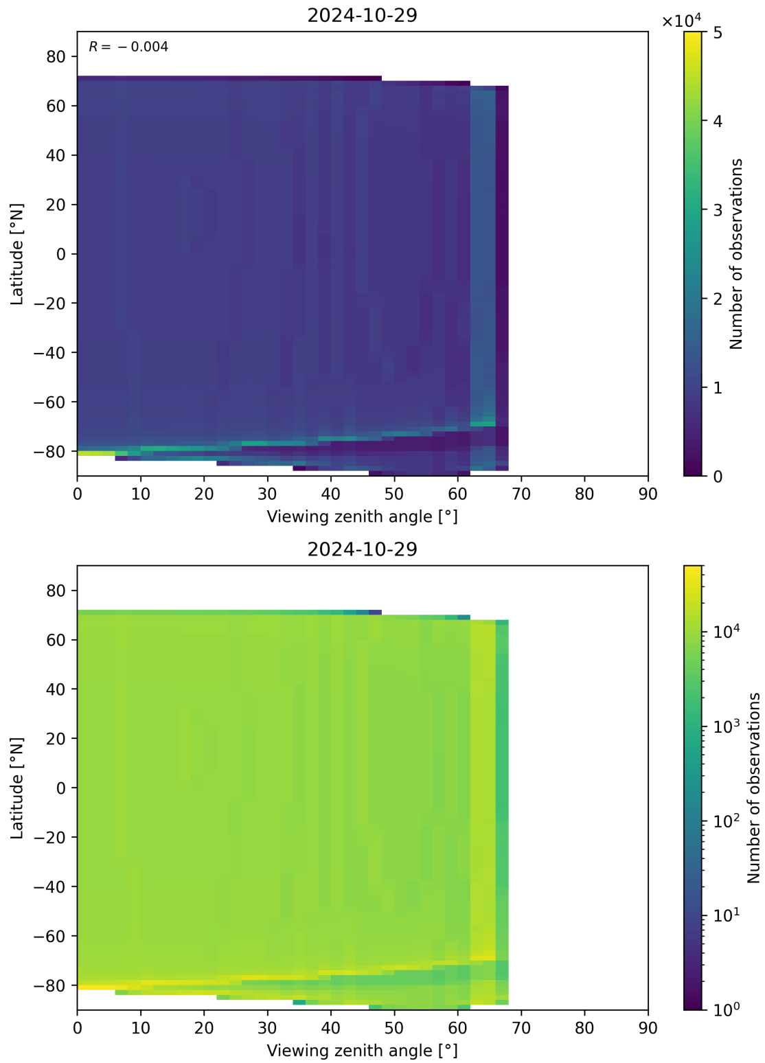
Figure 314: Scatter density plot of “Viewing zenith angle” against “Latitude” for 2024-10-29 to 2024-10-30.
