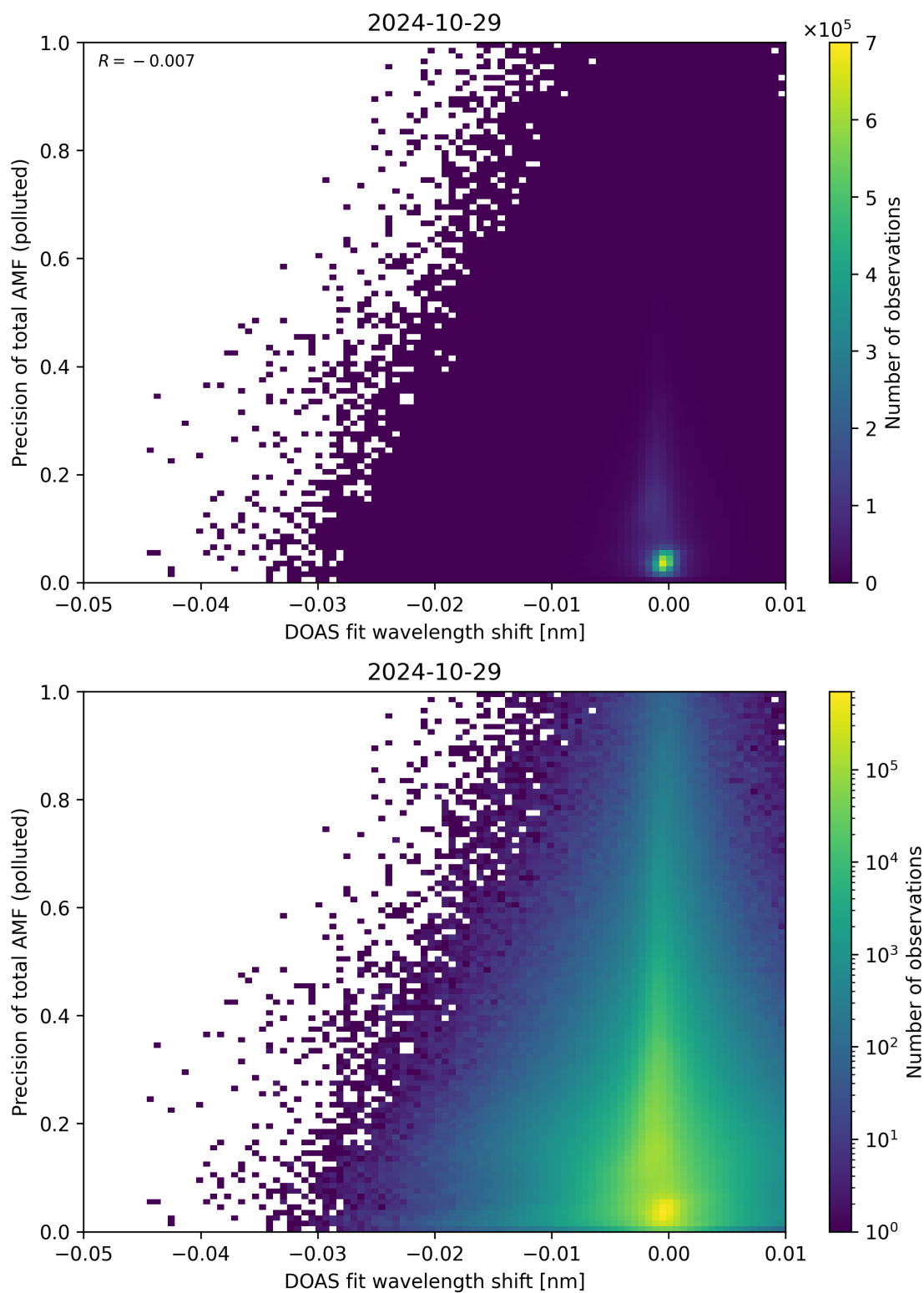
Figure 131: Scatter density plot of “DOAS fit wavelength shift” against “Precision of total AMF (polluted)” for 2024-10-29 to 2024-10-30.
