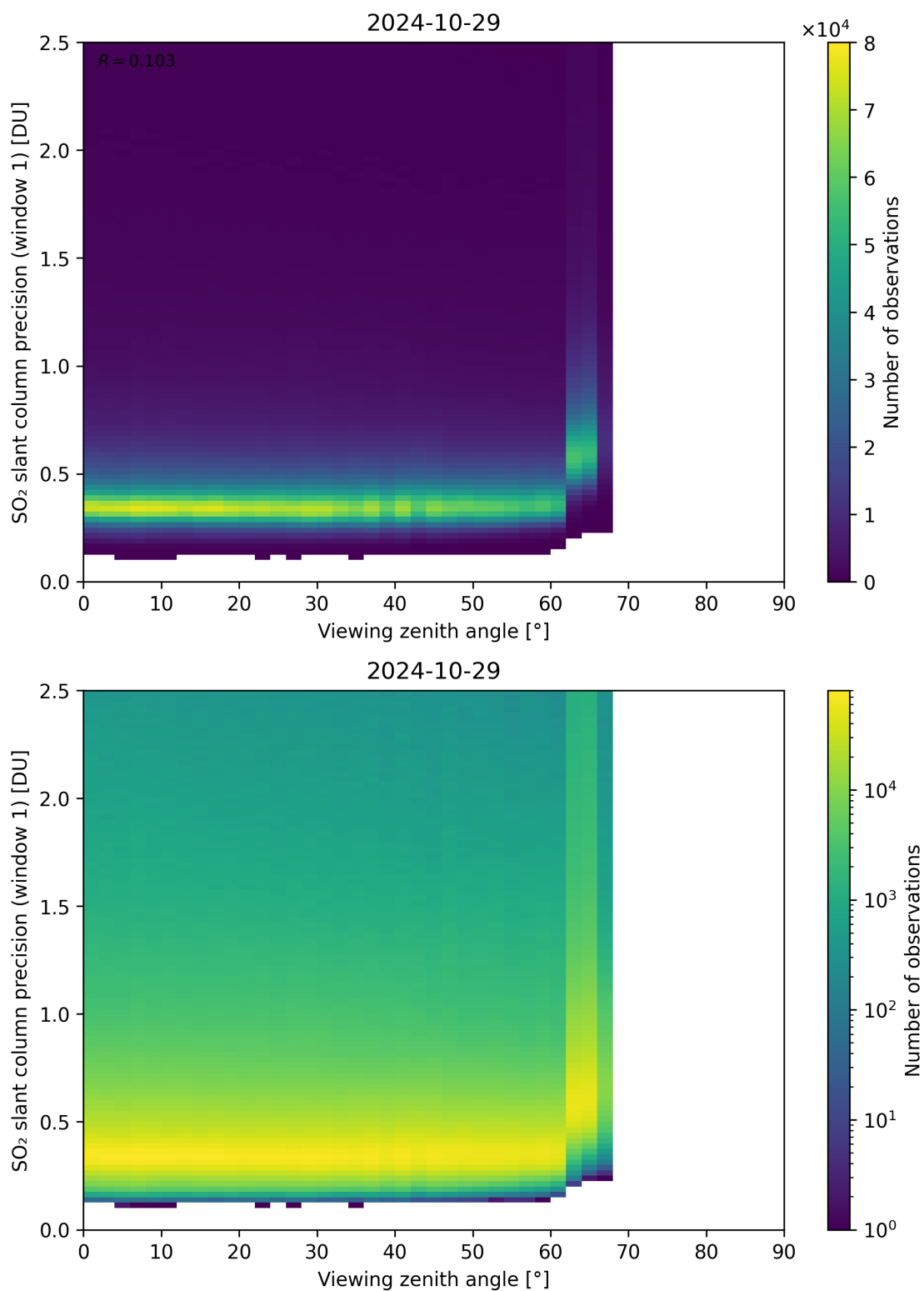
Figure 321: Scatter density plot of “Viewing zenith angle” against “SO 2 slant column precision (window 1)” for 2024-10-29 to 2024-10-30.
