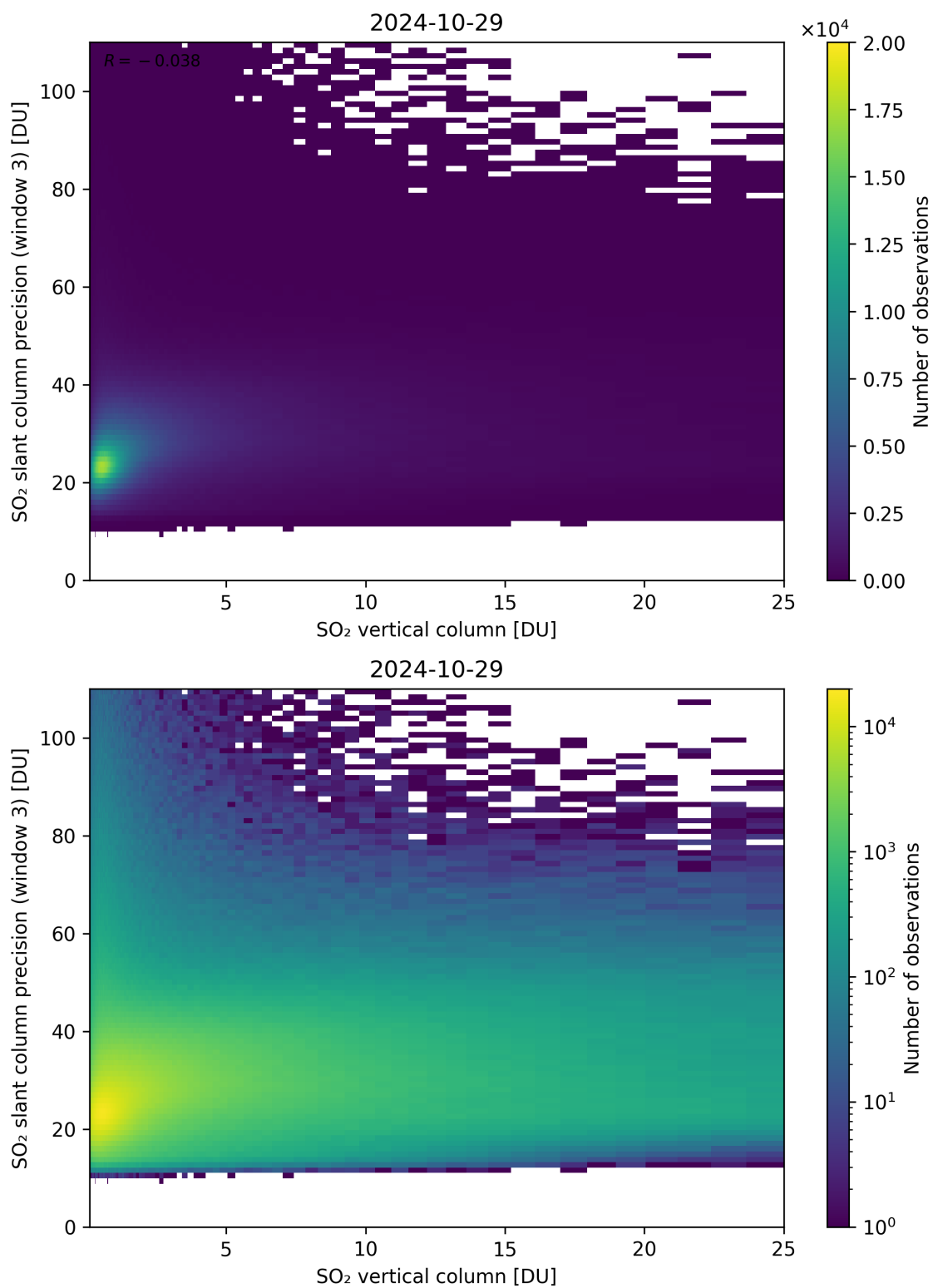
Figure 304: Scatter density plot of “SO 2 vertical column” against “SO 2 slant column precision (window 3)” for 2024-10-29 to 2024-10-30.
