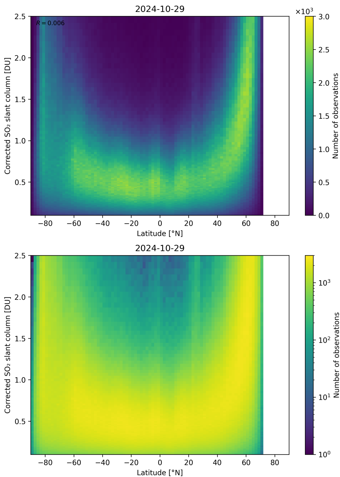
Figure 146: Scatter density plot of “Latitude” against “Corrected SO 2 slant column” for 2024-10-29 to 2024-10-30.
