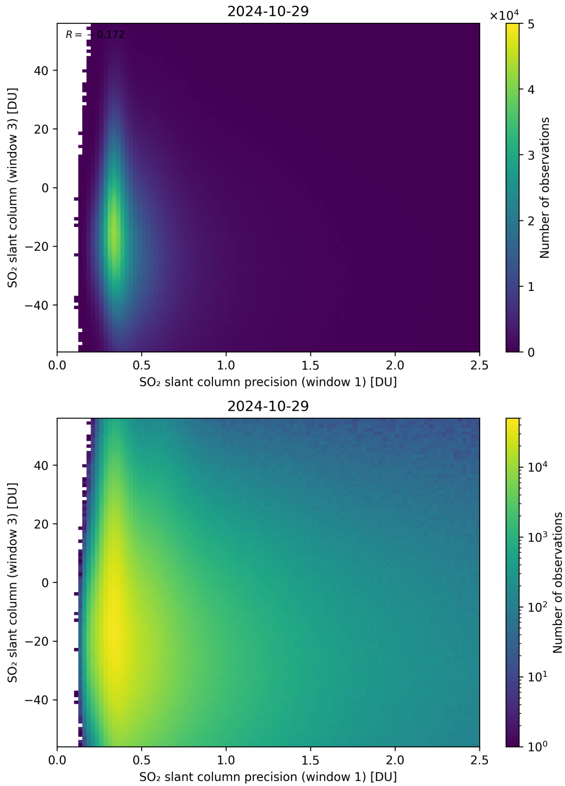
Figure 228: Scatter density plot of “SO 2 slant column precision (window 1)” against “SO 2 slant column (window 3)” for 2024-10-29 to 2024-10-30.
