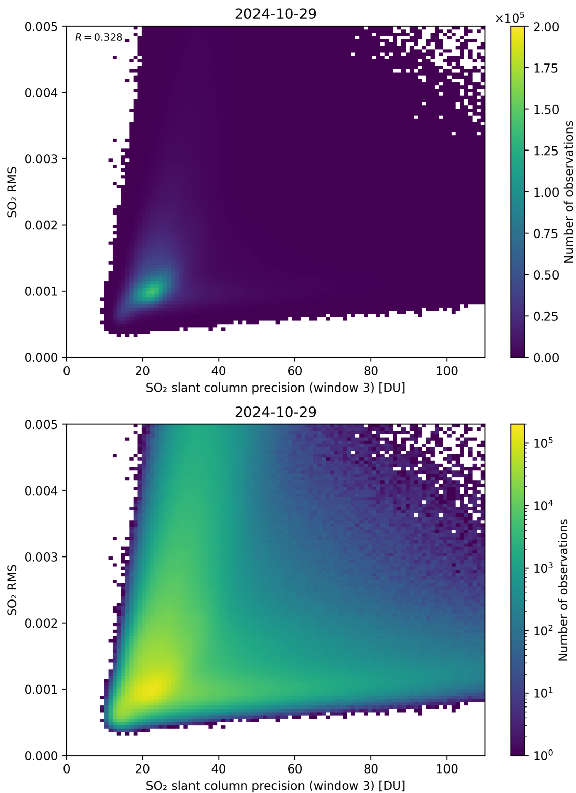
Figure 260: Scatter density plot of “SO 2 slant column precision (window 3)” against “SO 2 RMS” for 2024-10-29 to 2024-10-30.
