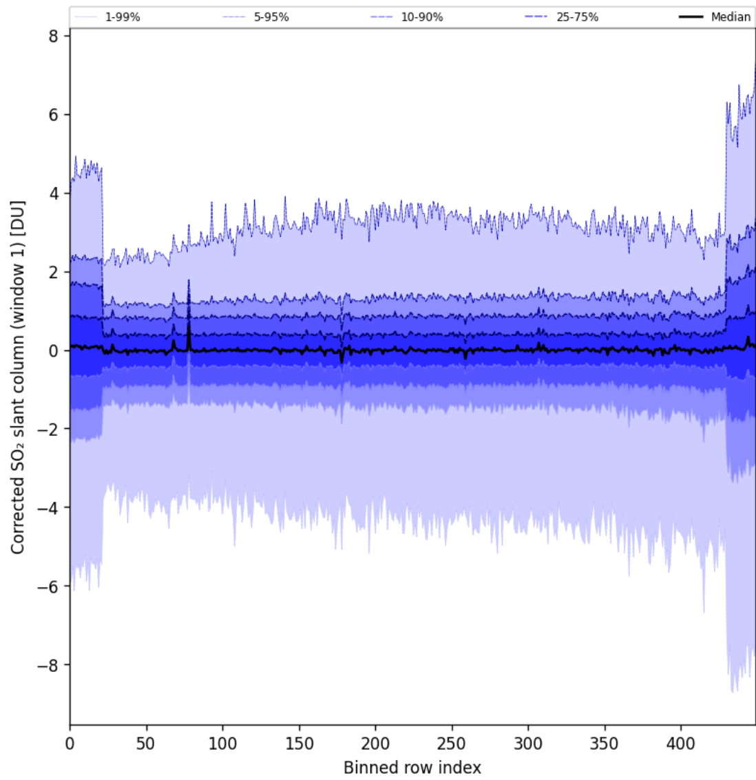
Figure 81: Along track statistics of “Corrected SO 2 slant column (window 1)” for 2024-10-29 to 2024-10-30
