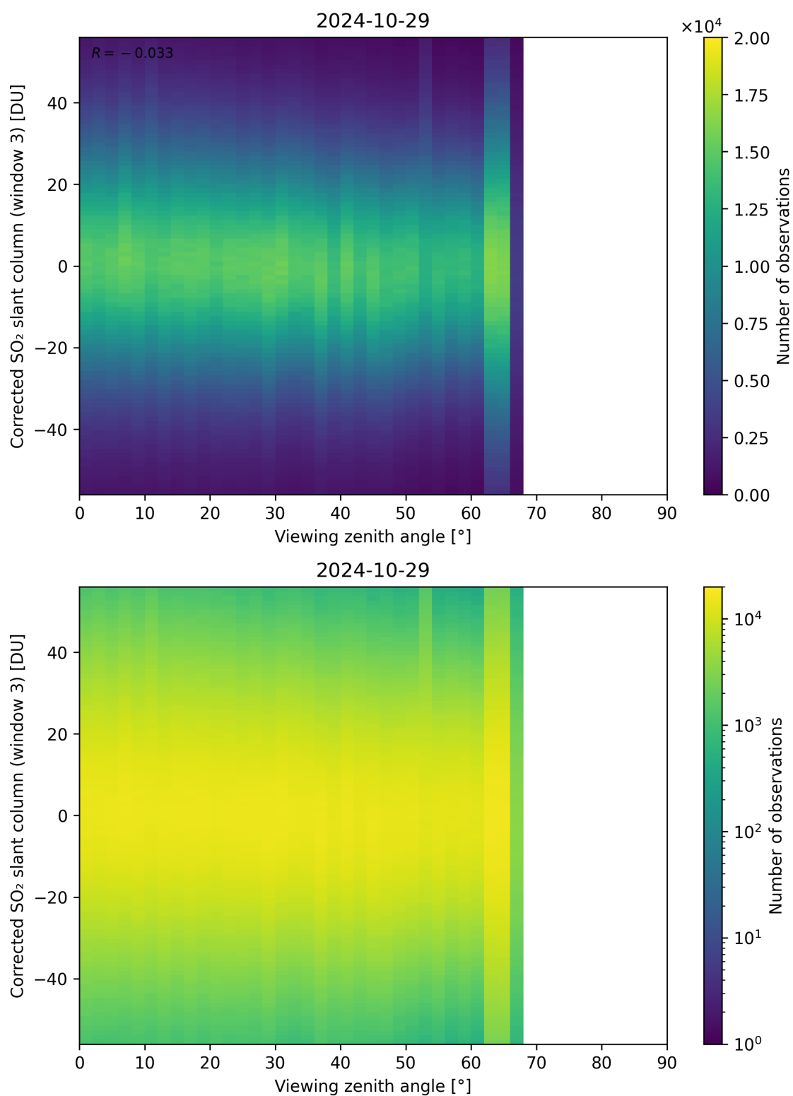
Figure 319: Scatter density plot of “Viewing zenith angle” against “Corrected SO 2 slant column (window 3)” for 2024-10-29 to 2024-10-30.
