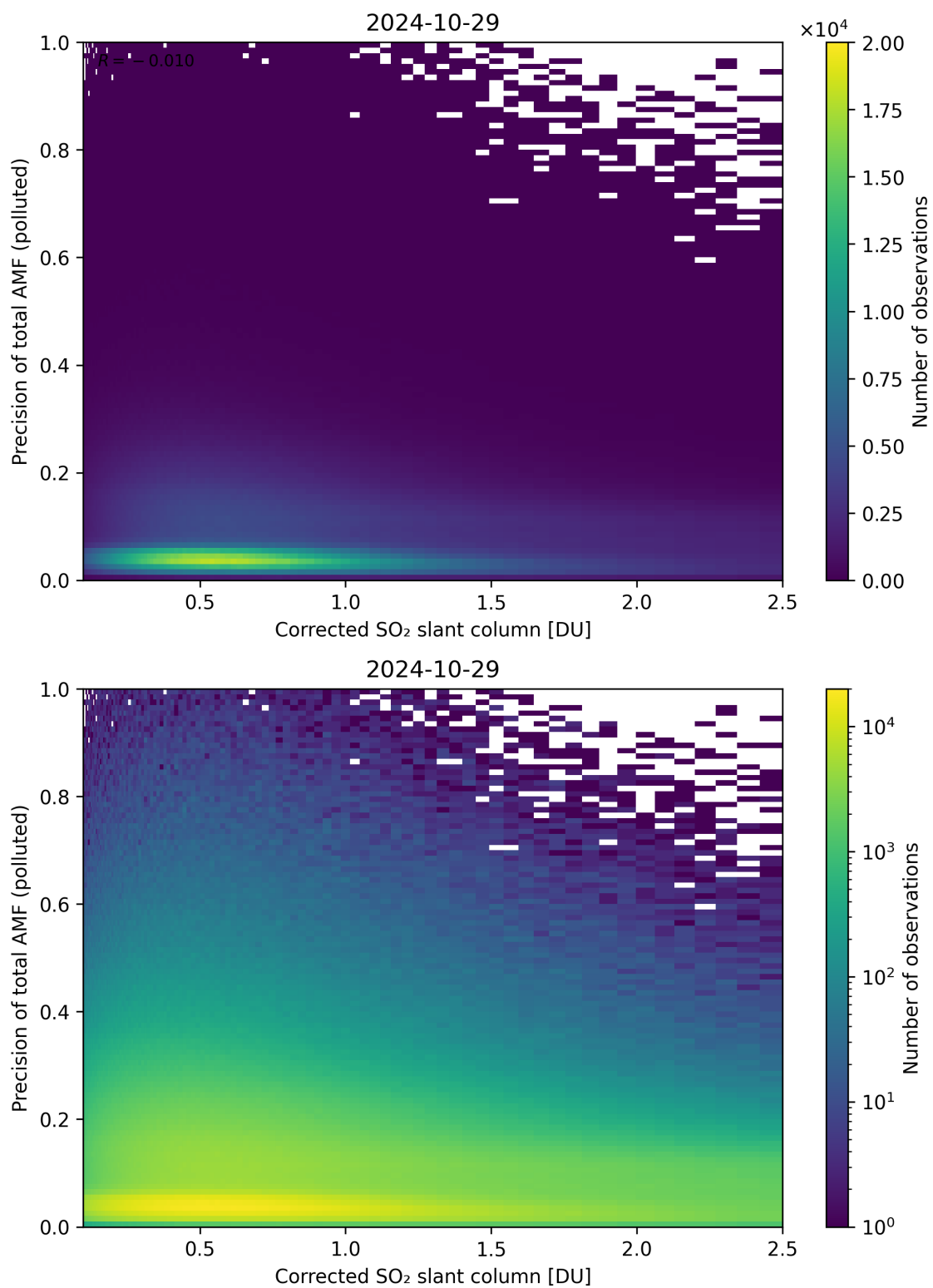
Figure 193: Scatter density plot of “Corrected SO 2 slant column” against “Precision of total AMF (polluted)” for 2024-10-29 to 2024-10-30.
