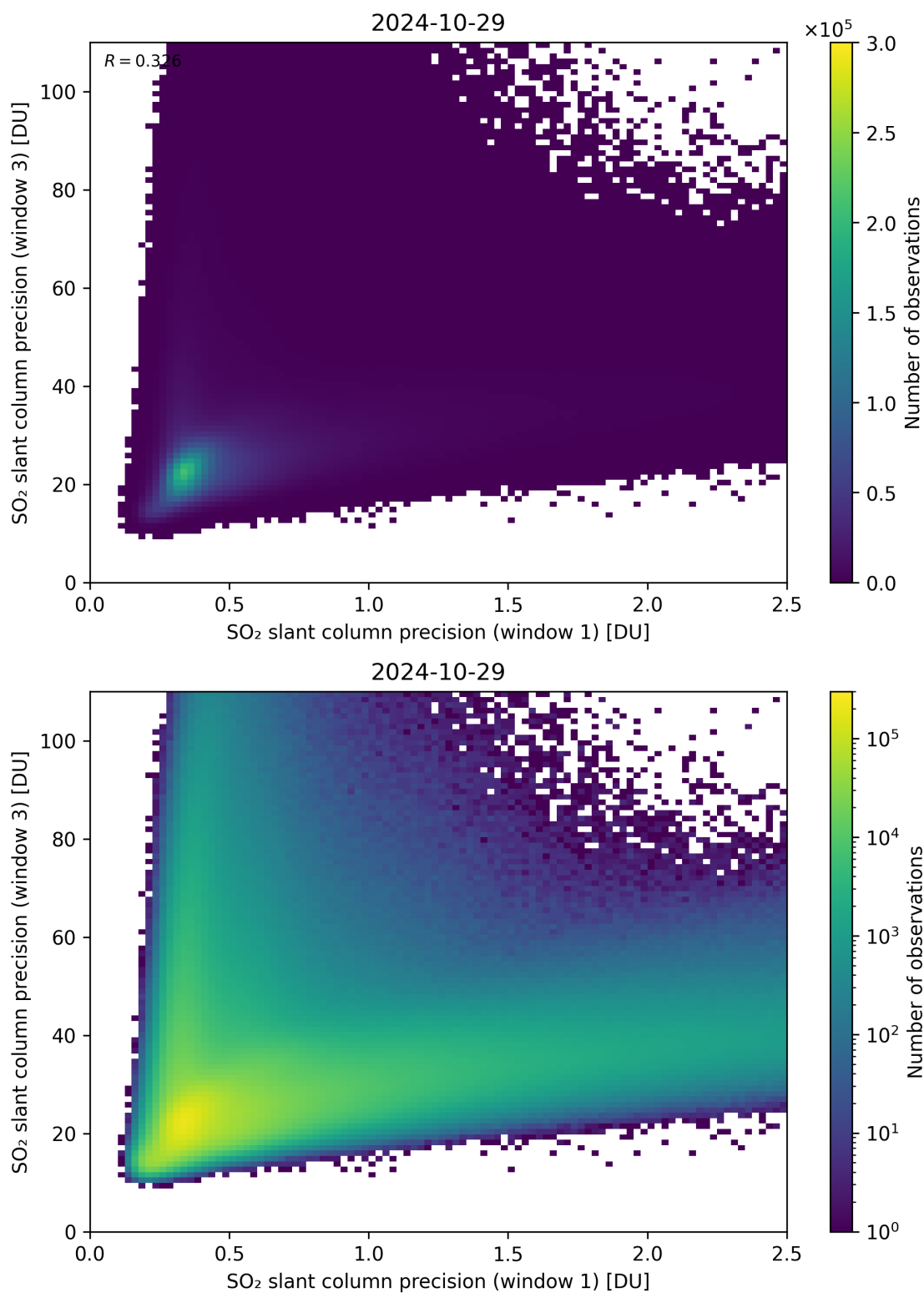
Figure 229: Scatter density plot of “SO 2 slant column precision (window 1)” against “SO 2 slant column precision (window 3)” for 2024-10-29 to 2024-10-30.
