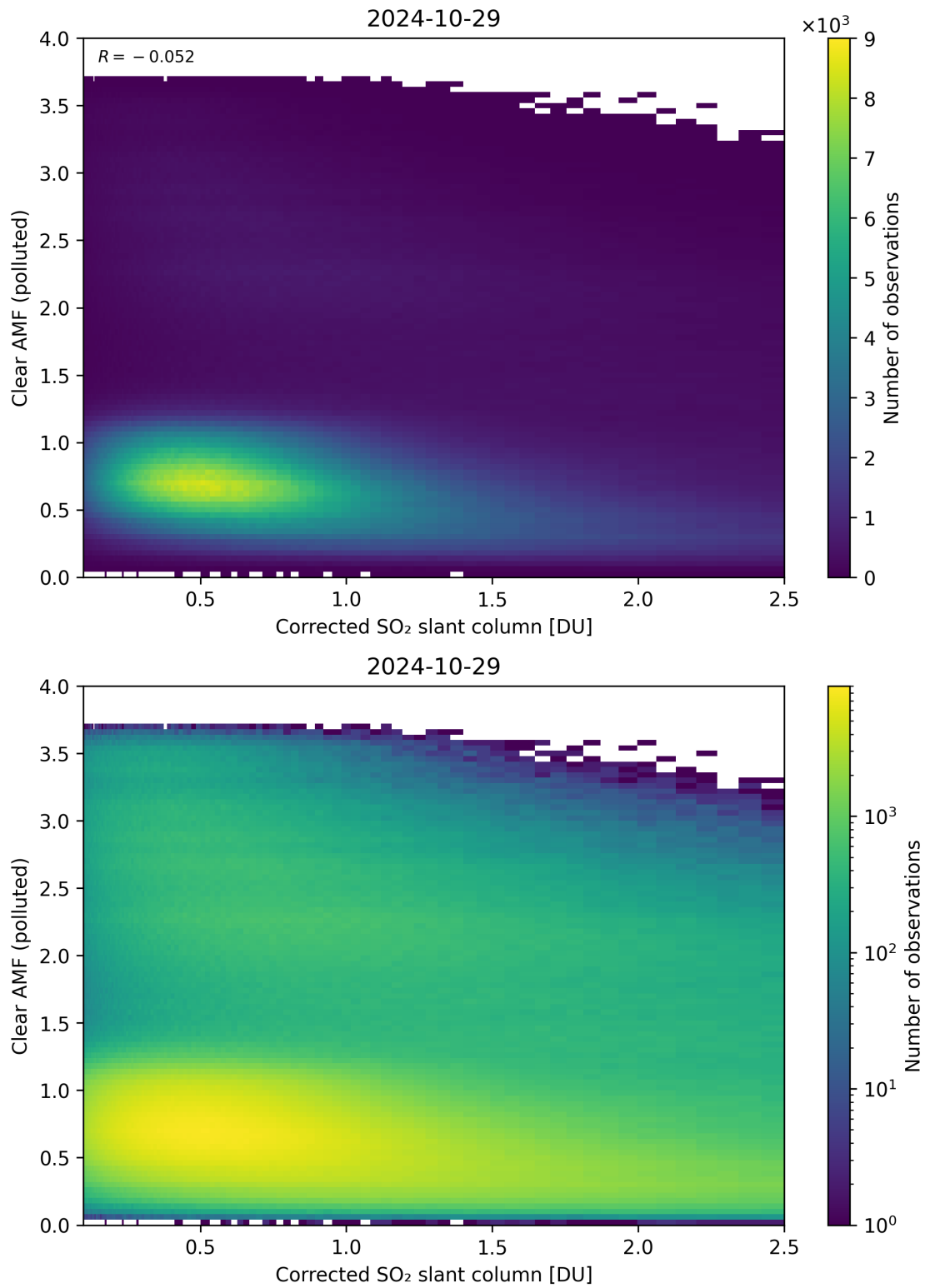
Figure 184: Scatter density plot of “Corrected SO 2 slant column” against “Clear AMF (polluted)” for 2024-10-29 to 2024-10-30.
