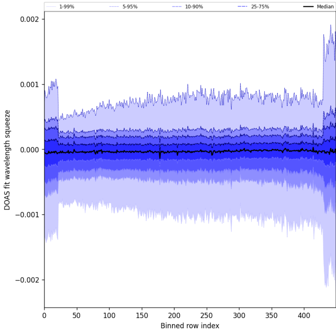
Figure 92: Along track statistics of “DOAS fit wavelength squeeze” for 2024-10-29 to 2024-10-30
