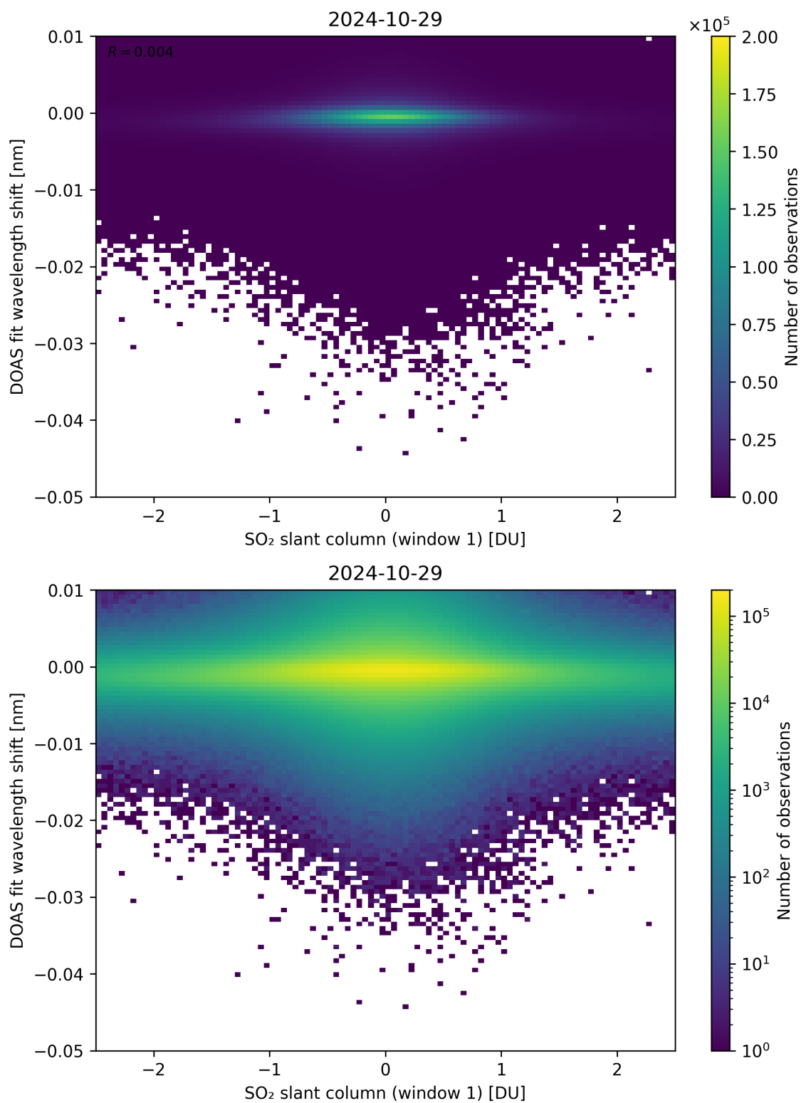
Figure 215: Scatter density plot of “SO 2 slant column (window 1)” against “DOAS fit wavelength shift” for 2024-10-29 to 2024-10-30.
