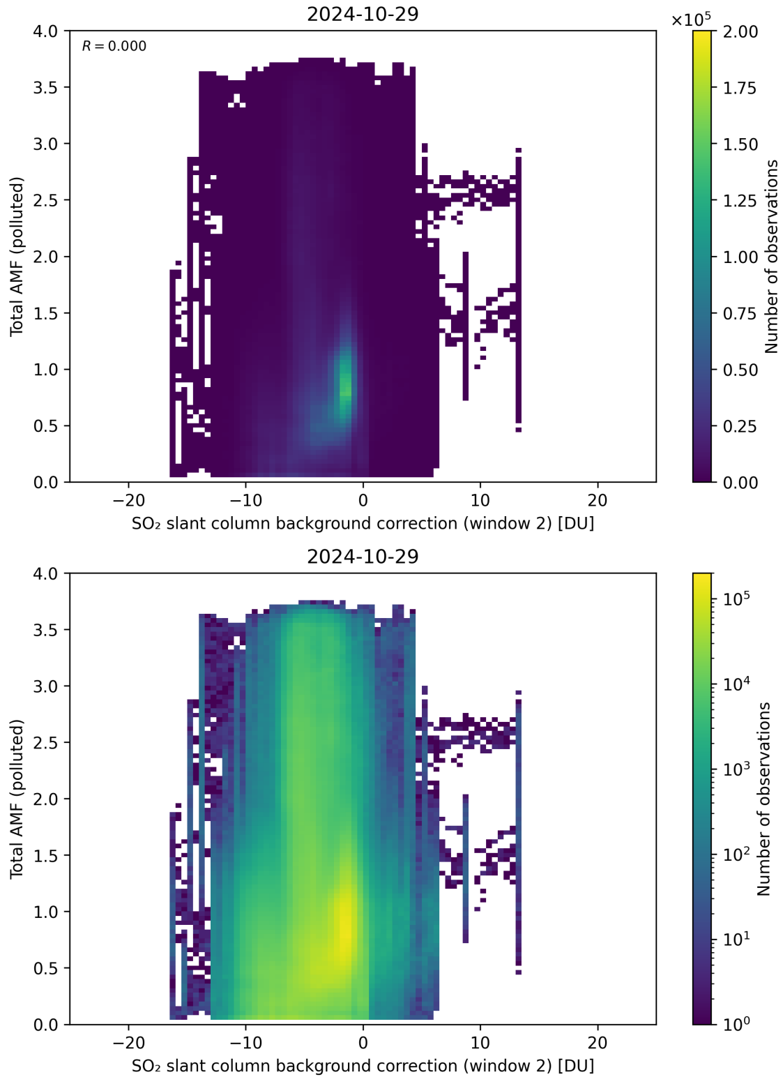
Figure 119: Scatter density plot of “SO 2 slant column background correction (window 2)” against “Total AMF (polluted)” for 2024-10-29 to 2024-10-30.
