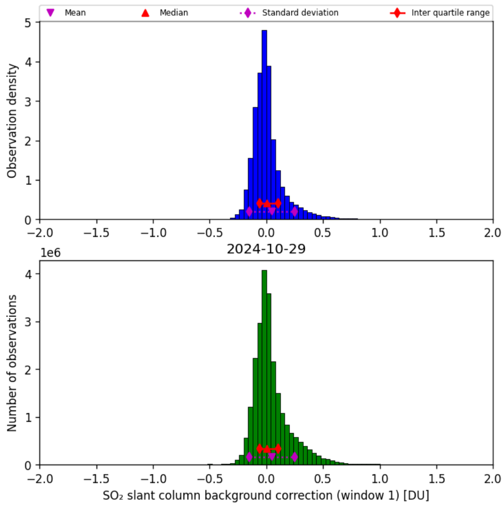
Figure 59: Histogram of “SO 2 slant column background correction (window 1)” for 2024-10-29 to 2024-10-30
