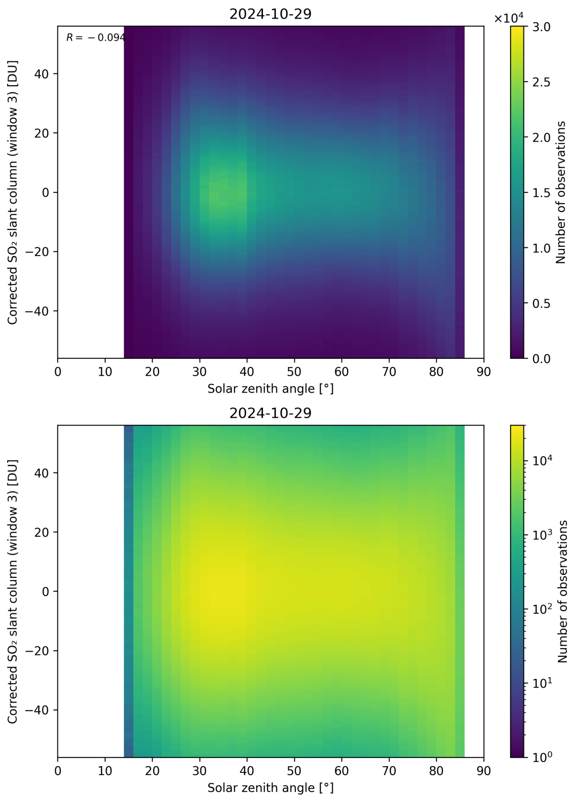
Figure 168: Scatter density plot of “Solar zenith angle” against “Corrected SO 2 slant column (window 3)” for 2024-10-29 to 2024-10-30.
