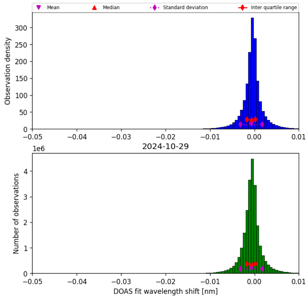
Figure 68: Histogram of “DOAS fit wavelength shift” for 2024-10-29 to 2024-10-30
