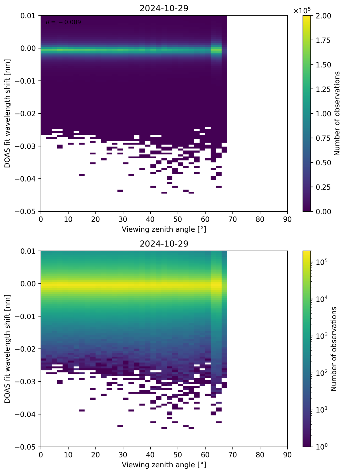
Figure 311: Scatter density plot of “Viewing zenith angle” against “DOAS fit wavelength shift” for 2024-10-29 to 2024-10-30.
