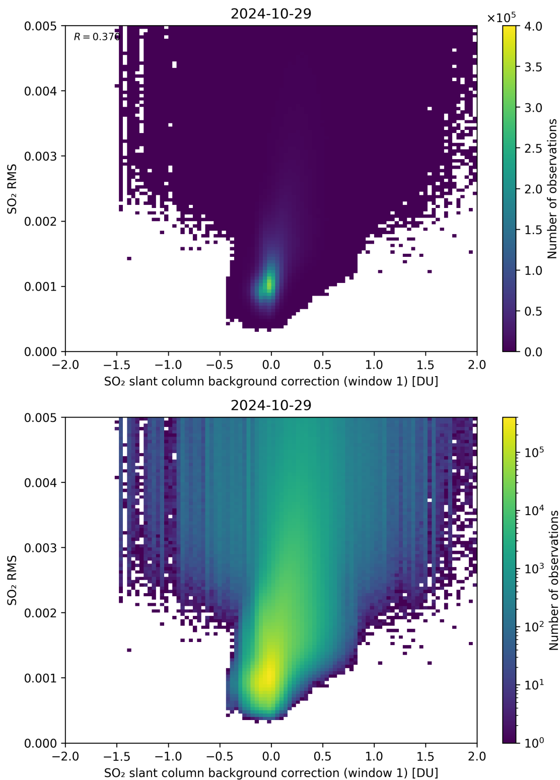
Figure 102: Scatter density plot of “SO 2 slant column background correction (window 1)” against “SO 2 RMS” for 2024-10-29 to 2024-10-30.
