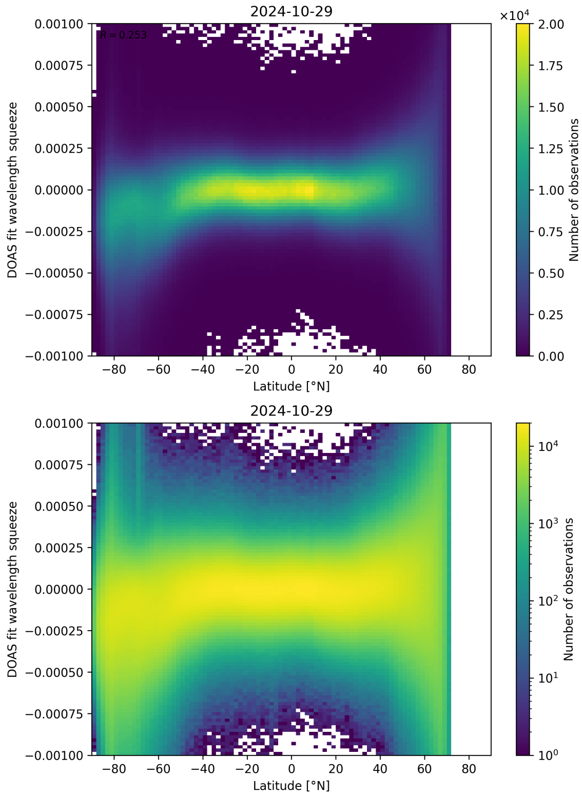
Figure 143: Scatter density plot of “Latitude” against “DOAS fit wavelength squeeze” for 2024-10-29 to 2024-10-30.
