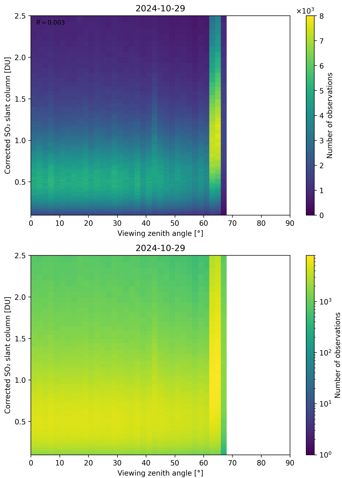
Figure 317: Scatter density plot of “Viewing zenith angle” against “Corrected SO 2 slant column” for 2024-10-29 to 2024-10-30.
