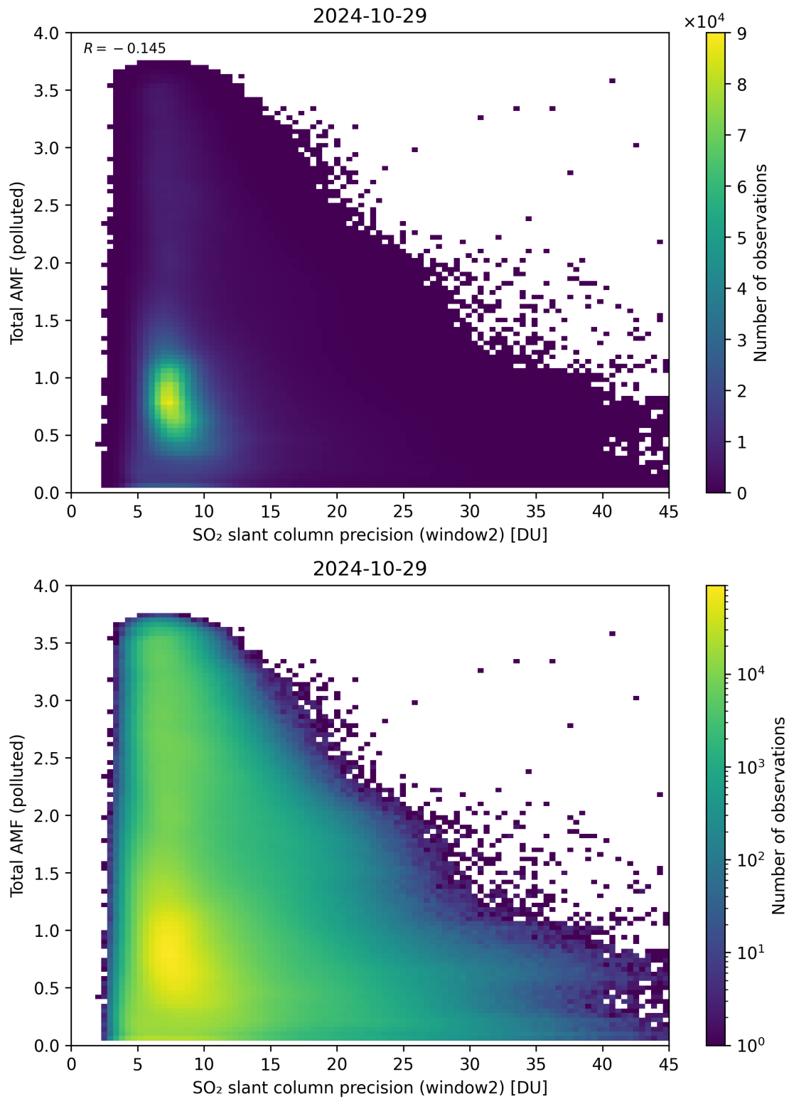
Figure 251: Scatter density plot of “SO 2 slant column precision (window2)” against “Total AMF (polluted)” for 2024-10-29 to 2024-10-30.
