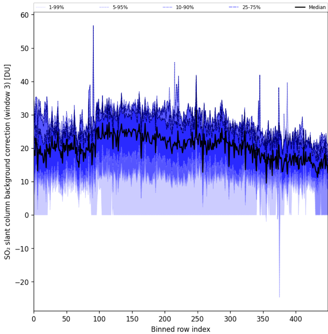
Figure 90: Along track statistics of “SO 2 slant column background correction (window 3)” for 2024-10-29 to 2024-10-30
