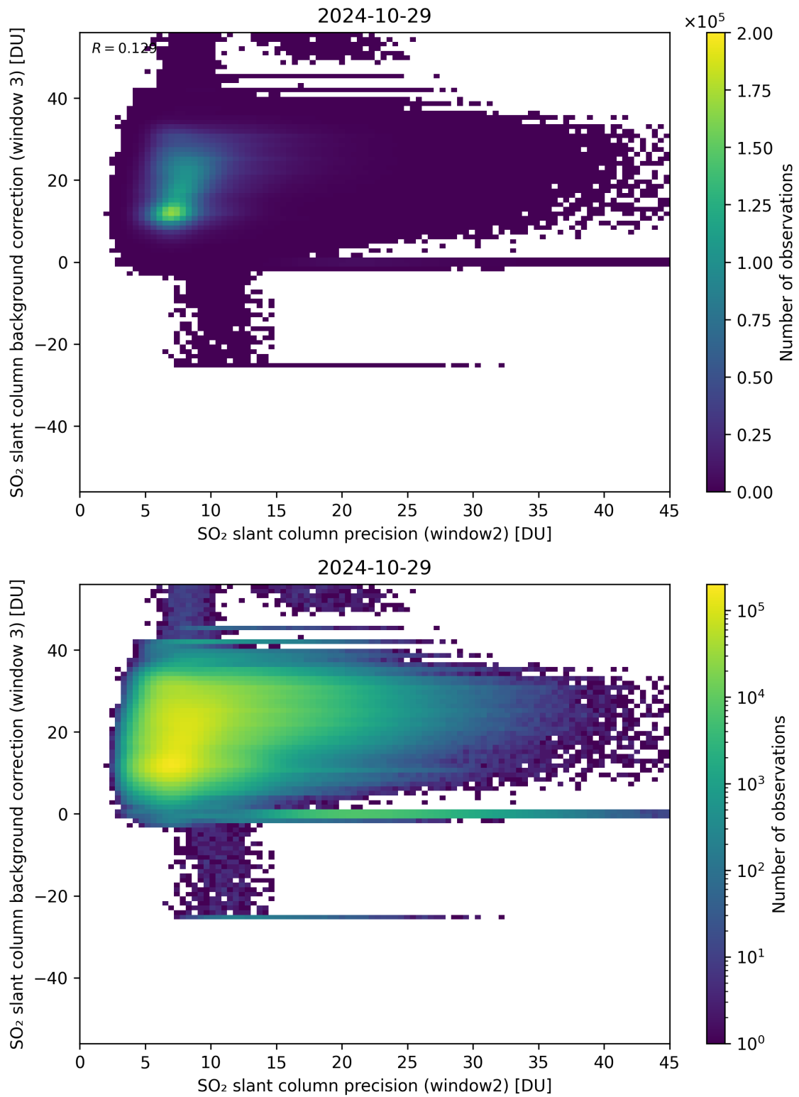
Figure 242: Scatter density plot of “SO 2 slant column precision (window2)” against “SO 2 slant column background correction (window 3)” for 2024-10-29 to 2024-10-30.
