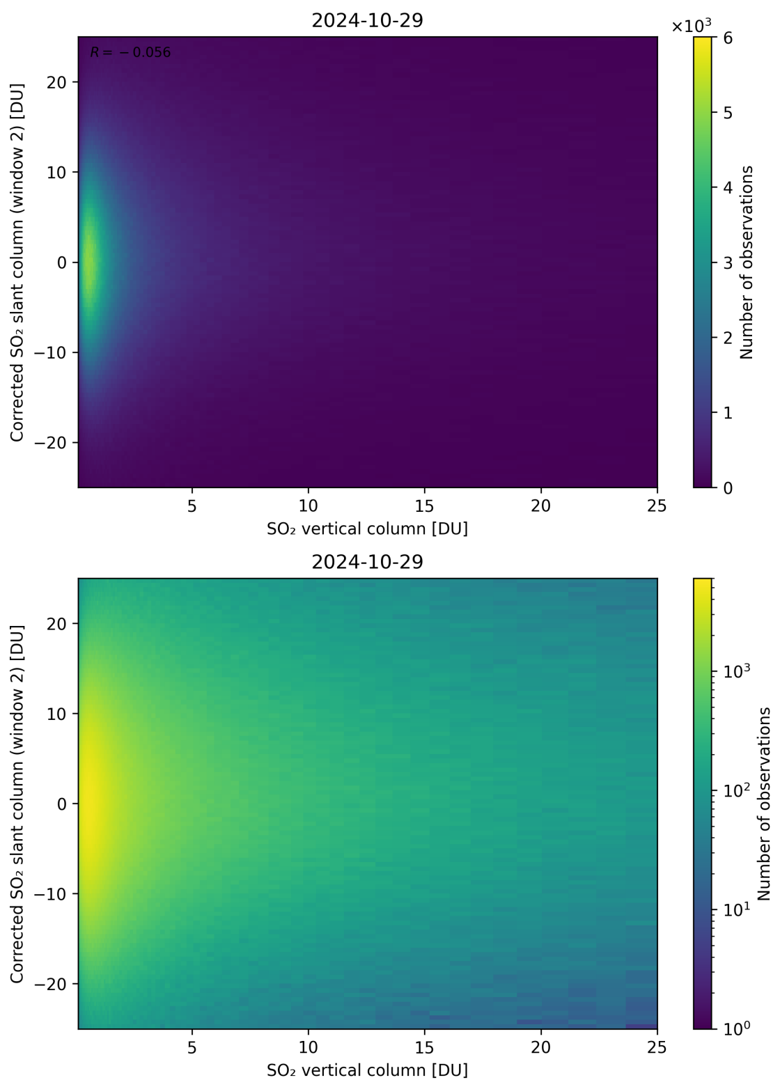
Figure 298: Scatter density plot of “SO 2 vertical column” against “Corrected SO 2 slant column (window 2)” for 2024-10-29 to 2024-10-30.
