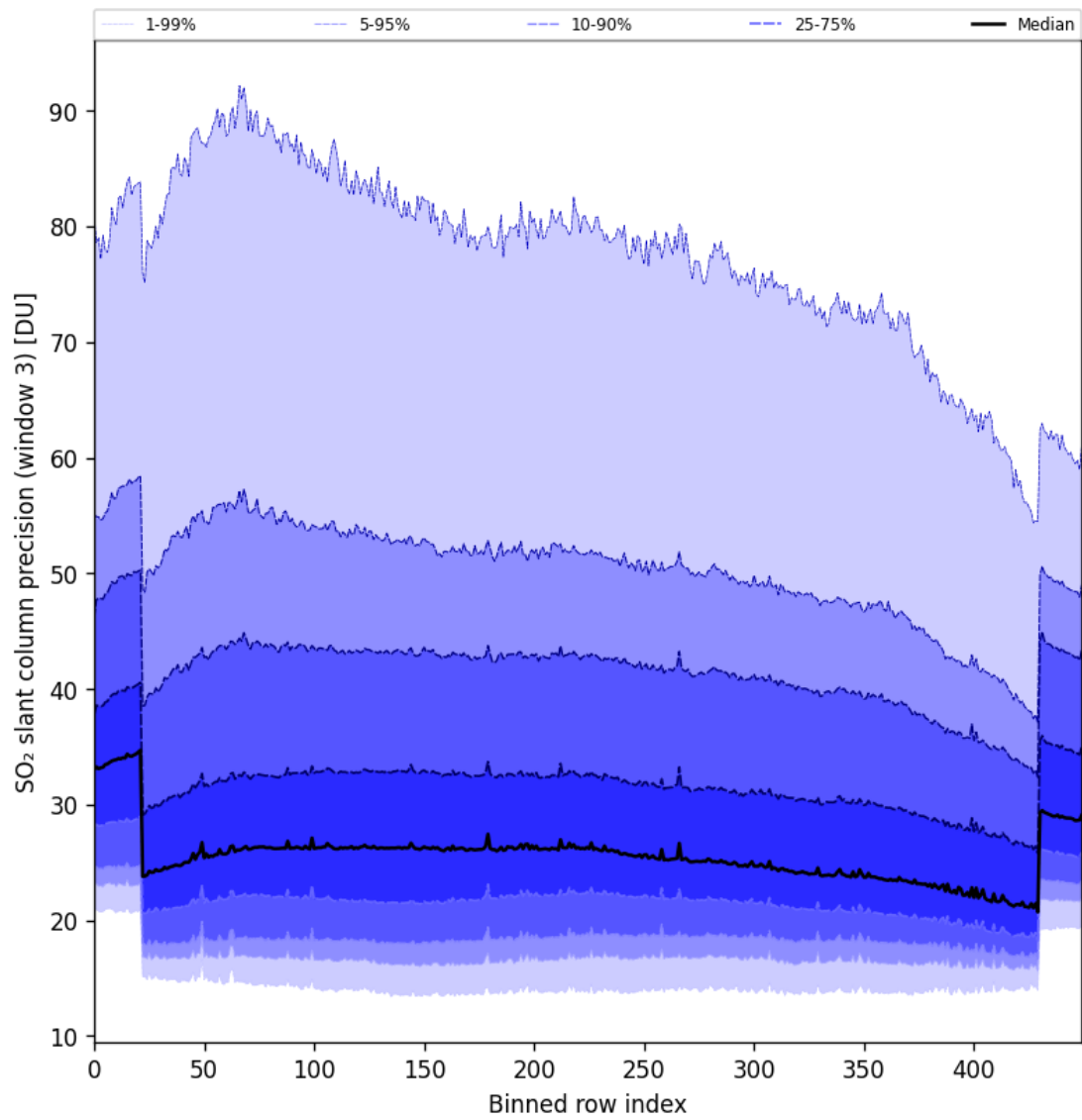
Figure 88: Along track statistics of “SO 2 slant column precision (window 3)” for 2024-10-29 to 2024-10-30
