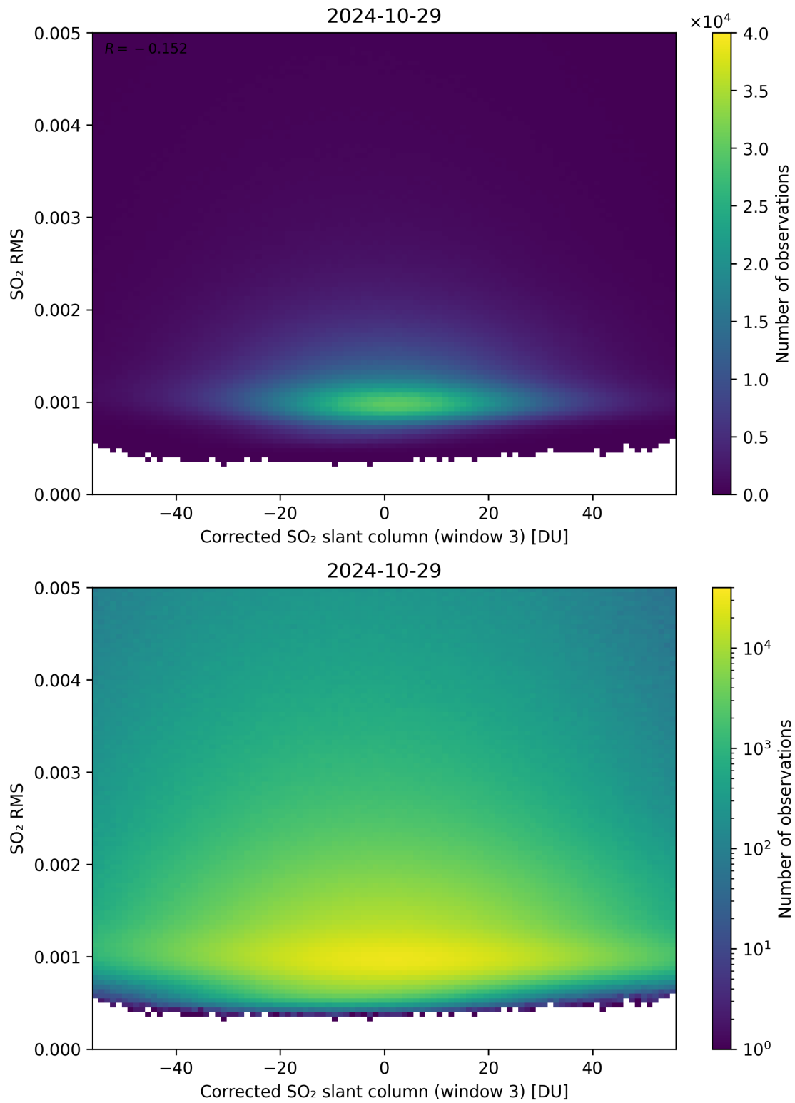
Figure 208: Scatter density plot of “Corrected SO 2 slant column (window 3)” against “SO 2 RMS” for 2024-10-29 to 2024-10-30.
