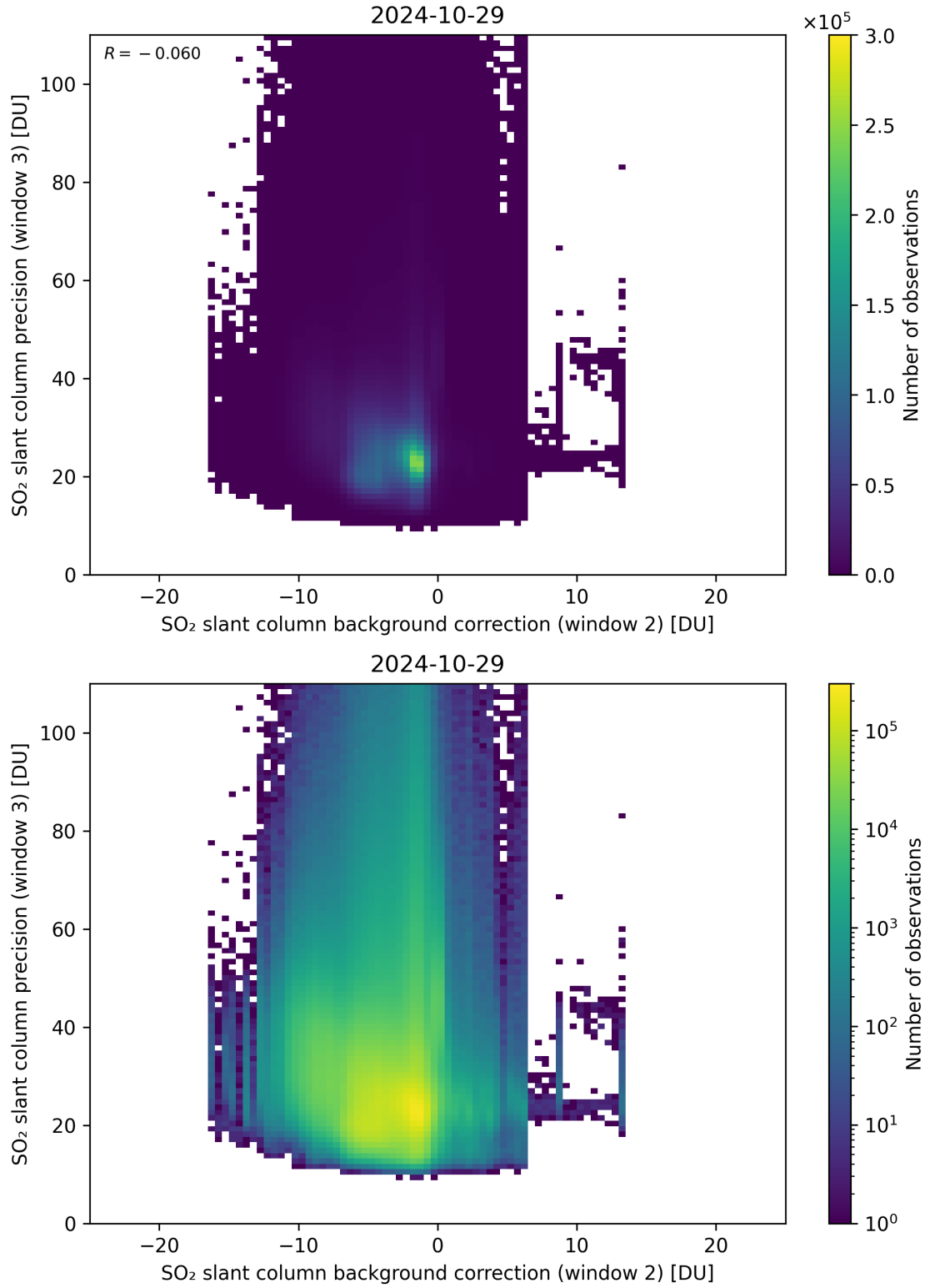
Figure 118: Scatter density plot of “SO 2 slant column background correction (window 2)” against “SO 2 slant column precision (window 3)” for 2024-10-29 to 2024-10-30.
