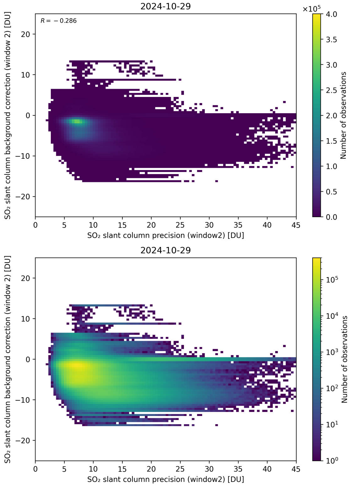
Figure 241: Scatter density plot of “SO 2 slant column precision (window2)” against “SO 2 slant column background correction (window 2)” for 2024-10-29 to 2024-10-30.
