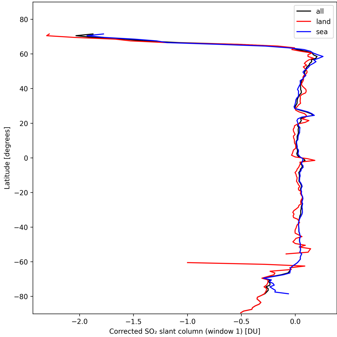
Figure 35: Zonal average of “Corrected SO 2 slant column (window 1)” for 2024-10-29 to 2024-10-30.
