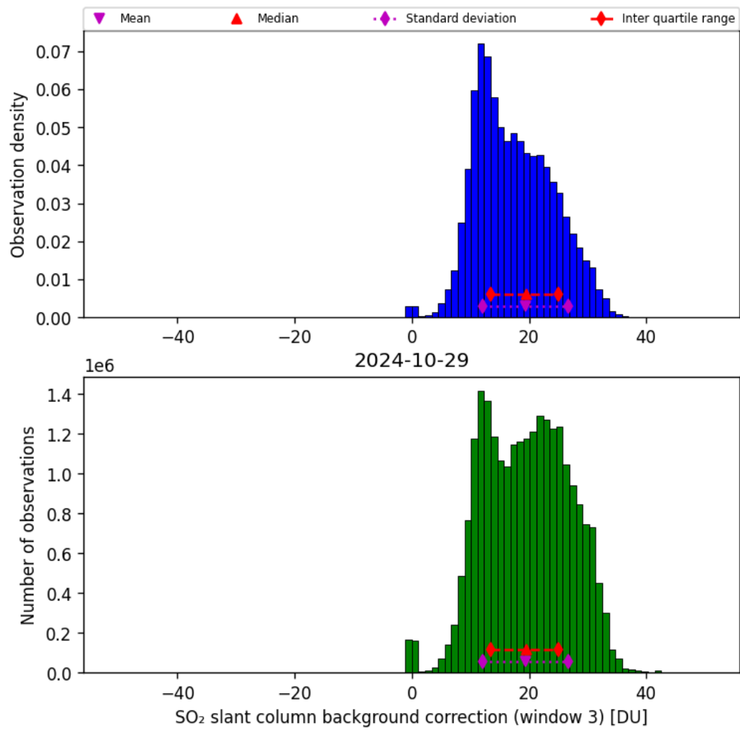
Figure 67: Histogram of “SO 2 slant column background correction (window 3)” for 2024-10-29 to 2024-10-30
