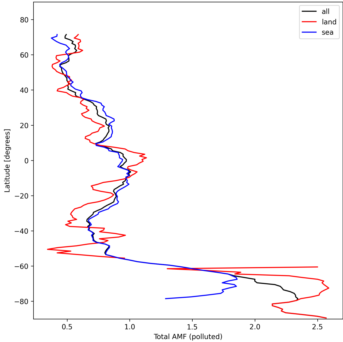
Figure 48: Zonal average of “Total AMF (polluted)” for 2024-10-29 to 2024-10-30.
