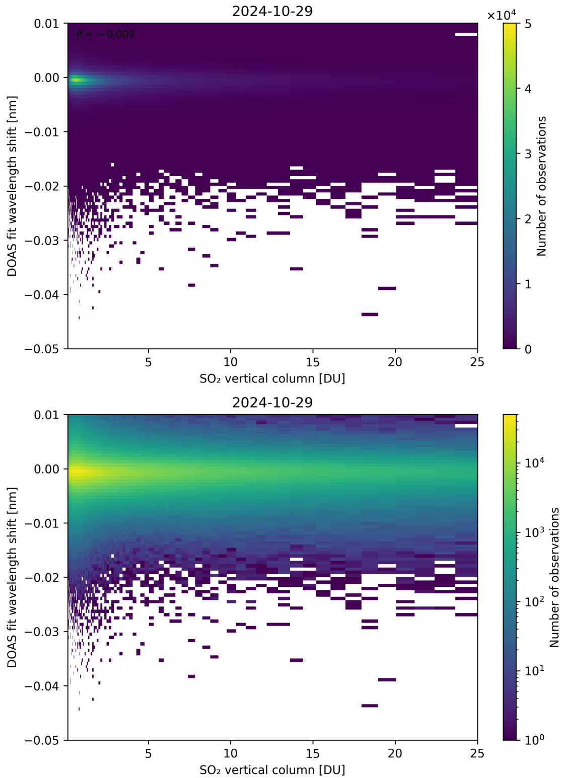
Figure 276: Scatter density plot of “SO 2 vertical column” against “DOAS fit wavelength shift” for 2024-10-29 to 2024-10-30.
