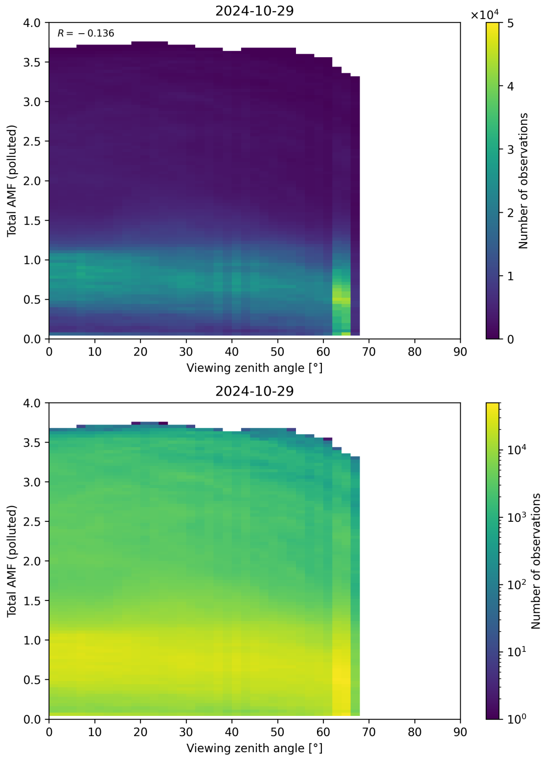
Figure 325: Scatter density plot of “Viewing zenith angle” against “Total AMF (polluted)” for 2024-10-29 to 2024-10-30.
