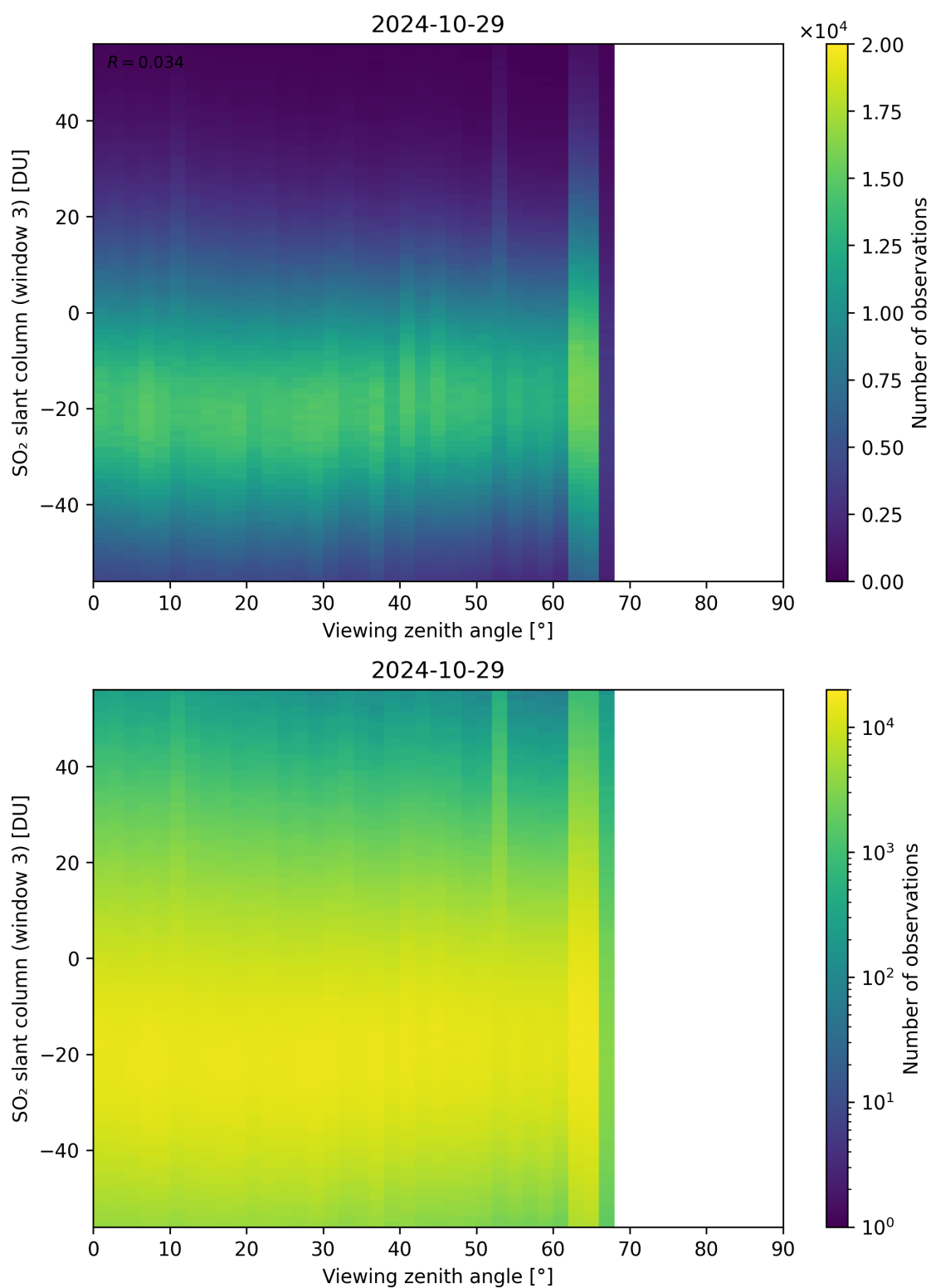
Figure 323: Scatter density plot of “Viewing zenith angle” against “SO 2 slant column (window 3)” for 2024-10-29 to 2024-10-30.
