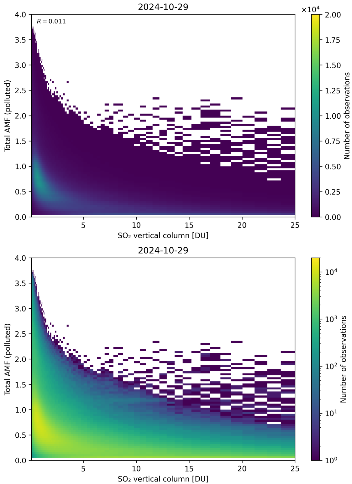
Figure 305: Scatter density plot of “SO 2 vertical column” against “Total AMF (polluted)” for 2024-10-29 to 2024-10-30.
