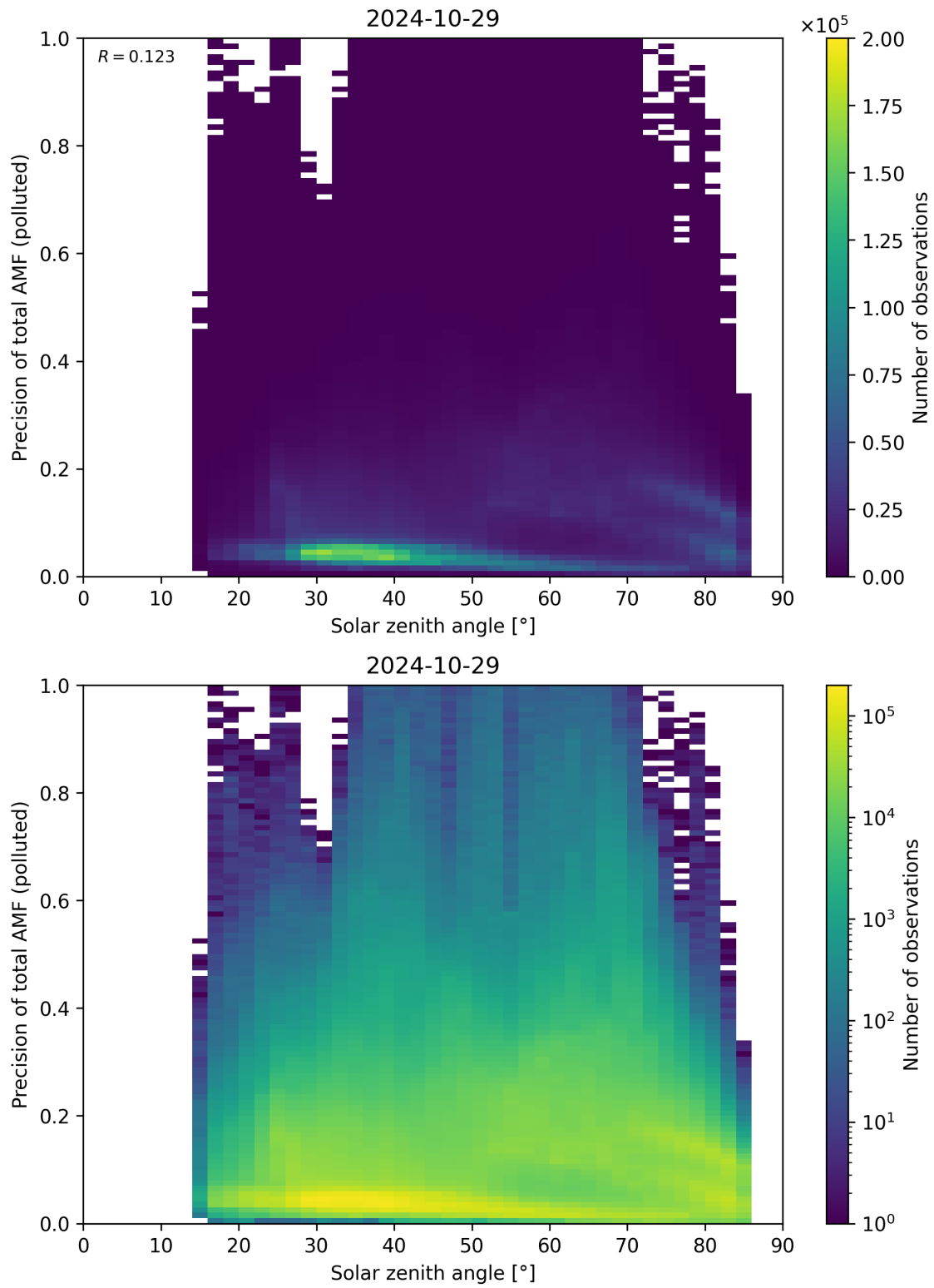
Figure 175: Scatter density plot of “Solar zenith angle” against “Precision of total AMF (polluted)” for 2024-10-29 to 2024-10-30.
