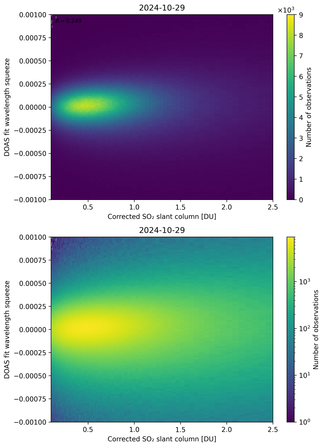
Figure 182: Scatter density plot of “Corrected SO 2 slant column” against “DOAS fit wavelength squeeze” for 2024-10-29 to 2024-10-30.
