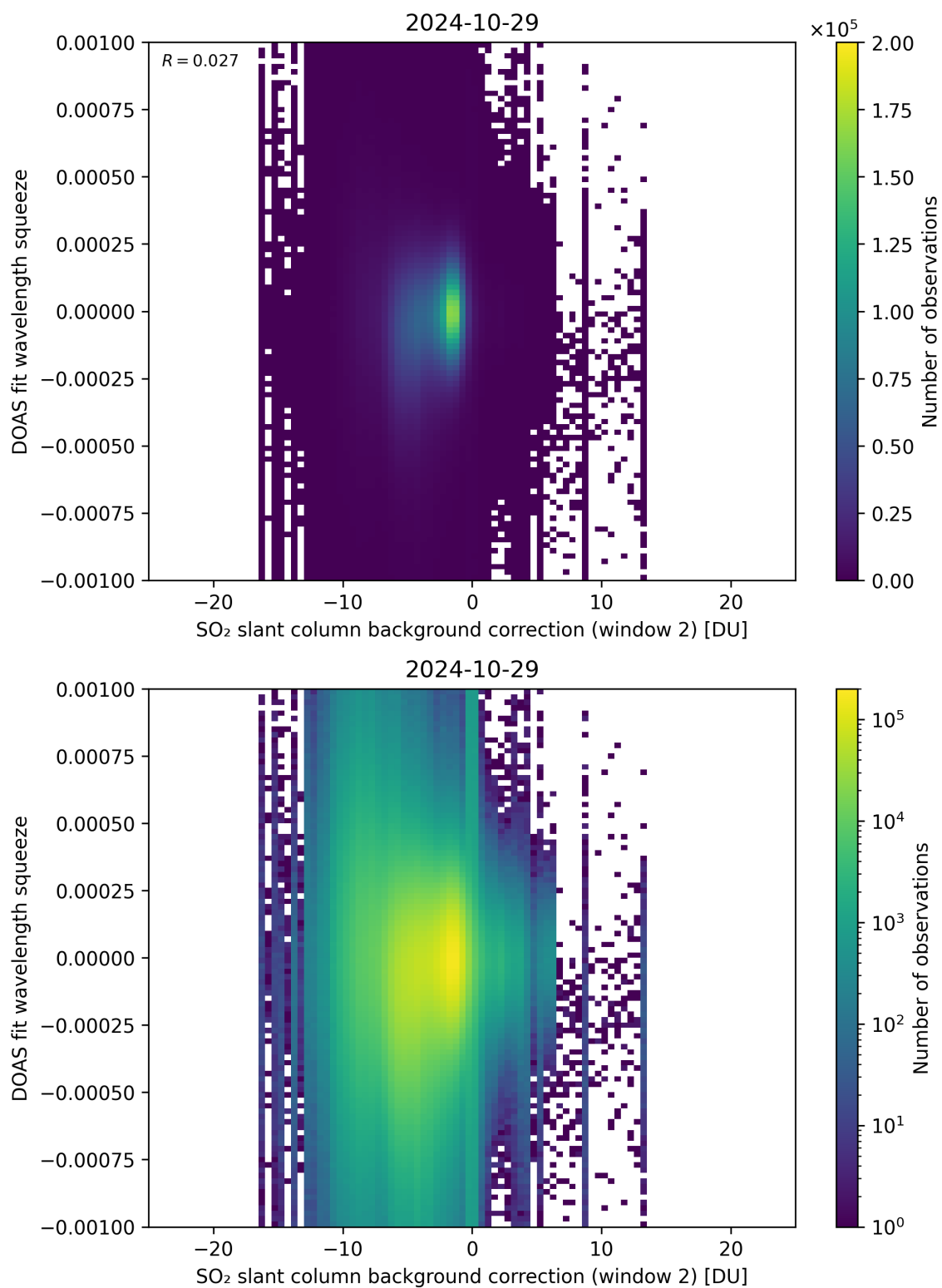
Figure 113: Scatter density plot of “SO 2 slant column background correction (window 2)” against “DOAS fit wavelength squeeze” for 2024-10-29 to 2024-10-30.
