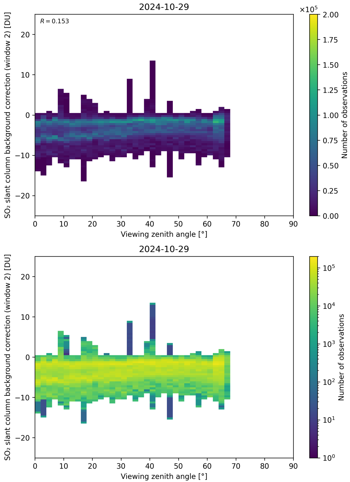
Figure 309: Scatter density plot of “Viewing zenith angle” against “SO 2 slant column background correction (window 2)” for 2024-10-29 to 2024-10-30.
