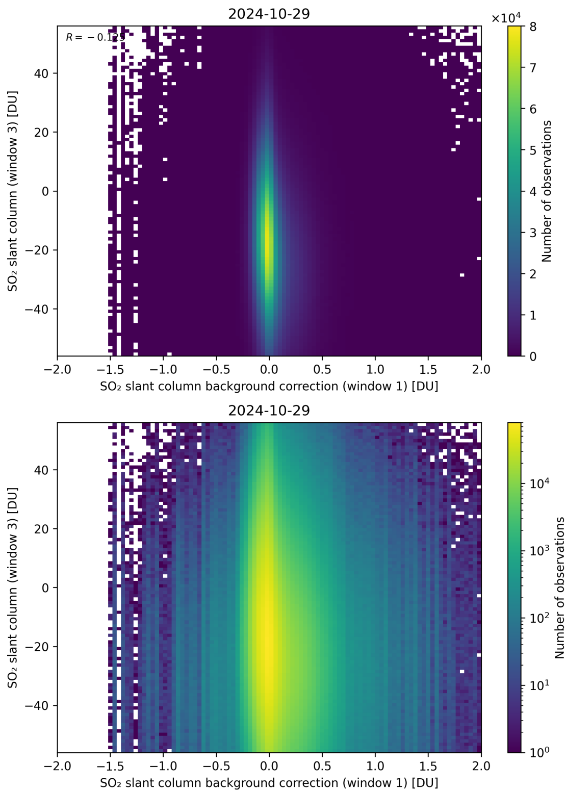
Figure 107: Scatter density plot of “SO 2 slant column background correction (window 1)” against “SO 2 slant column (window 3)” for 2024-10-29 to 2024-10-30.
