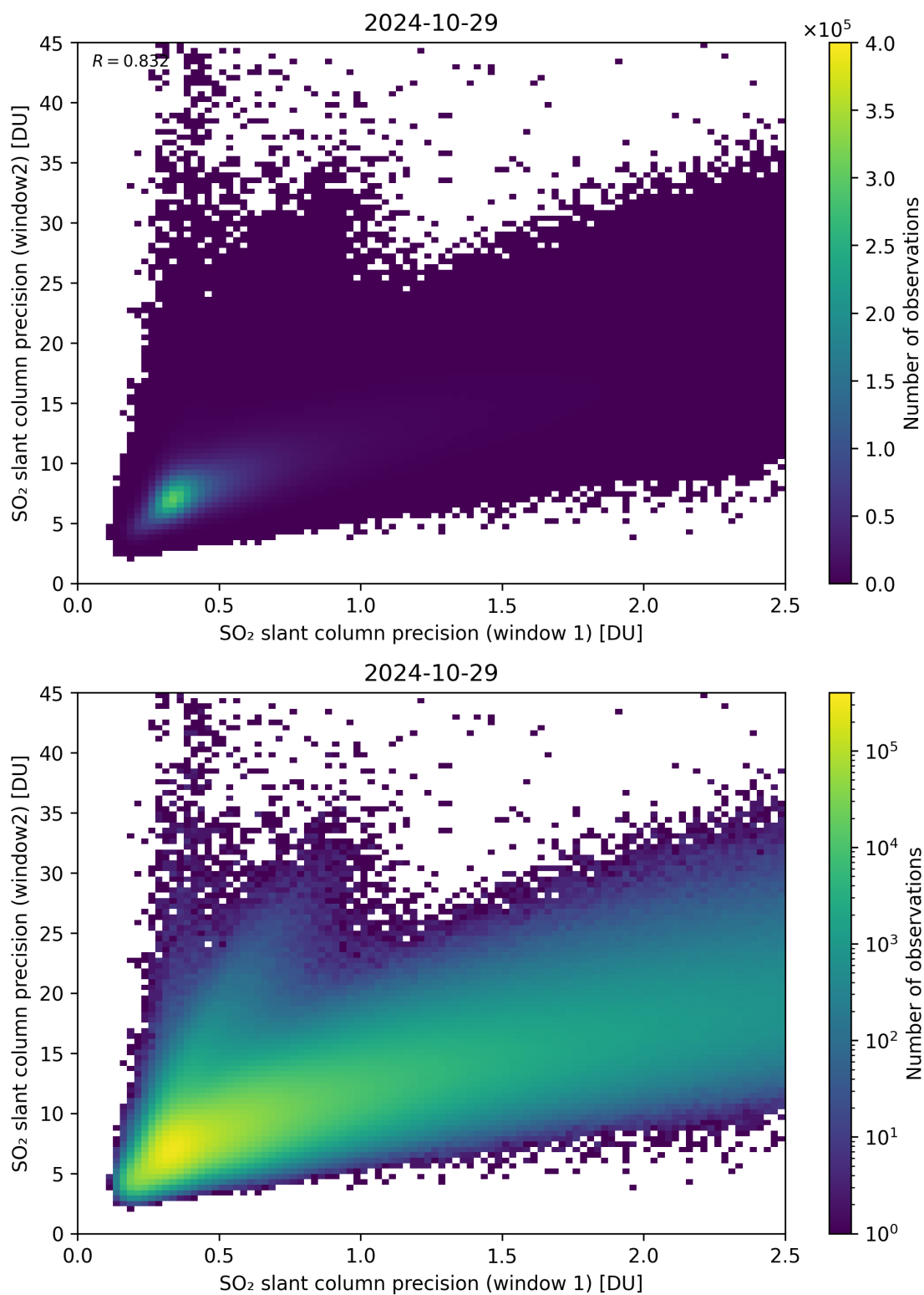
Figure 227: Scatter density plot of “SO 2 slant column precision (window 1)” against “SO 2 slant column precision (window 2)” for 2024-10-29 to 2024-10-30.
