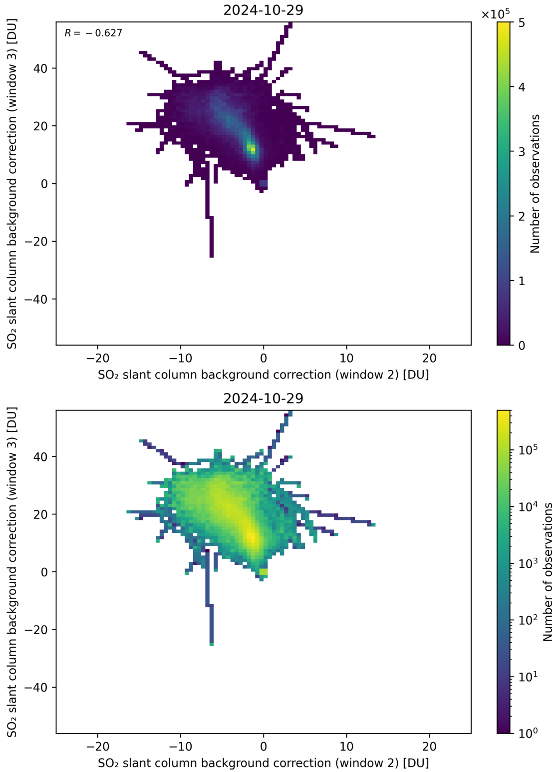
Figure 111: Scatter density plot of “SO 2 slant column background correction (window 2)” against “SO 2 slant column background correction (window 3)” for 2024-10-29 to 2024-10-30.
