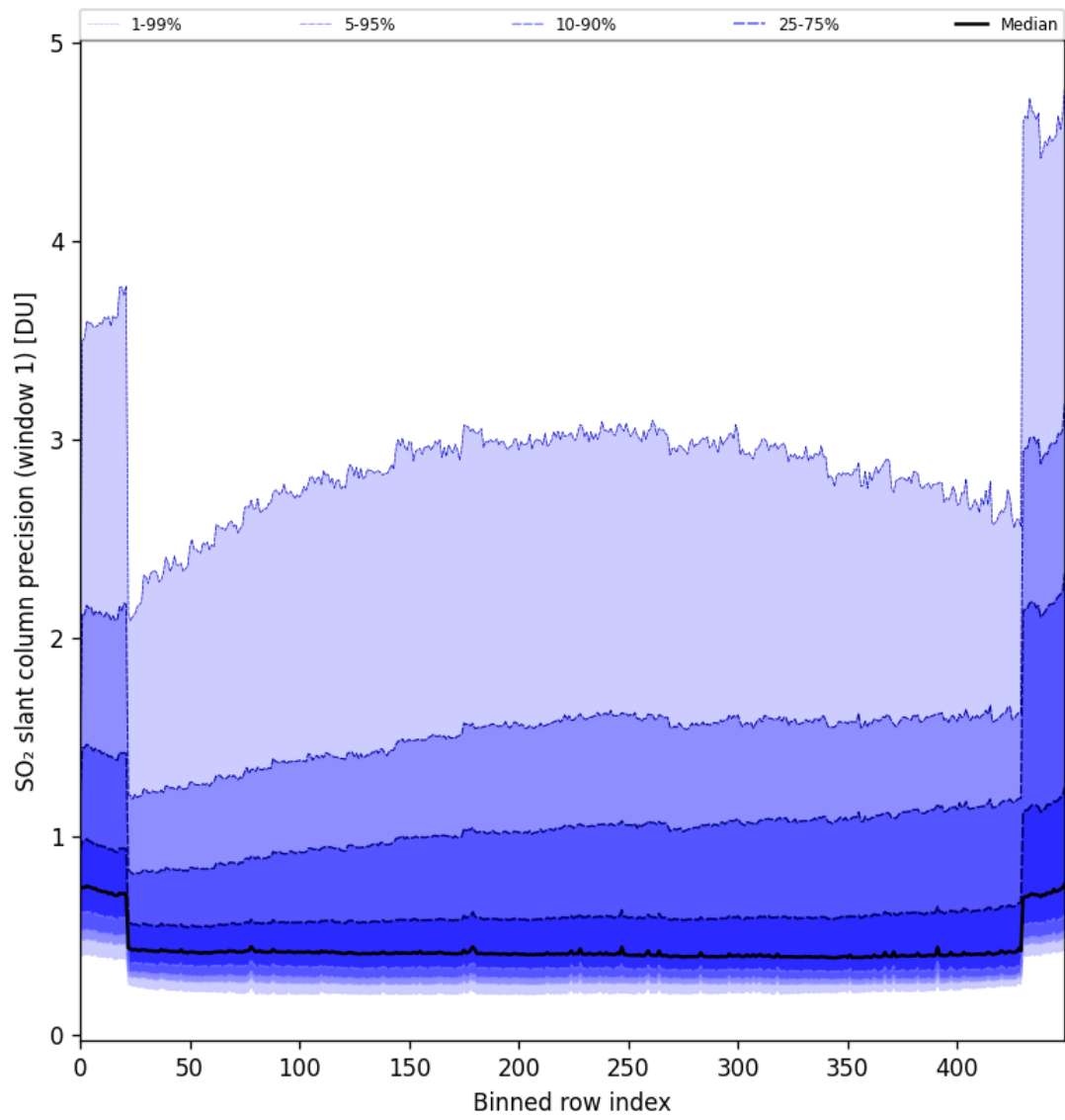
Figure 80: Along track statistics of "SO 2 slant column precision (window 1)" for 2024-10-29 to 2024-10-30
