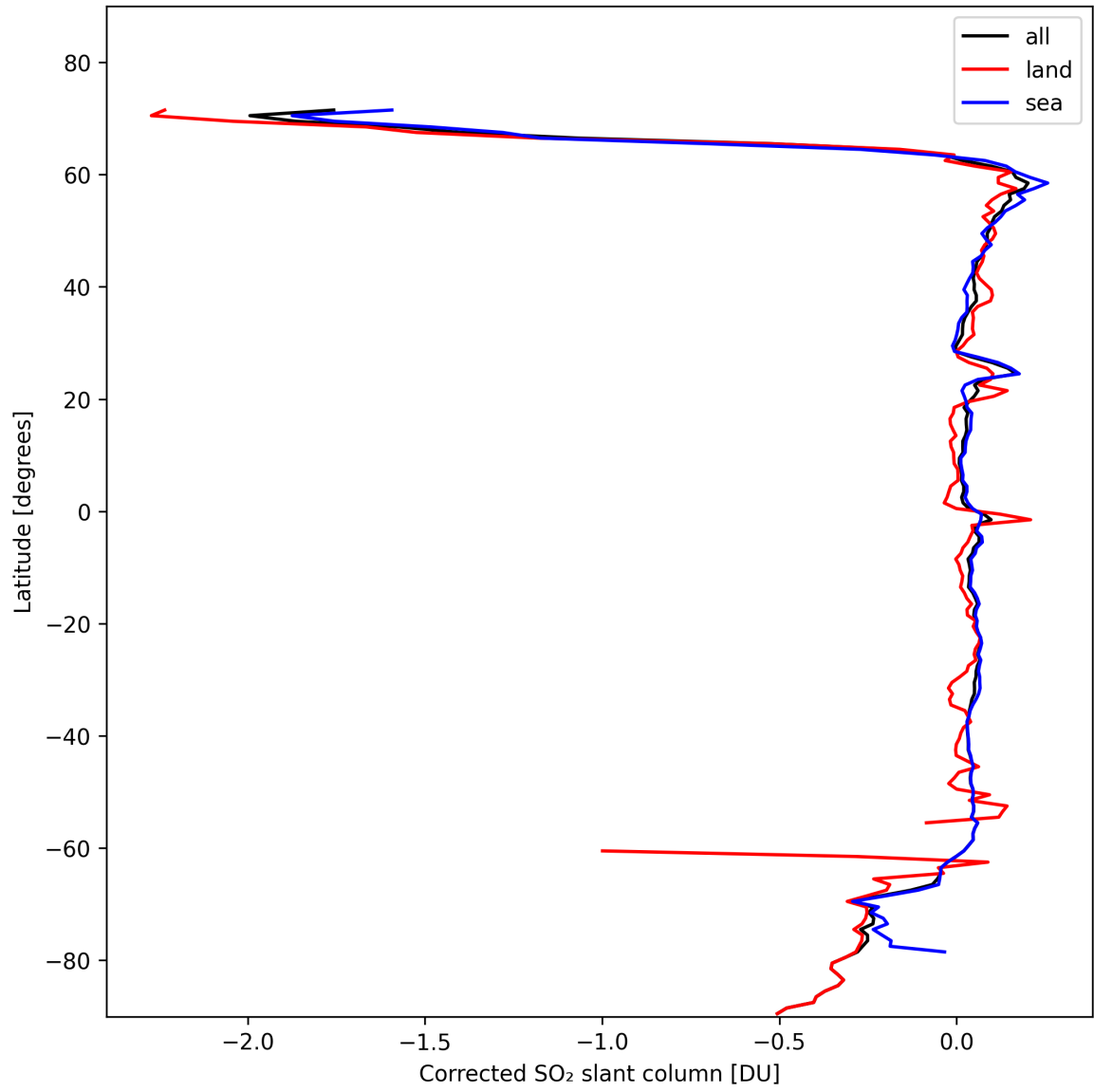
Figure 32: Zonal average of “Corrected SO 2 slant column” for 2024-10-29 to 2024-10-30.
