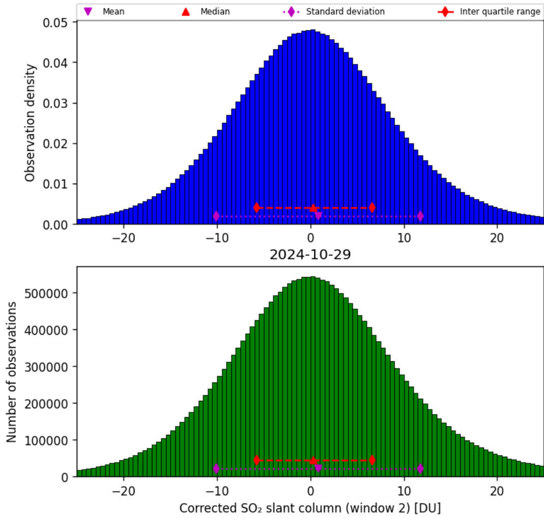
Figure 62: Histogram of “Corrected SO 2 slant column (window 2)” for 2024-10-29 to 2024-10-30
