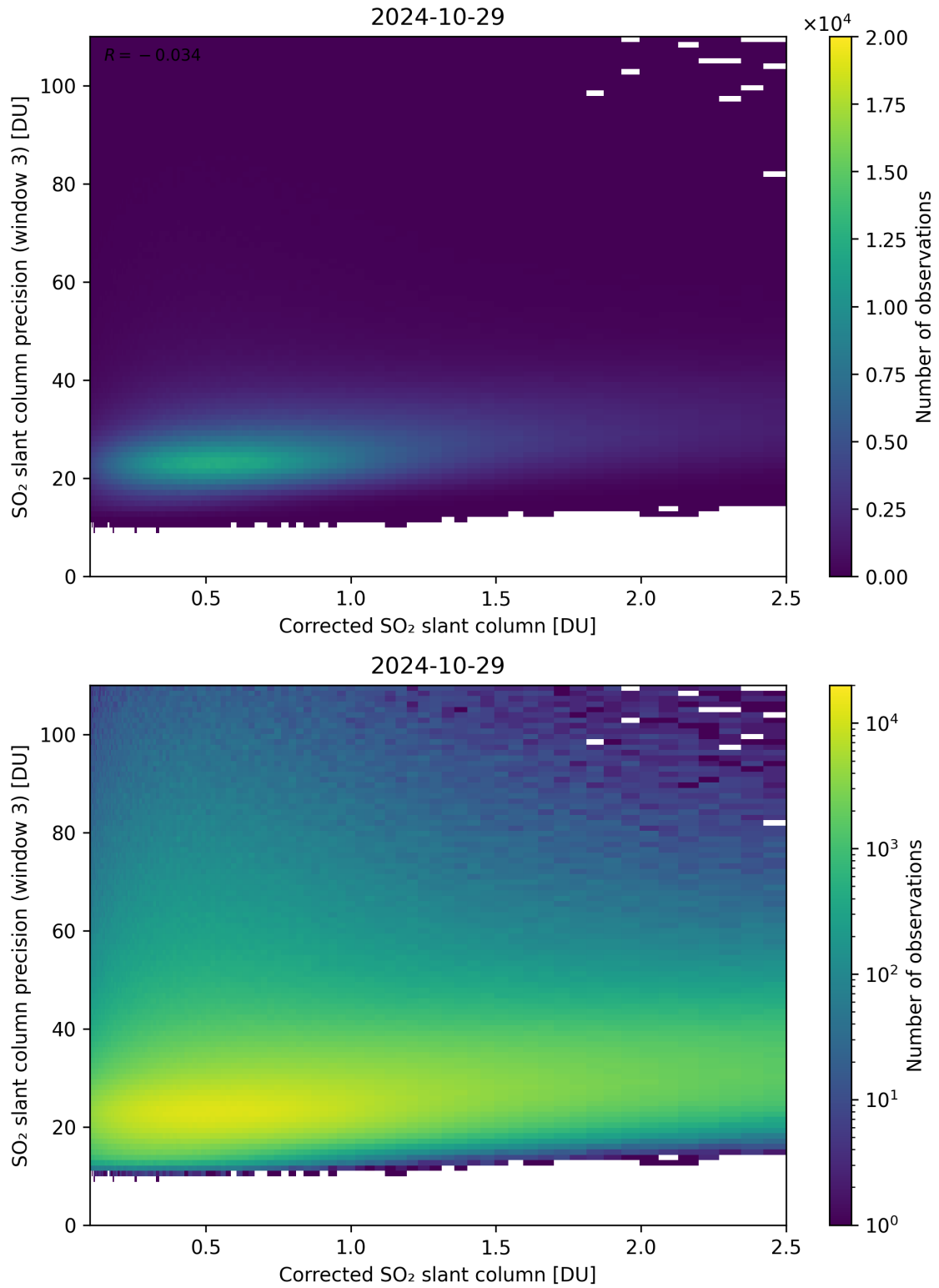
Figure 191: Scatter density plot of “Corrected SO 2 slant column” against “SO 2 slant column precision (window 3)” for 2024-10-29 to 2024-10-30.
