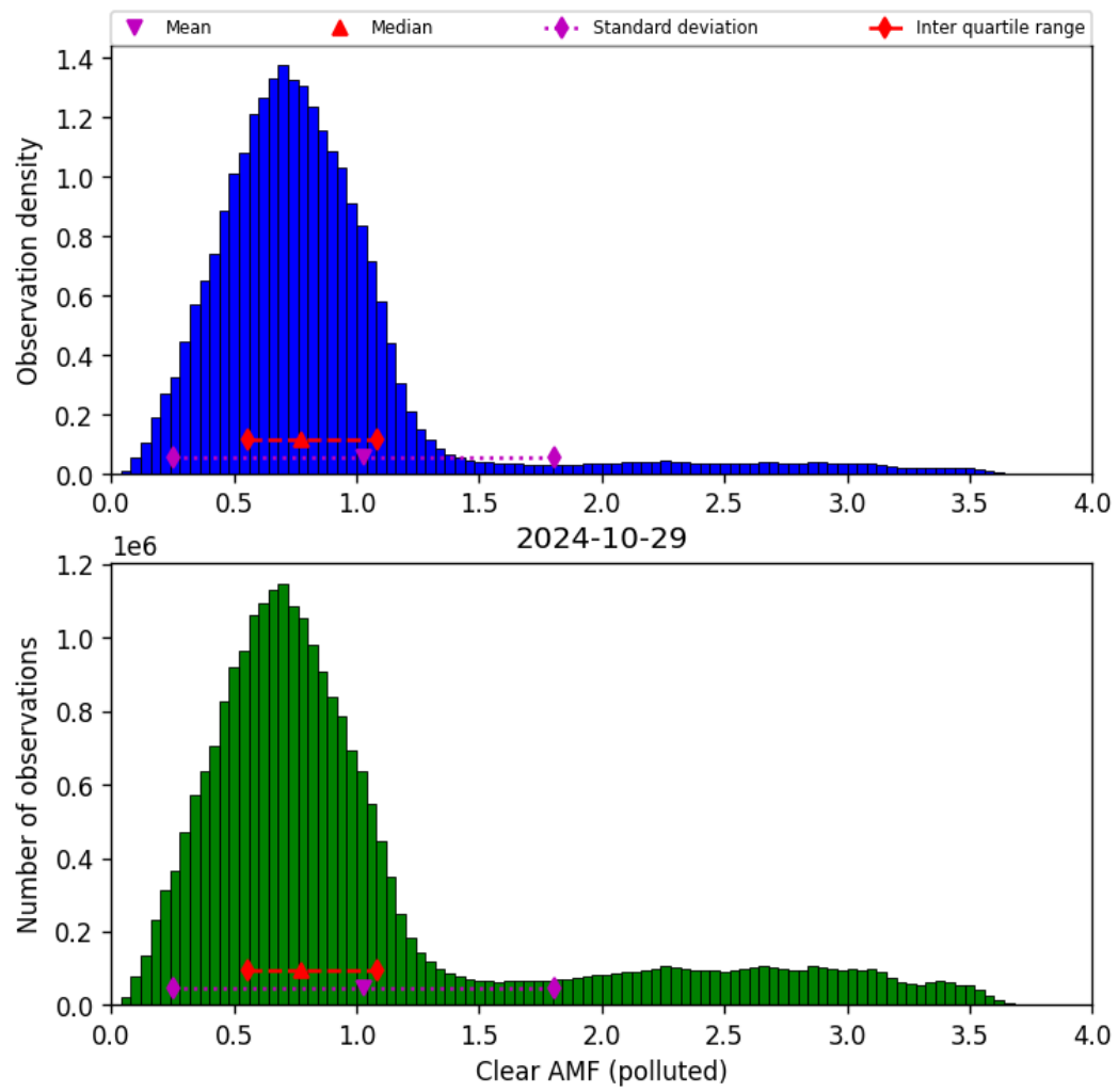
Figure 73: Histogram of “Clear AMF (polluted)” for 2024-10-29 to 2024-10-30
