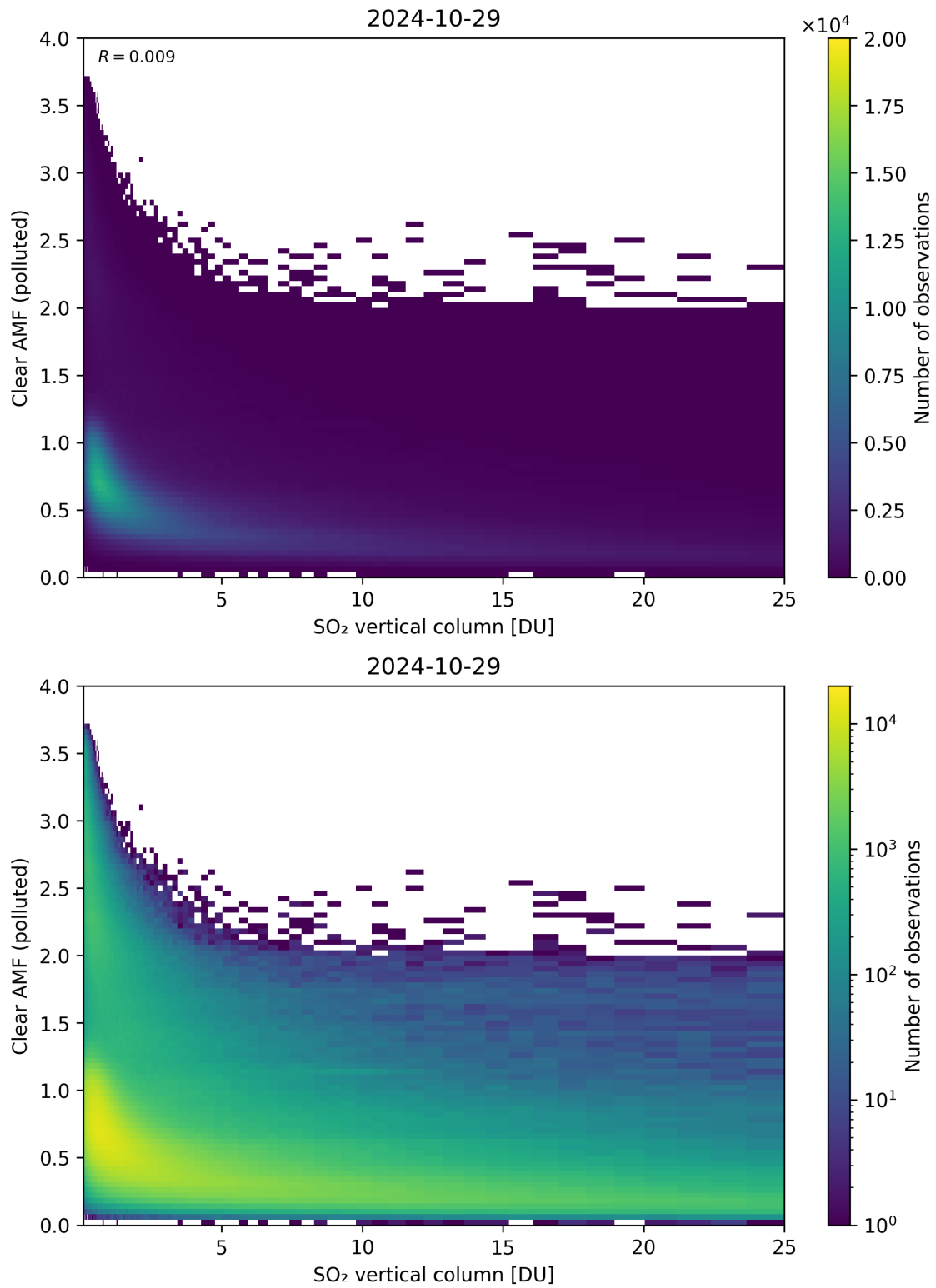
Figure 296: Scatter density plot of “SO 2 vertical column” against “Clear AMF (polluted)” for 2024-10-29 to 2024-10-30.
