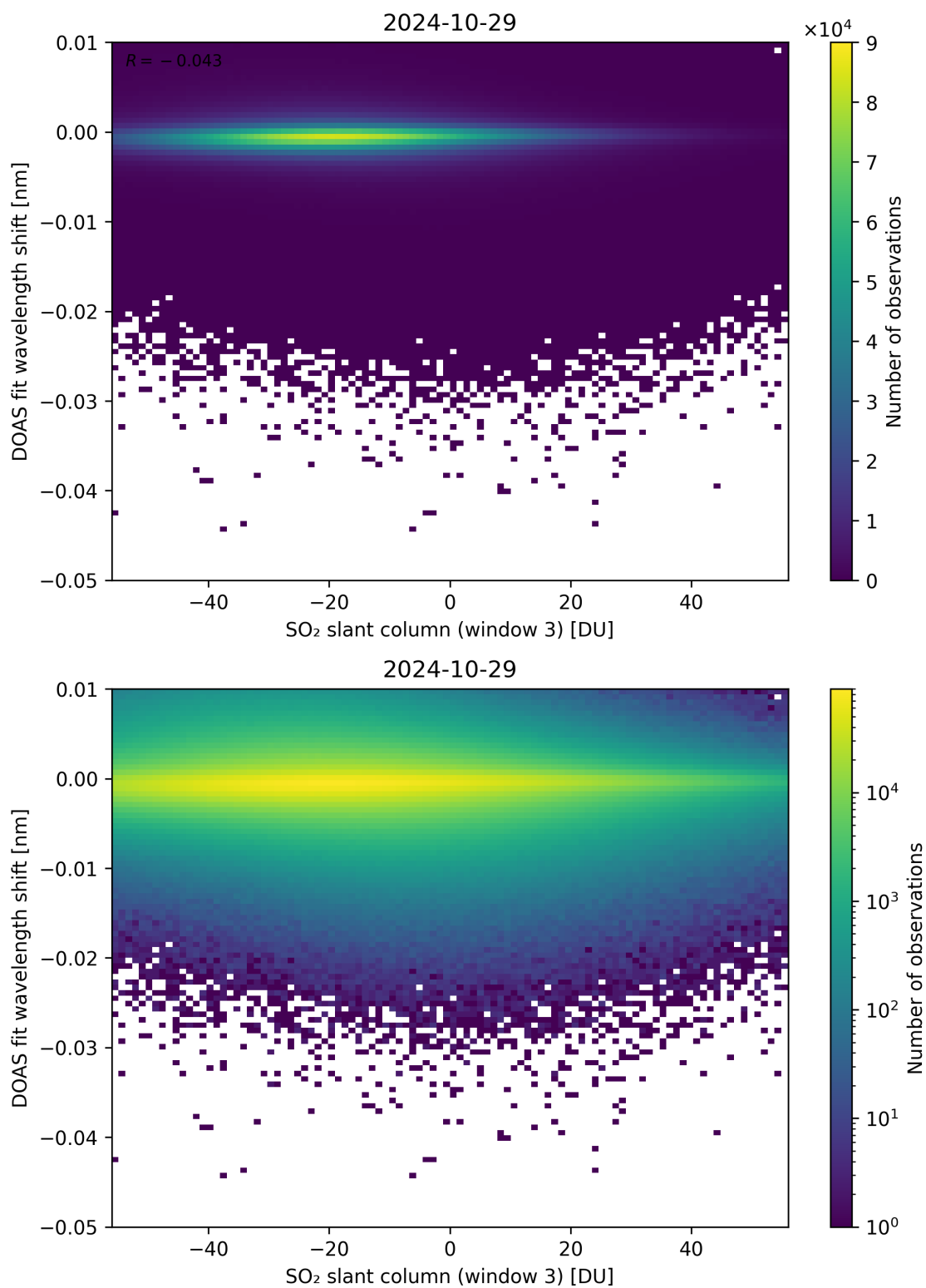
Figure 254: Scatter density plot of “SO 2 slant column (window 3)” against “DOAS fit wavelength shift” for 2024-10-29 to 2024-10-30.
