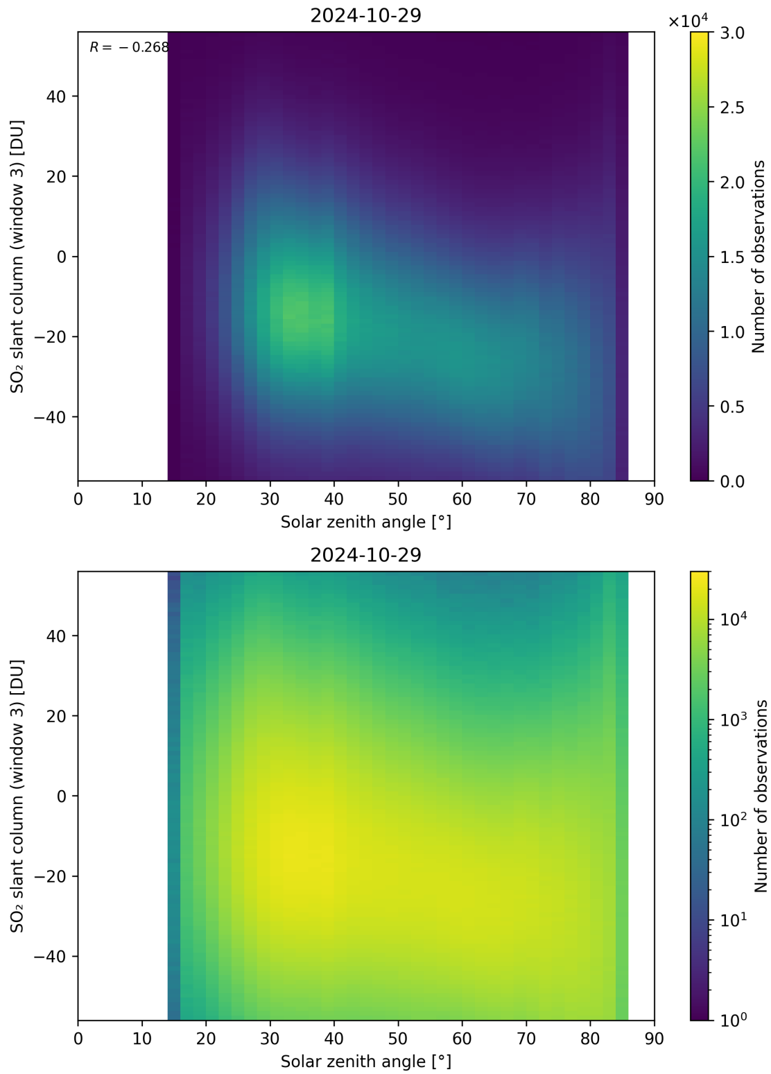
Figure 172: Scatter density plot of “Solar zenith angle” against “SO 2 slant column (window 3)” for 2024-10-29 to 2024-10-30.
