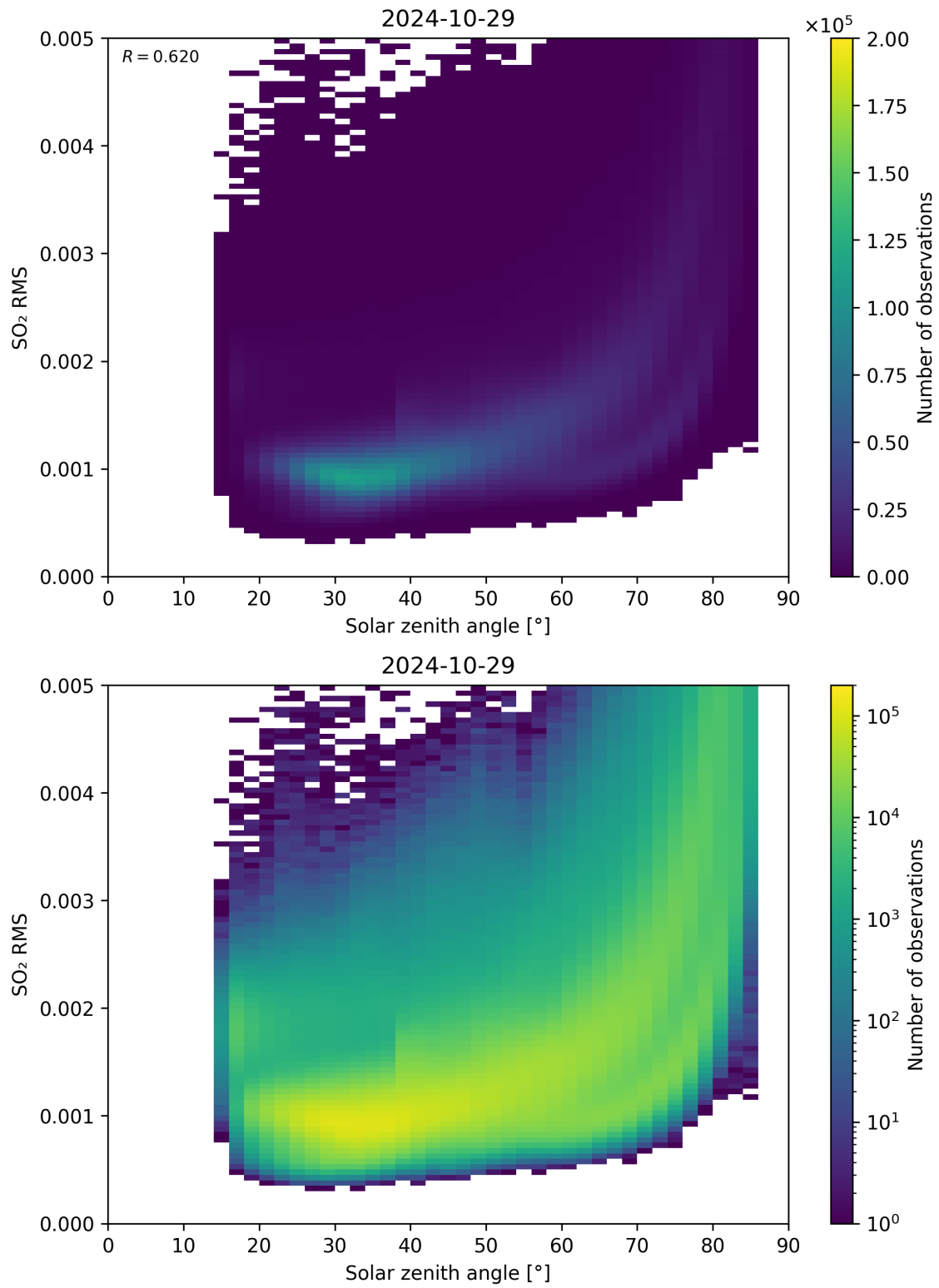
Figure 163: Scatter density plot of “Solar zenith angle” against “SO 2 RMS” for 2024-10-29 to 2024-10-30.
