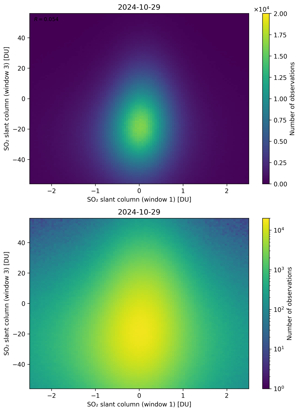
Figure 237: Scatter density plot of “SO 2 slant column (window 1)” against “SO 2 slant column (window 3)” for 2024-10-29 to 2024-10-30.
