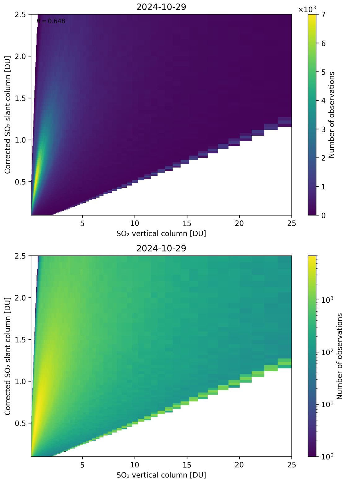
Figure 297: Scatter density plot of “SO 2 vertical column” against “Corrected SO 2 slant column” for 2024-10-29 to 2024-10-30.
