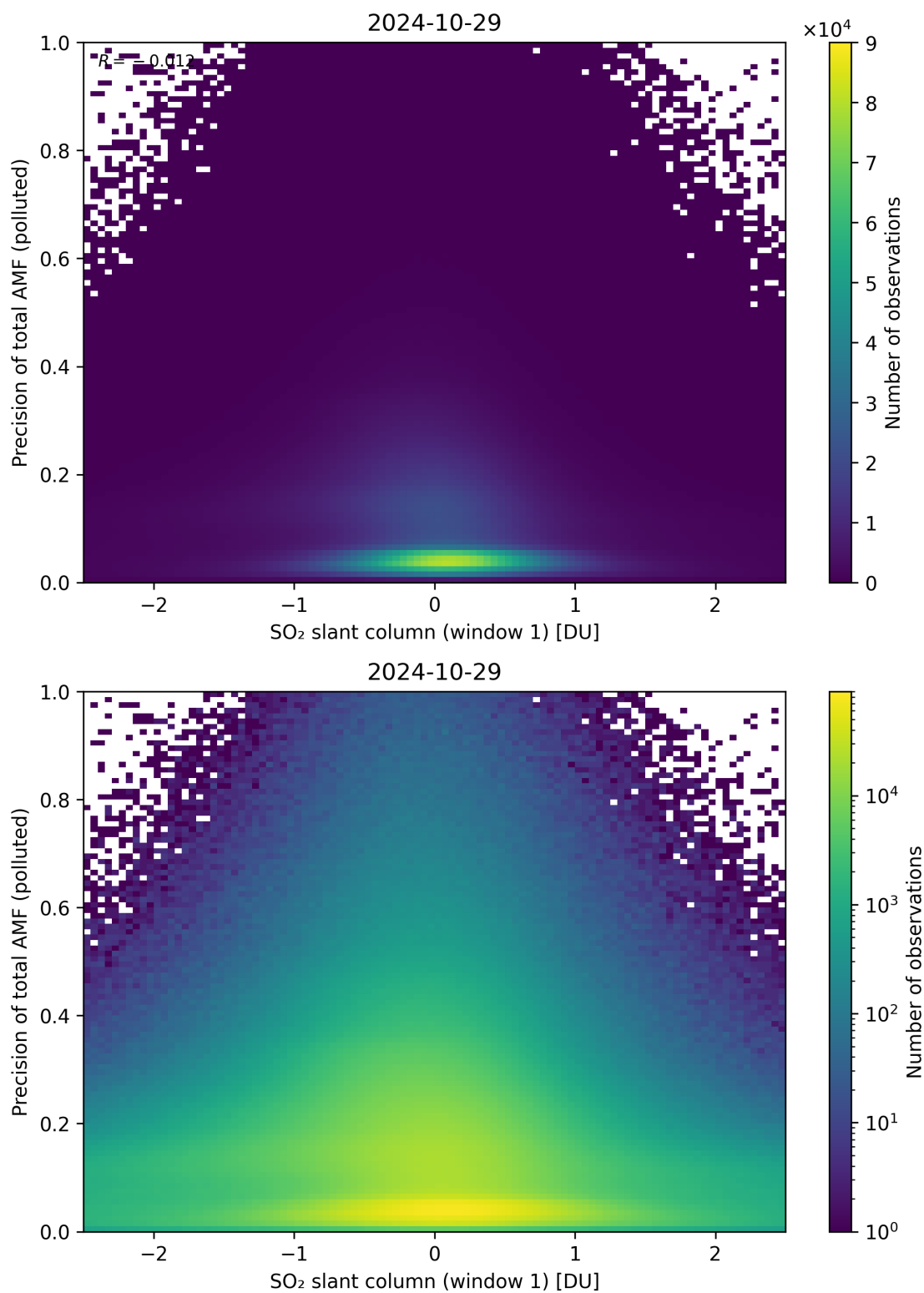
Figure 240: Scatter density plot of “SO 2 slant column (window 1)” against “Precision of total AMF (polluted)” for 2024-10-29 to 2024-10-30.
