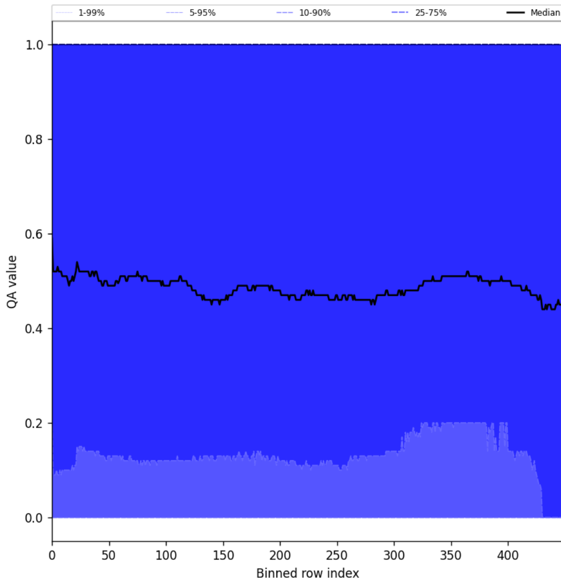
Figure 75: Along track statistics of “QA value” for 2024-10-29 to 2024-10-30
