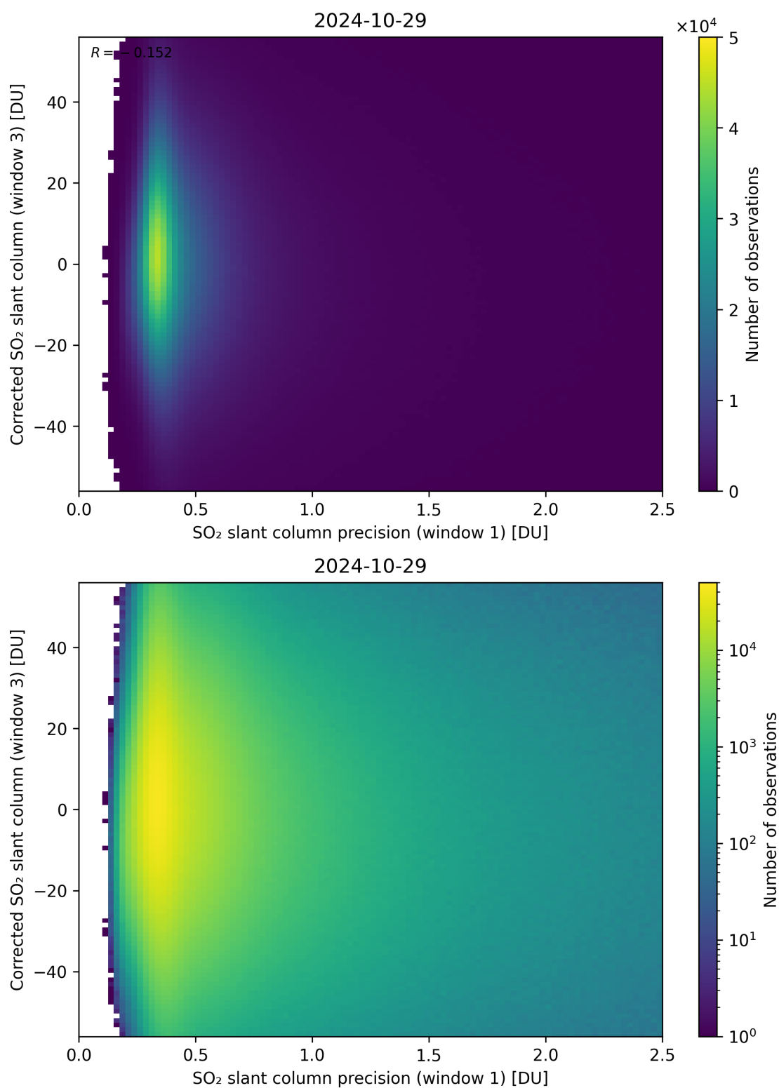
Figure 226: Scatter density plot of “SO 2 slant column precision (window 1)” against “Corrected SO 2 slant column (window 3)” for 2024-10-29 to 2024-10-30.
