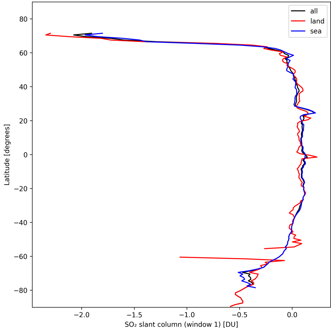
Figure 33: Zonal average of “SO 2 slant column (window 1)” for 2024-10-29 to 2024-10-30.
