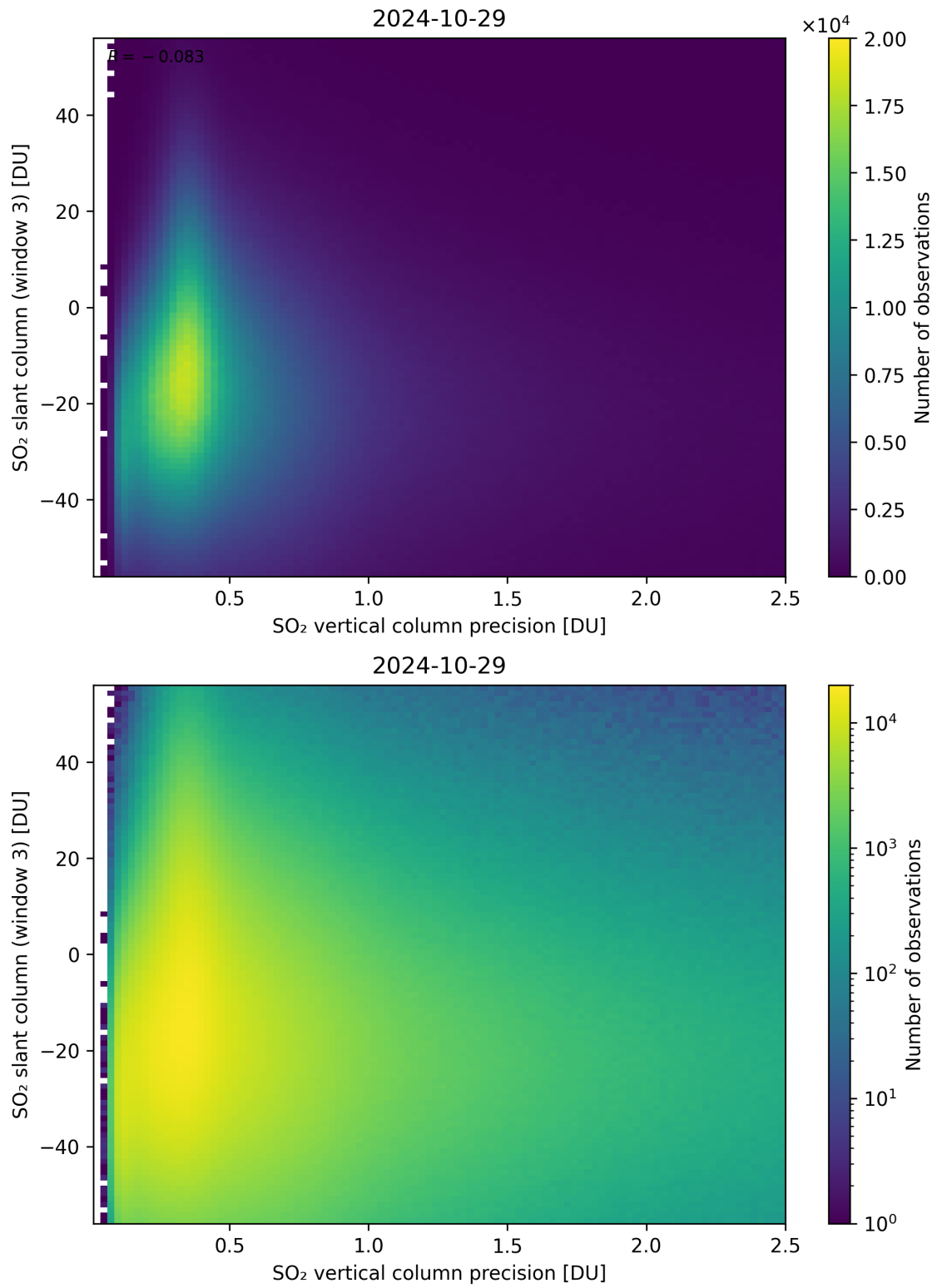
Figure 292: Scatter density plot of “SO 2 vertical column precision” against “SO 2 slant column (window 3)” for 2024-10-29 to 2024-10-30.
