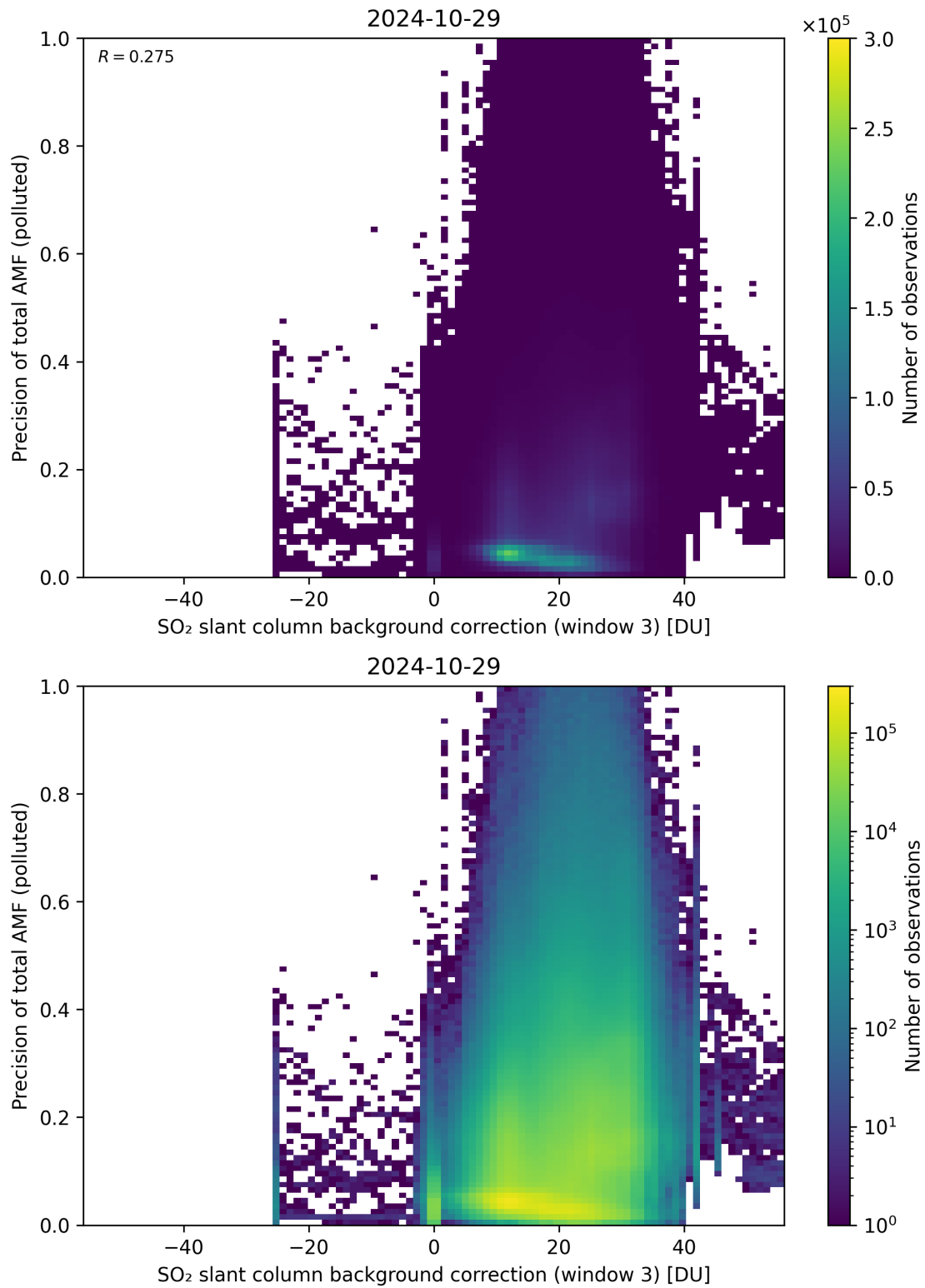
Figure 126: Scatter density plot of “SO 2 slant column background correction (window 3)” against “Precision of total AMF (polluted)” for 2024-10-29 to 2024-10-30.
