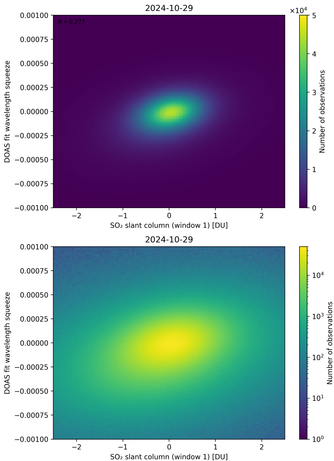
Figure 216: Scatter density plot of “SO 2 slant column (window 1)” against “DOAS fit wavelength squeeze” for 2024-10-29 to 2024-10-30.
