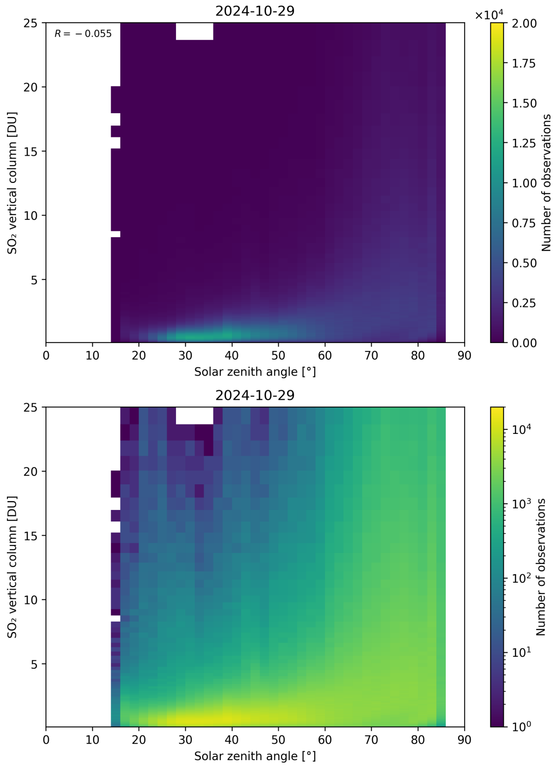
Figure 176: Scatter density plot of “Solar zenith angle” against “SO 2 vertical column” for 2024-10-29 to 2024-10-30.
