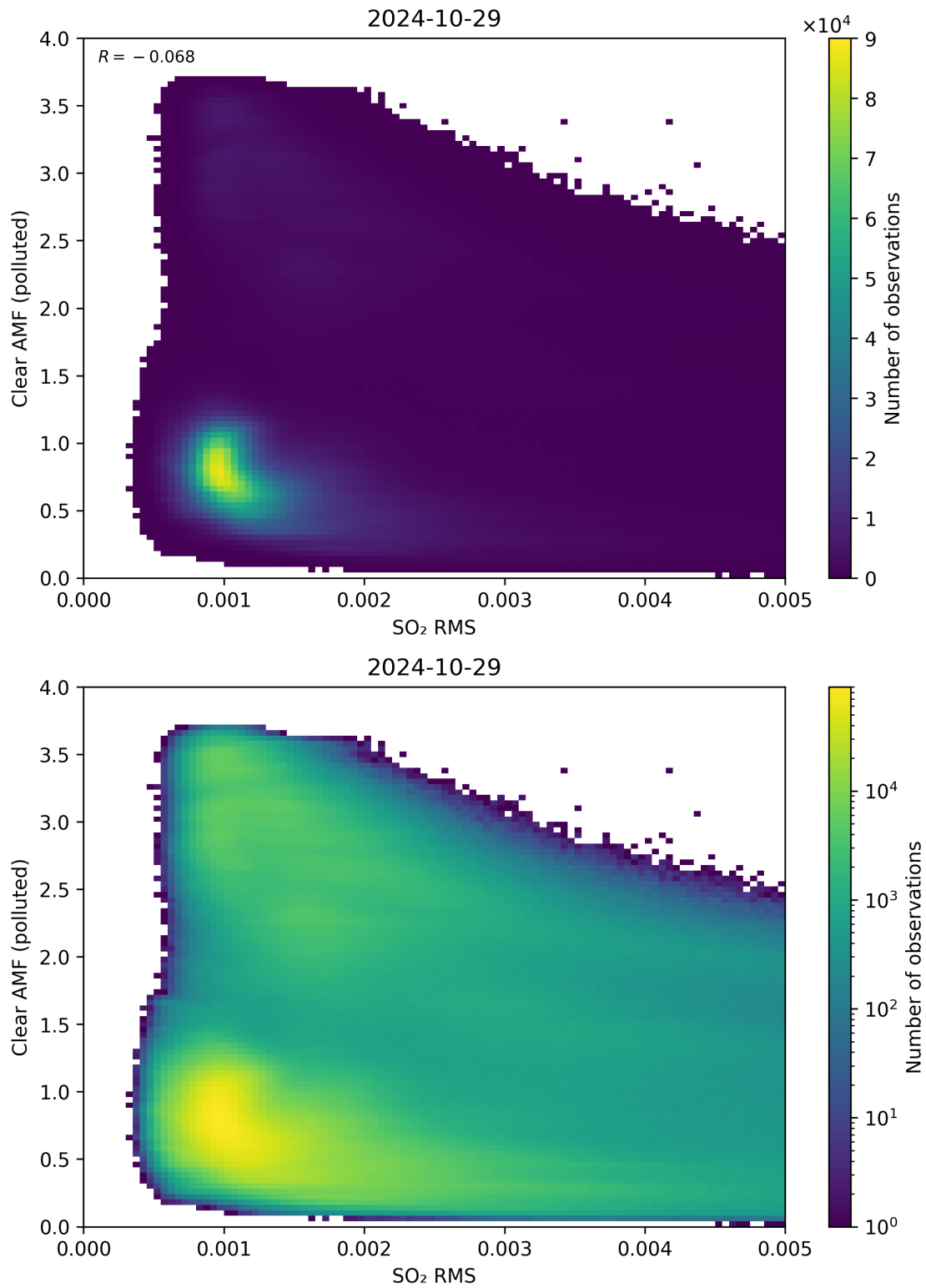
Figure 136: Scatter density plot of “SO 2 RMS” against “Clear AMF (polluted)” for 2024-10-29 to 2024-10-30.
