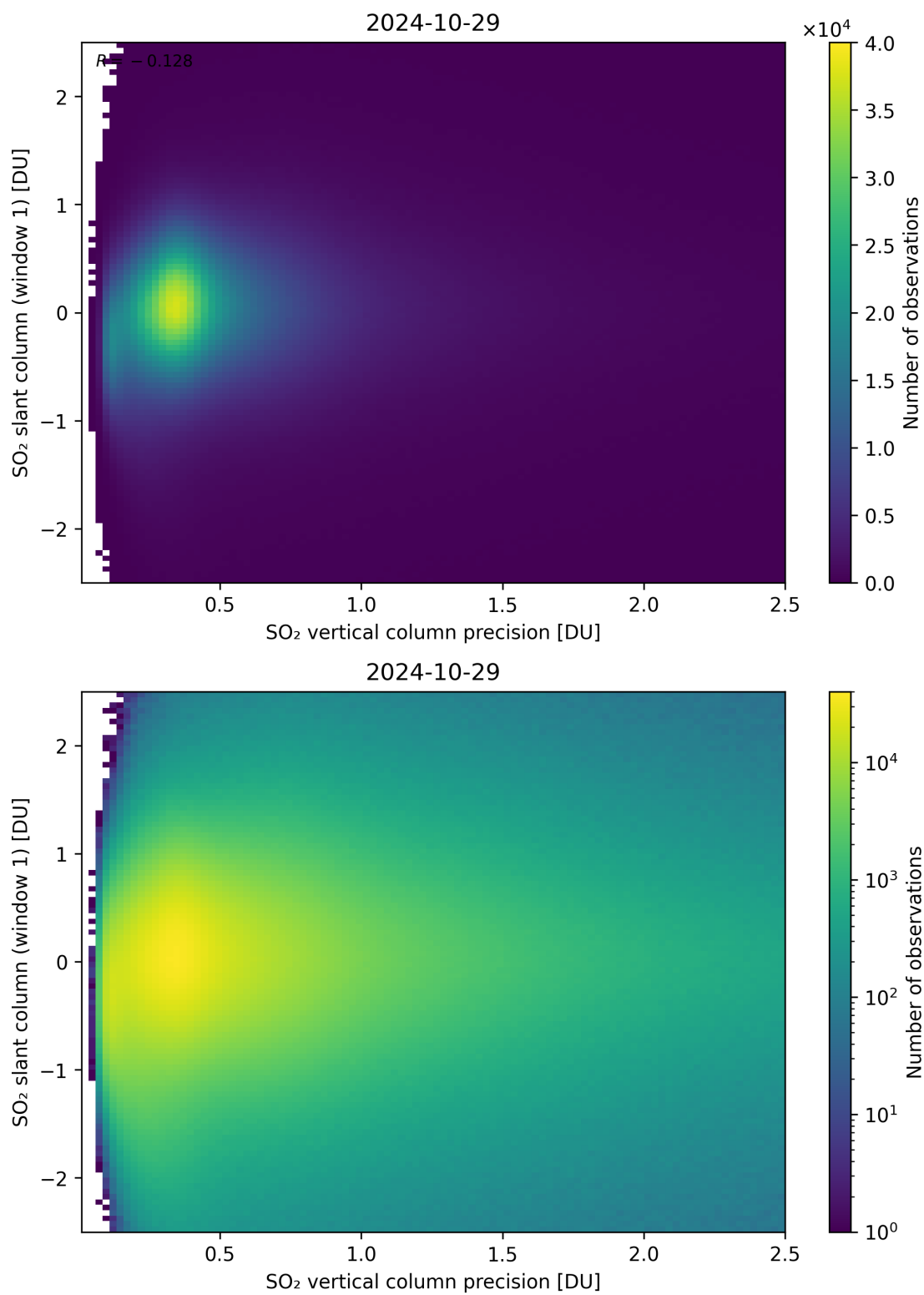
Figure 289: Scatter density plot of “SO 2 vertical column precision” against “SO 2 slant column (window 1)” for 2024-10-29 to 2024-10-30.
