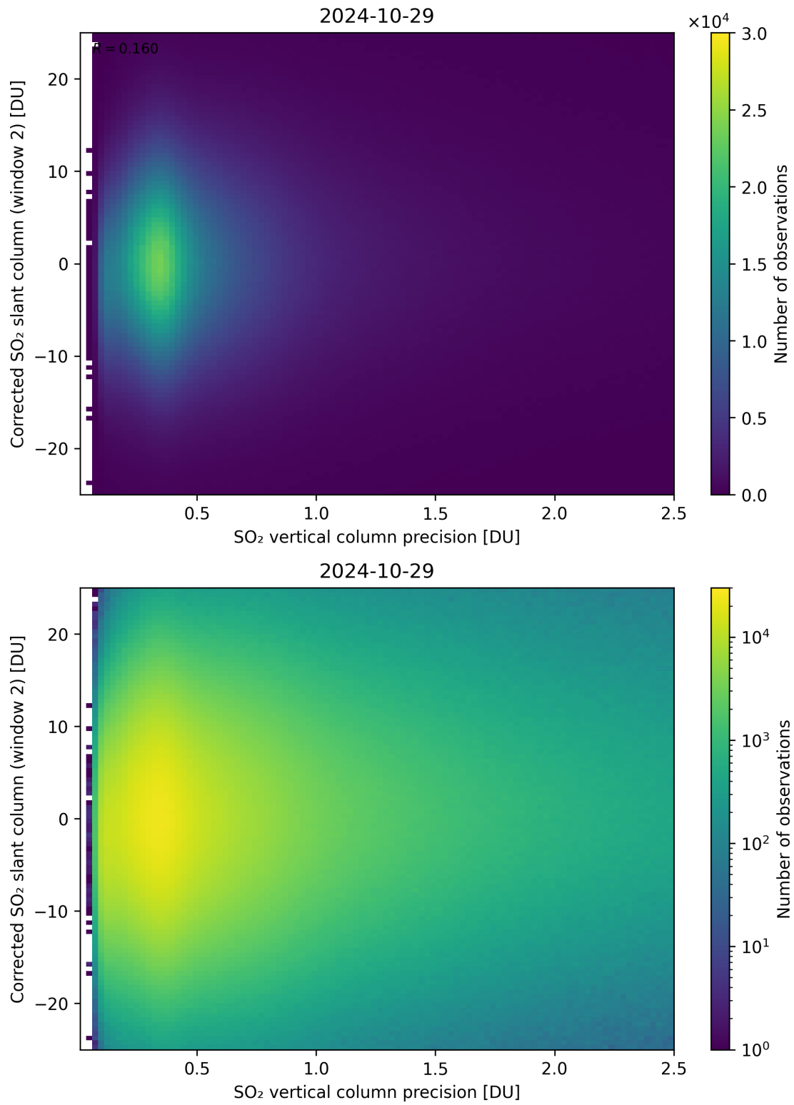
Figure 287: Scatter density plot of “SO 2 vertical column precision” against “Corrected SO 2 slant column (window 2)” for 2024-10-29 to 2024-10-30.
