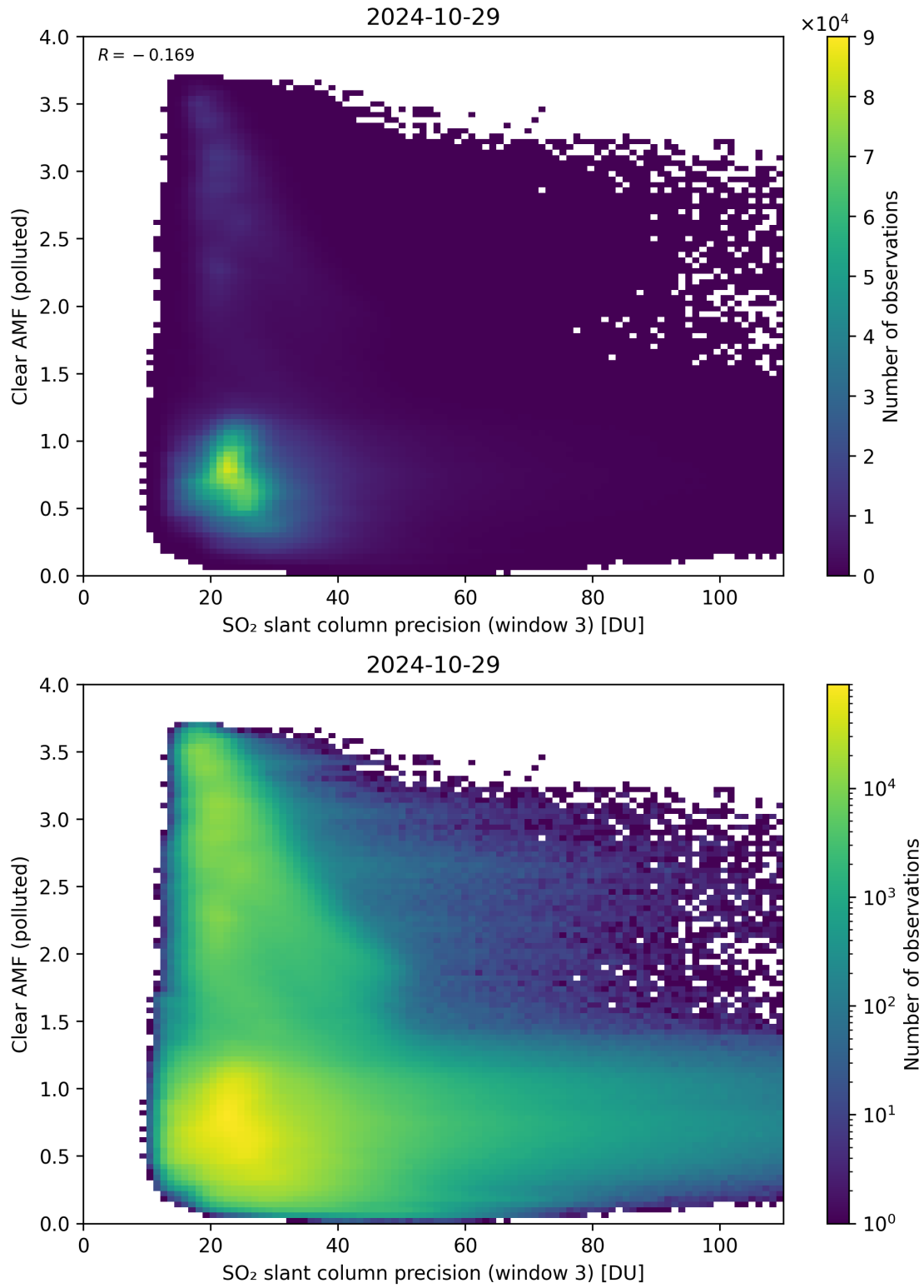
Figure 261: Scatter density plot of “SO 2 slant column precision (window 3)” against “Clear AMF (polluted)” for 2024-10-29 to 2024-10-30.
