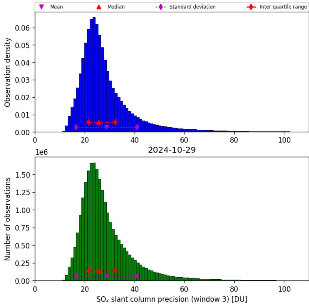
Figure 65: Histogram of “SO 2 slant column precision (window 3)” for 2024-10-29 to 2024-10-30
