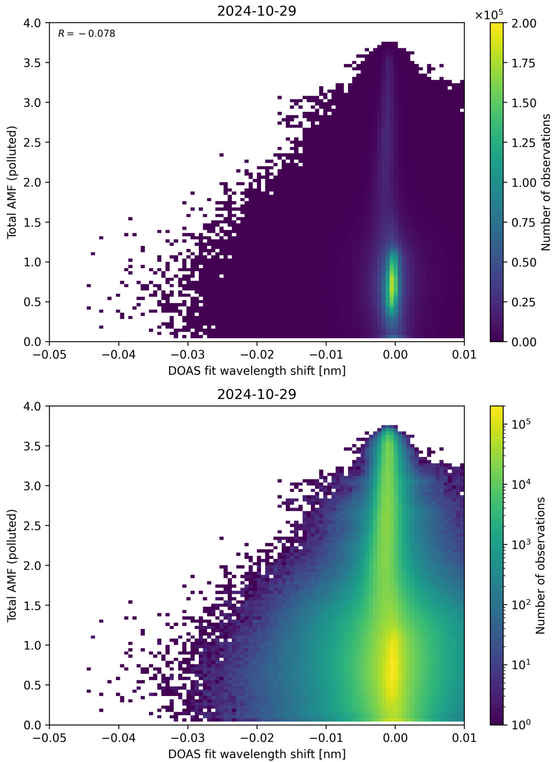
Figure 130: Scatter density plot of “DOAS fit wavelength shift” against “Total AMF (polluted)” for 2024-10-29 to 2024-10-30.
