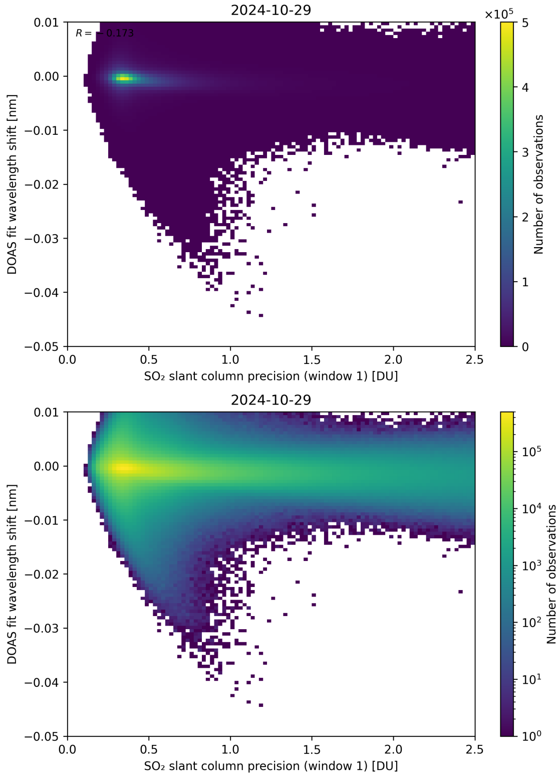
Figure 221: Scatter density plot of “SO 2 slant column precision (window 1)” against “DOAS fit wavelength shift” for 2024-10-29 to 2024-10-30.
