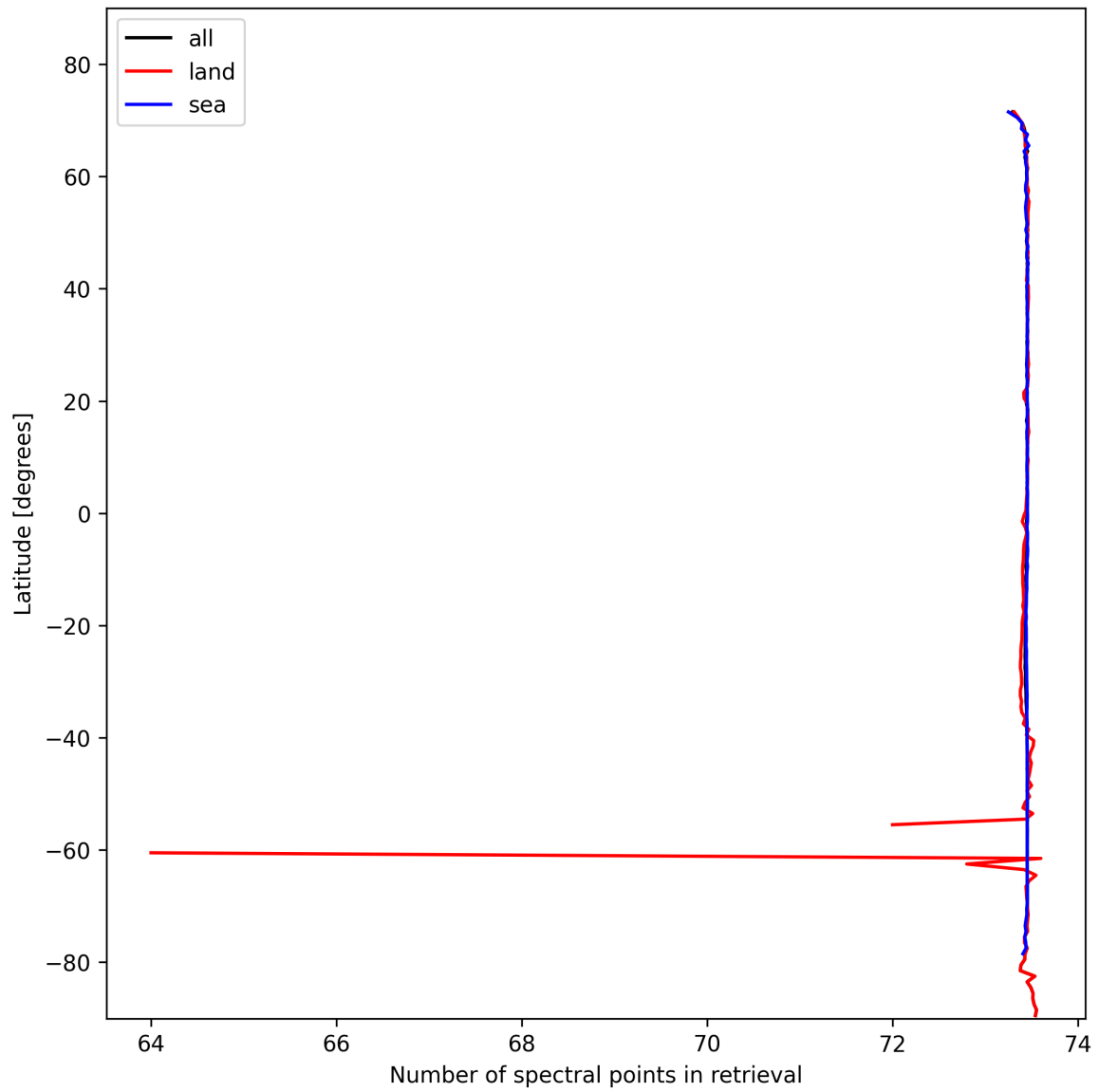
Figure 51: Zonal average of “Number of spectral points in retrieval” for 2024-10-29 to 2024-10-30.
