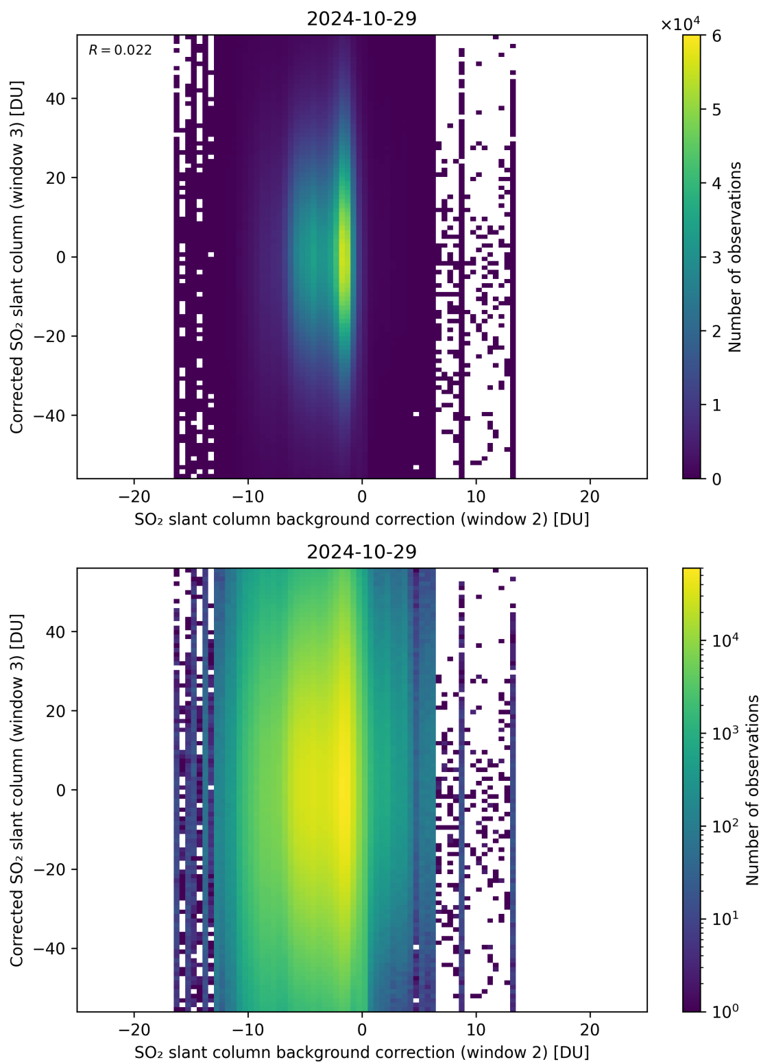
Figure 116: Scatter density plot of “SO 2 slant column background correction (window 2)” against “Corrected SO 2 slant column (window 3)” for 2024-10-29 to 2024-10-30.
