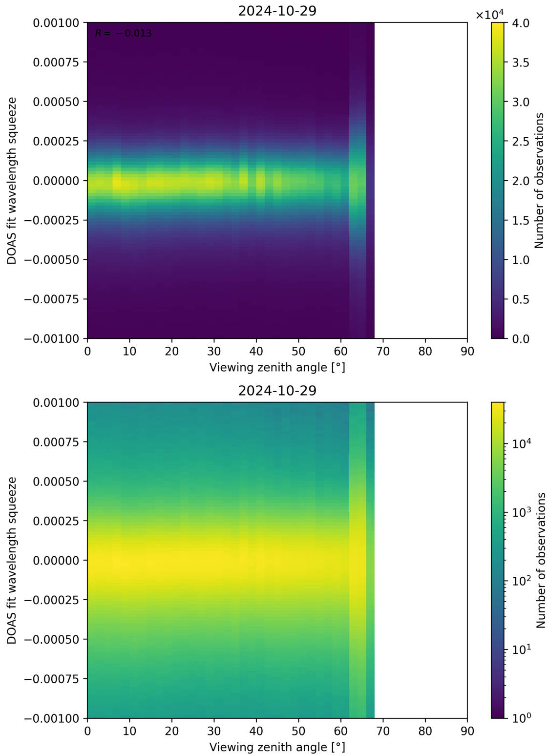
Figure 312: Scatter density plot of “Viewing zenith angle” against “DOAS fit wavelength squeeze” for 2024-10-29 to 2024-10-30.
