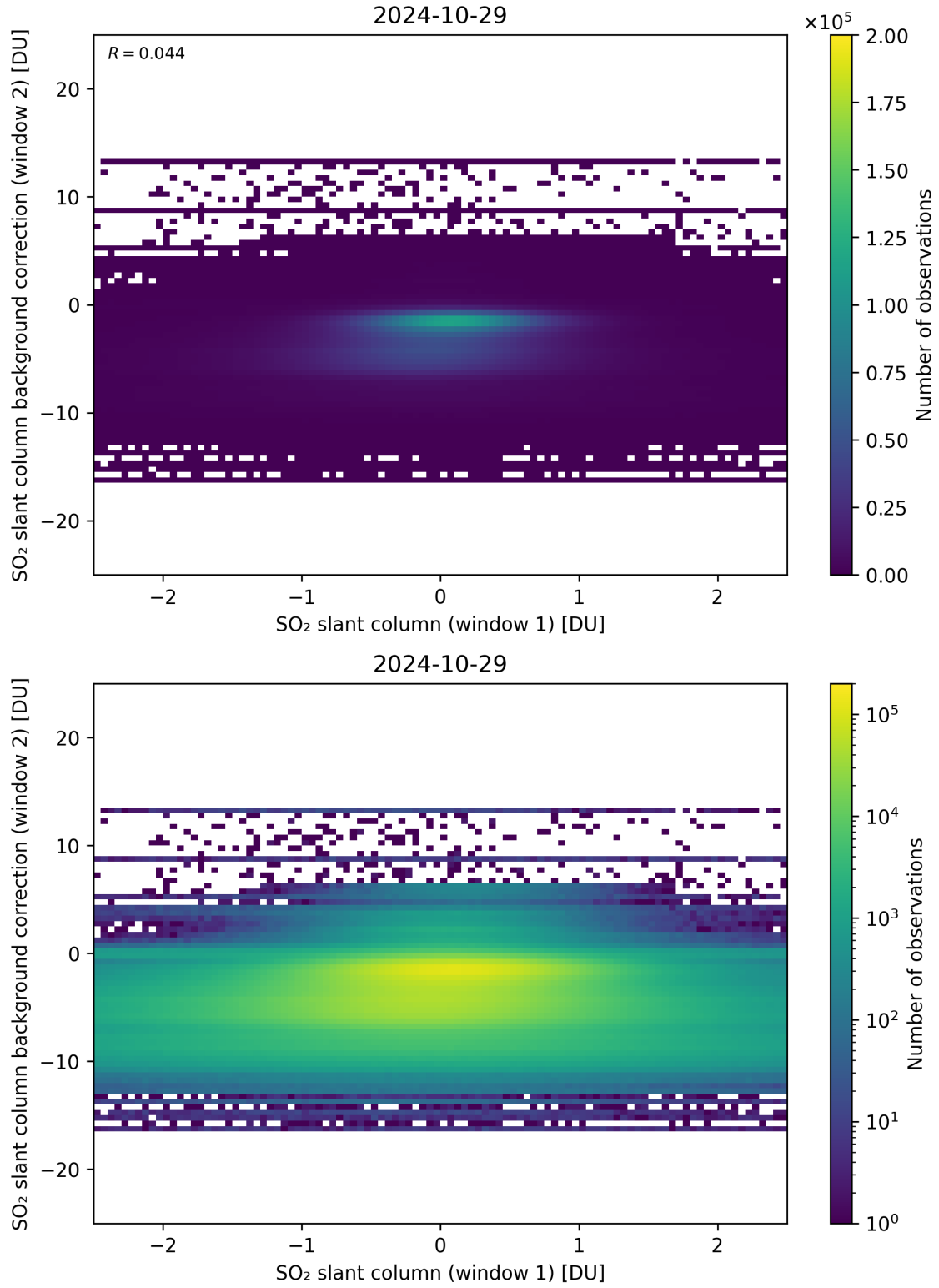
Figure 213: Scatter density plot of “SO 2 slant column (window 1)” against “SO 2 slant column background correction (window 2)” for 2024-10-29 to 2024-10-30.
