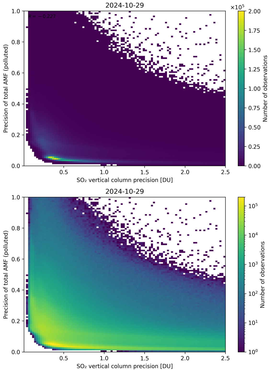
Figure 295: Scatter density plot of “SO 2 vertical column precision” against “Precision of total AMF (polluted)” for 2024-10-29 to 2024-10-30.
