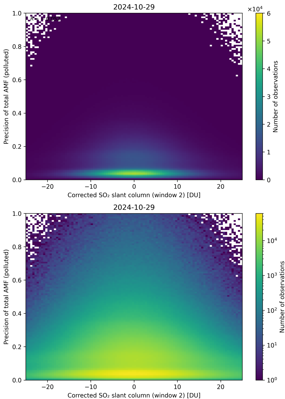
Figure 204: Scatter density plot of “Corrected SO 2 slant column (window 2)” against “Precision of total AMF (polluted)” for 2024-10-29 to 2024-10-30.
