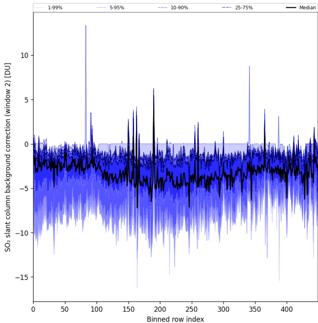
Figure 86: Along track statistics of “SO 2 slant column background correction (window 2)” for 2024-10-29 to 2024-10-30
