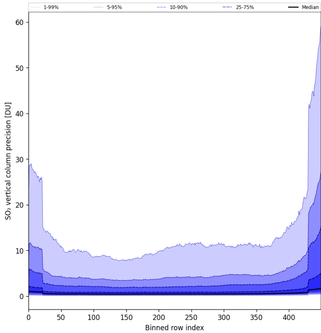
Figure 77: Along track statistics of “SO 2 vertical column precision” for 2024-10-29 to 2024-10-30
