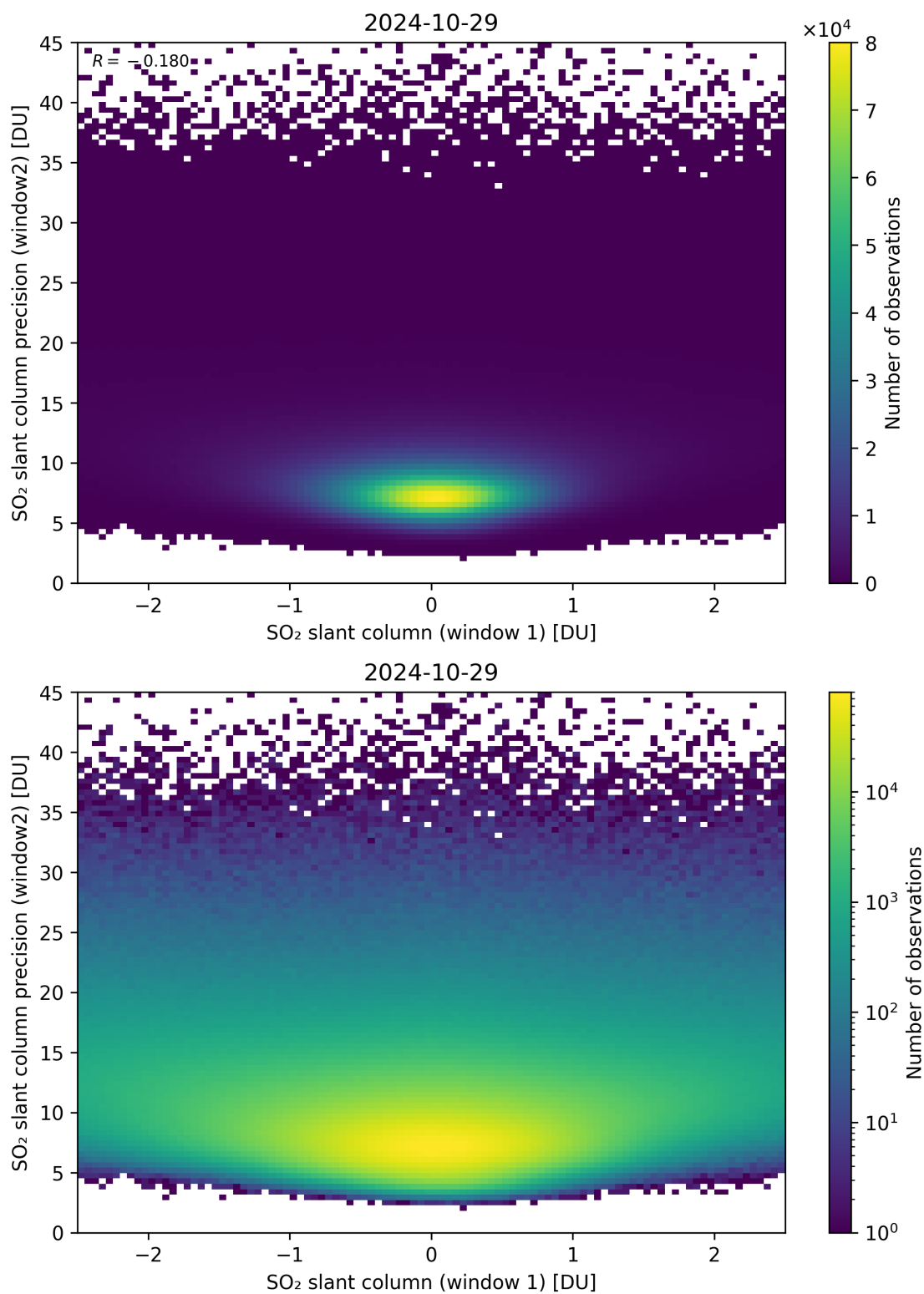
Figure 236: Scatter density plot of “SO 2 slant column (window 1)” against “SO 2 slant column precision (window2)” for 2024-10-29 to 2024-10-30.
