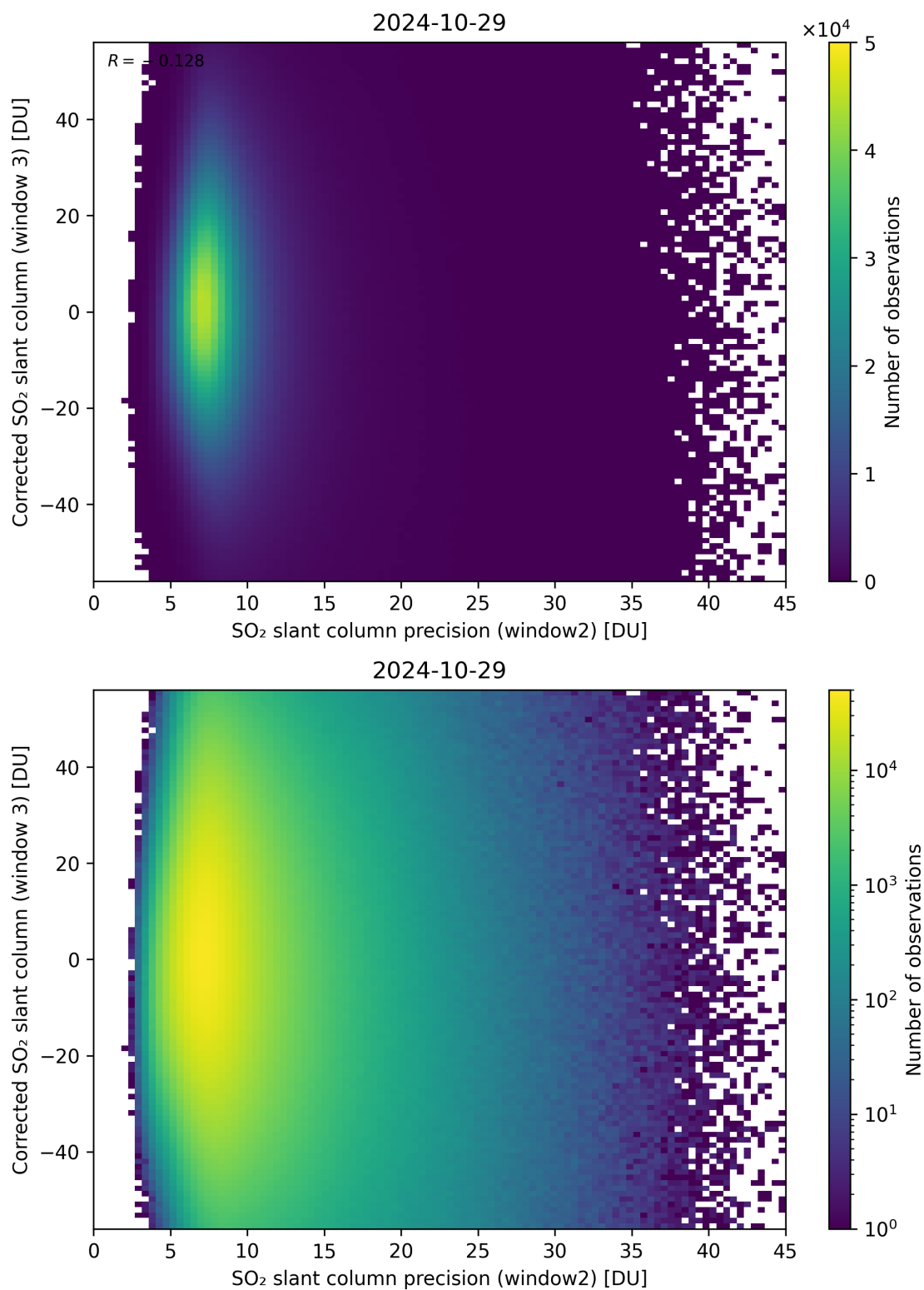
Figure 248: Scatter density plot of “SO 2 slant column precision (window2)” against “Corrected SO 2 slant column (window 3)” for 2024-10-29 to 2024-10-30.
