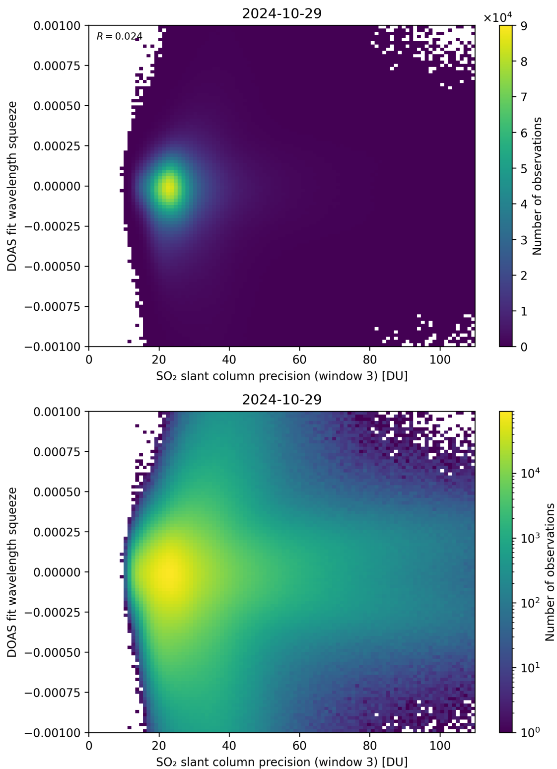
Figure 259: Scatter density plot of “SO 2 slant column precision (window 3)” against “DOAS fit wavelength squeeze” for 2024-10-29 to 2024-10-30.
