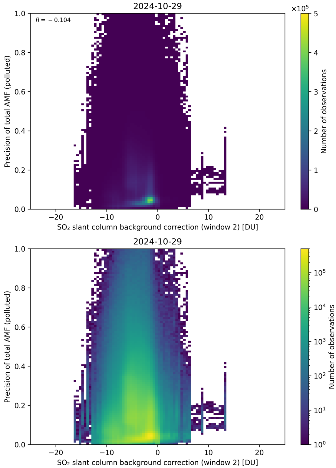
Figure 120: Scatter density plot of “SO 2 slant column background correction (window 2)” against “Precision of total AMF (polluted)” for 2024-10-29 to 2024-10-30.
