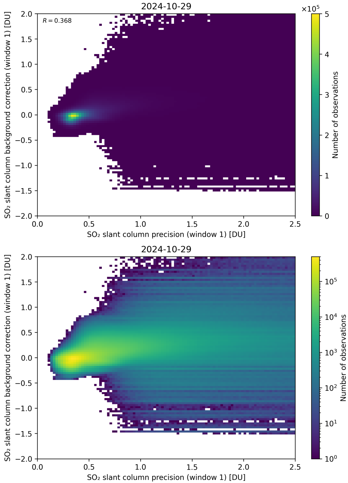
Figure 218: Scatter density plot of “SO 2 slant column precision (window 1)” against “SO 2 slant column background correction (window 1)” for 2024-10-29 to 2024-10-30.
