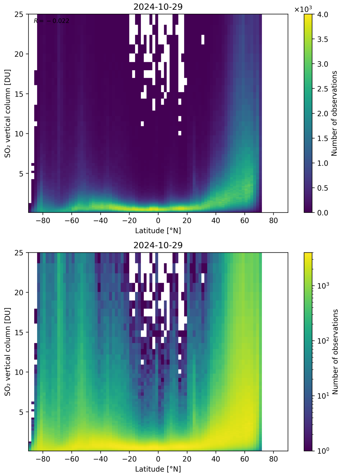
Figure 156: Scatter density plot of “Latitude” against “SO 2 vertical column” for 2024-10-29 to 2024-10-30.
