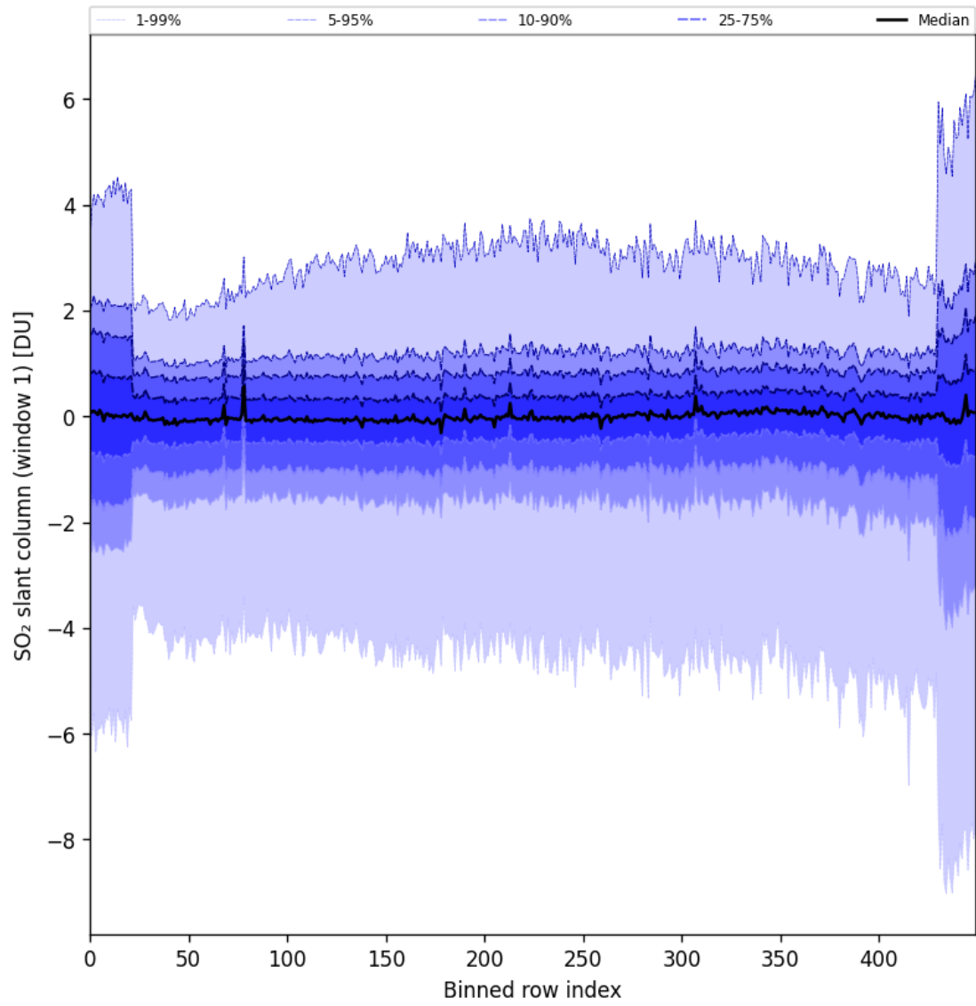
Figure 79: Along track statistics of “SO 2 slant column (window 1)” for 2024-10-29 to 2024-10-30
