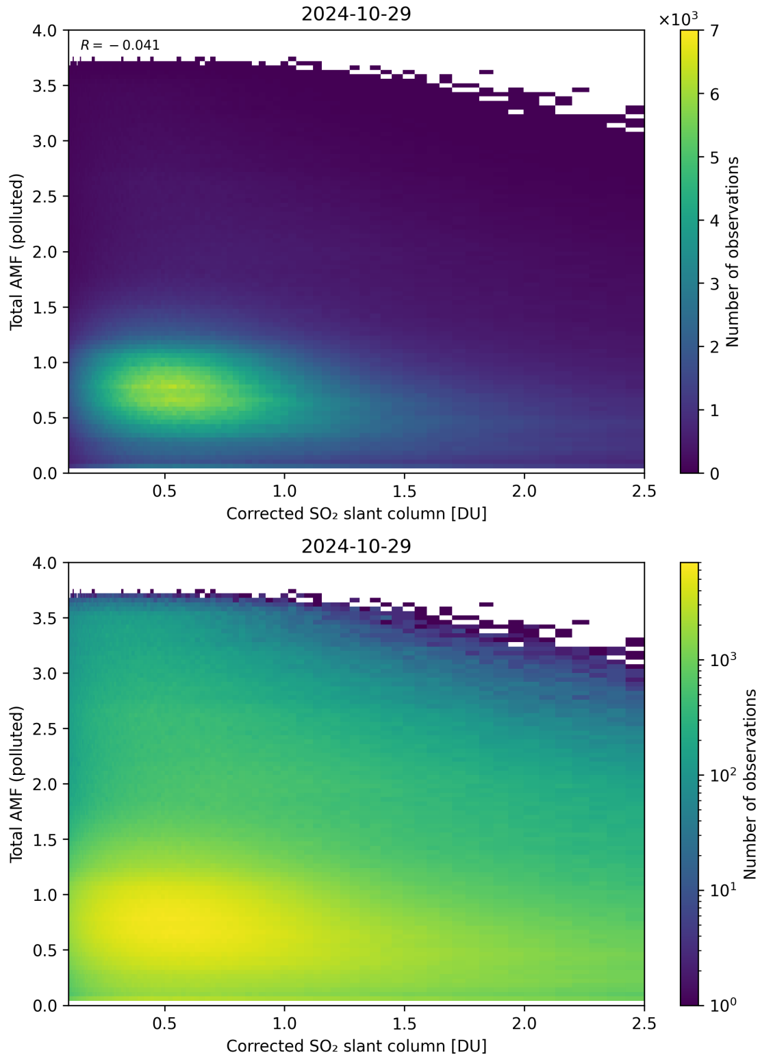
Figure 192: Scatter density plot of “Corrected SO 2 slant column” against “Total AMF (polluted)” for 2024-10-29 to 2024-10-30.
