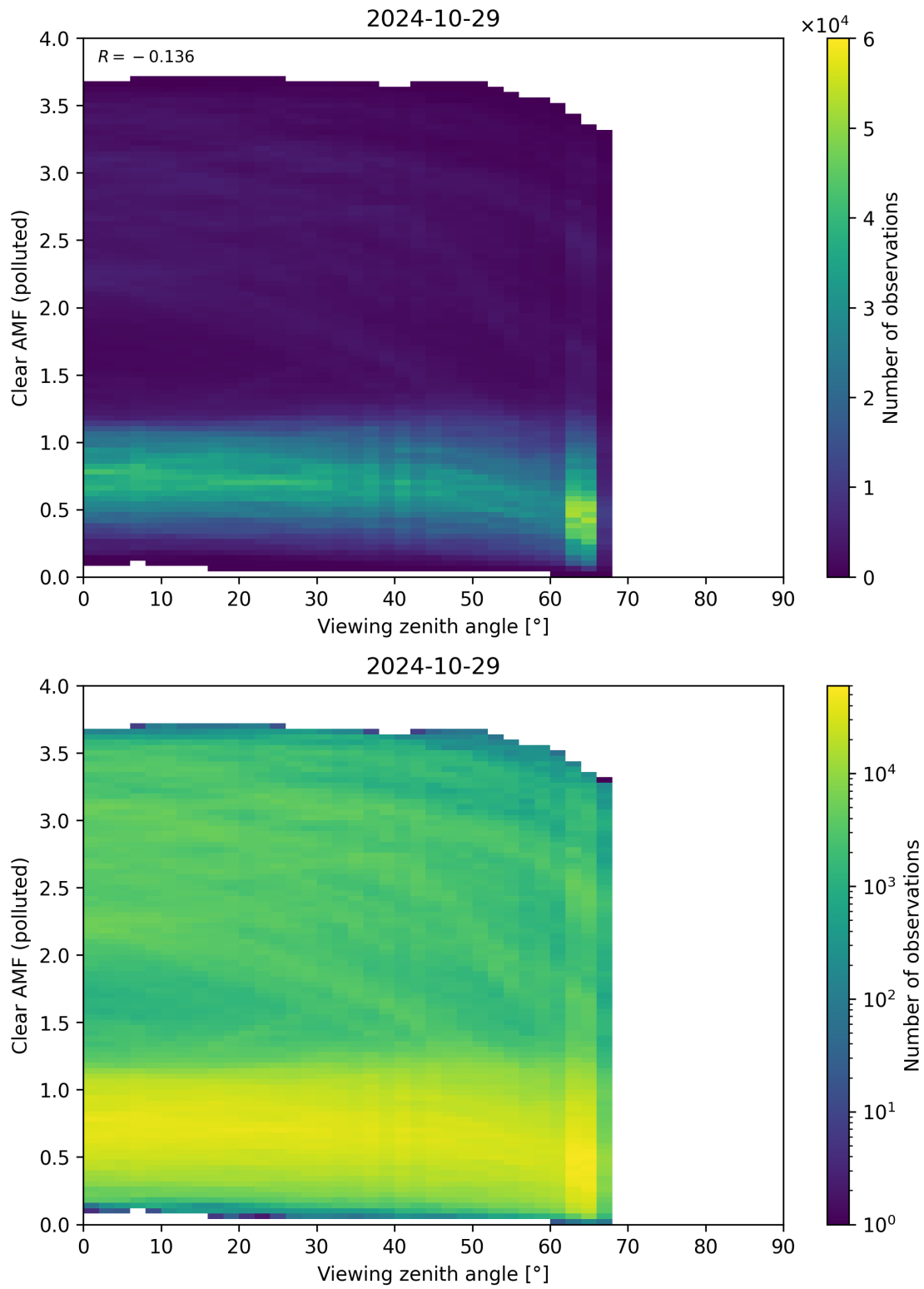
Figure 316: Scatter density plot of “Viewing zenith angle” against “Clear AMF (polluted)” for 2024-10-29 to 2024-10-30.
