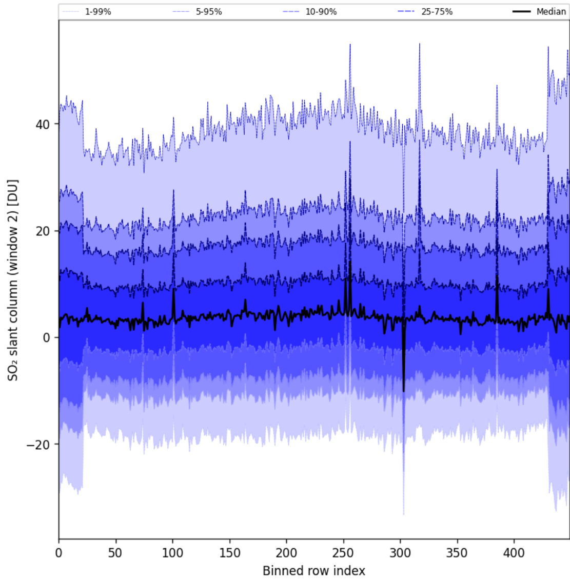
Figure 83: Along track statistics of “SO 2 slant column (window 2)” for 2024-10-29 to 2024-10-30
