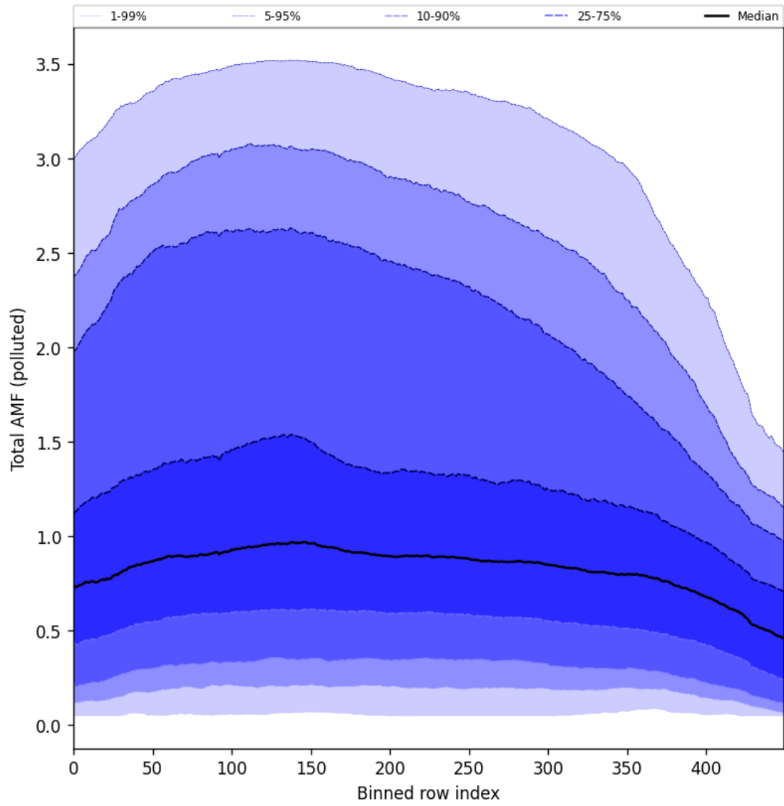
Figure 94: Along track statistics of “Total AMF (polluted)” for 2024-10-29 to 2024-10-30
