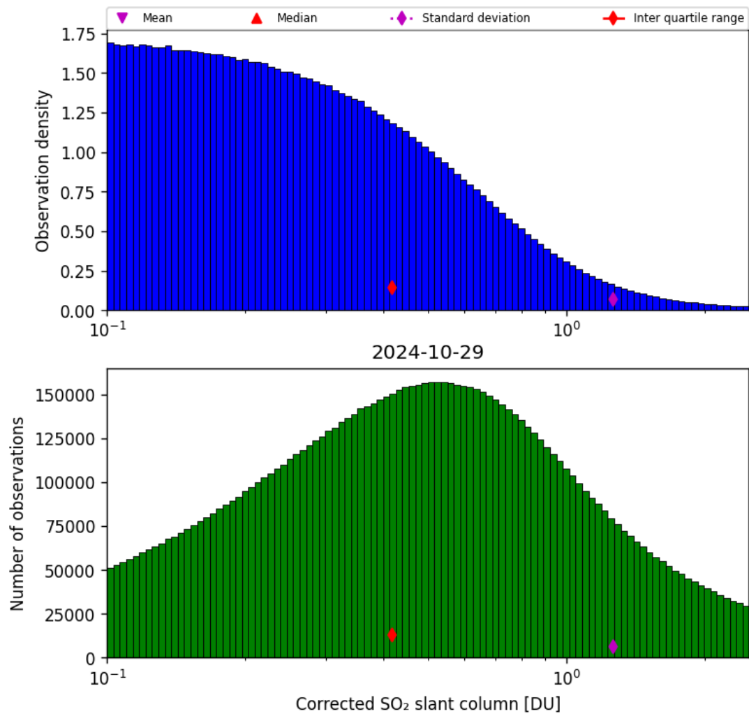
Figure 55: Histogram of "Corrected SO 2 slant column" for 2024-10-29 to 2024-10-30
