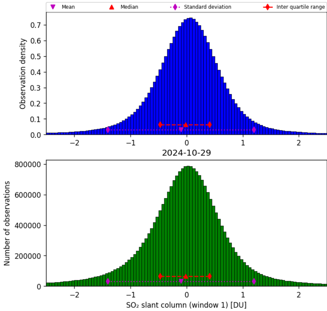
Figure 56: Histogram of “SO 2 slant column (window 1)” for 2024-10-29 to 2024-10-30
