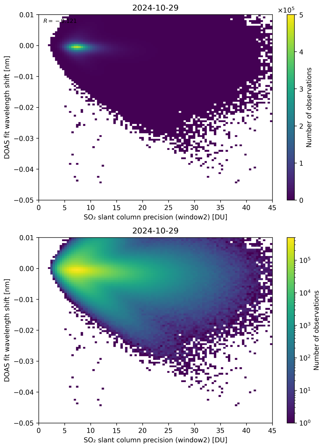
Figure 243: Scatter density plot of “SO 2 slant column precision (window2)” against “DOAS fit wavelength shift” for 2024-10-29 to 2024-10-30.
