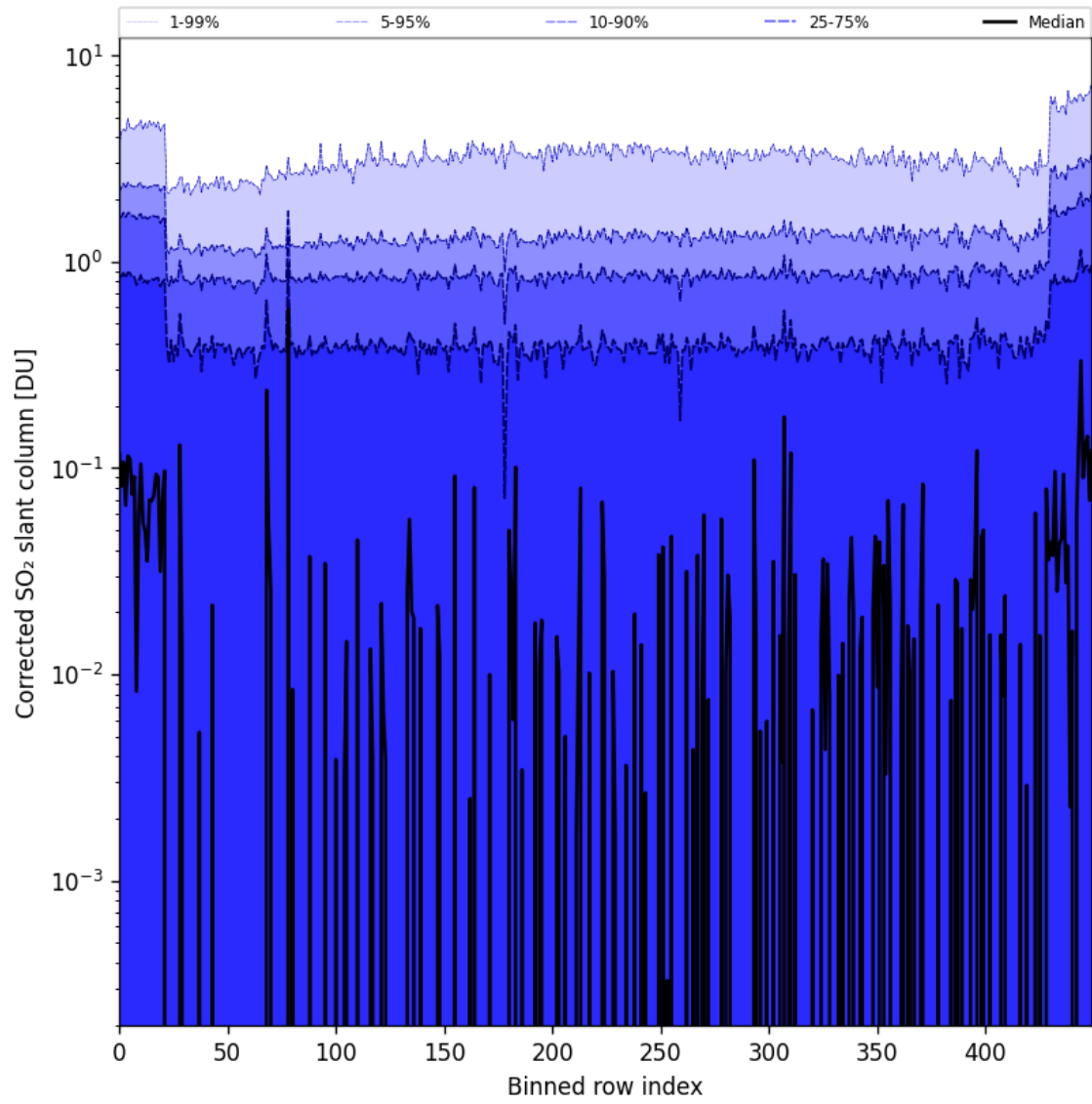
Figure 78: Along track statistics of “Corrected SO 2 slant column” for 2024-10-29 to 2024-10-30
