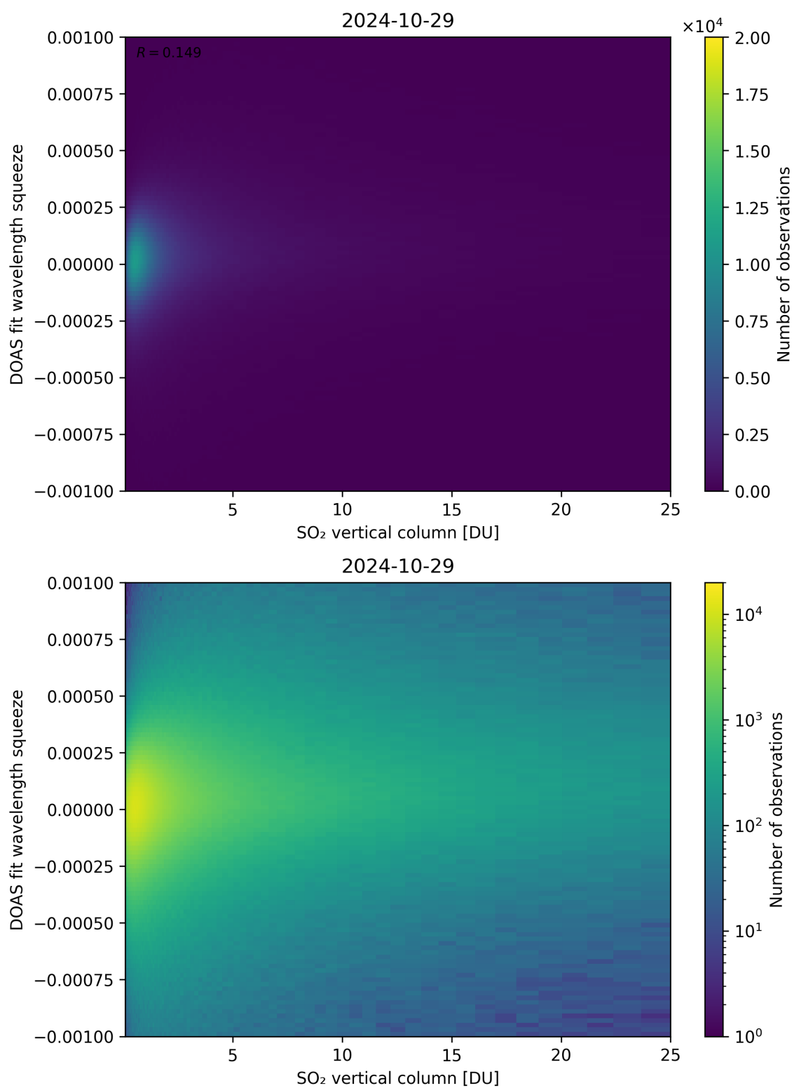
Figure 277: Scatter density plot of “SO 2 vertical column” against “DOAS fit wavelength squeeze” for 2024-10-29 to 2024-10-30.
