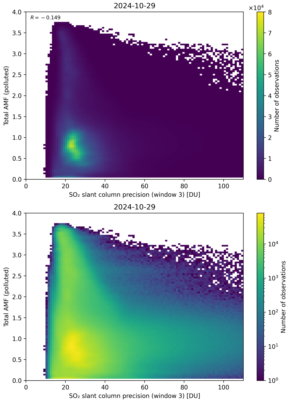
Figure 263: Scatter density plot of “SO 2 slant column precision (window 3)” against “Total AMF (polluted)” for 2024-10-29 to 2024-10-30.
