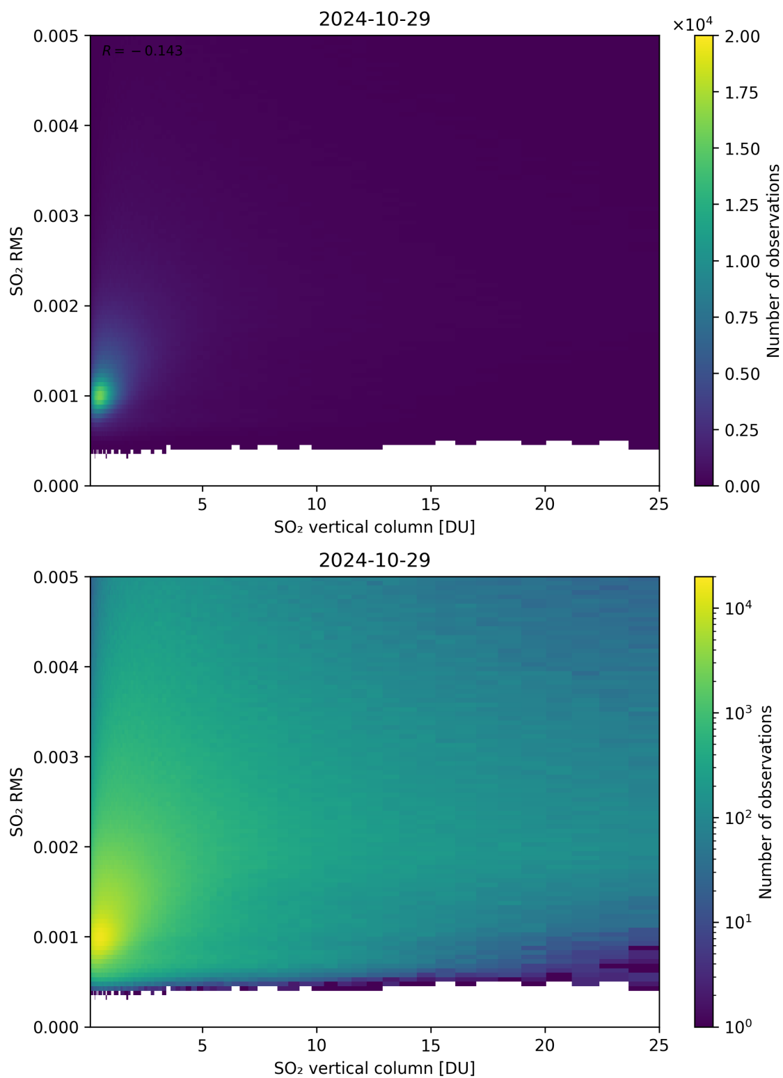
Figure 278: Scatter density plot of “SO 2 vertical column” against “SO 2 RMS” for 2024-10-29 to 2024-10-30.
