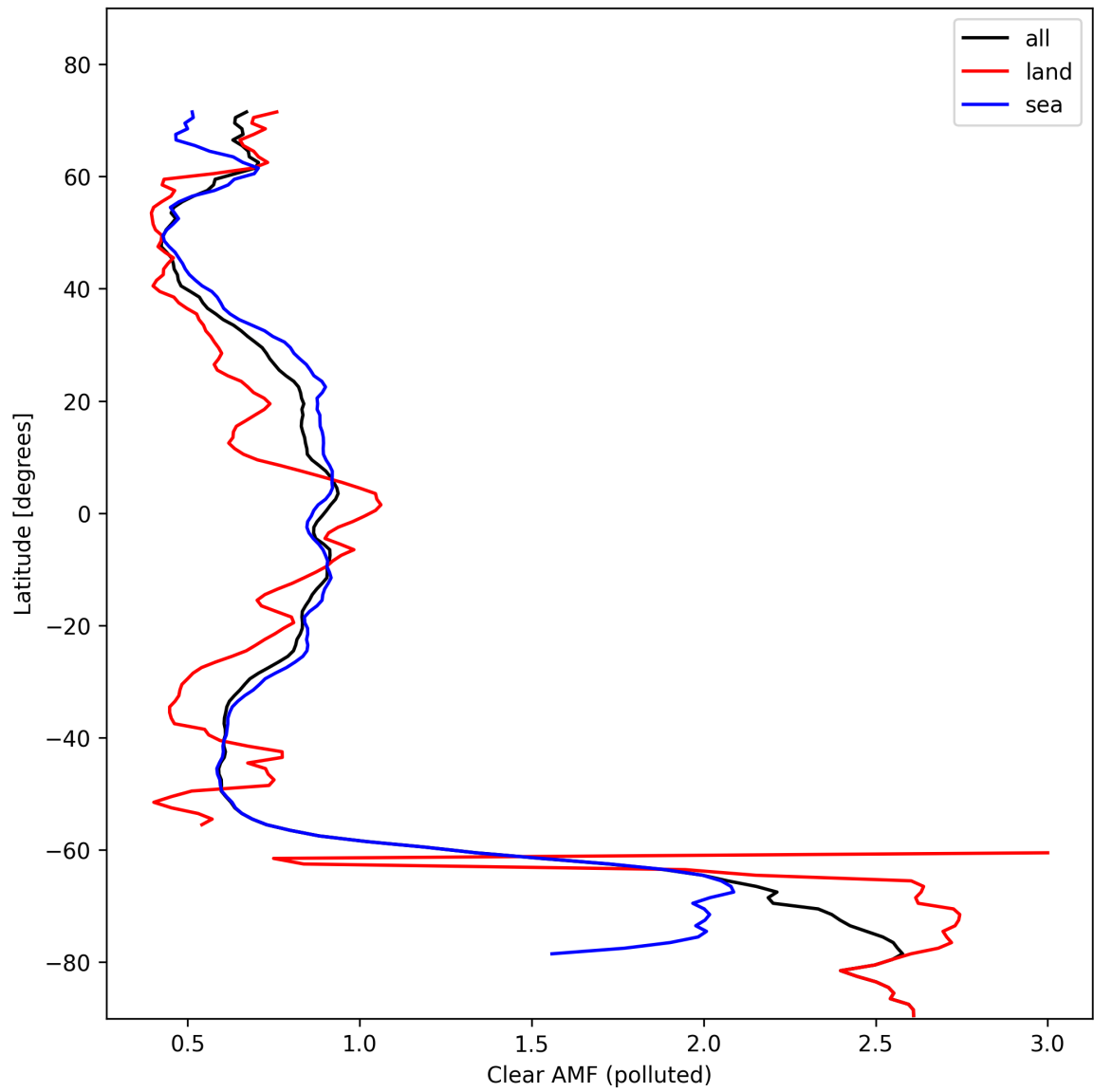
Figure 50: Zonal average of “Clear AMF (polluted)” for 2024-10-29 to 2024-10-30.
