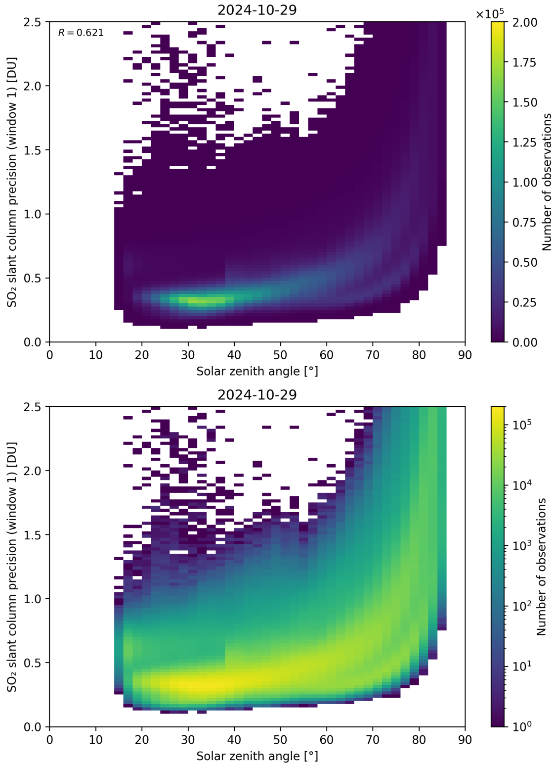
Figure 170: Scatter density plot of “Solar zenith angle” against “SO 2 slant column precision (window 1)” for 2024-10-29 to 2024-10-30.
