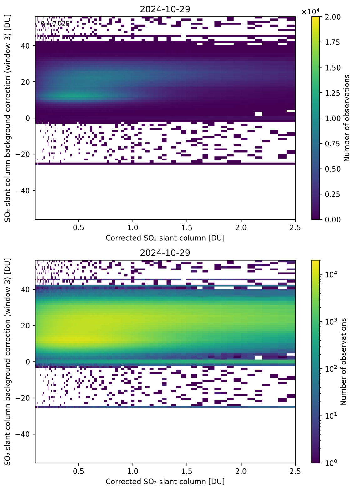
Figure 180: Scatter density plot of “Corrected SO 2 slant column” against “SO 2 slant column background correction (window 3)” for 2024-10-29 to 2024-10-30.
