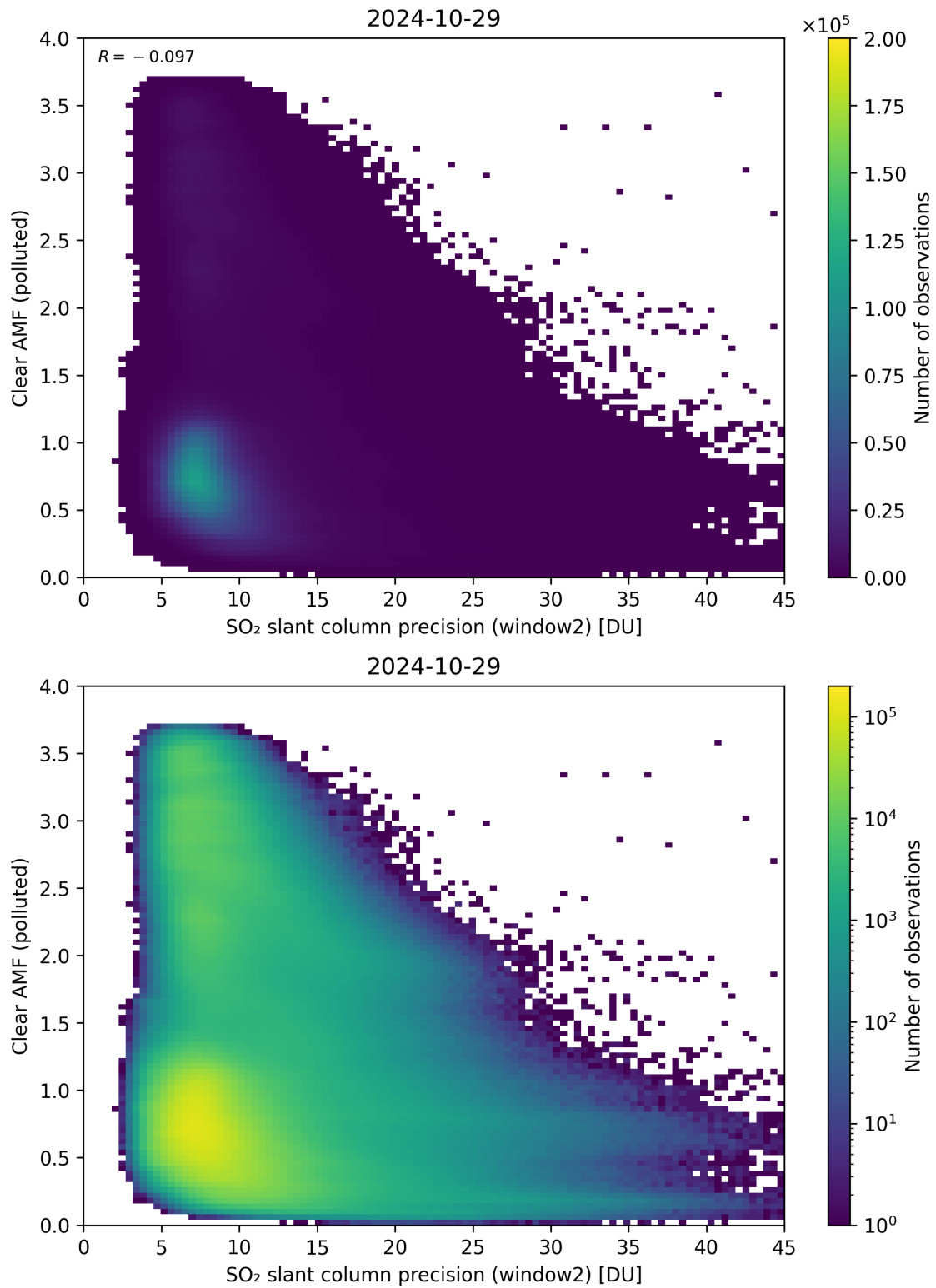
Figure 246: Scatter density plot of “SO 2 slant column precision (window2)” against “Clear AMF (polluted)” for 2024-10-29 to 2024-10-30.
