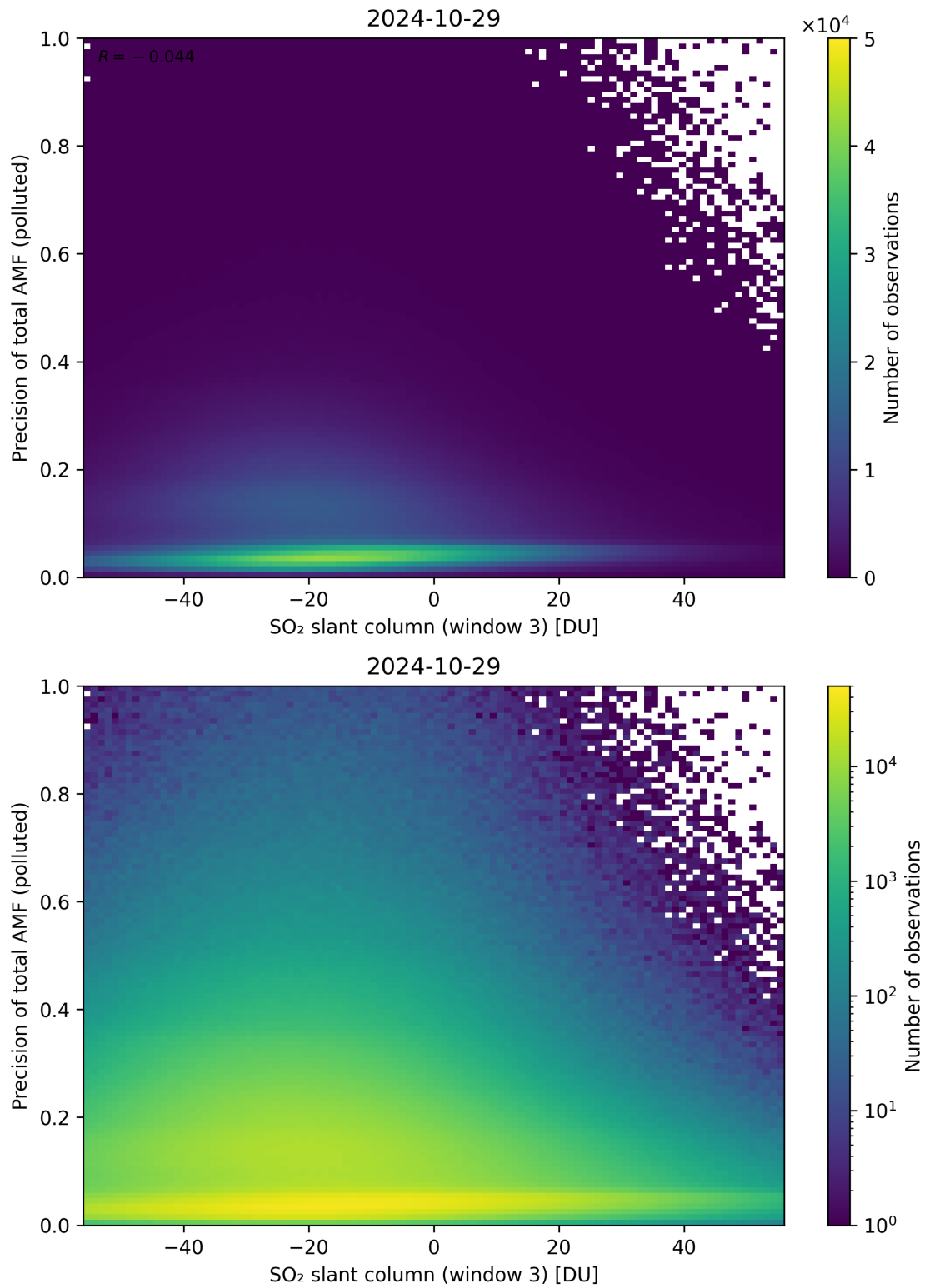
Figure 269: Scatter density plot of “SO 2 slant column (window 3)” against “Precision of total AMF (polluted)” for 2024-10-29 to 2024-10-30.
