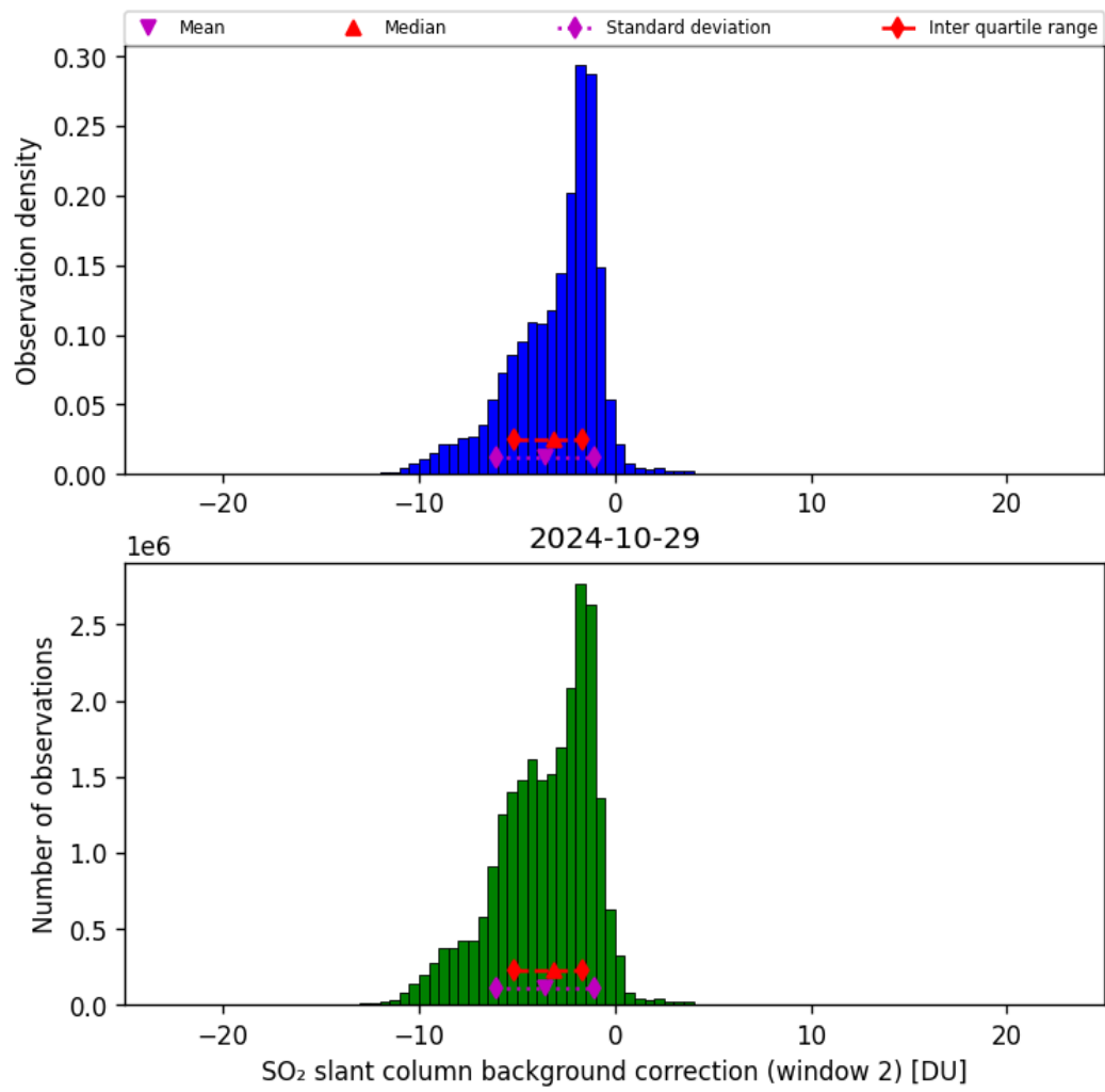
Figure 63: Histogram of “SO 2 slant column background correction (window 2)” for 2024-10-29 to 2024-10-30
