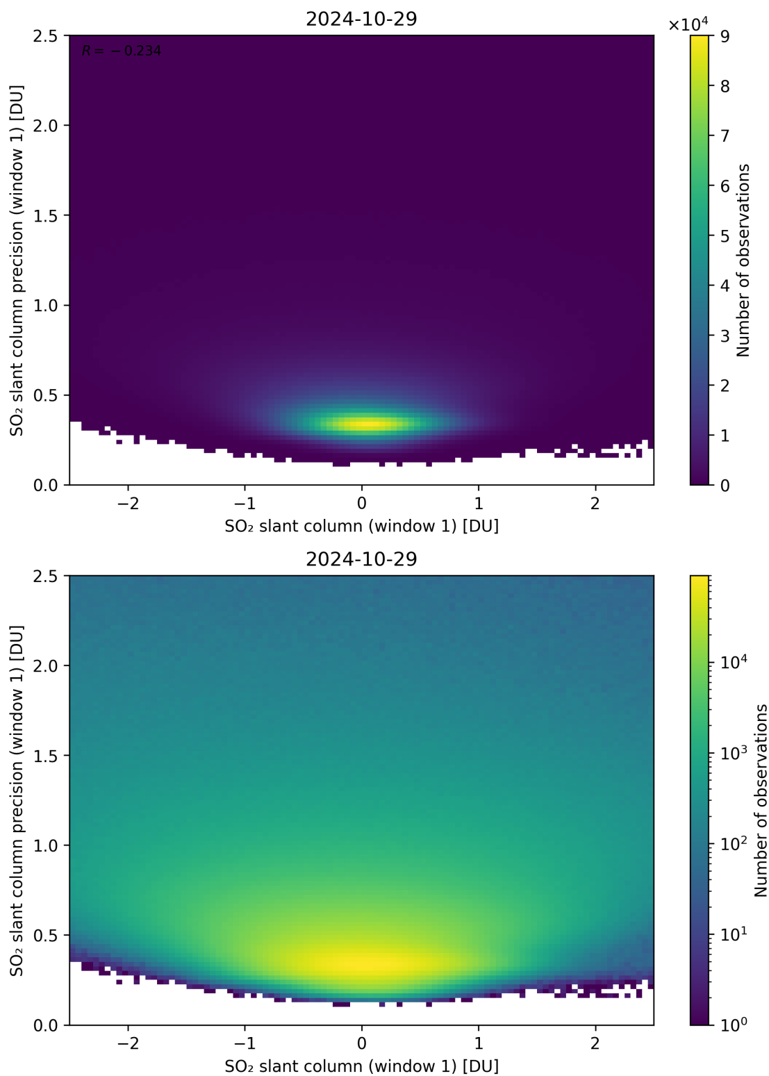
Figure 235: Scatter density plot of “SO 2 slant column (window 1)” against “SO 2 slant column precision (window 1)” for 2024-10-29 to 2024-10-30.
