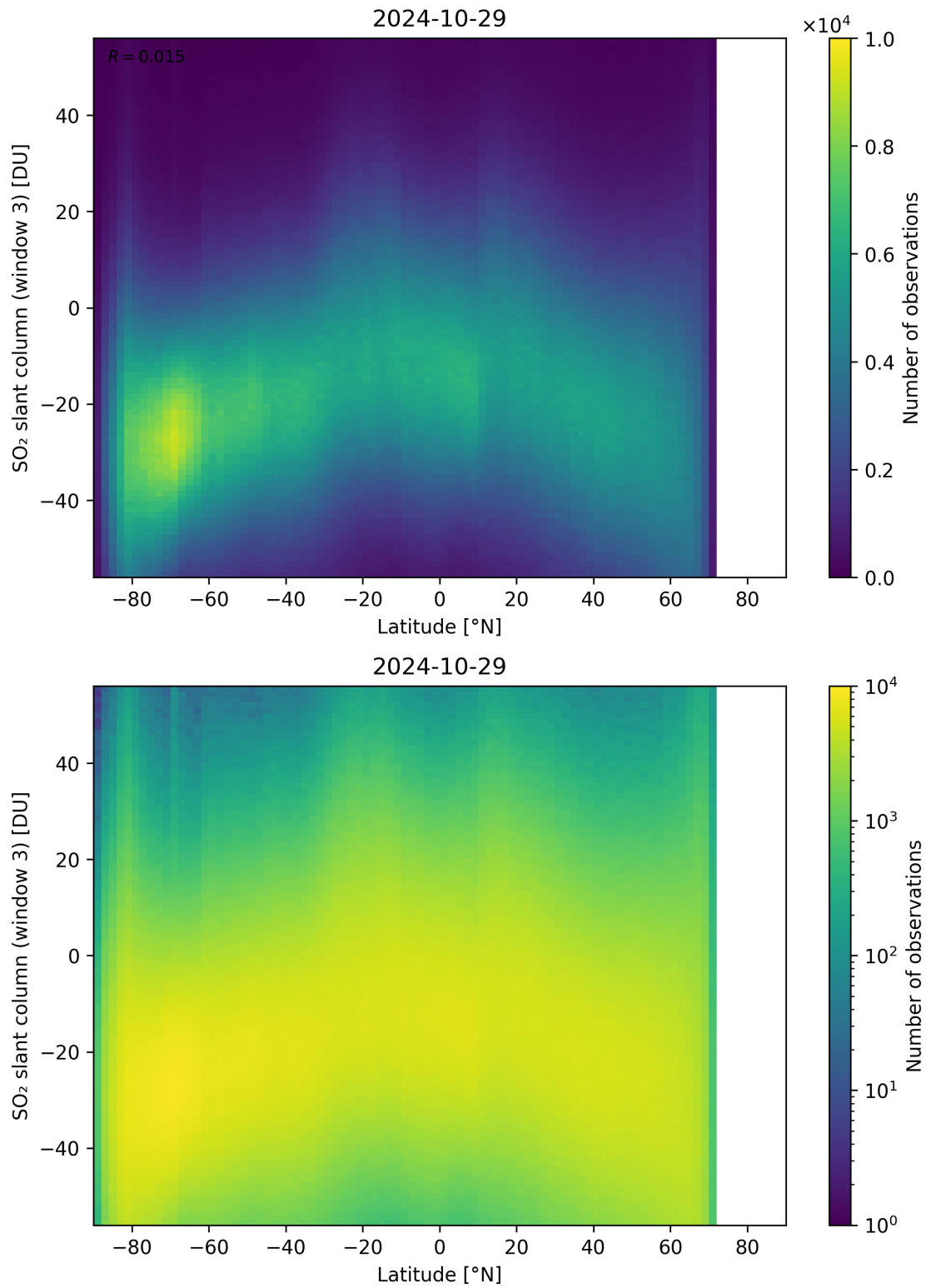
Figure 152: Scatter density plot of “Latitude” against “SO 2 slant column (window 3)” for 2024-10-29 to 2024-10-30.
