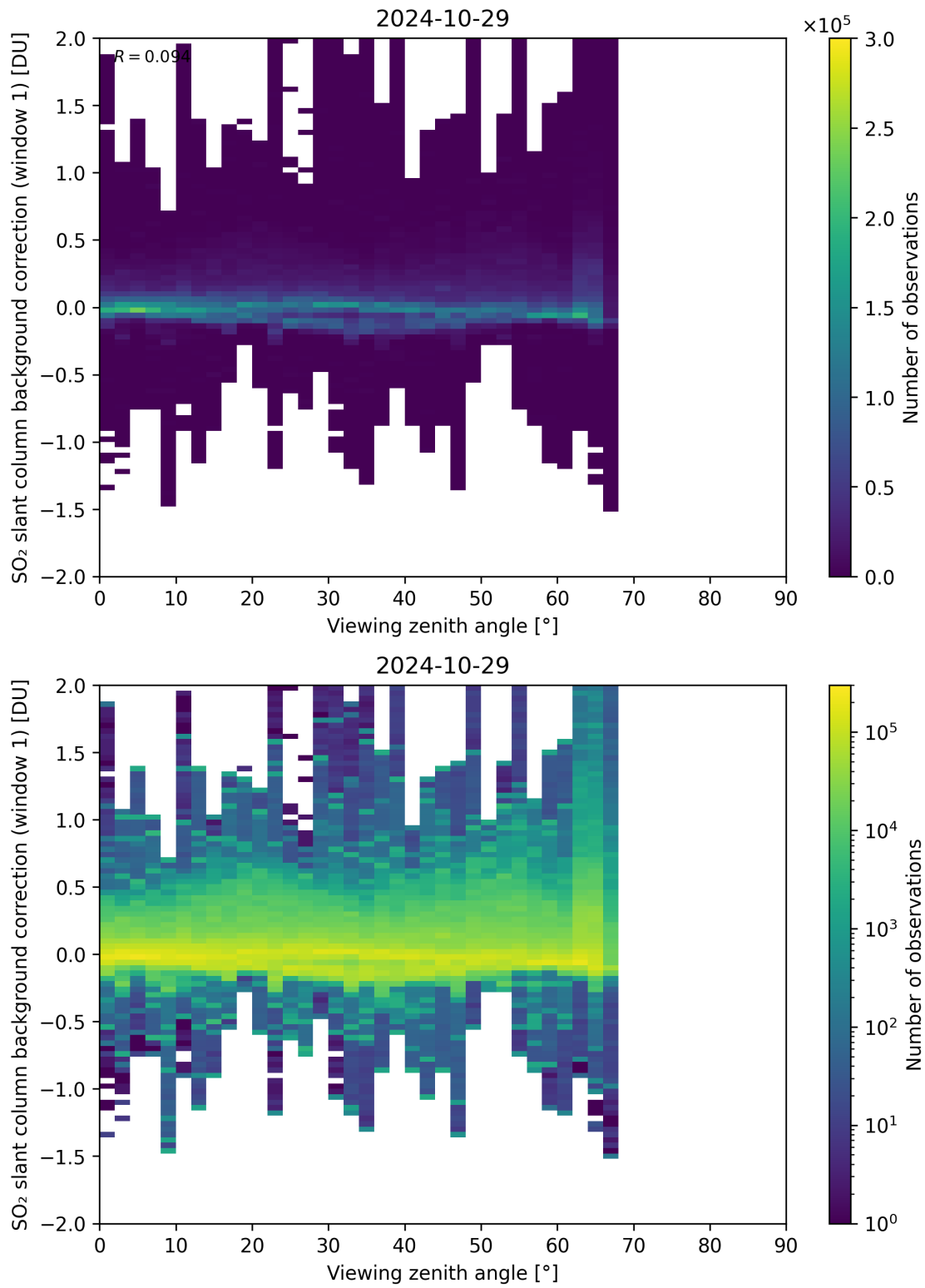
Figure 308: Scatter density plot of “Viewing zenith angle” against “SO 2 slant column background correction (window 1)” for 2024-10-29 to 2024-10-30.
