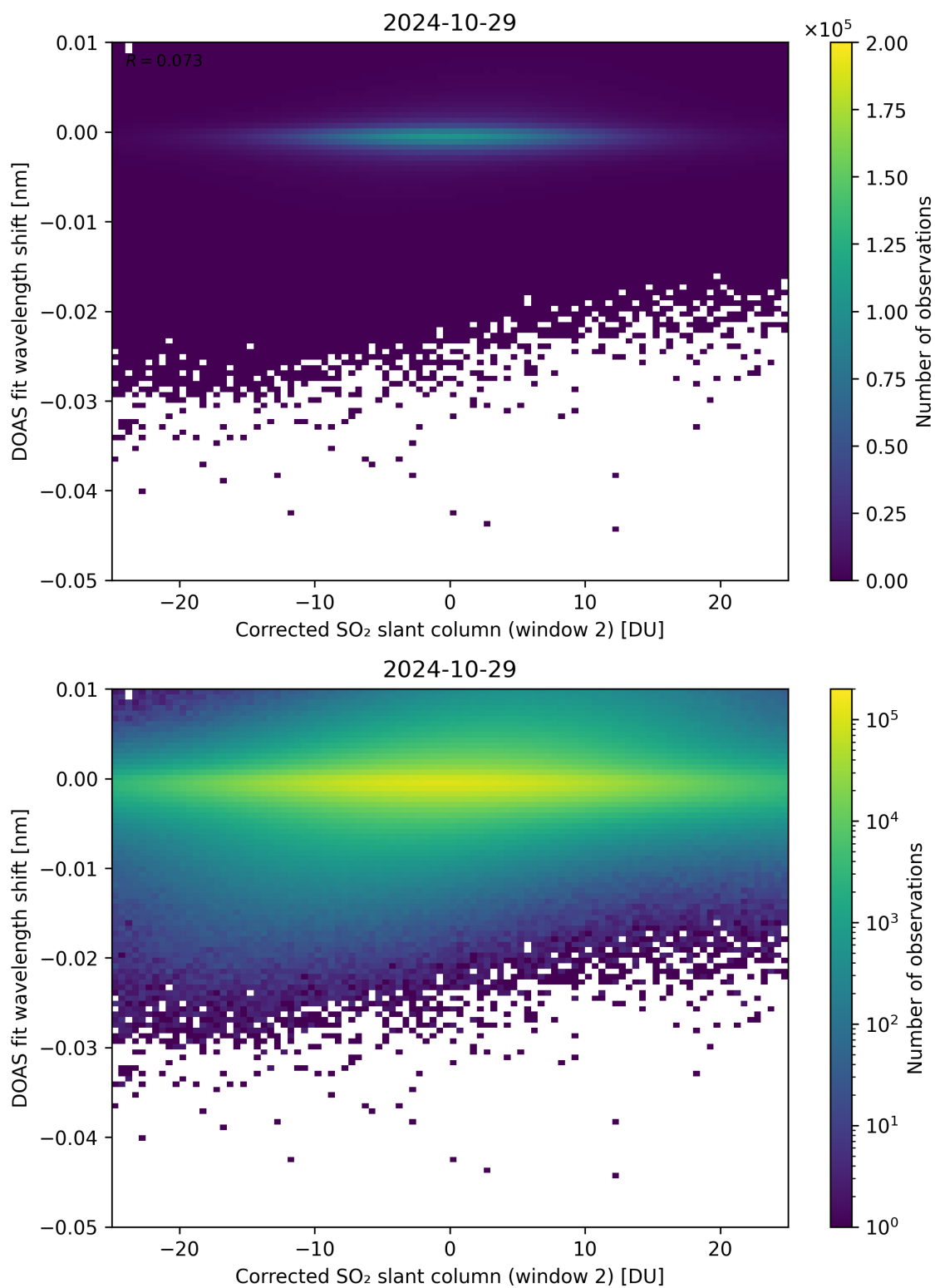
Figure 196: Scatter density plot of “Corrected SO 2 slant column (window 2)” against “DOAS fit wavelength shift” for 2024-10-29 to 2024-10-30.
