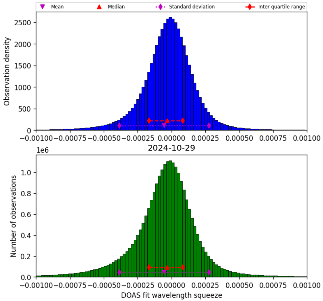
Figure 69: Histogram of “DOAS fit wavelength squeeze” for 2024-10-29 to 2024-10-30
