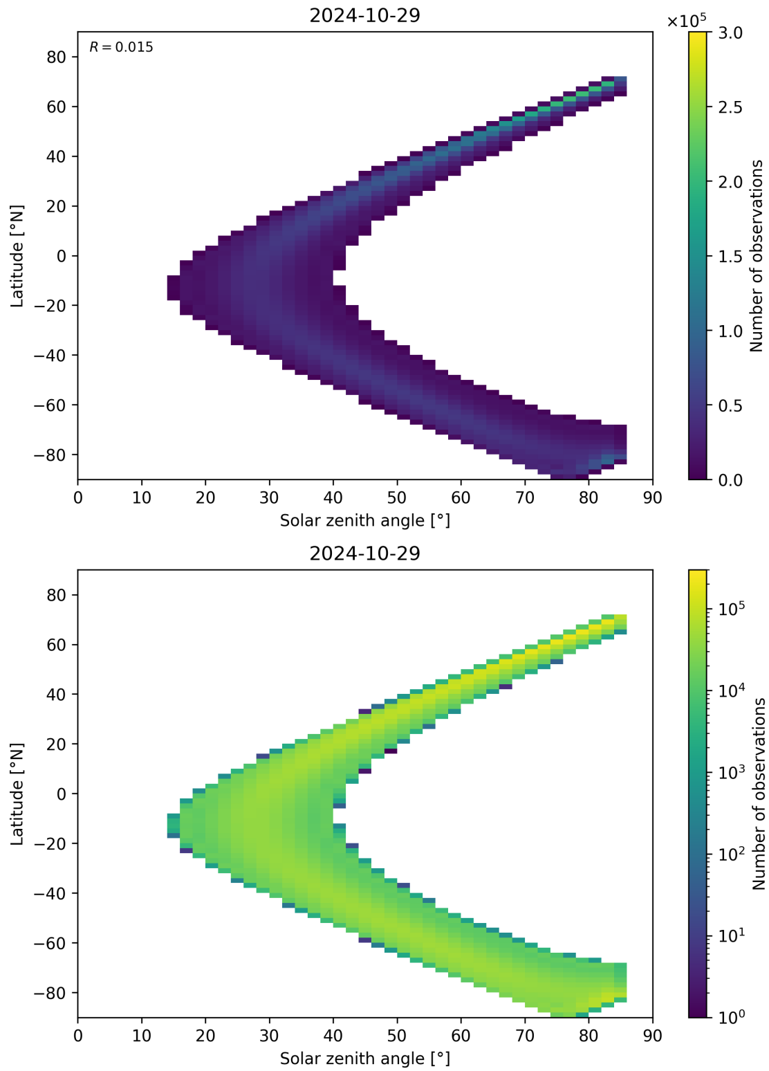
Figure 164: Scatter density plot of “Solar zenith angle” against “Latitude” for 2024-10-29 to 2024-10-30.
