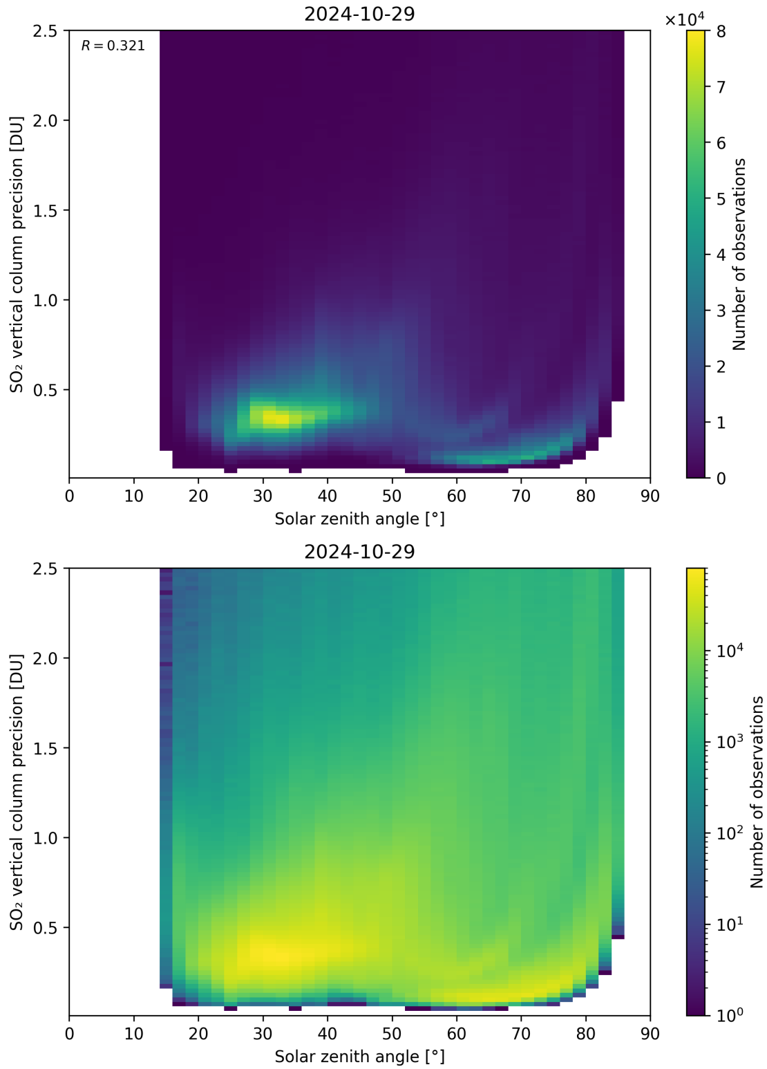
Figure 177: Scatter density plot of “Solar zenith angle” against “SO 2 vertical column precision” for 2024-10-29 to 2024-10-30.
