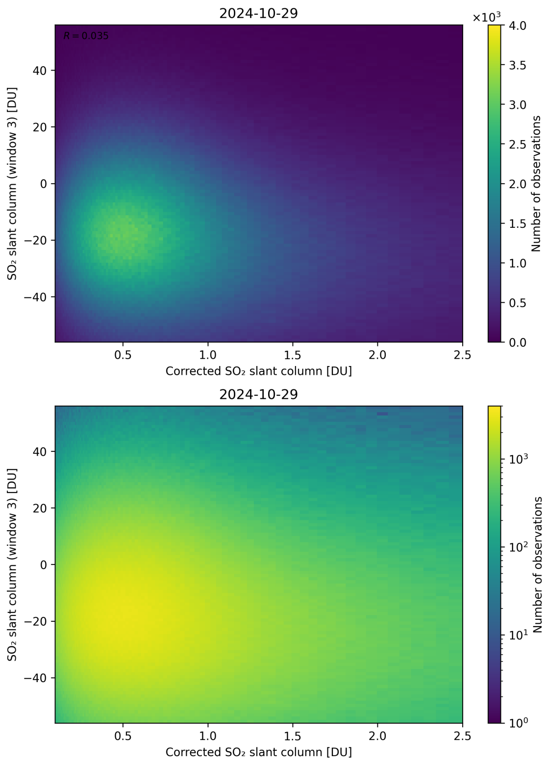
Figure 190: Scatter density plot of “Corrected SO 2 slant column” against “SO 2 slant column (window 3)” for 2024-10-29 to 2024-10-30.
