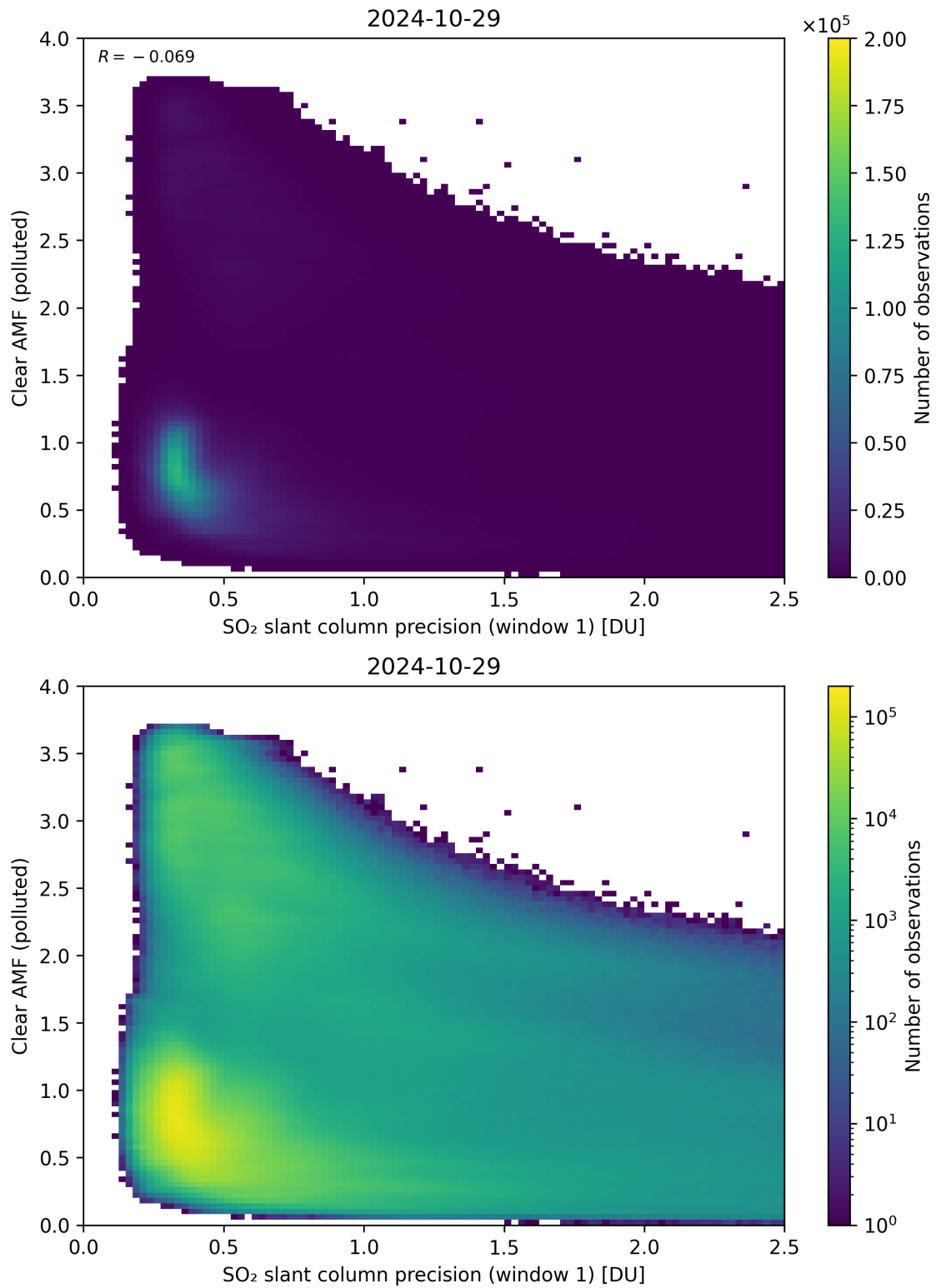
Figure 224: Scatter density plot of “SO 2 slant column precision (window 1)” against “Clear AMF (polluted)” for 2024-10-29 to 2024-10-30.
