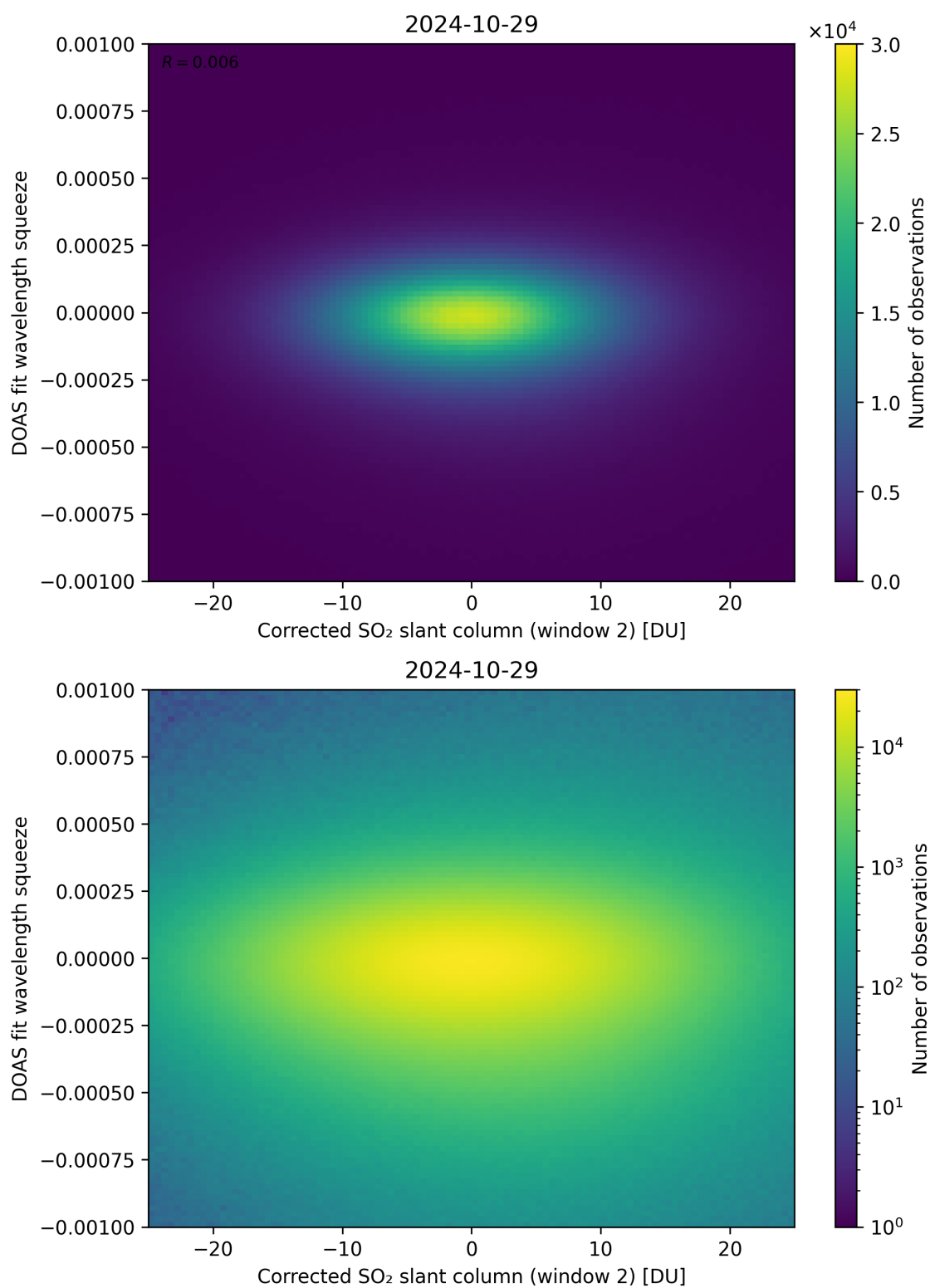
Figure 197: Scatter density plot of “Corrected SO 2 slant column (window 2)” against “DOAS fit wavelength squeeze” for 2024-10-29 to 2024-10-30.
