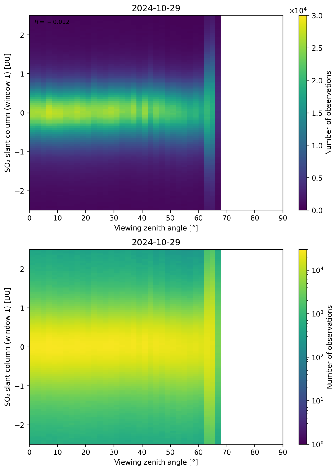
Figure 320: Scatter density plot of “Viewing zenith angle” against “SO 2 slant column (window 1)” for 2024-10-29 to 2024-10-30.
