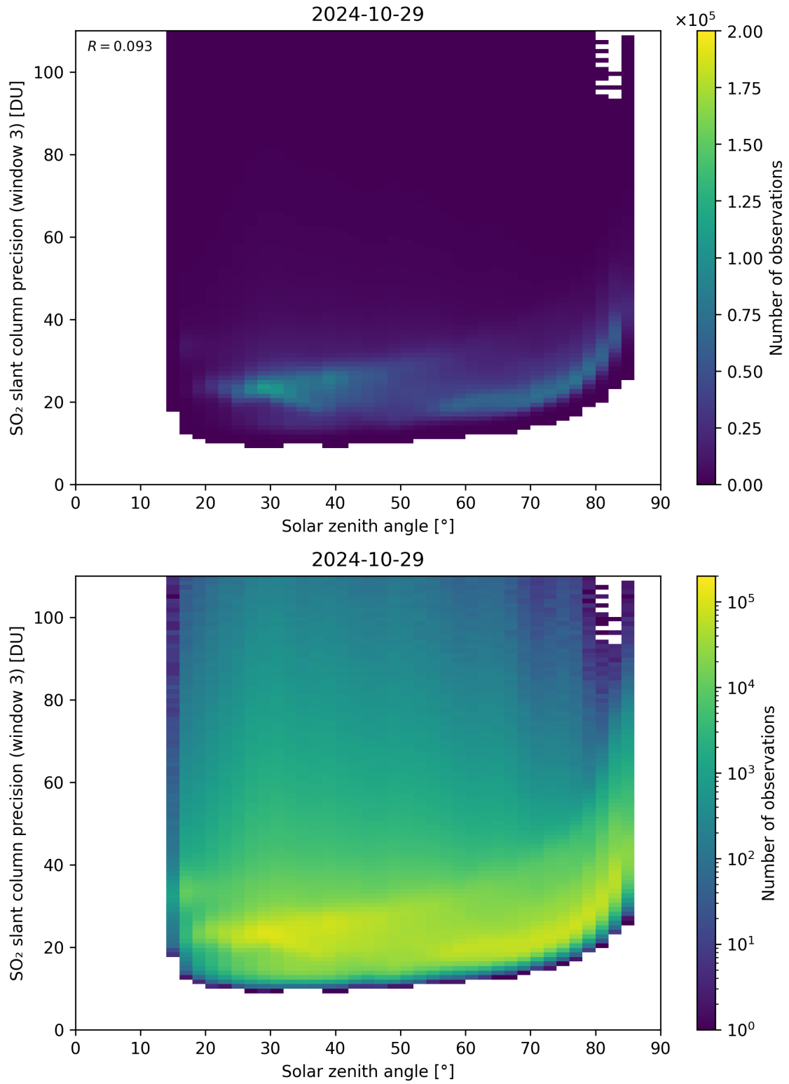
Figure 173: Scatter density plot of “Solar zenith angle” against “SO 2 slant column precision (window 3)” for 2024-10-29 to 2024-10-30.
