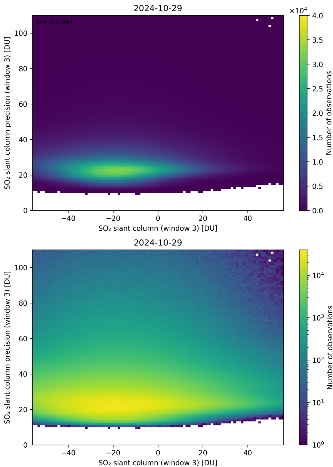
Figure 267: Scatter density plot of “SO 2 slant column (window 3)” against “SO 2 slant column precision (window 3)” for 2024-10-29 to 2024-10-30.
