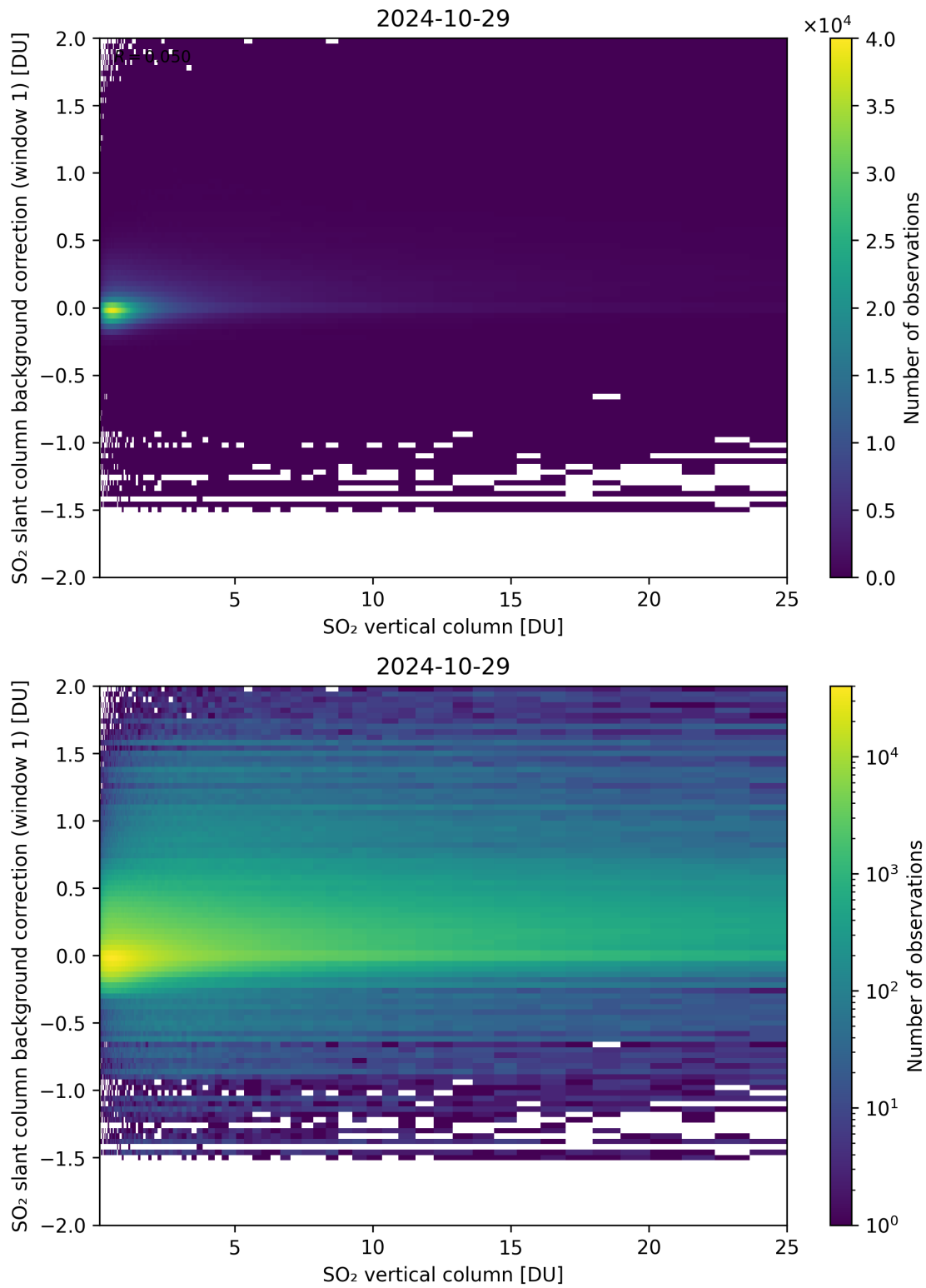
Figure 273: Scatter density plot of “SO 2 vertical column” against “SO 2 slant column background correction (window 1)” for 2024-10-29 to 2024-10-30.
