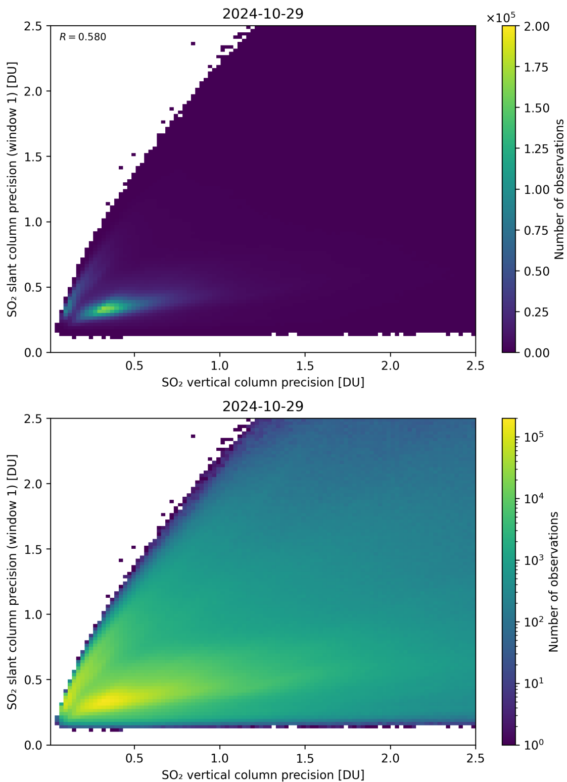
Figure 290: Scatter density plot of “SO 2 vertical column precision” against “SO 2 slant column precision (window 1)” for 2024-10-29 to 2024-10-30.
