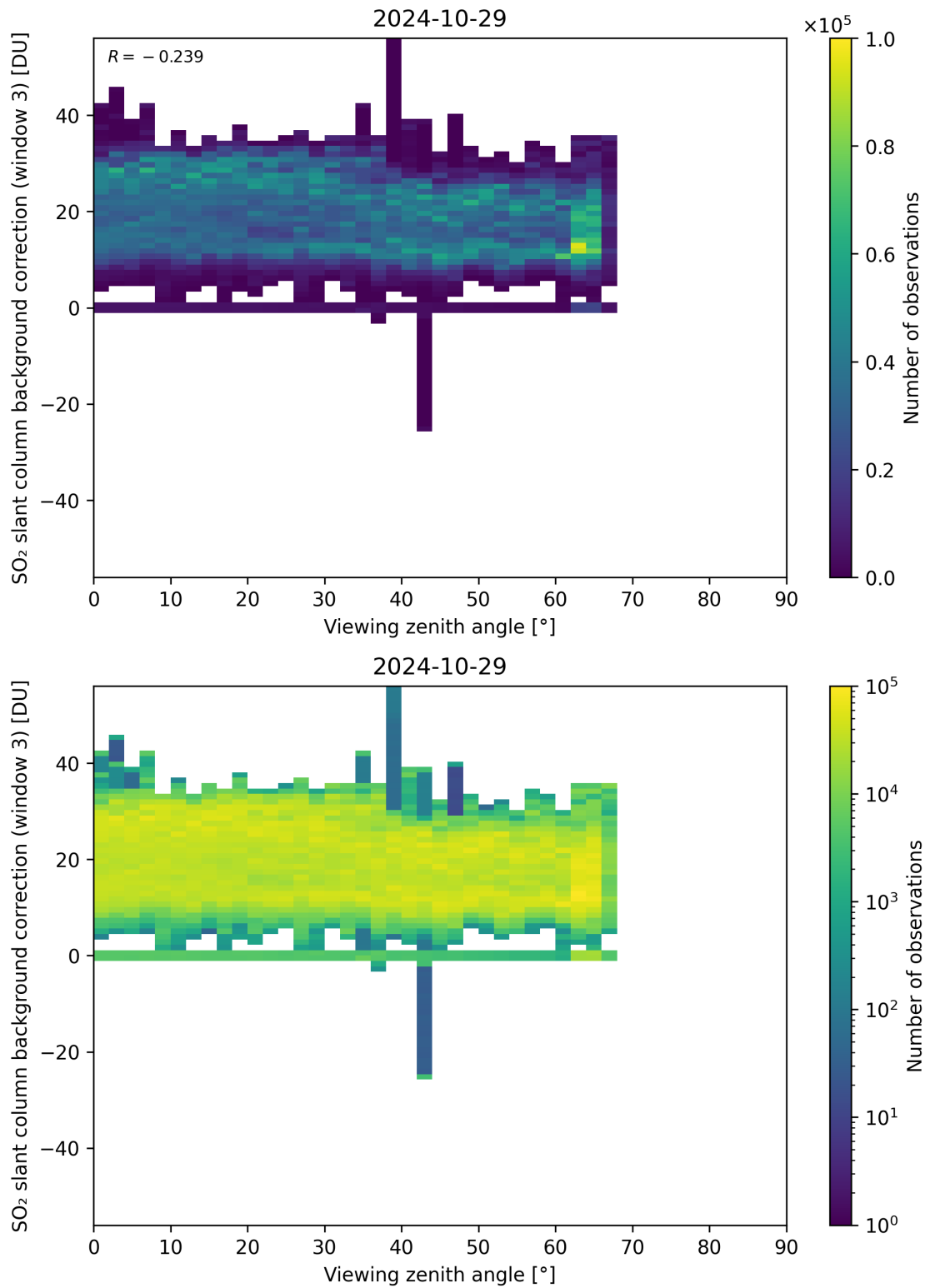
Figure 310: Scatter density plot of “Viewing zenith angle” against “SO 2 slant column background correction (window 3)” for 2024-10-29 to 2024-10-30.
