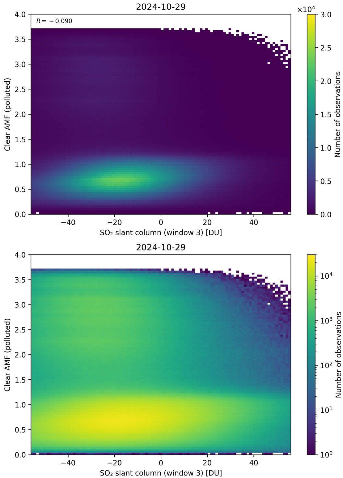
Figure 265: Scatter density plot of “SO 2 slant column (window 3)” against “Clear AMF (polluted)” for 2024-10-29 to 2024-10-30.
