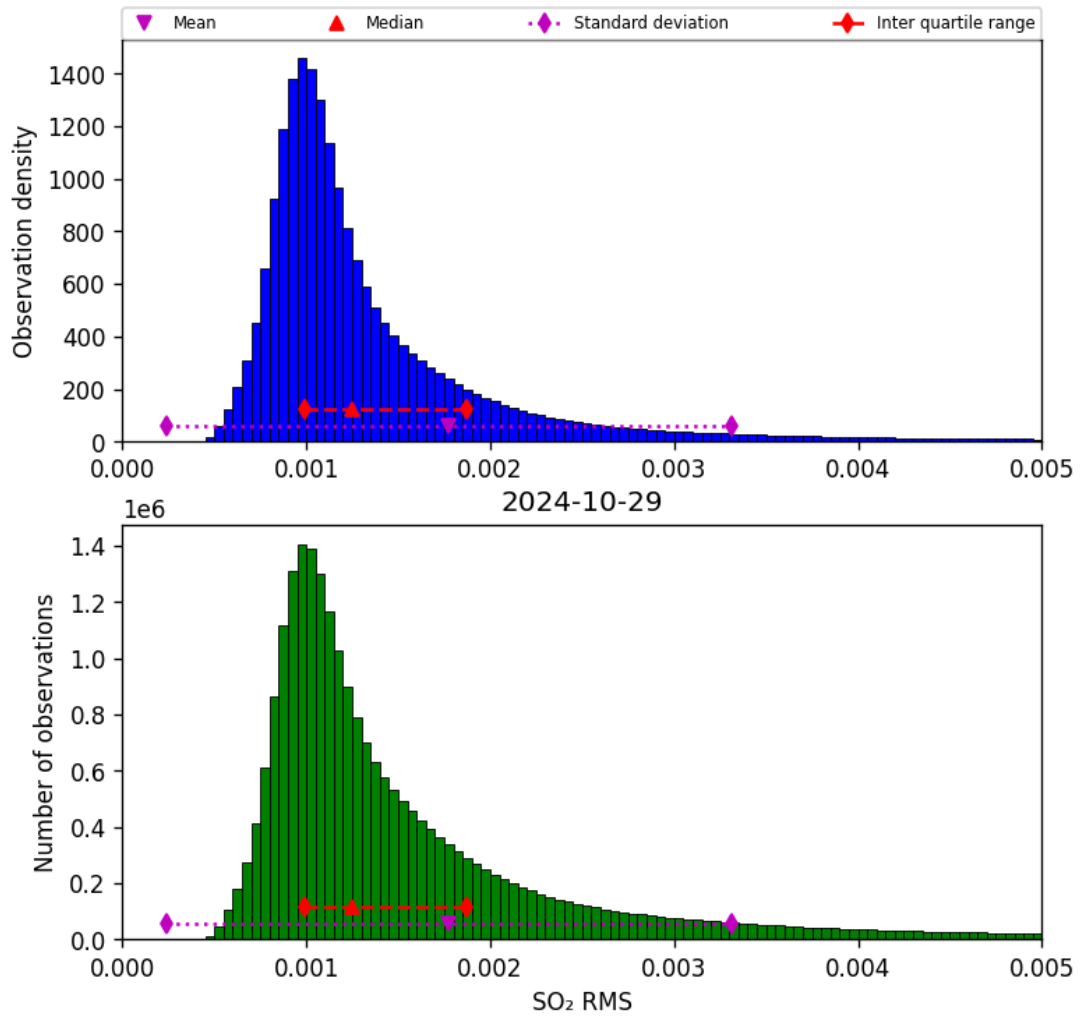
Figure 70: Histogram of “SO 2 RMS” for 2024-10-29 to 2024-10-30
