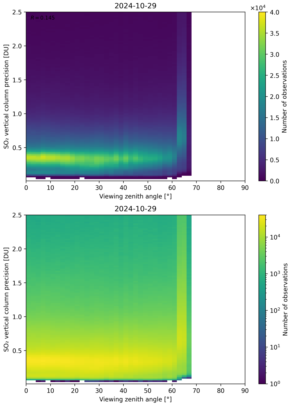
Figure 328: Scatter density plot of “Viewing zenith angle” against “SO 2 vertical column precision” for 2024-10-29 to 2024-10-30.
