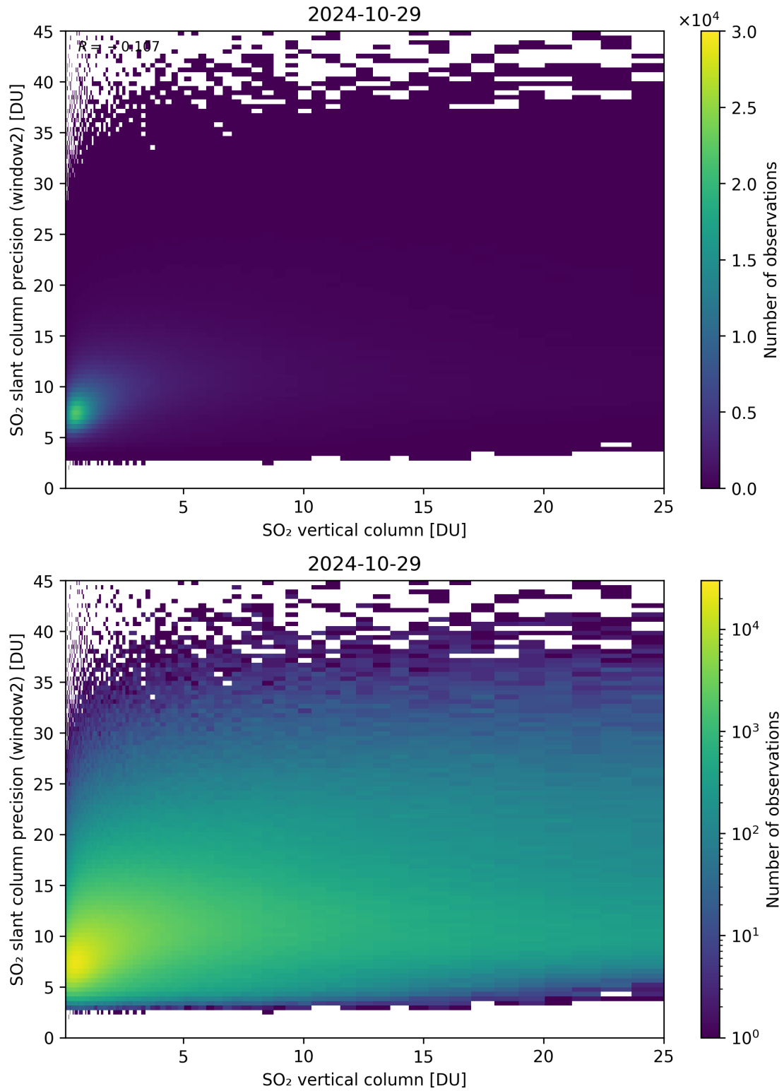
Figure 302: Scatter density plot of “SO 2 vertical column” against “SO 2 slant column precision (window2)” for 2024-10-29 to 2024-10-30.
