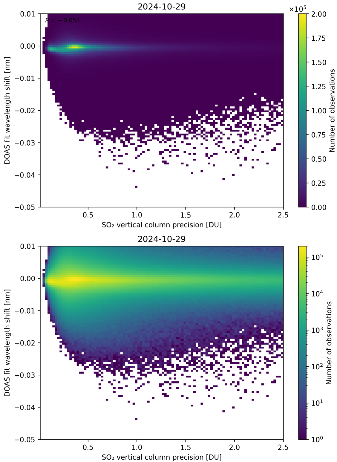
Figure 282: Scatter density plot of “SO 2 vertical column precision” against “DOAS fit wavelength shift” for 2024-10-29 to 2024-10-30.
