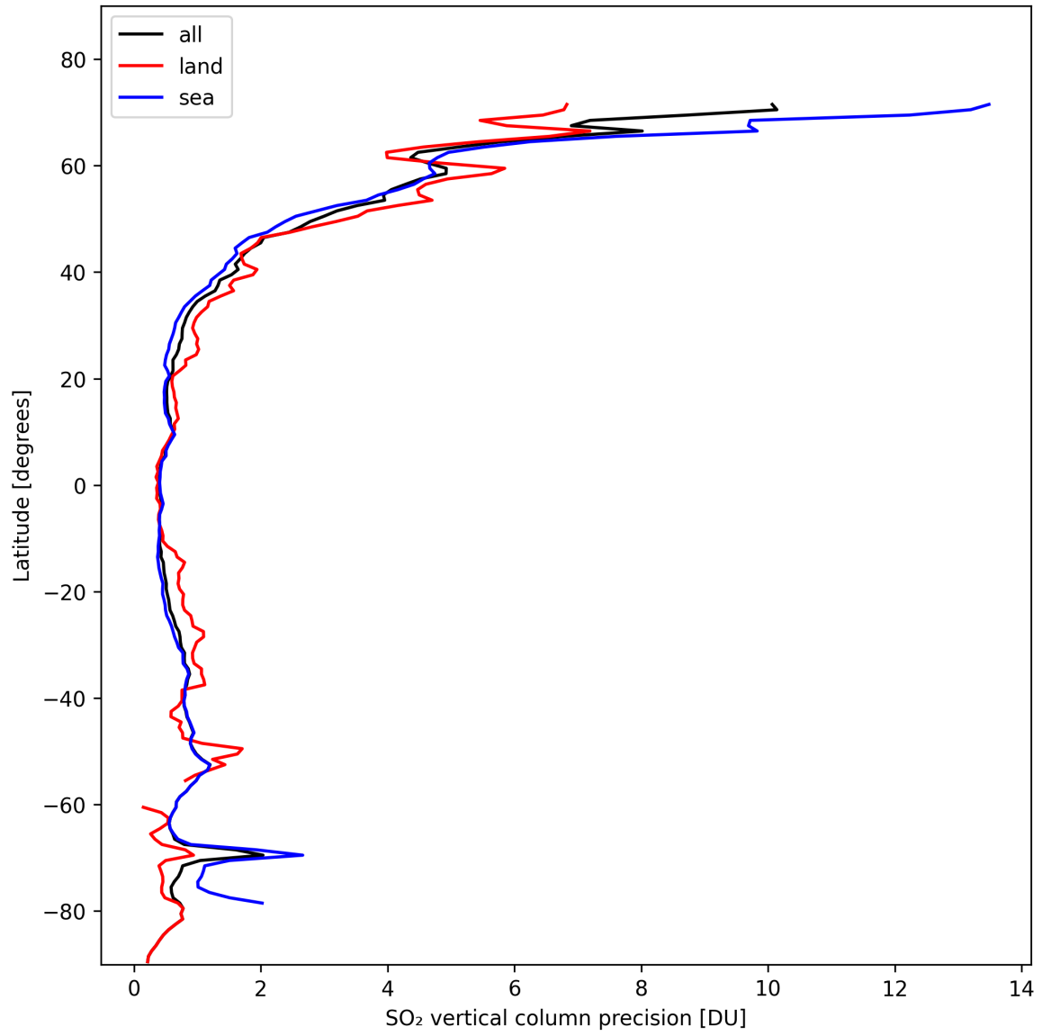
Figure 31: Zonal average of “SO 2 vertical column precision” for 2024-10-29 to 2024-10-30.
