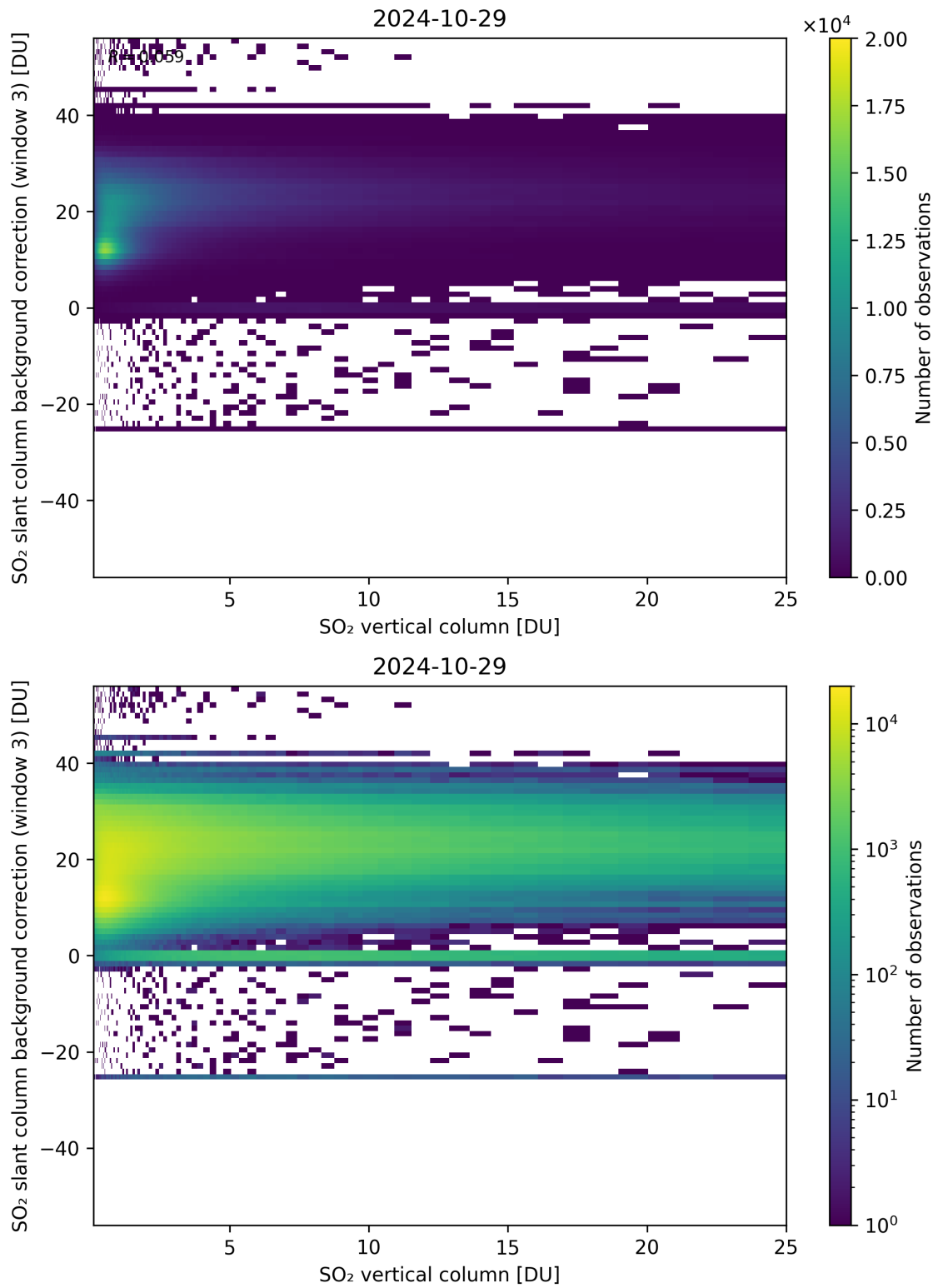
Figure 275: Scatter density plot of “SO 2 vertical column” against “SO 2 slant column background correction (window 3)” for 2024-10-29 to 2024-10-30.
