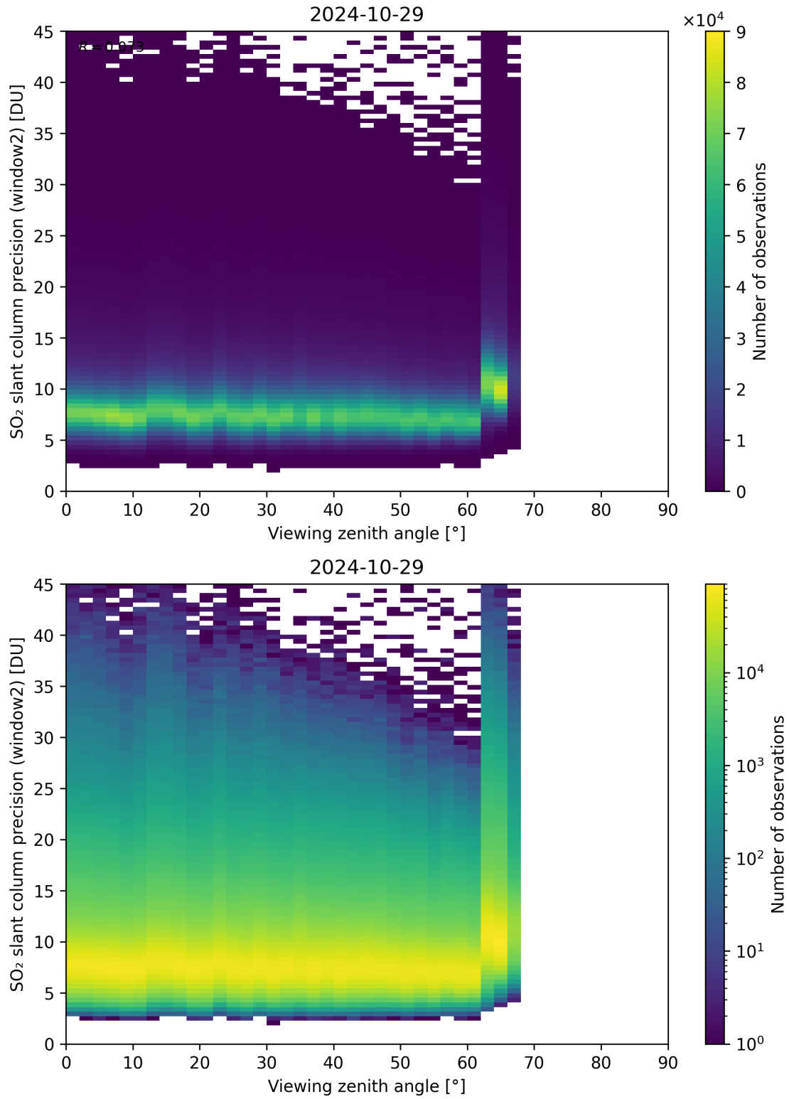
Figure 322: Scatter density plot of “Viewing zenith angle” against “SO 2 slant column precision (window2)” for 2024-10-29 to 2024-10-30.
