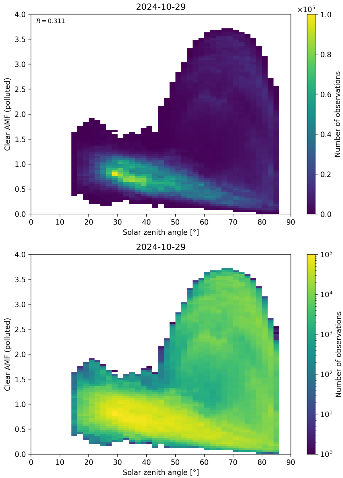
Figure 165: Scatter density plot of “Solar zenith angle” against “Clear AMF (polluted)” for 2024-10-29 to 2024-10-30.
