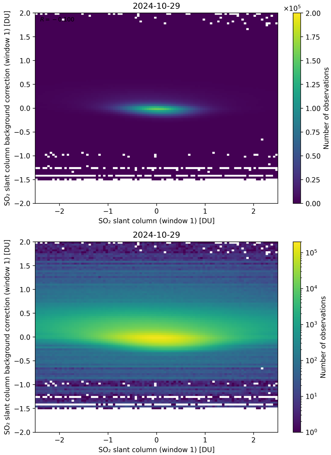
Figure 212: Scatter density plot of “SO 2 slant column (window 1)” against “SO 2 slant column background correction (window 1)” for 2024-10-29 to 2024-10-30.
