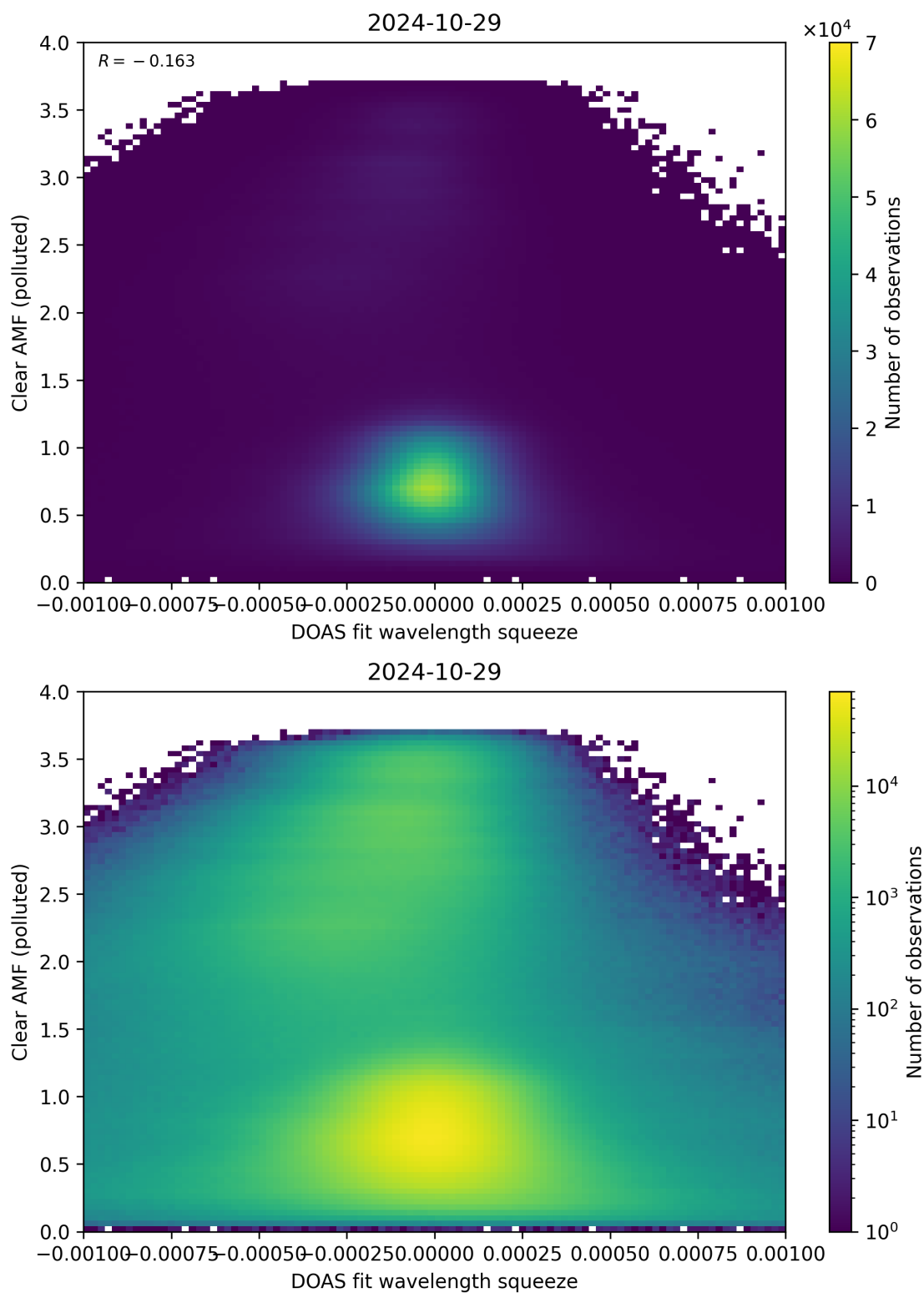
Figure 133: Scatter density plot of “DOAS fit wavelength squeeze” against “Clear AMF (polluted)” for 2024-10-29 to 2024-10-30.
