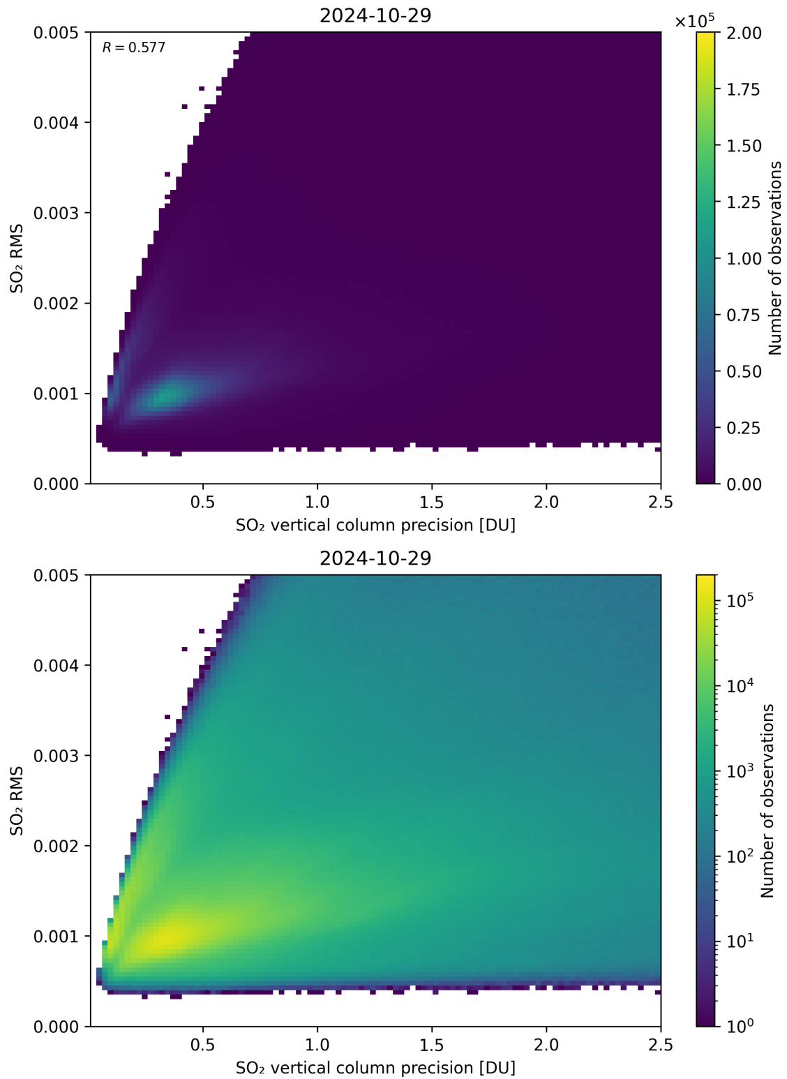
Figure 284: Scatter density plot of “SO 2 vertical column precision” against “SO 2 RMS” for 2024-10-29 to 2024-10-30.
