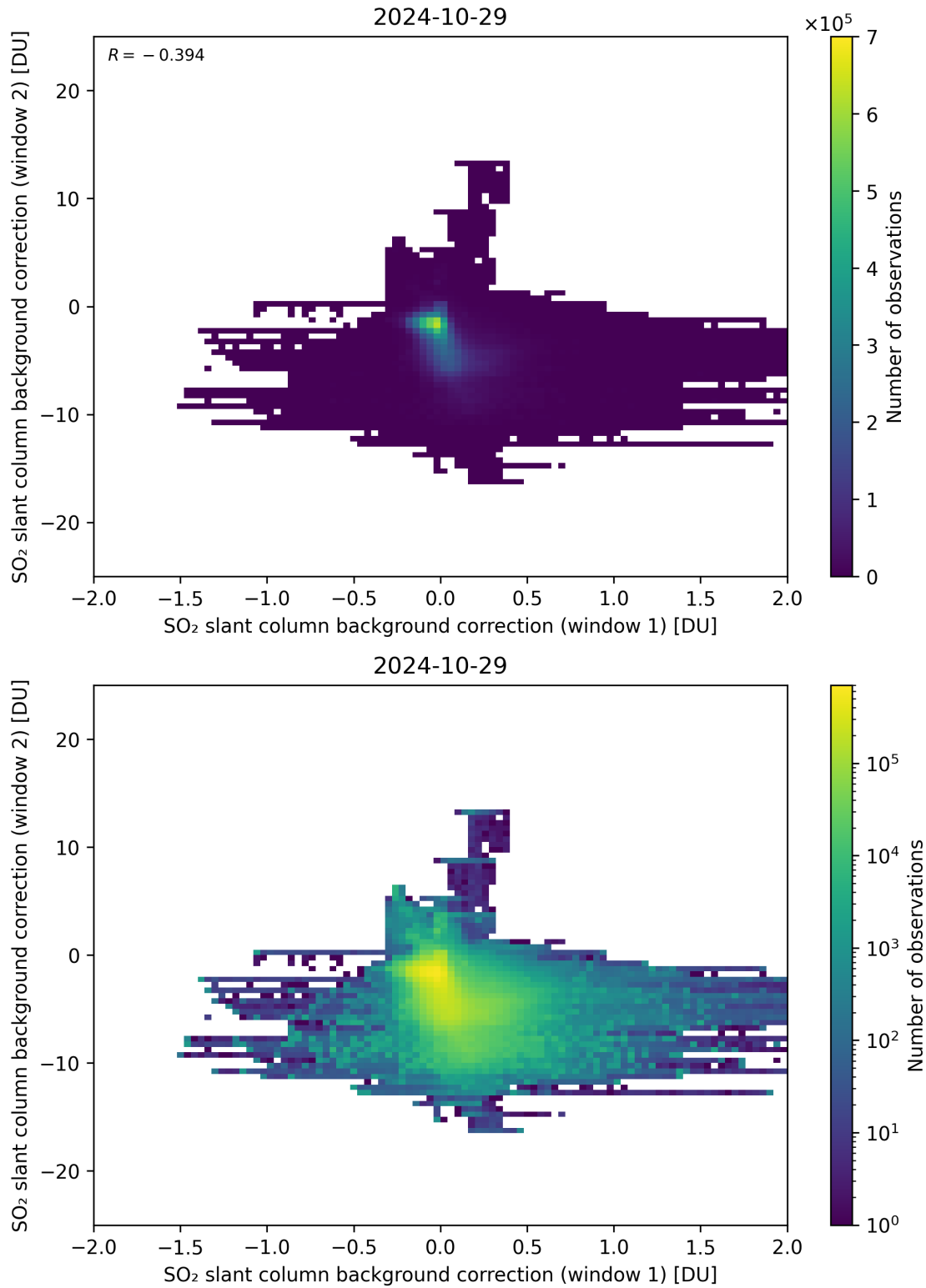
Figure 98: Scatter density plot of “SO 2 slant column background correction (window 1)” against “SO 2 slant column background correction (window 2)” for 2024-10-29 to 2024-10-30.
