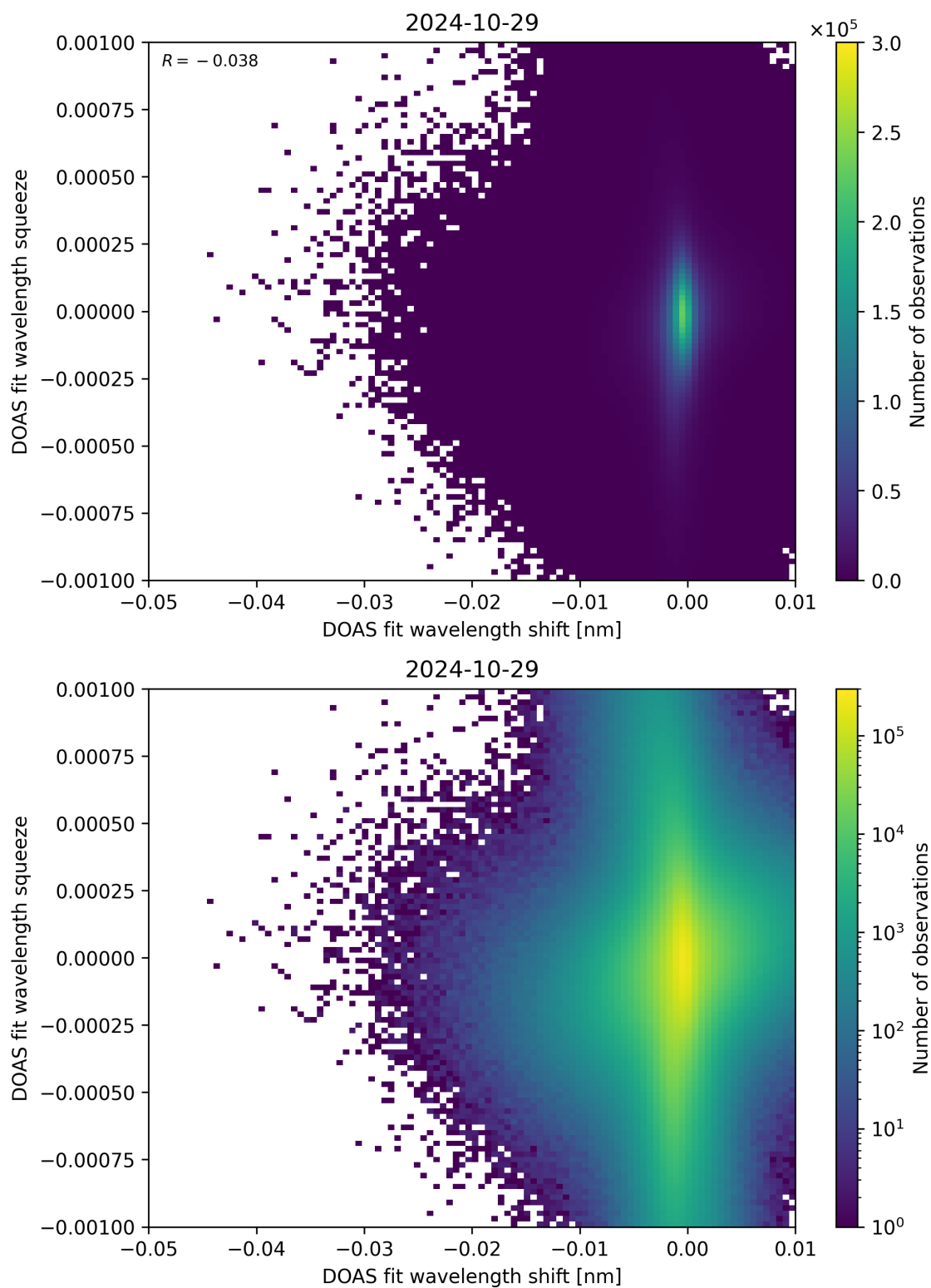
Figure 127: Scatter density plot of “DOAS fit wavelength shift” against “DOAS fit wavelength squeeze” for 2024-10-29 to 2024-10-30.
