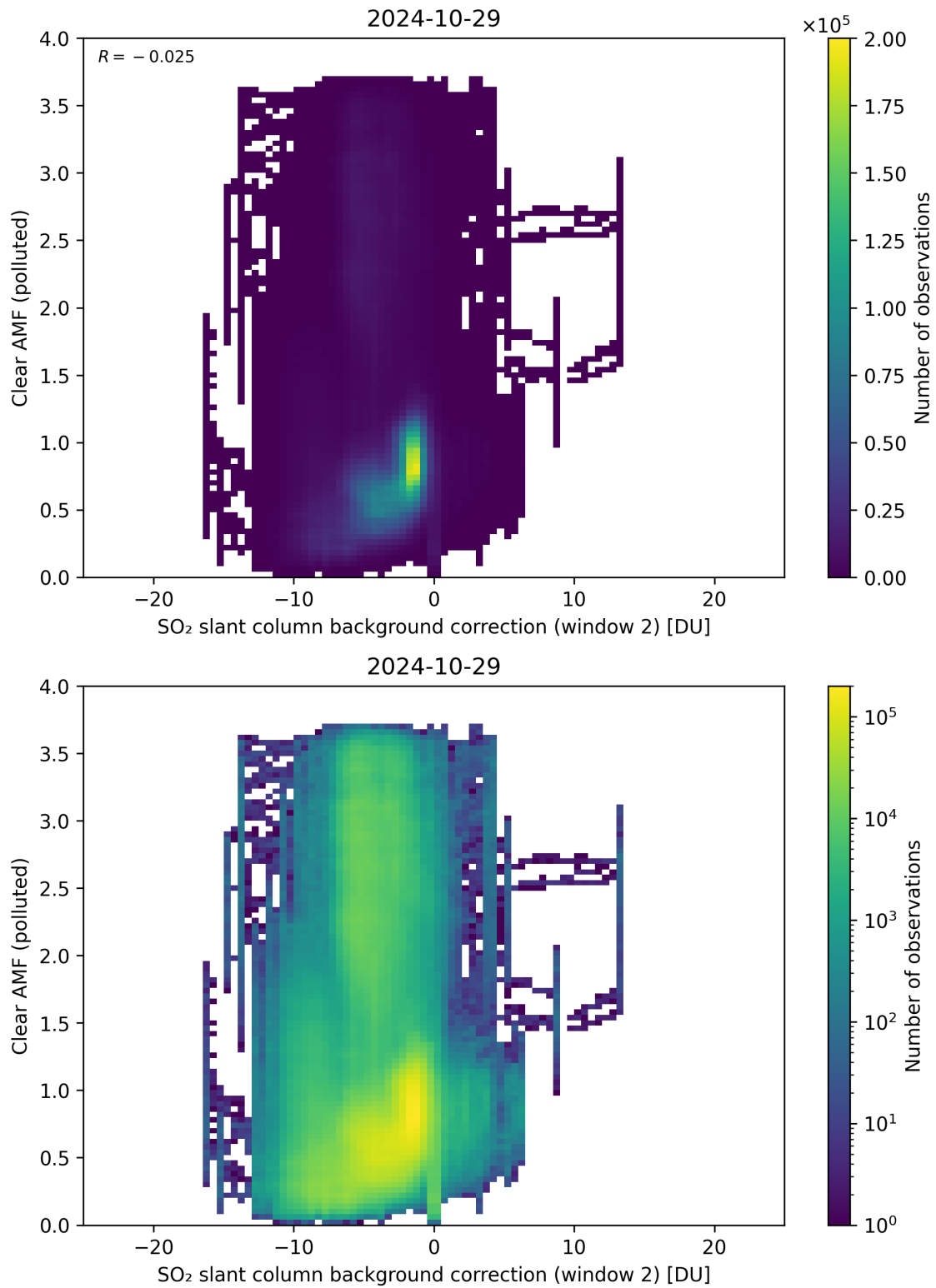
Figure 115: Scatter density plot of “SO 2 slant column background correction (window 2)” against “Clear AMF (polluted)” for 2024-10-29 to 2024-10-30.
