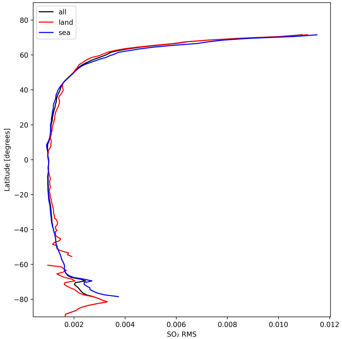
Figure 47: Zonal average of “SO 2 RMS” for 2024-10-29 to 2024-10-30.
