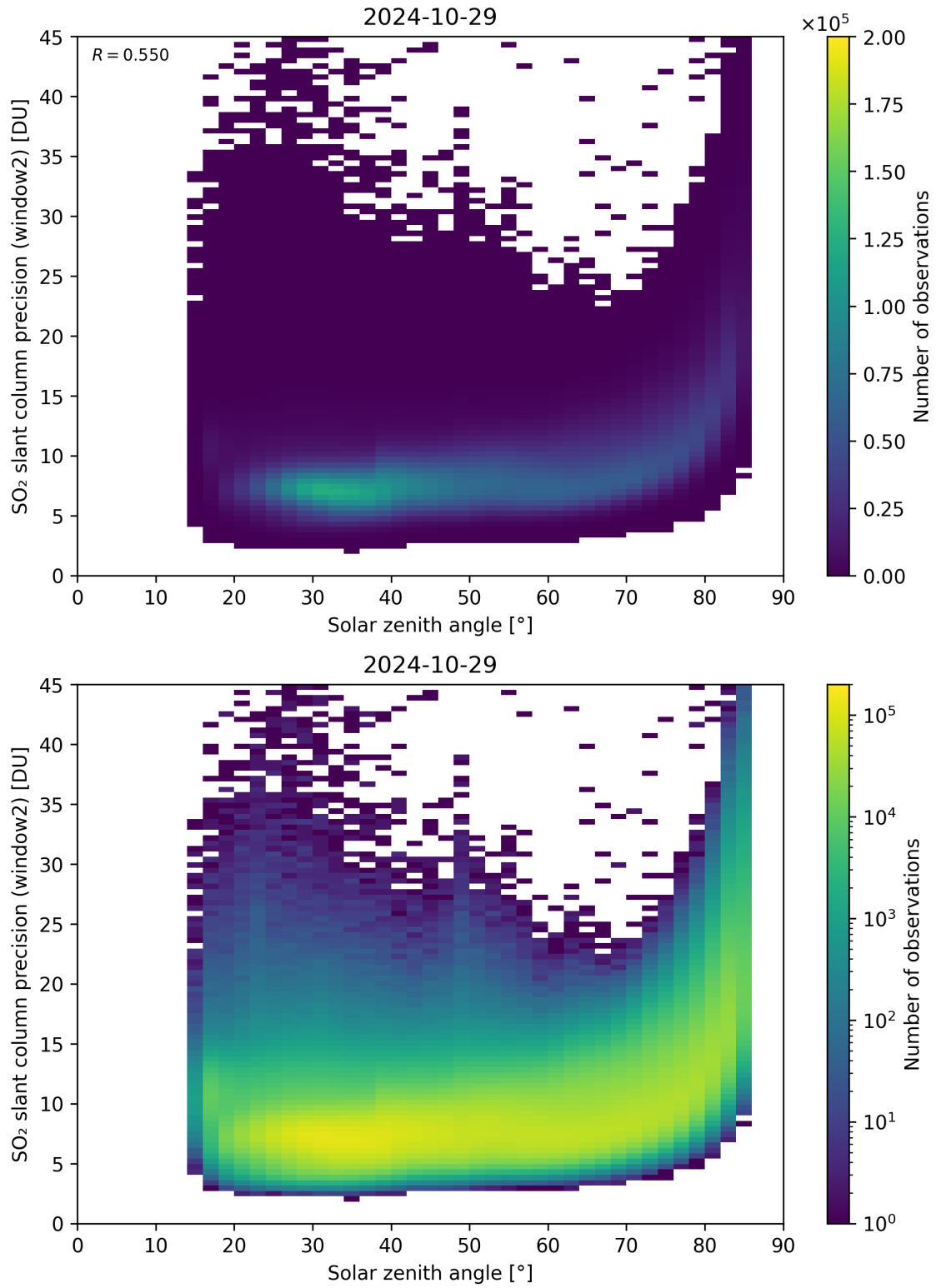
Figure 171: Scatter density plot of “Solar zenith angle” against “SO 2 slant column precision (window2)” for 2024-10-29 to 2024-10-30.
