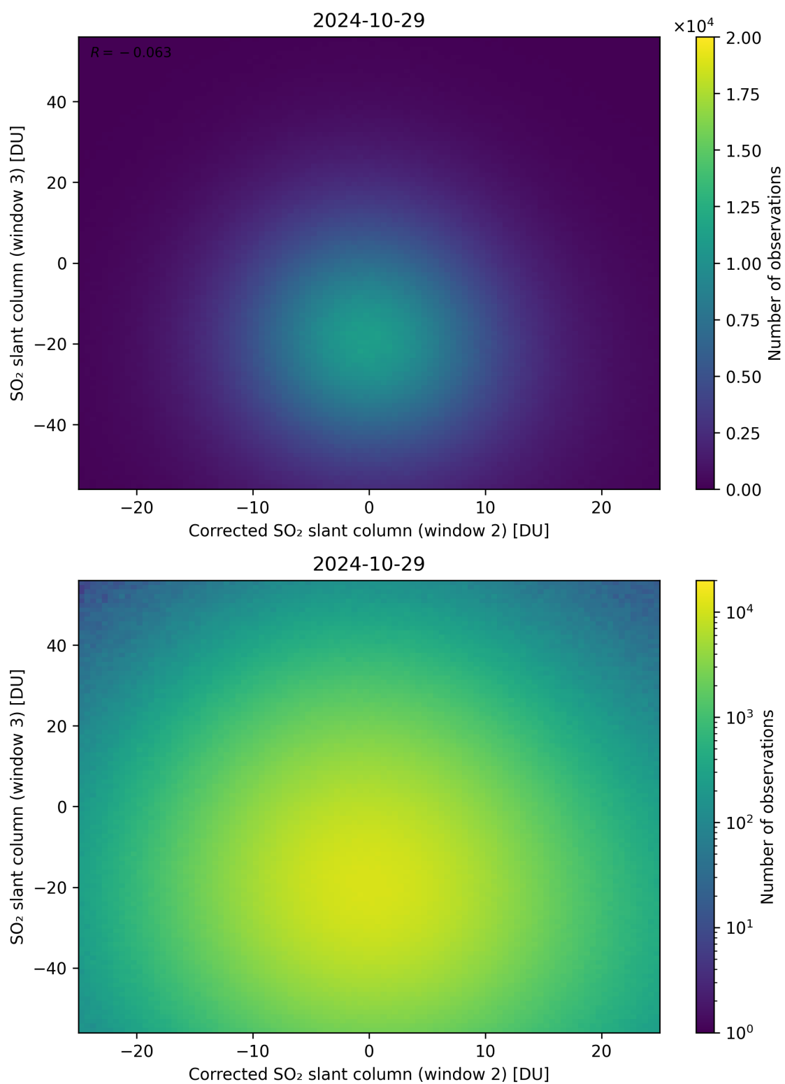
Figure 201: Scatter density plot of “Corrected SO 2 slant column (window 2)” against “SO 2 slant column (window 3)” for 2024-10-29 to 2024-10-30.
