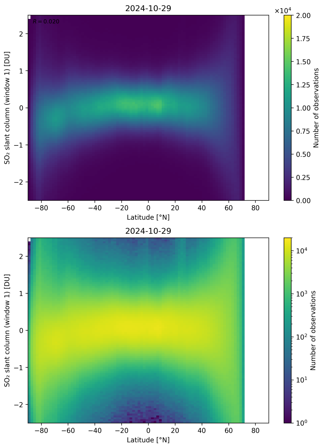
Figure 149: Scatter density plot of “Latitude” against “SO 2 slant column (window 1)” for 2024-10-29 to 2024-10-30.
