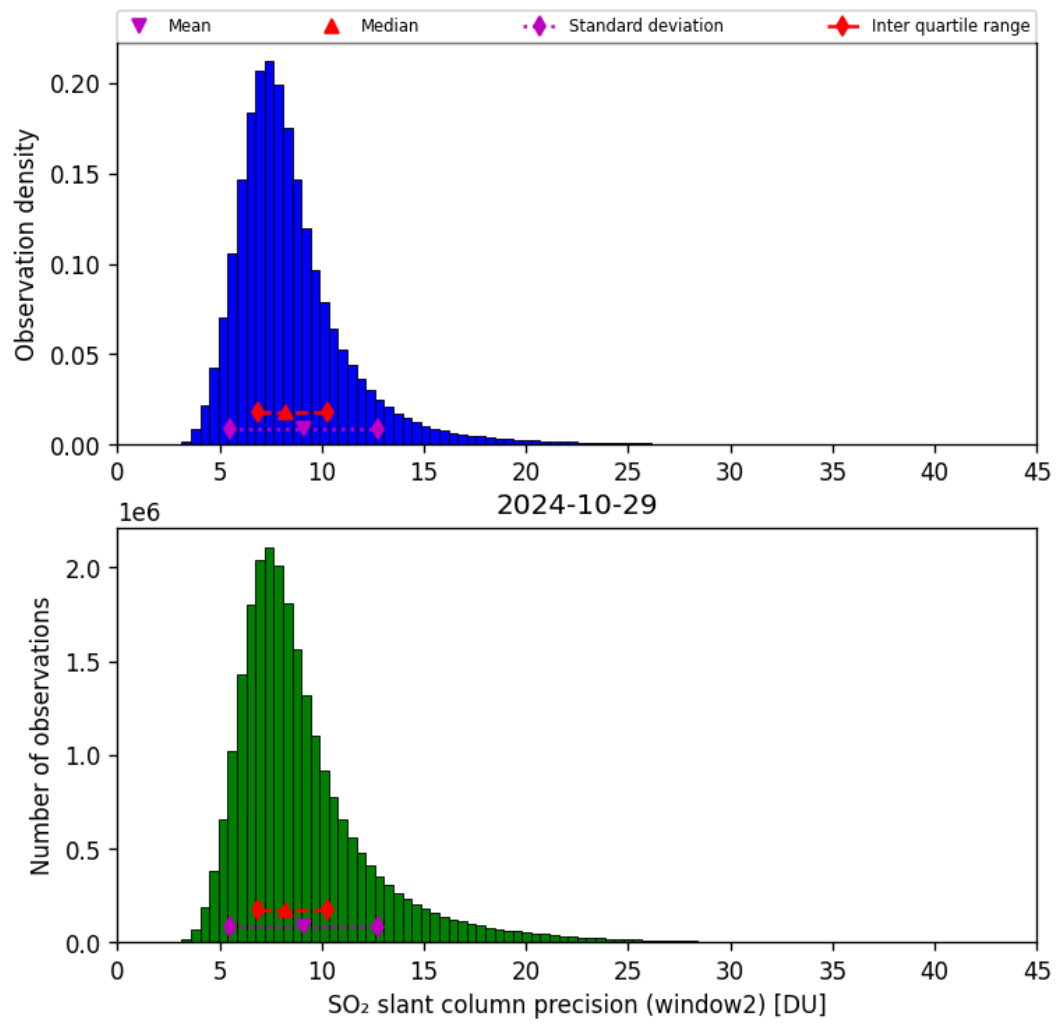
Figure 61: Histogram of “SO 2 slant column precision (window2)” for 2024-10-29 to 2024-10-30
