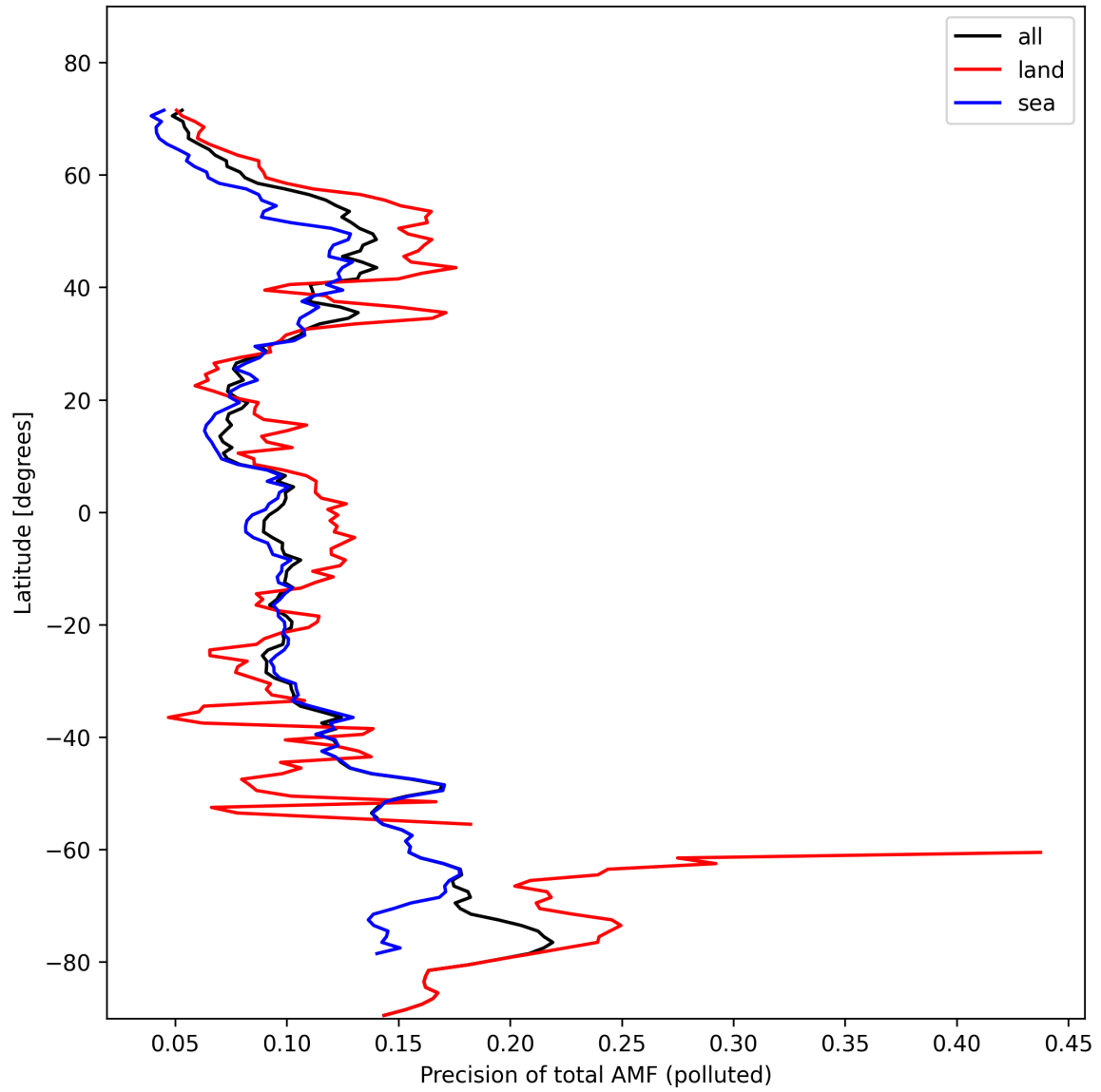
Figure 49: Zonal average of “Precision of total AMF (polluted)” for 2024-10-29 to 2024-10-30.
