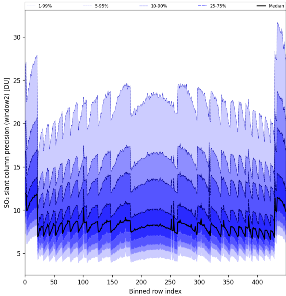
Figure 84: Along track statistics of “SO 2 slant column precision (window2)” for 2024-10-29 to 2024-10-30
