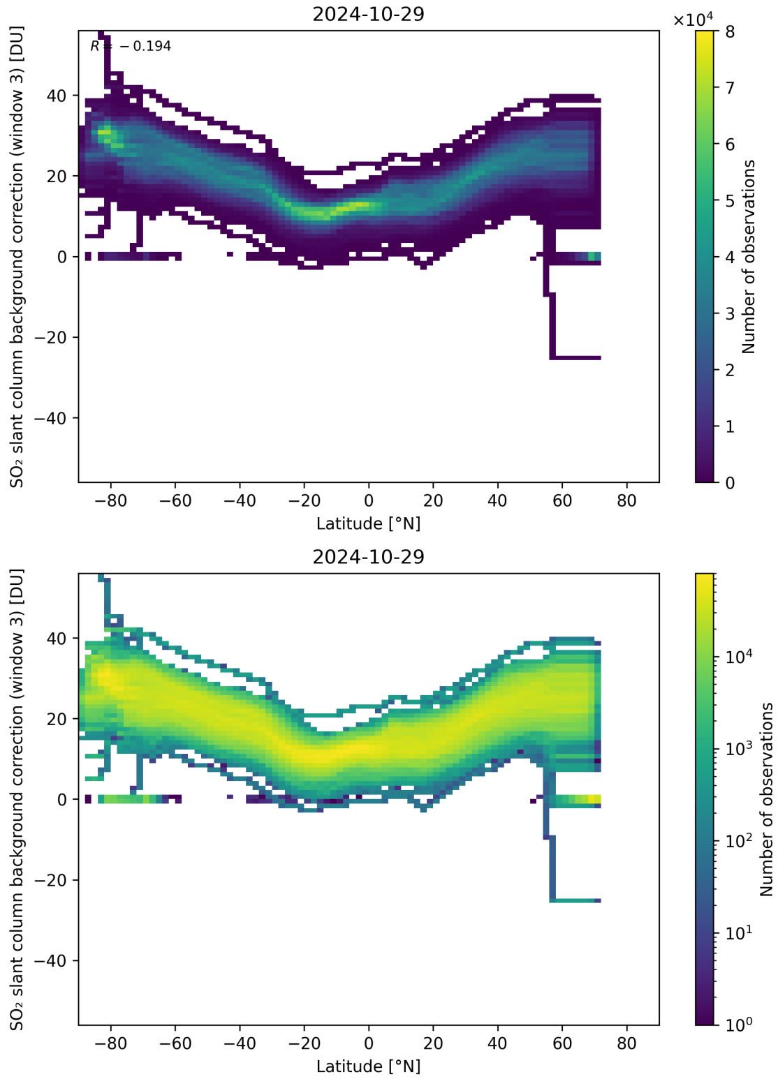
Figure 141: Scatter density plot of “Latitude” against “SO 2 slant column background correction (window 3)” for 2024-10-29 to 2024-10-30.
