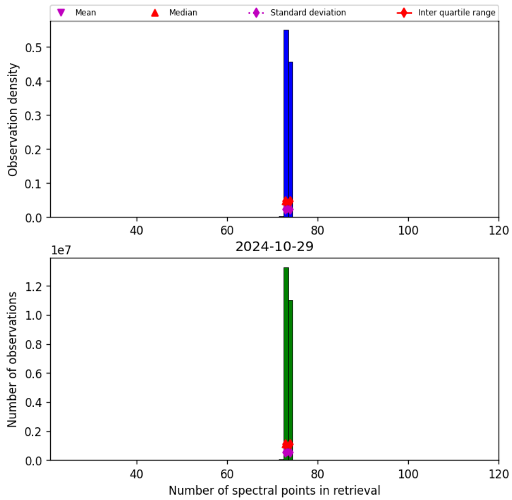
Figure 74: Histogram of “Number of spectral points in retrieval” for 2024-10-29 to 2024-10-30
