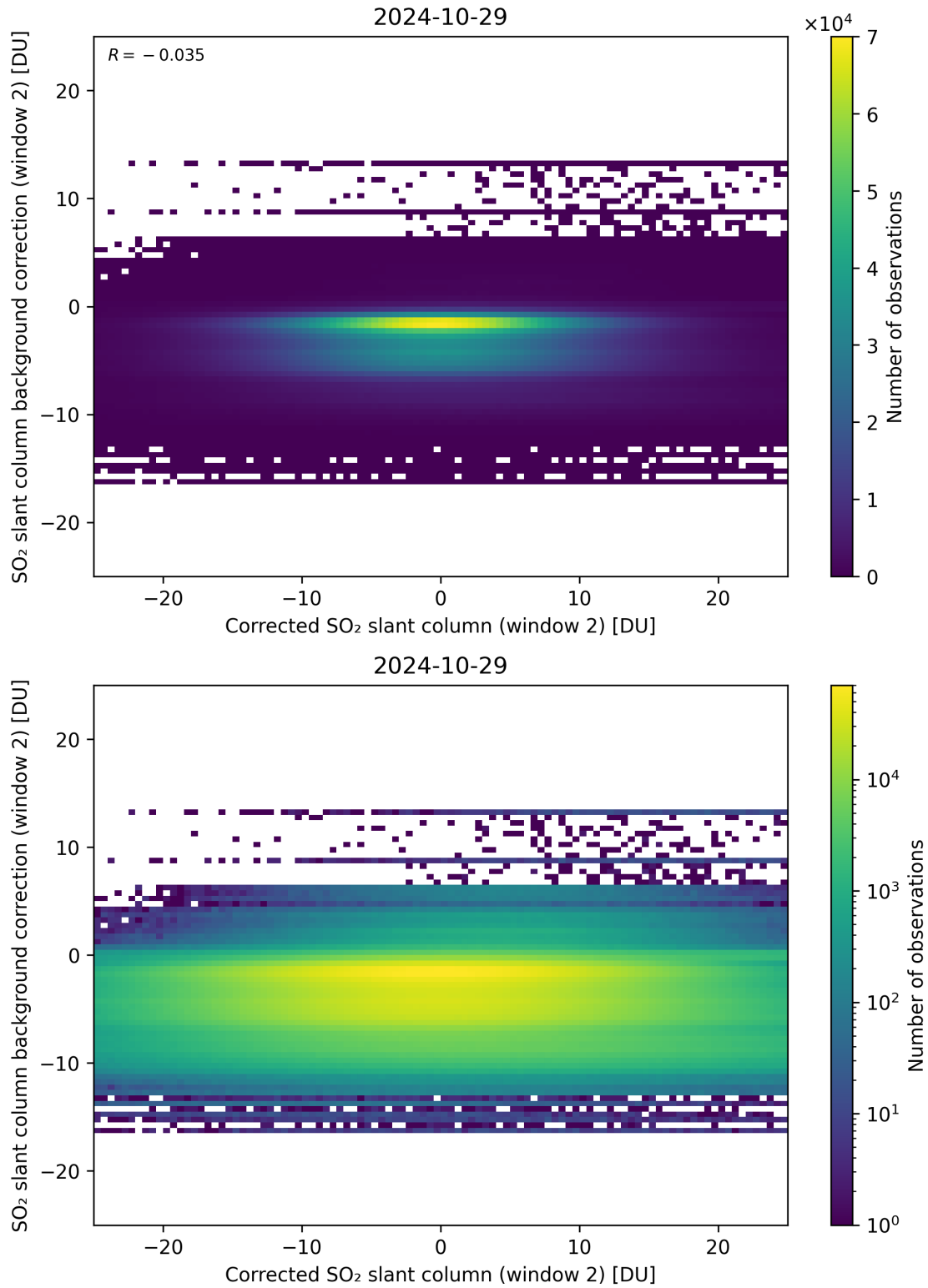
Figure 194: Scatter density plot of “Corrected SO 2 slant column (window 2)” against “SO 2 slant column background correction (window 2)” for 2024-10-29 to 2024-10-30.
