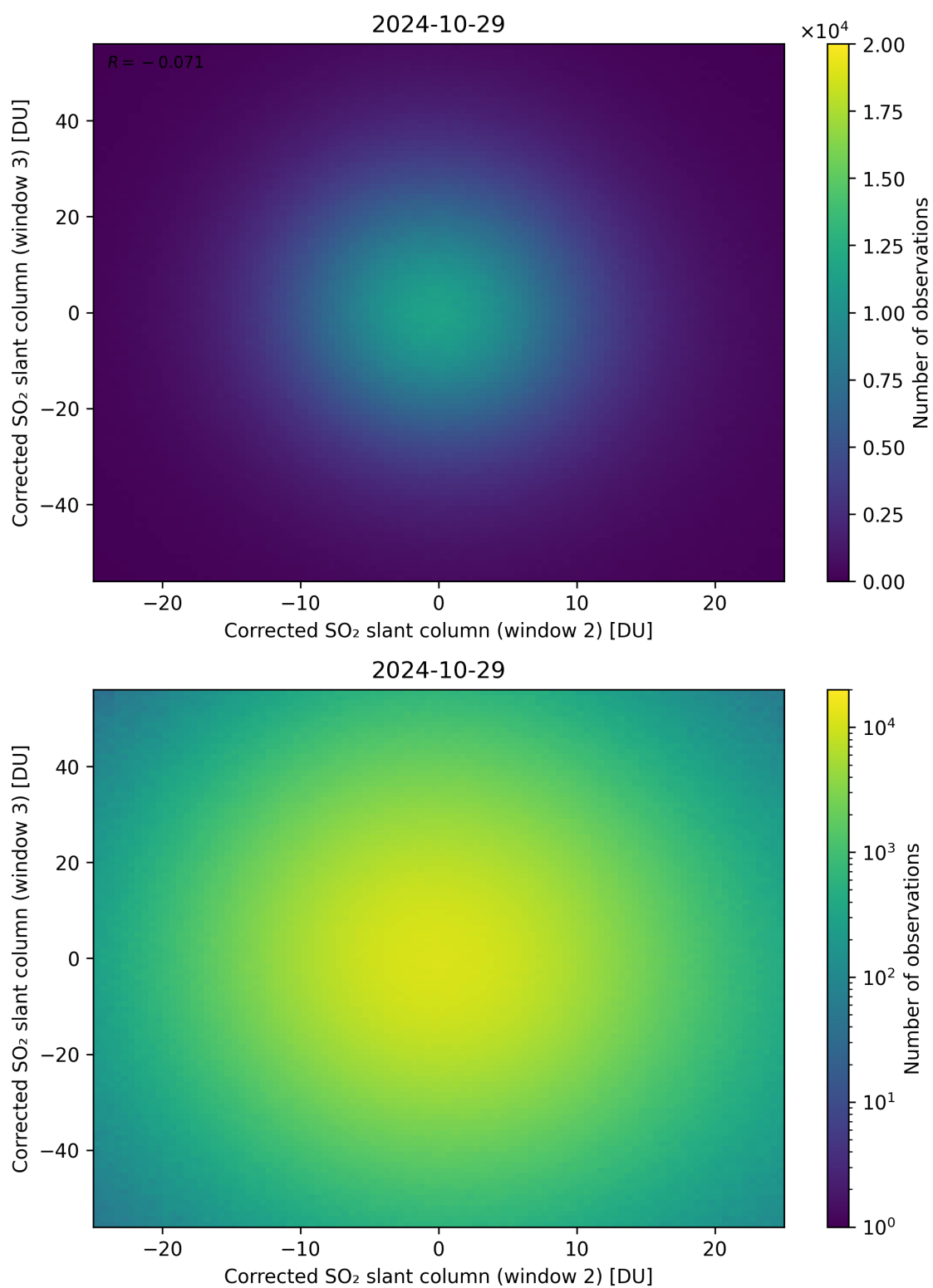
Figure 200: Scatter density plot of “Corrected SO 2 slant column (window 2)” against “Corrected SO 2 slant column (window 3)” for 2024-10-29 to 2024-10-30.
