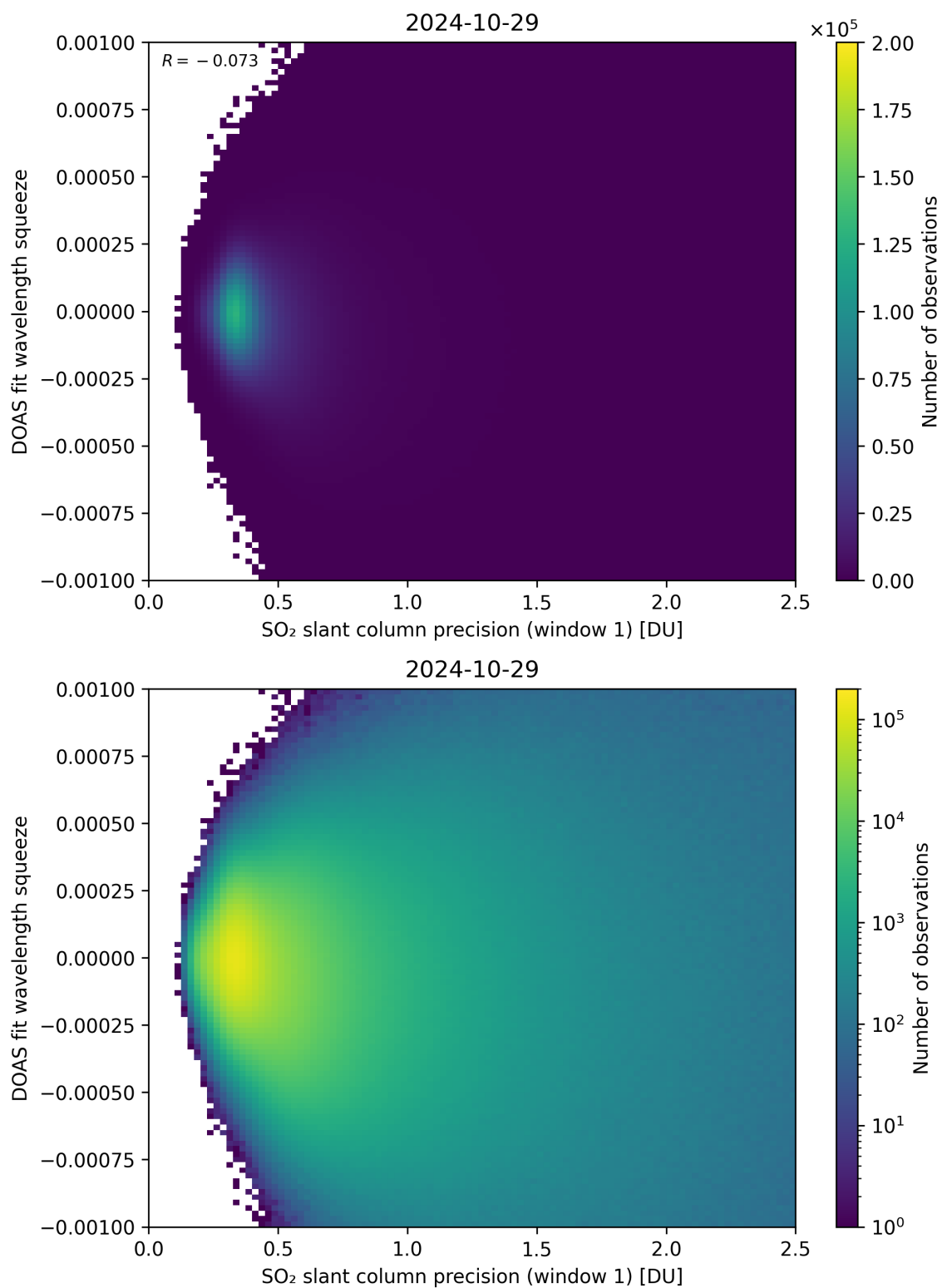
Figure 222: Scatter density plot of “SO 2 slant column precision (window 1)” against “DOAS fit wavelength squeeze” for 2024-10-29 to 2024-10-30.
