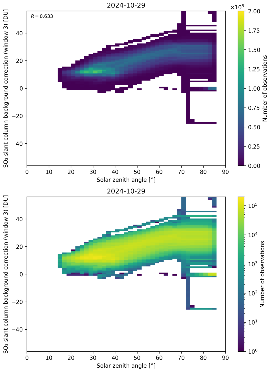
Figure 160: Scatter density plot of “Solar zenith angle” against “SO 2 slant column background correction (window 3)” for 2024-10-29 to 2024-10-30.
