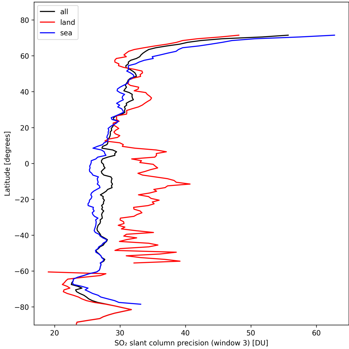
Figure 42: Zonal average of “SO 2 slant column precision (window 3)” for 2024-10-29 to 2024-10-30.
