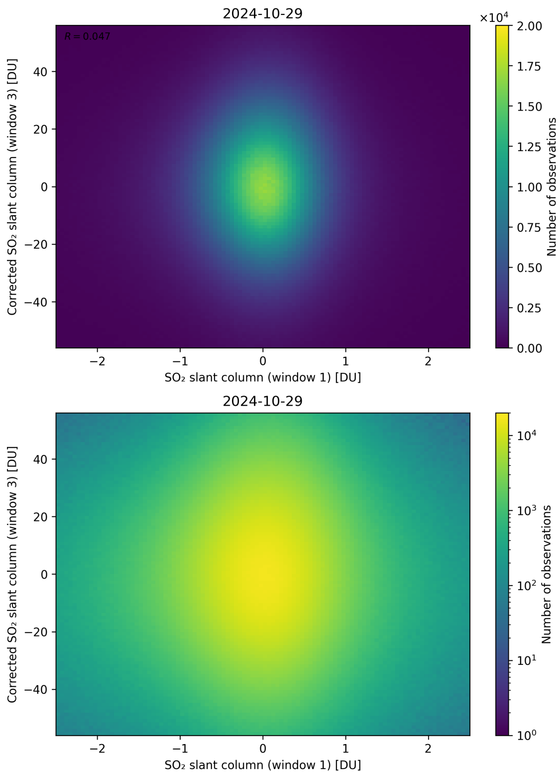
Figure 234: Scatter density plot of “SO 2 slant column (window 1)” against “Corrected SO 2 slant column (window 3)” for 2024-10-29 to 2024-10-30.
