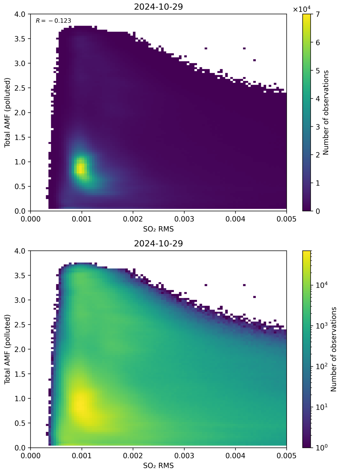
Figure 137: Scatter density plot of “SO 2 RMS” against “Total AMF (polluted)” for 2024-10-29 to 2024-10-30.
