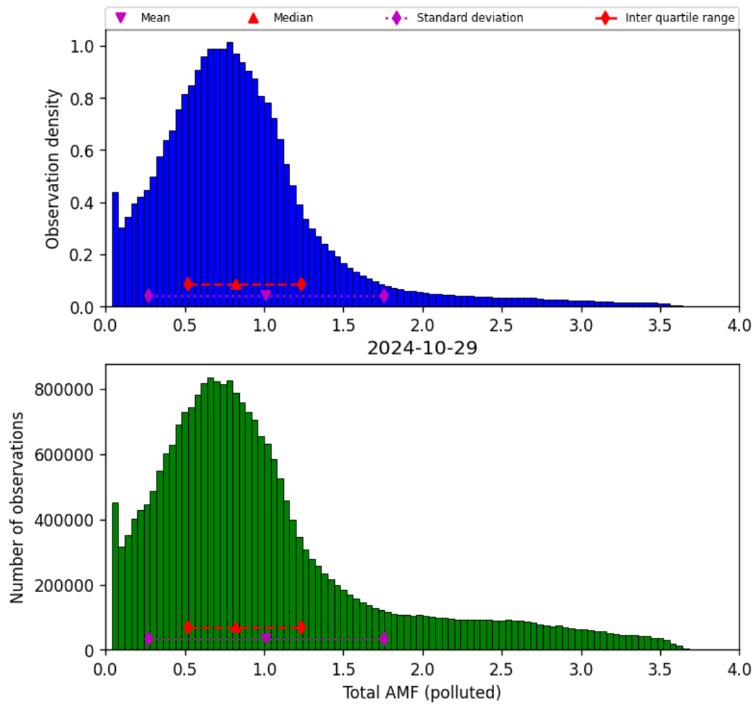
Figure 71: Histogram of “Total AMF (polluted)” for 2024-10-29 to 2024-10-30
