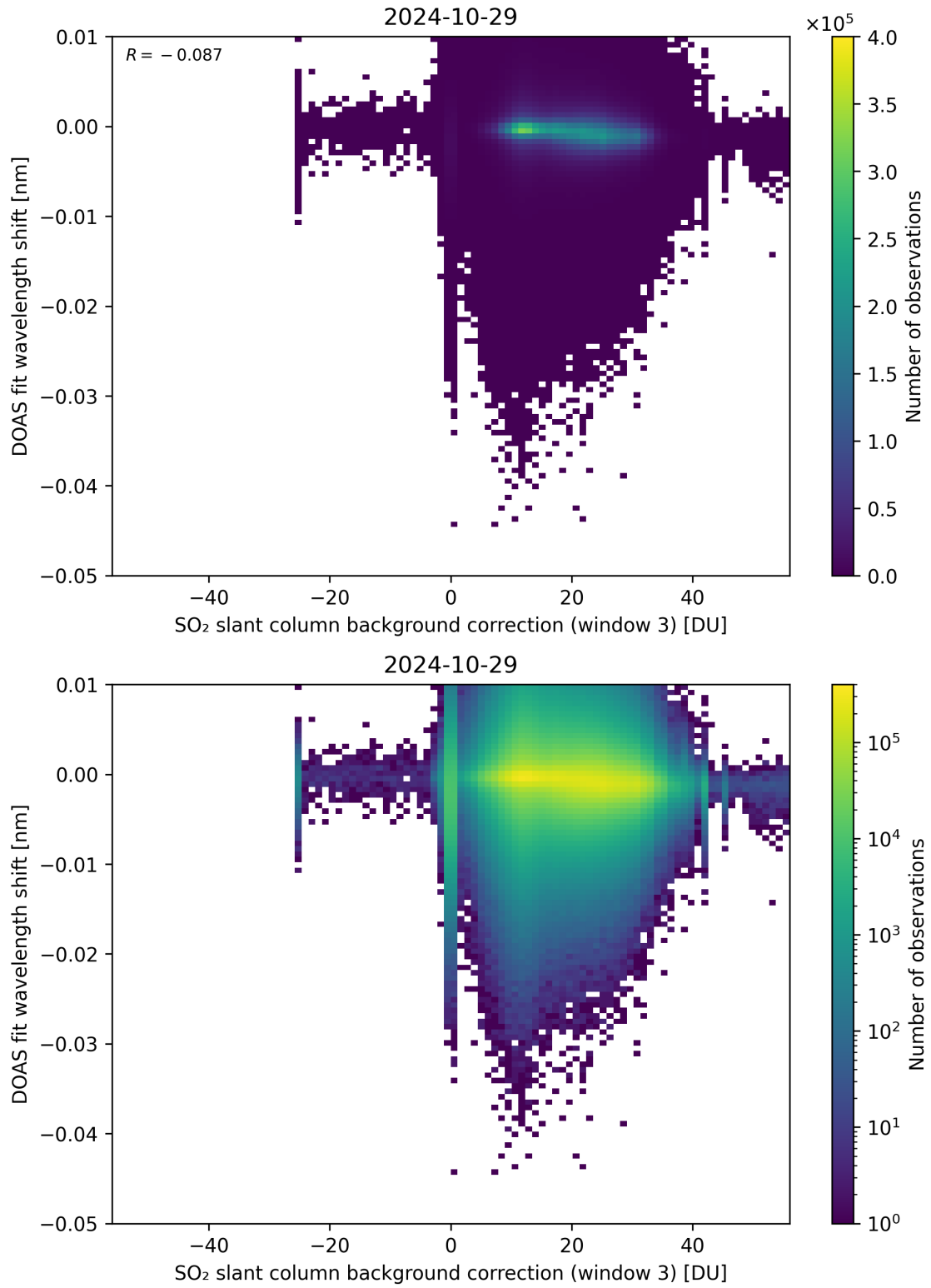
Figure 121: Scatter density plot of “SO 2 slant column background correction (window 3)” against “DOAS fit wavelength shift” for 2024-10-29 to 2024-10-30.
