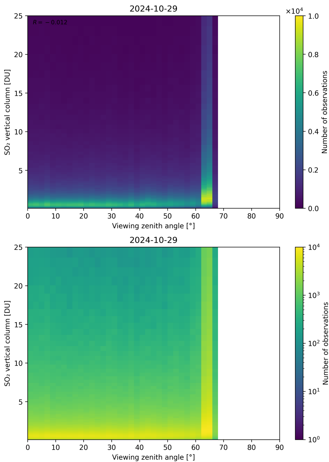
Figure 327: Scatter density plot of “Viewing zenith angle” against “SO 2 vertical column” for 2024-10-29 to 2024-10-30.
