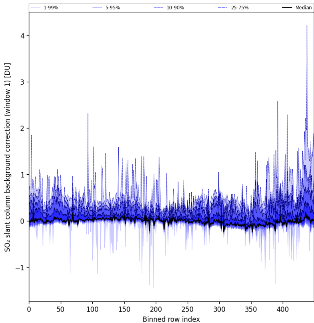
Figure 82: Along track statistics of “SO 2 slant column background correction (window 1)” for 2024-10-29 to 2024-10-30
