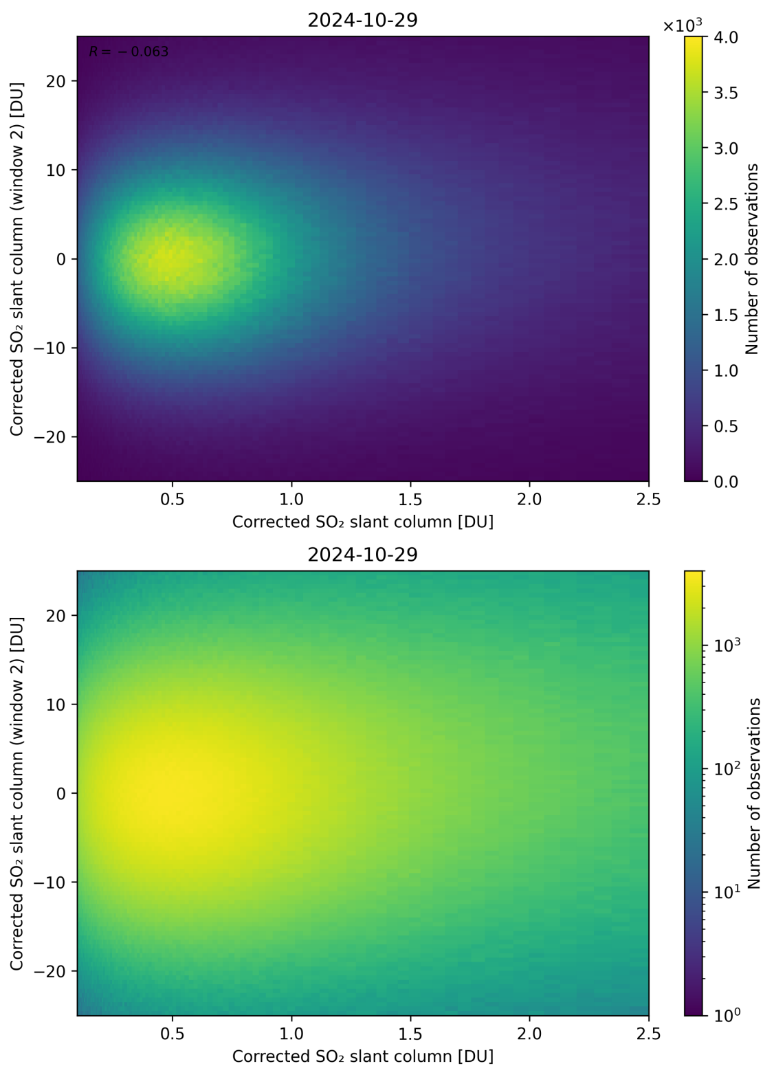
Figure 185: Scatter density plot of “Corrected SO 2 slant column” against “Corrected SO 2 slant column (window 2)” for 2024-10-29 to 2024-10-30.
