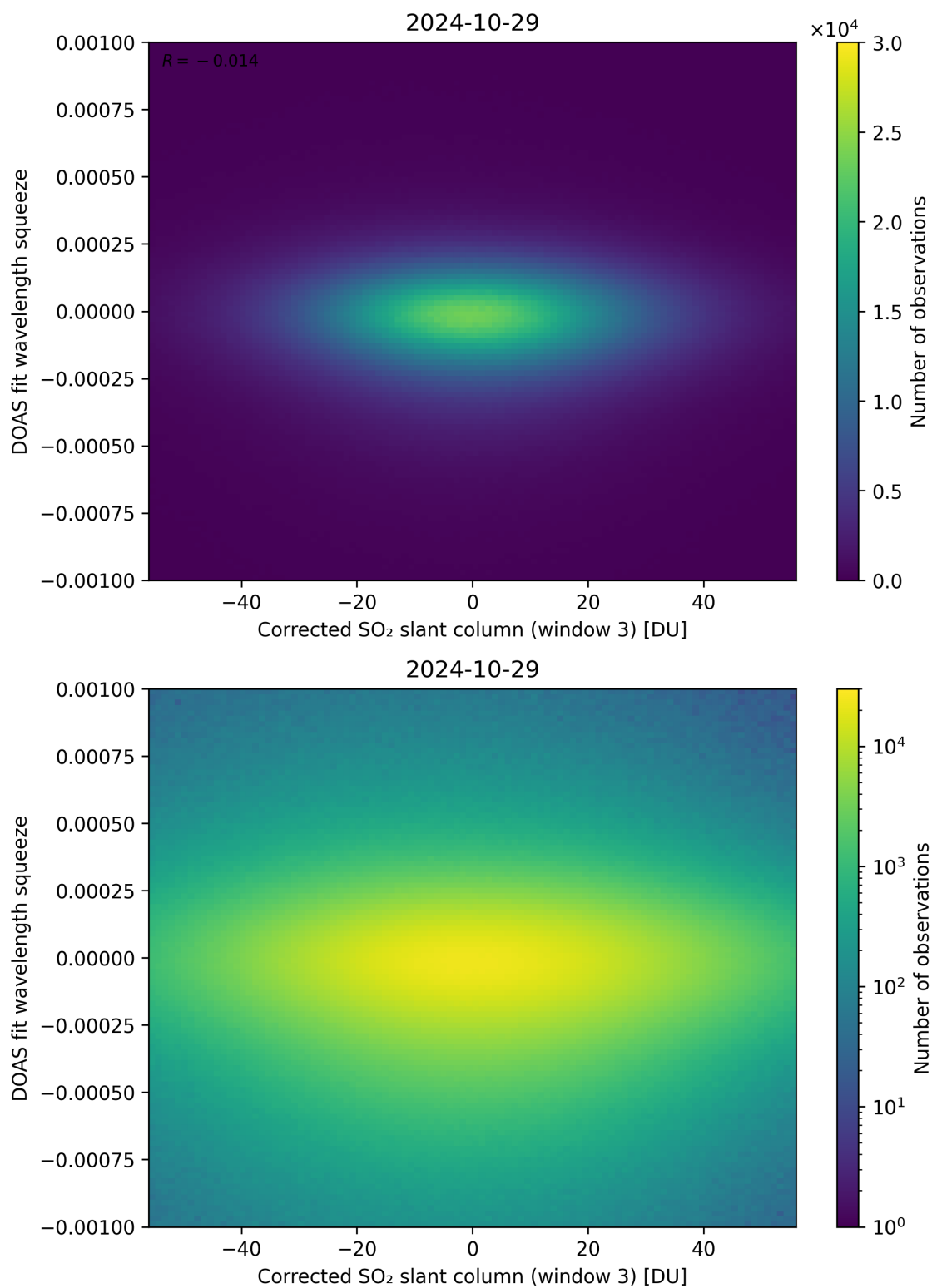
Figure 207: Scatter density plot of “Corrected SO 2 slant column (window 3)” against “DOAS fit wavelength squeeze” for 2024-10-29 to 2024-10-30.
