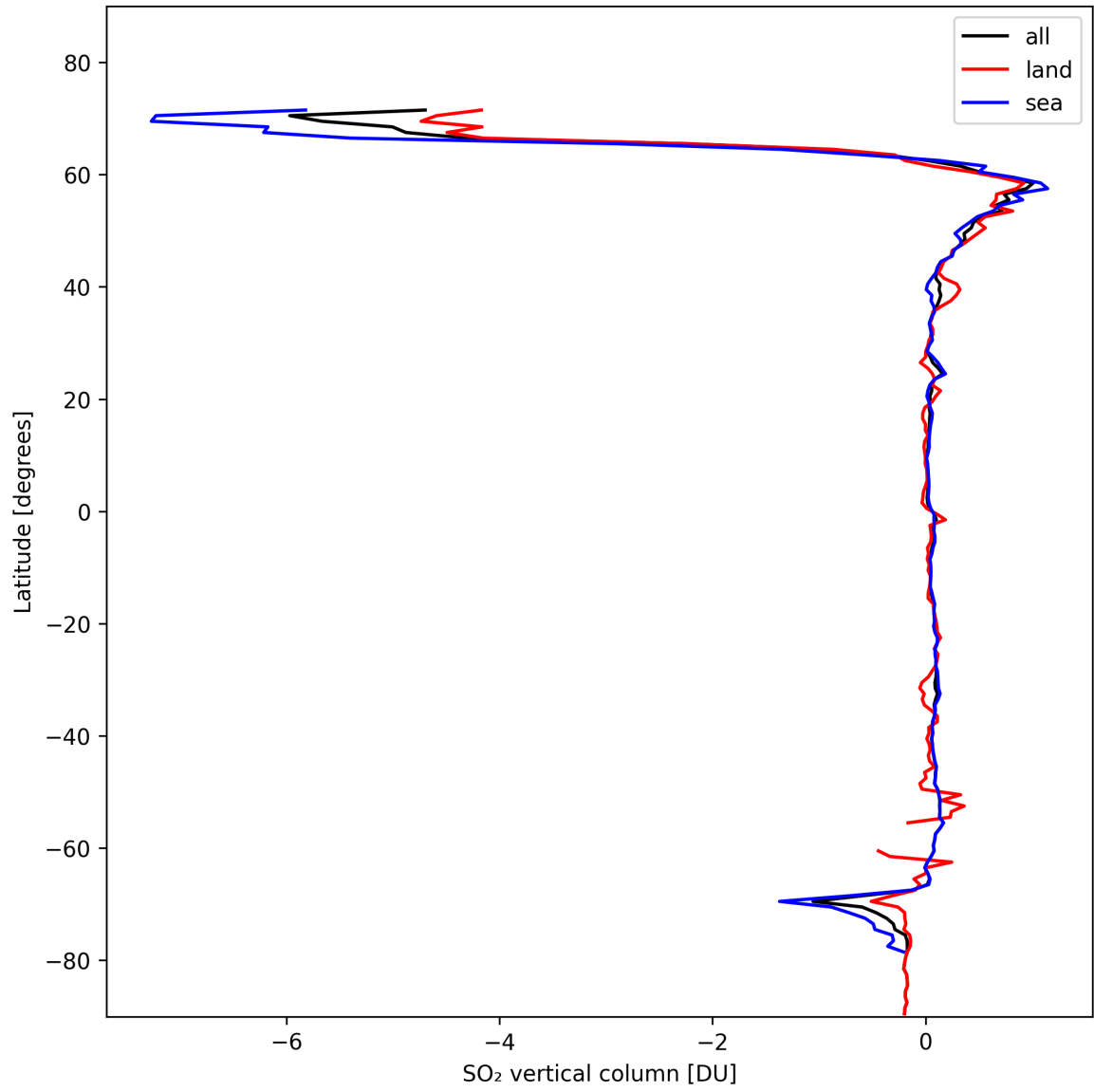
Figure 30: Zonal average of “SO 2 vertical column” for 2024-10-29 to 2024-10-30.
