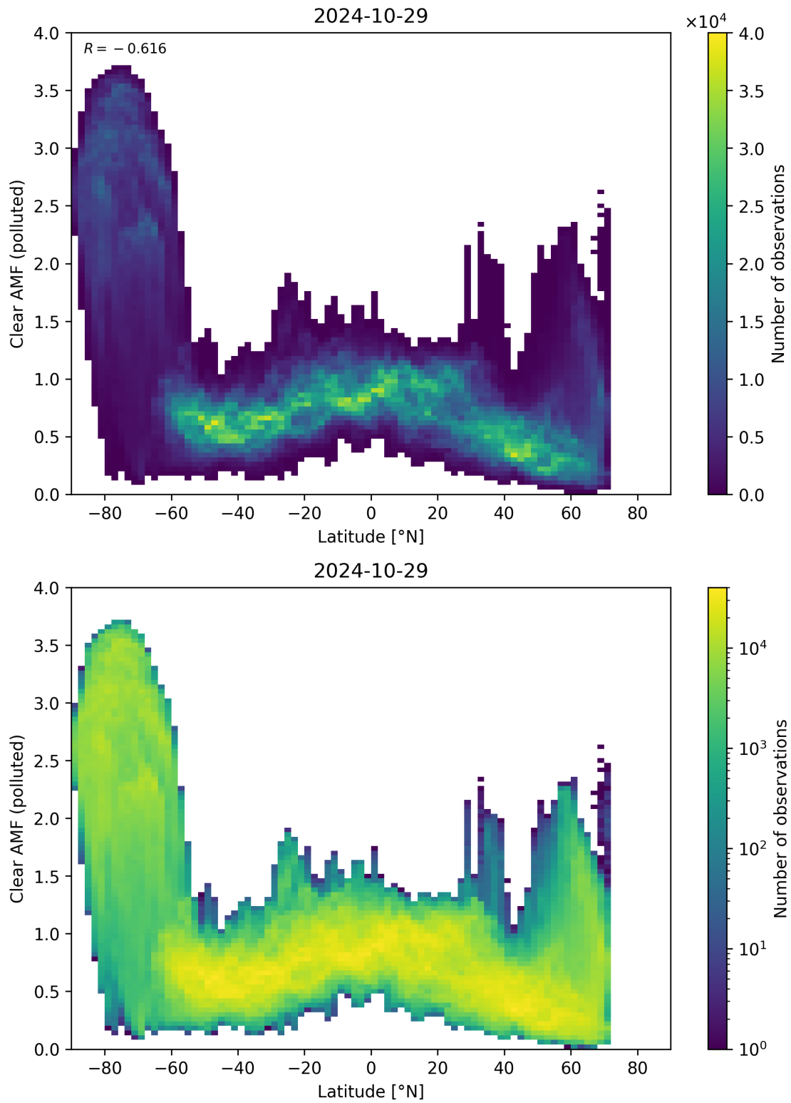
Figure 145: Scatter density plot of “Latitude” against “Clear AMF (polluted)” for 2024-10-29 to 2024-10-30.
