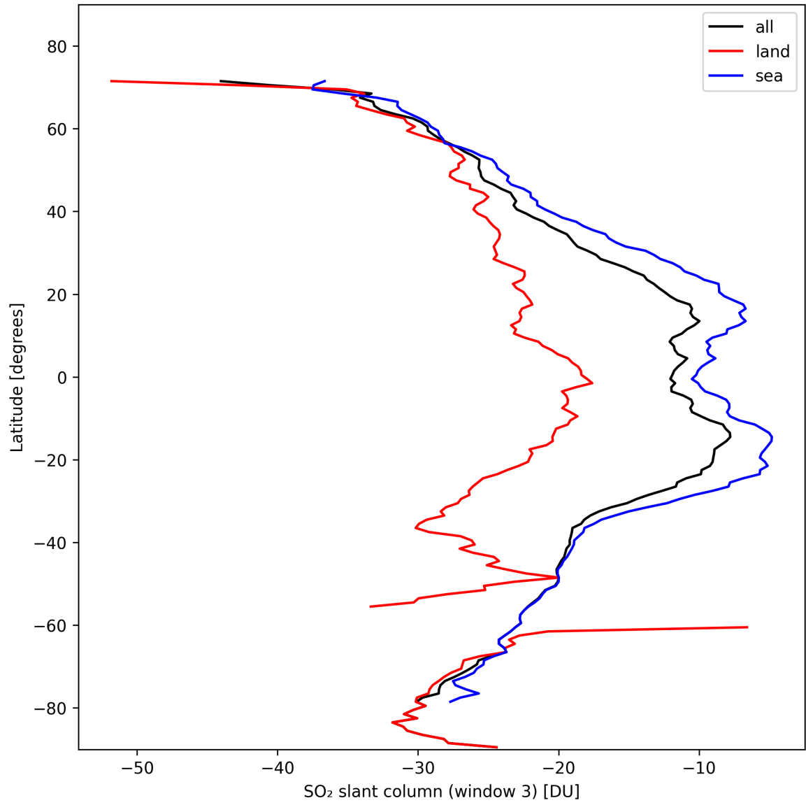
Figure 41: Zonal average of “SO 2 slant column (window 3)” for 2024-10-29 to 2024-10-30.
