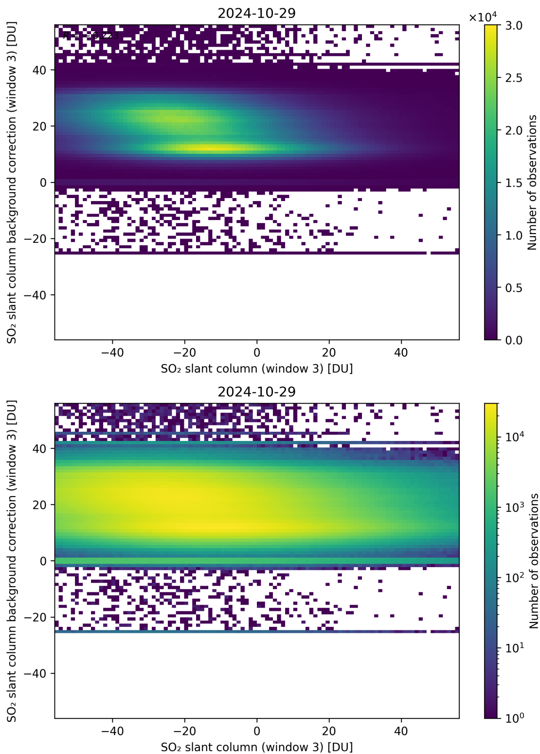
Figure 253: Scatter density plot of “SO 2 slant column (window 3)” against “SO 2 slant column background correction (window 3)” for 2024-10-29 to 2024-10-30.
