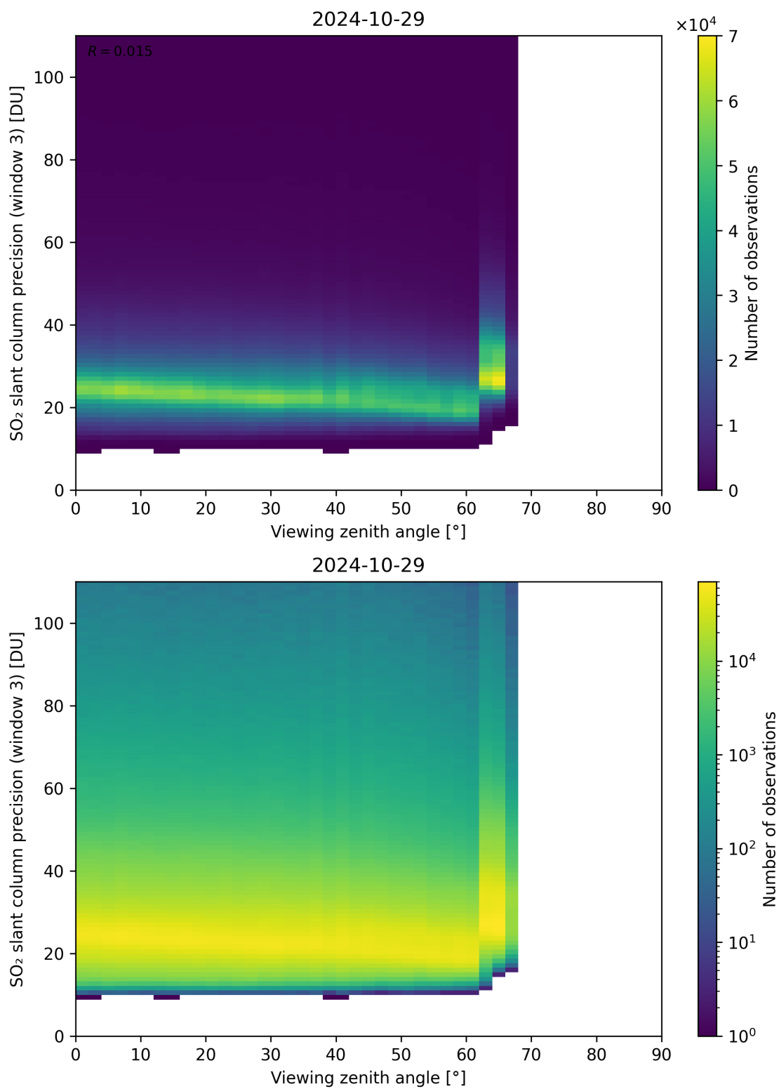
Figure 324: Scatter density plot of “Viewing zenith angle” against “SO 2 slant column precision (window 3)” for 2024-10-29 to 2024-10-30.
