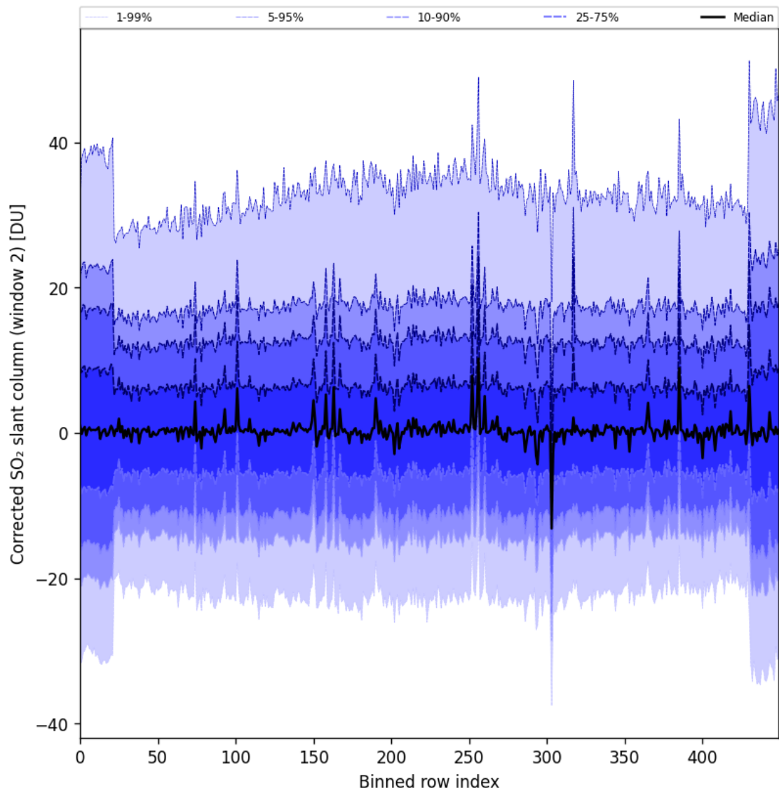
Figure 85: Along track statistics of “Corrected SO 2 slant column (window 2)” for 2024-10-29 to 2024-10-30
