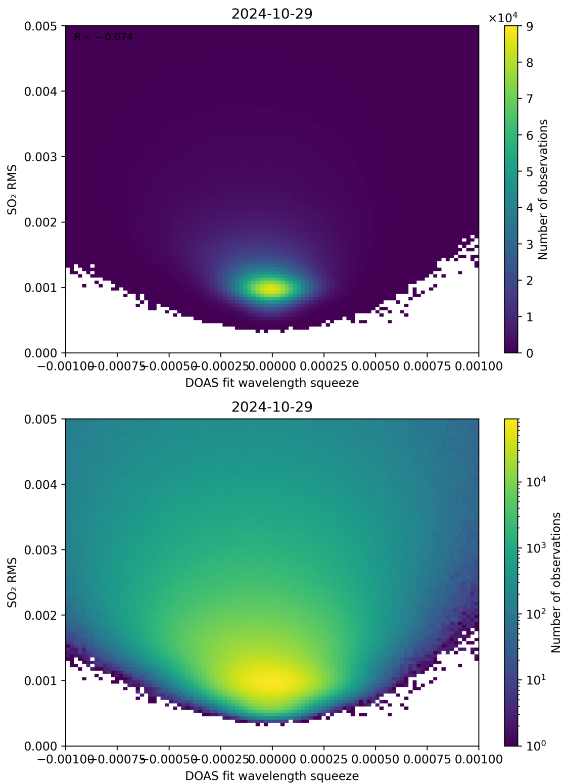
Figure 132: Scatter density plot of “DOAS fit wavelength squeeze” against “SO 2 RMS” for 2024-10-29 to 2024-10-30.
