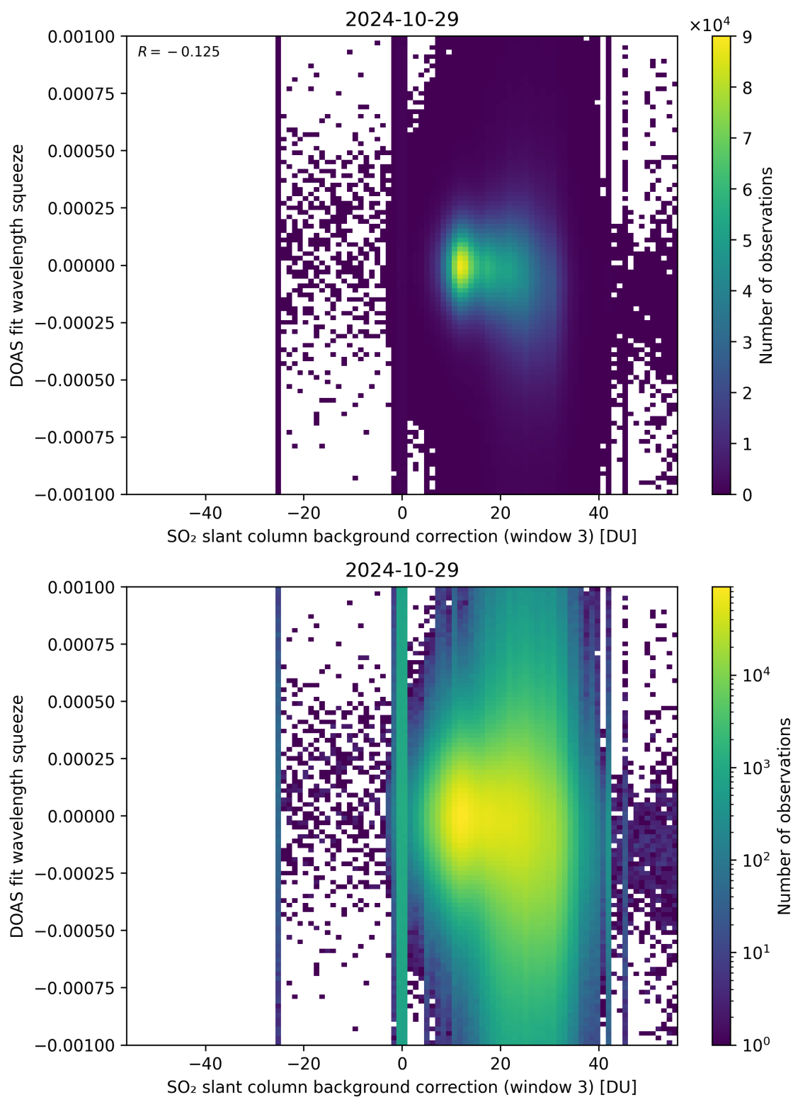
Figure 122: Scatter density plot of “SO 2 slant column background correction (window 3)” against “DOAS fit wavelength squeeze” for 2024-10-29 to 2024-10-30.
