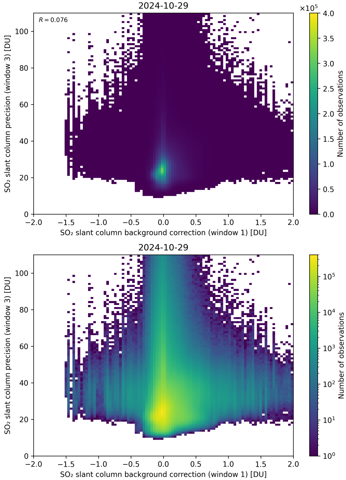
Figure 108: Scatter density plot of “SO 2 slant column background correction (window 1)” against “SO 2 slant column precision (window 3)” for 2024-10-29 to 2024-10-30.
