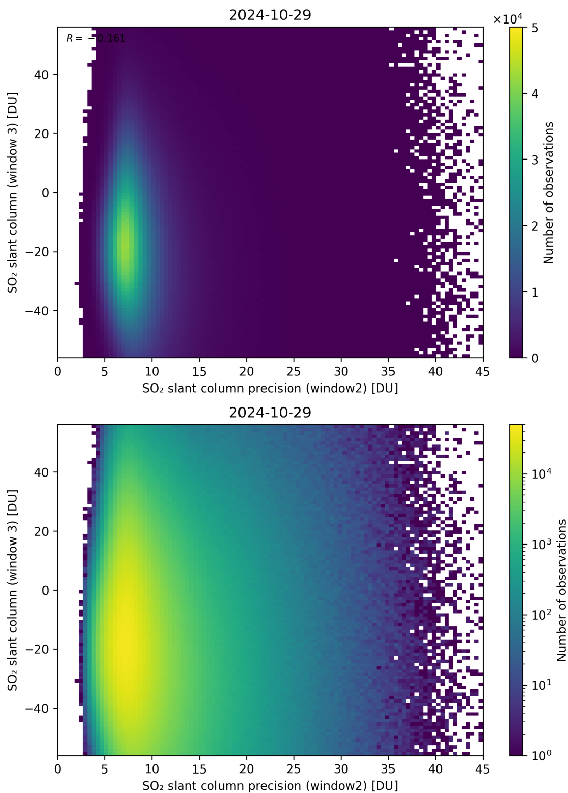
Figure 249: Scatter density plot of “SO 2 slant column precision (window2)” against “SO 2 slant column (window 3)” for 2024-10-29 to 2024-10-30.
