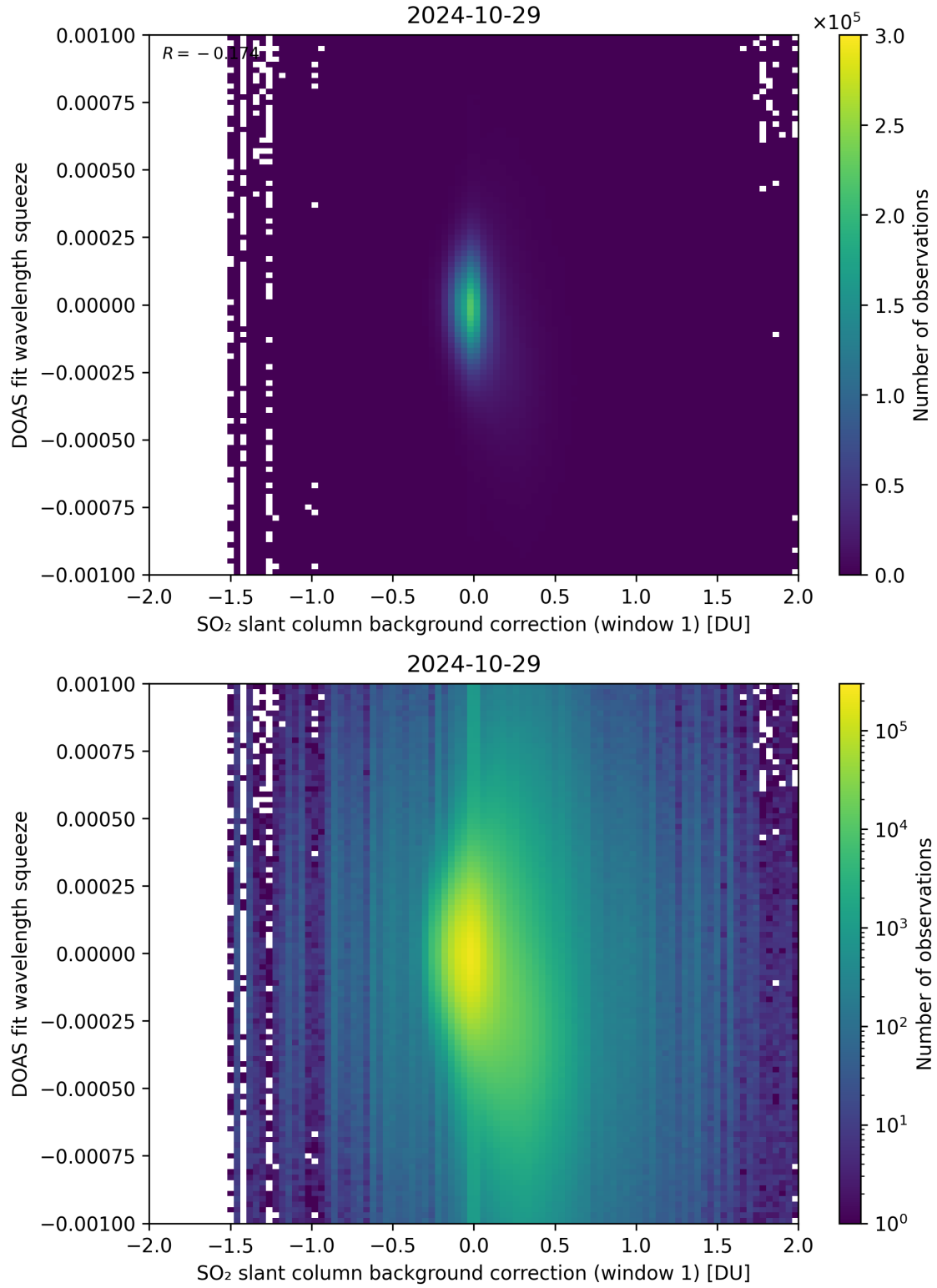
Figure 101: Scatter density plot of “SO 2 slant column background correction (window 1)” against “DOAS fit wavelength squeeze” for 2024-10-29 to 2024-10-30.
