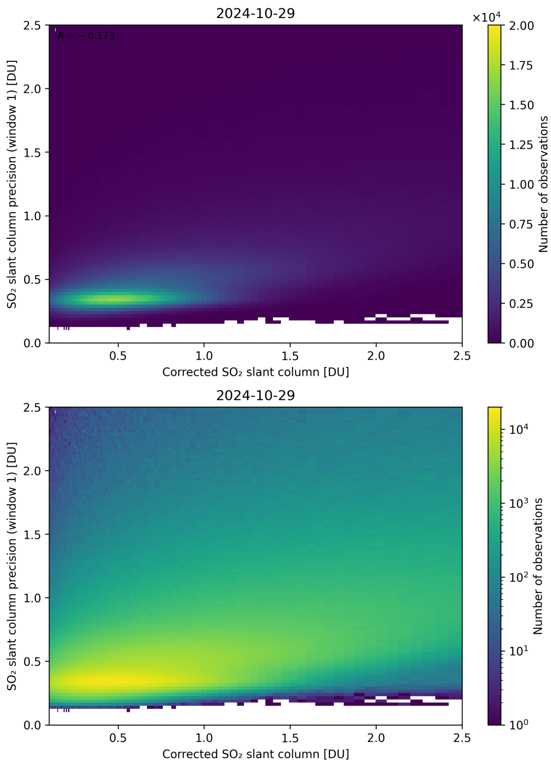
Figure 188: Scatter density plot of “Corrected SO 2 slant column” against “SO 2 slant column precision (window 1)” for 2024-10-29 to 2024-10-30.
