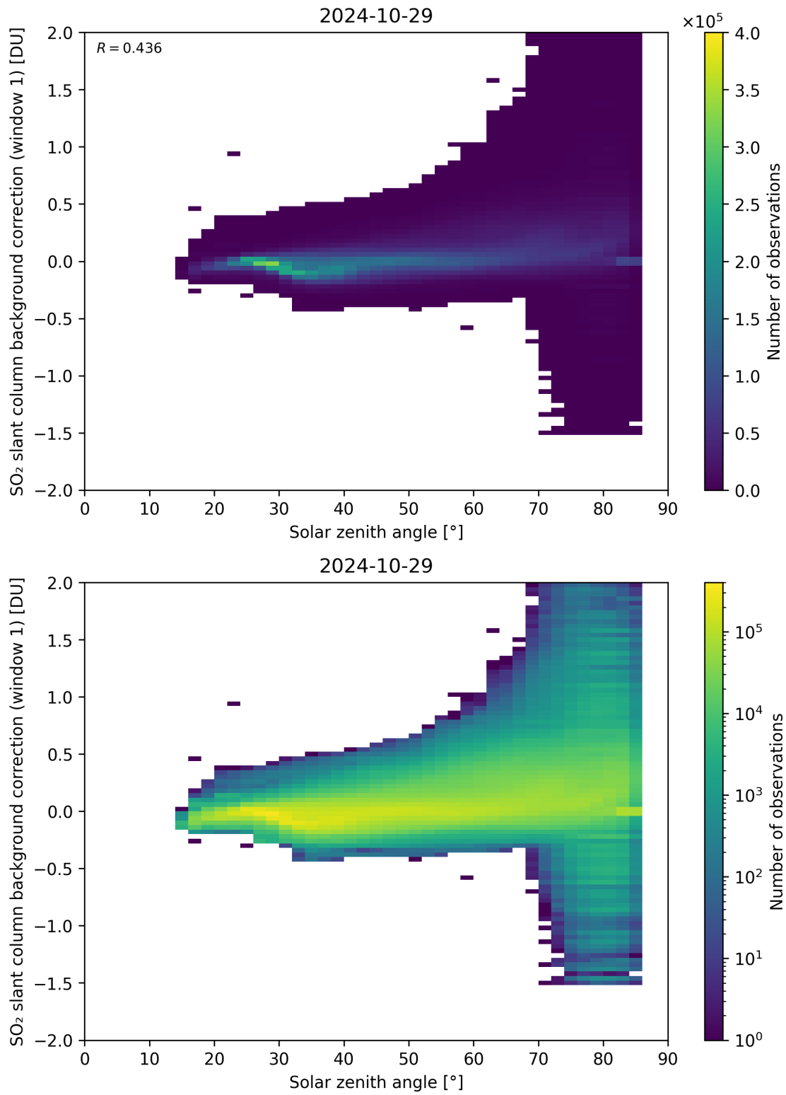
Figure 158: Scatter density plot of “Solar zenith angle” against “SO 2 slant column background correction (window 1)” for 2024-10-29 to 2024-10-30.
