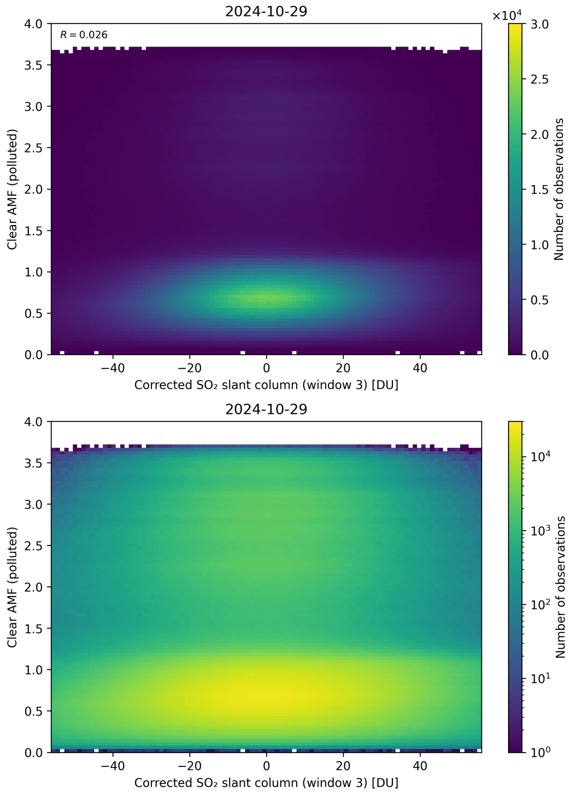
Figure 209: Scatter density plot of “Corrected SO 2 slant column (window 3)” against “Clear AMF (polluted)” for 2024-10-29 to 2024-10-30.
