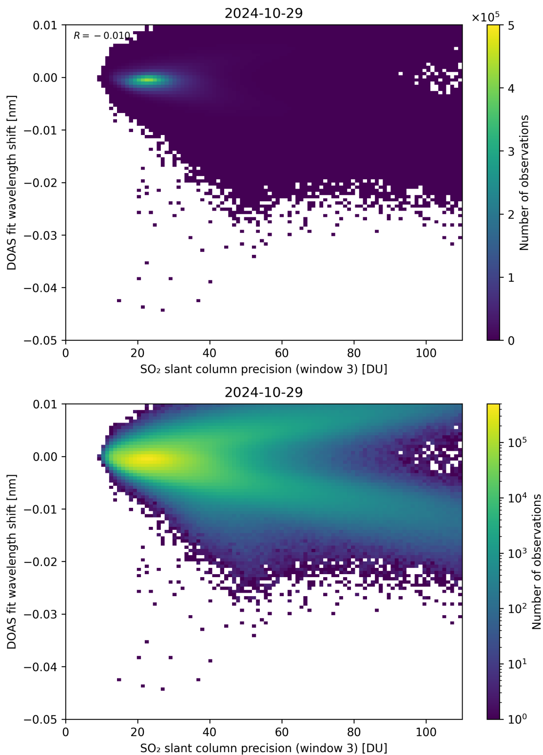
Figure 258: Scatter density plot of “SO 2 slant column precision (window 3)” against “DOAS fit wavelength shift” for 2024-10-29 to 2024-10-30.
