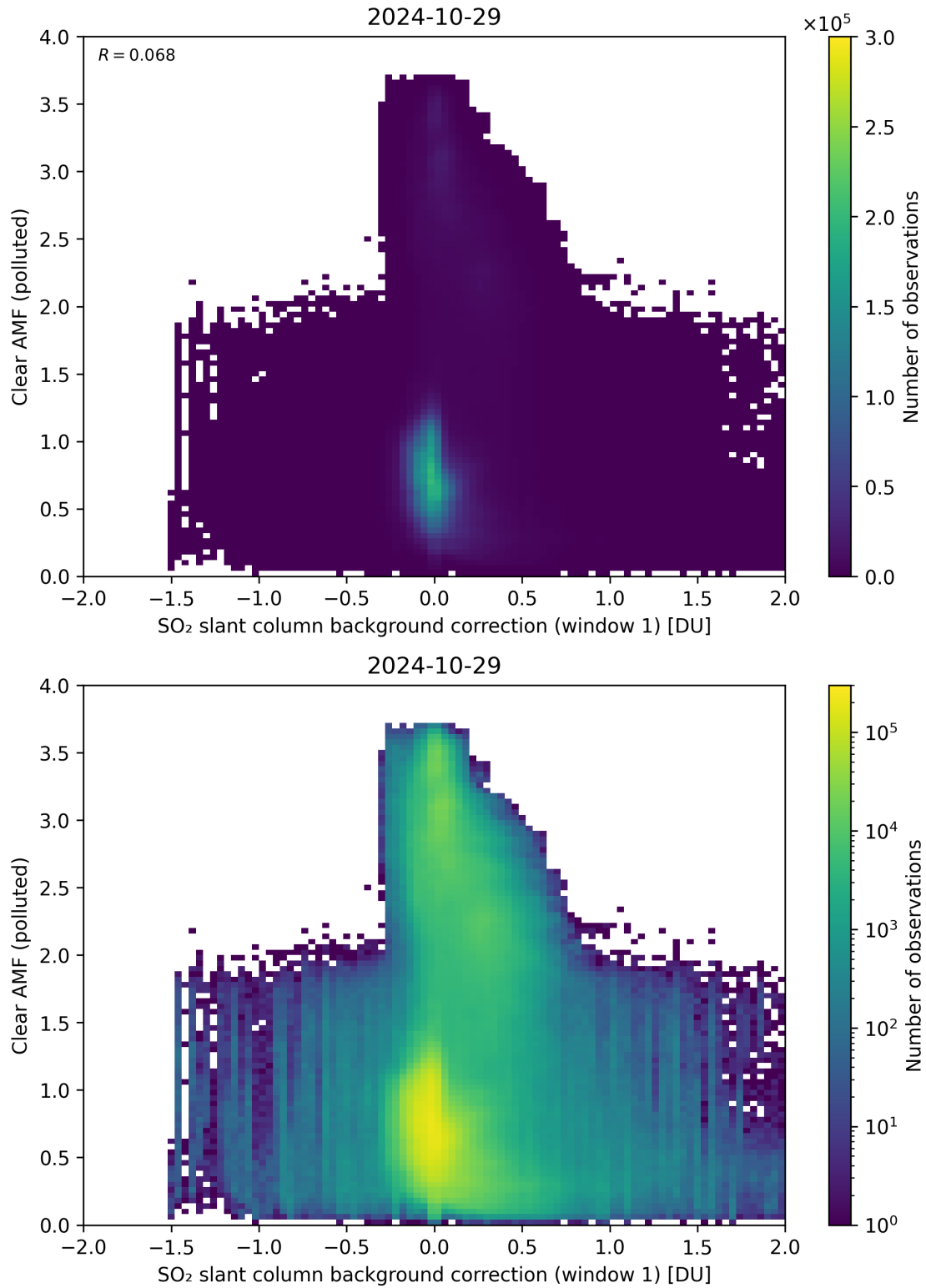
Figure 103: Scatter density plot of “SO 2 slant column background correction (window 1)” against “Clear AMF (polluted)” for 2024-10-29 to 2024-10-30.
