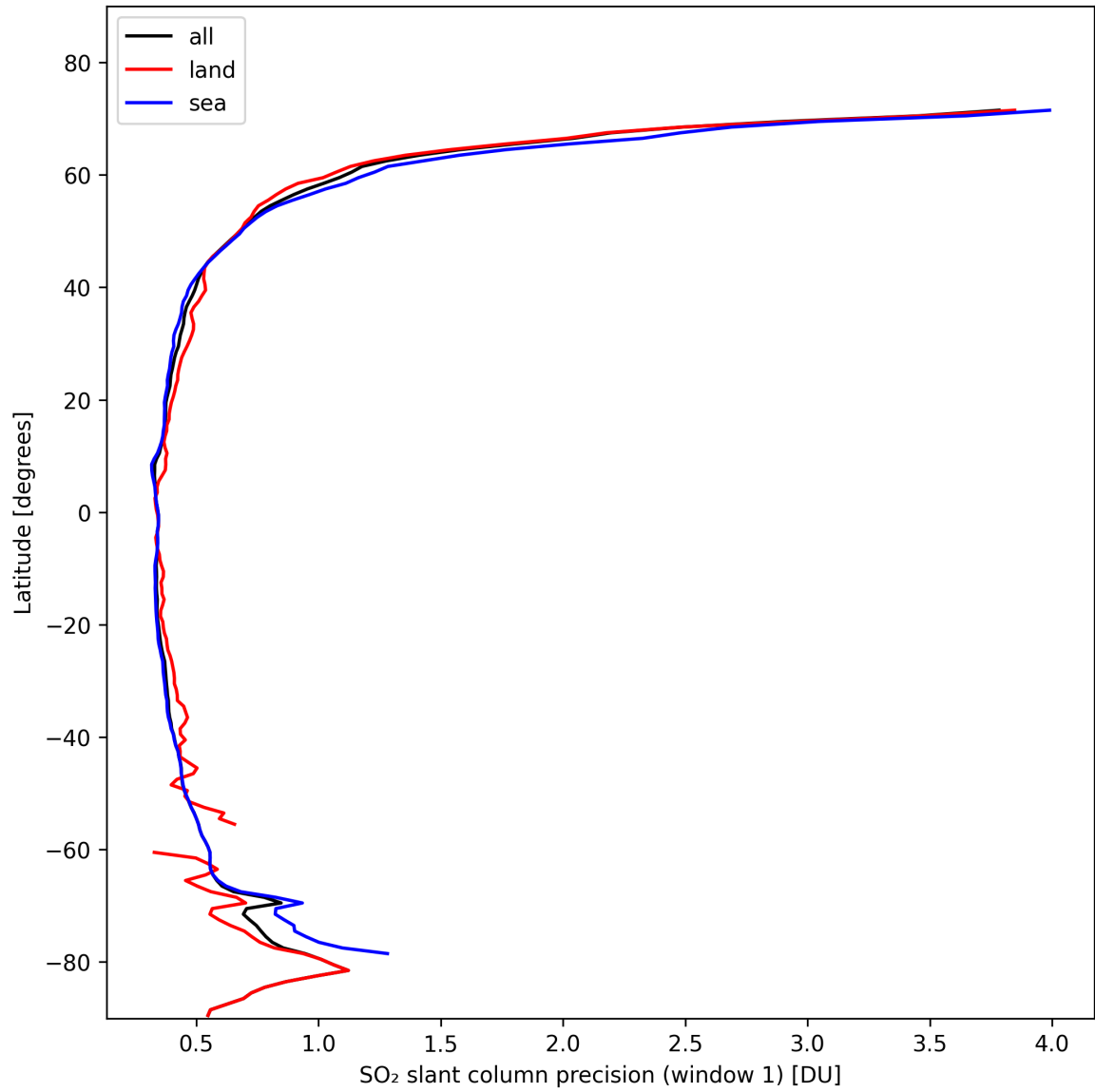
Figure 34: Zonal average of “SO 2 slant column precision (window 1)” for 2024-10-29 to 2024-10-30.
