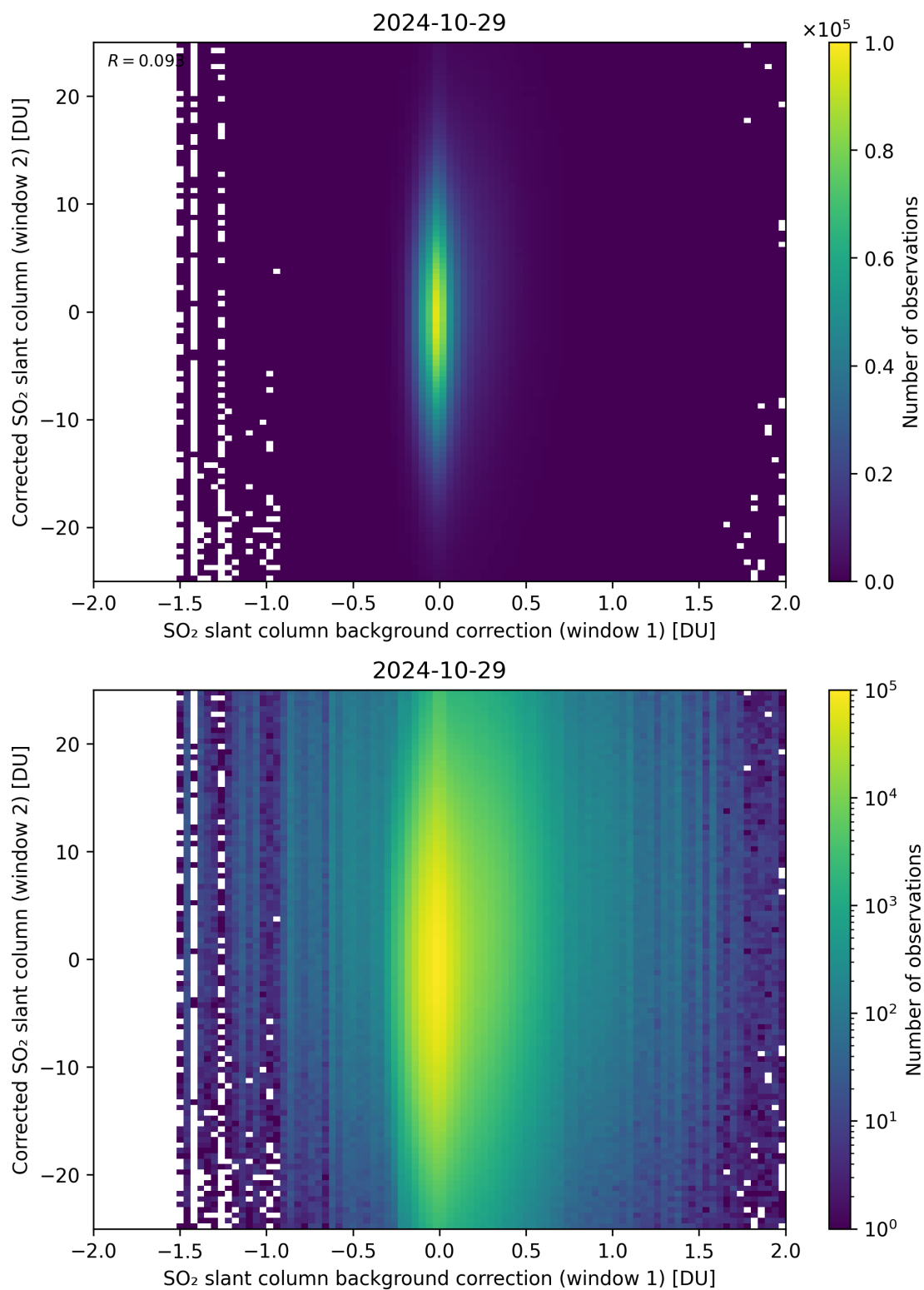
Figure 104: Scatter density plot of “SO 2 slant column background correction (window 1)” against “Corrected SO 2 slant column (window 2)” for 2024-10-29 to 2024-10-30.
