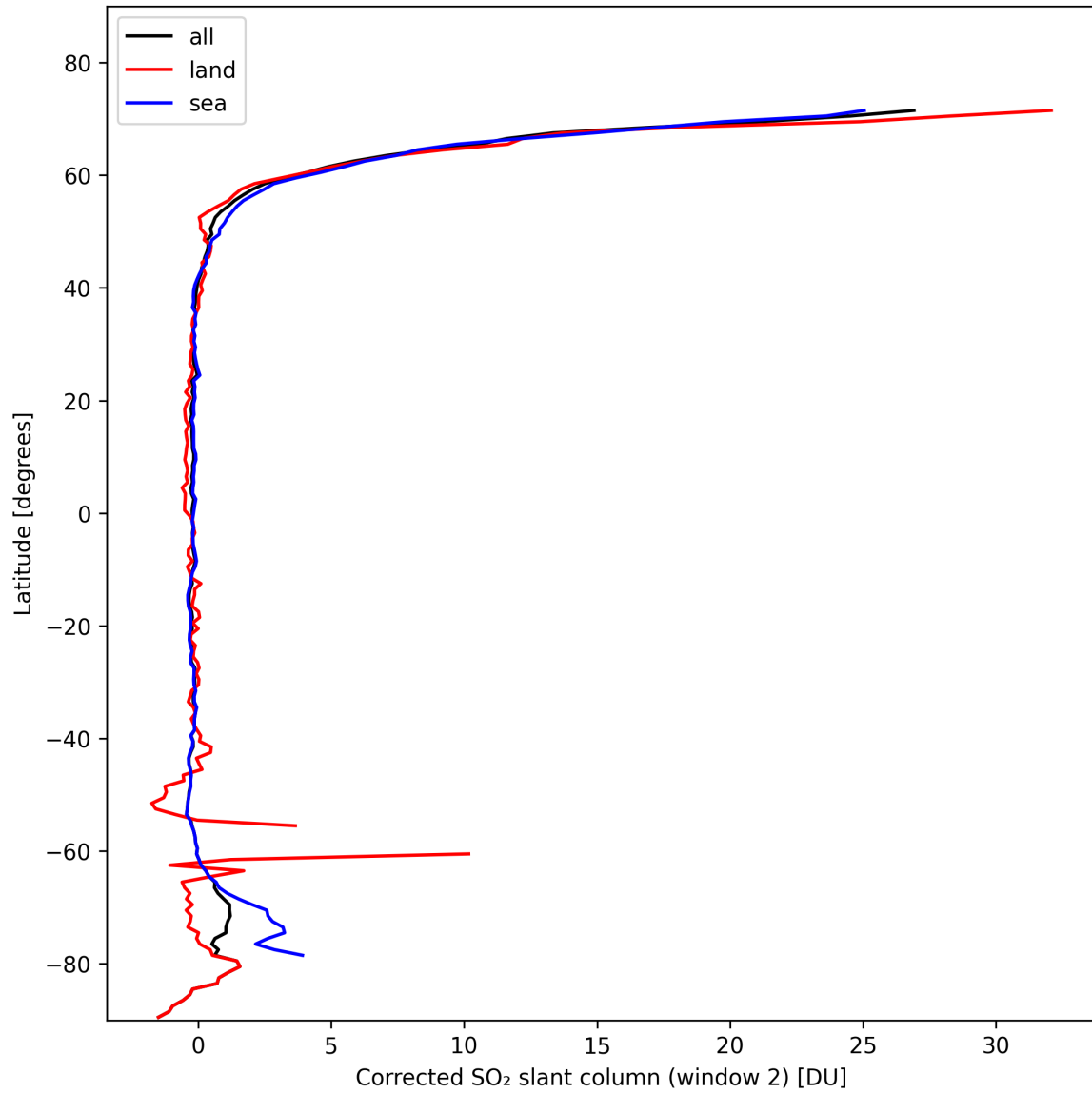
Figure 39: Zonal average of “Corrected SO 2 slant column (window 2)” for 2024-10-29 to 2024-10-30.
