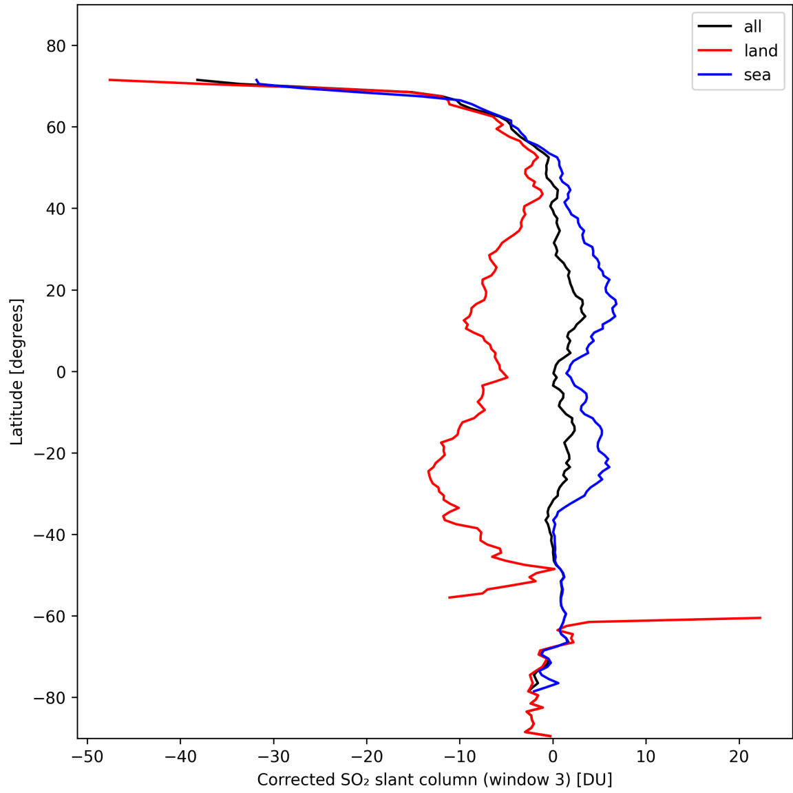
Figure 43: Zonal average of “Corrected SO 2 slant column (window 3)” for 2024-10-29 to 2024-10-30.
