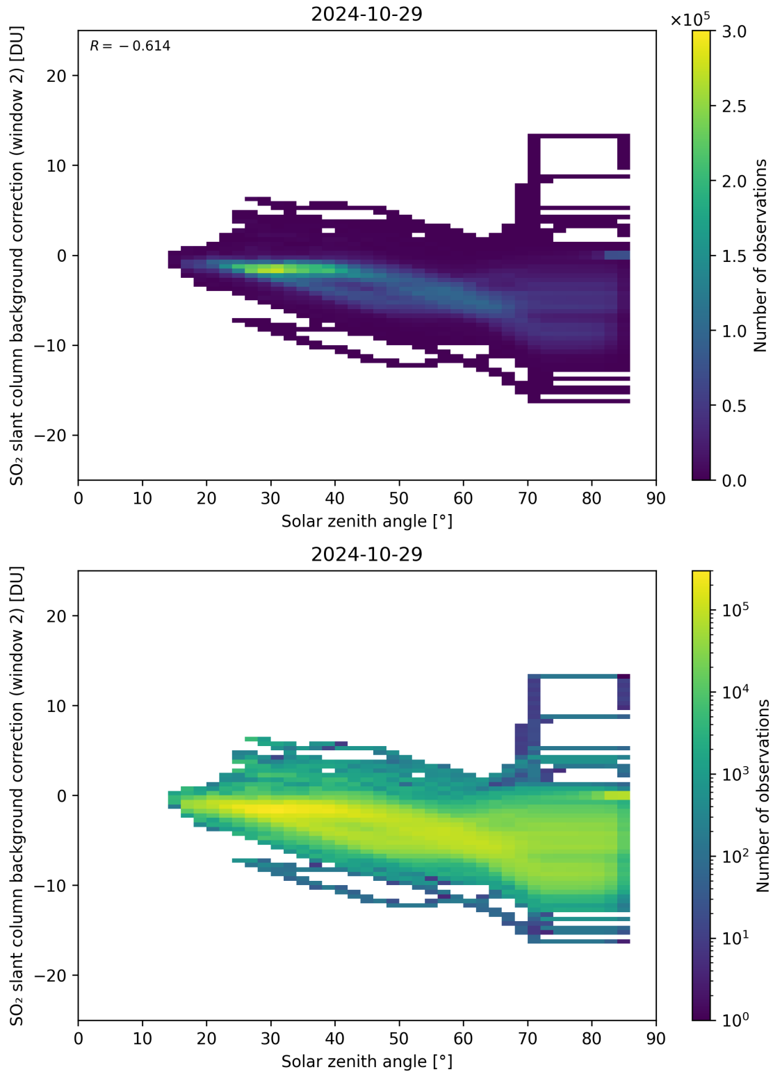
Figure 159: Scatter density plot of “Solar zenith angle” against “SO 2 slant column background correction (window 2)” for 2024-10-29 to 2024-10-30.
