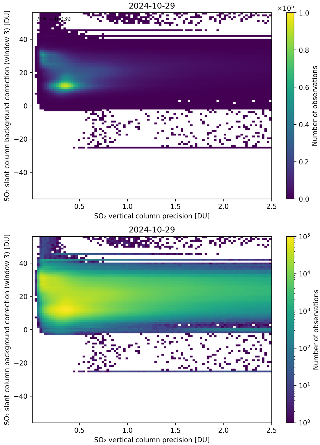
Figure 281: Scatter density plot of “SO 2 vertical column precision” against “SO 2 slant column background correction (window 3)” for 2024-10-29 to 2024-10-30.
