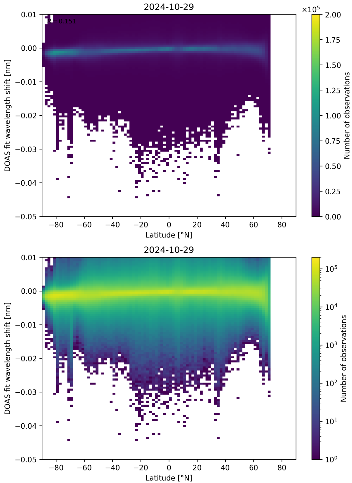
Figure 142: Scatter density plot of “Latitude” against “DOAS fit wavelength shift” for 2024-10-29 to 2024-10-30.
