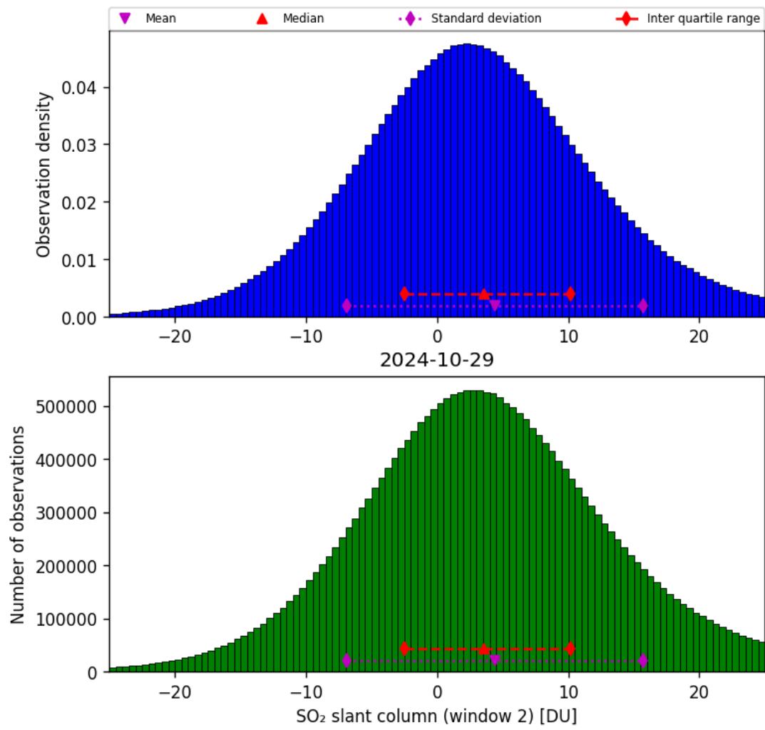
Figure 60: Histogram of “SO 2 slant column (window 2)” for 2024-10-29 to 2024-10-30
