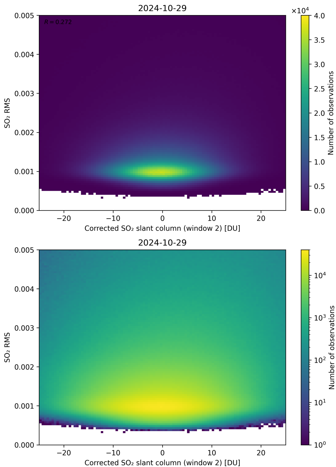
Figure 198: Scatter density plot of “Corrected SO 2 slant column (window 2)” against “SO 2 RMS” for 2024-10-29 to 2024-10-30.
