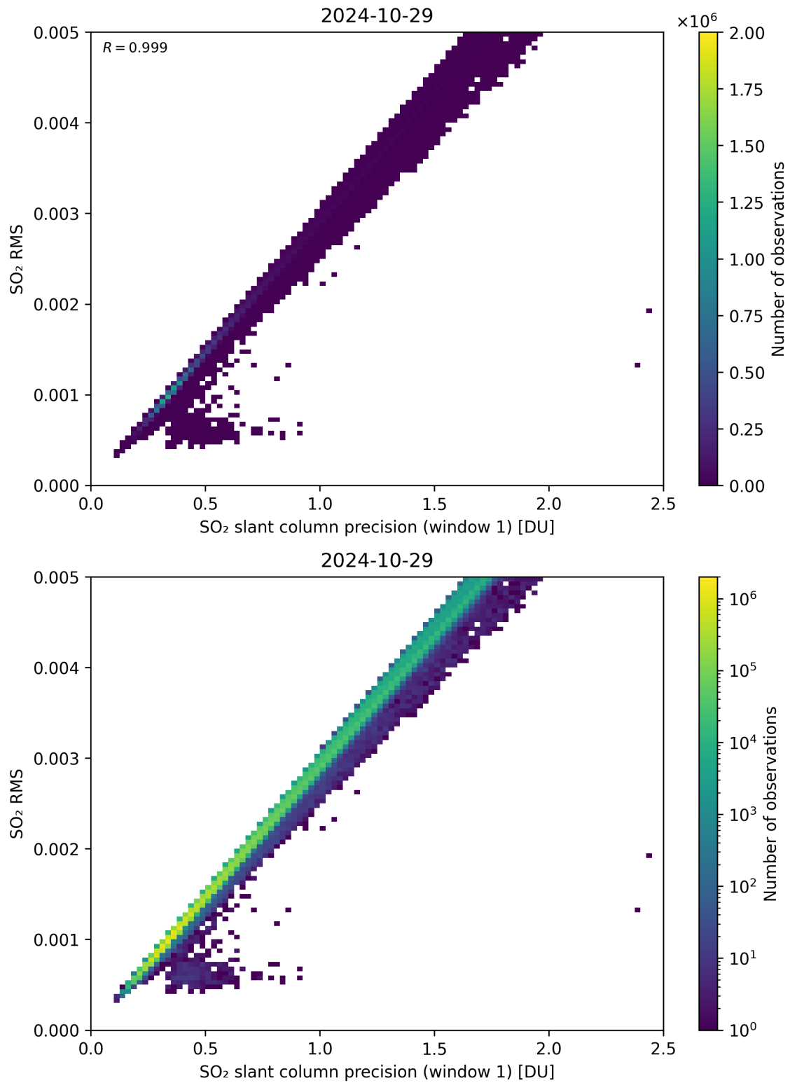
Figure 223: Scatter density plot of “SO 2 slant column precision (window 1)” against “SO 2 RMS” for 2024-10-29 to 2024-10-30.
