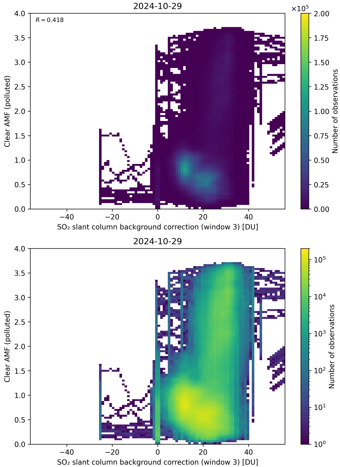
Figure 124: Scatter density plot of “SO 2 slant column background correction (window 3)” against “Clear AMF (polluted)” for 2024-10-29 to 2024-10-30.
