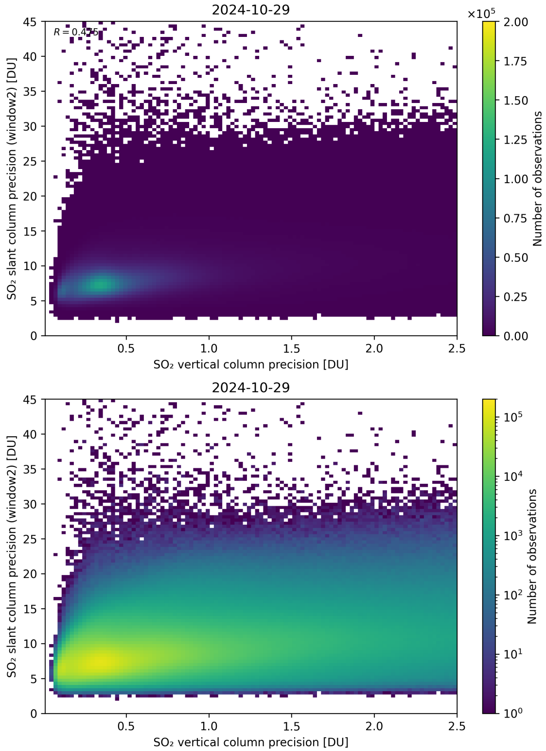
Figure 291: Scatter density plot of “SO 2 vertical column precision” against “SO 2 slant column precision (window2)” for 2024-10-29 to 2024-10-30.
