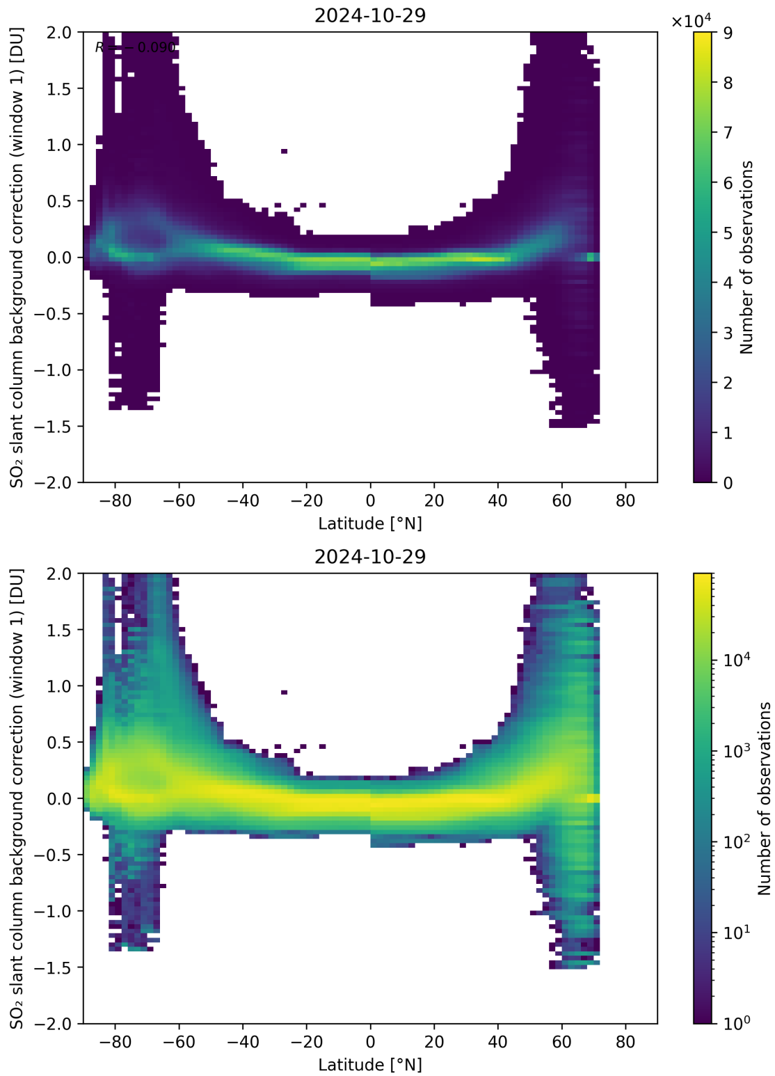
Figure 139: Scatter density plot of “Latitude” against “SO 2 slant column background correction (window 1)” for 2024-10-29 to 2024-10-30.
