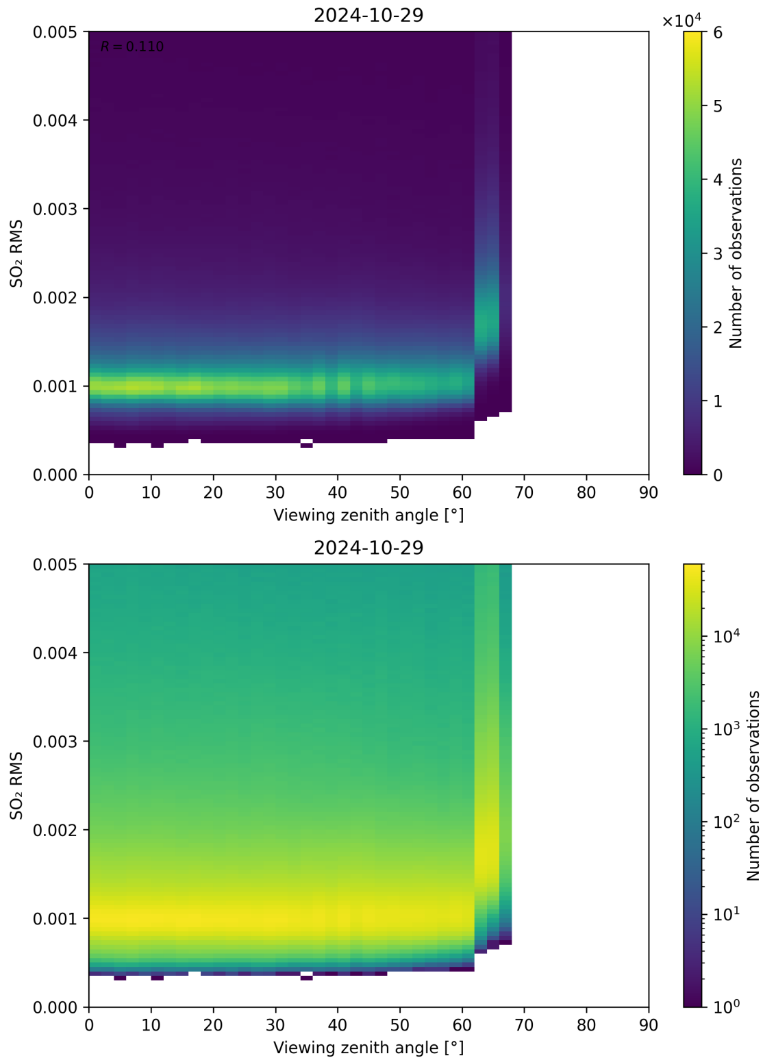
Figure 313: Scatter density plot of “Viewing zenith angle” against “SO 2 RMS” for 2024-10-29 to 2024-10-30.
