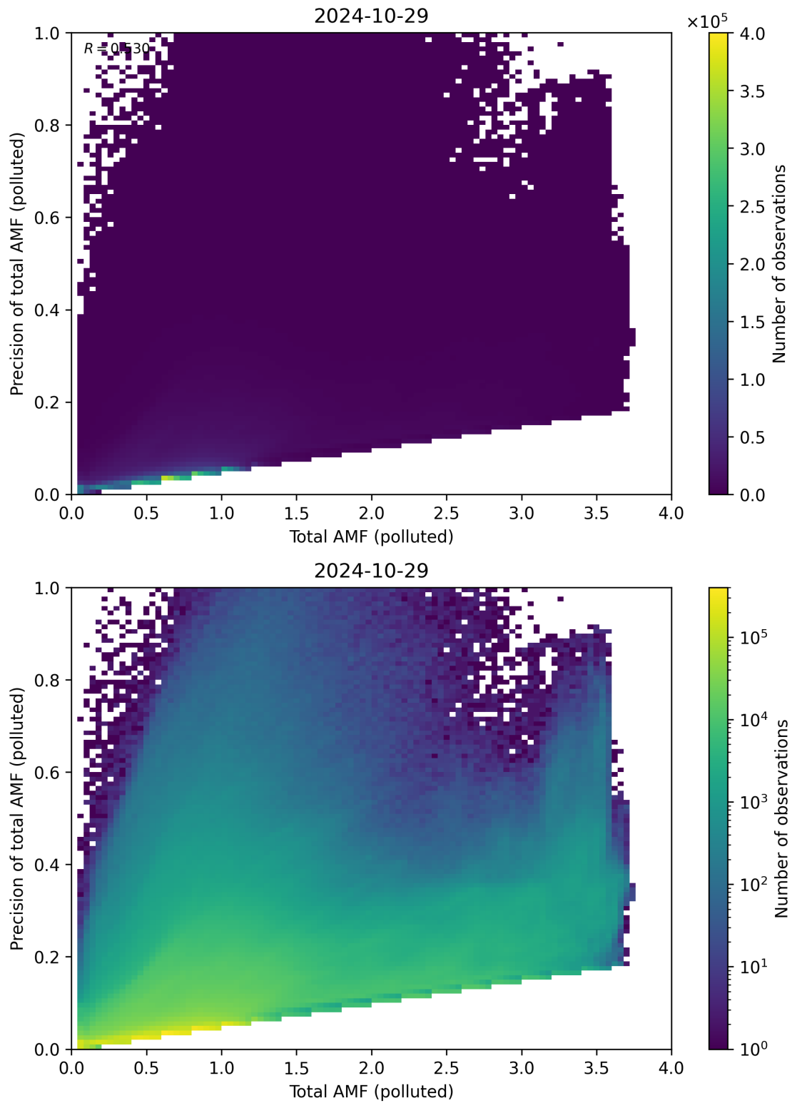
Figure 272: Scatter density plot of “Total AMF (polluted)” against “Precision of total AMF (polluted)” for 2024-10-29 to 2024-10-30.
