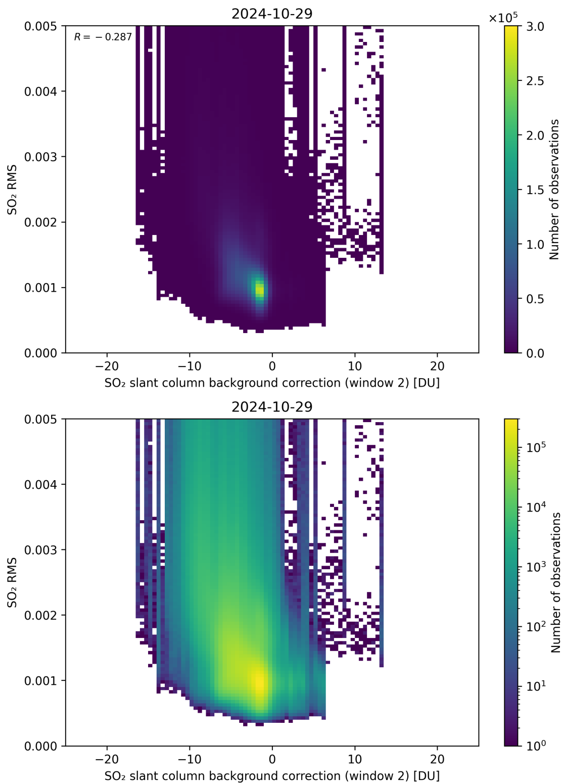
Figure 114: Scatter density plot of “SO 2 slant column background correction (window 2)” against “SO 2 RMS” for 2024-10-29 to 2024-10-30.
