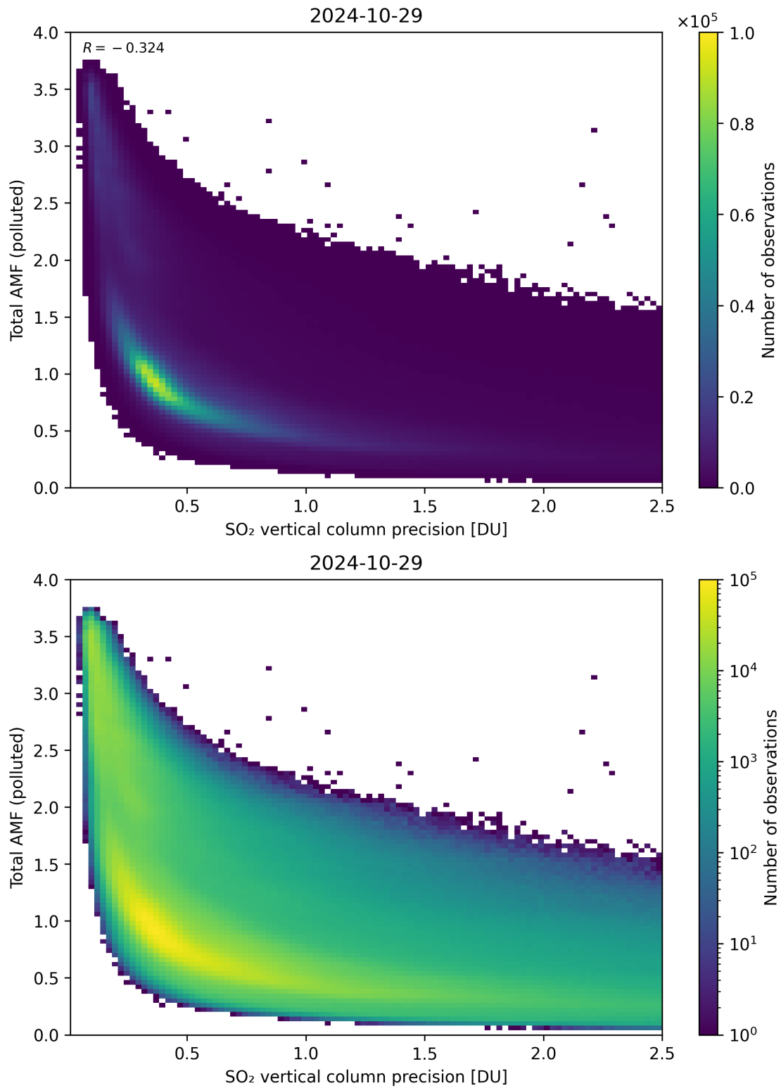
Figure 294: Scatter density plot of “SO 2 vertical column precision” against “Total AMF (polluted)” for 2024-10-29 to 2024-10-30.
