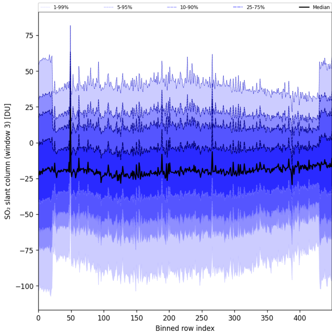
Figure 87: Along track statistics of “SO 2 slant column (window 3)” for 2024-10-29 to 2024-10-30
