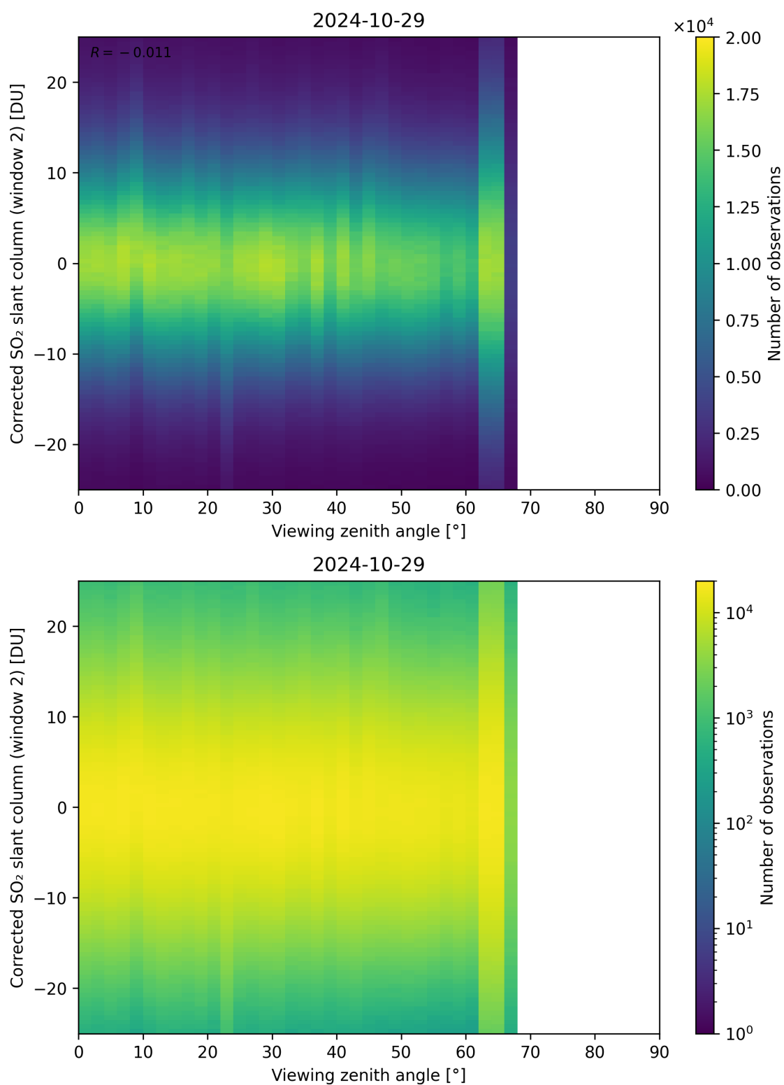
Figure 318: Scatter density plot of “Viewing zenith angle” against “Corrected SO 2 slant column (window 2)” for 2024-10-29 to 2024-10-30.
