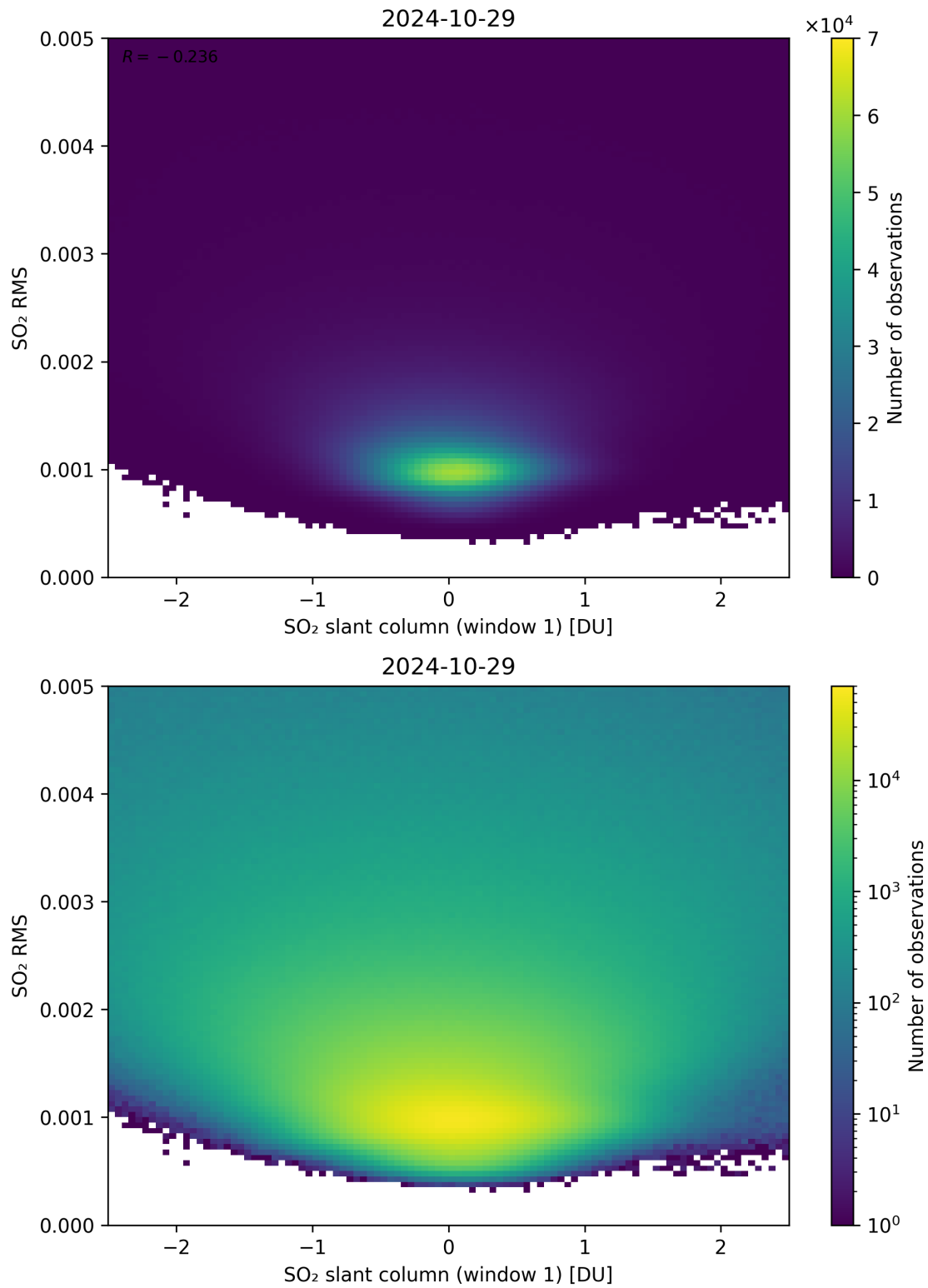
Figure 217: Scatter density plot of “SO 2 slant column (window 1)” against “SO 2 RMS” for 2024-10-29 to 2024-10-30.
