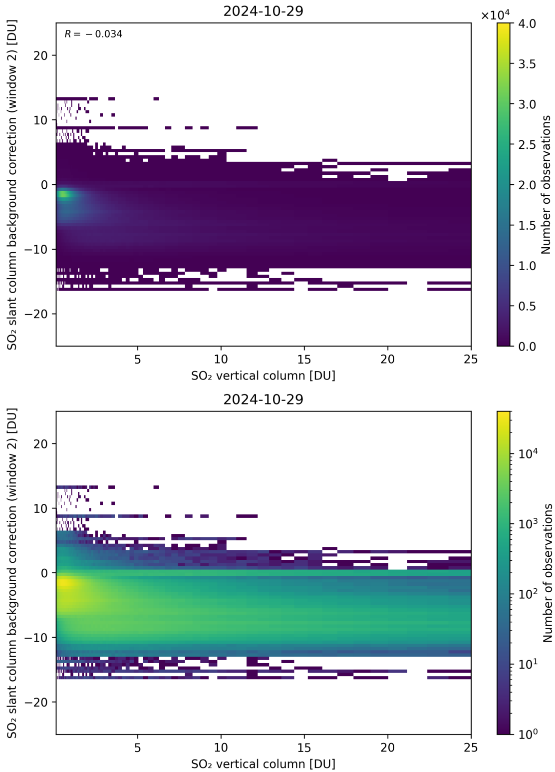
Figure 274: Scatter density plot of “SO 2 vertical column” against “SO 2 slant column background correction (window 2)” for 2024-10-29 to 2024-10-30.
