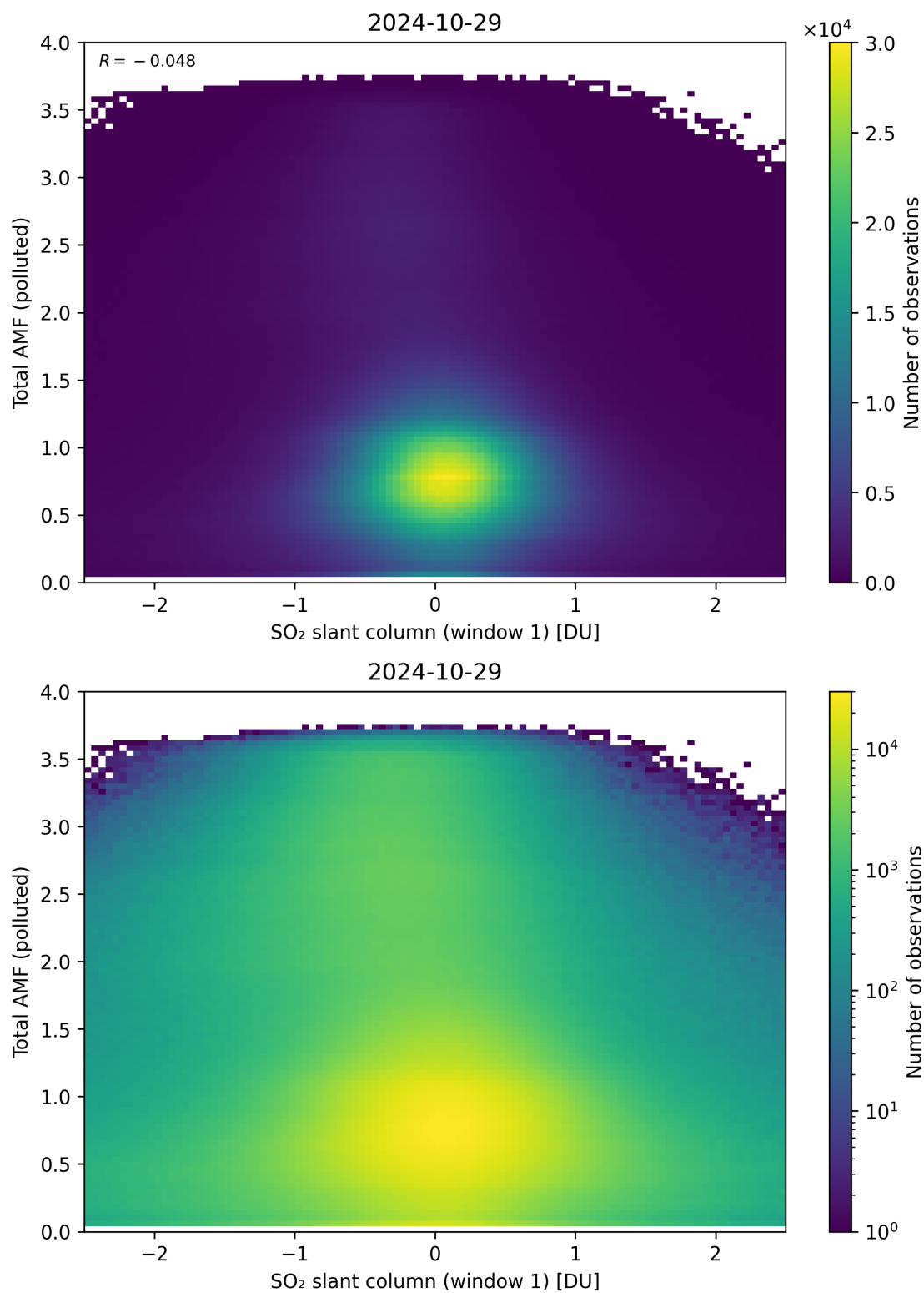
Figure 239: Scatter density plot of “SO 2 slant column (window 1)” against “Total AMF (polluted)” for 2024-10-29 to 2024-10-30.
