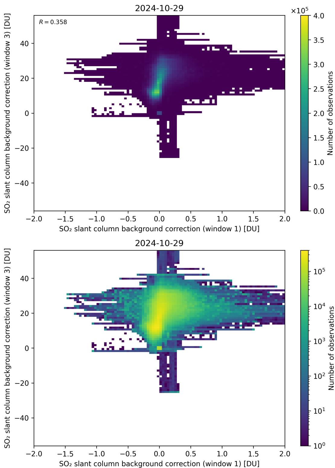
Figure 99: Scatter density plot of “SO 2 slant column background correction (window 1)” against “SO 2 slant column background correction (window 3)” for 2024-10-29 to 2024-10-30.
