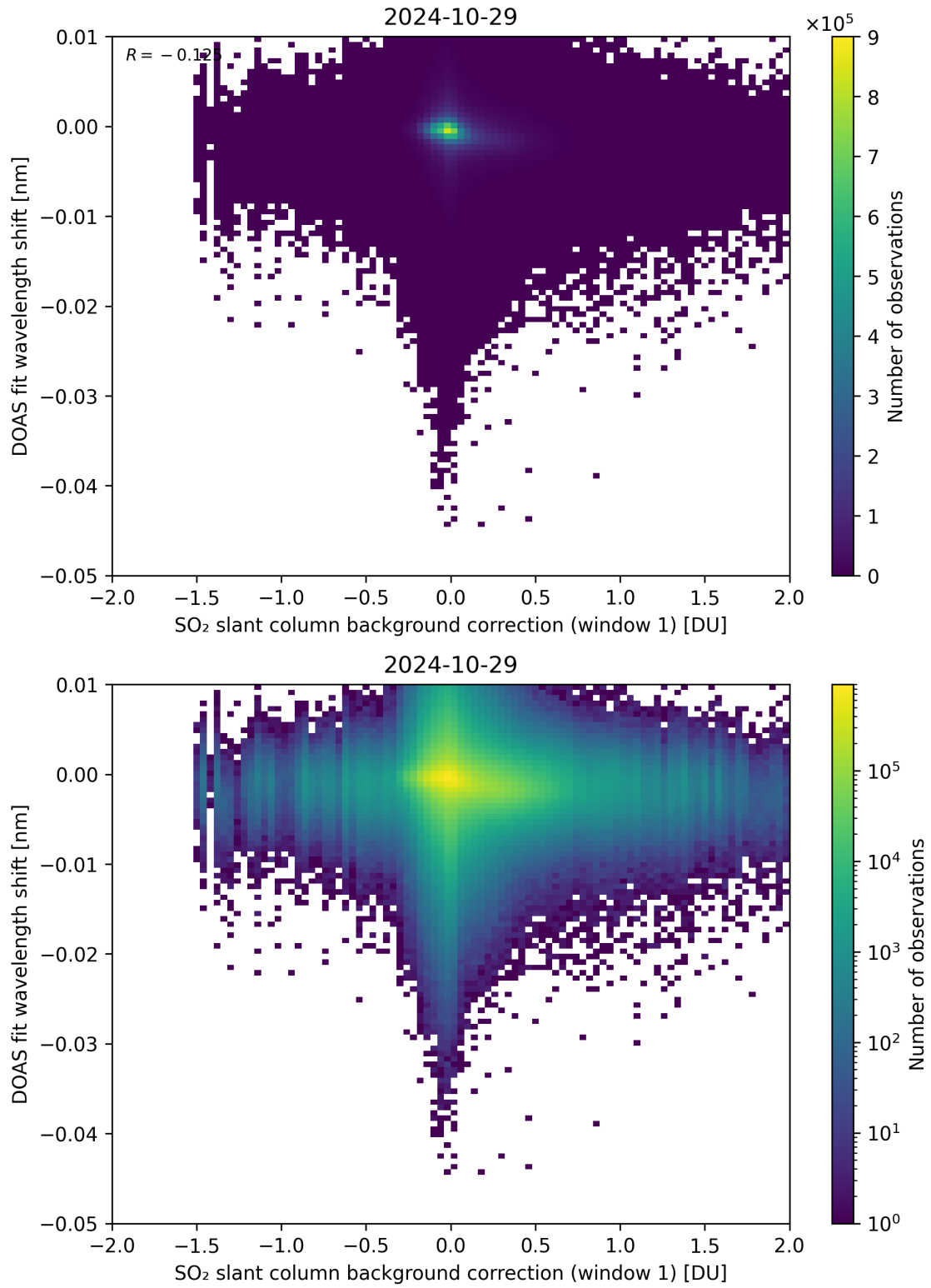
Figure 100: Scatter density plot of “SO 2 slant column background correction (window 1)” against “DOAS fit wavelength shift” for 2024-10-29 to 2024-10-30.
