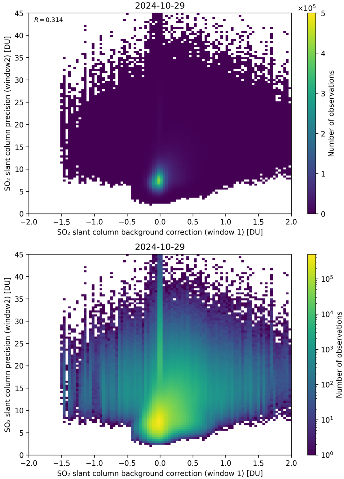
Figure 106: Scatter density plot of “SO 2 slant column background correction (window 1)” against “SO 2 slant column precision (window2)” for 2024-10-29 to 2024-10-30.
