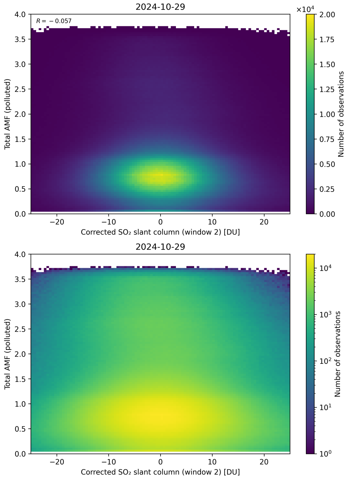
Figure 203: Scatter density plot of “Corrected SO 2 slant column (window 2)” against “Total AMF (polluted)” for 2024-10-29 to 2024-10-30.
