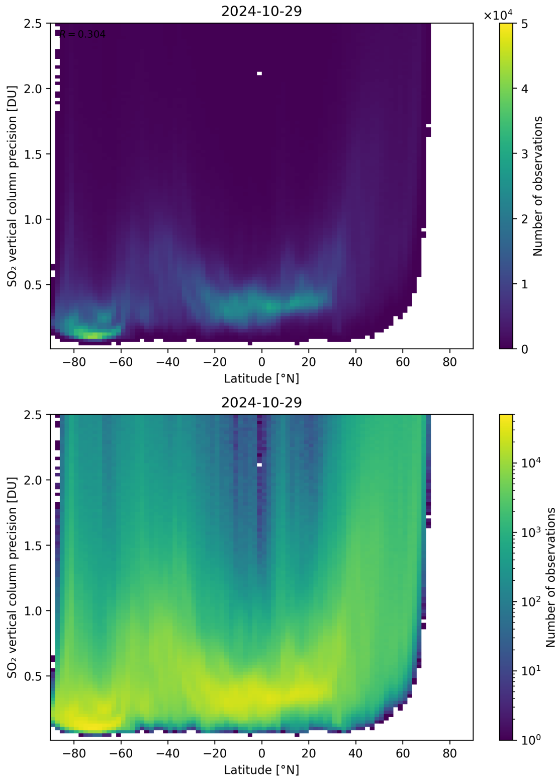
Figure 157: Scatter density plot of “Latitude” against “SO 2 vertical column precision” for 2024-10-29 to 2024-10-30.
