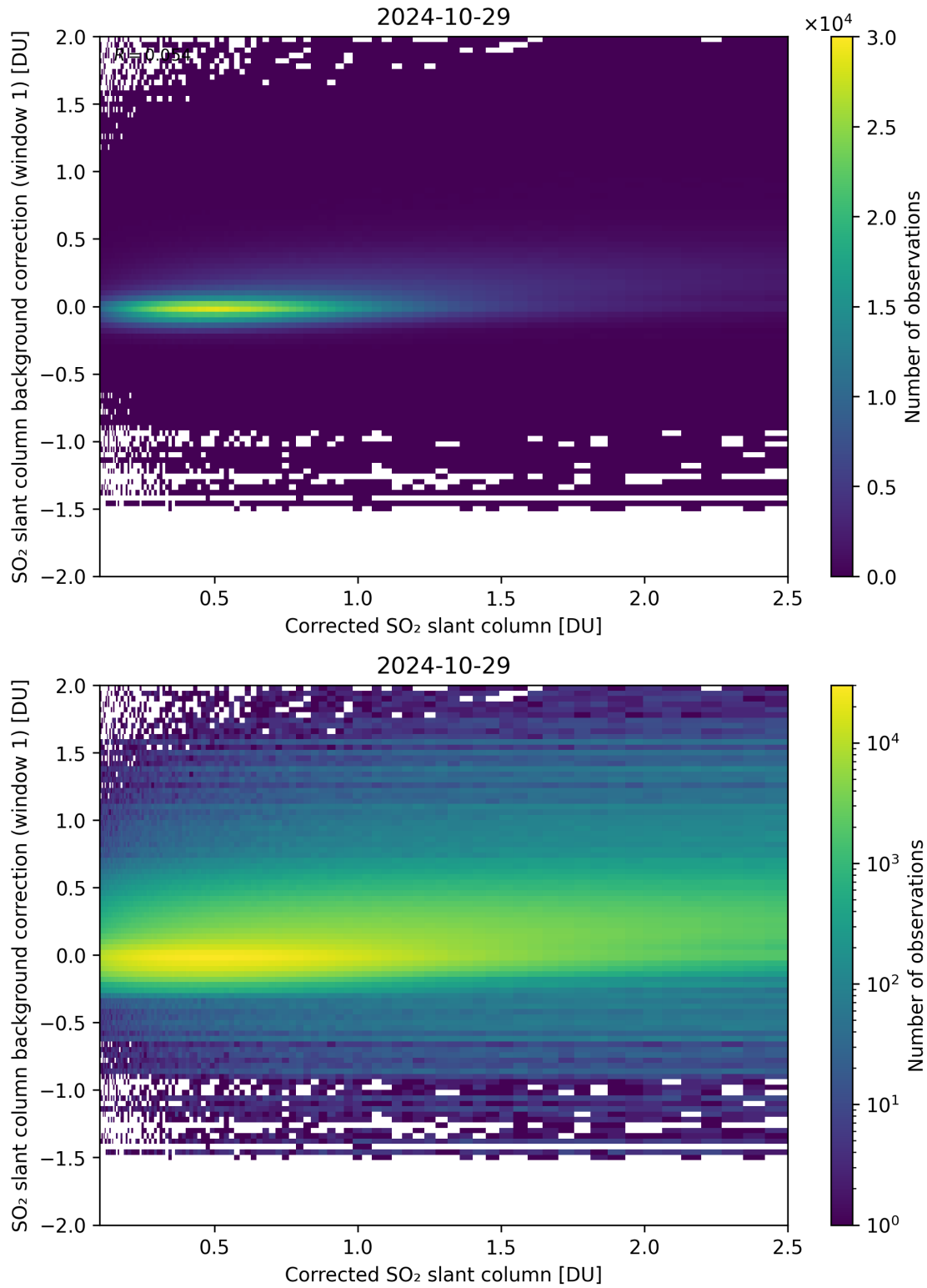
Figure 178: Scatter density plot of “Corrected SO 2 slant column” against “SO 2 slant column background correction (window 1)” for 2024-10-29 to 2024-10-30.
