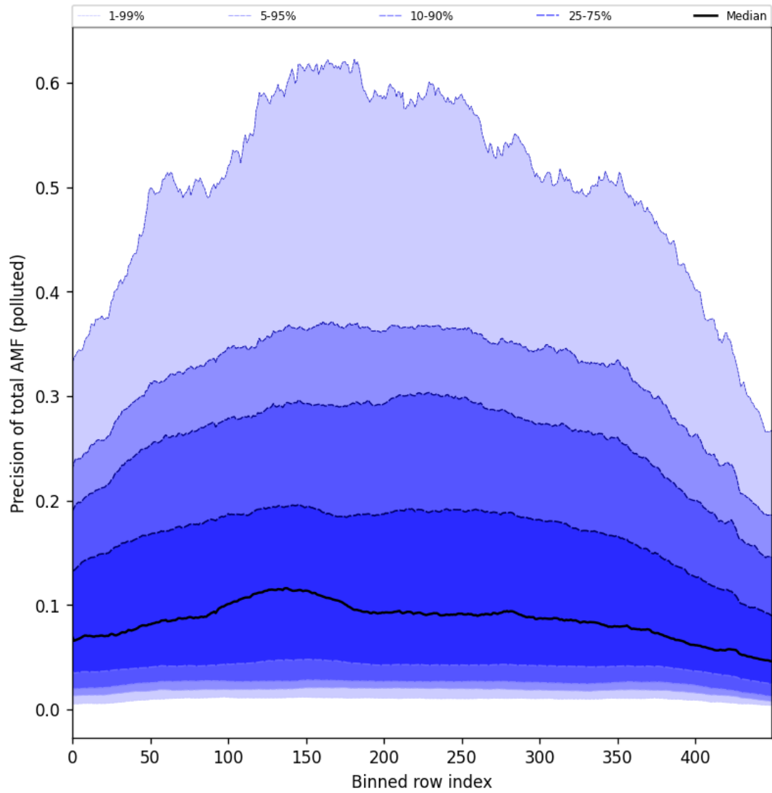
Figure 95: Along track statistics of “Precision of total AMF (polluted)” for 2024-10-29 to 2024-10-30
