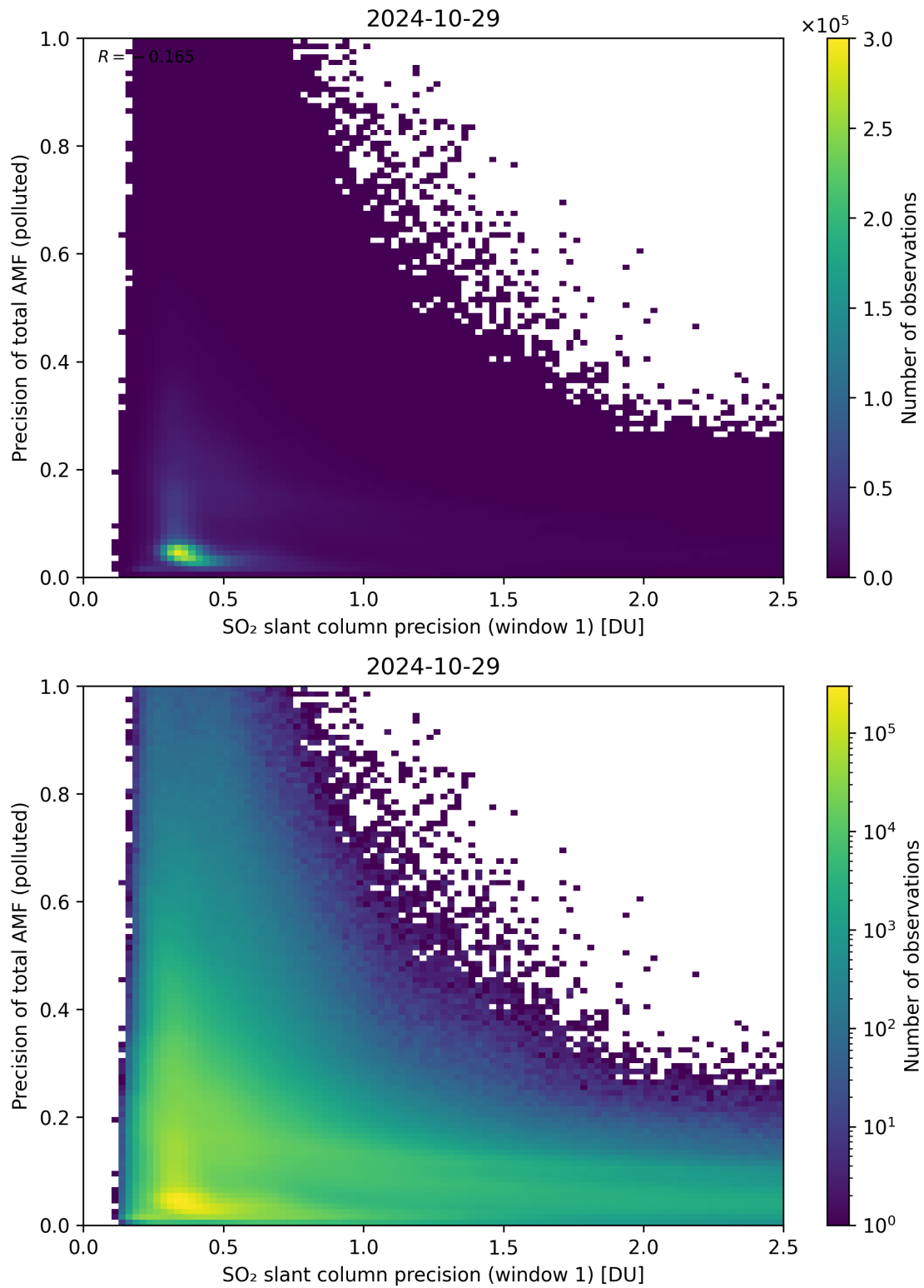
Figure 231: Scatter density plot of “SO 2 slant column precision (window 1)” against “Precision of total AMF (polluted)” for 2024-10-29 to 2024-10-30.
