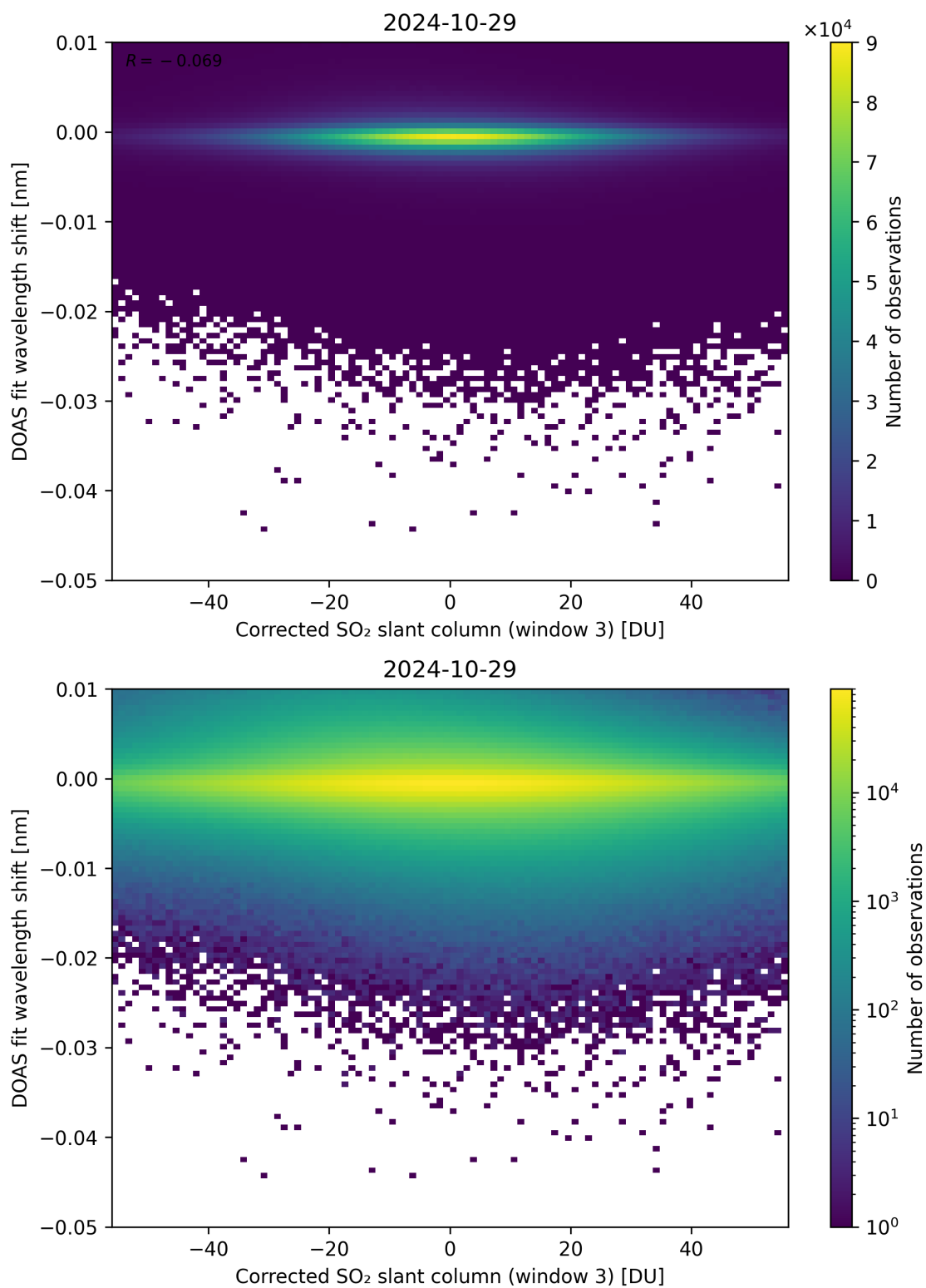
Figure 206: Scatter density plot of “Corrected SO 2 slant column (window 3)” against “DOAS fit wavelength shift” for 2024-10-29 to 2024-10-30.
