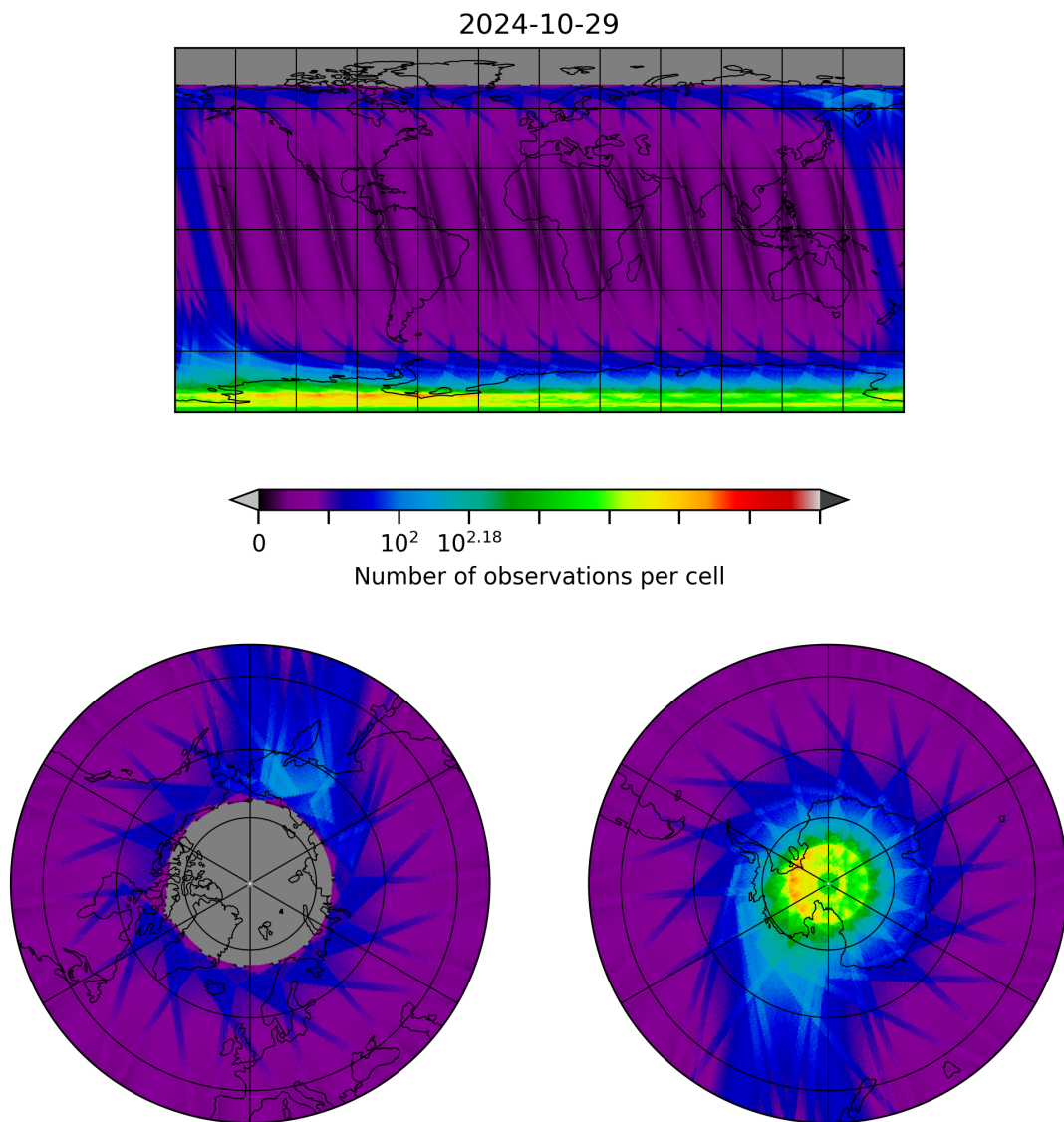
Figure 28: Map of the number of observations for 2024-10-29 to 2024-10-30
