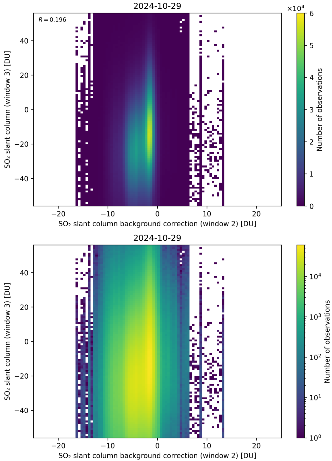
Figure 117: Scatter density plot of “SO 2 slant column background correction (window 2)” against “SO 2 slant column (window 3)” for 2024-10-29 to 2024-10-30.
