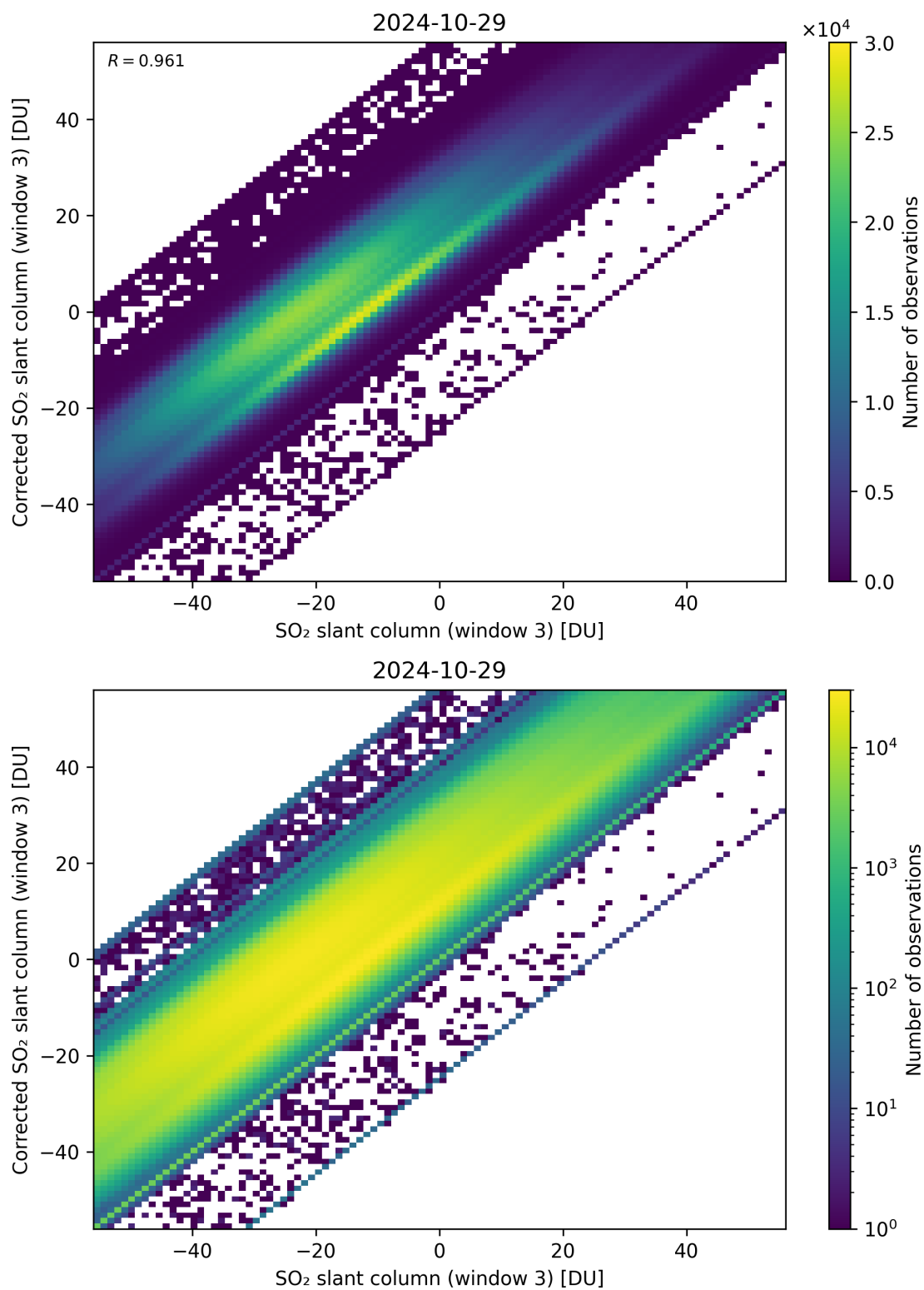
Figure 266: Scatter density plot of “SO 2 slant column (window 3)” against “Corrected SO 2 slant column (window 3)” for 2024-10-29 to 2024-10-30.
