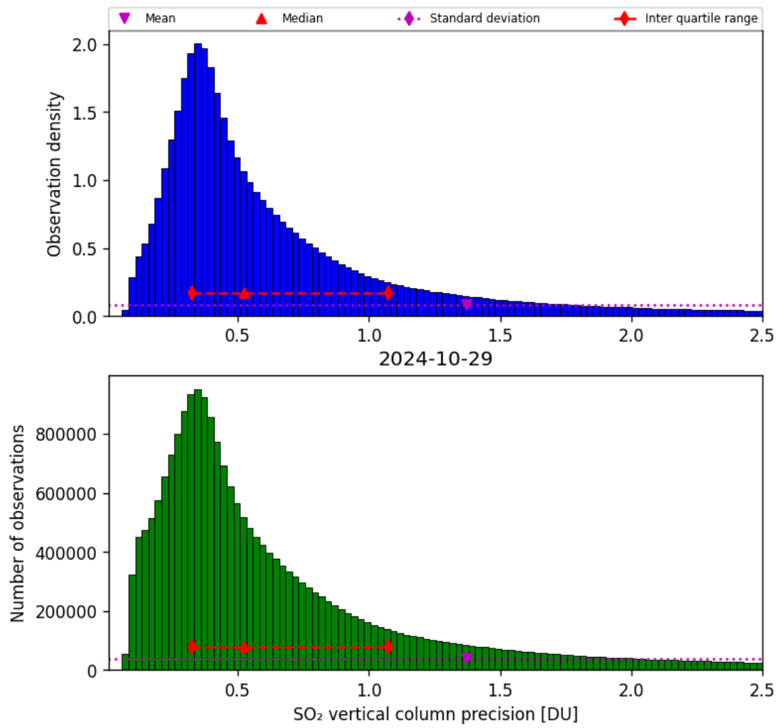
Figure 54: Histogram of “SO 2 vertical column precision” for 2024-10-29 to 2024-10-30
