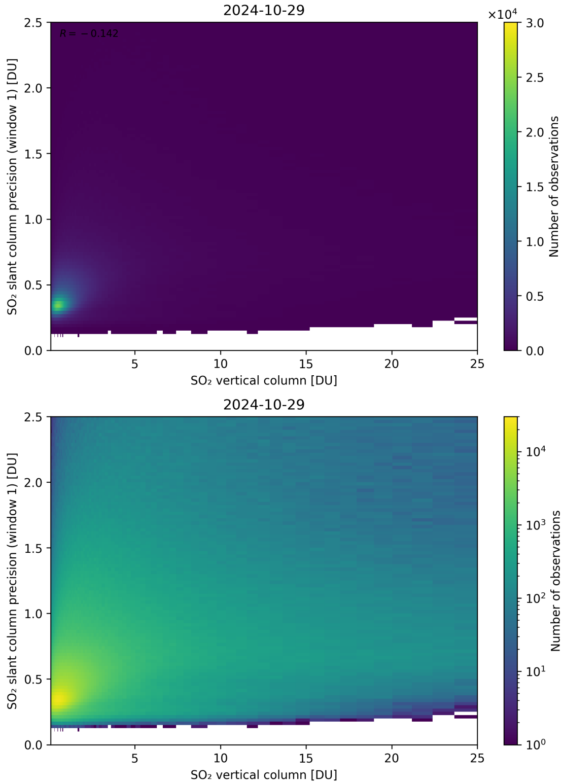
Figure 301: Scatter density plot of “SO 2 vertical column” against “SO 2 slant column precision (window 1)” for 2024-10-29 to 2024-10-30.
