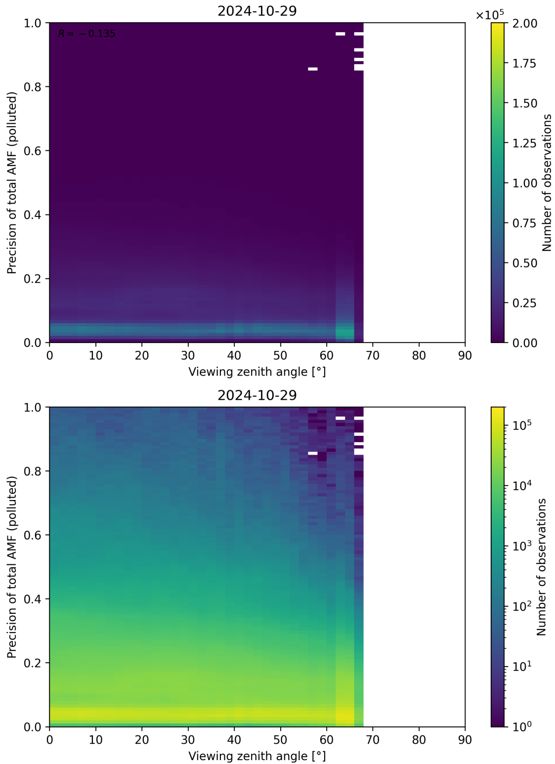
Figure 326: Scatter density plot of “Viewing zenith angle” against “Precision of total AMF (polluted)” for 2024-10-29 to 2024-10-30.
