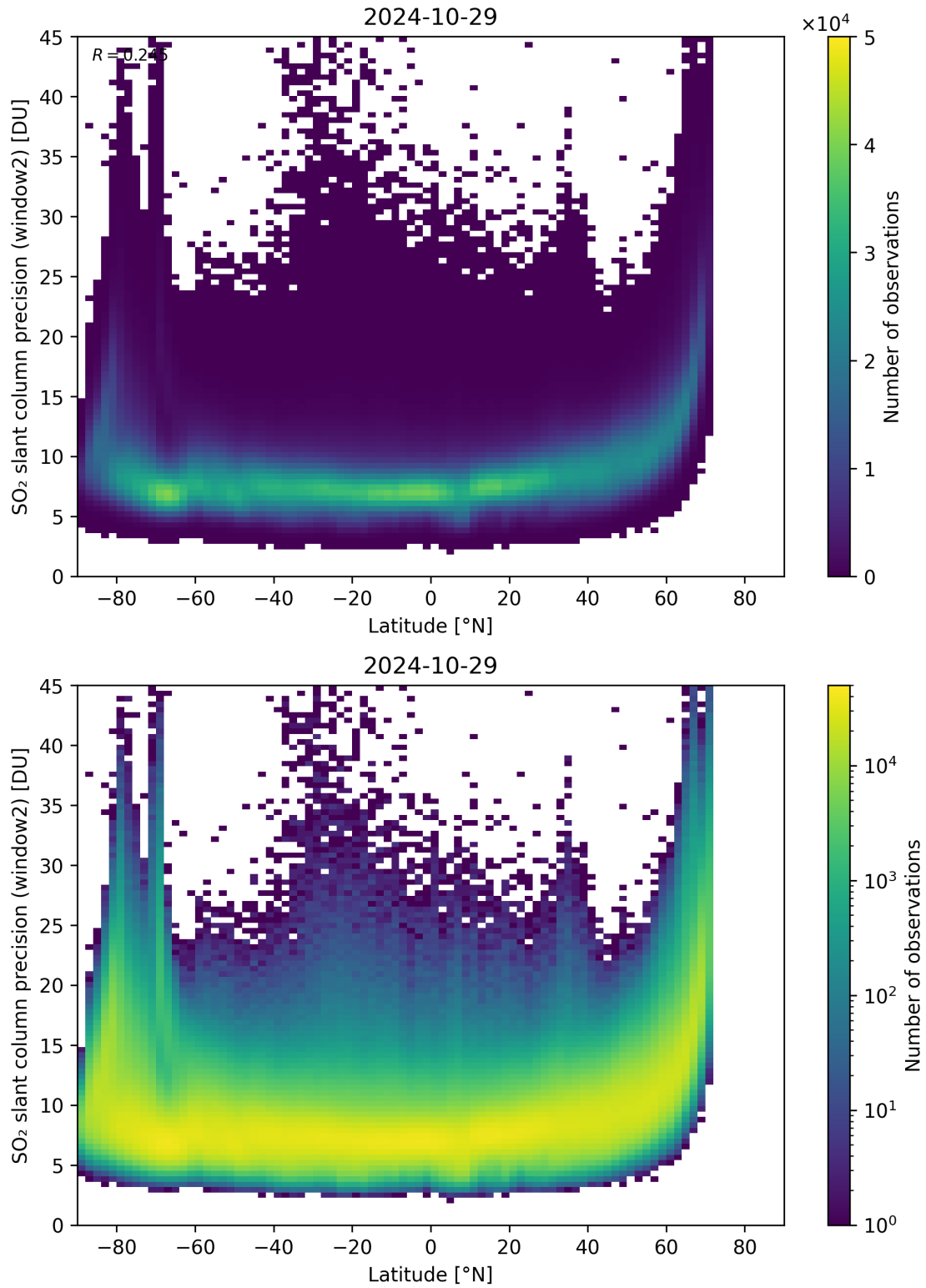
Figure 151: Scatter density plot of “Latitude” against “SO 2 slant column precision (window2)” for 2024-10-29 to 2024-10-30.
