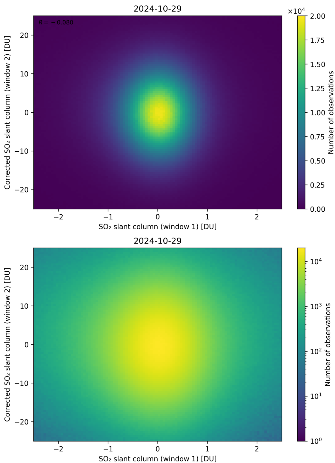
Figure 233: Scatter density plot of “SO 2 slant column (window 1)” against “Corrected SO 2 slant column (window 2)” for 2024-10-29 to 2024-10-30.
