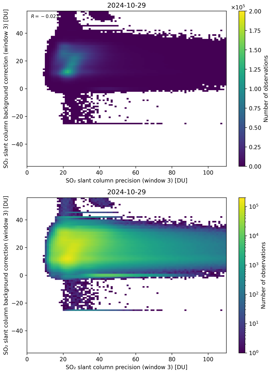
Figure 257: Scatter density plot of “SO 2 slant column precision (window 3)” against “SO 2 slant column background correction (window 3)” for 2024-10-29 to 2024-10-30.
