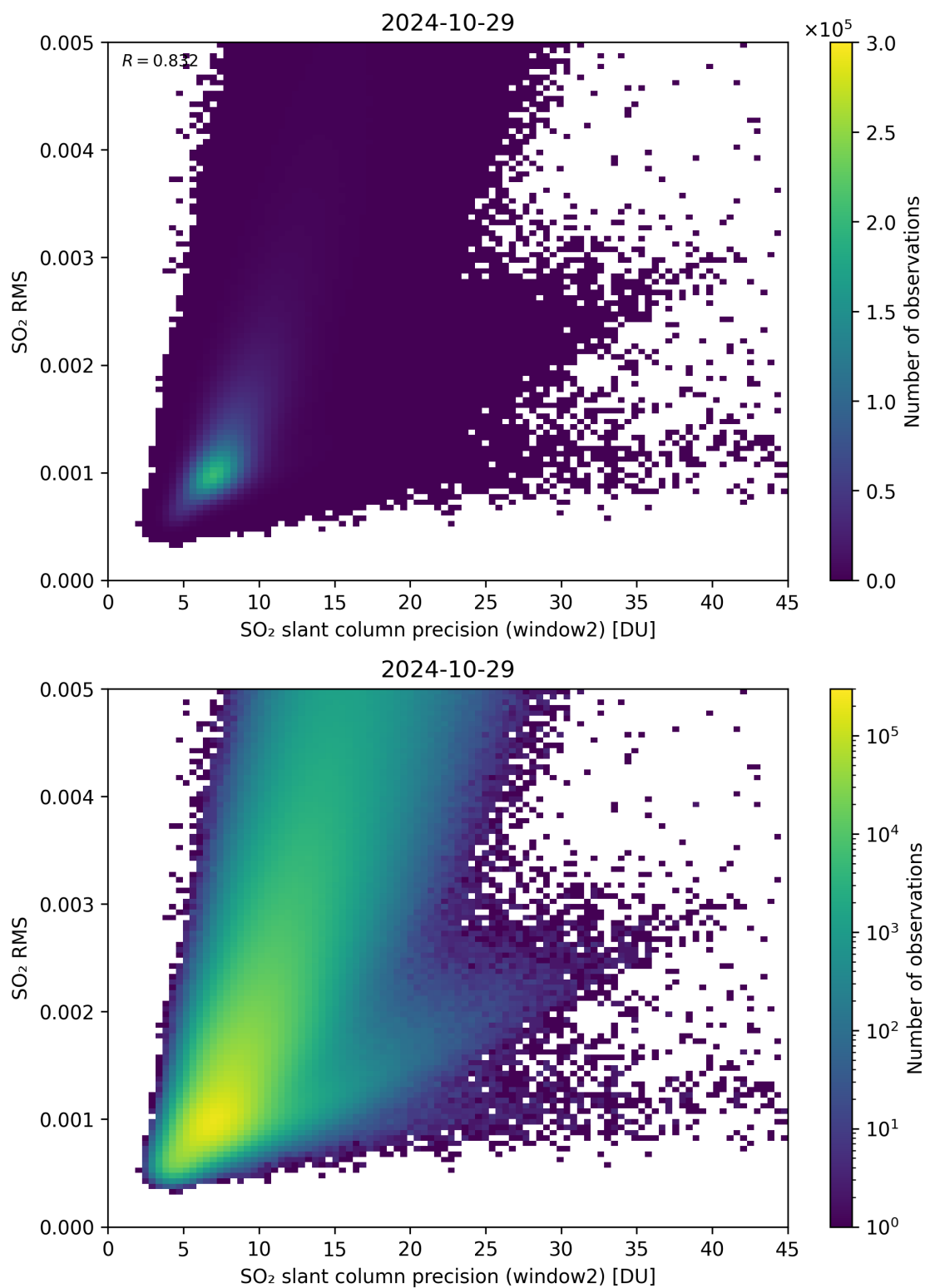
Figure 245: Scatter density plot of “SO 2 slant column precision (window2)” against “SO 2 RMS” for 2024-10-29 to 2024-10-30.
