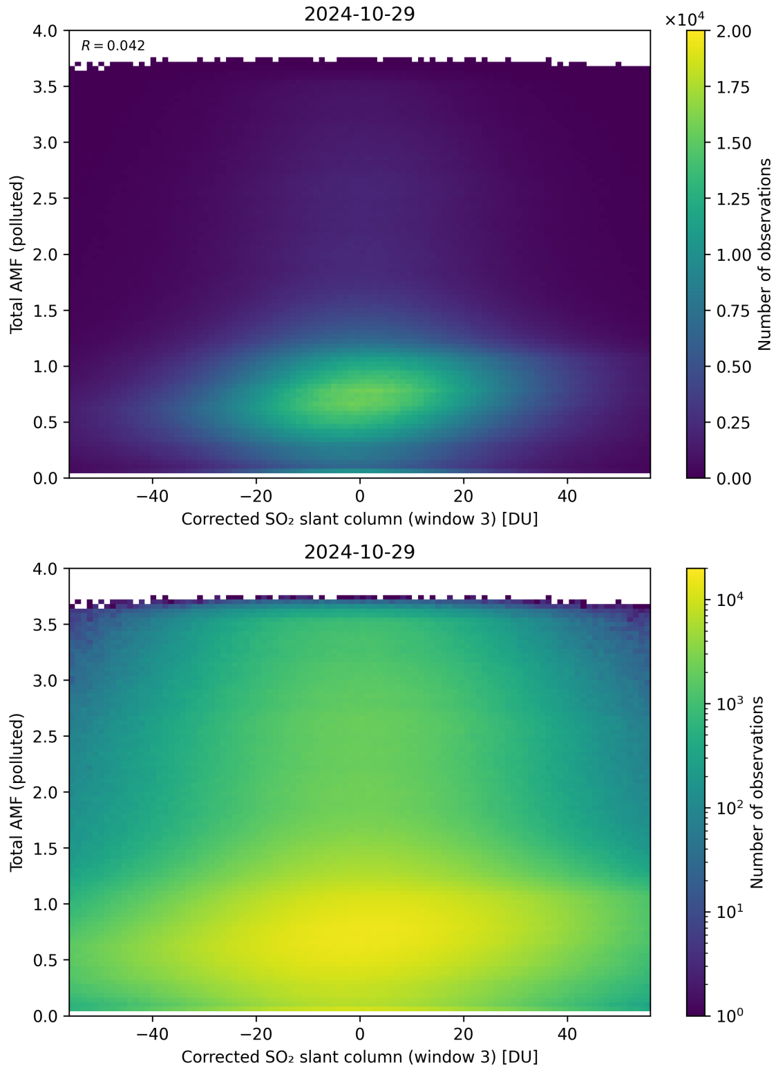
Figure 210: Scatter density plot of “Corrected SO 2 slant column (window 3)” against “Total AMF (polluted)” for 2024-10-29 to 2024-10-30.
