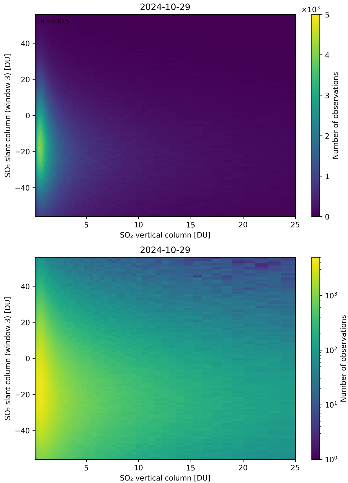
Figure 303: Scatter density plot of “SO 2 vertical column” against “SO 2 slant column (window 3)” for 2024-10-29 to 2024-10-30.
