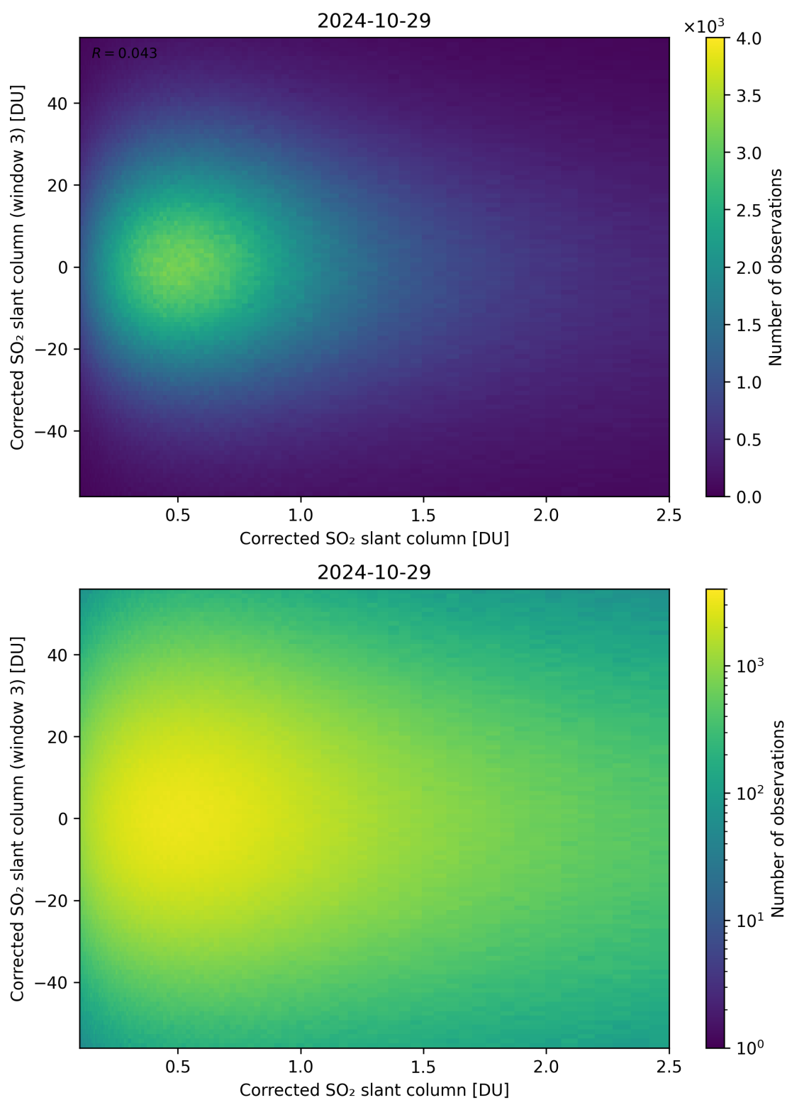
Figure 186: Scatter density plot of “Corrected SO 2 slant column” against “Corrected SO 2 slant column (window 3)” for 2024-10-29 to 2024-10-30.
