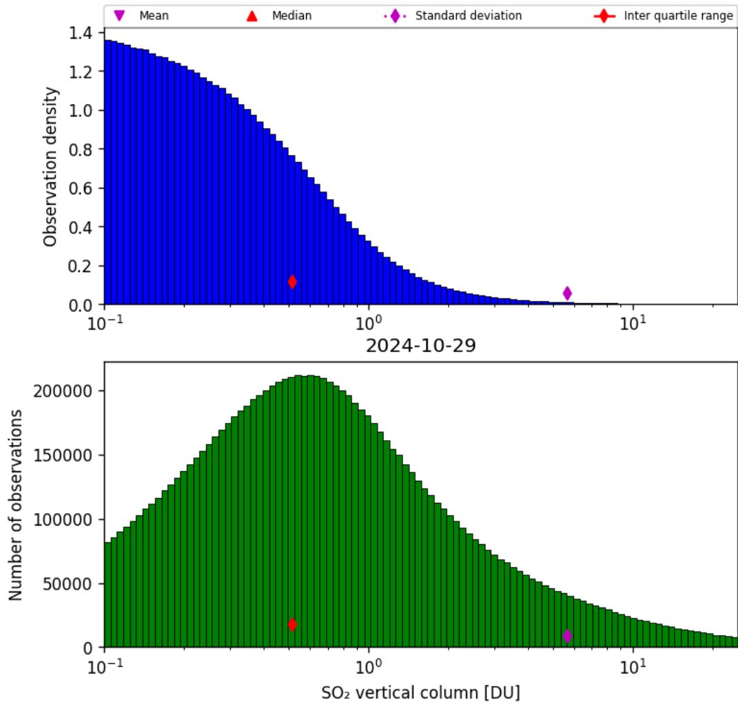
Figure 53: Histogram of “SO 2 vertical column” for 2024-10-29 to 2024-10-30
