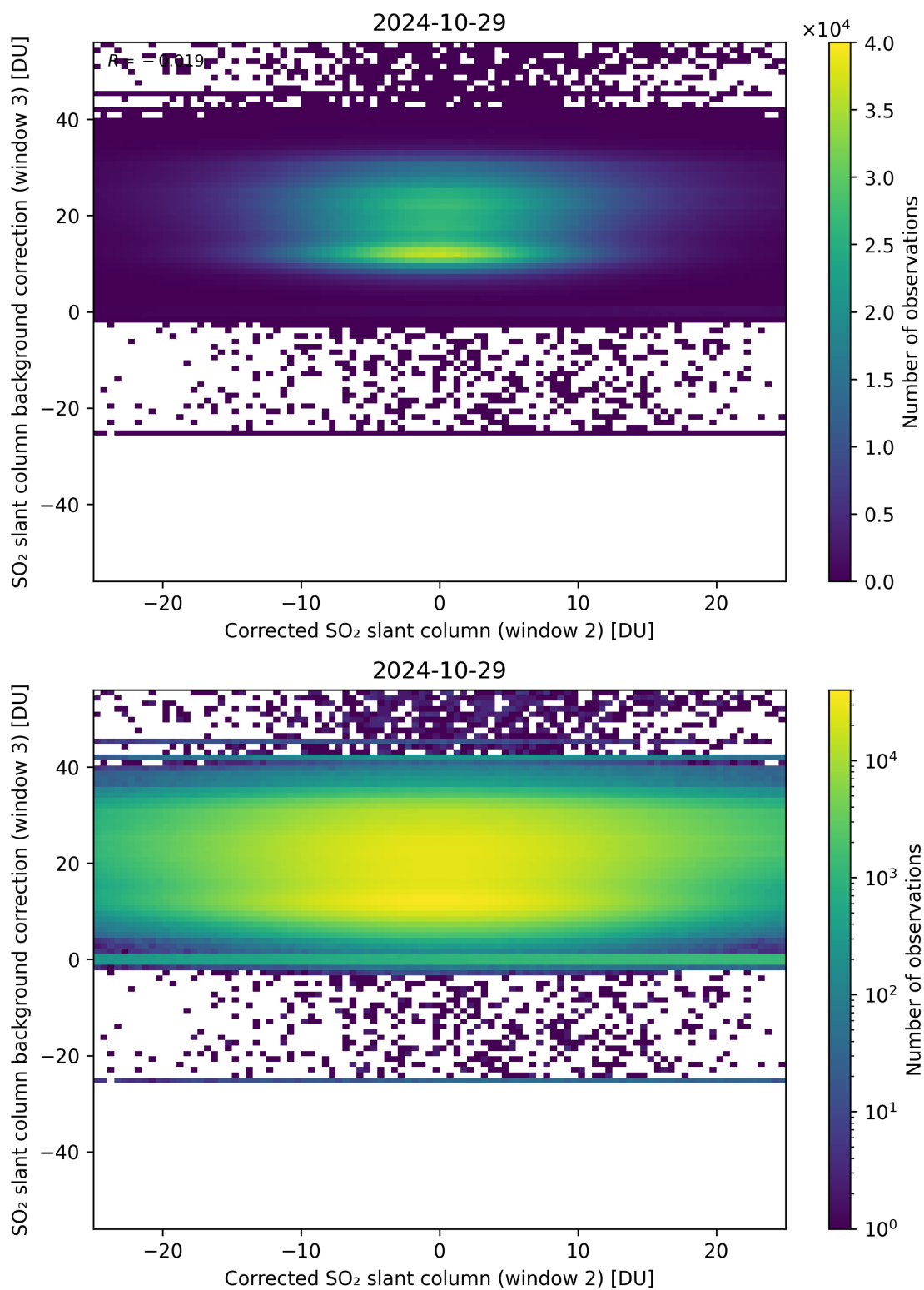
Figure 195: Scatter density plot of “Corrected SO 2 slant column (window 2)” against “SO 2 slant column background correction (window 3)” for 2024-10-29 to 2024-10-30.
