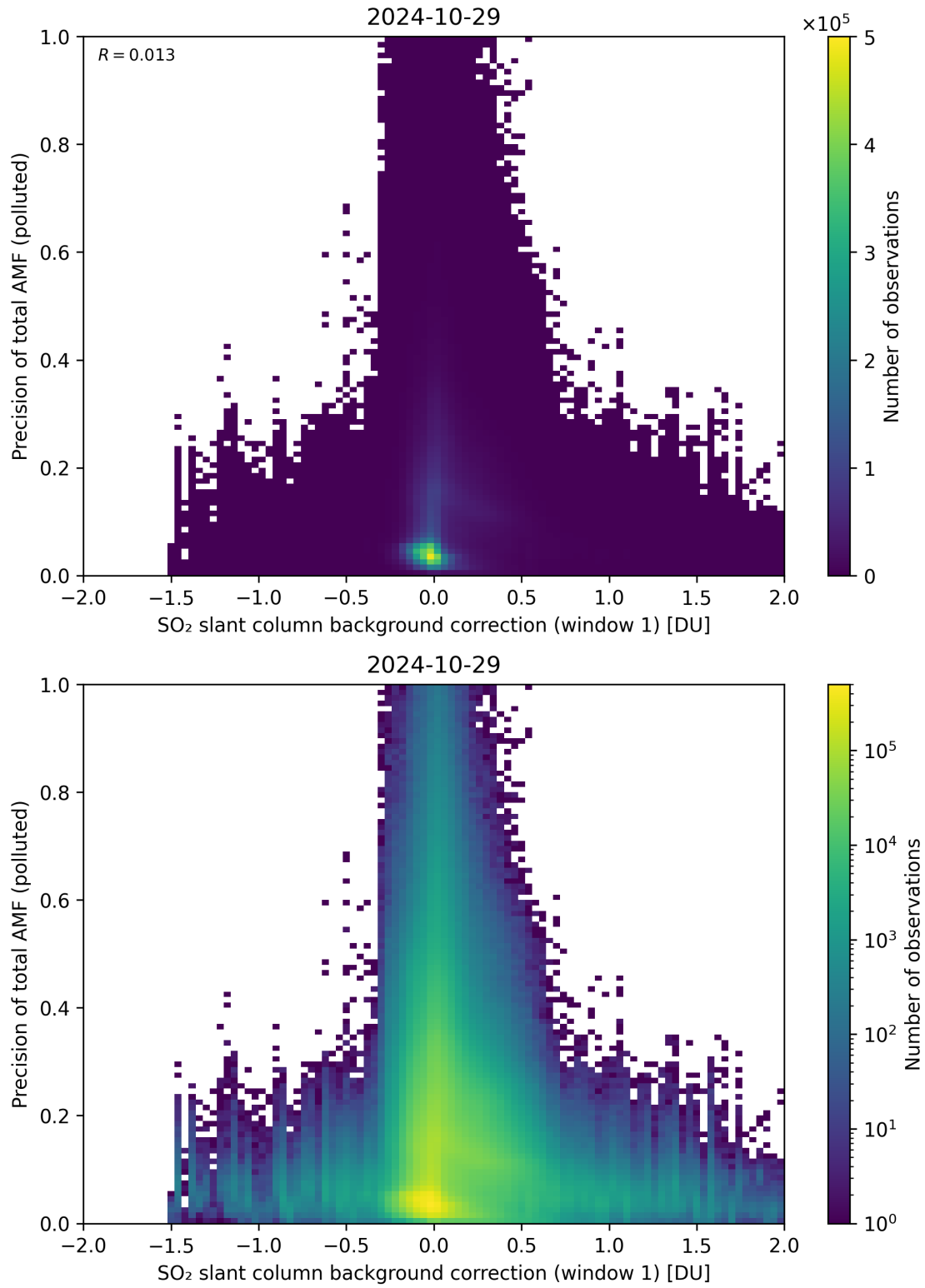
Figure 110: Scatter density plot of “SO 2 slant column background correction (window 1)” against “Precision of total AMF (polluted)” for 2024-10-29 to 2024-10-30.
