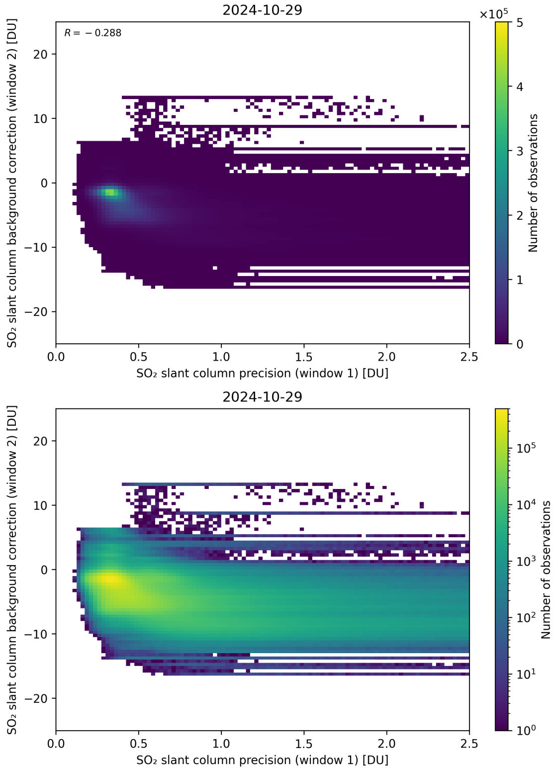
Figure 219: Scatter density plot of “SO 2 slant column precision (window 1)” against “SO 2 slant column background correction (window 2)” for 2024-10-29 to 2024-10-30.
