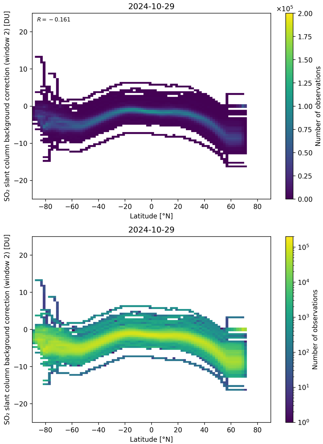
Figure 140: Scatter density plot of “Latitude” against “SO 2 slant column background correction (window 2)” for 2024-10-29 to 2024-10-30.
