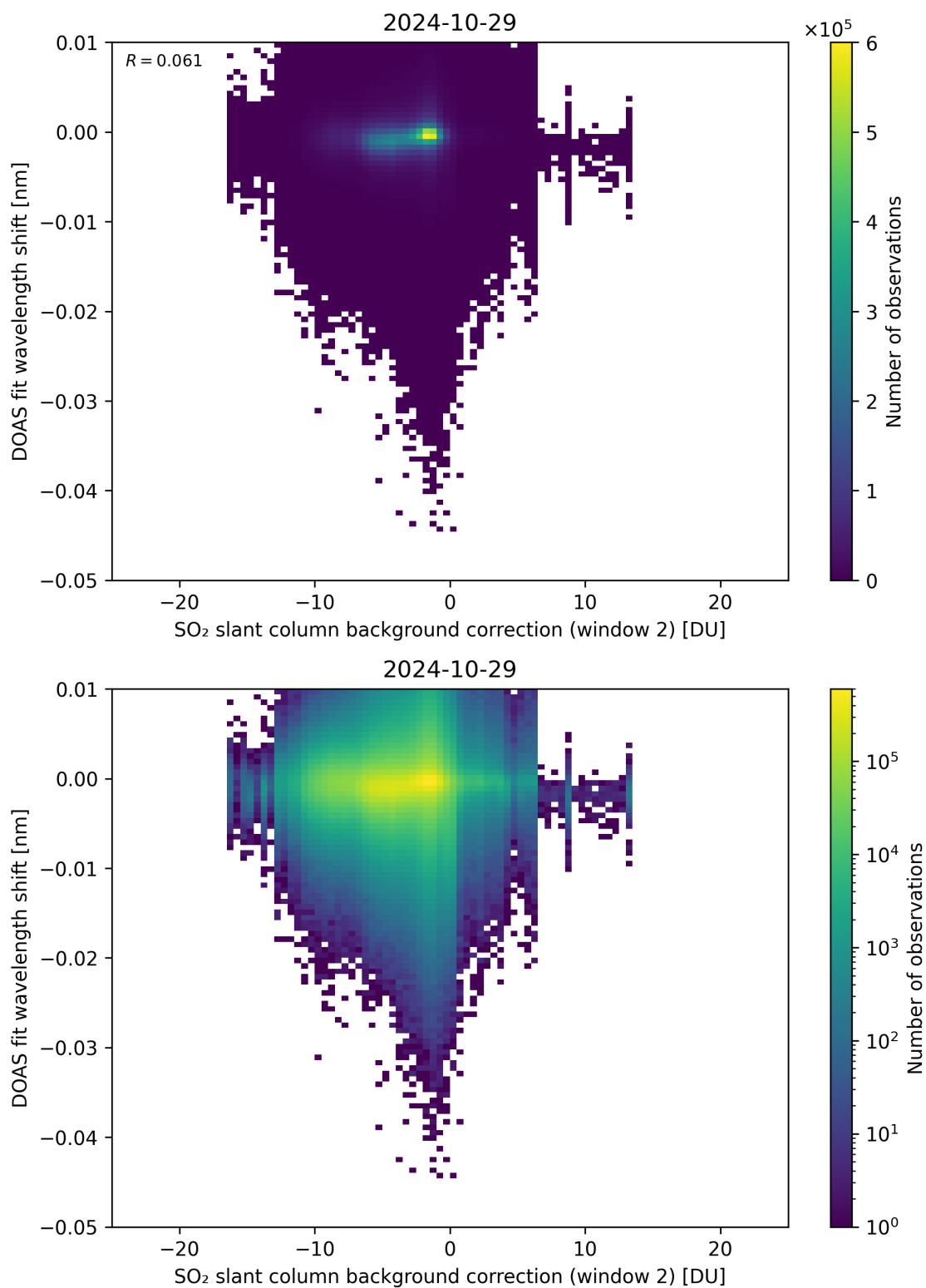
Figure 112: Scatter density plot of “SO 2 slant column background correction (window 2)” against “DOAS fit wavelength shift” for 2024-10-29 to 2024-10-30.
