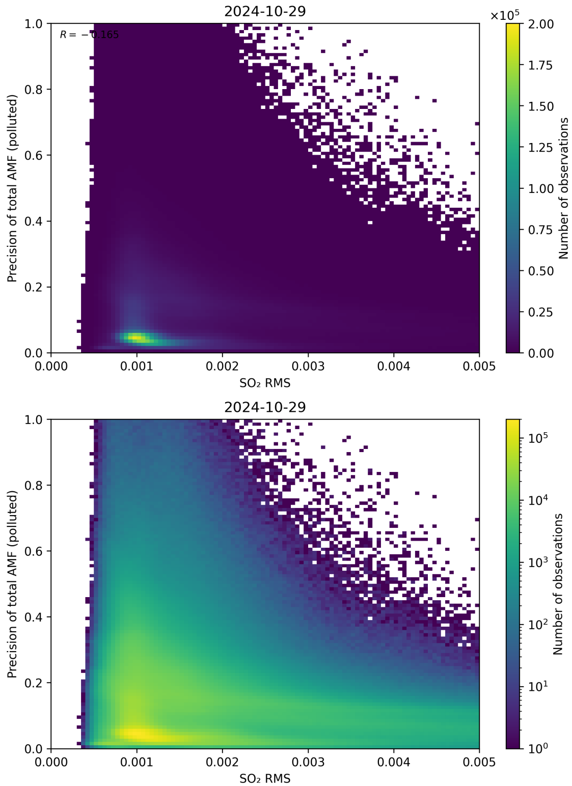
Figure 138: Scatter density plot of “SO 2 RMS” against “Precision of total AMF (polluted)” for 2024-10-29 to 2024-10-30.
