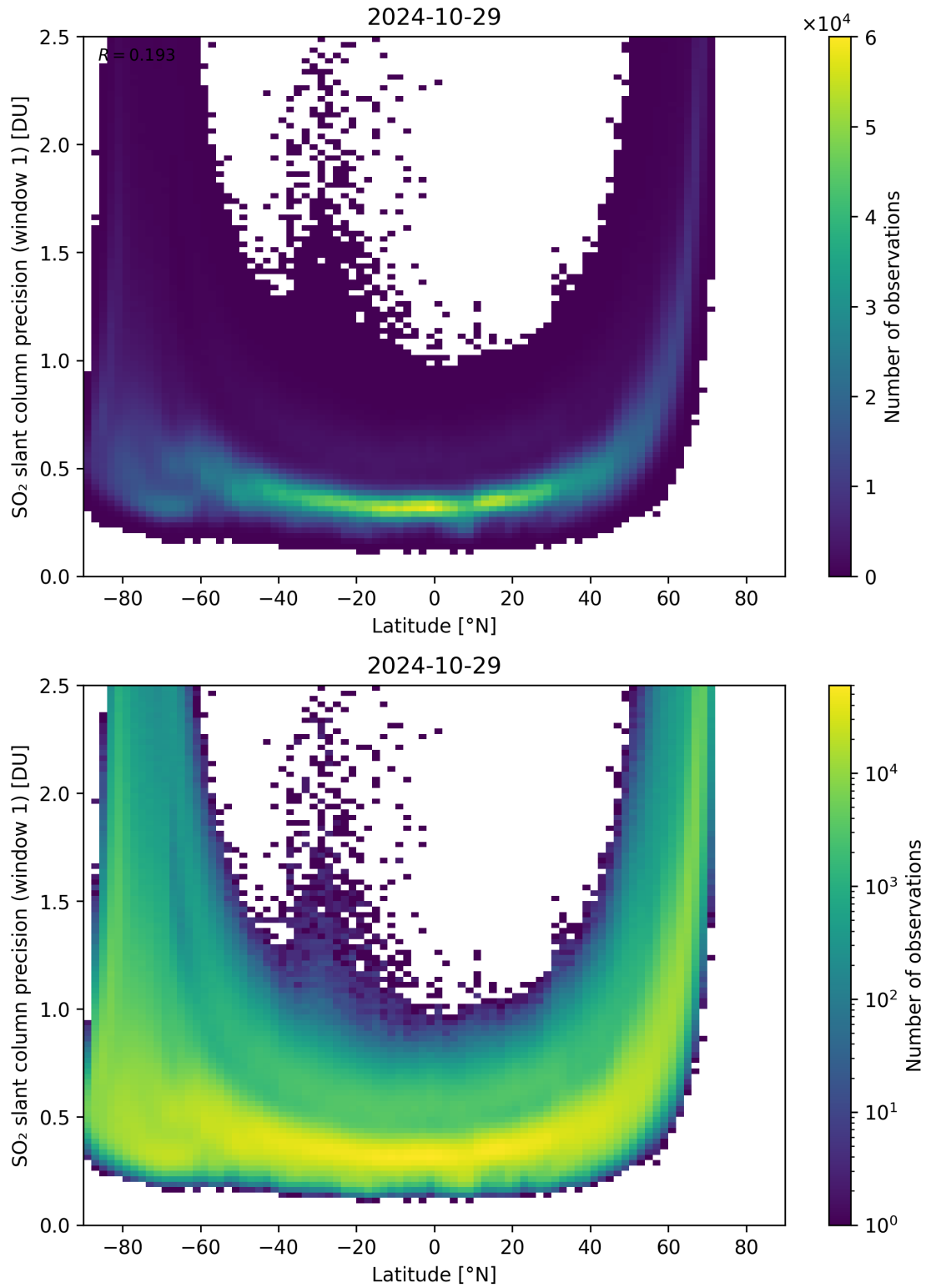
Figure 150: Scatter density plot of “Latitude” against “SO 2 slant column precision (window 1)” for 2024-10-29 to 2024-10-30.
