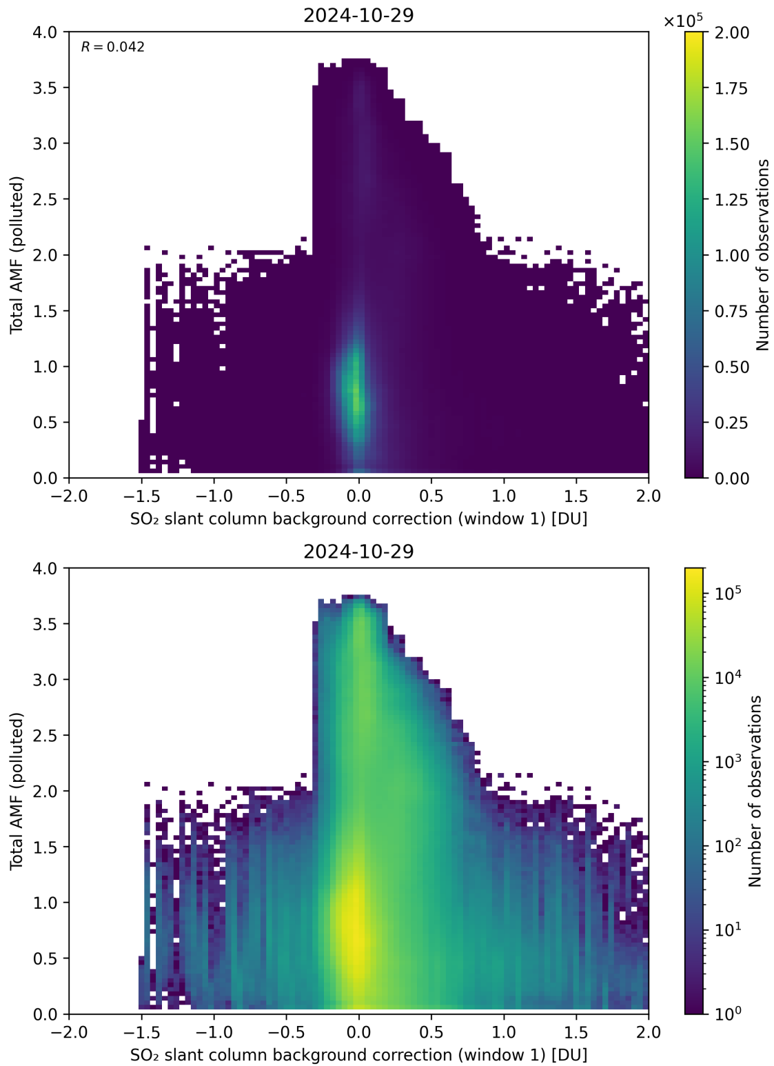
Figure 109: Scatter density plot of “SO 2 slant column background correction (window 1)” against “Total AMF (polluted)” for 2024-10-29 to 2024-10-30.
