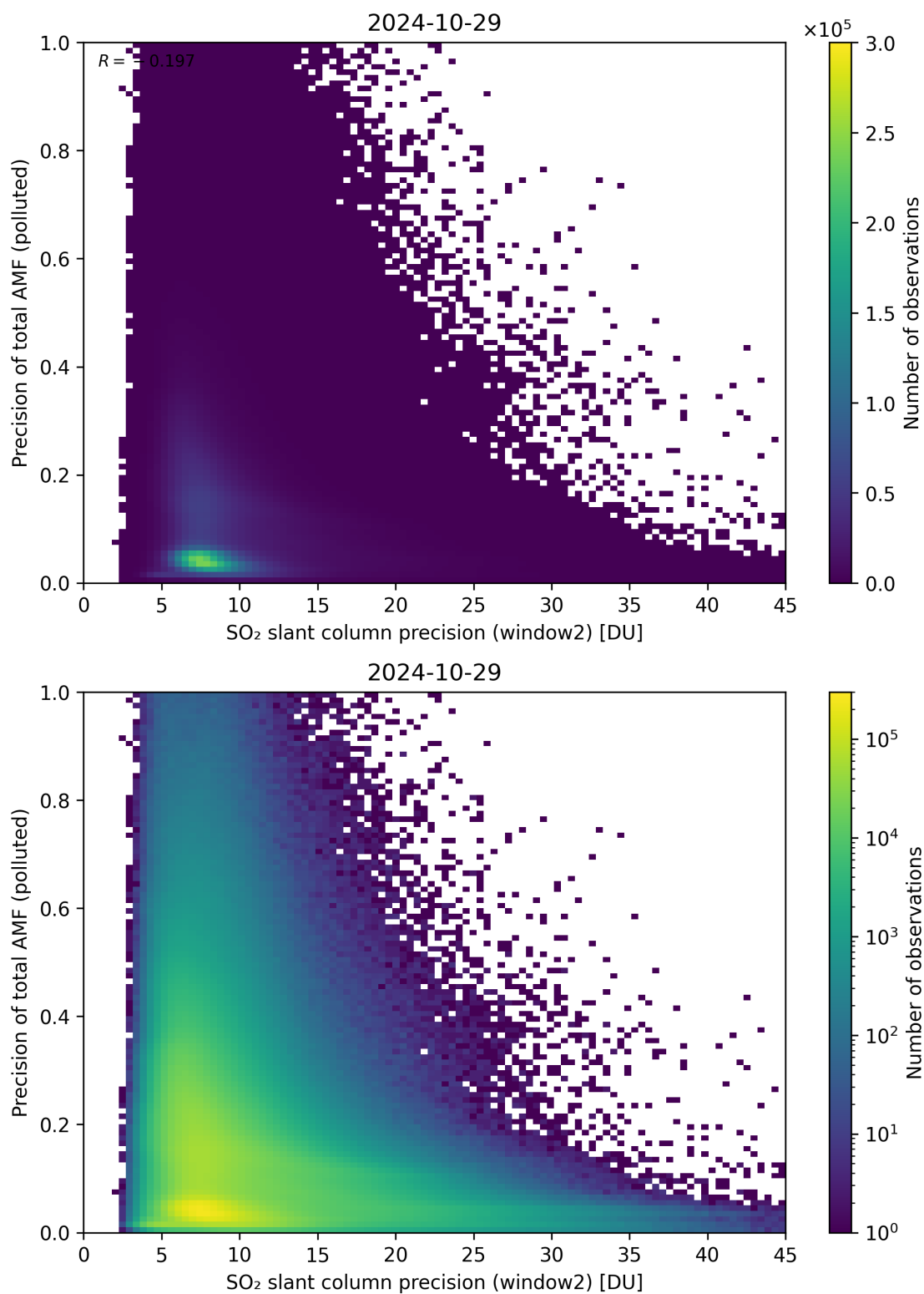
Figure 252: Scatter density plot of “SO 2 slant column precision (window2)” against “Precision of total AMF (polluted)” for 2024-10-29 to 2024-10-30.
