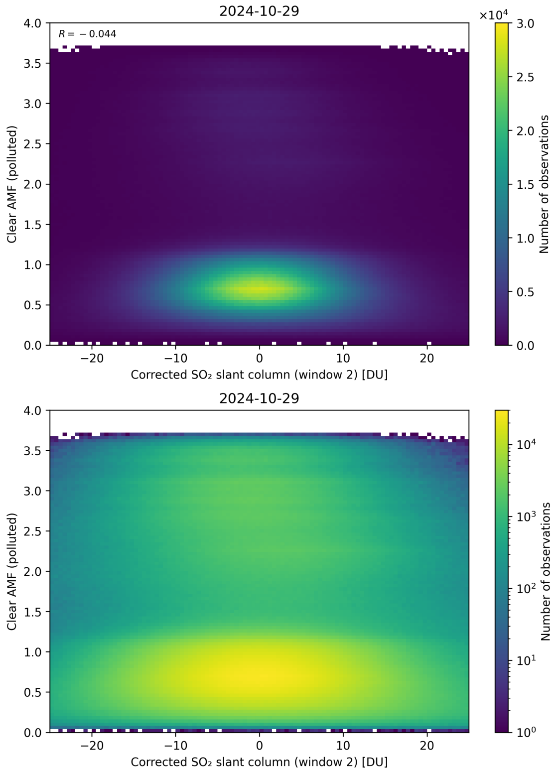
Figure 199: Scatter density plot of “Corrected SO 2 slant column (window 2)” against “Clear AMF (polluted)” for 2024-10-29 to 2024-10-30.
