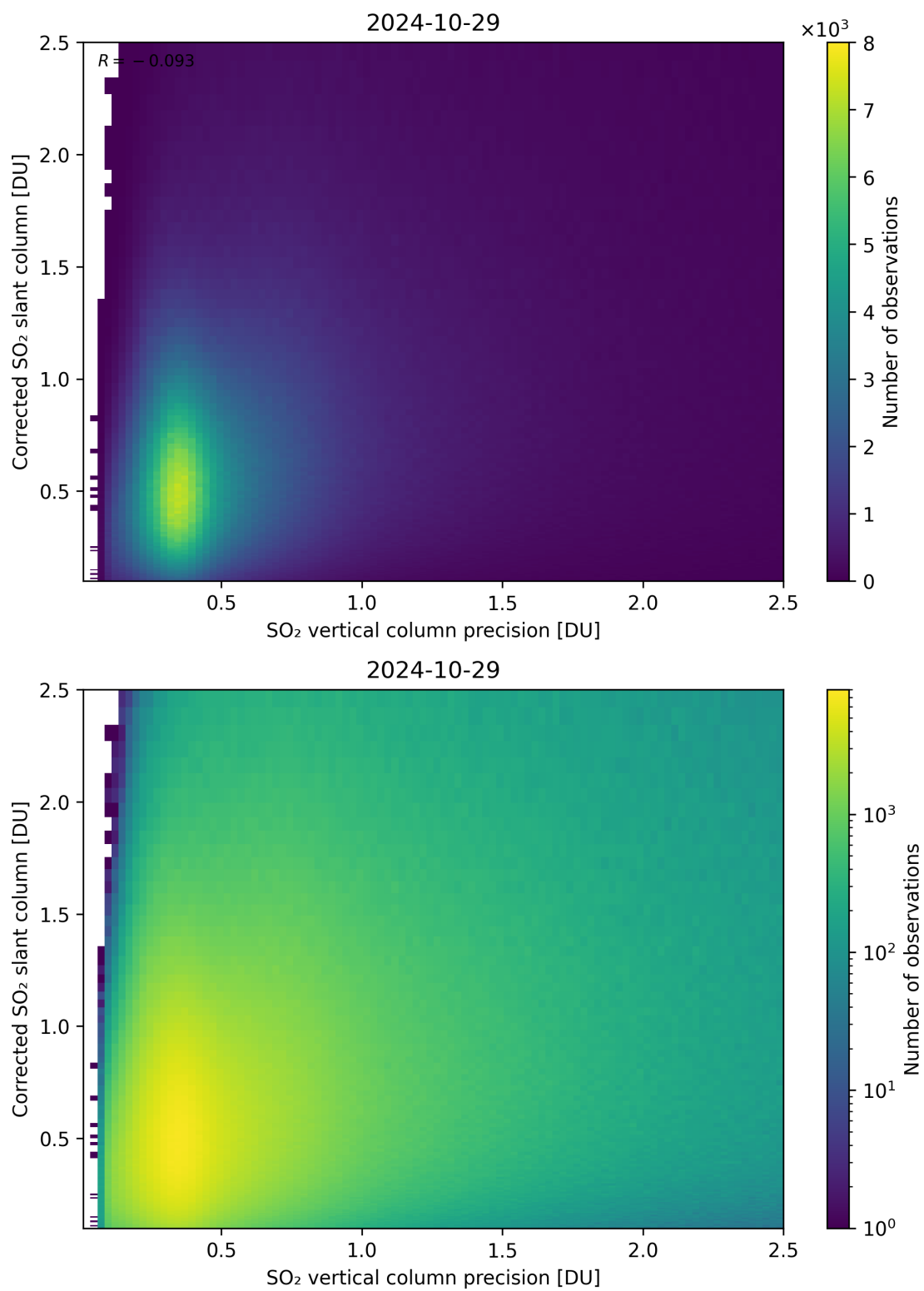
Figure 286: Scatter density plot of “SO 2 vertical column precision” against “Corrected SO 2 slant column” for 2024-10-29 to 2024-10-30.
