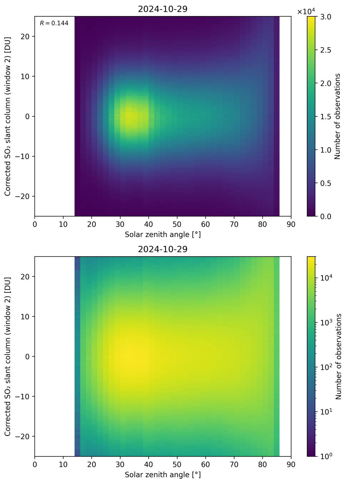
Figure 167: Scatter density plot of “Solar zenith angle” against “Corrected SO 2 slant column (window 2)” for 2024-10-29 to 2024-10-30.
