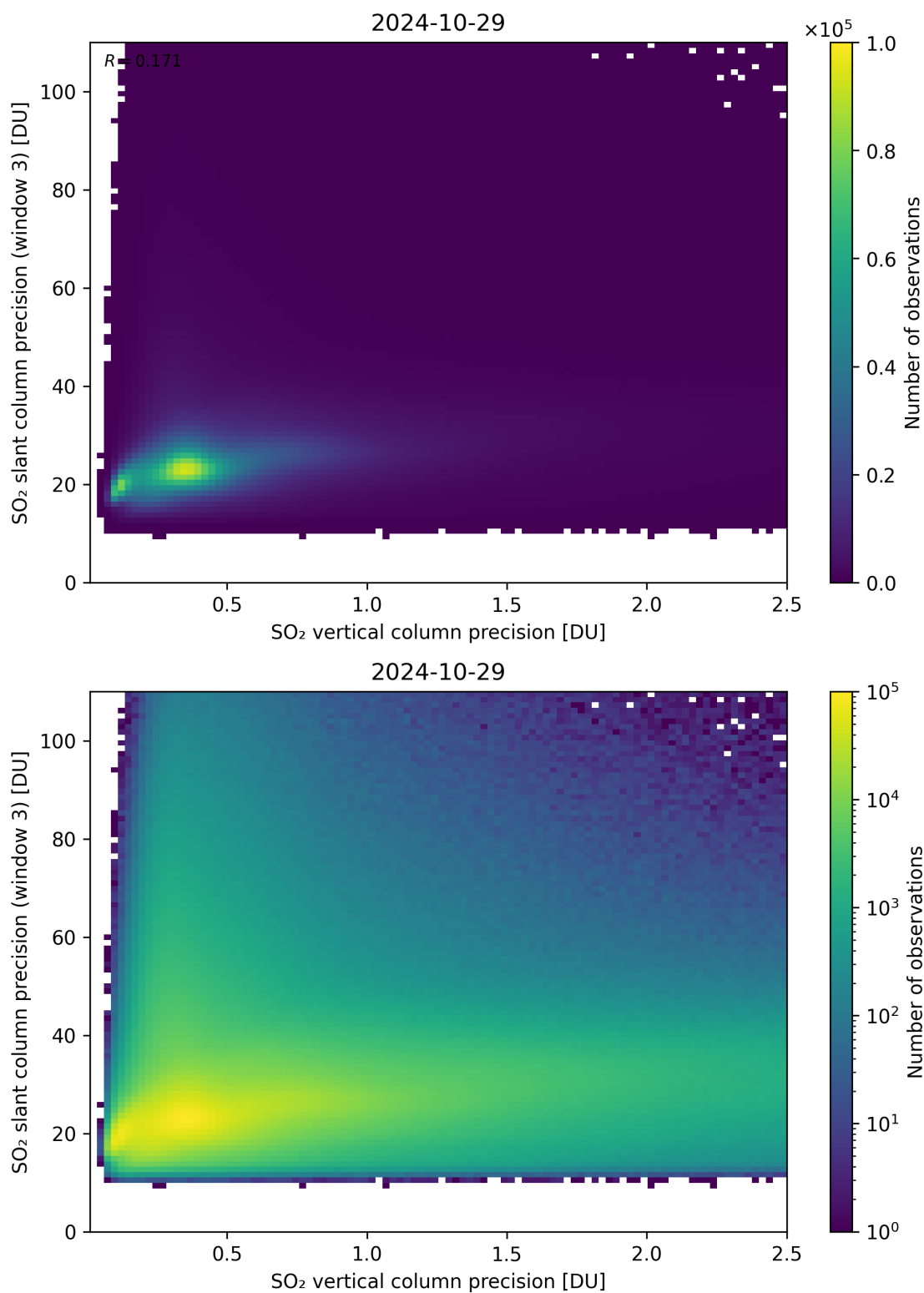
Figure 293: Scatter density plot of “SO 2 vertical column precision” against “SO 2 slant column precision (window 3)” for 2024-10-29 to 2024-10-30.
