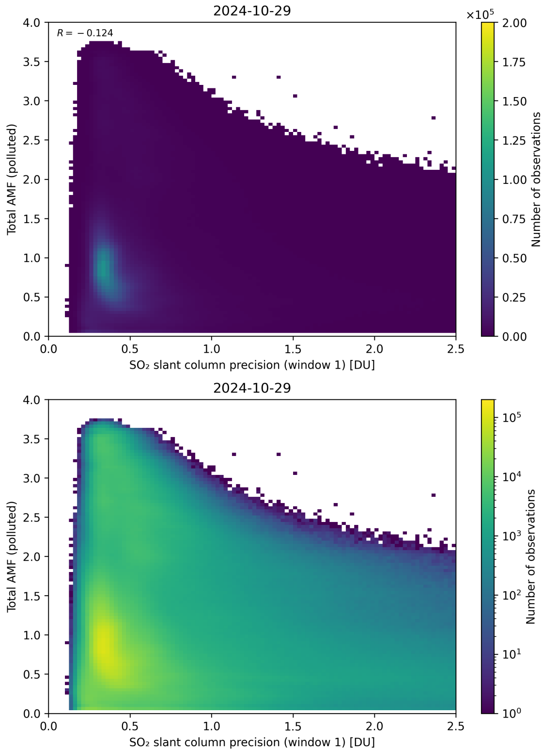
Figure 230: Scatter density plot of “SO 2 slant column precision (window 1)” against “Total AMF (polluted)” for 2024-10-29 to 2024-10-30.
