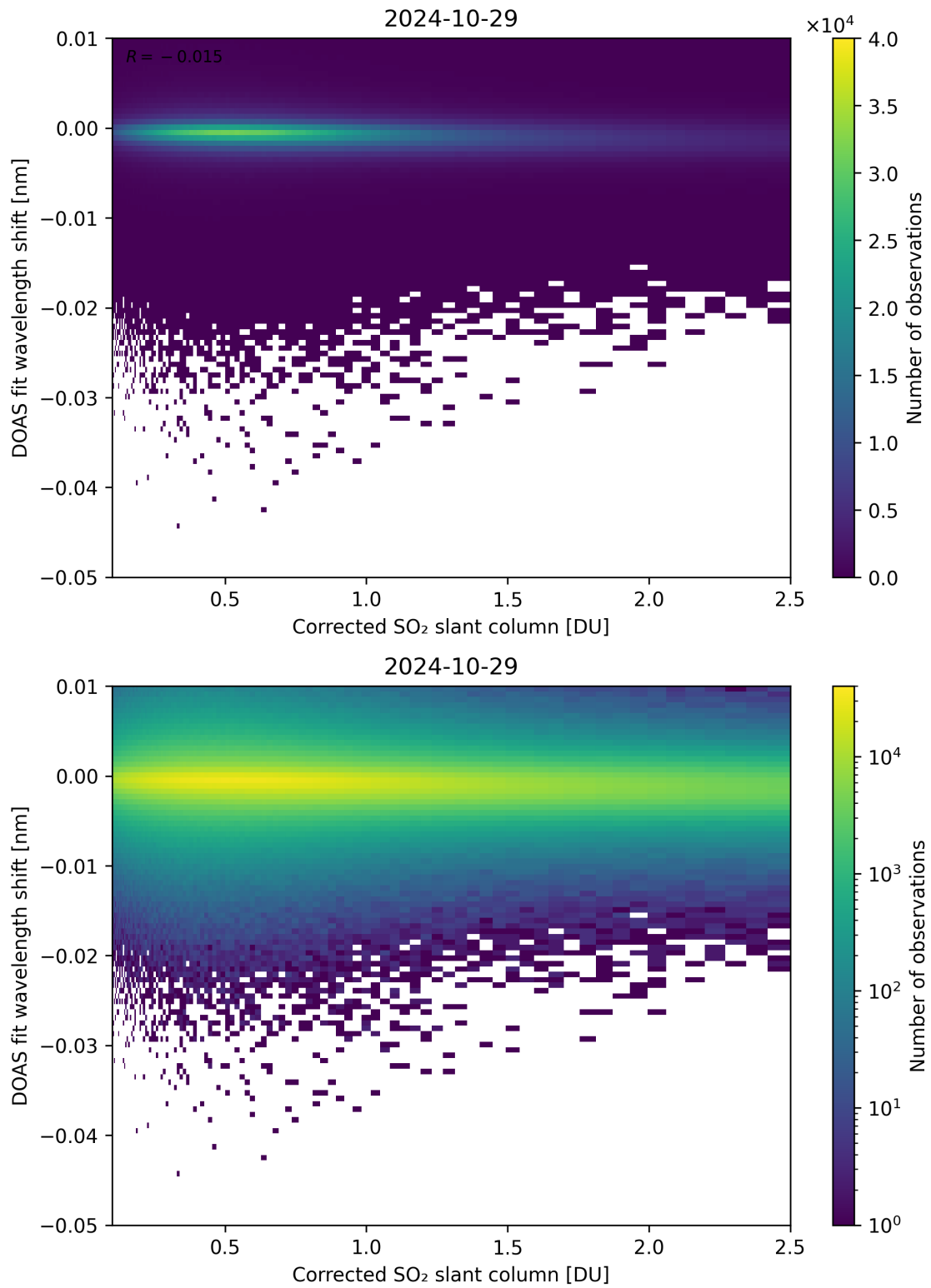
Figure 181: Scatter density plot of “Corrected SO 2 slant column” against “DOAS fit wavelength shift” for 2024-10-29 to 2024-10-30.
