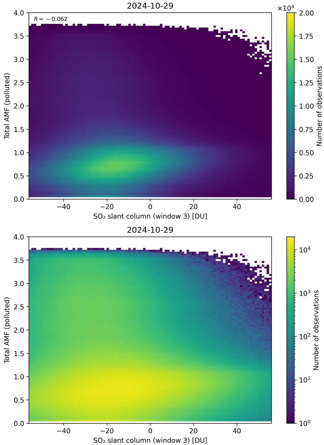
Figure 268: Scatter density plot of “SO 2 slant column (window 3)” against “Total AMF (polluted)” for 2024-10-29 to 2024-10-30.
