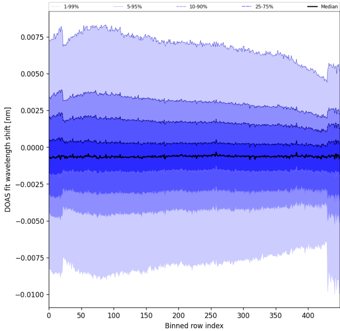
Figure 91: Along track statistics of “DOAS fit wavelength shift” for 2024-10-29 to 2024-10-30
