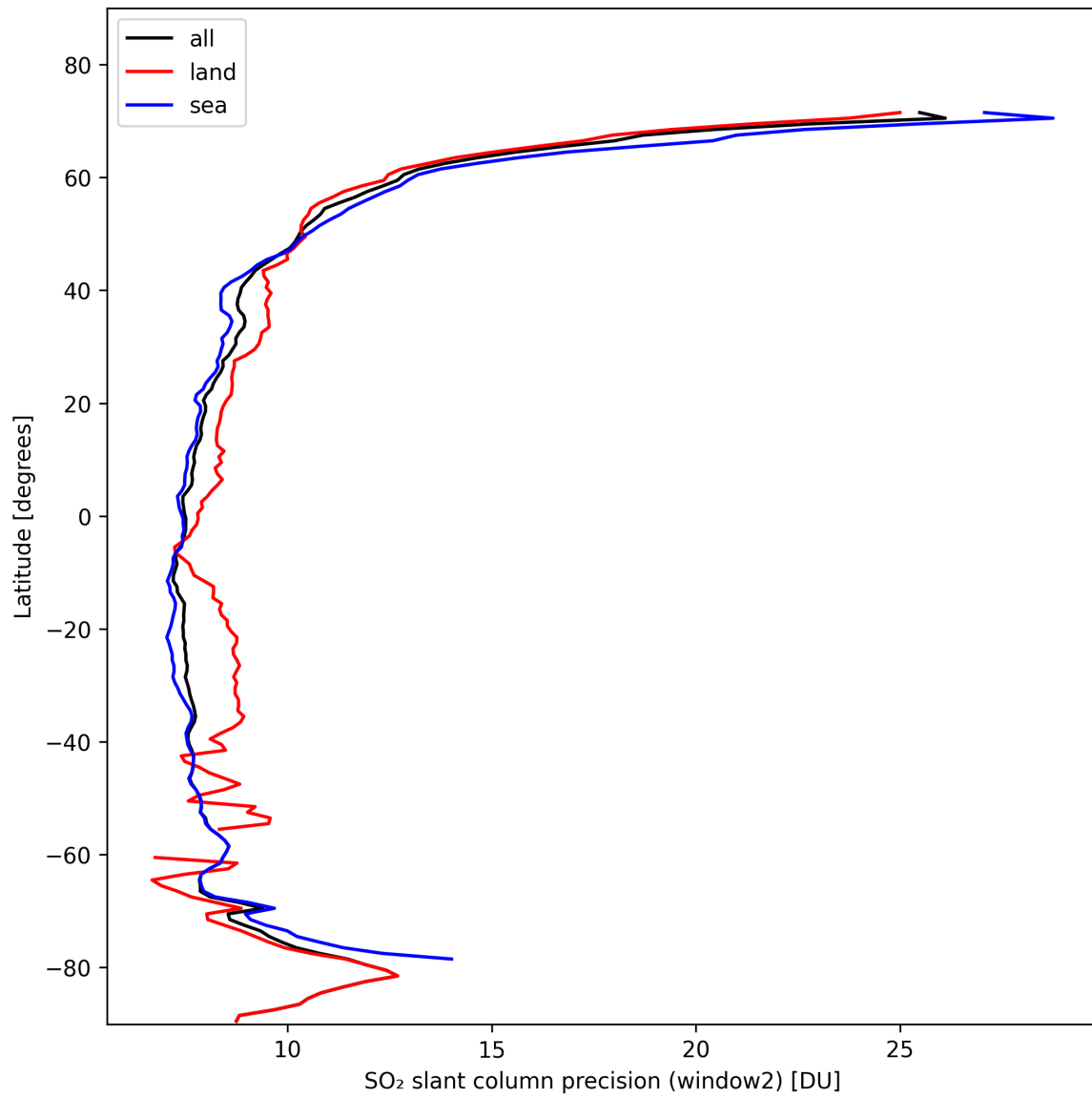
Figure 38: Zonal average of “SO 2 slant column precision (window2)” for 2024-10-30 to 2024-10-31.
