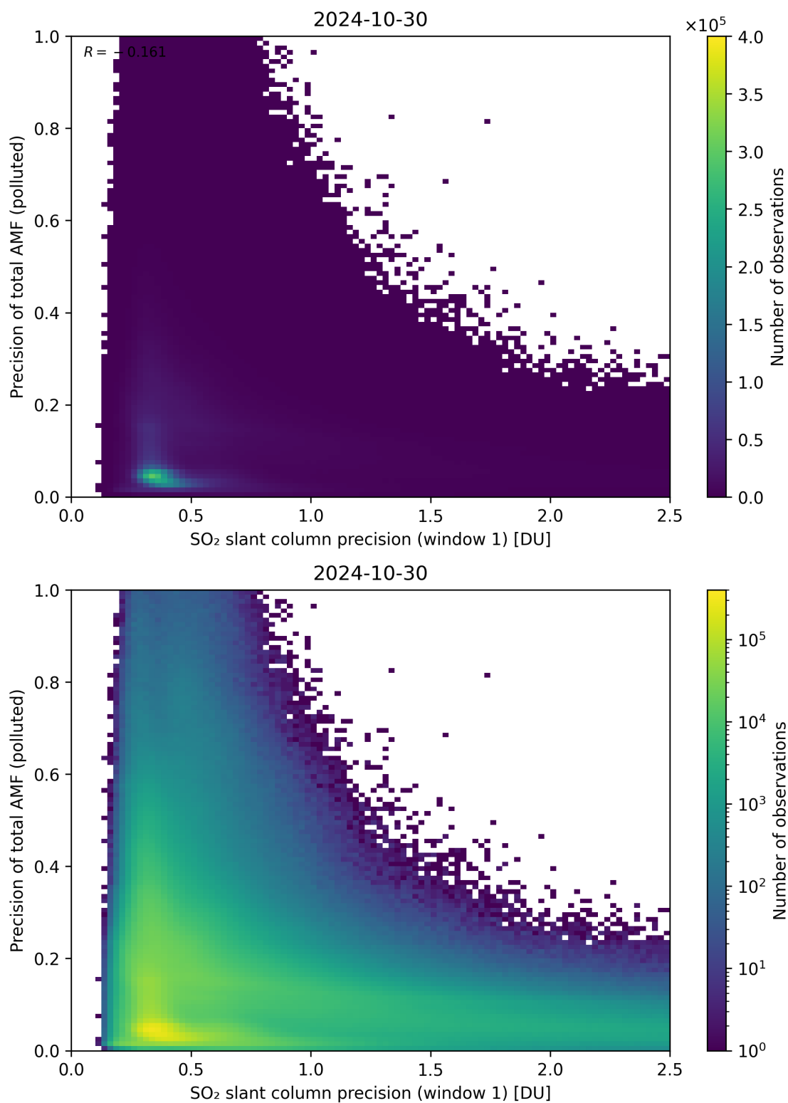
Figure 231: Scatter density plot of “SO 2 slant column precision (window 1)” against “Precision of total AMF (polluted)” for 2024-10-30 to 2024-10-31.
