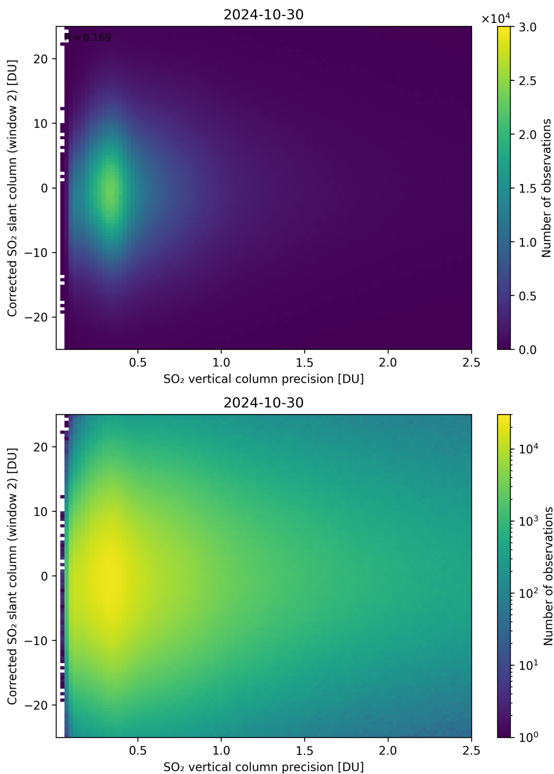
Figure 287: Scatter density plot of “SO 2 vertical column precision” against “Corrected SO 2 slant column (window 2)” for 2024-10-30 to 2024-10-31.
