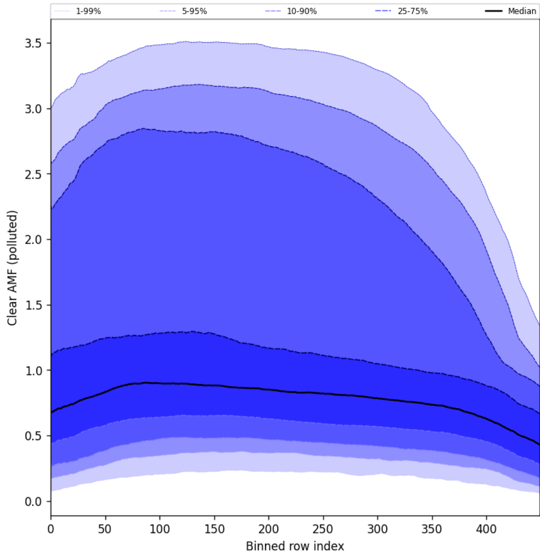
Figure 96: Along track statistics of “Clear AMF (polluted)” for 2024-10-30 to 2024-10-31
