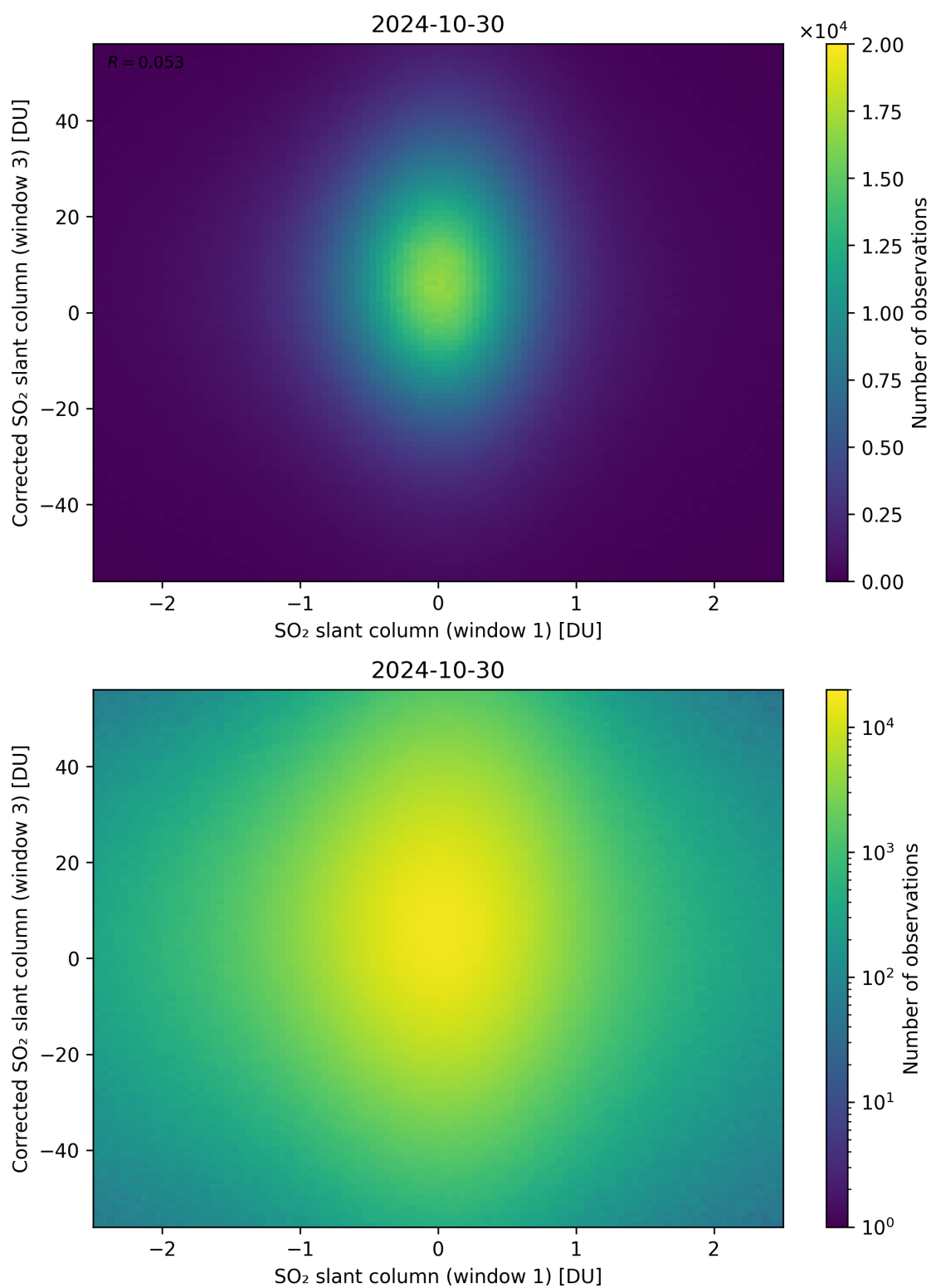
Figure 234: Scatter density plot of “SO 2 slant column (window 1)” against “Corrected SO 2 slant column (window 3)” for 2024-10-30 to 2024-10-31.
