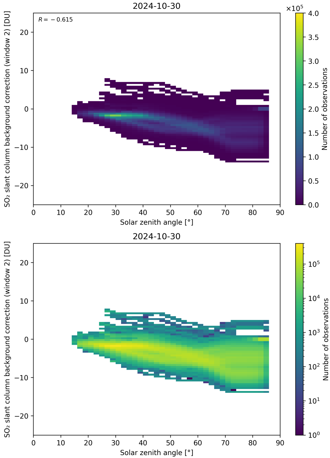
Figure 159: Scatter density plot of “Solar zenith angle” against “SO 2 slant column background correction (window 2)” for 2024-10-30 to 2024-10-31.
