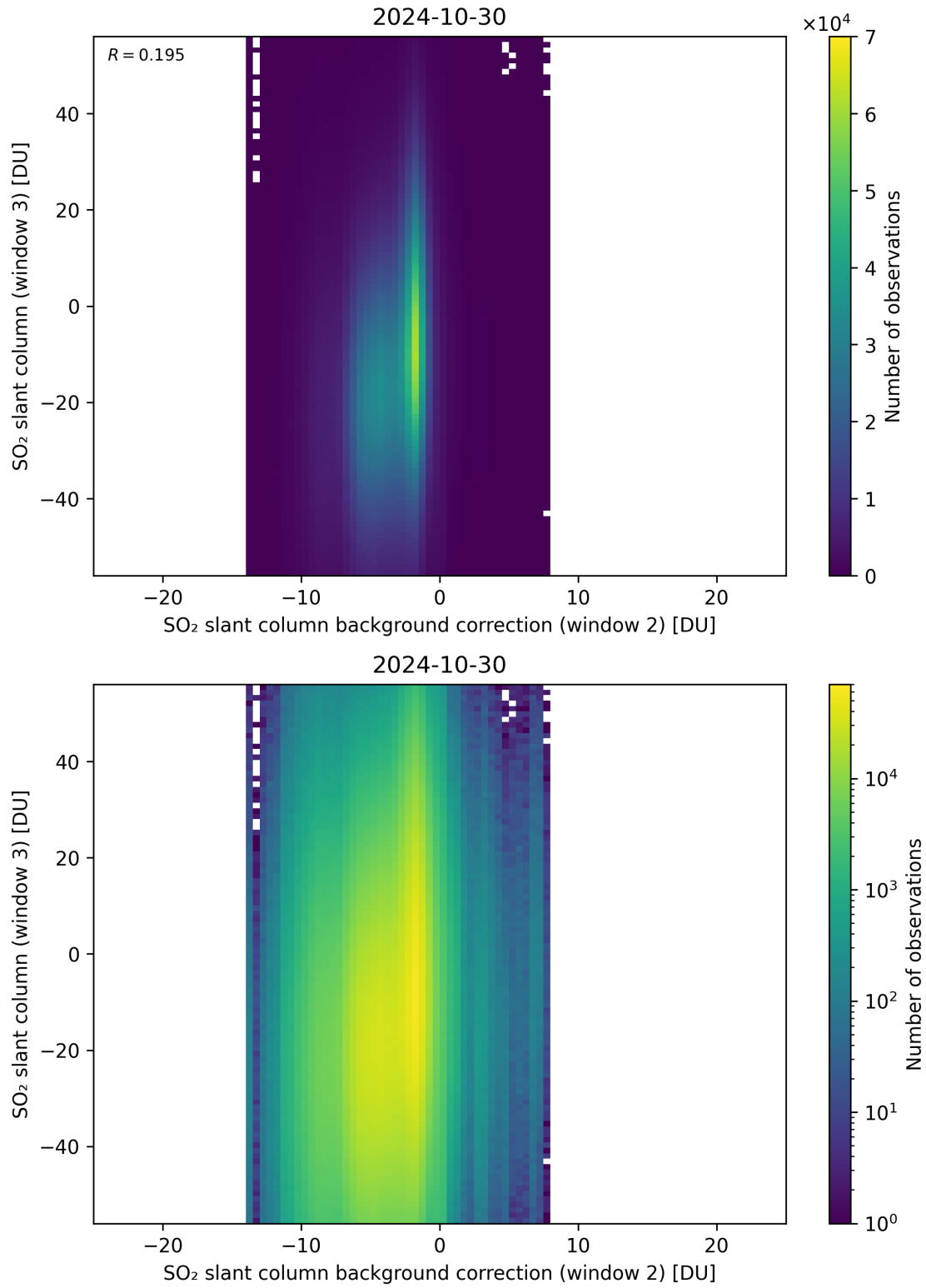
Figure 117: Scatter density plot of “SO 2 slant column background correction (window 2)” against “SO 2 slant column (window 3)” for 2024-10-30 to 2024-10-31.
