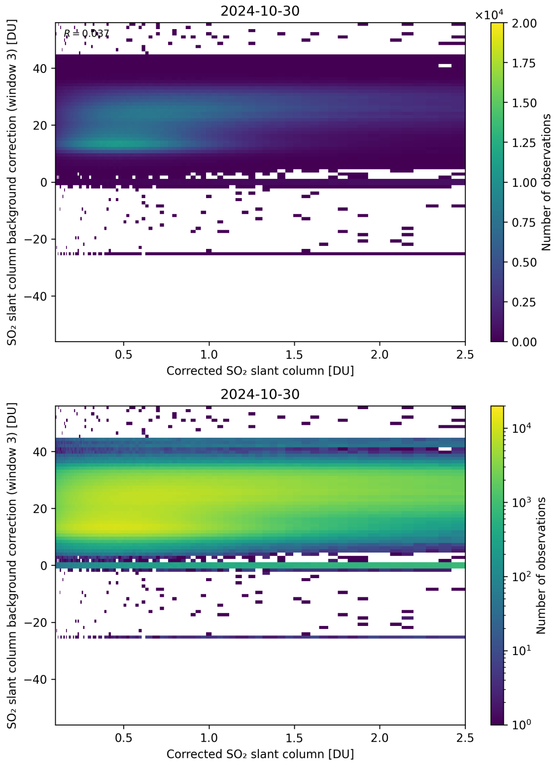
Figure 180: Scatter density plot of “Corrected SO 2 slant column” against “SO 2 slant column background correction (window 3)” for 2024-10-30 to 2024-10-31.
