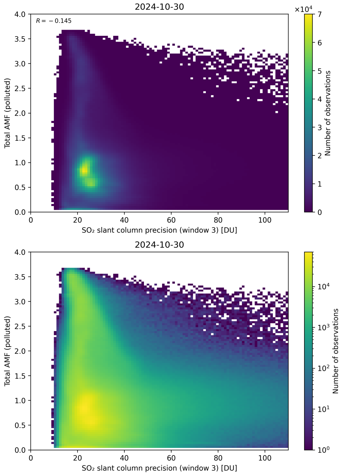
Figure 263: Scatter density plot of “SO 2 slant column precision (window 3)” against “Total AMF (polluted)” for 2024-10-30 to 2024-10-31.
