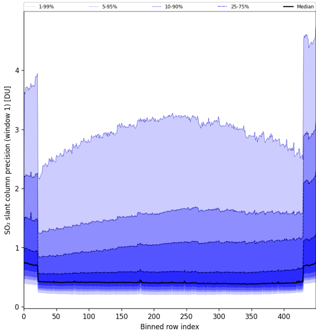
Figure 80: Along track statistics of “SO 2 slant column precision (window 1)” for 2024-10-30 to 2024-10-31
