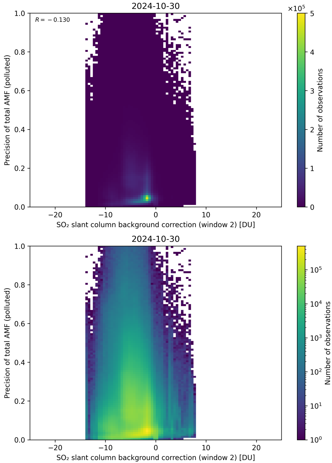
Figure 120: Scatter density plot of “SO 2 slant column background correction (window 2)” against “Precision of total AMF (polluted)” for 2024-10-30 to 2024-10-31.
