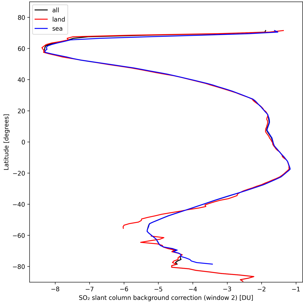
Figure 40: Zonal average of “SO 2 slant column background correction (window 2)” for 2024-10-30 to 2024-10-31.
