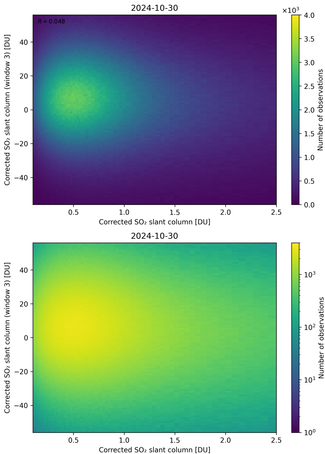
Figure 186: Scatter density plot of “Corrected SO 2 slant column” against “Corrected SO 2 slant column (window 3)” for 2024-10-30 to 2024-10-31.
