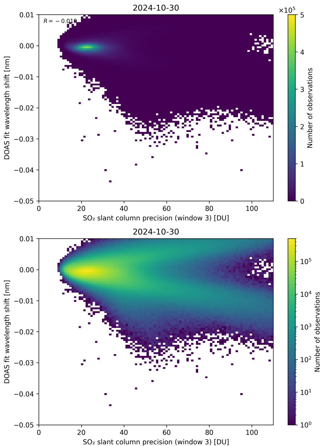
Figure 258: Scatter density plot of “SO 2 slant column precision (window 3)” against “DOAS fit wavelength shift” for 2024-10-30 to 2024-10-31.
