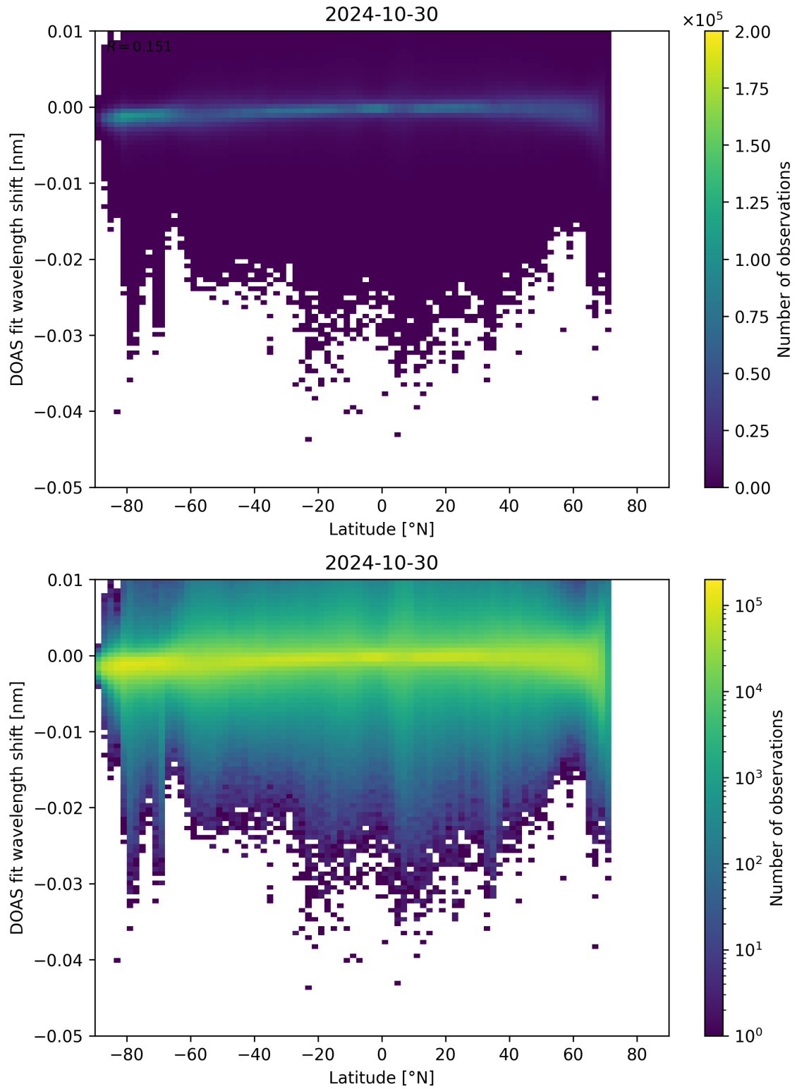
Figure 142: Scatter density plot of “Latitude” against “DOAS fit wavelength shift” for 2024-10-30 to 2024-10-31.
