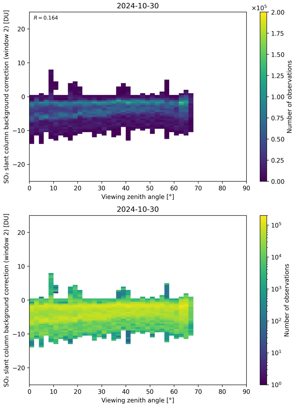
Figure 309: Scatter density plot of “Viewing zenith angle” against “SO 2 slant column background correction (window 2)” for 2024-10-30 to 2024-10-31.
