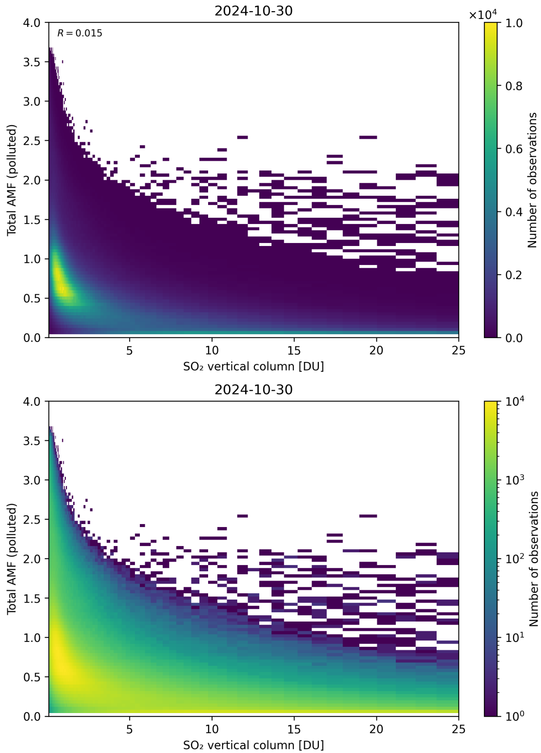
Figure 305: Scatter density plot of “SO 2 vertical column” against “Total AMF (polluted)” for 2024-10-30 to 2024-10-31.
