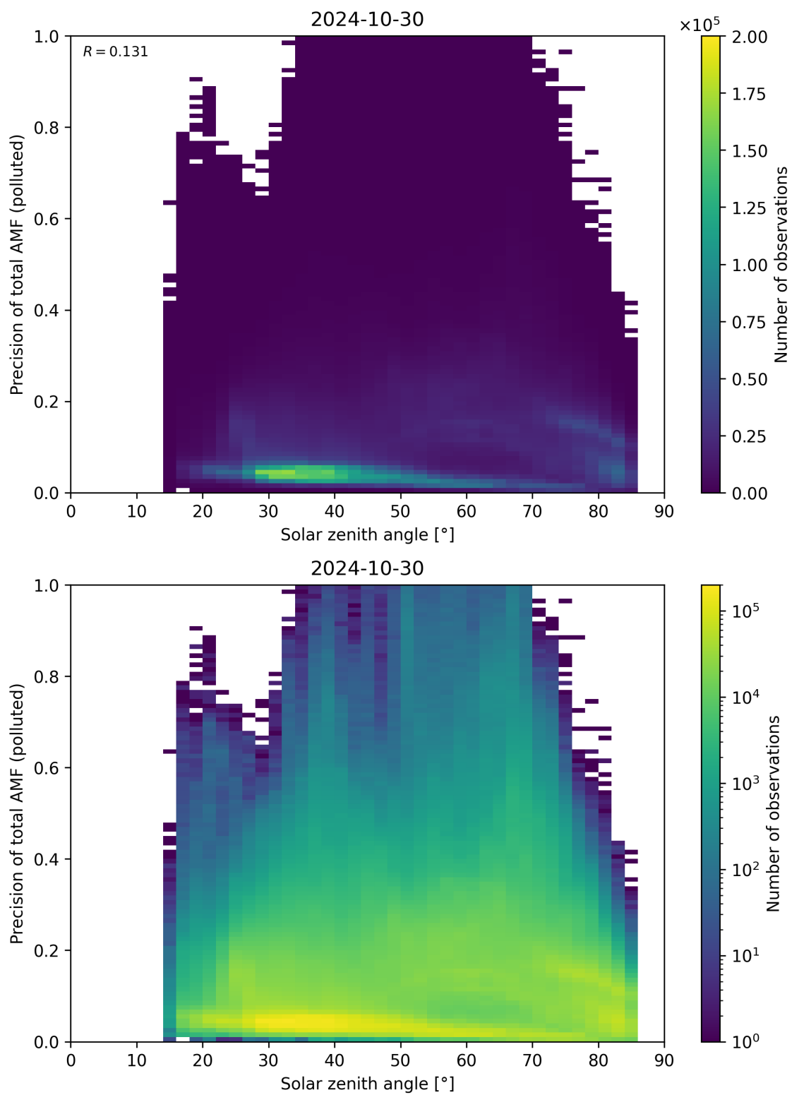
Figure 175: Scatter density plot of “Solar zenith angle” against “Precision of total AMF (polluted)” for 2024-10-30 to 2024-10-31.
