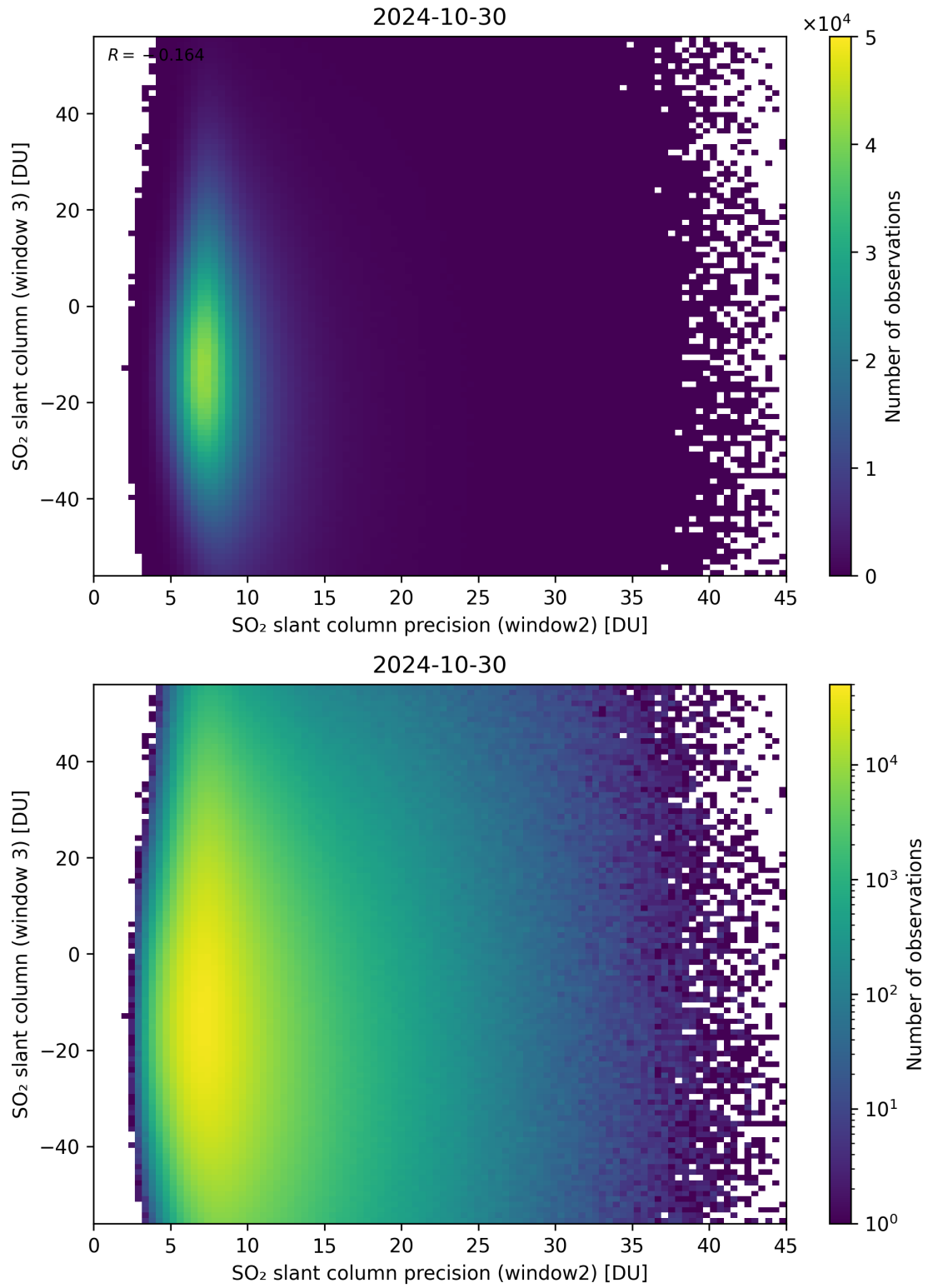
Figure 249: Scatter density plot of “SO 2 slant column precision (window2)” against “SO 2 slant column (window 3)” for 2024-10-30 to 2024-10-31.
