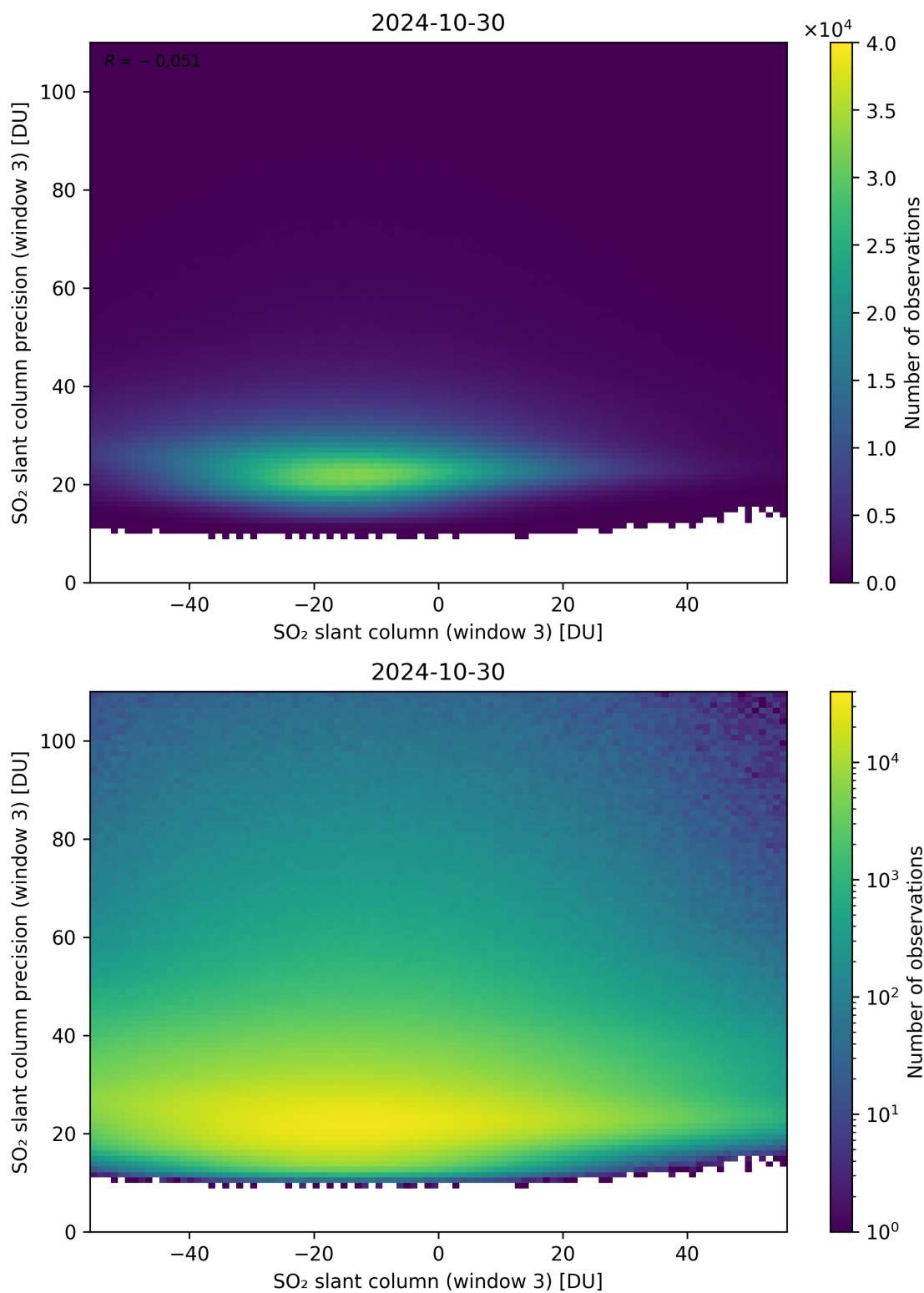
Figure 267: Scatter density plot of “SO 2 slant column (window 3)” against “SO 2 slant column precision (window 3)” for 2024-10-30 to 2024-10-31.
