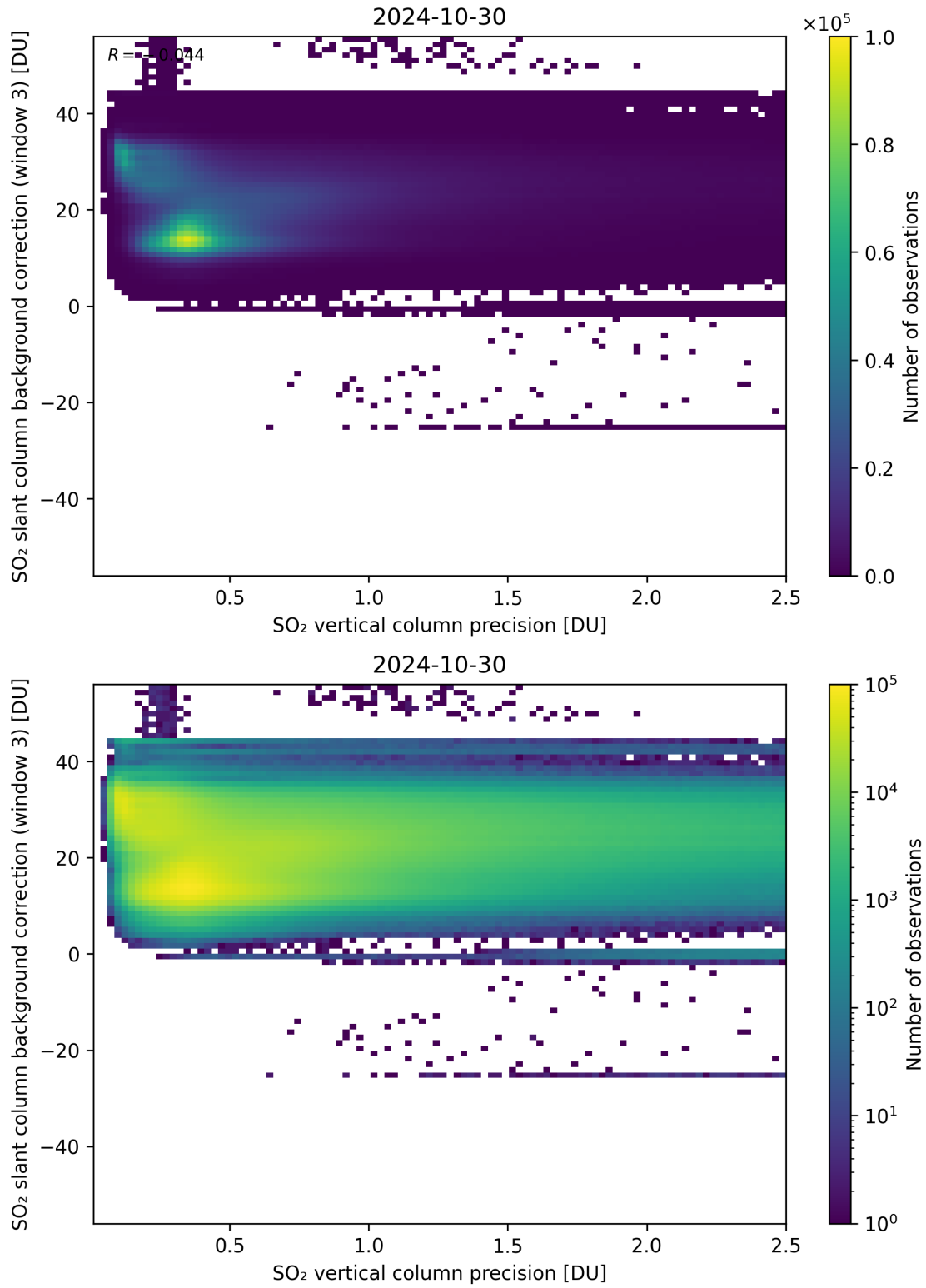
Figure 281: Scatter density plot of “SO 2 vertical column precision” against “SO 2 slant column background correction (window 3)” for 2024-10-30 to 2024-10-31.
