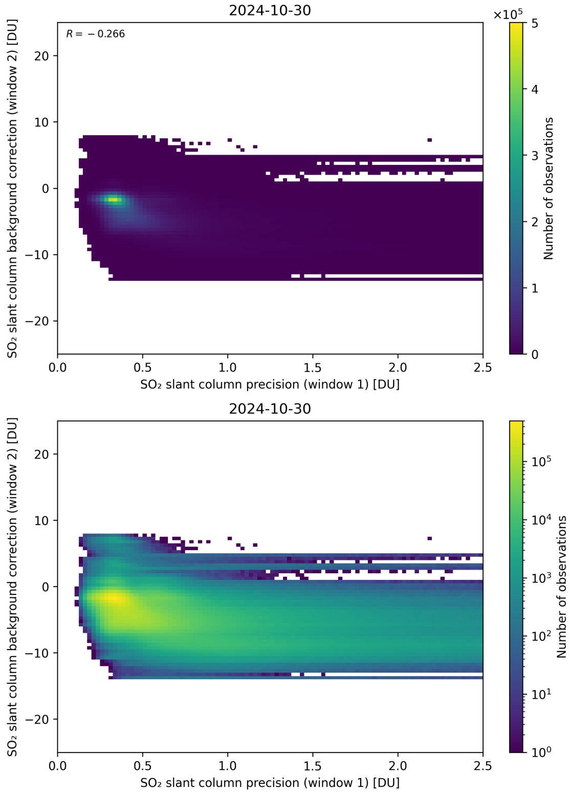
Figure 219: Scatter density plot of “SO 2 slant column precision (window 1)” against “SO 2 slant column background correction (window 2)” for 2024-10-30 to 2024-10-31.
