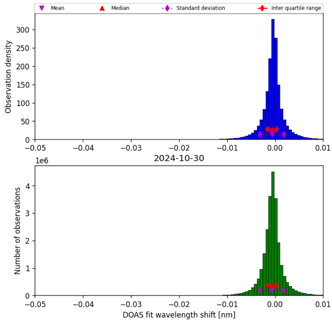
Figure 68: Histogram of “DOAS fit wavelength shift” for 2024-10-30 to 2024-10-31
