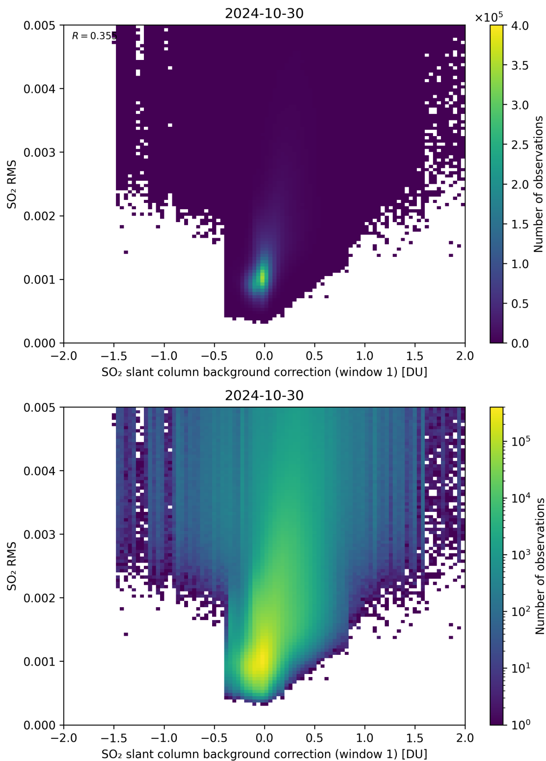
Figure 102: Scatter density plot of “SO 2 slant column background correction (window 1)” against “SO 2 RMS” for 2024-10-30 to 2024-10-31.
