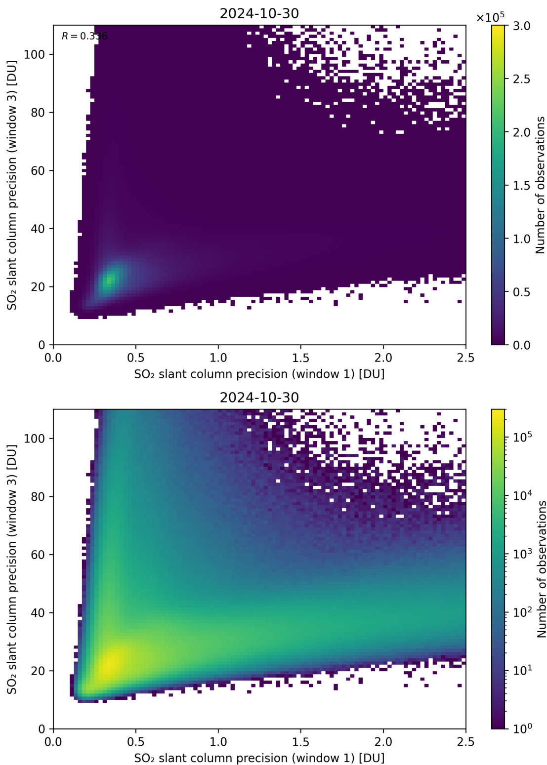
Figure 229: Scatter density plot of “SO 2 slant column precision (window 1)” against “SO 2 slant column precision (window 3)” for 2024-10-30 to 2024-10-31.
