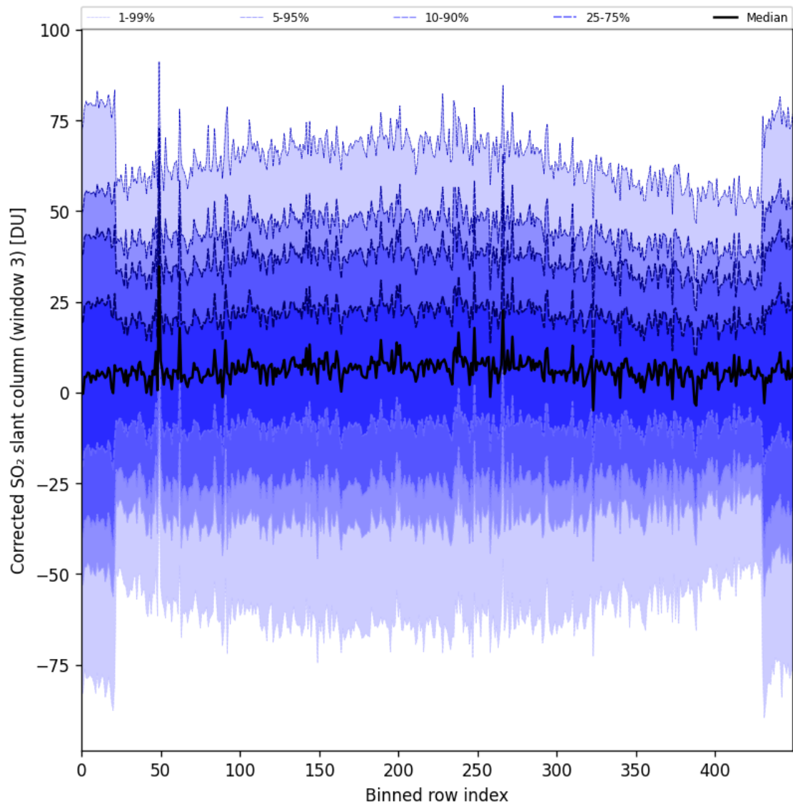
Figure 89: Along track statistics of “Corrected SO 2 slant column (window 3)” for 2024-10-30 to 2024-10-31
