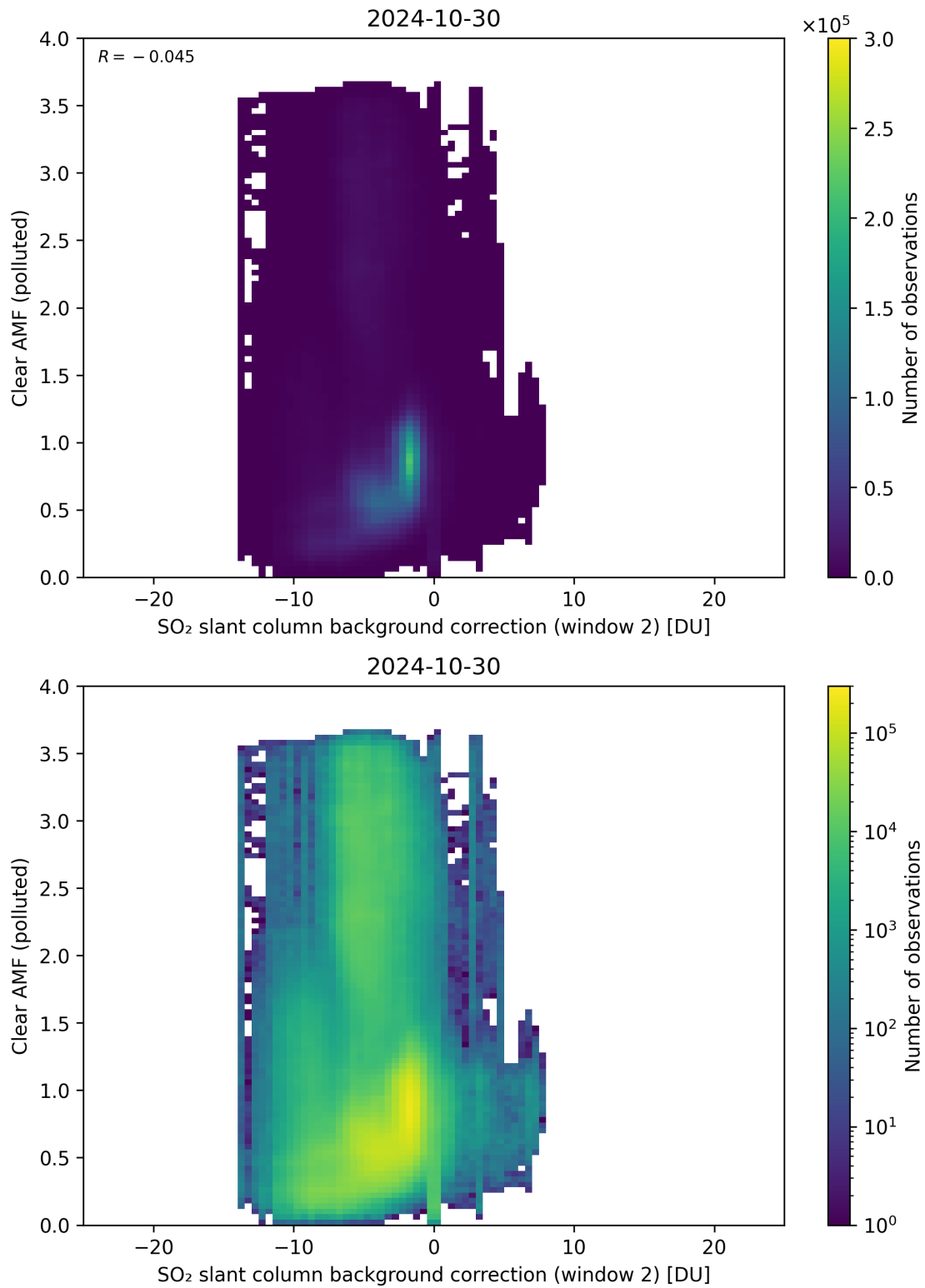
Figure 115: Scatter density plot of “SO 2 slant column background correction (window 2)” against “Clear AMF (polluted)” for 2024-10-30 to 2024-10-31.
