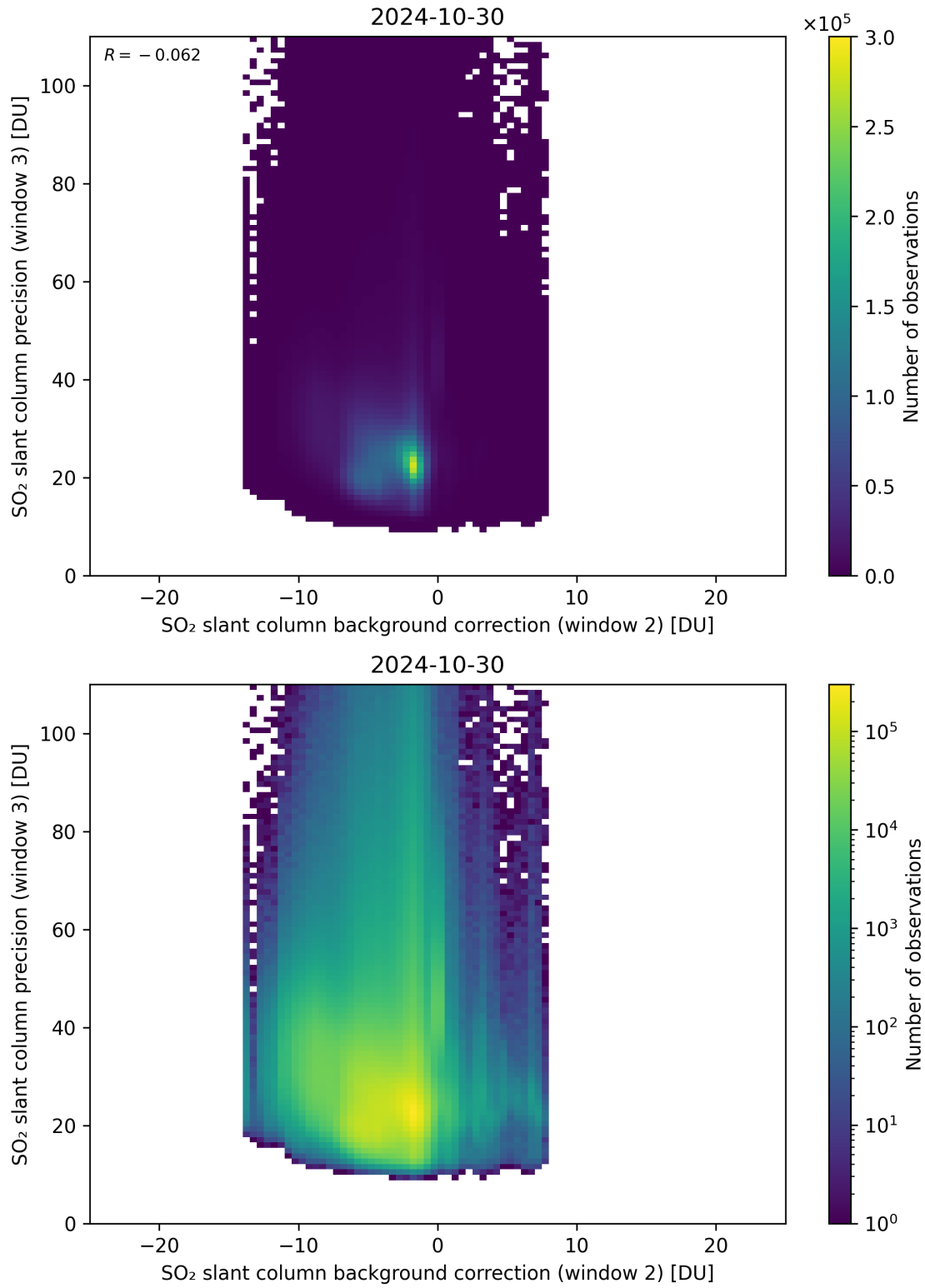
Figure 118: Scatter density plot of “SO 2 slant column background correction (window 2)” against “SO 2 slant column precision (window 3)” for 2024-10-30 to 2024-10-31.
