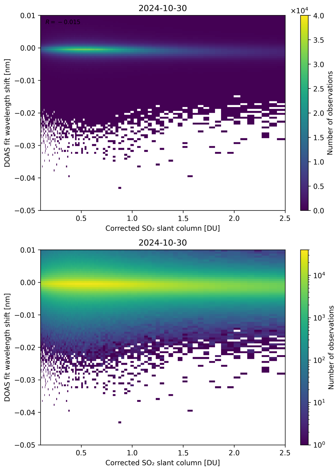
Figure 181: Scatter density plot of “Corrected SO 2 slant column” against “DOAS fit wavelength shift” for 2024-10-30 to 2024-10-31.
