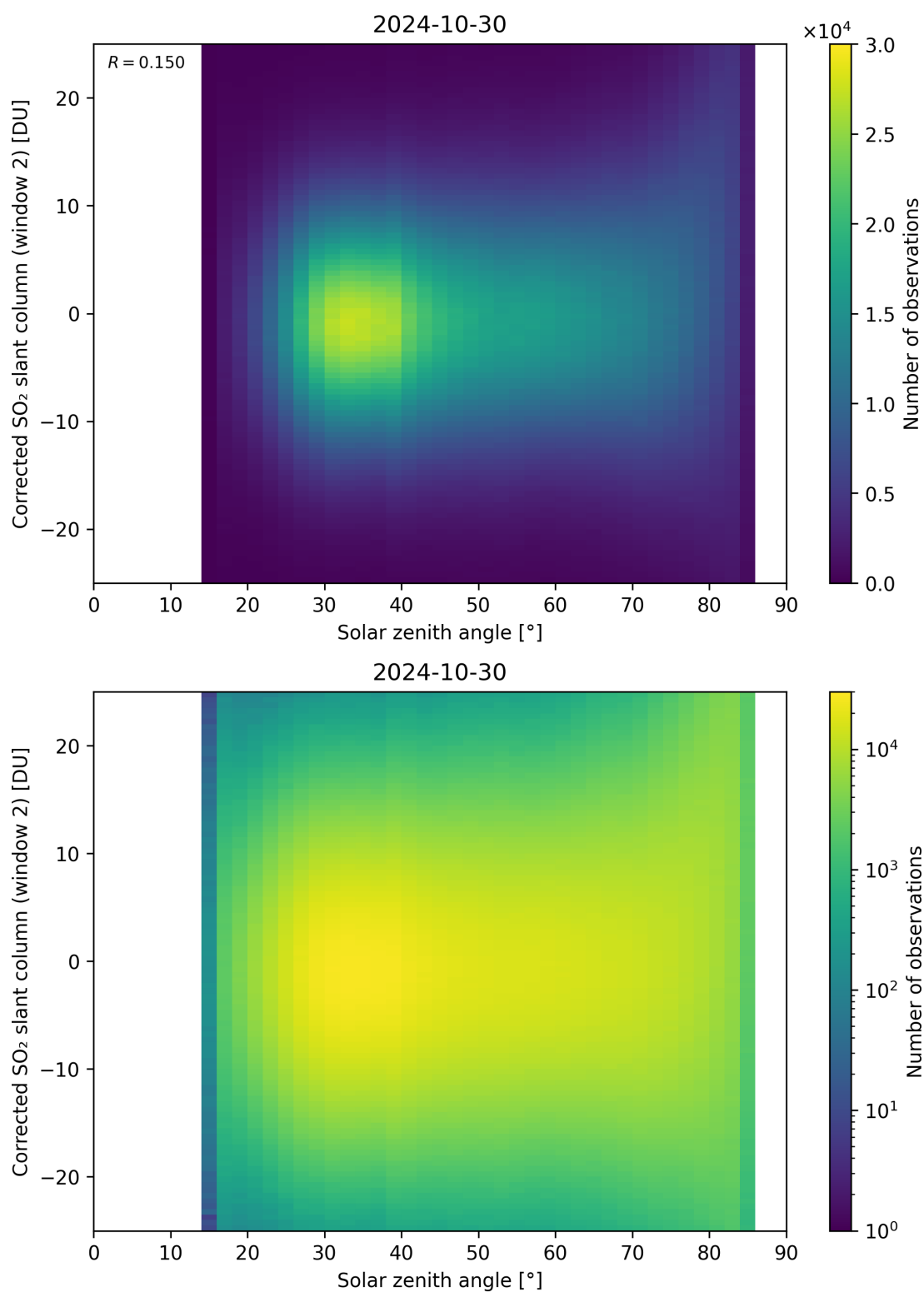
Figure 167: Scatter density plot of “Solar zenith angle” against “Corrected SO 2 slant column (window 2)” for 2024-10-30 to 2024-10-31.
