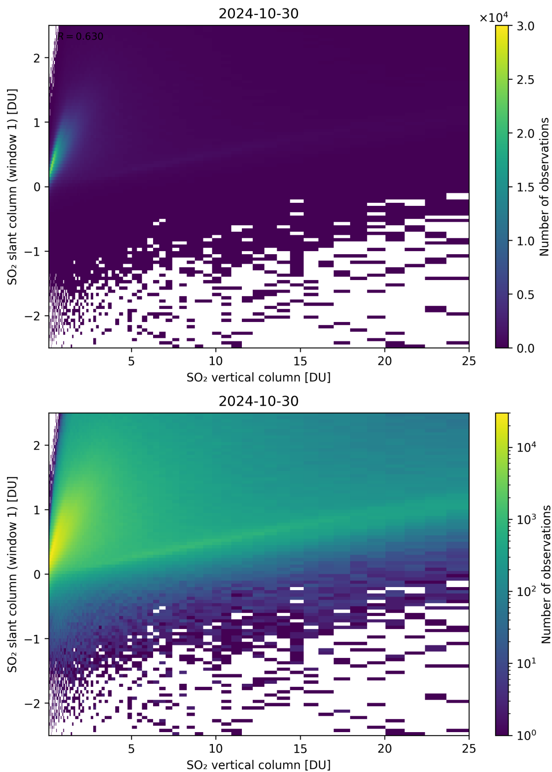
Figure 300: Scatter density plot of “SO 2 vertical column” against “SO 2 slant column (window 1)” for 2024-10-30 to 2024-10-31.
