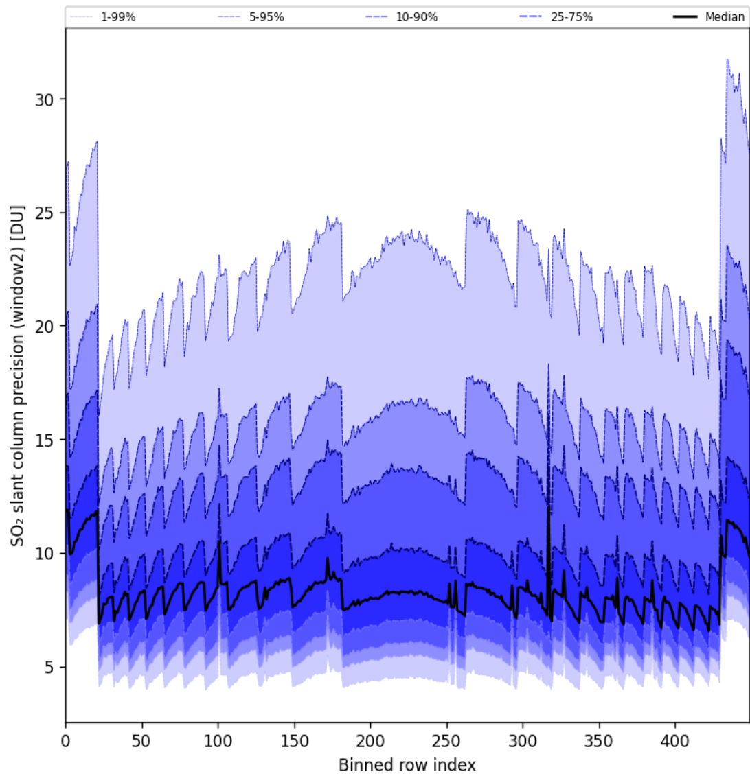
Figure 84: Along track statistics of “SO 2 slant column precision (window2)” for 2024-10-30 to 2024-10-31
