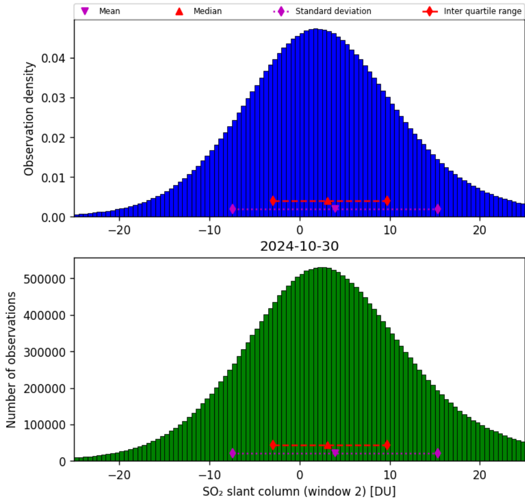
Figure 60: Histogram of “SO 2 slant column (window 2)” for 2024-10-30 to 2024-10-31
