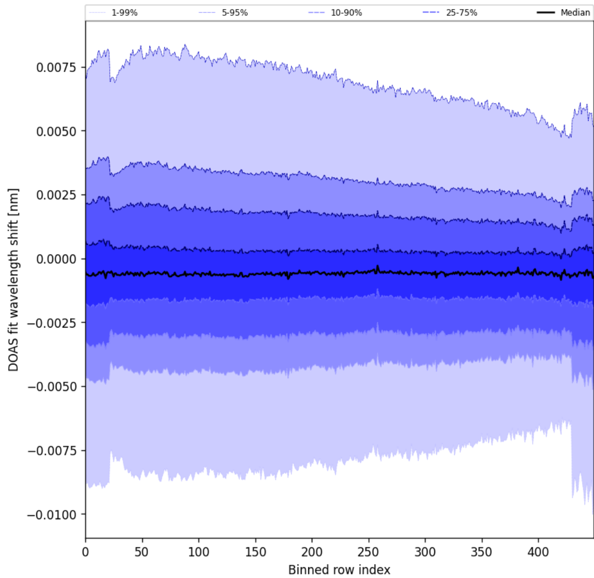
Figure 91: Along track statistics of “DOAS fit wavelength shift” for 2024-10-30 to 2024-10-31
