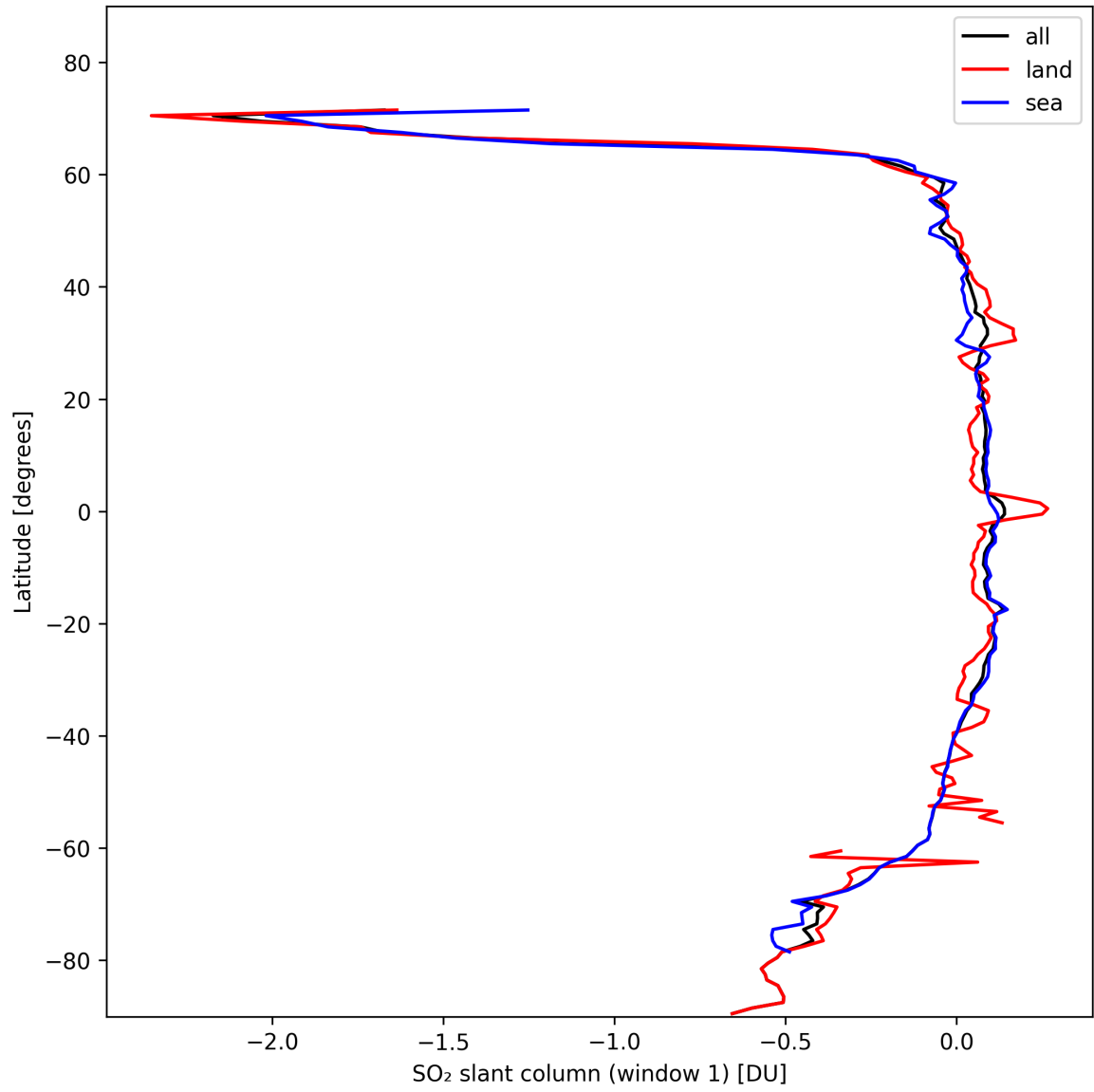
Figure 33: Zonal average of “SO 2 slant column (window 1)” for 2024-10-30 to 2024-10-31.
