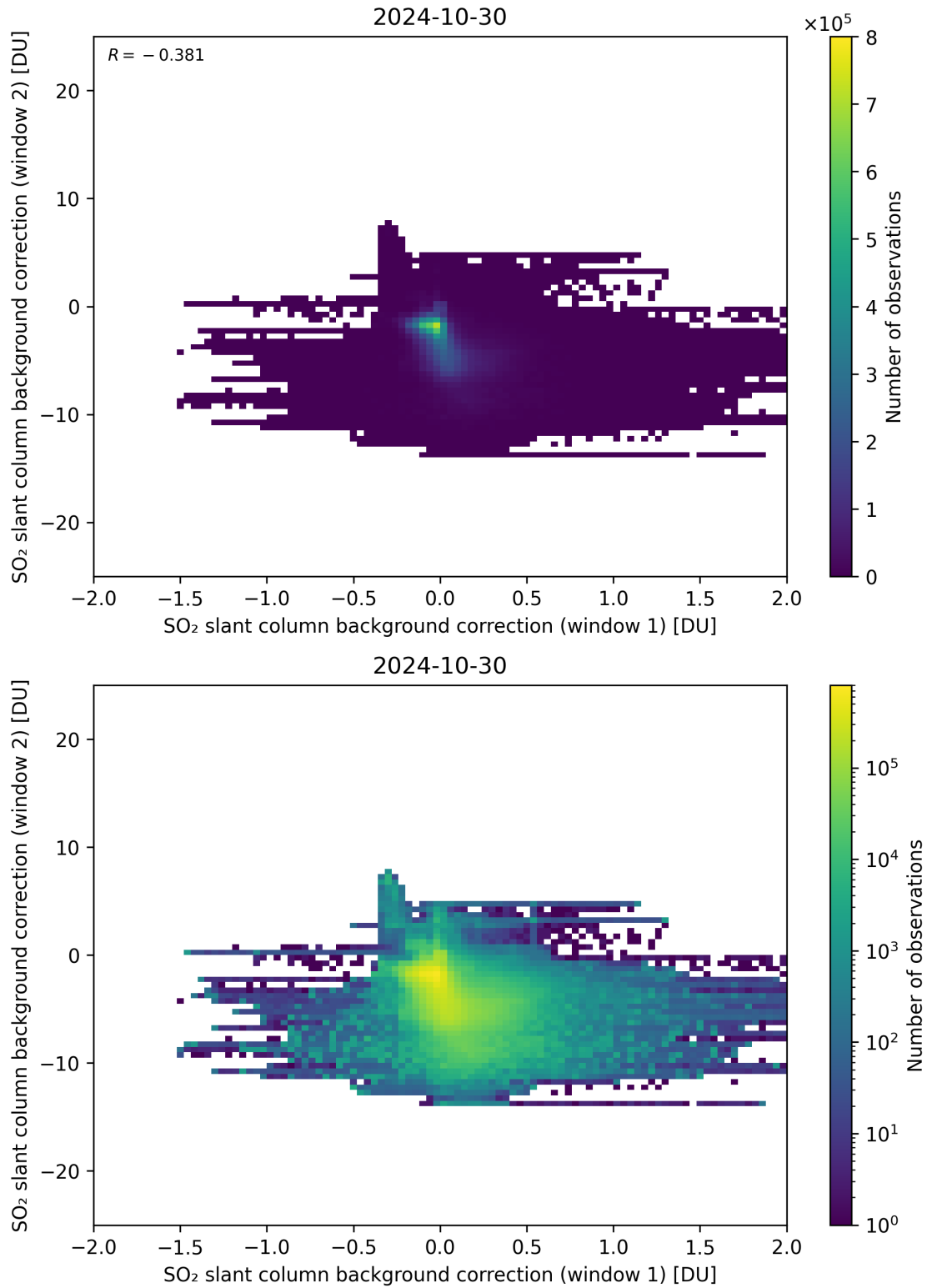
Figure 98: Scatter density plot of “SO 2 slant column background correction (window 1)” against “SO 2 slant column background correction (window 2)” for 2024-10-30 to 2024-10-31.
