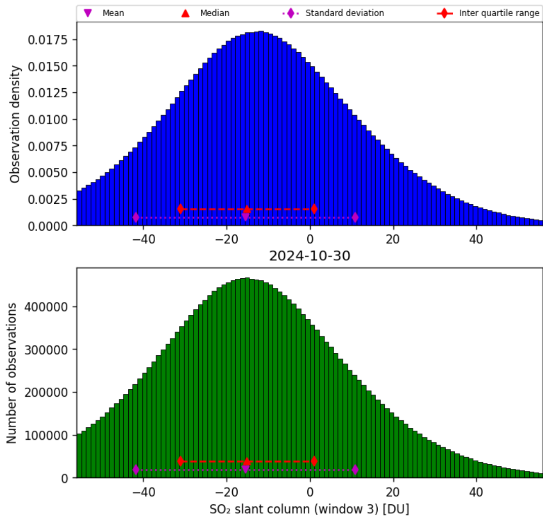
Figure 64: Histogram of “SO 2 slant column (window 3)” for 2024-10-30 to 2024-10-31
