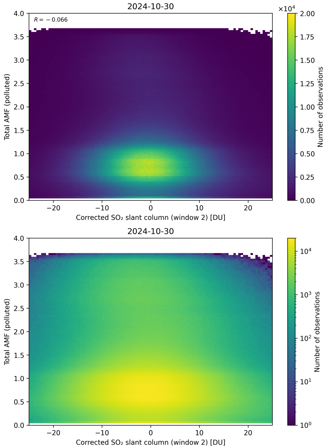
Figure 203: Scatter density plot of “Corrected SO 2 slant column (window 2)” against “Total AMF (polluted)” for 2024-10-30 to 2024-10-31.
