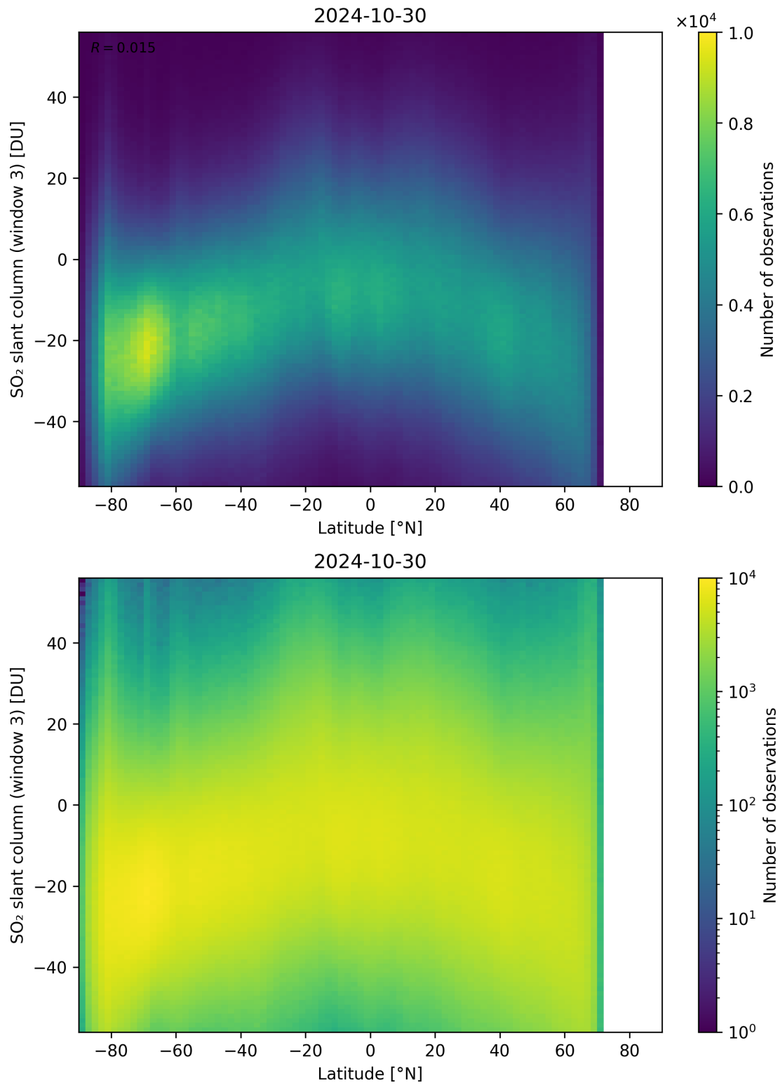
Figure 152: Scatter density plot of “Latitude” against “SO 2 slant column (window 3)” for 2024-10-30 to 2024-10-31.
