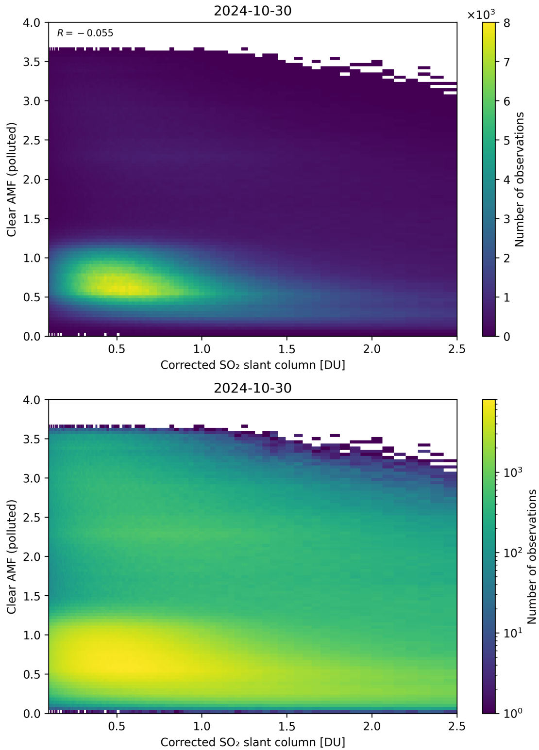
Figure 184: Scatter density plot of “Corrected SO 2 slant column” against “Clear AMF (polluted)” for 2024-10-30 to 2024-10-31.
