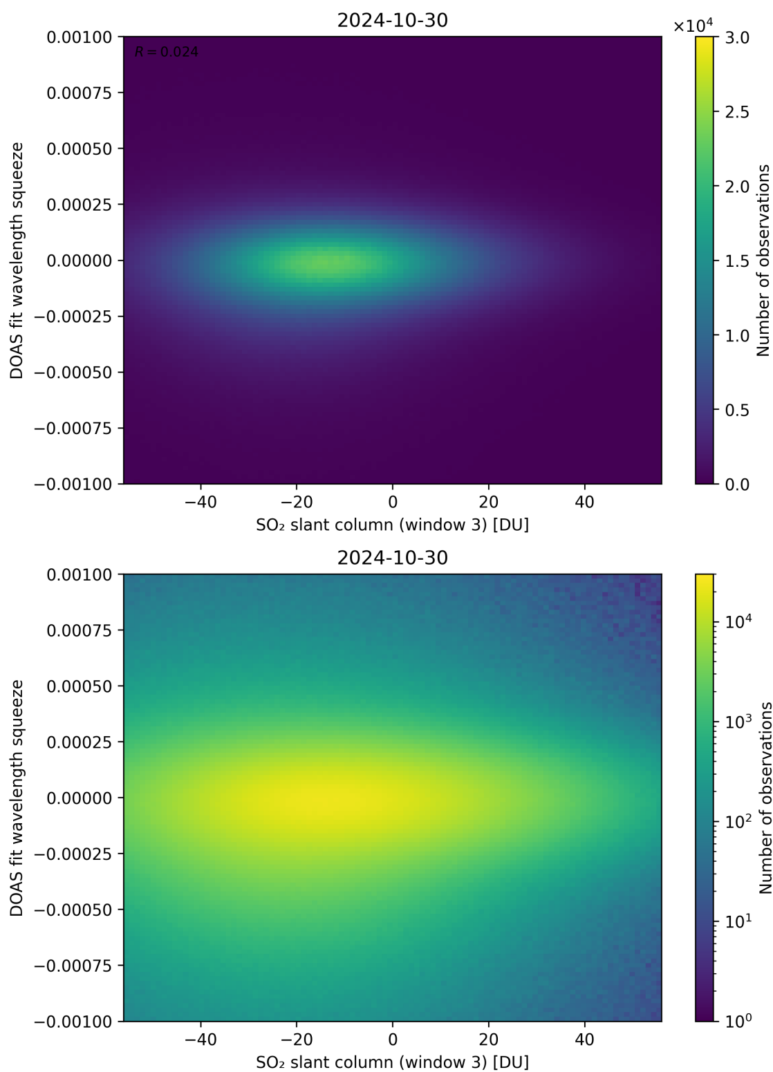
Figure 255: Scatter density plot of “SO 2 slant column (window 3)” against “DOAS fit wavelength squeeze” for 2024-10-30 to 2024-10-31.
