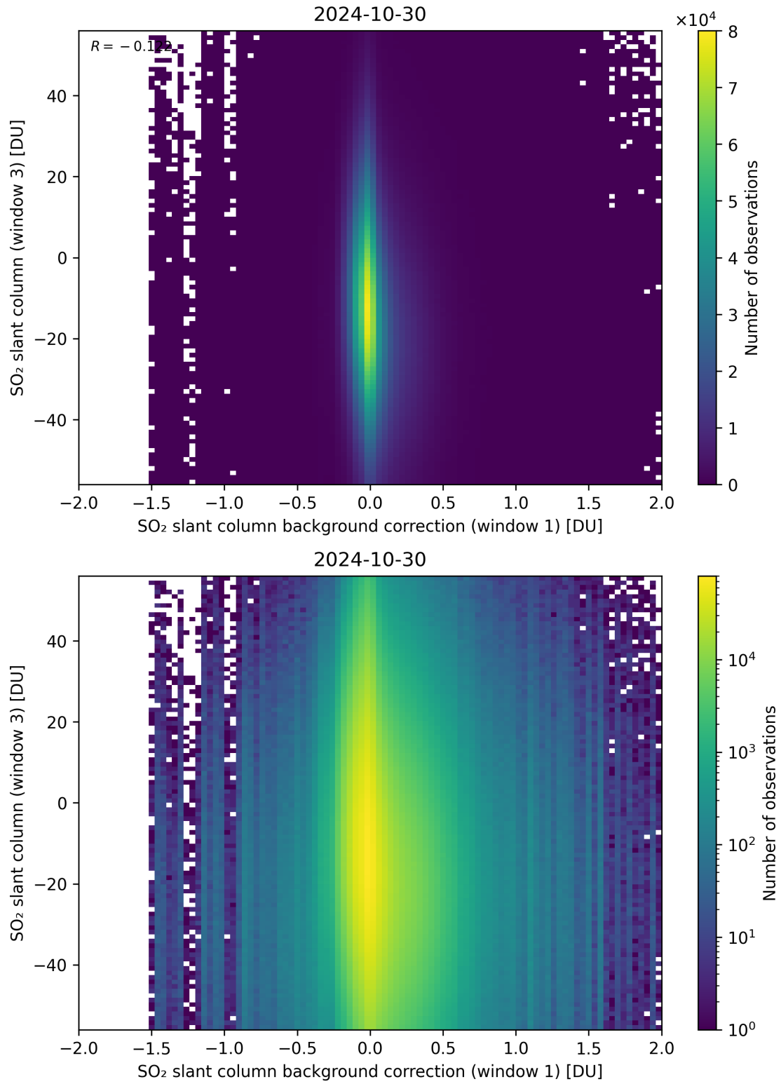
Figure 107: Scatter density plot of “SO 2 slant column background correction (window 1)” against “SO 2 slant column (window 3)” for 2024-10-30 to 2024-10-31.
