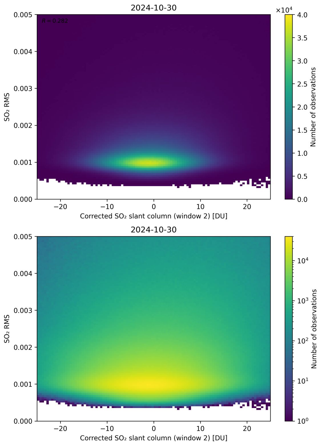
Figure 198: Scatter density plot of “Corrected SO 2 slant column (window 2)” against “SO 2 RMS” for 2024-10-30 to 2024-10-31.
