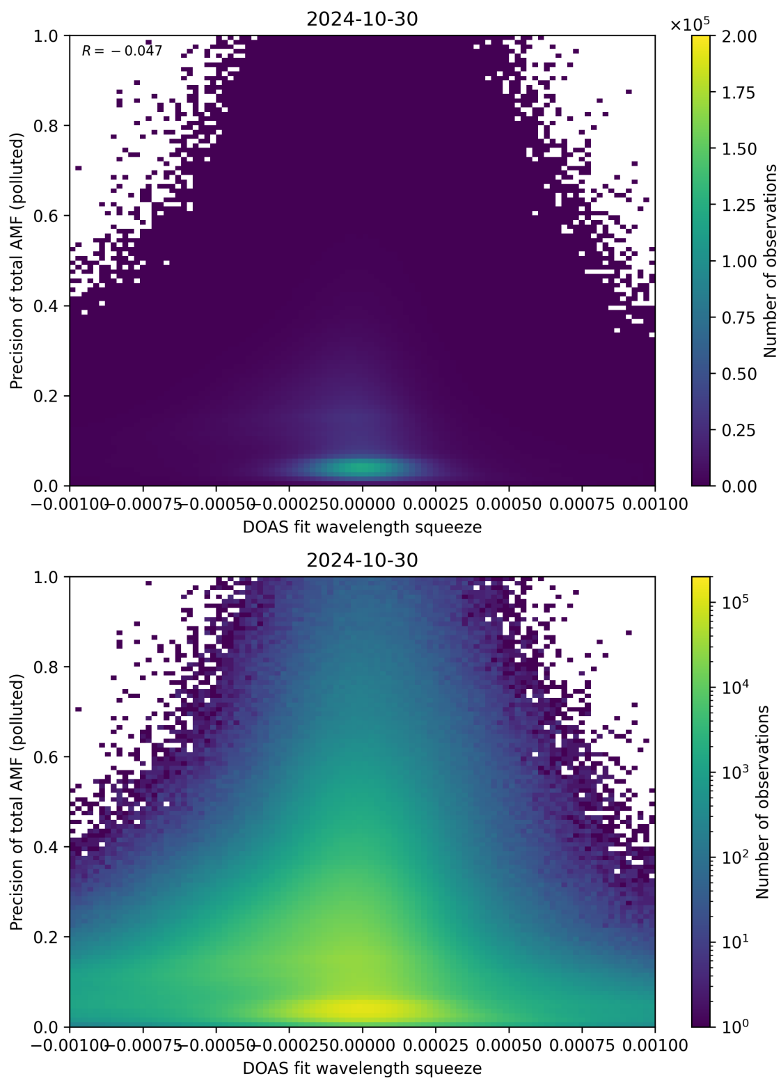
Figure 135: Scatter density plot of “DOAS fit wavelength squeeze” against “Precision of total AMF (polluted)” for 2024-10-30 to 2024-10-31.
