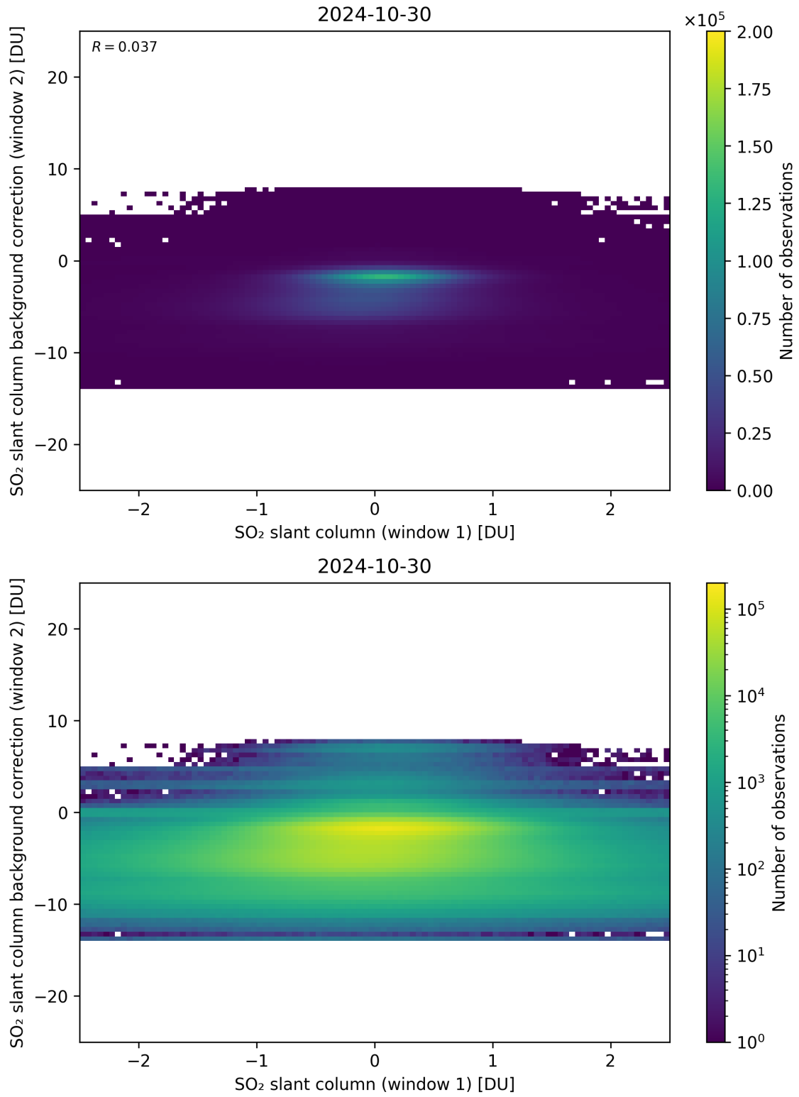
Figure 213: Scatter density plot of “SO 2 slant column (window 1)” against “SO 2 slant column background correction (window 2)” for 2024-10-30 to 2024-10-31.
