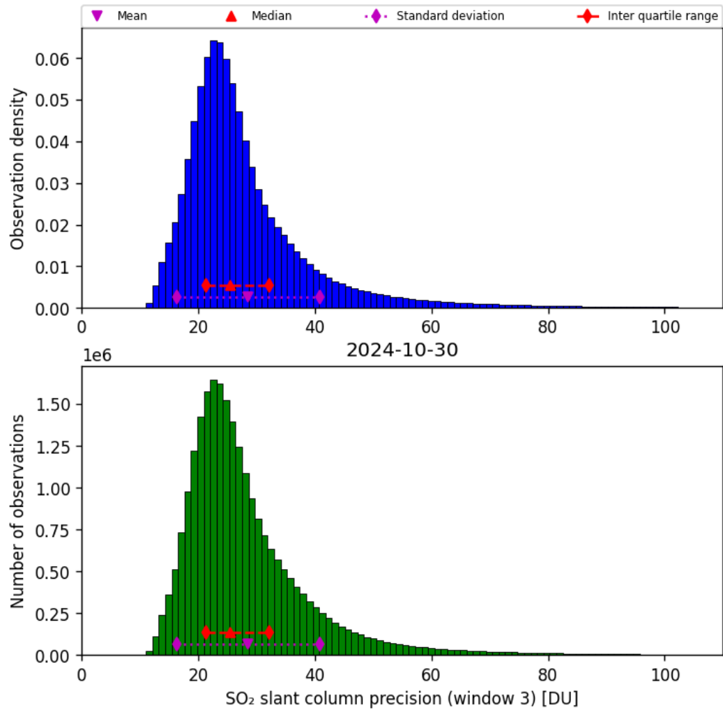
Figure 65: Histogram of “SO 2 slant column precision (window 3)” for 2024-10-30 to 2024-10-31
