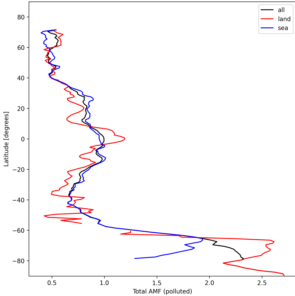
Figure 48: Zonal average of “Total AMF (polluted)” for 2024-10-30 to 2024-10-31.
