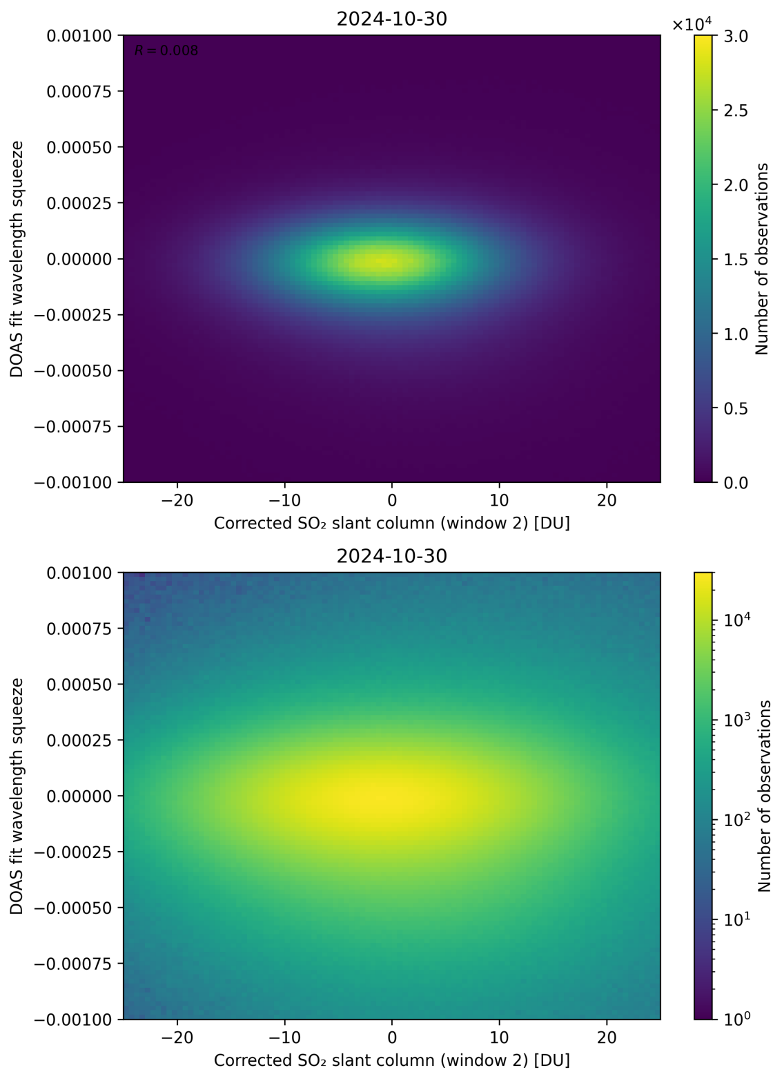
Figure 197: Scatter density plot of “Corrected SO 2 slant column (window 2)” against “DOAS fit wavelength squeeze” for 2024-10-30 to 2024-10-31.
