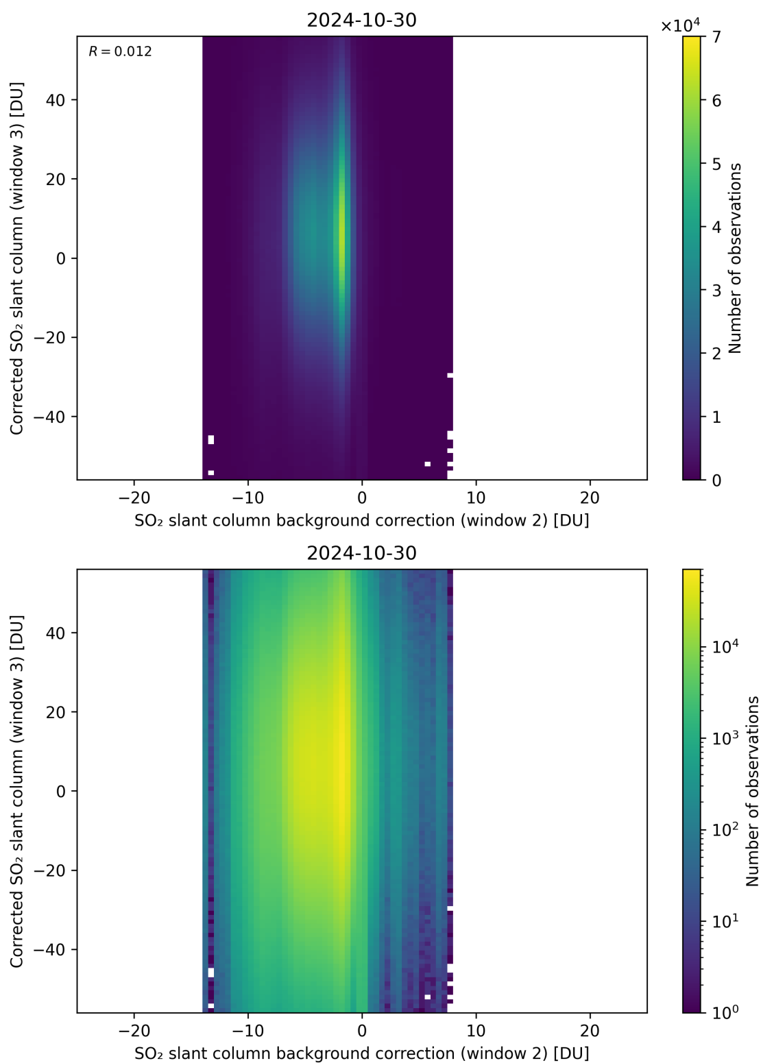
Figure 116: Scatter density plot of “SO 2 slant column background correction (window 2)” against “Corrected SO 2 slant column (window 3)” for 2024-10-30 to 2024-10-31.
