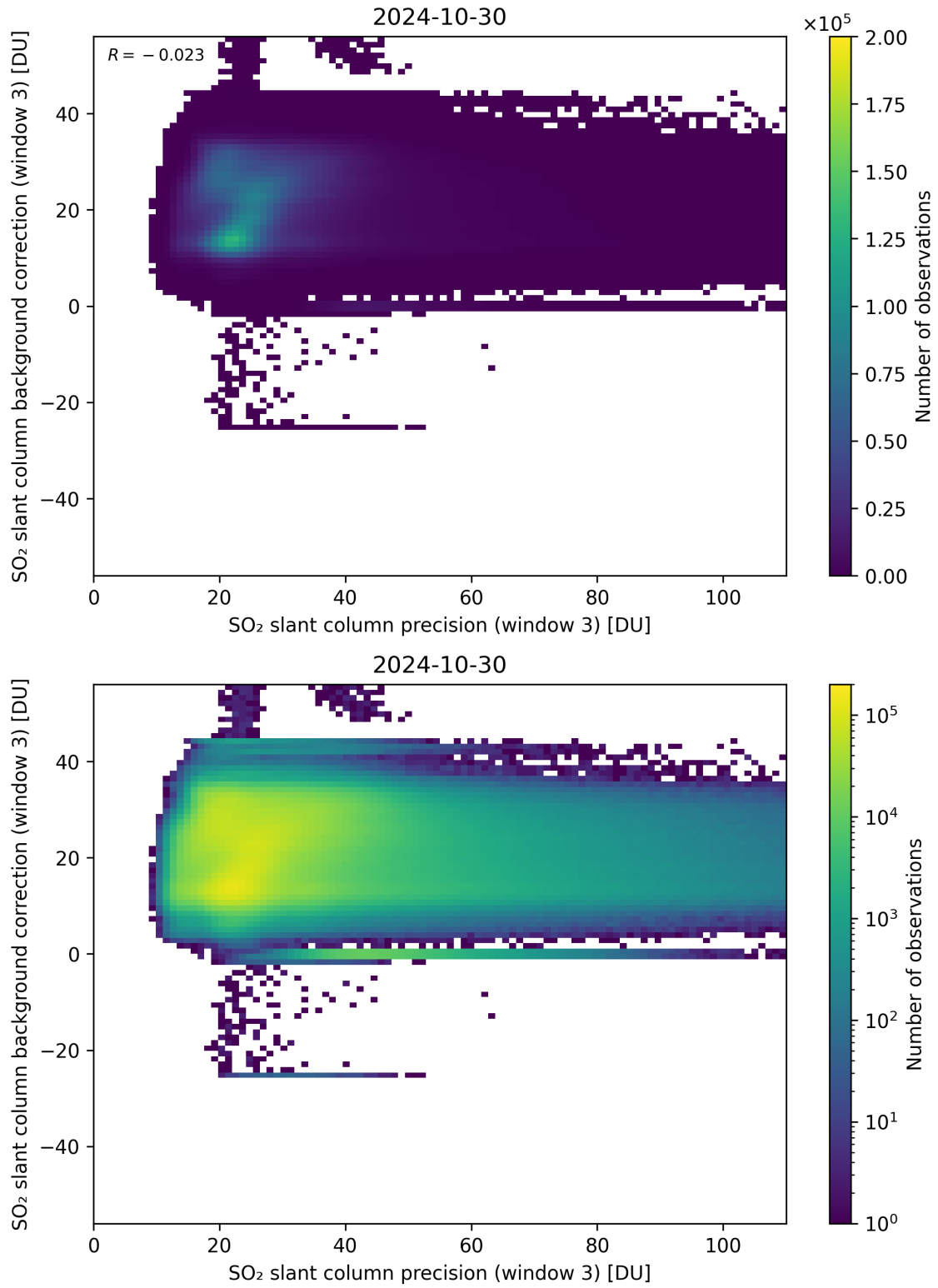
Figure 257: Scatter density plot of “SO 2 slant column precision (window 3)” against “SO 2 slant column background correction (window 3)” for 2024-10-30 to 2024-10-31.
