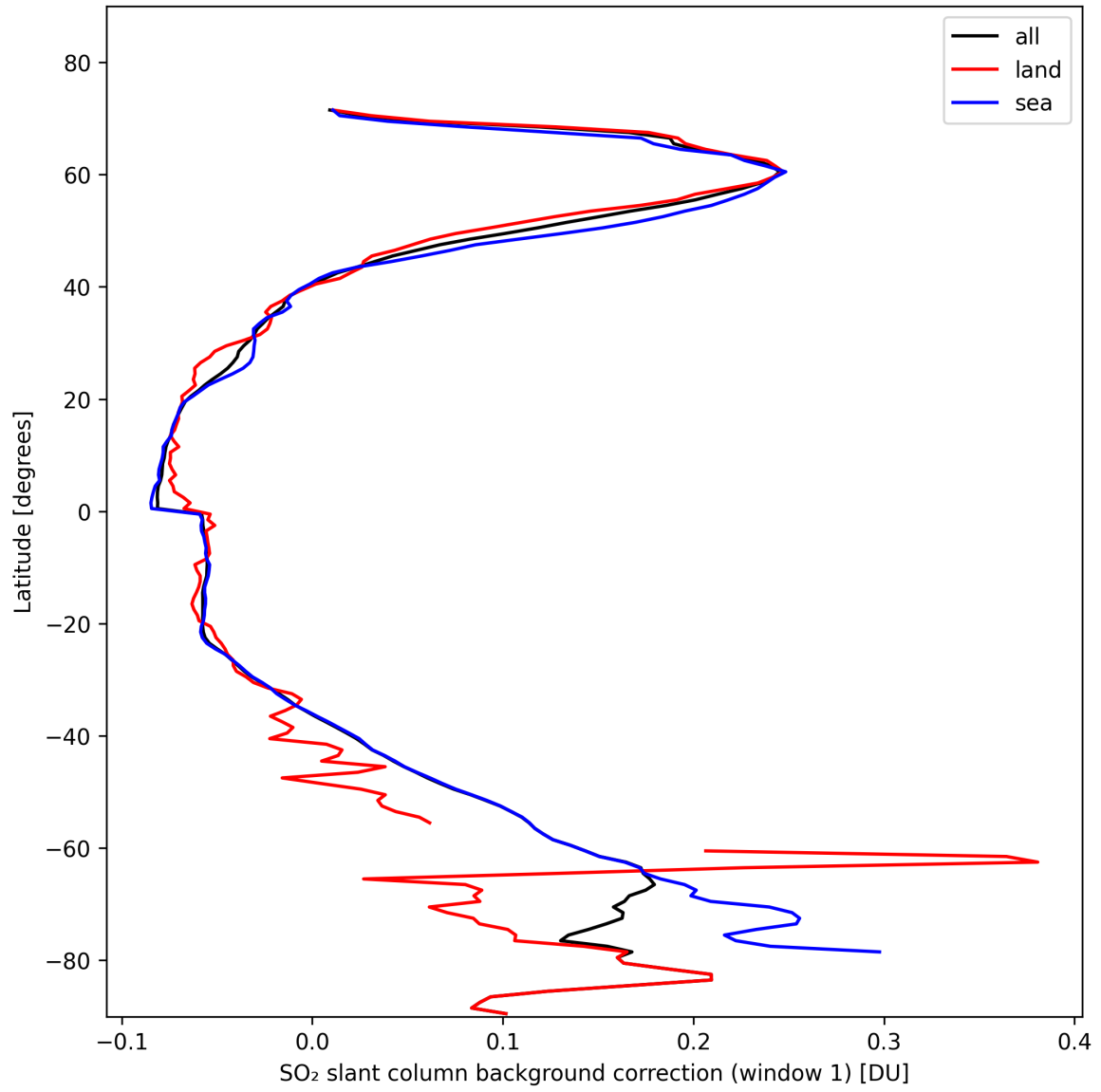
Figure 36: Zonal average of “SO 2 slant column background correction (window 1)” for 2024-10-30 to 2024-10-31.
