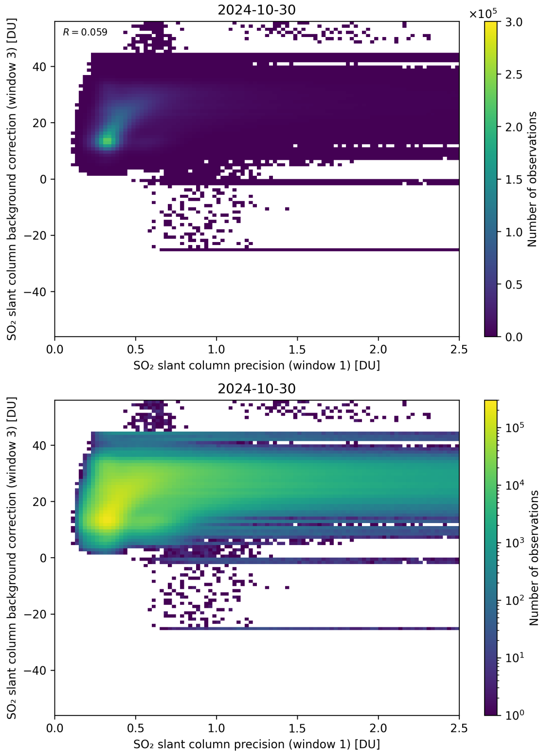
Figure 220: Scatter density plot of “SO 2 slant column precision (window 1)” against “SO 2 slant column background correction (window 3)” for 2024-10-30 to 2024-10-31.
