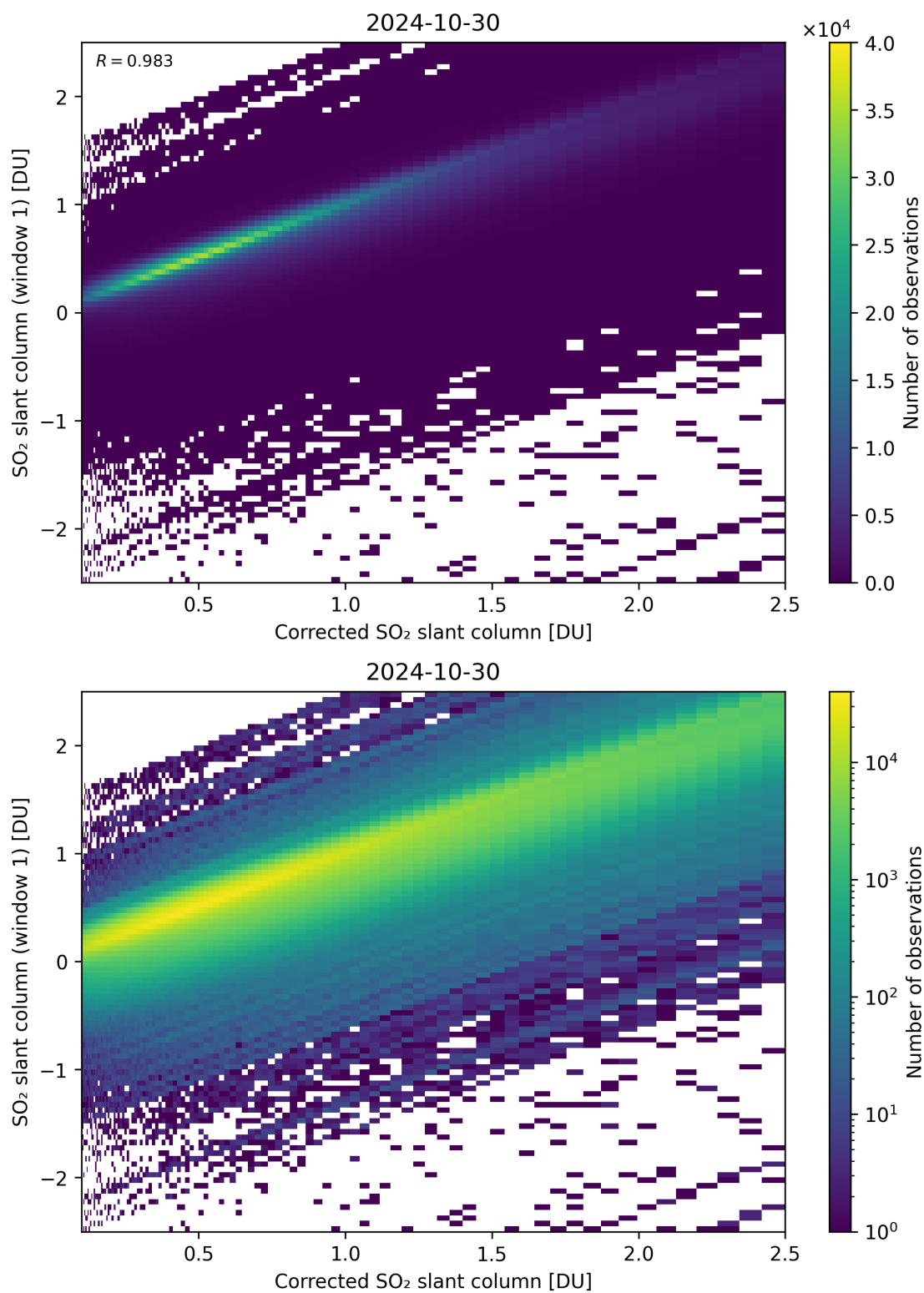
Figure 187: Scatter density plot of “Corrected SO 2 slant column” against “SO 2 slant column (window 1)” for 2024-10-30 to 2024-10-31.
