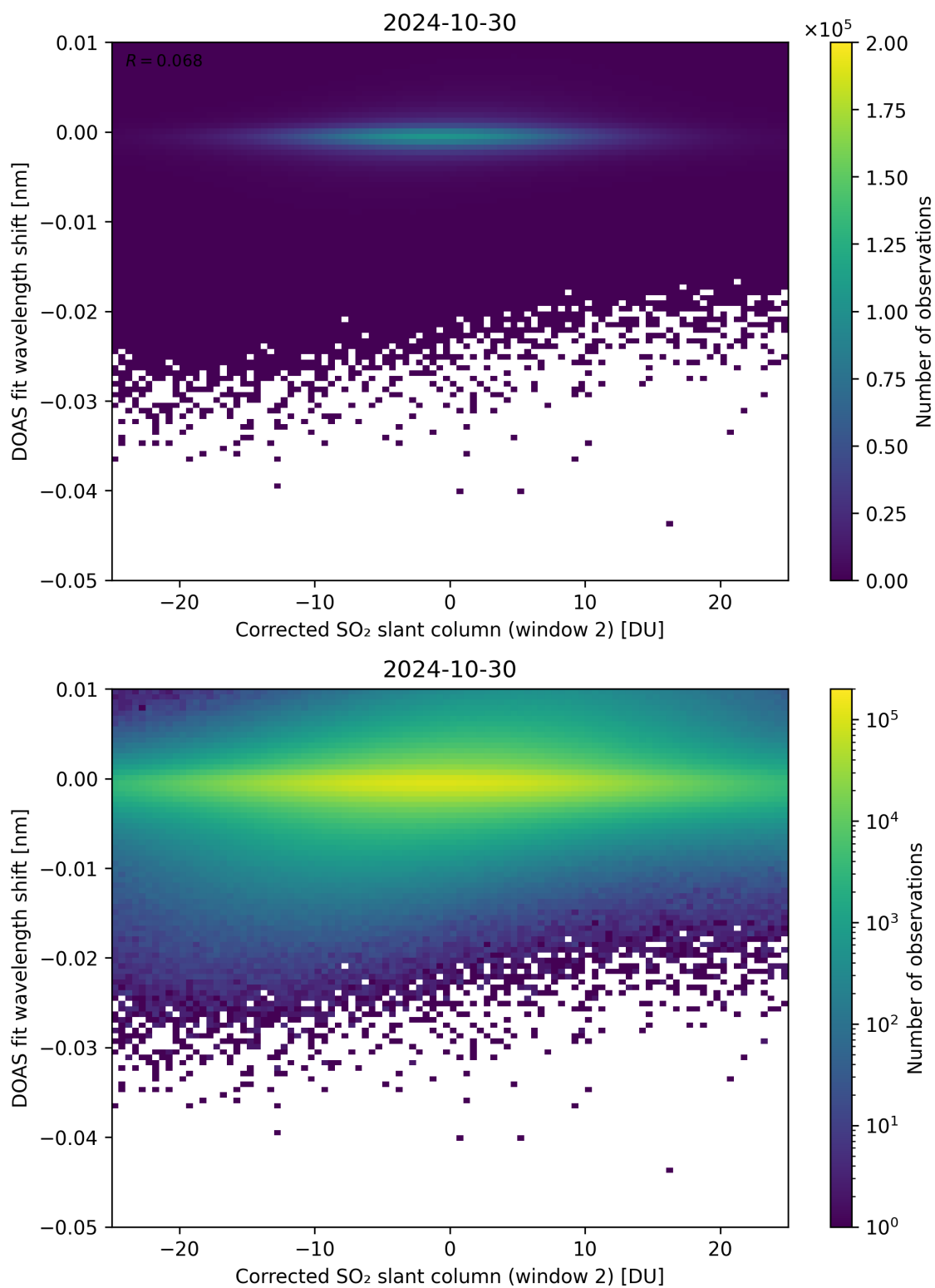
Figure 196: Scatter density plot of “Corrected SO 2 slant column (window 2)” against “DOAS fit wavelength shift” for 2024-10-30 to 2024-10-31.
