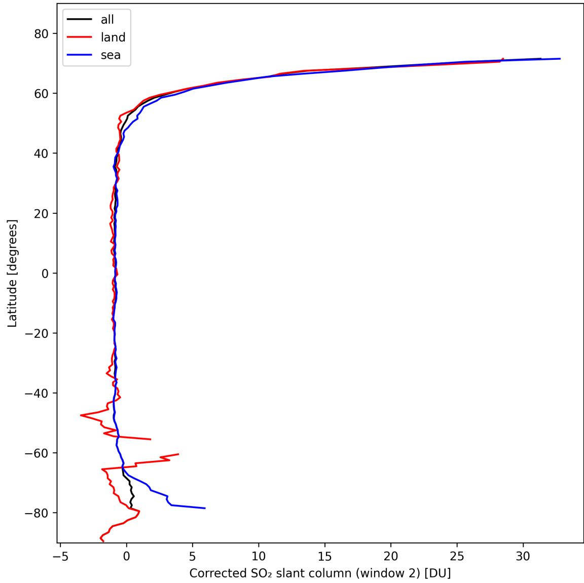
Figure 39: Zonal average of “Corrected SO 2 slant column (window 2)” for 2024-10-30 to 2024-10-31.
