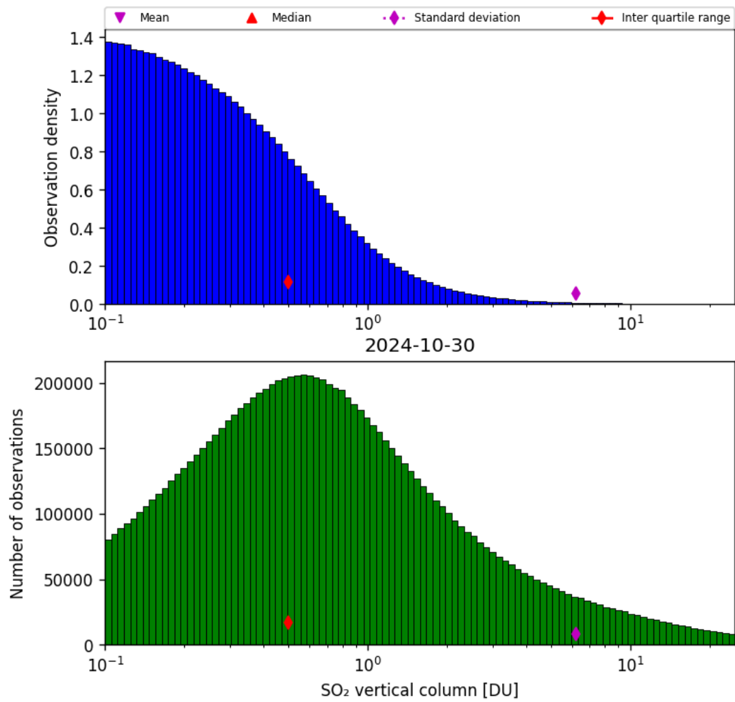
Figure 53: Histogram of “SO 2 vertical column” for 2024-10-30 to 2024-10-31
