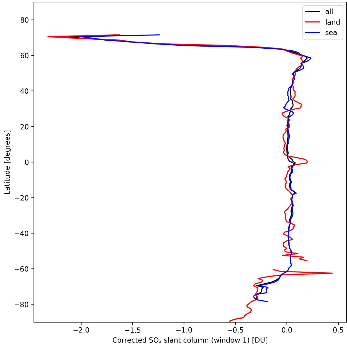
Figure 35: Zonal average of “Corrected SO 2 slant column (window 1)” for 2024-10-30 to 2024-10-31.
