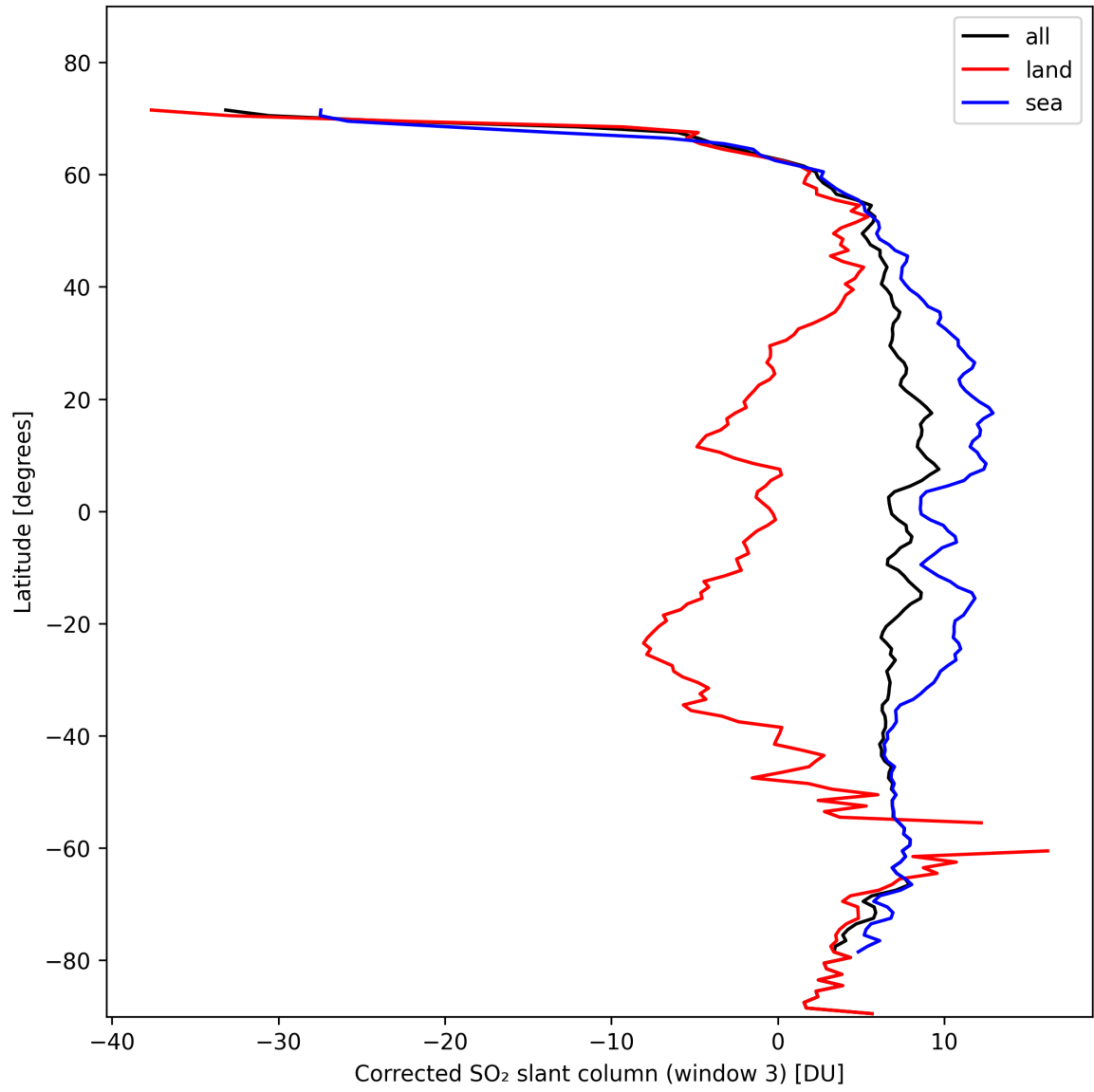
Figure 43: Zonal average of “Corrected SO 2 slant column (window 3)” for 2024-10-30 to 2024-10-31.
