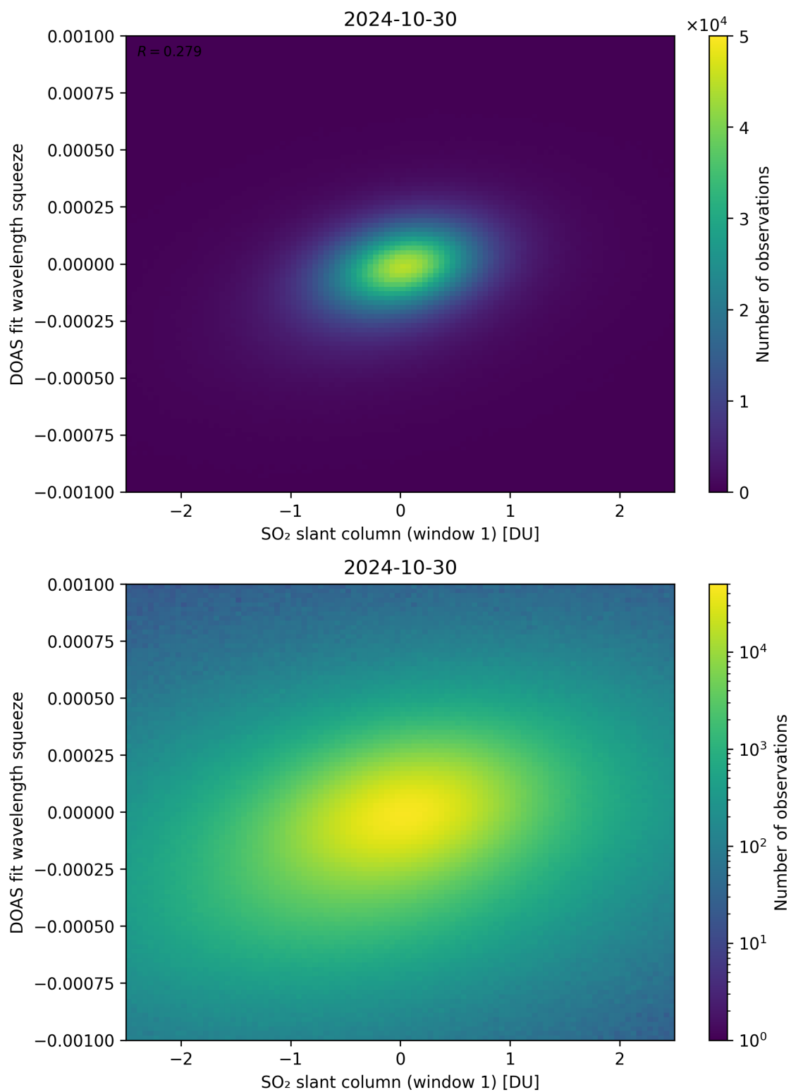
Figure 216: Scatter density plot of “SO 2 slant column (window 1)” against “DOAS fit wavelength squeeze” for 2024-10-30 to 2024-10-31.
