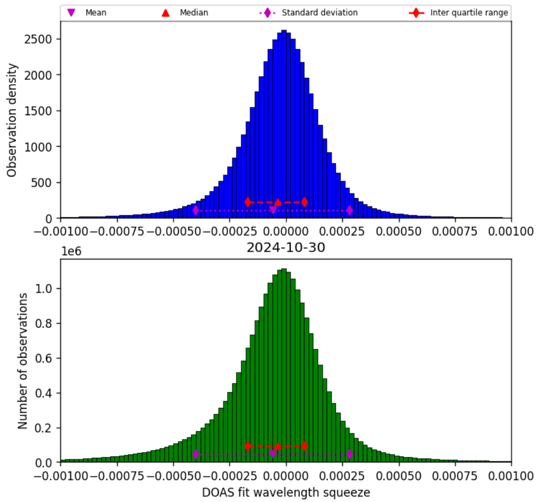
Figure 69: Histogram of “DOAS fit wavelength squeeze” for 2024-10-30 to 2024-10-31
