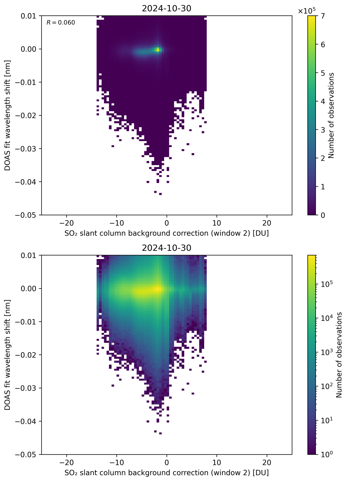
Figure 112: Scatter density plot of “SO 2 slant column background correction (window 2)” against “DOAS fit wavelength shift” for 2024-10-30 to 2024-10-31.
