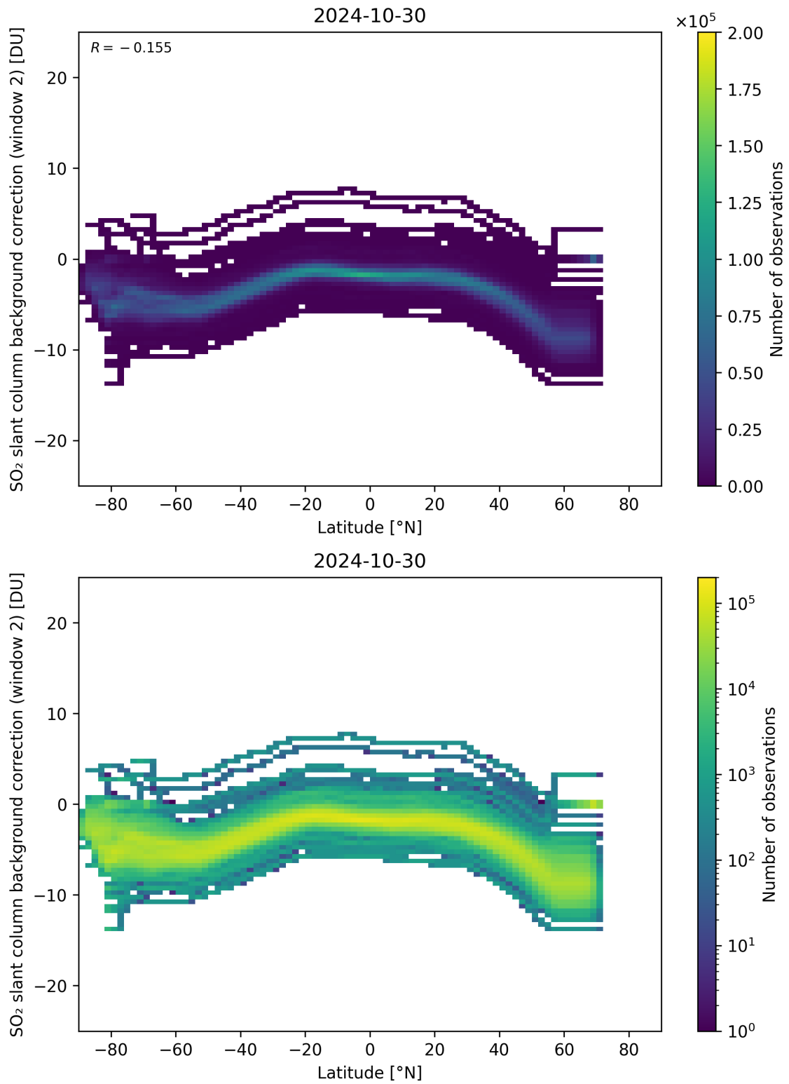
Figure 140: Scatter density plot of “Latitude” against “SO 2 slant column background correction (window 2)” for 2024-10-30 to 2024-10-31.
