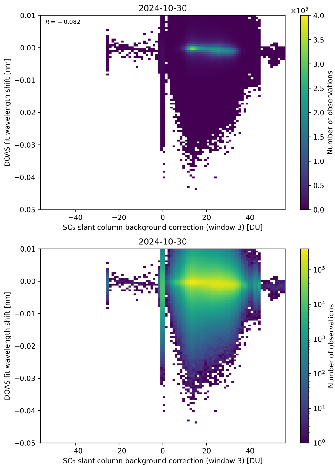
Figure 121: Scatter density plot of “SO 2 slant column background correction (window 3)” against “DOAS fit wavelength shift” for 2024-10-30 to 2024-10-31.
