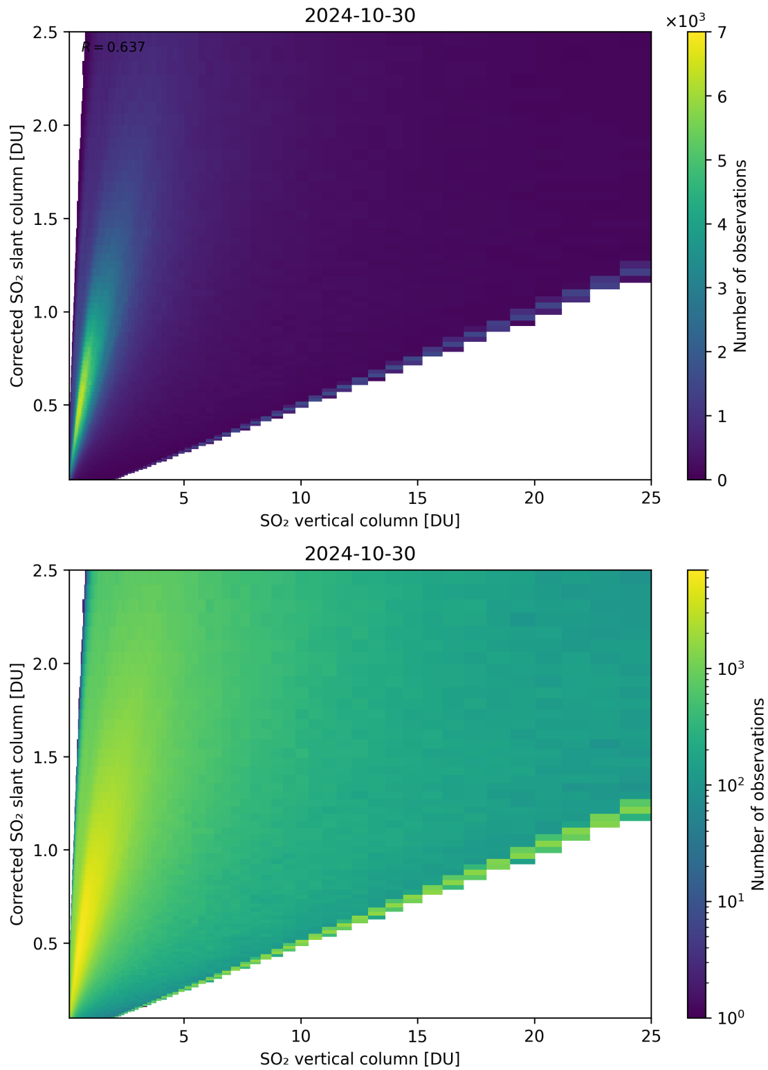
Figure 297: Scatter density plot of “SO 2 vertical column” against “Corrected SO 2 slant column” for 2024-10-30 to 2024-10-31.
