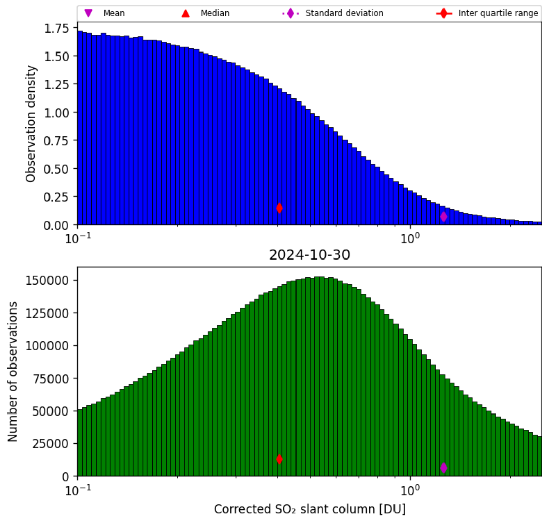
Figure 55: Histogram of “Corrected SO 2 slant column” for 2024-10-30 to 2024-10-31
