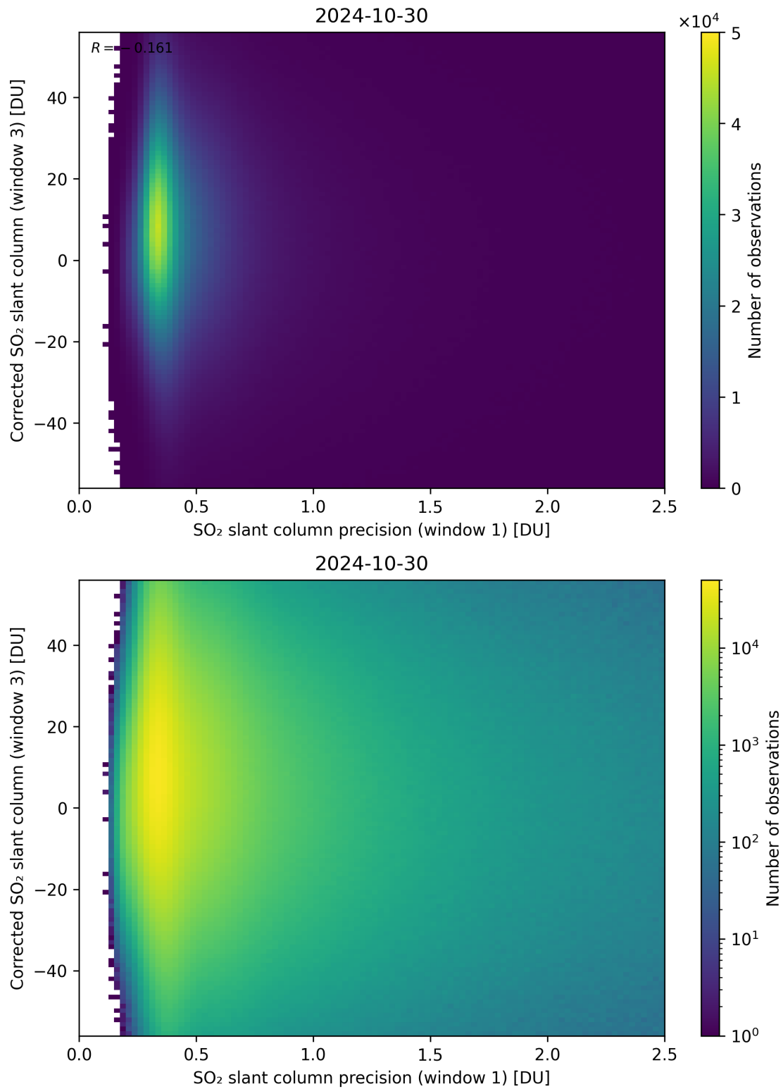
Figure 226: Scatter density plot of “SO 2 slant column precision (window 1)” against “Corrected SO 2 slant column (window 3)” for 2024-10-30 to 2024-10-31.
