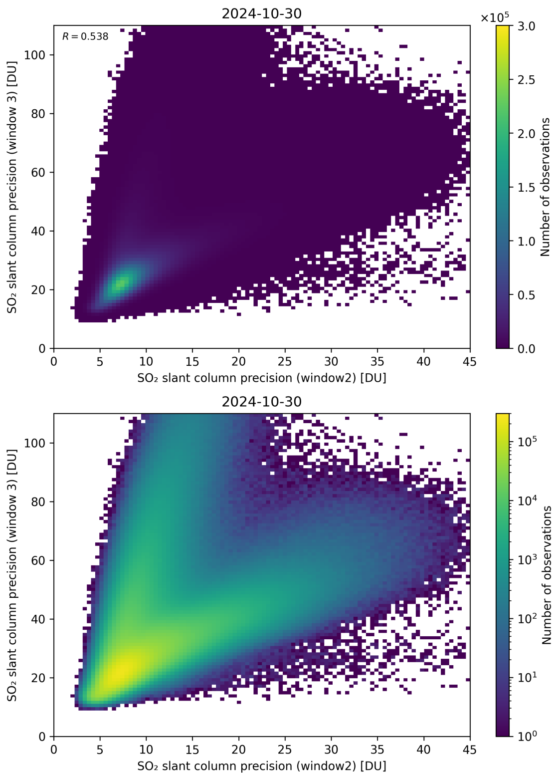
Figure 250: Scatter density plot of “SO 2 slant column precision (window2)” against “SO 2 slant column precision (window 3)” for 2024-10-30 to 2024-10-31.
