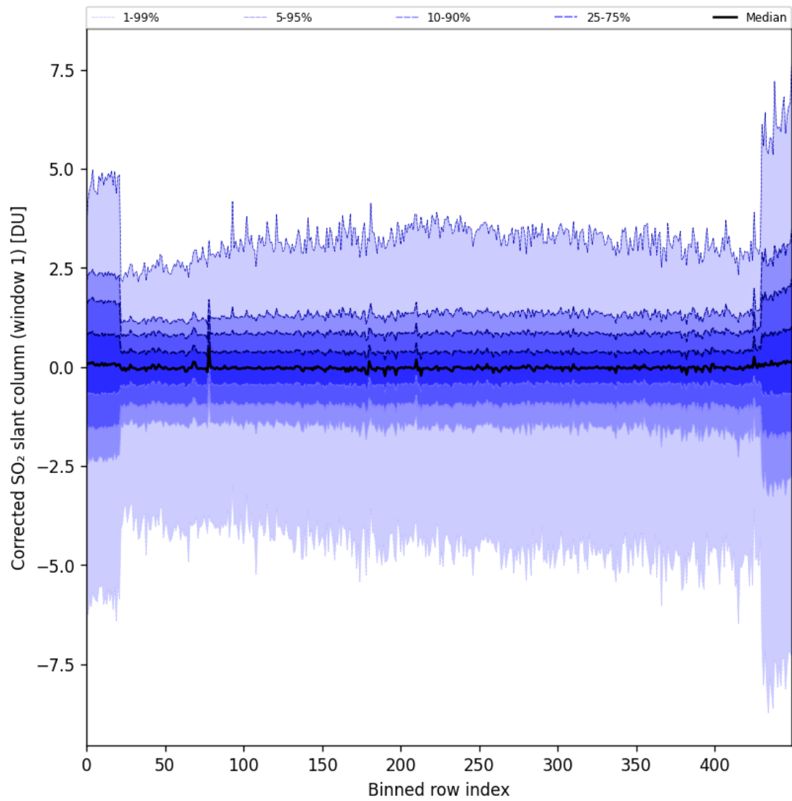
Figure 81: Along track statistics of “Corrected SO 2 slant column (window 1)” for 2024-10-30 to 2024-10-31
