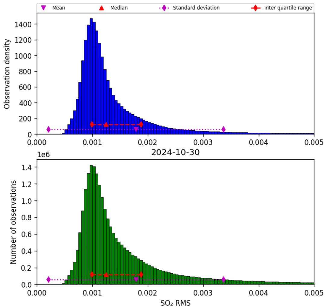
Figure 70: Histogram of “SO 2 RMS” for 2024-10-30 to 2024-10-31
