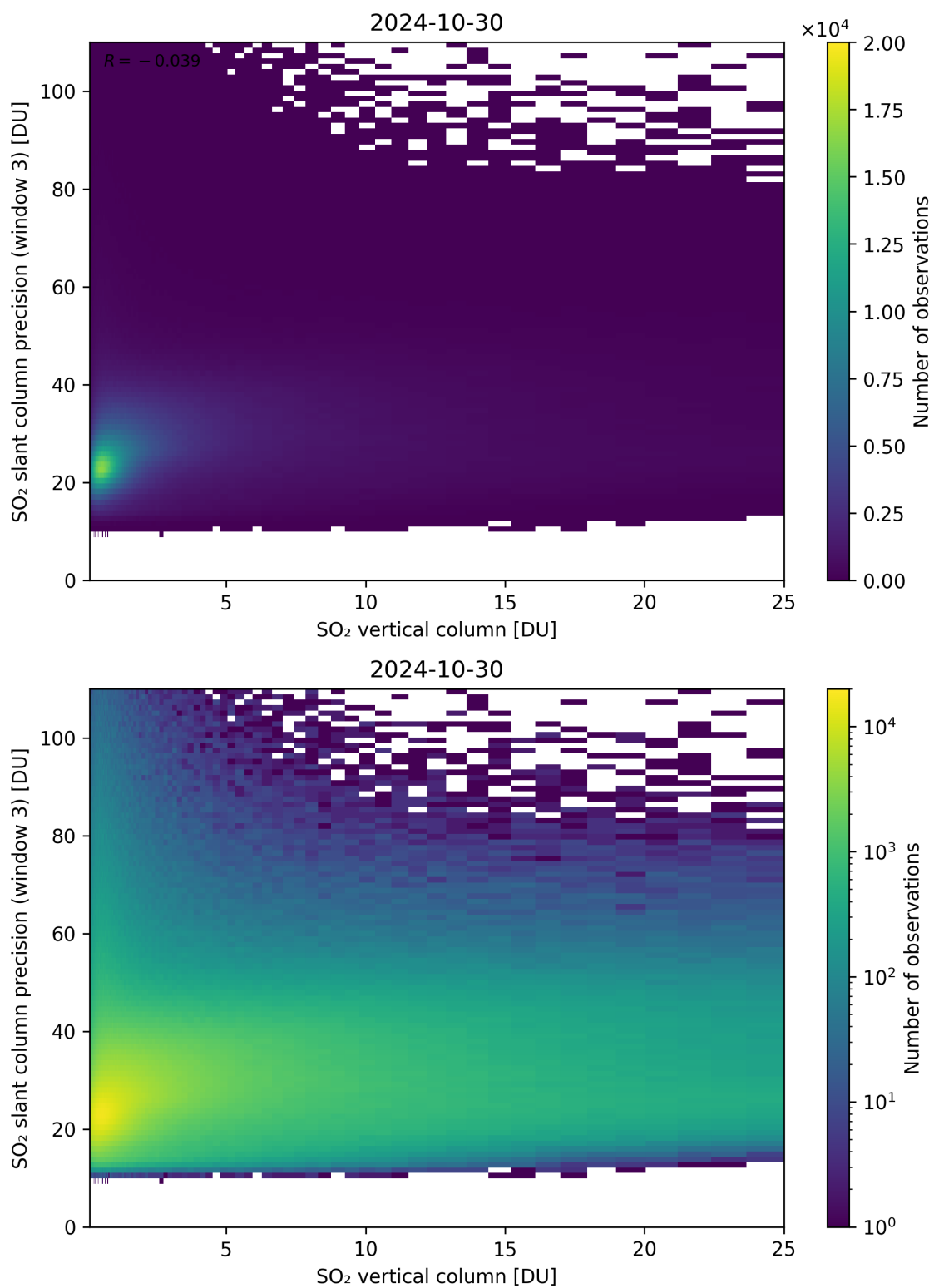
Figure 304: Scatter density plot of “SO 2 vertical column” against “SO 2 slant column precision (window 3)” for 2024-10-30 to 2024-10-31.
