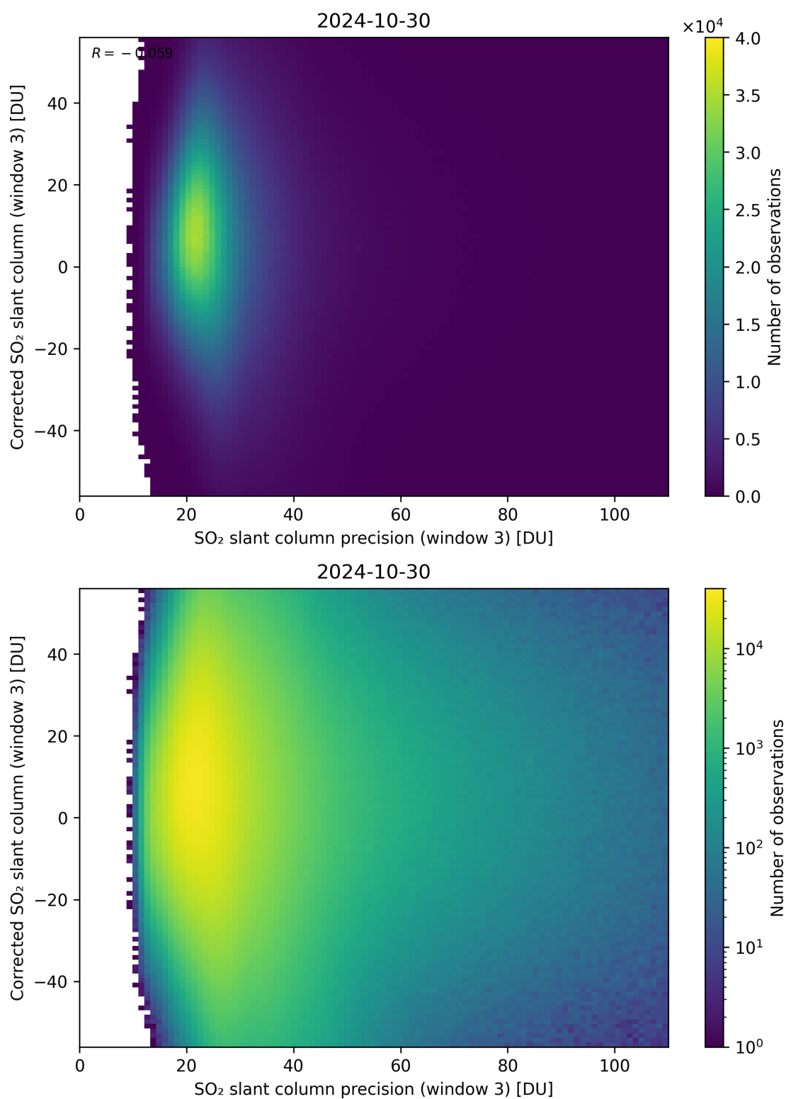
Figure 262: Scatter density plot of “SO 2 slant column precision (window 3)” against “Corrected SO 2 slant column (window 3)” for 2024-10-30 to 2024-10-31.
