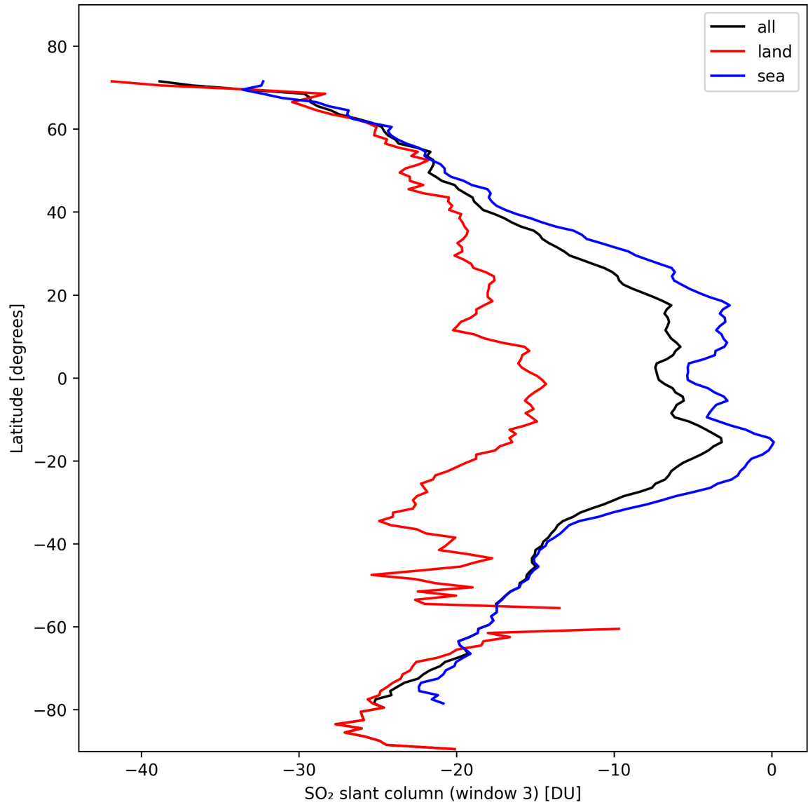
Figure 41: Zonal average of “SO 2 slant column (window 3)” for 2024-10-30 to 2024-10-31.
