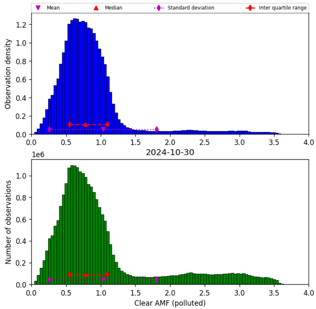
Figure 73: Histogram of “Clear AMF (polluted)” for 2024-10-30 to 2024-10-31
