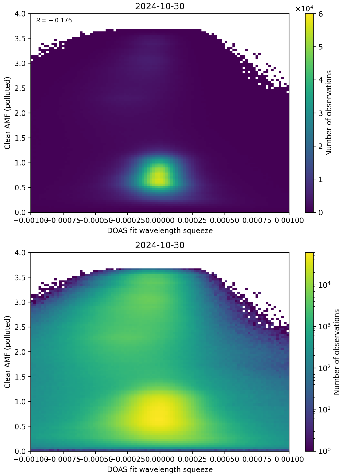
Figure 133: Scatter density plot of “DOAS fit wavelength squeeze” against “Clear AMF (polluted)” for 2024-10-30 to 2024-10-31.
