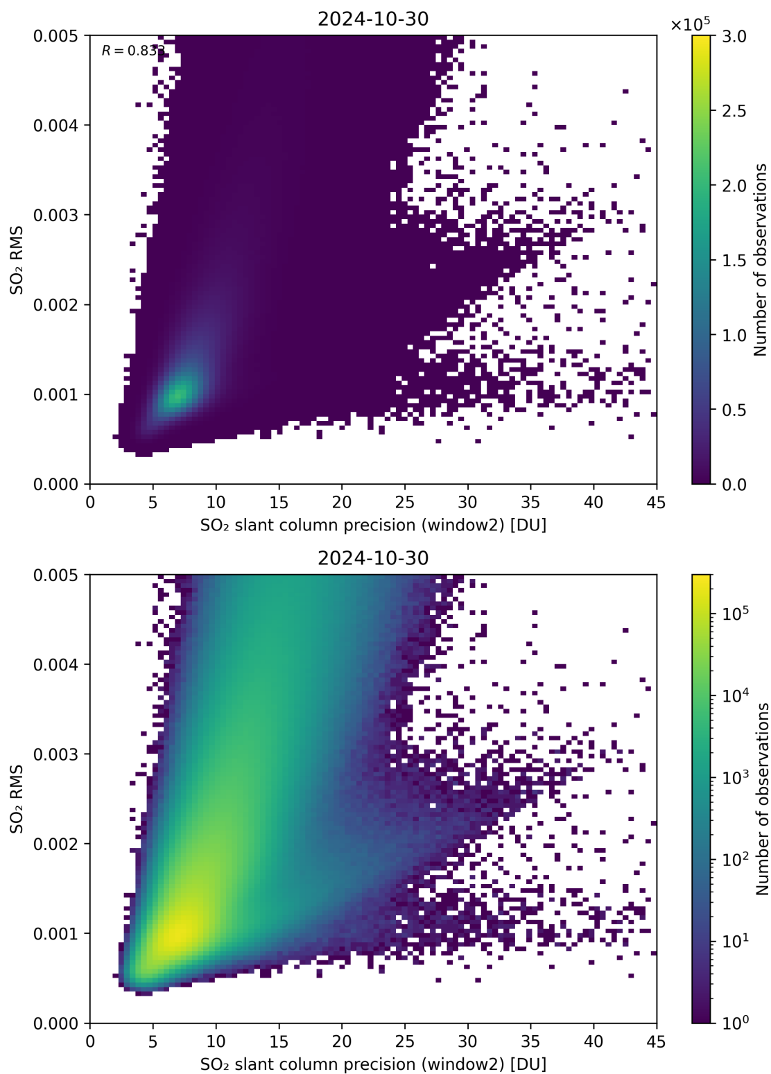
Figure 245: Scatter density plot of “SO 2 slant column precision (window2)” against “SO 2 RMS” for 2024-10-30 to 2024-10-31.
