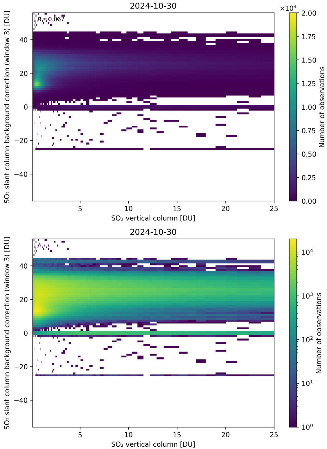
Figure 275: Scatter density plot of “SO 2 vertical column” against “SO 2 slant column background correction (window 3)” for 2024-10-30 to 2024-10-31.
