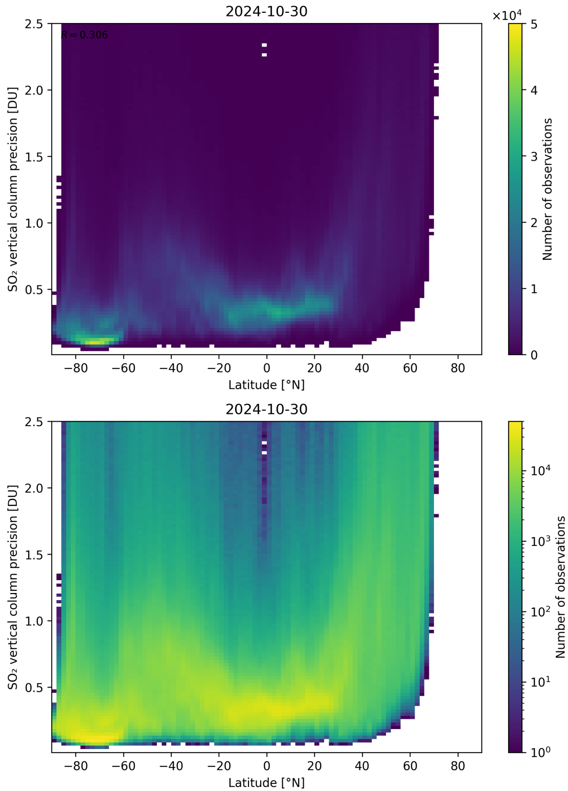
Figure 157: Scatter density plot of “Latitude” against “SO 2 vertical column precision” for 2024-10-30 to 2024-10-31.
