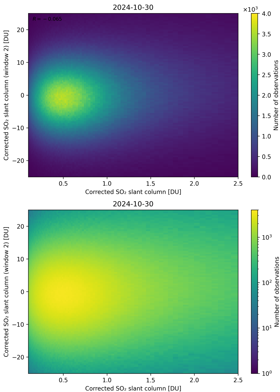
Figure 185: Scatter density plot of “Corrected SO 2 slant column” against “Corrected SO 2 slant column (window 2)” for 2024-10-30 to 2024-10-31.
