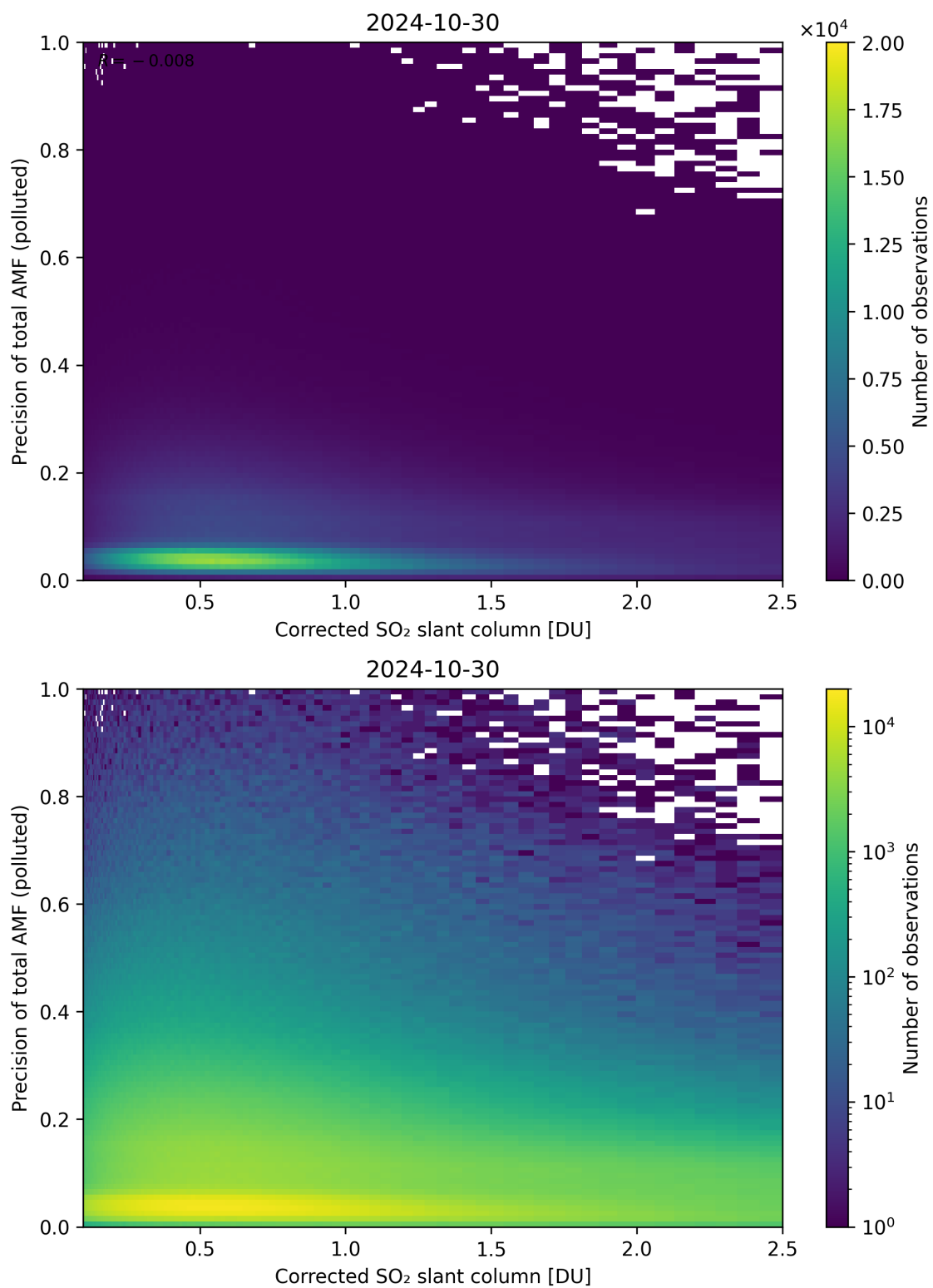
Figure 193: Scatter density plot of “Corrected SO 2 slant column” against “Precision of total AMF (polluted)” for 2024-10-30 to 2024-10-31.
