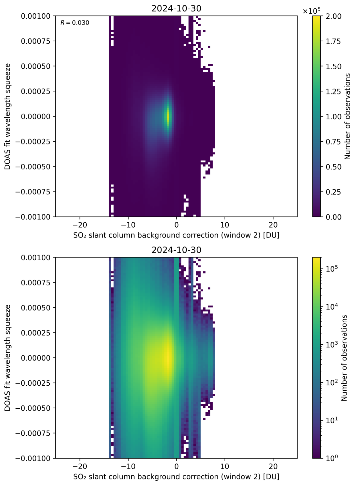
Figure 113: Scatter density plot of “SO 2 slant column background correction (window 2)” against “DOAS fit wavelength squeeze” for 2024-10-30 to 2024-10-31.
