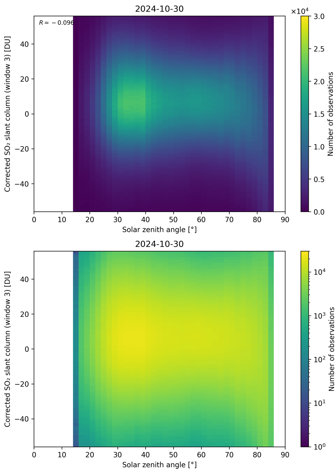
Figure 168: Scatter density plot of “Solar zenith angle” against “Corrected SO 2 slant column (window 3)” for 2024-10-30 to 2024-10-31.
