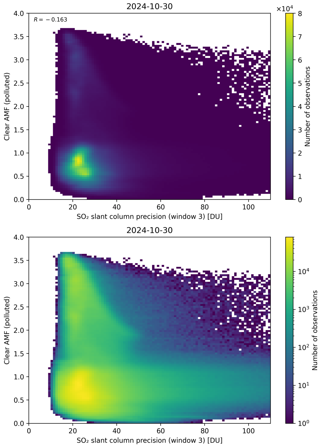
Figure 261: Scatter density plot of “SO 2 slant column precision (window 3)” against “Clear AMF (polluted)” for 2024-10-30 to 2024-10-31.
