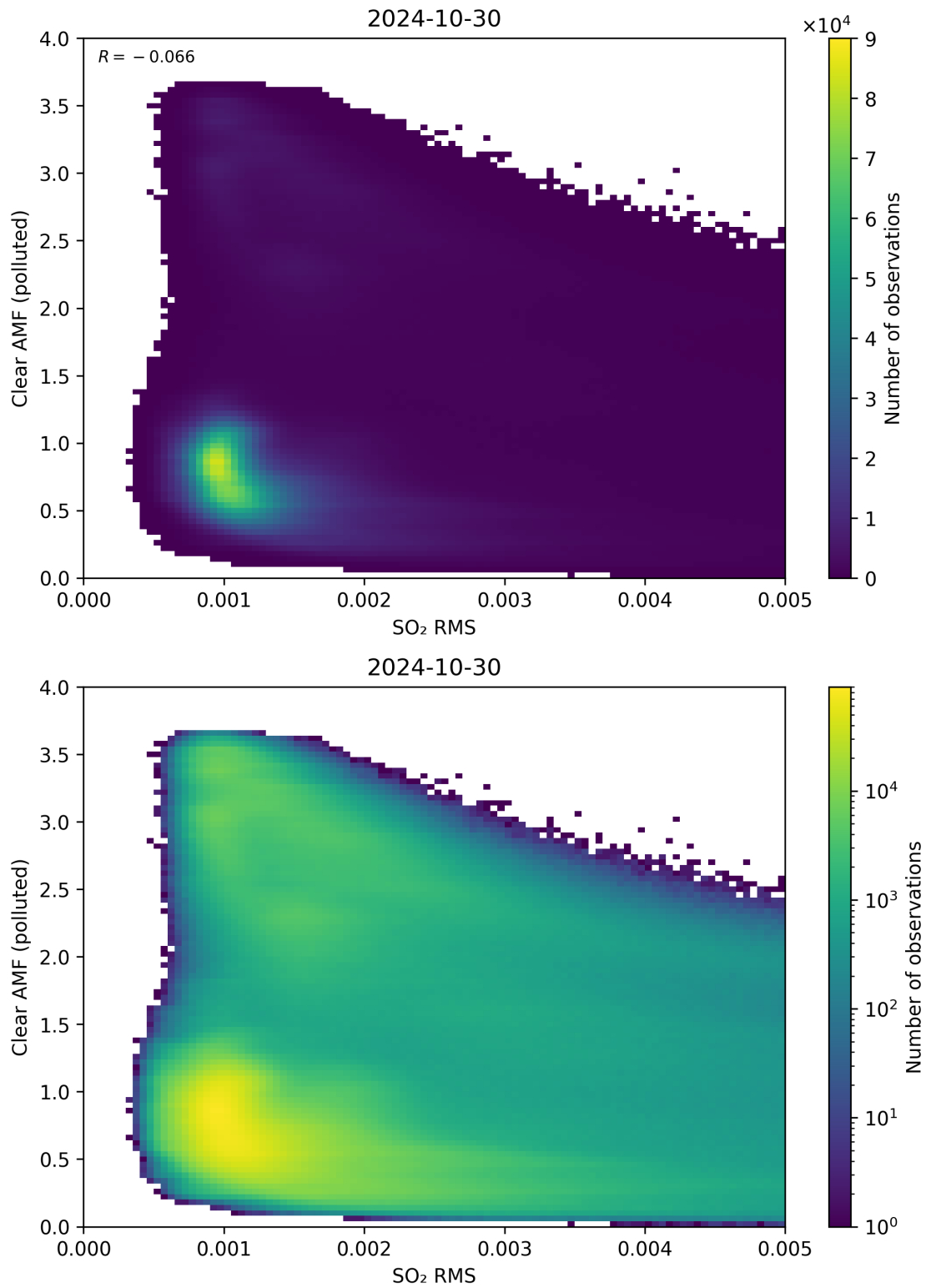
Figure 136: Scatter density plot of “SO 2 RMS” against “Clear AMF (polluted)” for 2024-10-30 to 2024-10-31.
