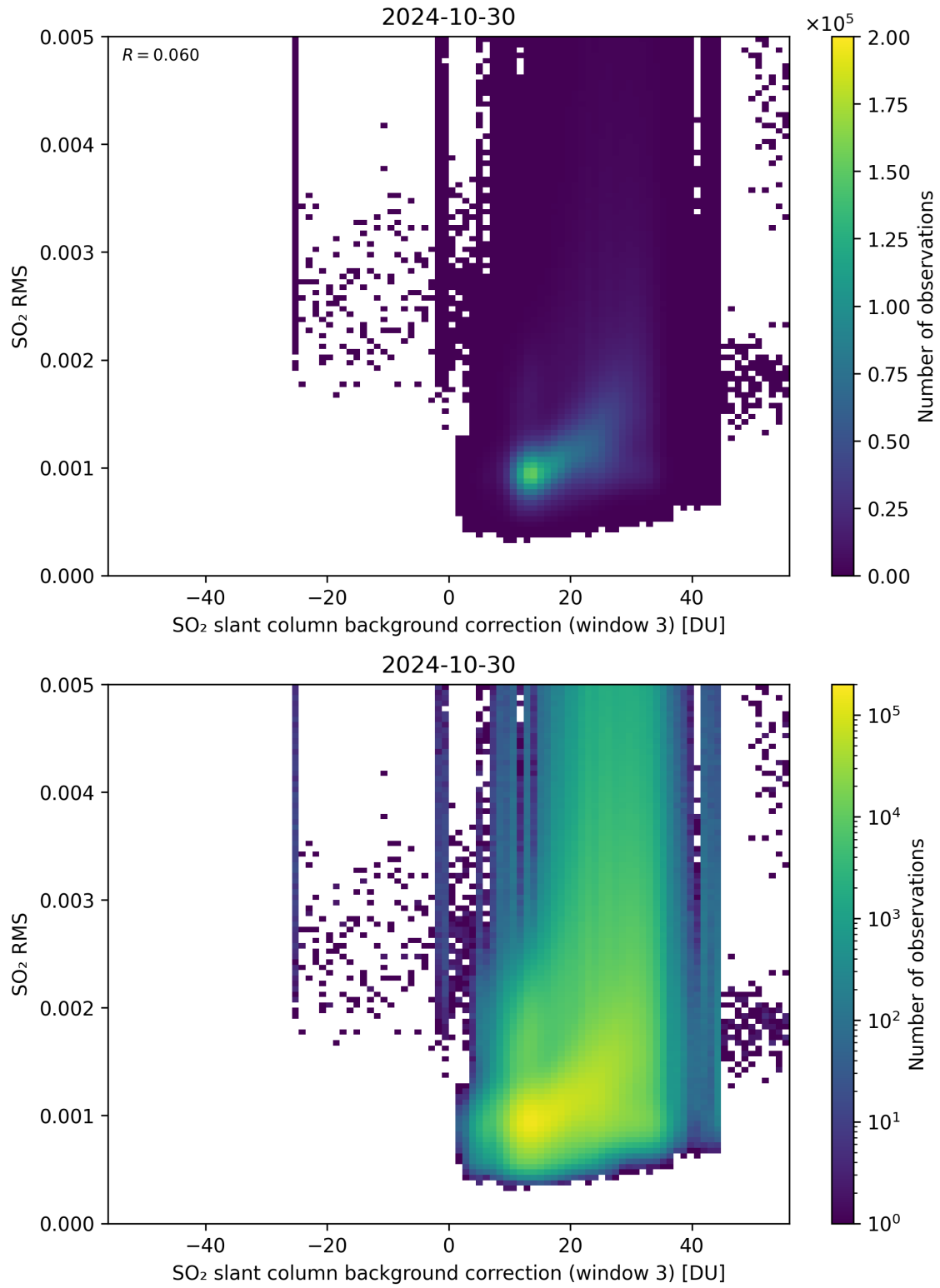
Figure 123: Scatter density plot of “SO 2 slant column background correction (window 3)” against “SO 2 RMS” for 2024-10-30 to 2024-10-31.
