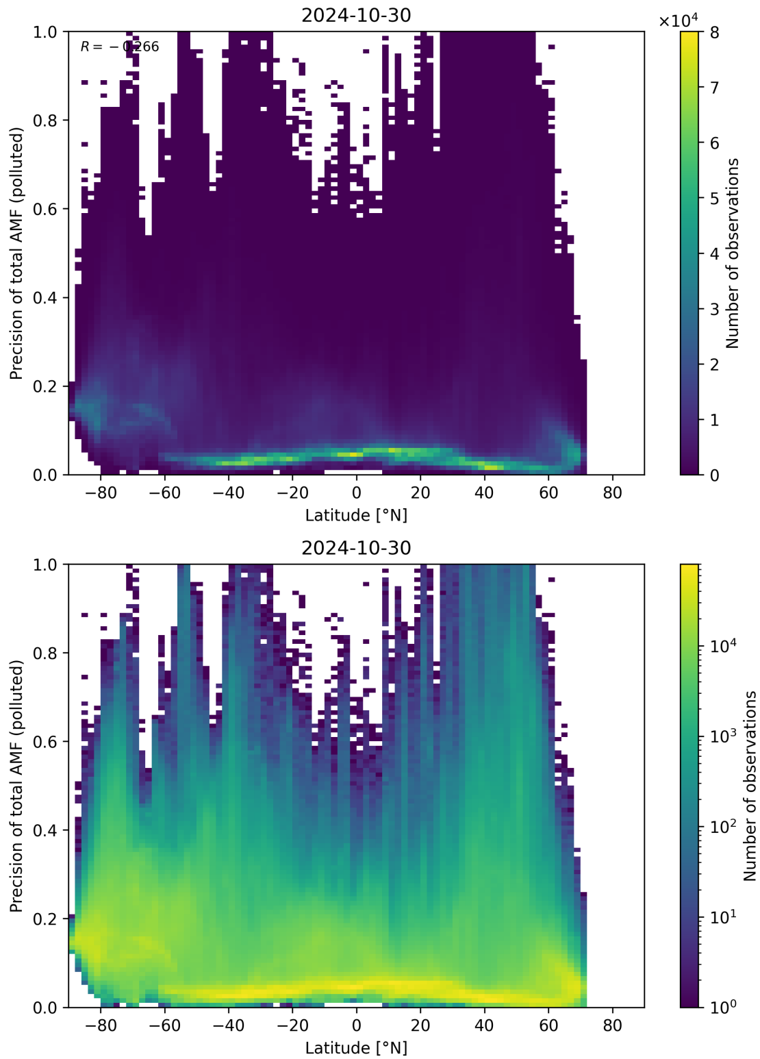
Figure 155: Scatter density plot of “Latitude” against “Precision of total AMF (polluted)” for 2024-10-30 to 2024-10-31.
