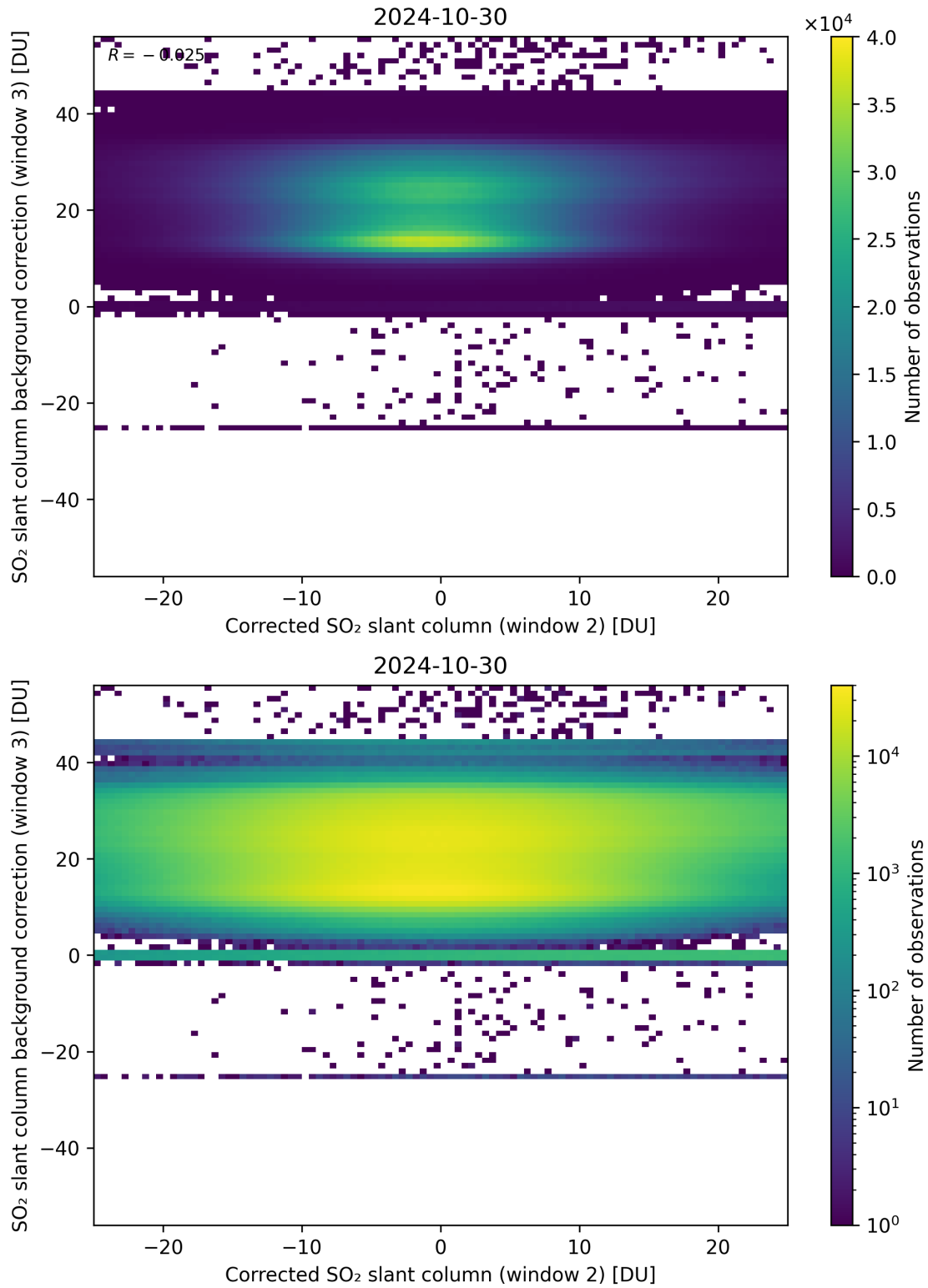
Figure 195: Scatter density plot of “Corrected SO 2 slant column (window 2)” against “SO 2 slant column background correction (window 3)” for 2024-10-30 to 2024-10-31.
