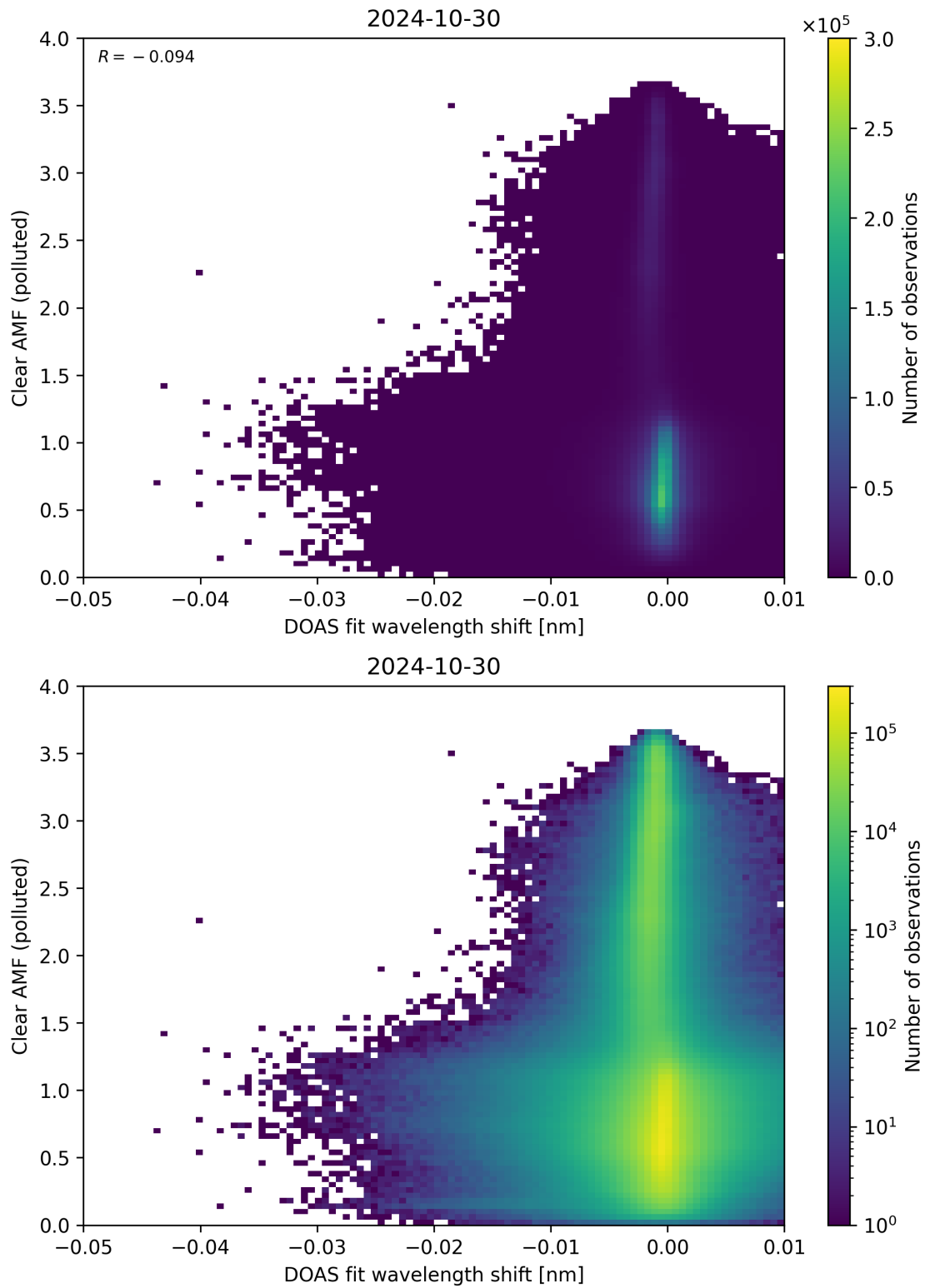
Figure 129: Scatter density plot of “DOAS fit wavelength shift” against “Clear AMF (polluted)” for 2024-10-30 to 2024-10-31.
