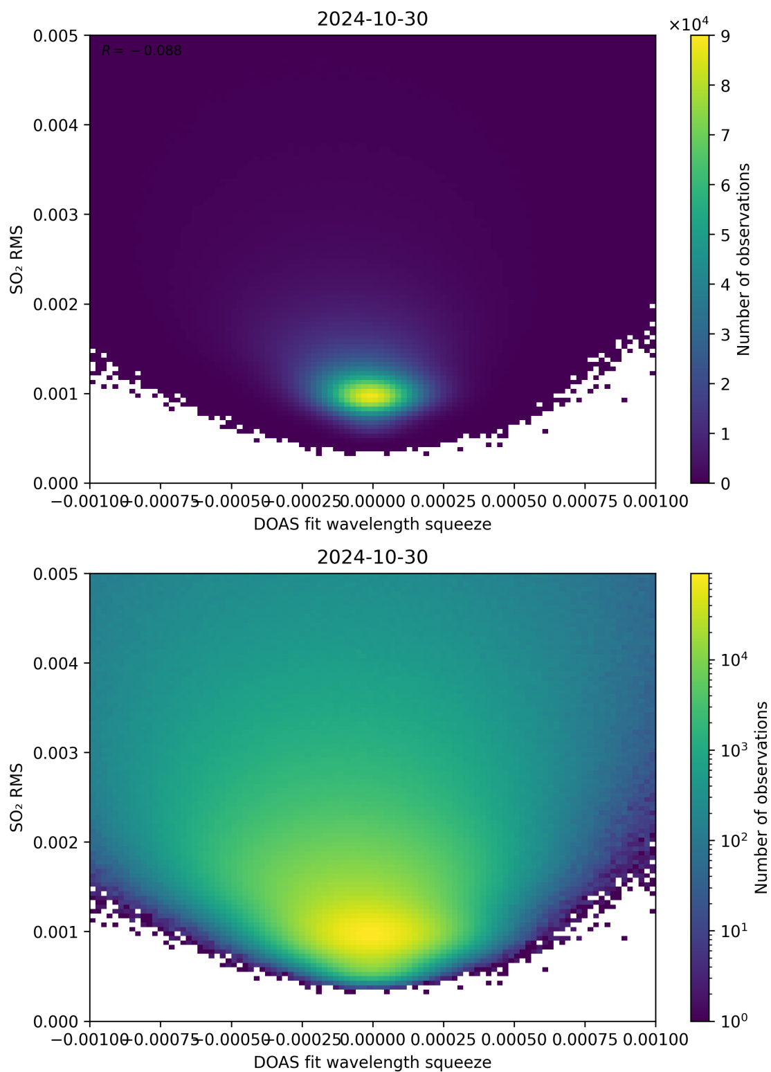
Figure 132: Scatter density plot of “DOAS fit wavelength squeeze” against “SO 2 RMS” for 2024-10-30 to 2024-10-31.
