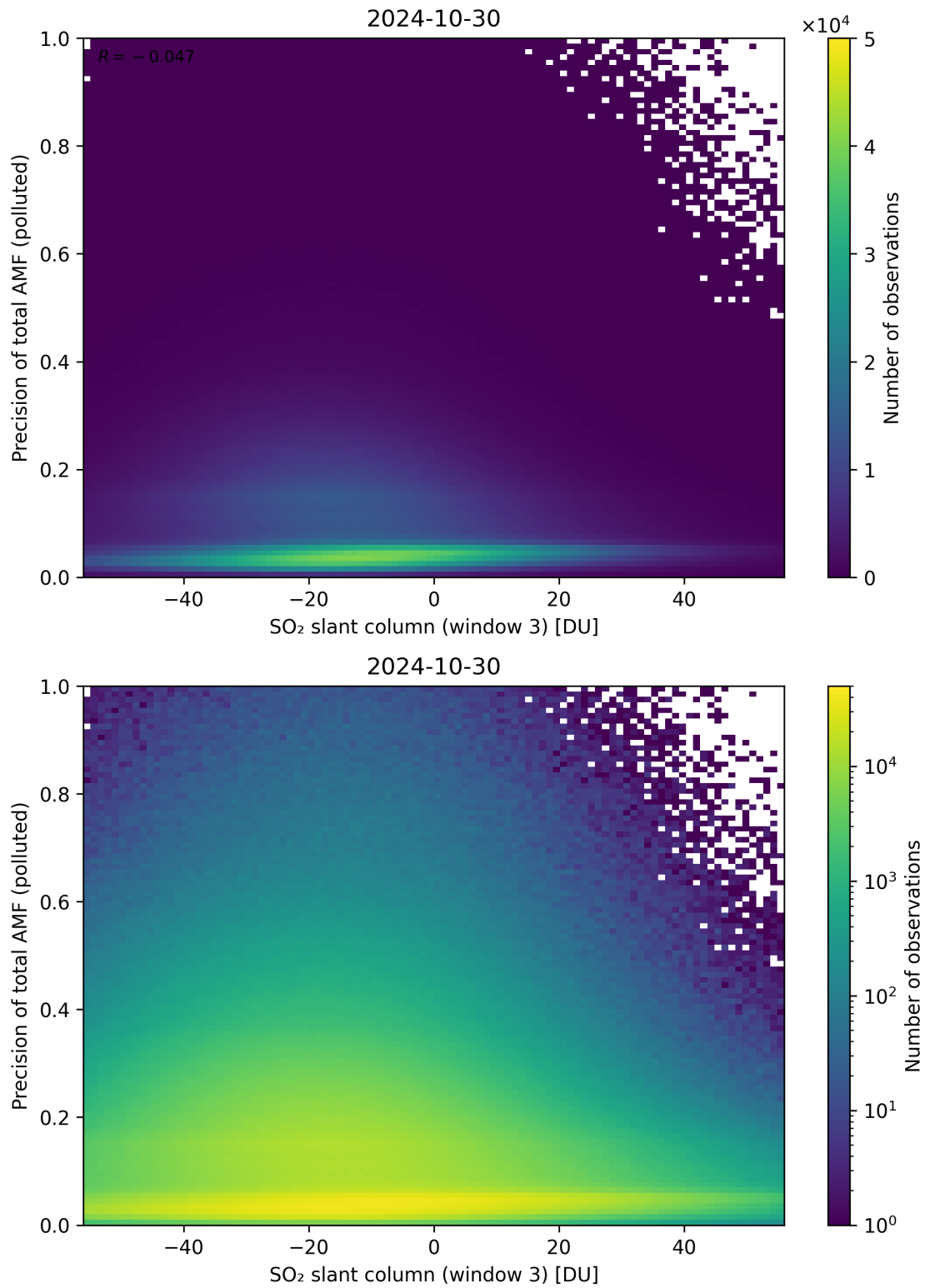
Figure 269: Scatter density plot of “SO 2 slant column (window 3)” against “Precision of total AMF (polluted)” for 2024-10-30 to 2024-10-31.
