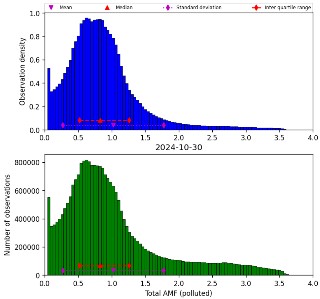
Figure 71: Histogram of “Total AMF (polluted)” for 2024-10-30 to 2024-10-31
