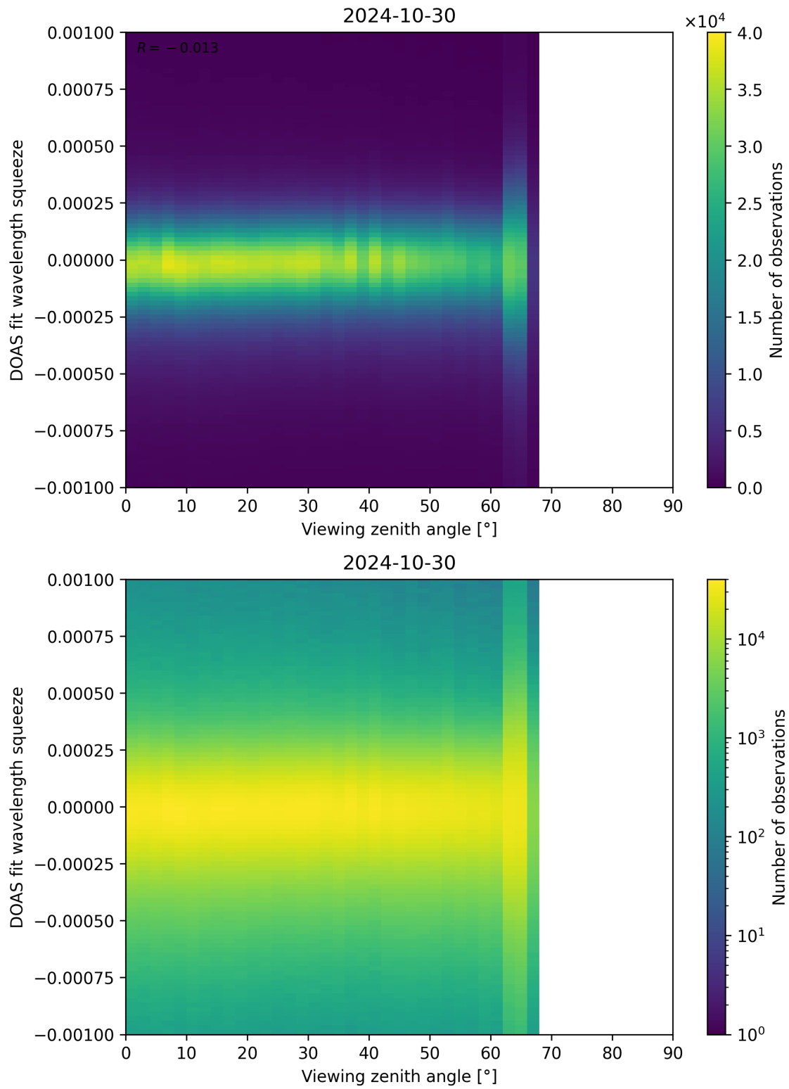
Figure 312: Scatter density plot of “Viewing zenith angle” against “DOAS fit wavelength squeeze” for 2024-10-30 to 2024-10-31.
