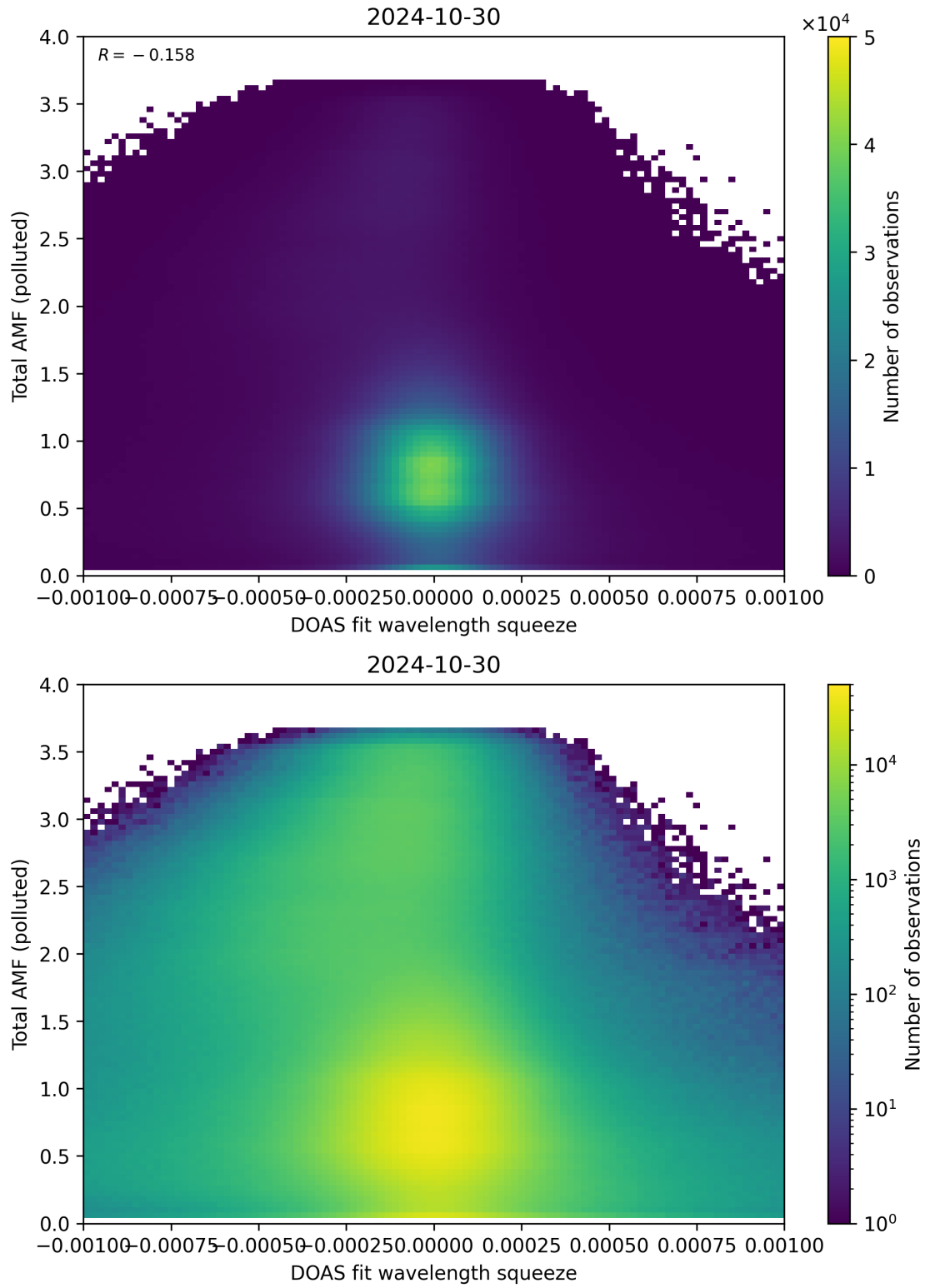
Figure 134: Scatter density plot of “DOAS fit wavelength squeeze” against “Total AMF (polluted)” for 2024-10-30 to 2024-10-31.
