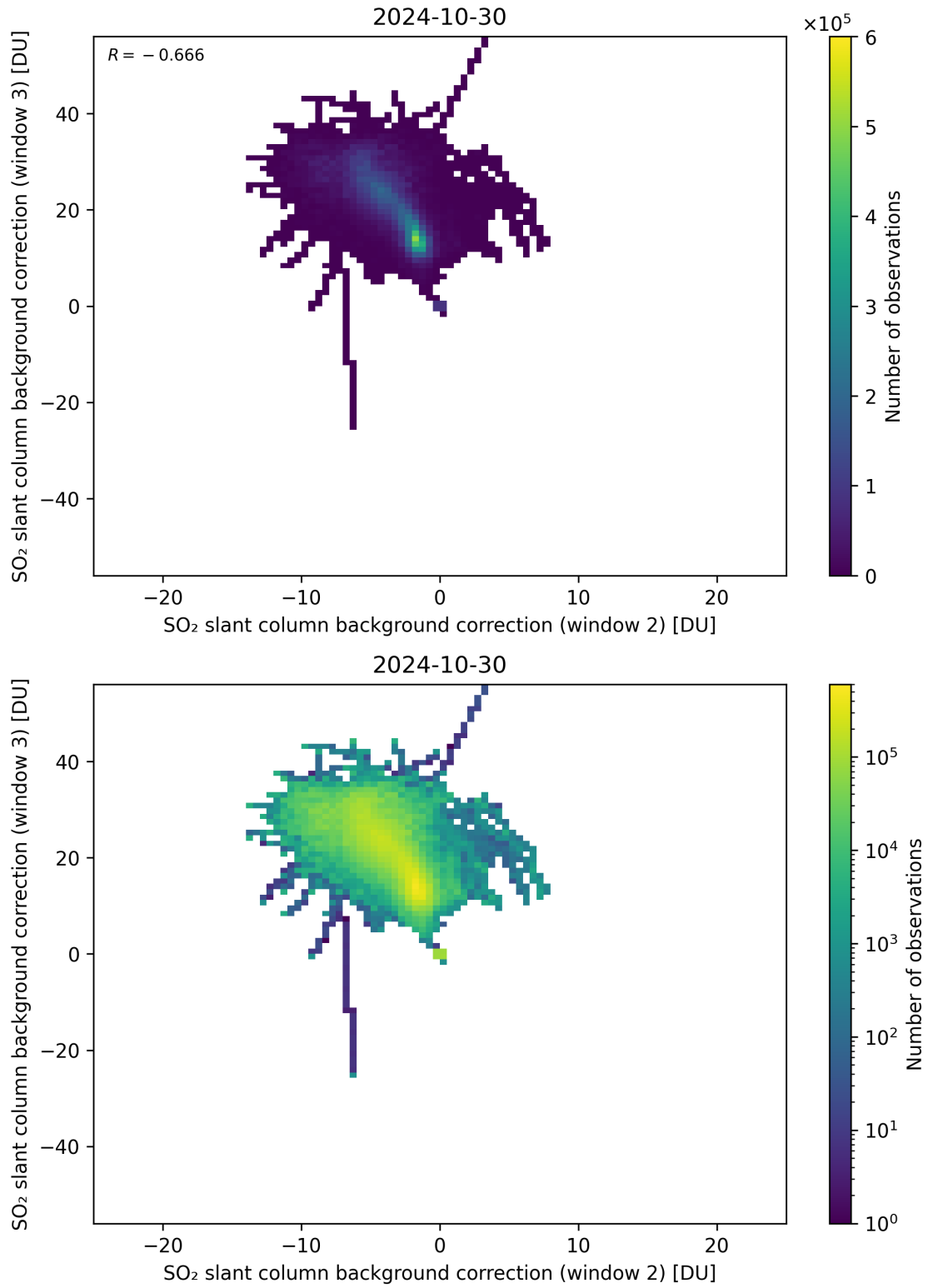
Figure 111: Scatter density plot of “SO 2 slant column background correction (window 2)” against “SO 2 slant column background correction (window 3)” for 2024-10-30 to 2024-10-31.
