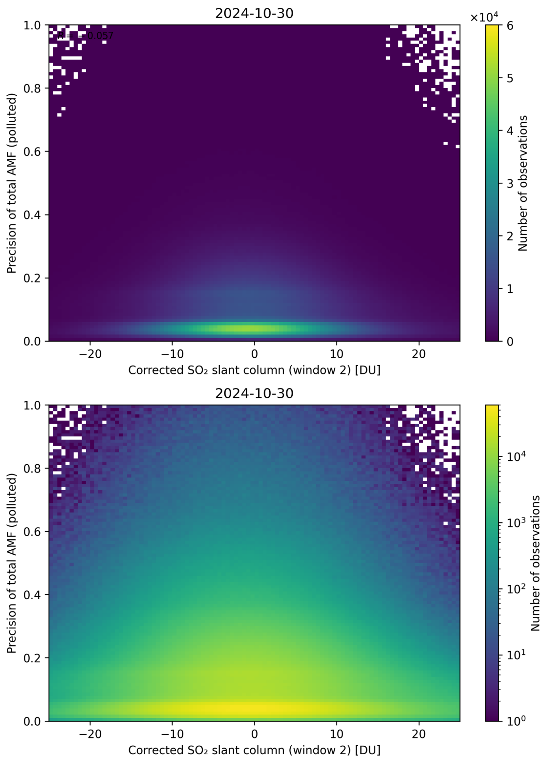
Figure 204: Scatter density plot of “Corrected SO 2 slant column (window 2)” against “Precision of total AMF (polluted)” for 2024-10-30 to 2024-10-31.
