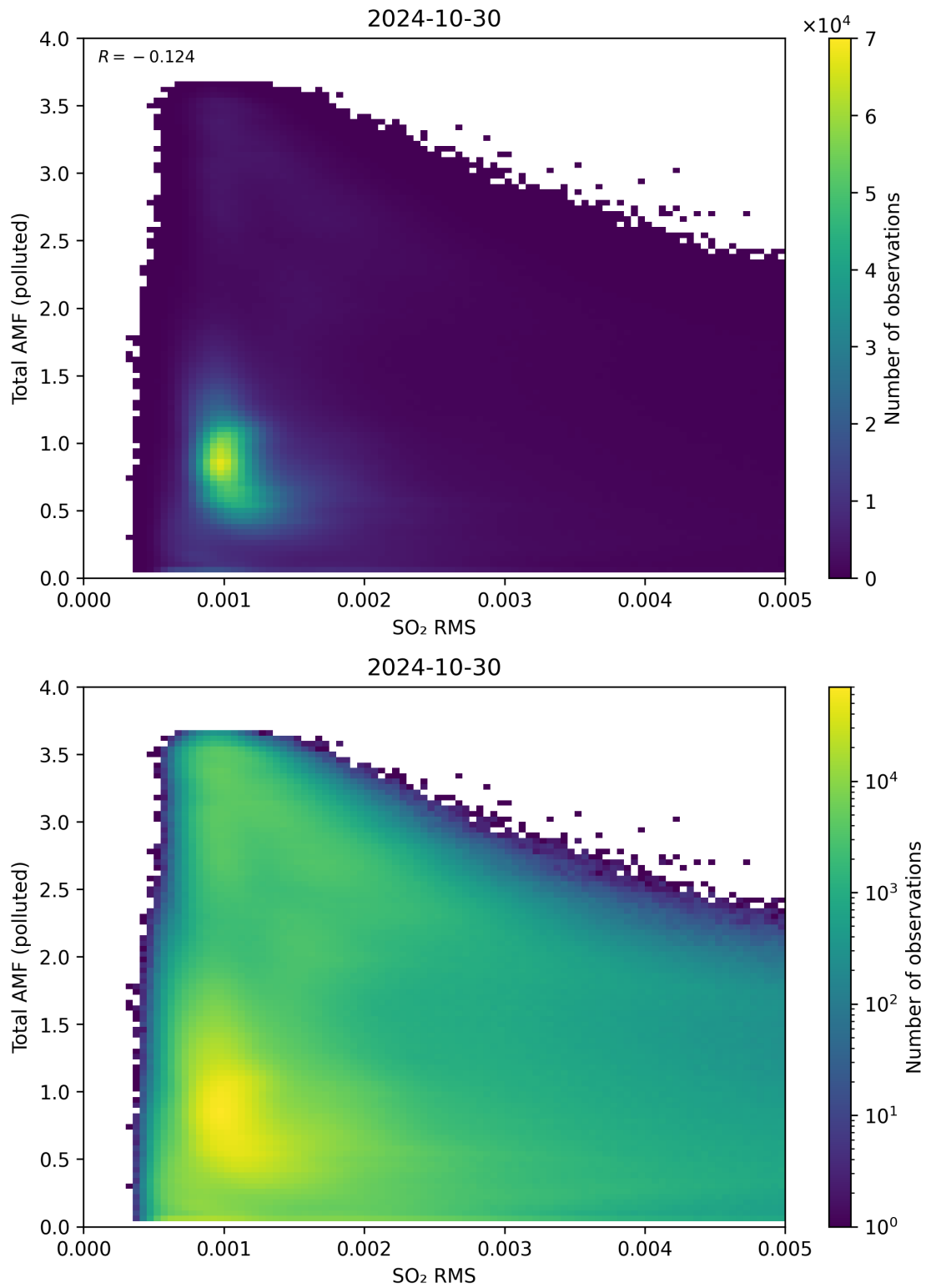
Figure 137: Scatter density plot of “SO 2 RMS” against “Total AMF (polluted)” for 2024-10-30 to 2024-10-31.
