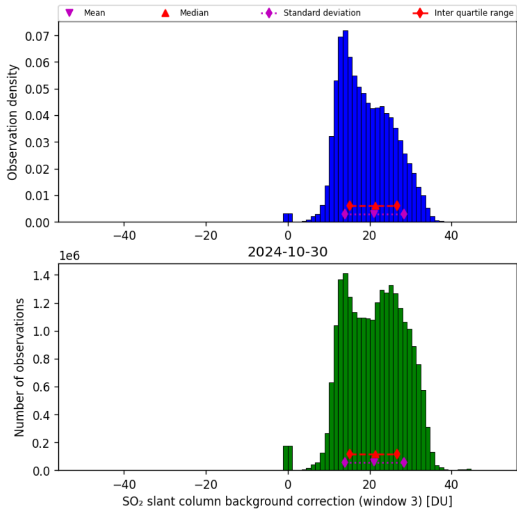
Figure 67: Histogram of “SO 2 slant column background correction (window 3)” for 2024-10-30 to 2024-10-31
