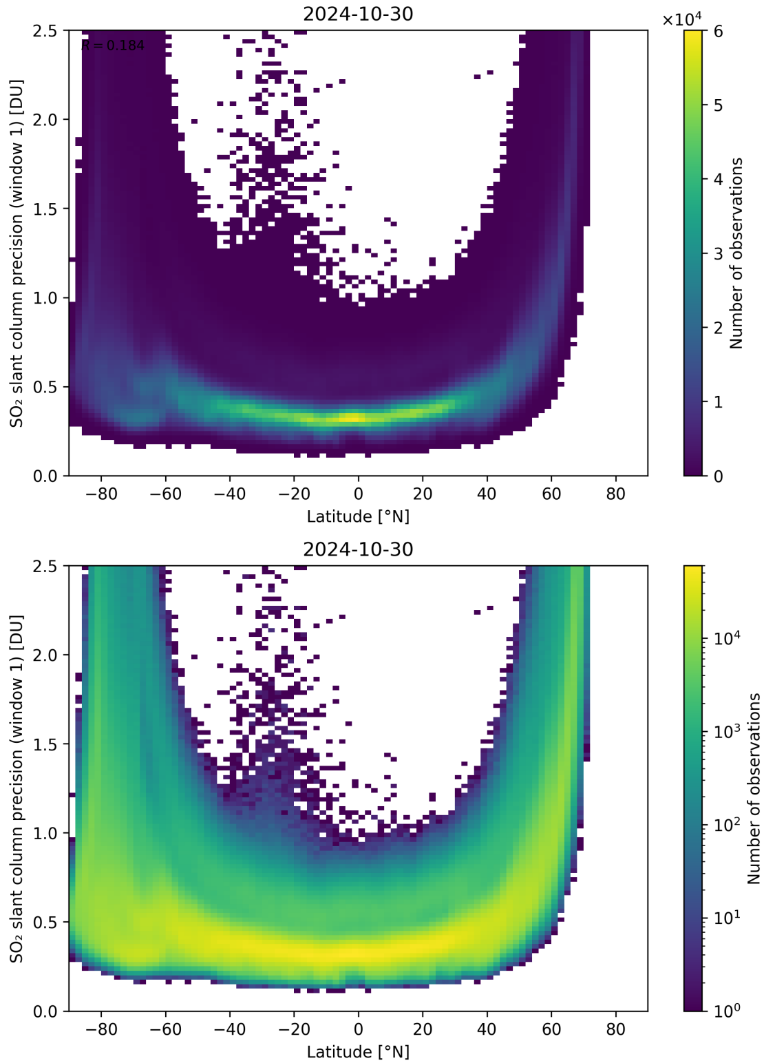
Figure 150: Scatter density plot of “Latitude” against “SO 2 slant column precision (window 1)” for 2024-10-30 to 2024-10-31.
