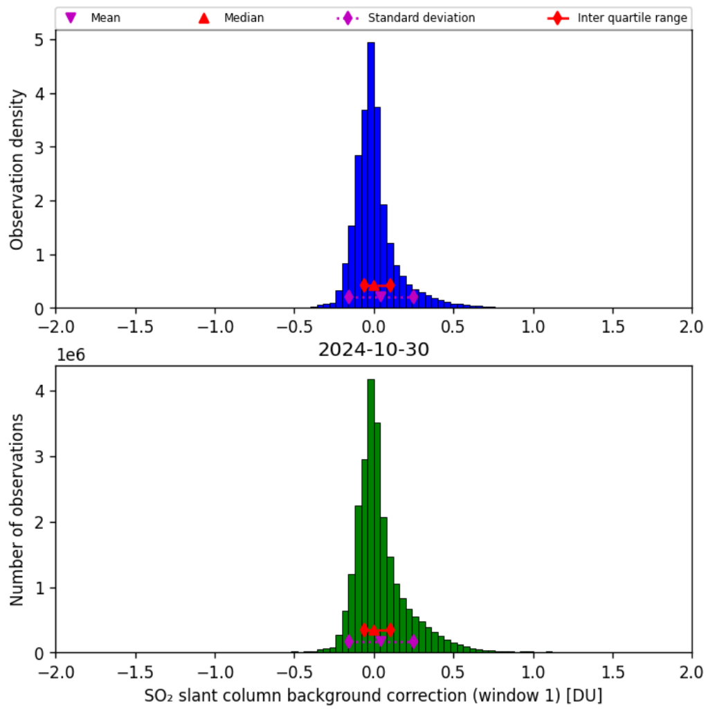
Figure 59: Histogram of “SO 2 slant column background correction (window 1)” for 2024-10-30 to 2024-10-31
