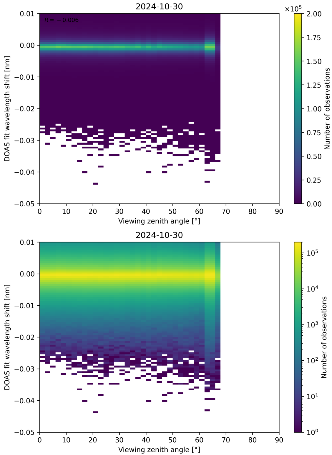
Figure 311: Scatter density plot of “Viewing zenith angle” against “DOAS fit wavelength shift” for 2024-10-30 to 2024-10-31.
