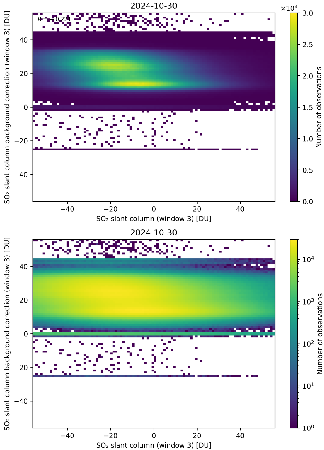
Figure 253: Scatter density plot of “SO 2 slant column (window 3)” against “SO 2 slant column background correction (window 3)” for 2024-10-30 to 2024-10-31.
