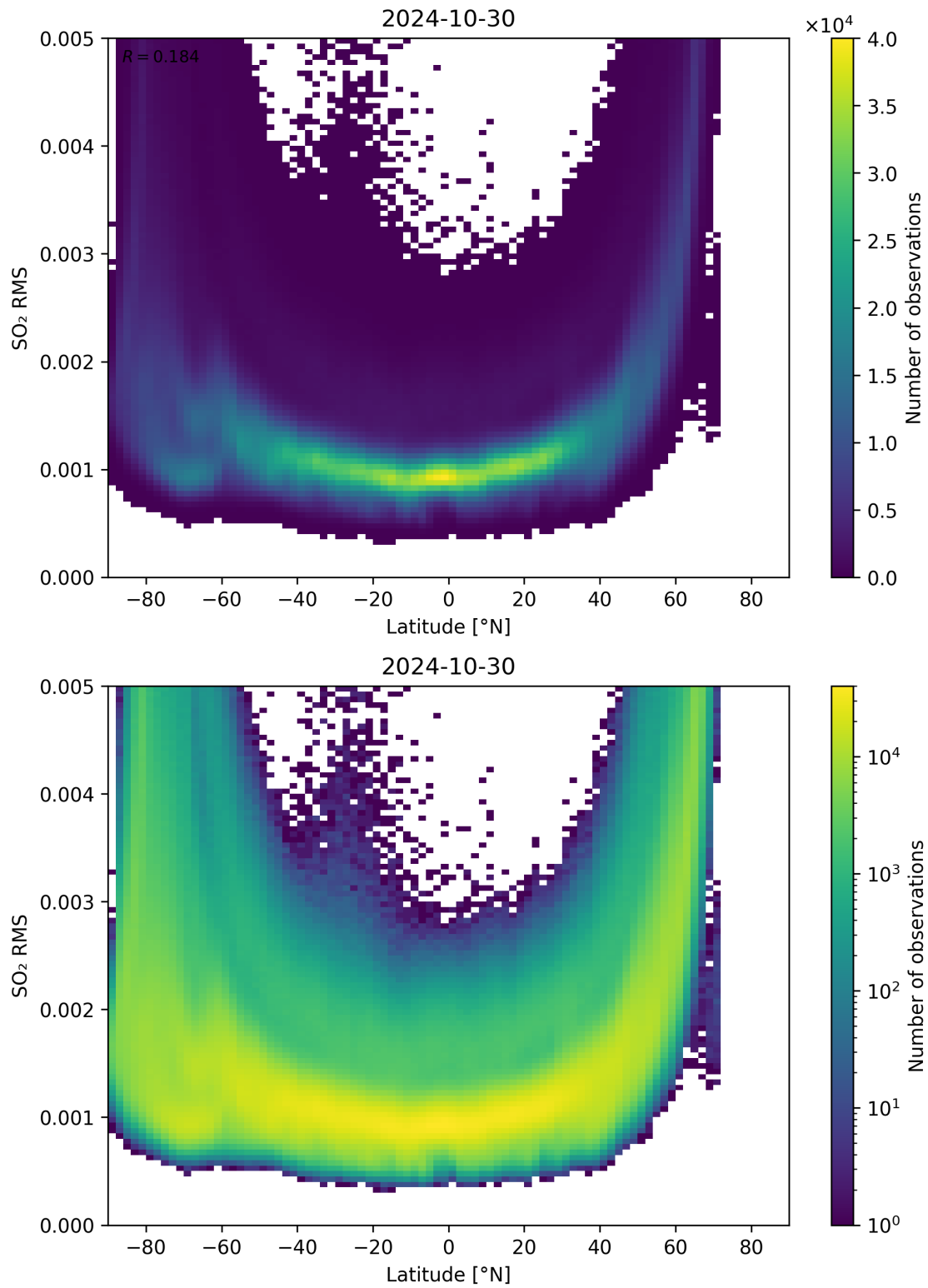
Figure 144: Scatter density plot of “Latitude” against “SO 2 RMS” for 2024-10-30 to 2024-10-31.
