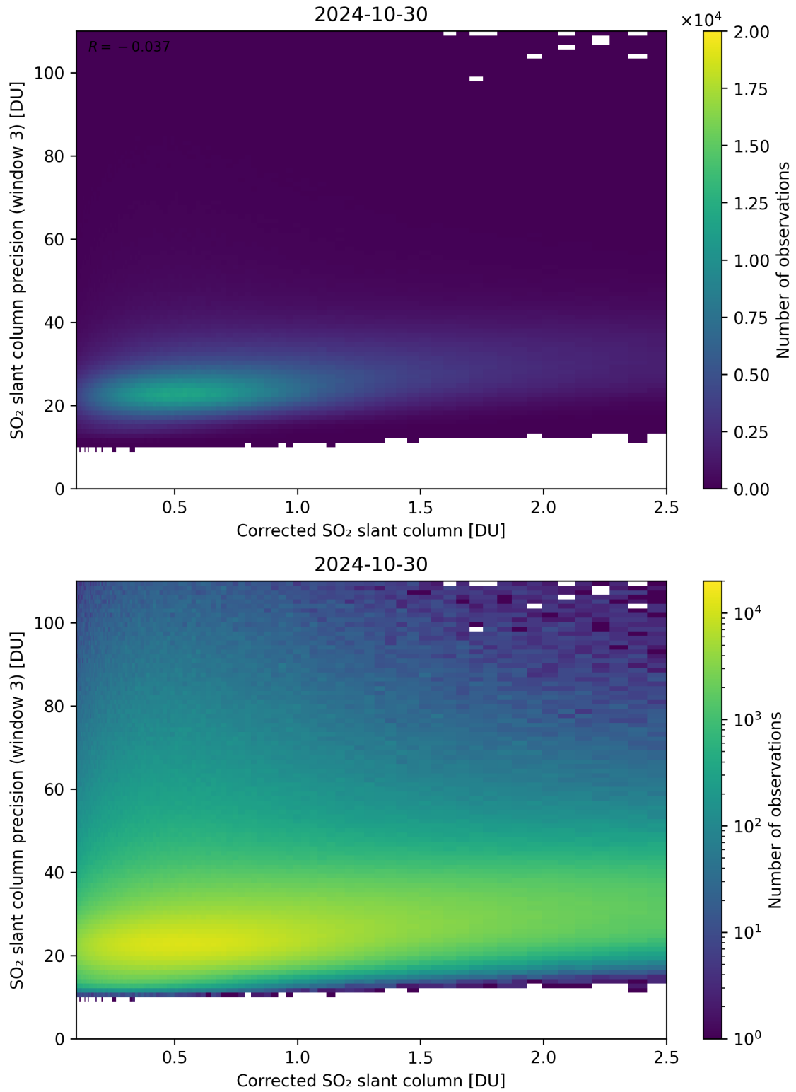
Figure 191: Scatter density plot of “Corrected SO 2 slant column” against “SO 2 slant column precision (window 3)” for 2024-10-30 to 2024-10-31.
