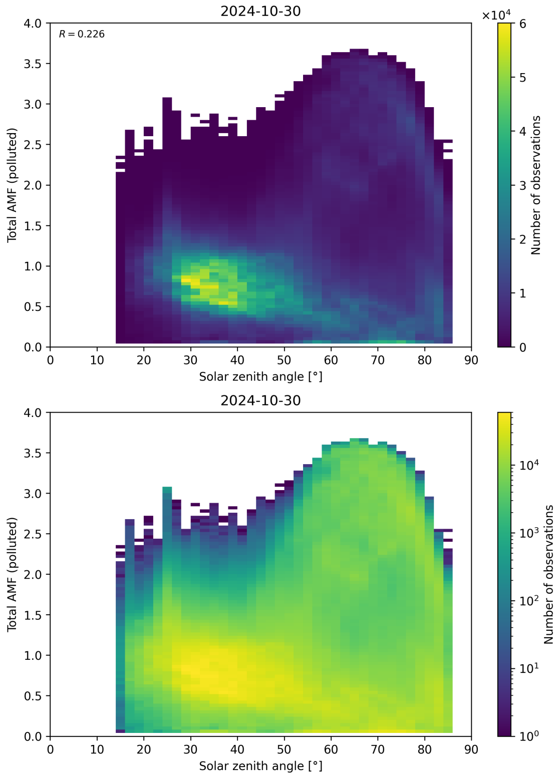
Figure 174: Scatter density plot of “Solar zenith angle” against “Total AMF (polluted)” for 2024-10-30 to 2024-10-31.
