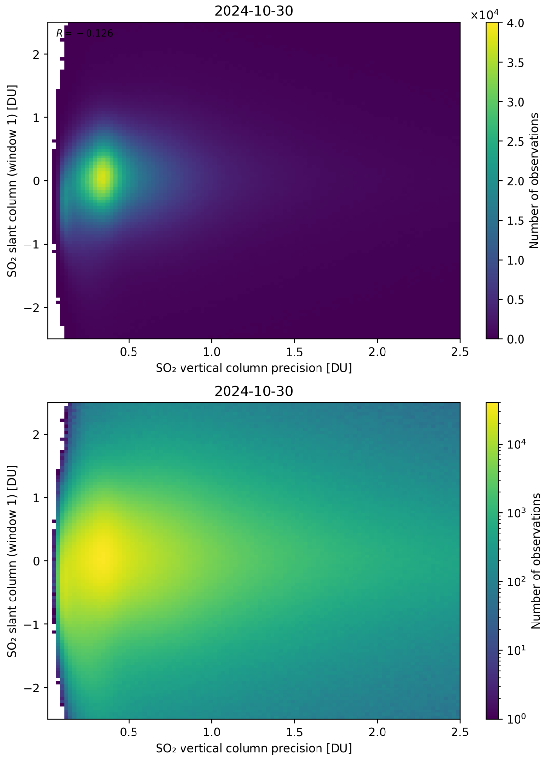
Figure 289: Scatter density plot of “SO 2 vertical column precision” against “SO 2 slant column (window 1)” for 2024-10-30 to 2024-10-31.
