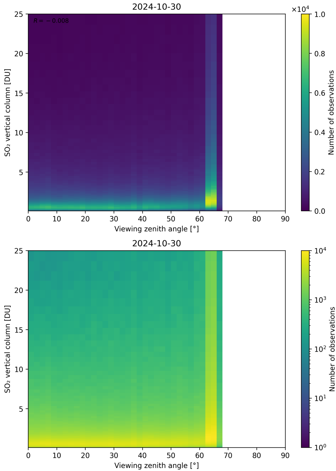
Figure 327: Scatter density plot of “Viewing zenith angle” against “SO 2 vertical column” for 2024-10-30 to 2024-10-31.
