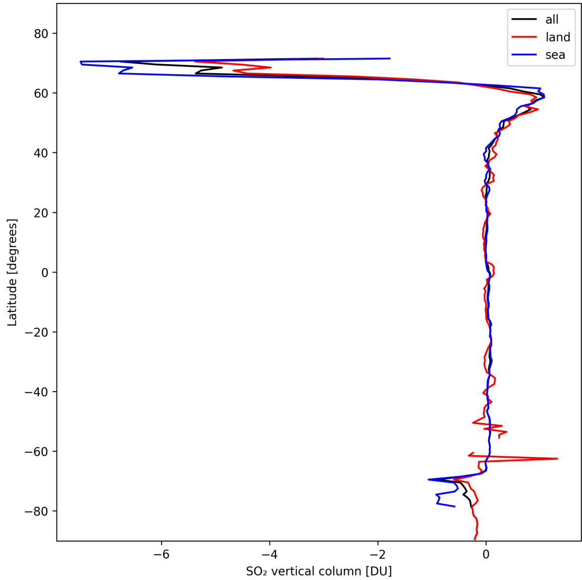
Figure 30: Zonal average of “SO 2 vertical column” for 2024-10-30 to 2024-10-31.
