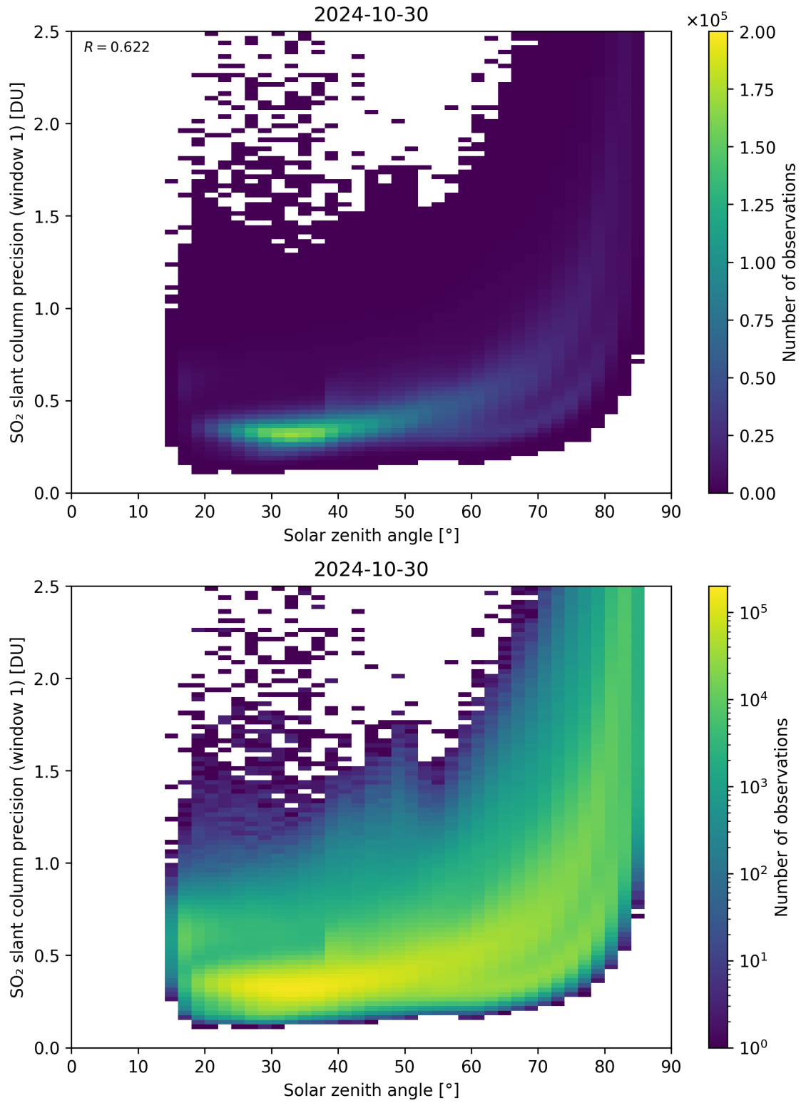
Figure 170: Scatter density plot of “Solar zenith angle” against “SO 2 slant column precision (window 1)” for 2024-10-30 to 2024-10-31.
