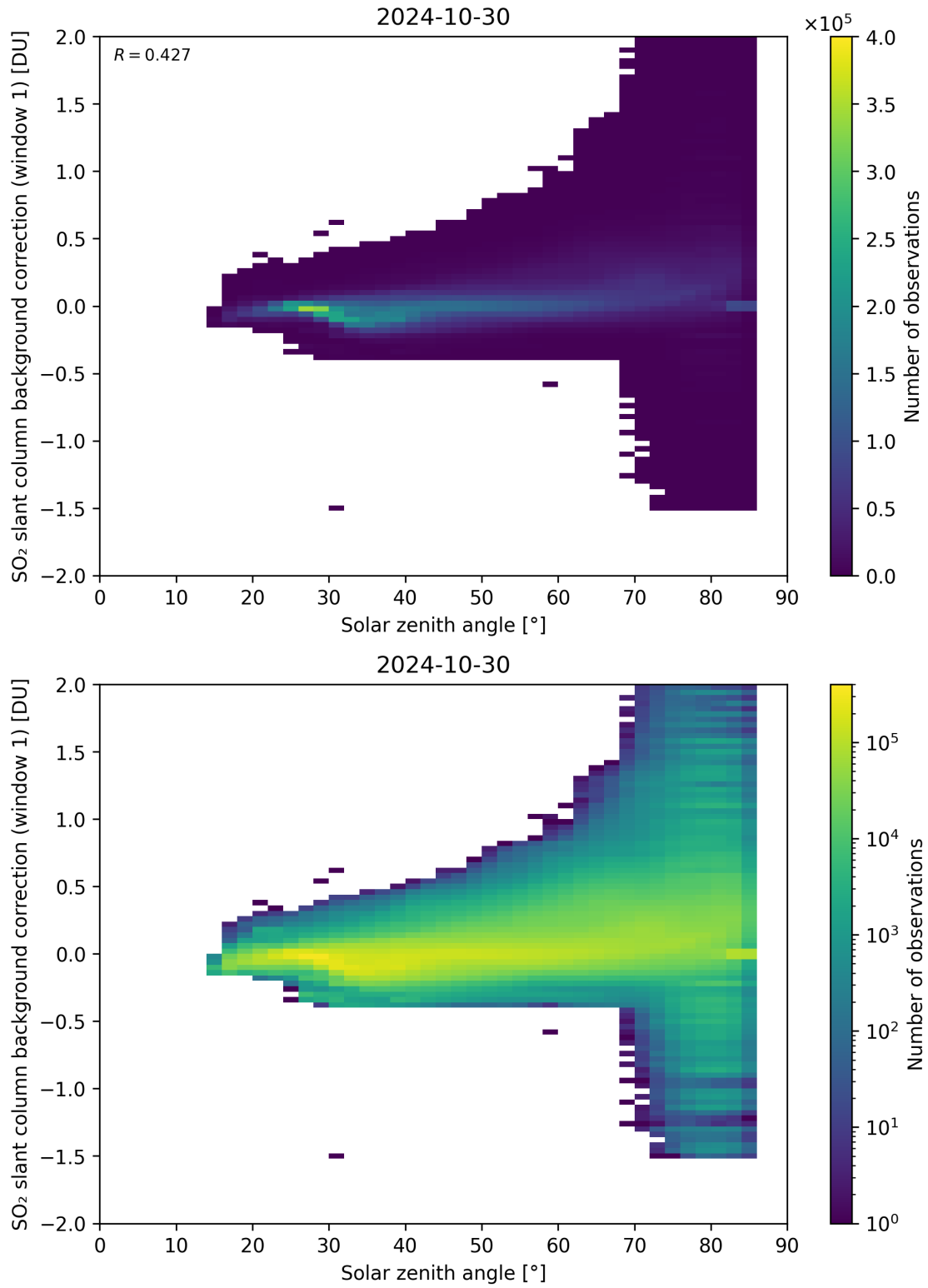
Figure 158: Scatter density plot of “Solar zenith angle” against “SO 2 slant column background correction (window 1)” for 2024-10-30 to 2024-10-31.
