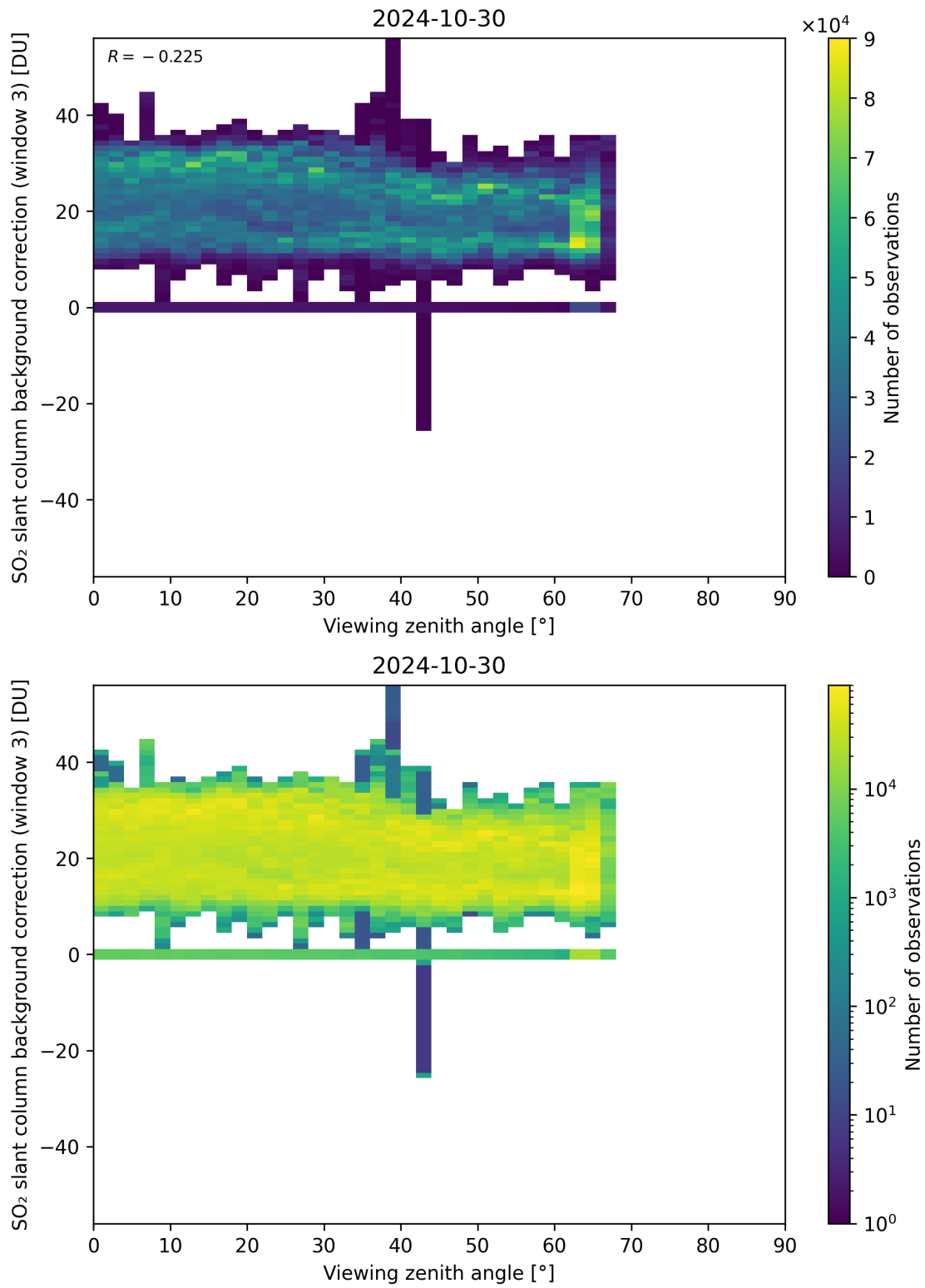
Figure 310: Scatter density plot of “Viewing zenith angle” against “SO 2 slant column background correction (window 3)” for 2024-10-30 to 2024-10-31.
