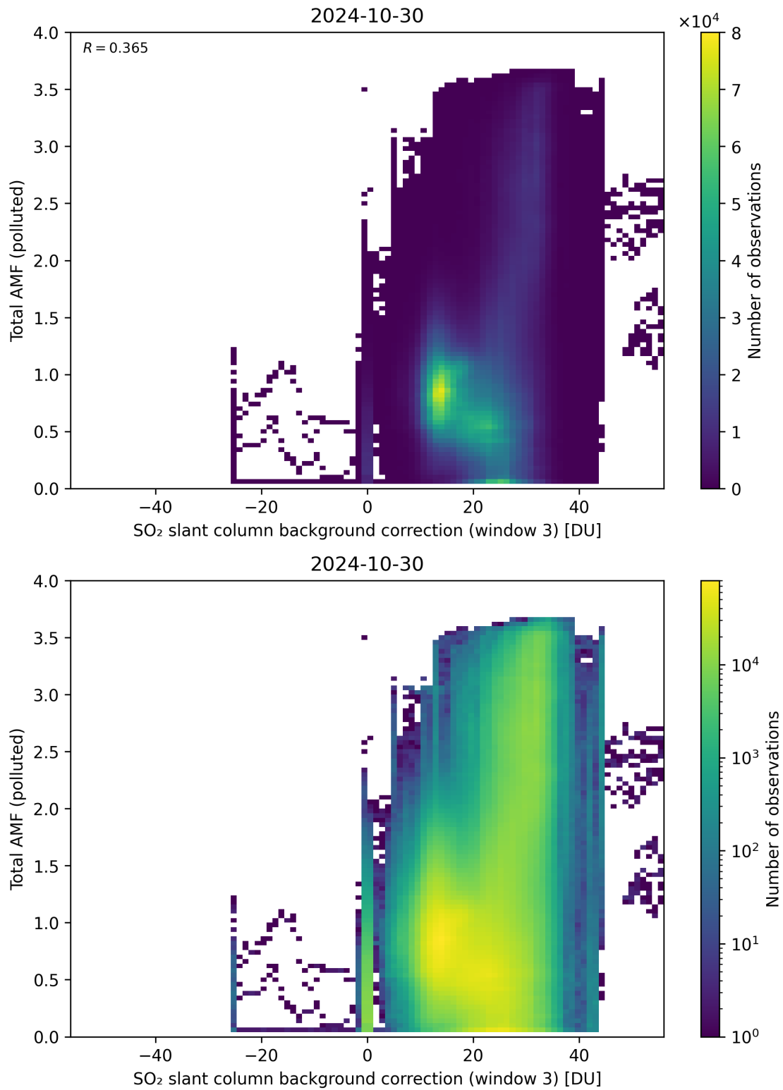
Figure 125: Scatter density plot of “SO 2 slant column background correction (window 3)” against “Total AMF (polluted)” for 2024-10-30 to 2024-10-31.
