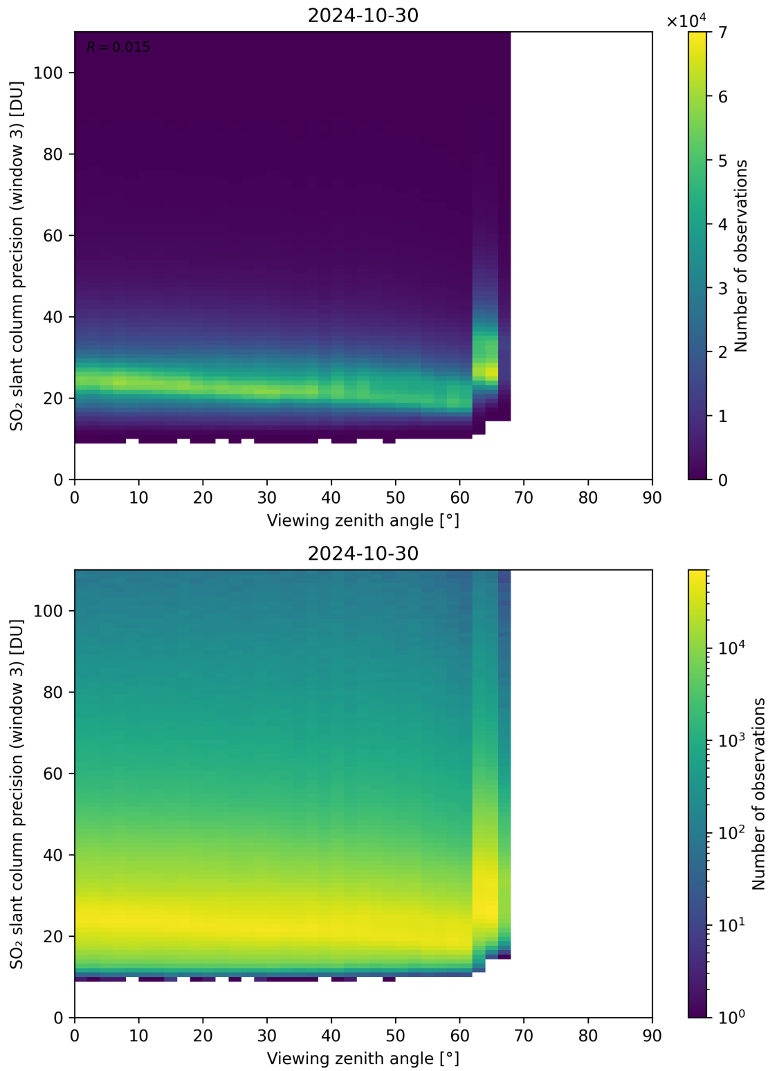
Figure 324: Scatter density plot of “Viewing zenith angle” against “SO 2 slant column precision (window 3)” for 2024-10-30 to 2024-10-31.
