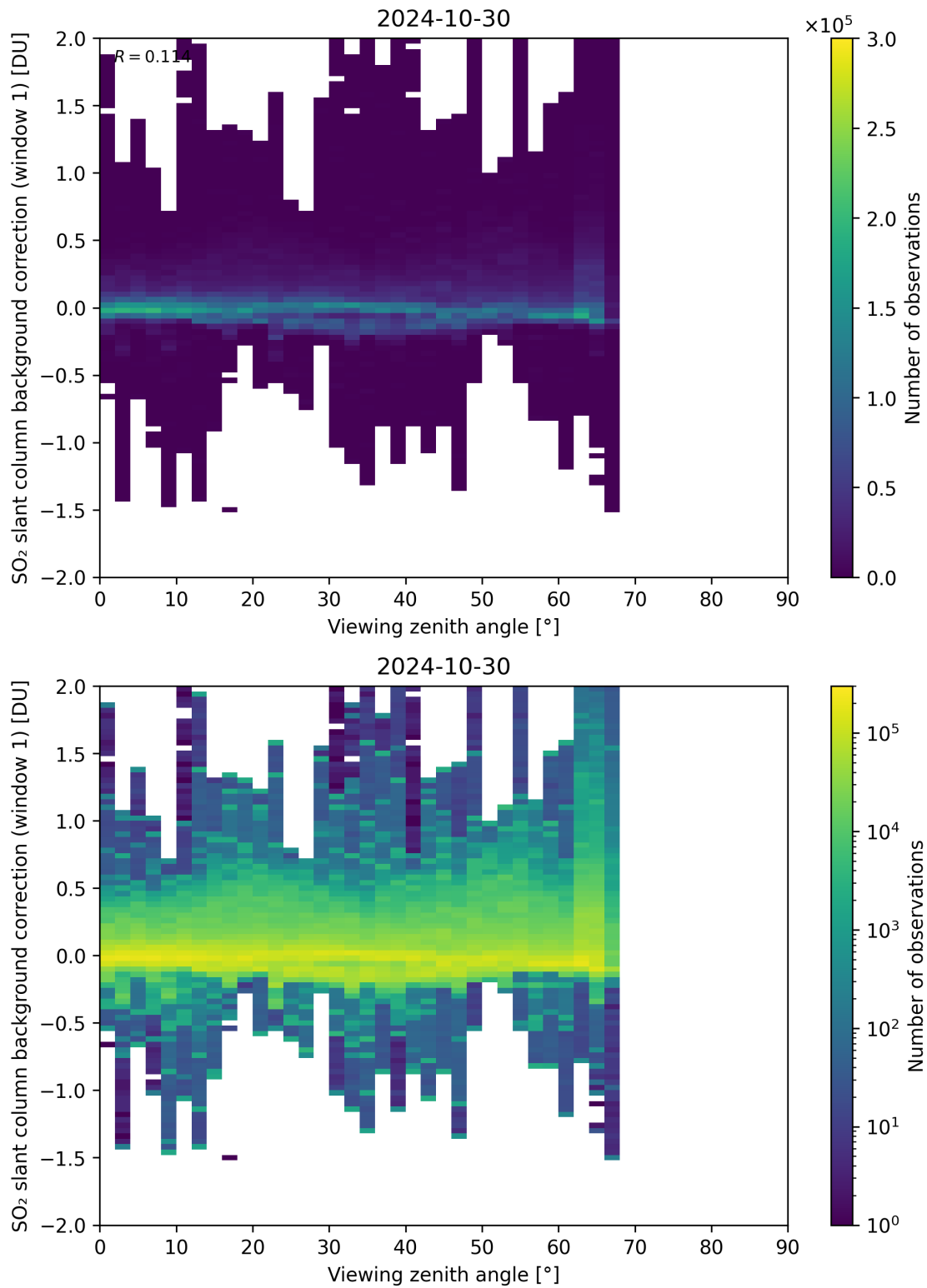
Figure 308: Scatter density plot of “Viewing zenith angle” against “SO 2 slant column background correction (window 1)” for 2024-10-30 to 2024-10-31.
