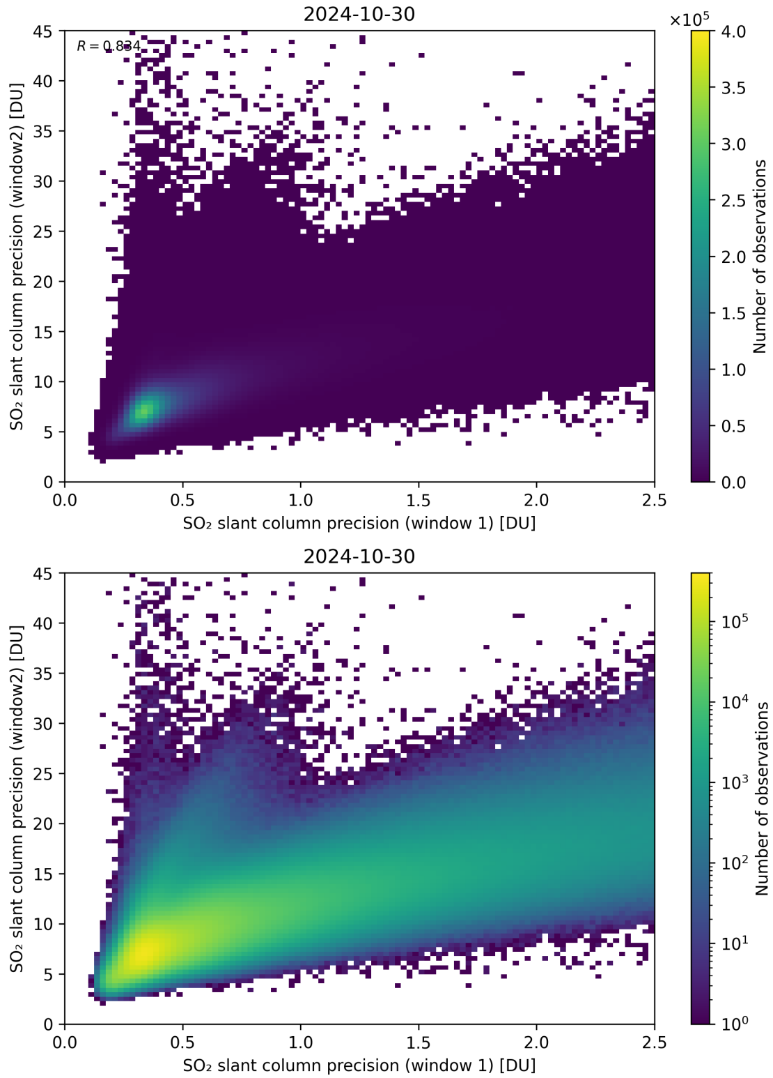
Figure 227: Scatter density plot of “SO 2 slant column precision (window 1)” against “SO 2 slant column precision (window2)” for 2024-10-30 to 2024-10-31.
