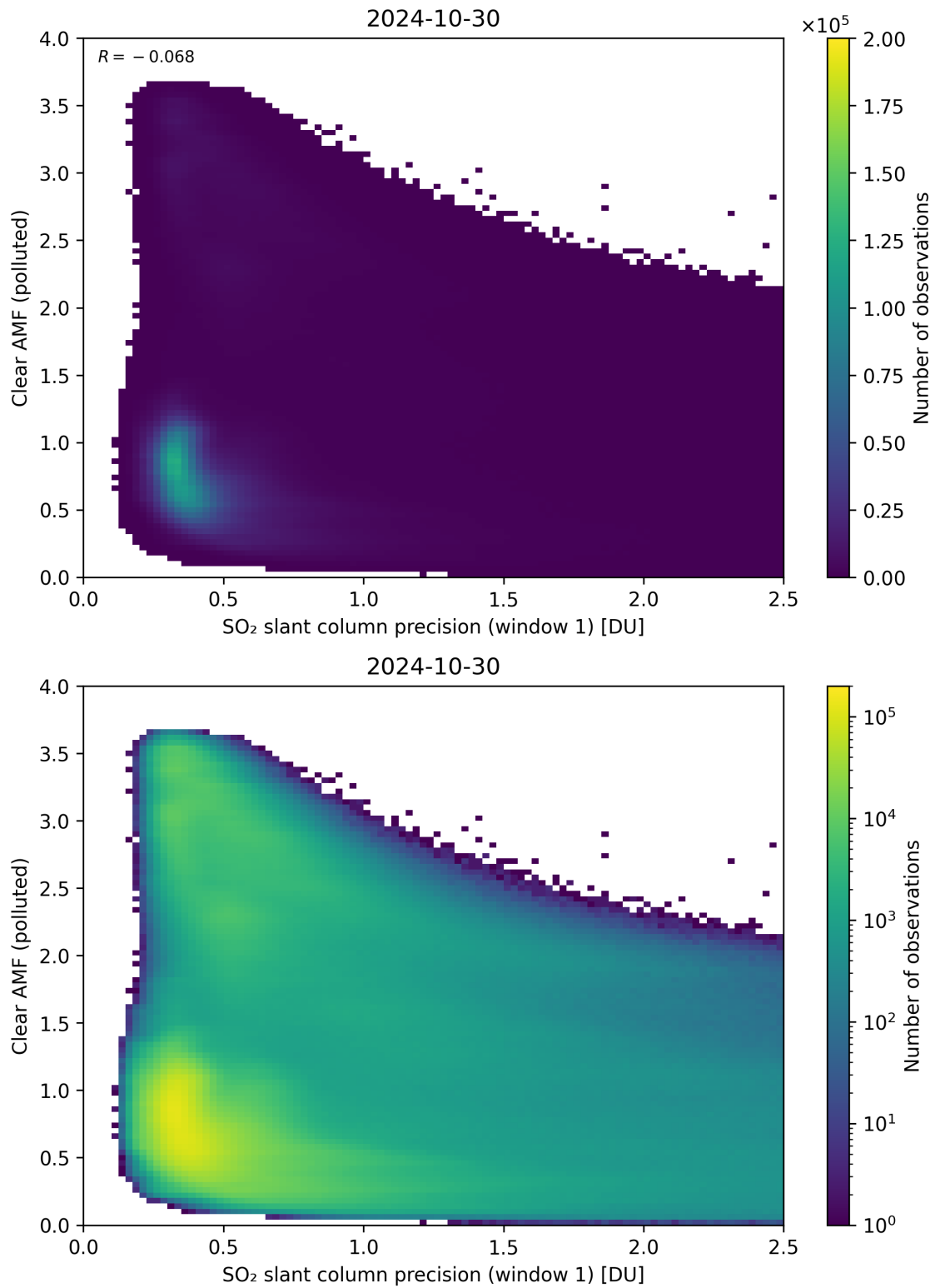
Figure 224: Scatter density plot of “SO 2 slant column precision (window 1)” against “Clear AMF (polluted)” for 2024-10-30 to 2024-10-31.
