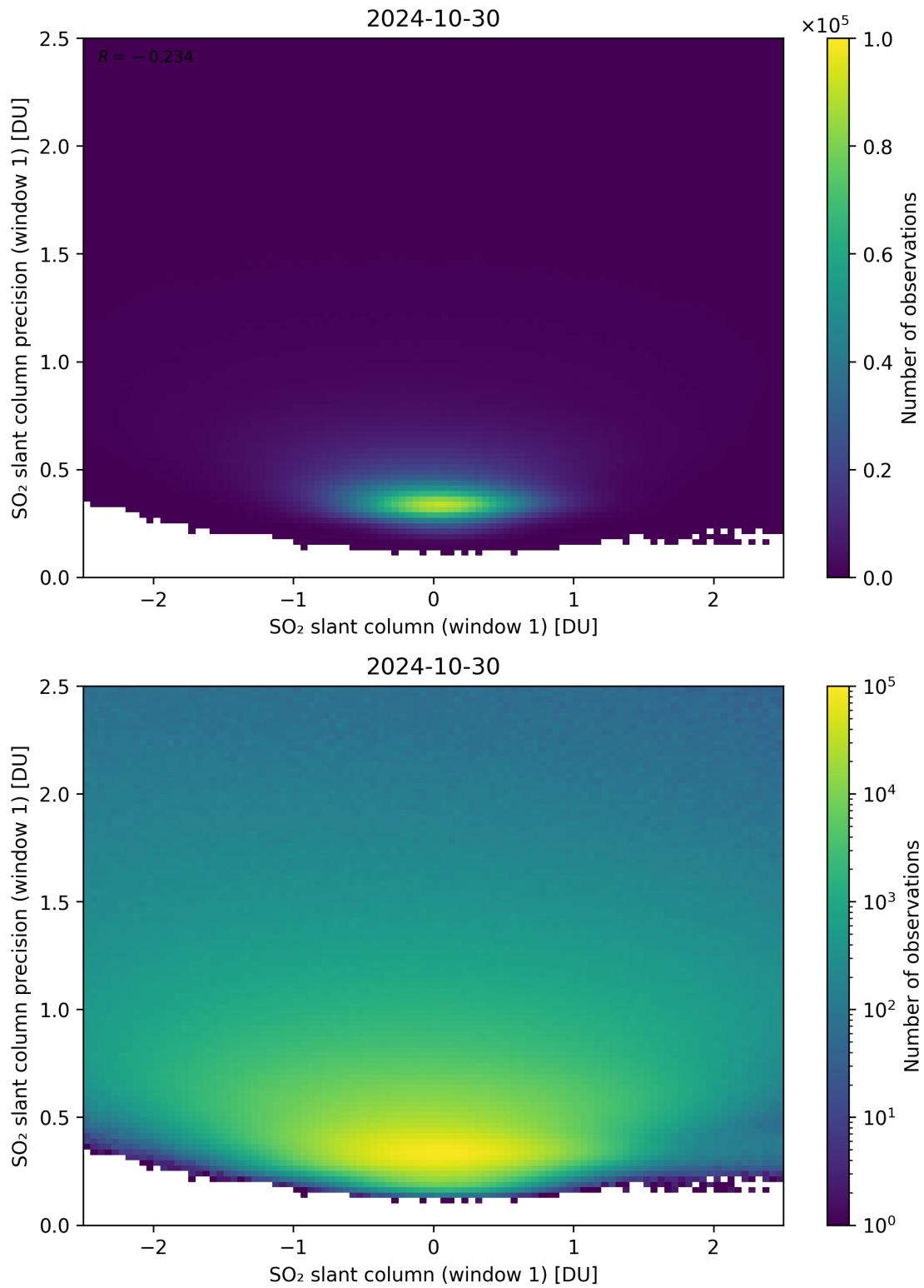
Figure 235: Scatter density plot of “SO 2 slant column (window 1)” against “SO 2 slant column precision (window 1)” for 2024-10-30 to 2024-10-31.
