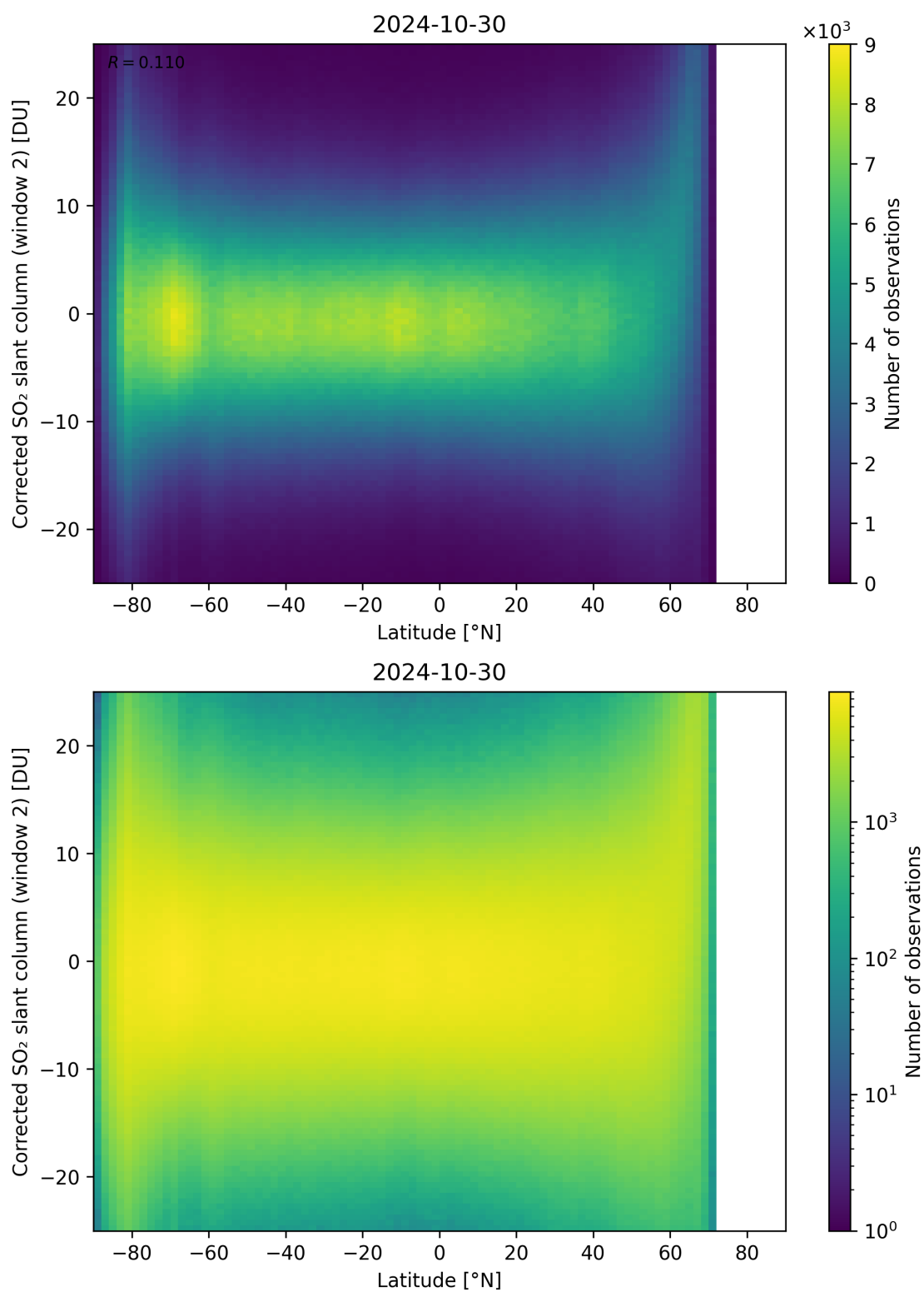
Figure 147: Scatter density plot of “Latitude” against “Corrected SO 2 slant column (window 2)” for 2024-10-30 to 2024-10-31.
