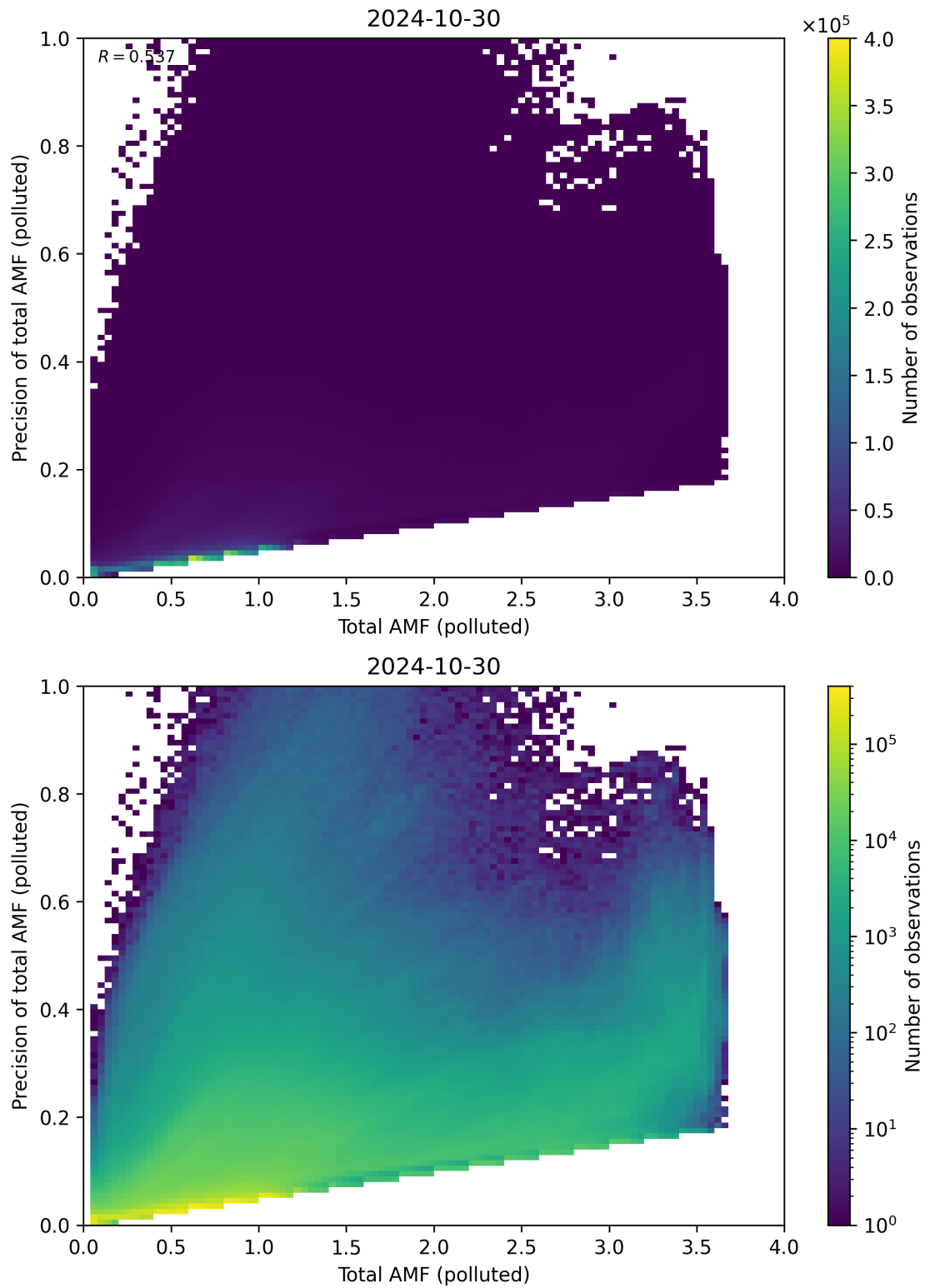
Figure 272: Scatter density plot of “Total AMF (polluted)” against “Precision of total AMF (polluted)” for 2024-10-30 to 2024-10-31.
