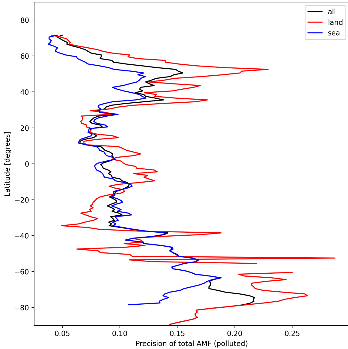
Figure 49: Zonal average of “Precision of total AMF (polluted)” for 2024-10-30 to 2024-10-31.
