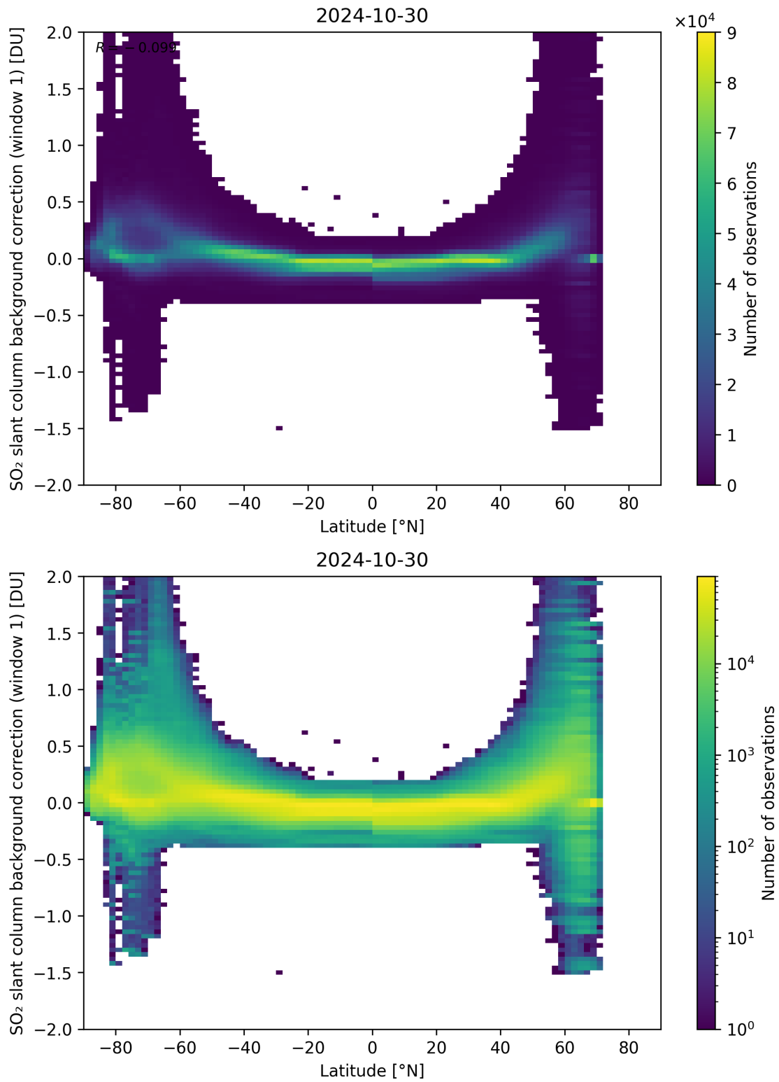
Figure 139: Scatter density plot of “Latitude” against “SO 2 slant column background correction (window 1)” for 2024-10-30 to 2024-10-31.
