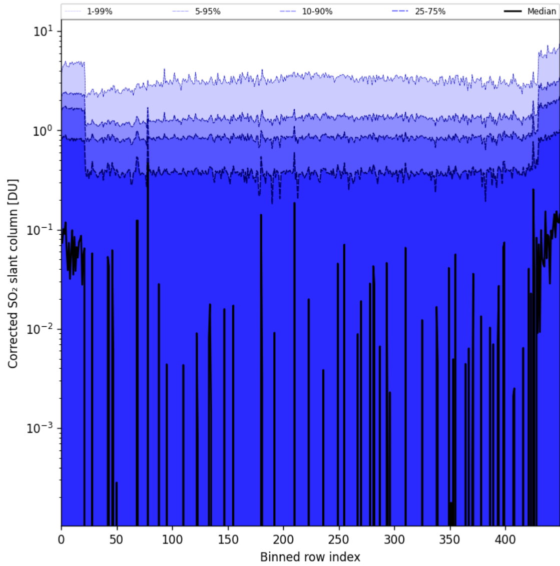
Figure 78: Along track statistics of “Corrected SO 2 slant column” for 2024-10-30 to 2024-10-31
