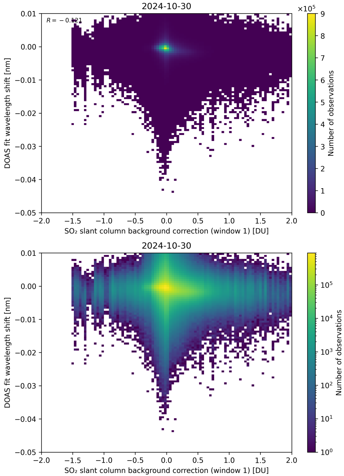
Figure 100: Scatter density plot of “SO 2 slant column background correction (window 1)” against “DOAS fit wavelength shift” for 2024-10-30 to 2024-10-31.
