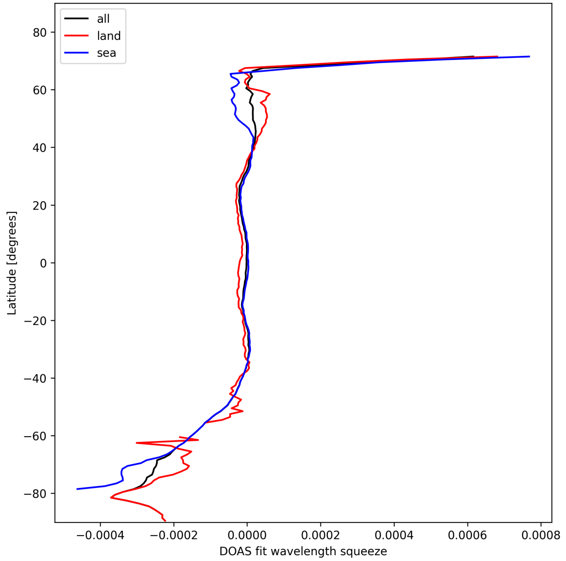
Figure 46: Zonal average of “DOAS fit wavelength squeeze” for 2024-10-30 to 2024-10-31.
