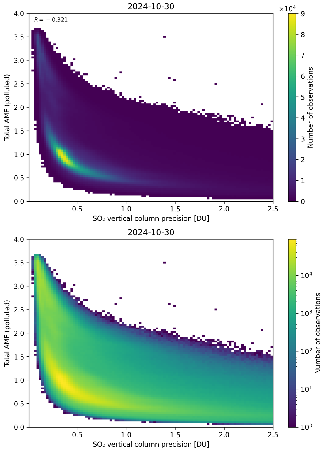
Figure 294: Scatter density plot of “SO 2 vertical column precision” against “Total AMF (polluted)” for 2024-10-30 to 2024-10-31.
