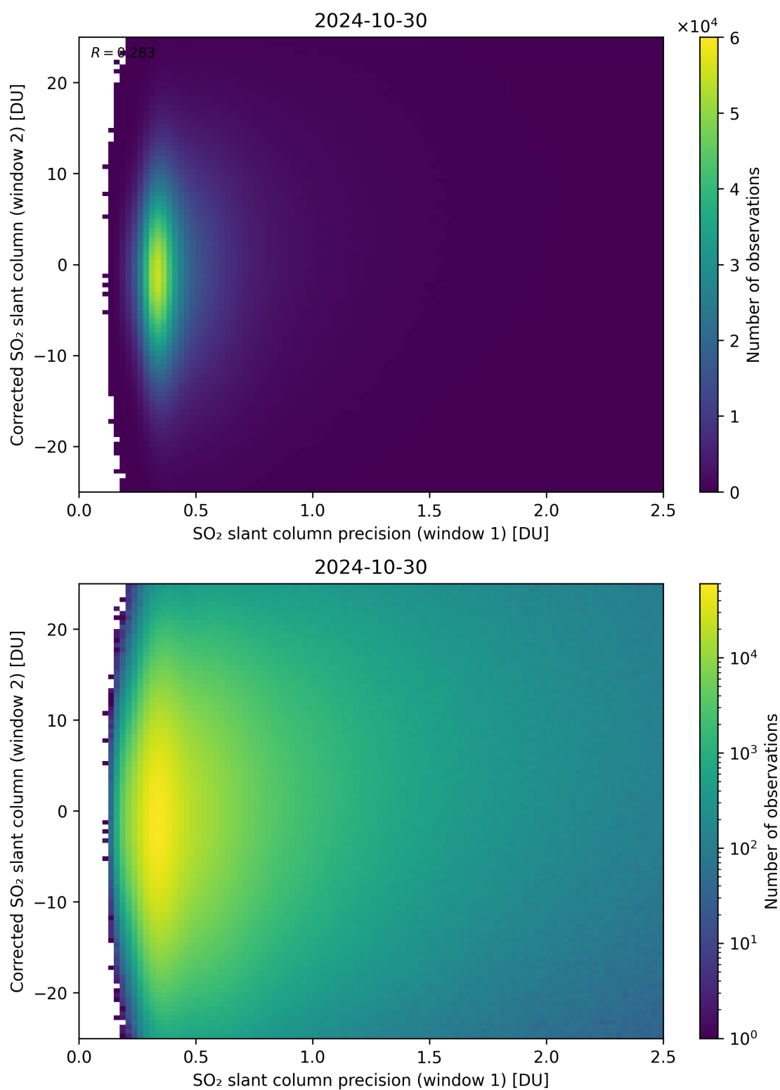
Figure 225: Scatter density plot of “SO 2 slant column precision (window 1)” against “Corrected SO 2 slant column (window 2)” for 2024-10-30 to 2024-10-31.
