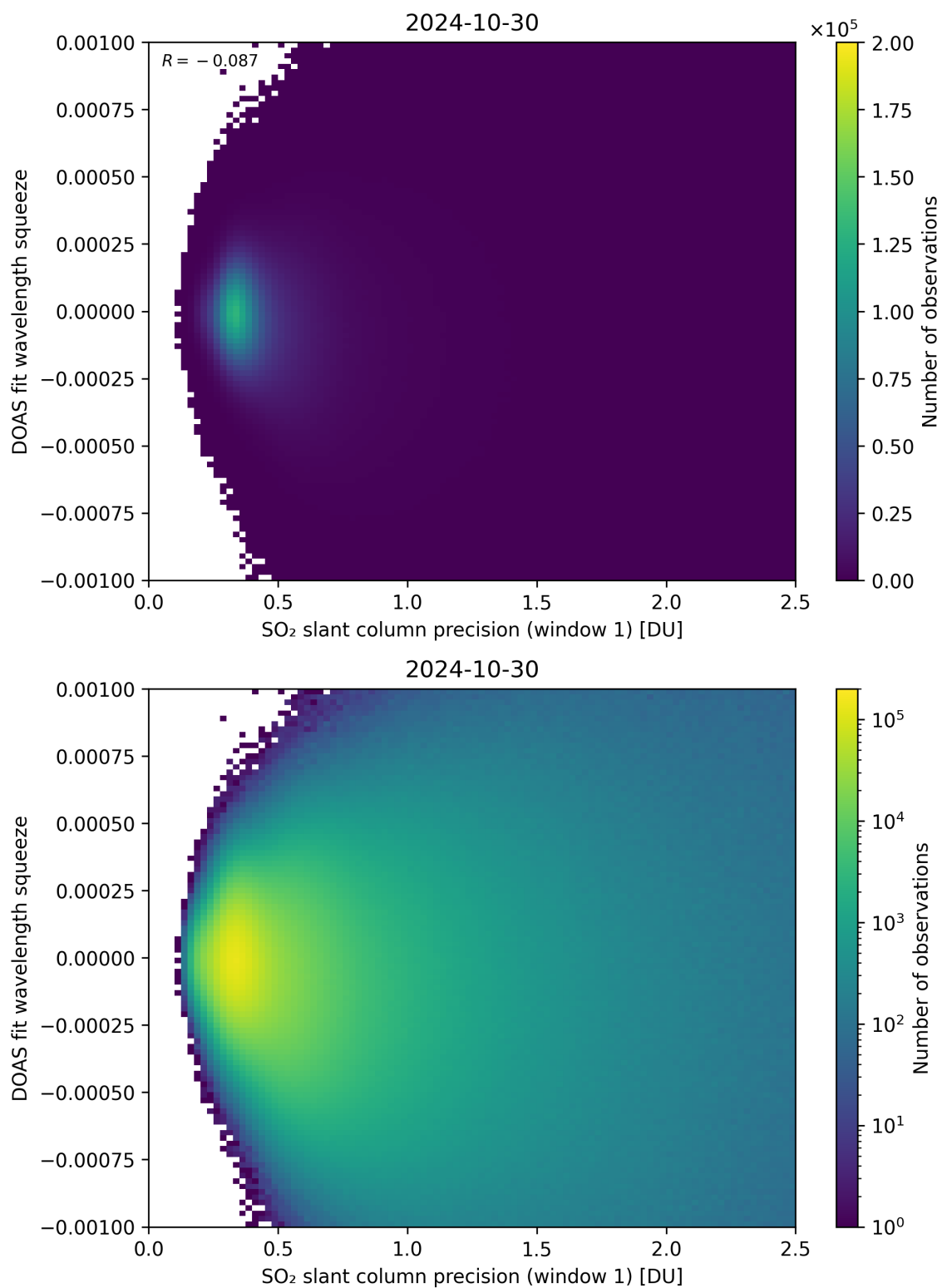
Figure 222: Scatter density plot of “SO 2 slant column precision (window 1)” against “DOAS fit wavelength squeeze” for 2024-10-30 to 2024-10-31.
