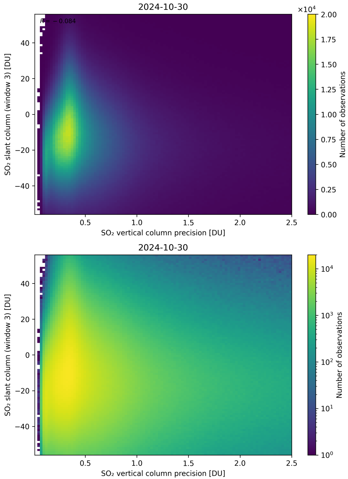
Figure 292: Scatter density plot of “SO 2 vertical column precision” against “SO 2 slant column (window 3)” for 2024-10-30 to 2024-10-31.
