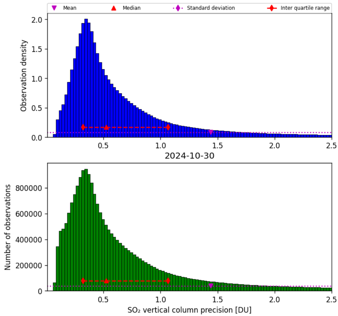
Figure 54: Histogram of “SO 2 vertical column precision” for 2024-10-30 to 2024-10-31
