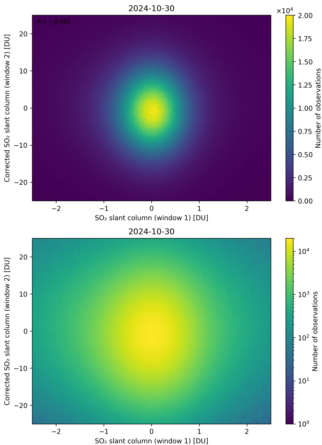
Figure 233: Scatter density plot of “SO 2 slant column (window 1)” against “Corrected SO 2 slant column (window 2)” for 2024-10-30 to 2024-10-31.
