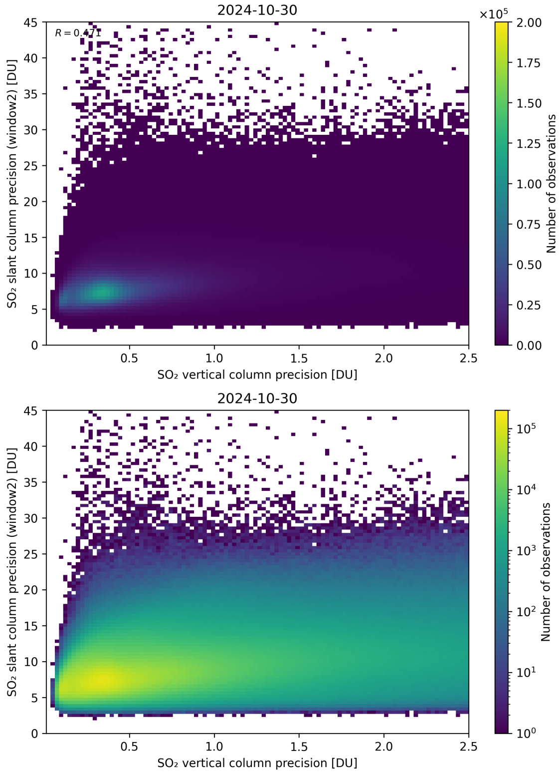
Figure 291: Scatter density plot of “SO 2 vertical column precision” against “SO 2 slant column precision (window2)” for 2024-10-30 to 2024-10-31.
