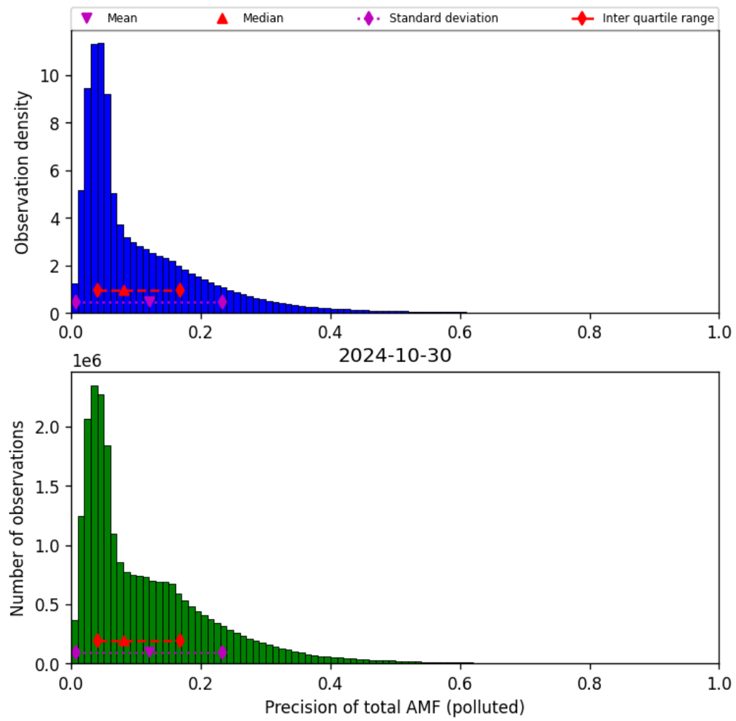
Figure 72: Histogram of “Precision of total AMF (polluted)” for 2024-10-30 to 2024-10-31
