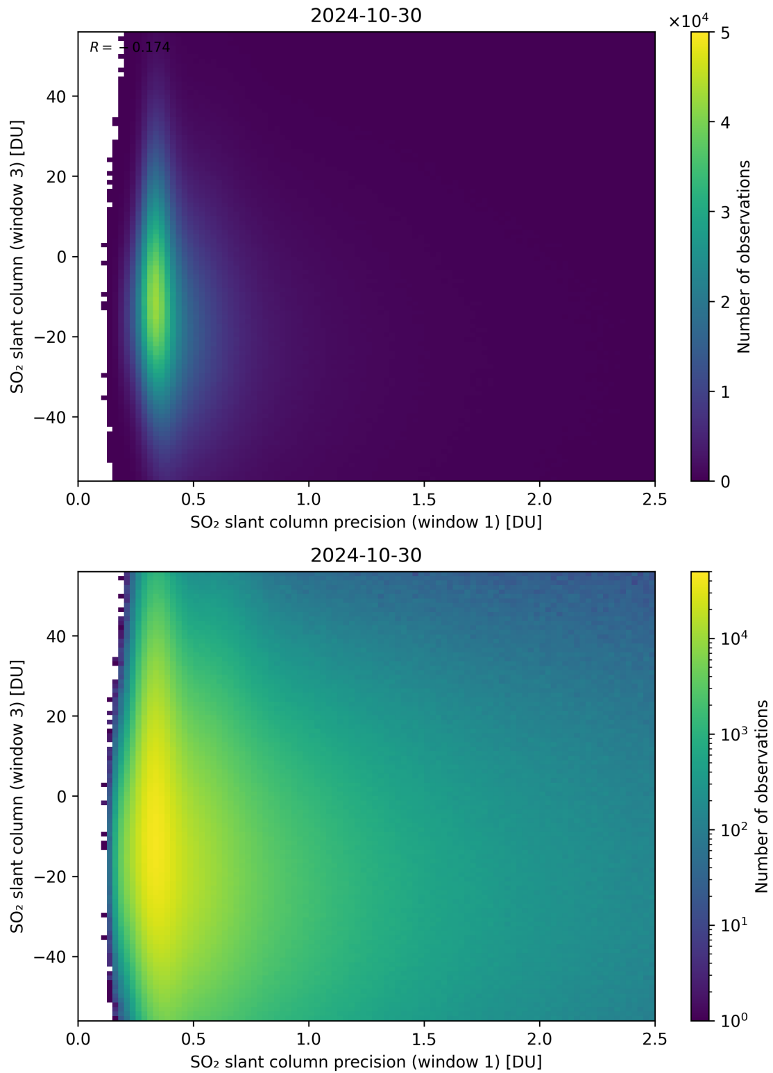
Figure 228: Scatter density plot of “SO 2 slant column precision (window 1)” against “SO 2 slant column (window 3)” for 2024-10-30 to 2024-10-31.
