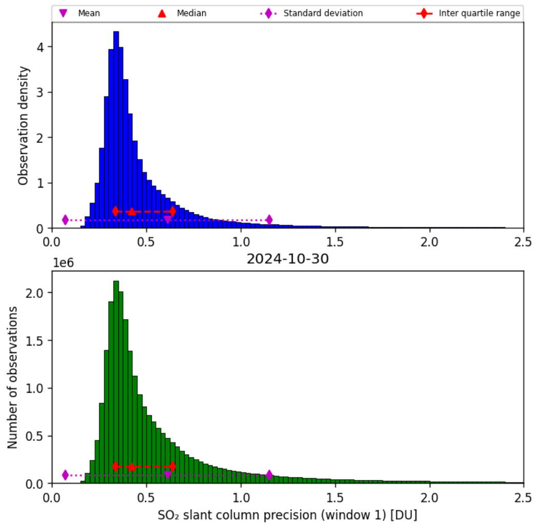
Figure 57: Histogram of “SO 2 slant column precision (window 1)” for 2024-10-30 to 2024-10-31
