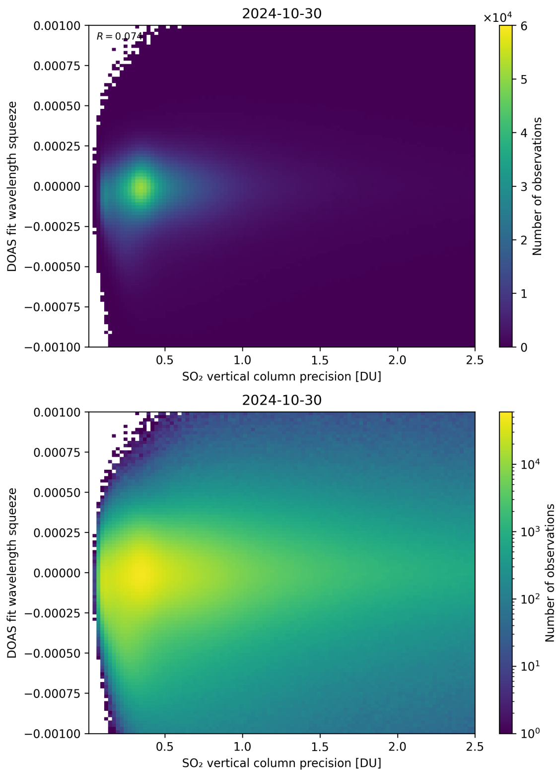
Figure 283: Scatter density plot of “SO 2 vertical column precision” against “DOAS fit wavelength squeeze” for 2024-10-30 to 2024-10-31.
