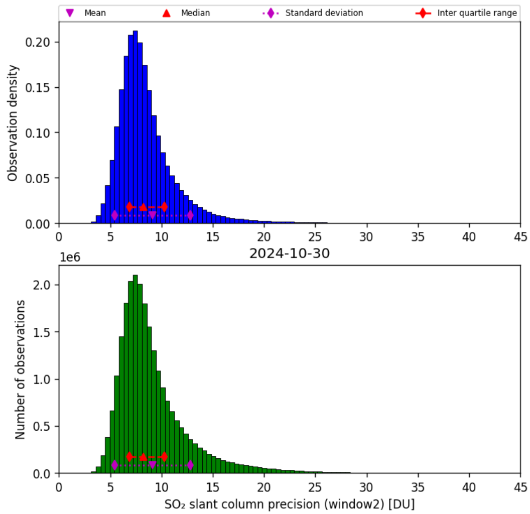
Figure 61: Histogram of “SO 2 slant column precision (window2)” for 2024-10-30 to 2024-10-31
