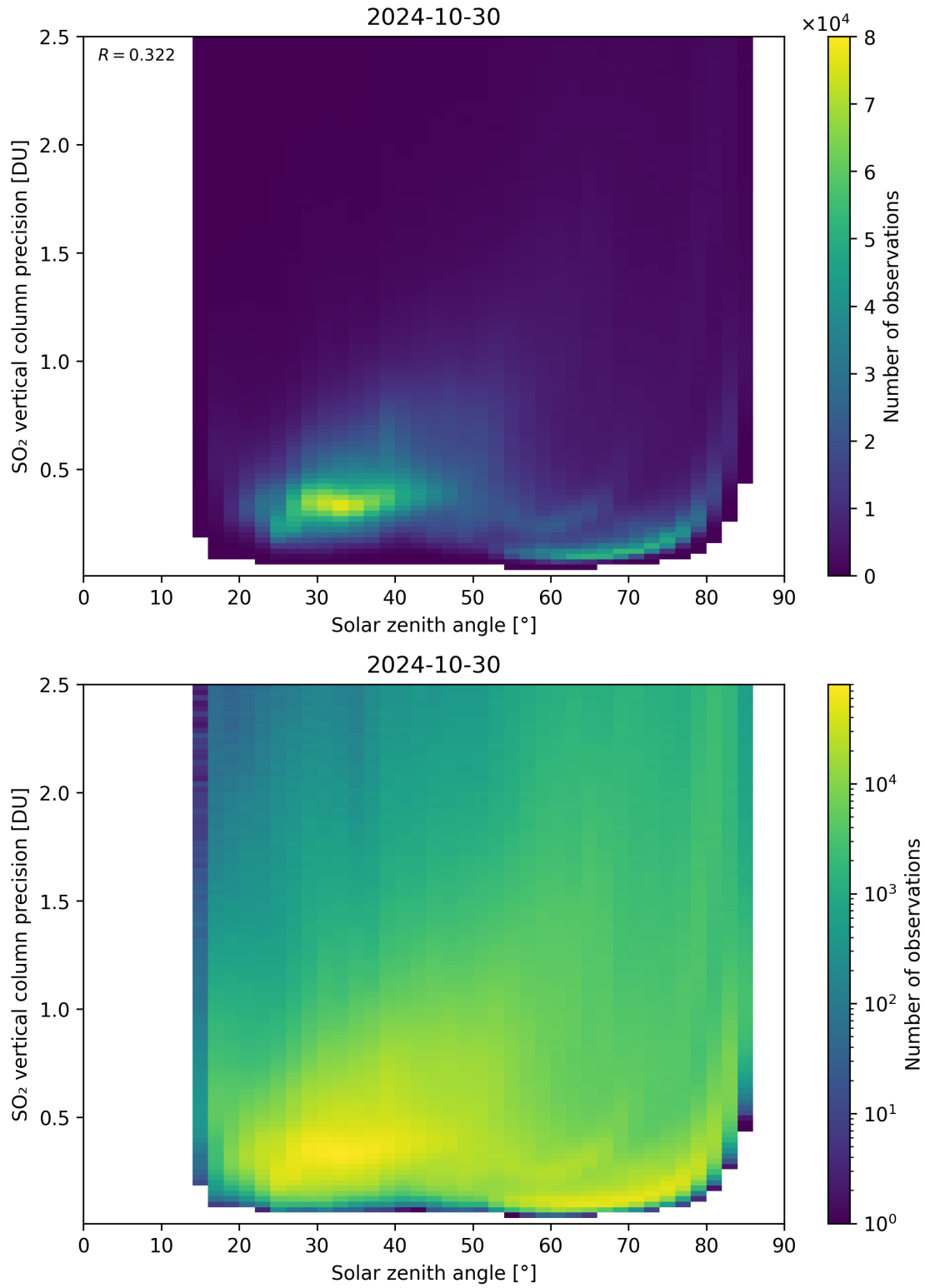
Figure 177: Scatter density plot of “Solar zenith angle” against “SO 2 vertical column precision” for 2024-10-30 to 2024-10-31.
