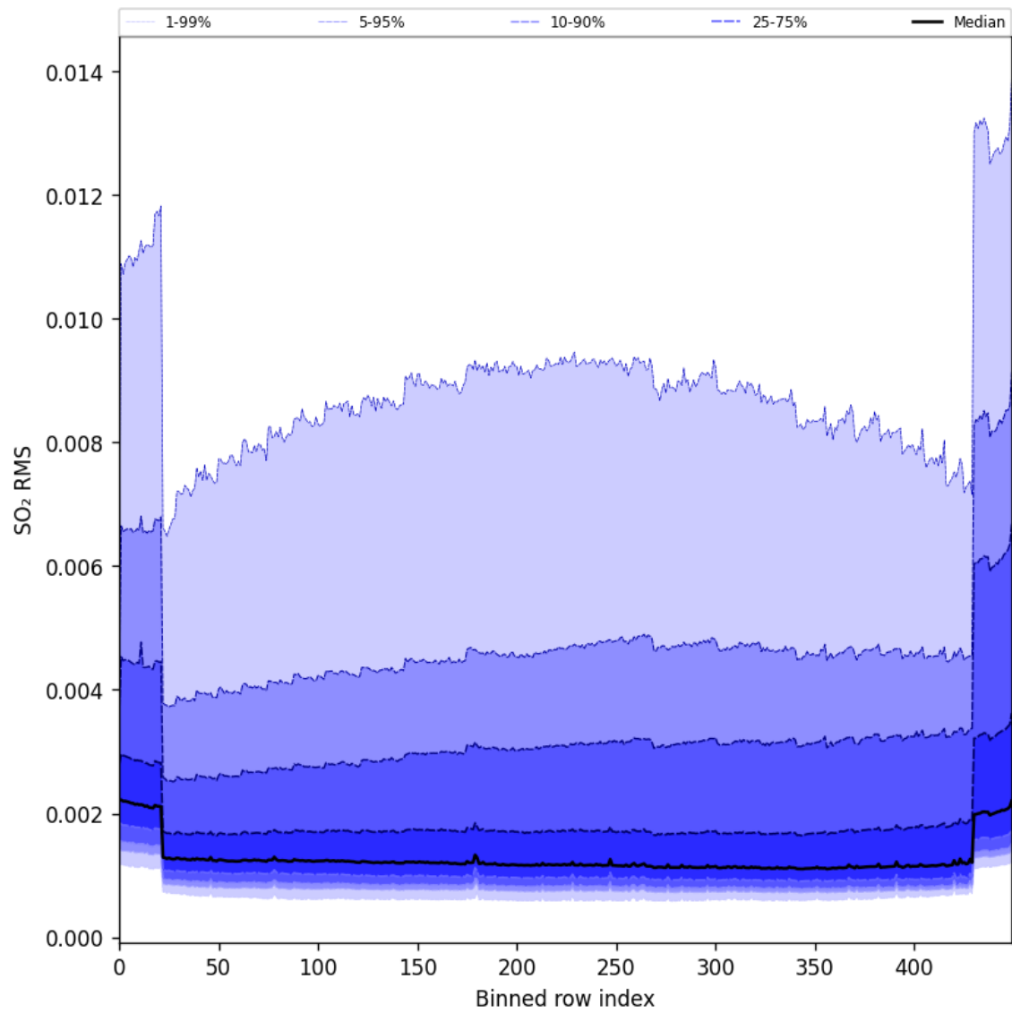
Figure 93: Along track statistics of “SO 2 RMS” for 2024-10-30 to 2024-10-31
