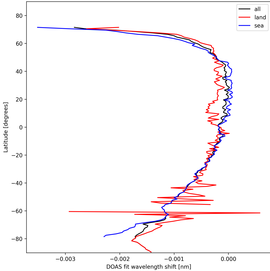
Figure 45: Zonal average of “DOAS fit wavelength shift” for 2024-10-30 to 2024-10-31.
