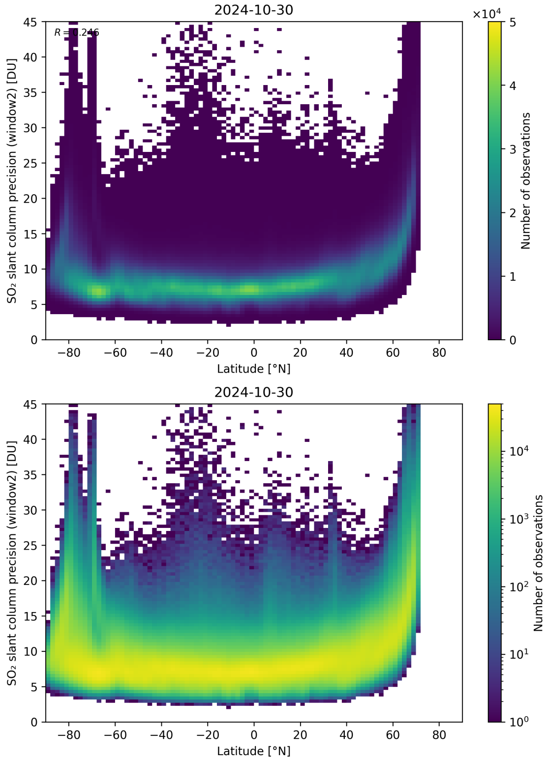
Figure 151: Scatter density plot of “Latitude” against “SO 2 slant column precision (window2)” for 2024-10-30 to 2024-10-31.
