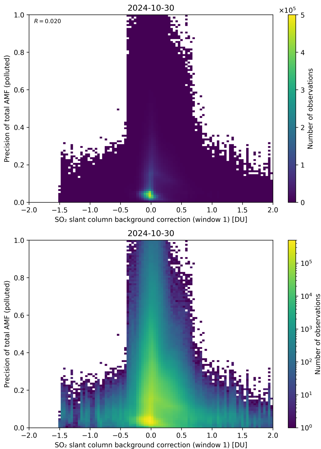
Figure 110: Scatter density plot of “SO 2 slant column background correction (window 1)” against “Precision of total AMF (polluted)” for 2024-10-30 to 2024-10-31.
