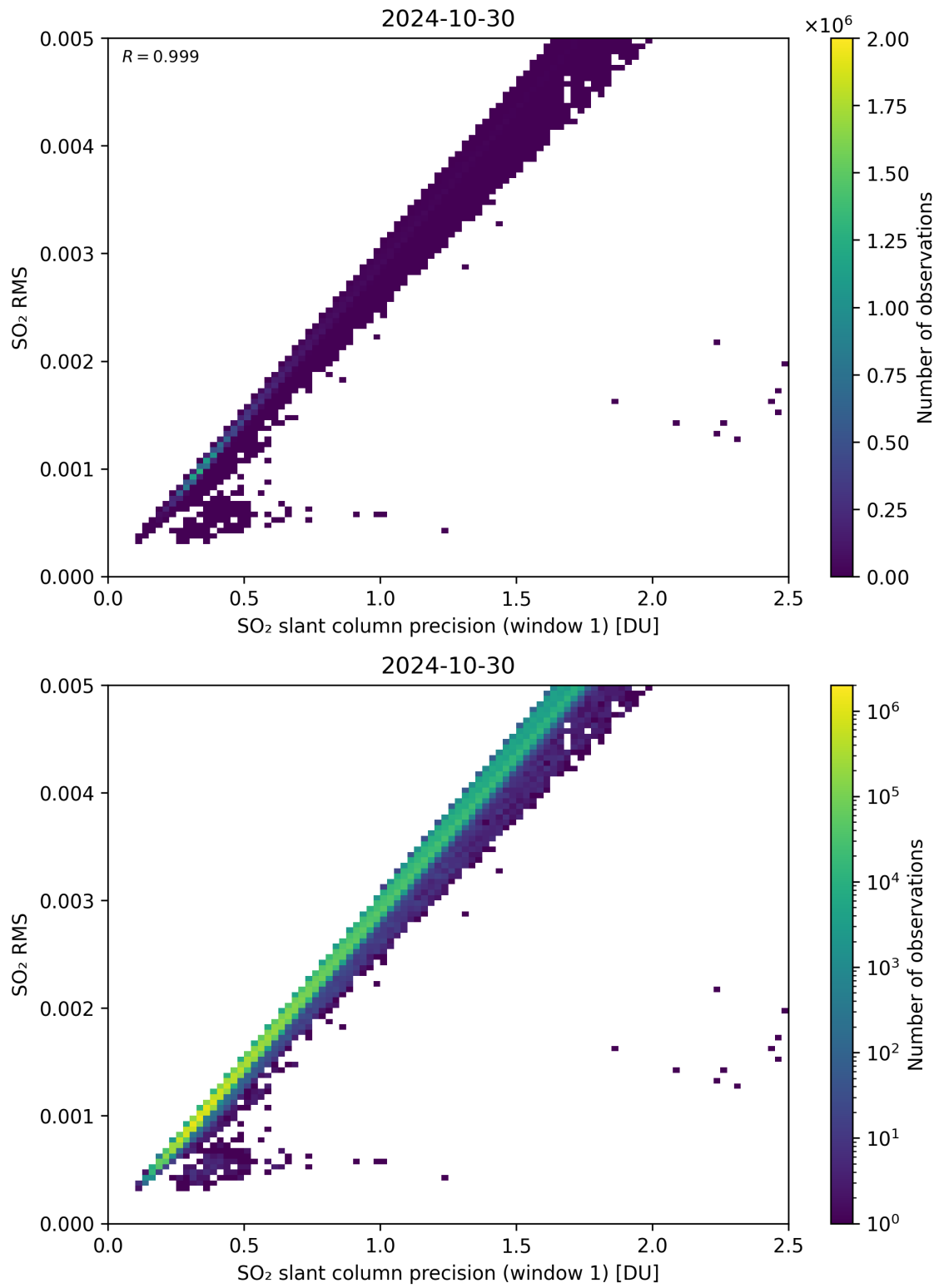
Figure 223: Scatter density plot of “SO 2 slant column precision (window 1)” against “SO 2 RMS” for 2024-10-30 to 2024-10-31.
