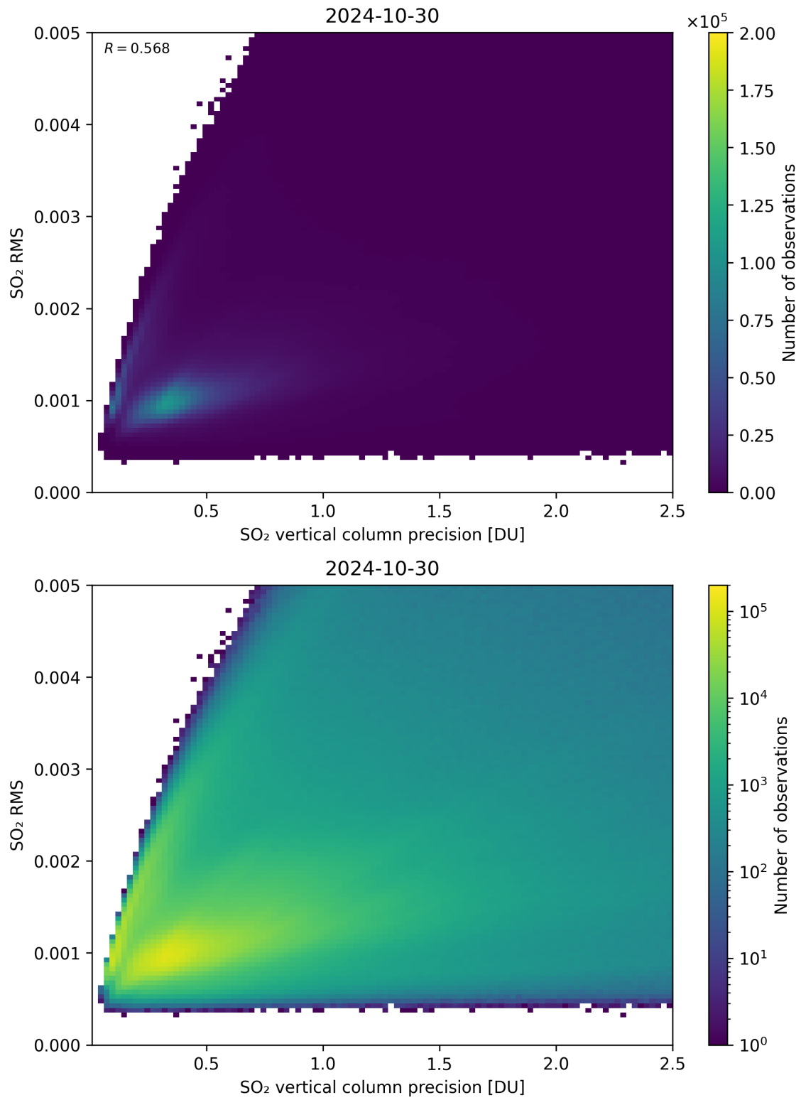
Figure 284: Scatter density plot of “SO 2 vertical column precision” against “SO 2 RMS” for 2024-10-30 to 2024-10-31.
