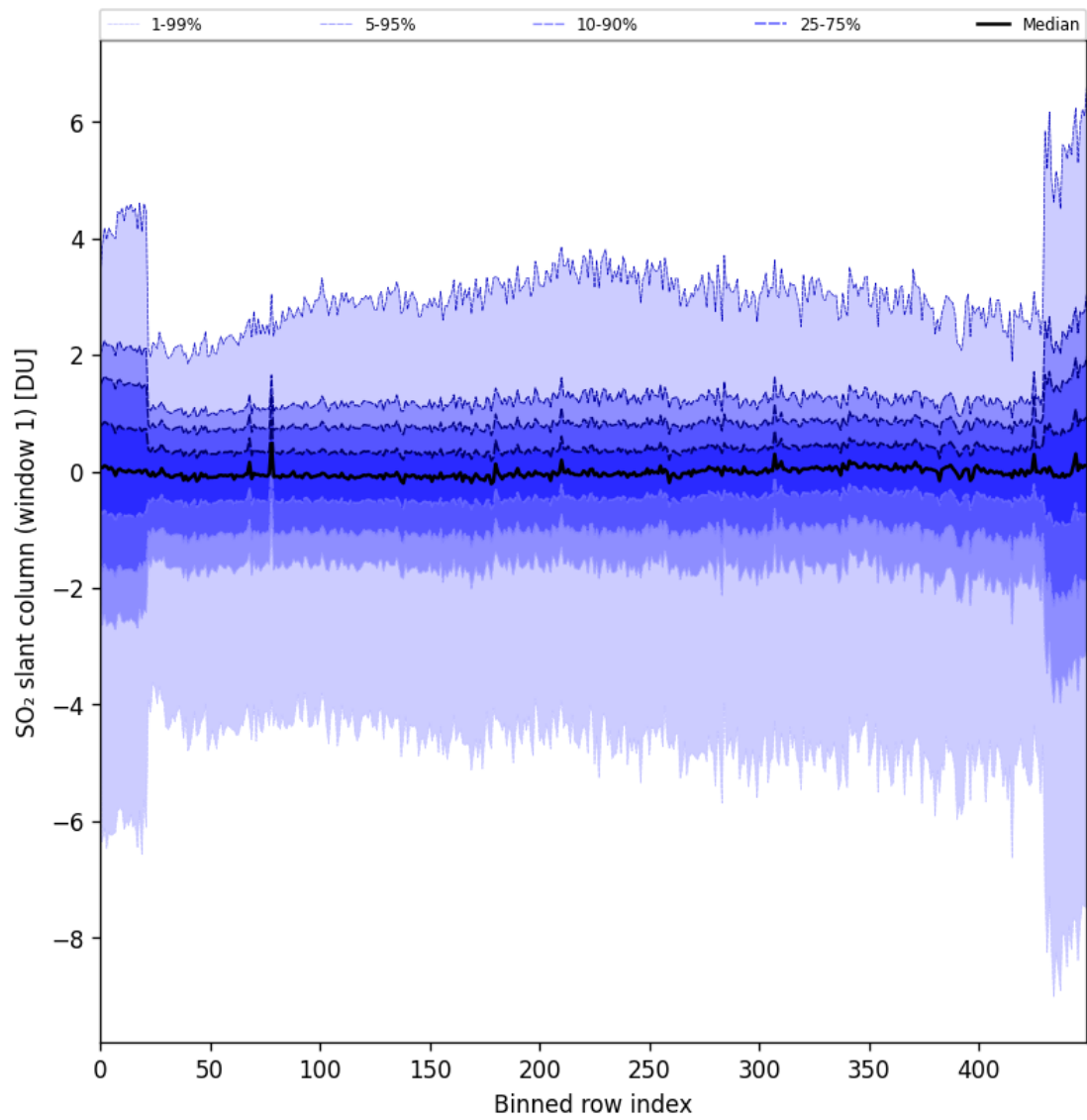
Figure 79: Along track statistics of “SO 2 slant column (window 1)” for 2024-10-30 to 2024-10-31
