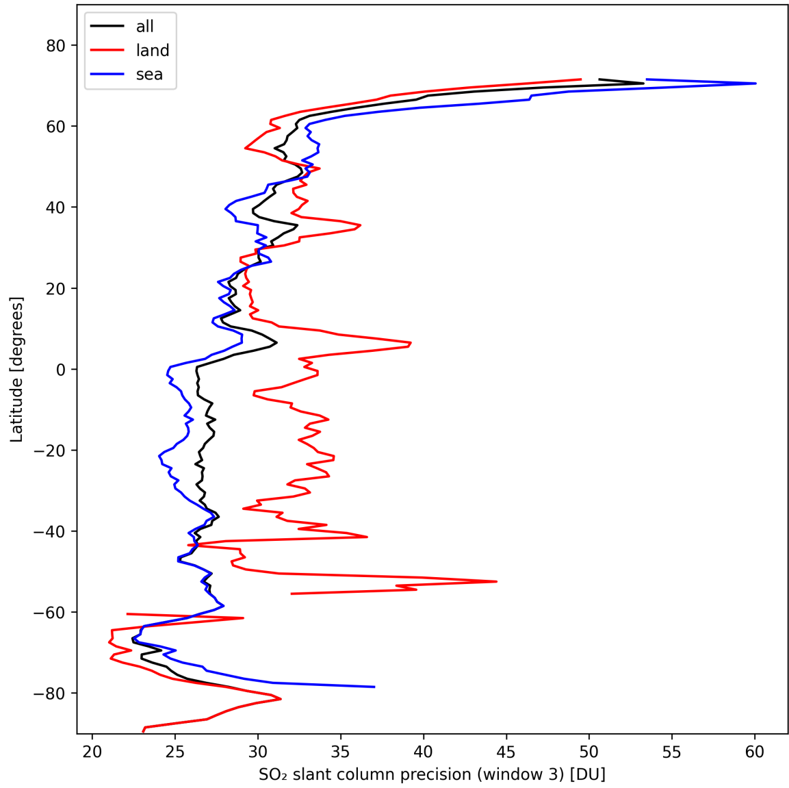
Figure 42: Zonal average of “SO 2 slant column precision (window 3)” for 2024-10-30 to 2024-10-31.
