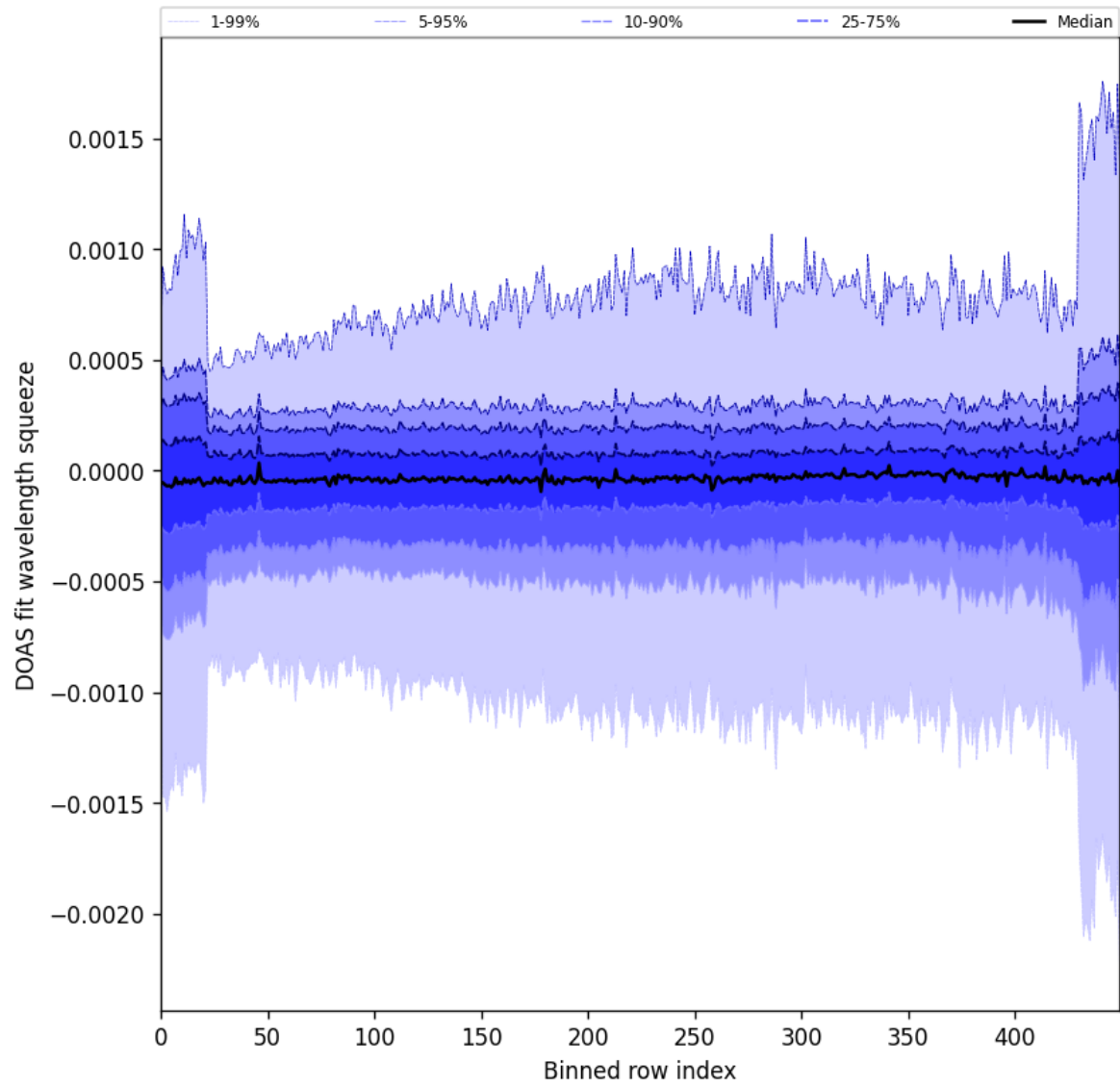
Figure 92: Along track statistics of “DOAS fit wavelength squeeze” for 2024-10-30 to 2024-10-31
