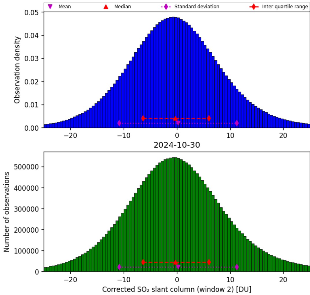
Figure 62: Histogram of “Corrected SO 2 slant column (window 2)” for 2024-10-30 to 2024-10-31
