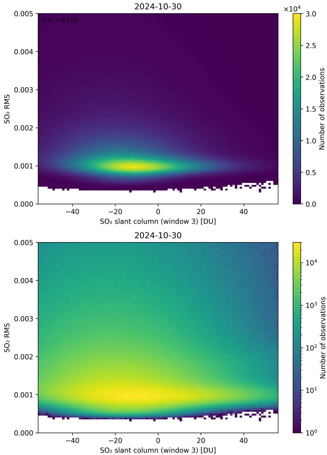
Figure 256: Scatter density plot of “SO 2 slant column (window 3)” against “SO 2 RMS” for 2024-10-30 to 2024-10-31.
