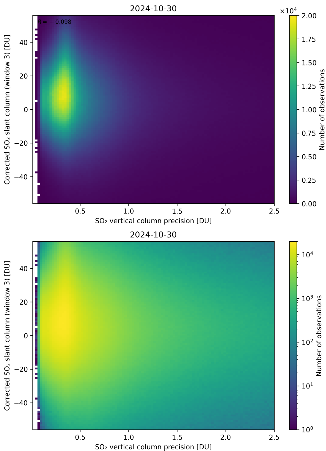
Figure 288: Scatter density plot of “SO 2 vertical column precision” against “Corrected SO 2 slant column (window 3)” for 2024-10-30 to 2024-10-31.
