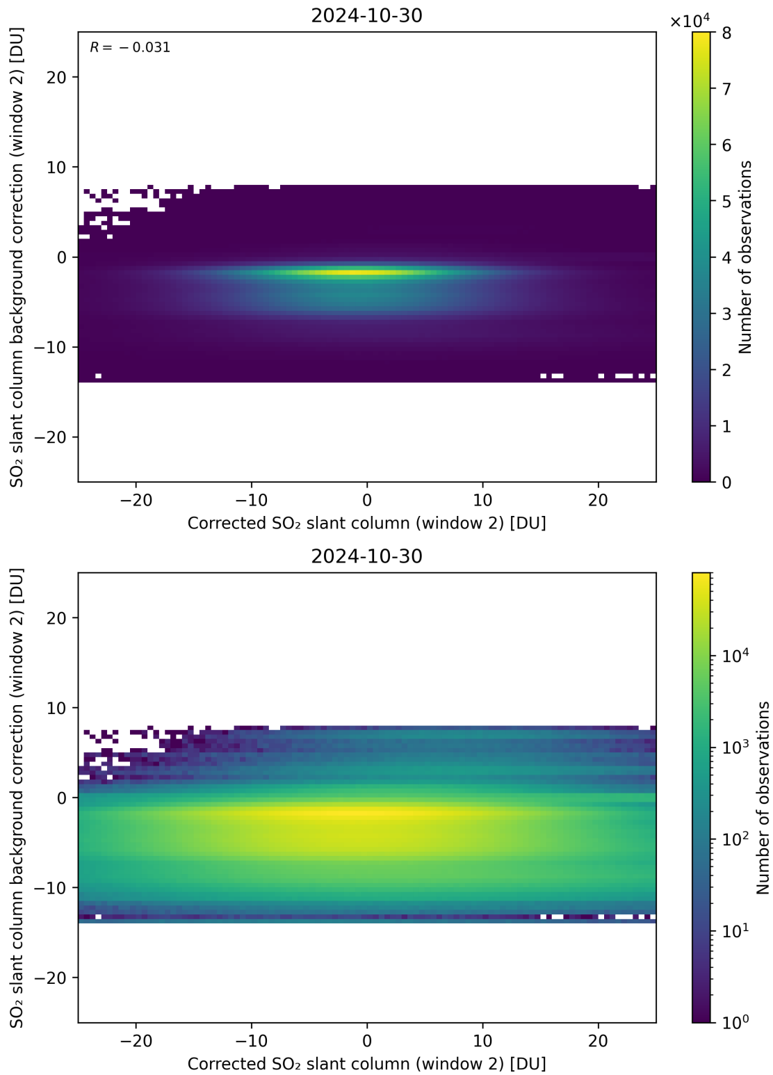
Figure 194: Scatter density plot of “Corrected SO 2 slant column (window 2)” against “SO 2 slant column background correction (window 2)” for 2024-10-30 to 2024-10-31.
