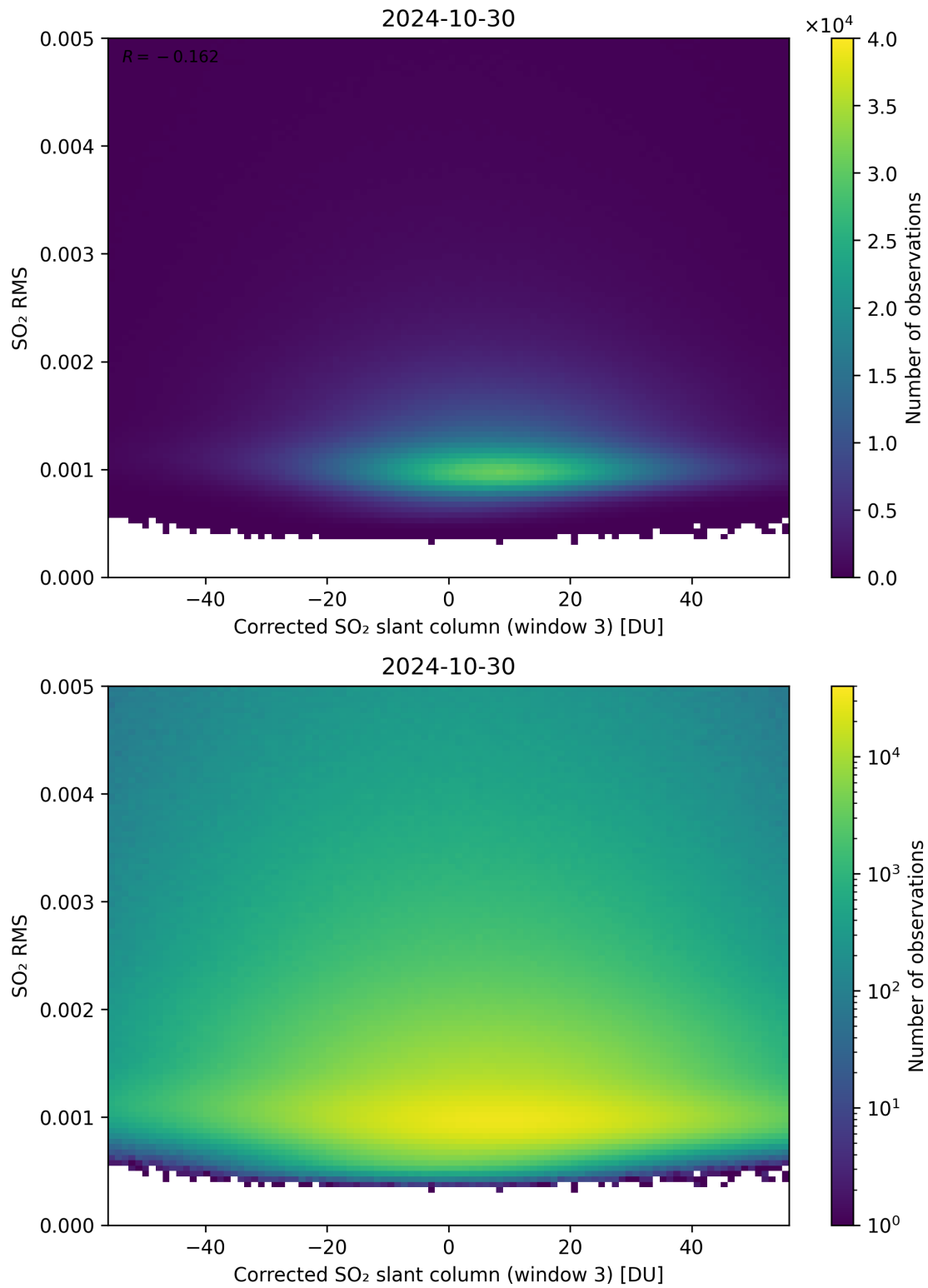
Figure 208: Scatter density plot of “Corrected SO 2 slant column (window 3)” against “SO 2 RMS” for 2024-10-30 to 2024-10-31.
