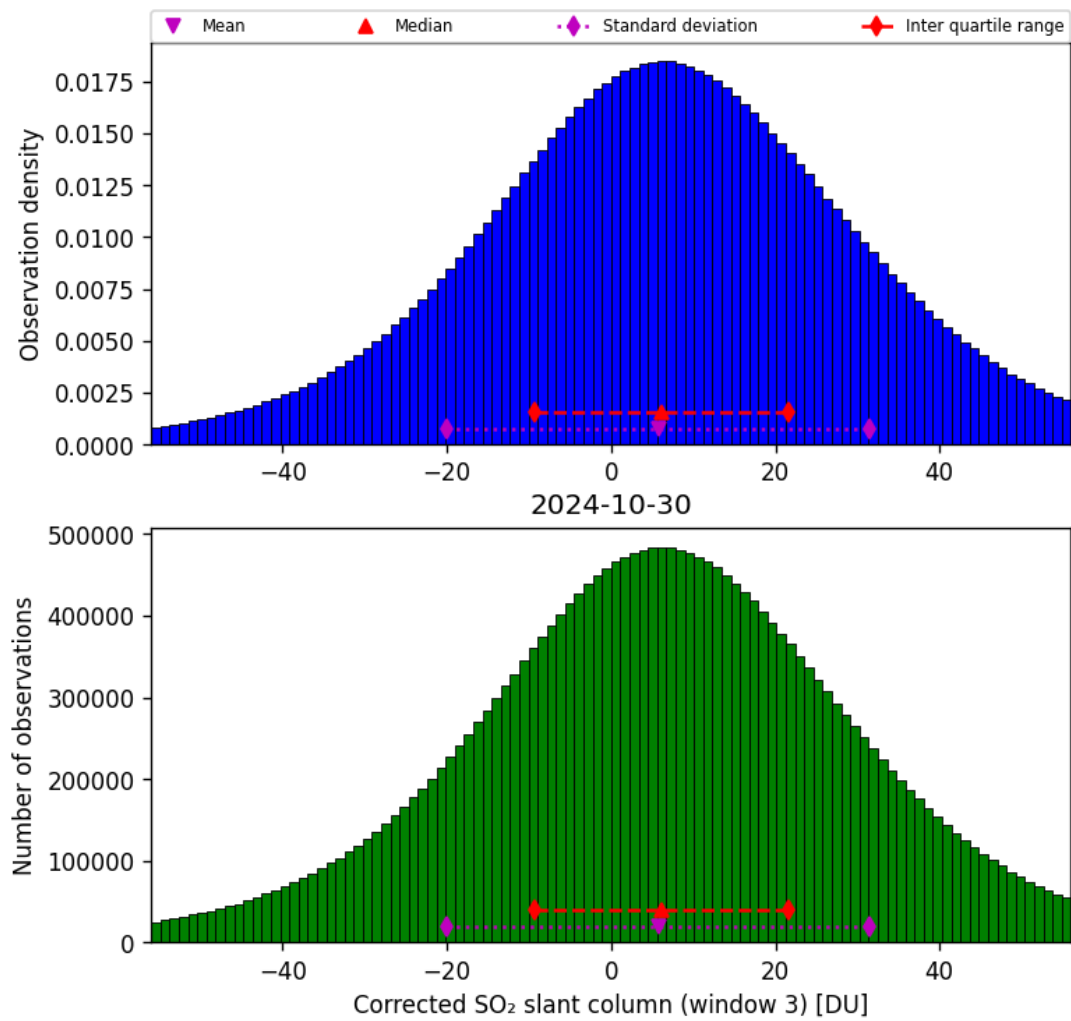
Figure 66: Histogram of “Corrected SO 2 slant column (window 3)” for 2024-10-30 to 2024-10-31
