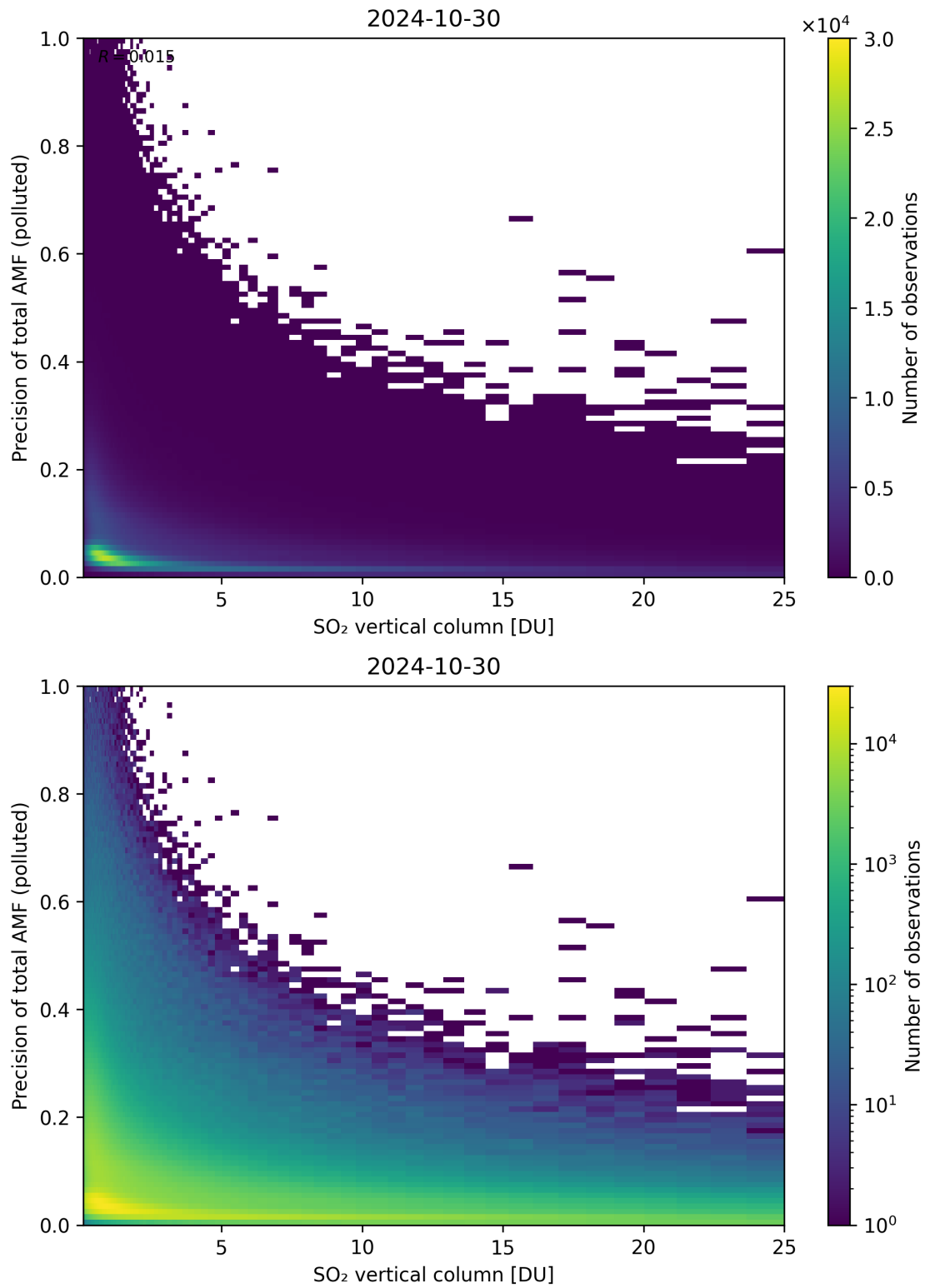
Figure 306: Scatter density plot of “SO 2 vertical column” against “Precision of total AMF (polluted)” for 2024-10-30 to 2024-10-31.
