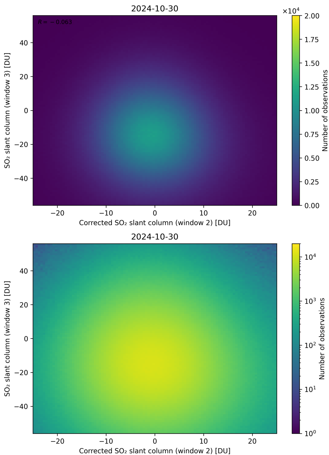
Figure 201: Scatter density plot of “Corrected SO 2 slant column (window 2)” against “SO 2 slant column (window 3)” for 2024-10-30 to 2024-10-31.
