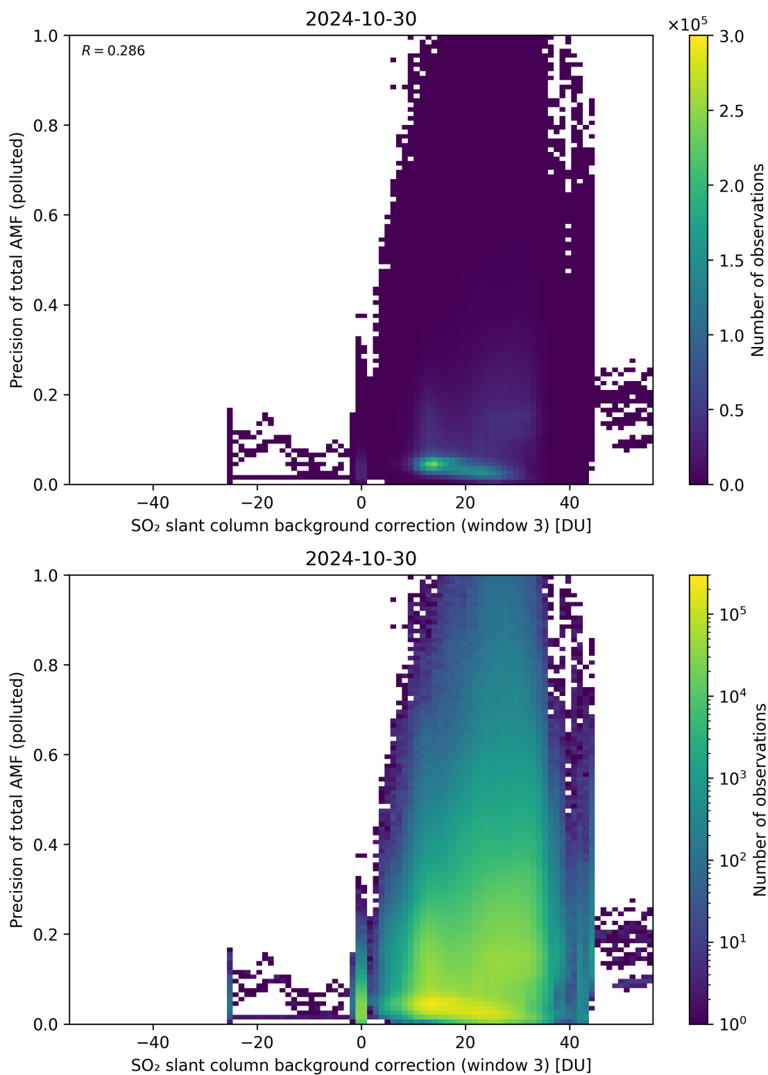
Figure 126: Scatter density plot of “SO 2 slant column background correction (window 3)” against “Precision of total AMF (polluted)” for 2024-10-30 to 2024-10-31.
