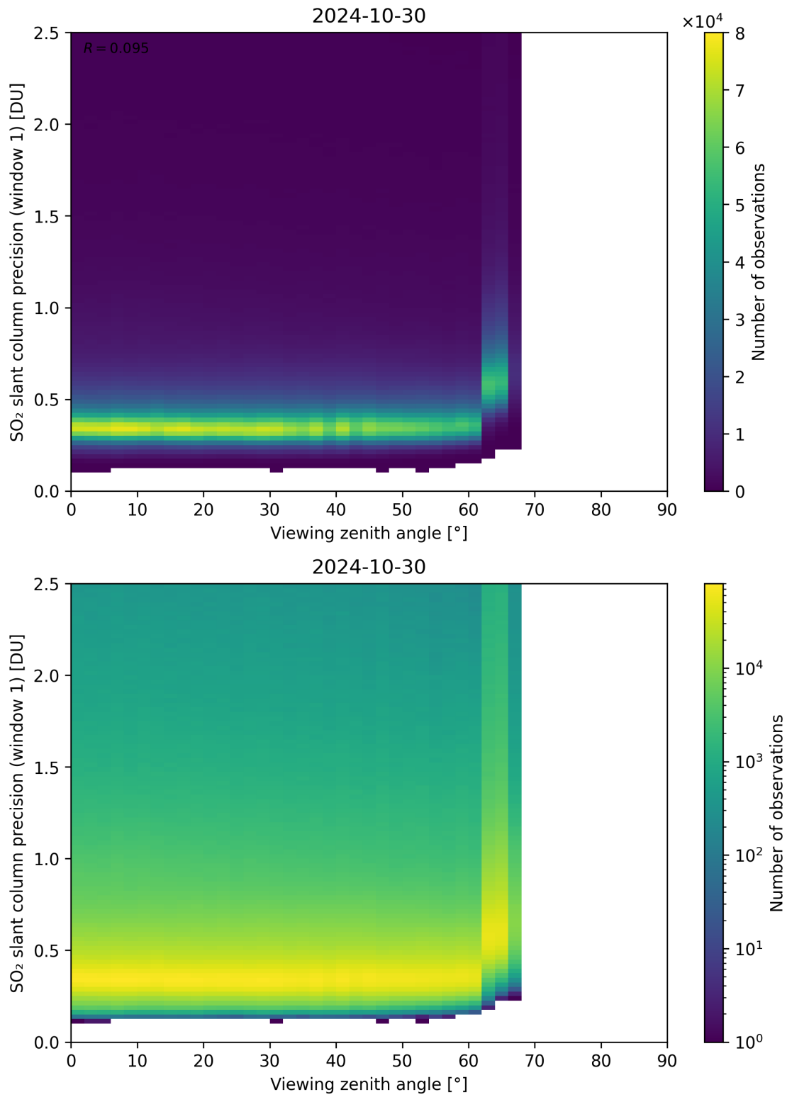
Figure 321: Scatter density plot of “Viewing zenith angle” against “SO 2 slant column precision (window 1)” for 2024-10-30 to 2024-10-31.
