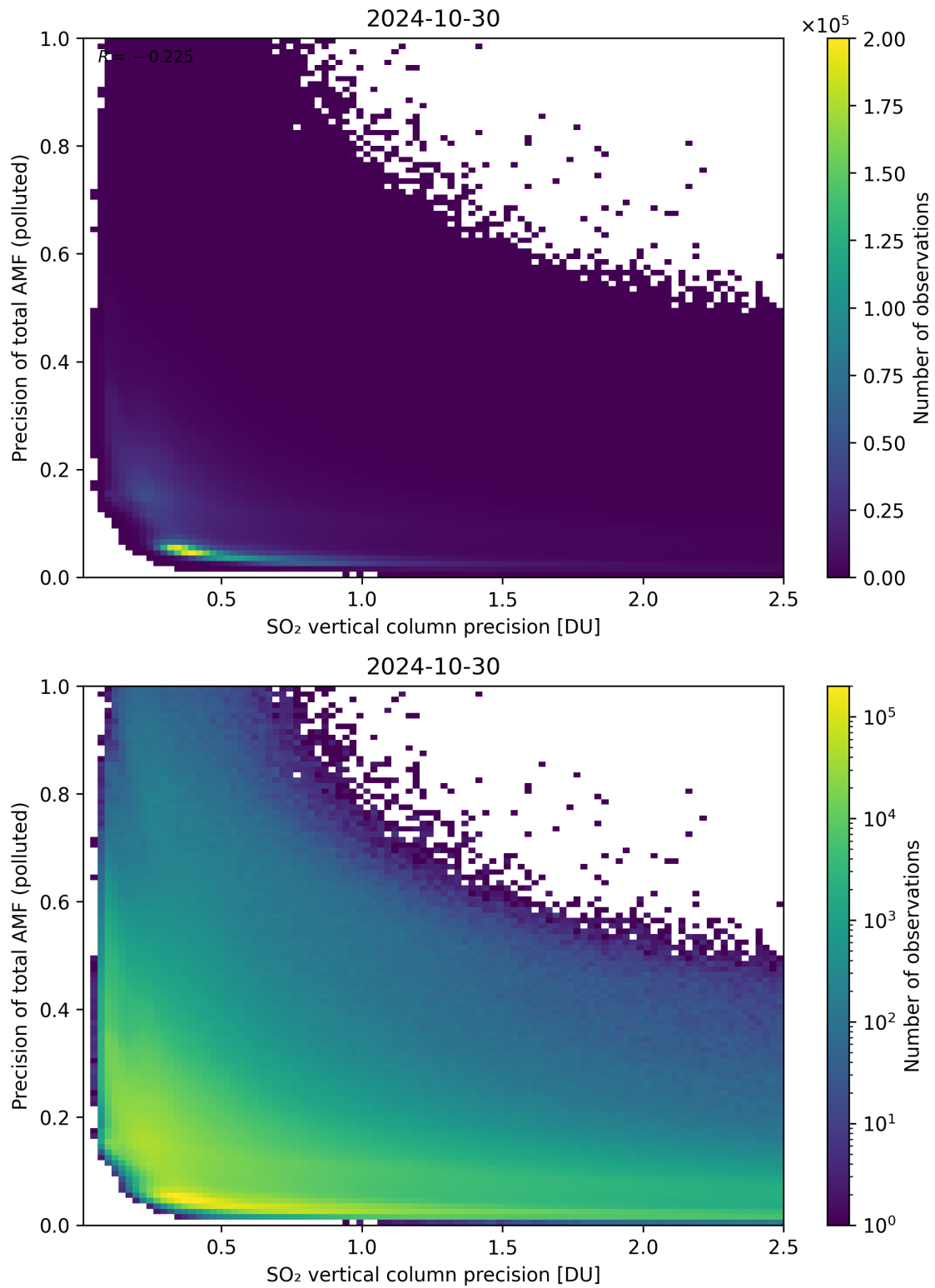
Figure 295: Scatter density plot of “SO 2 vertical column precision” against “Precision of total AMF (polluted)” for 2024-10-30 to 2024-10-31.
