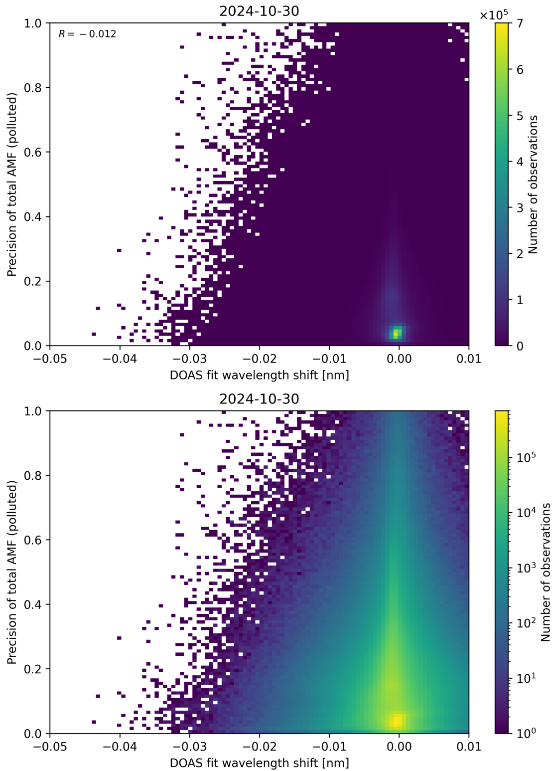
Figure 131: Scatter density plot of “DOAS fit wavelength shift” against “Precision of total AMF (polluted)” for 2024-10-30 to 2024-10-31.
