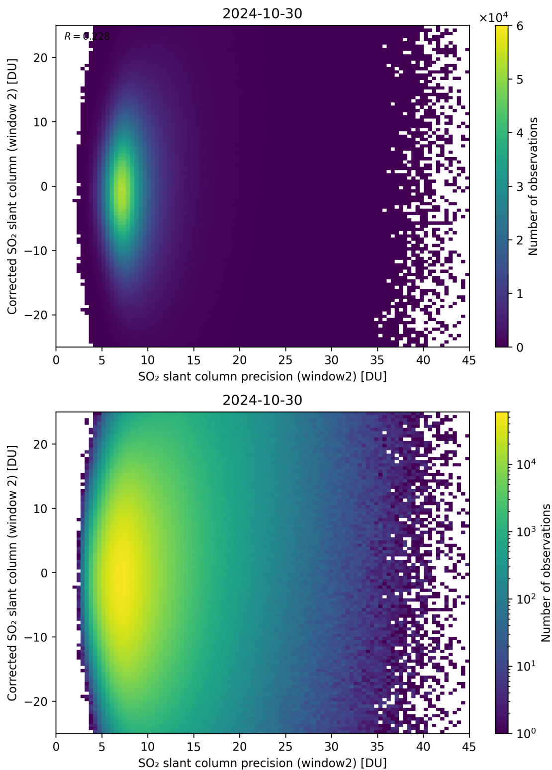
Figure 247: Scatter density plot of “SO 2 slant column precision (window2)” against “Corrected SO 2 slant column (window 2)” for 2024-10-30 to 2024-10-31.
