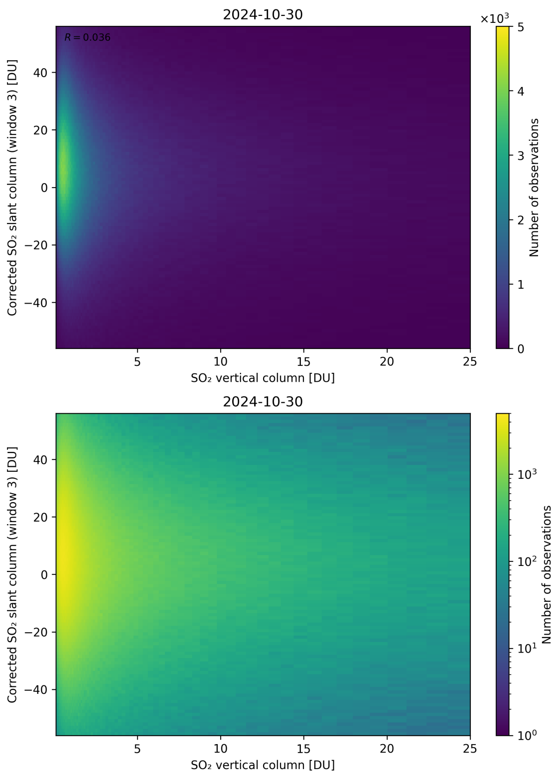
Figure 299: Scatter density plot of “SO 2 vertical column” against “Corrected SO 2 slant column (window 3)” for 2024-10-30 to 2024-10-31.
