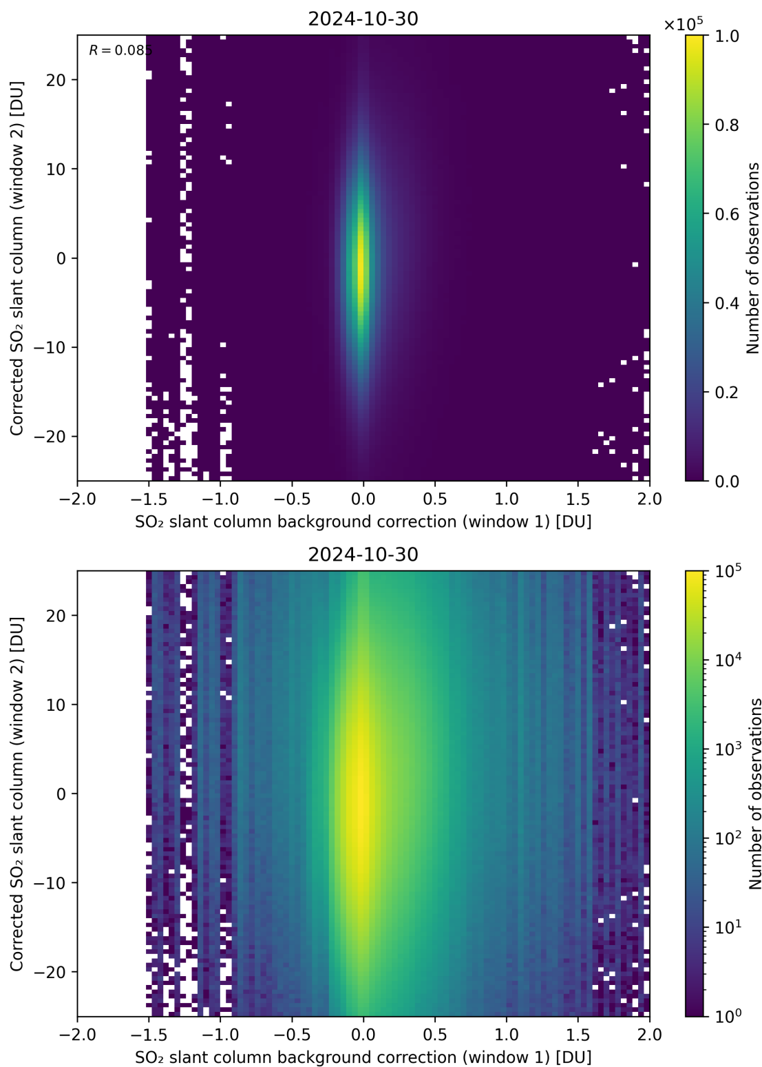
Figure 104: Scatter density plot of “SO 2 slant column background correction (window 1)” against “Corrected SO 2 slant column (window 2)” for 2024-10-30 to 2024-10-31.
