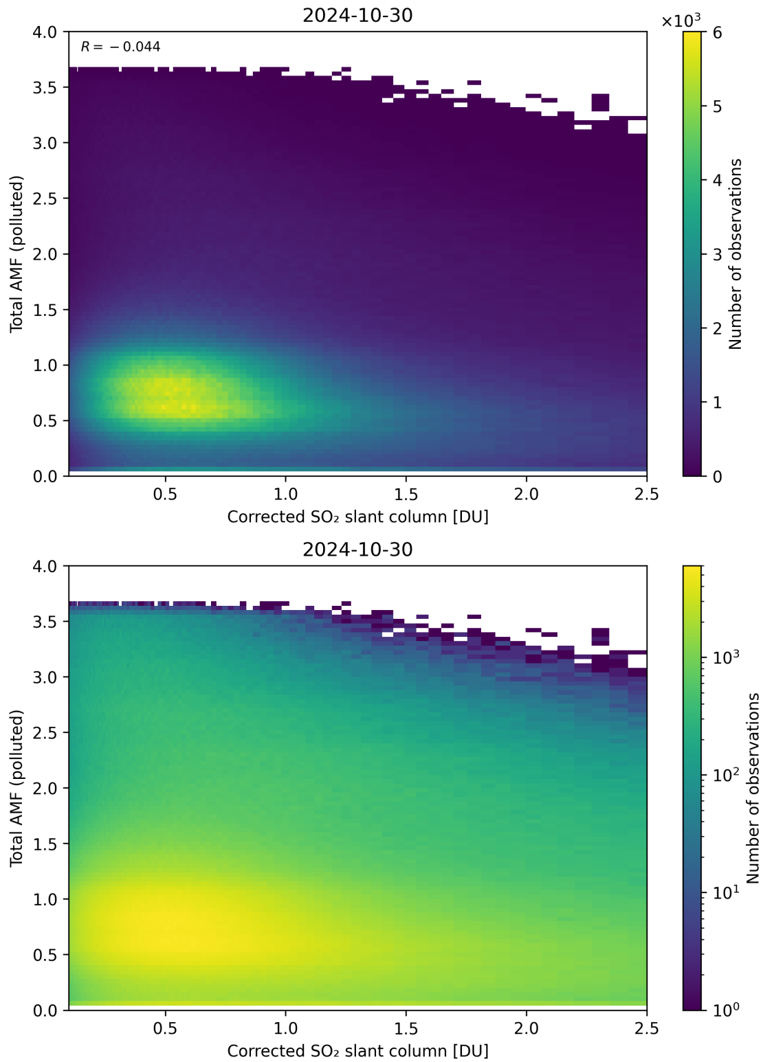
Figure 192: Scatter density plot of “Corrected SO 2 slant column” against “Total AMF (polluted)” for 2024-10-30 to 2024-10-31.
