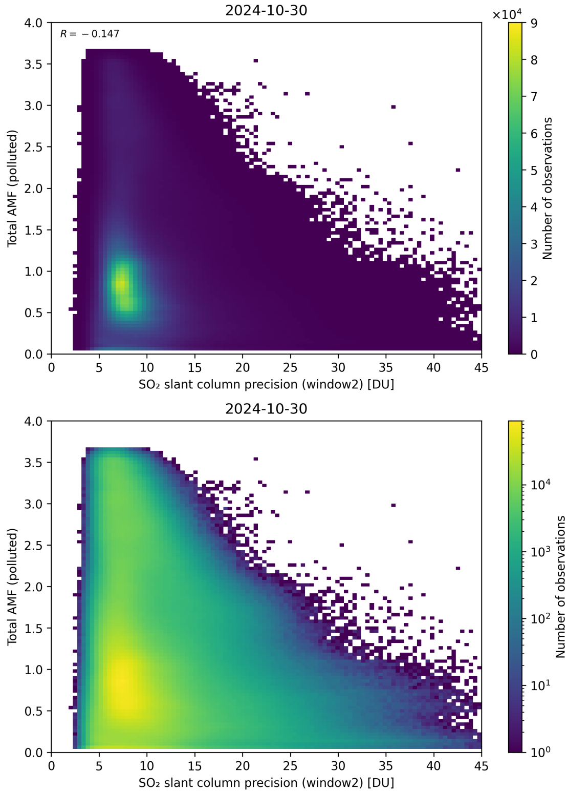
Figure 251: Scatter density plot of “SO 2 slant column precision (window2)” against “Total AMF (polluted)” for 2024-10-30 to 2024-10-31.
