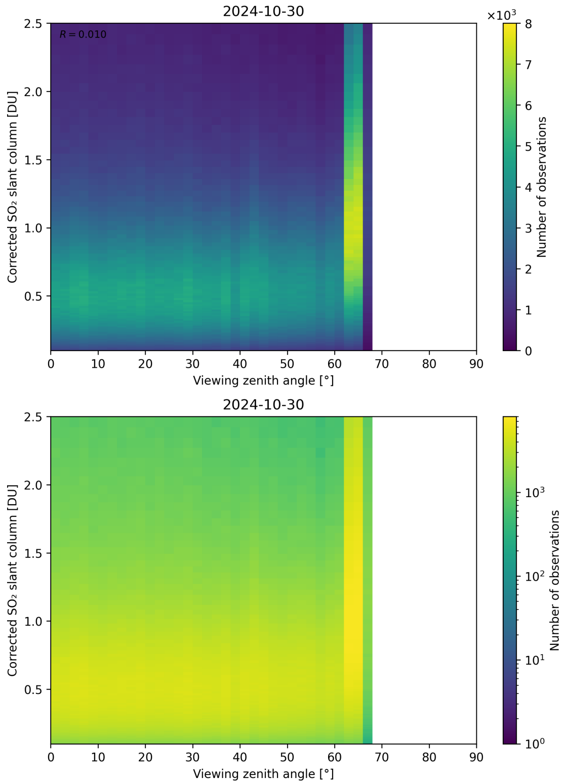
Figure 317: Scatter density plot of “Viewing zenith angle” against “Corrected SO 2 slant column” for 2024-10-30 to 2024-10-31.
