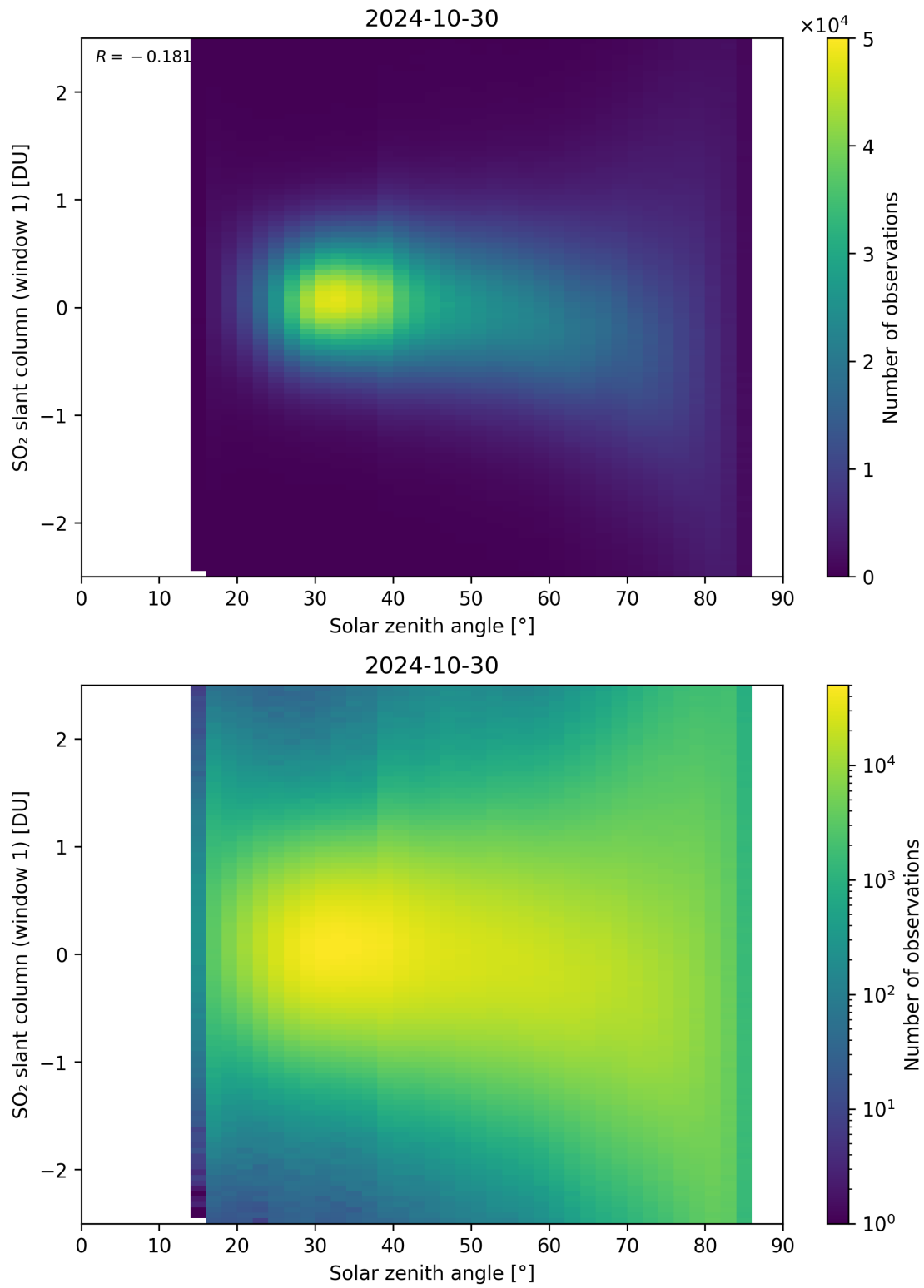
Figure 169: Scatter density plot of “Solar zenith angle” against “SO 2 slant column (window 1)” for 2024-10-30 to 2024-10-31.
