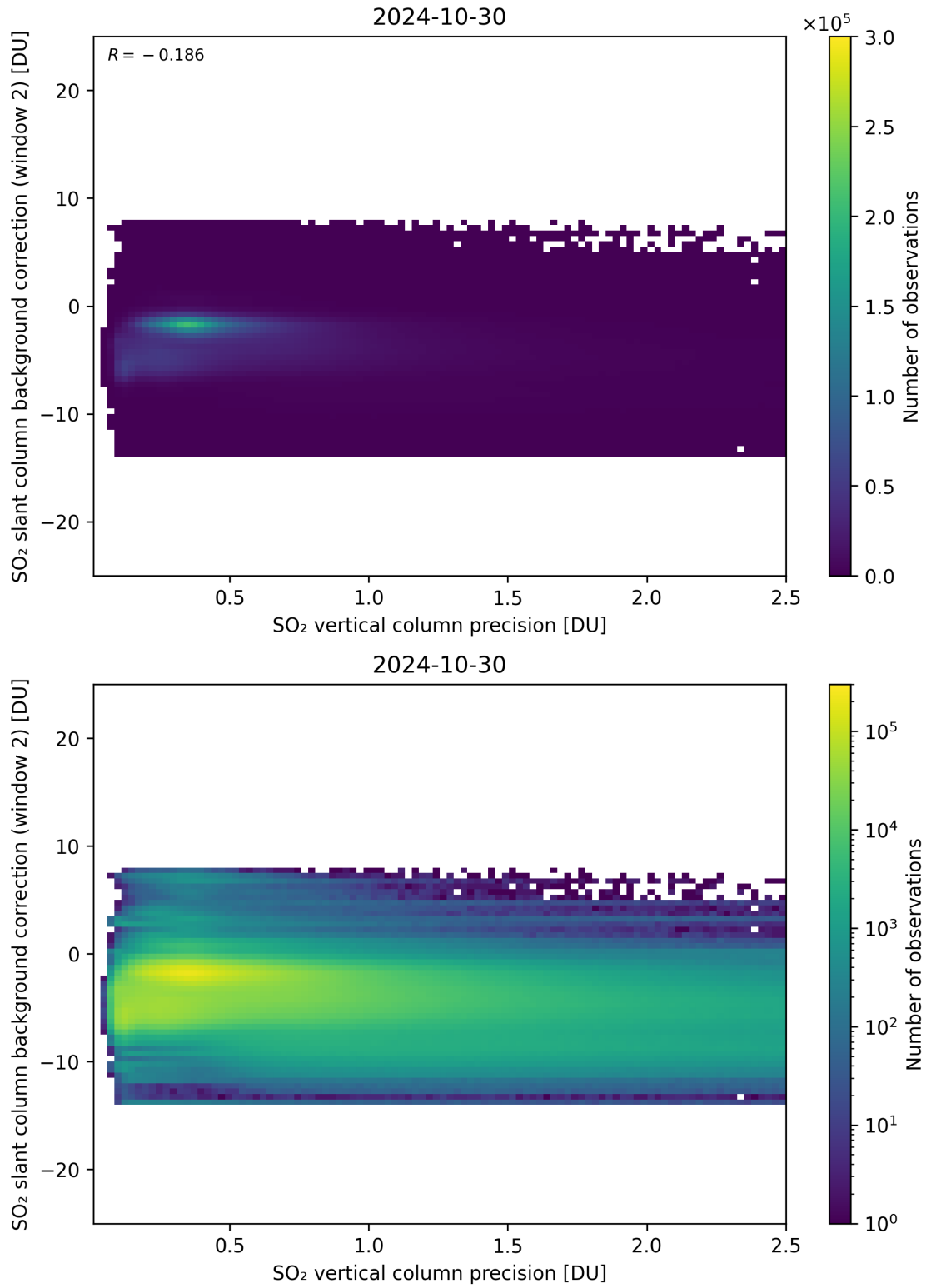
Figure 280: Scatter density plot of “SO 2 vertical column precision” against “SO 2 slant column background correction (window 2)” for 2024-10-30 to 2024-10-31.
