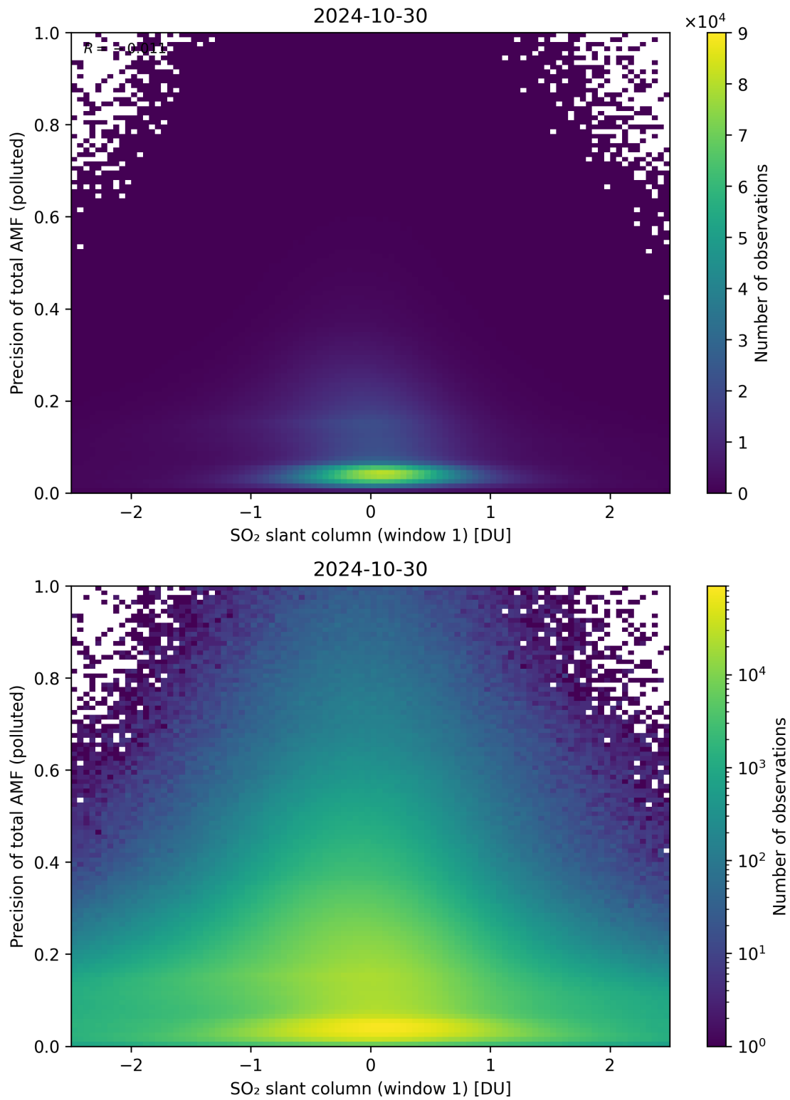
Figure 240: Scatter density plot of “SO 2 slant column (window 1)” against “Precision of total AMF (polluted)” for 2024-10-30 to 2024-10-31.
