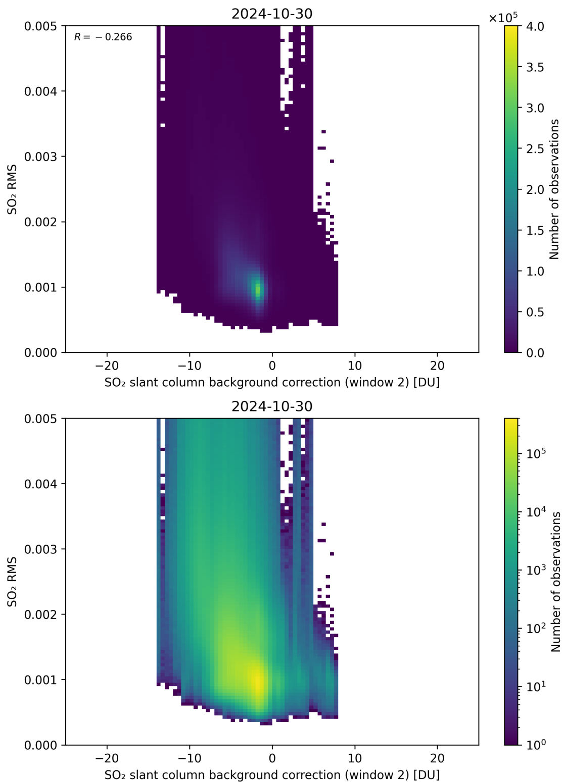
Figure 114: Scatter density plot of “SO 2 slant column background correction (window 2)” against “SO 2 RMS” for 2024-10-30 to 2024-10-31.
