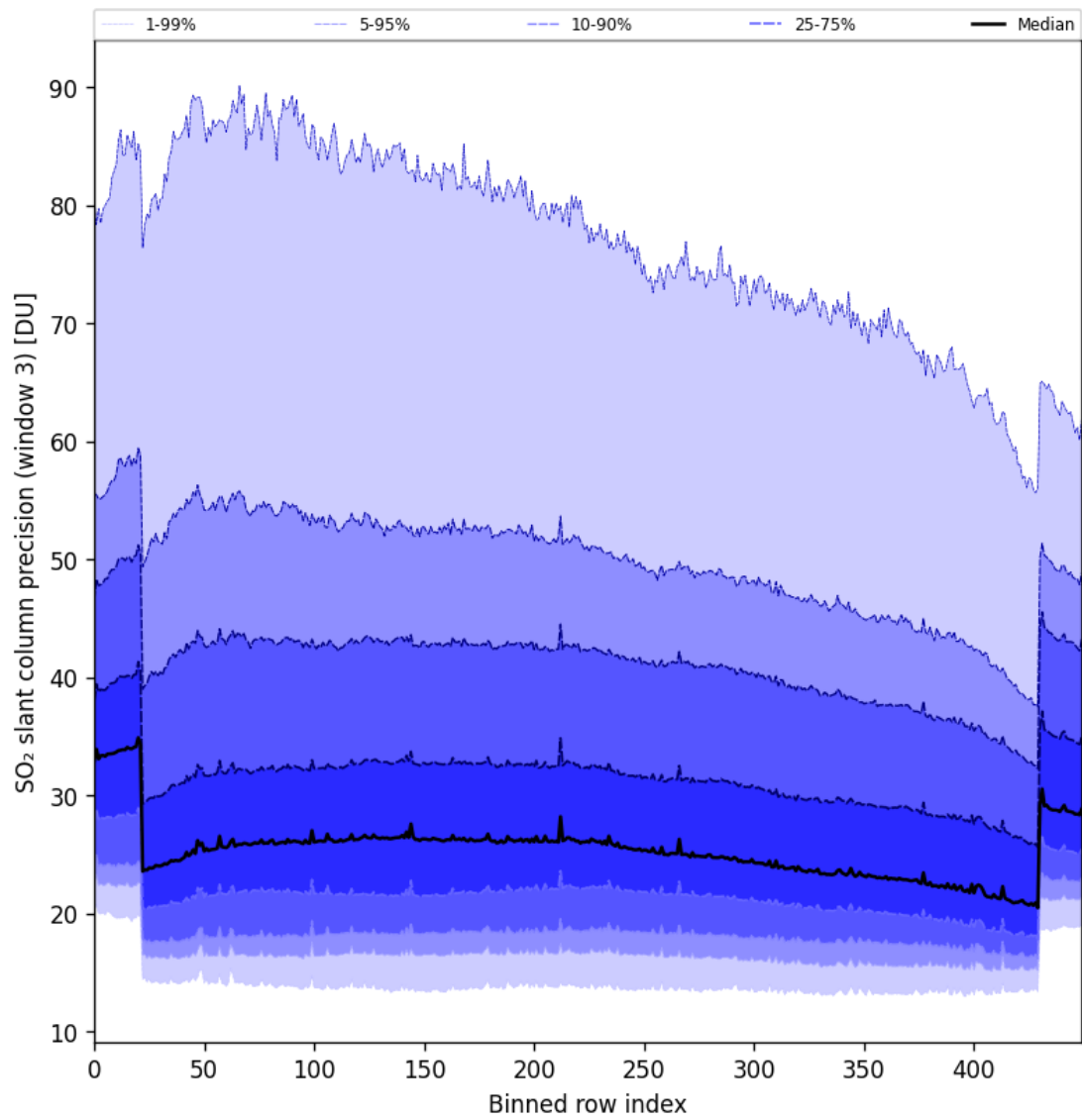
Figure 88: Along track statistics of “SO 2 slant column precision (window 3)” for 2024-10-30 to 2024-10-31
