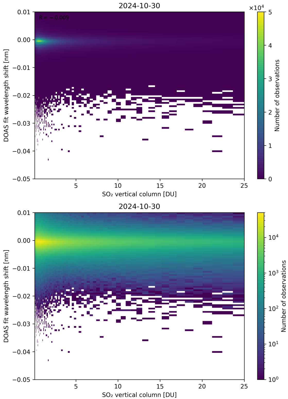
Figure 276: Scatter density plot of “SO 2 vertical column” against “DOAS fit wavelength shift” for 2024-10-30 to 2024-10-31.
