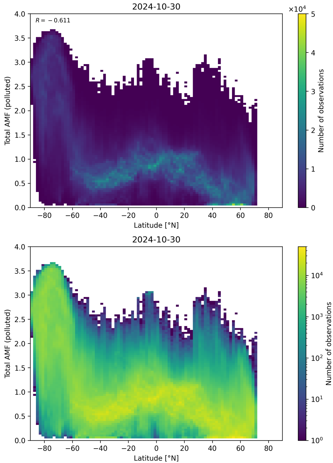
Figure 154: Scatter density plot of “Latitude” against “Total AMF (polluted)” for 2024-10-30 to 2024-10-31.
