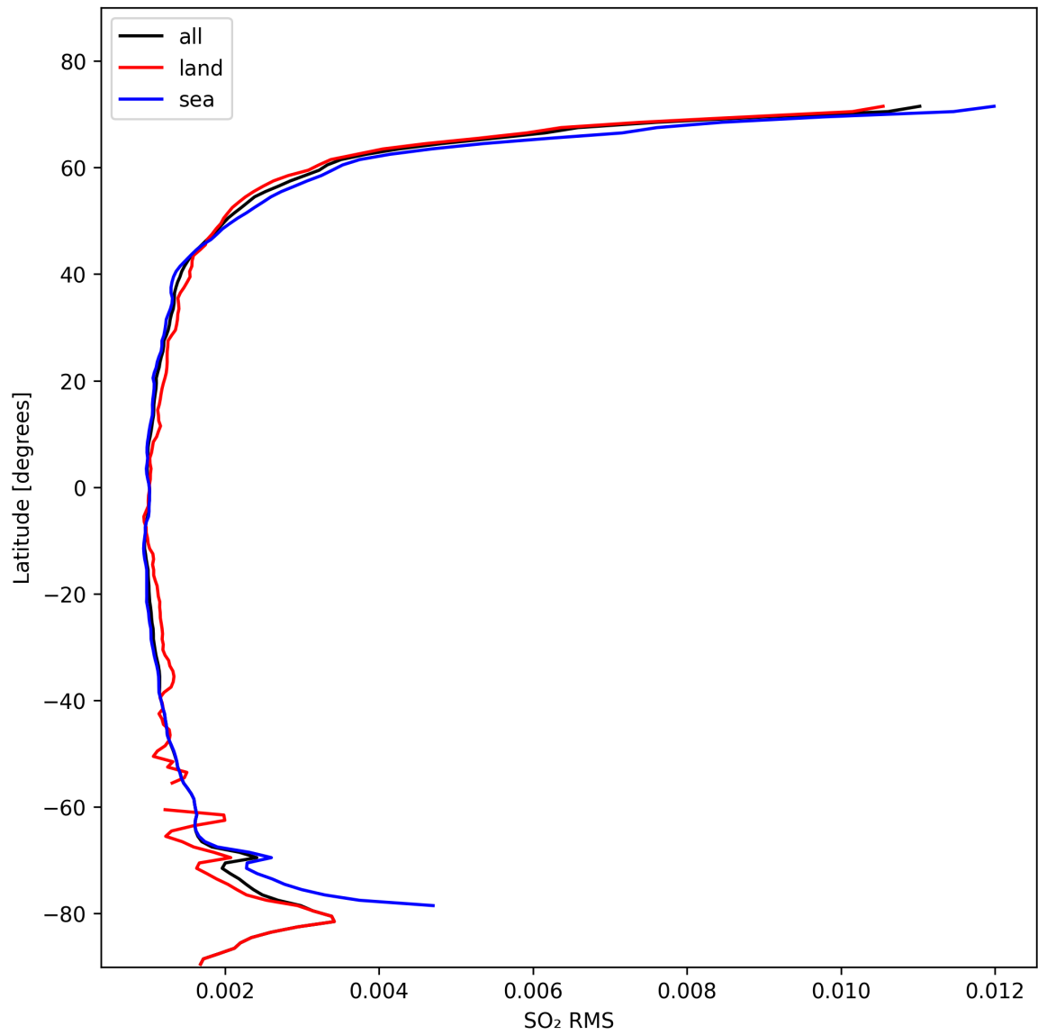
Figure 47: Zonal average of “SO 2 RMS” for 2024-10-30 to 2024-10-31.
