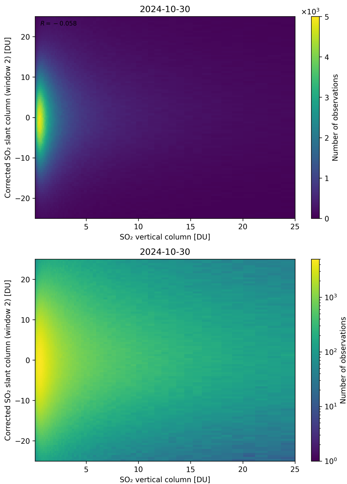
Figure 298: Scatter density plot of “SO 2 vertical column” against “Corrected SO 2 slant column (window 2)” for 2024-10-30 to 2024-10-31.
