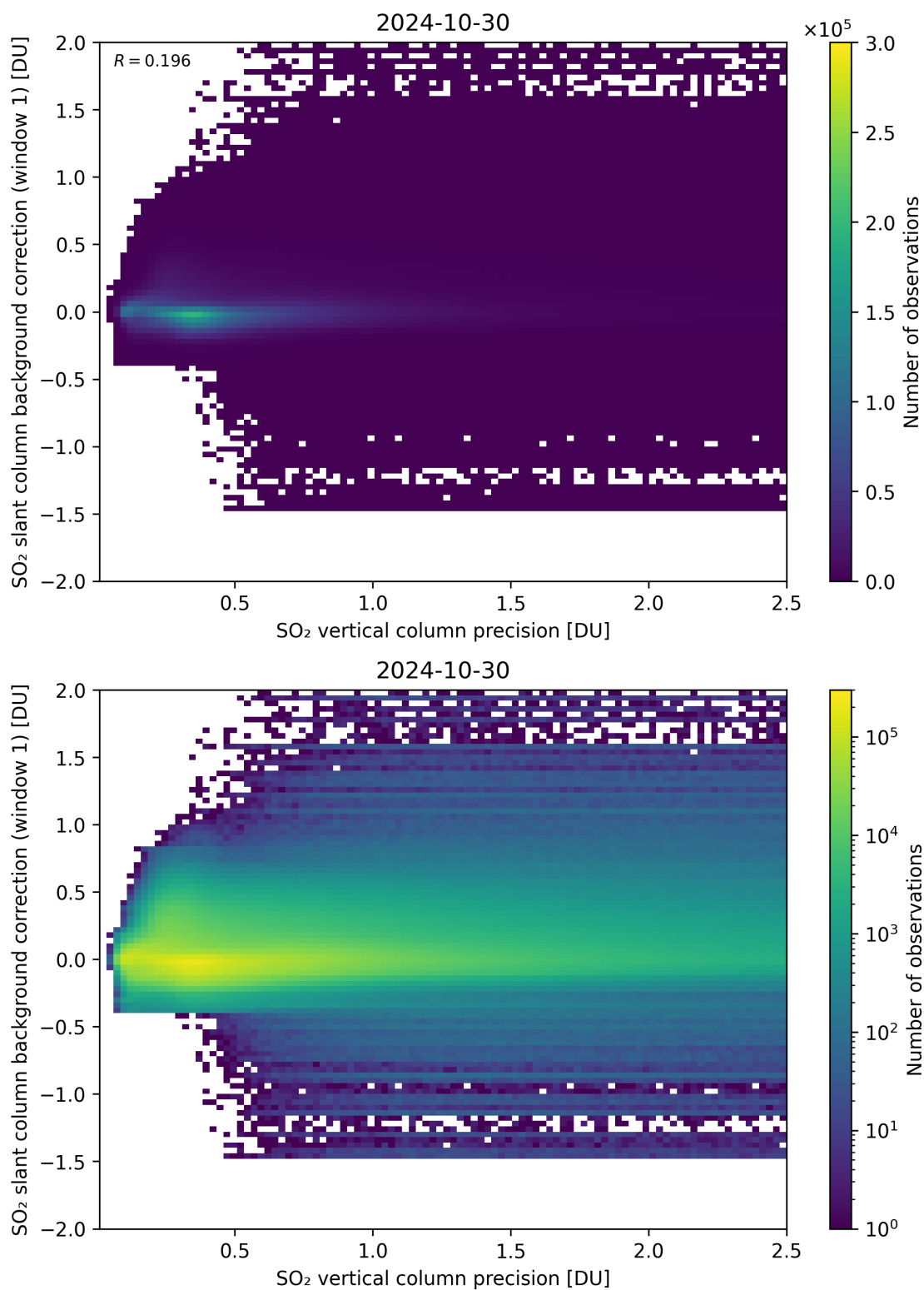
Figure 279: Scatter density plot of “SO 2 vertical column precision” against “SO 2 slant column background correction (window 1)” for 2024-10-30 to 2024-10-31.
