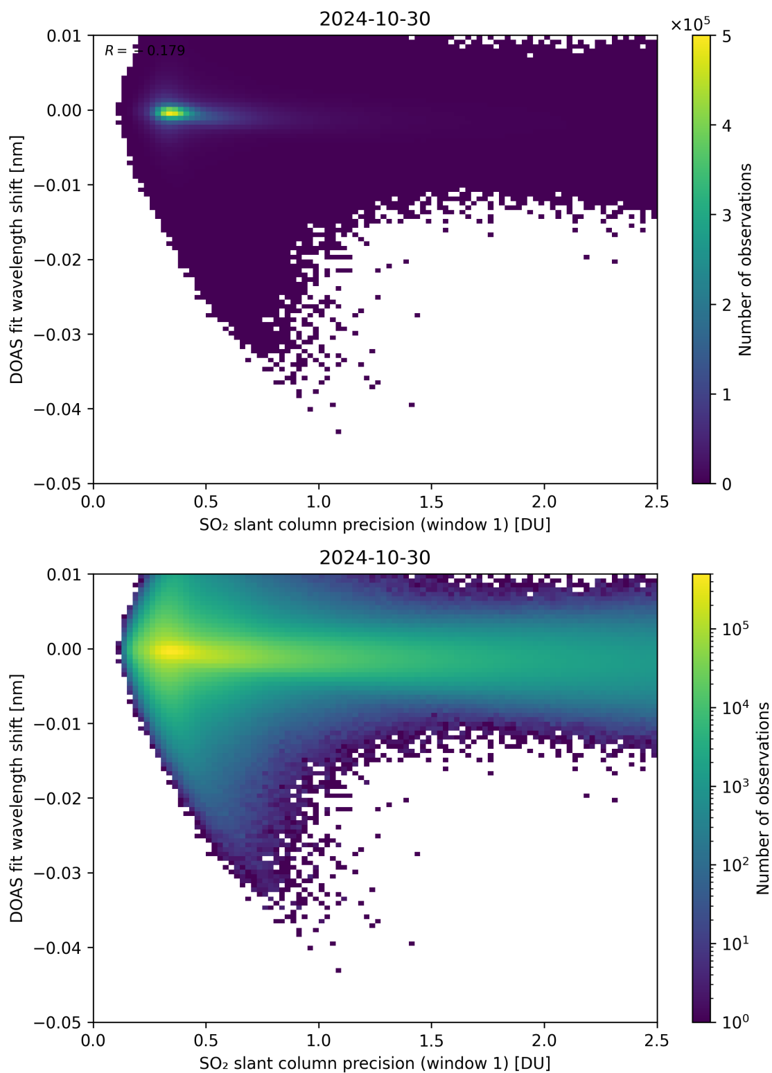
Figure 221: Scatter density plot of “SO 2 slant column precision (window 1)” against “DOAS fit wavelength shift” for 2024-10-30 to 2024-10-31.
