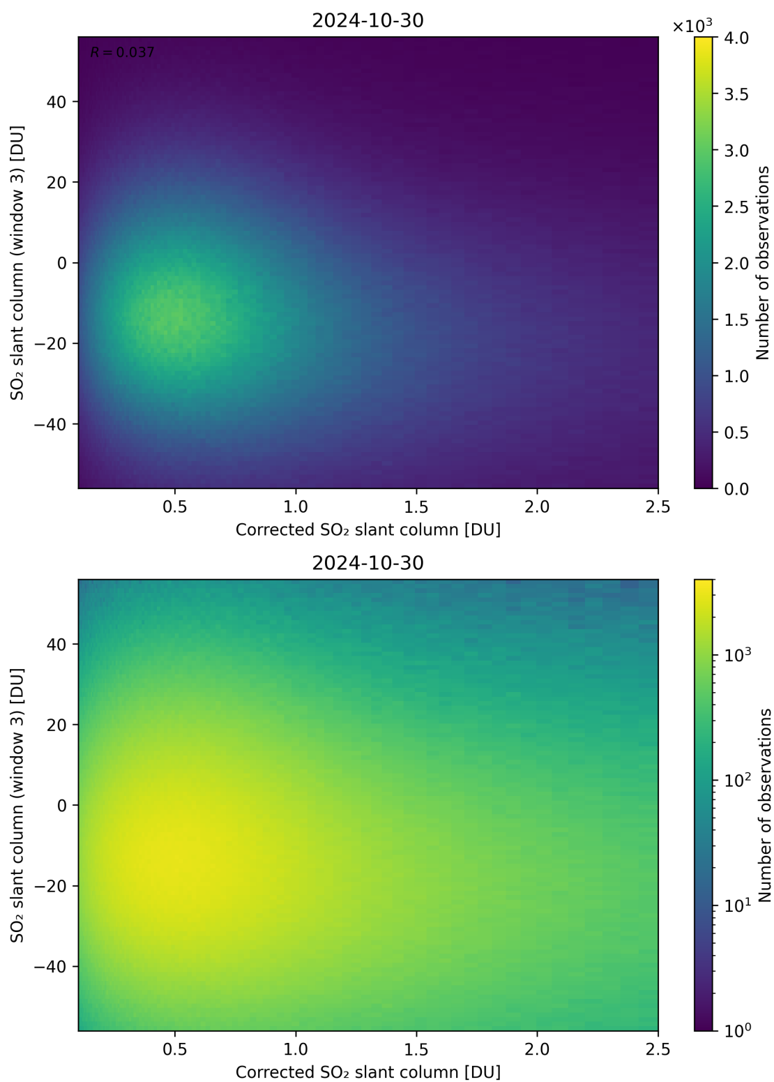
Figure 190: Scatter density plot of “Corrected SO 2 slant column” against “SO 2 slant column (window 3)” for 2024-10-30 to 2024-10-31.
