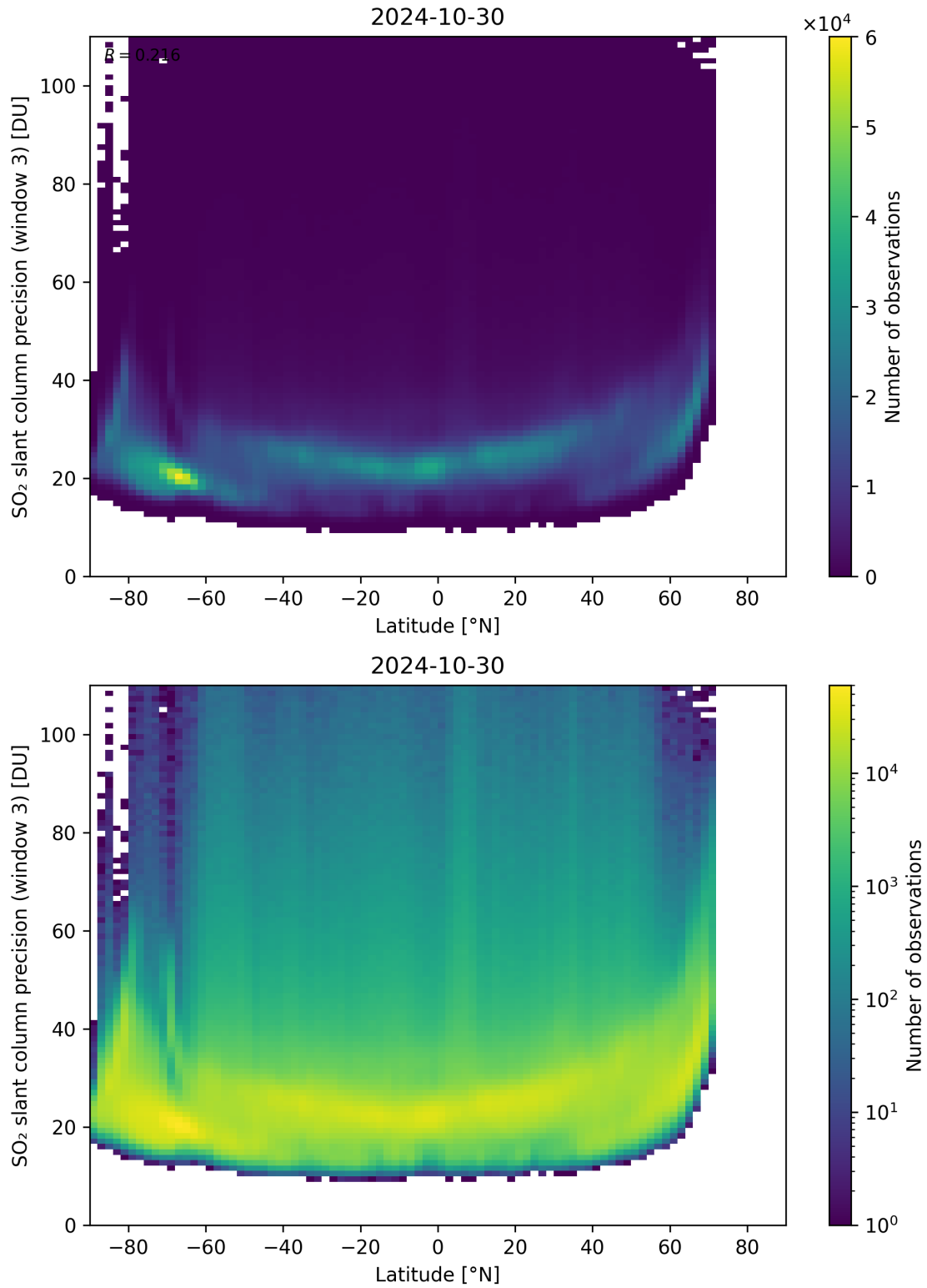
Figure 153: Scatter density plot of “Latitude” against “SO 2 slant column precision (window 3)” for 2024-10-30 to 2024-10-31.
