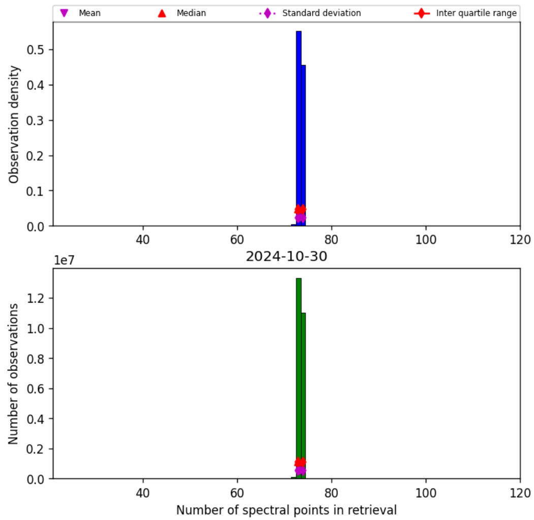
Figure 74: Histogram of “Number of spectral points in retrieval” for 2024-10-30 to 2024-10-31
