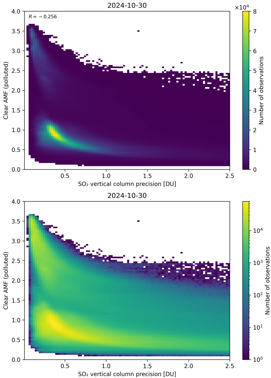
Figure 285: Scatter density plot of “SO 2 vertical column precision” against “Clear AMF (polluted)” for 2024-10-30 to 2024-10-31.
