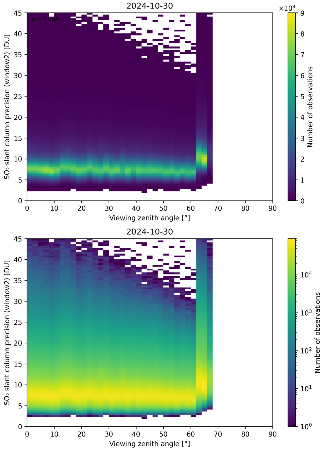
Figure 322: Scatter density plot of “Viewing zenith angle” against “SO 2 slant column precision (window2)” for 2024-10-30 to 2024-10-31.
