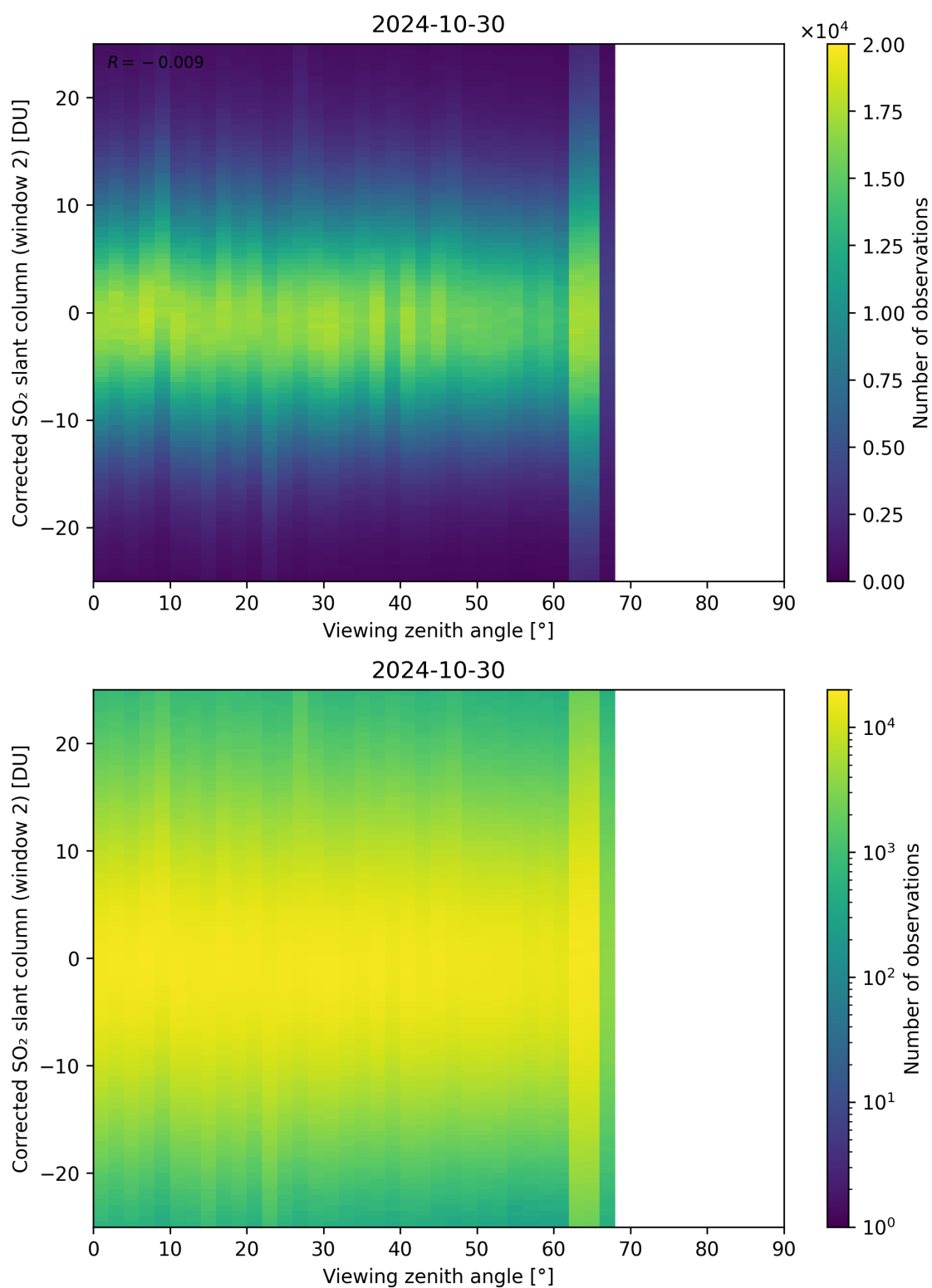
Figure 318: Scatter density plot of “Viewing zenith angle” against “Corrected SO 2 slant column (window 2)” for 2024-10-30 to 2024-10-31.
