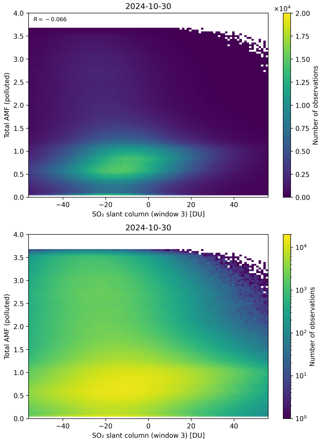
Figure 268: Scatter density plot of “SO 2 slant column (window 3)” against “Total AMF (polluted)” for 2024-10-30 to 2024-10-31.
