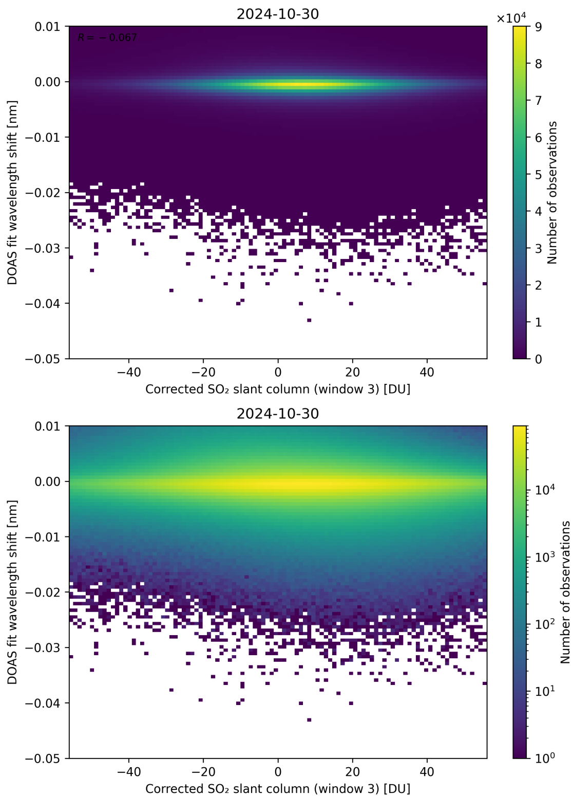
Figure 206: Scatter density plot of “Corrected SO 2 slant column (window 3)” against “DOAS fit wavelength shift” for 2024-10-30 to 2024-10-31.
