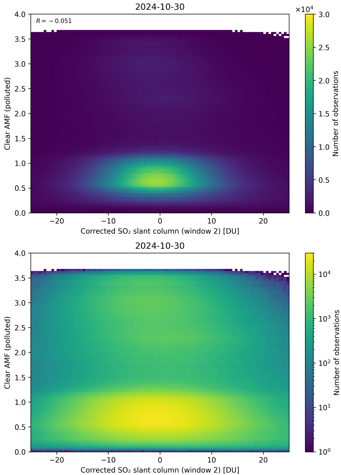
Figure 199: Scatter density plot of “Corrected SO 2 slant column (window 2)” against “Clear AMF (polluted)” for 2024-10-30 to 2024-10-31.
