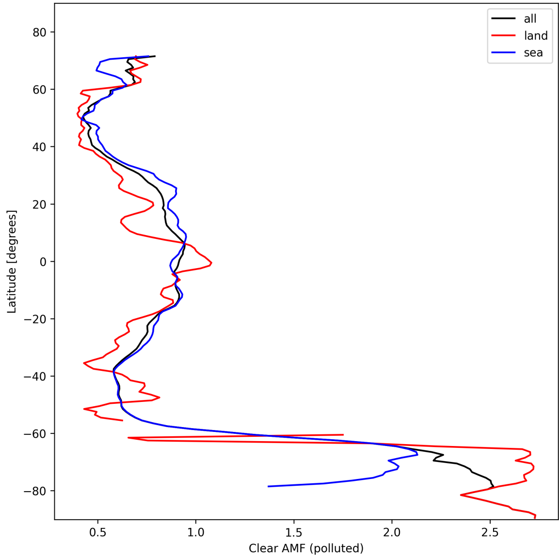
Figure 50: Zonal average of “Clear AMF (polluted)” for 2024-10-30 to 2024-10-31.
