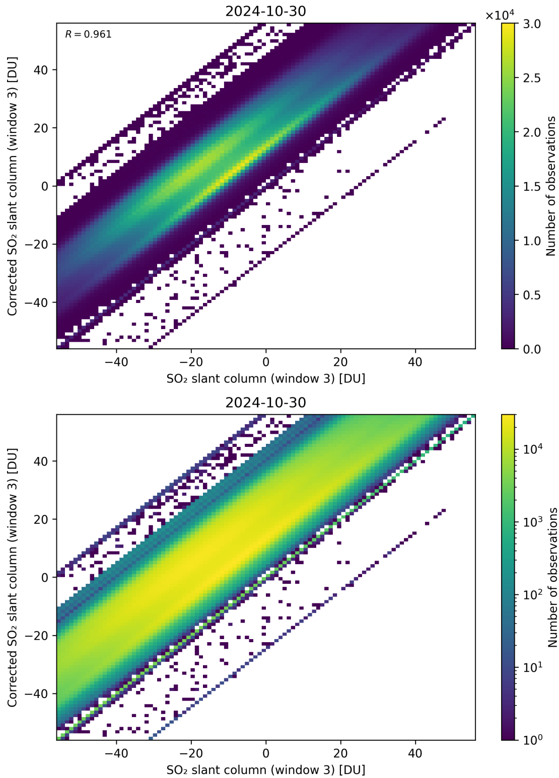
Figure 266: Scatter density plot of “SO 2 slant column (window 3)” against “Corrected SO 2 slant column (window 3)” for 2024-10-30 to 2024-10-31.
