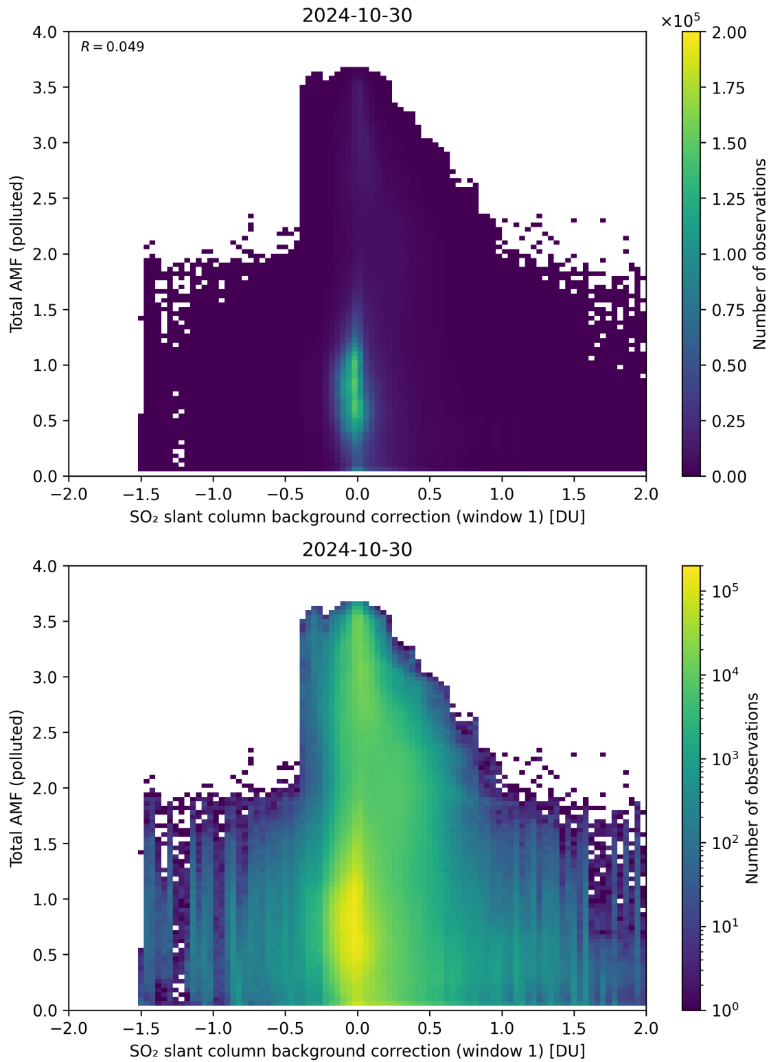
Figure 109: Scatter density plot of “SO 2 slant column background correction (window 1)” against “Total AMF (polluted)” for 2024-10-30 to 2024-10-31.
