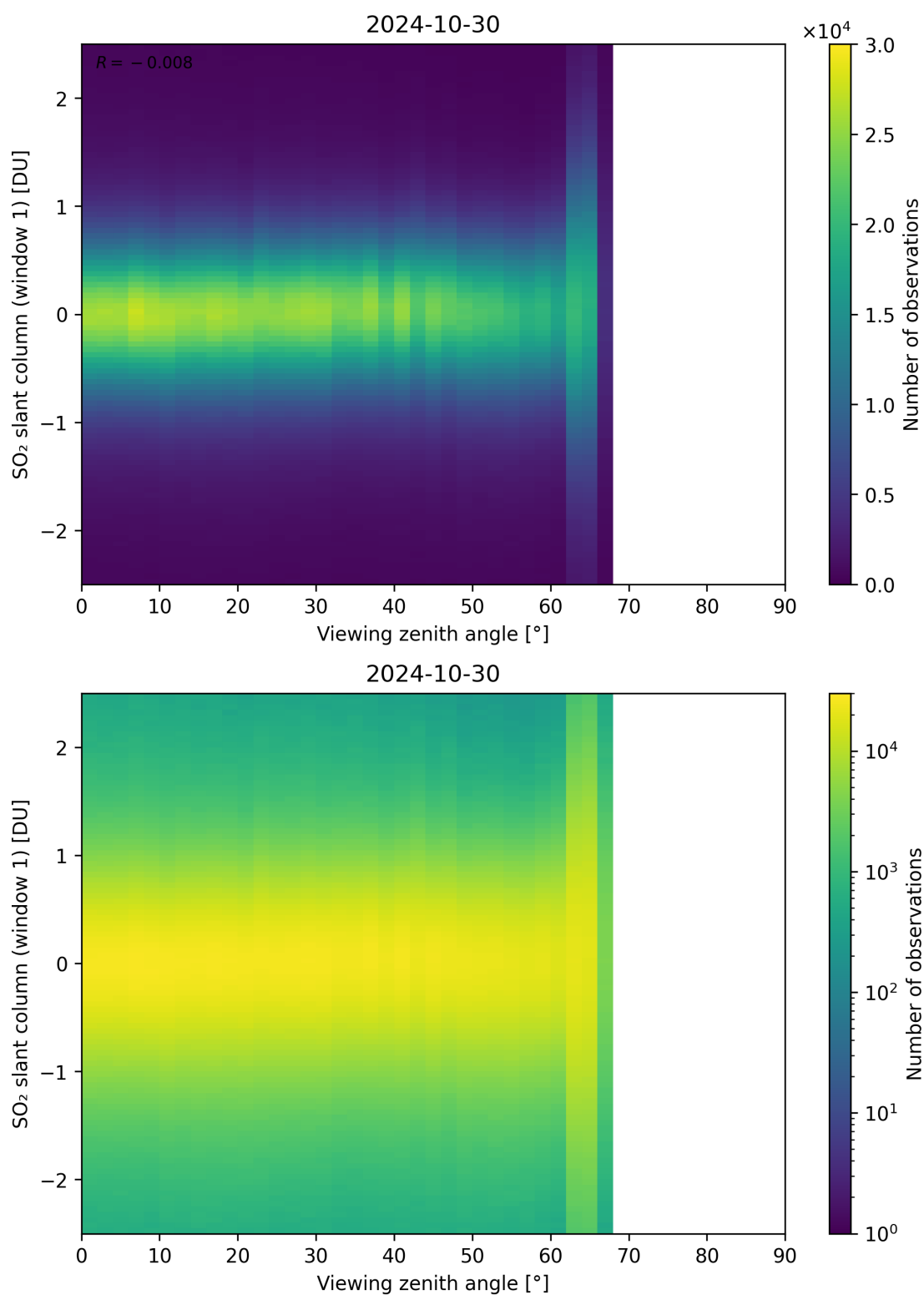
Figure 320: Scatter density plot of “Viewing zenith angle” against “SO 2 slant column (window 1)” for 2024-10-30 to 2024-10-31.
