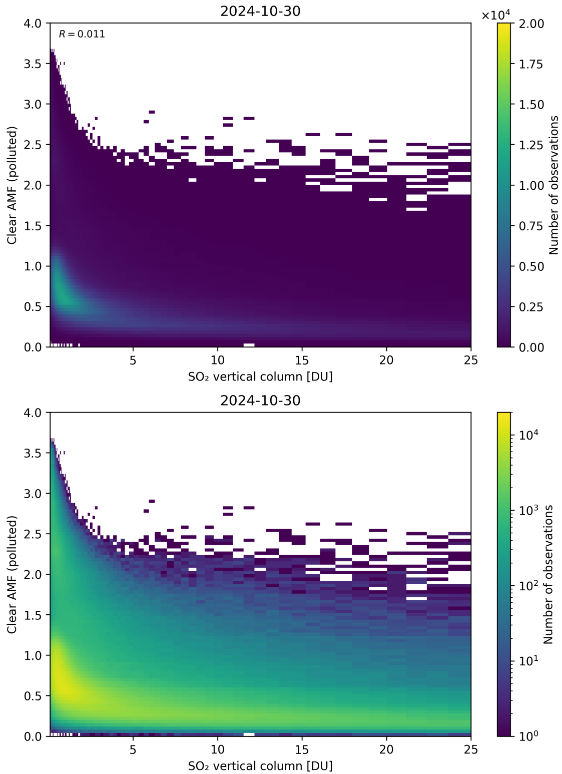
Figure 296: Scatter density plot of “SO 2 vertical column” against “Clear AMF (polluted)” for 2024-10-30 to 2024-10-31.
