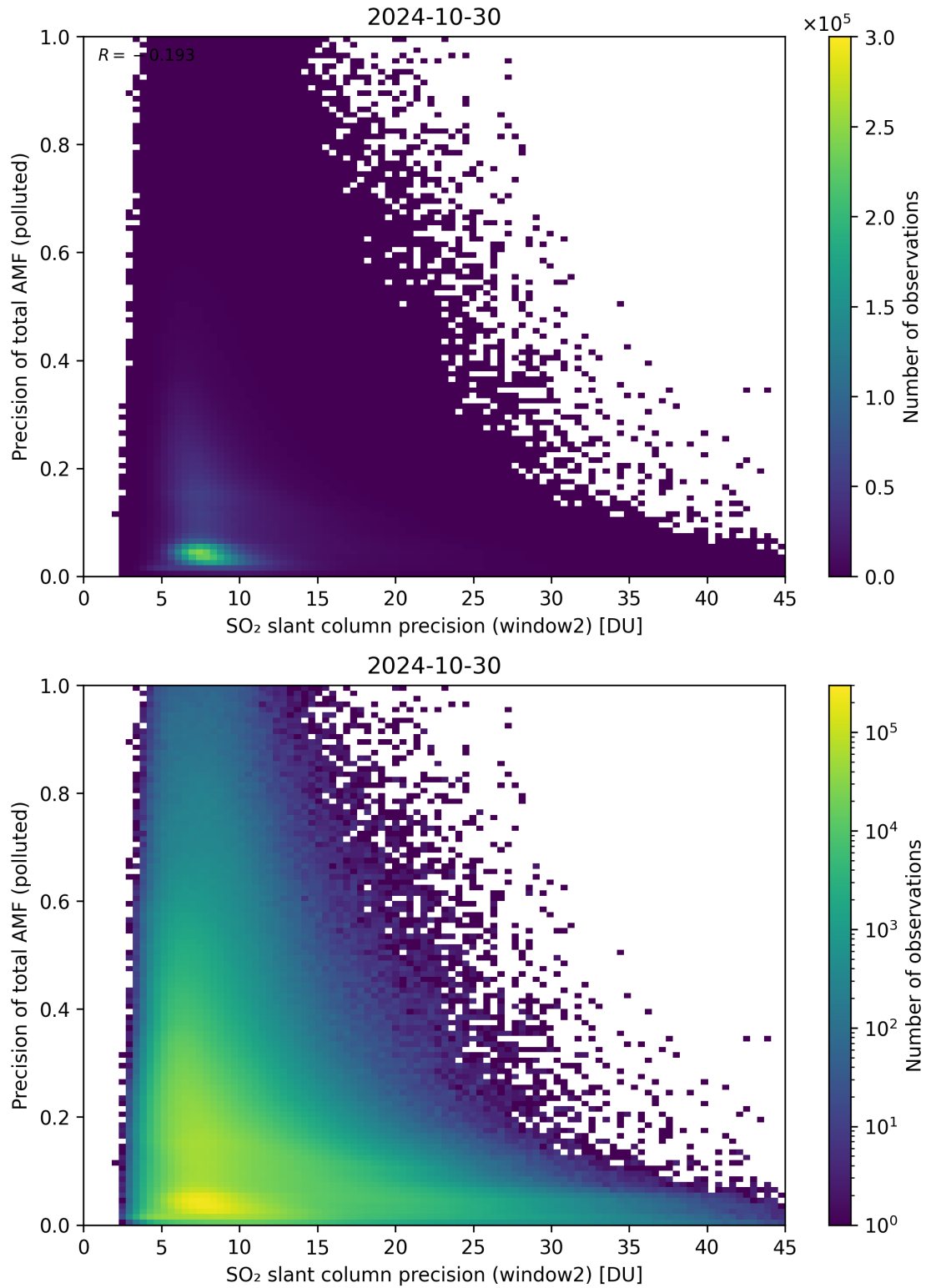
Figure 252: Scatter density plot of “SO 2 slant column precision (window2)” against “Precision of total AMF (polluted)” for 2024-10-30 to 2024-10-31.
