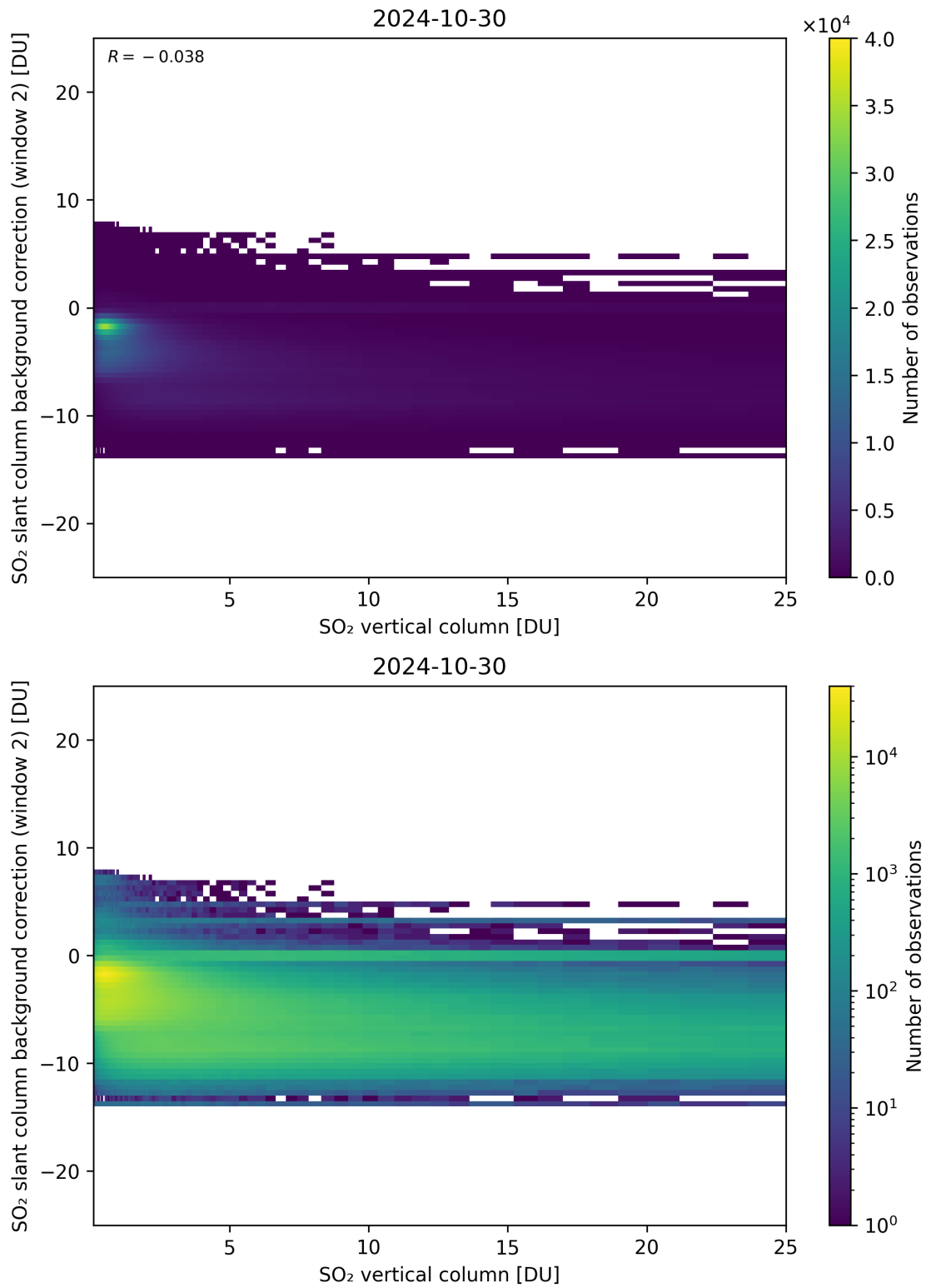
Figure 274: Scatter density plot of “SO 2 vertical column” against “SO 2 slant column background correction (window 2)” for 2024-10-30 to 2024-10-31.
