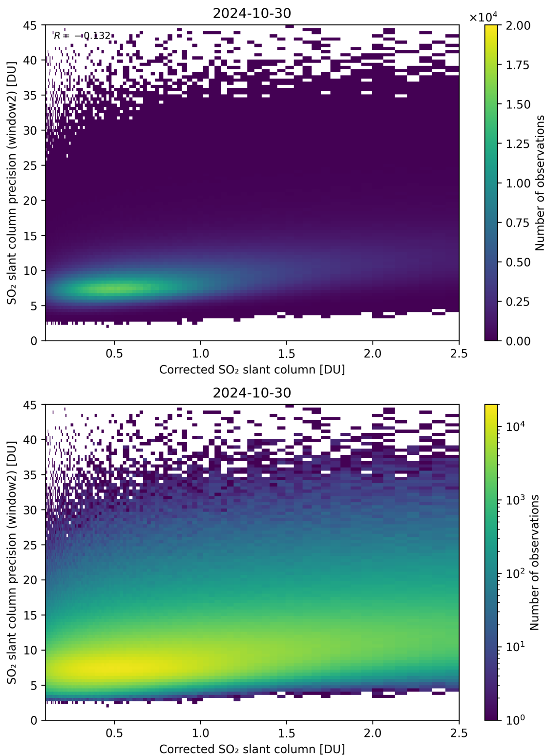
Figure 189: Scatter density plot of “Corrected SO 2 slant column” against “SO 2 slant column precision (window2)” for 2024-10-30 to 2024-10-31.
