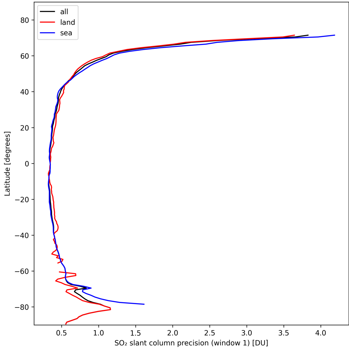
Figure 34: Zonal average of “SO 2 slant column precision (window 1)” for 2024-10-30 to 2024-10-31.
