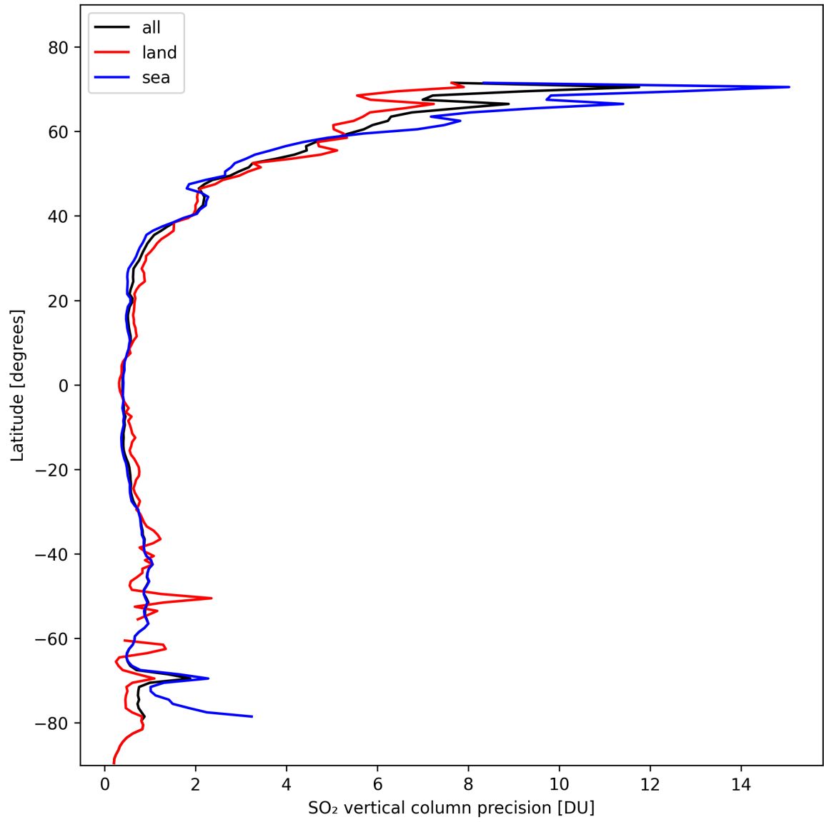
Figure 31: Zonal average of “SO 2 vertical column precision” for 2024-10-30 to 2024-10-31.
