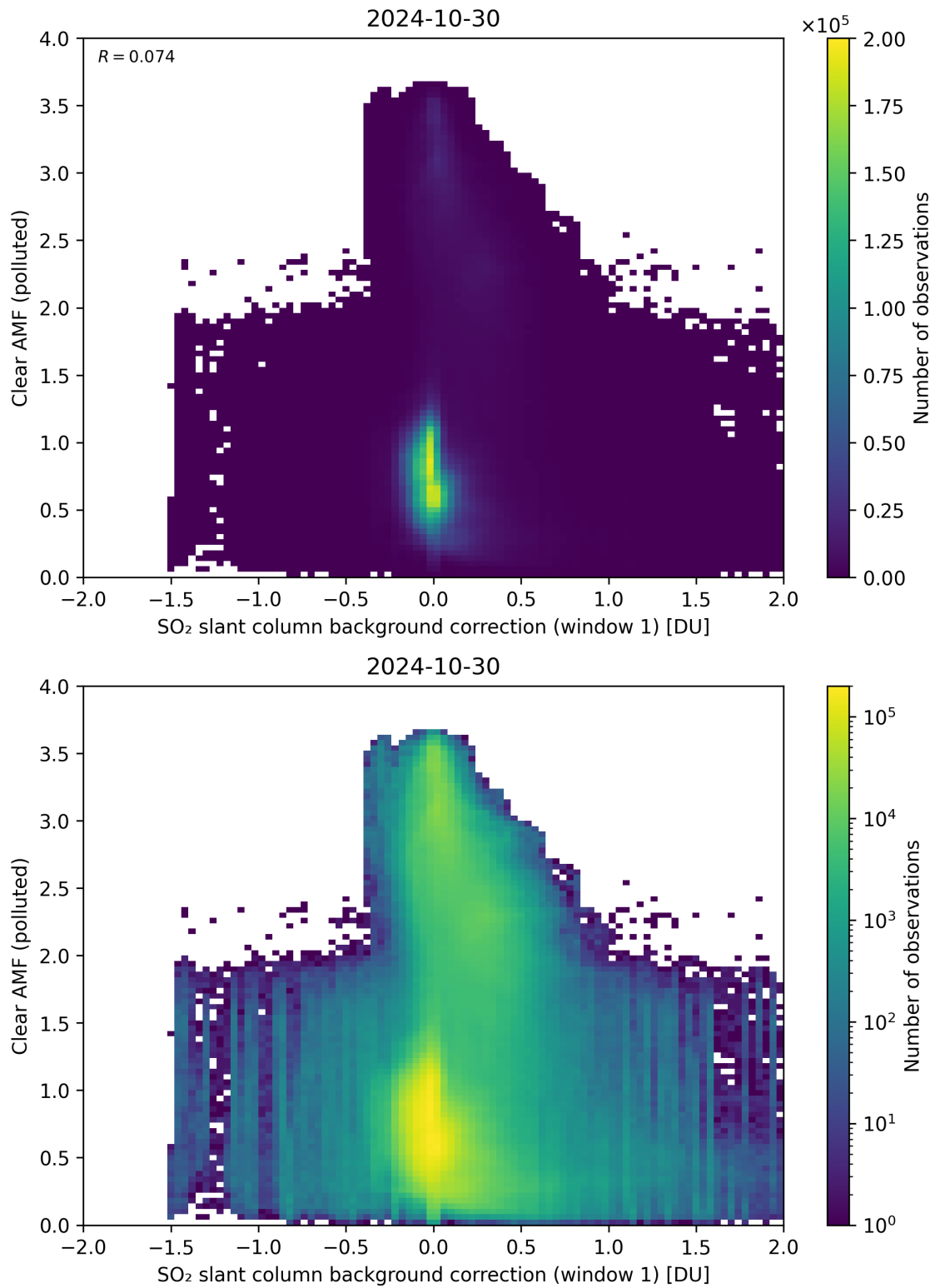
Figure 103: Scatter density plot of “SO 2 slant column background correction (window 1)” against “Clear AMF (polluted)” for 2024-10-30 to 2024-10-31.
