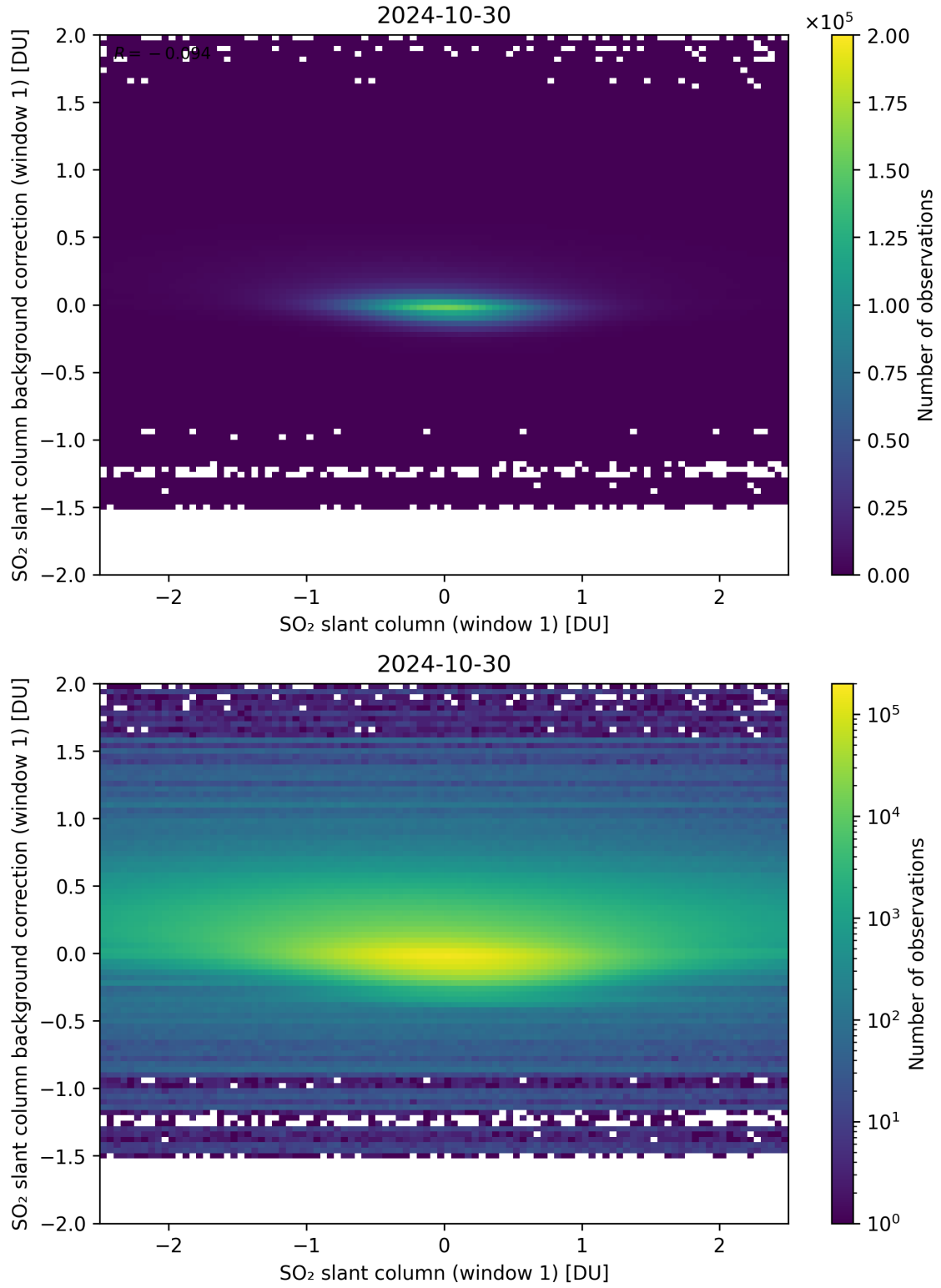
Figure 212: Scatter density plot of “SO 2 slant column (window 1)” against “SO 2 slant column background correction (window 1)” for 2024-10-30 to 2024-10-31.
