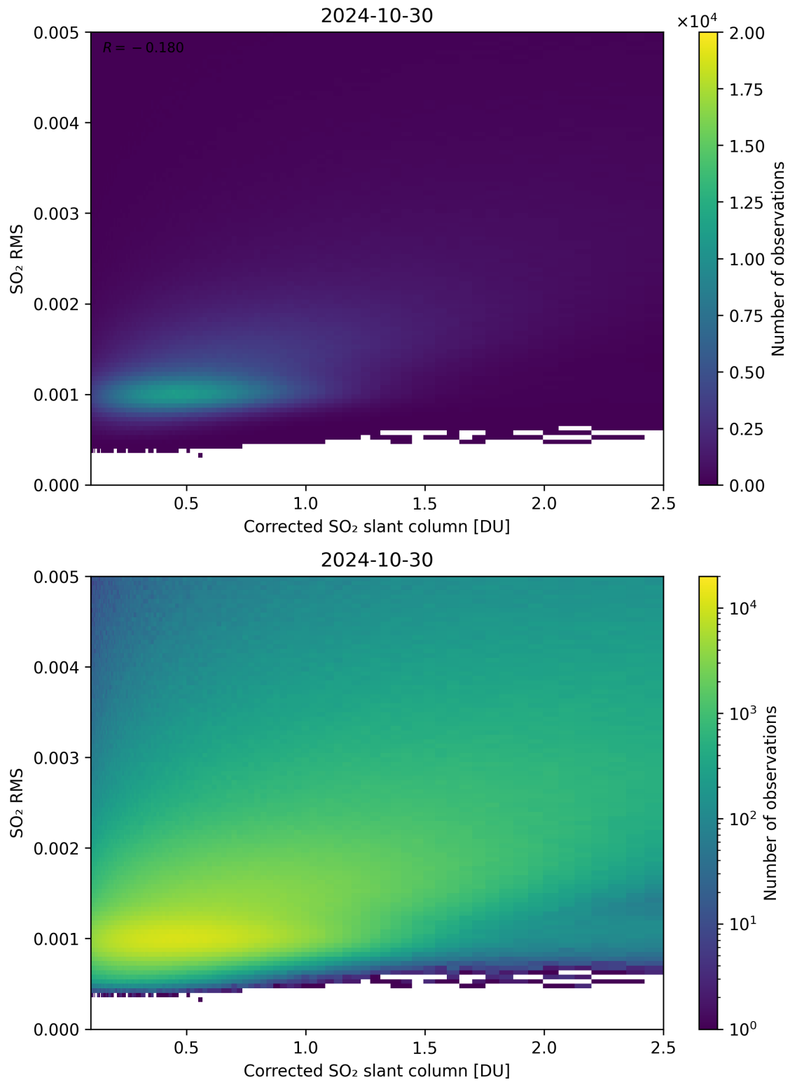
Figure 183: Scatter density plot of “Corrected SO 2 slant column” against “SO 2 RMS” for 2024-10-30 to 2024-10-31.
