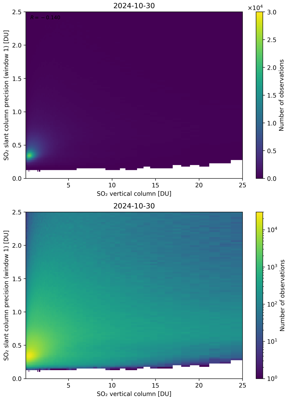
Figure 301: Scatter density plot of “SO 2 vertical column” against “SO 2 slant column precision (window 1)” for 2024-10-30 to 2024-10-31.
