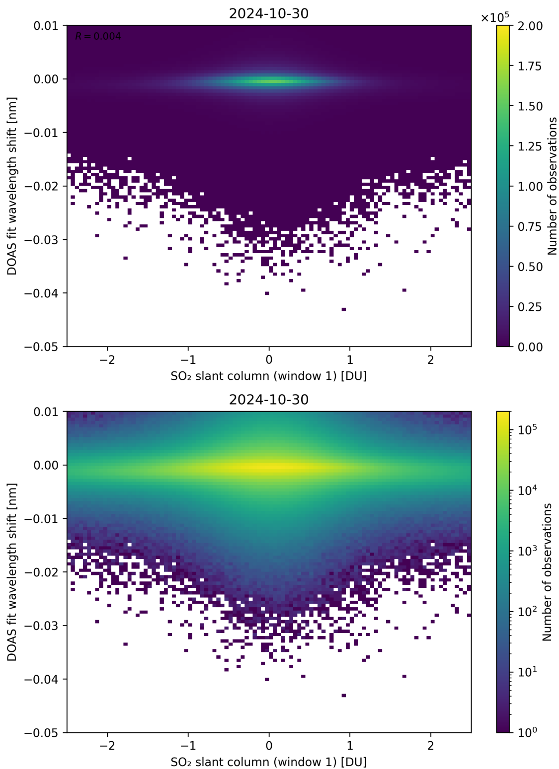
Figure 215: Scatter density plot of “SO 2 slant column (window 1)” against “DOAS fit wavelength shift” for 2024-10-30 to 2024-10-31.
