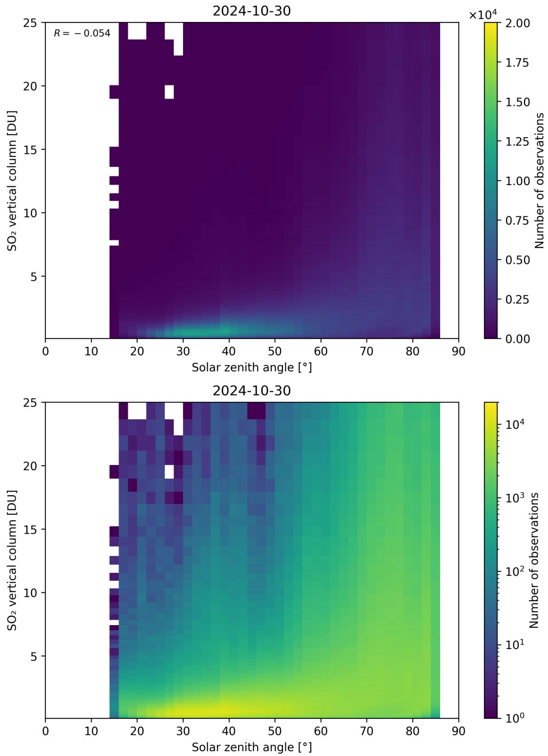
Figure 176: Scatter density plot of “Solar zenith angle” against “SO 2 vertical column” for 2024-10-30 to 2024-10-31.
