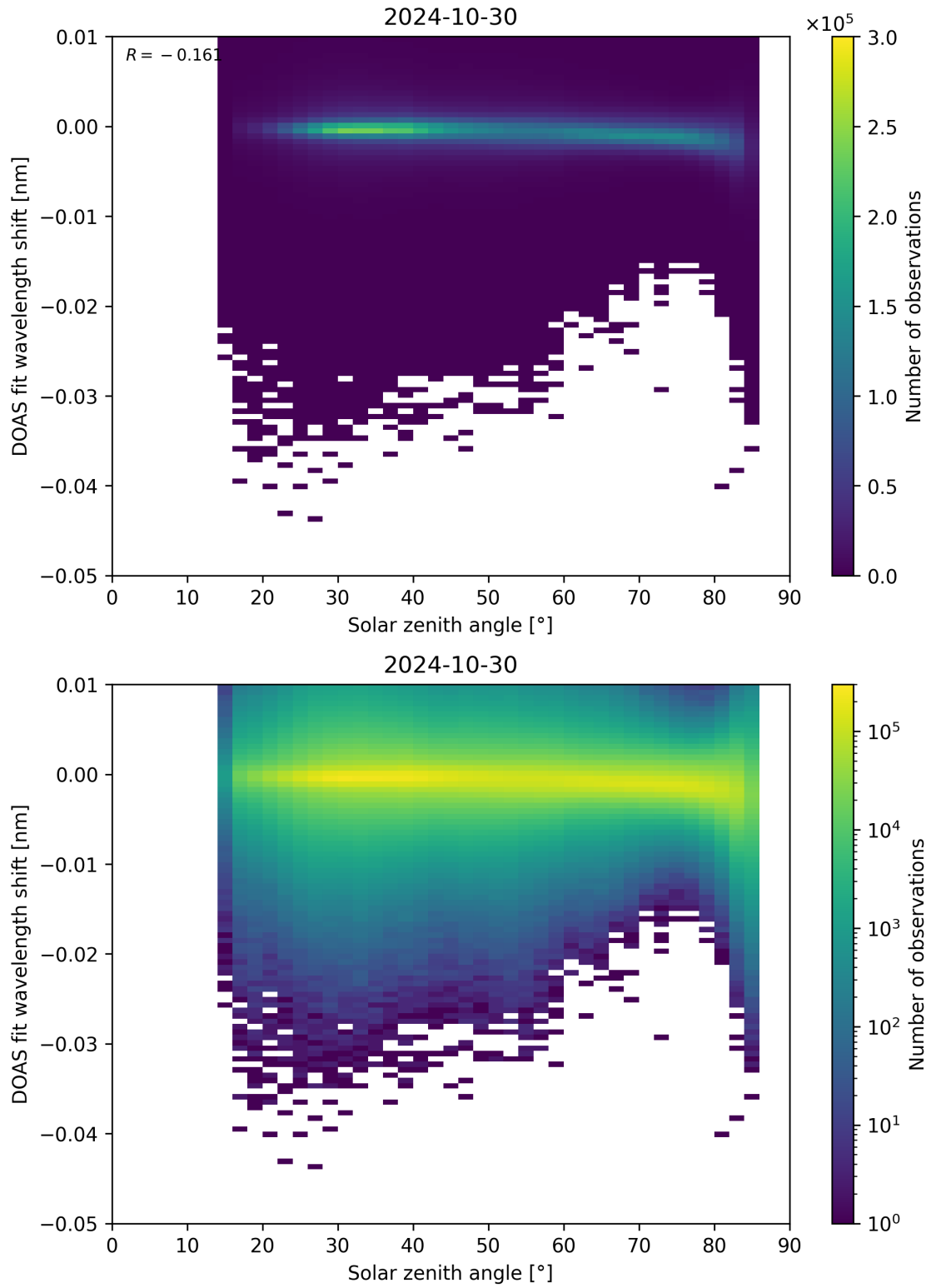
Figure 161: Scatter density plot of “Solar zenith angle” against “DOAS fit wavelength shift” for 2024-10-30 to 2024-10-31.
