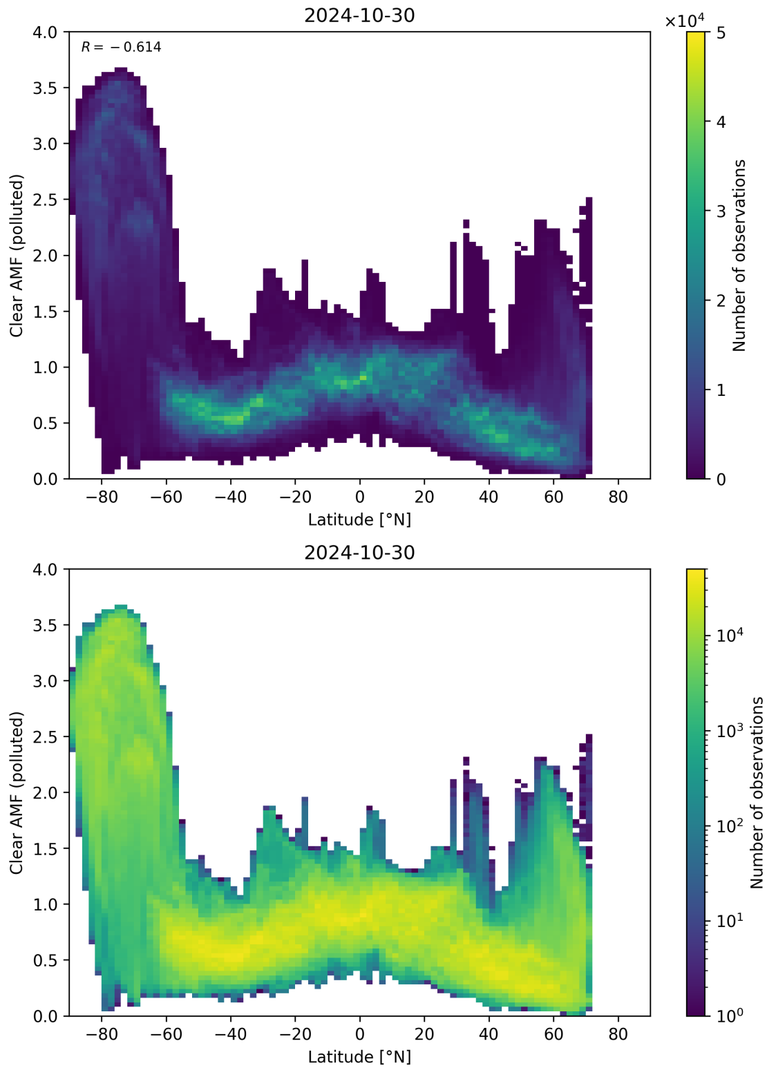
Figure 145: Scatter density plot of “Latitude” against “Clear AMF (polluted)” for 2024-10-30 to 2024-10-31.
