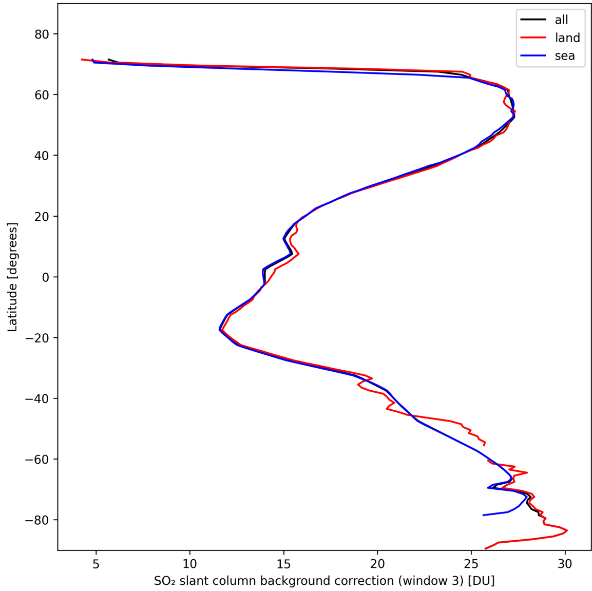
Figure 44: Zonal average of “SO 2 slant column background correction (window 3)” for 2024-10-30 to 2024-10-31.
