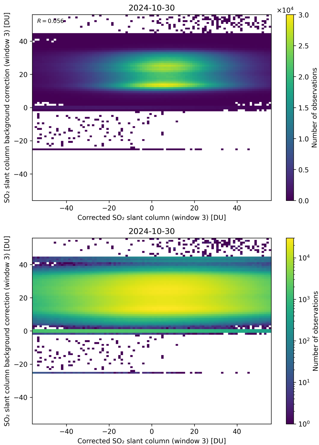
Figure 205: Scatter density plot of “Corrected SO 2 slant column (window 3)” against “SO 2 slant column background correction (window 3)” for 2024-10-30 to 2024-10-31.
