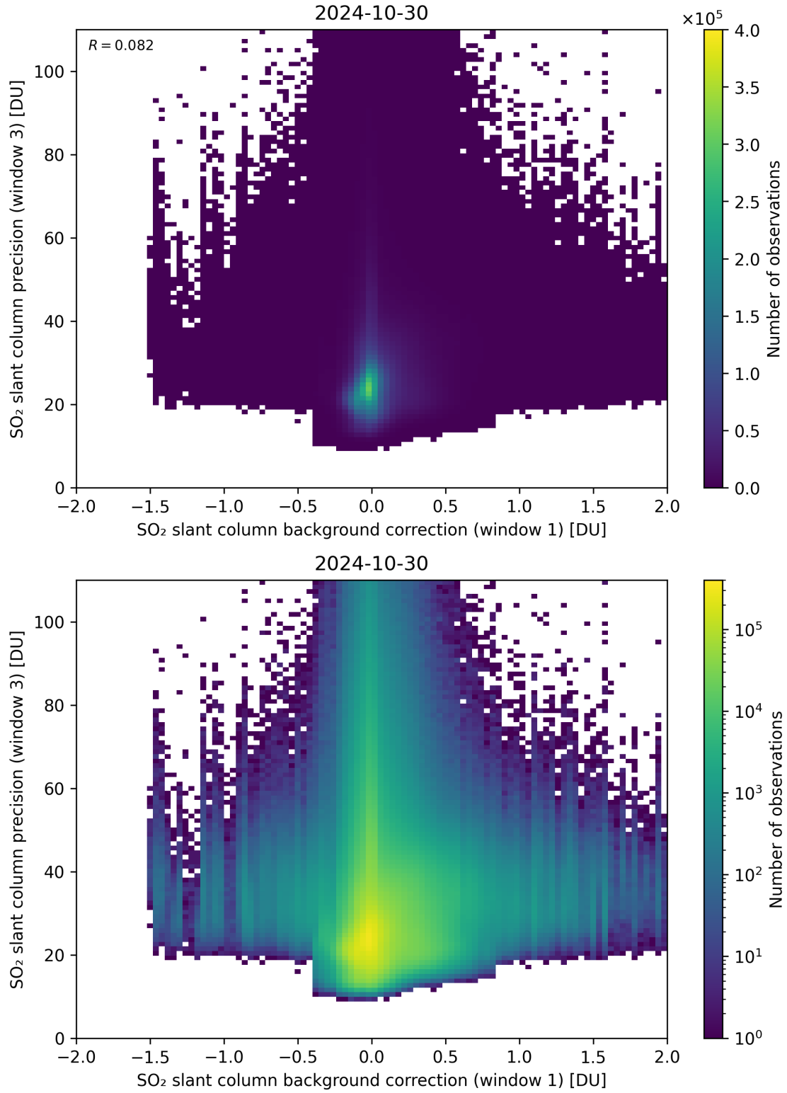
Figure 108: Scatter density plot of “SO 2 slant column background correction (window 1)” against “SO 2 slant column precision (window 3)” for 2024-10-30 to 2024-10-31.
