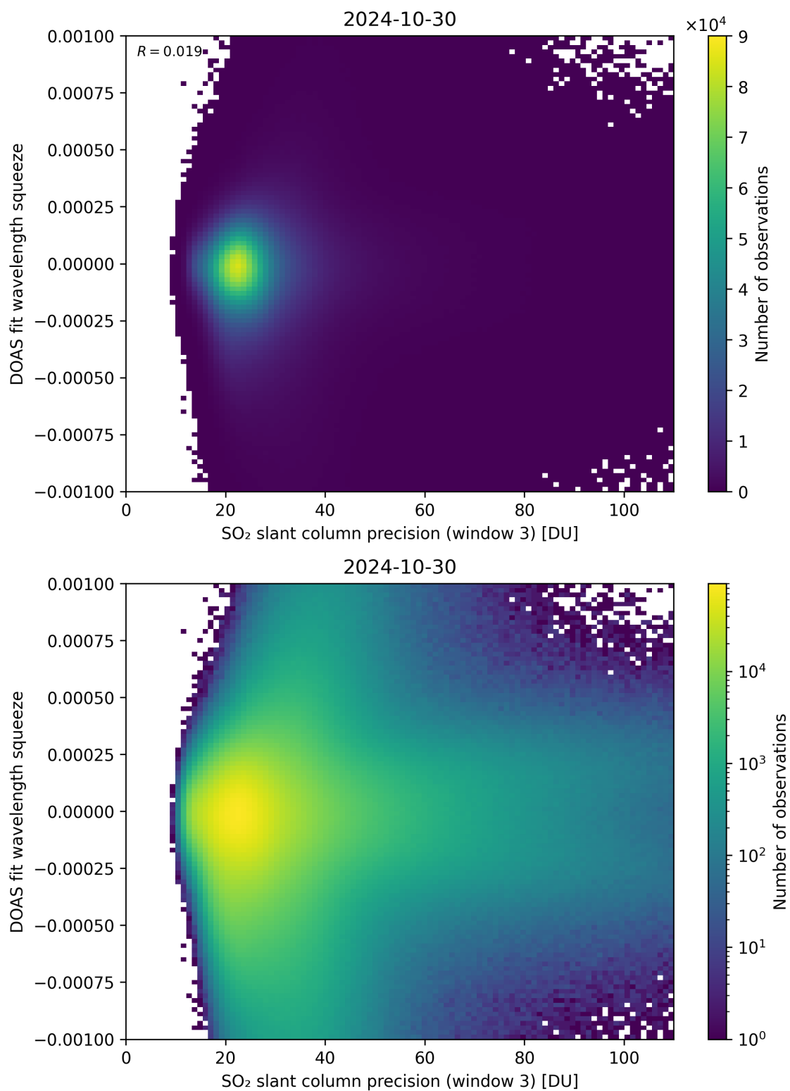
Figure 259: Scatter density plot of “SO 2 slant column precision (window 3)” against “DOAS fit wavelength squeeze” for 2024-10-30 to 2024-10-31.
