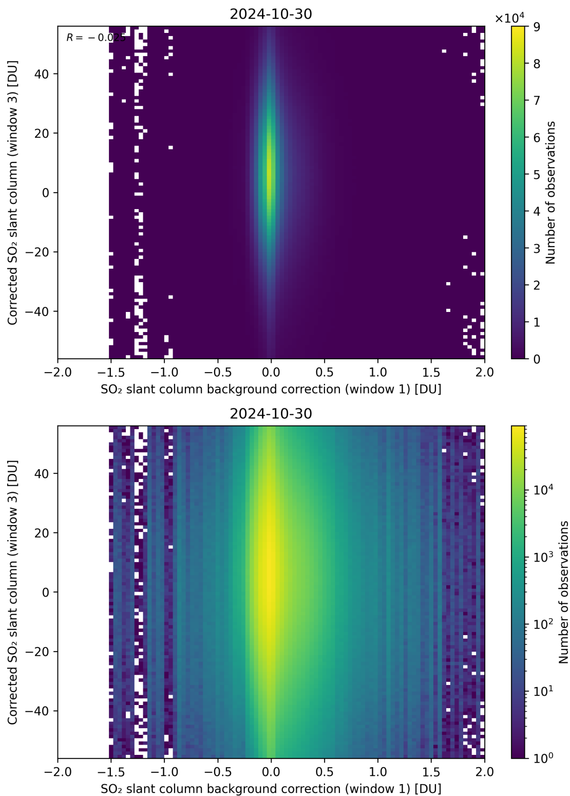
Figure 105: Scatter density plot of “SO 2 slant column background correction (window 1)” against “Corrected SO 2 slant column (window 3)” for 2024-10-30 to 2024-10-31.
