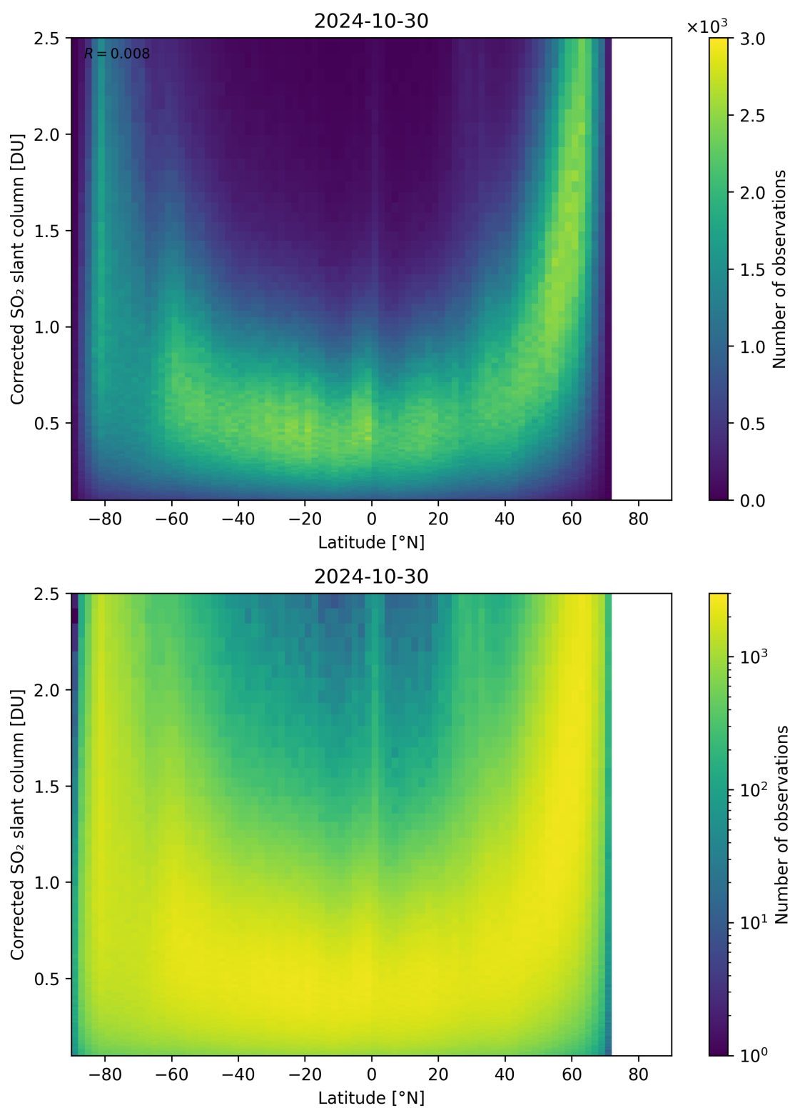
Figure 146: Scatter density plot of “Latitude” against “Corrected SO 2 slant column” for 2024-10-30 to 2024-10-31.
