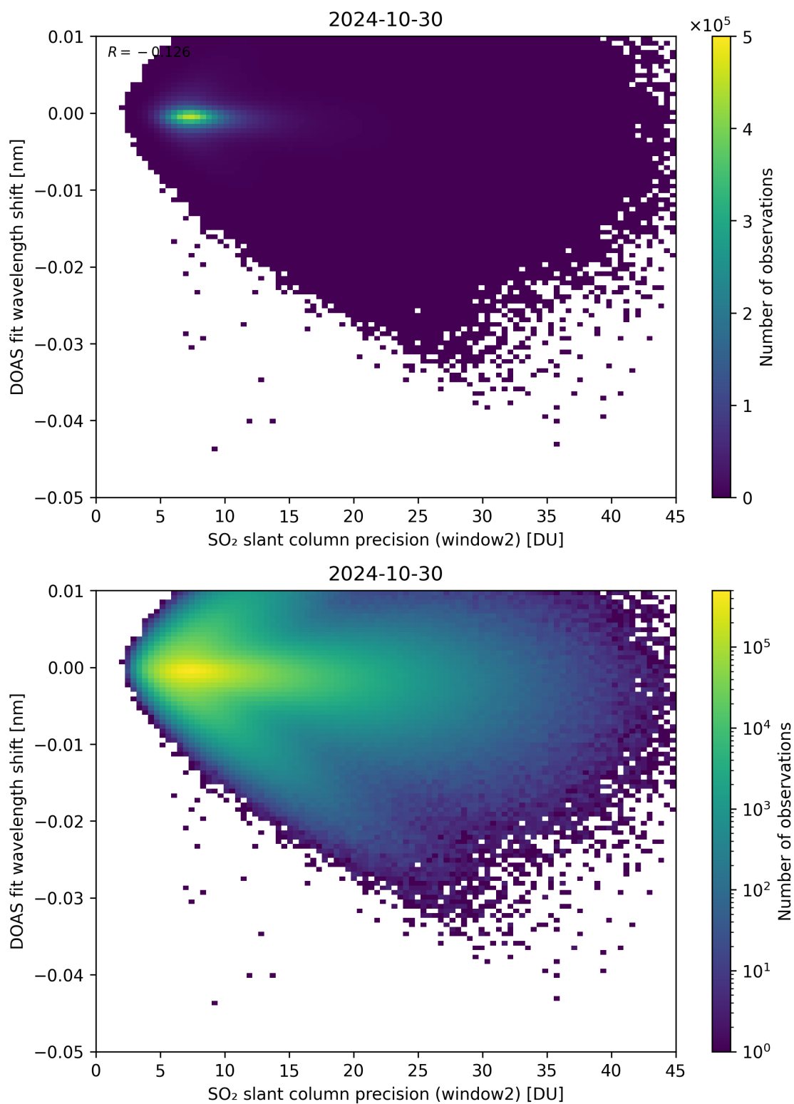
Figure 243: Scatter density plot of “SO 2 slant column precision (window2)” against “DOAS fit wavelength shift” for 2024-10-30 to 2024-10-31.
