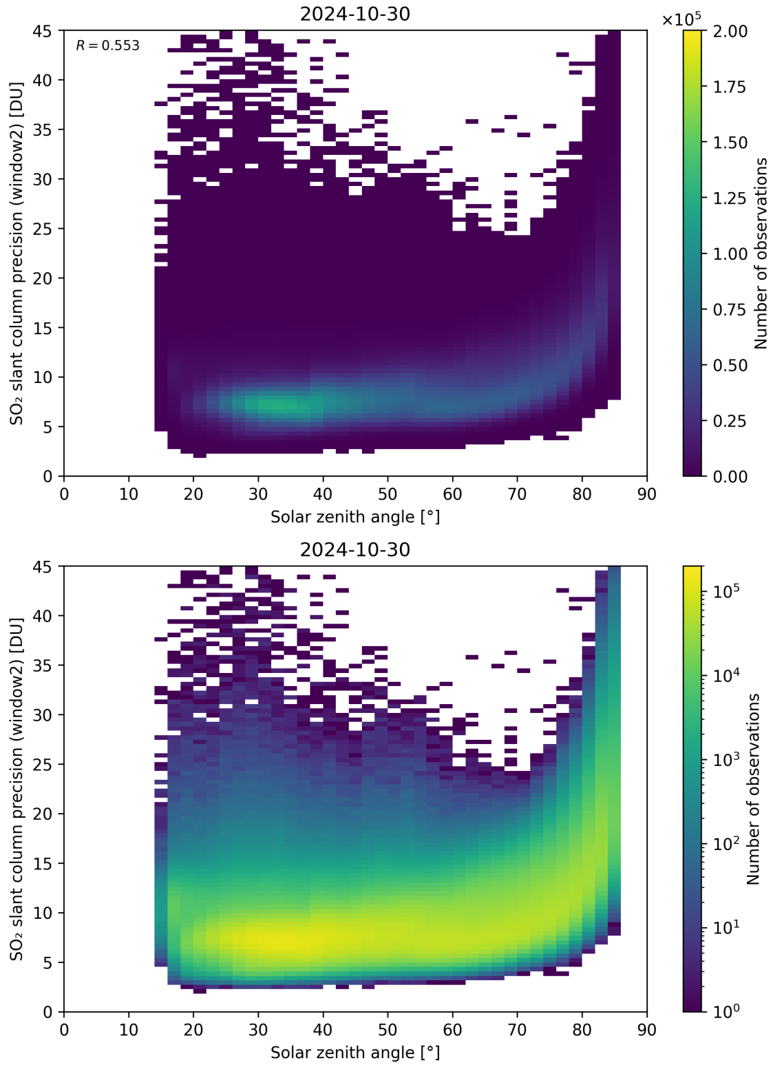
Figure 171: Scatter density plot of “Solar zenith angle” against “SO 2 slant column precision (window2)” for 2024-10-30 to 2024-10-31.
