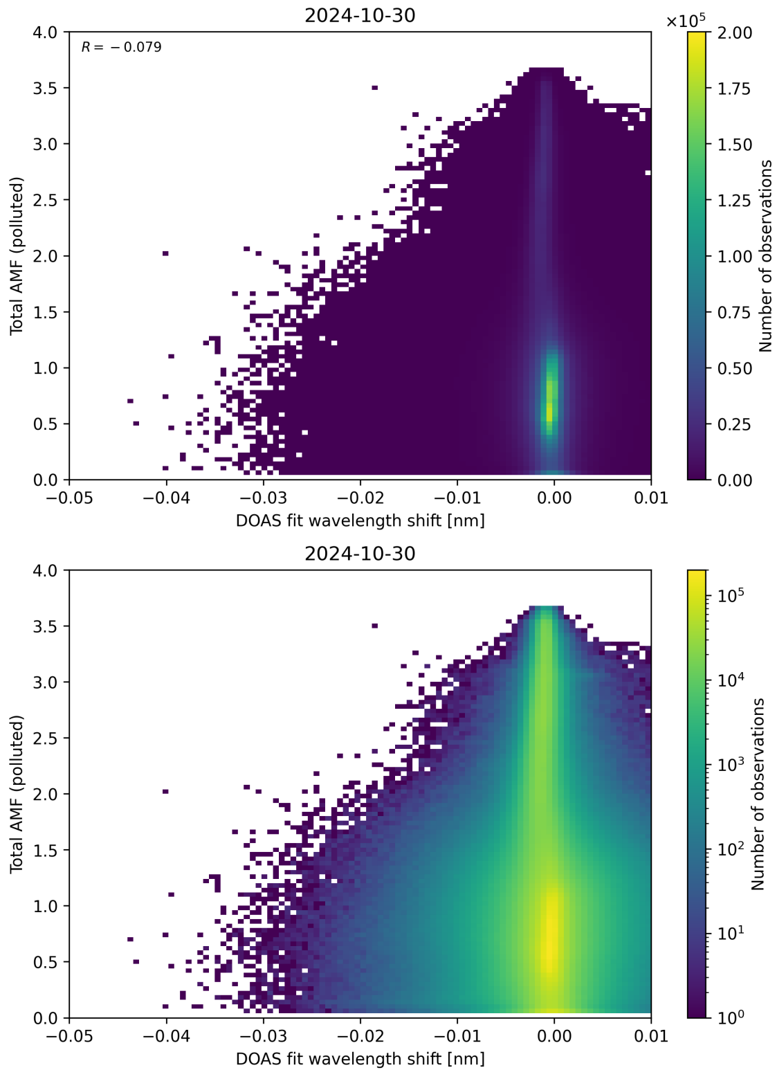
Figure 130: Scatter density plot of “DOAS fit wavelength shift” against “Total AMF (polluted)” for 2024-10-30 to 2024-10-31.
