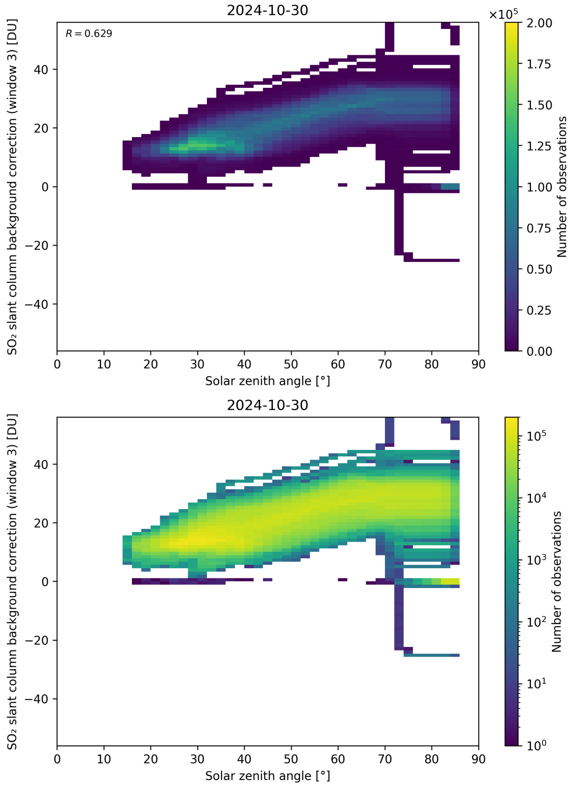
Figure 160: Scatter density plot of “Solar zenith angle” against “SO 2 slant column background correction (window 3)” for 2024-10-30 to 2024-10-31.
