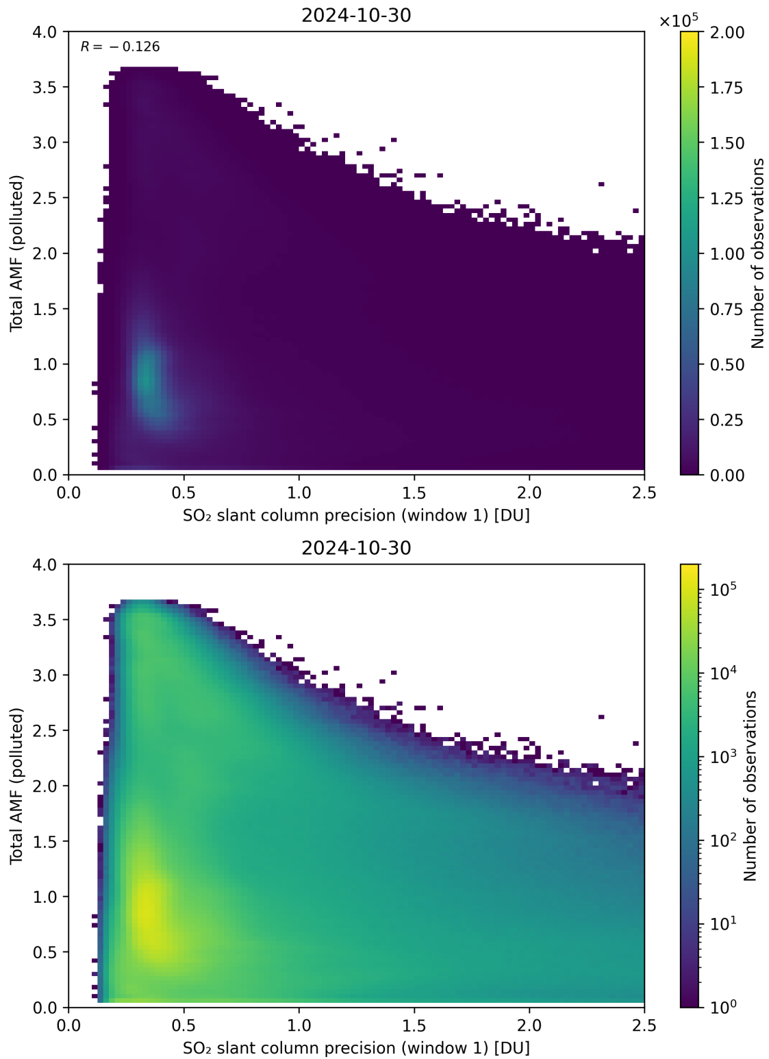
Figure 230: Scatter density plot of “SO 2 slant column precision (window 1)” against “Total AMF (polluted)” for 2024-10-30 to 2024-10-31.
