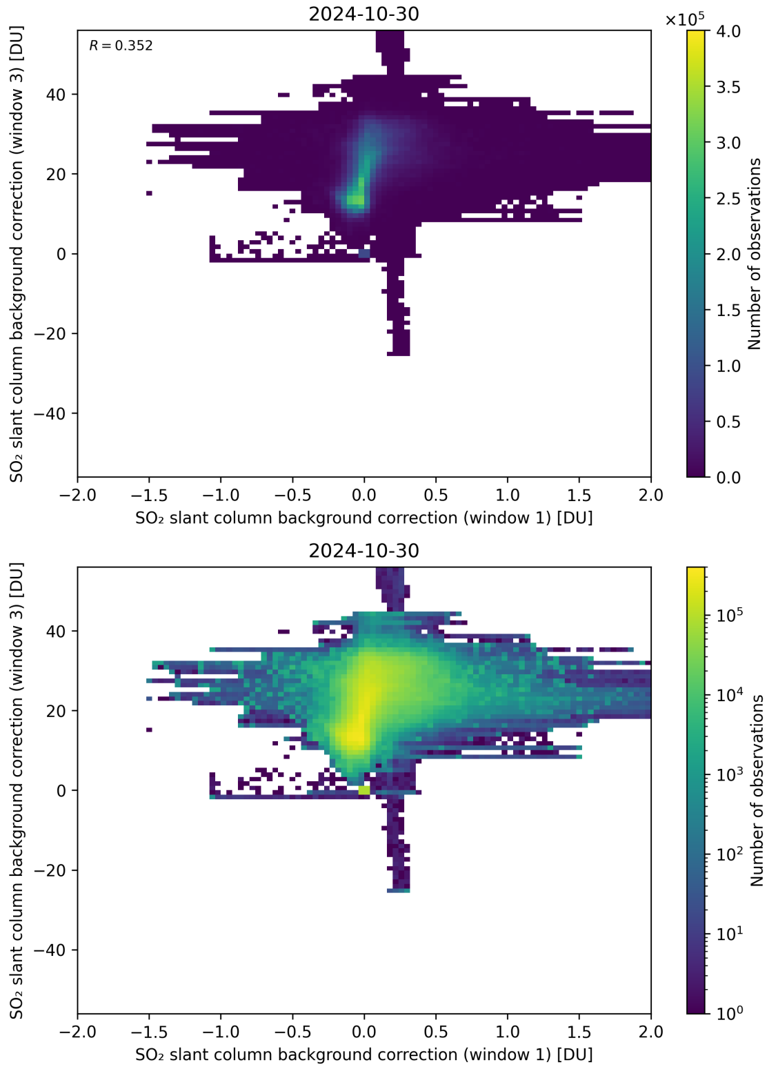
Figure 99: Scatter density plot of “SO 2 slant column background correction (window 1)” against “SO 2 slant column background correction (window 3)” for 2024-10-30 to 2024-10-31.
