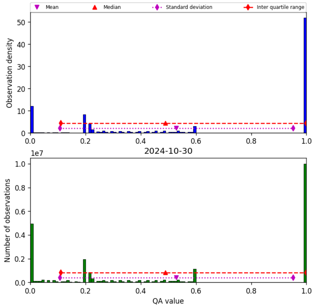
Figure 52: Histogram of “QA value” for 2024-10-30 to 2024-10-31
