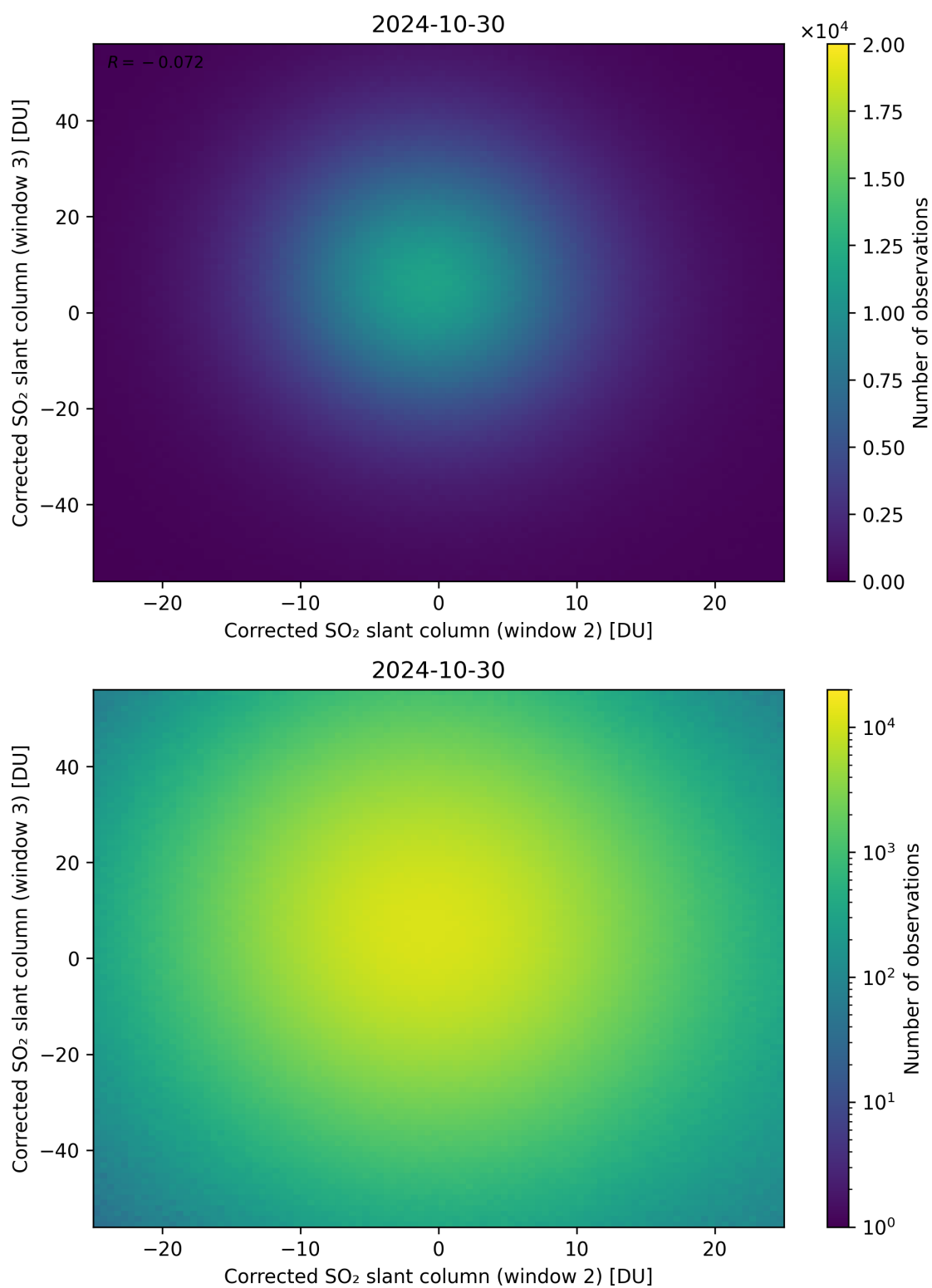
Figure 200: Scatter density plot of “Corrected SO 2 slant column (window 2)” against “Corrected SO 2 slant column (window 3)” for 2024-10-30 to 2024-10-31.
