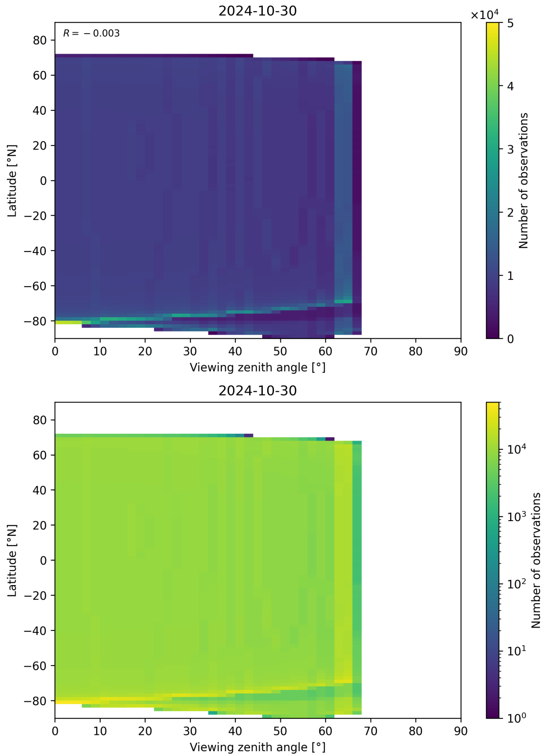
Figure 314: Scatter density plot of “Viewing zenith angle” against “Latitude” for 2024-10-30 to 2024-10-31.
