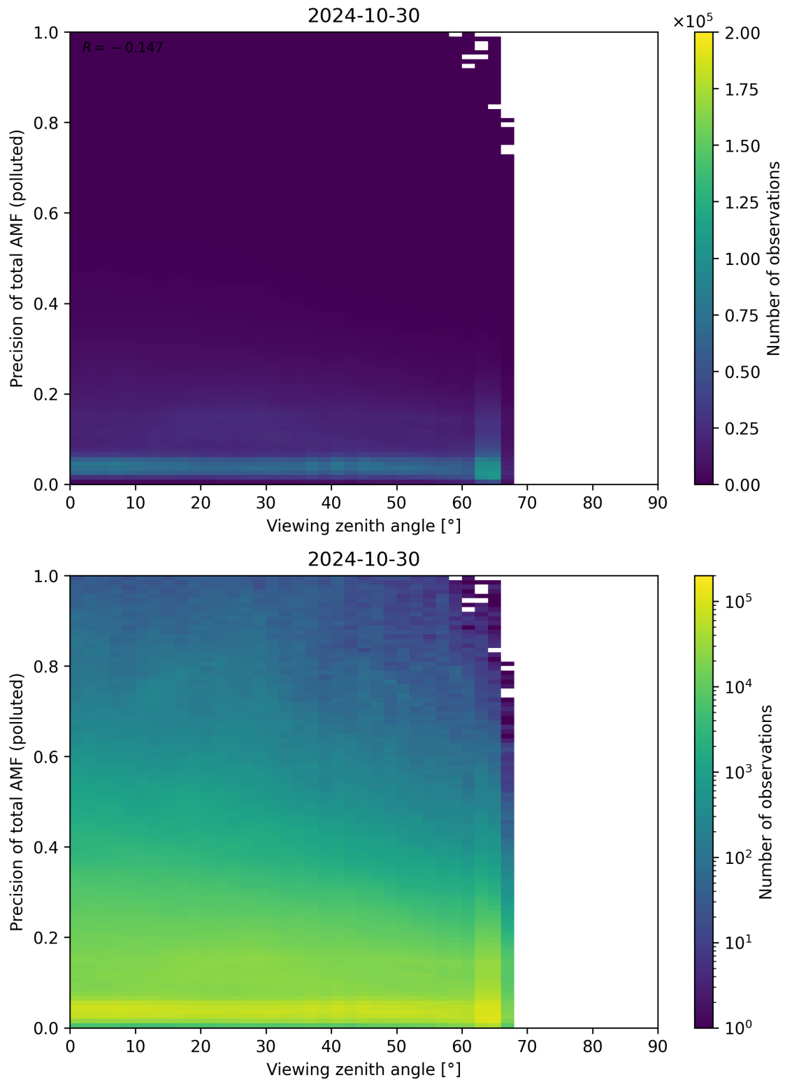
Figure 326: Scatter density plot of “Viewing zenith angle” against “Precision of total AMF (polluted)” for 2024-10-30 to 2024-10-31.
