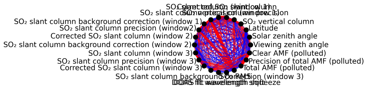
Figure 1: Map of correlation graph for 2024-10-30 to 2024-10-31.
