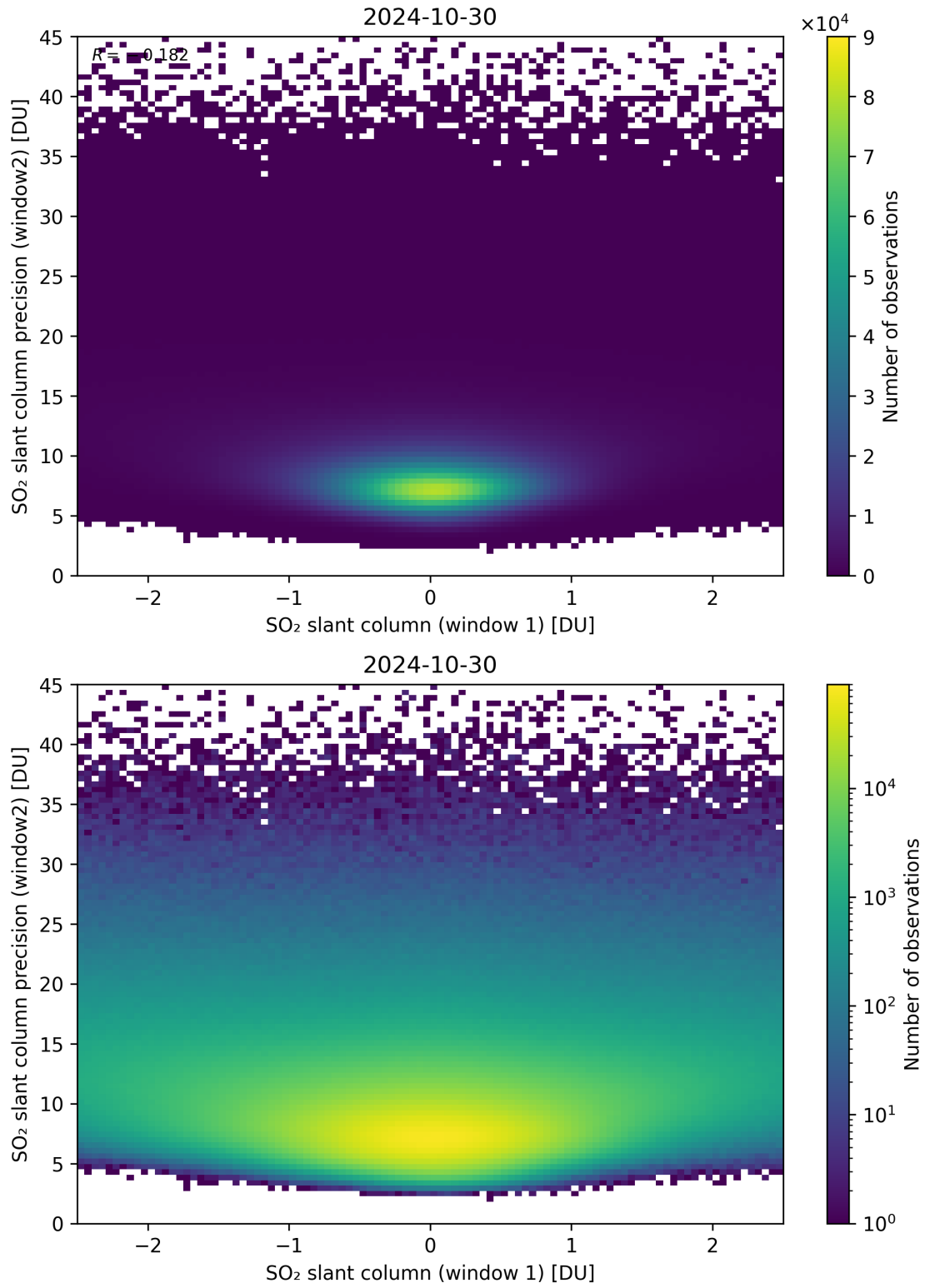
Figure 236: Scatter density plot of “SO 2 slant column (window 1)” against “SO 2 slant column precision (window2)” for 2024-10-30 to 2024-10-31.
