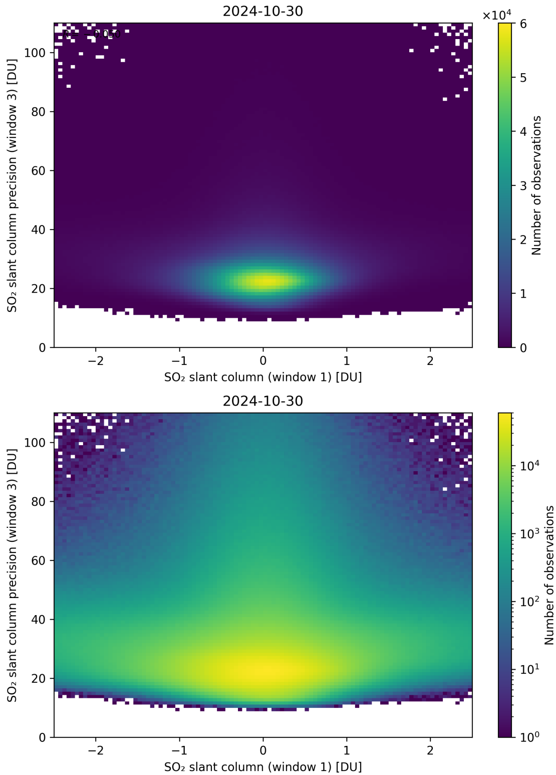
Figure 238: Scatter density plot of “SO 2 slant column (window 1)” against “SO 2 slant column precision (window 3)” for 2024-10-30 to 2024-10-31.
