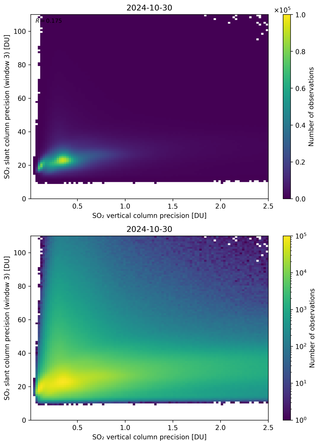
Figure 293: Scatter density plot of “SO 2 vertical column precision” against “SO 2 slant column precision (window 3)” for 2024-10-30 to 2024-10-31.
