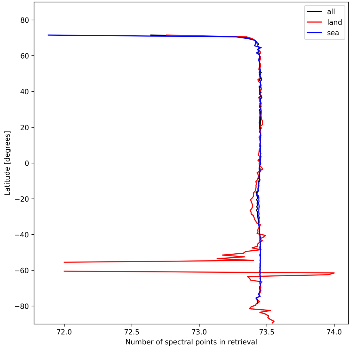
Figure 51: Zonal average of “Number of spectral points in retrieval” for 2024-10-30 to 2024-10-31.
