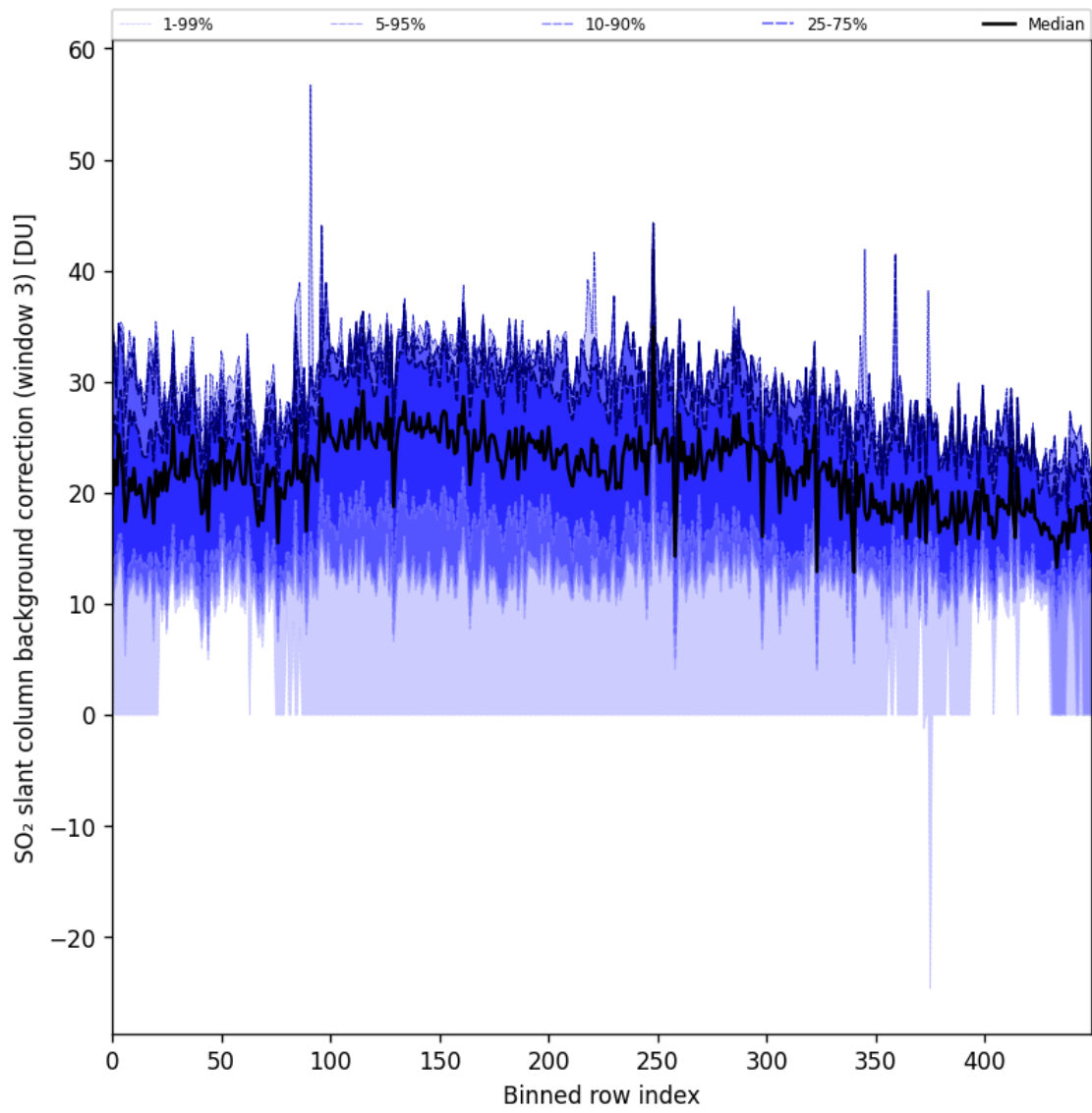
Figure 90: Along track statistics of “SO 2 slant column background correction (window 3)” for 2024-10-30 to 2024-10-31
