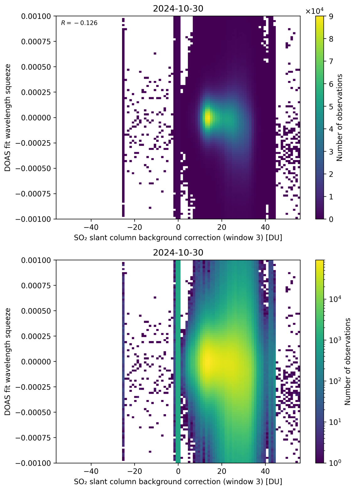
Figure 122: Scatter density plot of “SO 2 slant column background correction (window 3)” against “DOAS fit wavelength squeeze” for 2024-10-30 to 2024-10-31.
