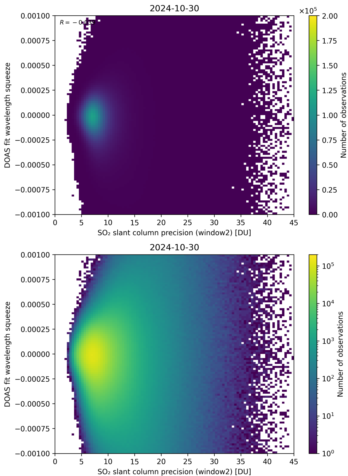
Figure 244: Scatter density plot of “SO 2 slant column precision (window2)” against “DOAS fit wavelength squeeze” for 2024-10-30 to 2024-10-31.
