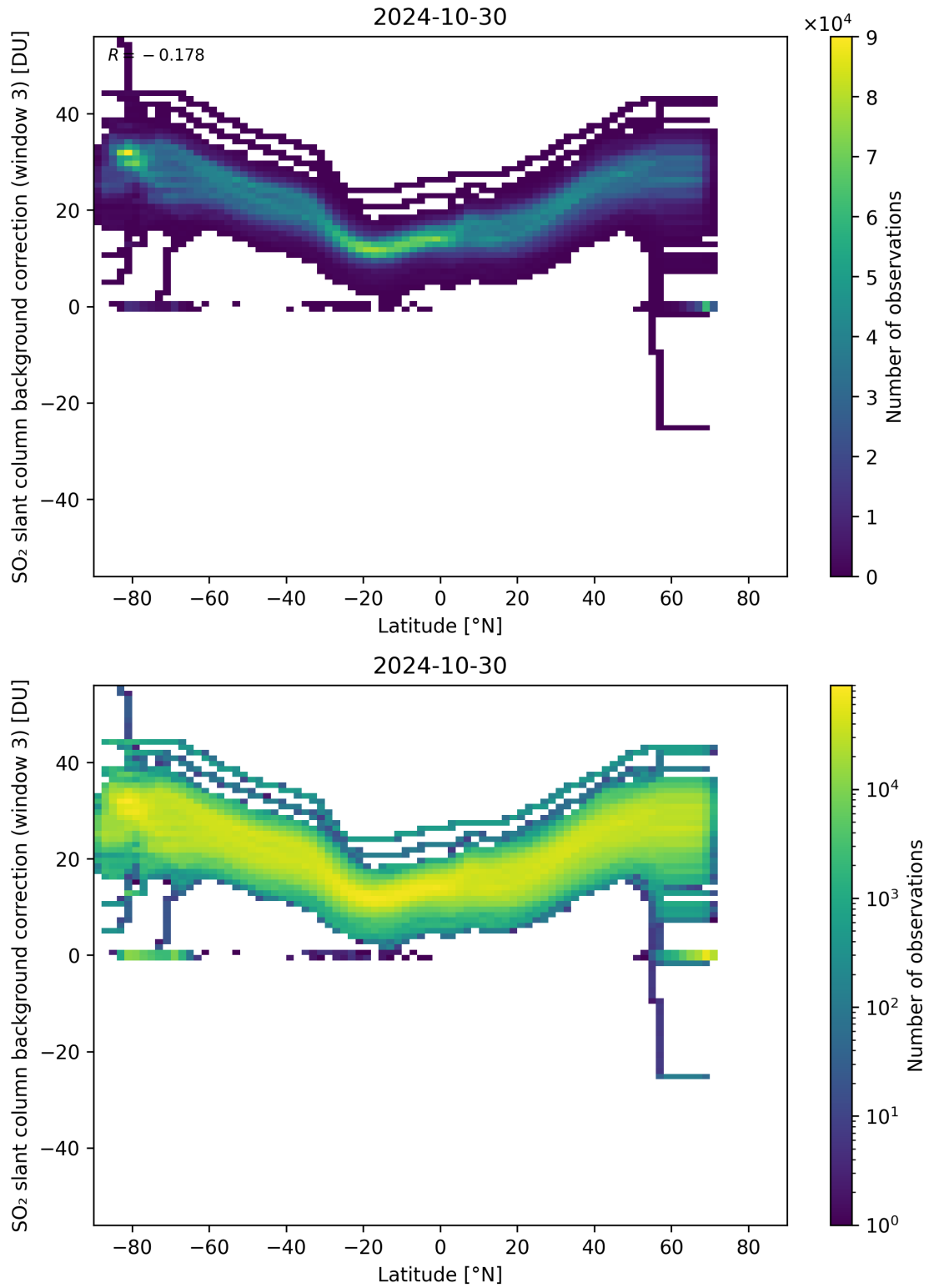
Figure 141: Scatter density plot of “Latitude” against “SO 2 slant column background correction (window 3)” for 2024-10-30 to 2024-10-31.
