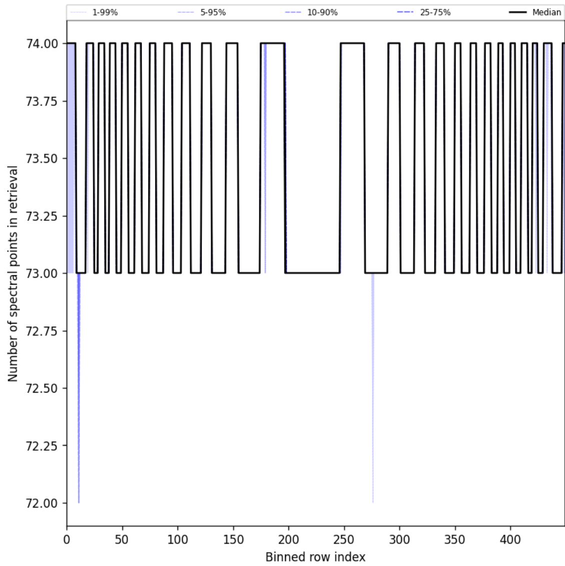
Figure 97: Along track statistics of “Number of spectral points in retrieval” for 2024-10-30 to 2024-10-31
