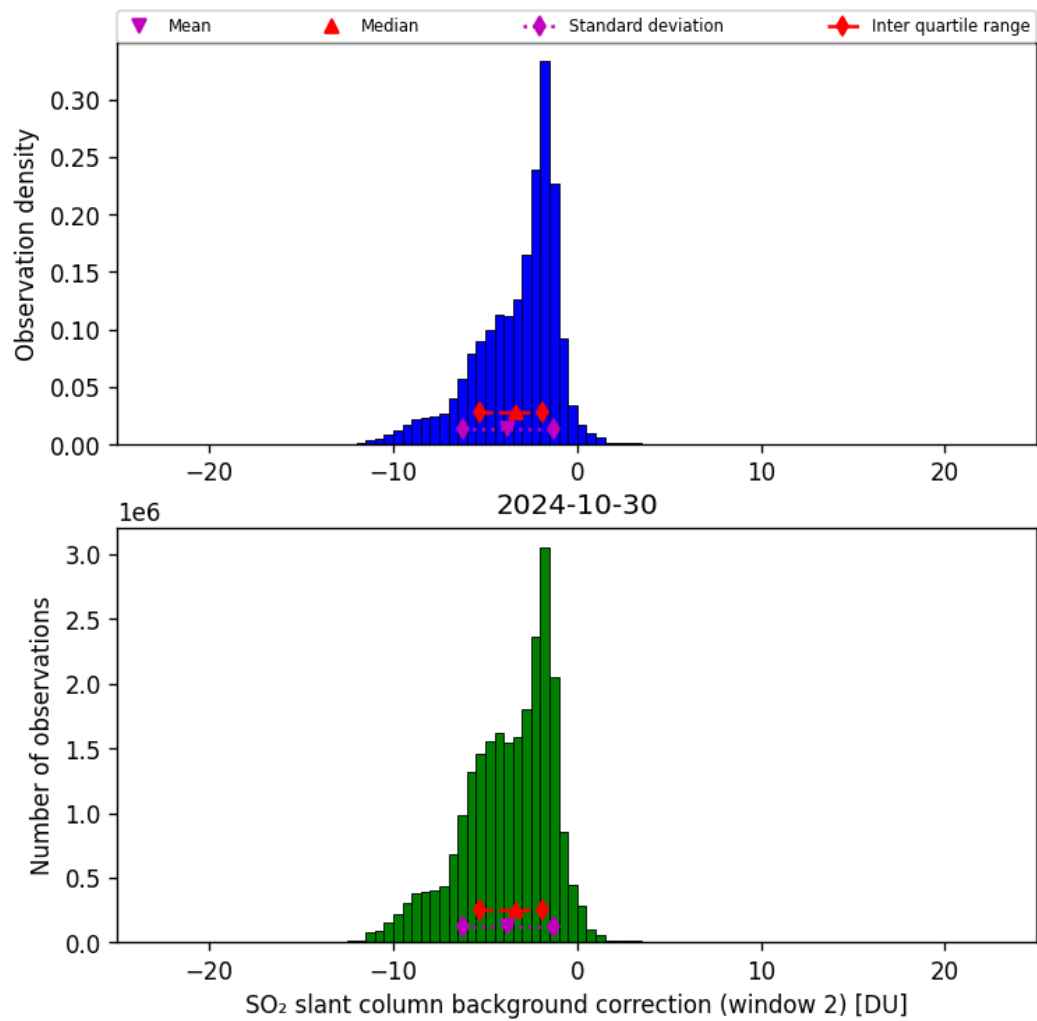
Figure 63: Histogram of “SO 2 slant column background correction (window 2)” for 2024-10-30 to 2024-10-31
