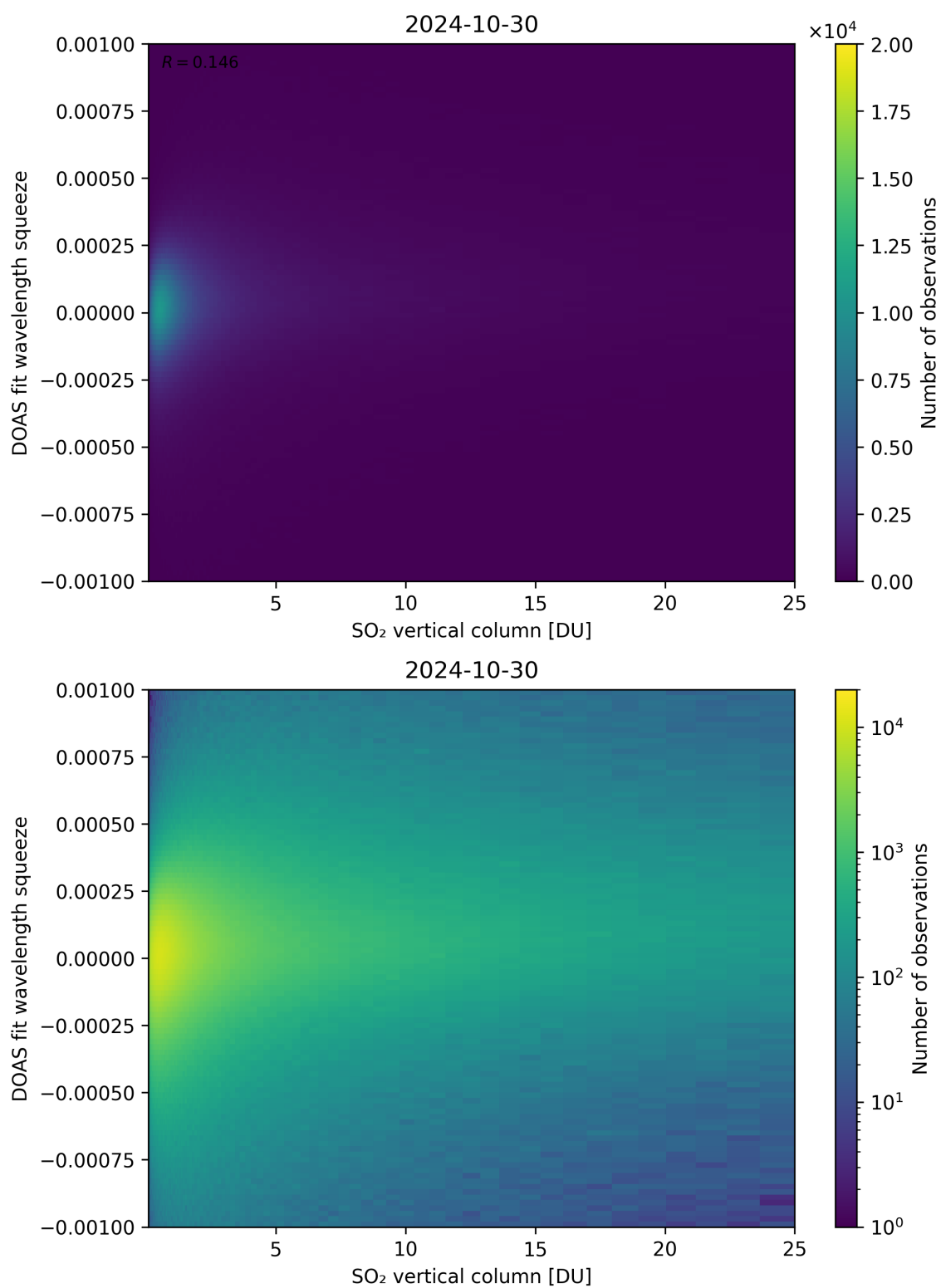
Figure 277: Scatter density plot of “SO 2 vertical column” against “DOAS fit wavelength squeeze” for 2024-10-30 to 2024-10-31.
