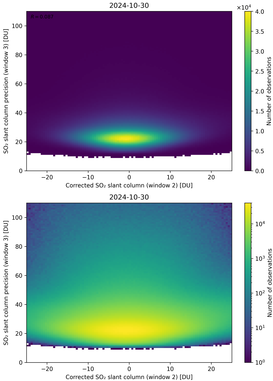
Figure 202: Scatter density plot of “Corrected SO 2 slant column (window 2)” against “SO 2 slant column precision (window 3)” for 2024-10-30 to 2024-10-31.
