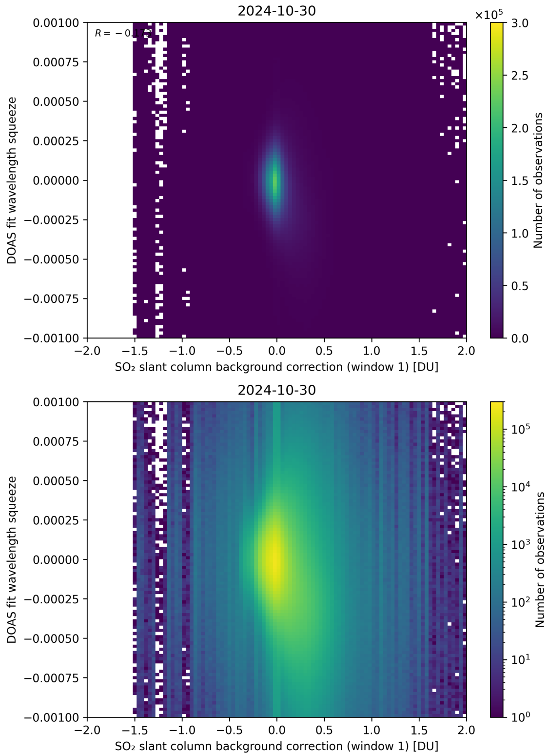
Figure 101: Scatter density plot of “SO 2 slant column background correction (window 1)” against “DOAS fit wavelength squeeze” for 2024-10-30 to 2024-10-31.
