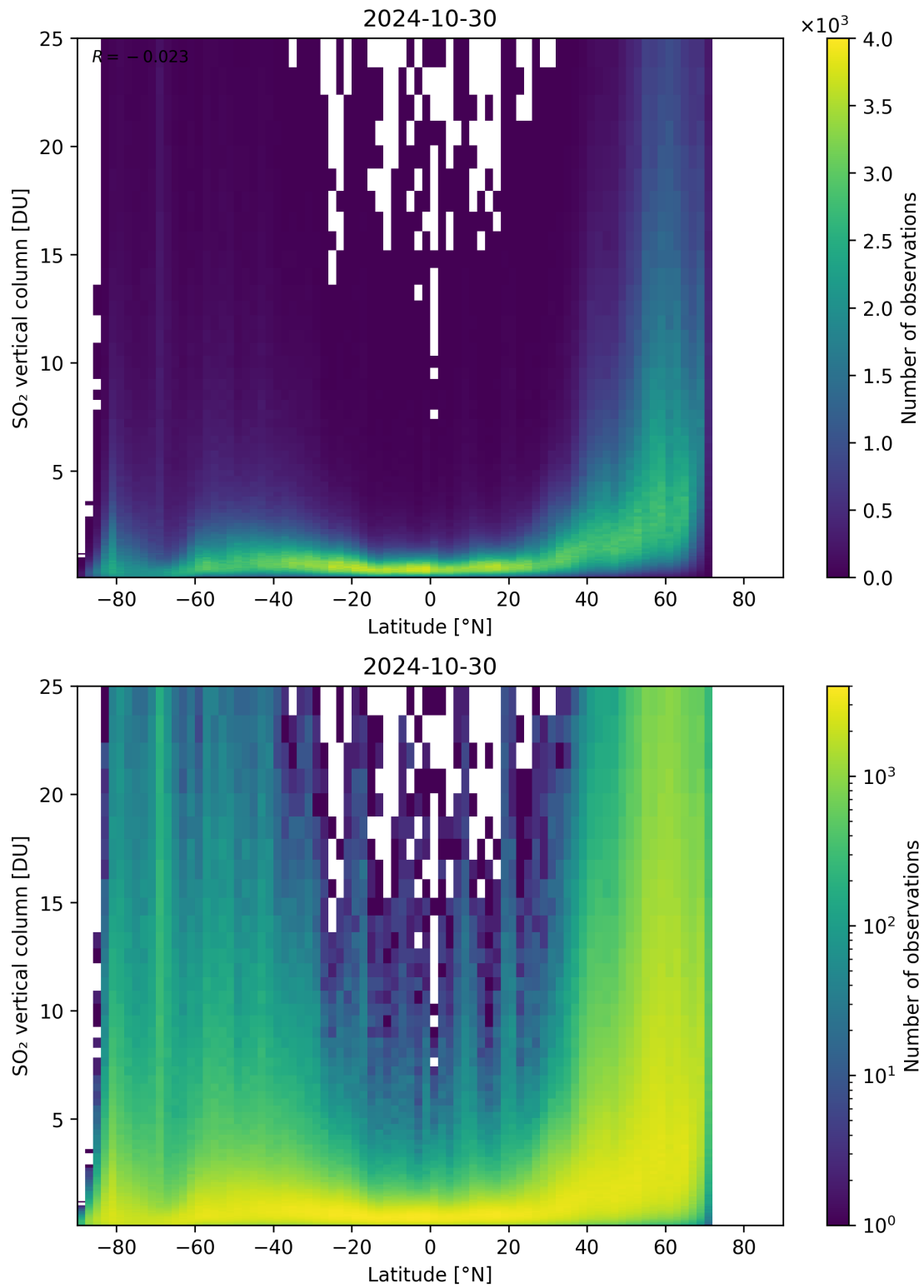
Figure 156: Scatter density plot of “Latitude” against “SO 2 vertical column” for 2024-10-30 to 2024-10-31.
