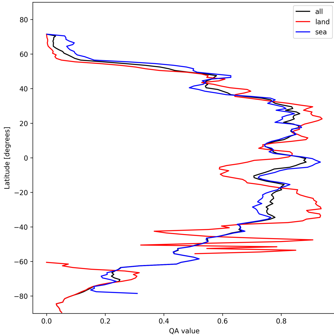
Figure 29: Zonal average of “QA value” for 2024-10-30 to 2024-10-31.
