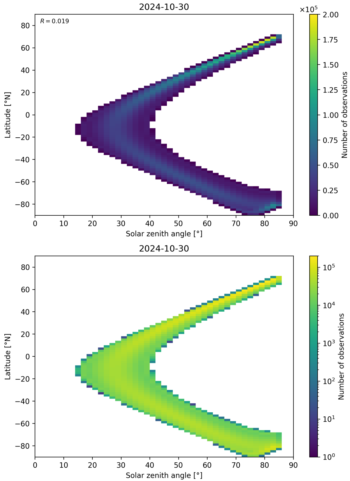
Figure 164: Scatter density plot of “Solar zenith angle” against “Latitude” for 2024-10-30 to 2024-10-31.
