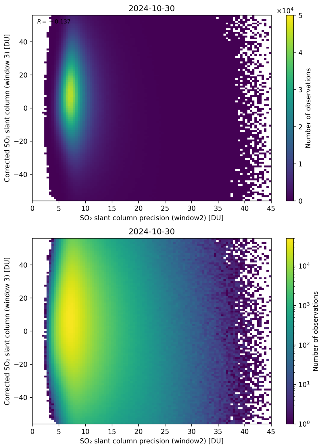
Figure 248: Scatter density plot of “SO 2 slant column precision (window2)” against “Corrected SO 2 slant column (window 3)” for 2024-10-30 to 2024-10-31.
