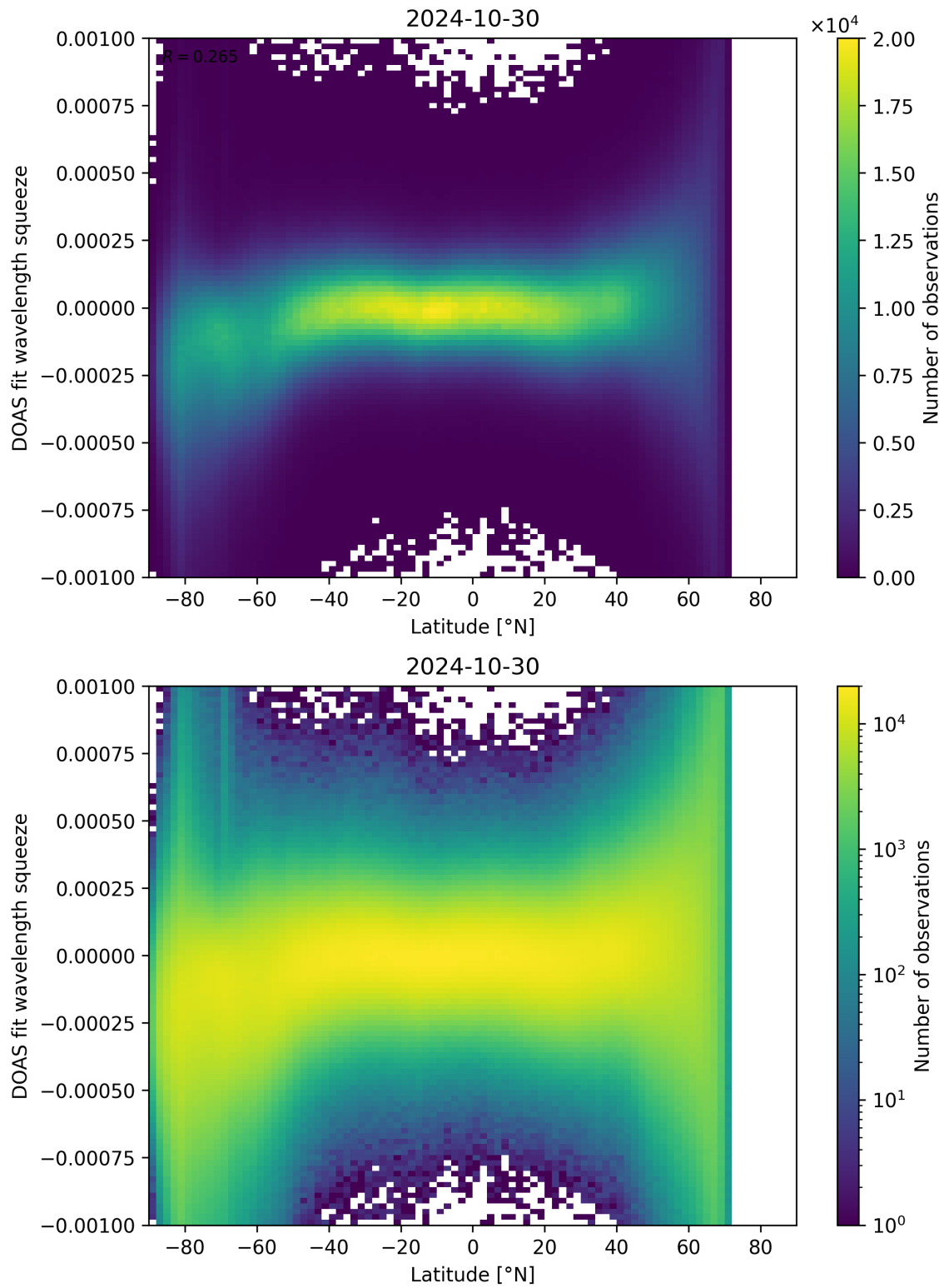
Figure 143: Scatter density plot of “Latitude” against “DOAS fit wavelength squeeze” for 2024-10-30 to 2024-10-31.
