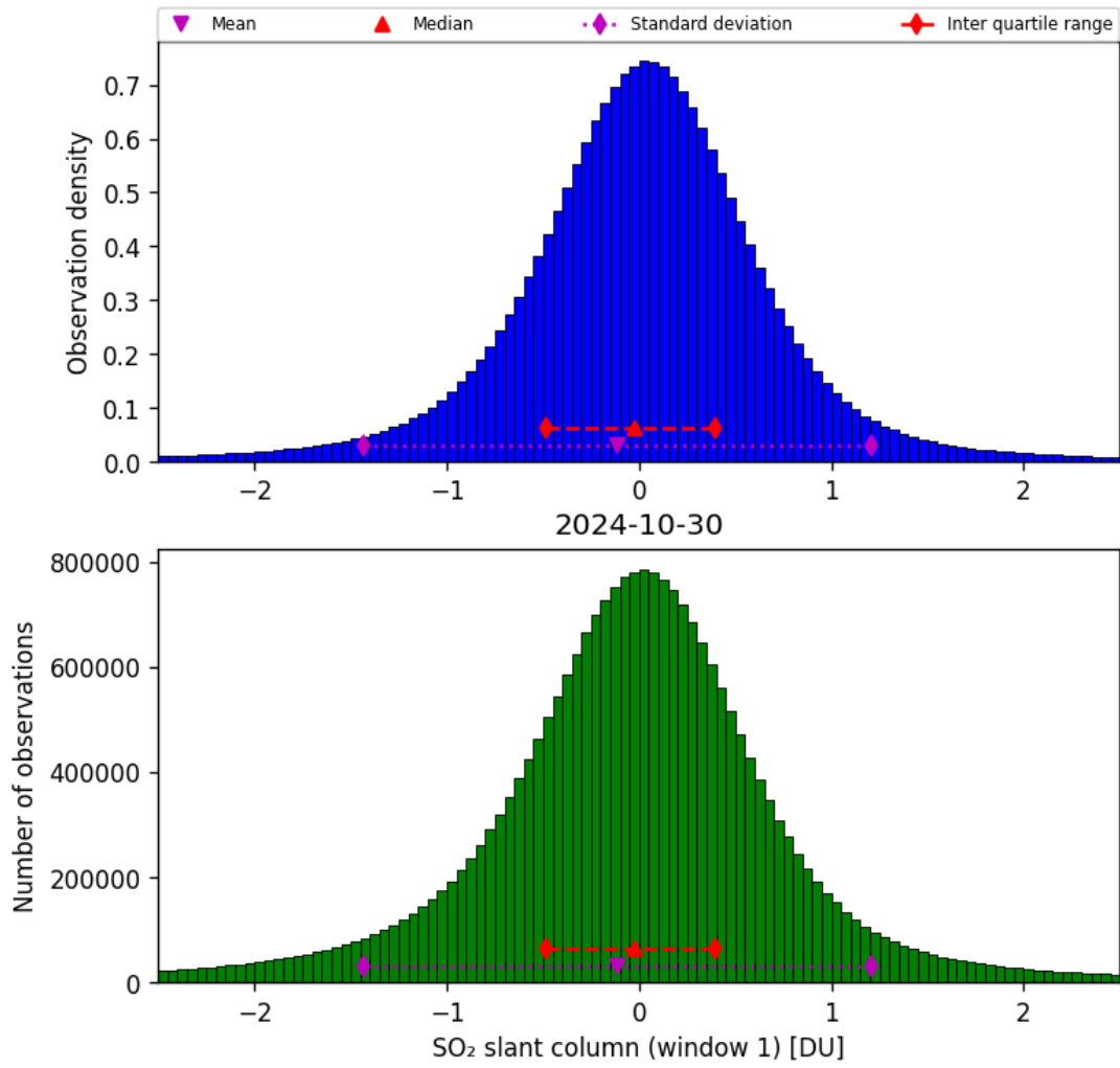
Figure 56: Histogram of “SO 2 slant column (window 1)” for 2024-10-30 to 2024-10-31
