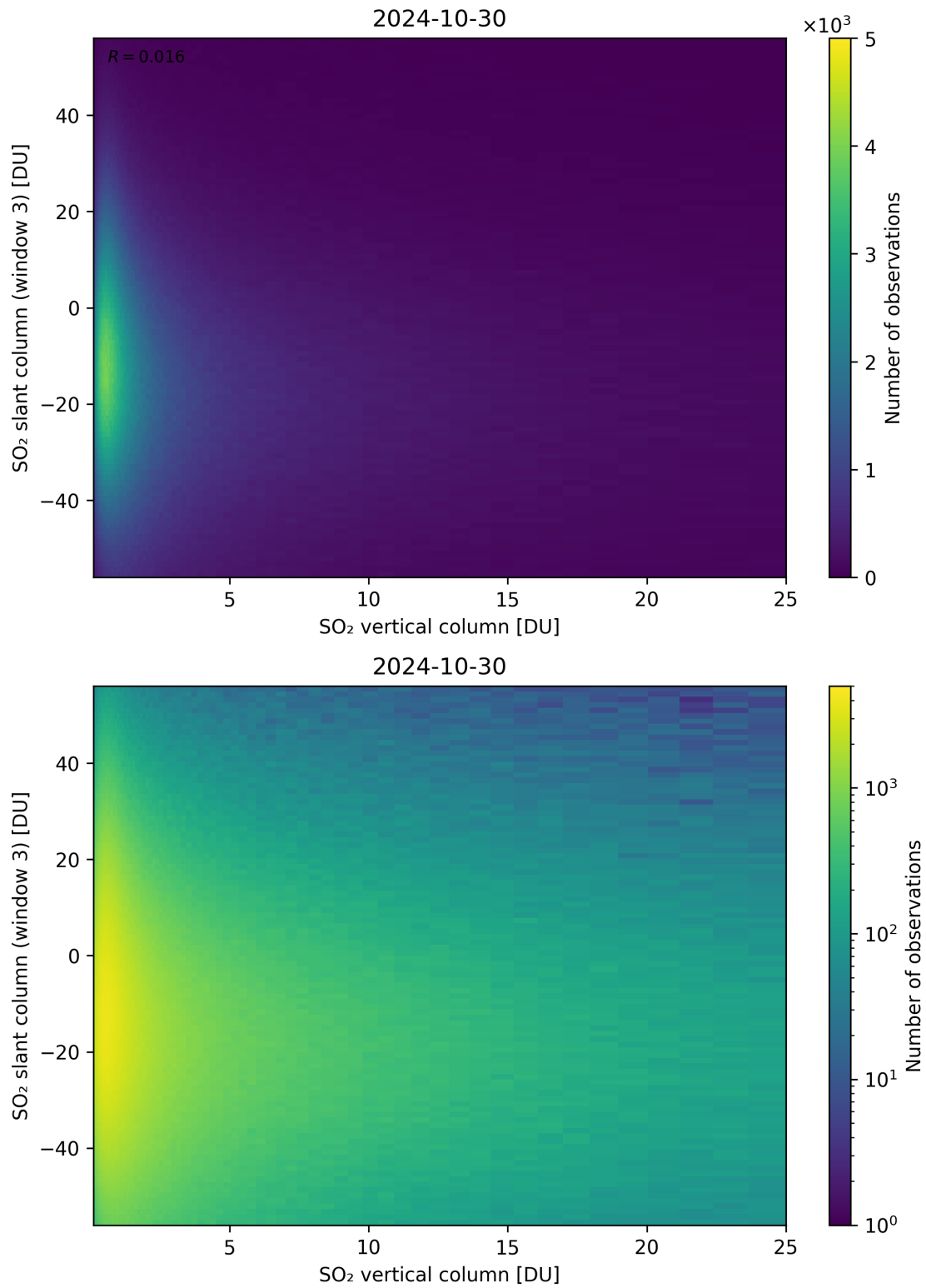
Figure 303: Scatter density plot of “SO 2 vertical column” against “SO 2 slant column (window 3)” for 2024-10-30 to 2024-10-31.
