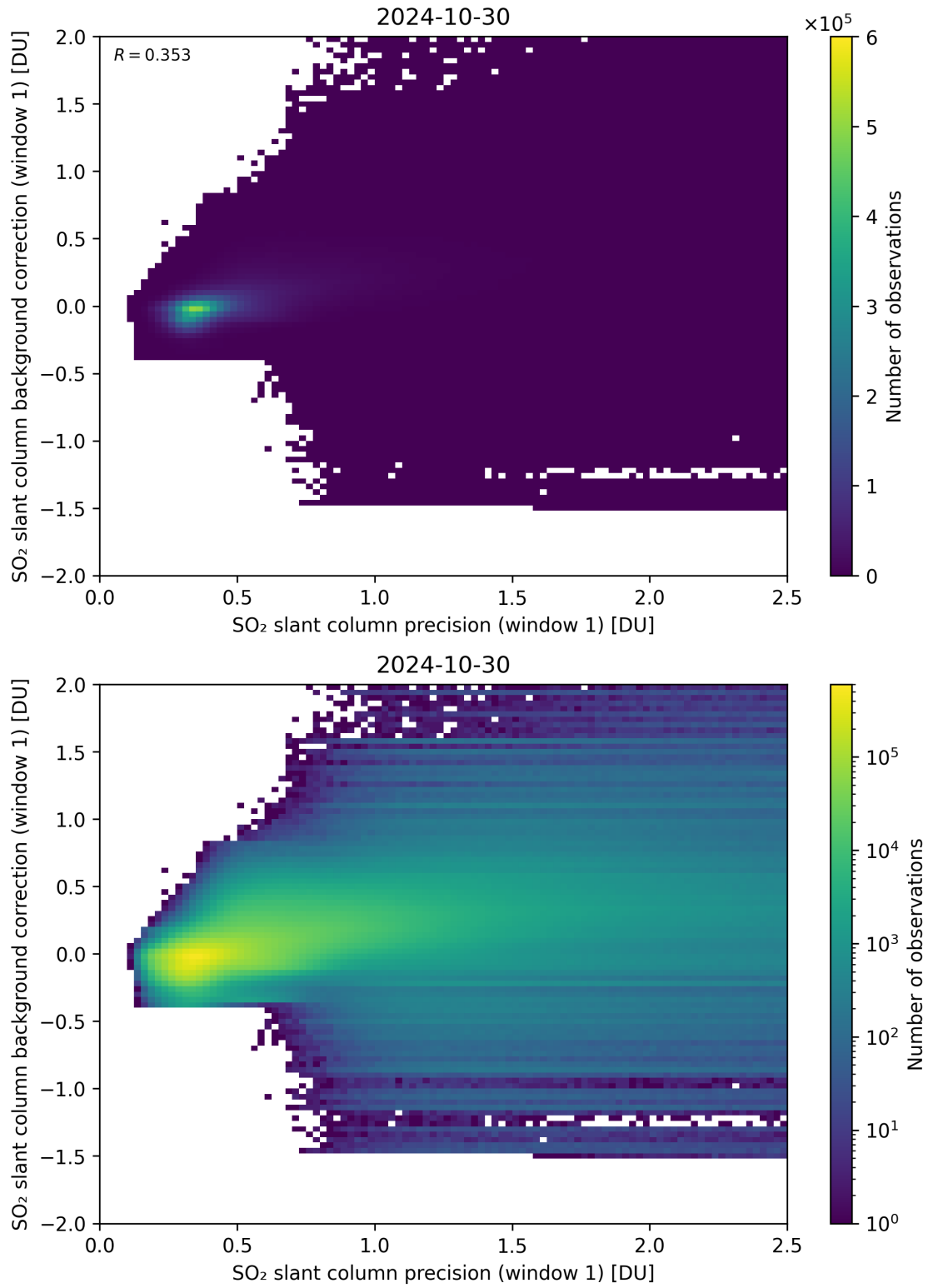
Figure 218: Scatter density plot of “SO 2 slant column precision (window 1)” against “SO 2 slant column background correction (window 1)” for 2024-10-30 to 2024-10-31.
