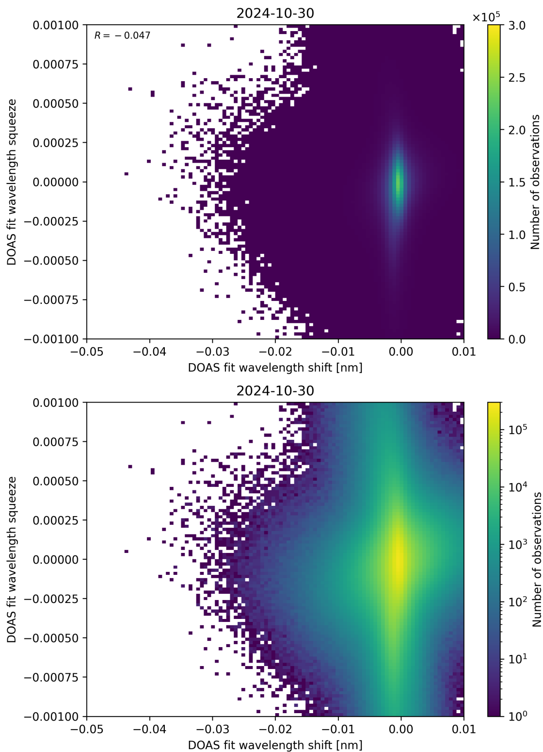
Figure 127: Scatter density plot of “DOAS fit wavelength shift” against “DOAS fit wavelength squeeze” for 2024-10-30 to 2024-10-31.
