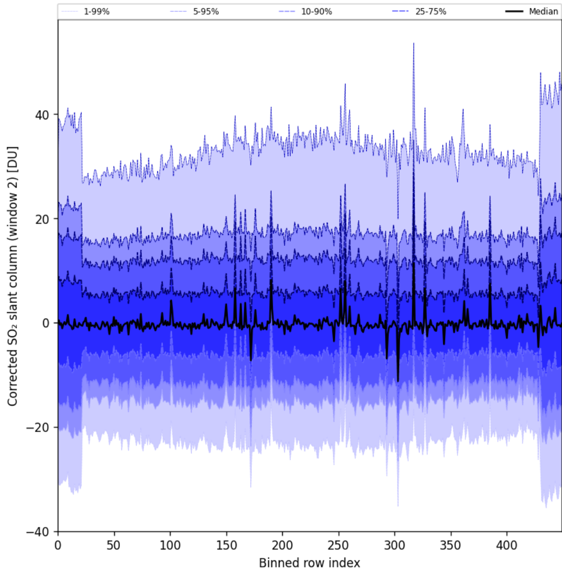
Figure 85: Along track statistics of “Corrected SO 2 slant column (window 2)” for 2024-10-30 to 2024-10-31
