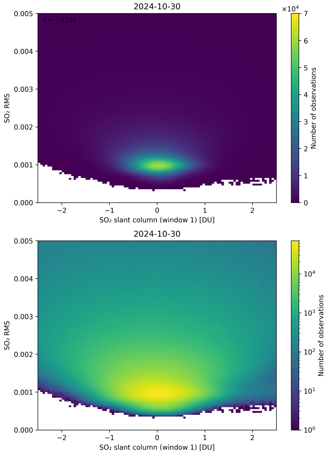
Figure 217: Scatter density plot of “SO 2 slant column (window 1)” against “SO 2 RMS” for 2024-10-30 to 2024-10-31.
