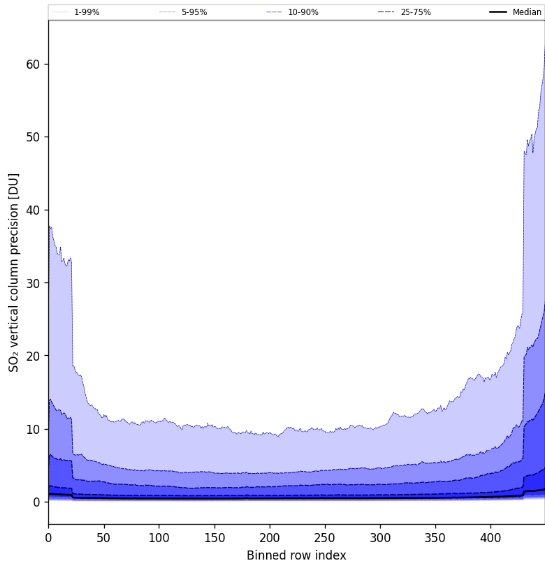
Figure 77: Along track statistics of “SO 2 vertical column precision” for 2024-10-30 to 2024-10-31
