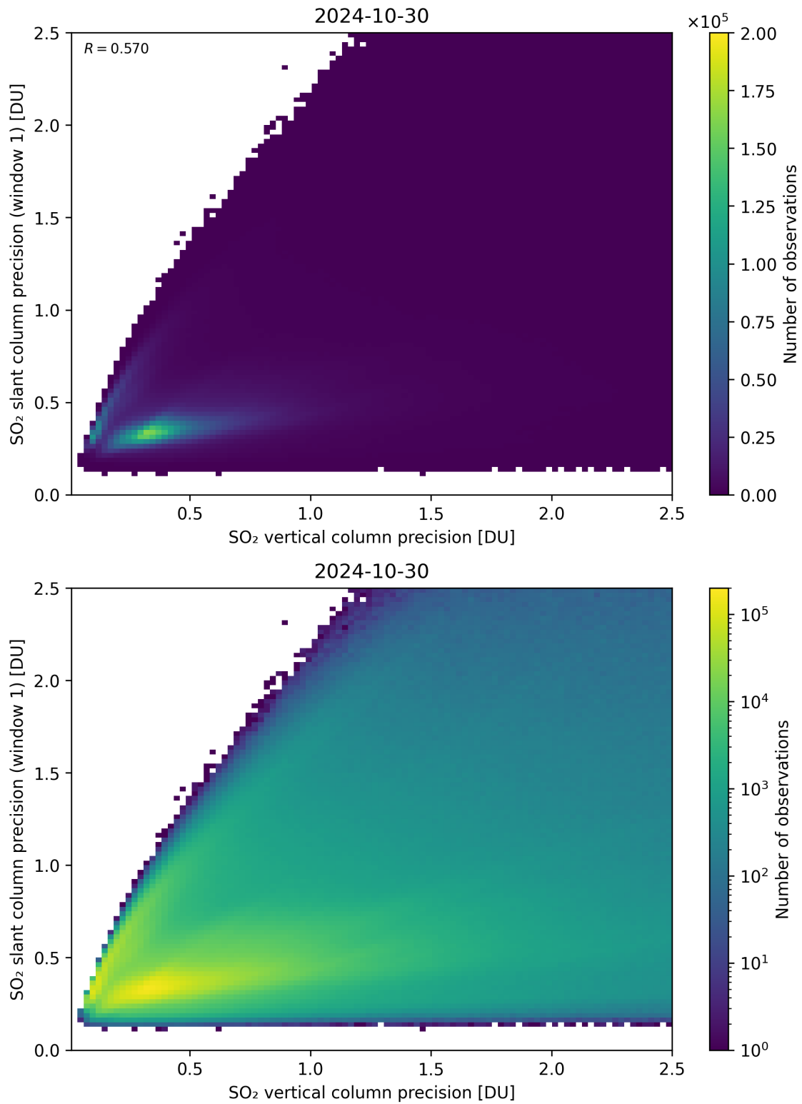
Figure 290: Scatter density plot of “SO 2 vertical column precision” against “SO 2 slant column precision (window 1)” for 2024-10-30 to 2024-10-31.
