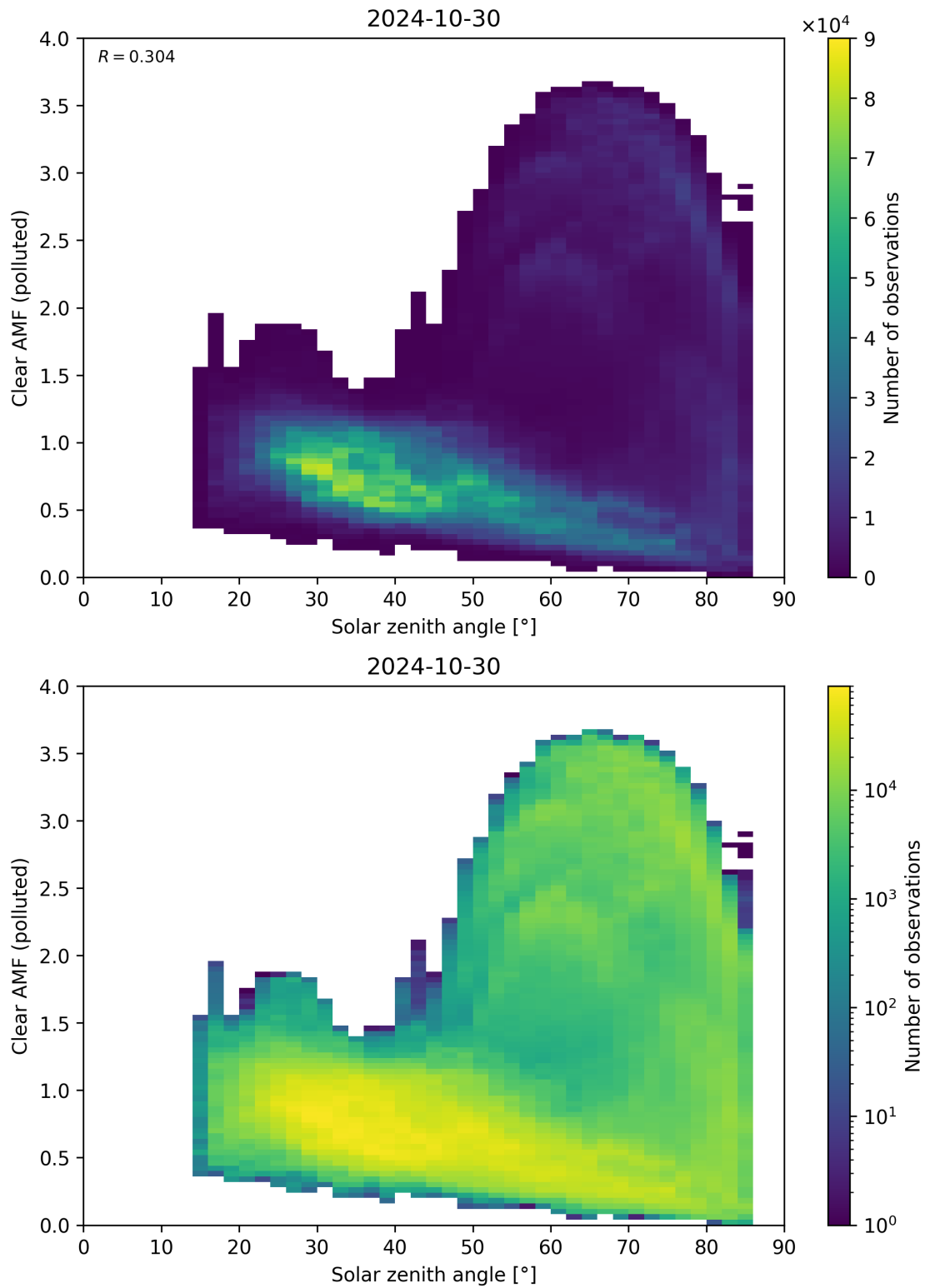
Figure 165: Scatter density plot of “Solar zenith angle” against “Clear AMF (polluted)” for 2024-10-30 to 2024-10-31.
