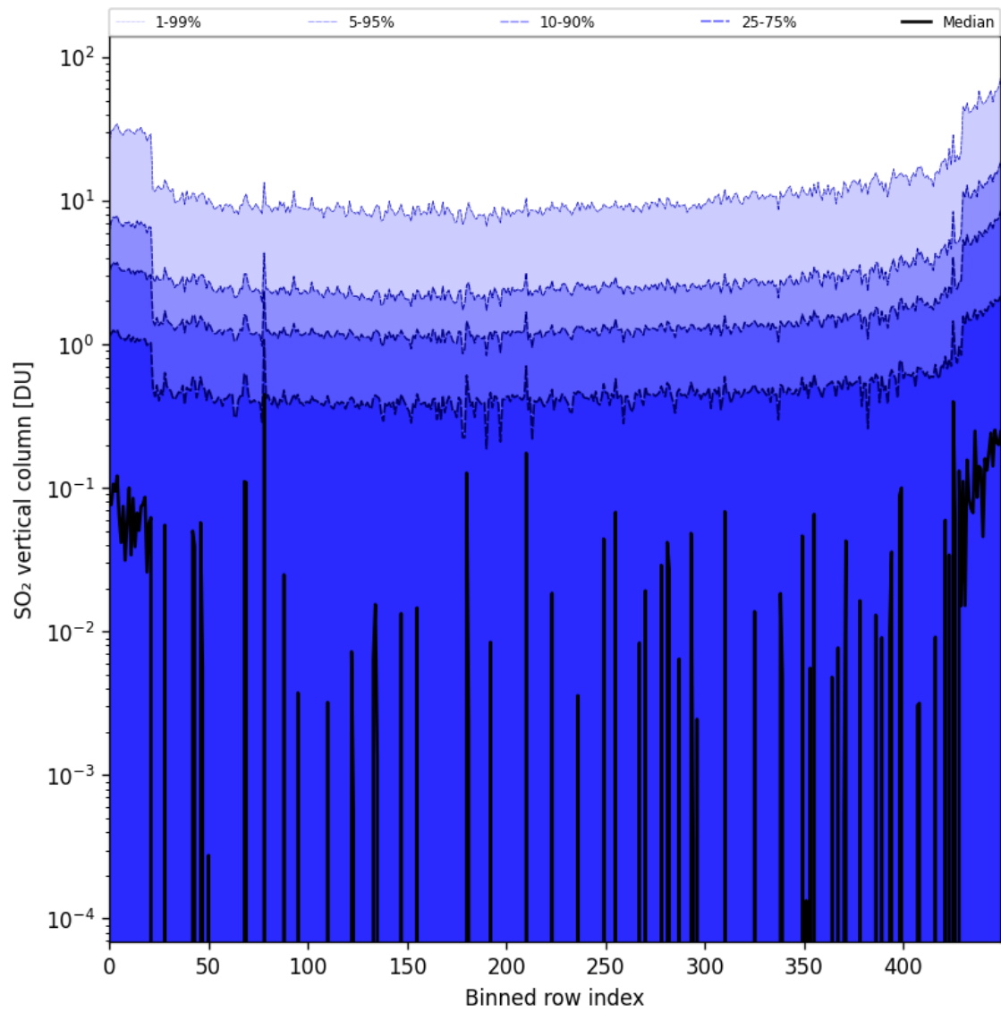
Figure 76: Along track statistics of “SO 2 vertical column” for 2024-10-30 to 2024-10-31
