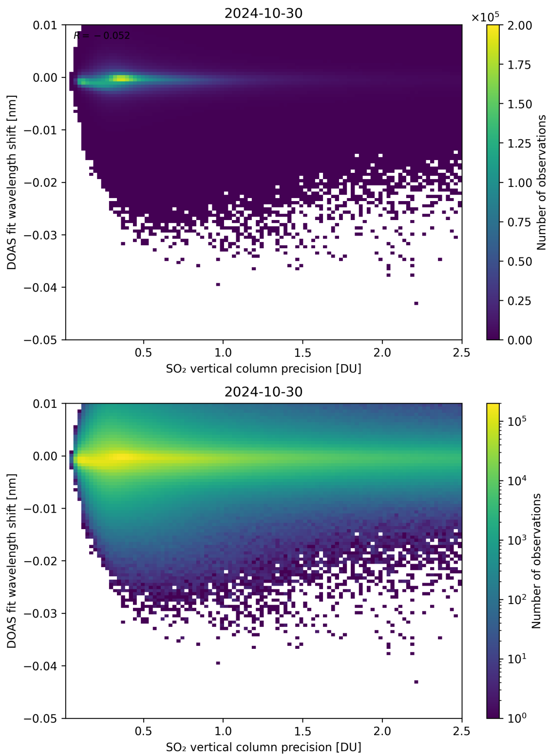
Figure 282: Scatter density plot of “SO 2 vertical column precision” against “DOAS fit wavelength shift” for 2024-10-30 to 2024-10-31.
