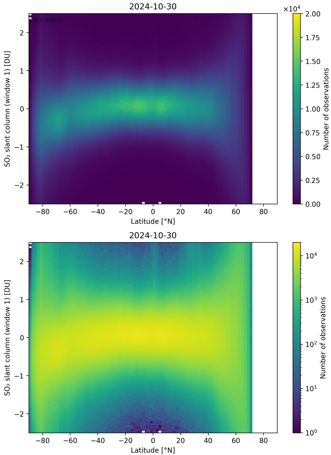
Figure 149: Scatter density plot of “Latitude” against “SO 2 slant column (window 1)” for 2024-10-30 to 2024-10-31.
