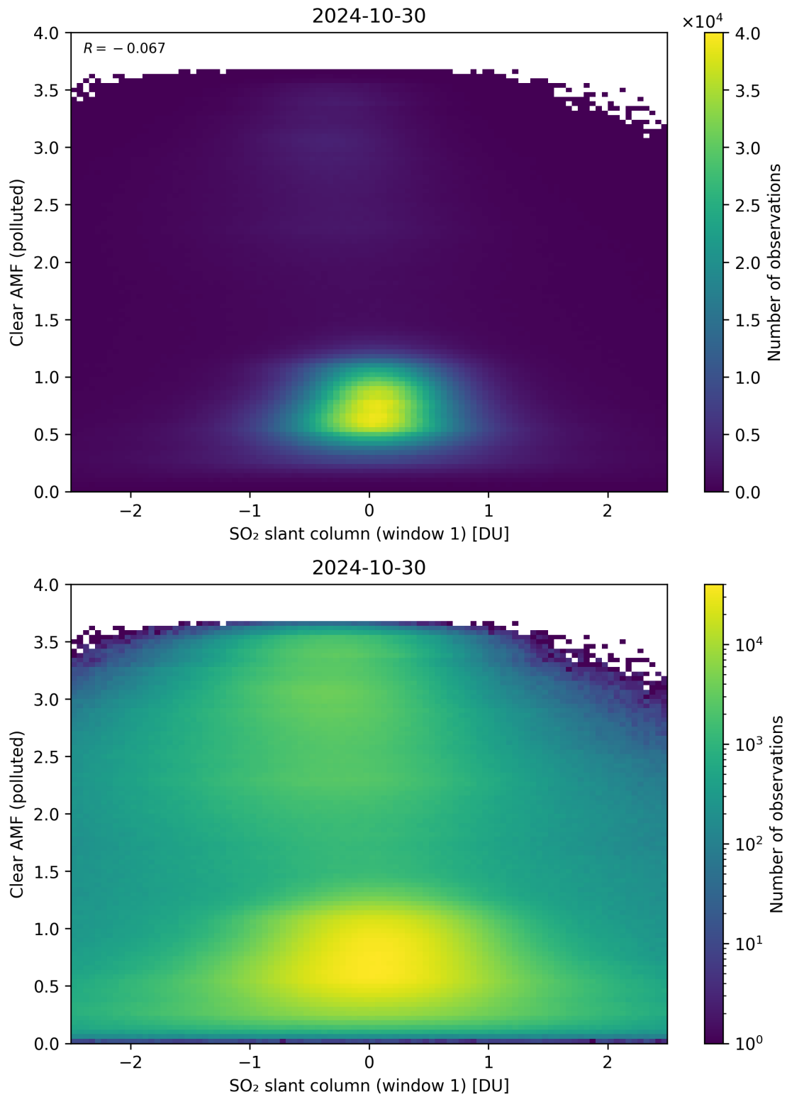
Figure 232: Scatter density plot of “SO 2 slant column (window 1)” against “Clear AMF (polluted)” for 2024-10-30 to 2024-10-31.
