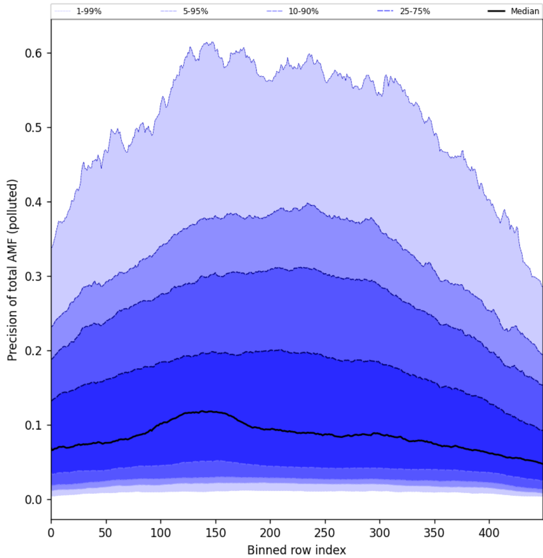
Figure 95: Along track statistics of “Precision of total AMF (polluted)” for 2024-10-30 to 2024-10-31
