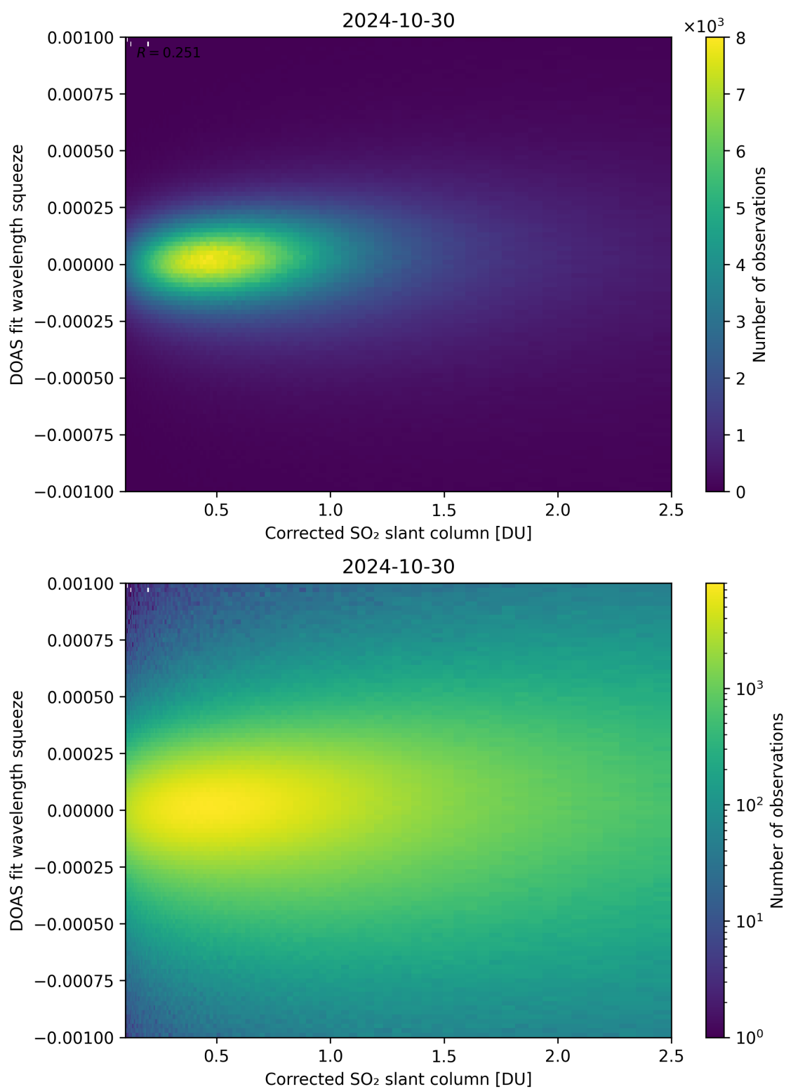
Figure 182: Scatter density plot of “Corrected SO 2 slant column” against “DOAS fit wavelength squeeze” for 2024-10-30 to 2024-10-31.
