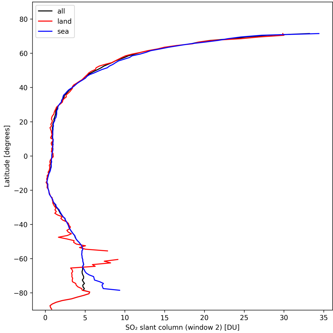
Figure 37: Zonal average of “SO 2 slant column (window 2)” for 2024-10-30 to 2024-10-31.
