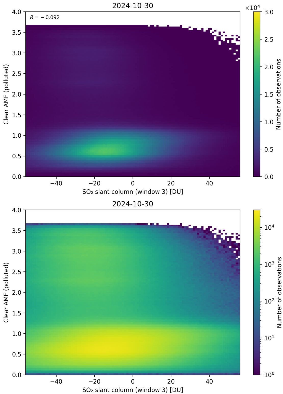
Figure 265: Scatter density plot of “SO 2 slant column (window 3)” against “Clear AMF (polluted)” for 2024-10-30 to 2024-10-31.
