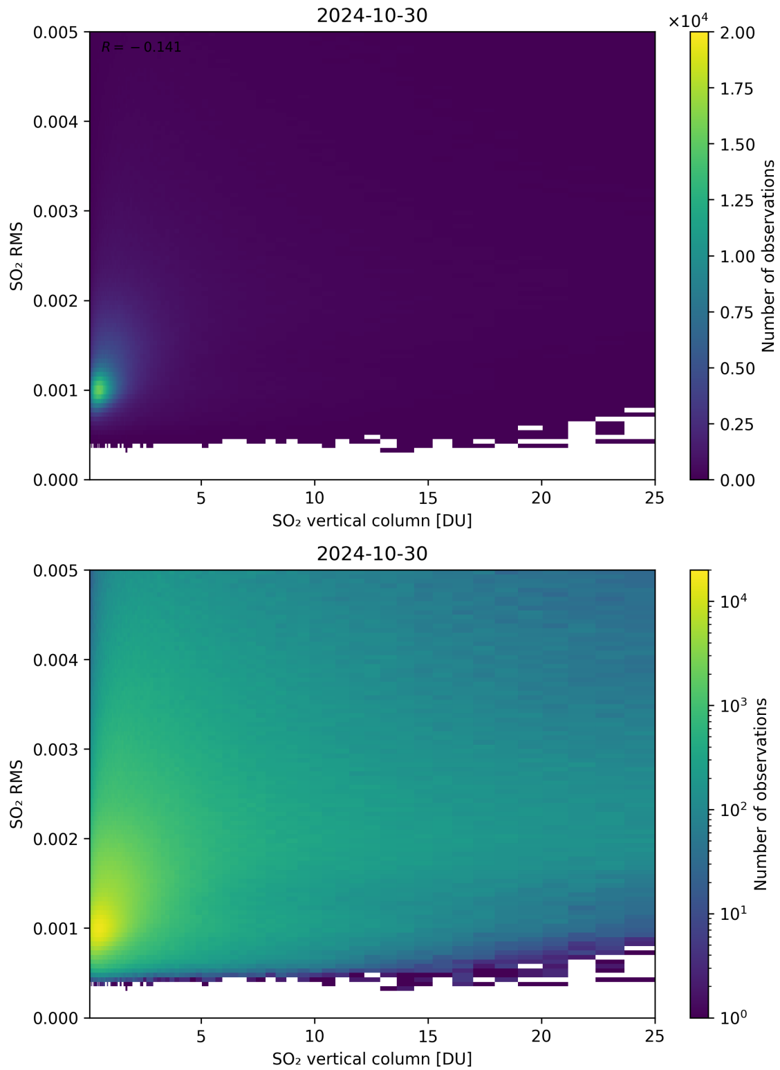
Figure 278: Scatter density plot of “SO 2 vertical column” against “SO 2 RMS” for 2024-10-30 to 2024-10-31.
