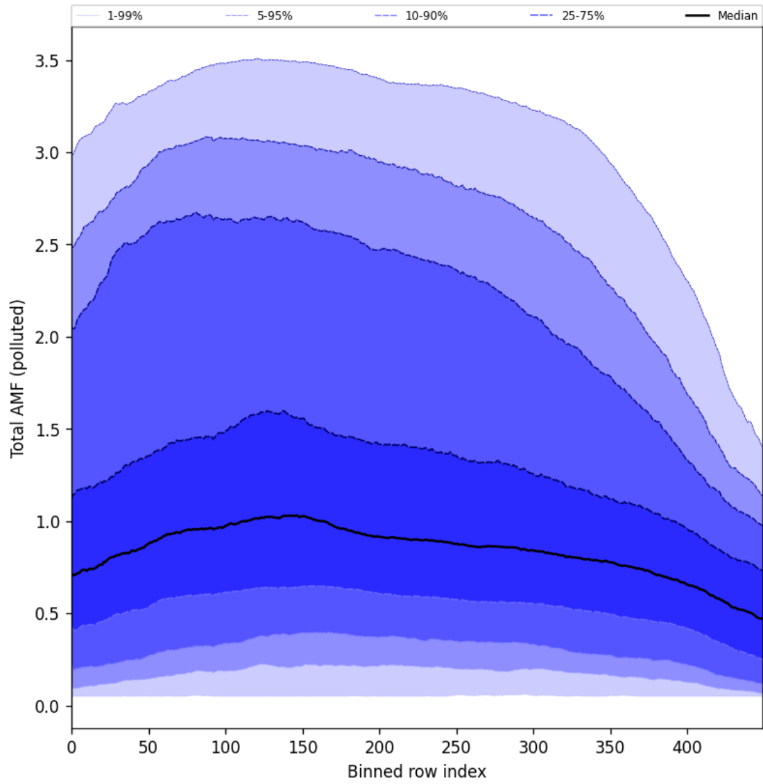
Figure 94: Along track statistics of “Total AMF (polluted)” for 2024-10-30 to 2024-10-31
