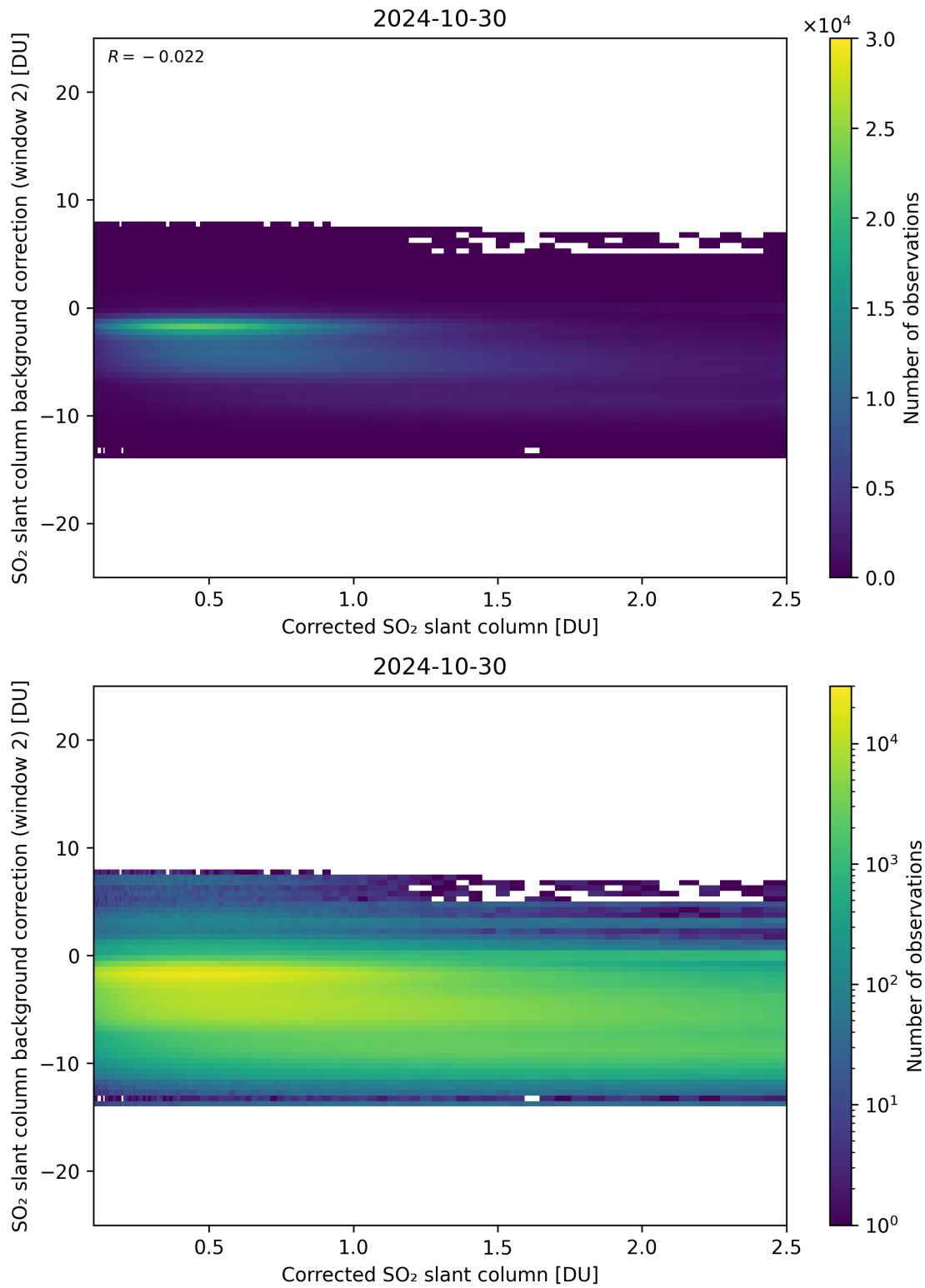
Figure 179: Scatter density plot of “Corrected SO 2 slant column” against “SO 2 slant column background correction (window 2)” for 2024-10-30 to 2024-10-31.
