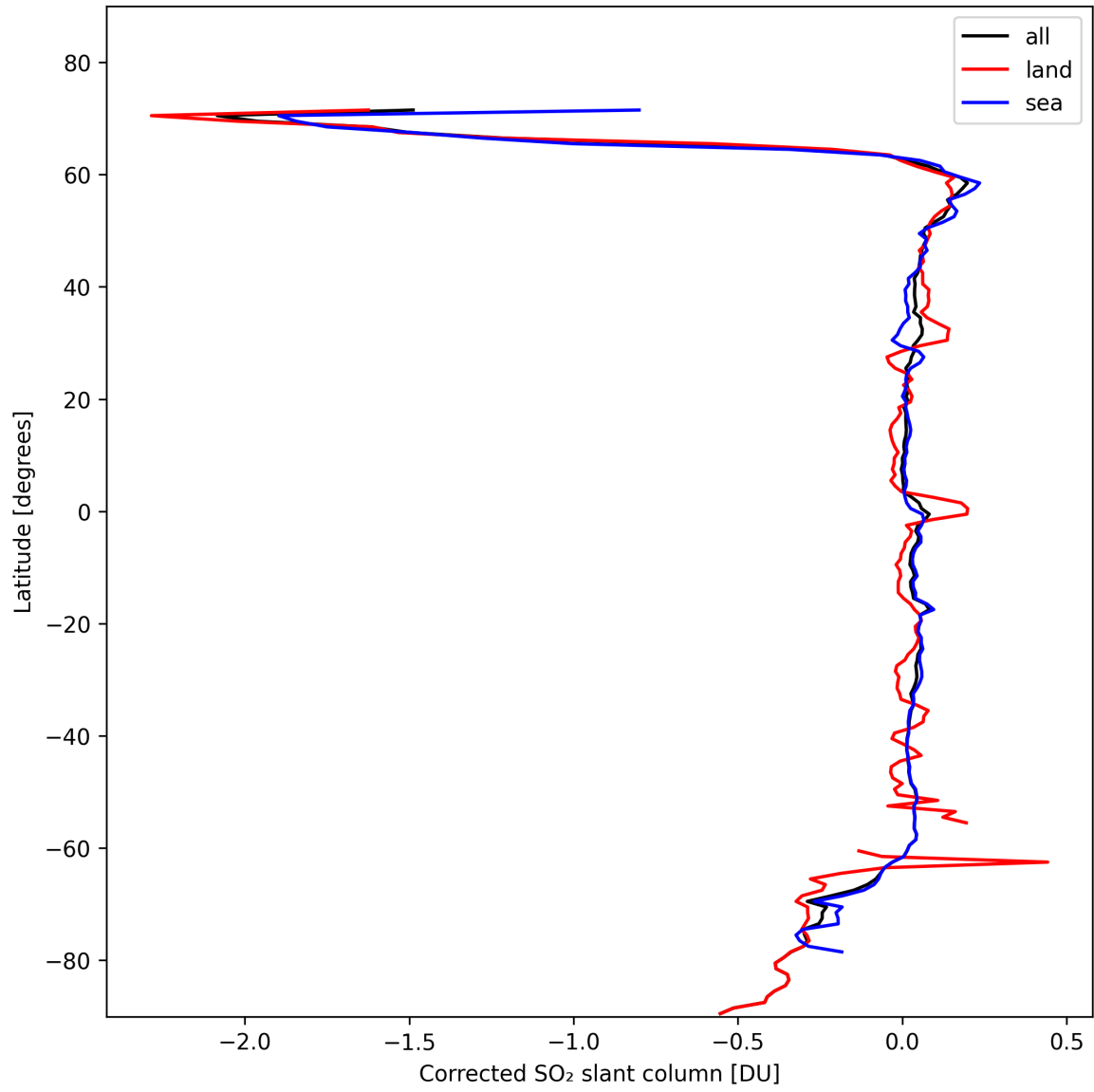
Figure 32: Zonal average of “Corrected SO 2 slant column” for 2024-10-30 to 2024-10-31.
