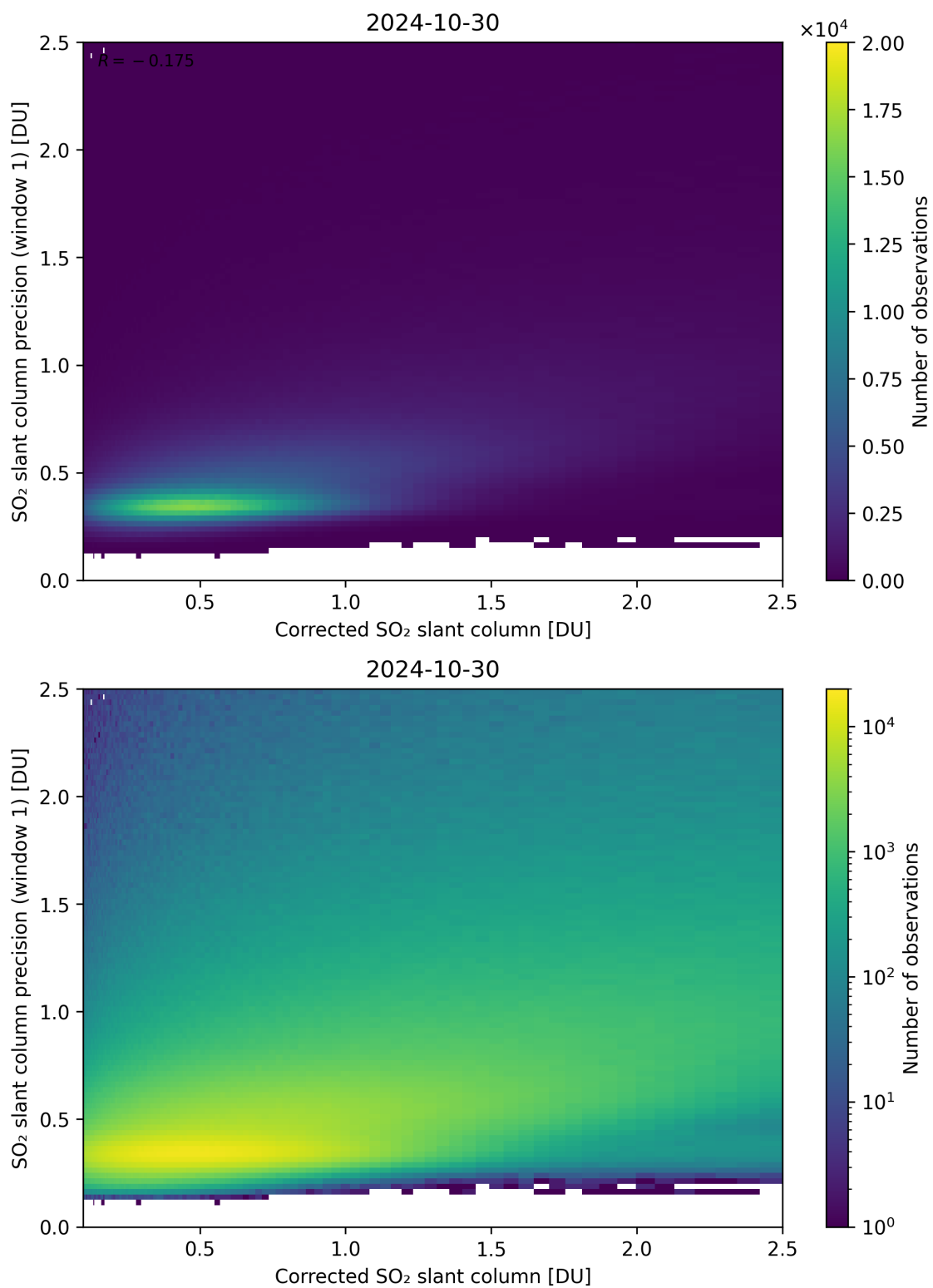
Figure 188: Scatter density plot of “Corrected SO 2 slant column” against “SO 2 slant column precision (window 1)” for 2024-10-30 to 2024-10-31.
