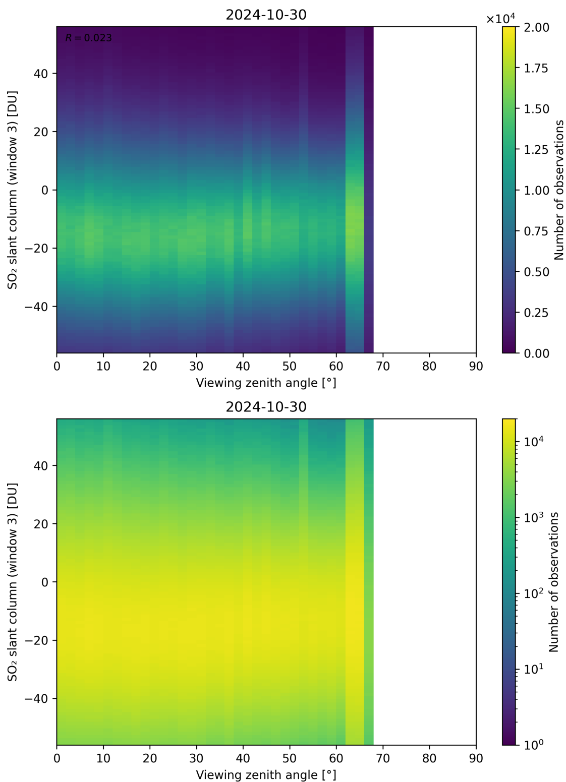
Figure 323: Scatter density plot of “Viewing zenith angle” against “SO 2 slant column (window 3)” for 2024-10-30 to 2024-10-31.
