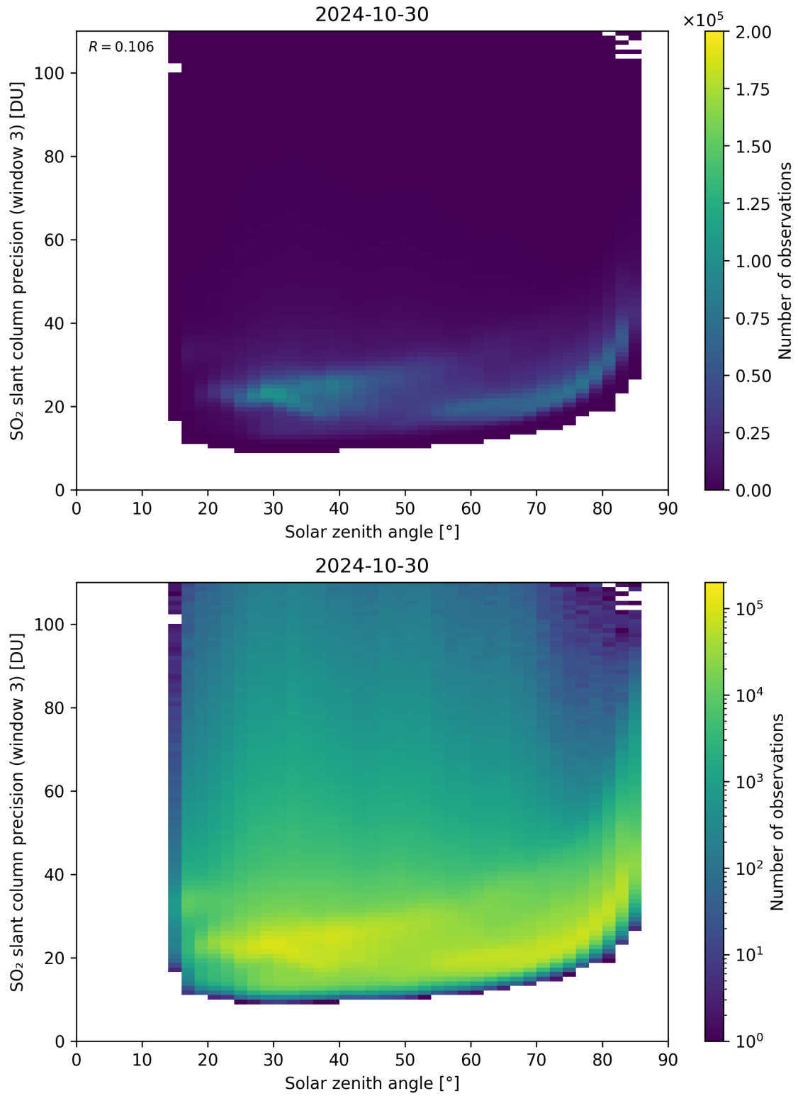
Figure 173: Scatter density plot of “Solar zenith angle” against “SO 2 slant column precision (window 3)” for 2024-10-30 to 2024-10-31.
