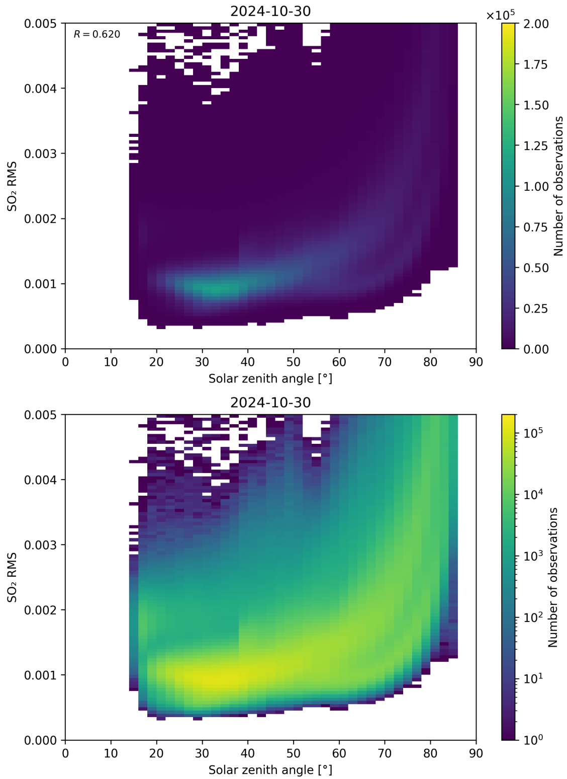
Figure 163: Scatter density plot of “Solar zenith angle” against “SO 2 RMS” for 2024-10-30 to 2024-10-31.
