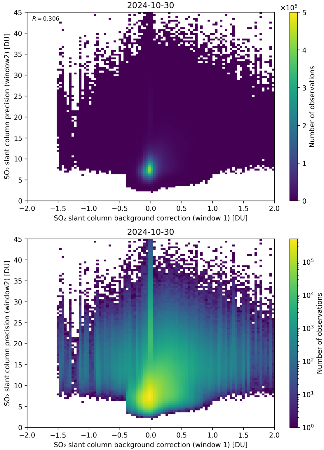
Figure 106: Scatter density plot of “SO 2 slant column background correction (window 1)” against “SO 2 slant column precision (window2)” for 2024-10-30 to 2024-10-31.
