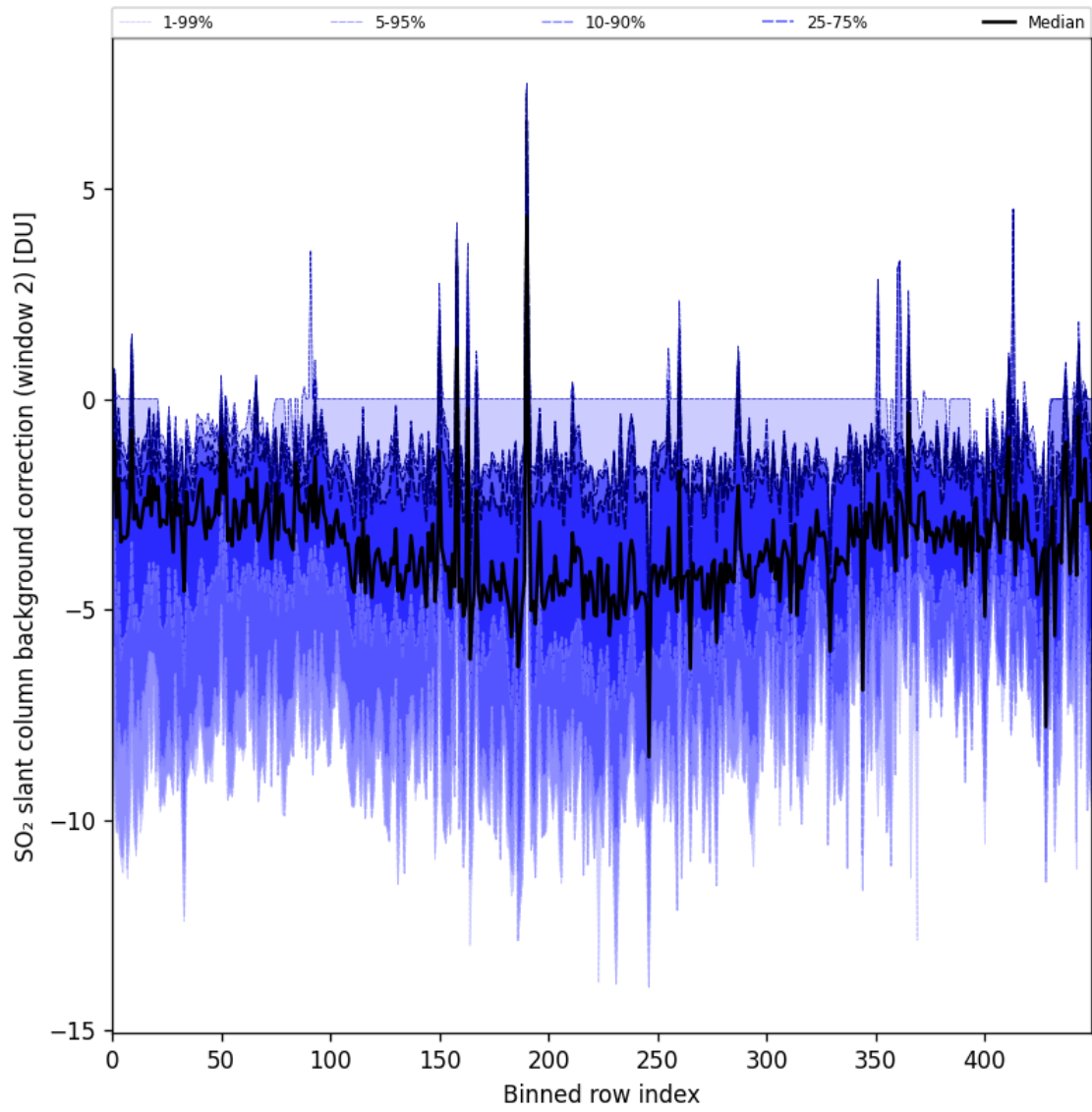
Figure 86: Along track statistics of “SO 2 slant column background correction (window 2)” for 2024-10-30 to 2024-10-31
