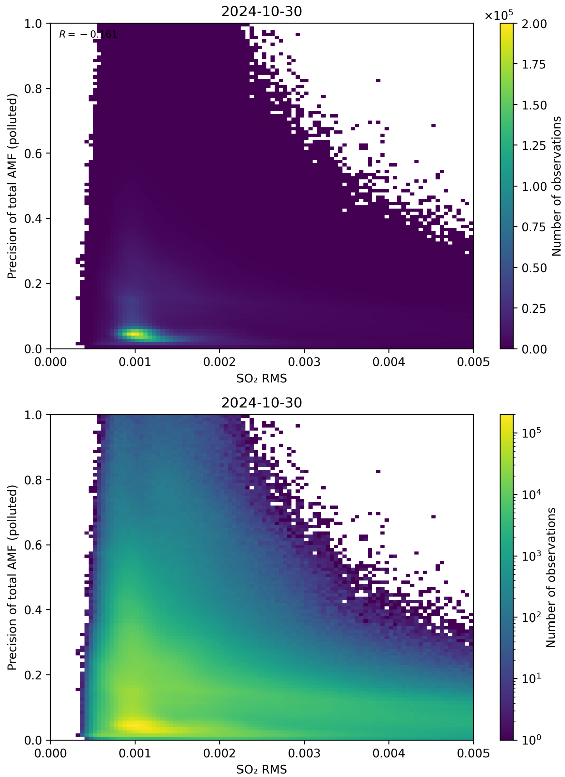
Figure 138: Scatter density plot of “SO 2 RMS” against “Precision of total AMF (polluted)” for 2024-10-30 to 2024-10-31.
