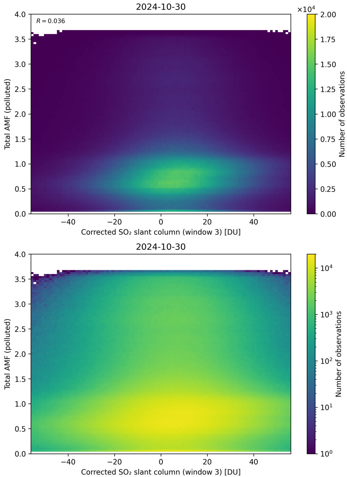
Figure 210: Scatter density plot of “Corrected SO 2 slant column (window 3)” against “Total AMF (polluted)” for 2024-10-30 to 2024-10-31.
