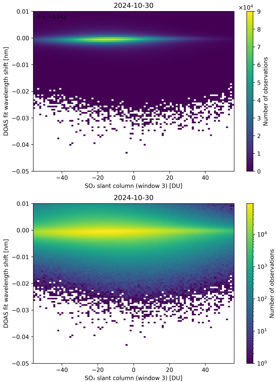
Figure 254: Scatter density plot of “SO 2 slant column (window 3)” against “DOAS fit wavelength shift” for 2024-10-30 to 2024-10-31.
