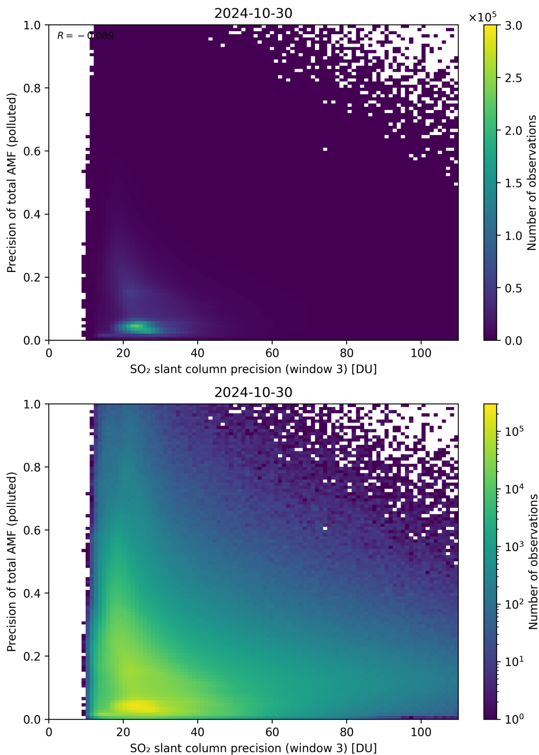
Figure 264: Scatter density plot of “SO 2 slant column precision (window 3)” against “Precision of total AMF (polluted)” for 2024-10-30 to 2024-10-31.
