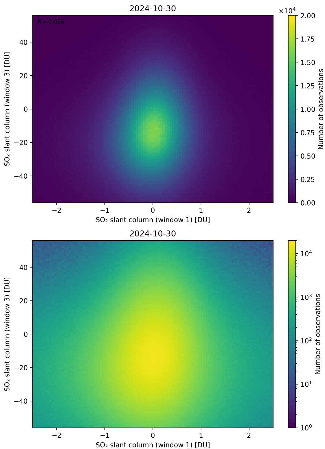
Figure 237: Scatter density plot of “SO 2 slant column (window 1)” against “SO 2 slant column (window 3)” for 2024-10-30 to 2024-10-31.
