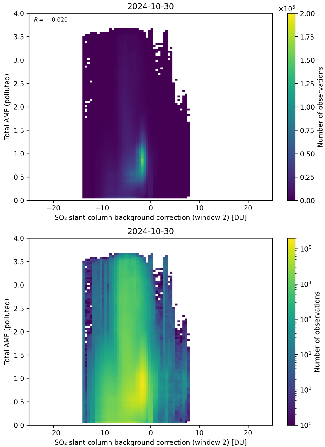
Figure 119: Scatter density plot of “SO 2 slant column background correction (window 2)” against “Total AMF (polluted)” for 2024-10-30 to 2024-10-31.
