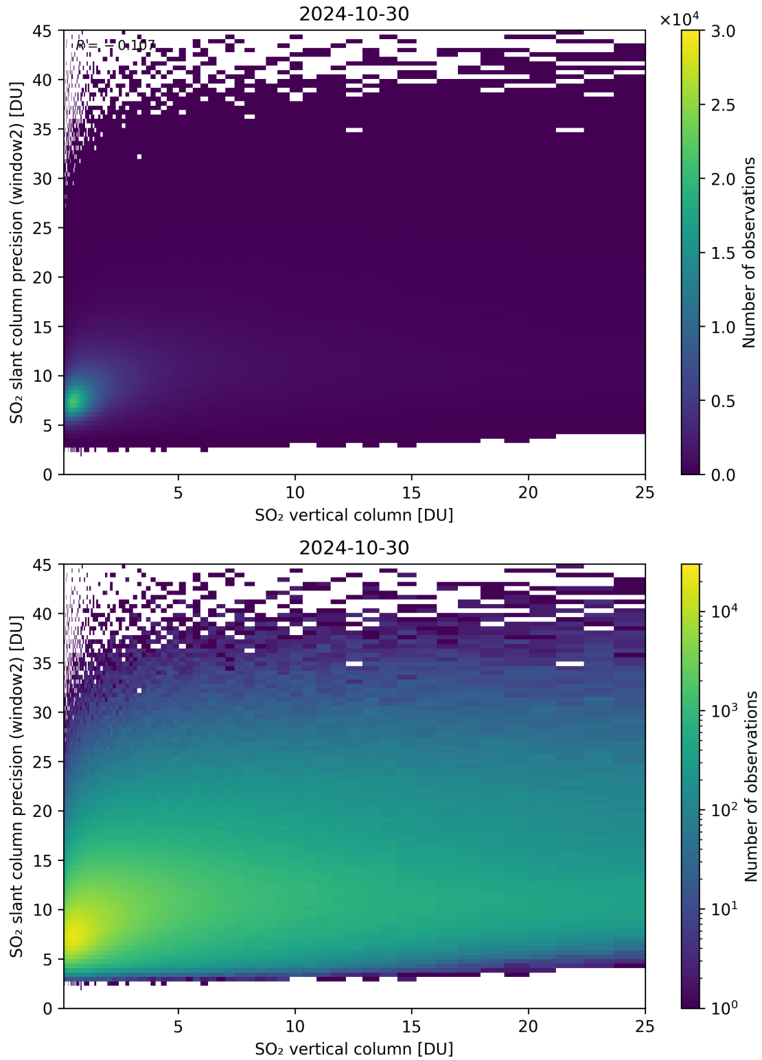
Figure 302: Scatter density plot of “SO 2 vertical column” against “SO 2 slant column precision (window2)” for 2024-10-30 to 2024-10-31.
