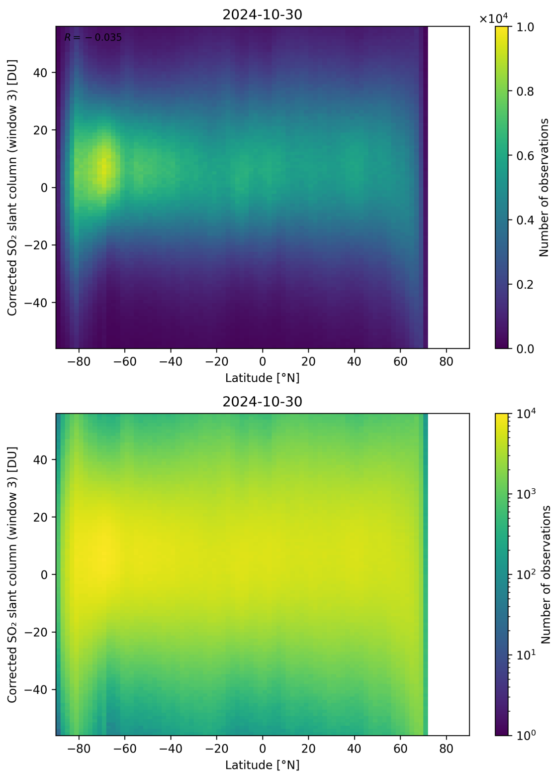
Figure 148: Scatter density plot of “Latitude” against “Corrected SO 2 slant column (window 3)” for 2024-10-30 to 2024-10-31.
