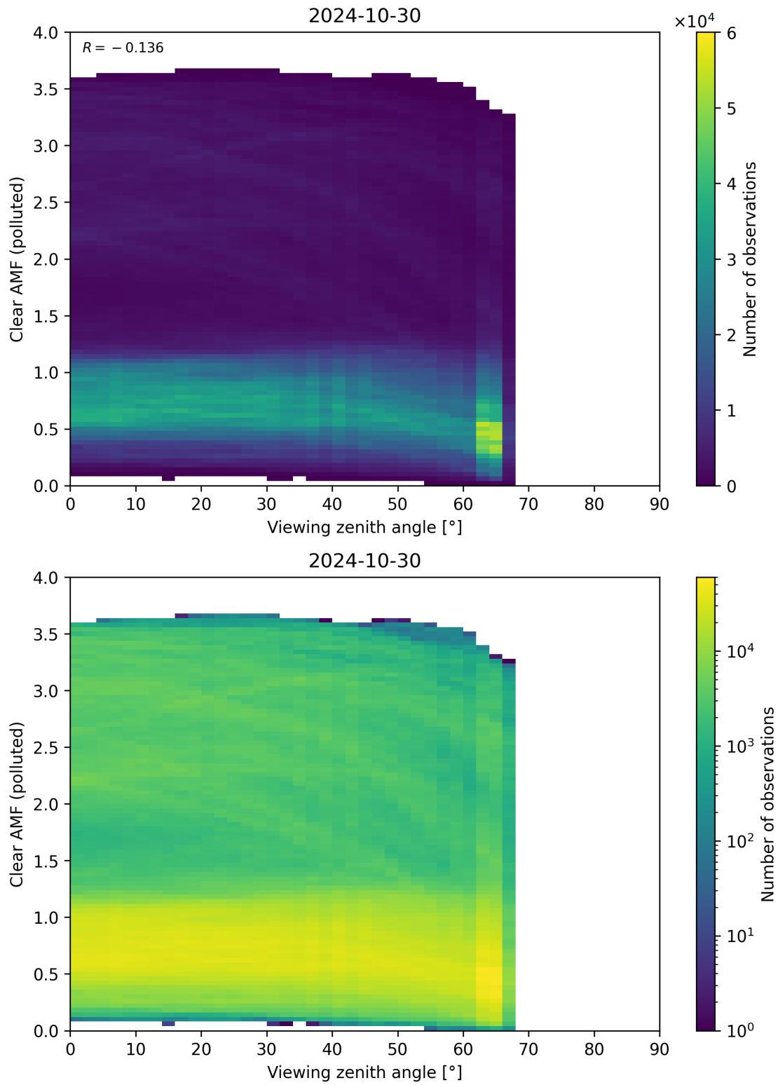
Figure 316: Scatter density plot of “Viewing zenith angle” against “Clear AMF (polluted)” for 2024-10-30 to 2024-10-31.
