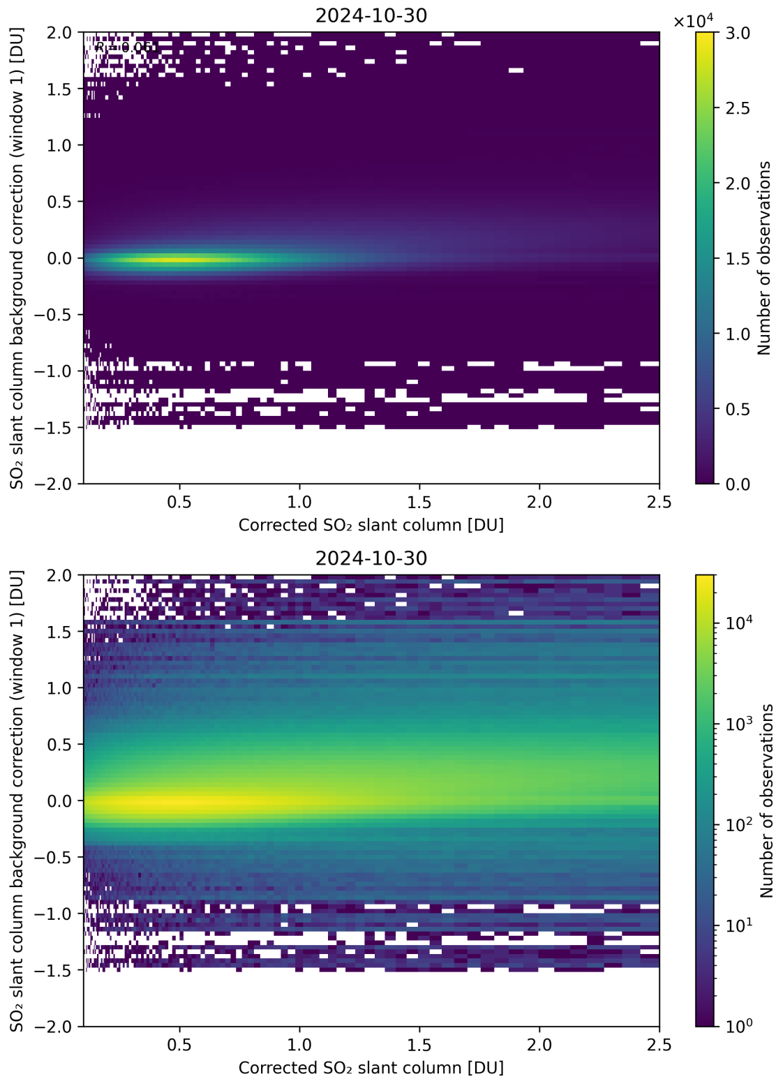
Figure 178: Scatter density plot of “Corrected SO 2 slant column” against “SO 2 slant column background correction (window 1)” for 2024-10-30 to 2024-10-31.
