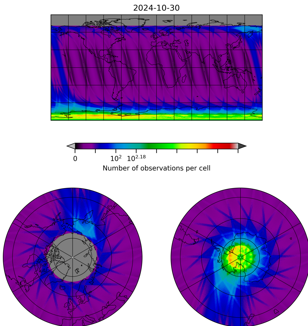
Figure 28: Map of the number of observations for 2024-10-30 to 2024-10-31
