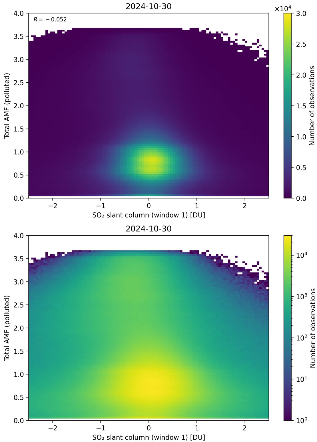
Figure 239: Scatter density plot of “SO 2 slant column (window 1)” against “Total AMF (polluted)” for 2024-10-30 to 2024-10-31.
