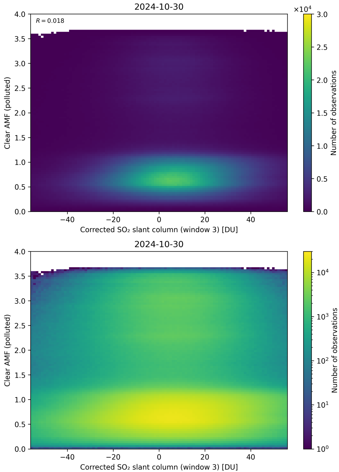
Figure 209: Scatter density plot of “Corrected SO 2 slant column (window 3)” against “Clear AMF (polluted)” for 2024-10-30 to 2024-10-31.
