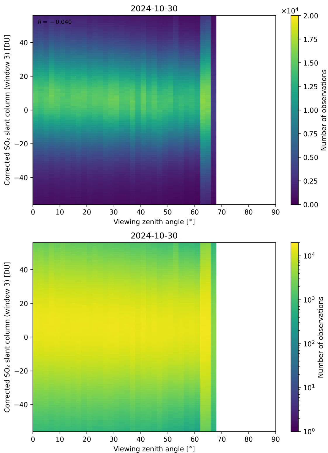
Figure 319: Scatter density plot of “Viewing zenith angle” against “Corrected SO 2 slant column (window 3)” for 2024-10-30 to 2024-10-31.
