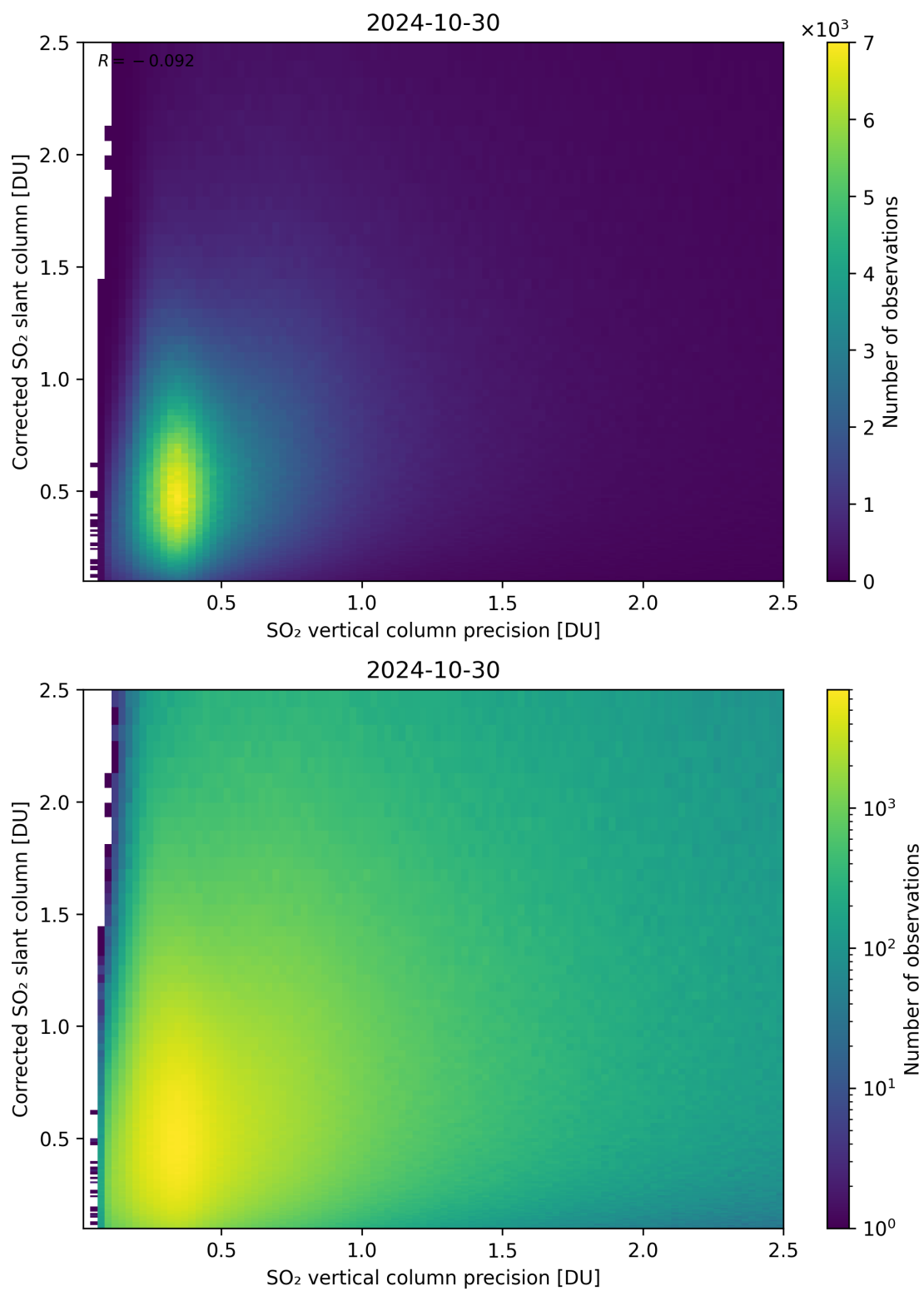
Figure 286: Scatter density plot of “SO 2 vertical column precision” against “Corrected SO 2 slant column” for 2024-10-30 to 2024-10-31.
