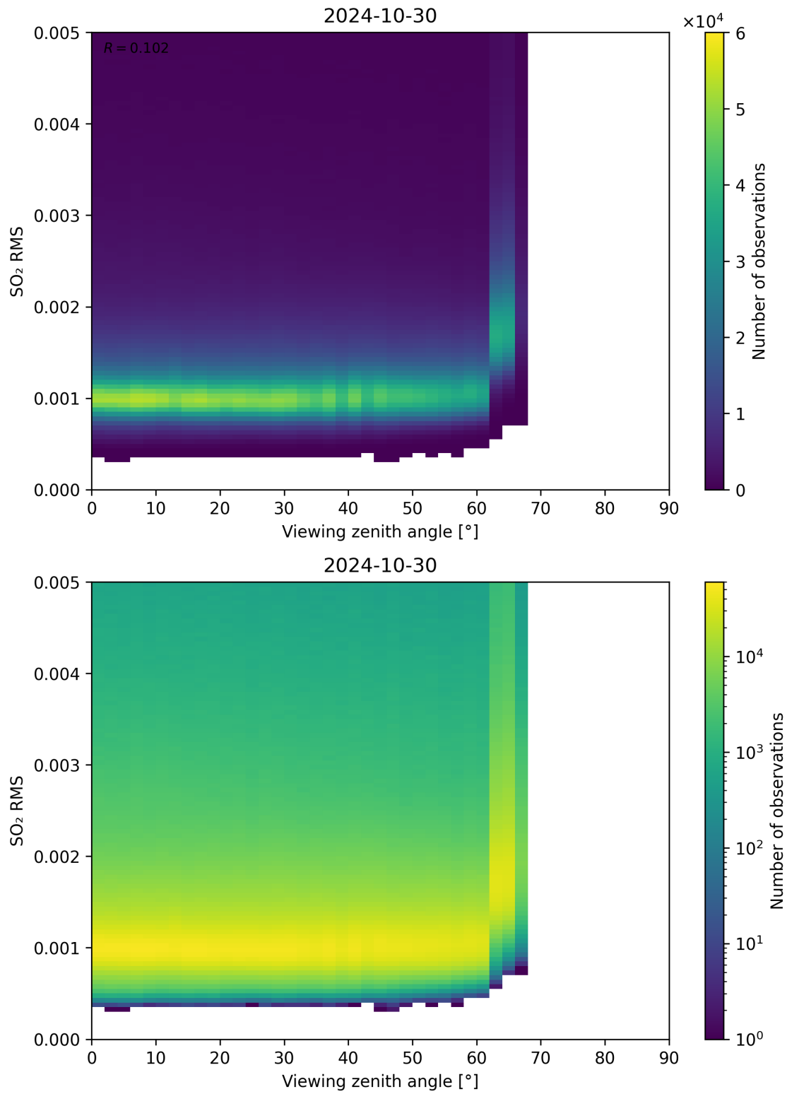
Figure 313: Scatter density plot of “Viewing zenith angle” against “SO 2 RMS” for 2024-10-30 to 2024-10-31.
