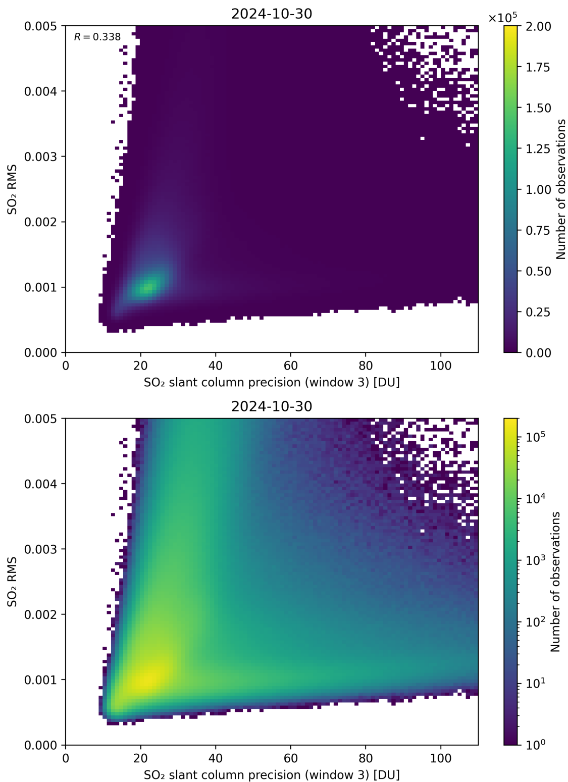
Figure 260: Scatter density plot of “SO 2 slant column precision (window 3)” against “SO 2 RMS” for 2024-10-30 to 2024-10-31.
