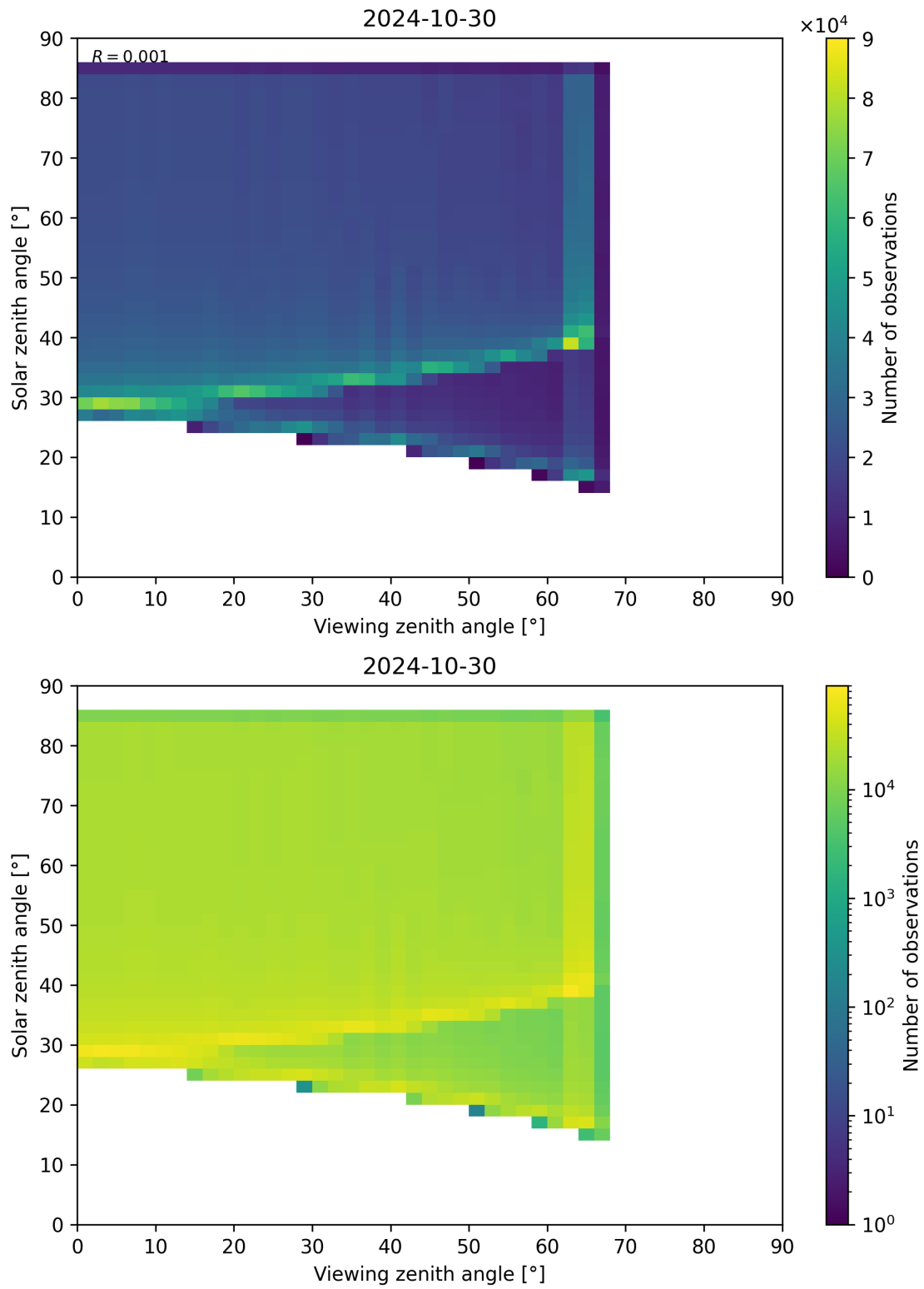
Figure 315: Scatter density plot of “Viewing zenith angle” against “Solar zenith angle” for 2024-10-30 to 2024-10-31.
