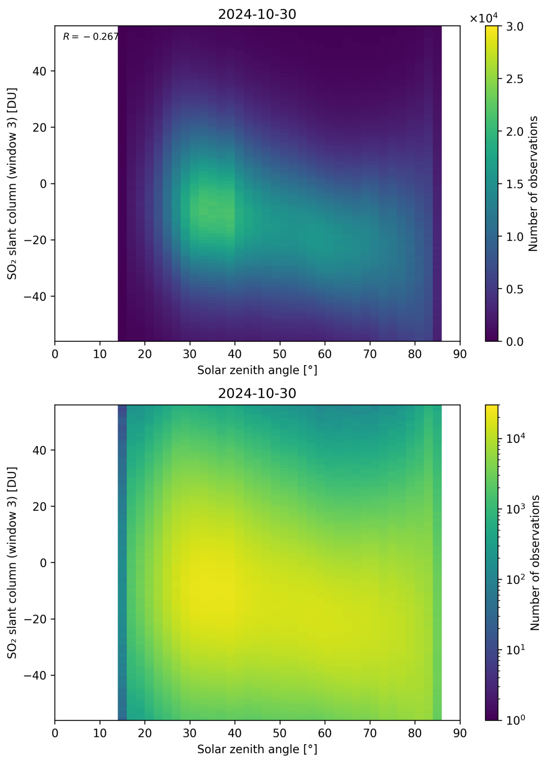
Figure 172: Scatter density plot of “Solar zenith angle” against “SO 2 slant column (window 3)” for 2024-10-30 to 2024-10-31.
