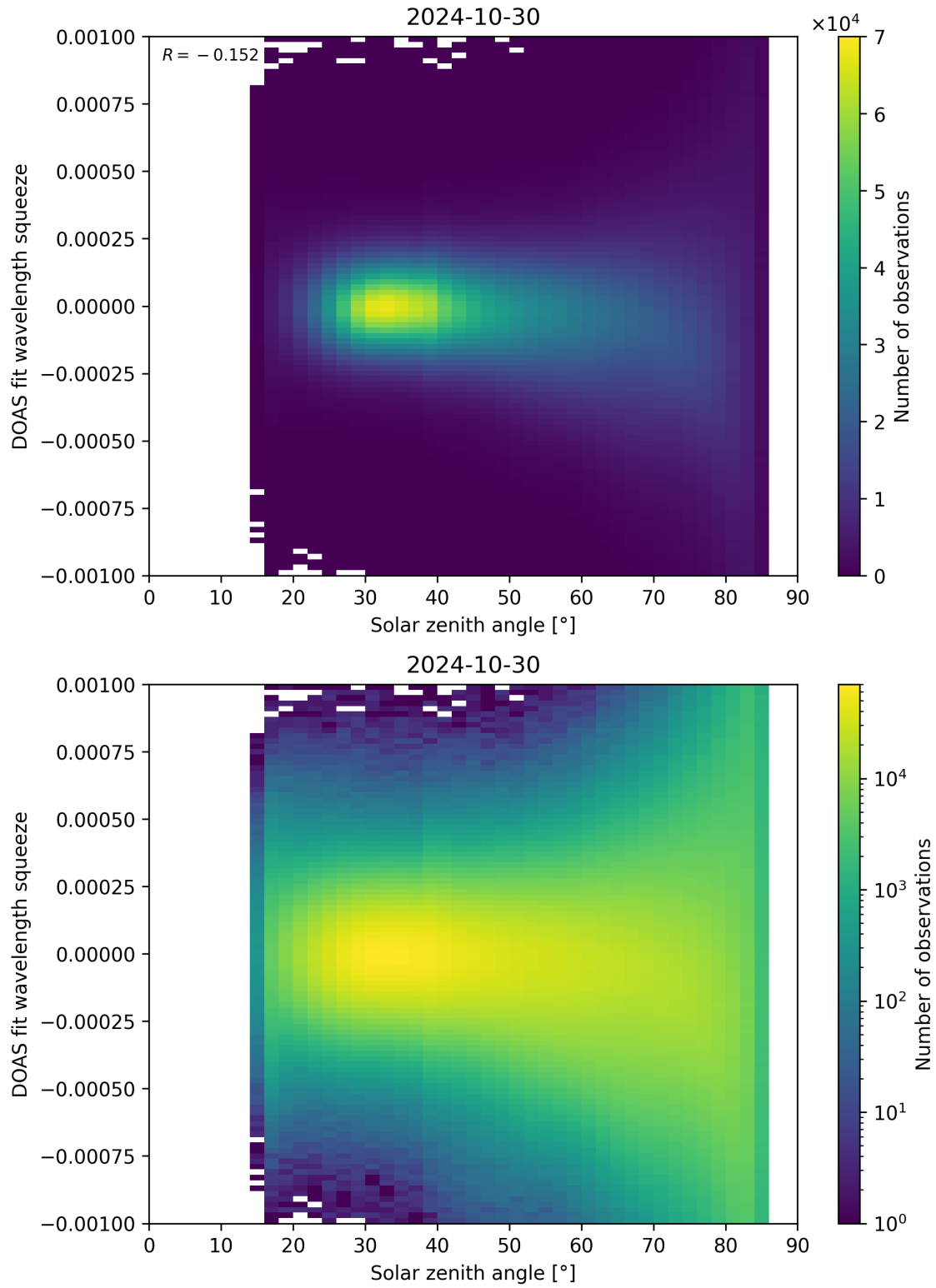
Figure 162: Scatter density plot of “Solar zenith angle” against “DOAS fit wavelength squeeze” for 2024-10-30 to 2024-10-31.
