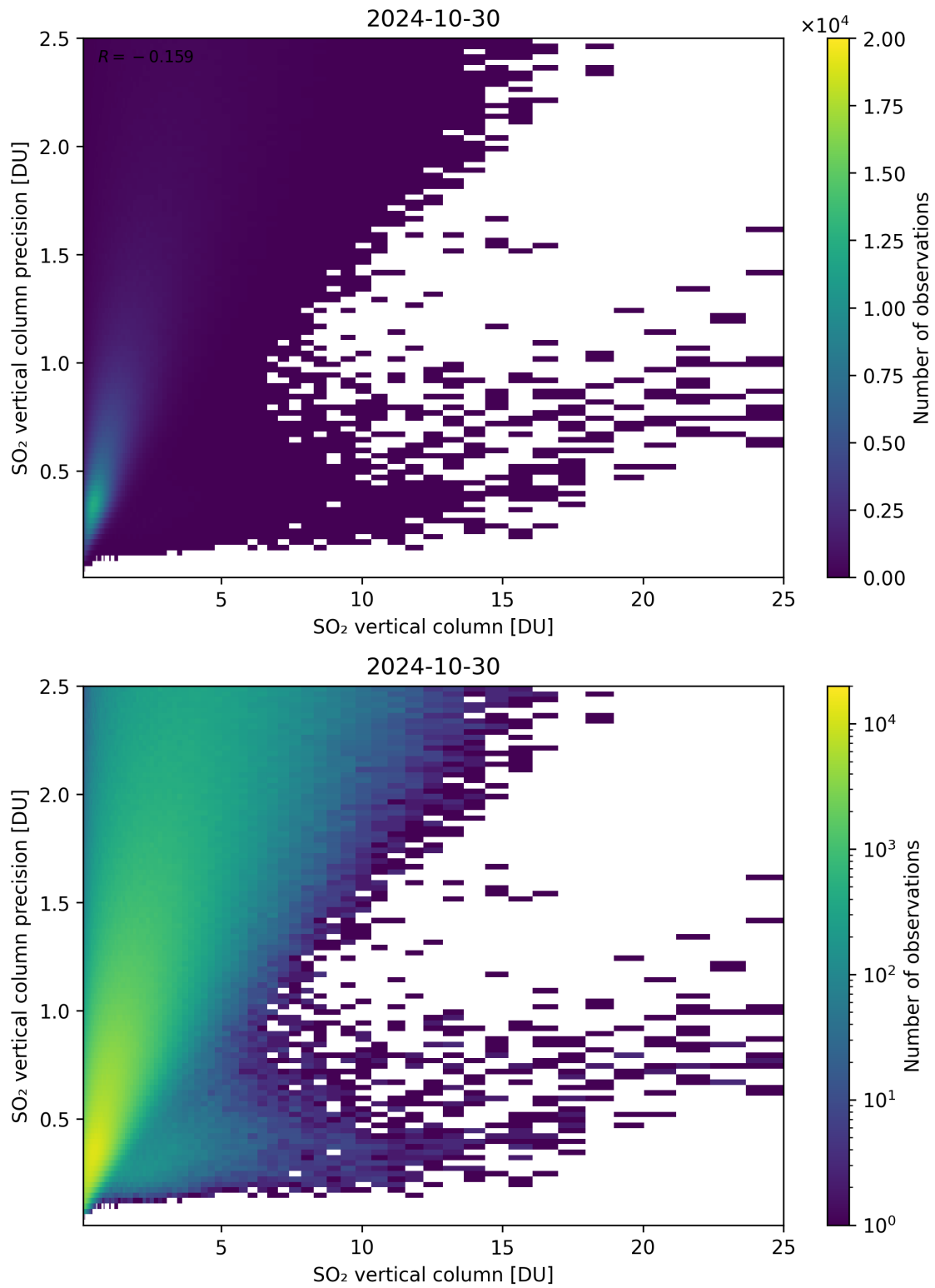
Figure 307: Scatter density plot of “SO 2 vertical column” against “SO 2 vertical column precision” for 2024-10-30 to 2024-10-31.
