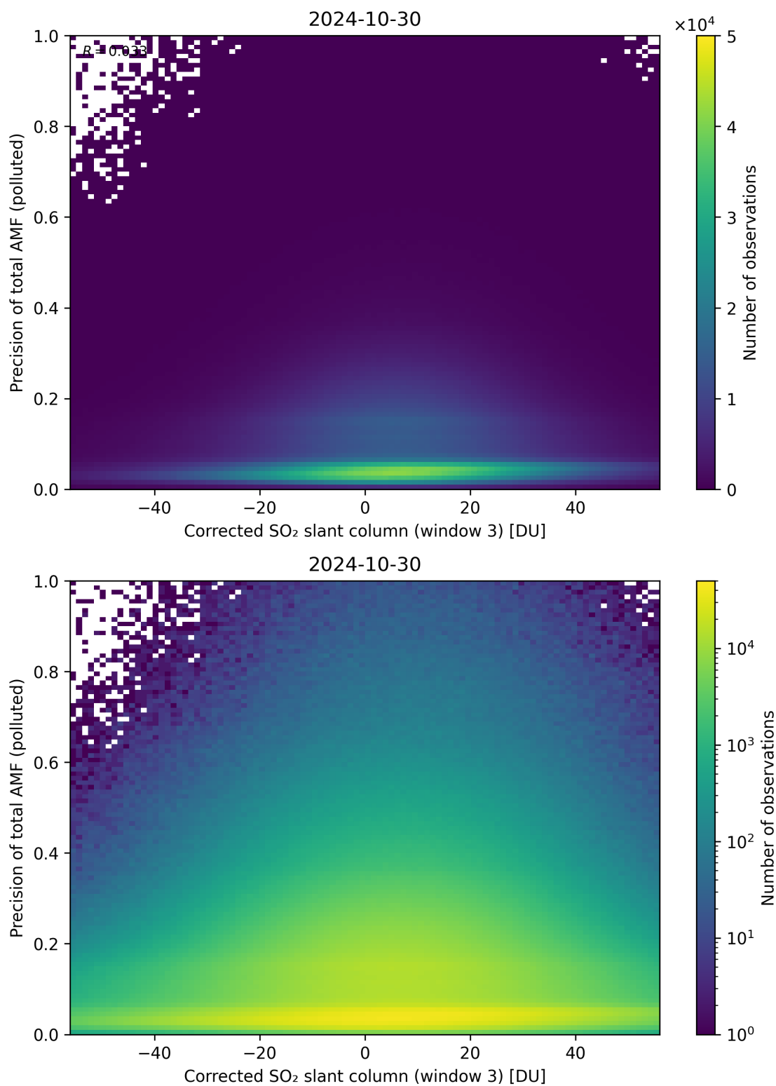
Figure 211: Scatter density plot of “Corrected SO 2 slant column (window 3)” against “Precision of total AMF (polluted)” for 2024-10-30 to 2024-10-31.
