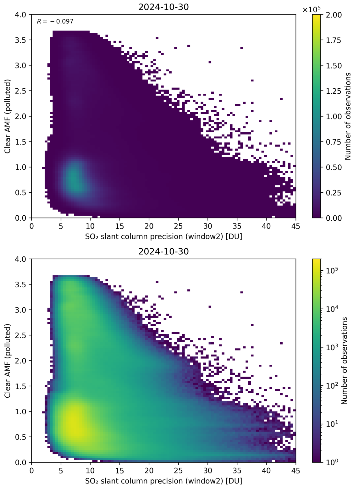
Figure 246: Scatter density plot of “SO 2 slant column precision (window2)” against “Clear AMF (polluted)” for 2024-10-30 to 2024-10-31.
