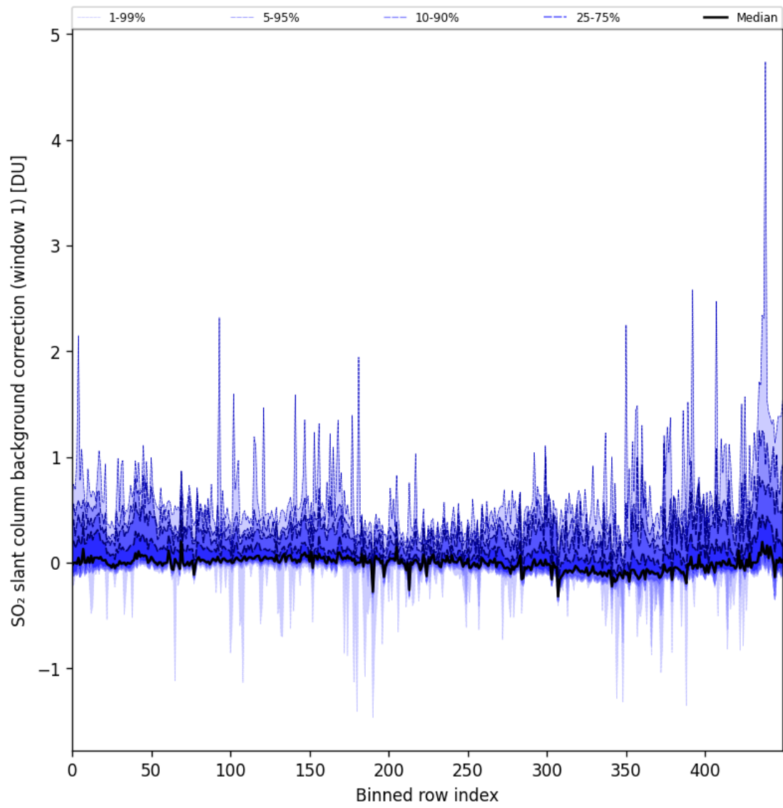
Figure 82: Along track statistics of “SO 2 slant column background correction (window 1)” for 2024-10-30 to 2024-10-31
