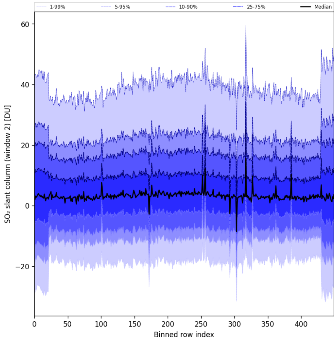
Figure 83: Along track statistics of “SO 2 slant column (window 2)” for 2024-10-30 to 2024-10-31
