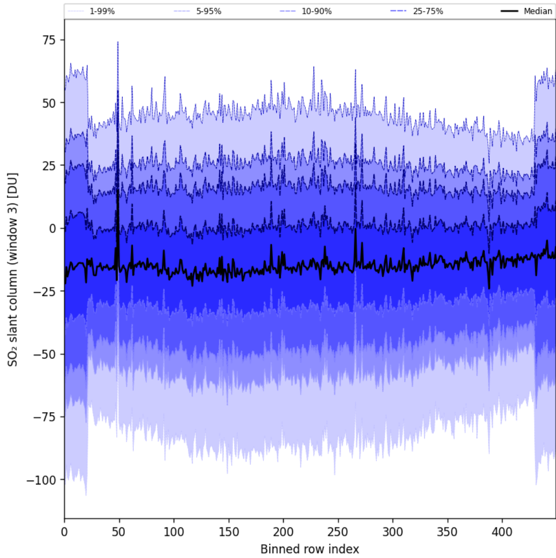
Figure 87: Along track statistics of “SO 2 slant column (window 3)” for 2024-10-30 to 2024-10-31
