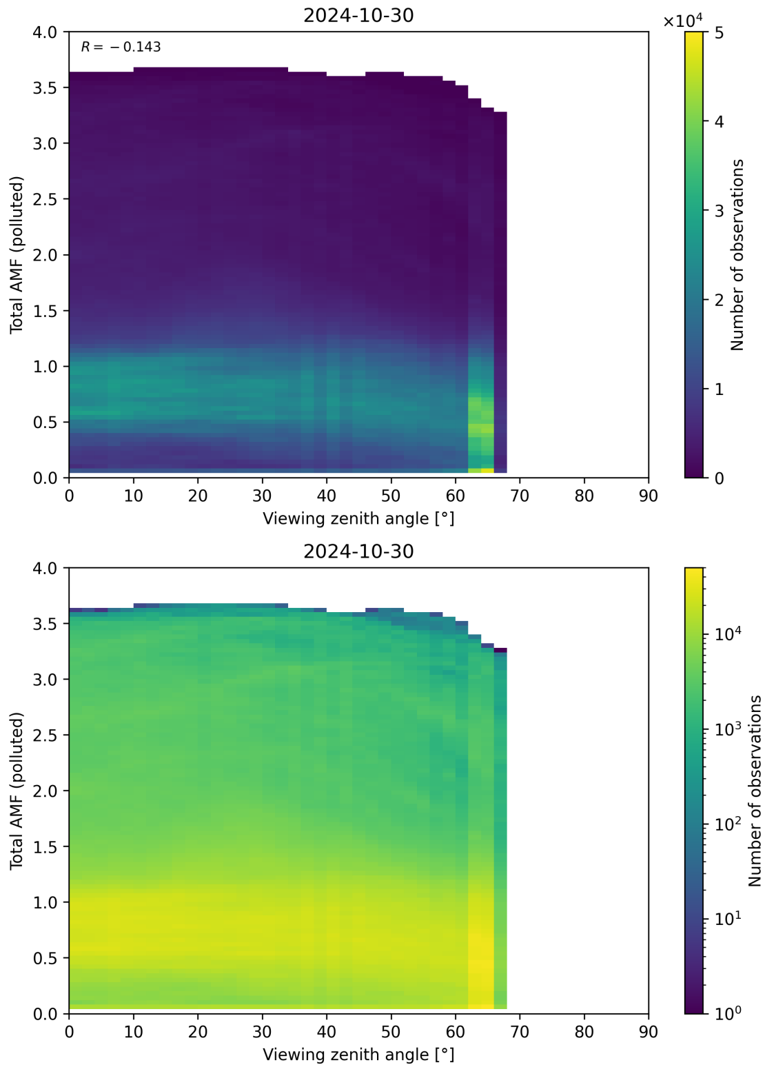
Figure 325: Scatter density plot of “Viewing zenith angle” against “Total AMF (polluted)” for 2024-10-30 to 2024-10-31.
