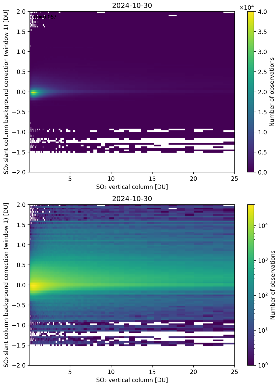
Figure 273: Scatter density plot of “SO 2 vertical column” against “SO 2 slant column background correction (window 1)” for 2024-10-30 to 2024-10-31.
