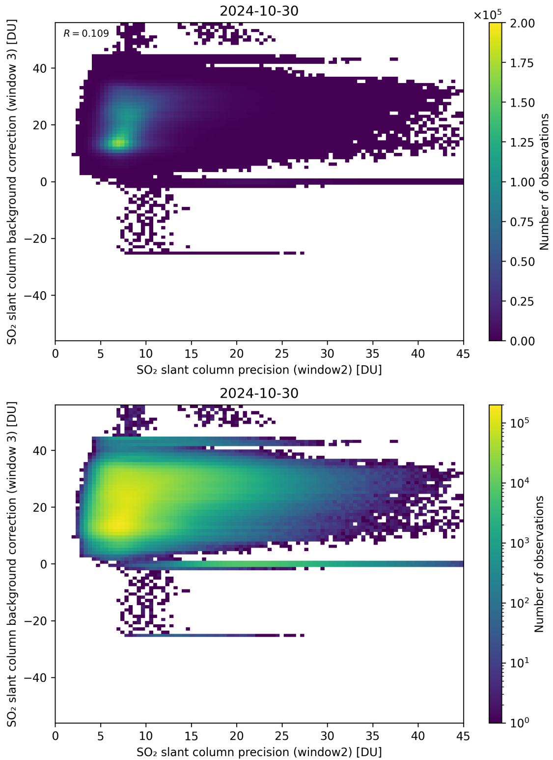
Figure 242: Scatter density plot of “SO 2 slant column precision (window2)” against “SO 2 slant column background correction (window 3)” for 2024-10-30 to 2024-10-31.
