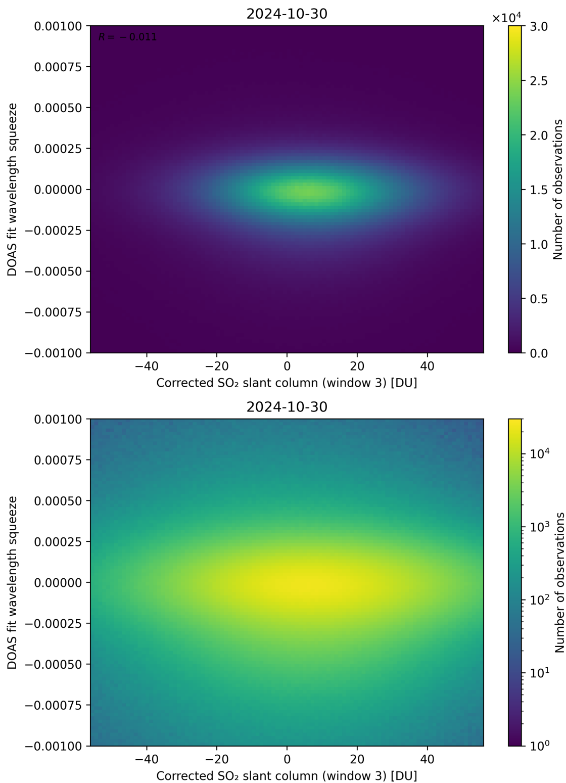
Figure 207: Scatter density plot of “Corrected SO 2 slant column (window 3)” against “DOAS fit wavelength squeeze” for 2024-10-30 to 2024-10-31.
