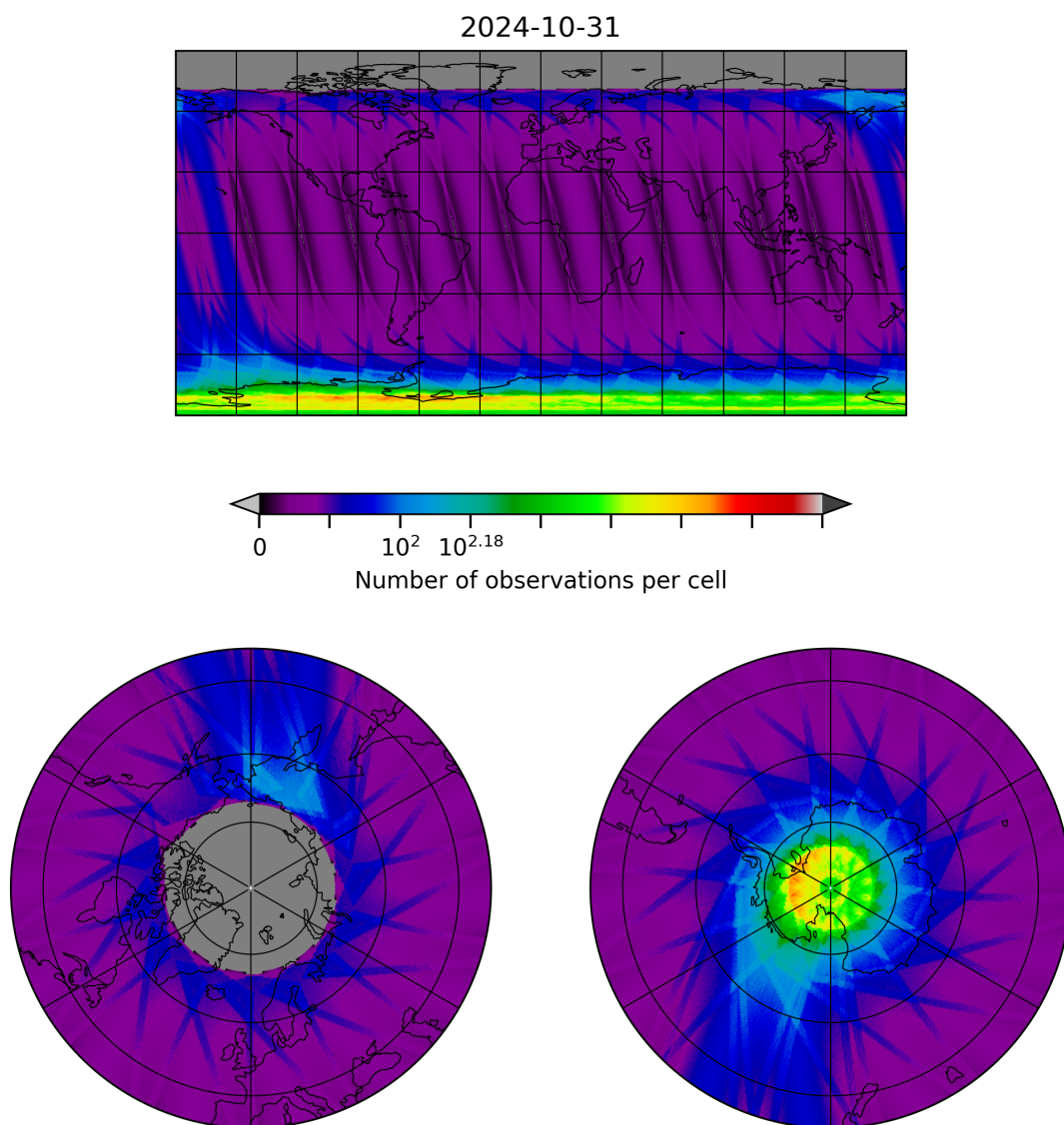
Figure 28: Map of the number of observations for 2024-10-30 to 2024-11-01
