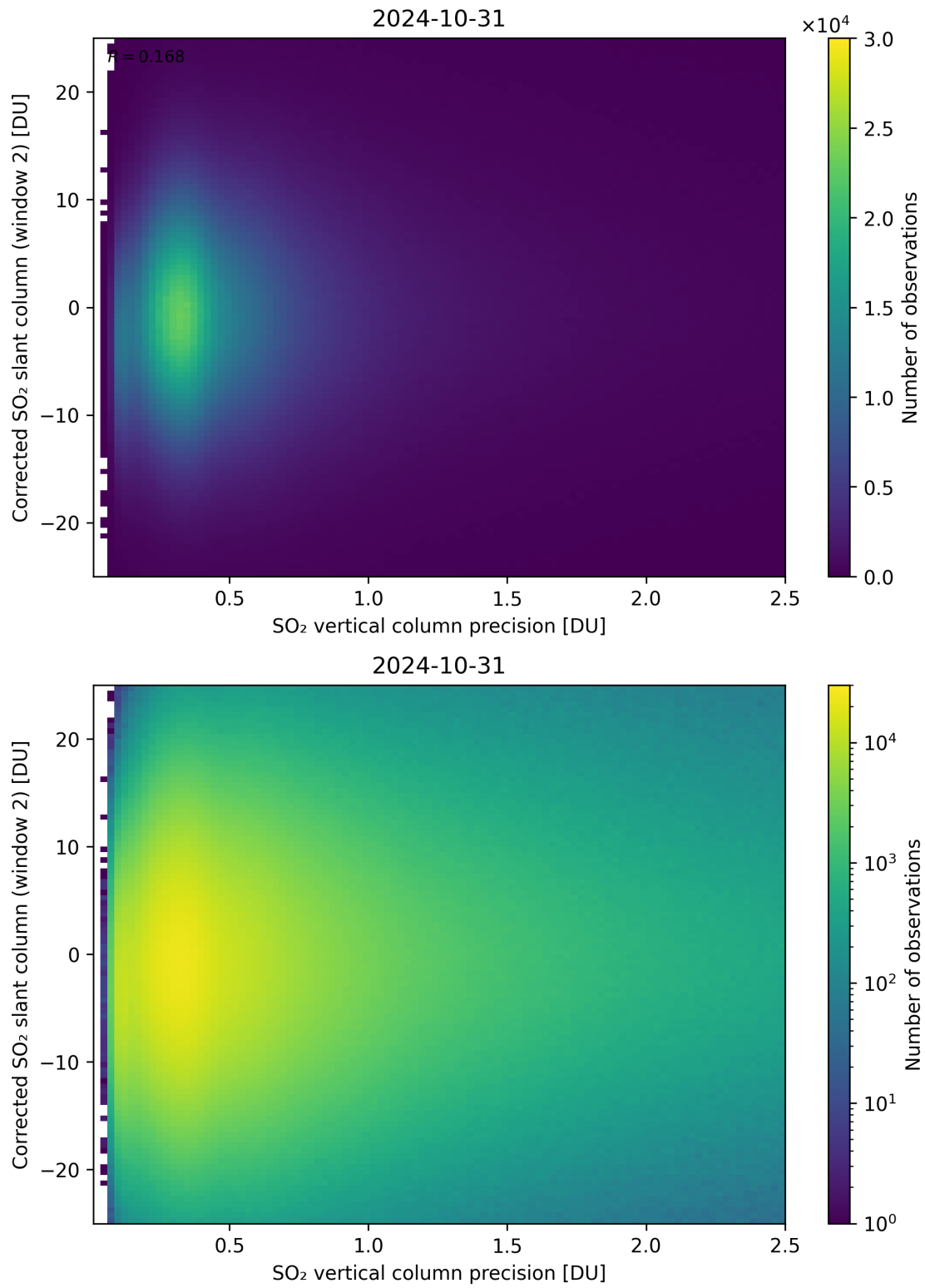
Figure 287: Scatter density plot of “SO 2 vertical column precision” against “Corrected SO 2 slant column (window 2)” for 2024-10-30 to 2024-11-01.
