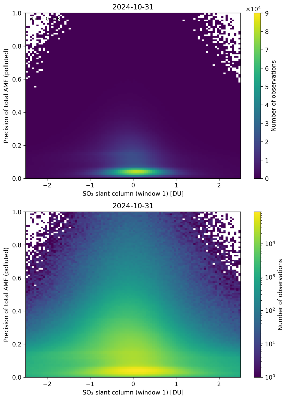
Figure 240: Scatter density plot of “SO 2 slant column (window 1)” against “Precision of total AMF (polluted)” for 2024-10-30 to 2024-11-01.
