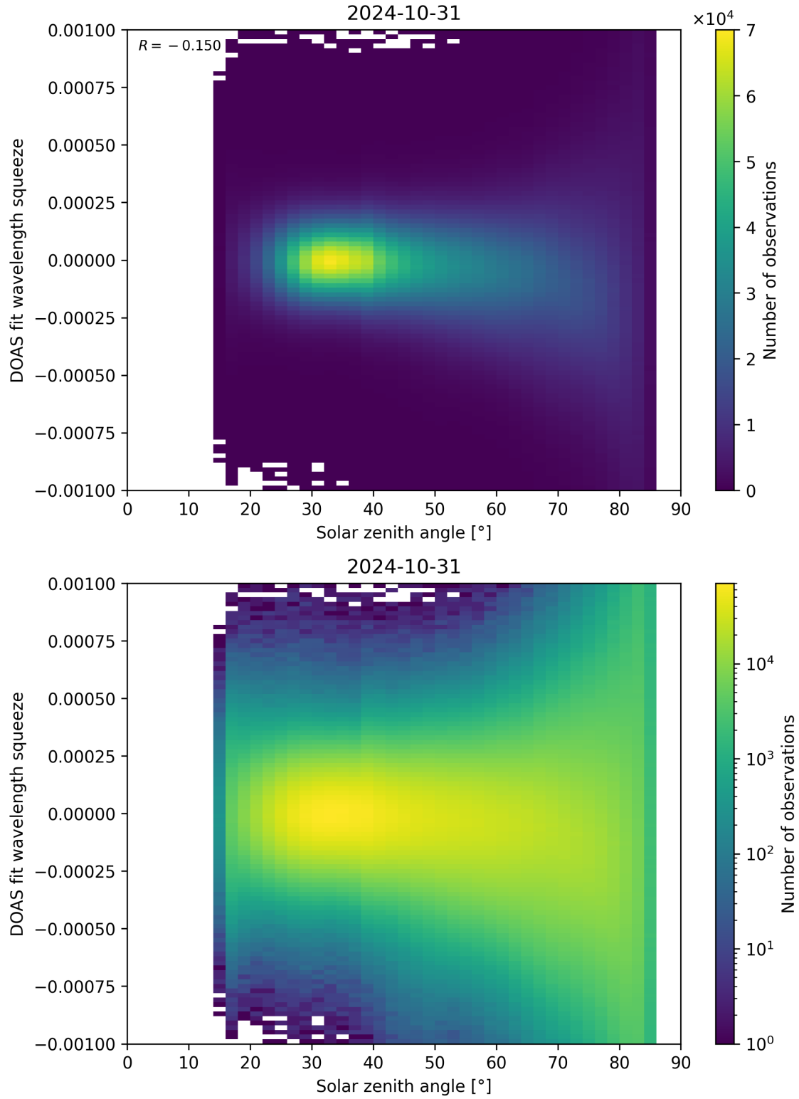
Figure 162: Scatter density plot of “Solar zenith angle” against “DOAS fit wavelength squeeze” for 2024-10-30 to 2024-11-01.
