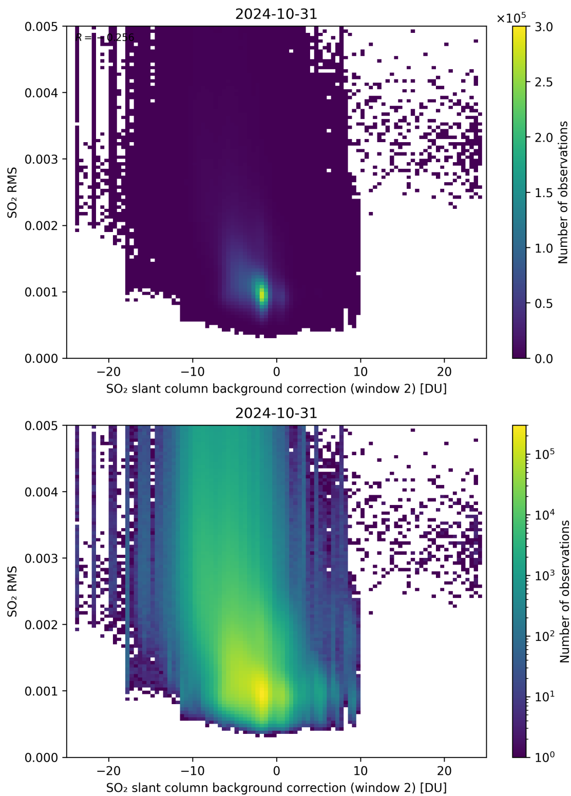
Figure 114: Scatter density plot of “SO 2 slant column background correction (window 2)” against “SO 2 RMS” for 2024-10-30 to 2024-11-01.
