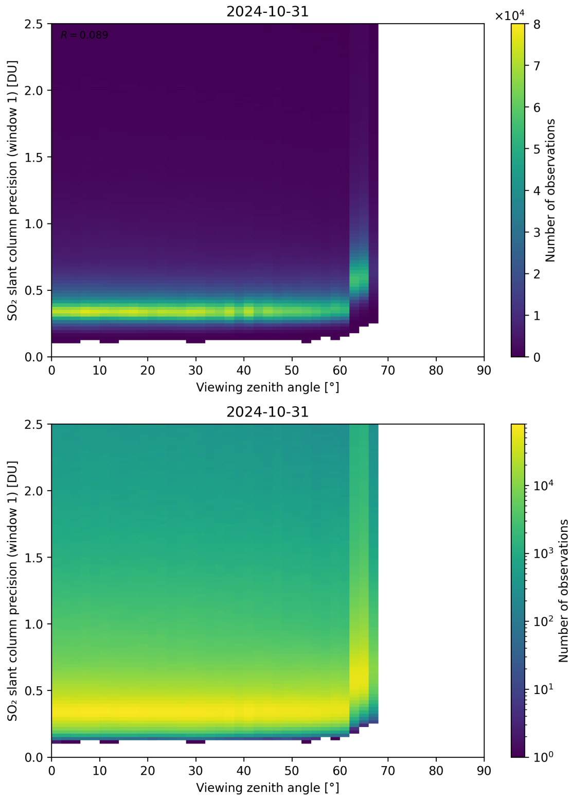
Figure 321: Scatter density plot of “Viewing zenith angle” against “SO 2 slant column precision (window 1)” for 2024-10-30 to 2024-11-01.
