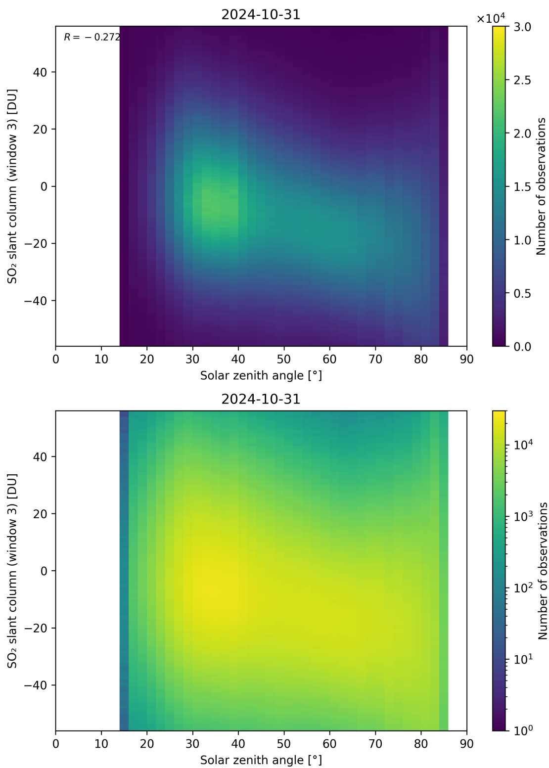
Figure 172: Scatter density plot of “Solar zenith angle” against “SO 2 slant column (window 3)” for 2024-10-30 to 2024-11-01.
