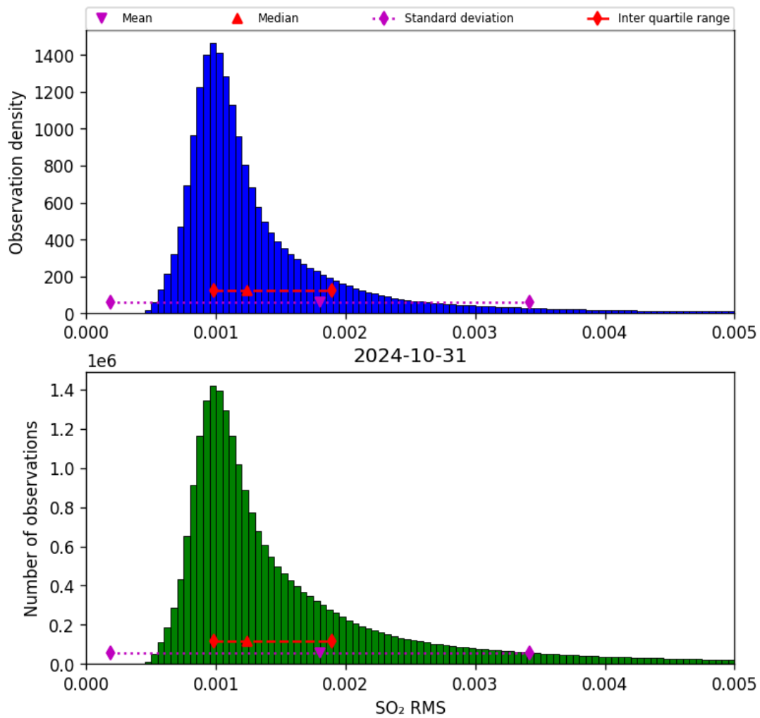
Figure 70: Histogram of “SO 2 RMS” for 2024-10-30 to 2024-11-01
