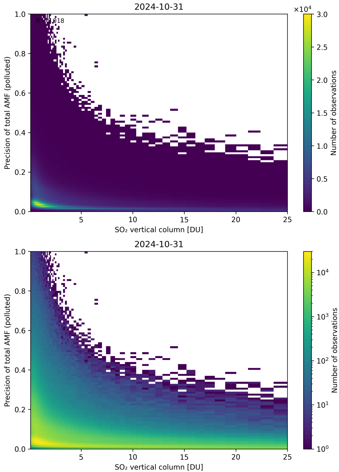
Figure 306: Scatter density plot of “SO 2 vertical column” against “Precision of total AMF (polluted)” for 2024-10-30 to 2024-11-01.
