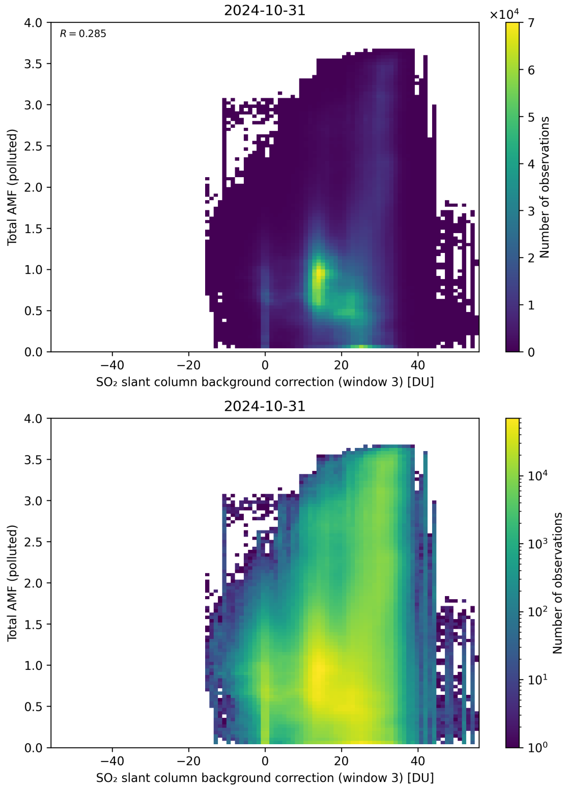
Figure 125: Scatter density plot of “SO 2 slant column background correction (window 3)” against “Total AMF (polluted)” for 2024-10-30 to 2024-11-01.
