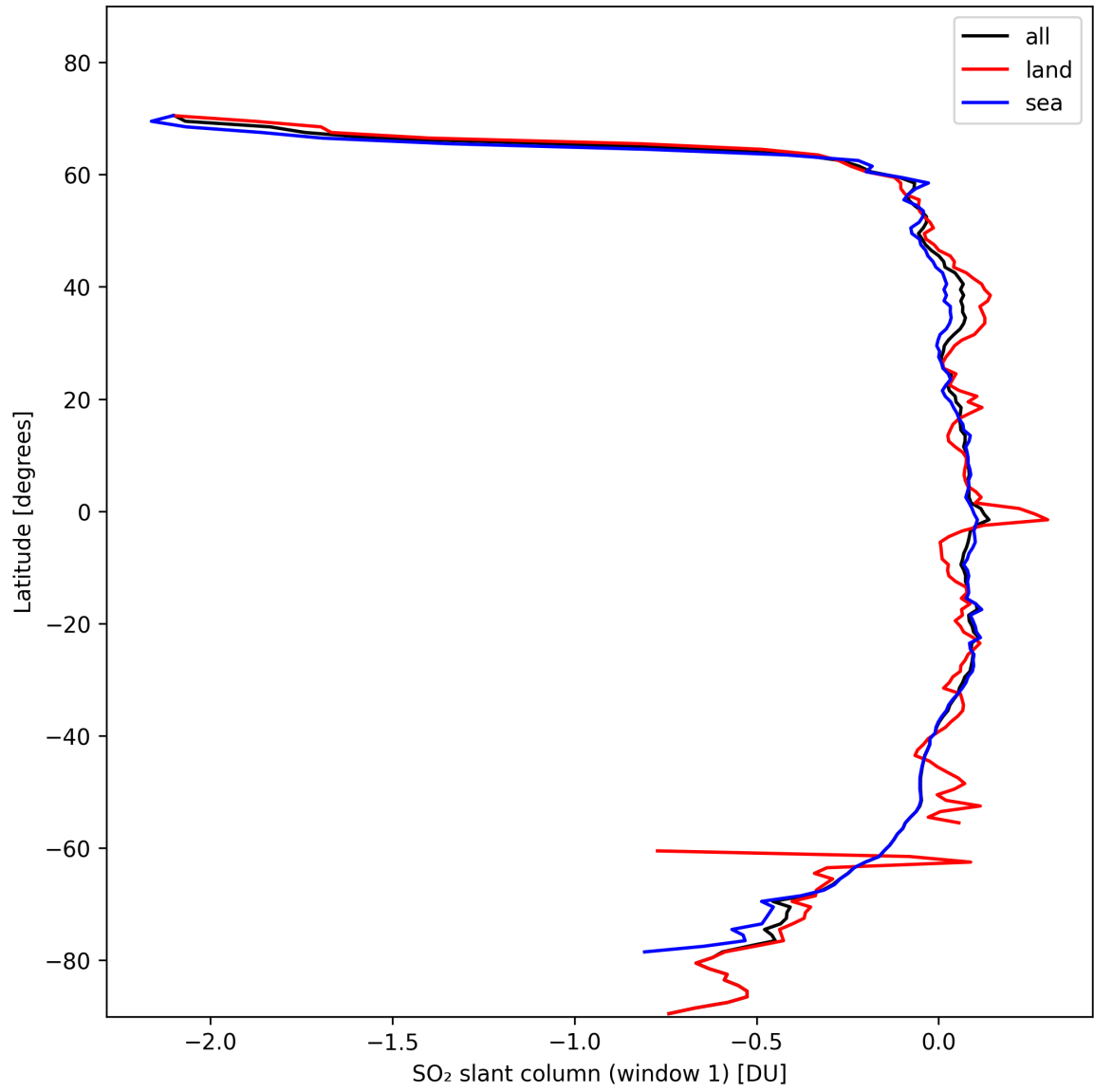
Figure 33: Zonal average of “SO 2 slant column (window 1)” for 2024-10-30 to 2024-11-01.
