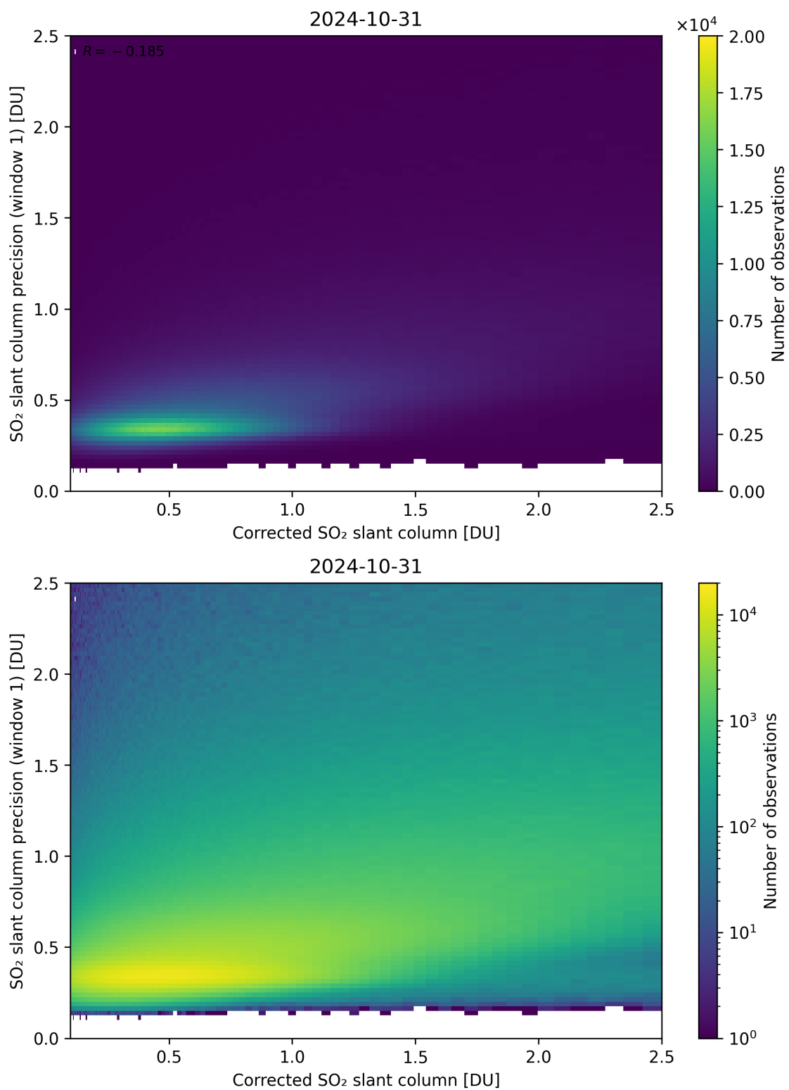
Figure 188: Scatter density plot of “Corrected SO 2 slant column” against “SO 2 slant column precision (window 1)” for 2024-10-30 to 2024-11-01.
