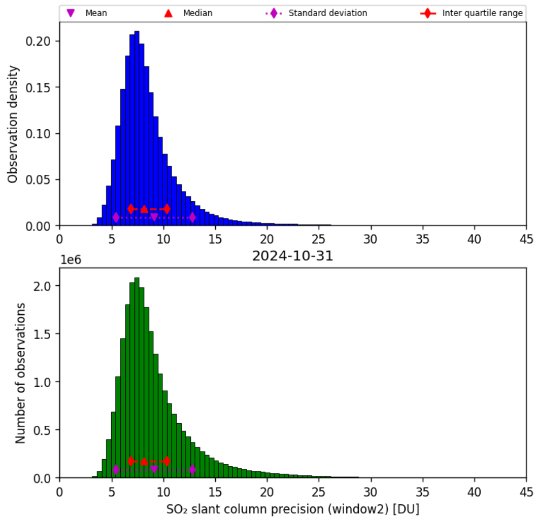
Figure 61: Histogram of “SO 2 slant column precision (window2)” for 2024-10-30 to 2024-11-01
