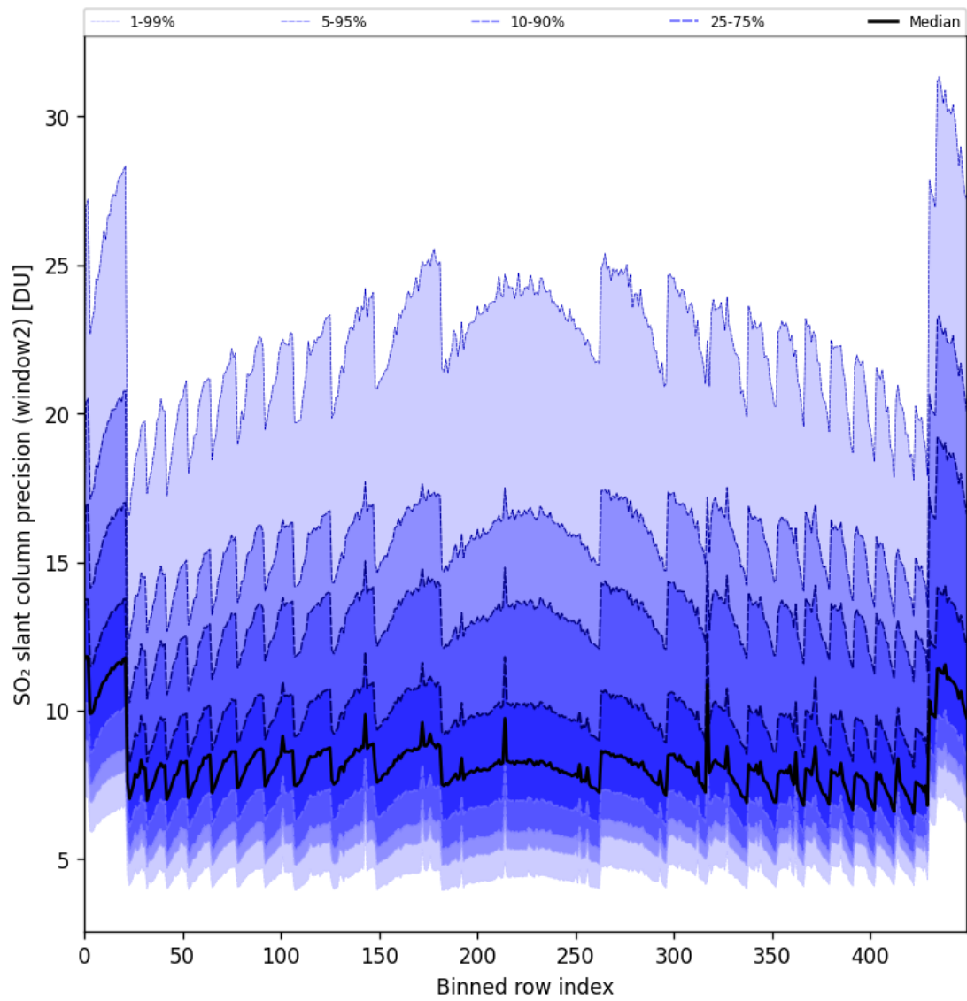
Figure 84: Along track statistics of “SO 2 slant column precision (window2)” for 2024-10-30 to 2024-11-01
