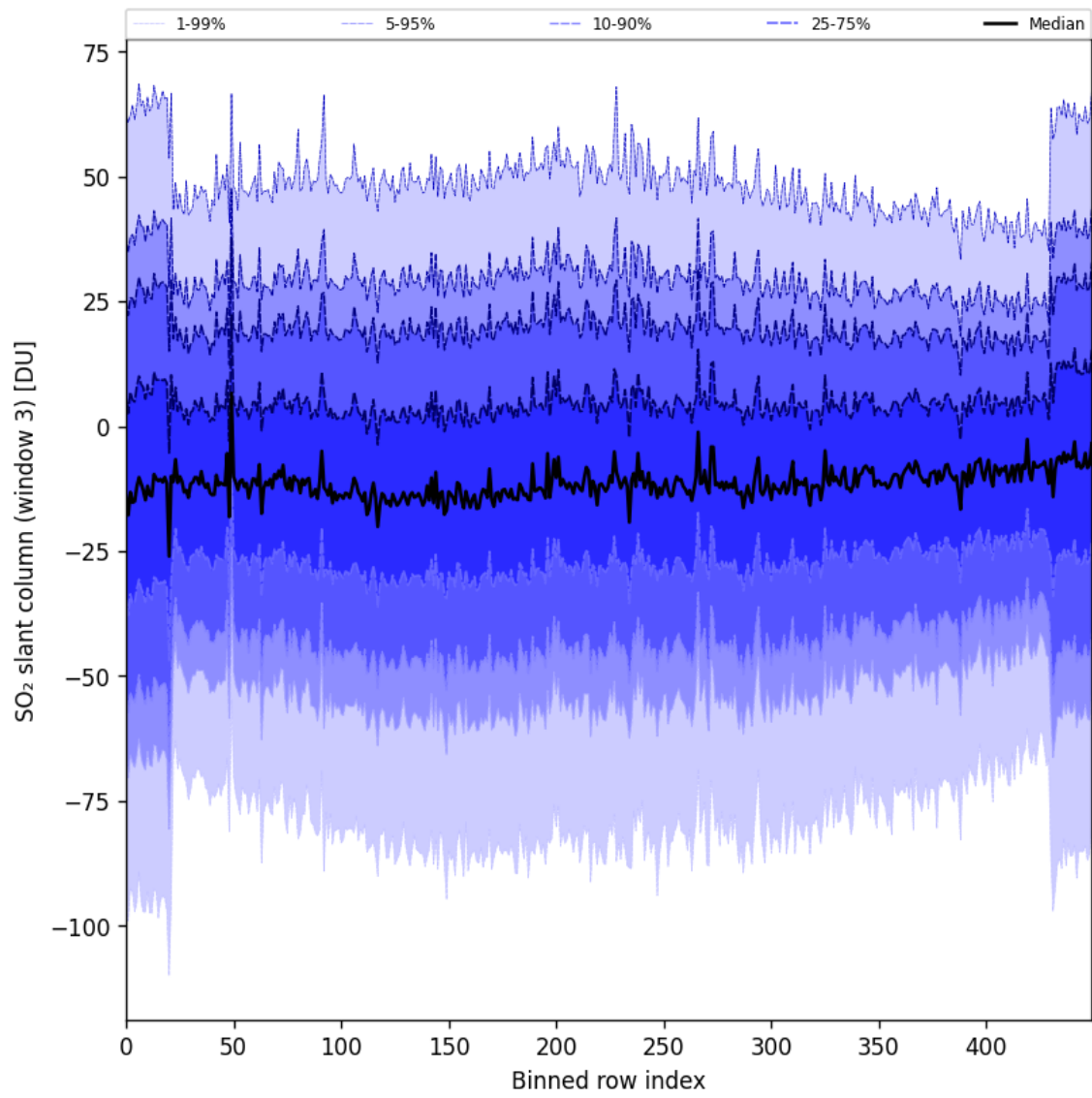
Figure 87: Along track statistics of “SO 2 slant column (window 3)” for 2024-10-30 to 2024-11-01
