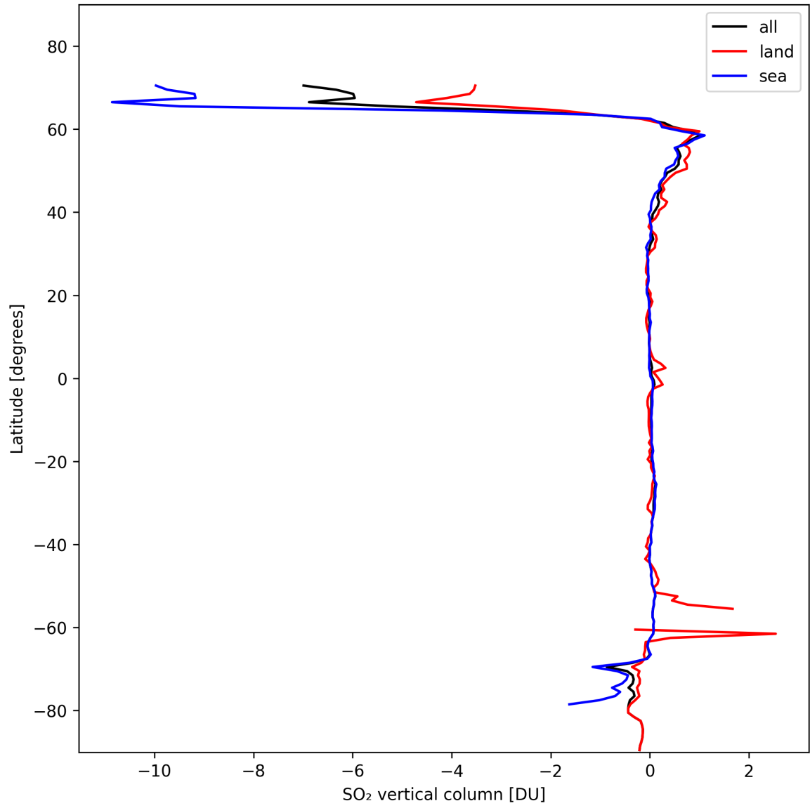
Figure 30: Zonal average of “SO 2 vertical column” for 2024-10-30 to 2024-11-01.
