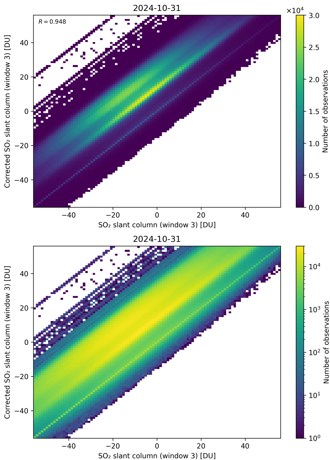
Figure 266: Scatter density plot of “SO 2 slant column (window 3)” against “Corrected SO 2 slant column (window 3)” for 2024-10-30 to 2024-11-01.
