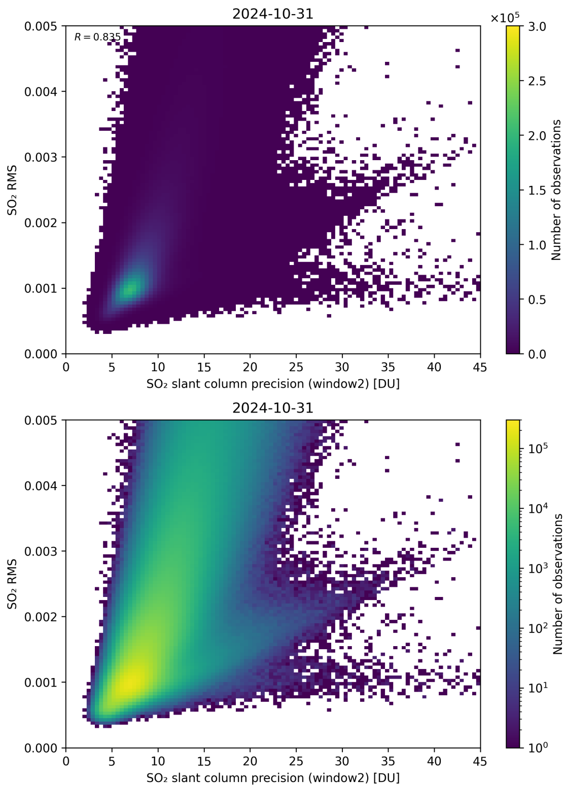
Figure 245: Scatter density plot of “SO 2 slant column precision (window2)” against “SO 2 RMS” for 2024-10-30 to 2024-11-01.
