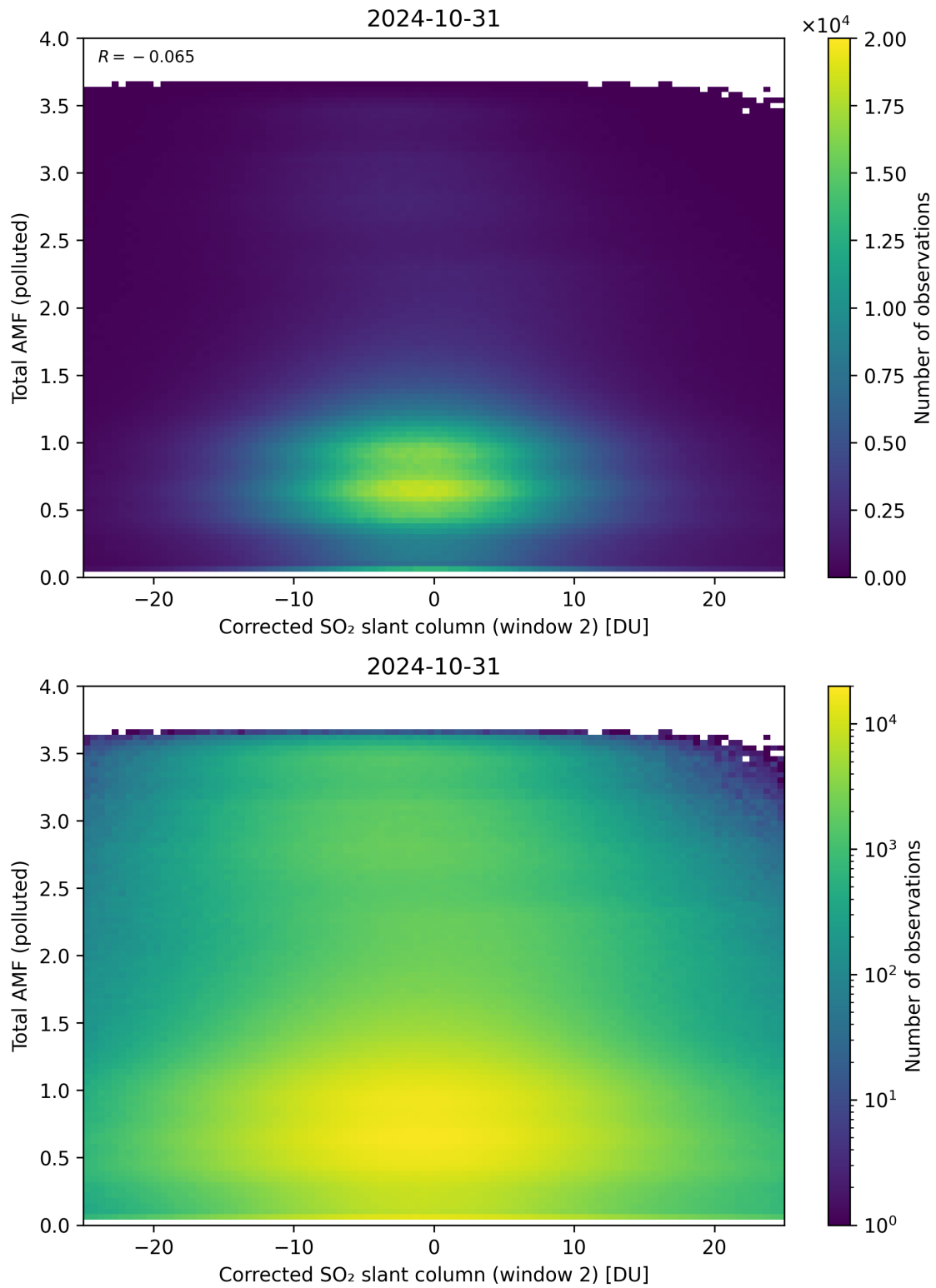
Figure 203: Scatter density plot of “Corrected SO 2 slant column (window 2)” against “Total AMF (polluted)” for 2024-10-30 to 2024-11-01.
