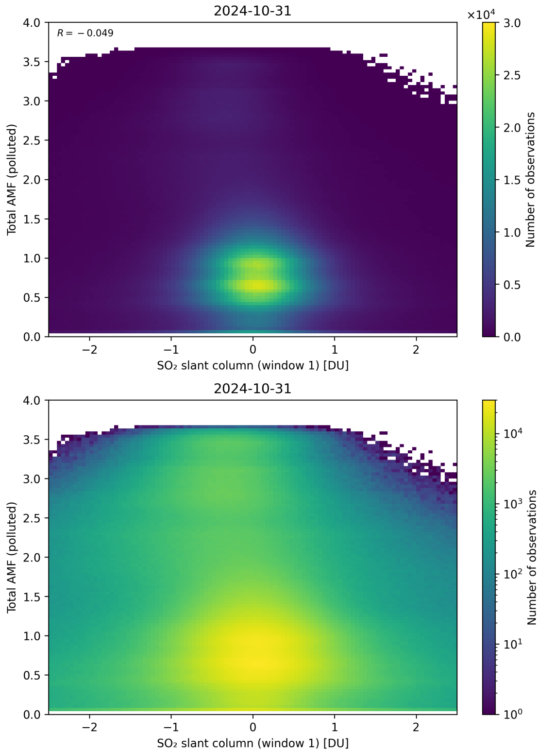
Figure 239: Scatter density plot of “SO 2 slant column (window 1)” against “Total AMF (polluted)” for 2024-10-30 to 2024-11-01.
