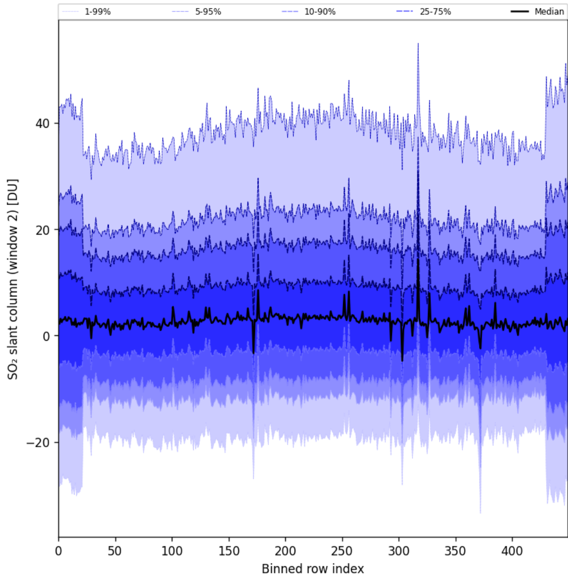
Figure 83: Along track statistics of “SO 2 slant column (window 2)” for 2024-10-30 to 2024-11-01
