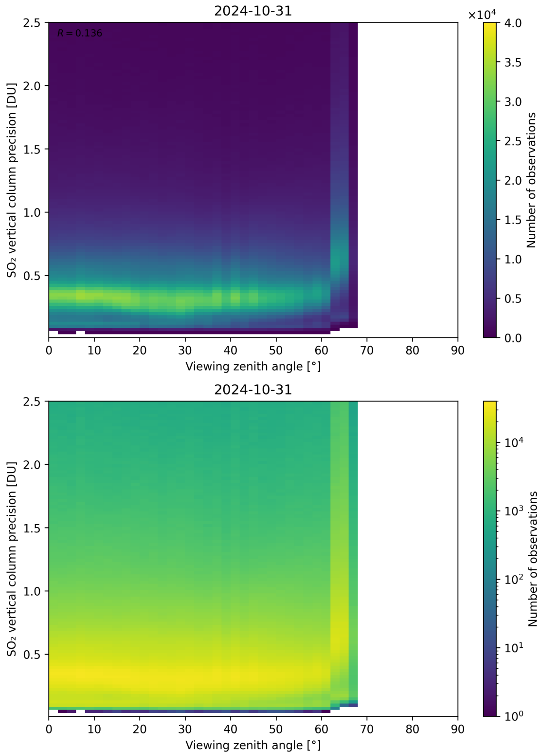
Figure 328: Scatter density plot of “Viewing zenith angle” against “SO 2 vertical column precision” for 2024-10-30 to 2024-11-01.
