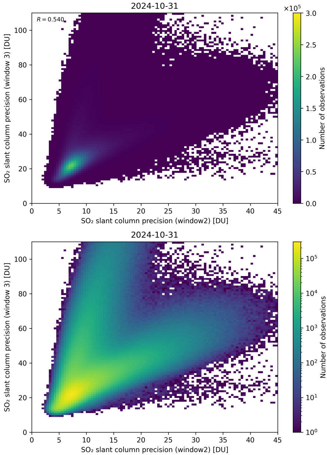
Figure 250: Scatter density plot of “SO 2 slant column precision (window2)” against “SO 2 slant column precision (window 3)” for 2024-10-30 to 2024-11-01.
