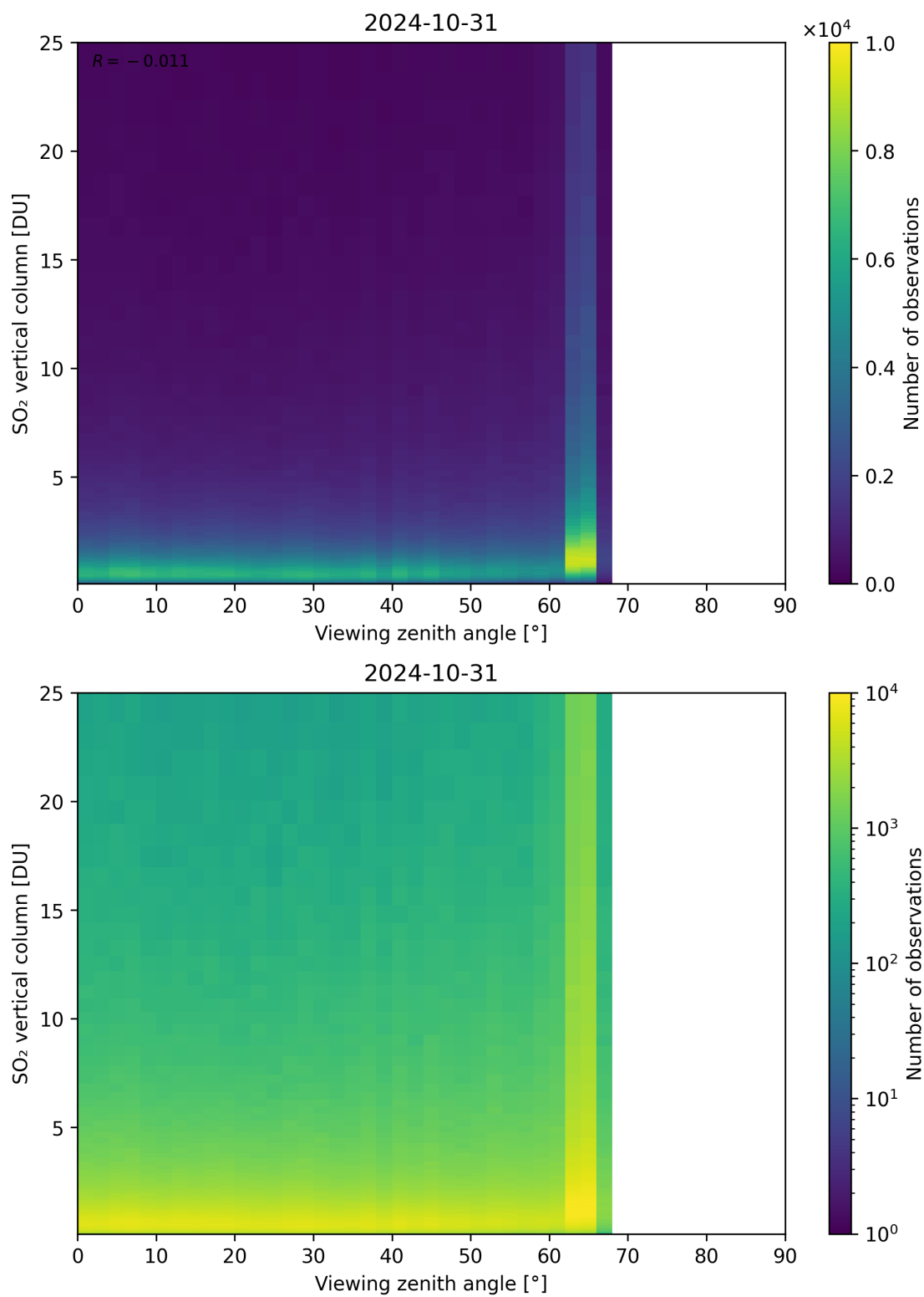
Figure 327: Scatter density plot of “Viewing zenith angle” against “SO 2 vertical column” for 2024-10-30 to 2024-11-01.
