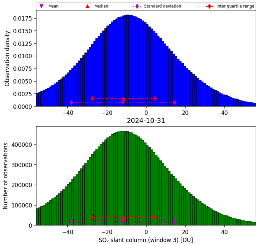
Figure 64: Histogram of “SO 2 slant column (window 3)” for 2024-10-30 to 2024-11-01
