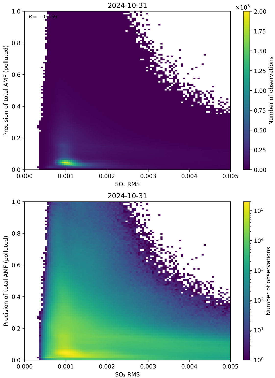
Figure 138: Scatter density plot of “SO 2 RMS” against “Precision of total AMF (polluted)” for 2024-10-30 to 2024-11-01.
