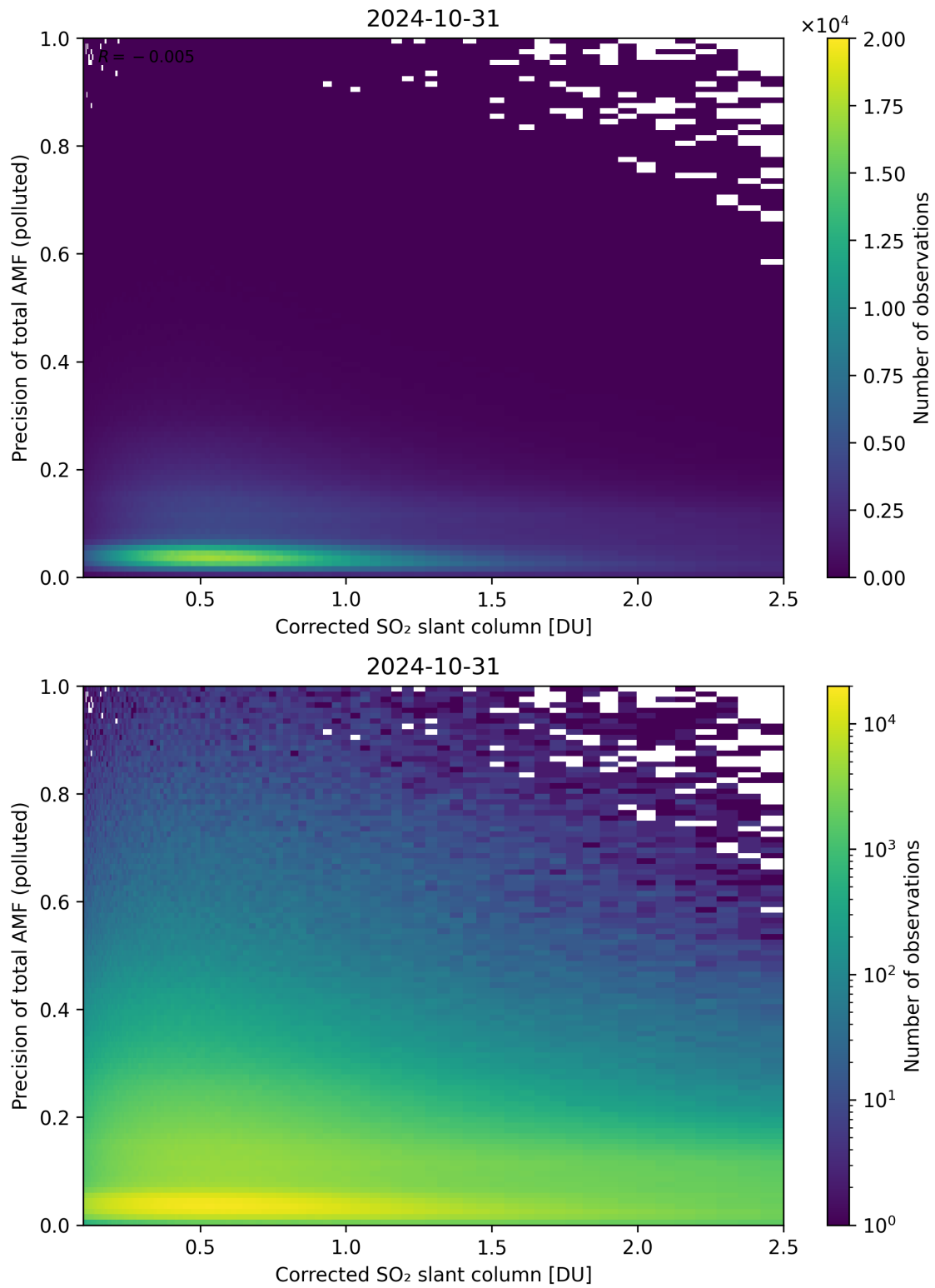
Figure 193: Scatter density plot of “Corrected SO 2 slant column” against “Precision of total AMF (polluted)” for 2024-10-30 to 2024-11-01.
