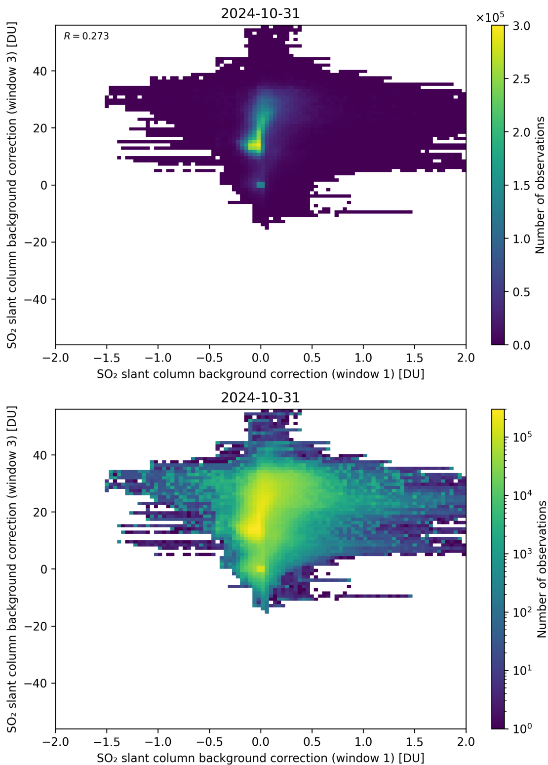
Figure 99: Scatter density plot of “SO 2 slant column background correction (window 1)” against “SO 2 slant column background correction (window 3)” for 2024-10-30 to 2024-11-01.
