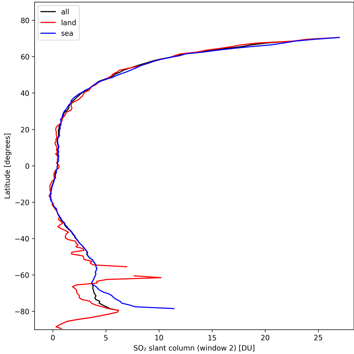
Figure 37: Zonal average of “SO 2 slant column (window 2)” for 2024-10-30 to 2024-11-01.
