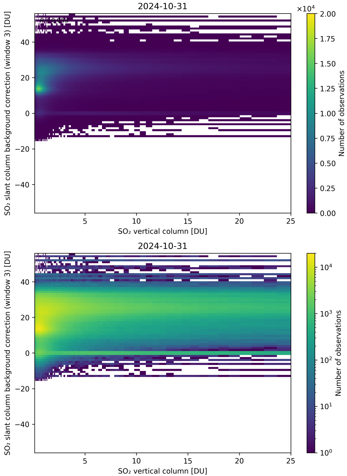
Figure 275: Scatter density plot of “SO 2 vertical column” against “SO 2 slant column background correction (window 3)” for 2024-10-30 to 2024-11-01.
