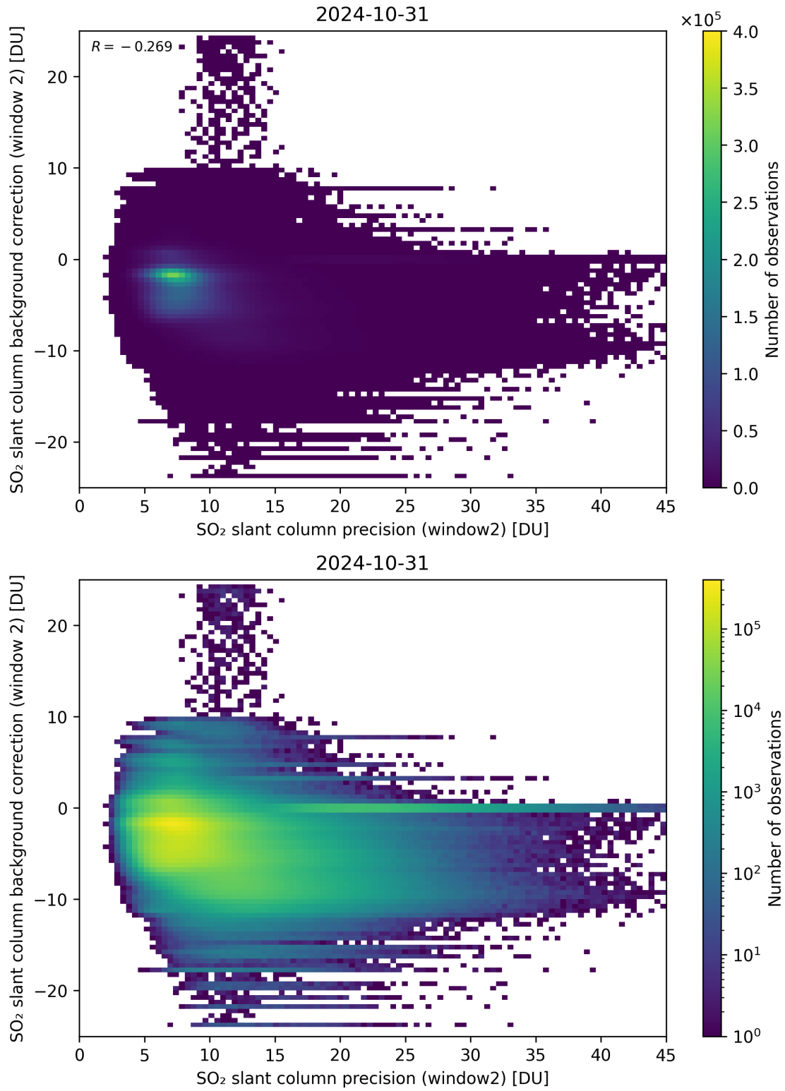
Figure 241: Scatter density plot of “SO 2 slant column precision (window2)” against “SO 2 slant column background correction (window 2)” for 2024-10-30 to 2024-11-01.
