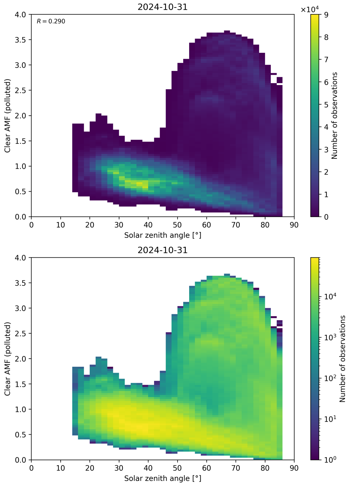
Figure 165: Scatter density plot of “Solar zenith angle” against “Clear AMF (polluted)” for 2024-10-30 to 2024-11-01.
