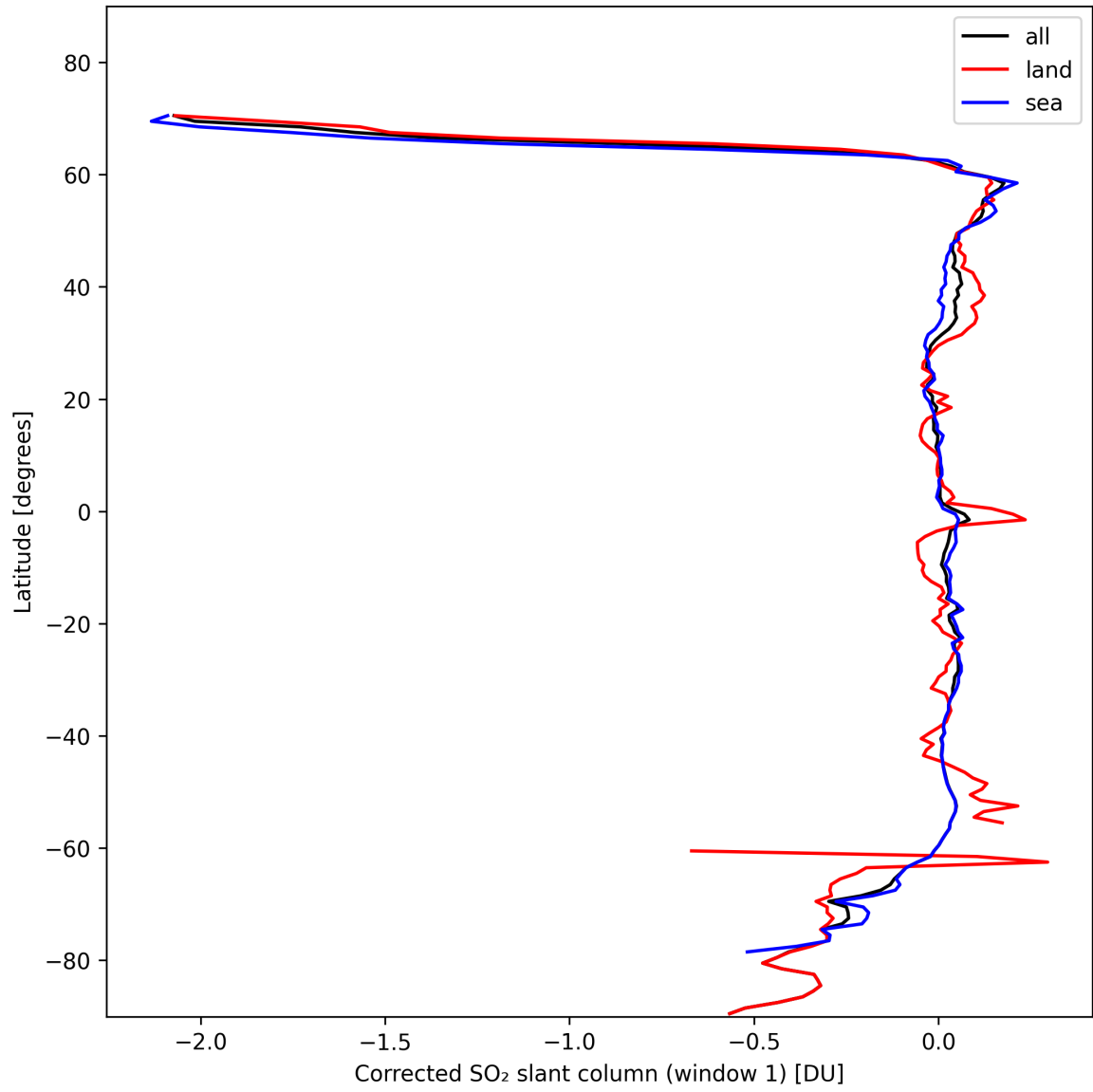
Figure 35: Zonal average of “Corrected SO 2 slant column (window 1)” for 2024-10-30 to 2024-11-01.
