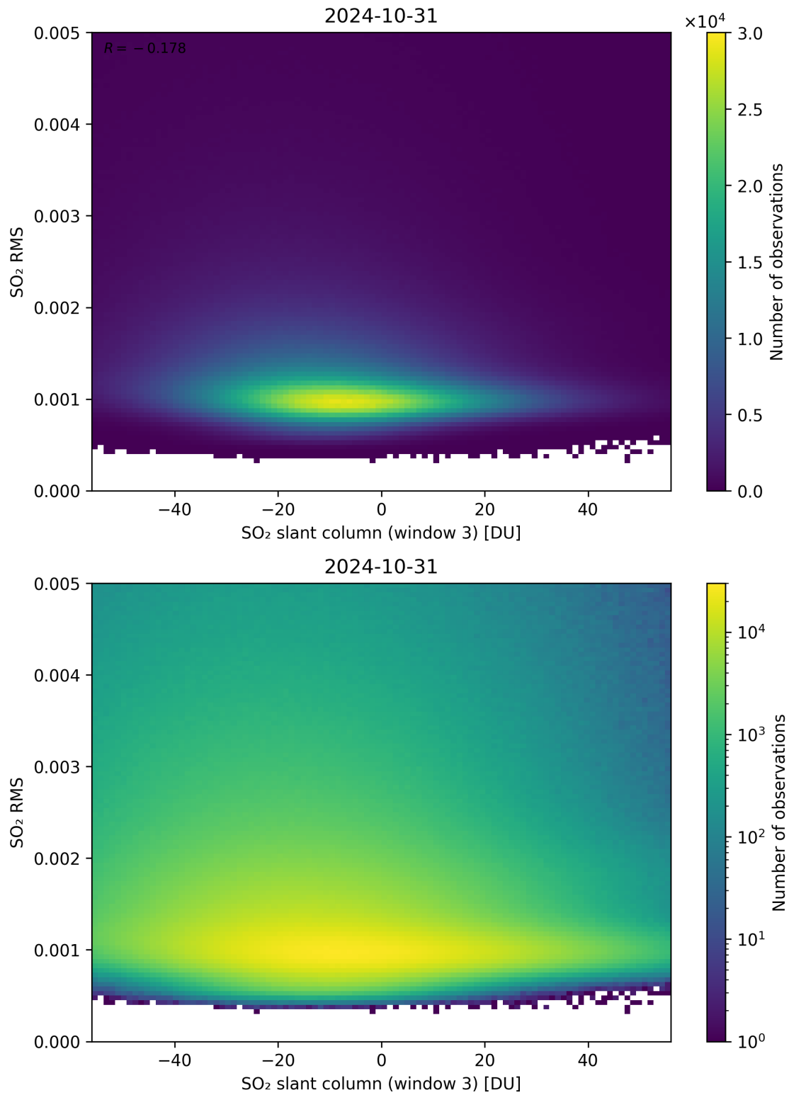
Figure 256: Scatter density plot of “SO 2 slant column (window 3)” against “SO 2 RMS” for 2024-10-30 to 2024-11-01.
