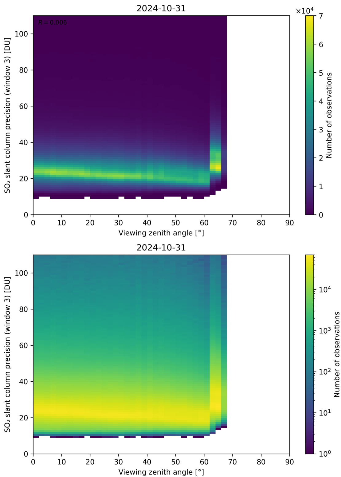
Figure 324: Scatter density plot of “Viewing zenith angle” against “SO 2 slant column precision (window 3)” for 2024-10-30 to 2024-11-01.
