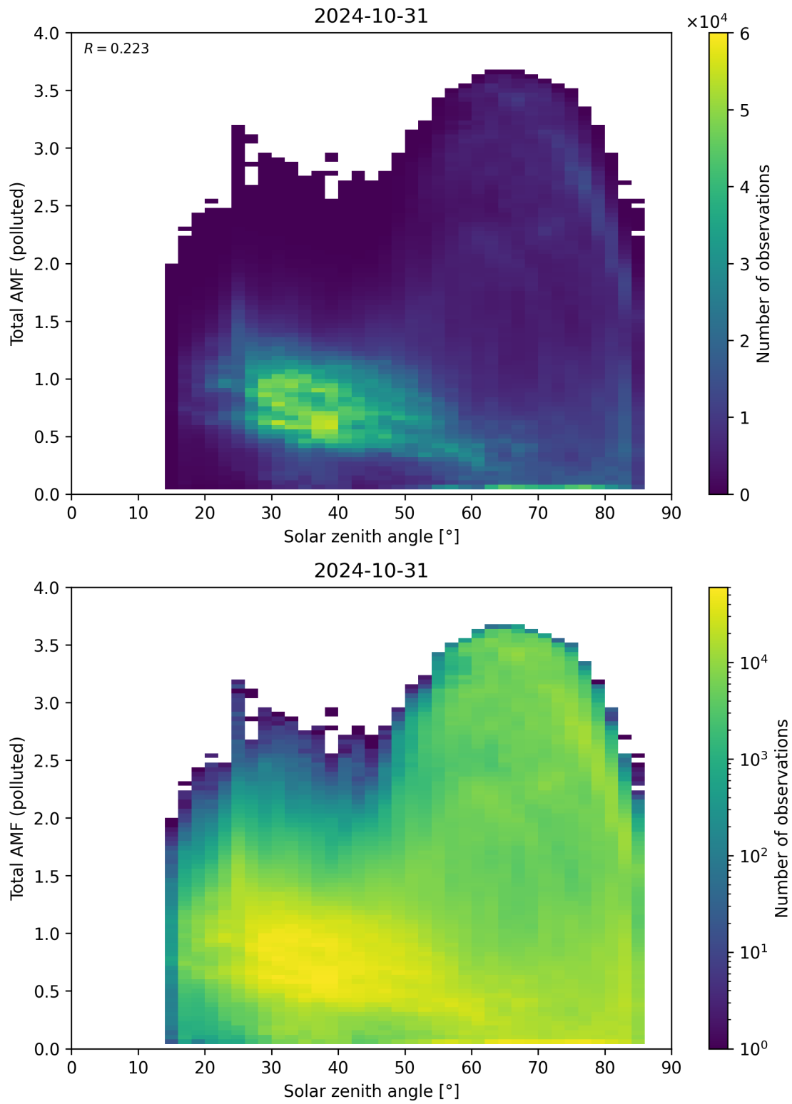
Figure 174: Scatter density plot of “Solar zenith angle” against “Total AMF (polluted)” for 2024-10-30 to 2024-11-01.
