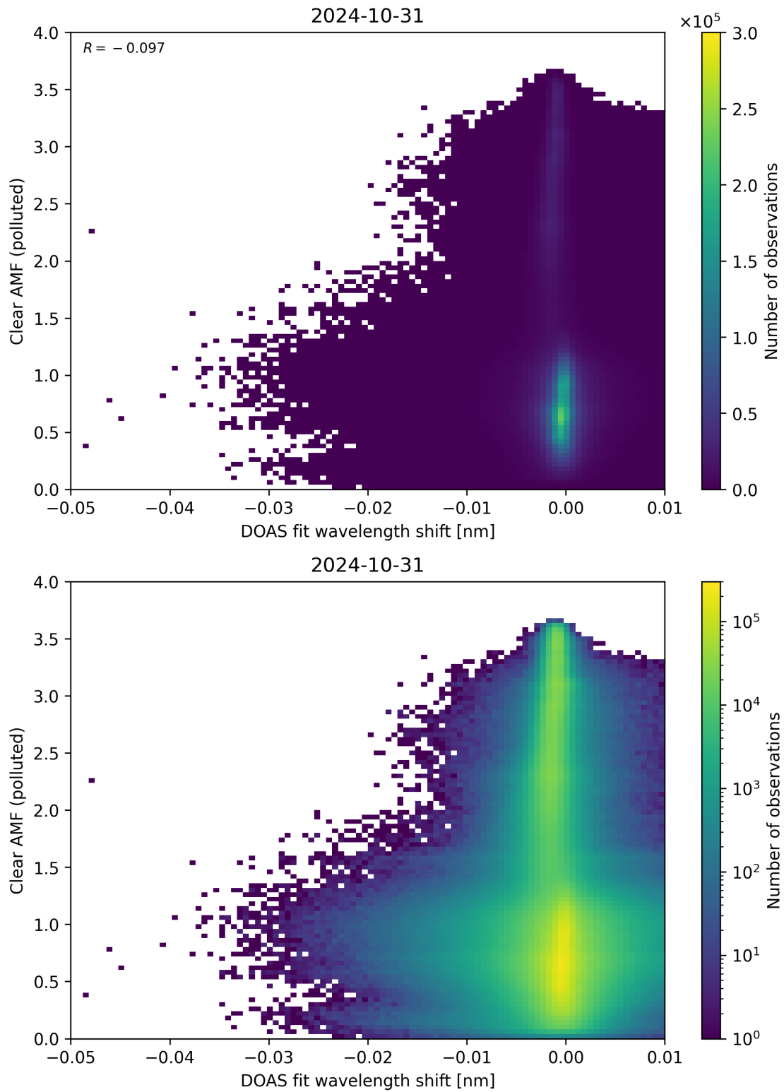
Figure 129: Scatter density plot of “DOAS fit wavelength shift” against “Clear AMF (polluted)” for 2024-10-30 to 2024-11-01.
