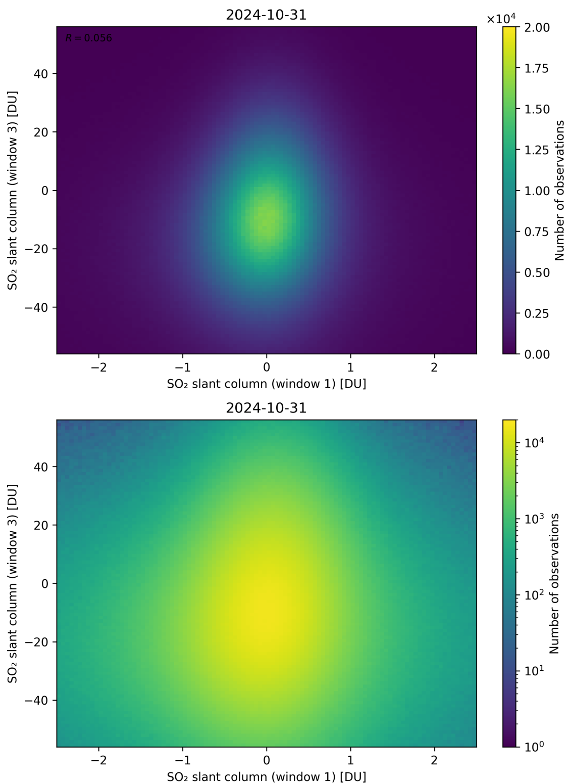
Figure 237: Scatter density plot of “SO 2 slant column (window 1)” against “SO 2 slant column (window 3)” for 2024-10-30 to 2024-11-01.
