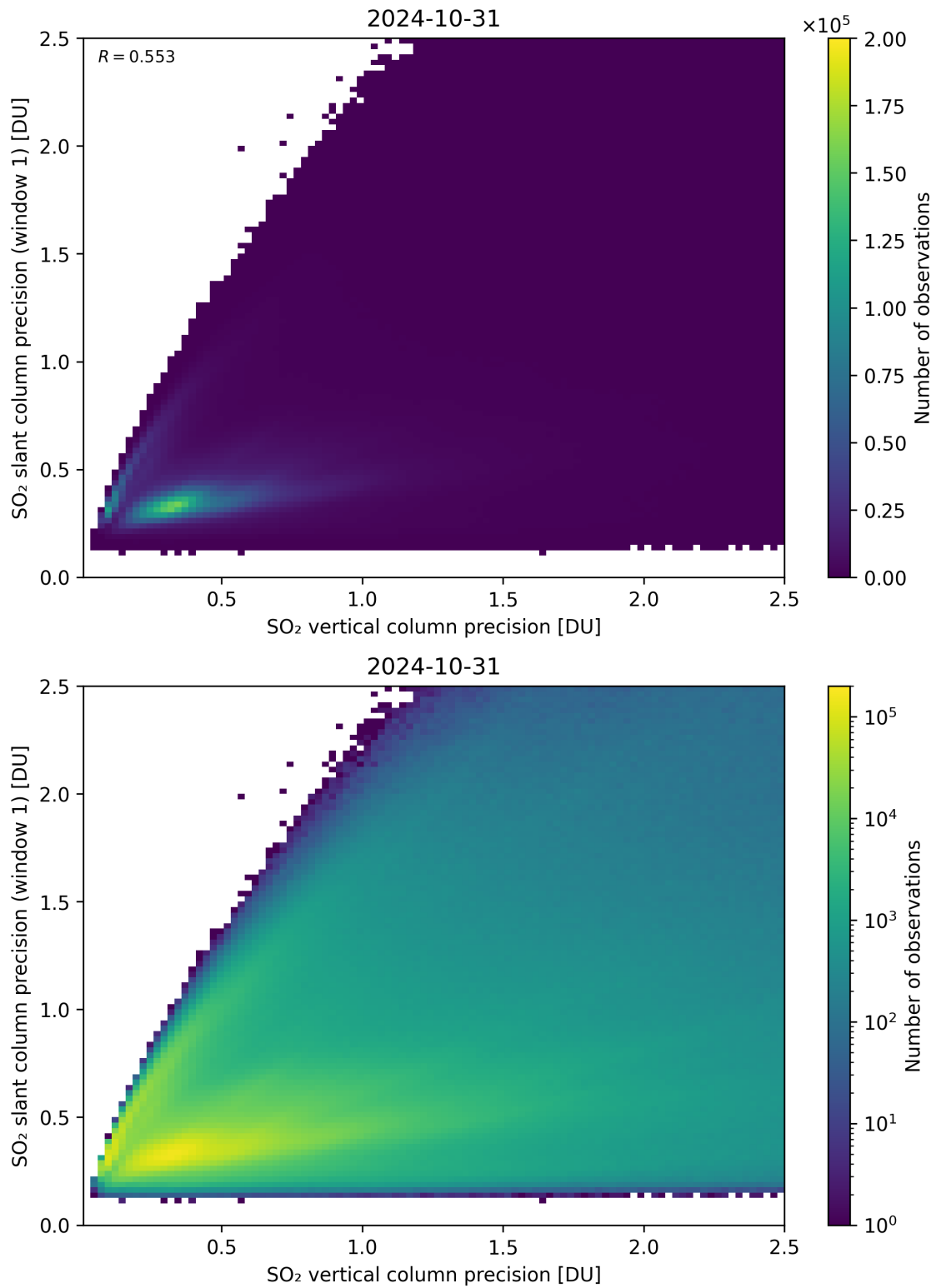
Figure 290: Scatter density plot of “SO 2 vertical column precision” against “SO 2 slant column precision (window 1)” for 2024-10-30 to 2024-11-01.
