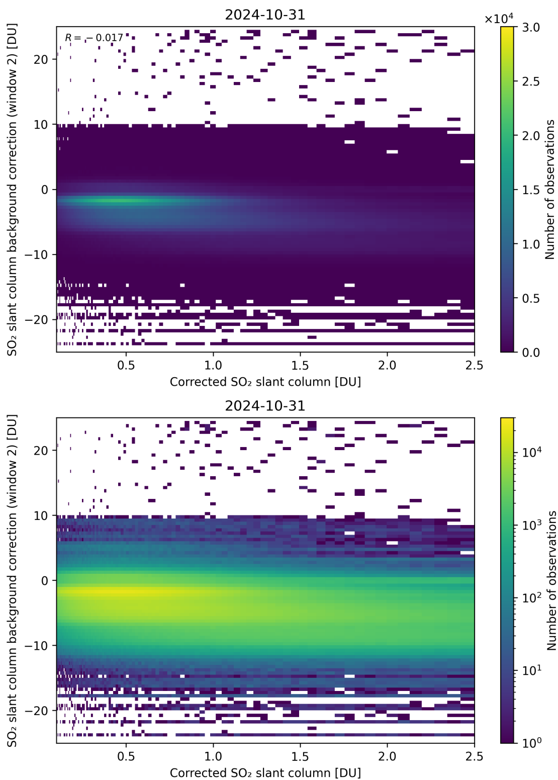
Figure 179: Scatter density plot of “Corrected SO 2 slant column” against “SO 2 slant column background correction (window 2)” for 2024-10-30 to 2024-11-01.
