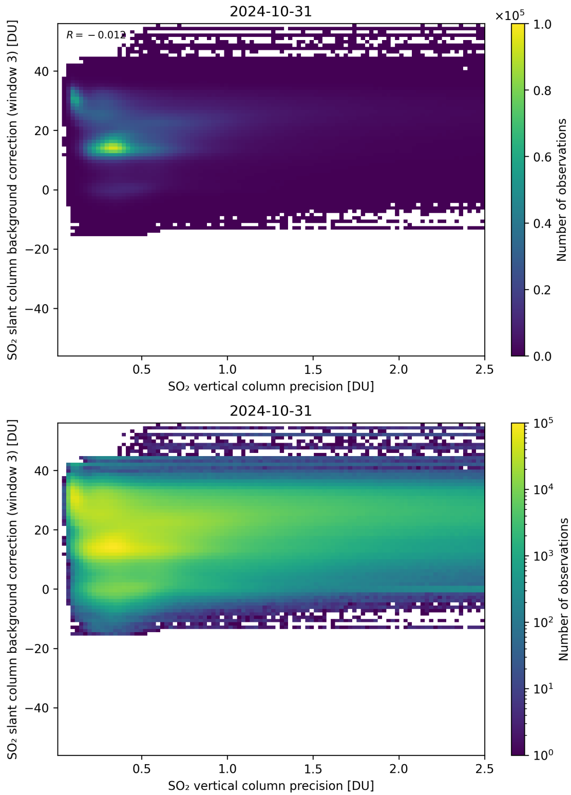
Figure 281: Scatter density plot of “SO 2 vertical column precision” against “SO 2 slant column background correction (window 3)” for 2024-10-30 to 2024-11-01.
