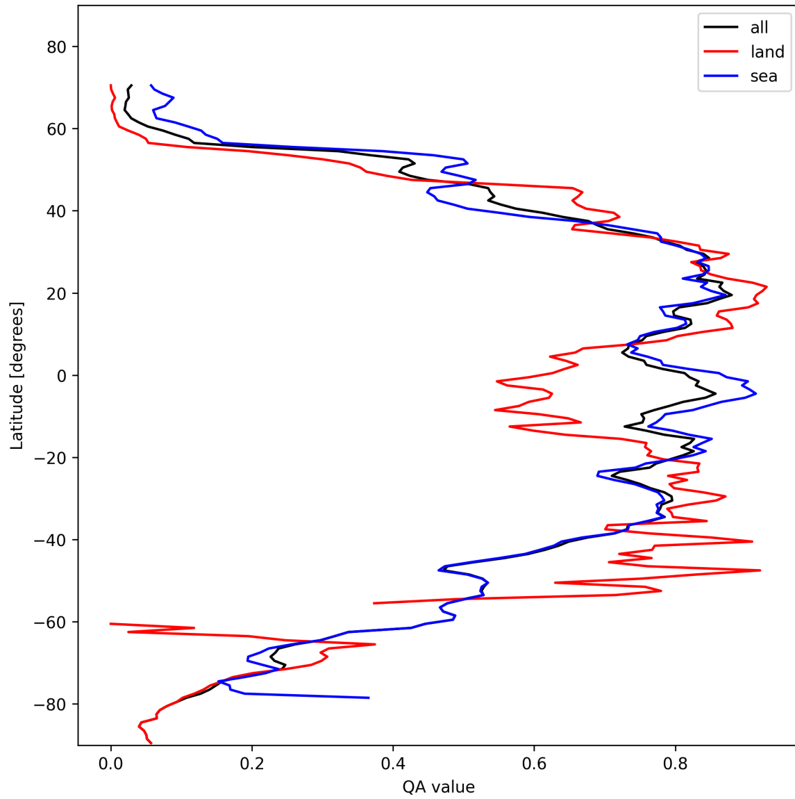
Figure 29: Zonal average of “QA value” for 2024-10-30 to 2024-11-01.
