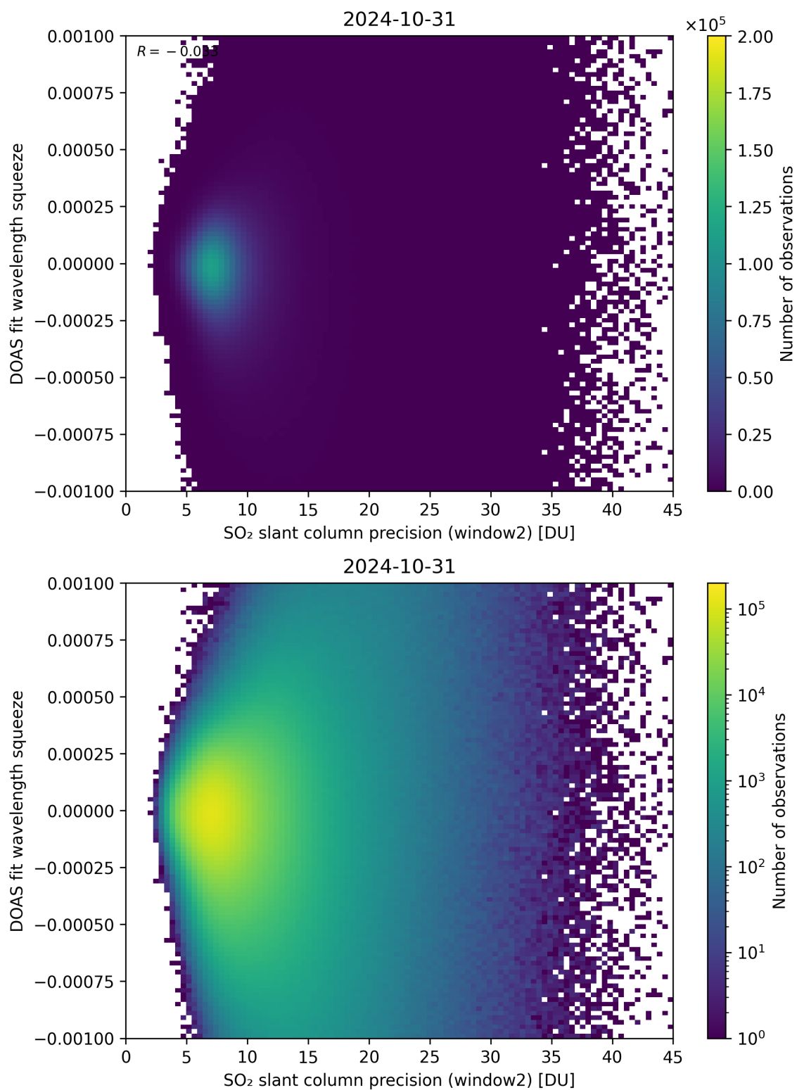
Figure 244: Scatter density plot of “SO 2 slant column precision (window2)” against “DOAS fit wavelength squeeze” for 2024-10-30 to 2024-11-01.
