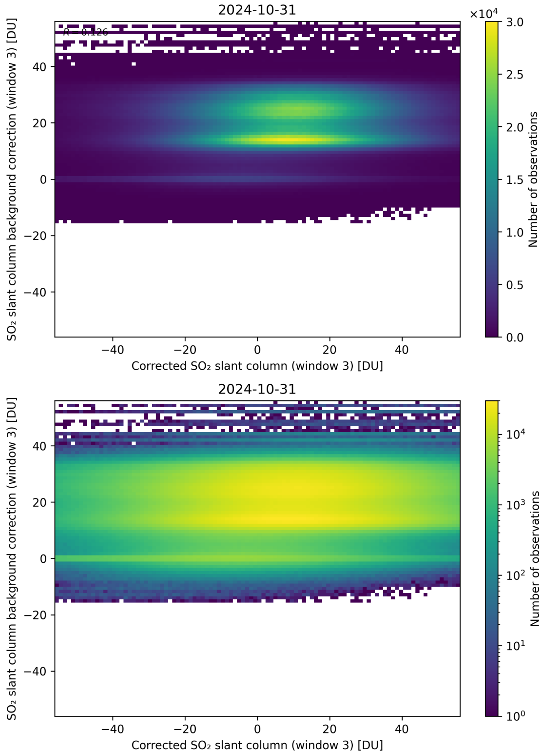
Figure 205: Scatter density plot of “Corrected SO 2 slant column (window 3)” against “SO 2 slant column background correction (window 3)” for 2024-10-30 to 2024-11-01.
