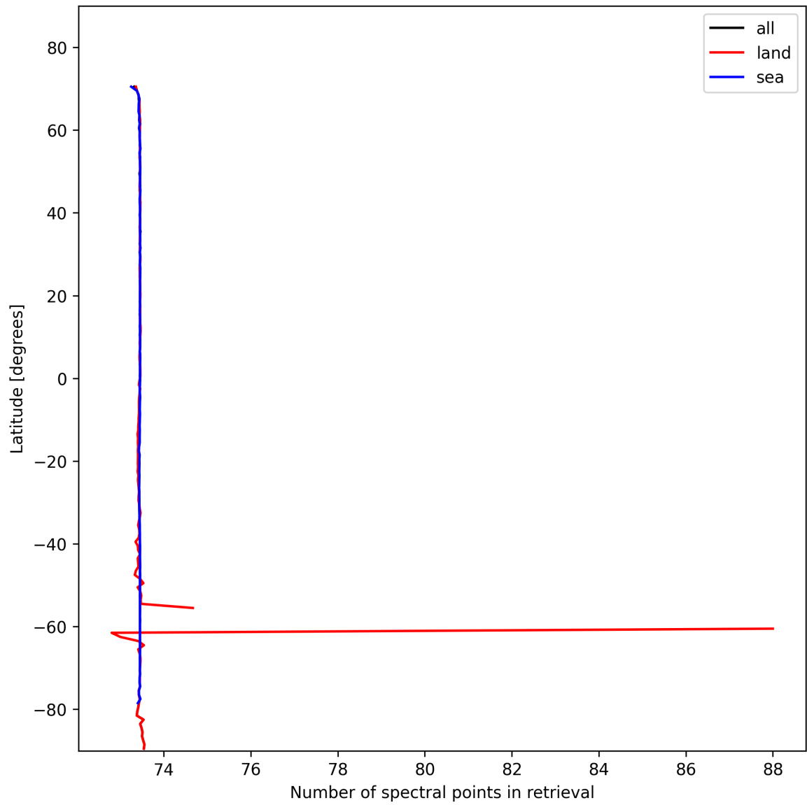
Figure 51: Zonal average of “Number of spectral points in retrieval” for 2024-10-30 to 2024-11-01.
