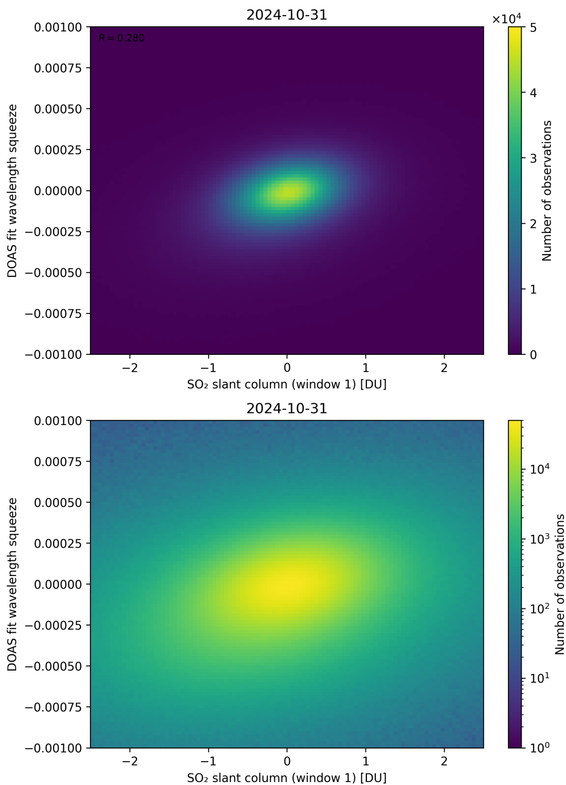
Figure 216: Scatter density plot of “SO 2 slant column (window 1)” against “DOAS fit wavelength squeeze” for 2024-10-30 to 2024-11-01.
