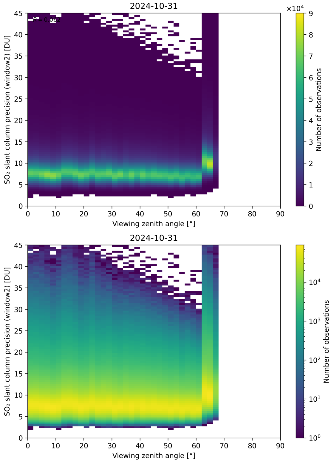
Figure 322: Scatter density plot of “Viewing zenith angle” against “SO 2 slant column precision (window2)” for 2024-10-30 to 2024-11-01.
