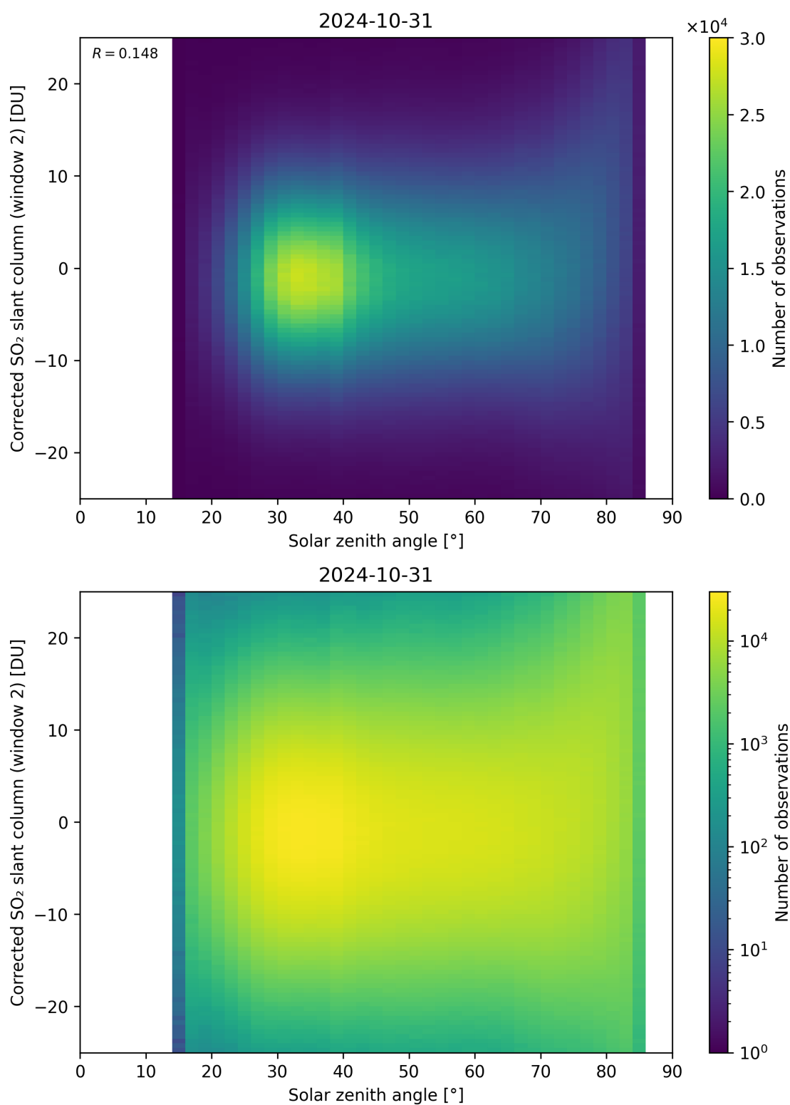
Figure 167: Scatter density plot of “Solar zenith angle” against “Corrected SO 2 slant column (window 2)” for 2024-10-30 to 2024-11-01.
