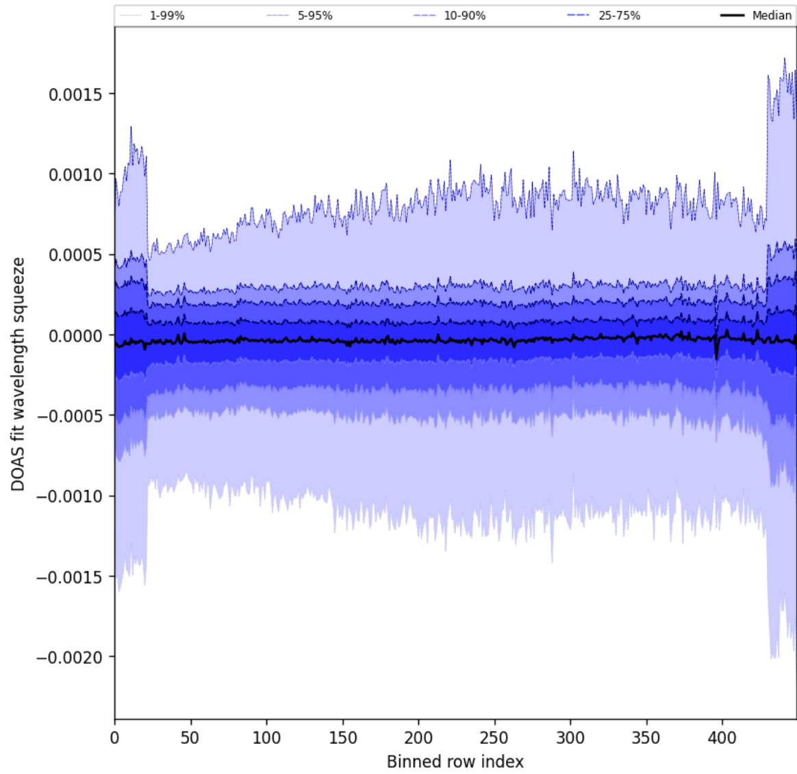
Figure 92: Along track statistics of “DOAS fit wavelength squeeze” for 2024-10-30 to 2024-11-01
