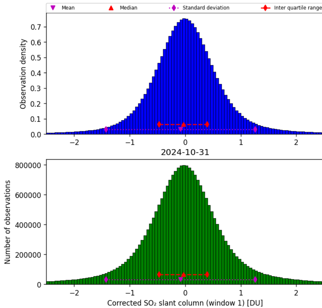
Figure 58: Histogram of “Corrected SO 2 slant column (window 1)” for 2024-10-30 to 2024-11-01
