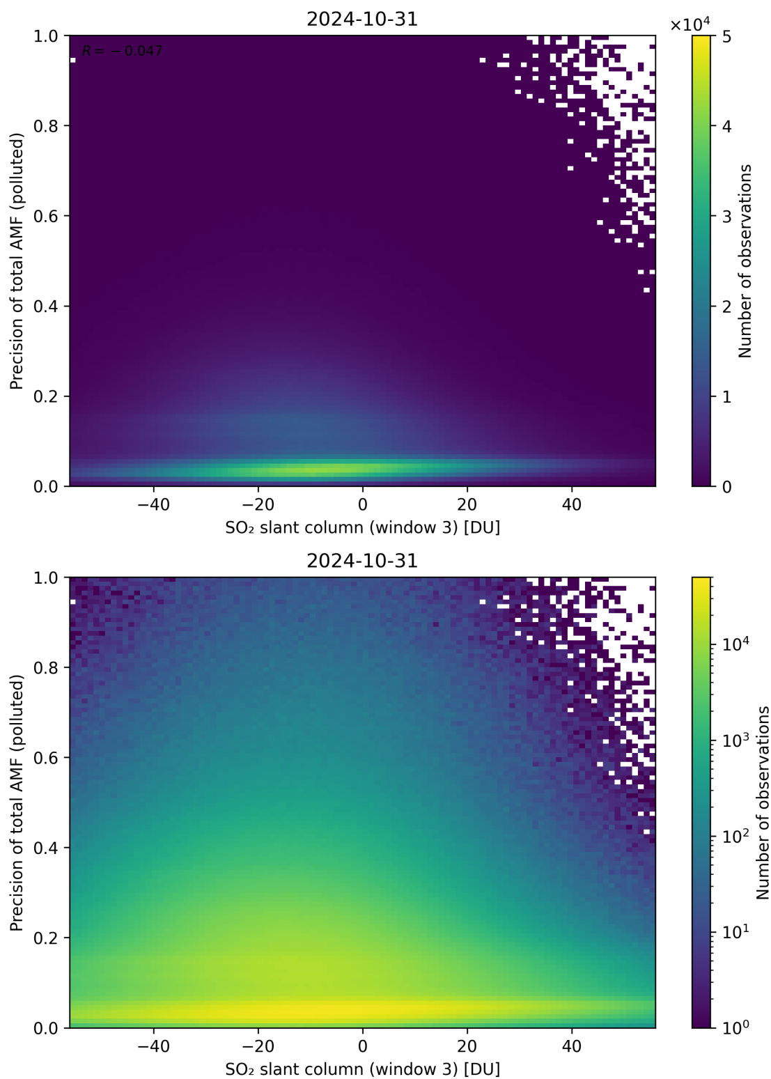
Figure 269: Scatter density plot of “SO 2 slant column (window 3)” against “Precision of total AMF (polluted)” for 2024-10-30 to 2024-11-01.
