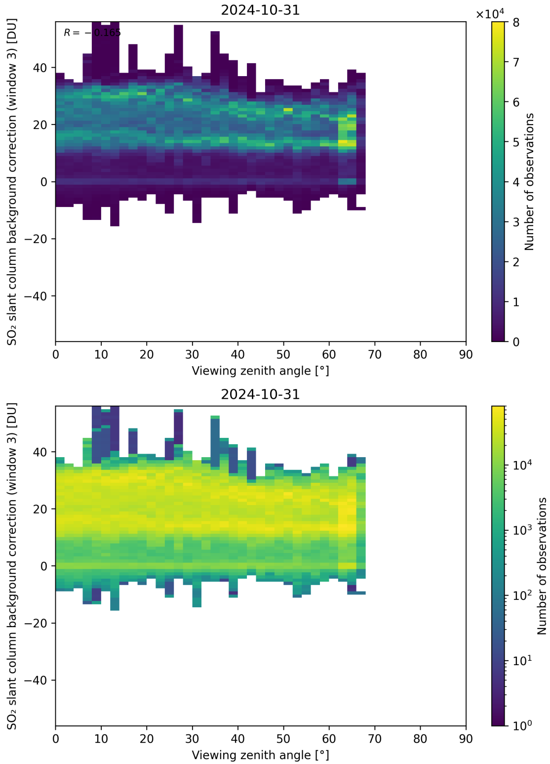
Figure 310: Scatter density plot of “Viewing zenith angle” against “SO 2 slant column background correction (window 3)” for 2024-10-30 to 2024-11-01.
