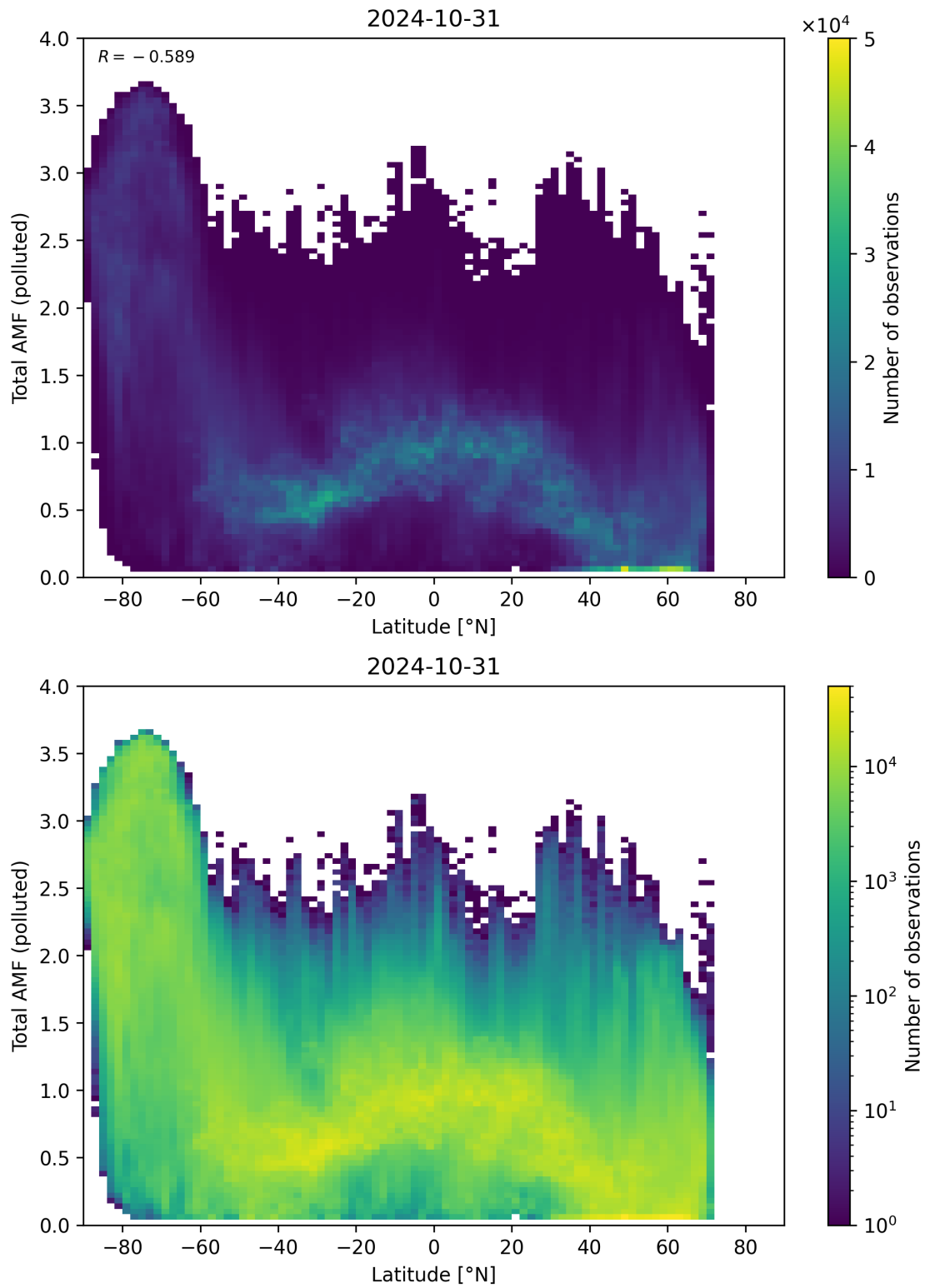
Figure 154: Scatter density plot of “Latitude” against “Total AMF (polluted)” for 2024-10-30 to 2024-11-01.
