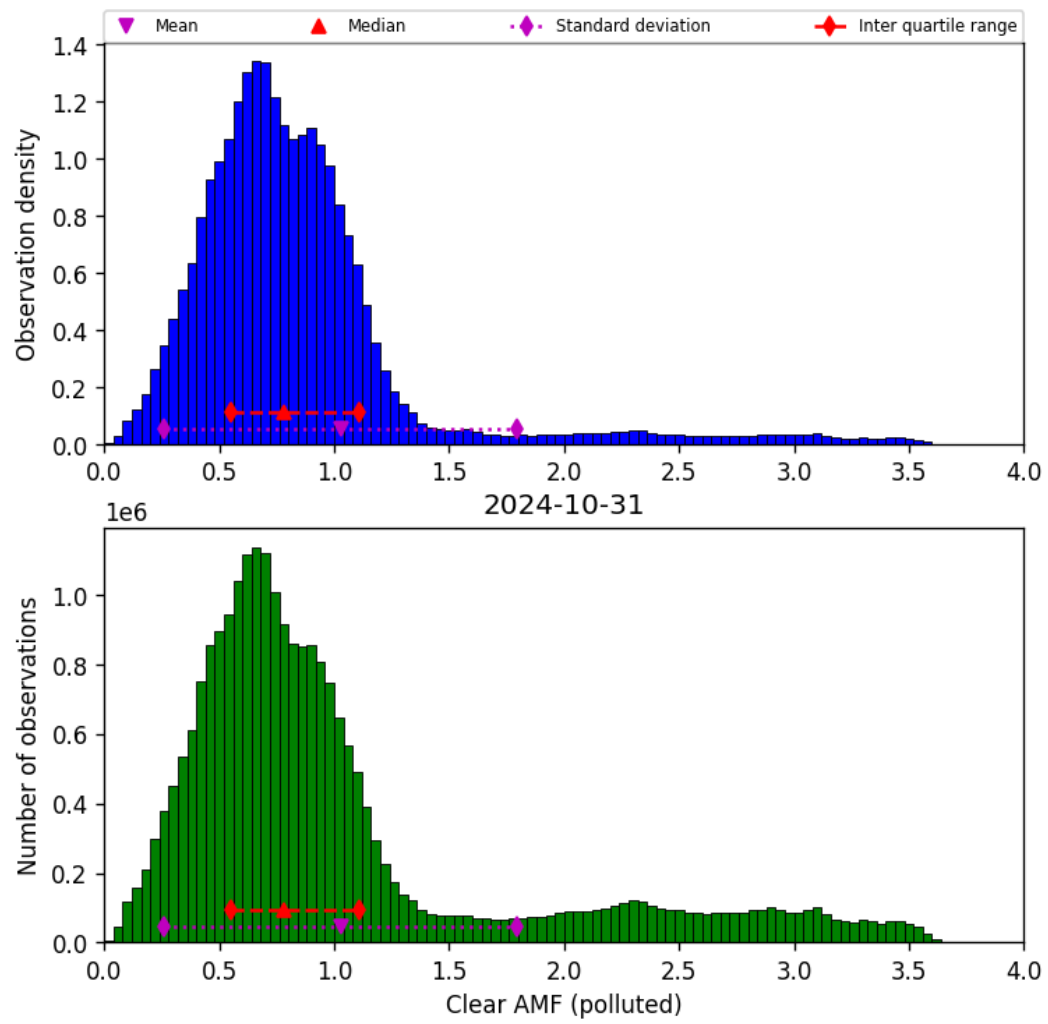
Figure 73: Histogram of “Clear AMF (polluted)” for 2024-10-30 to 2024-11-01
