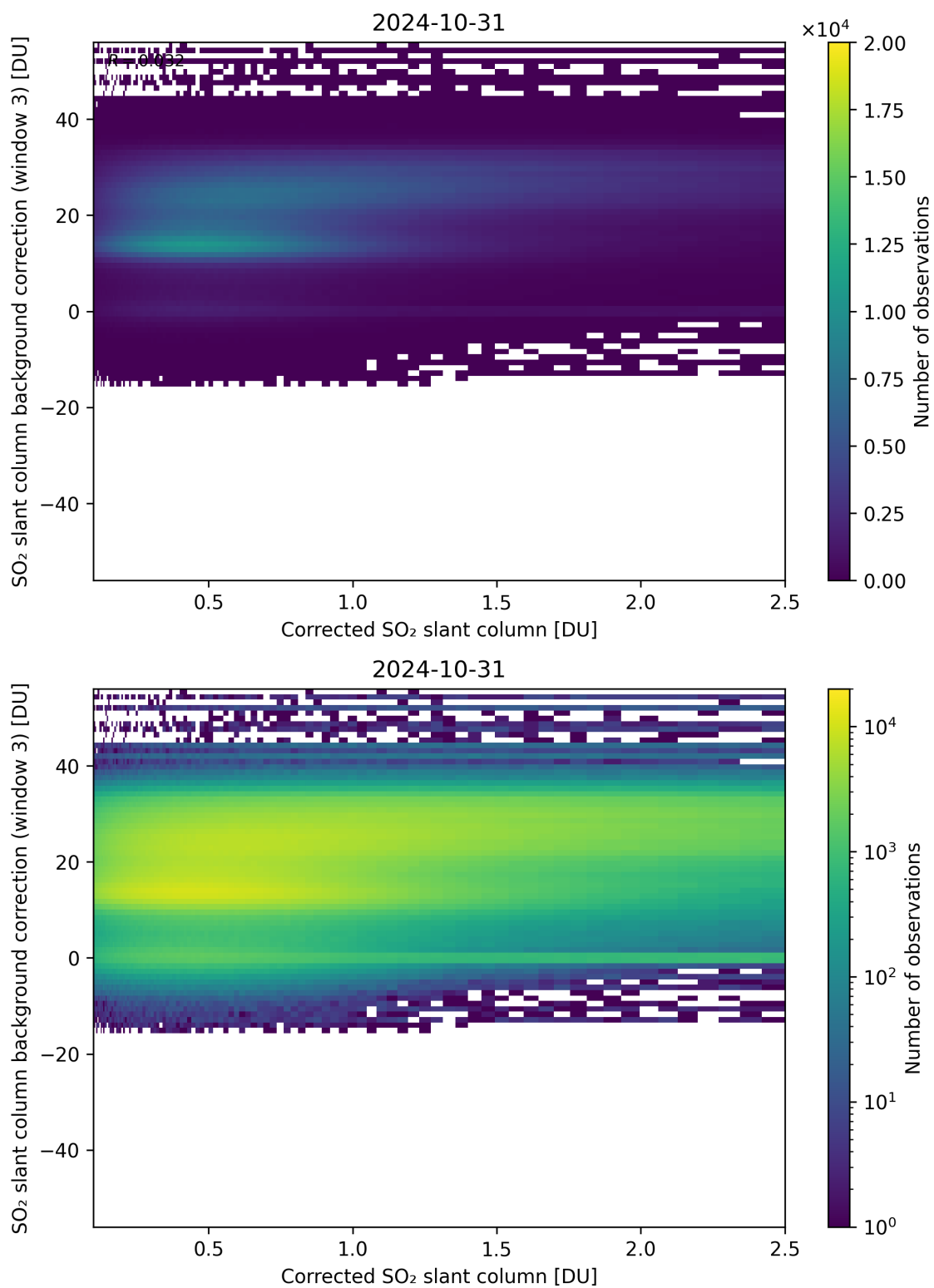
Figure 180: Scatter density plot of “Corrected SO 2 slant column” against “SO 2 slant column background correction (window 3)” for 2024-10-30 to 2024-11-01.
