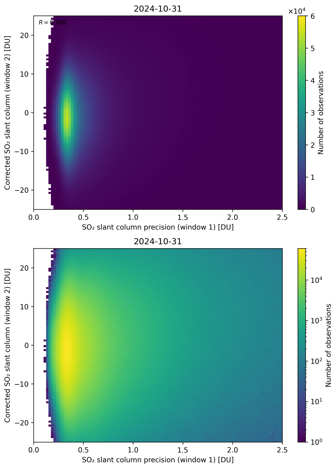
Figure 225: Scatter density plot of “SO 2 slant column precision (window 1)” against “Corrected SO 2 slant column (window 2)” for 2024-10-30 to 2024-11-01.
