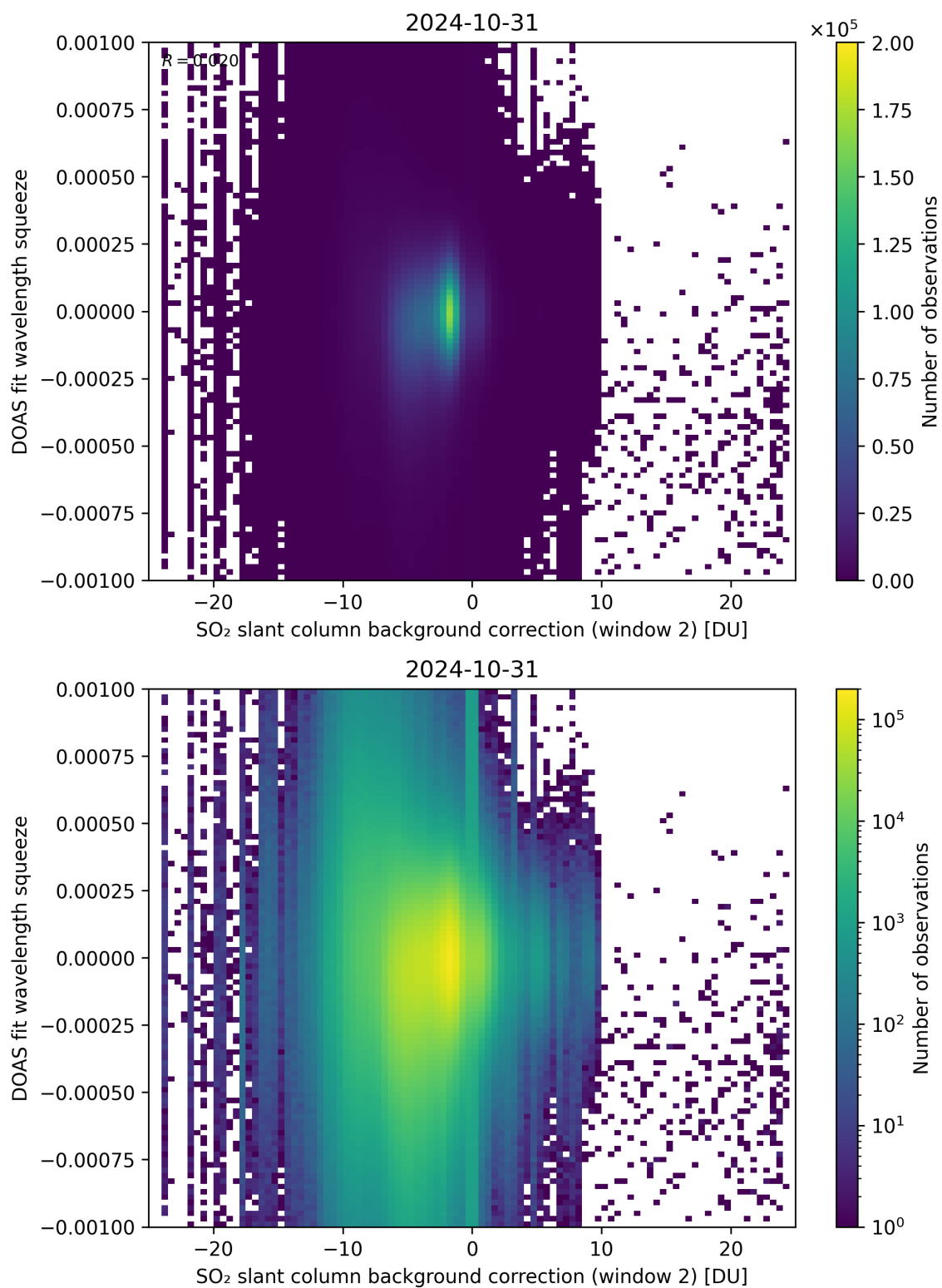
Figure 113: Scatter density plot of “SO 2 slant column background correction (window 2)” against “DOAS fit wavelength squeeze” for 2024-10-30 to 2024-11-01.
