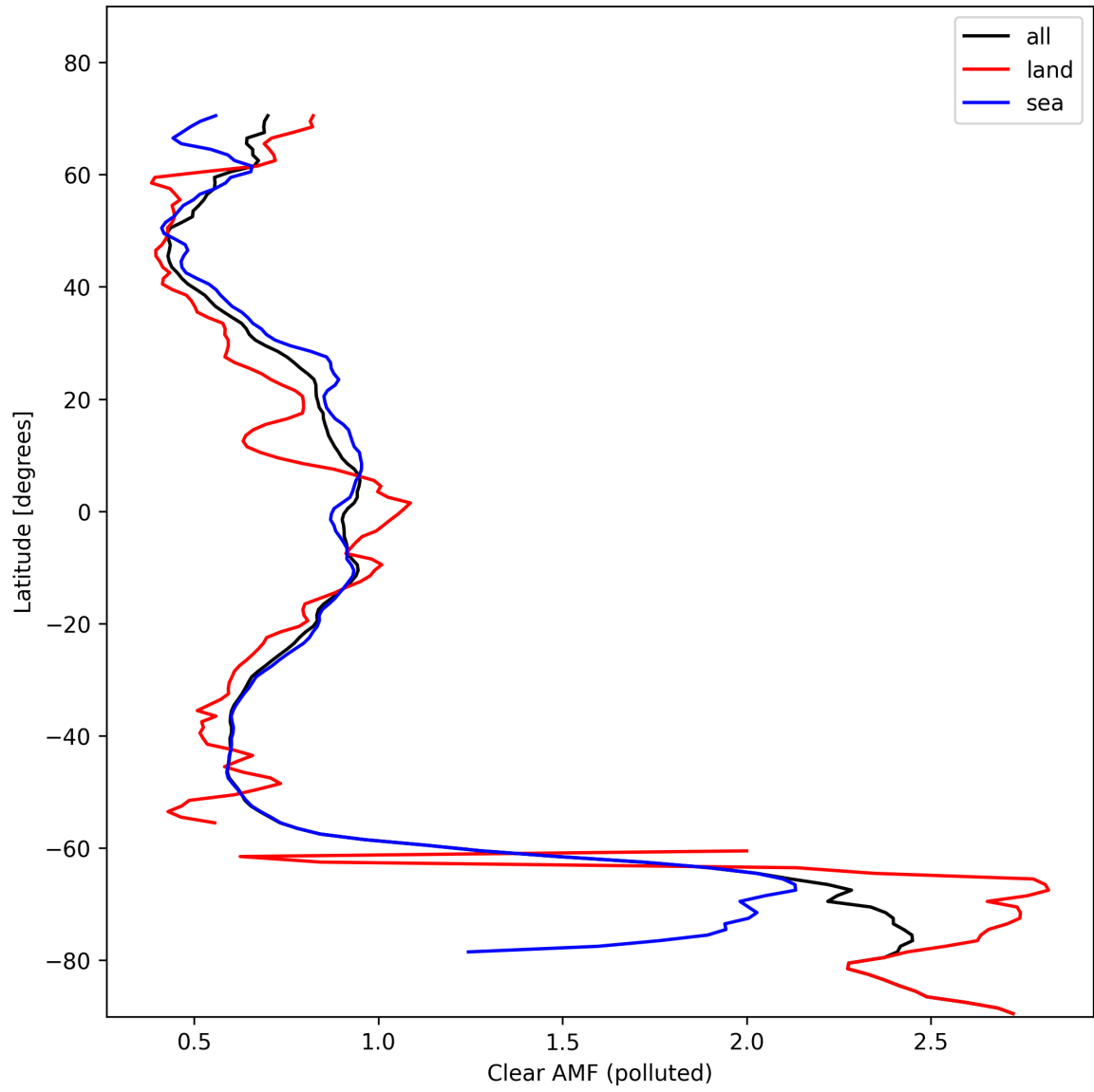
Figure 50: Zonal average of “Clear AMF (polluted)” for 2024-10-30 to 2024-11-01.
