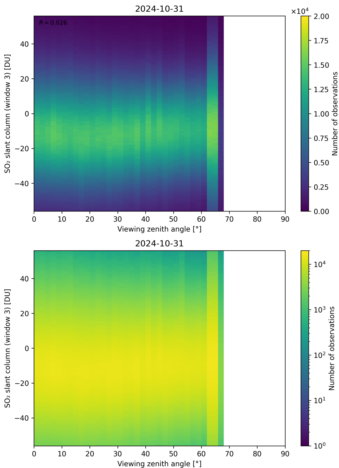
Figure 323: Scatter density plot of “Viewing zenith angle” against “SO 2 slant column (window 3)” for 2024-10-30 to 2024-11-01.
