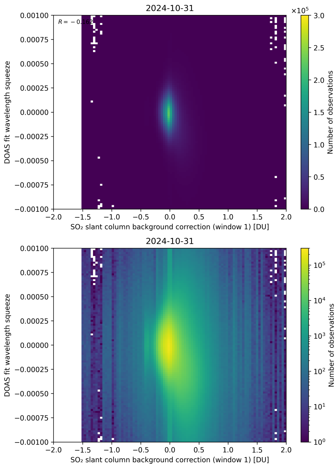
Figure 101: Scatter density plot of “SO 2 slant column background correction (window 1)” against “DOAS fit wavelength squeeze” for 2024-10-30 to 2024-11-01.
