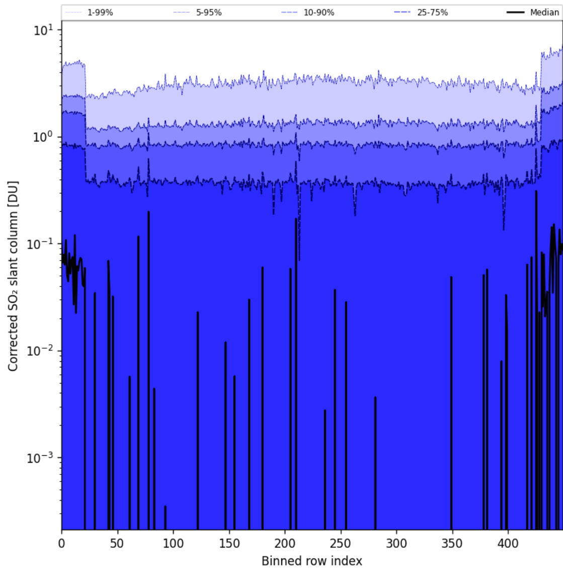
Figure 78: Along track statistics of “Corrected SO 2 slant column” for 2024-10-30 to 2024-11-01
