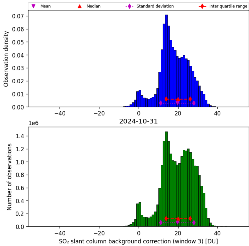
Figure 67: Histogram of “SO 2 slant column background correction (window 3)” for 2024-10-30 to 2024-11-01
