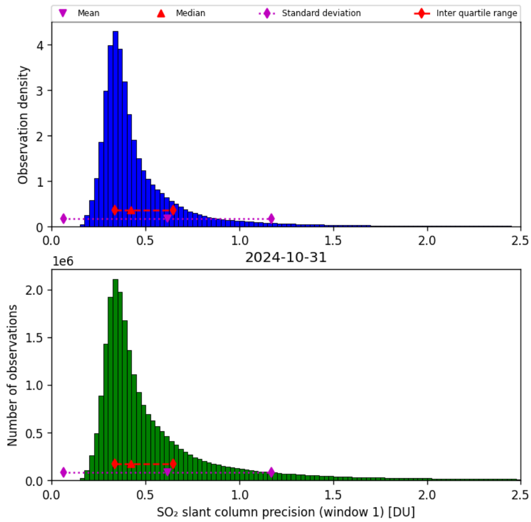
Figure 57: Histogram of “SO 2 slant column precision (window 1)” for 2024-10-30 to 2024-11-01
