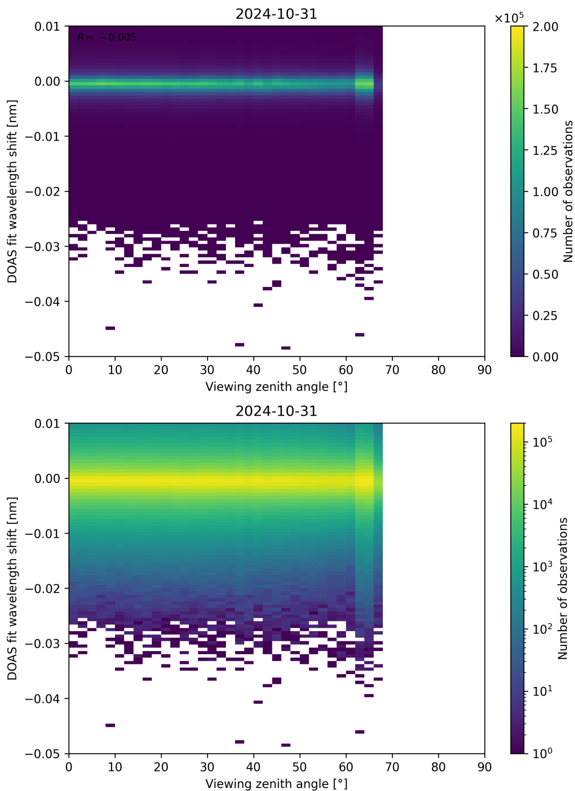
Figure 311: Scatter density plot of “Viewing zenith angle” against “DOAS fit wavelength shift” for 2024-10-30 to 2024-11-01.
