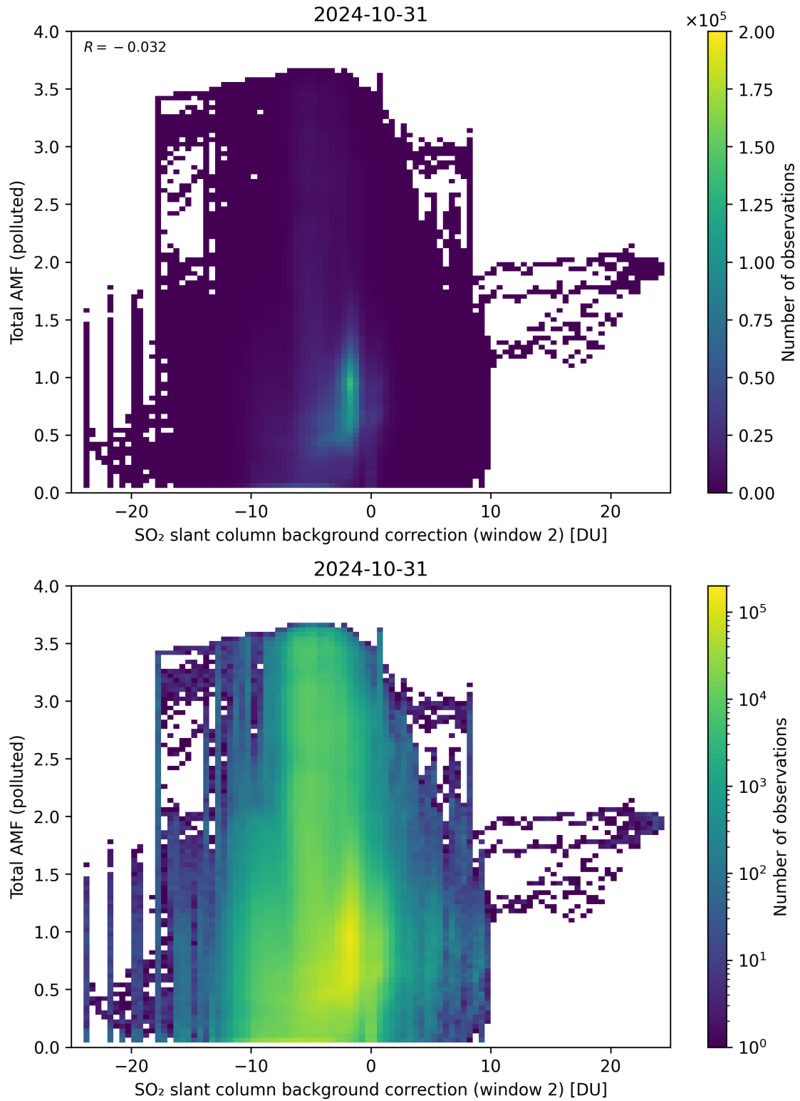
Figure 119: Scatter density plot of “SO 2 slant column background correction (window 2)” against “Total AMF (polluted)” for 2024-10-30 to 2024-11-01.
