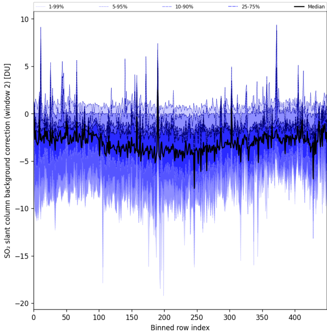
Figure 86: Along track statistics of “SO 2 slant column background correction (window 2)” for 2024-10-30 to 2024-11-01
