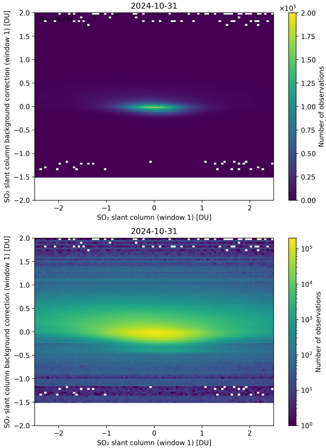
Figure 212: Scatter density plot of “SO 2 slant column (window 1)” against “SO 2 slant column background correction (window 1)” for 2024-10-30 to 2024-11-01.
