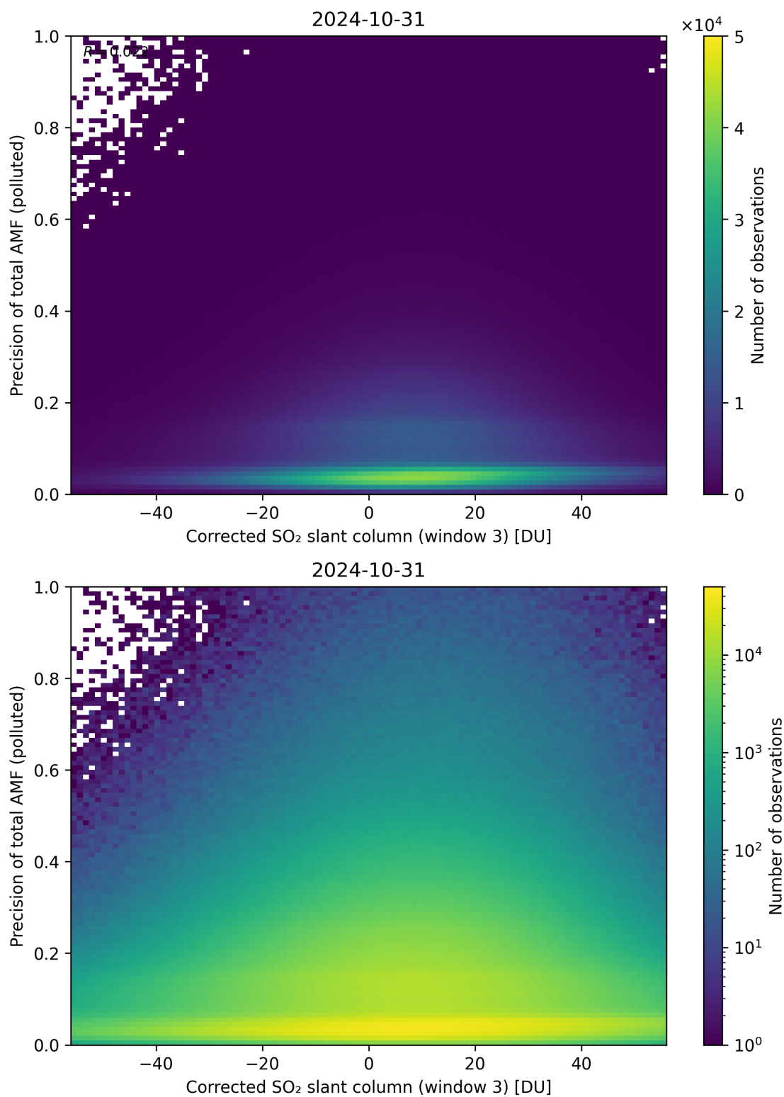
Figure 211: Scatter density plot of “Corrected SO 2 slant column (window 3)” against “Precision of total AMF (polluted)” for 2024-10-30 to 2024-11-01.
