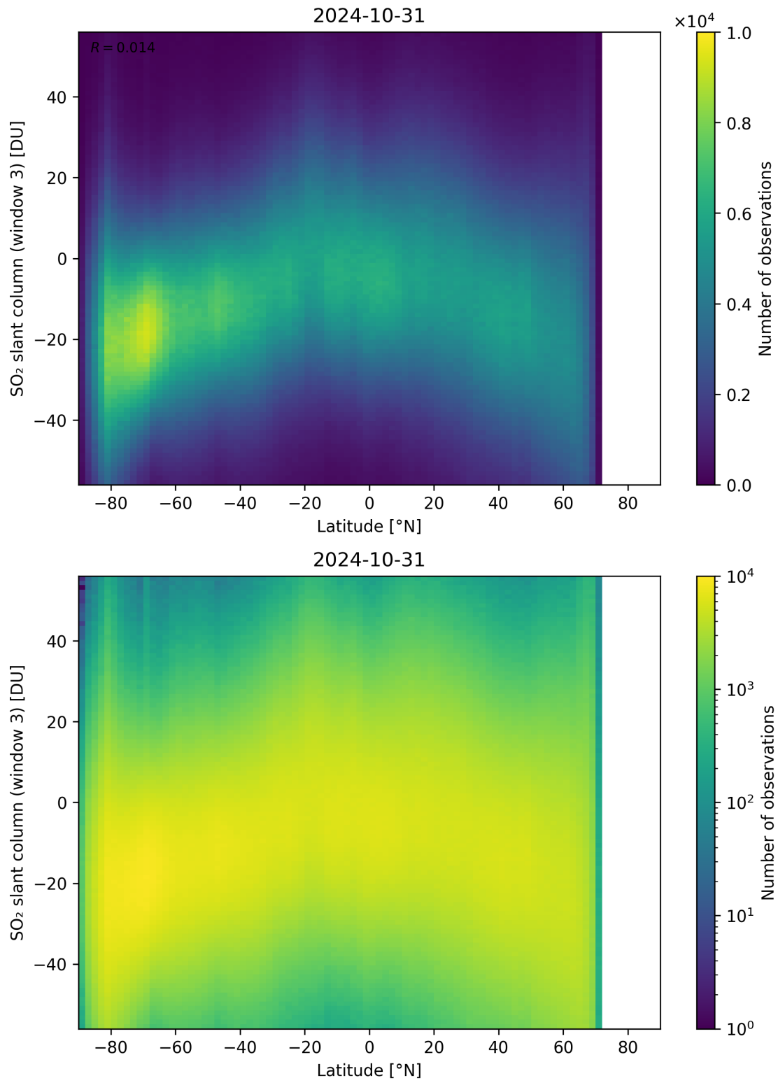
Figure 152: Scatter density plot of “Latitude” against “SO 2 slant column (window 3)” for 2024-10-30 to 2024-11-01.
