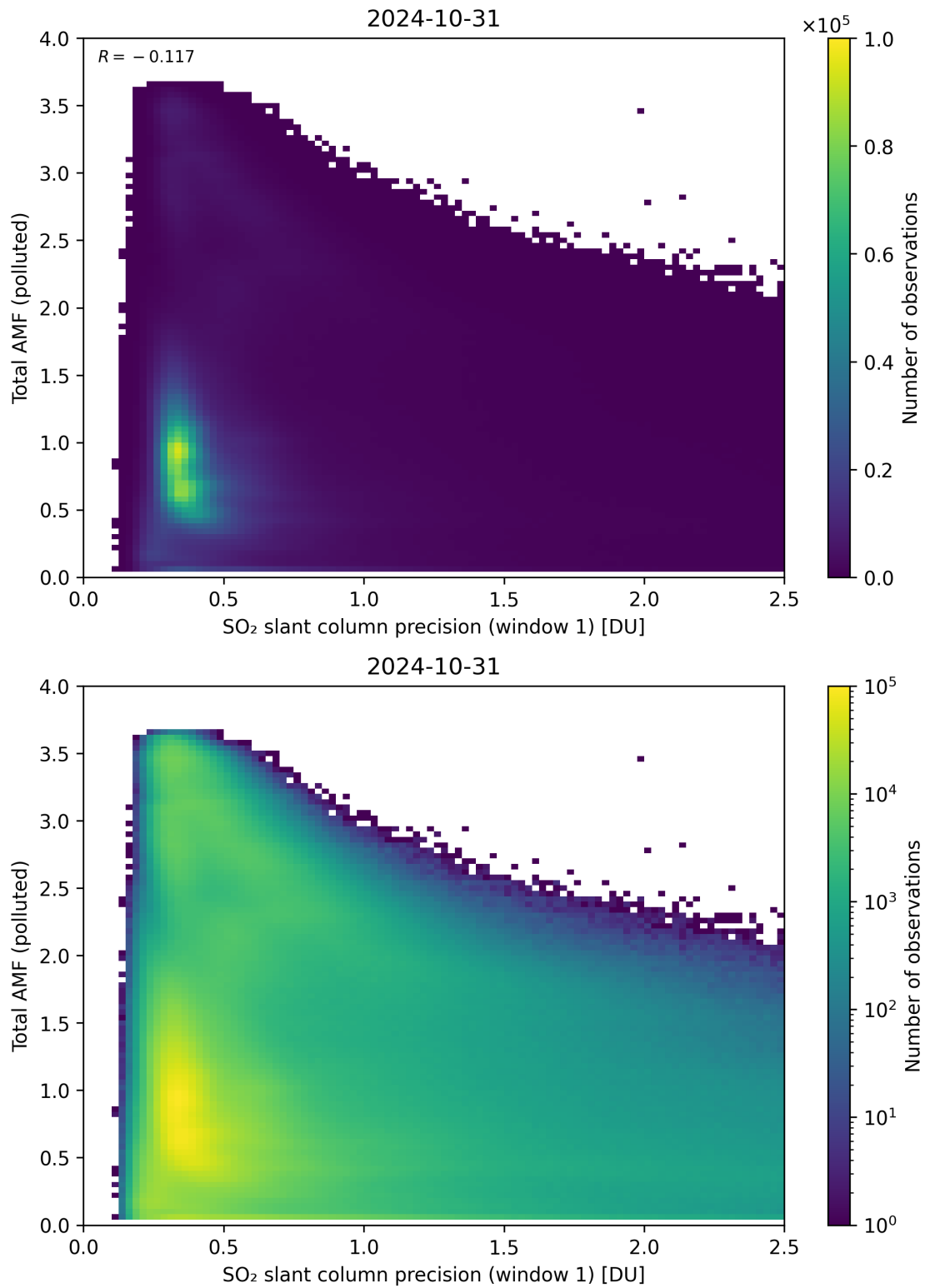
Figure 230: Scatter density plot of “SO 2 slant column precision (window 1)” against “Total AMF (polluted)” for 2024-10-30 to 2024-11-01.
