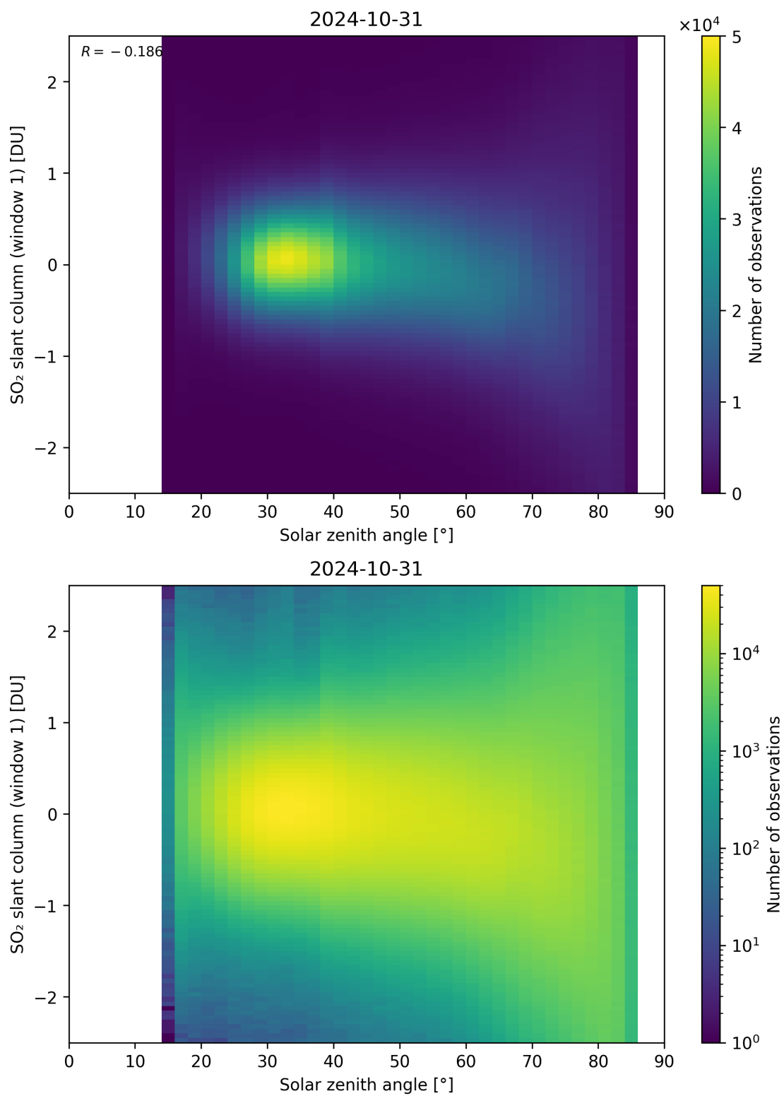
Figure 169: Scatter density plot of “Solar zenith angle” against “SO 2 slant column (window 1)” for 2024-10-30 to 2024-11-01.
