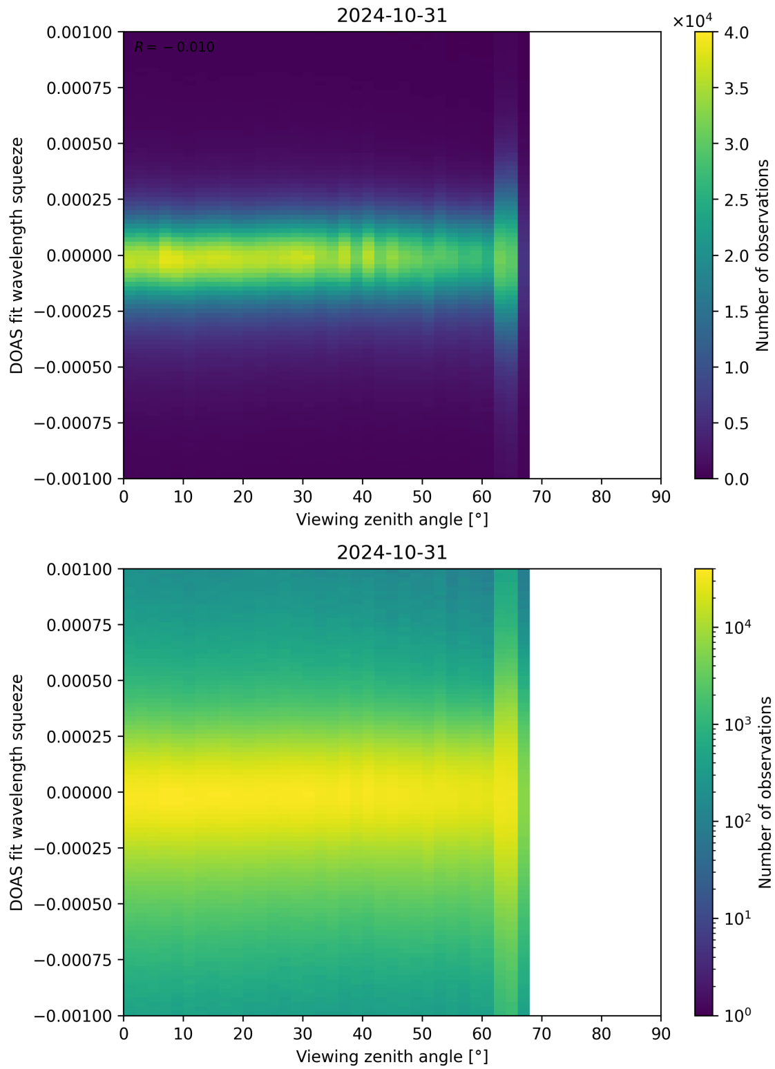
Figure 312: Scatter density plot of “Viewing zenith angle” against “DOAS fit wavelength squeeze” for 2024-10-30 to 2024-11-01.
