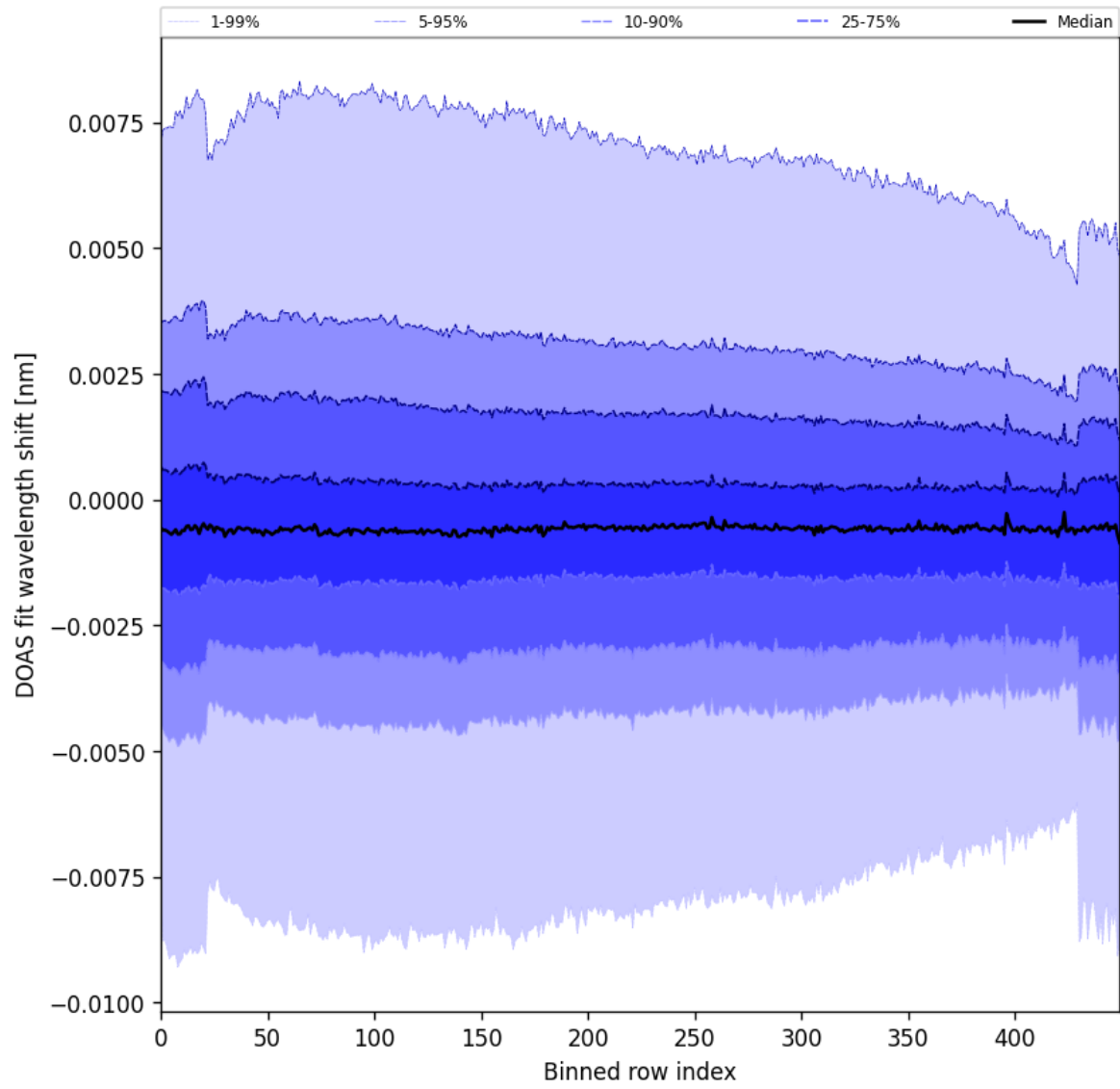
Figure 91: Along track statistics of “DOAS fit wavelength shift” for 2024-10-30 to 2024-11-01
