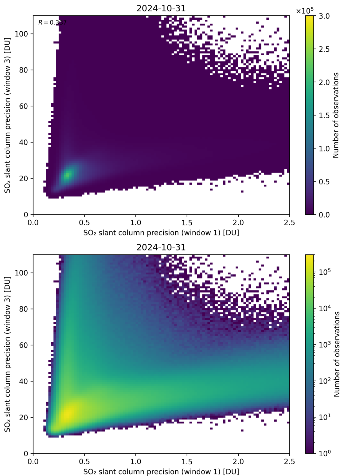
Figure 229: Scatter density plot of “SO 2 slant column precision (window 1)” against “SO 2 slant column precision (window 3)” for 2024-10-30 to 2024-11-01.
