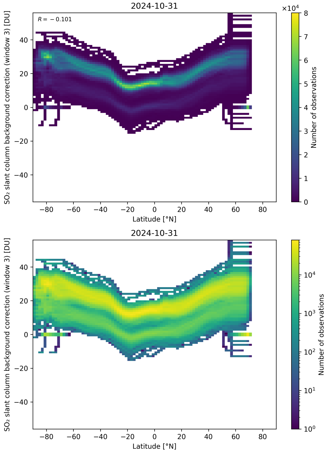
Figure 141: Scatter density plot of “Latitude” against “SO 2 slant column background correction (window 3)” for 2024-10-30 to 2024-11-01.
