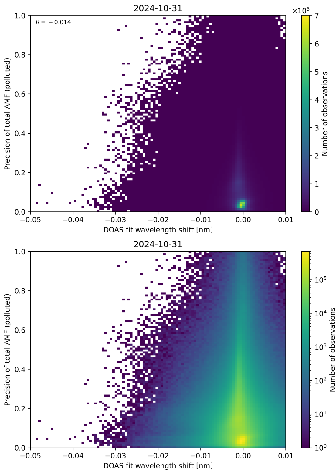
Figure 131: Scatter density plot of “DOAS fit wavelength shift” against “Precision of total AMF (polluted)” for 2024-10-30 to 2024-11-01.
