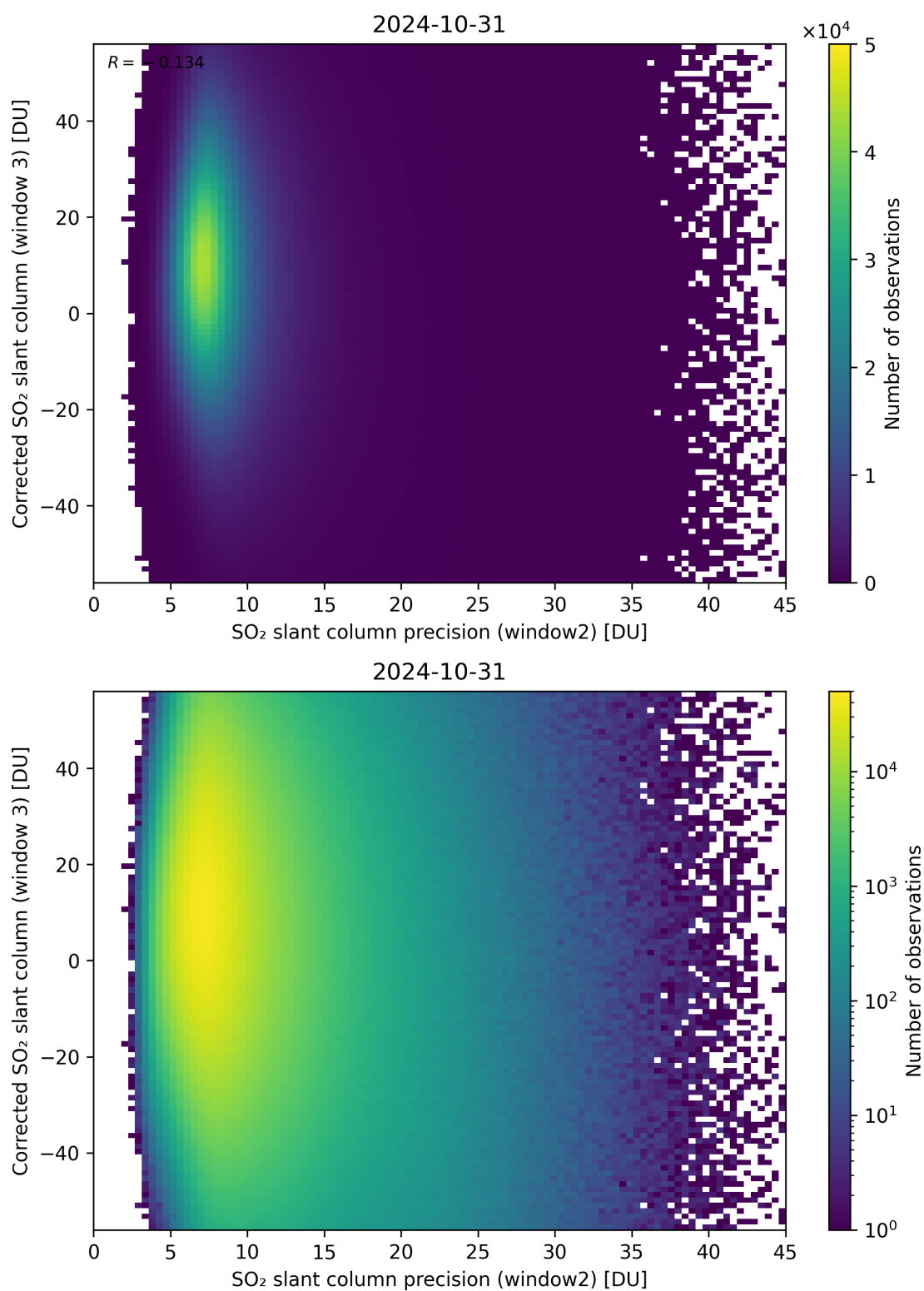
Figure 248: Scatter density plot of “SO 2 slant column precision (window2)” against “Corrected SO 2 slant column (window 3)” for 2024-10-30 to 2024-11-01.
