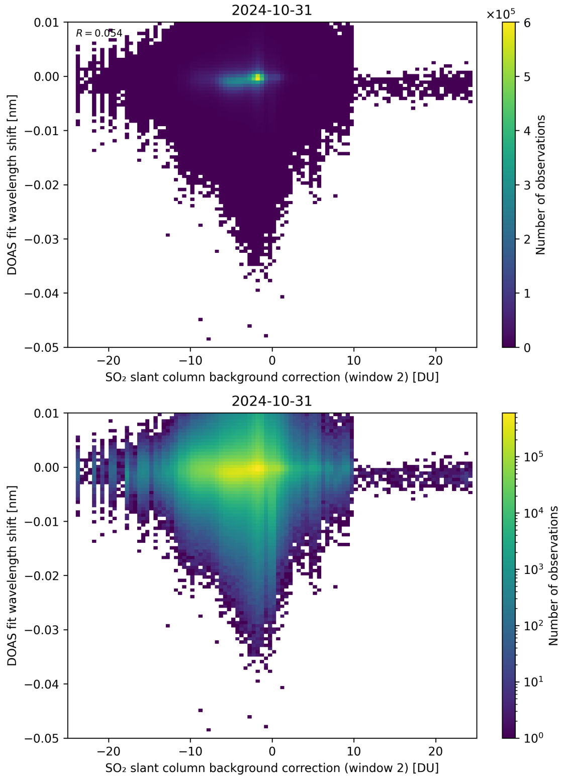
Figure 112: Scatter density plot of “SO 2 slant column background correction (window 2)” against “DOAS fit wavelength shift” for 2024-10-30 to 2024-11-01.
