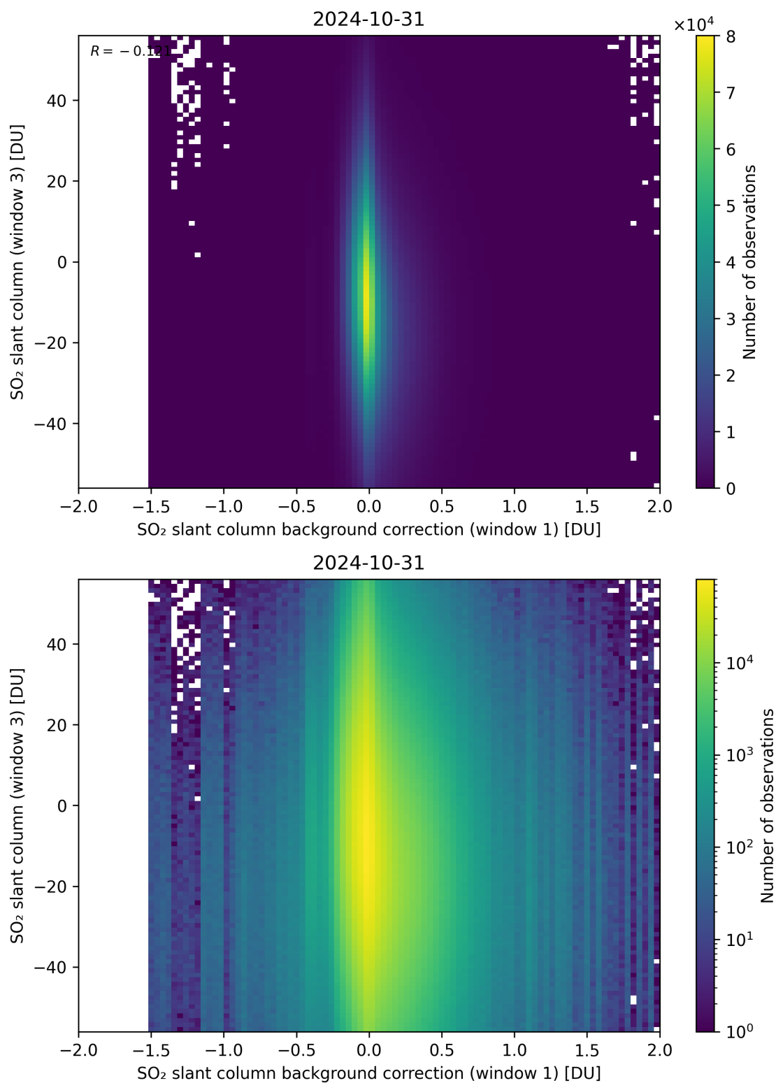
Figure 107: Scatter density plot of “SO 2 slant column background correction (window 1)” against “SO 2 slant column (window 3)” for 2024-10-30 to 2024-11-01.
