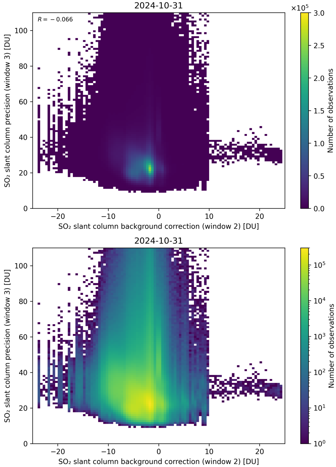
Figure 118: Scatter density plot of “SO 2 slant column background correction (window 2)” against “SO 2 slant column precision (window 3)” for 2024-10-30 to 2024-11-01.
