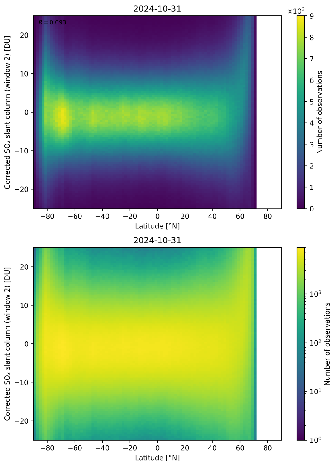
Figure 147: Scatter density plot of “Latitude” against “Corrected SO 2 slant column (window 2)” for 2024-10-30 to 2024-11-01.
