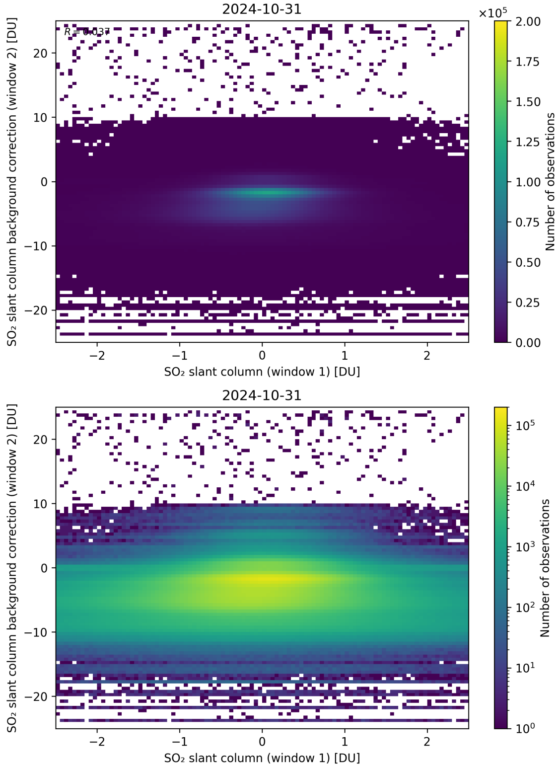
Figure 213: Scatter density plot of “SO 2 slant column (window 1)” against “SO 2 slant column background correction (window 2)” for 2024-10-30 to 2024-11-01.
