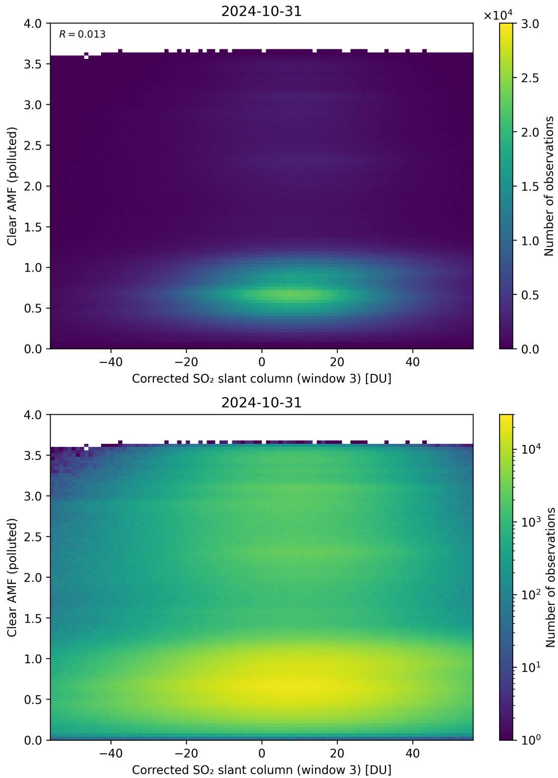
Figure 209: Scatter density plot of “Corrected SO 2 slant column (window 3)” against “Clear AMF (polluted)” for 2024-10-30 to 2024-11-01.
