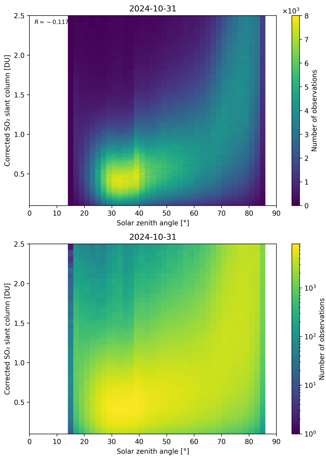
Figure 166: Scatter density plot of “Solar zenith angle” against “Corrected SO 2 slant column” for 2024-10-30 to 2024-11-01.
