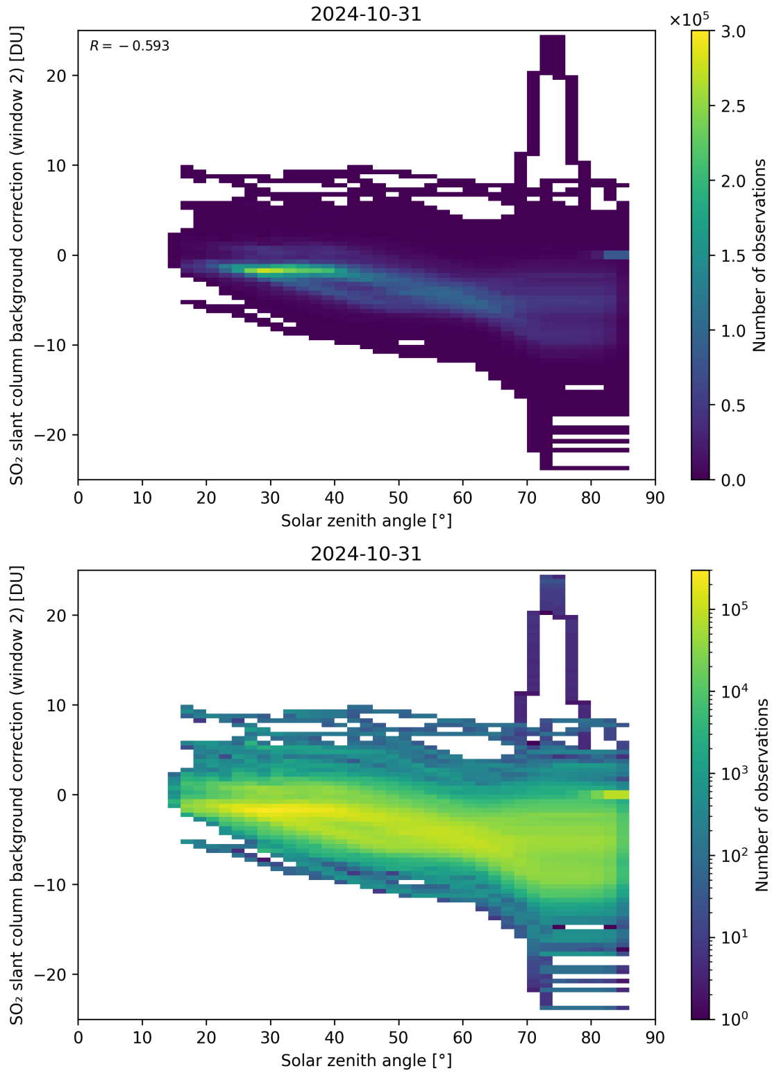
Figure 159: Scatter density plot of “Solar zenith angle” against “SO 2 slant column background correction (window 2)” for 2024-10-30 to 2024-11-01.
