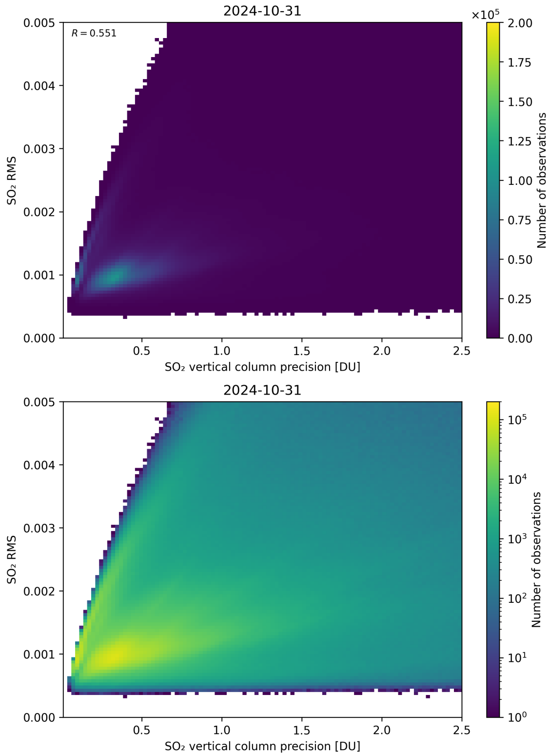
Figure 284: Scatter density plot of “SO 2 vertical column precision” against “SO 2 RMS” for 2024-10-30 to 2024-11-01.
