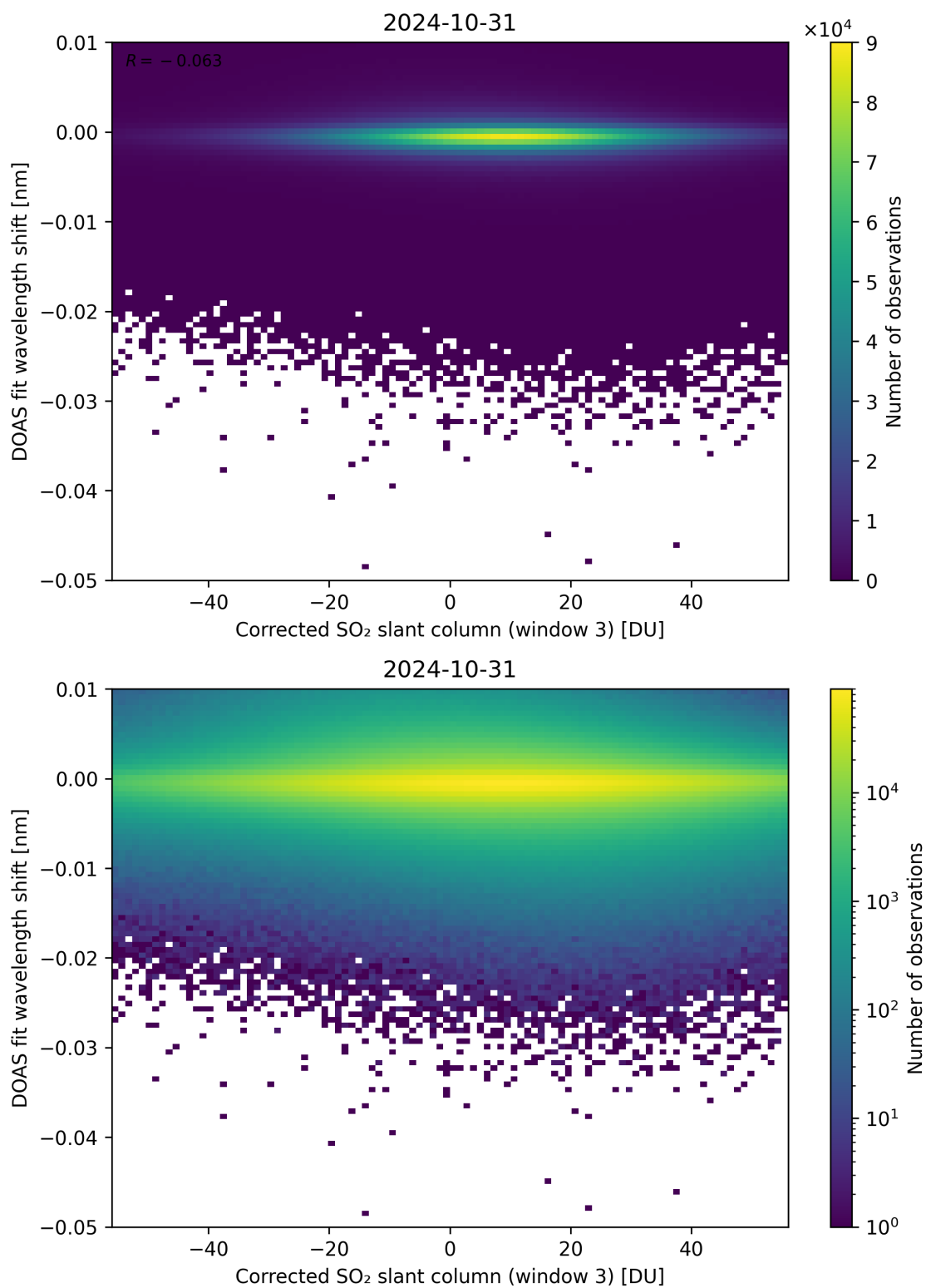
Figure 206: Scatter density plot of “Corrected SO 2 slant column (window 3)” against “DOAS fit wavelength shift” for 2024-10-30 to 2024-11-01.
