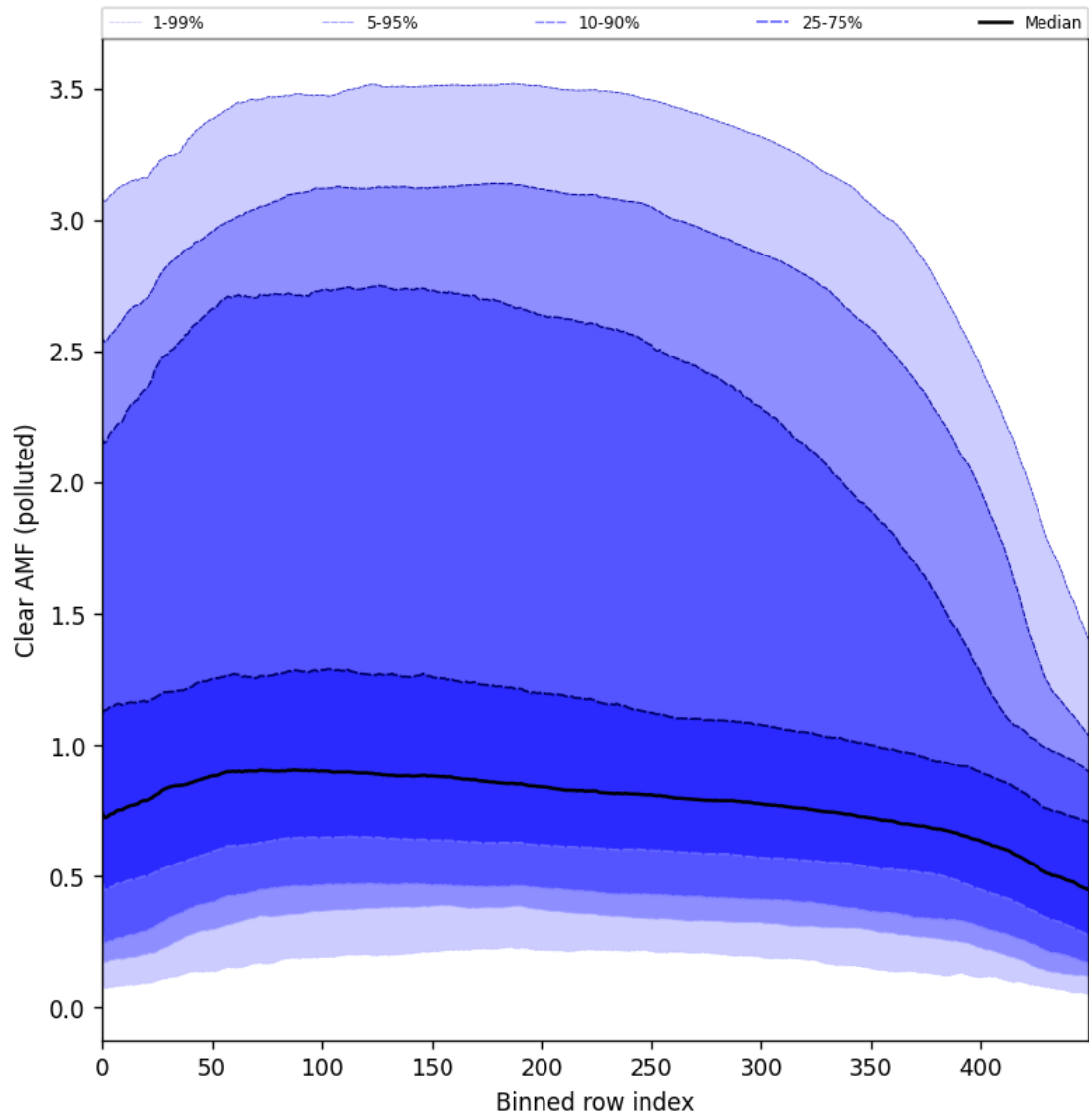
Figure 96: Along track statistics of “Clear AMF (polluted)” for 2024-10-30 to 2024-11-01
