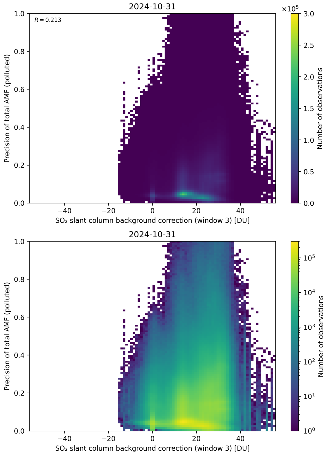
Figure 126: Scatter density plot of “SO 2 slant column background correction (window 3)” against “Precision of total AMF (polluted)” for 2024-10-30 to 2024-11-01.
