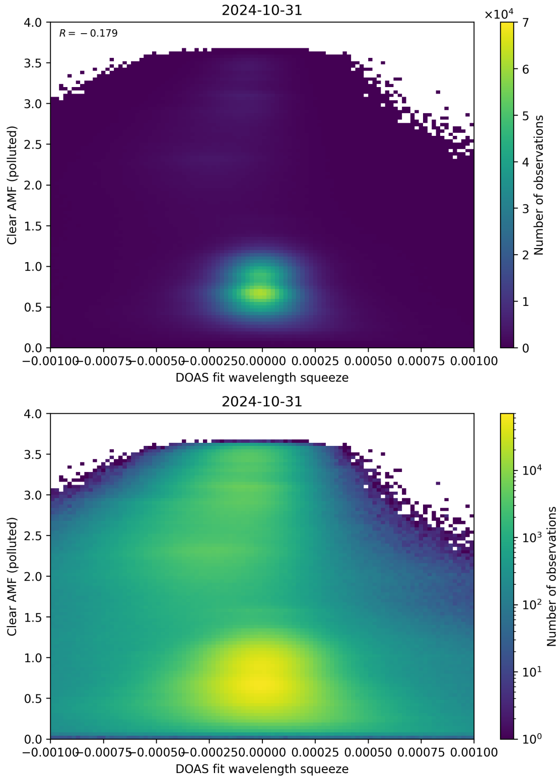
Figure 133: Scatter density plot of “DOAS fit wavelength squeeze” against “Clear AMF (polluted)” for 2024-10-30 to 2024-11-01.
