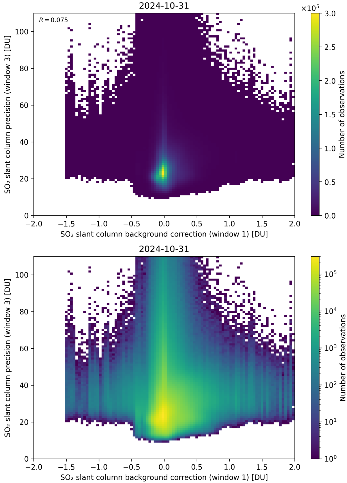
Figure 108: Scatter density plot of “SO 2 slant column background correction (window 1)” against “SO 2 slant column precision (window 3)” for 2024-10-30 to 2024-11-01.
