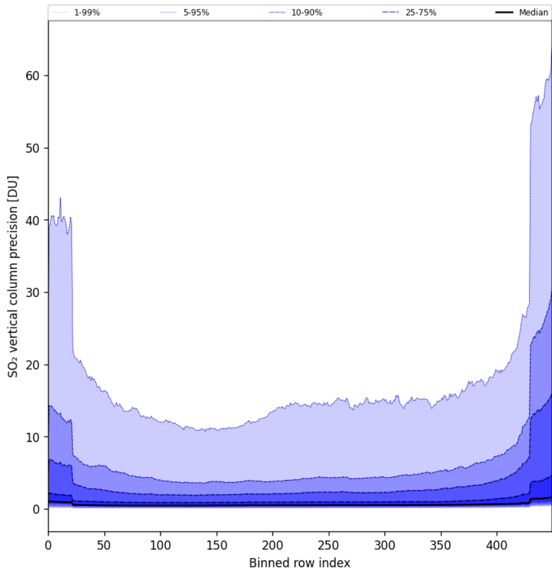
Figure 77: Along track statistics of “SO 2 vertical column precision” for 2024-10-30 to 2024-11-01
