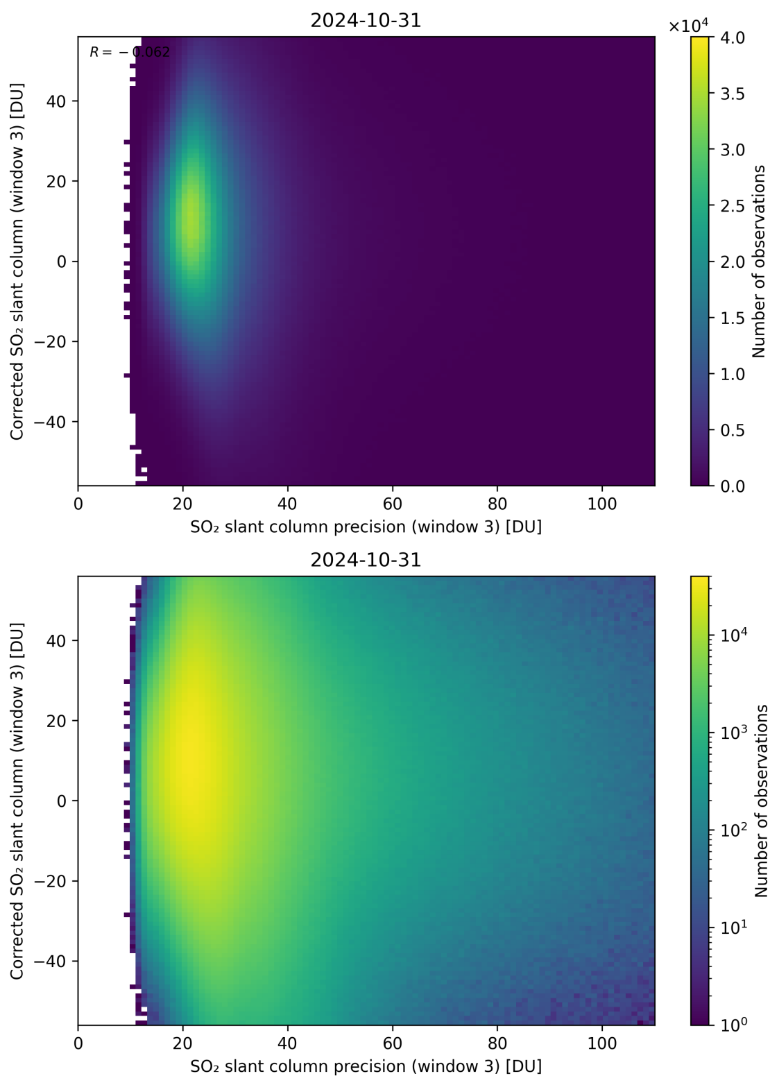
Figure 262: Scatter density plot of “SO 2 slant column precision (window 3)” against “Corrected SO 2 slant column (window 3)” for 2024-10-30 to 2024-11-01.
