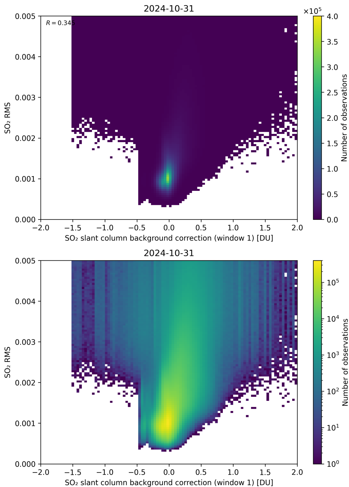
Figure 102: Scatter density plot of “SO 2 slant column background correction (window 1)” against “SO 2 RMS” for 2024-10-30 to 2024-11-01.
