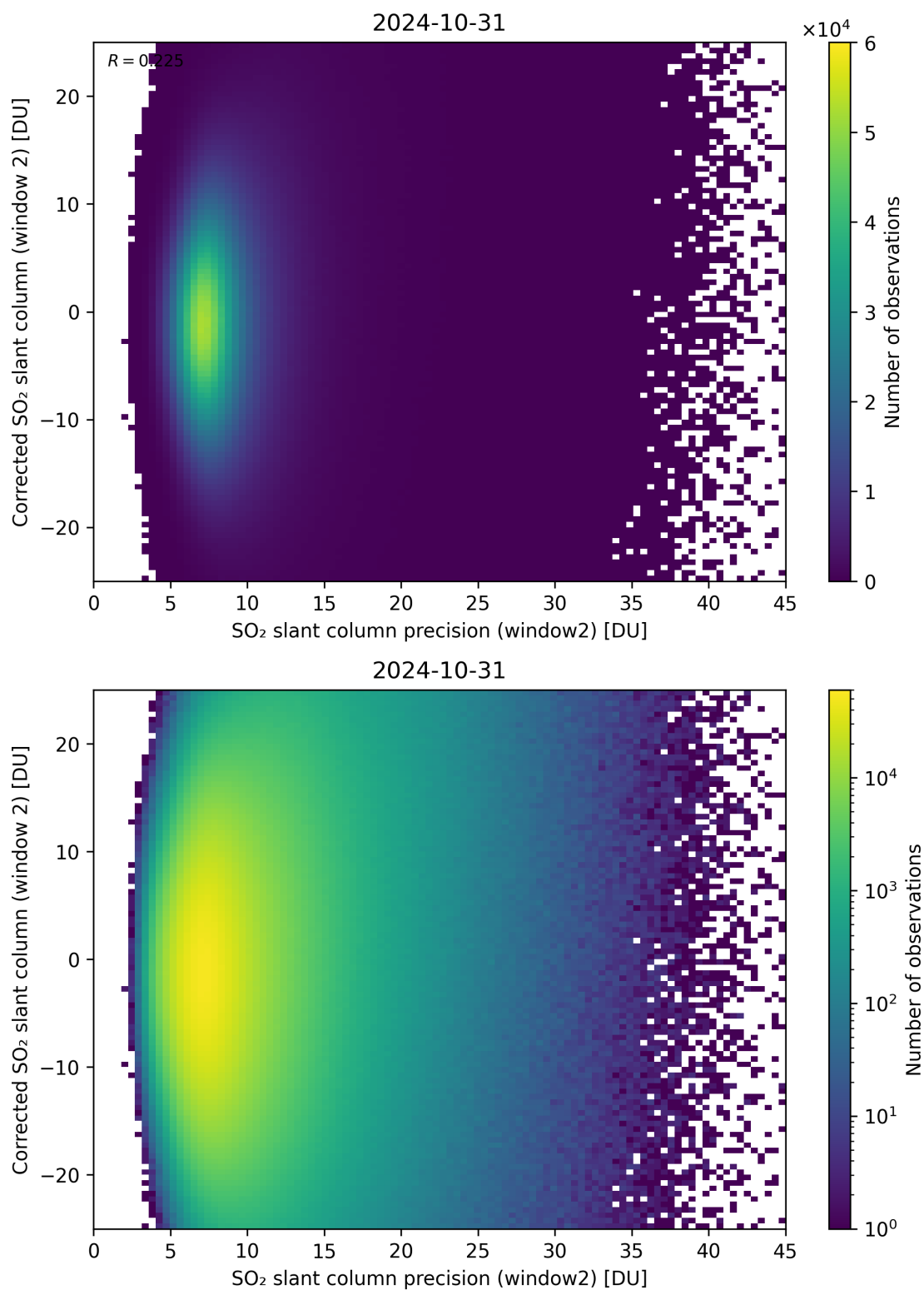
Figure 247: Scatter density plot of “SO 2 slant column precision (window2)” against “Corrected SO 2 slant column (window 2)” for 2024-10-30 to 2024-11-01.
