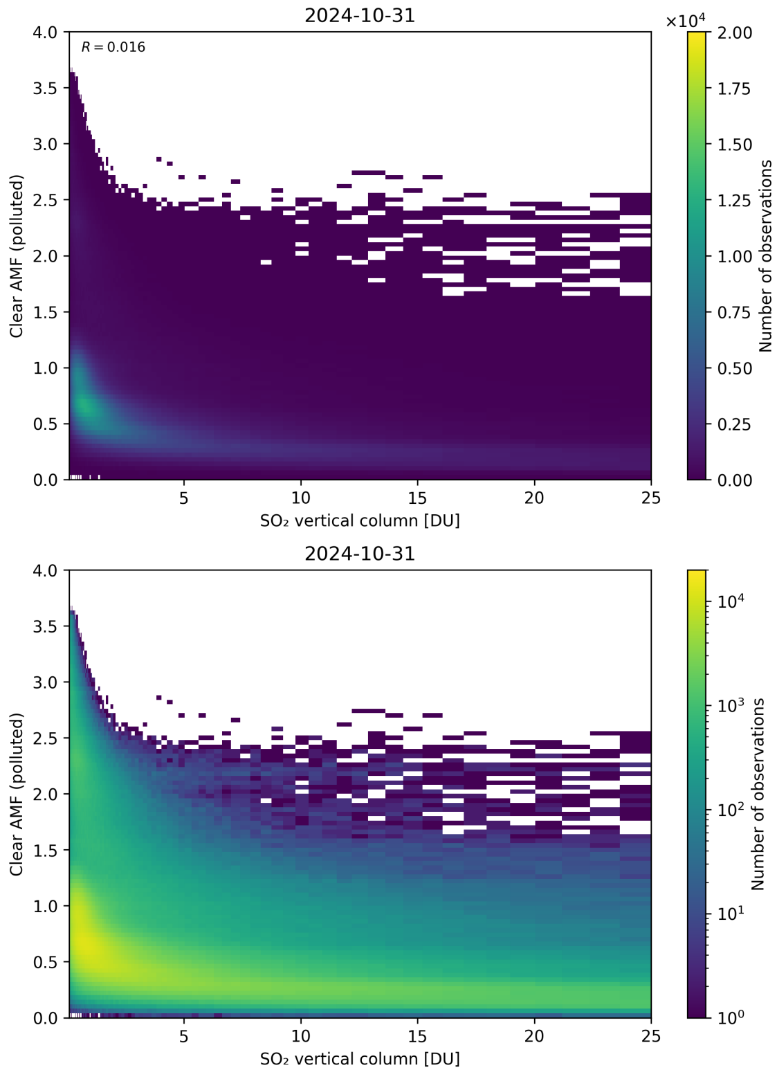
Figure 296: Scatter density plot of “SO 2 vertical column” against “Clear AMF (polluted)” for 2024-10-30 to 2024-11-01.
