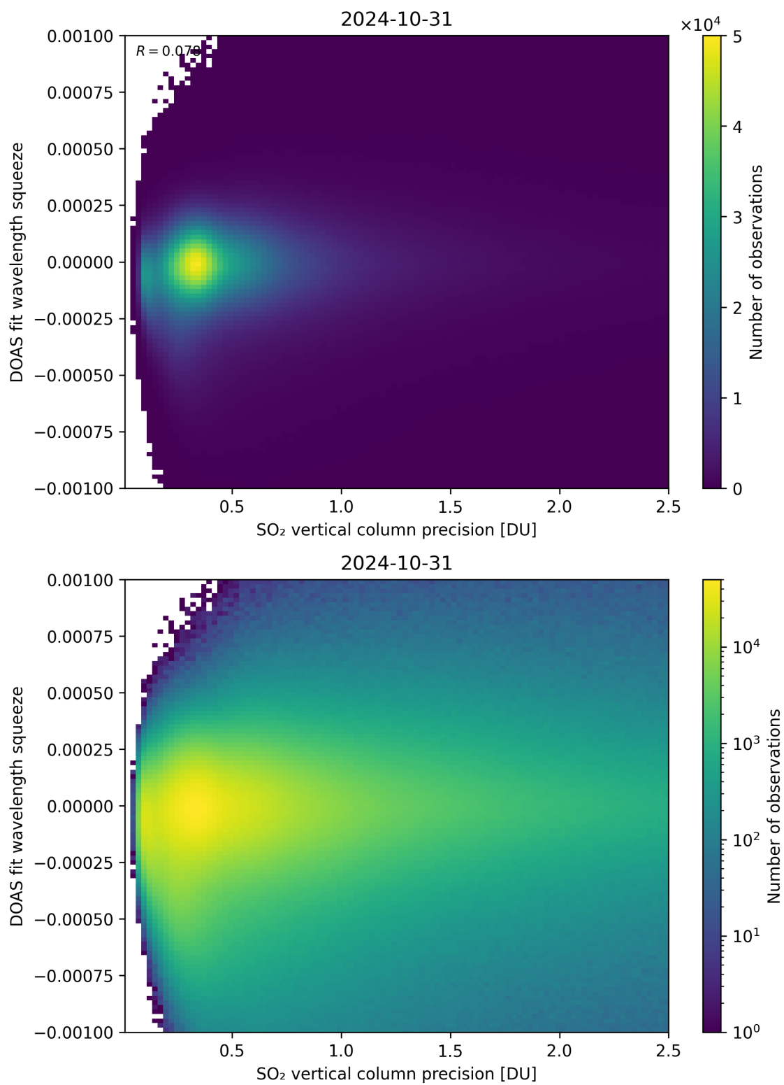
Figure 283: Scatter density plot of “SO 2 vertical column precision” against “DOAS fit wavelength squeeze” for 2024-10-30 to 2024-11-01.
