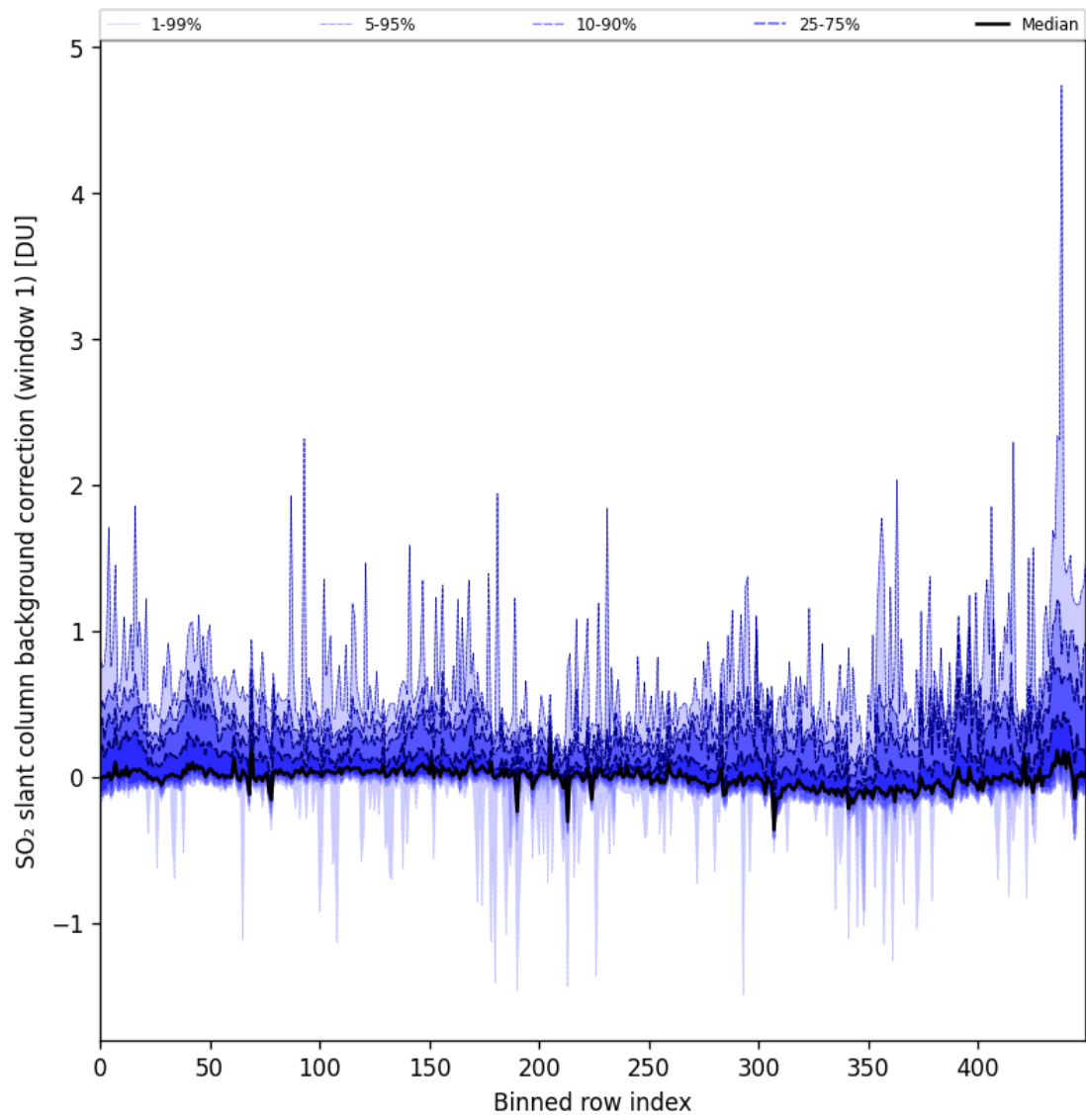
Figure 82: Along track statistics of “SO 2 slant column background correction (window 1)” for 2024-10-30 to 2024-11-01
