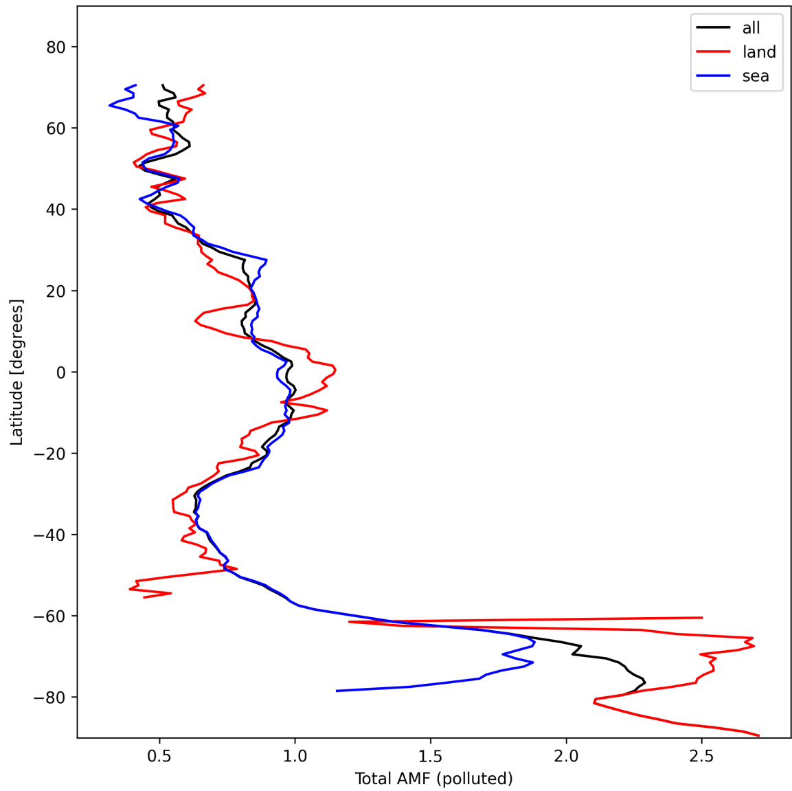
Figure 48: Zonal average of “Total AMF (polluted)” for 2024-10-30 to 2024-11-01.
