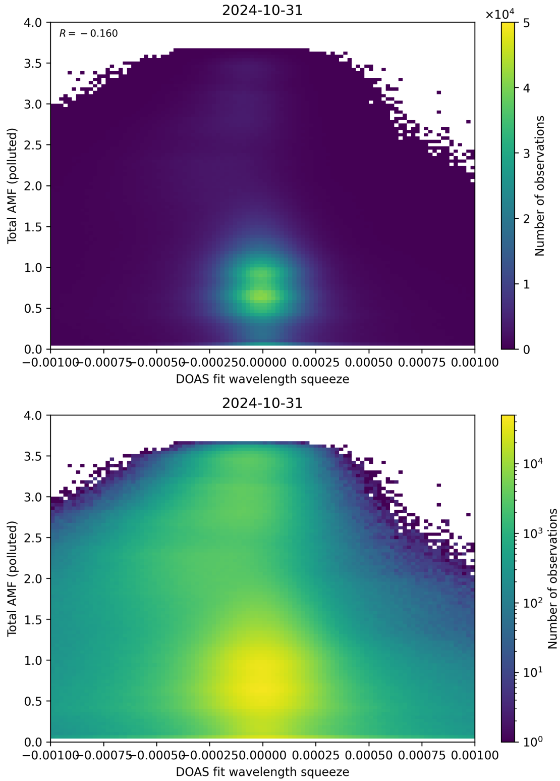
Figure 134: Scatter density plot of “DOAS fit wavelength squeeze” against “Total AMF (polluted)” for 2024-10-30 to 2024-11-01.
