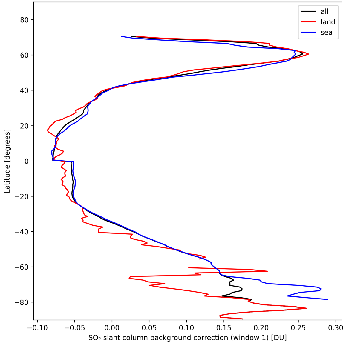
Figure 36: Zonal average of “SO 2 slant column background correction (window 1)” for 2024-10-30 to 2024-11-01.
