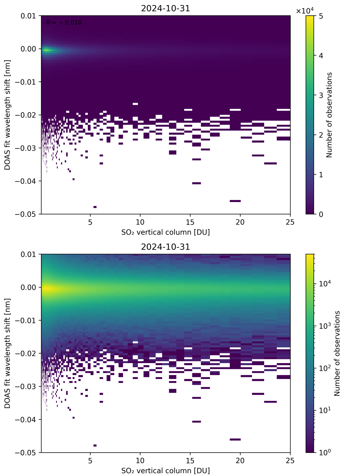
Figure 276: Scatter density plot of “SO 2 vertical column” against “DOAS fit wavelength shift” for 2024-10-30 to 2024-11-01.
