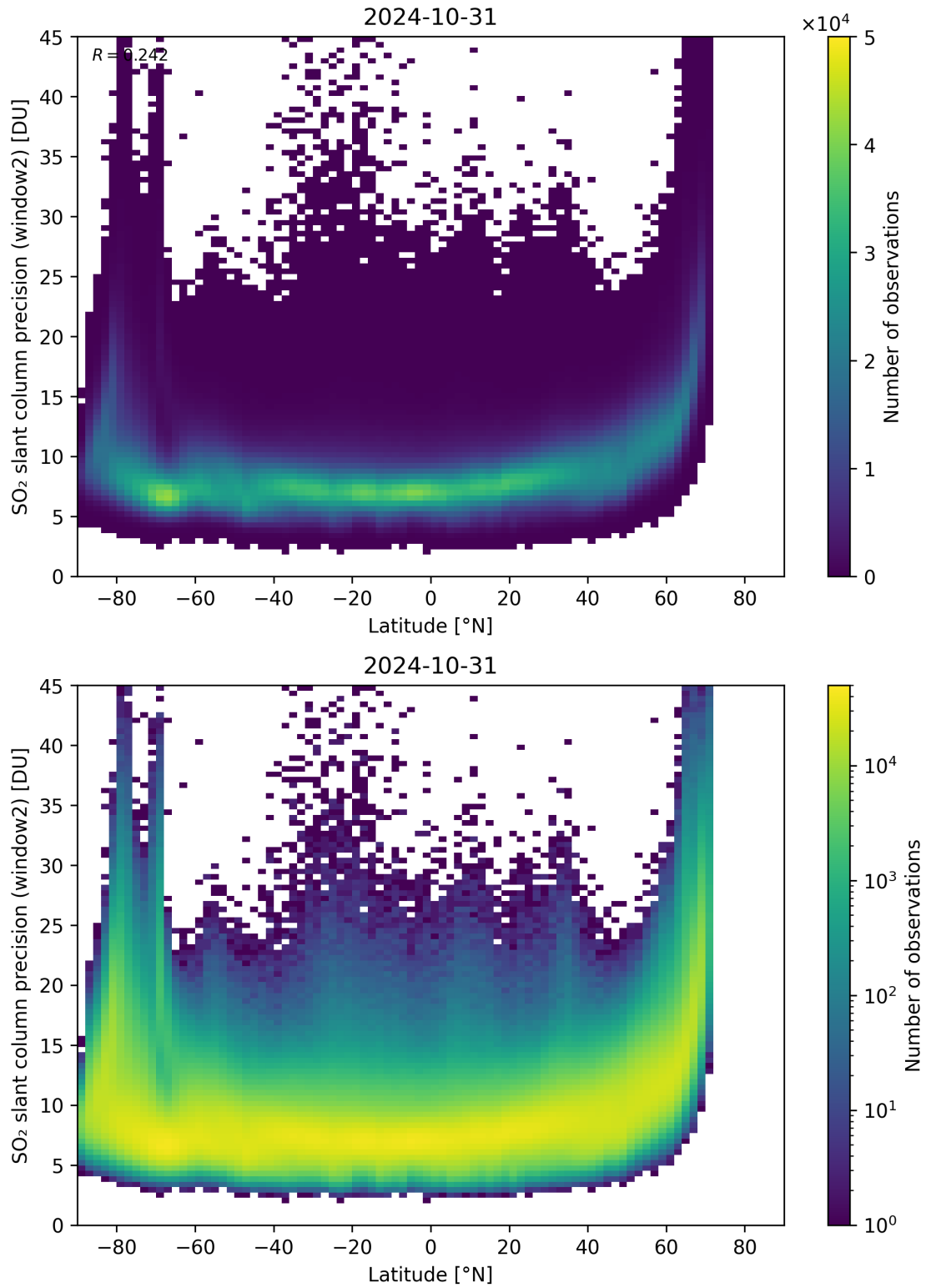
Figure 151: Scatter density plot of “Latitude” against “SO 2 slant column precision (window2)” for 2024-10-30 to 2024-11-01.
