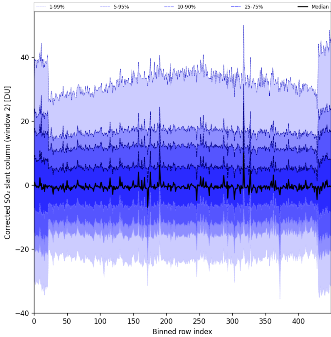
Figure 85: Along track statistics of “Corrected SO 2 slant column (window 2)” for 2024-10-30 to 2024-11-01
