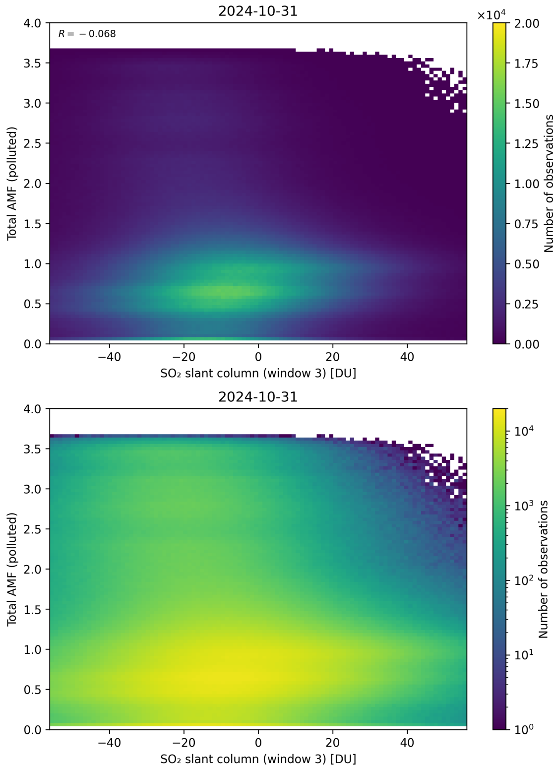
Figure 268: Scatter density plot of “SO 2 slant column (window 3)” against “Total AMF (polluted)” for 2024-10-30 to 2024-11-01.
