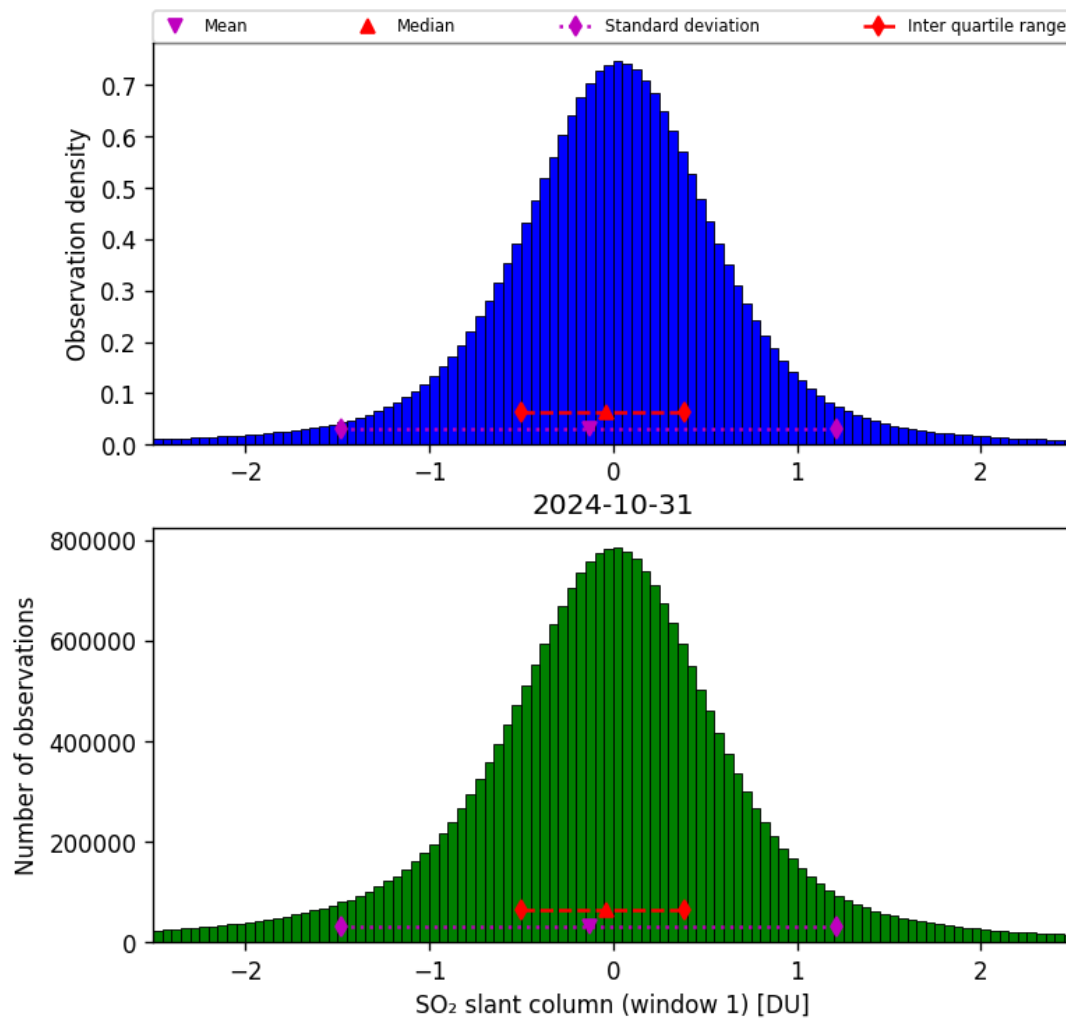
Figure 56: Histogram of “SO 2 slant column (window 1)” for 2024-10-30 to 2024-11-01
