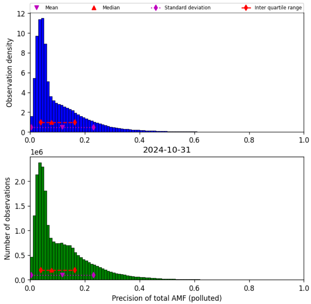
Figure 72: Histogram of “Precision of total AMF (polluted)” for 2024-10-30 to 2024-11-01
