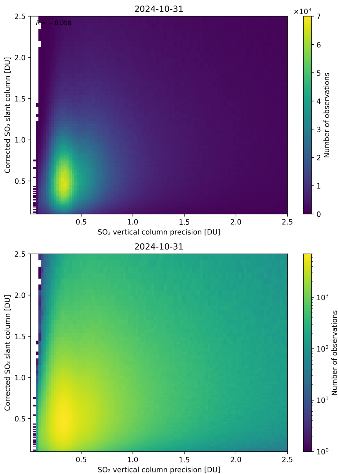
Figure 286: Scatter density plot of “SO 2 vertical column precision” against “Corrected SO 2 slant column” for 2024-10-30 to 2024-11-01.
