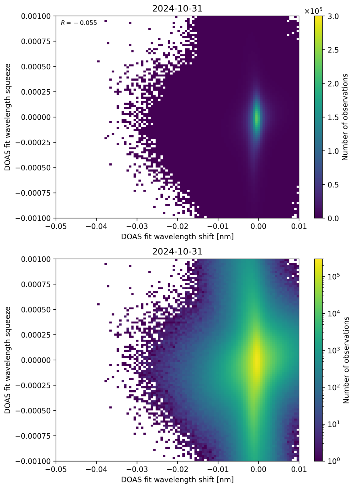
Figure 127: Scatter density plot of “DOAS fit wavelength shift” against “DOAS fit wavelength squeeze” for 2024-10-30 to 2024-11-01.
