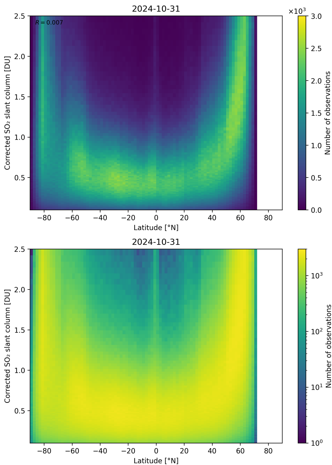
Figure 146: Scatter density plot of “Latitude” against “Corrected SO 2 slant column” for 2024-10-30 to 2024-11-01.
