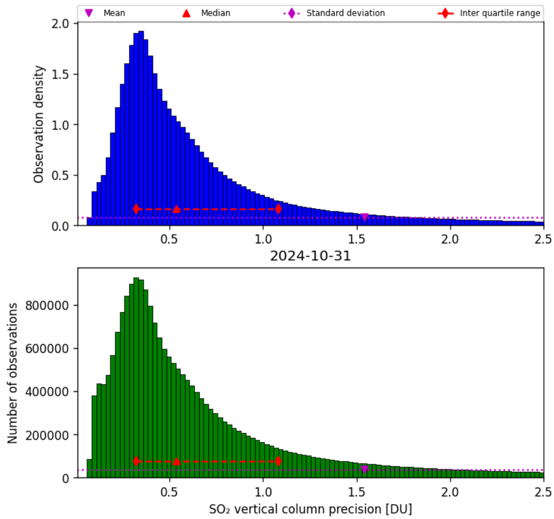
Figure 54: Histogram of “SO 2 vertical column precision” for 2024-10-30 to 2024-11-01
