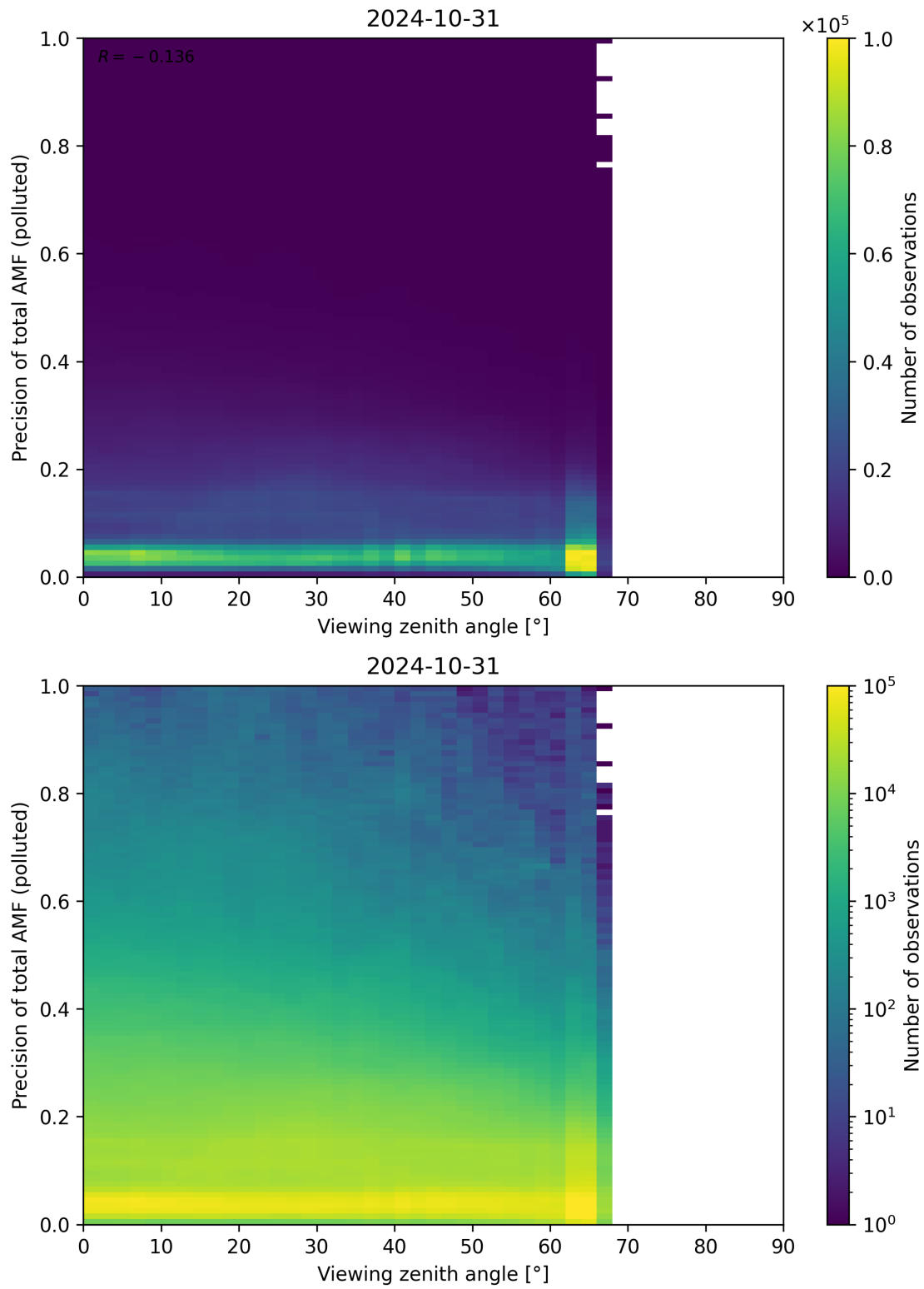
Figure 326: Scatter density plot of “Viewing zenith angle” against “Precision of total AMF (polluted)” for 2024-10-30 to 2024-11-01.
