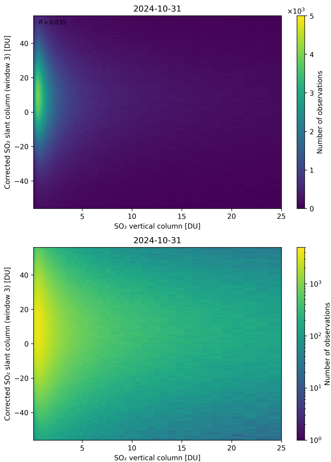
Figure 299: Scatter density plot of “SO 2 vertical column” against “Corrected SO 2 slant column (window 3)” for 2024-10-30 to 2024-11-01.
