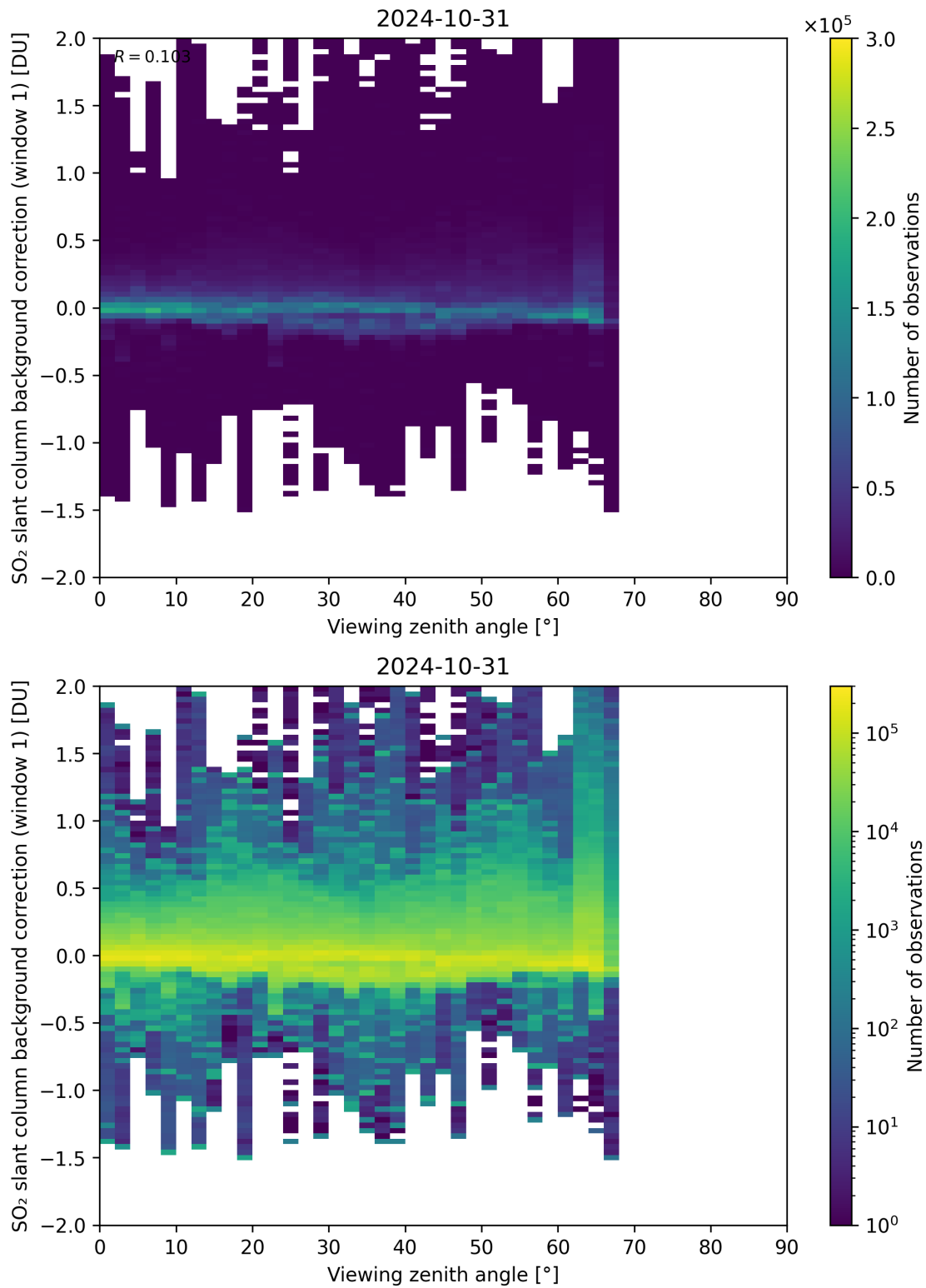
Figure 308: Scatter density plot of “Viewing zenith angle” against “SO 2 slant column background correction (window 1)” for 2024-10-30 to 2024-11-01.
