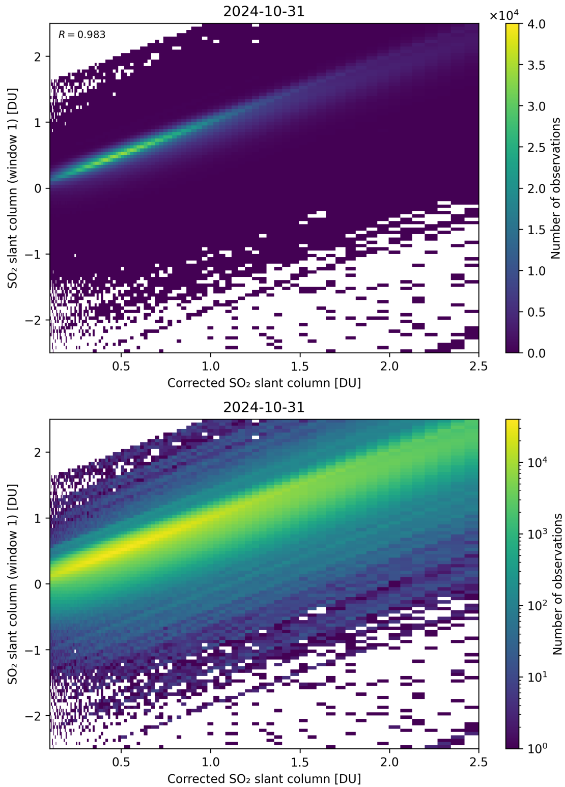
Figure 187: Scatter density plot of “Corrected SO 2 slant column” against “SO 2 slant column (window 1)” for 2024-10-30 to 2024-11-01.
