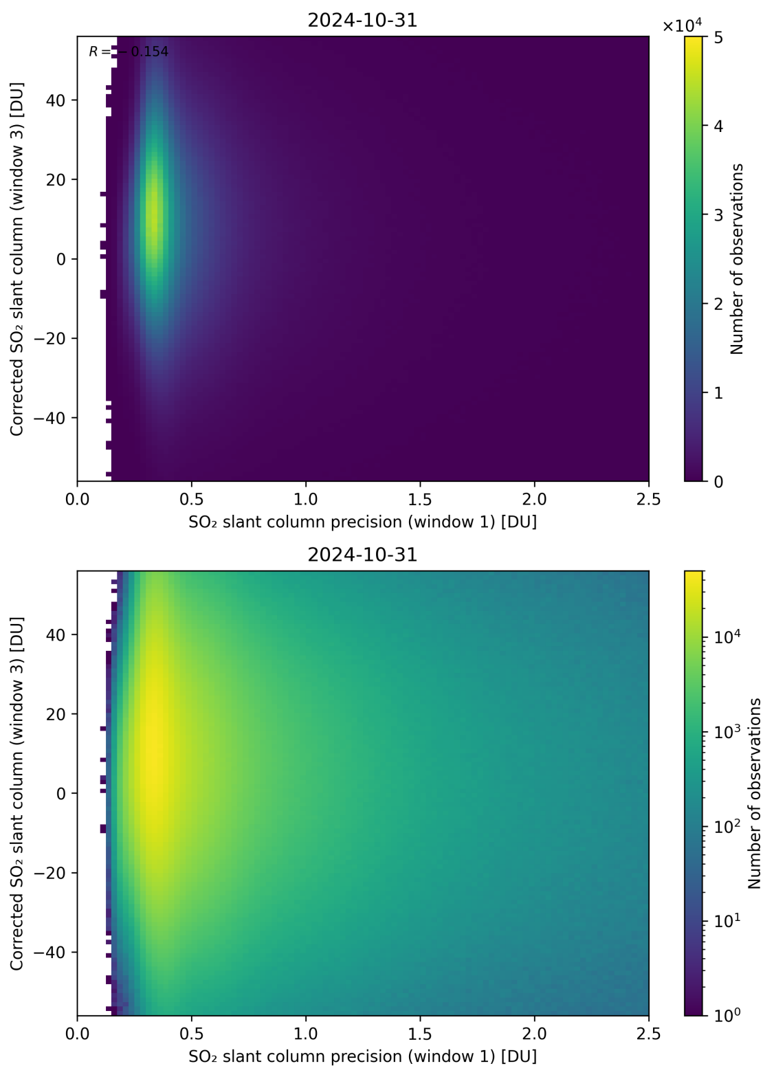
Figure 226: Scatter density plot of “SO 2 slant column precision (window 1)” against “Corrected SO 2 slant column (window 3)” for 2024-10-30 to 2024-11-01.
