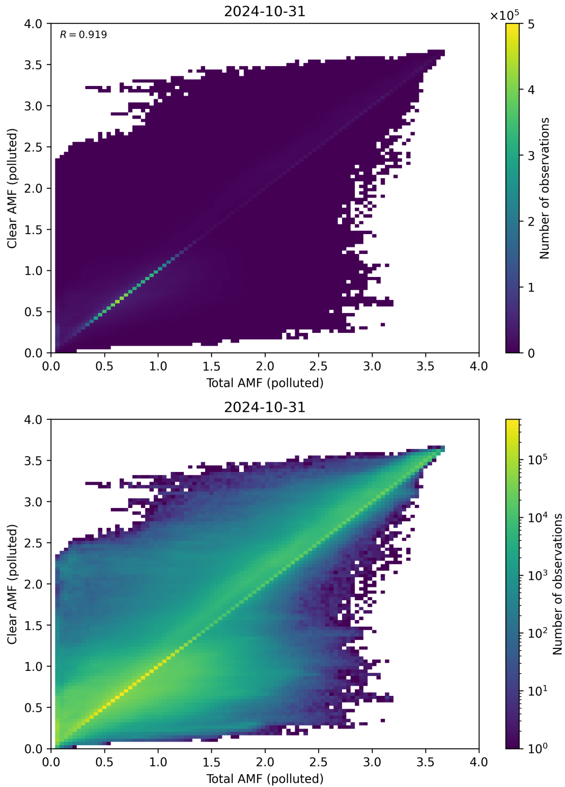
Figure 271: Scatter density plot of “Total AMF (polluted)” against “Clear AMF (polluted)” for 2024-10-30 to 2024-11-01.
