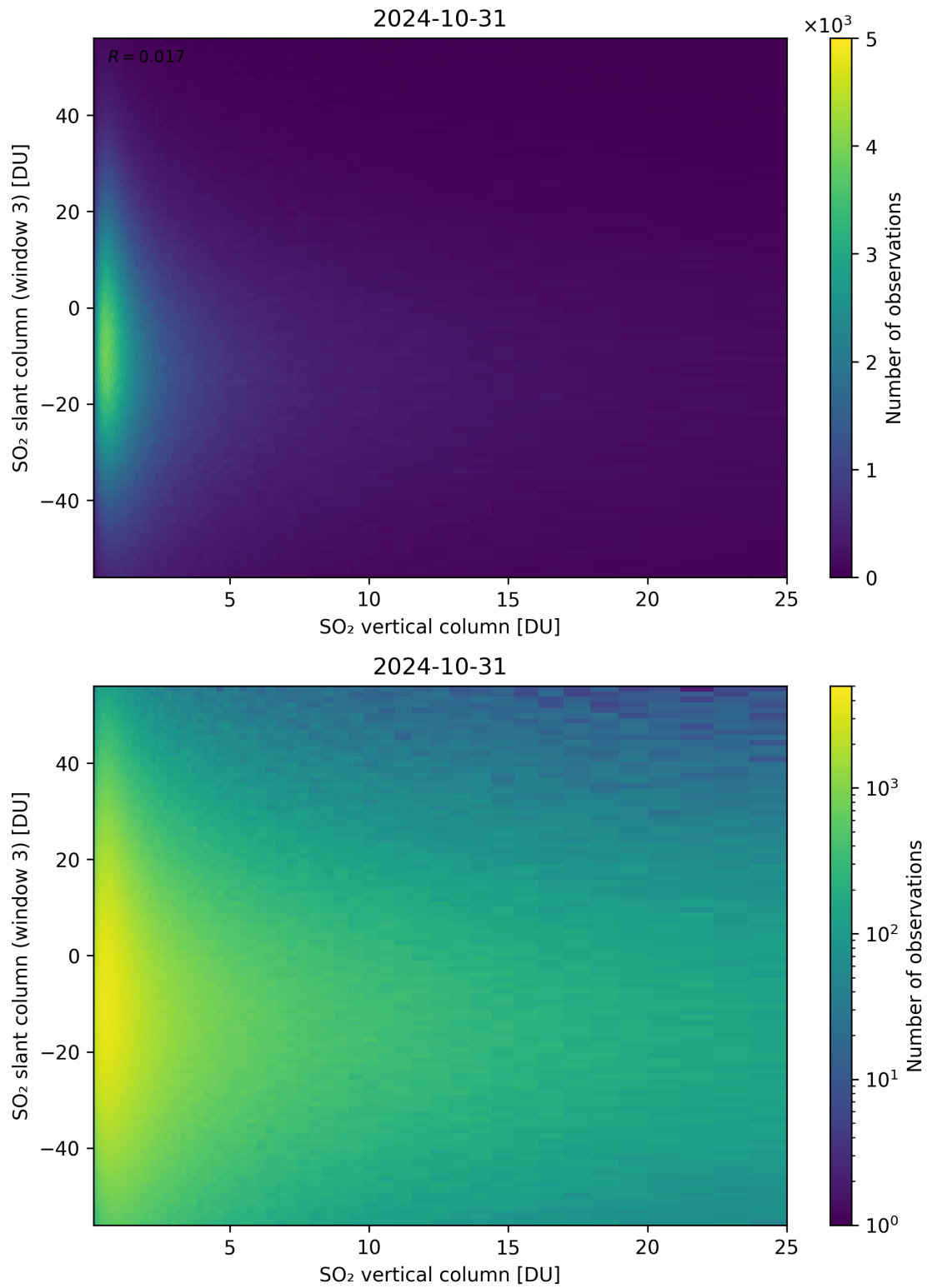
Figure 303: Scatter density plot of “SO 2 vertical column” against “SO 2 slant column (window 3)” for 2024-10-30 to 2024-11-01.
