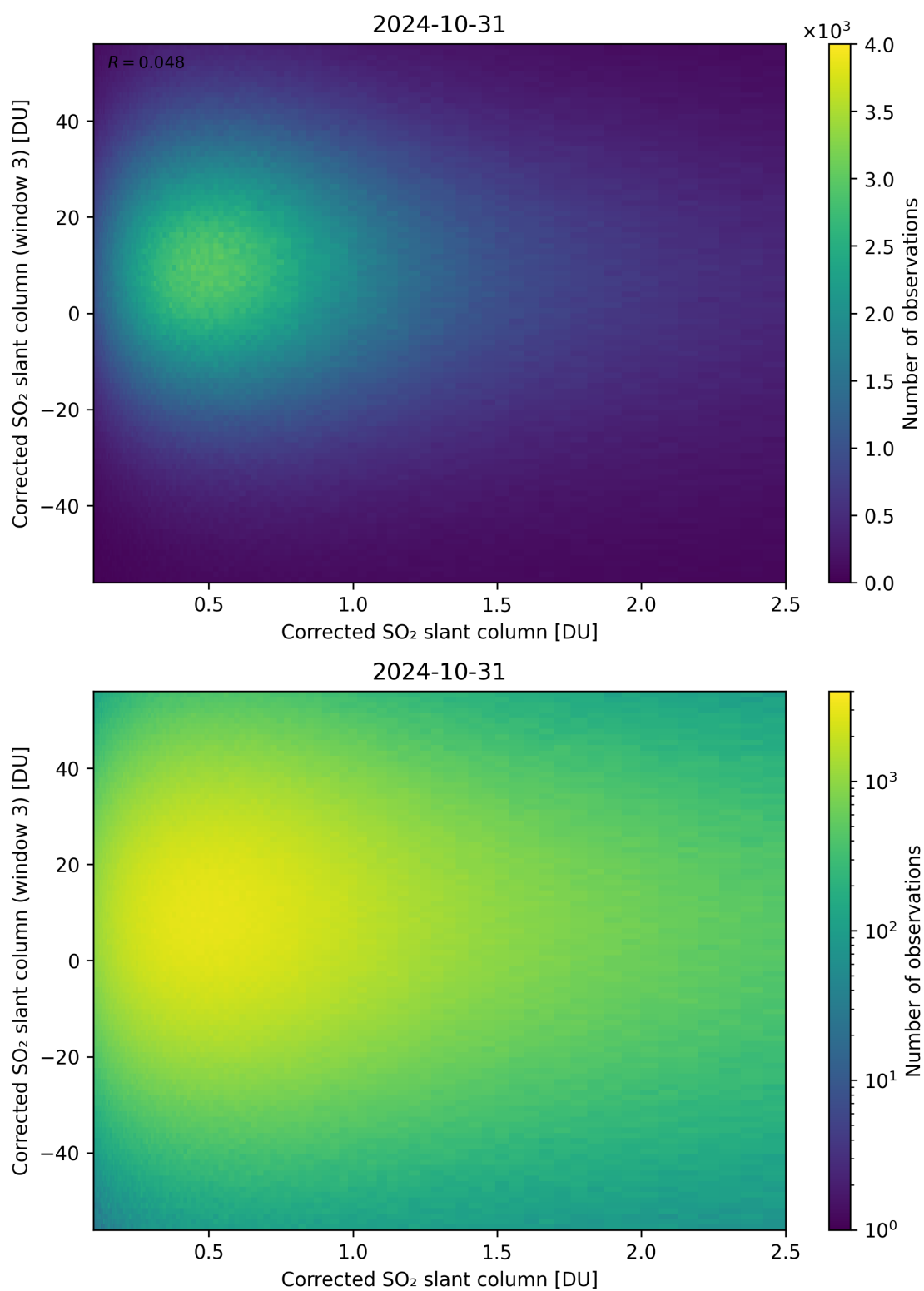
Figure 186: Scatter density plot of “Corrected SO 2 slant column” against “Corrected SO 2 slant column (window 3)” for 2024-10-30 to 2024-11-01.
