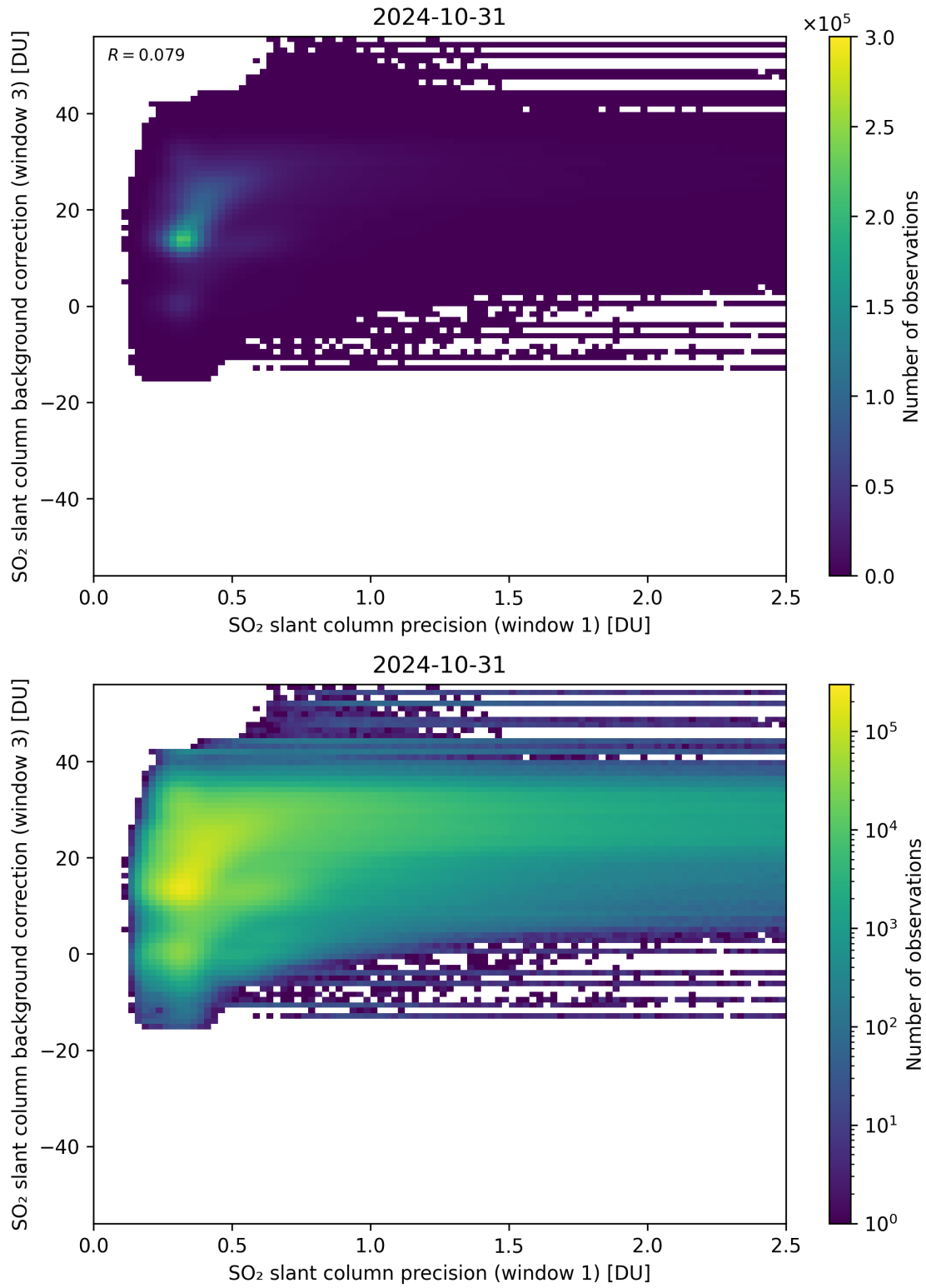
Figure 220: Scatter density plot of “SO 2 slant column precision (window 1)” against “SO 2 slant column background correction (window 3)” for 2024-10-30 to 2024-11-01.
