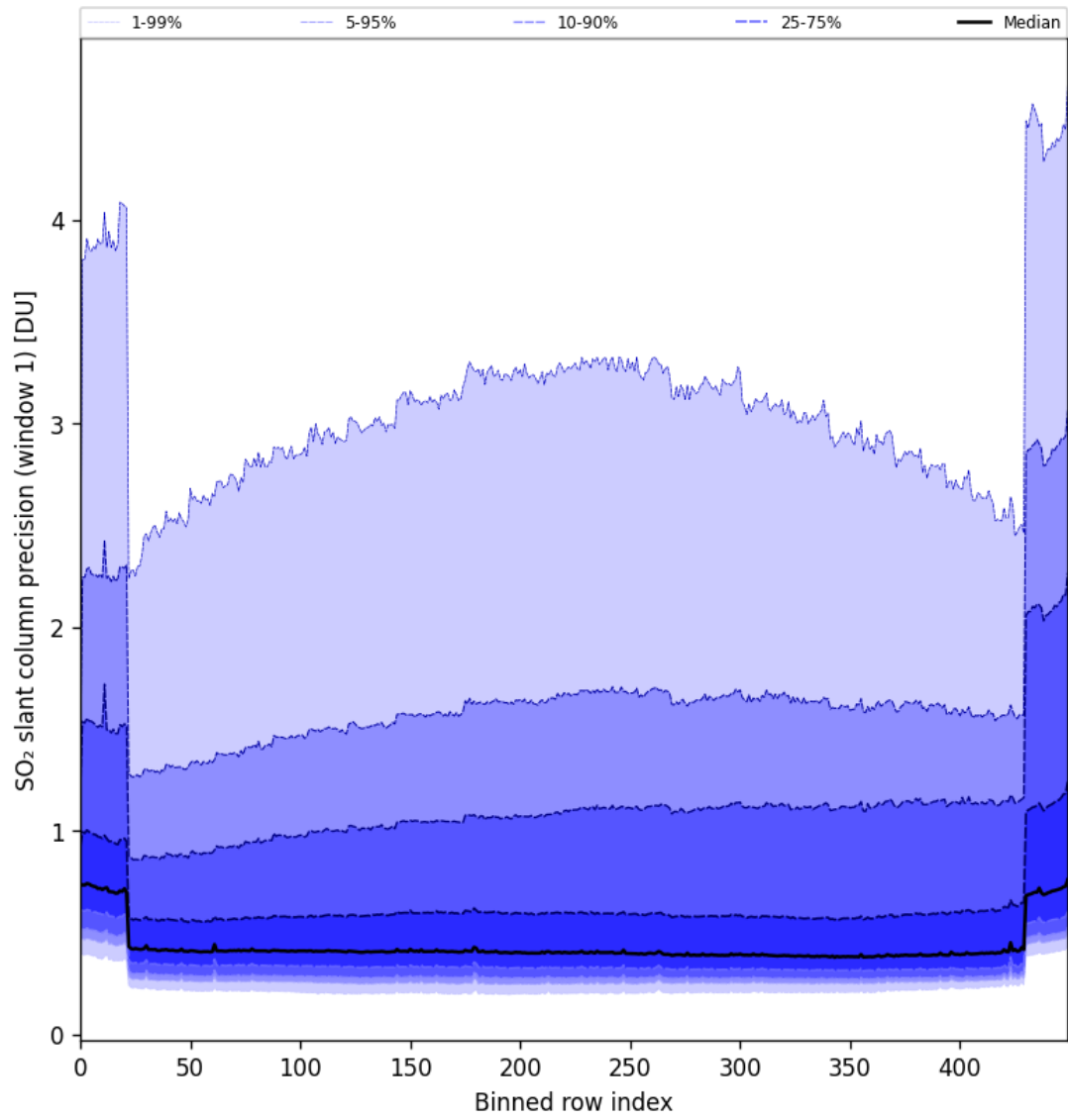
Figure 80: Along track statistics of “SO 2 slant column precision (window 1)” for 2024-10-30 to 2024-11-01
