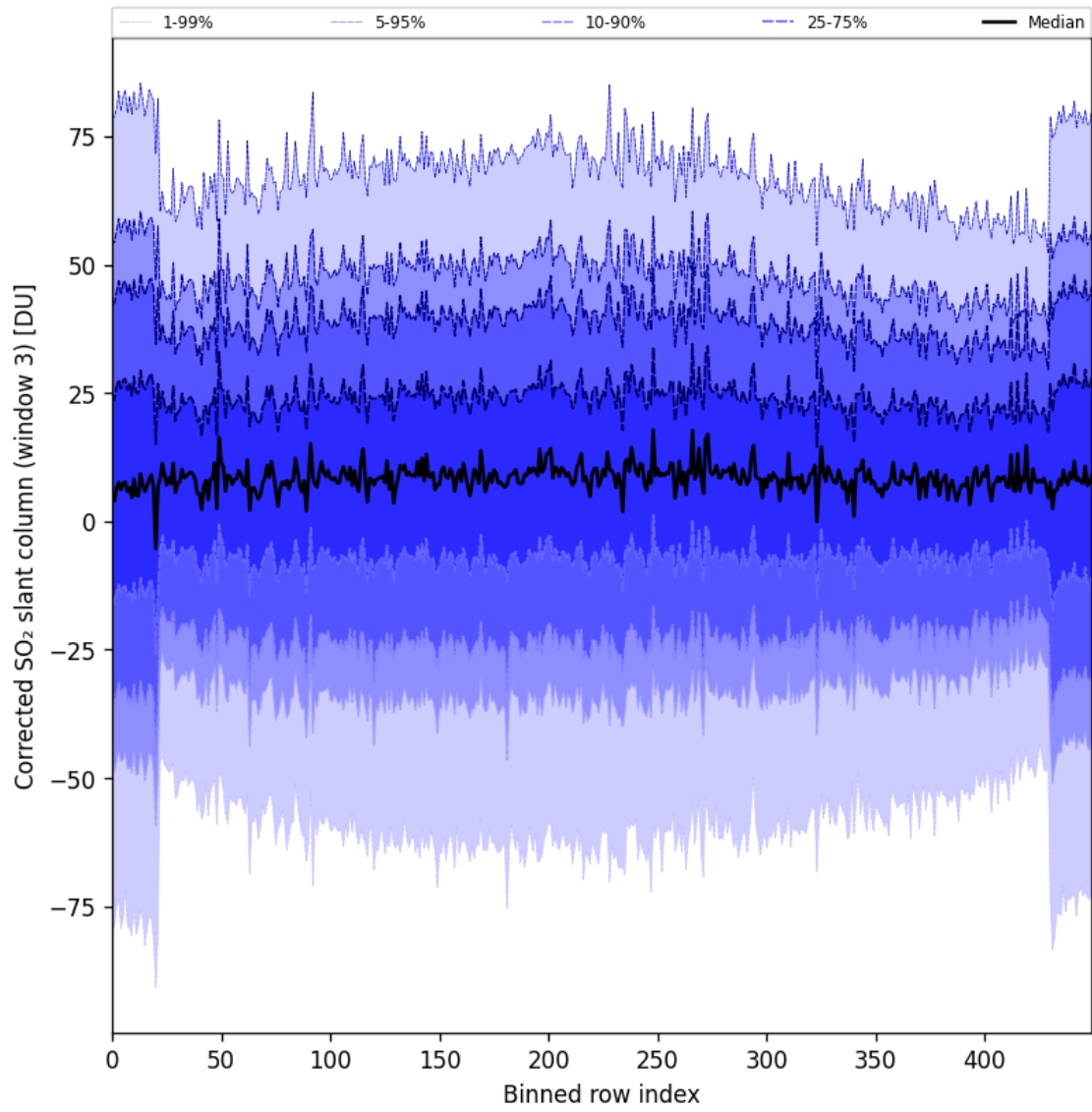
Figure 89: Along track statistics of “Corrected SO 2 slant column (window 3)” for 2024-10-30 to 2024-11-01
