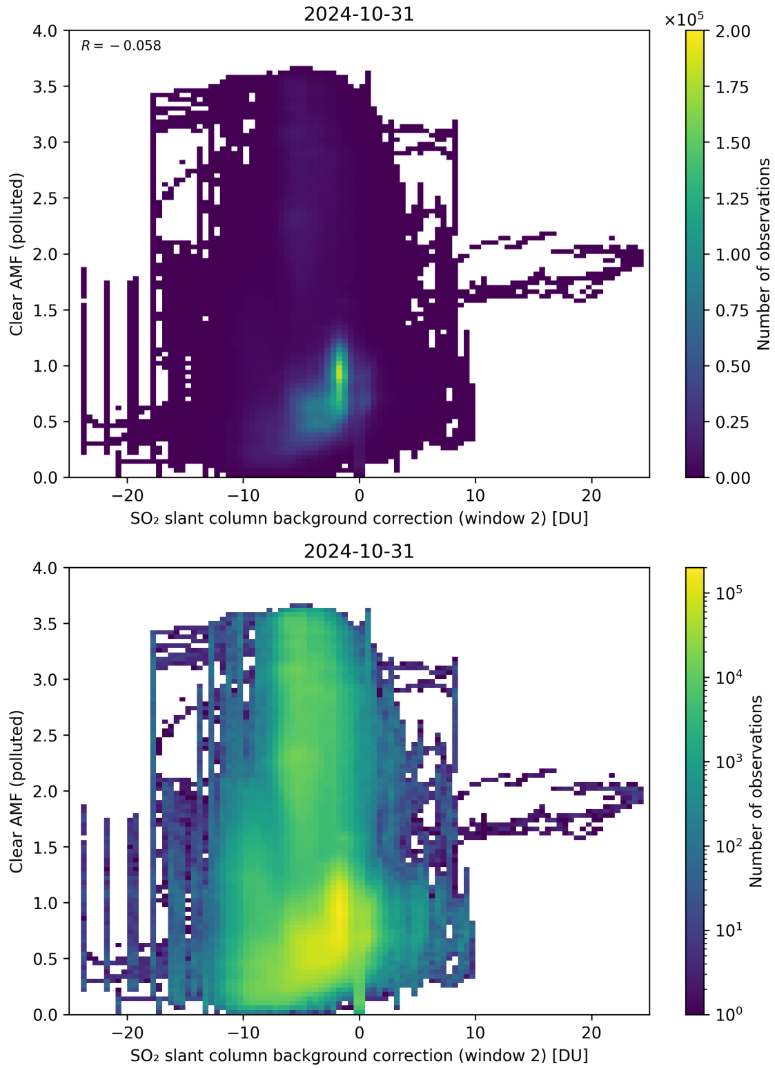
Figure 115: Scatter density plot of “SO 2 slant column background correction (window 2)” against “Clear AMF (polluted)” for 2024-10-30 to 2024-11-01.
