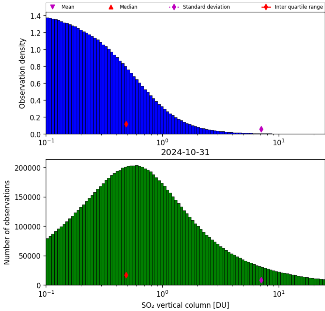
Figure 53: Histogram of “SO 2 vertical column” for 2024-10-30 to 2024-11-01
