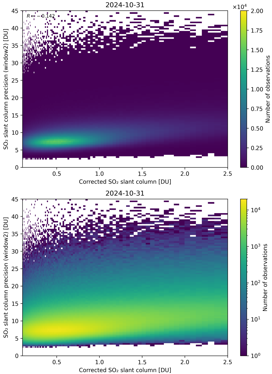
Figure 189: Scatter density plot of “Corrected SO 2 slant column” against “SO 2 slant column precision (window2)” for 2024-10-30 to 2024-11-01.
