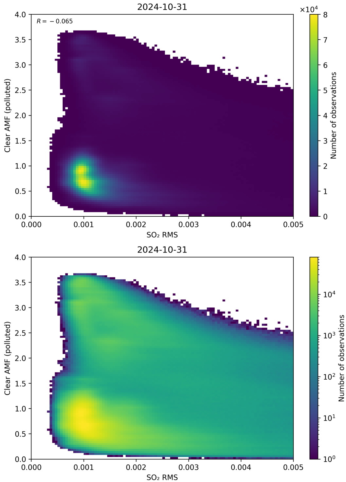
Figure 136: Scatter density plot of “SO 2 RMS” against “Clear AMF (polluted)” for 2024-10-30 to 2024-11-01.
