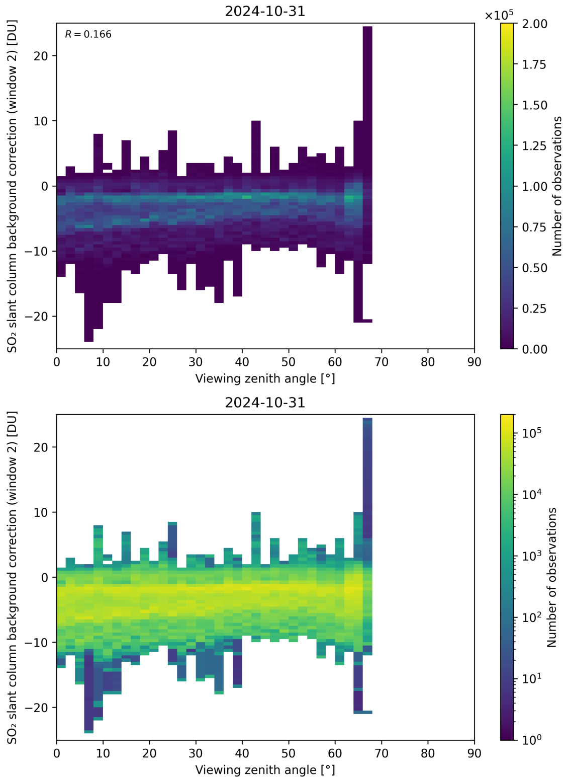
Figure 309: Scatter density plot of “Viewing zenith angle” against “SO 2 slant column background correction (window 2)” for 2024-10-30 to 2024-11-01.
