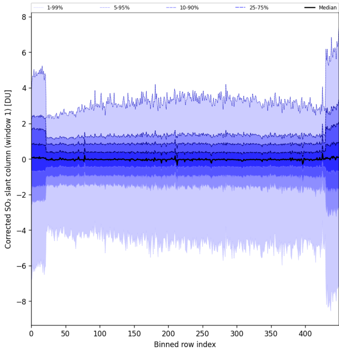
Figure 81: Along track statistics of “Corrected SO 2 slant column (window 1)” for 2024-10-30 to 2024-11-01
