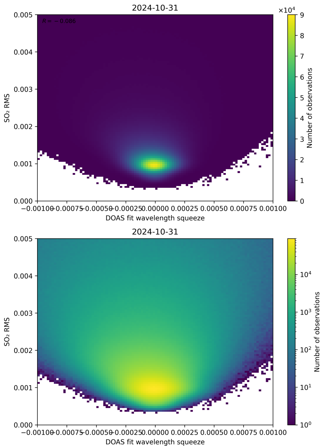
Figure 132: Scatter density plot of “DOAS fit wavelength squeeze” against “SO 2 RMS” for 2024-10-30 to 2024-11-01.
