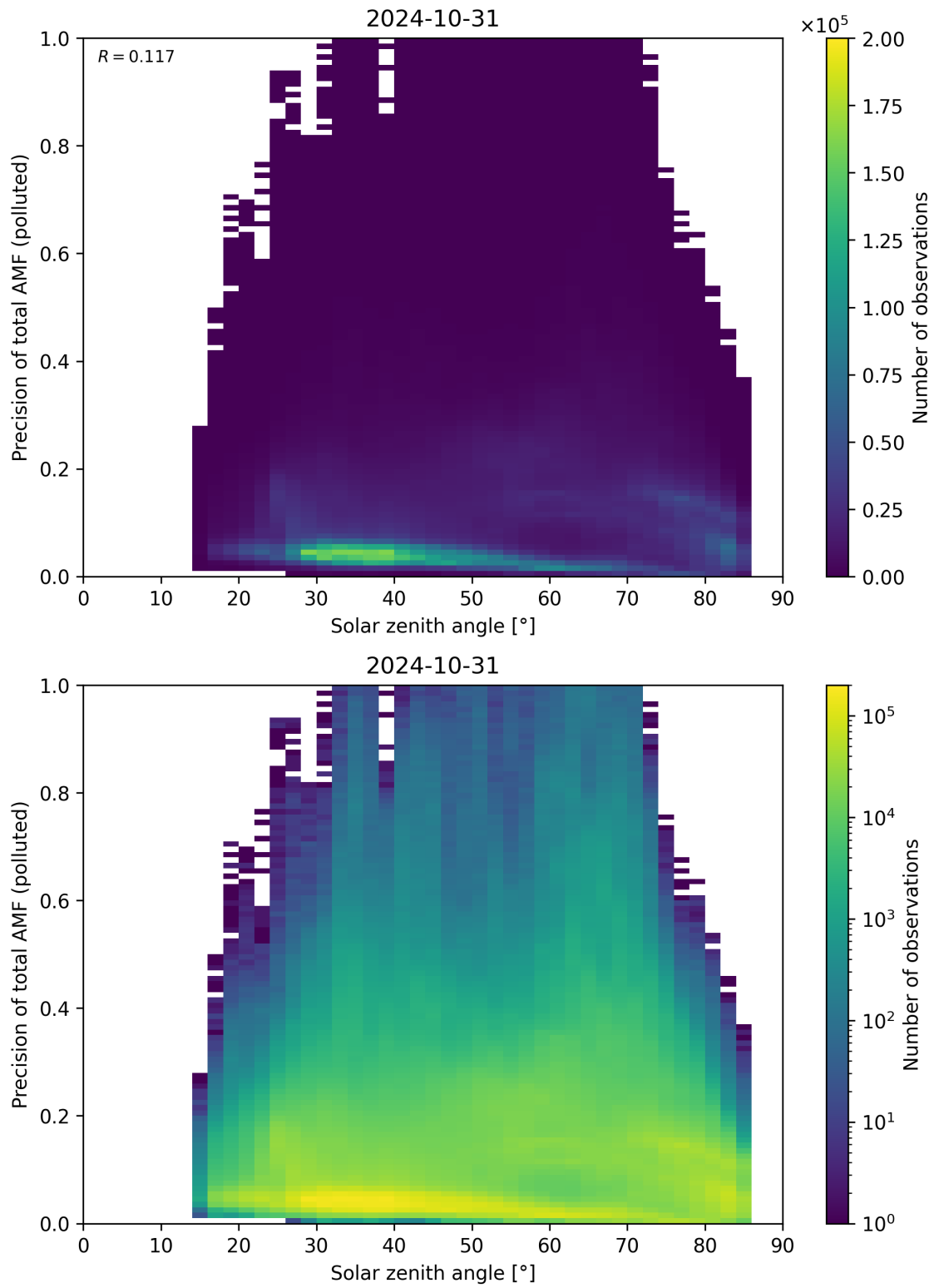
Figure 175: Scatter density plot of “Solar zenith angle” against “Precision of total AMF (polluted)” for 2024-10-30 to 2024-11-01.
