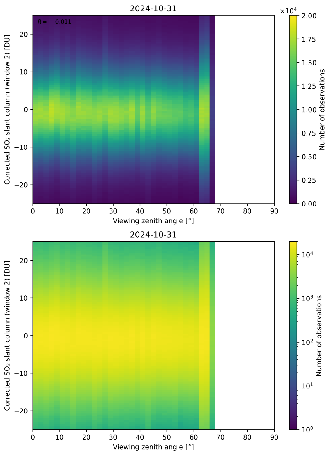
Figure 318: Scatter density plot of “Viewing zenith angle” against “Corrected SO 2 slant column (window 2)” for 2024-10-30 to 2024-11-01.
