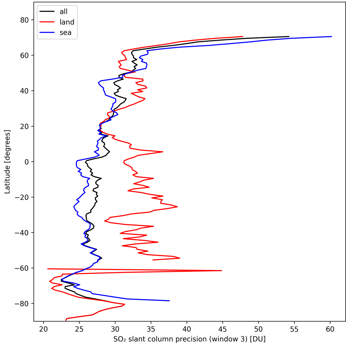
Figure 42: Zonal average of “SO 2 slant column precision (window 3)” for 2024-10-30 to 2024-11-01.
