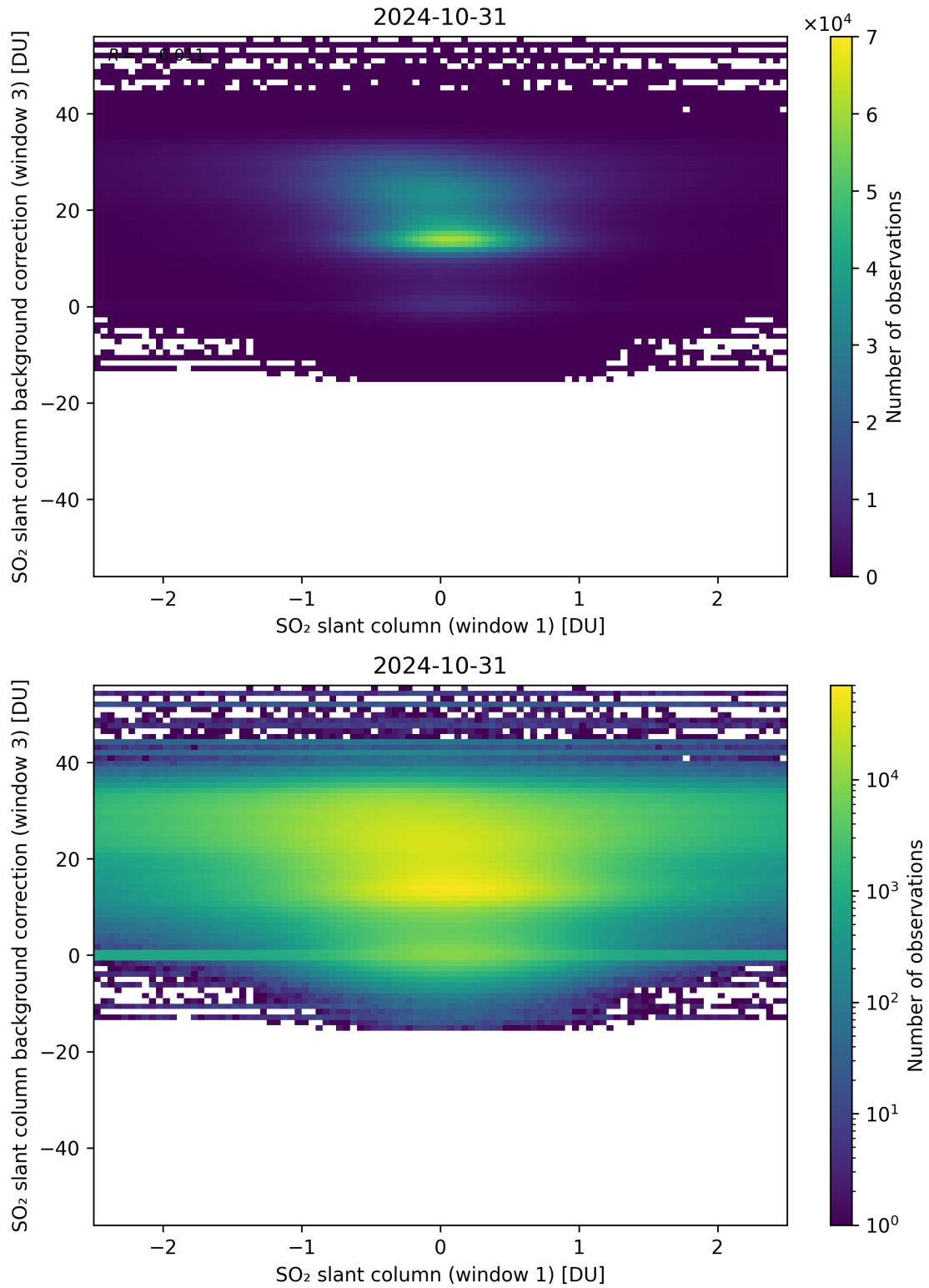
Figure 214: Scatter density plot of “SO 2 slant column (window 1)” against “SO 2 slant column background correction (window 3)” for 2024-10-30 to 2024-11-01.
