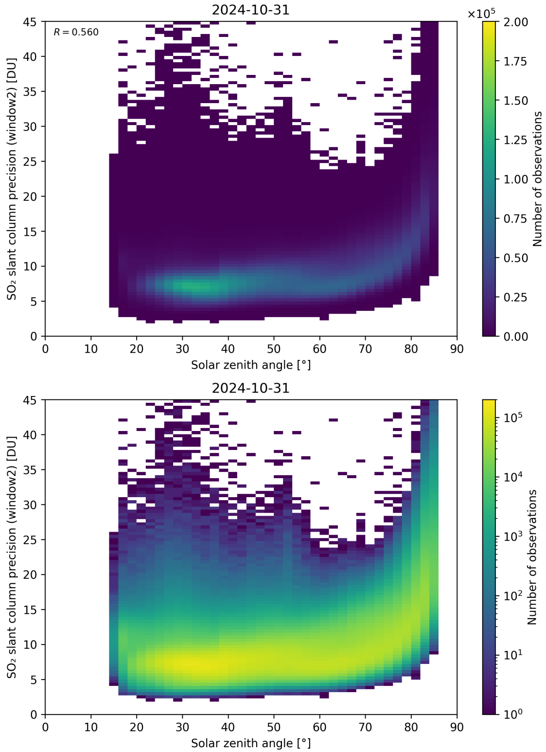
Figure 171: Scatter density plot of “Solar zenith angle” against “SO 2 slant column precision (window2)” for 2024-10-30 to 2024-11-01.
