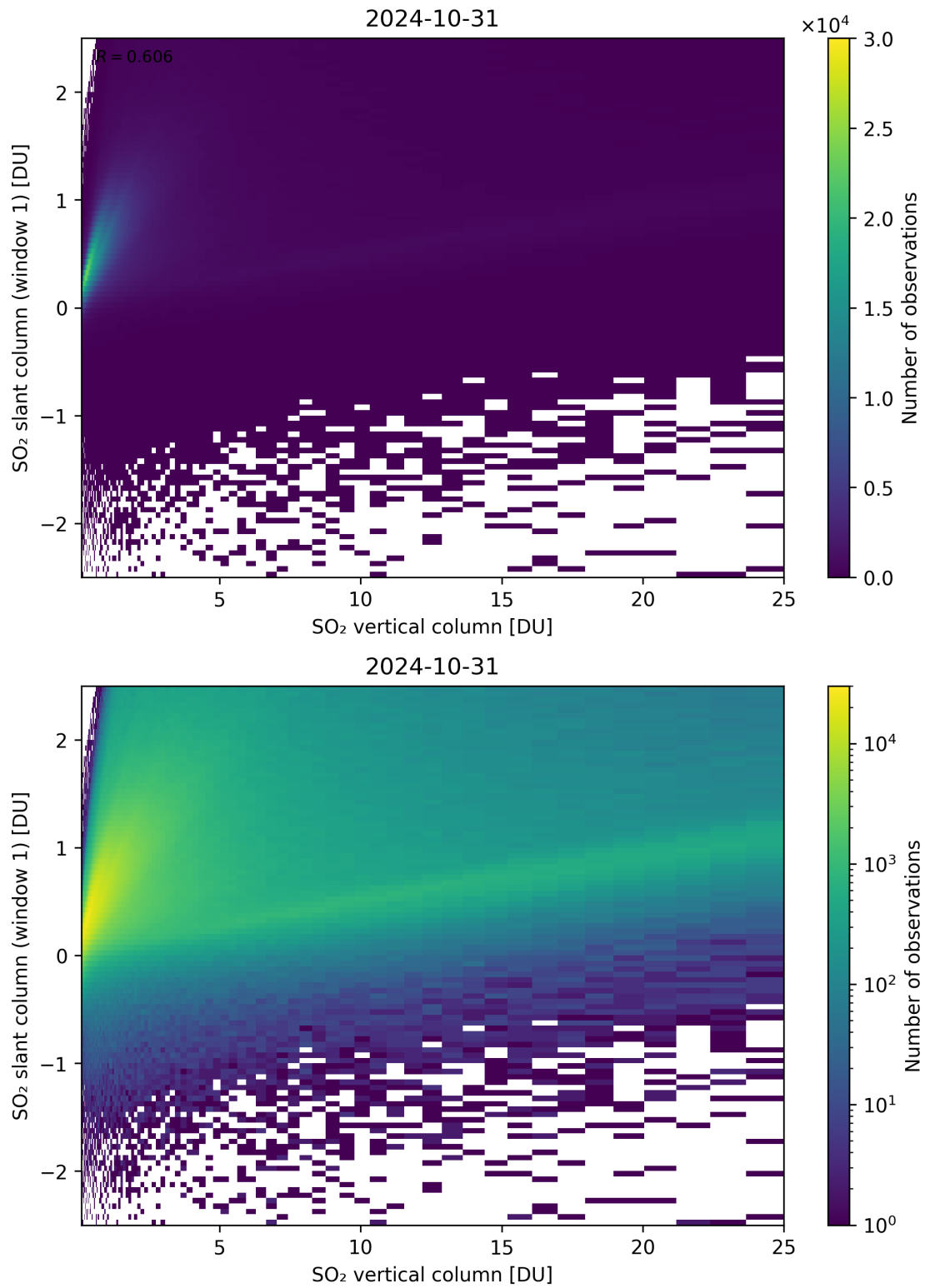
Figure 300: Scatter density plot of “SO 2 vertical column” against “SO 2 slant column (window 1)” for 2024-10-30 to 2024-11-01.
