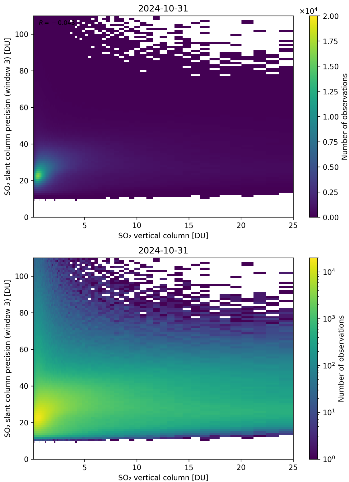
Figure 304: Scatter density plot of “SO 2 vertical column” against “SO 2 slant column precision (window 3)” for 2024-10-30 to 2024-11-01.
