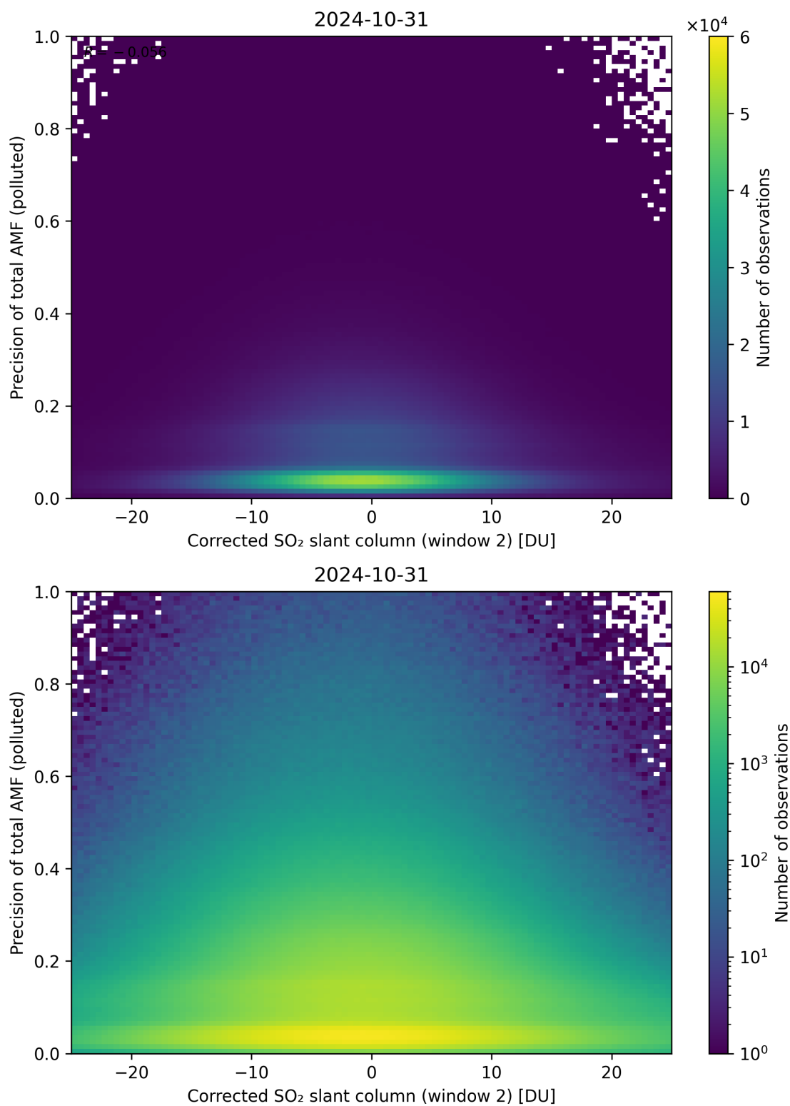
Figure 204: Scatter density plot of “Corrected SO 2 slant column (window 2)” against “Precision of total AMF (polluted)” for 2024-10-30 to 2024-11-01.
