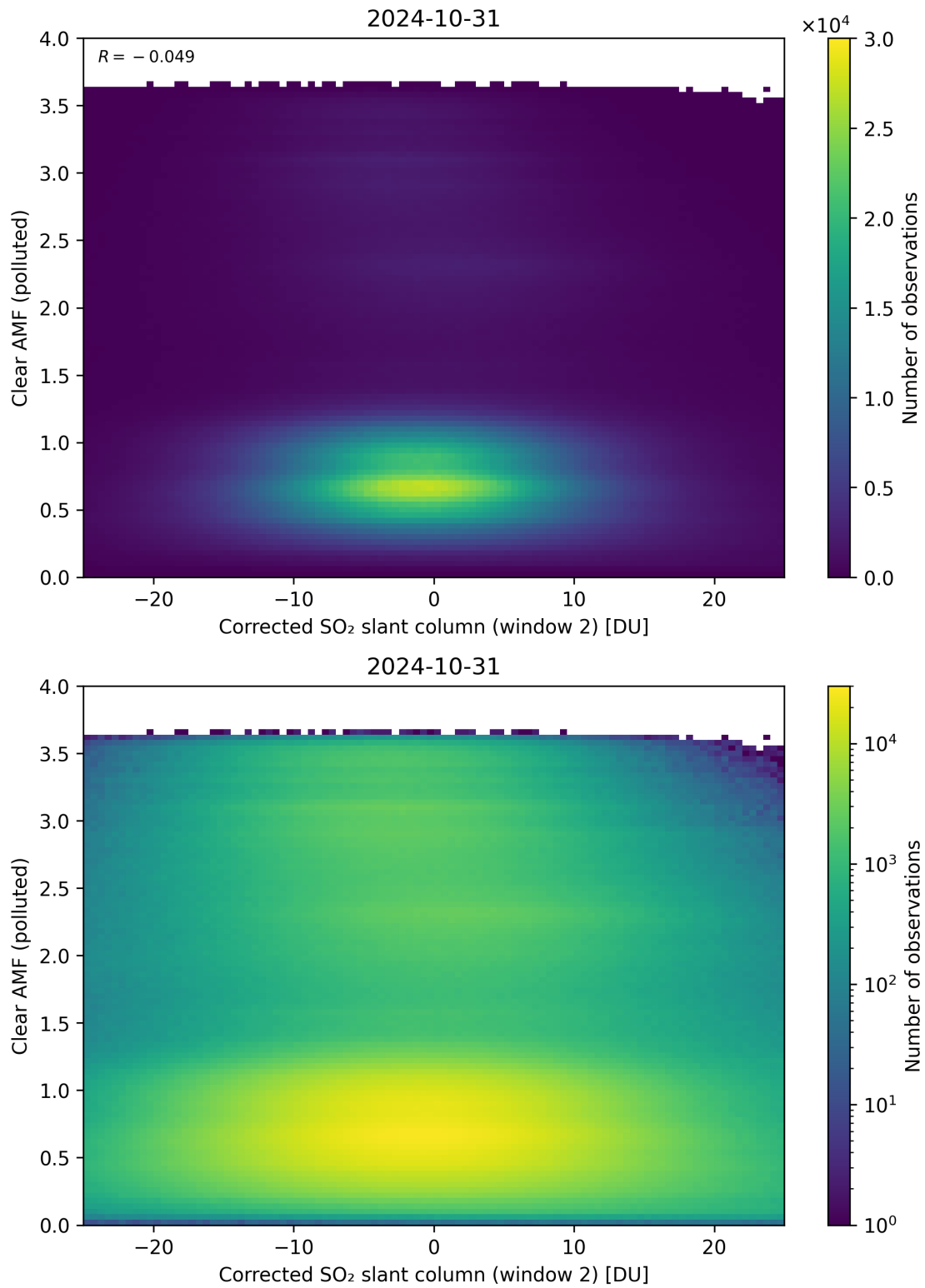
Figure 199: Scatter density plot of “Corrected SO 2 slant column (window 2)” against “Clear AMF (polluted)” for 2024-10-30 to 2024-11-01.
