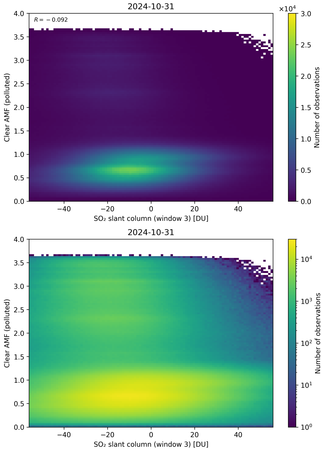
Figure 265: Scatter density plot of “SO 2 slant column (window 3)” against “Clear AMF (polluted)” for 2024-10-30 to 2024-11-01.
