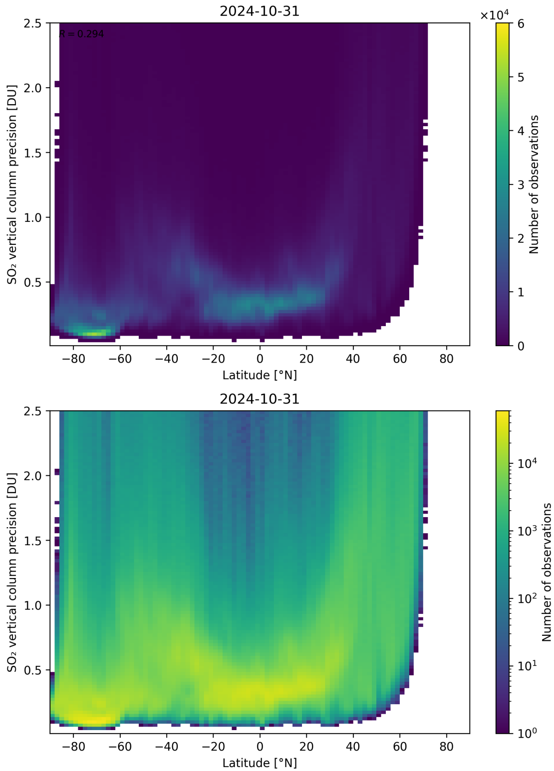
Figure 157: Scatter density plot of “Latitude” against “SO 2 vertical column precision” for 2024-10-30 to 2024-11-01.
