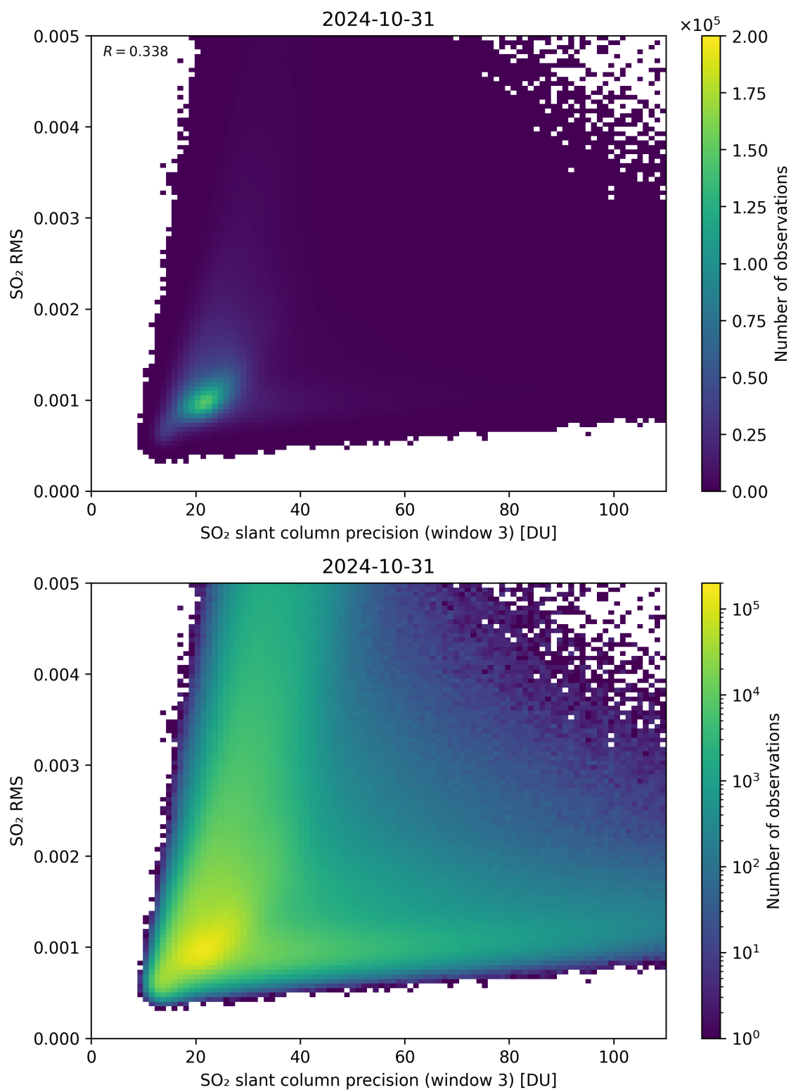
Figure 260: Scatter density plot of “SO 2 slant column precision (window 3)” against “SO 2 RMS” for 2024-10-30 to 2024-11-01.
