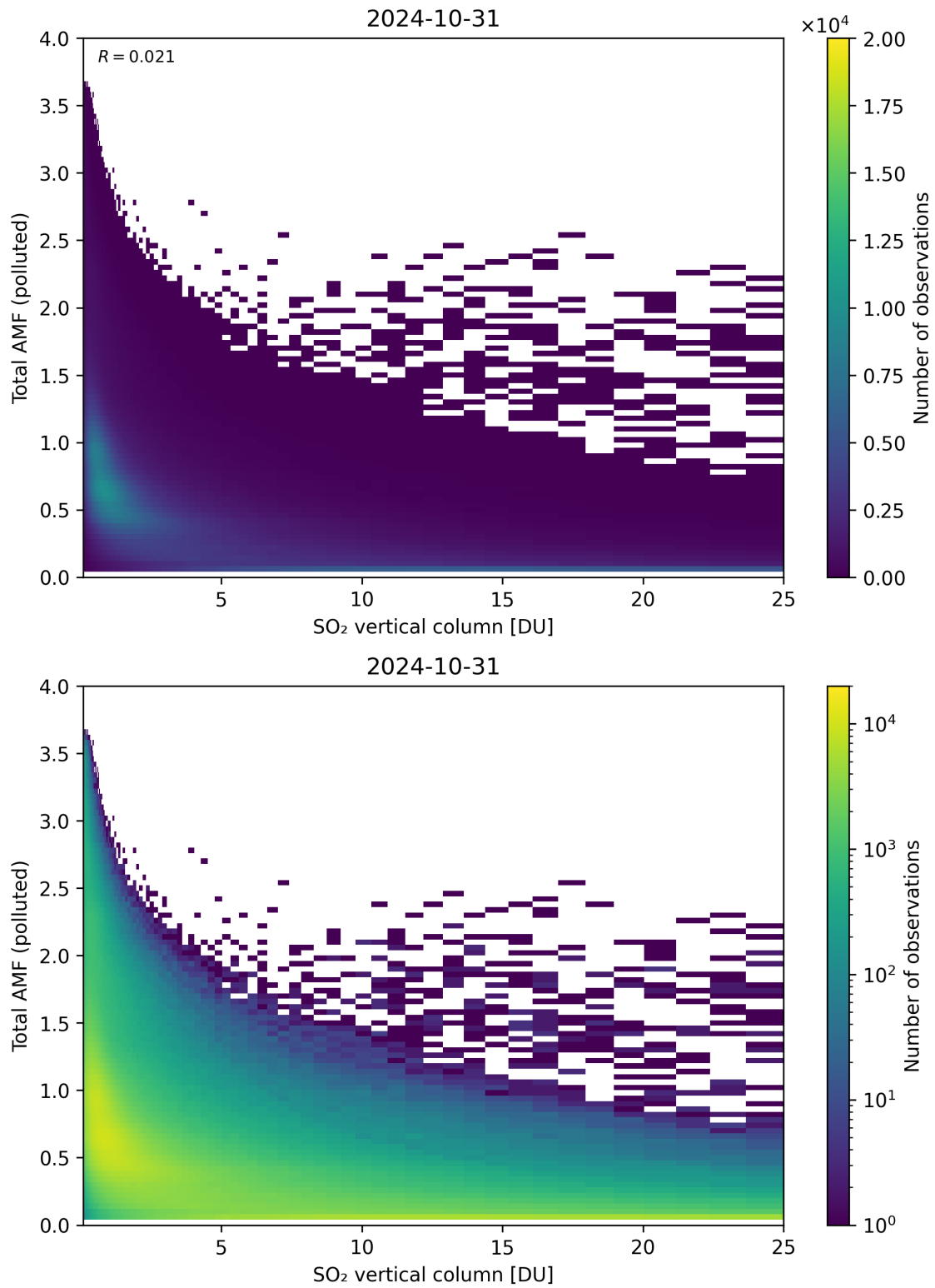
Figure 305: Scatter density plot of “SO 2 vertical column” against “Total AMF (polluted)” for 2024-10-30 to 2024-11-01.
