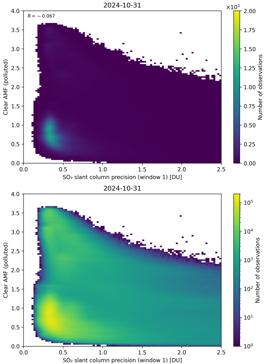
Figure 224: Scatter density plot of “SO 2 slant column precision (window 1)” against “Clear AMF (polluted)” for 2024-10-30 to 2024-11-01.
