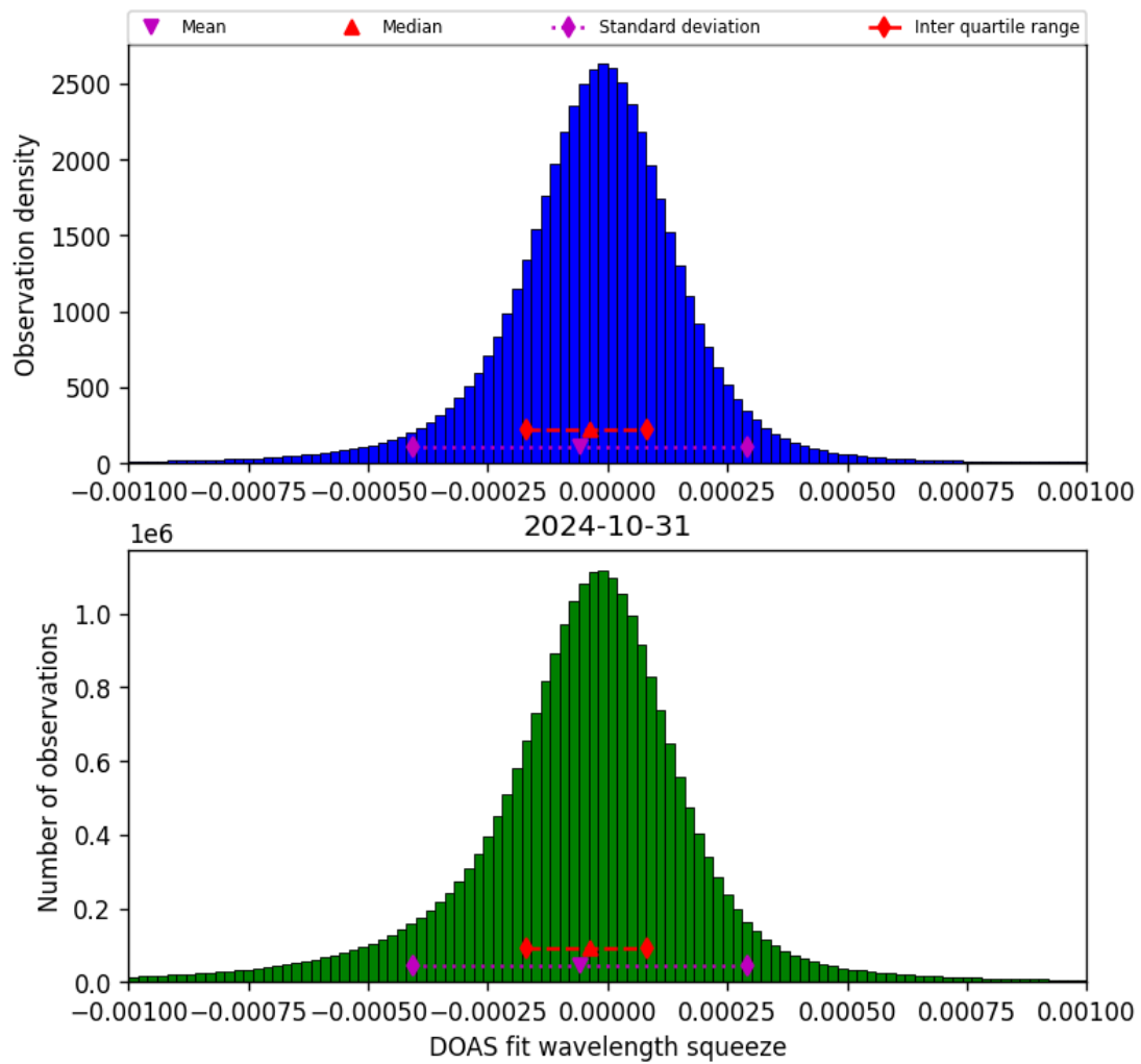
Figure 69: Histogram of “DOAS fit wavelength squeeze” for 2024-10-30 to 2024-11-01
