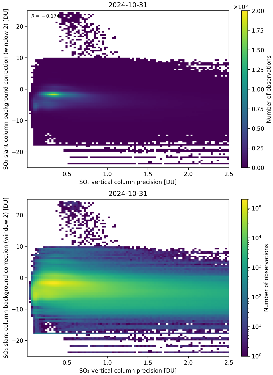
Figure 280: Scatter density plot of “SO 2 vertical column precision” against “SO 2 slant column background correction (window 2)” for 2024-10-30 to 2024-11-01.
