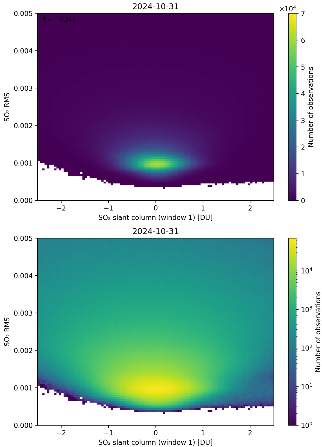
Figure 217: Scatter density plot of “SO 2 slant column (window 1)” against “SO 2 RMS” for 2024-10-30 to 2024-11-01.
