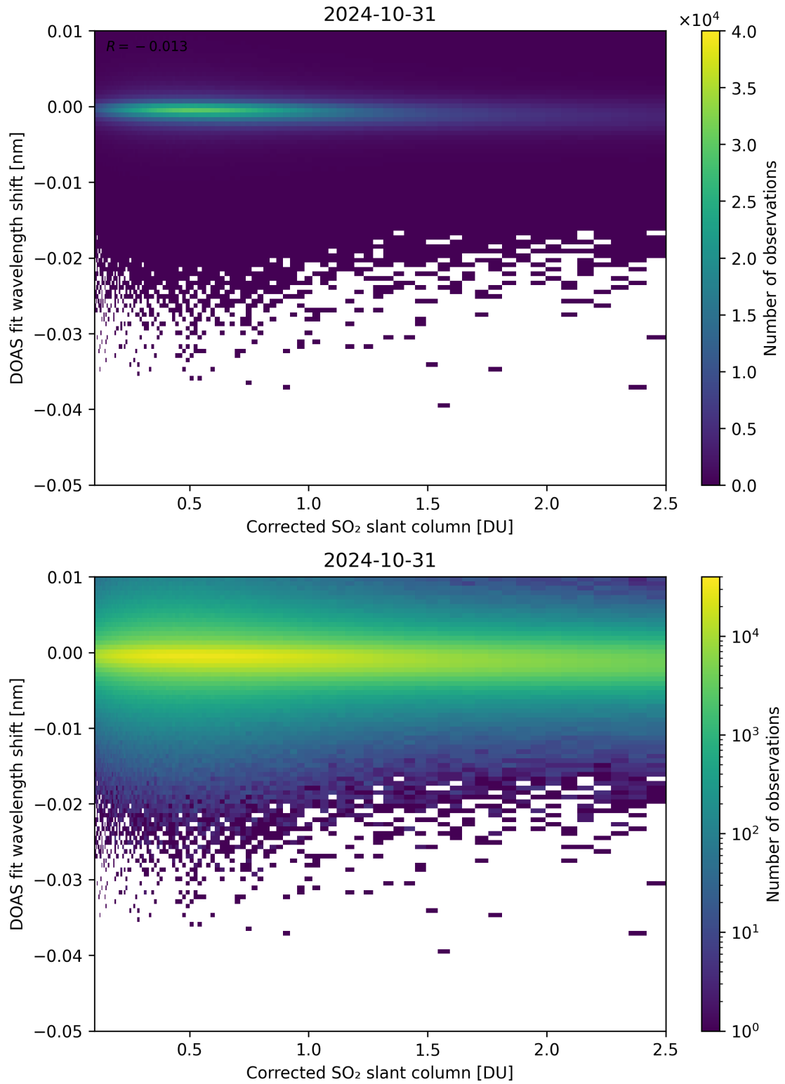
Figure 181: Scatter density plot of “Corrected SO 2 slant column” against “DOAS fit wavelength shift” for 2024-10-30 to 2024-11-01.
