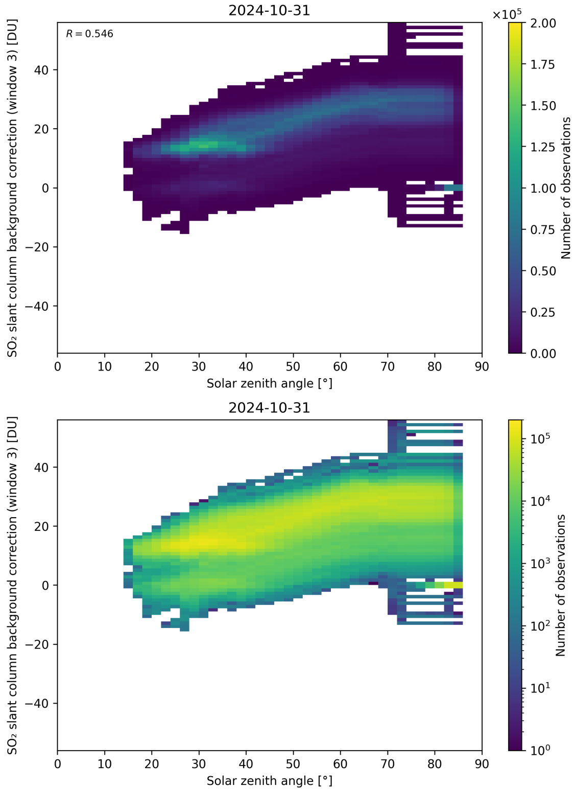
Figure 160: Scatter density plot of “Solar zenith angle” against “SO 2 slant column background correction (window 3)” for 2024-10-30 to 2024-11-01.
