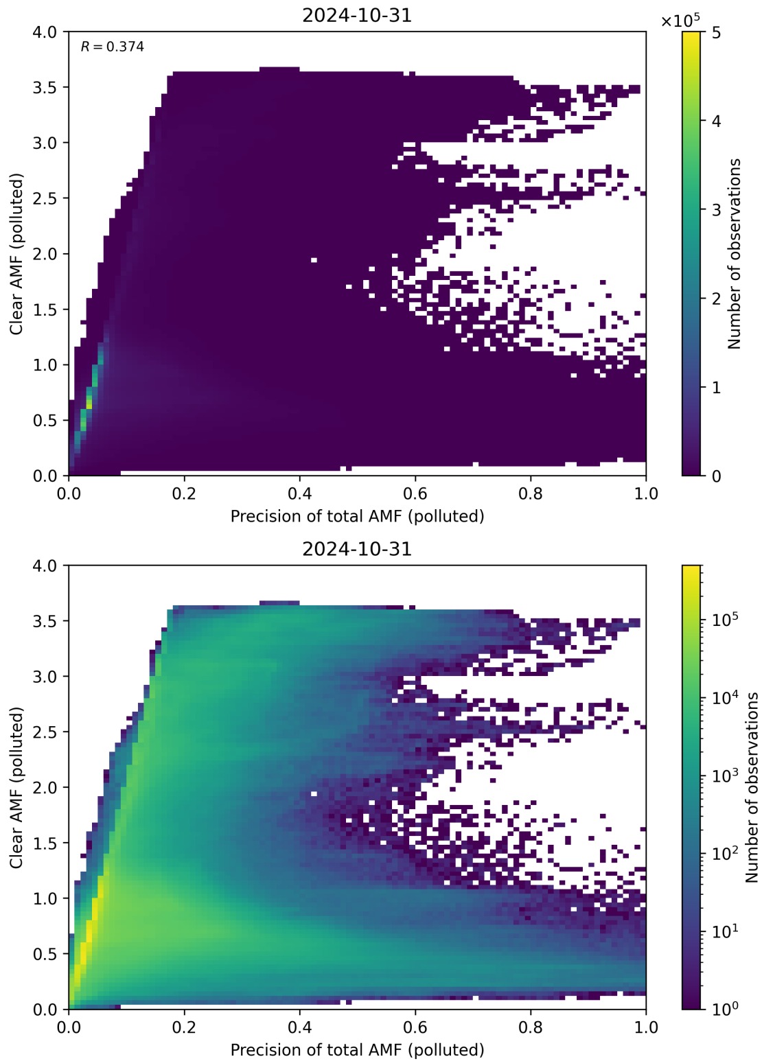
Figure 270: Scatter density plot of “Precision of total AMF (polluted)” against “Clear AMF (polluted)” for 2024-10-30 to 2024-11-01.
