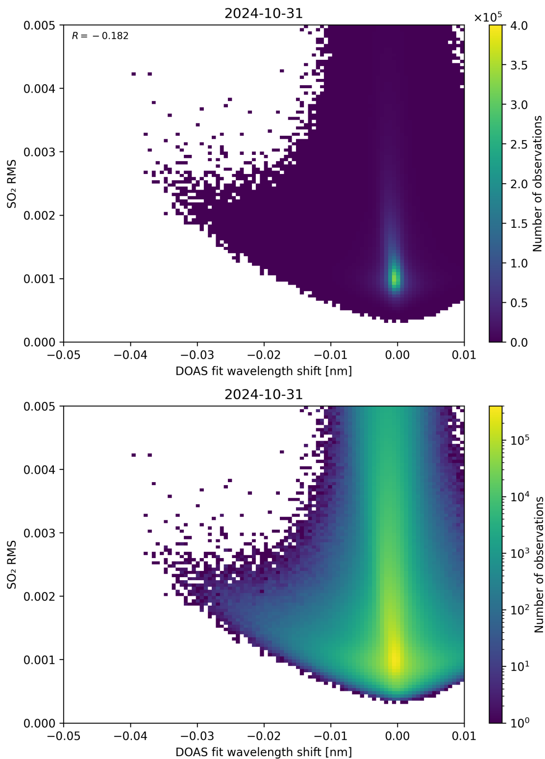
Figure 128: Scatter density plot of “DOAS fit wavelength shift” against “SO 2 RMS” for 2024-10-30 to 2024-11-01.
