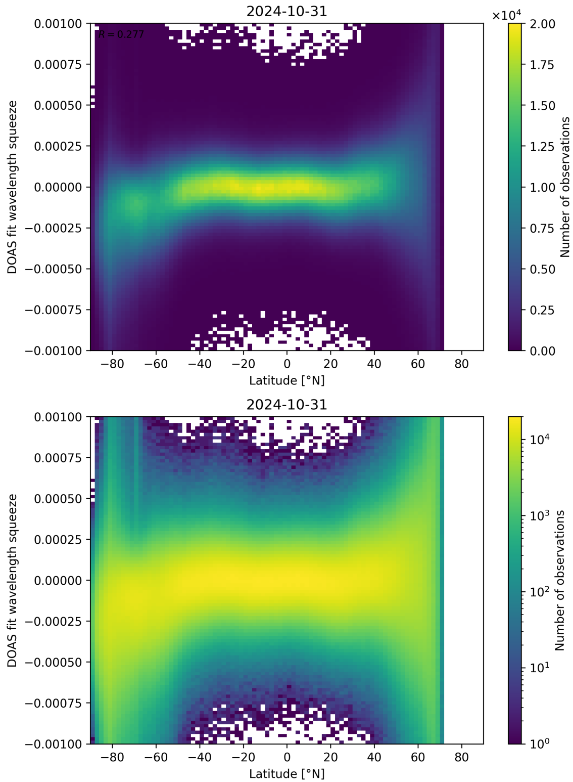
Figure 143: Scatter density plot of “Latitude” against “DOAS fit wavelength squeeze” for 2024-10-30 to 2024-11-01.
