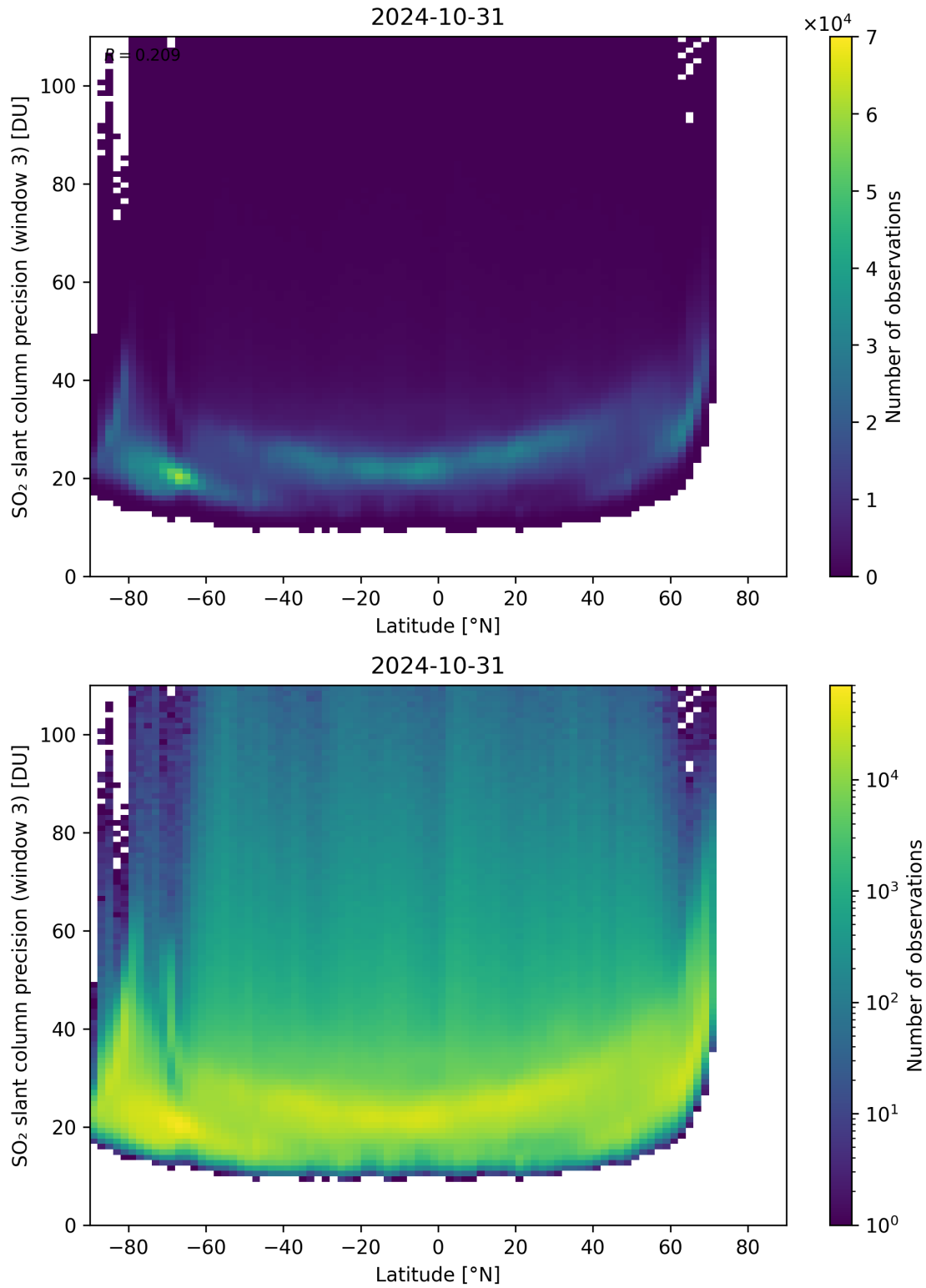
Figure 153: Scatter density plot of “Latitude” against “SO 2 slant column precision (window 3)” for 2024-10-30 to 2024-11-01.
