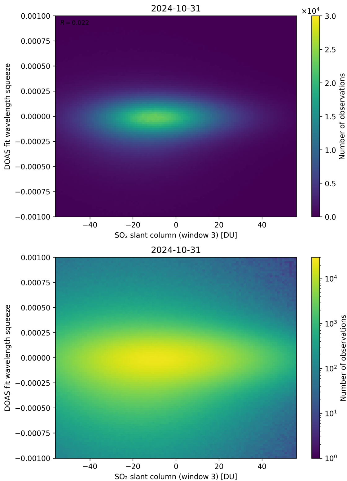
Figure 255: Scatter density plot of “SO 2 slant column (window 3)” against “DOAS fit wavelength squeeze” for 2024-10-30 to 2024-11-01.
