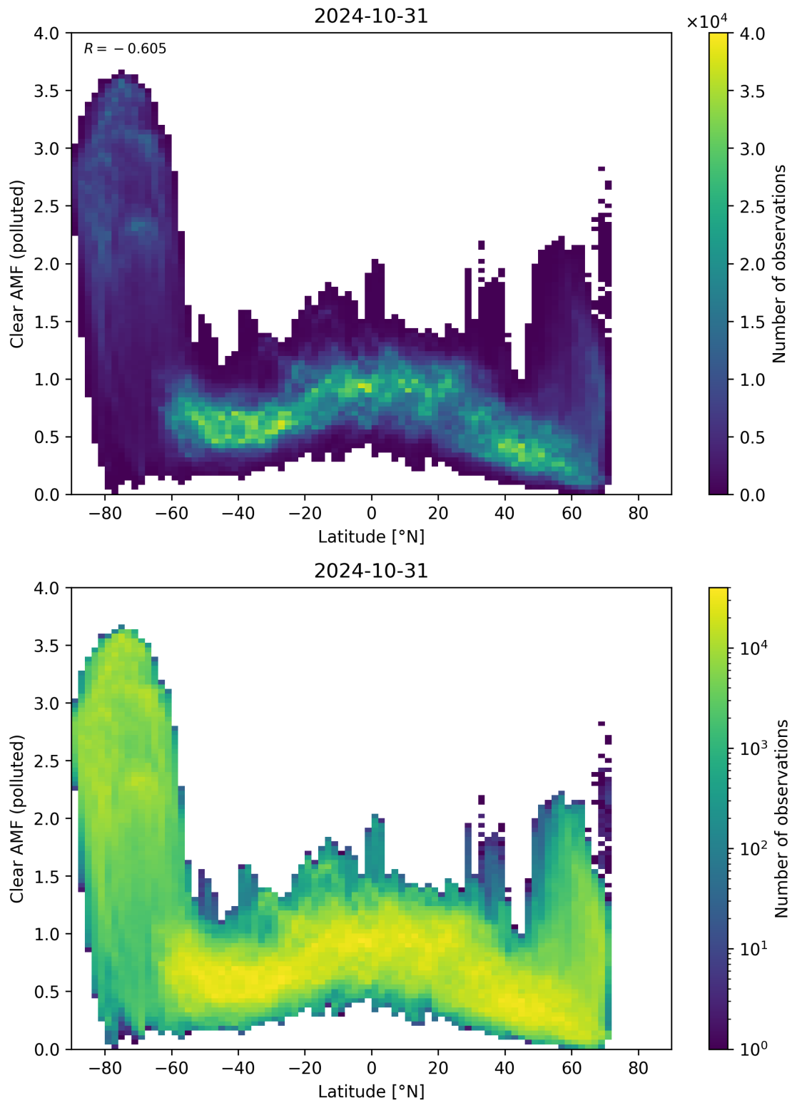
Figure 145: Scatter density plot of “Latitude” against “Clear AMF (polluted)” for 2024-10-30 to 2024-11-01.
