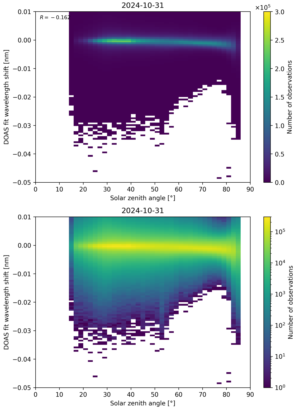
Figure 161: Scatter density plot of “Solar zenith angle” against “DOAS fit wavelength shift” for 2024-10-30 to 2024-11-01.
