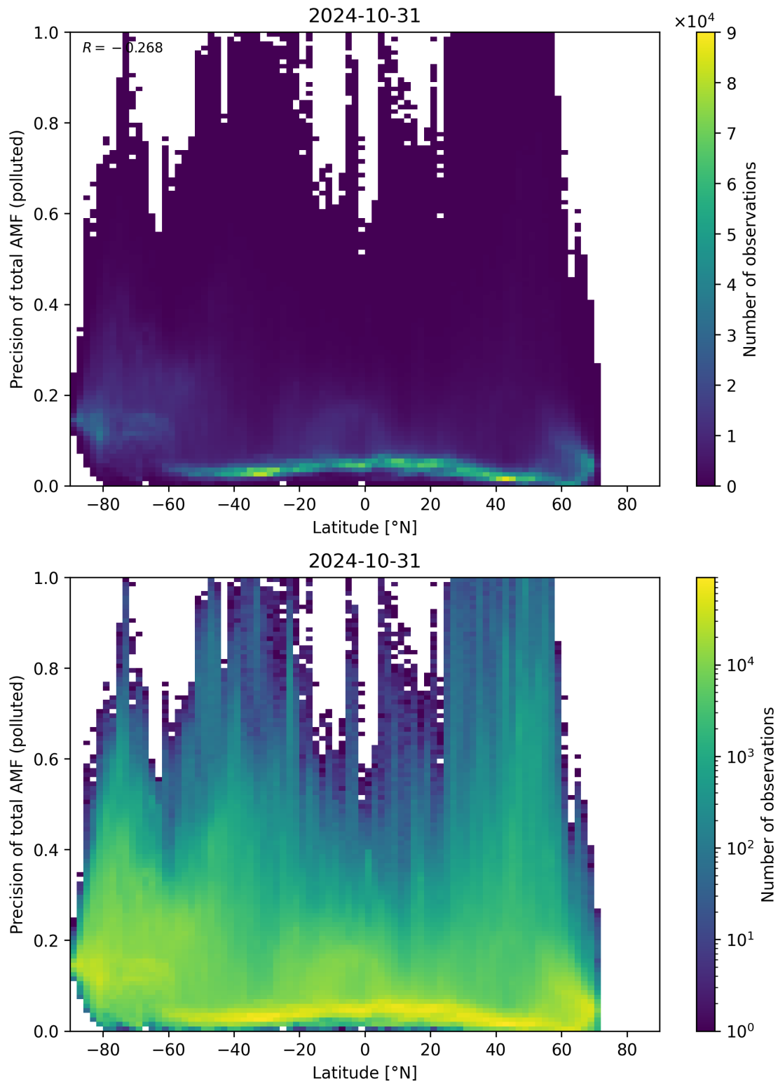
Figure 155: Scatter density plot of “Latitude” against “Precision of total AMF (polluted)” for 2024-10-30 to 2024-11-01.
