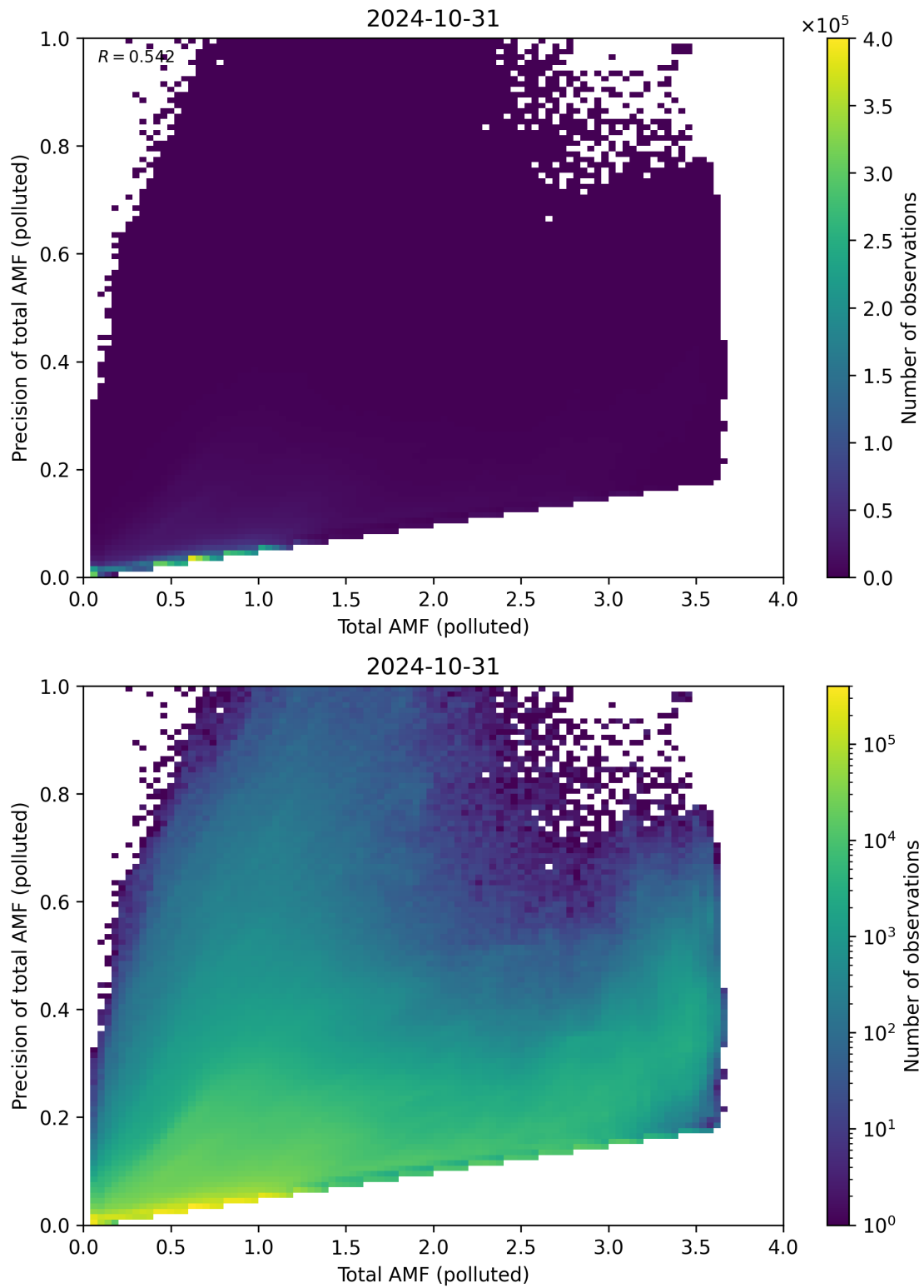
Figure 272: Scatter density plot of “Total AMF (polluted)” against “Precision of total AMF (polluted)” for 2024-10-30 to 2024-11-01.
