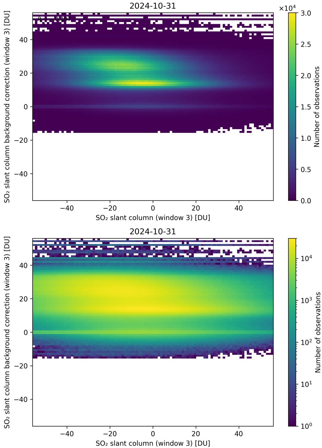
Figure 253: Scatter density plot of “SO 2 slant column (window 3)” against “SO 2 slant column background correction (window 3)” for 2024-10-30 to 2024-11-01.
