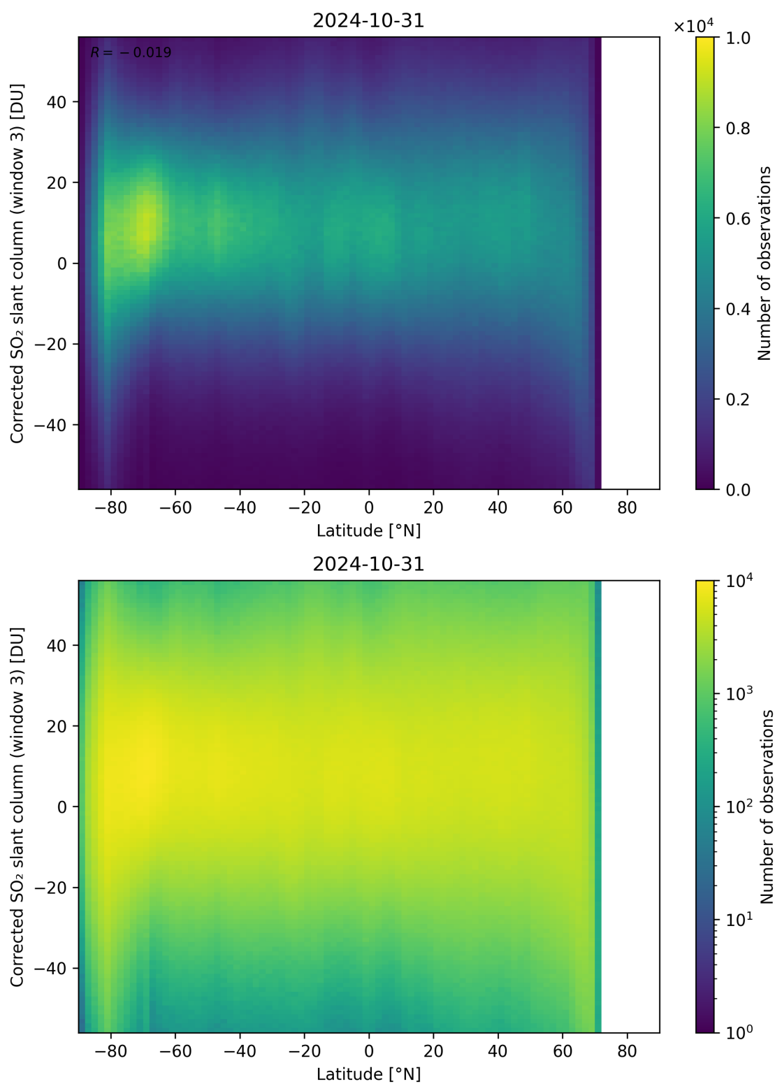
Figure 148: Scatter density plot of “Latitude” against “Corrected SO 2 slant column (window 3)” for 2024-10-30 to 2024-11-01.
