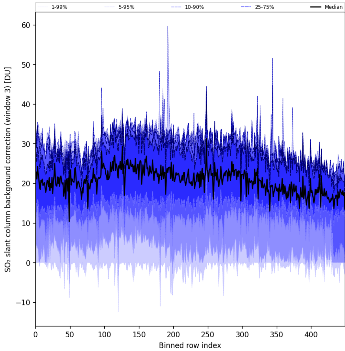
Figure 90: Along track statistics of “SO 2 slant column background correction (window 3)” for 2024-10-30 to 2024-11-01
