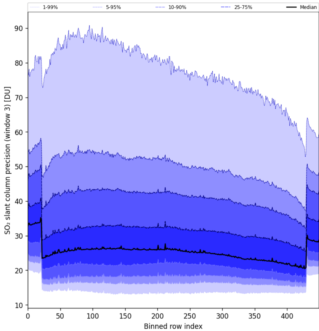
Figure 88: Along track statistics of “SO 2 slant column precision (window 3)” for 2024-10-30 to 2024-11-01
