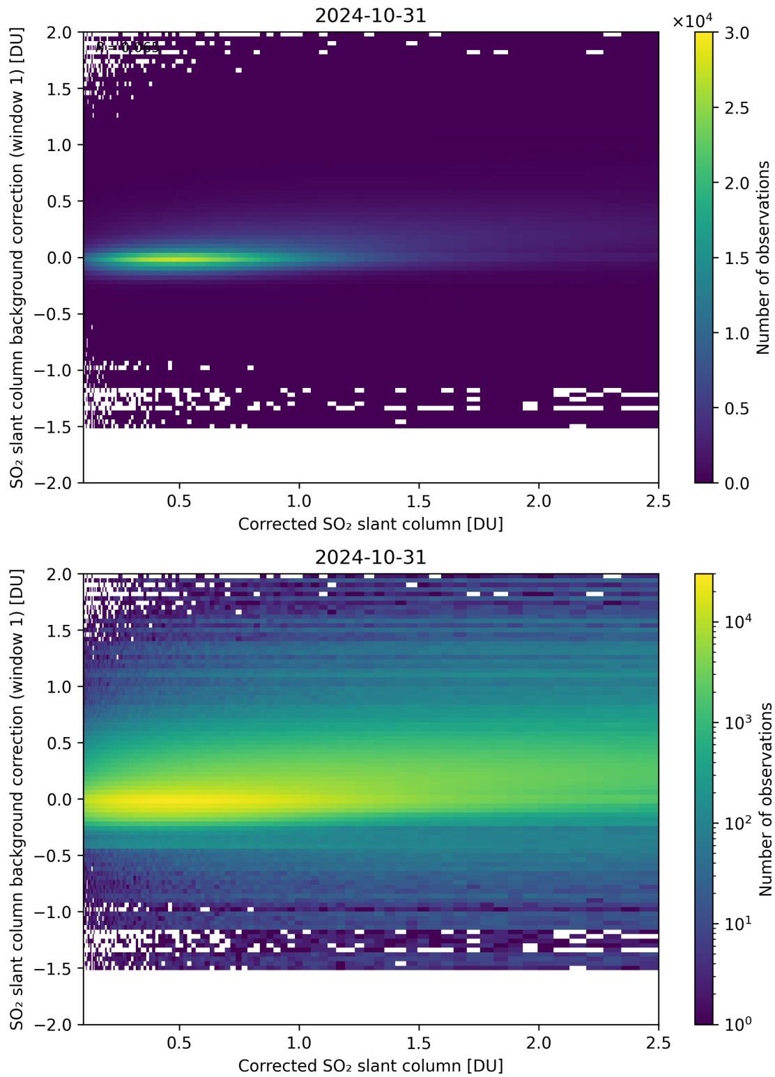
Figure 178: Scatter density plot of “Corrected SO 2 slant column” against “SO 2 slant column background correction (window 1)” for 2024-10-30 to 2024-11-01.
