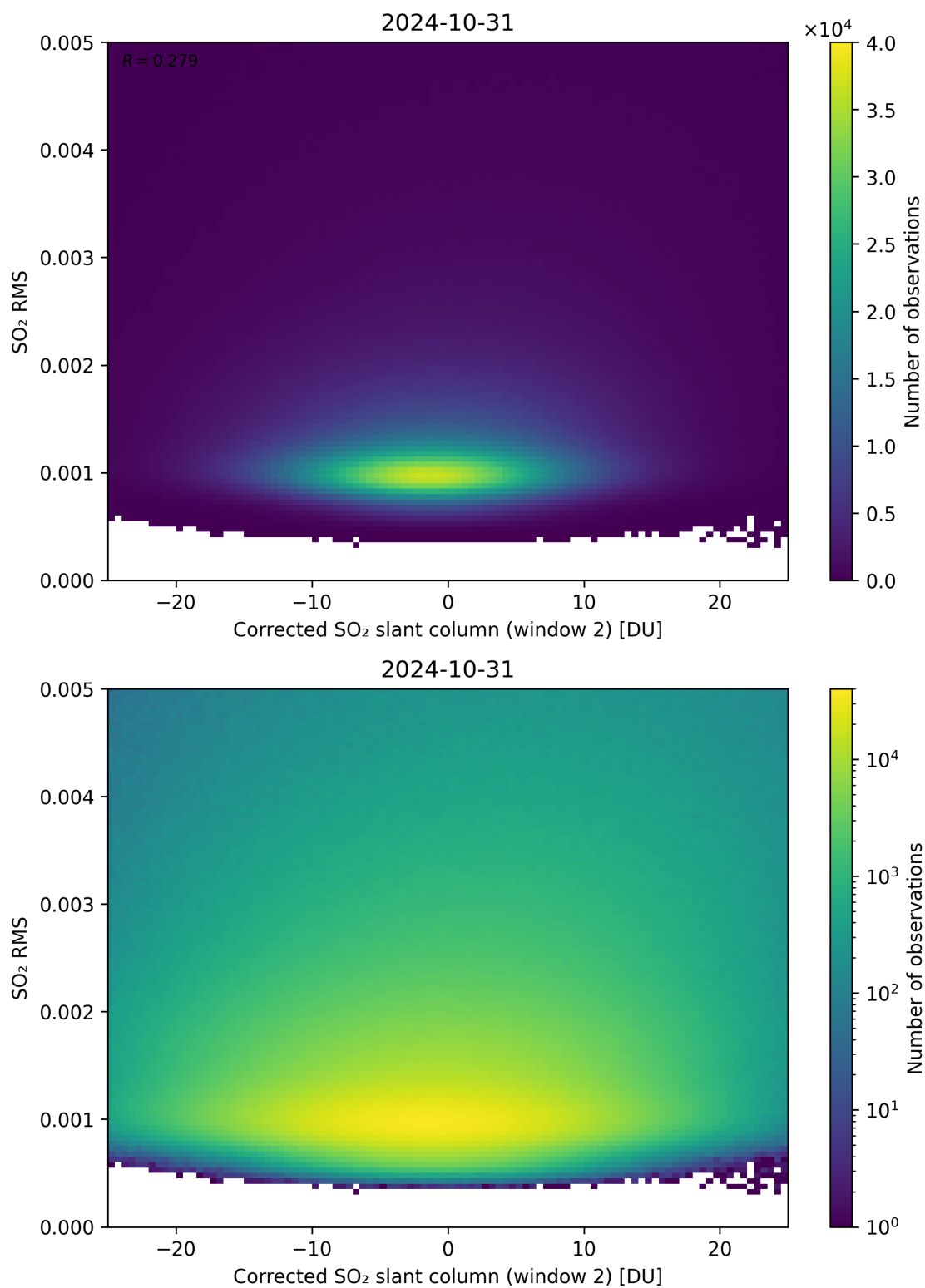
Figure 198: Scatter density plot of “Corrected SO 2 slant column (window 2)” against “SO 2 RMS” for 2024-10-30 to 2024-11-01.
