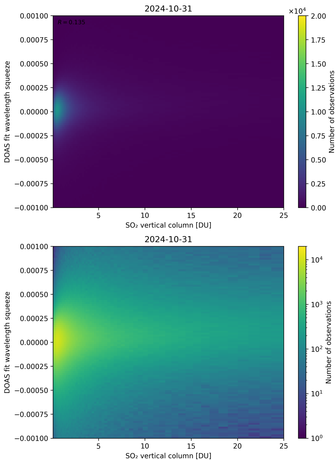
Figure 277: Scatter density plot of “SO 2 vertical column” against “DOAS fit wavelength squeeze” for 2024-10-30 to 2024-11-01.
