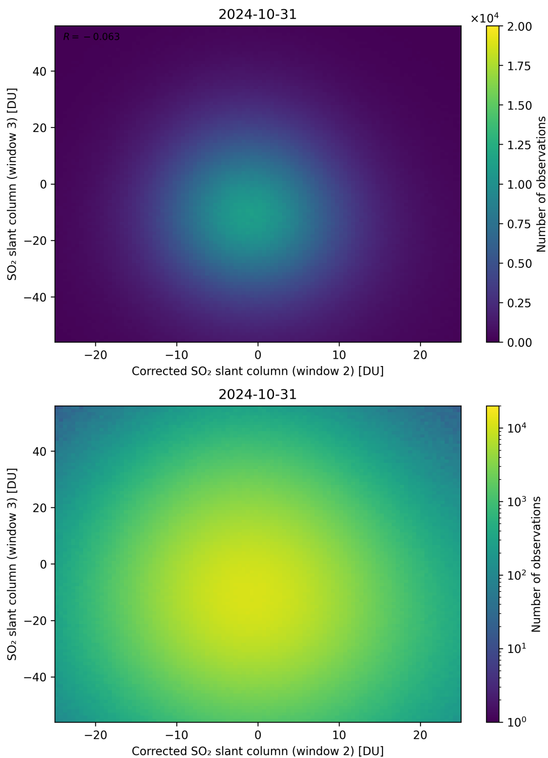
Figure 201: Scatter density plot of “Corrected SO 2 slant column (window 2)” against “SO 2 slant column (window 3)” for 2024-10-30 to 2024-11-01.
