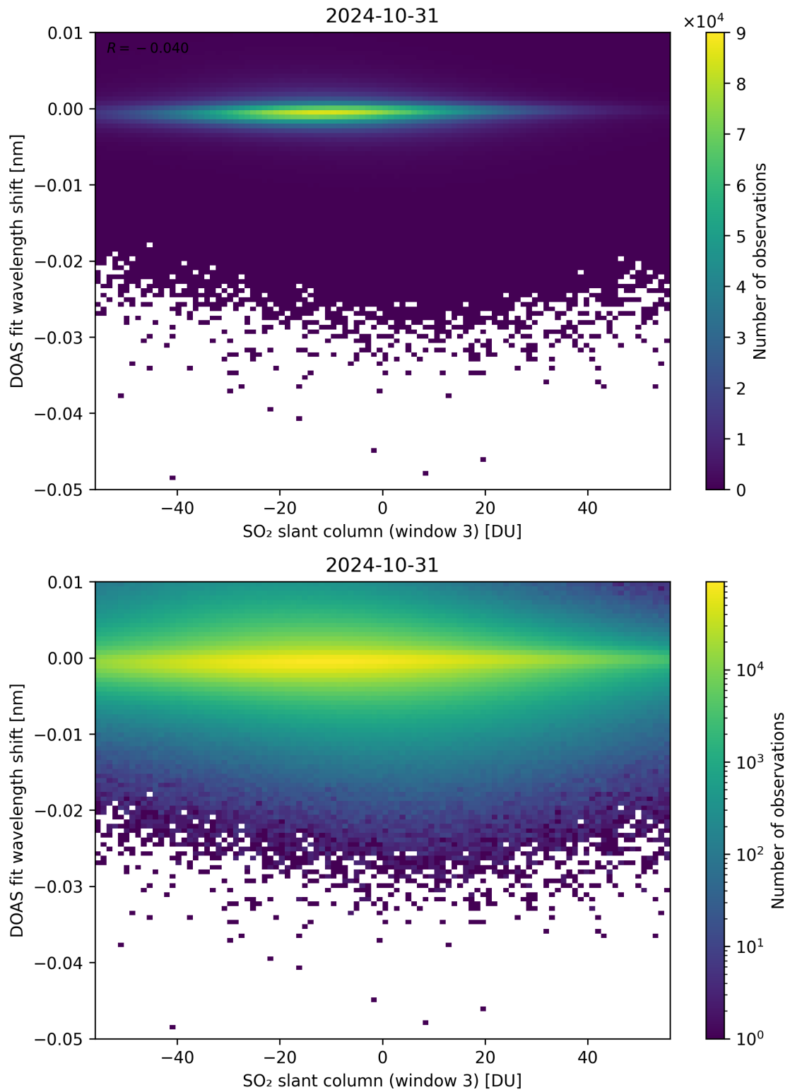
Figure 254: Scatter density plot of “SO 2 slant column (window 3)” against “DOAS fit wavelength shift” for 2024-10-30 to 2024-11-01.
