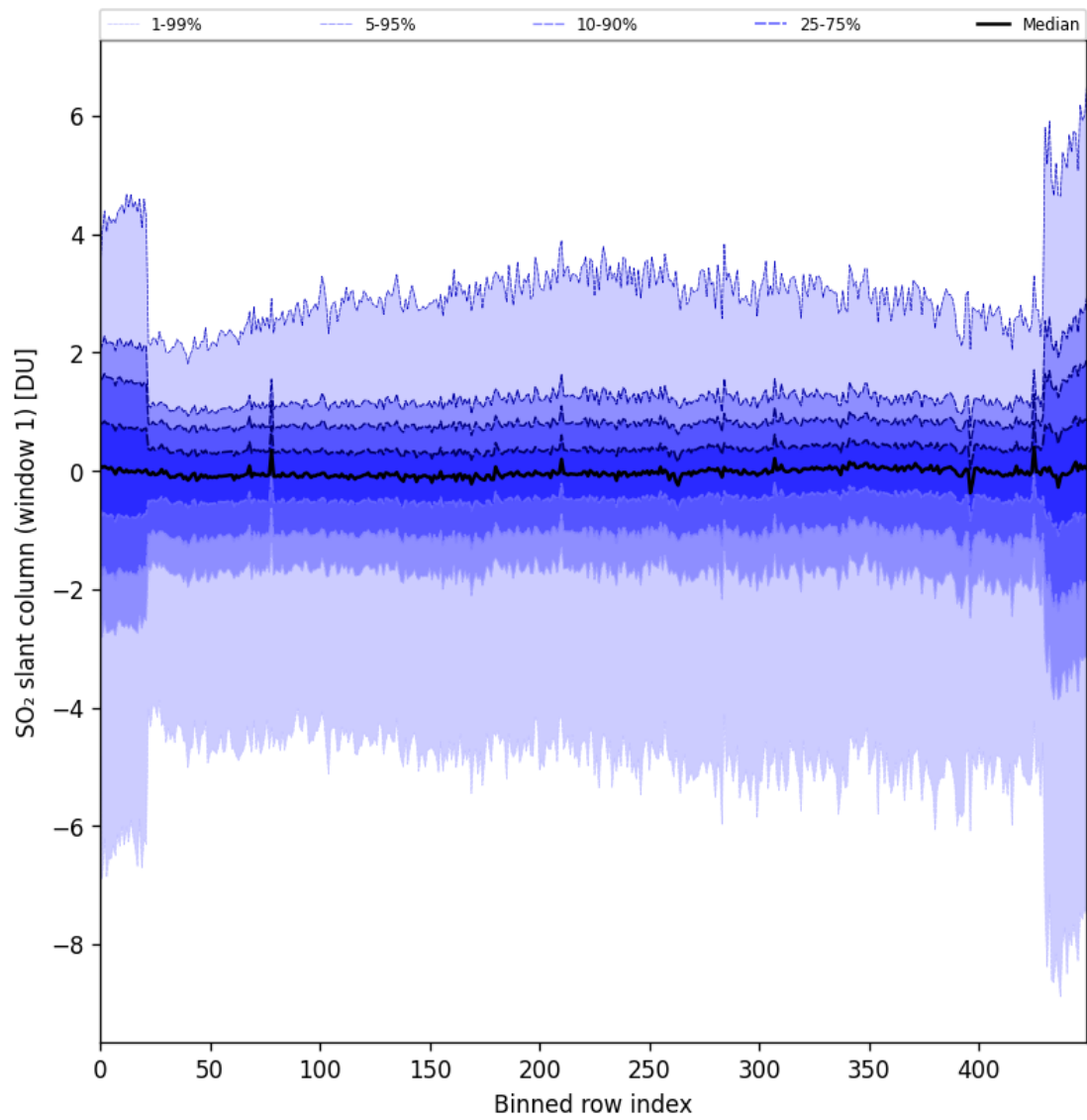
Figure 79: Along track statistics of "SO 2 slant column (window 1)" for 2024-10-30 to 2024-11-01
