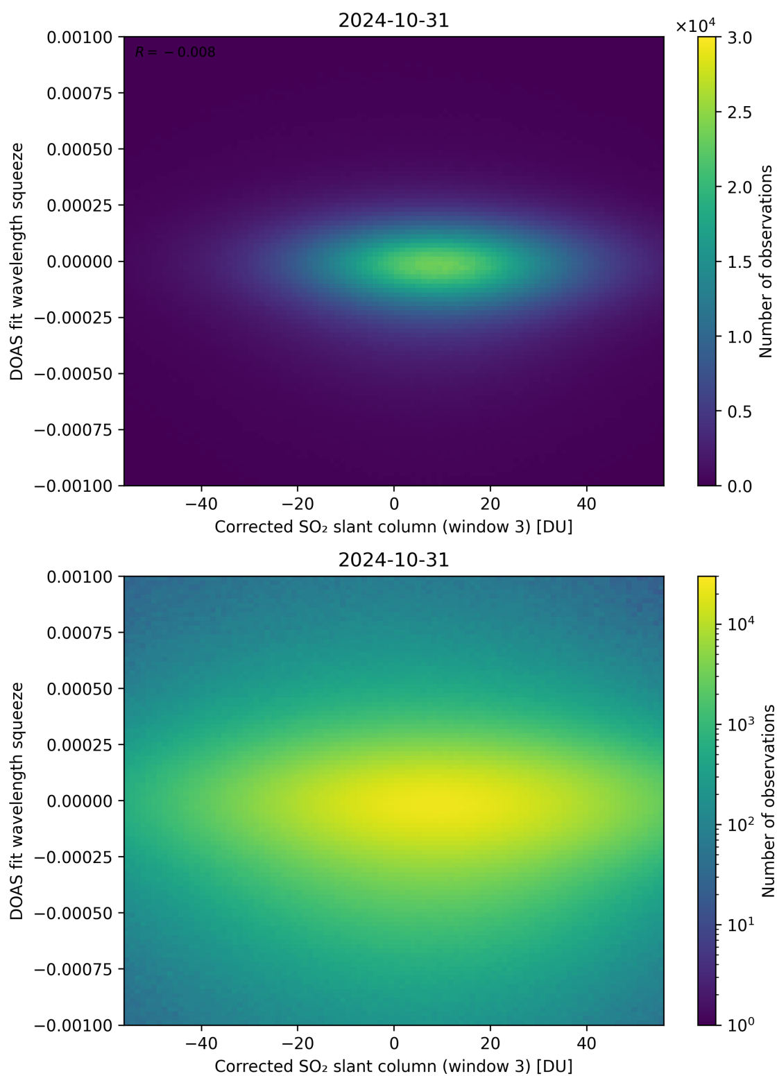
Figure 207: Scatter density plot of “Corrected SO 2 slant column (window 3)” against “DOAS fit wavelength squeeze” for 2024-10-30 to 2024-11-01.
