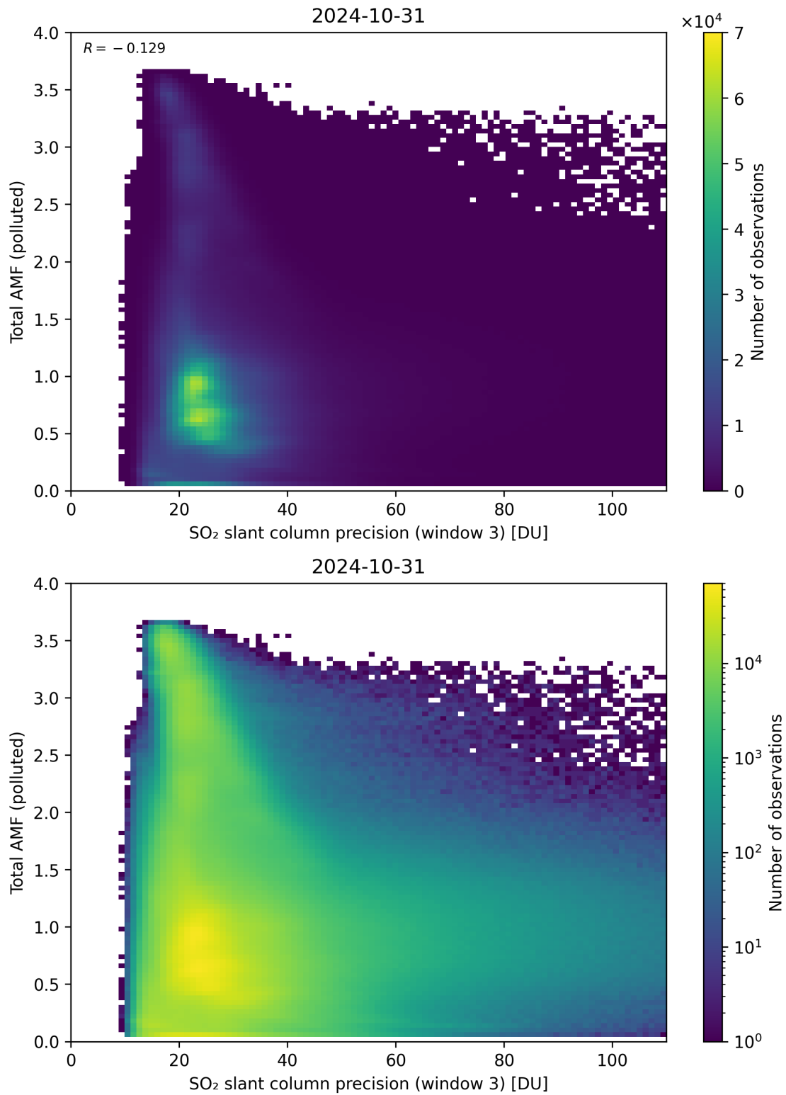
Figure 263: Scatter density plot of “SO 2 slant column precision (window 3)” against “Total AMF (polluted)” for 2024-10-30 to 2024-11-01.
