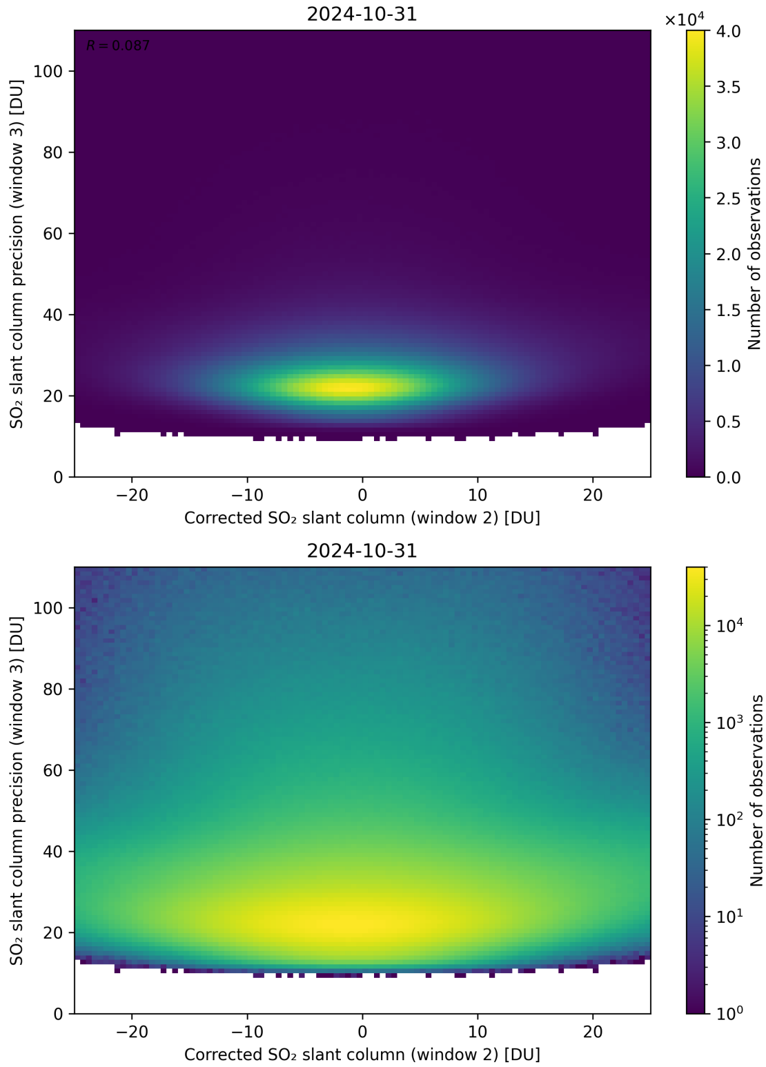
Figure 202: Scatter density plot of “Corrected SO 2 slant column (window 2)” against “SO 2 slant column precision (window 3)” for 2024-10-30 to 2024-11-01.
