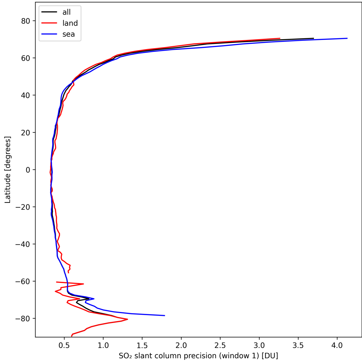
Figure 34: Zonal average of “SO 2 slant column precision (window 1)” for 2024-10-30 to 2024-11-01.
