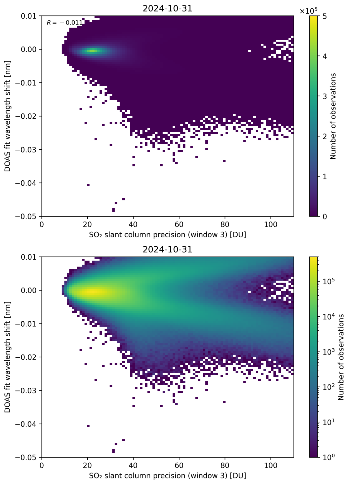
Figure 258: Scatter density plot of “SO 2 slant column precision (window 3)” against “DOAS fit wavelength shift” for 2024-10-30 to 2024-11-01.
