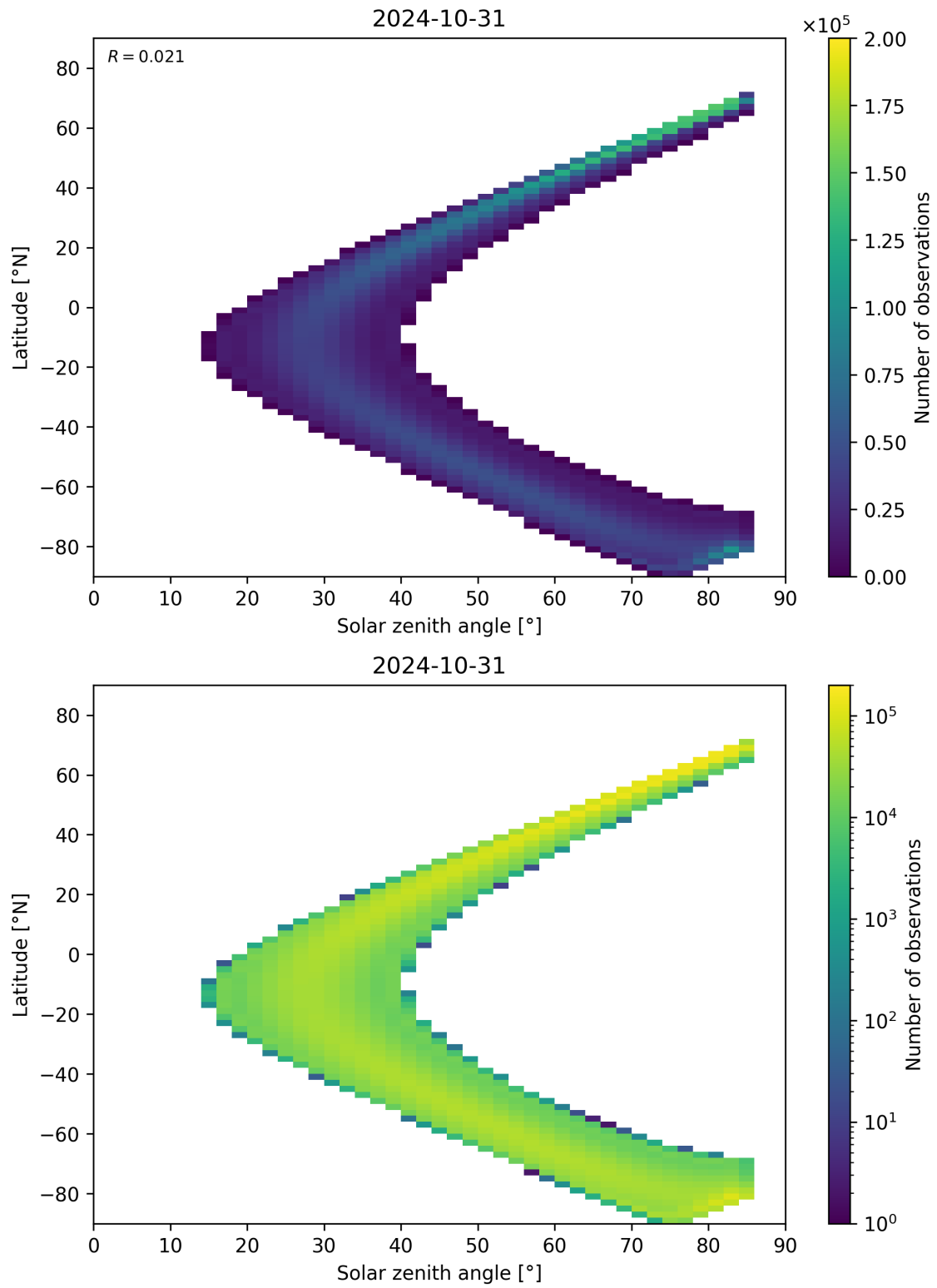
Figure 164: Scatter density plot of “Solar zenith angle” against “Latitude” for 2024-10-30 to 2024-11-01.
