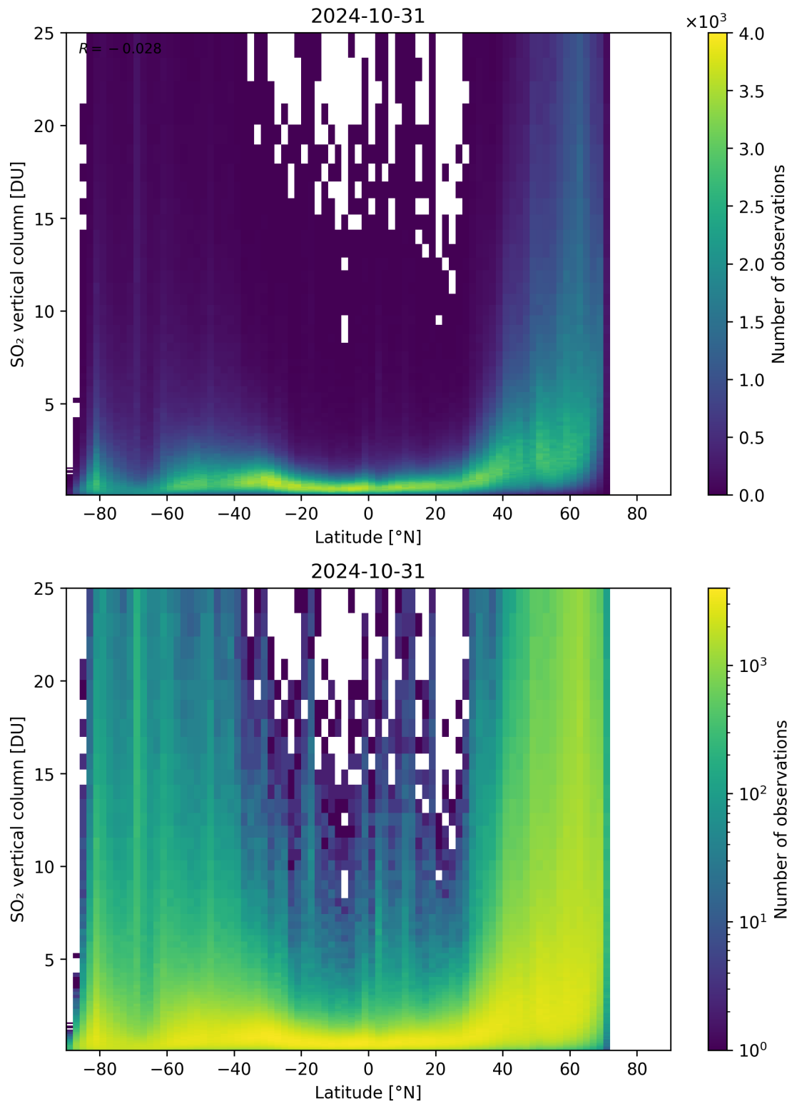
Figure 156: Scatter density plot of “Latitude” against “SO 2 vertical column” for 2024-10-30 to 2024-11-01.
