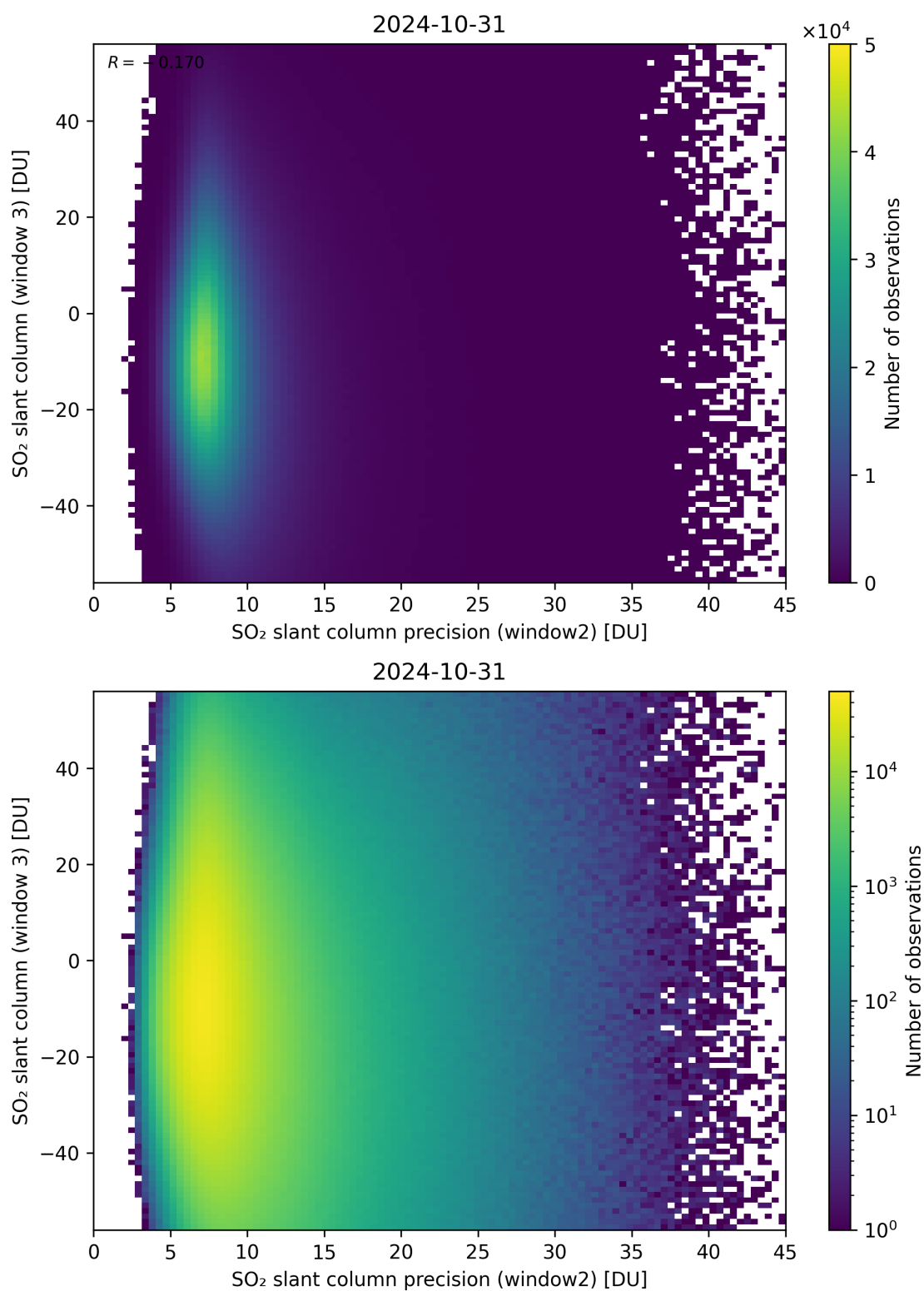
Figure 249: Scatter density plot of “SO 2 slant column precision (window2)” against “SO 2 slant column (window 3)” for 2024-10-30 to 2024-11-01.
