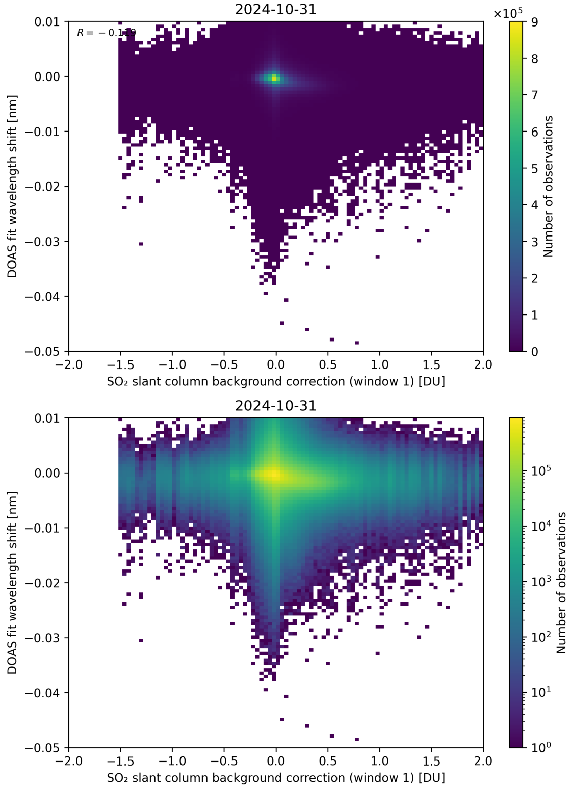
Figure 100: Scatter density plot of “SO 2 slant column background correction (window 1)” against “DOAS fit wavelength shift” for 2024-10-30 to 2024-11-01.
