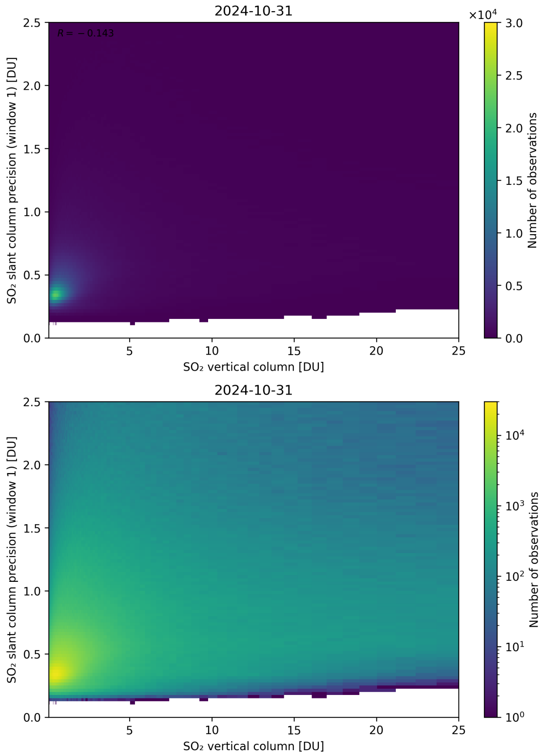
Figure 301: Scatter density plot of “SO 2 vertical column” against “SO 2 slant column precision (window 1)” for 2024-10-30 to 2024-11-01.
