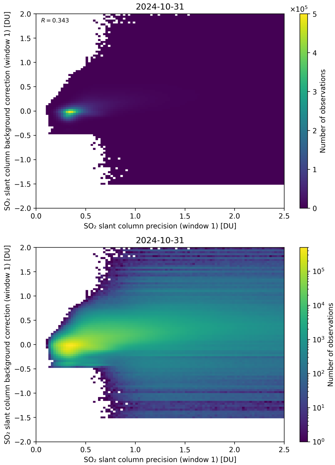
Figure 218: Scatter density plot of “SO 2 slant column precision (window 1)” against “SO 2 slant column background correction (window 1)” for 2024-10-30 to 2024-11-01.
