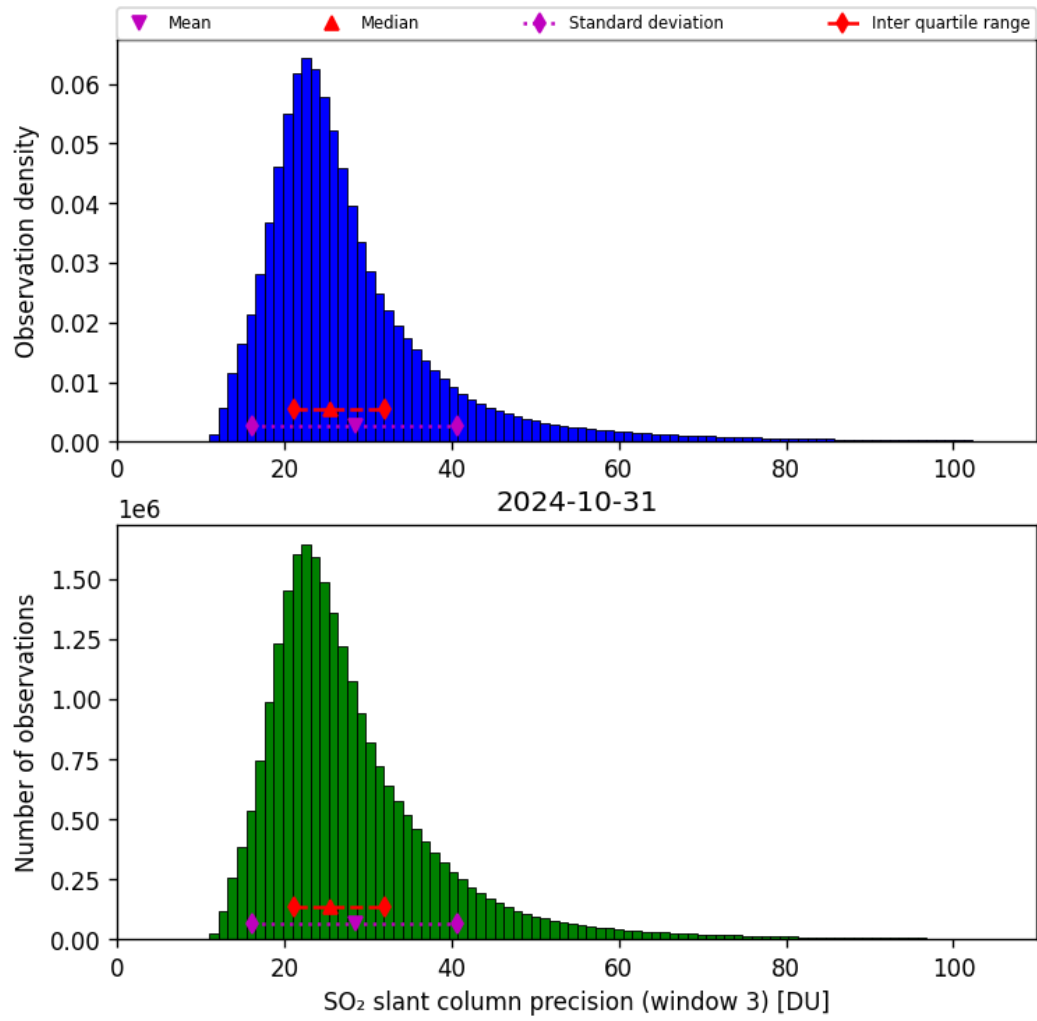
Figure 65: Histogram of “SO 2 slant column precision (window 3)” for 2024-10-30 to 2024-11-01
