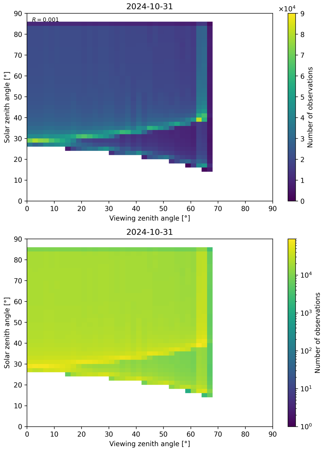
Figure 315: Scatter density plot of “Viewing zenith angle” against “Solar zenith angle” for 2024-10-30 to 2024-11-01.
