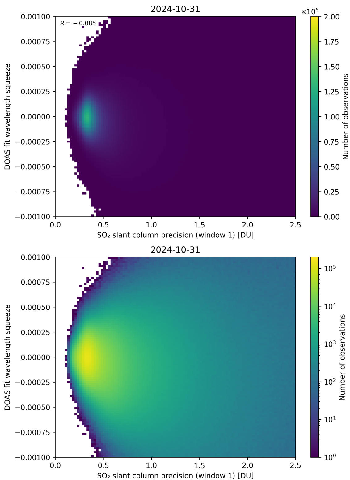
Figure 222: Scatter density plot of “SO 2 slant column precision (window 1)” against “DOAS fit wavelength squeeze” for 2024-10-30 to 2024-11-01.
