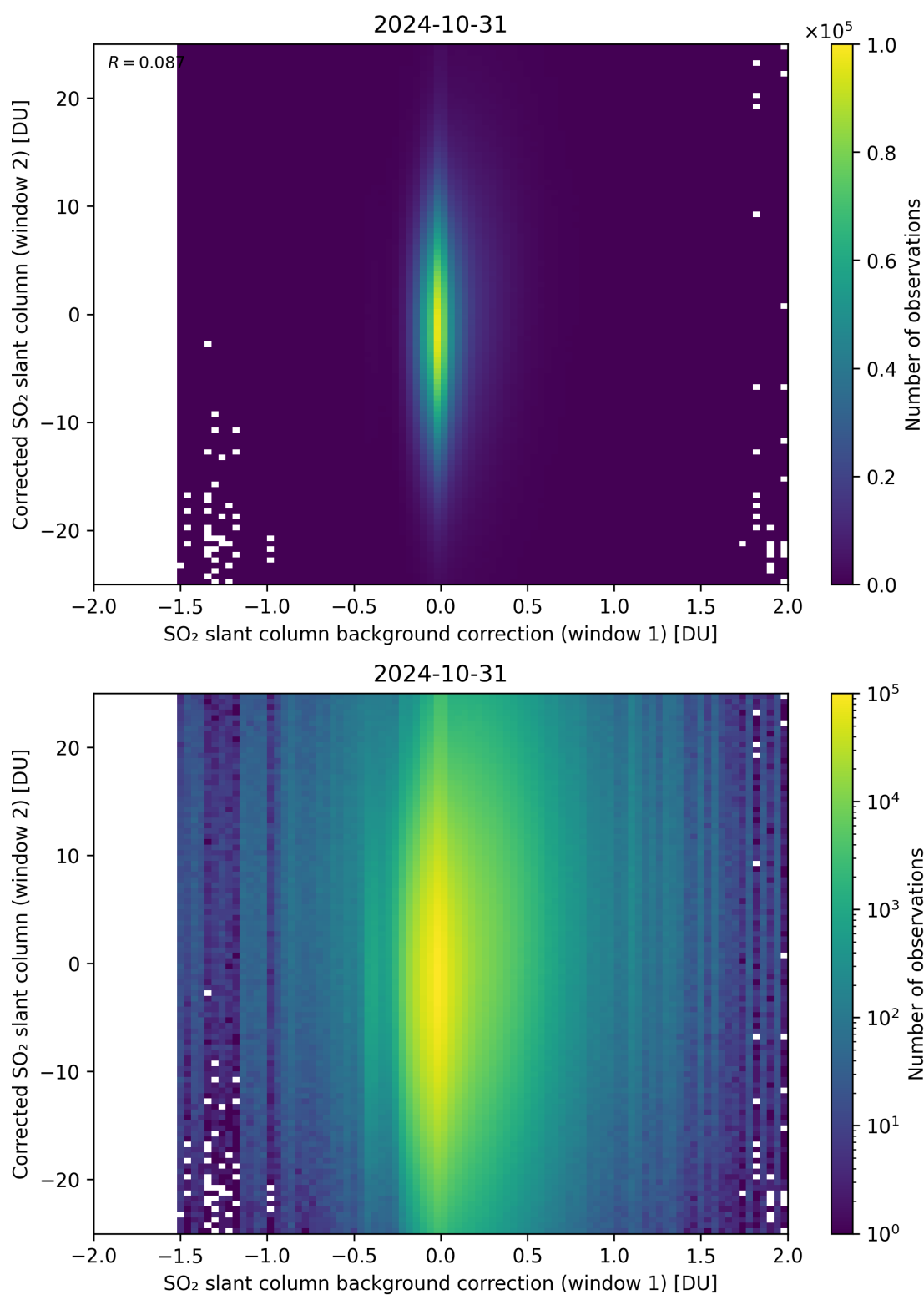
Figure 104: Scatter density plot of “SO 2 slant column background correction (window 1)” against “Corrected SO 2 slant column (window 2)” for 2024-10-30 to 2024-11-01.
