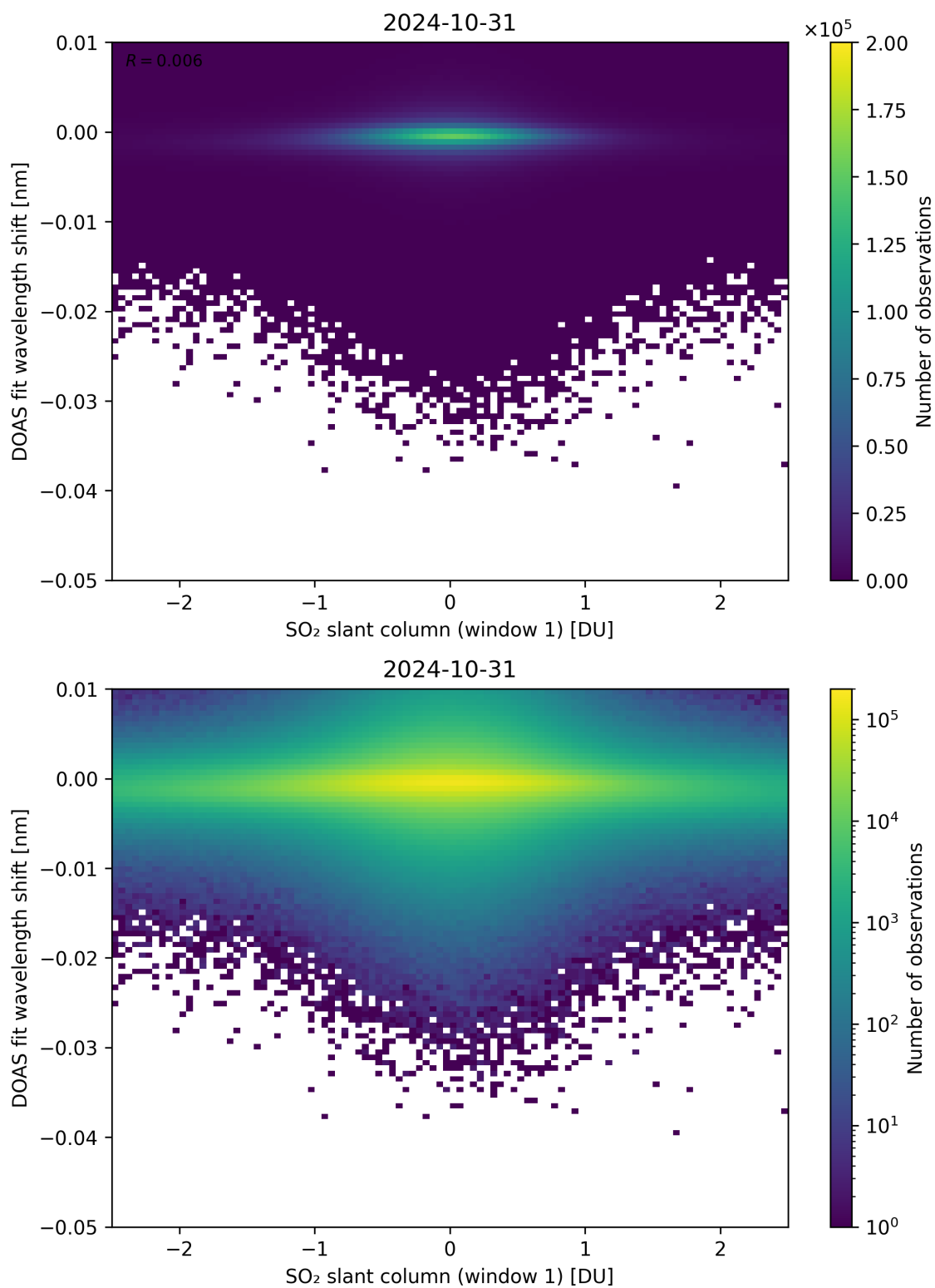
Figure 215: Scatter density plot of “SO 2 slant column (window 1)” against “DOAS fit wavelength shift” for 2024-10-30 to 2024-11-01.
