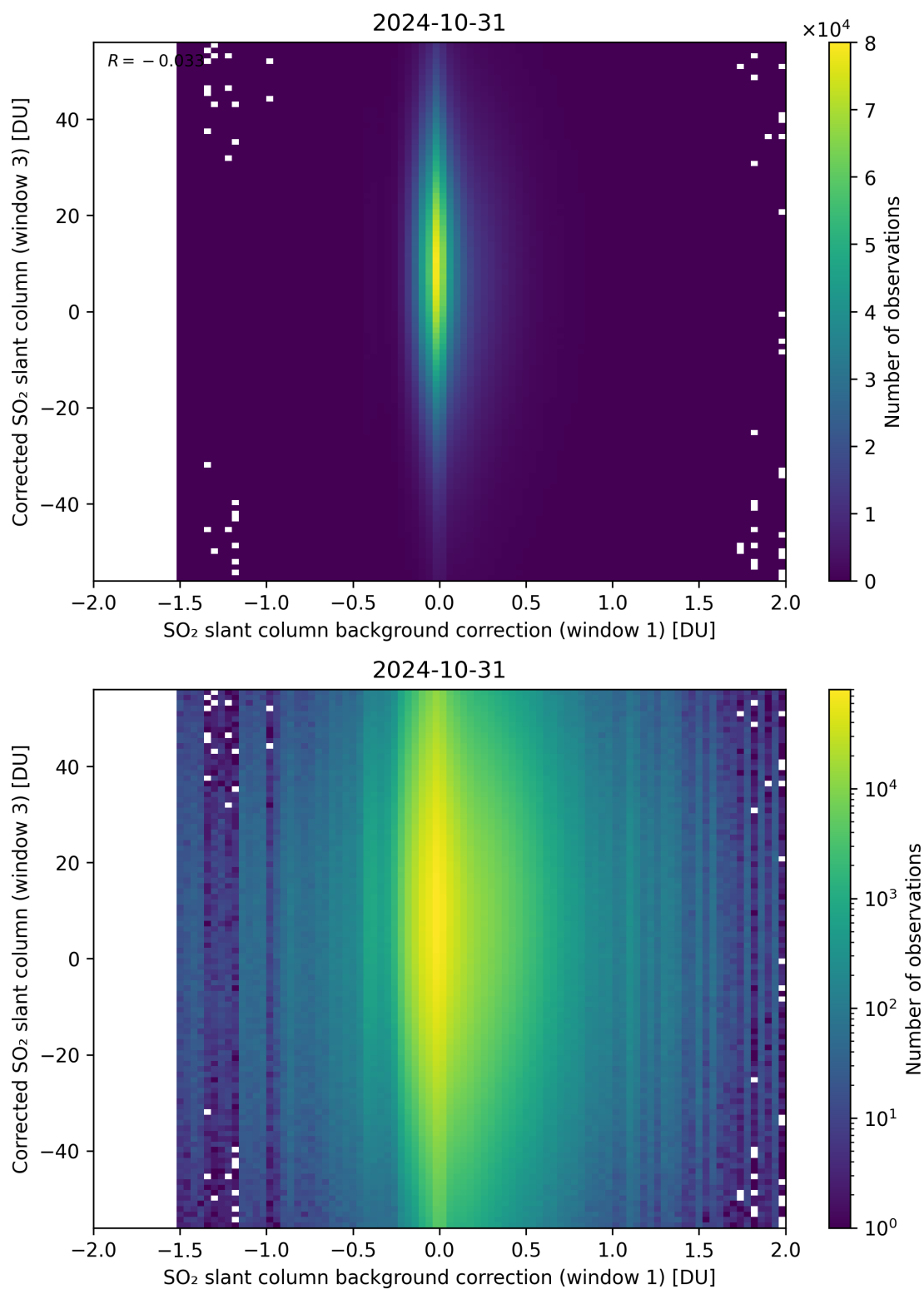
Figure 105: Scatter density plot of “SO 2 slant column background correction (window 1)” against “Corrected SO 2 slant column (window 3)” for 2024-10-30 to 2024-11-01.
