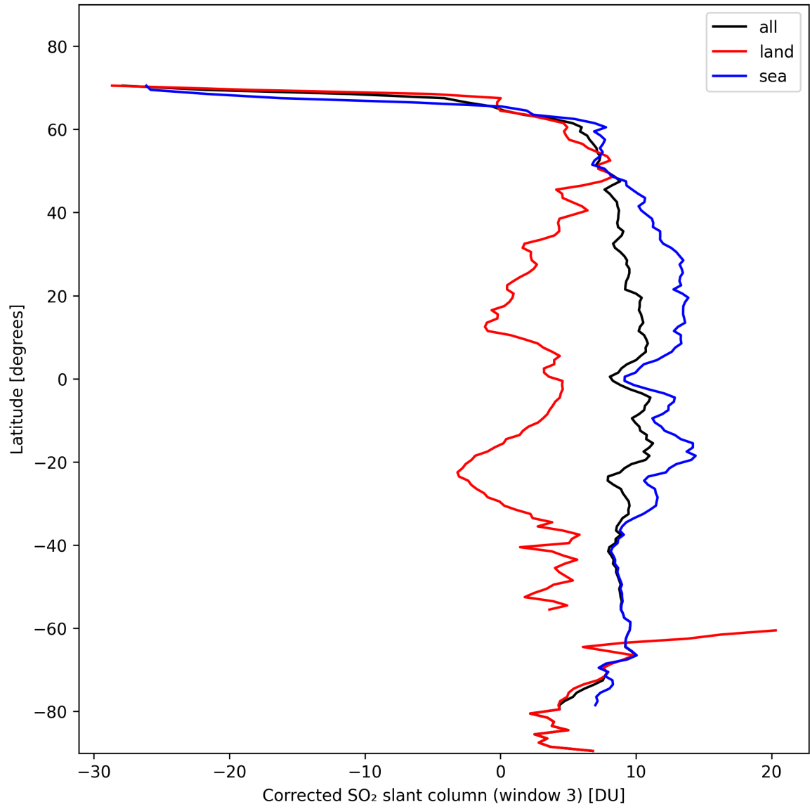
Figure 43: Zonal average of “Corrected SO 2 slant column (window 3)” for 2024-10-30 to 2024-11-01.
