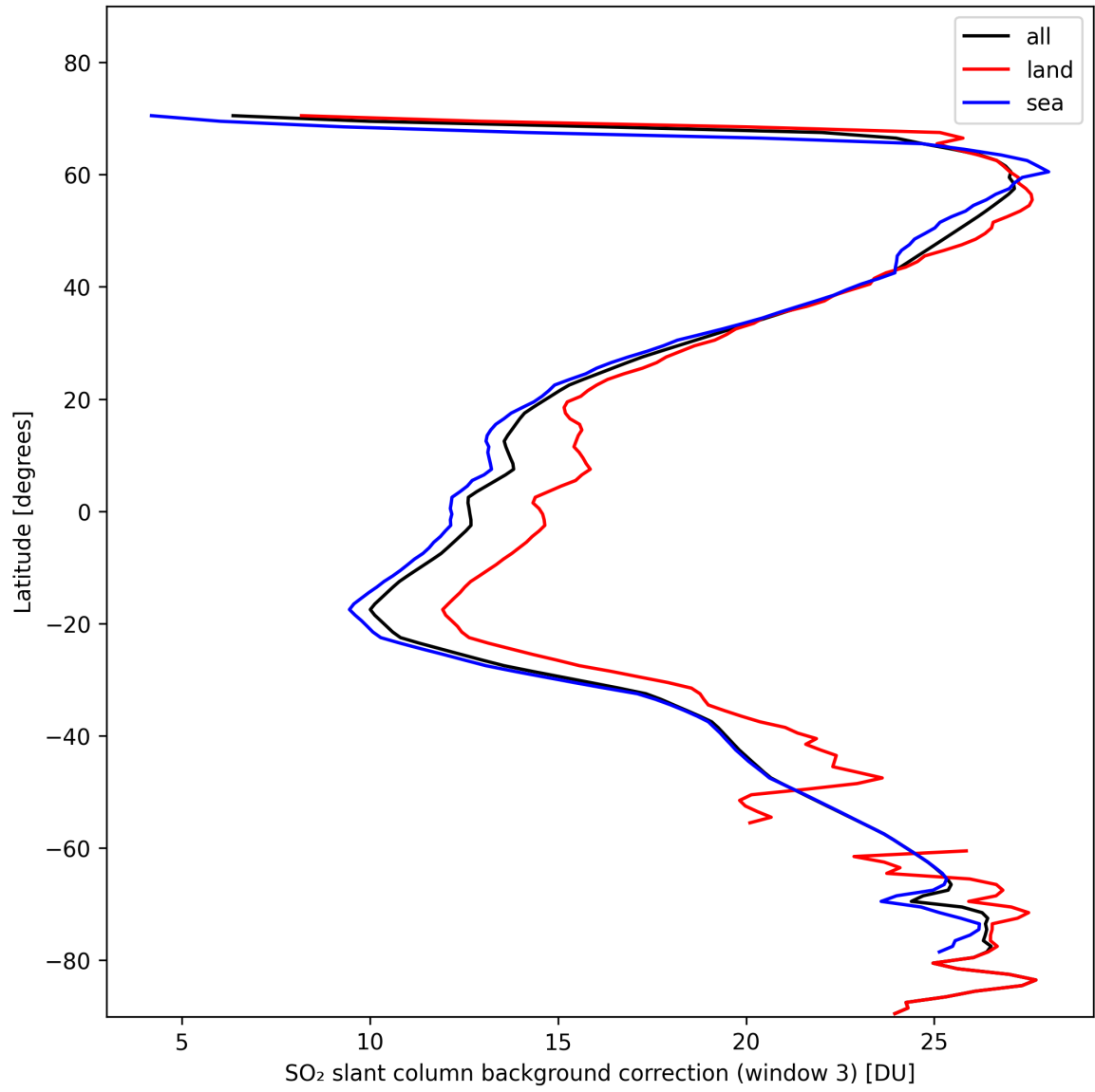
Figure 44: Zonal average of “SO 2 slant column background correction (window 3)” for 2024-10-30 to 2024-11-01.
