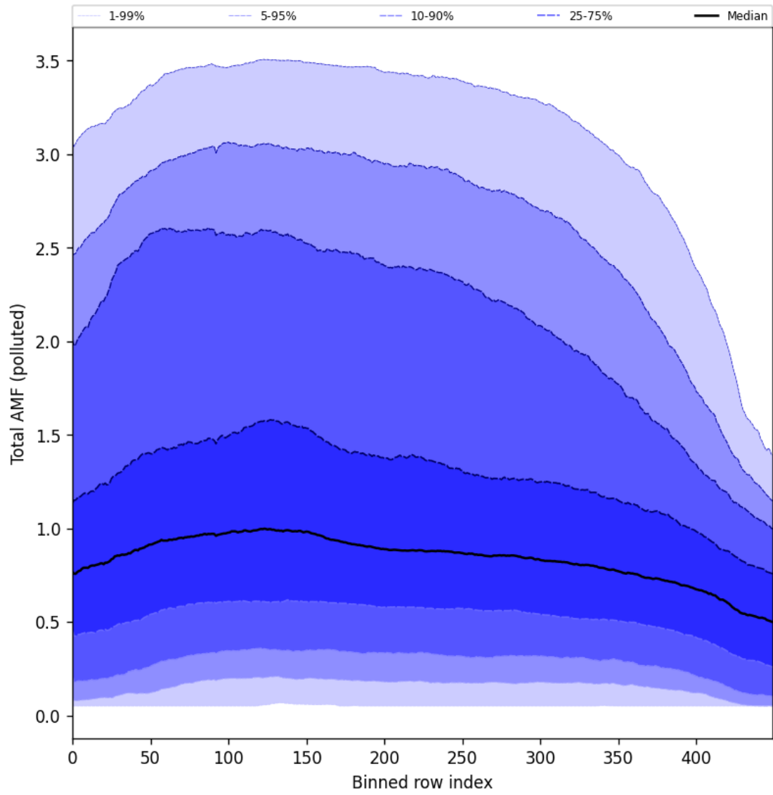
Figure 94: Along track statistics of “Total AMF (polluted)” for 2024-10-30 to 2024-11-01
