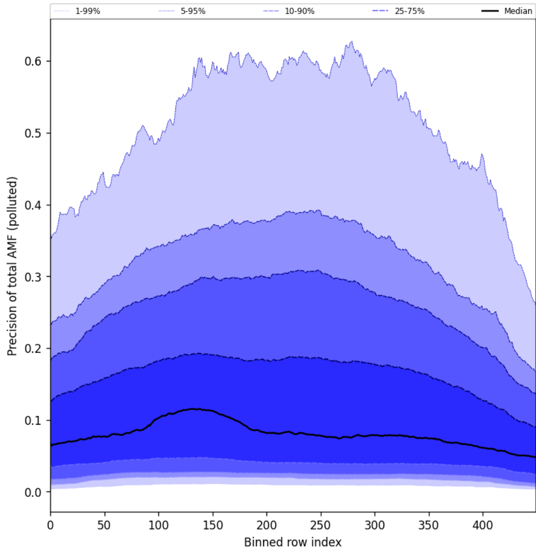
Figure 95: Along track statistics of “Precision of total AMF (polluted)” for 2024-10-30 to 2024-11-01
