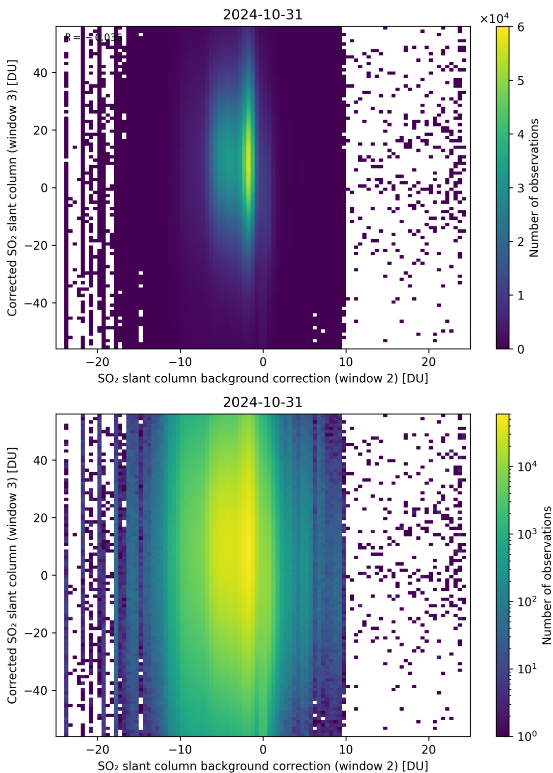
Figure 116: Scatter density plot of “SO 2 slant column background correction (window 2)” against “Corrected SO 2 slant column (window 3)” for 2024-10-30 to 2024-11-01.
