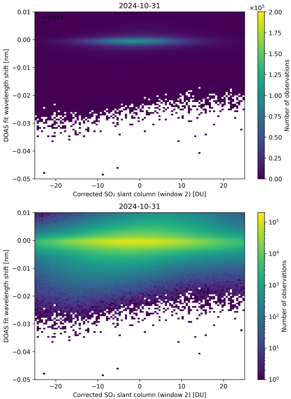
Figure 196: Scatter density plot of “Corrected SO 2 slant column (window 2)” against “DOAS fit wavelength shift” for 2024-10-30 to 2024-11-01.
