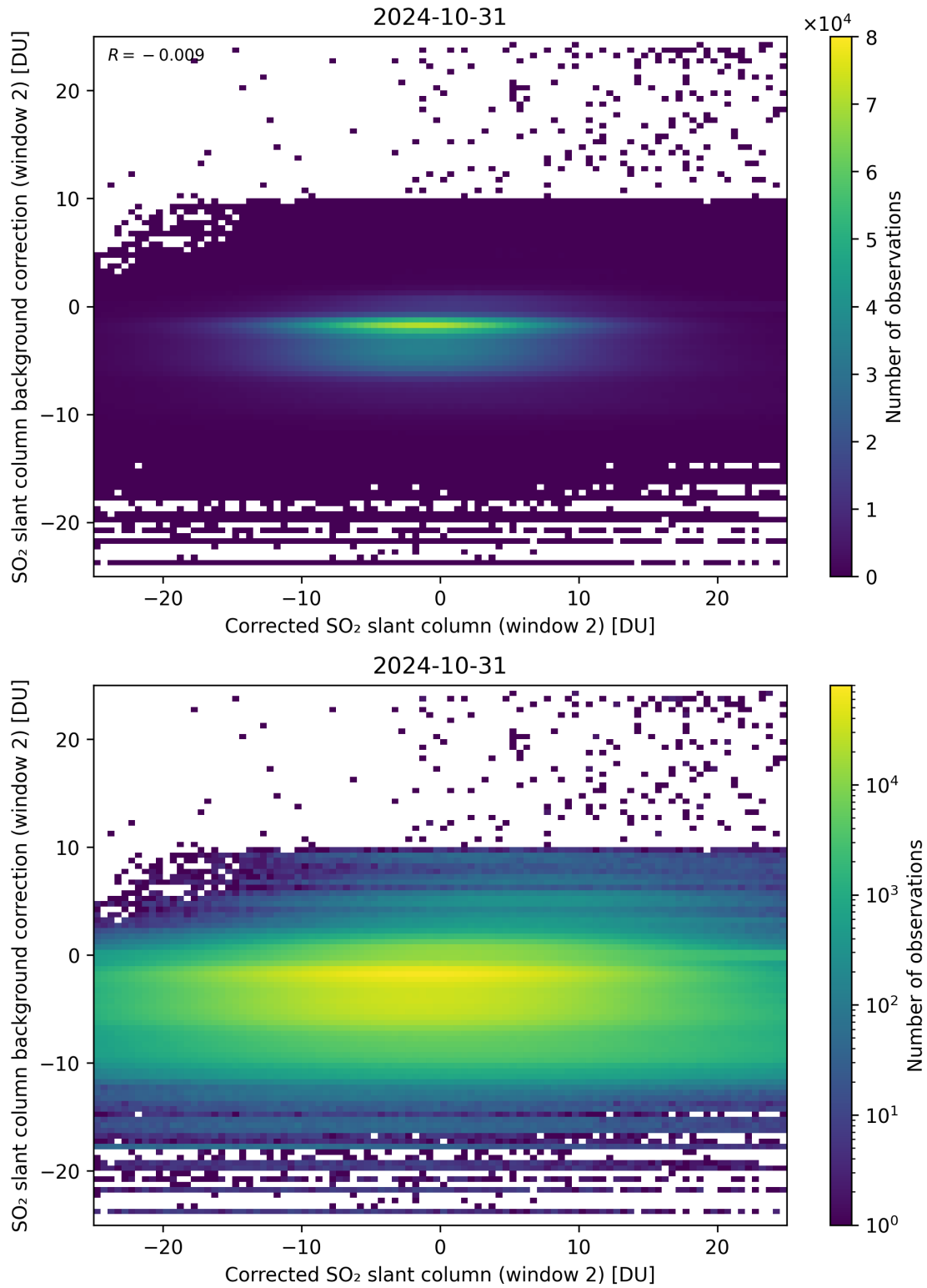
Figure 194: Scatter density plot of “Corrected SO 2 slant column (window 2)” against “SO 2 slant column background correction (window 2)” for 2024-10-30 to 2024-11-01.
