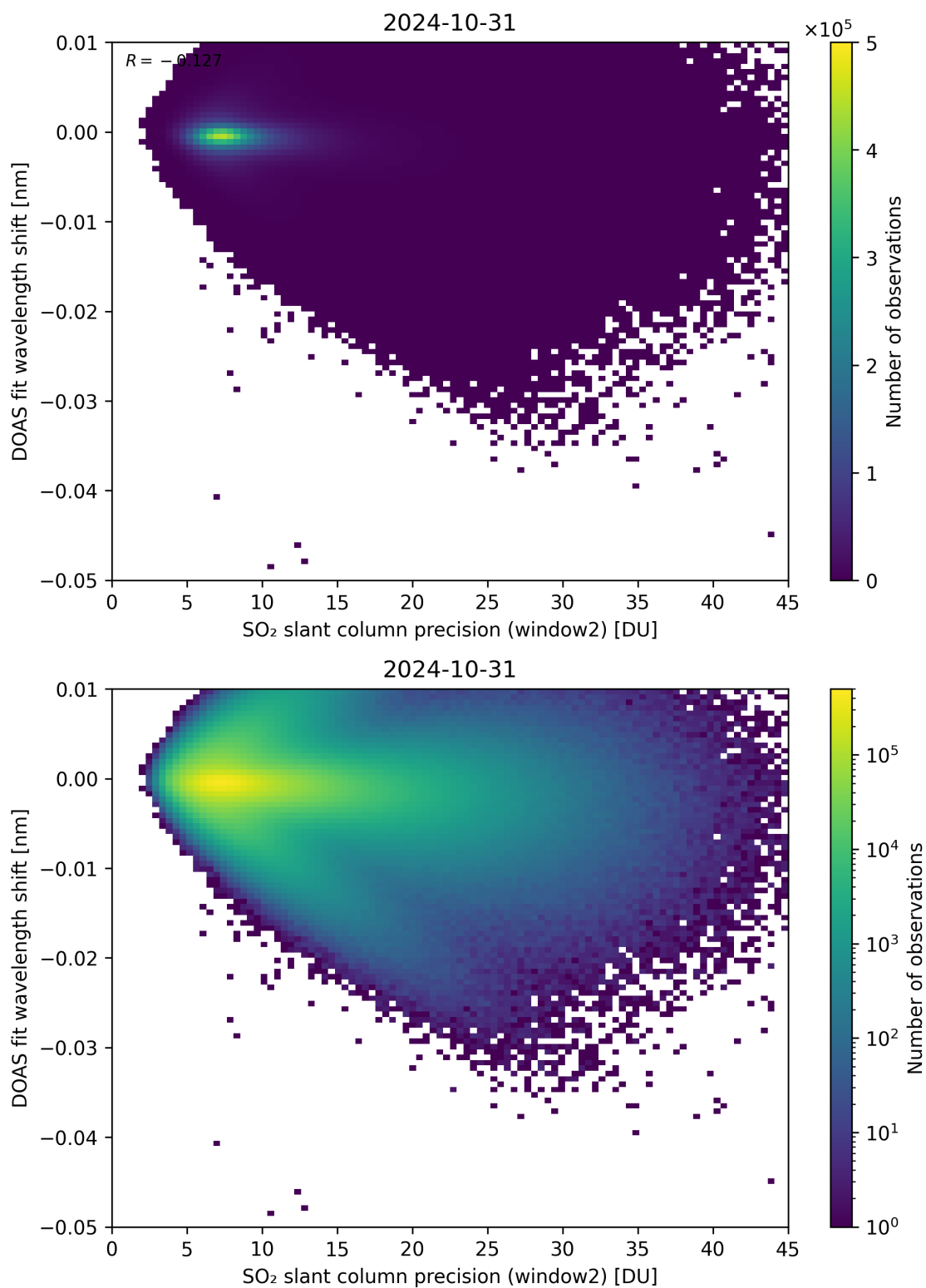
Figure 243: Scatter density plot of “SO 2 slant column precision (window2)” against “DOAS fit wavelength shift” for 2024-10-30 to 2024-11-01.
