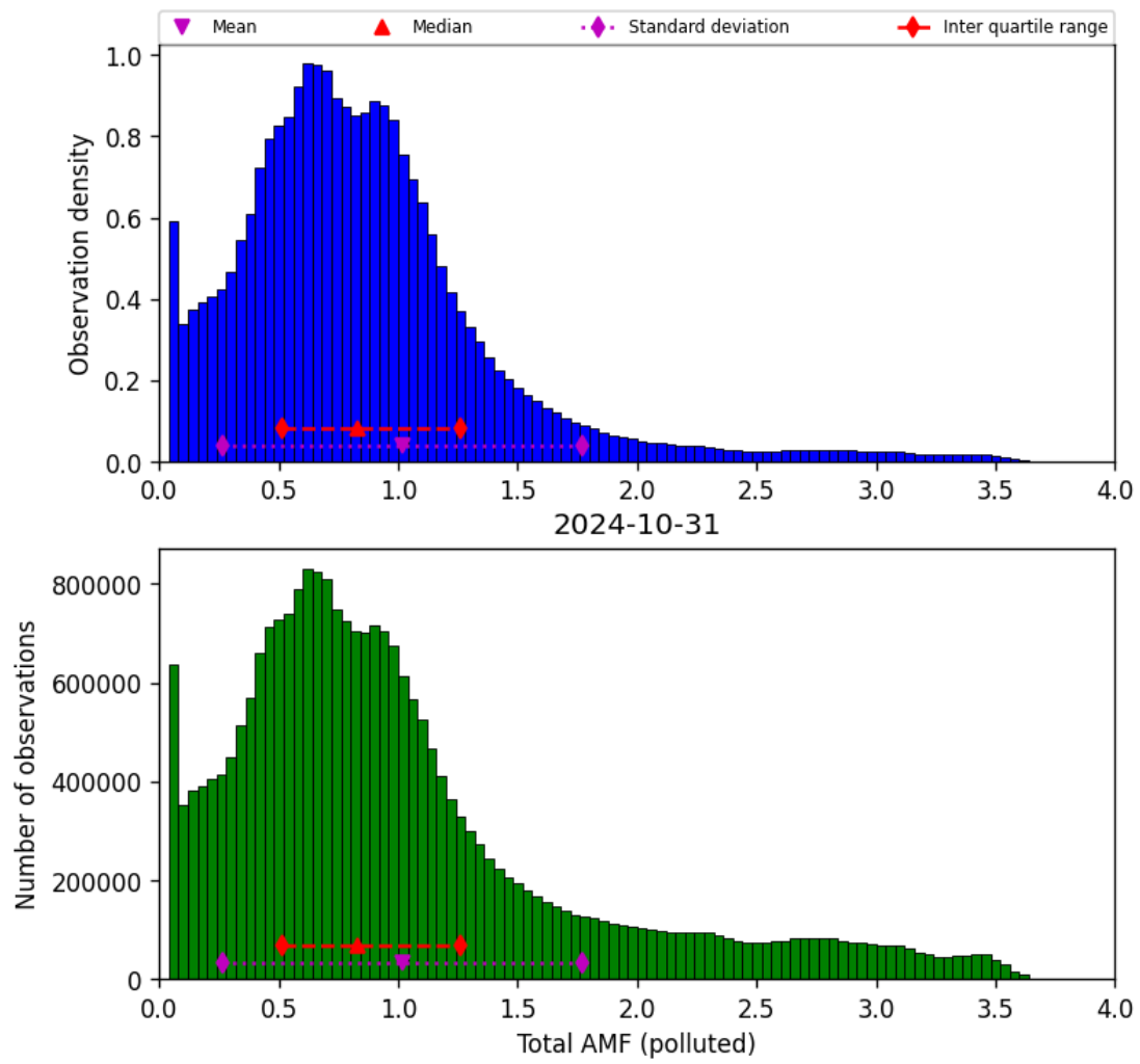
Figure 71: Histogram of “Total AMF (polluted)” for 2024-10-30 to 2024-11-01
