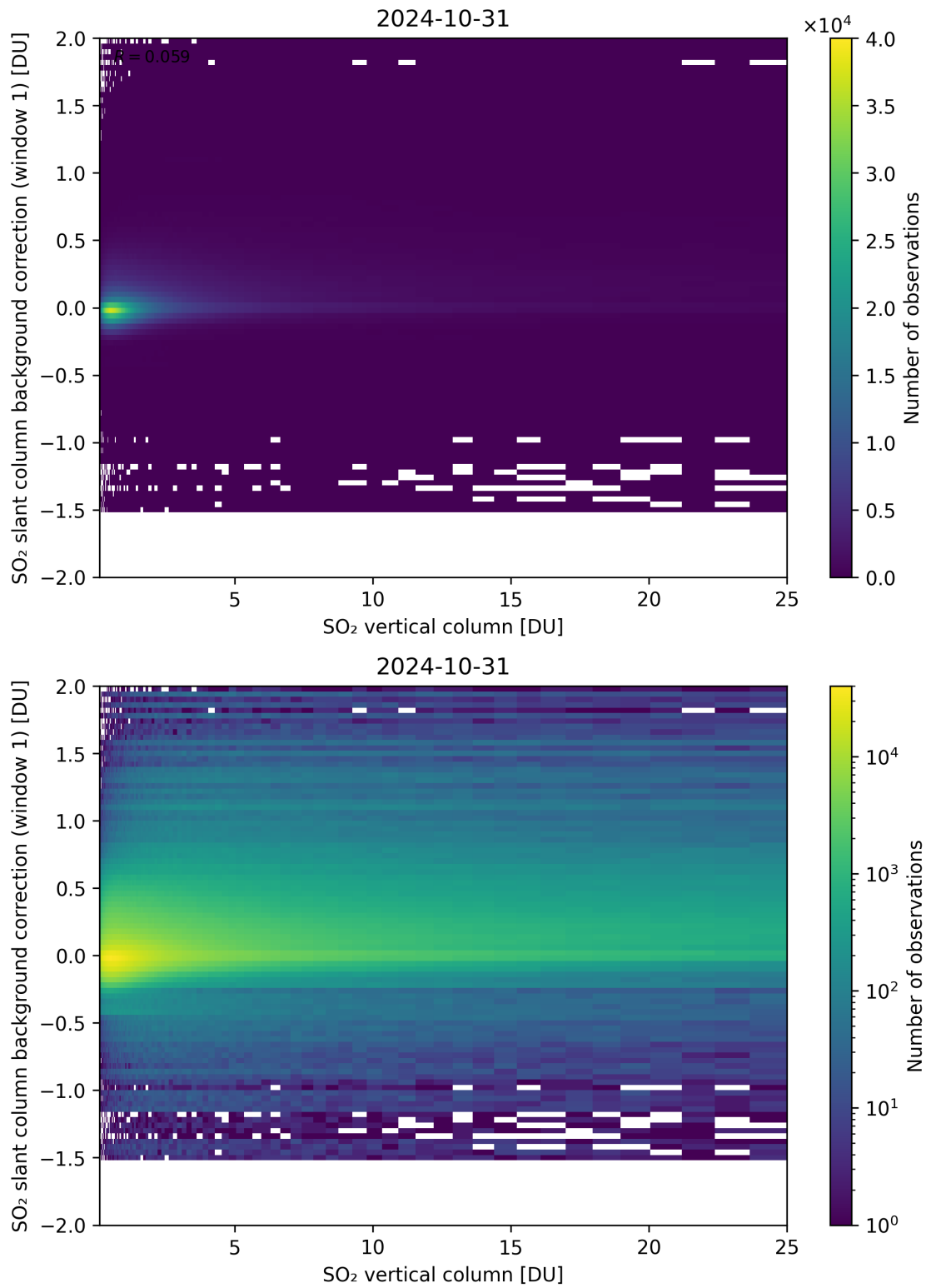
Figure 273: Scatter density plot of “SO 2 vertical column” against “SO 2 slant column background correction (window 1)” for 2024-10-30 to 2024-11-01.
