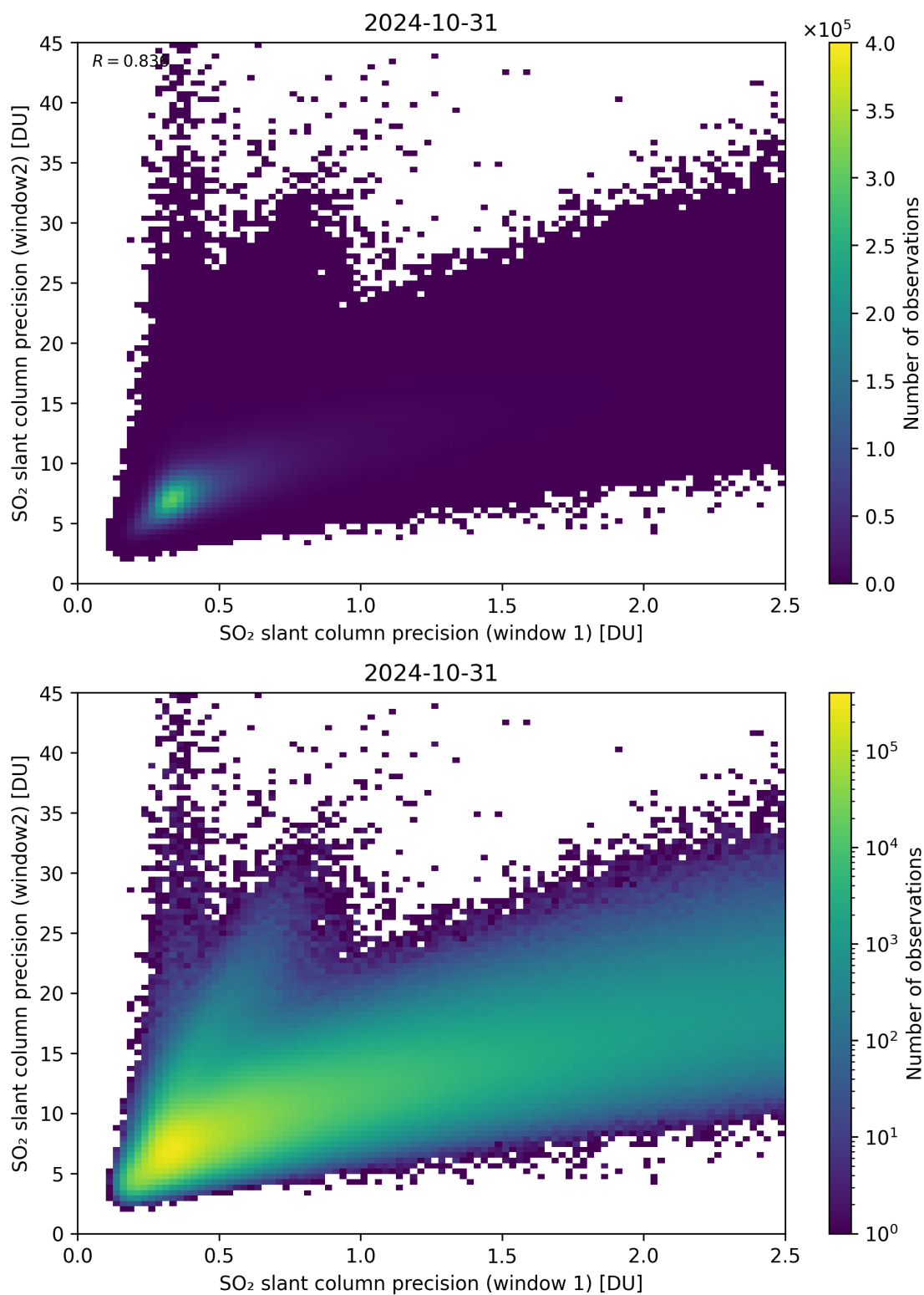
Figure 227: Scatter density plot of “SO 2 slant column precision (window 1)” against “SO 2 slant column precision (window2)” for 2024-10-30 to 2024-11-01.
