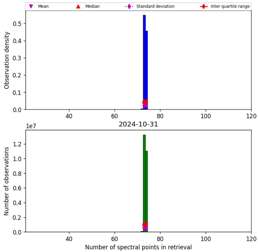
Figure 74: Histogram of “Number of spectral points in retrieval” for 2024-10-30 to 2024-11-01
