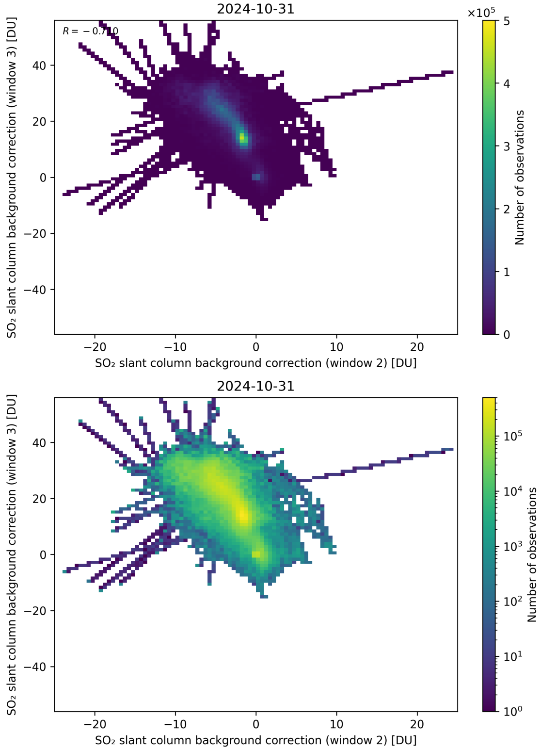
Figure 111: Scatter density plot of “SO 2 slant column background correction (window 2)” against “SO 2 slant column background correction (window 3)” for 2024-10-30 to 2024-11-01.
