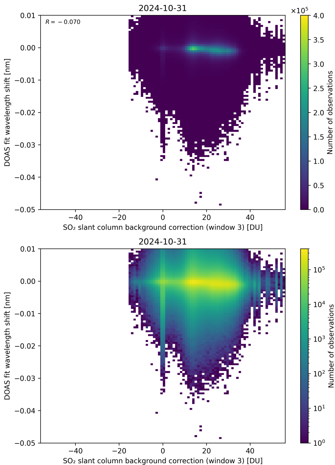
Figure 121: Scatter density plot of “SO 2 slant column background correction (window 3)” against “DOAS fit wavelength shift” for 2024-10-30 to 2024-11-01.
