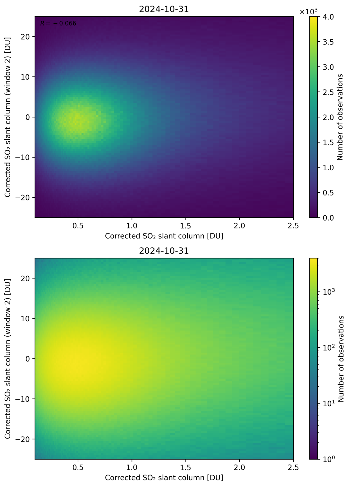
Figure 185: Scatter density plot of “Corrected SO 2 slant column” against “Corrected SO 2 slant column (window 2)” for 2024-10-30 to 2024-11-01.
