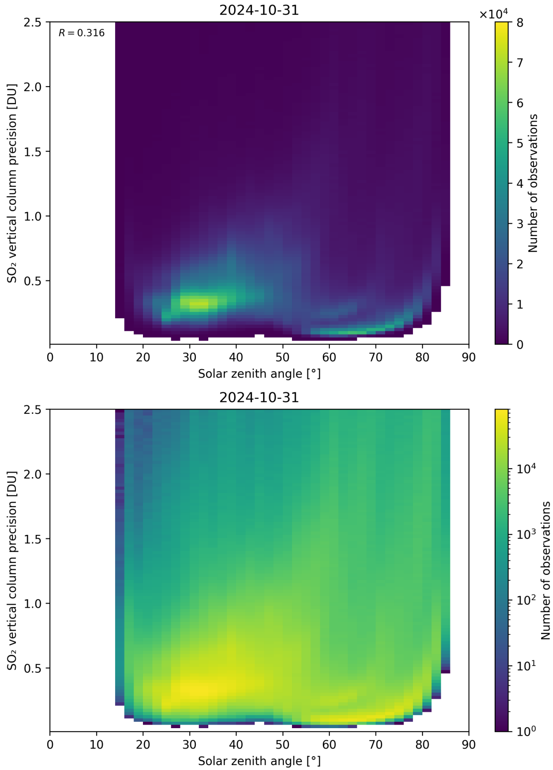
Figure 177: Scatter density plot of “Solar zenith angle” against “SO 2 vertical column precision” for 2024-10-30 to 2024-11-01.
