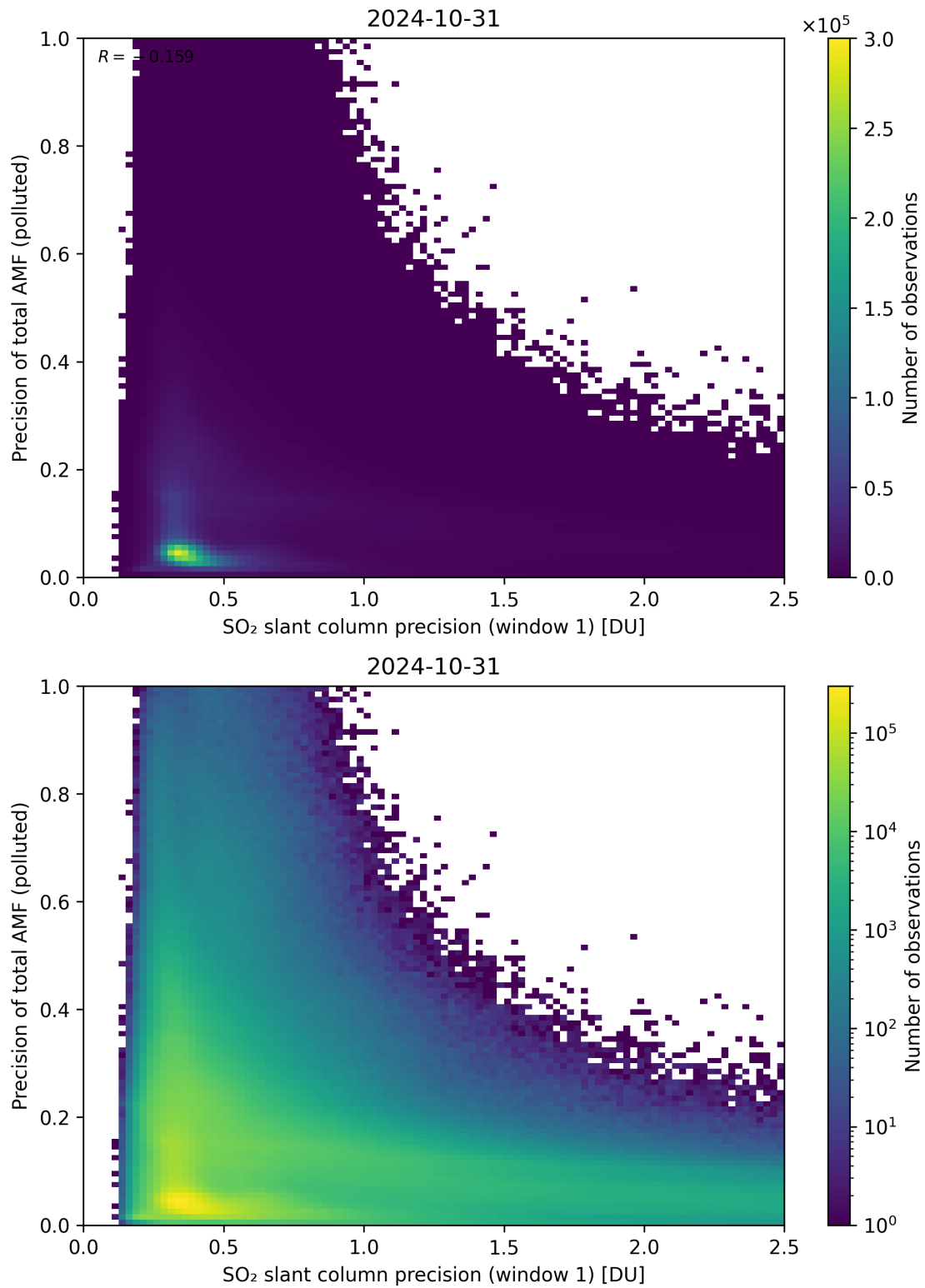
Figure 231: Scatter density plot of “SO 2 slant column precision (window 1)” against “Precision of total AMF (polluted)” for 2024-10-30 to 2024-11-01.
