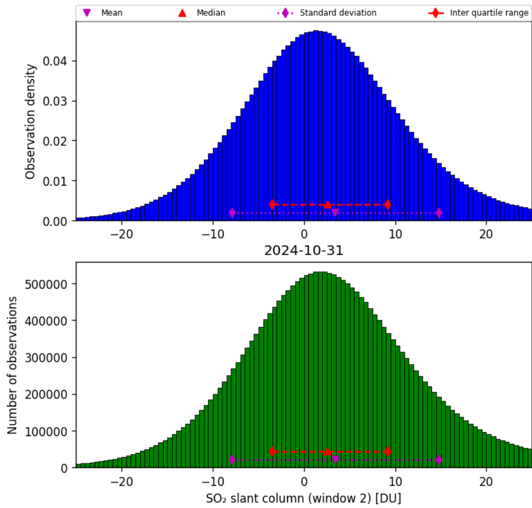
Figure 60: Histogram of “SO 2 slant column (window 2)” for 2024-10-30 to 2024-11-01
