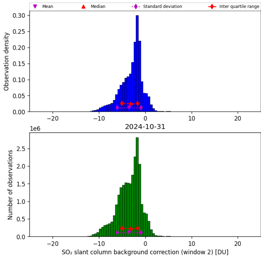
Figure 63: Histogram of “SO 2 slant column background correction (window 2)” for 2024-10-30 to 2024-11-01
