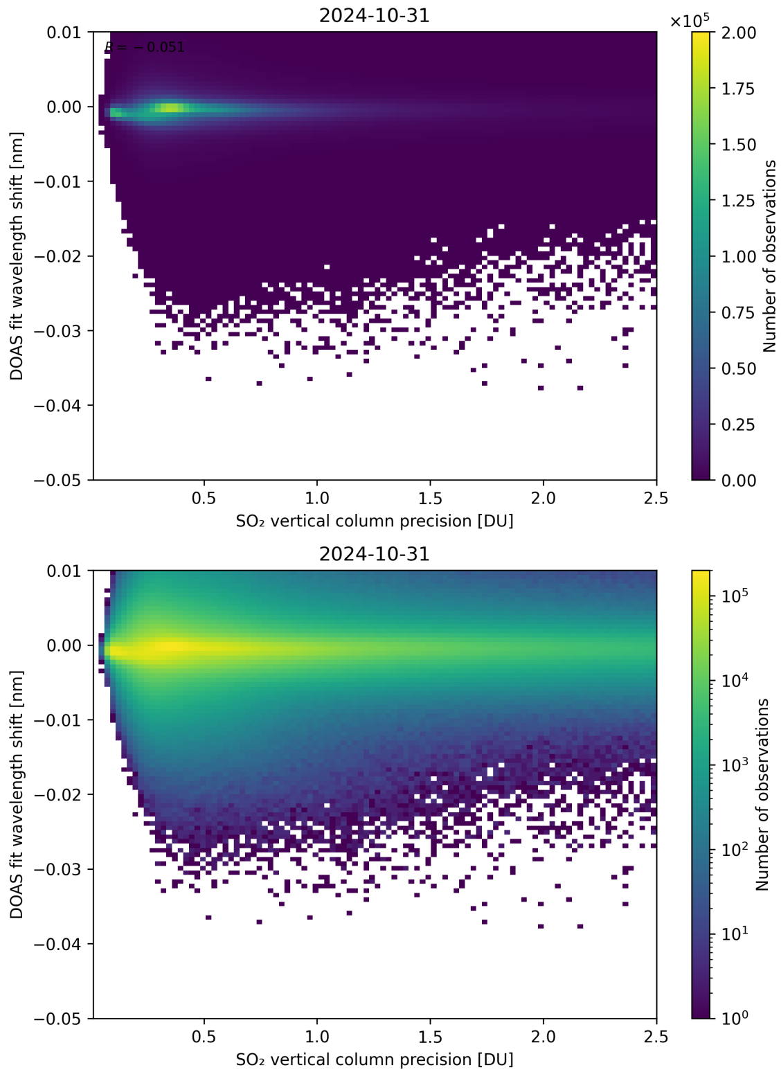
Figure 282: Scatter density plot of “SO 2 vertical column precision” against “DOAS fit wavelength shift” for 2024-10-30 to 2024-11-01.
