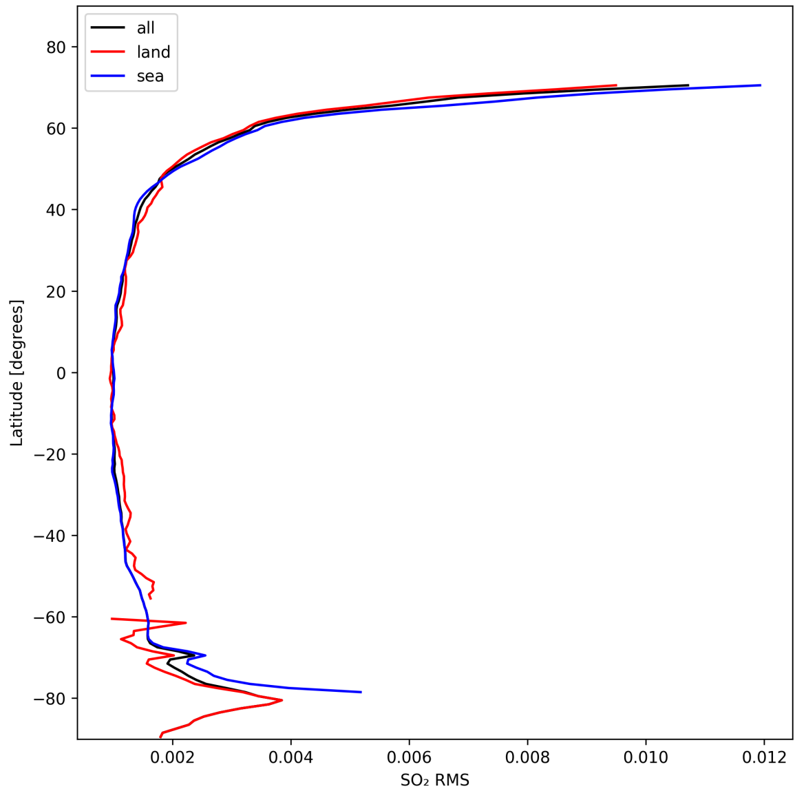
Figure 47: Zonal average of “SO 2 RMS” for 2024-10-30 to 2024-11-01.
