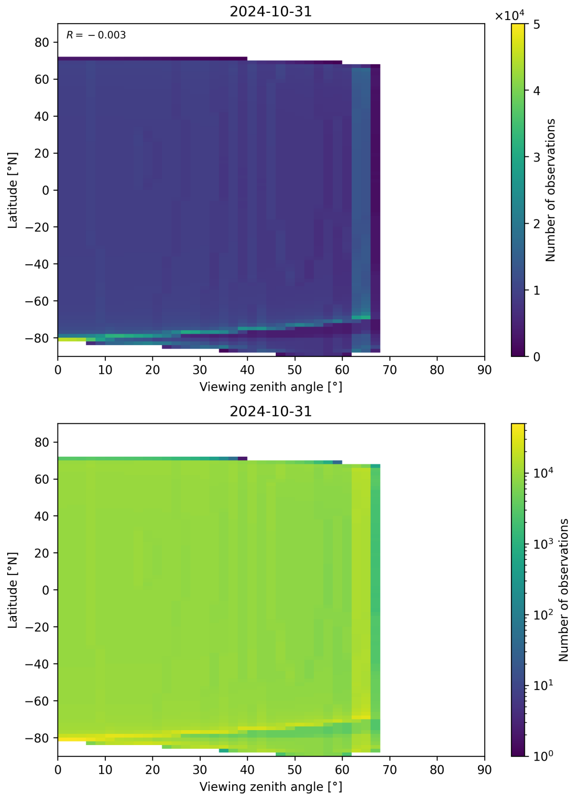
Figure 314: Scatter density plot of “Viewing zenith angle” against “Latitude” for 2024-10-30 to 2024-11-01.
