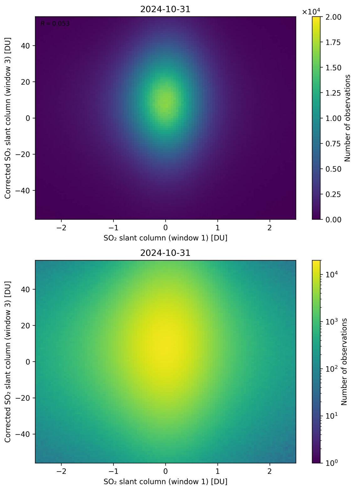
Figure 234: Scatter density plot of “SO 2 slant column (window 1)” against “Corrected SO 2 slant column (window 3)” for 2024-10-30 to 2024-11-01.
