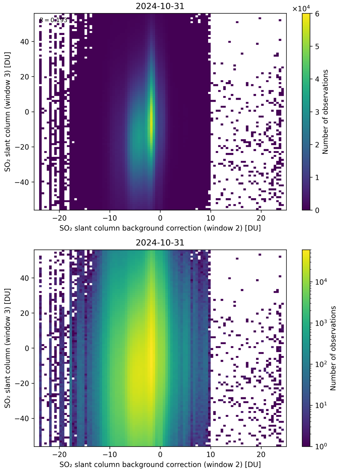
Figure 117: Scatter density plot of “SO 2 slant column background correction (window 2)” against “SO 2 slant column (window 3)” for 2024-10-30 to 2024-11-01.
