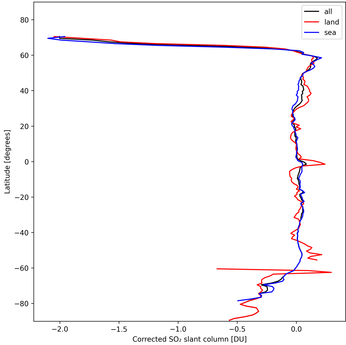
Figure 32: Zonal average of “Corrected SO 2 slant column” for 2024-10-30 to 2024-11-01.
