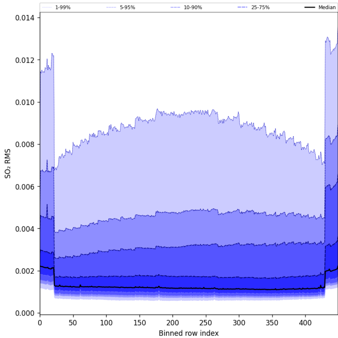
Figure 93: Along track statistics of “SO 2 RMS” for 2024-10-30 to 2024-11-01
