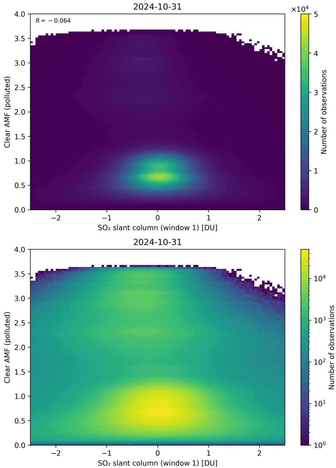
Figure 232: Scatter density plot of “SO 2 slant column (window 1)” against “Clear AMF (polluted)” for 2024-10-30 to 2024-11-01.
