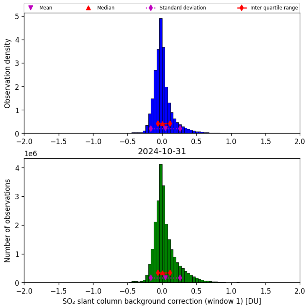
Figure 59: Histogram of “SO 2 slant column background correction (window 1)” for 2024-10-30 to 2024-11-01
