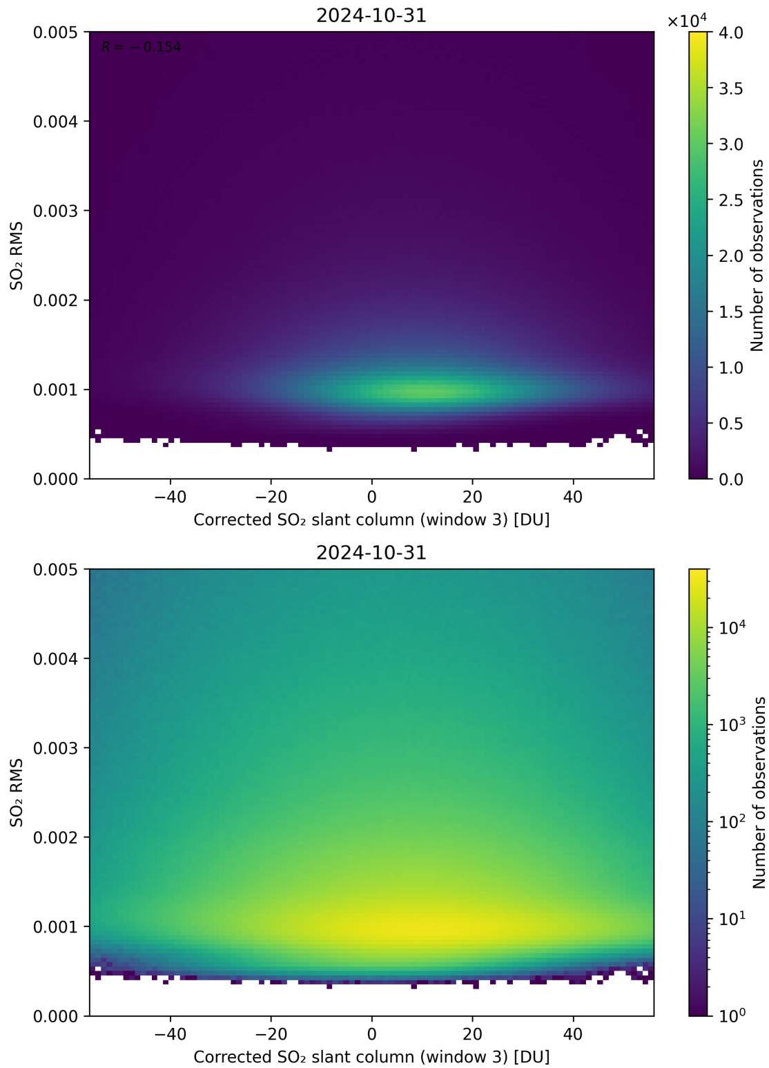
Figure 208: Scatter density plot of “Corrected SO 2 slant column (window 3)” against “SO 2 RMS” for 2024-10-30 to 2024-11-01.
