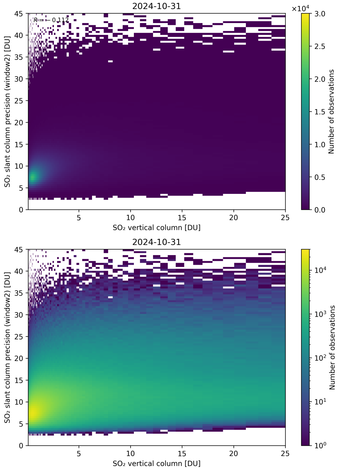
Figure 302: Scatter density plot of “SO 2 vertical column” against “SO 2 slant column precision (window2)” for 2024-10-30 to 2024-11-01.
