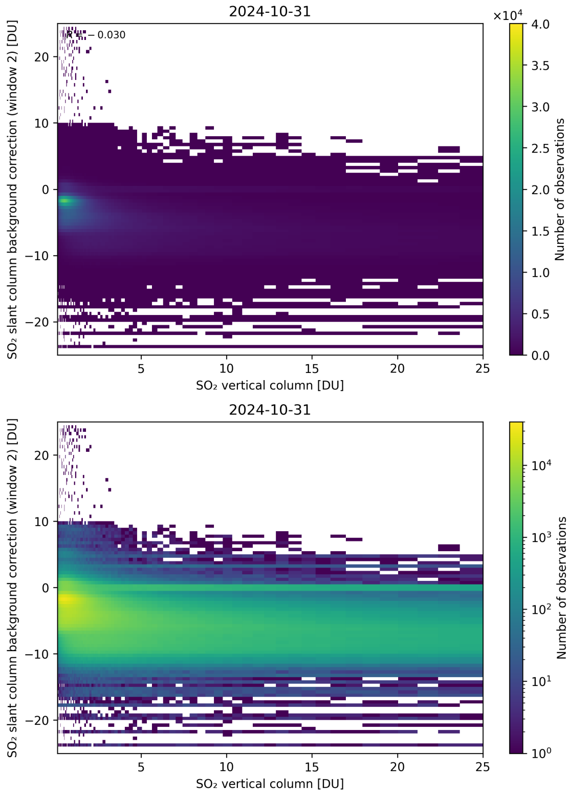
Figure 274: Scatter density plot of “SO 2 vertical column” against “SO 2 slant column background correction (window 2)” for 2024-10-30 to 2024-11-01.
