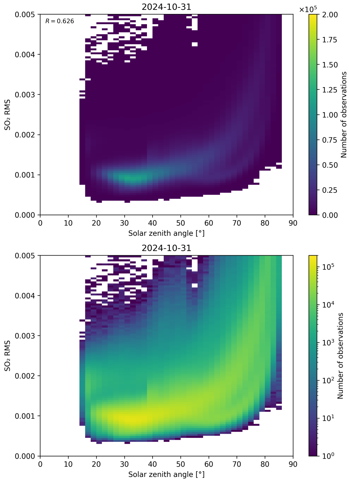
Figure 163: Scatter density plot of “Solar zenith angle” against “SO 2 RMS” for 2024-10-30 to 2024-11-01.
