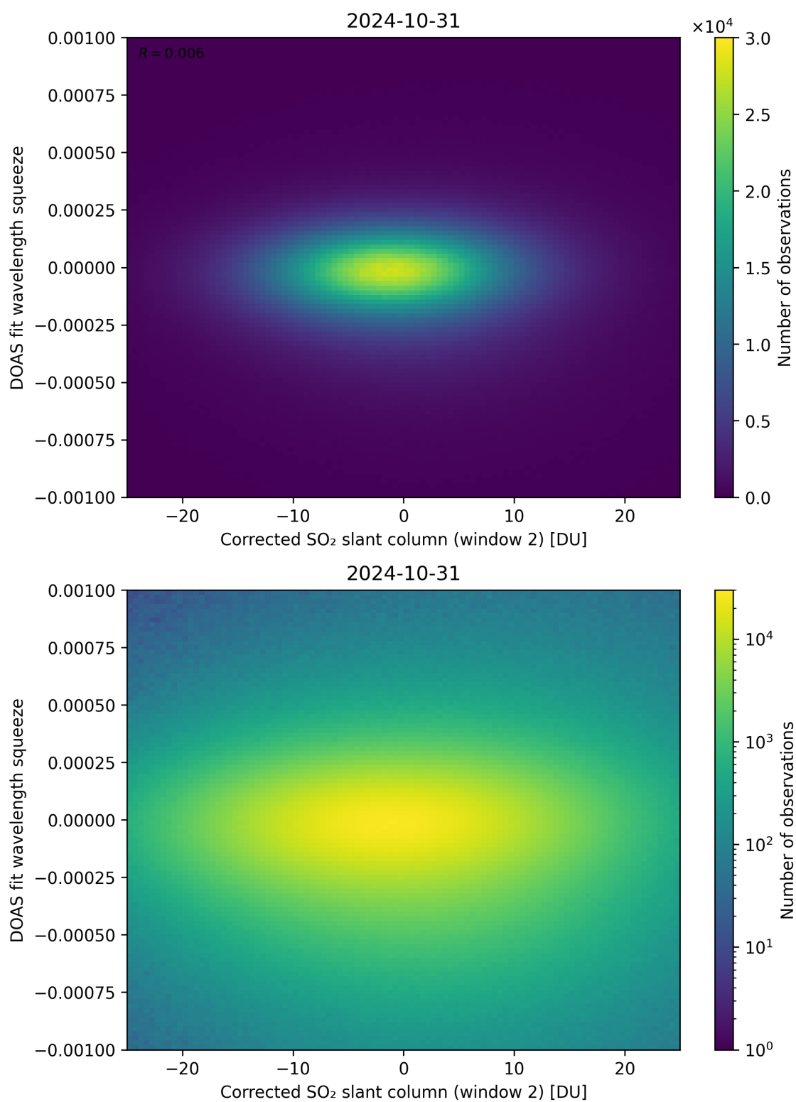
Figure 197: Scatter density plot of “Corrected SO 2 slant column (window 2)” against “DOAS fit wavelength squeeze” for 2024-10-30 to 2024-11-01.
