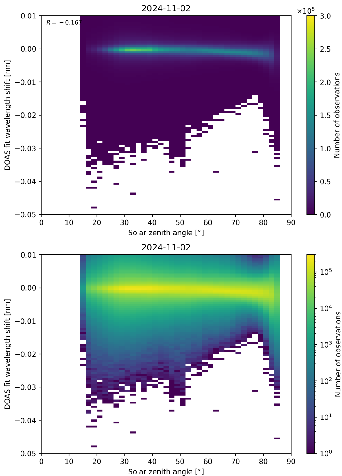
Figure 161: Scatter density plot of “Solar zenith angle” against “DOAS fit wavelength shift” for 2024-11-01 to 2024-11-03.
