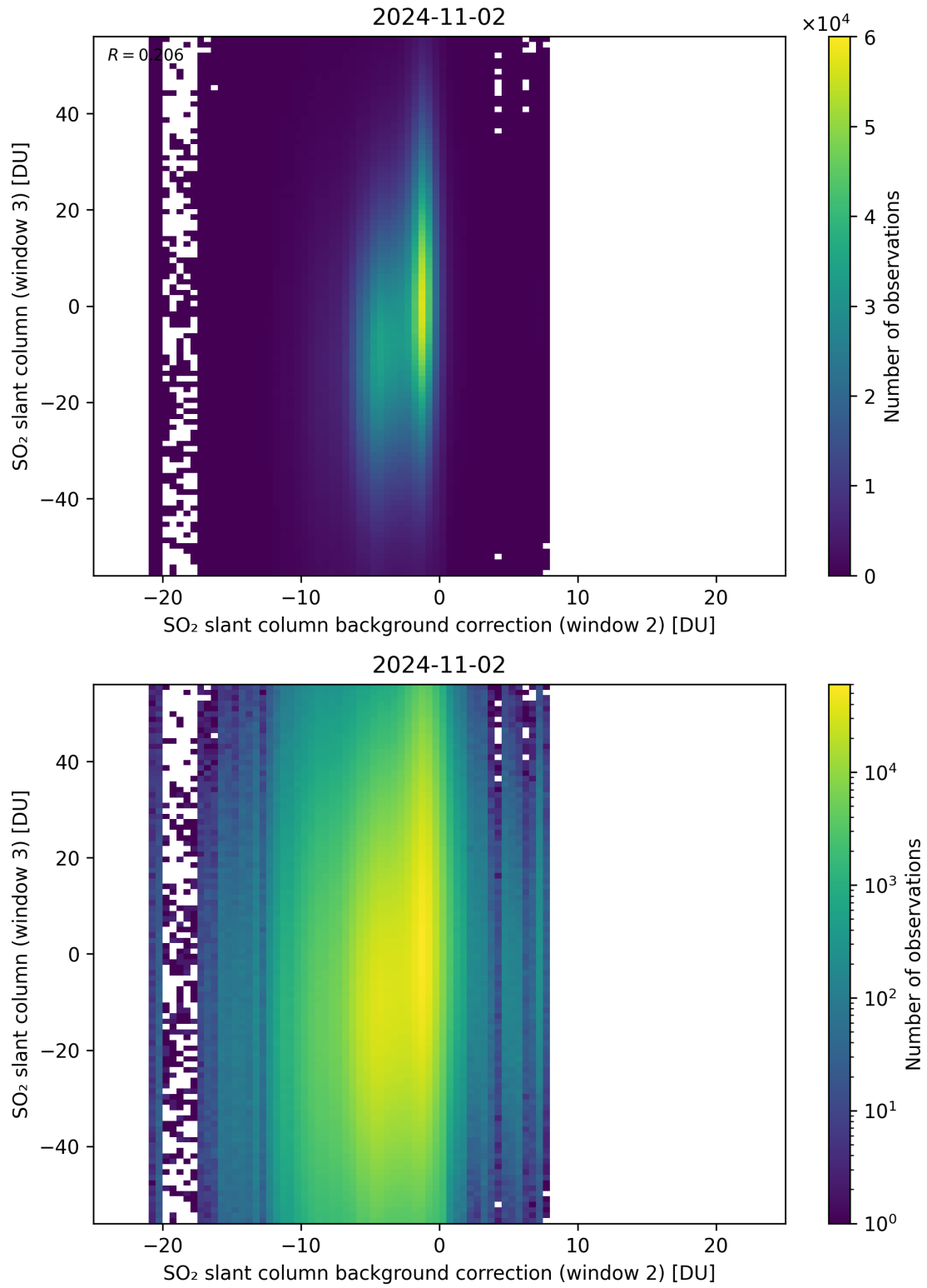
Figure 117: Scatter density plot of “SO 2 slant column background correction (window 2)” against “SO 2 slant column (window 3)” for 2024-11-01 to 2024-11-03.
