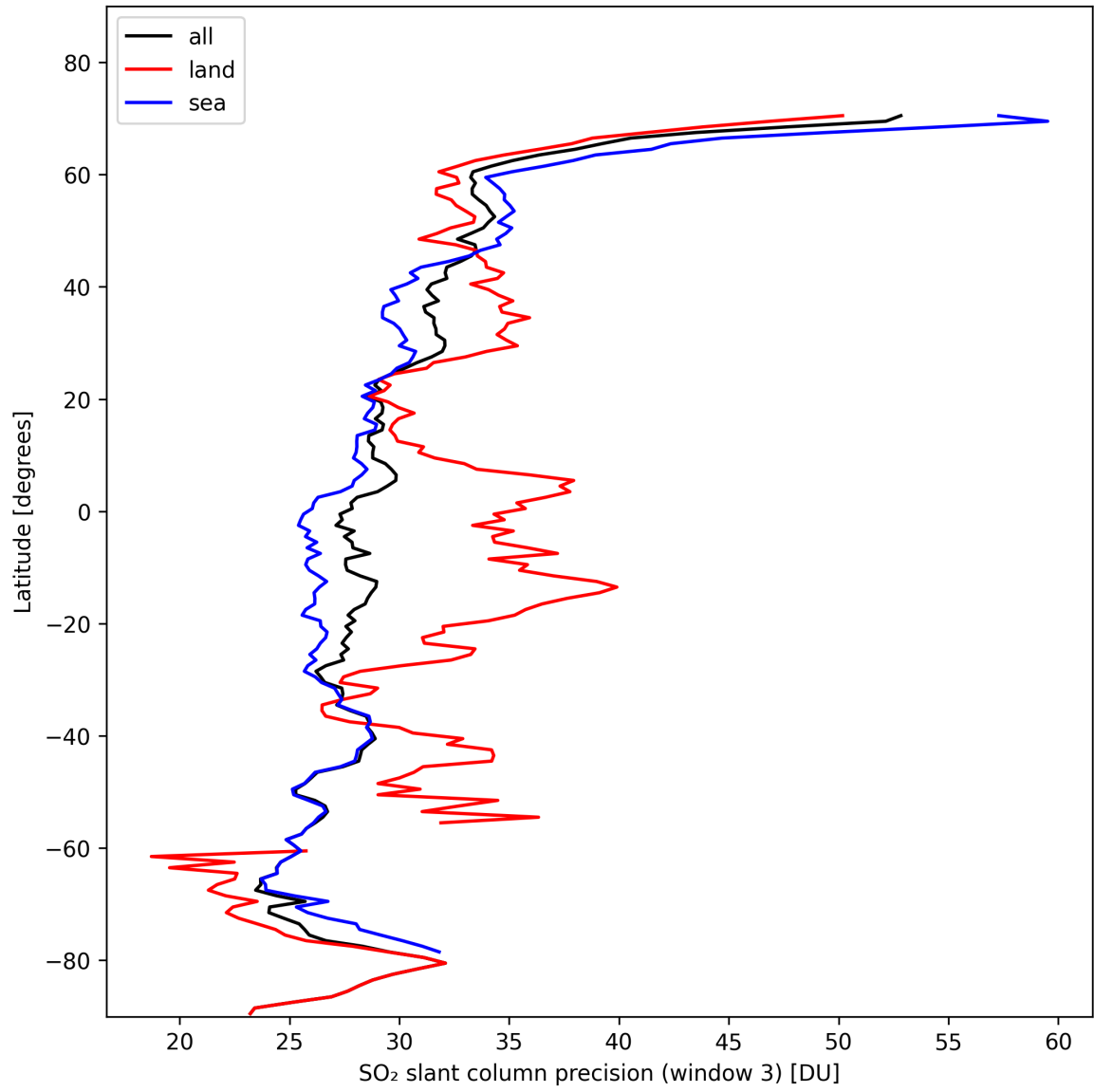
Figure 42: Zonal average of “SO 2 slant column precision (window 3)” for 2024-11-01 to 2024-11-03.
