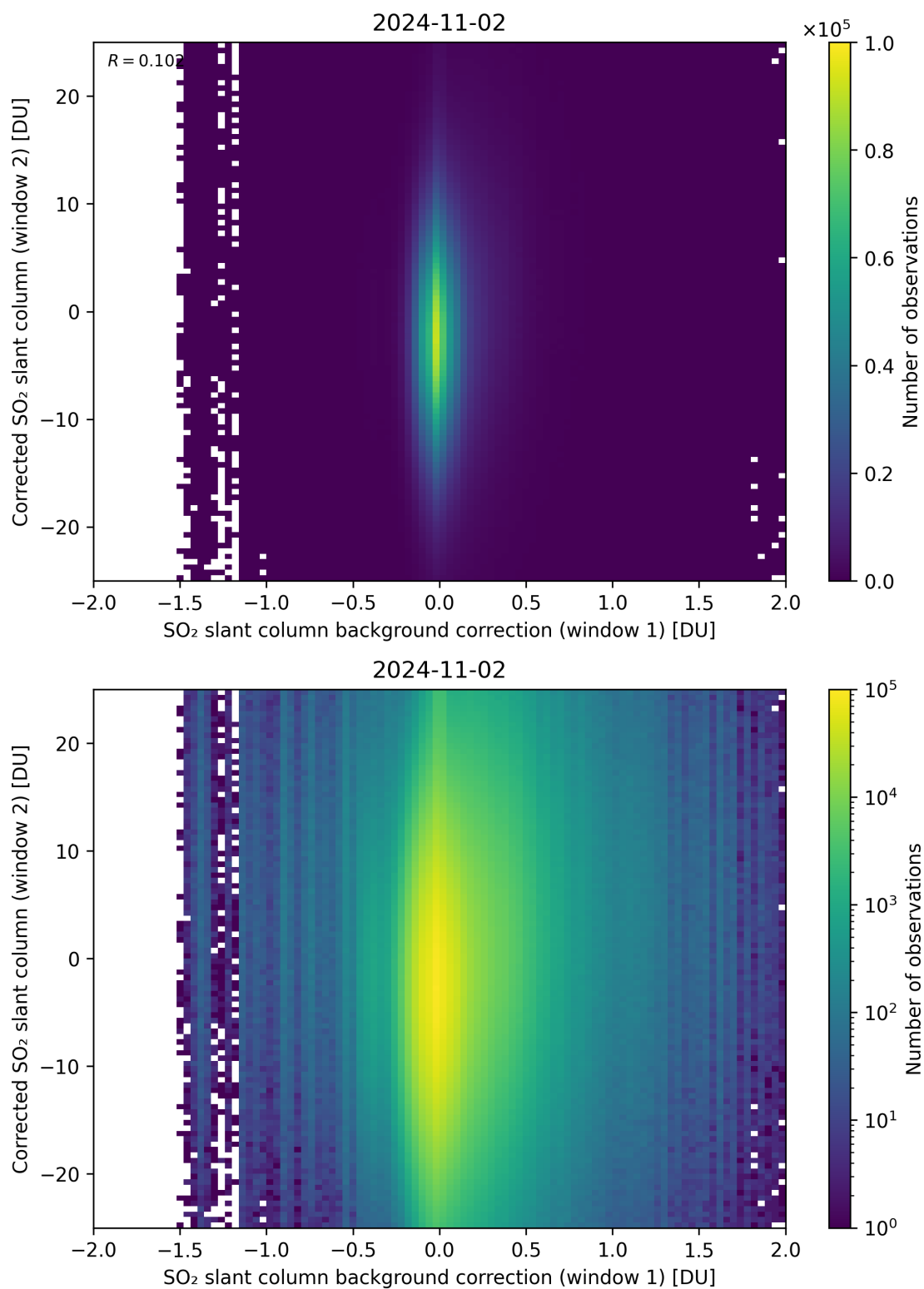
Figure 104: Scatter density plot of “SO 2 slant column background correction (window 1)” against “Corrected SO 2 slant column (window 2)” for 2024-11-01 to 2024-11-03.
