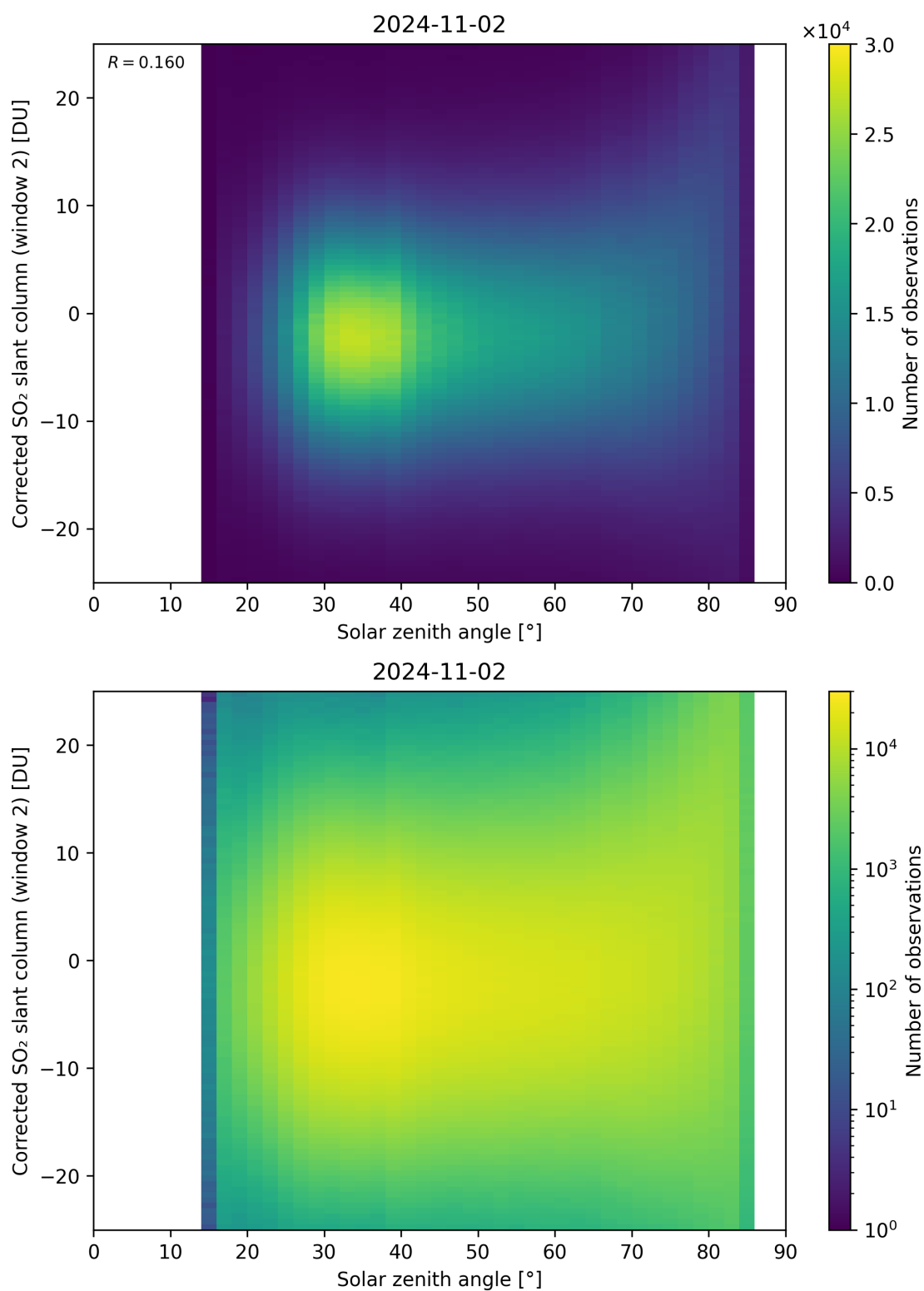
Figure 167: Scatter density plot of “Solar zenith angle” against “Corrected SO 2 slant column (window 2)” for 2024-11-01 to 2024-11-03.
