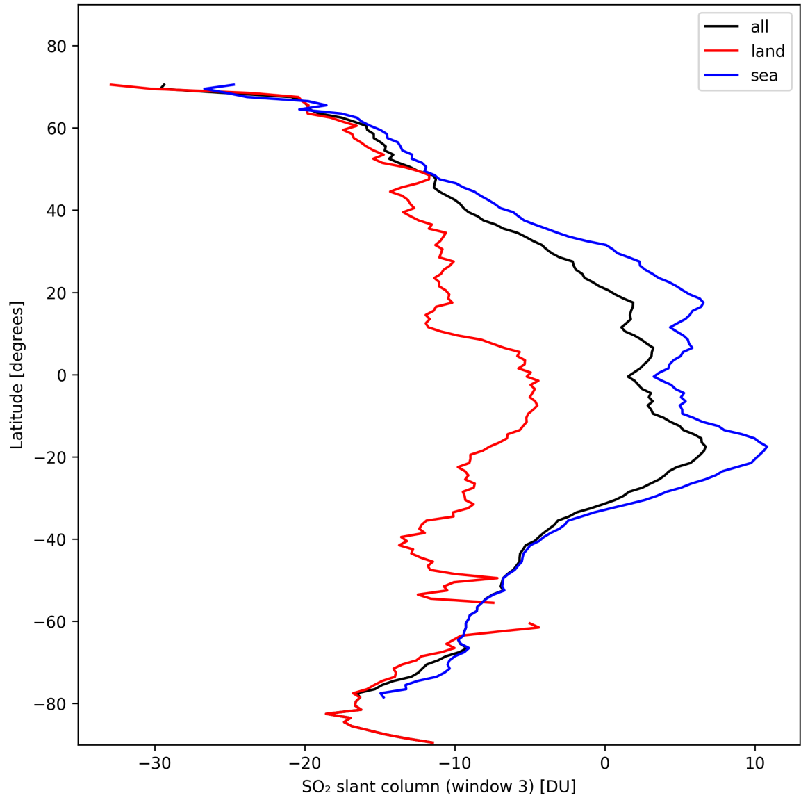
Figure 41: Zonal average of “SO 2 slant column (window 3)” for 2024-11-01 to 2024-11-03.
