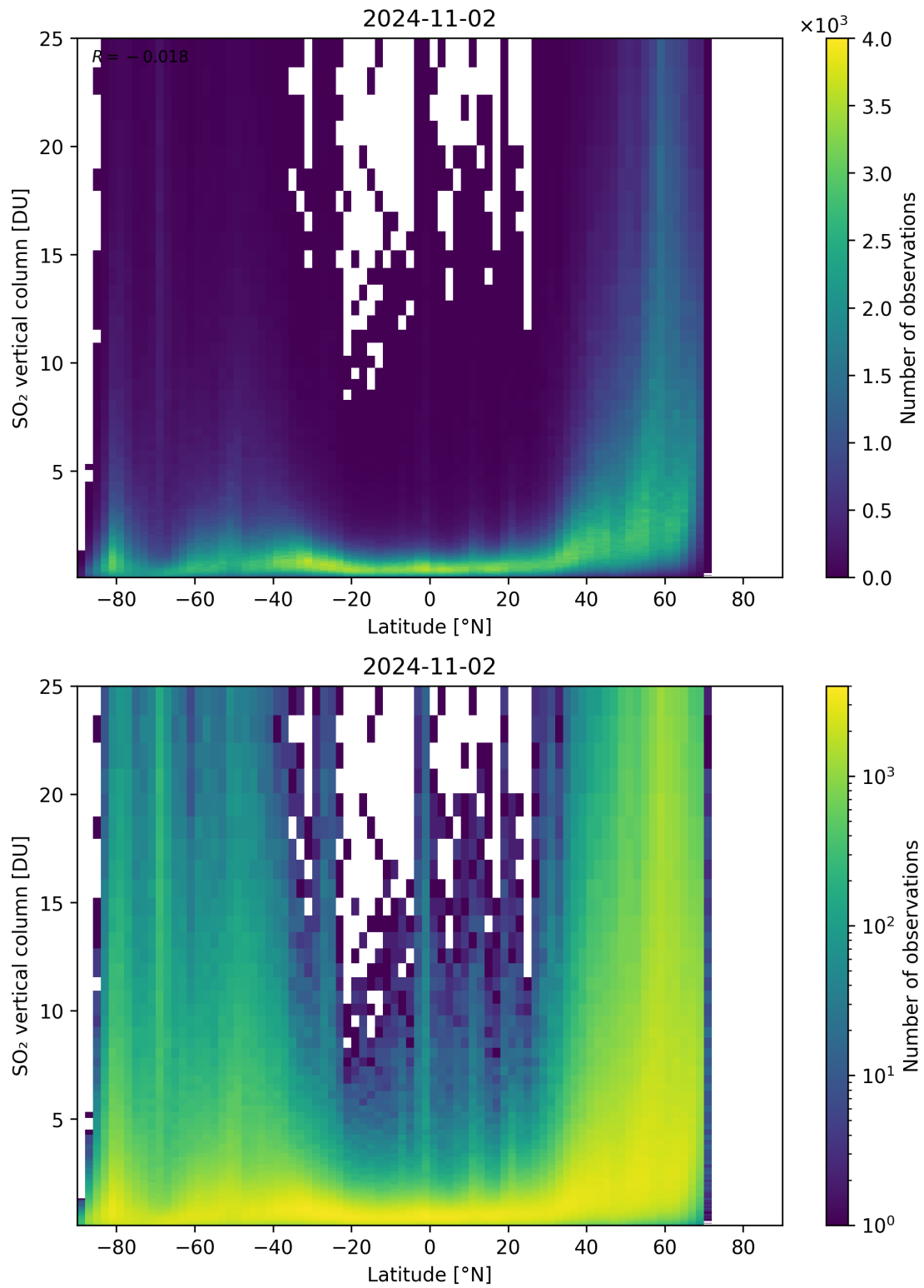
Figure 156: Scatter density plot of “Latitude” against “SO 2 vertical column” for 2024-11-01 to 2024-11-03.
