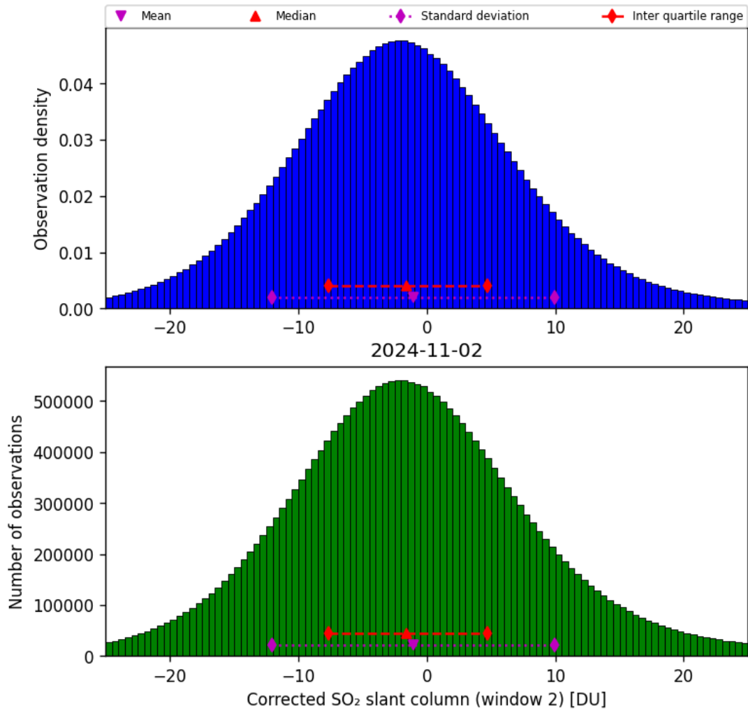
Figure 62: Histogram of “Corrected SO 2 slant column (window 2)” for 2024-11-01 to 2024-11-03
