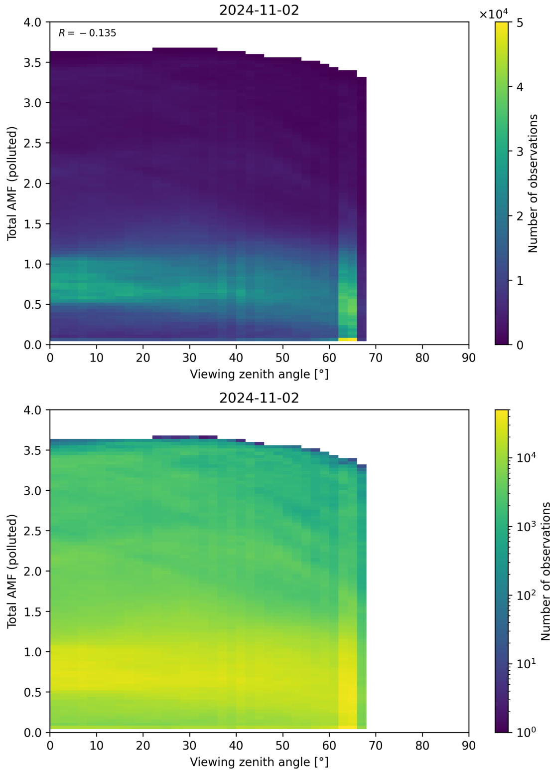
Figure 325: Scatter density plot of “Viewing zenith angle” against “Total AMF (polluted)” for 2024-11-01 to 2024-11-03.
