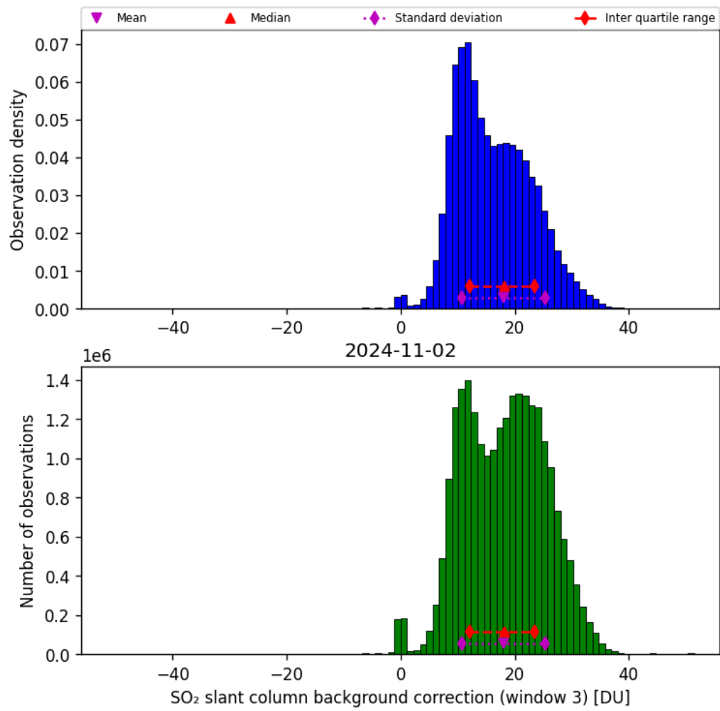
Figure 67: Histogram of “SO 2 slant column background correction (window 3)” for 2024-11-01 to 2024-11-03
