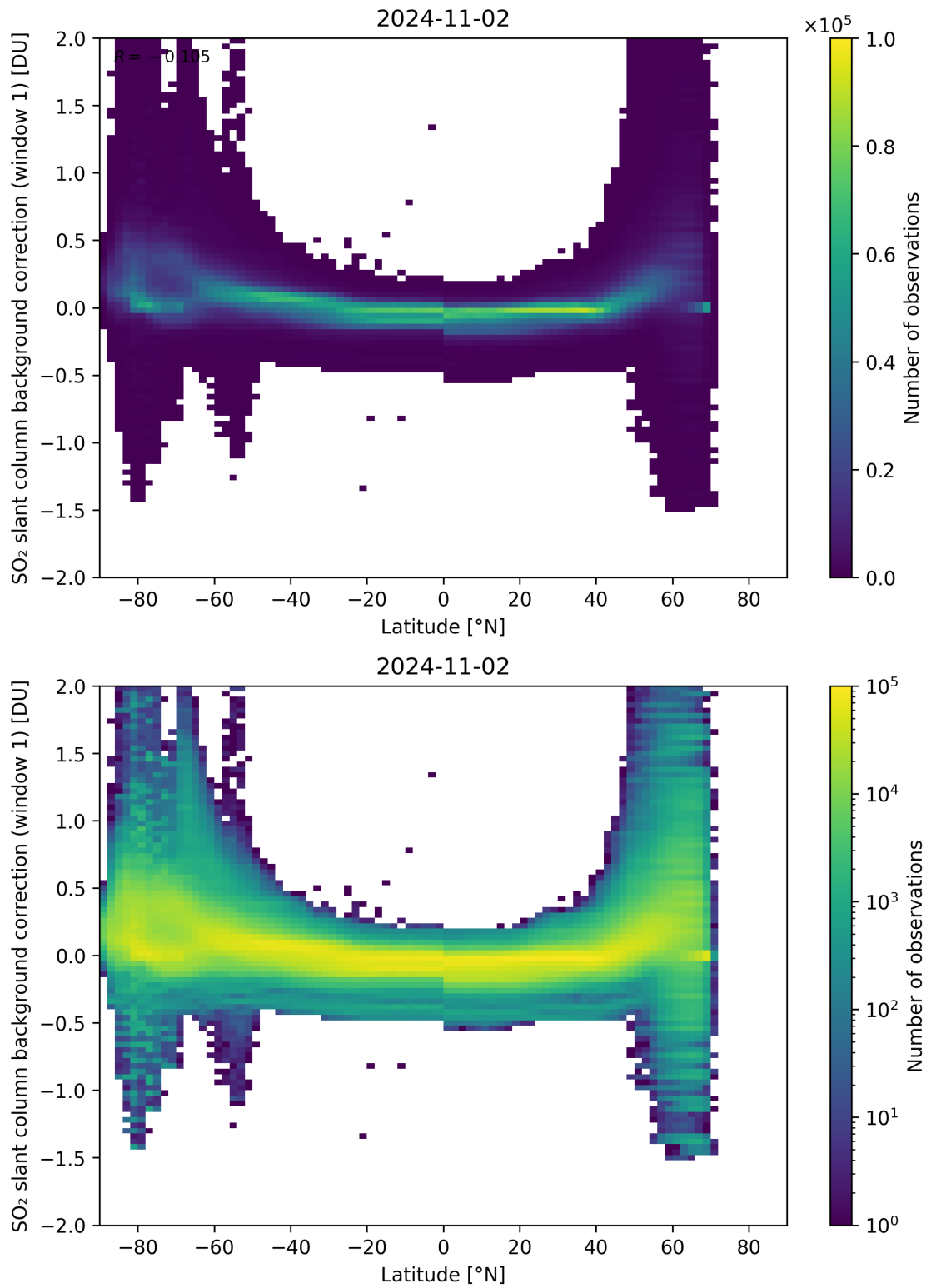
Figure 139: Scatter density plot of “Latitude” against “SO 2 slant column background correction (window 1)” for 2024-11-01 to 2024-11-03.
