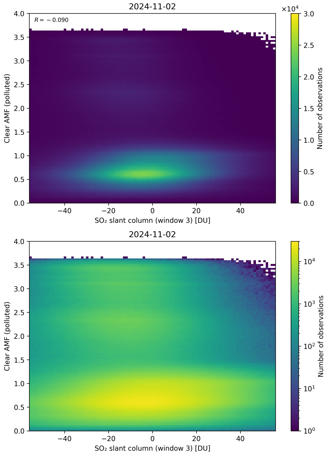
Figure 265: Scatter density plot of “SO 2 slant column (window 3)” against “Clear AMF (polluted)” for 2024-11-01 to 2024-11-03.
