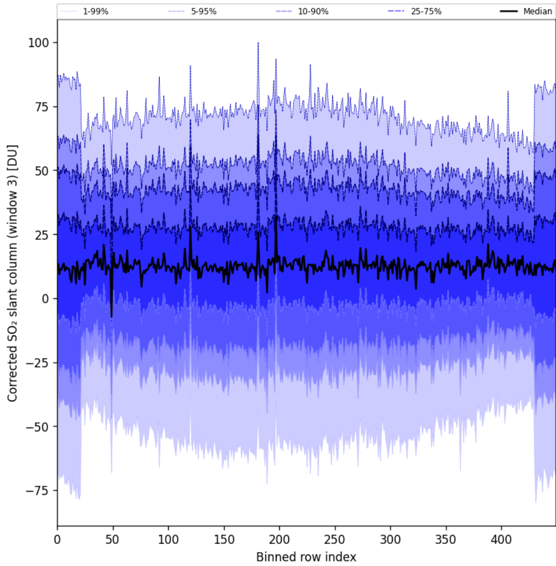
Figure 89: Along track statistics of “Corrected SO 2 slant column (window 3)” for 2024-11-01 to 2024-11-03
