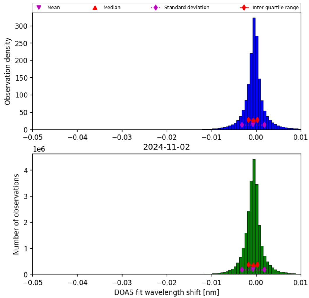
Figure 68: Histogram of “DOAS fit wavelength shift” for 2024-11-01 to 2024-11-03
