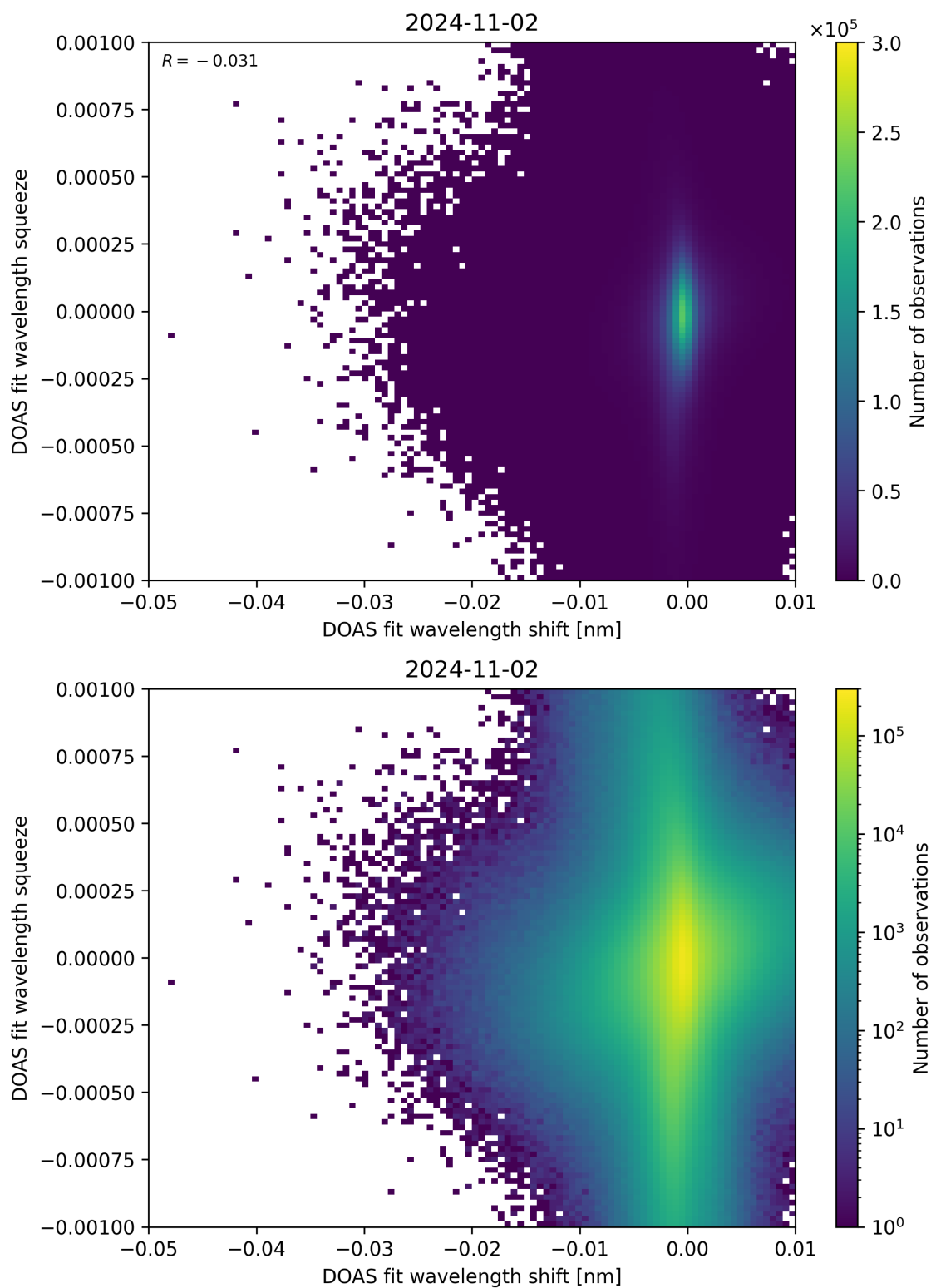
Figure 127: Scatter density plot of “DOAS fit wavelength shift” against “DOAS fit wavelength squeeze” for 2024-11-01 to 2024-11-03.
