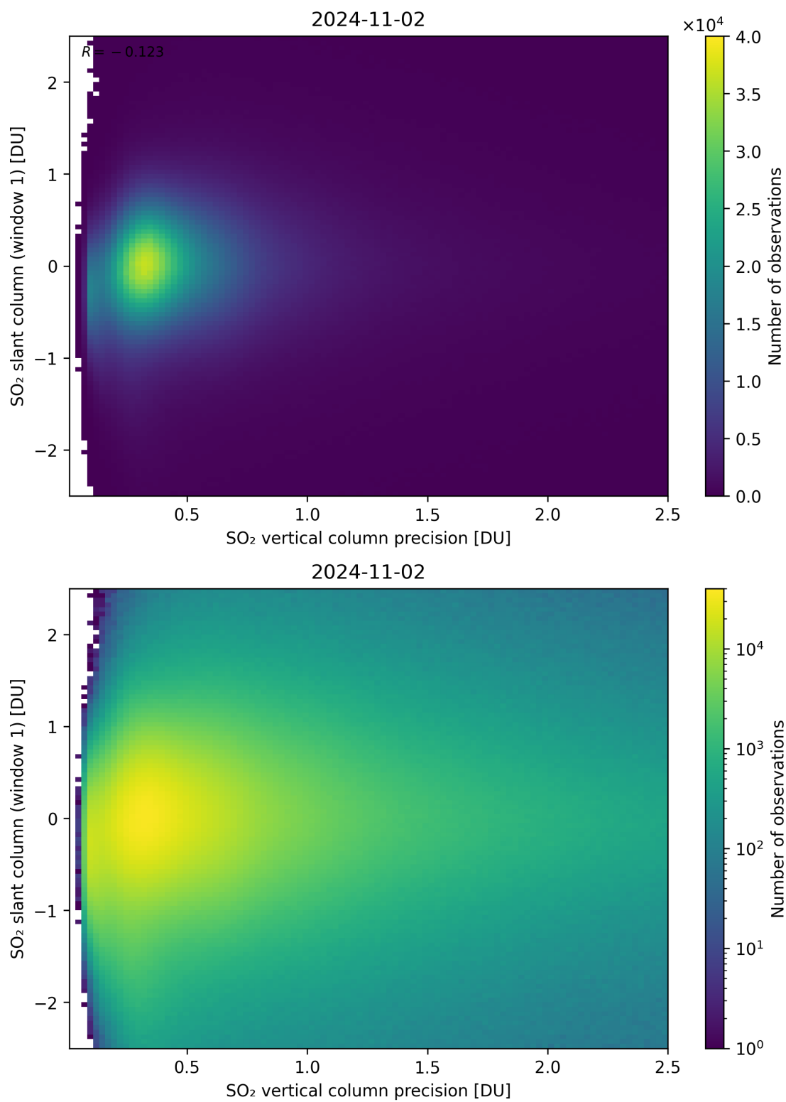
Figure 289: Scatter density plot of “SO 2 vertical column precision” against “SO 2 slant column (window 1)” for 2024-11-01 to 2024-11-03.
