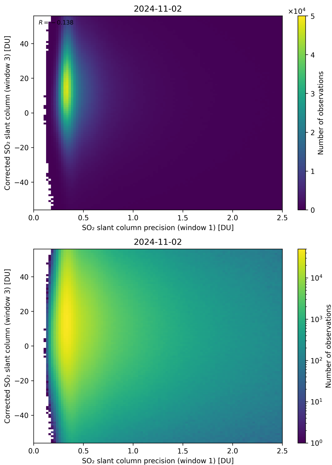
Figure 226: Scatter density plot of “SO 2 slant column precision (window 1)” against “Corrected SO 2 slant column (window 3)” for 2024-11-01 to 2024-11-03.
