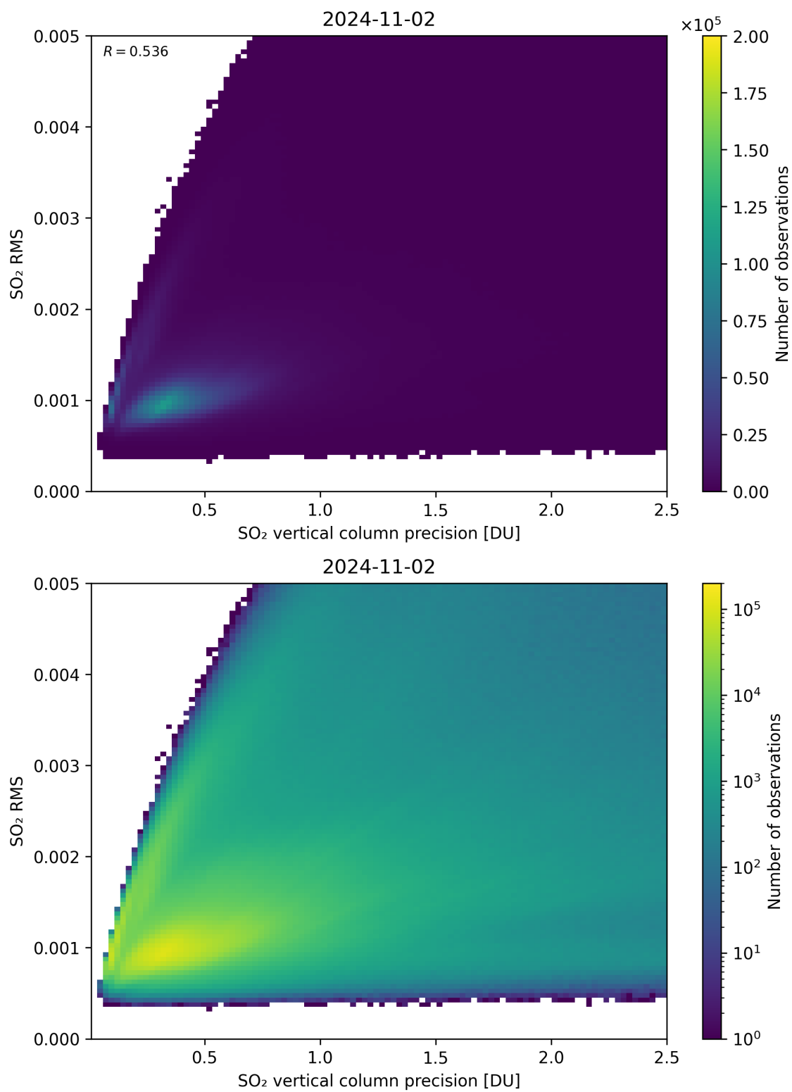
Figure 284: Scatter density plot of “SO 2 vertical column precision” against “SO 2 RMS” for 2024-11-01 to 2024-11-03.
