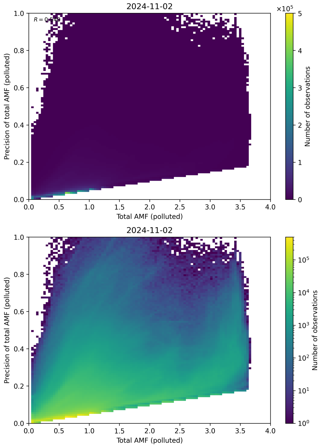
Figure 272: Scatter density plot of “Total AMF (polluted)” against “Precision of total AMF (polluted)” for 2024-11-01 to 2024-11-03.
