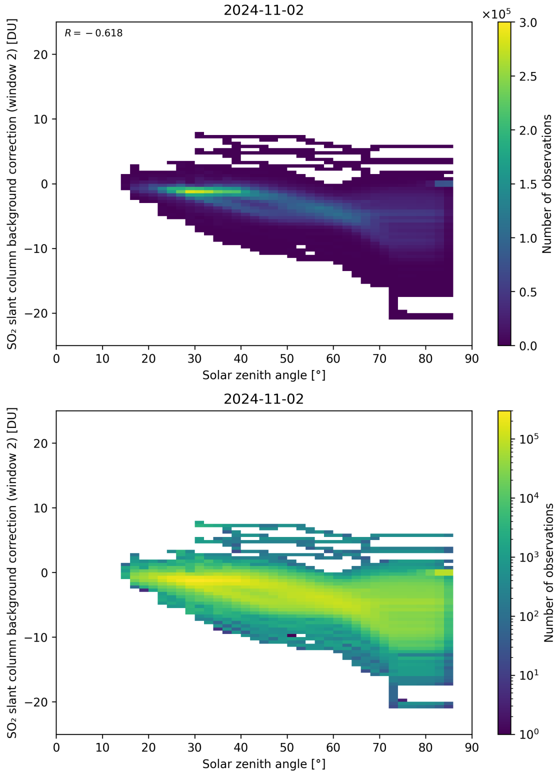
Figure 159: Scatter density plot of “Solar zenith angle” against “SO 2 slant column background correction (window 2)” for 2024-11-01 to 2024-11-03.
