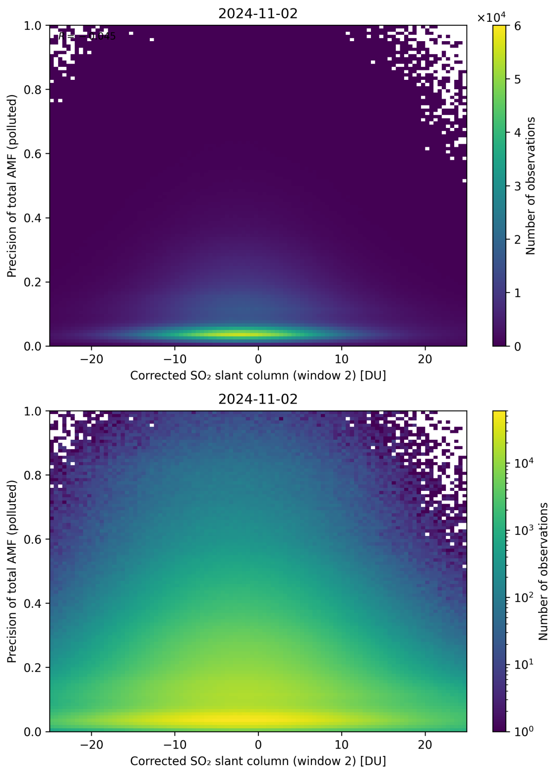
Figure 204: Scatter density plot of “Corrected SO 2 slant column (window 2)” against “Precision of total AMF (polluted)” for 2024-11-01 to 2024-11-03.
