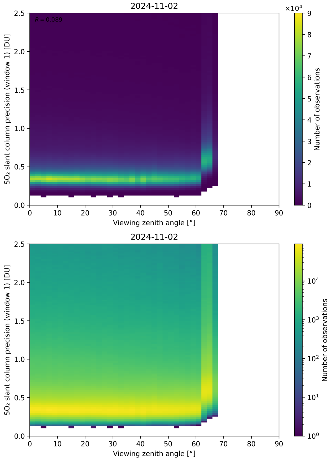
Figure 321: Scatter density plot of “Viewing zenith angle” against “SO 2 slant column precision (window 1)” for 2024-11-01 to 2024-11-03.
