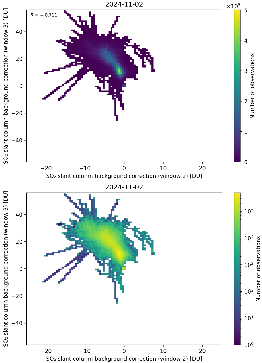
Figure 111: Scatter density plot of “SO 2 slant column background correction (window 2)” against “SO 2 slant column background correction (window 3)” for 2024-11-01 to 2024-11-03.
