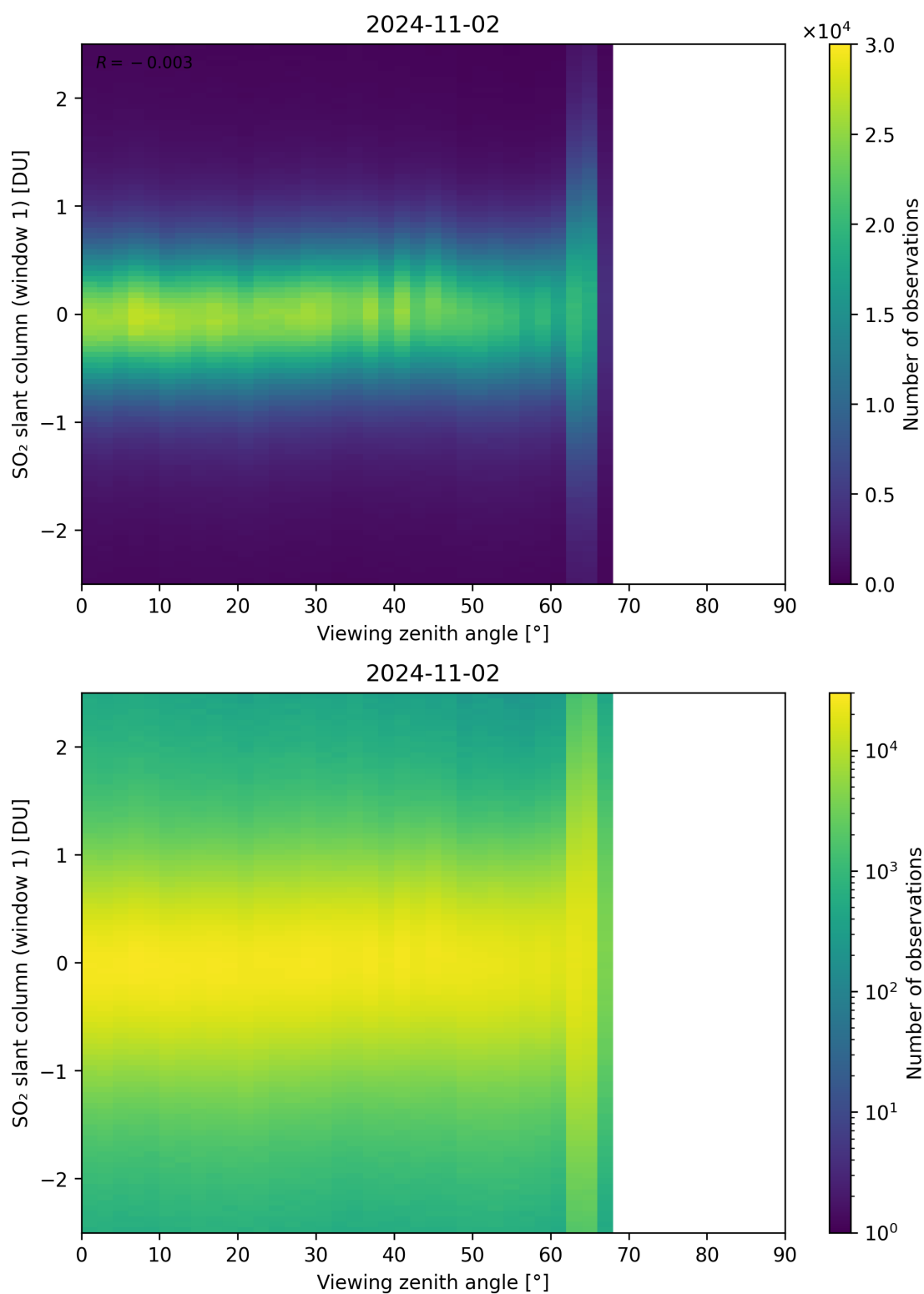
Figure 320: Scatter density plot of “Viewing zenith angle” against “SO 2 slant column (window 1)” for 2024-11-01 to 2024-11-03.
