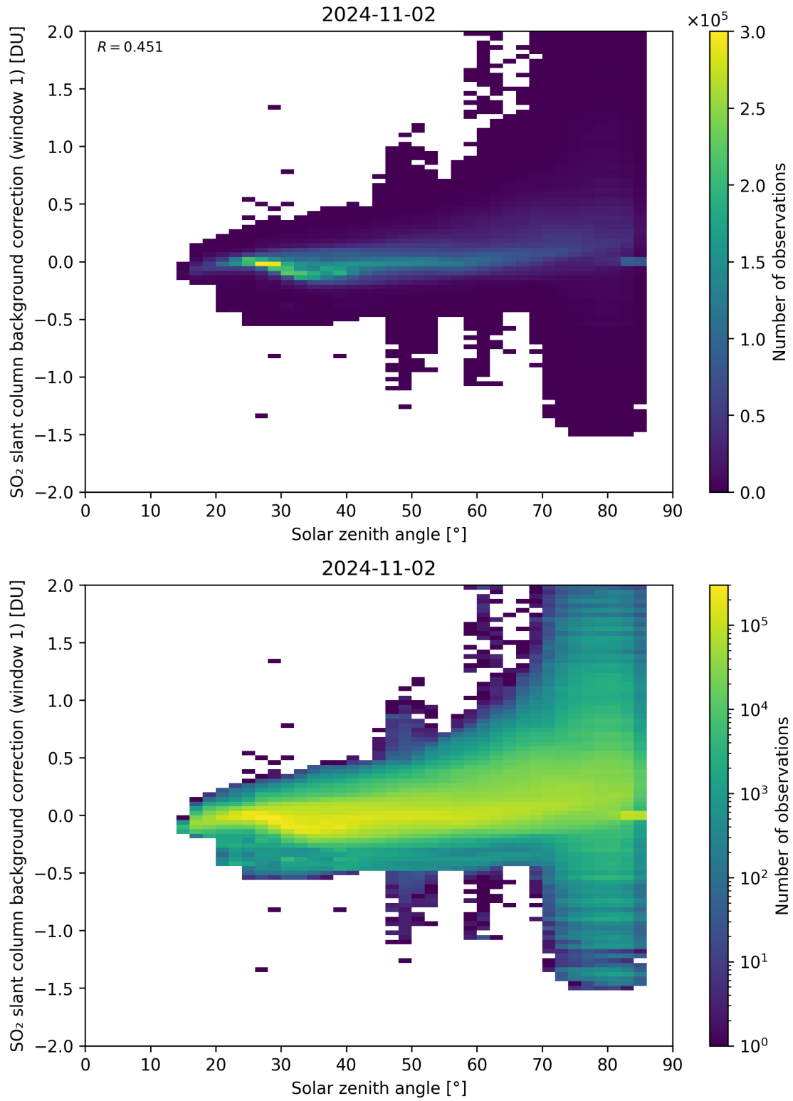
Figure 158: Scatter density plot of “Solar zenith angle” against “SO 2 slant column background correction (window 1)” for 2024-11-01 to 2024-11-03.
