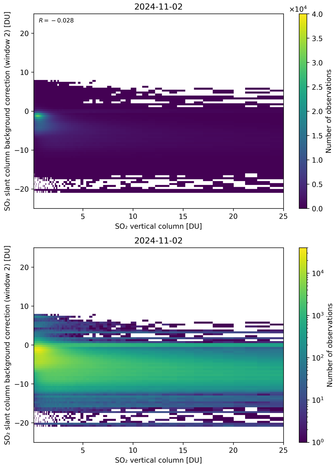
Figure 274: Scatter density plot of “SO 2 vertical column” against “SO 2 slant column background correction (window 2)” for 2024-11-01 to 2024-11-03.
