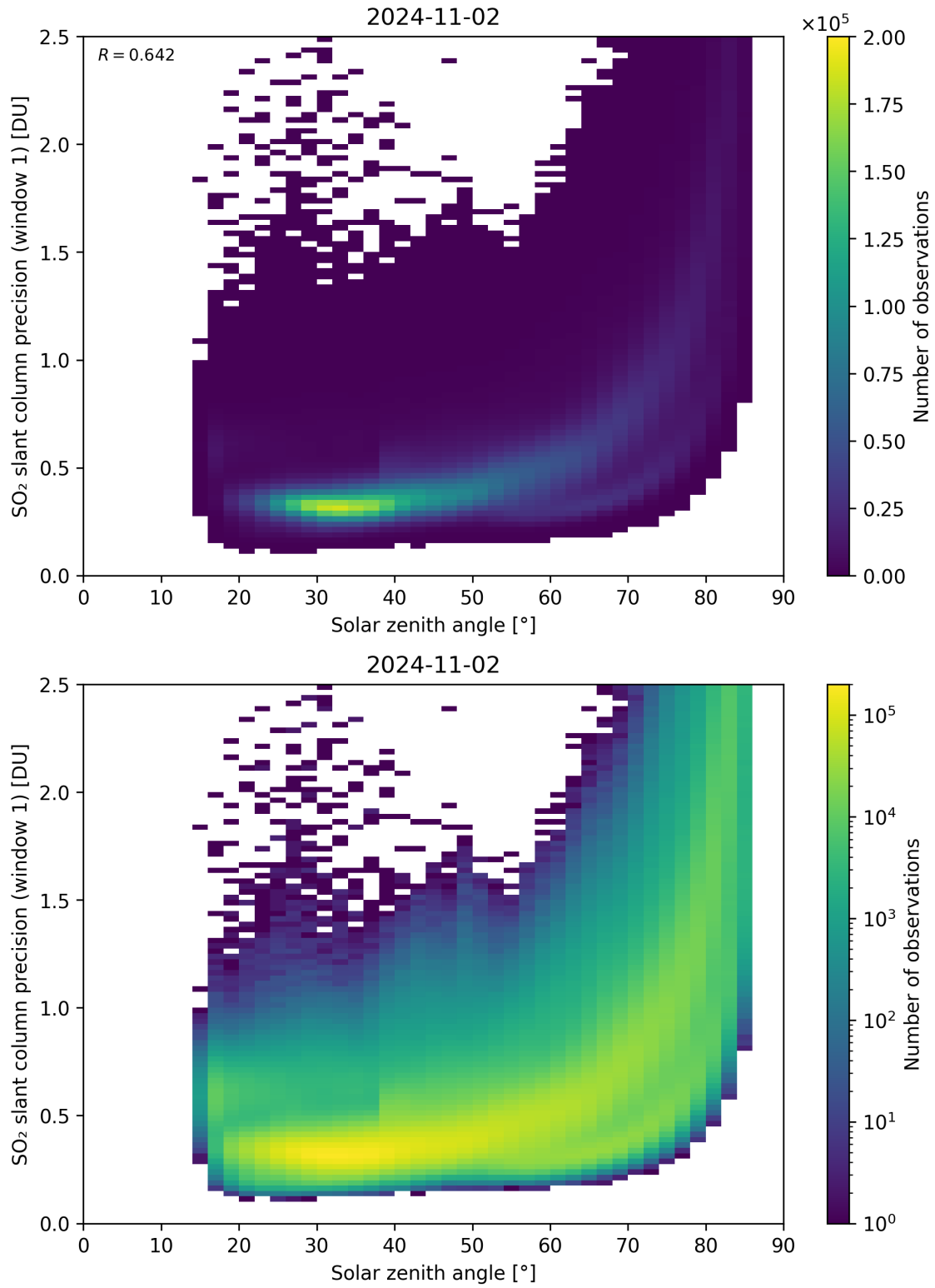
Figure 170: Scatter density plot of “Solar zenith angle” against “SO 2 slant column precision (window 1)” for 2024-11-01 to 2024-11-03.
