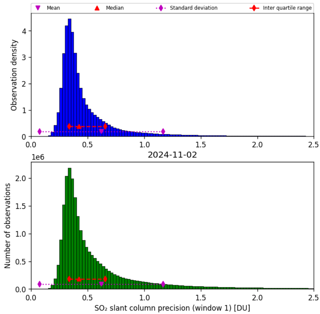
Figure 57: Histogram of “SO 2 slant column precision (window 1)” for 2024-11-01 to 2024-11-03
