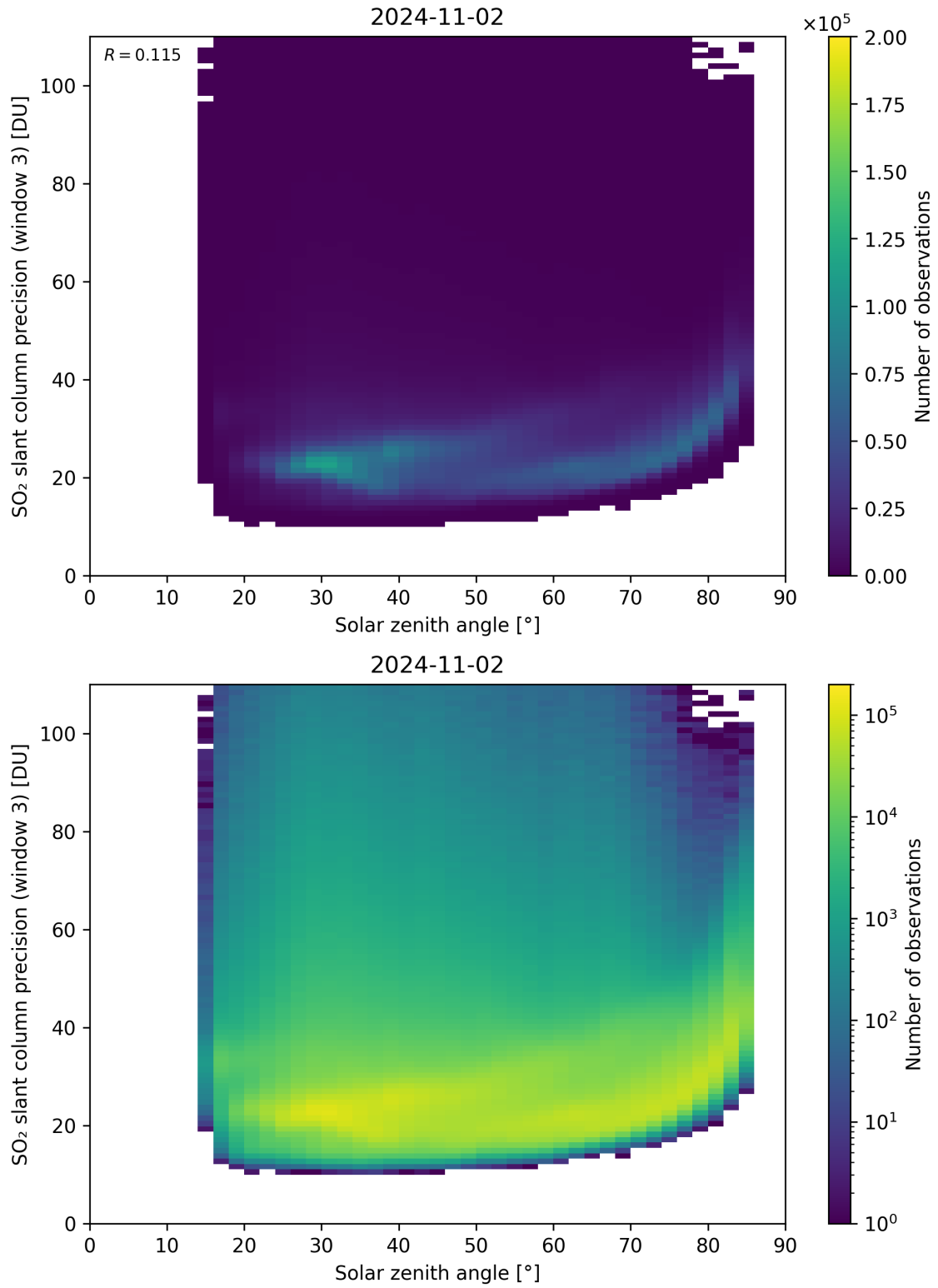
Figure 173: Scatter density plot of “Solar zenith angle” against “SO 2 slant column precision (window 3)” for 2024-11-01 to 2024-11-03.
