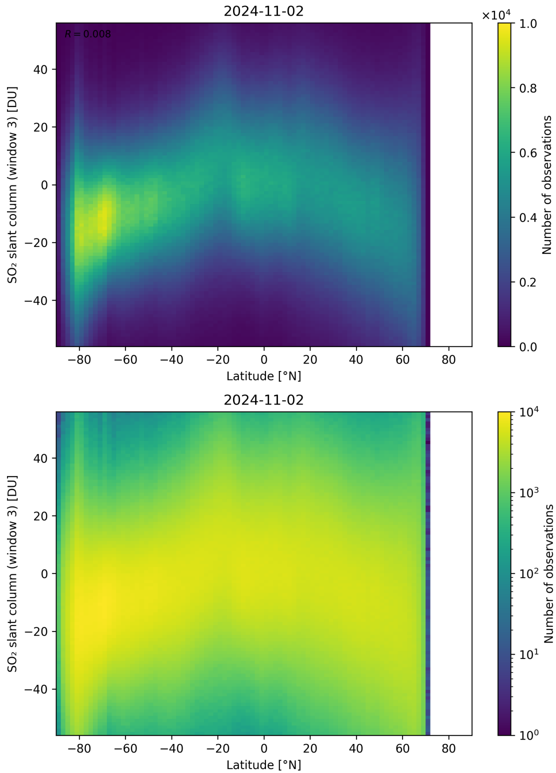
Figure 152: Scatter density plot of “Latitude” against “SO 2 slant column (window 3)” for 2024-11-01 to 2024-11-03.
