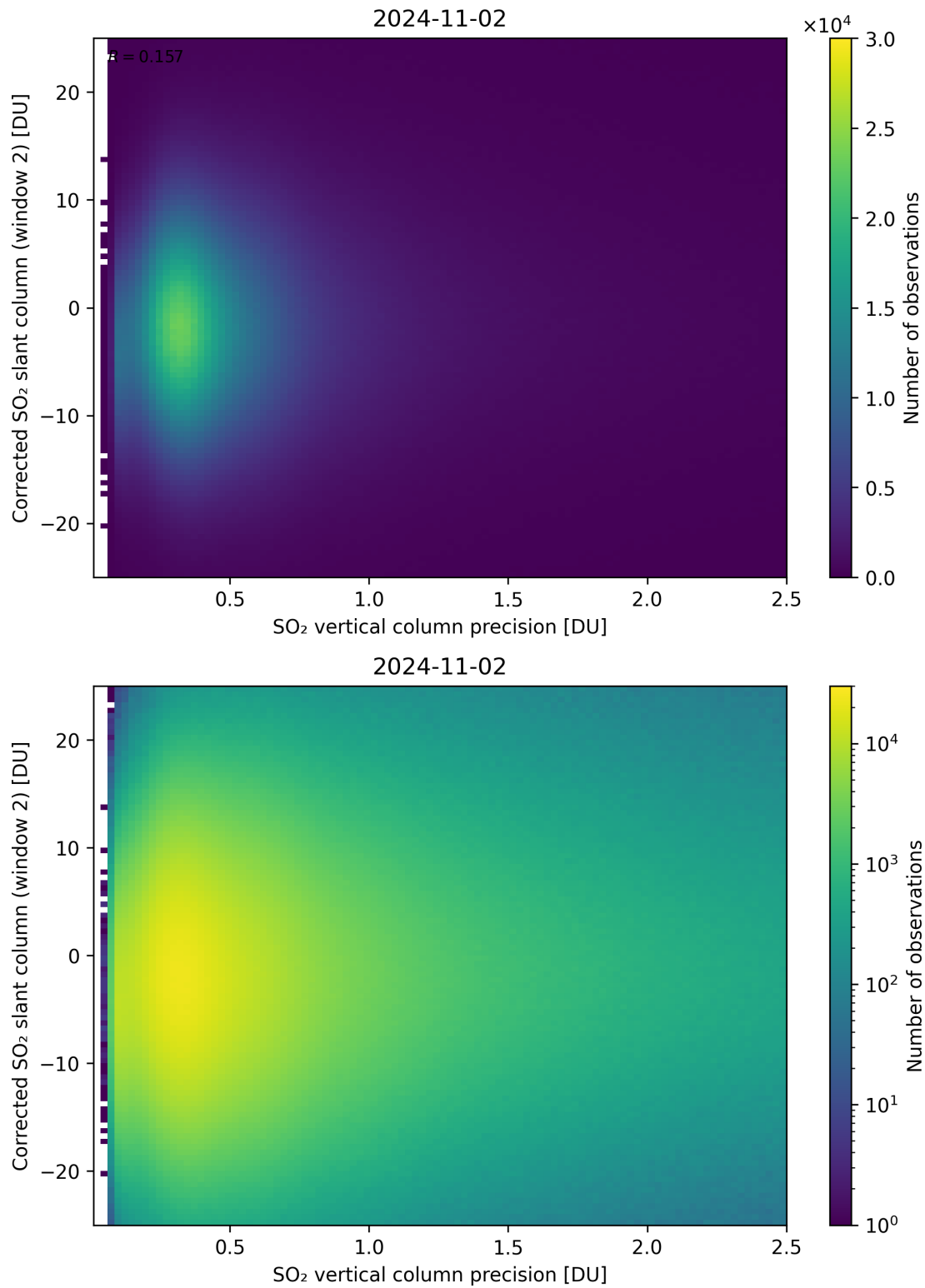
Figure 287: Scatter density plot of “SO 2 vertical column precision” against “Corrected SO 2 slant column (window 2)” for 2024-11-01 to 2024-11-03.
