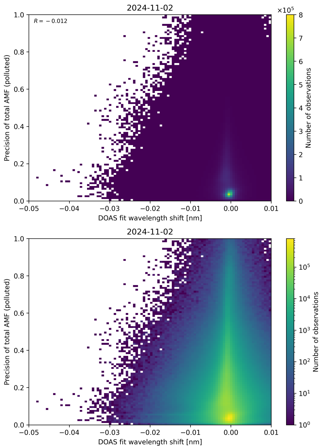
Figure 131: Scatter density plot of “DOAS fit wavelength shift” against “Precision of total AMF (polluted)” for 2024-11-01 to 2024-11-03.
