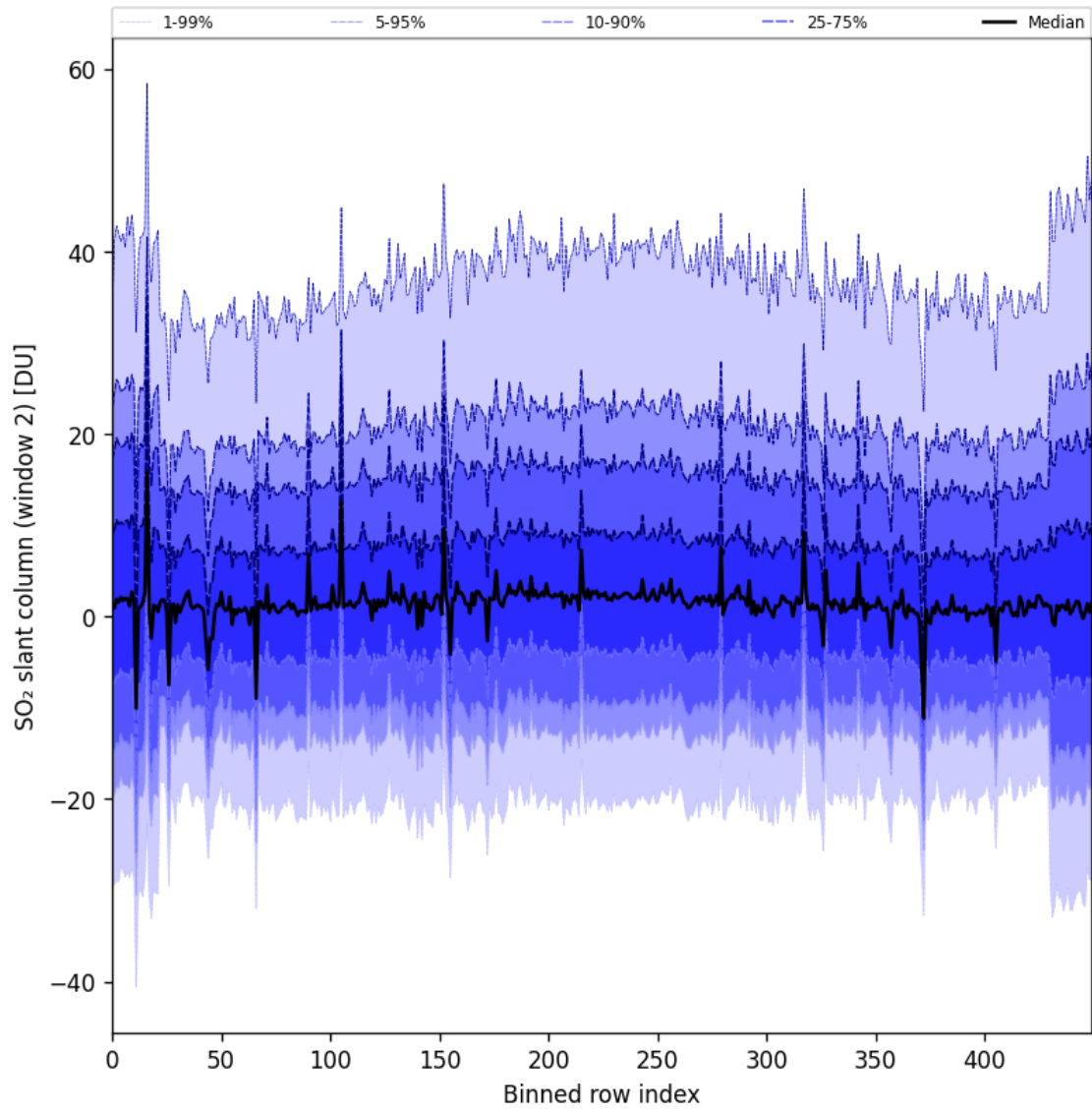
Figure 83: Along track statistics of “SO 2 slant column (window 2)” for 2024-11-01 to 2024-11-03
