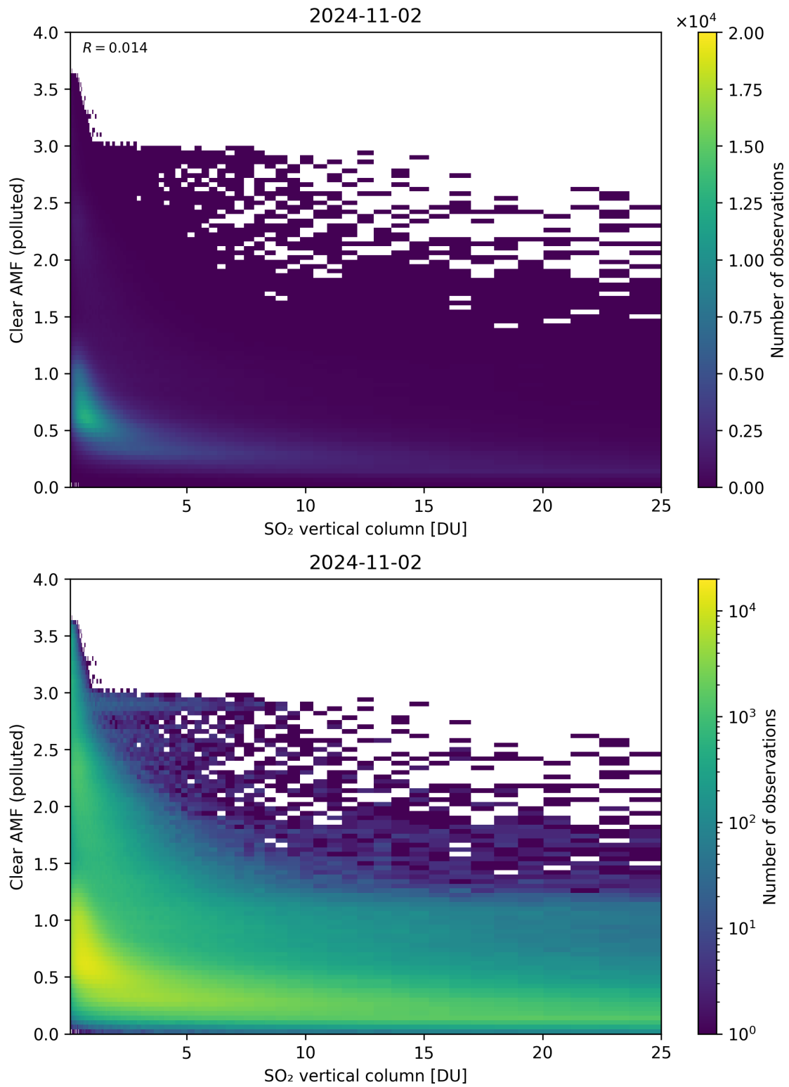
Figure 296: Scatter density plot of “SO 2 vertical column” against “Clear AMF (polluted)” for 2024-11-01 to 2024-11-03.
