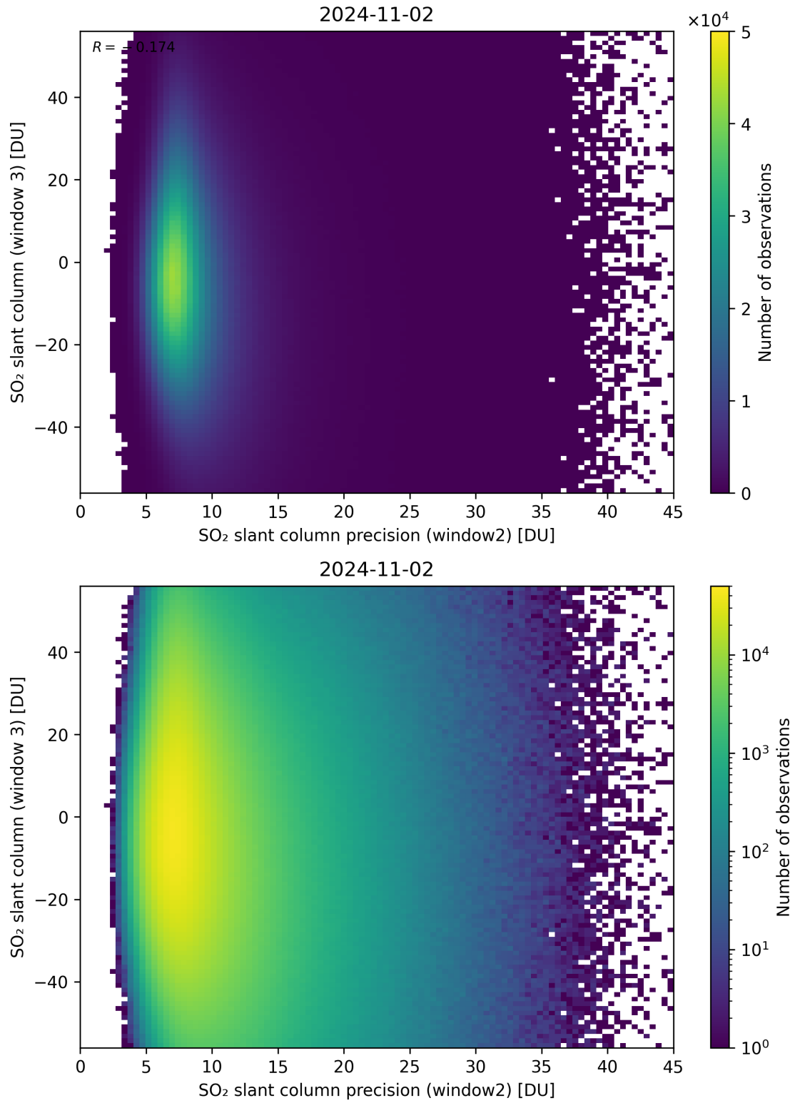
Figure 249: Scatter density plot of “SO 2 slant column precision (window2)” against “SO 2 slant column (window 3)” for 2024-11-01 to 2024-11-03.
