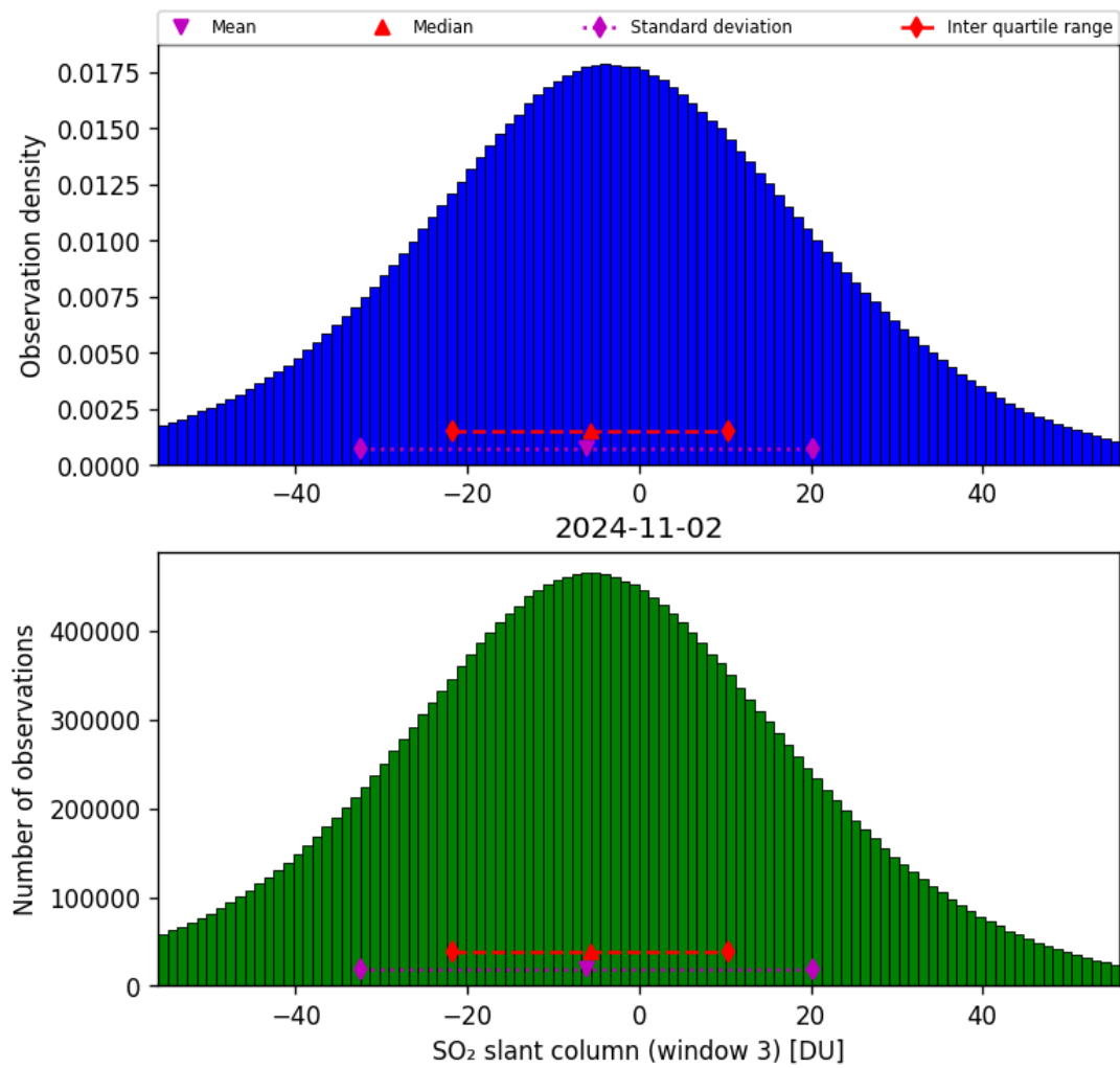
Figure 64: Histogram of “SO 2 slant column (window 3)” for 2024-11-01 to 2024-11-03
