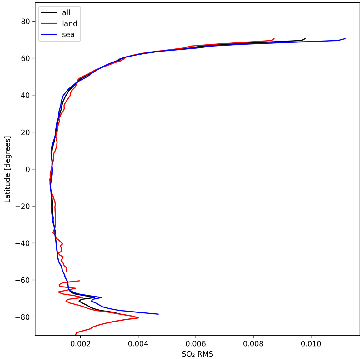
Figure 47: Zonal average of “SO 2 RMS” for 2024-11-01 to 2024-11-03.
