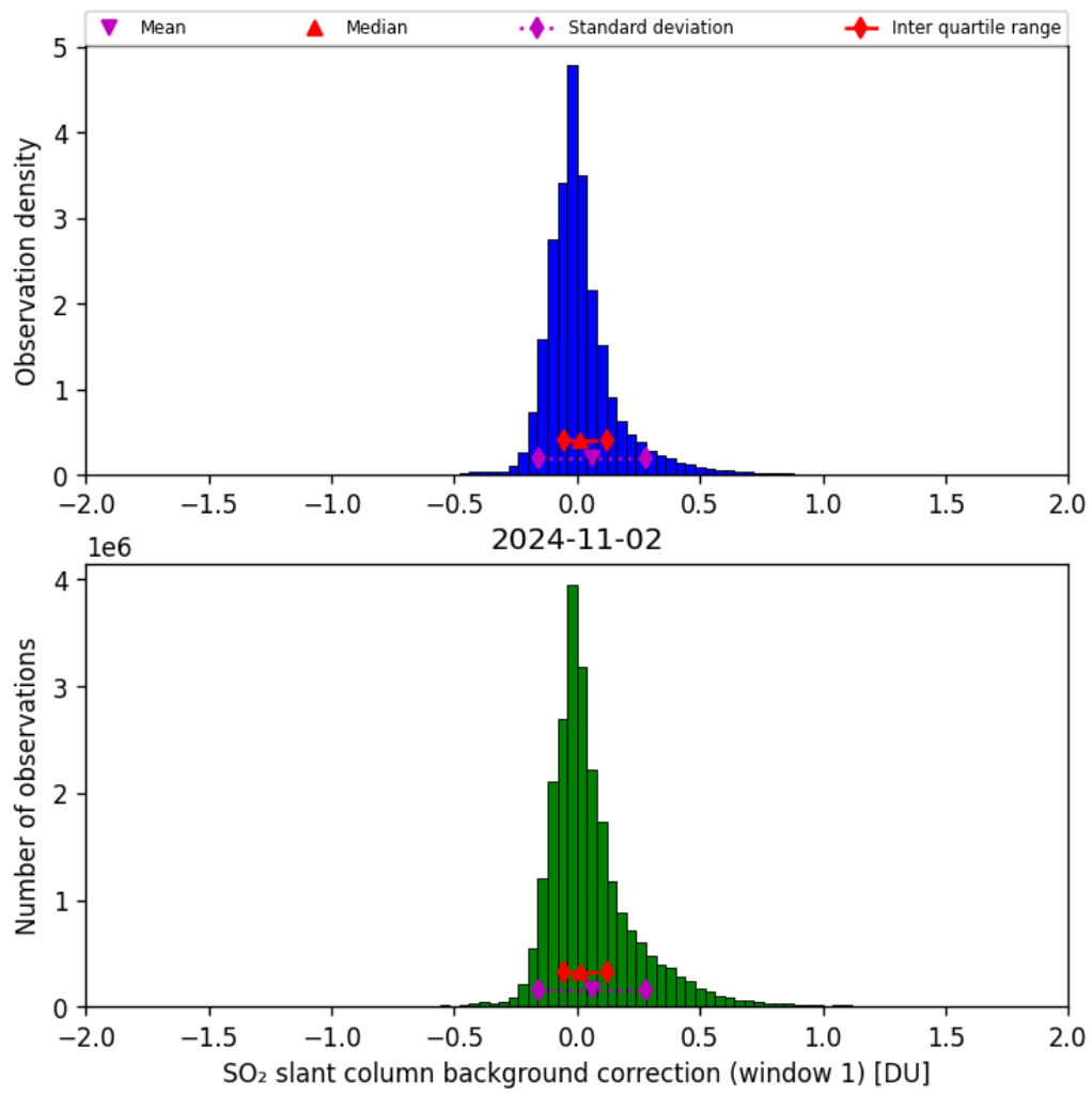
Figure 59: Histogram of “SO 2 slant column background correction (window 1)” for 2024-11-01 to 2024-11-03
