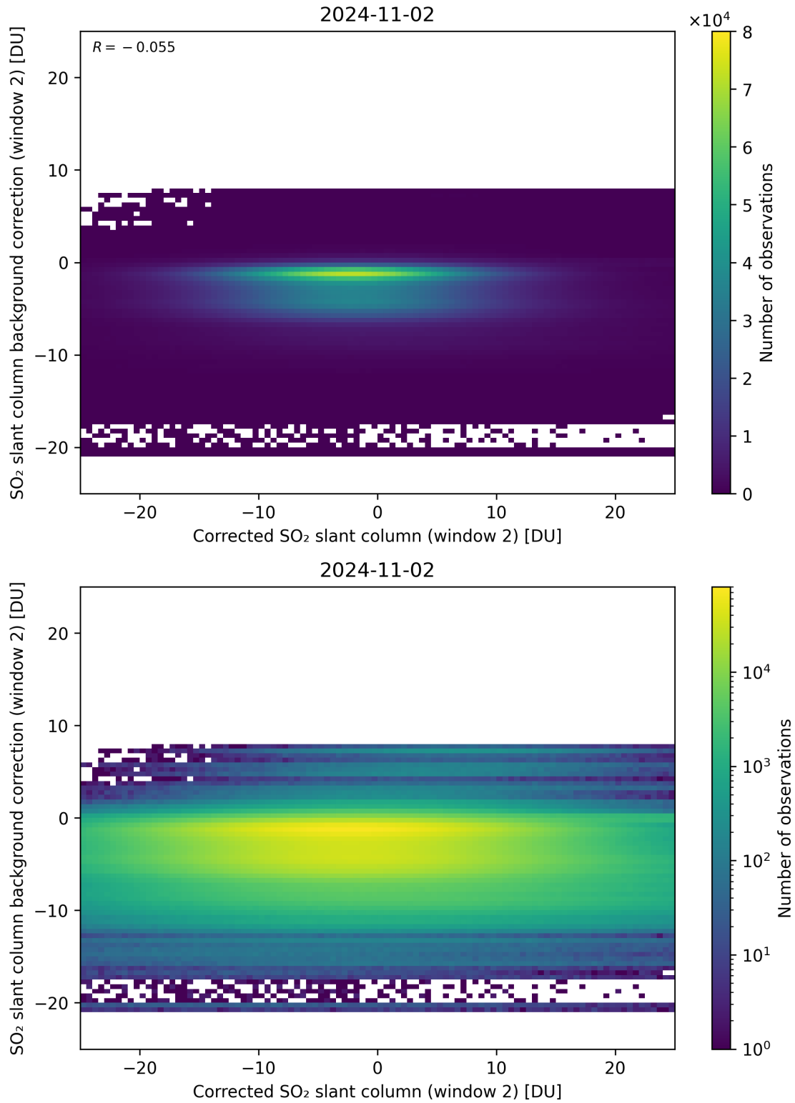
Figure 194: Scatter density plot of “Corrected SO 2 slant column (window 2)” against “SO 2 slant column background correction (window 2)” for 2024-11-01 to 2024-11-03.
