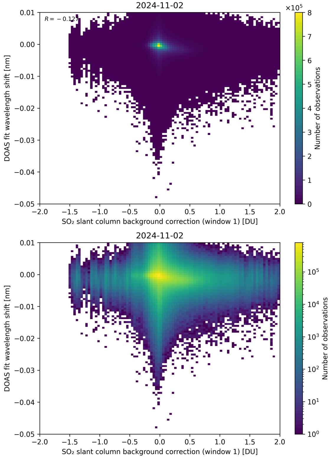
Figure 100: Scatter density plot of “SO 2 slant column background correction (window 1)” against “DOAS fit wavelength shift” for 2024-11-01 to 2024-11-03.
