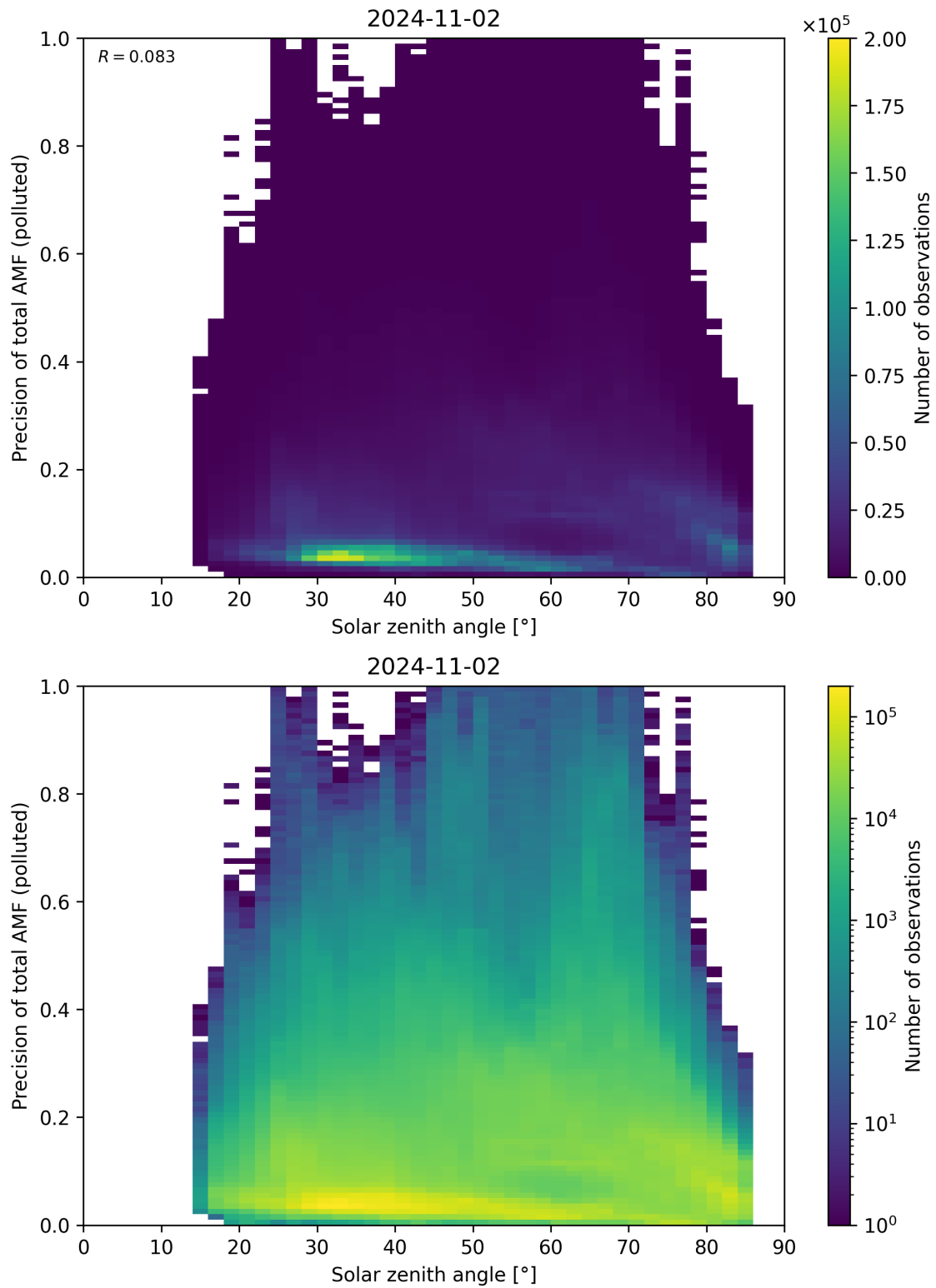
Figure 175: Scatter density plot of “Solar zenith angle” against “Precision of total AMF (polluted)” for 2024-11-01 to 2024-11-03.
