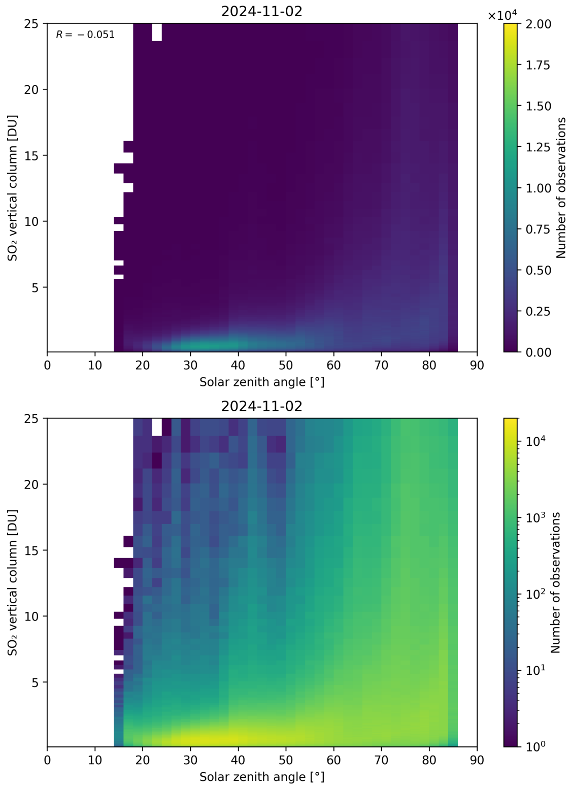
Figure 176: Scatter density plot of “Solar zenith angle” against “SO 2 vertical column” for 2024-11-01 to 2024-11-03.
