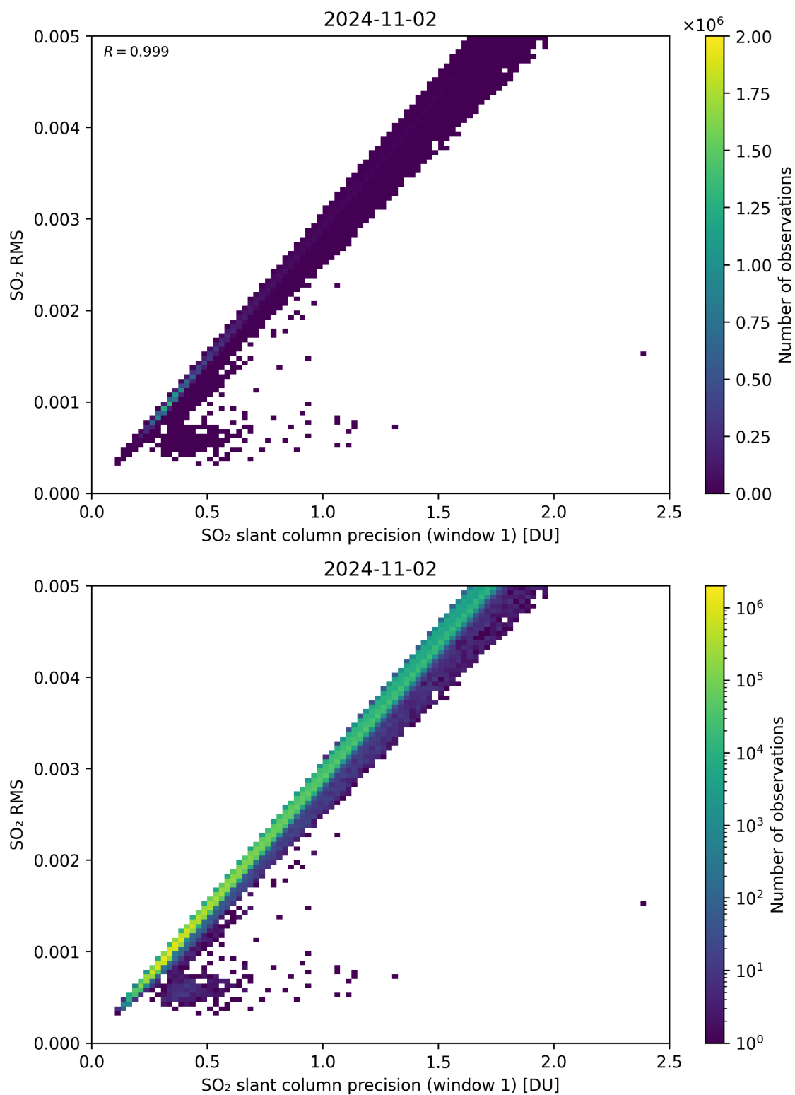
Figure 223: Scatter density plot of “SO 2 slant column precision (window 1)” against “SO 2 RMS” for 2024-11-01 to 2024-11-03.
