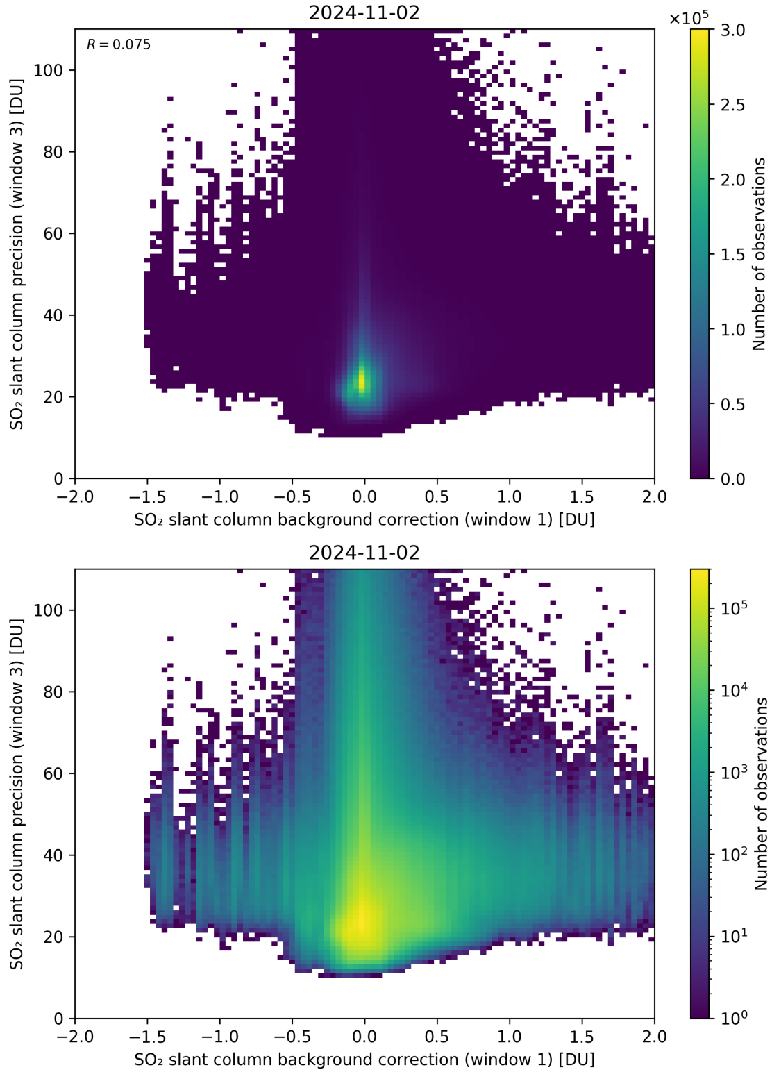
Figure 108: Scatter density plot of “SO 2 slant column background correction (window 1)” against “SO 2 slant column precision (window 3)” for 2024-11-01 to 2024-11-03.
