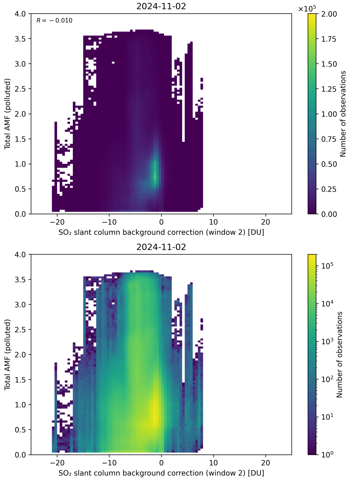
Figure 119: Scatter density plot of “SO 2 slant column background correction (window 2)” against “Total AMF (polluted)” for 2024-11-01 to 2024-11-03.
