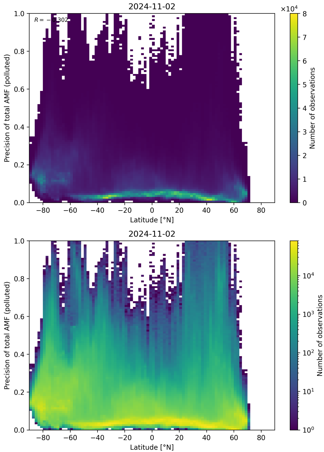
Figure 155: Scatter density plot of “Latitude” against “Precision of total AMF (polluted)” for 2024-11-01 to 2024-11-03.
