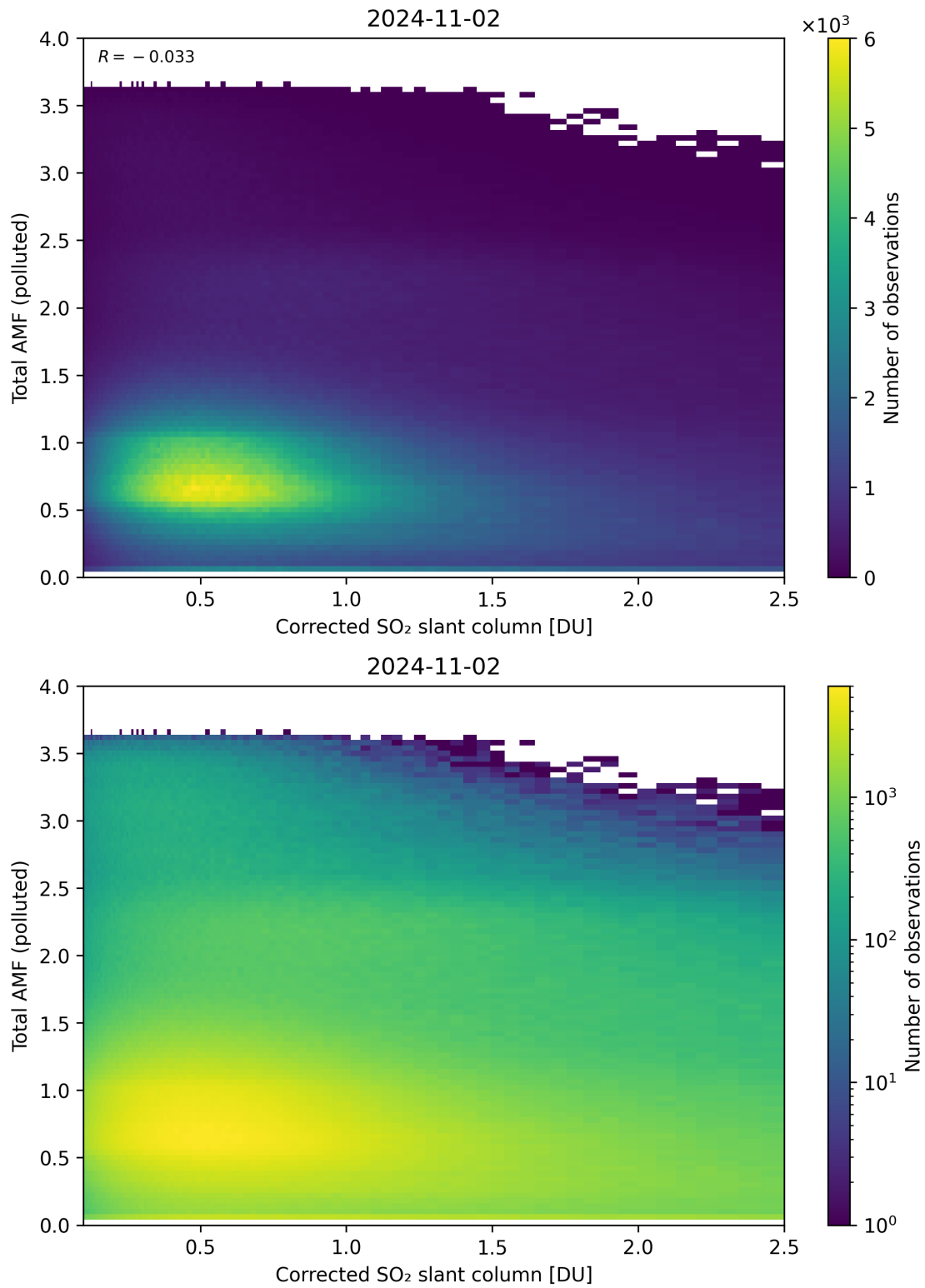
Figure 192: Scatter density plot of “Corrected SO 2 slant column” against “Total AMF (polluted)” for 2024-11-01 to 2024-11-03.
