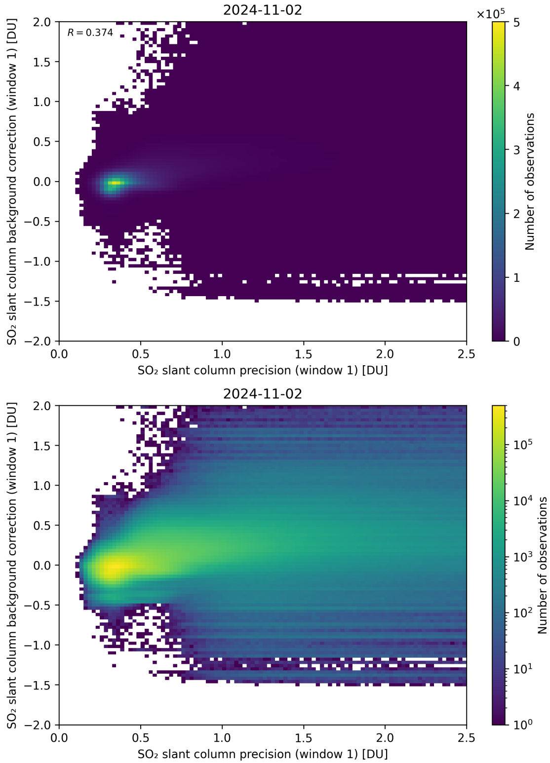
Figure 218: Scatter density plot of “SO 2 slant column precision (window 1)” against “SO 2 slant column background correction (window 1)” for 2024-11-01 to 2024-11-03.
