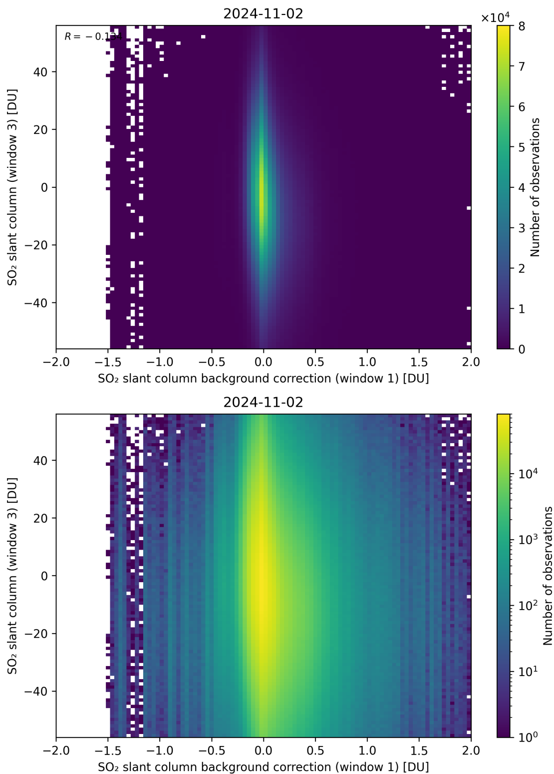
Figure 107: Scatter density plot of “SO 2 slant column background correction (window 1)” against “SO 2 slant column (window 3)” for 2024-11-01 to 2024-11-03.
