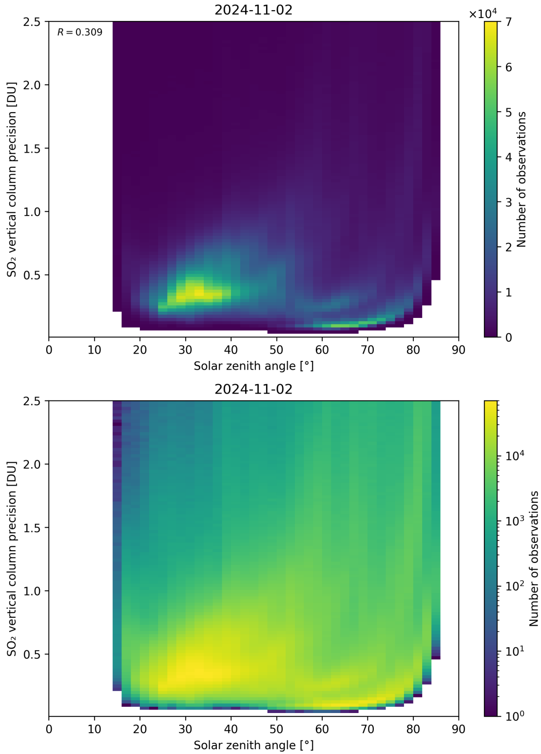
Figure 177: Scatter density plot of “Solar zenith angle” against “SO 2 vertical column precision” for 2024-11-01 to 2024-11-03.
