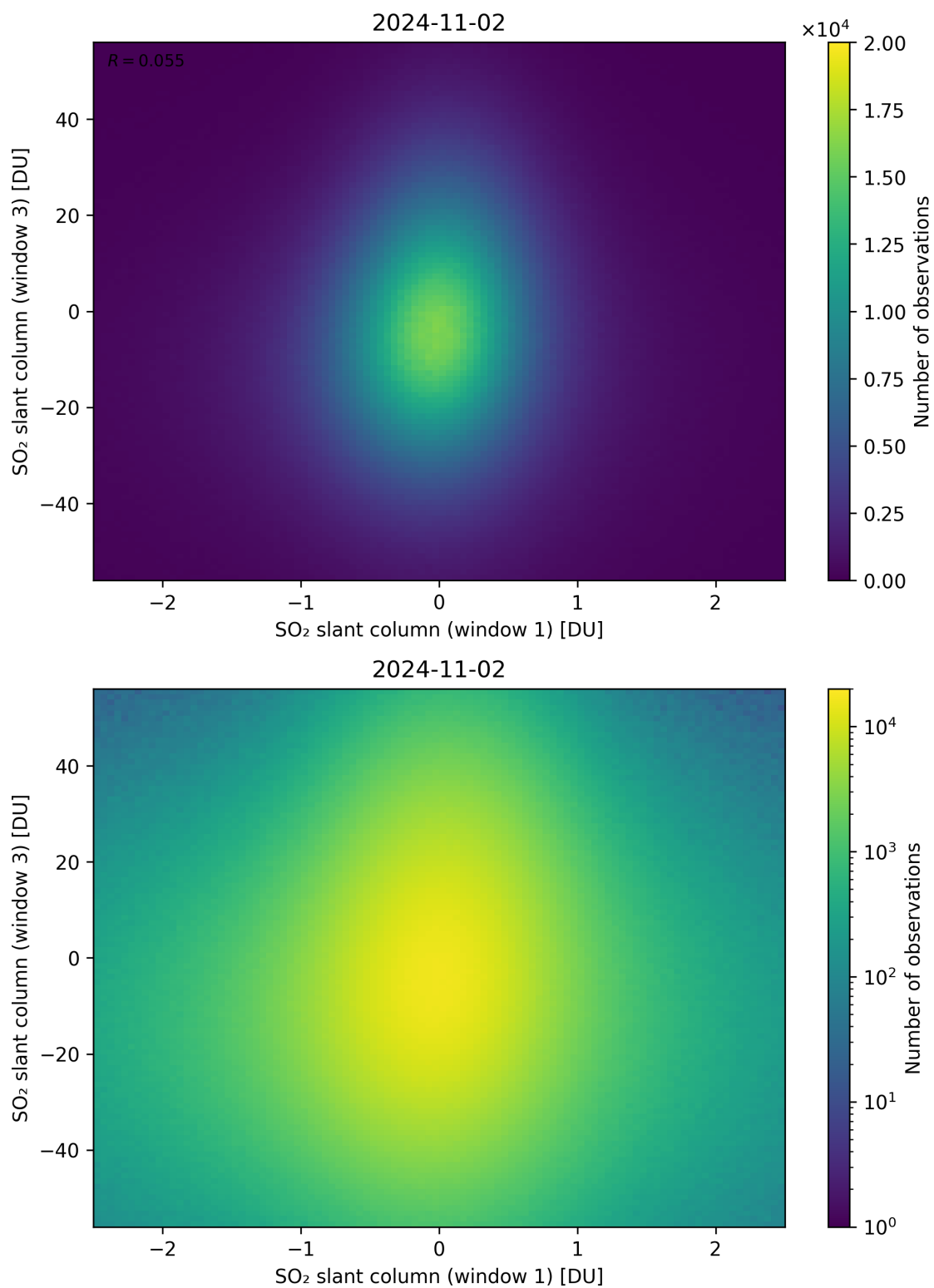
Figure 237: Scatter density plot of “SO 2 slant column (window 1)” against “SO 2 slant column (window 3)” for 2024-11-01 to 2024-11-03.
