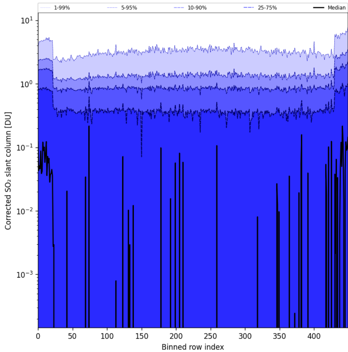
Figure 78: Along track statistics of “Corrected SO 2 slant column” for 2024-11-01 to 2024-11-03
