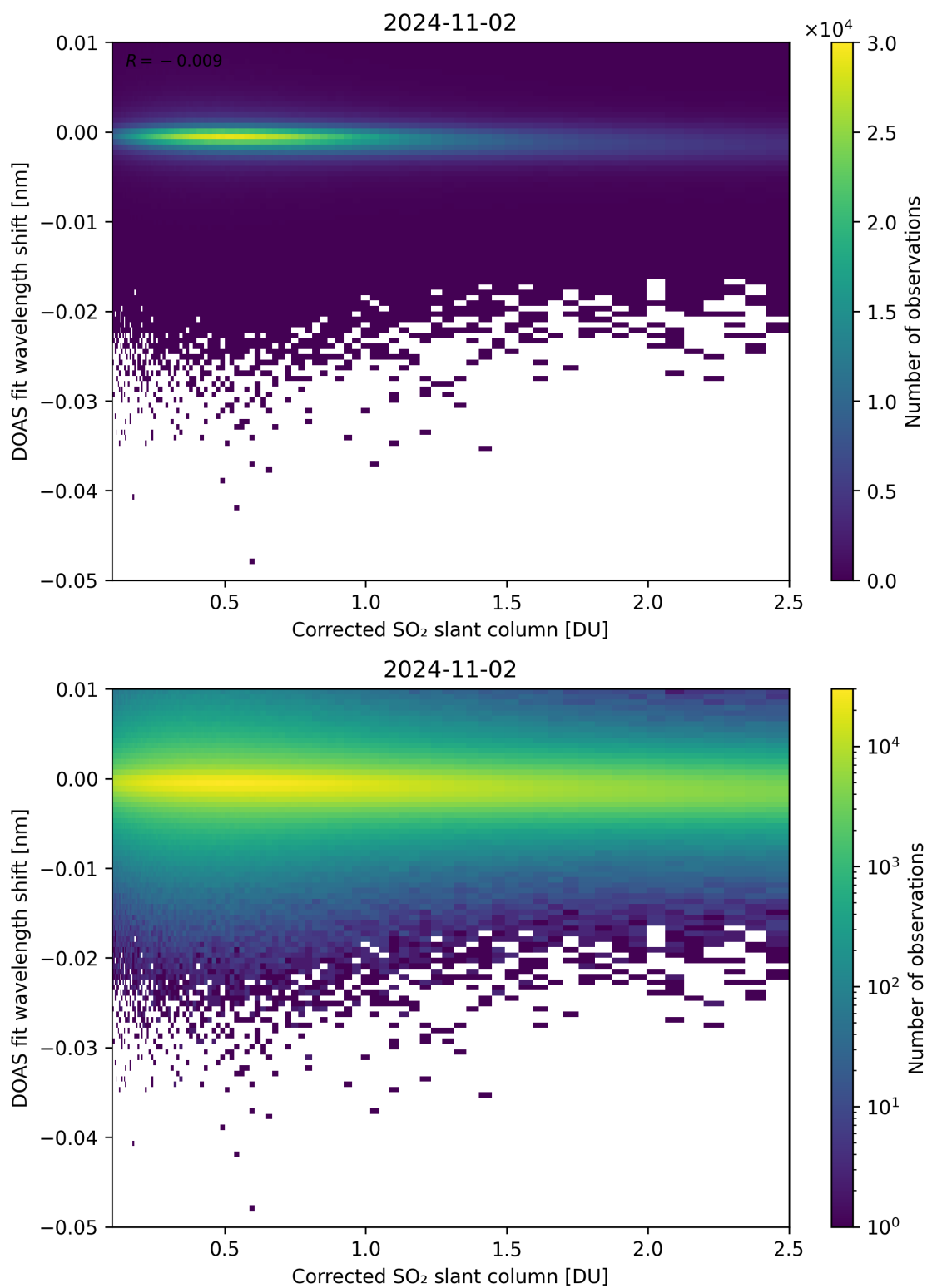
Figure 181: Scatter density plot of “Corrected SO 2 slant column” against “DOAS fit wavelength shift” for 2024-11-01 to 2024-11-03.
