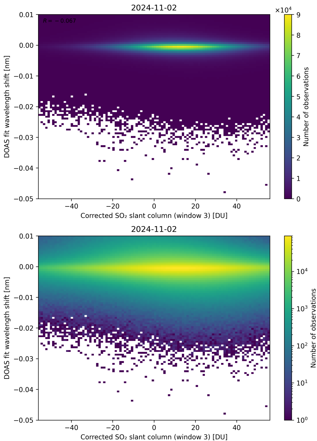
Figure 206: Scatter density plot of “Corrected SO 2 slant column (window 3)” against “DOAS fit wavelength shift” for 2024-11-01 to 2024-11-03.
