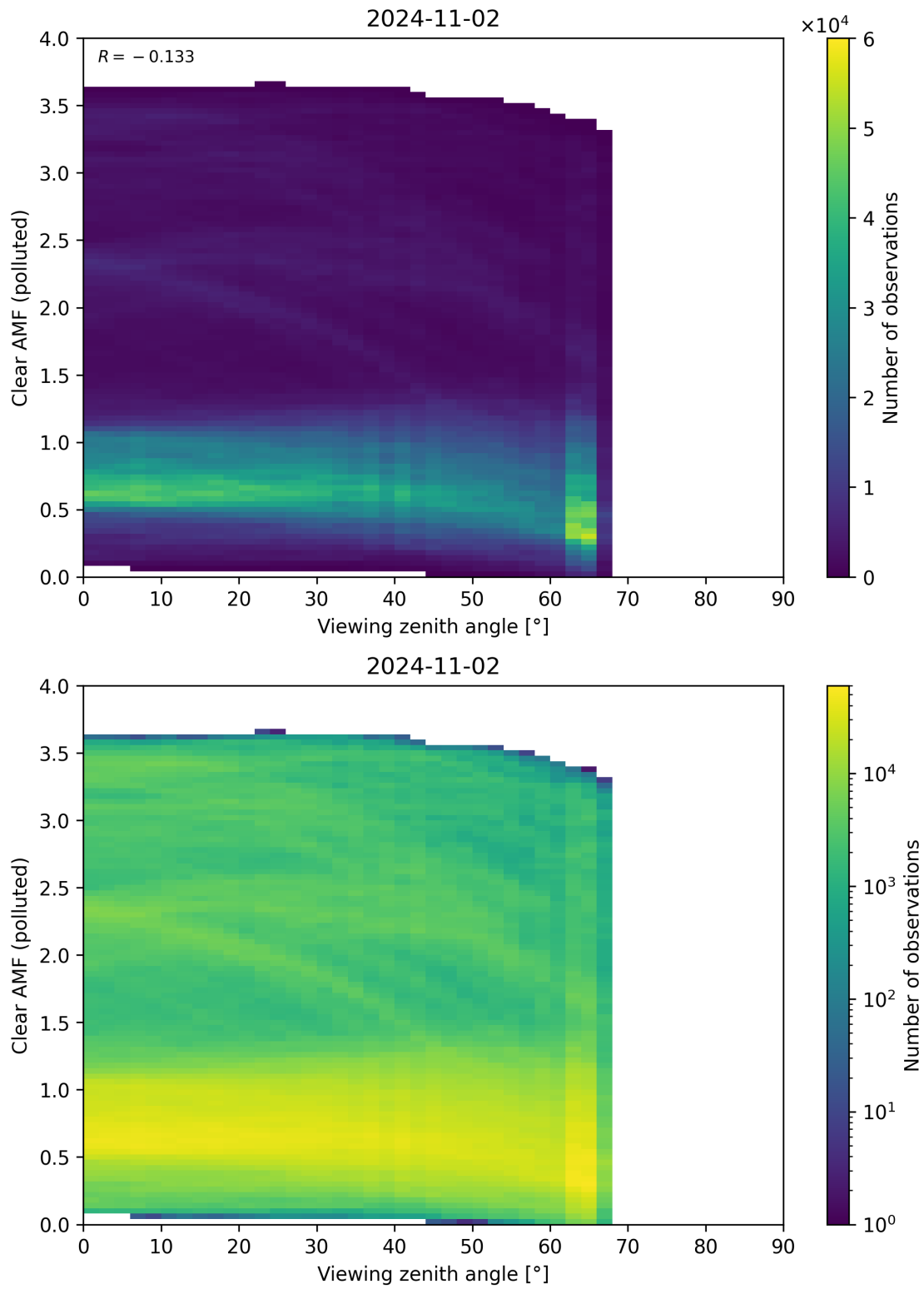
Figure 316: Scatter density plot of “Viewing zenith angle” against “Clear AMF (polluted)” for 2024-11-01 to 2024-11-03.
