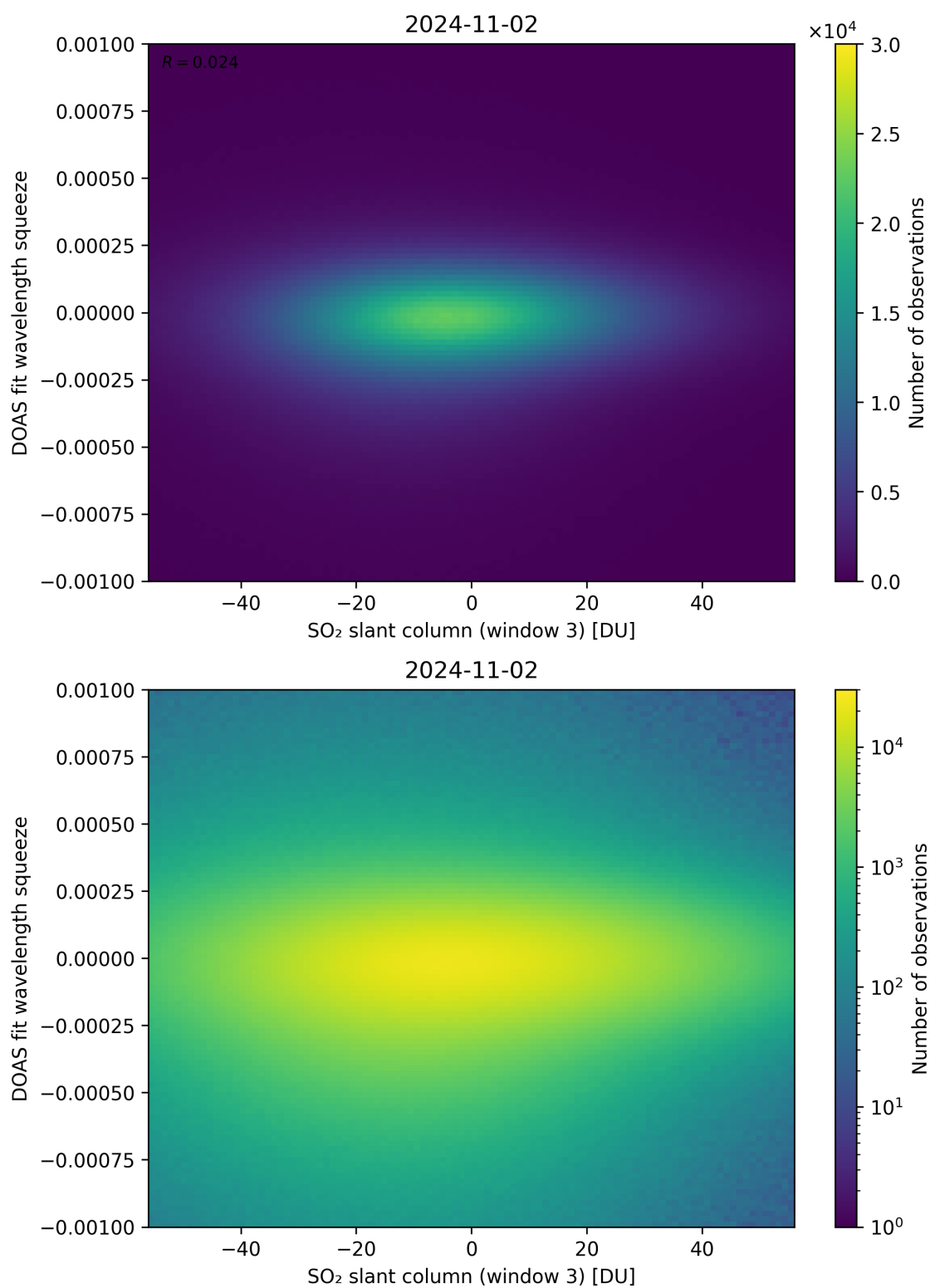
Figure 255: Scatter density plot of “SO 2 slant column (window 3)” against “DOAS fit wavelength squeeze” for 2024-11-01 to 2024-11-03.
