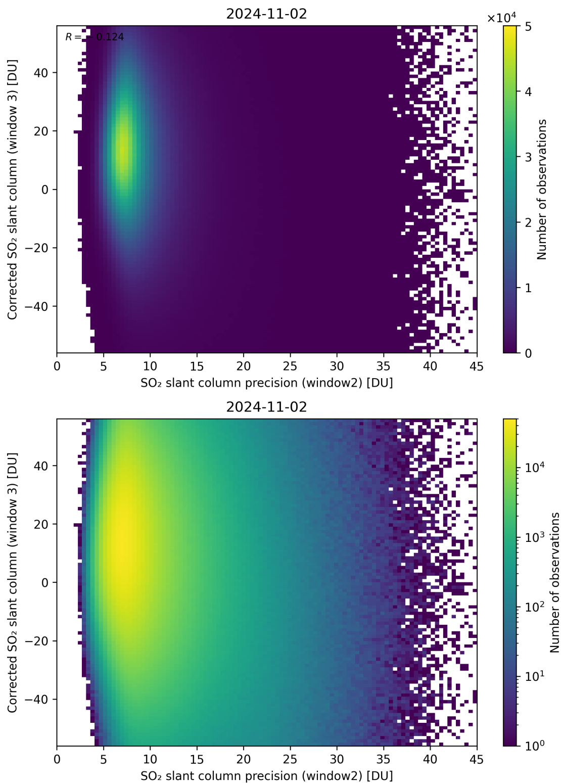
Figure 248: Scatter density plot of “SO 2 slant column precision (window2)” against “Corrected SO 2 slant column (window 3)” for 2024-11-01 to 2024-11-03.
