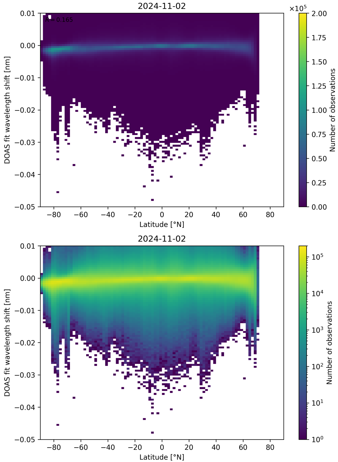
Figure 142: Scatter density plot of “Latitude” against “DOAS fit wavelength shift” for 2024-11-01 to 2024-11-03.
