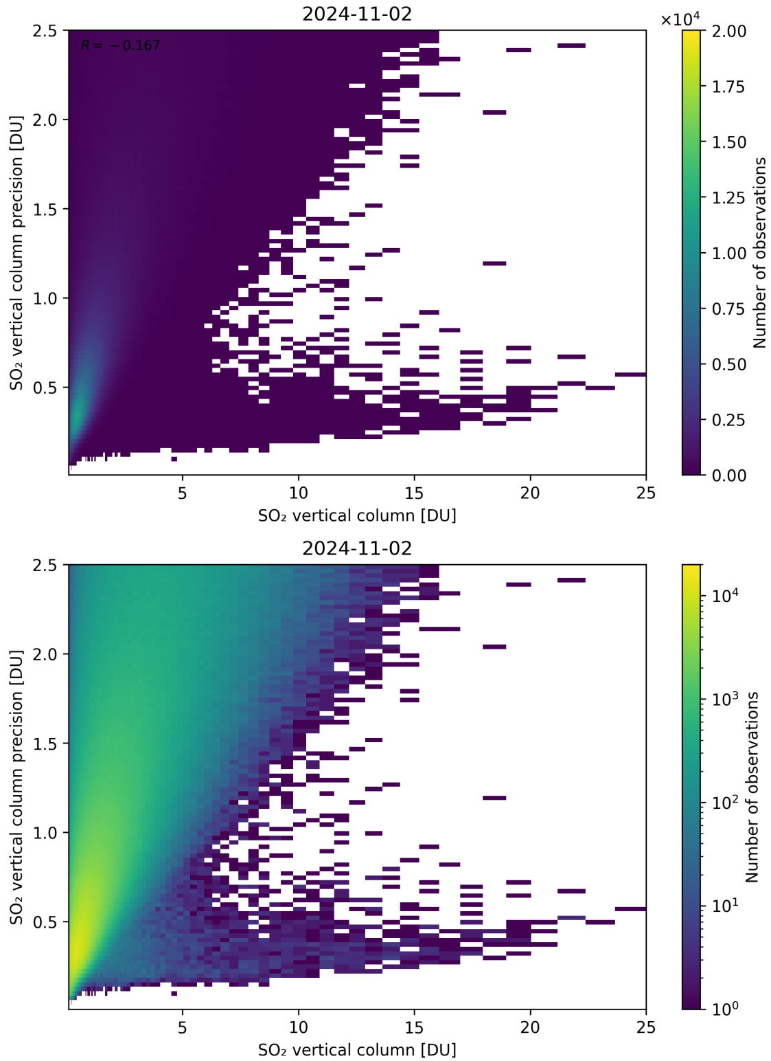
Figure 307: Scatter density plot of “SO 2 vertical column” against “SO 2 vertical column precision” for 2024-11-01 to 2024-11-03.
