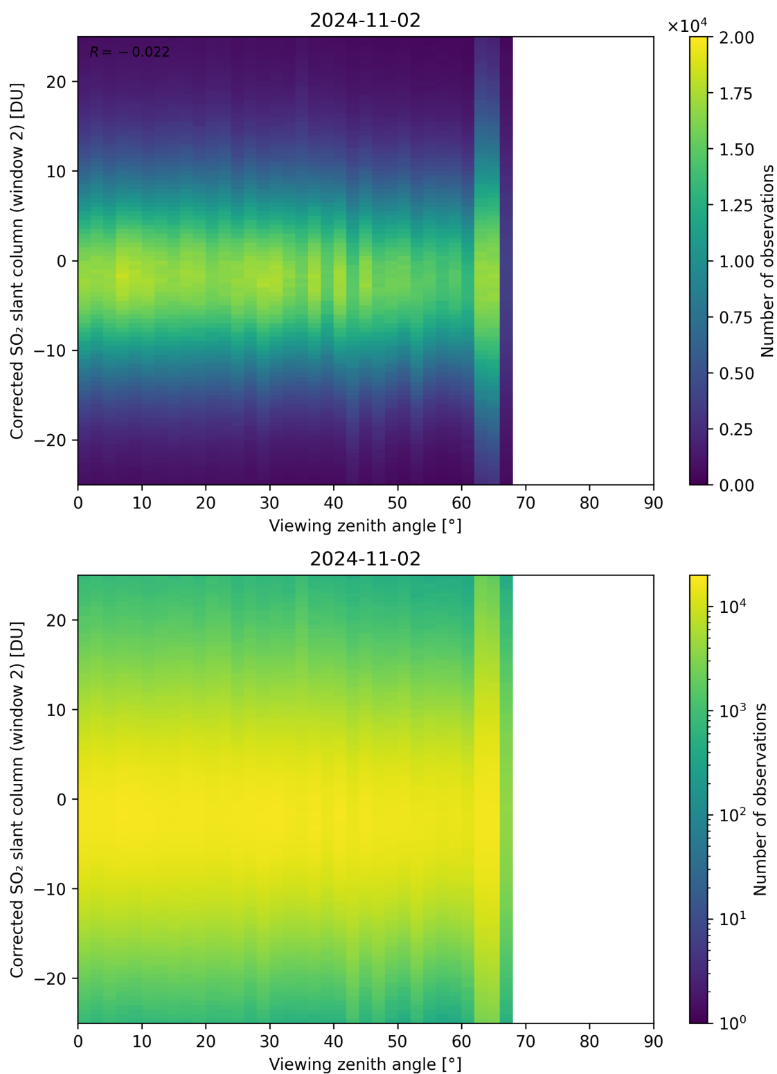
Figure 318: Scatter density plot of “Viewing zenith angle” against “Corrected SO 2 slant column (window 2)” for 2024-11-01 to 2024-11-03.
