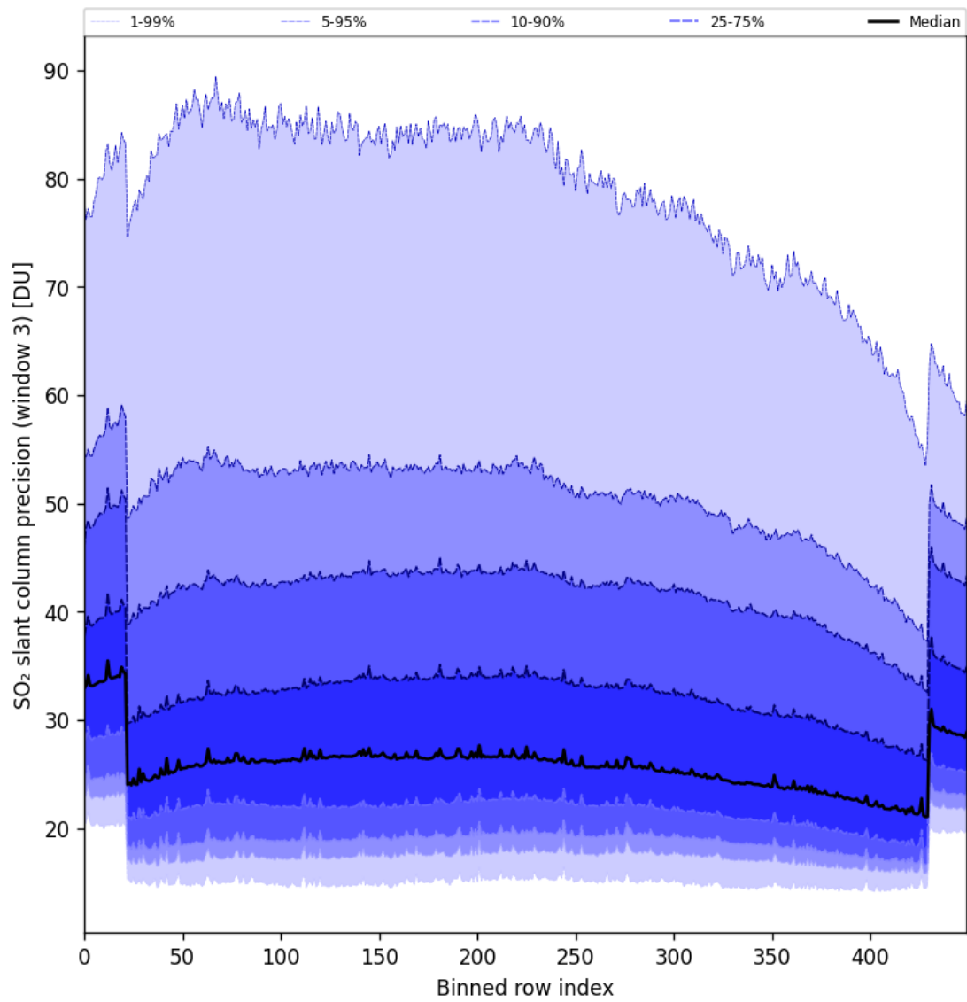
Figure 88: Along track statistics of “SO 2 slant column precision (window 3)” for 2024-11-01 to 2024-11-03
