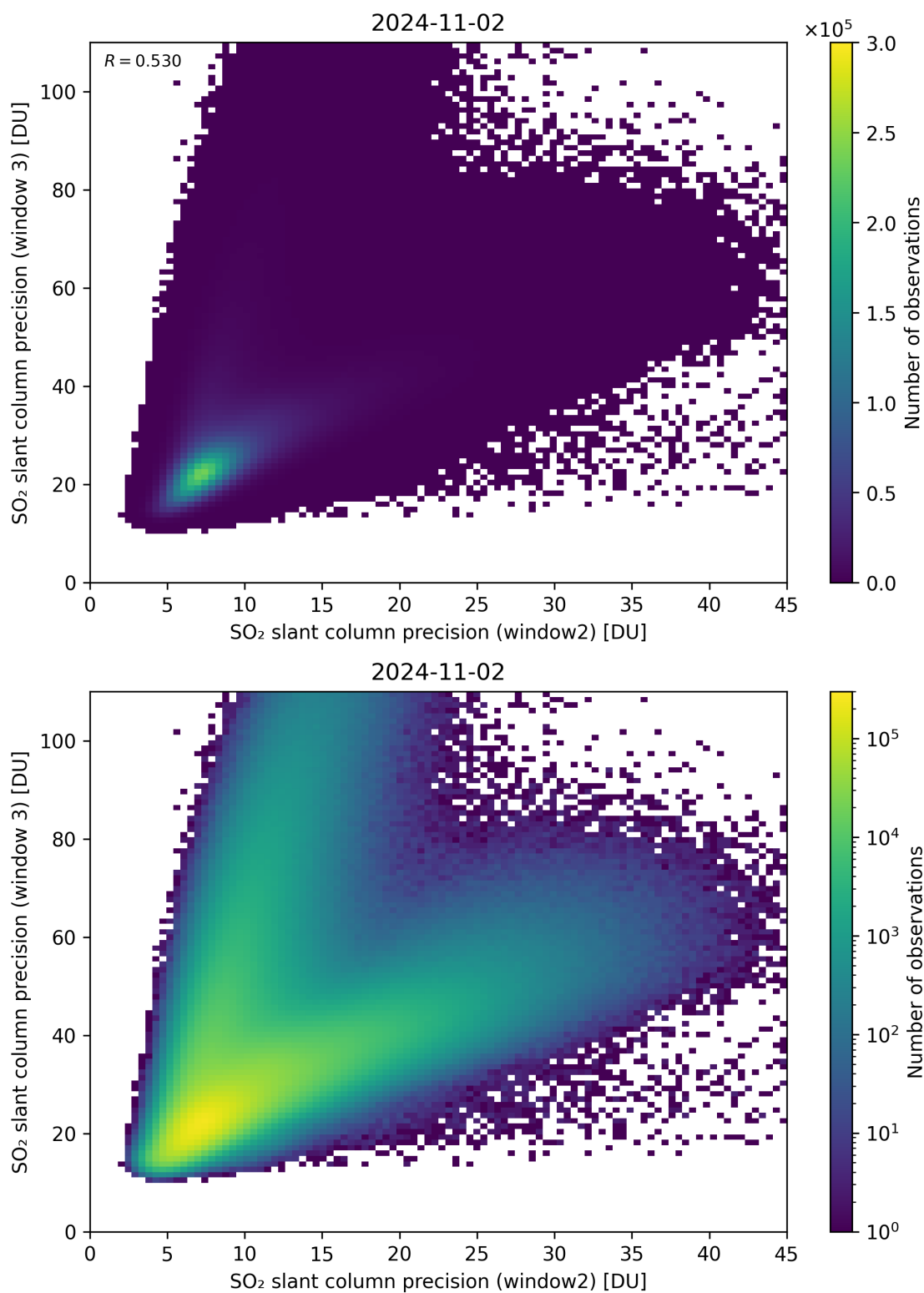
Figure 250: Scatter density plot of “SO 2 slant column precision (window2)” against “SO 2 slant column precision (window 3)” for 2024-11-01 to 2024-11-03.
