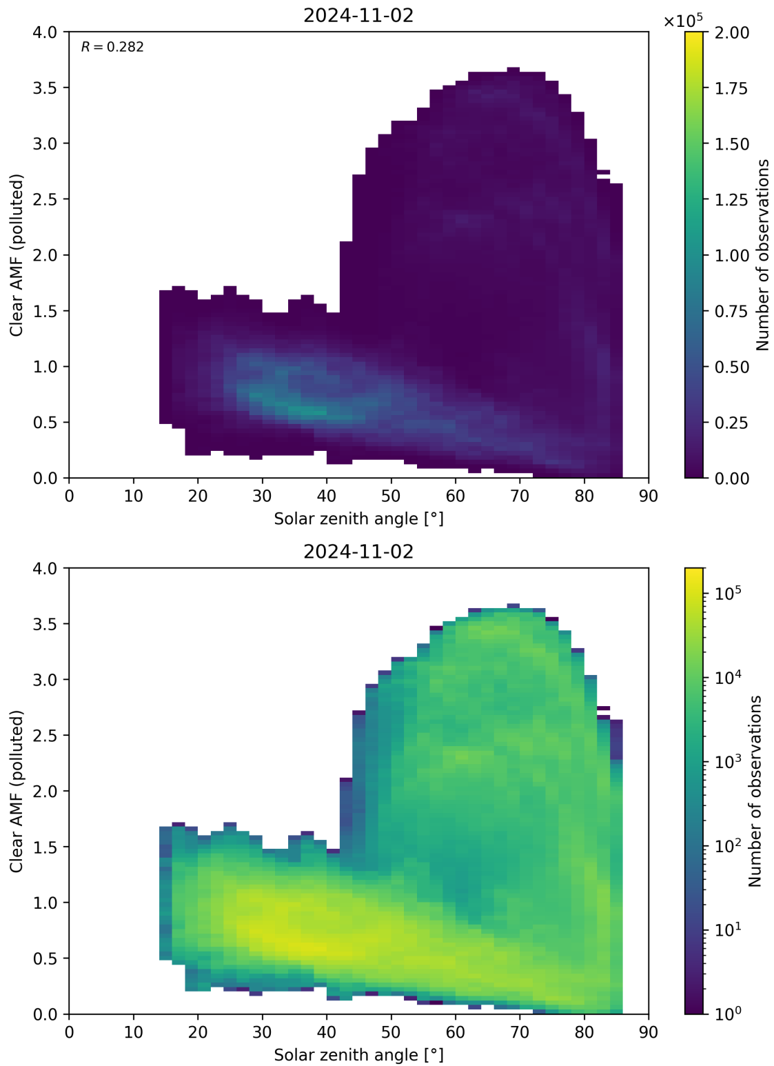
Figure 165: Scatter density plot of “Solar zenith angle” against “Clear AMF (polluted)” for 2024-11-01 to 2024-11-03.
