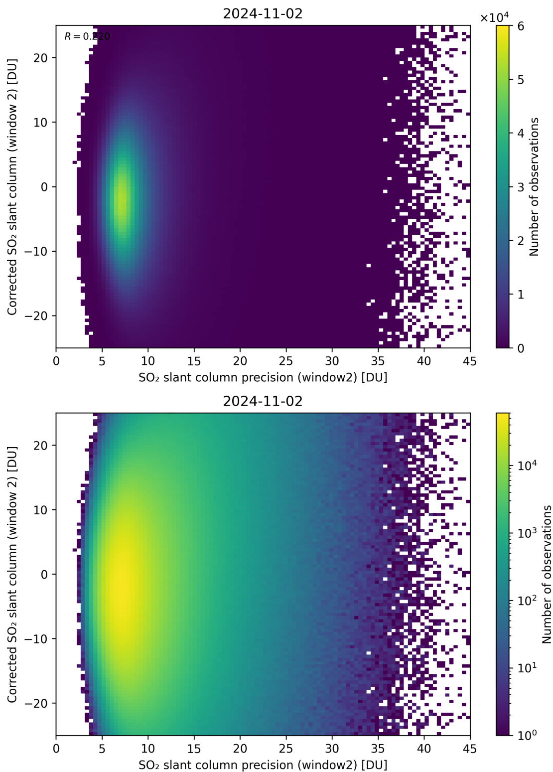
Figure 247: Scatter density plot of “SO 2 slant column precision (window2)” against “Corrected SO 2 slant column (window 2)” for 2024-11-01 to 2024-11-03.
