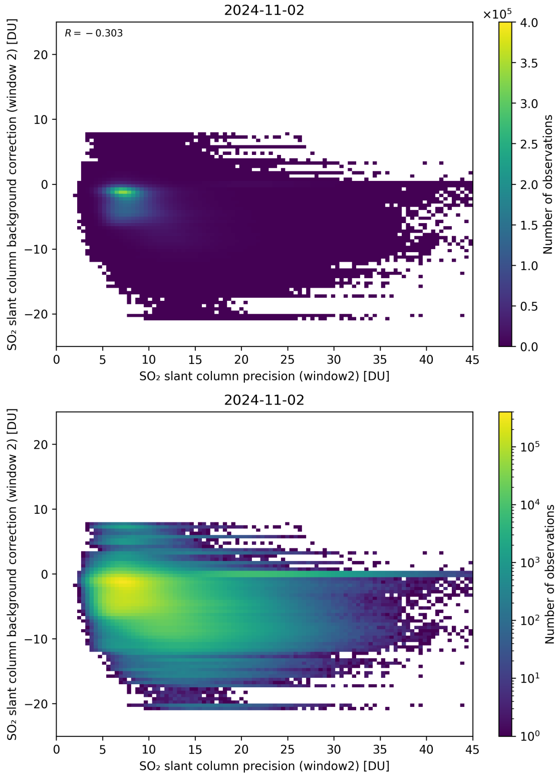
Figure 241: Scatter density plot of “SO 2 slant column precision (window2)” against “SO 2 slant column background correction (window 2)” for 2024-11-01 to 2024-11-03.
