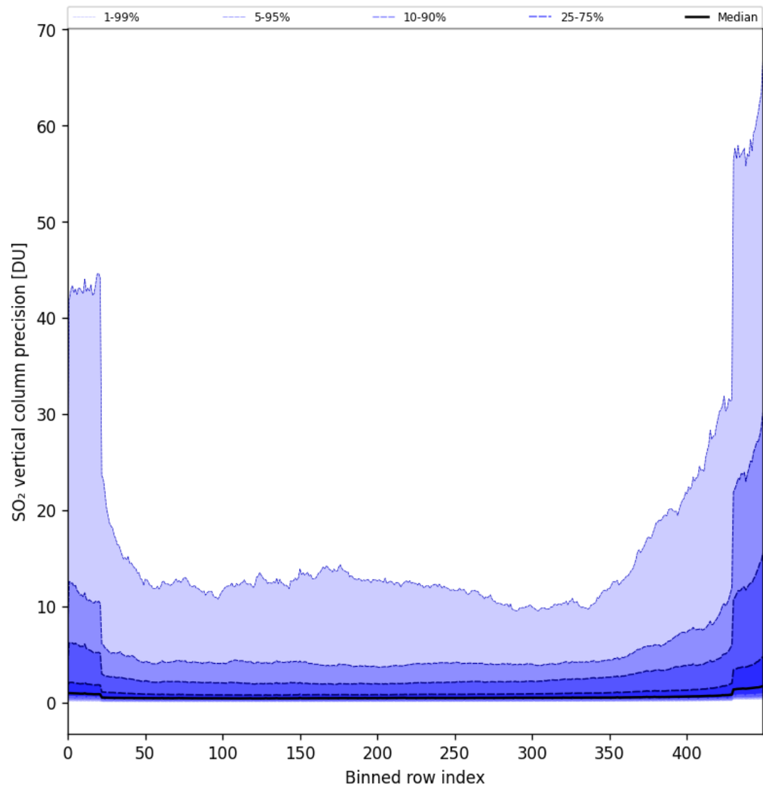
Figure 77: Along track statistics of “SO 2 vertical column precision” for 2024-11-01 to 2024-11-03
