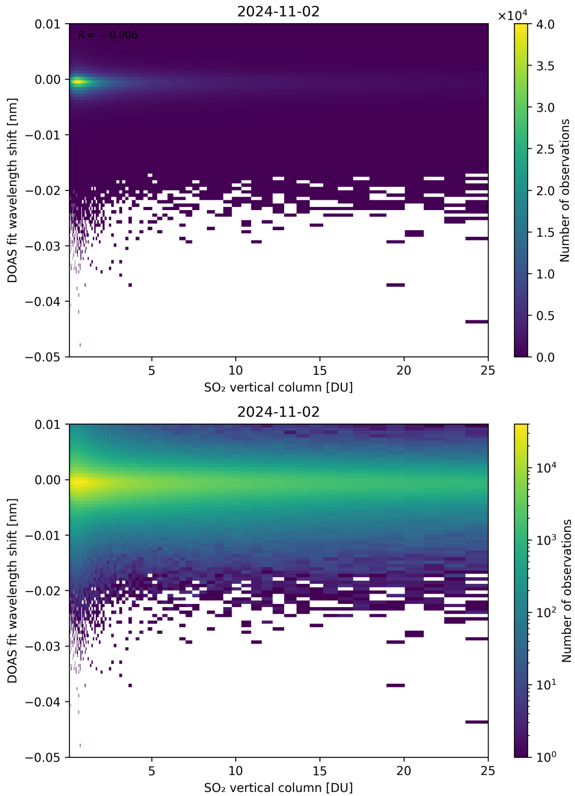
Figure 276: Scatter density plot of “SO 2 vertical column” against “DOAS fit wavelength shift” for 2024-11-01 to 2024-11-03.
