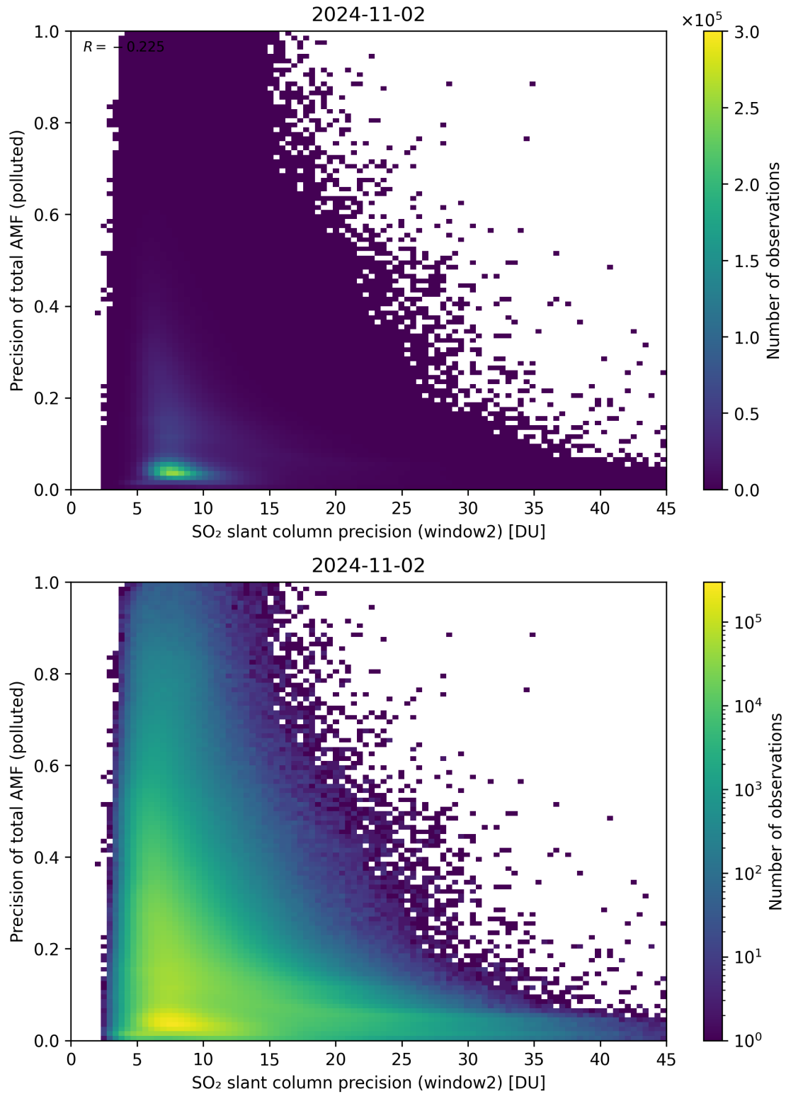
Figure 252: Scatter density plot of “SO 2 slant column precision (window2)” against “Precision of total AMF (polluted)” for 2024-11-01 to 2024-11-03.
