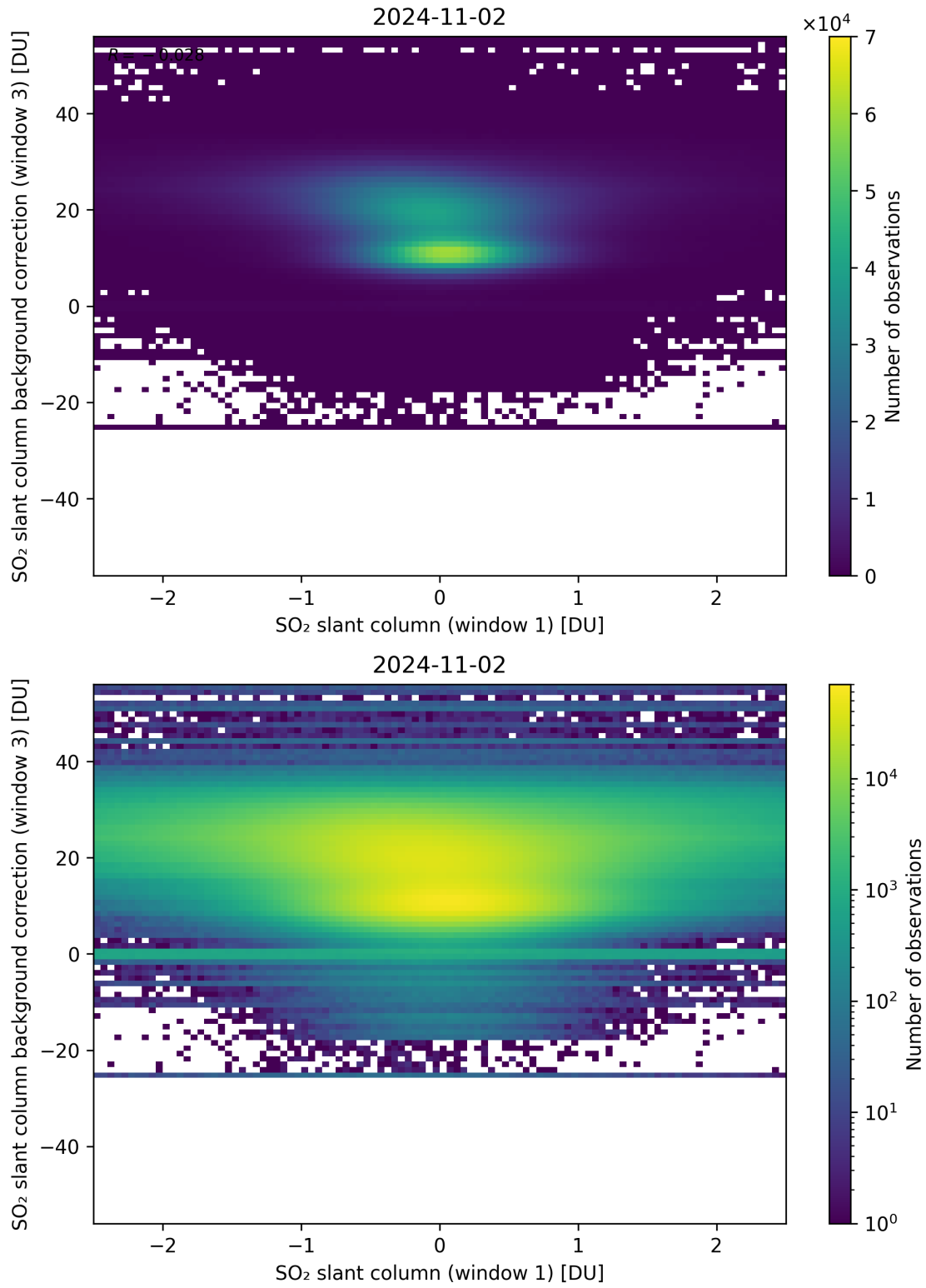
Figure 214: Scatter density plot of “SO 2 slant column (window 1)” against “SO 2 slant column background correction (window 3)” for 2024-11-01 to 2024-11-03.
