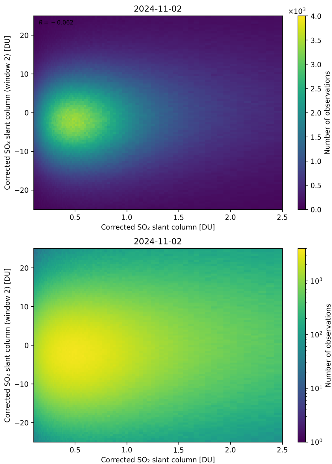
Figure 185: Scatter density plot of “Corrected SO 2 slant column” against “Corrected SO 2 slant column (window 2)” for 2024-11-01 to 2024-11-03.
