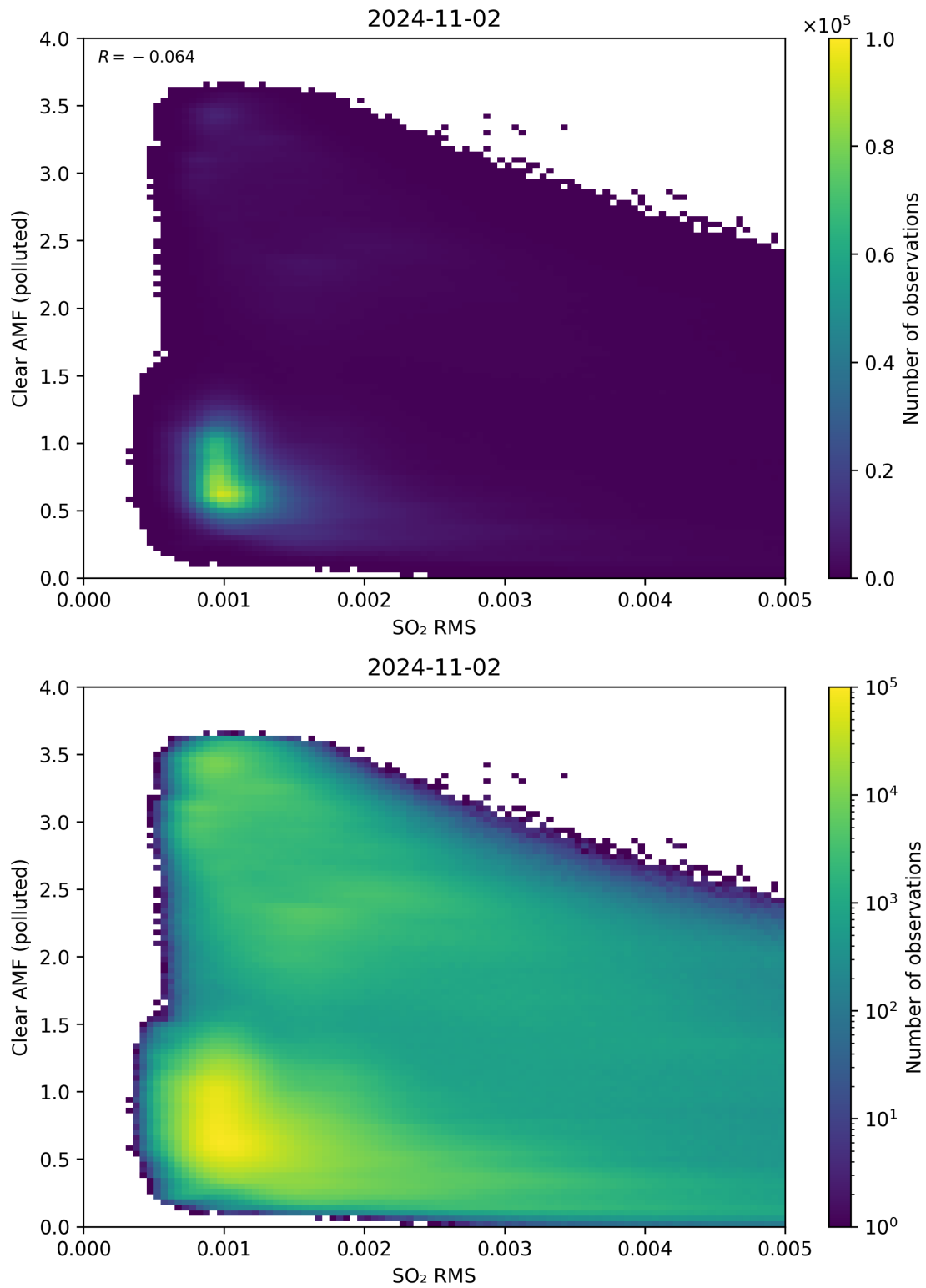
Figure 136: Scatter density plot of “SO 2 RMS” against “Clear AMF (polluted)” for 2024-11-01 to 2024-11-03.
