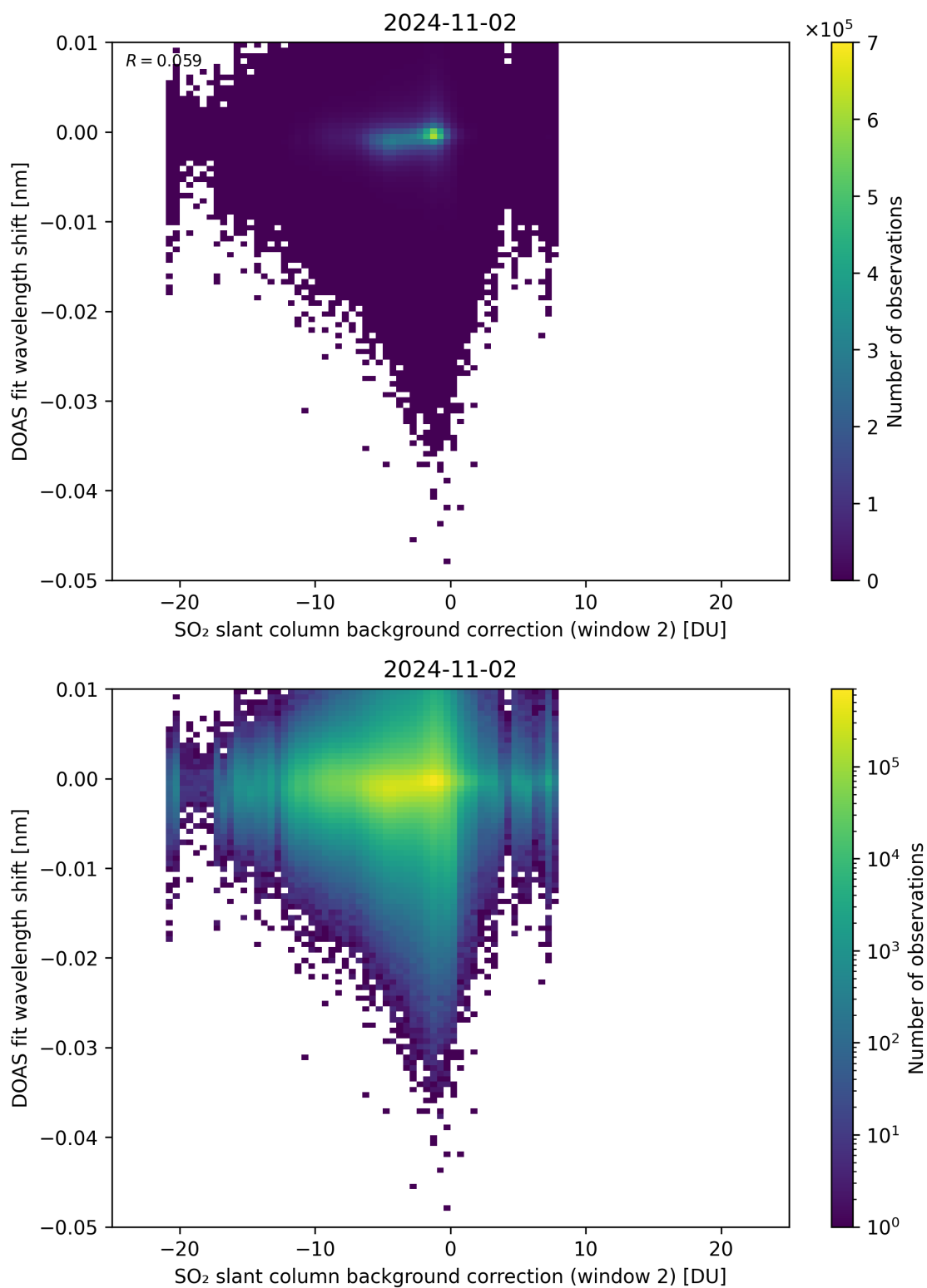
Figure 112: Scatter density plot of “SO 2 slant column background correction (window 2)” against “DOAS fit wavelength shift” for 2024-11-01 to 2024-11-03.
