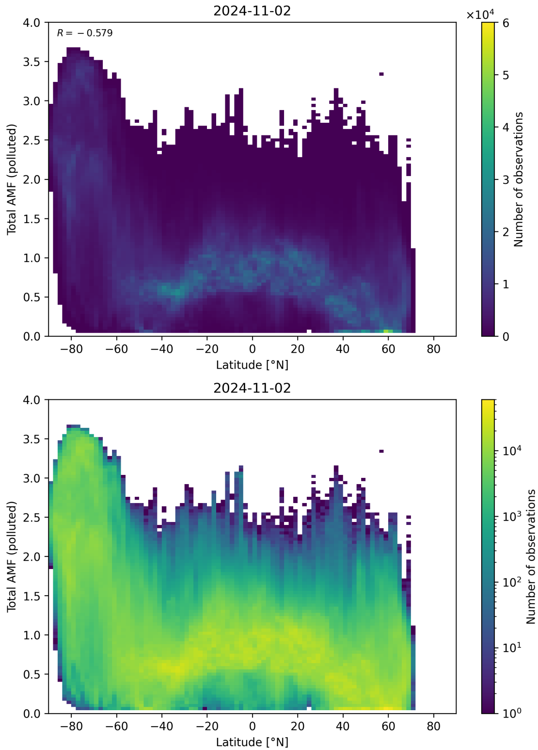
Figure 154: Scatter density plot of “Latitude” against “Total AMF (polluted)” for 2024-11-01 to 2024-11-03.
