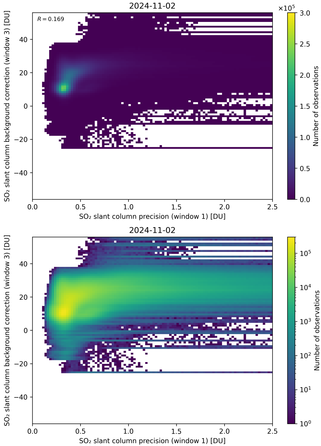
Figure 220: Scatter density plot of “SO 2 slant column precision (window 1)” against “SO 2 slant column background correction (window 3)” for 2024-11-01 to 2024-11-03.
