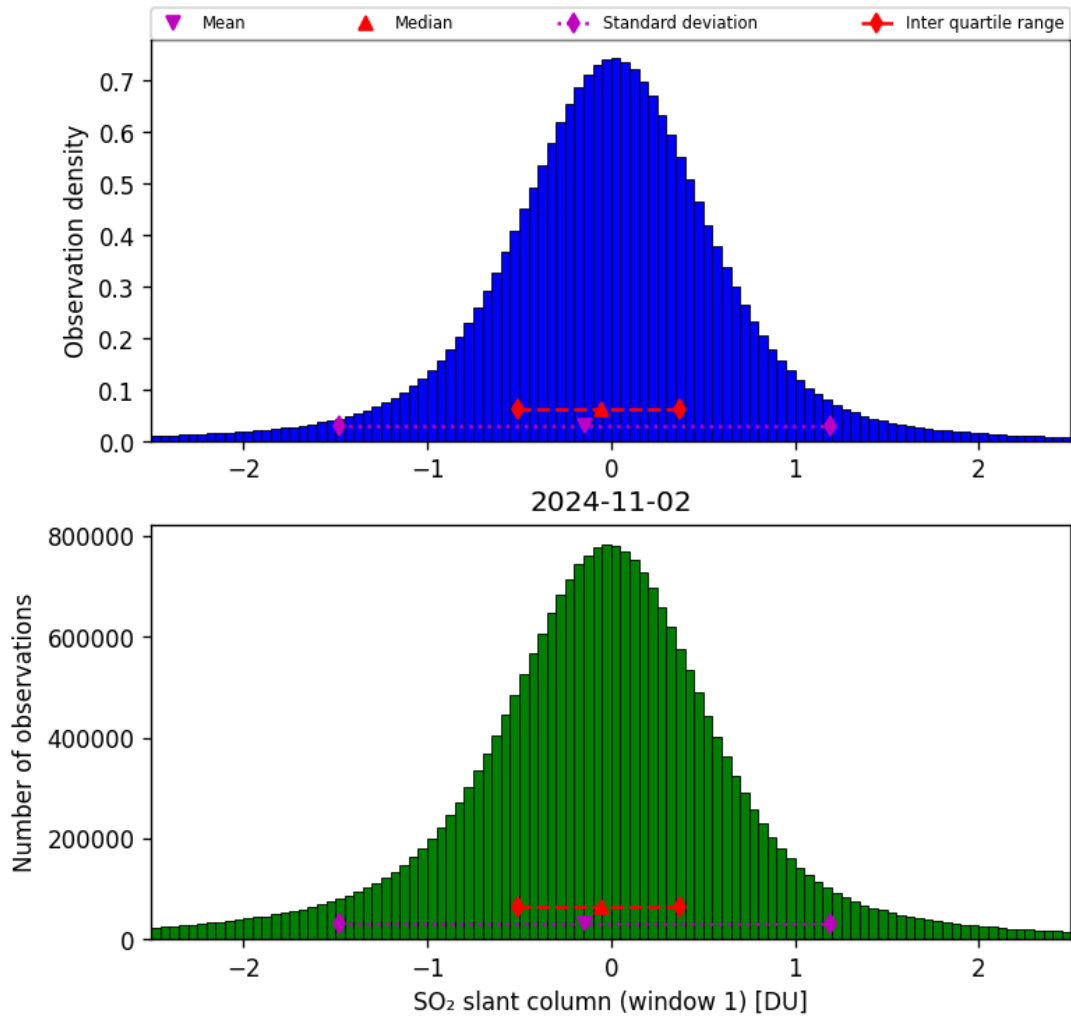
Figure 56: Histogram of “SO 2 slant column (window 1)” for 2024-11-01 to 2024-11-03
