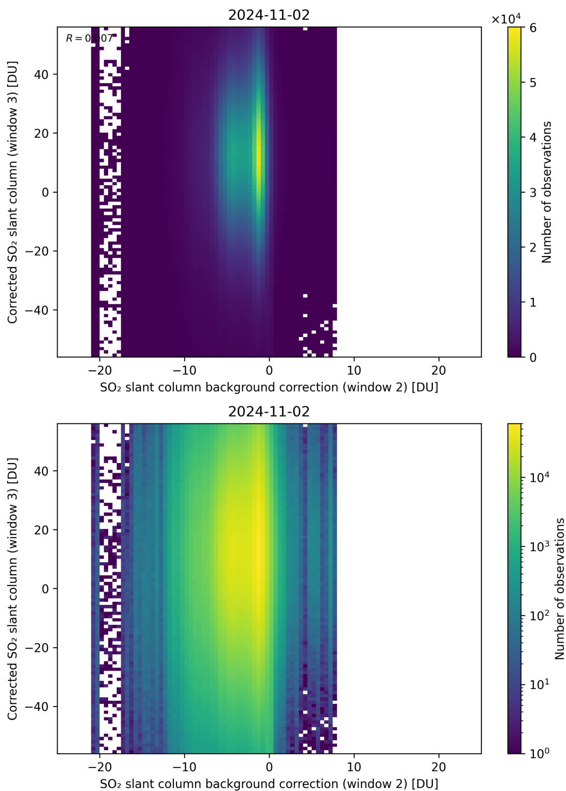
Figure 116: Scatter density plot of “SO 2 slant column background correction (window 2)” against “Corrected SO 2 slant column (window 3)” for 2024-11-01 to 2024-11-03.
