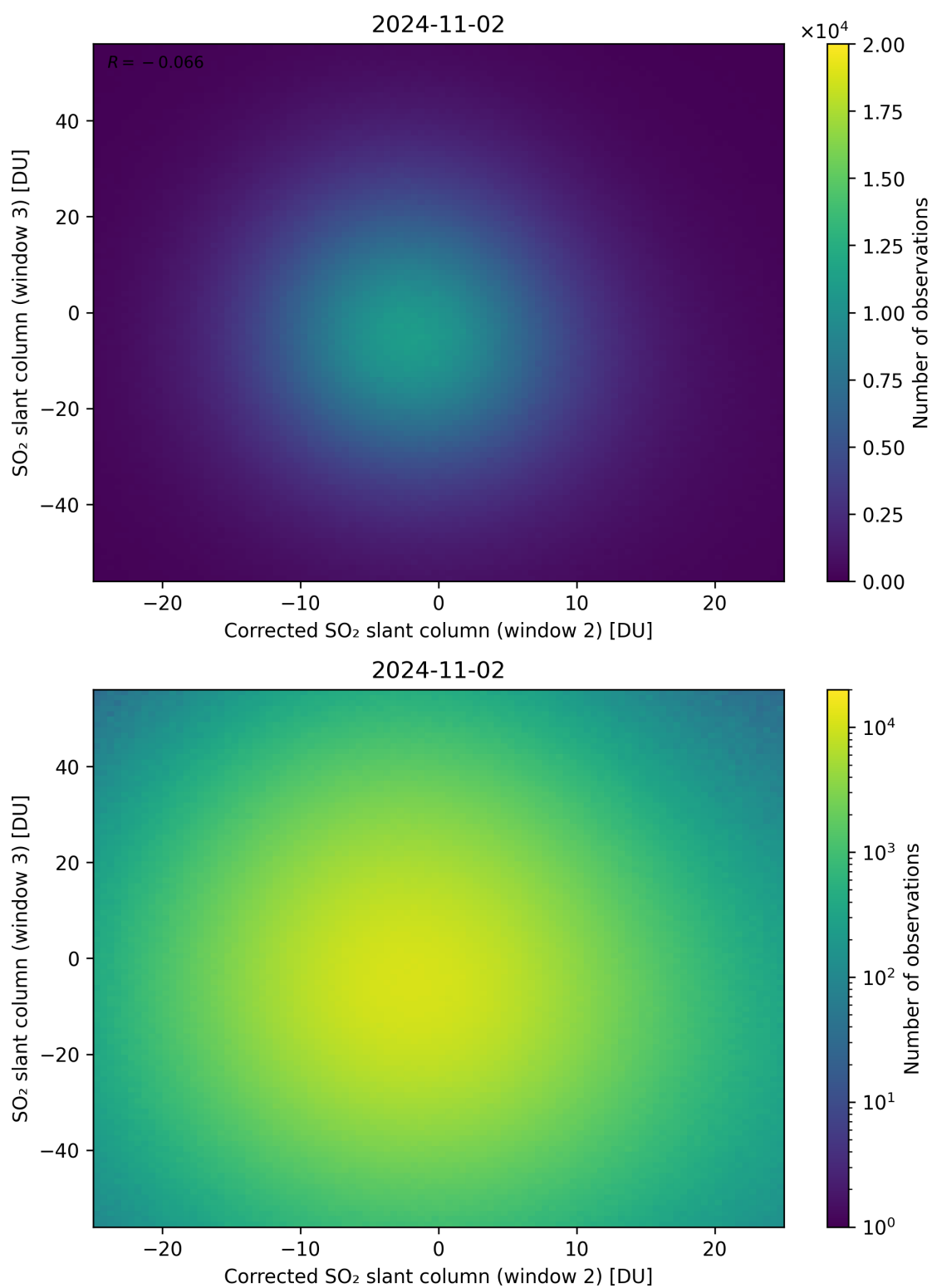
Figure 201: Scatter density plot of “Corrected SO 2 slant column (window 2)” against “SO 2 slant column (window 3)” for 2024-11-01 to 2024-11-03.
