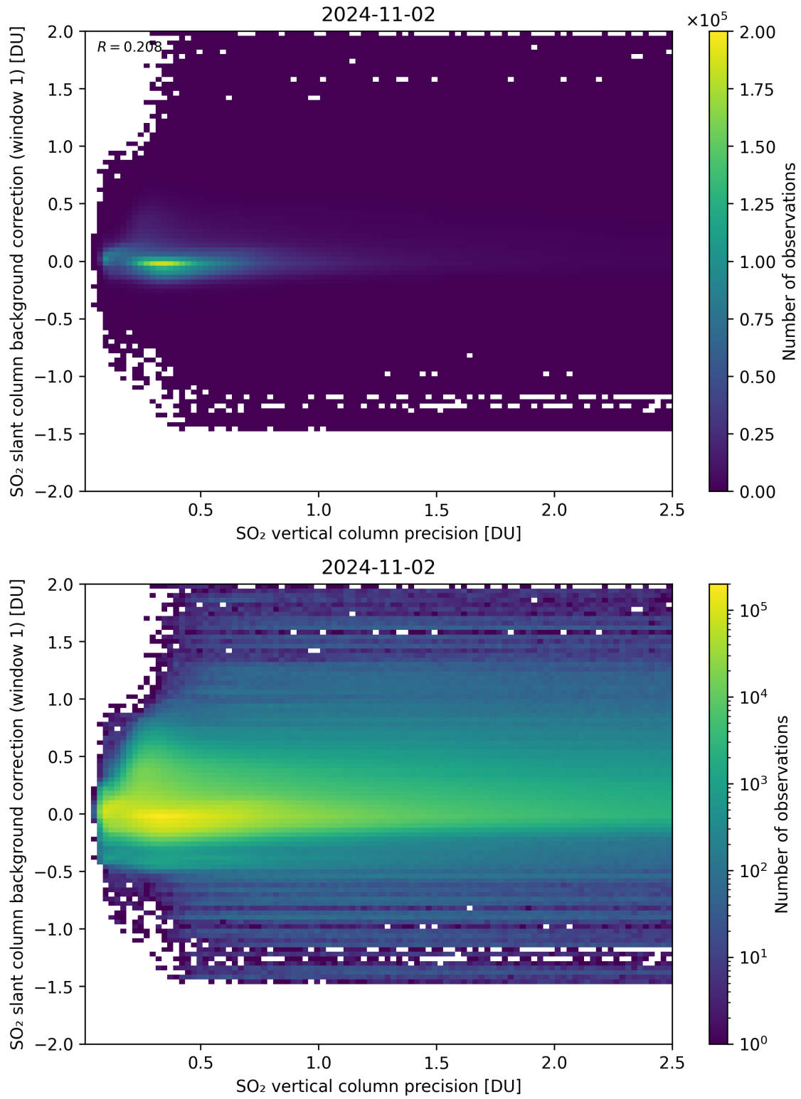
Figure 279: Scatter density plot of “SO 2 vertical column precision” against “SO 2 slant column background correction (window 1)” for 2024-11-01 to 2024-11-03.
