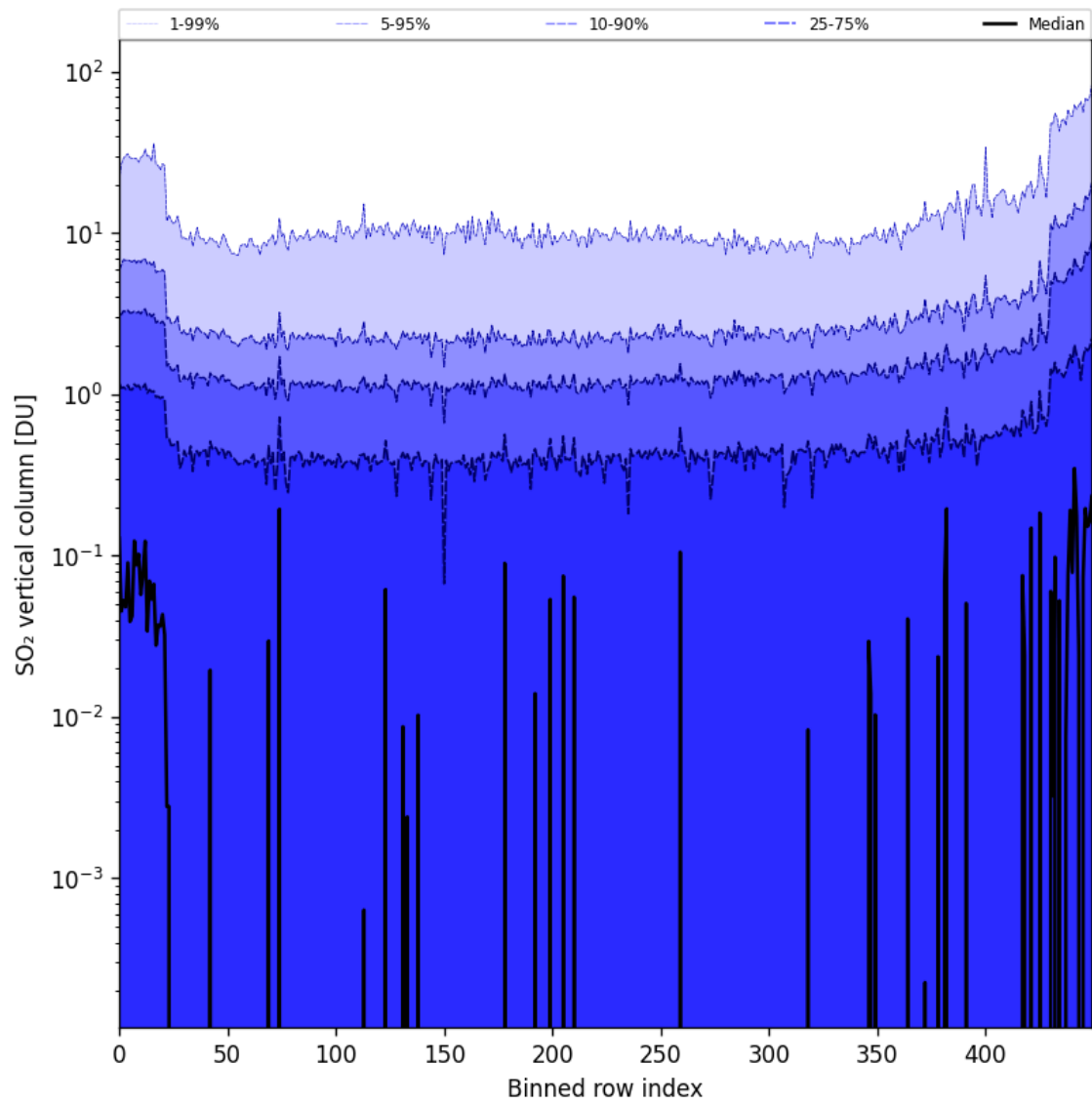
Figure 76: Along track statistics of “SO 2 vertical column” for 2024-11-01 to 2024-11-03
