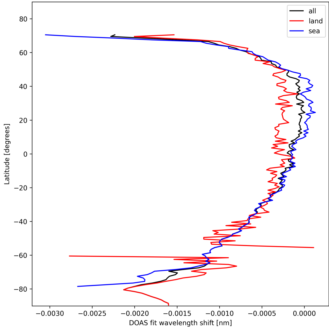
Figure 45: Zonal average of “DOAS fit wavelength shift” for 2024-11-01 to 2024-11-03.
