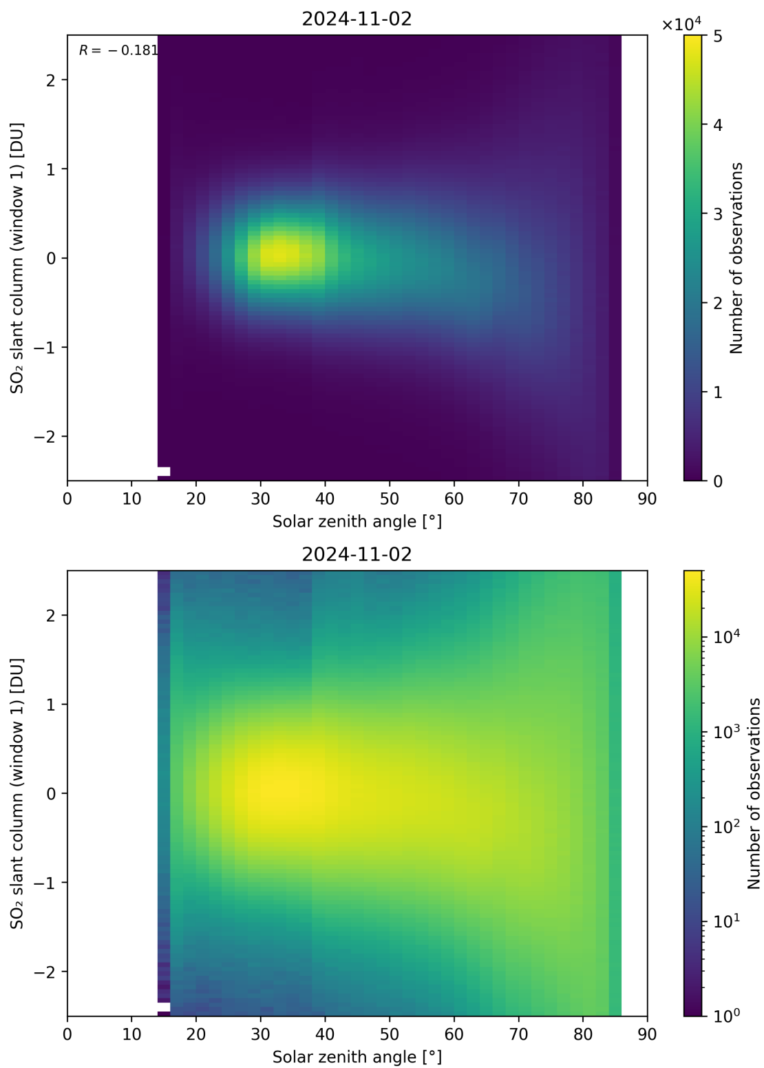
Figure 169: Scatter density plot of “Solar zenith angle” against “SO 2 slant column (window 1)” for 2024-11-01 to 2024-11-03.
