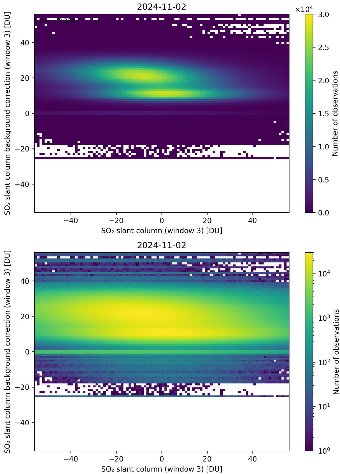
Figure 253: Scatter density plot of “SO 2 slant column (window 3)” against “SO 2 slant column background correction (window 3)” for 2024-11-01 to 2024-11-03.
