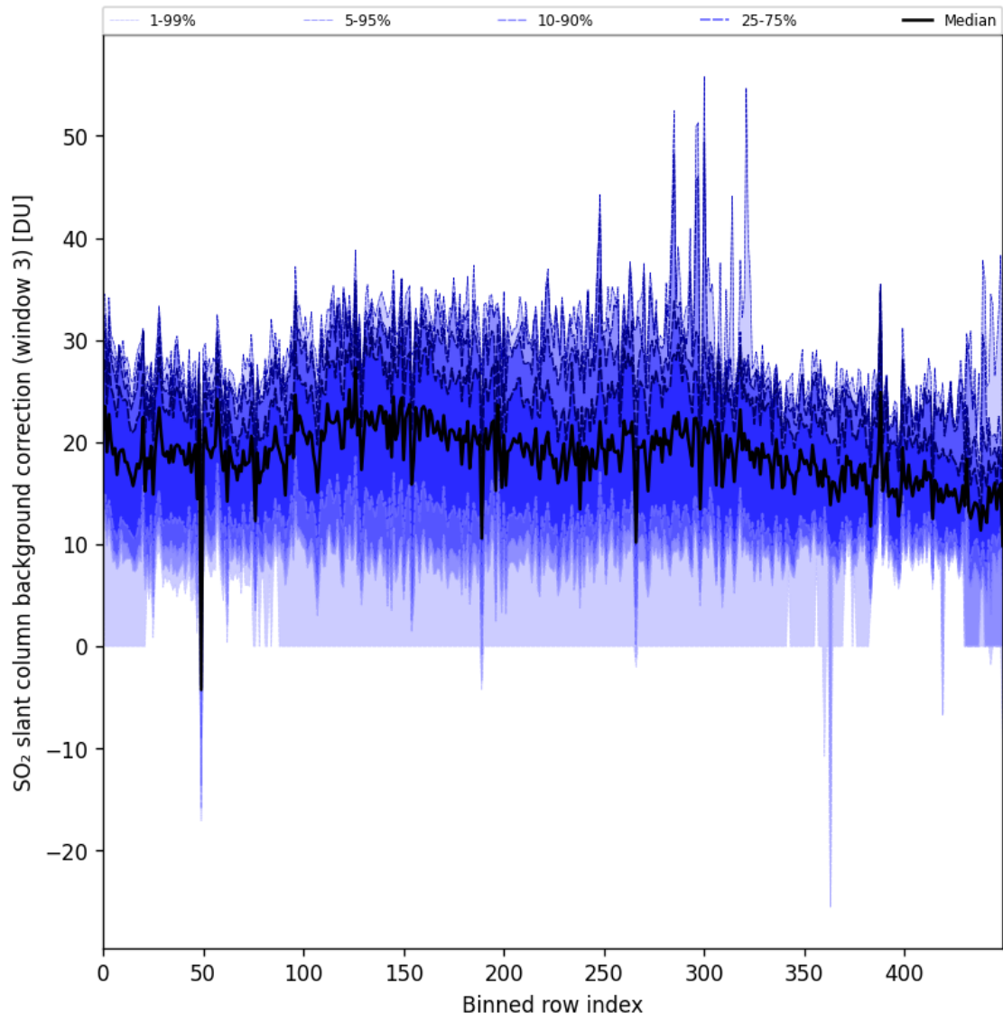
Figure 90: Along track statistics of “SO 2 slant column background correction (window 3)” for 2024-11-01 to 2024-11-03
