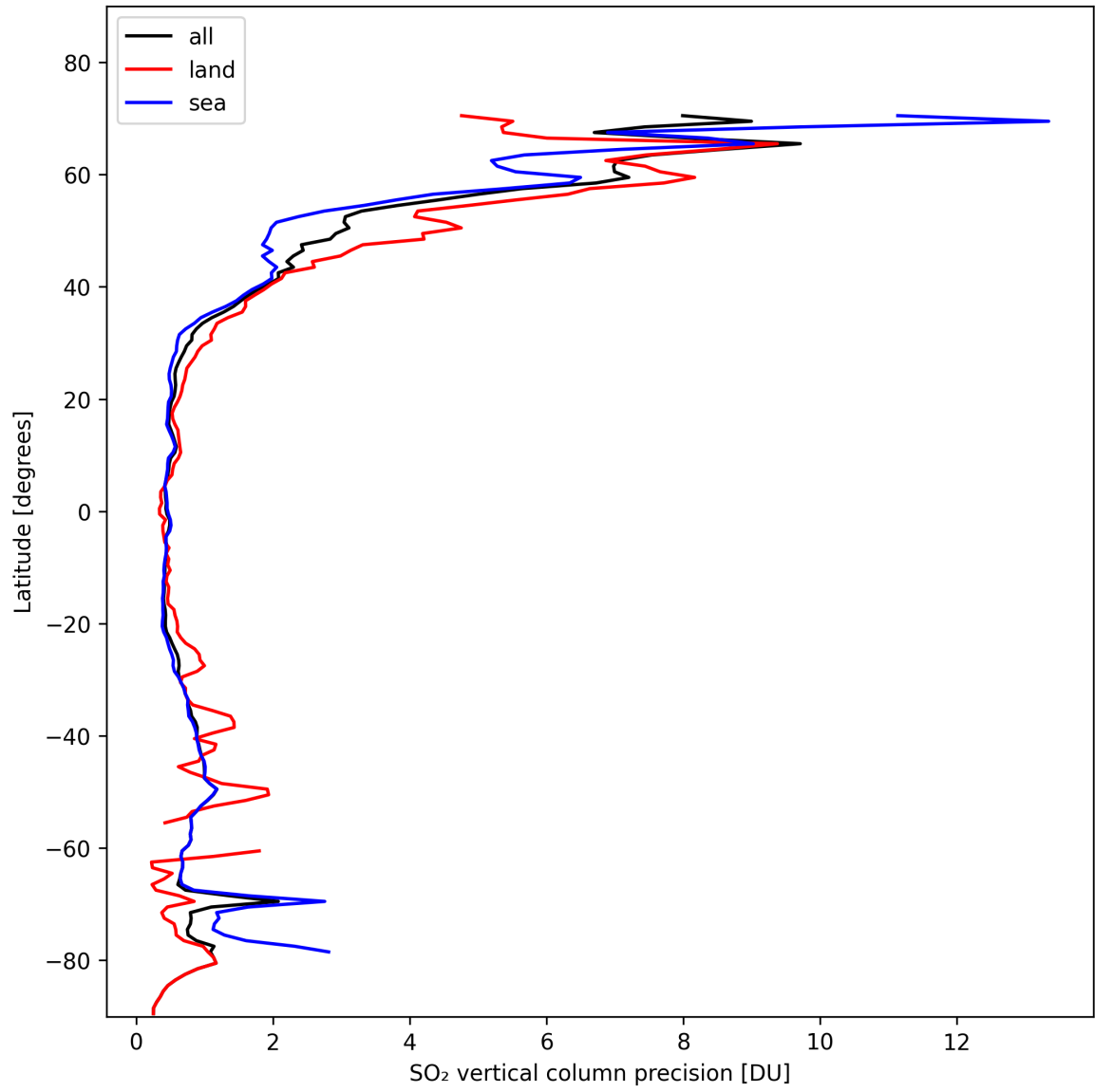
Figure 31: Zonal average of “SO 2 vertical column precision” for 2024-11-01 to 2024-11-03.
