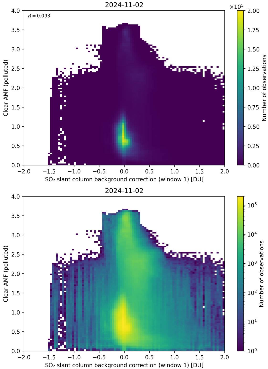
Figure 103: Scatter density plot of “SO 2 slant column background correction (window 1)” against “Clear AMF (polluted)” for 2024-11-01 to 2024-11-03.
