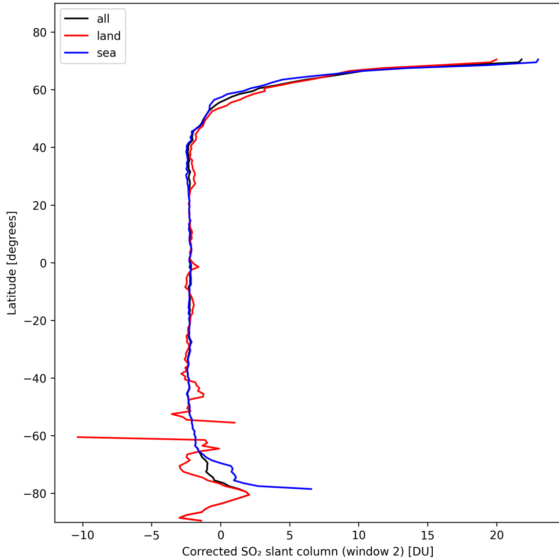
Figure 39: Zonal average of “Corrected SO 2 slant column (window 2)” for 2024-11-01 to 2024-11-03.
