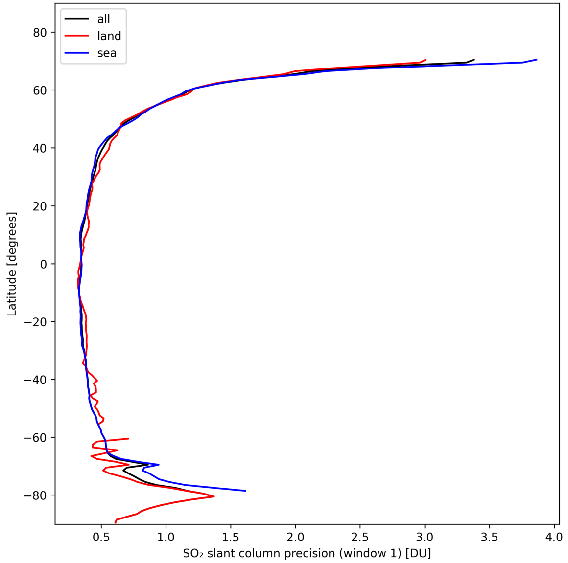
Figure 34: Zonal average of “SO 2 slant column precision (window 1)” for 2024-11-01 to 2024-11-03.
