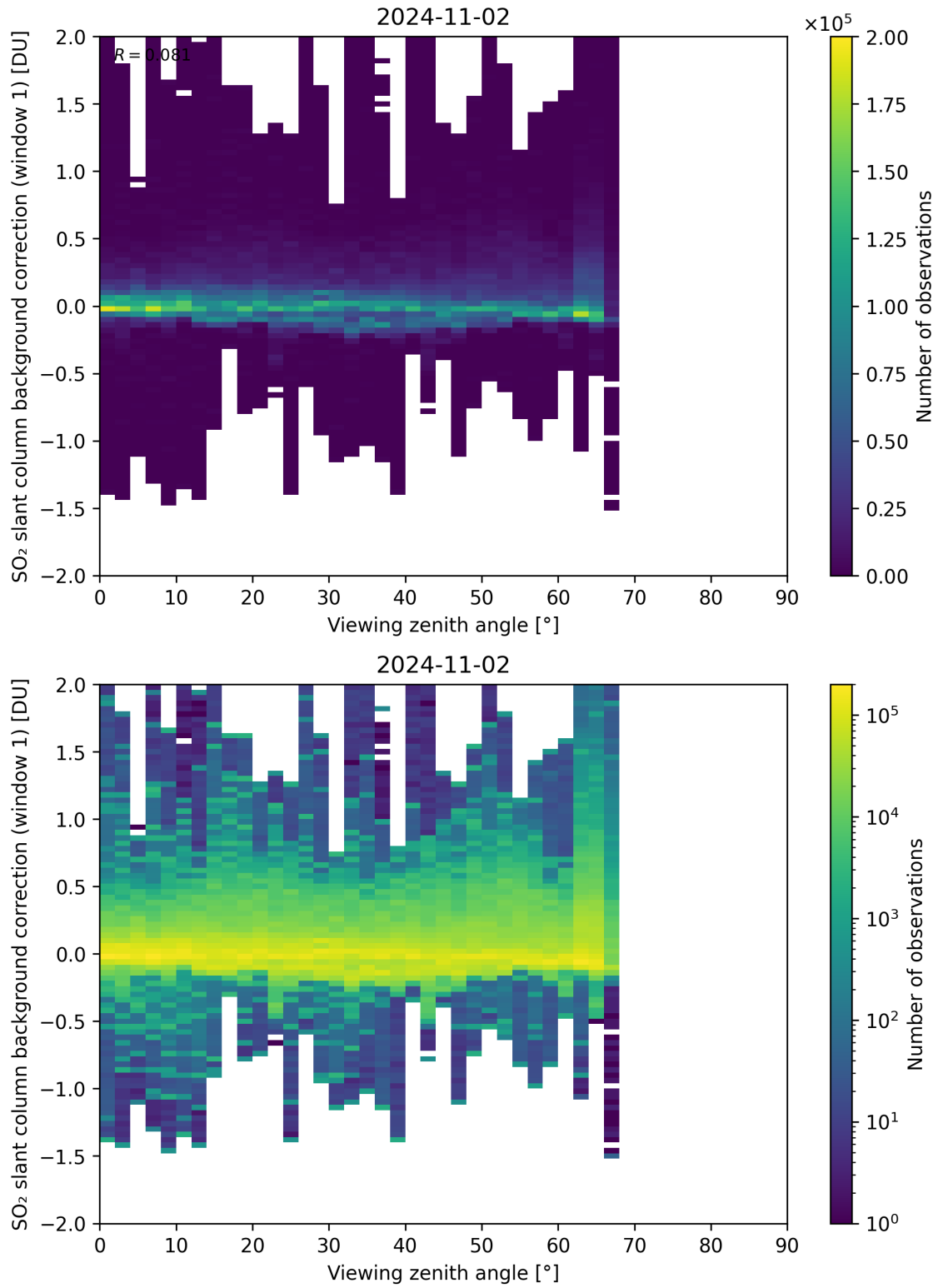
Figure 308: Scatter density plot of “Viewing zenith angle” against “SO 2 slant column background correction (window 1)” for 2024-11-01 to 2024-11-03.
