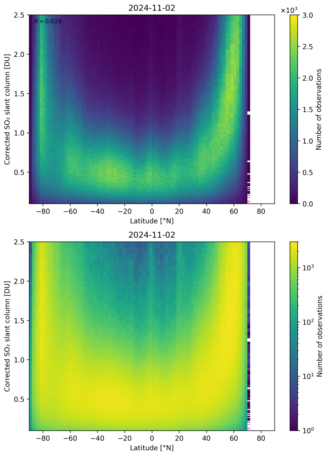
Figure 146: Scatter density plot of “Latitude” against “Corrected SO 2 slant column” for 2024-11-01 to 2024-11-03.
