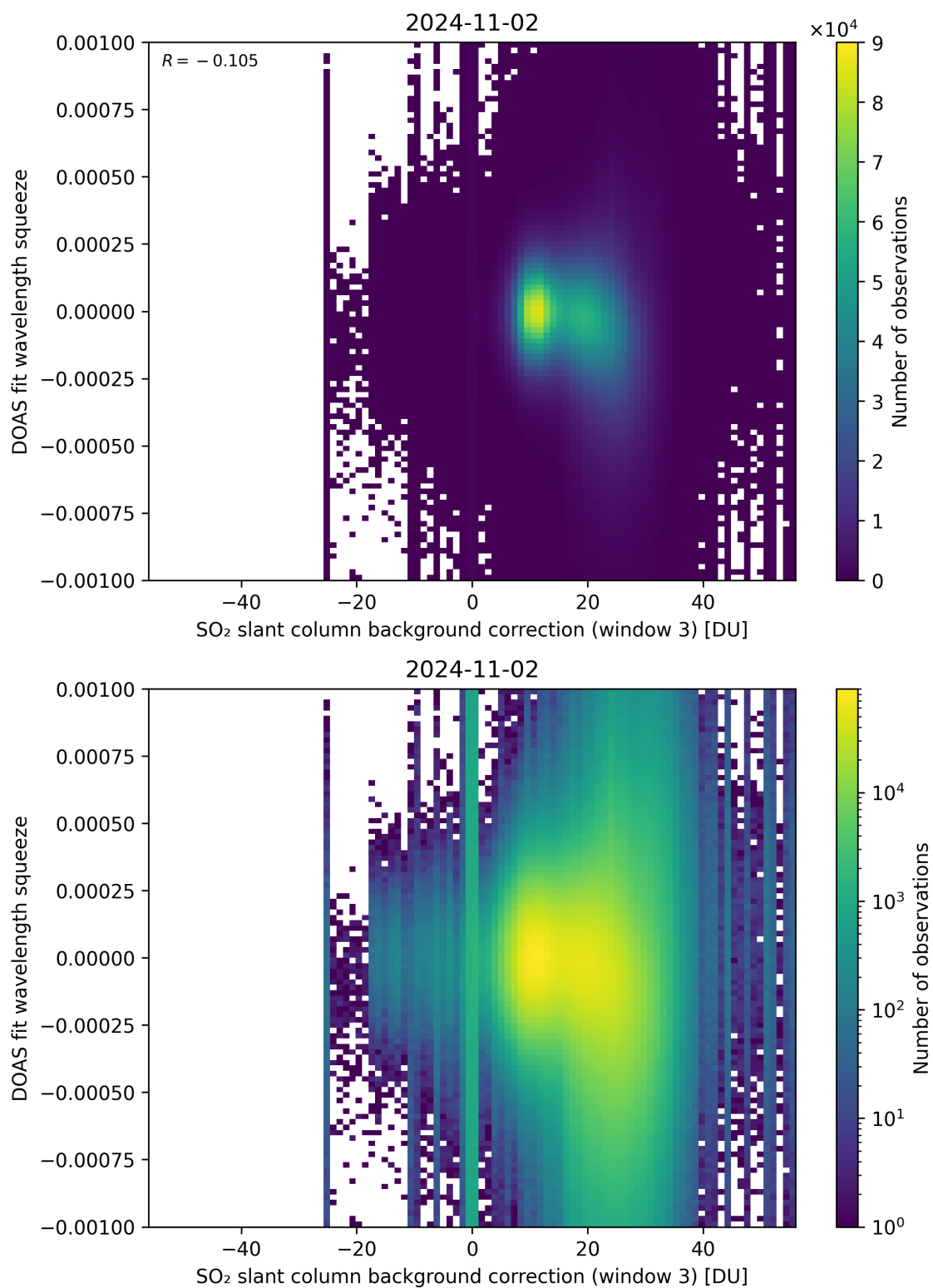
Figure 122: Scatter density plot of “SO 2 slant column background correction (window 3)” against “DOAS fit wavelength squeeze” for 2024-11-01 to 2024-11-03.
