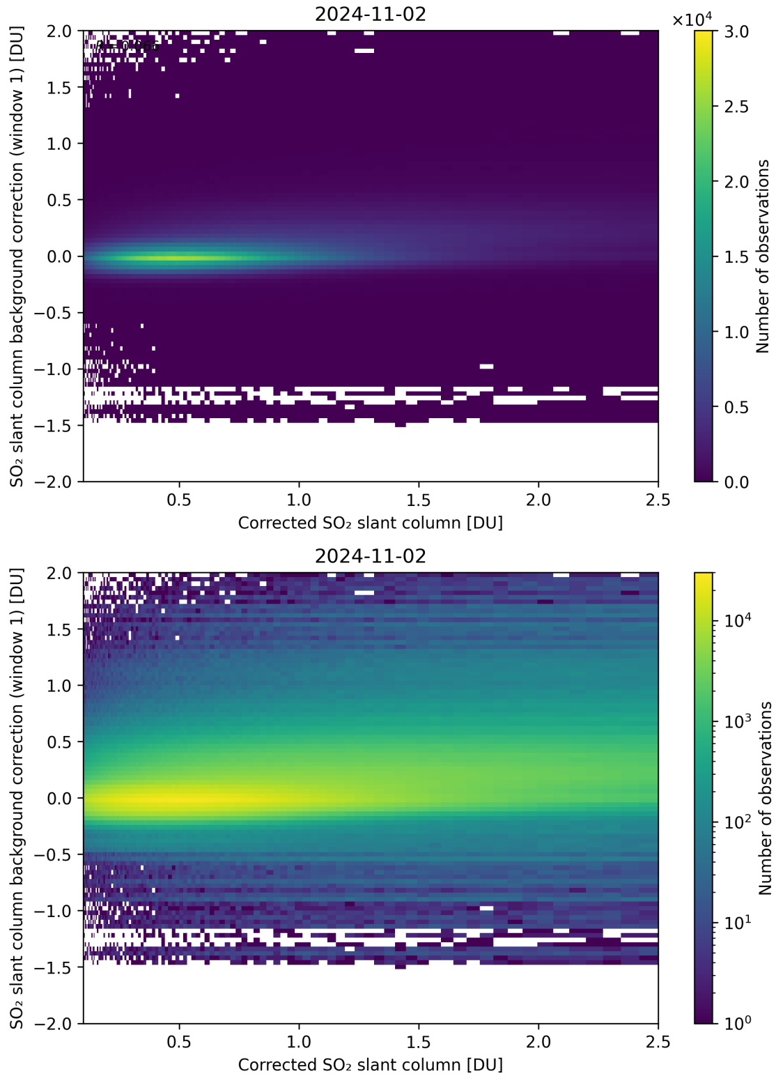
Figure 178: Scatter density plot of “Corrected SO 2 slant column” against “SO 2 slant column background correction (window 1)” for 2024-11-01 to 2024-11-03.
