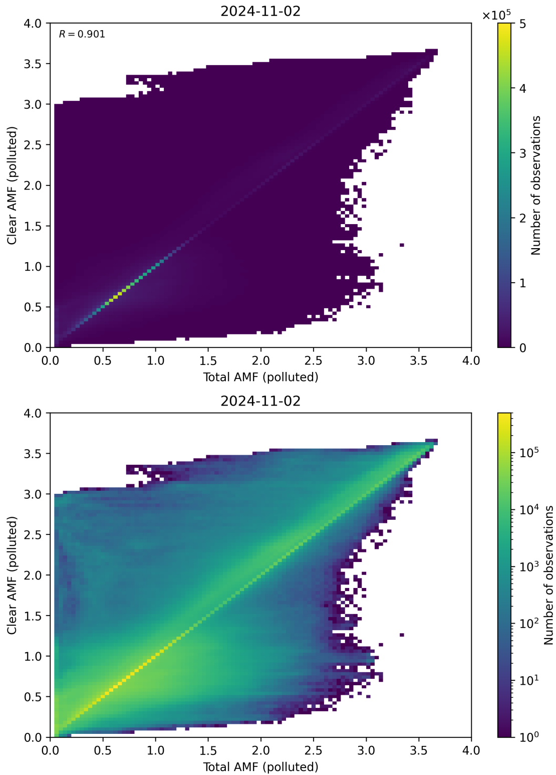
Figure 271: Scatter density plot of “Total AMF (polluted)” against “Clear AMF (polluted)” for 2024-11-01 to 2024-11-03.
