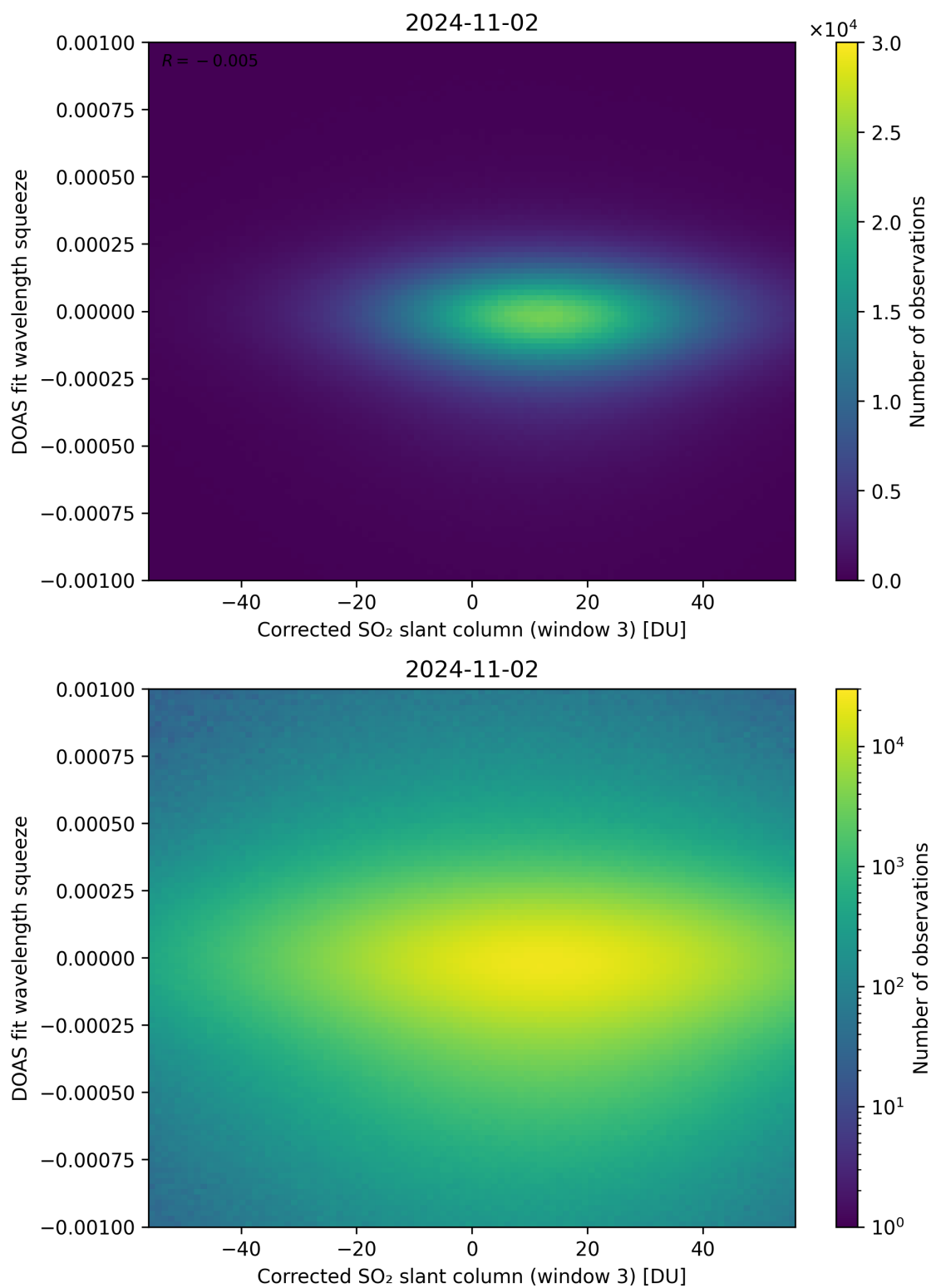
Figure 207: Scatter density plot of “Corrected SO 2 slant column (window 3)” against “DOAS fit wavelength squeeze” for 2024-11-01 to 2024-11-03.
