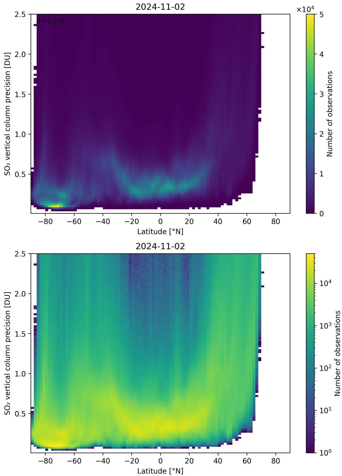
Figure 157: Scatter density plot of “Latitude” against “SO 2 vertical column precision” for 2024-11-01 to 2024-11-03.
