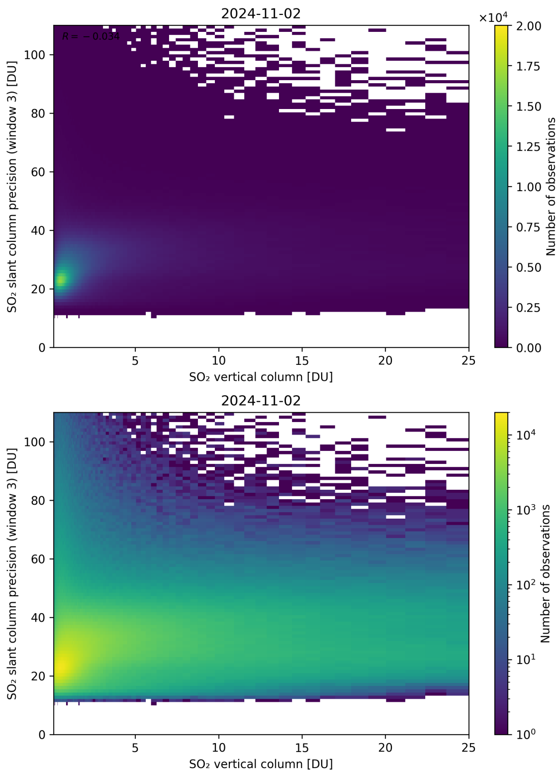
Figure 304: Scatter density plot of “SO 2 vertical column” against “SO 2 slant column precision (window 3)” for 2024-11-01 to 2024-11-03.
