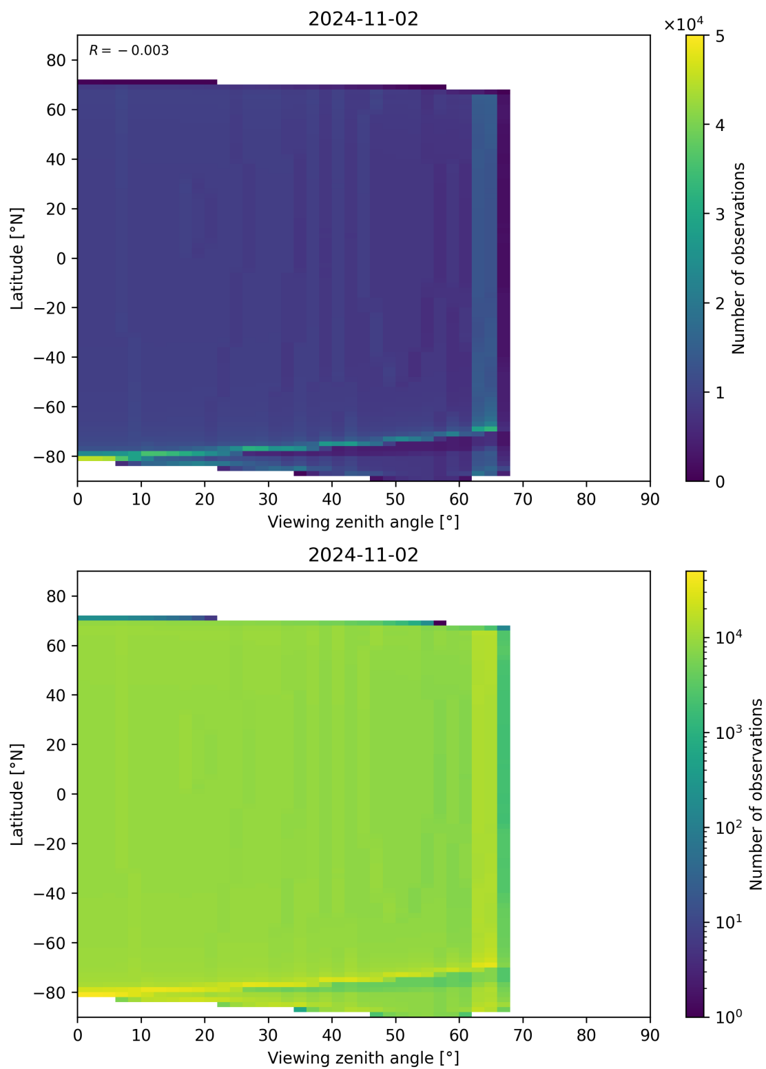
Figure 314: Scatter density plot of “Viewing zenith angle” against “Latitude” for 2024-11-01 to 2024-11-03.
