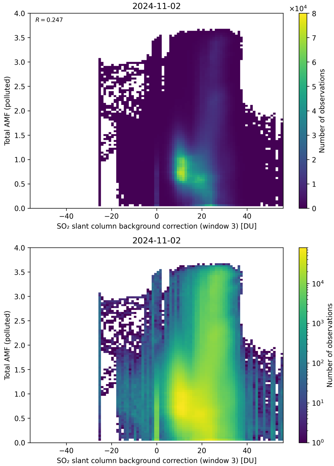
Figure 125: Scatter density plot of “SO 2 slant column background correction (window 3)” against “Total AMF (polluted)” for 2024-11-01 to 2024-11-03.
