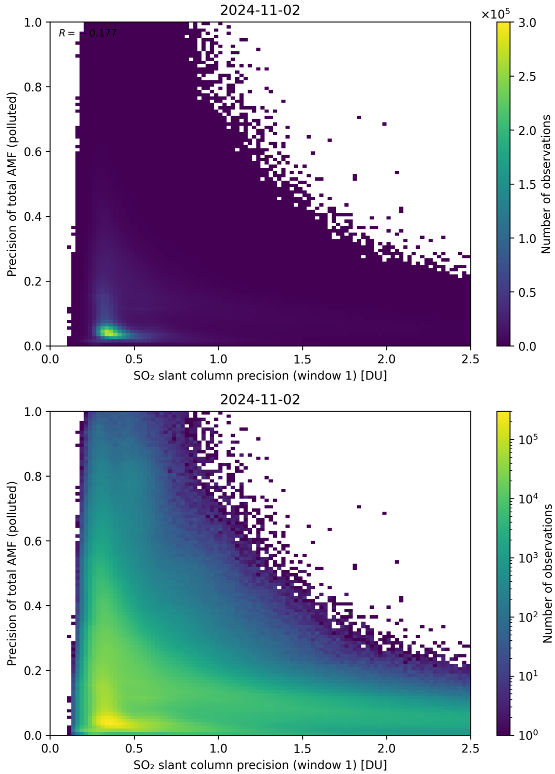
Figure 231: Scatter density plot of “SO 2 slant column precision (window 1)” against “Precision of total AMF (polluted)” for 2024-11-01 to 2024-11-03.
