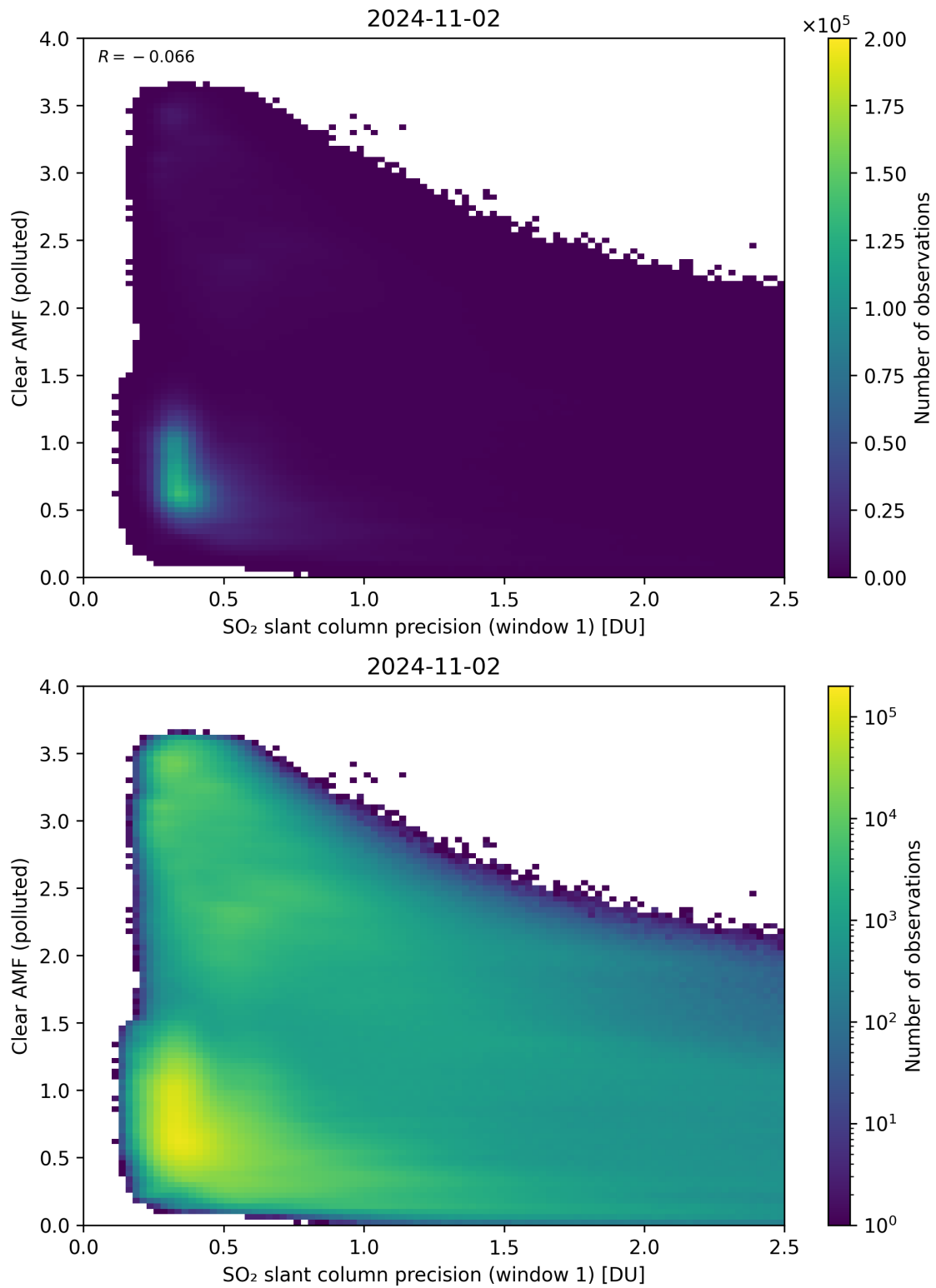
Figure 224: Scatter density plot of “SO 2 slant column precision (window 1)” against “Clear AMF (polluted)” for 2024-11-01 to 2024-11-03.
