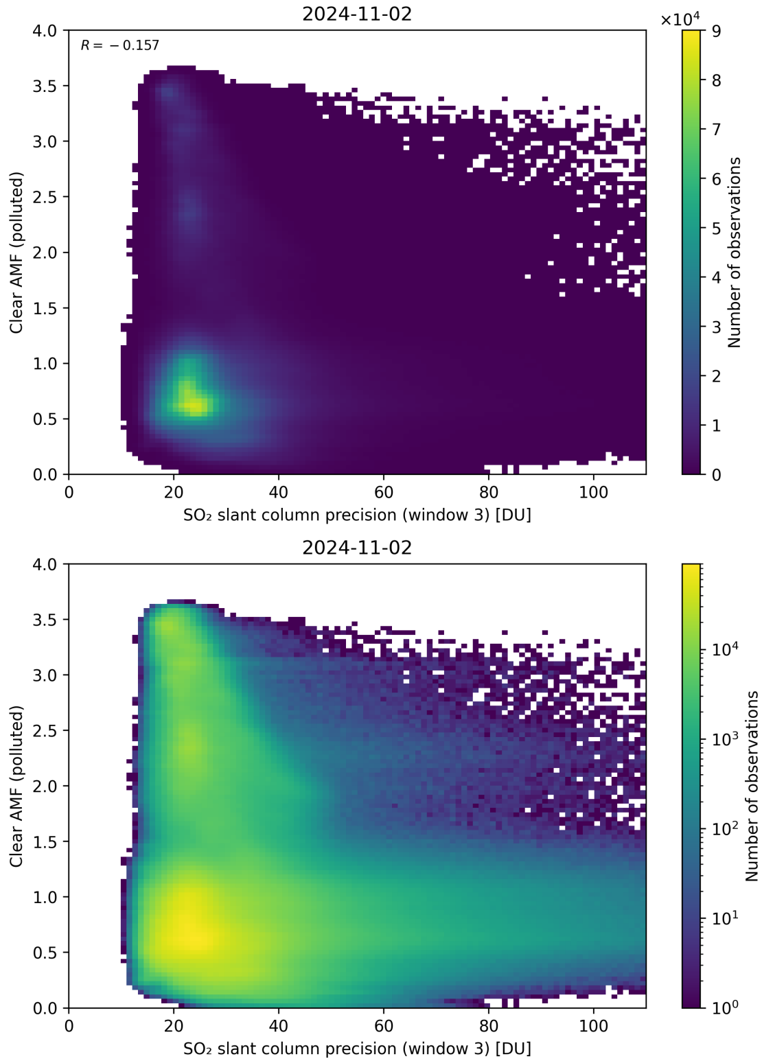
Figure 261: Scatter density plot of “SO 2 slant column precision (window 3)” against “Clear AMF (polluted)” for 2024-11-01 to 2024-11-03.
