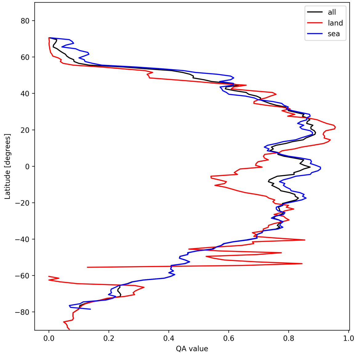
Figure 29: Zonal average of “QA value” for 2024-11-01 to 2024-11-03.
