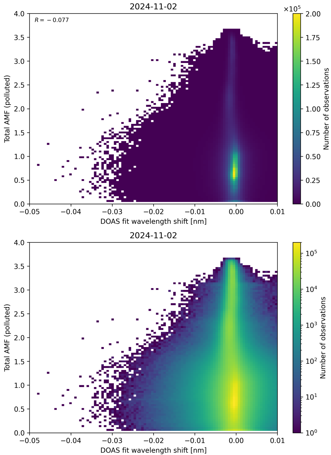
Figure 130: Scatter density plot of “DOAS fit wavelength shift” against “Total AMF (polluted)” for 2024-11-01 to 2024-11-03.
