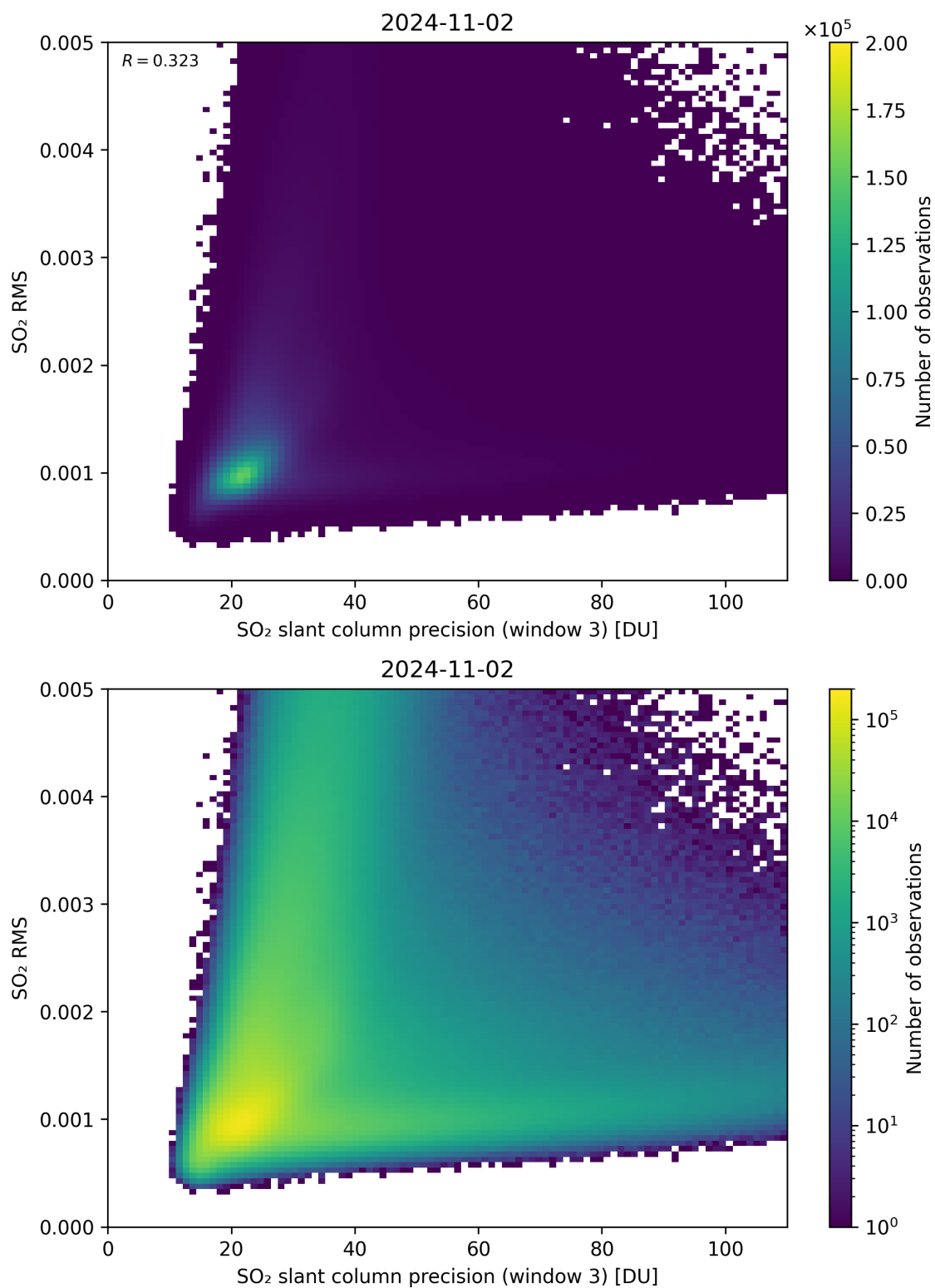
Figure 260: Scatter density plot of “SO 2 slant column precision (window 3)” against “SO 2 RMS” for 2024-11-01 to 2024-11-03.
