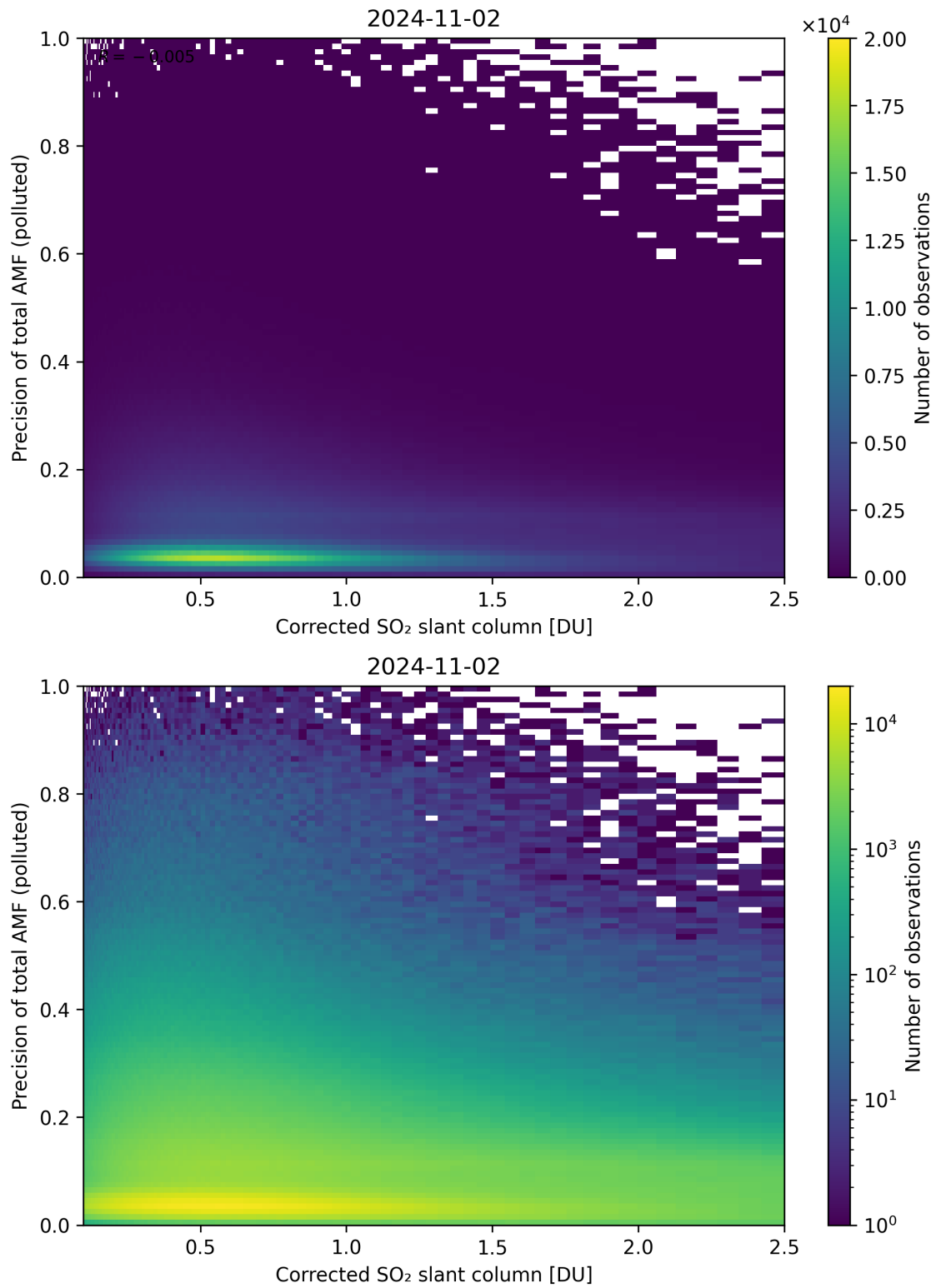
Figure 193: Scatter density plot of “Corrected SO 2 slant column” against “Precision of total AMF (polluted)” for 2024-11-01 to 2024-11-03.
