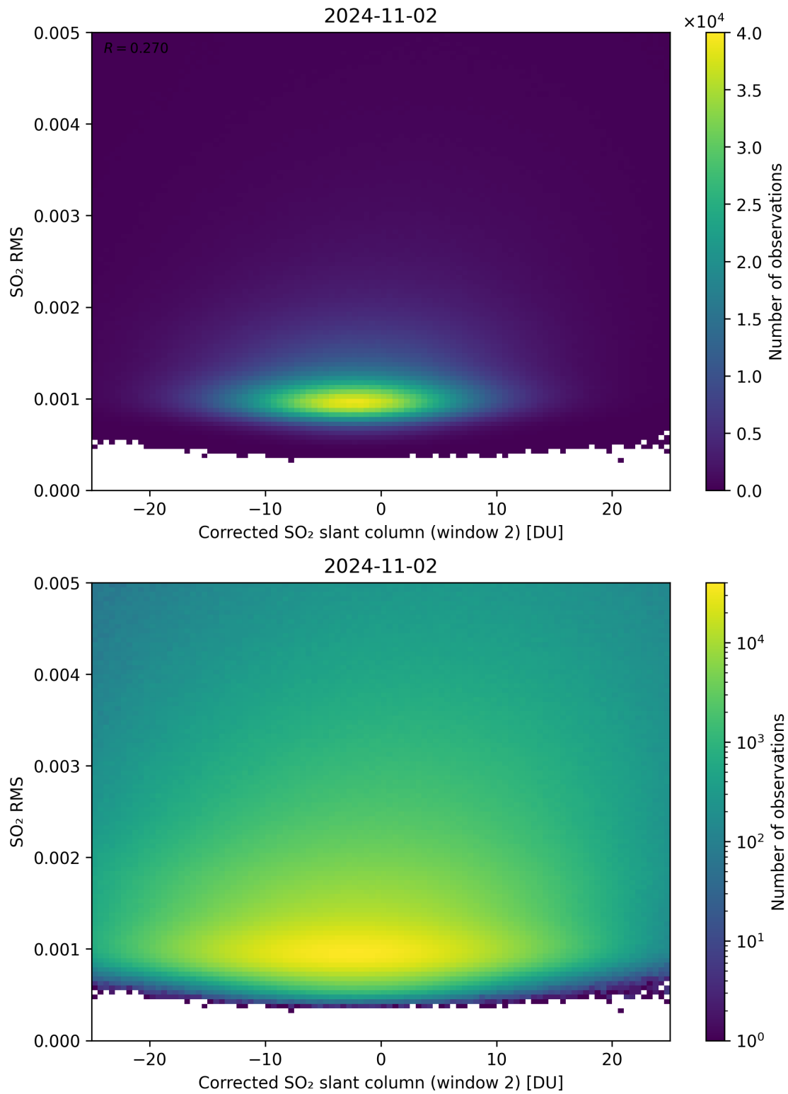
Figure 198: Scatter density plot of “Corrected SO 2 slant column (window 2)” against “SO 2 RMS” for 2024-11-01 to 2024-11-03.
