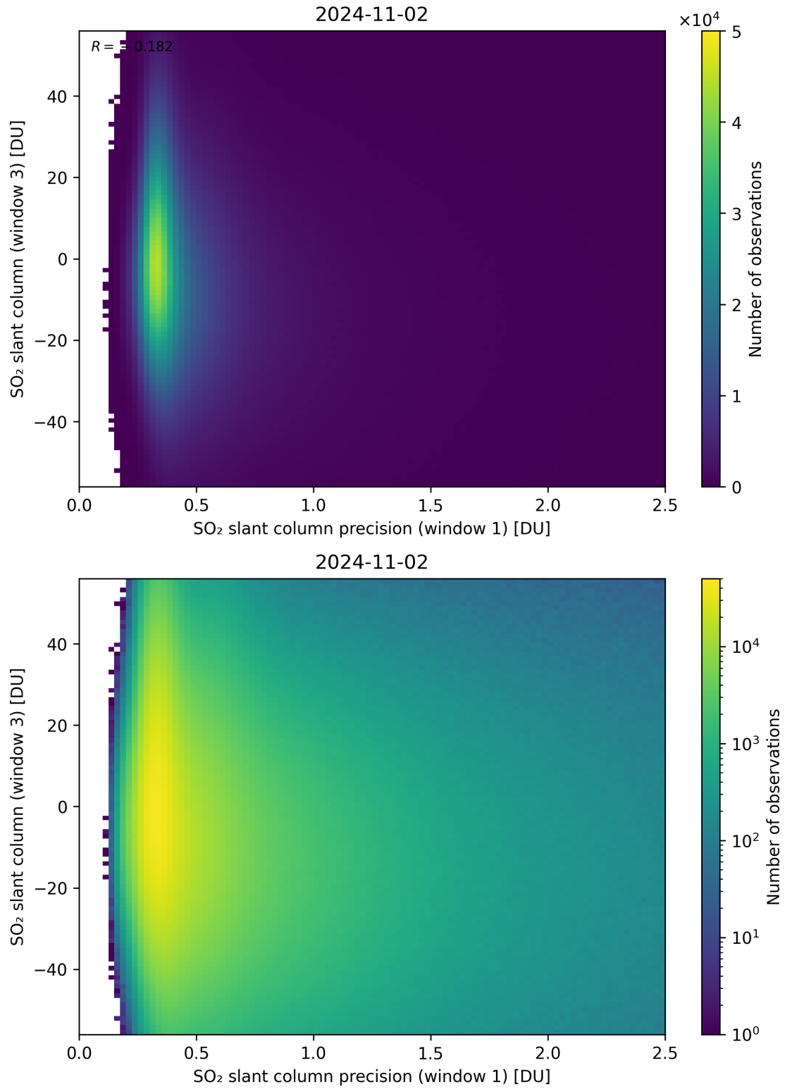
Figure 228: Scatter density plot of “SO 2 slant column precision (window 1)” against “SO 2 slant column (window 3)” for 2024-11-01 to 2024-11-03.
