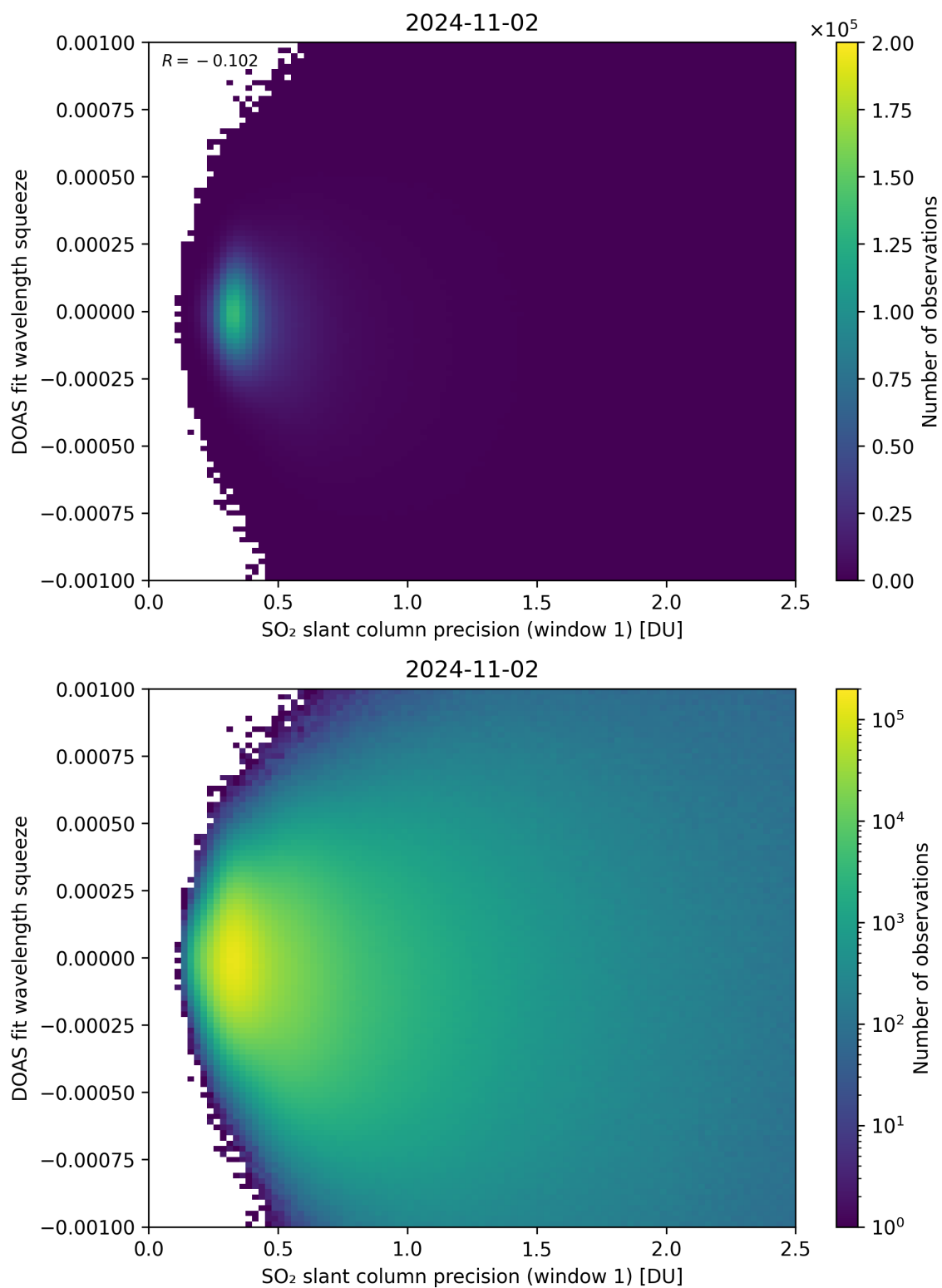
Figure 222: Scatter density plot of “SO 2 slant column precision (window 1)” against “DOAS fit wavelength squeeze” for 2024-11-01 to 2024-11-03.
