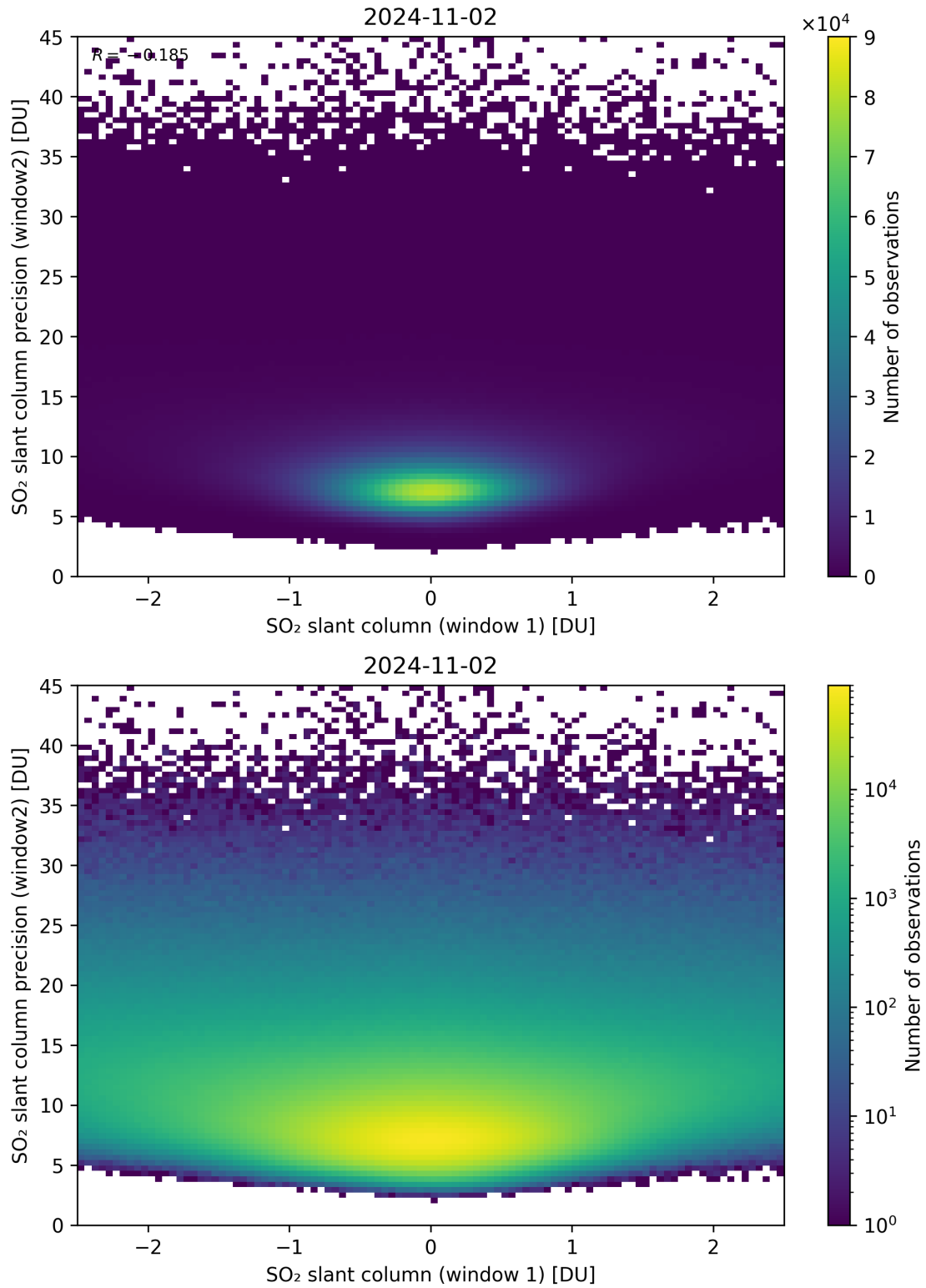
Figure 236: Scatter density plot of “SO 2 slant column (window 1)” against “SO 2 slant column precision (window2)” for 2024-11-01 to 2024-11-03.
