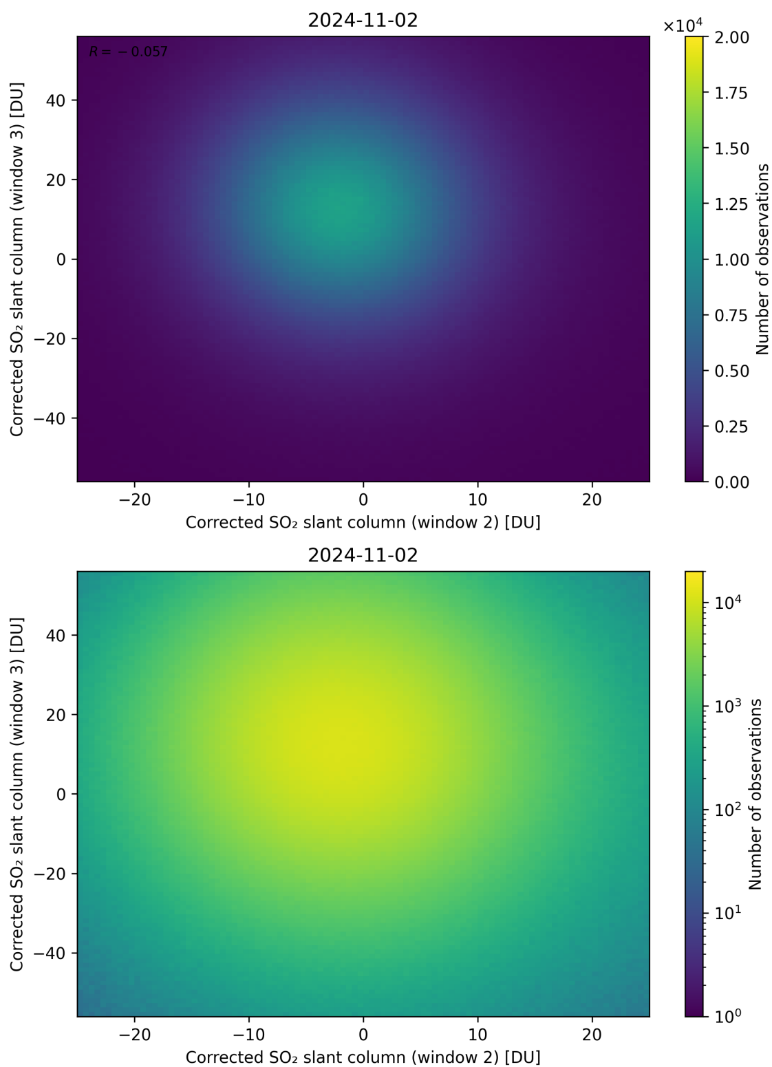
Figure 200: Scatter density plot of “Corrected SO 2 slant column (window 2)” against “Corrected SO 2 slant column (window 3)” for 2024-11-01 to 2024-11-03.
