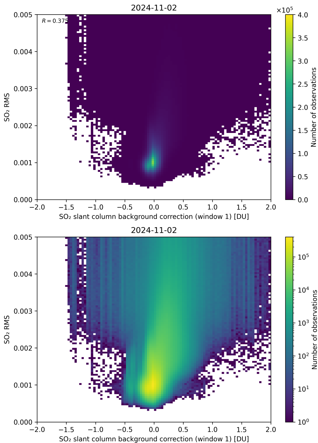
Figure 102: Scatter density plot of “SO 2 slant column background correction (window 1)” against “SO 2 RMS” for 2024-11-01 to 2024-11-03.
