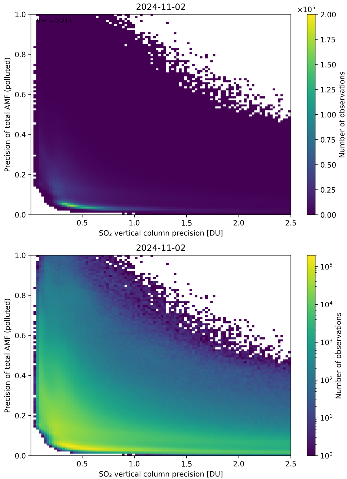
Figure 295: Scatter density plot of “SO 2 vertical column precision” against “Precision of total AMF (polluted)” for 2024-11-01 to 2024-11-03.
