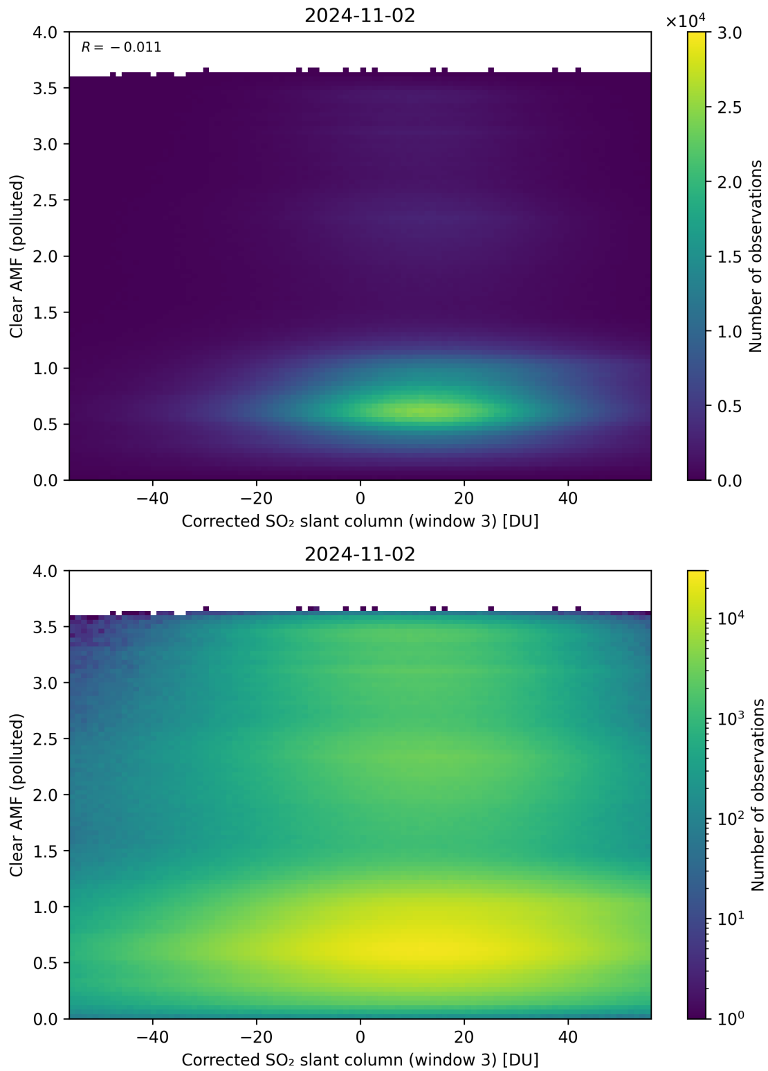
Figure 209: Scatter density plot of “Corrected SO 2 slant column (window 3)” against “Clear AMF (polluted)” for 2024-11-01 to 2024-11-03.
