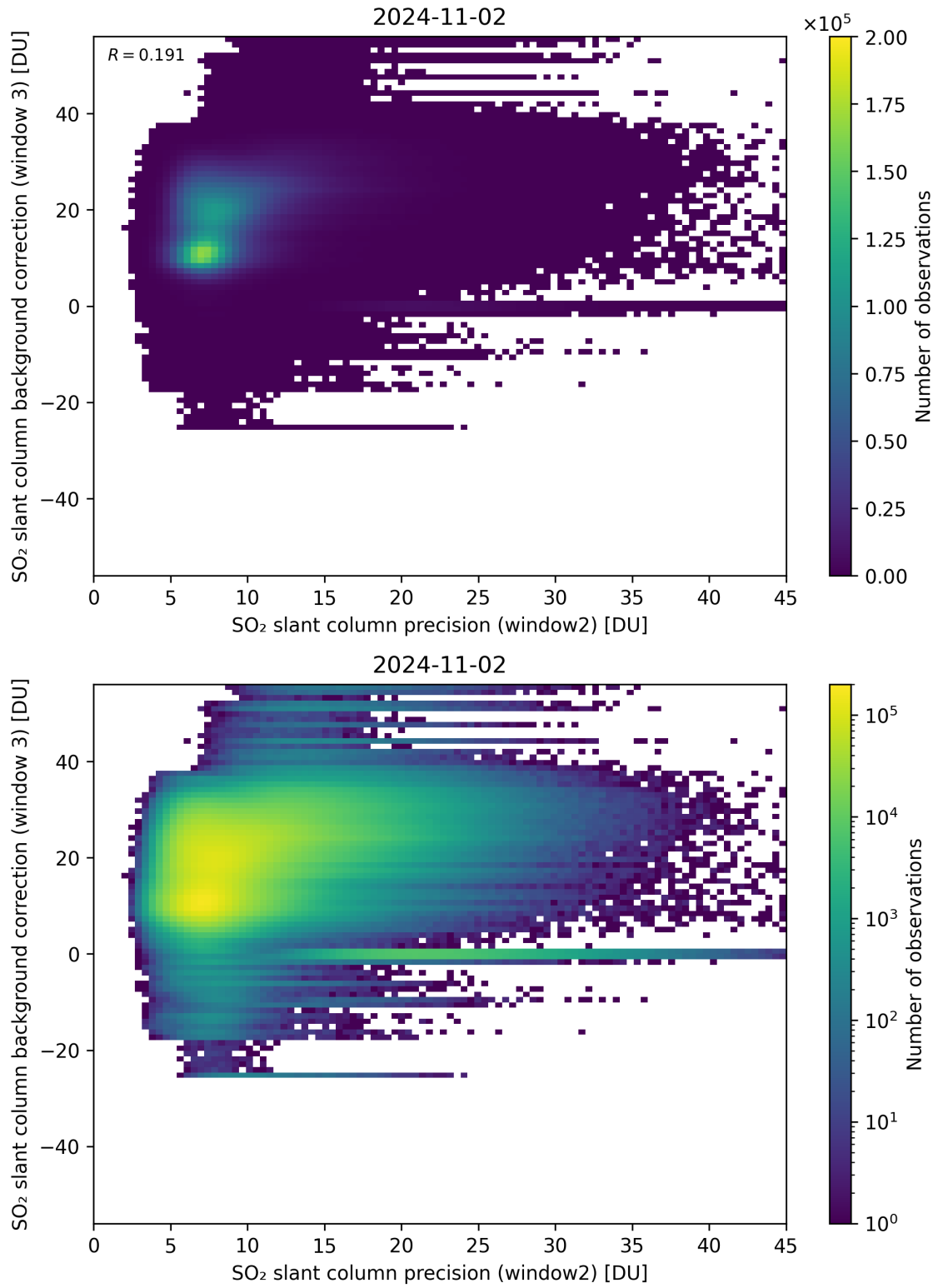
Figure 242: Scatter density plot of “SO 2 slant column precision (window2)” against “SO 2 slant column background correction (window 3)” for 2024-11-01 to 2024-11-03.
