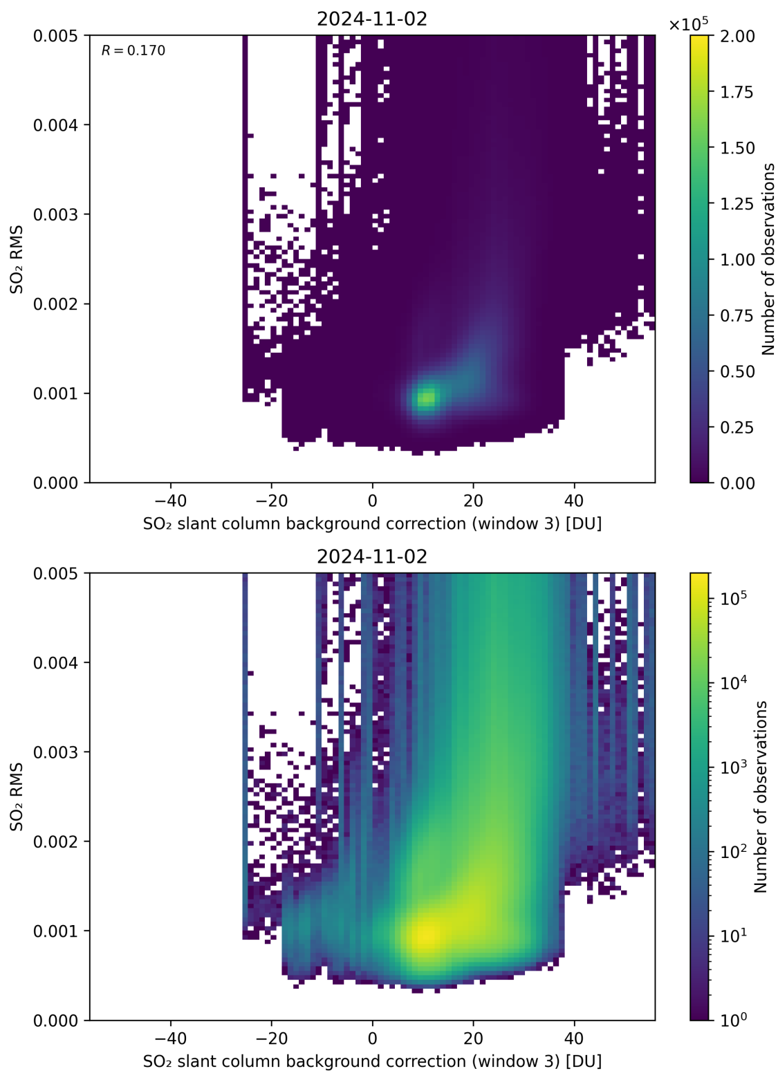
Figure 123: Scatter density plot of “SO 2 slant column background correction (window 3)” against “SO 2 RMS” for 2024-11-01 to 2024-11-03.
