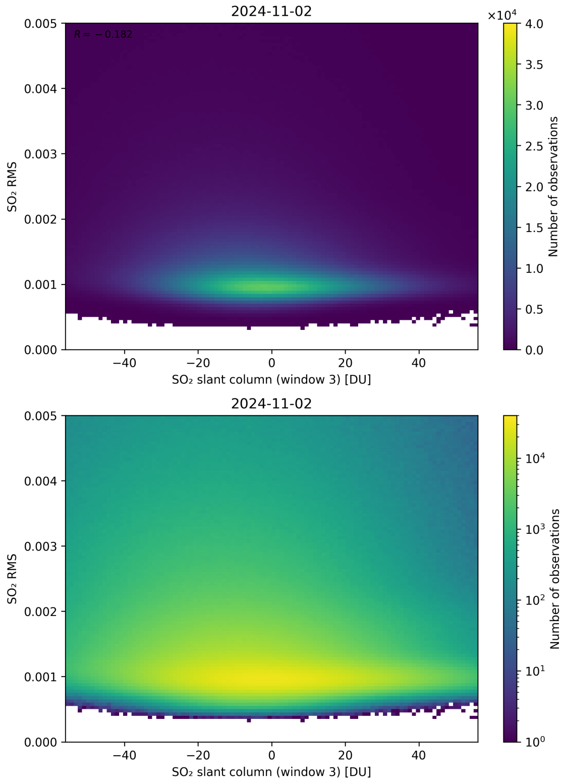
Figure 256: Scatter density plot of “SO 2 slant column (window 3)” against “SO 2 RMS” for 2024-11-01 to 2024-11-03.
