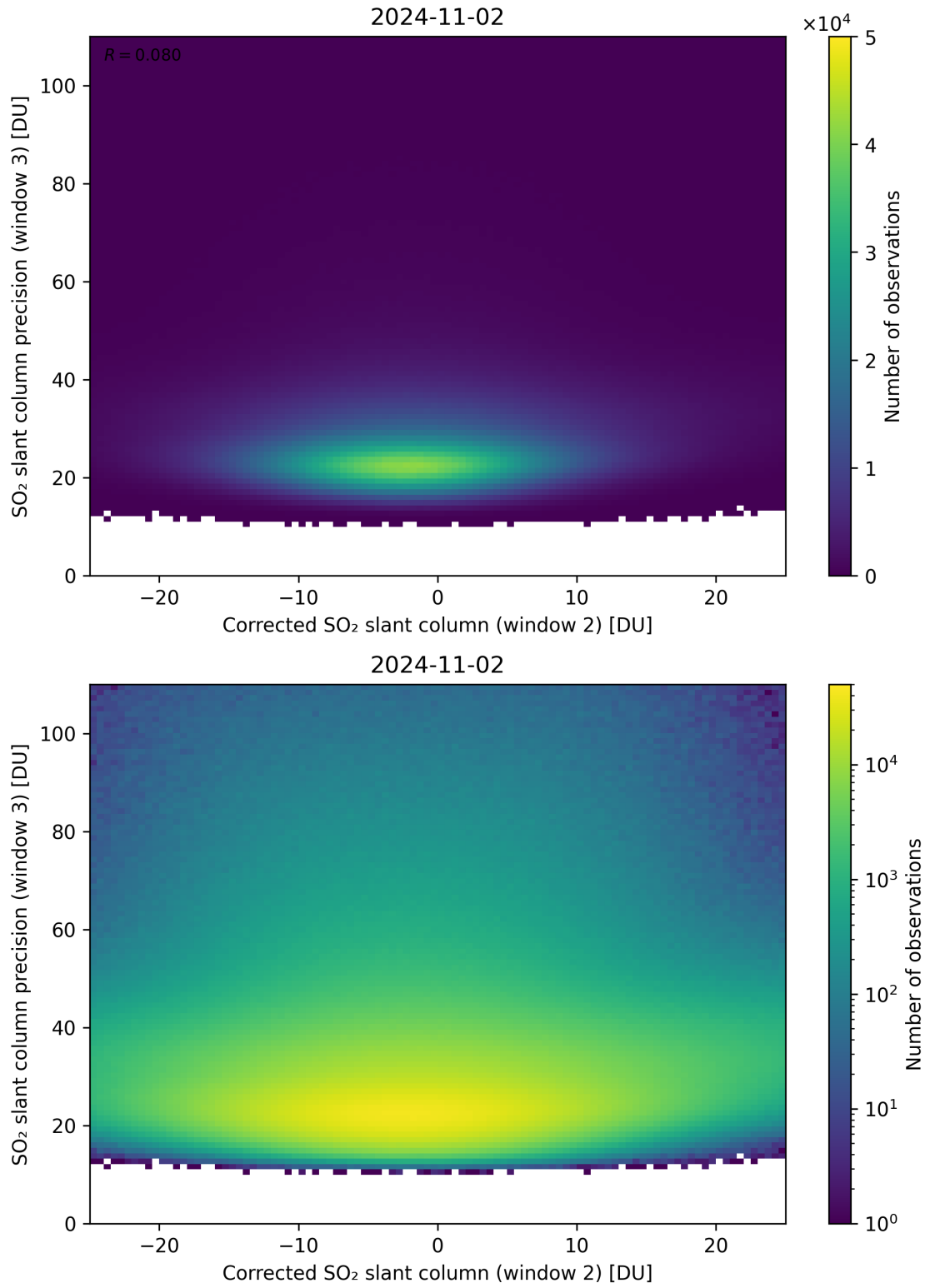
Figure 202: Scatter density plot of “Corrected SO 2 slant column (window 2)” against “SO 2 slant column precision (window 3)” for 2024-11-01 to 2024-11-03.
