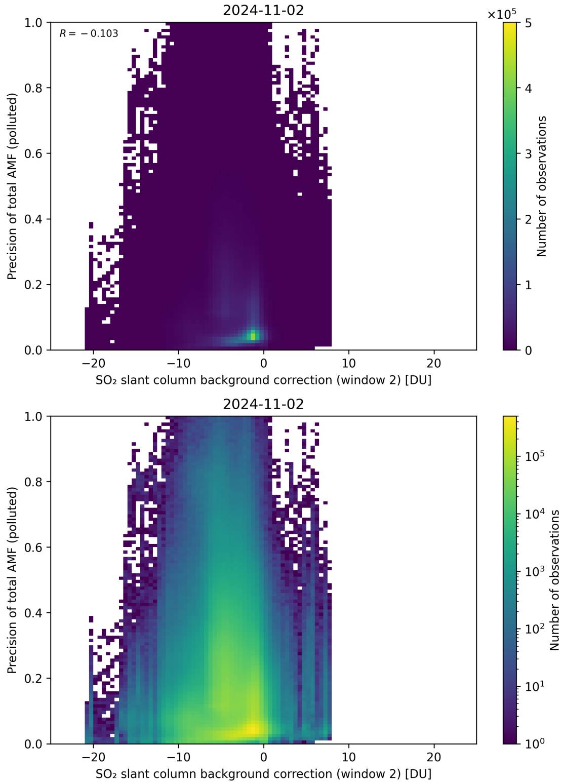
Figure 120: Scatter density plot of “SO 2 slant column background correction (window 2)” against “Precision of total AMF (polluted)” for 2024-11-01 to 2024-11-03.
