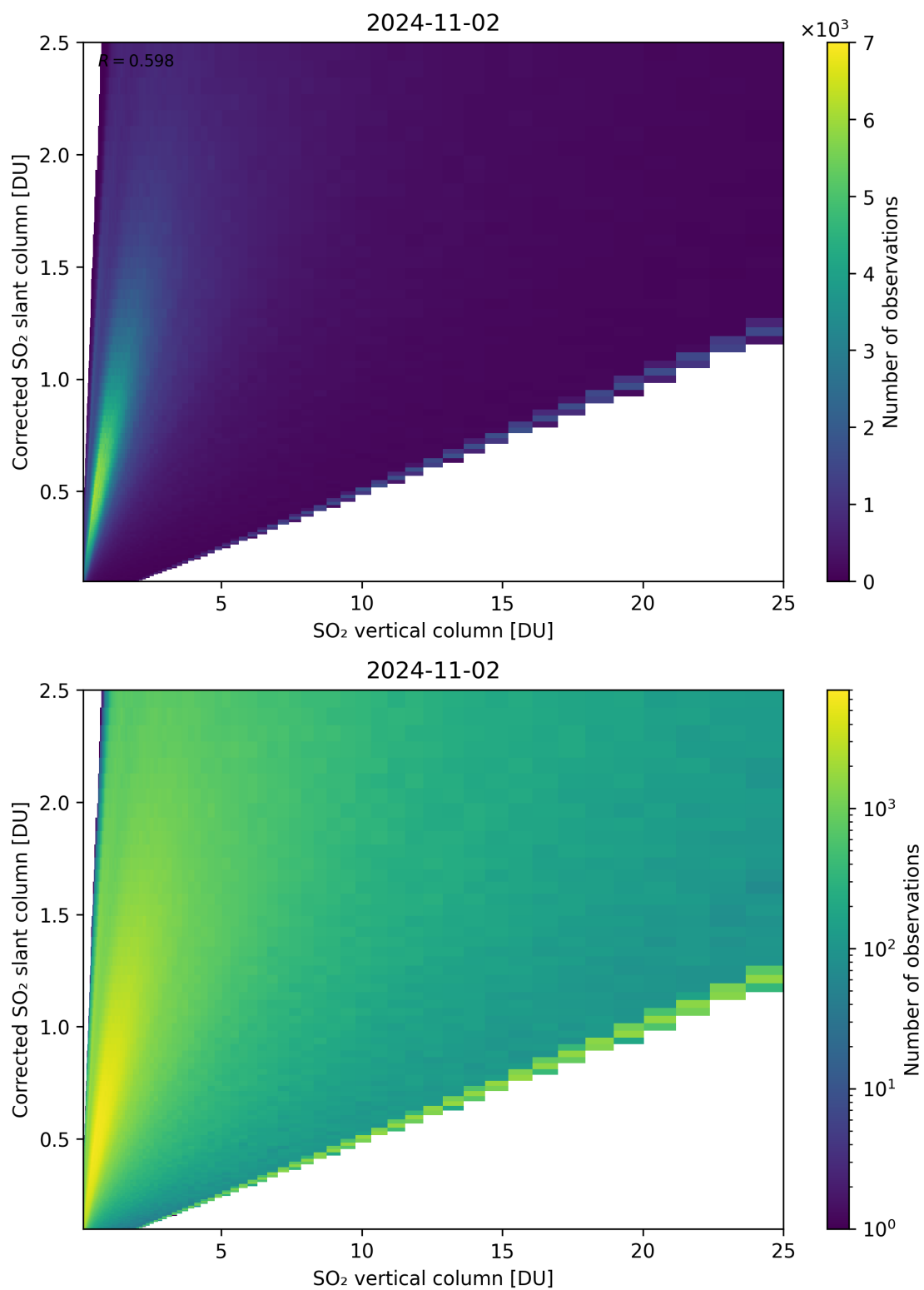
Figure 297: Scatter density plot of “SO 2 vertical column” against “Corrected SO 2 slant column” for 2024-11-01 to 2024-11-03.
