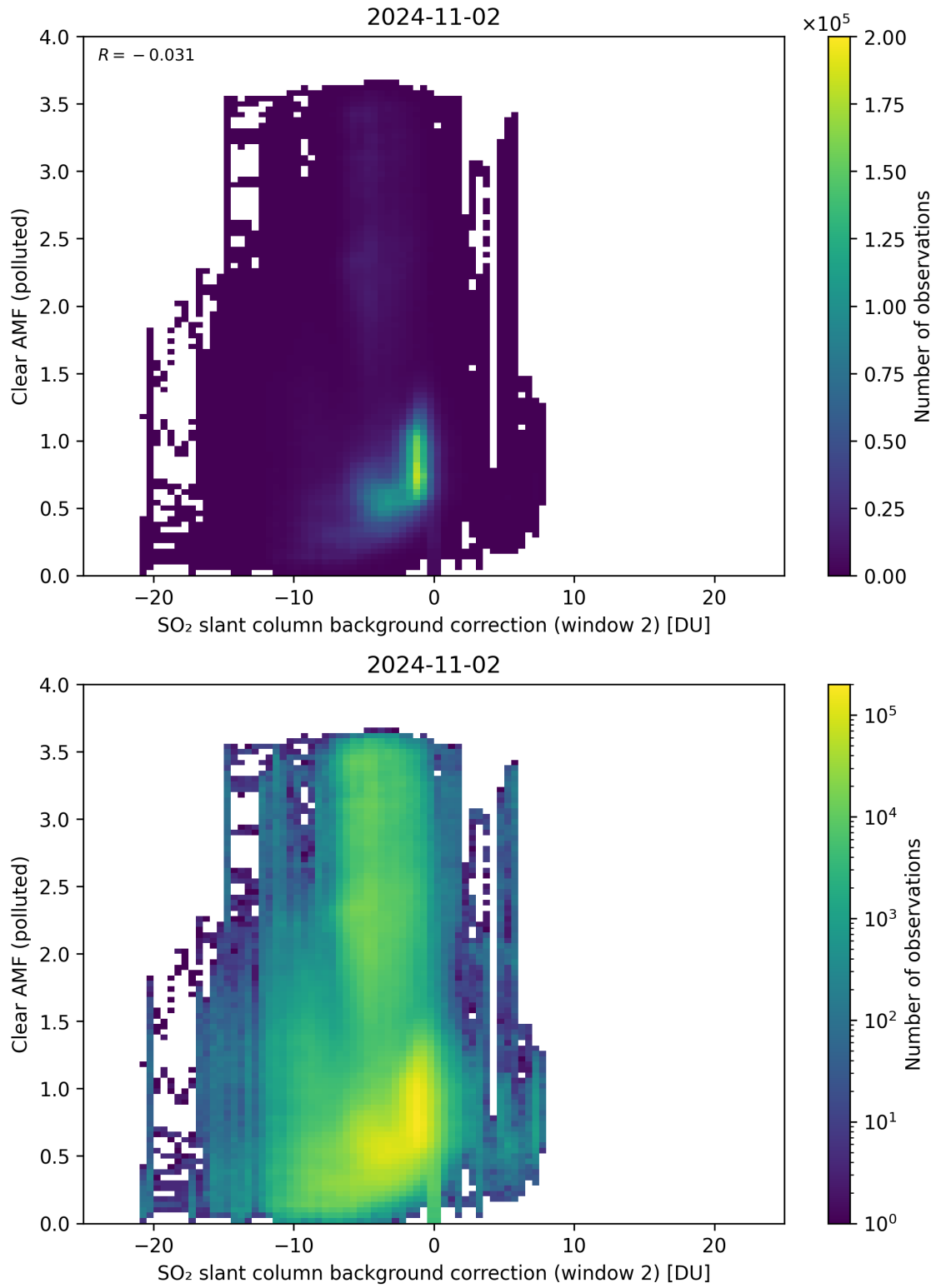
Figure 115: Scatter density plot of “SO 2 slant column background correction (window 2)” against “Clear AMF (polluted)” for 2024-11-01 to 2024-11-03.
