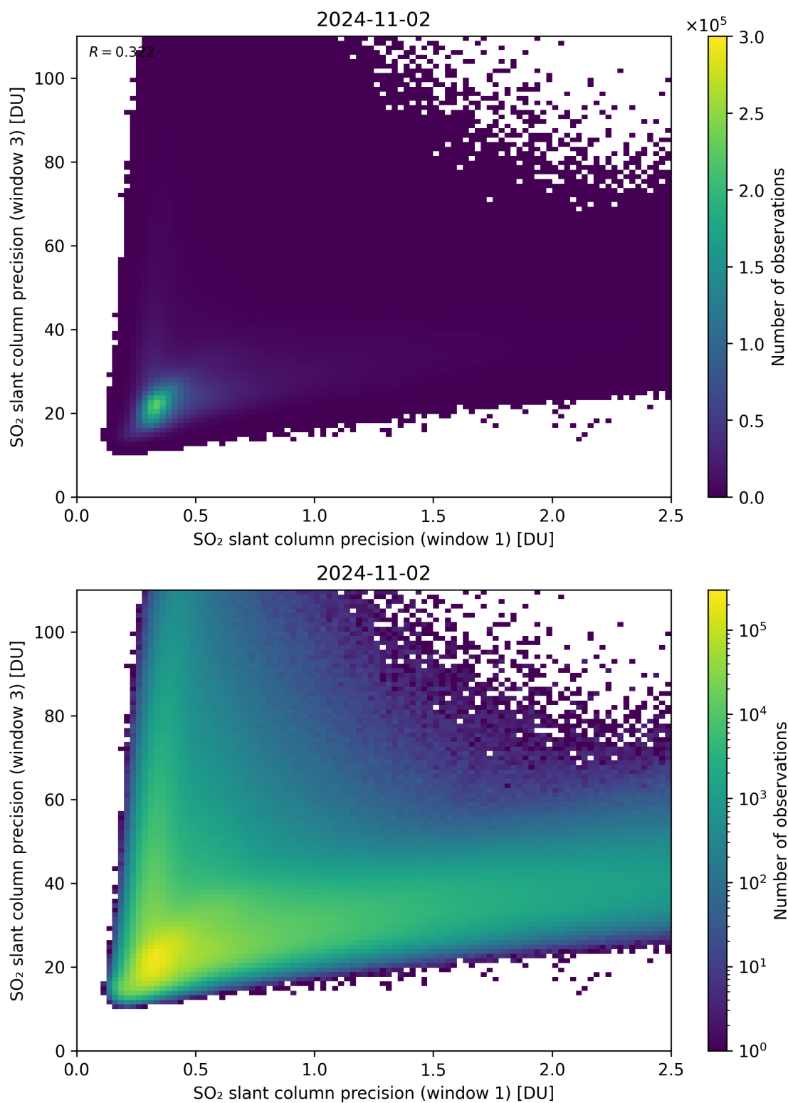
Figure 229: Scatter density plot of “SO 2 slant column precision (window 1)” against “SO 2 slant column precision (window 3)” for 2024-11-01 to 2024-11-03.
