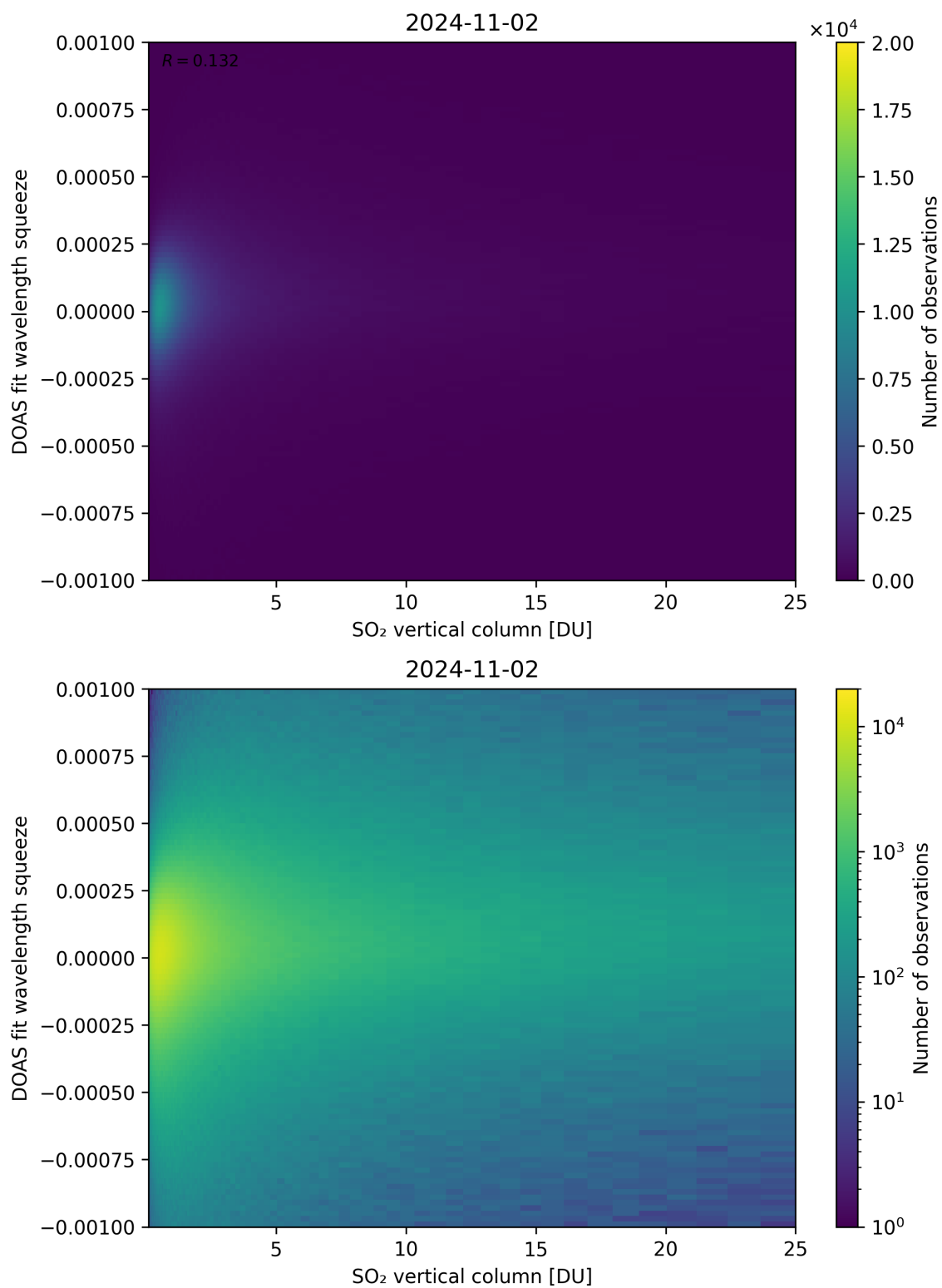
Figure 277: Scatter density plot of “SO 2 vertical column” against “DOAS fit wavelength squeeze” for 2024-11-01 to 2024-11-03.
