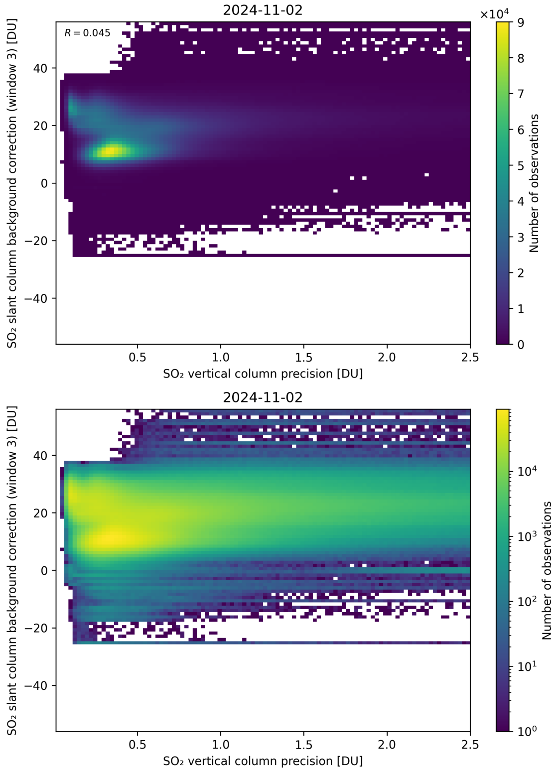
Figure 281: Scatter density plot of “SO 2 vertical column precision” against “SO 2 slant column background correction (window 3)” for 2024-11-01 to 2024-11-03.
