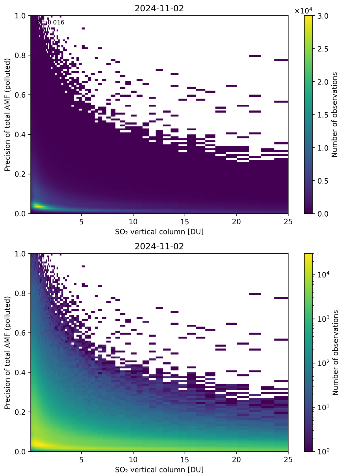
Figure 306: Scatter density plot of “SO 2 vertical column” against “Precision of total AMF (polluted)” for 2024-11-01 to 2024-11-03.
