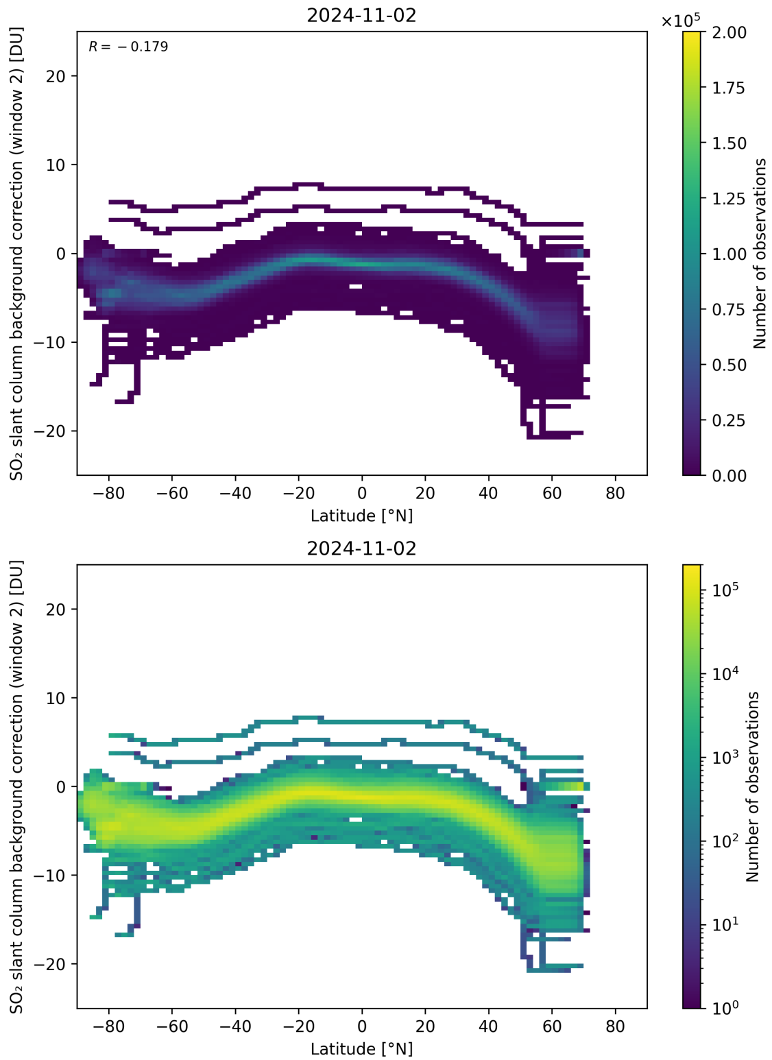
Figure 140: Scatter density plot of “Latitude” against “SO 2 slant column background correction (window 2)” for 2024-11-01 to 2024-11-03.
