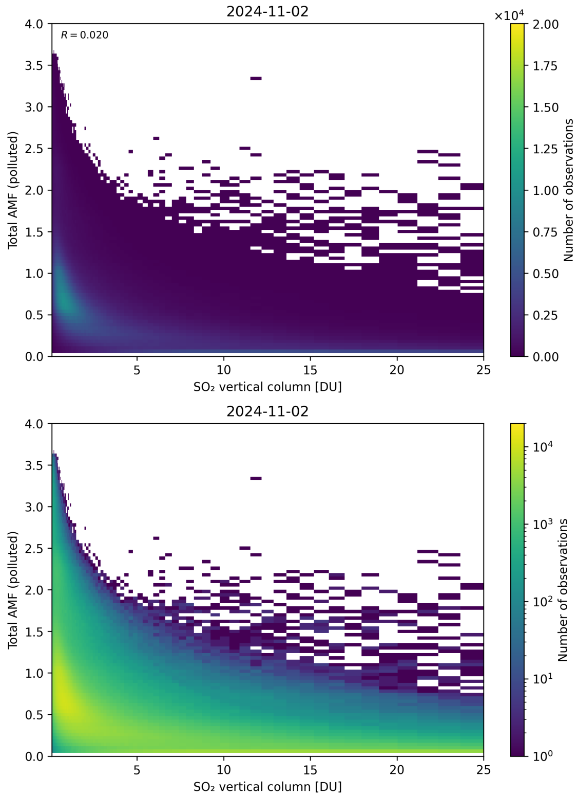
Figure 305: Scatter density plot of “SO 2 vertical column” against “Total AMF (polluted)” for 2024-11-01 to 2024-11-03.
