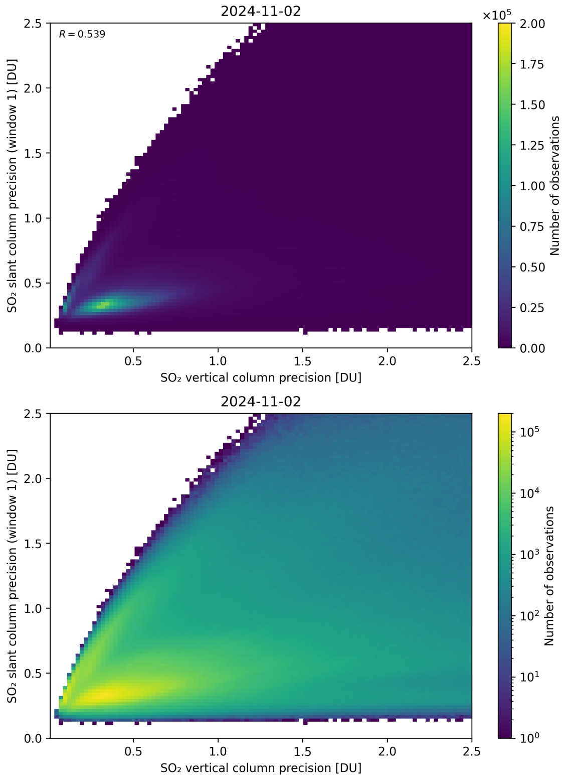
Figure 290: Scatter density plot of “SO 2 vertical column precision” against “SO 2 slant column precision (window 1)” for 2024-11-01 to 2024-11-03.
