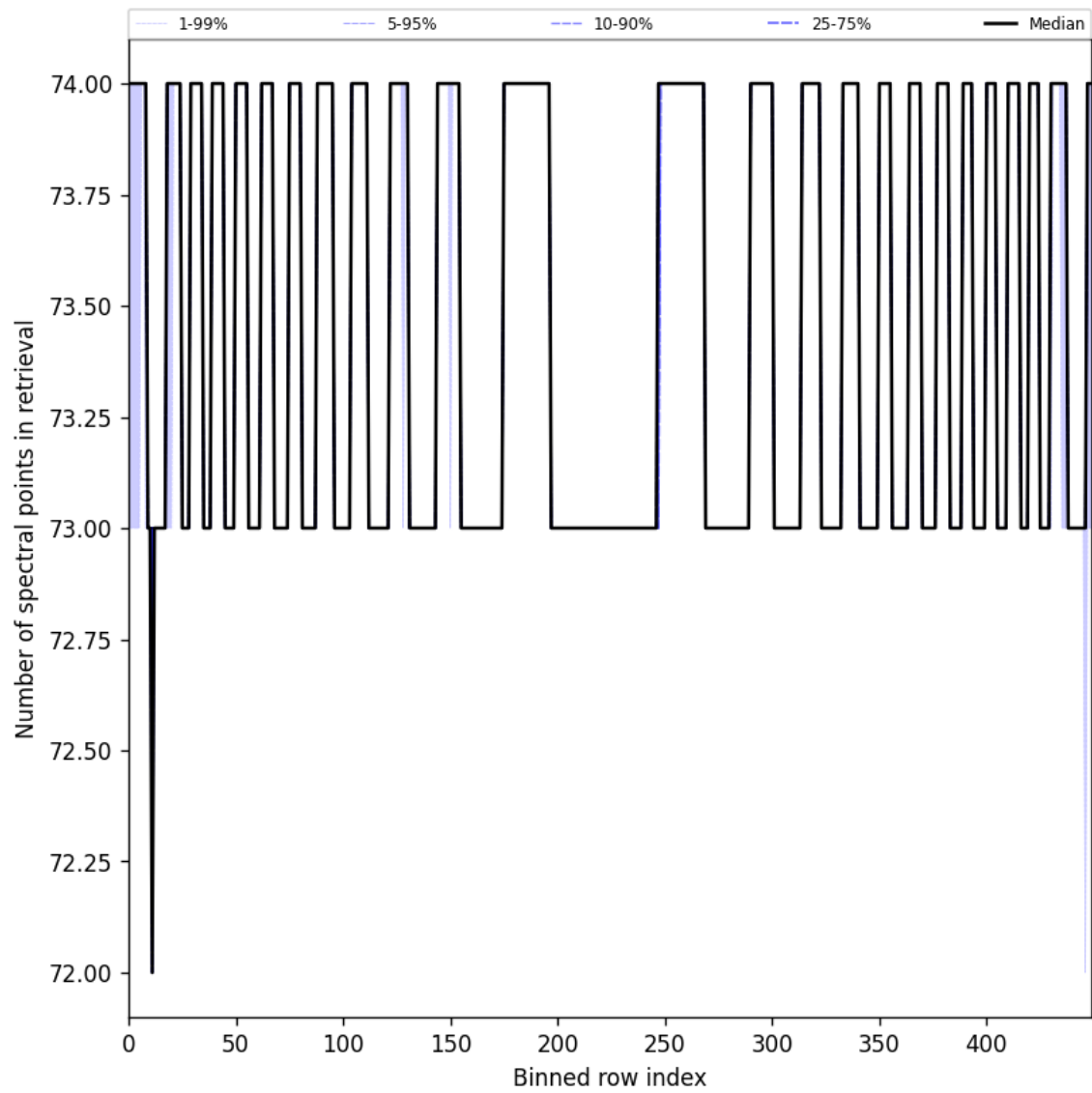
Figure 97: Along track statistics of “Number of spectral points in retrieval” for 2024-11-01 to 2024-11-03
