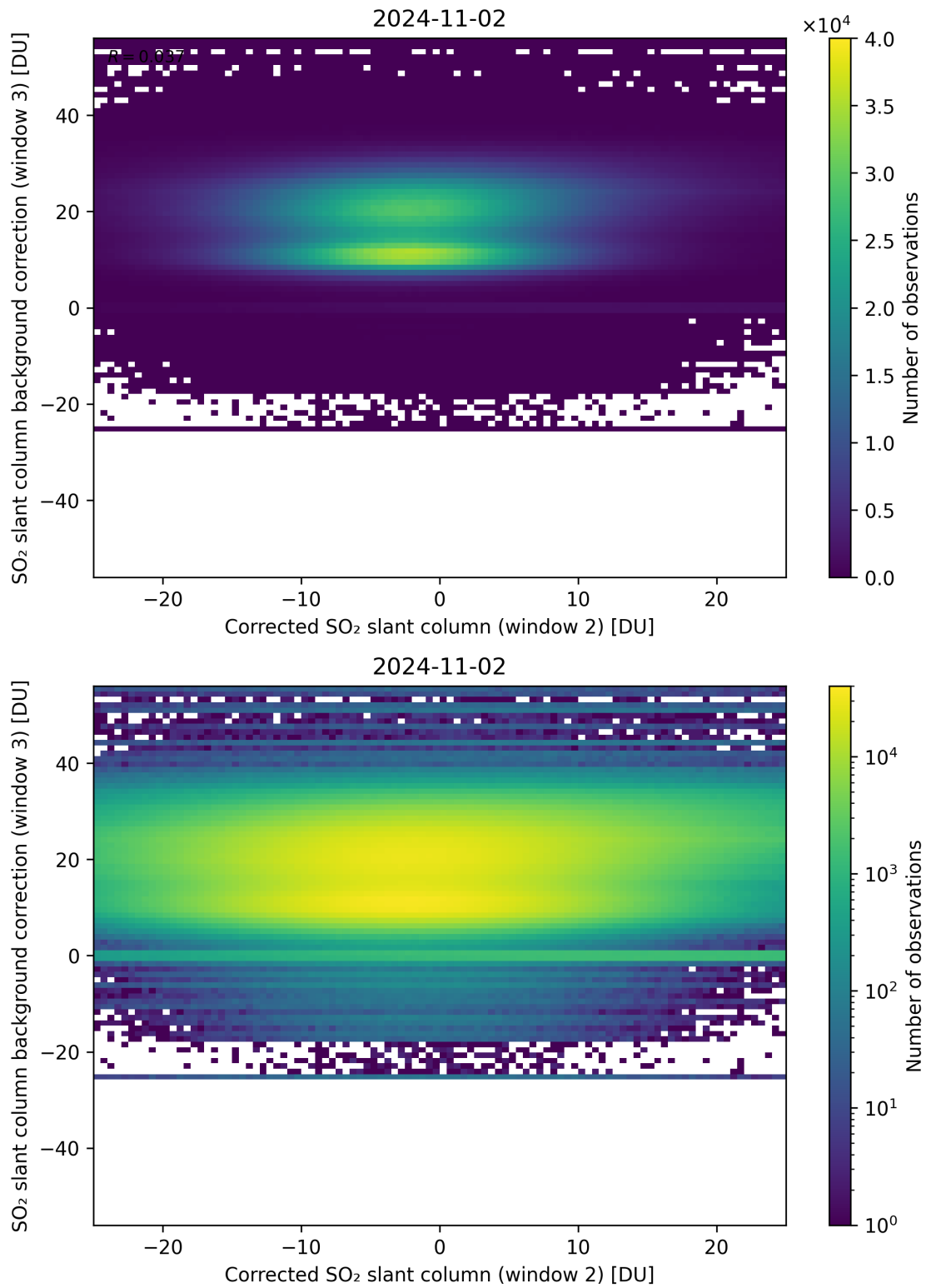
Figure 195: Scatter density plot of “Corrected SO 2 slant column (window 2)” against “SO 2 slant column background correction (window 3)” for 2024-11-01 to 2024-11-03.
