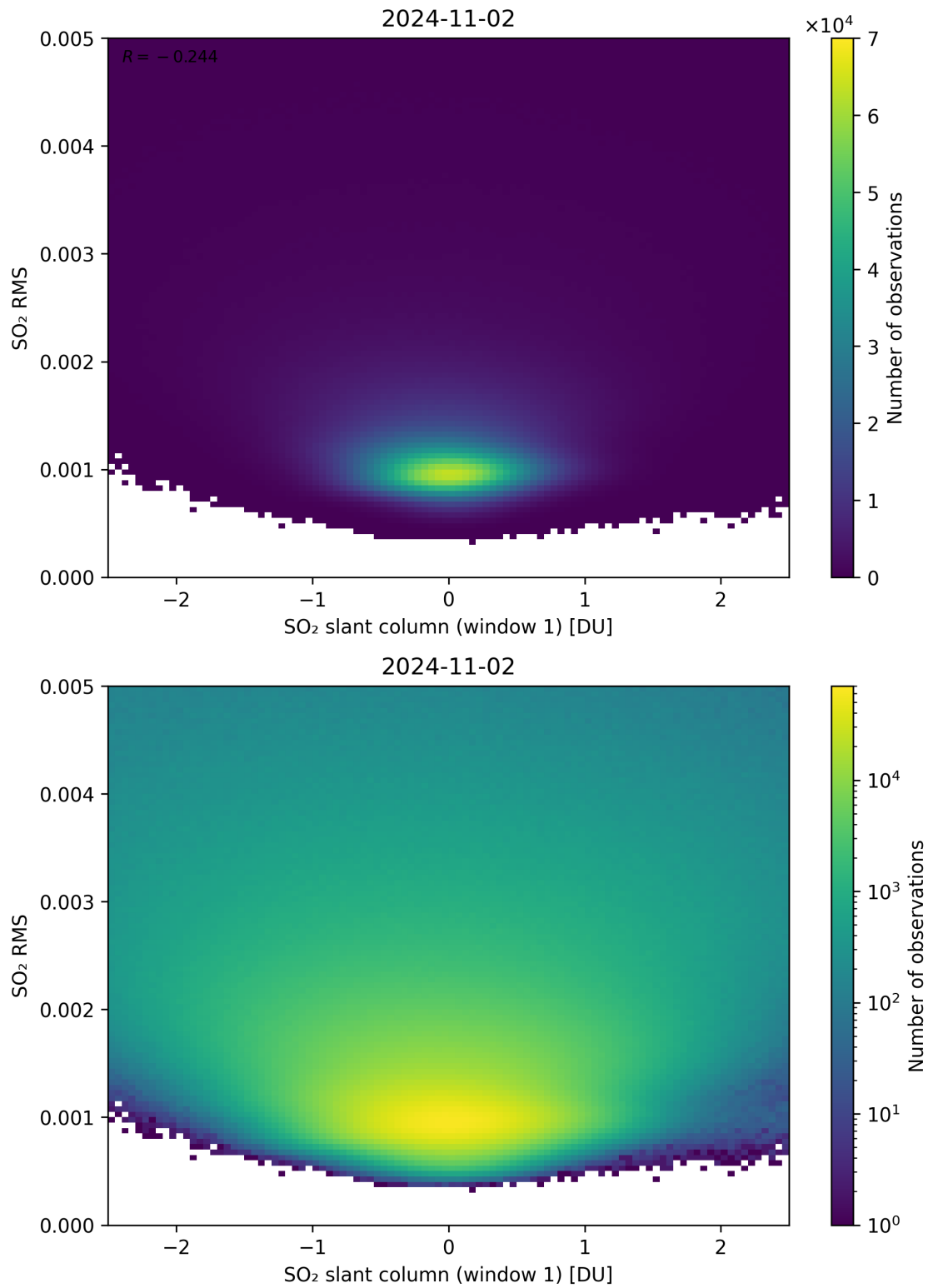
Figure 217: Scatter density plot of “SO 2 slant column (window 1)” against “SO 2 RMS” for 2024-11-01 to 2024-11-03.
