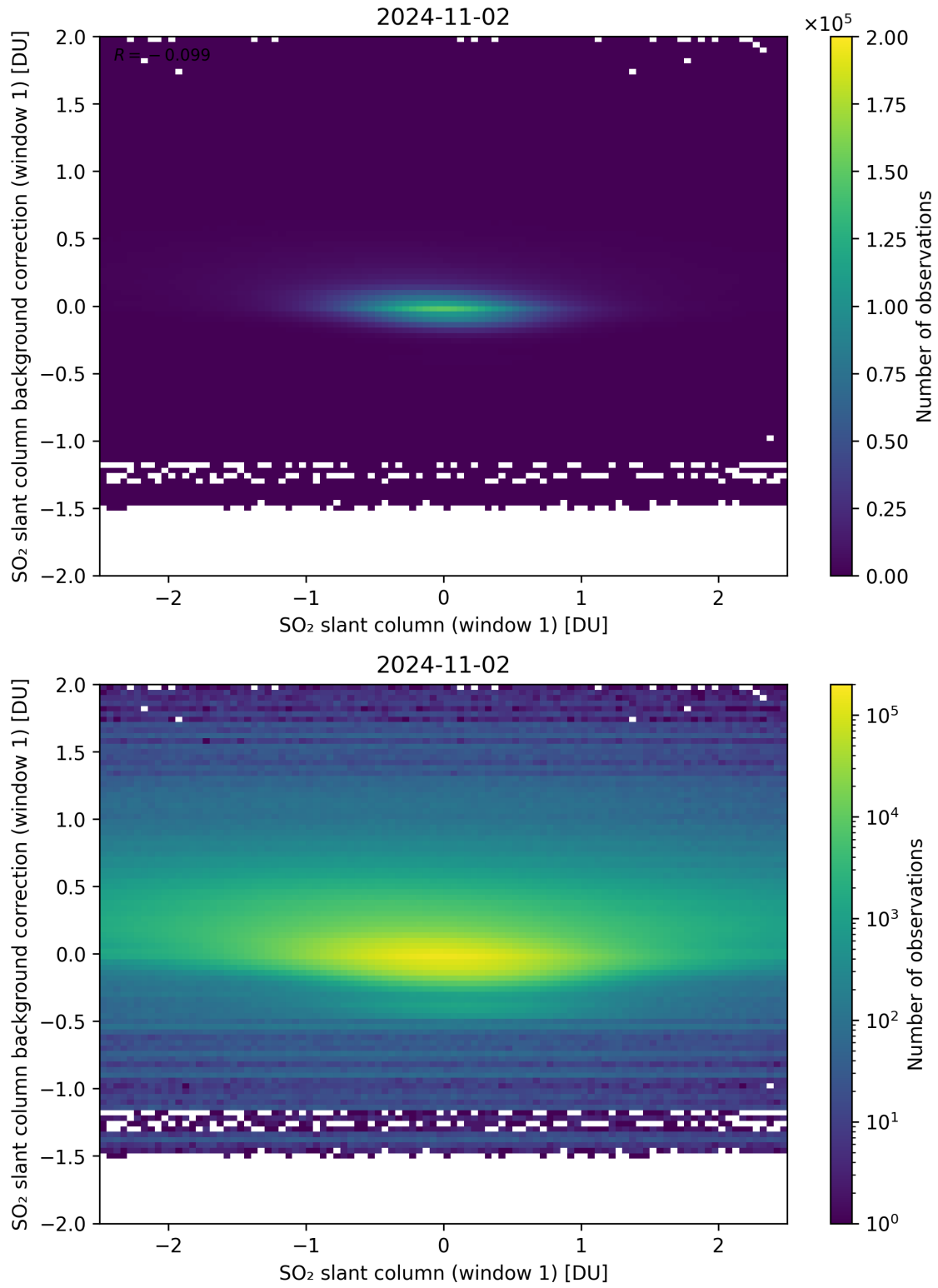
Figure 212: Scatter density plot of “SO 2 slant column (window 1)” against “SO 2 slant column background correction (window 1)” for 2024-11-01 to 2024-11-03.
