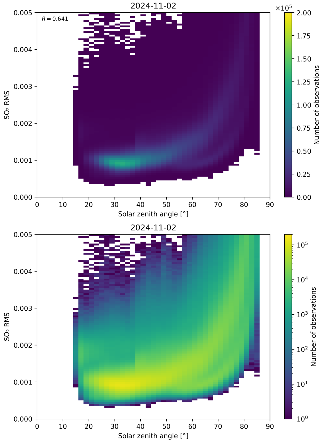
Figure 163: Scatter density plot of “Solar zenith angle” against “SO 2 RMS” for 2024-11-01 to 2024-11-03.
