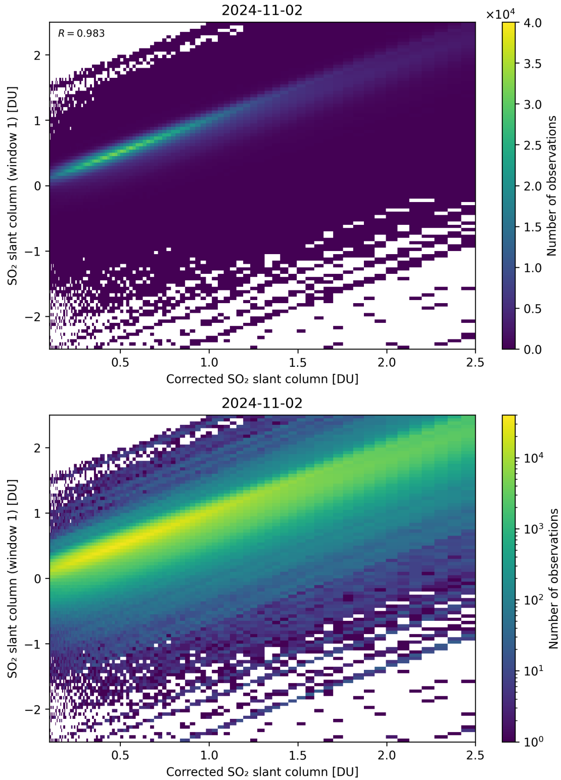
Figure 187: Scatter density plot of “Corrected SO 2 slant column” against “SO 2 slant column (window 1)” for 2024-11-01 to 2024-11-03.
