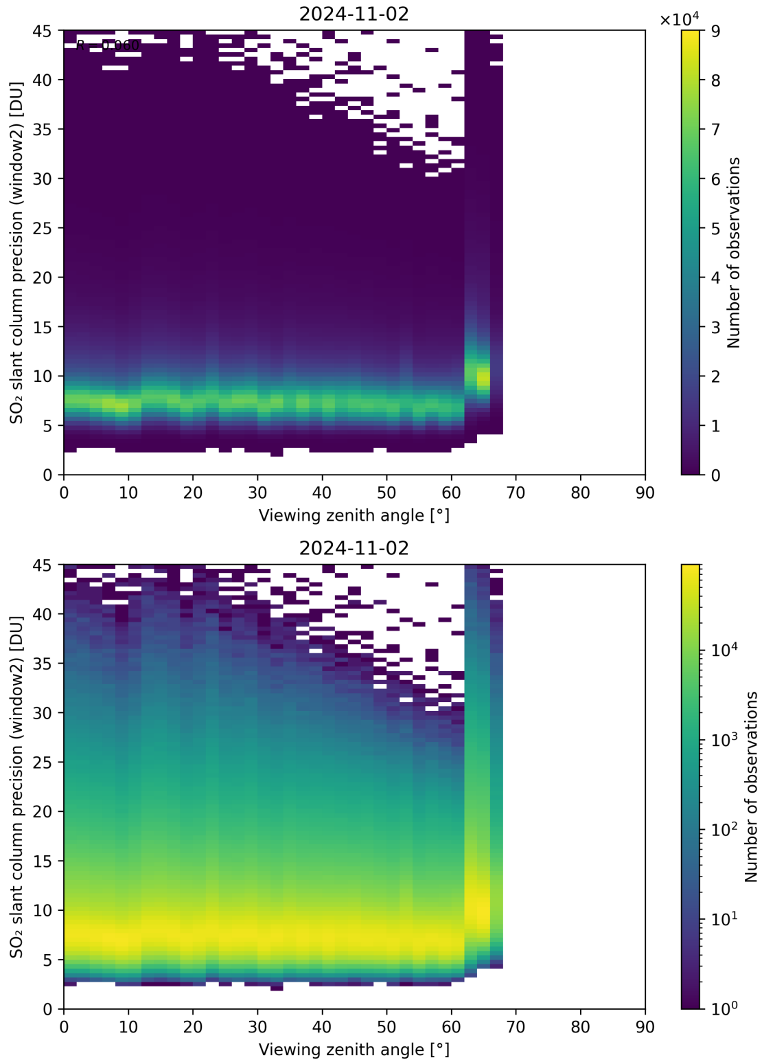
Figure 322: Scatter density plot of “Viewing zenith angle” against “SO 2 slant column precision (window2)” for 2024-11-01 to 2024-11-03.
