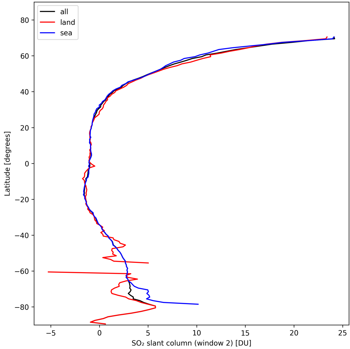
Figure 37: Zonal average of “SO 2 slant column (window 2)” for 2024-11-01 to 2024-11-03.
