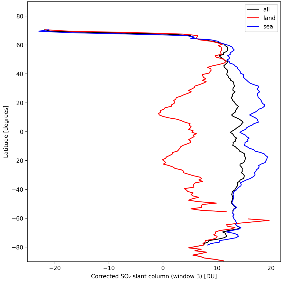
Figure 43: Zonal average of “Corrected SO 2 slant column (window 3)” for 2024-11-01 to 2024-11-03.
