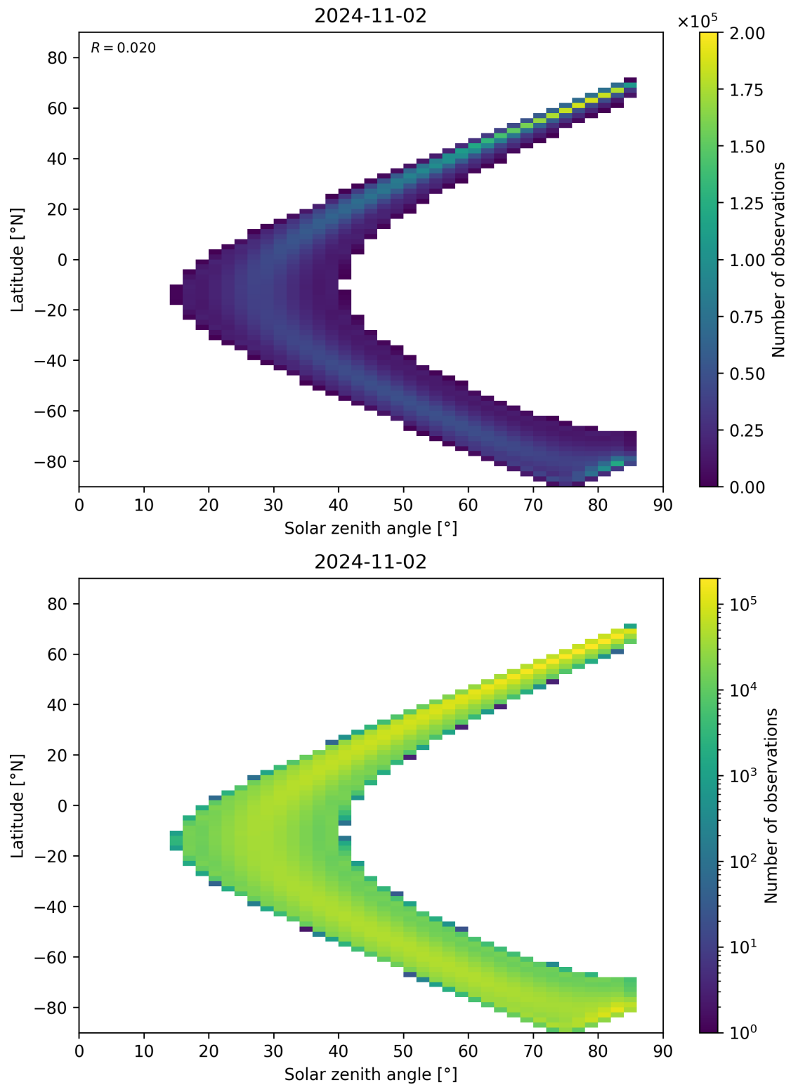
Figure 164: Scatter density plot of “Solar zenith angle” against “Latitude” for 2024-11-01 to 2024-11-03.
