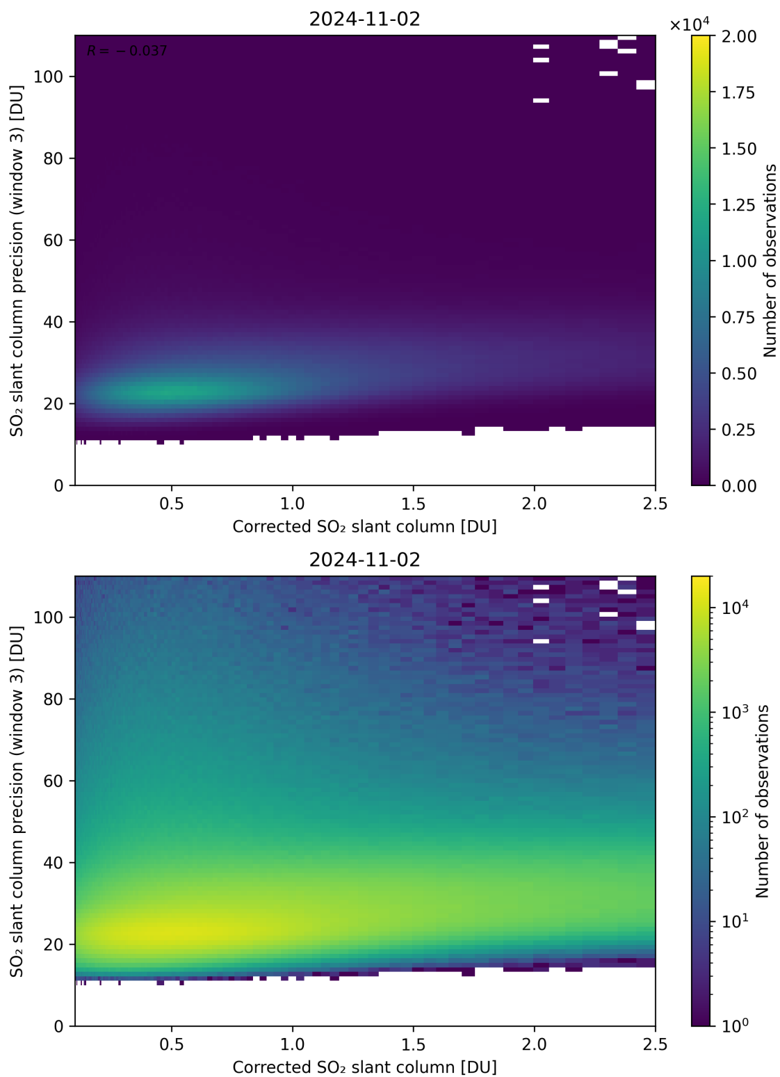
Figure 191: Scatter density plot of “Corrected SO 2 slant column” against “SO 2 slant column precision (window 3)” for 2024-11-01 to 2024-11-03.
