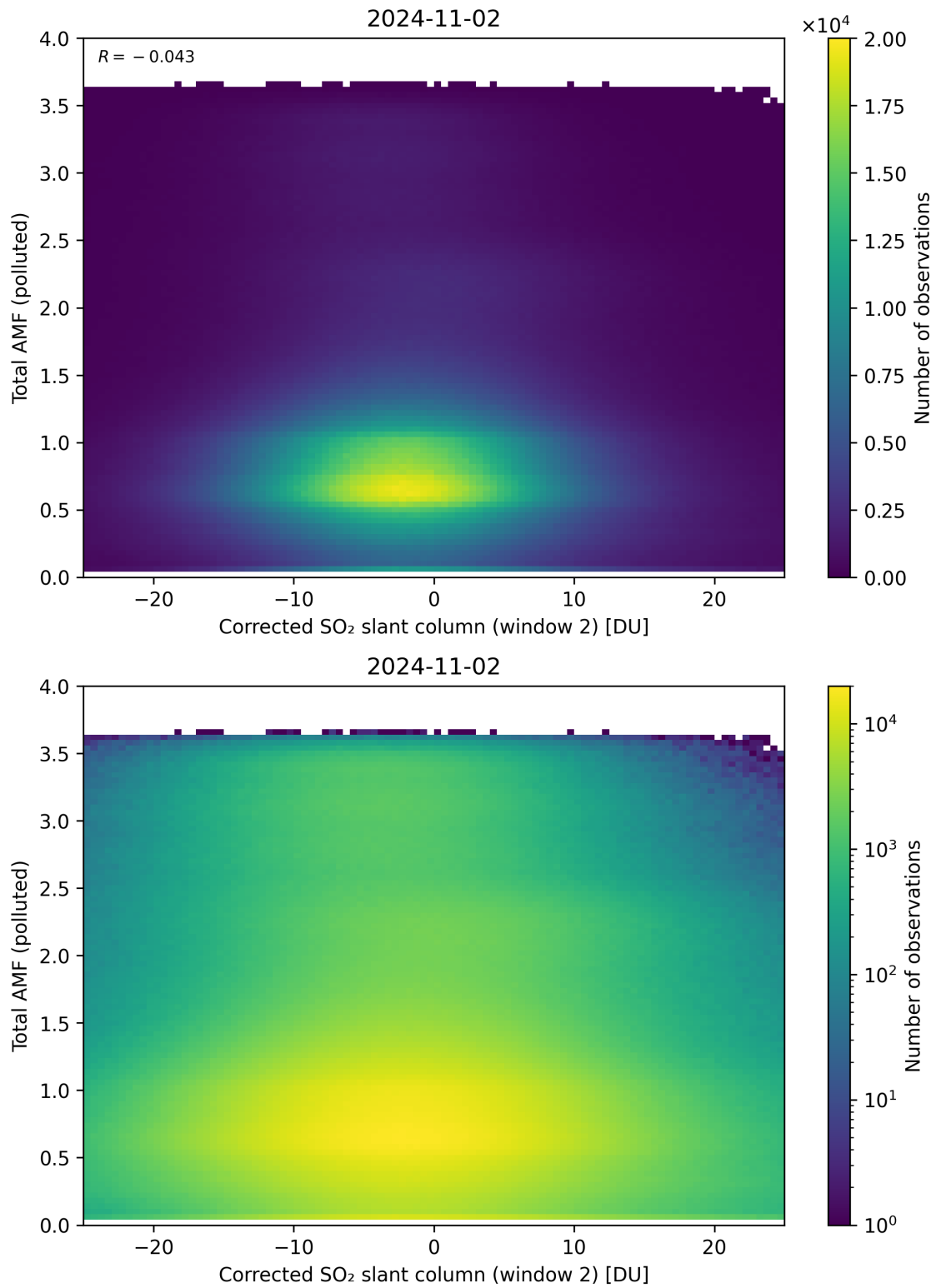
Figure 203: Scatter density plot of “Corrected SO 2 slant column (window 2)” against “Total AMF (polluted)” for 2024-11-01 to 2024-11-03.
