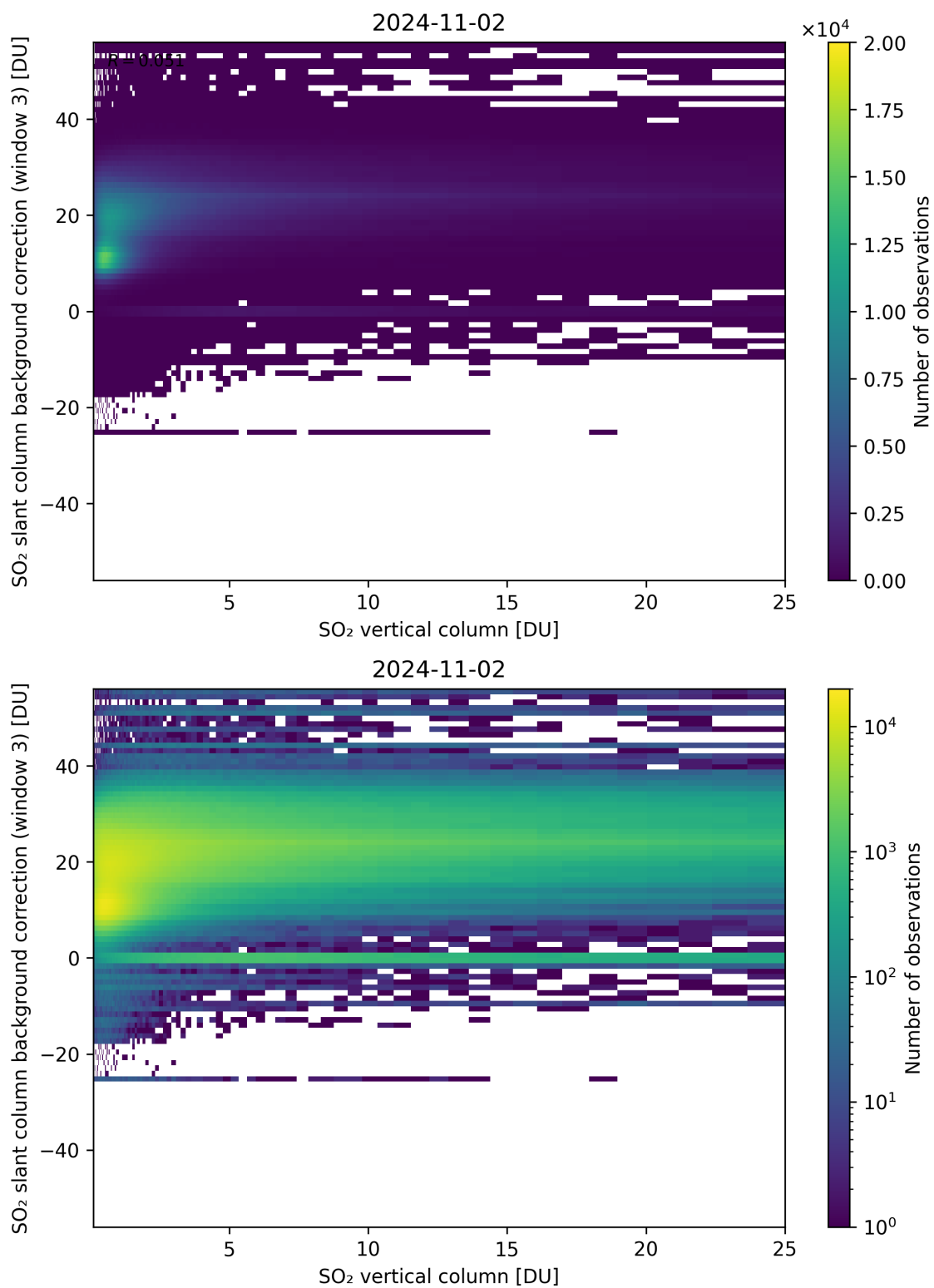
Figure 275: Scatter density plot of “SO 2 vertical column” against “SO 2 slant column background correction (window 3)” for 2024-11-01 to 2024-11-03.
