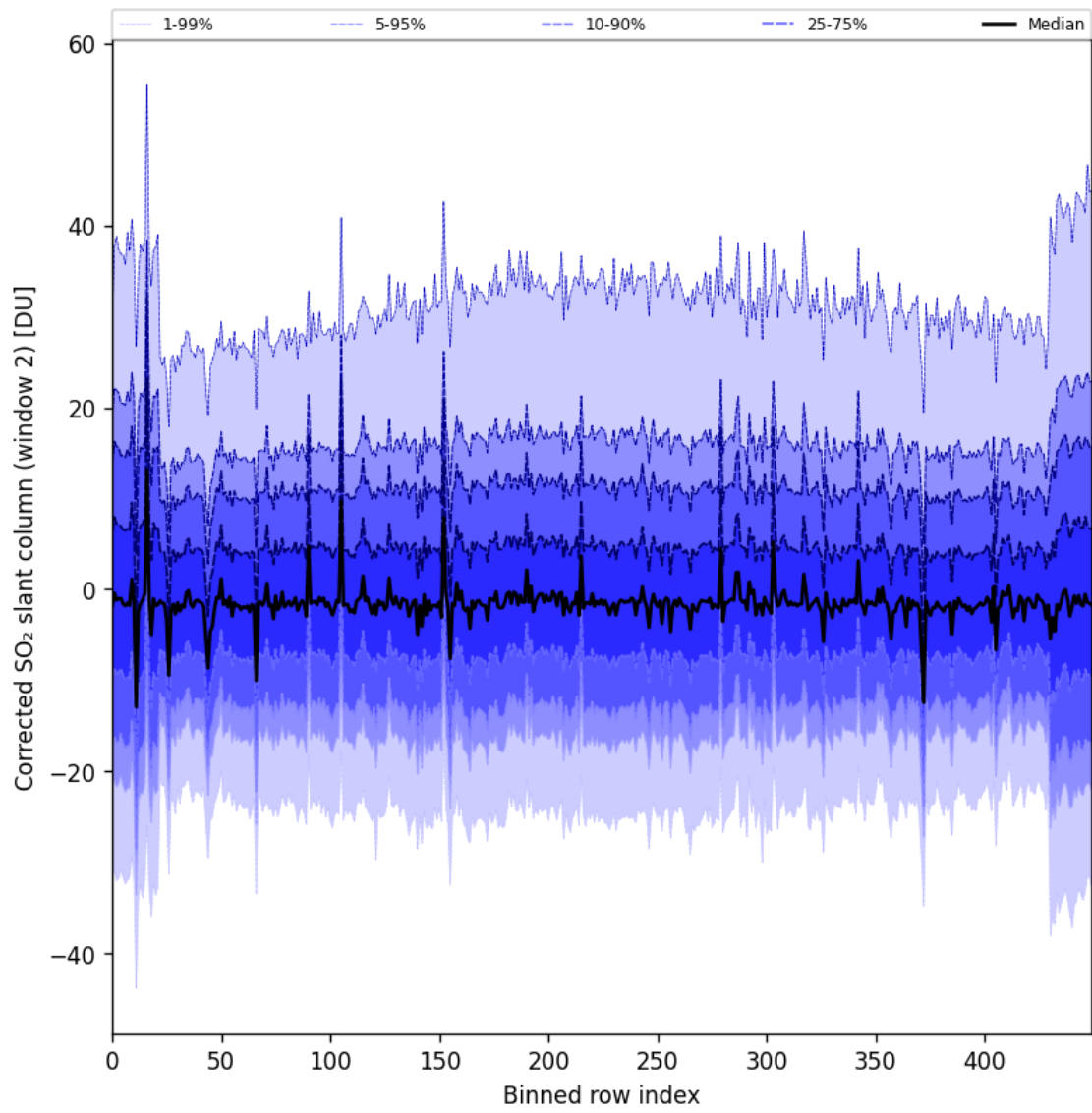
Figure 85: Along track statistics of “Corrected SO 2 slant column (window 2)” for 2024-11-01 to 2024-11-03
