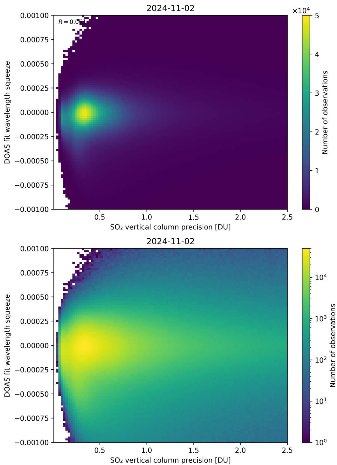
Figure 283: Scatter density plot of “SO 2 vertical column precision” against “DOAS fit wavelength squeeze” for 2024-11-01 to 2024-11-03.
