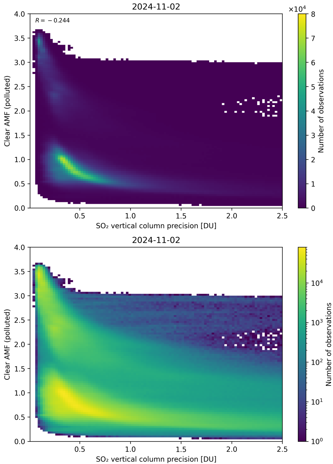
Figure 285: Scatter density plot of “SO 2 vertical column precision” against “Clear AMF (polluted)” for 2024-11-01 to 2024-11-03.
