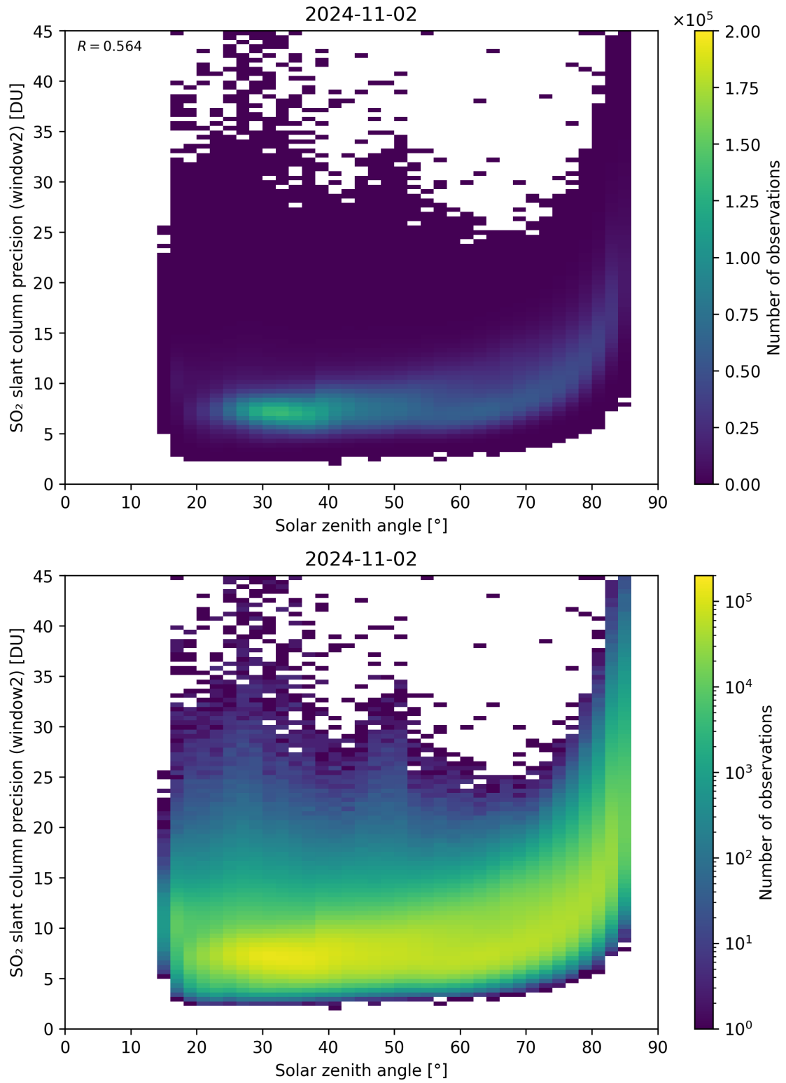
Figure 171: Scatter density plot of “Solar zenith angle” against “SO 2 slant column precision (window2)” for 2024-11-01 to 2024-11-03.
