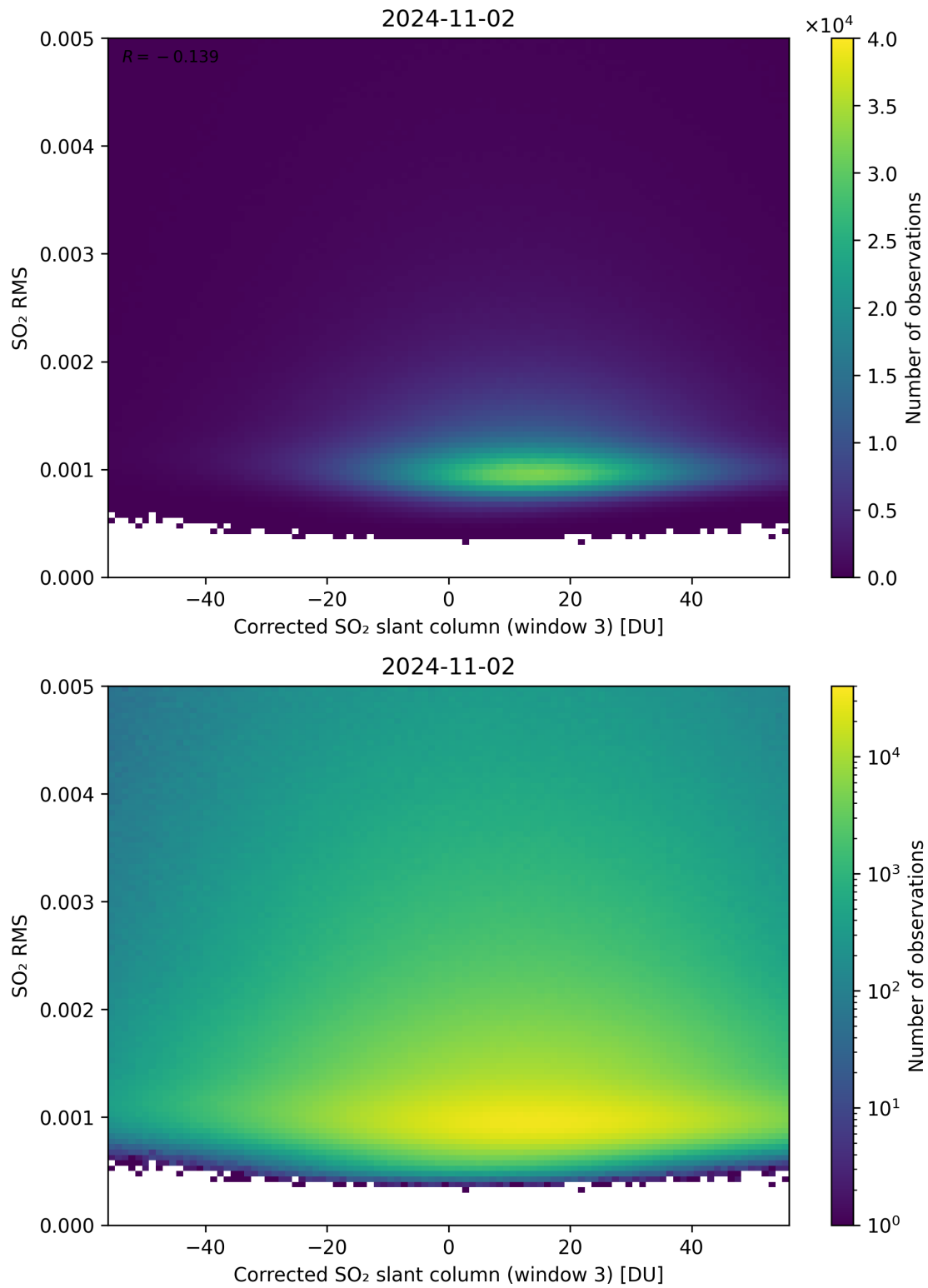
Figure 208: Scatter density plot of “Corrected SO 2 slant column (window 3)” against “SO 2 RMS” for 2024-11-01 to 2024-11-03.
