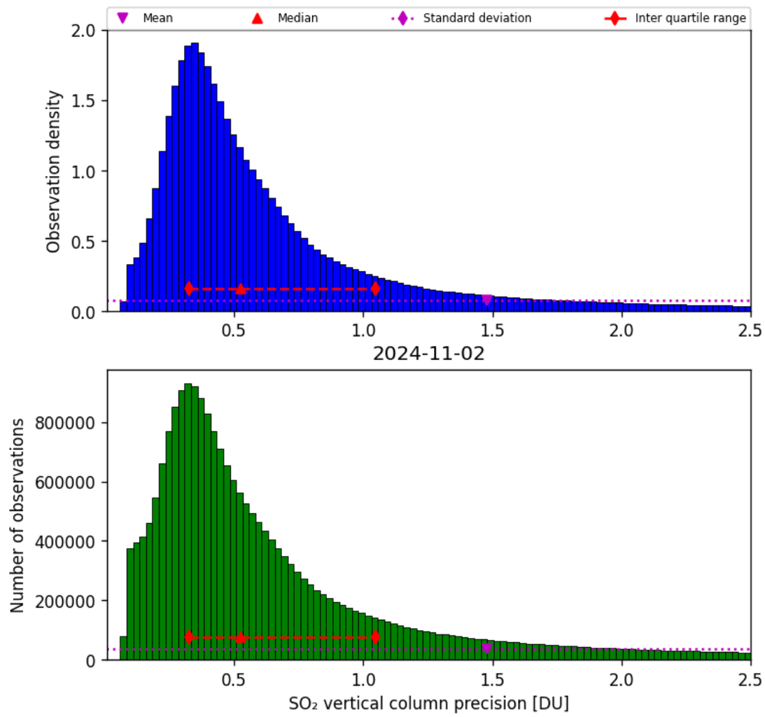
Figure 54: Histogram of “SO 2 vertical column precision” for 2024-11-01 to 2024-11-03
