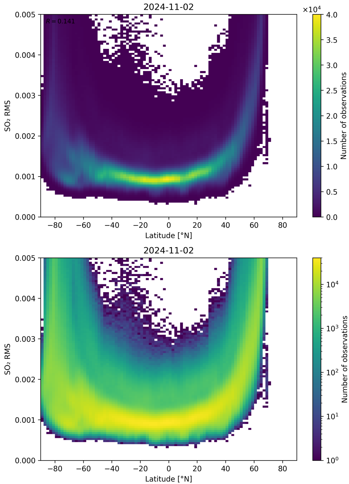
Figure 144: Scatter density plot of “Latitude” against “SO 2 RMS” for 2024-11-01 to 2024-11-03.
