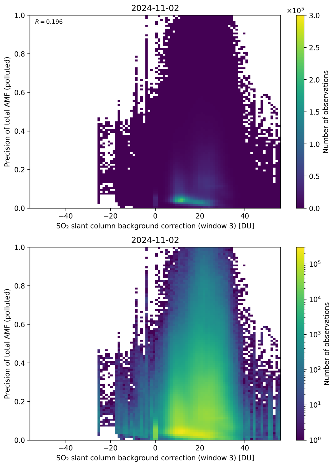
Figure 126: Scatter density plot of “SO 2 slant column background correction (window 3)” against “Precision of total AMF (polluted)” for 2024-11-01 to 2024-11-03.
