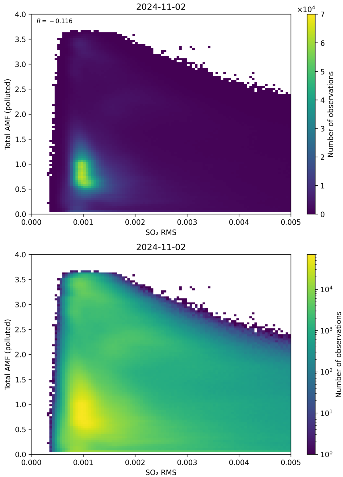
Figure 137: Scatter density plot of “SO 2 RMS” against “Total AMF (polluted)” for 2024-11-01 to 2024-11-03.
