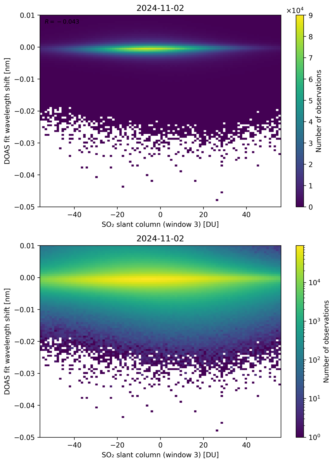
Figure 254: Scatter density plot of “SO 2 slant column (window 3)” against “DOAS fit wavelength shift” for 2024-11-01 to 2024-11-03.
