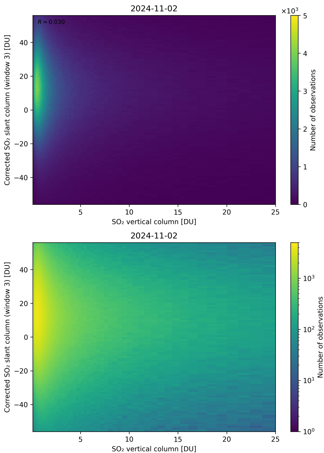
Figure 299: Scatter density plot of “SO 2 vertical column” against “Corrected SO 2 slant column (window 3)” for 2024-11-01 to 2024-11-03.
