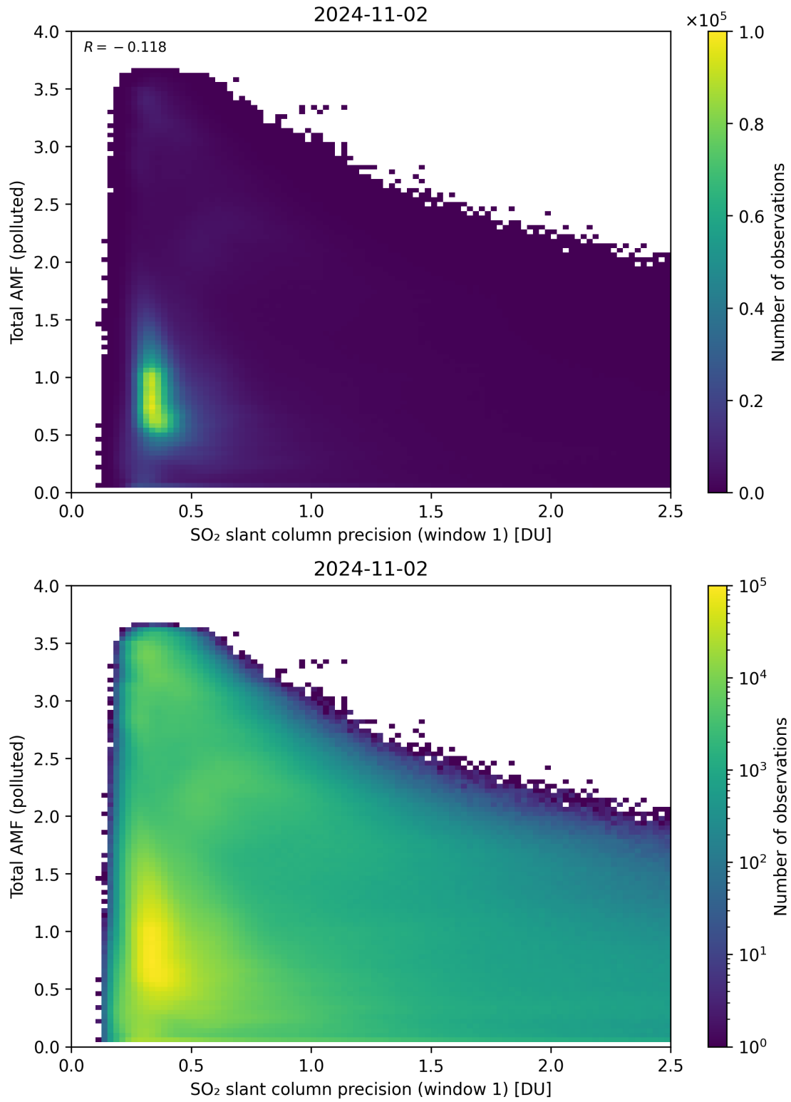
Figure 230: Scatter density plot of “SO 2 slant column precision (window 1)” against “Total AMF (polluted)” for 2024-11-01 to 2024-11-03.
