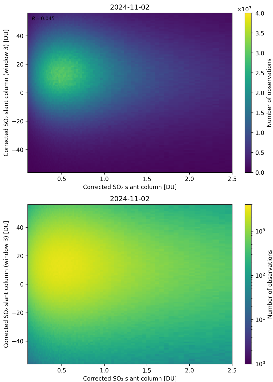
Figure 186: Scatter density plot of “Corrected SO 2 slant column” against “Corrected SO 2 slant column (window 3)” for 2024-11-01 to 2024-11-03.
