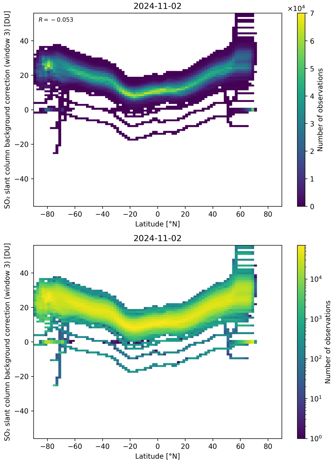
Figure 141: Scatter density plot of “Latitude” against “SO 2 slant column background correction (window 3)” for 2024-11-01 to 2024-11-03.
