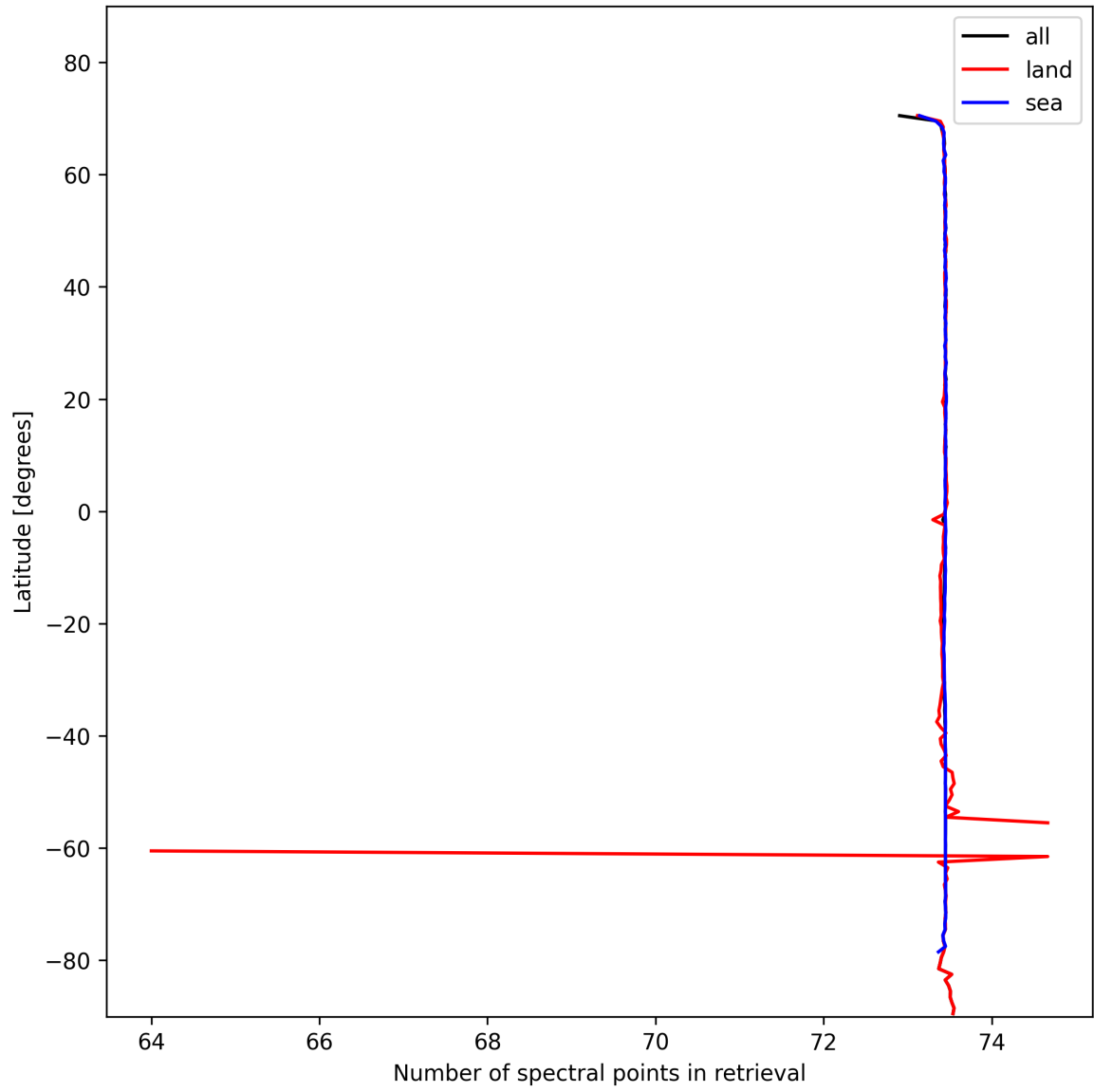
Figure 51: Zonal average of “Number of spectral points in retrieval” for 2024-11-01 to 2024-11-03.
