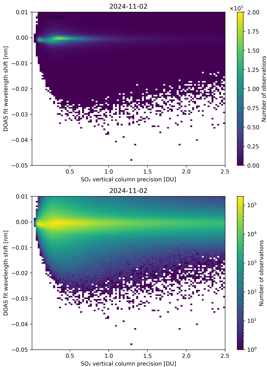
Figure 282: Scatter density plot of “SO 2 vertical column precision” against “DOAS fit wavelength shift” for 2024-11-01 to 2024-11-03.
