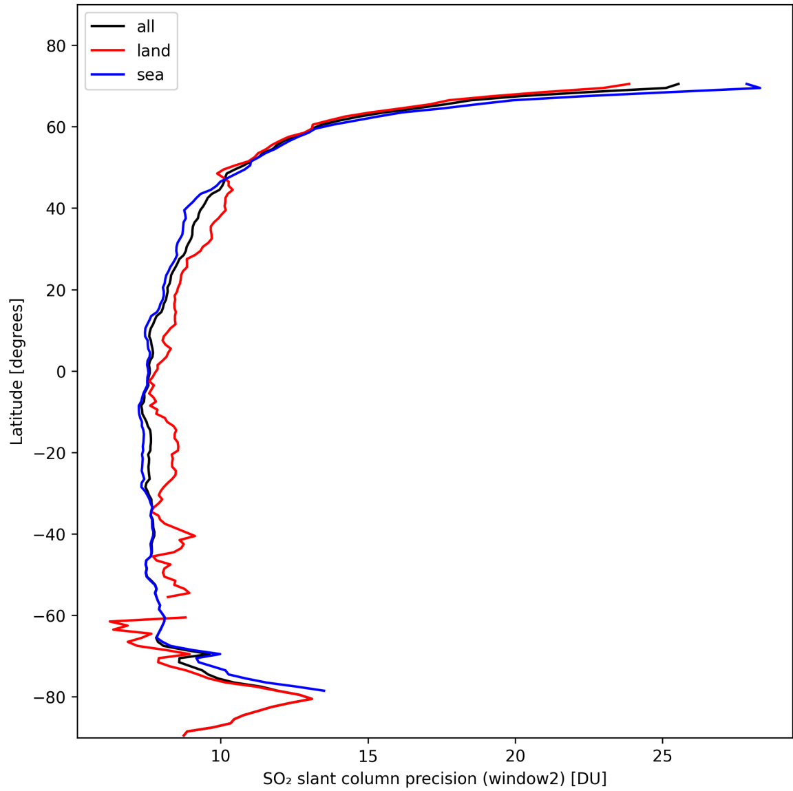
Figure 38: Zonal average of “SO 2 slant column precision (window2)” for 2024-11-01 to 2024-11-03.
