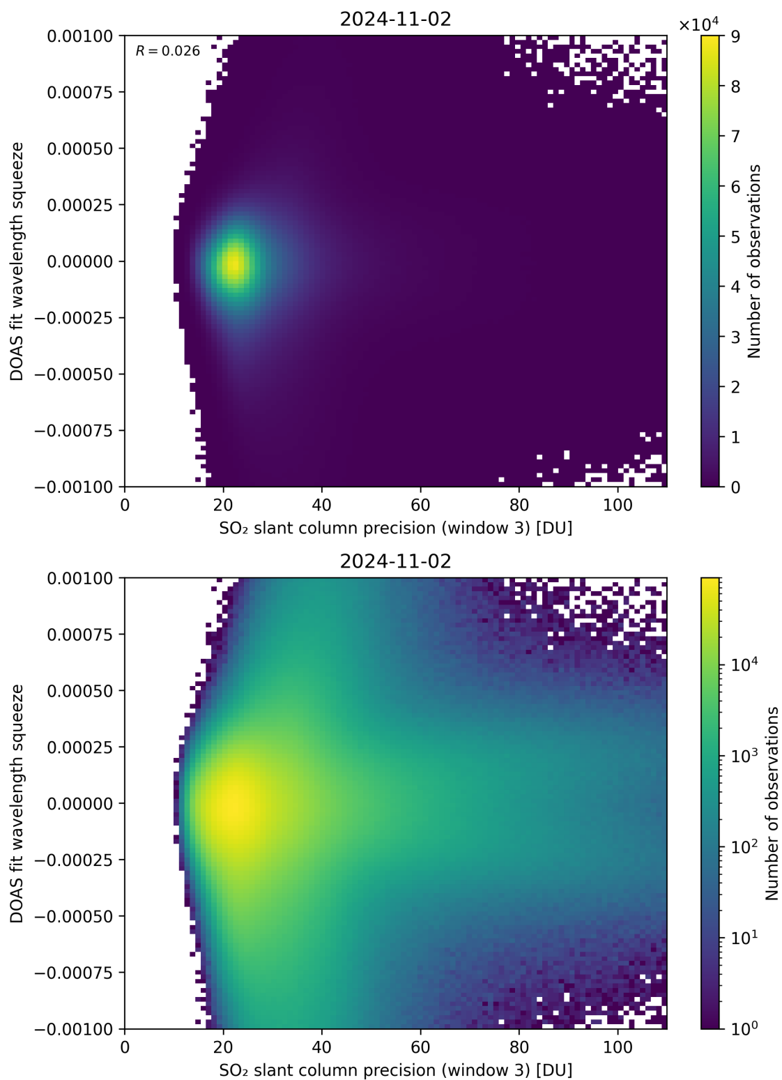
Figure 259: Scatter density plot of “SO 2 slant column precision (window 3)” against “DOAS fit wavelength squeeze” for 2024-11-01 to 2024-11-03.
