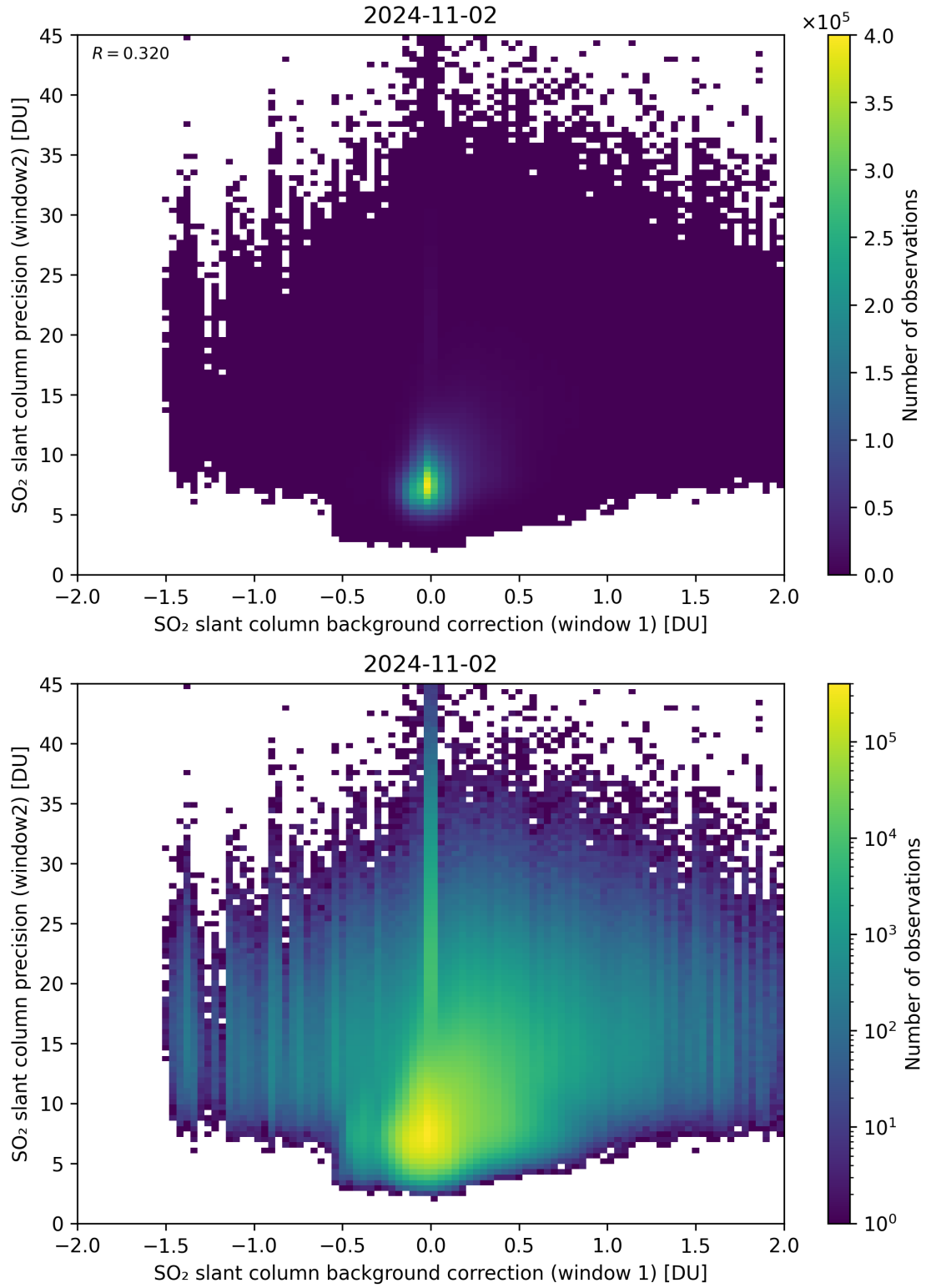
Figure 106: Scatter density plot of “SO 2 slant column background correction (window 1)” against “SO 2 slant column precision (window2)” for 2024-11-01 to 2024-11-03.
