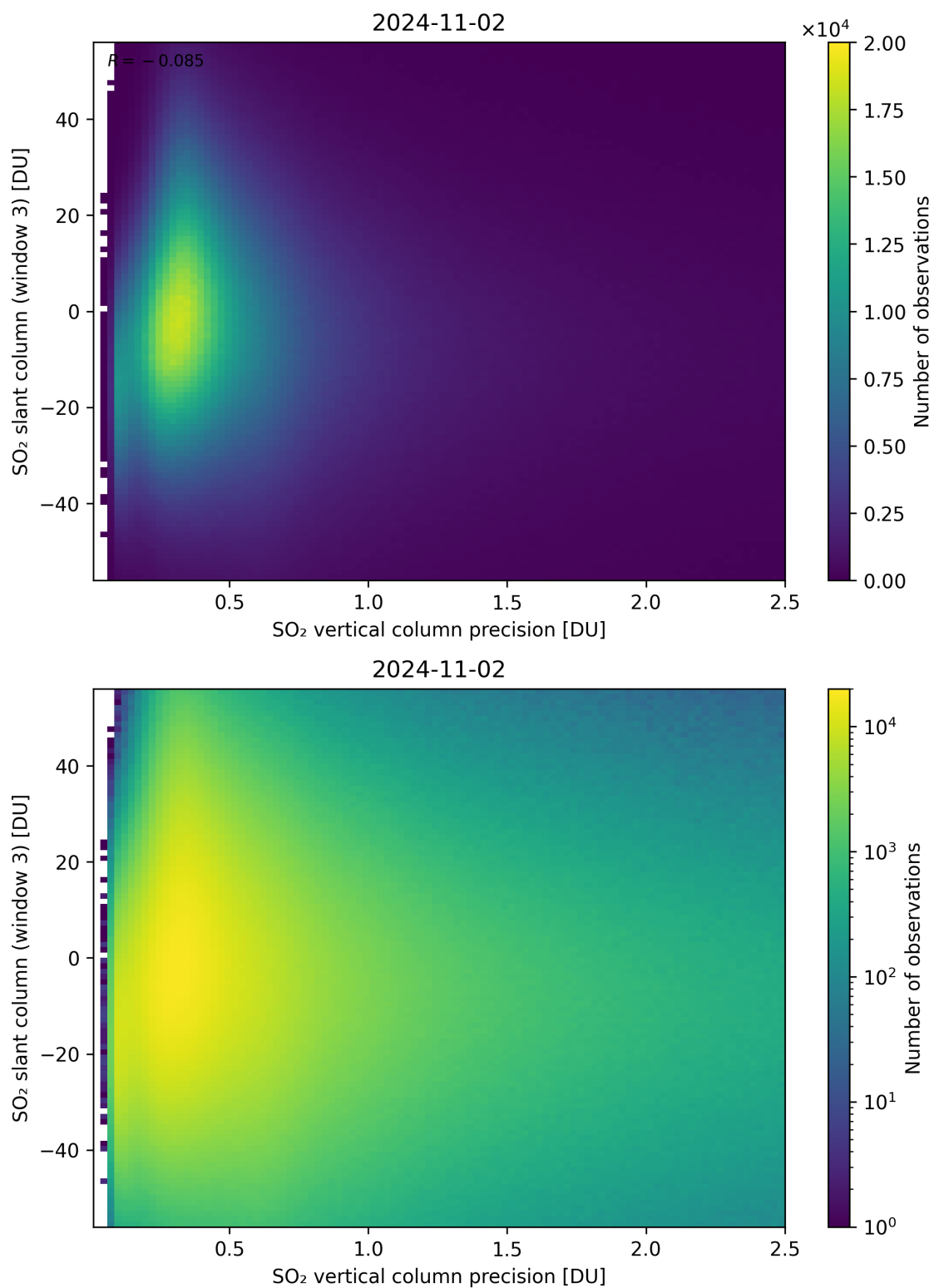
Figure 292: Scatter density plot of “SO 2 vertical column precision” against “SO 2 slant column (window 3)” for 2024-11-01 to 2024-11-03.
