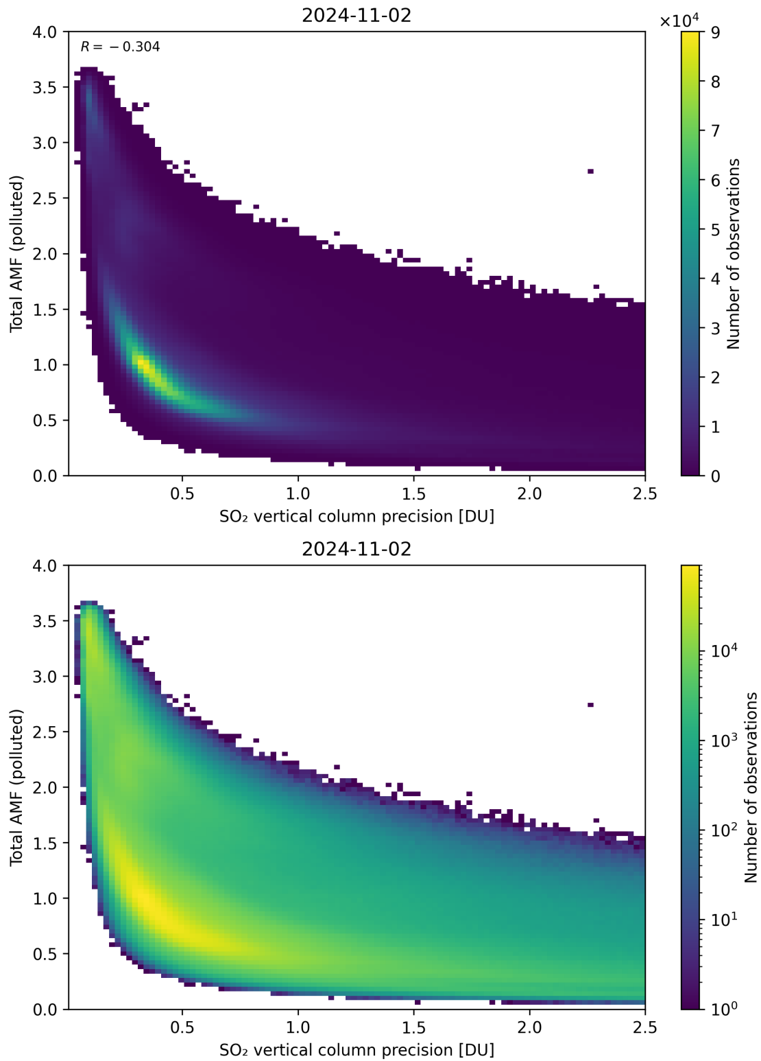
Figure 294: Scatter density plot of “SO 2 vertical column precision” against “Total AMF (polluted)” for 2024-11-01 to 2024-11-03.
