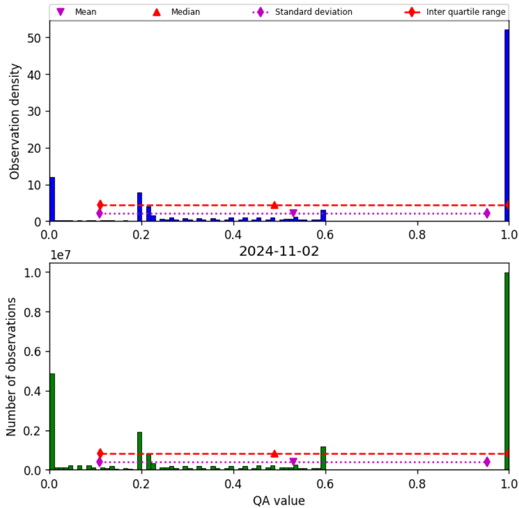
Figure 52: Histogram of “QA value” for 2024-11-01 to 2024-11-03
