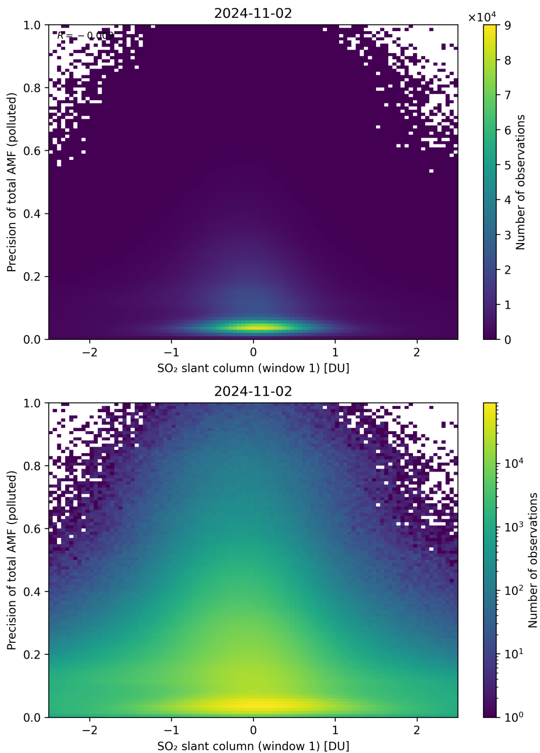
Figure 240: Scatter density plot of “SO 2 slant column (window 1)” against “Precision of total AMF (polluted)” for 2024-11-01 to 2024-11-03.
