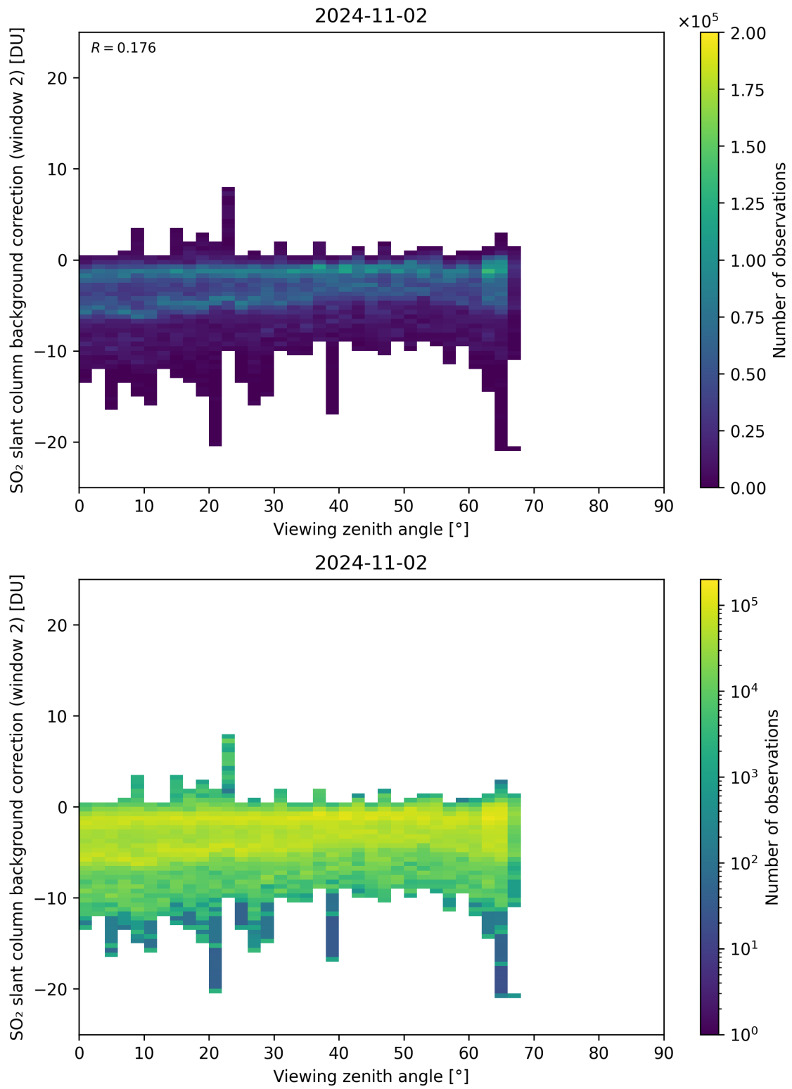
Figure 309: Scatter density plot of “Viewing zenith angle” against “SO 2 slant column background correction (window 2)” for 2024-11-01 to 2024-11-03.
