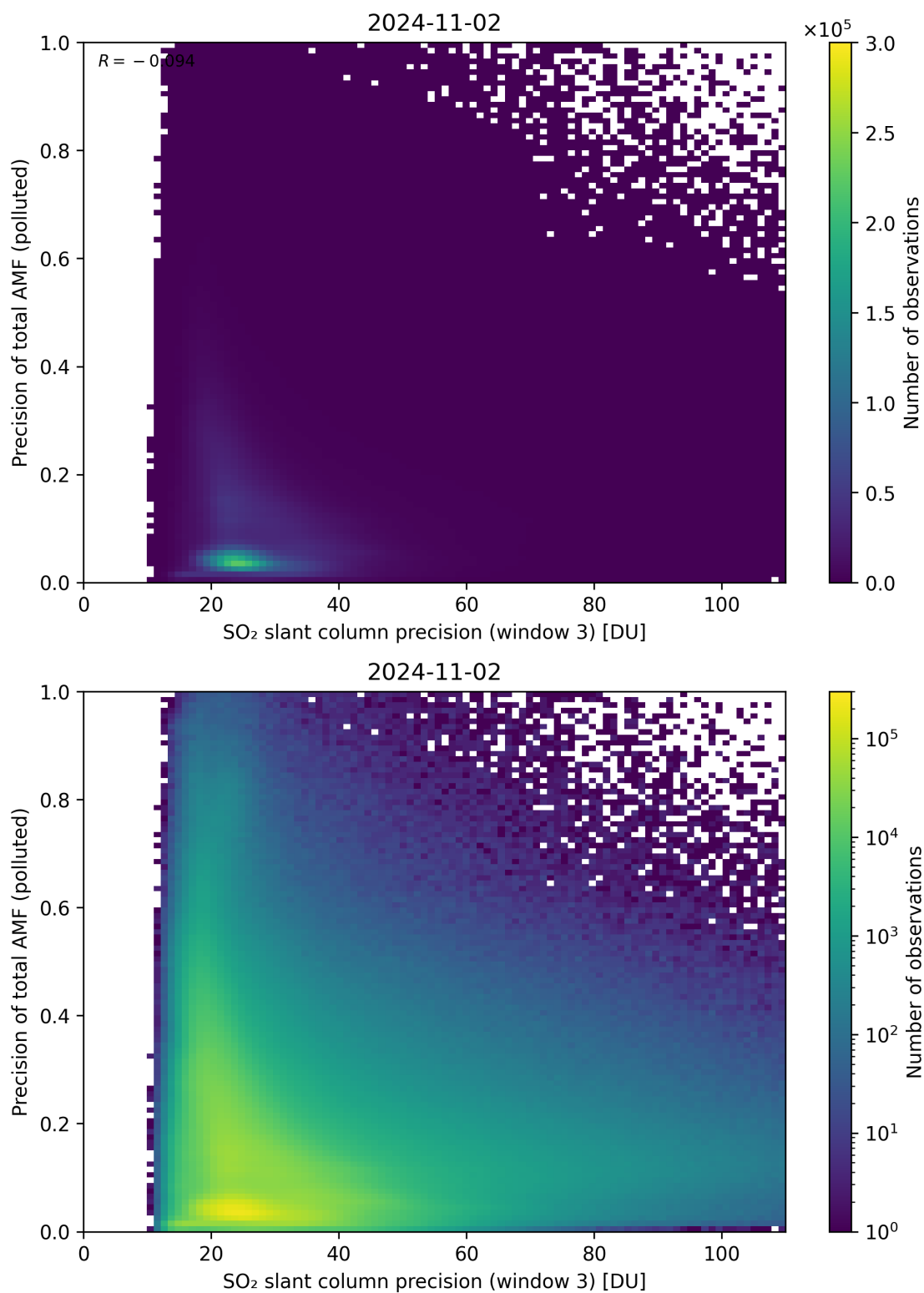
Figure 264: Scatter density plot of “SO 2 slant column precision (window 3)” against “Precision of total AMF (polluted)” for 2024-11-01 to 2024-11-03.
