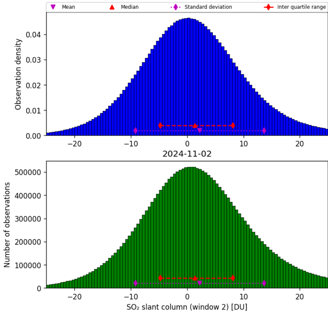
Figure 60: Histogram of “SO 2 slant column (window 2)” for 2024-11-01 to 2024-11-03
