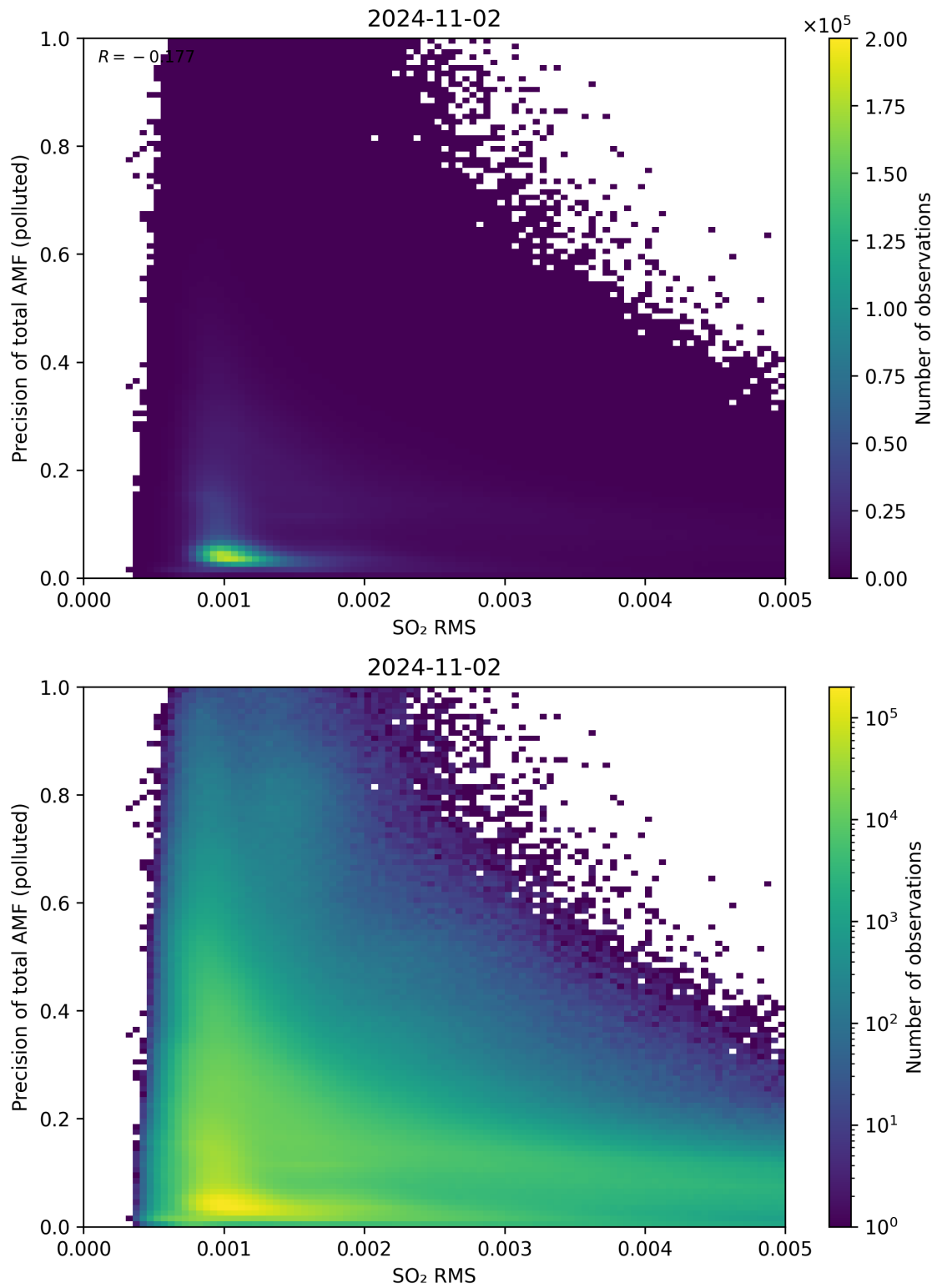
Figure 138: Scatter density plot of “SO 2 RMS” against “Precision of total AMF (polluted)” for 2024-11-01 to 2024-11-03.
