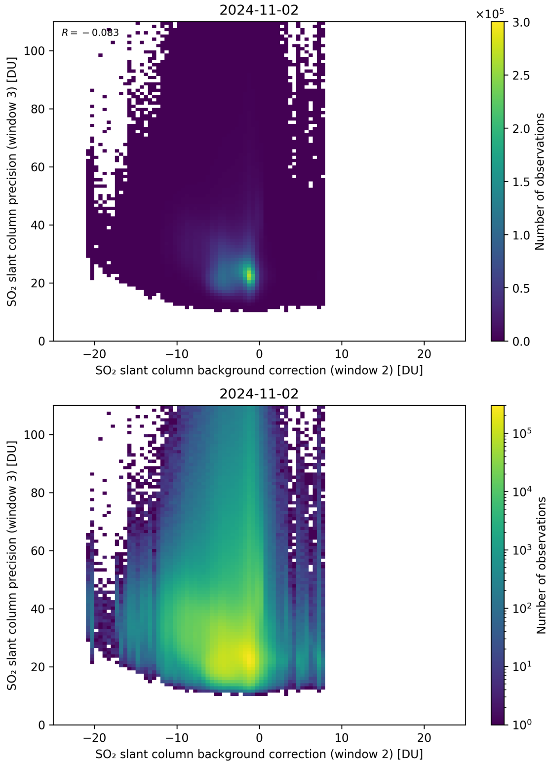
Figure 118: Scatter density plot of “SO 2 slant column background correction (window 2)” against “SO 2 slant column precision (window 3)” for 2024-11-01 to 2024-11-03.
