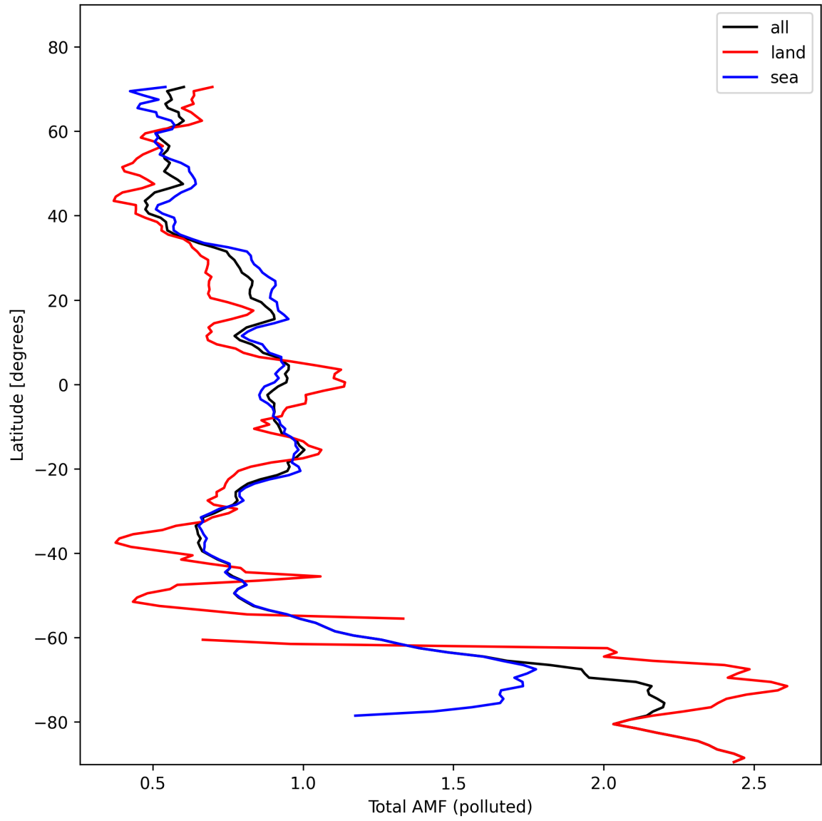
Figure 48: Zonal average of “Total AMF (polluted)” for 2024-11-01 to 2024-11-03.
