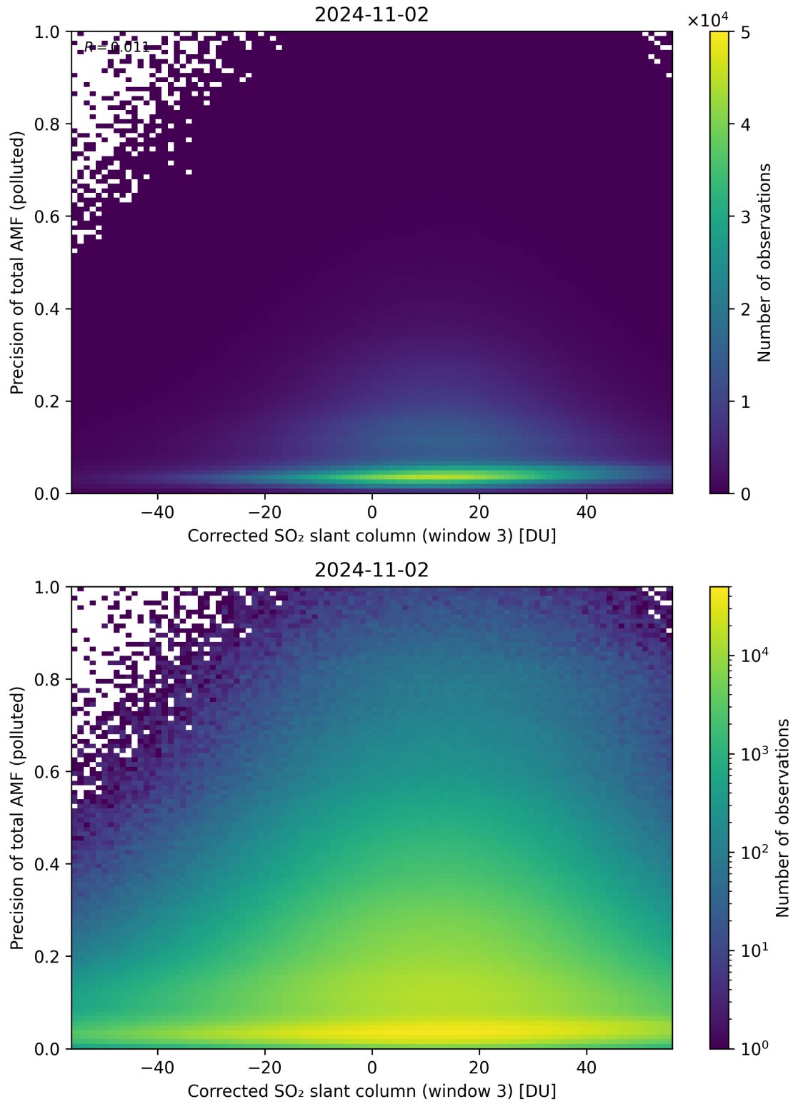
Figure 211: Scatter density plot of “Corrected SO 2 slant column (window 3)” against “Precision of total AMF (polluted)” for 2024-11-01 to 2024-11-03.
