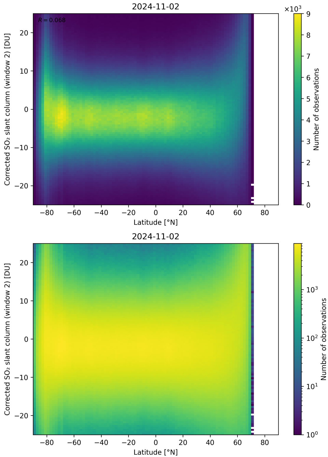
Figure 147: Scatter density plot of “Latitude” against “Corrected SO 2 slant column (window 2)” for 2024-11-01 to 2024-11-03.
