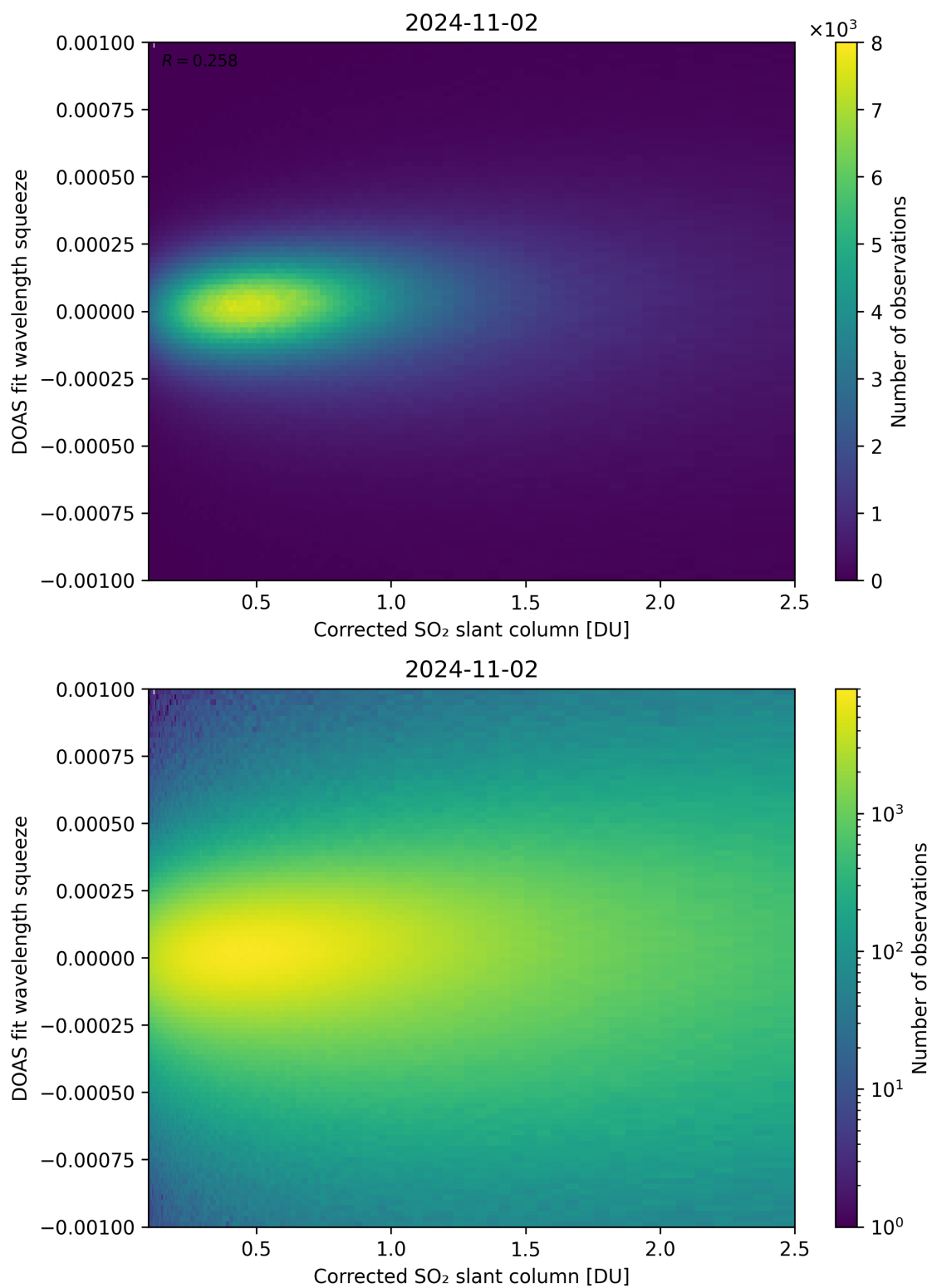
Figure 182: Scatter density plot of "Corrected SO 2 slant column" against "DOAS fit wavelength squeeze" for 2024-11-01 to 2024-11-03.
