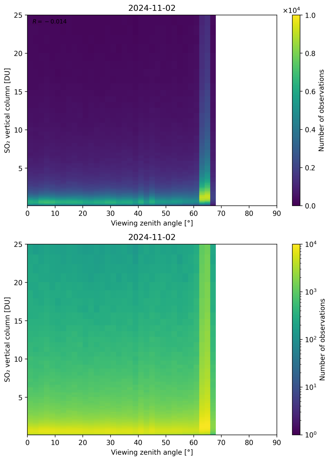
Figure 327: Scatter density plot of “Viewing zenith angle” against “SO 2 vertical column” for 2024-11-01 to 2024-11-03.
