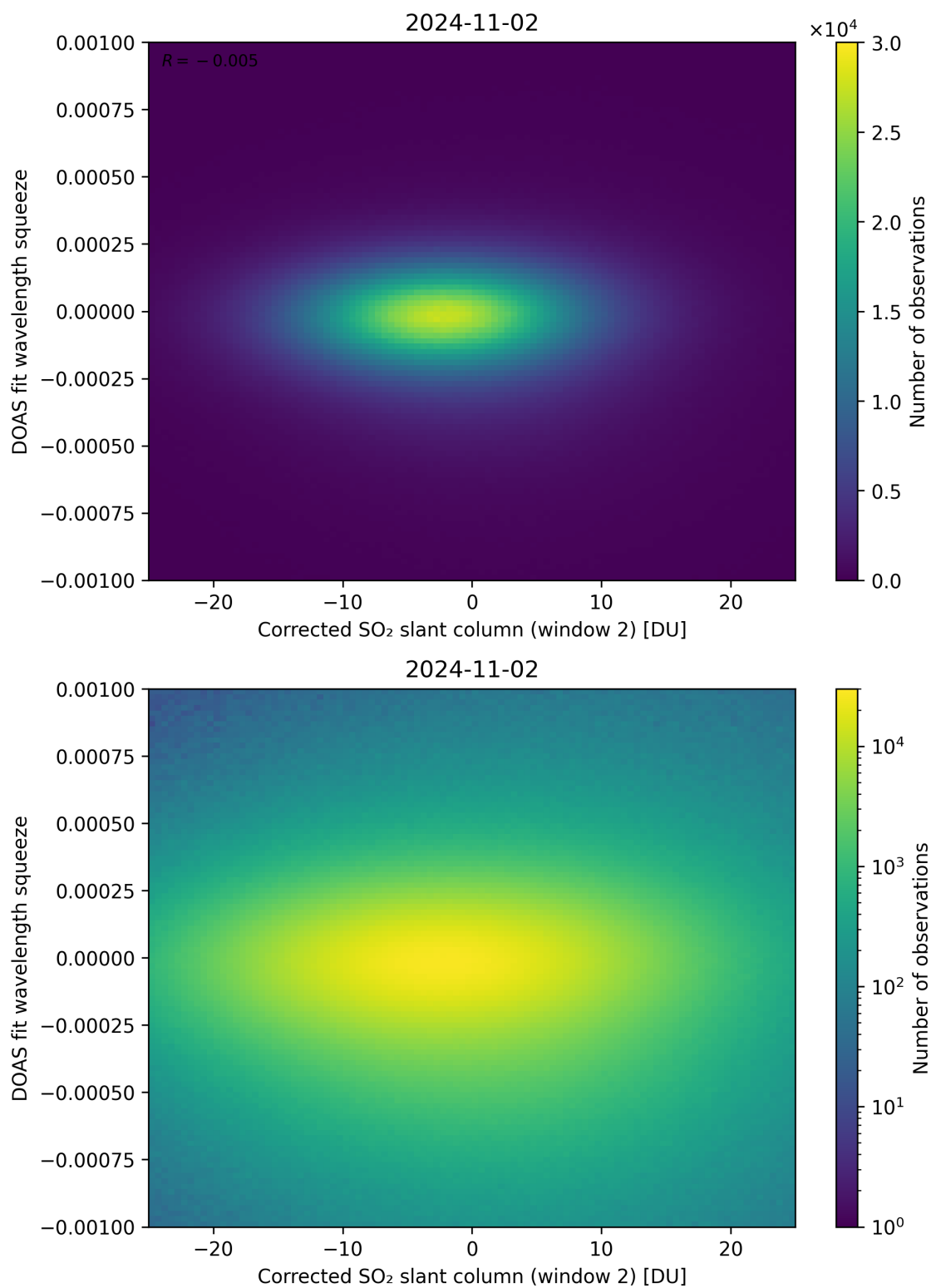
Figure 197: Scatter density plot of “Corrected SO 2 slant column (window 2)” against “DOAS fit wavelength squeeze” for 2024-11-01 to 2024-11-03.
