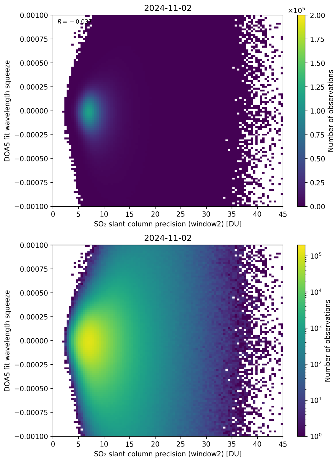
Figure 244: Scatter density plot of “SO 2 slant column precision (window2)” against “DOAS fit wavelength squeeze” for 2024-11-01 to 2024-11-03.
