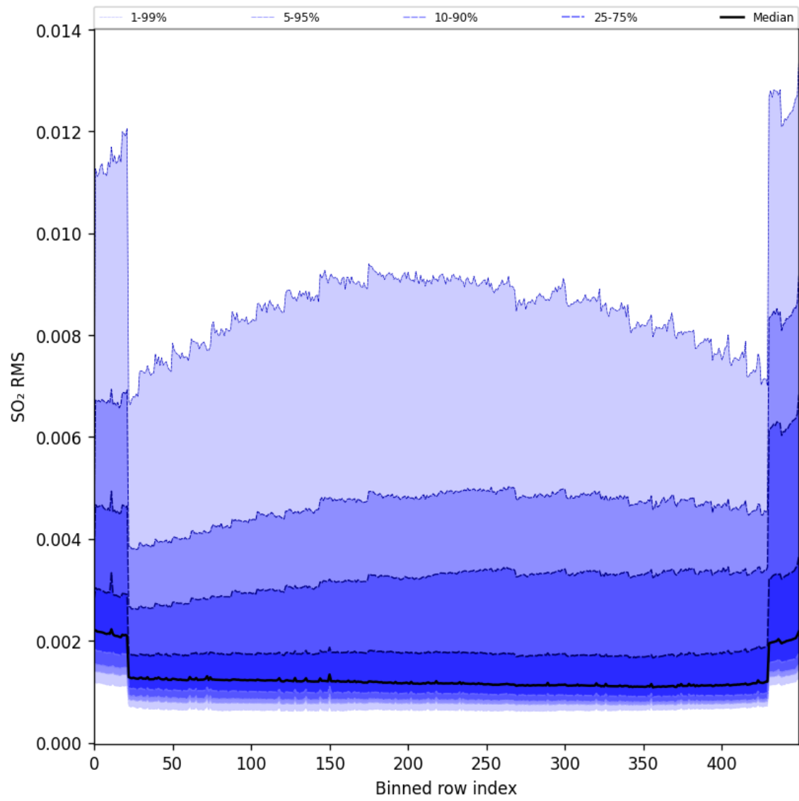
Figure 93: Along track statistics of “SO 2 RMS” for 2024-11-01 to 2024-11-03
