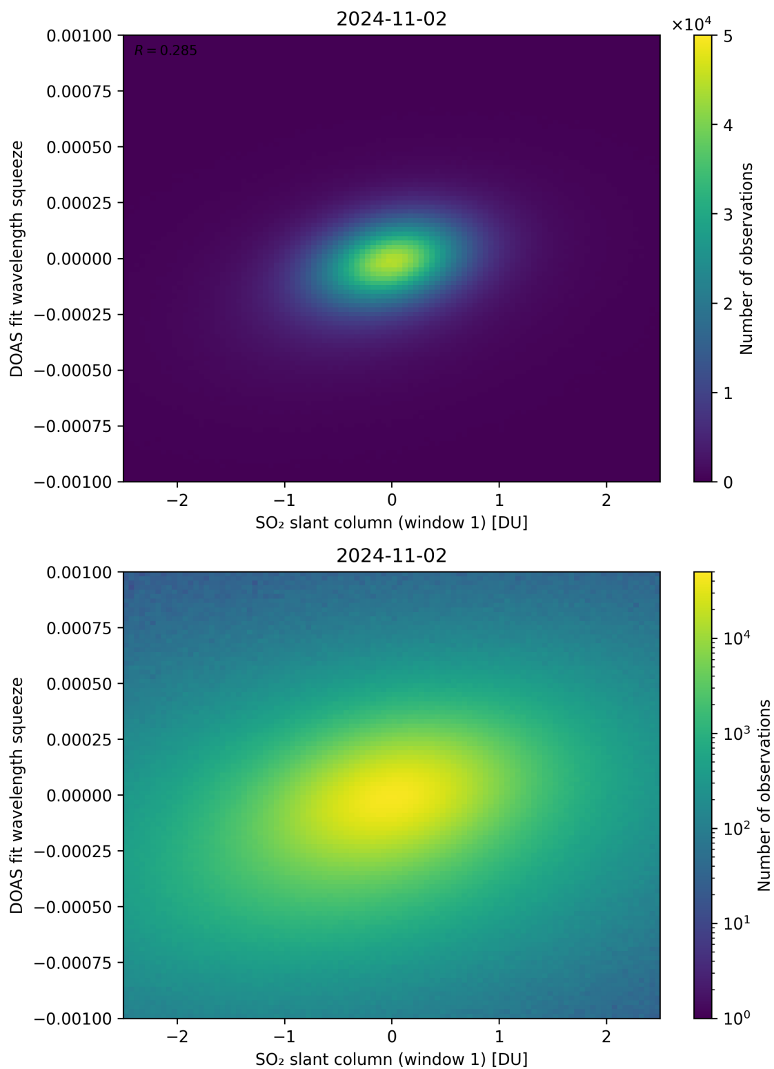
Figure 216: Scatter density plot of “SO 2 slant column (window 1)” against “DOAS fit wavelength squeeze” for 2024-11-01 to 2024-11-03.
