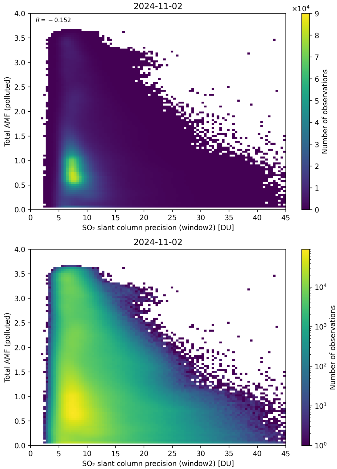
Figure 251: Scatter density plot of “SO 2 slant column precision (window2)” against “Total AMF (polluted)” for 2024-11-01 to 2024-11-03.
