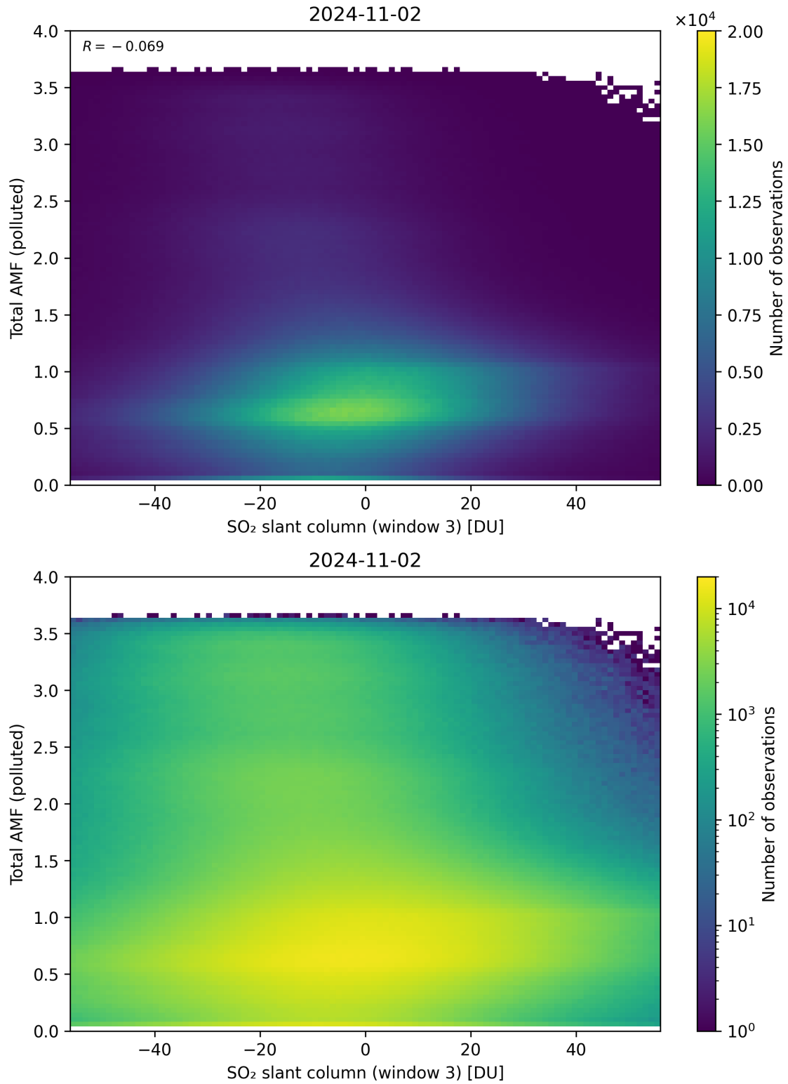
Figure 268: Scatter density plot of “SO 2 slant column (window 3)” against “Total AMF (polluted)” for 2024-11-01 to 2024-11-03.
