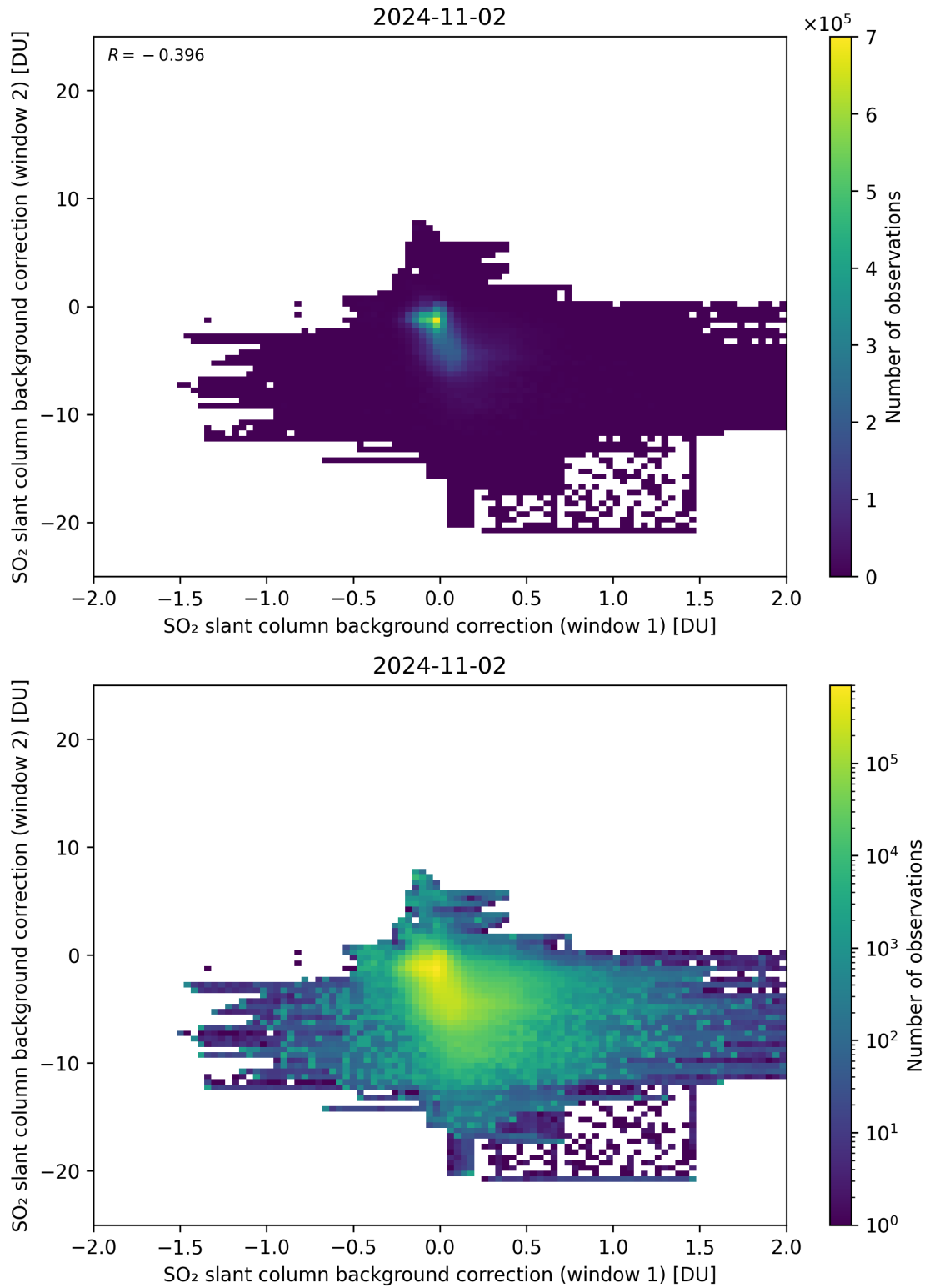
Figure 98: Scatter density plot of “SO 2 slant column background correction (window 1)” against “SO 2 slant column background correction (window 2)” for 2024-11-01 to 2024-11-03.
