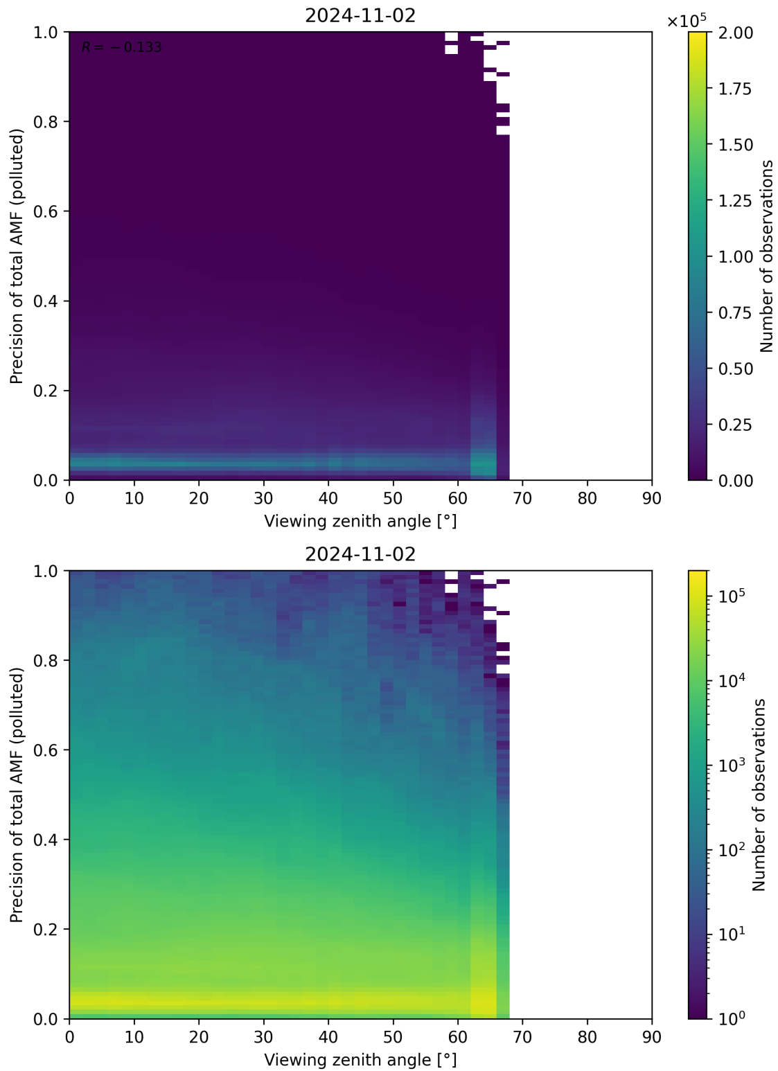
Figure 326: Scatter density plot of “Viewing zenith angle” against “Precision of total AMF (polluted)” for 2024-11-01 to 2024-11-03.
