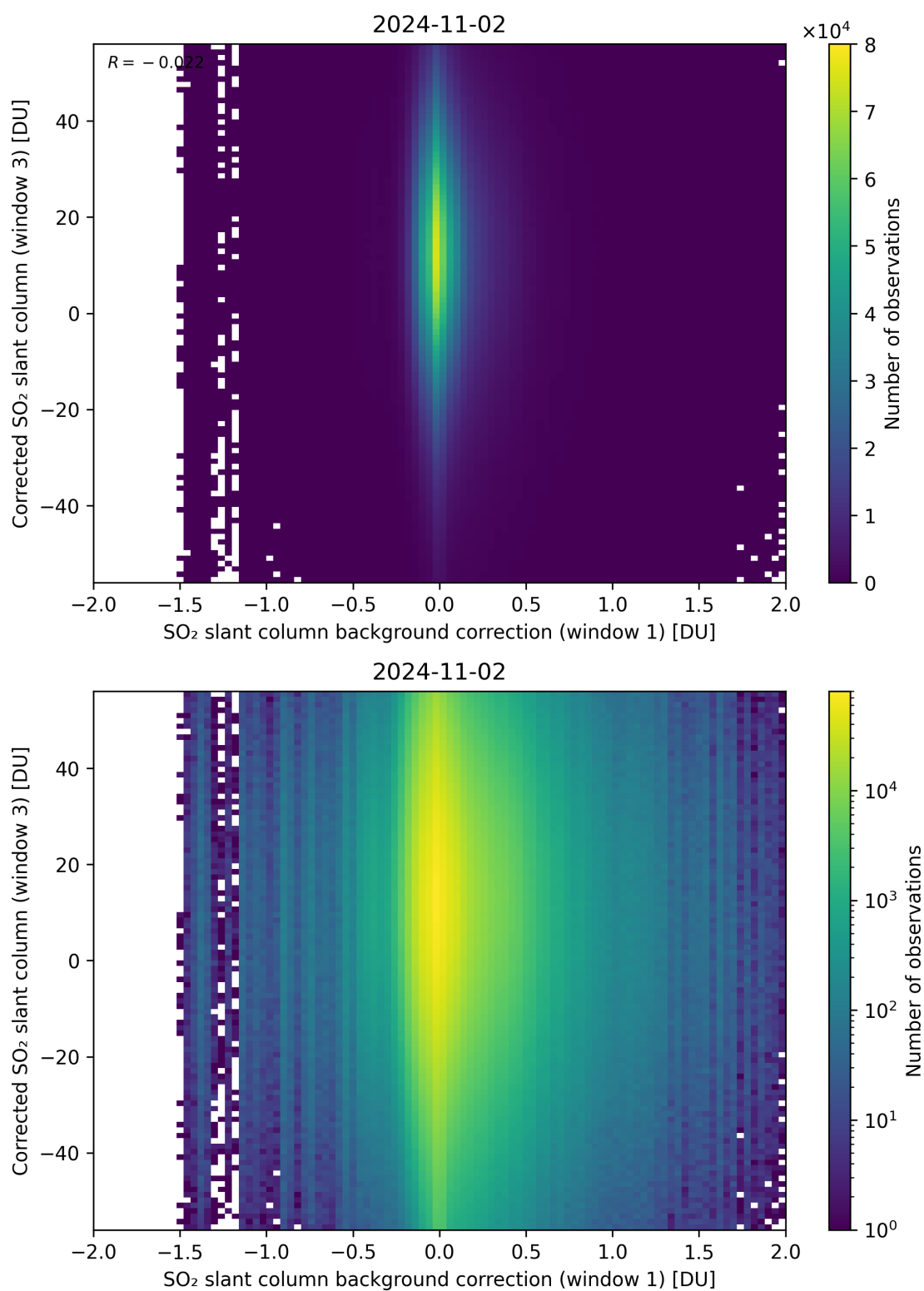
Figure 105: Scatter density plot of “SO 2 slant column background correction (window 1)” against “Corrected SO 2 slant column (window 3)” for 2024-11-01 to 2024-11-03.
