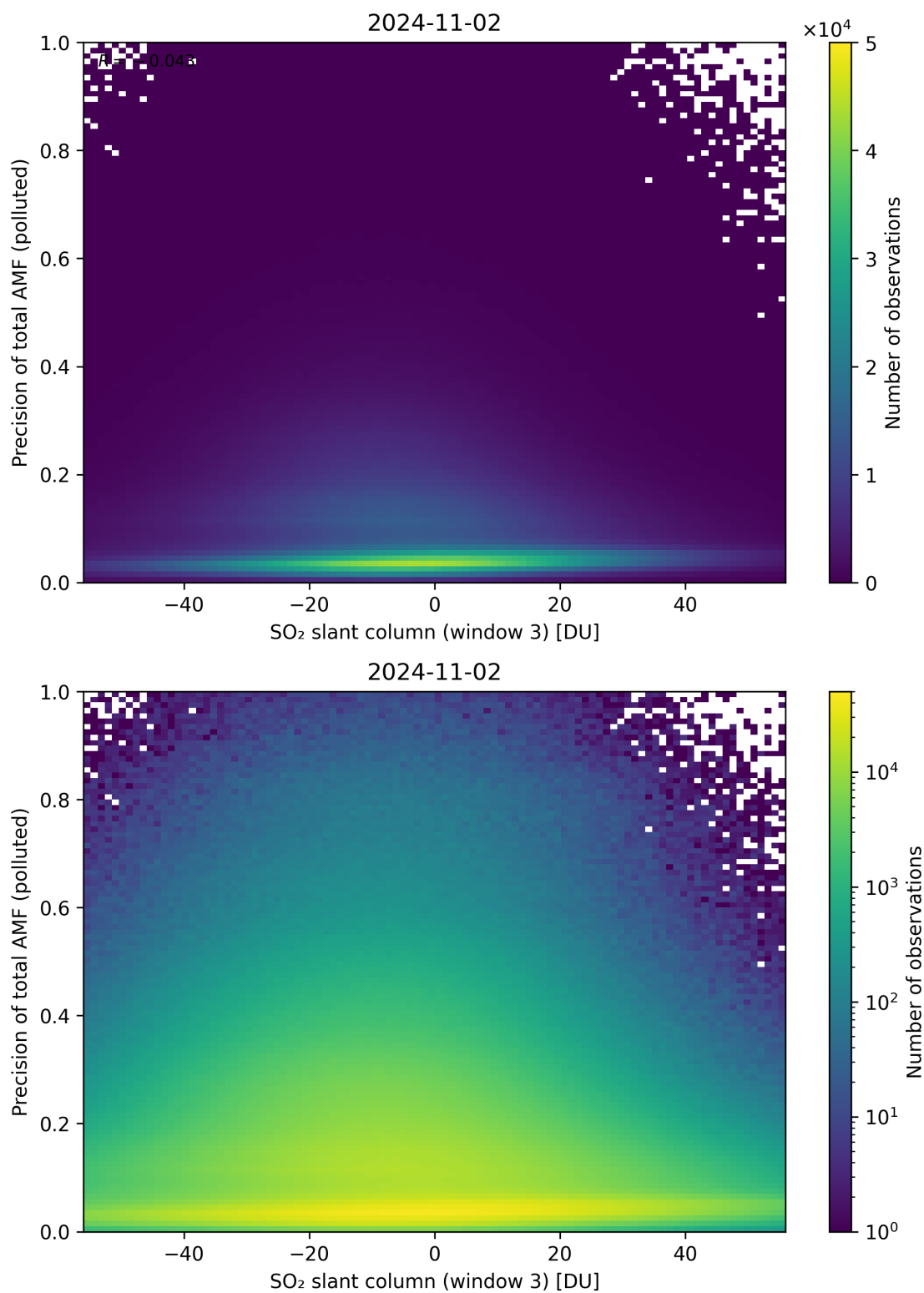
Figure 269: Scatter density plot of “SO 2 slant column (window 3)” against “Precision of total AMF (polluted)” for 2024-11-01 to 2024-11-03.
