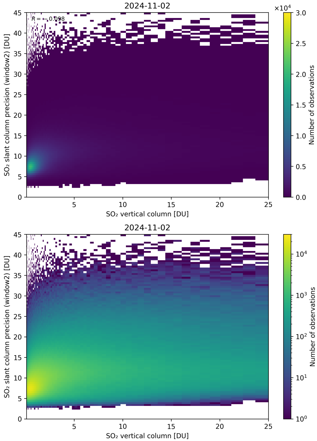
Figure 302: Scatter density plot of “SO 2 vertical column” against “SO 2 slant column precision (window2)” for 2024-11-01 to 2024-11-03.
