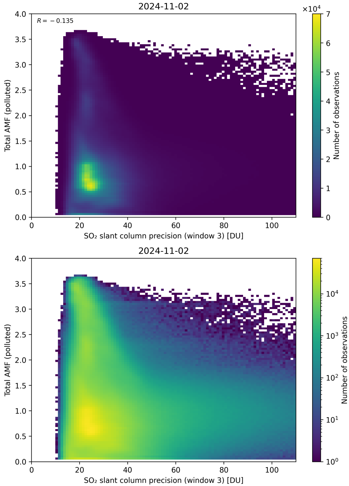
Figure 263: Scatter density plot of “SO 2 slant column precision (window 3)” against “Total AMF (polluted)” for 2024-11-01 to 2024-11-03.
