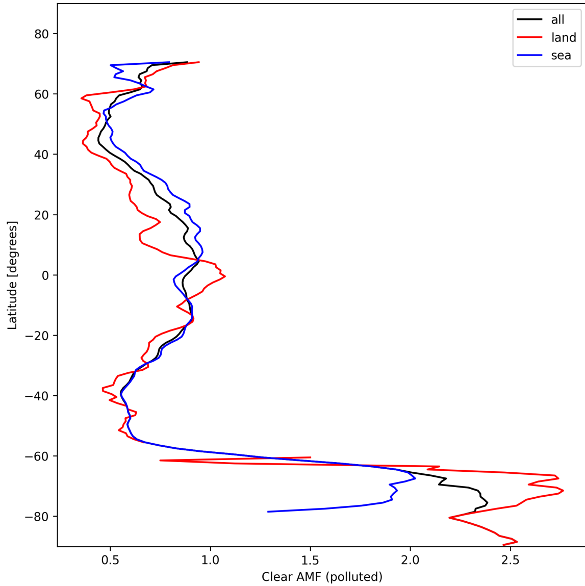
Figure 50: Zonal average of “Clear AMF (polluted)” for 2024-11-01 to 2024-11-03.
