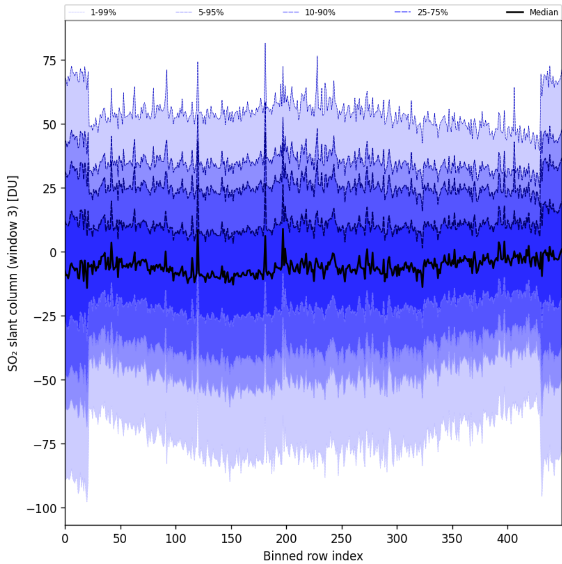
Figure 87: Along track statistics of “SO 2 slant column (window 3)” for 2024-11-01 to 2024-11-03
