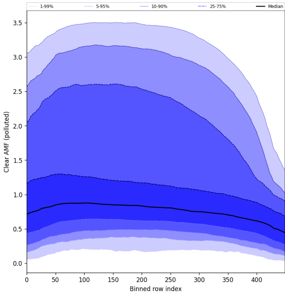
Figure 96: Along track statistics of “Clear AMF (polluted)” for 2024-11-01 to 2024-11-03
