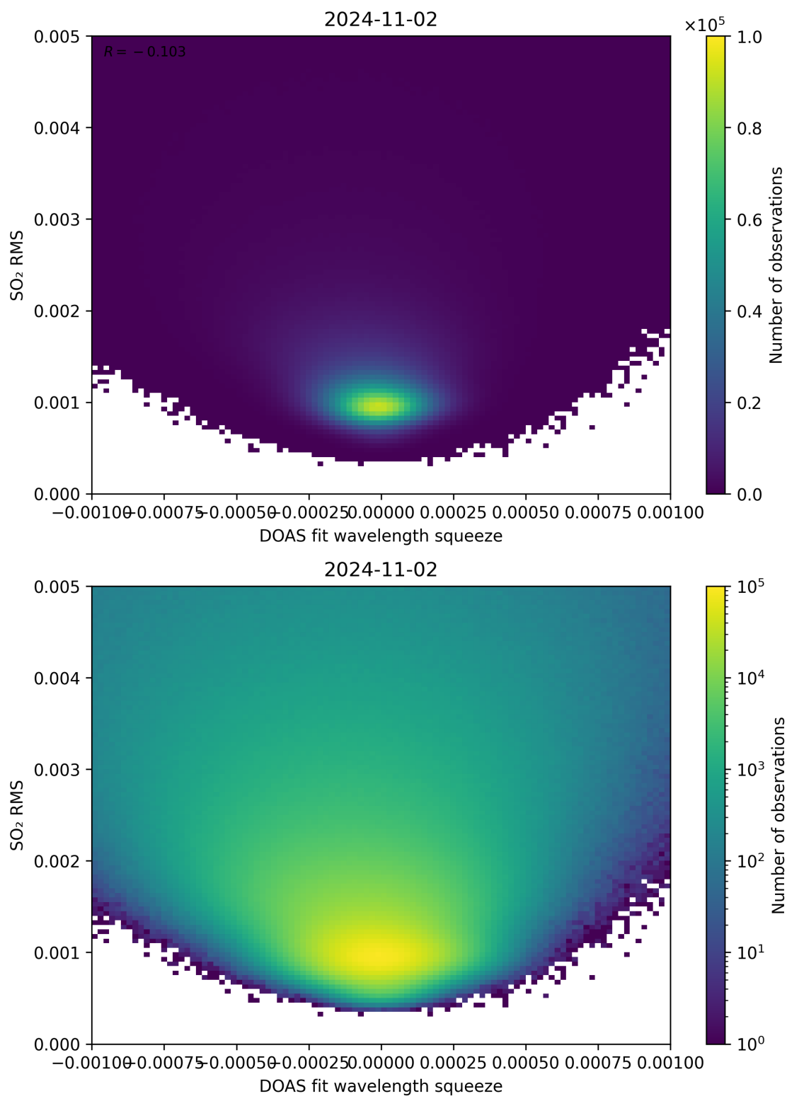
Figure 132: Scatter density plot of “DOAS fit wavelength squeeze” against “SO 2 RMS” for 2024-11-01 to 2024-11-03.
