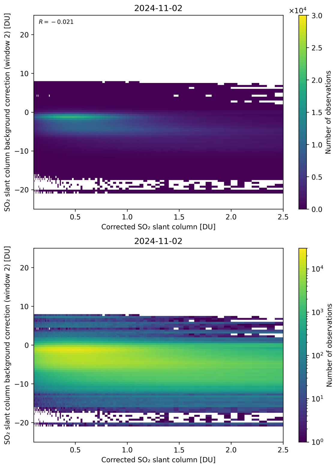
Figure 179: Scatter density plot of “Corrected SO 2 slant column” against “SO 2 slant column background correction (window 2)” for 2024-11-01 to 2024-11-03.
