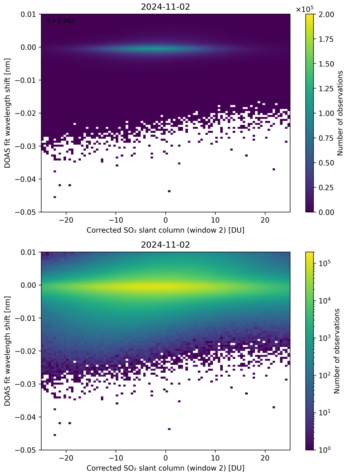
Figure 196: Scatter density plot of “Corrected SO 2 slant column (window 2)” against “DOAS fit wavelength shift” for 2024-11-01 to 2024-11-03.
