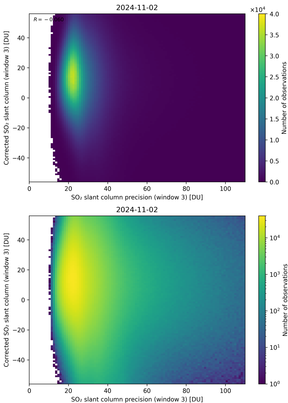
Figure 262: Scatter density plot of “SO 2 slant column precision (window 3)” against “Corrected SO 2 slant column (window 3)” for 2024-11-01 to 2024-11-03.
