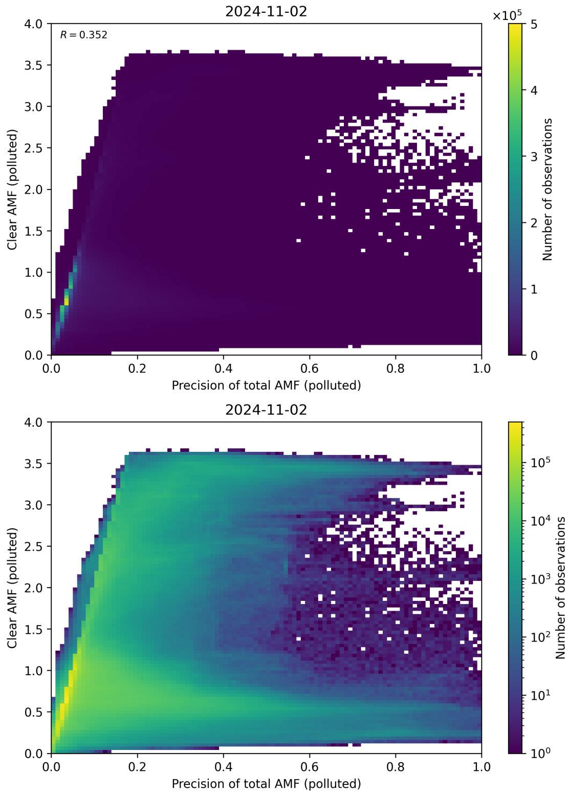
Figure 270: Scatter density plot of “Precision of total AMF (polluted)” against “Clear AMF (polluted)” for 2024-11-01 to 2024-11-03.
