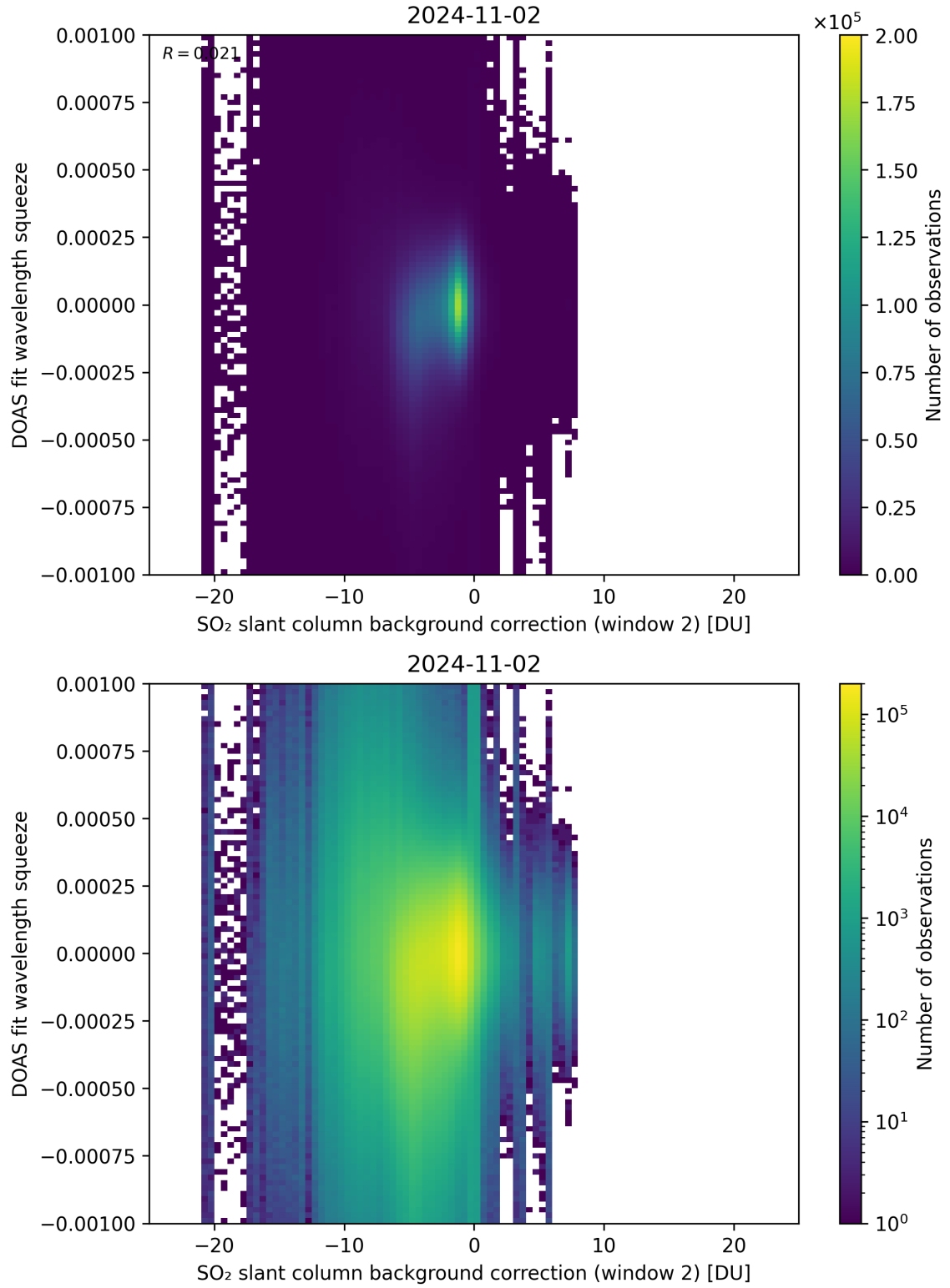
Figure 113: Scatter density plot of "SO 2 slant column background correction (window 2)" against "DOAS fit wavelength squeeze" for 2024-11-01 to 2024-11-03.
