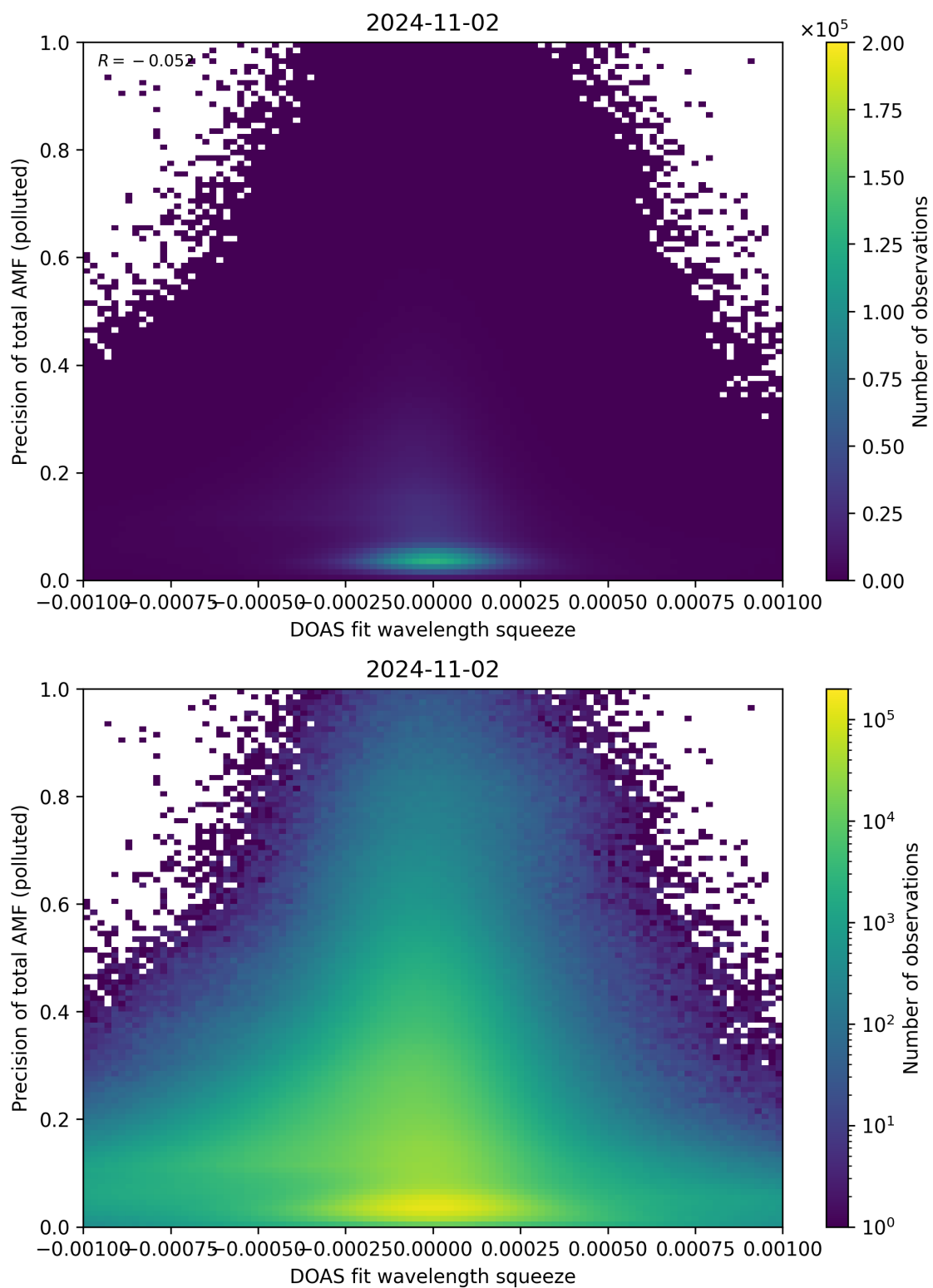
Figure 135: Scatter density plot of “DOAS fit wavelength squeeze” against “Precision of total AMF (polluted)” for 2024-11-01 to 2024-11-03.
