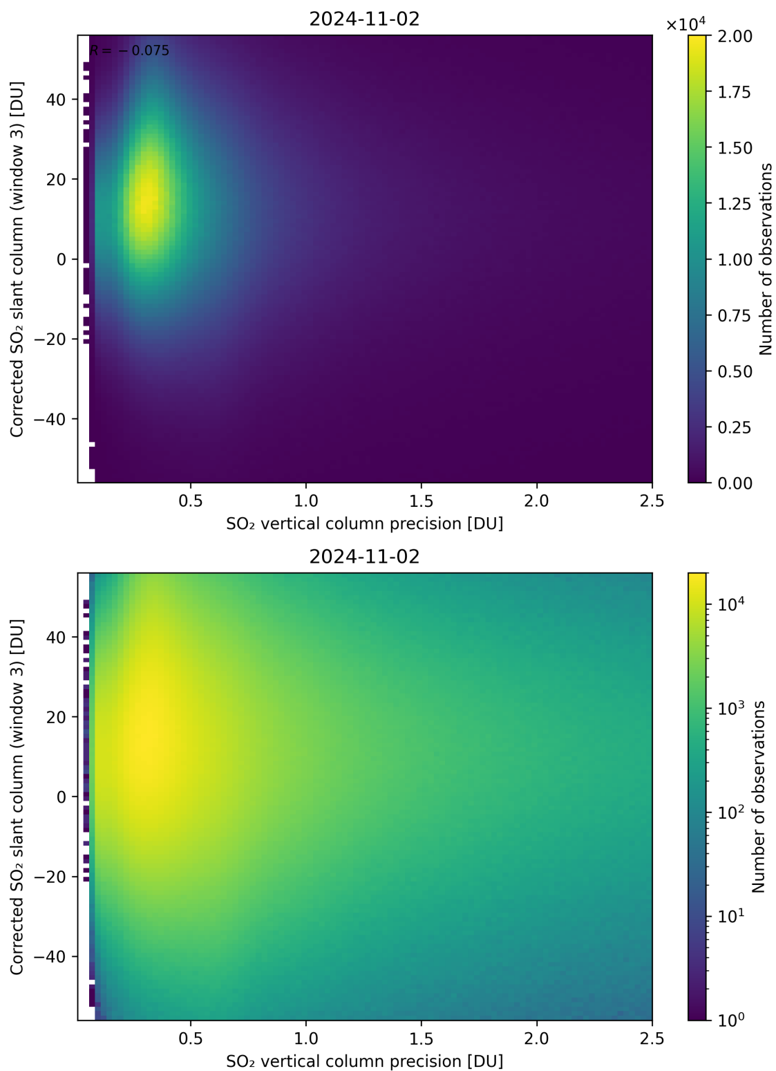
Figure 288: Scatter density plot of “SO 2 vertical column precision” against “Corrected SO 2 slant column (window 3)” for 2024-11-01 to 2024-11-03.
