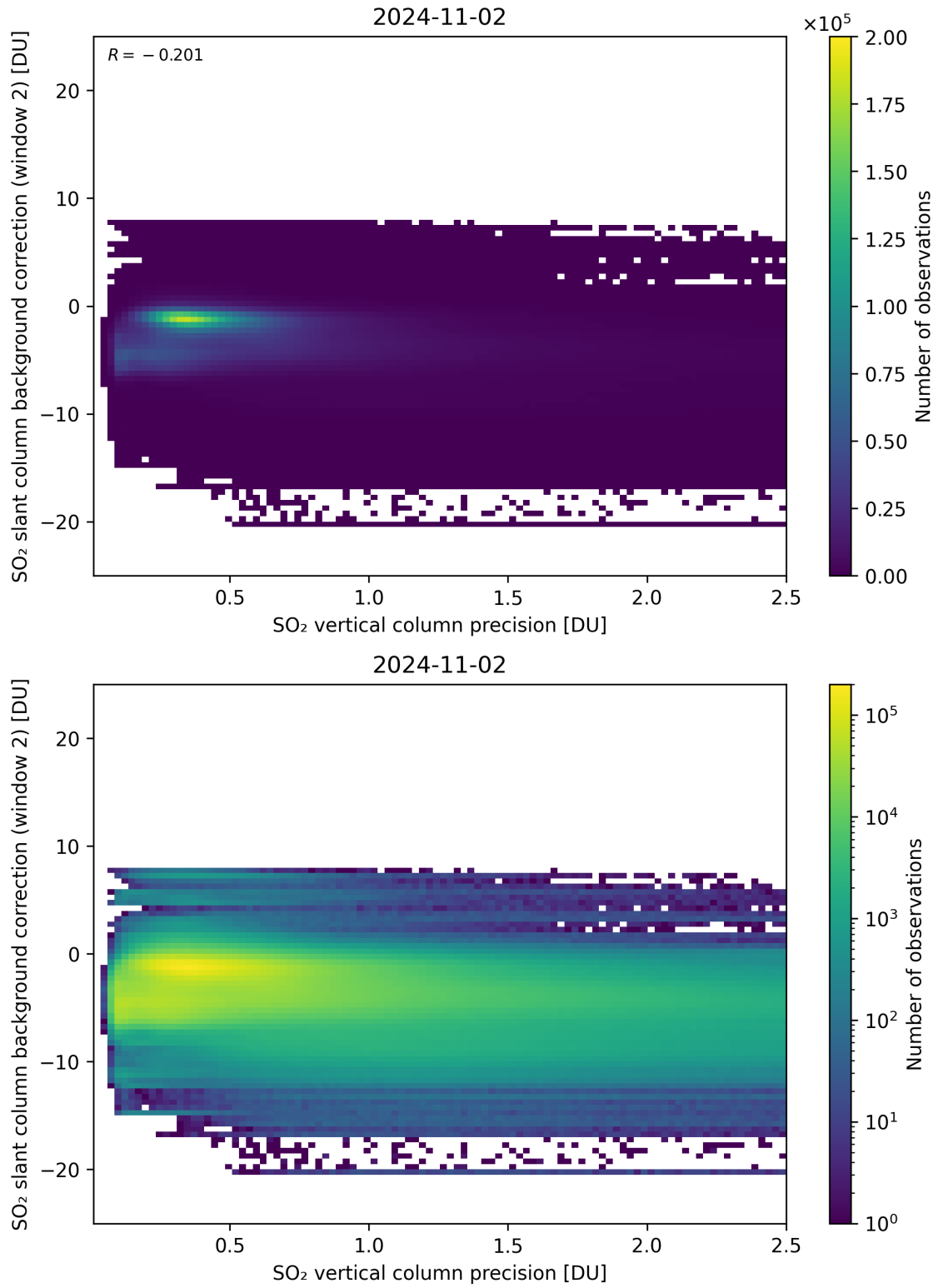
Figure 280: Scatter density plot of “SO 2 vertical column precision” against “SO 2 slant column background correction (window 2)” for 2024-11-01 to 2024-11-03.
