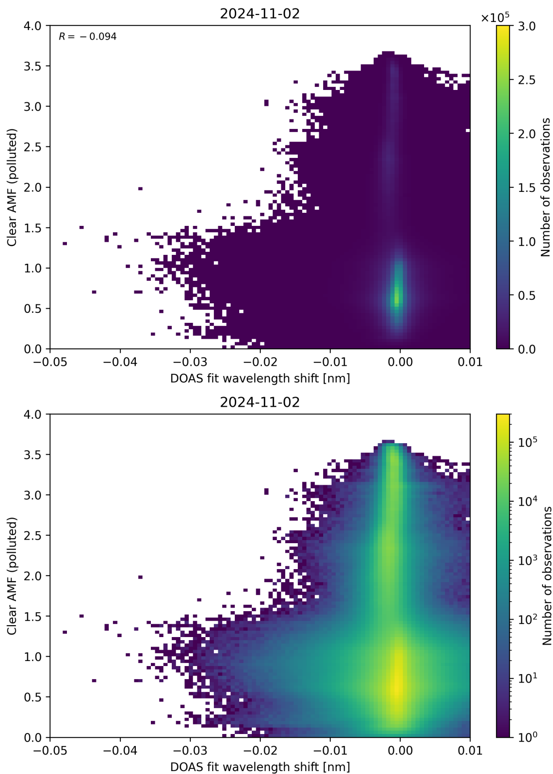
Figure 129: Scatter density plot of “DOAS fit wavelength shift” against “Clear AMF (polluted)” for 2024-11-01 to 2024-11-03.
