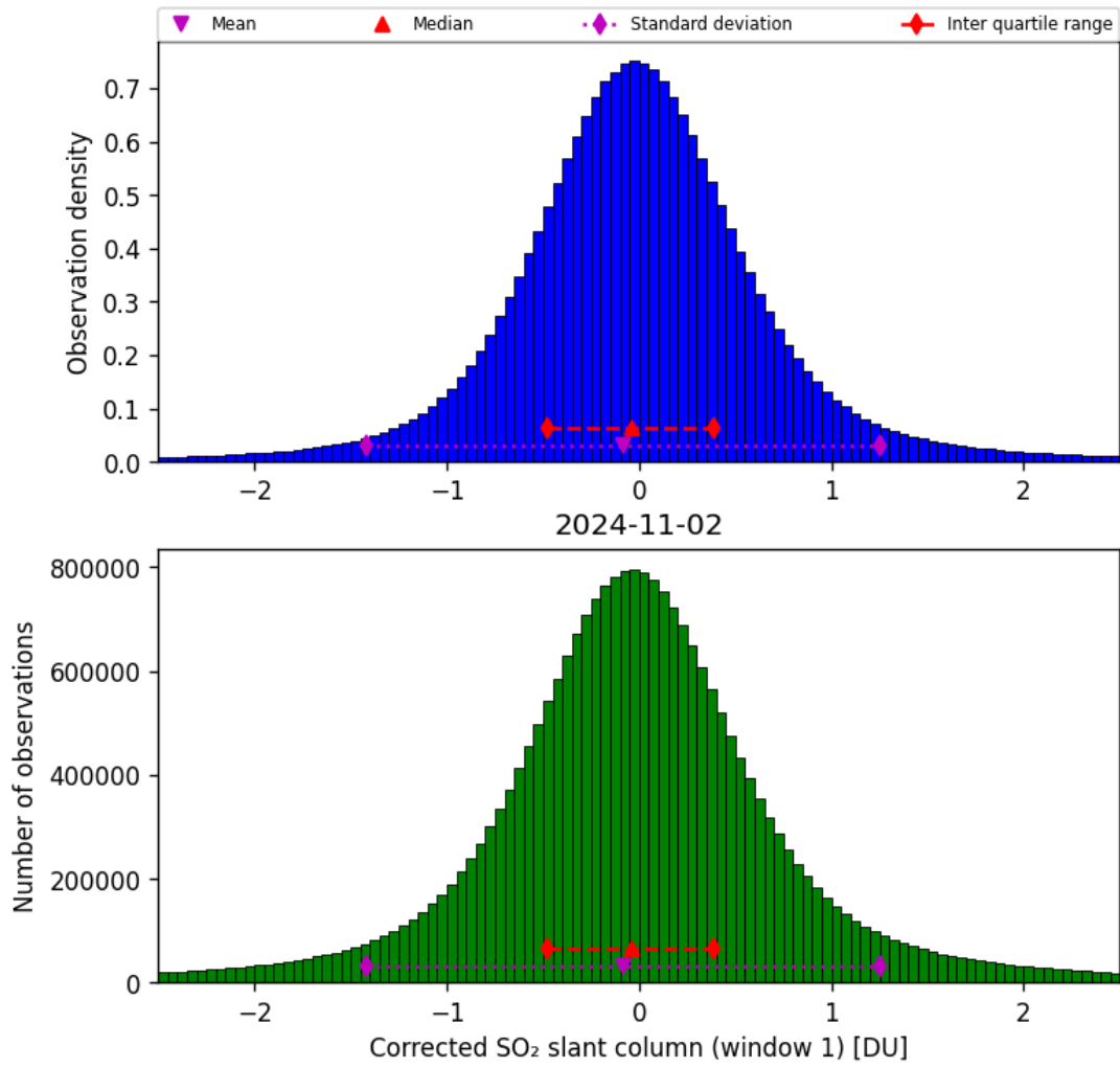
Figure 58: Histogram of “Corrected SO 2 slant column (window 1)” for 2024-11-01 to 2024-11-03
