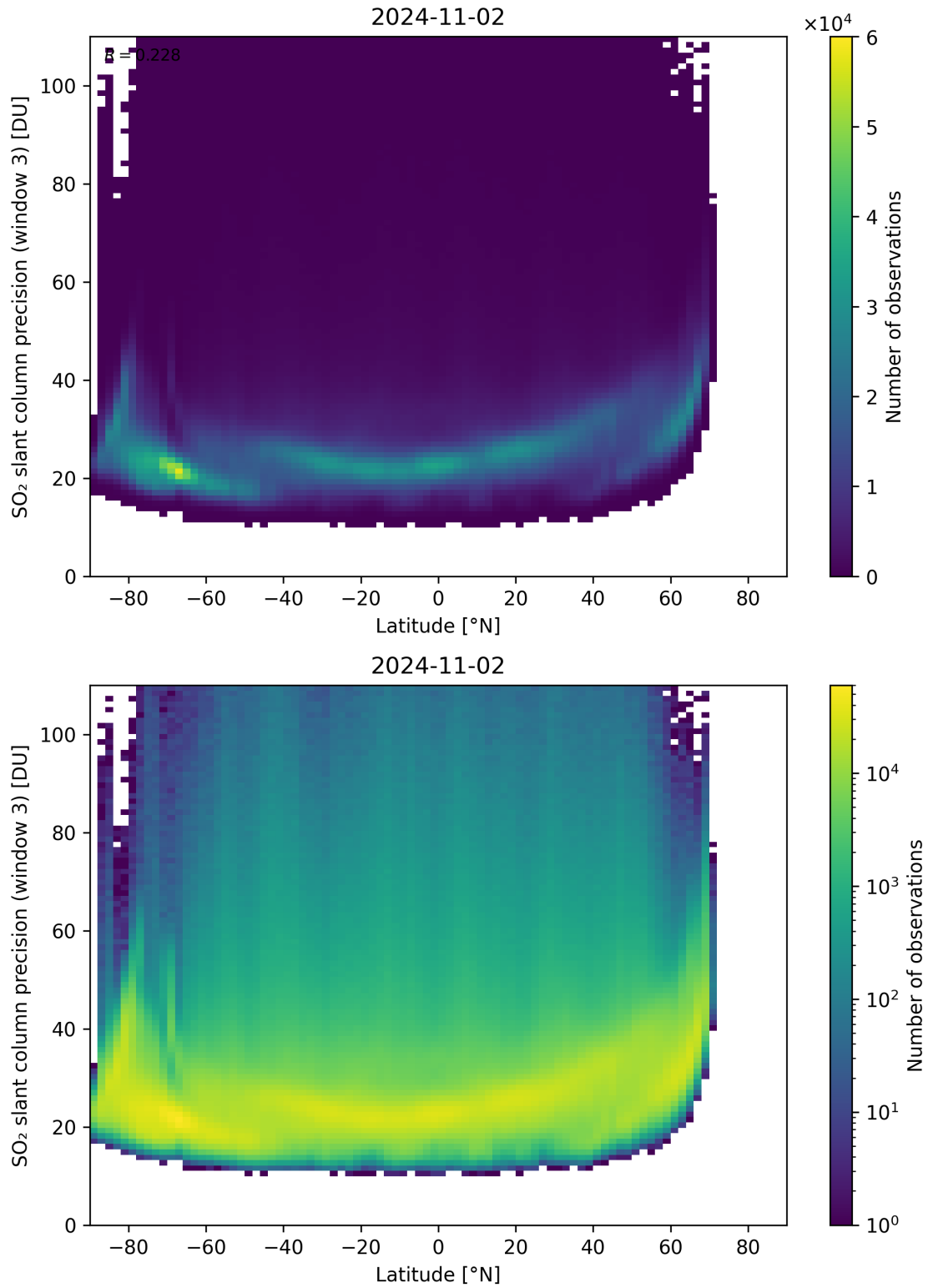
Figure 153: Scatter density plot of “Latitude” against “SO 2 slant column precision (window 3)” for 2024-11-01 to 2024-11-03.
