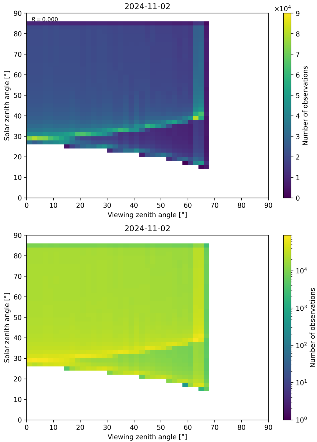
Figure 315: Scatter density plot of “Viewing zenith angle” against “Solar zenith angle” for 2024-11-01 to 2024-11-03.
