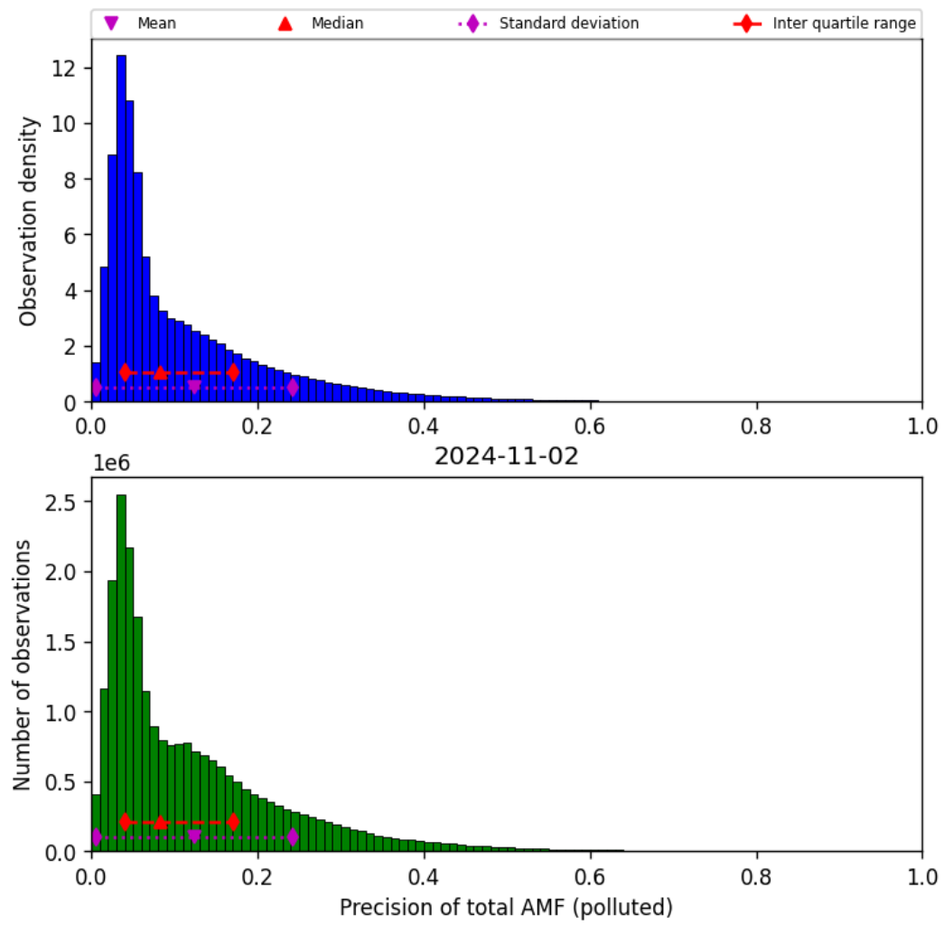
Figure 72: Histogram of “Precision of total AMF (polluted)” for 2024-11-01 to 2024-11-03
