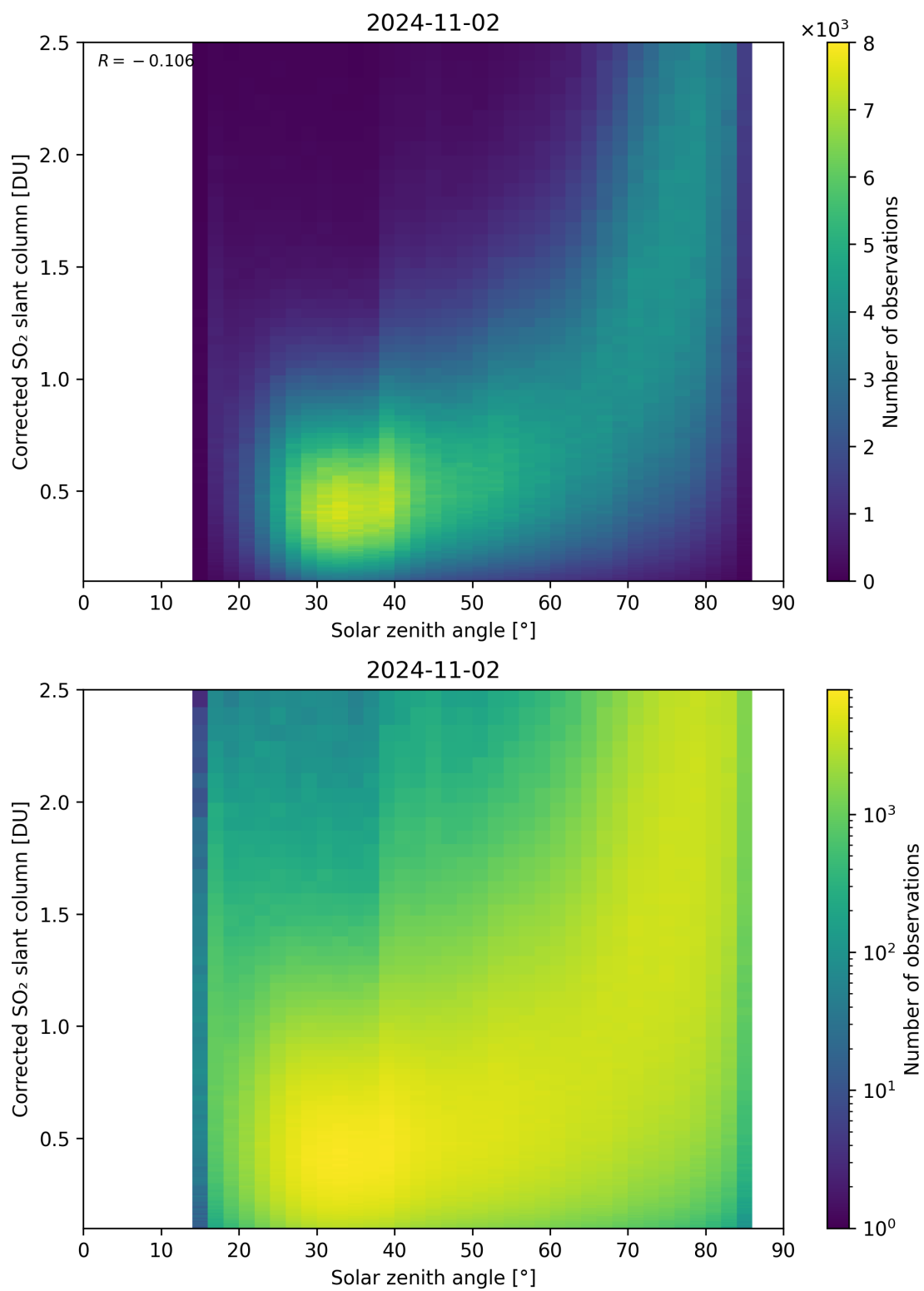
Figure 166: Scatter density plot of “Solar zenith angle” against “Corrected SO 2 slant column” for 2024-11-01 to 2024-11-03.
