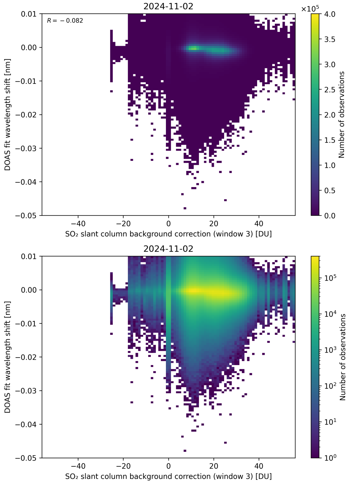
Figure 121: Scatter density plot of “SO 2 slant column background correction (window 3)” against “DOAS fit wavelength shift” for 2024-11-01 to 2024-11-03.
