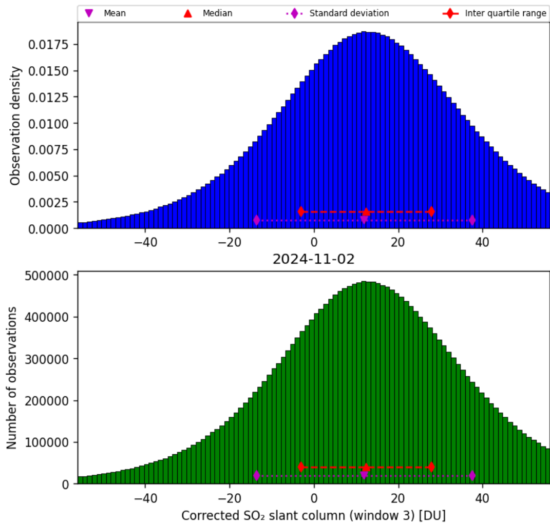
Figure 66: Histogram of “Corrected SO 2 slant column (window 3)” for 2024-11-01 to 2024-11-03
