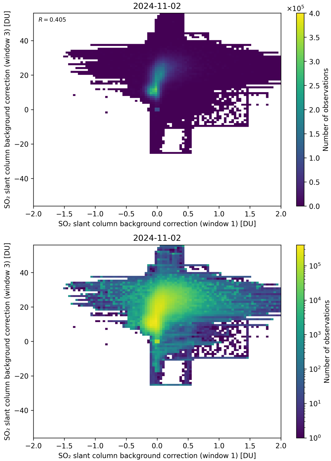
Figure 99: Scatter density plot of “SO 2 slant column background correction (window 1)” against “SO 2 slant column background correction (window 3)” for 2024-11-01 to 2024-11-03.
