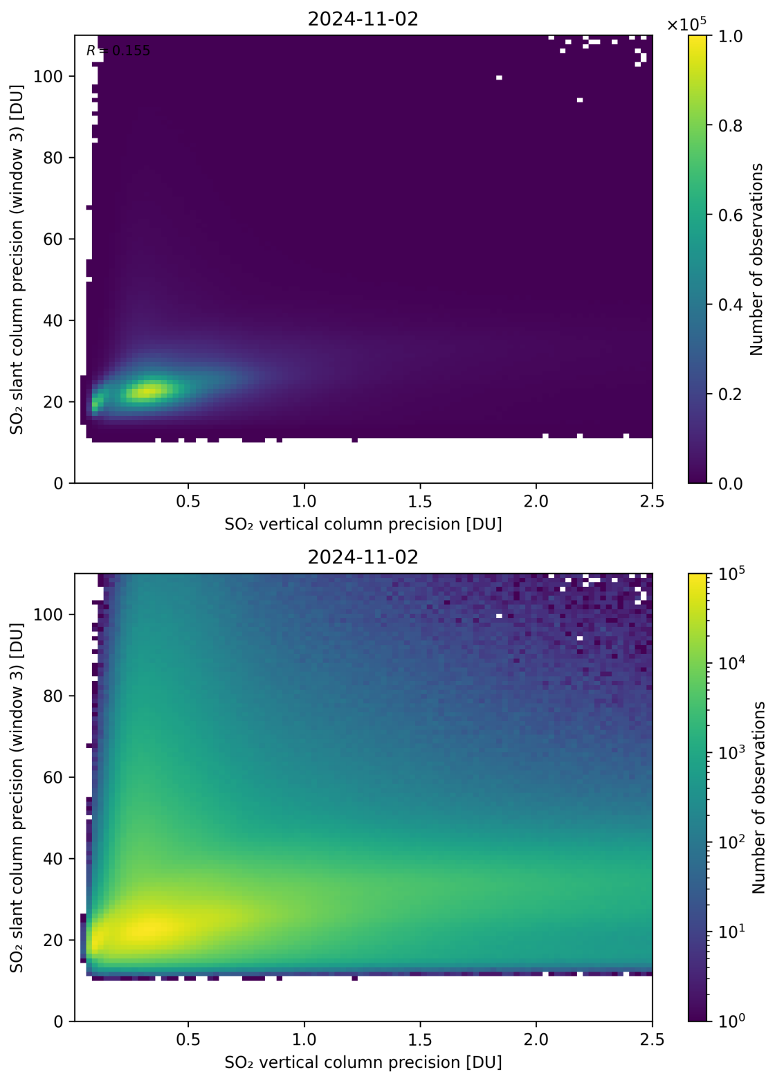
Figure 293: Scatter density plot of “SO 2 vertical column precision” against “SO 2 slant column precision (window 3)” for 2024-11-01 to 2024-11-03.
