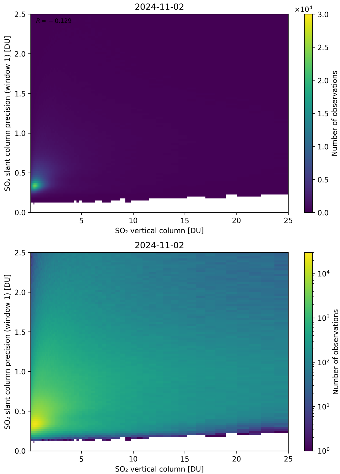
Figure 301: Scatter density plot of “SO 2 vertical column” against “SO 2 slant column precision (window 1)” for 2024-11-01 to 2024-11-03.
