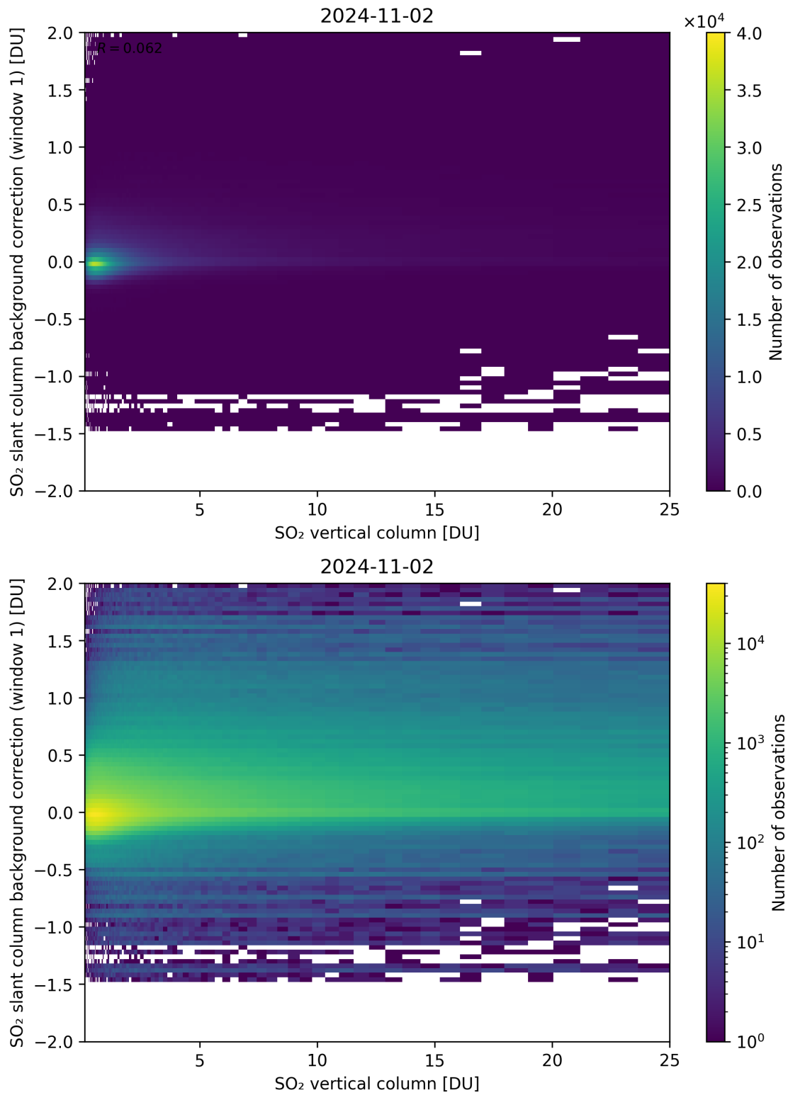
Figure 273: Scatter density plot of “SO 2 vertical column” against “SO 2 slant column background correction (window 1)” for 2024-11-01 to 2024-11-03.
