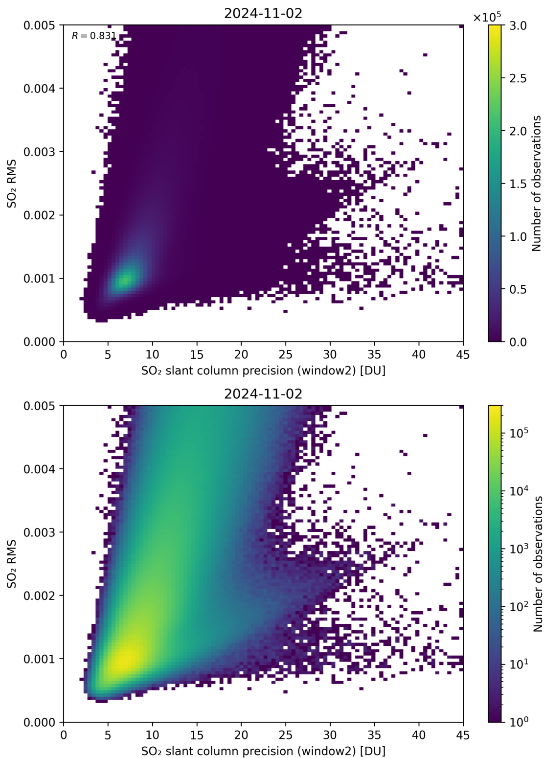
Figure 245: Scatter density plot of “SO 2 slant column precision (window2)” against “SO 2 RMS” for 2024-11-01 to 2024-11-03.
