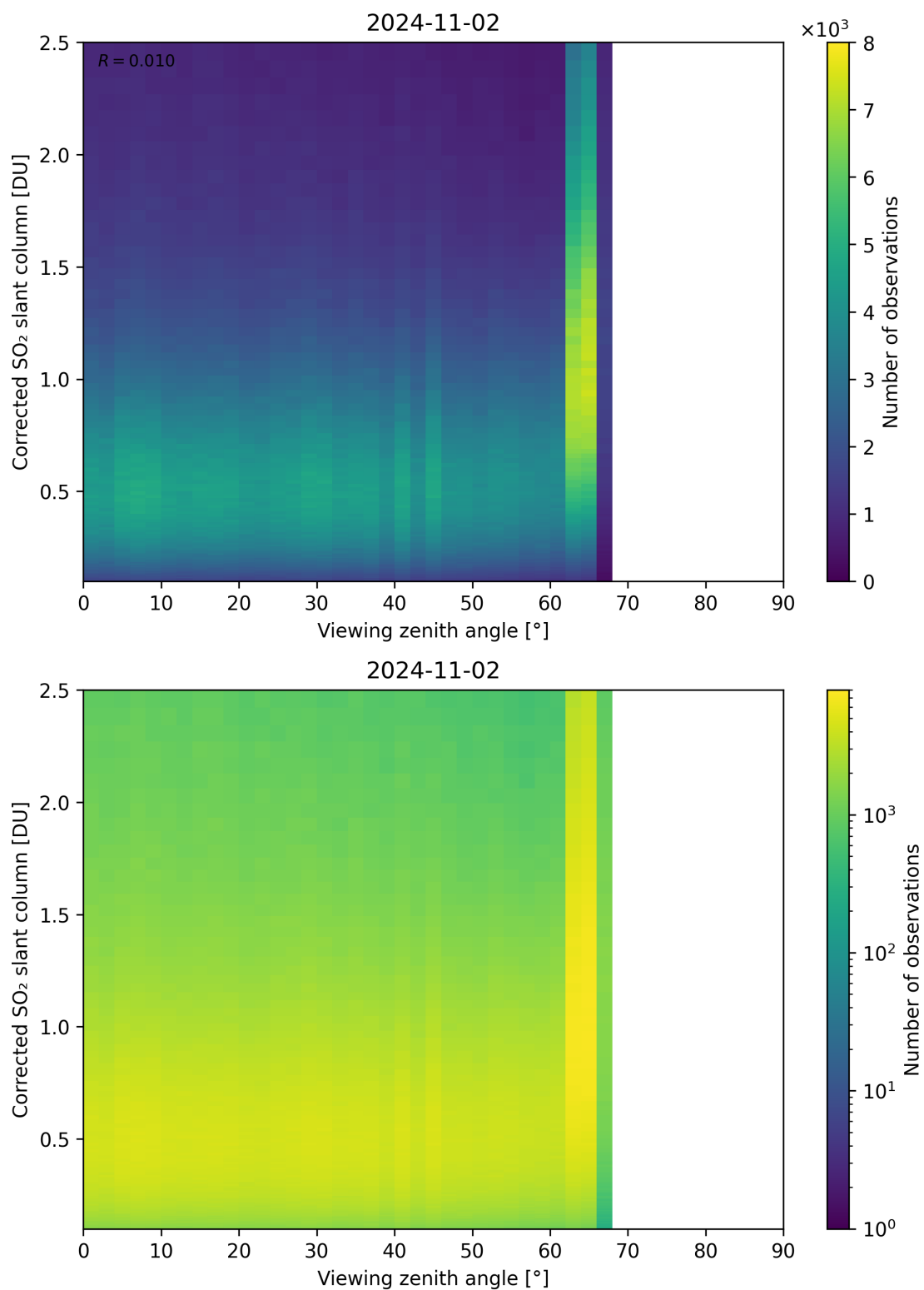
Figure 317: Scatter density plot of “Viewing zenith angle” against “Corrected SO 2 slant column” for 2024-11-01 to 2024-11-03.
