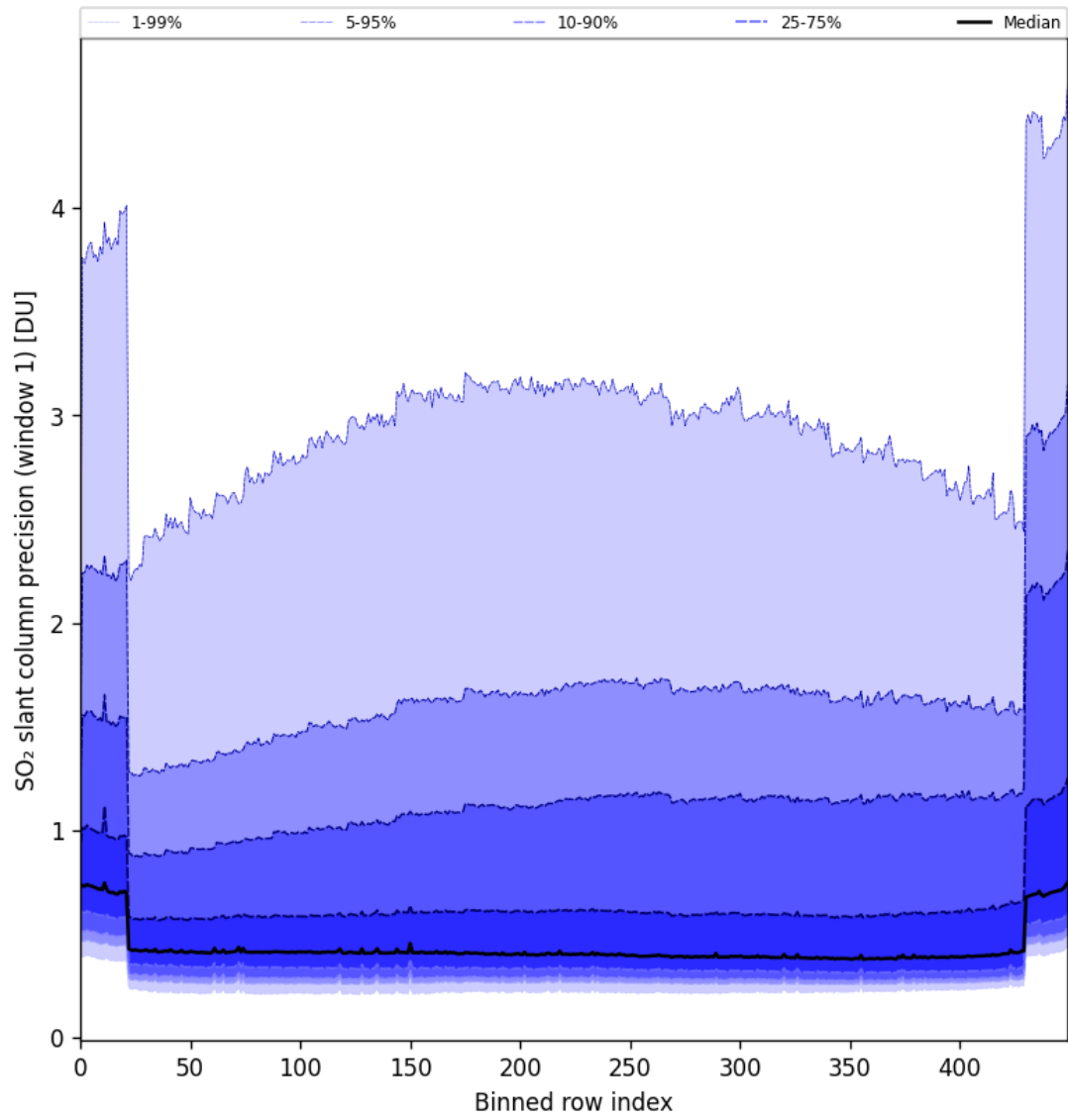
Figure 80: Along track statistics of “SO 2 slant column precision (window 1)” for 2024-11-01 to 2024-11-03
