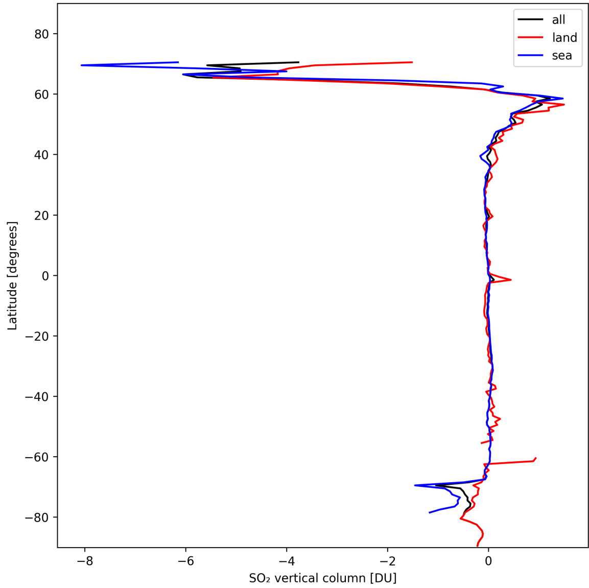
Figure 30: Zonal average of “SO 2 vertical column” for 2024-11-01 to 2024-11-03.
