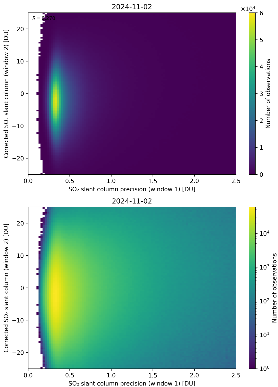
Figure 225: Scatter density plot of “SO 2 slant column precision (window 1)” against “Corrected SO 2 slant column (window 2)” for 2024-11-01 to 2024-11-03.
