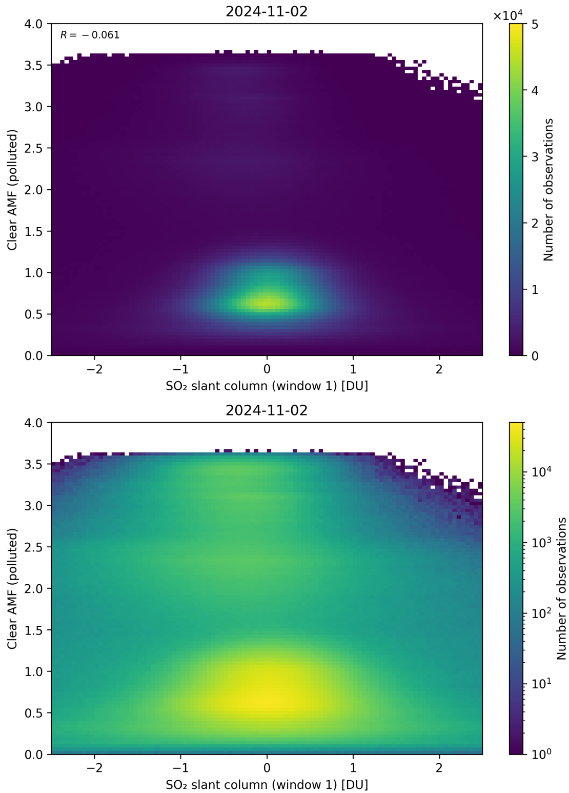
Figure 232: Scatter density plot of “SO 2 slant column (window 1)” against “Clear AMF (polluted)” for 2024-11-01 to 2024-11-03.
