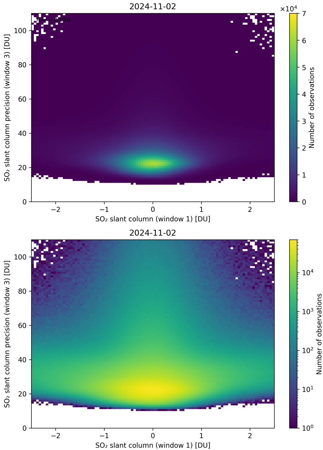
Figure 238: Scatter density plot of “SO 2 slant column (window 1)” against “SO 2 slant column precision (window 3)” for 2024-11-01 to 2024-11-03.
