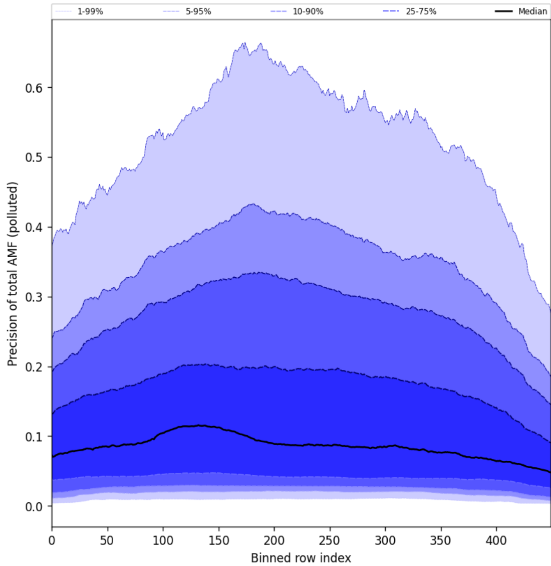
Figure 95: Along track statistics of “Precision of total AMF (polluted)” for 2024-11-01 to 2024-11-03
