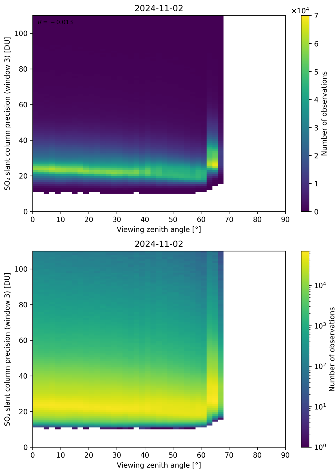
Figure 324: Scatter density plot of “Viewing zenith angle” against “SO 2 slant column precision (window 3)” for 2024-11-01 to 2024-11-03.
