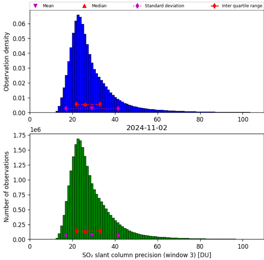
Figure 65: Histogram of “SO 2 slant column precision (window 3)” for 2024-11-01 to 2024-11-03
