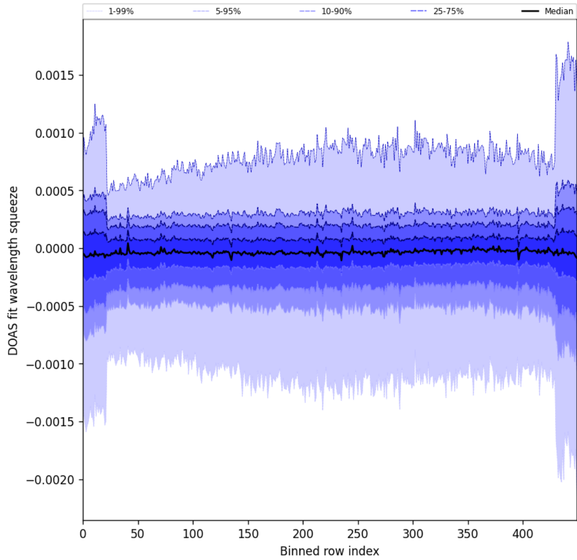
Figure 92: Along track statistics of “DOAS fit wavelength squeeze” for 2024-11-01 to 2024-11-03
