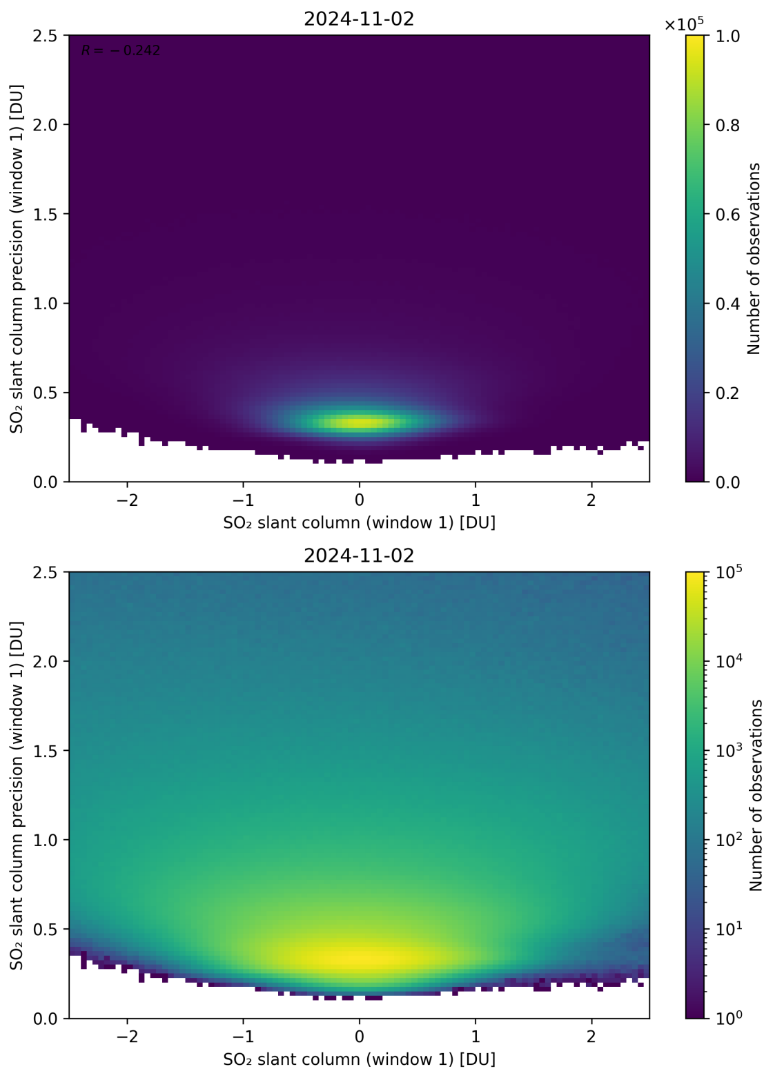
Figure 235: Scatter density plot of “SO 2 slant column (window 1)” against “SO 2 slant column precision (window 1)” for 2024-11-01 to 2024-11-03.
