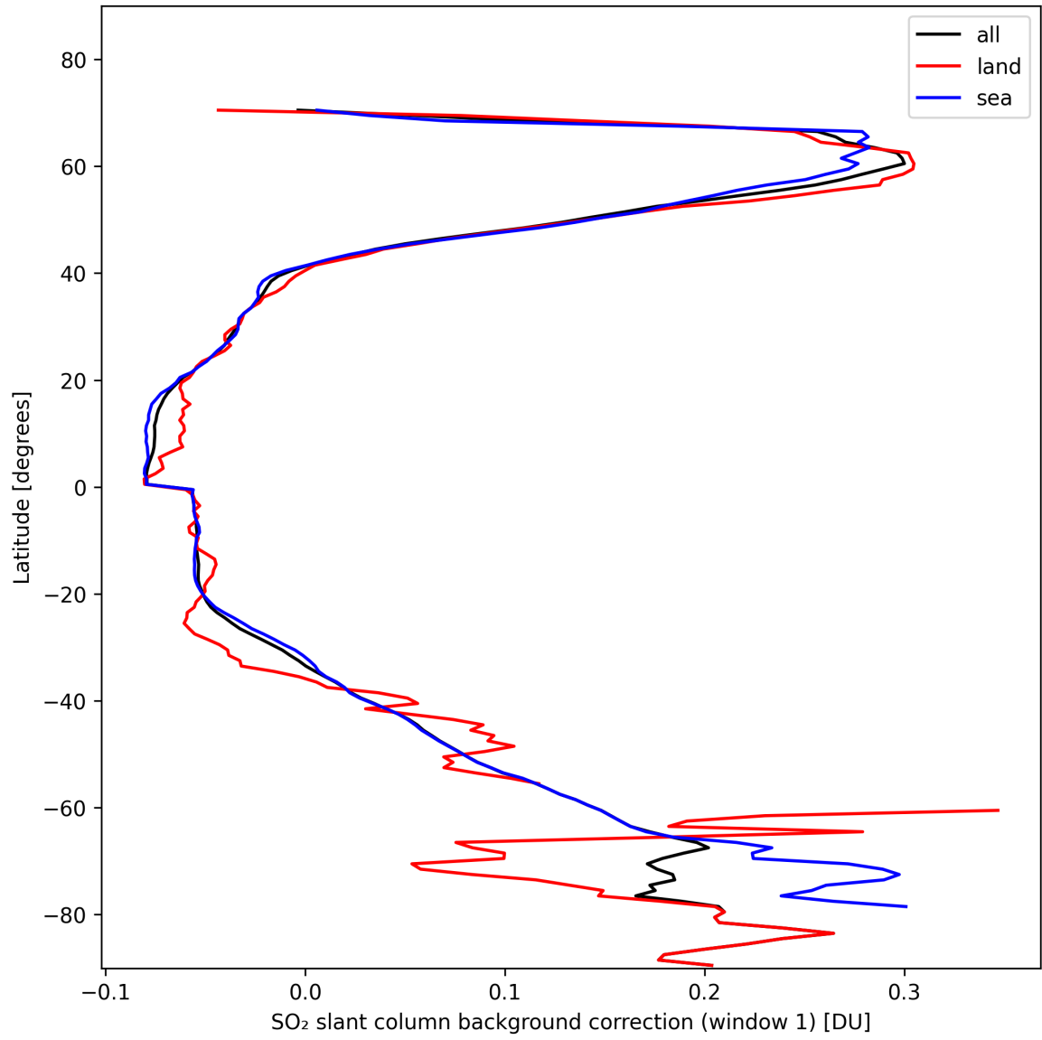
Figure 36: Zonal average of “SO 2 slant column background correction (window 1)” for 2024-11-01 to 2024-11-03.
