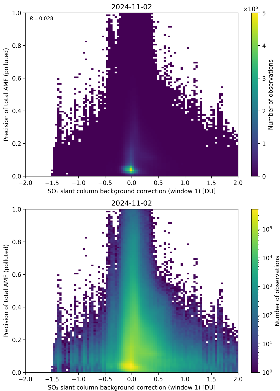
Figure 110: Scatter density plot of “SO 2 slant column background correction (window 1)” against “Precision of total AMF (polluted)” for 2024-11-01 to 2024-11-03.
