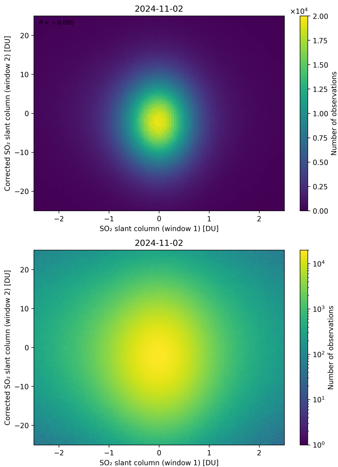
Figure 233: Scatter density plot of “SO 2 slant column (window 1)” against “Corrected SO 2 slant column (window 2)” for 2024-11-01 to 2024-11-03.
