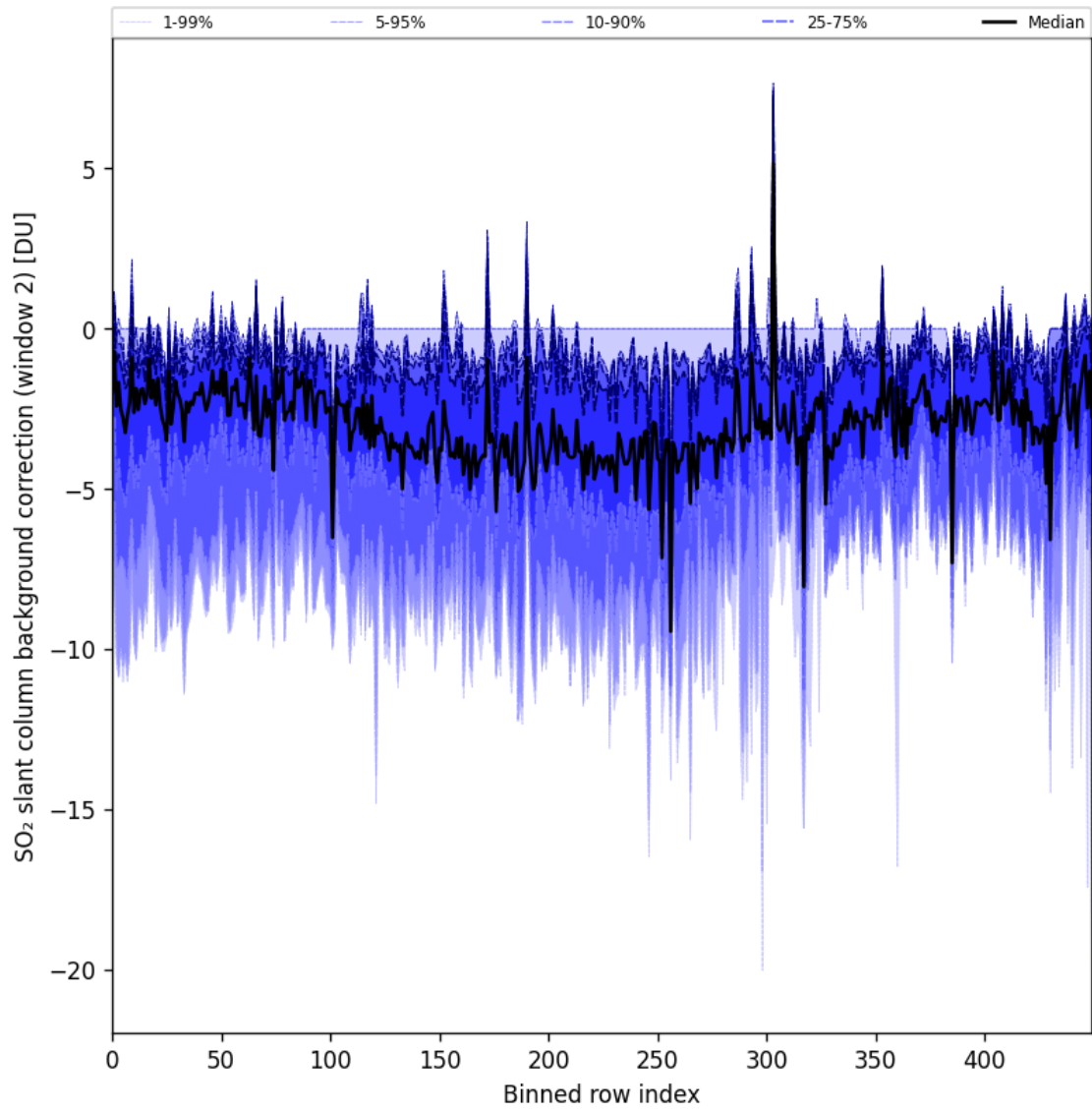
Figure 86: Along track statistics of “SO 2 slant column background correction (window 2)” for 2024-11-01 to 2024-11-03
