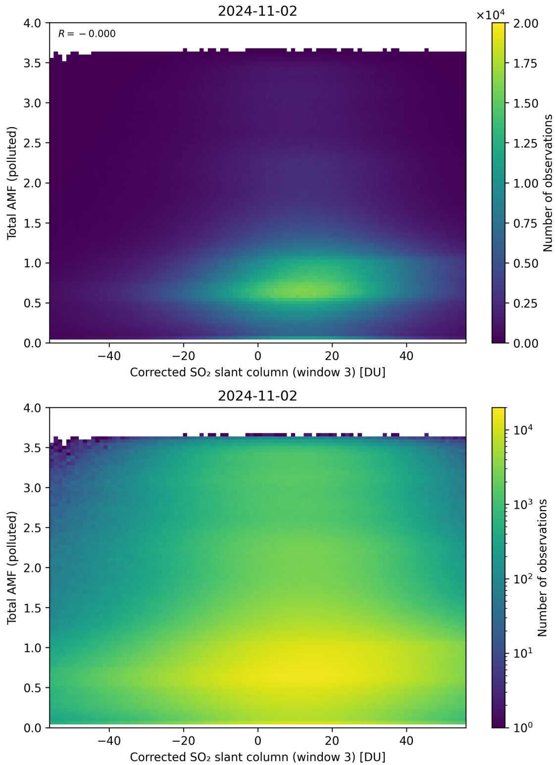
Figure 210: Scatter density plot of “Corrected SO 2 slant column (window 3)” against “Total AMF (polluted)” for 2024-11-01 to 2024-11-03.
