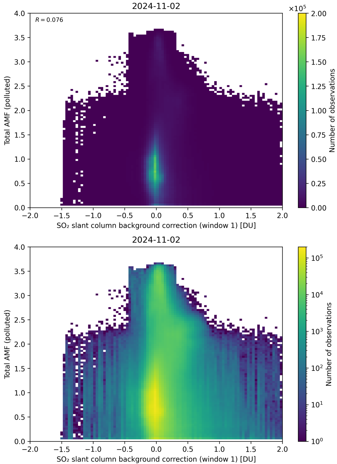
Figure 109: Scatter density plot of “SO 2 slant column background correction (window 1)” against “Total AMF (polluted)” for 2024-11-01 to 2024-11-03.
