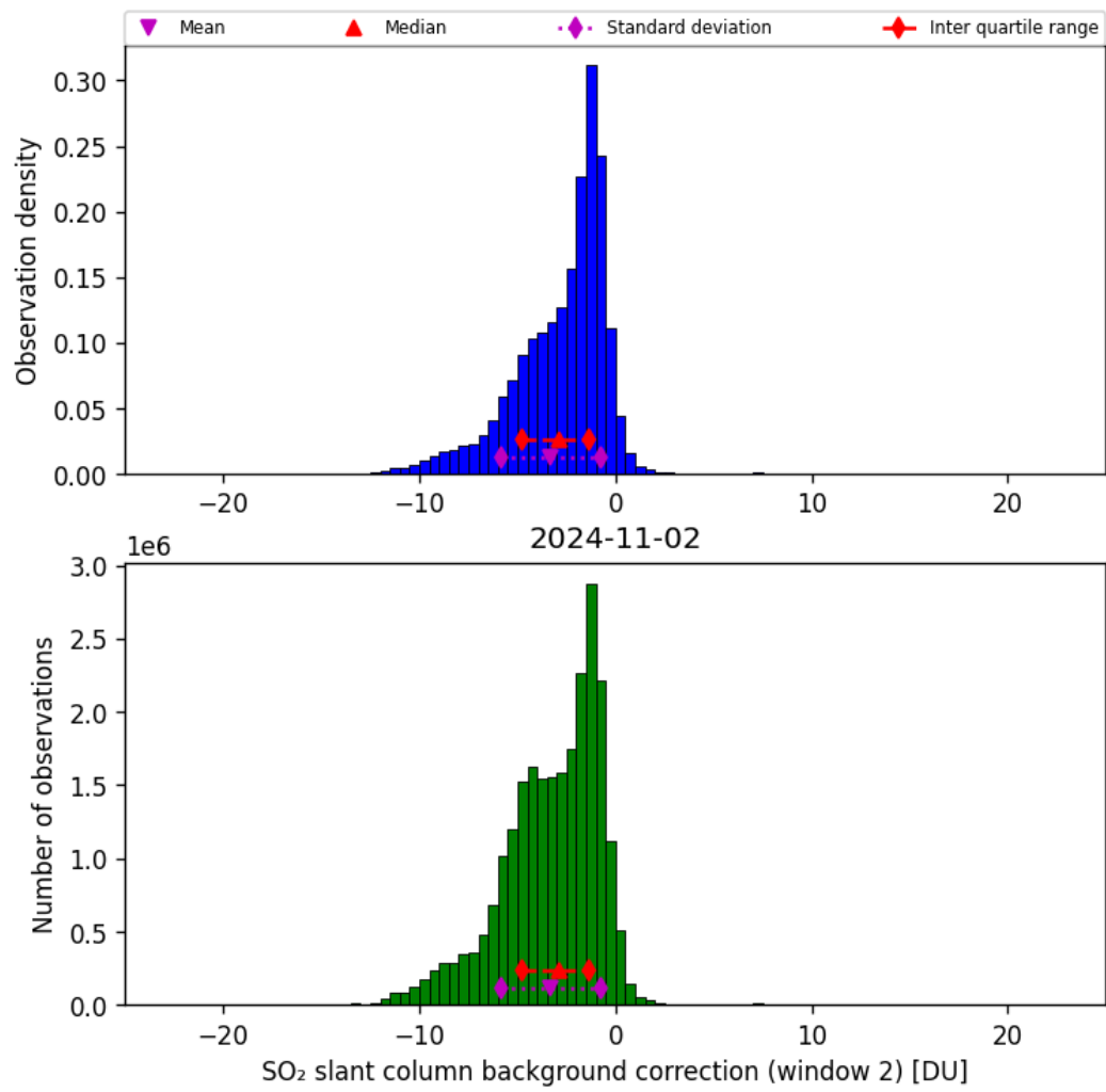
Figure 63: Histogram of “SO 2 slant column background correction (window 2)” for 2024-11-01 to 2024-11-03
