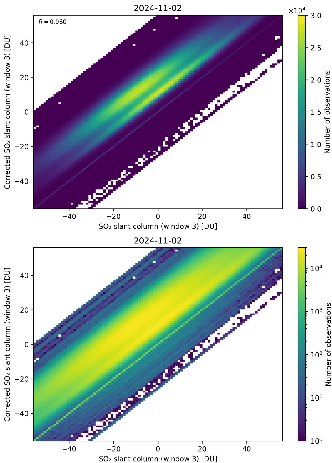
Figure 266: Scatter density plot of “SO 2 slant column (window 3)” against “Corrected SO 2 slant column (window 3)” for 2024-11-01 to 2024-11-03.
