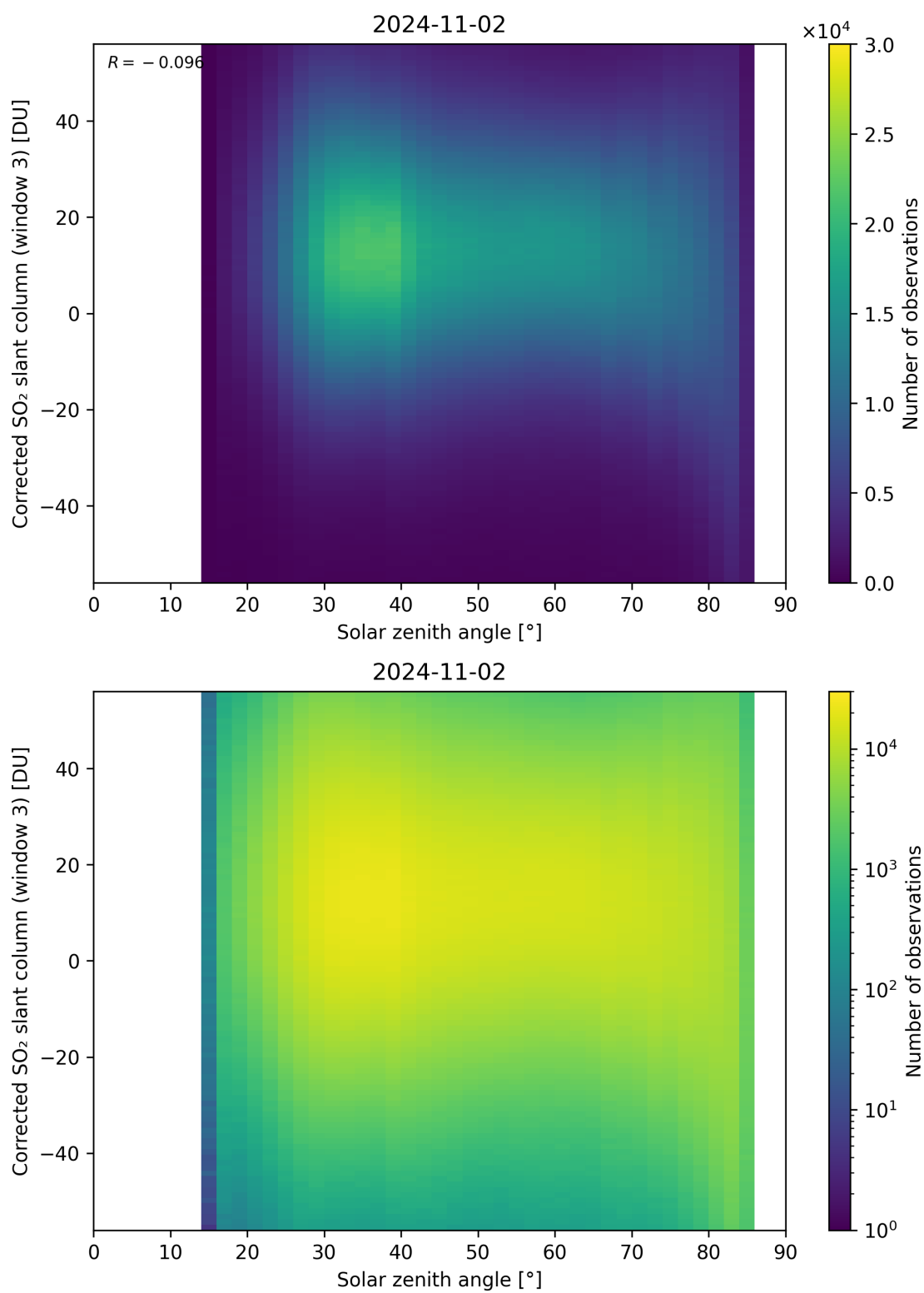
Figure 168: Scatter density plot of “Solar zenith angle” against “Corrected SO 2 slant column (window 3)” for 2024-11-01 to 2024-11-03.
