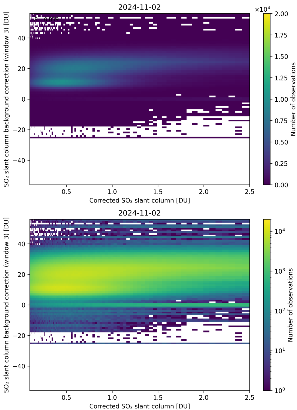
Figure 180: Scatter density plot of “Corrected SO 2 slant column” against “SO 2 slant column background correction (window 3)” for 2024-11-01 to 2024-11-03.
