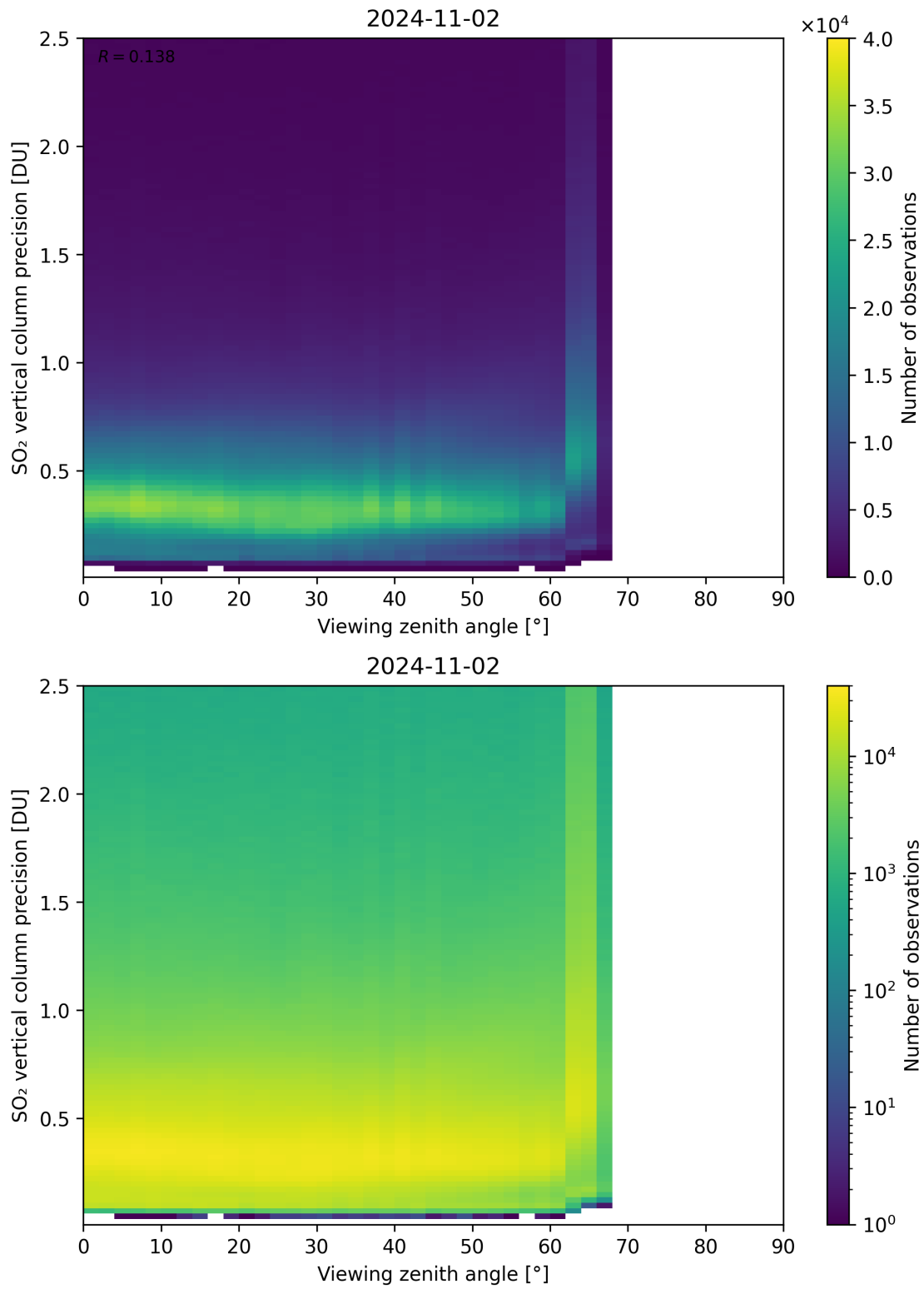
Figure 328: Scatter density plot of “Viewing zenith angle” against “SO 2 vertical column precision” for 2024-11-01 to 2024-11-03.
