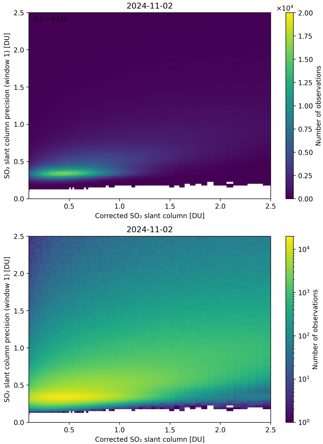
Figure 188: Scatter density plot of “Corrected SO 2 slant column” against “SO 2 slant column precision (window 1)” for 2024-11-01 to 2024-11-03.
