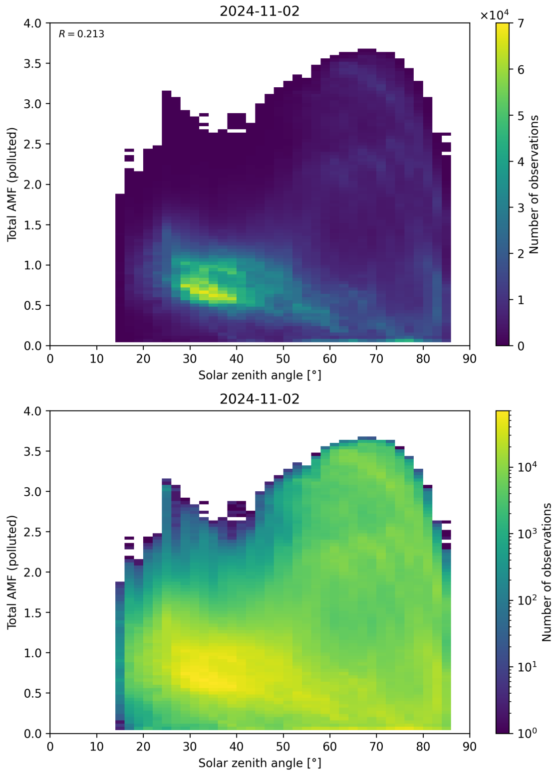
Figure 174: Scatter density plot of “Solar zenith angle” against “Total AMF (polluted)” for 2024-11-01 to 2024-11-03.
