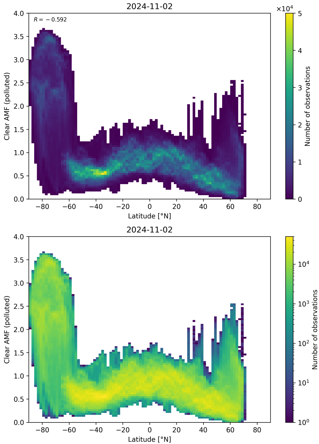
Figure 145: Scatter density plot of “Latitude” against “Clear AMF (polluted)” for 2024-11-01 to 2024-11-03.
