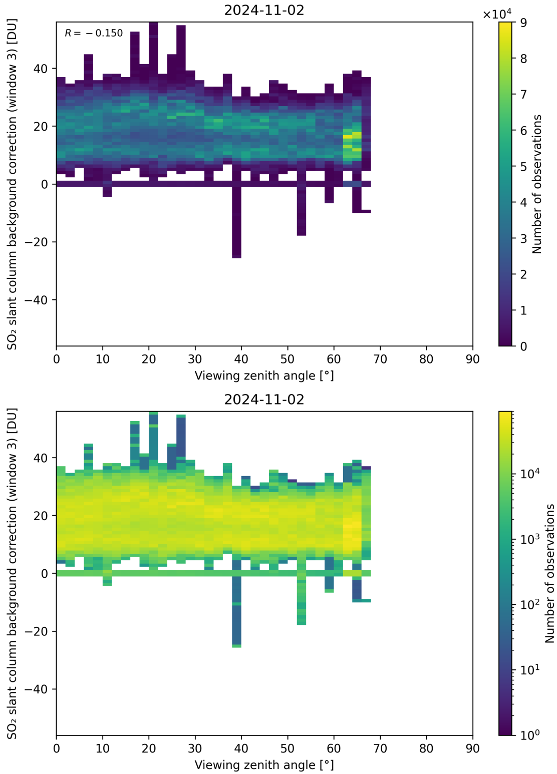
Figure 310: Scatter density plot of “Viewing zenith angle” against “SO 2 slant column background correction (window 3)” for 2024-11-01 to 2024-11-03.
