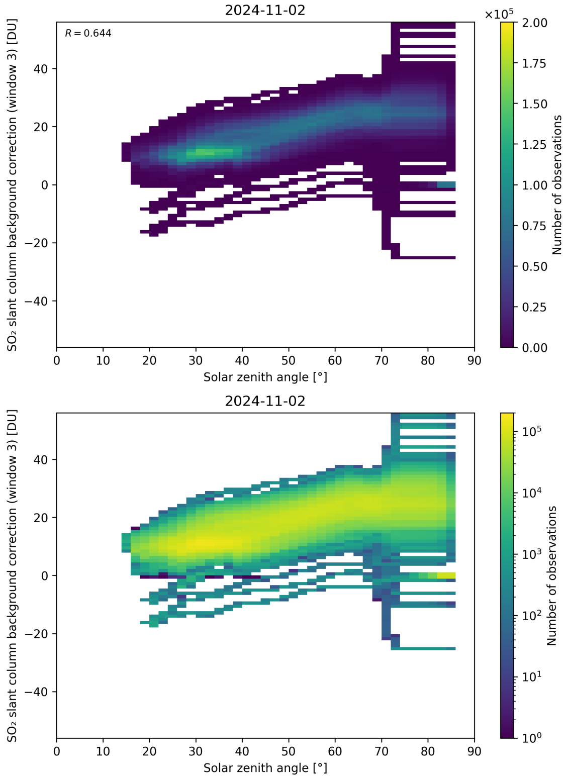
Figure 160: Scatter density plot of “Solar zenith angle” against “SO 2 slant column background correction (window 3)” for 2024-11-01 to 2024-11-03.
