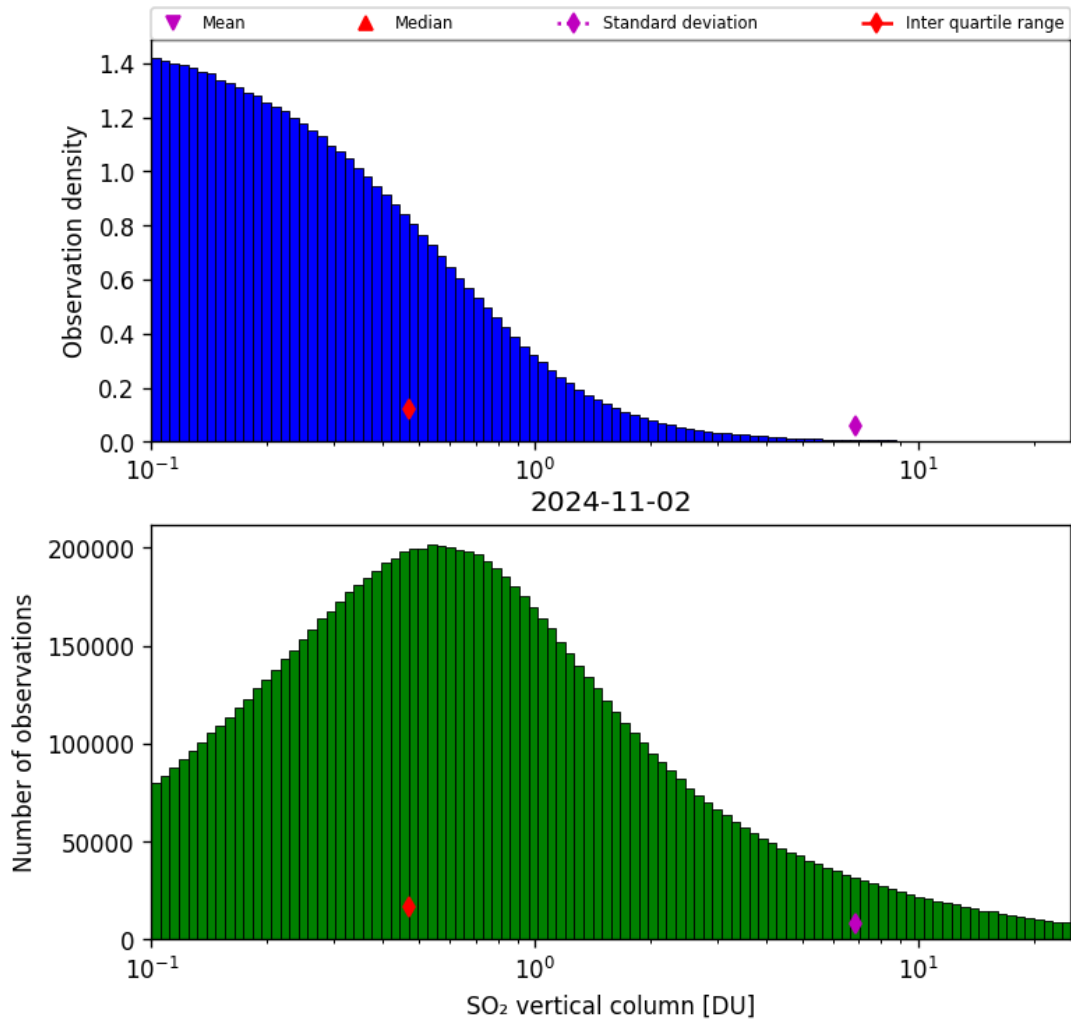
Figure 53: Histogram of “SO 2 vertical column” for 2024-11-01 to 2024-11-03
