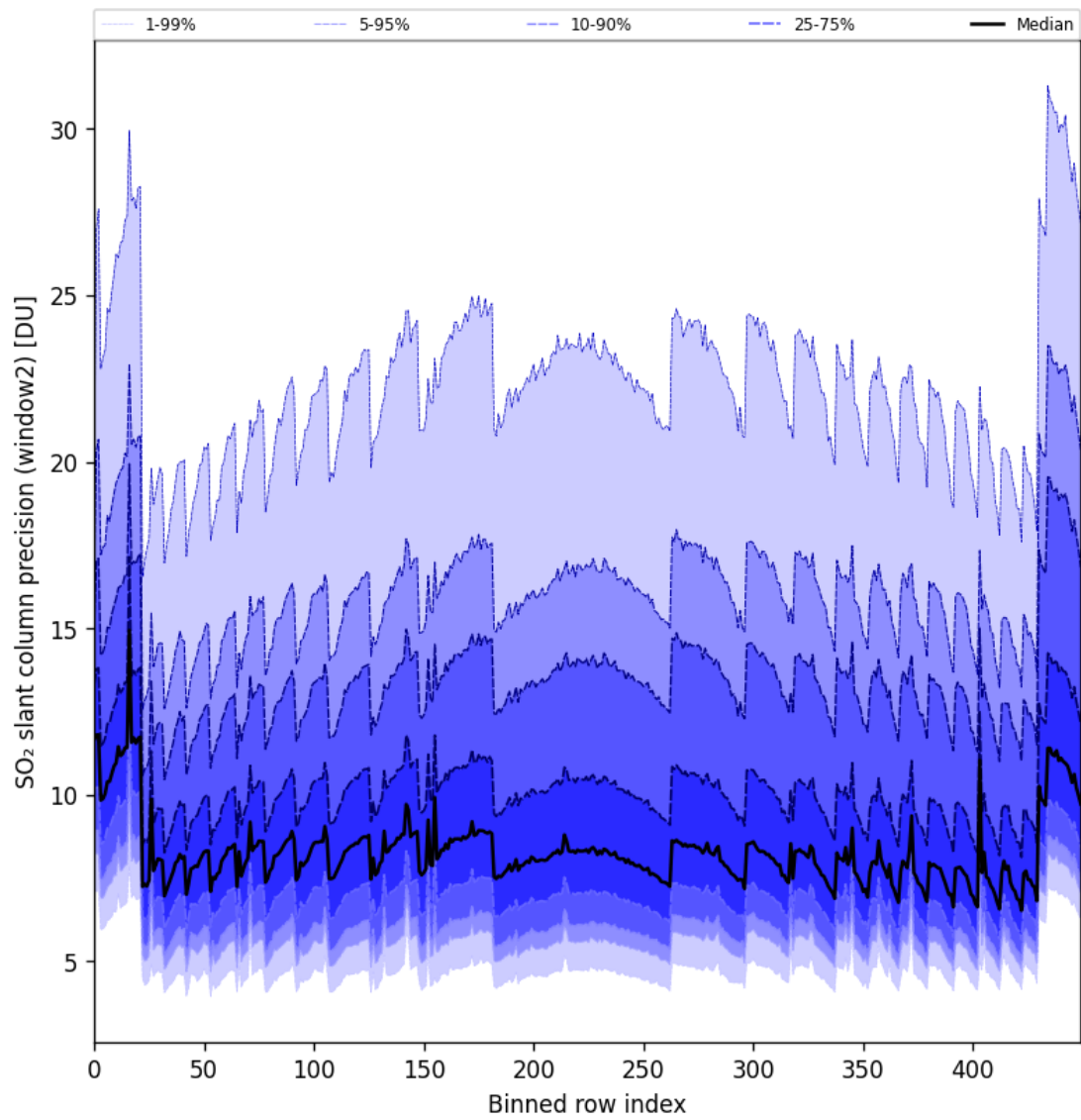
Figure 84: Along track statistics of “SO 2 slant column precision (window2)” for 2024-11-01 to 2024-11-03
