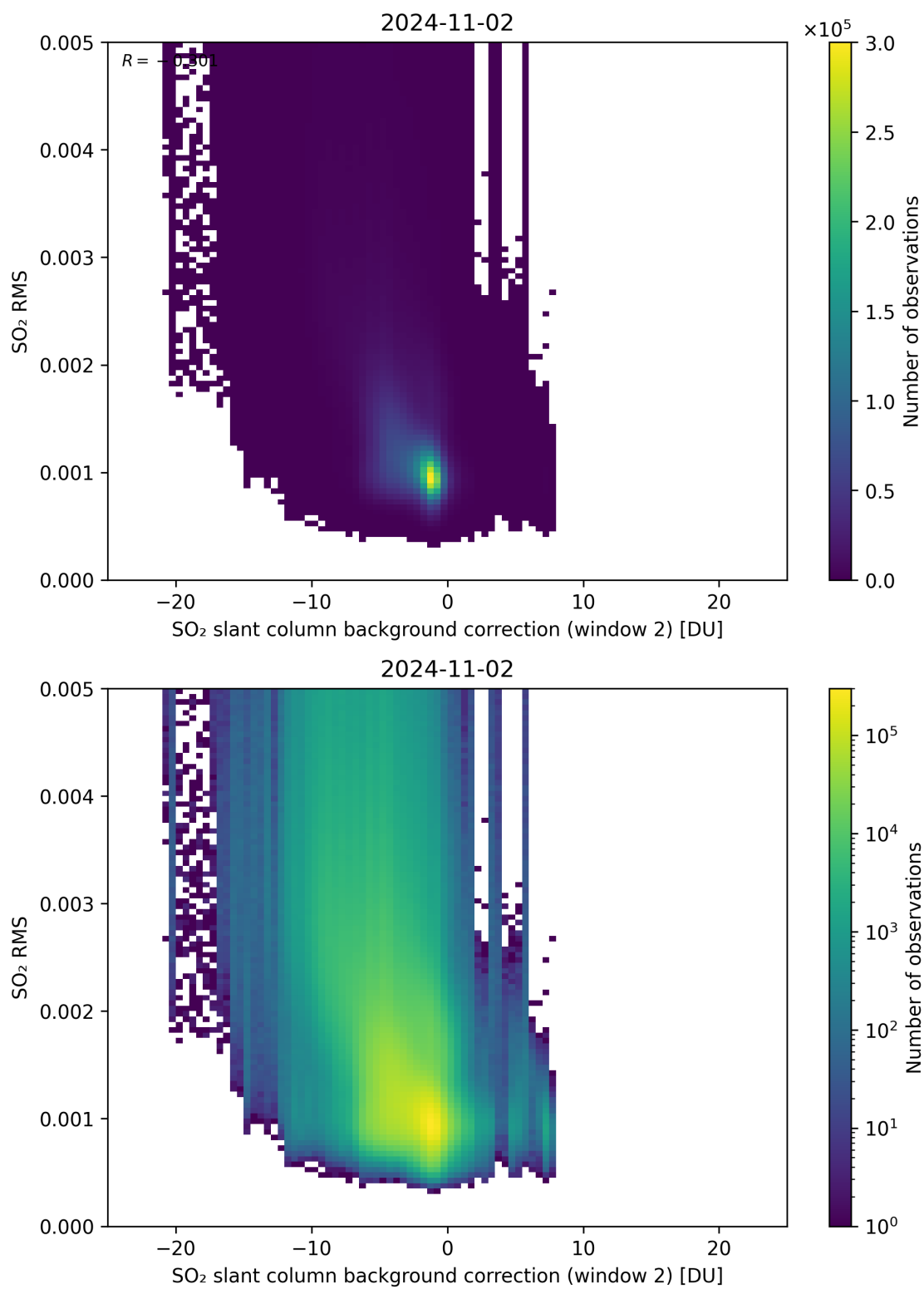
Figure 114: Scatter density plot of “SO 2 slant column background correction (window 2)” against “SO 2 RMS” for 2024-11-01 to 2024-11-03.
