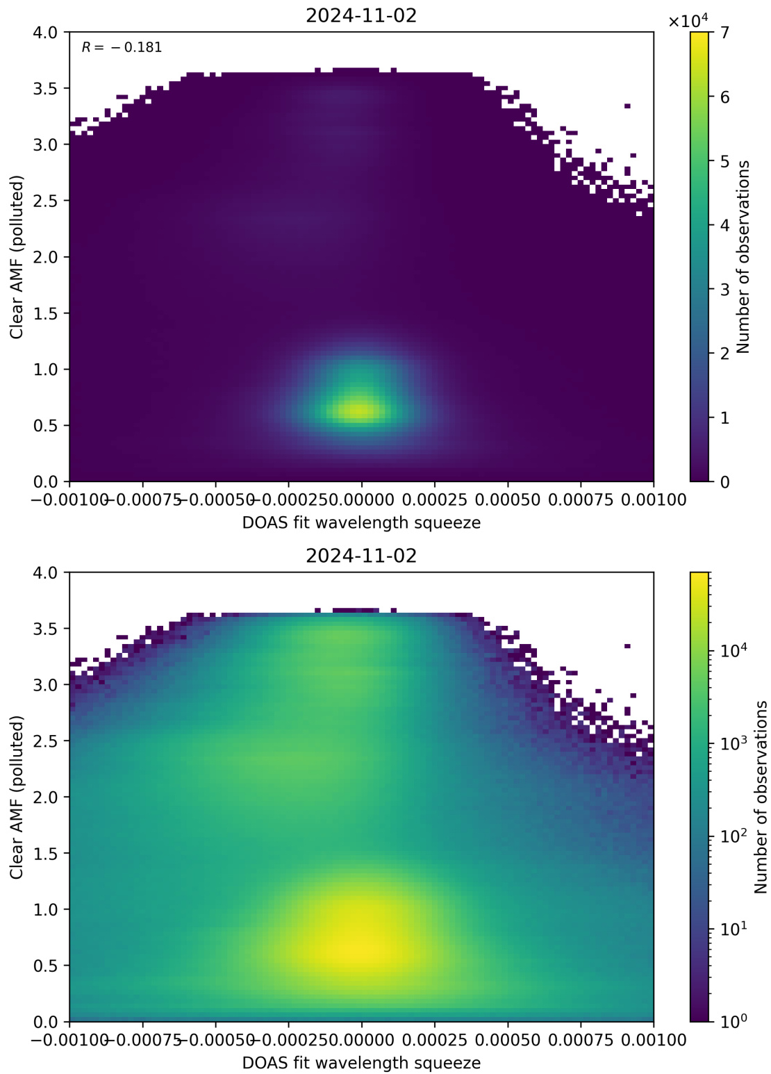
Figure 133: Scatter density plot of “DOAS fit wavelength squeeze” against “Clear AMF (polluted)” for 2024-11-01 to 2024-11-03.
