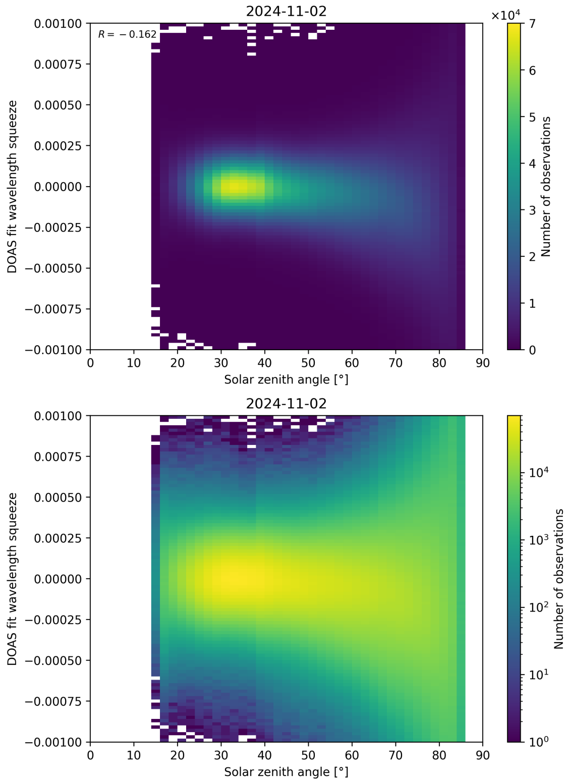
Figure 162: Scatter density plot of “Solar zenith angle” against “DOAS fit wavelength squeeze” for 2024-11-01 to 2024-11-03.
