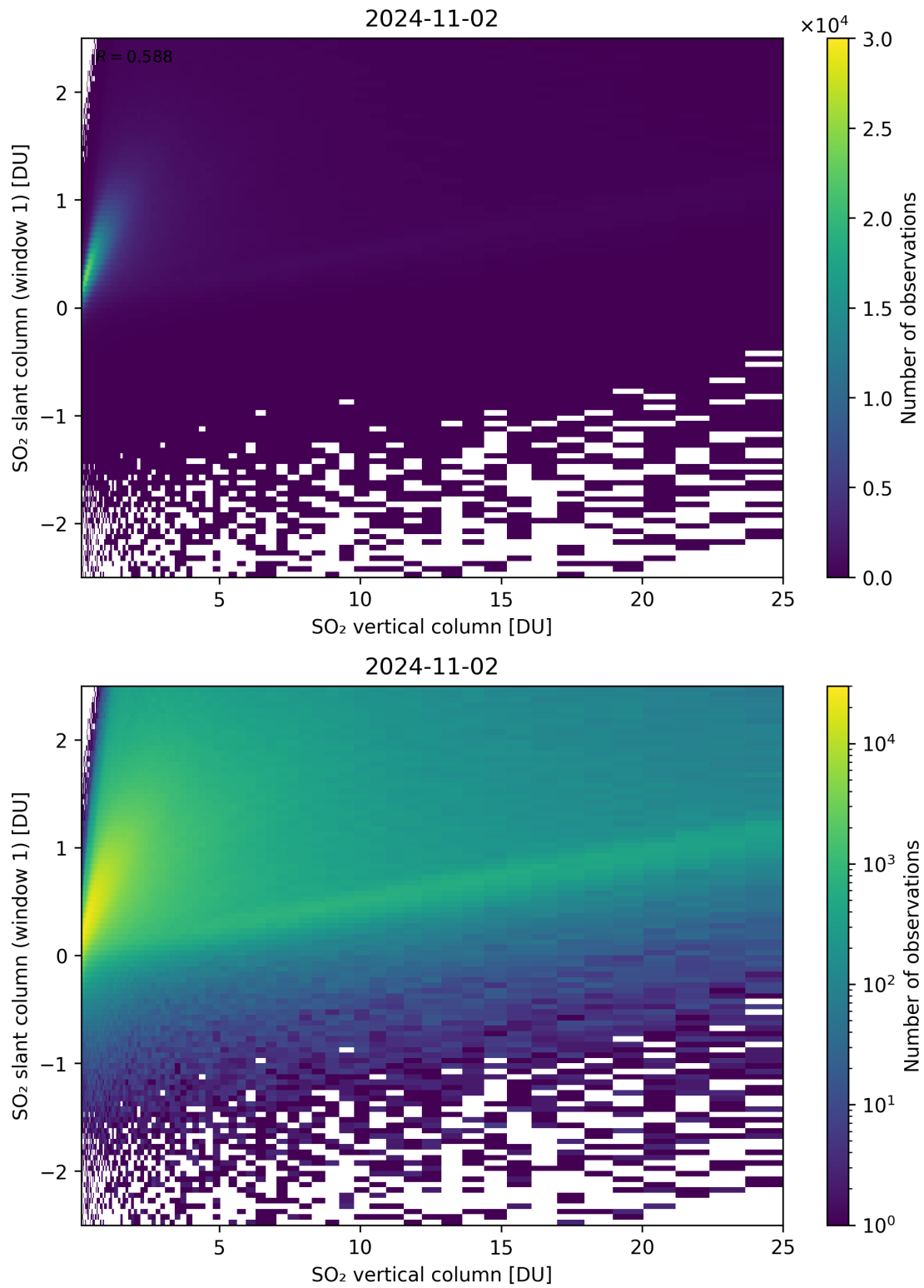
Figure 300: Scatter density plot of “SO 2 vertical column” against “SO 2 slant column (window 1)” for 2024-11-01 to 2024-11-03.
