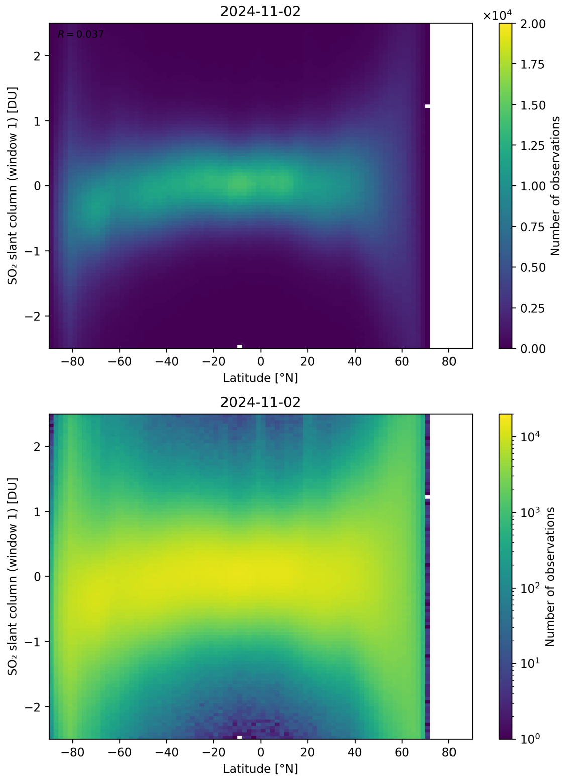
Figure 149: Scatter density plot of “Latitude” against “SO 2 slant column (window 1)” for 2024-11-01 to 2024-11-03.
