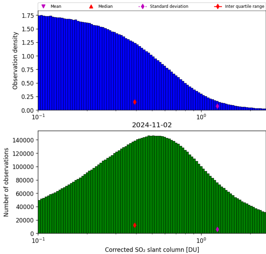
Figure 55: Histogram of “Corrected SO 2 slant column” for 2024-11-01 to 2024-11-03
