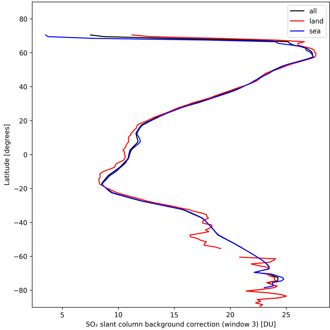
Figure 44: Zonal average of “SO 2 slant column background correction (window 3)” for 2024-11-01 to 2024-11-03.
