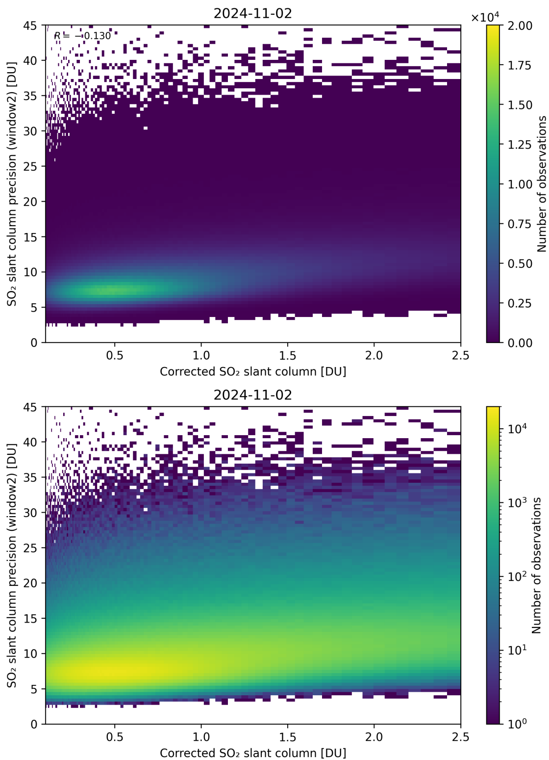
Figure 189: Scatter density plot of “Corrected SO 2 slant column” against “SO 2 slant column precision (window2)” for 2024-11-01 to 2024-11-03.
