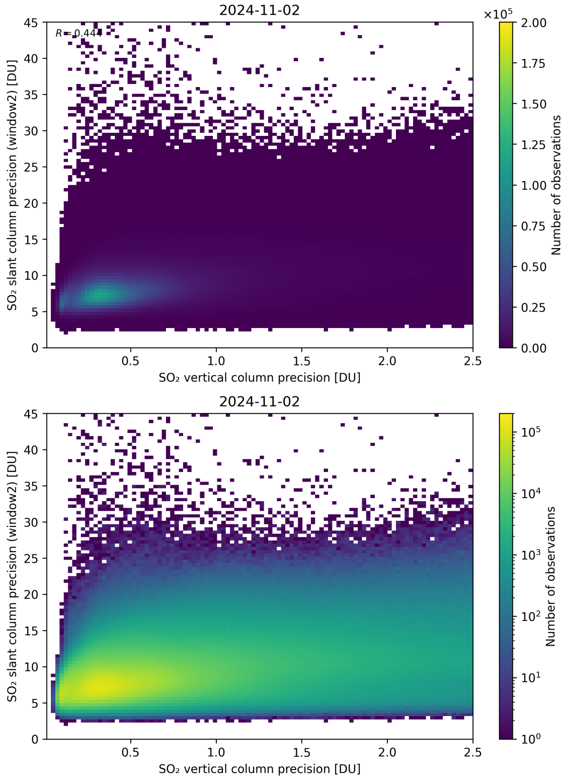
Figure 291: Scatter density plot of “SO 2 vertical column precision” against “SO 2 slant column precision (window2)” for 2024-11-01 to 2024-11-03.
