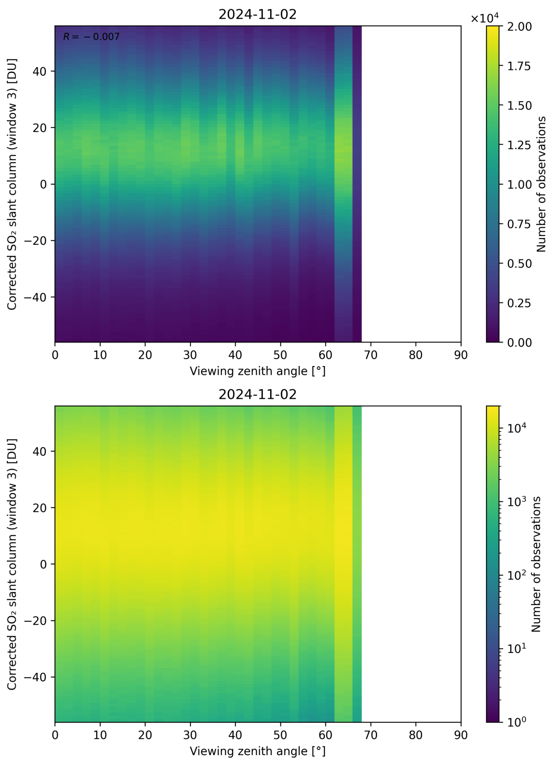
Figure 319: Scatter density plot of “Viewing zenith angle” against “Corrected SO 2 slant column (window 3)” for 2024-11-01 to 2024-11-03.
