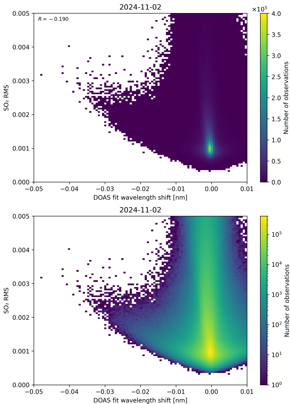
Figure 128: Scatter density plot of “DOAS fit wavelength shift” against “SO 2 RMS” for 2024-11-01 to 2024-11-03.
