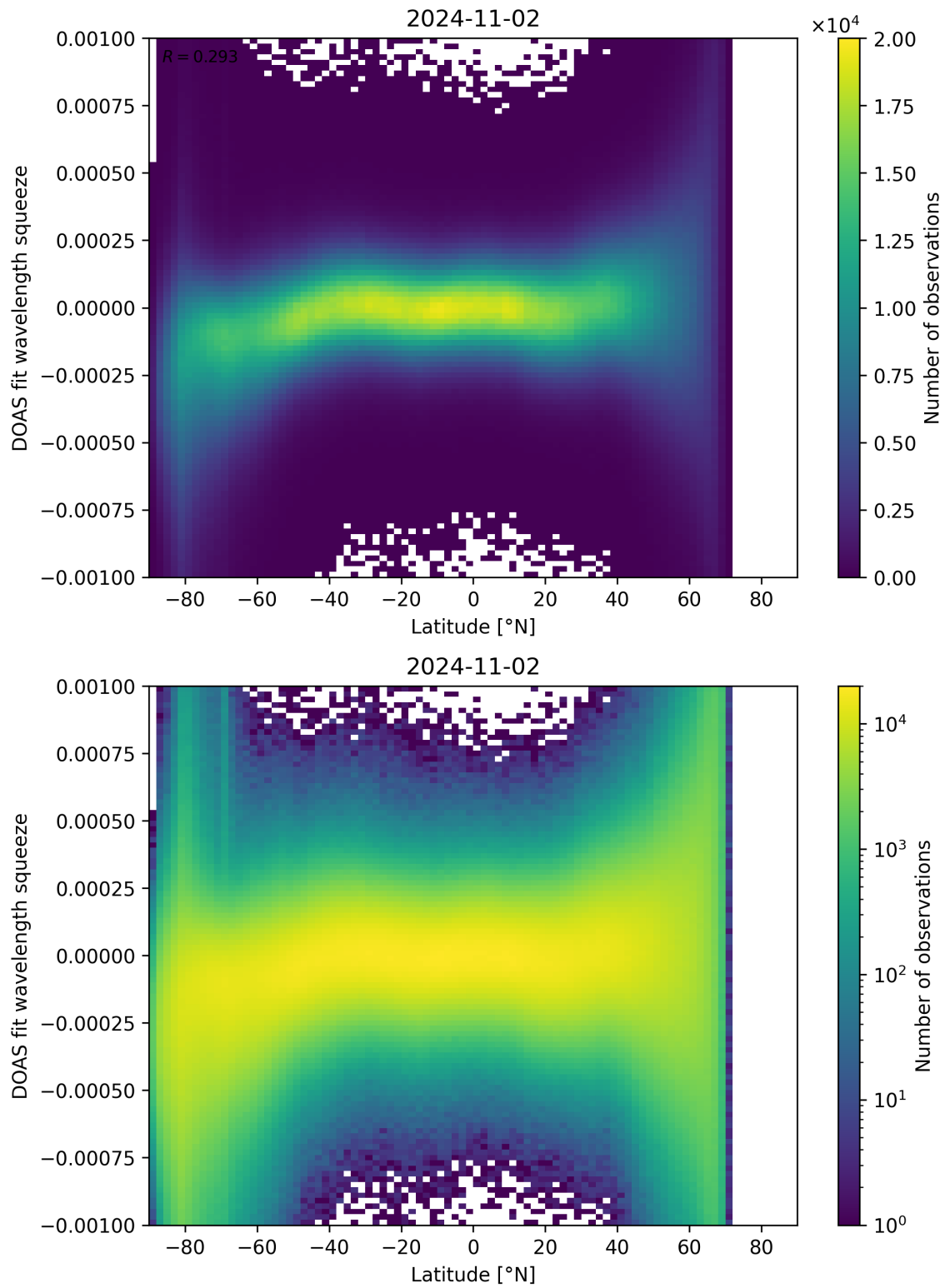
Figure 143: Scatter density plot of “Latitude” against “DOAS fit wavelength squeeze” for 2024-11-01 to 2024-11-03.
