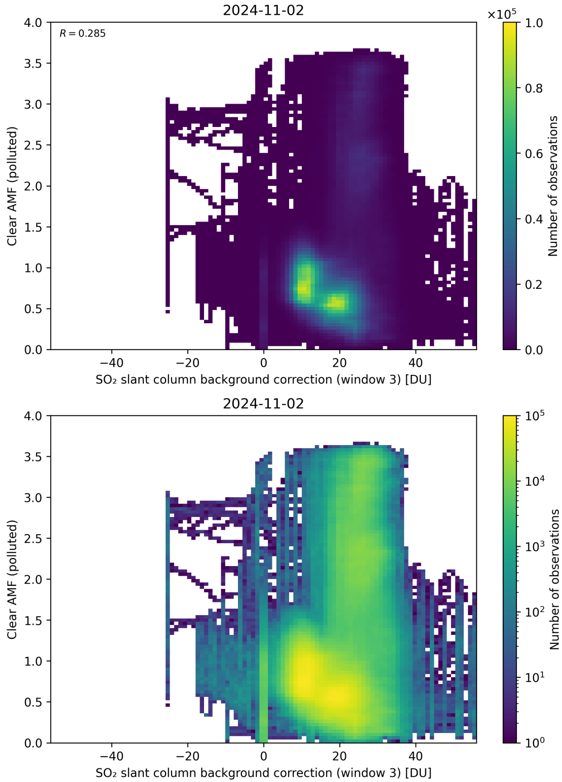
Figure 124: Scatter density plot of “SO 2 slant column background correction (window 3)” against “Clear AMF (polluted)” for 2024-11-01 to 2024-11-03.
