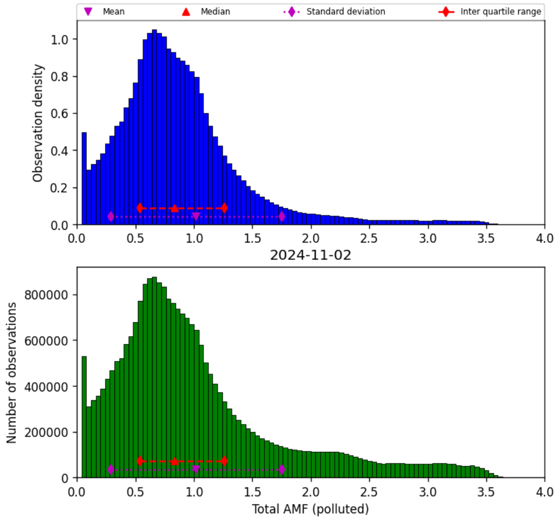
Figure 71: Histogram of “Total AMF (polluted)” for 2024-11-01 to 2024-11-03
