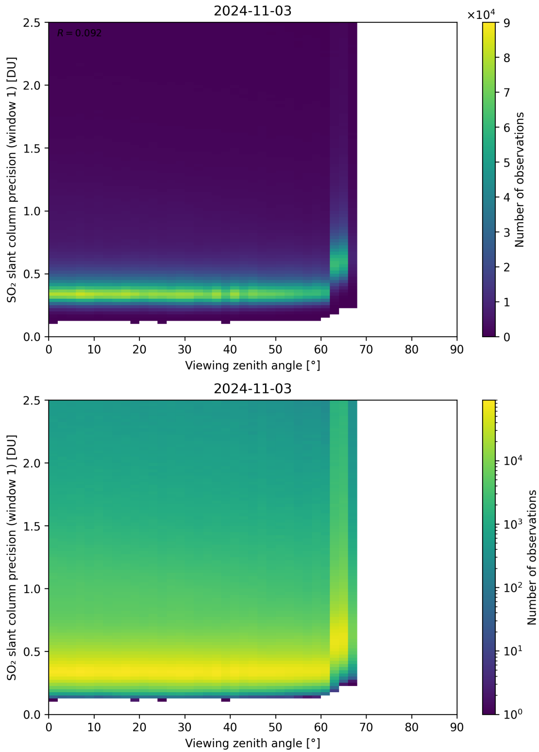
Figure 321: Scatter density plot of “Viewing zenith angle” against “SO 2 slant column precision (window 1)” for 2024-11-02 to 2024-11-04.
