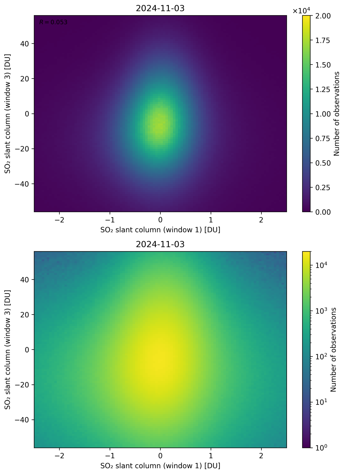
Figure 237: Scatter density plot of “SO 2 slant column (window 1)” against “SO 2 slant column (window 3)” for 2024-11-02 to 2024-11-04.
