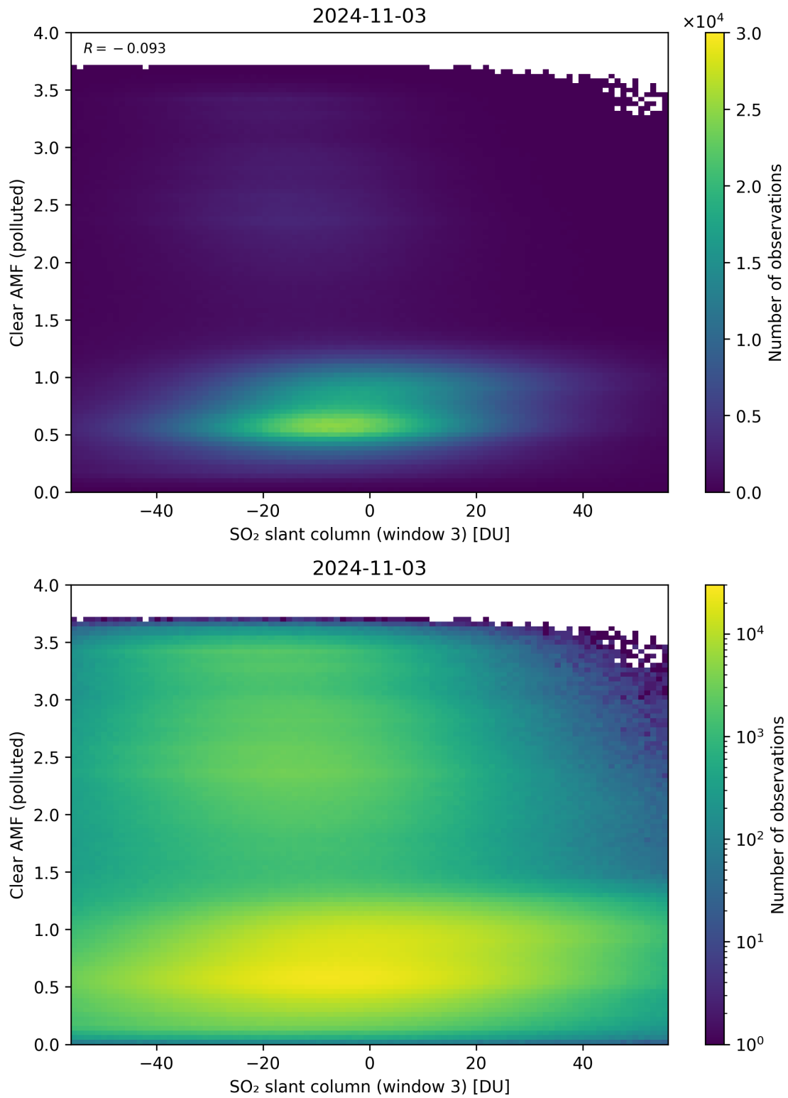
Figure 265: Scatter density plot of “SO 2 slant column (window 3)” against “Clear AMF (polluted)” for 2024-11-02 to 2024-11-04.
