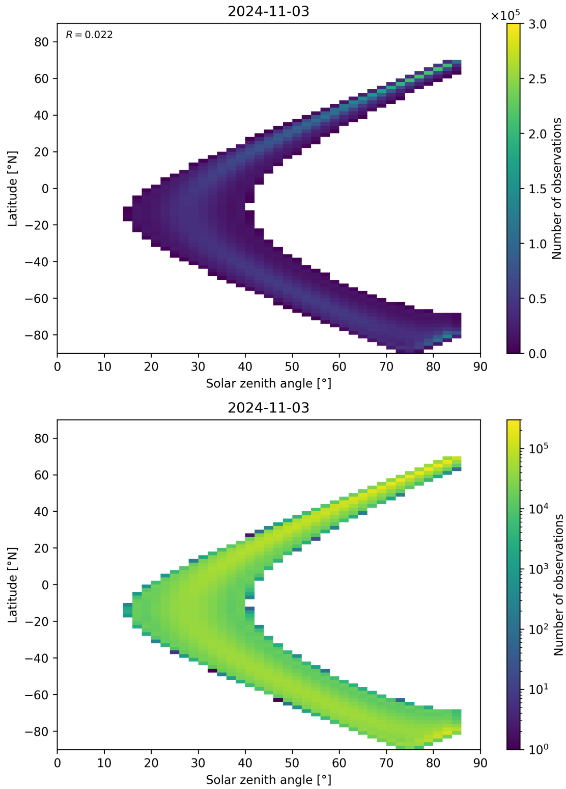
Figure 164: Scatter density plot of “Solar zenith angle” against “Latitude” for 2024-11-02 to 2024-11-04.
