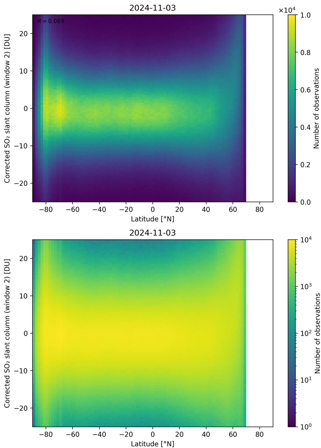
Figure 147: Scatter density plot of “Latitude” against “Corrected SO 2 slant column (window 2)” for 2024-11-02 to 2024-11-04.
