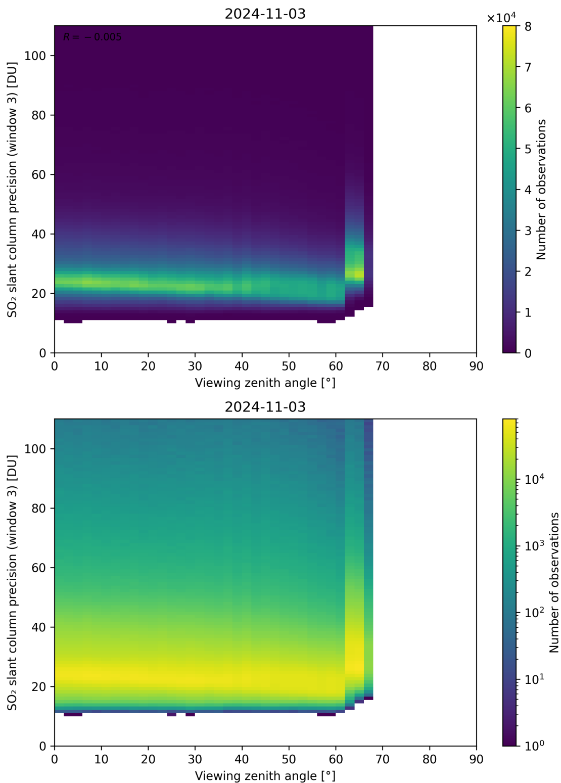
Figure 324: Scatter density plot of “Viewing zenith angle” against “SO 2 slant column precision (window 3)” for 2024-11-02 to 2024-11-04.
