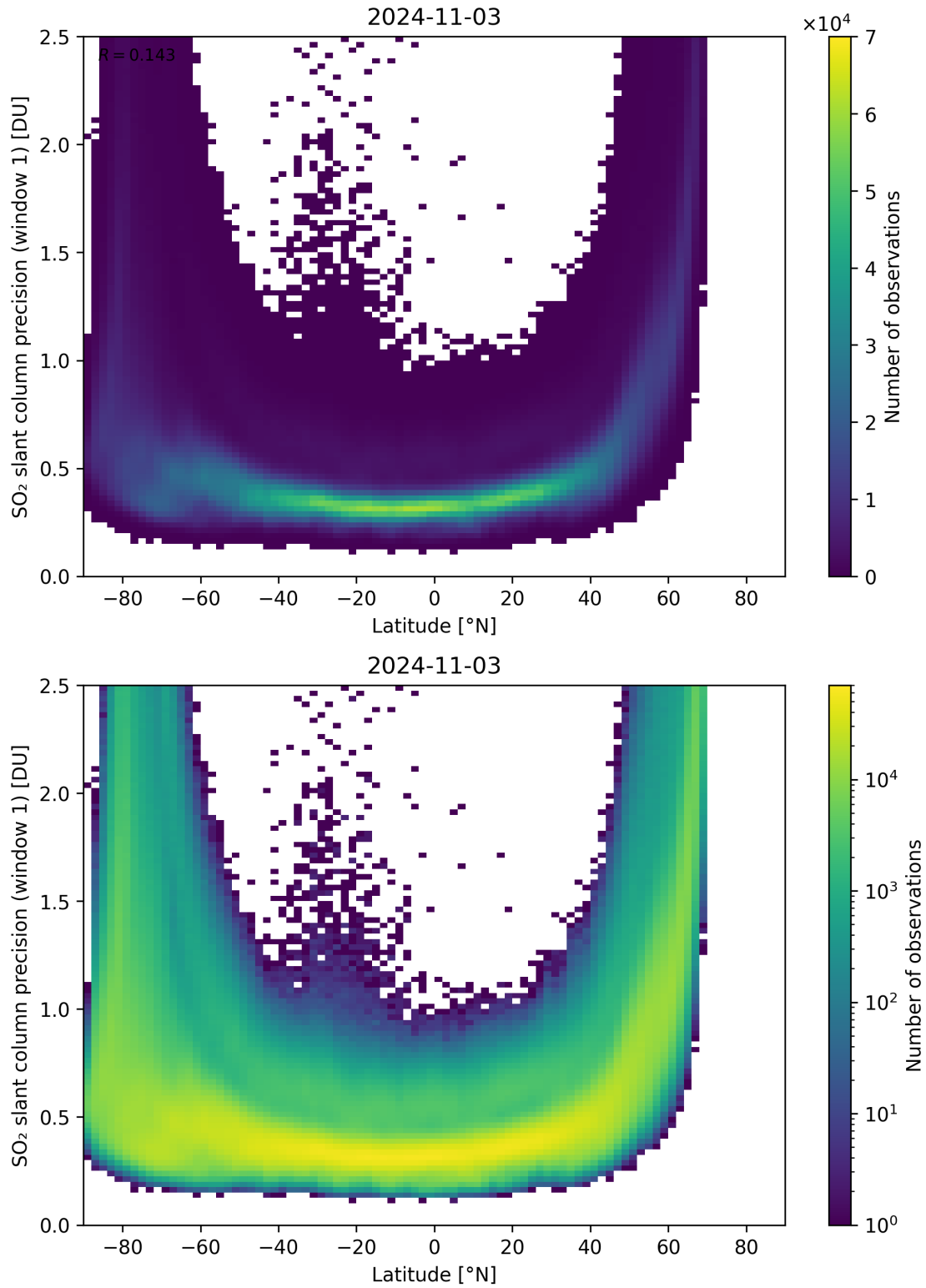
Figure 150: Scatter density plot of “Latitude” against “SO 2 slant column precision (window 1)” for 2024-11-02 to 2024-11-04.
