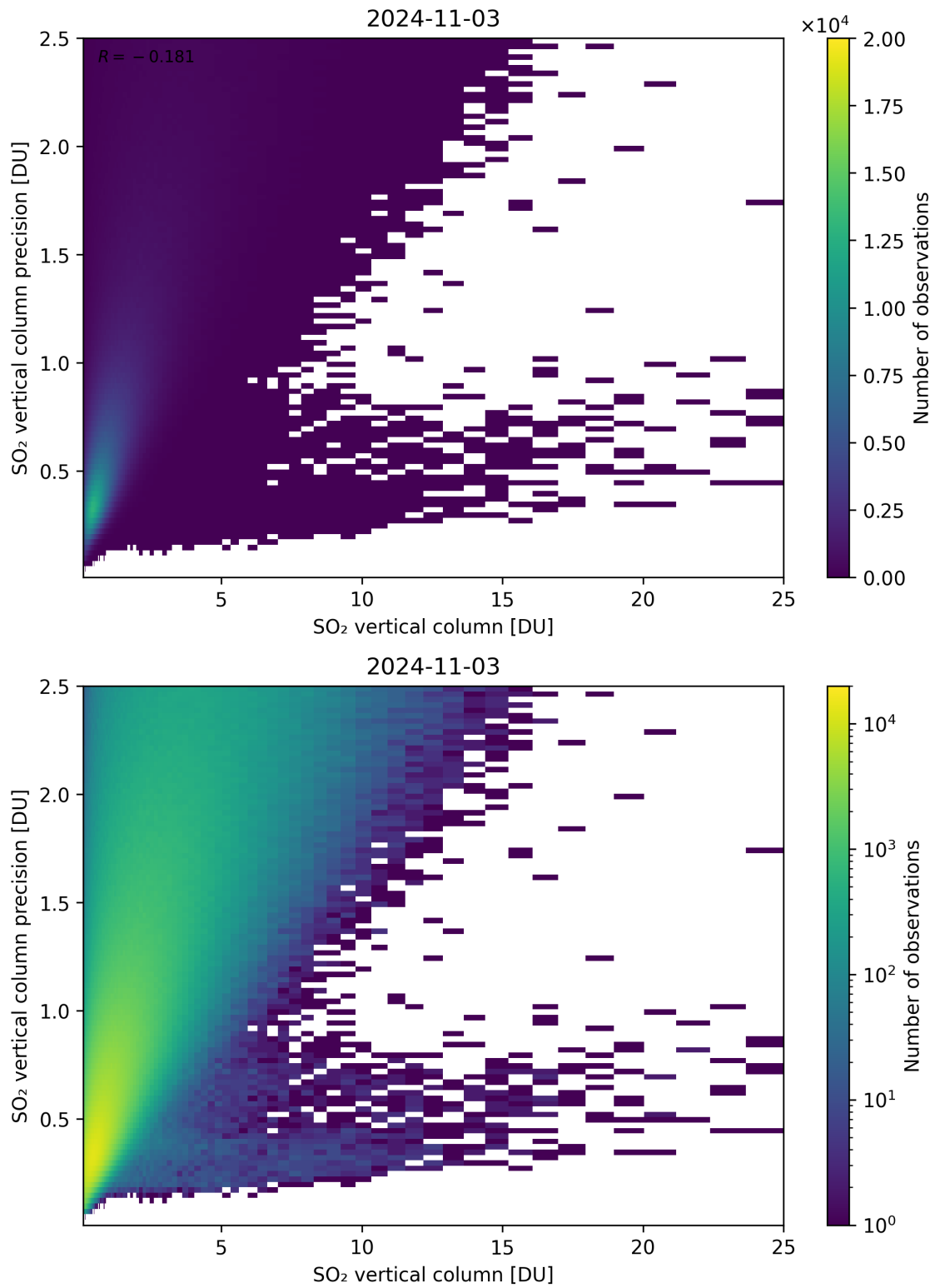
Figure 307: Scatter density plot of “SO 2 vertical column” against “SO 2 vertical column precision” for 2024-11-02 to 2024-11-04.
