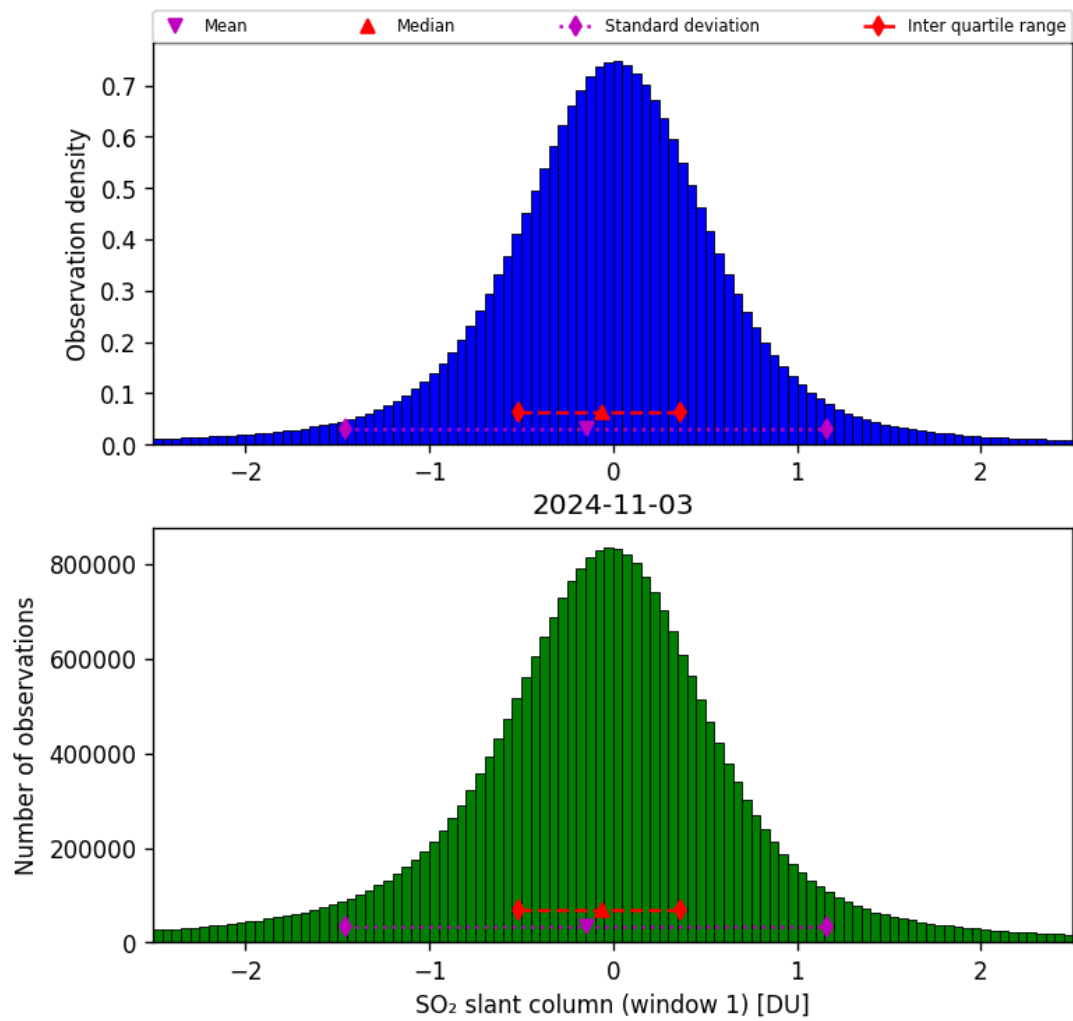
Figure 56: Histogram of “SO 2 slant column (window 1)” for 2024-11-02 to 2024-11-04
