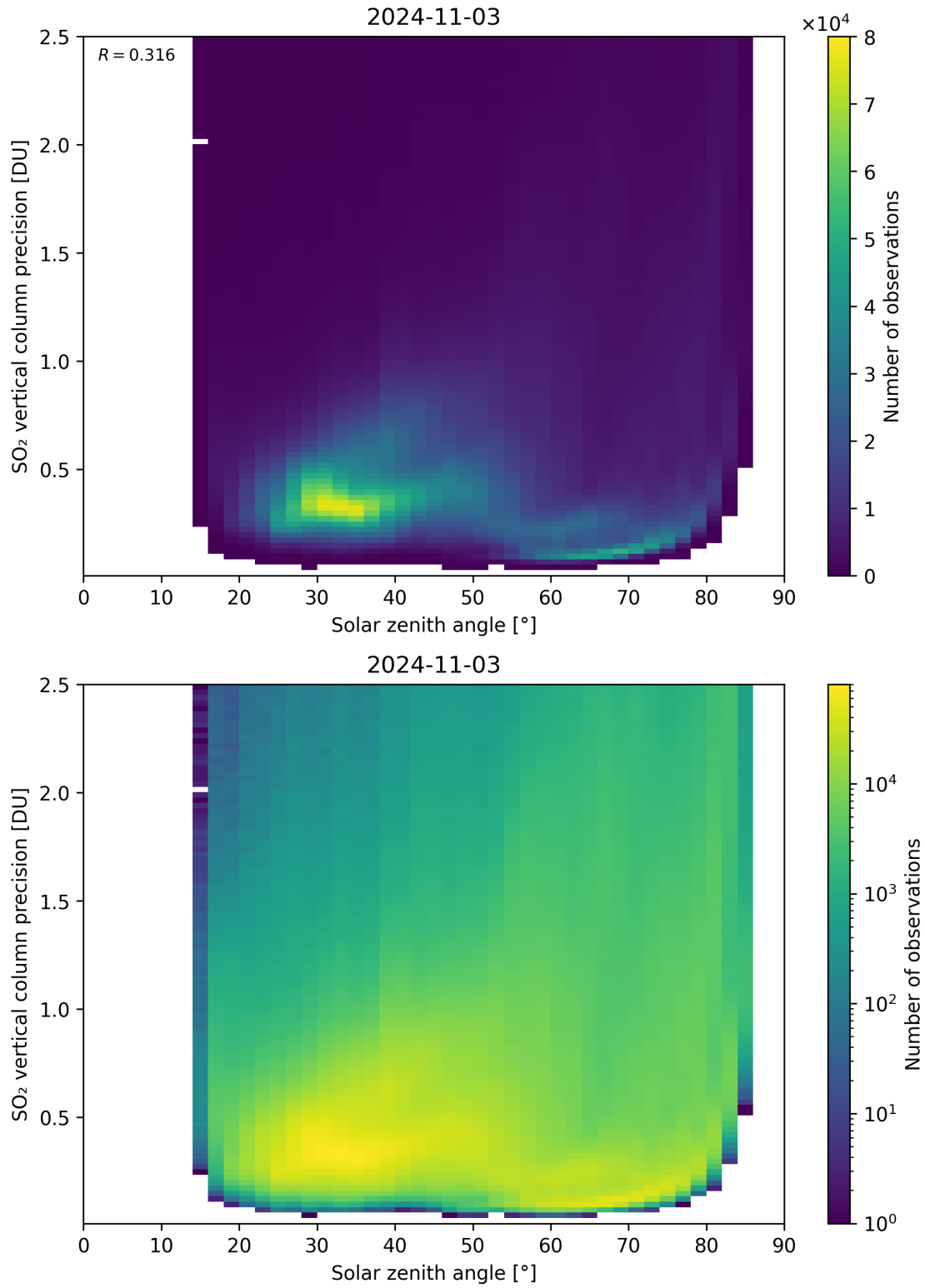
Figure 177: Scatter density plot of “Solar zenith angle” against “SO 2 vertical column precision” for 2024-11-02 to 2024-11-04.
