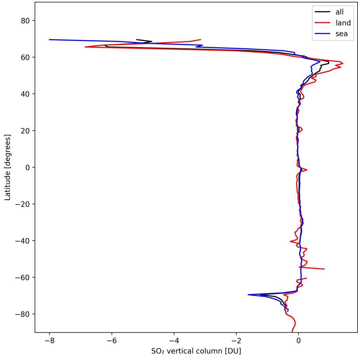
Figure 30: Zonal average of “SO 2 vertical column” for 2024-11-02 to 2024-11-04.
