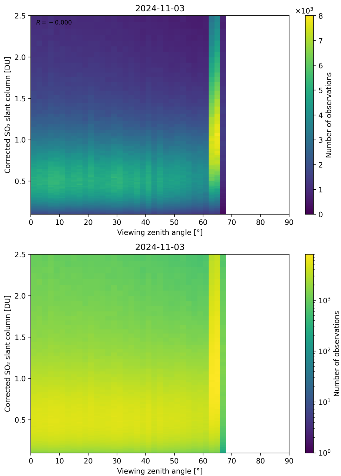
Figure 317: Scatter density plot of “Viewing zenith angle” against “Corrected SO 2 slant column” for 2024-11-02 to 2024-11-04.
