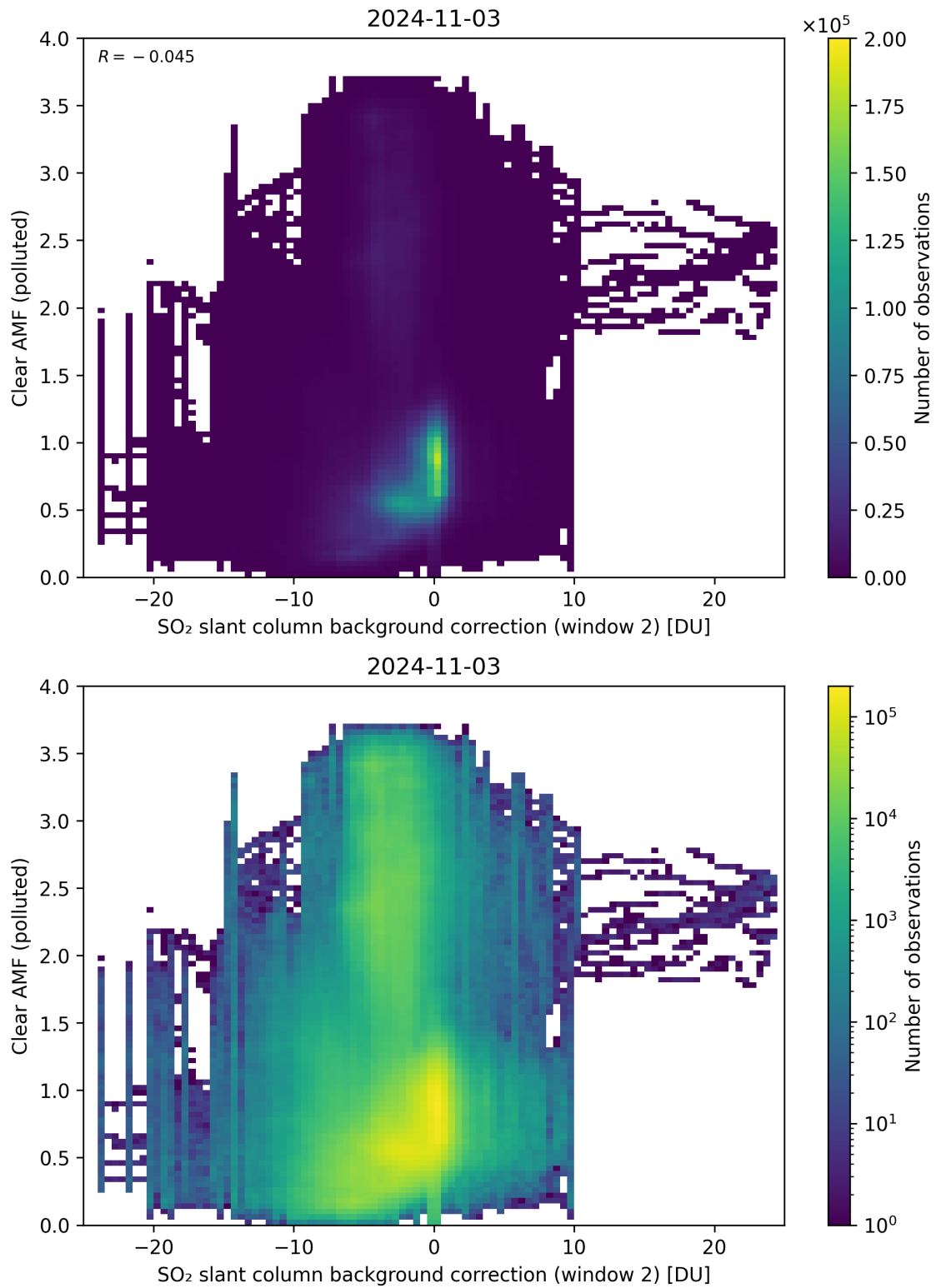
Figure 115: Scatter density plot of “SO 2 slant column background correction (window 2)” against “Clear AMF (polluted)” for 2024-11-02 to 2024-11-04.
