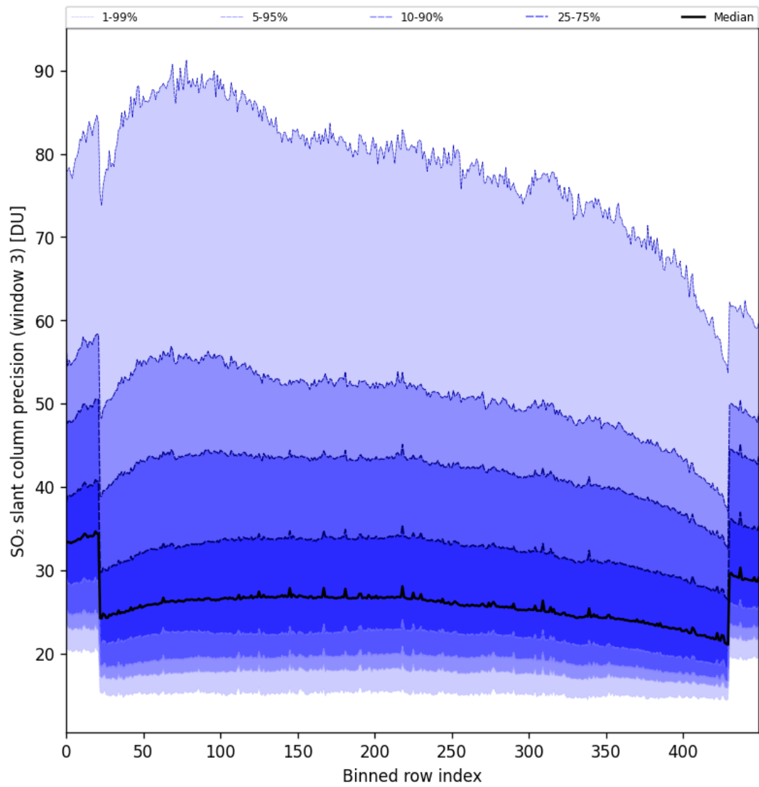
Figure 88: Along track statistics of “SO 2 slant column precision (window 3)” for 2024-11-02 to 2024-11-04
