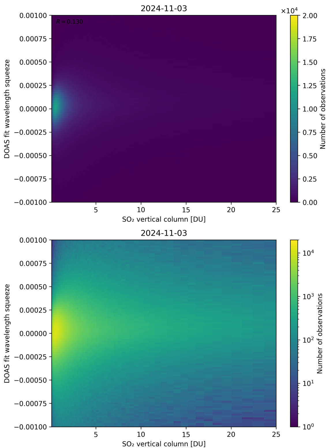
Figure 277: Scatter density plot of “SO 2 vertical column” against “DOAS fit wavelength squeeze” for 2024-11-02 to 2024-11-04.
