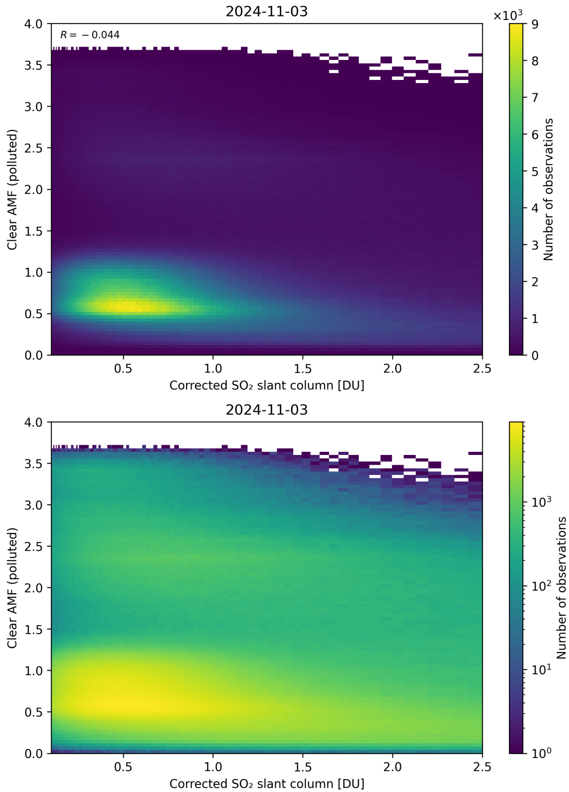
Figure 184: Scatter density plot of “Corrected SO 2 slant column” against “Clear AMF (polluted)” for 2024-11-02 to 2024-11-04.
