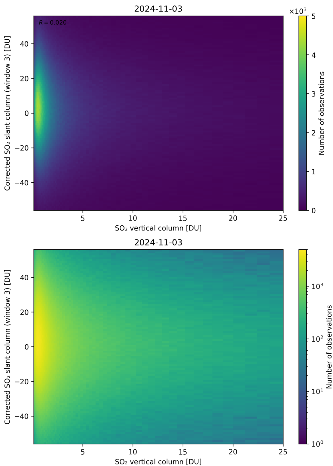
Figure 299: Scatter density plot of “SO 2 vertical column” against “Corrected SO 2 slant column (window 3)” for 2024-11-02 to 2024-11-04.
