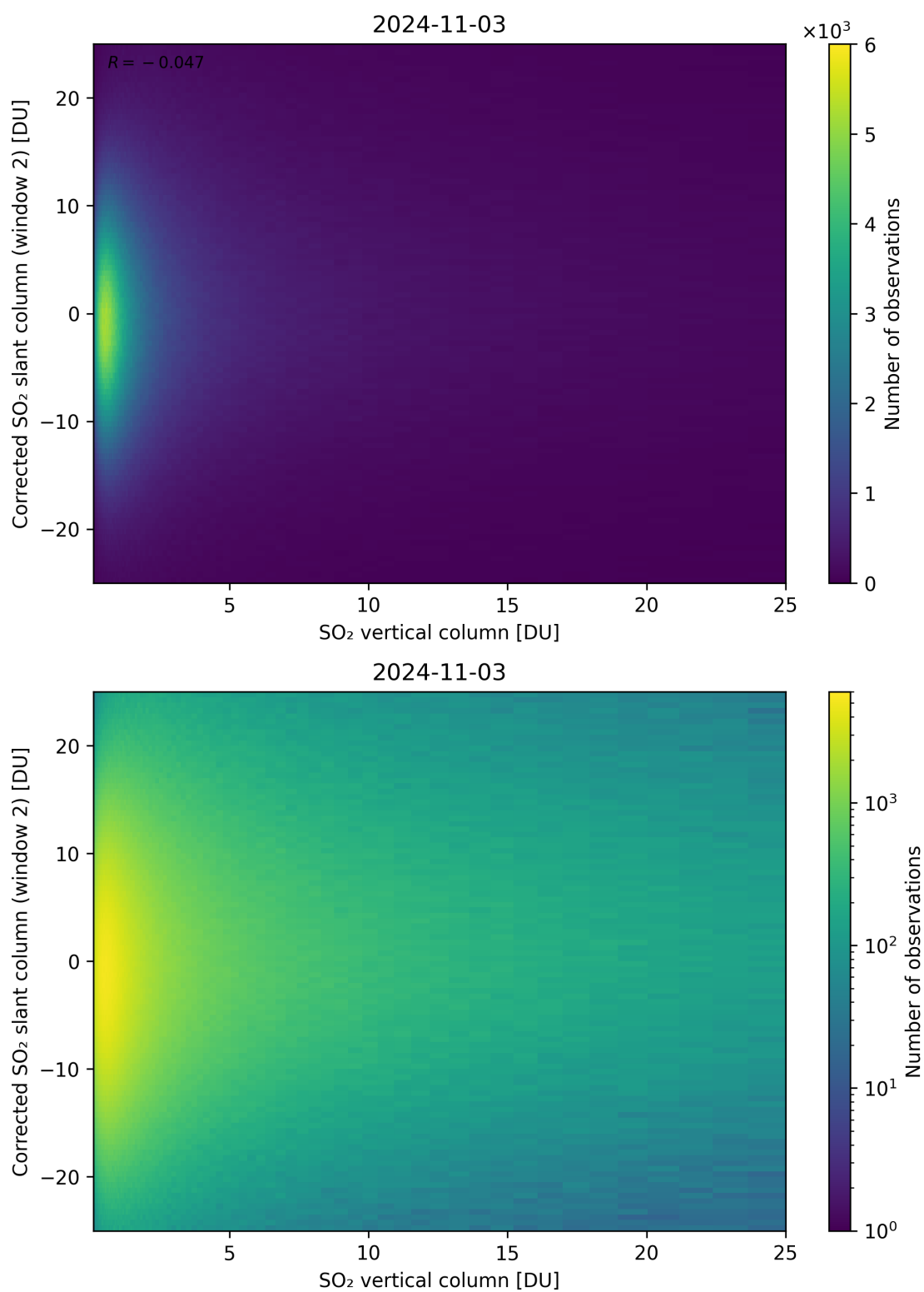
Figure 298: Scatter density plot of “SO 2 vertical column” against “Corrected SO 2 slant column (window 2)” for 2024-11-02 to 2024-11-04.
