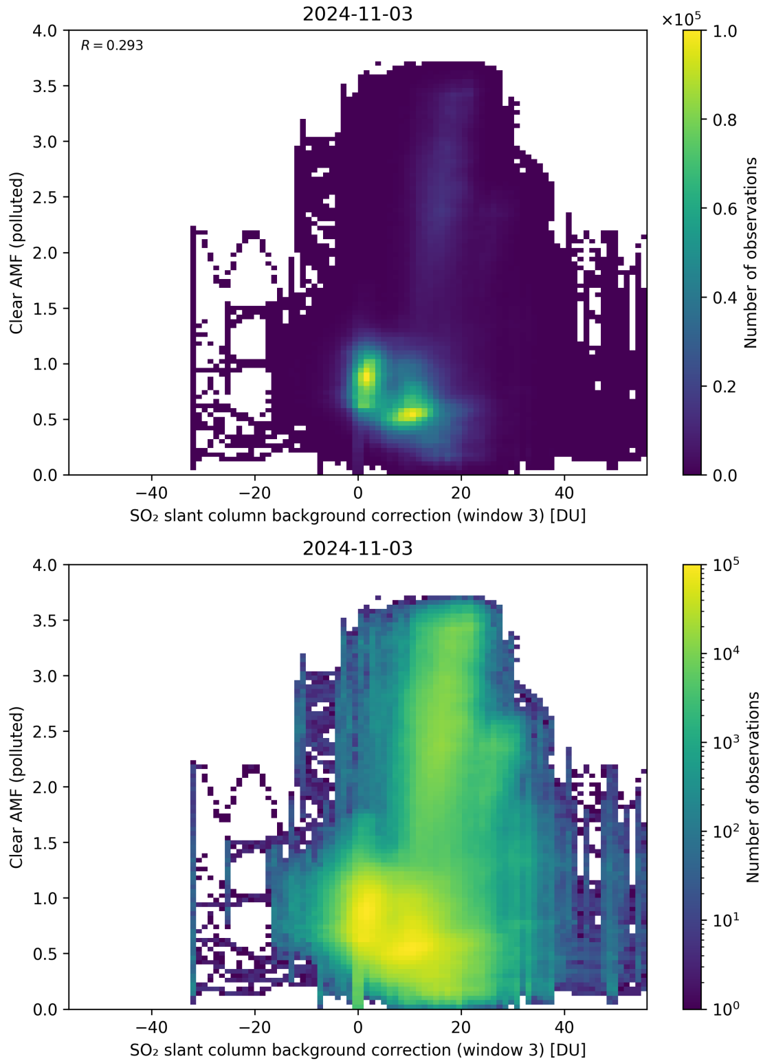
Figure 124: Scatter density plot of “SO 2 slant column background correction (window 3)” against “Clear AMF (polluted)” for 2024-11-02 to 2024-11-04.
