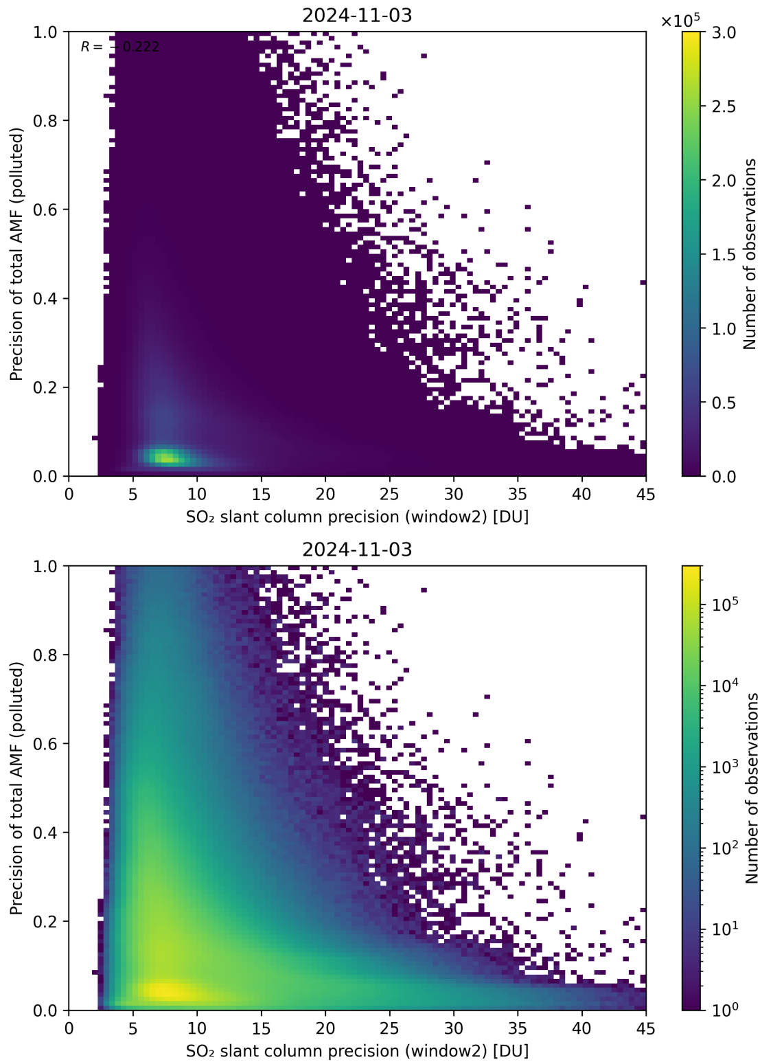
Figure 252: Scatter density plot of “SO 2 slant column precision (window2)” against “Precision of total AMF (polluted)” for 2024-11-02 to 2024-11-04.
