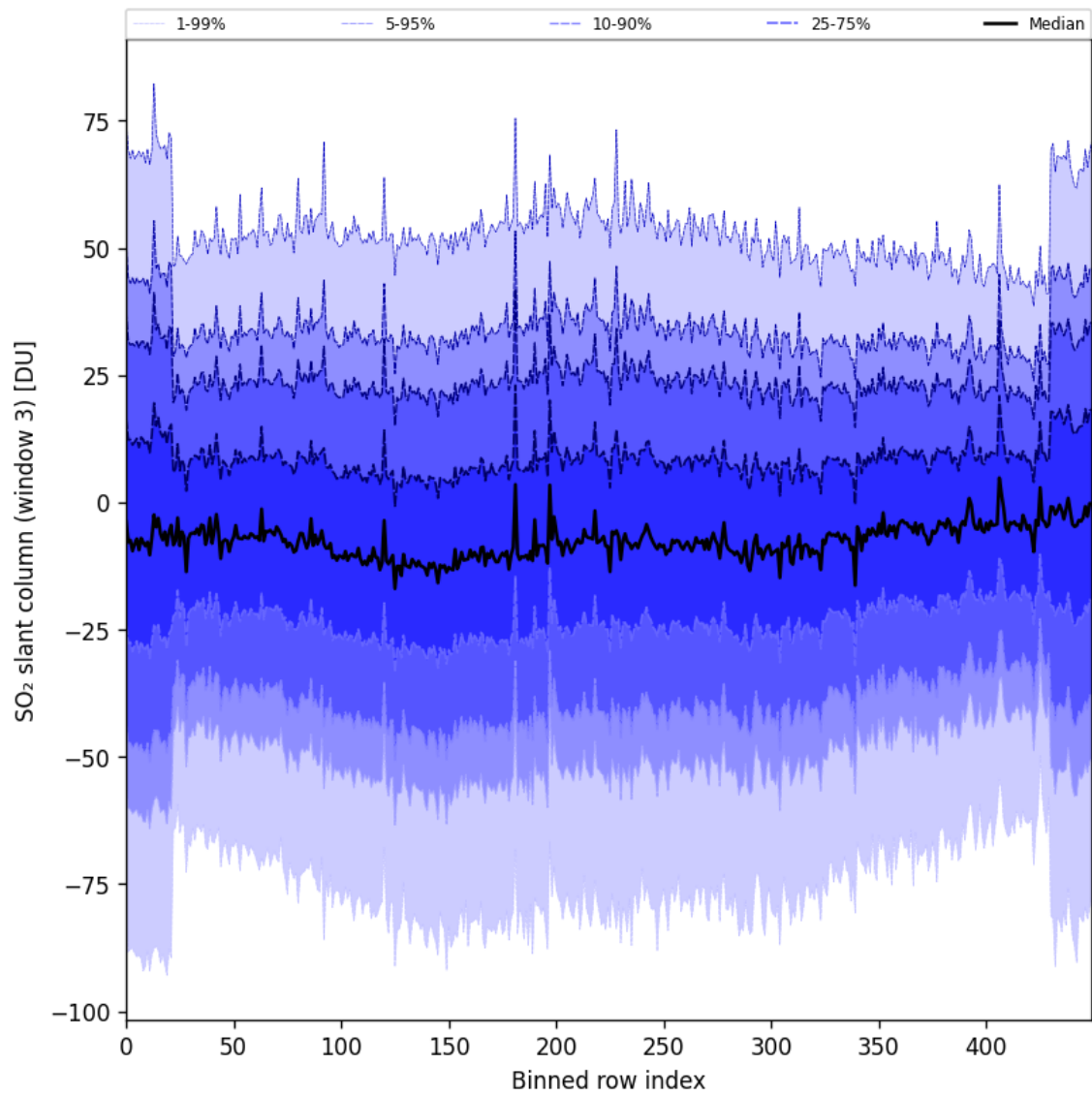
Figure 87: Along track statistics of “SO 2 slant column (window 3)” for 2024-11-02 to 2024-11-04
