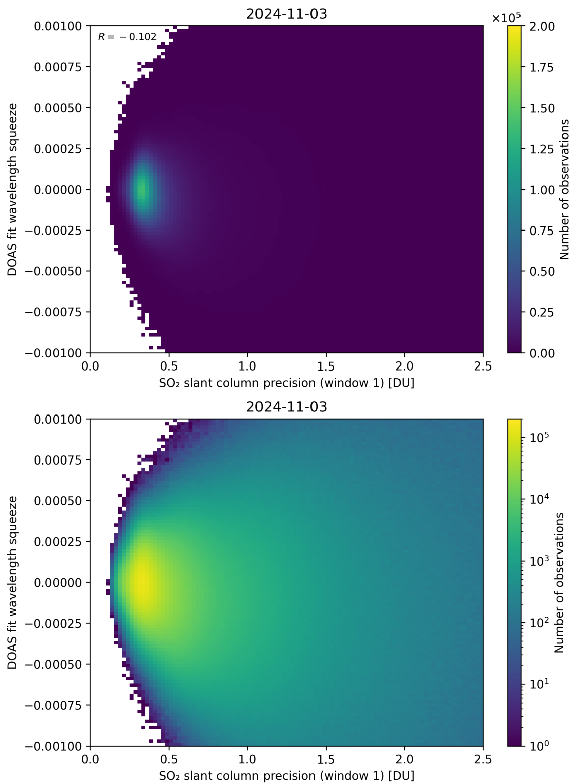
Figure 222: Scatter density plot of “SO 2 slant column precision (window 1)” against “DOAS fit wavelength squeeze” for 2024-11-02 to 2024-11-04.
