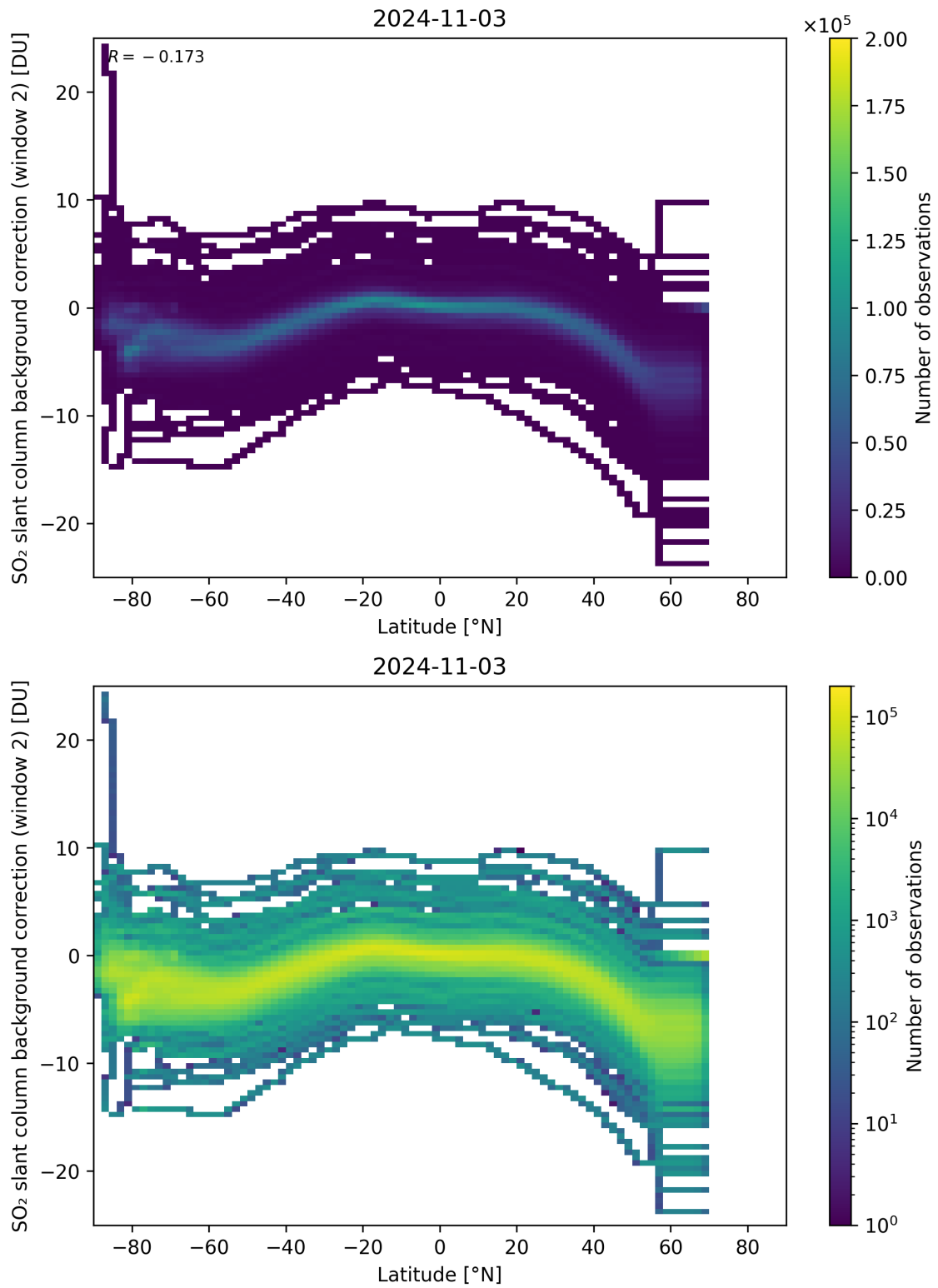
Figure 140: Scatter density plot of “Latitude” against “SO 2 slant column background correction (window 2)” for 2024-11-02 to 2024-11-04.
