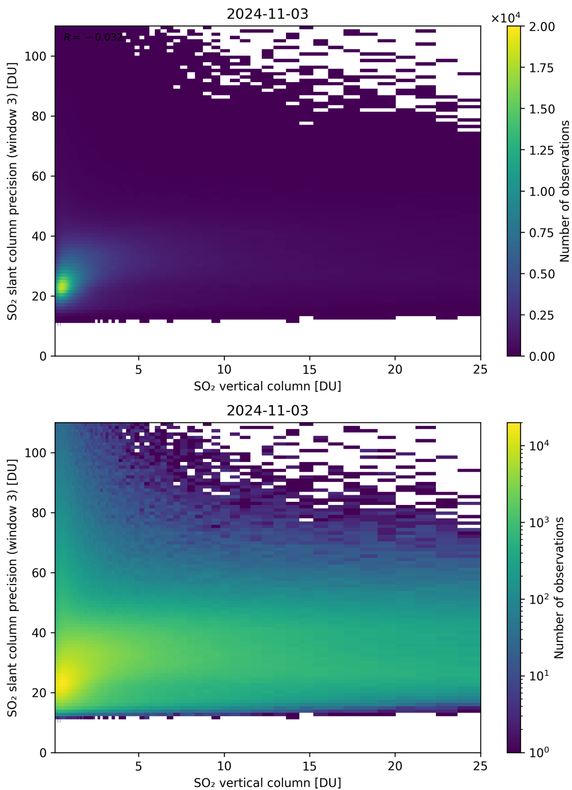
Figure 304: Scatter density plot of “SO 2 vertical column” against “SO 2 slant column precision (window 3)” for 2024-11-02 to 2024-11-04.
