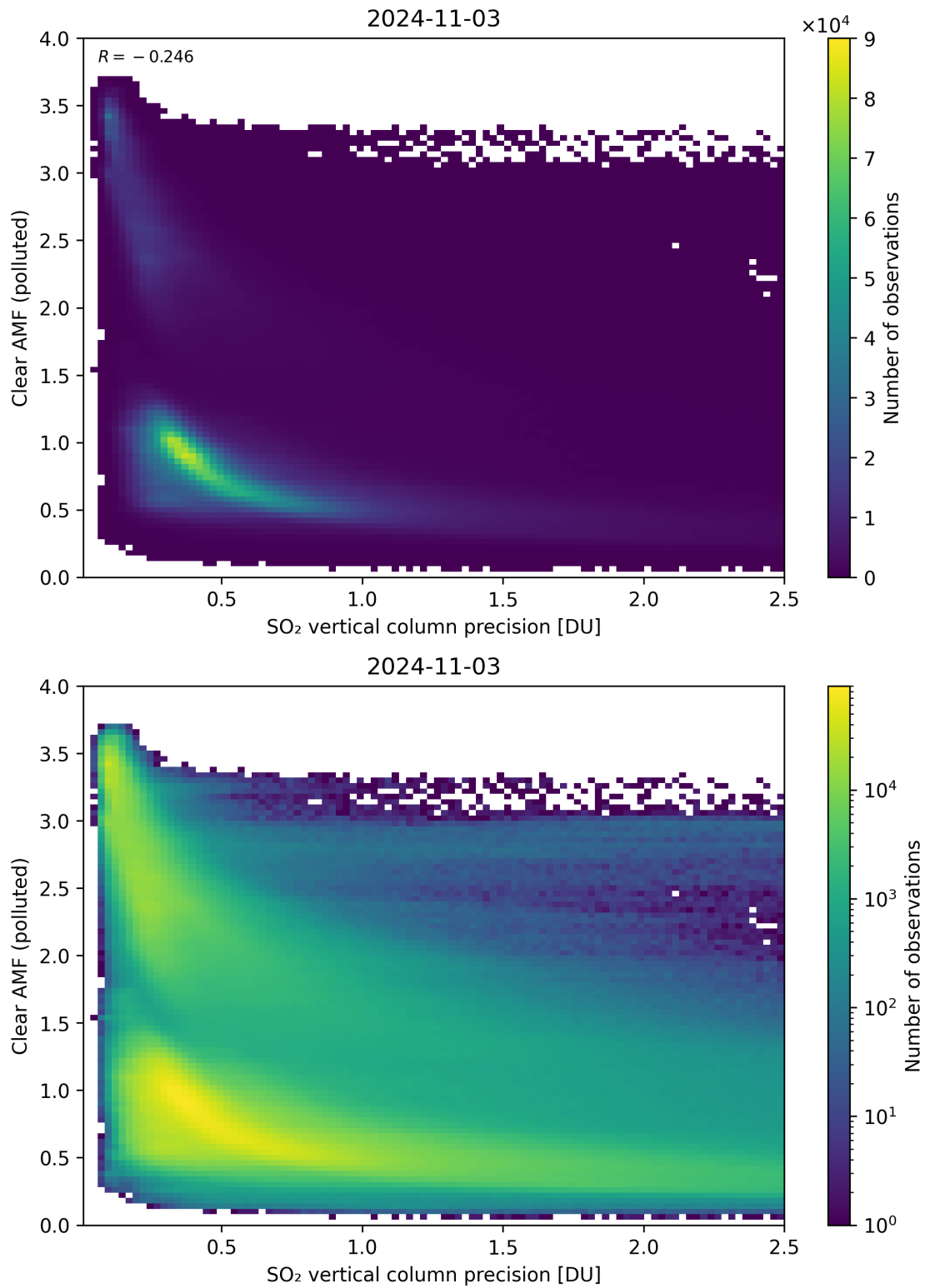
Figure 285: Scatter density plot of “SO 2 vertical column precision” against “Clear AMF (polluted)” for 2024-11-02 to 2024-11-04.
