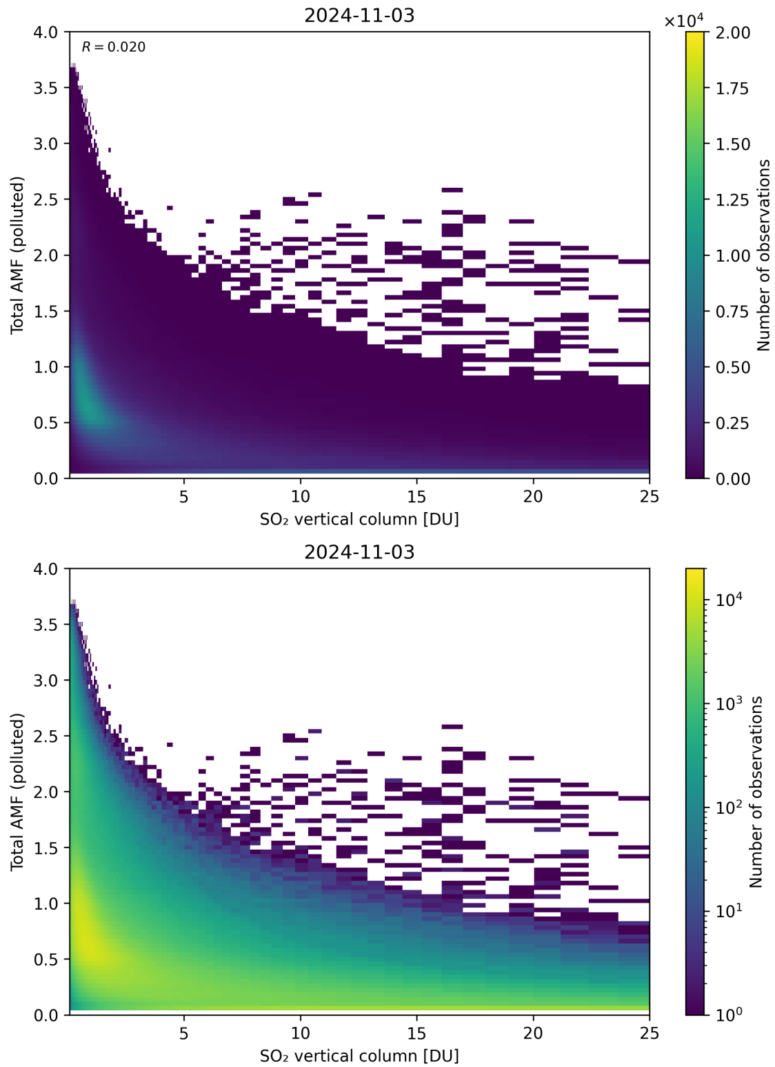
Figure 305: Scatter density plot of “SO 2 vertical column” against “Total AMF (polluted)” for 2024-11-02 to 2024-11-04.
