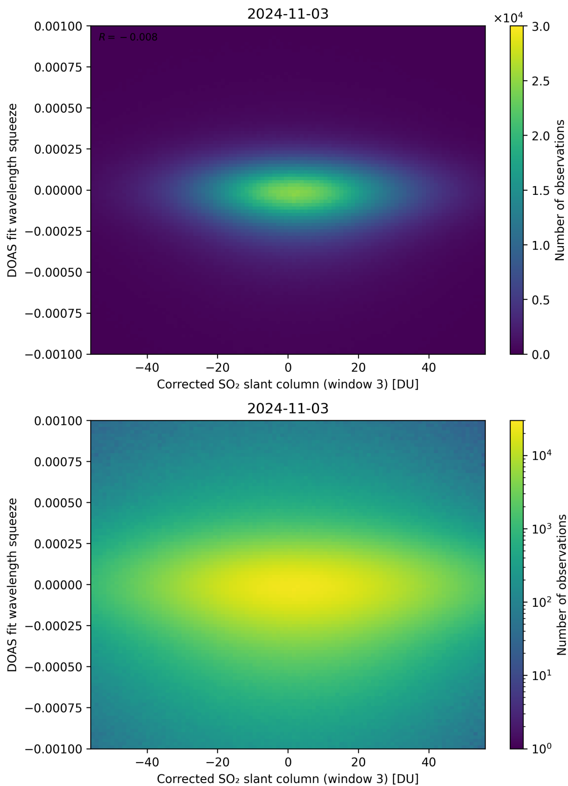
Figure 207: Scatter density plot of “Corrected SO 2 slant column (window 3)” against “DOAS fit wavelength squeeze” for 2024-11-02 to 2024-11-04.
