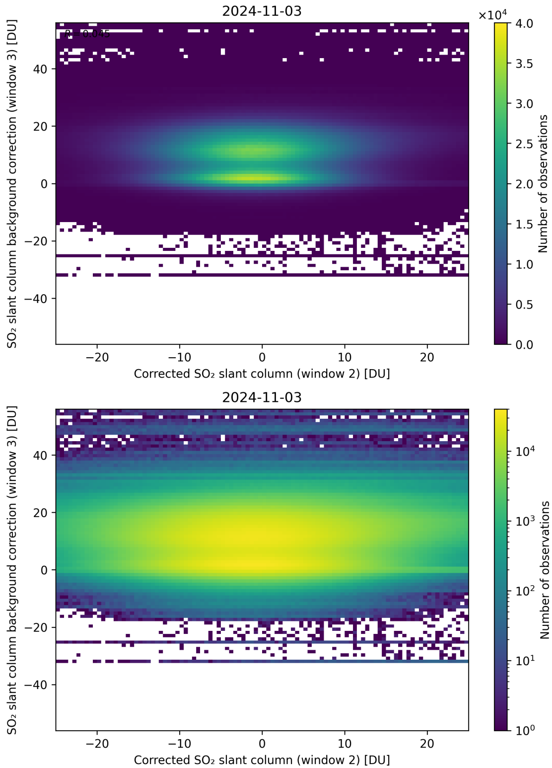
Figure 195: Scatter density plot of “Corrected SO 2 slant column (window 2)” against “SO 2 slant column background correction (window 3)” for 2024-11-02 to 2024-11-04.
