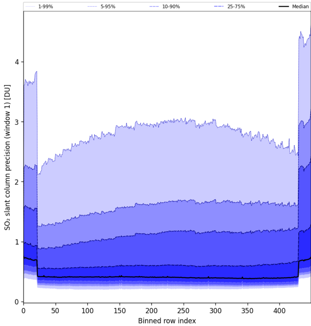
Figure 80: Along track statistics of “SO 2 slant column precision (window 1)” for 2024-11-02 to 2024-11-04
