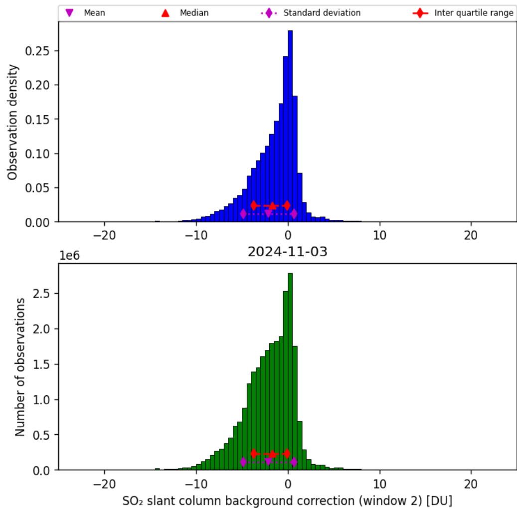
Figure 63: Histogram of “SO 2 slant column background correction (window 2)” for 2024-11-02 to 2024-11-04
