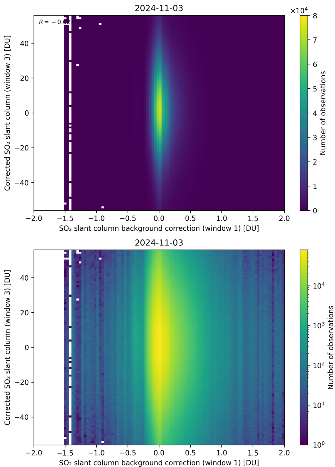
Figure 105: Scatter density plot of “SO 2 slant column background correction (window 1)” against “Corrected SO 2 slant column (window 3)” for 2024-11-02 to 2024-11-04.
