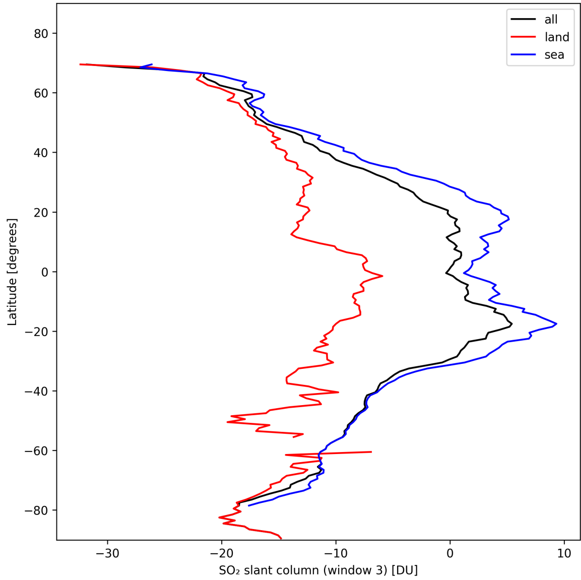
Figure 41: Zonal average of “SO 2 slant column (window 3)” for 2024-11-02 to 2024-11-04.
