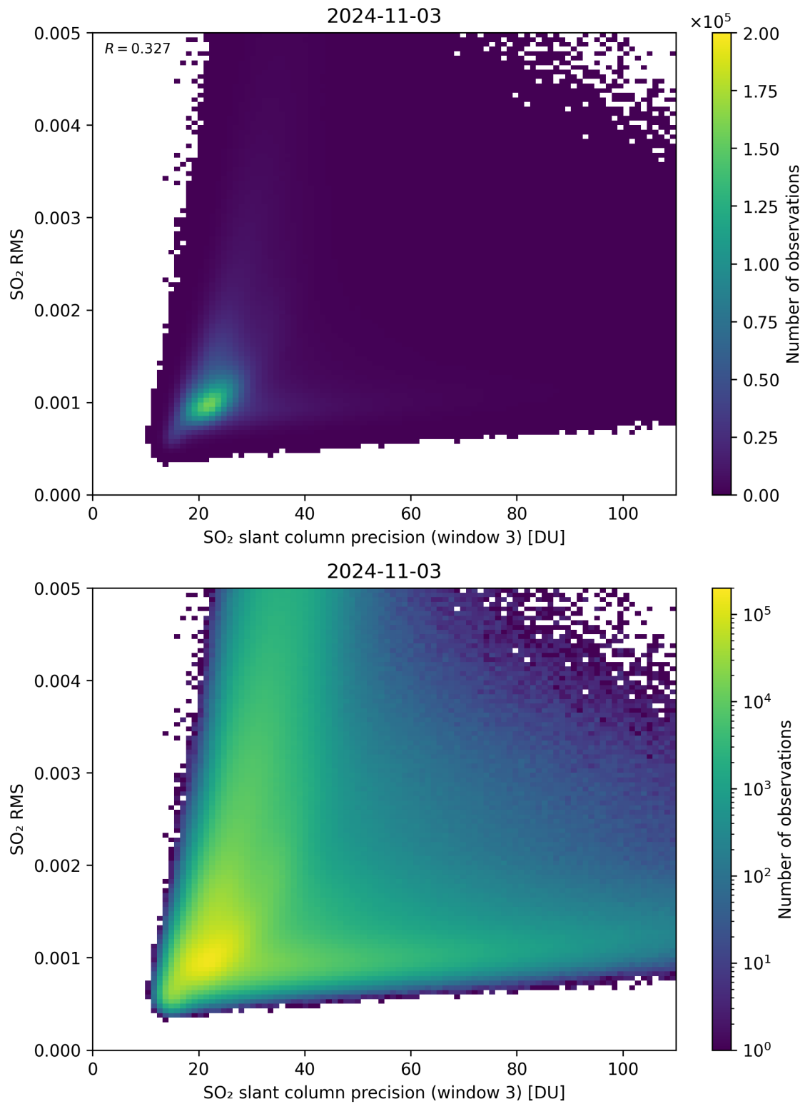
Figure 260: Scatter density plot of “SO 2 slant column precision (window 3)” against “SO 2 RMS” for 2024-11-02 to 2024-11-04.
