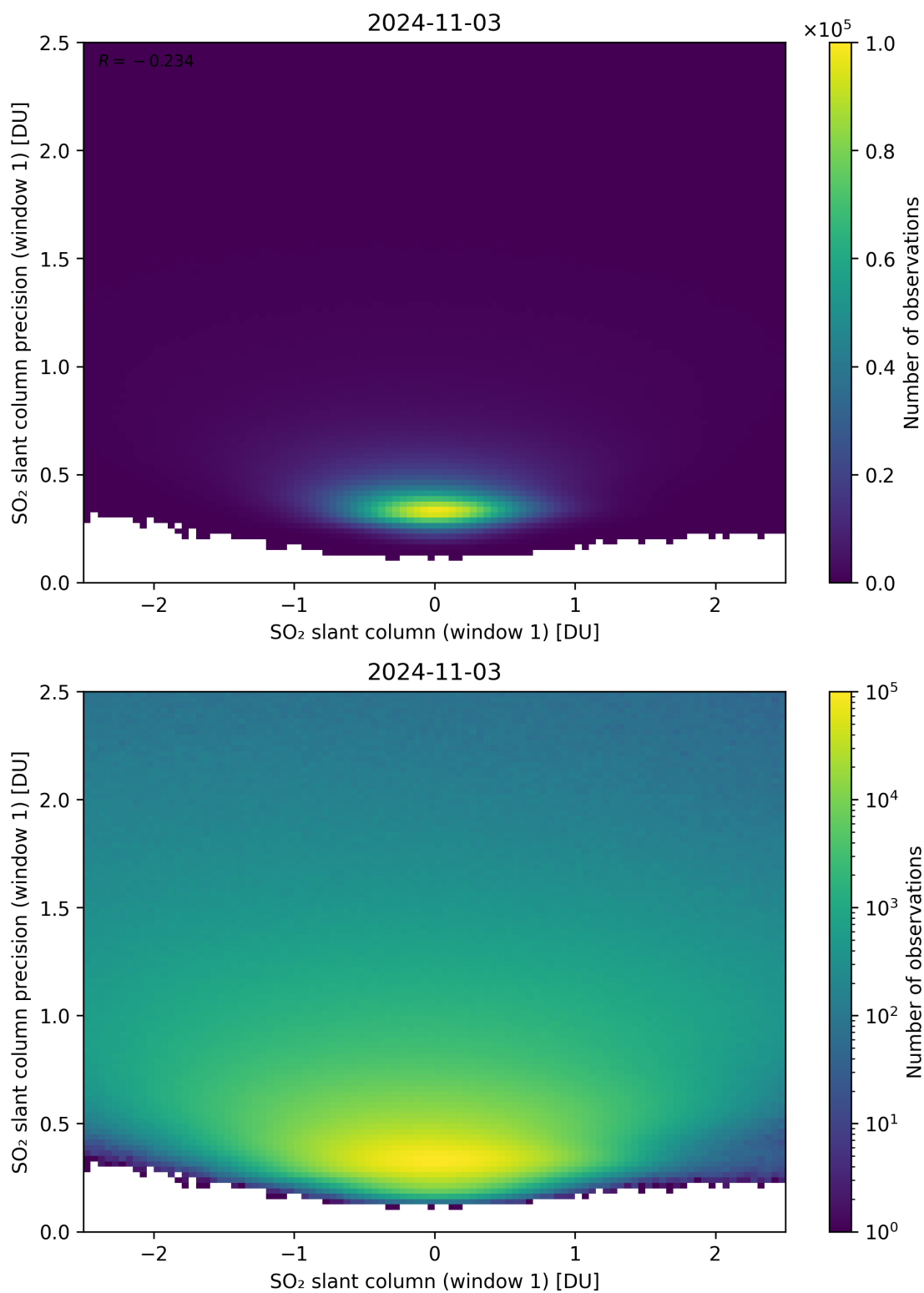
Figure 235: Scatter density plot of “SO 2 slant column (window 1)” against “SO 2 slant column precision (window 1)” for 2024-11-02 to 2024-11-04.
