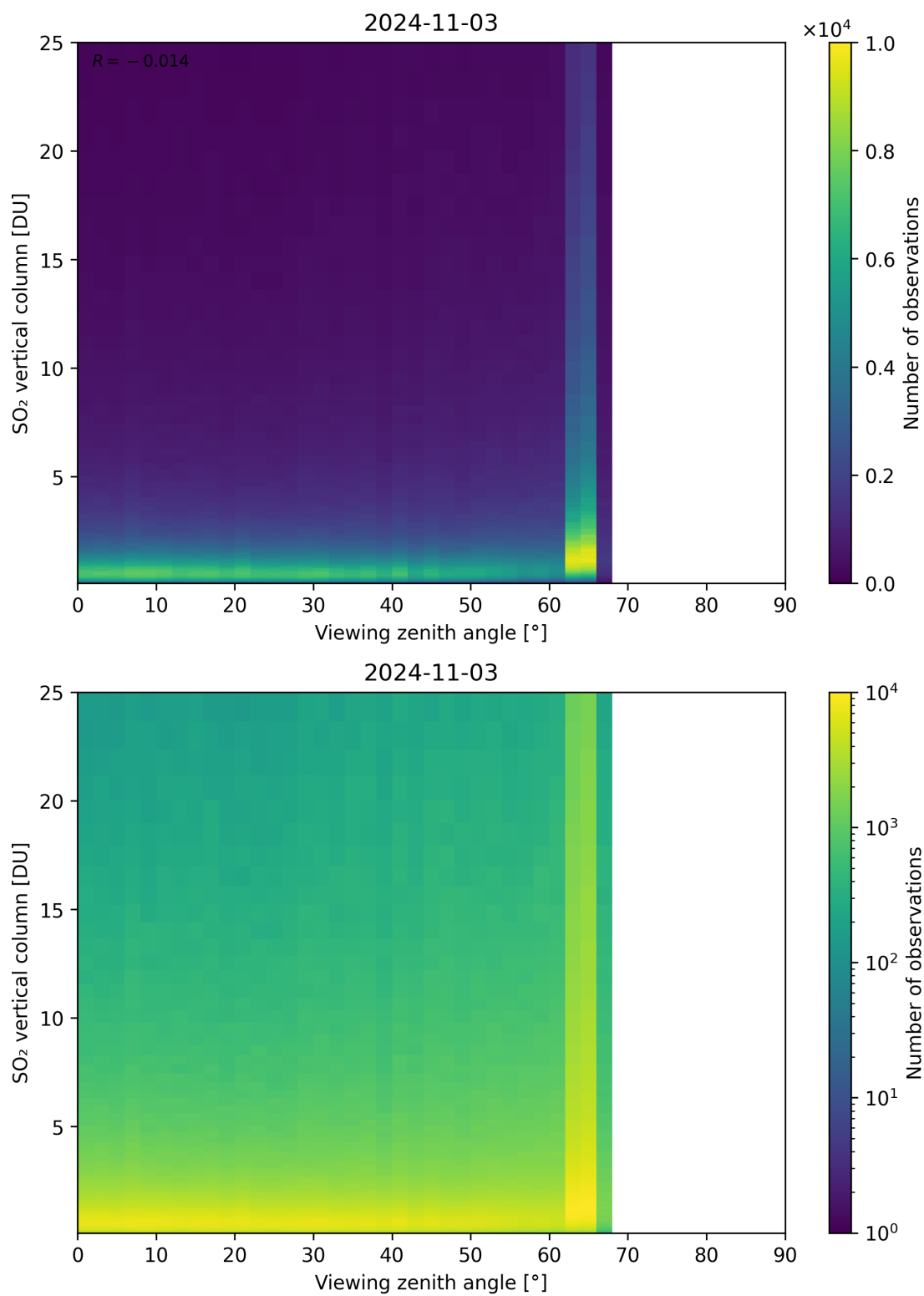
Figure 327: Scatter density plot of “Viewing zenith angle” against “SO 2 vertical column” for 2024-11-02 to 2024-11-04.
