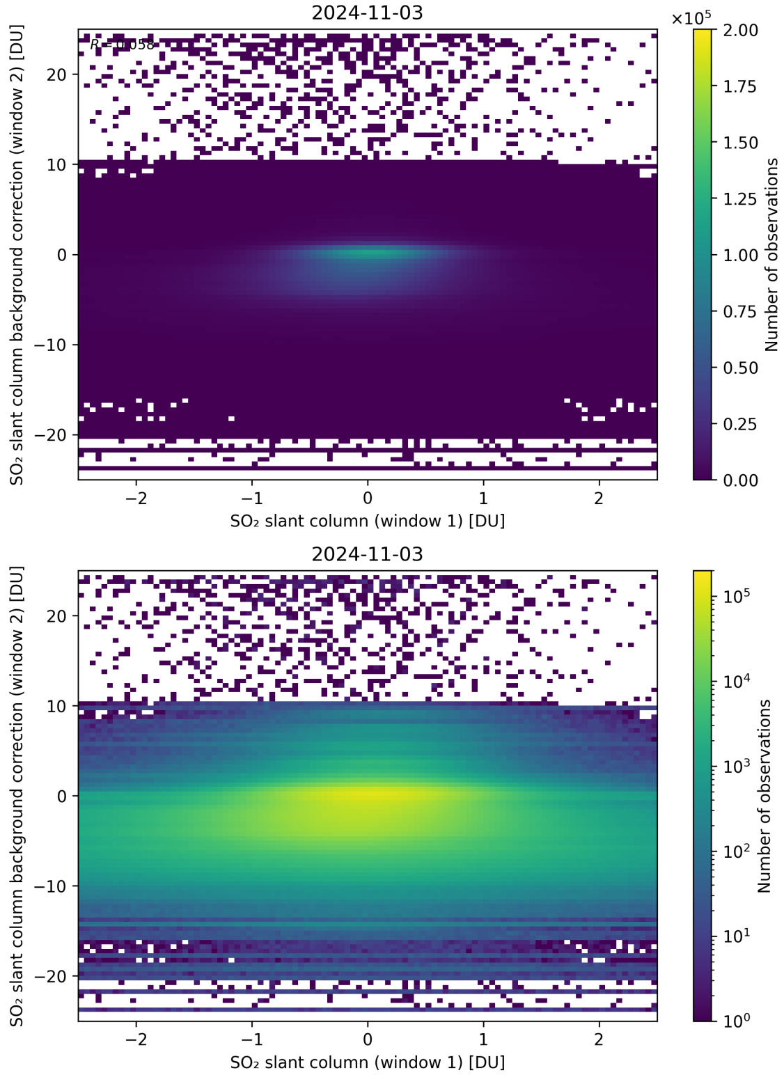
Figure 213: Scatter density plot of “SO 2 slant column (window 1)” against “SO 2 slant column background correction (window 2)” for 2024-11-02 to 2024-11-04.
