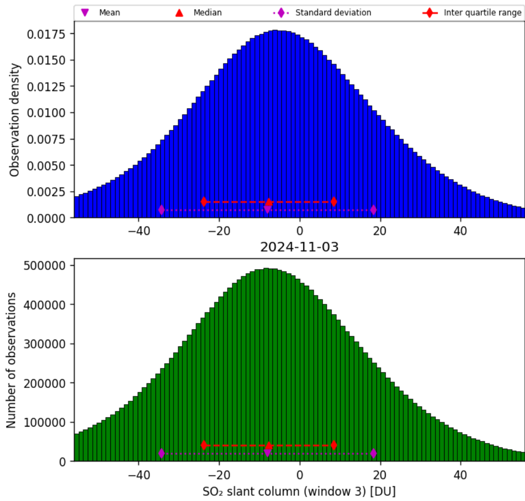
Figure 64: Histogram of “SO 2 slant column (window 3)” for 2024-11-02 to 2024-11-04
