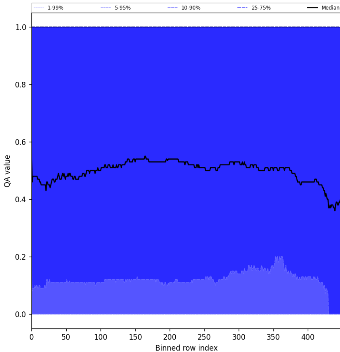
Figure 75: Along track statistics of “QA value” for 2024-11-02 to 2024-11-04
