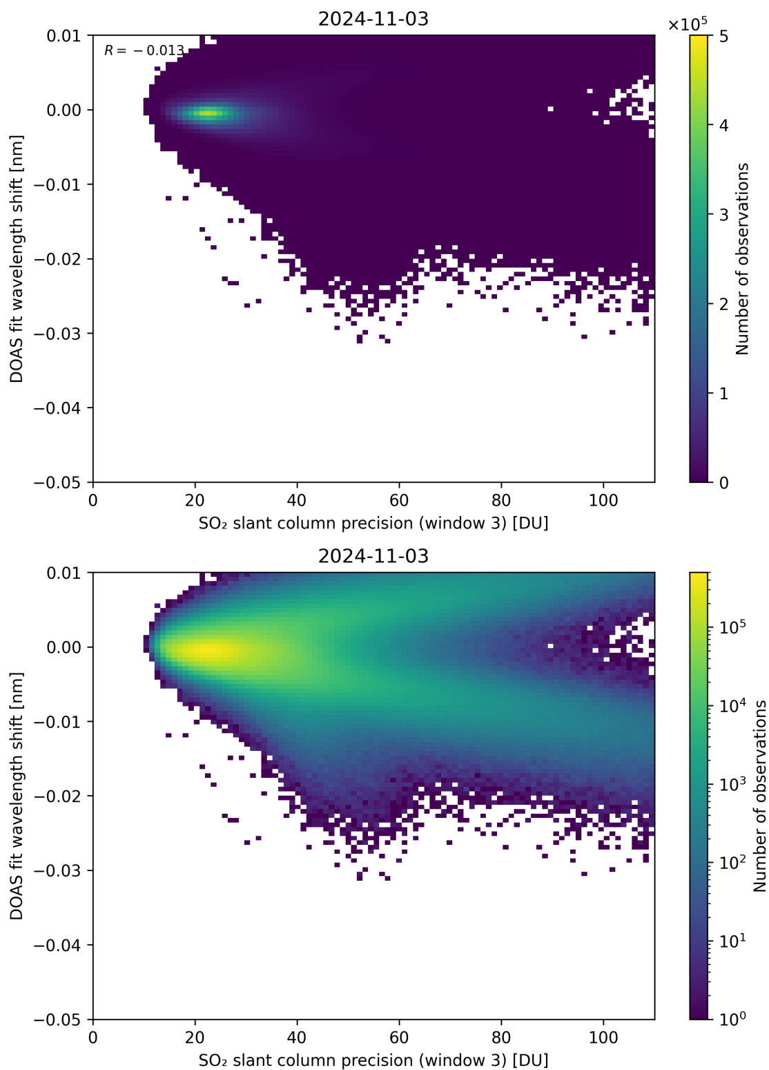
Figure 258: Scatter density plot of “SO 2 slant column precision (window 3)” against “DOAS fit wavelength shift” for 2024-11-02 to 2024-11-04.
