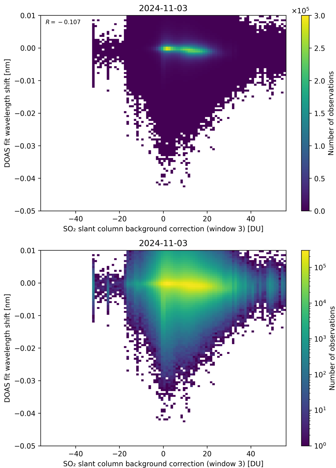
Figure 121: Scatter density plot of “SO 2 slant column background correction (window 3)” against “DOAS fit wavelength shift” for 2024-11-02 to 2024-11-04.
