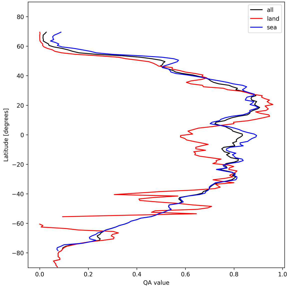
Figure 29: Zonal average of “QA value” for 2024-11-02 to 2024-11-04.
