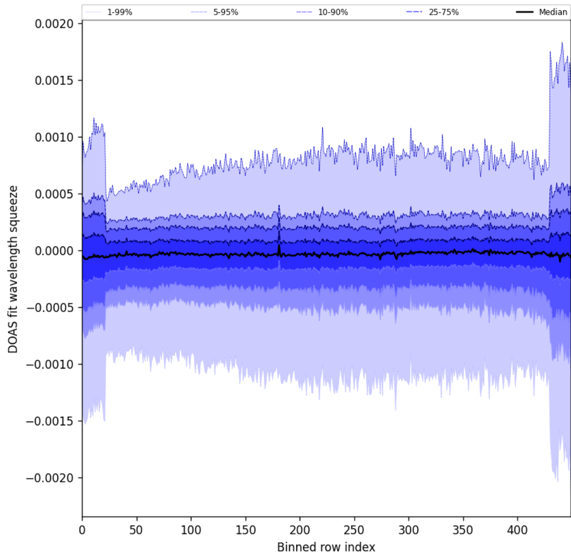
Figure 92: Along track statistics of “DOAS fit wavelength squeeze” for 2024-11-02 to 2024-11-04
