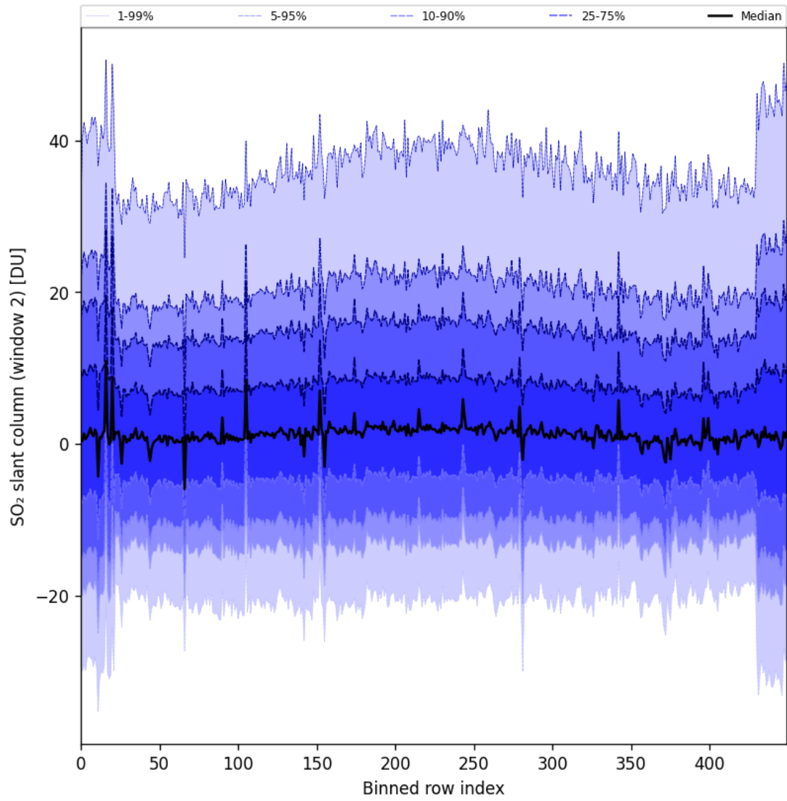
Figure 83: Along track statistics of “SO 2 slant column (window 2)” for 2024-11-02 to 2024-11-04
