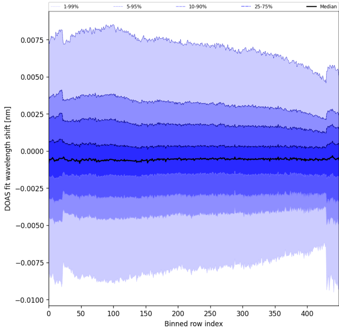
Figure 91: Along track statistics of “DOAS fit wavelength shift” for 2024-11-02 to 2024-11-04
