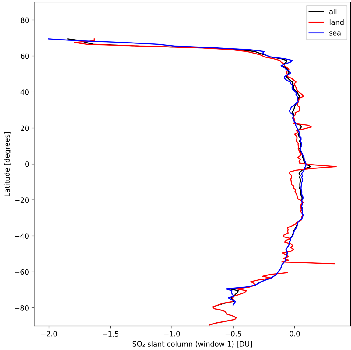
Figure 33: Zonal average of “SO 2 slant column (window 1)” for 2024-11-02 to 2024-11-04.
