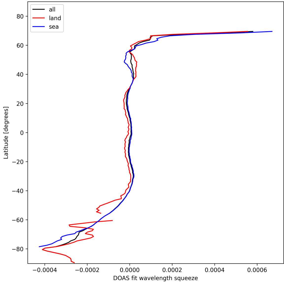
Figure 46: Zonal average of “DOAS fit wavelength squeeze” for 2024-11-02 to 2024-11-04.
