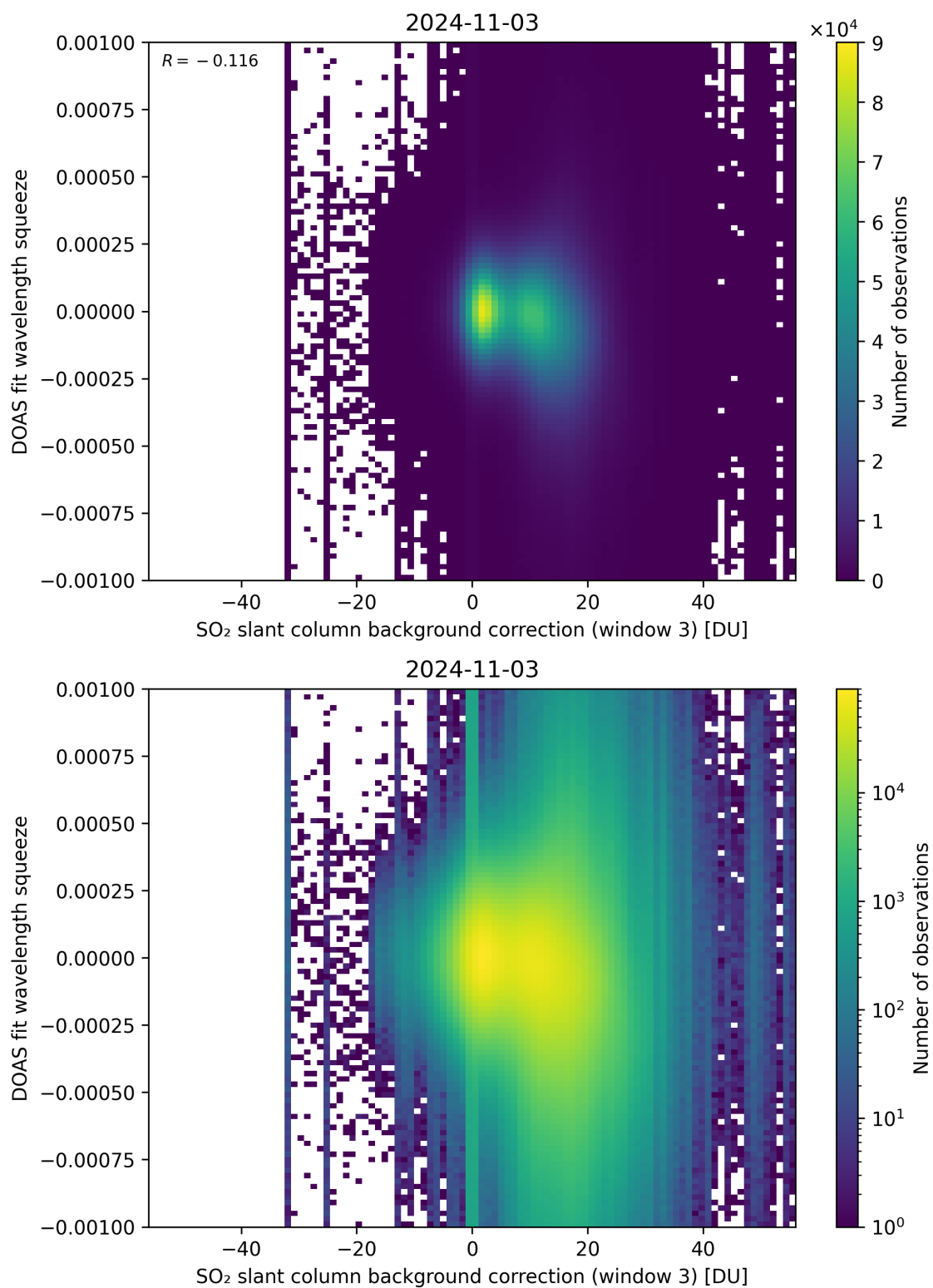
Figure 122: Scatter density plot of “SO 2 slant column background correction (window 3)” against “DOAS fit wavelength squeeze” for 2024-11-02 to 2024-11-04.
