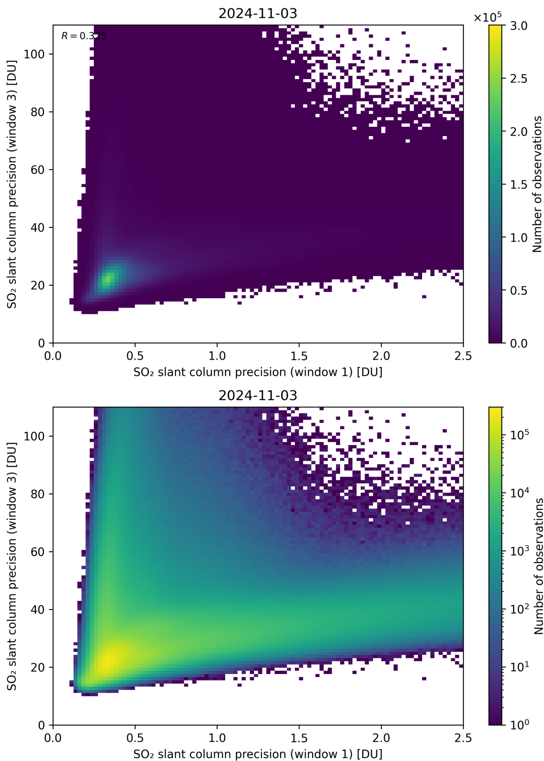
Figure 229: Scatter density plot of “SO 2 slant column precision (window 1)” against “SO 2 slant column precision (window 3)” for 2024-11-02 to 2024-11-04.
