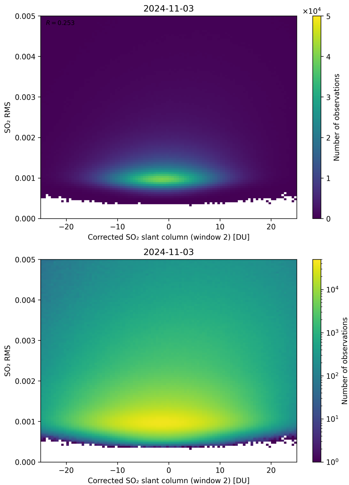
Figure 198: Scatter density plot of “Corrected SO 2 slant column (window 2)” against “SO 2 RMS” for 2024-11-02 to 2024-11-04.
