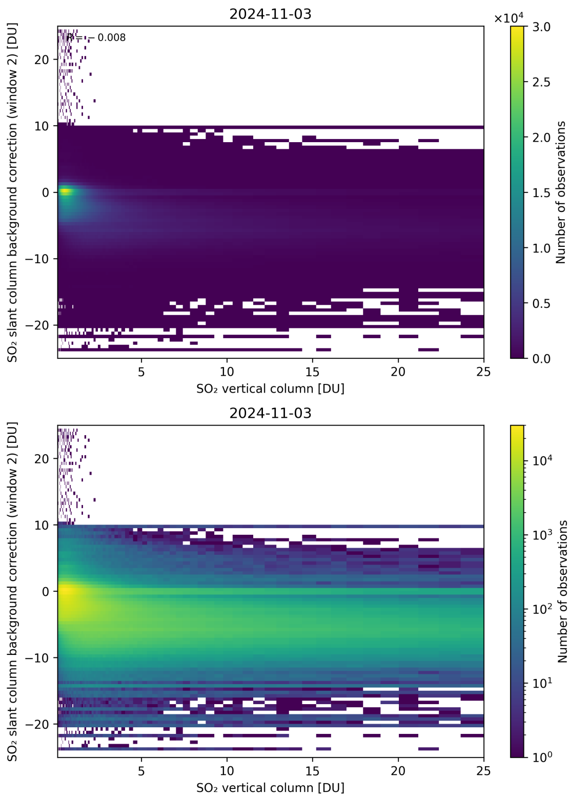
Figure 274: Scatter density plot of “SO 2 vertical column” against “SO 2 slant column background correction (window 2)” for 2024-11-02 to 2024-11-04.
