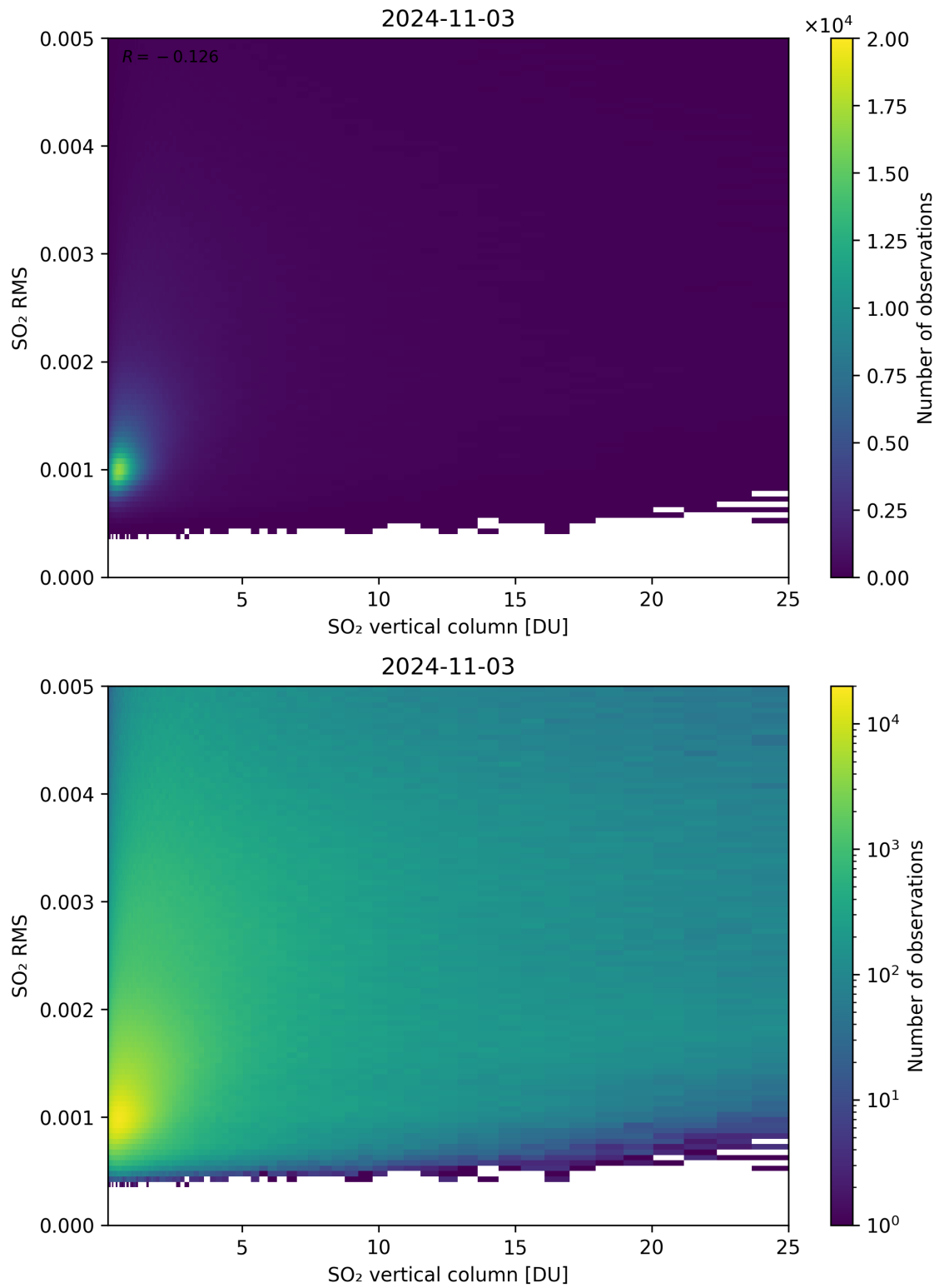
Figure 278: Scatter density plot of “SO 2 vertical column” against “SO 2 RMS” for 2024-11-02 to 2024-11-04.
