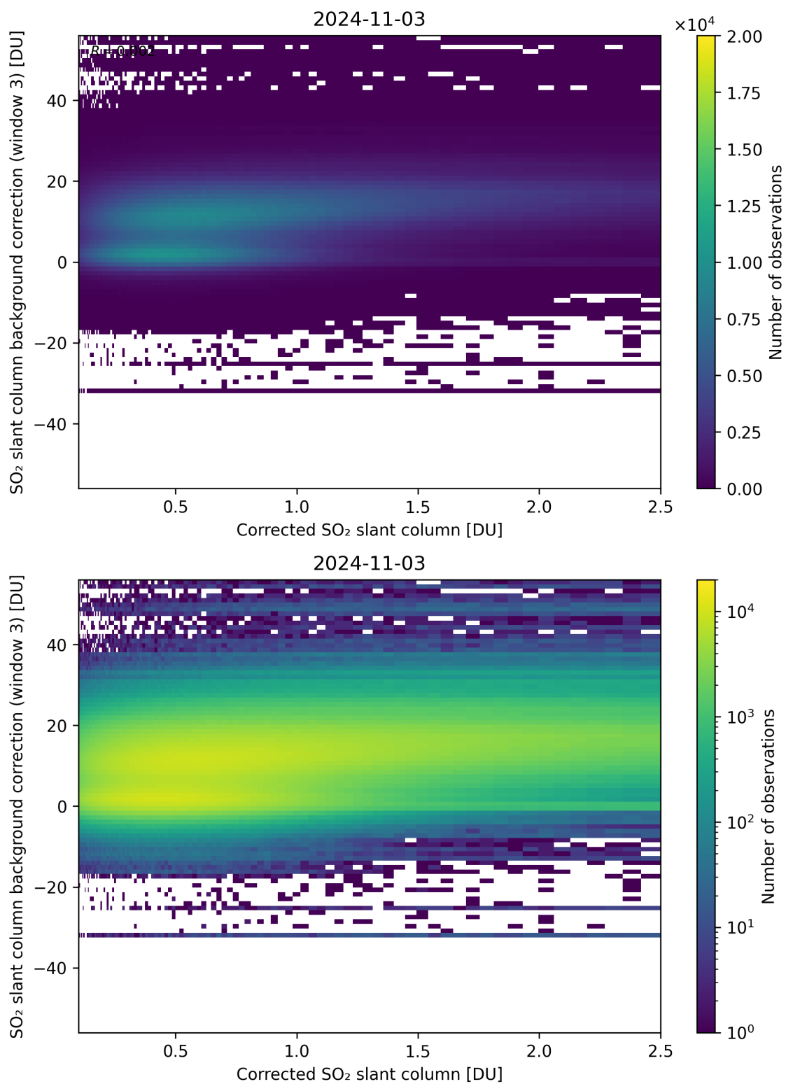
Figure 180: Scatter density plot of “Corrected SO 2 slant column” against “SO 2 slant column background correction (window 3)” for 2024-11-02 to 2024-11-04.
