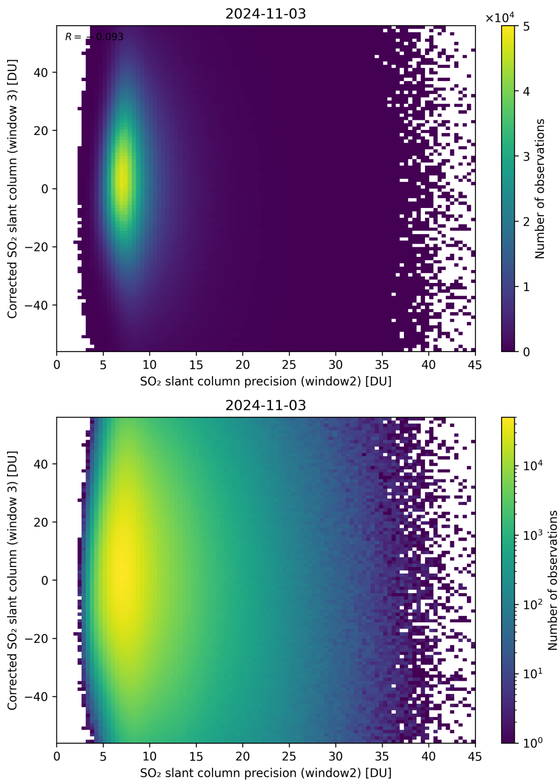
Figure 248: Scatter density plot of “SO 2 slant column precision (window2)” against “Corrected SO 2 slant column (window 3)” for 2024-11-02 to 2024-11-04.
