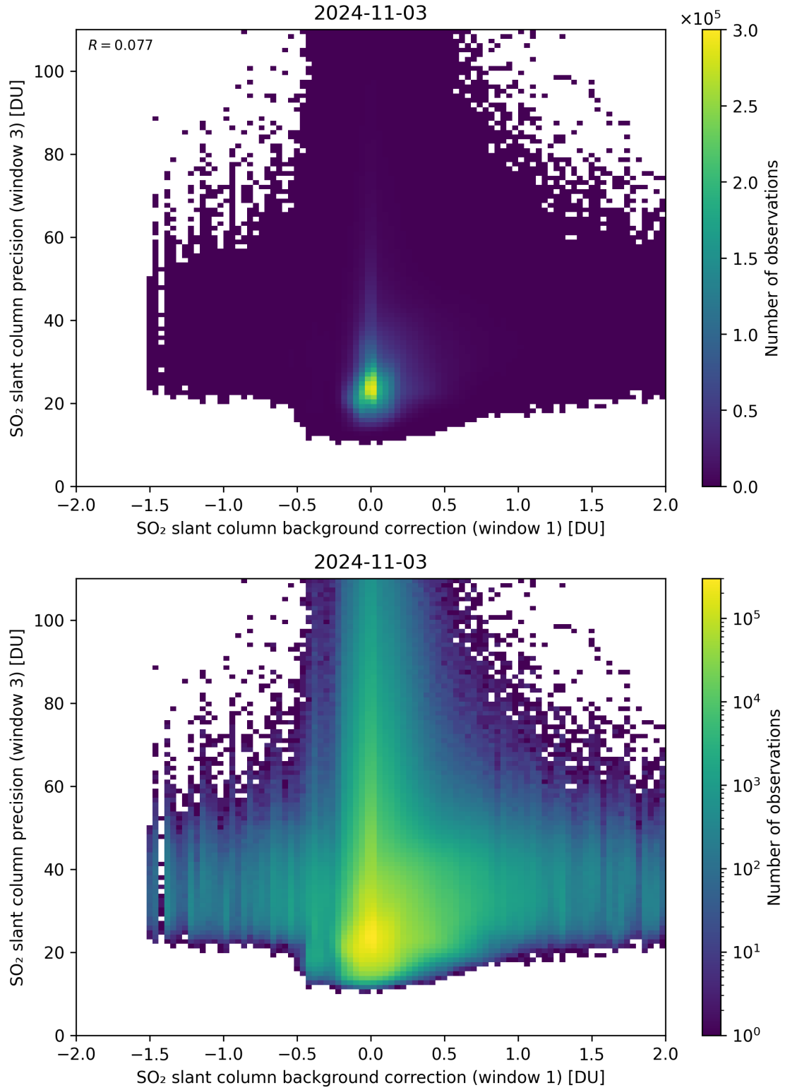
Figure 108: Scatter density plot of “SO 2 slant column background correction (window 1)” against “SO 2 slant column precision (window 3)” for 2024-11-02 to 2024-11-04.
