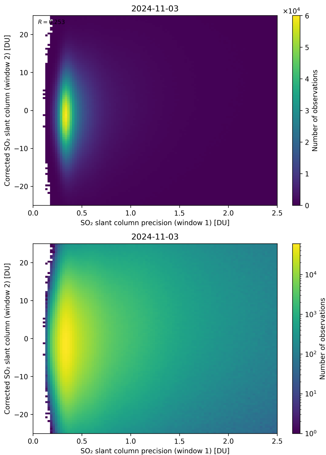
Figure 225: Scatter density plot of “SO 2 slant column precision (window 1)” against “Corrected SO 2 slant column (window 2)” for 2024-11-02 to 2024-11-04.
