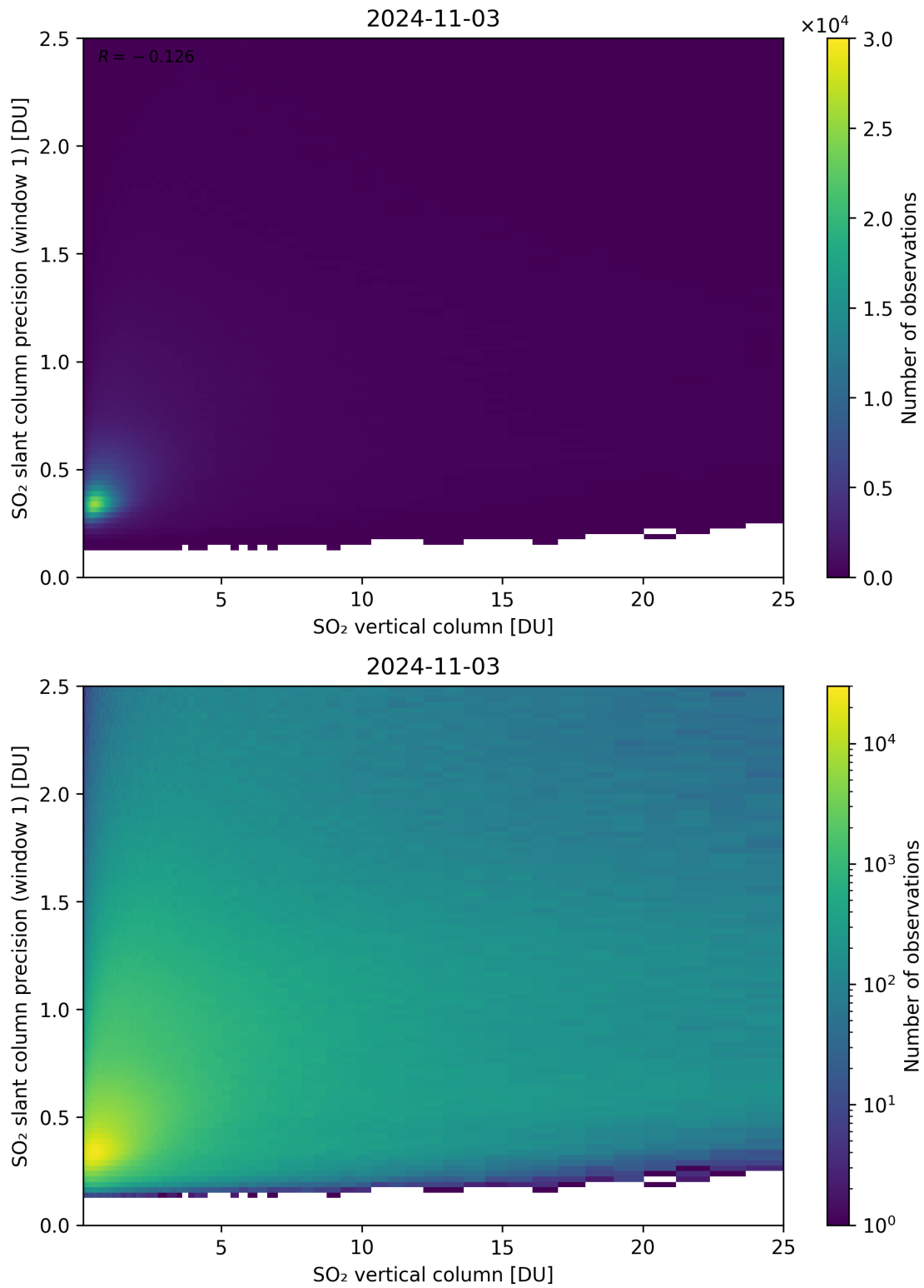
Figure 301: Scatter density plot of “SO 2 vertical column” against “SO 2 slant column precision (window 1)” for 2024-11-02 to 2024-11-04.
