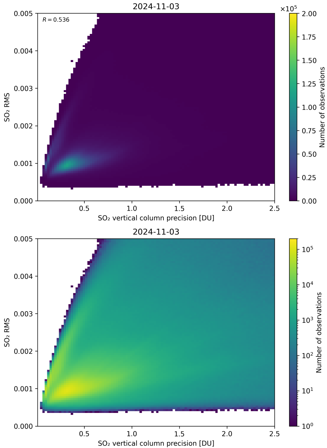
Figure 284: Scatter density plot of “SO 2 vertical column precision” against “SO 2 RMS” for 2024-11-02 to 2024-11-04.
