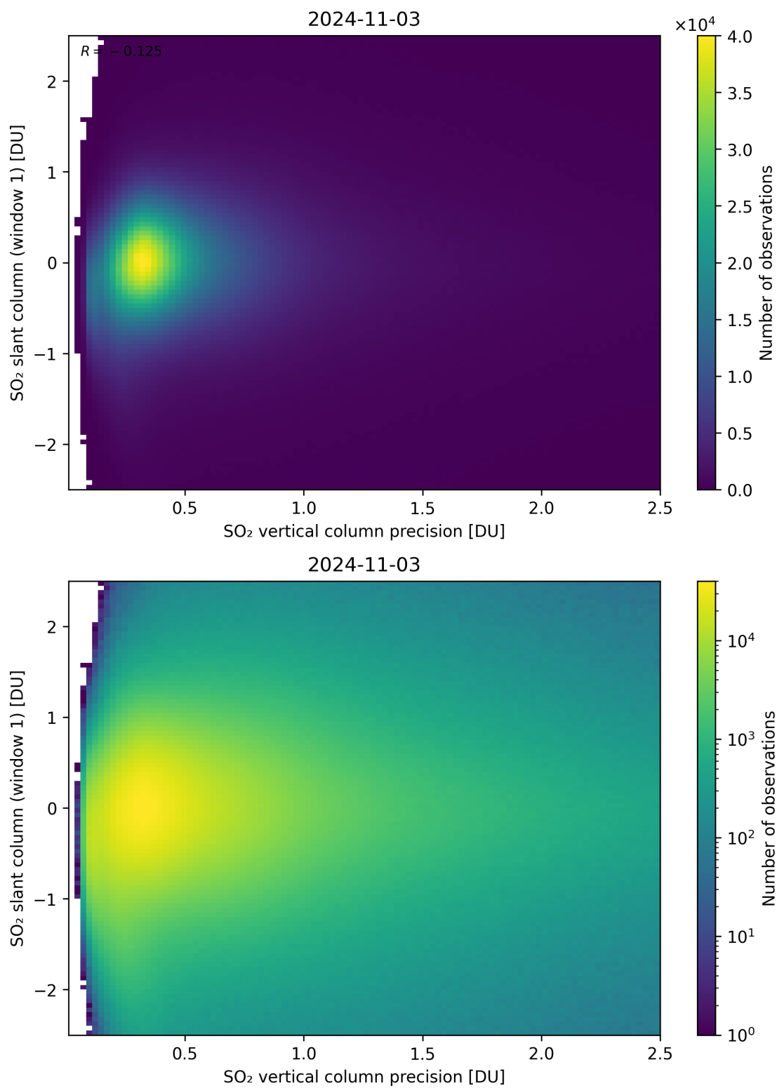
Figure 289: Scatter density plot of “SO 2 vertical column precision” against “SO 2 slant column (window 1)” for 2024-11-02 to 2024-11-04.
