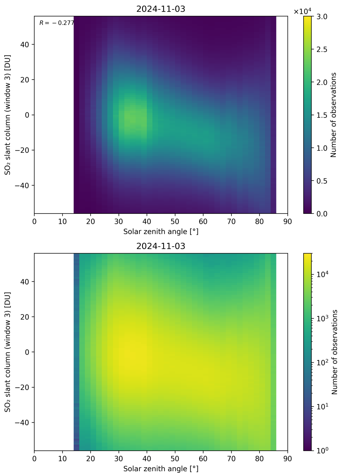
Figure 172: Scatter density plot of “Solar zenith angle” against “SO 2 slant column (window 3)” for 2024-11-02 to 2024-11-04.
