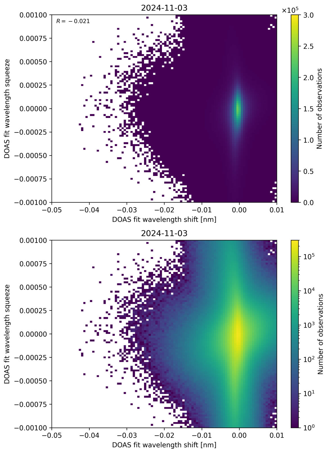
Figure 127: Scatter density plot of “DOAS fit wavelength shift” against “DOAS fit wavelength squeeze” for 2024-11-02 to 2024-11-04.
