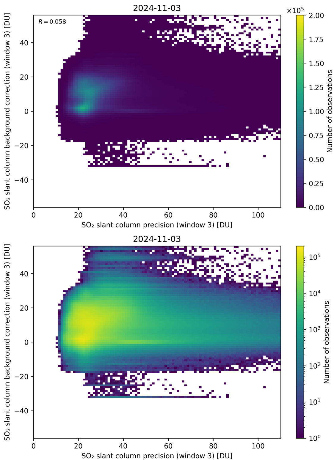
Figure 257: Scatter density plot of “SO 2 slant column precision (window 3)” against “SO 2 slant column background correction (window 3)” for 2024-11-02 to 2024-11-04.
