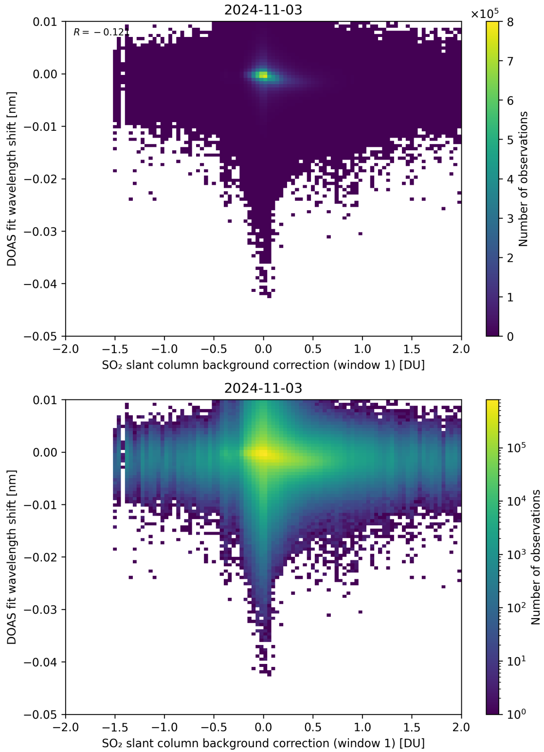
Figure 100: Scatter density plot of “SO 2 slant column background correction (window 1)” against “DOAS fit wavelength shift” for 2024-11-02 to 2024-11-04.
