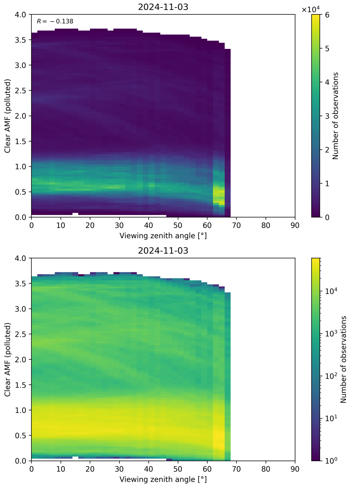
Figure 316: Scatter density plot of “Viewing zenith angle” against “Clear AMF (polluted)” for 2024-11-02 to 2024-11-04.
