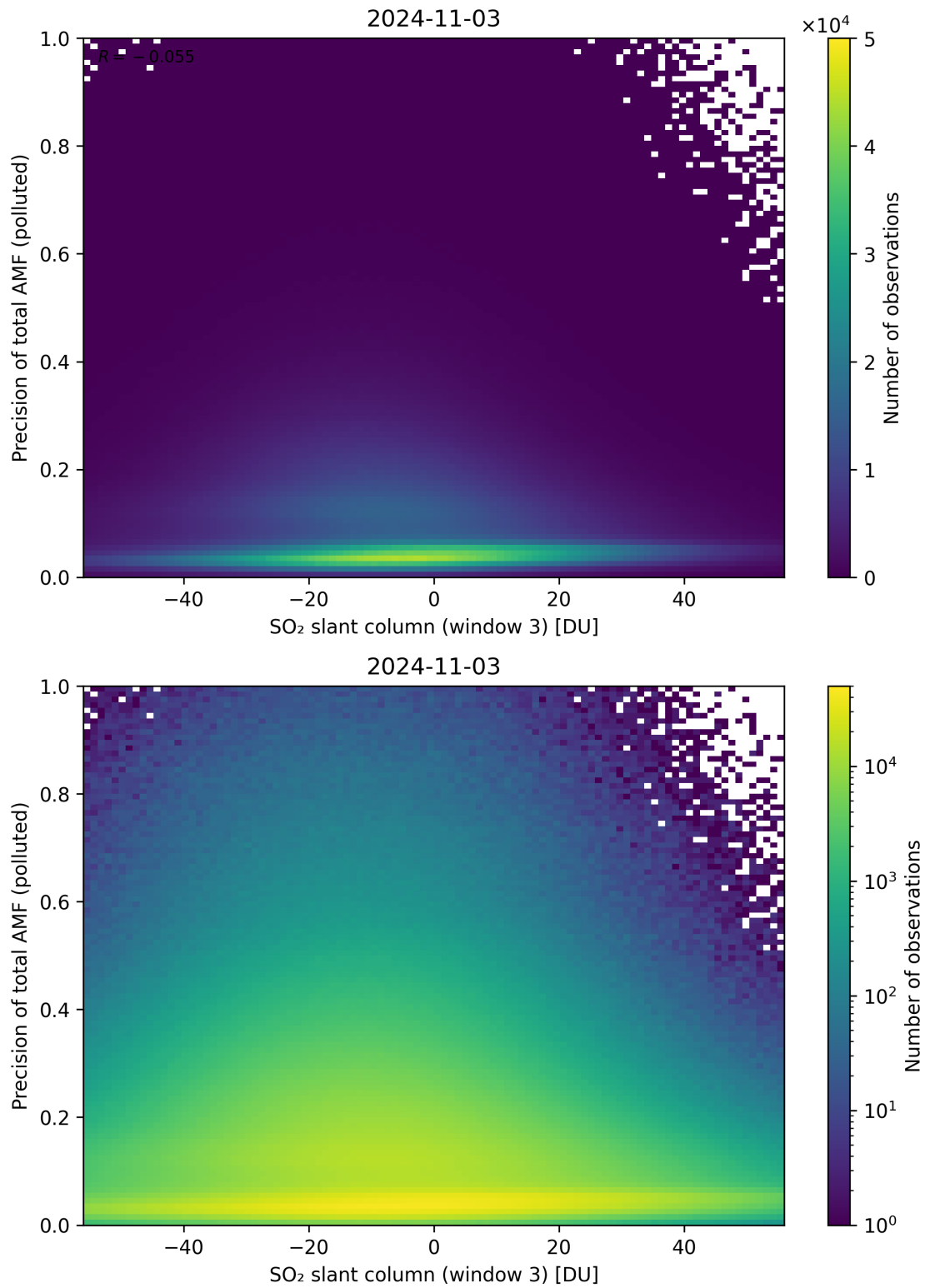
Figure 269: Scatter density plot of “SO 2 slant column (window 3)” against “Precision of total AMF (polluted)” for 2024-11-02 to 2024-11-04.
