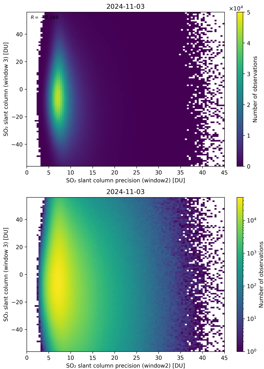
Figure 249: Scatter density plot of “SO 2 slant column precision (window2)” against “SO 2 slant column (window 3)” for 2024-11-02 to 2024-11-04.
