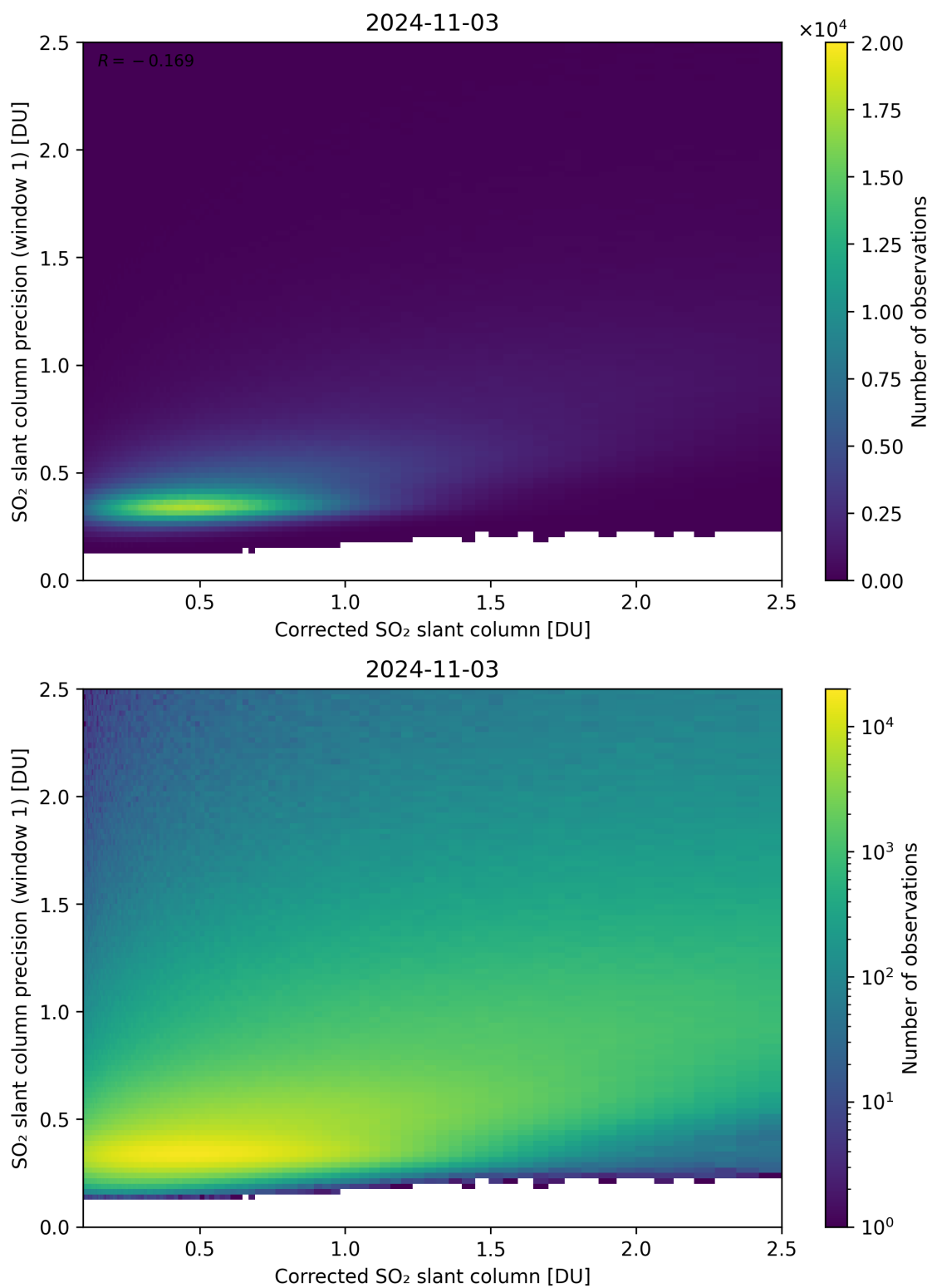
Figure 188: Scatter density plot of “Corrected SO 2 slant column” against “SO 2 slant column precision (window 1)” for 2024-11-02 to 2024-11-04.
