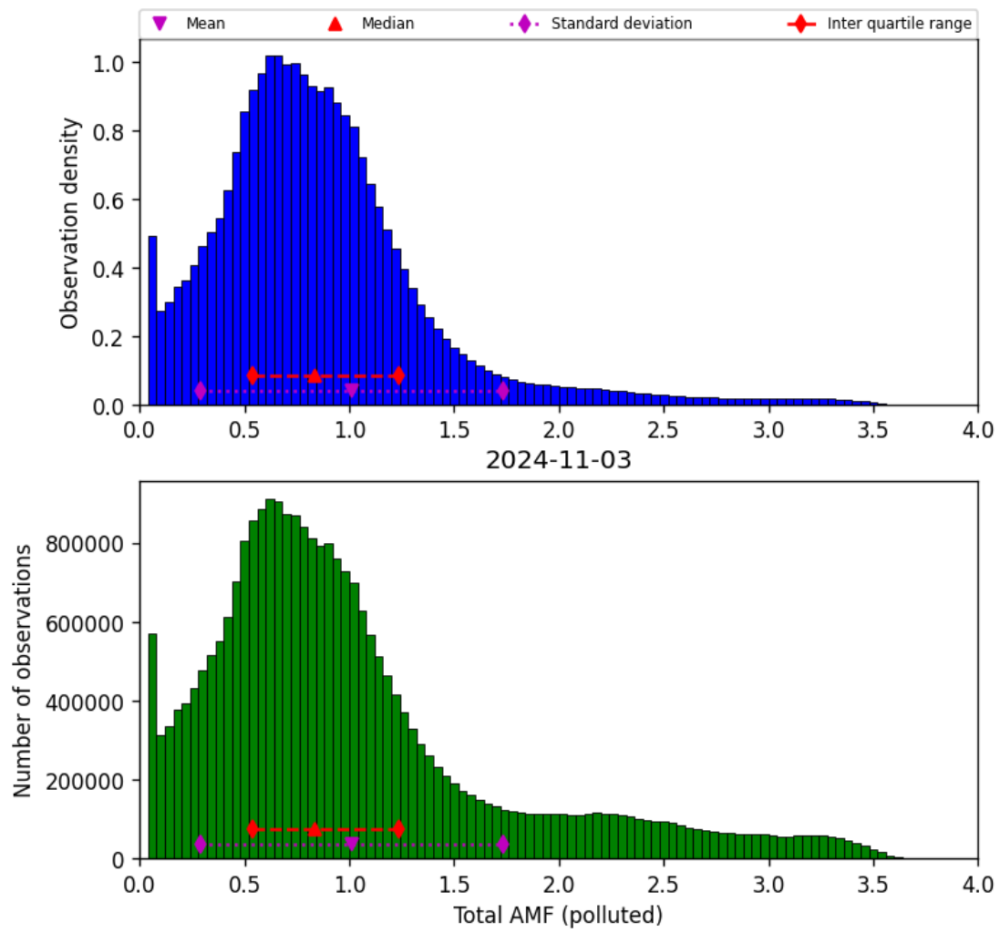
Figure 71: Histogram of “Total AMF (polluted)” for 2024-11-02 to 2024-11-04
