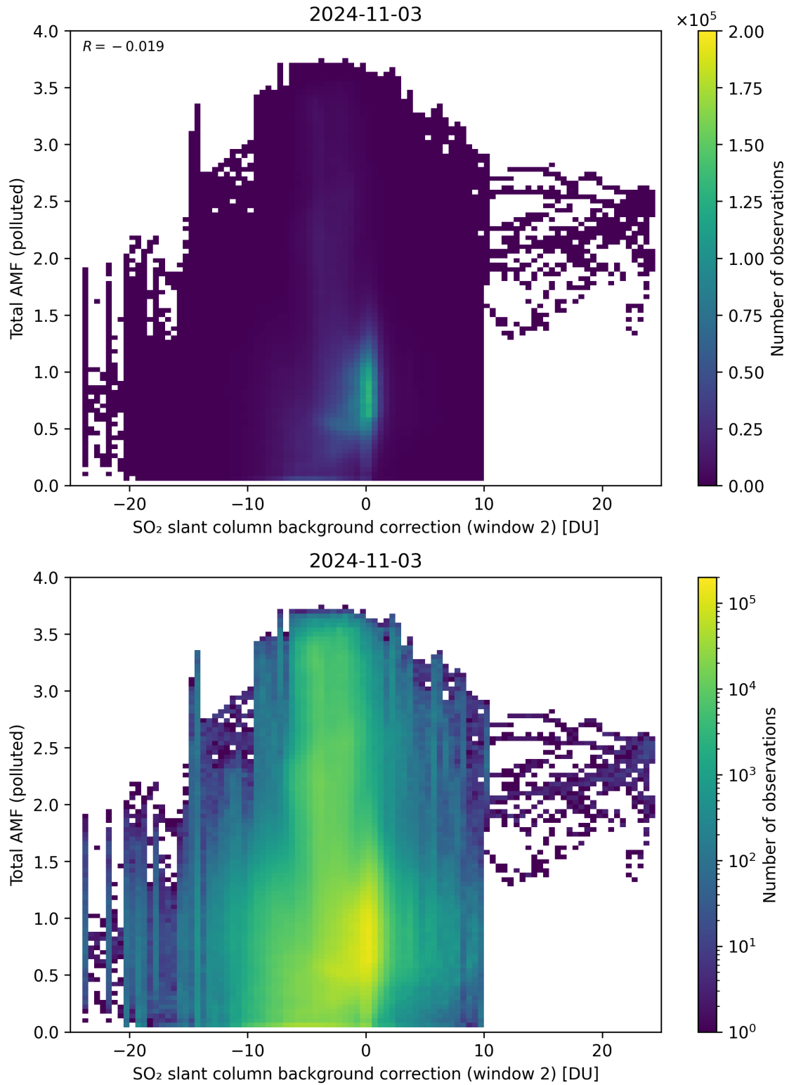
Figure 119: Scatter density plot of “SO 2 slant column background correction (window 2)” against “Total AMF (polluted)” for 2024-11-02 to 2024-11-04.
