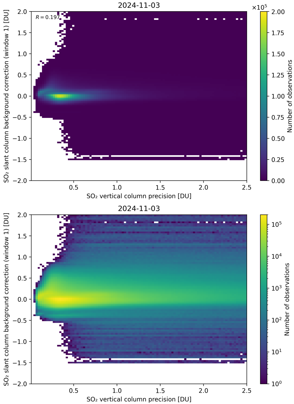
Figure 279: Scatter density plot of “SO 2 vertical column precision” against “SO 2 slant column background correction (window 1)” for 2024-11-02 to 2024-11-04.
