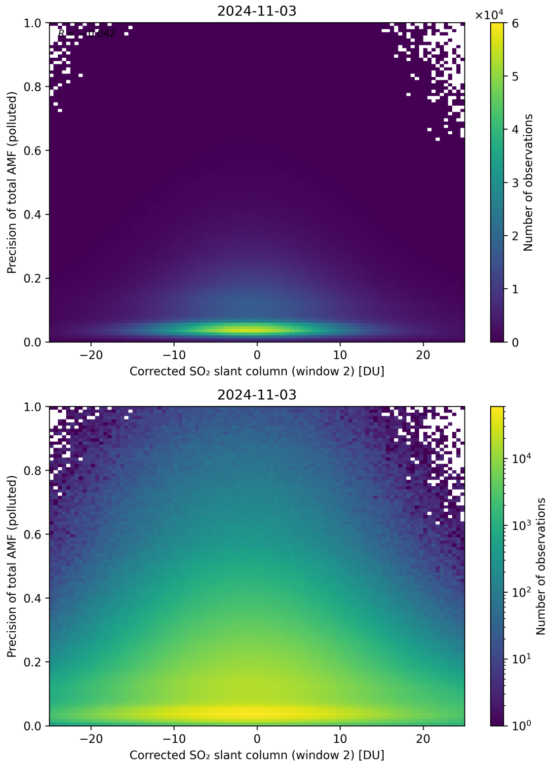
Figure 204: Scatter density plot of “Corrected SO 2 slant column (window 2)” against “Precision of total AMF (polluted)” for 2024-11-02 to 2024-11-04.
