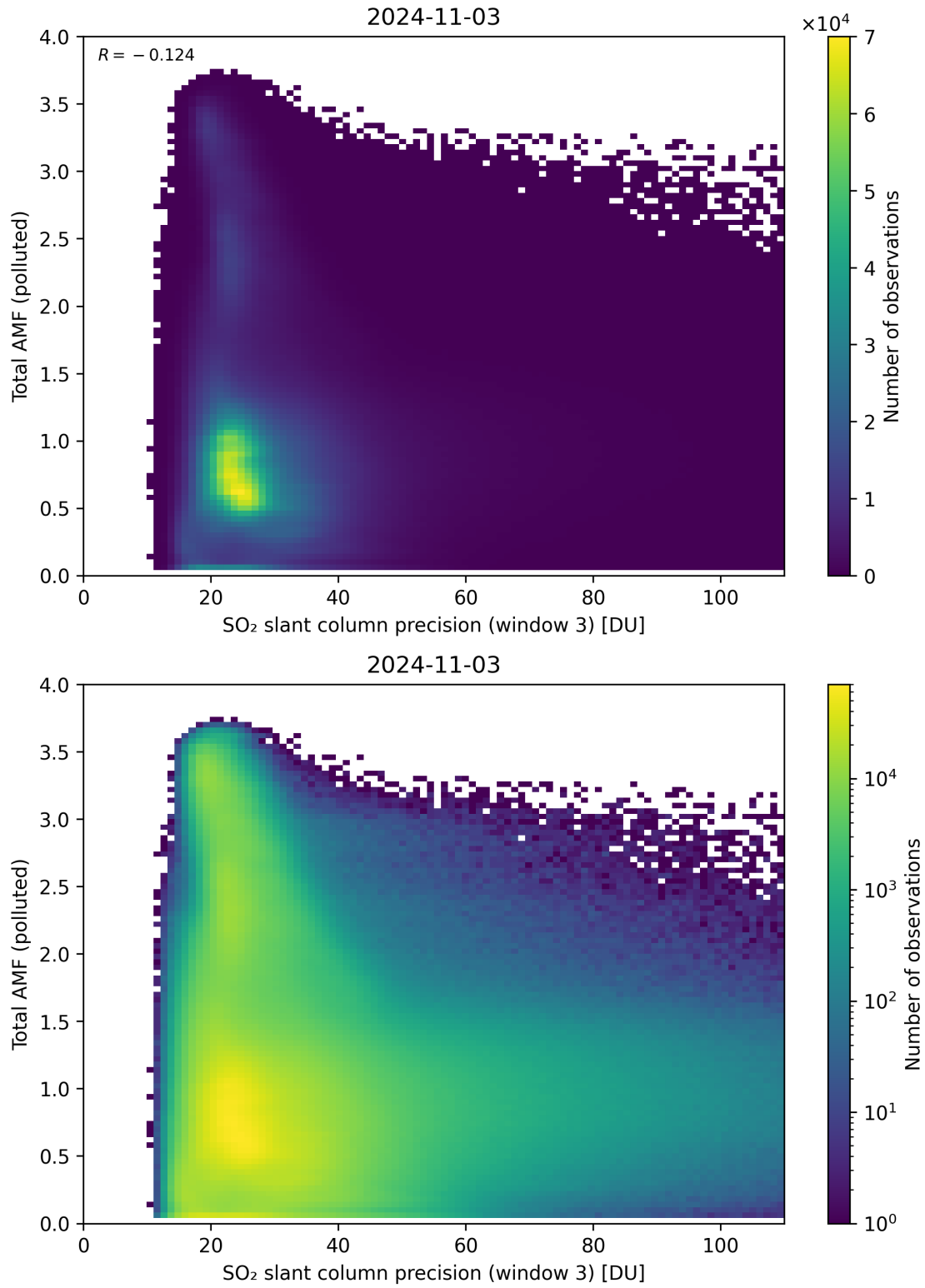
Figure 263: Scatter density plot of “SO 2 slant column precision (window 3)” against “Total AMF (polluted)” for 2024-11-02 to 2024-11-04.
