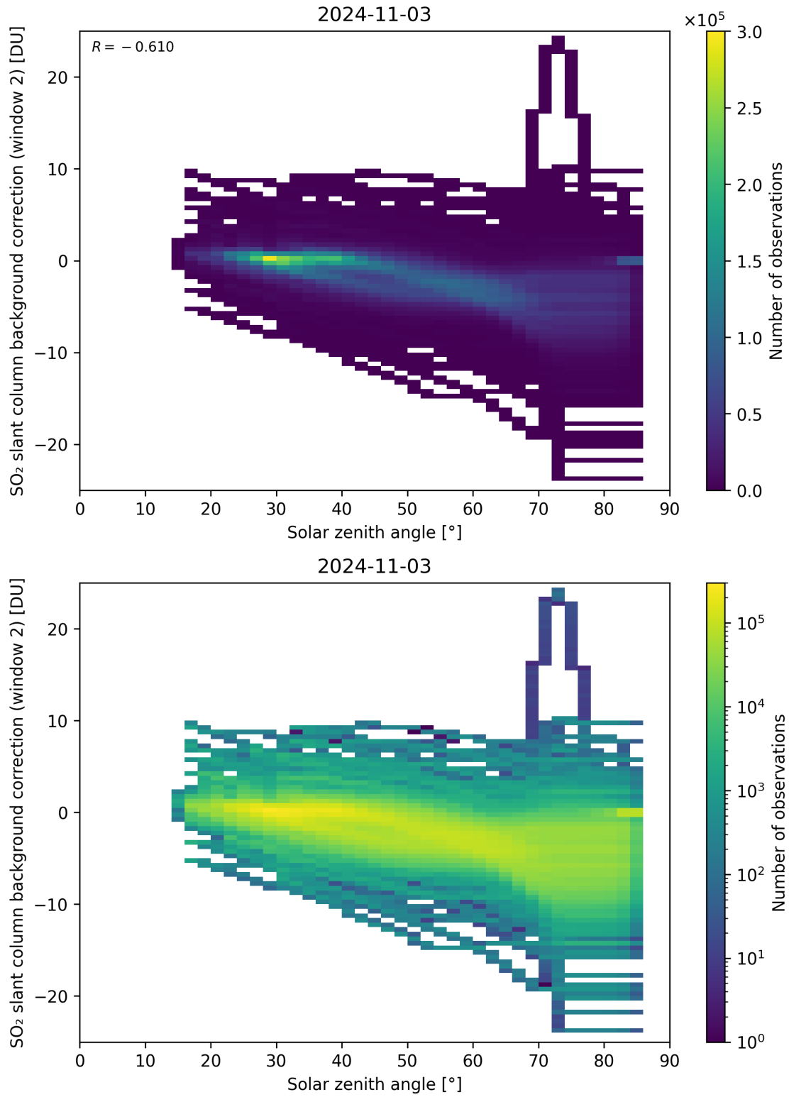
Figure 159: Scatter density plot of “Solar zenith angle” against “SO 2 slant column background correction (window 2)” for 2024-11-02 to 2024-11-04.
