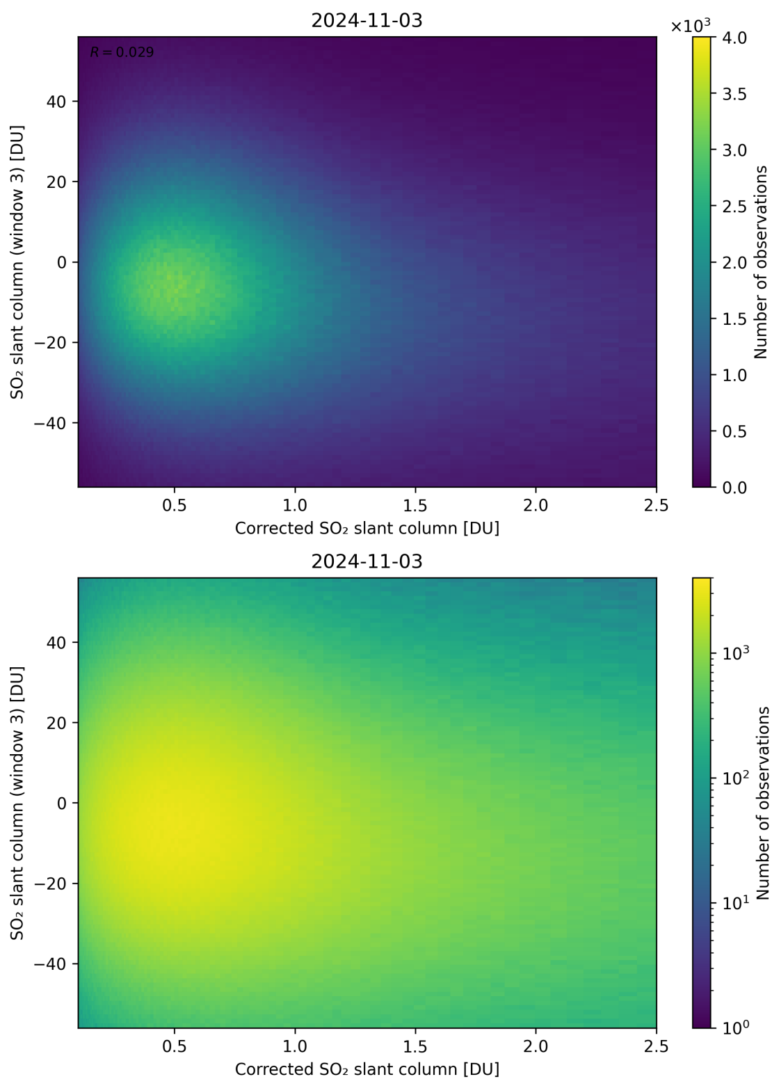
Figure 190: Scatter density plot of “Corrected SO 2 slant column” against “SO 2 slant column (window 3)” for 2024-11-02 to 2024-11-04.
