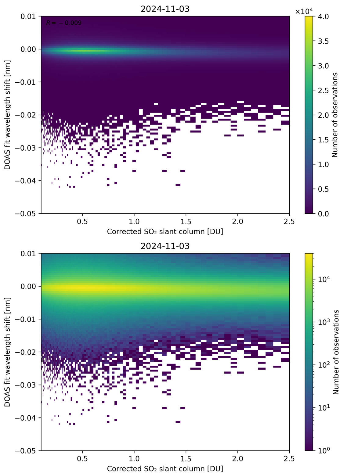
Figure 181: Scatter density plot of “Corrected SO 2 slant column” against “DOAS fit wavelength shift” for 2024-11-02 to 2024-11-04.
