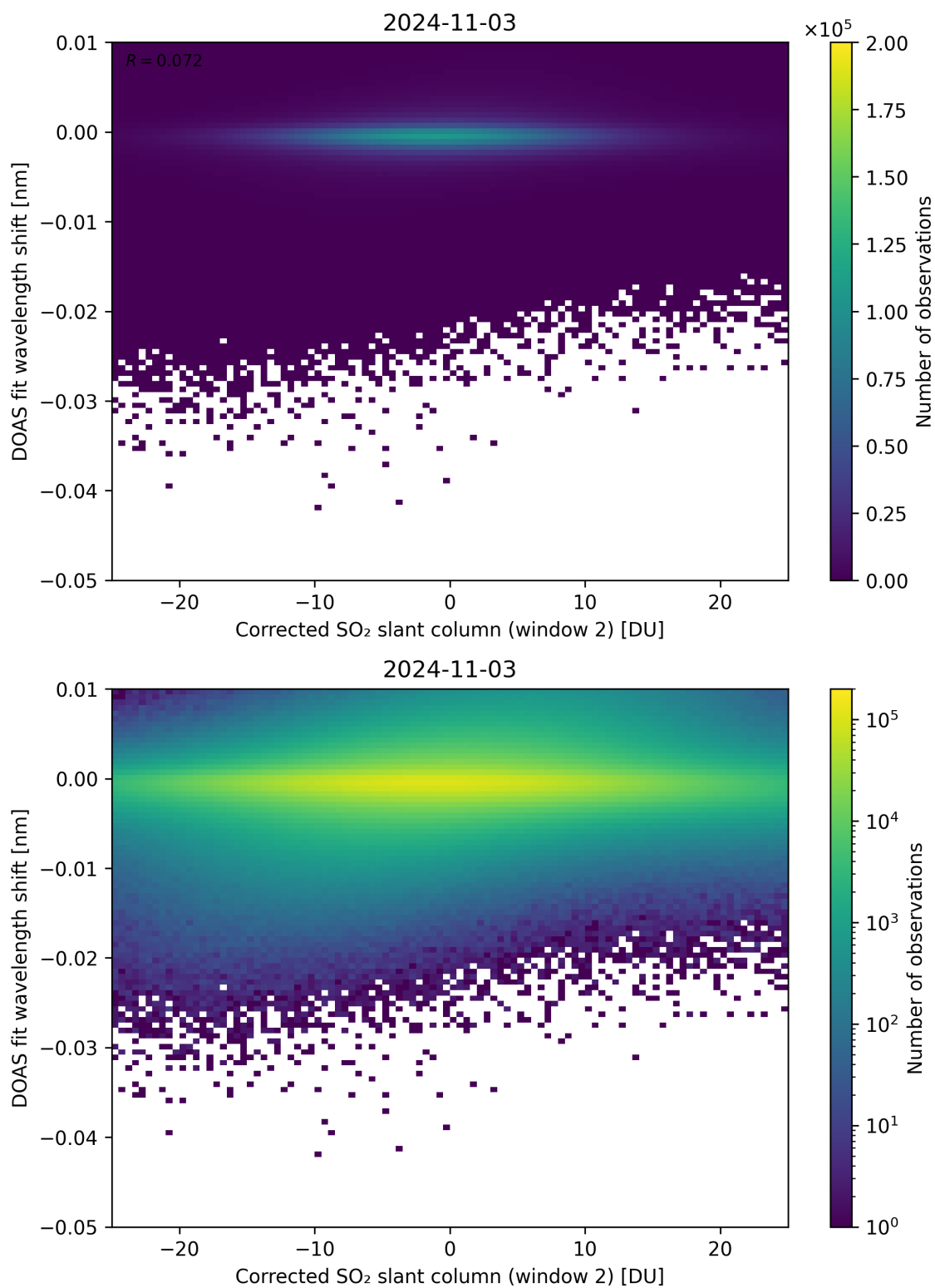
Figure 196: Scatter density plot of “Corrected SO 2 slant column (window 2)” against “DOAS fit wavelength shift” for 2024-11-02 to 2024-11-04.
