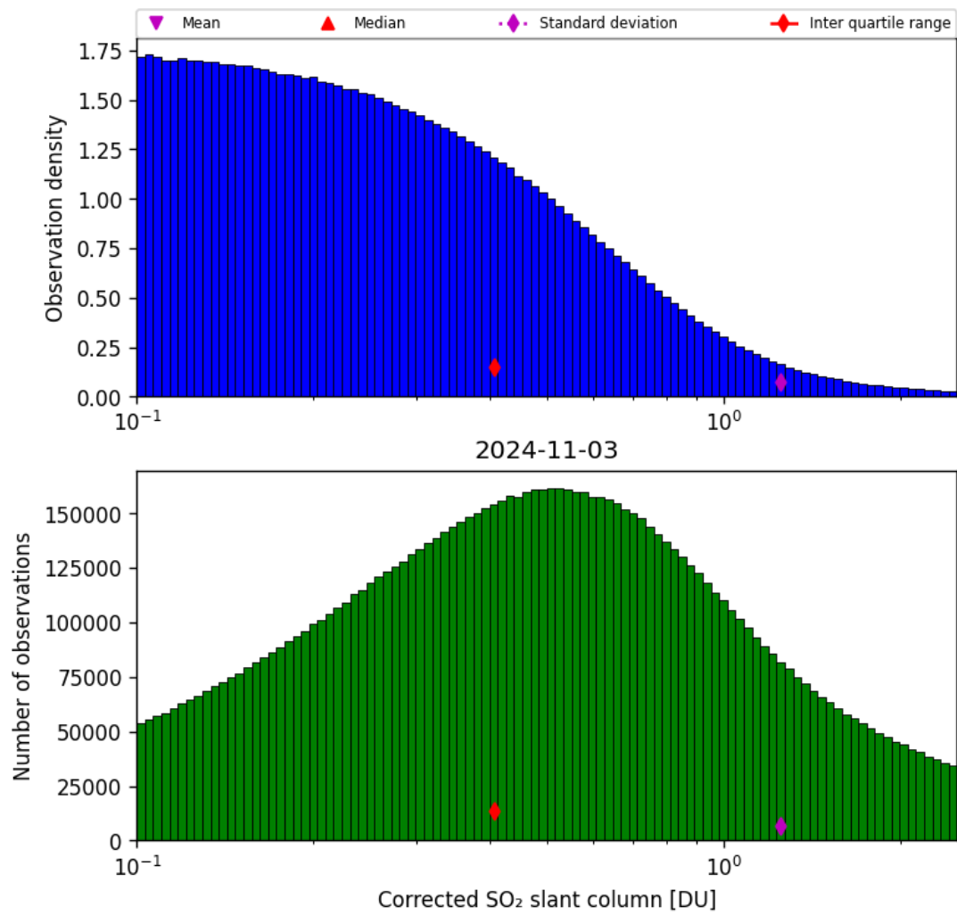
Figure 55: Histogram of “Corrected SO 2 slant column” for 2024-11-02 to 2024-11-04
