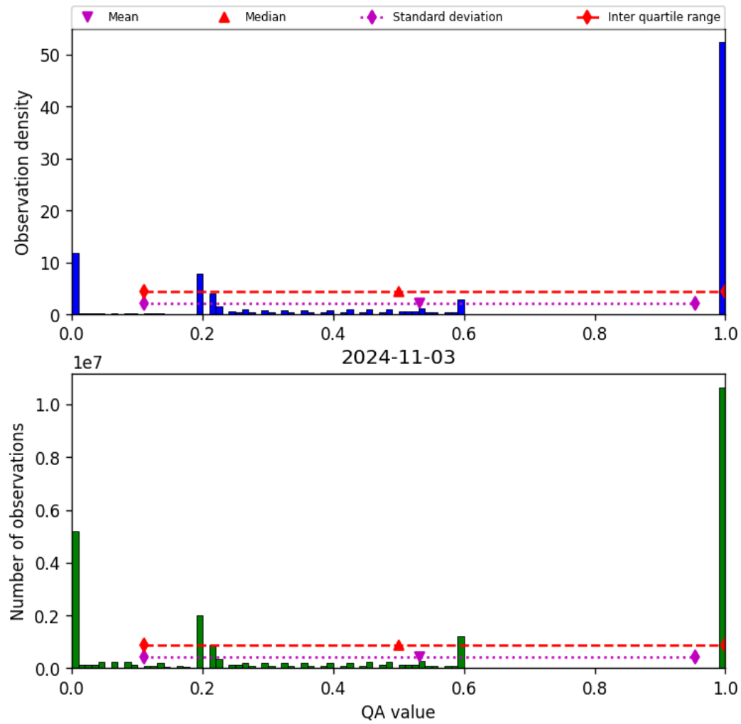
Figure 52: Histogram of “QA value” for 2024-11-02 to 2024-11-04
