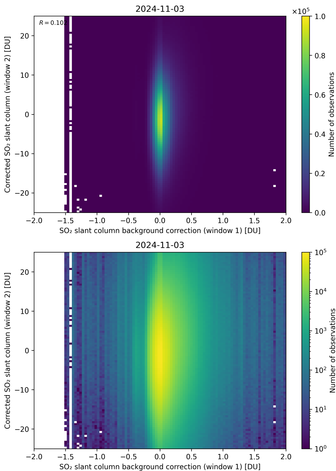
Figure 104: Scatter density plot of “SO 2 slant column background correction (window 1)” against “Corrected SO 2 slant column (window 2)” for 2024-11-02 to 2024-11-04.
