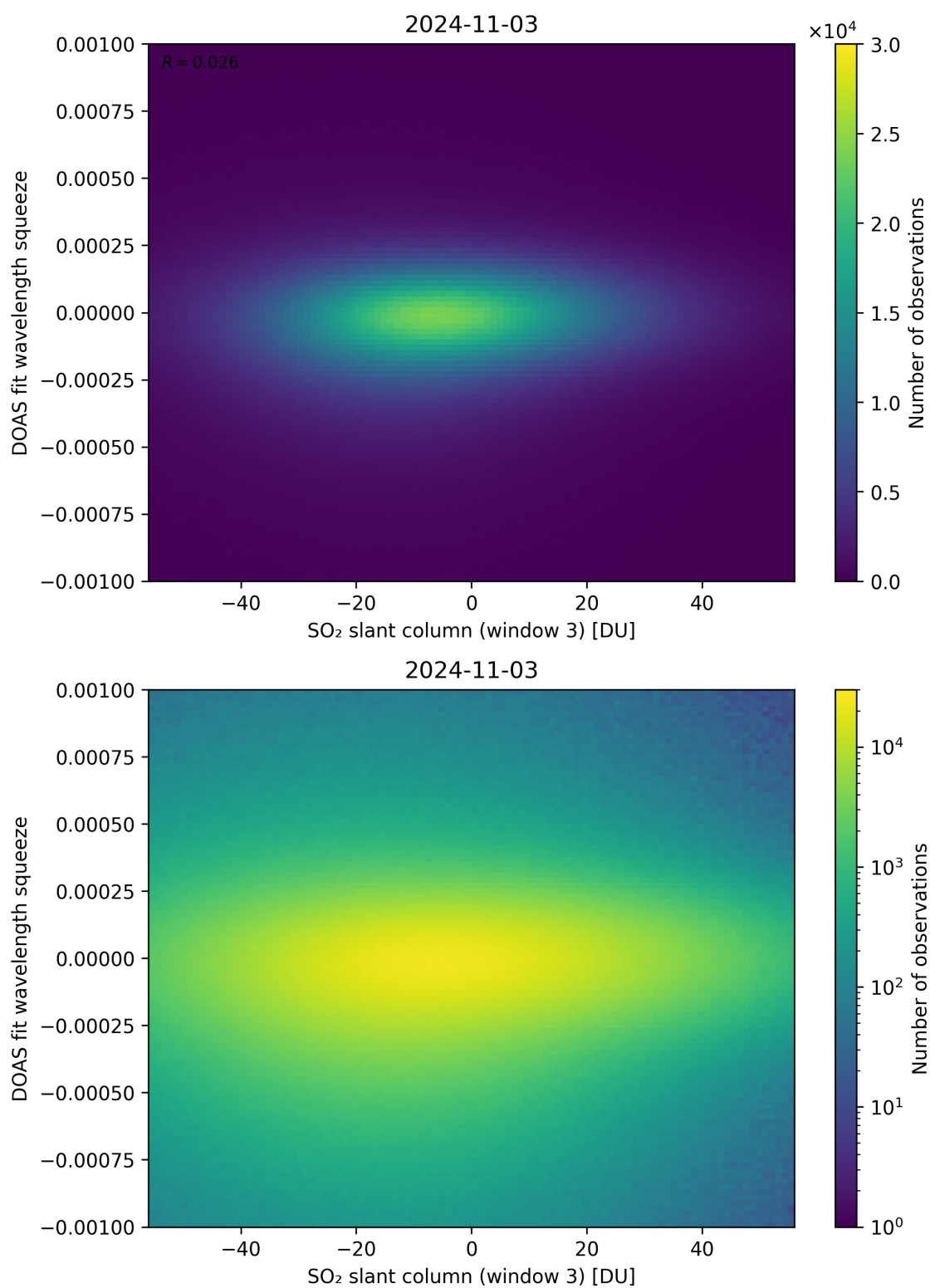
Figure 255: Scatter density plot of “SO 2 slant column (window 3)” against “DOAS fit wavelength squeeze” for 2024-11-02 to 2024-11-04.
