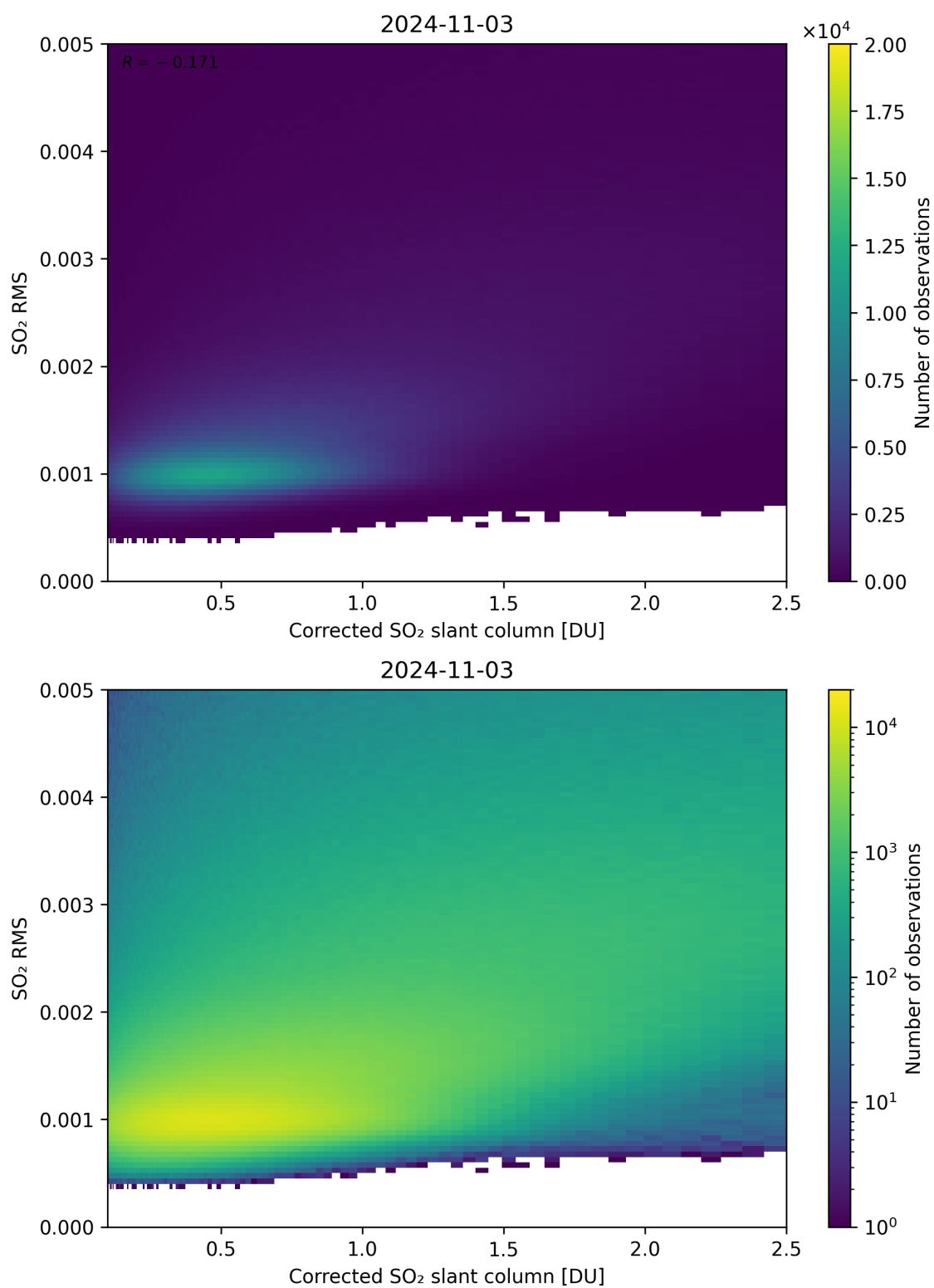
Figure 183: Scatter density plot of “Corrected SO 2 slant column” against “SO 2 RMS” for 2024-11-02 to 2024-11-04.
