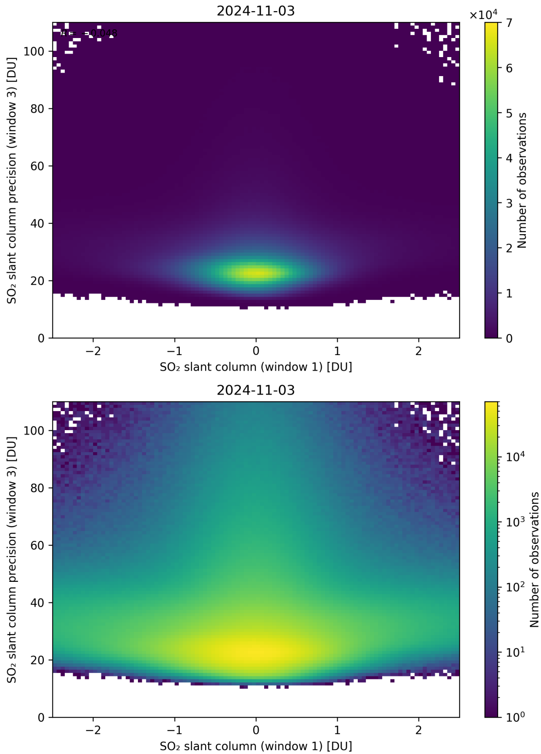
Figure 238: Scatter density plot of “SO 2 slant column (window 1)” against “SO 2 slant column precision (window 3)” for 2024-11-02 to 2024-11-04.
