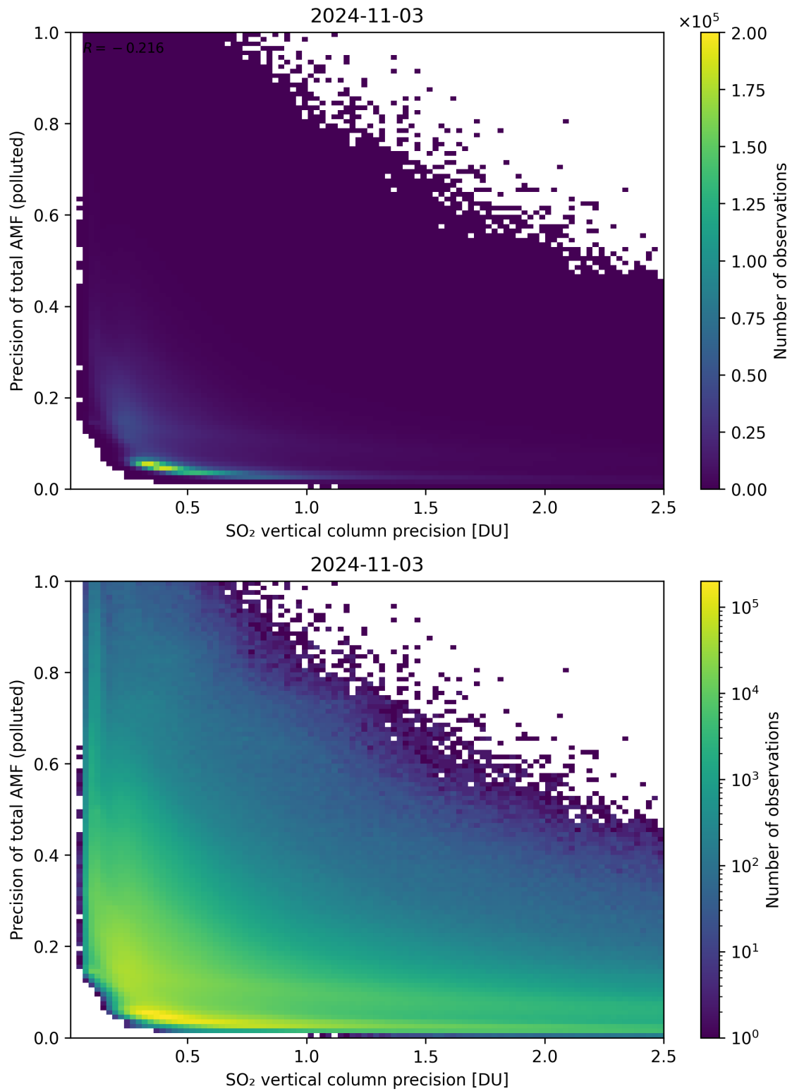
Figure 295: Scatter density plot of “SO 2 vertical column precision” against “Precision of total AMF (polluted)” for 2024-11-02 to 2024-11-04.
