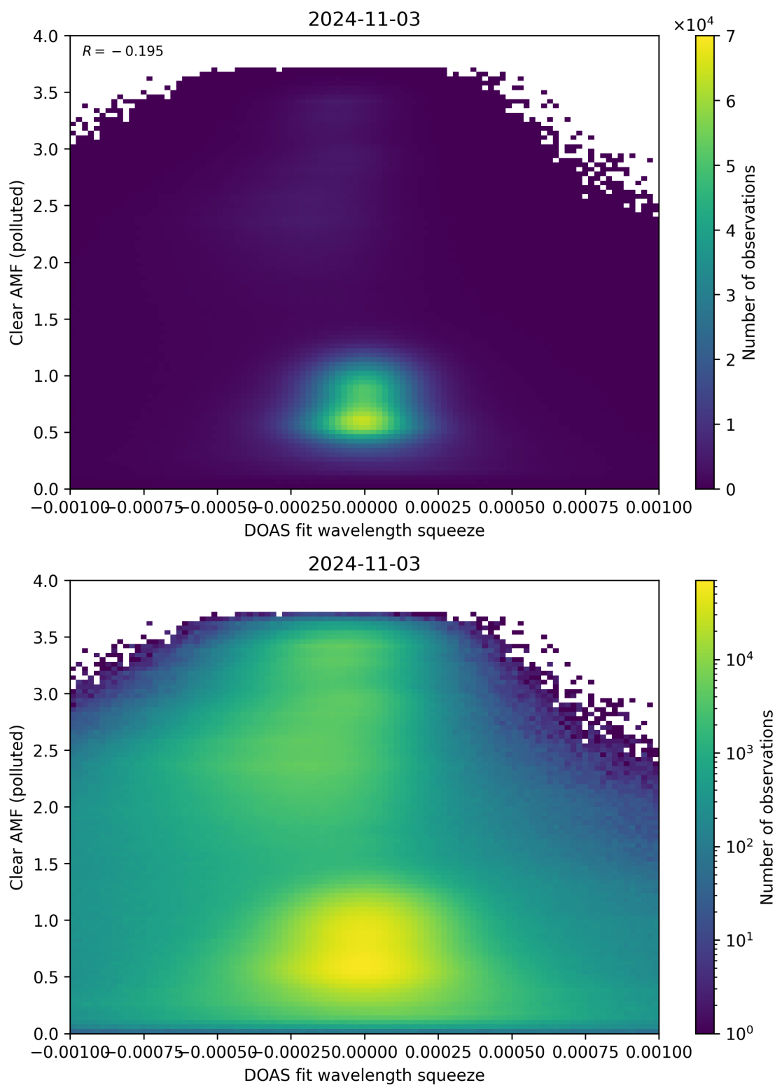
Figure 133: Scatter density plot of “DOAS fit wavelength squeeze” against “Clear AMF (polluted)” for 2024-11-02 to 2024-11-04.
