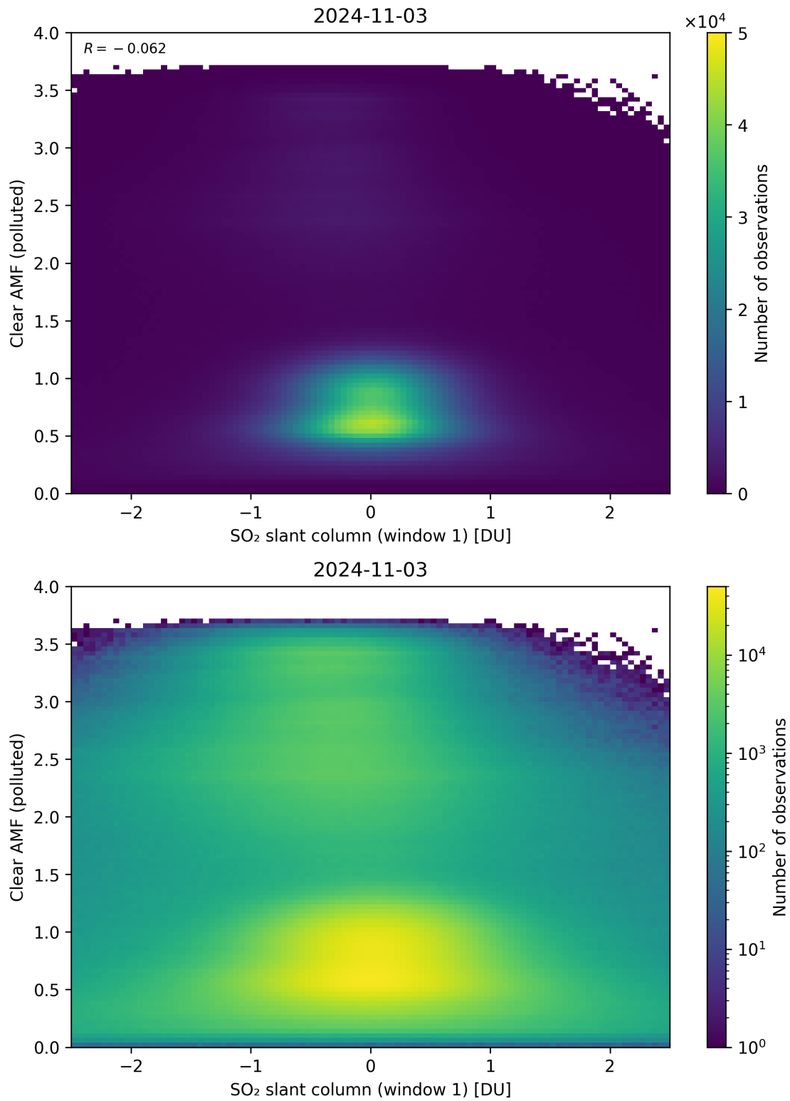
Figure 232: Scatter density plot of “SO 2 slant column (window 1)” against “Clear AMF (polluted)” for 2024-11-02 to 2024-11-04.
