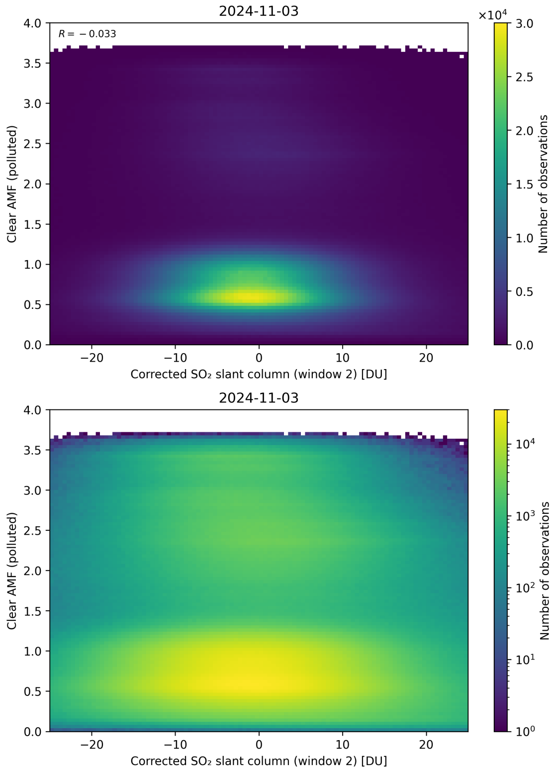
Figure 199: Scatter density plot of “Corrected SO 2 slant column (window 2)” against “Clear AMF (polluted)” for 2024-11-02 to 2024-11-04.
