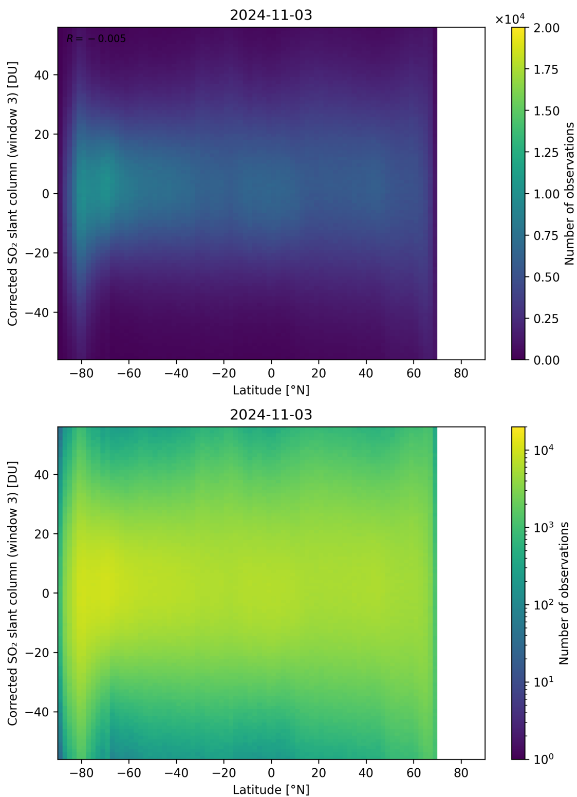
Figure 148: Scatter density plot of “Latitude” against “Corrected SO 2 slant column (window 3)” for 2024-11-02 to 2024-11-04.
