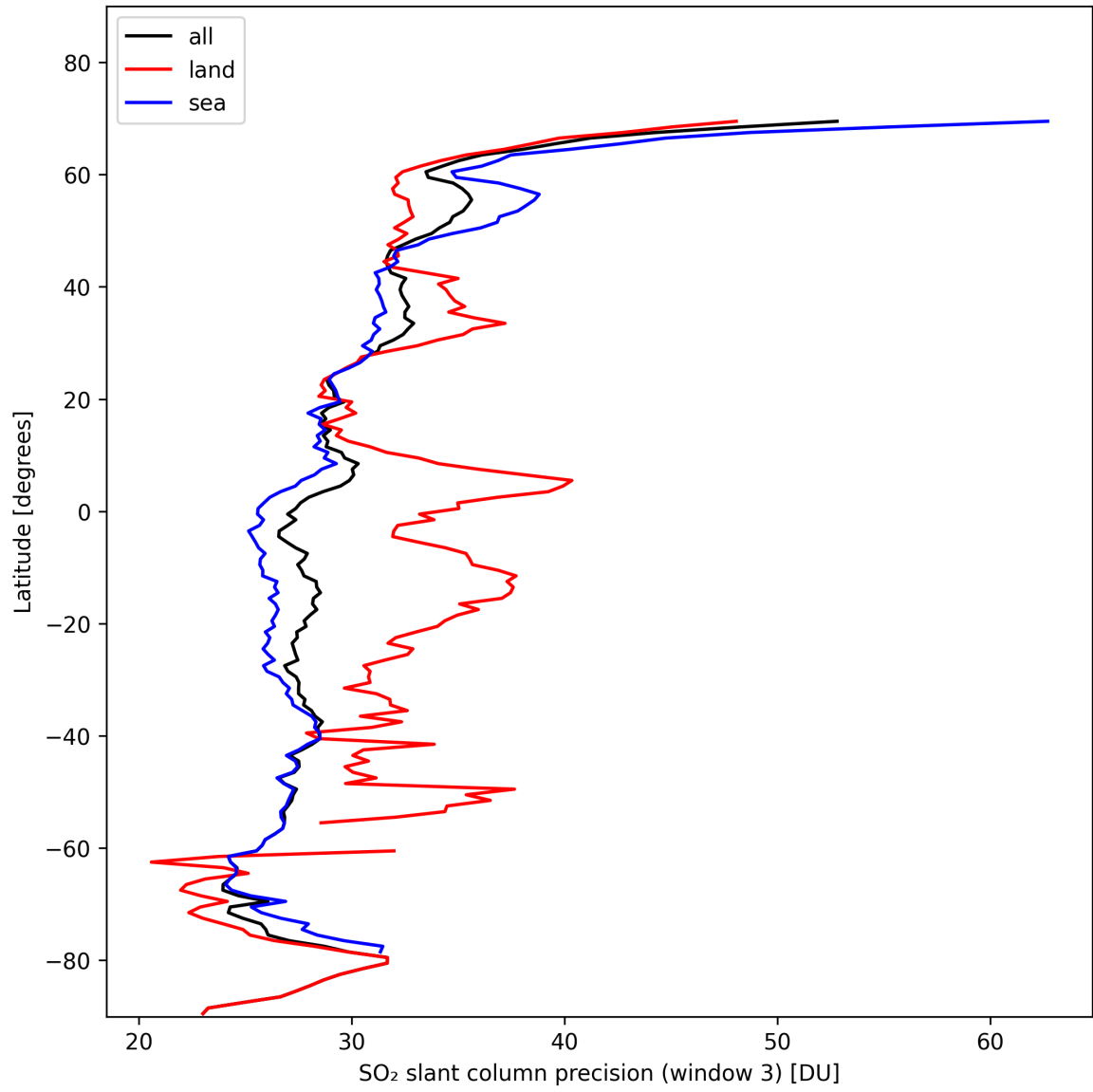
Figure 42: Zonal average of “SO 2 slant column precision (window 3)” for 2024-11-02 to 2024-11-04.
