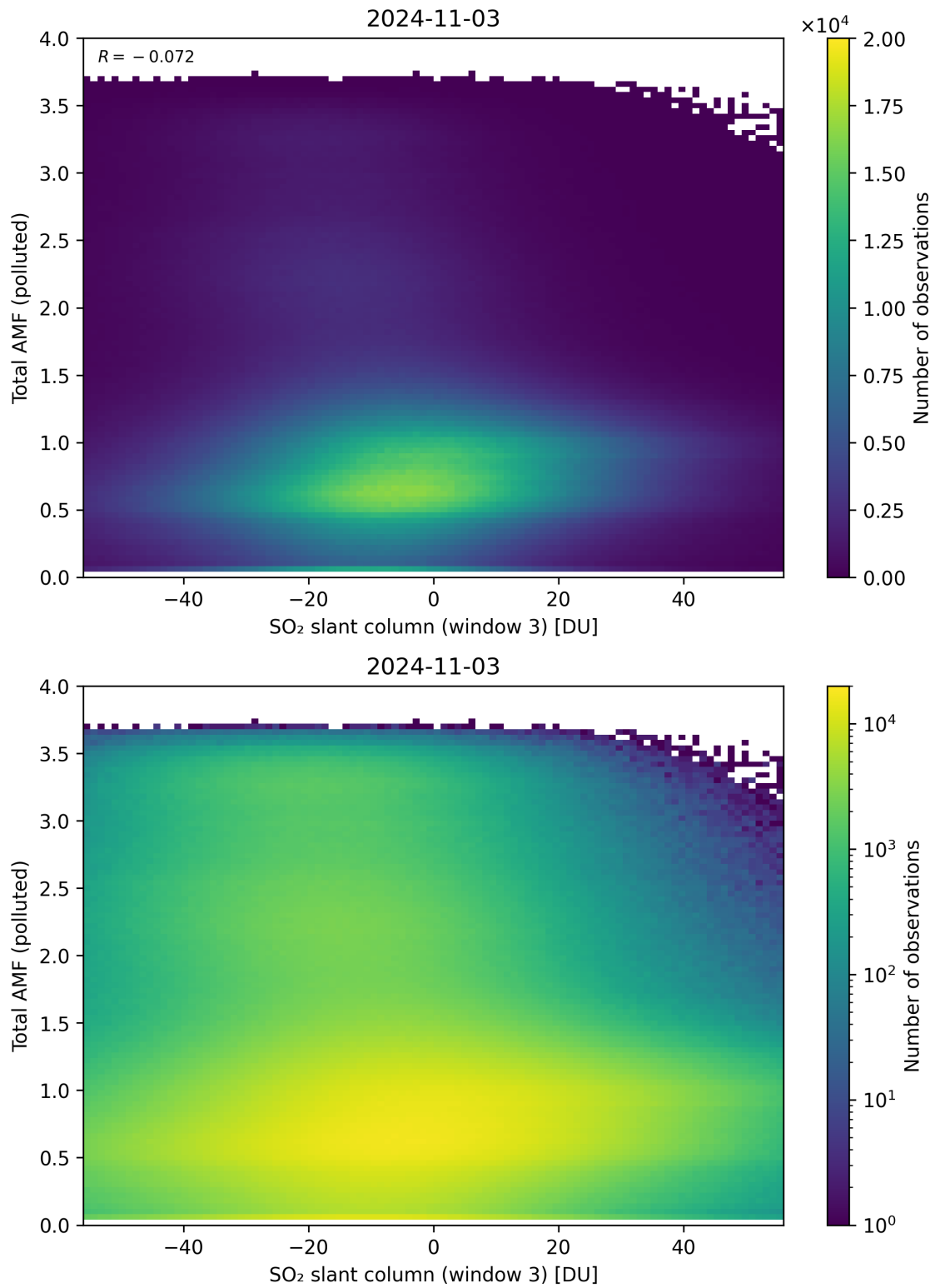
Figure 268: Scatter density plot of “SO 2 slant column (window 3)” against “Total AMF (polluted)” for 2024-11-02 to 2024-11-04.
