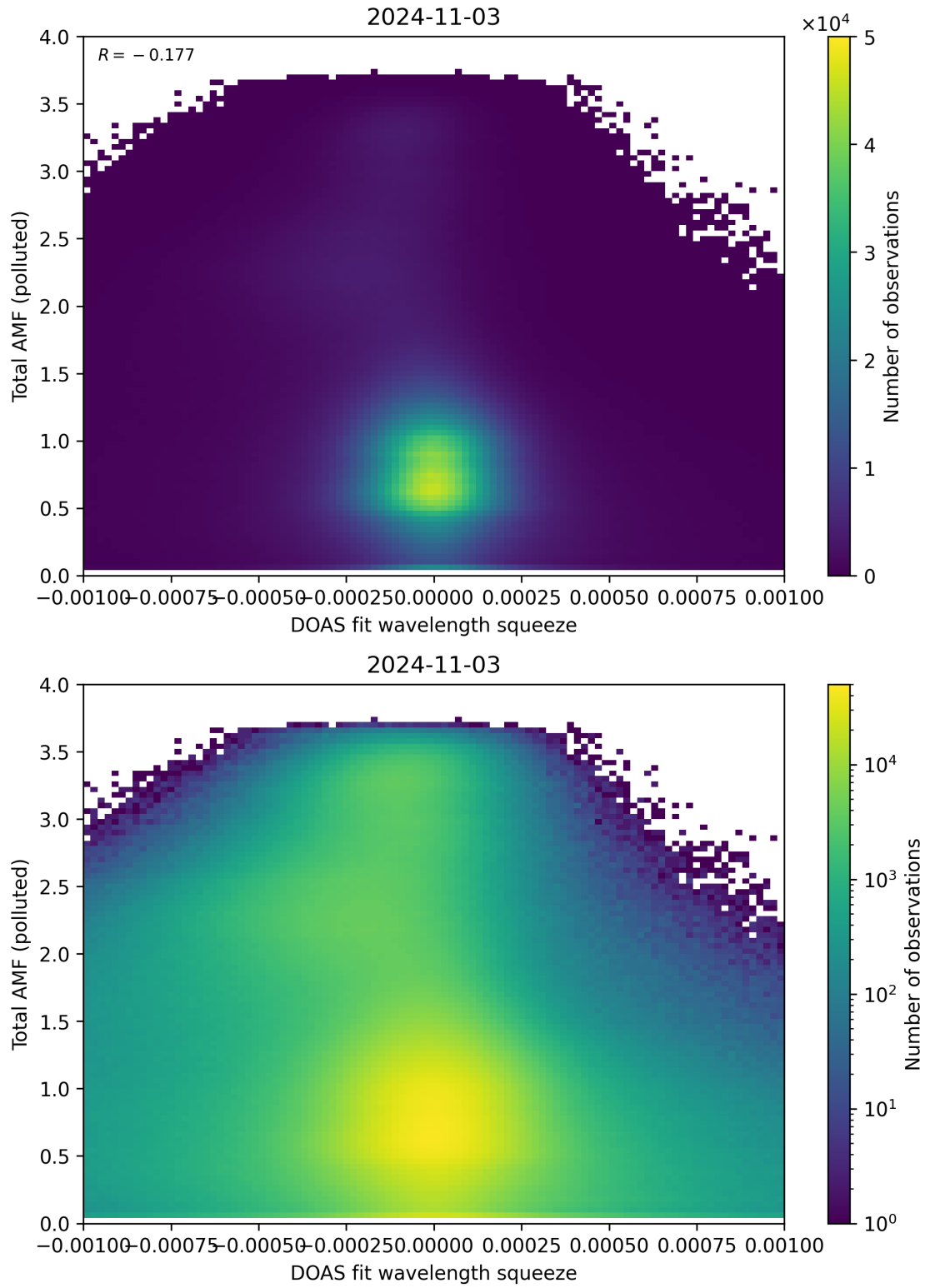
Figure 134: Scatter density plot of “DOAS fit wavelength squeeze” against “Total AMF (polluted)” for 2024-11-02 to 2024-11-04.
