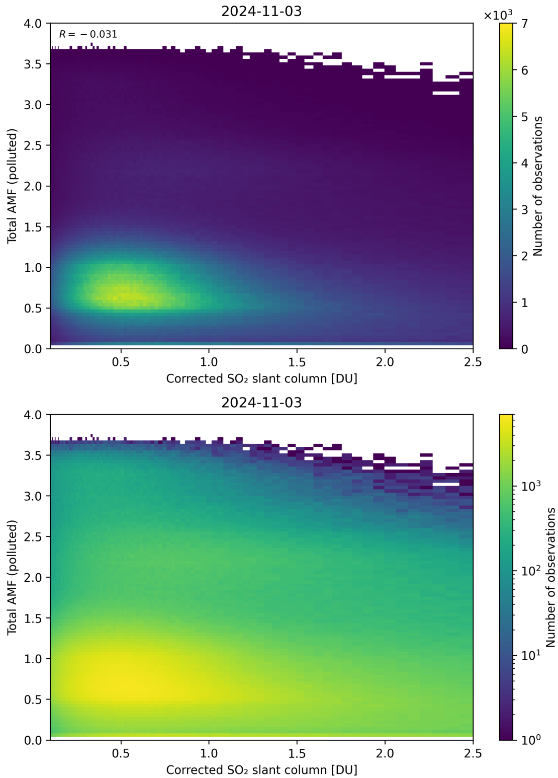
Figure 192: Scatter density plot of “Corrected SO 2 slant column” against “Total AMF (polluted)” for 2024-11-02 to 2024-11-04.
