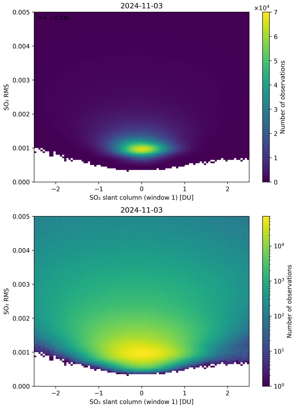
Figure 217: Scatter density plot of “SO 2 slant column (window 1)” against “SO 2 RMS” for 2024-11-02 to 2024-11-04.
