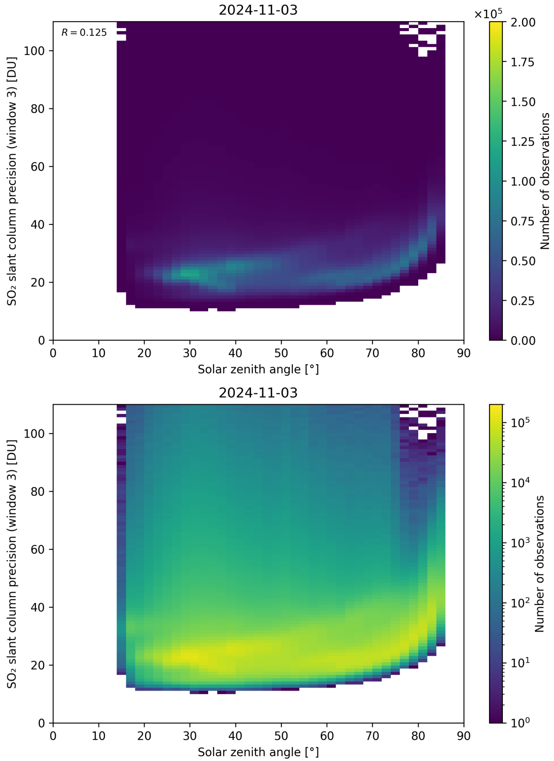
Figure 173: Scatter density plot of “Solar zenith angle” against “SO 2 slant column precision (window 3)” for 2024-11-02 to 2024-11-04.
