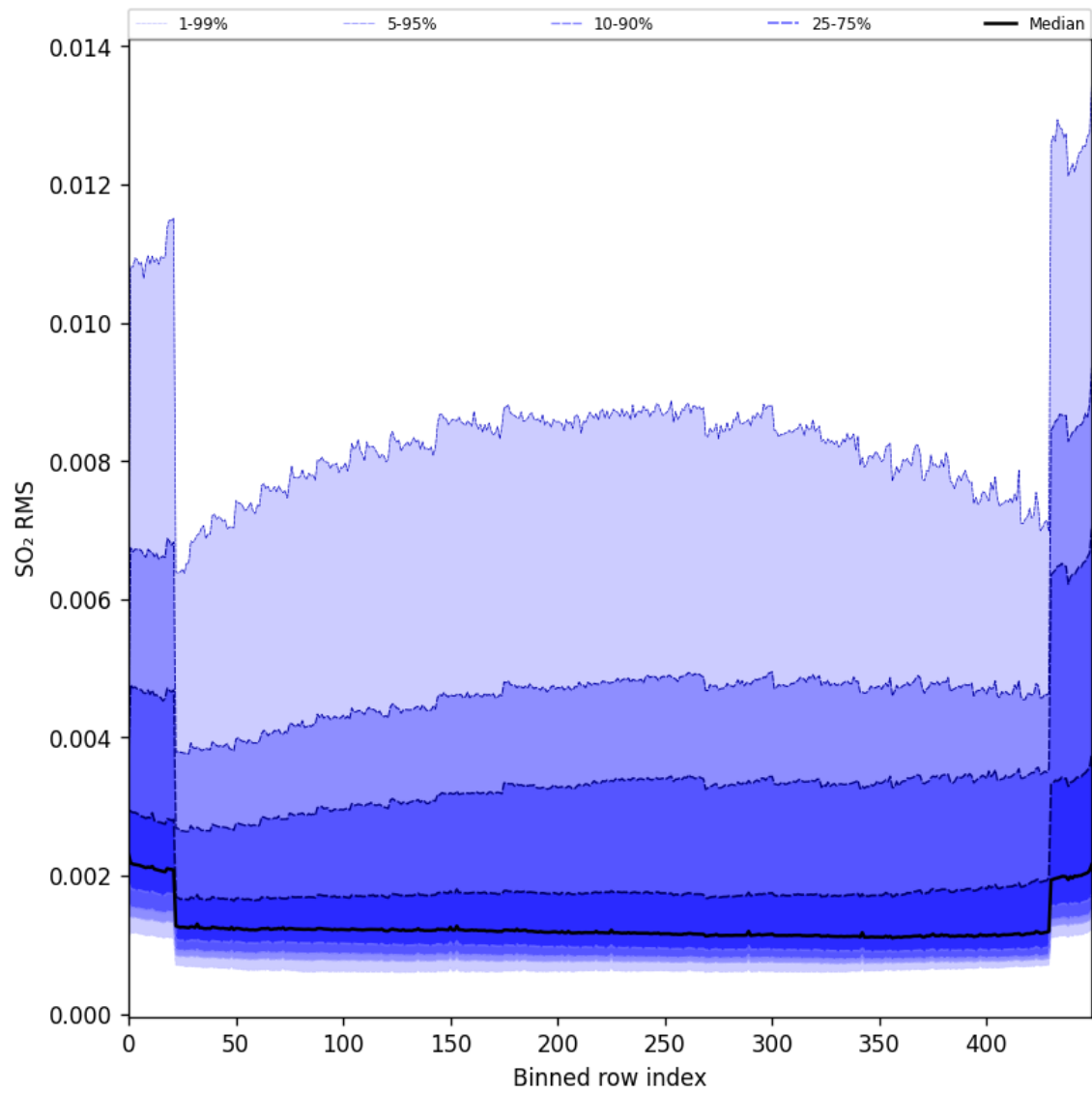
Figure 93: Along track statistics of “SO 2 RMS” for 2024-11-02 to 2024-11-04
