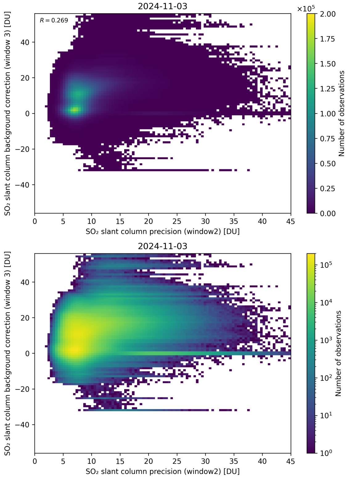
Figure 242: Scatter density plot of “SO 2 slant column precision (window2)” against “SO 2 slant column background correction (window 3)” for 2024-11-02 to 2024-11-04.
