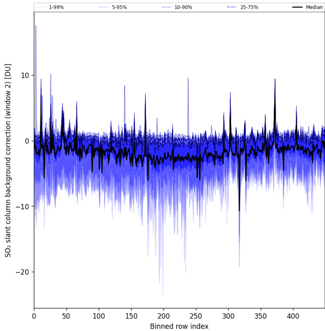
Figure 86: Along track statistics of “SO 2 slant column background correction (window 2)” for 2024-11-02 to 2024-11-04
