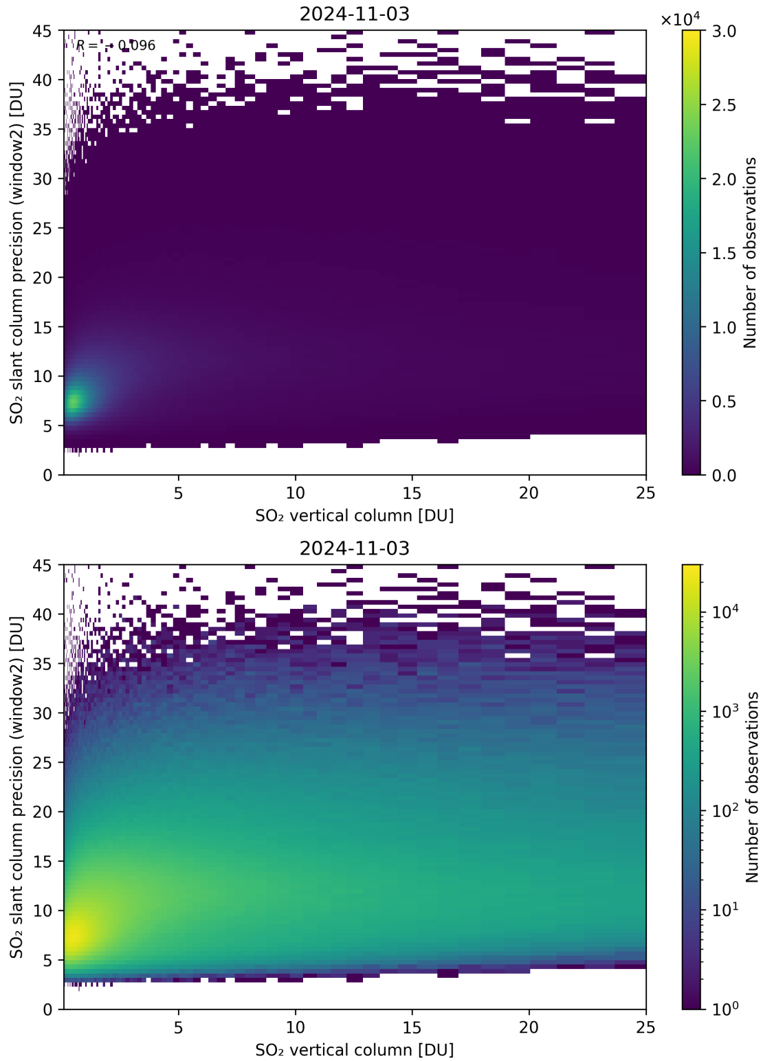
Figure 302: Scatter density plot of “SO 2 vertical column” against “SO 2 slant column precision (window2)” for 2024-11-02 to 2024-11-04.
