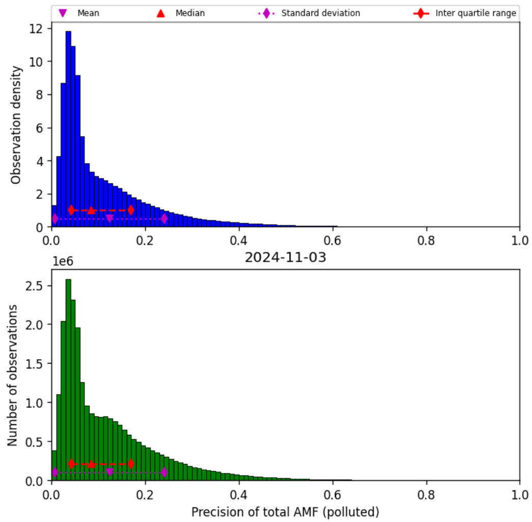
Figure 72: Histogram of “Precision of total AMF (polluted)” for 2024-11-02 to 2024-11-04
