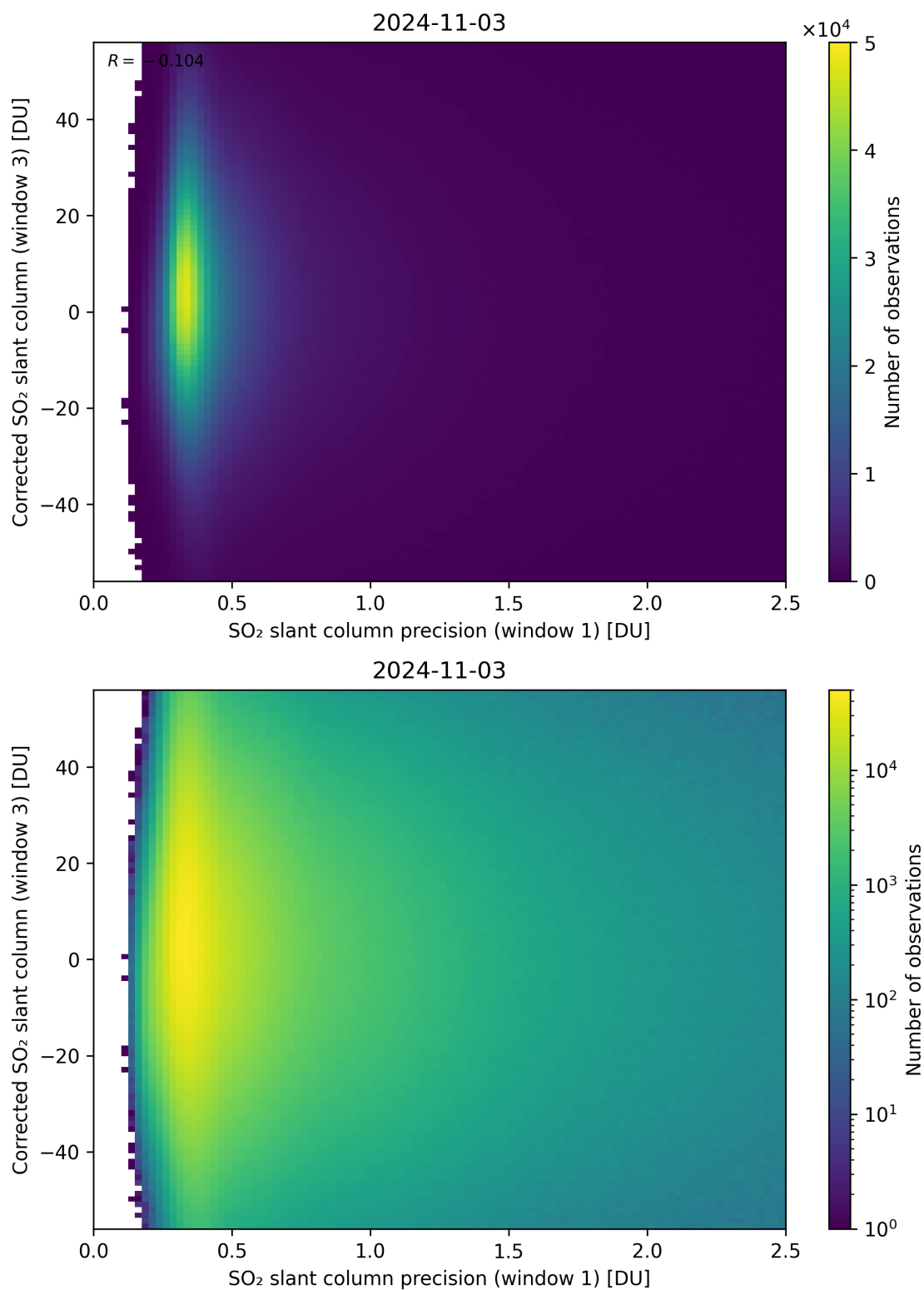
Figure 226: Scatter density plot of “SO 2 slant column precision (window 1)” against “Corrected SO 2 slant column (window 3)” for 2024-11-02 to 2024-11-04.
