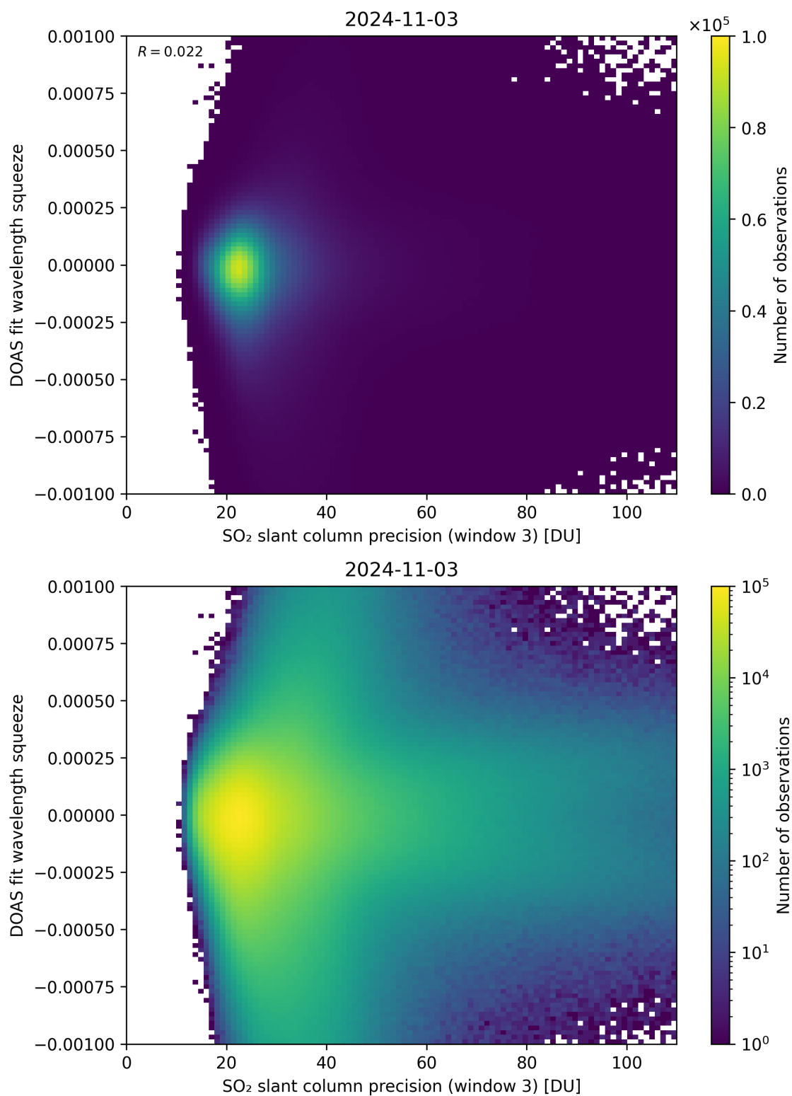
Figure 259: Scatter density plot of “SO 2 slant column precision (window 3)” against “DOAS fit wavelength squeeze” for 2024-11-02 to 2024-11-04.
