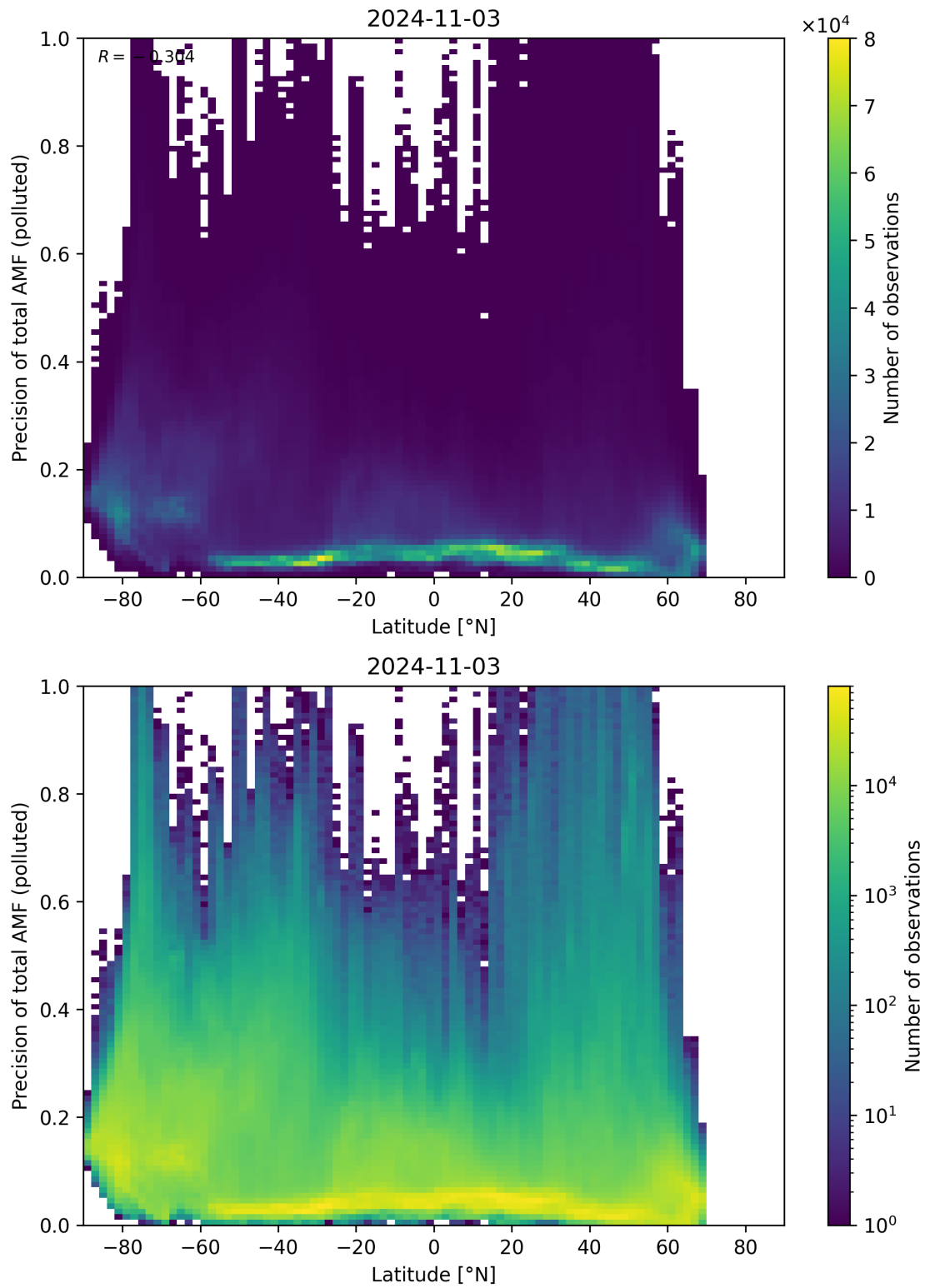
Figure 155: Scatter density plot of “Latitude” against “Precision of total AMF (polluted)” for 2024-11-02 to 2024-11-04.
