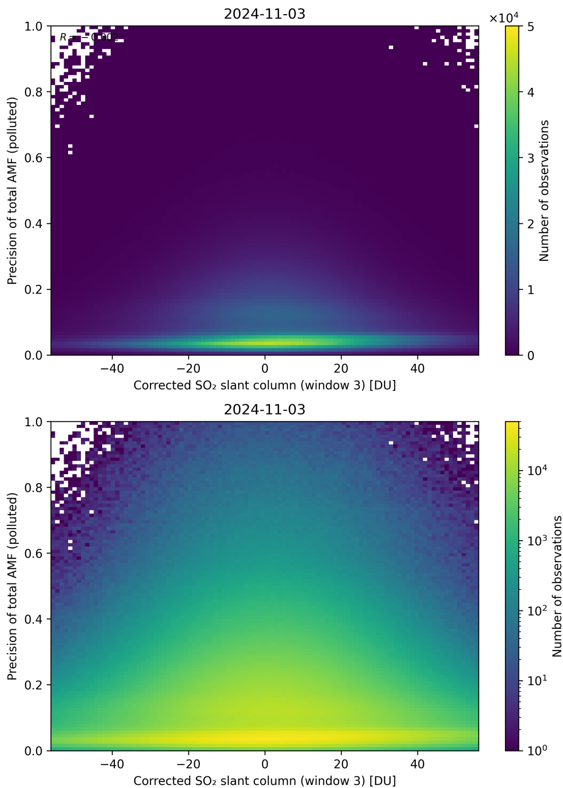
Figure 211: Scatter density plot of “Corrected SO 2 slant column (window 3)” against “Precision of total AMF (polluted)” for 2024-11-02 to 2024-11-04.
