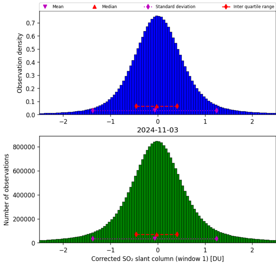
Figure 58: Histogram of “Corrected SO 2 slant column (window 1)” for 2024-11-02 to 2024-11-04
