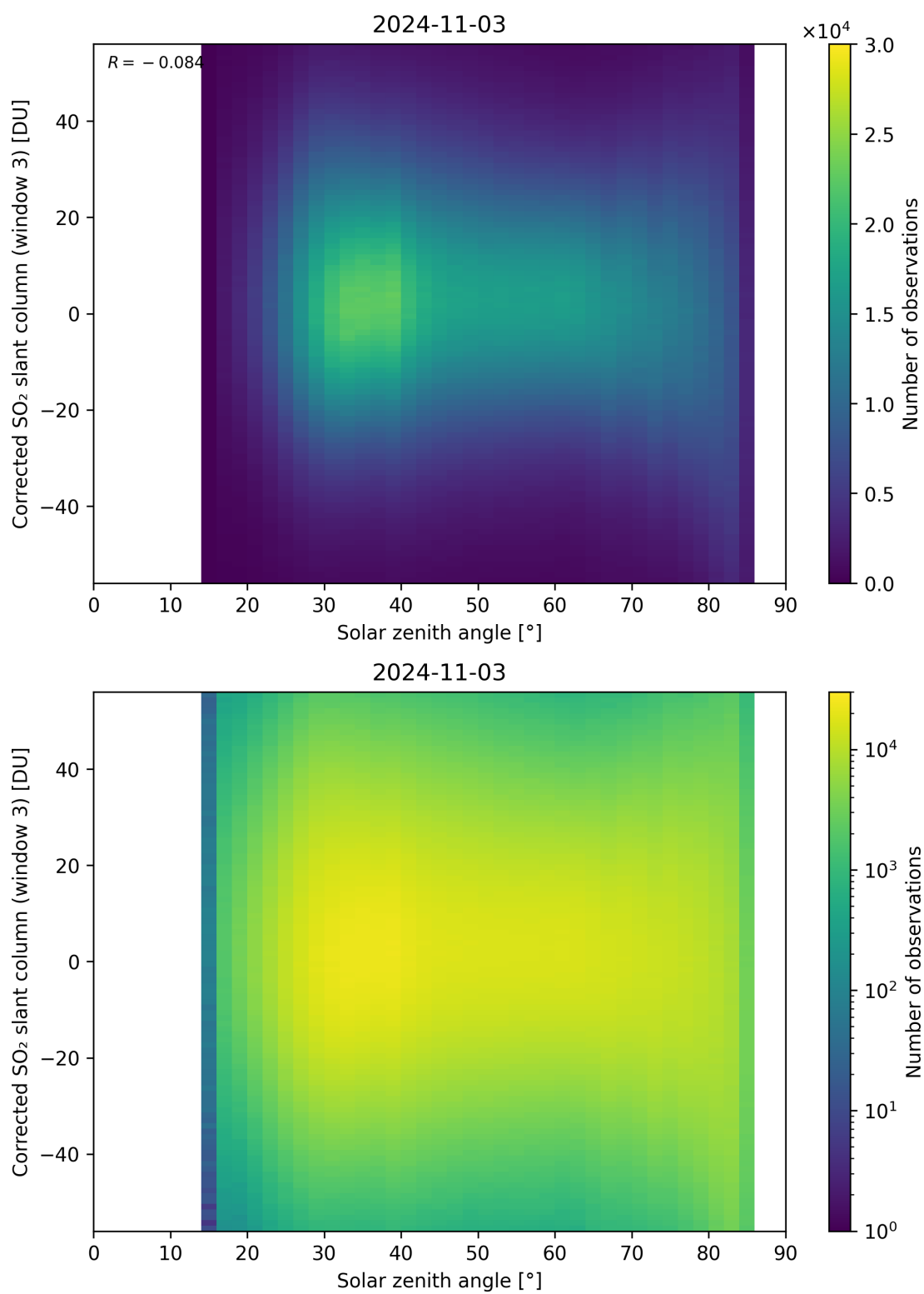
Figure 168: Scatter density plot of “Solar zenith angle” against “Corrected SO 2 slant column (window 3)” for 2024-11-02 to 2024-11-04.
