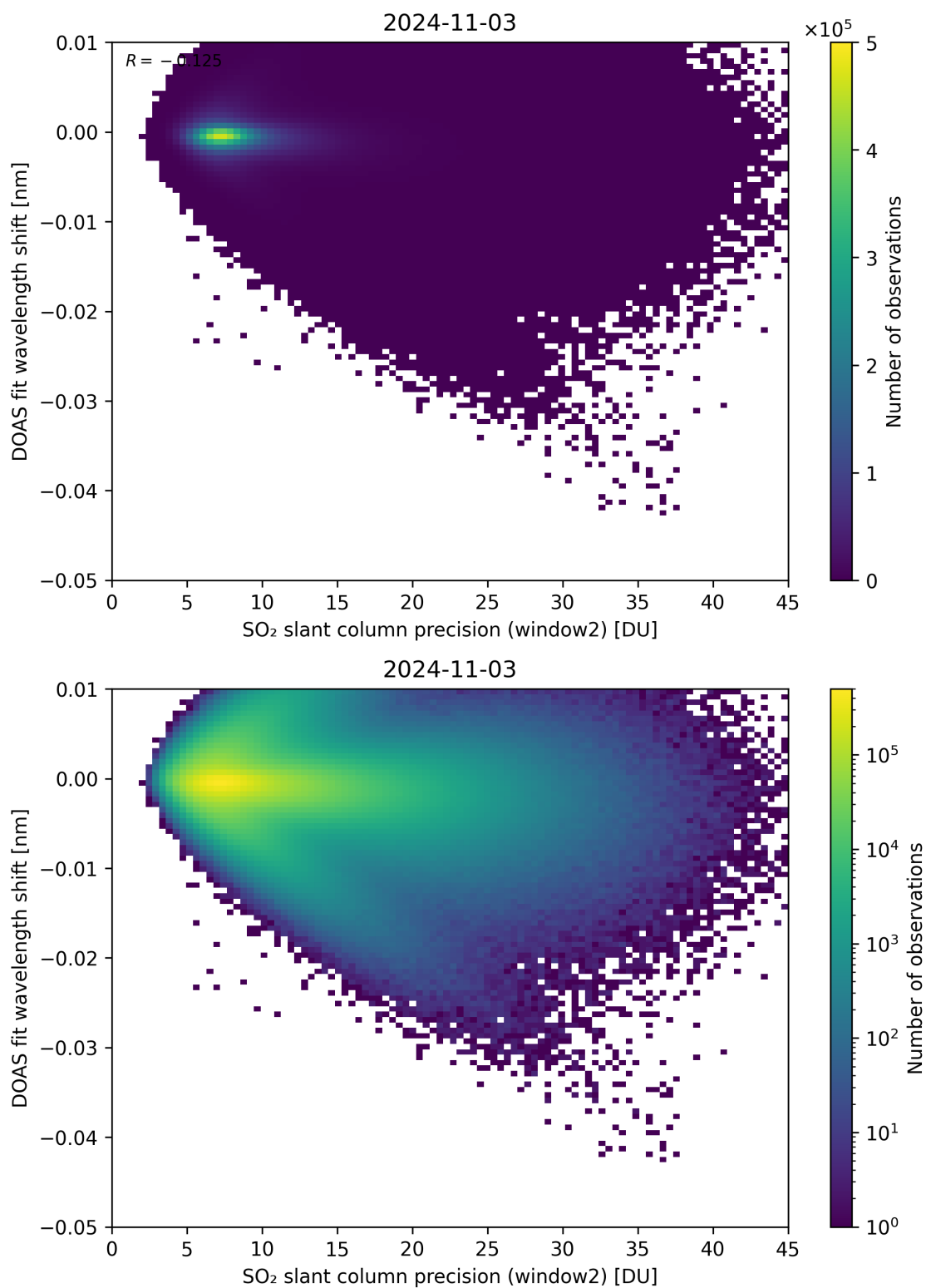
Figure 243: Scatter density plot of “SO 2 slant column precision (window2)” against “DOAS fit wavelength shift” for 2024-11-02 to 2024-11-04.
