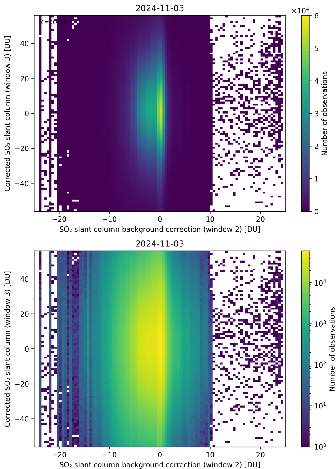
Figure 116: Scatter density plot of “SO 2 slant column background correction (window 2)” against “Corrected SO 2 slant column (window 3)” for 2024-11-02 to 2024-11-04.
