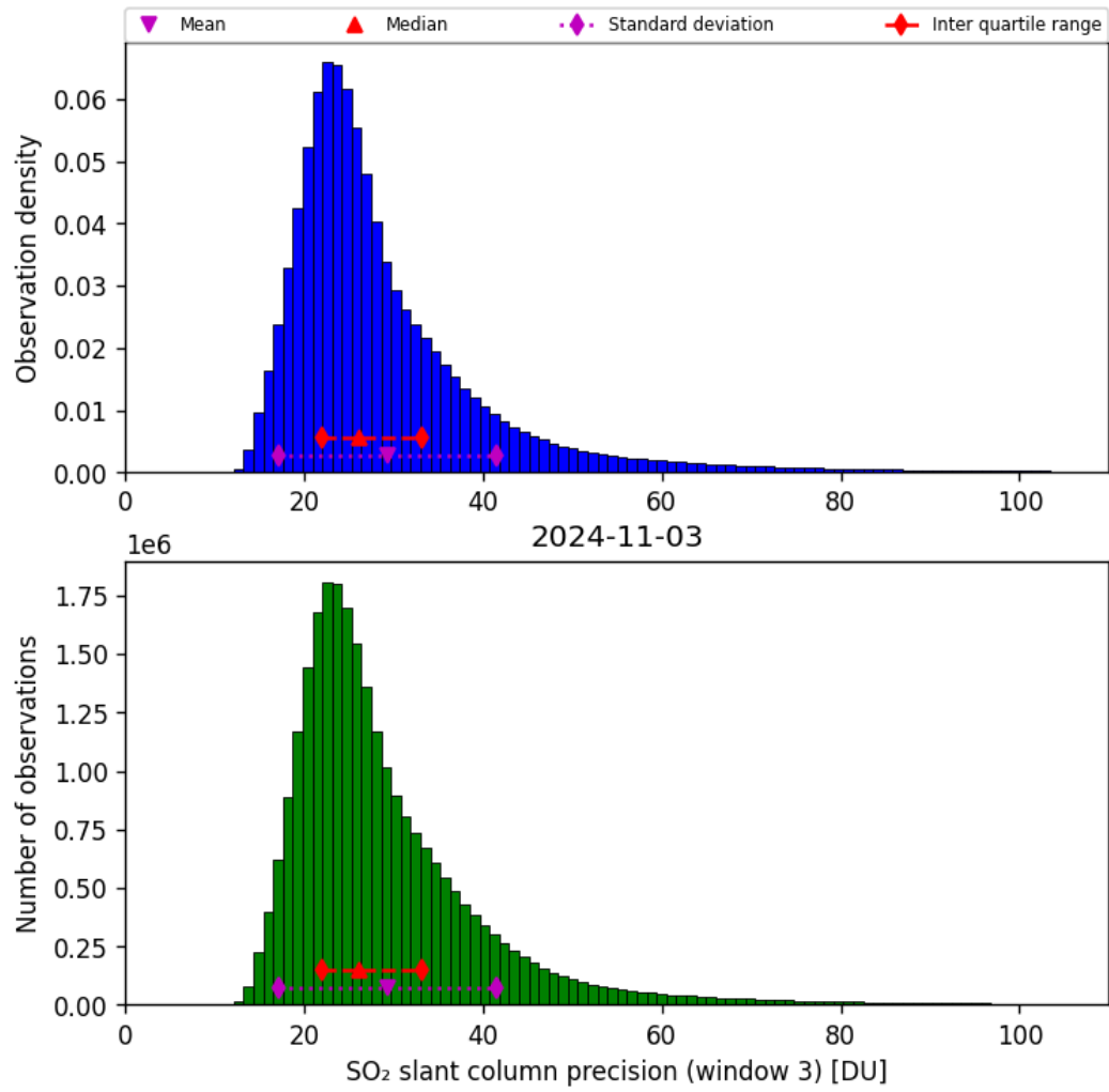
Figure 65: Histogram of “SO 2 slant column precision (window 3)” for 2024-11-02 to 2024-11-04
