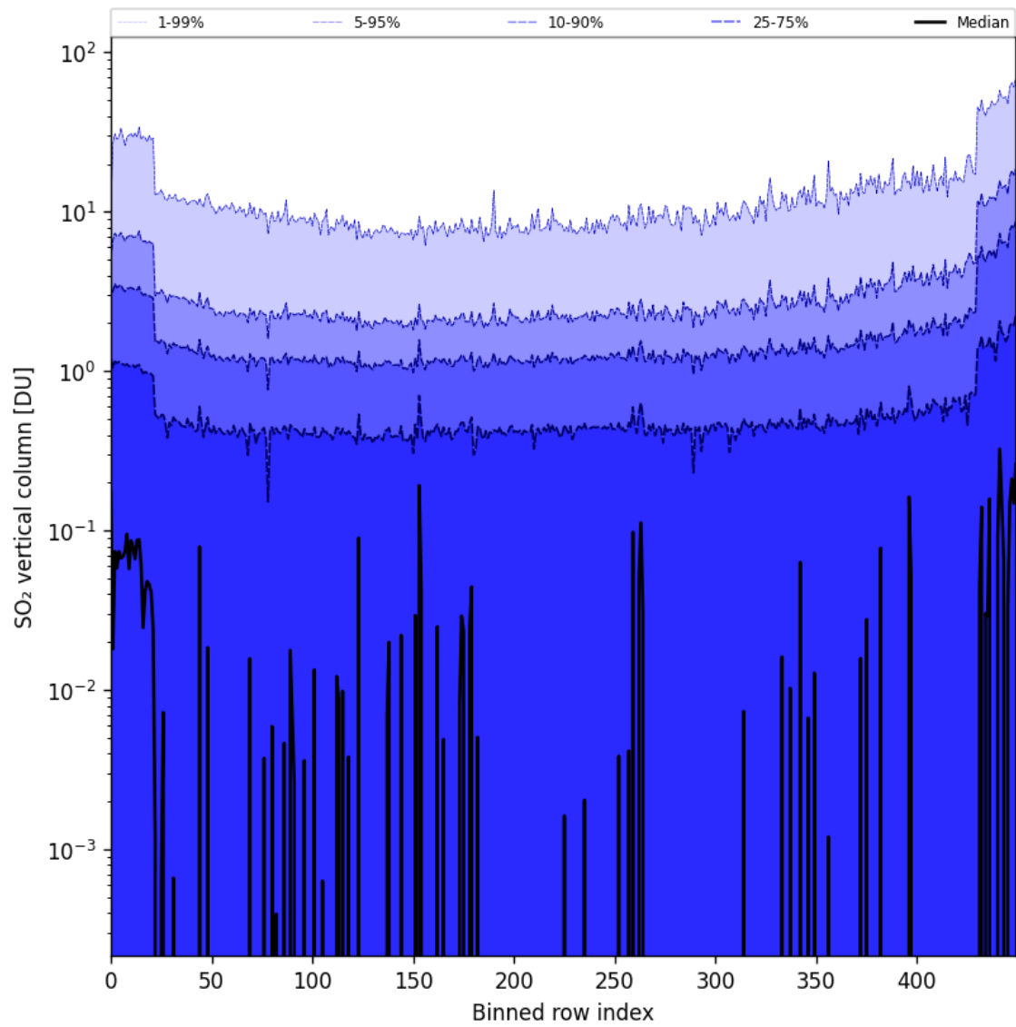
Figure 76: Along track statistics of “SO 2 vertical column” for 2024-11-02 to 2024-11-04
