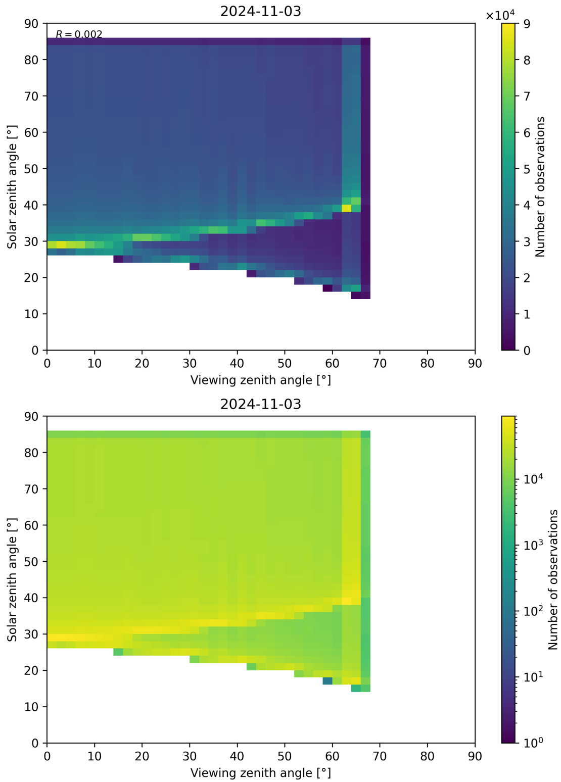
Figure 315: Scatter density plot of “Viewing zenith angle” against “Solar zenith angle” for 2024-11-02 to 2024-11-04.
