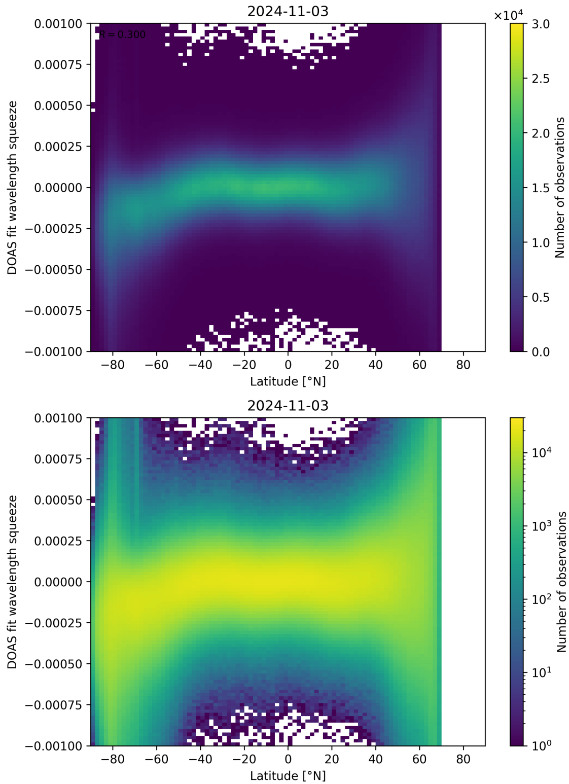
Figure 143: Scatter density plot of “Latitude” against “DOAS fit wavelength squeeze” for 2024-11-02 to 2024-11-04.
