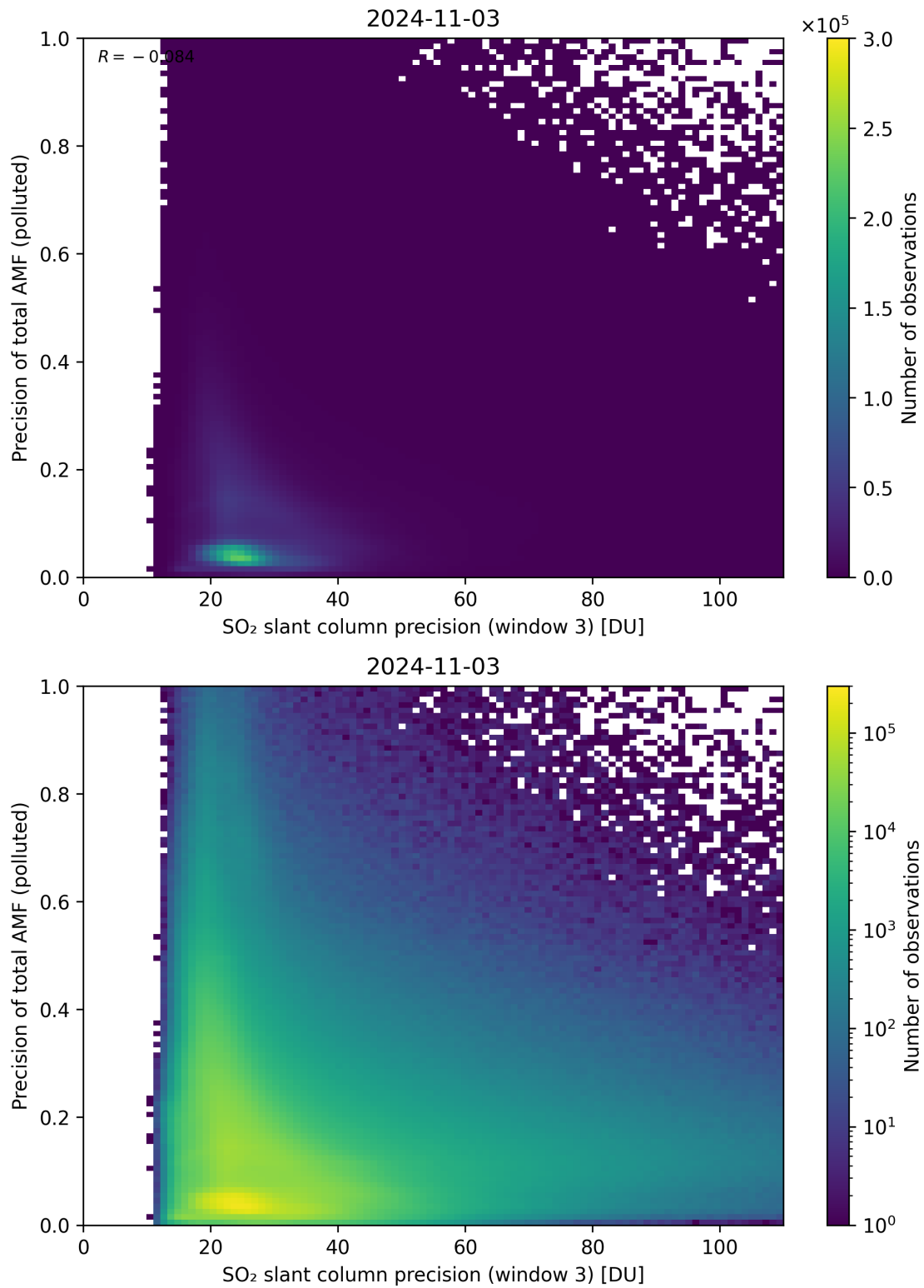
Figure 264: Scatter density plot of “SO 2 slant column precision (window 3)” against “Precision of total AMF (polluted)” for 2024-11-02 to 2024-11-04.
