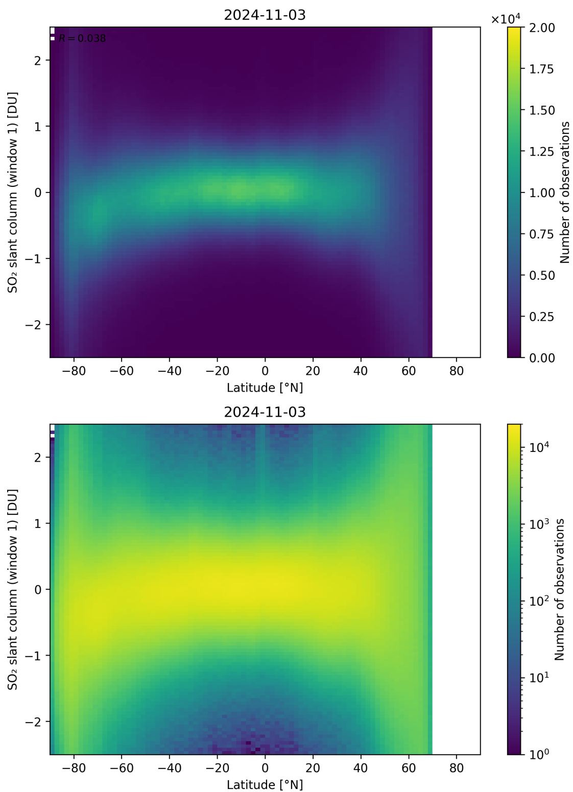
Figure 149: Scatter density plot of “Latitude” against “SO 2 slant column (window 1)” for 2024-11-02 to 2024-11-04.
