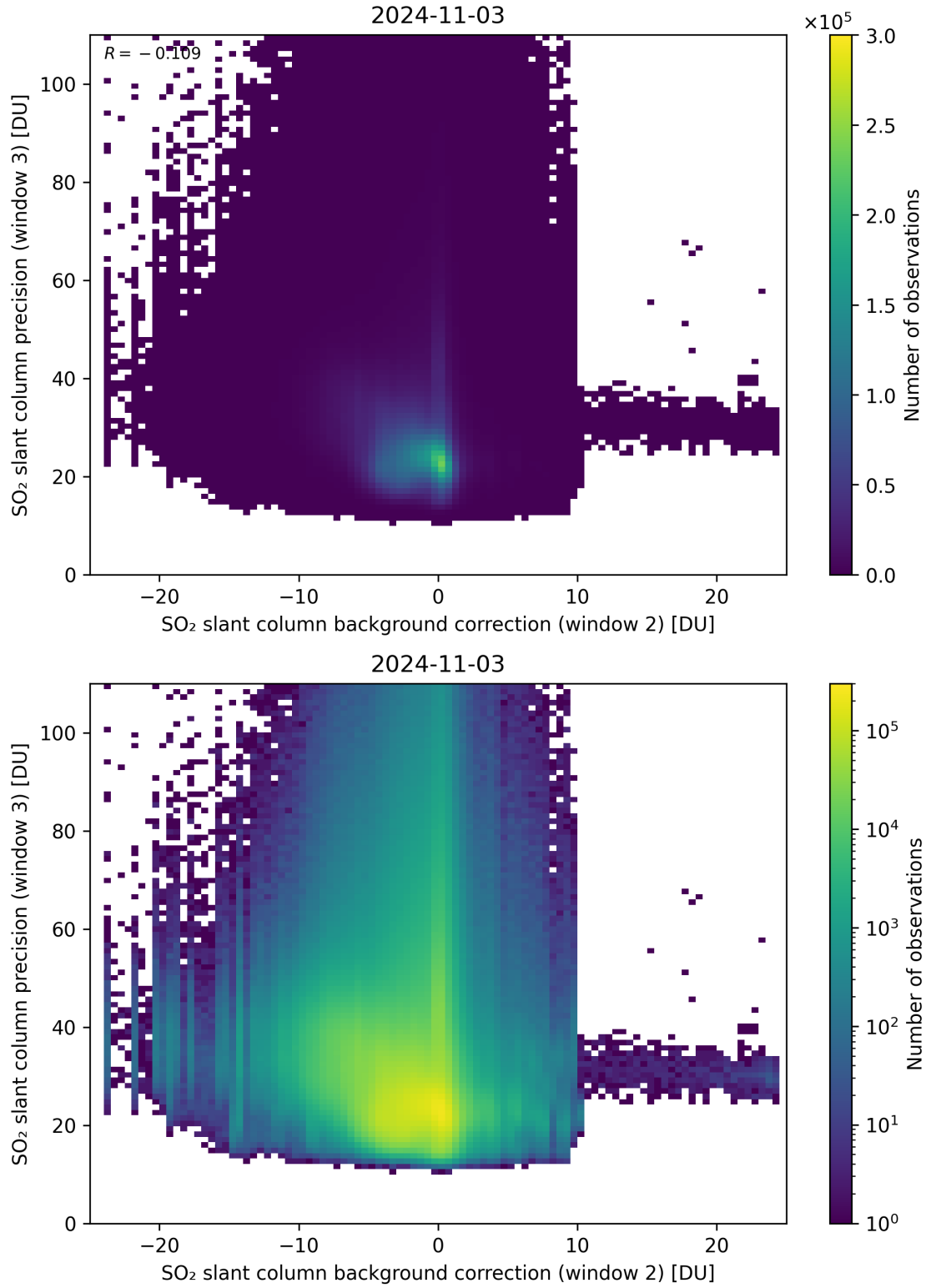
Figure 118: Scatter density plot of “SO 2 slant column background correction (window 2)” against “SO 2 slant column precision (window 3)” for 2024-11-02 to 2024-11-04.
