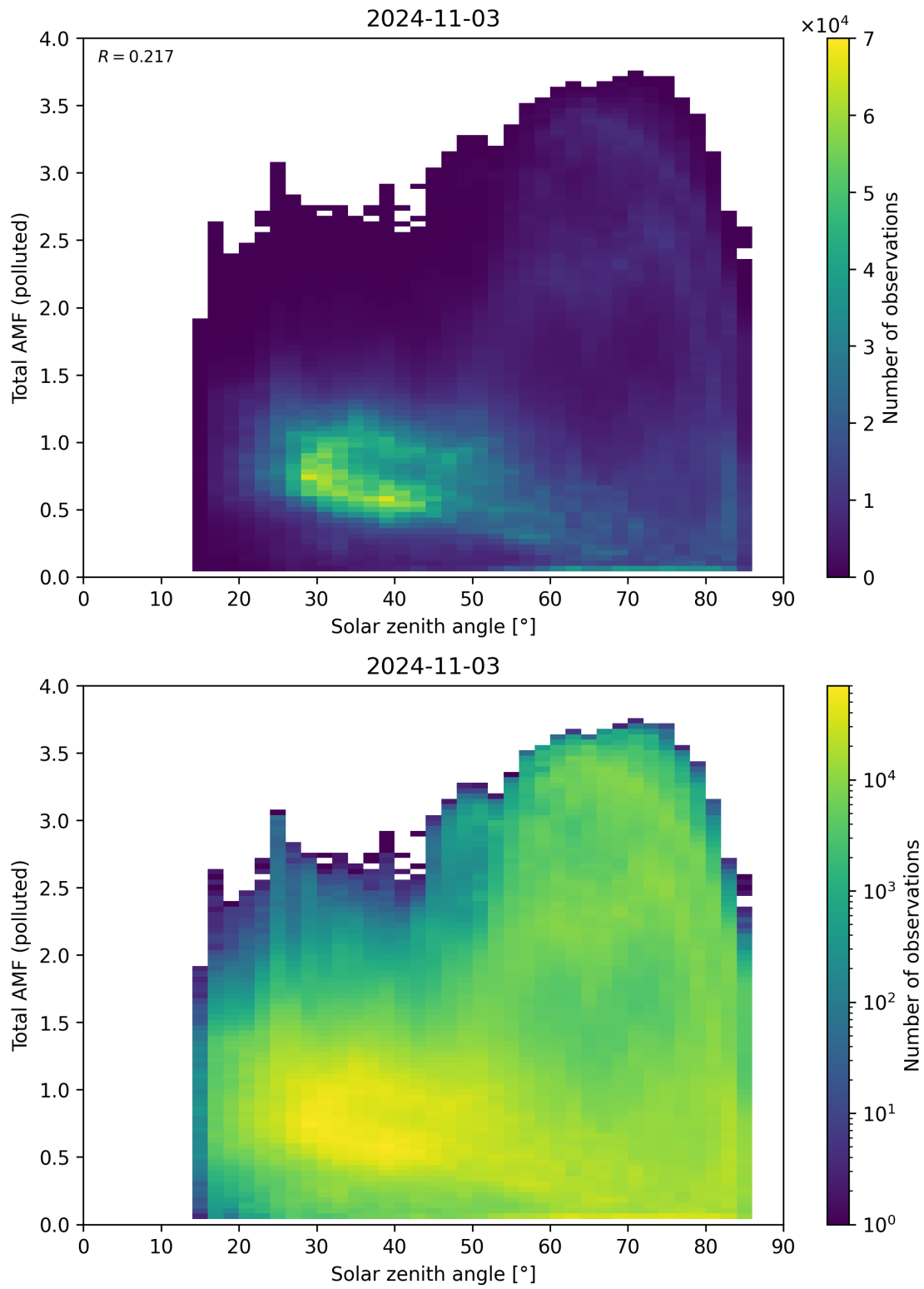
Figure 174: Scatter density plot of “Solar zenith angle” against “Total AMF (polluted)” for 2024-11-02 to 2024-11-04.
