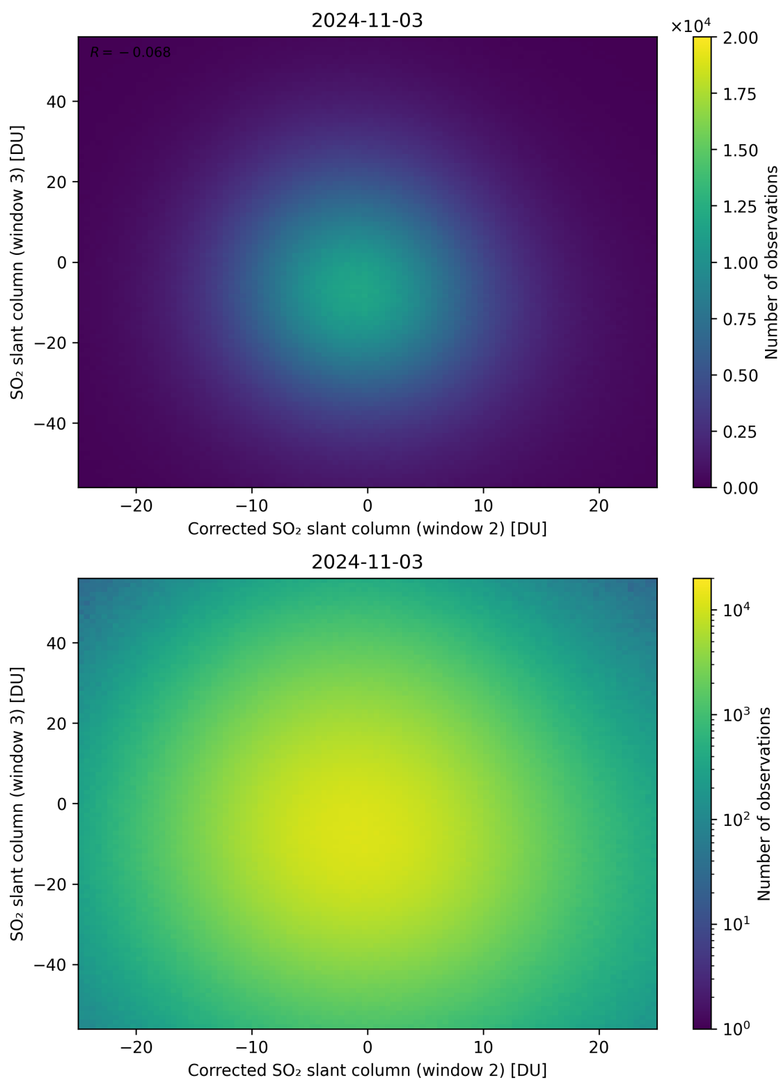
Figure 201: Scatter density plot of “Corrected SO 2 slant column (window 2)” against “SO 2 slant column (window 3)” for 2024-11-02 to 2024-11-04.
