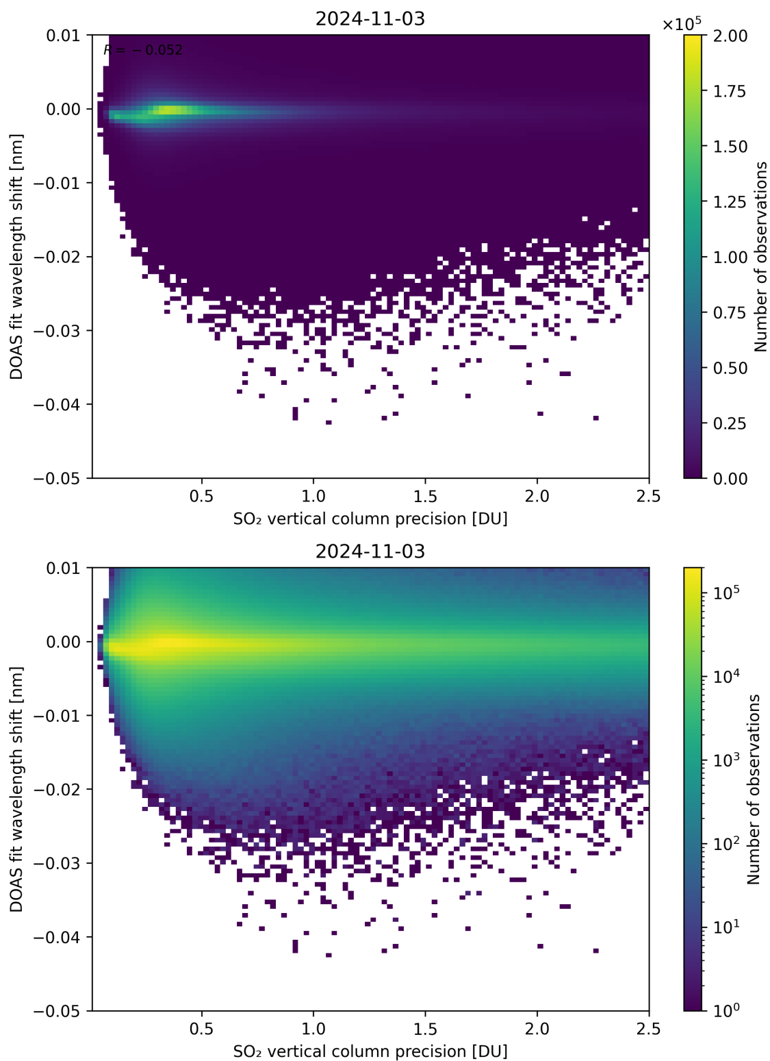
Figure 282: Scatter density plot of “SO 2 vertical column precision” against “DOAS fit wavelength shift” for 2024-11-02 to 2024-11-04.
