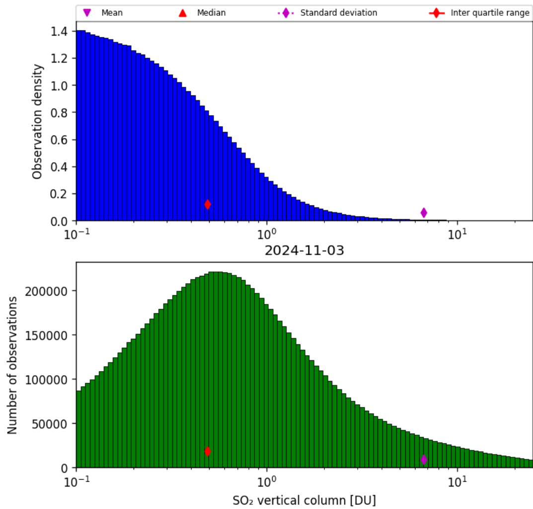
Figure 53: Histogram of “SO 2 vertical column” for 2024-11-02 to 2024-11-04
