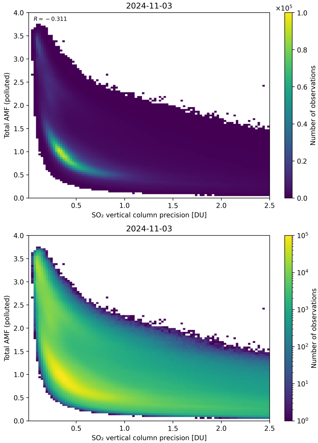
Figure 294: Scatter density plot of “SO 2 vertical column precision” against “Total AMF (polluted)” for 2024-11-02 to 2024-11-04.
