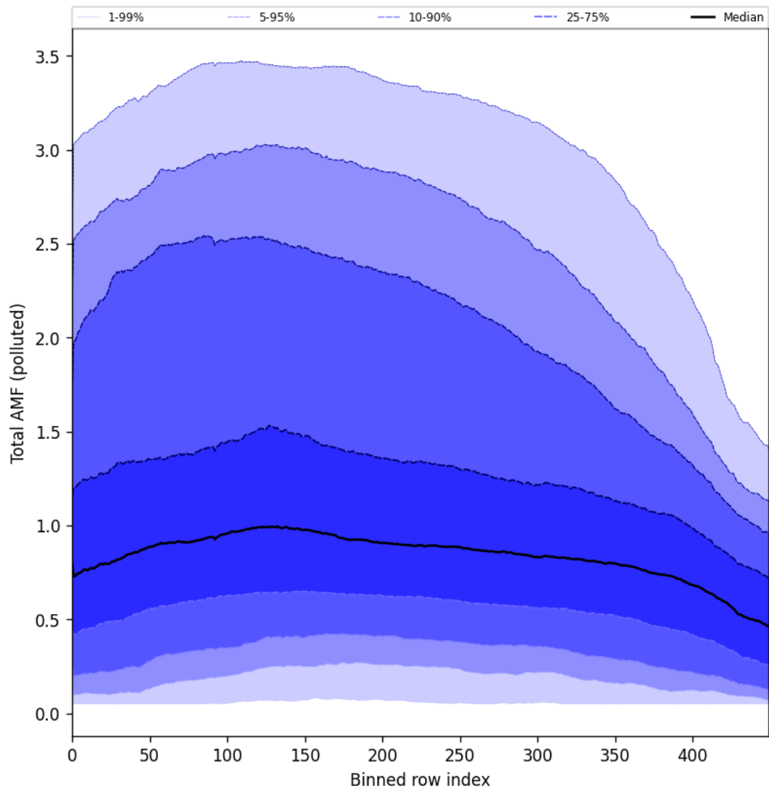
Figure 94: Along track statistics of “Total AMF (polluted)” for 2024-11-02 to 2024-11-04
