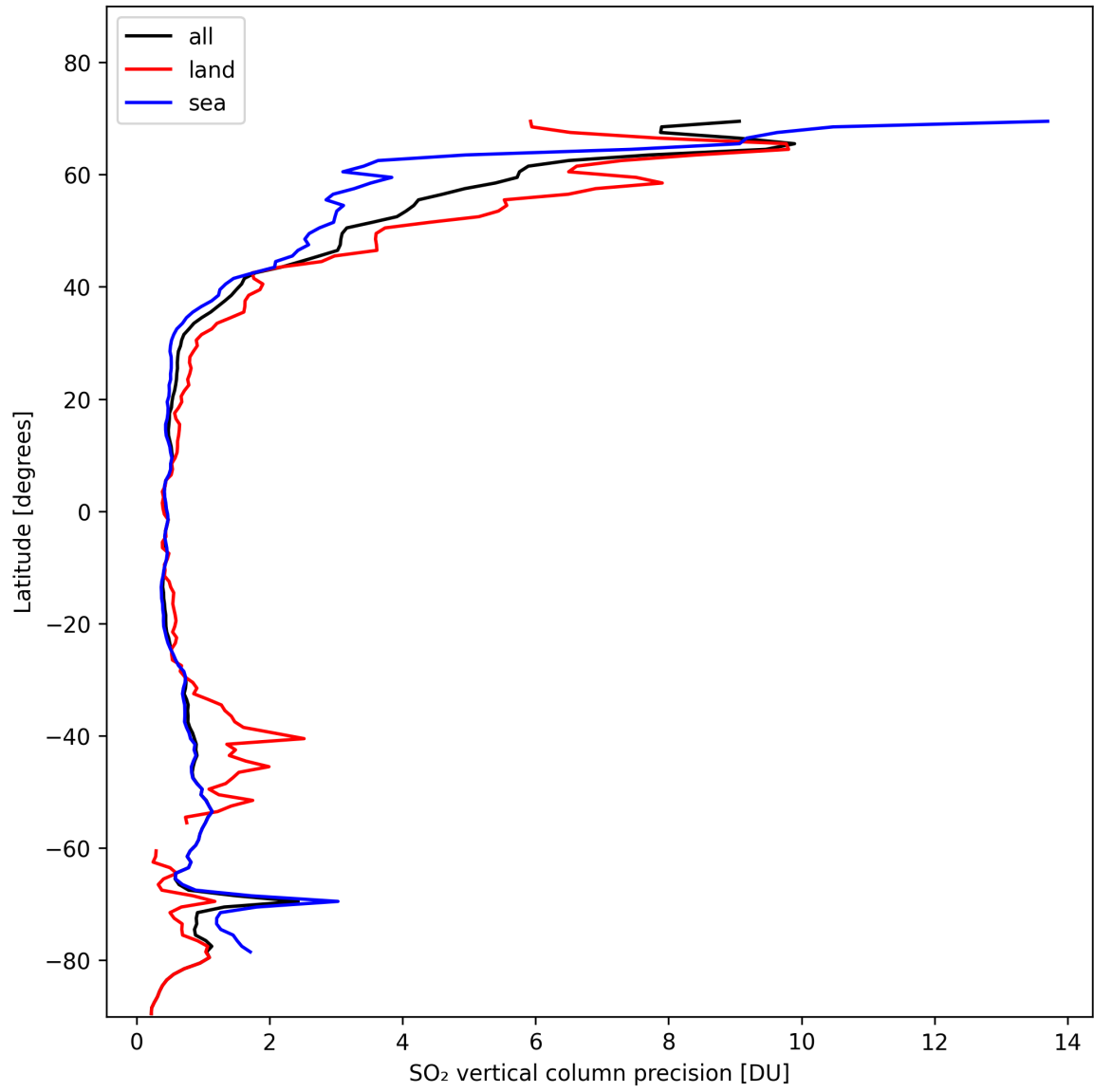
Figure 31: Zonal average of “SO 2 vertical column precision” for 2024-11-02 to 2024-11-04.
