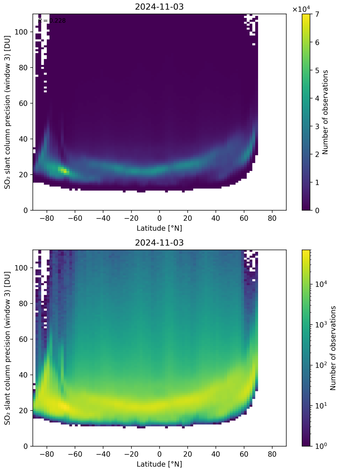
Figure 153: Scatter density plot of “Latitude” against “SO 2 slant column precision (window 3)” for 2024-11-02 to 2024-11-04.
