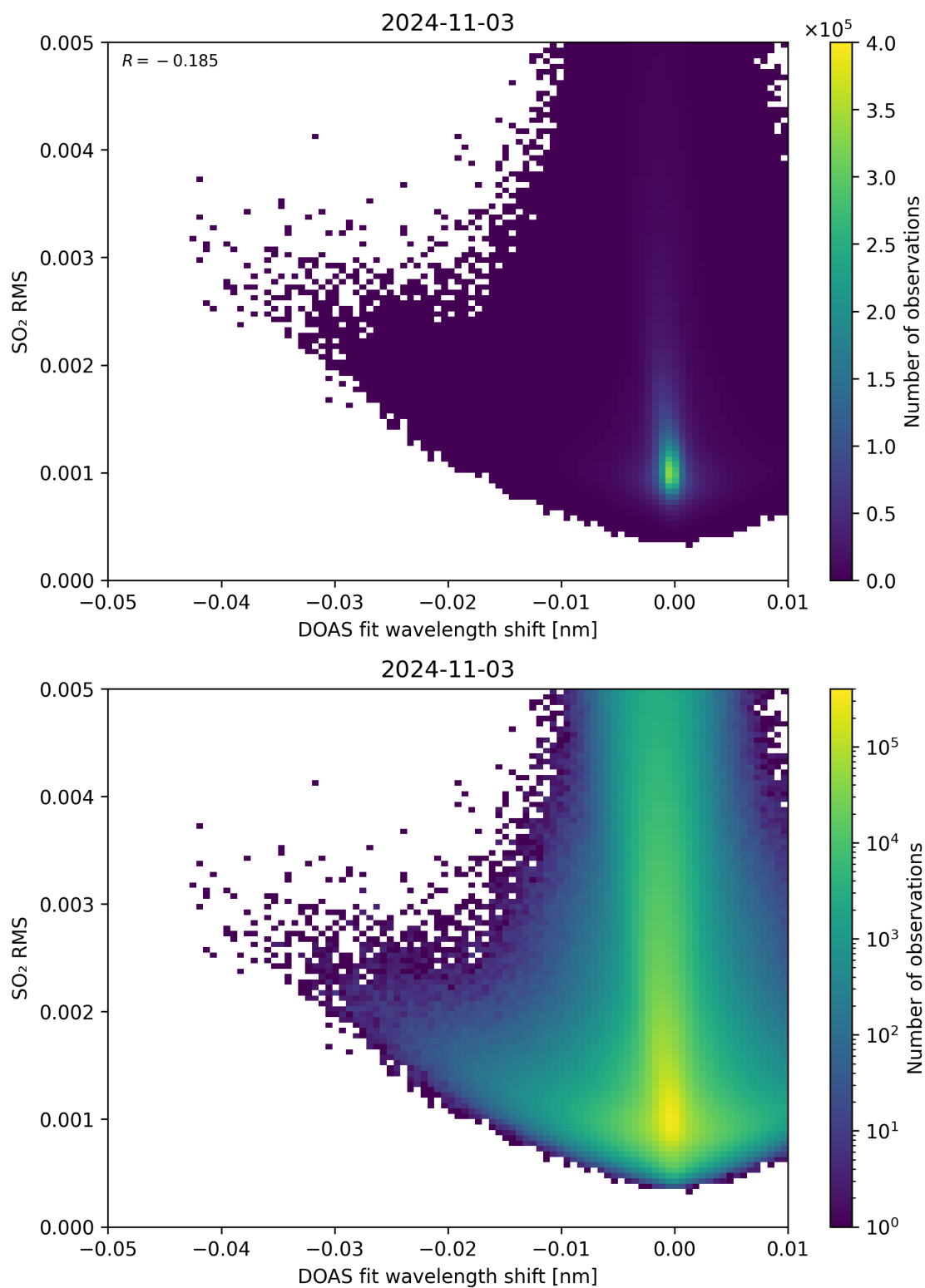
Figure 128: Scatter density plot of “DOAS fit wavelength shift” against “SO 2 RMS” for 2024-11-02 to 2024-11-04.
