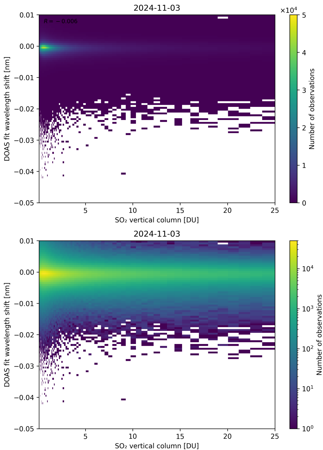
Figure 276: Scatter density plot of “SO 2 vertical column” against “DOAS fit wavelength shift” for 2024-11-02 to 2024-11-04.
