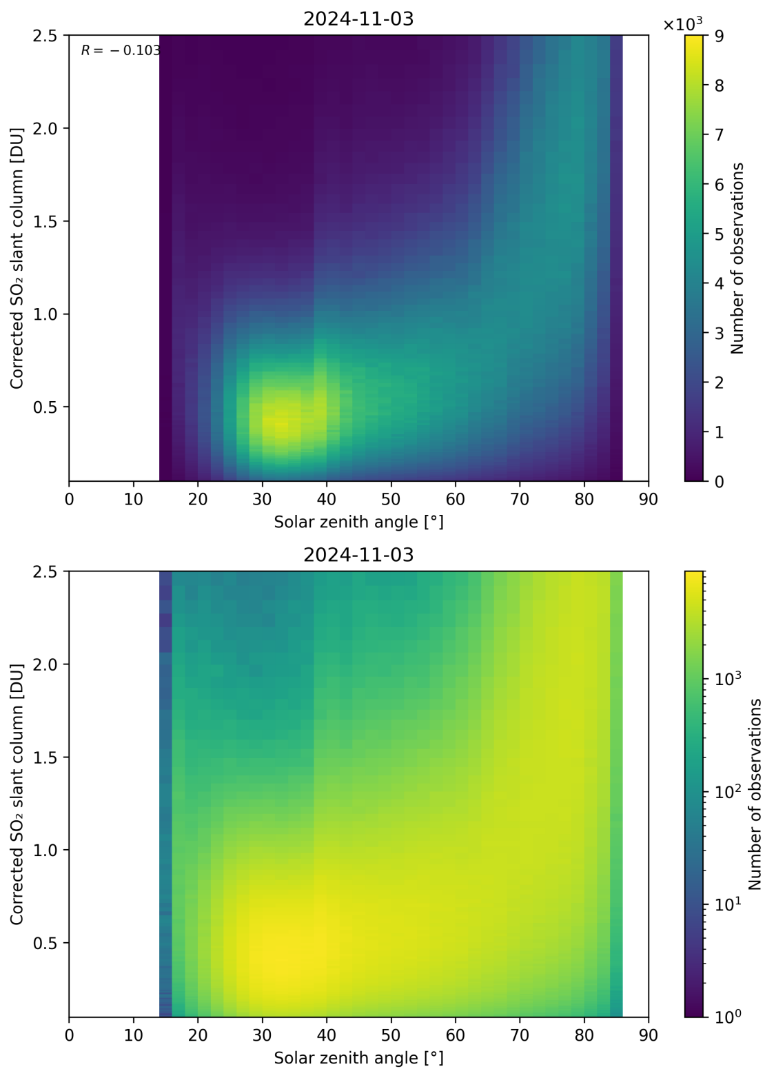
Figure 166: Scatter density plot of “Solar zenith angle” against “Corrected SO 2 slant column” for 2024-11-02 to 2024-11-04.
