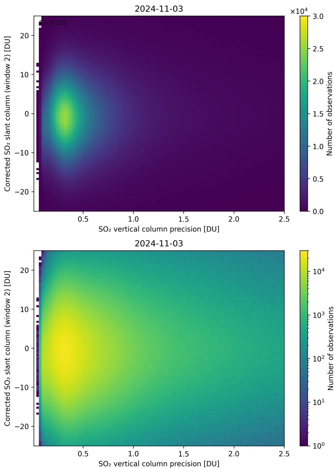
Figure 287: Scatter density plot of “SO 2 vertical column precision” against “Corrected SO 2 slant column (window 2)” for 2024-11-02 to 2024-11-04.
