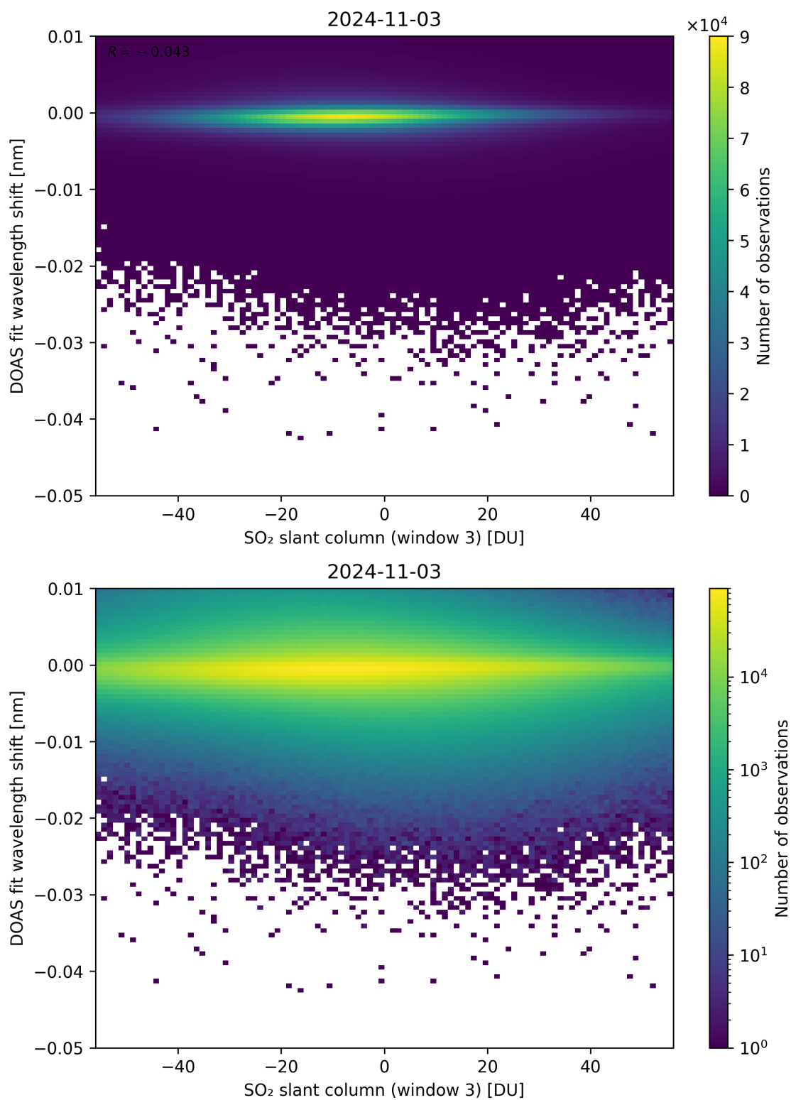
Figure 254: Scatter density plot of “SO 2 slant column (window 3)” against “DOAS fit wavelength shift” for 2024-11-02 to 2024-11-04.
