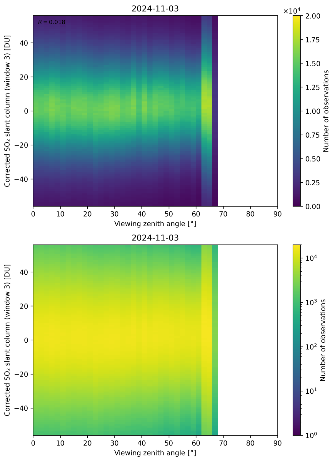
Figure 319: Scatter density plot of “Viewing zenith angle” against “Corrected SO 2 slant column (window 3)” for 2024-11-02 to 2024-11-04.
