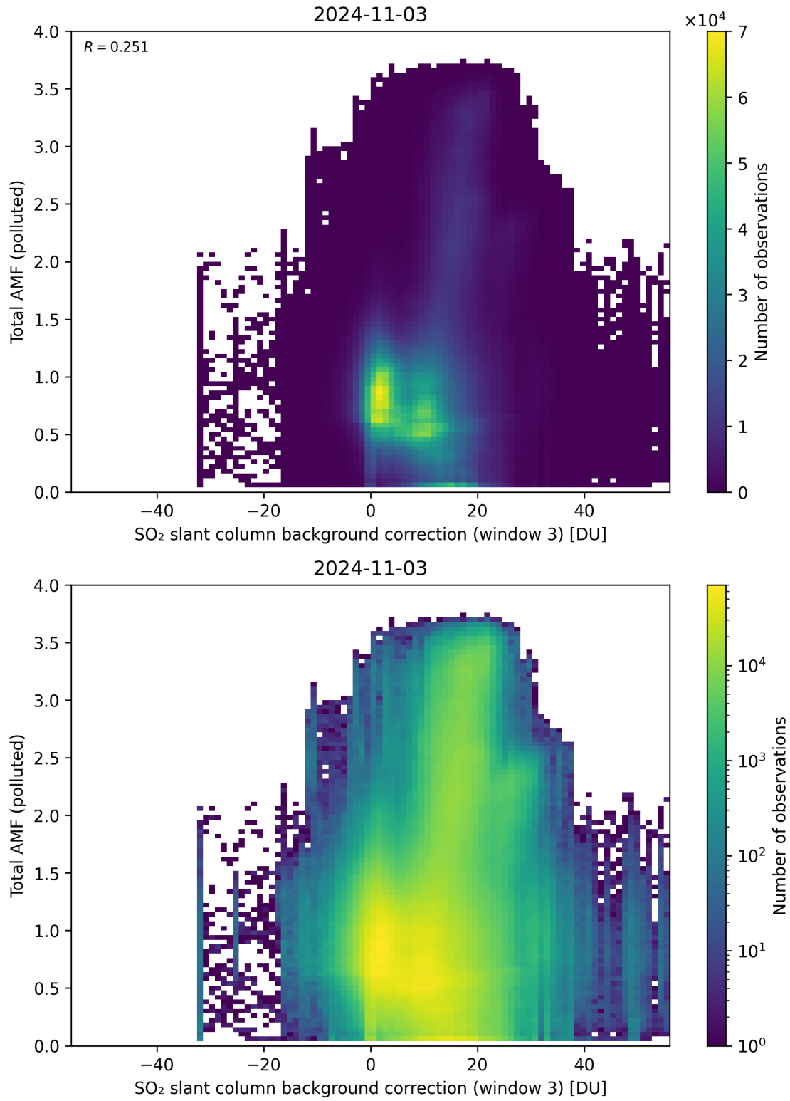
Figure 125: Scatter density plot of “SO 2 slant column background correction (window 3)” against “Total AMF (polluted)” for 2024-11-02 to 2024-11-04.
