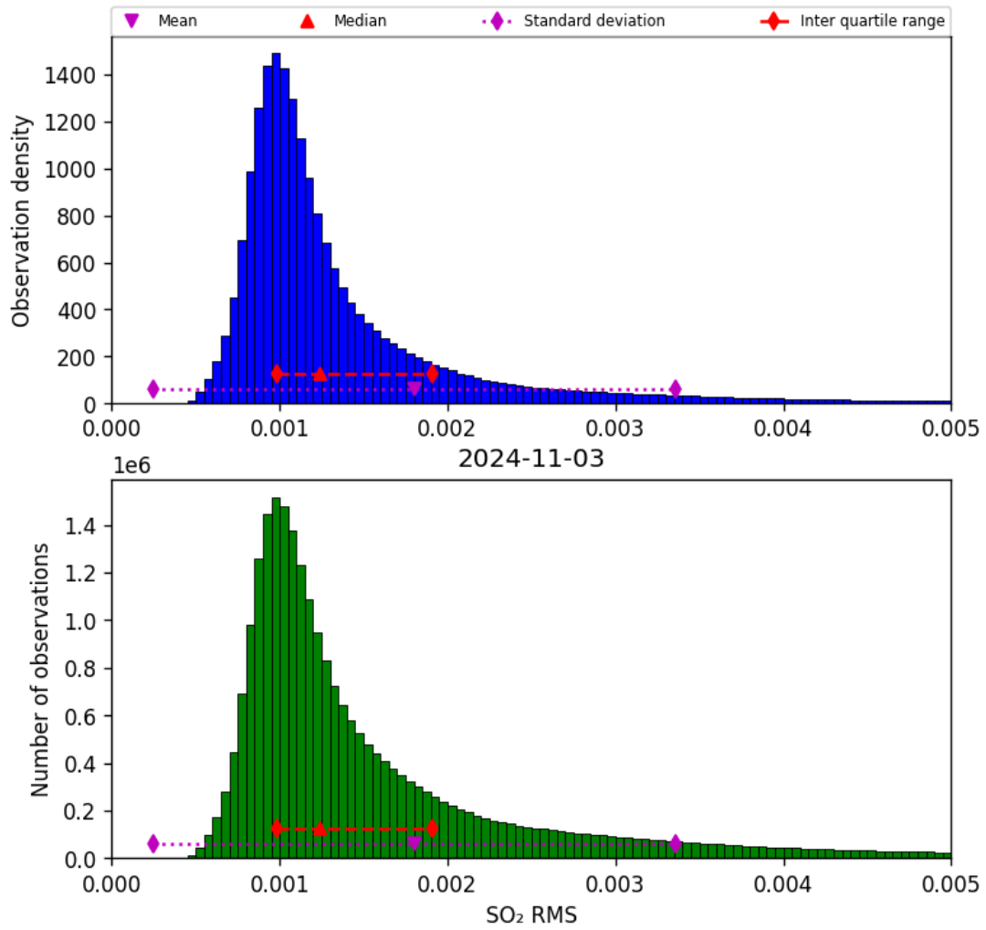
Figure 70: Histogram of “SO 2 RMS” for 2024-11-02 to 2024-11-04
