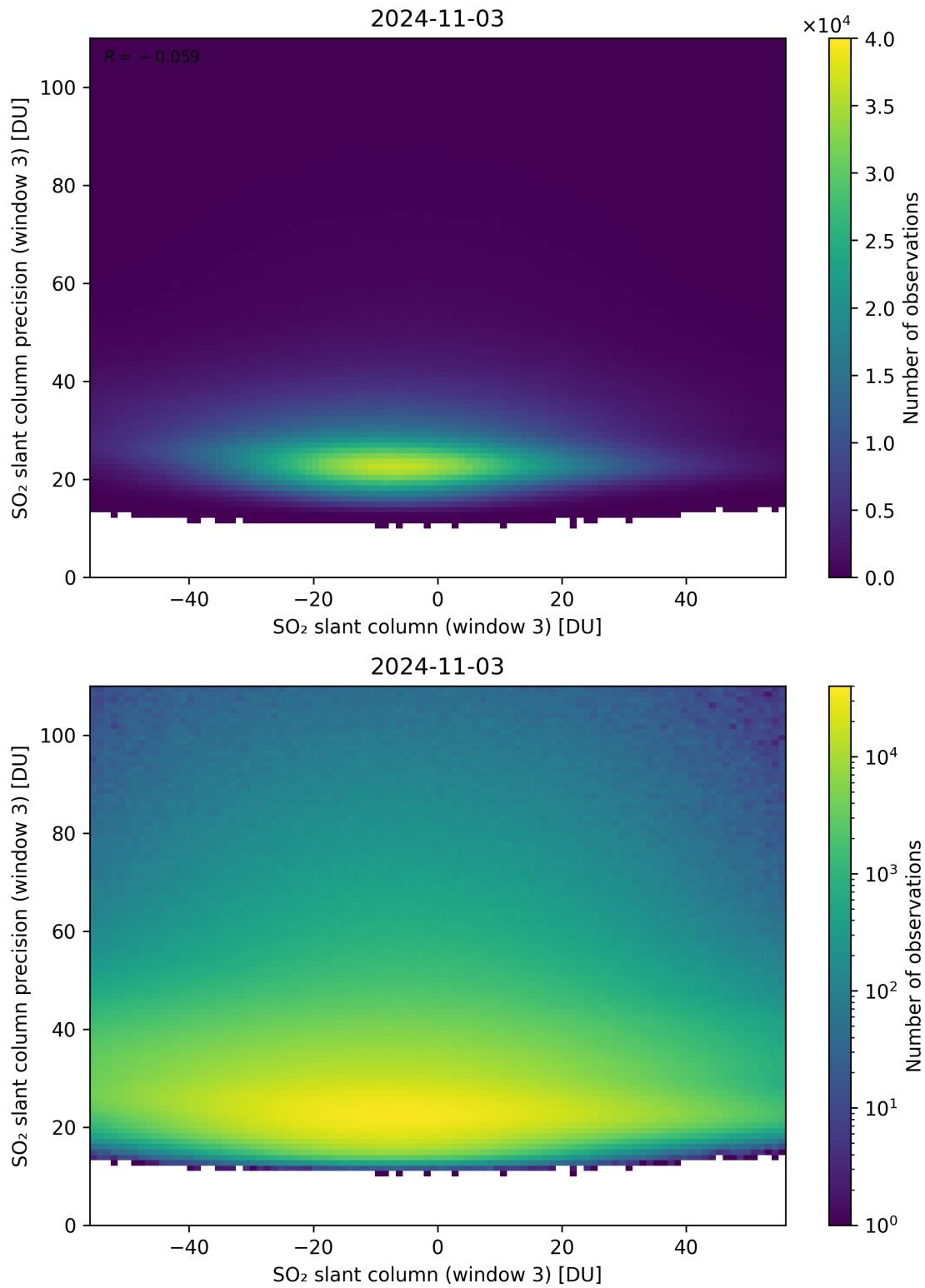
Figure 267: Scatter density plot of “SO 2 slant column (window 3)” against “SO 2 slant column precision (window 3)” for 2024-11-02 to 2024-11-04.
