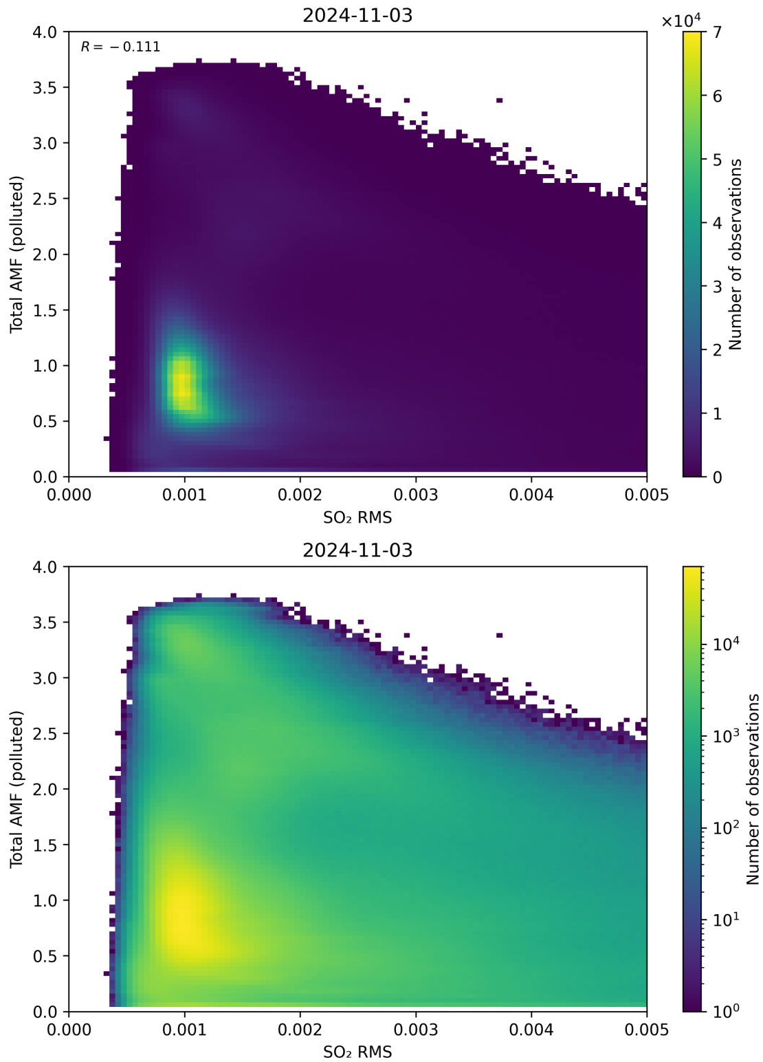
Figure 137: Scatter density plot of “SO 2 RMS” against “Total AMF (polluted)” for 2024-11-02 to 2024-11-04.
