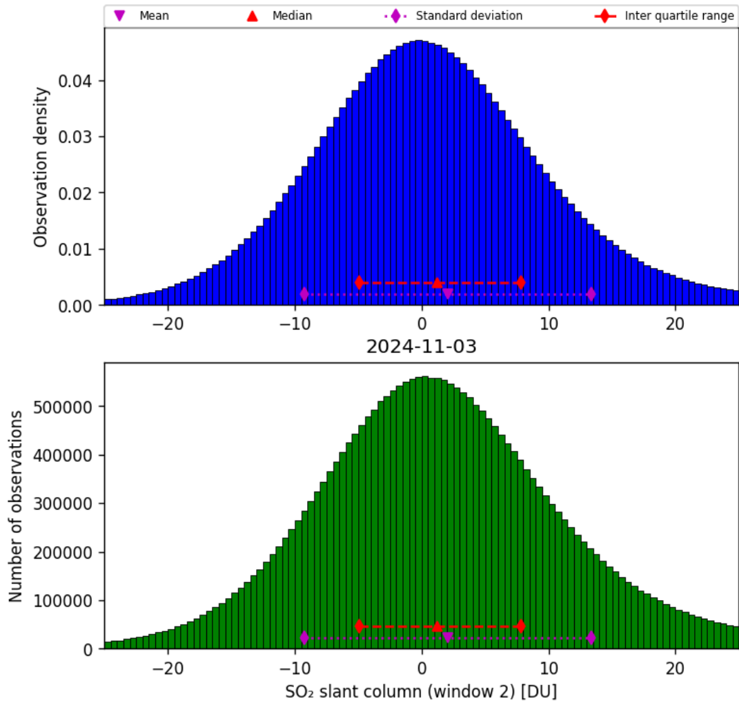
Figure 60: Histogram of “SO 2 slant column (window 2)” for 2024-11-02 to 2024-11-04
