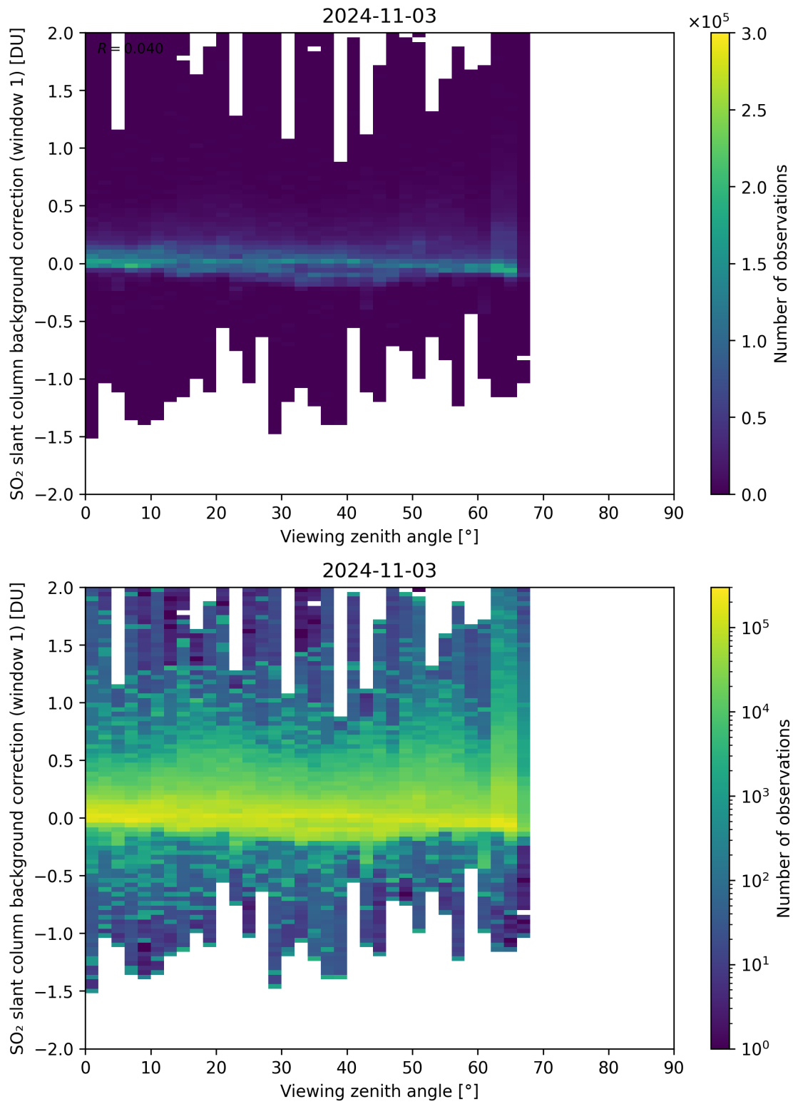
Figure 308: Scatter density plot of “Viewing zenith angle” against “SO 2 slant column background correction (window 1)” for 2024-11-02 to 2024-11-04.
