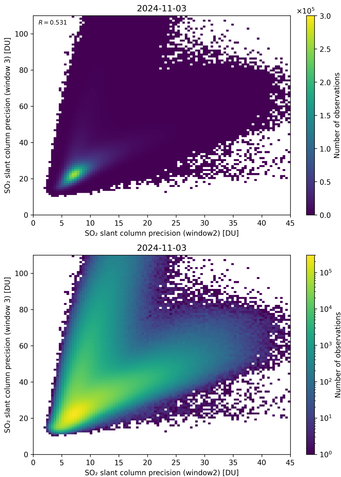
Figure 250: Scatter density plot of “SO 2 slant column precision (window2)” against “SO 2 slant column precision (window 3)” for 2024-11-02 to 2024-11-04.
