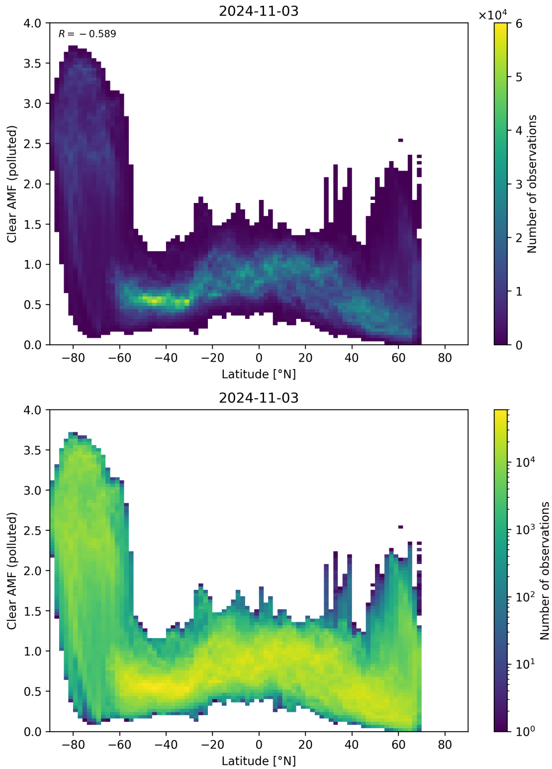
Figure 145: Scatter density plot of “Latitude” against “Clear AMF (polluted)” for 2024-11-02 to 2024-11-04.
