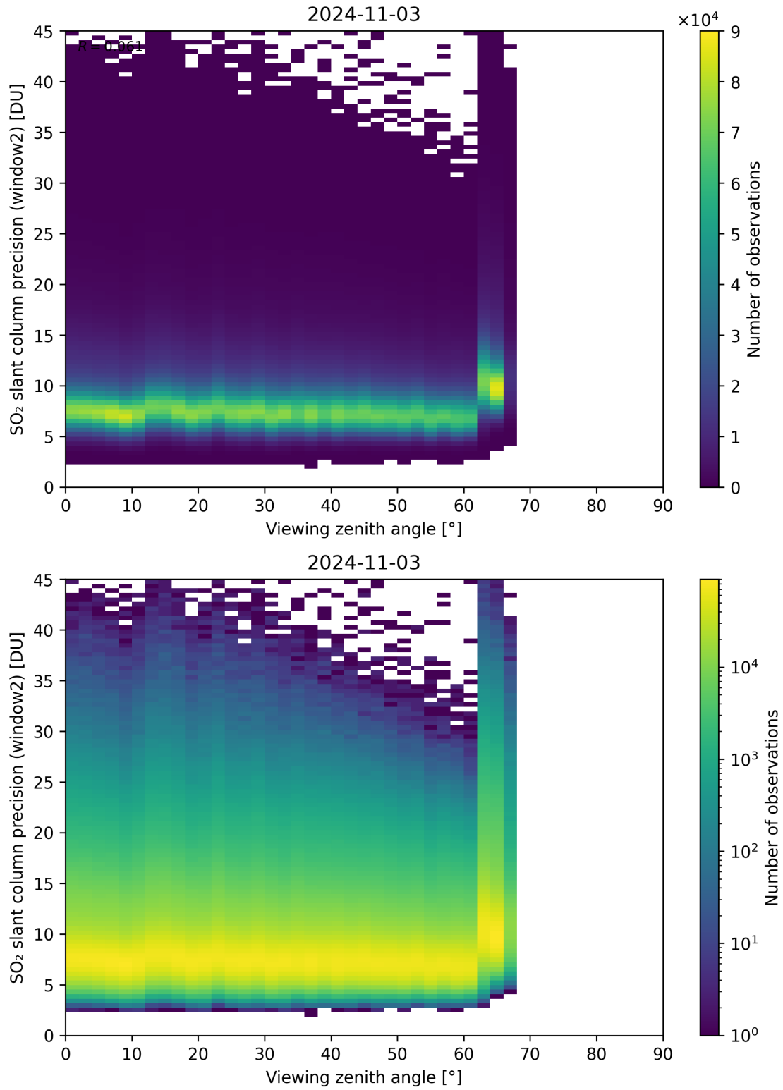
Figure 322: Scatter density plot of “Viewing zenith angle” against “SO 2 slant column precision (window2)” for 2024-11-02 to 2024-11-04.
