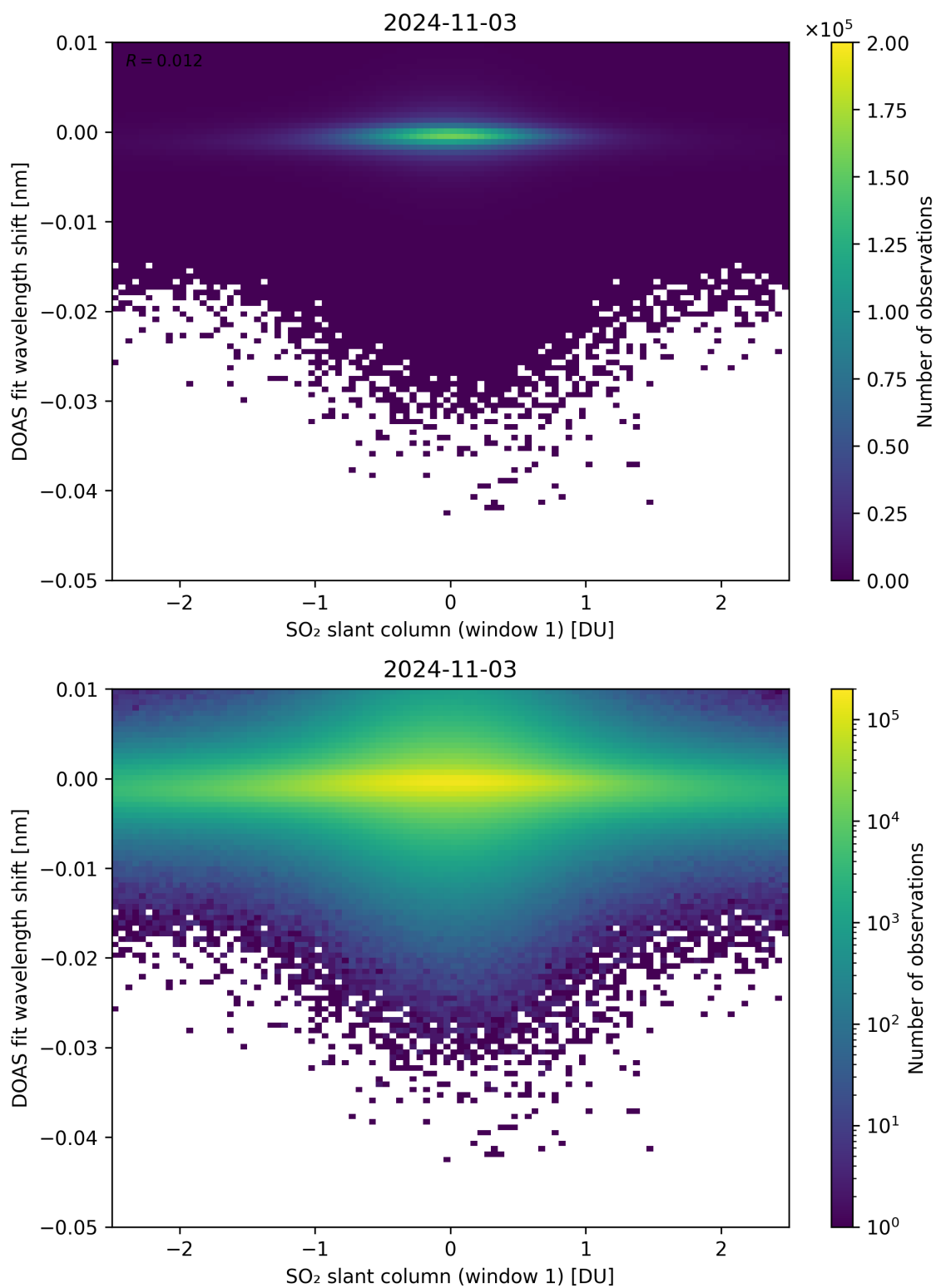
Figure 215: Scatter density plot of “SO 2 slant column (window 1)” against “DOAS fit wavelength shift” for 2024-11-02 to 2024-11-04.
