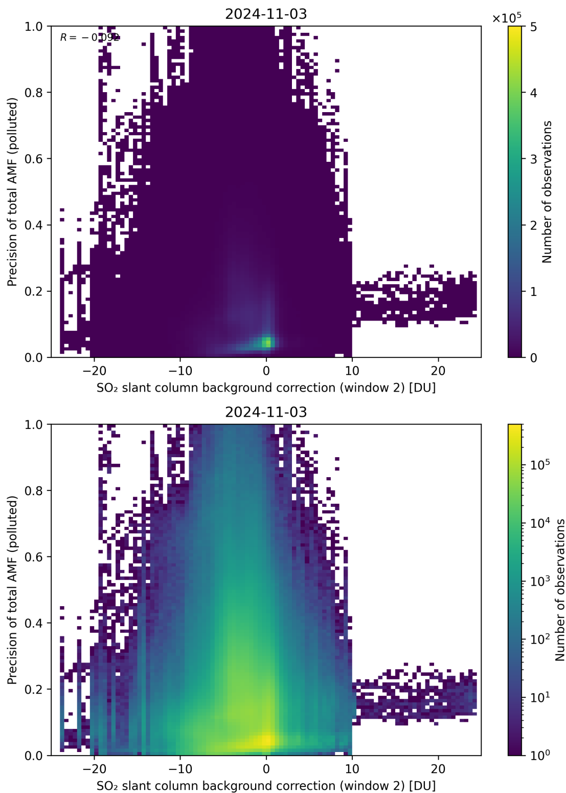
Figure 120: Scatter density plot of “SO 2 slant column background correction (window 2)” against “Precision of total AMF (polluted)” for 2024-11-02 to 2024-11-04.
