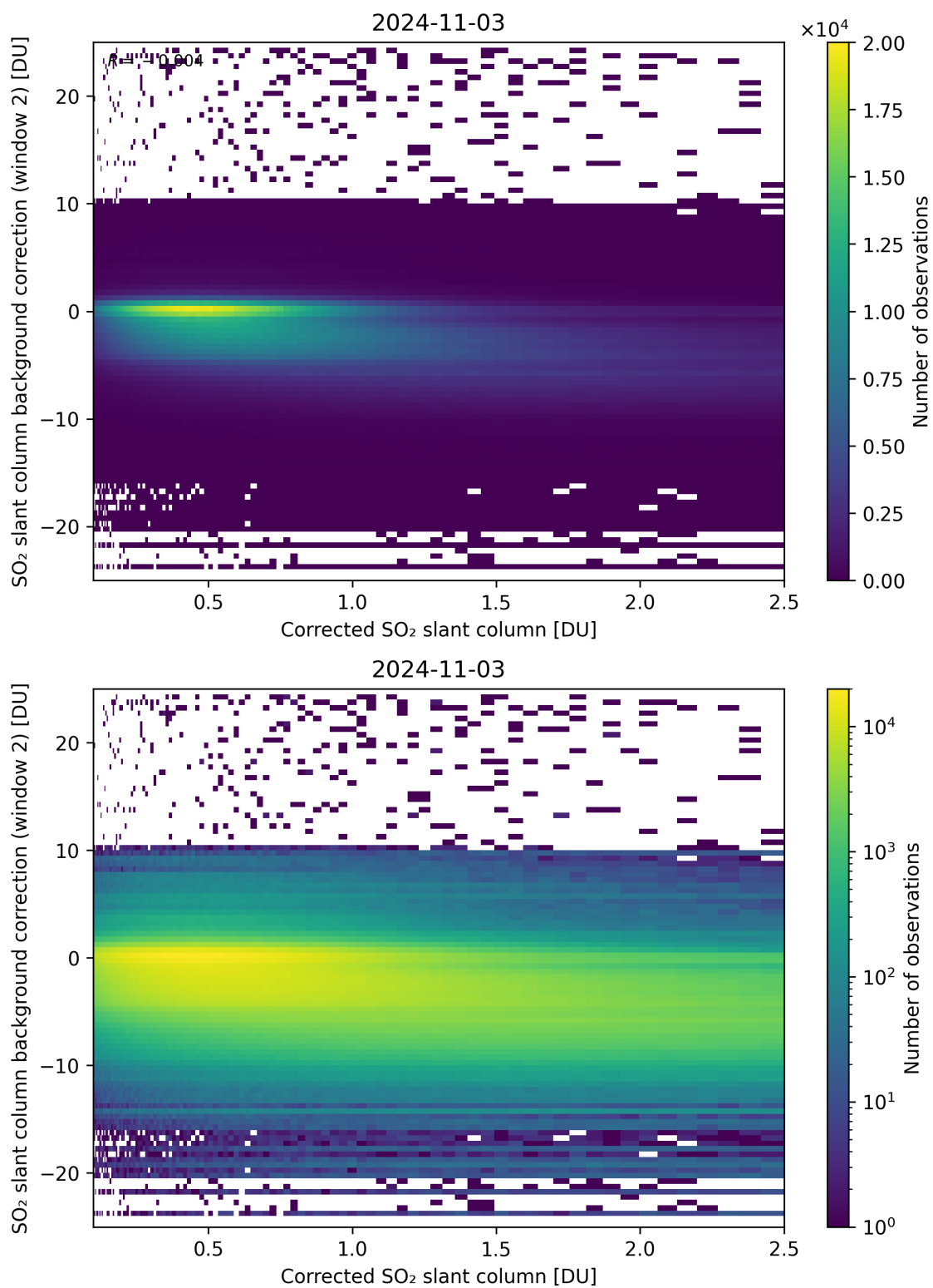
Figure 179: Scatter density plot of “Corrected SO 2 slant column” against “SO 2 slant column background correction (window 2)” for 2024-11-02 to 2024-11-04.
