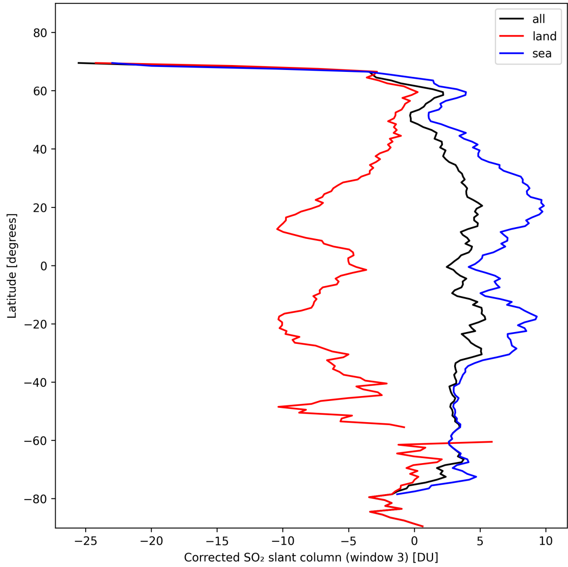
Figure 43: Zonal average of “Corrected SO 2 slant column (window 3)” for 2024-11-02 to 2024-11-04.
