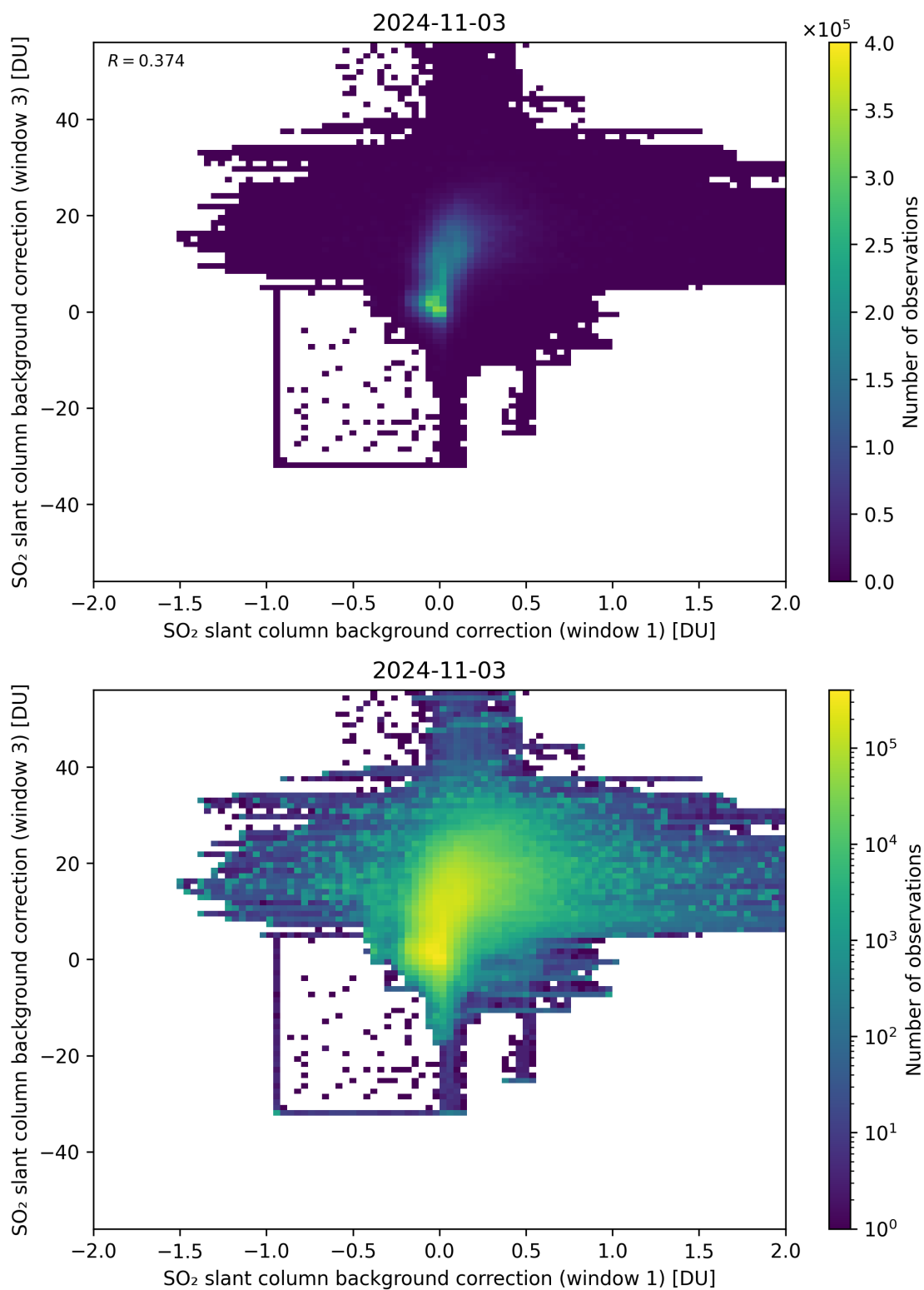
Figure 99: Scatter density plot of “SO 2 slant column background correction (window 1)” against “SO 2 slant column background correction (window 3)” for 2024-11-02 to 2024-11-04.
