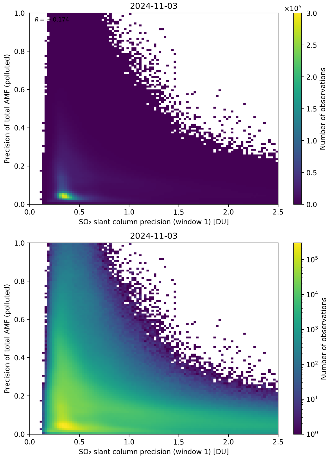
Figure 231: Scatter density plot of “SO 2 slant column precision (window 1)” against “Precision of total AMF (polluted)” for 2024-11-02 to 2024-11-04.
