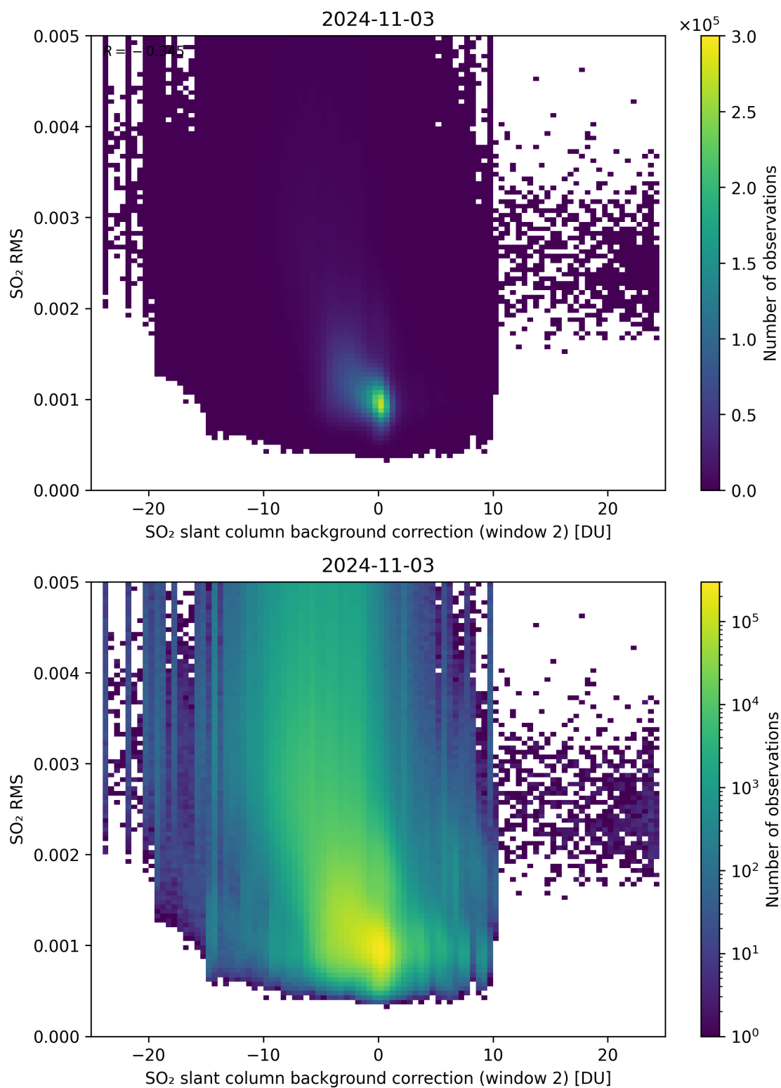
Figure 114: Scatter density plot of “SO 2 slant column background correction (window 2)” against “SO 2 RMS” for 2024-11-02 to 2024-11-04.
