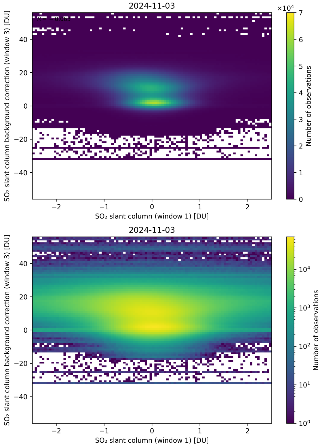
Figure 214: Scatter density plot of “SO 2 slant column (window 1)” against “SO 2 slant column background correction (window 3)” for 2024-11-02 to 2024-11-04.
