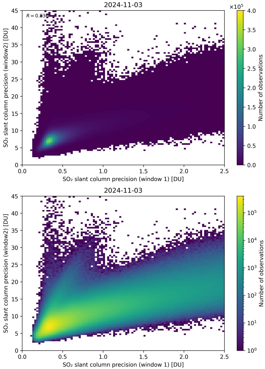
Figure 227: Scatter density plot of “SO 2 slant column precision (window 1)” against “SO 2 slant column precision (window2)” for 2024-11-02 to 2024-11-04.
