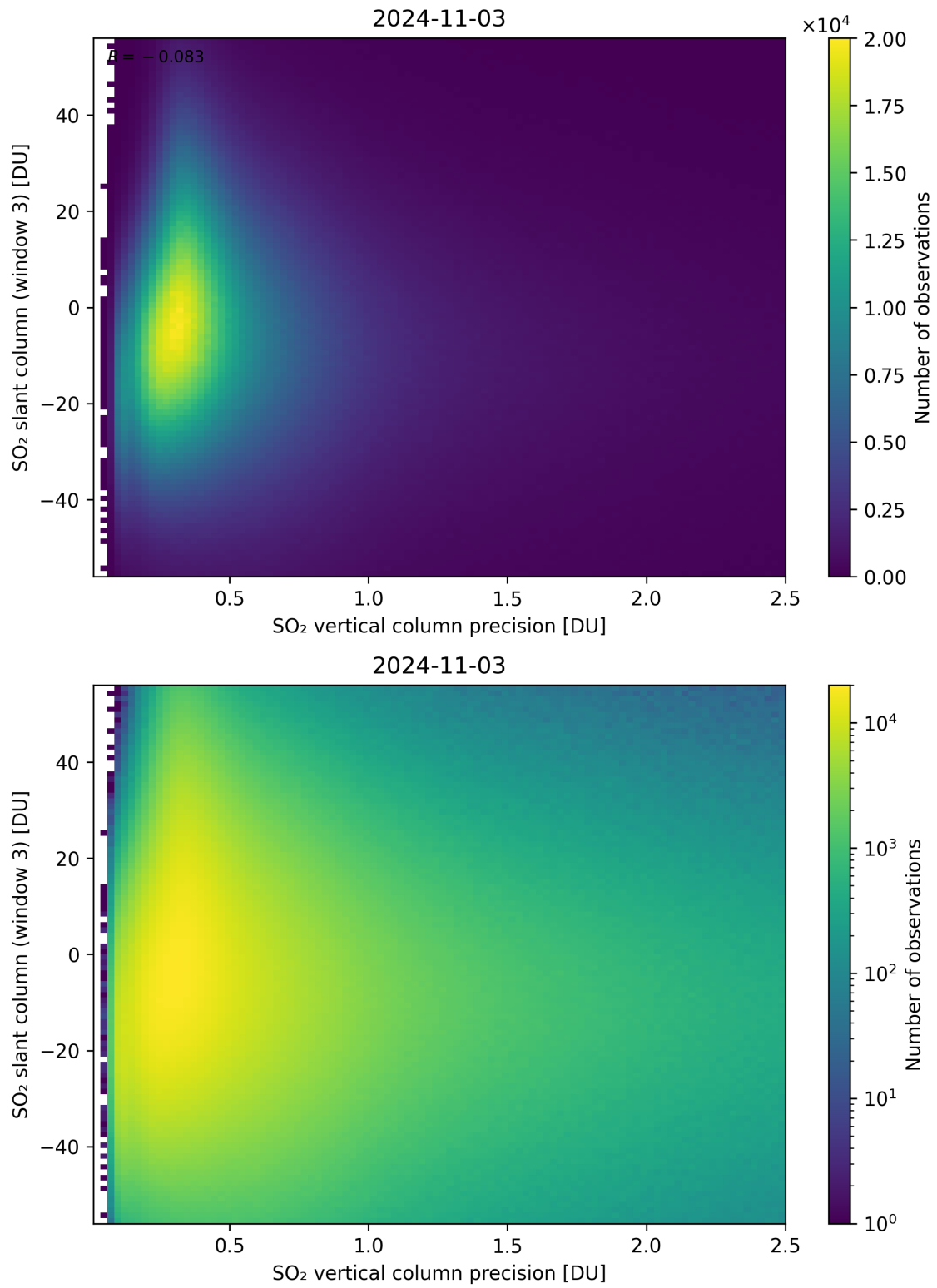
Figure 292: Scatter density plot of “SO 2 vertical column precision” against “SO 2 slant column (window 3)” for 2024-11-02 to 2024-11-04.
