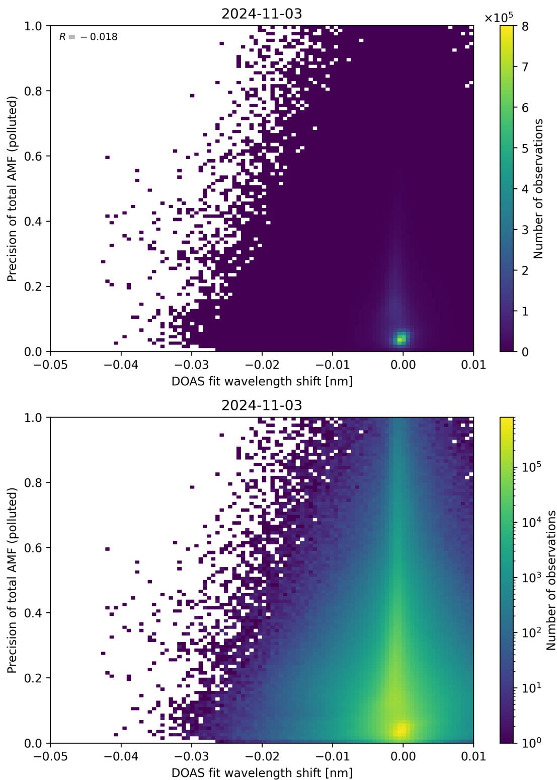
Figure 131: Scatter density plot of “DOAS fit wavelength shift” against “Precision of total AMF (polluted)” for 2024-11-02 to 2024-11-04.
