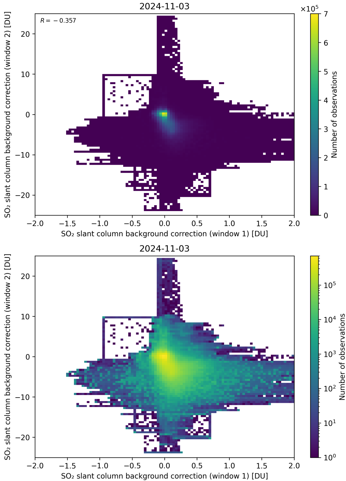
Figure 98: Scatter density plot of “SO 2 slant column background correction (window 1)” against “SO 2 slant column background correction (window 2)” for 2024-11-02 to 2024-11-04.
