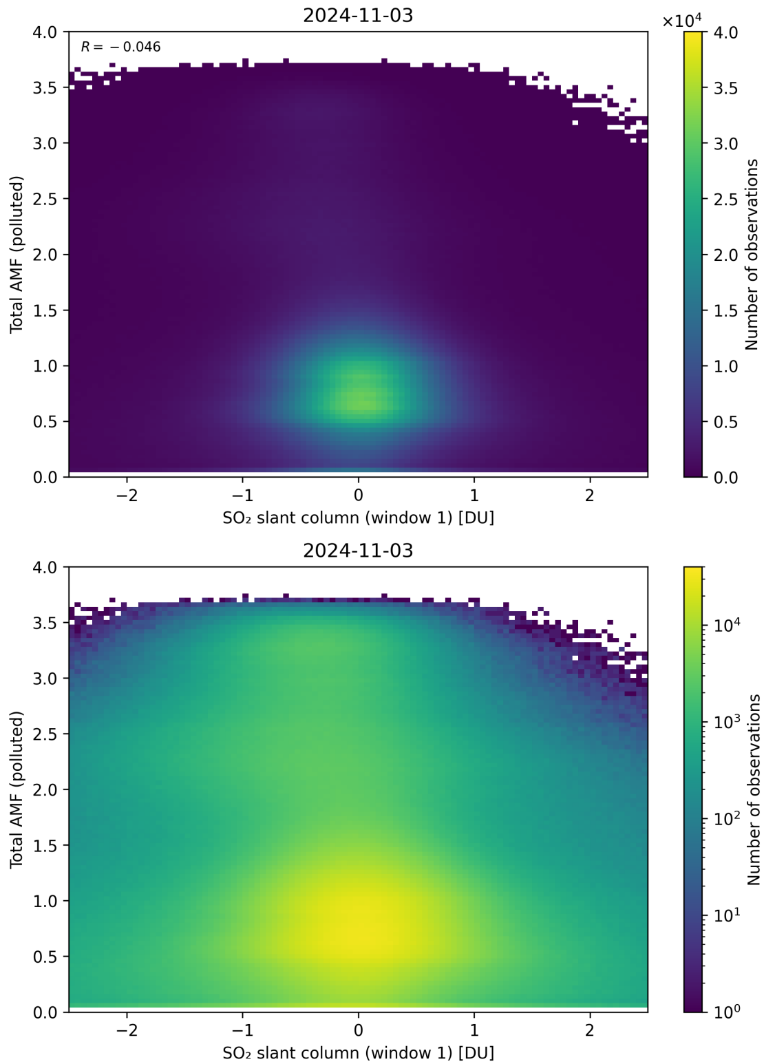
Figure 239: Scatter density plot of “SO 2 slant column (window 1)” against “Total AMF (polluted)” for 2024-11-02 to 2024-11-04.
