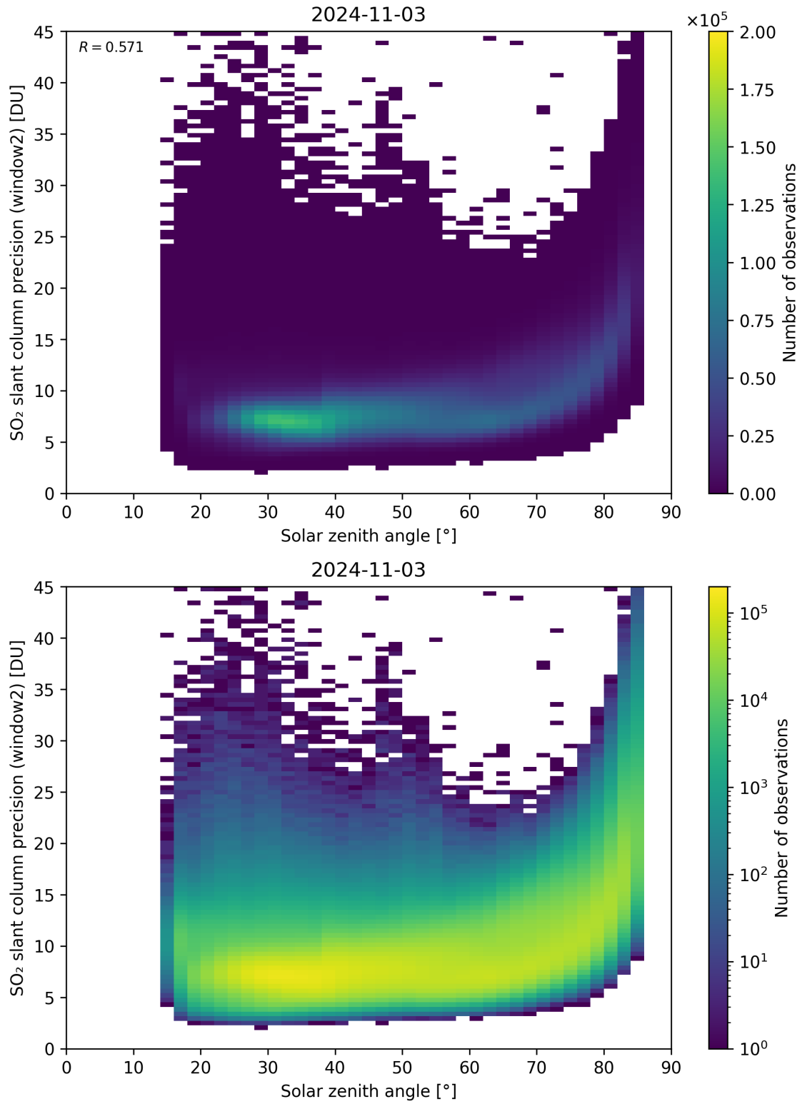
Figure 171: Scatter density plot of “Solar zenith angle” against “SO 2 slant column precision (window2)” for 2024-11-02 to 2024-11-04.
