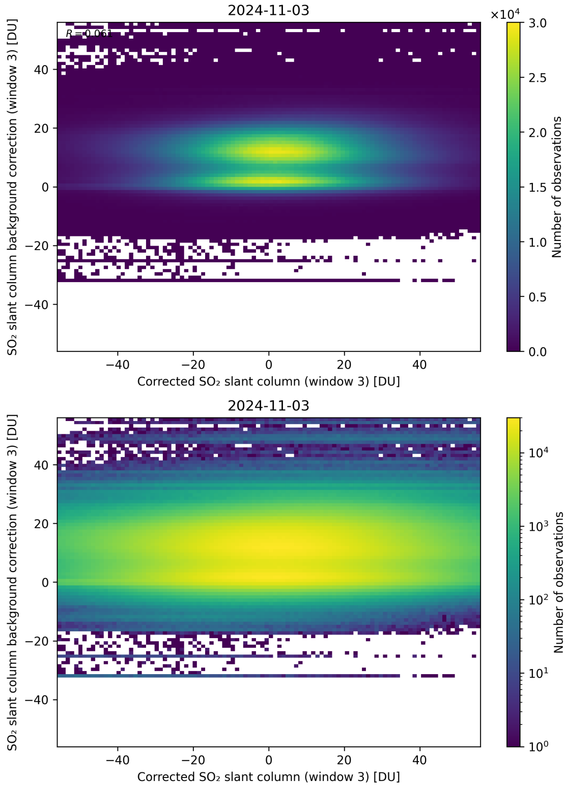
Figure 205: Scatter density plot of “Corrected SO 2 slant column (window 3)” against “SO 2 slant column background correction (window 3)” for 2024-11-02 to 2024-11-04.
