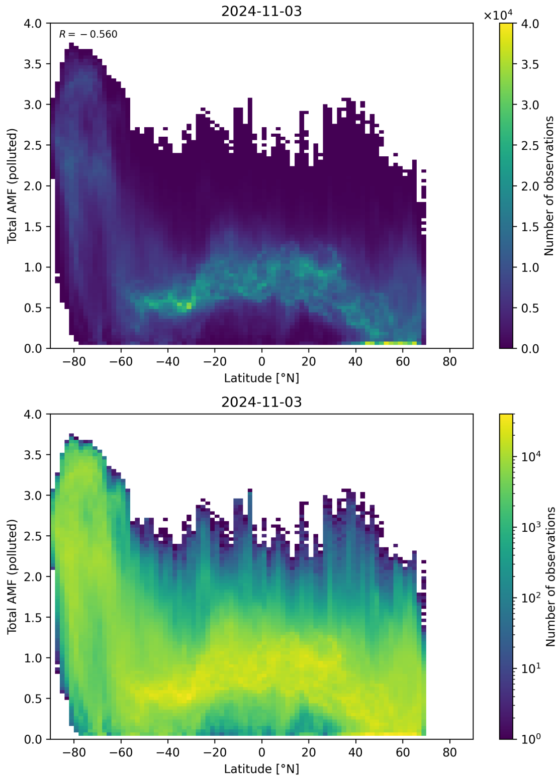
Figure 154: Scatter density plot of “Latitude” against “Total AMF (polluted)” for 2024-11-02 to 2024-11-04.
