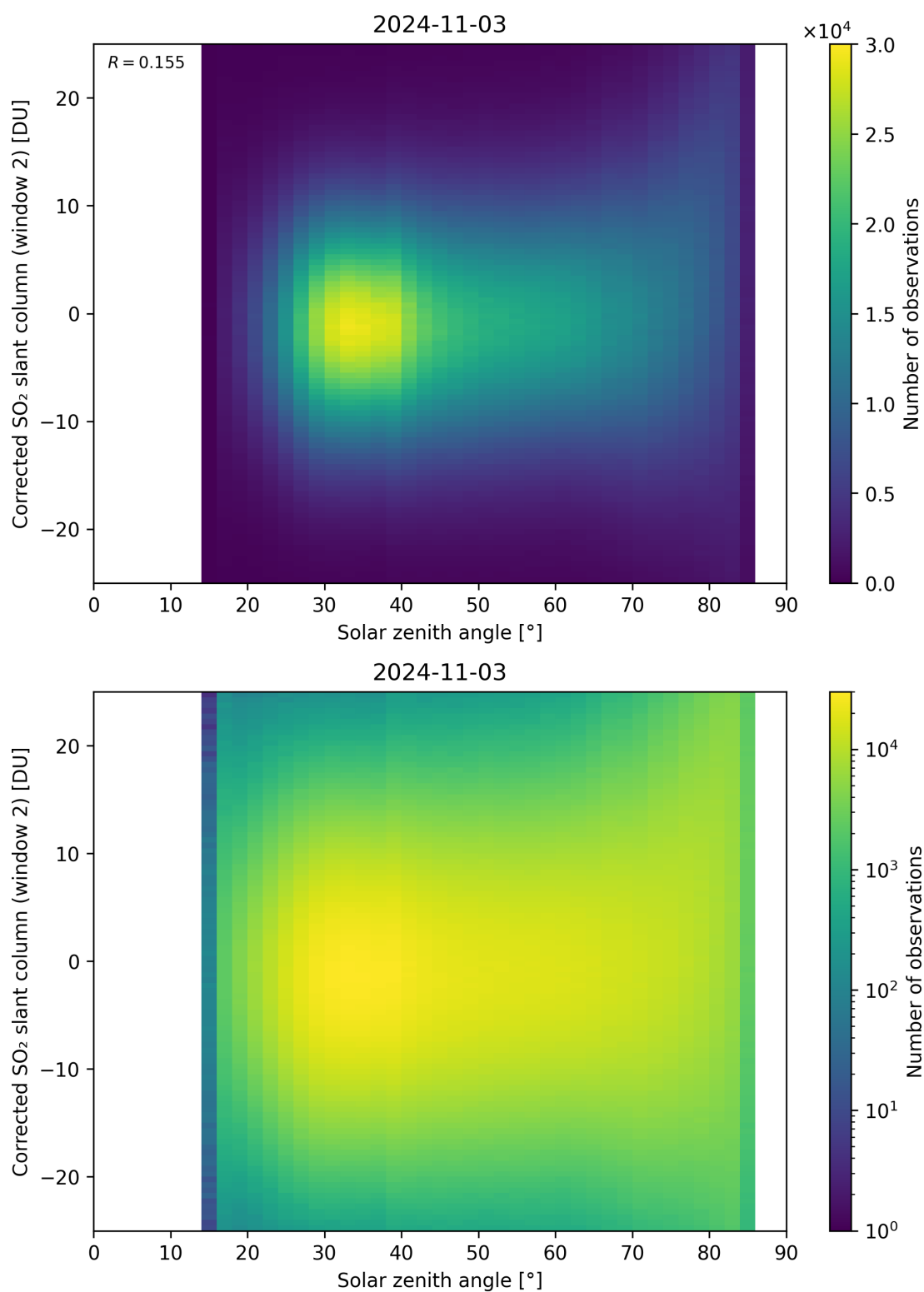
Figure 167: Scatter density plot of “Solar zenith angle” against “Corrected SO 2 slant column (window 2)” for 2024-11-02 to 2024-11-04.
