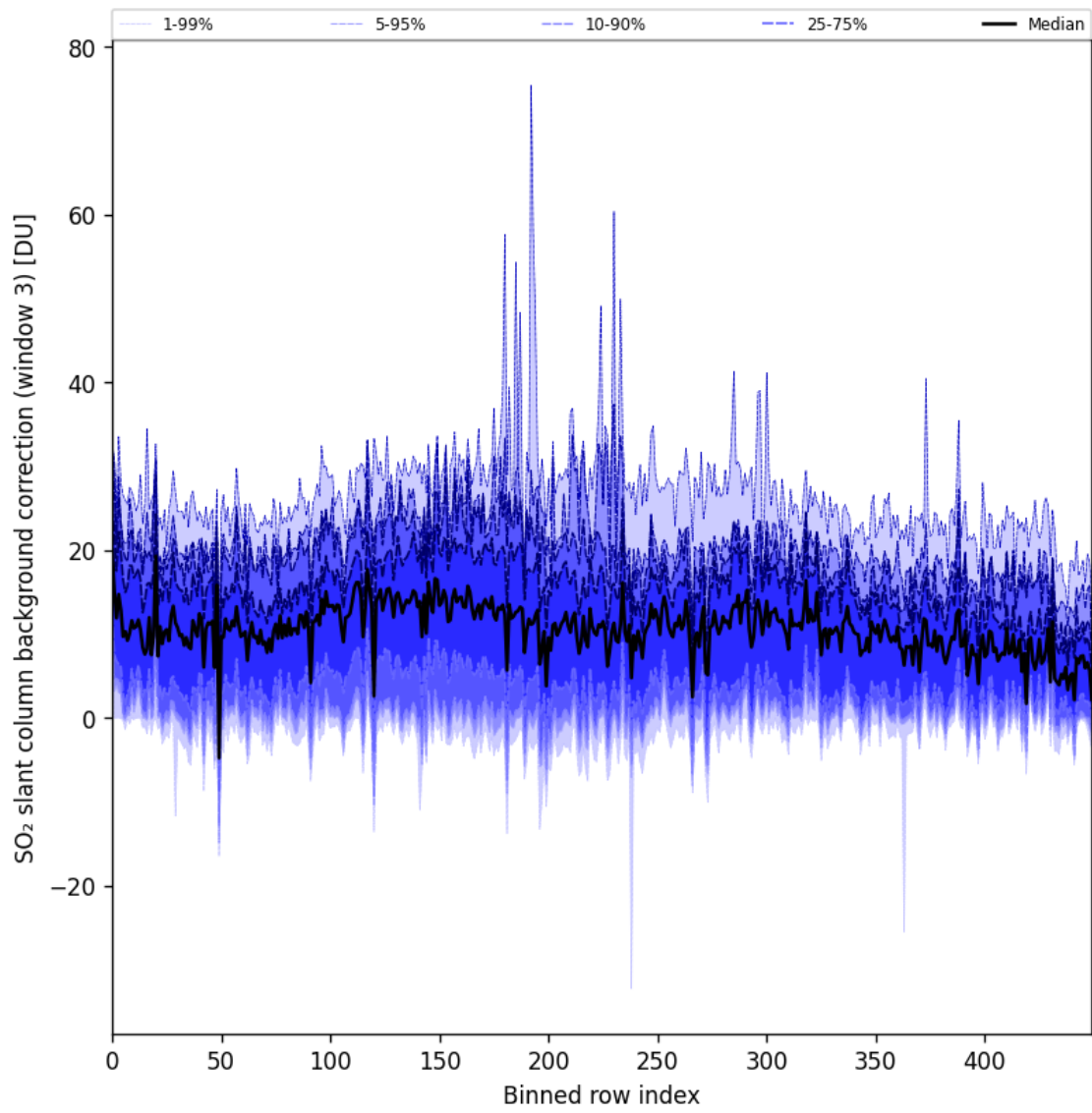
Figure 90: Along track statistics of “SO 2 slant column background correction (window 3)” for 2024-11-02 to 2024-11-04
