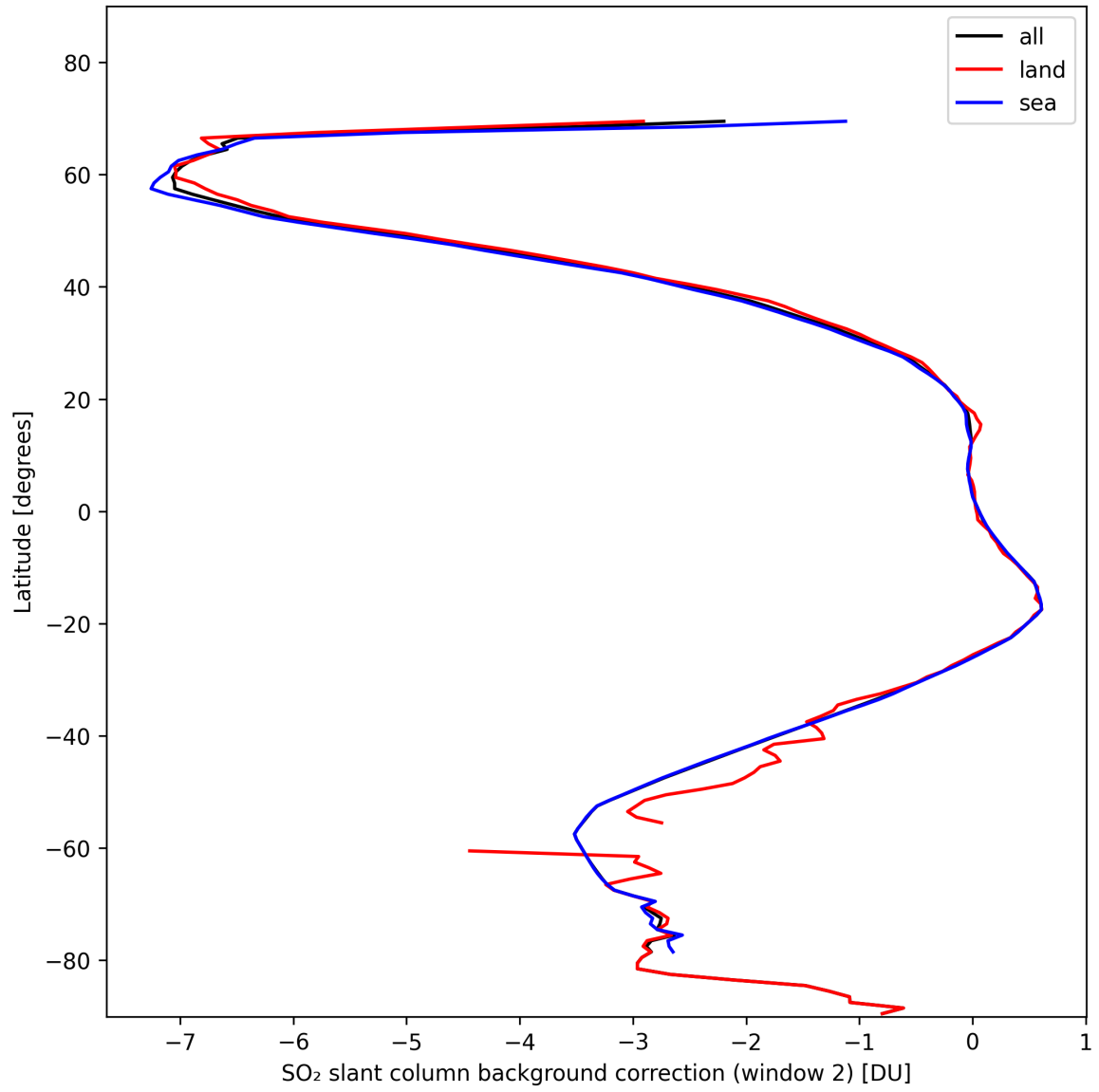
Figure 40: Zonal average of “SO 2 slant column background correction (window 2)” for 2024-11-02 to 2024-11-04.
