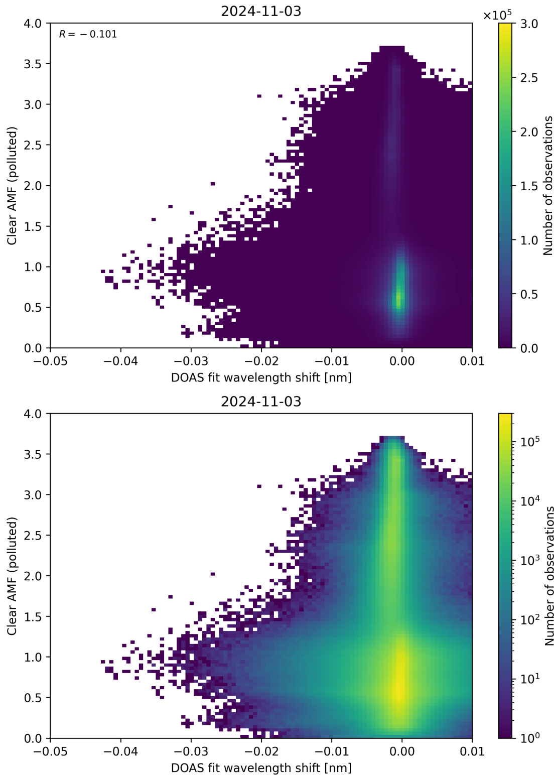
Figure 129: Scatter density plot of “DOAS fit wavelength shift” against “Clear AMF (polluted)” for 2024-11-02 to 2024-11-04.
