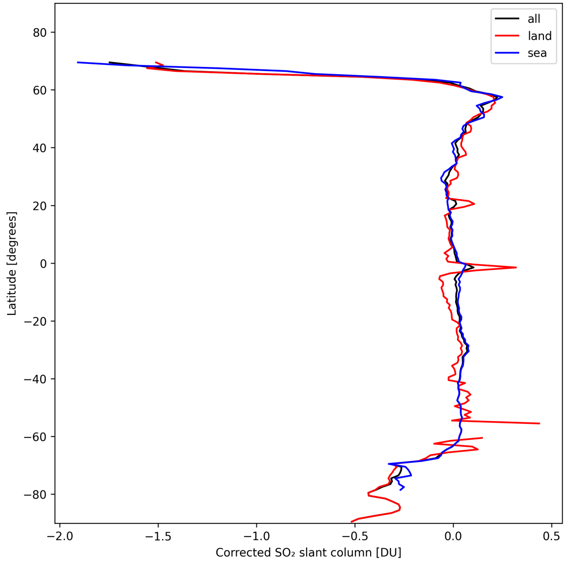
Figure 32: Zonal average of “Corrected SO 2 slant column” for 2024-11-02 to 2024-11-04.
