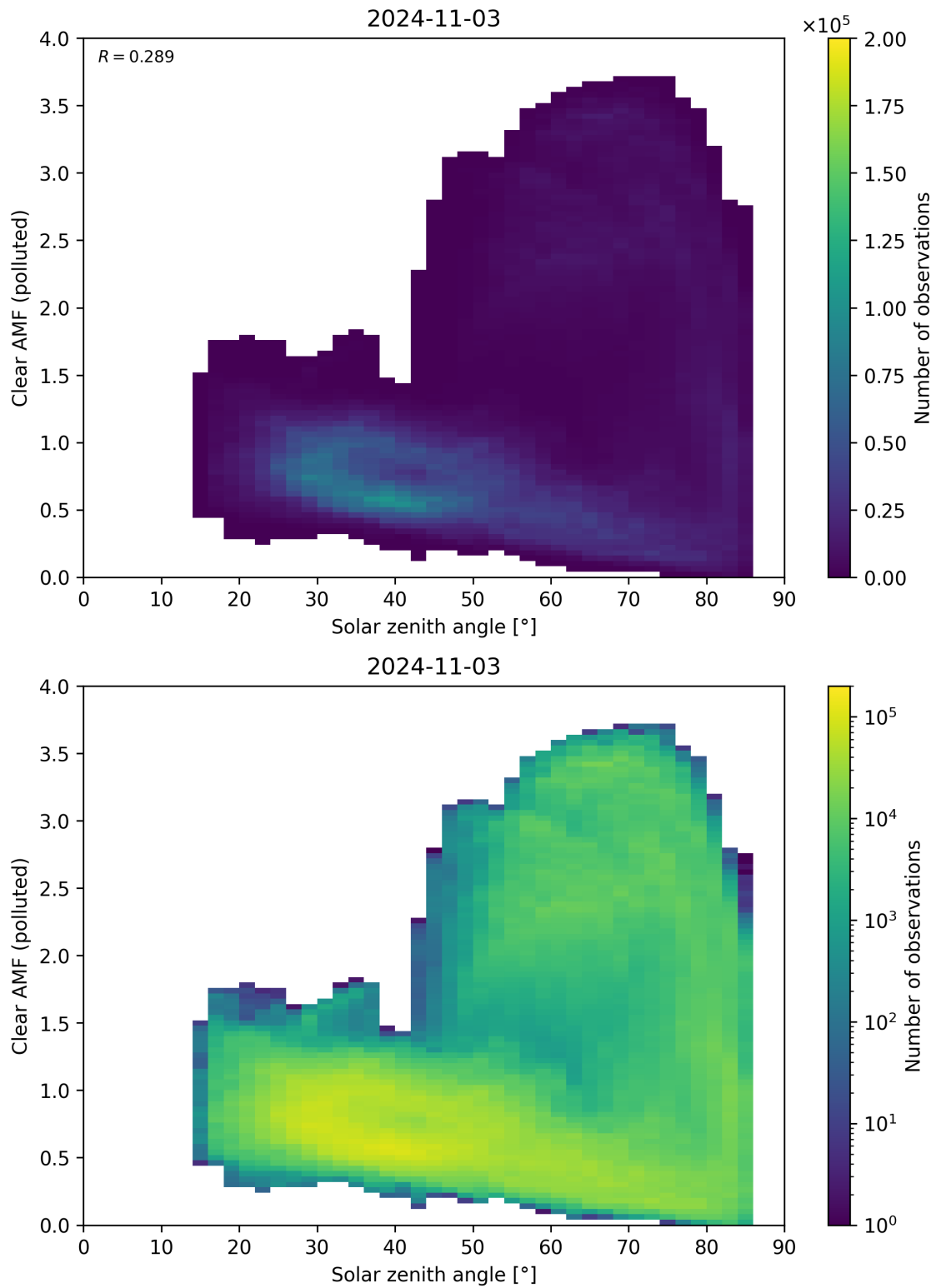
Figure 165: Scatter density plot of “Solar zenith angle” against “Clear AMF (polluted)” for 2024-11-02 to 2024-11-04.
