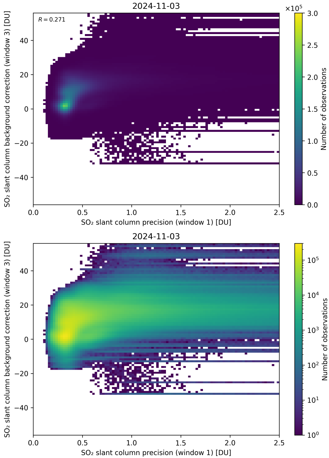
Figure 220: Scatter density plot of “SO 2 slant column precision (window 1)” against “SO 2 slant column background correction (window 3)” for 2024-11-02 to 2024-11-04.
