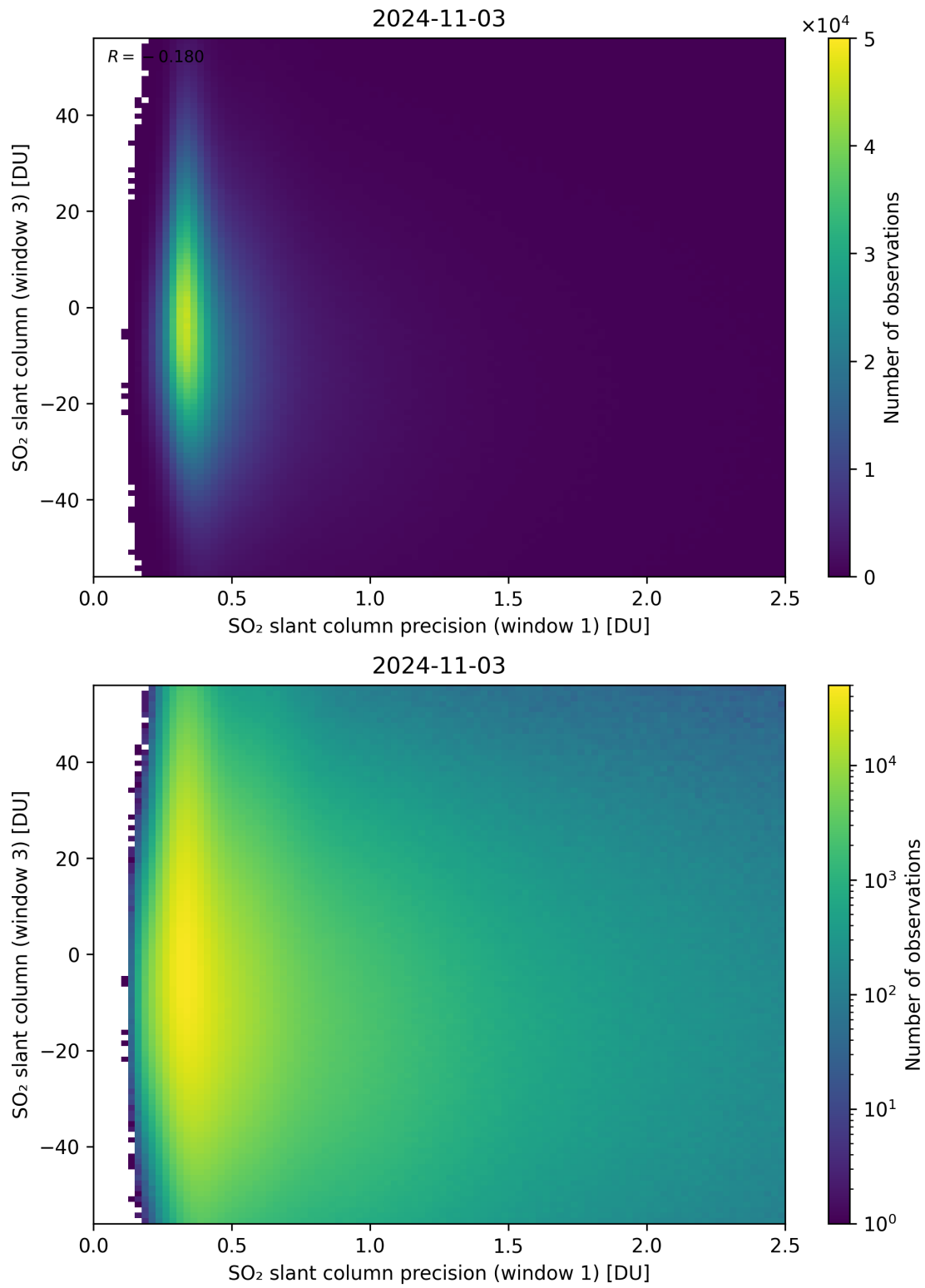
Figure 228: Scatter density plot of “SO 2 slant column precision (window 1)” against “SO 2 slant column (window 3)” for 2024-11-02 to 2024-11-04.
