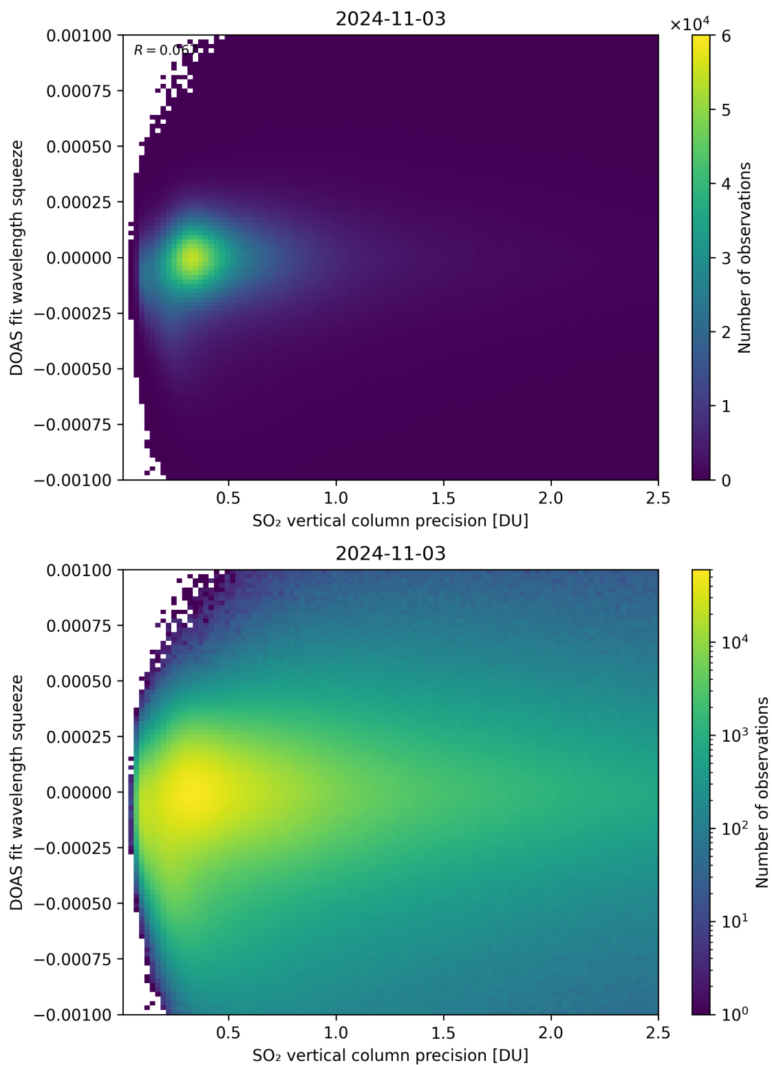
Figure 283: Scatter density plot of “SO 2 vertical column precision” against “DOAS fit wavelength squeeze” for 2024-11-02 to 2024-11-04.
