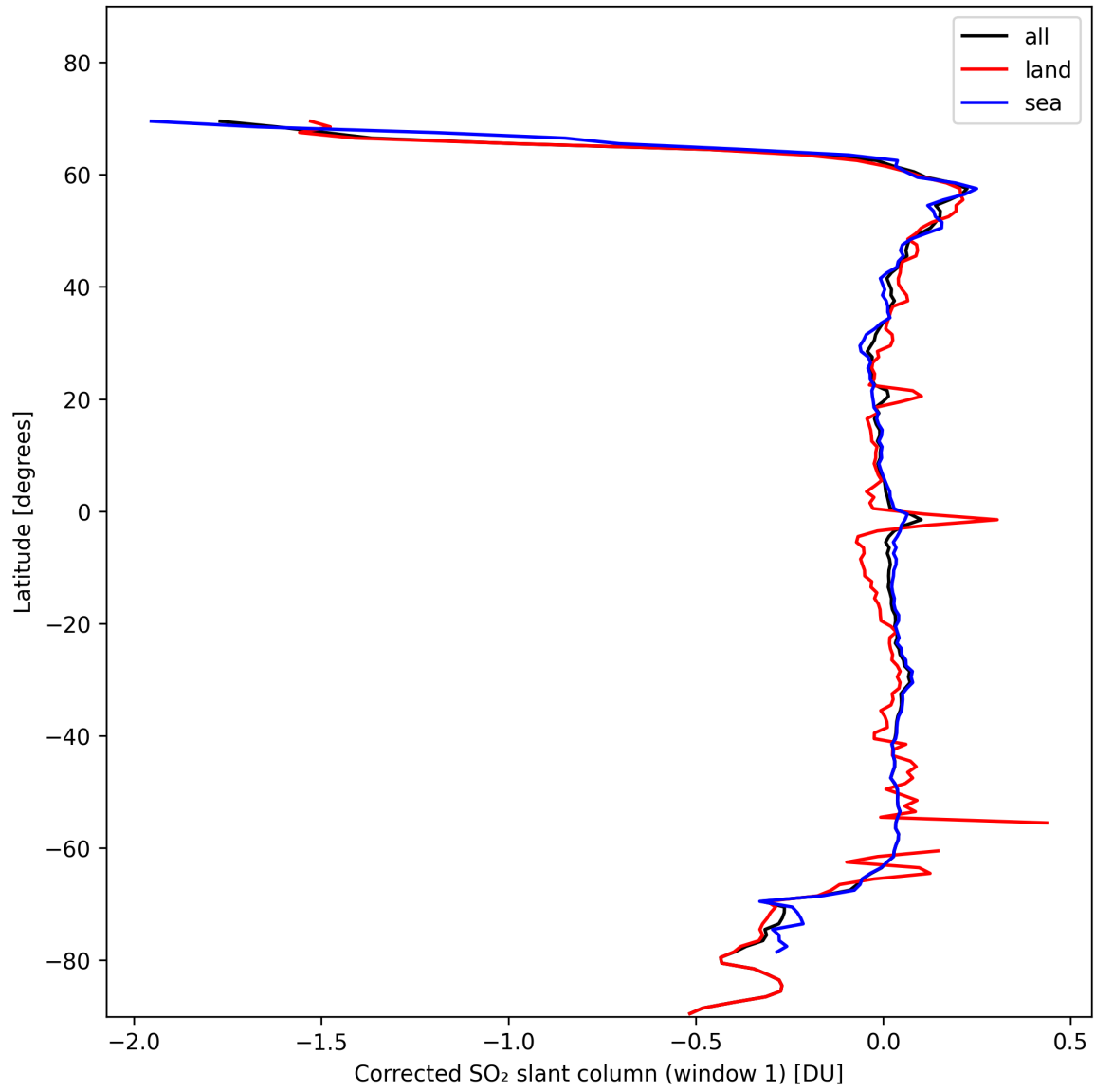
Figure 35: Zonal average of “Corrected SO 2 slant column (window 1)” for 2024-11-02 to 2024-11-04.
