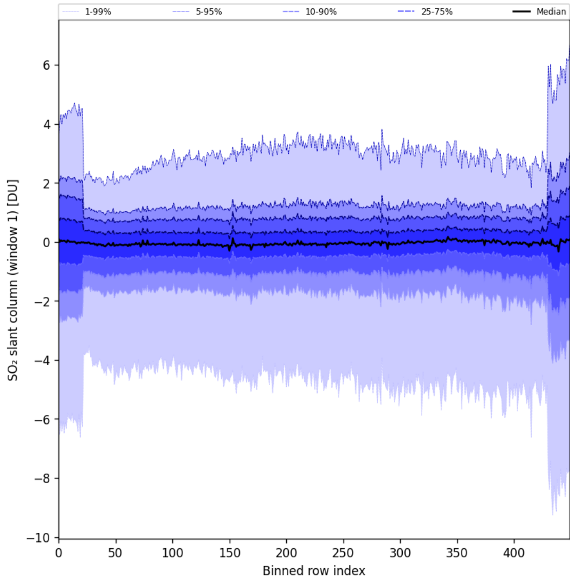
Figure 79: Along track statistics of “SO 2 slant column (window 1)” for 2024-11-02 to 2024-11-04
