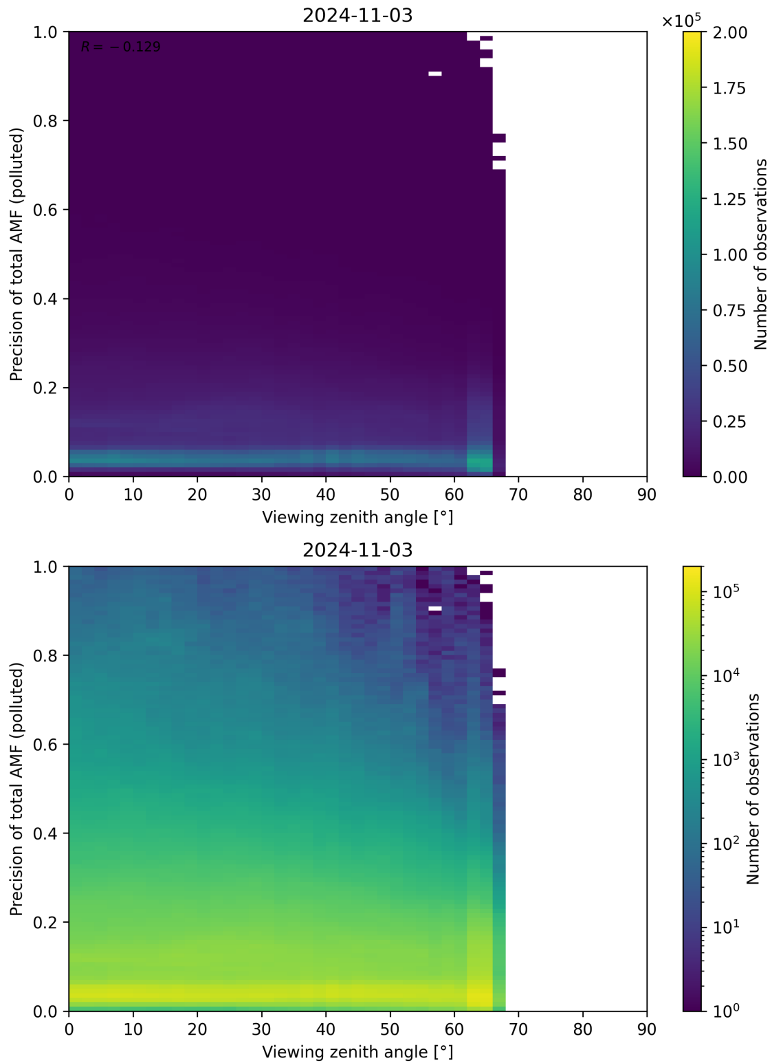
Figure 326: Scatter density plot of “Viewing zenith angle” against “Precision of total AMF (polluted)” for 2024-11-02 to 2024-11-04.
