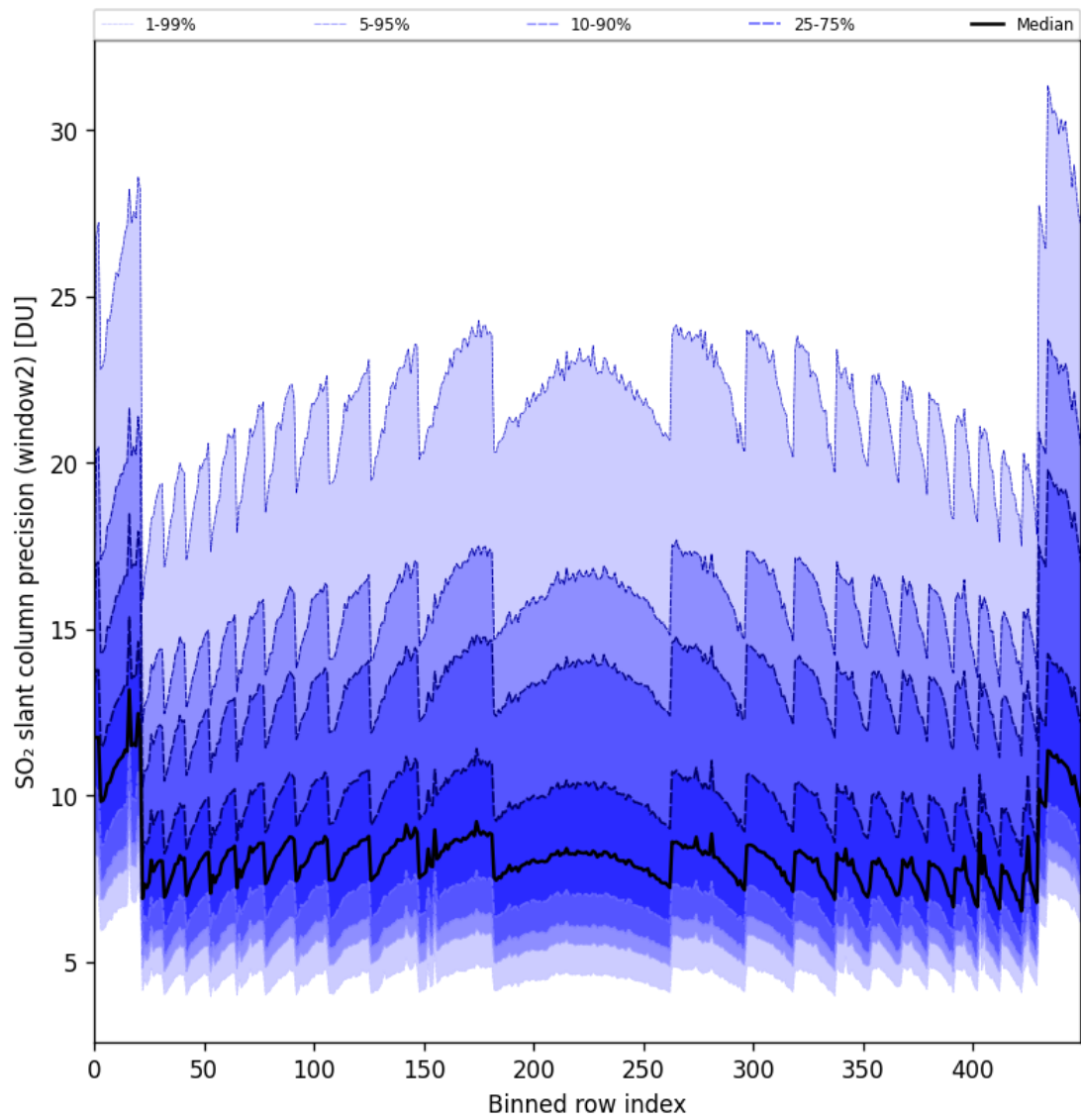
Figure 84: Along track statistics of “SO 2 slant column precision (window2)” for 2024-11-02 to 2024-11-04
