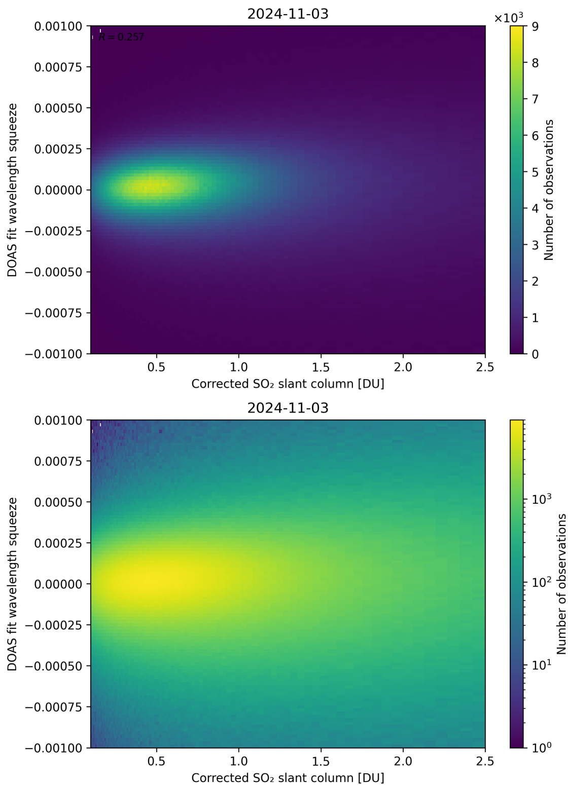
Figure 182: Scatter density plot of “Corrected SO 2 slant column” against “DOAS fit wavelength squeeze” for 2024-11-02 to 2024-11-04.
