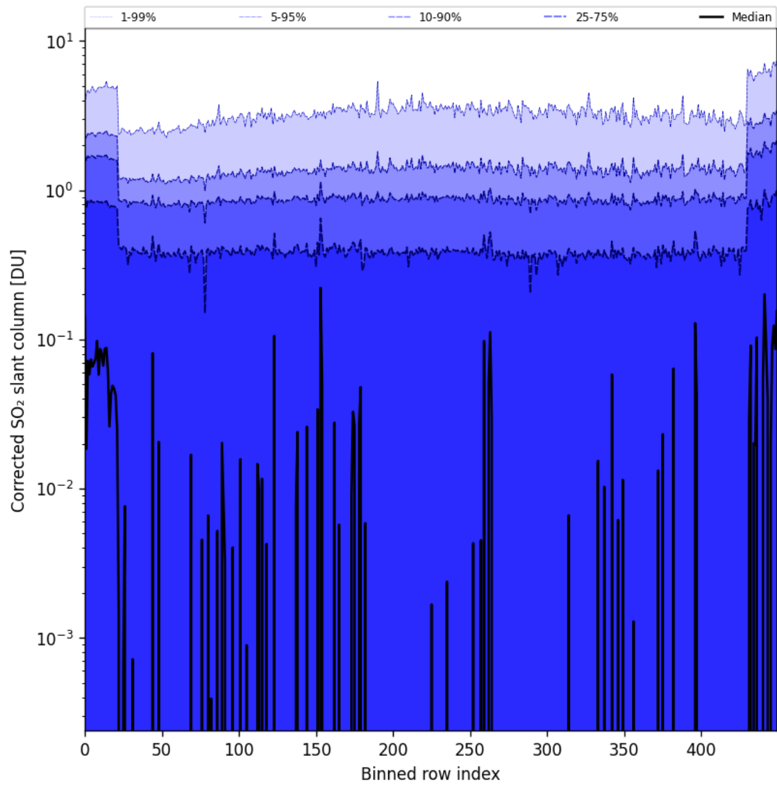
Figure 78: Along track statistics of “Corrected SO 2 slant column” for 2024-11-02 to 2024-11-04
