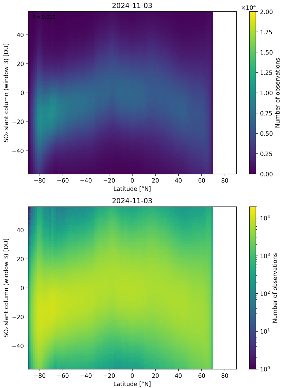
Figure 152: Scatter density plot of “Latitude” against “SO 2 slant column (window 3)” for 2024-11-02 to 2024-11-04.
