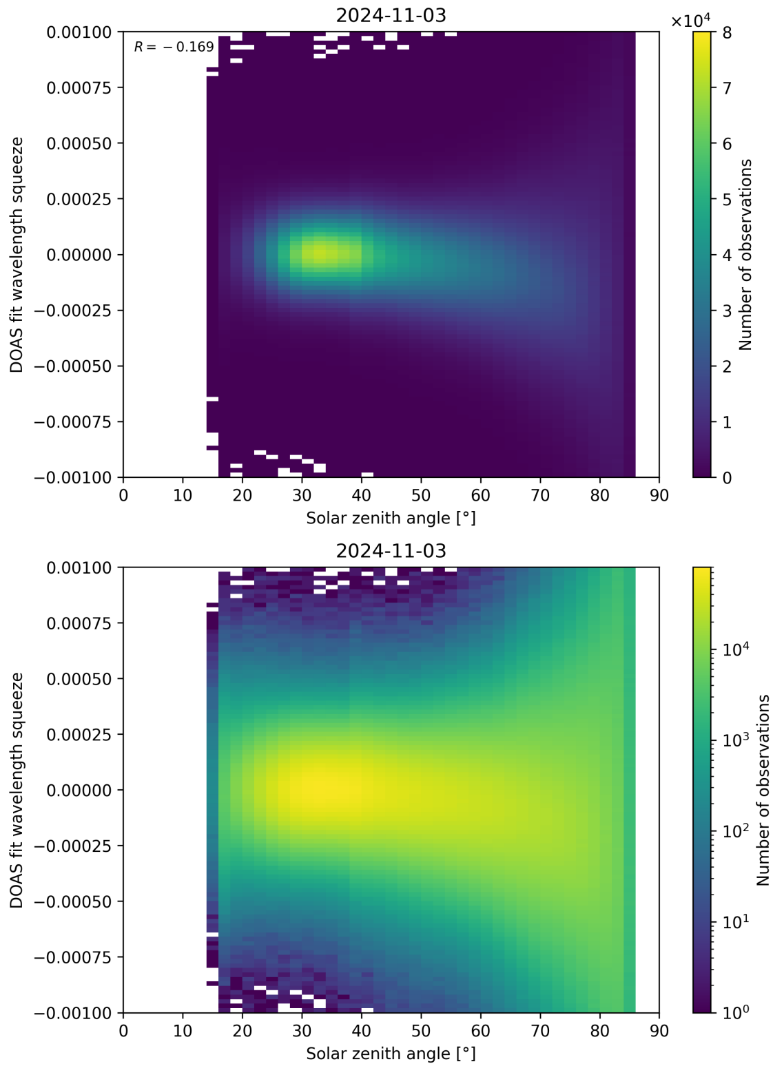
Figure 162: Scatter density plot of “Solar zenith angle” against “DOAS fit wavelength squeeze” for 2024-11-02 to 2024-11-04.
