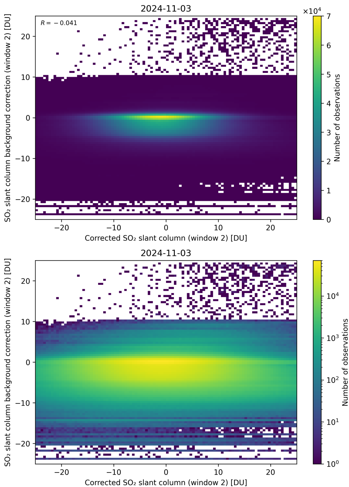
Figure 194: Scatter density plot of “Corrected SO 2 slant column (window 2)” against “SO 2 slant column background correction (window 2)” for 2024-11-02 to 2024-11-04.
