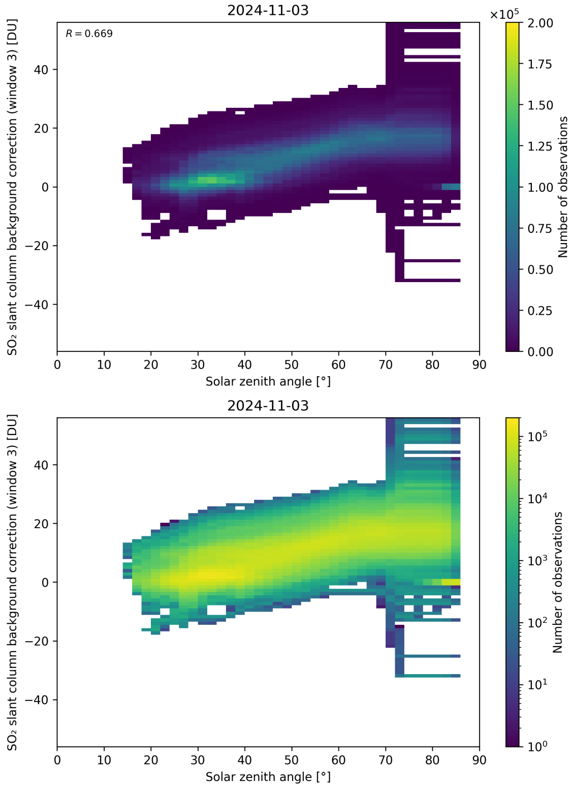
Figure 160: Scatter density plot of “Solar zenith angle” against “SO 2 slant column background correction (window 3)” for 2024-11-02 to 2024-11-04.
