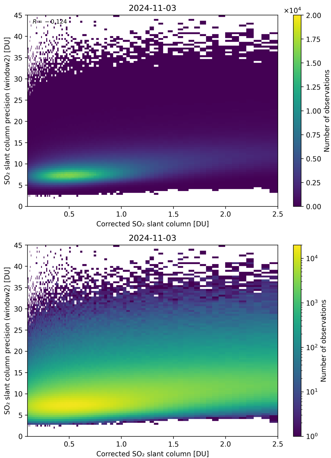
Figure 189: Scatter density plot of “Corrected SO 2 slant column” against “SO 2 slant column precision (window2)” for 2024-11-02 to 2024-11-04.
