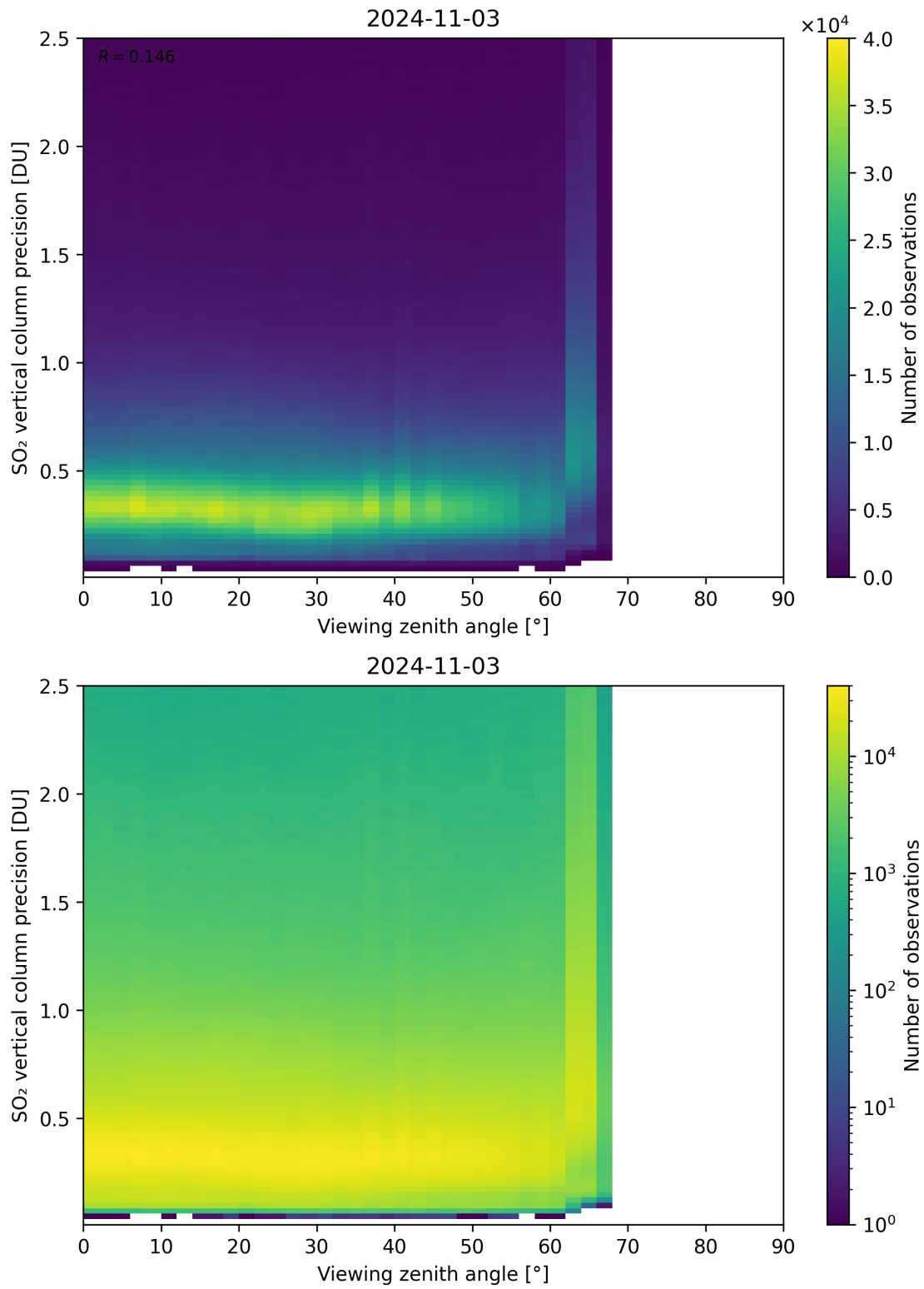
Figure 328: Scatter density plot of “Viewing zenith angle” against “SO 2 vertical column precision” for 2024-11-02 to 2024-11-04.
