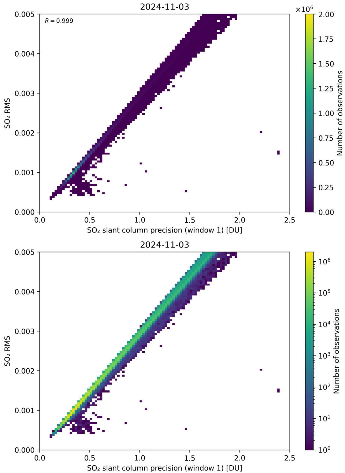
Figure 223: Scatter density plot of “SO 2 slant column precision (window 1)” against “SO 2 RMS” for 2024-11-02 to 2024-11-04.
