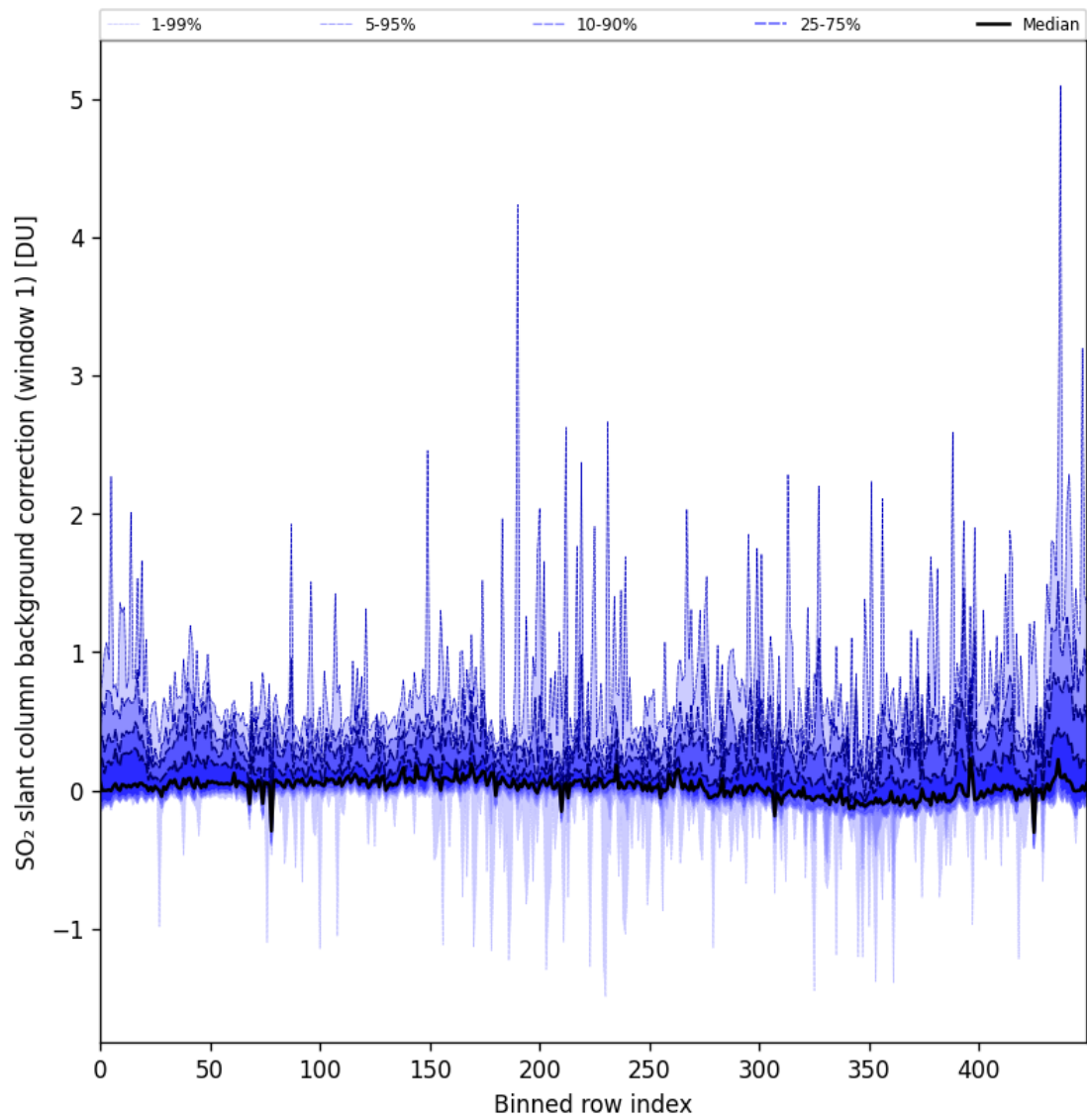
Figure 82: Along track statistics of “SO 2 slant column background correction (window 1)” for 2024-11-02 to 2024-11-04
