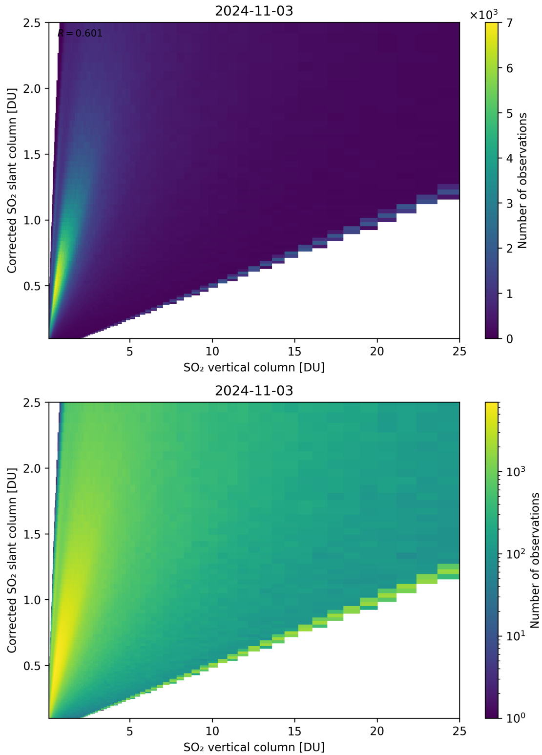
Figure 297: Scatter density plot of “SO 2 vertical column” against “Corrected SO 2 slant column” for 2024-11-02 to 2024-11-04.
