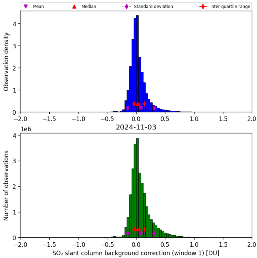
Figure 59: Histogram of “SO 2 slant column background correction (window 1)” for 2024-11-02 to 2024-11-04
