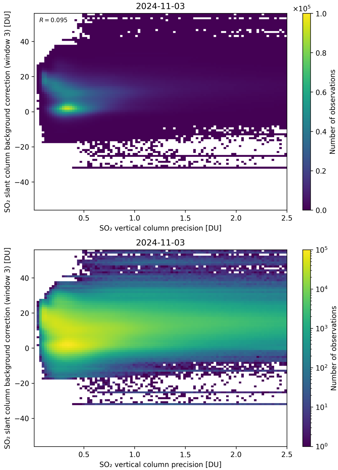
Figure 281: Scatter density plot of “SO 2 vertical column precision” against “SO 2 slant column background correction (window 3)” for 2024-11-02 to 2024-11-04.
