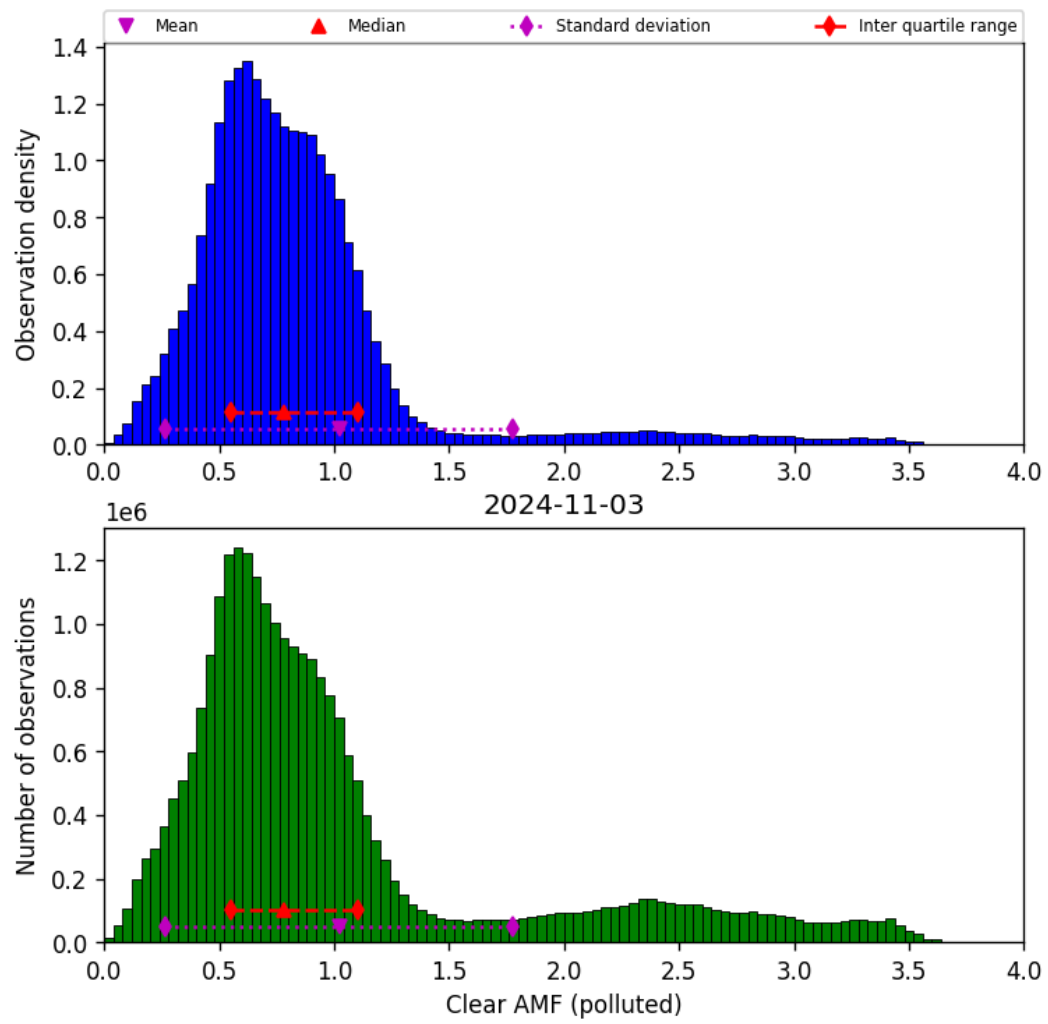
Figure 73: Histogram of “Clear AMF (polluted)” for 2024-11-02 to 2024-11-04
