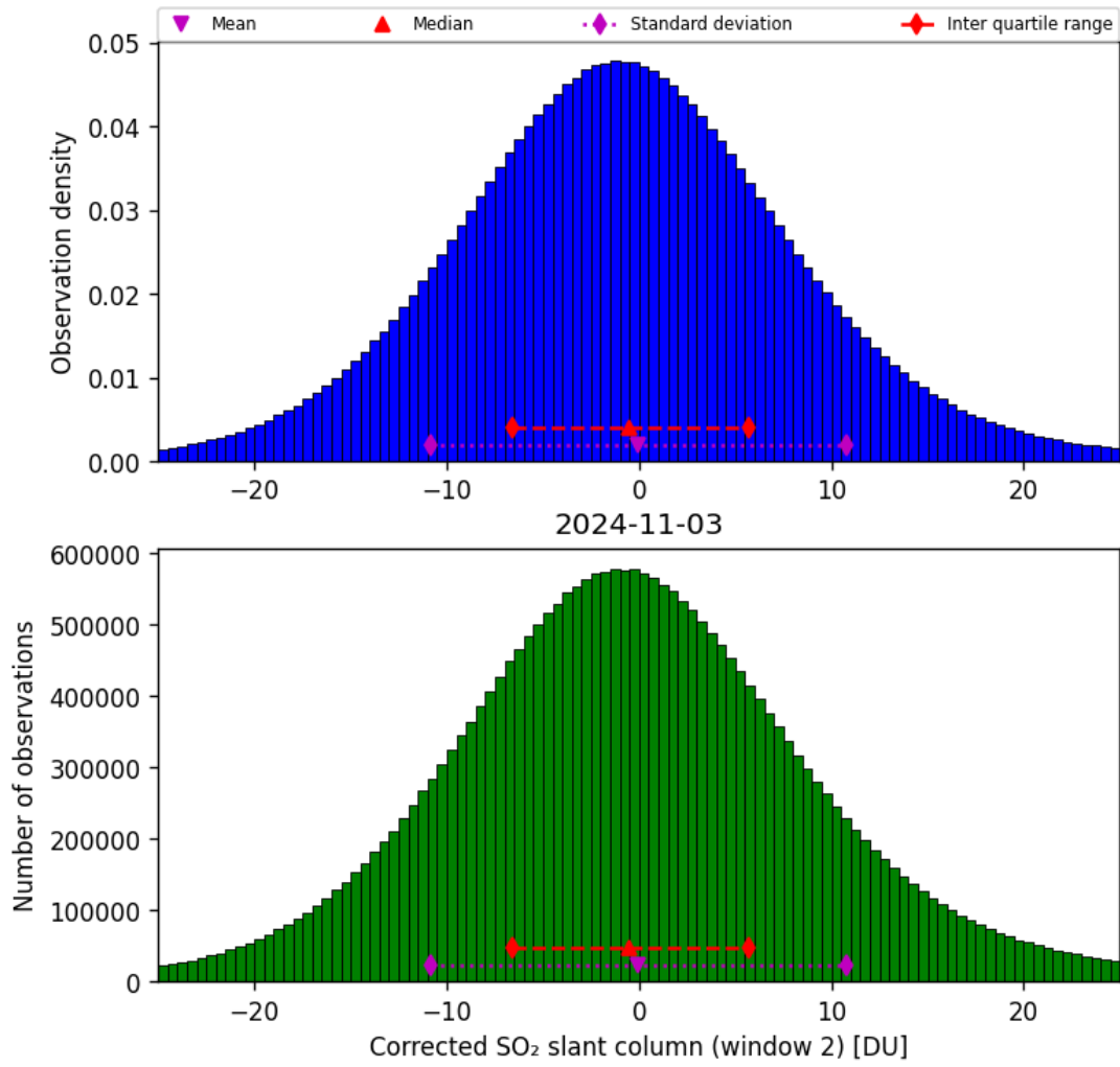
Figure 62: Histogram of “Corrected SO 2 slant column (window 2)” for 2024-11-02 to 2024-11-04
