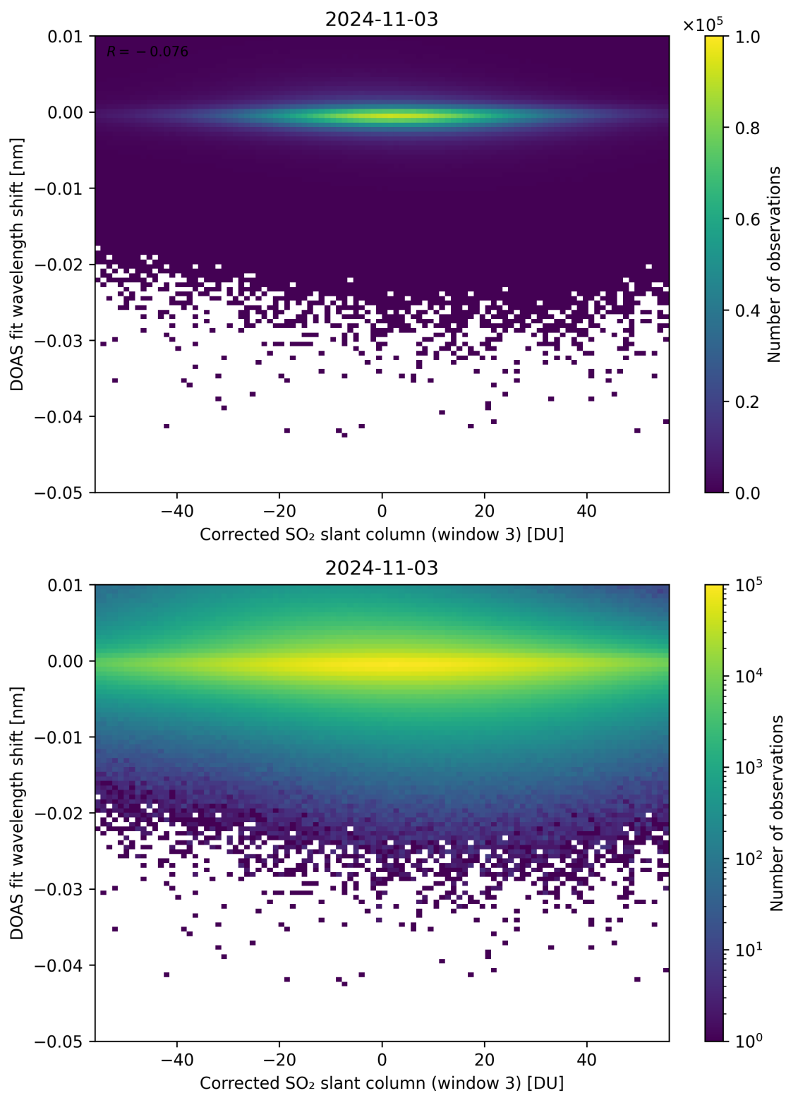
Figure 206: Scatter density plot of “Corrected SO 2 slant column (window 3)” against “DOAS fit wavelength shift” for 2024-11-02 to 2024-11-04.
