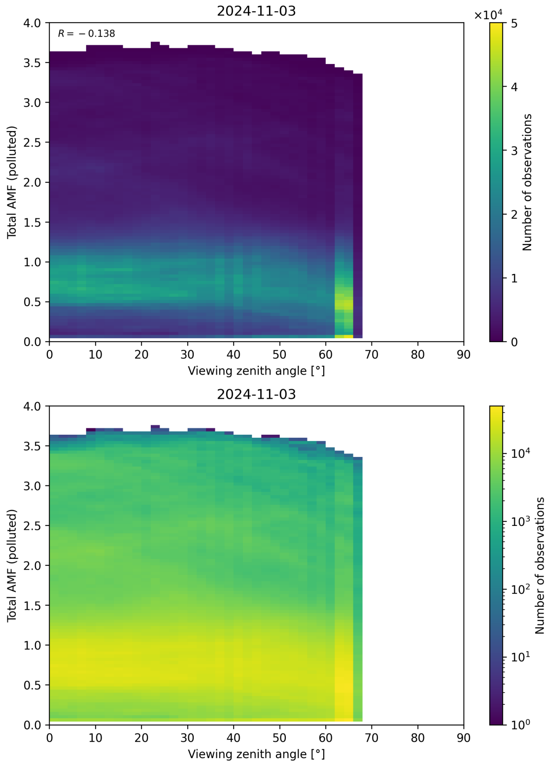
Figure 325: Scatter density plot of “Viewing zenith angle” against “Total AMF (polluted)” for 2024-11-02 to 2024-11-04.
