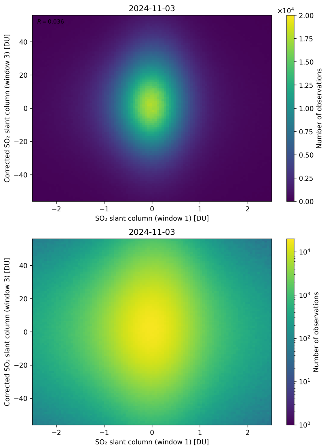
Figure 234: Scatter density plot of “SO 2 slant column (window 1)” against “Corrected SO 2 slant column (window 3)” for 2024-11-02 to 2024-11-04.
