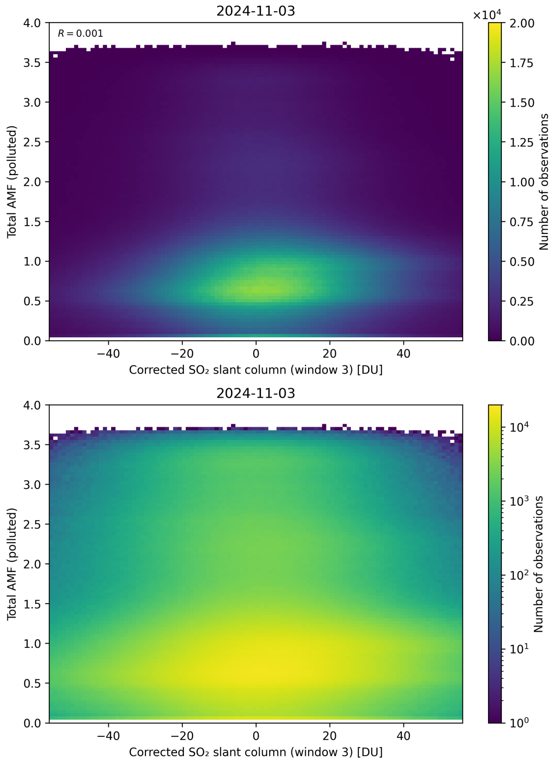
Figure 210: Scatter density plot of “Corrected SO 2 slant column (window 3)” against “Total AMF (polluted)” for 2024-11-02 to 2024-11-04.
