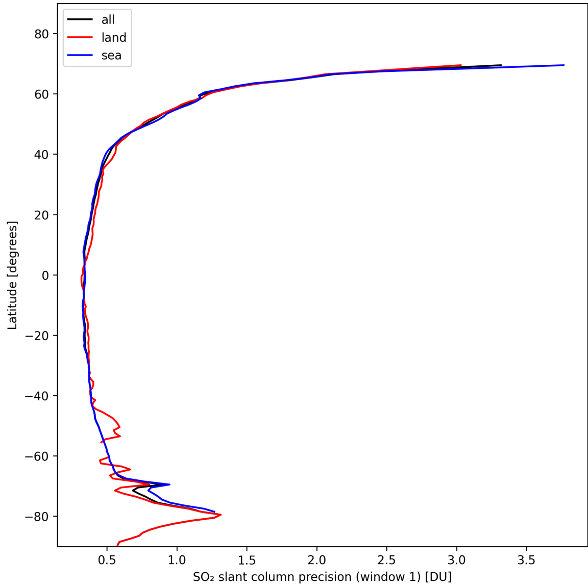
Figure 34: Zonal average of “SO 2 slant column precision (window 1)” for 2024-11-02 to 2024-11-04.
