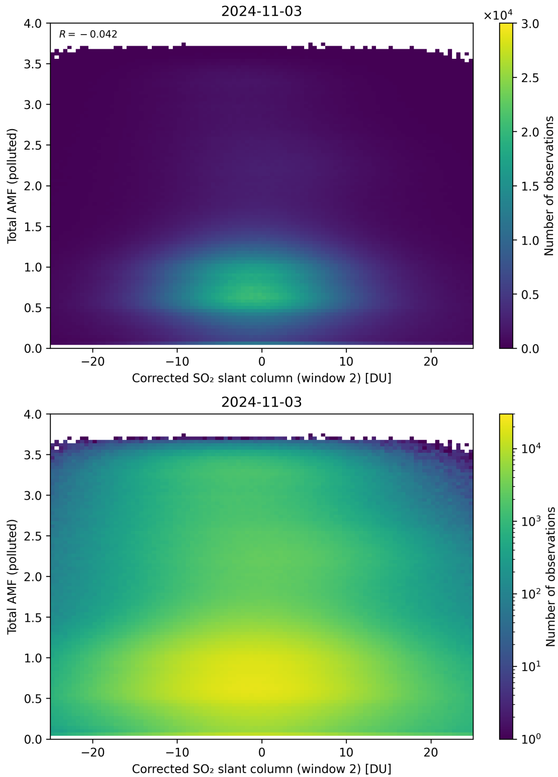
Figure 203: Scatter density plot of “Corrected SO 2 slant column (window 2)” against “Total AMF (polluted)” for 2024-11-02 to 2024-11-04.
