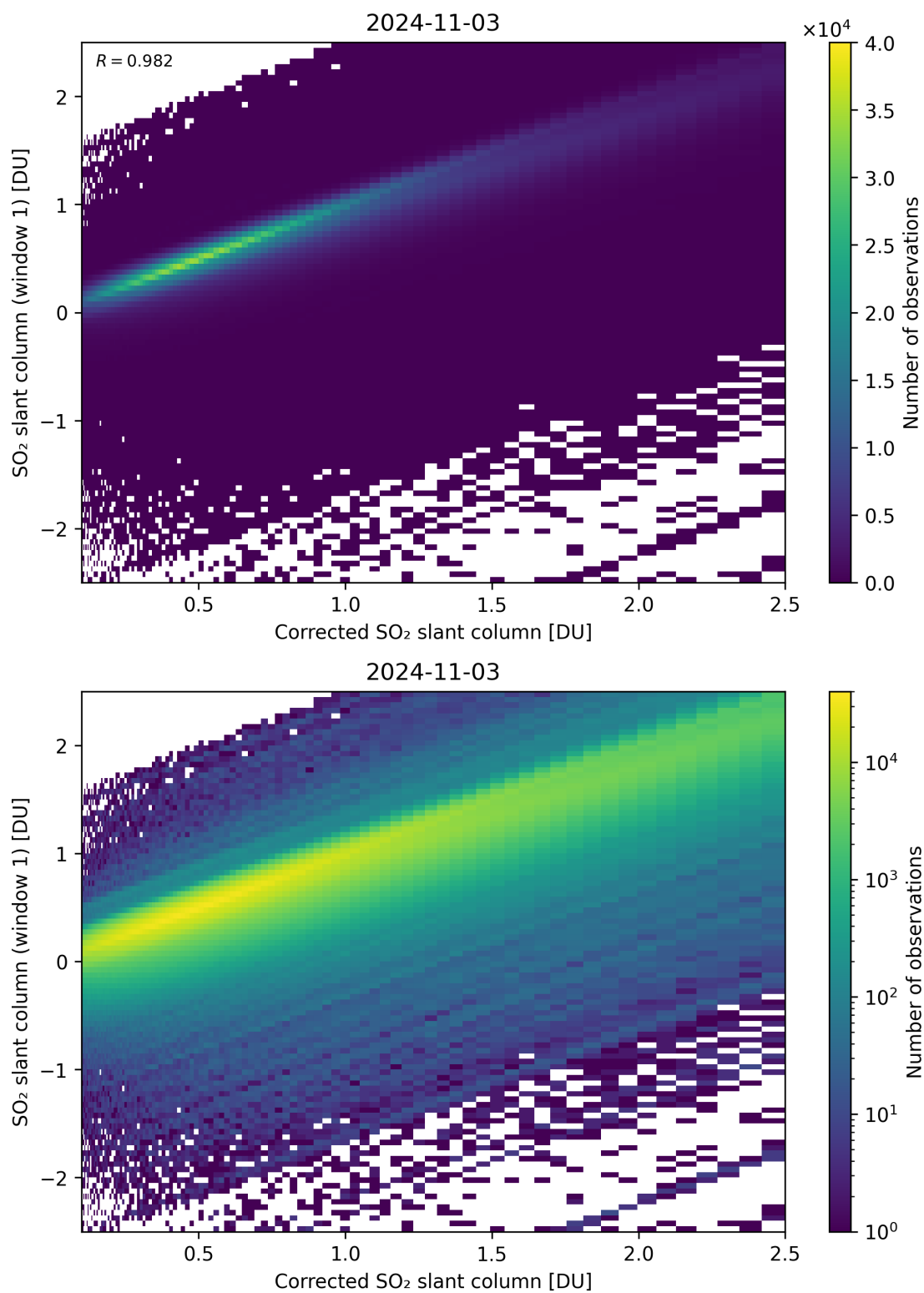
Figure 187: Scatter density plot of “Corrected SO 2 slant column” against “SO 2 slant column (window 1)” for 2024-11-02 to 2024-11-04.
