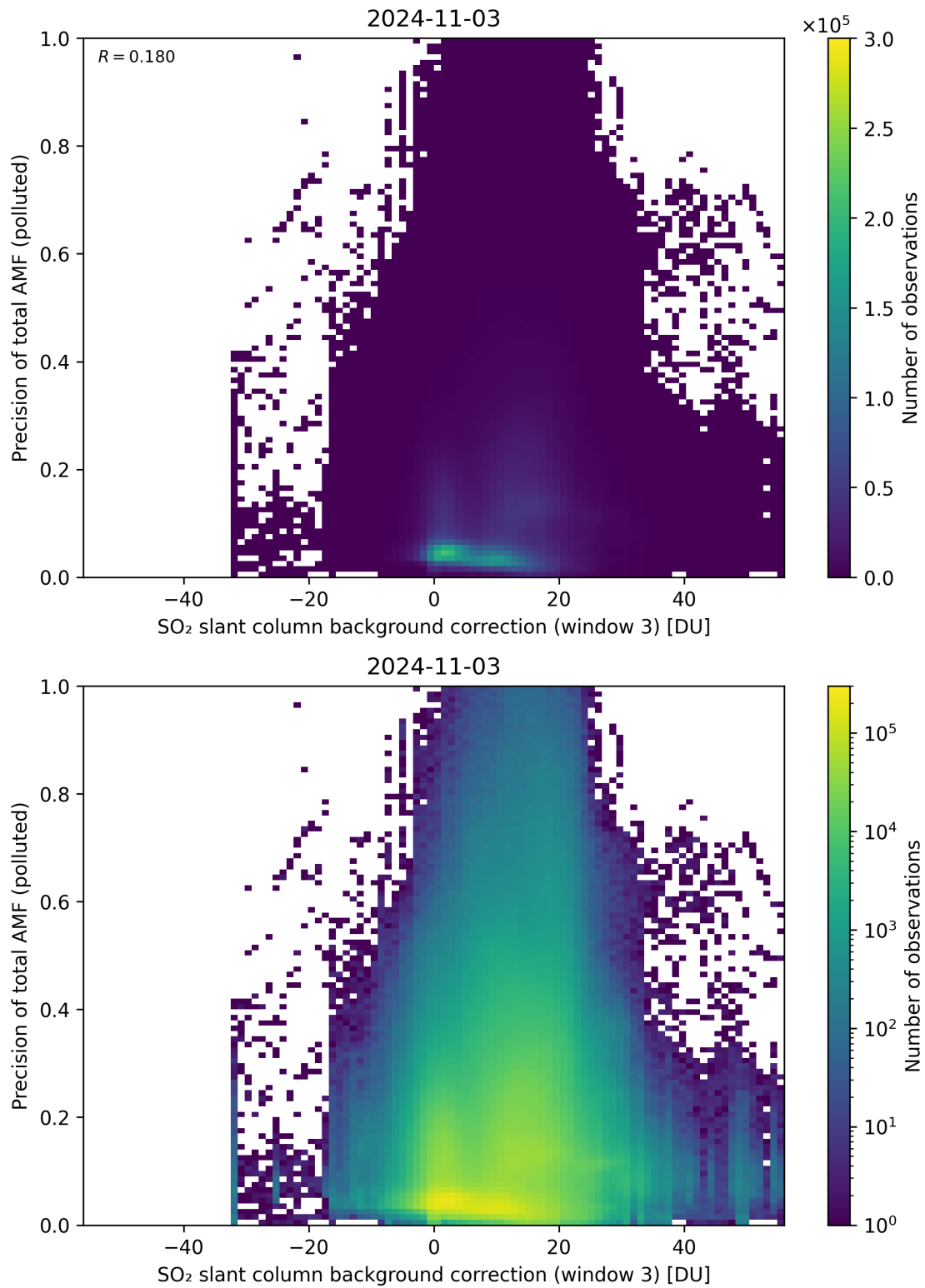
Figure 126: Scatter density plot of “SO 2 slant column background correction (window 3)” against “Precision of total AMF (polluted)” for 2024-11-02 to 2024-11-04.
