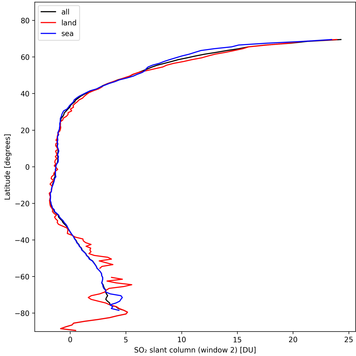
Figure 37: Zonal average of “SO 2 slant column (window 2)” for 2024-11-02 to 2024-11-04.
