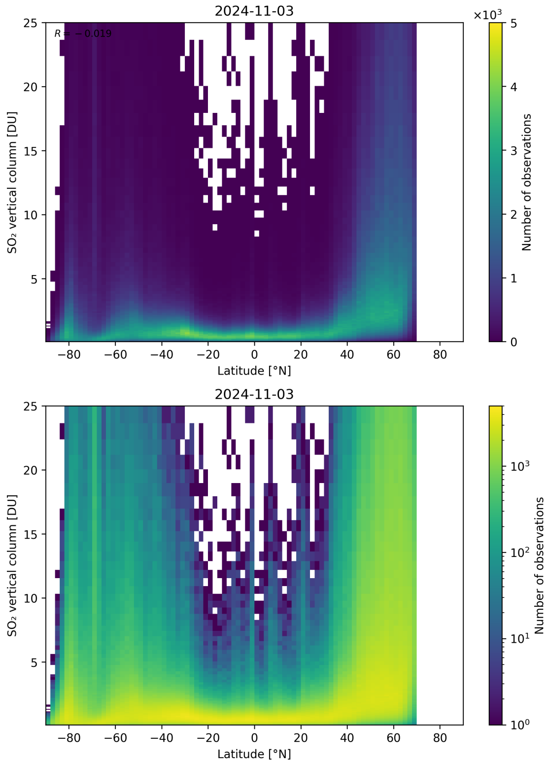
Figure 156: Scatter density plot of “Latitude” against “SO 2 vertical column” for 2024-11-02 to 2024-11-04.
