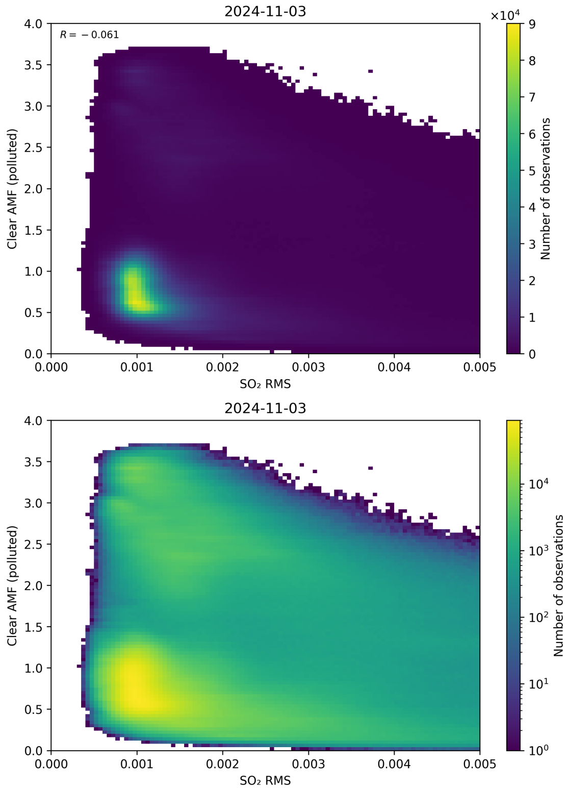
Figure 136: Scatter density plot of “SO 2 RMS” against “Clear AMF (polluted)” for 2024-11-02 to 2024-11-04.
