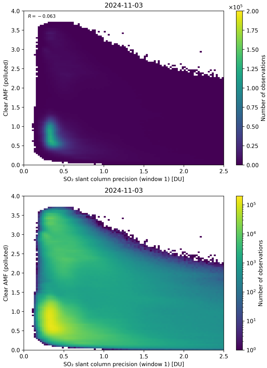
Figure 224: Scatter density plot of “SO 2 slant column precision (window 1)” against “Clear AMF (polluted)” for 2024-11-02 to 2024-11-04.
