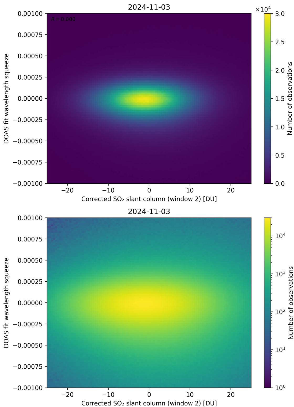
Figure 197: Scatter density plot of “Corrected SO 2 slant column (window 2)” against “DOAS fit wavelength squeeze” for 2024-11-02 to 2024-11-04.
