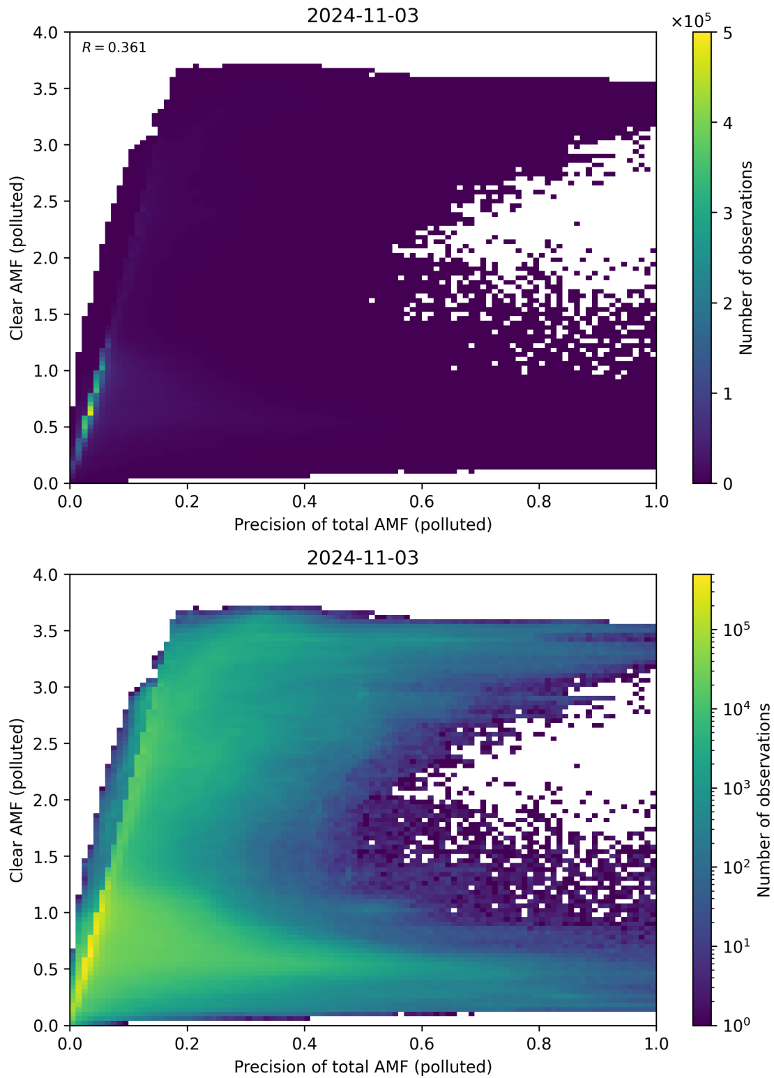
Figure 270: Scatter density plot of “Precision of total AMF (polluted)” against “Clear AMF (polluted)” for 2024-11-02 to 2024-11-04.
