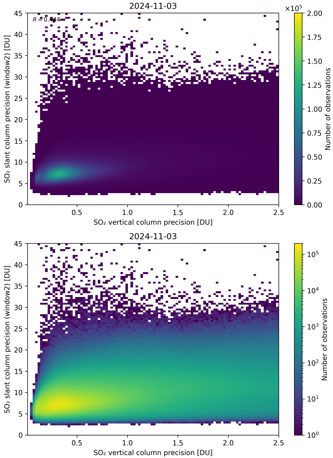
Figure 291: Scatter density plot of “SO 2 vertical column precision” against “SO 2 slant column precision (window2)” for 2024-11-02 to 2024-11-04.
