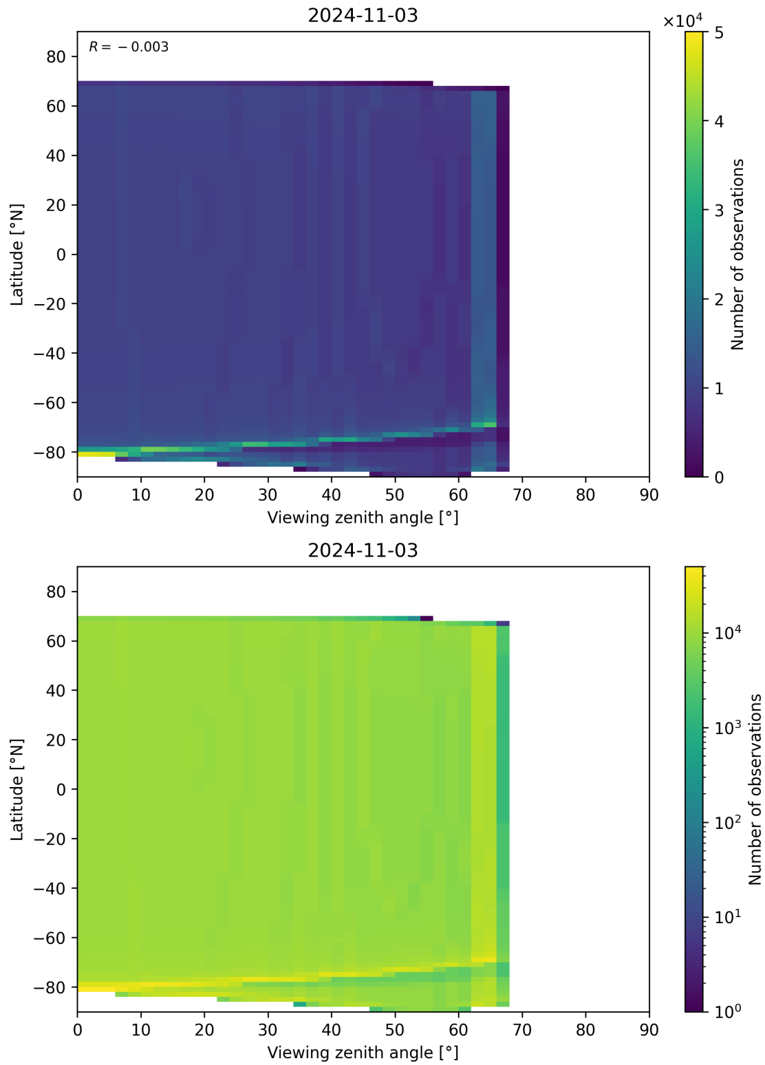
Figure 314: Scatter density plot of “Viewing zenith angle” against “Latitude” for 2024-11-02 to 2024-11-04.
