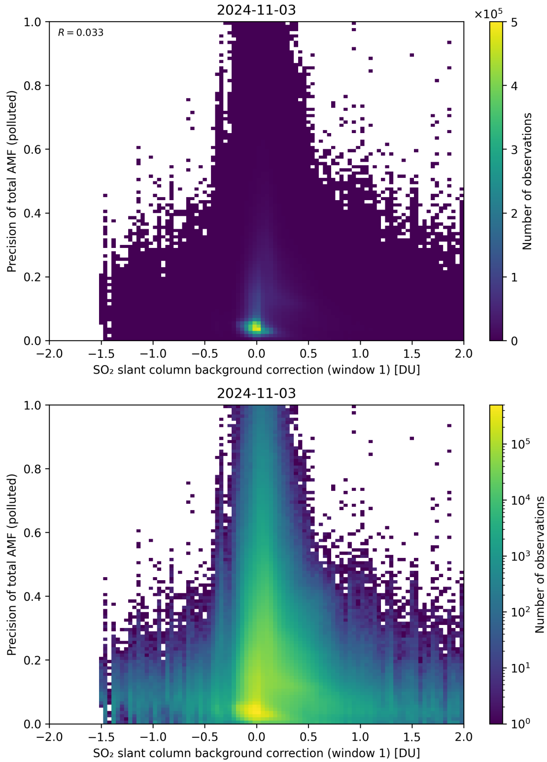
Figure 110: Scatter density plot of “SO 2 slant column background correction (window 1)” against “Precision of total AMF (polluted)” for 2024-11-02 to 2024-11-04.
