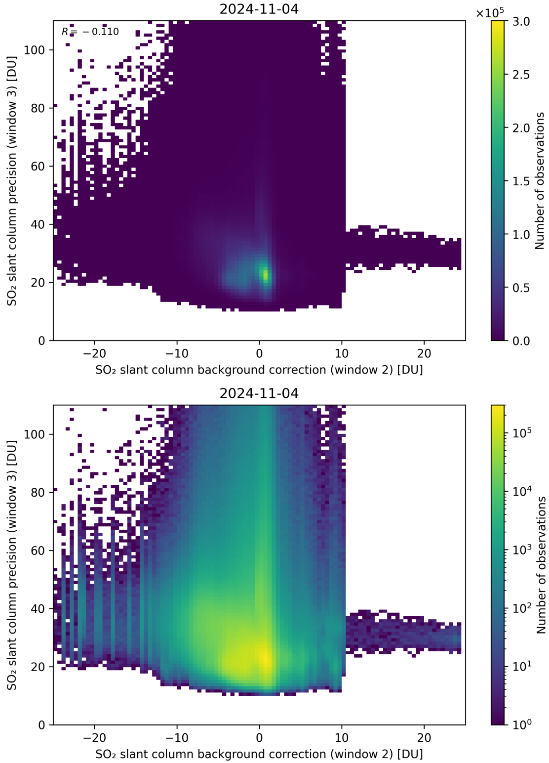
Figure 118: Scatter density plot of “SO 2 slant column background correction (window 2)” against “SO 2 slant column precision (window 3)” for 2024-11-04 to 2024-11-05.
