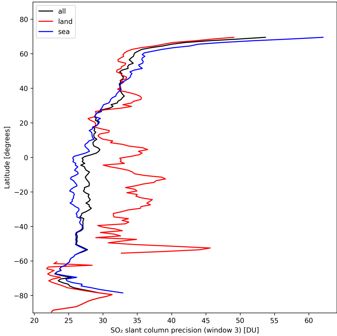
Figure 42: Zonal average of “SO 2 slant column precision (window 3)” for 2024-11-04 to 2024-11-05.
