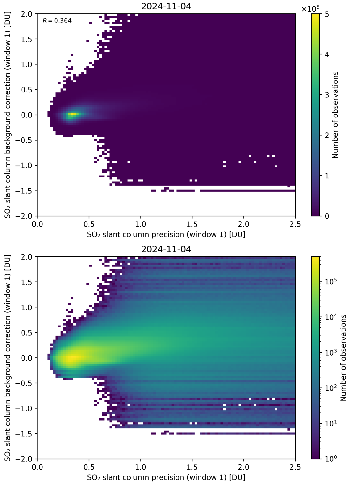
Figure 218: Scatter density plot of “SO 2 slant column precision (window 1)” against “SO 2 slant column background correction (window 1)” for 2024-11-04 to 2024-11-05.
