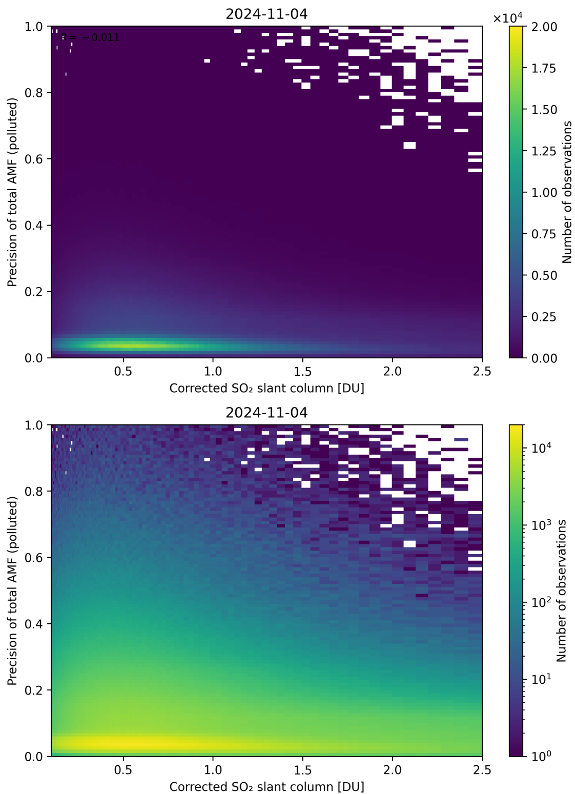
Figure 193: Scatter density plot of “Corrected SO 2 slant column” against “Precision of total AMF (polluted)” for 2024-11-04 to 2024-11-05.
