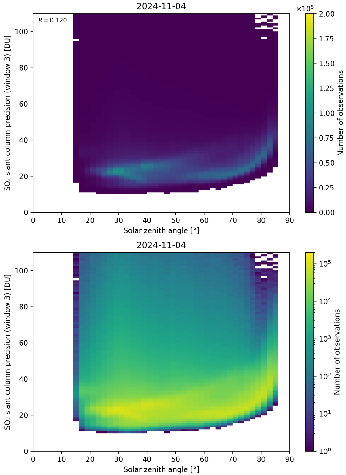
Figure 173: Scatter density plot of “Solar zenith angle” against “SO 2 slant column precision (window 3)” for 2024-11-04 to 2024-11-05.
