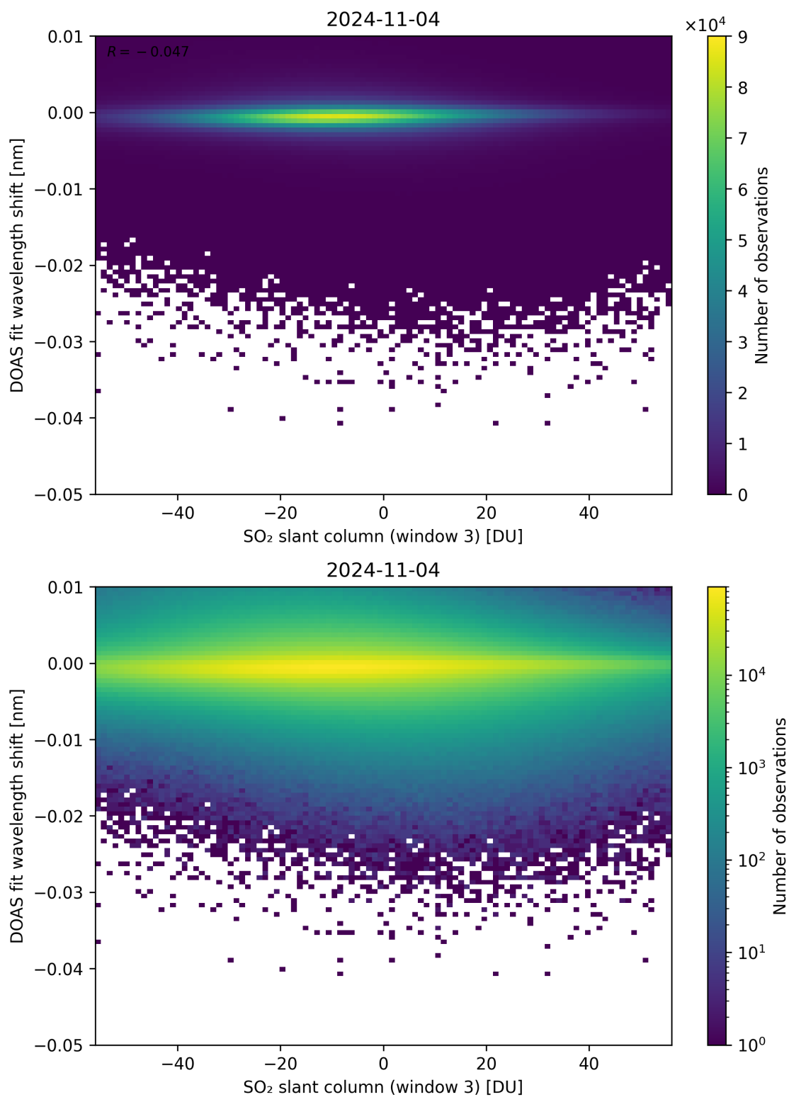
Figure 254: Scatter density plot of “SO 2 slant column (window 3)” against “DOAS fit wavelength shift” for 2024-11-04 to 2024-11-05.
