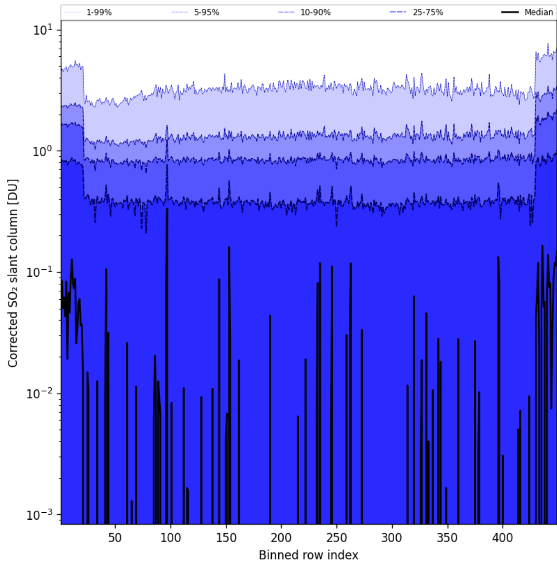
Figure 78: Along track statistics of “Corrected SO 2 slant column” for 2024-11-04 to 2024-11-05
