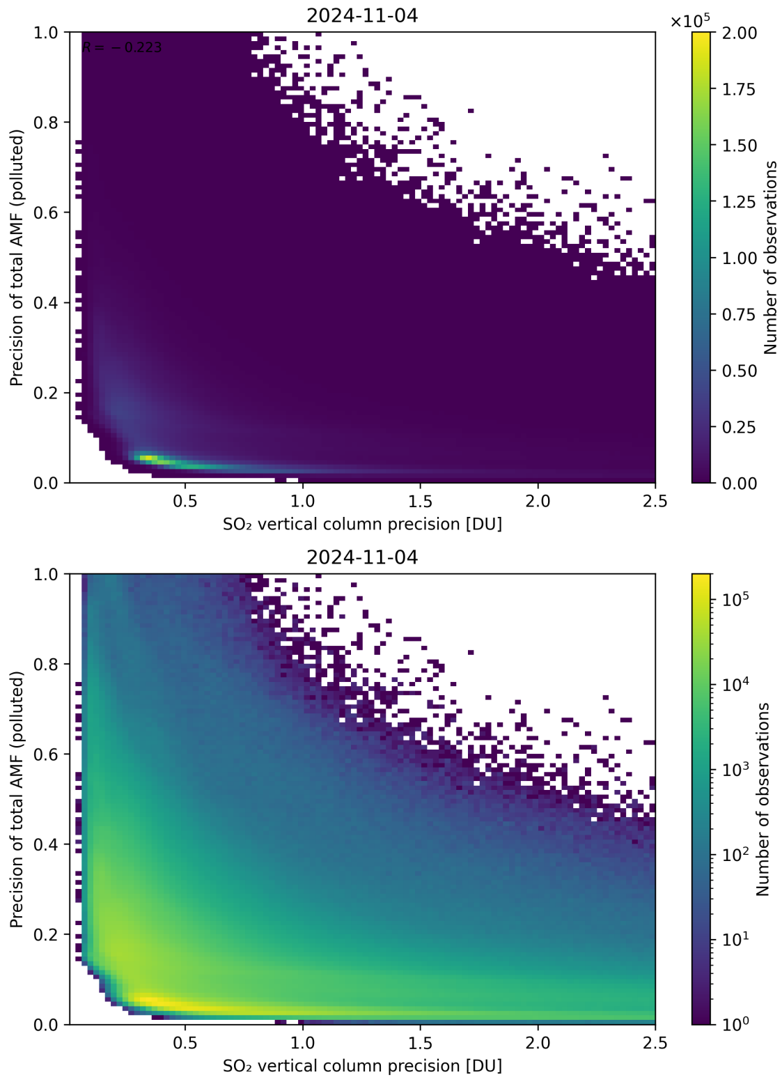
Figure 295: Scatter density plot of “SO 2 vertical column precision” against “Precision of total AMF (polluted)” for 2024-11-04 to 2024-11-05.
