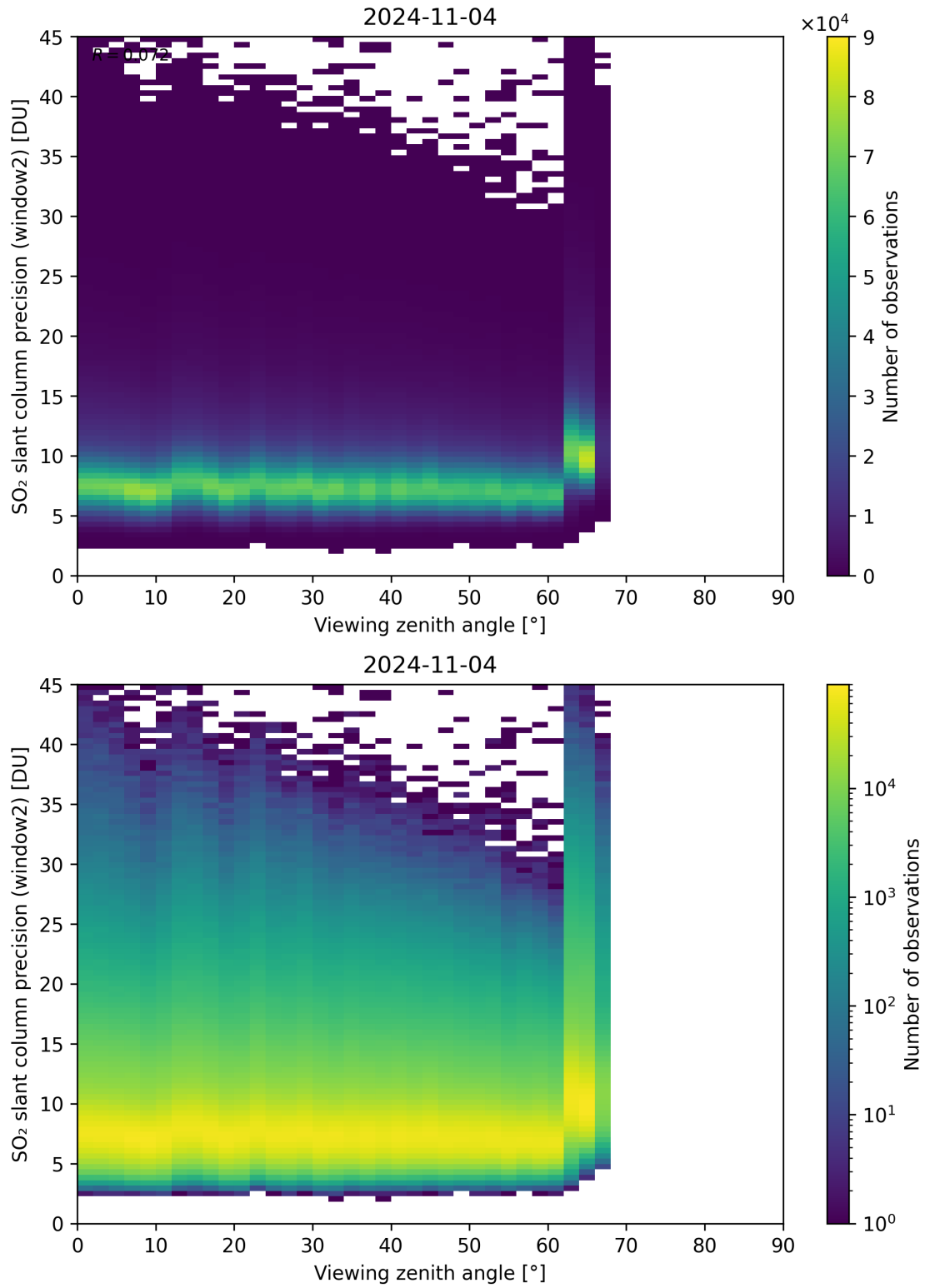
Figure 322: Scatter density plot of “Viewing zenith angle” against “SO 2 slant column precision (window2)” for 2024-11-04 to 2024-11-05.
