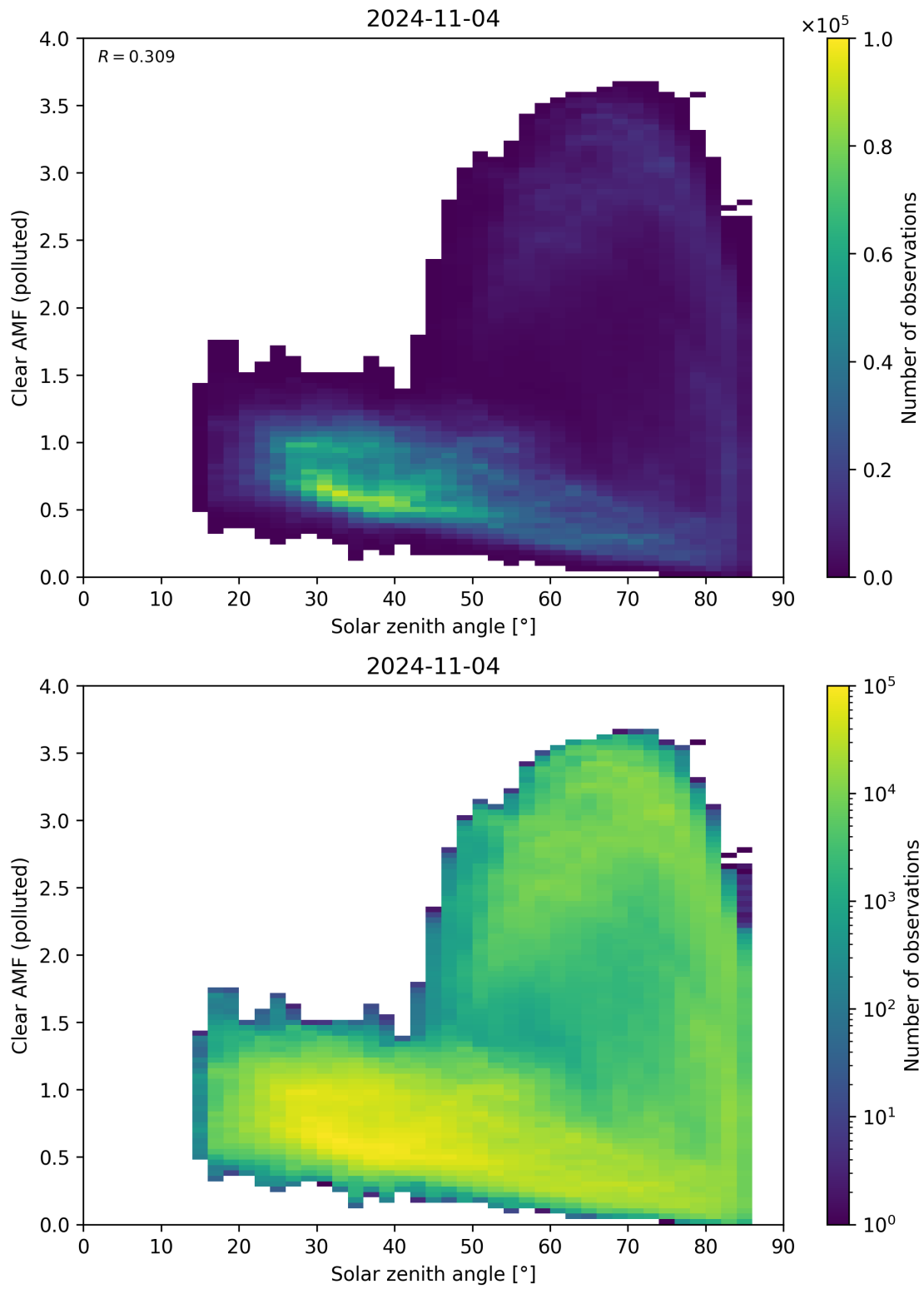
Figure 165: Scatter density plot of “Solar zenith angle” against “Clear AMF (polluted)” for 2024-11-04 to 2024-11-05.
