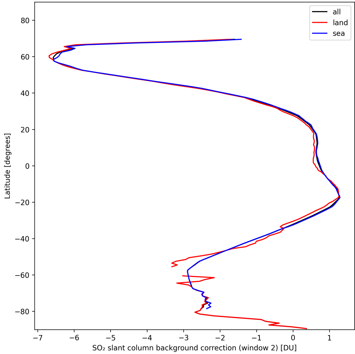
Figure 40: Zonal average of “SO 2 slant column background correction (window 2)” for 2024-11-04 to 2024-11-05.
