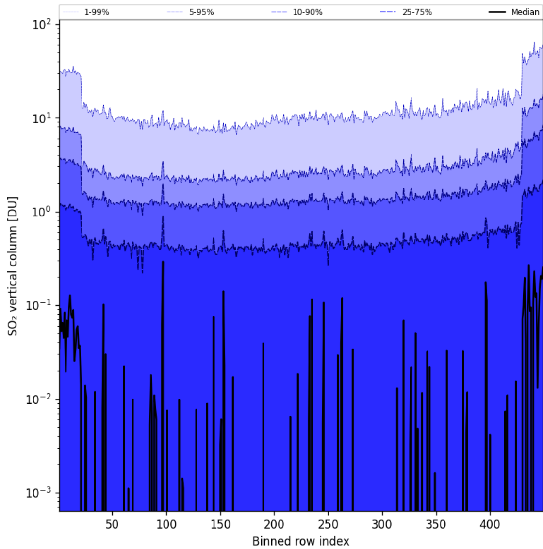
Figure 76: Along track statistics of “SO 2 vertical column” for 2024-11-04 to 2024-11-05
