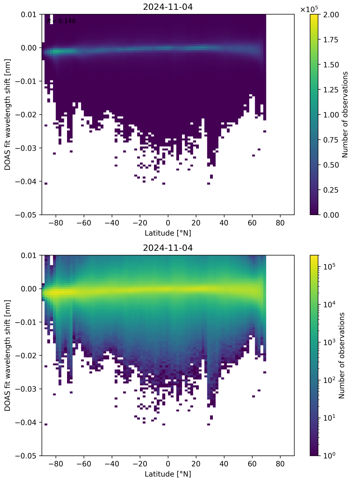
Figure 142: Scatter density plot of “Latitude” against “DOAS fit wavelength shift” for 2024-11-04 to 2024-11-05.
