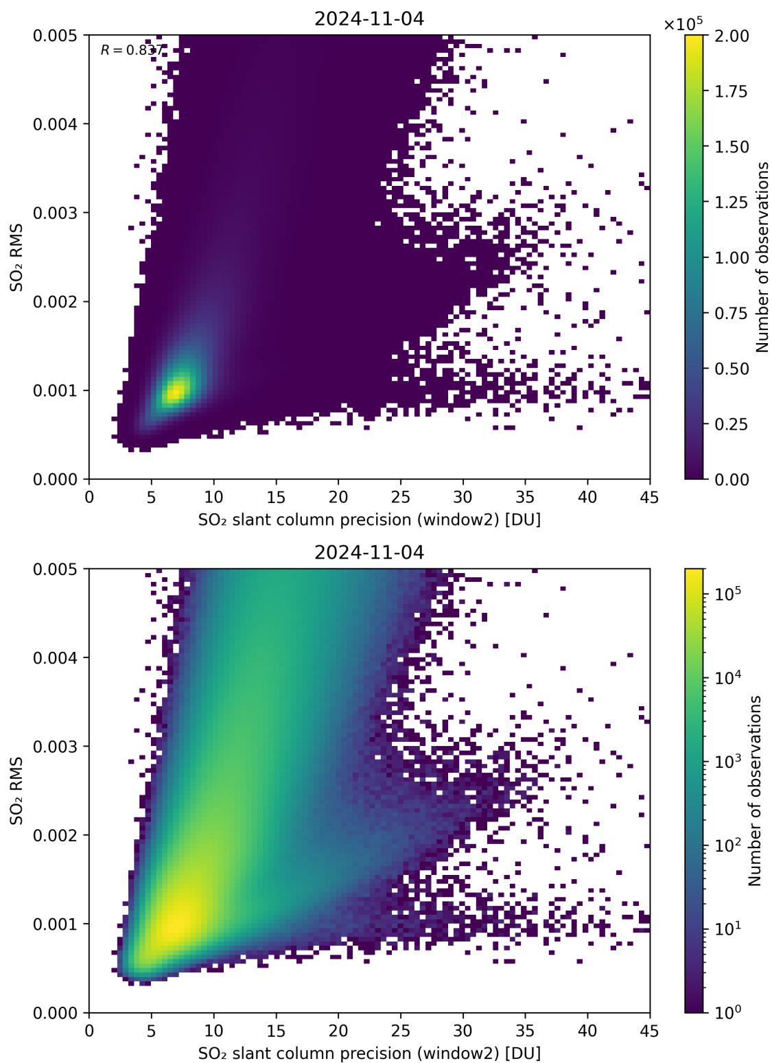
Figure 245: Scatter density plot of “SO 2 slant column precision (window2)” against “SO 2 RMS” for 2024-11-04 to 2024-11-05.
