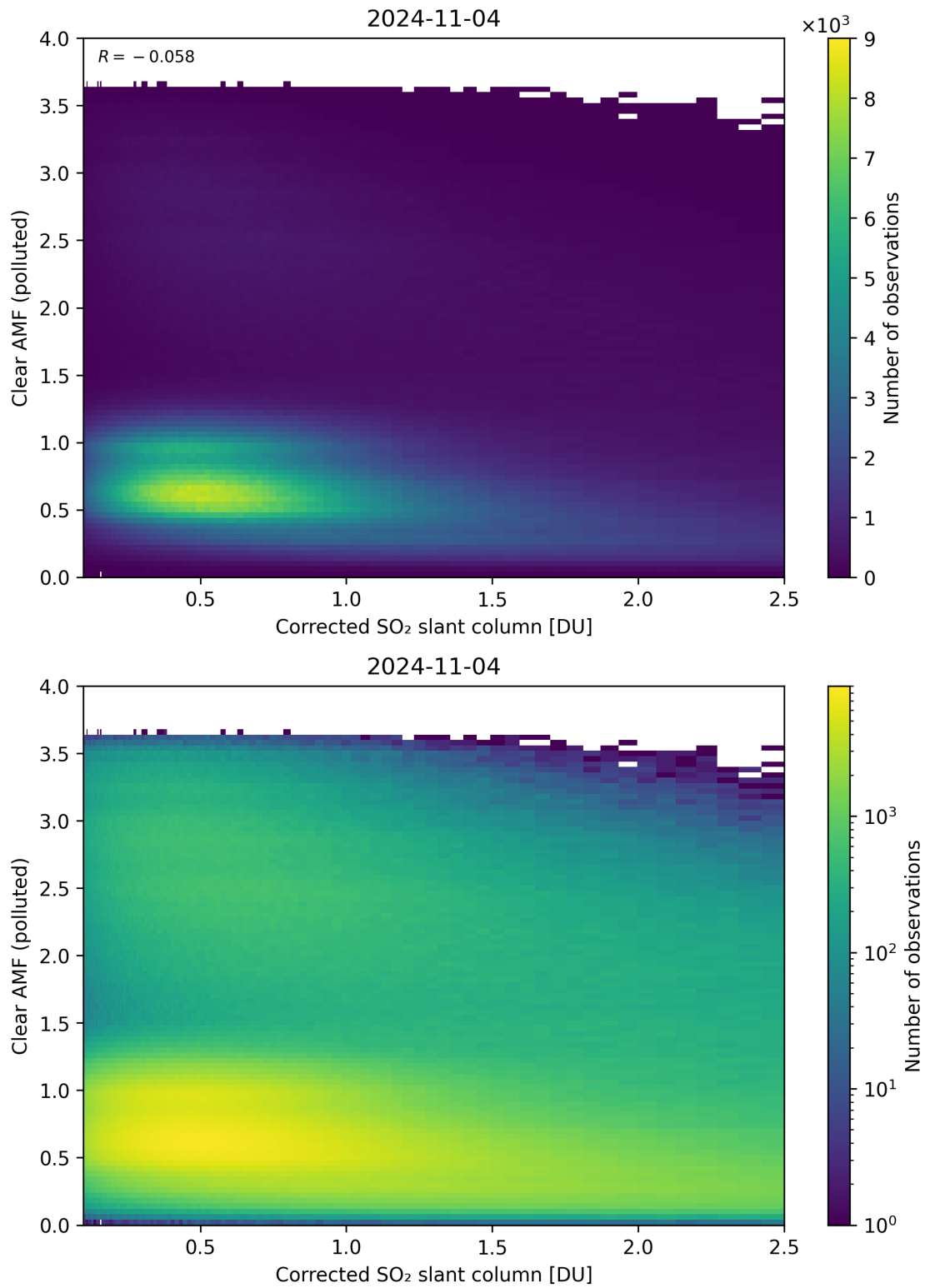
Figure 184: Scatter density plot of “Corrected SO 2 slant column” against “Clear AMF (polluted)” for 2024-11-04 to 2024-11-05.
