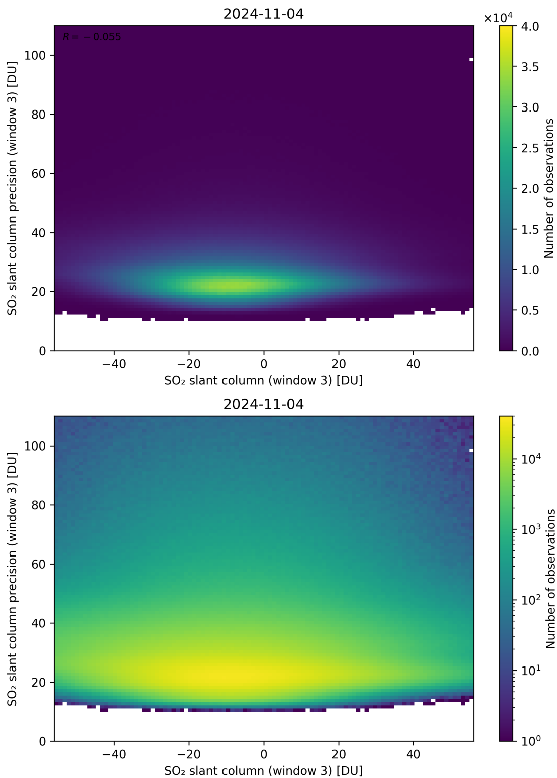
Figure 267: Scatter density plot of “SO 2 slant column (window 3)” against “SO 2 slant column precision (window 3)” for 2024-11-04 to 2024-11-05.
