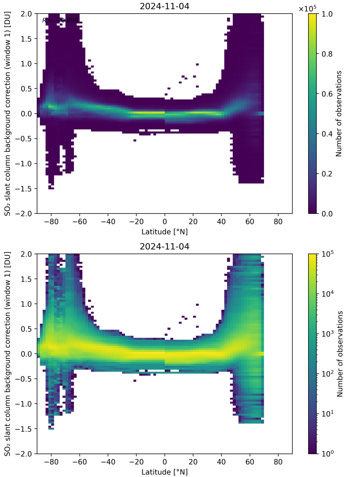
Figure 139: Scatter density plot of “Latitude” against “SO 2 slant column background correction (window 1)” for 2024-11-04 to 2024-11-05.
