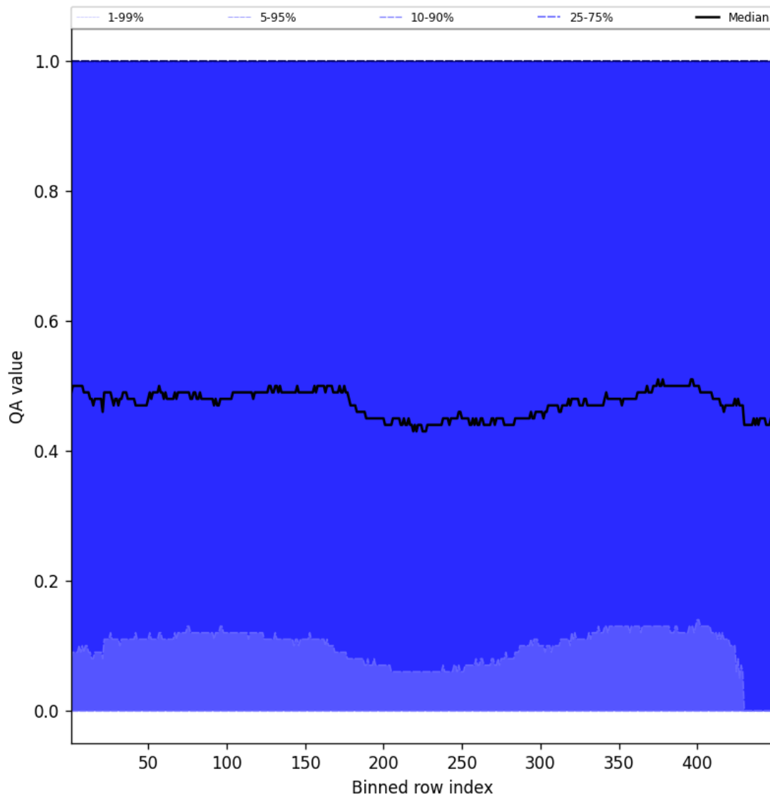
Figure 75: Along track statistics of “QA value” for 2024-11-04 to 2024-11-05
