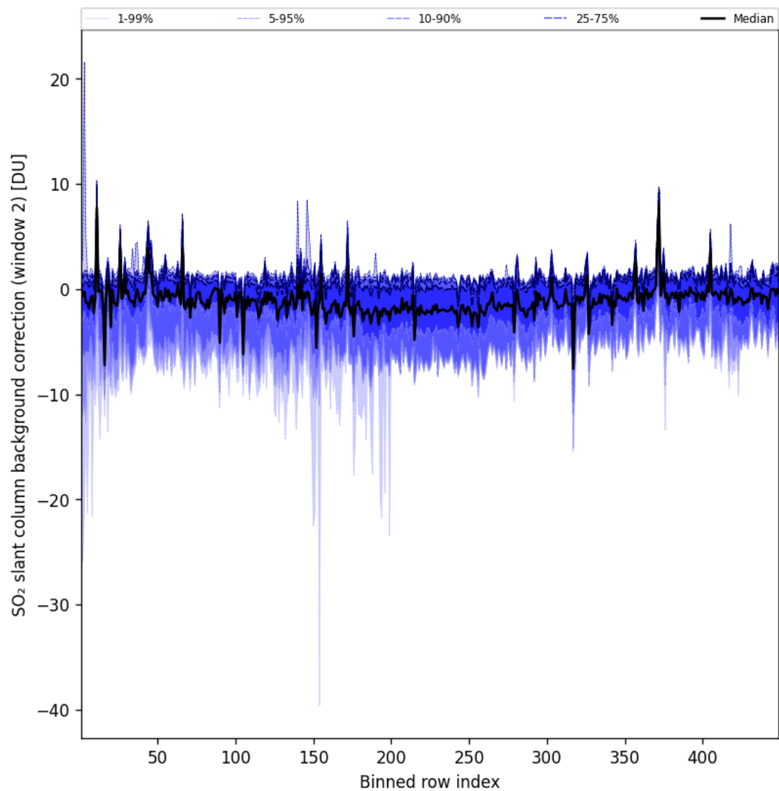
Figure 86: Along track statistics of “SO 2 slant column background correction (window 2)” for 2024-11-04 to 2024-11-05
