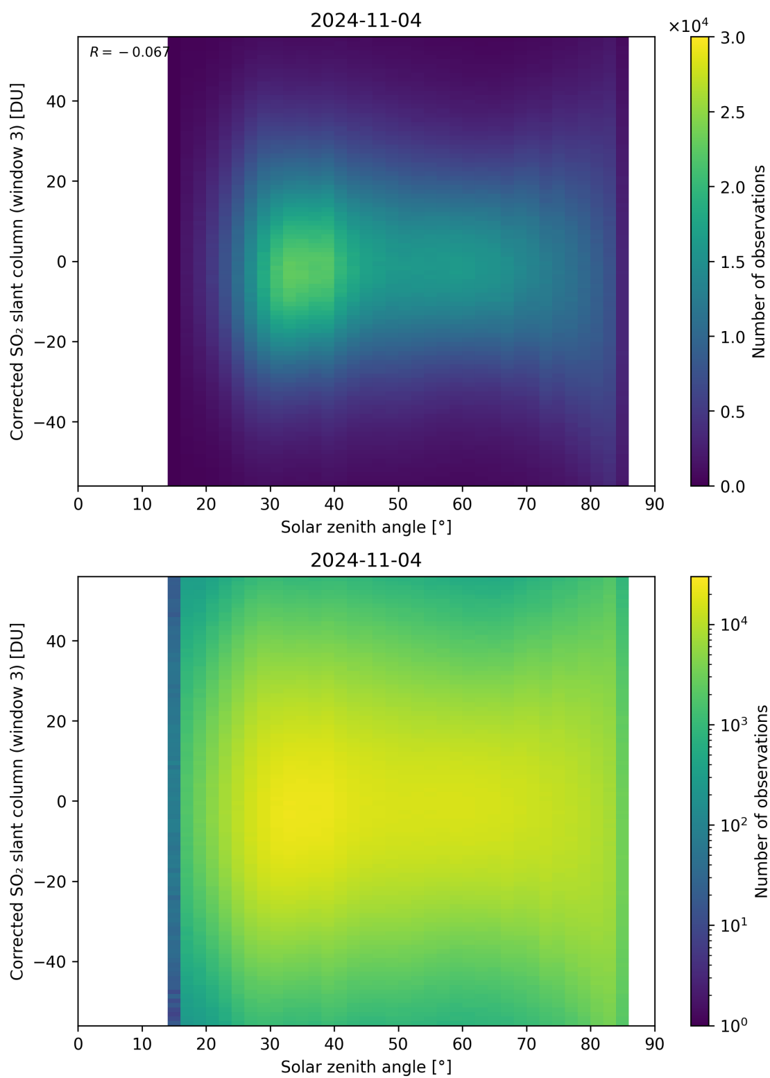
Figure 168: Scatter density plot of “Solar zenith angle” against “Corrected SO 2 slant column (window 3)” for 2024-11-04 to 2024-11-05.
