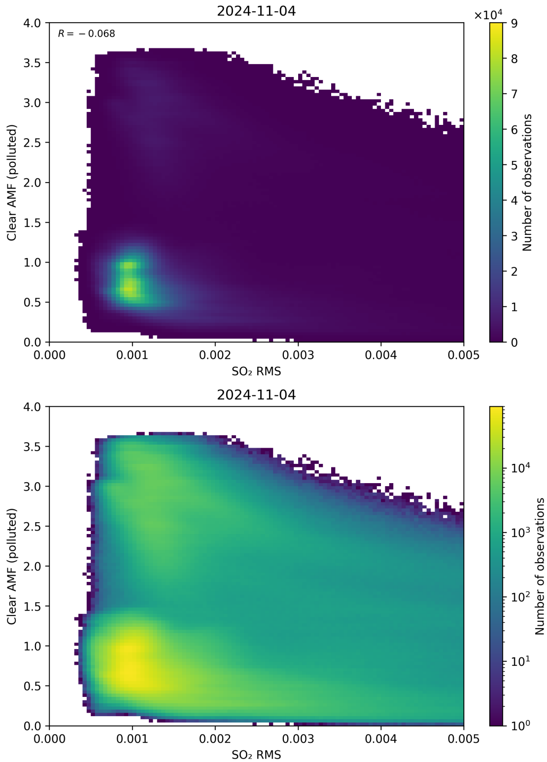
Figure 136: Scatter density plot of “SO 2 RMS” against “Clear AMF (polluted)” for 2024-11-04 to 2024-11-05.
