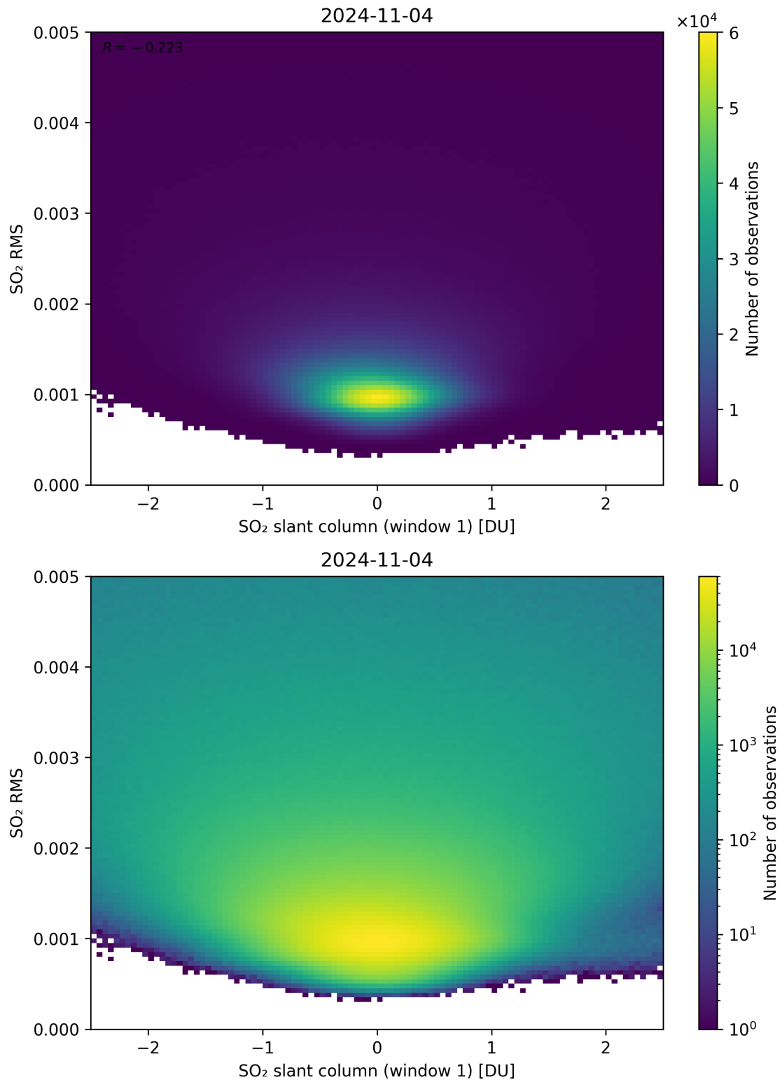
Figure 217: Scatter density plot of “SO 2 slant column (window 1)” against “SO 2 RMS” for 2024-11-04 to 2024-11-05.
