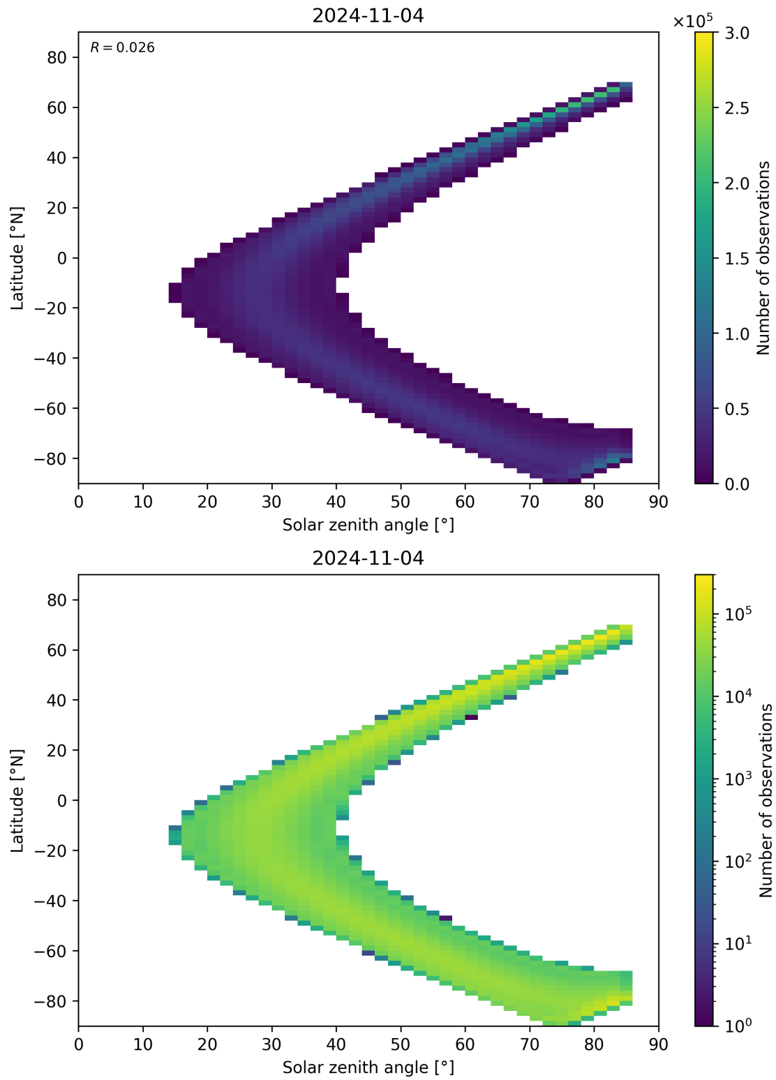
Figure 164: Scatter density plot of “Solar zenith angle” against “Latitude” for 2024-11-04 to 2024-11-05.
