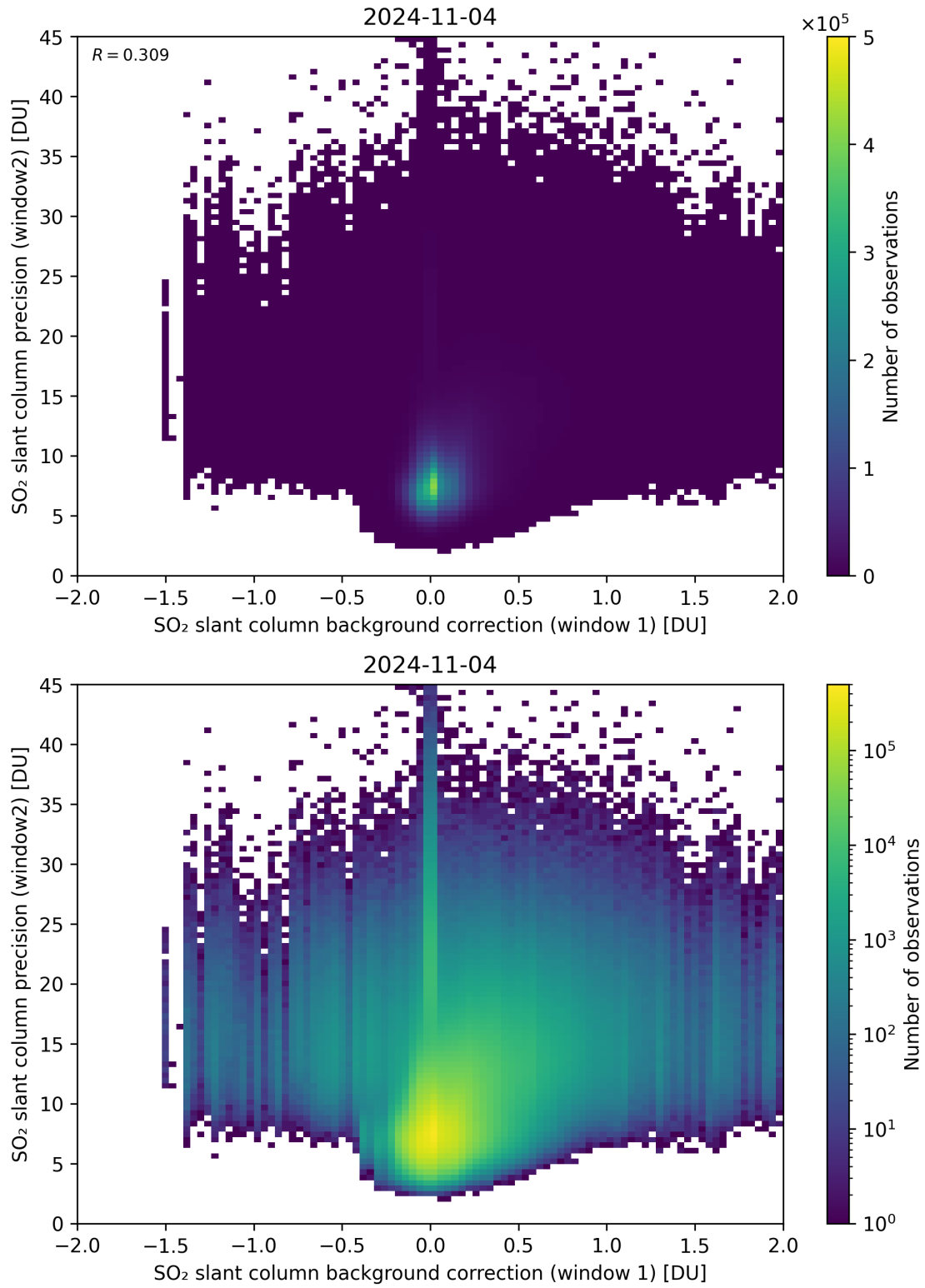
Figure 106: Scatter density plot of “SO 2 slant column background correction (window 1)” against “SO 2 slant column precision (window2)” for 2024-11-04 to 2024-11-05.
