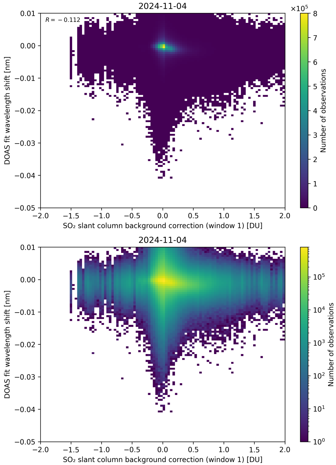
Figure 100: Scatter density plot of “SO 2 slant column background correction (window 1)” against “DOAS fit wavelength shift” for 2024-11-04 to 2024-11-05.
