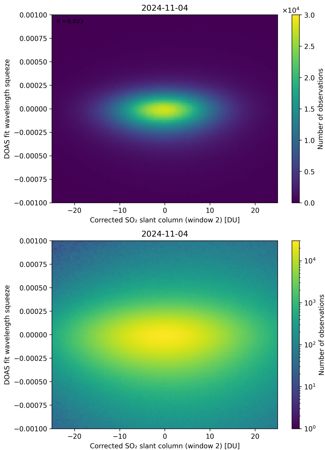
Figure 197: Scatter density plot of “Corrected SO 2 slant column (window 2)” against “DOAS fit wavelength squeeze” for 2024-11-04 to 2024-11-05.
