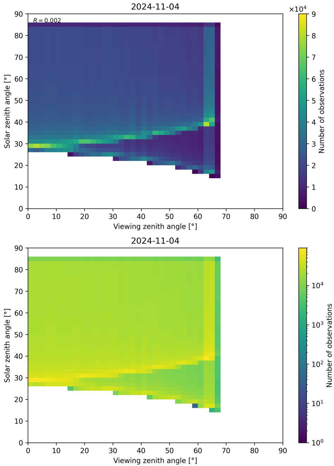
Figure 315: Scatter density plot of “Viewing zenith angle” against “Solar zenith angle” for 2024-11-04 to 2024-11-05.
