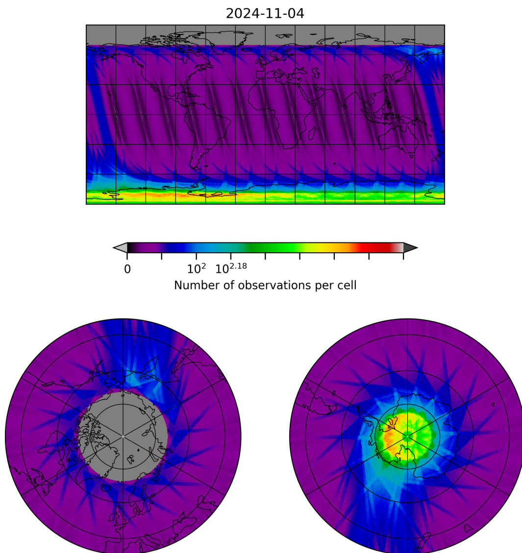
Figure 28: Map of the number of observations for 2024-11-04 to 2024-11-05
