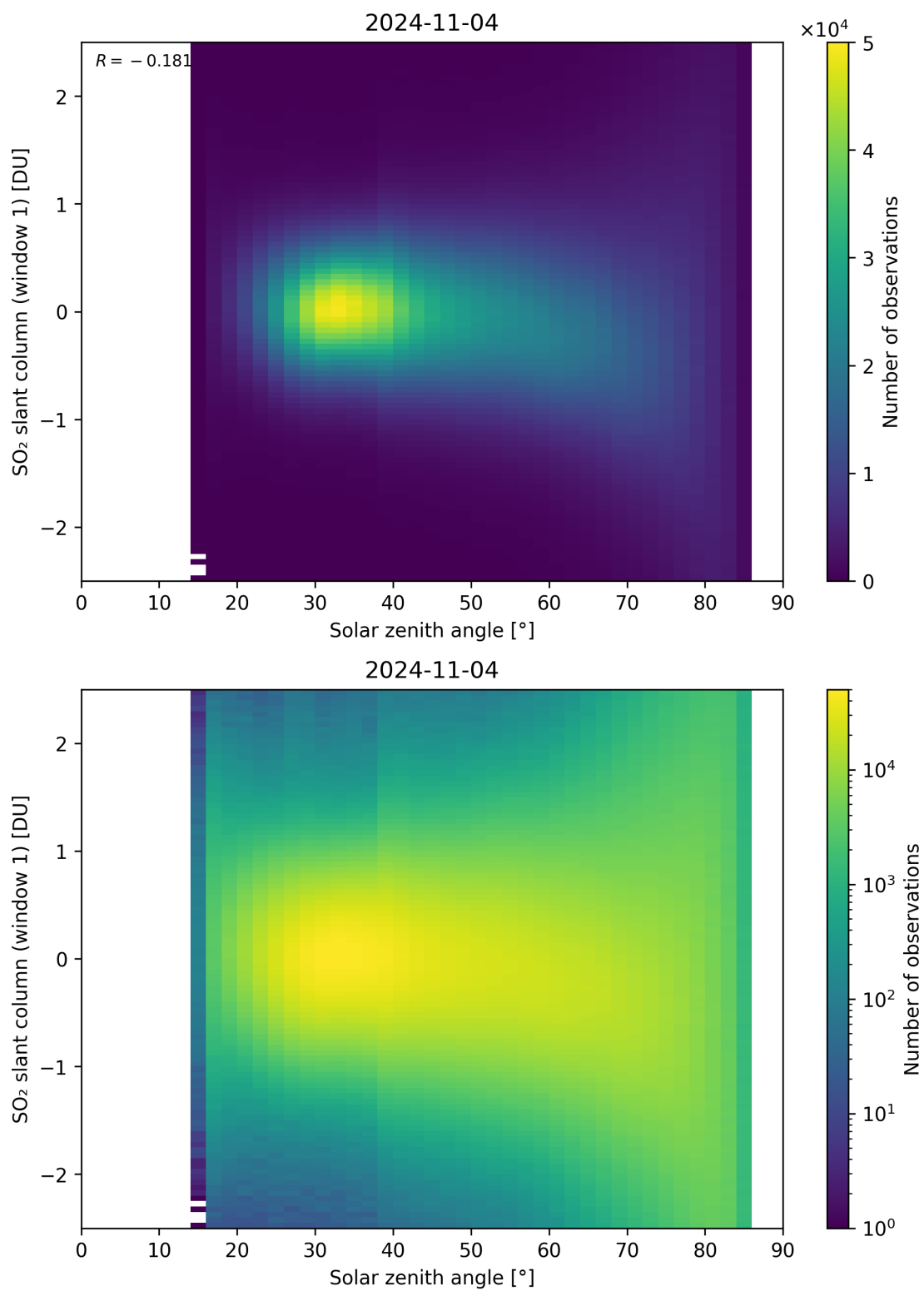
Figure 169: Scatter density plot of “Solar zenith angle” against “SO 2 slant column (window 1)” for 2024-11-04 to 2024-11-05.
