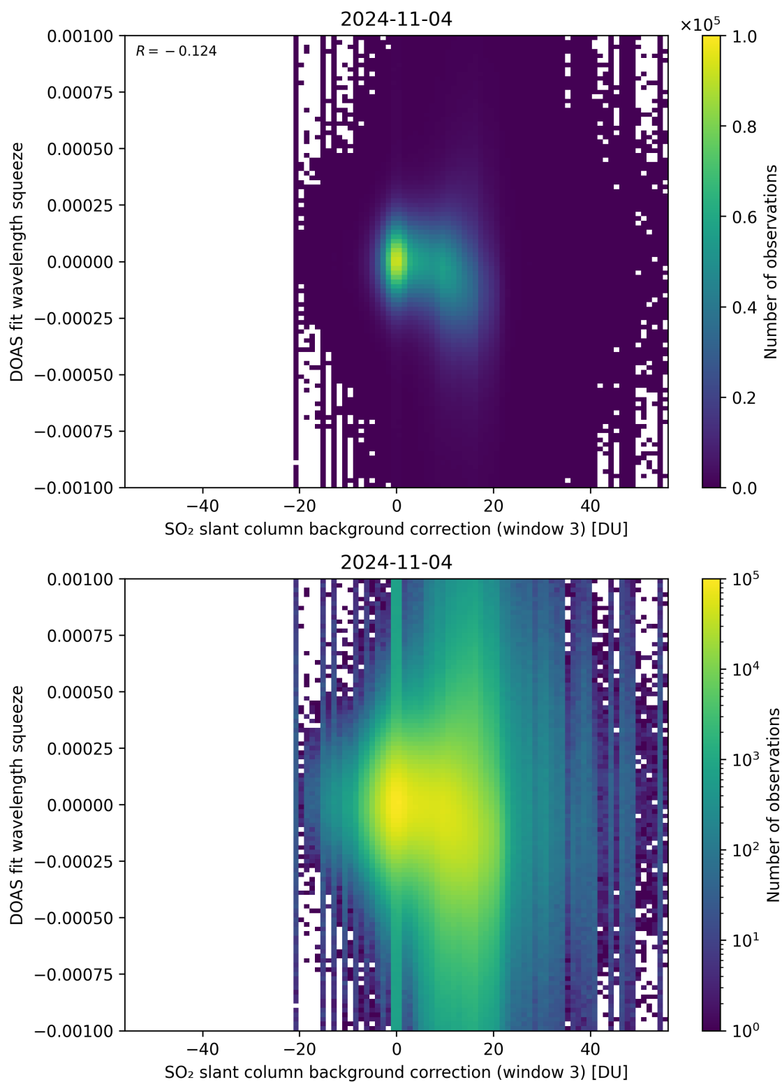
Figure 122: Scatter density plot of “SO 2 slant column background correction (window 3)” against “DOAS fit wavelength squeeze” for 2024-11-04 to 2024-11-05.
