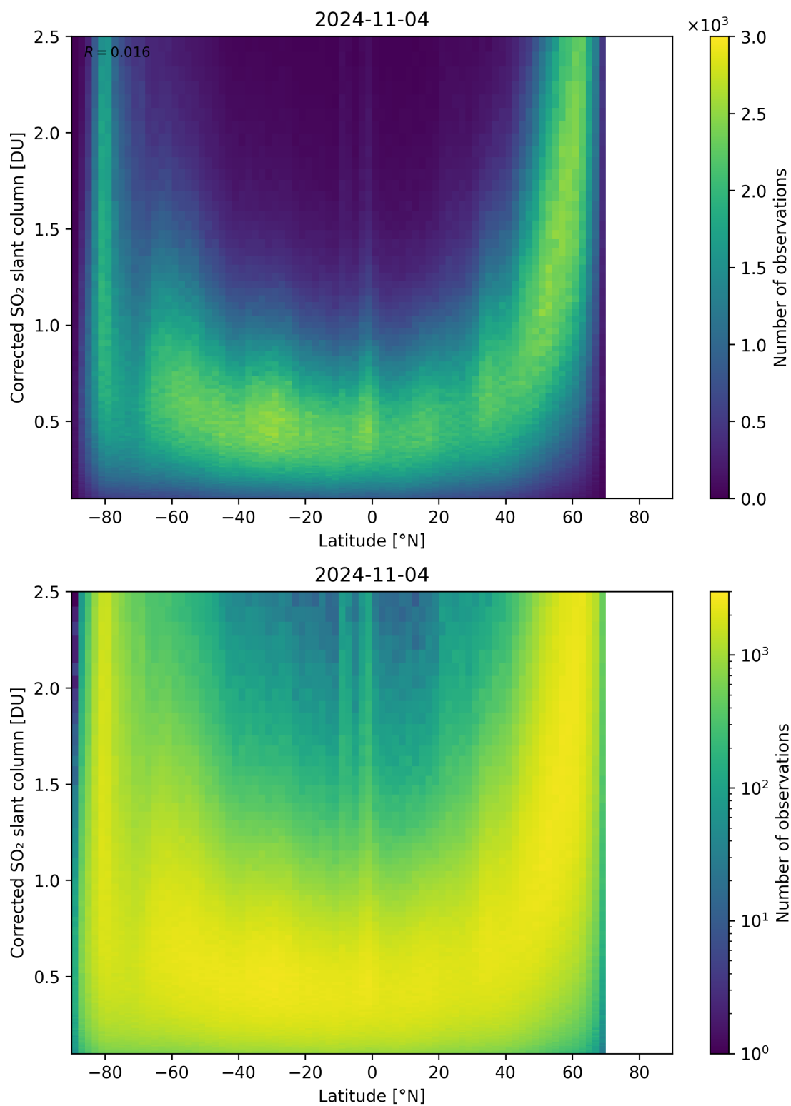
Figure 146: Scatter density plot of “Latitude” against “Corrected SO 2 slant column” for 2024-11-04 to 2024-11-05.
