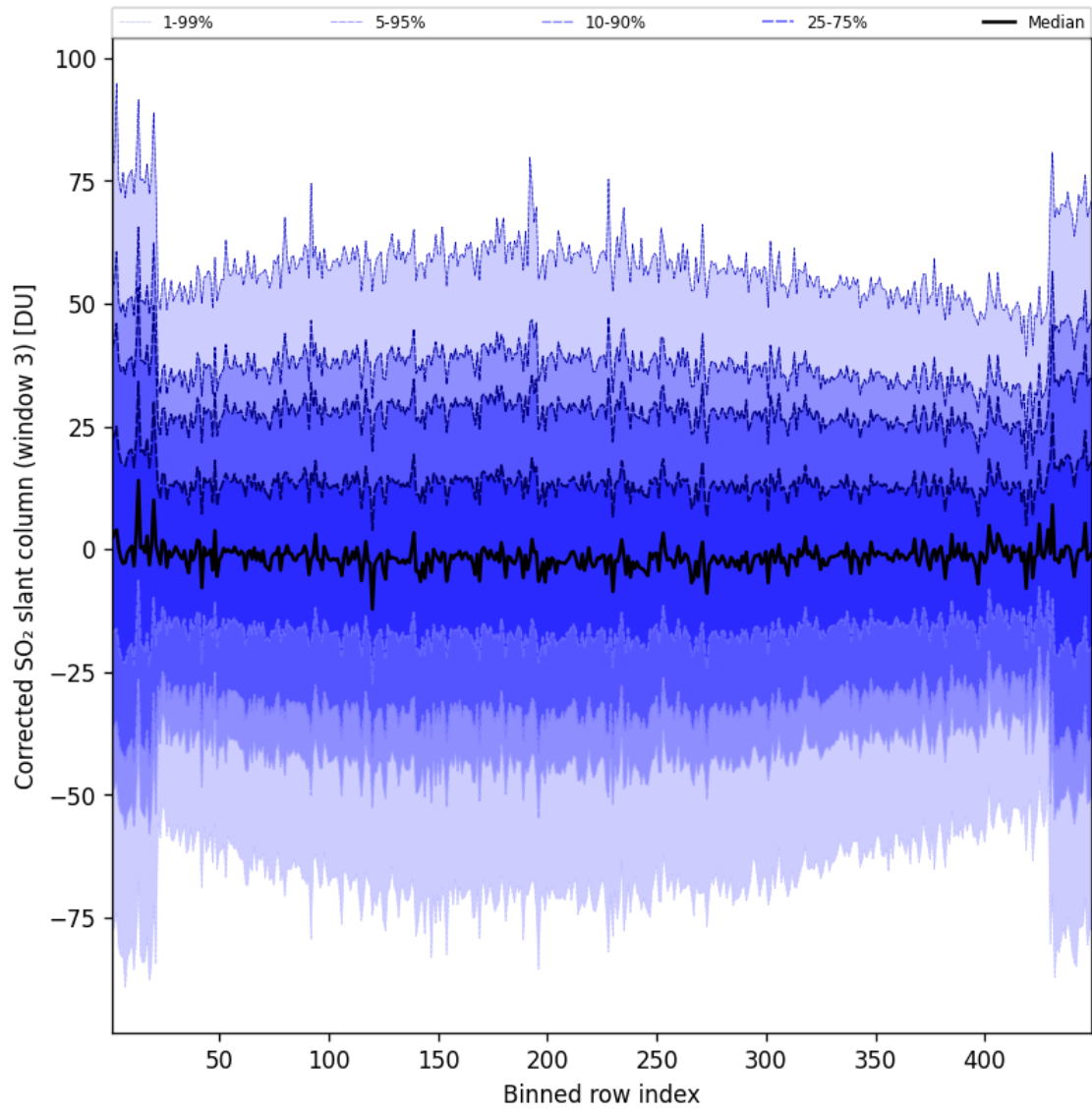
Figure 89: Along track statistics of “Corrected SO 2 slant column (window 3)” for 2024-11-04 to 2024-11-05
