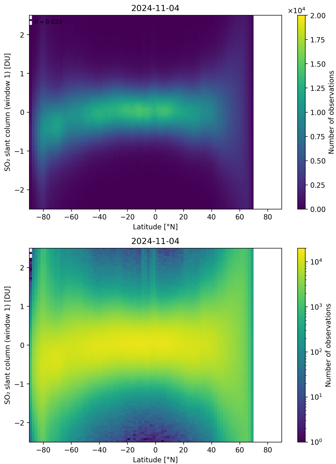
Figure 149: Scatter density plot of “Latitude” against “SO 2 slant column (window 1)” for 2024-11-04 to 2024-11-05.
