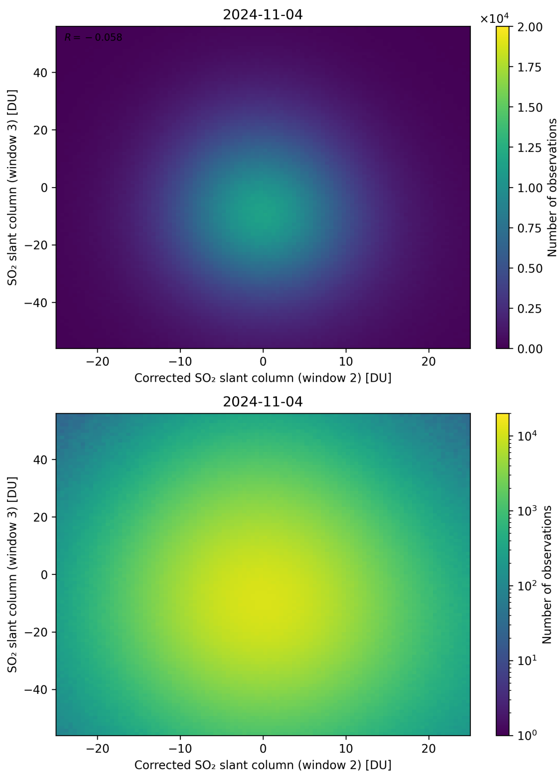
Figure 201: Scatter density plot of “Corrected SO 2 slant column (window 2)” against “SO 2 slant column (window 3)” for 2024-11-04 to 2024-11-05.
