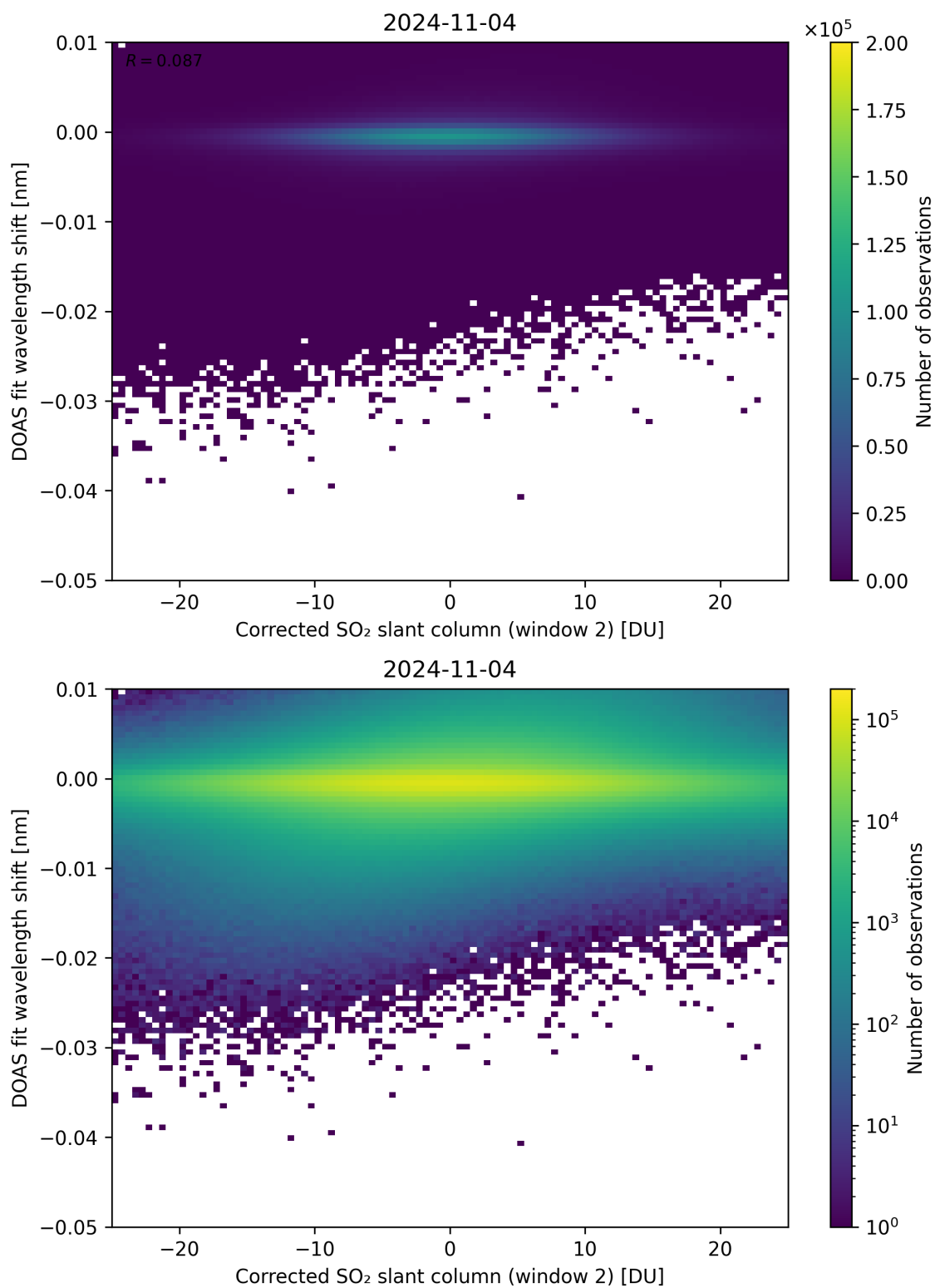
Figure 196: Scatter density plot of “Corrected SO 2 slant column (window 2)” against “DOAS fit wavelength shift” for 2024-11-04 to 2024-11-05.
