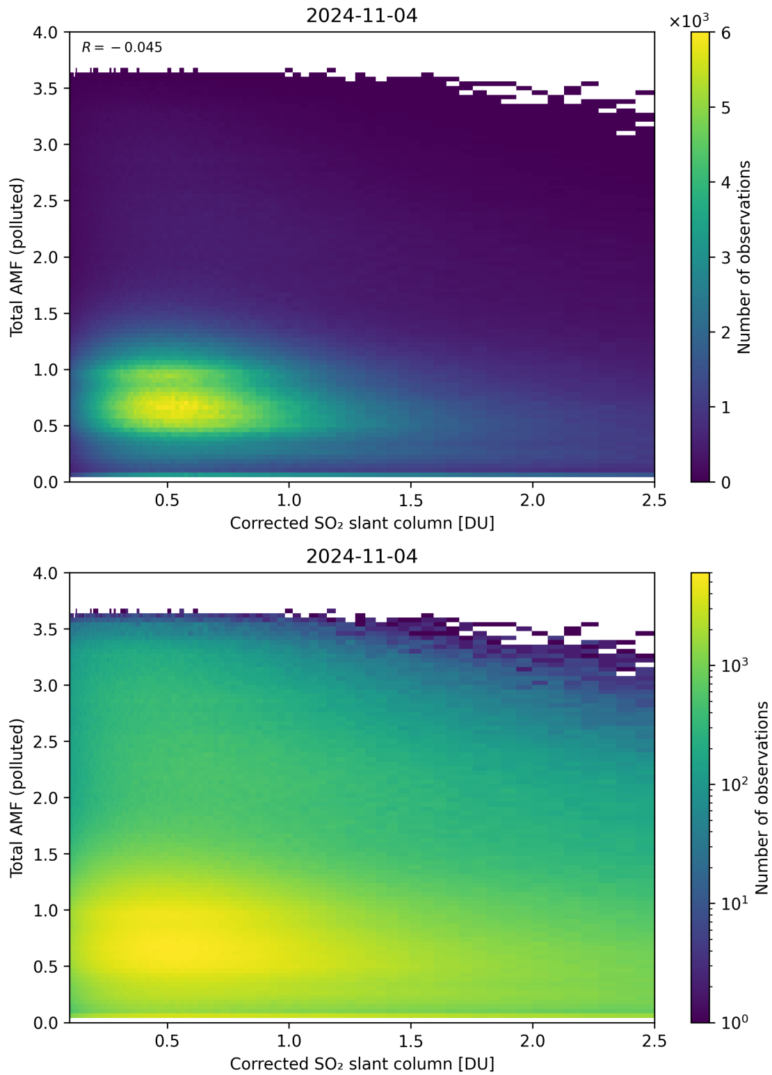
Figure 192: Scatter density plot of “Corrected SO 2 slant column” against “Total AMF (polluted)” for 2024-11-04 to 2024-11-05.
