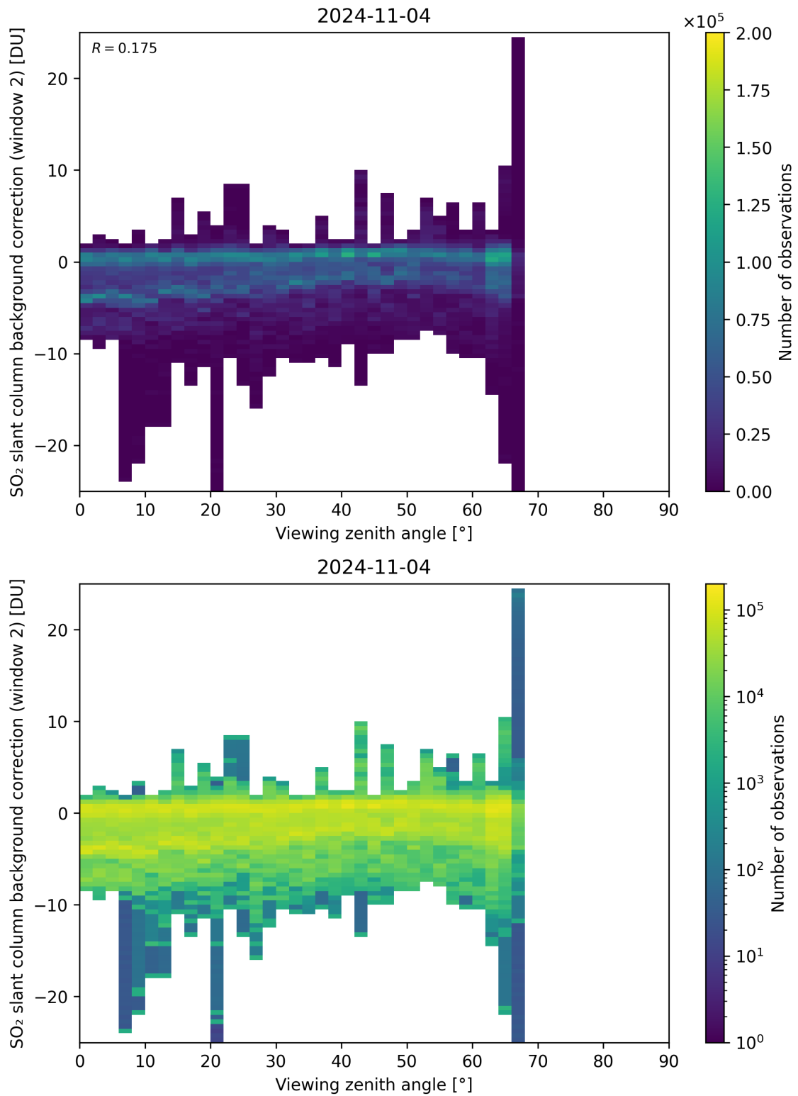
Figure 309: Scatter density plot of “Viewing zenith angle” against “SO 2 slant column background correction (window 2)” for 2024-11-04 to 2024-11-05.
