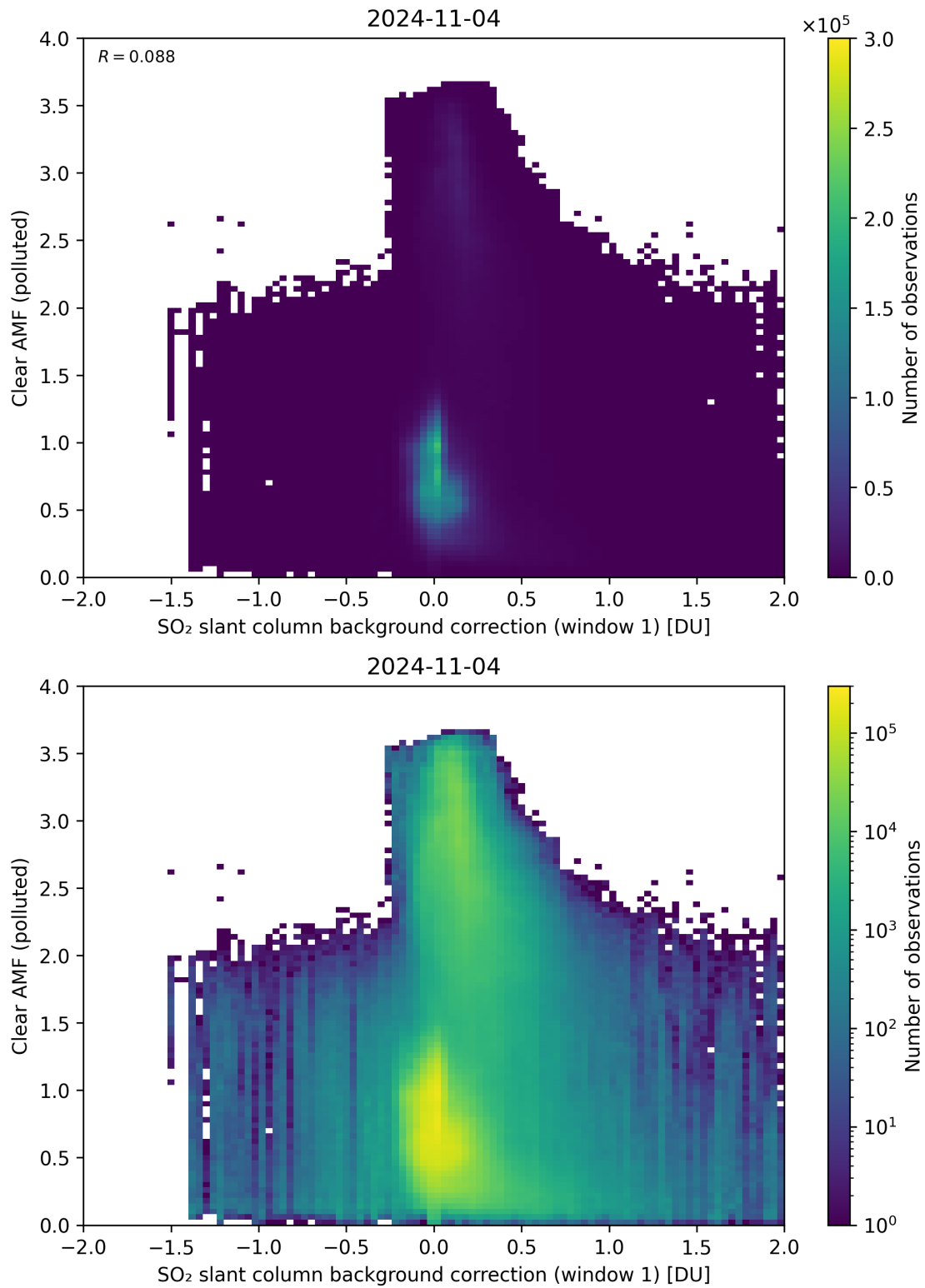
Figure 103: Scatter density plot of “SO 2 slant column background correction (window 1)” against “Clear AMF (polluted)” for 2024-11-04 to 2024-11-05.
