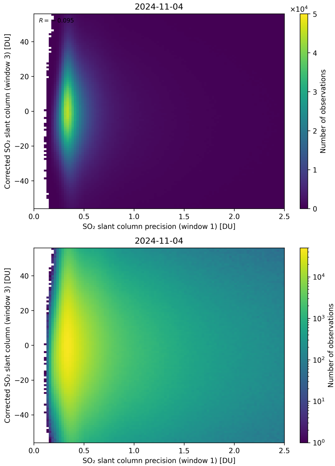
Figure 226: Scatter density plot of “SO 2 slant column precision (window 1)” against “Corrected SO 2 slant column (window 3)” for 2024-11-04 to 2024-11-05.
