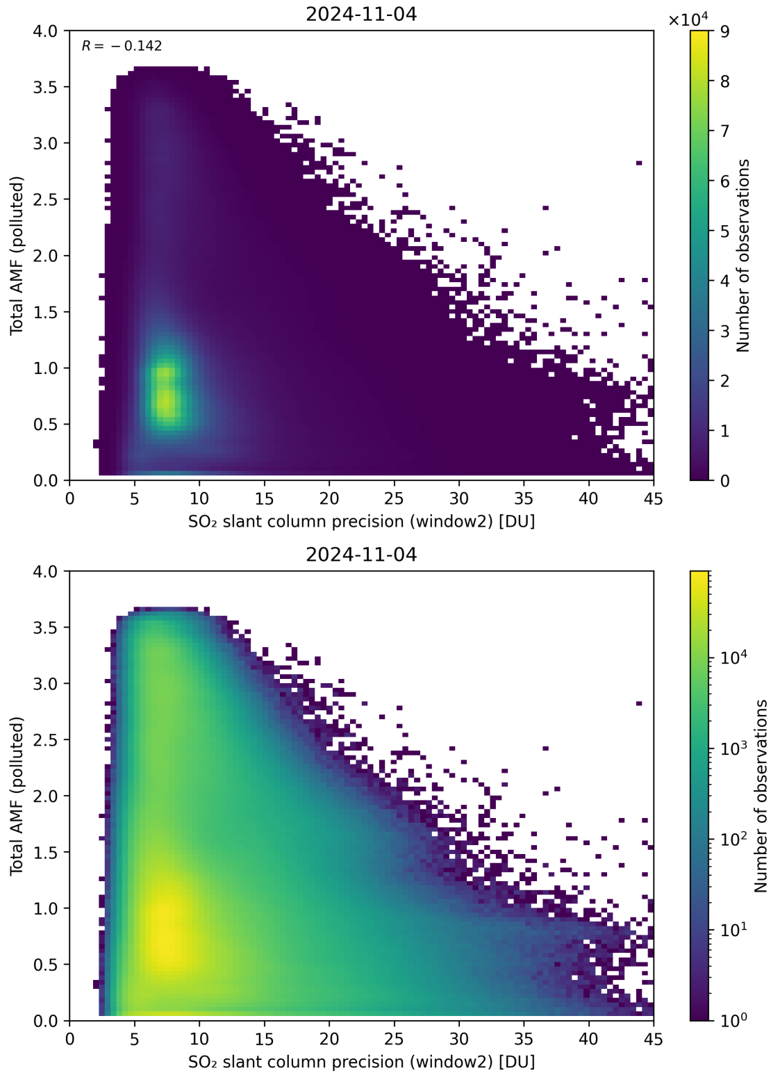
Figure 251: Scatter density plot of “SO 2 slant column precision (window2)” against “Total AMF (polluted)” for 2024-11-04 to 2024-11-05.
