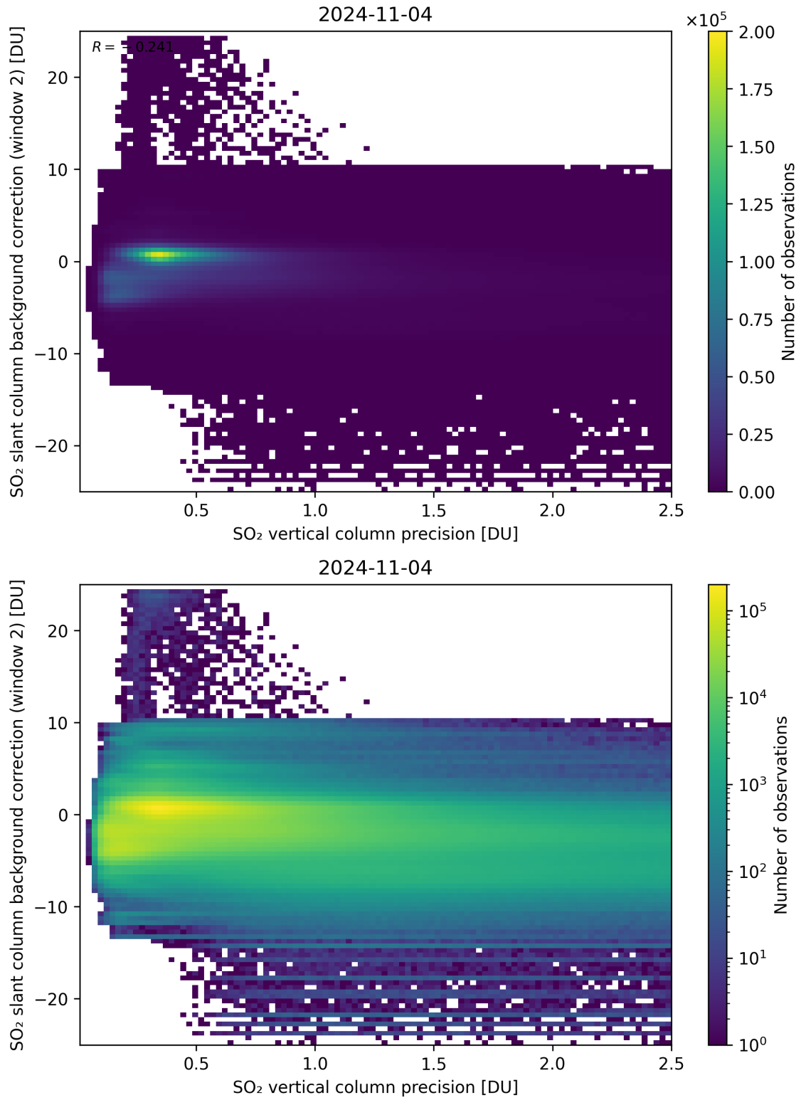
Figure 280: Scatter density plot of “SO 2 vertical column precision” against “SO 2 slant column background correction (window 2)” for 2024-11-04 to 2024-11-05.
