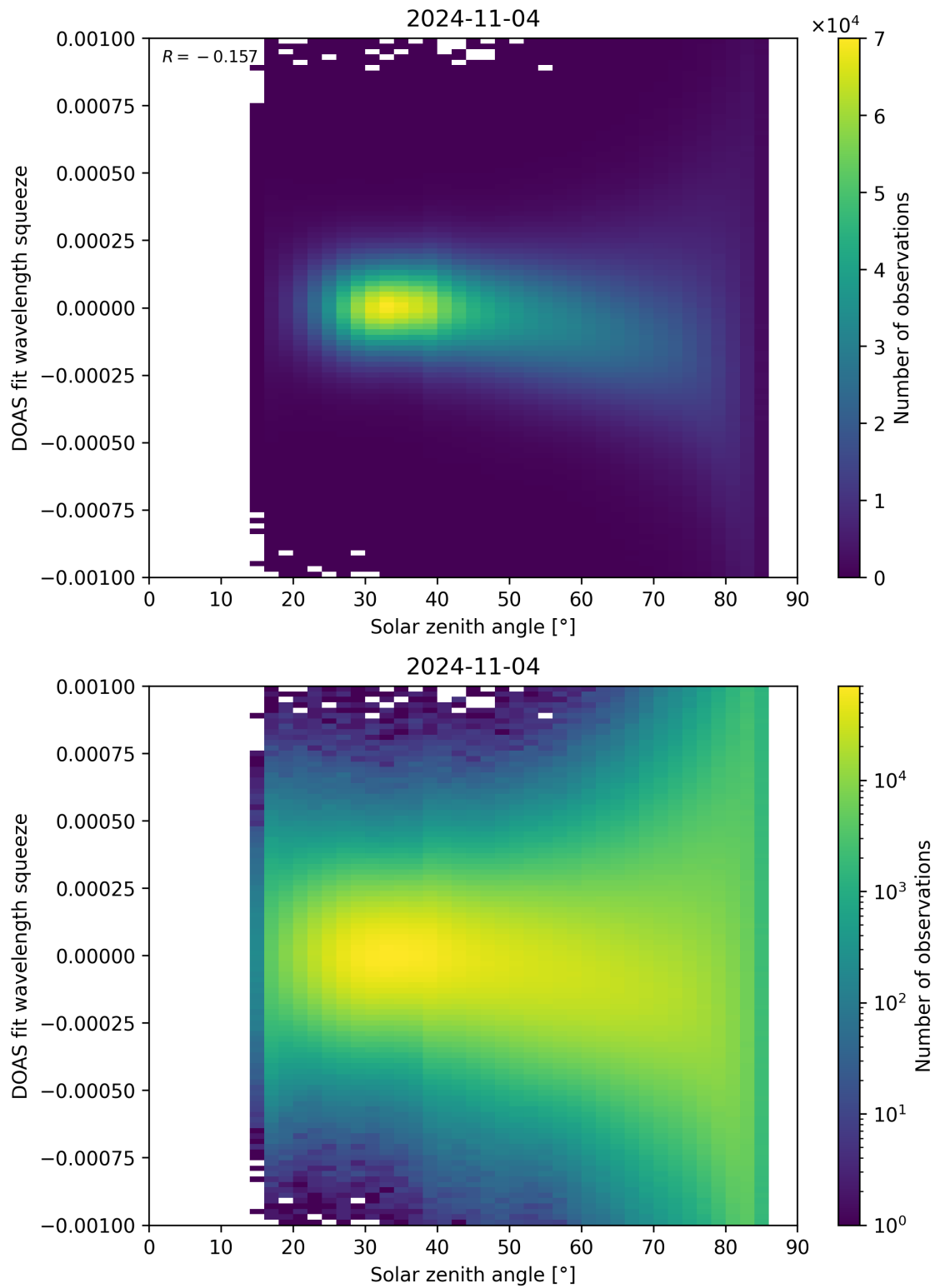
Figure 162: Scatter density plot of “Solar zenith angle” against “DOAS fit wavelength squeeze” for 2024-11-04 to 2024-11-05.
