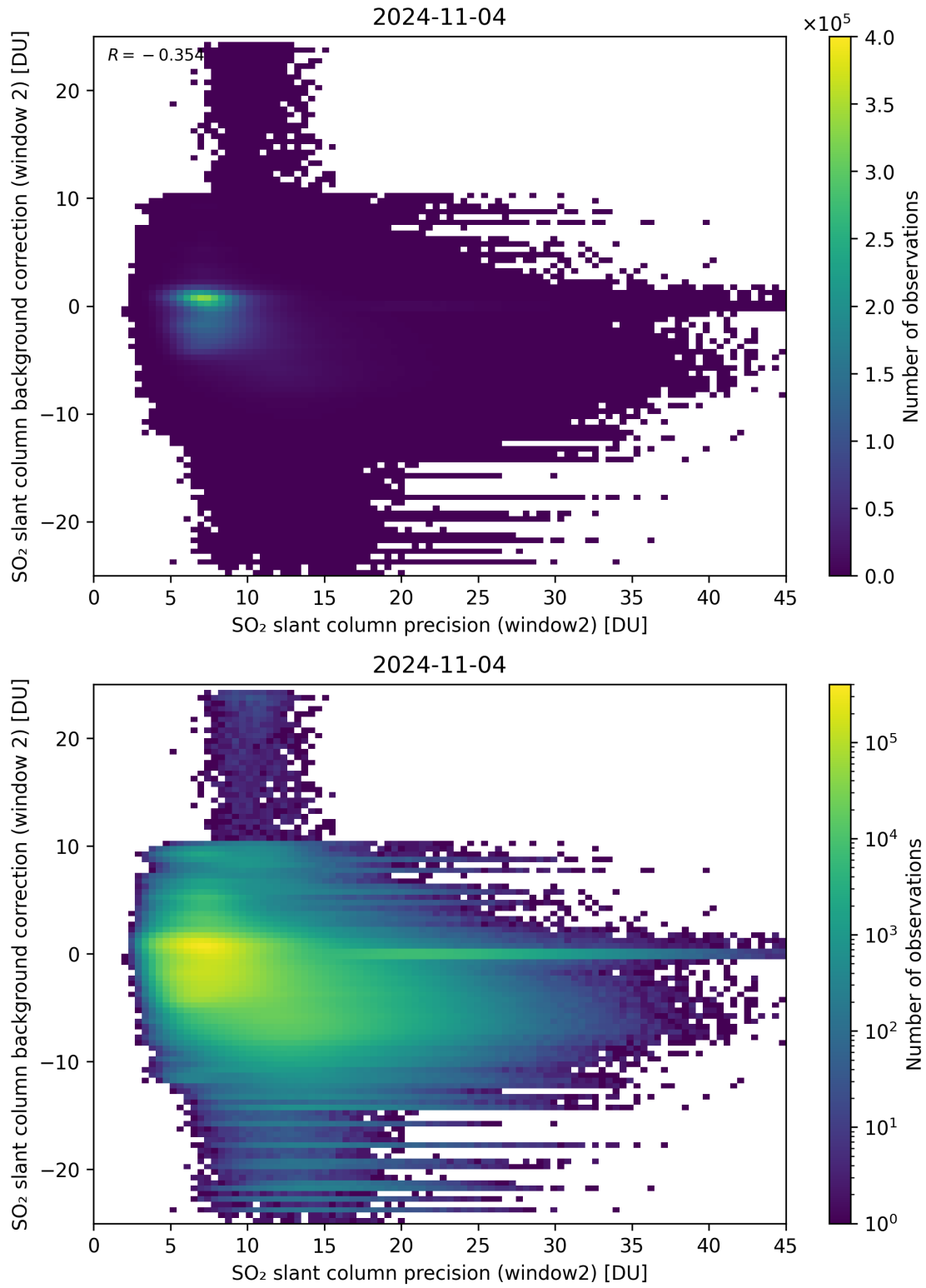
Figure 241: Scatter density plot of “SO 2 slant column precision (window2)” against “SO 2 slant column background correction (window 2)” for 2024-11-04 to 2024-11-05.
