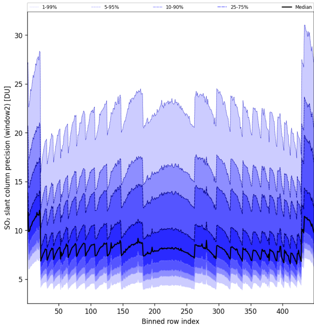
Figure 84: Along track statistics of “SO 2 slant column precision (window2)” for 2024-11-04 to 2024-11-05
