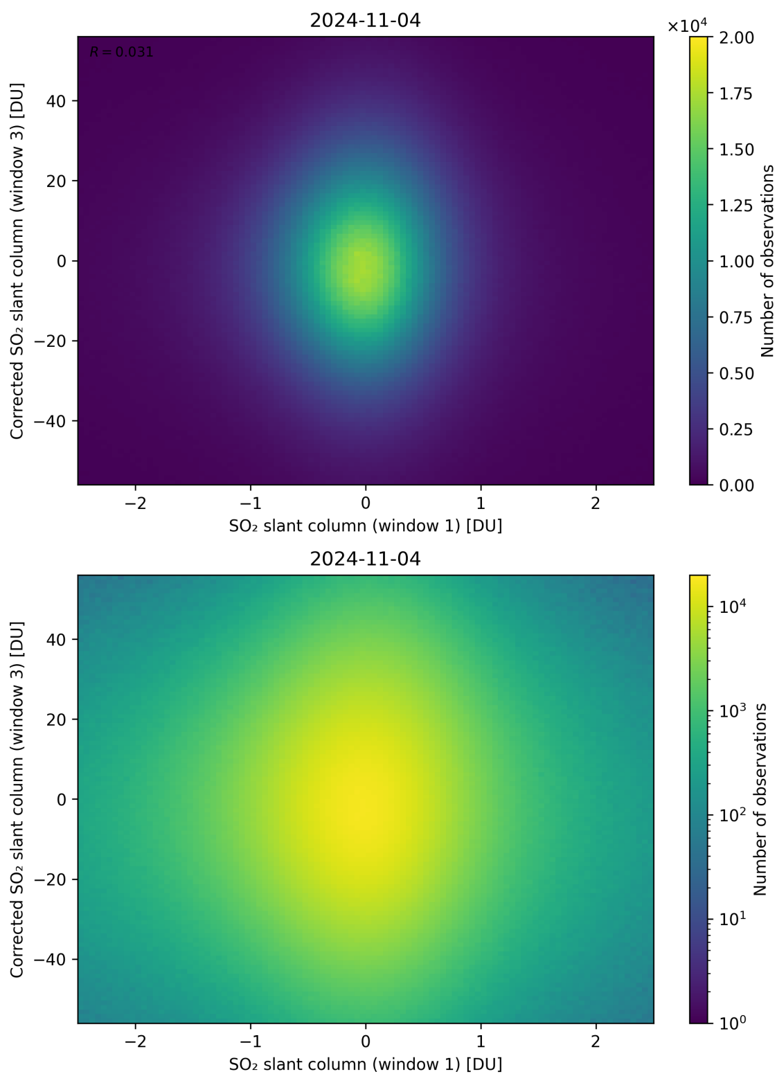
Figure 234: Scatter density plot of “SO 2 slant column (window 1)” against “Corrected SO 2 slant column (window 3)” for 2024-11-04 to 2024-11-05.
