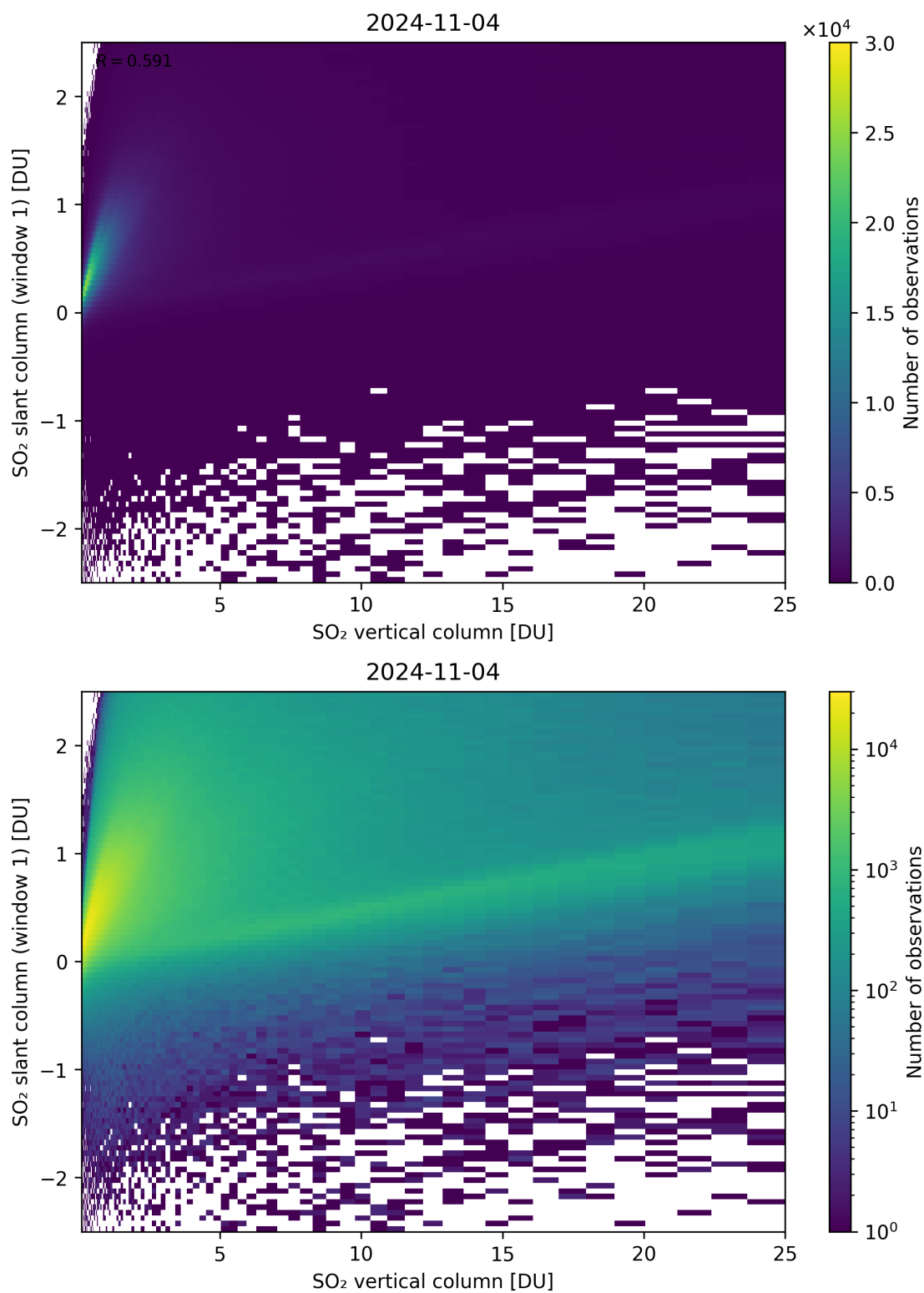
Figure 300: Scatter density plot of “SO 2 vertical column” against “SO 2 slant column (window 1)” for 2024-11-04 to 2024-11-05.
