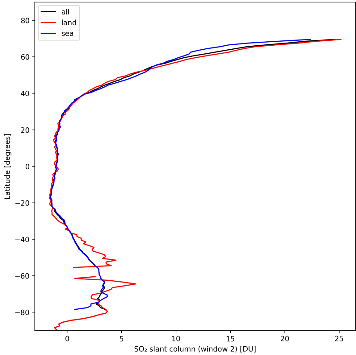
Figure 37: Zonal average of “SO 2 slant column (window 2)” for 2024-11-04 to 2024-11-05.
