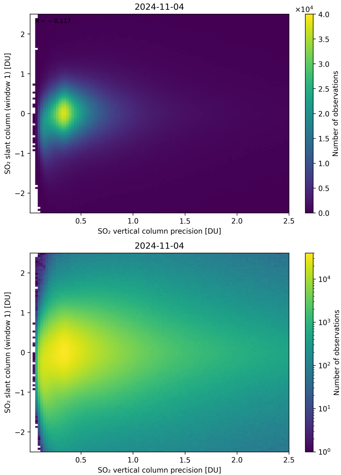
Figure 289: Scatter density plot of “SO 2 vertical column precision” against “SO 2 slant column (window 1)” for 2024-11-04 to 2024-11-05.
