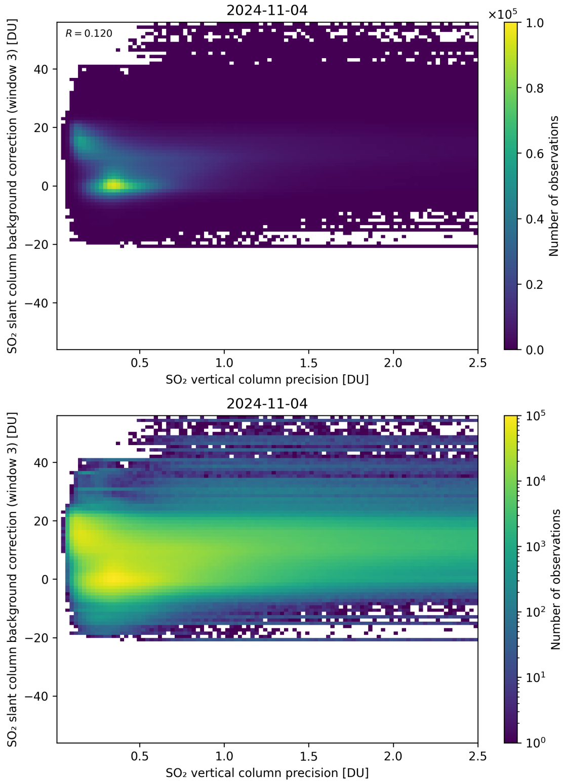
Figure 281: Scatter density plot of “SO 2 vertical column precision” against “SO 2 slant column background correction (window 3)” for 2024-11-04 to 2024-11-05.
