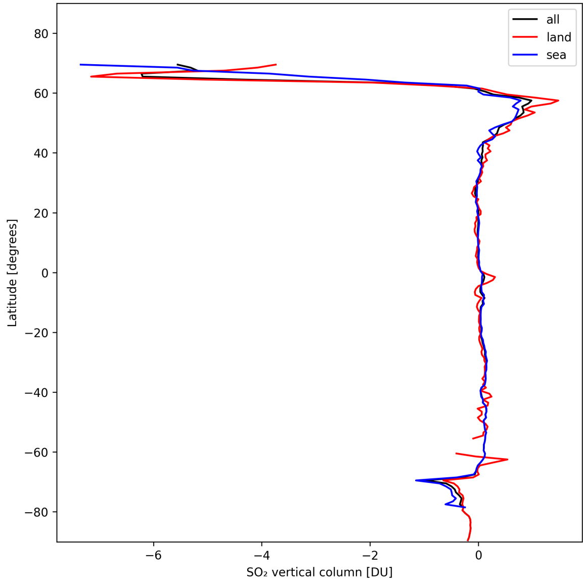
Figure 30: Zonal average of “SO 2 vertical column” for 2024-11-04 to 2024-11-05.
