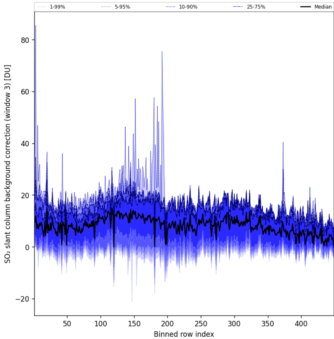
Figure 90: Along track statistics of “SO 2 slant column background correction (window 3)” for 2024-11-04 to 2024-11-05
