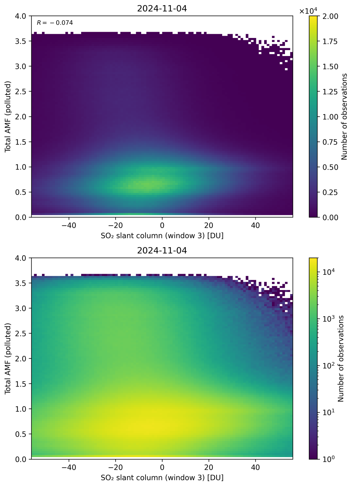
Figure 268: Scatter density plot of “SO 2 slant column (window 3)” against “Total AMF (polluted)” for 2024-11-04 to 2024-11-05.
