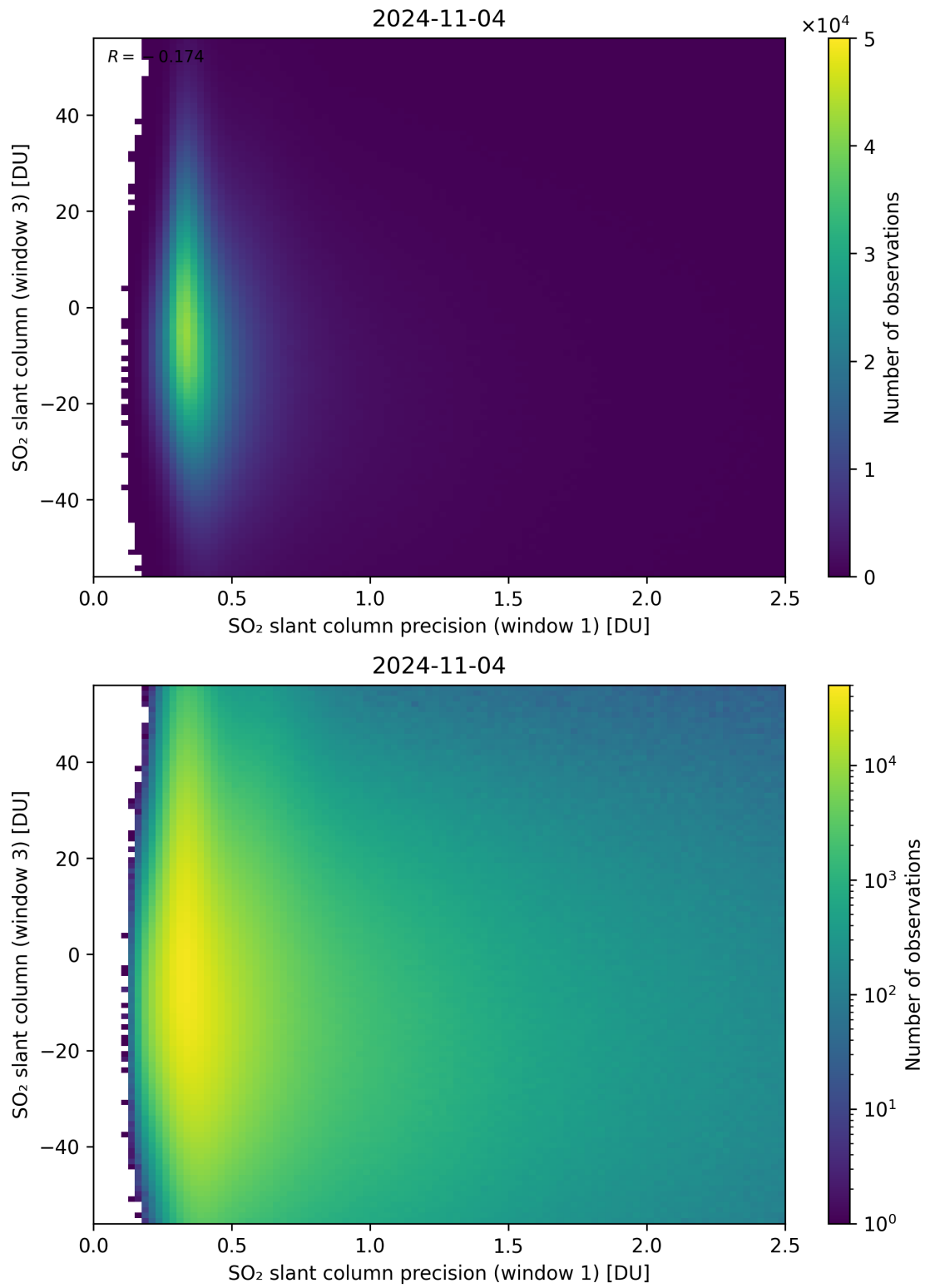
Figure 228: Scatter density plot of “SO 2 slant column precision (window 1)” against “SO 2 slant column (window 3)” for 2024-11-04 to 2024-11-05.
