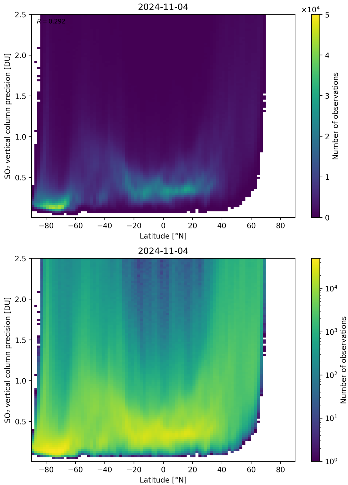
Figure 157: Scatter density plot of “Latitude” against “SO 2 vertical column precision” for 2024-11-04 to 2024-11-05.
