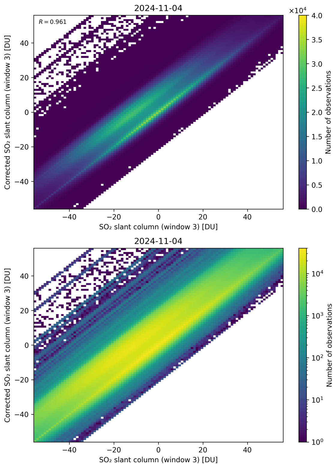
Figure 266: Scatter density plot of “SO 2 slant column (window 3)” against “Corrected SO 2 slant column (window 3)” for 2024-11-04 to 2024-11-05.
