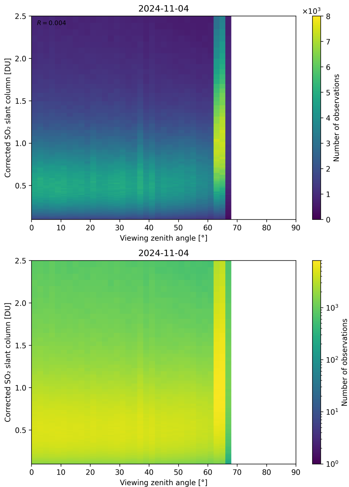
Figure 317: Scatter density plot of “Viewing zenith angle” against “Corrected SO 2 slant column” for 2024-11-04 to 2024-11-05.
