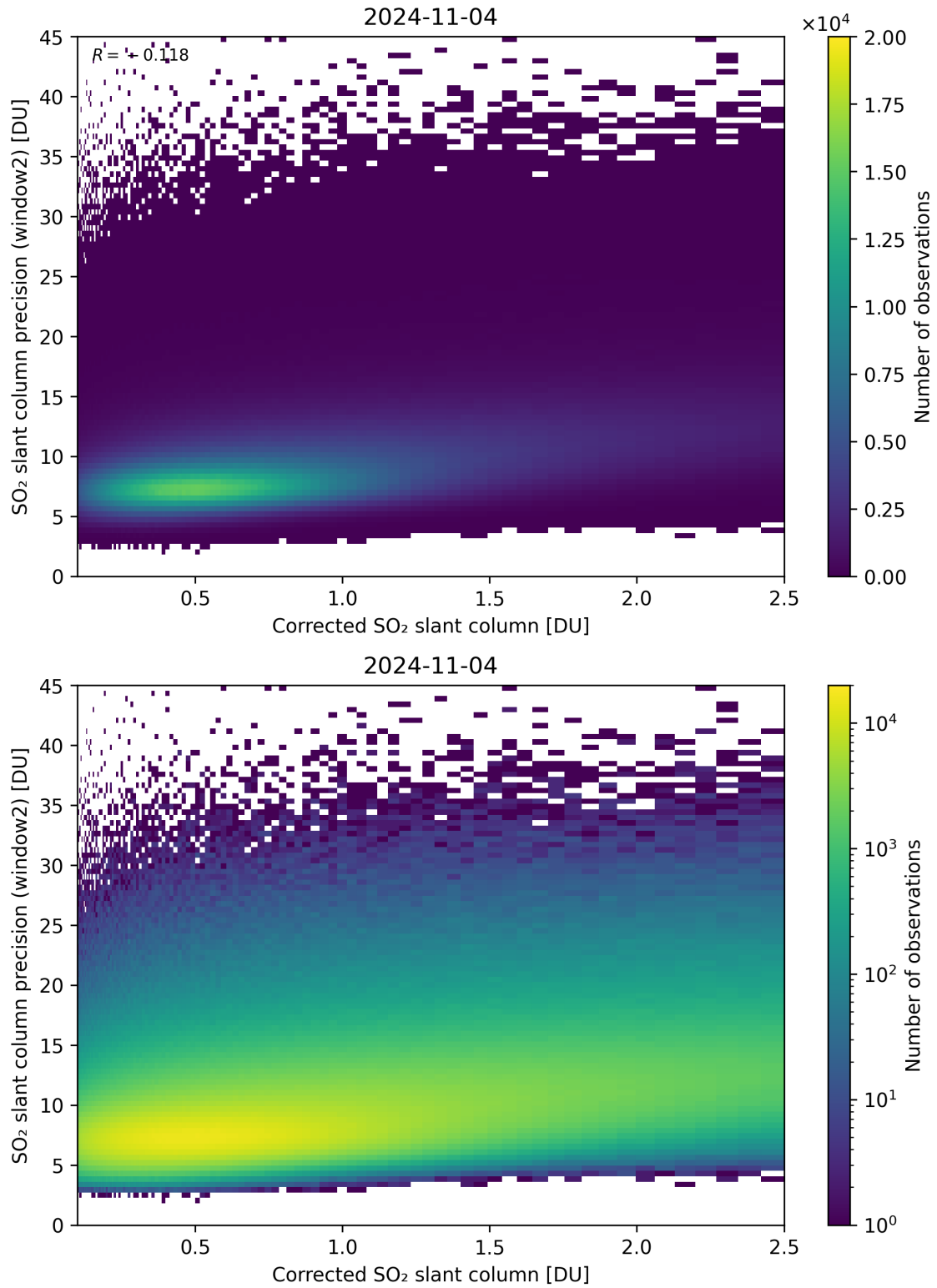
Figure 189: Scatter density plot of “Corrected SO 2 slant column” against “SO 2 slant column precision (window2)” for 2024-11-04 to 2024-11-05.
