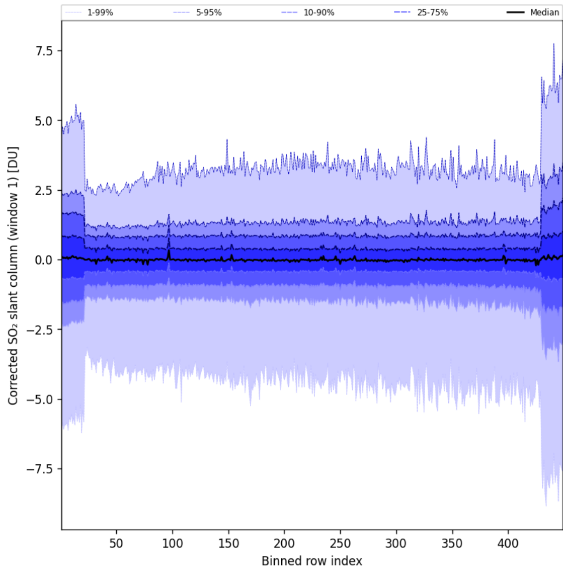
Figure 81: Along track statistics of “Corrected SO 2 slant column (window 1)” for 2024-11-04 to 2024-11-05
