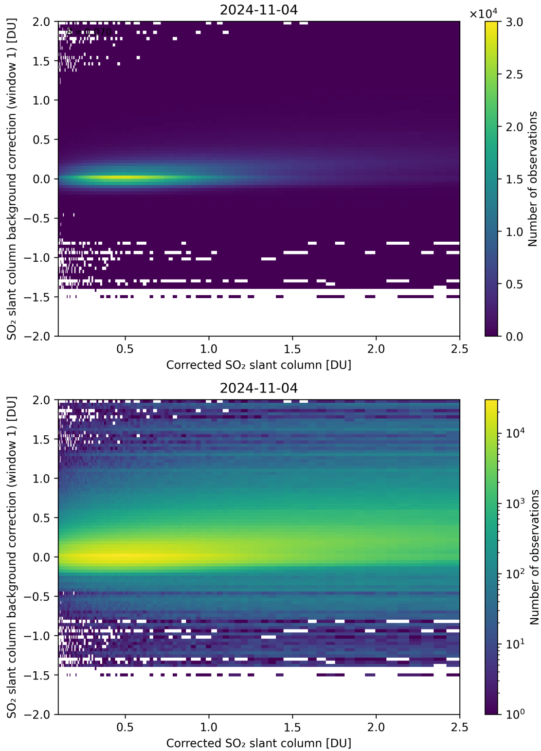
Figure 178: Scatter density plot of “Corrected SO 2 slant column” against “SO 2 slant column background correction (window 1)” for 2024-11-04 to 2024-11-05.
