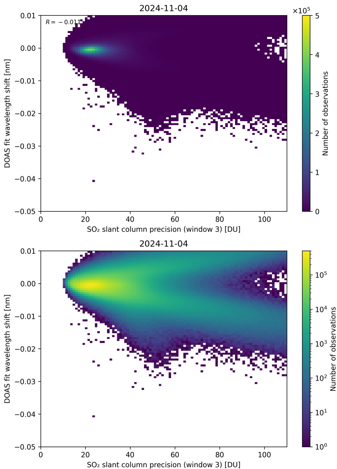
Figure 258: Scatter density plot of “SO 2 slant column precision (window 3)” against “DOAS fit wavelength shift” for 2024-11-04 to 2024-11-05.
