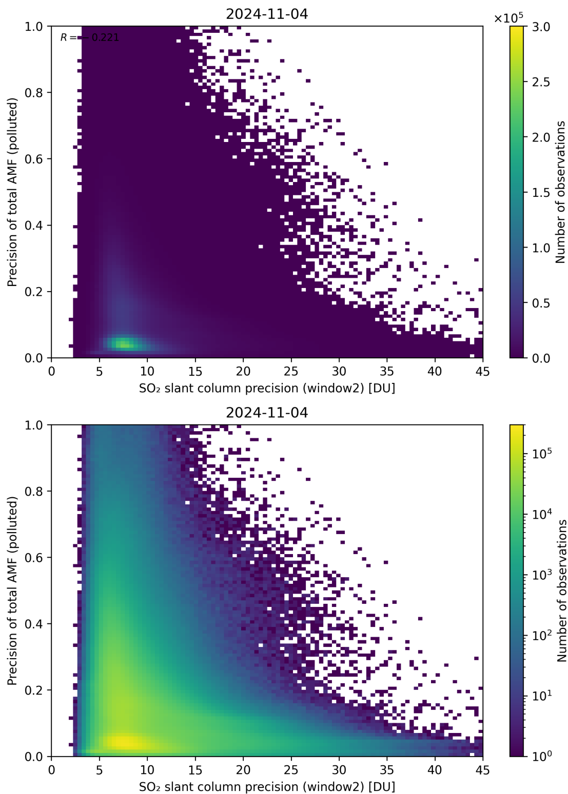
Figure 252: Scatter density plot of “SO 2 slant column precision (window2)” against “Precision of total AMF (polluted)” for 2024-11-04 to 2024-11-05.
