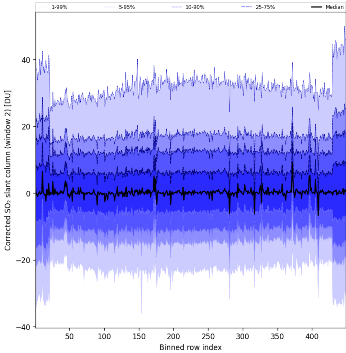
Figure 85: Along track statistics of “Corrected SO 2 slant column (window 2)” for 2024-11-04 to 2024-11-05
