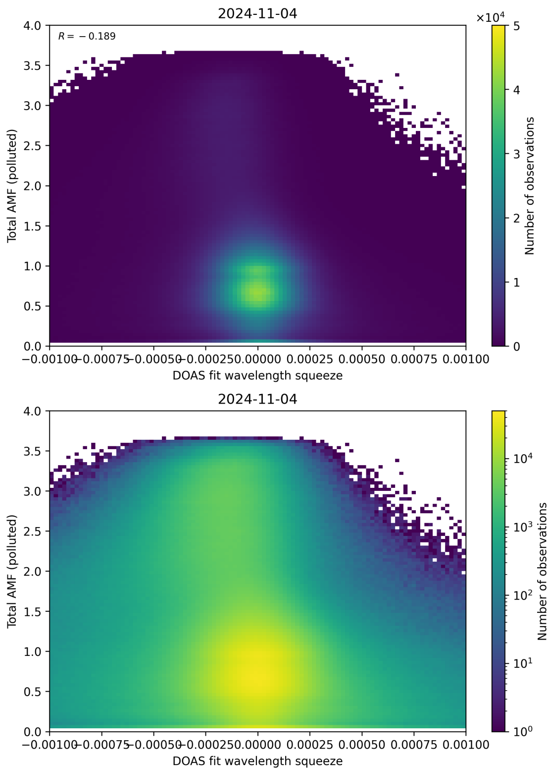
Figure 134: Scatter density plot of “DOAS fit wavelength squeeze” against “Total AMF (polluted)” for 2024-11-04 to 2024-11-05.
