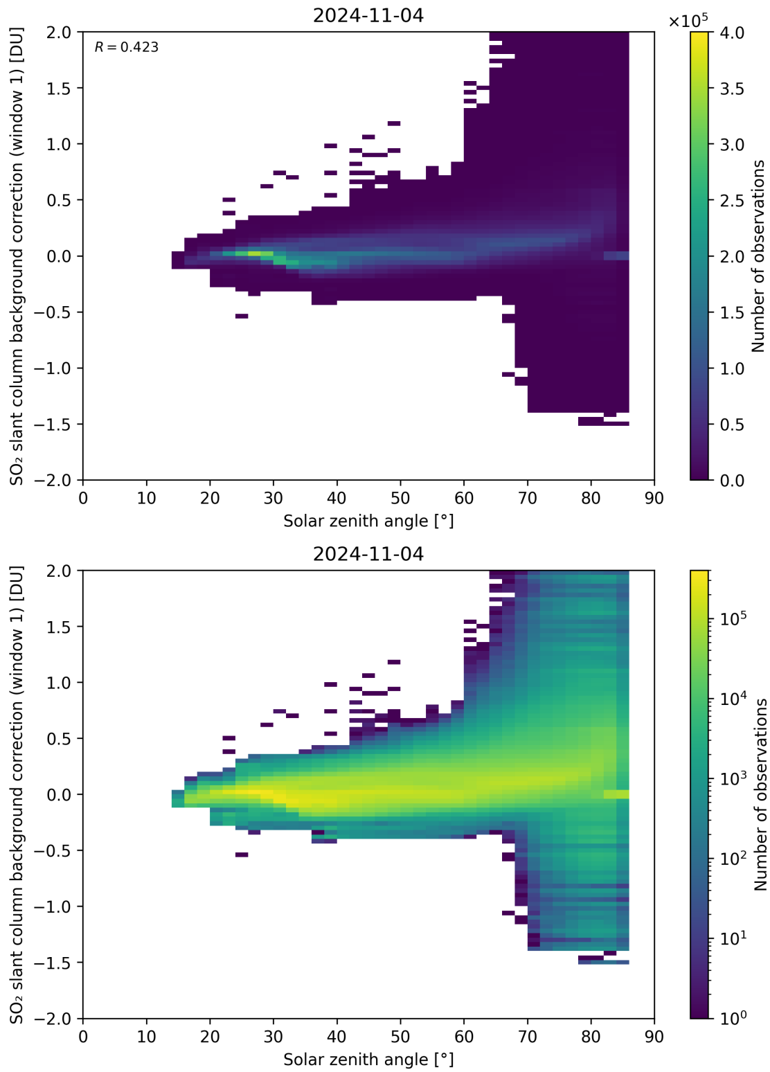
Figure 158: Scatter density plot of “Solar zenith angle” against “SO 2 slant column background correction (window 1)” for 2024-11-04 to 2024-11-05.
