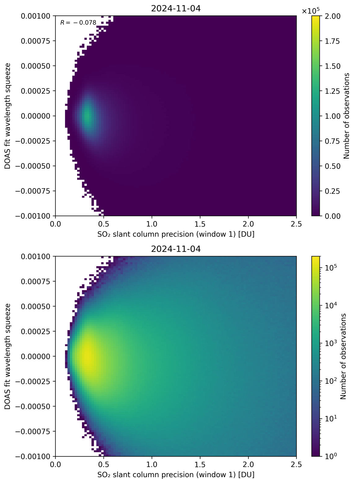
Figure 222: Scatter density plot of “SO 2 slant column precision (window 1)” against “DOAS fit wavelength squeeze” for 2024-11-04 to 2024-11-05.
