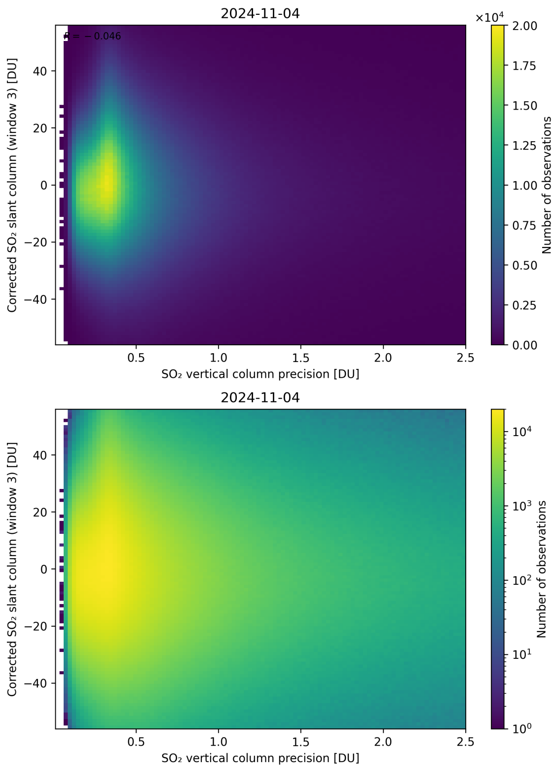
Figure 288: Scatter density plot of “SO 2 vertical column precision” against “Corrected SO 2 slant column (window 3)” for 2024-11-04 to 2024-11-05.
