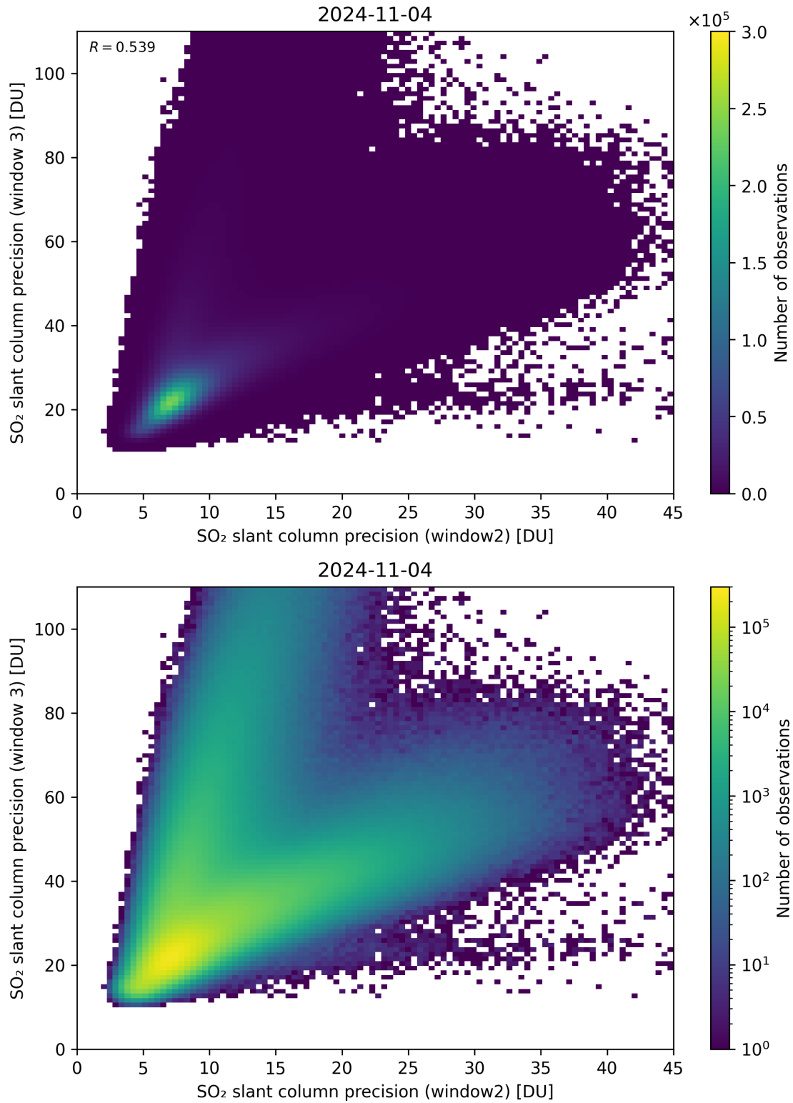
Figure 250: Scatter density plot of “SO 2 slant column precision (window2)” against “SO 2 slant column precision (window 3)” for 2024-11-04 to 2024-11-05.
