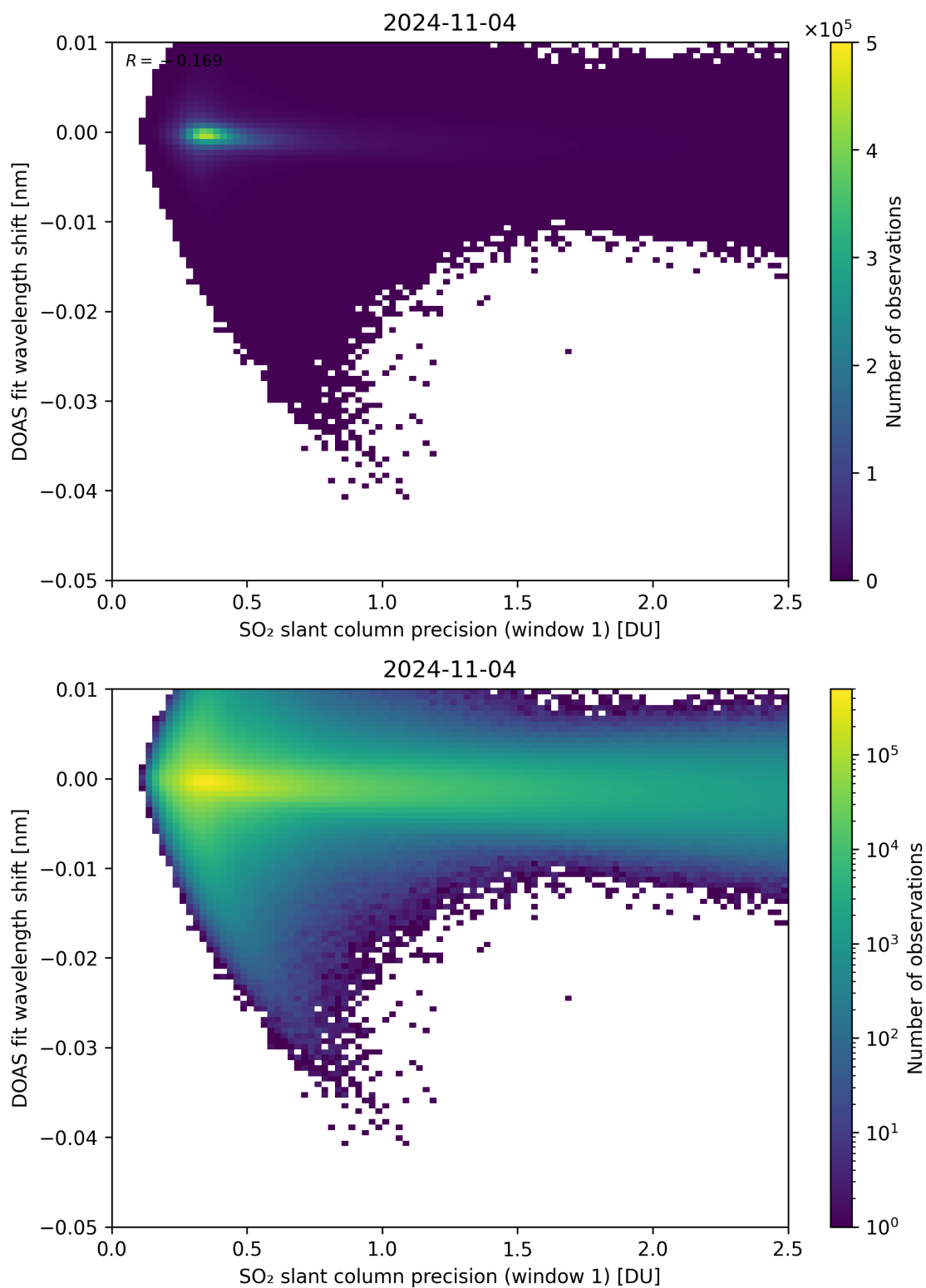
Figure 221: Scatter density plot of “SO 2 slant column precision (window 1)” against “DOAS fit wavelength shift” for 2024-11-04 to 2024-11-05.
