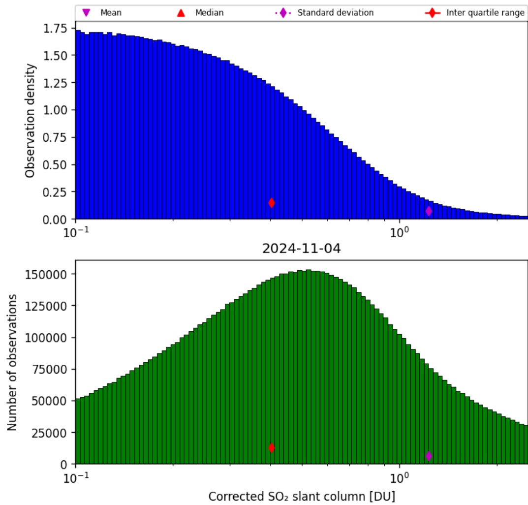
Figure 55: Histogram of “Corrected SO 2 slant column” for 2024-11-04 to 2024-11-05
