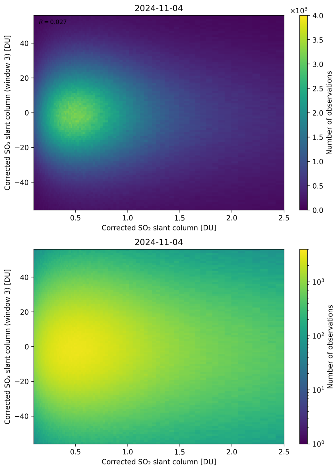
Figure 186: Scatter density plot of “Corrected SO 2 slant column” against “Corrected SO 2 slant column (window 3)” for 2024-11-04 to 2024-11-05.
