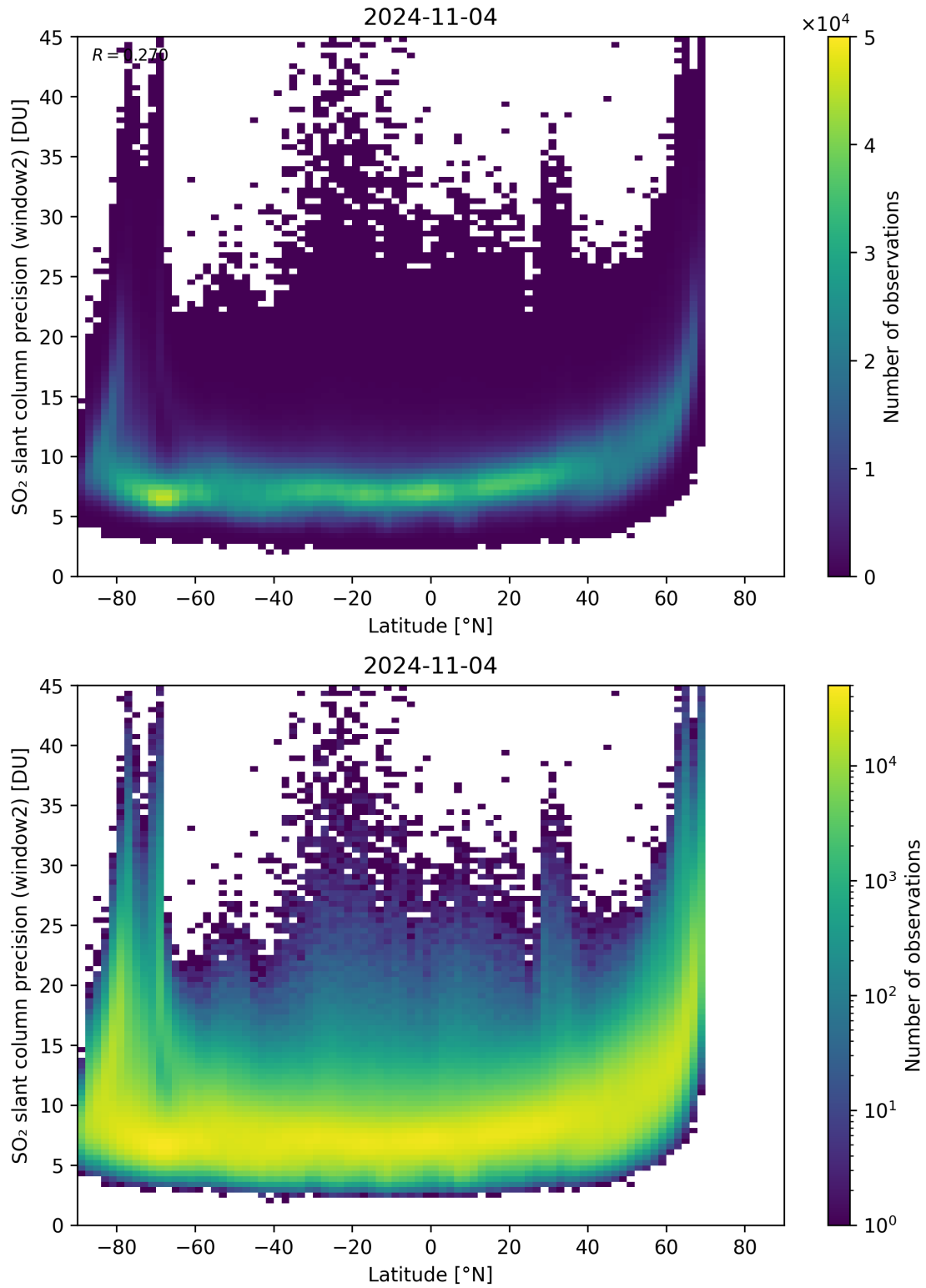
Figure 151: Scatter density plot of “Latitude” against “SO 2 slant column precision (window2)” for 2024-11-04 to 2024-11-05.
