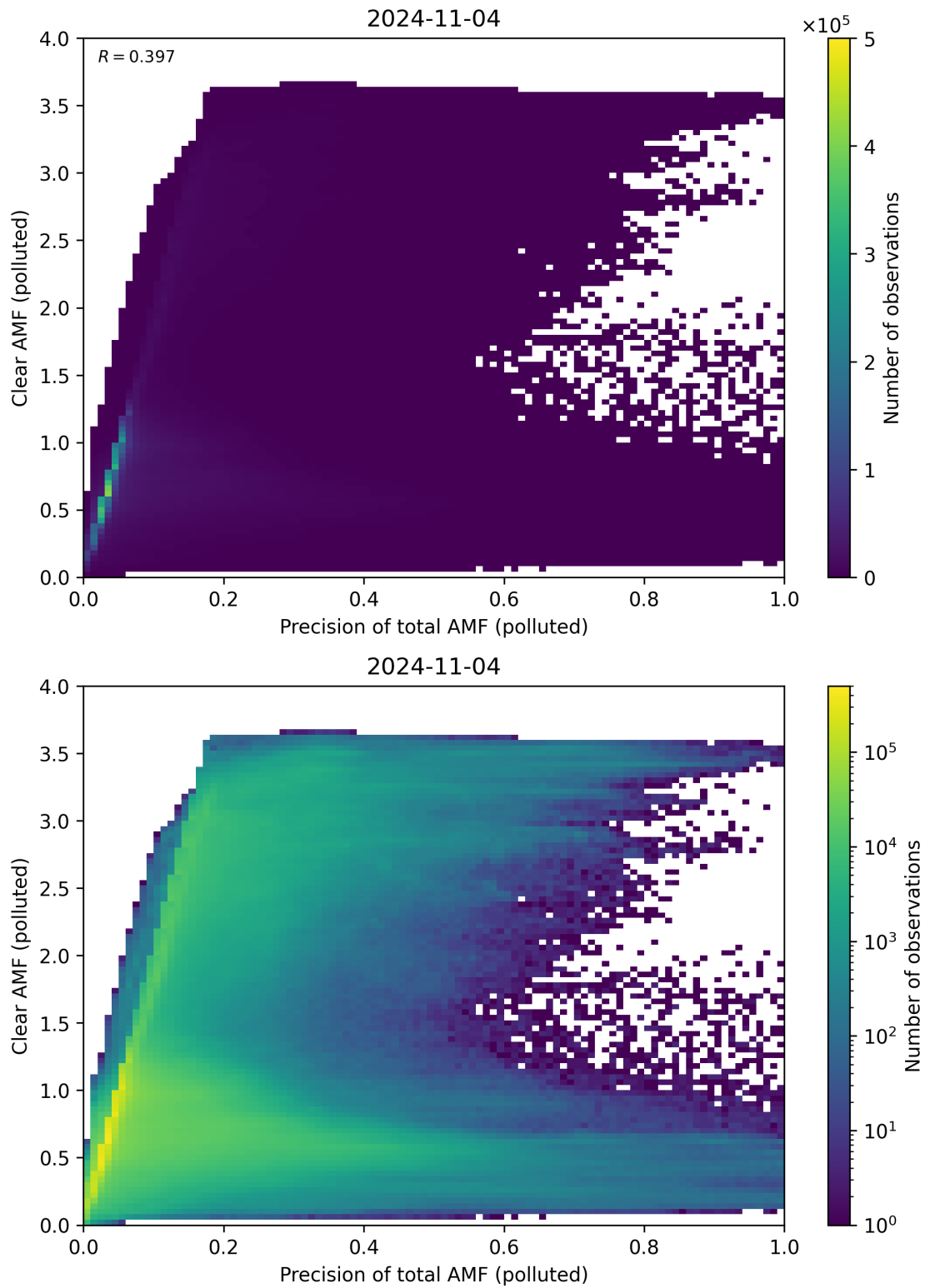
Figure 270: Scatter density plot of “Precision of total AMF (polluted)” against “Clear AMF (polluted)” for 2024-11-04 to 2024-11-05.
