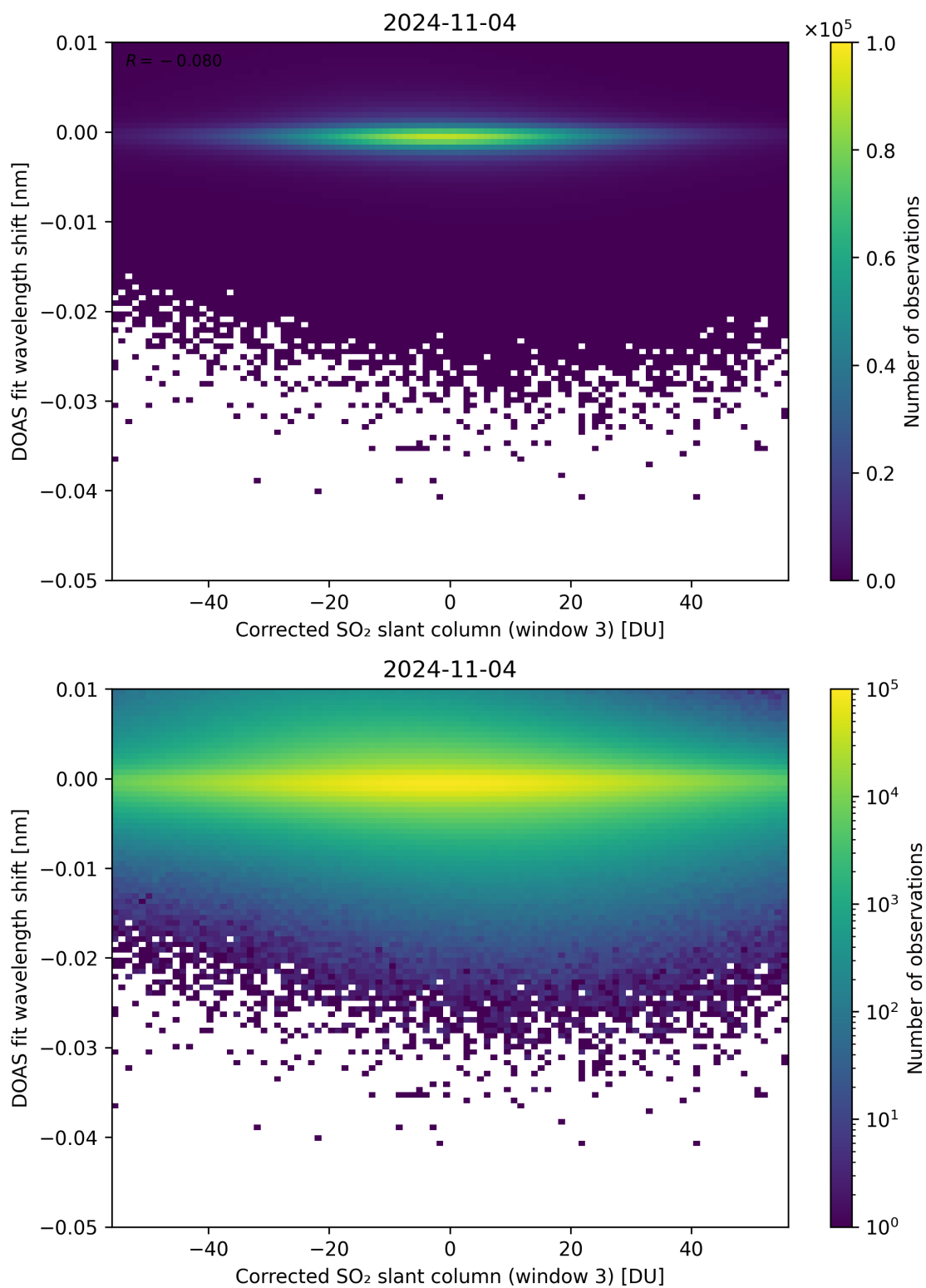
Figure 206: Scatter density plot of “Corrected SO 2 slant column (window 3)” against “DOAS fit wavelength shift” for 2024-11-04 to 2024-11-05.
