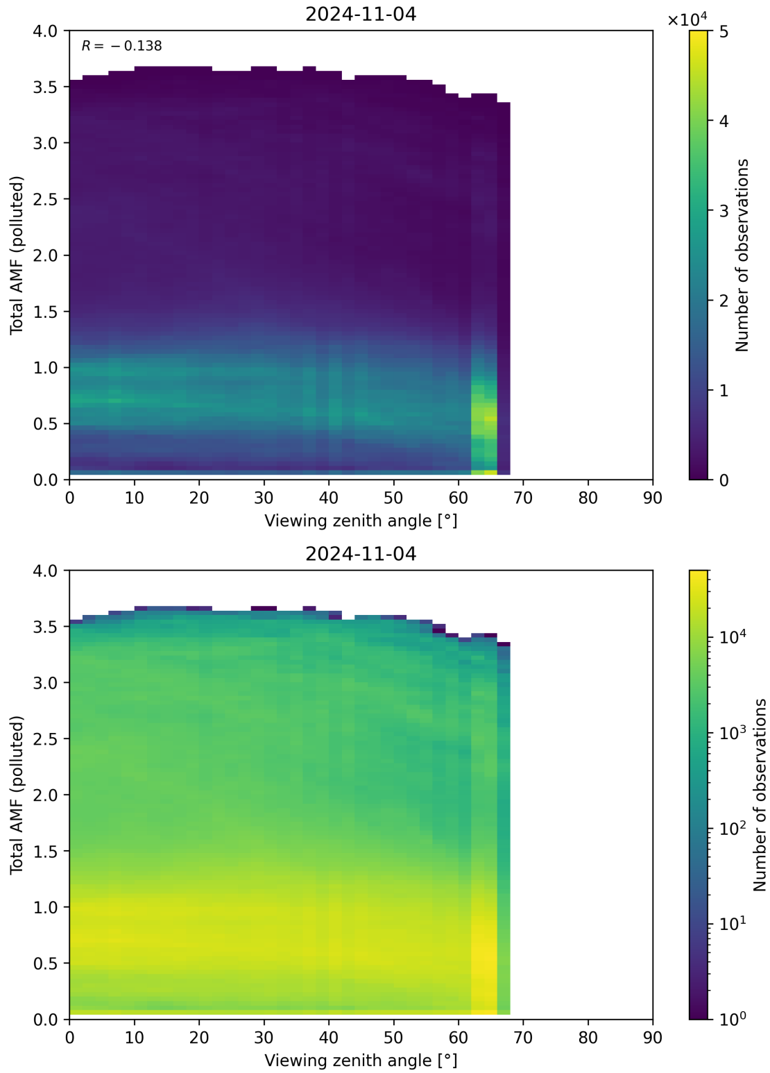
Figure 325: Scatter density plot of “Viewing zenith angle” against “Total AMF (polluted)” for 2024-11-04 to 2024-11-05.
