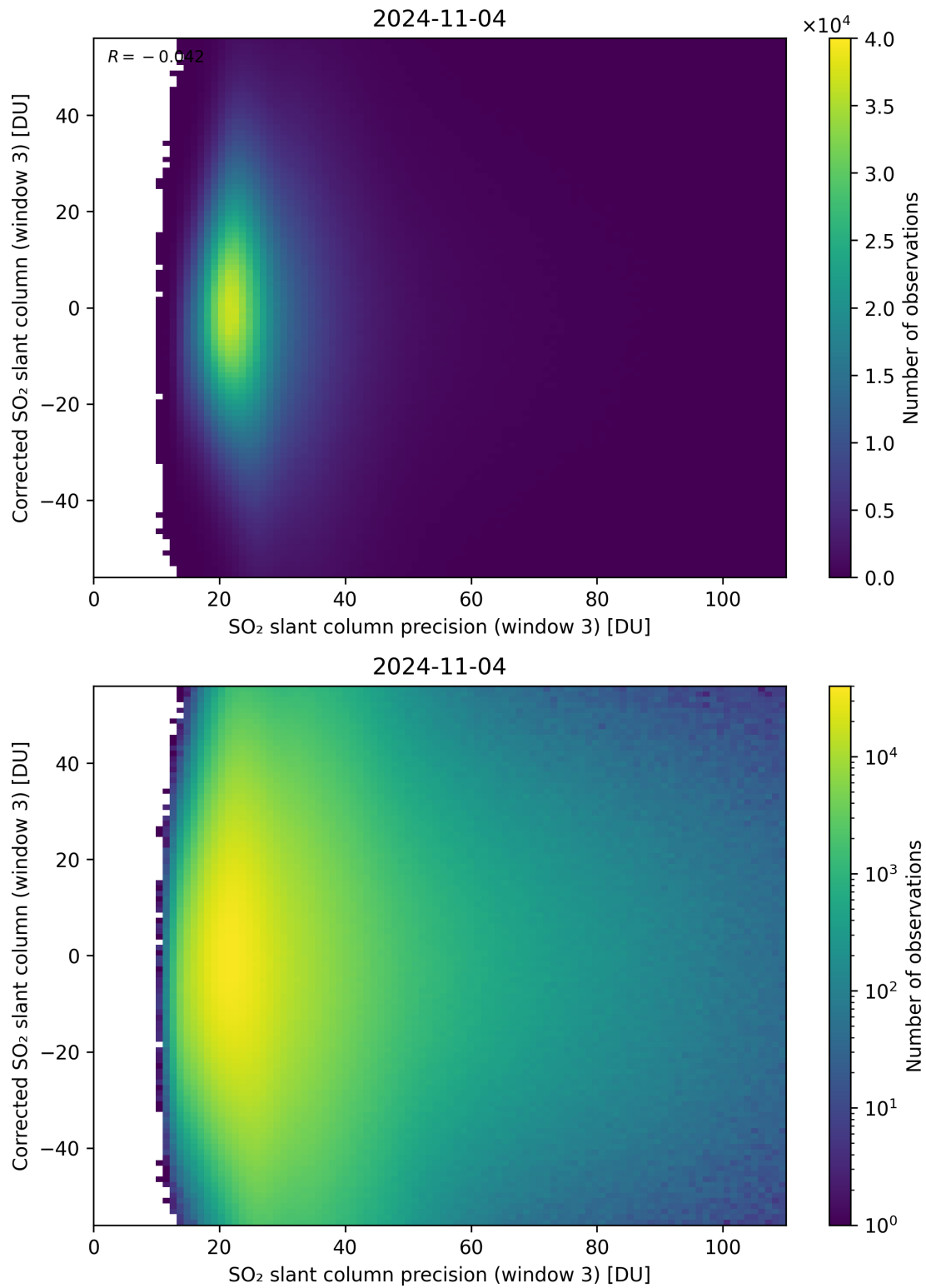
Figure 262: Scatter density plot of “SO 2 slant column precision (window 3)” against “Corrected SO 2 slant column (window 3)” for 2024-11-04 to 2024-11-05.
