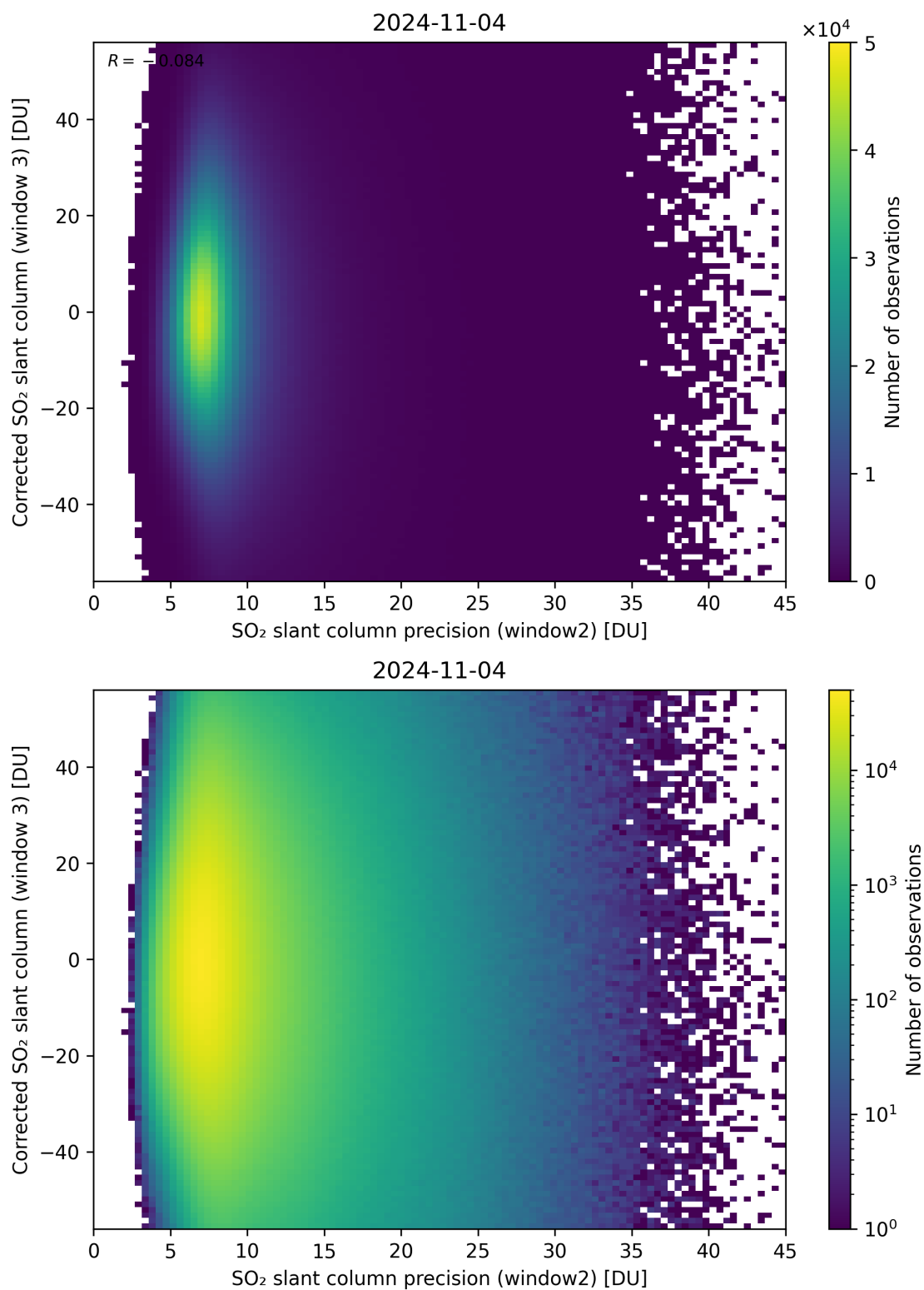
Figure 248: Scatter density plot of “SO 2 slant column precision (window2)” against “Corrected SO 2 slant column (window 3)” for 2024-11-04 to 2024-11-05.
