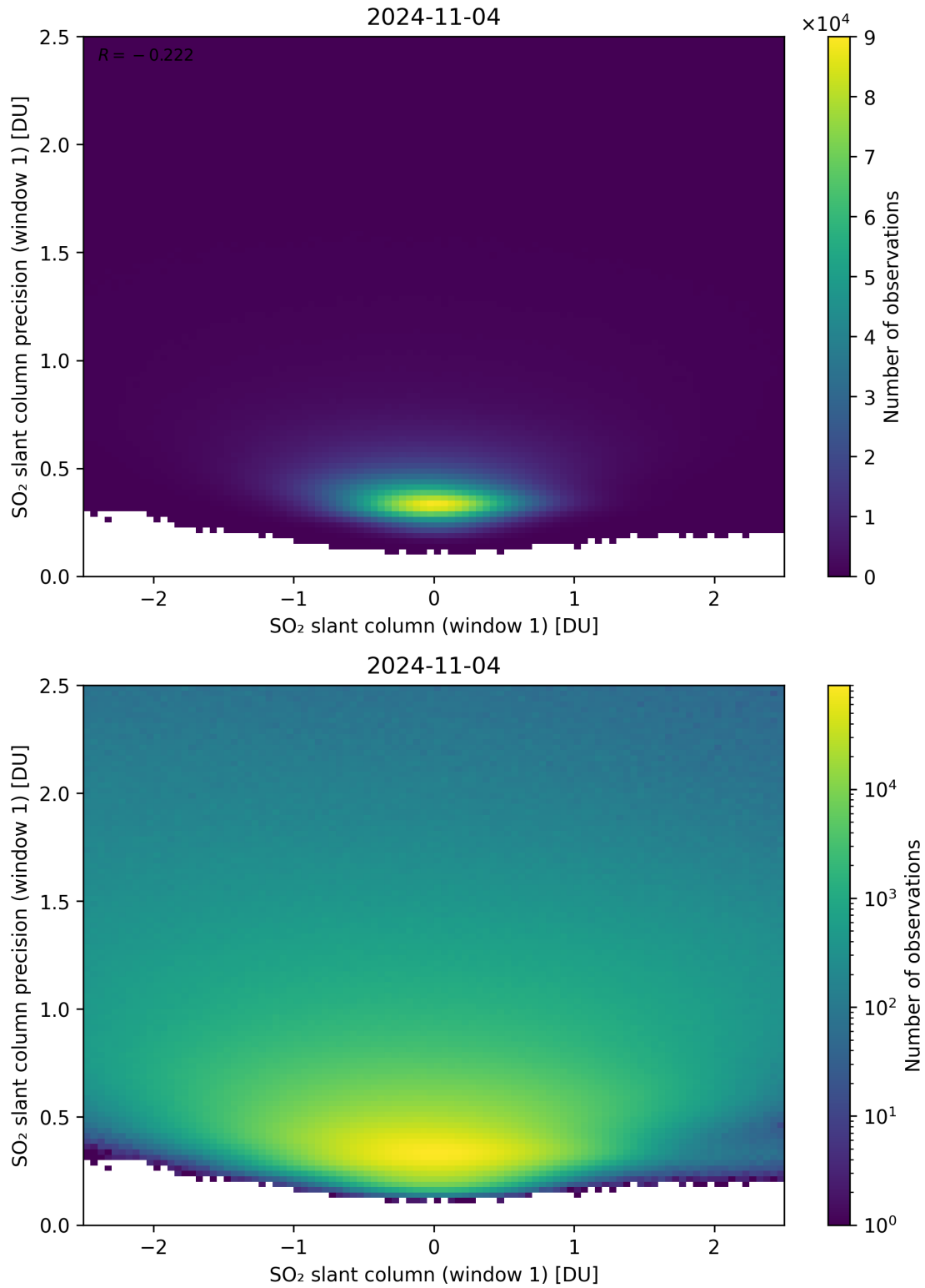
Figure 235: Scatter density plot of “SO 2 slant column (window 1)” against “SO 2 slant column precision (window 1)” for 2024-11-04 to 2024-11-05.
