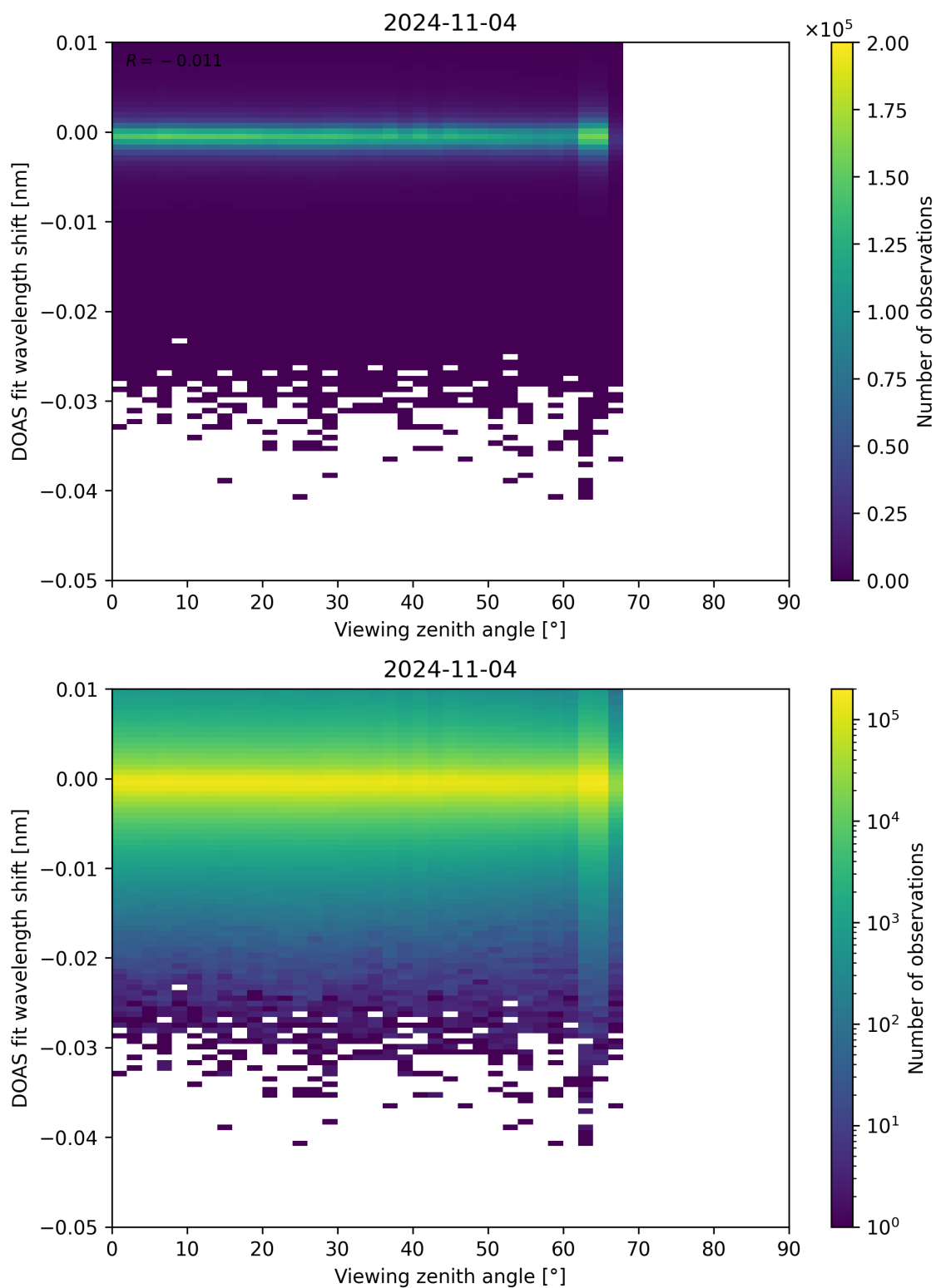
Figure 311: Scatter density plot of “Viewing zenith angle” against “DOAS fit wavelength shift” for 2024-11-04 to 2024-11-05.
