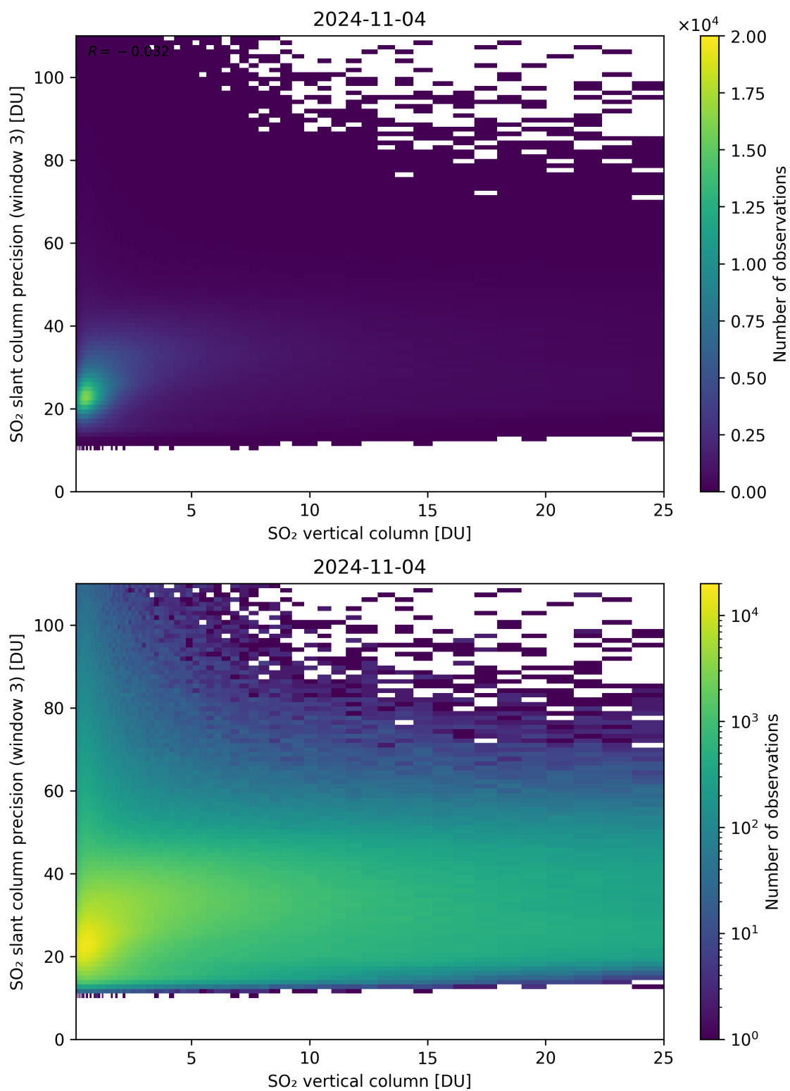
Figure 304: Scatter density plot of “SO 2 vertical column” against “SO 2 slant column precision (window 3)” for 2024-11-04 to 2024-11-05.
