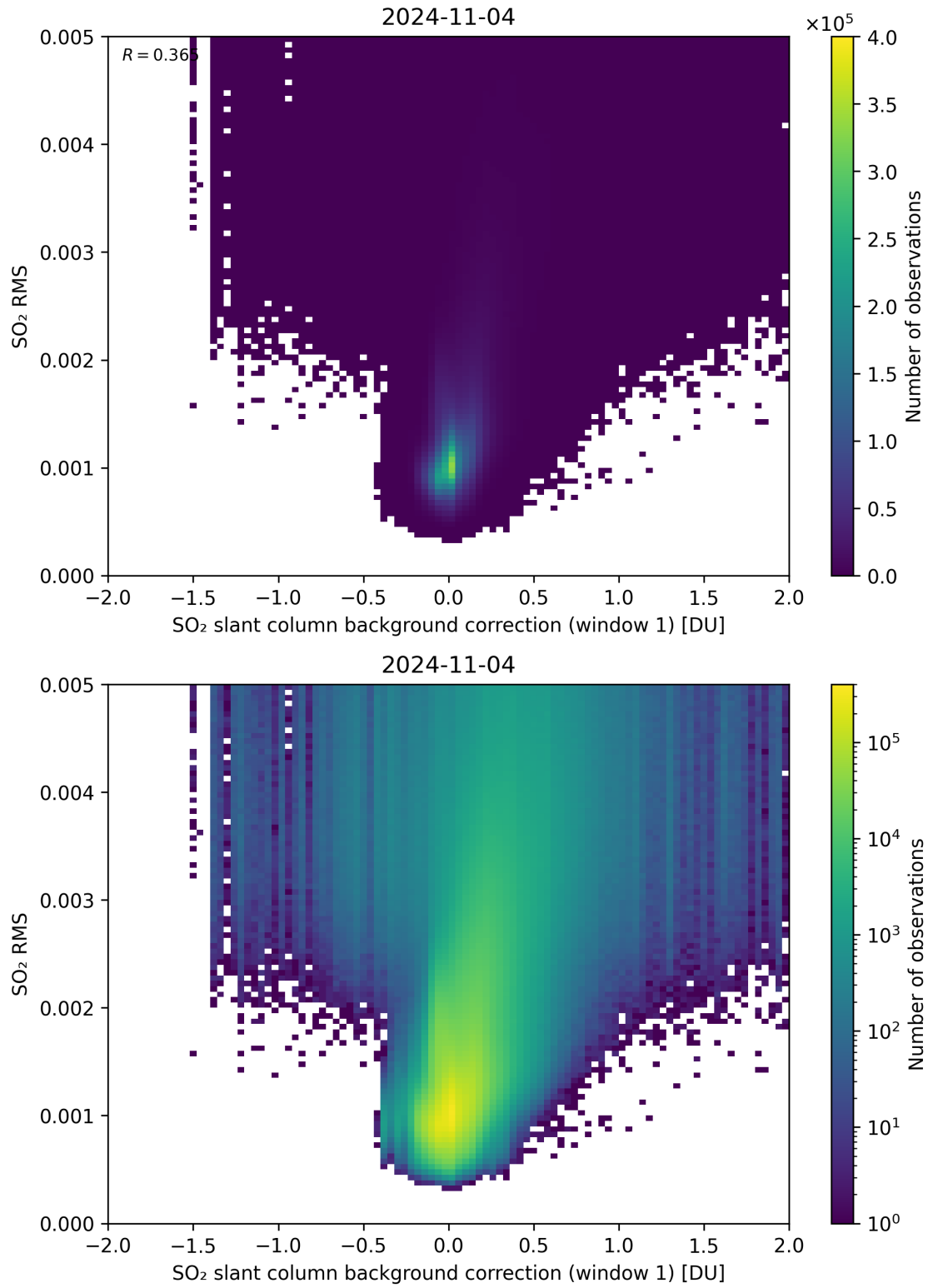
Figure 102: Scatter density plot of “SO 2 slant column background correction (window 1)” against “SO 2 RMS” for 2024-11-04 to 2024-11-05.
