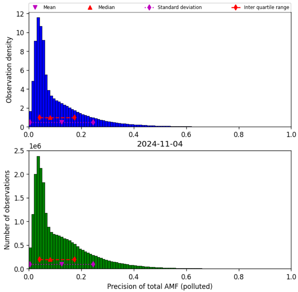
Figure 72: Histogram of “Precision of total AMF (polluted)” for 2024-11-04 to 2024-11-05
