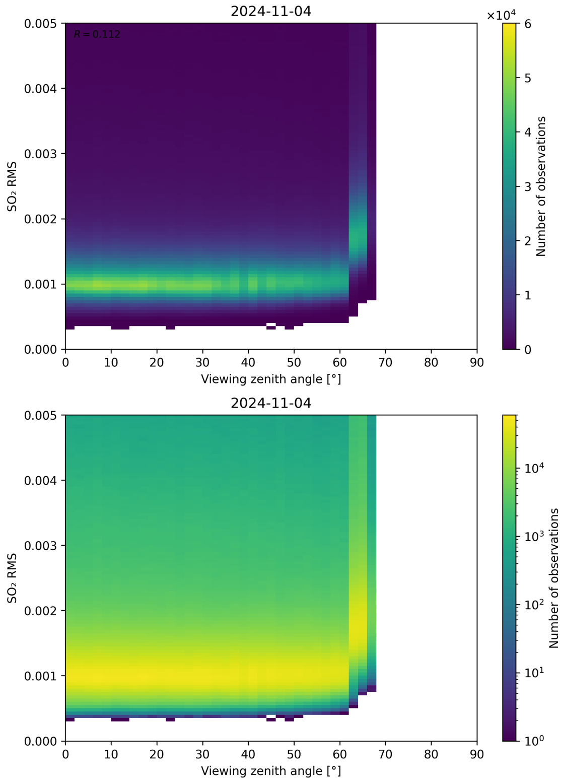
Figure 313: Scatter density plot of “Viewing zenith angle” against “SO 2 RMS” for 2024-11-04 to 2024-11-05.
