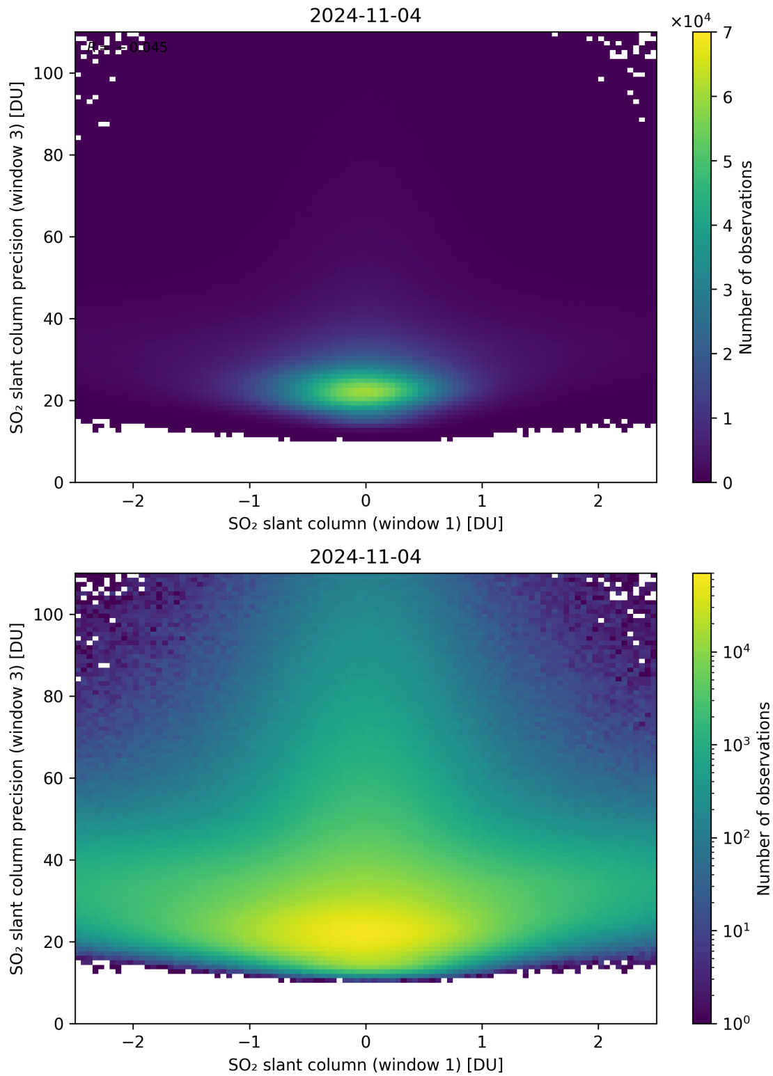
Figure 238: Scatter density plot of “SO 2 slant column (window 1)” against “SO 2 slant column precision (window 3)” for 2024-11-04 to 2024-11-05.
