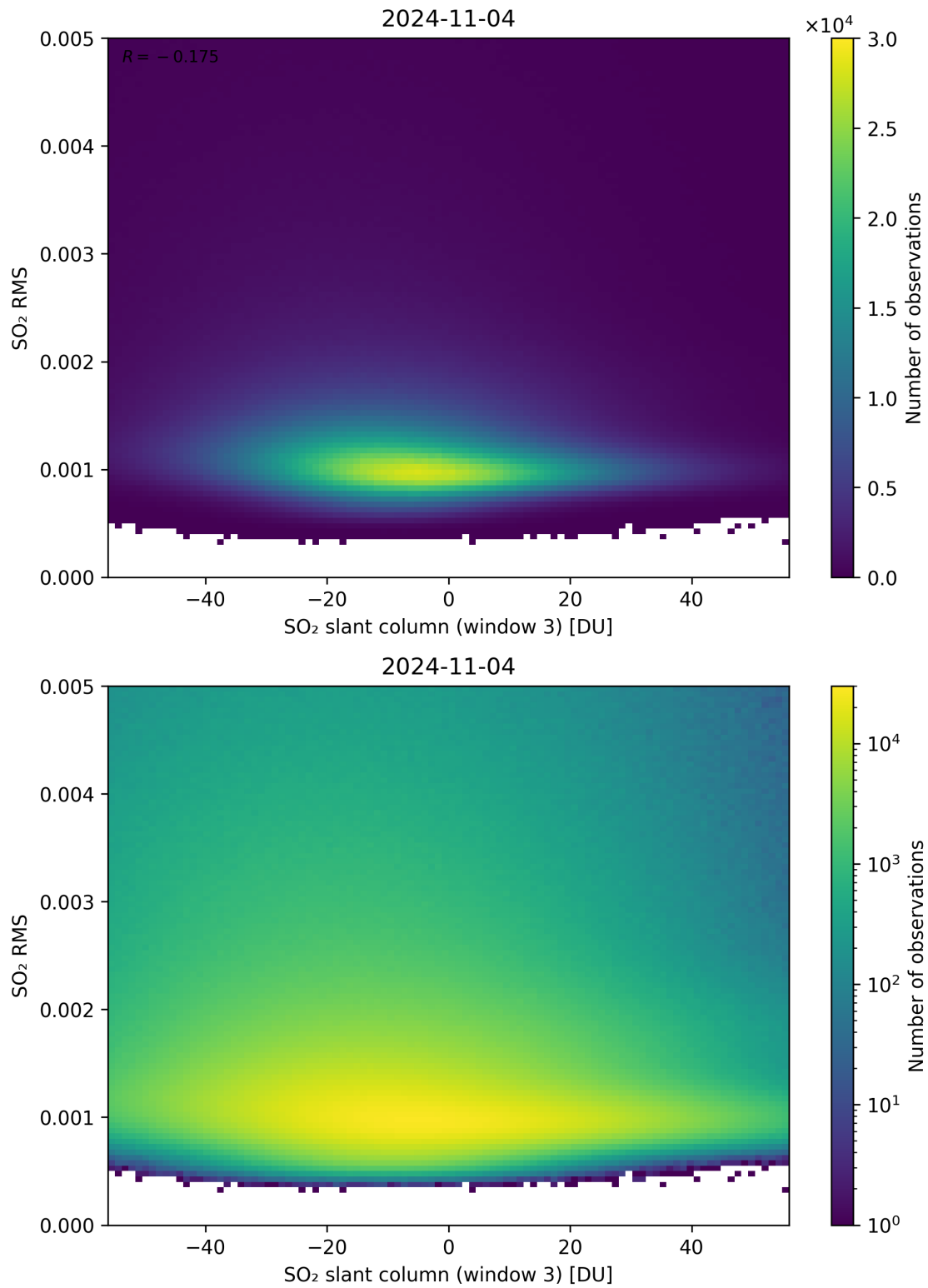
Figure 256: Scatter density plot of “SO 2 slant column (window 3)” against “SO 2 RMS” for 2024-11-04 to 2024-11-05.
