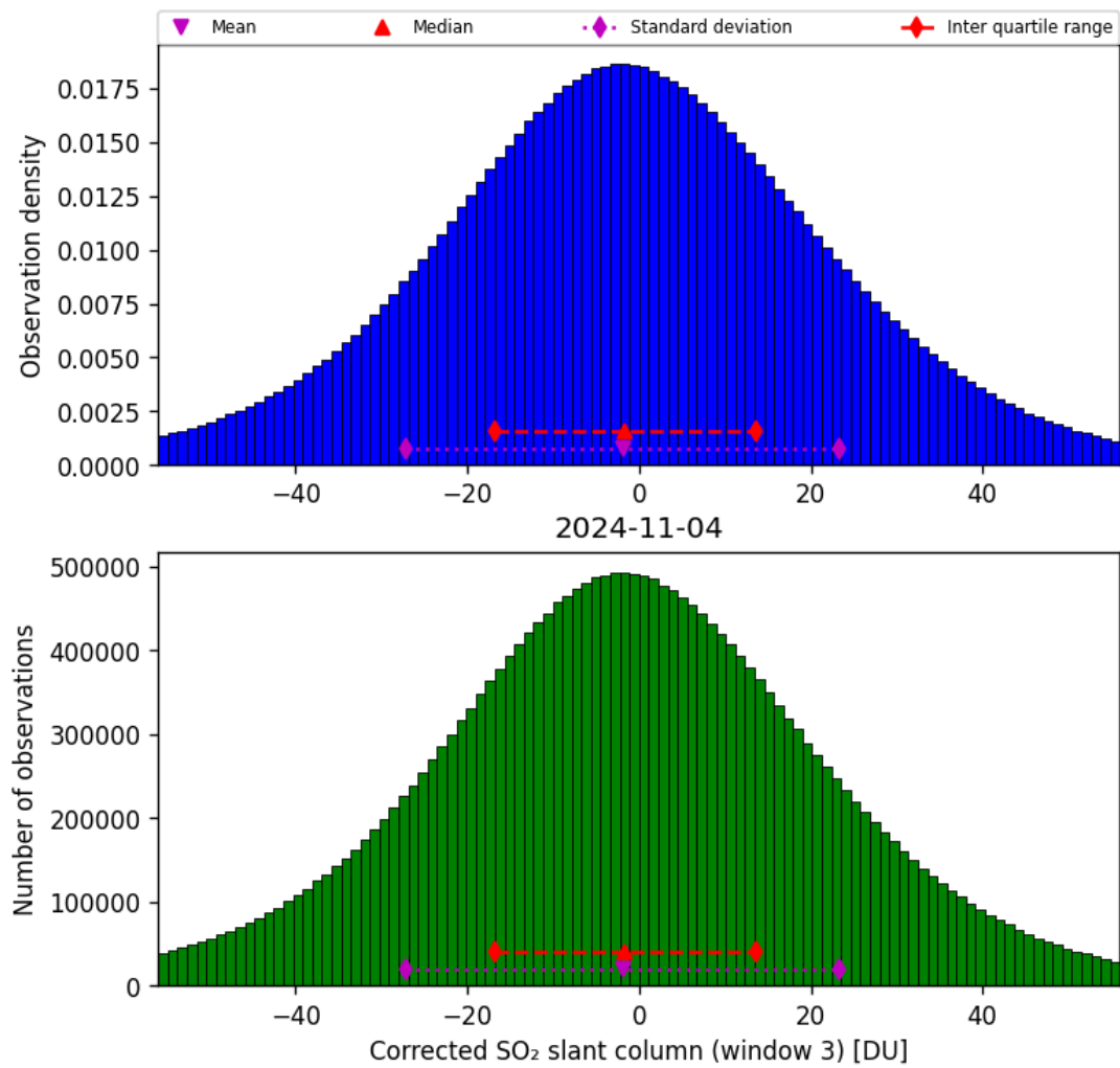
Figure 66: Histogram of “Corrected SO 2 slant column (window 3)” for 2024-11-04 to 2024-11-05
