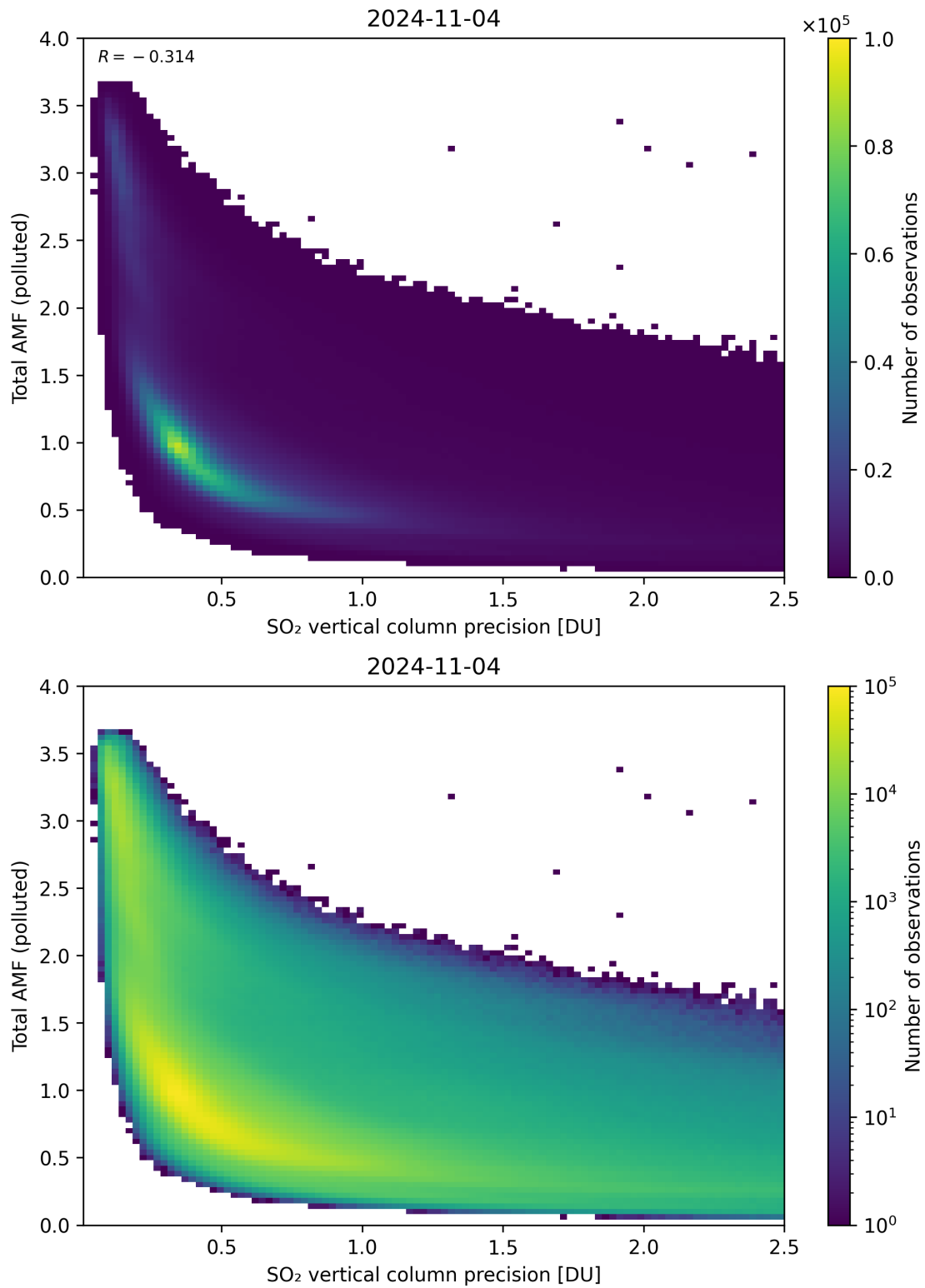
Figure 294: Scatter density plot of “SO 2 vertical column precision” against “Total AMF (polluted)” for 2024-11-04 to 2024-11-05.
