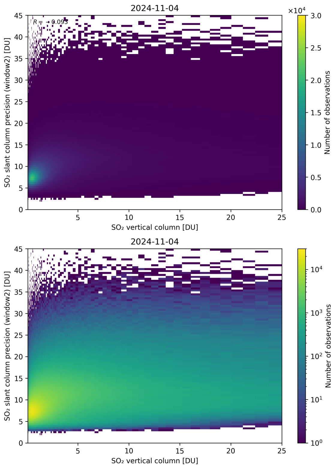
Figure 302: Scatter density plot of “SO 2 vertical column” against “SO 2 slant column precision (window2)” for 2024-11-04 to 2024-11-05.
