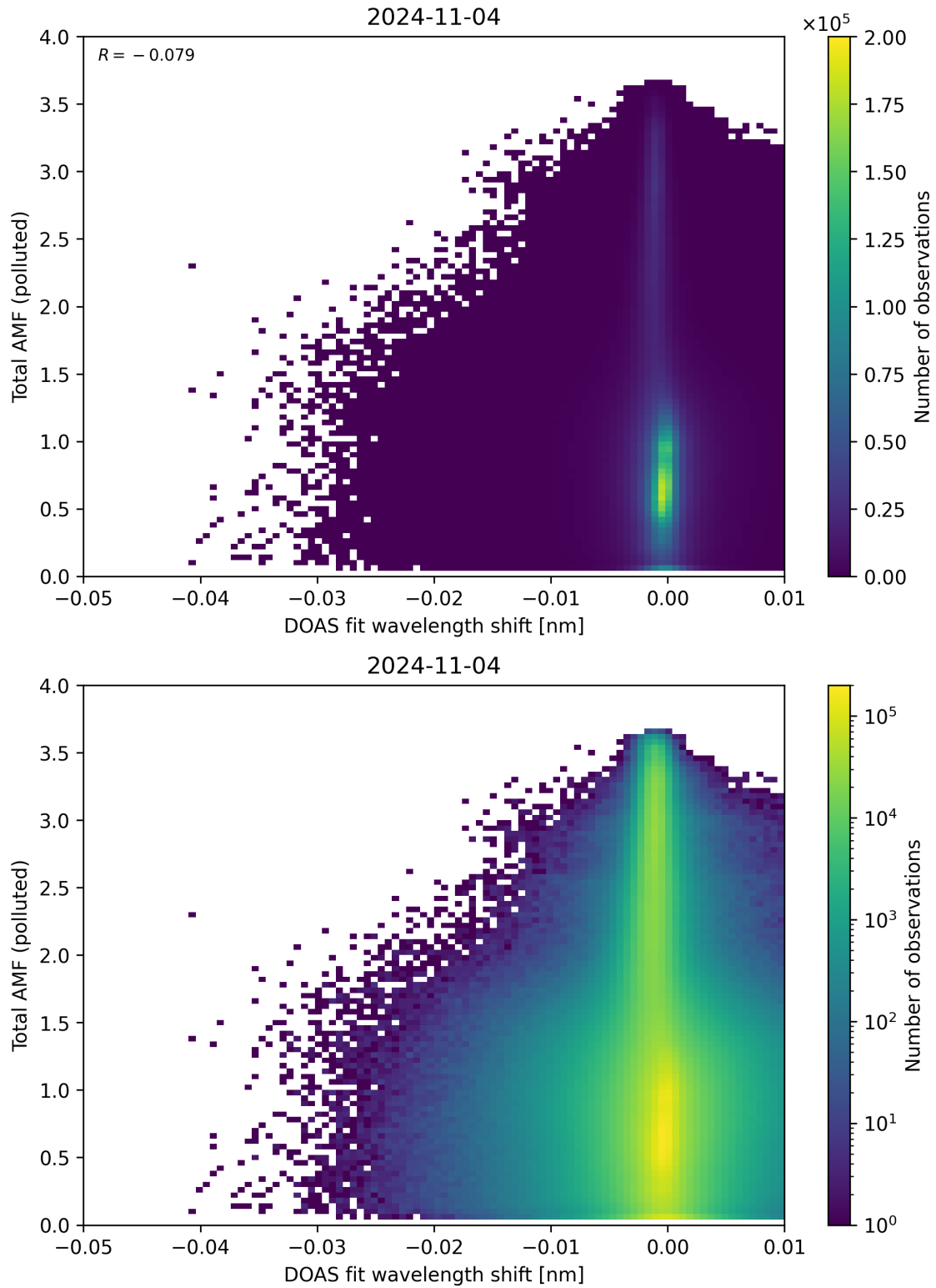
Figure 130: Scatter density plot of “DOAS fit wavelength shift” against “Total AMF (polluted)” for 2024-11-04 to 2024-11-05.
