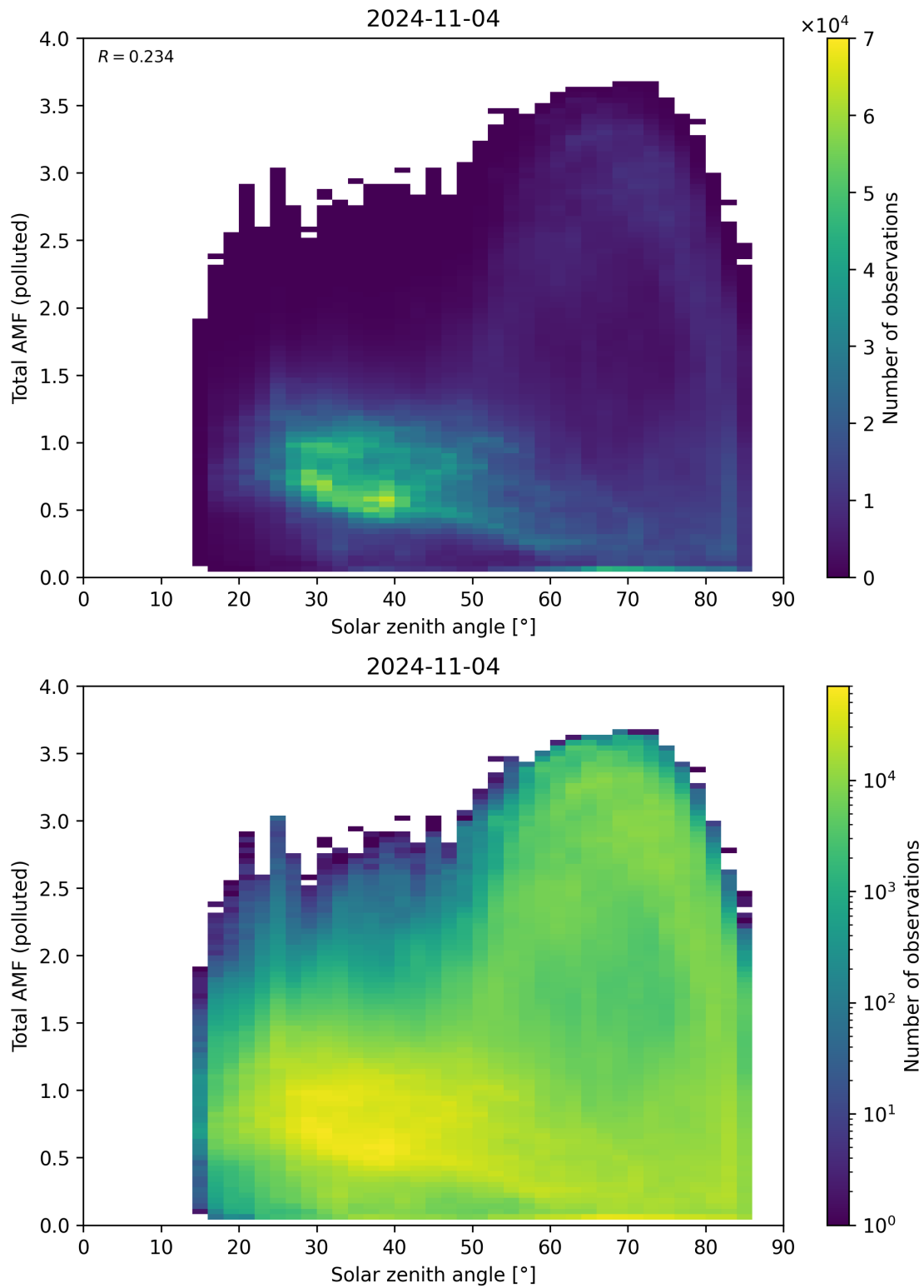
Figure 174: Scatter density plot of “Solar zenith angle” against “Total AMF (polluted)” for 2024-11-04 to 2024-11-05.
