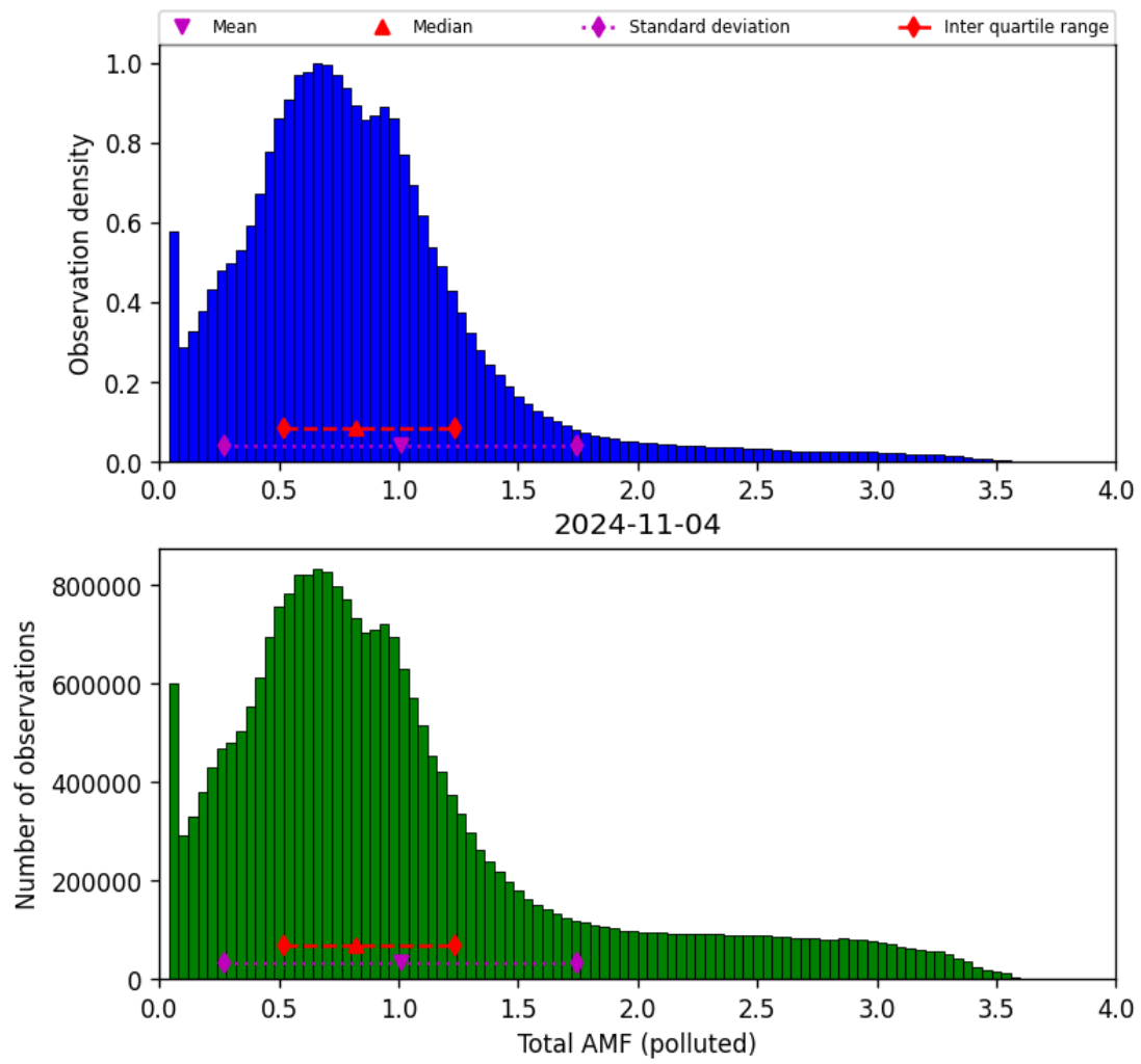
Figure 71: Histogram of “Total AMF (polluted)” for 2024-11-04 to 2024-11-05
