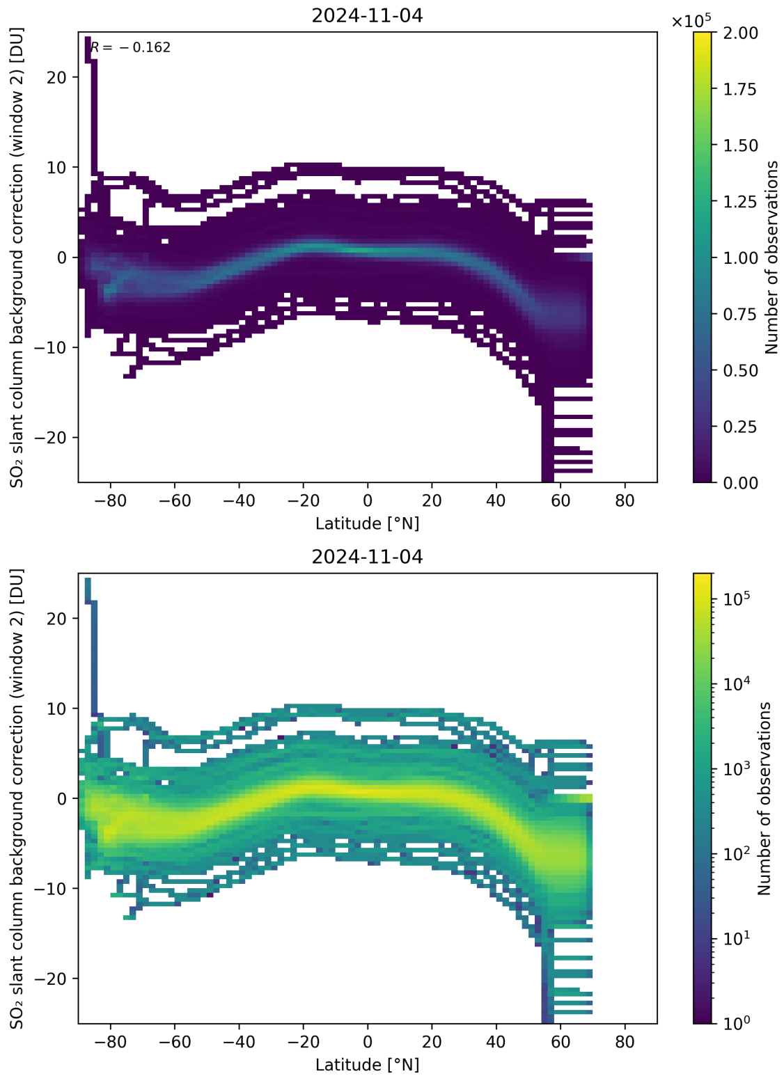
Figure 140: Scatter density plot of “Latitude” against “SO 2 slant column background correction (window 2)” for 2024-11-04 to 2024-11-05.
