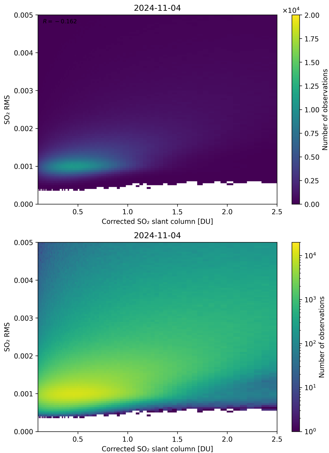
Figure 183: Scatter density plot of “Corrected SO 2 slant column” against “SO 2 RMS” for 2024-11-04 to 2024-11-05.
