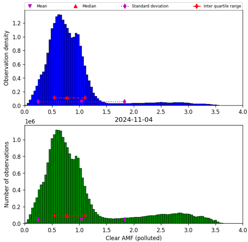
Figure 73: Histogram of “Clear AMF (polluted)” for 2024-11-04 to 2024-11-05
