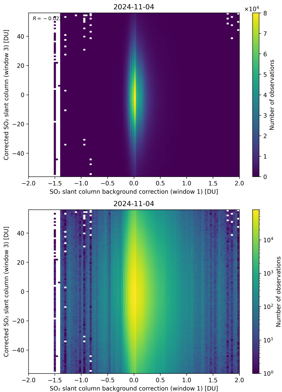
Figure 105: Scatter density plot of “SO 2 slant column background correction (window 1)” against “Corrected SO 2 slant column (window 3)” for 2024-11-04 to 2024-11-05.
