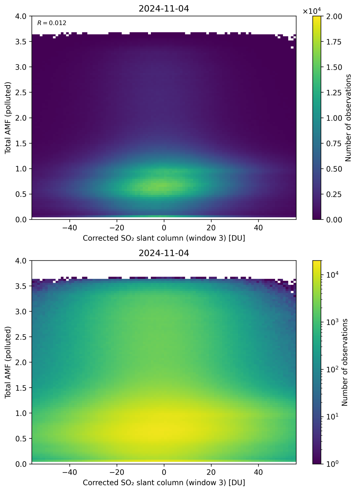
Figure 210: Scatter density plot of “Corrected SO 2 slant column (window 3)” against “Total AMF (polluted)” for 2024-11-04 to 2024-11-05.
