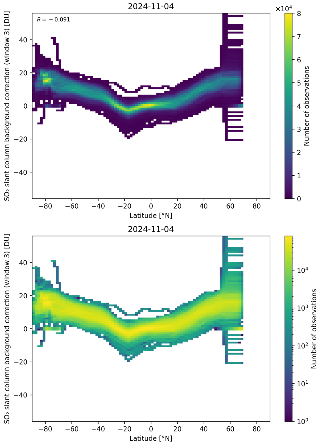
Figure 141: Scatter density plot of “Latitude” against “SO 2 slant column background correction (window 3)” for 2024-11-04 to 2024-11-05.
