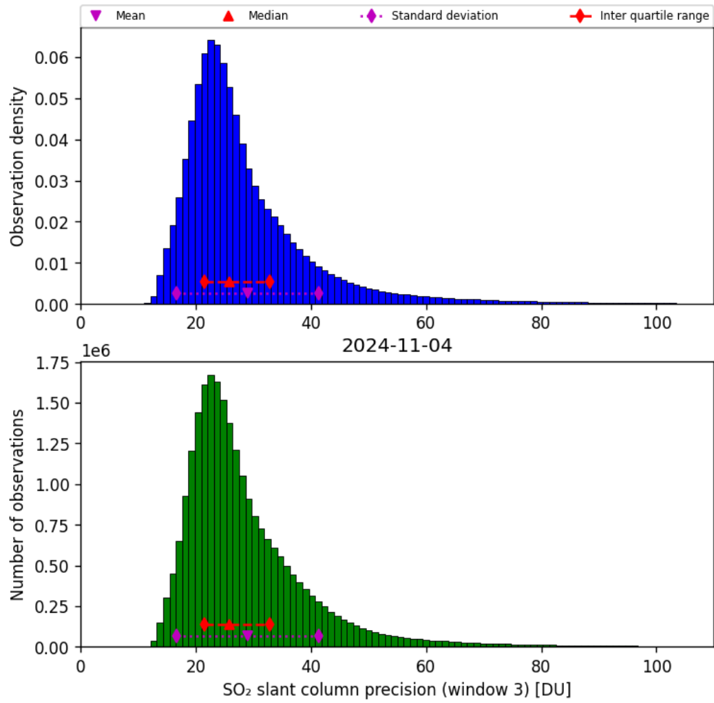
Figure 65: Histogram of “SO 2 slant column precision (window 3)” for 2024-11-04 to 2024-11-05
