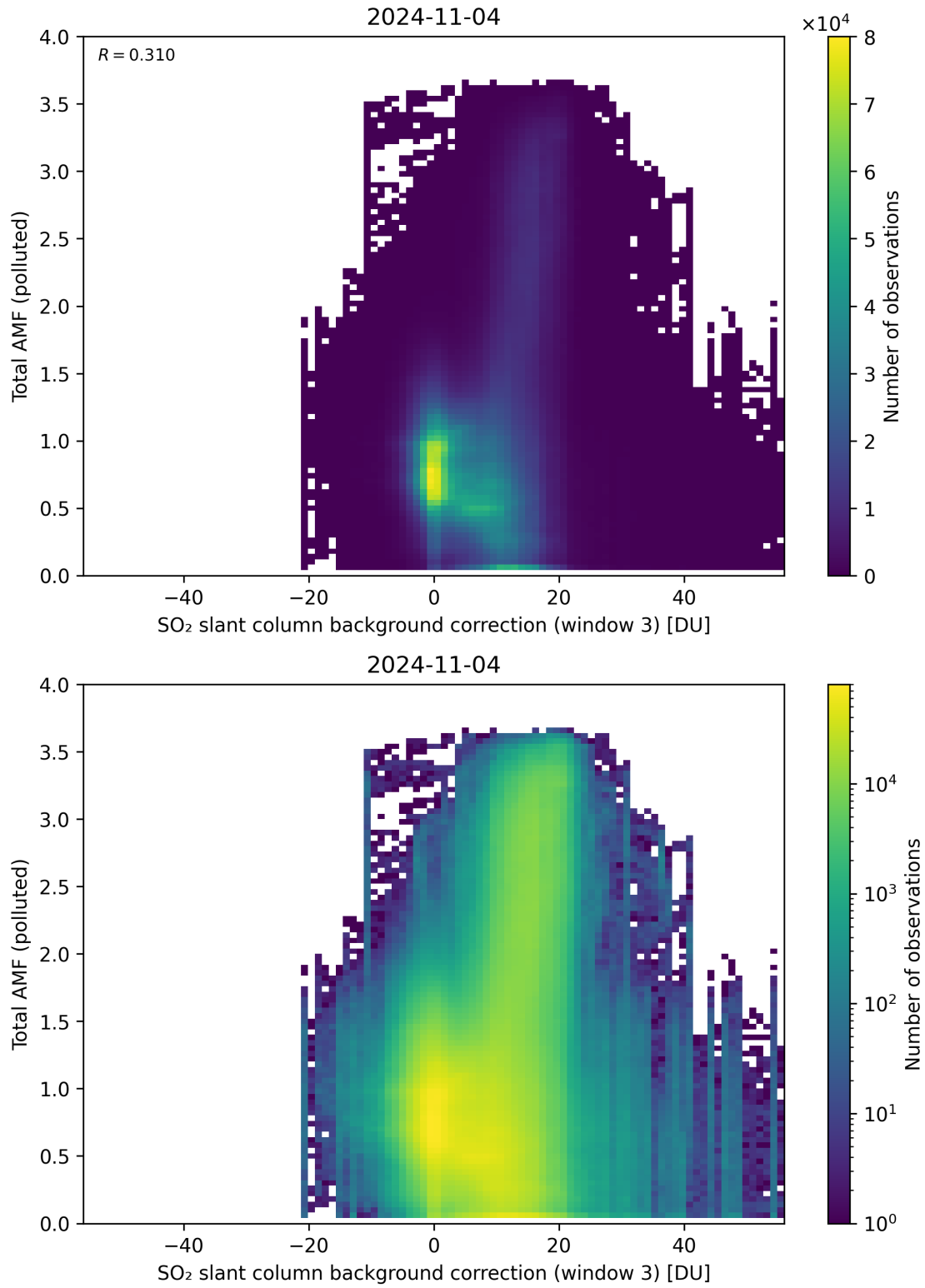
Figure 125: Scatter density plot of “SO 2 slant column background correction (window 3)” against “Total AMF (polluted)” for 2024-11-04 to 2024-11-05.
