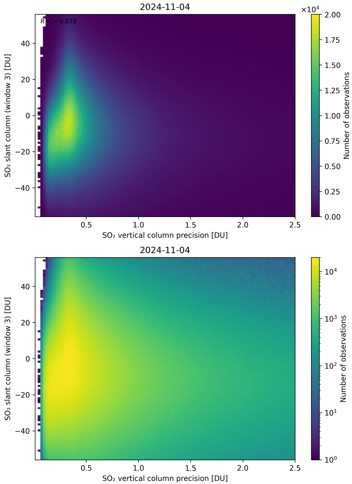
Figure 292: Scatter density plot of “SO 2 vertical column precision” against “SO 2 slant column (window 3)” for 2024-11-04 to 2024-11-05.
