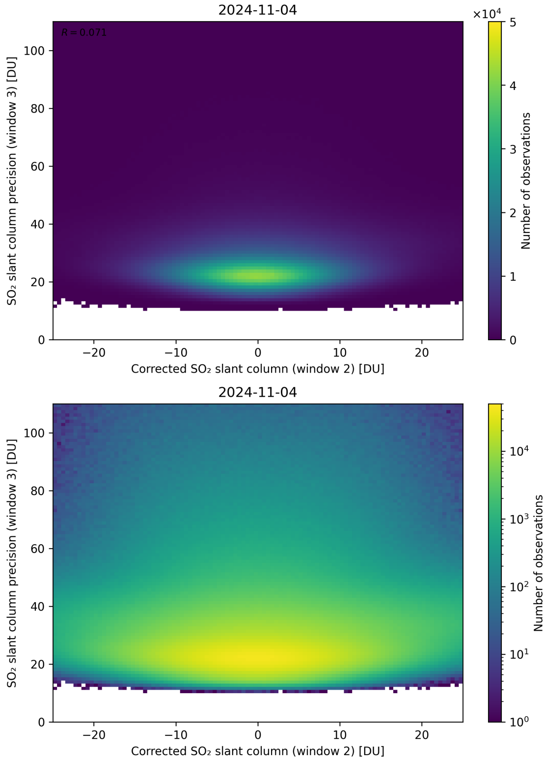
Figure 202: Scatter density plot of “Corrected SO 2 slant column (window 2)” against “SO 2 slant column precision (window 3)” for 2024-11-04 to 2024-11-05.
