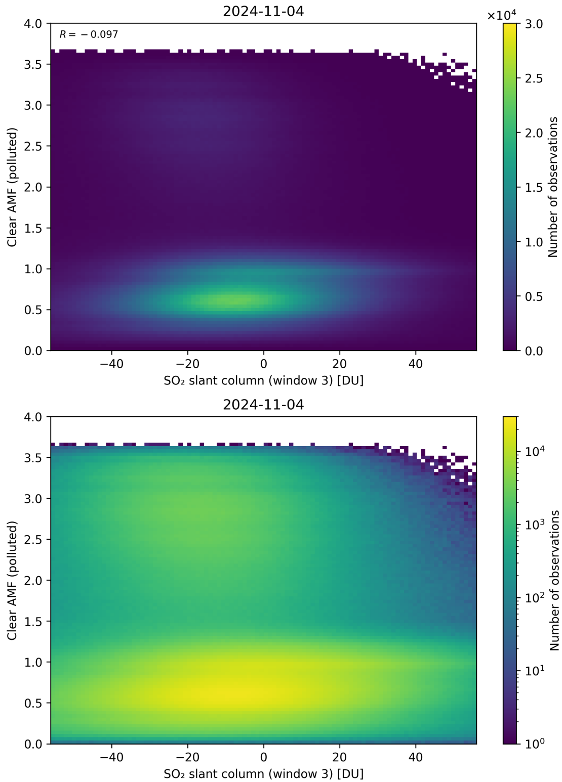
Figure 265: Scatter density plot of “SO 2 slant column (window 3)” against “Clear AMF (polluted)” for 2024-11-04 to 2024-11-05.
