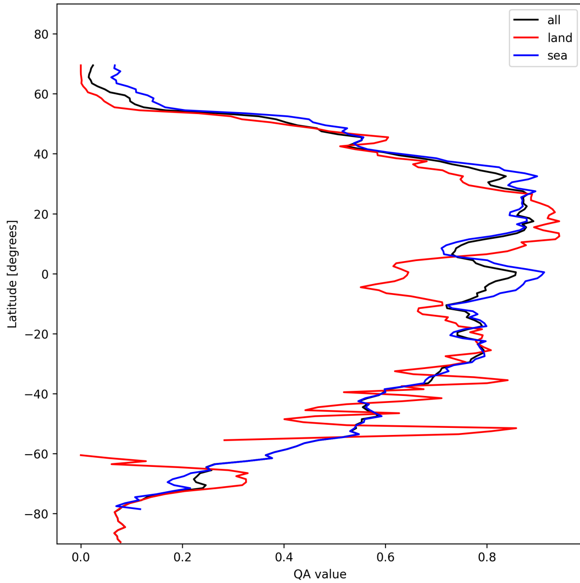
Figure 29: Zonal average of “QA value” for 2024-11-04 to 2024-11-05.
