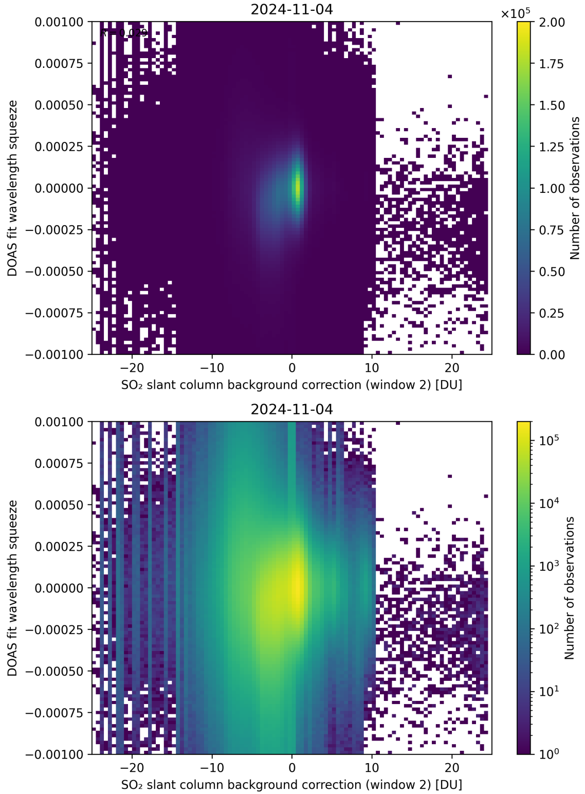
Figure 113: Scatter density plot of “SO 2 slant column background correction (window 2)” against “DOAS fit wavelength squeeze” for 2024-11-04 to 2024-11-05.
