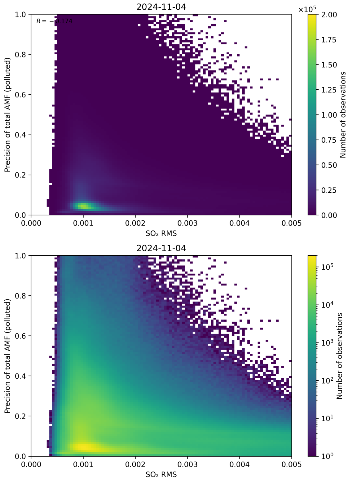
Figure 138: Scatter density plot of “SO 2 RMS” against “Precision of total AMF (polluted)” for 2024-11-04 to 2024-11-05.
