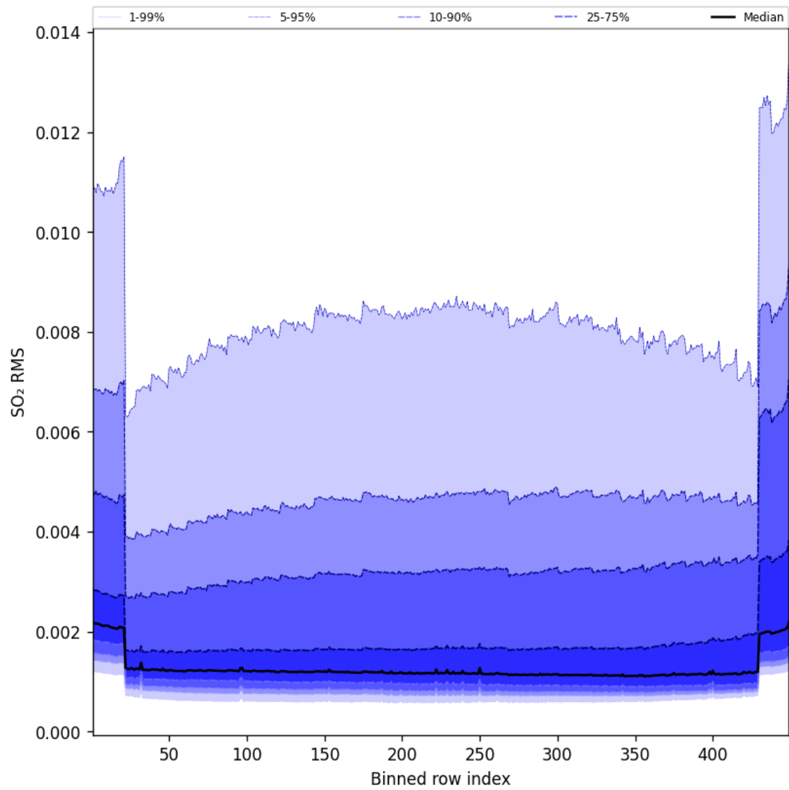
Figure 93: Along track statistics of “SO 2 RMS” for 2024-11-04 to 2024-11-05
