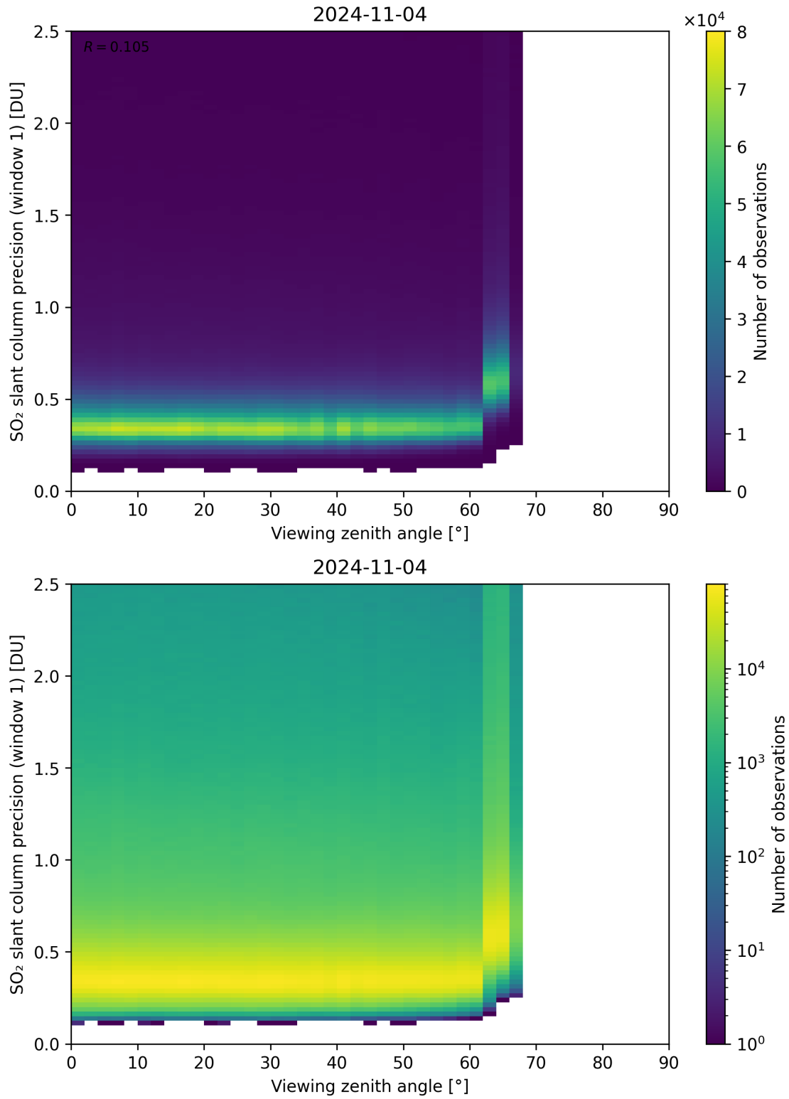
Figure 321: Scatter density plot of “Viewing zenith angle” against “SO 2 slant column precision (window 1)” for 2024-11-04 to 2024-11-05.
