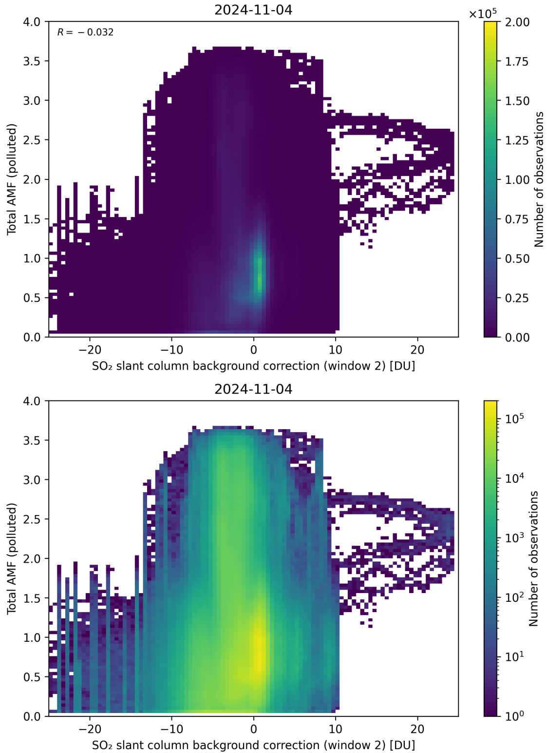
Figure 119: Scatter density plot of “SO 2 slant column background correction (window 2)” against “Total AMF (polluted)” for 2024-11-04 to 2024-11-05.
