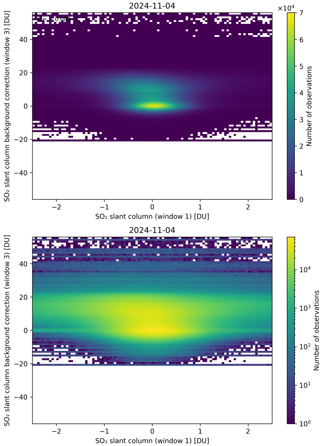
Figure 214: Scatter density plot of “SO 2 slant column (window 1)” against “SO 2 slant column background correction (window 3)” for 2024-11-04 to 2024-11-05.
