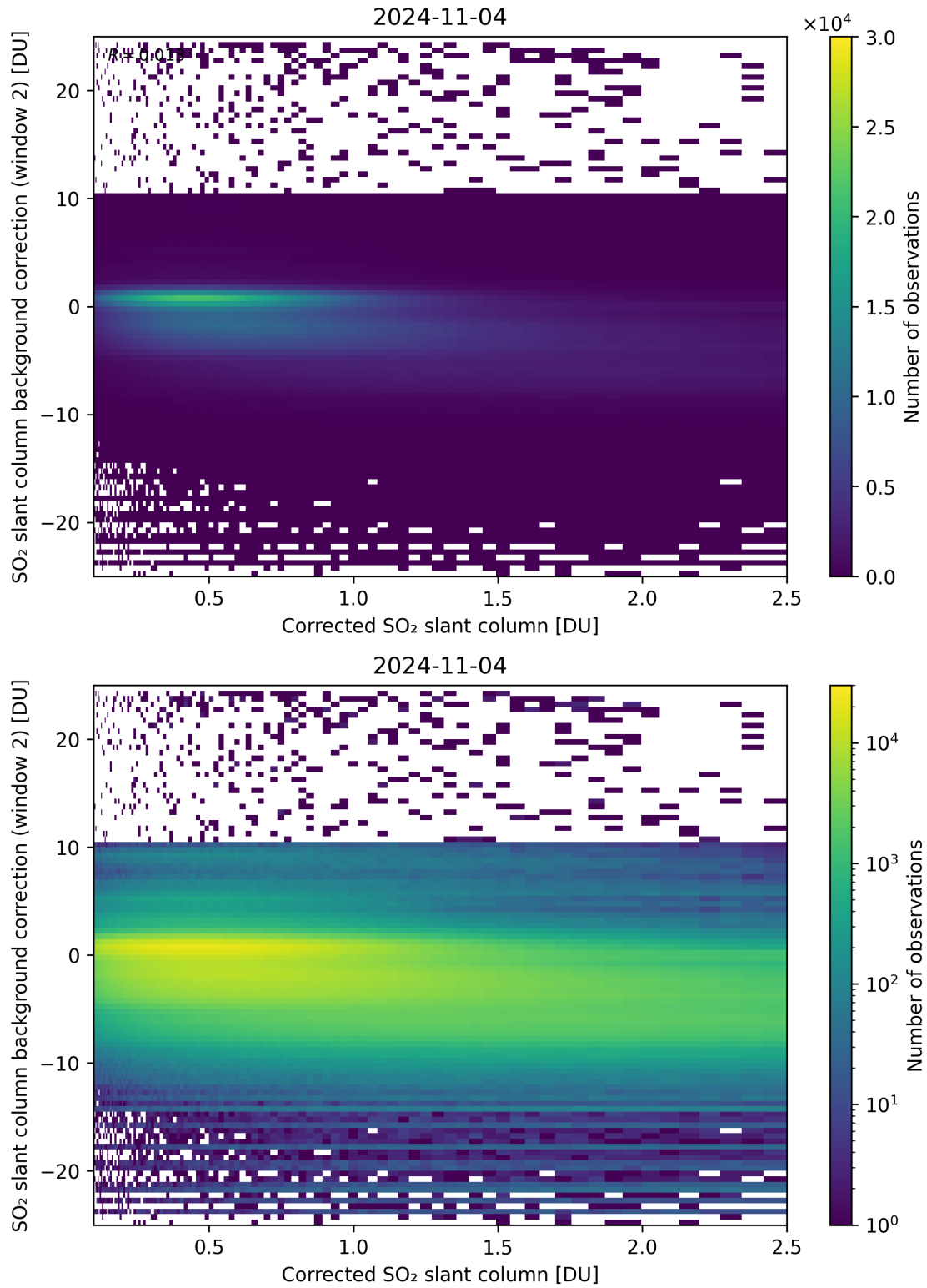
Figure 179: Scatter density plot of “Corrected SO 2 slant column” against “SO 2 slant column background correction (window 2)” for 2024-11-04 to 2024-11-05.
