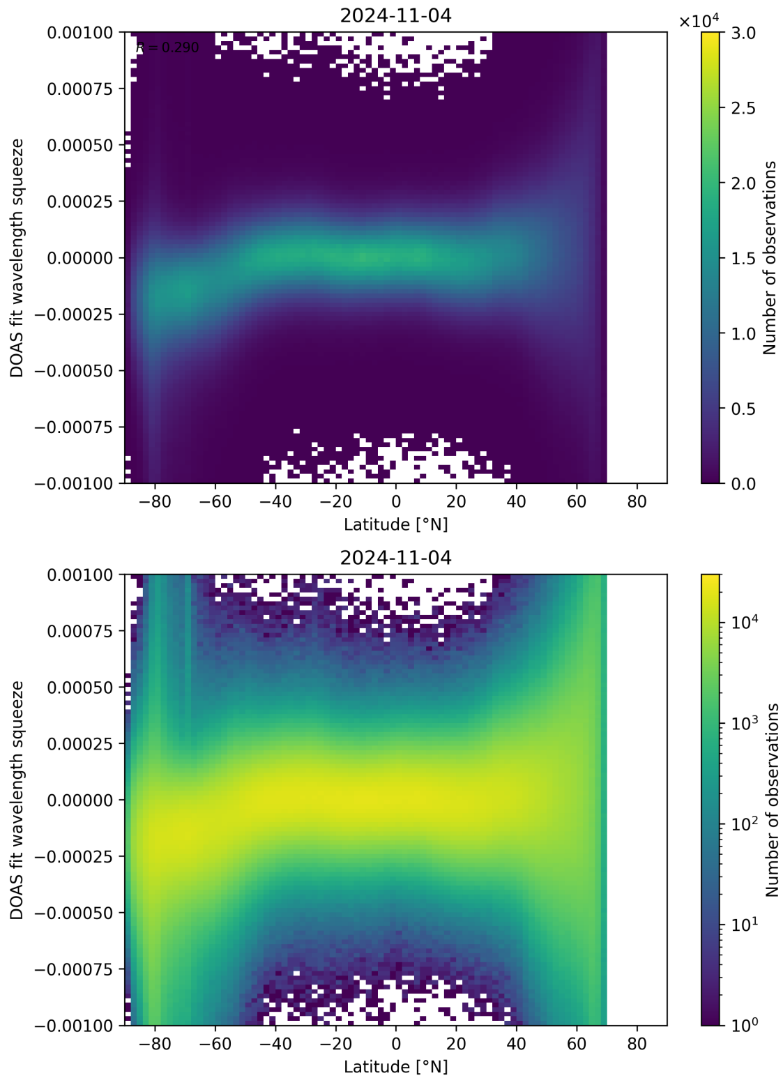
Figure 143: Scatter density plot of “Latitude” against “DOAS fit wavelength squeeze” for 2024-11-04 to 2024-11-05.
