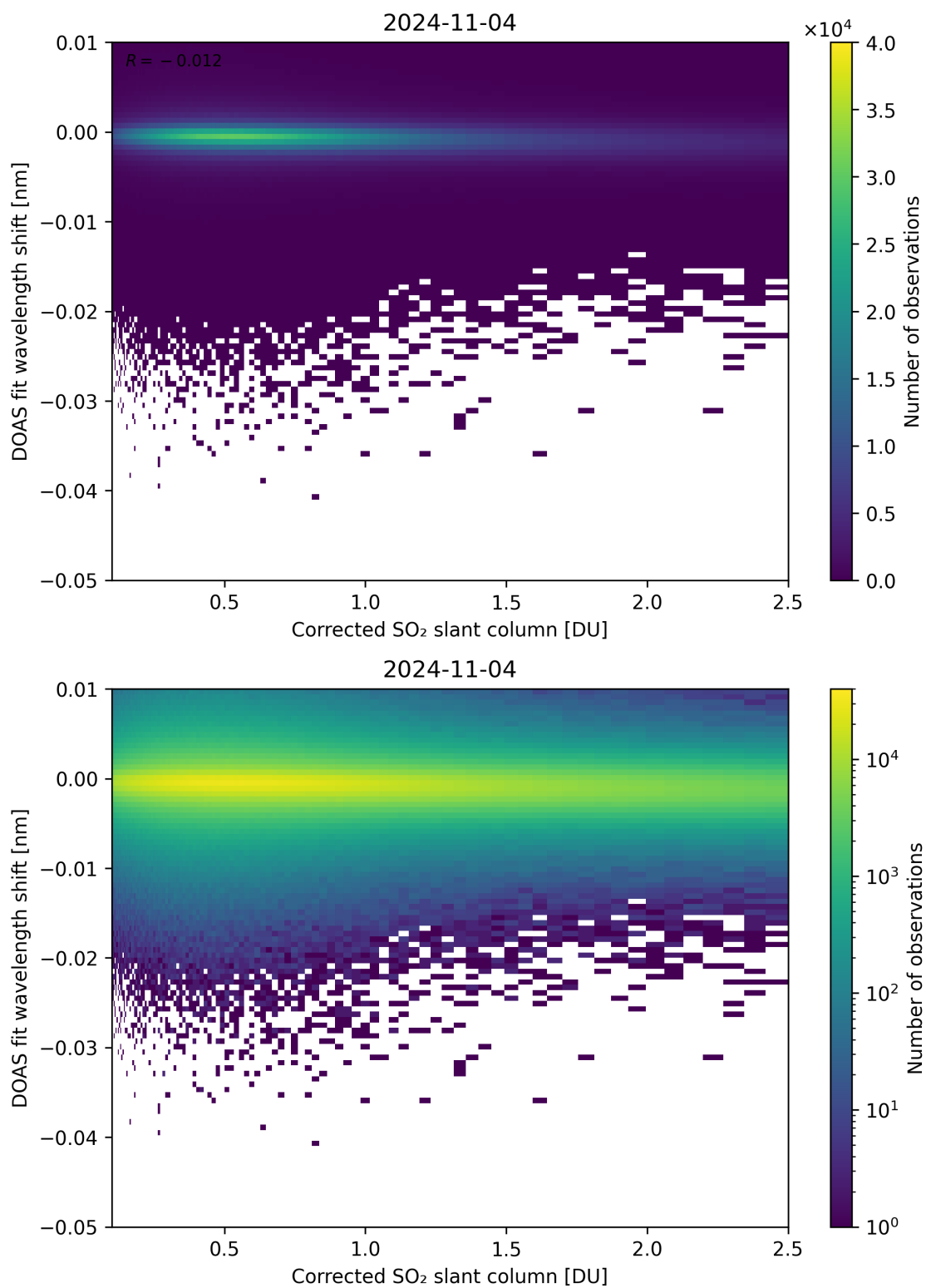
Figure 181: Scatter density plot of “Corrected SO 2 slant column” against “DOAS fit wavelength shift” for 2024-11-04 to 2024-11-05.
