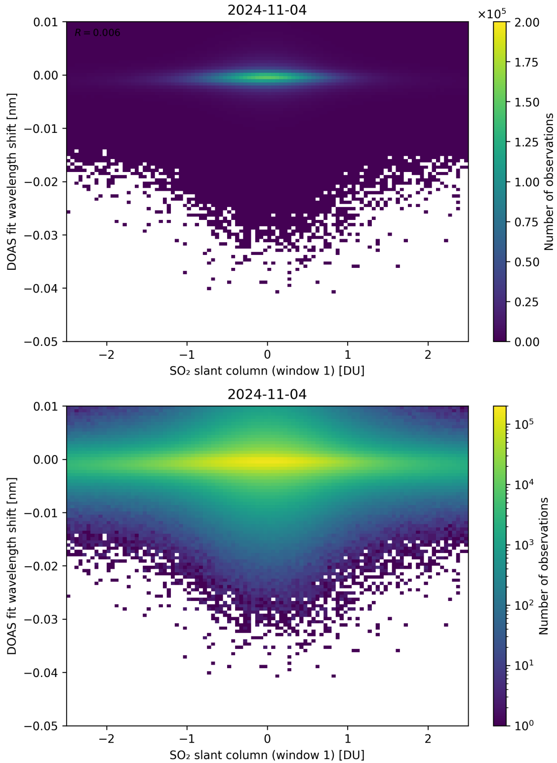
Figure 215: Scatter density plot of “SO 2 slant column (window 1)” against “DOAS fit wavelength shift” for 2024-11-04 to 2024-11-05.
