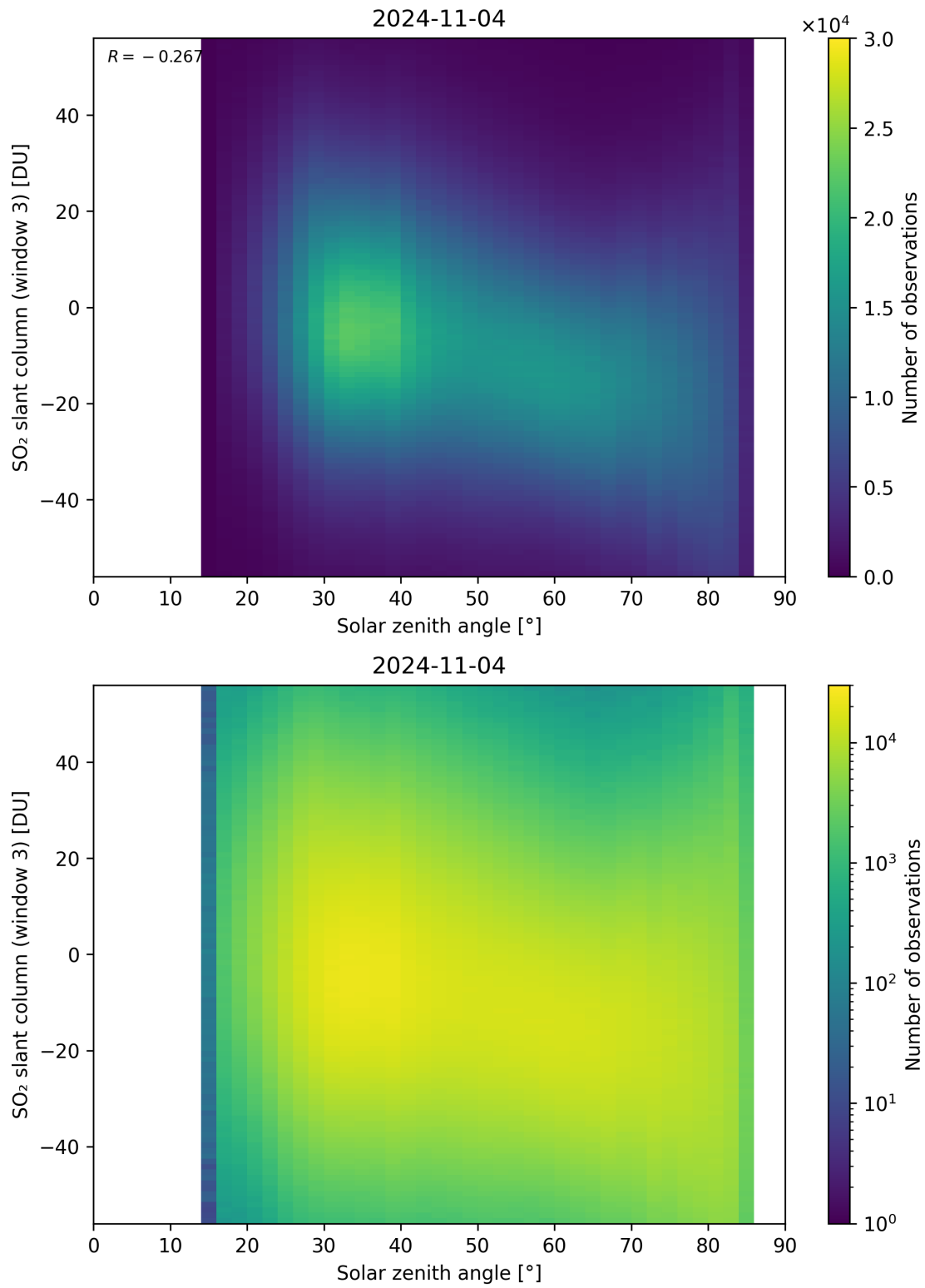
Figure 172: Scatter density plot of “Solar zenith angle” against “SO 2 slant column (window 3)” for 2024-11-04 to 2024-11-05.
