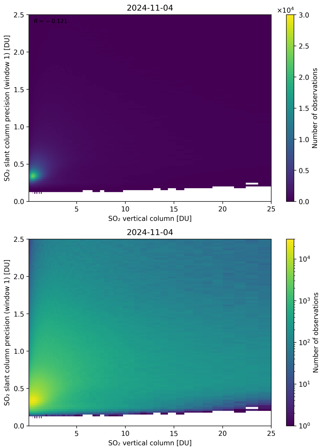
Figure 301: Scatter density plot of “SO 2 vertical column” against “SO 2 slant column precision (window 1)” for 2024-11-04 to 2024-11-05.
