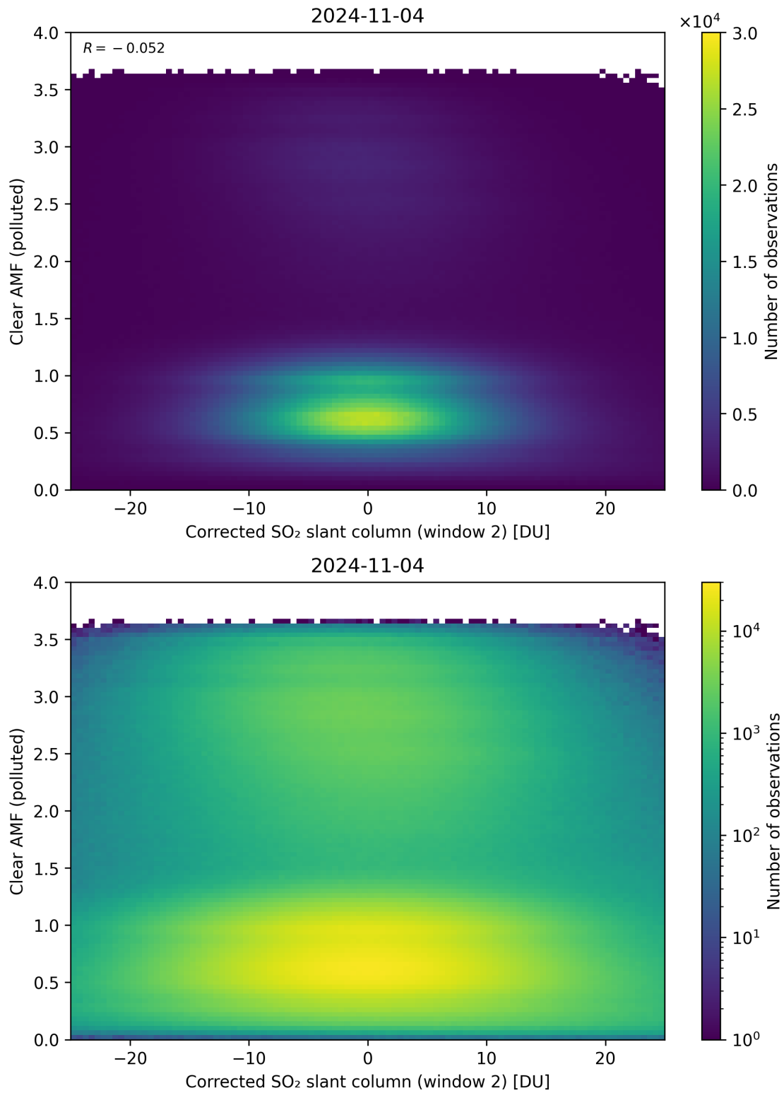
Figure 199: Scatter density plot of “Corrected SO 2 slant column (window 2)” against “Clear AMF (polluted)” for 2024-11-04 to 2024-11-05.
