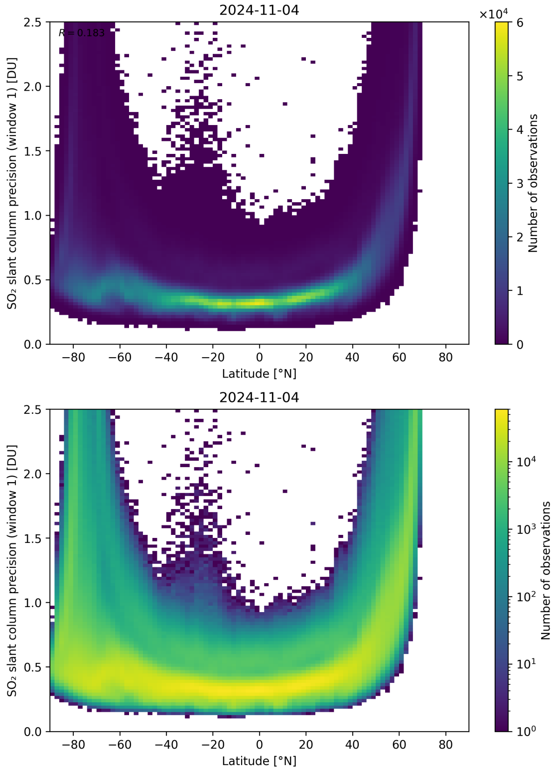
Figure 150: Scatter density plot of “Latitude” against “SO 2 slant column precision (window 1)” for 2024-11-04 to 2024-11-05.
