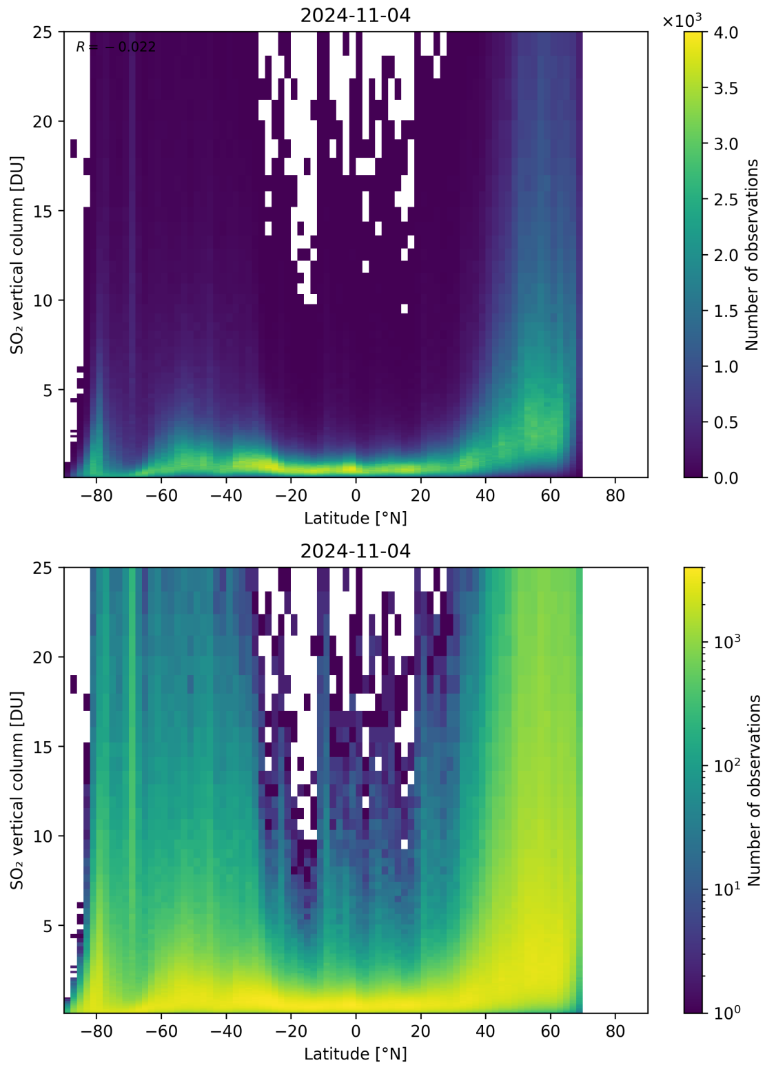
Figure 156: Scatter density plot of “Latitude” against “SO 2 vertical column” for 2024-11-04 to 2024-11-05.
