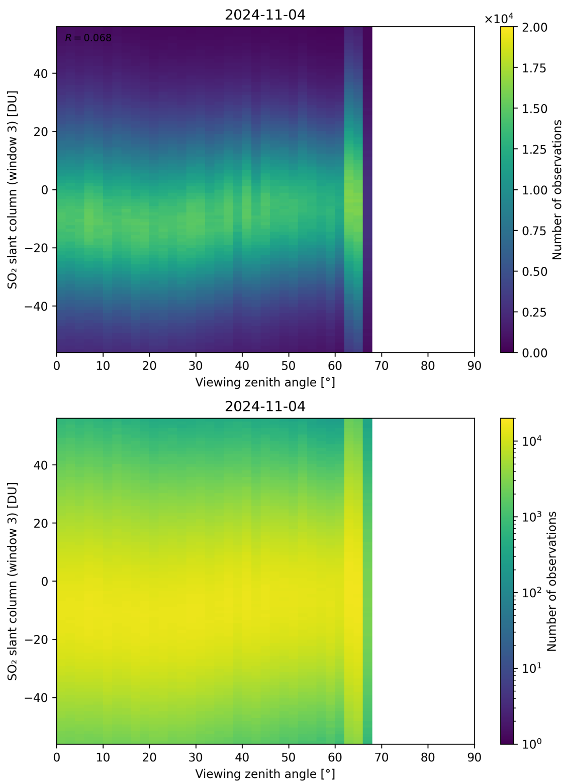
Figure 323: Scatter density plot of “Viewing zenith angle” against “SO 2 slant column (window 3)” for 2024-11-04 to 2024-11-05.
