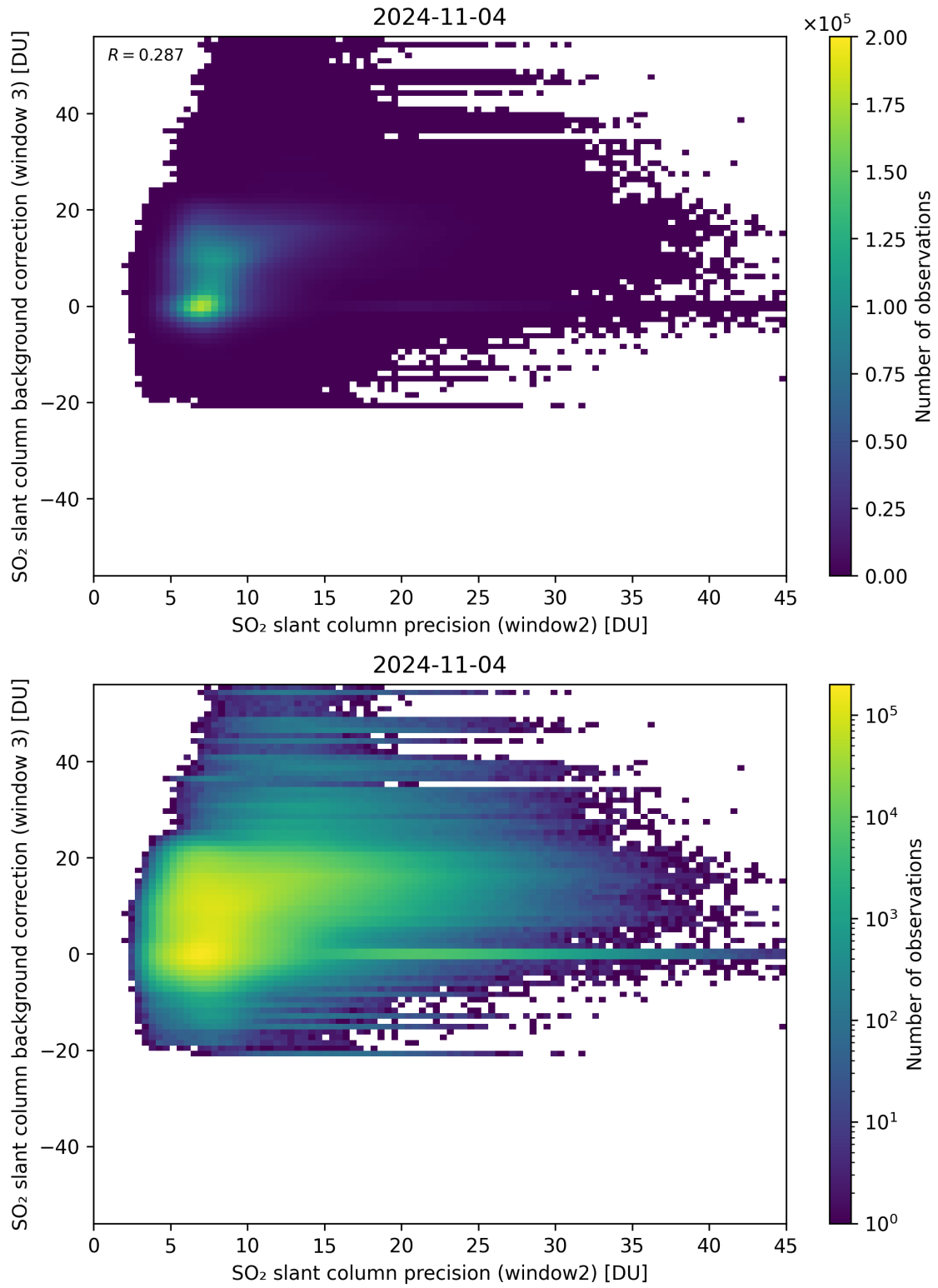
Figure 242: Scatter density plot of “SO 2 slant column precision (window2)” against “SO 2 slant column background correction (window 3)” for 2024-11-04 to 2024-11-05.
