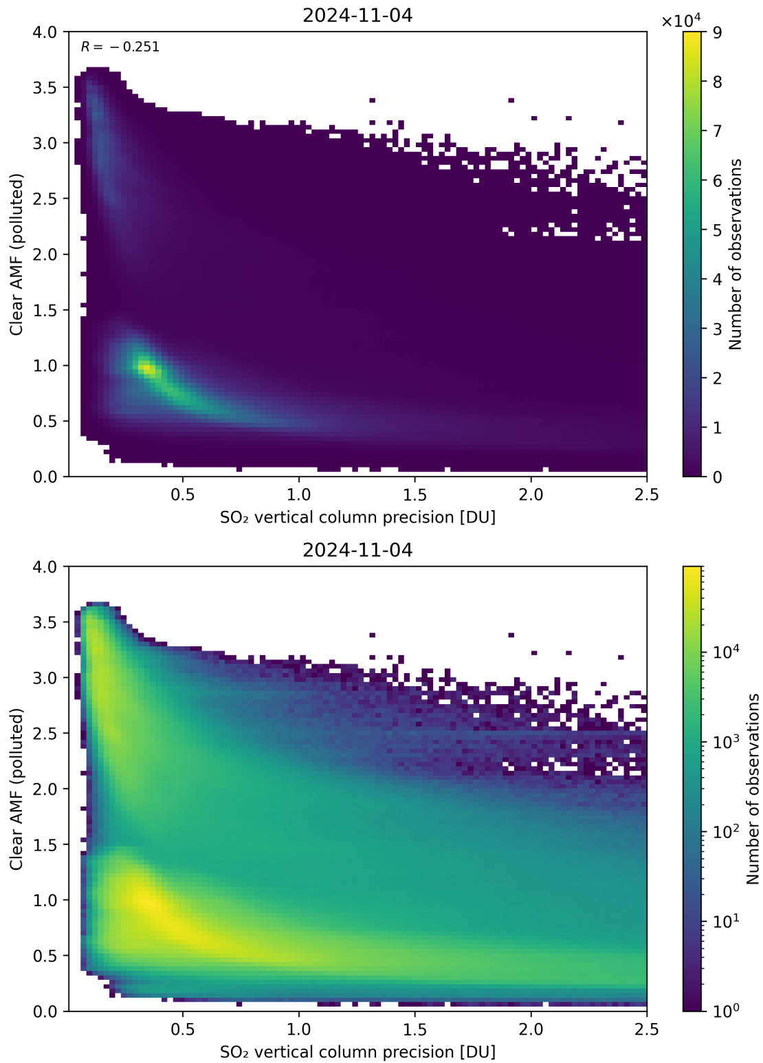
Figure 285: Scatter density plot of “SO 2 vertical column precision” against “Clear AMF (polluted)” for 2024-11-04 to 2024-11-05.
