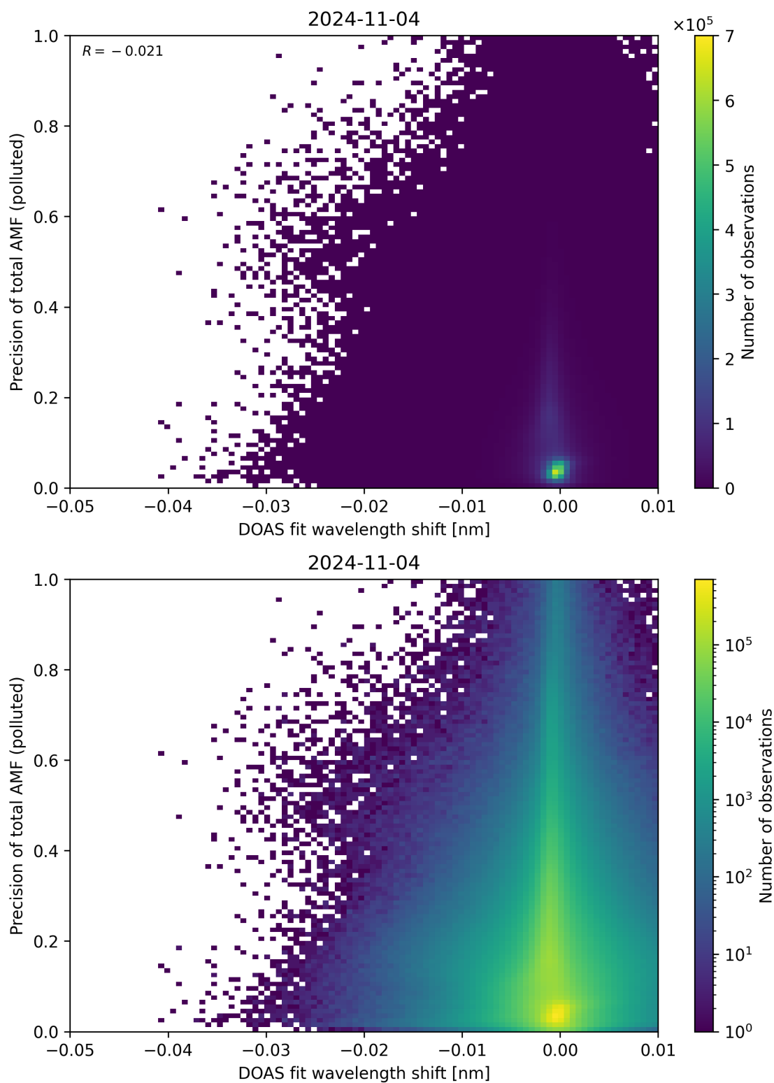
Figure 131: Scatter density plot of “DOAS fit wavelength shift” against “Precision of total AMF (polluted)” for 2024-11-04 to 2024-11-05.
