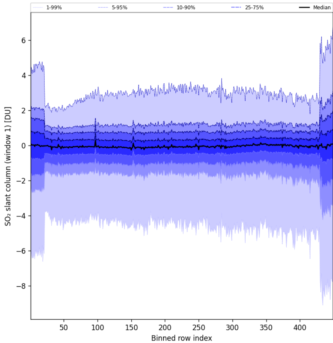
Figure 79: Along track statistics of “SO 2 slant column (window 1)” for 2024-11-04 to 2024-11-05
