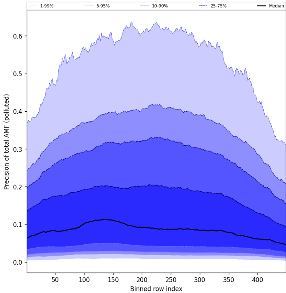
Figure 95: Along track statistics of “Precision of total AMF (polluted)” for 2024-11-04 to 2024-11-05
