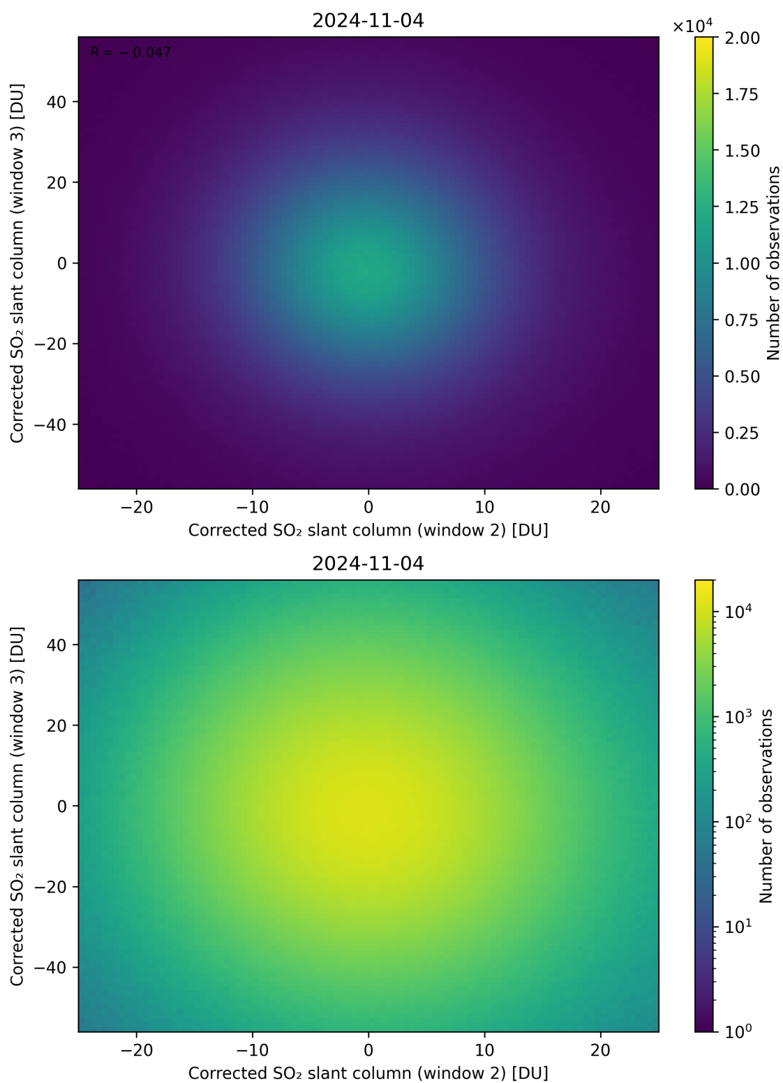
Figure 200: Scatter density plot of “Corrected SO 2 slant column (window 2)” against “Corrected SO 2 slant column (window 3)” for 2024-11-04 to 2024-11-05.
