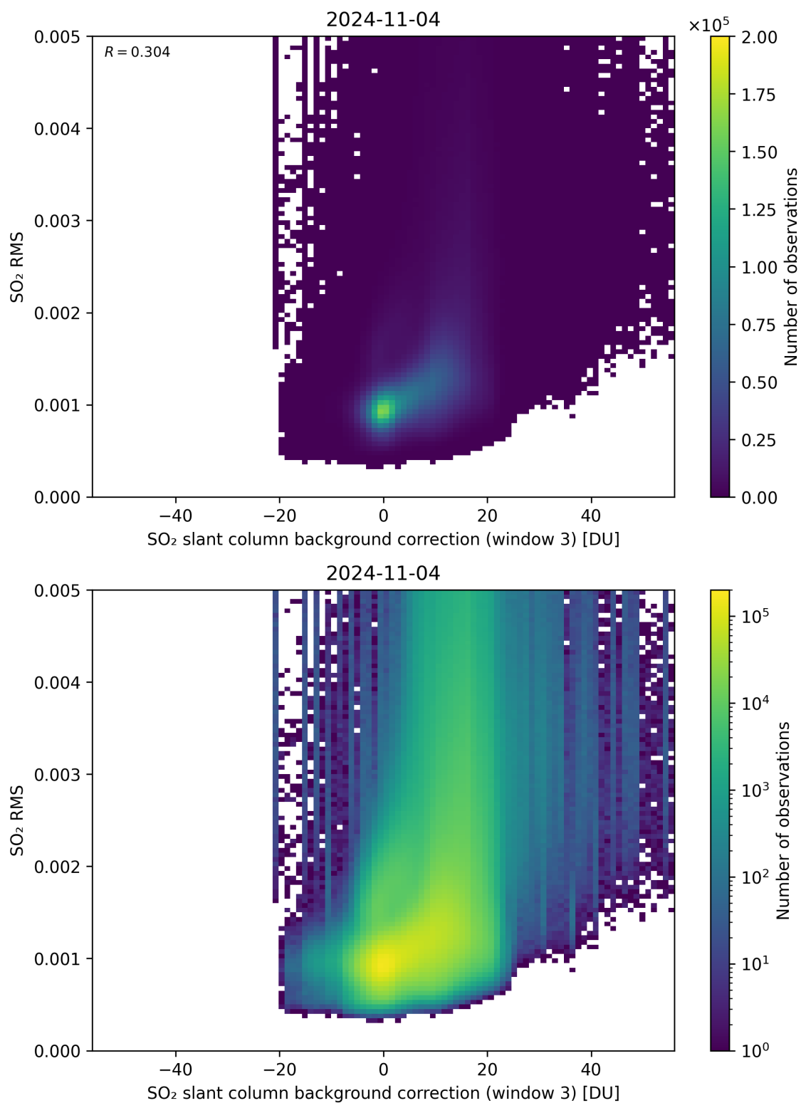
Figure 123: Scatter density plot of “SO 2 slant column background correction (window 3)” against “SO 2 RMS” for 2024-11-04 to 2024-11-05.
