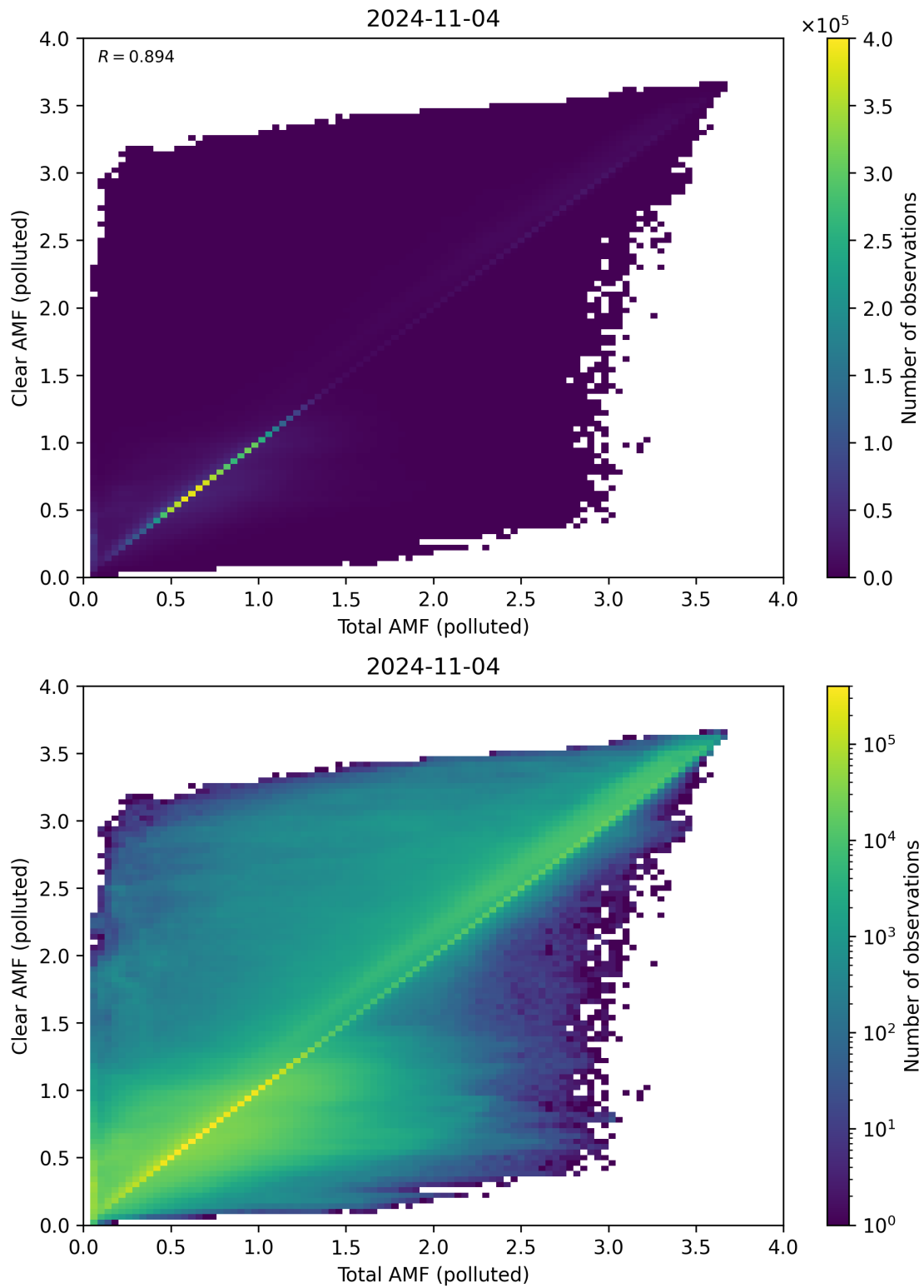
Figure 271: Scatter density plot of “Total AMF (polluted)” against “Clear AMF (polluted)” for 2024-11-04 to 2024-11-05.
