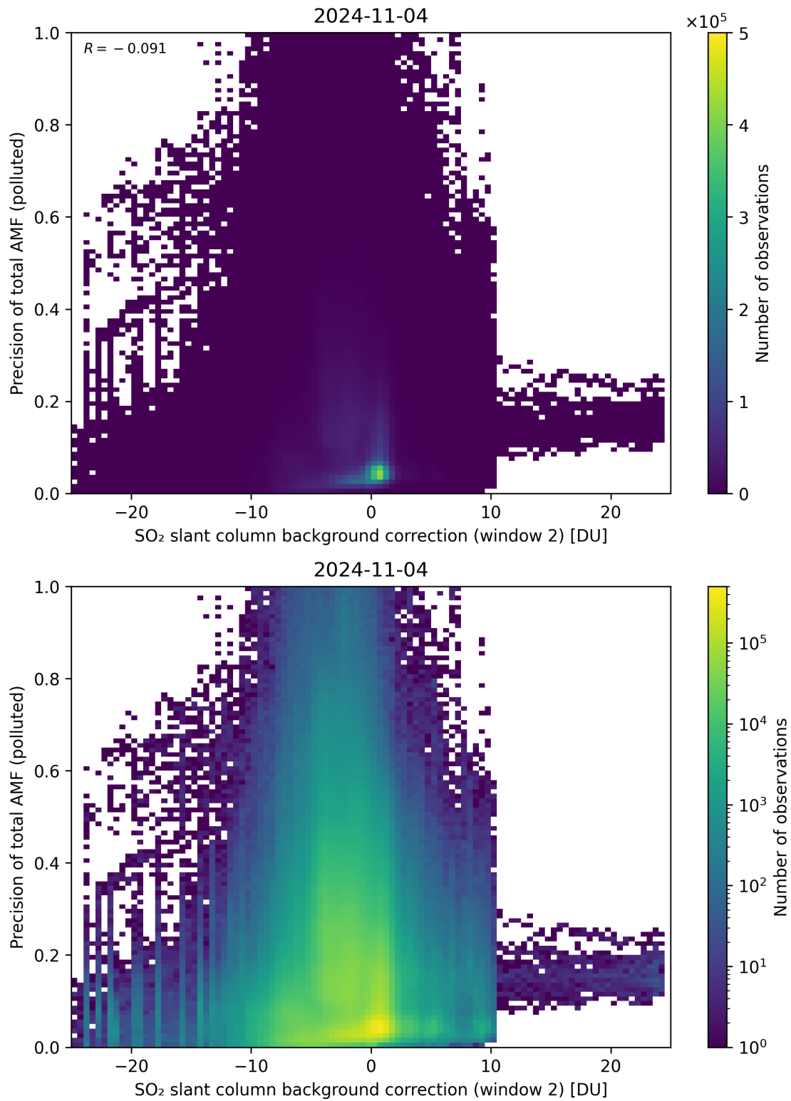
Figure 120: Scatter density plot of “SO 2 slant column background correction (window 2)” against “Precision of total AMF (polluted)” for 2024-11-04 to 2024-11-05.
