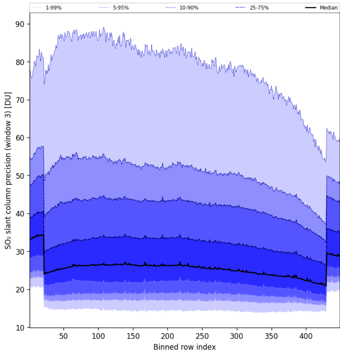
Figure 88: Along track statistics of “SO 2 slant column precision (window 3)” for 2024-11-04 to 2024-11-05
