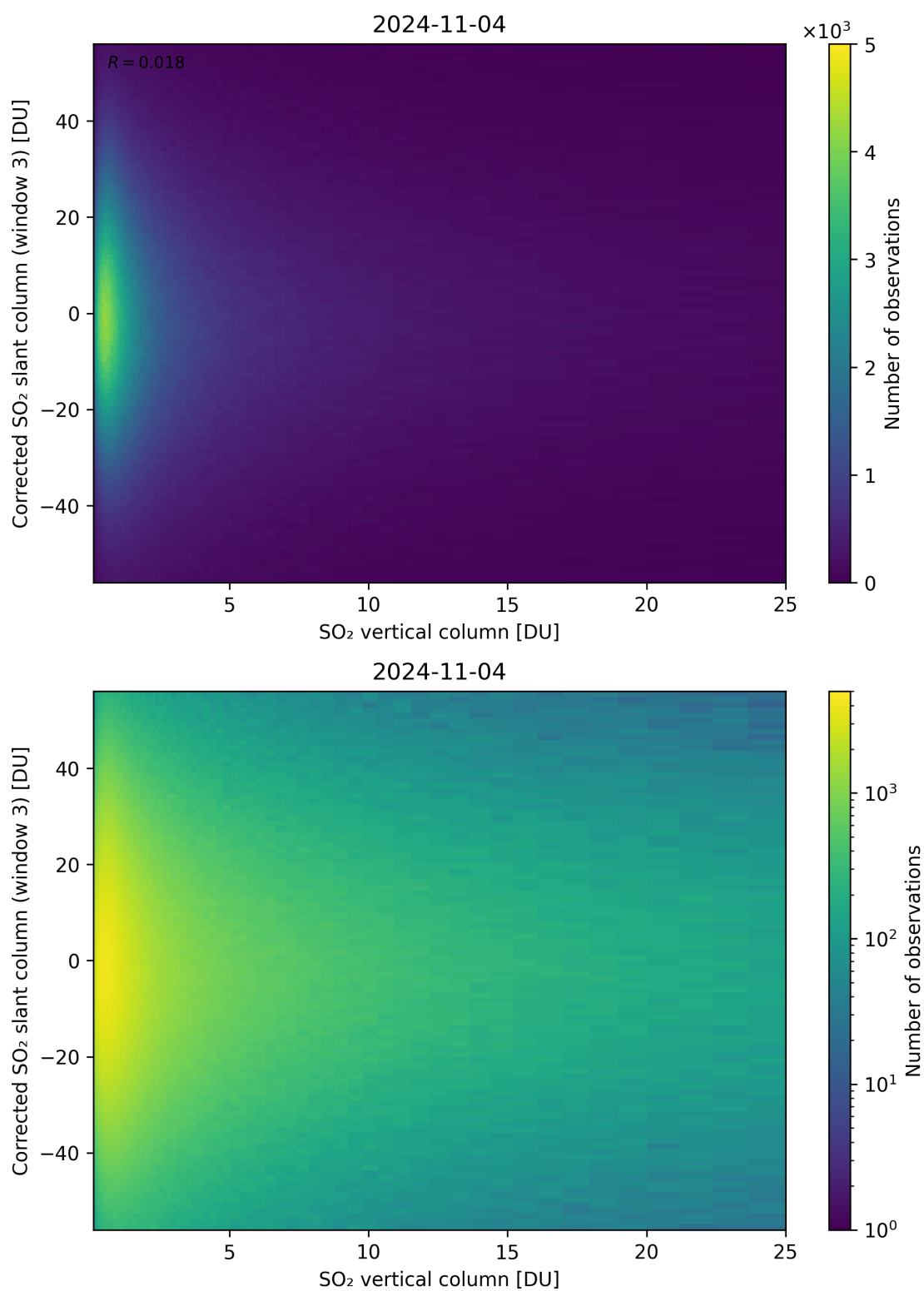
Figure 299: Scatter density plot of “SO 2 vertical column” against “Corrected SO 2 slant column (window 3)” for 2024-11-04 to 2024-11-05.
