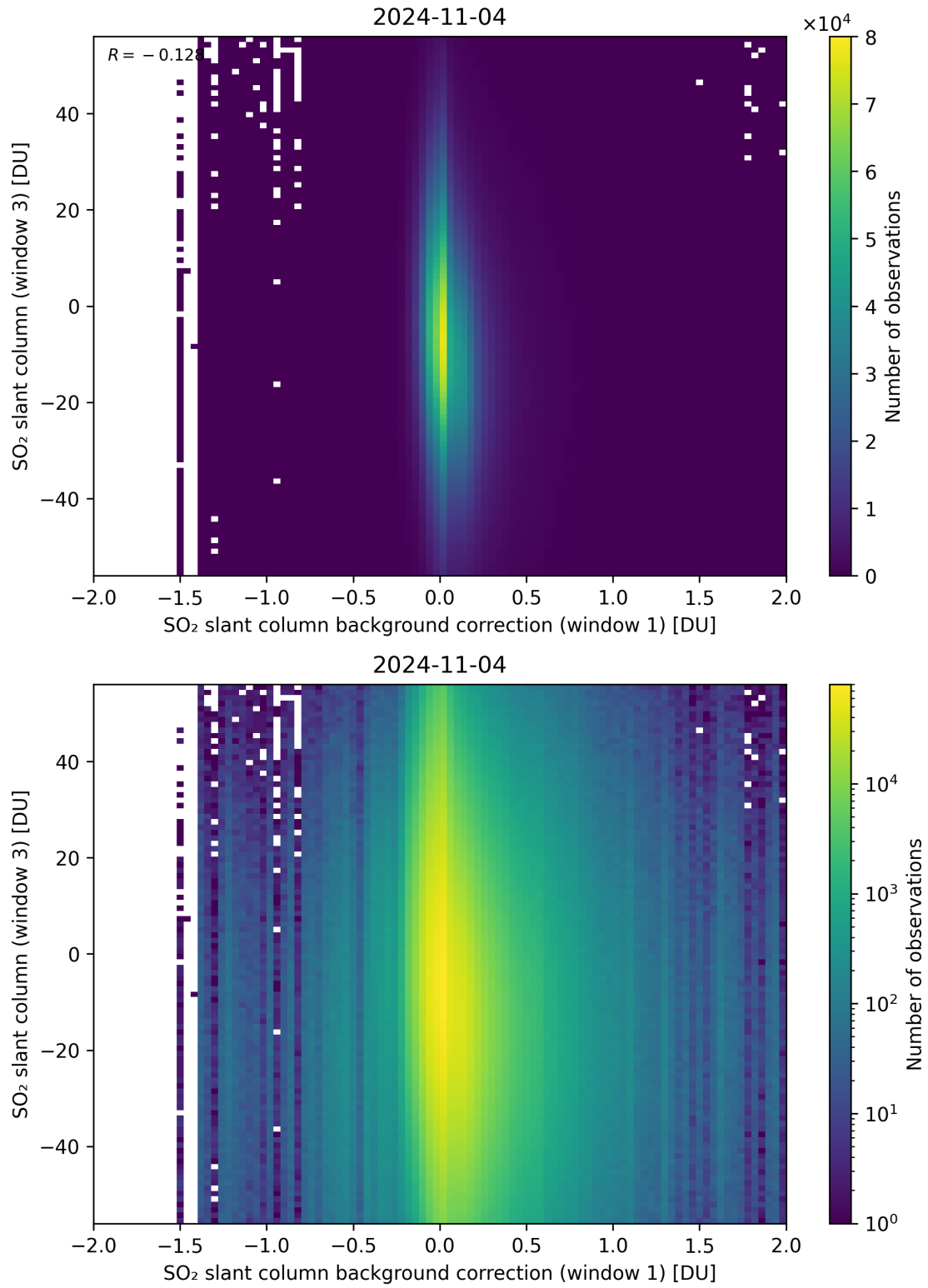
Figure 107: Scatter density plot of “SO 2 slant column background correction (window 1)” against “SO 2 slant column (window 3)” for 2024-11-04 to 2024-11-05.
