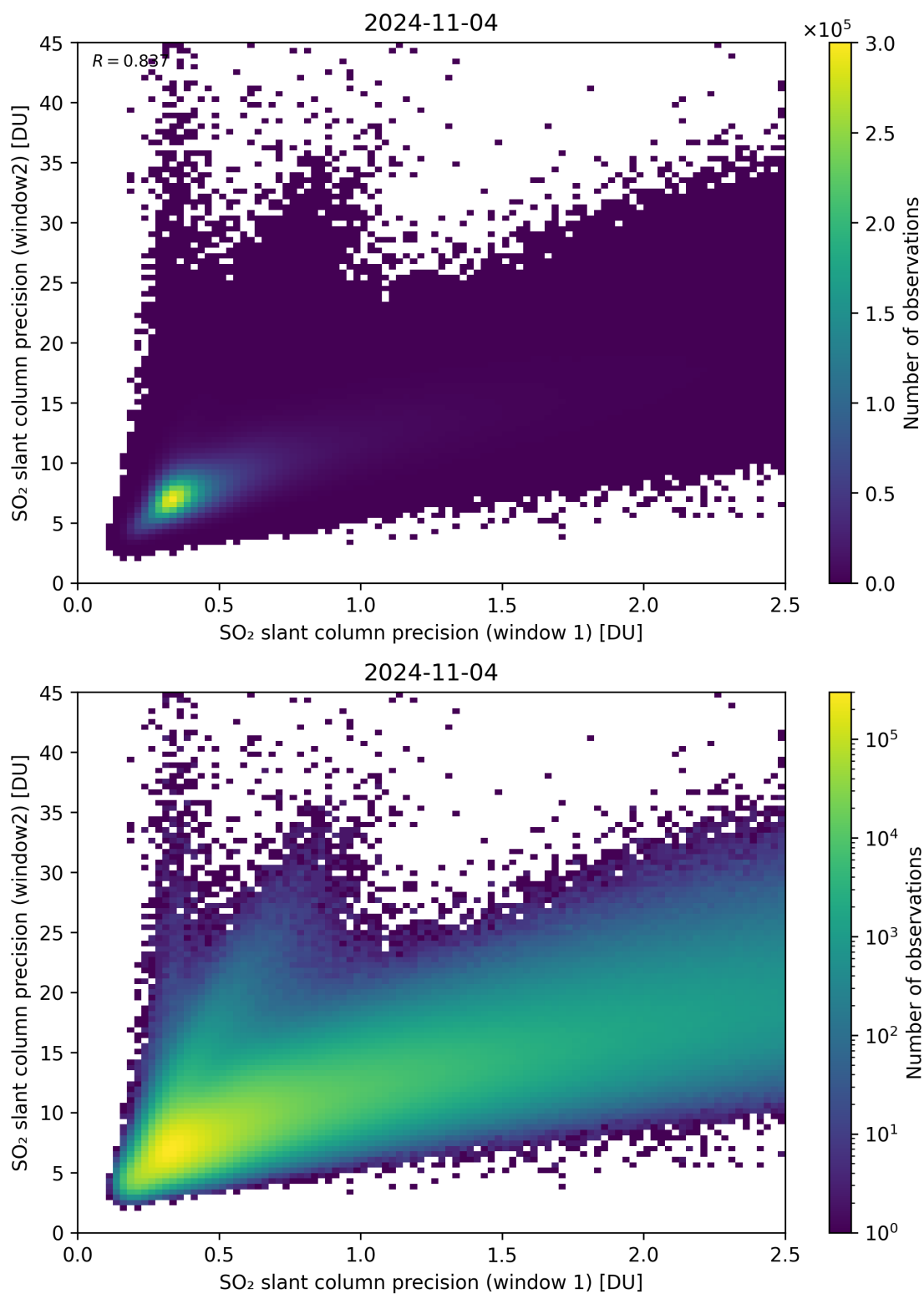
Figure 227: Scatter density plot of “SO 2 slant column precision (window 1)” against “SO 2 slant column precision (window2)” for 2024-11-04 to 2024-11-05.
