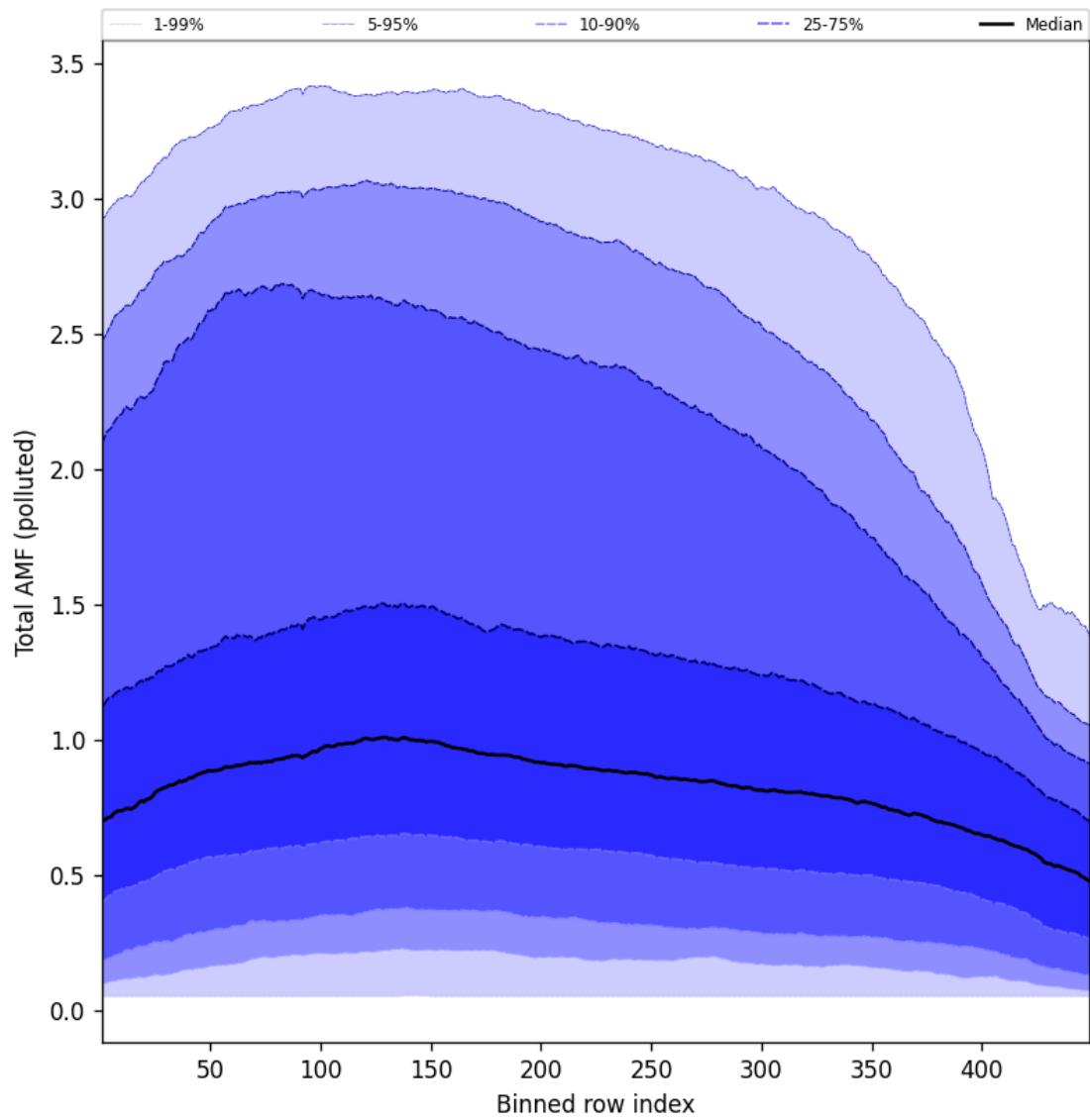
Figure 94: Along track statistics of “Total AMF (polluted)” for 2024-11-04 to 2024-11-05
