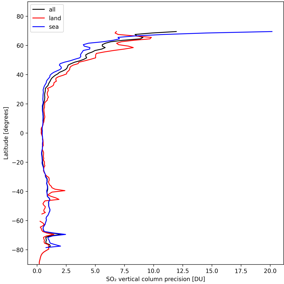
Figure 31: Zonal average of “SO 2 vertical column precision” for 2024-11-04 to 2024-11-05.
