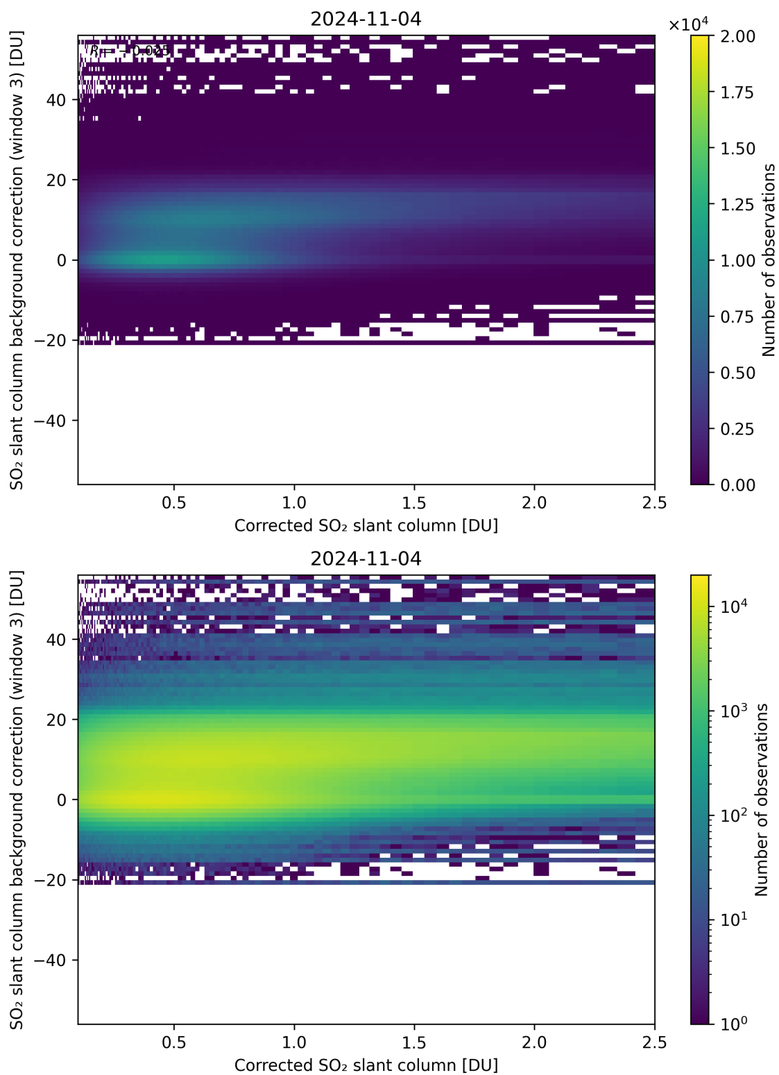
Figure 180: Scatter density plot of “Corrected SO 2 slant column” against “SO 2 slant column background correction (window 3)” for 2024-11-04 to 2024-11-05.
