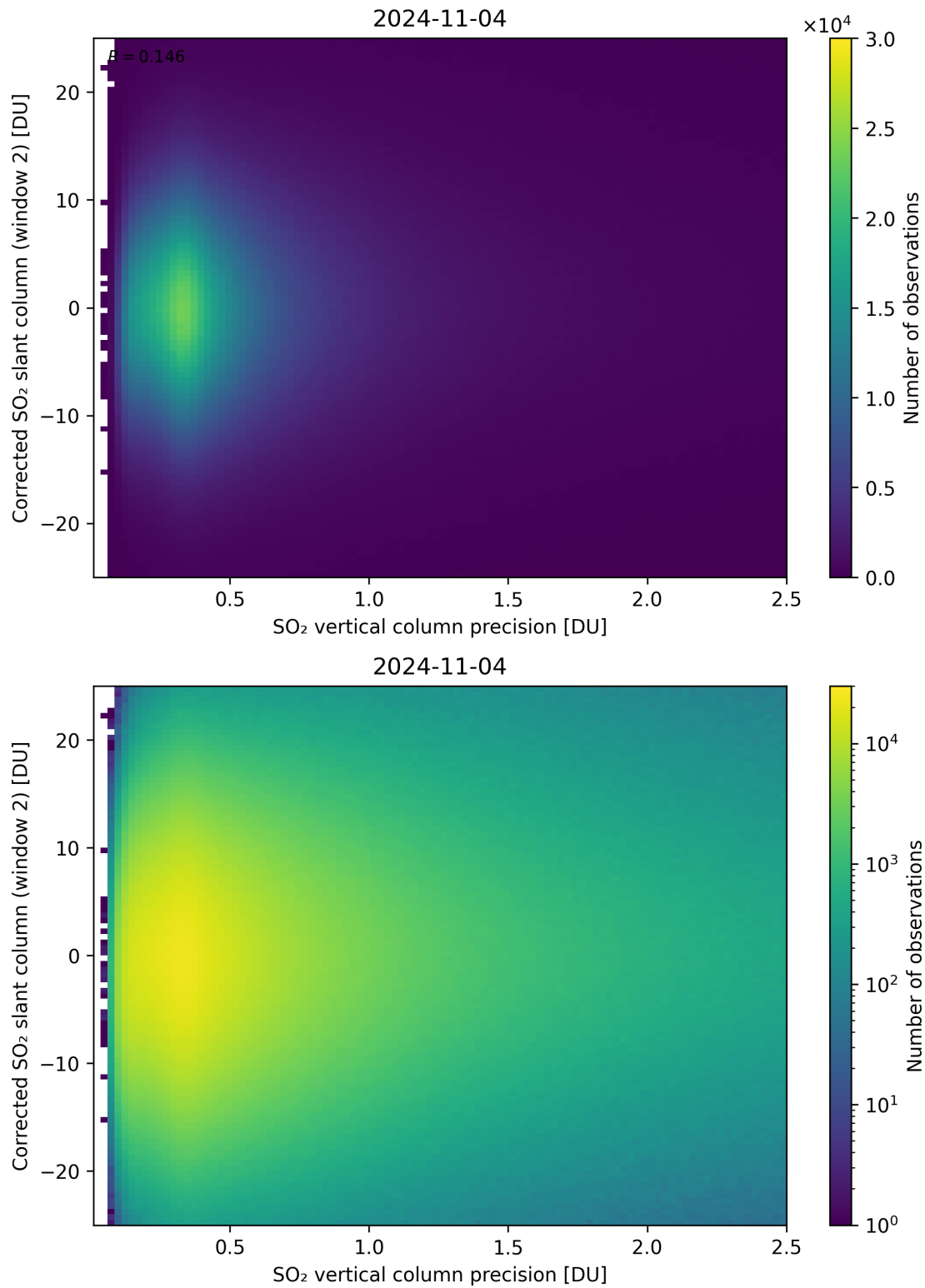
Figure 287: Scatter density plot of “SO 2 vertical column precision” against “Corrected SO 2 slant column (window 2)” for 2024-11-04 to 2024-11-05.
