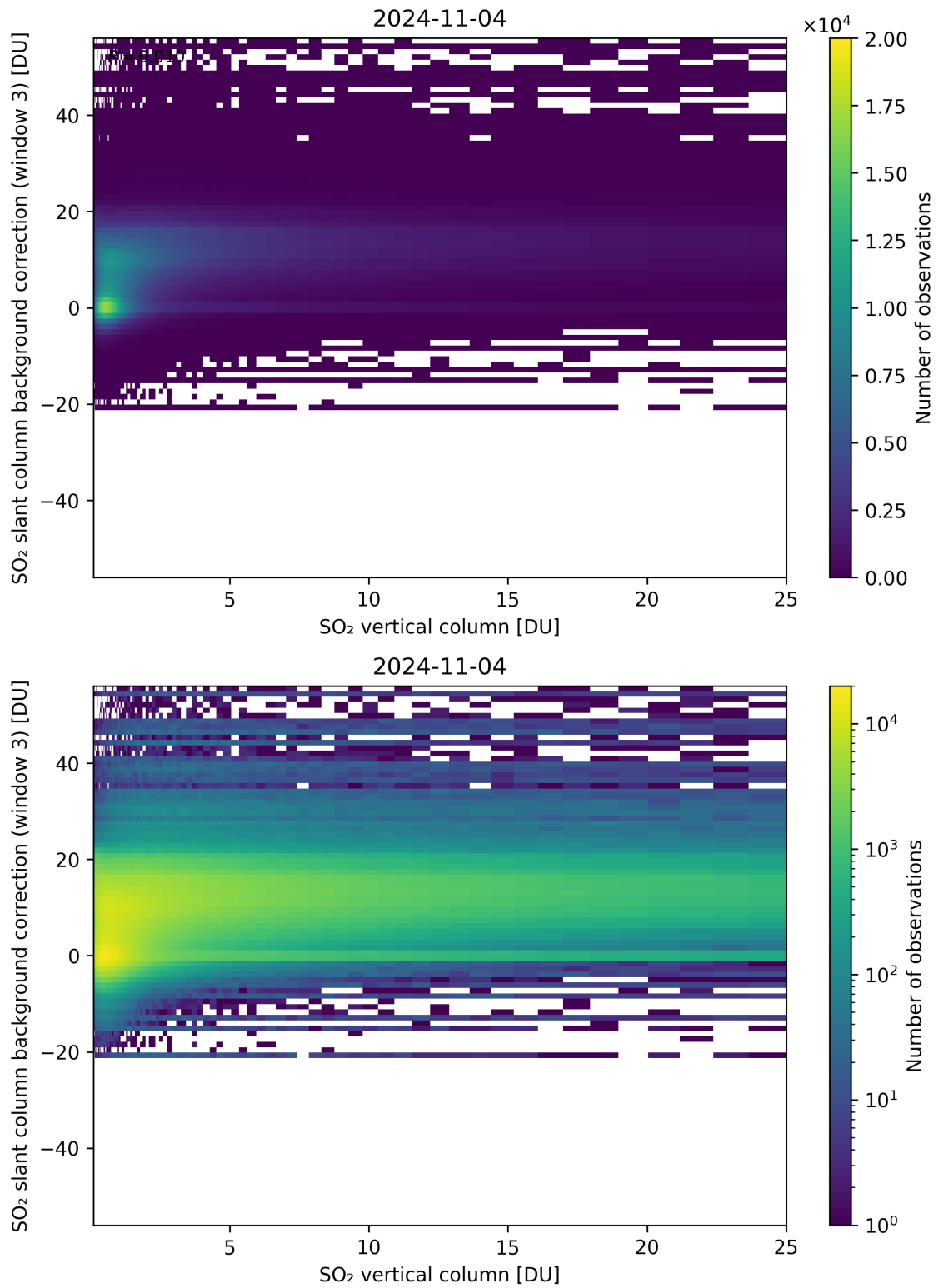
Figure 275: Scatter density plot of “SO 2 vertical column” against “SO 2 slant column background correction (window 3)” for 2024-11-04 to 2024-11-05.
