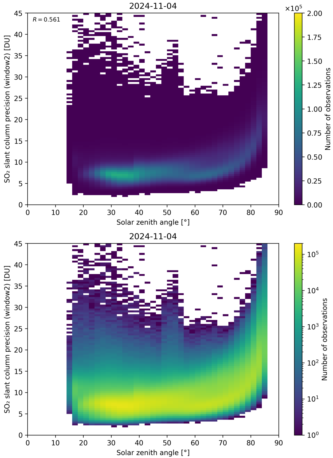
Figure 171: Scatter density plot of “Solar zenith angle” against “SO 2 slant column precision (window2)” for 2024-11-04 to 2024-11-05.
