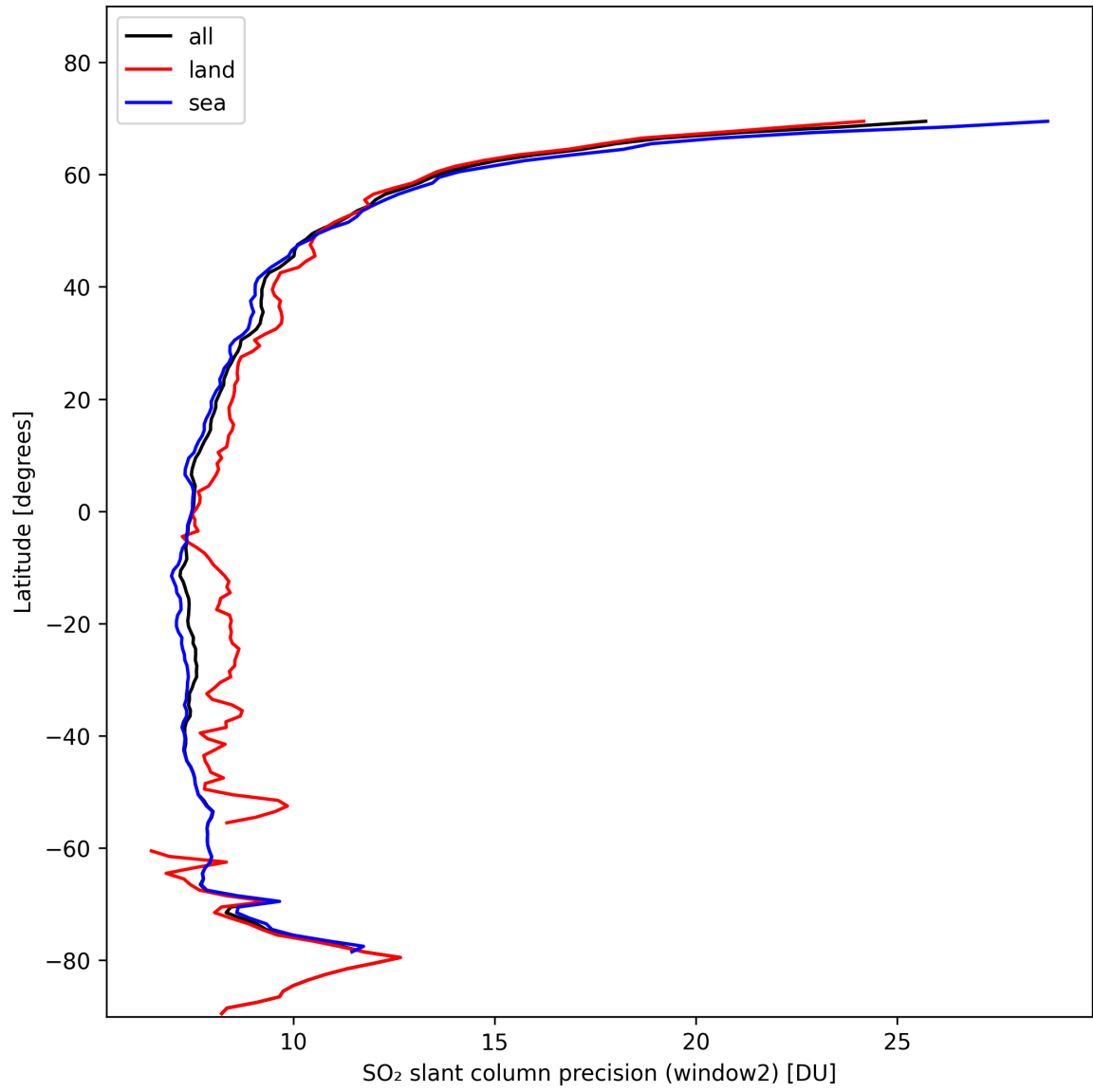
Figure 38: Zonal average of “SO 2 slant column precision (window2)” for 2024-11-04 to 2024-11-05.
