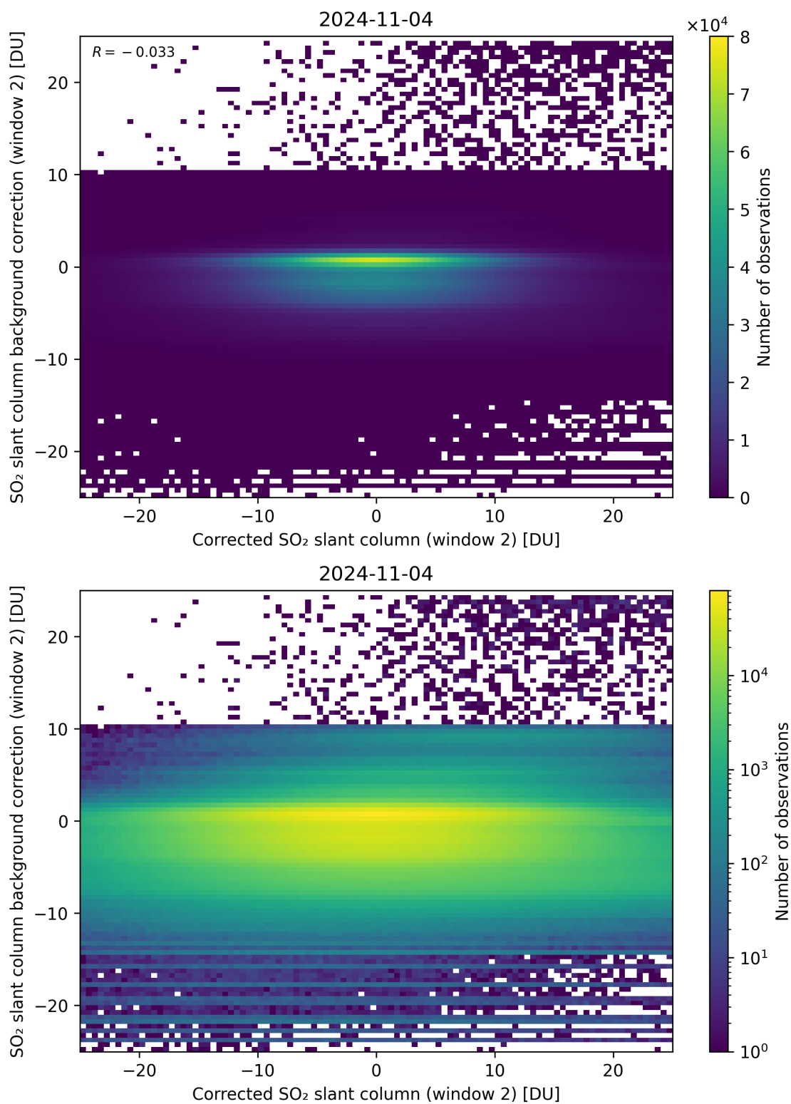
Figure 194: Scatter density plot of “Corrected SO 2 slant column (window 2)” against “SO 2 slant column background correction (window 2)” for 2024-11-04 to 2024-11-05.
