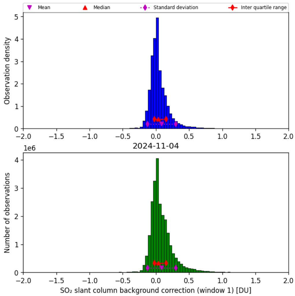
Figure 59: Histogram of “SO 2 slant column background correction (window 1)” for 2024-11-04 to 2024-11-05
