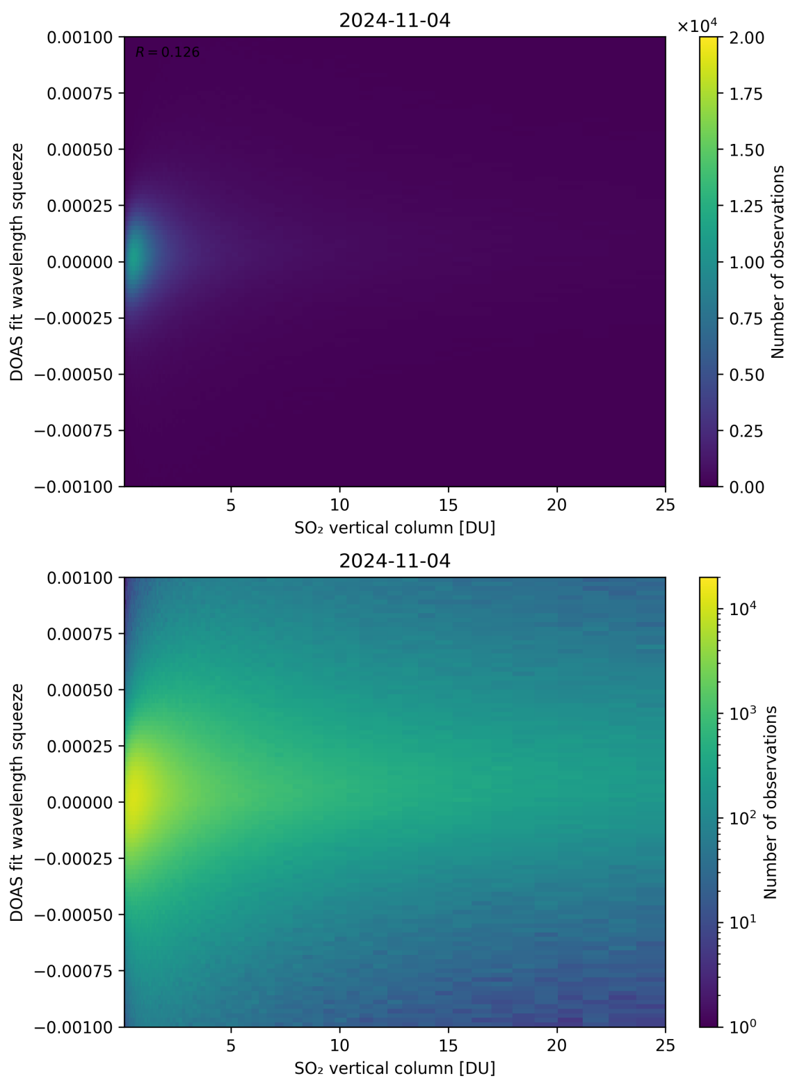
Figure 277: Scatter density plot of “SO 2 vertical column” against “DOAS fit wavelength squeeze” for 2024-11-04 to 2024-11-05.
