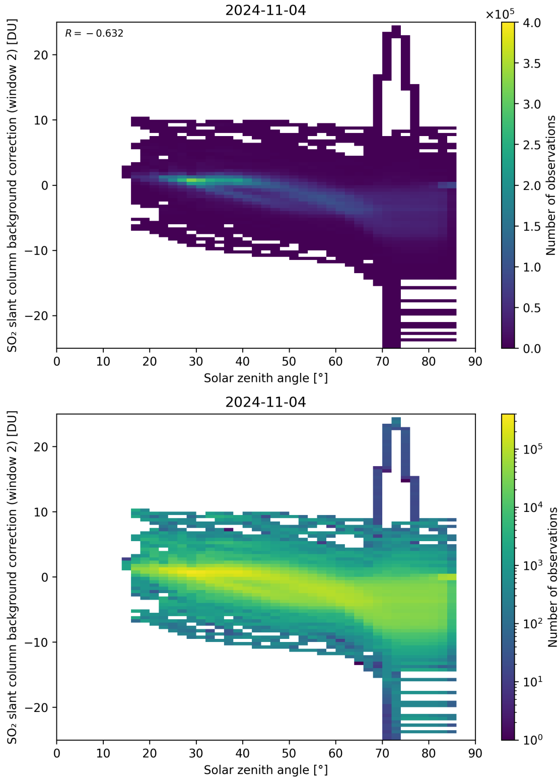
Figure 159: Scatter density plot of “Solar zenith angle” against “SO 2 slant column background correction (window 2)” for 2024-11-04 to 2024-11-05.
