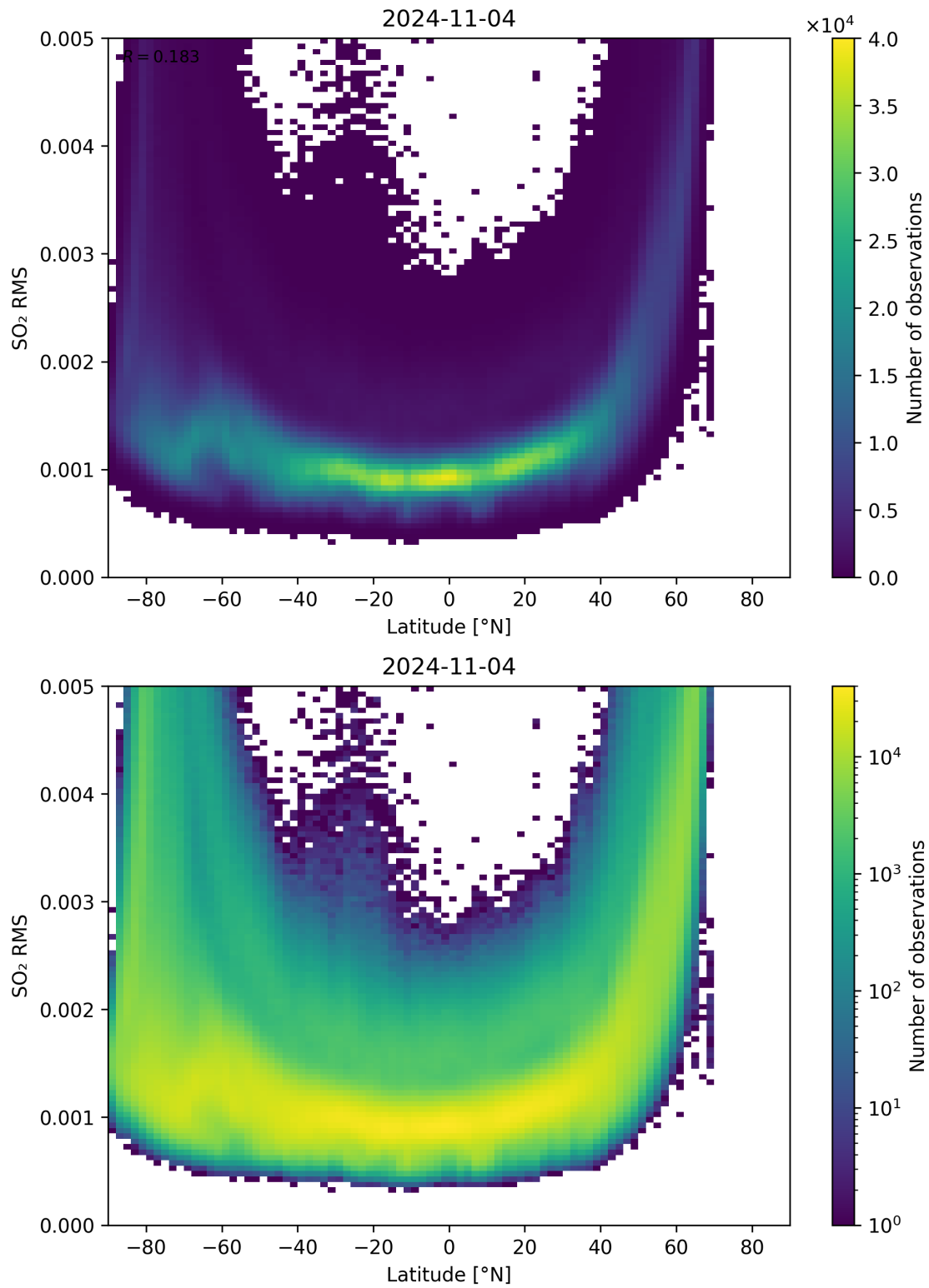
Figure 144: Scatter density plot of “Latitude” against “SO 2 RMS” for 2024-11-04 to 2024-11-05.
