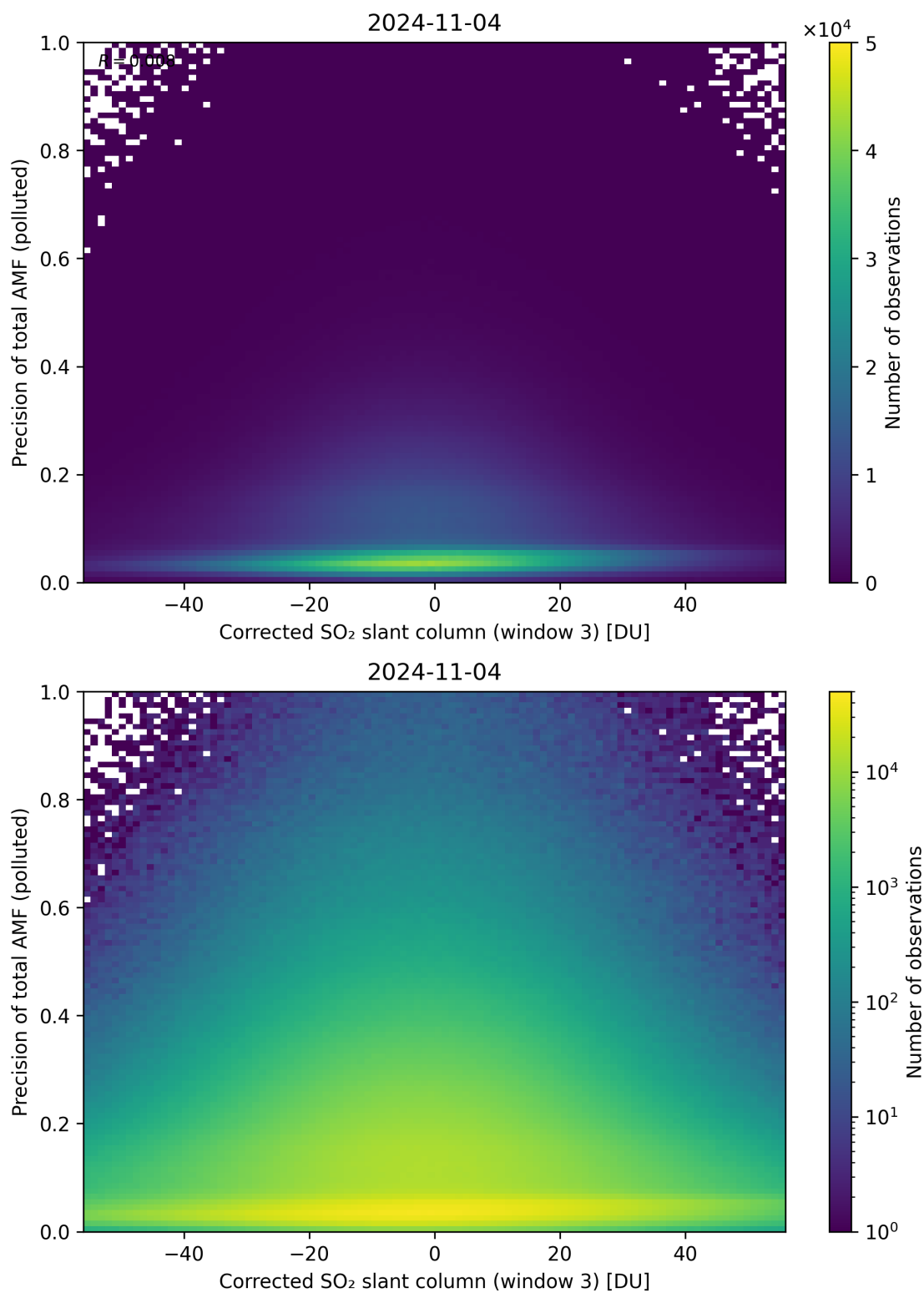
Figure 211: Scatter density plot of “Corrected SO 2 slant column (window 3)” against “Precision of total AMF (polluted)” for 2024-11-04 to 2024-11-05.
