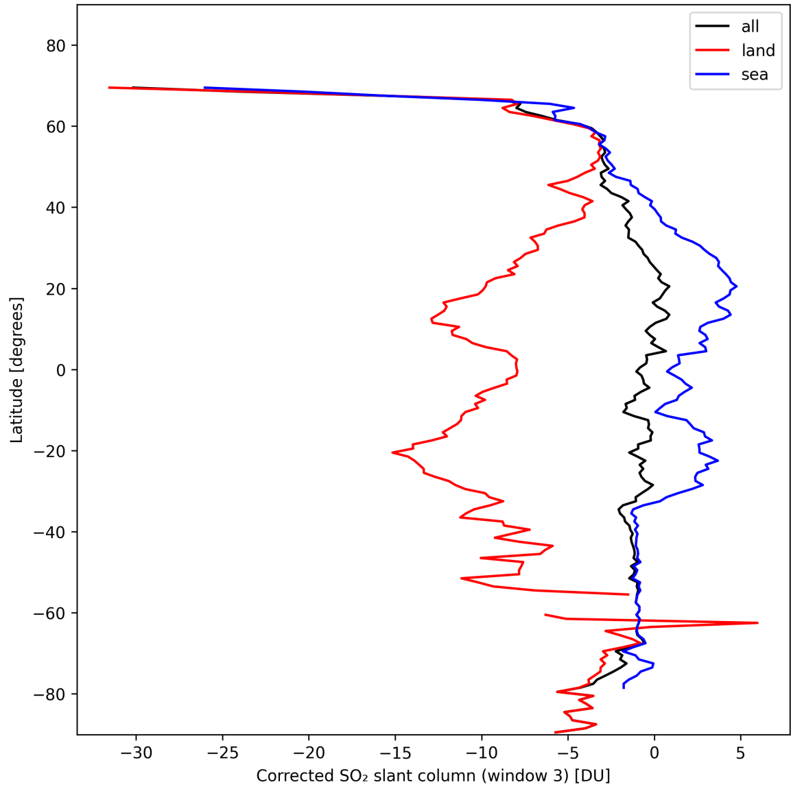
Figure 43: Zonal average of “Corrected SO 2 slant column (window 3)” for 2024-11-04 to 2024-11-05.
