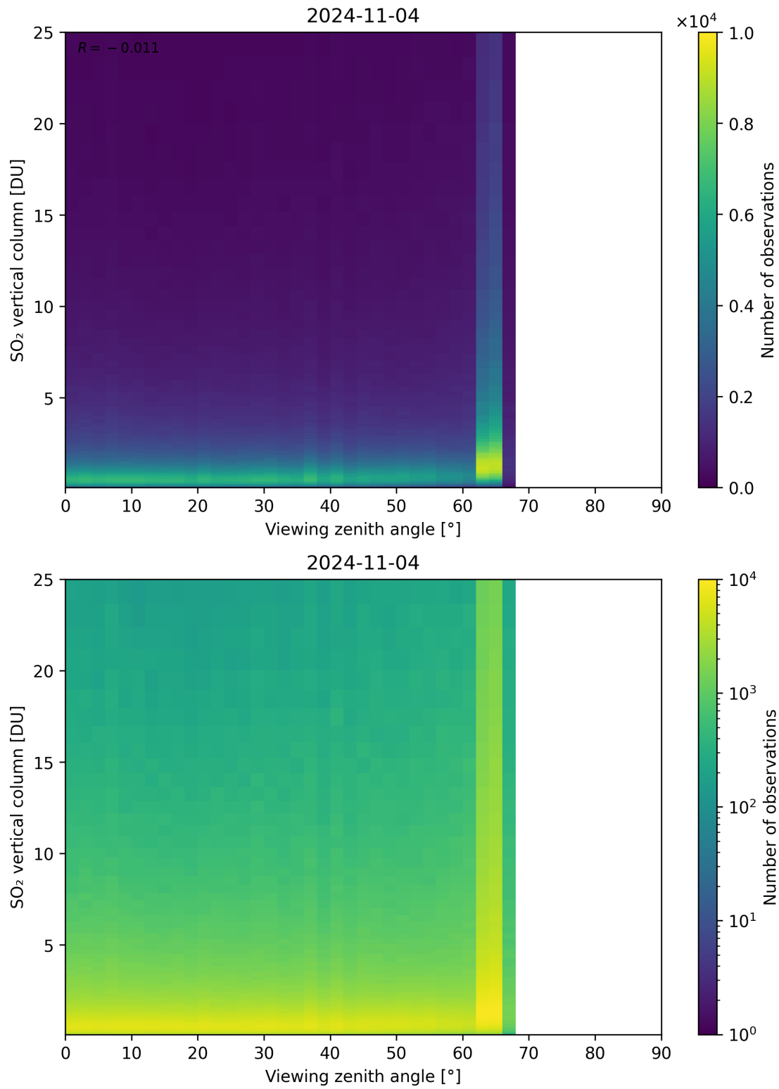
Figure 327: Scatter density plot of “Viewing zenith angle” against “SO 2 vertical column” for 2024-11-04 to 2024-11-05.
