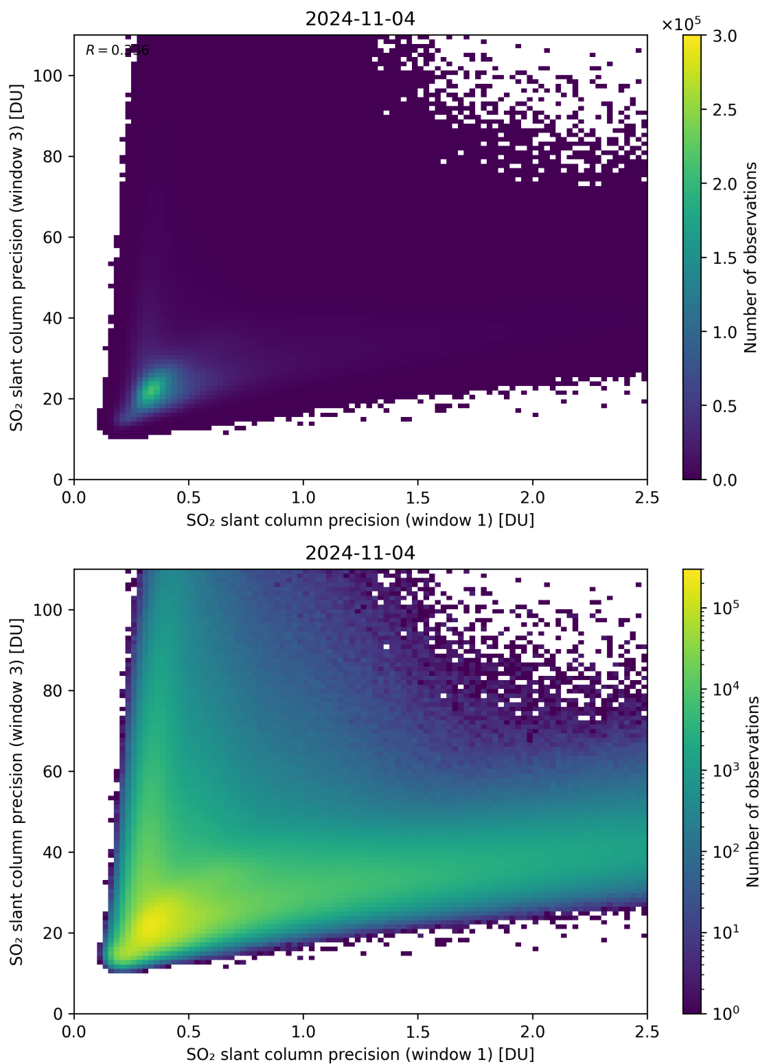
Figure 229: Scatter density plot of “SO 2 slant column precision (window 1)” against “SO 2 slant column precision (window 3)” for 2024-11-04 to 2024-11-05.
