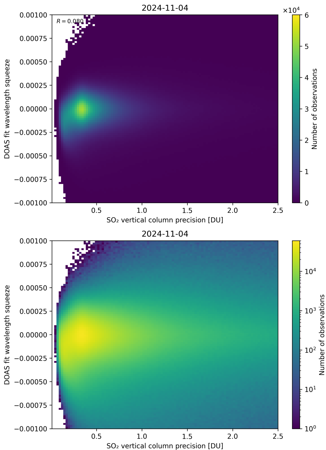
Figure 283: Scatter density plot of “SO 2 vertical column precision” against “DOAS fit wavelength squeeze” for 2024-11-04 to 2024-11-05.
