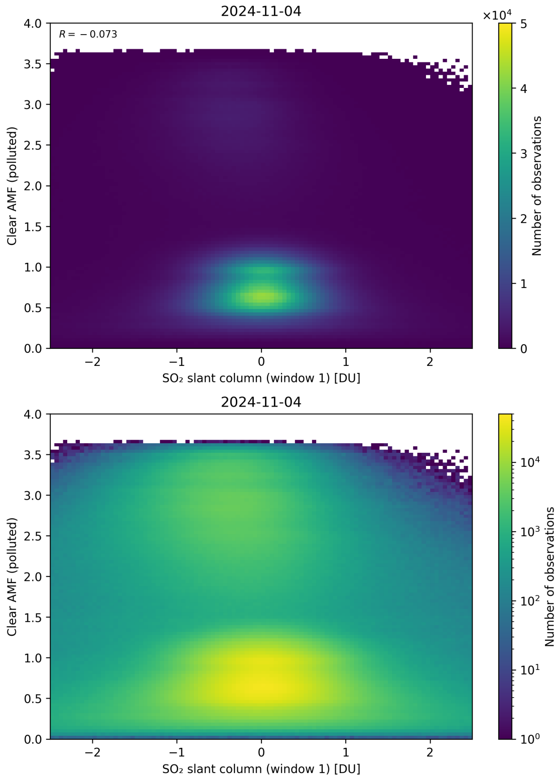
Figure 232: Scatter density plot of “SO 2 slant column (window 1)” against “Clear AMF (polluted)” for 2024-11-04 to 2024-11-05.
