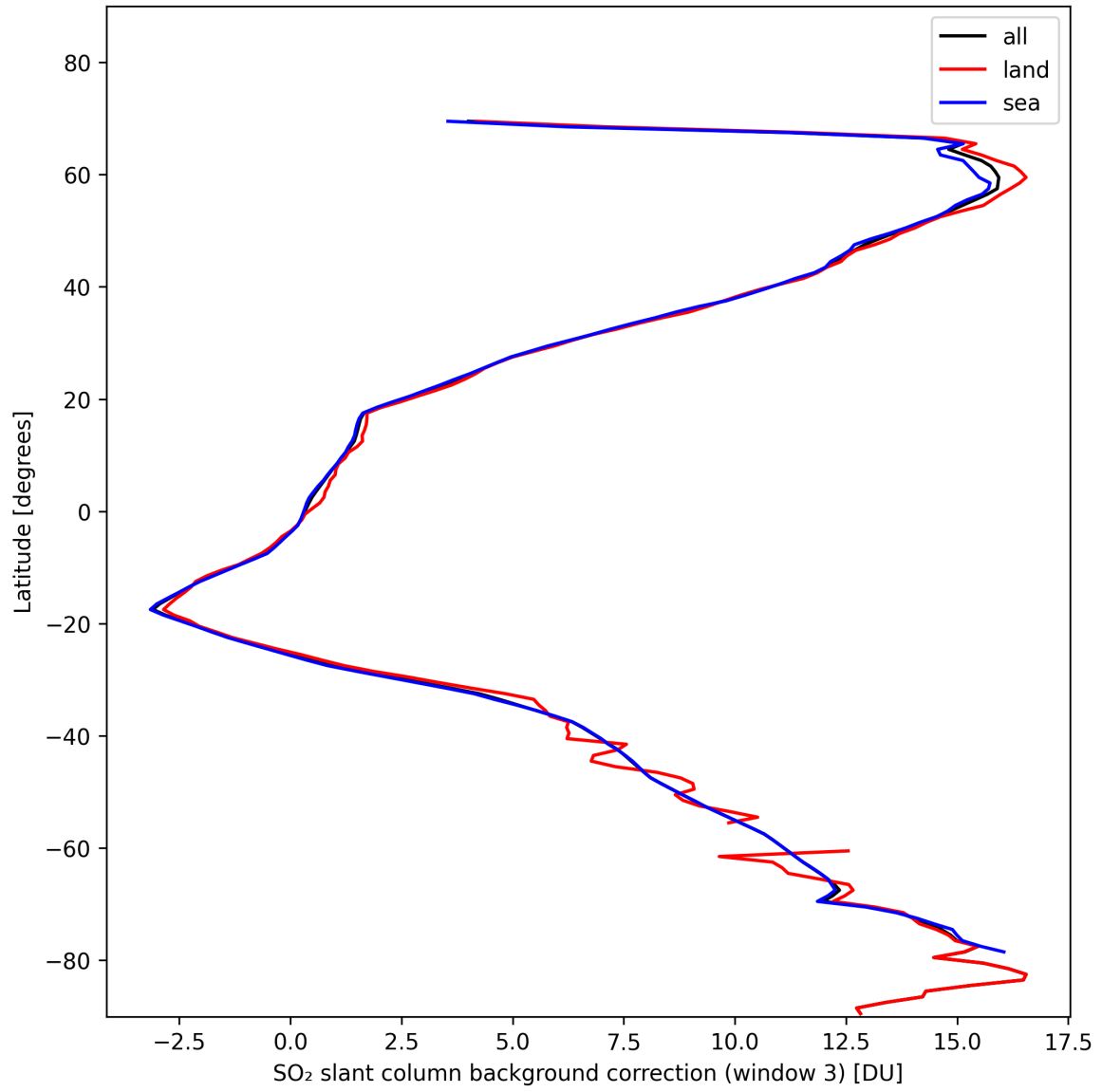
Figure 44: Zonal average of “SO 2 slant column background correction (window 3)” for 2024-11-04 to 2024-11-05.
