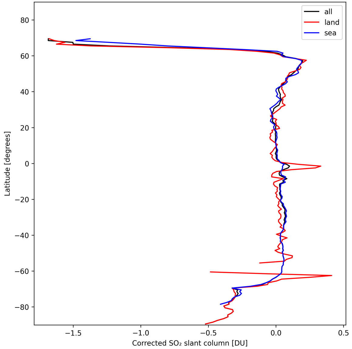
Figure 32: Zonal average of “Corrected SO 2 slant column” for 2024-11-04 to 2024-11-05.
