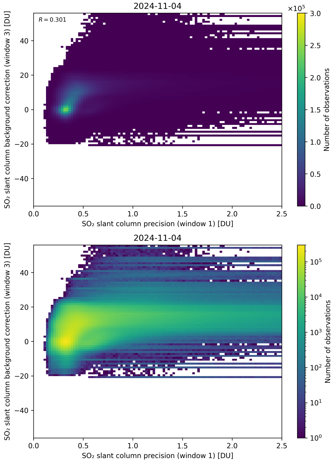
Figure 220: Scatter density plot of “SO 2 slant column precision (window 1)” against “SO 2 slant column background correction (window 3)” for 2024-11-04 to 2024-11-05.
