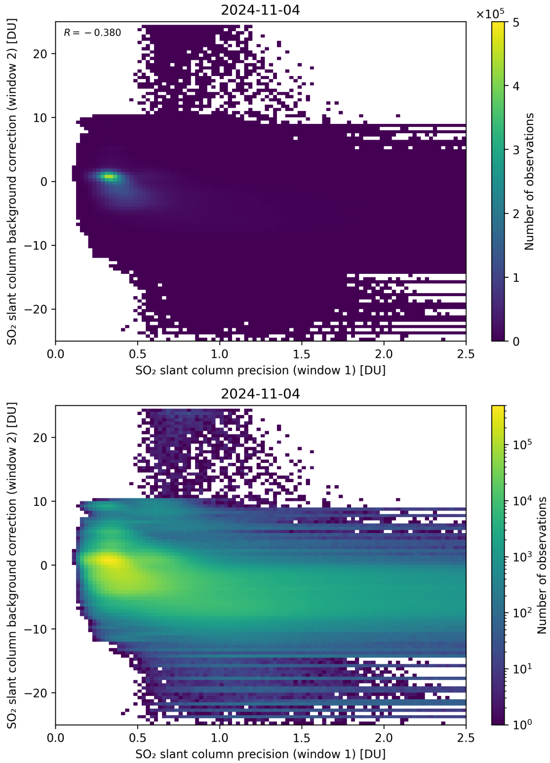
Figure 219: Scatter density plot of “SO 2 slant column precision (window 1)” against “SO 2 slant column background correction (window 2)” for 2024-11-04 to 2024-11-05.
