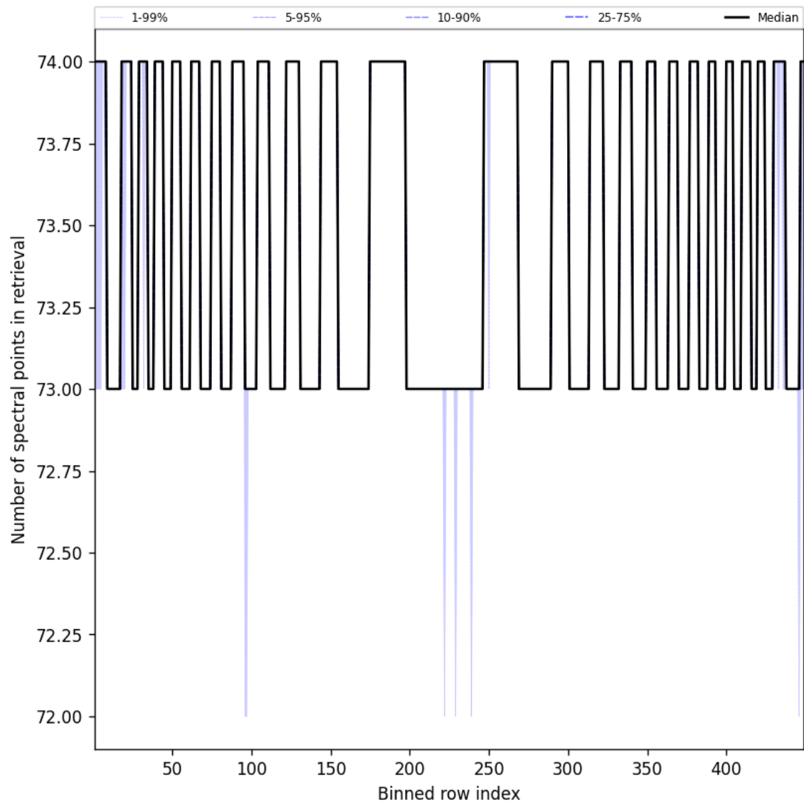
Figure 97: Along track statistics of “Number of spectral points in retrieval” for 2024-11-04 to 2024-11-05
