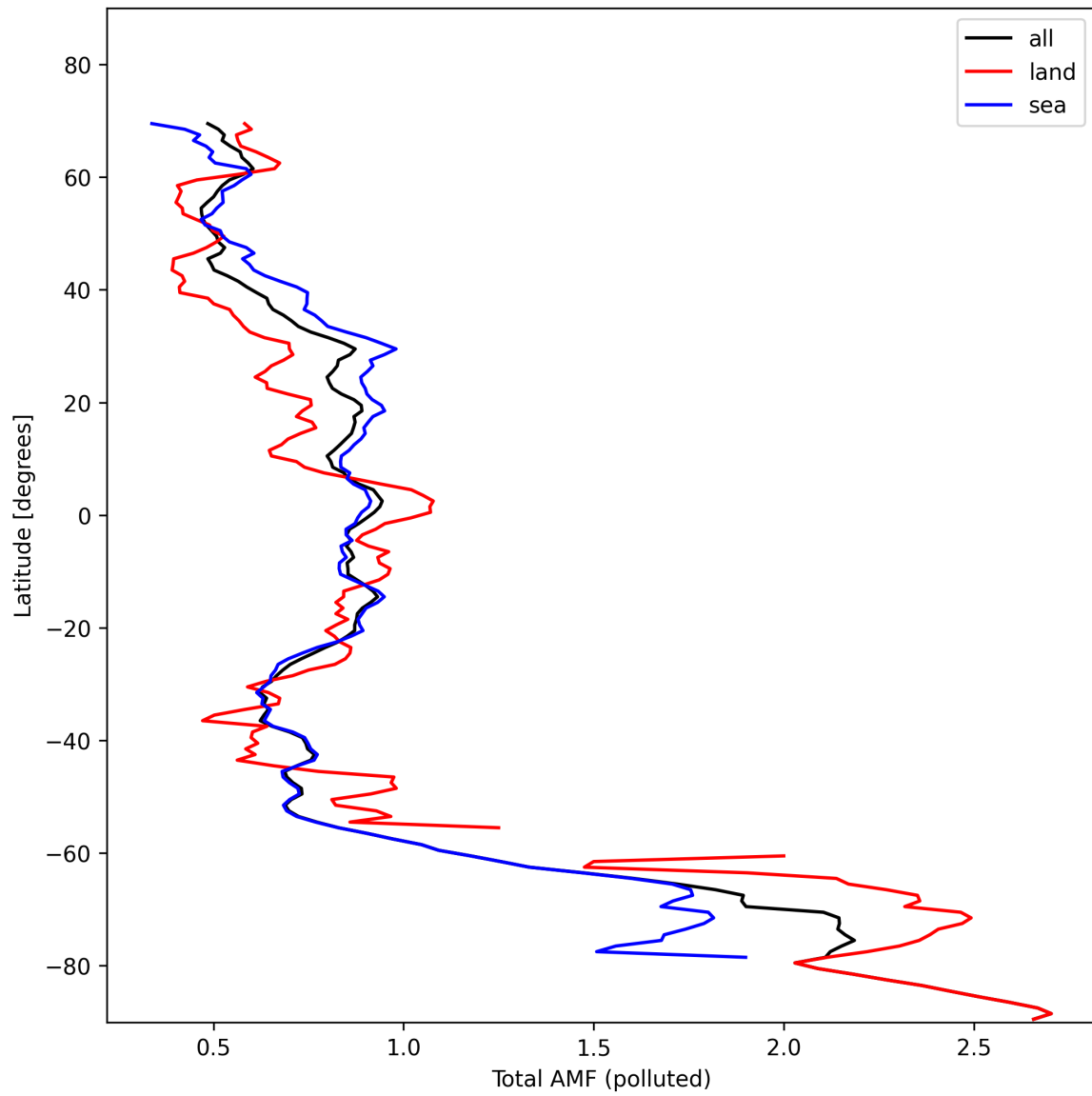
Figure 48: Zonal average of “Total AMF (polluted)” for 2024-11-04 to 2024-11-05.
