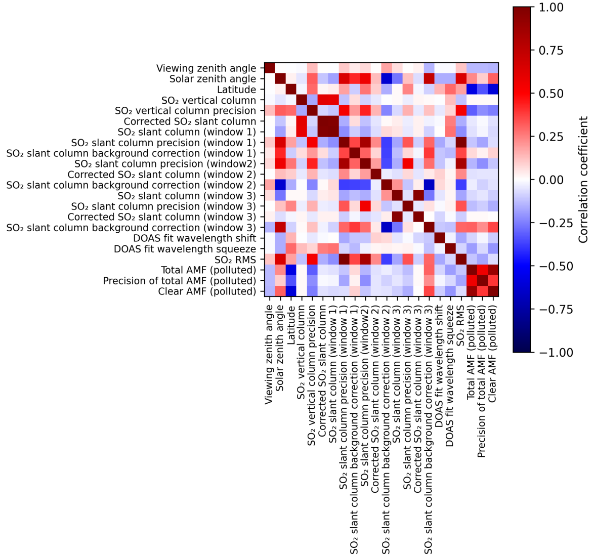
Figure 2: Map of correlation matrix for 2024-11-04 to 2024-11-05.
