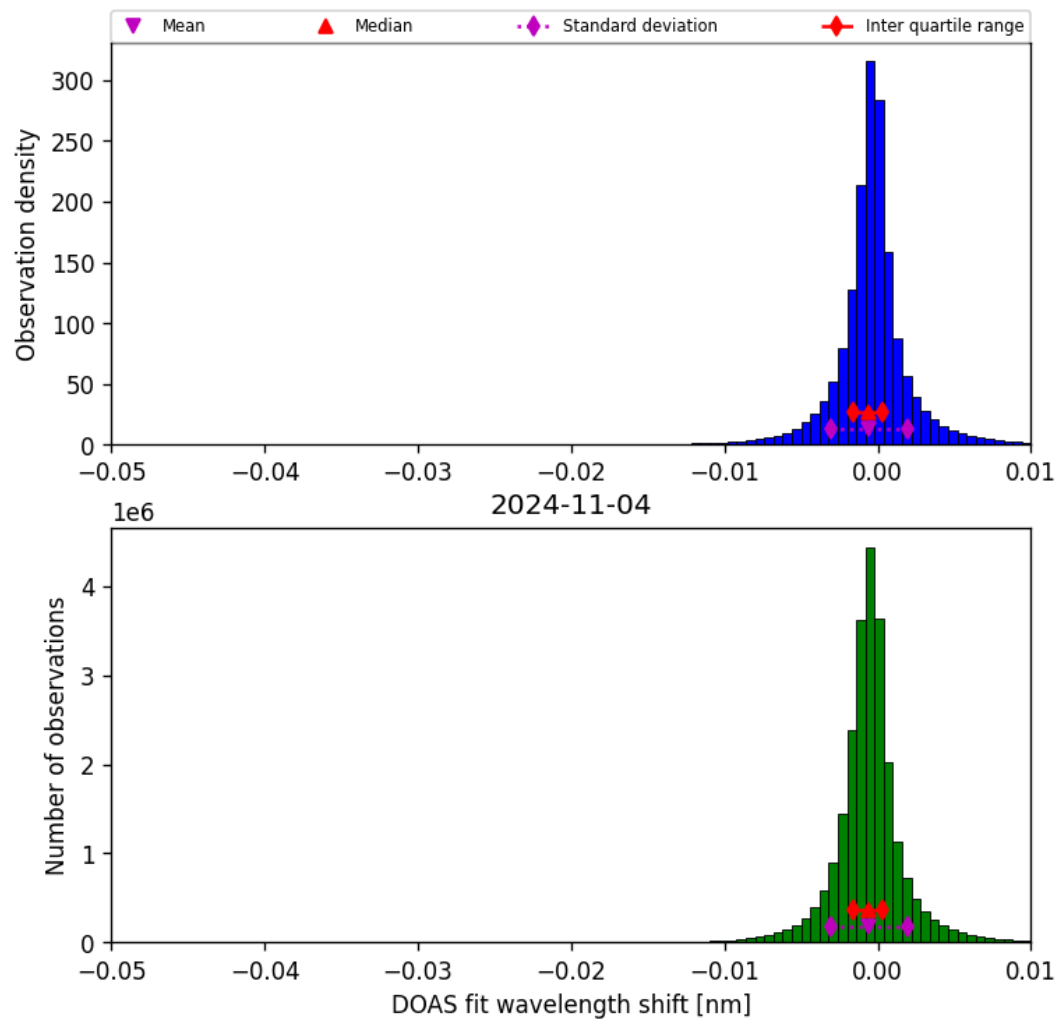
Figure 68: Histogram of “DOAS fit wavelength shift” for 2024-11-04 to 2024-11-05
