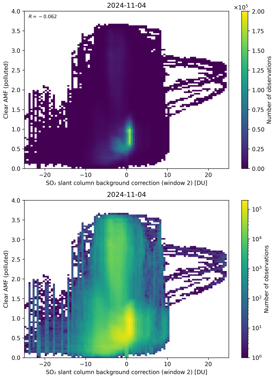
Figure 115: Scatter density plot of “SO 2 slant column background correction (window 2)” against “Clear AMF (polluted)” for 2024-11-04 to 2024-11-05.
