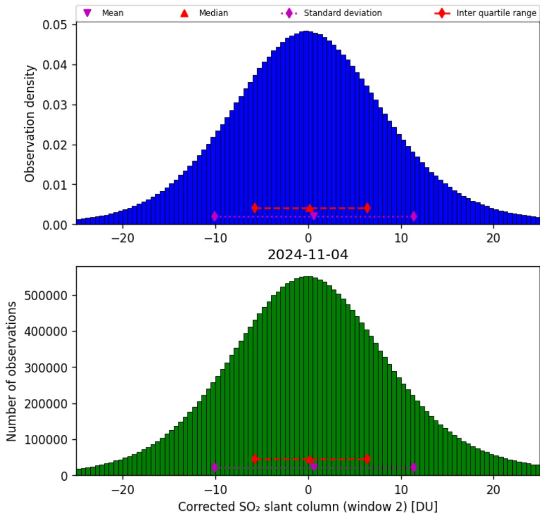
Figure 62: Histogram of “Corrected SO 2 slant column (window 2)” for 2024-11-04 to 2024-11-05
