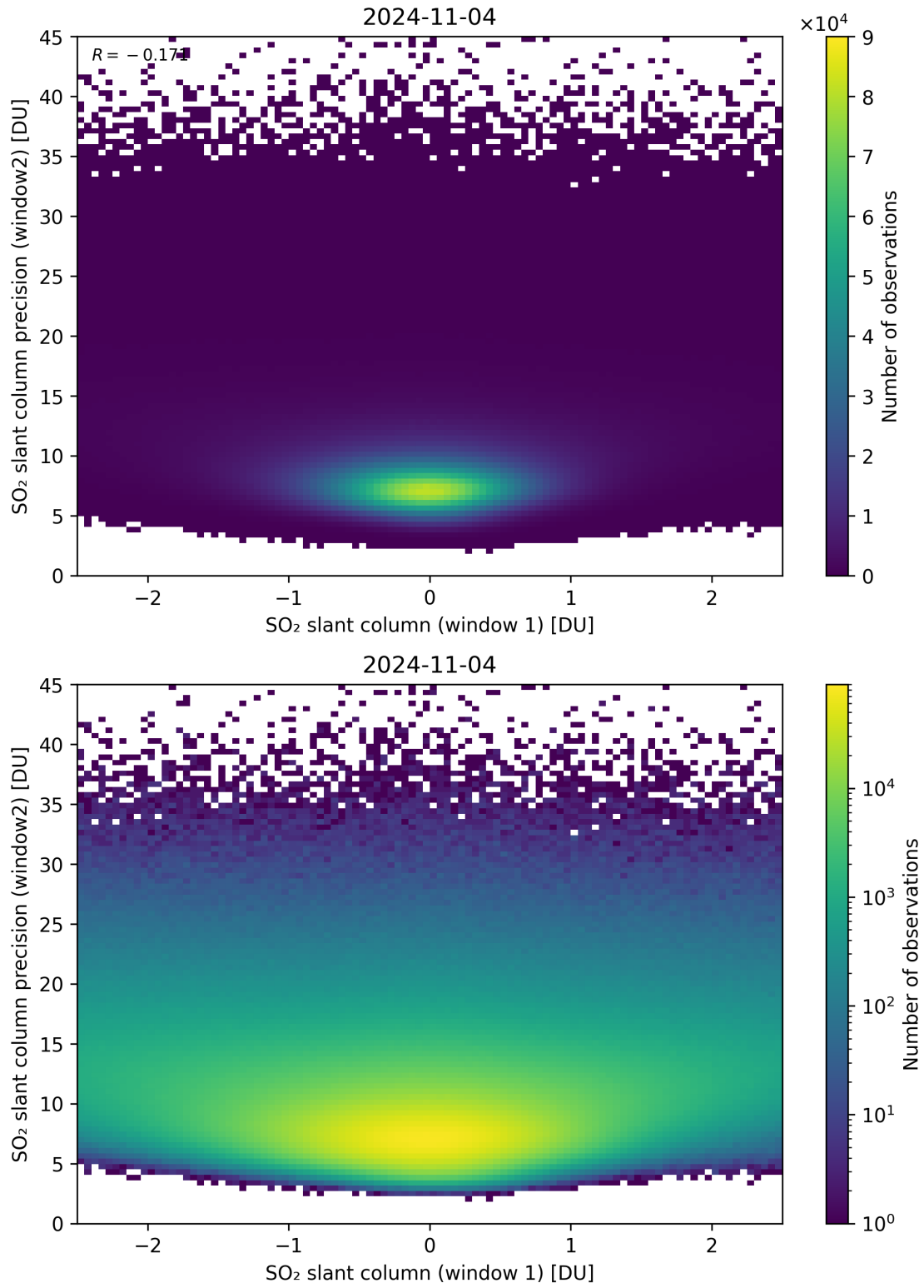
Figure 236: Scatter density plot of “SO 2 slant column (window 1)” against “SO 2 slant column precision (window2)” for 2024-11-04 to 2024-11-05.
