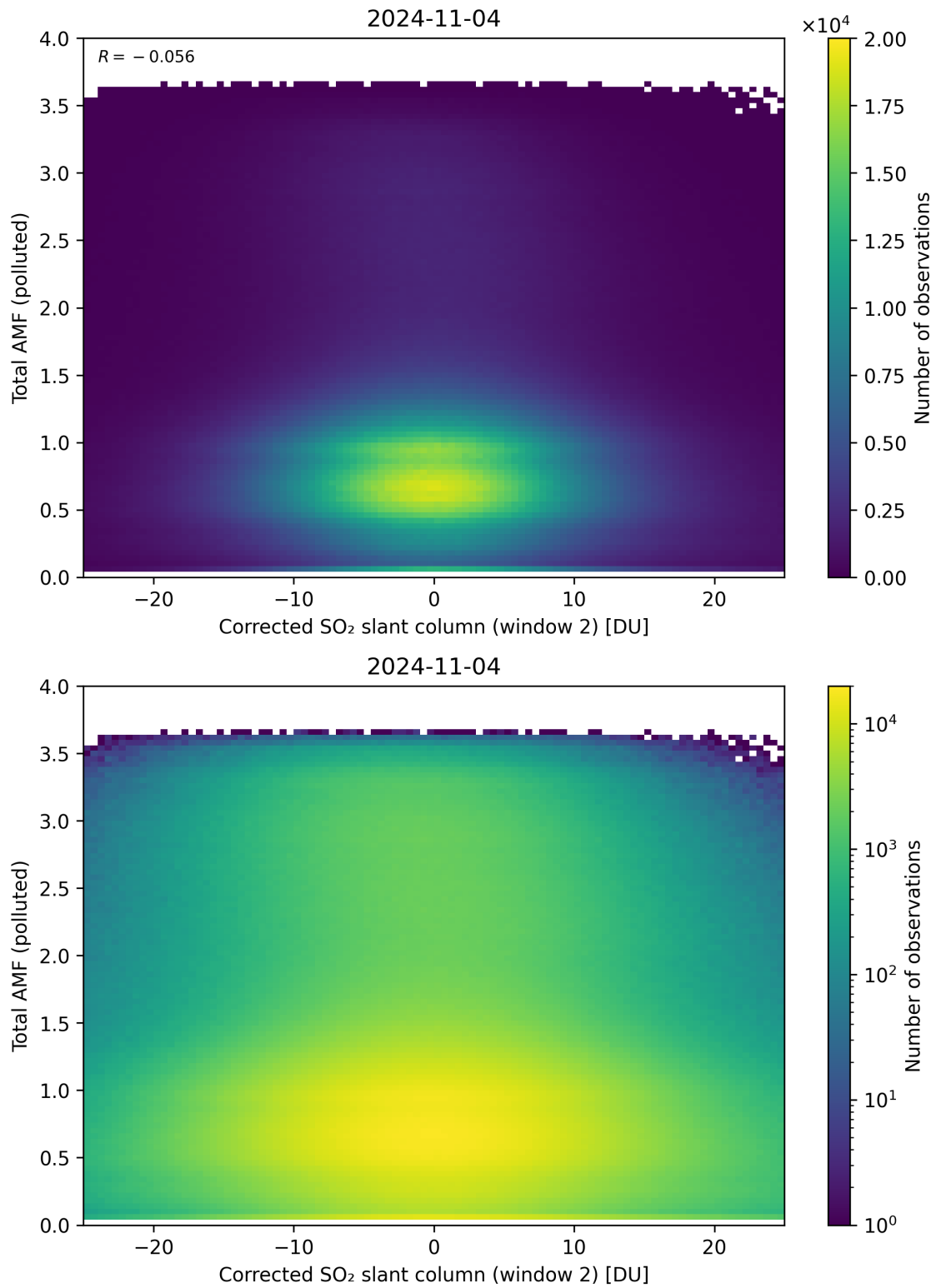
Figure 203: Scatter density plot of “Corrected SO 2 slant column (window 2)” against “Total AMF (polluted)” for 2024-11-04 to 2024-11-05.
