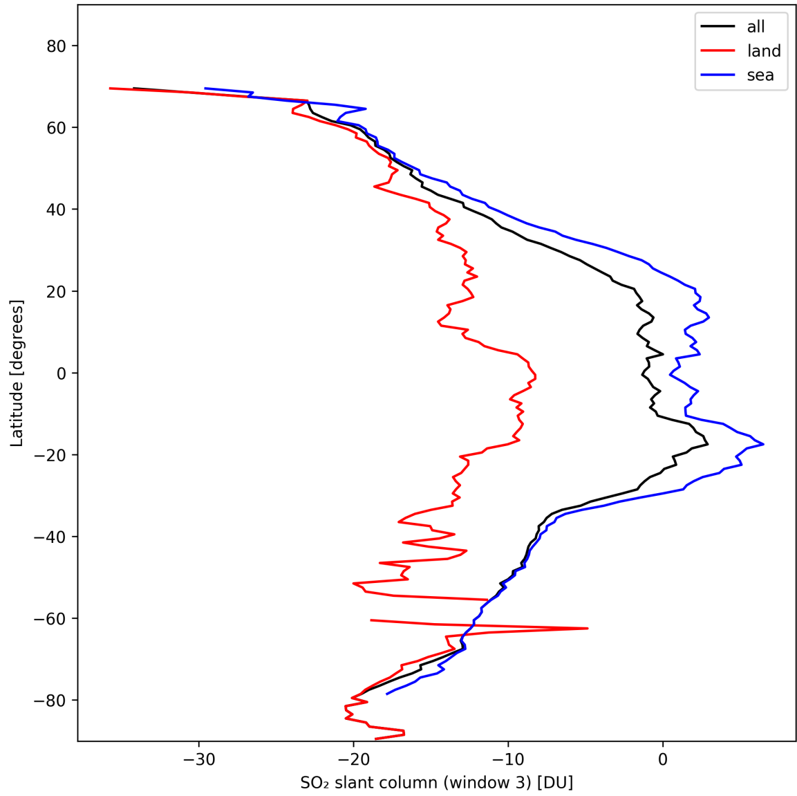
Figure 41: Zonal average of “SO 2 slant column (window 3)” for 2024-11-04 to 2024-11-05.
