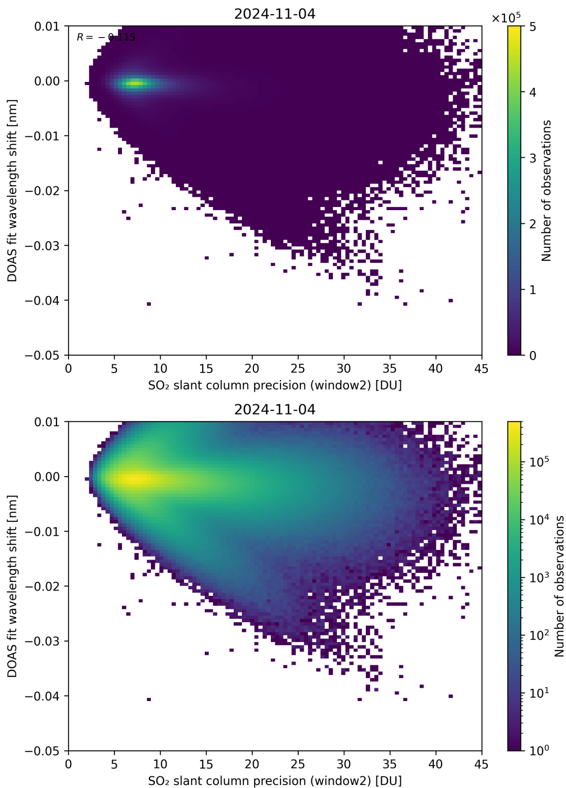
Figure 243: Scatter density plot of “SO 2 slant column precision (window2)” against “DOAS fit wavelength shift” for 2024-11-04 to 2024-11-05.
