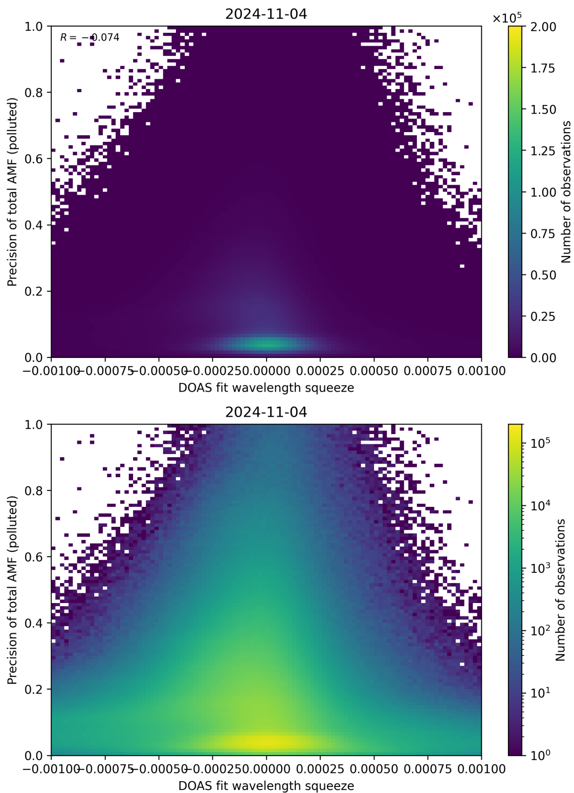
Figure 135: Scatter density plot of “DOAS fit wavelength squeeze” against “Precision of total AMF (polluted)” for 2024-11-04 to 2024-11-05.
