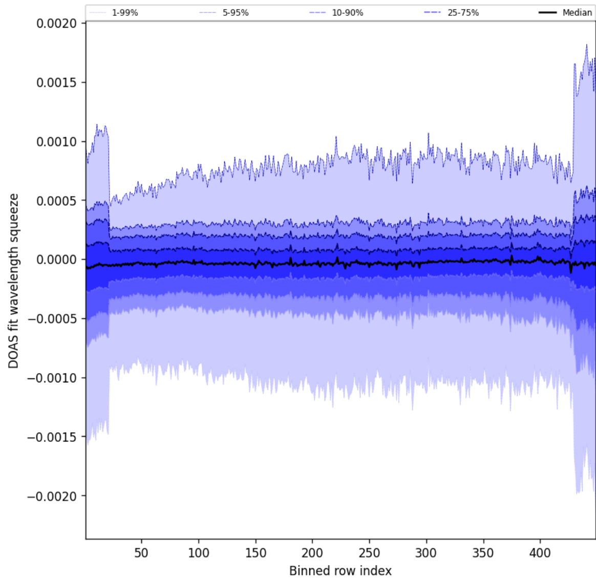
Figure 92: Along track statistics of “DOAS fit wavelength squeeze” for 2024-11-04 to 2024-11-05
