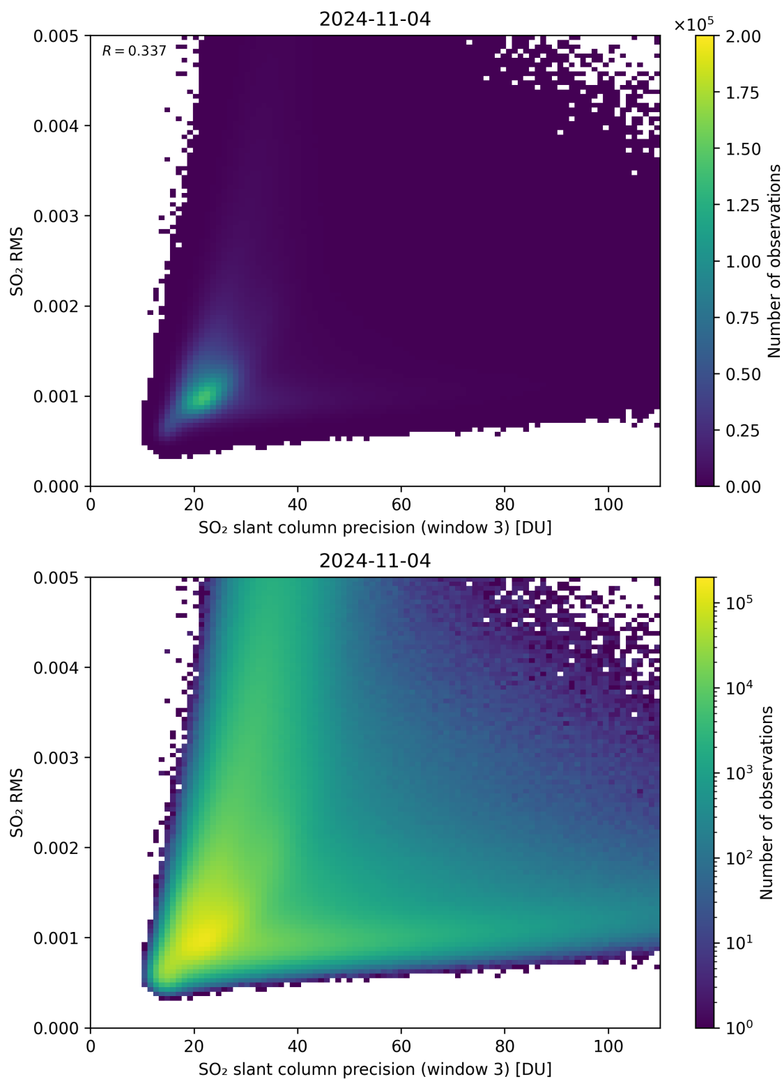
Figure 260: Scatter density plot of “SO 2 slant column precision (window 3)” against “SO 2 RMS” for 2024-11-04 to 2024-11-05.
