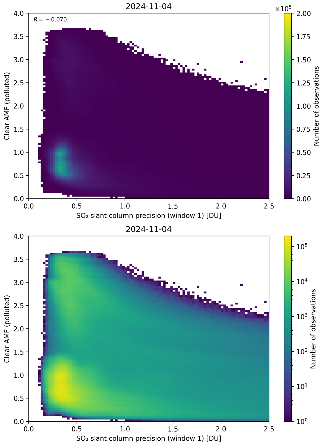
Figure 224: Scatter density plot of “SO 2 slant column precision (window 1)” against “Clear AMF (polluted)” for 2024-11-04 to 2024-11-05.
