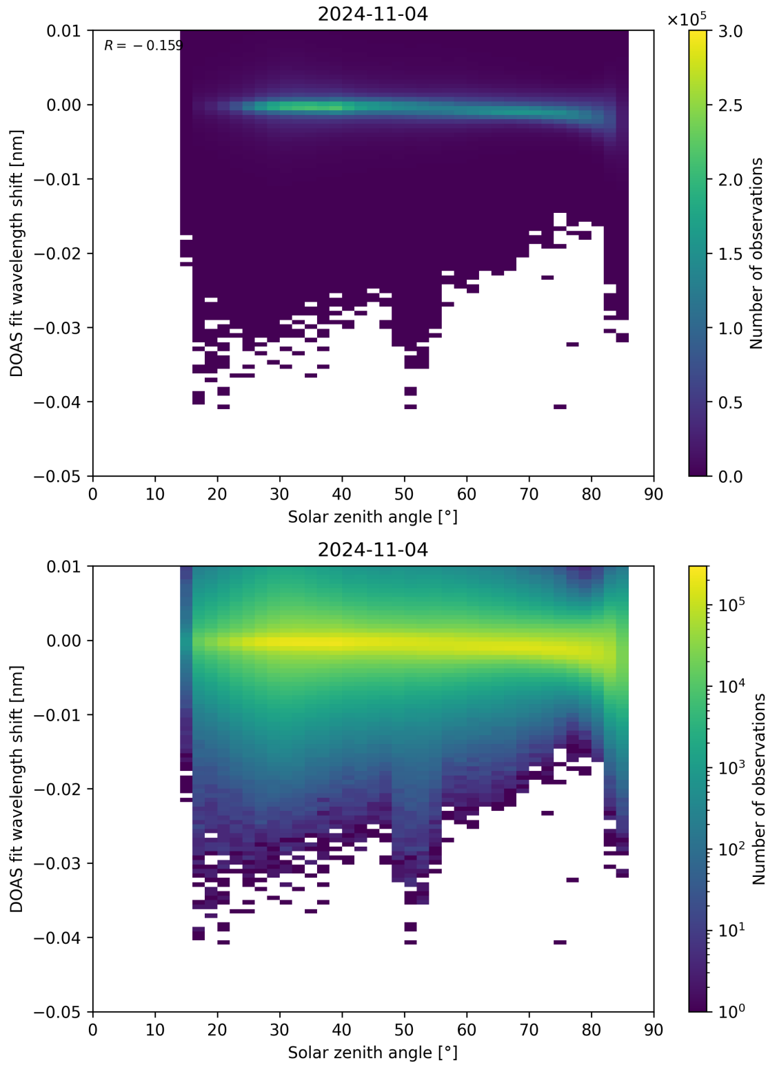
Figure 161: Scatter density plot of “Solar zenith angle” against “DOAS fit wavelength shift” for 2024-11-04 to 2024-11-05.
