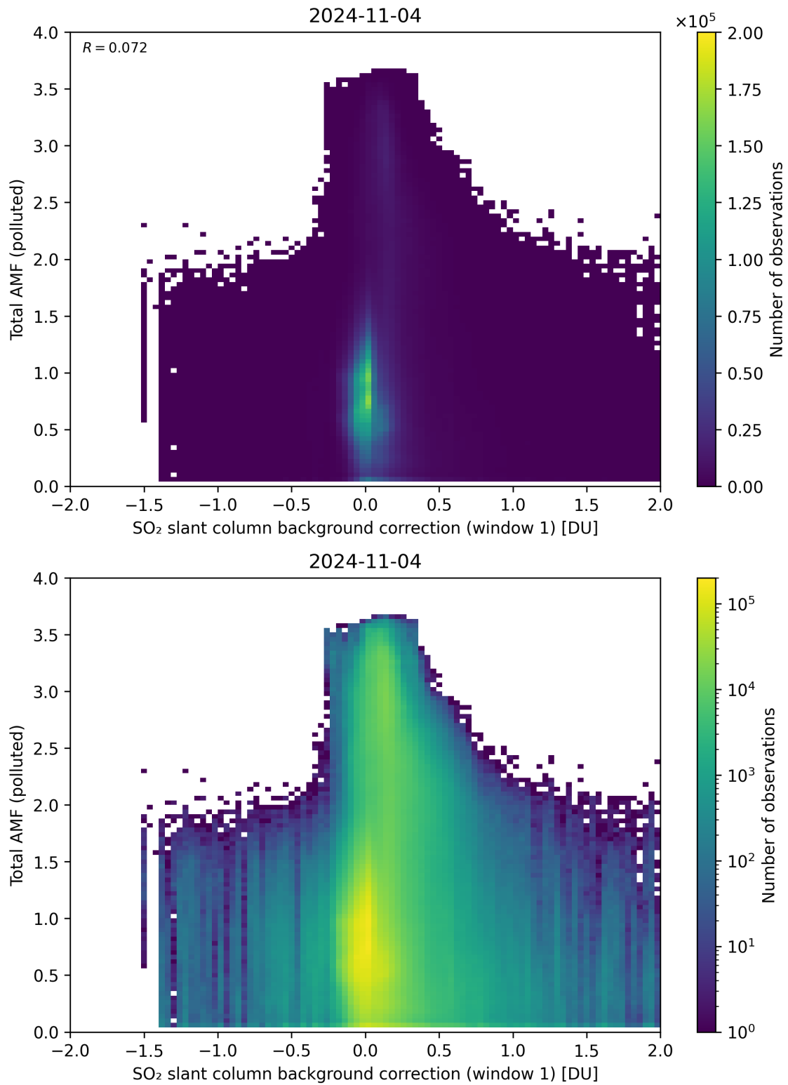
Figure 109: Scatter density plot of “SO 2 slant column background correction (window 1)” against “Total AMF (polluted)” for 2024-11-04 to 2024-11-05.
