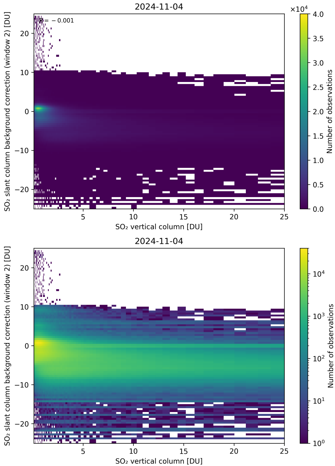
Figure 274: Scatter density plot of “SO 2 vertical column” against “SO 2 slant column background correction (window 2)” for 2024-11-04 to 2024-11-05.
