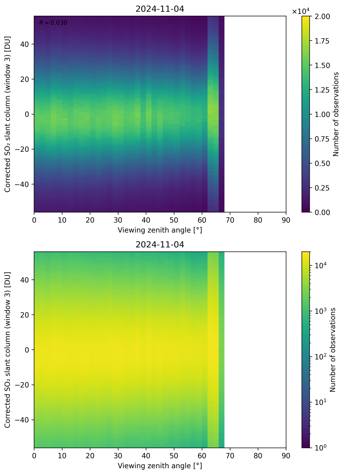
Figure 319: Scatter density plot of “Viewing zenith angle” against “Corrected SO 2 slant column (window 3)” for 2024-11-04 to 2024-11-05.
