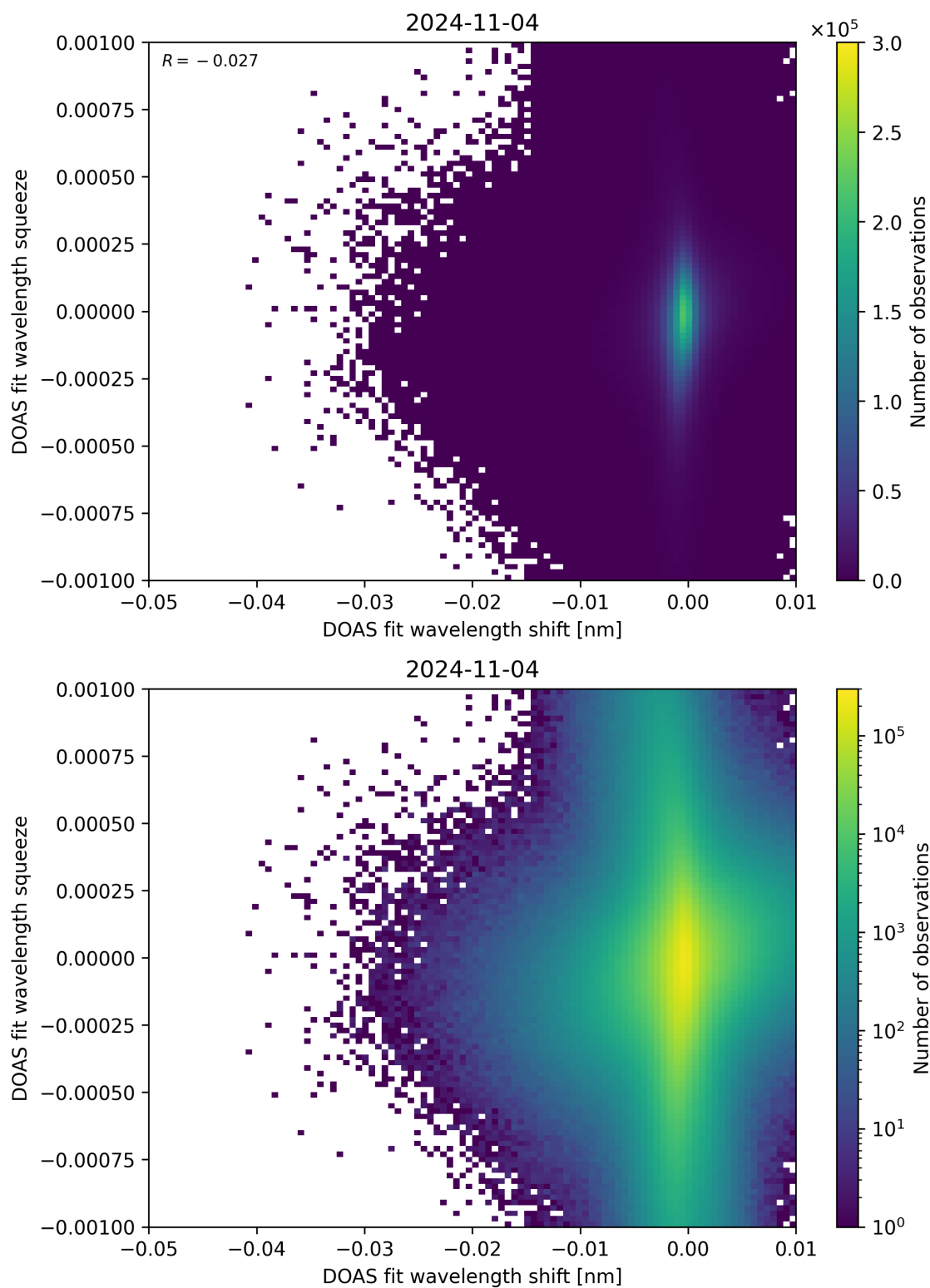
Figure 127: Scatter density plot of “DOAS fit wavelength shift” against “DOAS fit wavelength squeeze” for 2024-11-04 to 2024-11-05.
