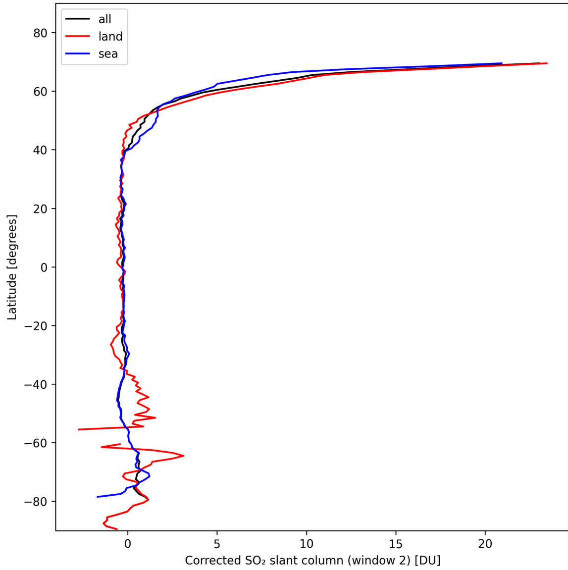
Figure 39: Zonal average of “Corrected SO 2 slant column (window 2)” for 2024-11-04 to 2024-11-05.
