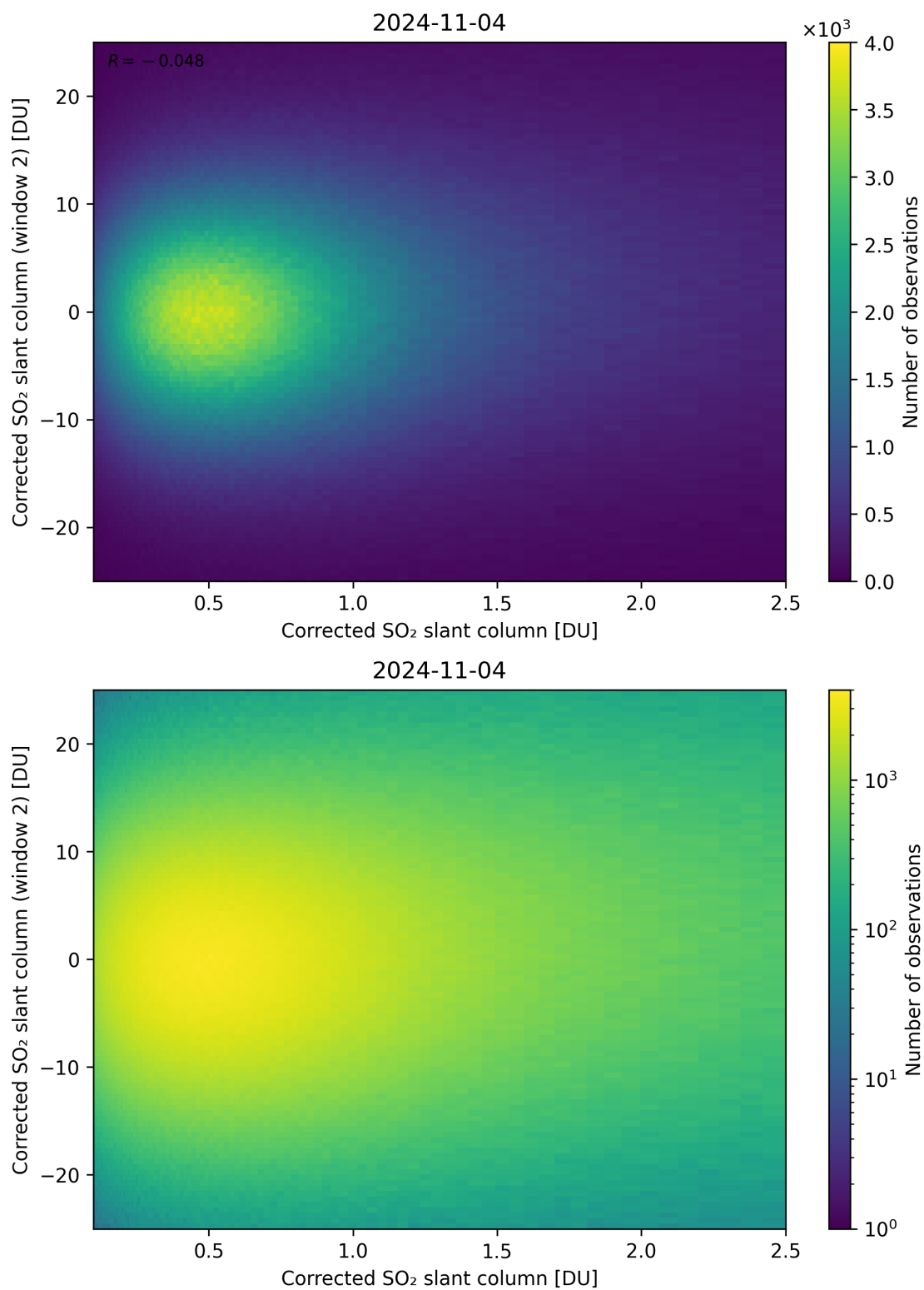
Figure 185: Scatter density plot of “Corrected SO 2 slant column” against “Corrected SO 2 slant column (window 2)” for 2024-11-04 to 2024-11-05.
