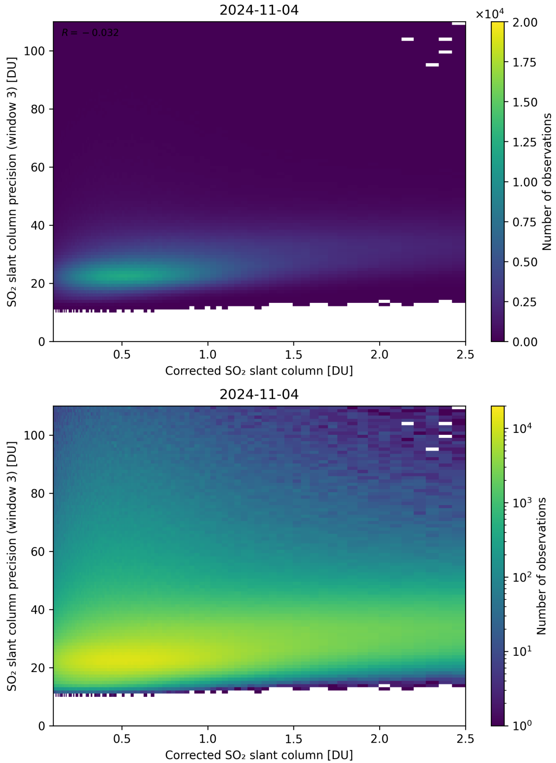
Figure 191: Scatter density plot of “Corrected SO 2 slant column” against “SO 2 slant column precision (window 3)” for 2024-11-04 to 2024-11-05.
