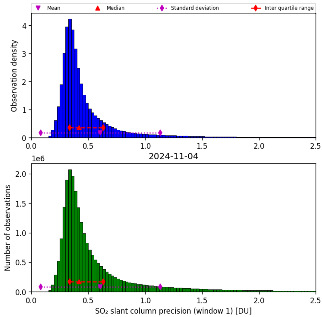
Figure 57: Histogram of “SO 2 slant column precision (window 1)” for 2024-11-04 to 2024-11-05
