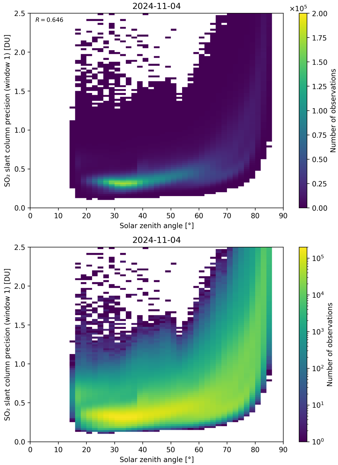
Figure 170: Scatter density plot of “Solar zenith angle” against “SO 2 slant column precision (window 1)” for 2024-11-04 to 2024-11-05.
