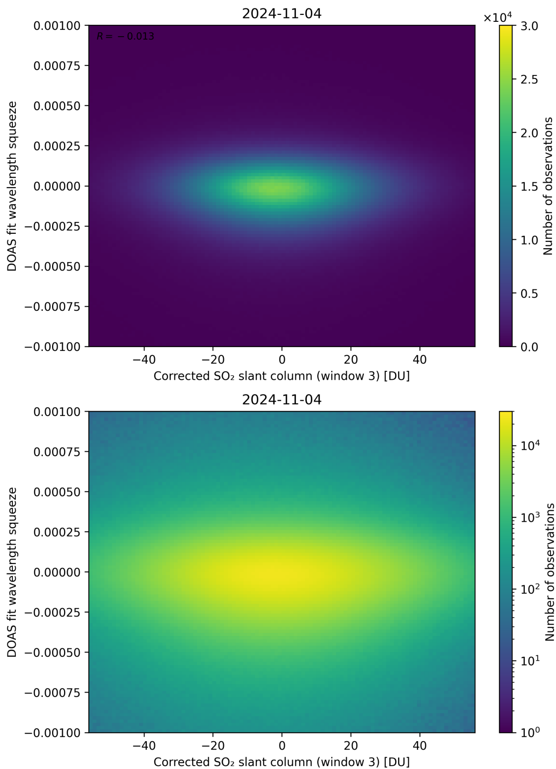
Figure 207: Scatter density plot of “Corrected SO 2 slant column (window 3)” against “DOAS fit wavelength squeeze” for 2024-11-04 to 2024-11-05.
