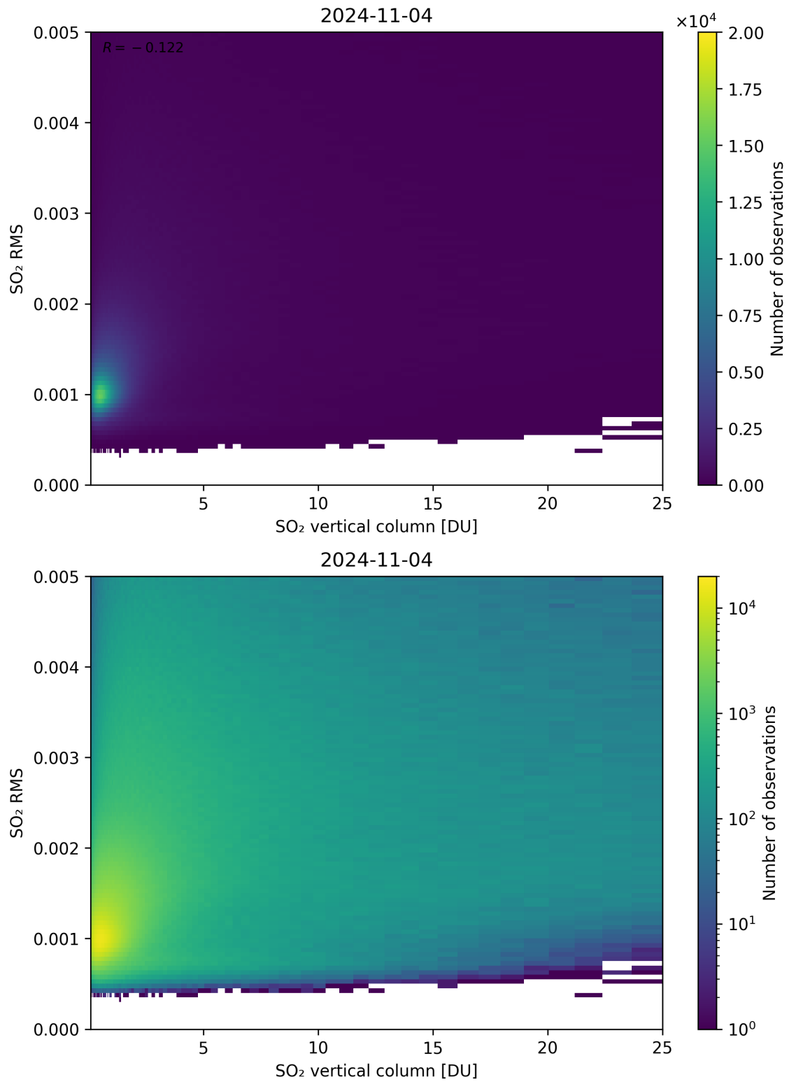
Figure 278: Scatter density plot of “SO 2 vertical column” against “SO 2 RMS” for 2024-11-04 to 2024-11-05.
