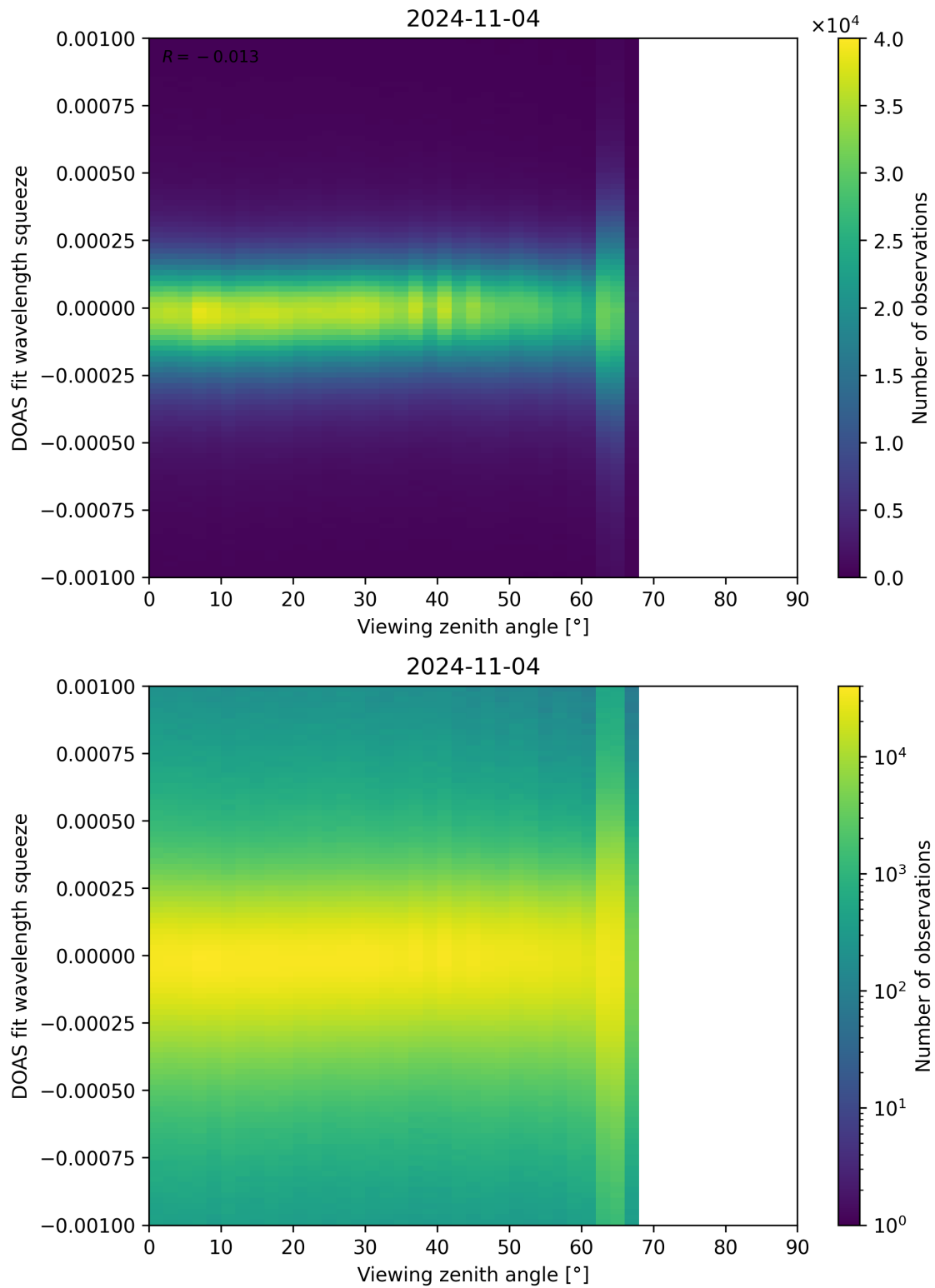
Figure 312: Scatter density plot of “Viewing zenith angle” against “DOAS fit wavelength squeeze” for 2024-11-04 to 2024-11-05.
