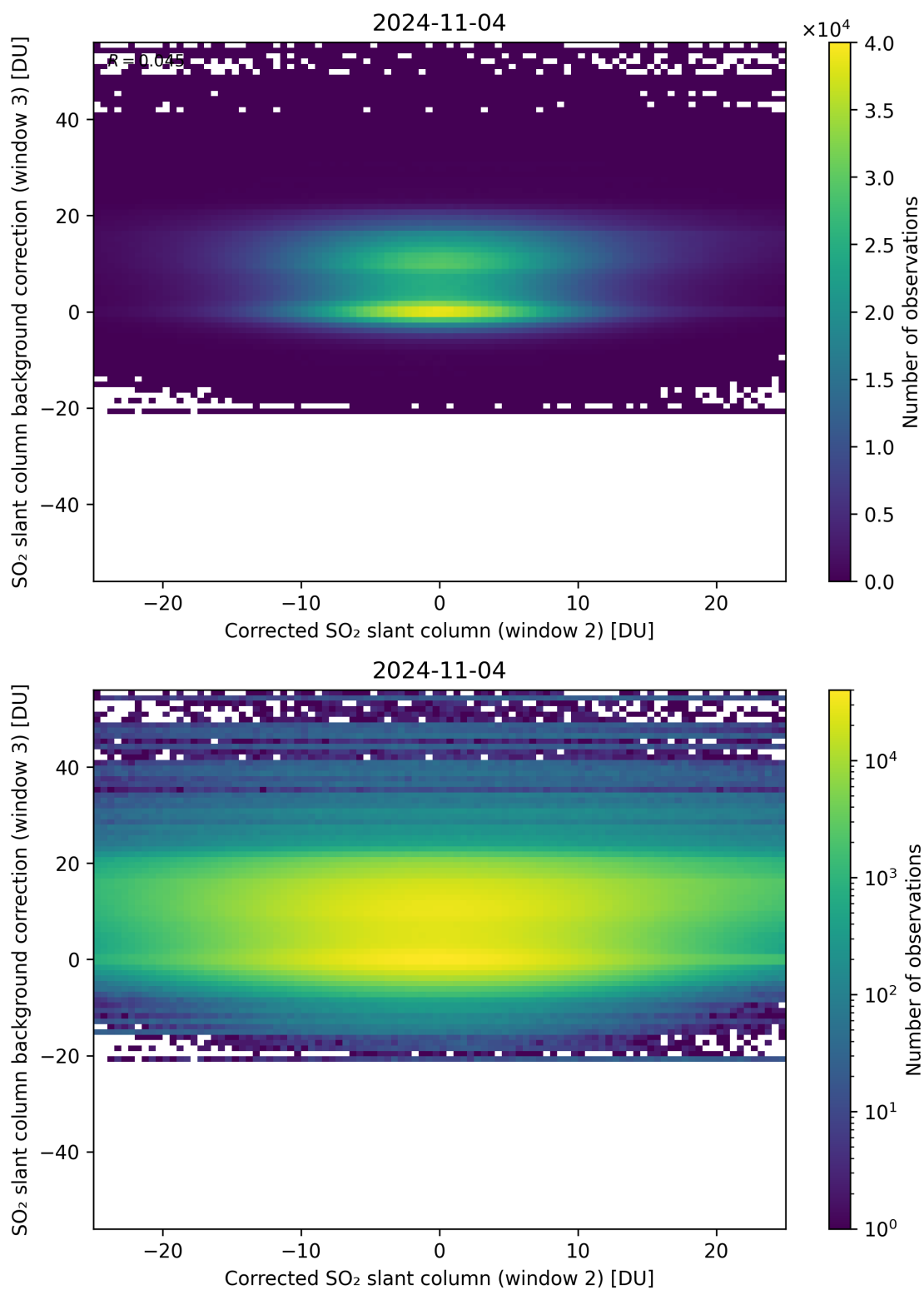
Figure 195: Scatter density plot of “Corrected SO 2 slant column (window 2)” against “SO 2 slant column background correction (window 3)” for 2024-11-04 to 2024-11-05.
