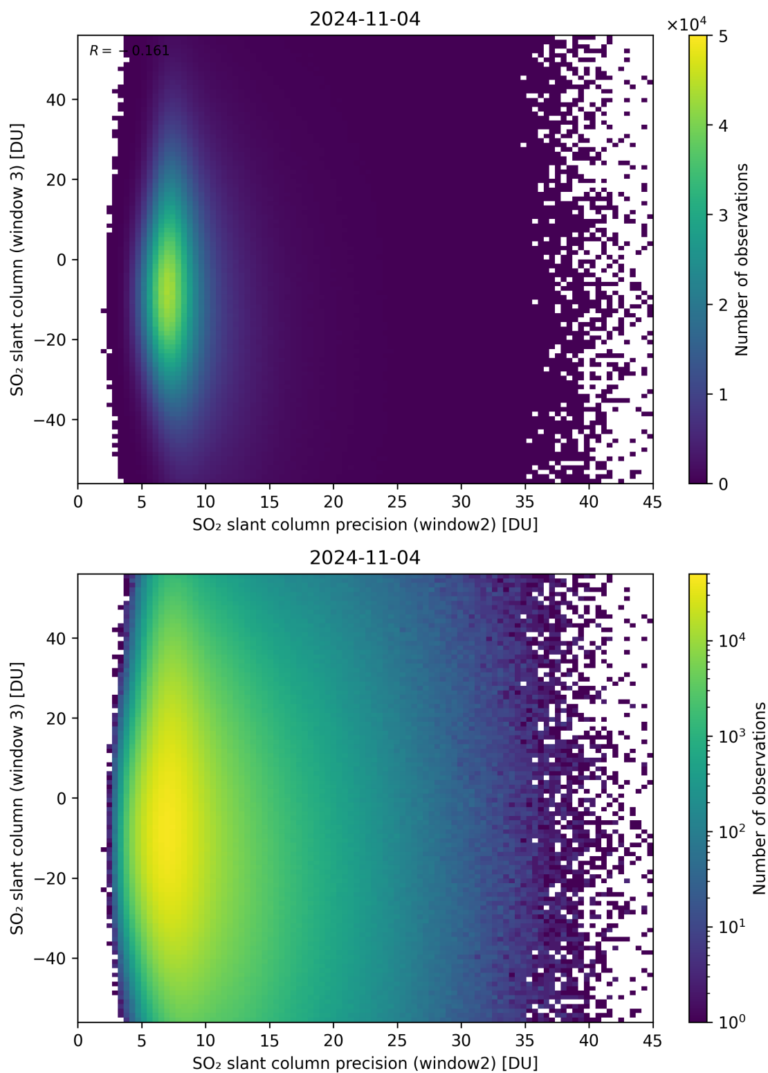
Figure 249: Scatter density plot of “SO 2 slant column precision (window2)” against “SO 2 slant column (window 3)” for 2024-11-04 to 2024-11-05.
