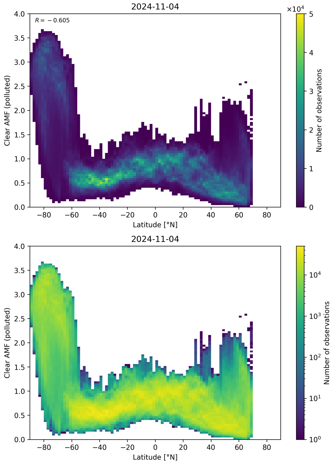
Figure 145: Scatter density plot of “Latitude” against “Clear AMF (polluted)” for 2024-11-04 to 2024-11-05.
