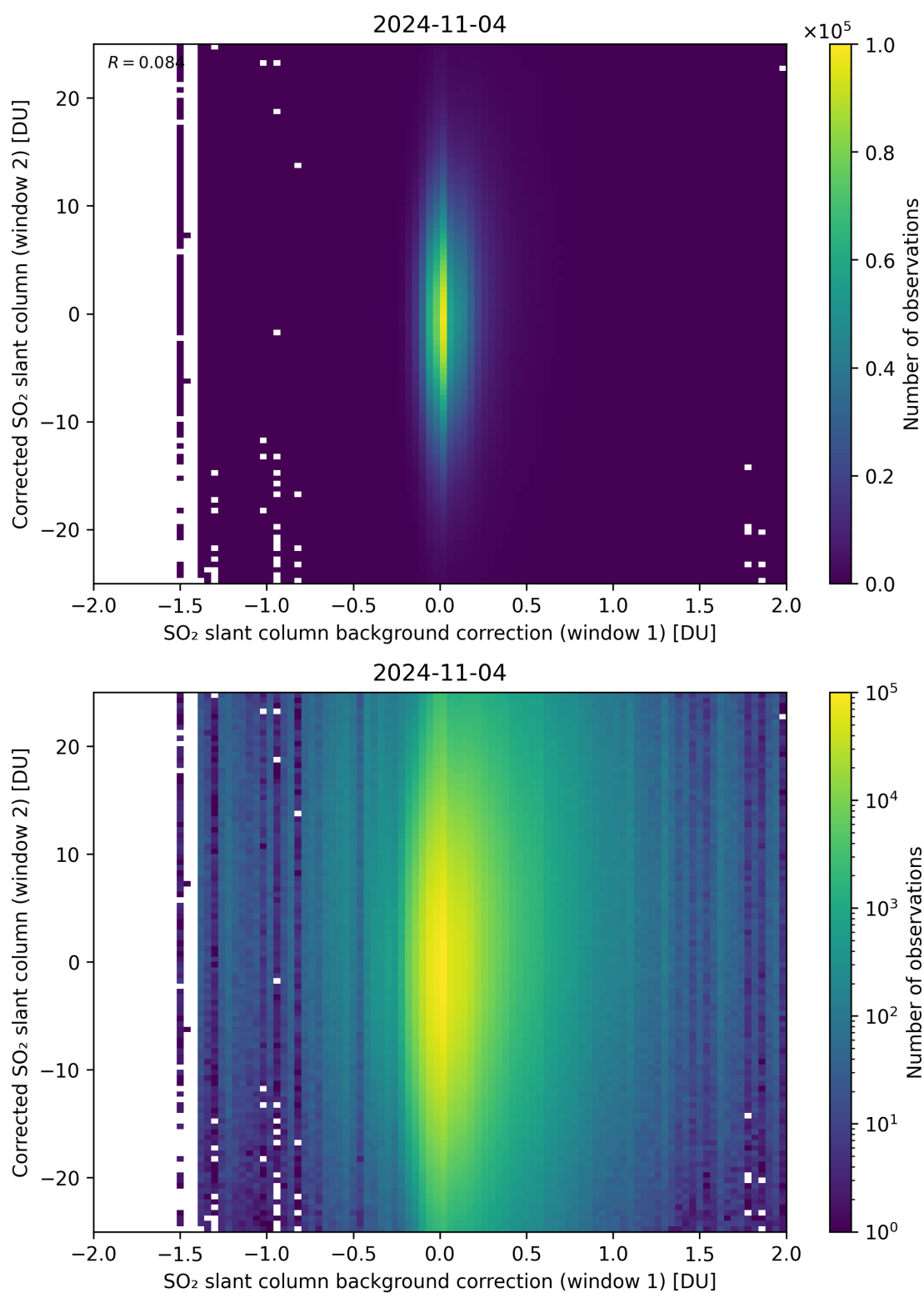
Figure 104: Scatter density plot of “SO 2 slant column background correction (window 1)” against “Corrected SO 2 slant column (window 2)” for 2024-11-04 to 2024-11-05.
