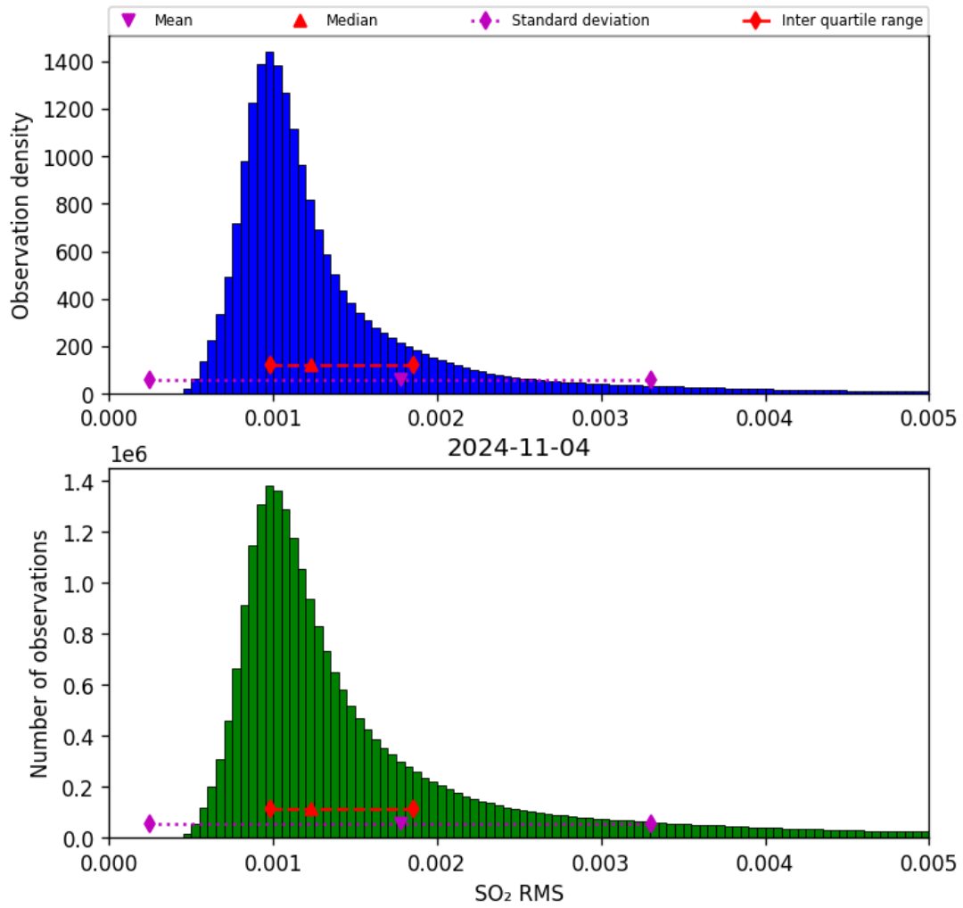
Figure 70: Histogram of “SO 2 RMS” for 2024-11-04 to 2024-11-05
