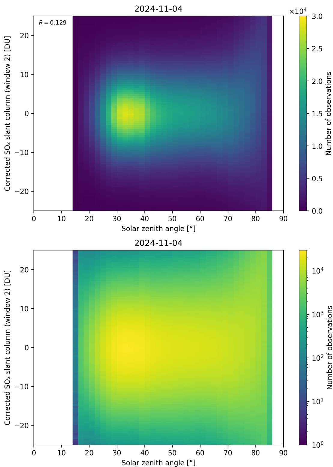
Figure 167: Scatter density plot of “Solar zenith angle” against “Corrected SO 2 slant column (window 2)” for 2024-11-04 to 2024-11-05.
