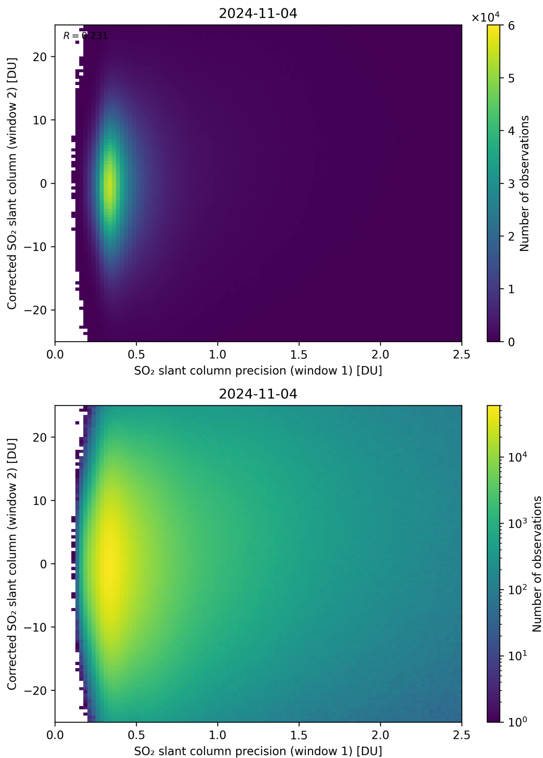
Figure 225: Scatter density plot of “SO 2 slant column precision (window 1)” against “Corrected SO 2 slant column (window 2)” for 2024-11-04 to 2024-11-05.
