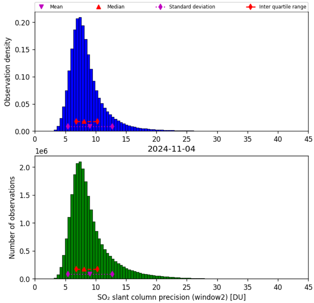
Figure 61: Histogram of “SO 2 slant column precision (window2)” for 2024-11-04 to 2024-11-05
