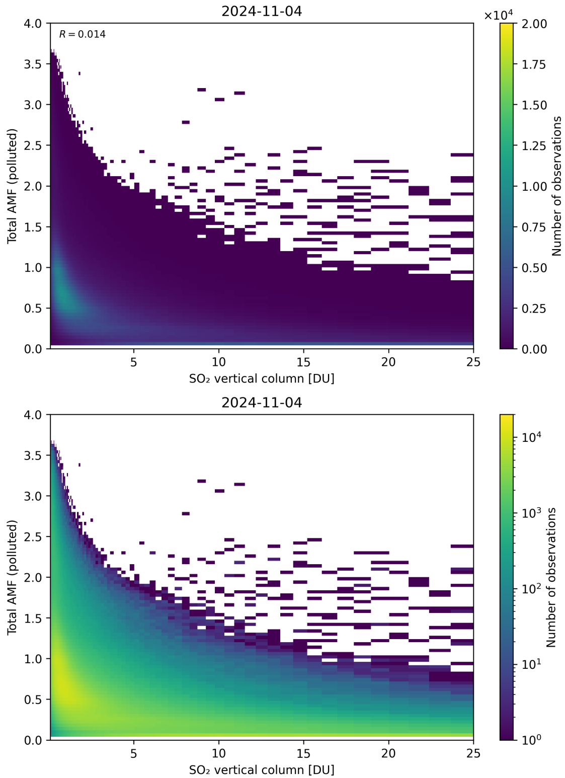
Figure 305: Scatter density plot of “SO 2 vertical column” against “Total AMF (polluted)” for 2024-11-04 to 2024-11-05.
