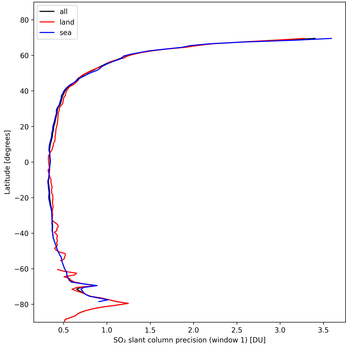
Figure 34: Zonal average of “SO 2 slant column precision (window 1)” for 2024-11-04 to 2024-11-05.
