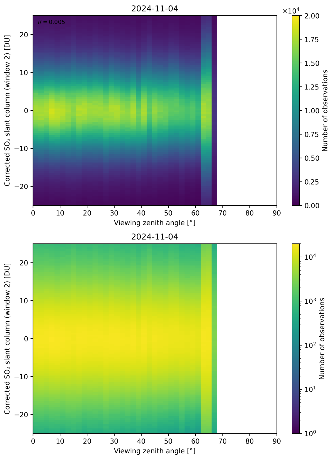
Figure 318: Scatter density plot of “Viewing zenith angle” against “Corrected SO 2 slant column (window 2)” for 2024-11-04 to 2024-11-05.
