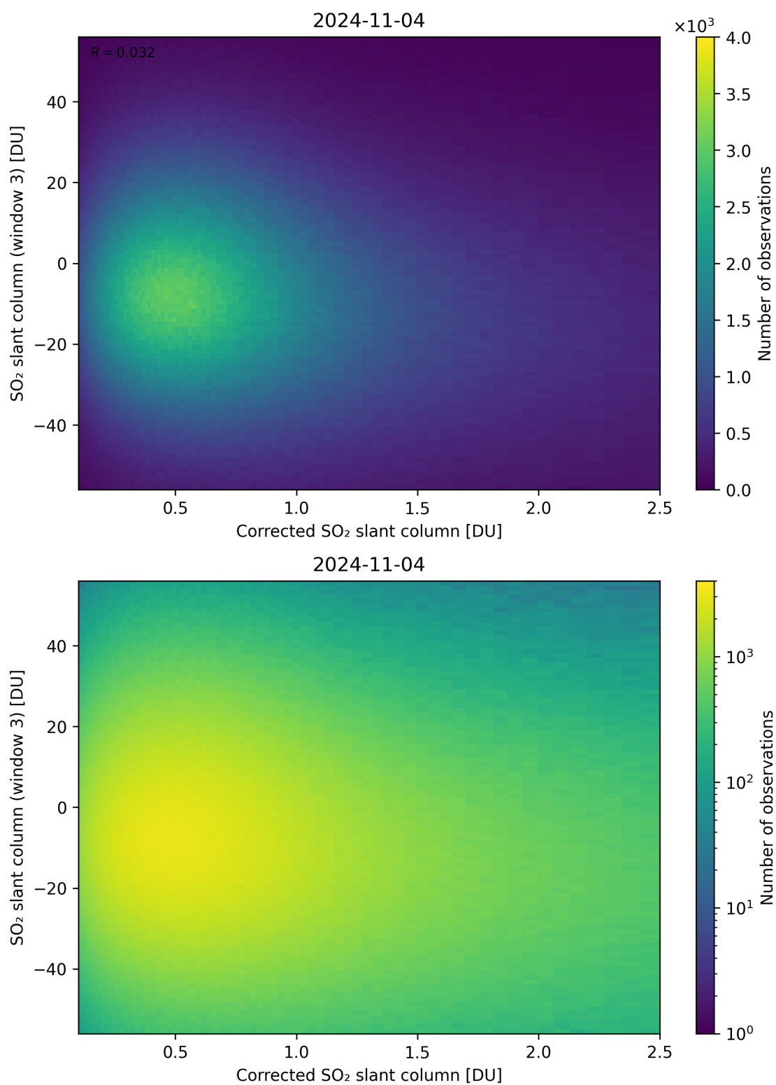
Figure 190: Scatter density plot of “Corrected SO 2 slant column” against “SO 2 slant column (window 3)” for 2024-11-04 to 2024-11-05.
