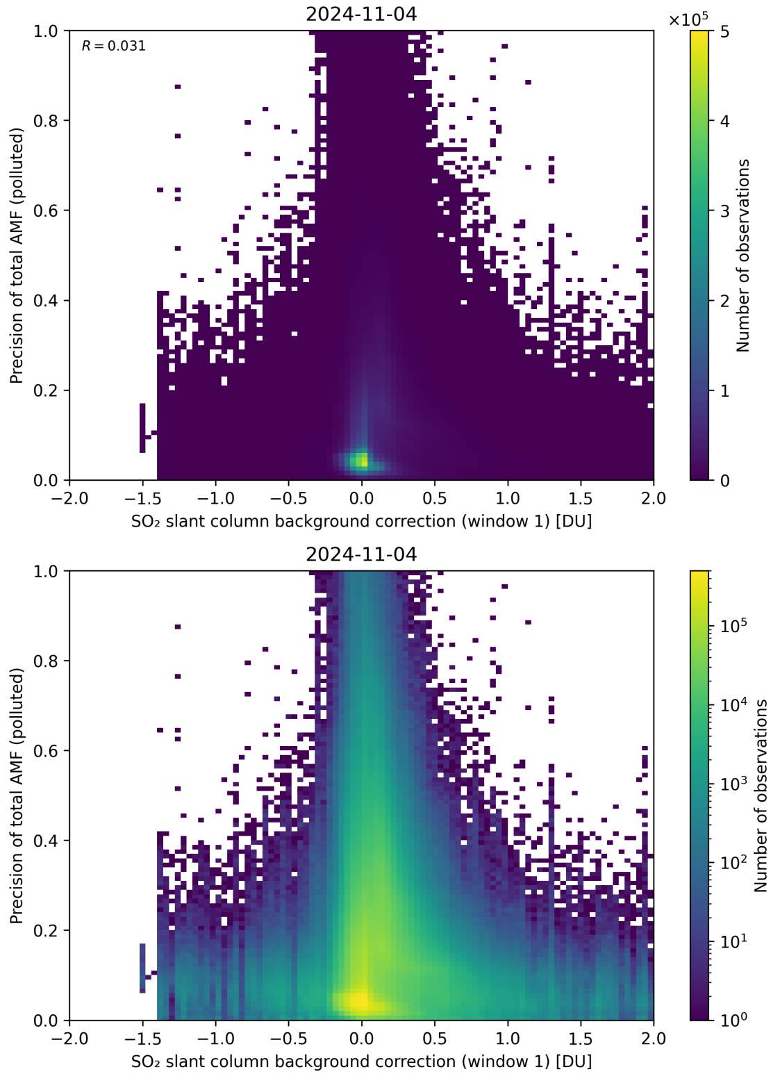
Figure 110: Scatter density plot of “SO 2 slant column background correction (window 1)” against “Precision of total AMF (polluted)” for 2024-11-04 to 2024-11-05.
