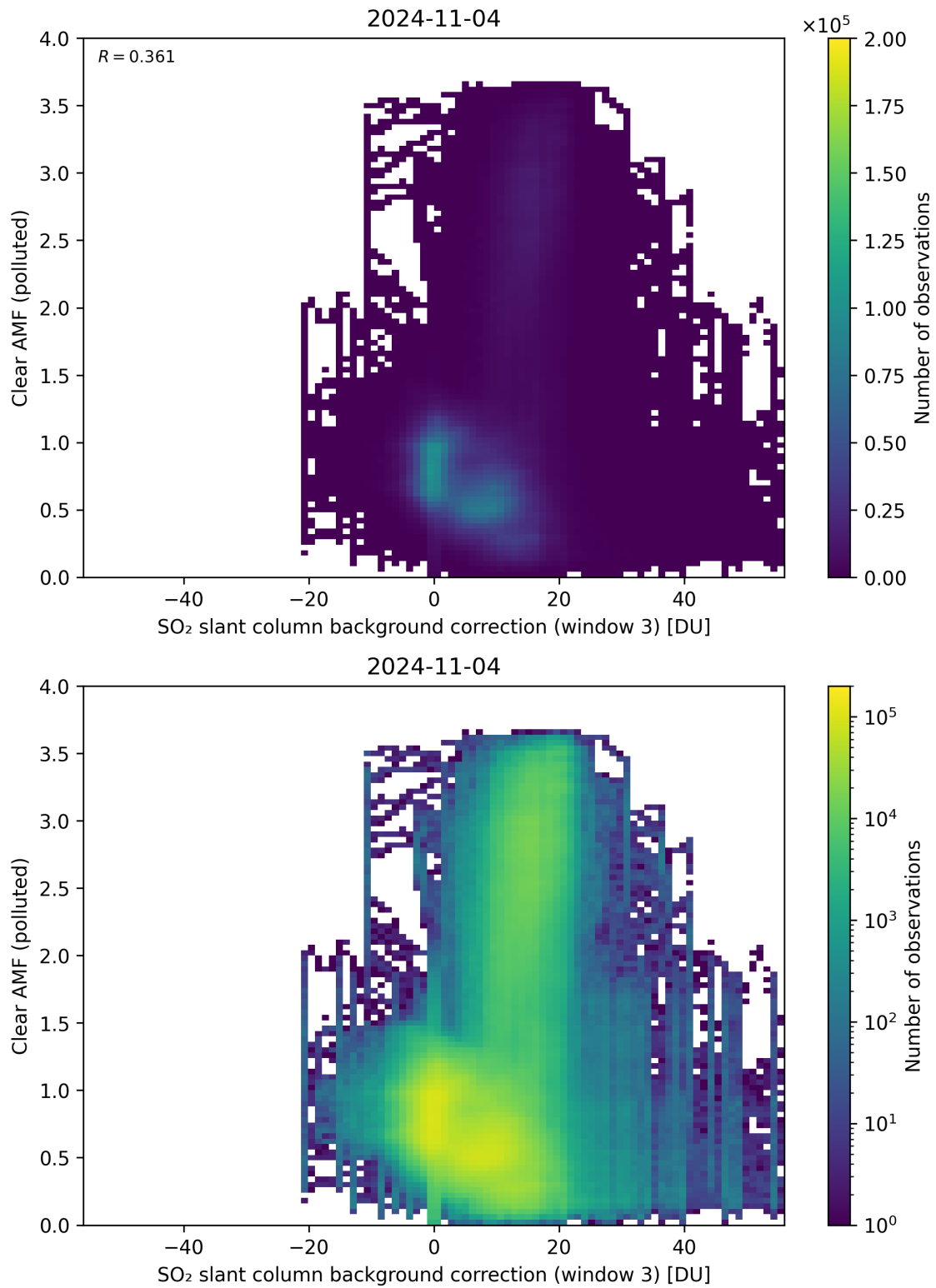
Figure 124: Scatter density plot of “SO 2 slant column background correction (window 3)” against “Clear AMF (polluted)” for 2024-11-04 to 2024-11-05.
