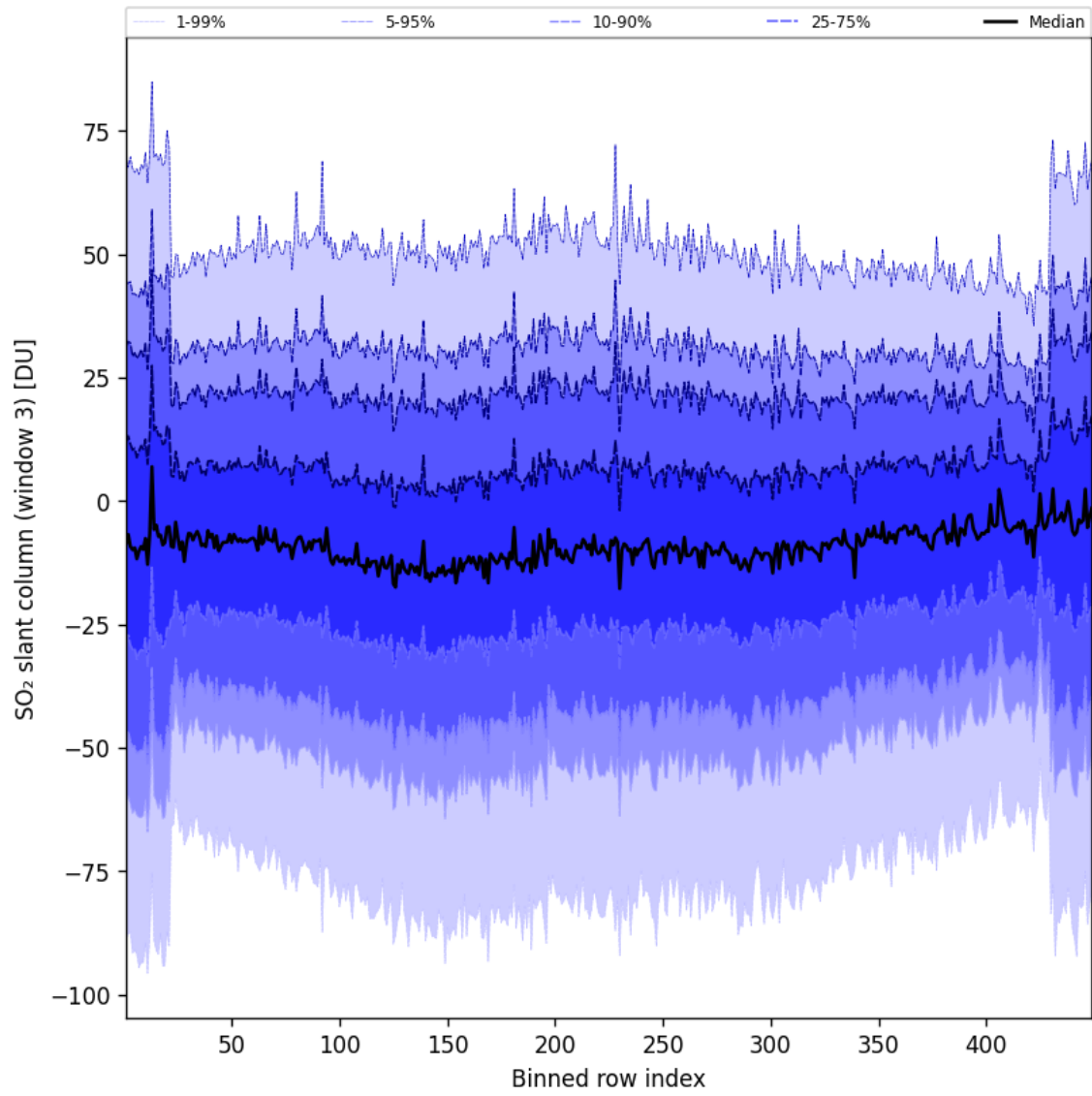
Figure 87: Along track statistics of “SO 2 slant column (window 3)” for 2024-11-04 to 2024-11-05
