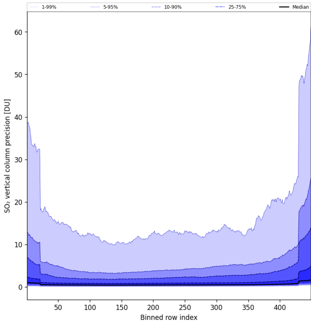
Figure 77: Along track statistics of “SO 2 vertical column precision” for 2024-11-04 to 2024-11-05
