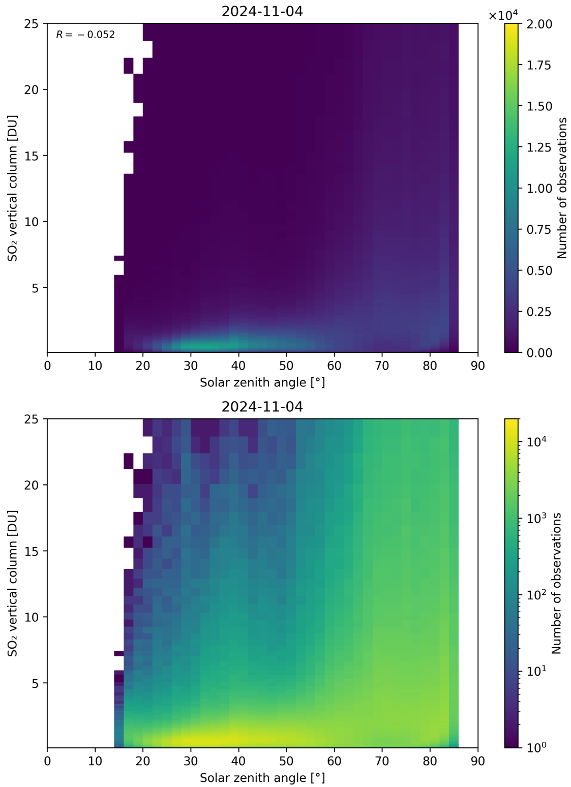
Figure 176: Scatter density plot of “Solar zenith angle” against “SO 2 vertical column” for 2024-11-04 to 2024-11-05.
