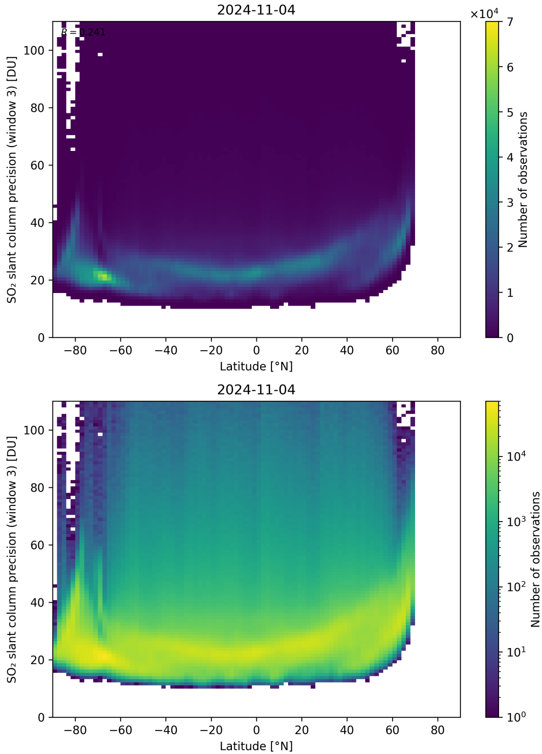
Figure 153: Scatter density plot of “Latitude” against “SO 2 slant column precision (window 3)” for 2024-11-04 to 2024-11-05.
