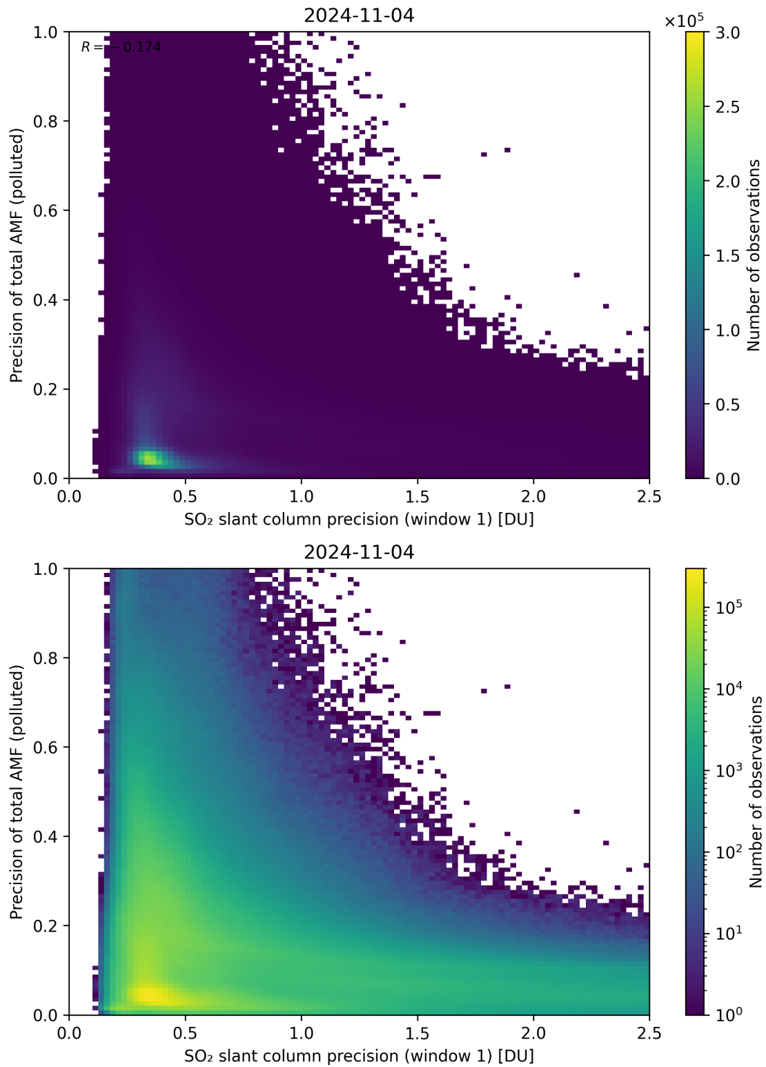
Figure 231: Scatter density plot of “SO 2 slant column precision (window 1)” against “Precision of total AMF (polluted)” for 2024-11-04 to 2024-11-05.
