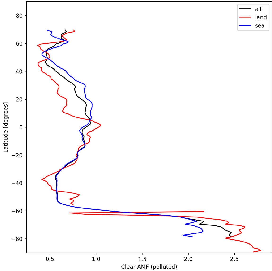
Figure 50: Zonal average of “Clear AMF (polluted)” for 2024-11-04 to 2024-11-05.
