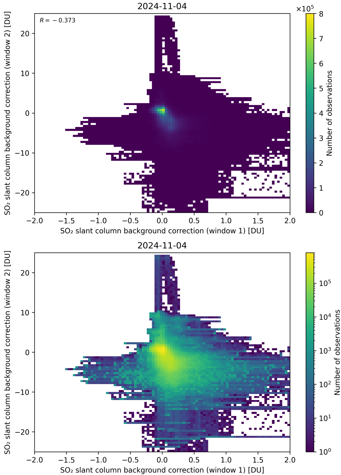
Figure 98: Scatter density plot of “SO 2 slant column background correction (window 1)” against “SO 2 slant column background correction (window 2)” for 2024-11-04 to 2024-11-05.
