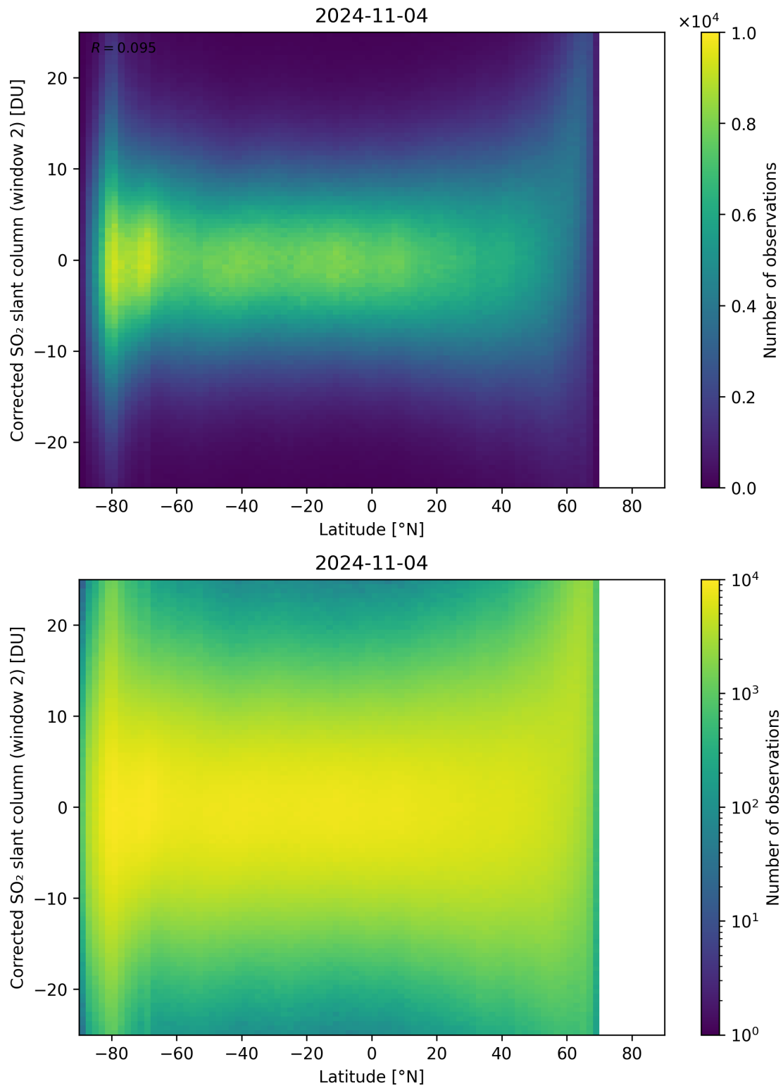
Figure 147: Scatter density plot of “Latitude” against “Corrected SO 2 slant column (window 2)” for 2024-11-04 to 2024-11-05.
