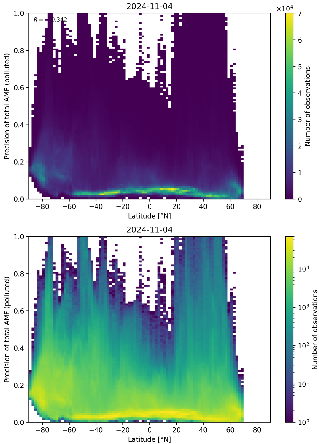
Figure 155: Scatter density plot of “Latitude” against “Precision of total AMF (polluted)” for 2024-11-04 to 2024-11-05.
