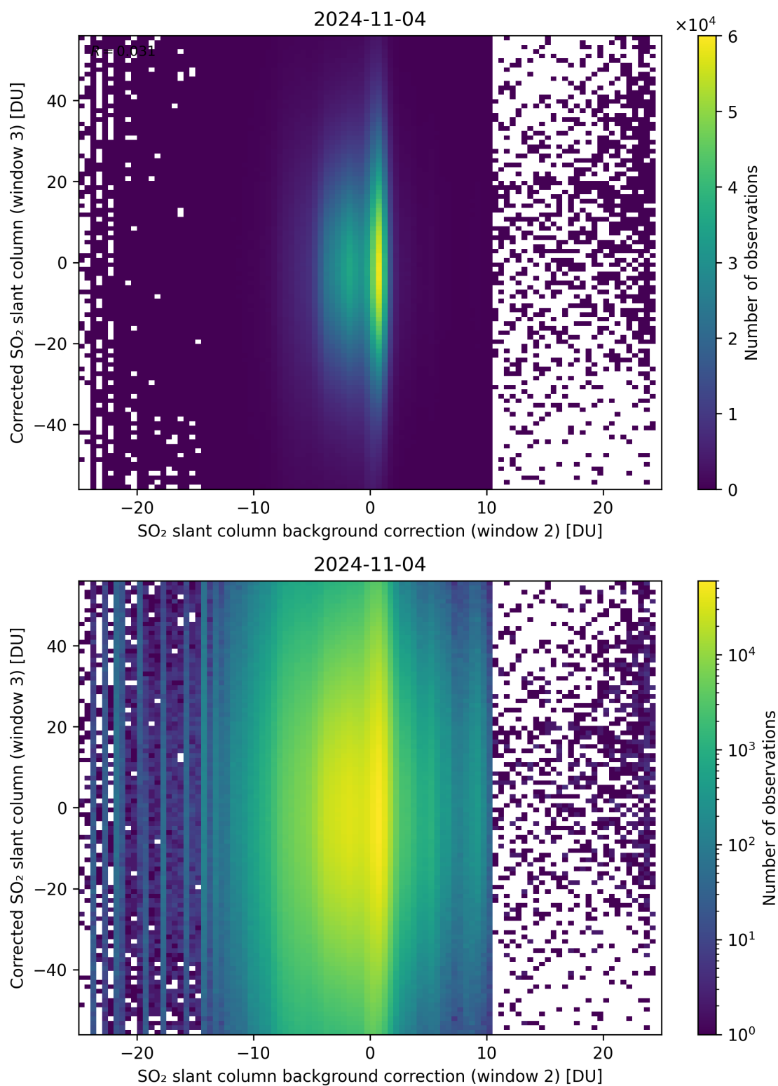
Figure 116: Scatter density plot of “SO 2 slant column background correction (window 2)” against “Corrected SO 2 slant column (window 3)” for 2024-11-04 to 2024-11-05.
