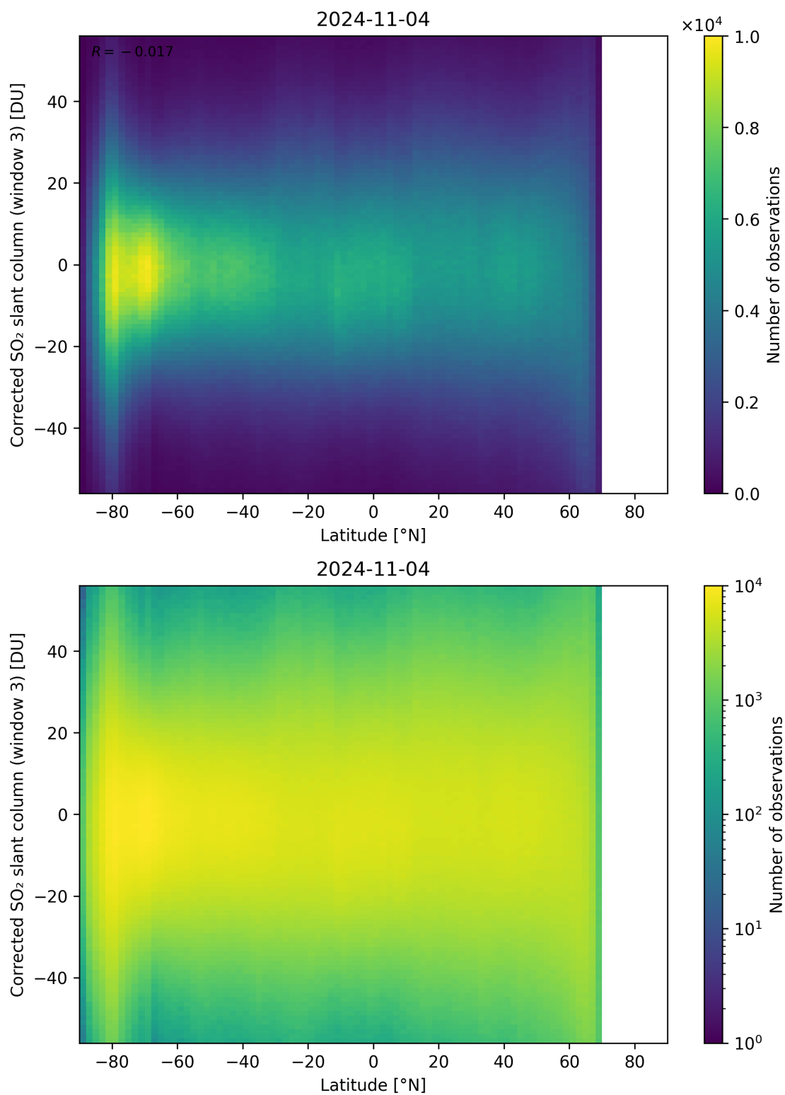
Figure 148: Scatter density plot of “Latitude” against “Corrected SO 2 slant column (window 3)” for 2024-11-04 to 2024-11-05.
