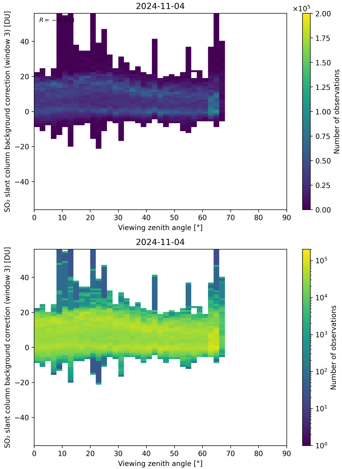
Figure 310: Scatter density plot of “Viewing zenith angle” against “SO 2 slant column background correction (window 3)” for 2024-11-04 to 2024-11-05.
