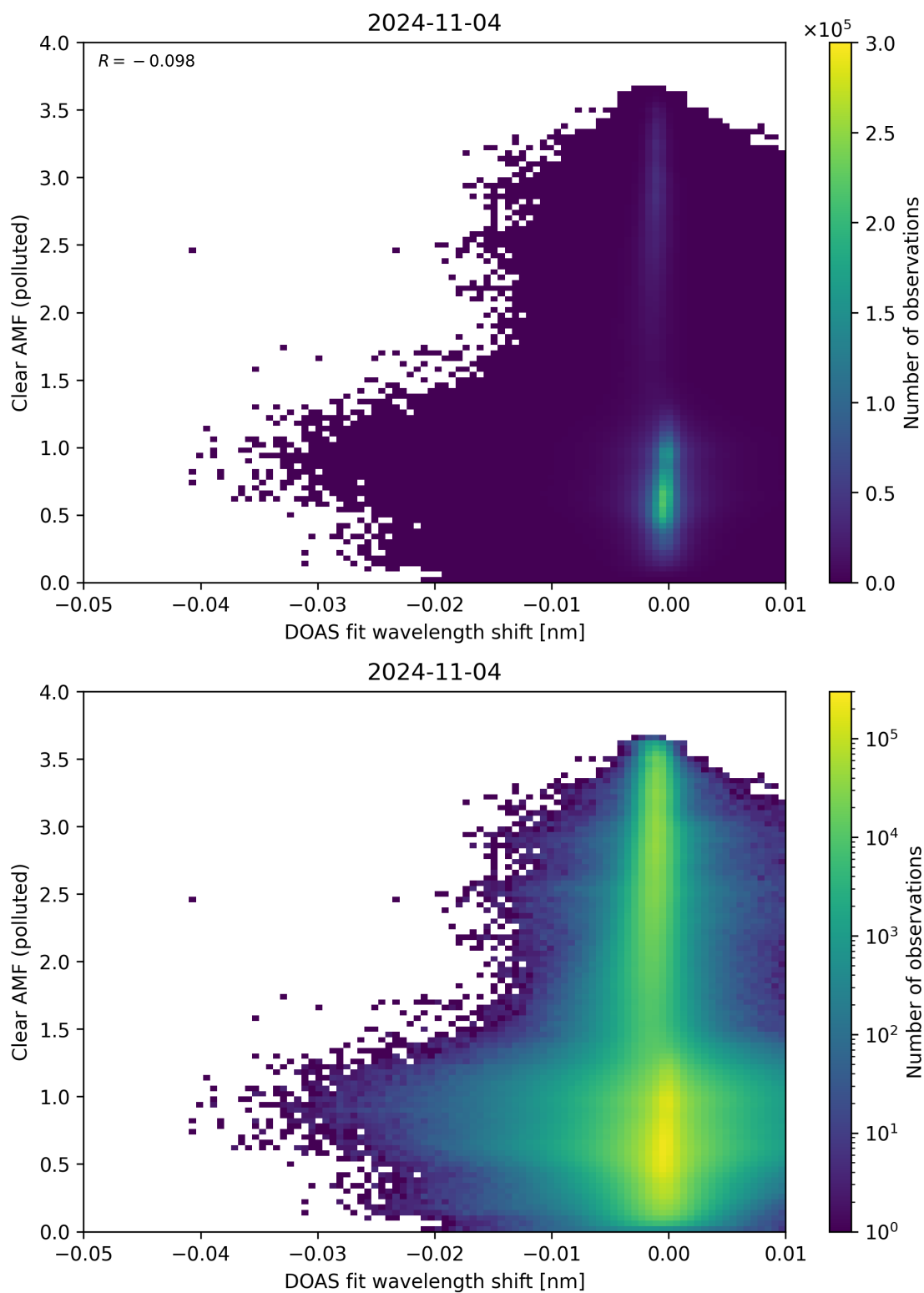
Figure 129: Scatter density plot of “DOAS fit wavelength shift” against “Clear AMF (polluted)” for 2024-11-04 to 2024-11-05.
