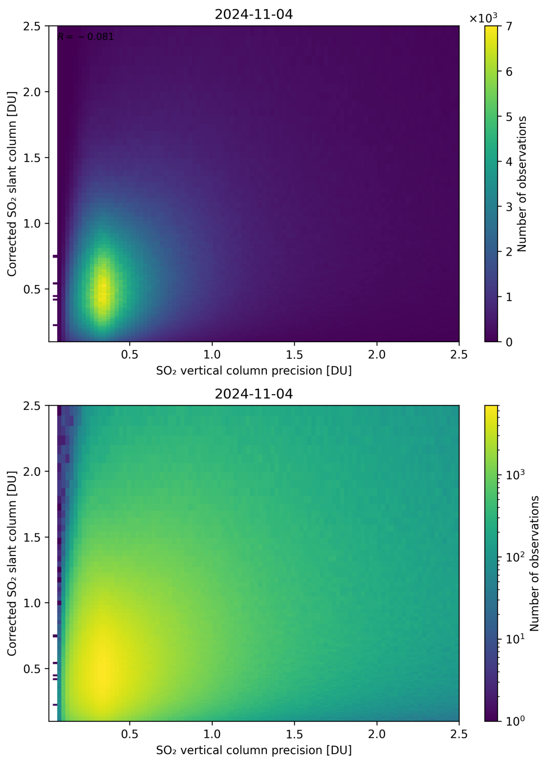
Figure 286: Scatter density plot of “SO 2 vertical column precision” against “Corrected SO 2 slant column” for 2024-11-04 to 2024-11-05.
