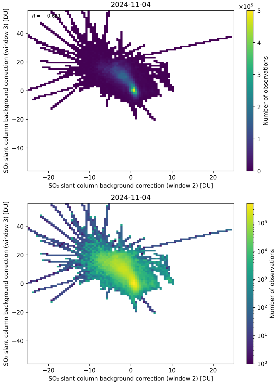
Figure 111: Scatter density plot of “SO 2 slant column background correction (window 2)” against “SO 2 slant column background correction (window 3)” for 2024-11-04 to 2024-11-05.
