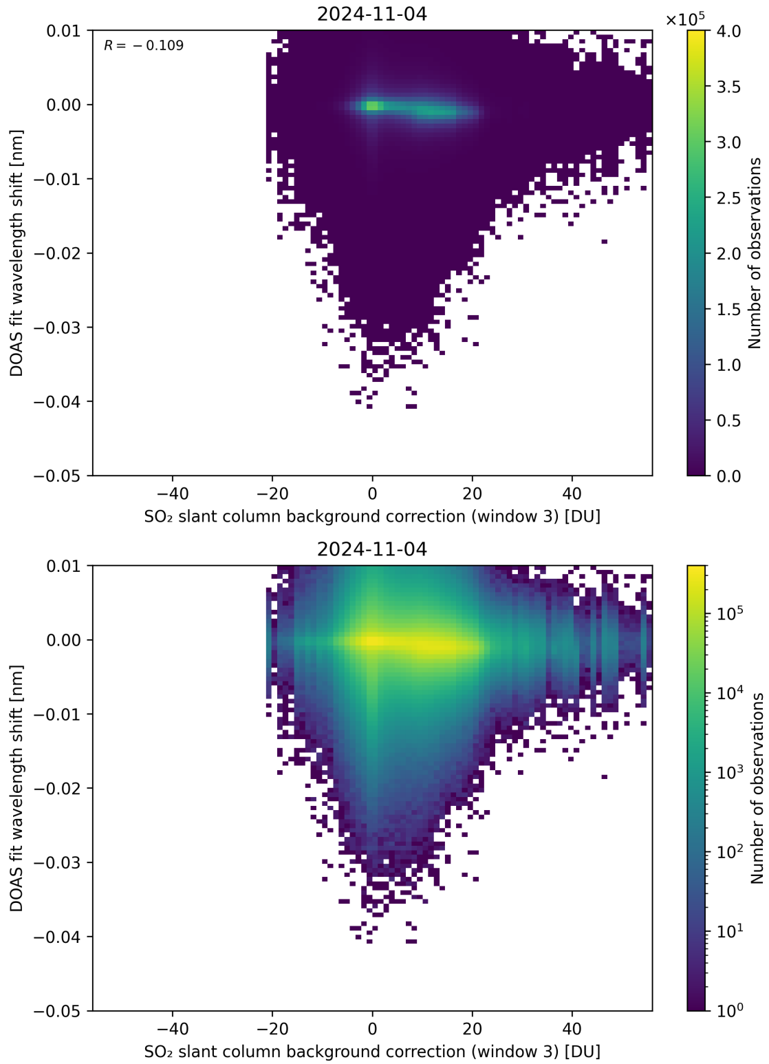
Figure 121: Scatter density plot of “SO 2 slant column background correction (window 3)” against “DOAS fit wavelength shift” for 2024-11-04 to 2024-11-05.
