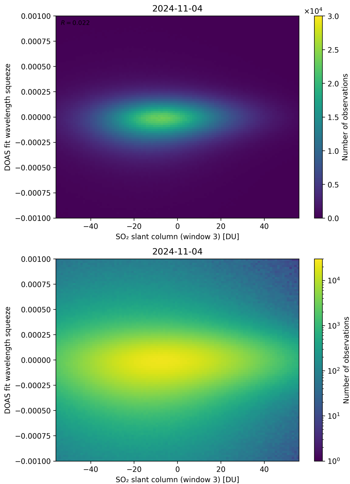
Figure 255: Scatter density plot of “SO 2 slant column (window 3)” against “DOAS fit wavelength squeeze” for 2024-11-04 to 2024-11-05.
