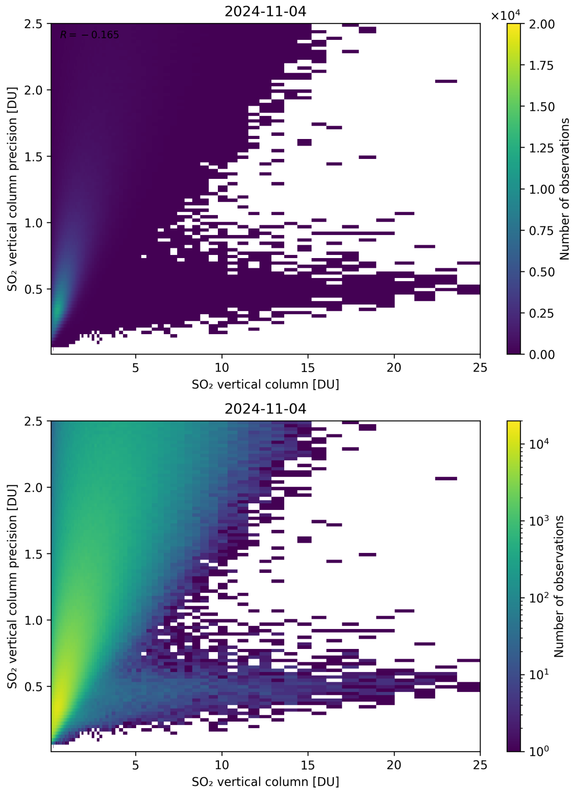
Figure 307: Scatter density plot of “SO 2 vertical column” against “SO 2 vertical column precision” for 2024-11-04 to 2024-11-05.
