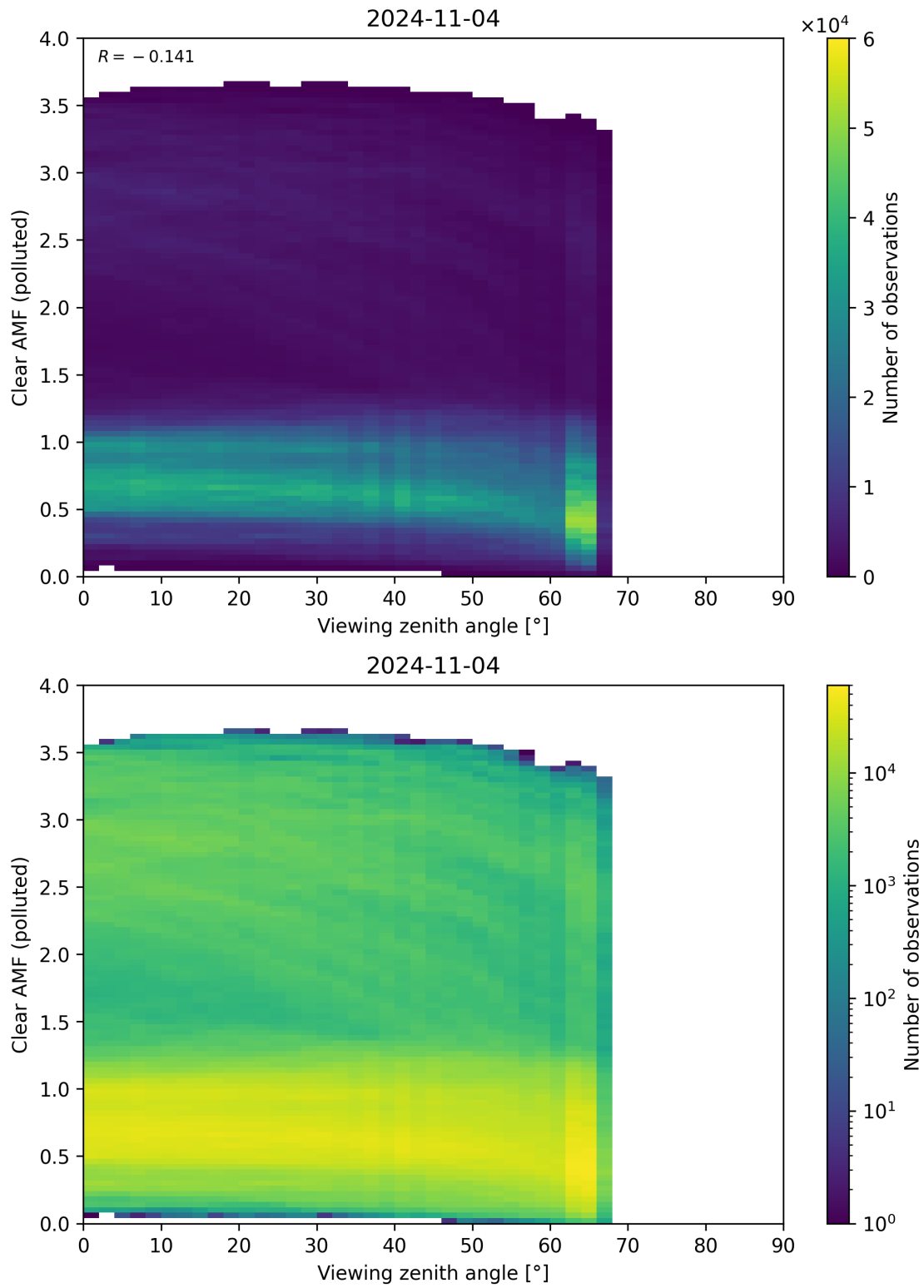
Figure 316: Scatter density plot of “Viewing zenith angle” against “Clear AMF (polluted)” for 2024-11-04 to 2024-11-05.
