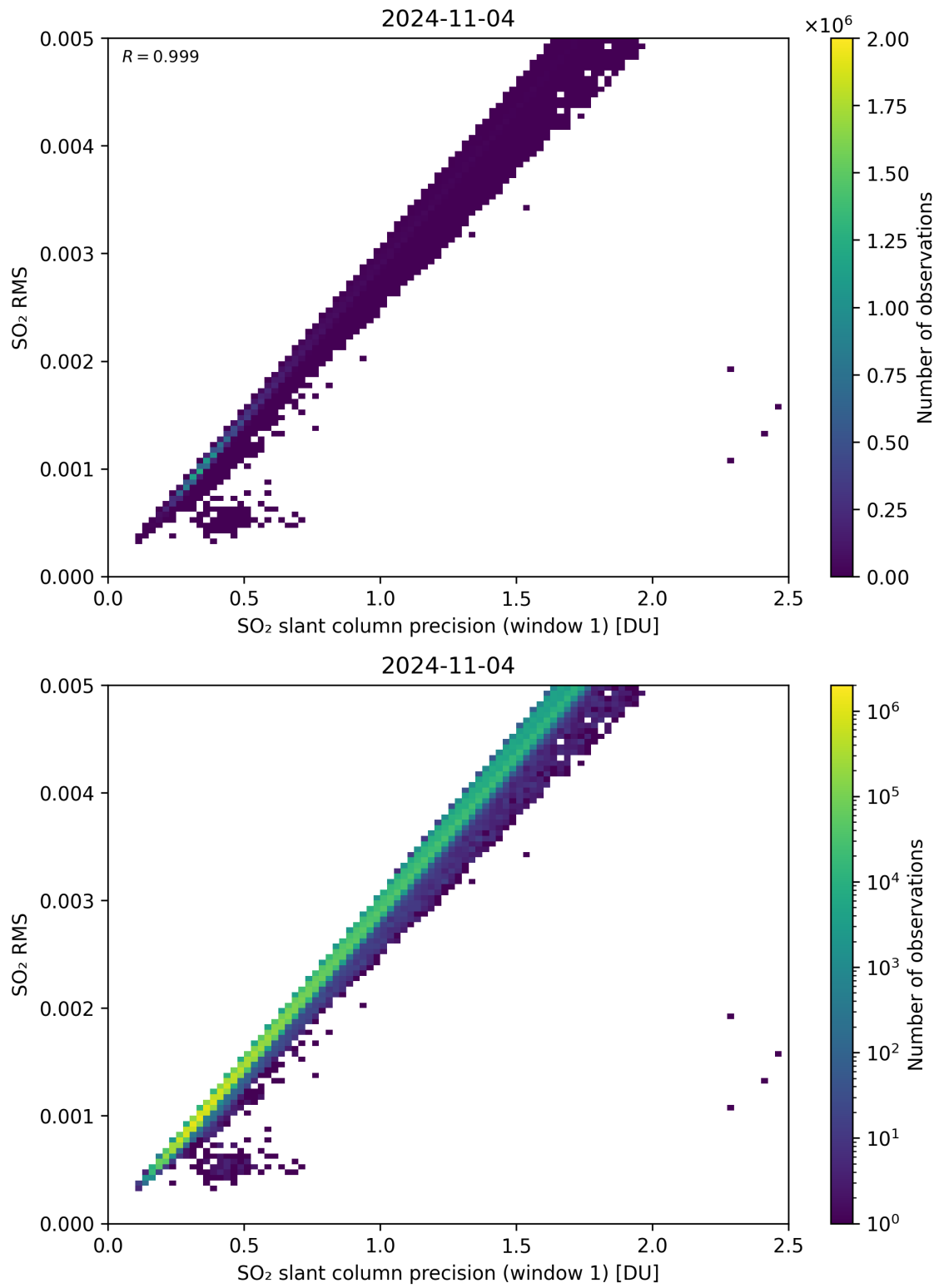
Figure 223: Scatter density plot of “SO 2 slant column precision (window 1)” against “SO 2 RMS” for 2024-11-04 to 2024-11-05.
