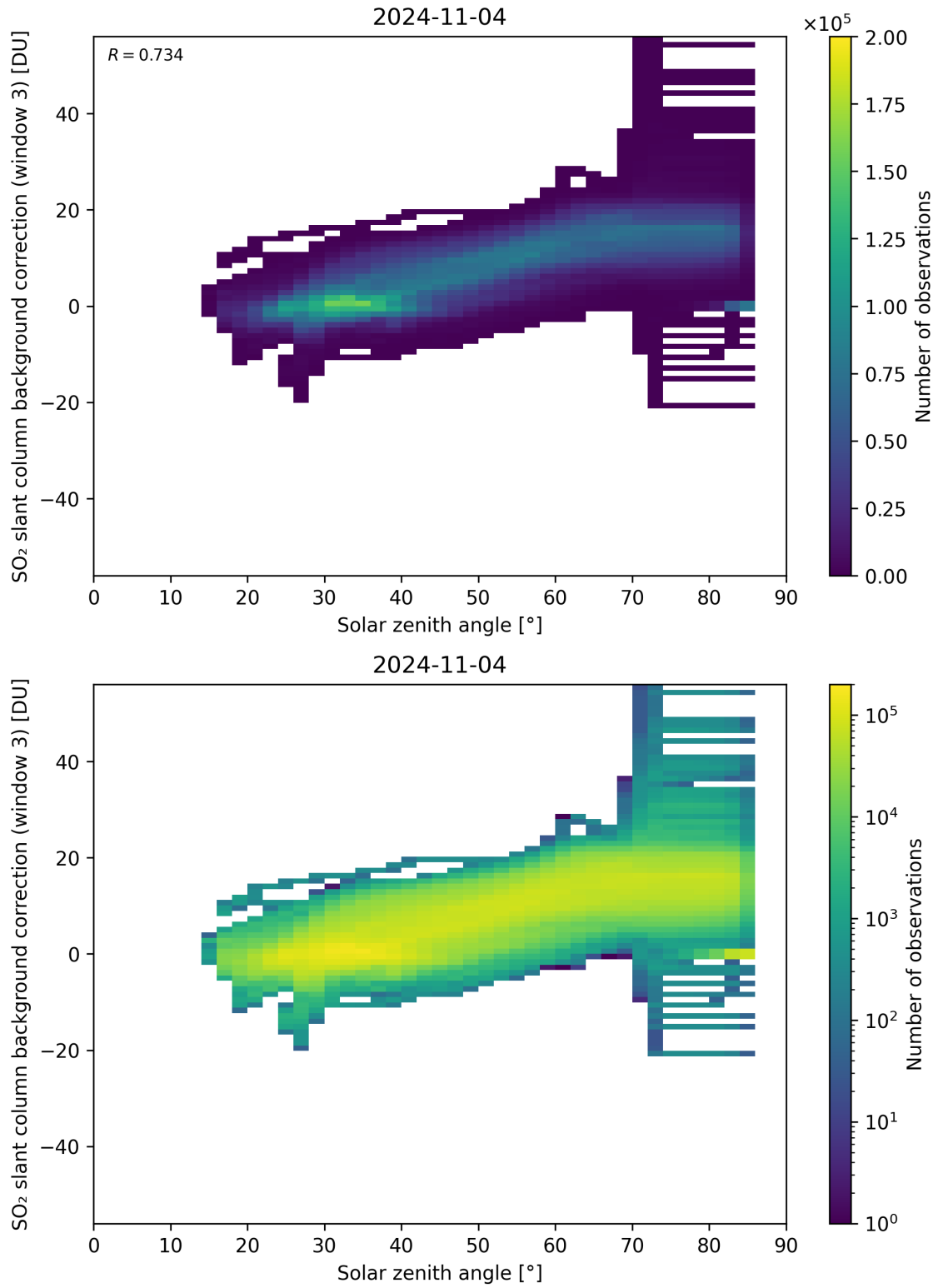
Figure 160: Scatter density plot of “Solar zenith angle” against “SO 2 slant column background correction (window 3)” for 2024-11-04 to 2024-11-05.
