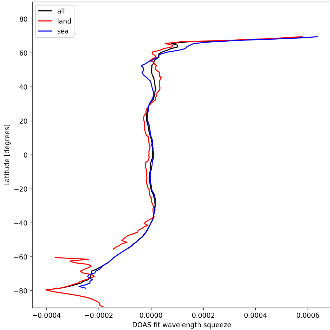
Figure 46: Zonal average of “DOAS fit wavelength squeeze” for 2024-11-04 to 2024-11-05.
