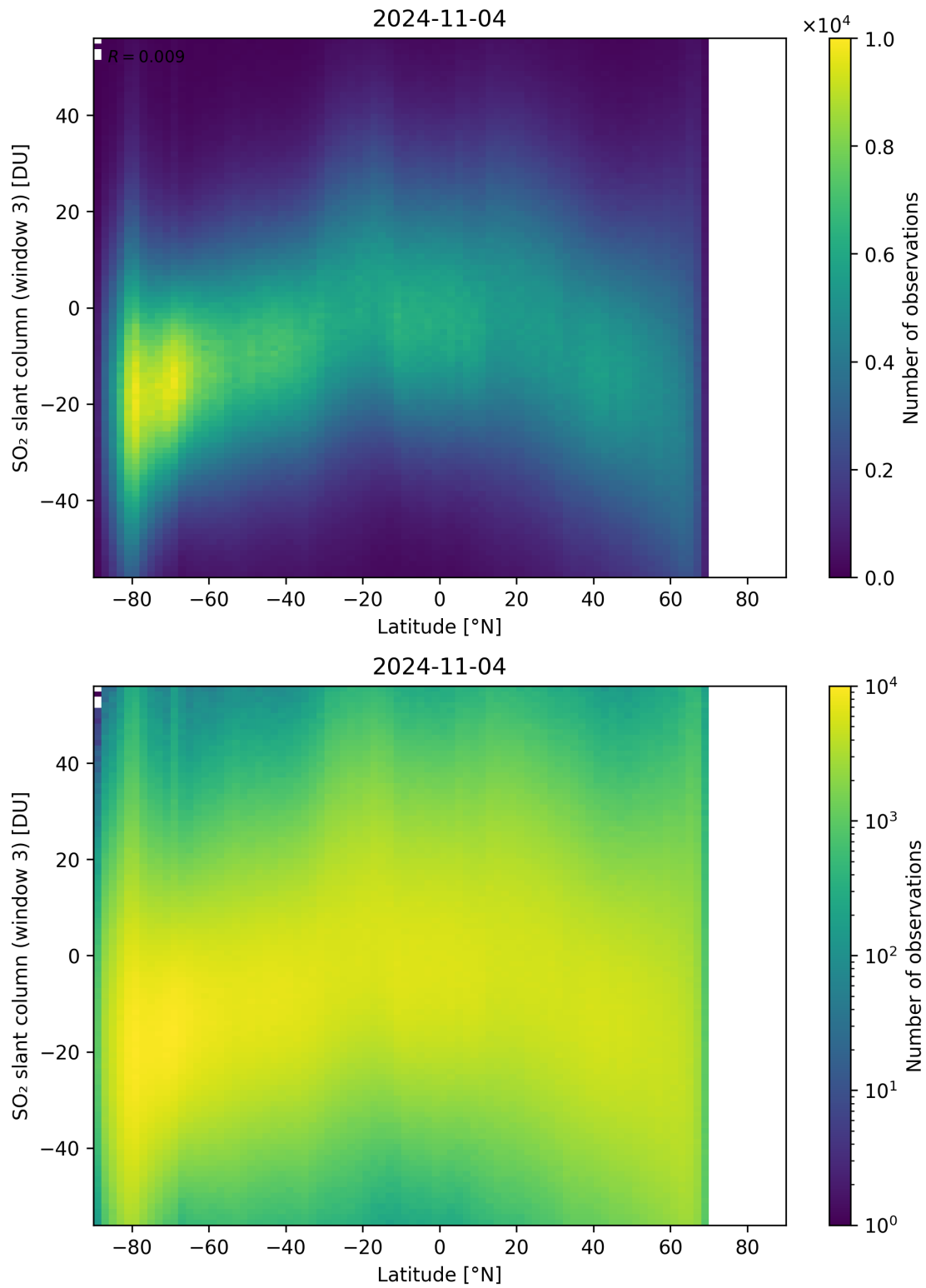
Figure 152: Scatter density plot of “Latitude” against “SO 2 slant column (window 3)” for 2024-11-04 to 2024-11-05.
