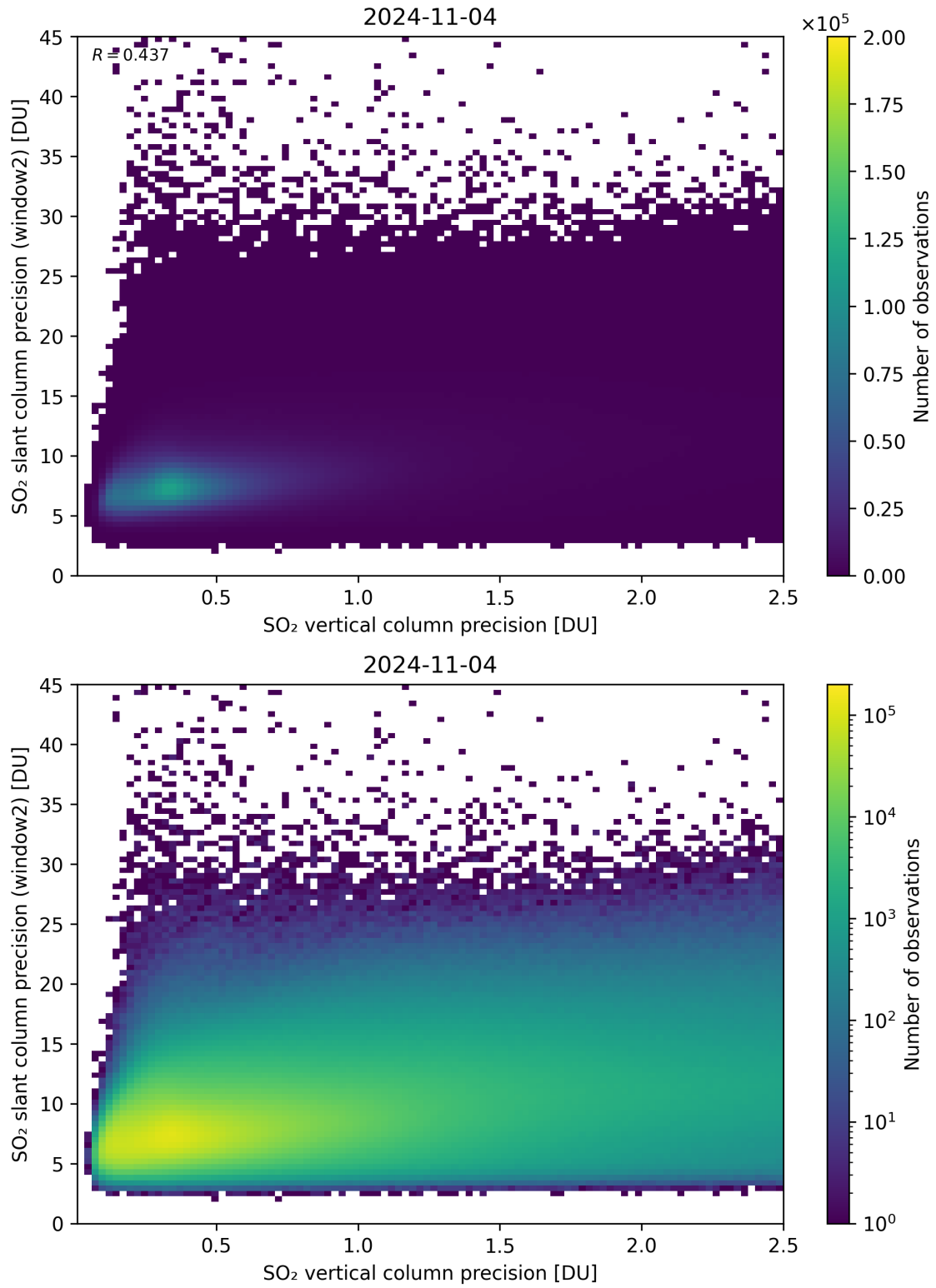
Figure 291: Scatter density plot of “SO 2 vertical column precision” against “SO 2 slant column precision (window2)” for 2024-11-04 to 2024-11-05.
