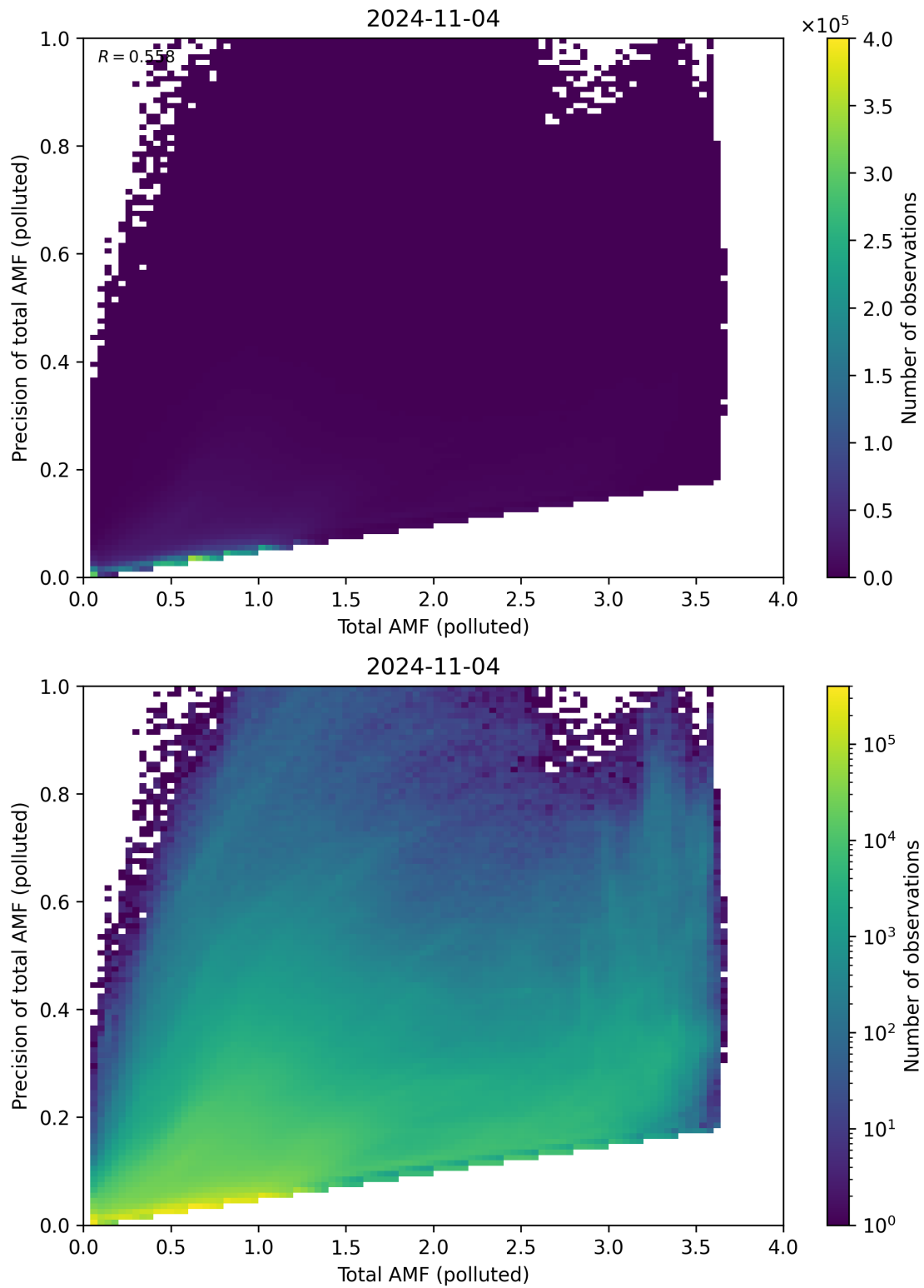
Figure 272: Scatter density plot of “Total AMF (polluted)” against “Precision of total AMF (polluted)” for 2024-11-04 to 2024-11-05.
