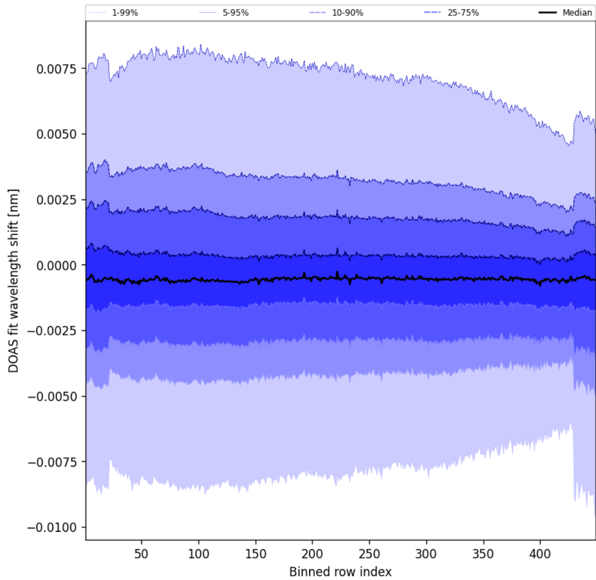
Figure 91: Along track statistics of “DOAS fit wavelength shift” for 2024-11-04 to 2024-11-05
