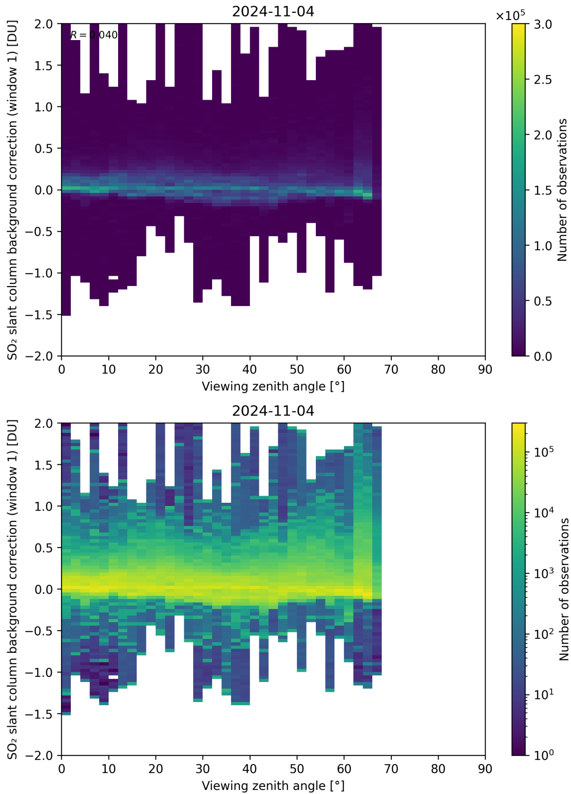
Figure 308: Scatter density plot of “Viewing zenith angle” against “SO 2 slant column background correction (window 1)” for 2024-11-04 to 2024-11-05.
