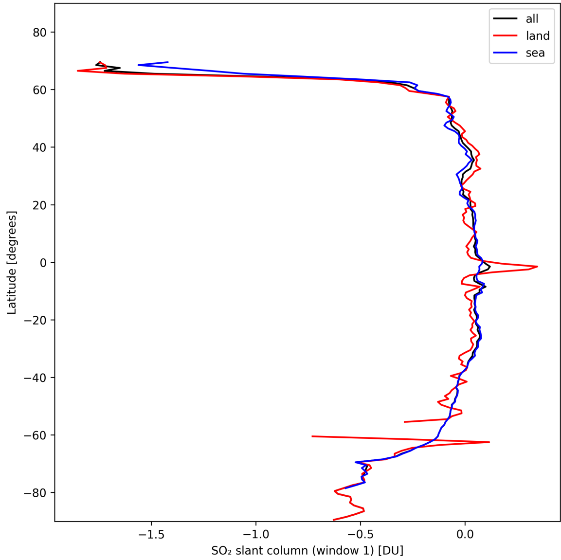
Figure 33: Zonal average of “SO 2 slant column (window 1)” for 2024-11-04 to 2024-11-05.
