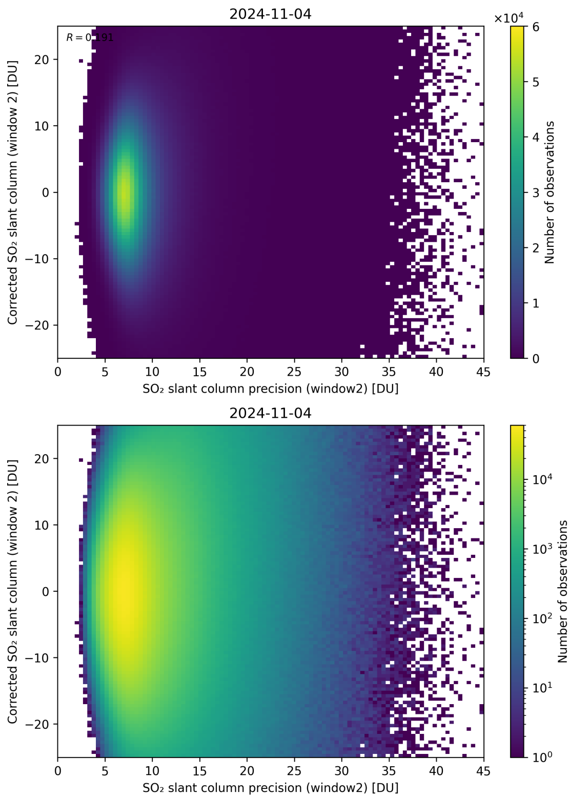
Figure 247: Scatter density plot of “SO 2 slant column precision (window2)” against “Corrected SO 2 slant column (window 2)” for 2024-11-04 to 2024-11-05.
