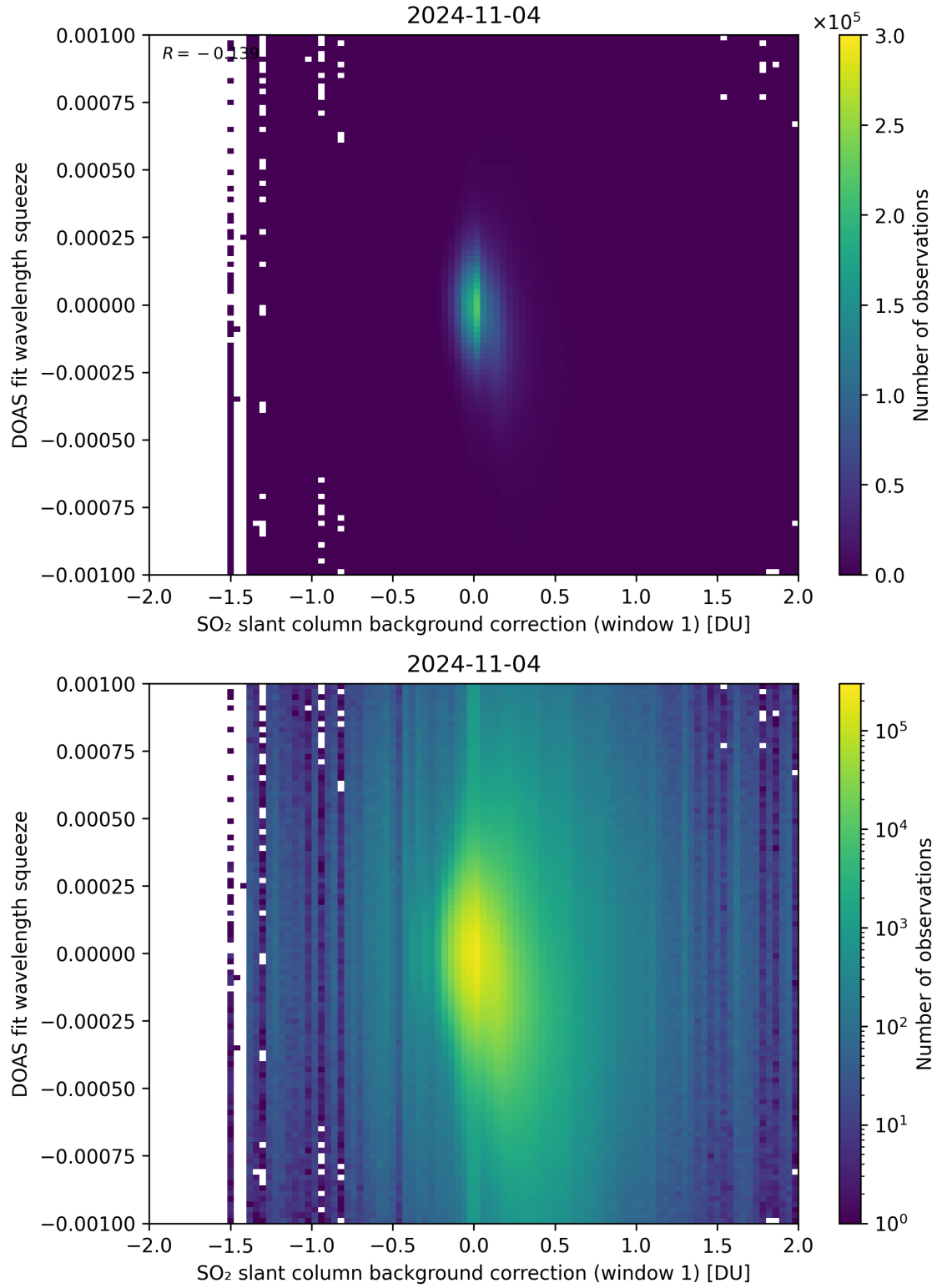
Figure 101: Scatter density plot of “SO 2 slant column background correction (window 1)” against “DOAS fit wavelength squeeze” for 2024-11-04 to 2024-11-05.
