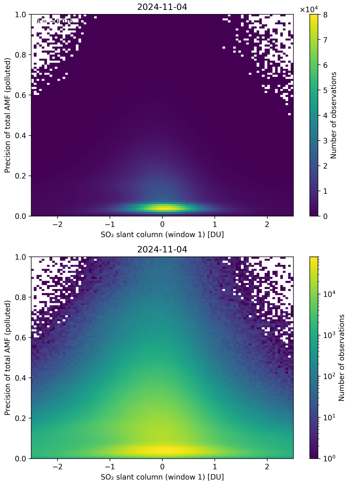
Figure 240: Scatter density plot of “SO 2 slant column (window 1)” against “Precision of total AMF (polluted)” for 2024-11-04 to 2024-11-05.
