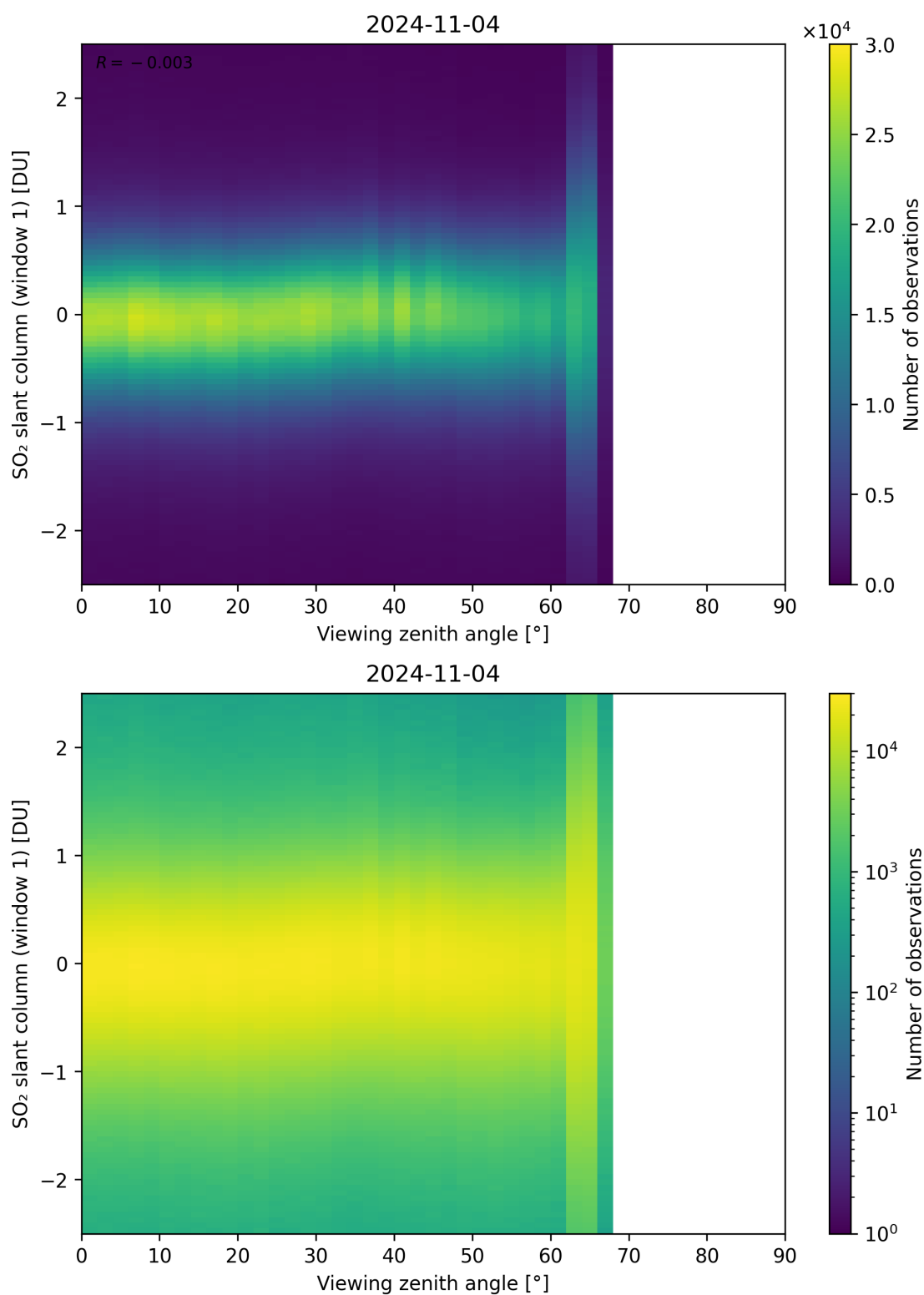
Figure 320: Scatter density plot of “Viewing zenith angle” against “SO 2 slant column (window 1)” for 2024-11-04 to 2024-11-05.
