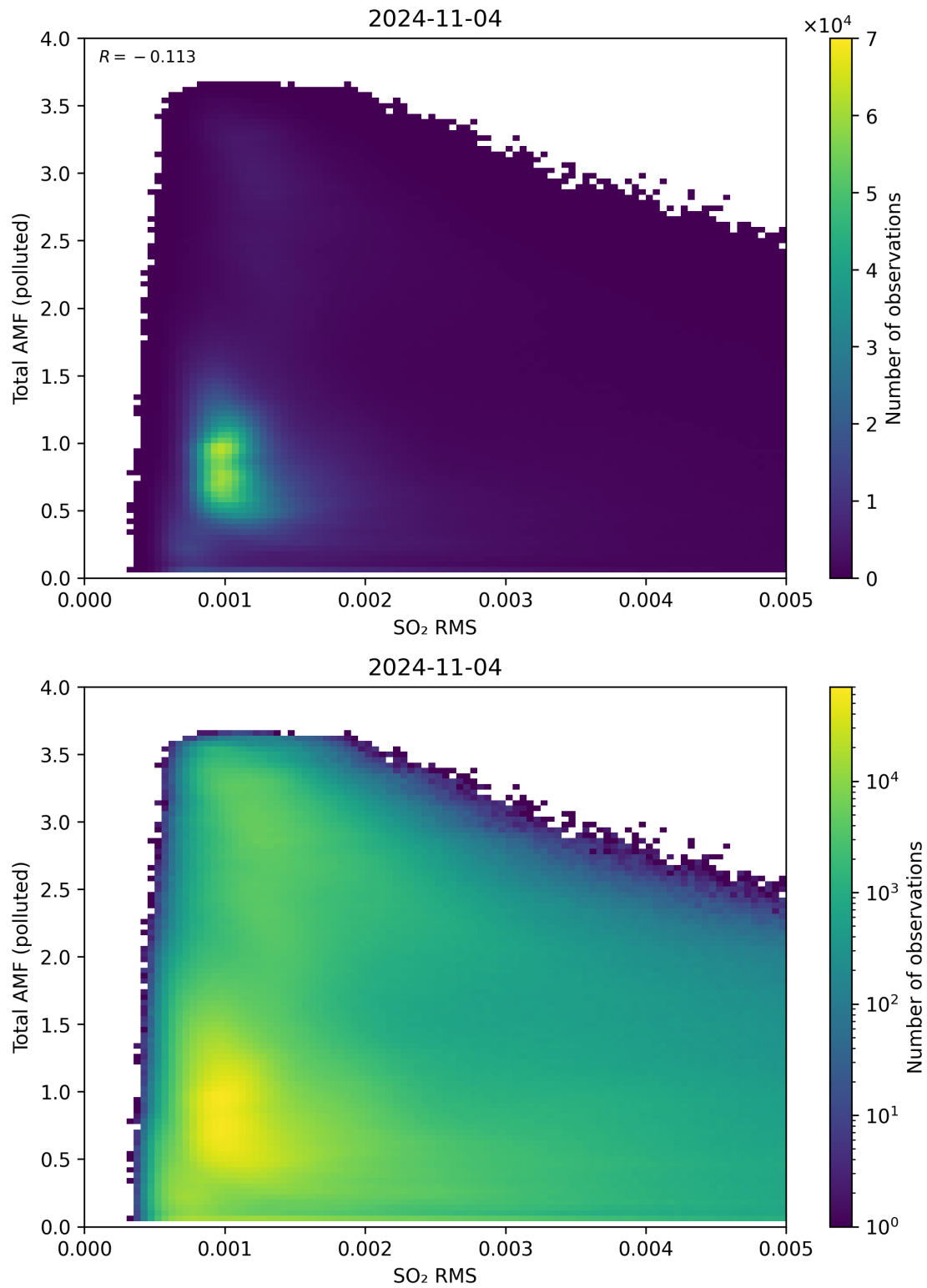
Figure 137: Scatter density plot of “SO 2 RMS” against “Total AMF (polluted)” for 2024-11-04 to 2024-11-05.
