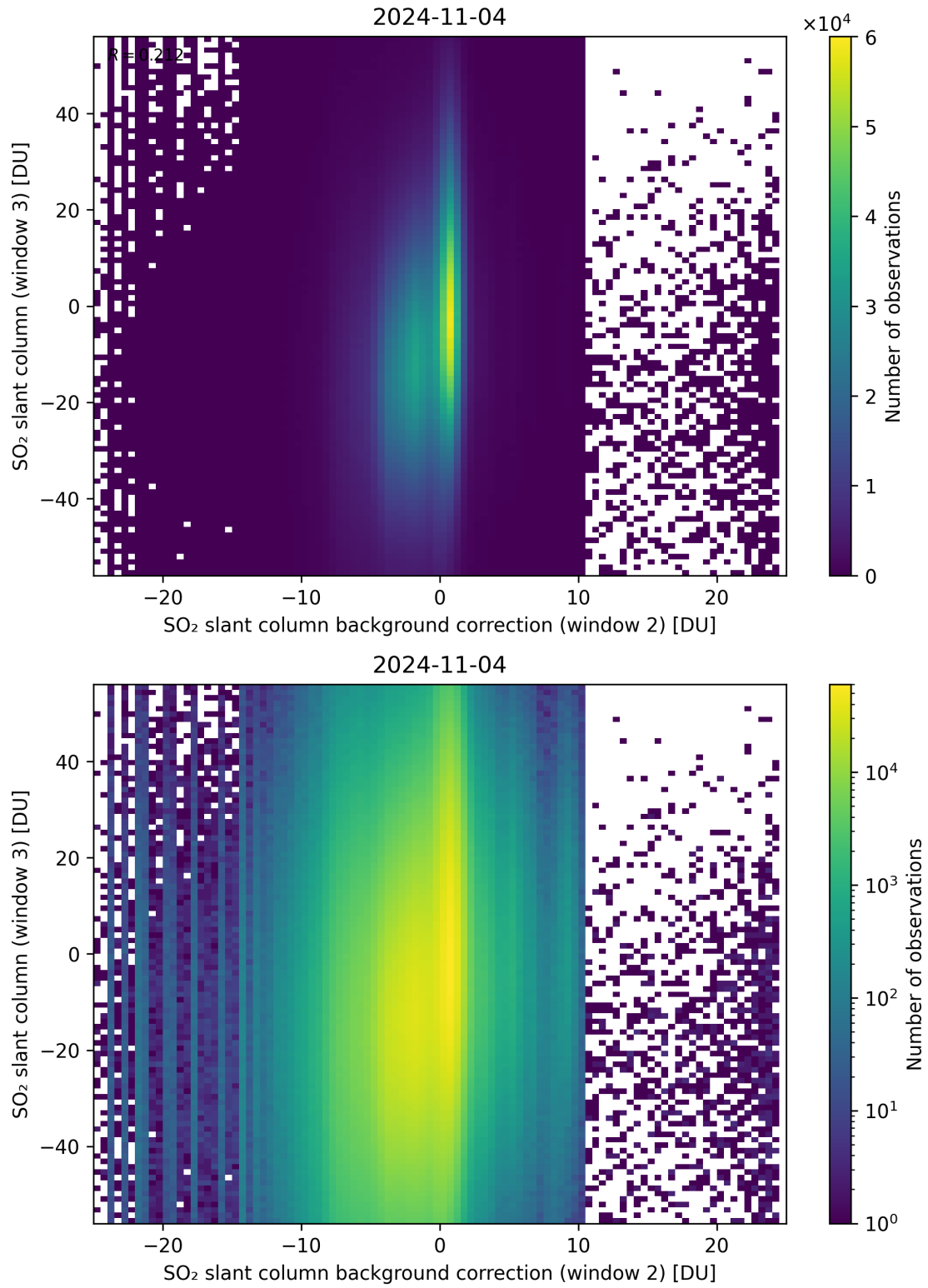
Figure 117: Scatter density plot of “SO 2 slant column background correction (window 2)” against “SO 2 slant column (window 3)” for 2024-11-04 to 2024-11-05.
