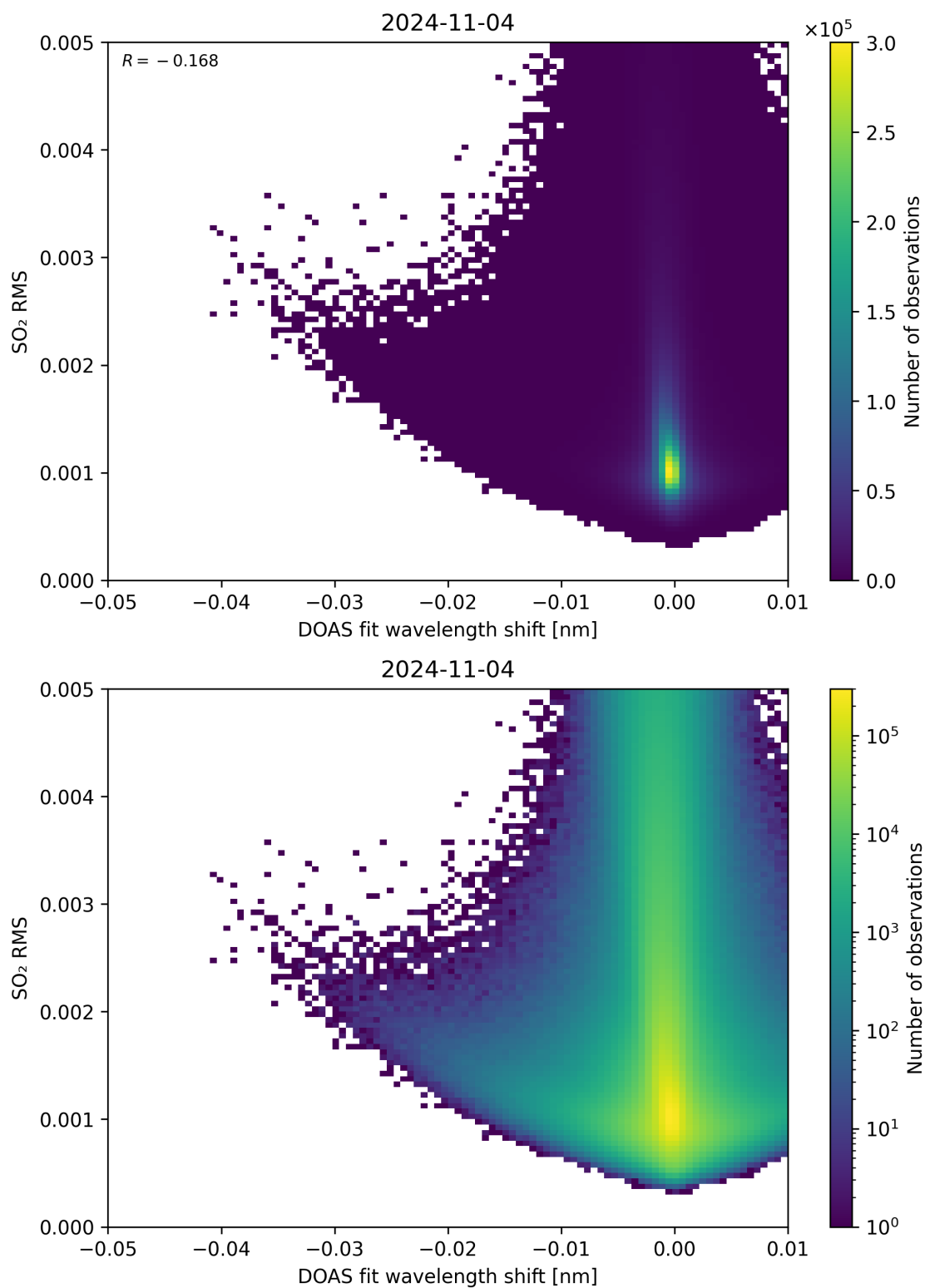
Figure 128: Scatter density plot of “DOAS fit wavelength shift” against “SO 2 RMS” for 2024-11-04 to 2024-11-05.
