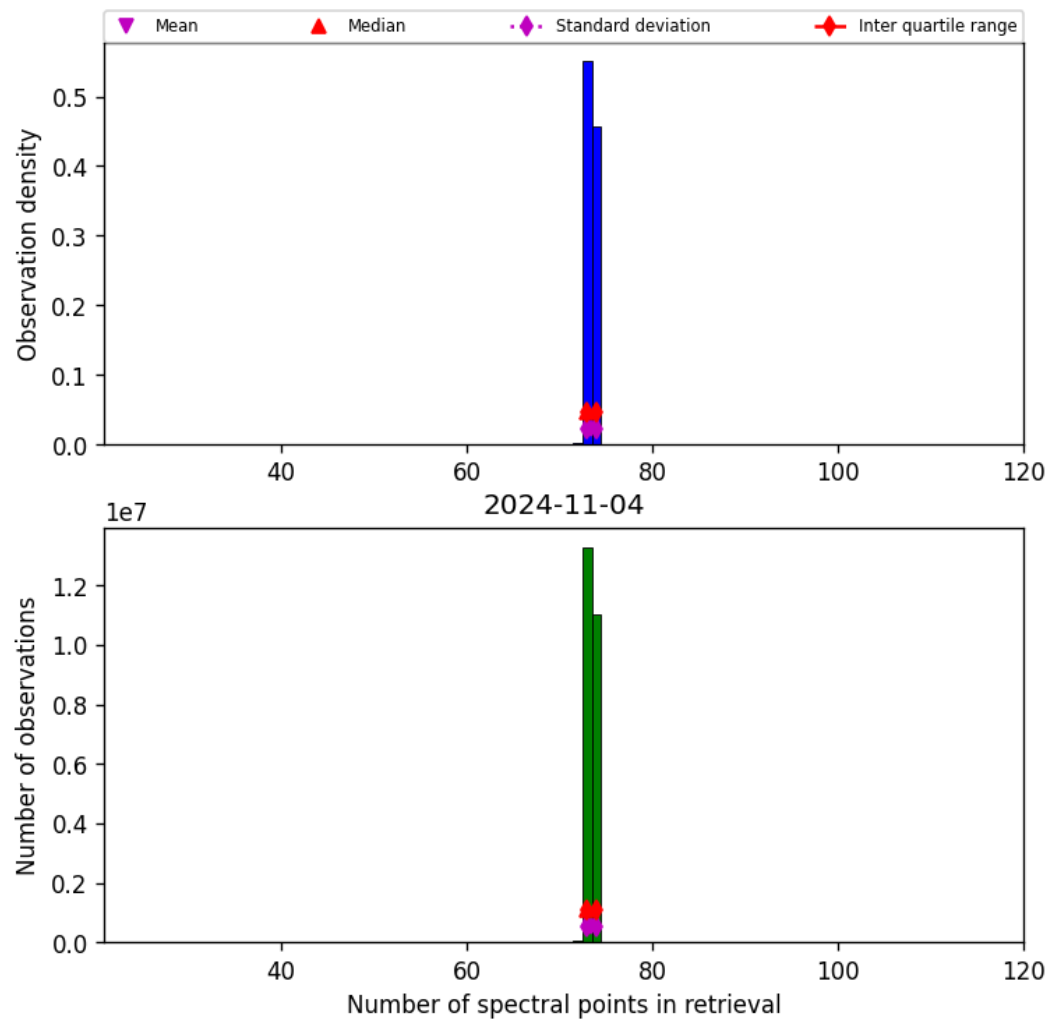
Figure 74: Histogram of “Number of spectral points in retrieval” for 2024-11-04 to 2024-11-05
