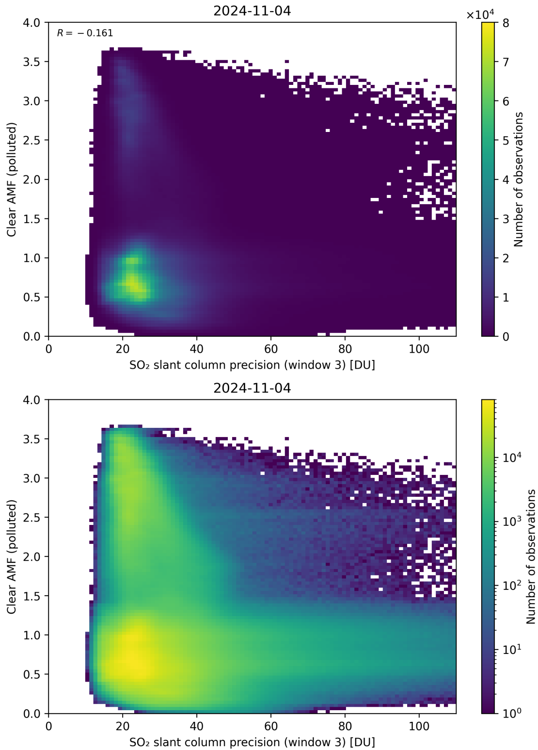
Figure 261: Scatter density plot of “SO 2 slant column precision (window 3)” against “Clear AMF (polluted)” for 2024-11-04 to 2024-11-05.
