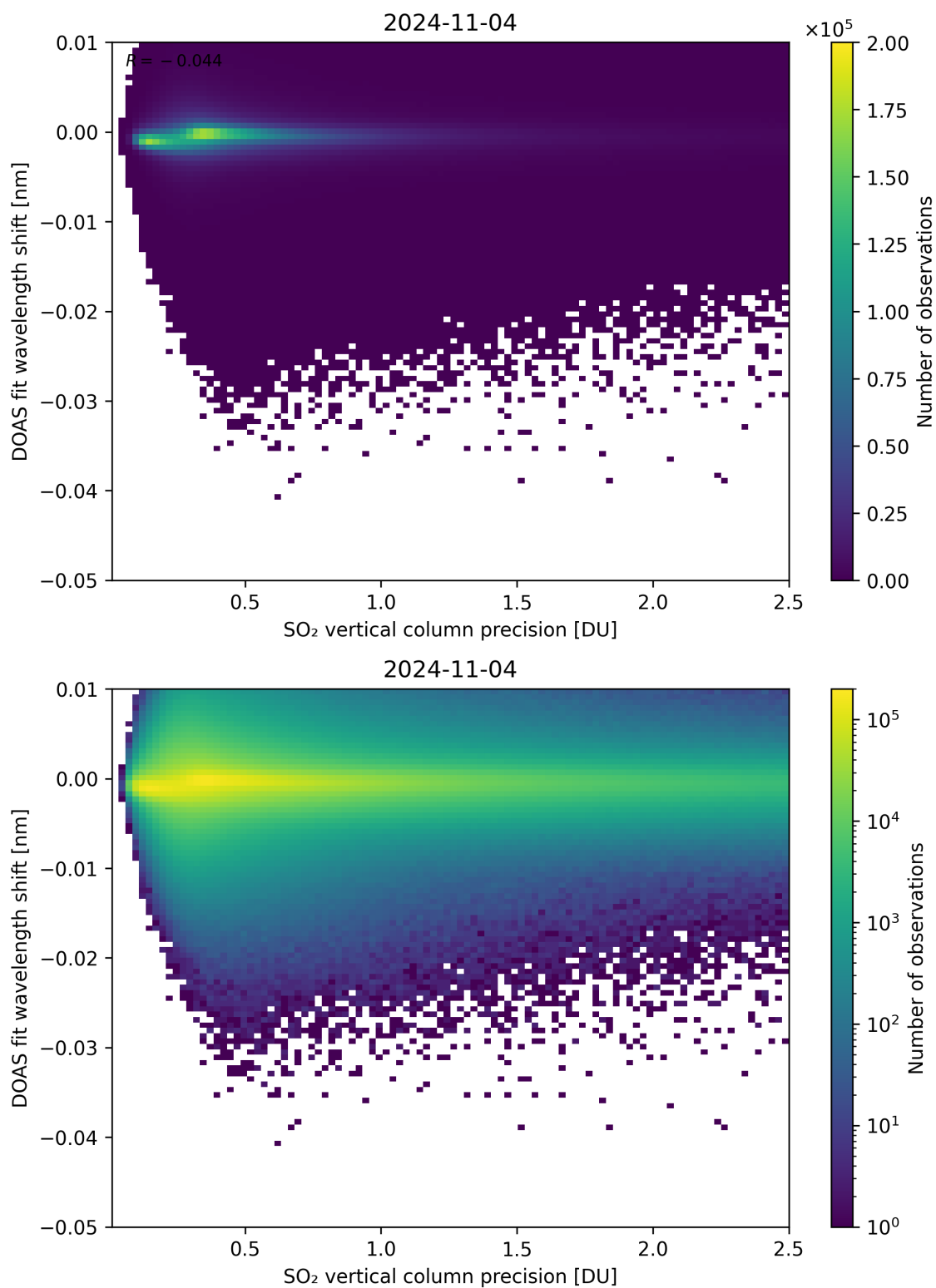
Figure 282: Scatter density plot of “SO 2 vertical column precision” against “DOAS fit wavelength shift” for 2024-11-04 to 2024-11-05.
