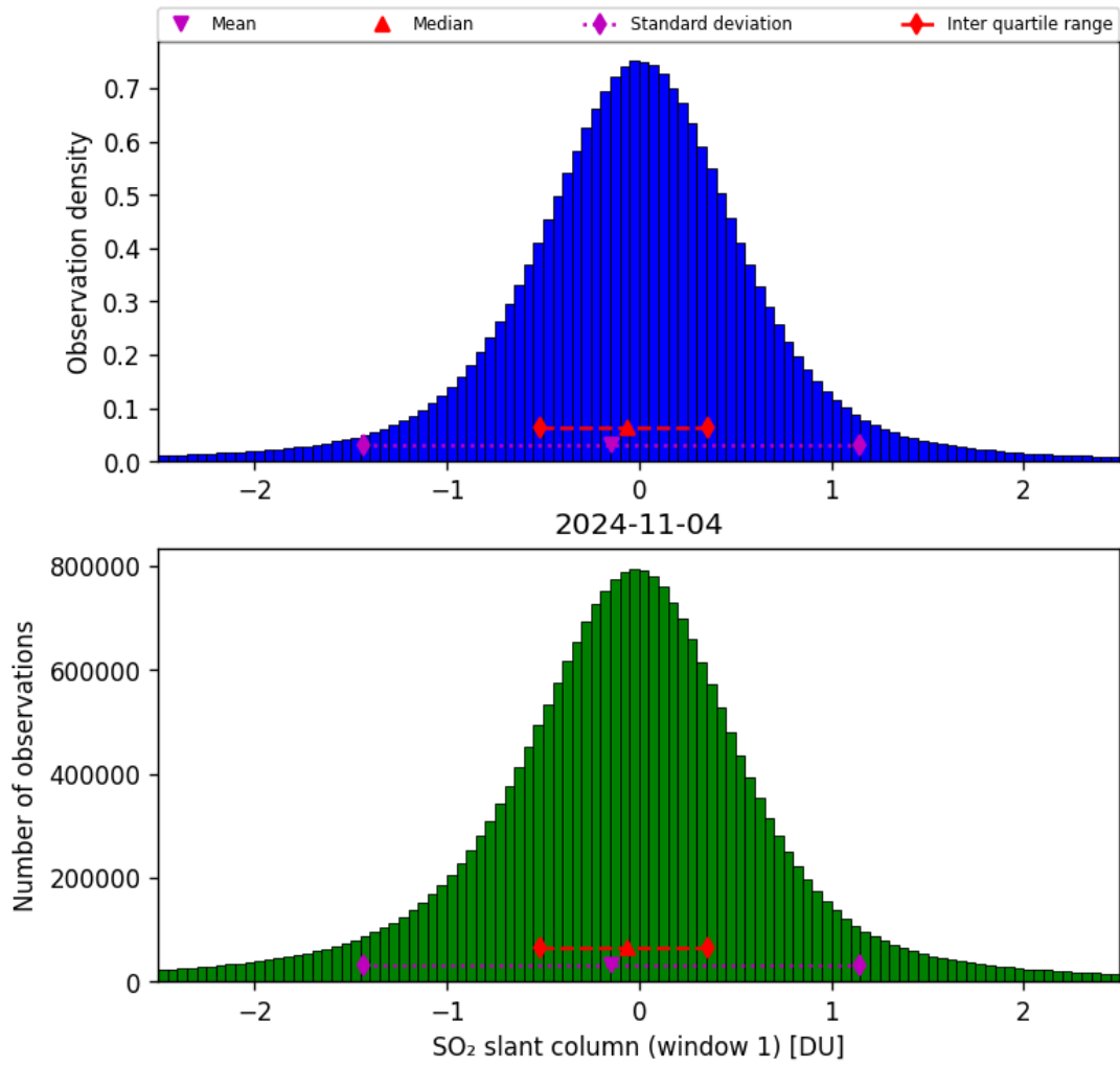
Figure 56: Histogram of “SO 2 slant column (window 1)” for 2024-11-04 to 2024-11-05
