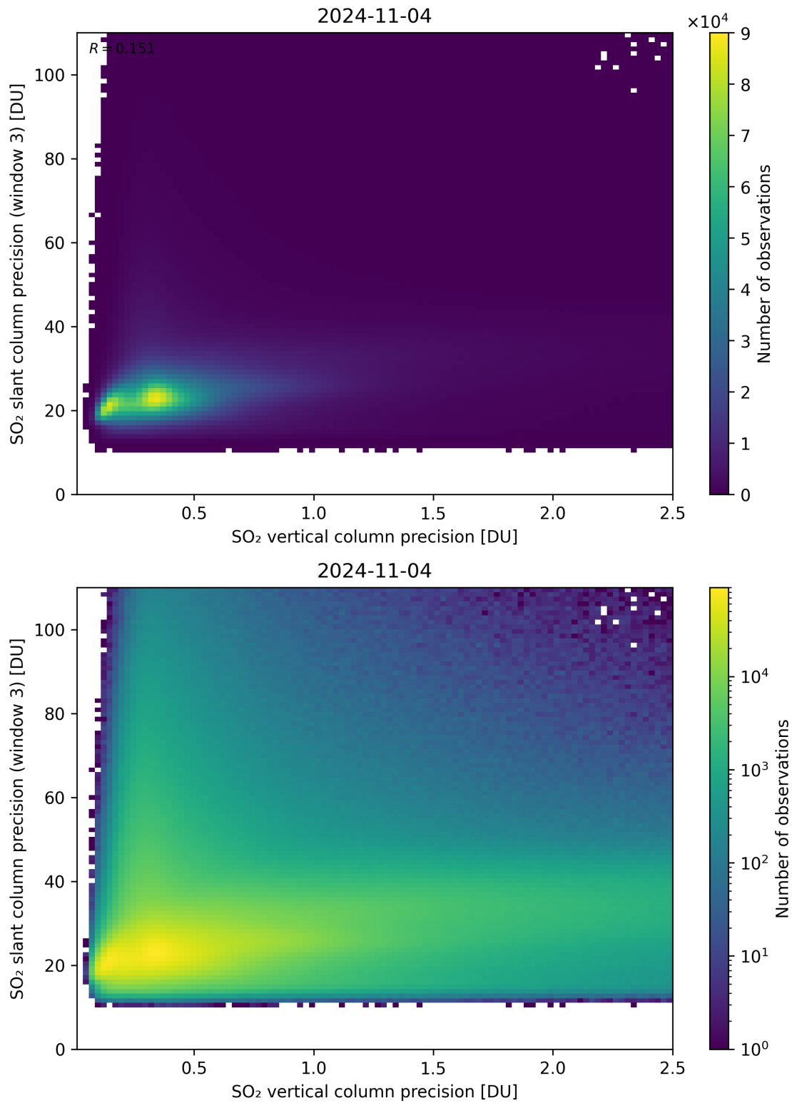
Figure 293: Scatter density plot of “SO 2 vertical column precision” against “SO 2 slant column precision (window 3)” for 2024-11-04 to 2024-11-05.
