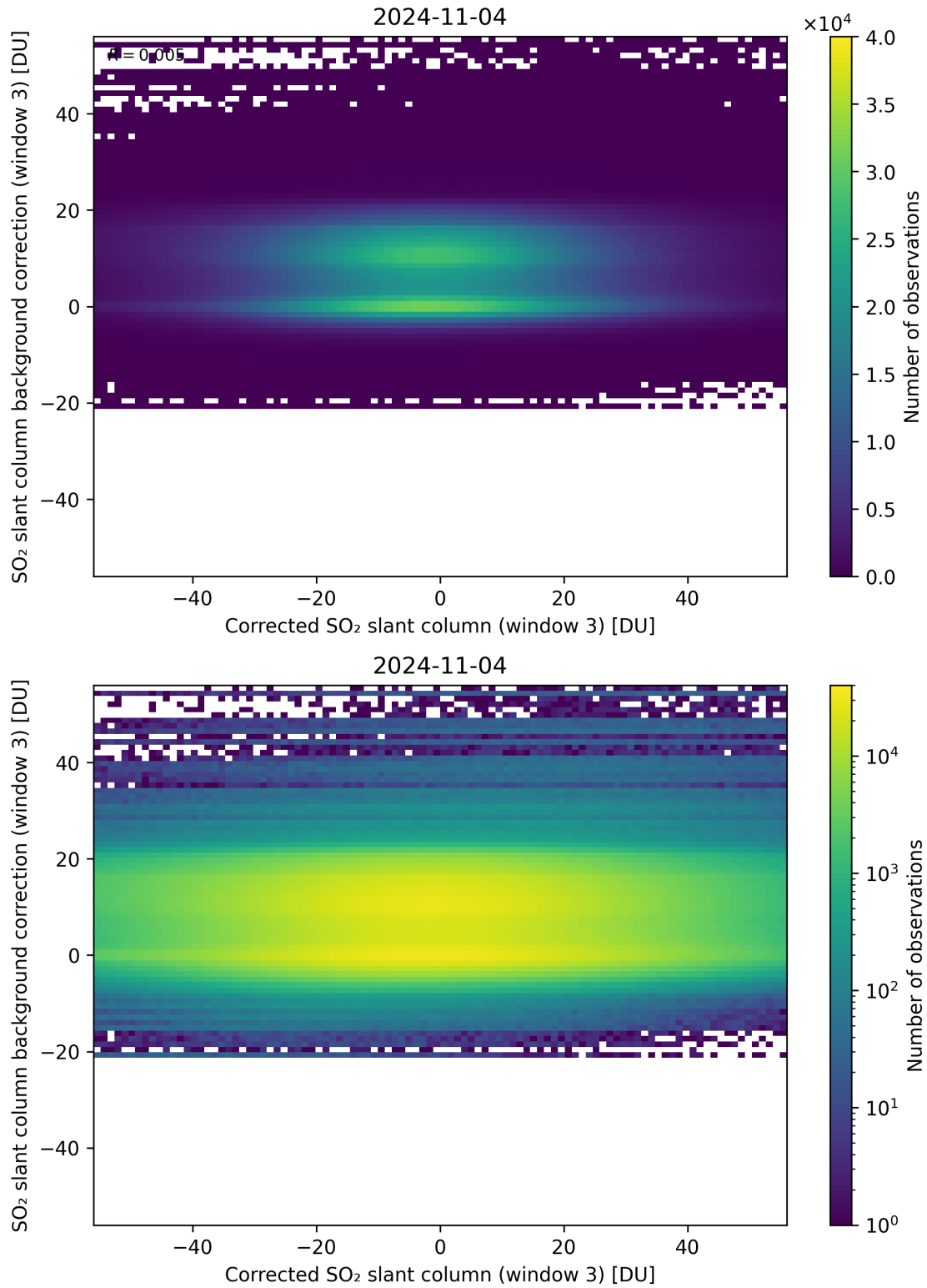
Figure 205: Scatter density plot of “Corrected SO 2 slant column (window 3)” against “SO 2 slant column background correction (window 3)” for 2024-11-04 to 2024-11-05.
