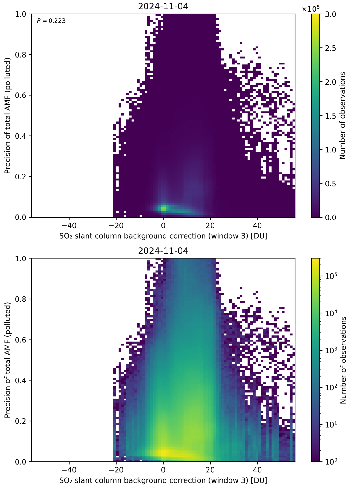
Figure 126: Scatter density plot of “SO 2 slant column background correction (window 3)” against “Precision of total AMF (polluted)” for 2024-11-04 to 2024-11-05.
