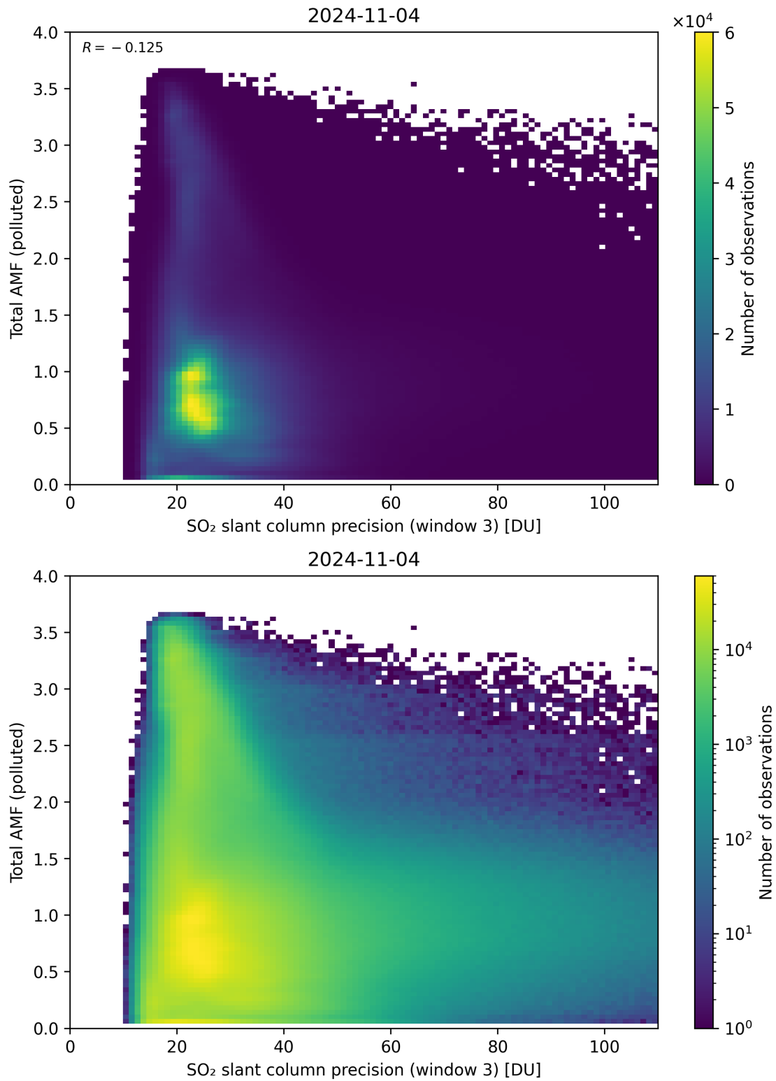
Figure 263: Scatter density plot of “SO 2 slant column precision (window 3)” against “Total AMF (polluted)” for 2024-11-04 to 2024-11-05.
