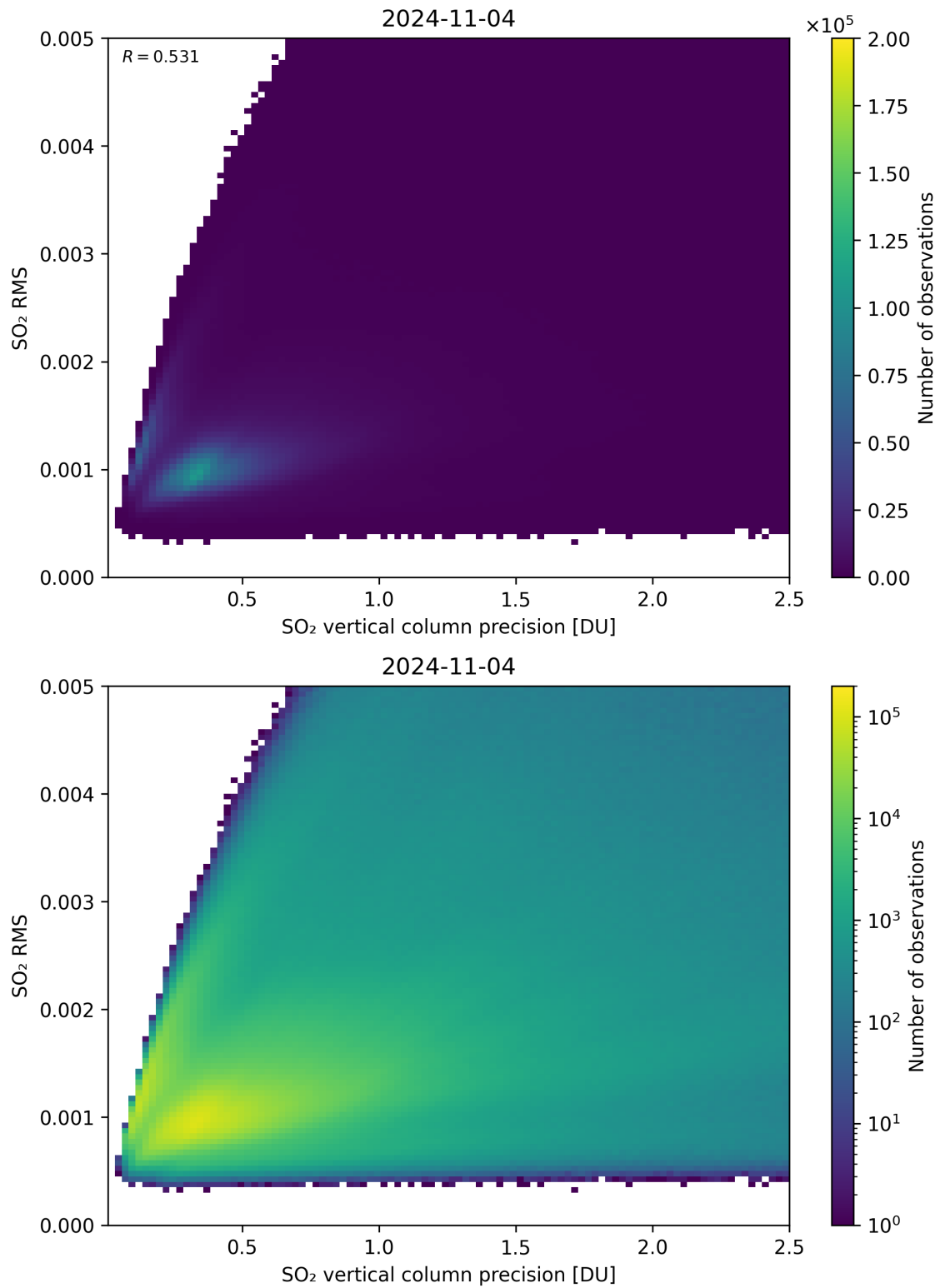
Figure 284: Scatter density plot of “SO 2 vertical column precision” against “SO 2 RMS” for 2024-11-04 to 2024-11-05.
