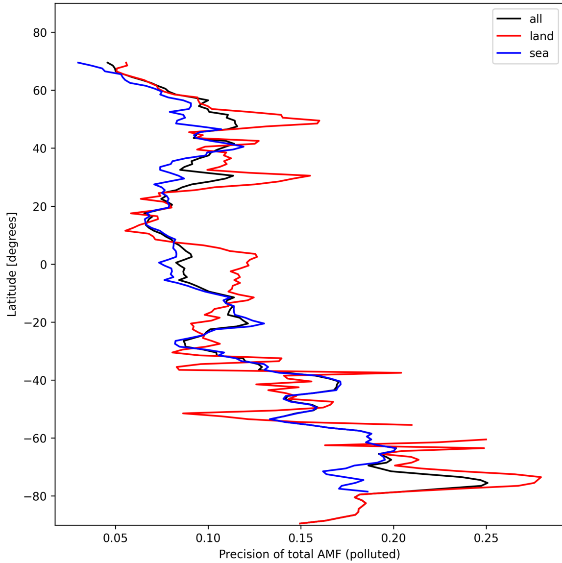
Figure 49: Zonal average of “Precision of total AMF (polluted)” for 2024-11-04 to 2024-11-05.
