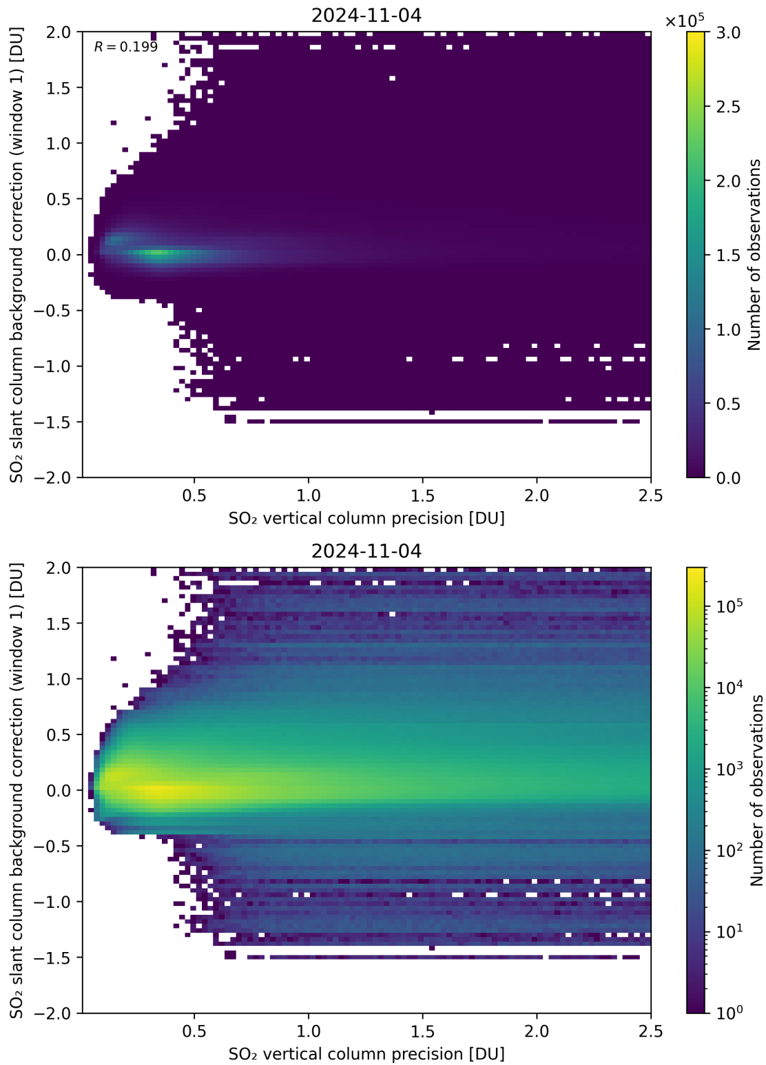
Figure 279: Scatter density plot of “SO 2 vertical column precision” against “SO 2 slant column background correction (window 1)” for 2024-11-04 to 2024-11-05.
