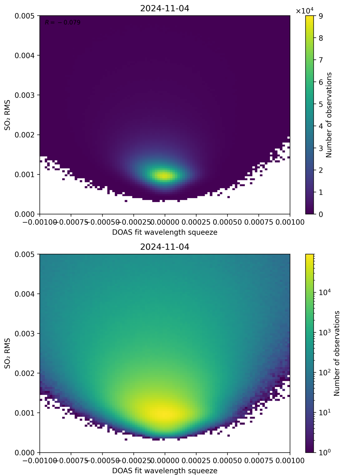
Figure 132: Scatter density plot of “DOAS fit wavelength squeeze” against “SO 2 RMS” for 2024-11-04 to 2024-11-05.
