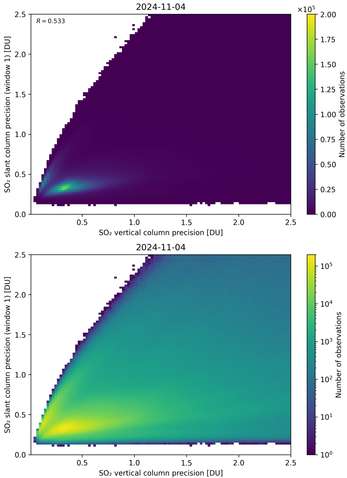
Figure 290: Scatter density plot of “SO 2 vertical column precision” against “SO 2 slant column precision (window 1)” for 2024-11-04 to 2024-11-05.
