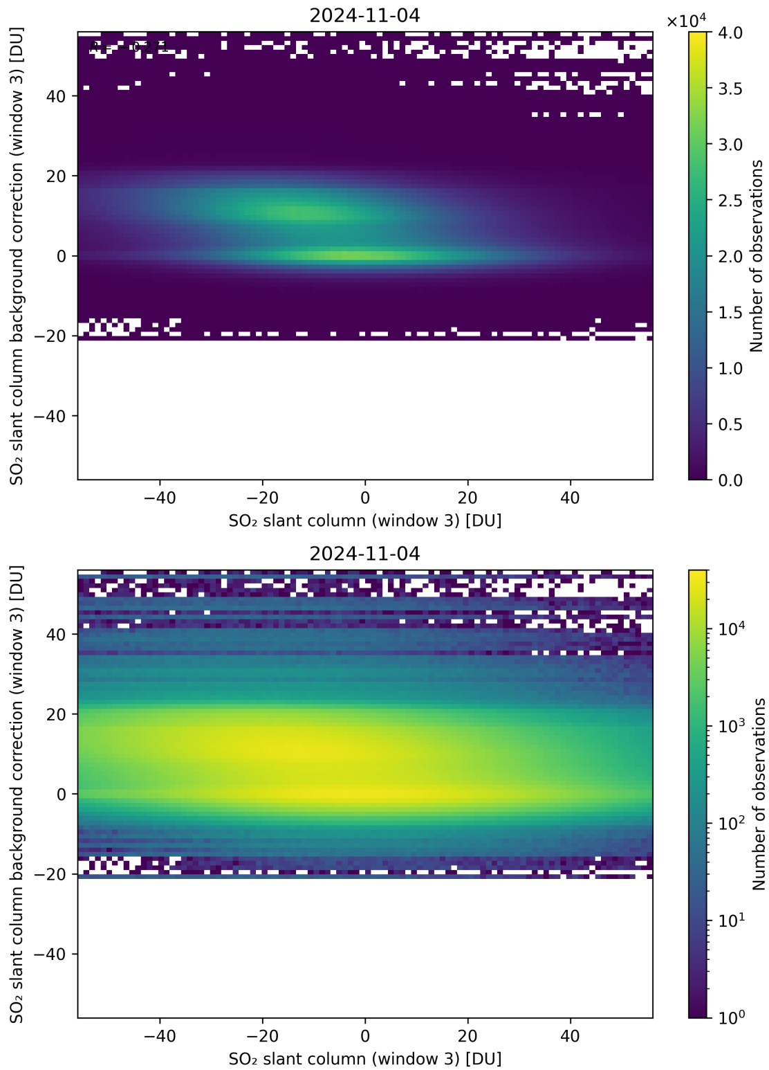
Figure 253: Scatter density plot of “SO 2 slant column (window 3)” against “SO 2 slant column background correction (window 3)” for 2024-11-04 to 2024-11-05.
