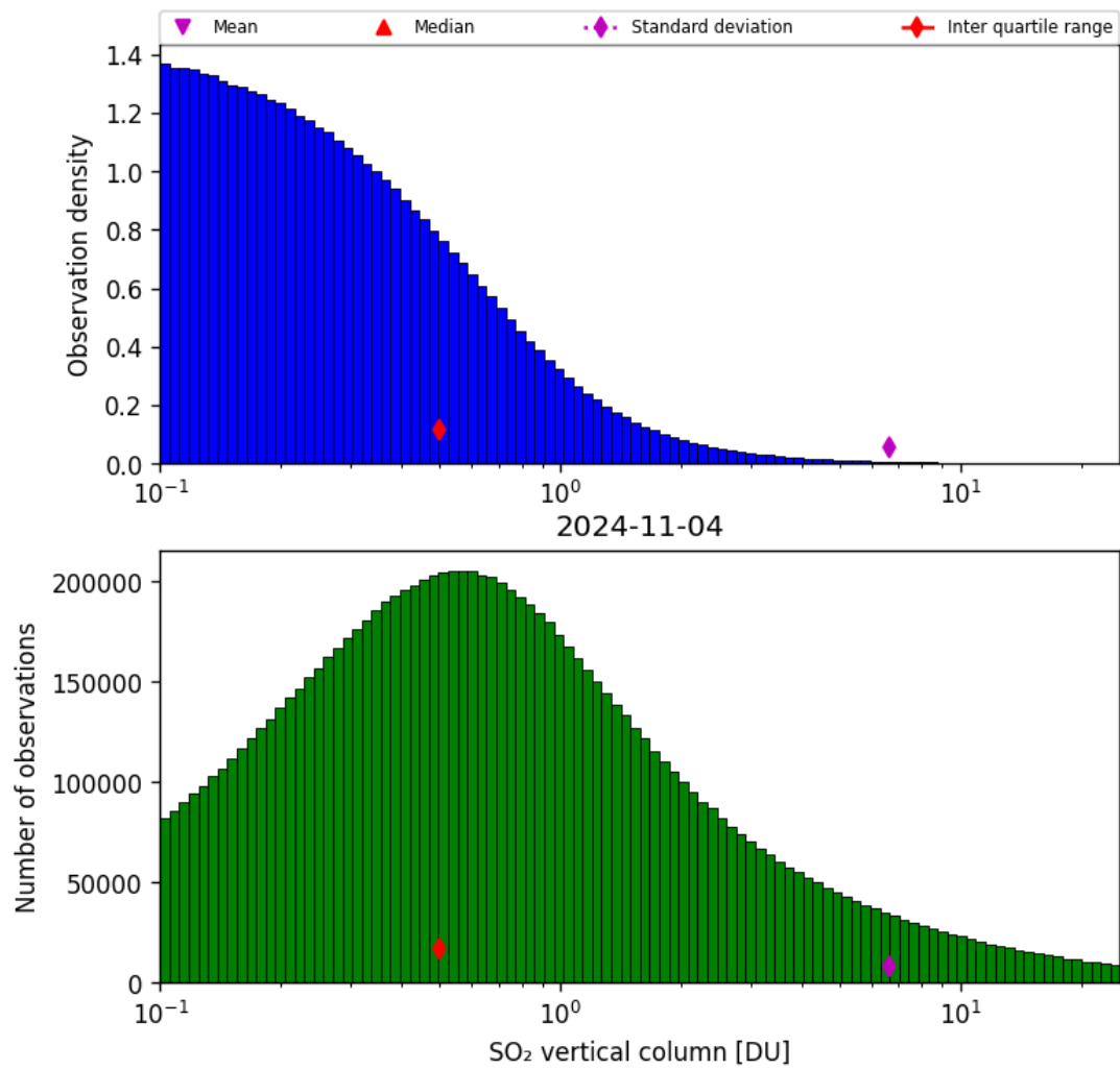
Figure 53: Histogram of “SO 2 vertical column” for 2024-11-04 to 2024-11-05
