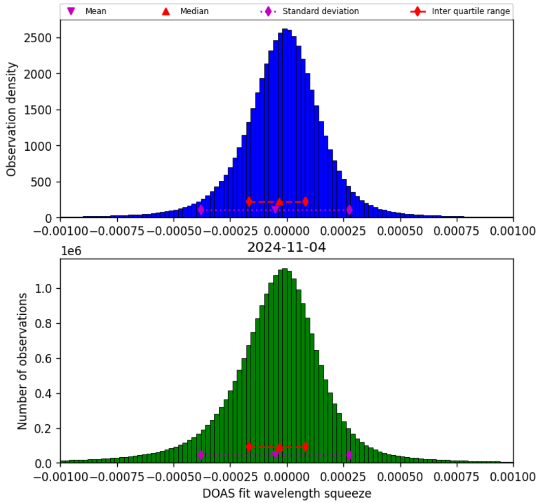
Figure 69: Histogram of “DOAS fit wavelength squeeze” for 2024-11-04 to 2024-11-05
