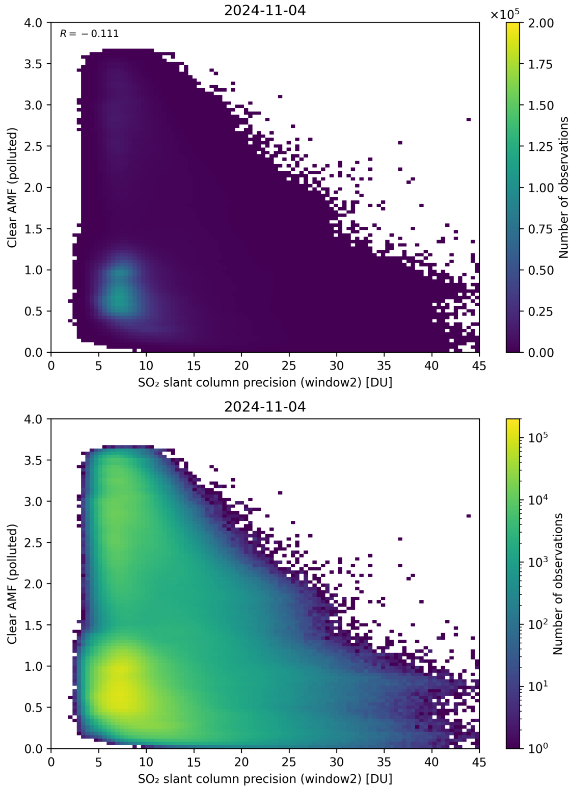
Figure 246: Scatter density plot of “SO 2 slant column precision (window2)” against “Clear AMF (polluted)” for 2024-11-04 to 2024-11-05.
