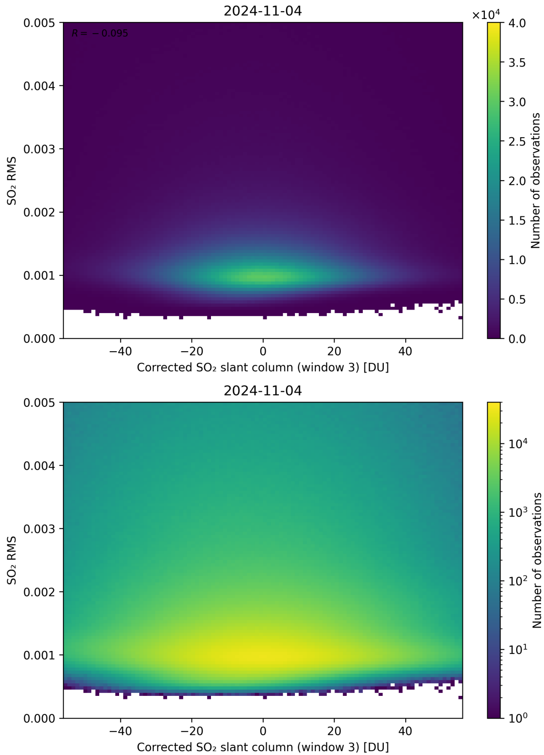
Figure 208: Scatter density plot of “Corrected SO 2 slant column (window 3)” against “SO 2 RMS” for 2024-11-04 to 2024-11-05.
