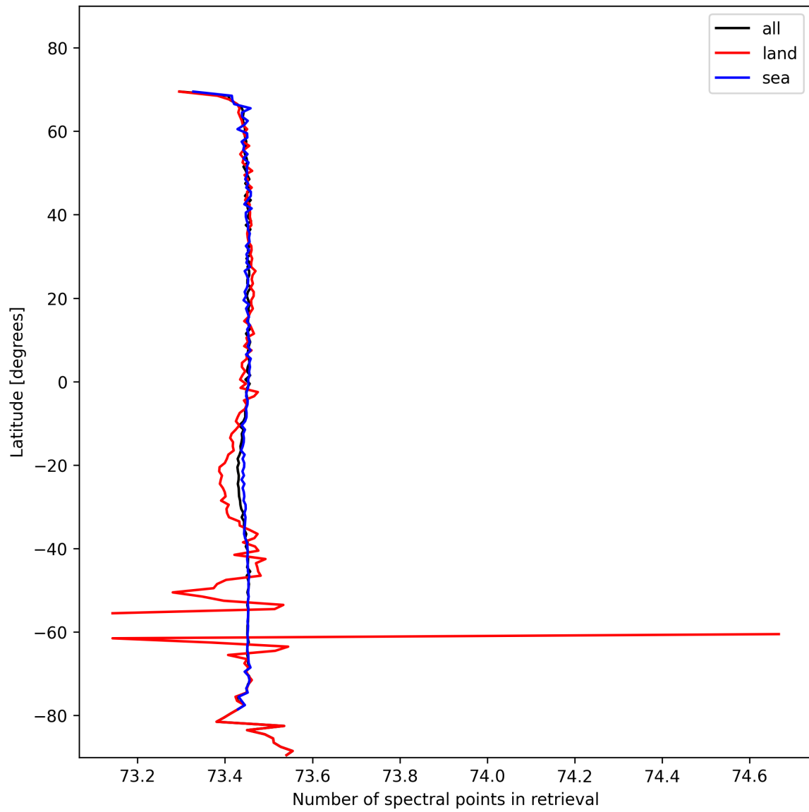
Figure 51: Zonal average of “Number of spectral points in retrieval” for 2024-11-04 to 2024-11-05.
