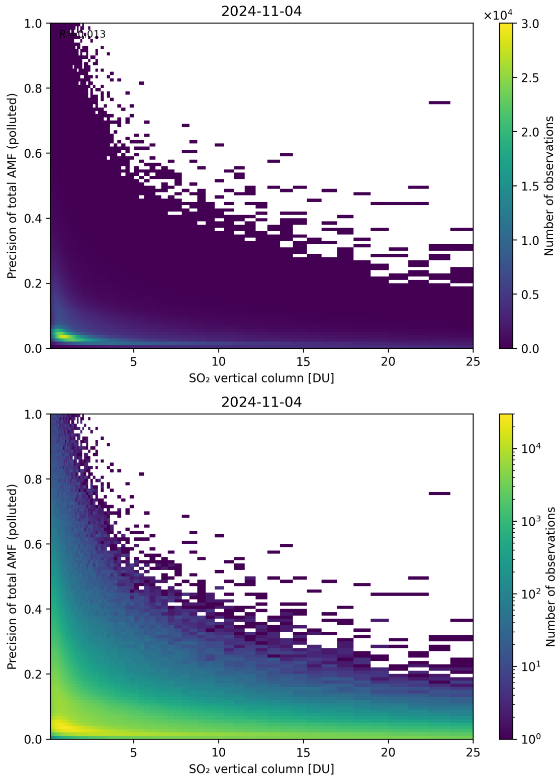
Figure 306: Scatter density plot of “SO 2 vertical column” against “Precision of total AMF (polluted)” for 2024-11-04 to 2024-11-05.
