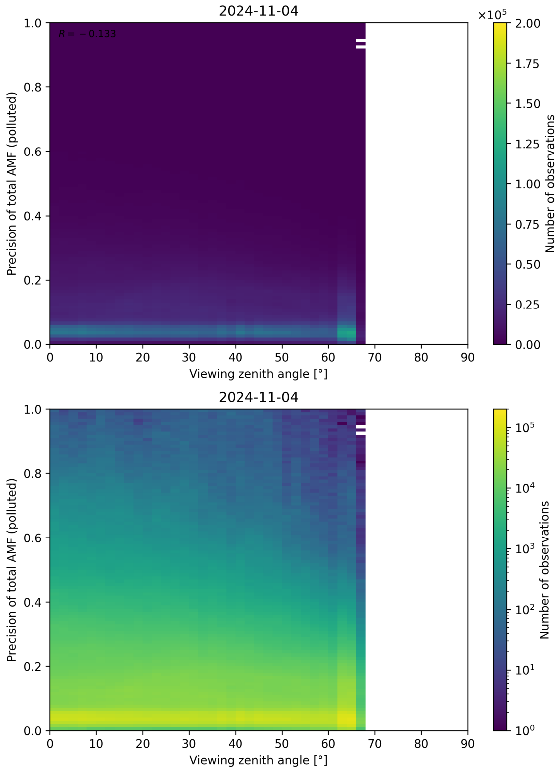
Figure 326: Scatter density plot of “Viewing zenith angle” against “Precision of total AMF (polluted)” for 2024-11-04 to 2024-11-05.
