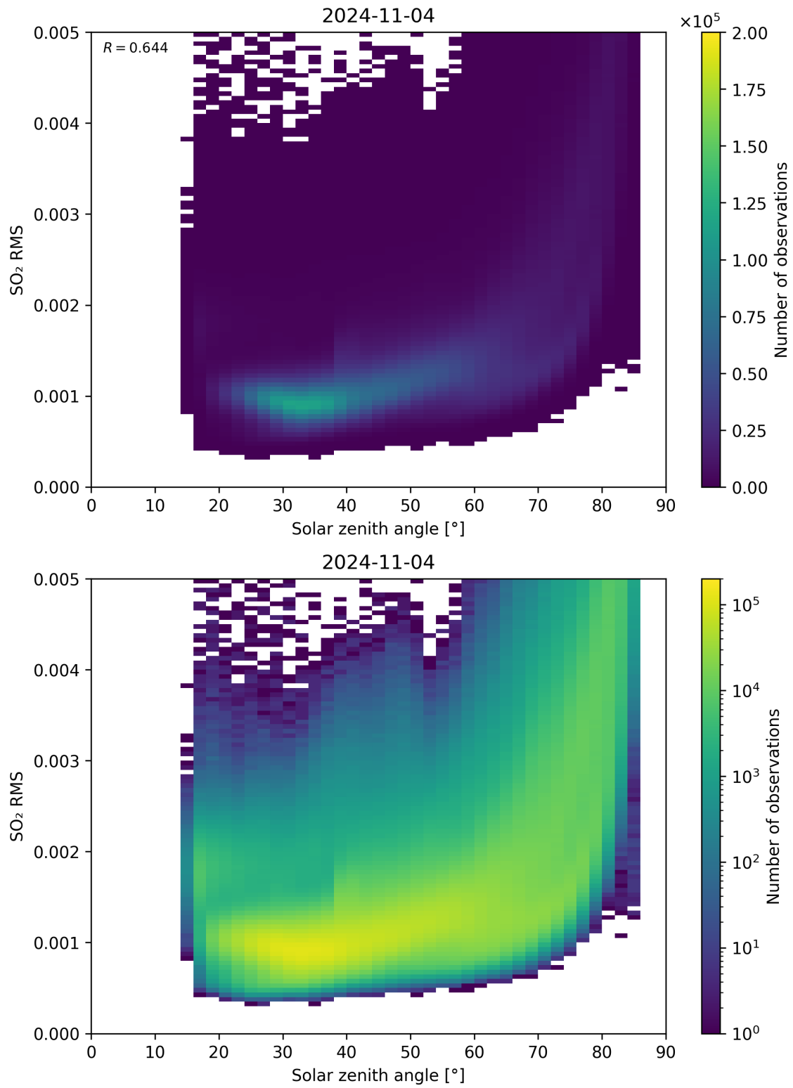
Figure 163: Scatter density plot of “Solar zenith angle” against “SO 2 RMS” for 2024-11-04 to 2024-11-05.
