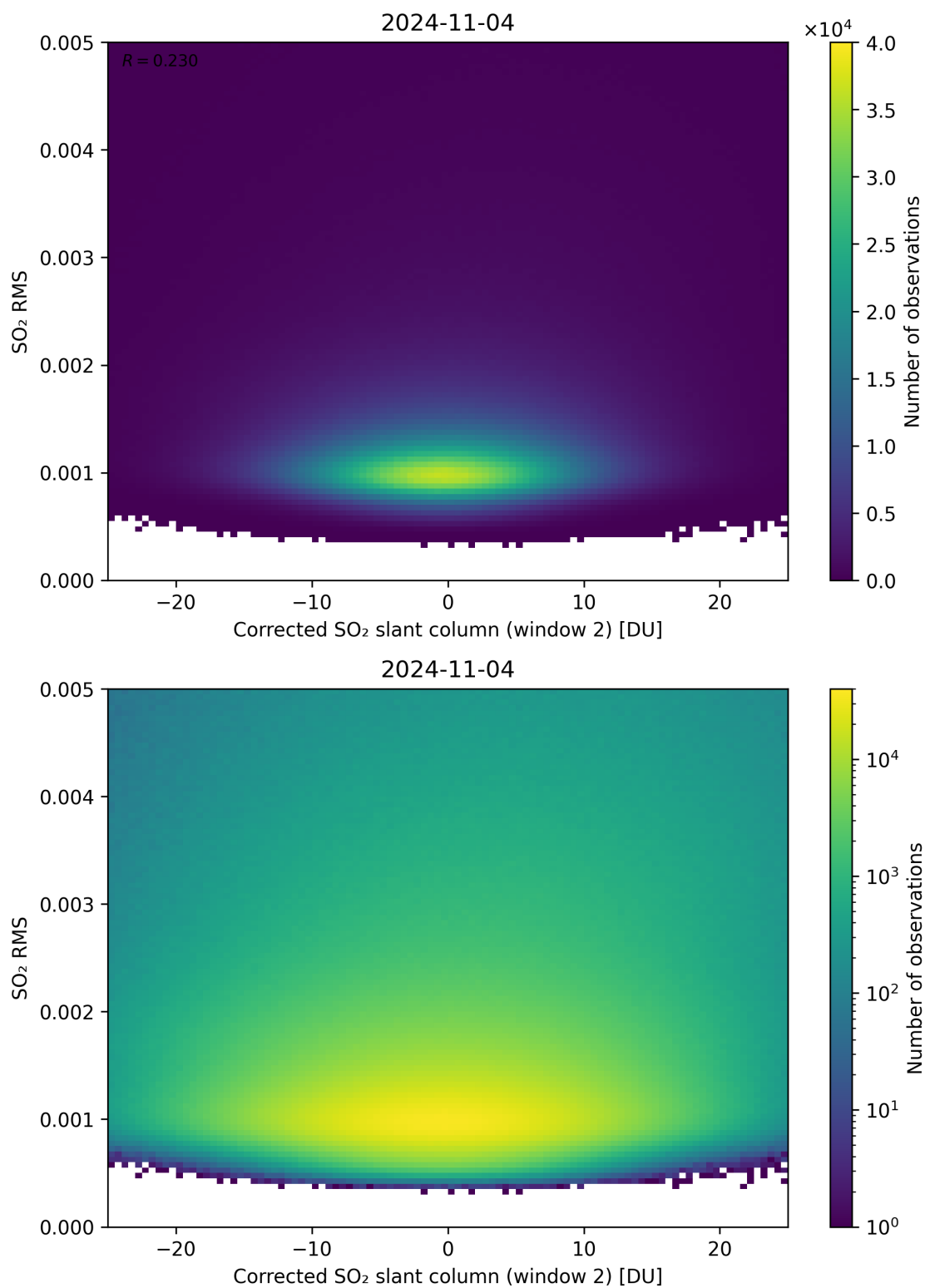
Figure 198: Scatter density plot of “Corrected SO 2 slant column (window 2)” against “SO 2 RMS” for 2024-11-04 to 2024-11-05.
