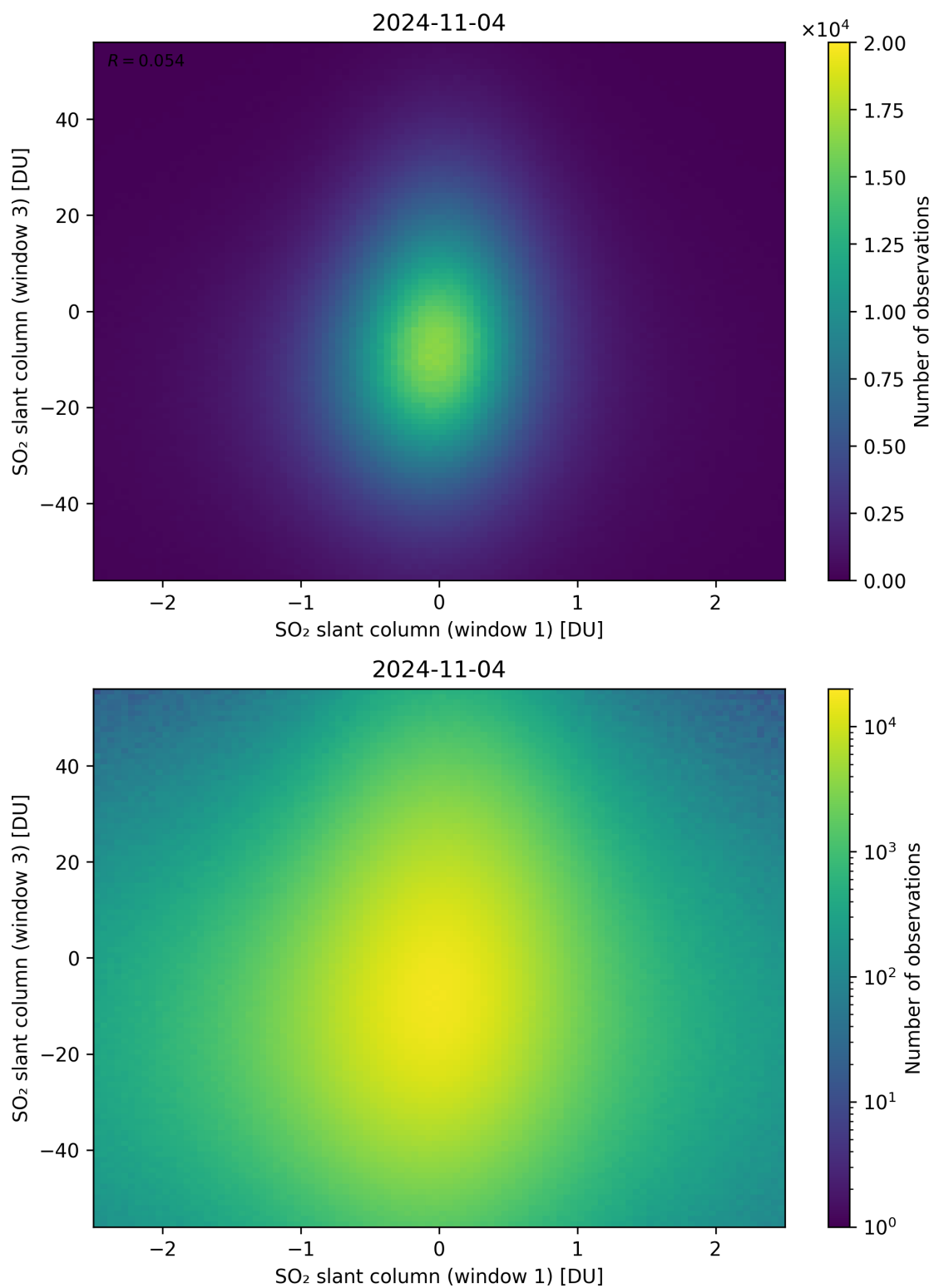
Figure 237: Scatter density plot of “SO 2 slant column (window 1)” against “SO 2 slant column (window 3)” for 2024-11-04 to 2024-11-05.
