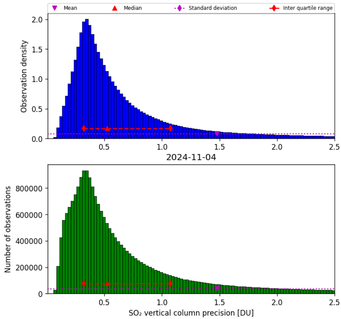
Figure 54: Histogram of “SO 2 vertical column precision” for 2024-11-04 to 2024-11-05
