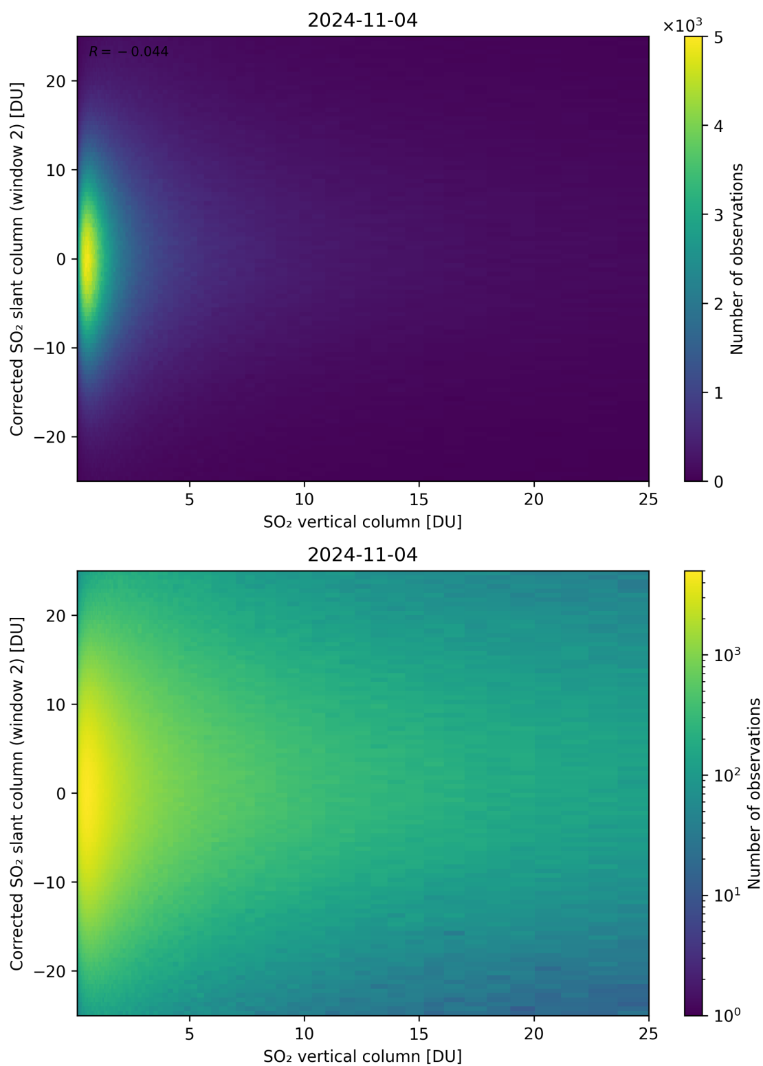
Figure 298: Scatter density plot of “SO 2 vertical column” against “Corrected SO 2 slant column (window 2)” for 2024-11-04 to 2024-11-05.
