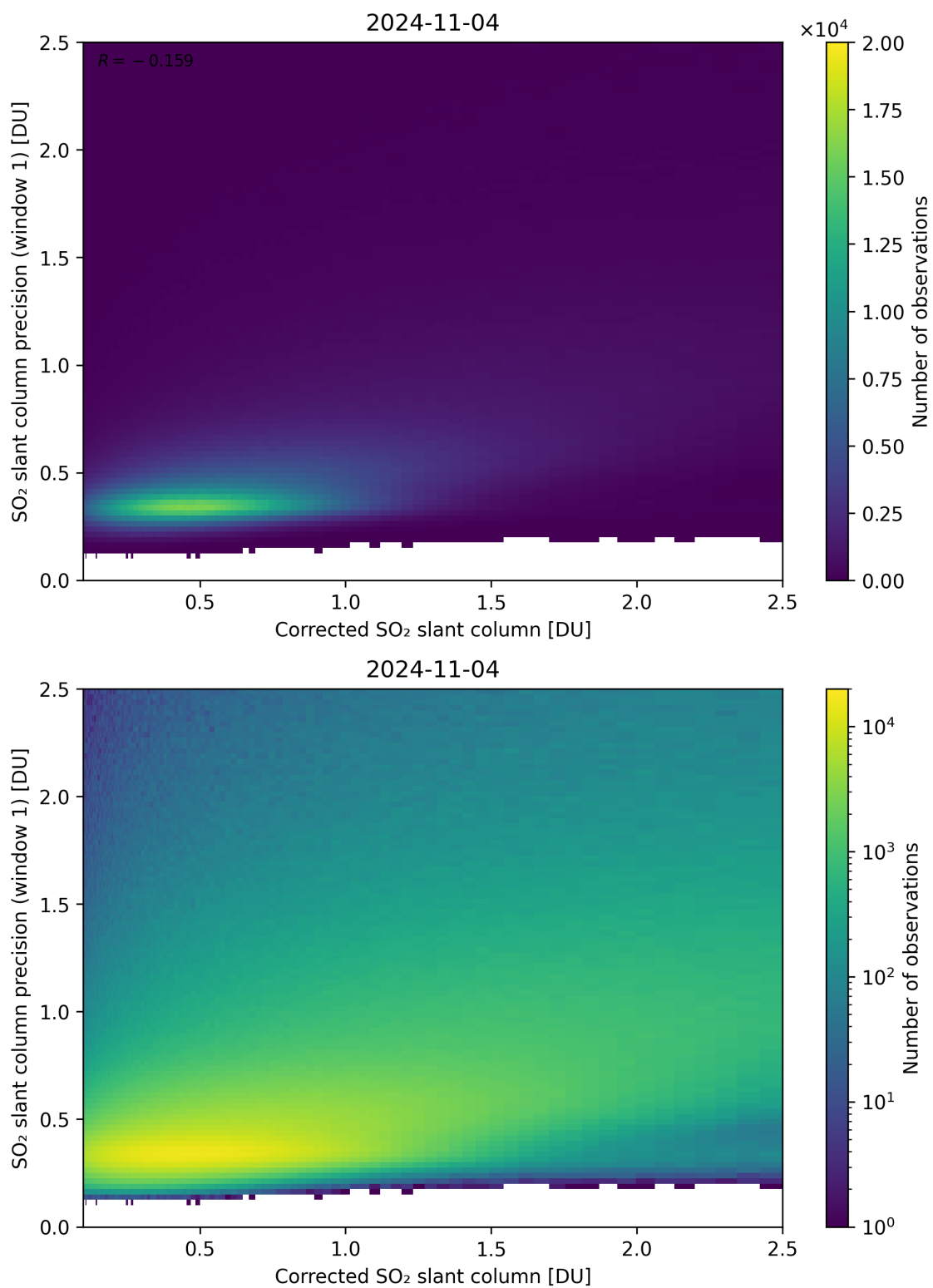
Figure 188: Scatter density plot of “Corrected SO 2 slant column” against “SO 2 slant column precision (window 1)” for 2024-11-04 to 2024-11-05.
