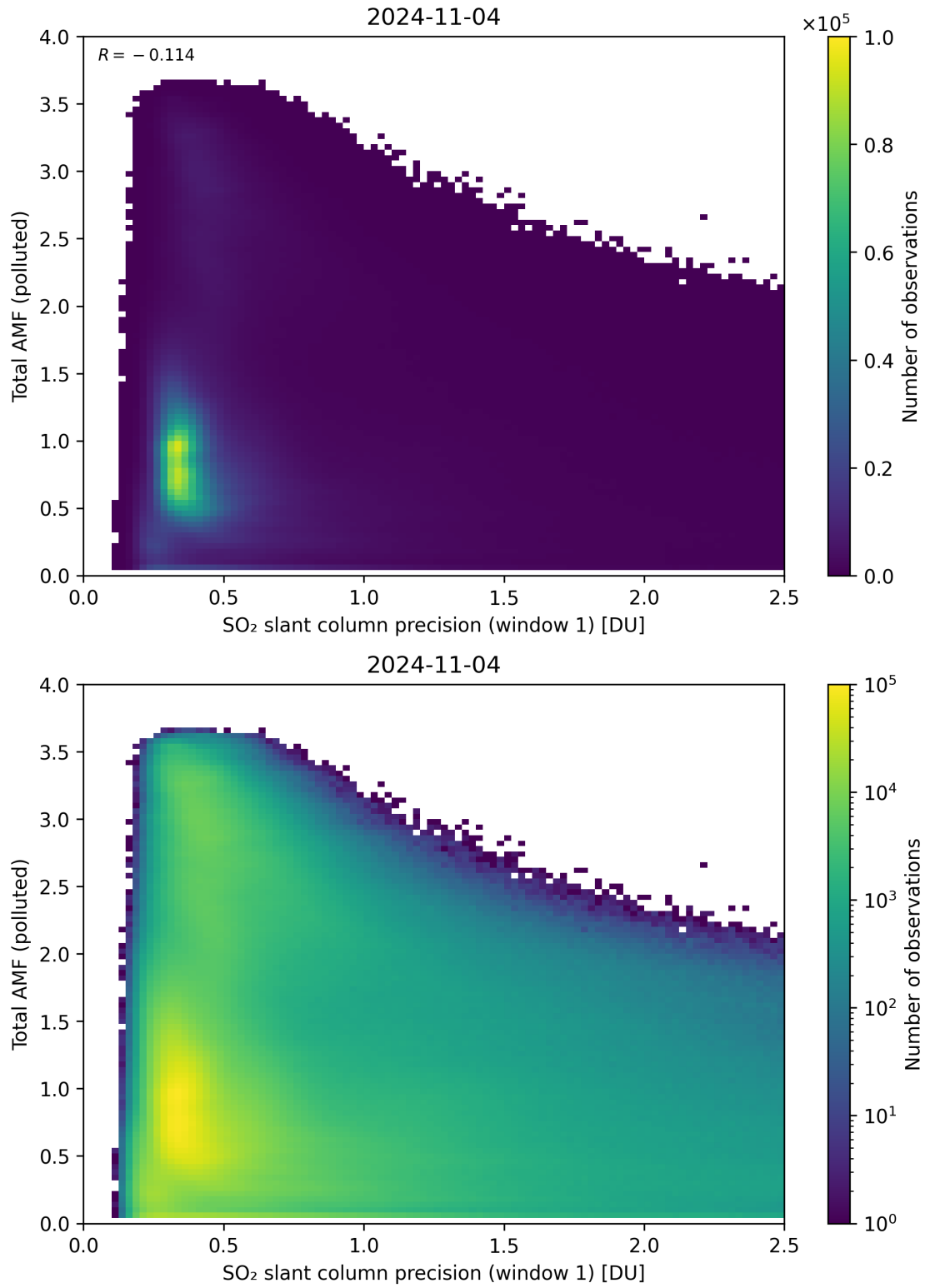
Figure 230: Scatter density plot of “SO 2 slant column precision (window 1)” against “Total AMF (polluted)” for 2024-11-04 to 2024-11-05.
