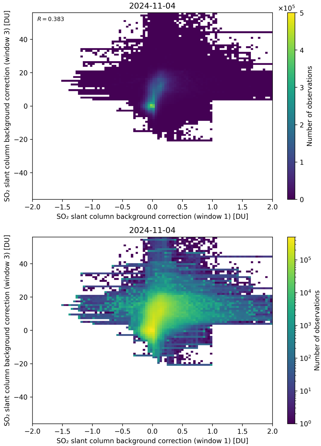
Figure 99: Scatter density plot of “SO 2 slant column background correction (window 1)” against “SO 2 slant column background correction (window 3)” for 2024-11-04 to 2024-11-05.
