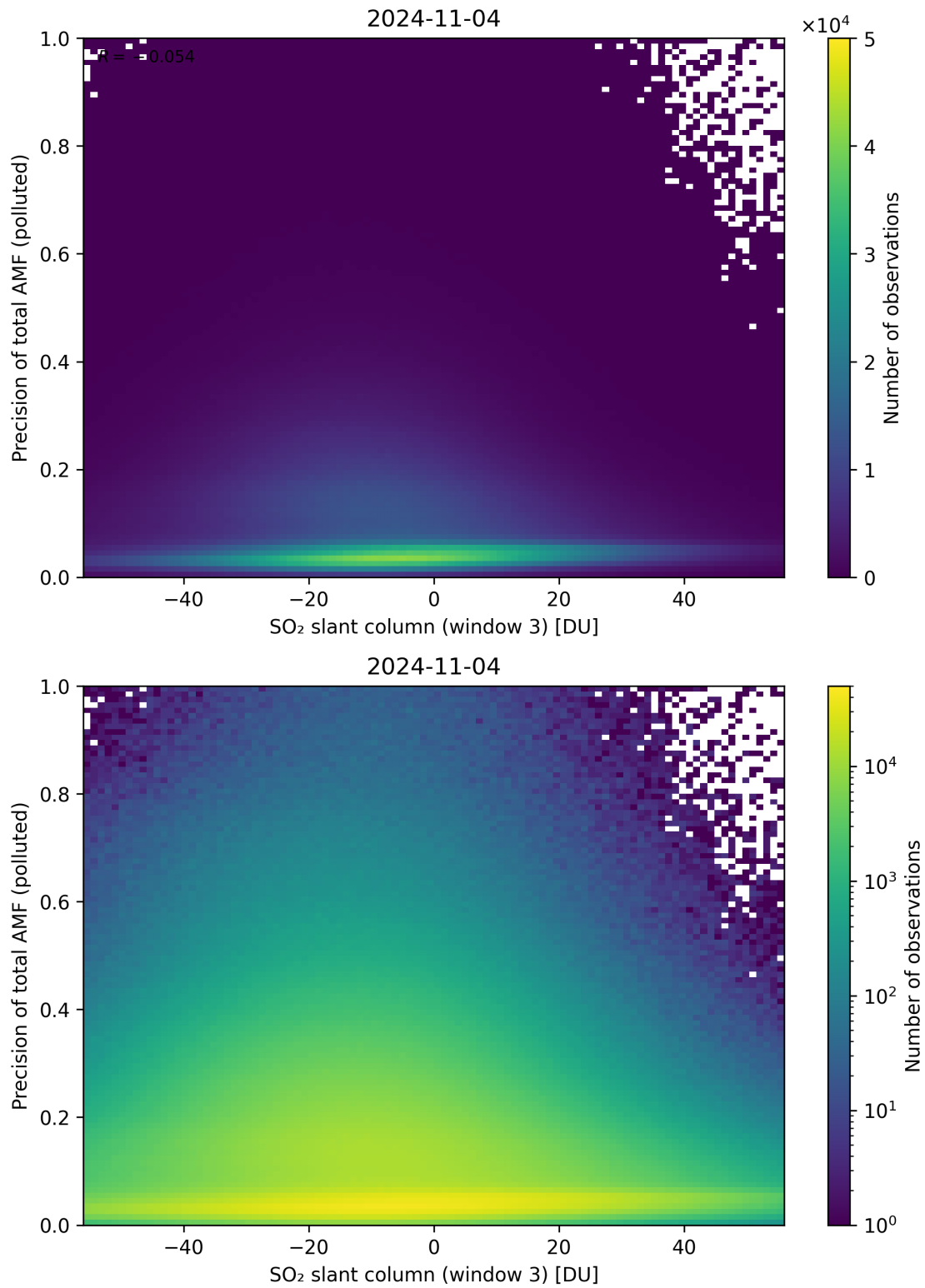
Figure 269: Scatter density plot of “SO 2 slant column (window 3)” against “Precision of total AMF (polluted)” for 2024-11-04 to 2024-11-05.
