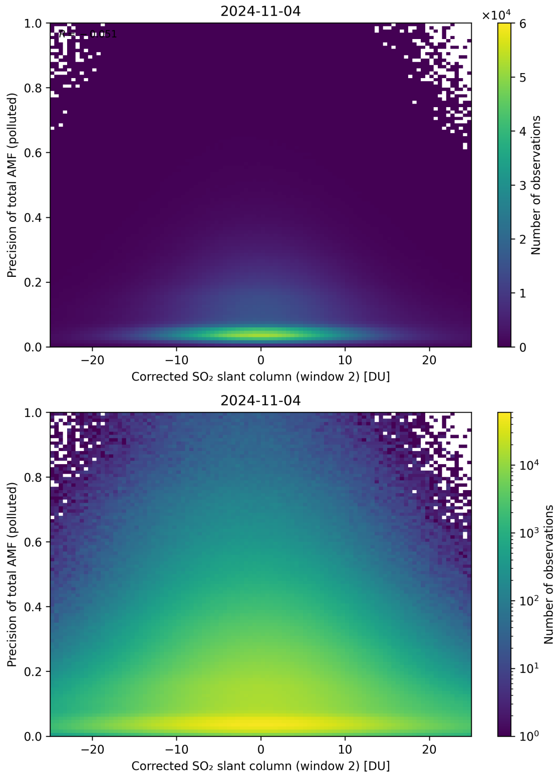
Figure 204: Scatter density plot of “Corrected SO 2 slant column (window 2)” against “Precision of total AMF (polluted)” for 2024-11-04 to 2024-11-05.
