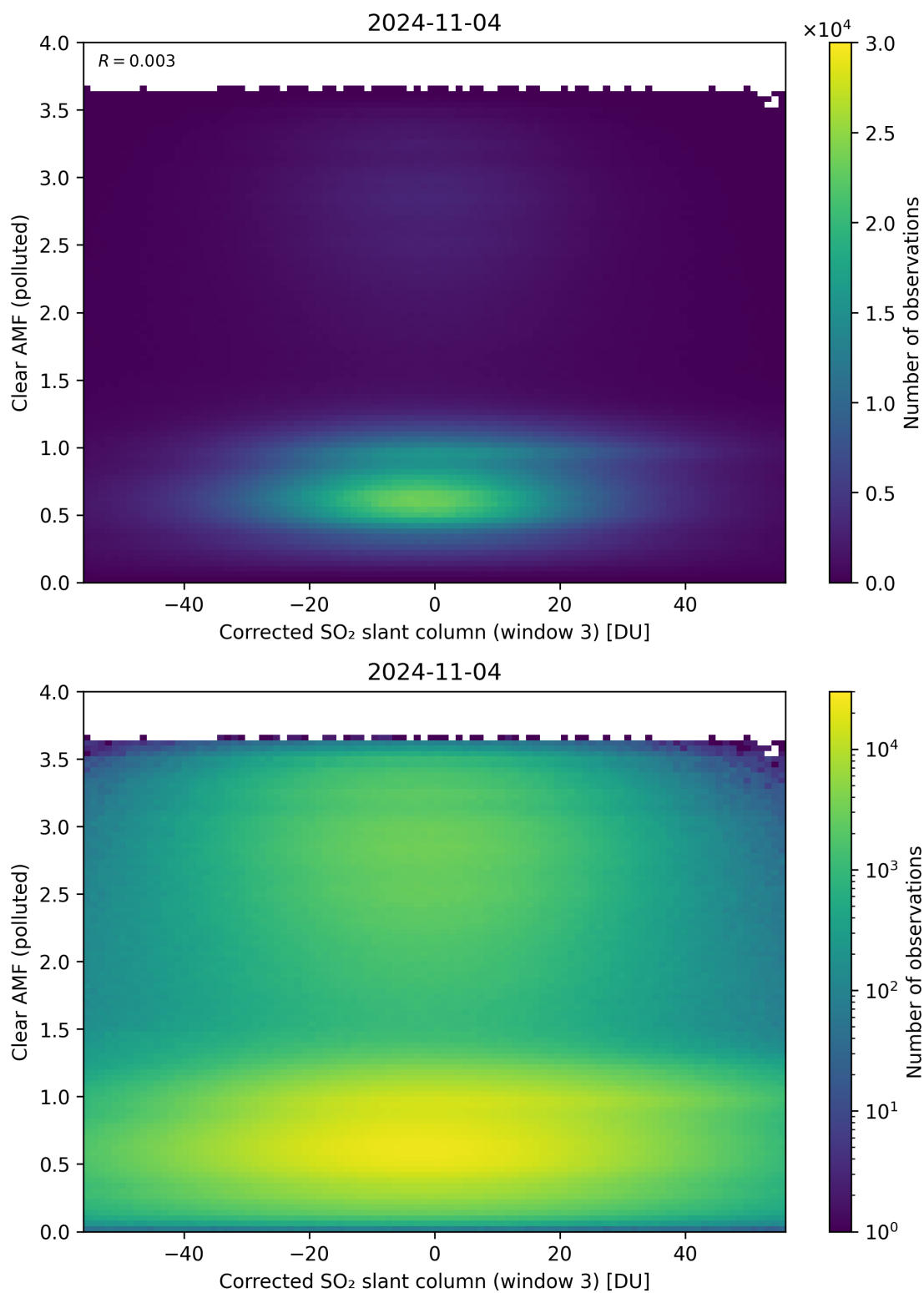
Figure 209: Scatter density plot of “Corrected SO 2 slant column (window 3)” against “Clear AMF (polluted)” for 2024-11-04 to 2024-11-05.
