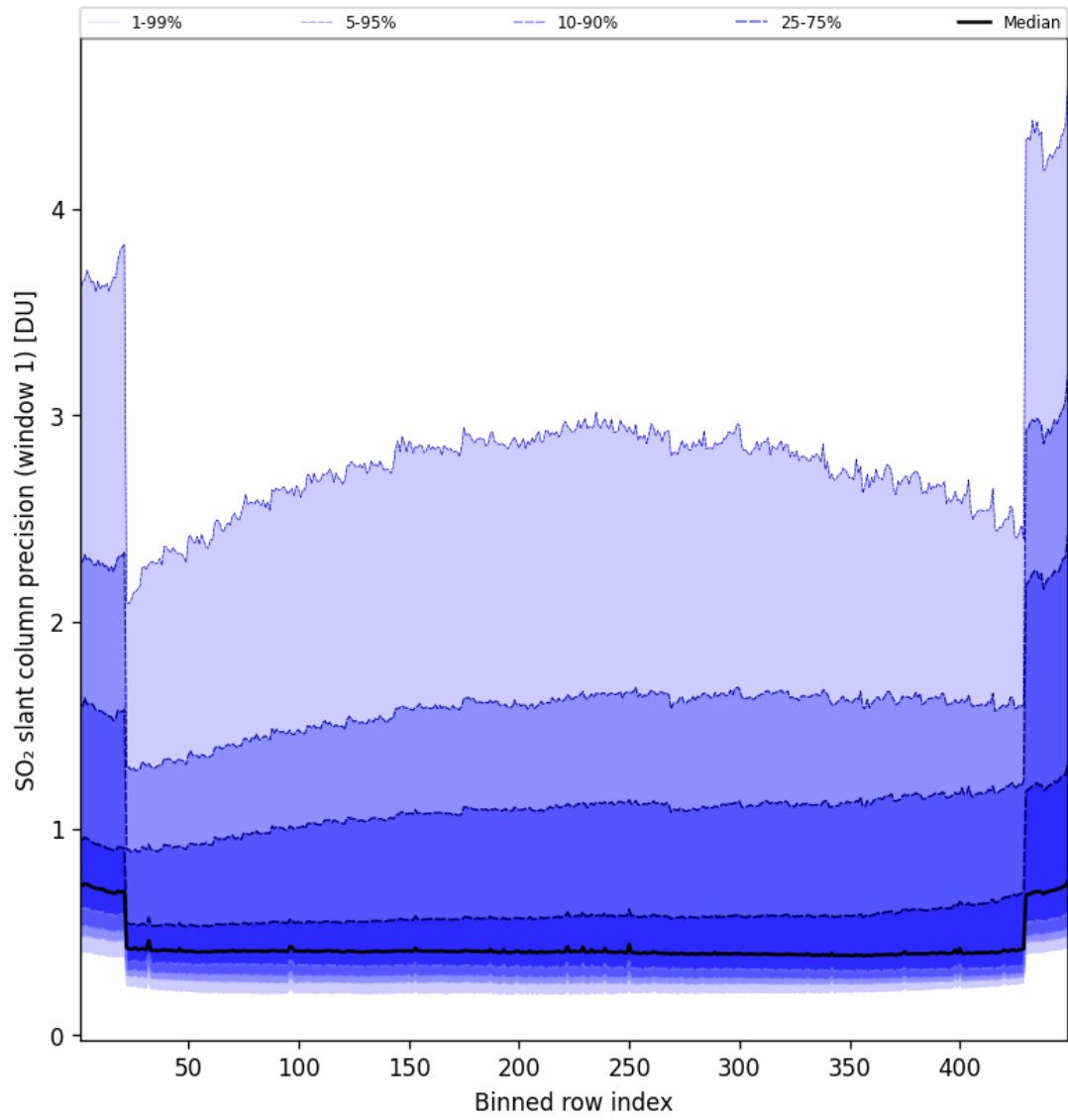
Figure 80: Along track statistics of “SO 2 slant column precision (window 1)” for 2024-11-04 to 2024-11-05
