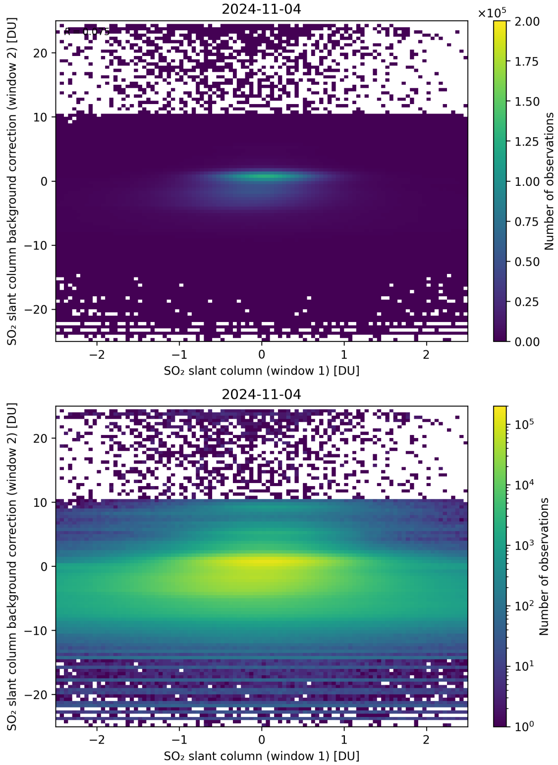
Figure 213: Scatter density plot of “SO 2 slant column (window 1)” against “SO 2 slant column background correction (window 2)” for 2024-11-04 to 2024-11-05.
