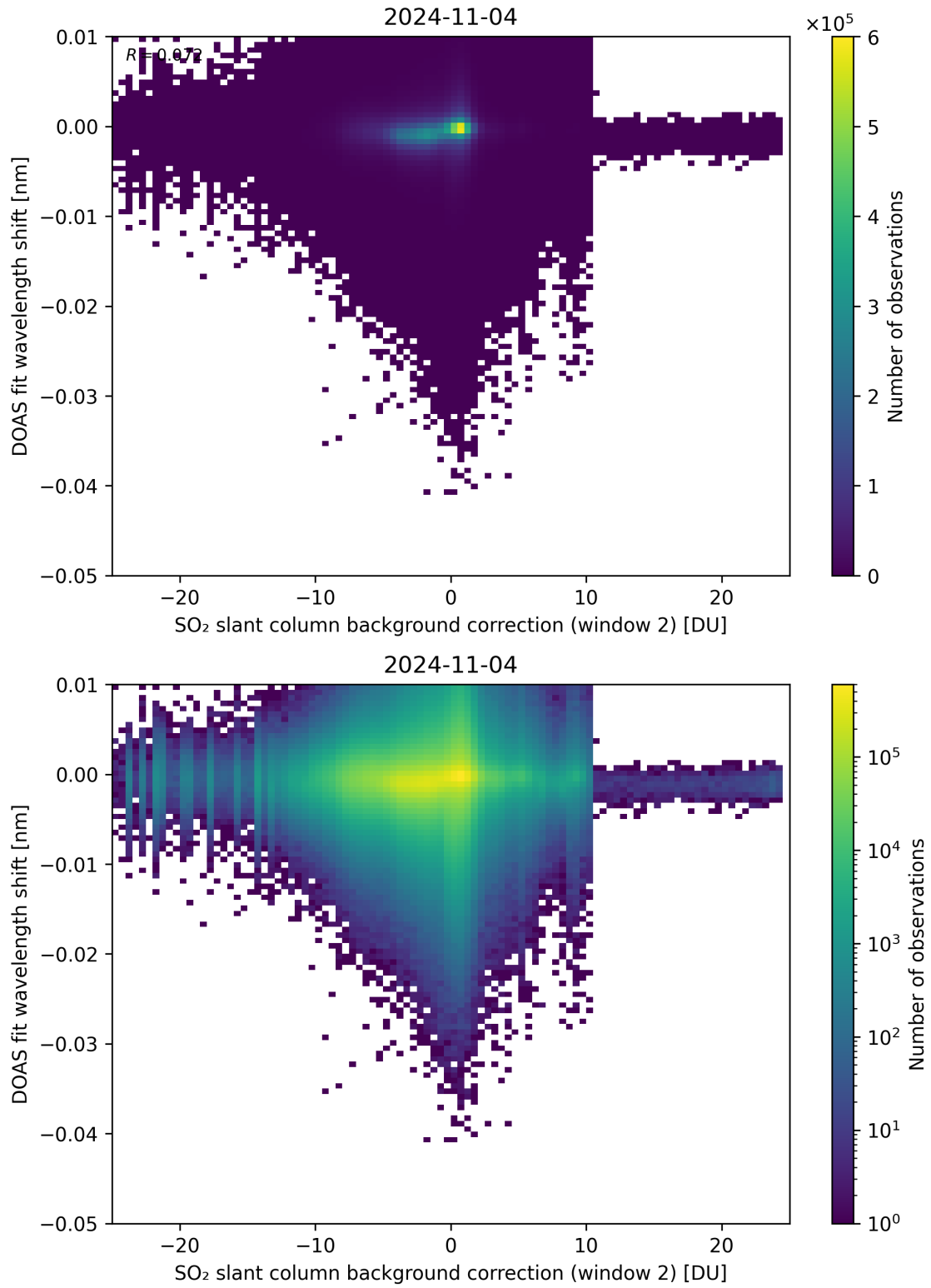
Figure 112: Scatter density plot of “SO 2 slant column background correction (window 2)” against “DOAS fit wavelength shift” for 2024-11-04 to 2024-11-05.
