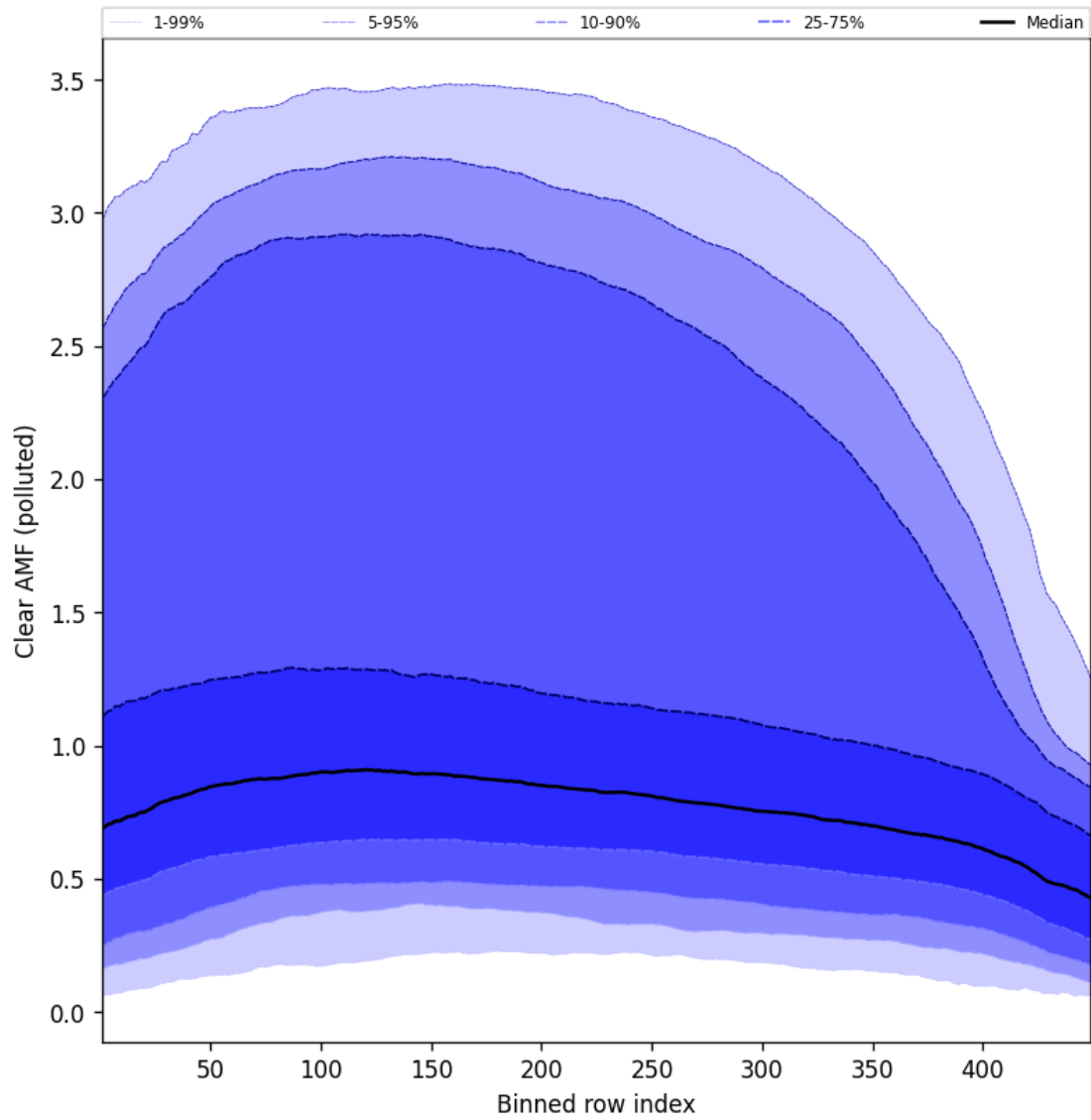
Figure 96: Along track statistics of “Clear AMF (polluted)” for 2024-11-04 to 2024-11-05
