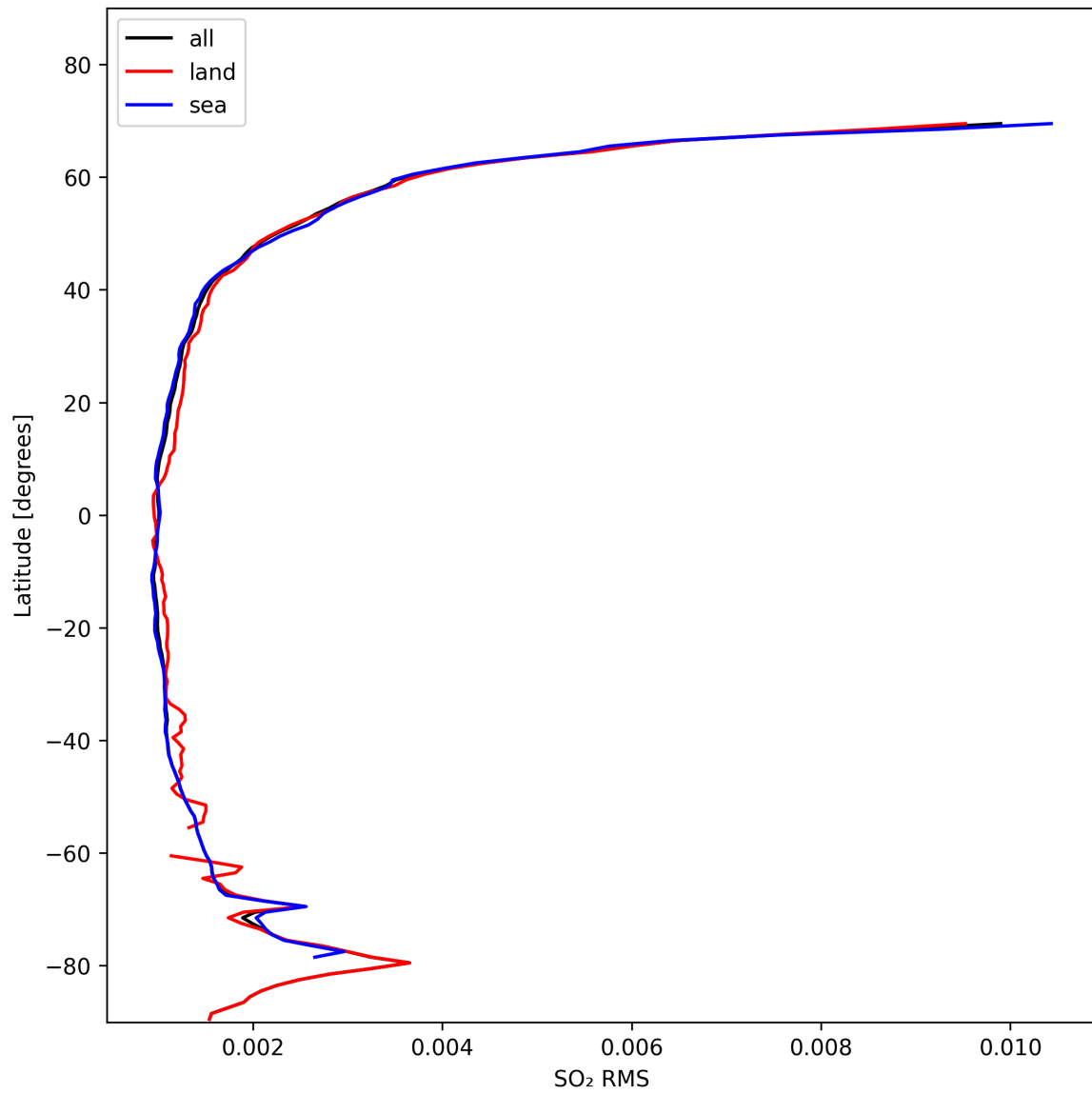
Figure 47: Zonal average of “SO 2 RMS” for 2024-11-04 to 2024-11-05.
