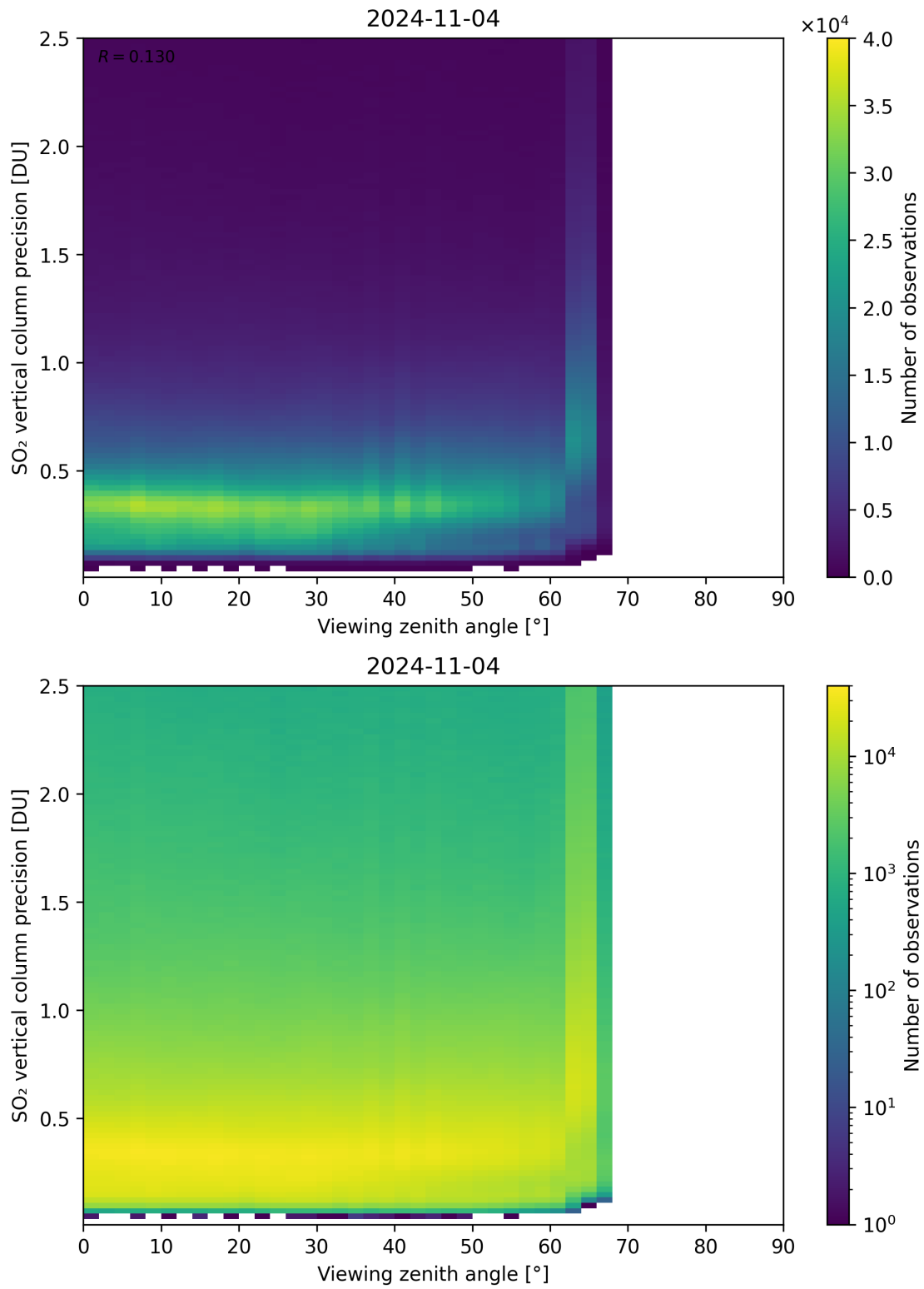
Figure 328: Scatter density plot of “Viewing zenith angle” against “SO 2 vertical column precision” for 2024-11-04 to 2024-11-05.
