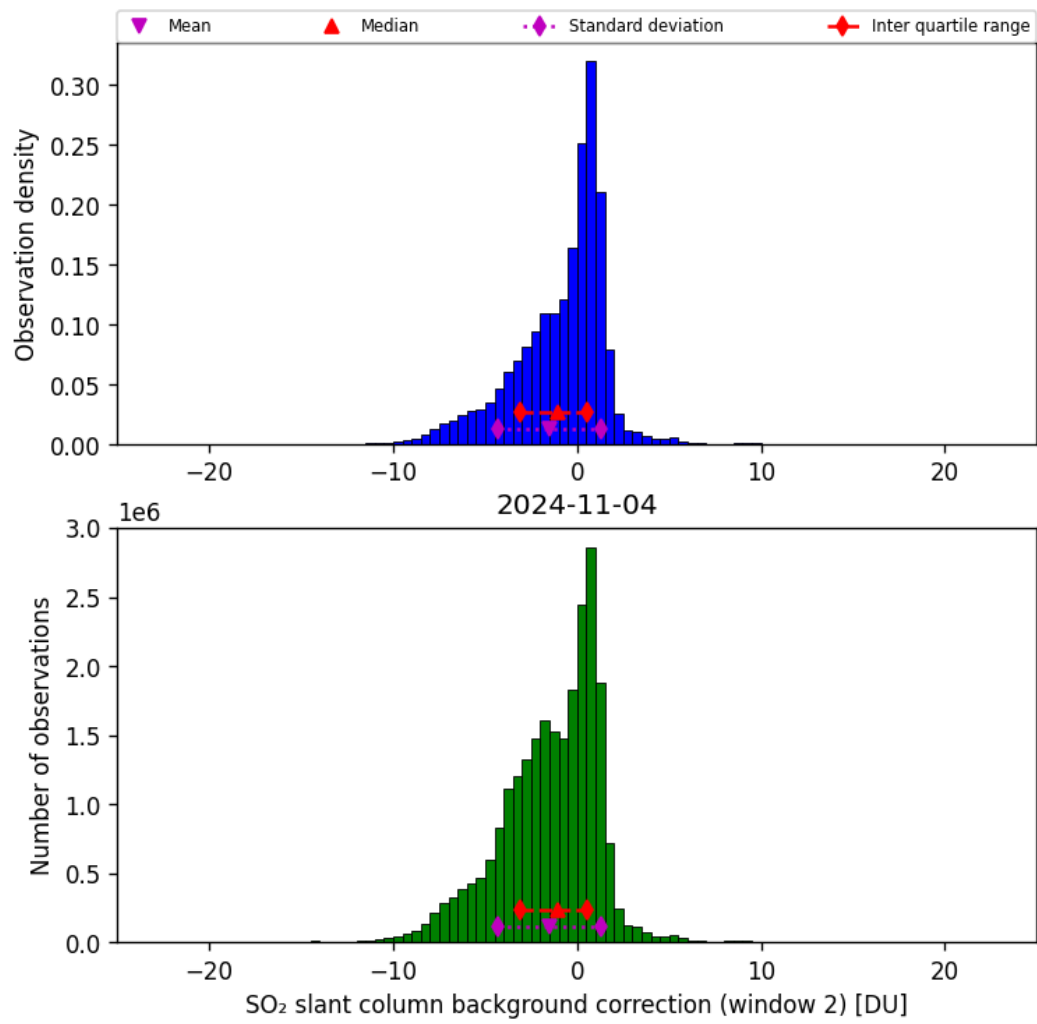
Figure 63: Histogram of “SO 2 slant column background correction (window 2)” for 2024-11-04 to 2024-11-05
