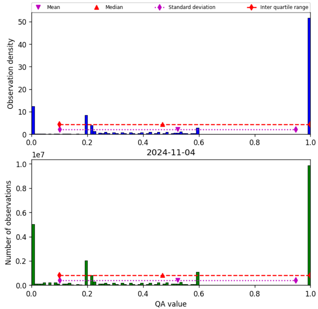
Figure 52: Histogram of “QA value” for 2024-11-04 to 2024-11-05
