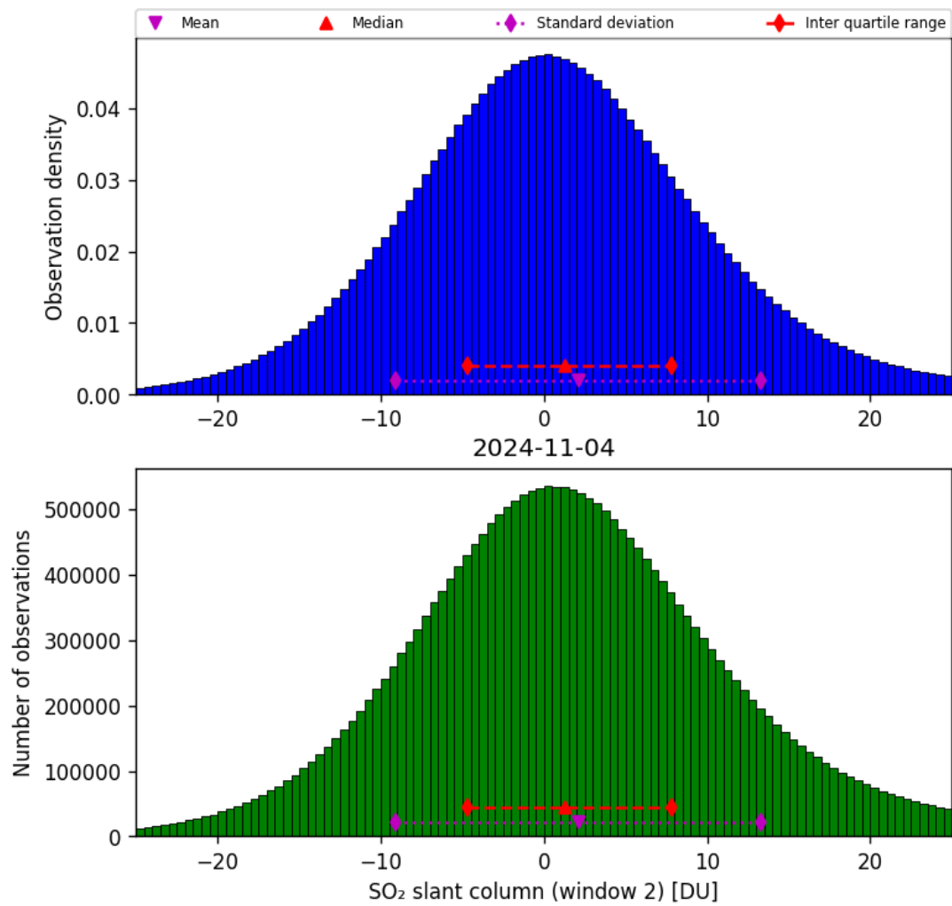
Figure 60: Histogram of “SO 2 slant column (window 2)” for 2024-11-04 to 2024-11-05
