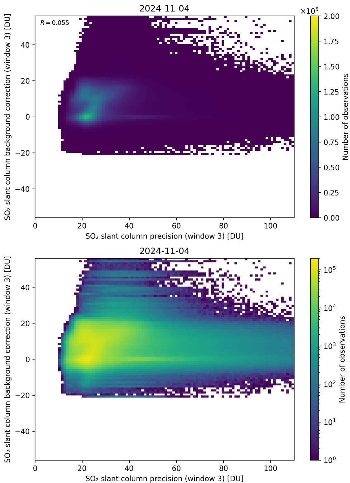
Figure 257: Scatter density plot of “SO 2 slant column precision (window 3)” against “SO 2 slant column background correction (window 3)” for 2024-11-04 to 2024-11-05.
