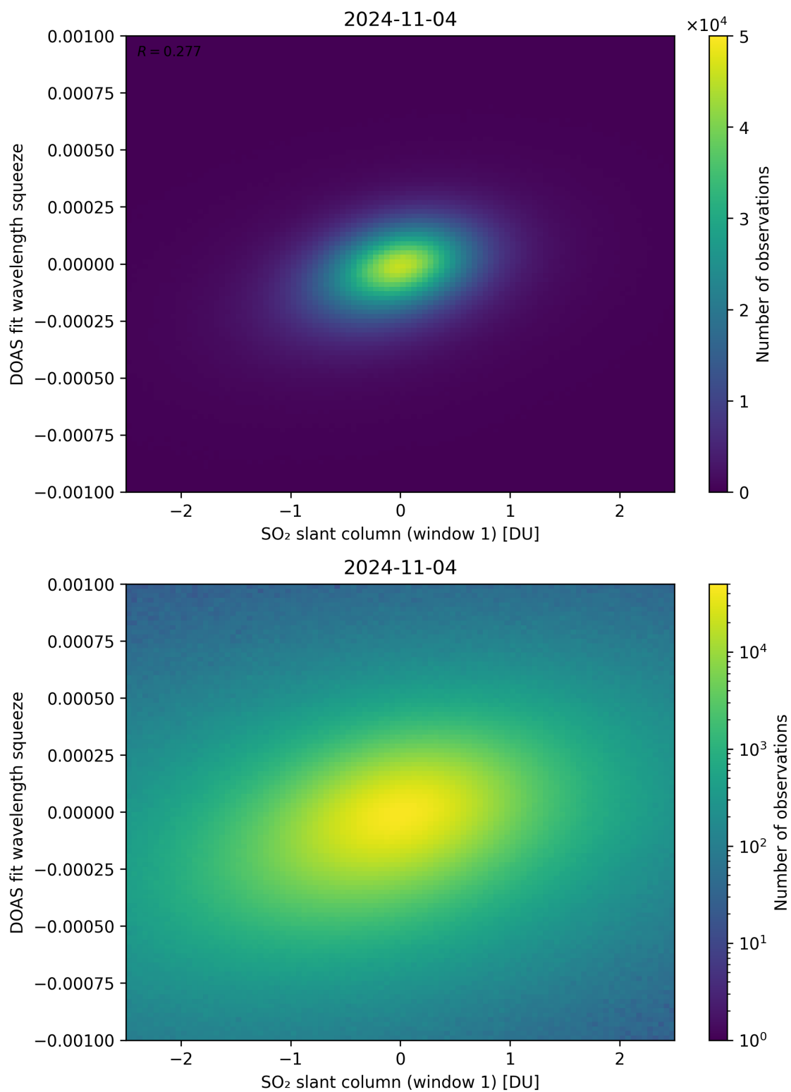
Figure 216: Scatter density plot of “SO 2 slant column (window 1)” against “DOAS fit wavelength squeeze” for 2024-11-04 to 2024-11-05.
