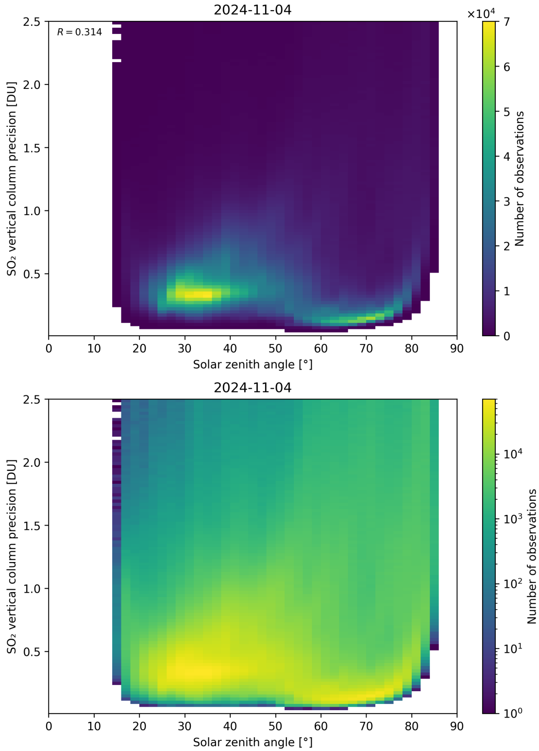
Figure 177: Scatter density plot of “Solar zenith angle” against “SO 2 vertical column precision” for 2024-11-04 to 2024-11-05.
