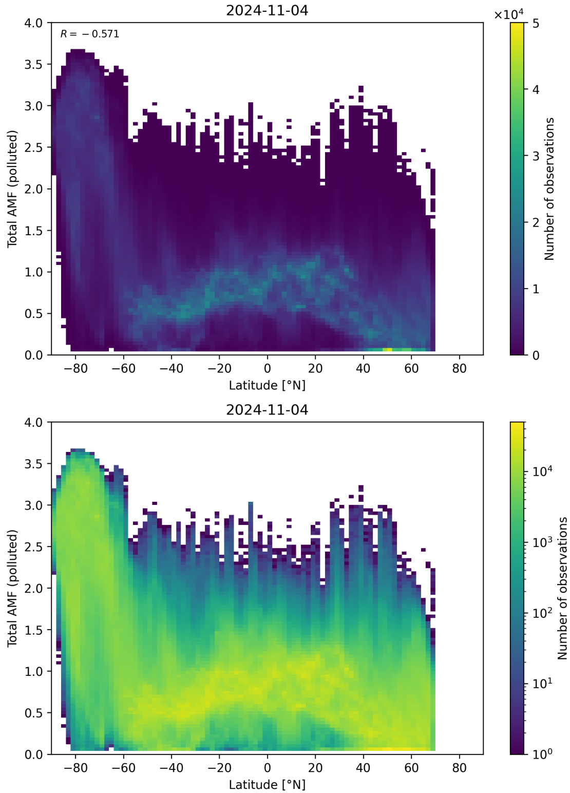
Figure 154: Scatter density plot of “Latitude” against “Total AMF (polluted)” for 2024-11-04 to 2024-11-05.
