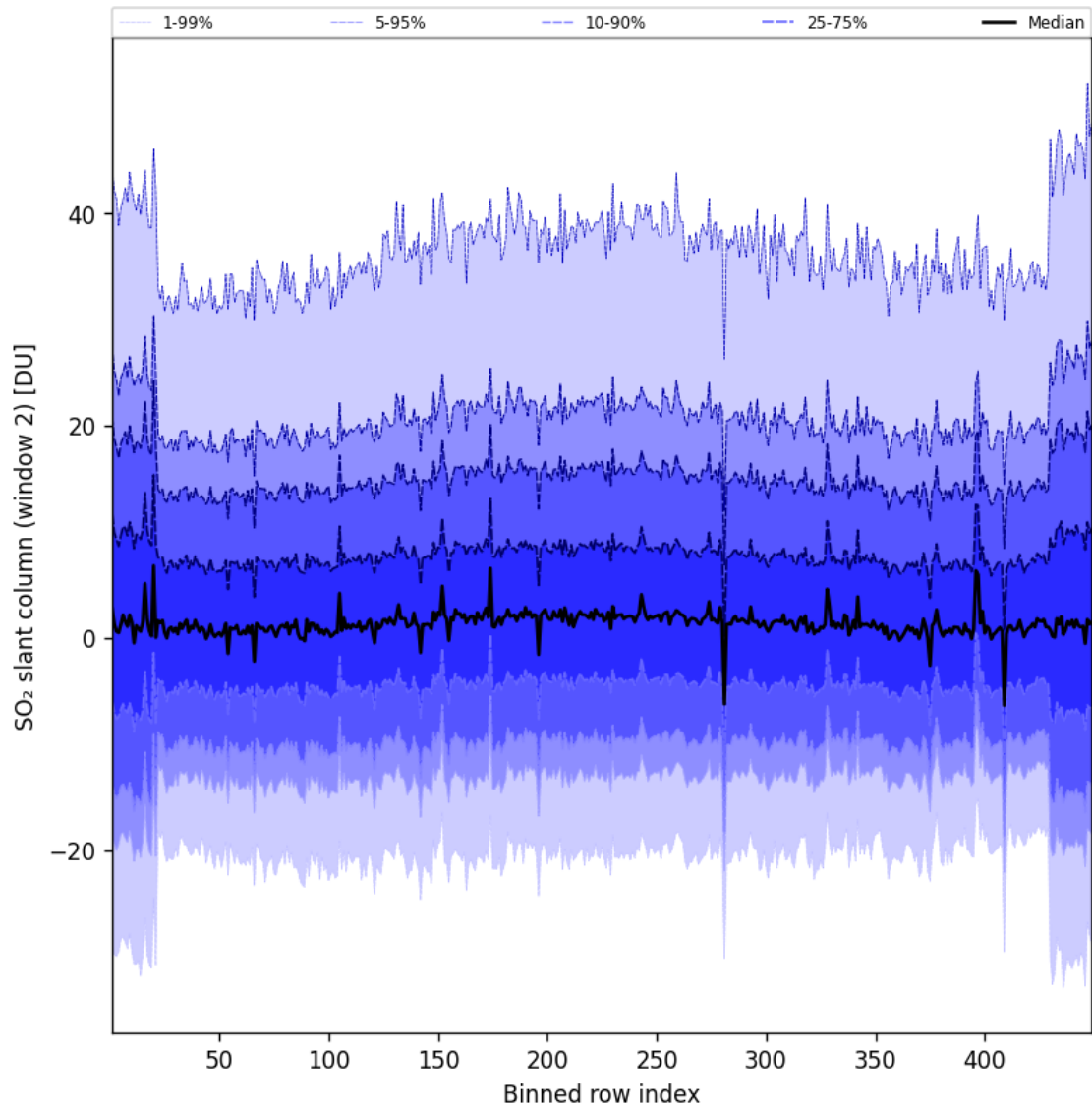
Figure 83: Along track statistics of “SO 2 slant column (window 2)” for 2024-11-04 to 2024-11-05
