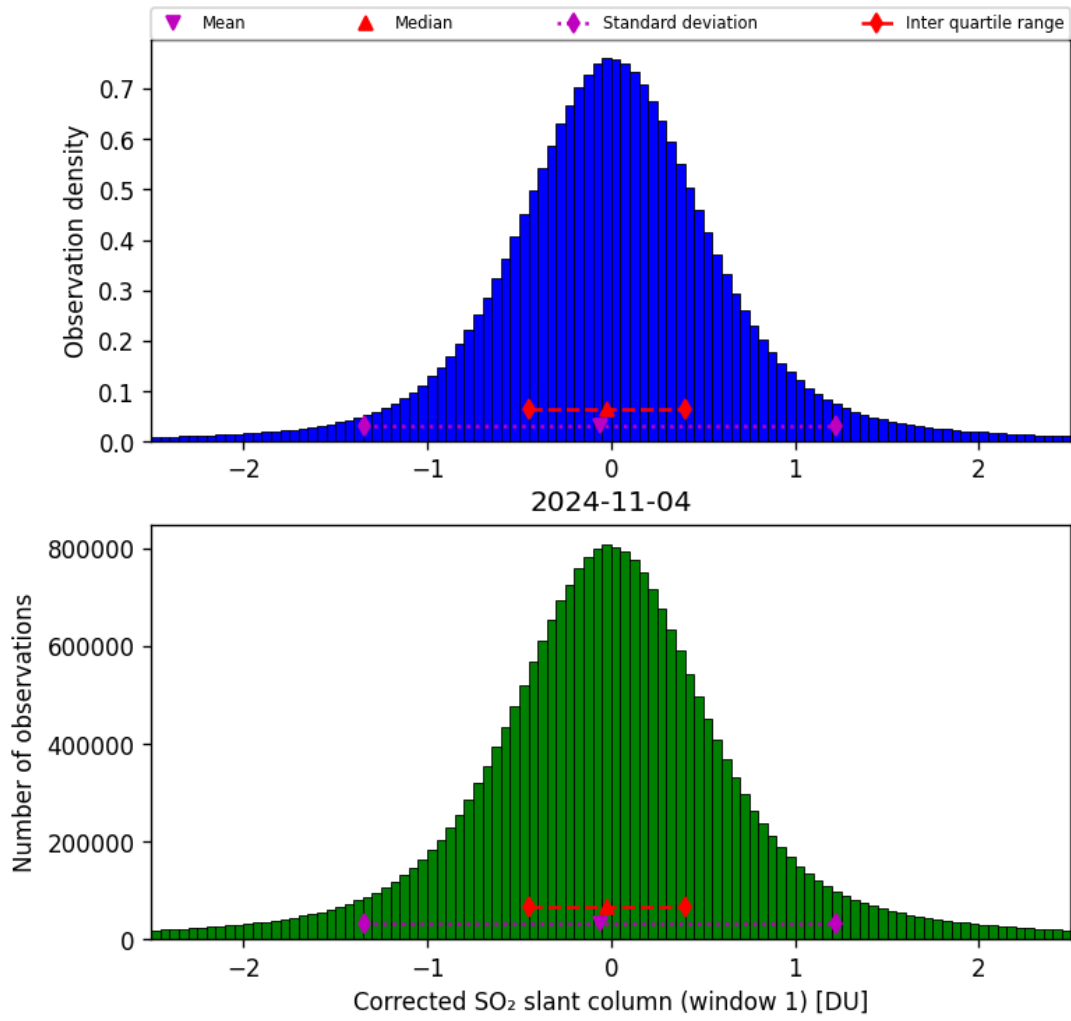
Figure 58: Histogram of “Corrected SO 2 slant column (window 1)” for 2024-11-04 to 2024-11-05
