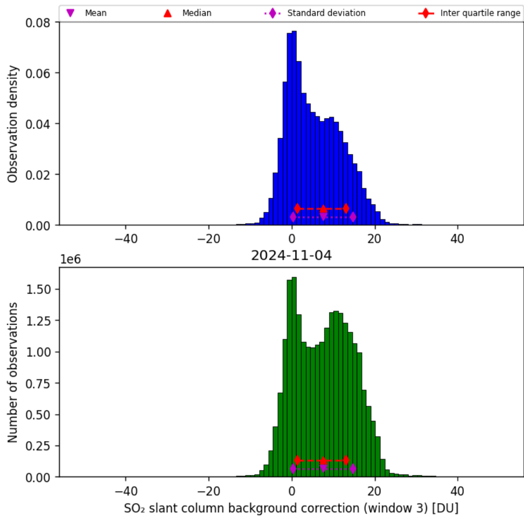
Figure 67: Histogram of “SO 2 slant column background correction (window 3)” for 2024-11-04 to 2024-11-05
