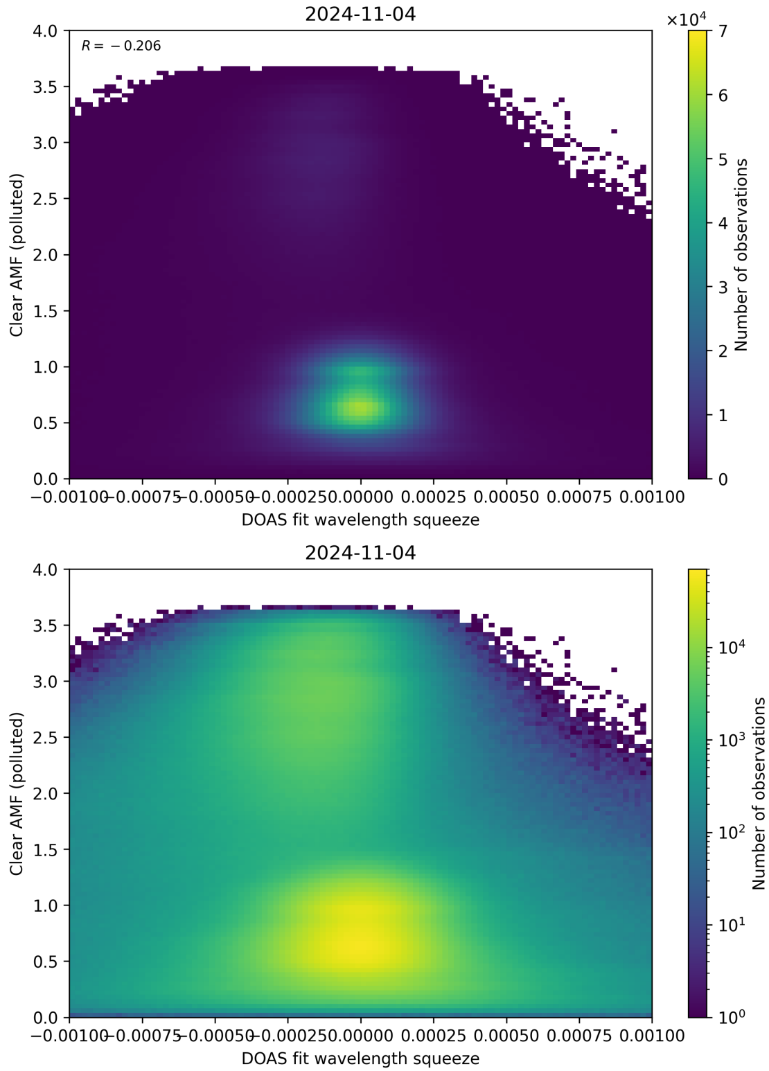
Figure 133: Scatter density plot of “DOAS fit wavelength squeeze” against “Clear AMF (polluted)” for 2024-11-04 to 2024-11-05.
