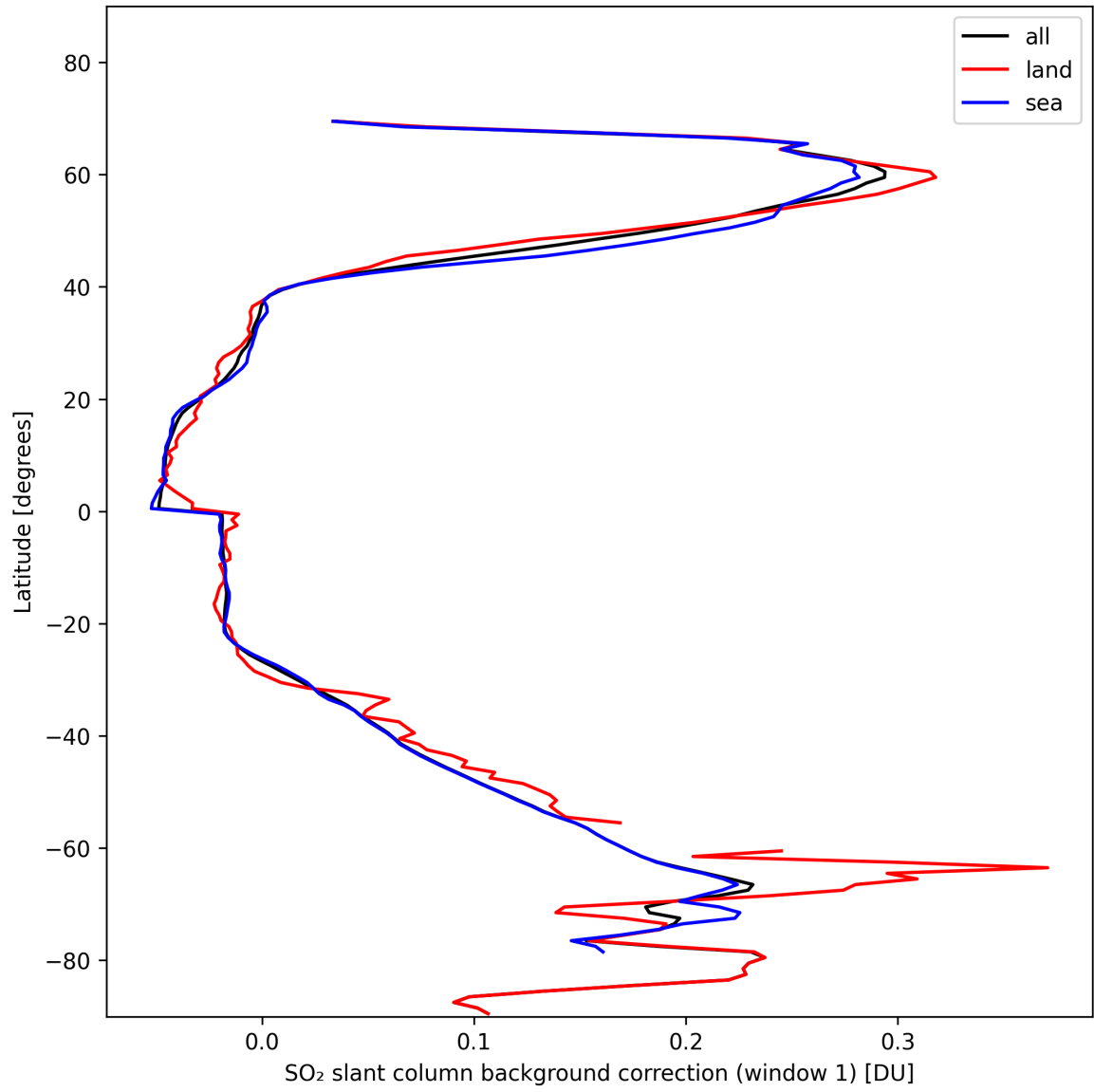
Figure 36: Zonal average of “SO 2 slant column background correction (window 1)” for 2024-11-04 to 2024-11-05.
