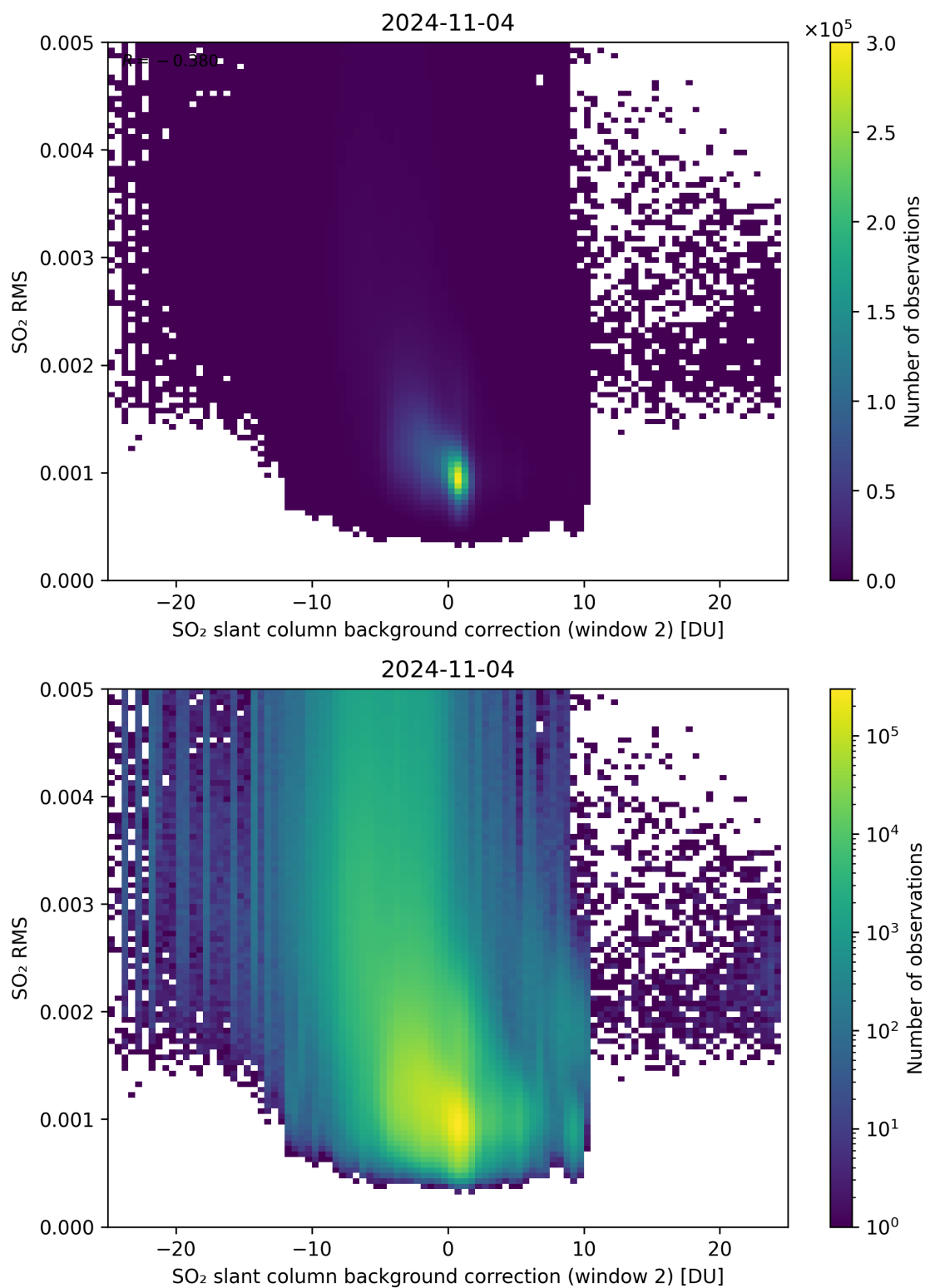
Figure 114: Scatter density plot of “SO 2 slant column background correction (window 2)” against “SO 2 RMS” for 2024-11-04 to 2024-11-05.
