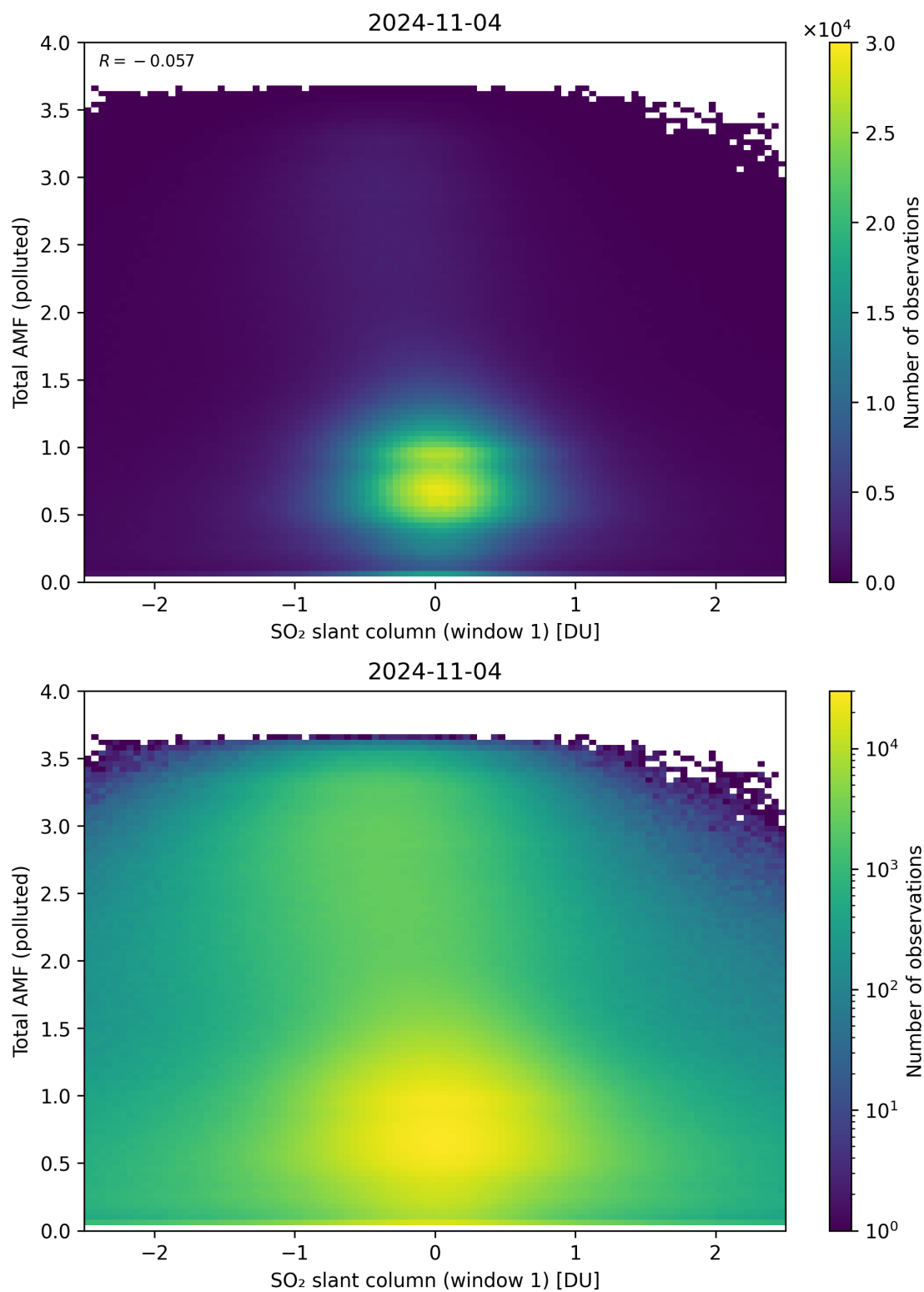
Figure 239: Scatter density plot of “SO 2 slant column (window 1)” against “Total AMF (polluted)” for 2024-11-04 to 2024-11-05.
