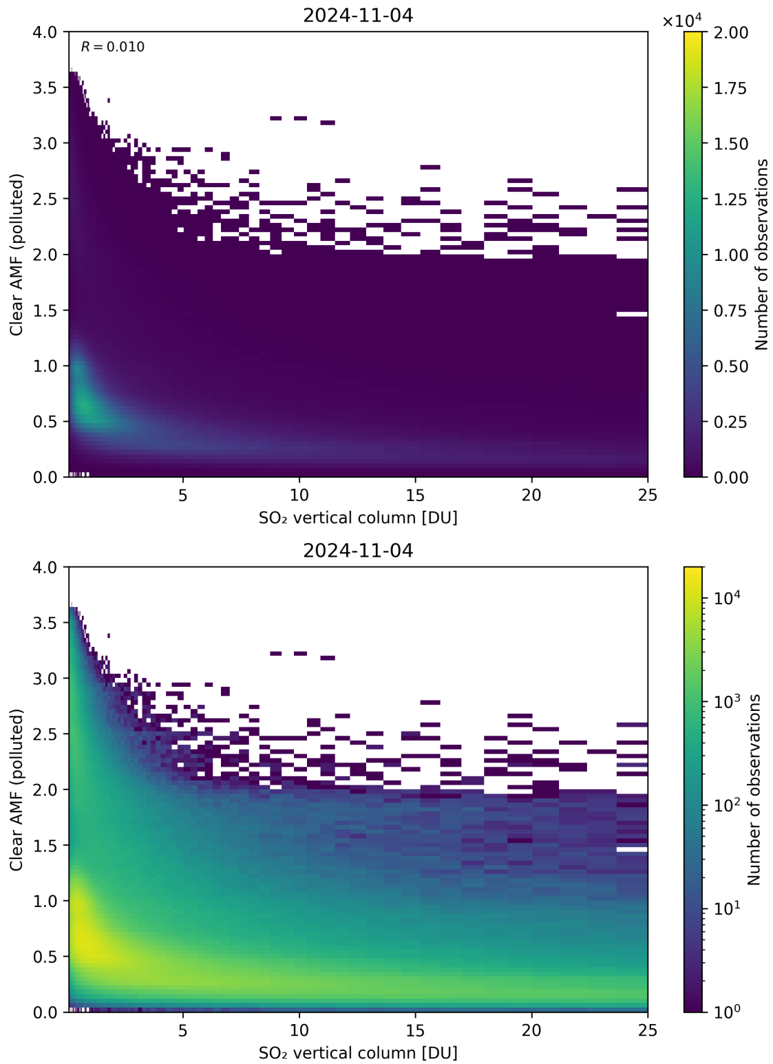
Figure 296: Scatter density plot of “SO 2 vertical column” against “Clear AMF (polluted)” for 2024-11-04 to 2024-11-05.
