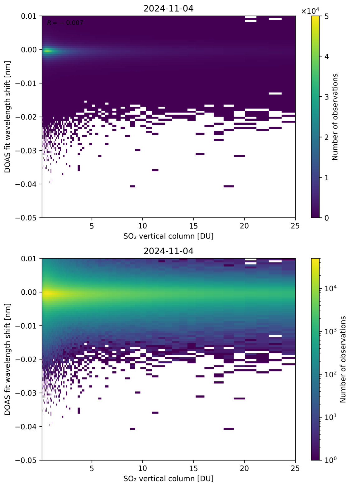
Figure 276: Scatter density plot of “SO 2 vertical column” against “DOAS fit wavelength shift” for 2024-11-04 to 2024-11-05.
