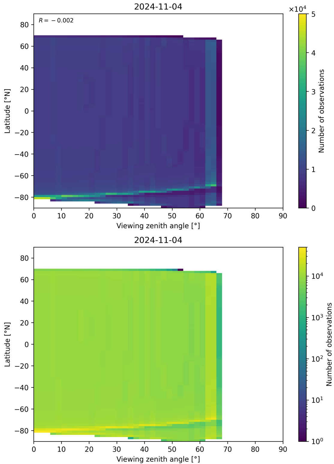
Figure 314: Scatter density plot of “Viewing zenith angle” against “Latitude” for 2024-11-04 to 2024-11-05.
