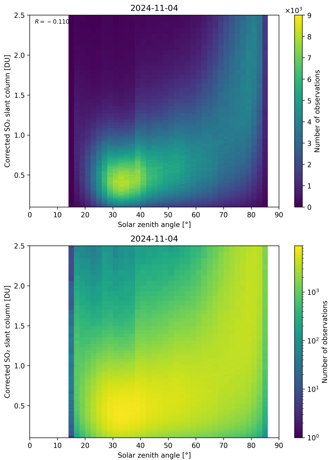
Figure 166: Scatter density plot of “Solar zenith angle” against “Corrected SO 2 slant column” for 2024-11-04 to 2024-11-05.
