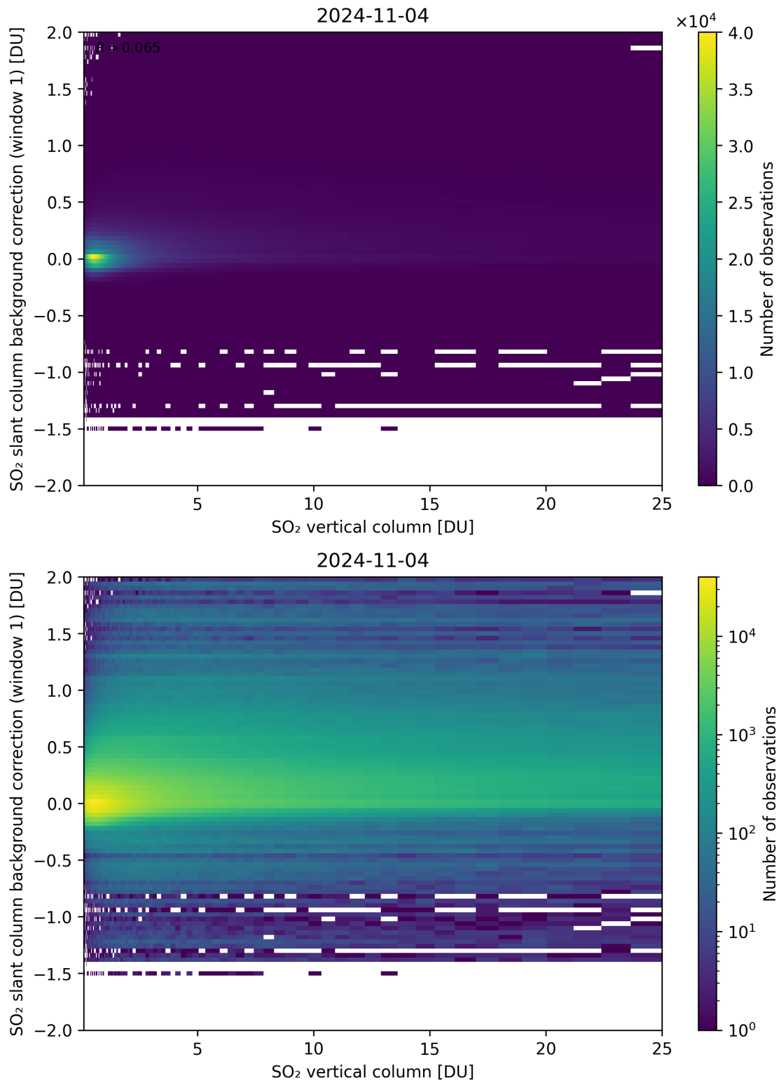
Figure 273: Scatter density plot of “SO 2 vertical column” against “SO 2 slant column background correction (window 1)” for 2024-11-04 to 2024-11-05.
