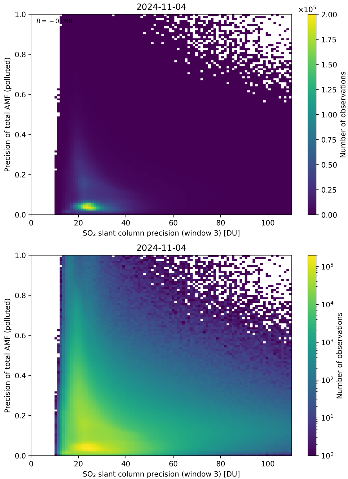
Figure 264: Scatter density plot of “SO 2 slant column precision (window 3)” against “Precision of total AMF (polluted)” for 2024-11-04 to 2024-11-05.
