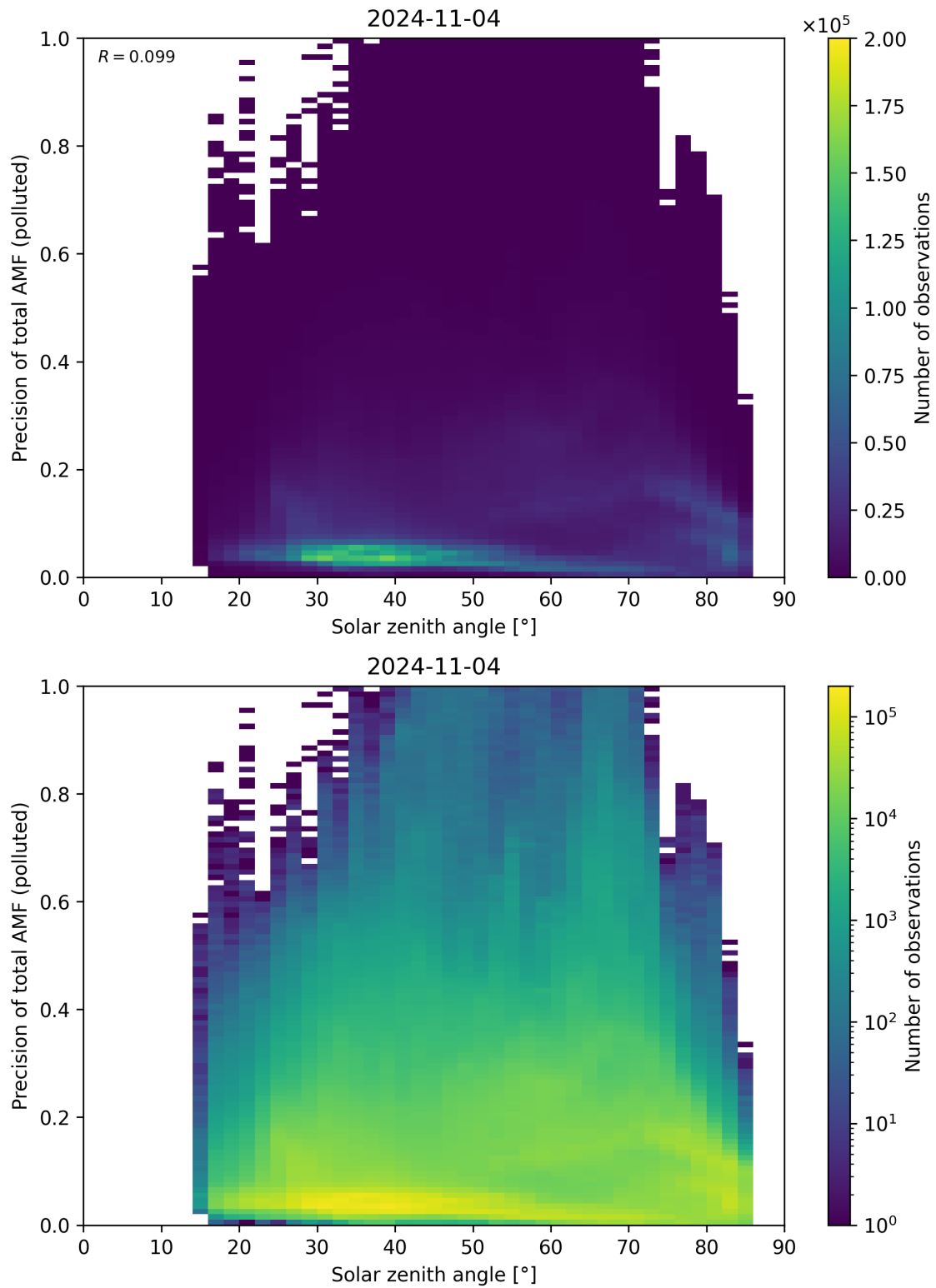
Figure 175: Scatter density plot of “Solar zenith angle” against “Precision of total AMF (polluted)” for 2024-11-04 to 2024-11-05.
