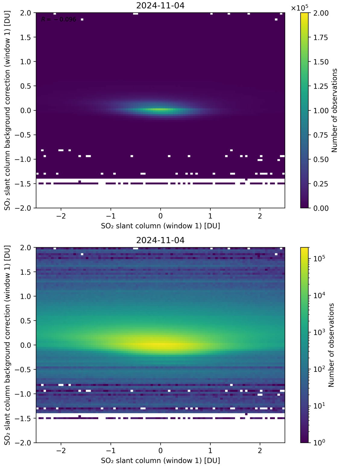
Figure 212: Scatter density plot of “SO 2 slant column (window 1)” against “SO 2 slant column background correction (window 1)” for 2024-11-04 to 2024-11-05.
