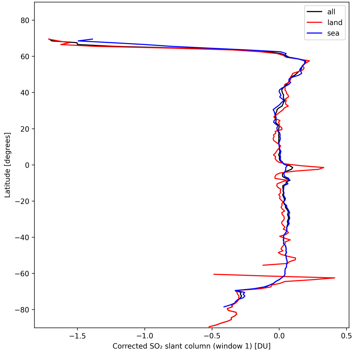
Figure 35: Zonal average of “Corrected SO 2 slant column (window 1)” for 2024-11-04 to 2024-11-05.
