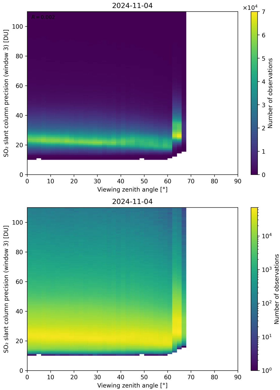
Figure 324: Scatter density plot of “Viewing zenith angle” against “SO 2 slant column precision (window 3)” for 2024-11-04 to 2024-11-05.
