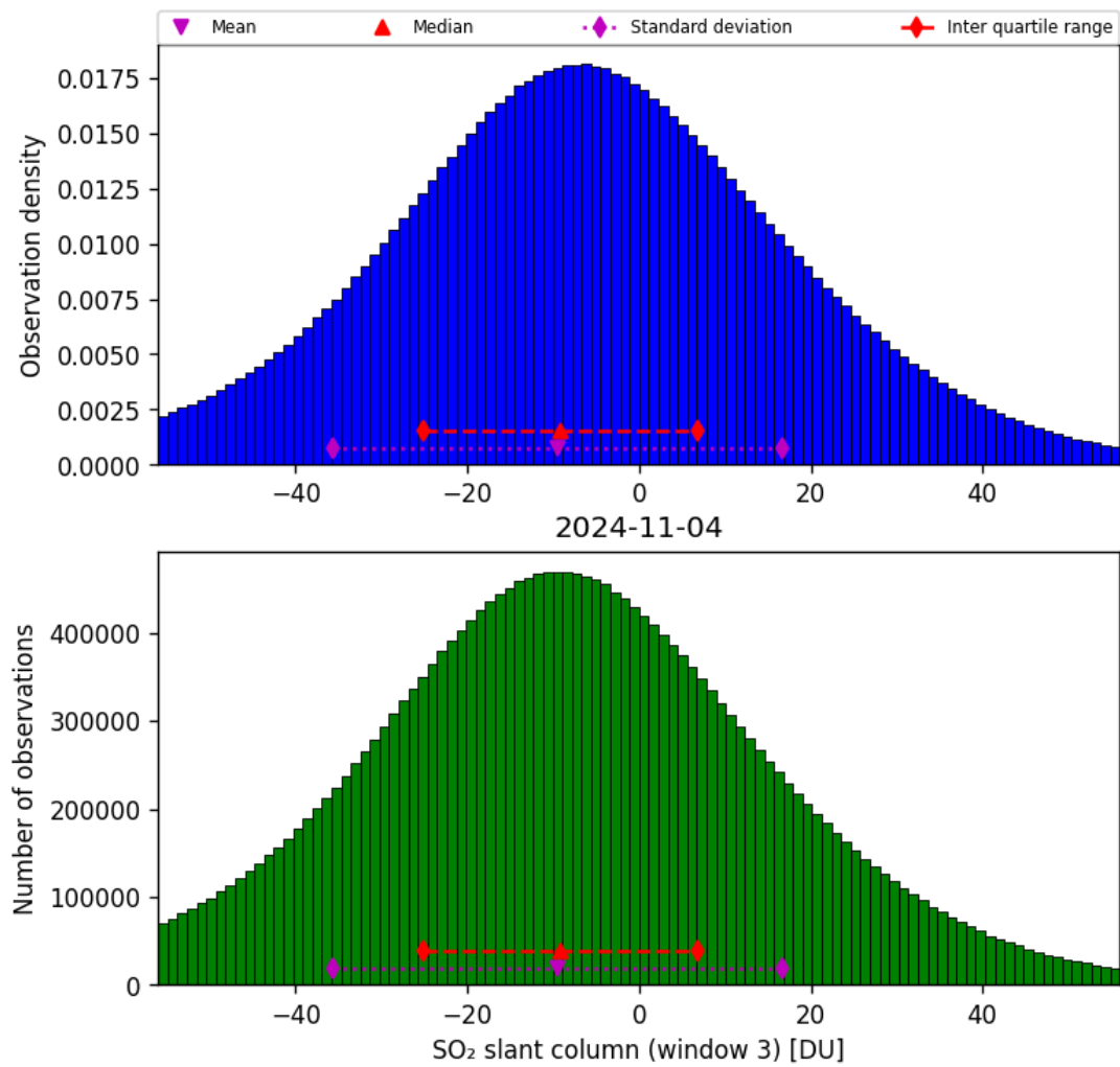
Figure 64: Histogram of “SO 2 slant column (window 3)” for 2024-11-04 to 2024-11-05
