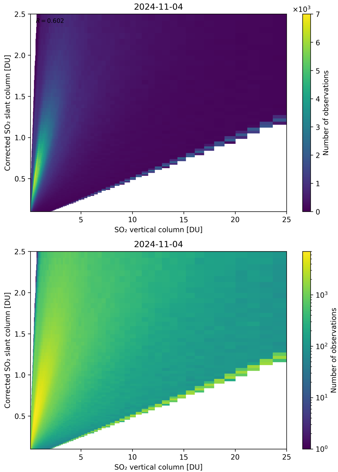
Figure 297: Scatter density plot of “SO 2 vertical column” against “Corrected SO 2 slant column” for 2024-11-04 to 2024-11-05.
