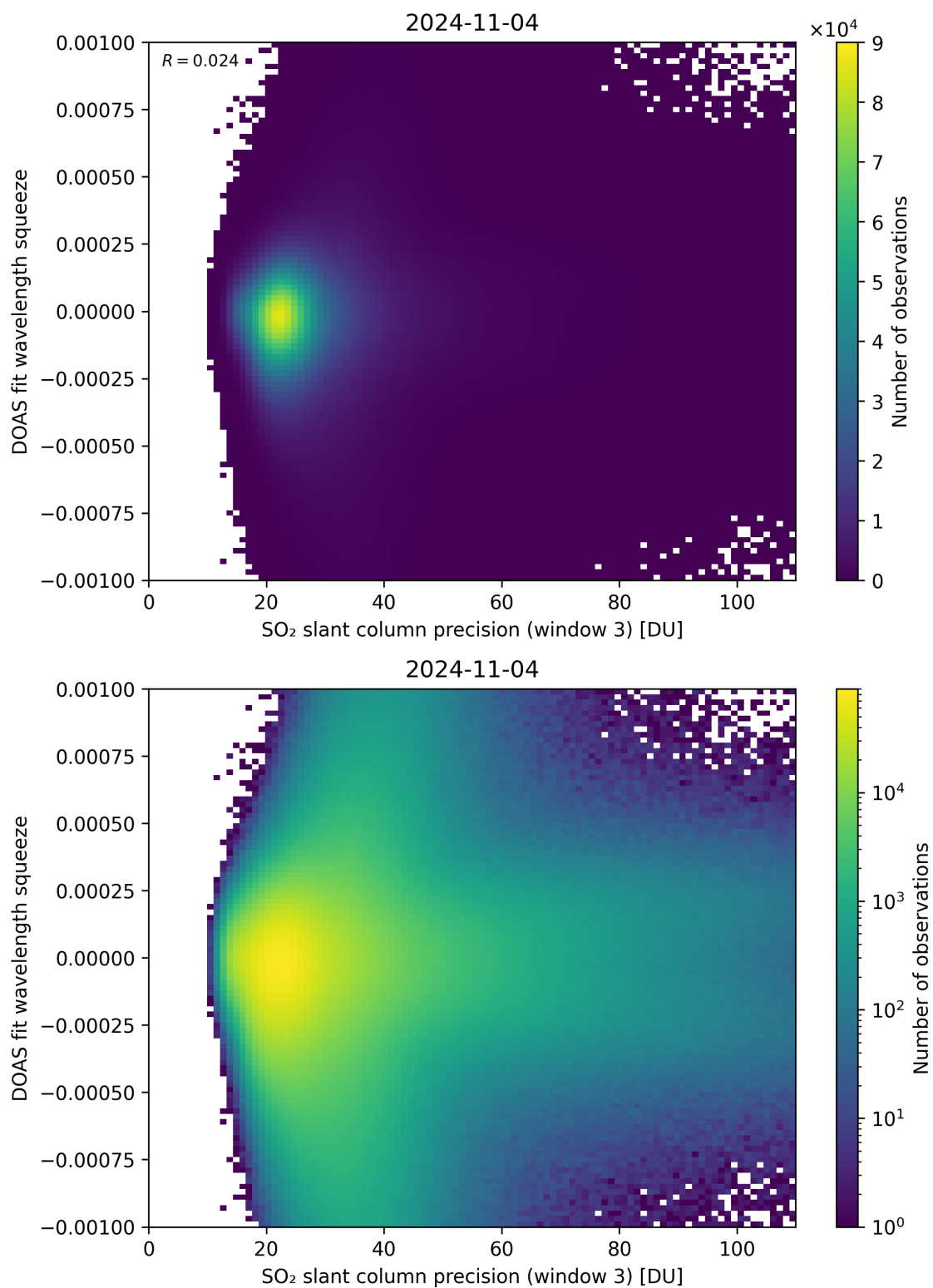
Figure 259: Scatter density plot of “SO 2 slant column precision (window 3)” against “DOAS fit wavelength squeeze” for 2024-11-04 to 2024-11-05.
