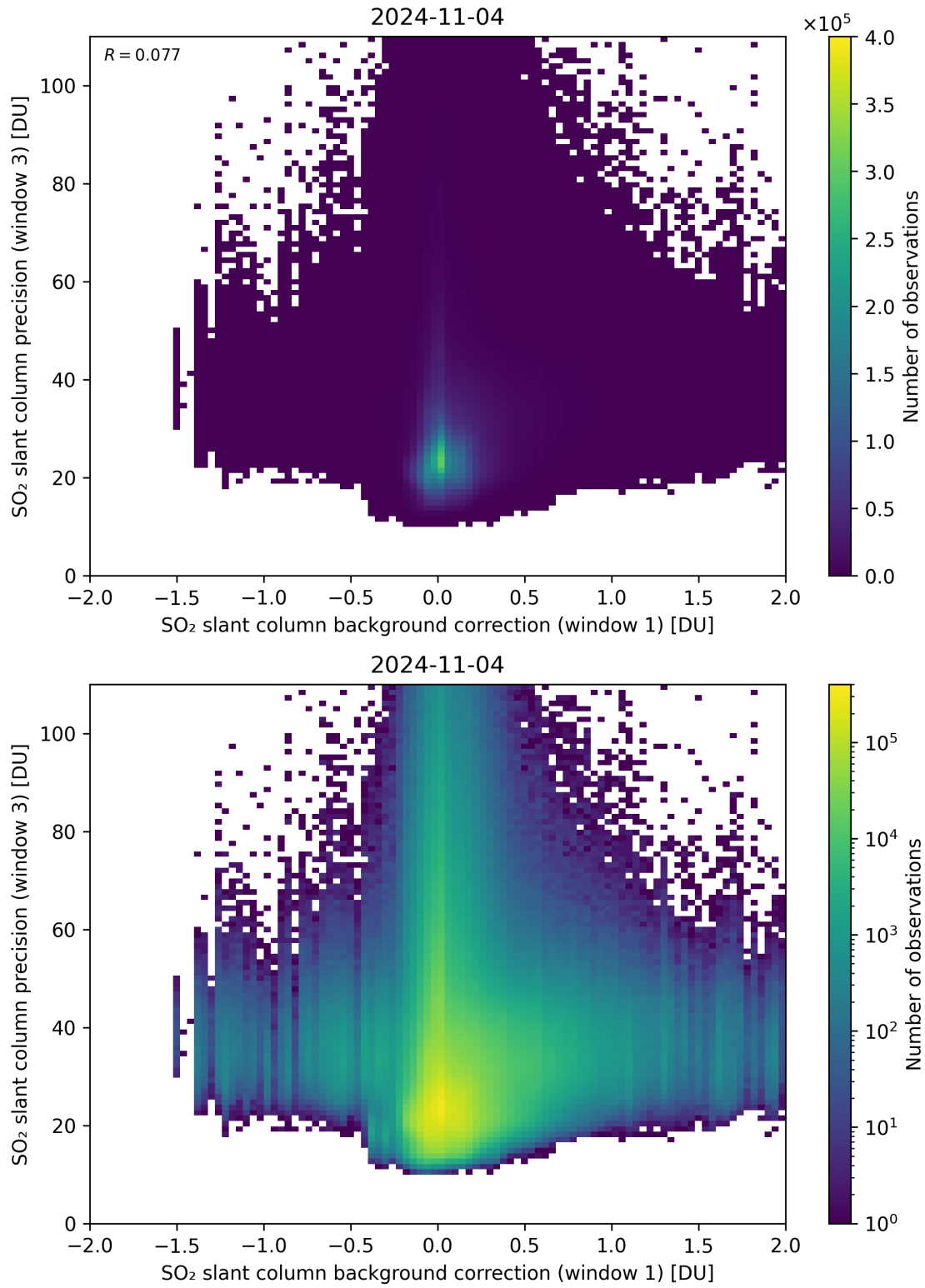
Figure 108: Scatter density plot of “SO 2 slant column background correction (window 1)” against “SO 2 slant column precision (window 3)” for 2024-11-04 to 2024-11-05.
