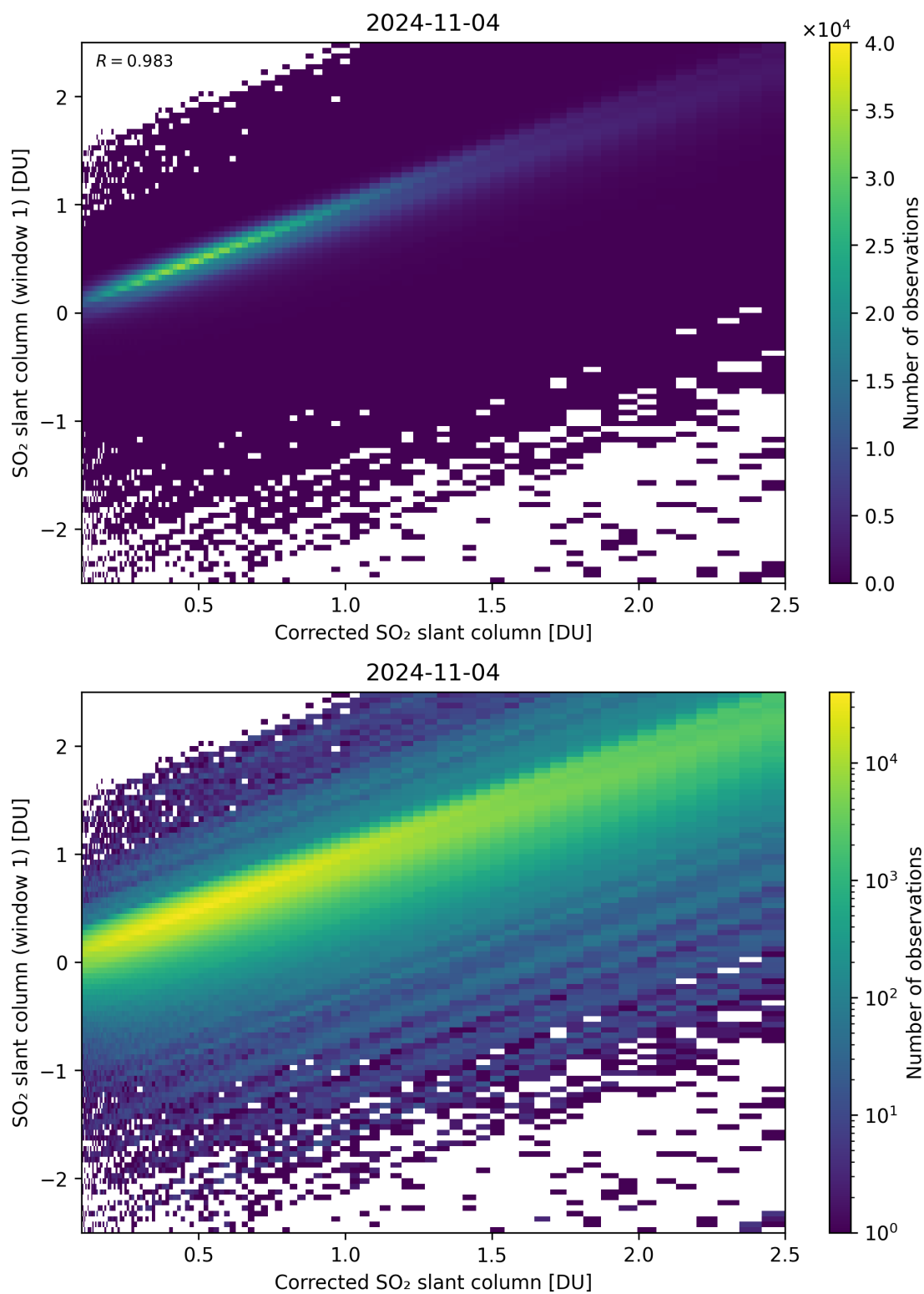
Figure 187: Scatter density plot of “Corrected SO 2 slant column” against “SO 2 slant column (window 1)” for 2024-11-04 to 2024-11-05.
