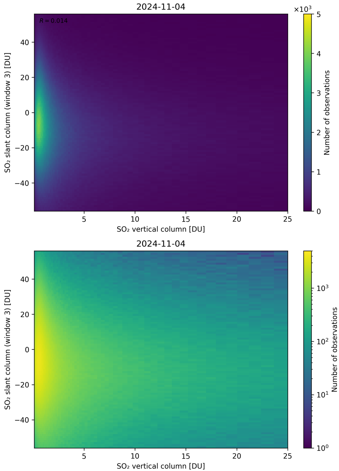
Figure 303: Scatter density plot of “SO 2 vertical column” against “SO 2 slant column (window 3)” for 2024-11-04 to 2024-11-05.
