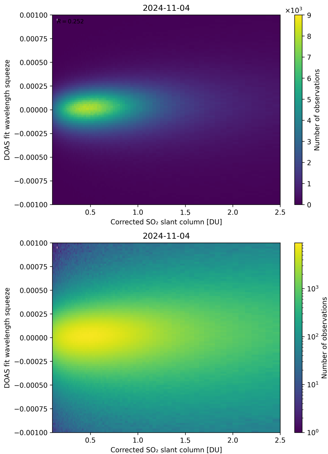
Figure 182: Scatter density plot of “Corrected SO 2 slant column” against “DOAS fit wavelength squeeze” for 2024-11-04 to 2024-11-05.
