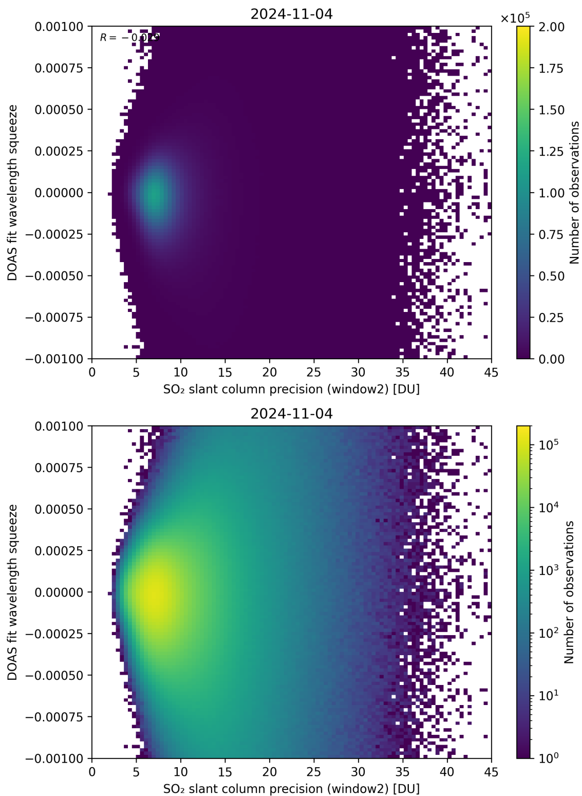
Figure 244: Scatter density plot of “SO 2 slant column precision (window2)” against “DOAS fit wavelength squeeze” for 2024-11-04 to 2024-11-05.
