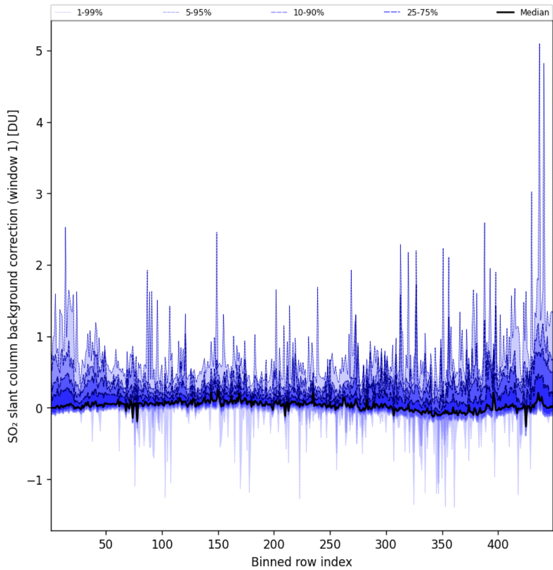
Figure 82: Along track statistics of “SO 2 slant column background correction (window 1)” for 2024-11-04 to 2024-11-05
