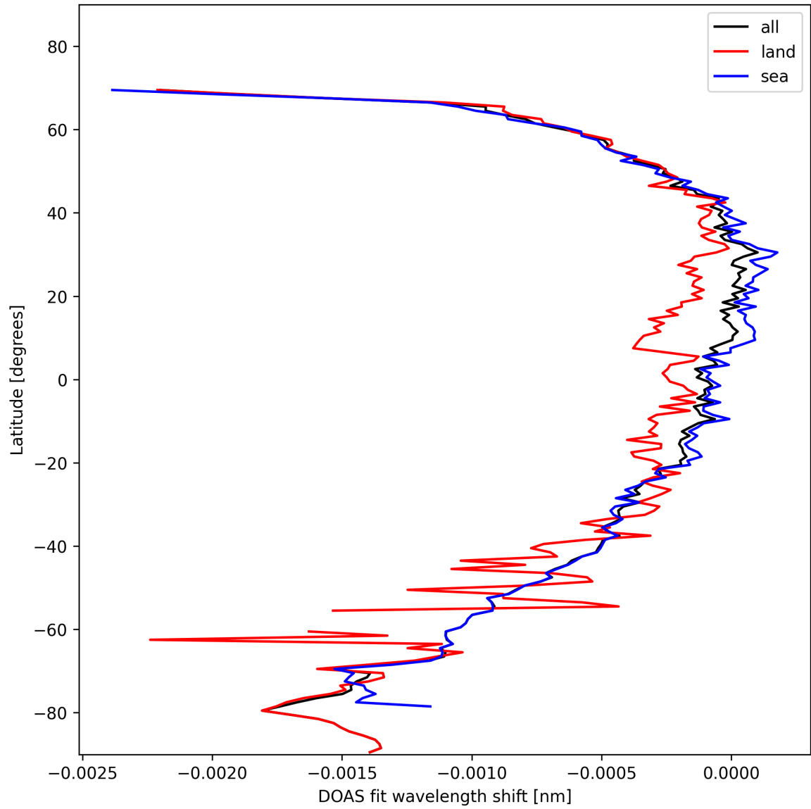
Figure 45: Zonal average of “DOAS fit wavelength shift” for 2024-11-04 to 2024-11-05.
