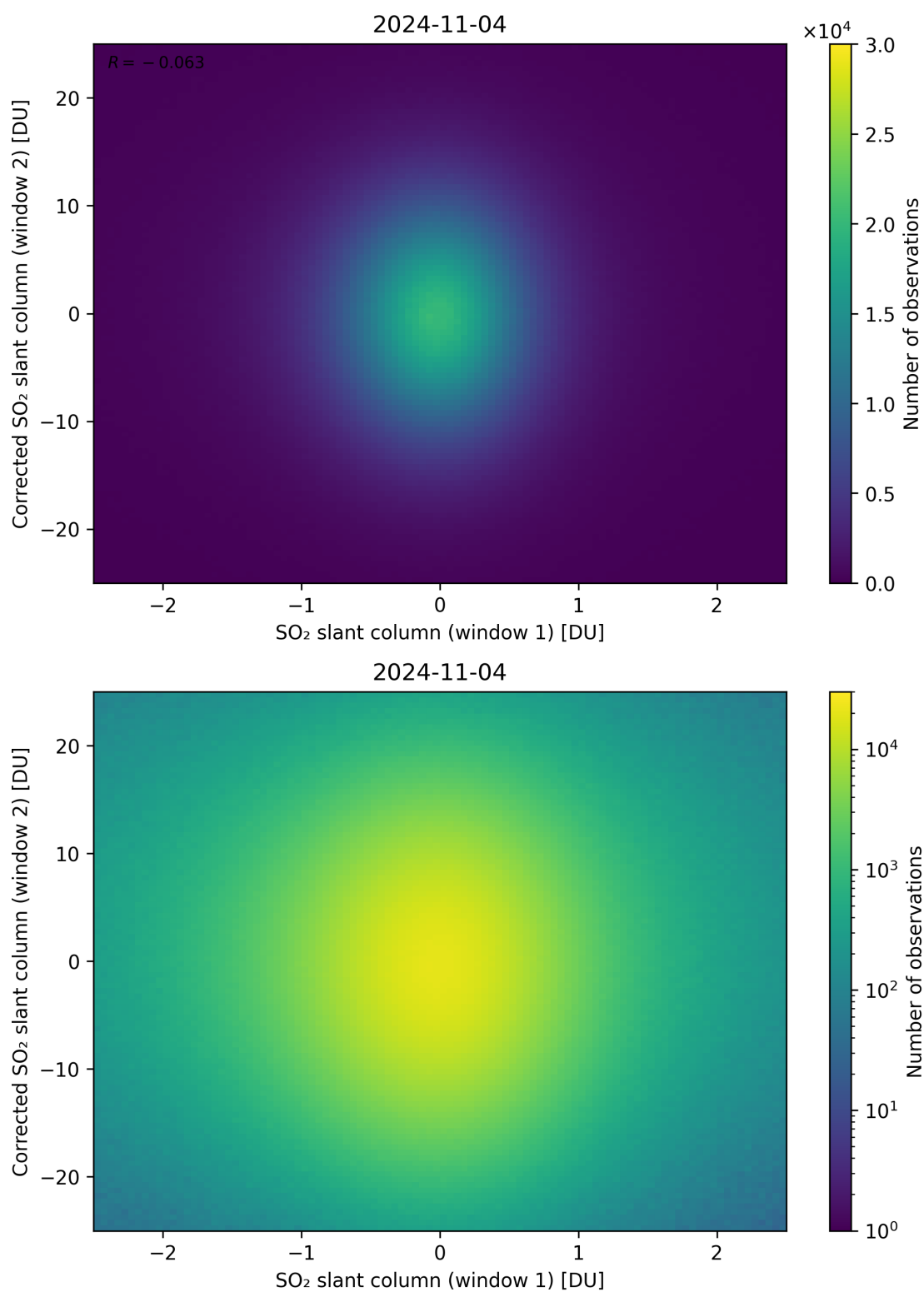
Figure 233: Scatter density plot of “SO 2 slant column (window 1)” against “Corrected SO 2 slant column (window 2)” for 2024-11-04 to 2024-11-05.
