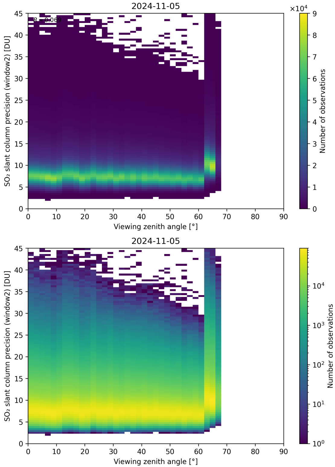
Figure 322: Scatter density plot of “Viewing zenith angle” against “SO 2 slant column precision (window2)” for 2024-11-04 to 2024-11-06.
