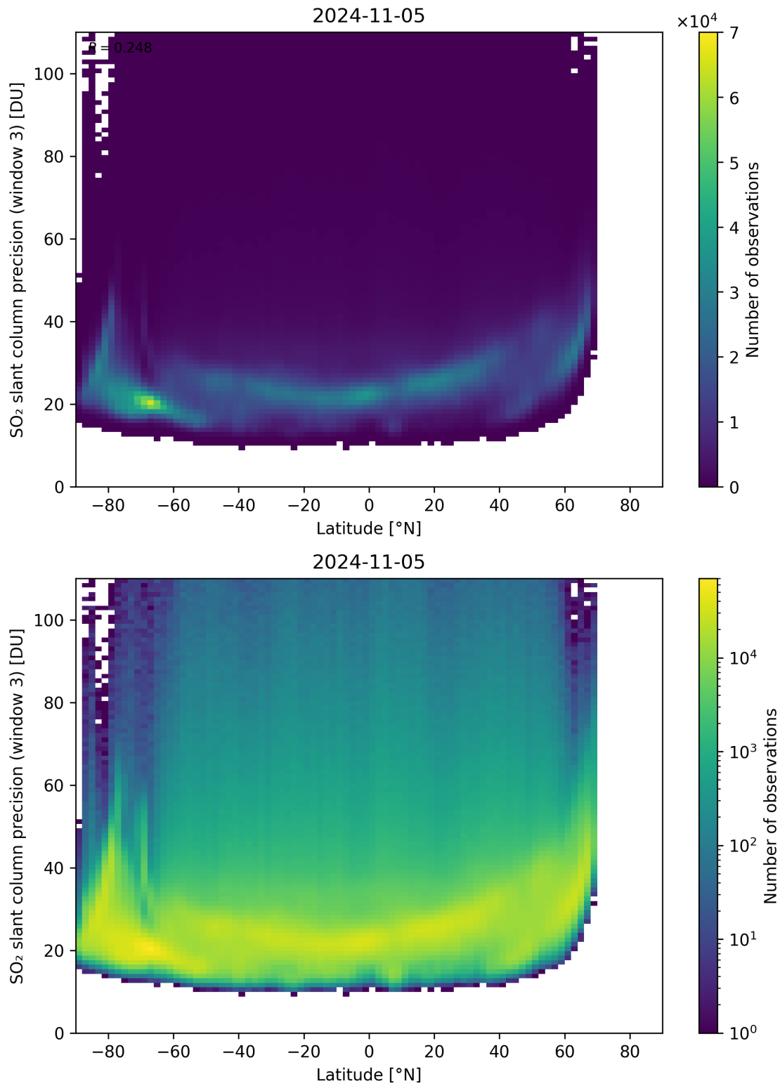
Figure 153: Scatter density plot of “Latitude” against “SO 2 slant column precision (window 3)” for 2024-11-04 to 2024-11-06.
