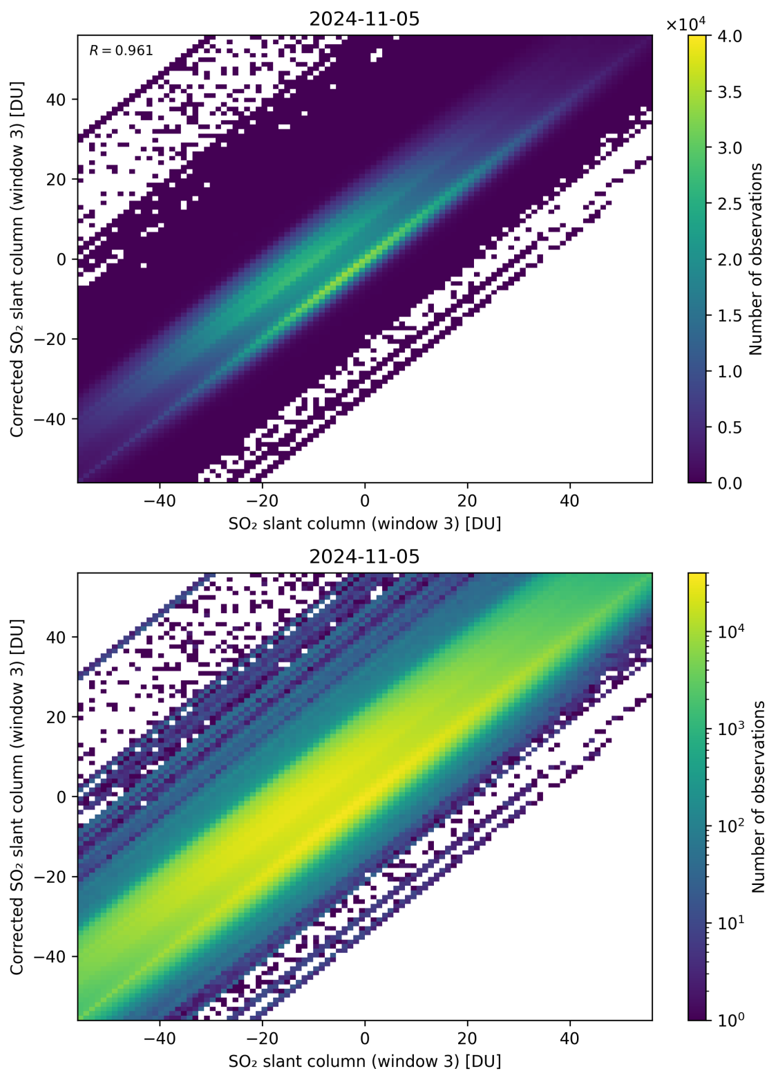
Figure 266: Scatter density plot of “SO 2 slant column (window 3)” against “Corrected SO 2 slant column (window 3)” for 2024-11-04 to 2024-11-06.
