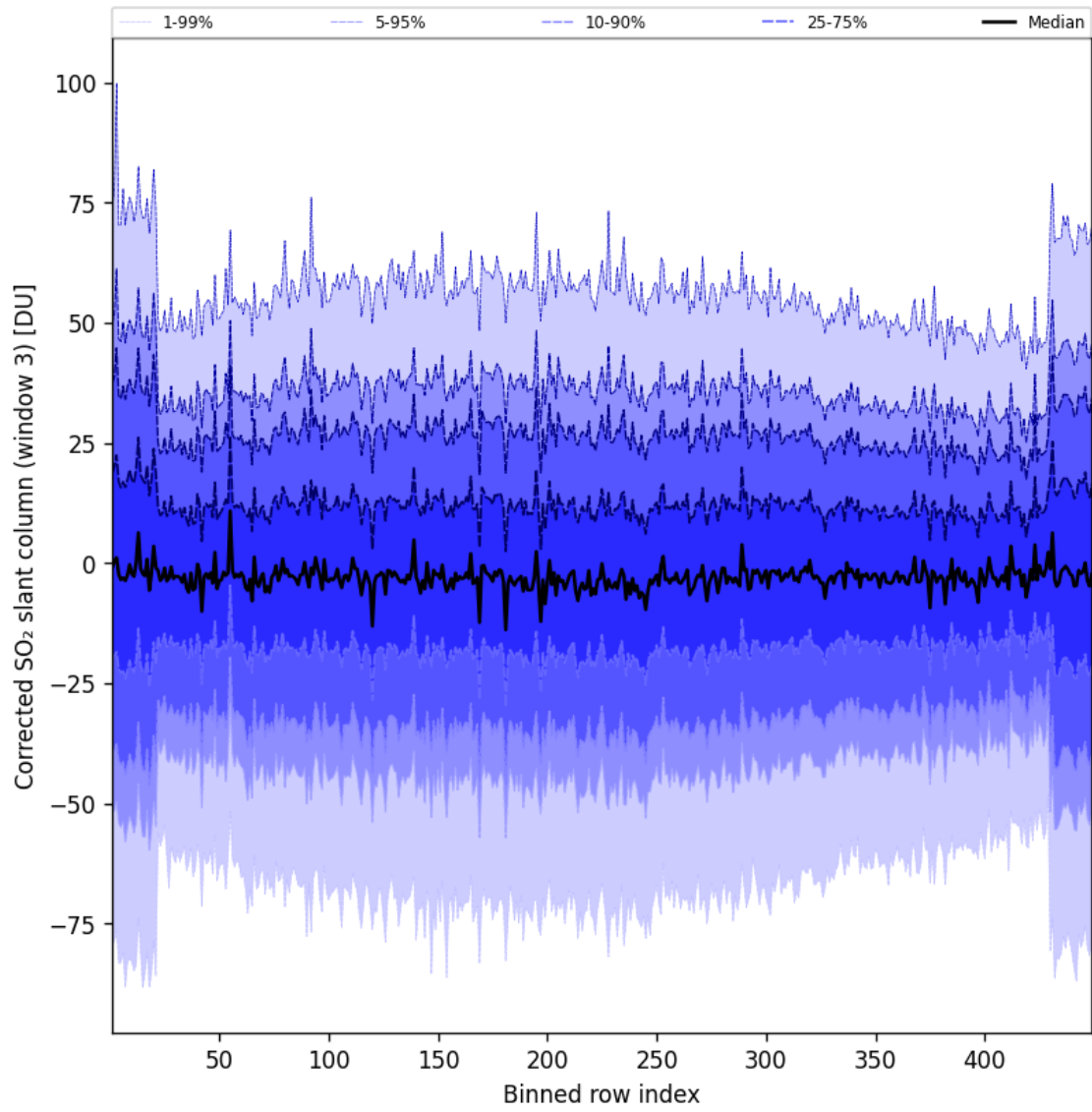
Figure 89: Along track statistics of “Corrected SO 2 slant column (window 3)” for 2024-11-04 to 2024-11-06
