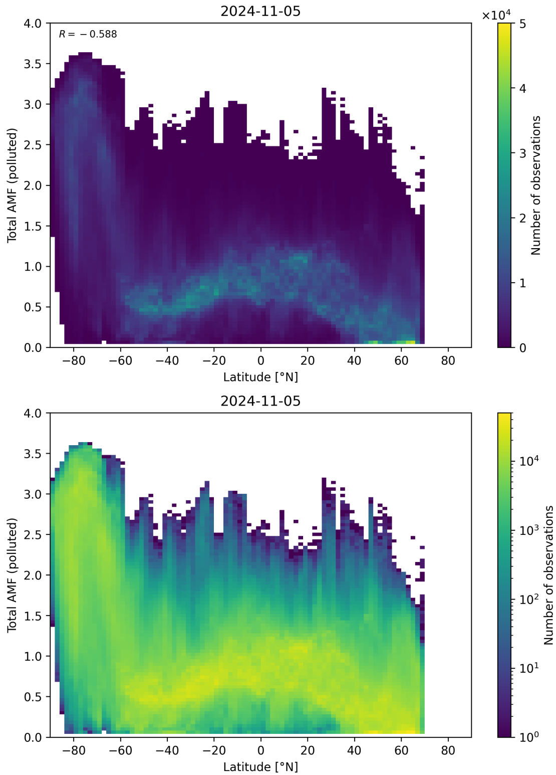
Figure 154: Scatter density plot of “Latitude” against “Total AMF (polluted)” for 2024-11-04 to 2024-11-06.
