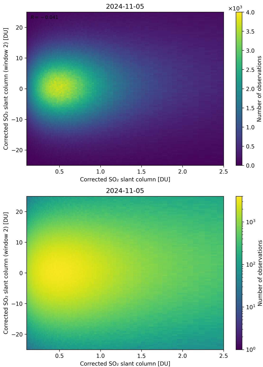
Figure 185: Scatter density plot of “Corrected SO 2 slant column” against “Corrected SO 2 slant column (window 2)” for 2024-11-04 to 2024-11-06.
