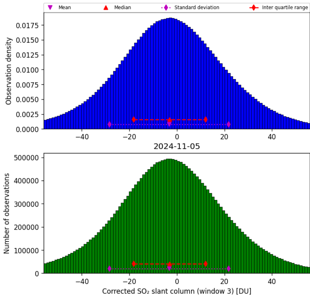
Figure 66: Histogram of “Corrected SO 2 slant column (window 3)” for 2024-11-04 to 2024-11-06
