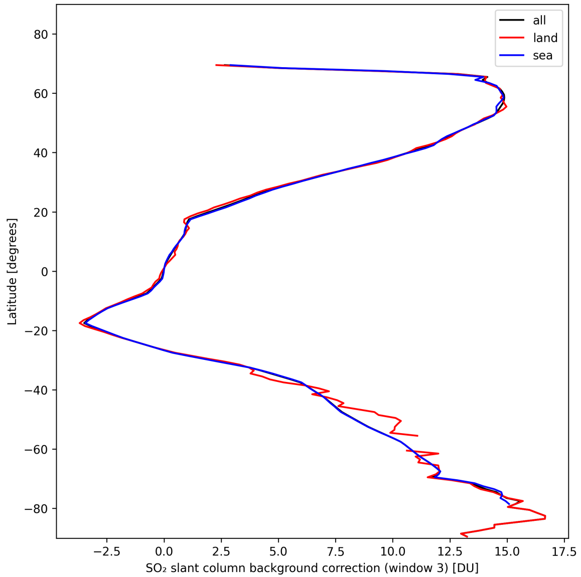
Figure 44: Zonal average of “SO 2 slant column background correction (window 3)” for 2024-11-04 to 2024-11-06.
