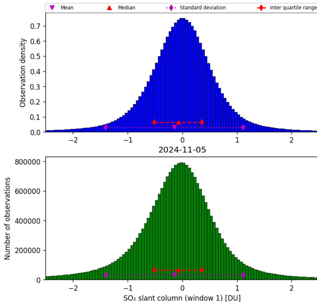
Figure 56: Histogram of “SO 2 slant column (window 1)” for 2024-11-04 to 2024-11-06
