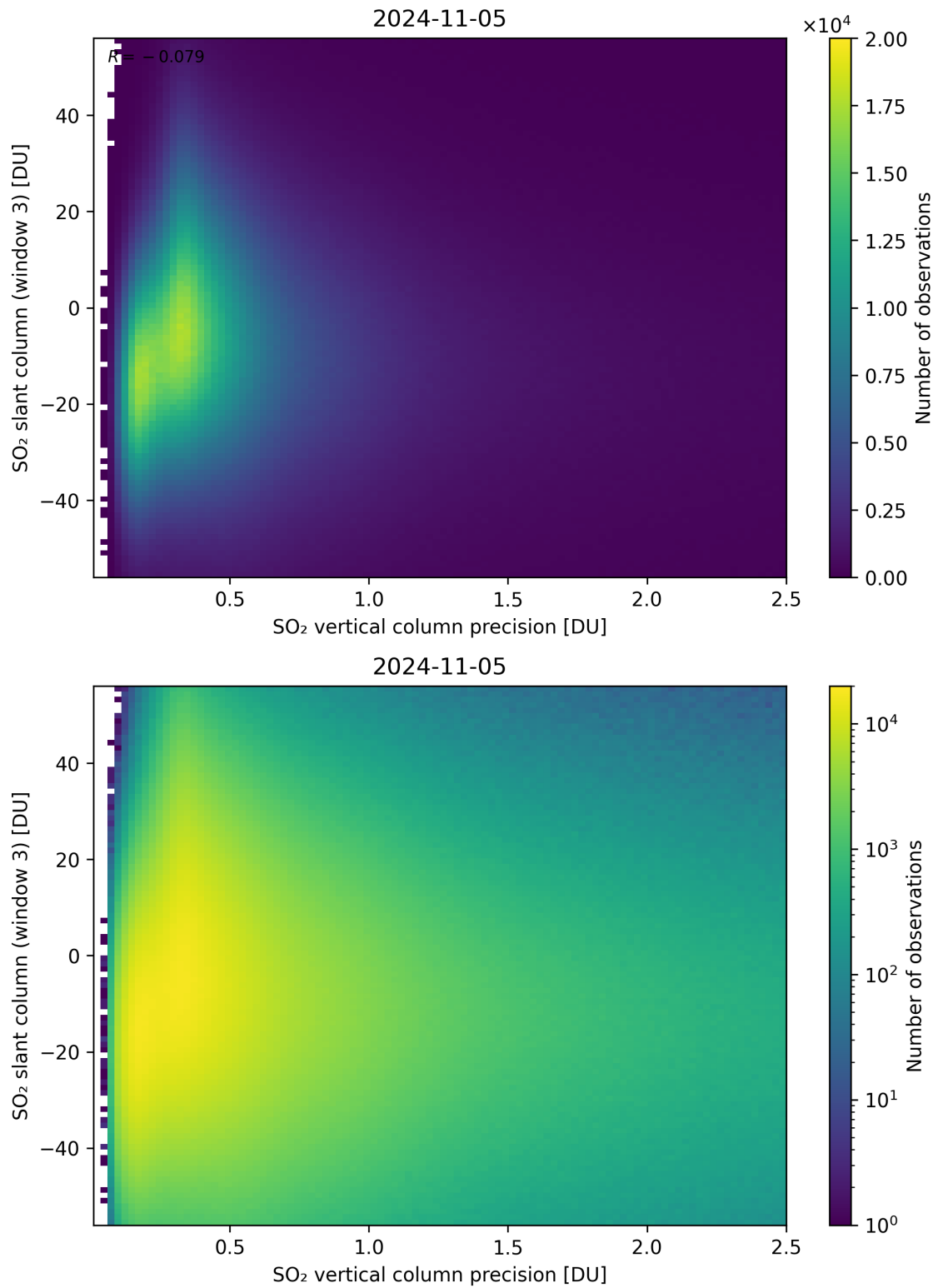
Figure 292: Scatter density plot of “SO 2 vertical column precision” against “SO 2 slant column (window 3)” for 2024-11-04 to 2024-11-06.
