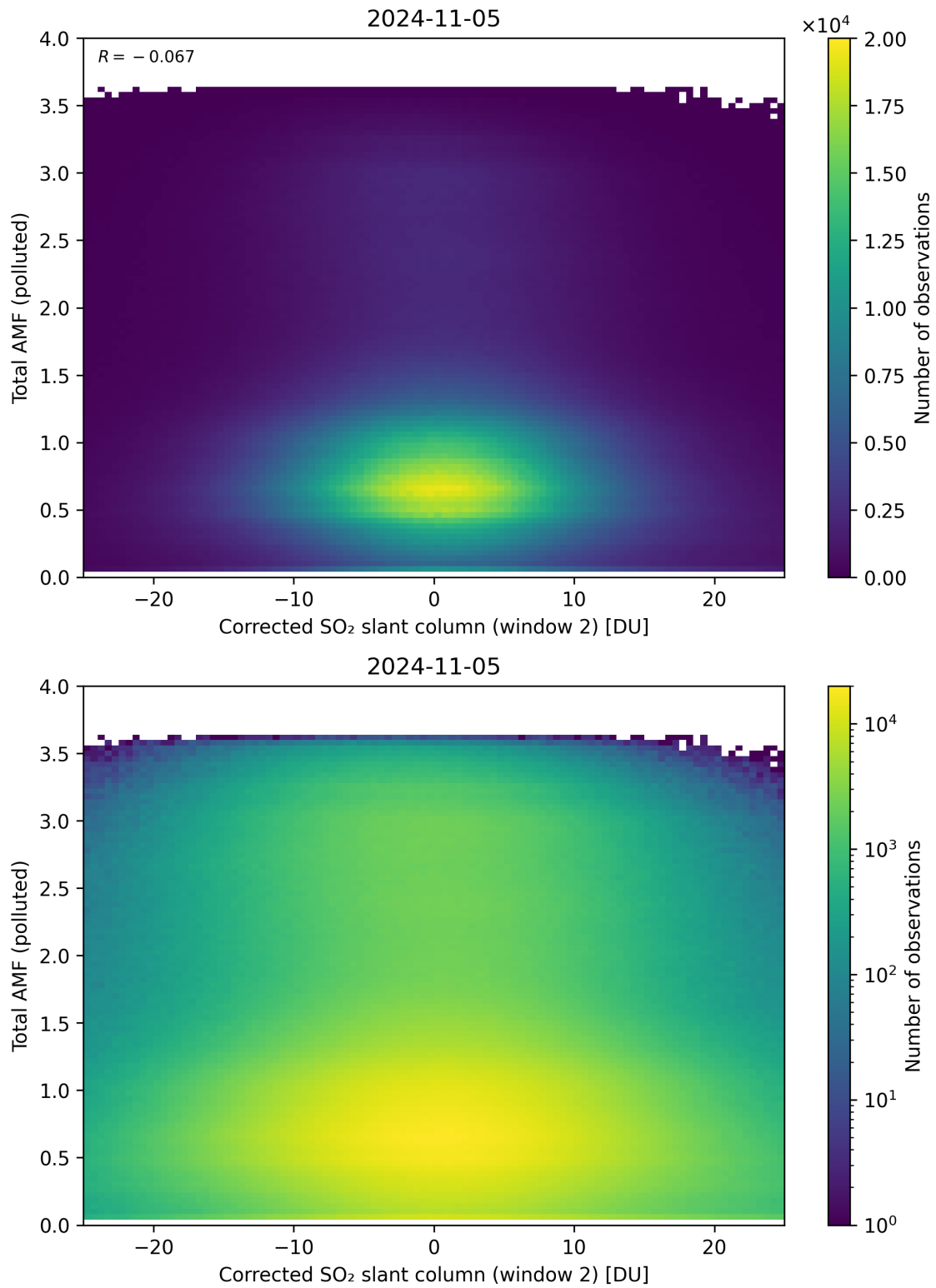
Figure 203: Scatter density plot of “Corrected SO 2 slant column (window 2)” against “Total AMF (polluted)” for 2024-11-04 to 2024-11-06.
