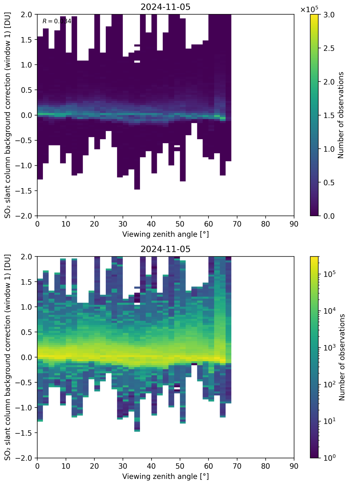
Figure 308: Scatter density plot of “Viewing zenith angle” against “SO 2 slant column background correction (window 1)” for 2024-11-04 to 2024-11-06.
