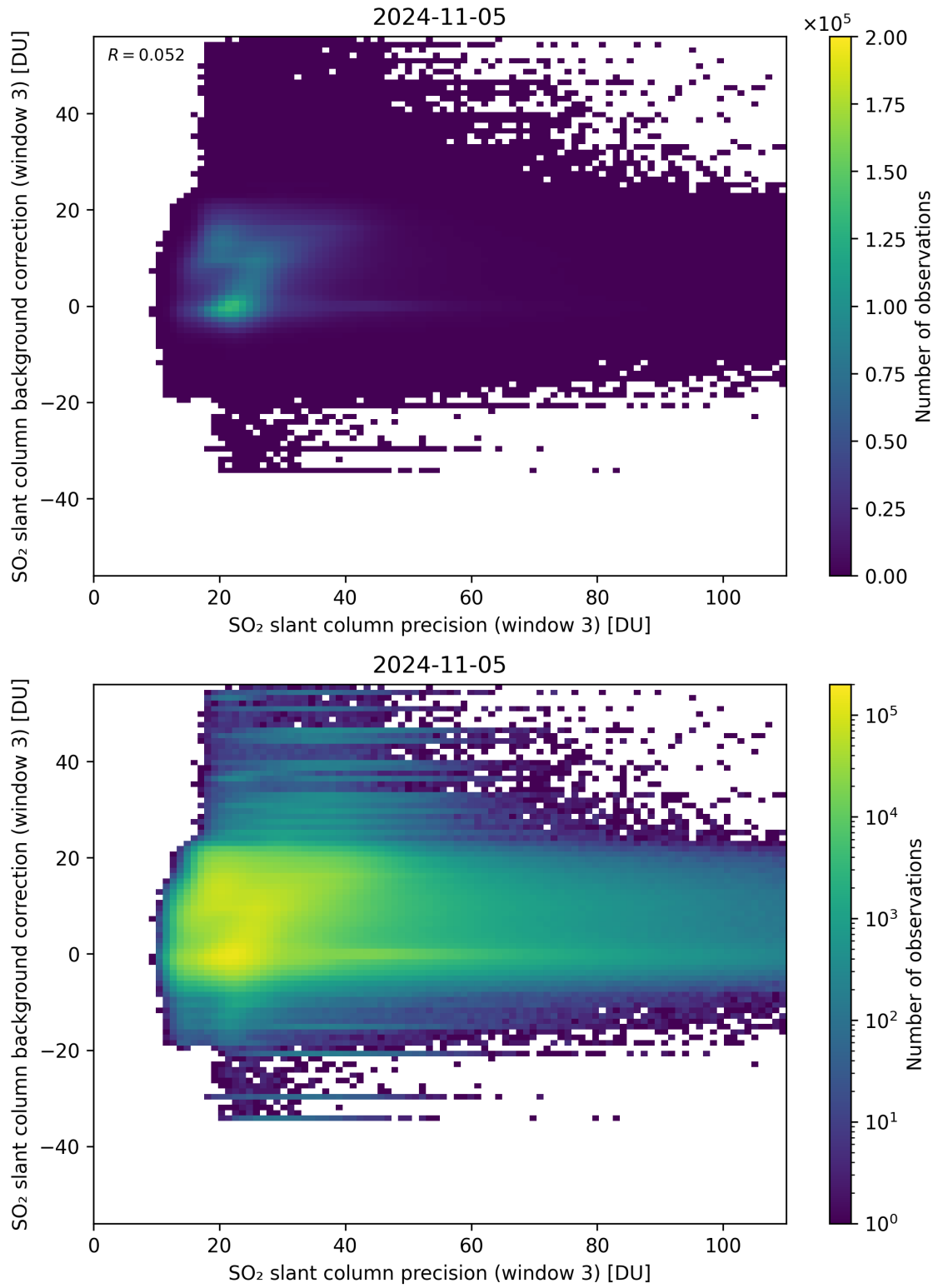
Figure 257: Scatter density plot of “SO 2 slant column precision (window 3)” against “SO 2 slant column background correction (window 3)” for 2024-11-04 to 2024-11-06.
