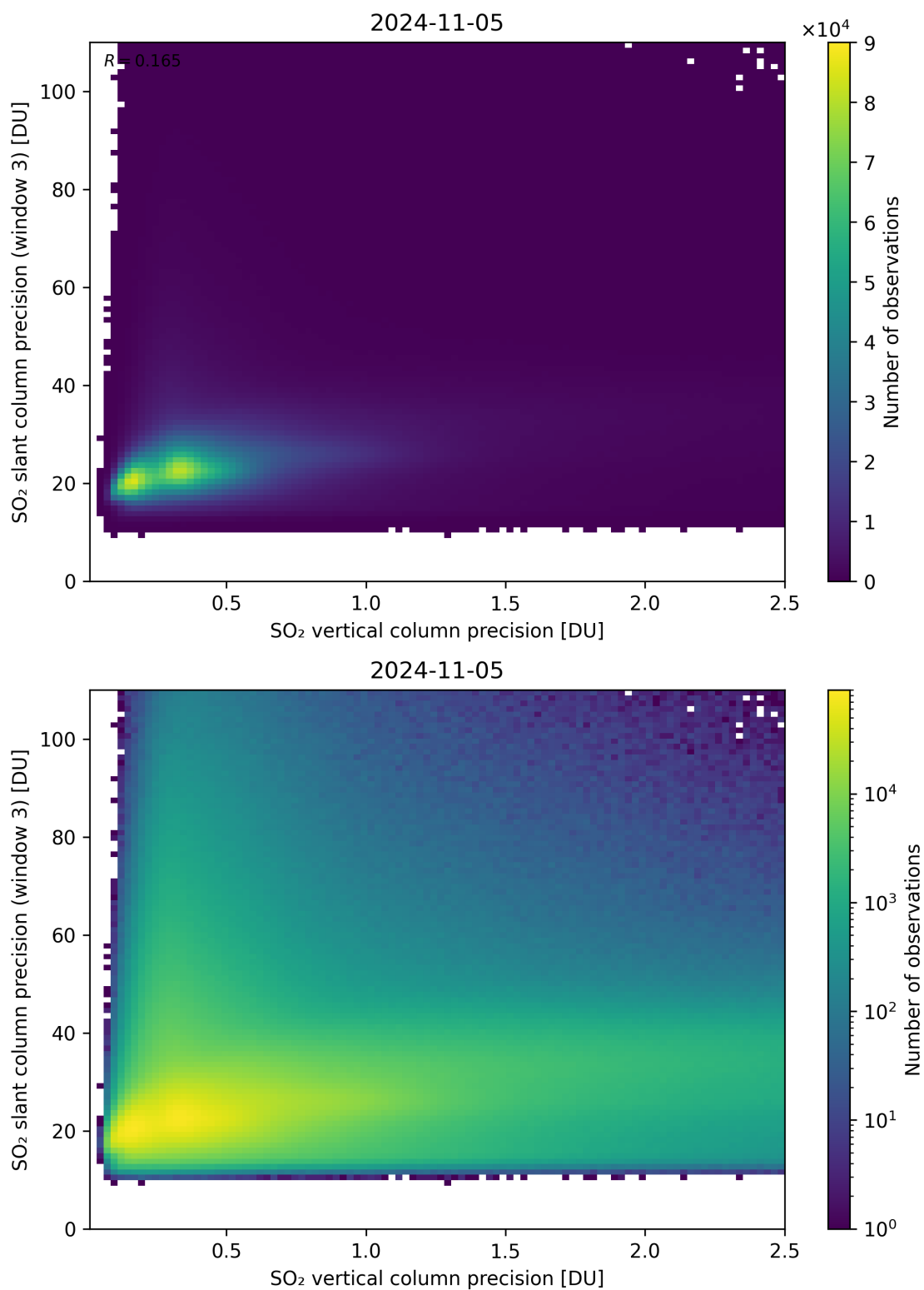
Figure 293: Scatter density plot of “SO 2 vertical column precision” against “SO 2 slant column precision (window 3)” for 2024-11-04 to 2024-11-06.
