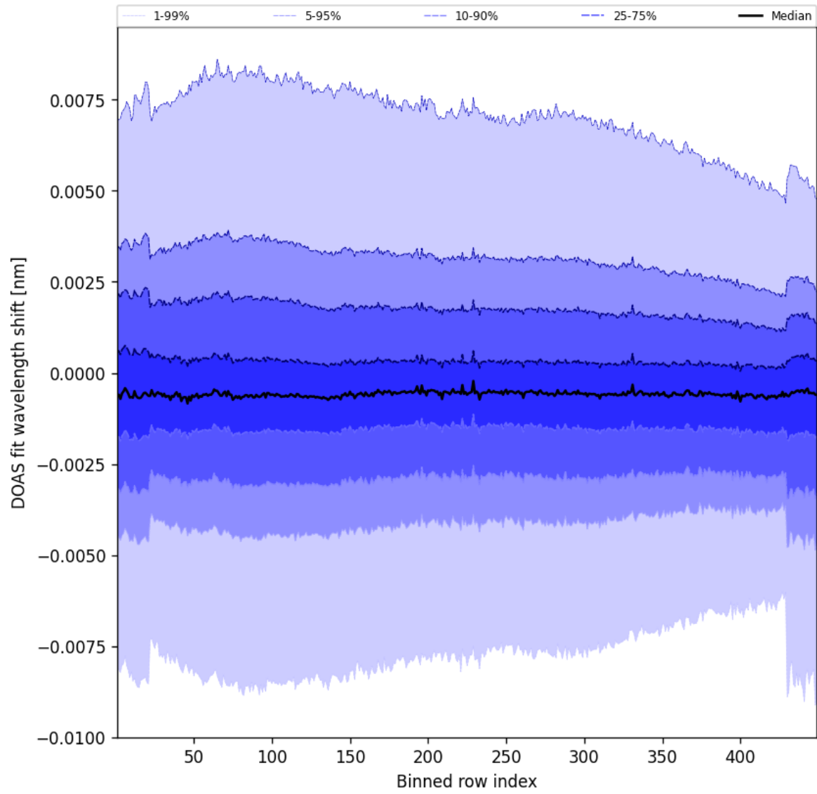
Figure 91: Along track statistics of “DOAS fit wavelength shift” for 2024-11-04 to 2024-11-06
