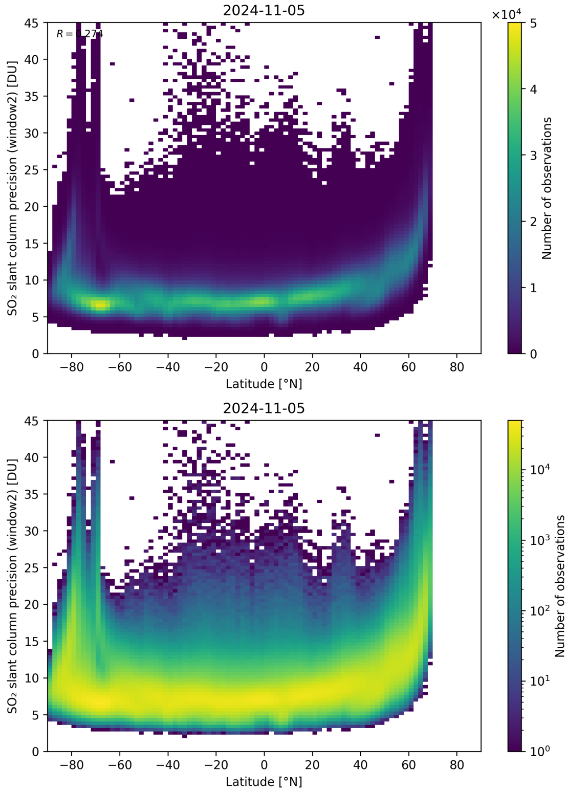
Figure 151: Scatter density plot of “Latitude” against “SO 2 slant column precision (window2)” for 2024-11-04 to 2024-11-06.
