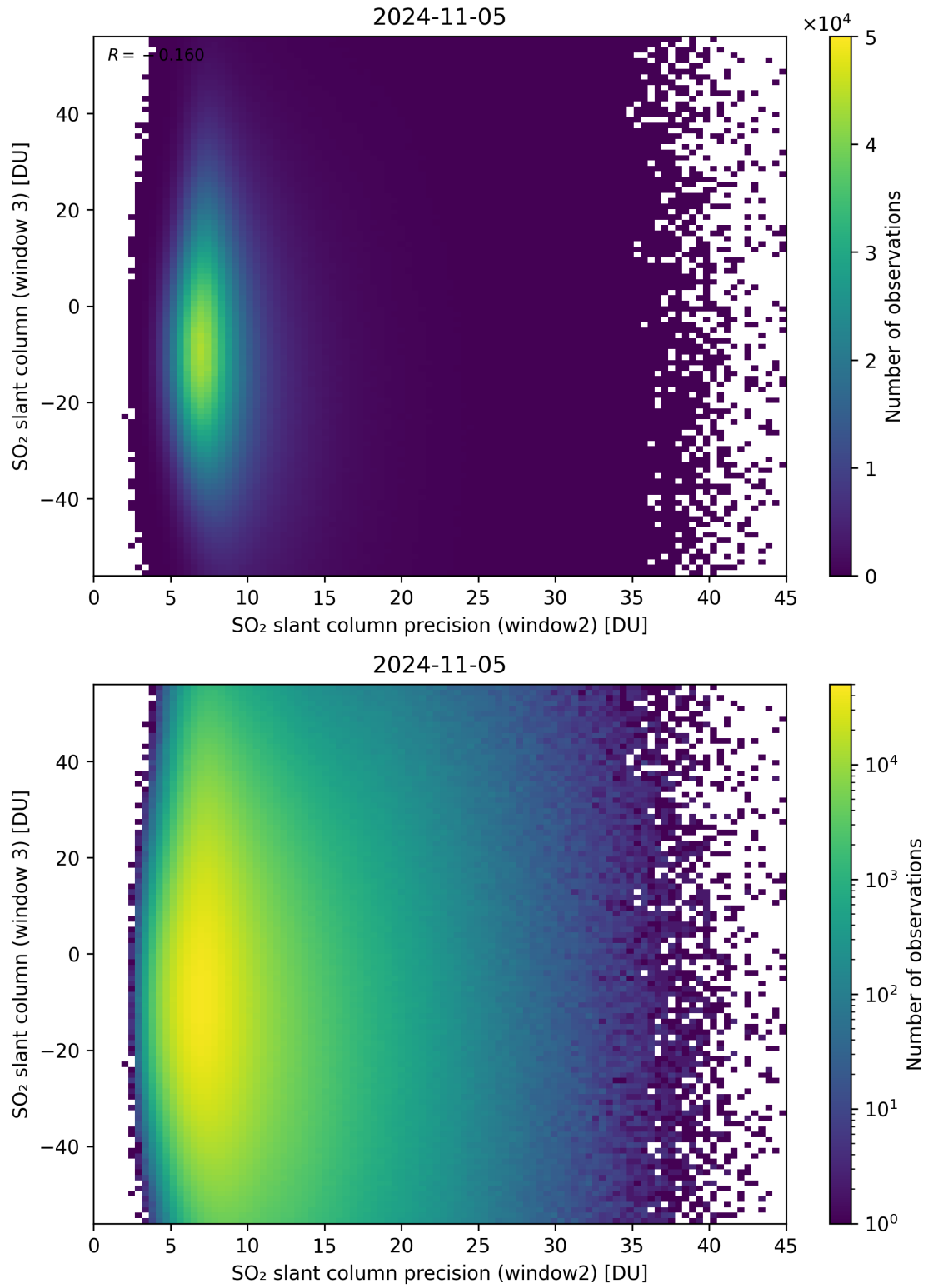
Figure 249: Scatter density plot of “SO 2 slant column precision (window2)” against “SO 2 slant column (window 3)” for 2024-11-04 to 2024-11-06.
