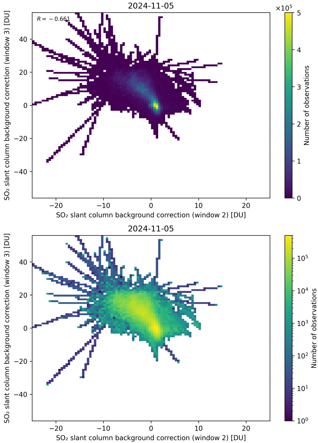
Figure 111: Scatter density plot of “SO 2 slant column background correction (window 2)” against “SO 2 slant column background correction (window 3)” for 2024-11-04 to 2024-11-06.
