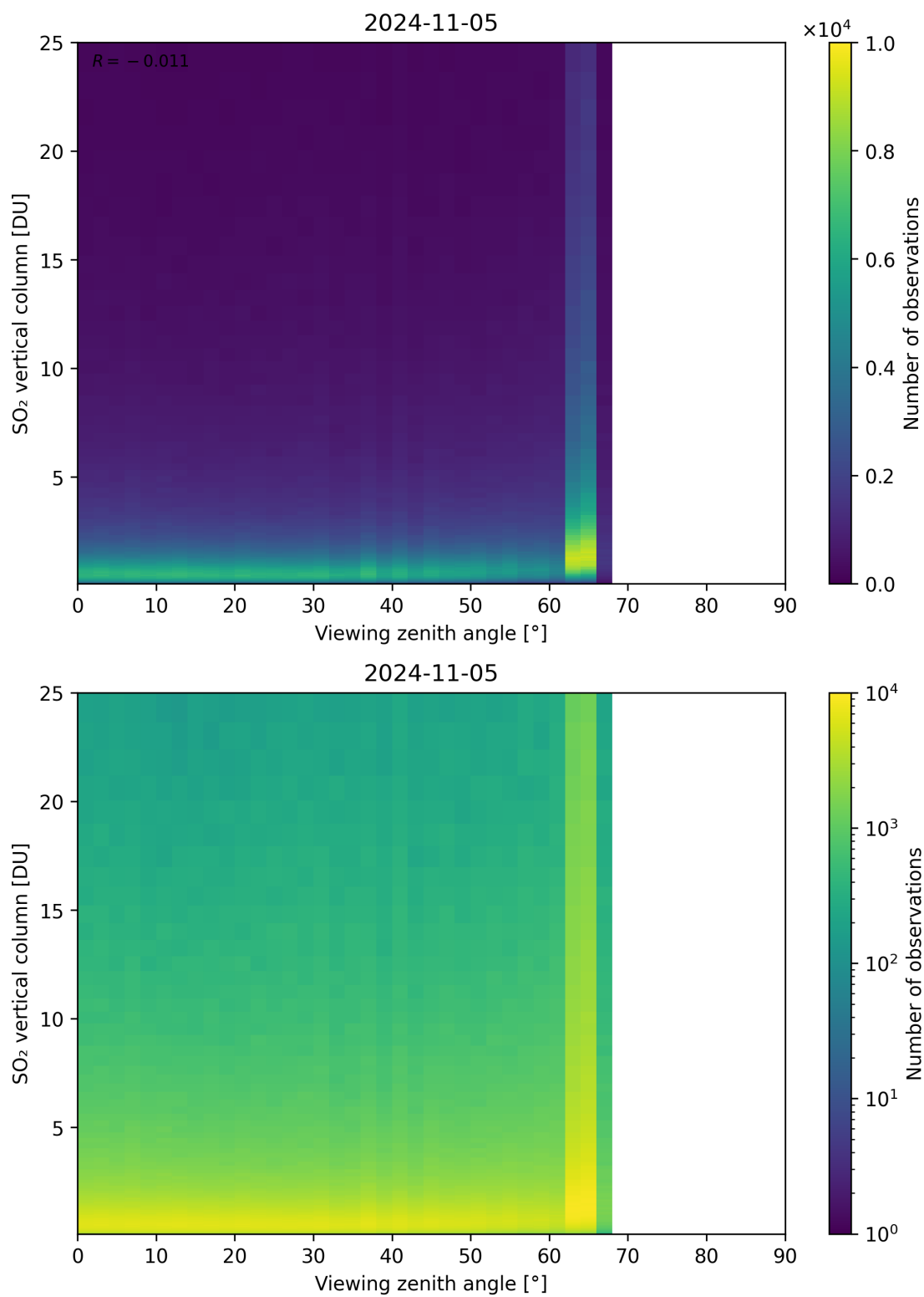
Figure 327: Scatter density plot of “Viewing zenith angle” against “SO 2 vertical column” for 2024-11-04 to 2024-11-06.
