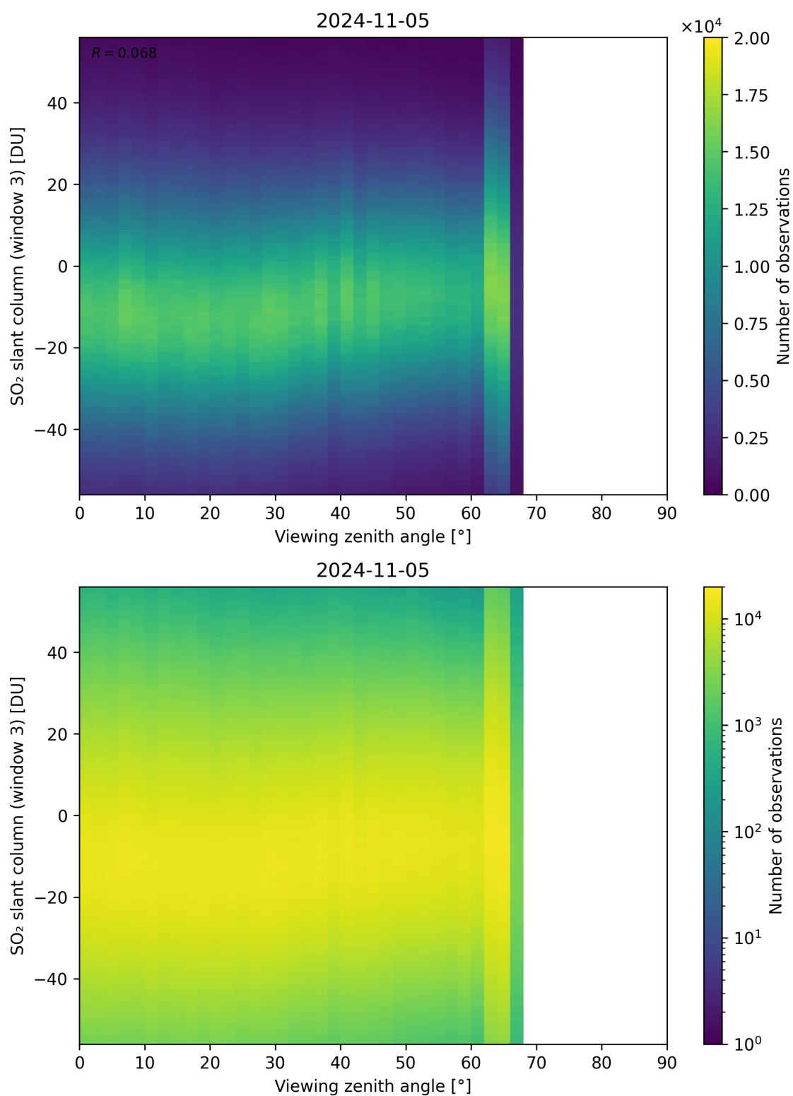
Figure 323: Scatter density plot of “Viewing zenith angle” against “SO 2 slant column (window 3)” for 2024-11-04 to 2024-11-06.
