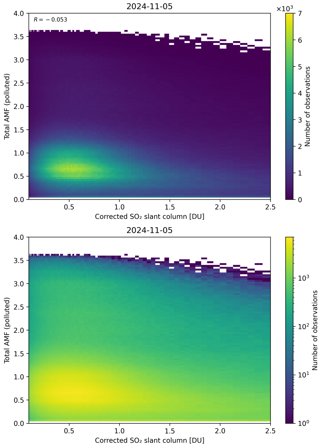
Figure 192: Scatter density plot of “Corrected SO 2 slant column” against “Total AMF (polluted)” for 2024-11-04 to 2024-11-06.
