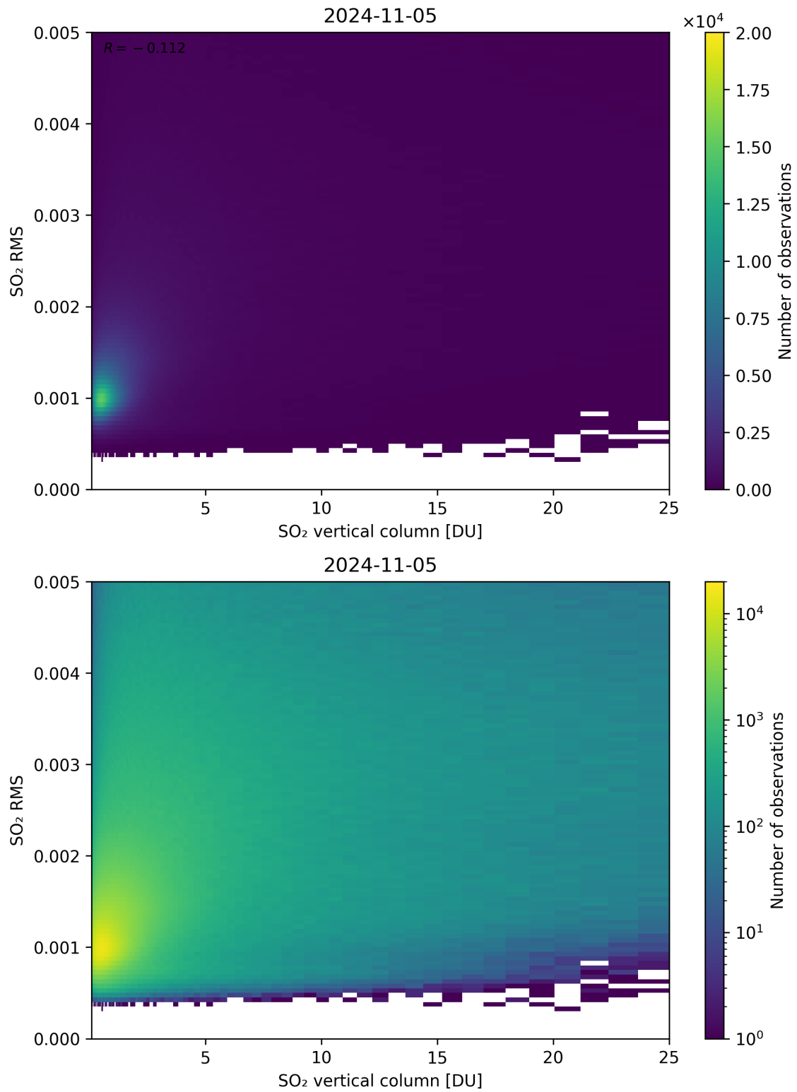
Figure 278: Scatter density plot of “SO 2 vertical column” against “SO 2 RMS” for 2024-11-04 to 2024-11-06.
