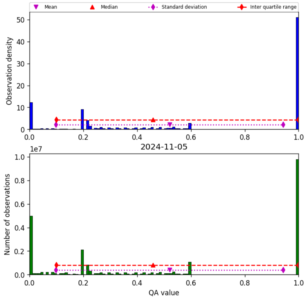
Figure 52: Histogram of “QA value” for 2024-11-04 to 2024-11-06
