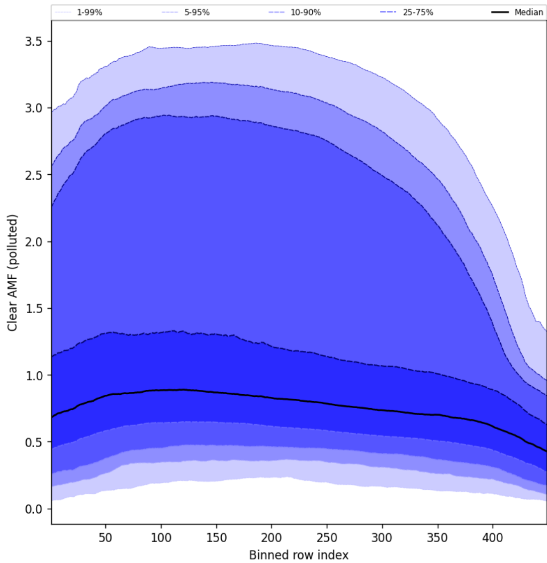
Figure 96: Along track statistics of “Clear AMF (polluted)” for 2024-11-04 to 2024-11-06
