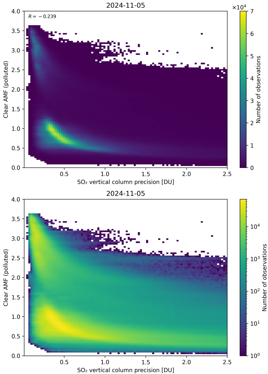
Figure 285: Scatter density plot of “SO 2 vertical column precision” against “Clear AMF (polluted)” for 2024-11-04 to 2024-11-06.
