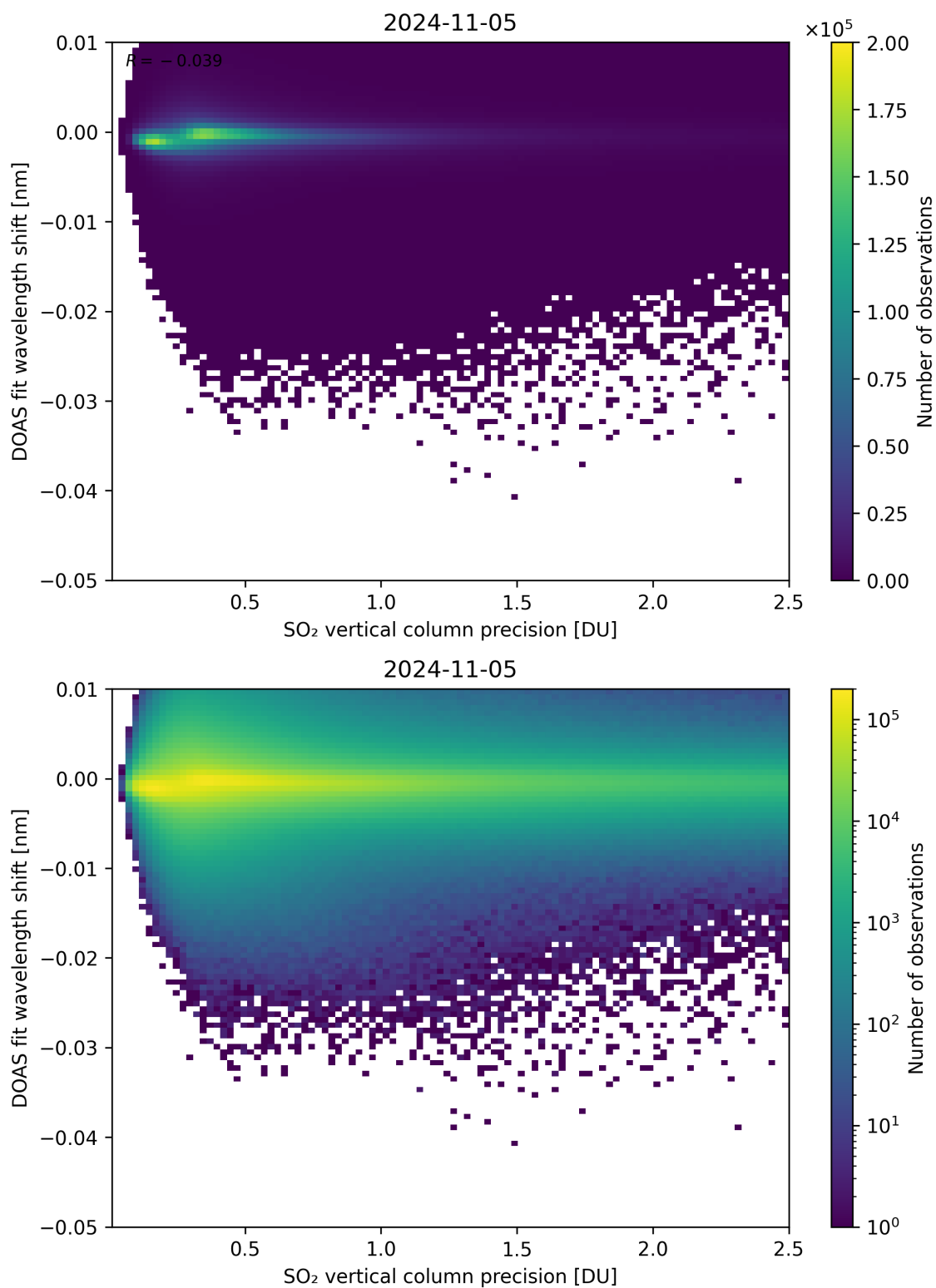
Figure 282: Scatter density plot of “SO 2 vertical column precision” against “DOAS fit wavelength shift” for 2024-11-04 to 2024-11-06.
