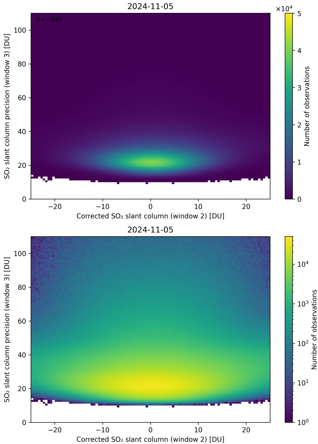
Figure 202: Scatter density plot of “Corrected SO 2 slant column (window 2)” against “SO 2 slant column precision (window 3)” for 2024-11-04 to 2024-11-06.
