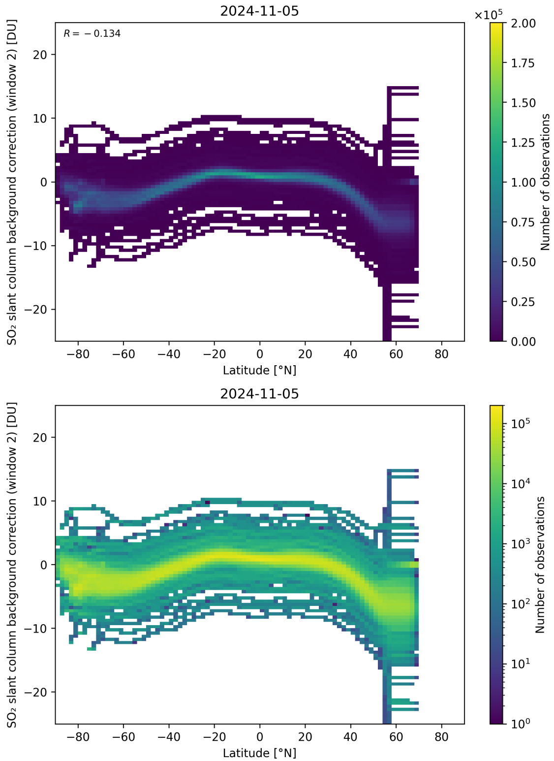
Figure 140: Scatter density plot of “Latitude” against “SO 2 slant column background correction (window 2)” for 2024-11-04 to 2024-11-06.
