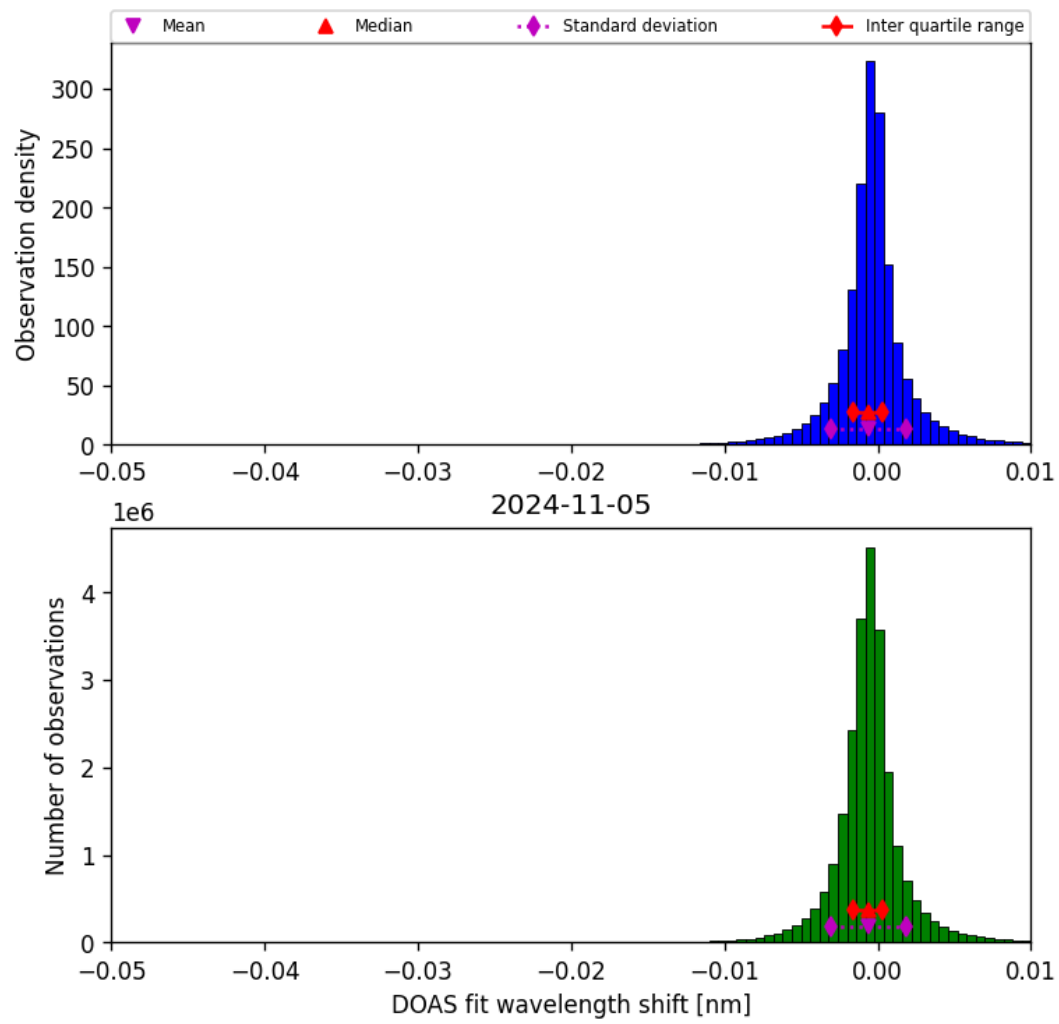
Figure 68: Histogram of “DOAS fit wavelength shift” for 2024-11-04 to 2024-11-06
