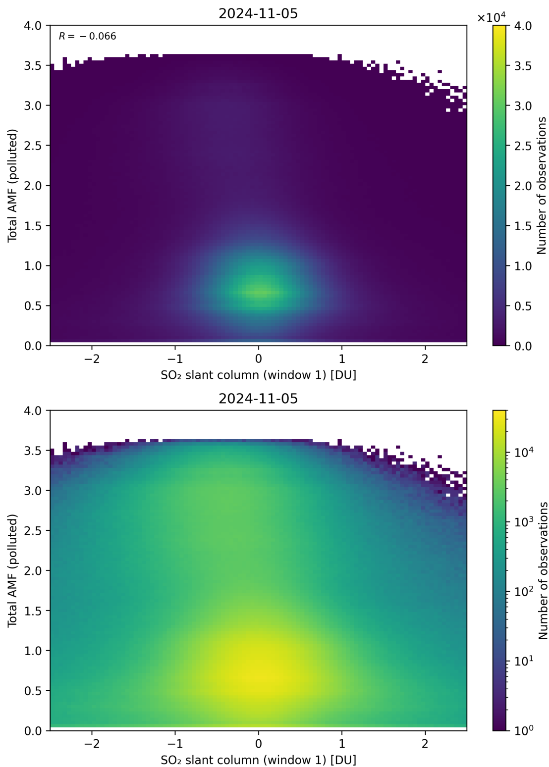
Figure 239: Scatter density plot of “SO 2 slant column (window 1)” against “Total AMF (polluted)” for 2024-11-04 to 2024-11-06.
