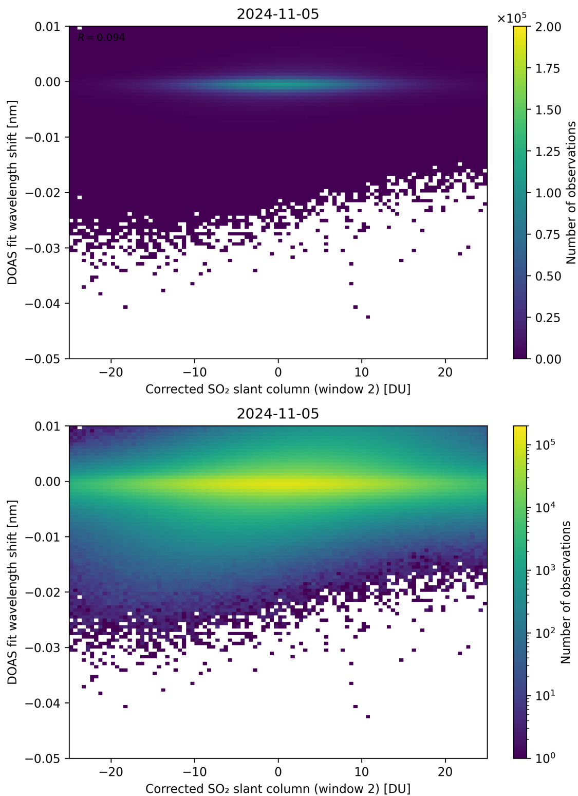
Figure 196: Scatter density plot of “Corrected SO 2 slant column (window 2)” against “DOAS fit wavelength shift” for 2024-11-04 to 2024-11-06.
