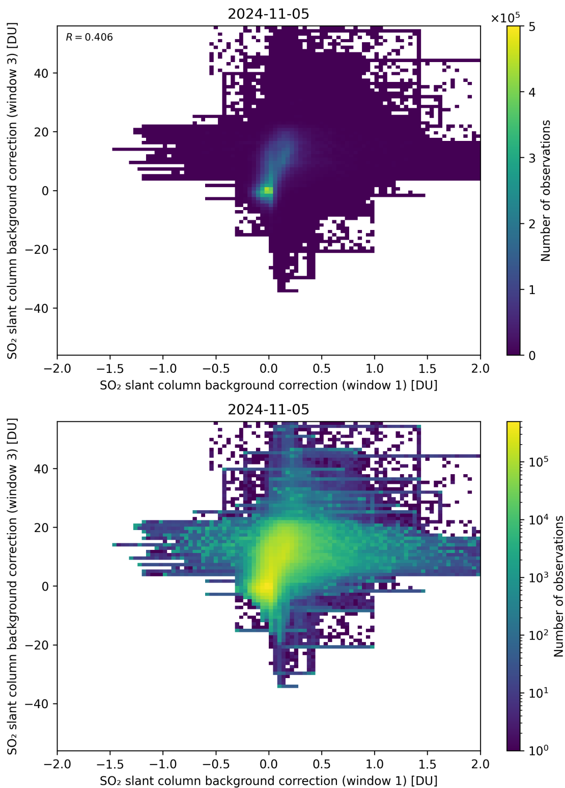
Figure 99: Scatter density plot of “SO 2 slant column background correction (window 1)” against “SO 2 slant column background correction (window 3)” for 2024-11-04 to 2024-11-06.
