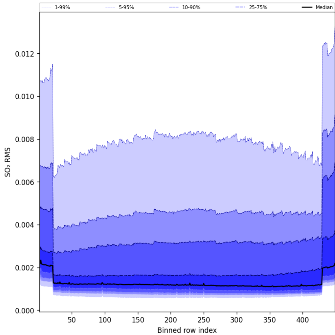
Figure 93: Along track statistics of “SO 2 RMS” for 2024-11-04 to 2024-11-06
