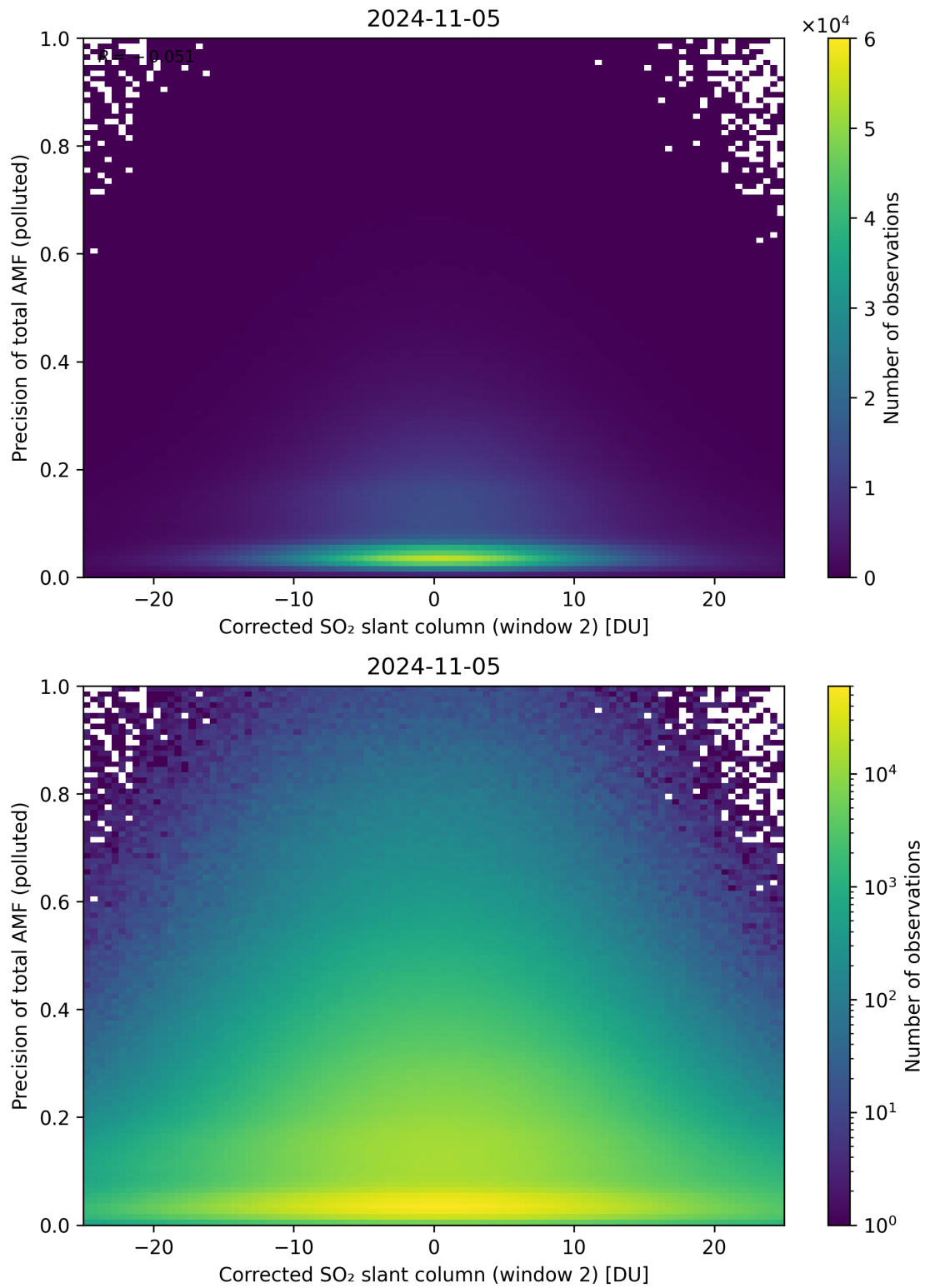
Figure 204: Scatter density plot of “Corrected SO 2 slant column (window 2)” against “Precision of total AMF (polluted)” for 2024-11-04 to 2024-11-06.
