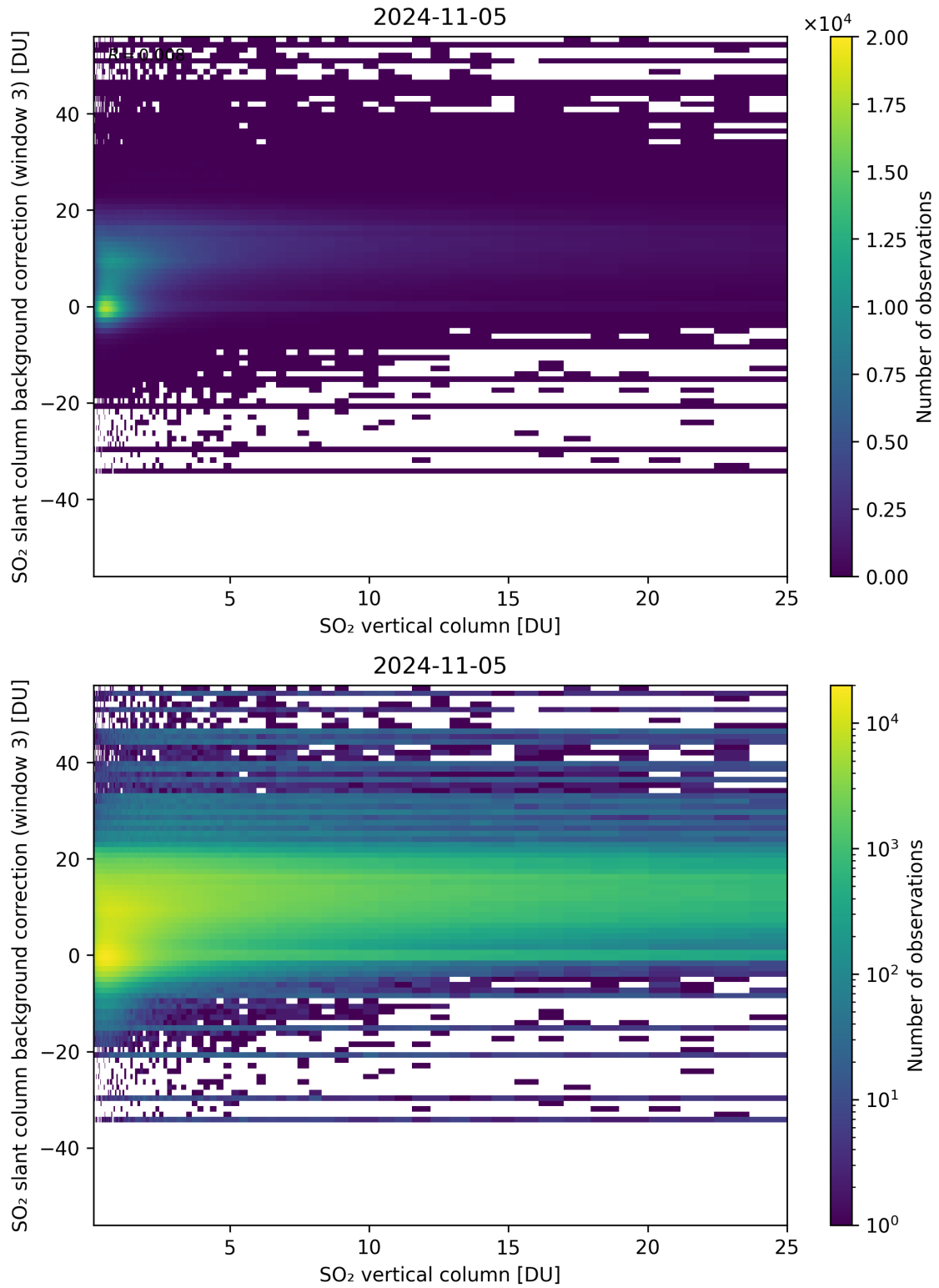
Figure 275: Scatter density plot of “SO 2 vertical column” against “SO 2 slant column background correction (window 3)” for 2024-11-04 to 2024-11-06.
