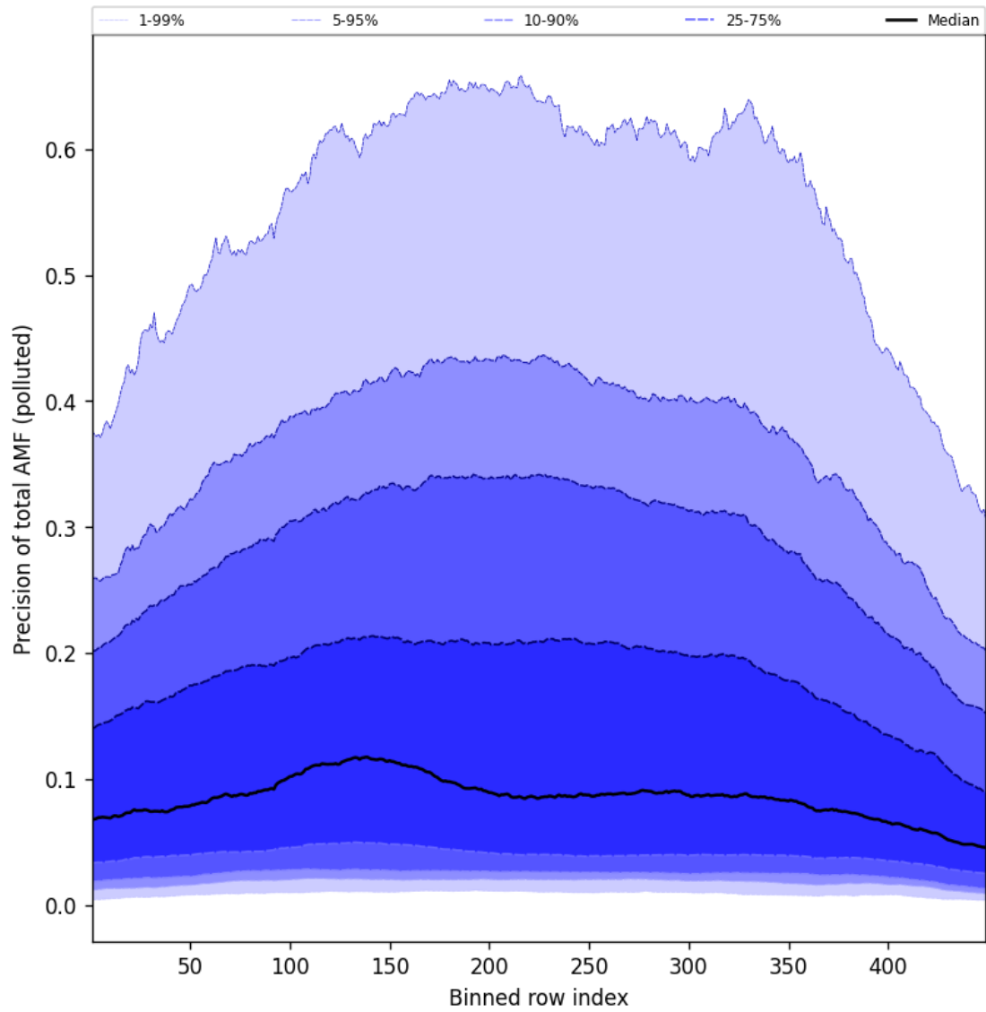
Figure 95: Along track statistics of “Precision of total AMF (polluted)” for 2024-11-04 to 2024-11-06
