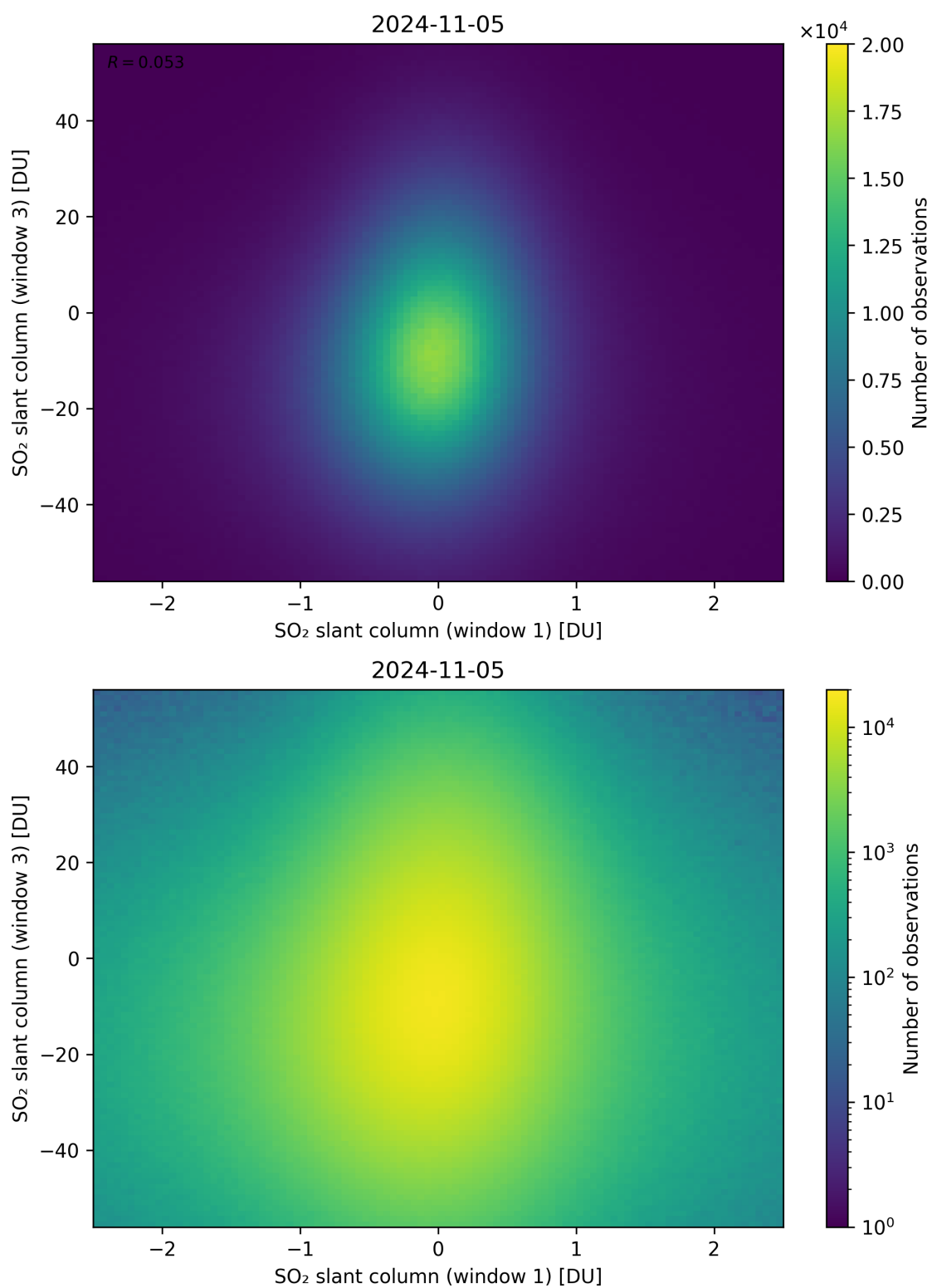
Figure 237: Scatter density plot of “SO 2 slant column (window 1)” against “SO 2 slant column (window 3)” for 2024-11-04 to 2024-11-06.
