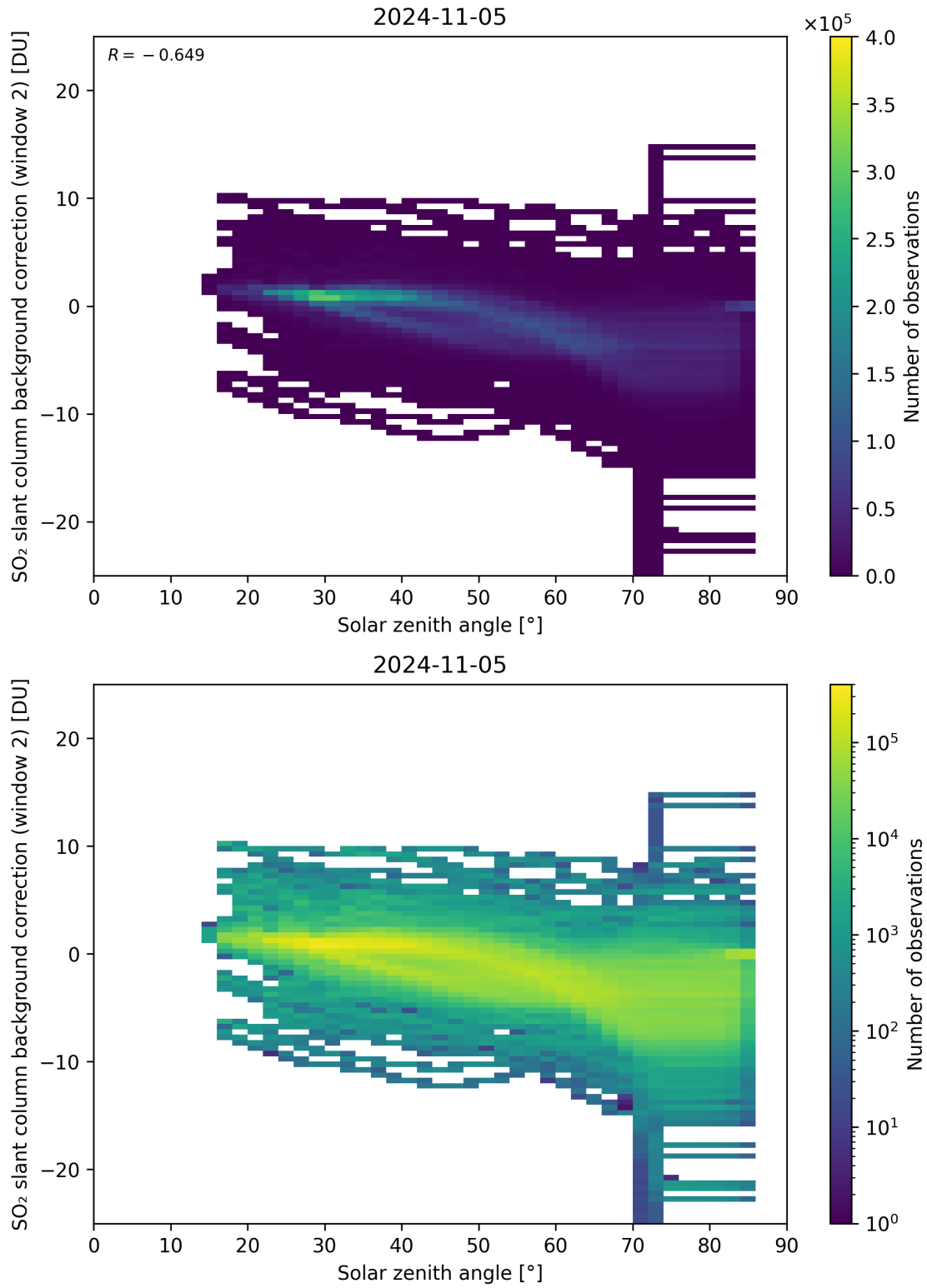
Figure 159: Scatter density plot of “Solar zenith angle” against “SO 2 slant column background correction (window 2)” for 2024-11-04 to 2024-11-06.
