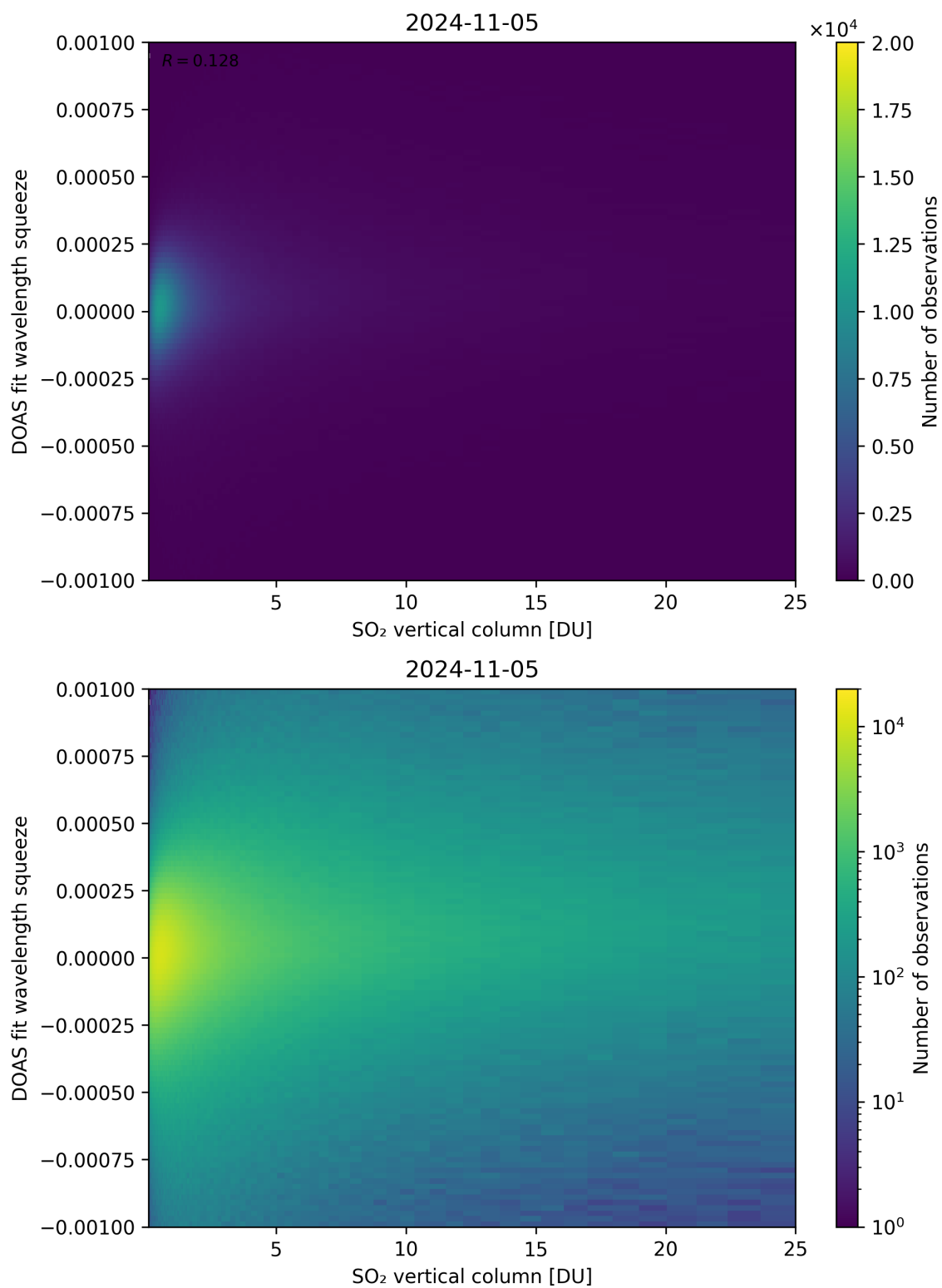
Figure 277: Scatter density plot of “SO 2 vertical column” against “DOAS fit wavelength squeeze” for 2024-11-04 to 2024-11-06.
