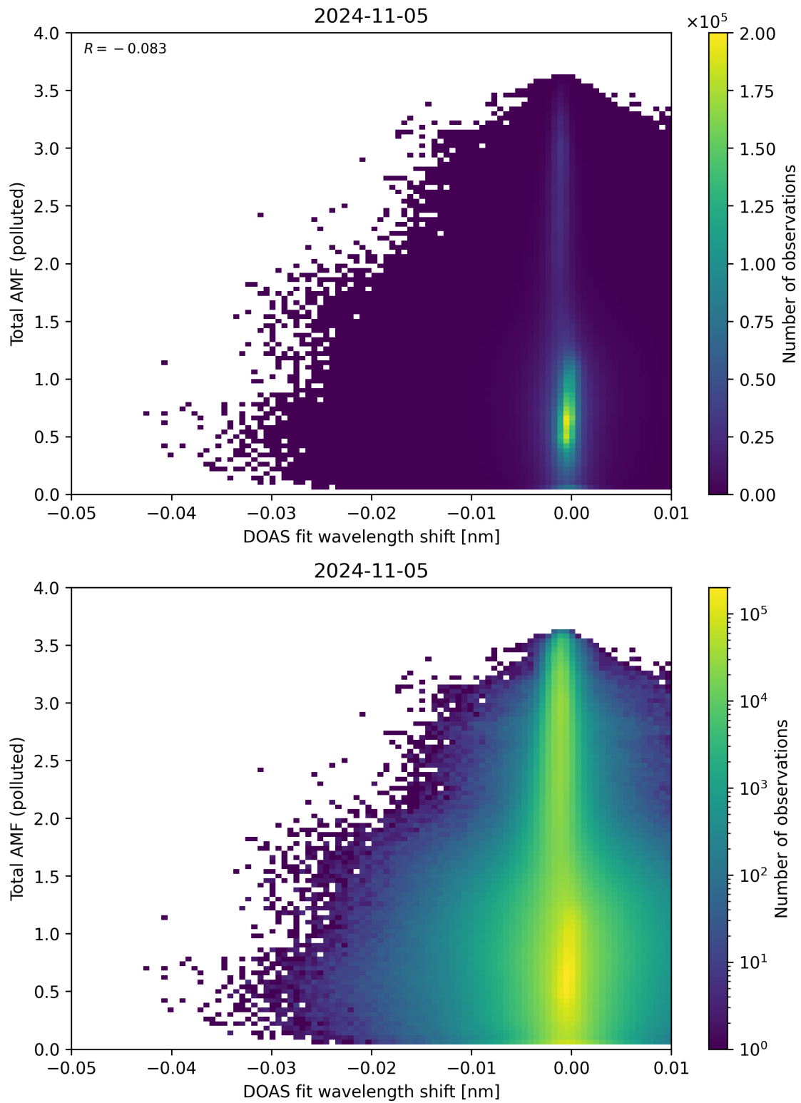
Figure 130: Scatter density plot of “DOAS fit wavelength shift” against “Total AMF (polluted)” for 2024-11-04 to 2024-11-06.
