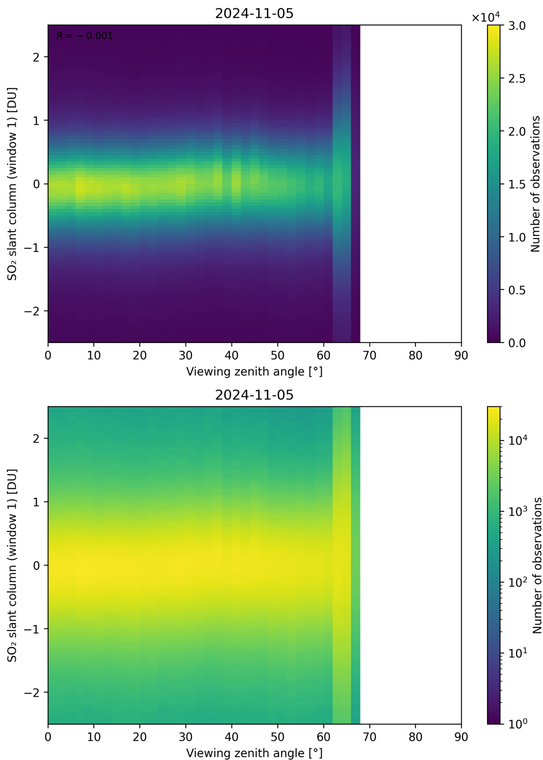
Figure 320: Scatter density plot of “Viewing zenith angle” against “SO 2 slant column (window 1)” for 2024-11-04 to 2024-11-06.
