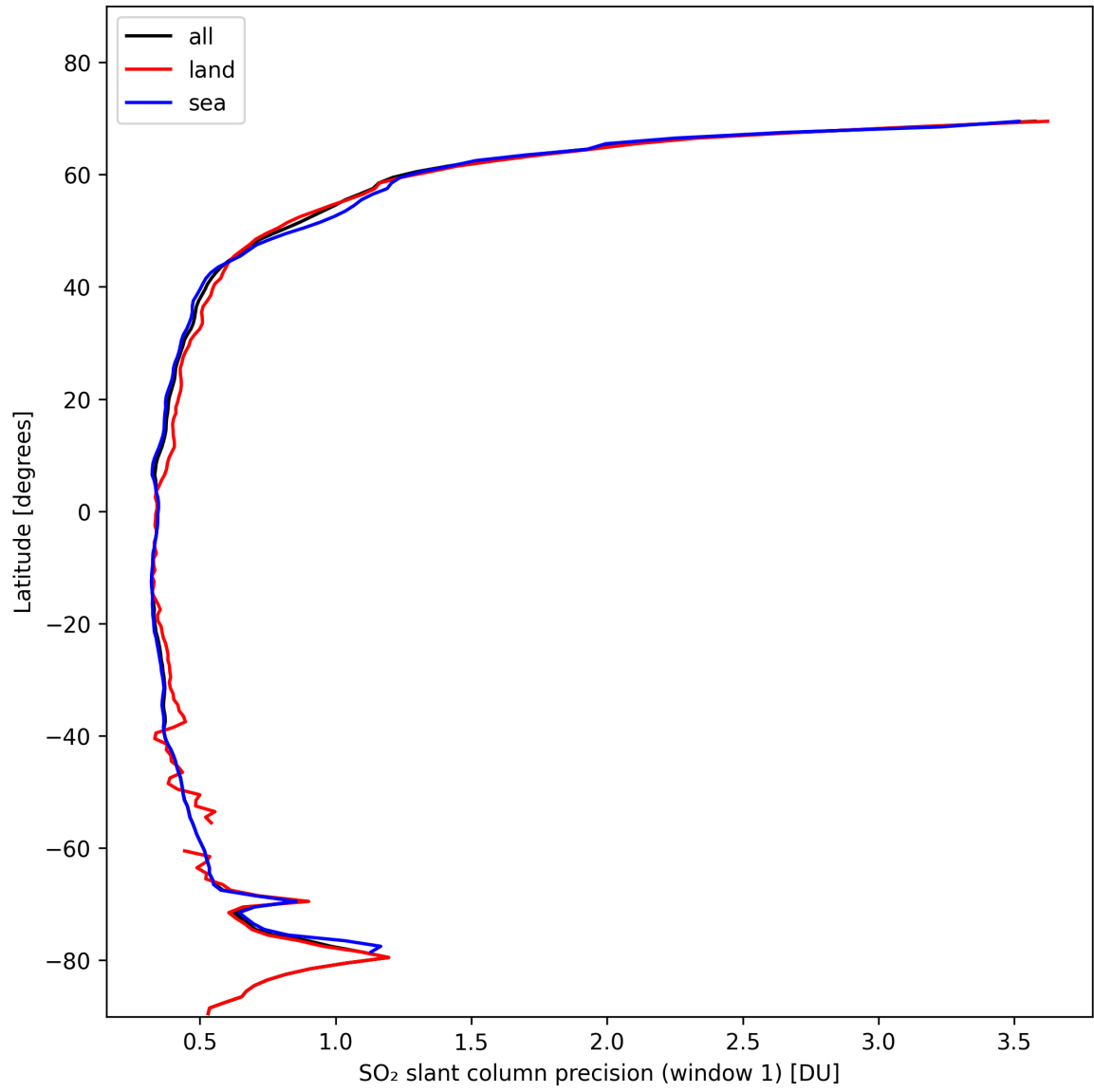
Figure 34: Zonal average of “SO 2 slant column precision (window 1)” for 2024-11-04 to 2024-11-06.
