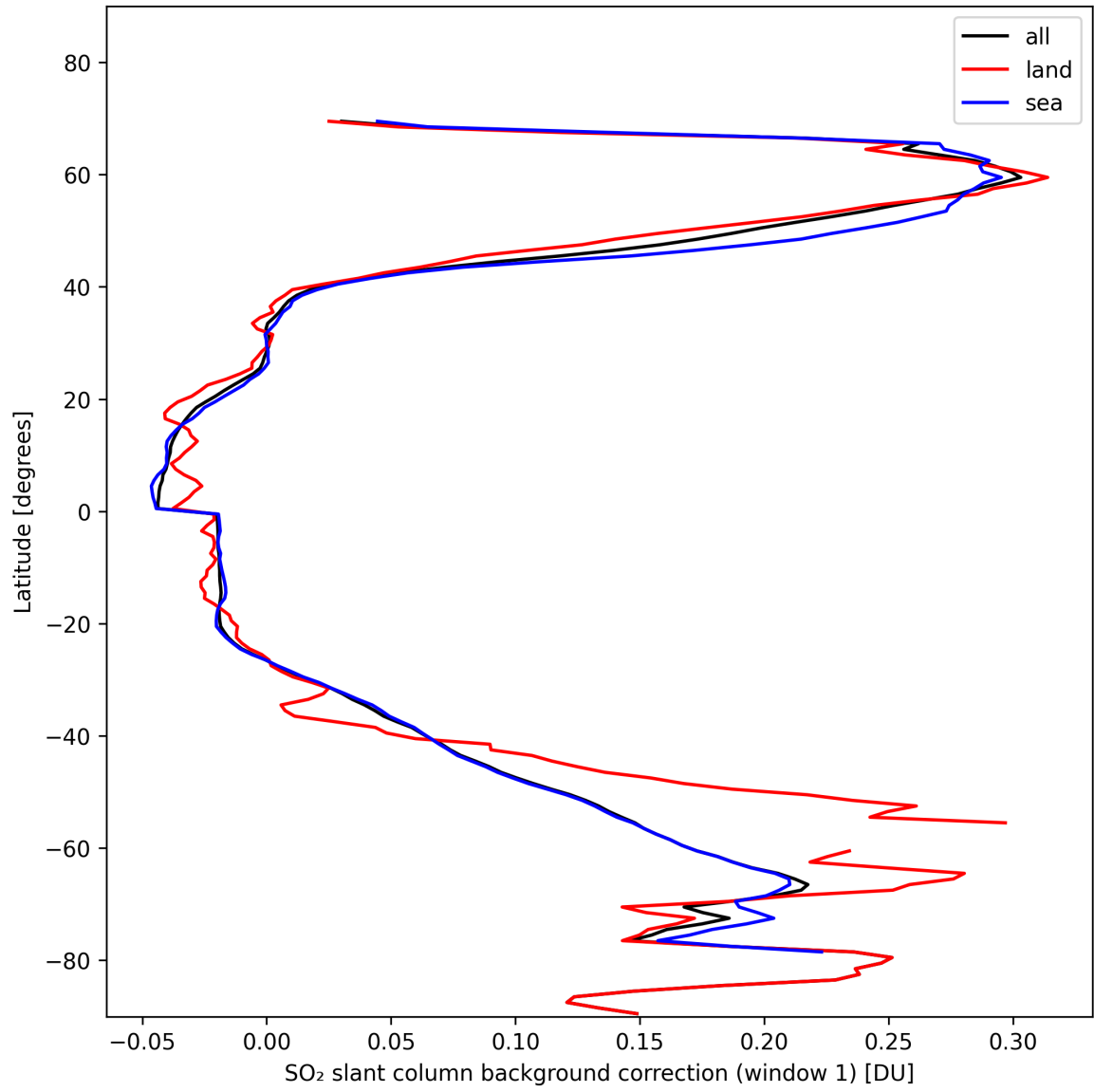
Figure 36: Zonal average of “SO 2 slant column background correction (window 1)” for 2024-11-04 to 2024-11-06.
