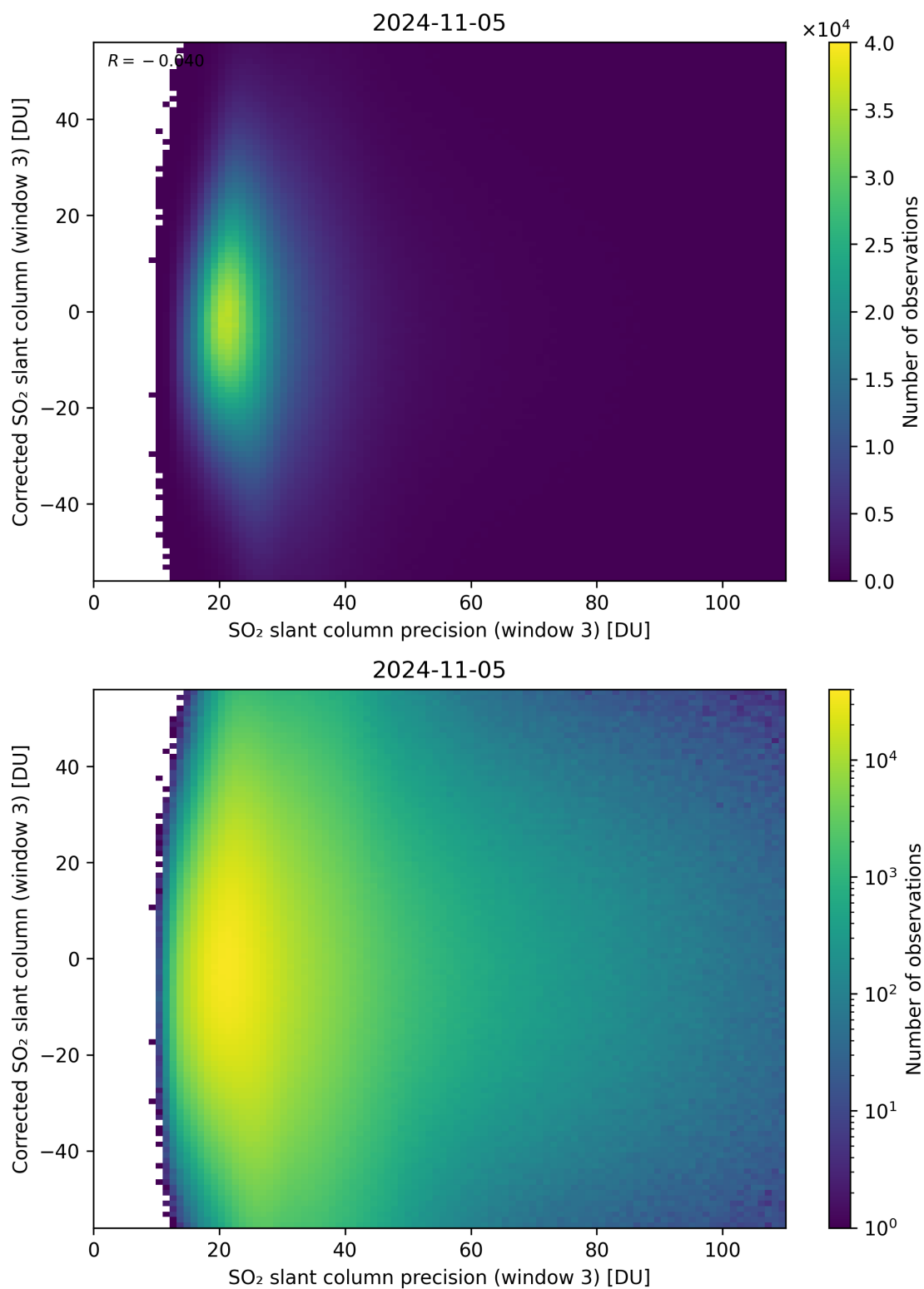
Figure 262: Scatter density plot of “SO 2 slant column precision (window 3)” against “Corrected SO 2 slant column (window 3)” for 2024-11-04 to 2024-11-06.
