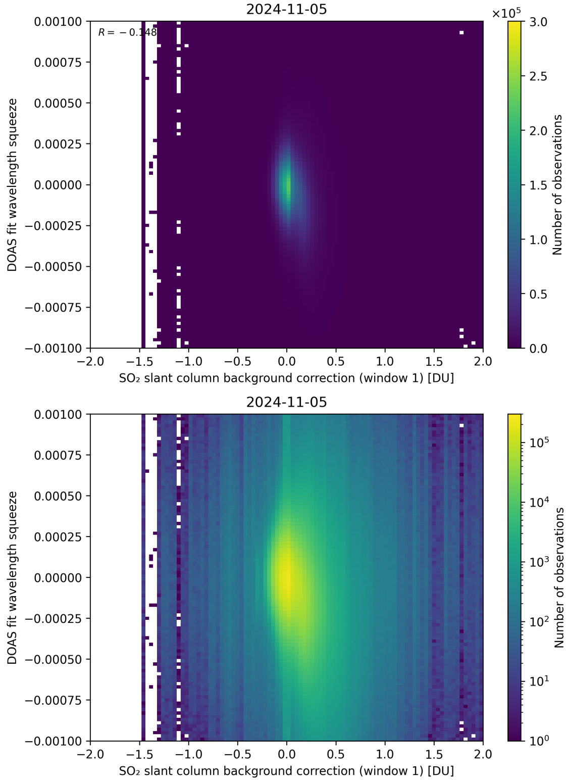
Figure 101: Scatter density plot of “SO 2 slant column background correction (window 1)” against “DOAS fit wavelength squeeze” for 2024-11-04 to 2024-11-06.
