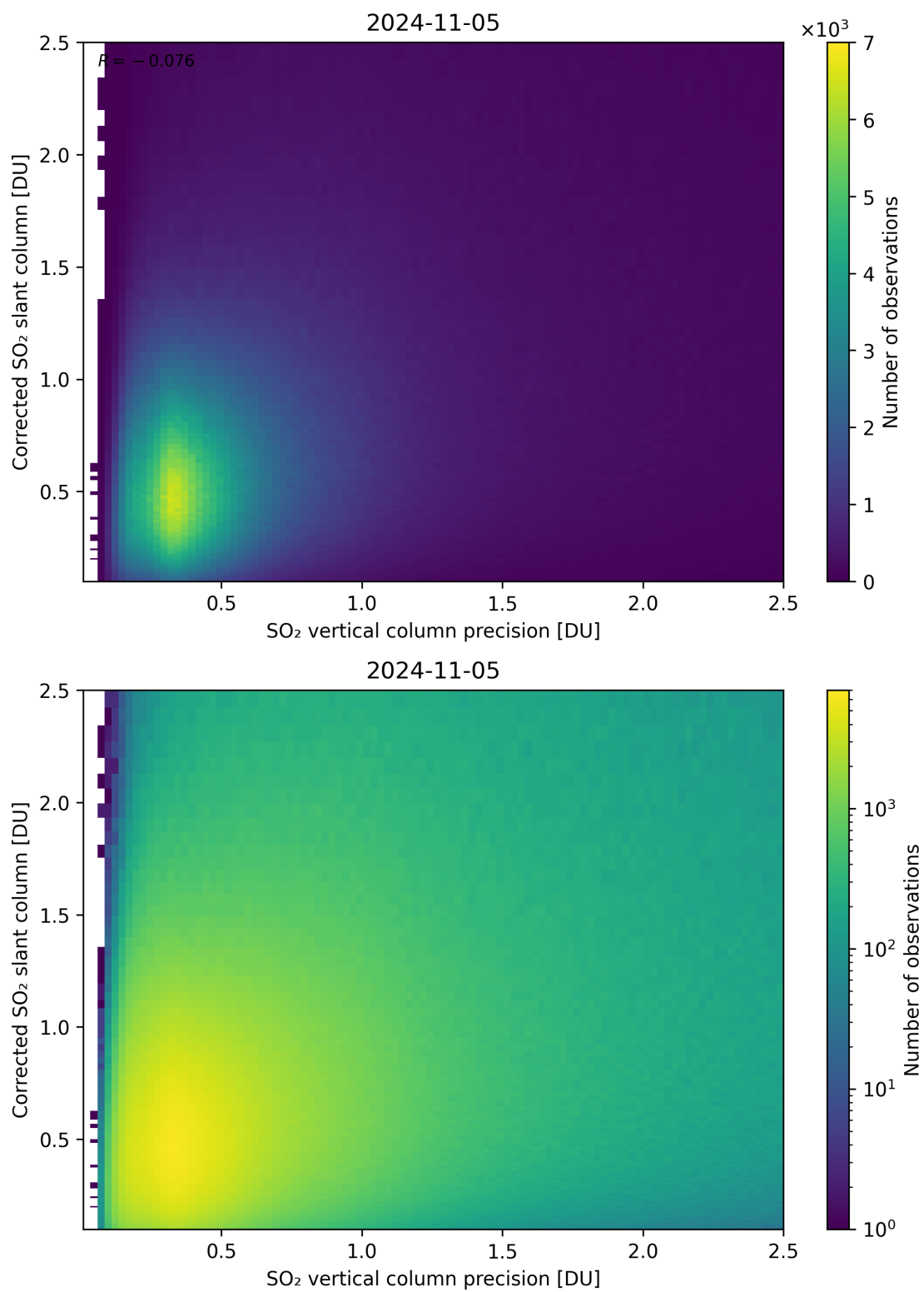
Figure 286: Scatter density plot of “SO 2 vertical column precision” against “Corrected SO 2 slant column” for 2024-11-04 to 2024-11-06.
