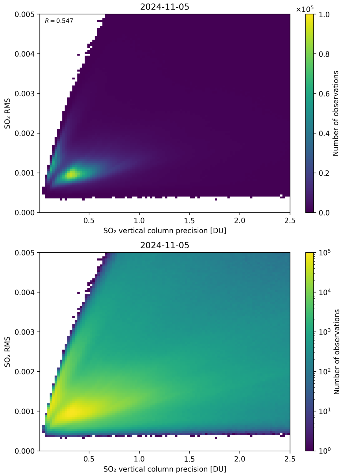
Figure 284: Scatter density plot of “SO 2 vertical column precision” against “SO 2 RMS” for 2024-11-04 to 2024-11-06.
