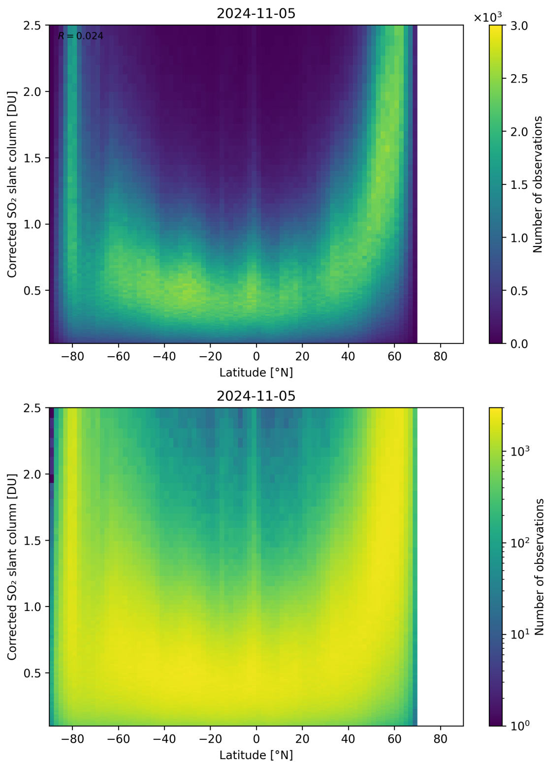
Figure 146: Scatter density plot of “Latitude” against “Corrected SO 2 slant column” for 2024-11-04 to 2024-11-06.
