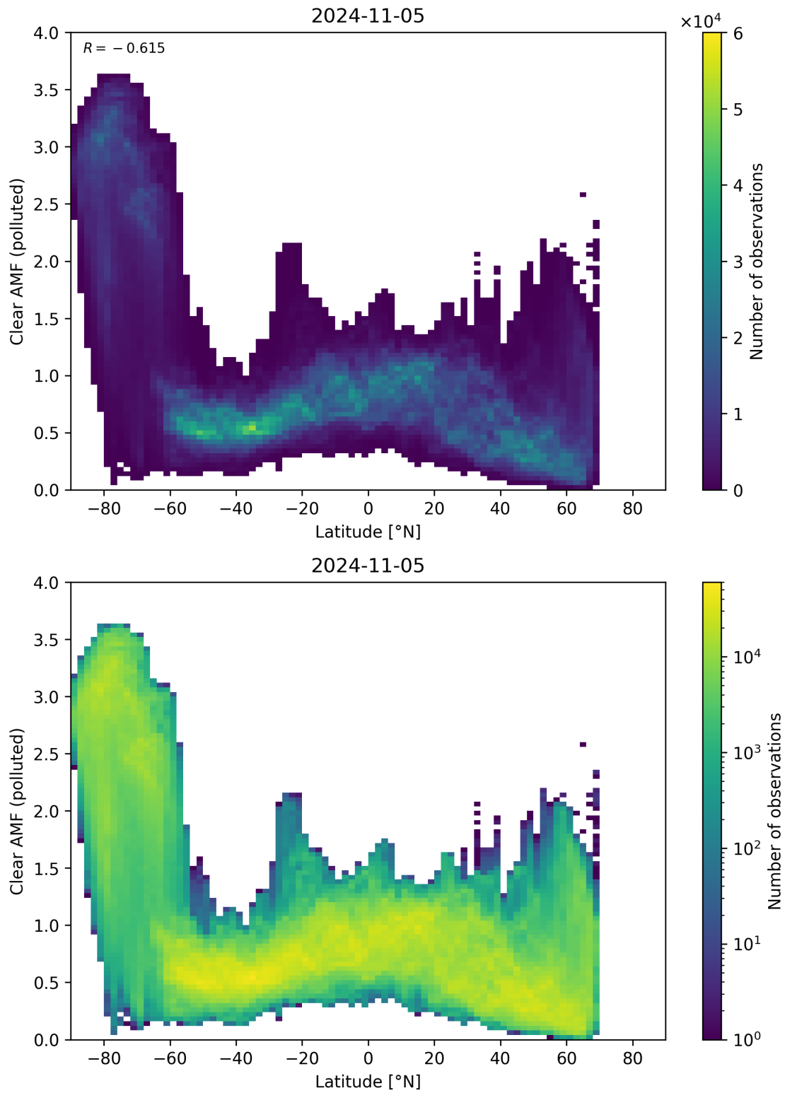
Figure 145: Scatter density plot of “Latitude” against “Clear AMF (polluted)” for 2024-11-04 to 2024-11-06.
