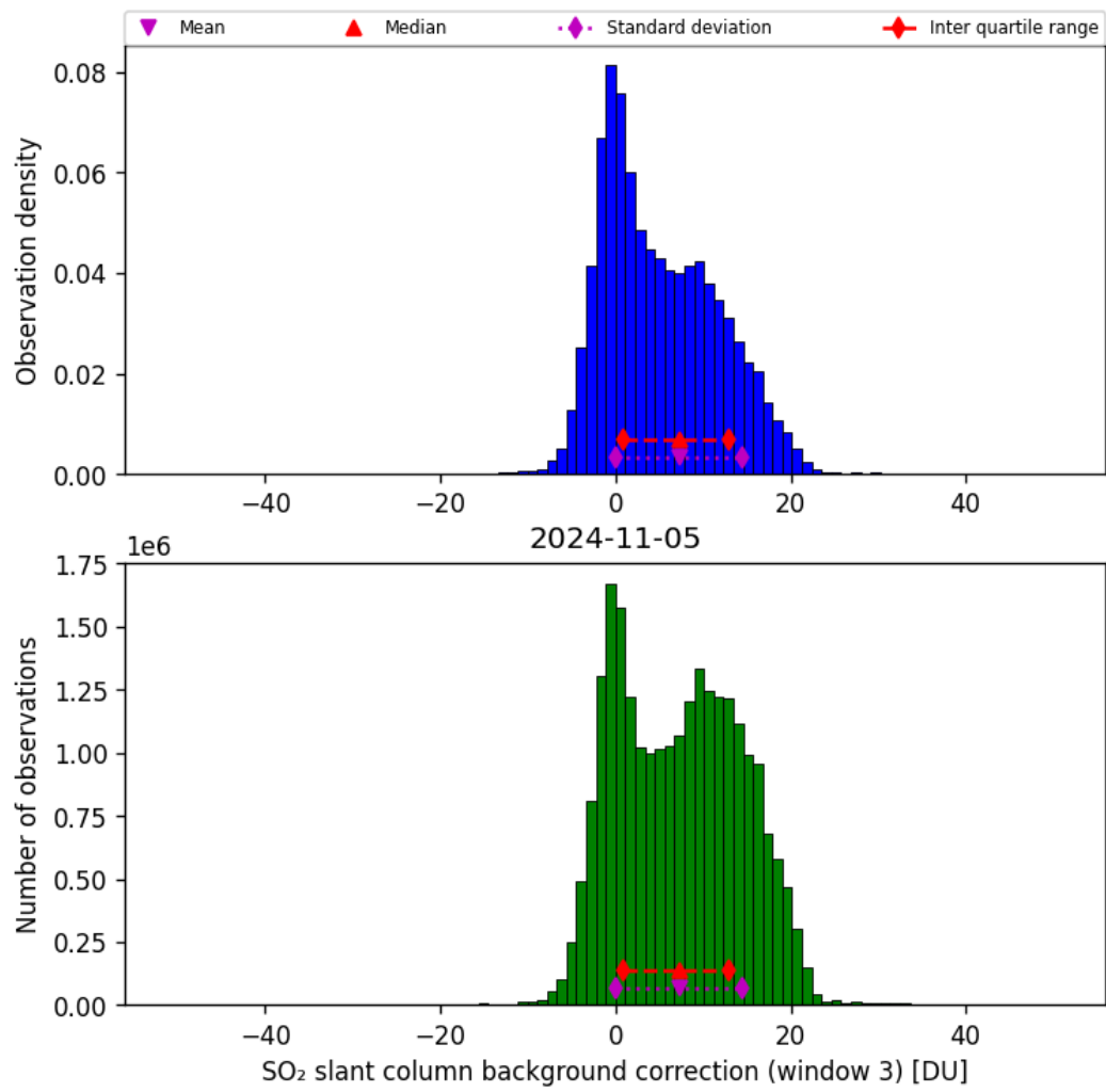
Figure 67: Histogram of “SO 2 slant column background correction (window 3)” for 2024-11-04 to 2024-11-06
