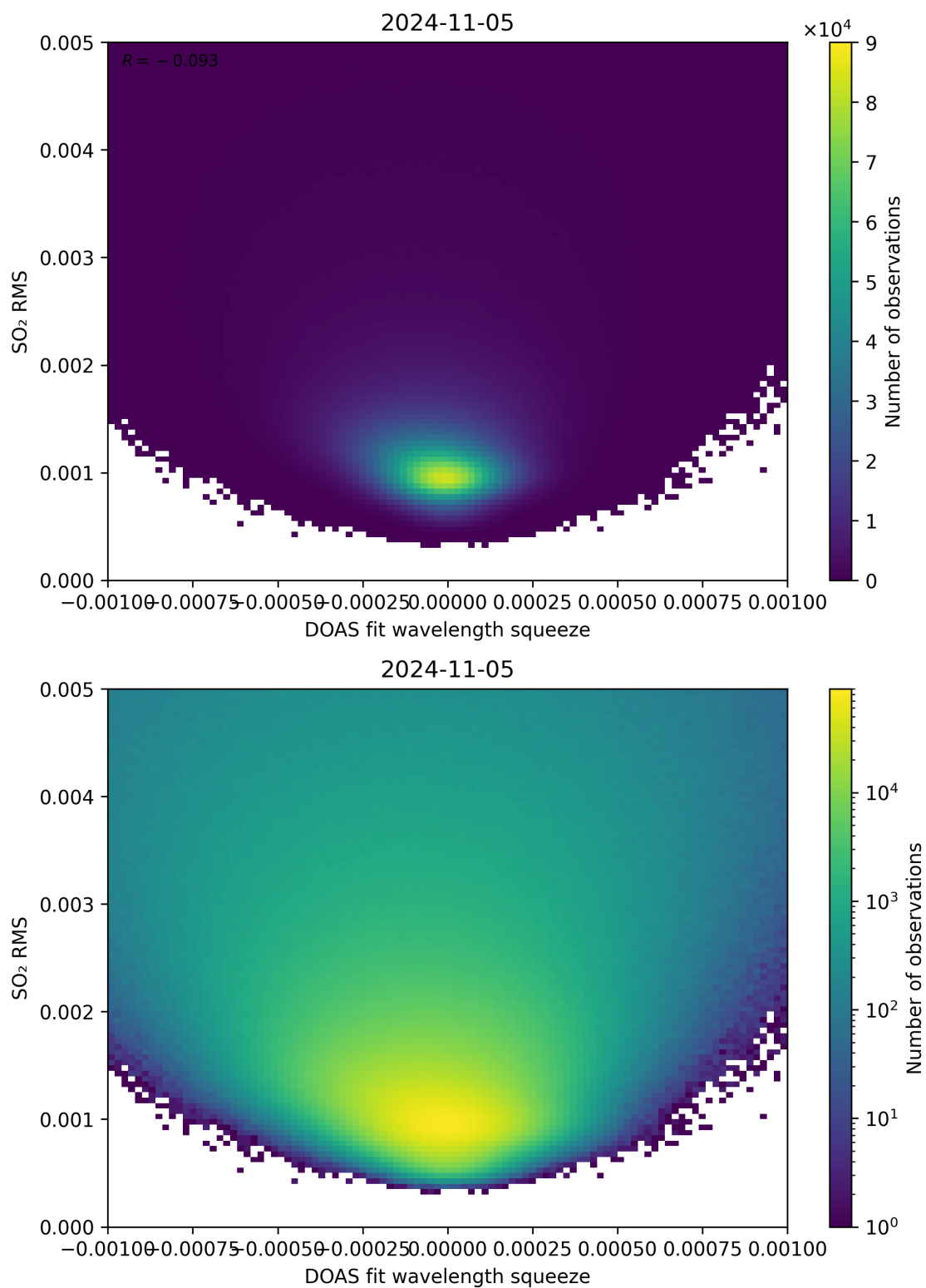
Figure 132: Scatter density plot of “DOAS fit wavelength squeeze” against “SO 2 RMS” for 2024-11-04 to 2024-11-06.
