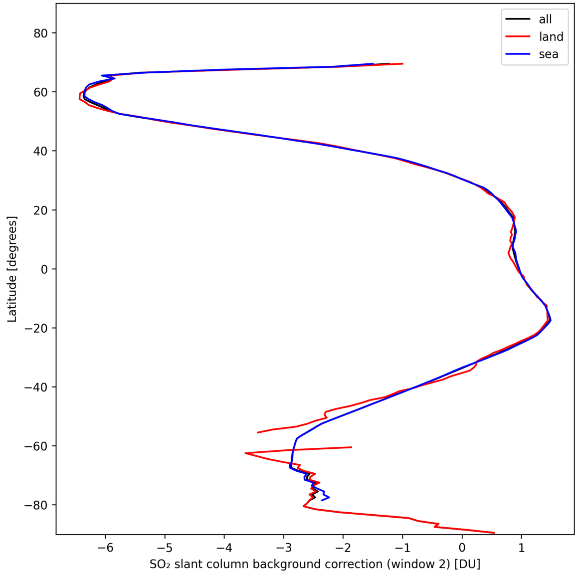
Figure 40: Zonal average of “SO 2 slant column background correction (window 2)” for 2024-11-04 to 2024-11-06.
