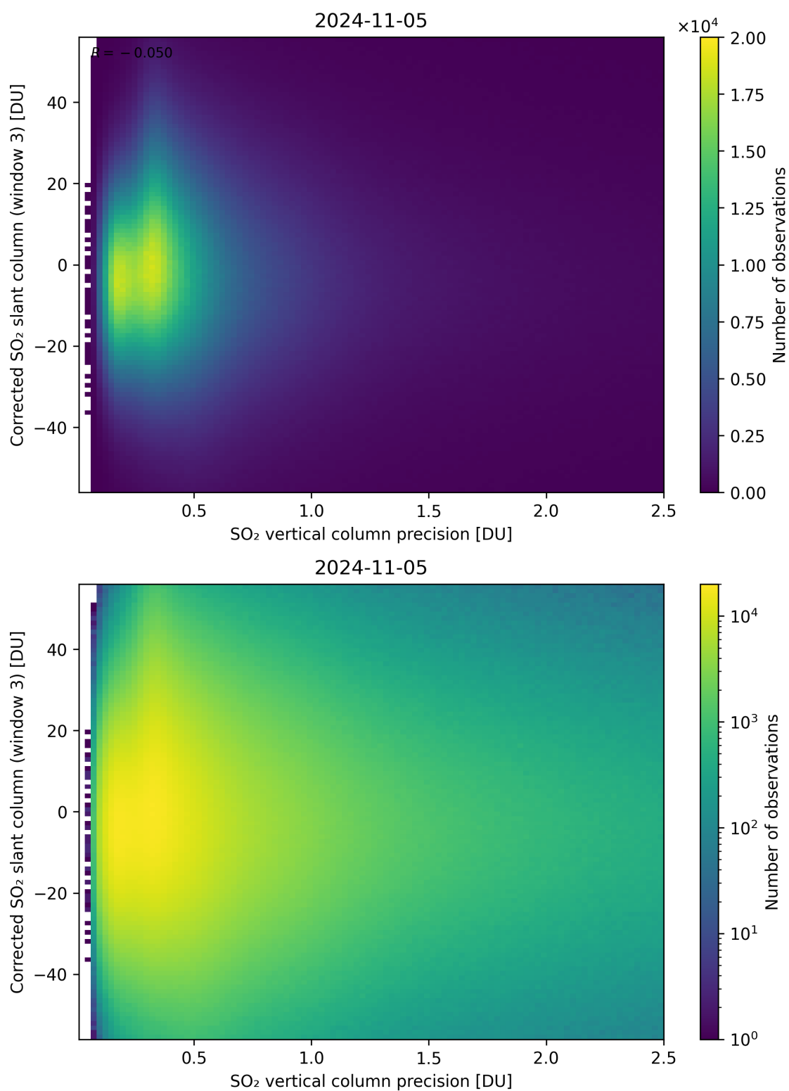
Figure 288: Scatter density plot of “SO 2 vertical column precision” against “Corrected SO 2 slant column (window 3)” for 2024-11-04 to 2024-11-06.
