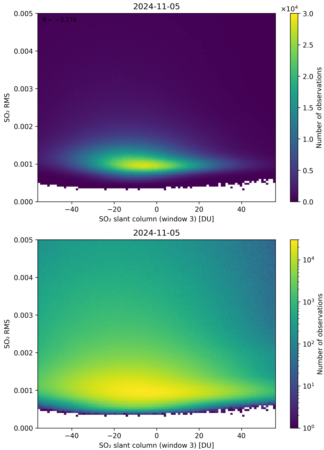
Figure 256: Scatter density plot of “SO 2 slant column (window 3)” against “SO 2 RMS” for 2024-11-04 to 2024-11-06.
