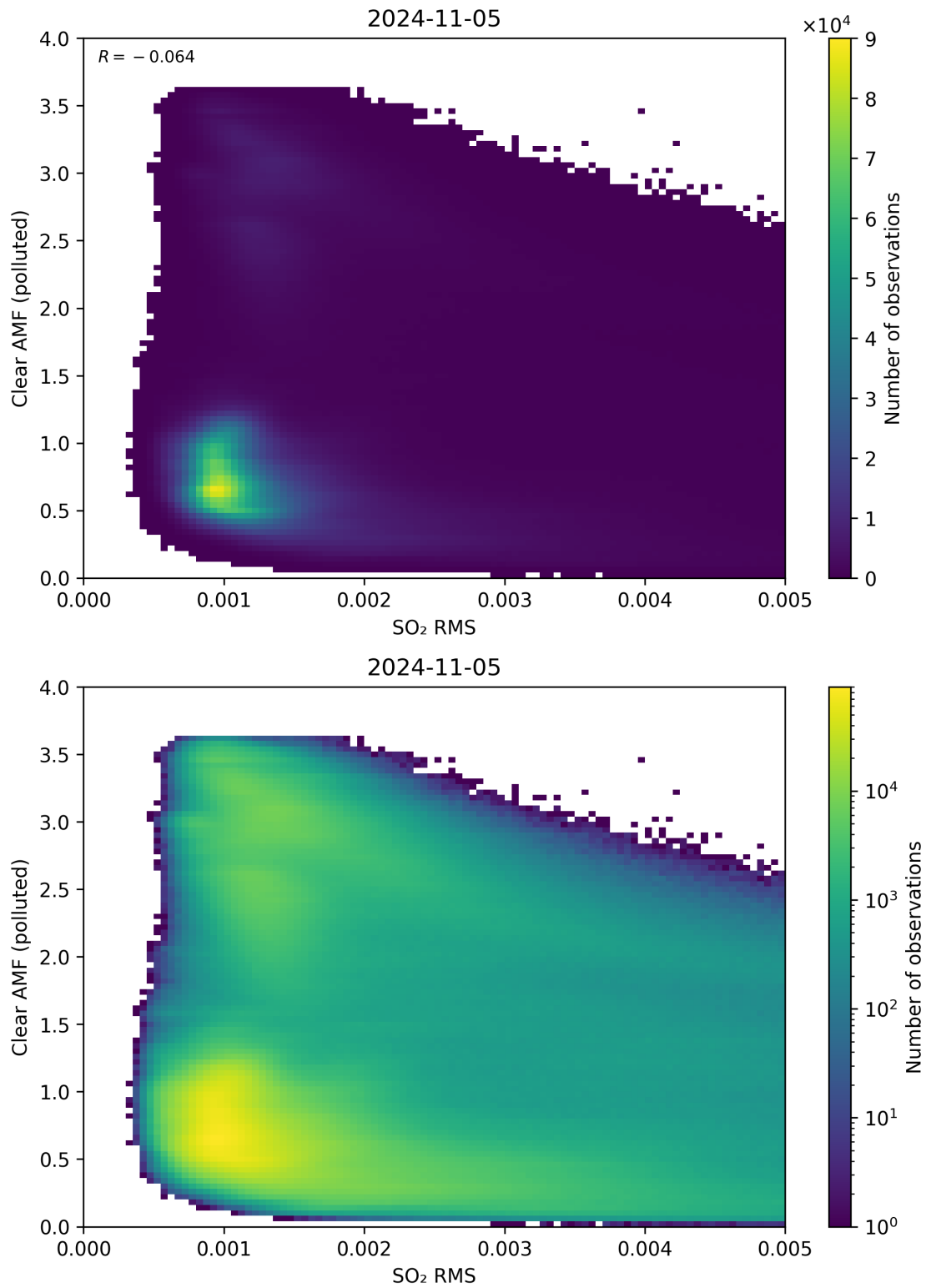
Figure 136: Scatter density plot of “SO 2 RMS” against “Clear AMF (polluted)” for 2024-11-04 to 2024-11-06.
