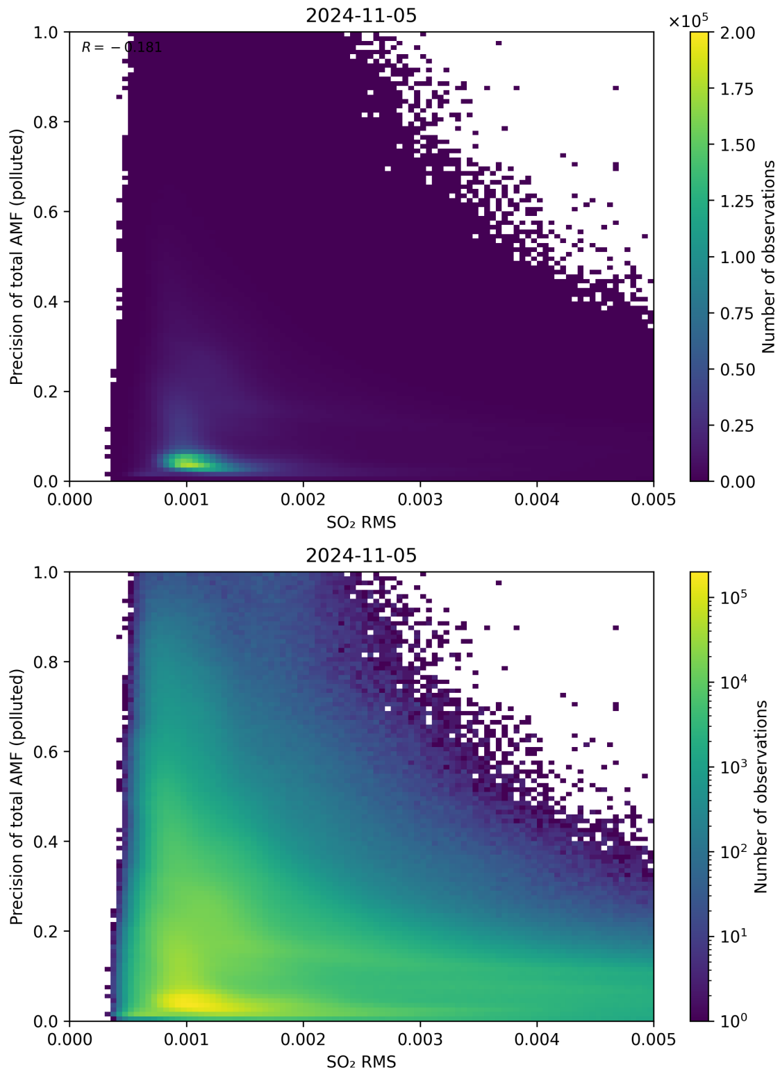
Figure 138: Scatter density plot of “SO 2 RMS” against “Precision of total AMF (polluted)” for 2024-11-04 to 2024-11-06.
