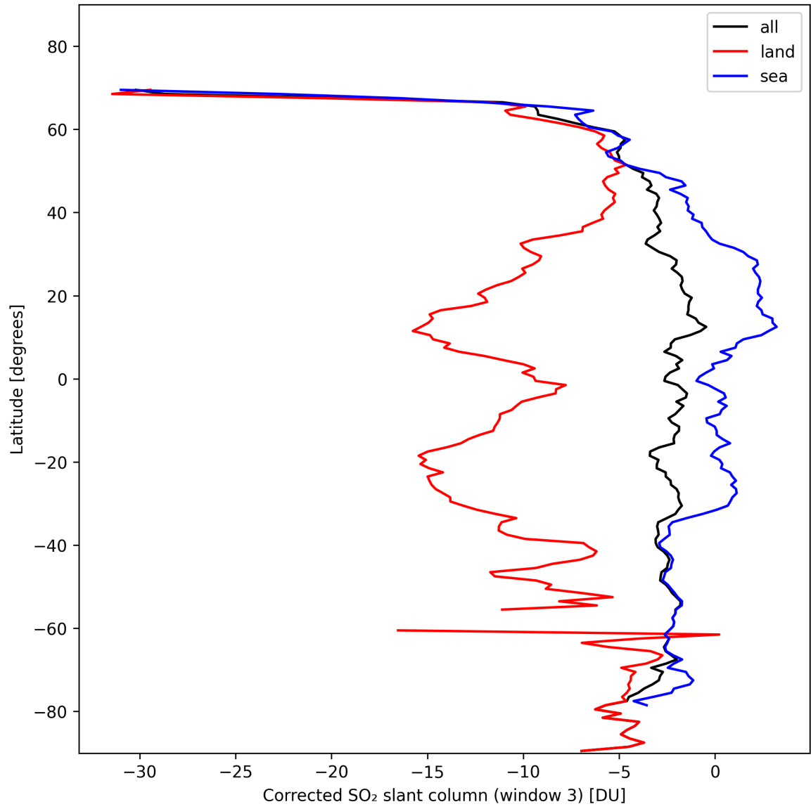
Figure 43: Zonal average of “Corrected SO 2 slant column (window 3)” for 2024-11-04 to 2024-11-06.
