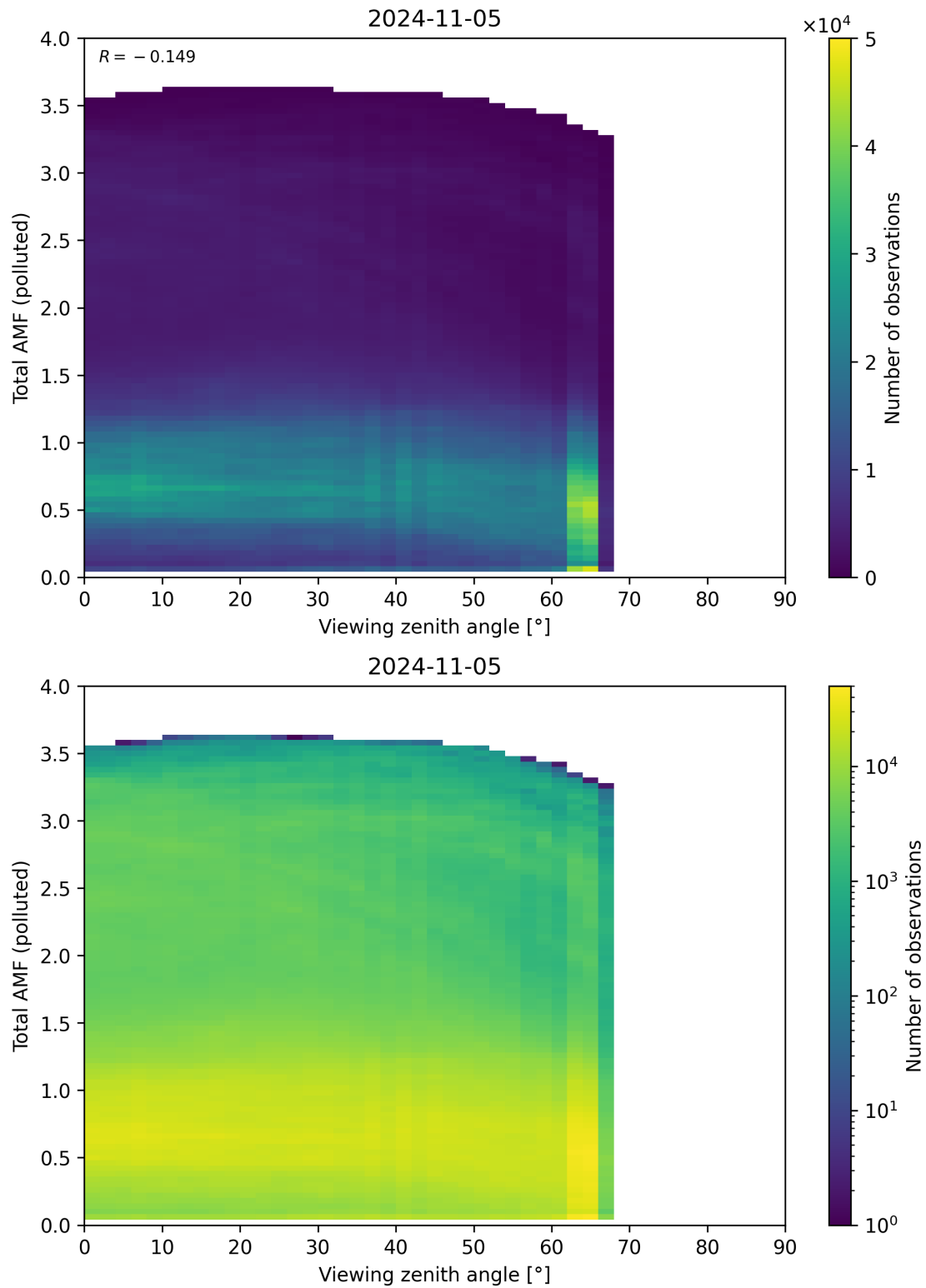
Figure 325: Scatter density plot of “Viewing zenith angle” against “Total AMF (polluted)” for 2024-11-04 to 2024-11-06.
