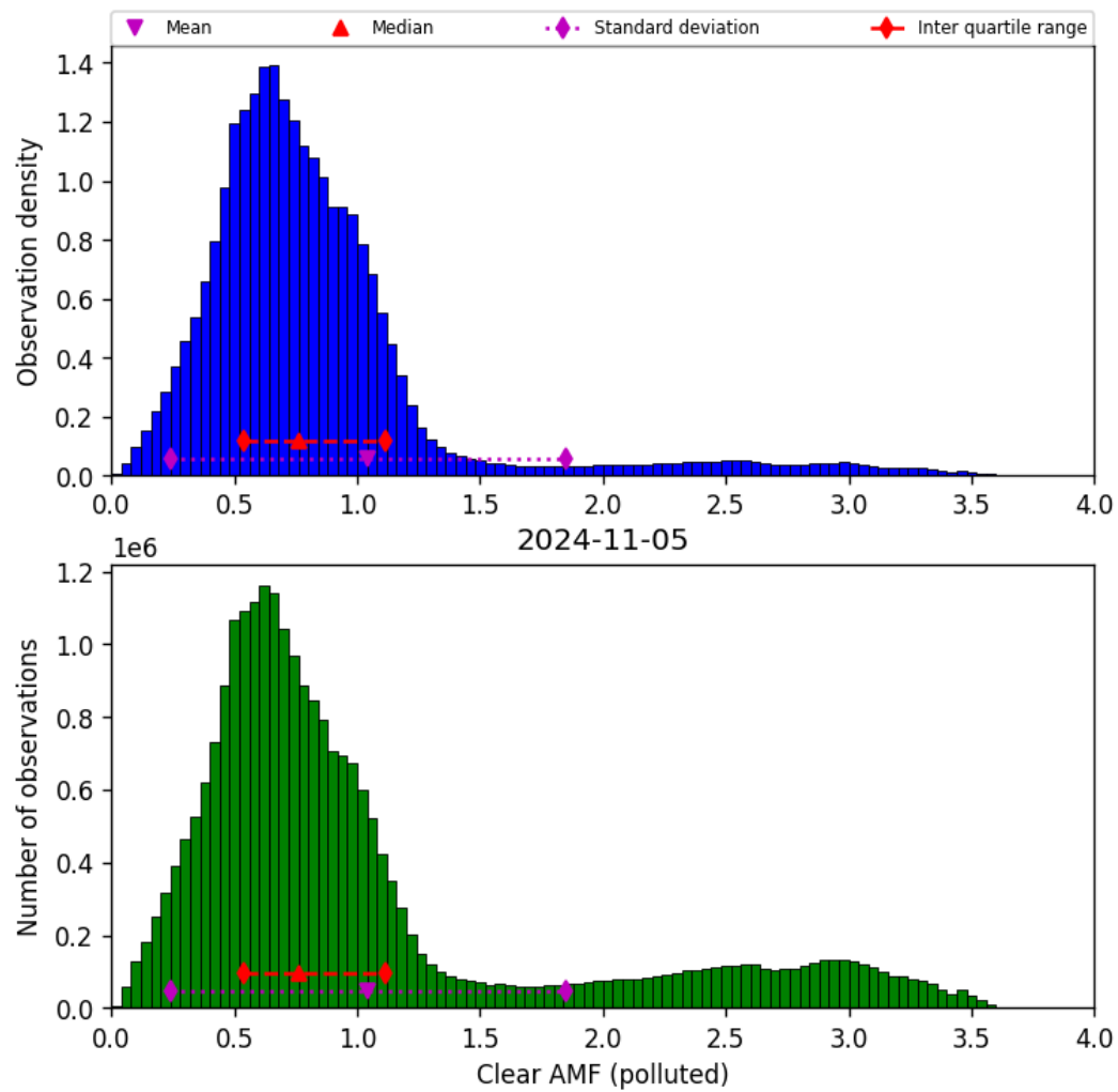
Figure 73: Histogram of “Clear AMF (polluted)” for 2024-11-04 to 2024-11-06
