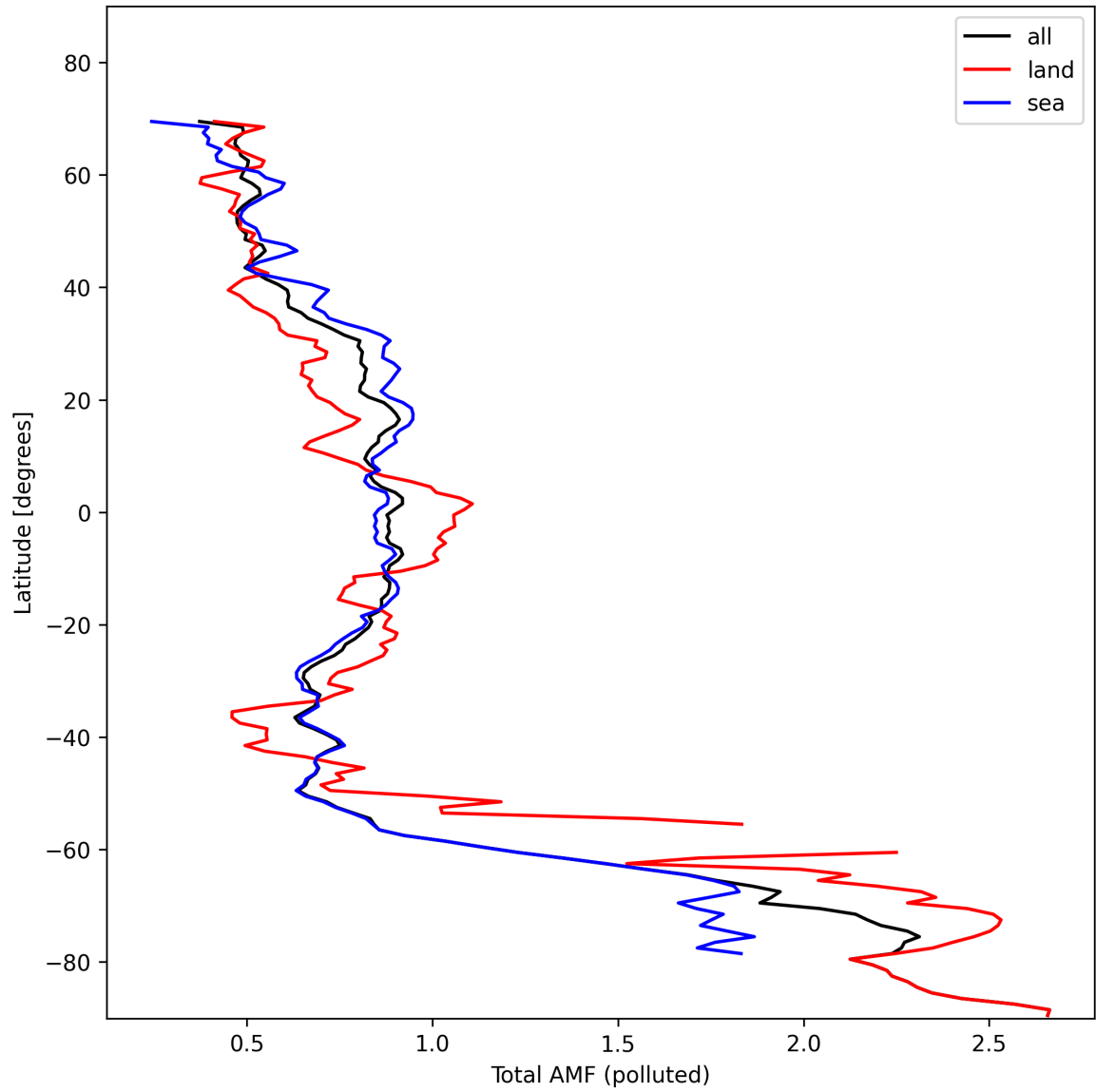
Figure 48: Zonal average of “Total AMF (polluted)” for 2024-11-04 to 2024-11-06.
