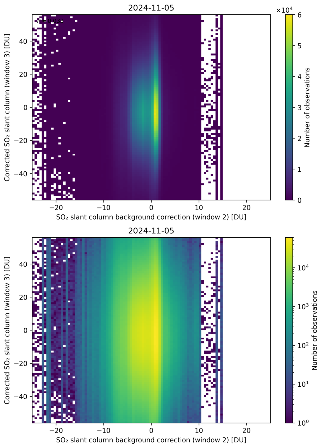
Figure 116: Scatter density plot of “SO 2 slant column background correction (window 2)” against “Corrected SO 2 slant column (window 3)” for 2024-11-04 to 2024-11-06.
