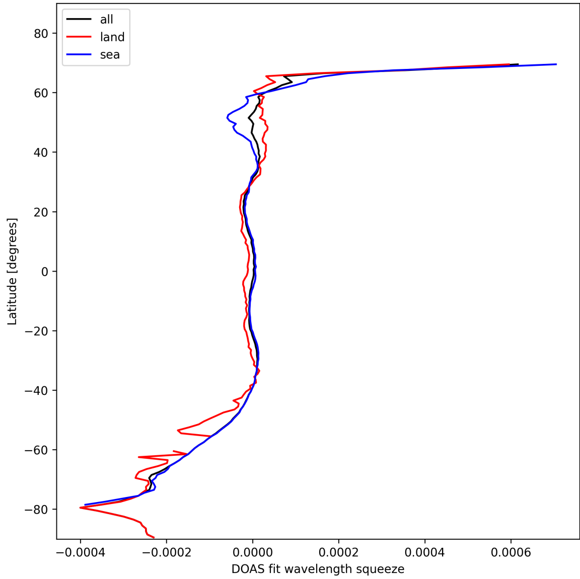
Figure 46: Zonal average of “DOAS fit wavelength squeeze” for 2024-11-04 to 2024-11-06.
