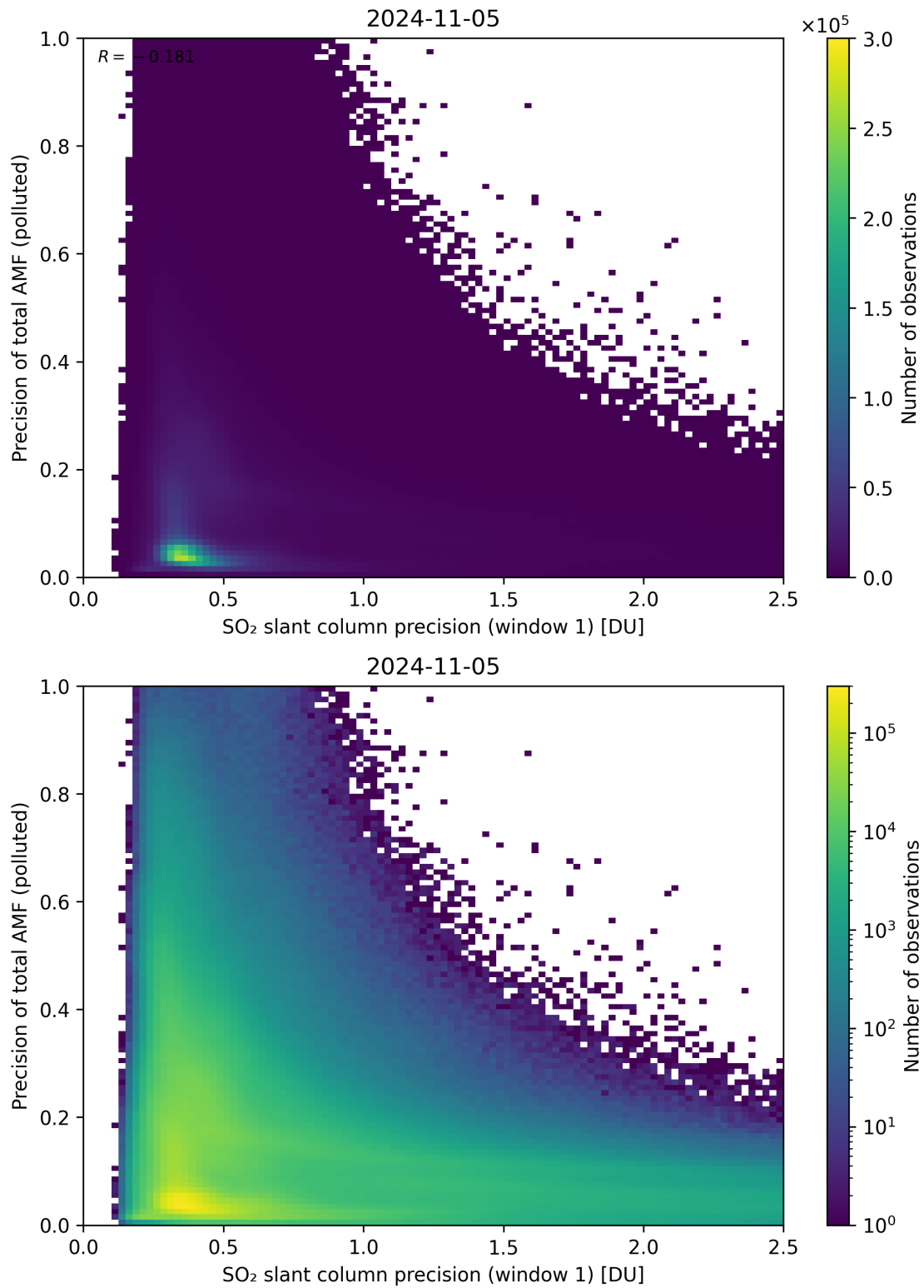
Figure 231: Scatter density plot of “SO 2 slant column precision (window 1)” against “Precision of total AMF (polluted)” for 2024-11-04 to 2024-11-06.
