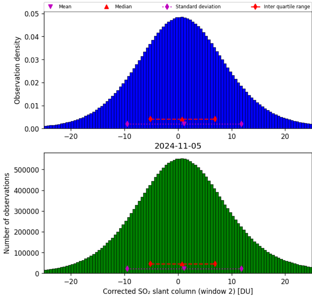
Figure 62: Histogram of “Corrected SO 2 slant column (window 2)” for 2024-11-04 to 2024-11-06
