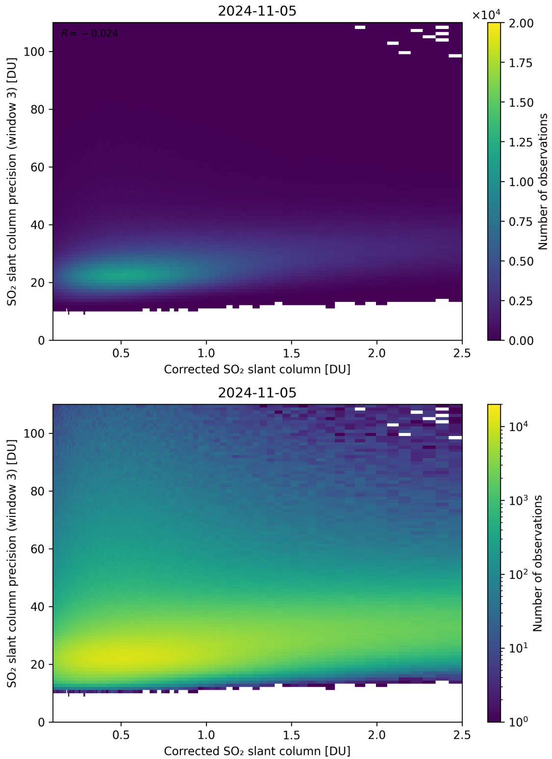
Figure 191: Scatter density plot of “Corrected SO 2 slant column” against “SO 2 slant column precision (window 3)” for 2024-11-04 to 2024-11-06.
