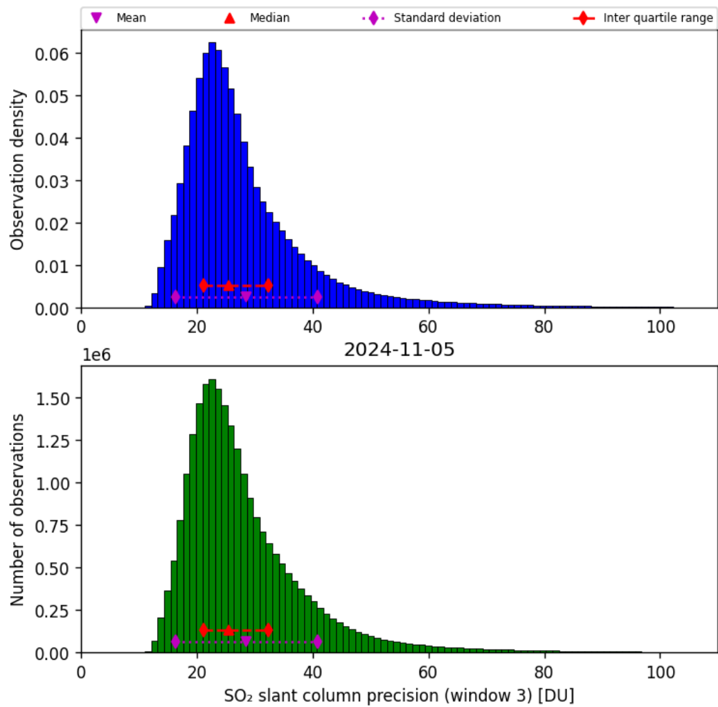
Figure 65: Histogram of “SO 2 slant column precision (window 3)” for 2024-11-04 to 2024-11-06
