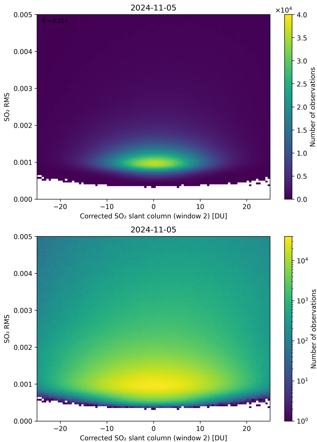
Figure 198: Scatter density plot of “Corrected SO 2 slant column (window 2)” against “SO 2 RMS” for 2024-11-04 to 2024-11-06.
