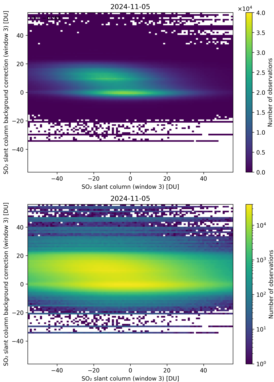
Figure 253: Scatter density plot of “SO 2 slant column (window 3)” against “SO 2 slant column background correction (window 3)” for 2024-11-04 to 2024-11-06.
