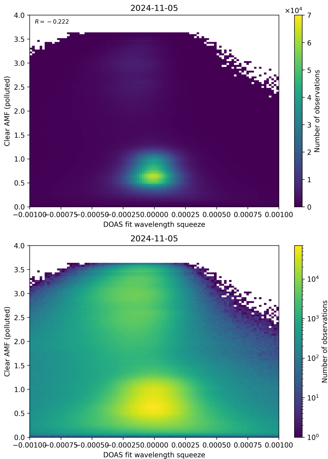
Figure 133: Scatter density plot of “DOAS fit wavelength squeeze” against “Clear AMF (polluted)” for 2024-11-04 to 2024-11-06.
