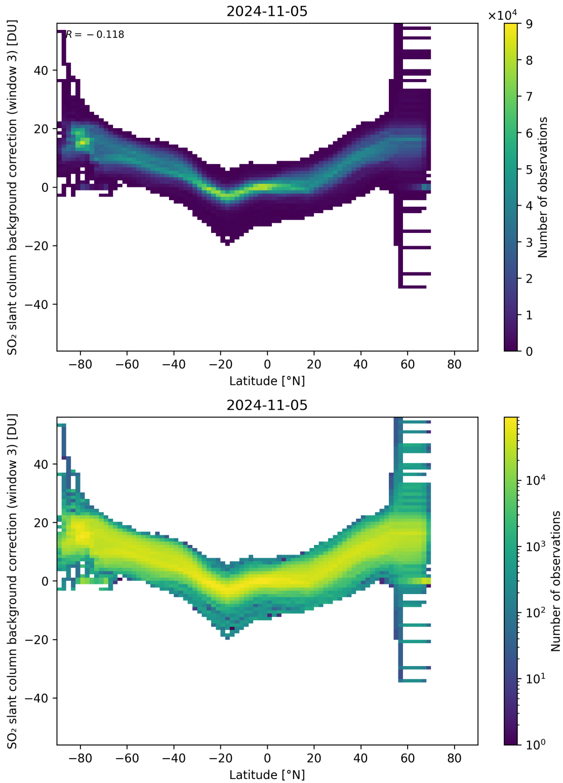
Figure 141: Scatter density plot of “Latitude” against “SO 2 slant column background correction (window 3)” for 2024-11-04 to 2024-11-06.
