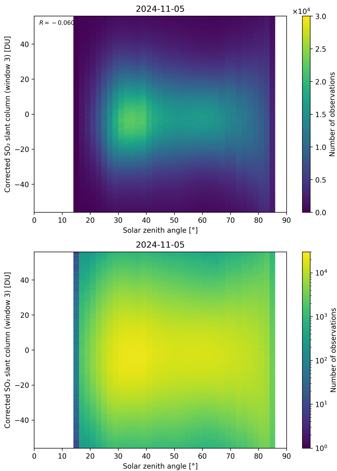
Figure 168: Scatter density plot of “Solar zenith angle” against “Corrected SO 2 slant column (window 3)” for 2024-11-04 to 2024-11-06.
