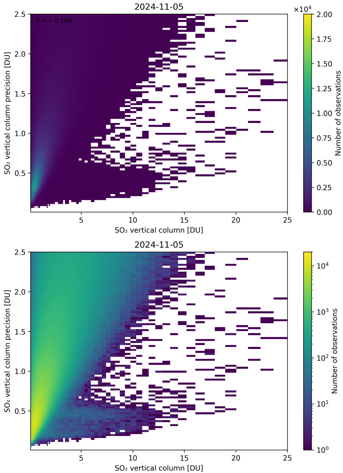
Figure 307: Scatter density plot of “SO 2 vertical column” against “SO 2 vertical column precision” for 2024-11-04 to 2024-11-06.
