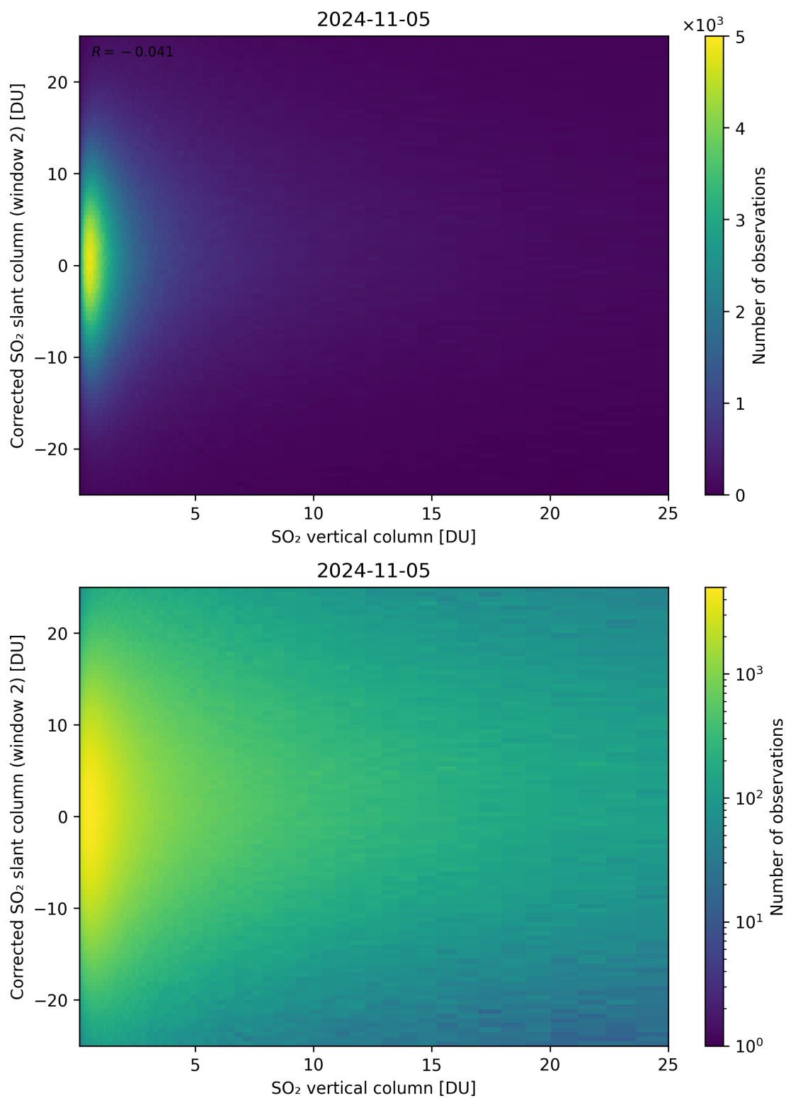
Figure 298: Scatter density plot of “SO 2 vertical column” against “Corrected SO 2 slant column (window 2)” for 2024-11-04 to 2024-11-06.
