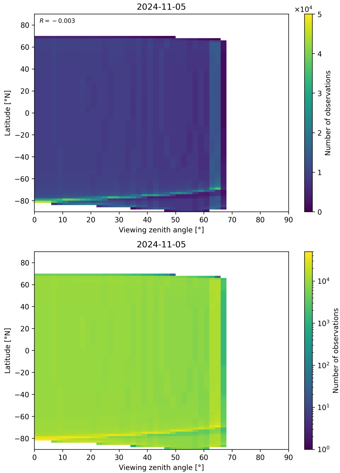
Figure 314: Scatter density plot of “Viewing zenith angle” against “Latitude” for 2024-11-04 to 2024-11-06.
