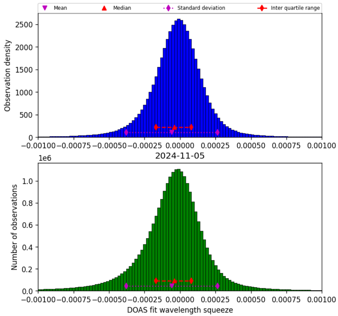
Figure 69: Histogram of “DOAS fit wavelength squeeze” for 2024-11-04 to 2024-11-06
