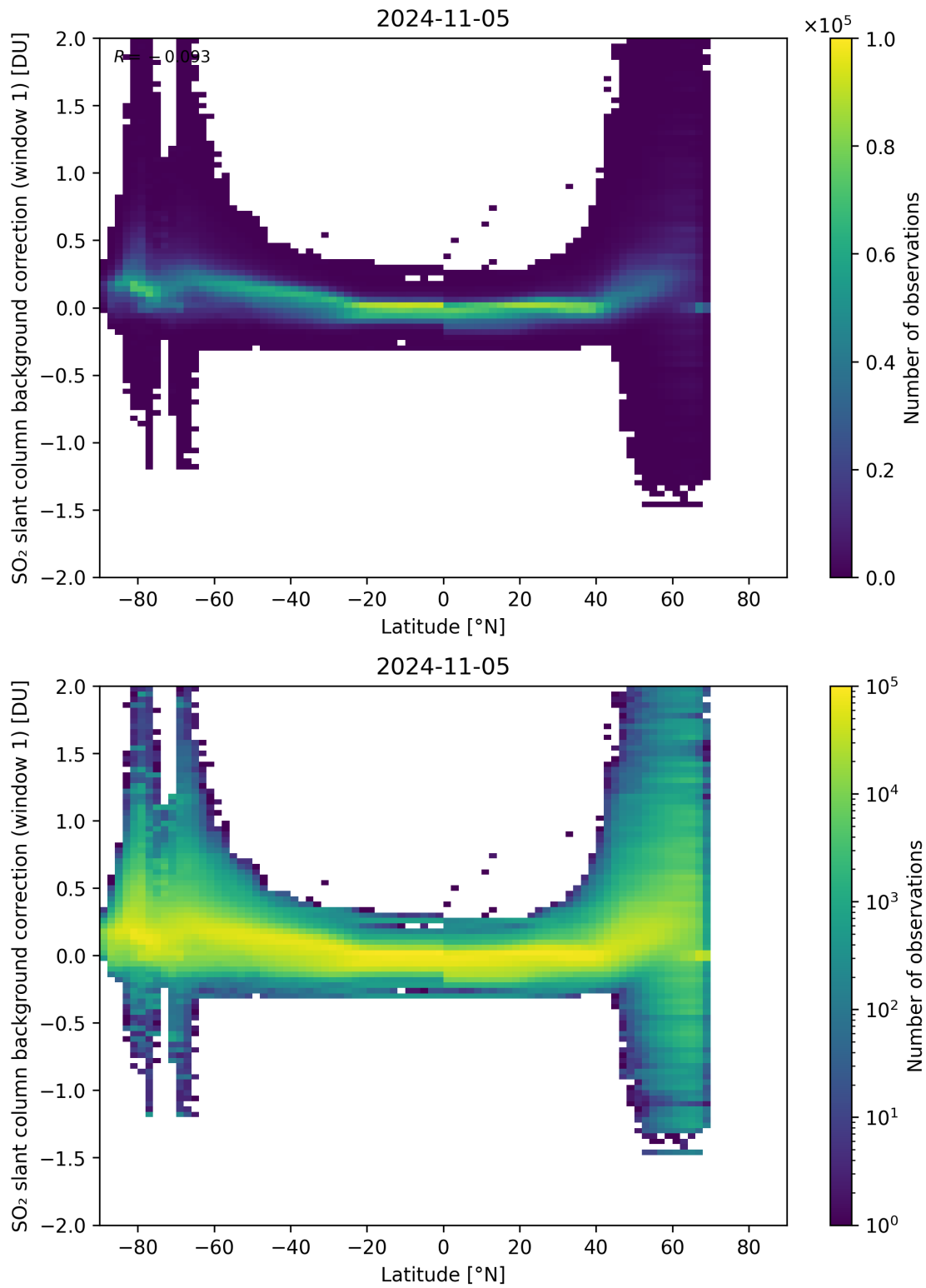
Figure 139: Scatter density plot of “Latitude” against “SO 2 slant column background correction (window 1)” for 2024-11-04 to 2024-11-06.
