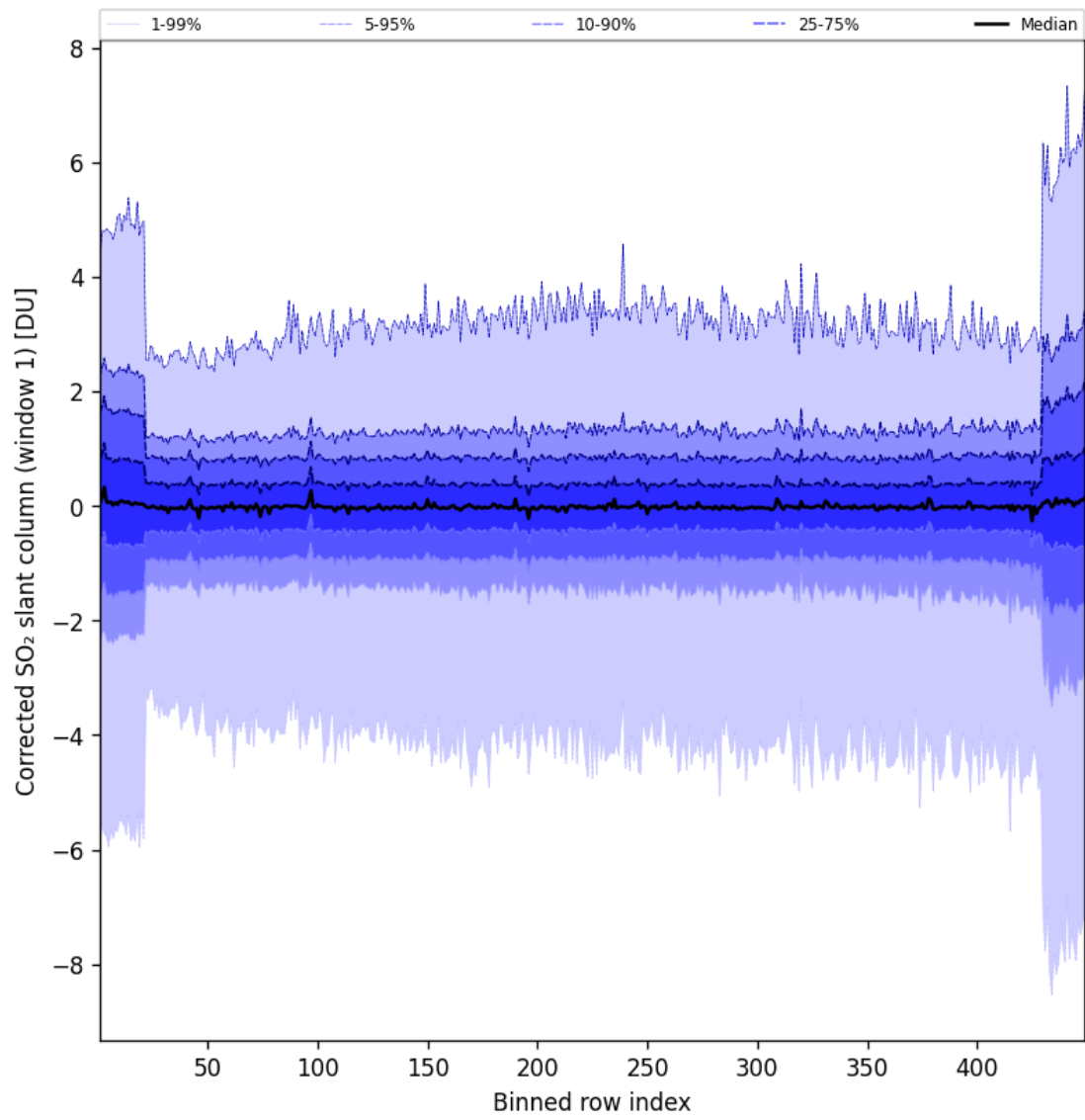
Figure 81: Along track statistics of “Corrected SO 2 slant column (window 1)” for 2024-11-04 to 2024-11-06
