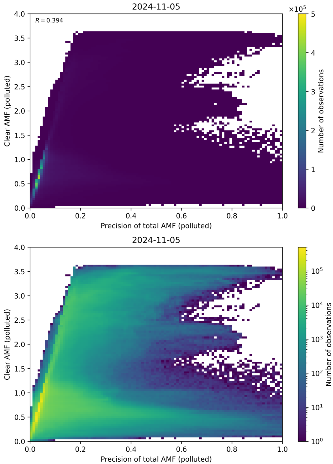
Figure 270: Scatter density plot of “Precision of total AMF (polluted)” against “Clear AMF (polluted)” for 2024-11-04 to 2024-11-06.
