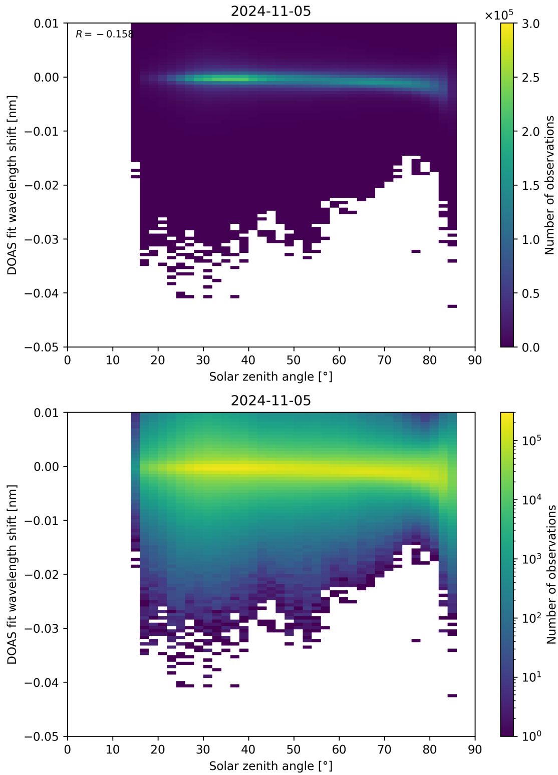
Figure 161: Scatter density plot of “Solar zenith angle” against “DOAS fit wavelength shift” for 2024-11-04 to 2024-11-06.
