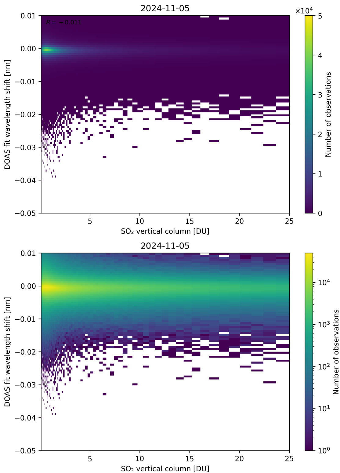
Figure 276: Scatter density plot of “SO 2 vertical column” against “DOAS fit wavelength shift” for 2024-11-04 to 2024-11-06.
