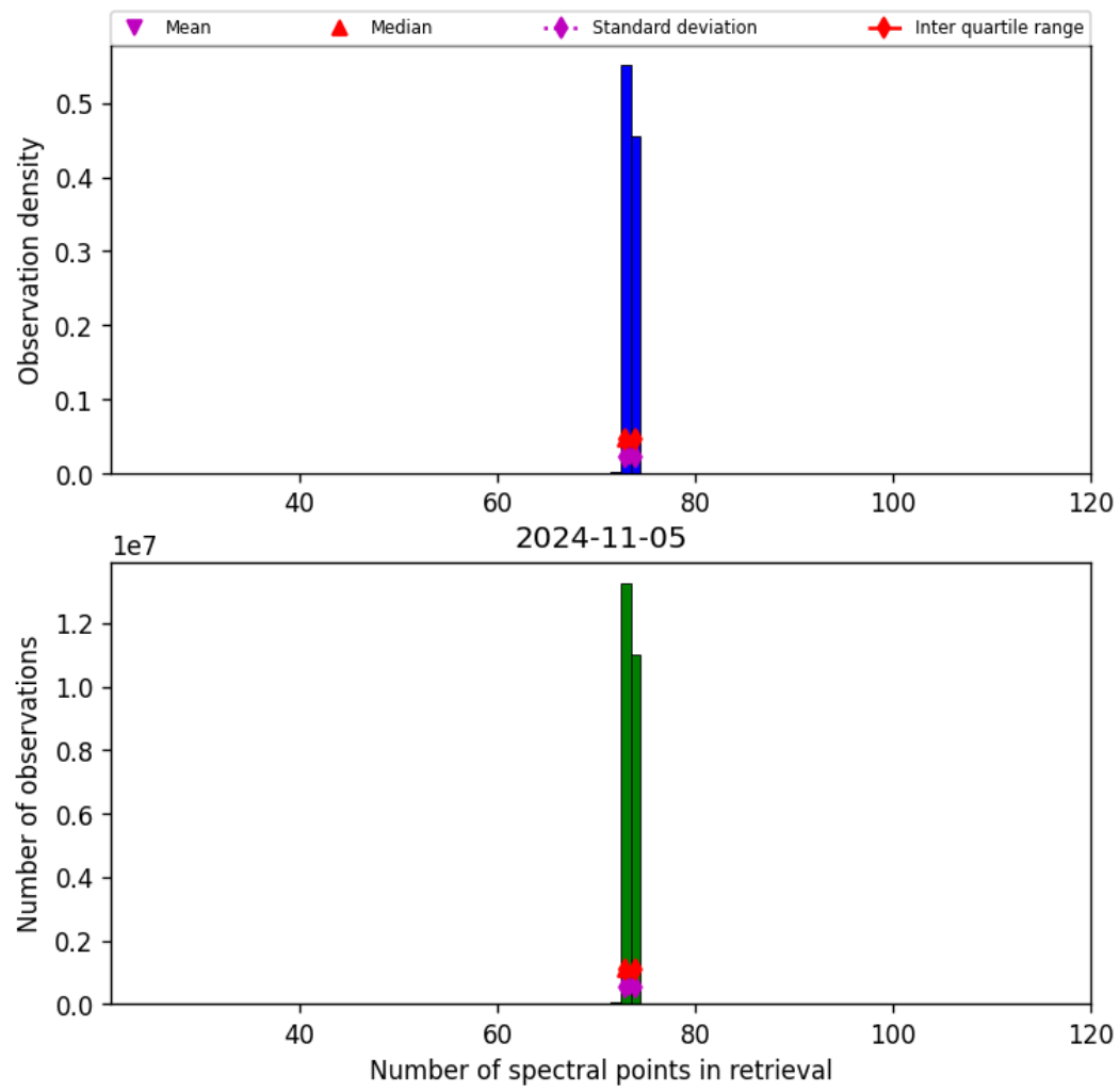
Figure 74: Histogram of “Number of spectral points in retrieval” for 2024-11-04 to 2024-11-06
