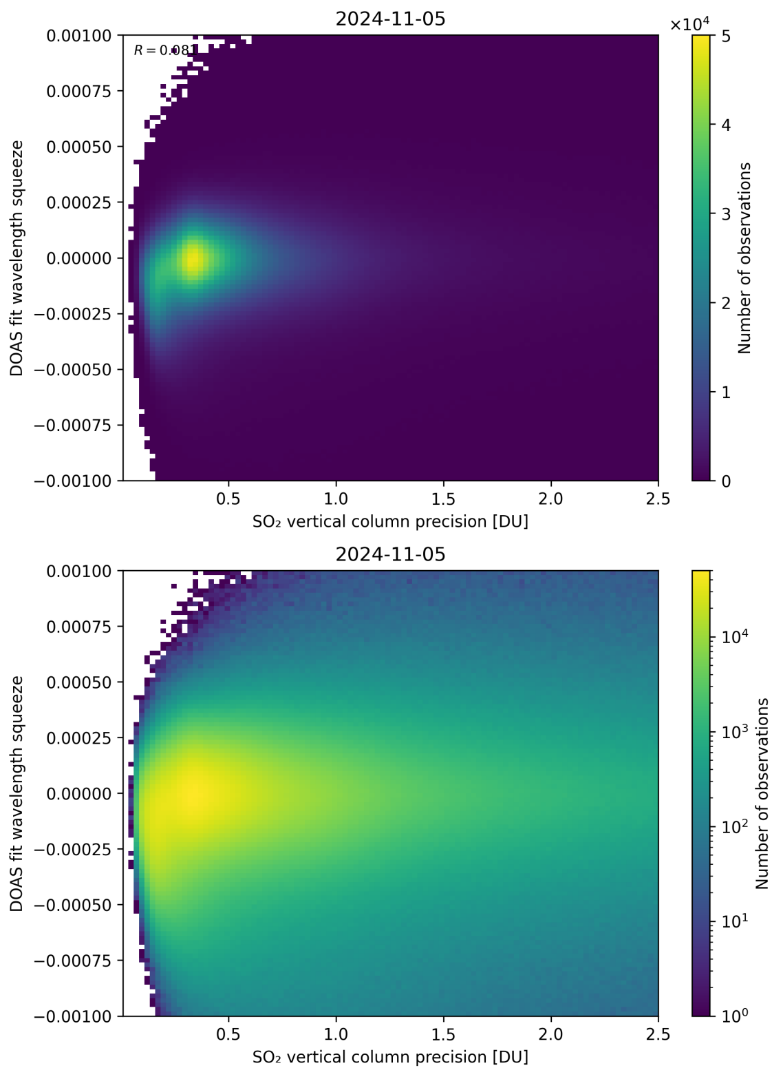
Figure 283: Scatter density plot of “SO 2 vertical column precision” against “DOAS fit wavelength squeeze” for 2024-11-04 to 2024-11-06.
