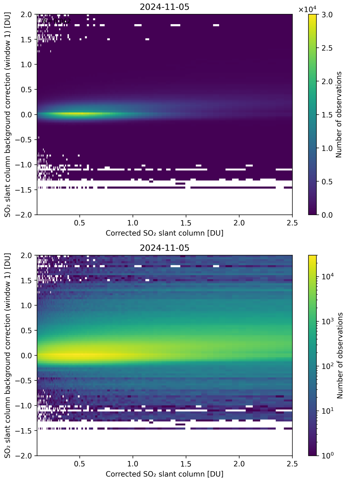
Figure 178: Scatter density plot of “Corrected SO 2 slant column” against “SO 2 slant column background correction (window 1)” for 2024-11-04 to 2024-11-06.
