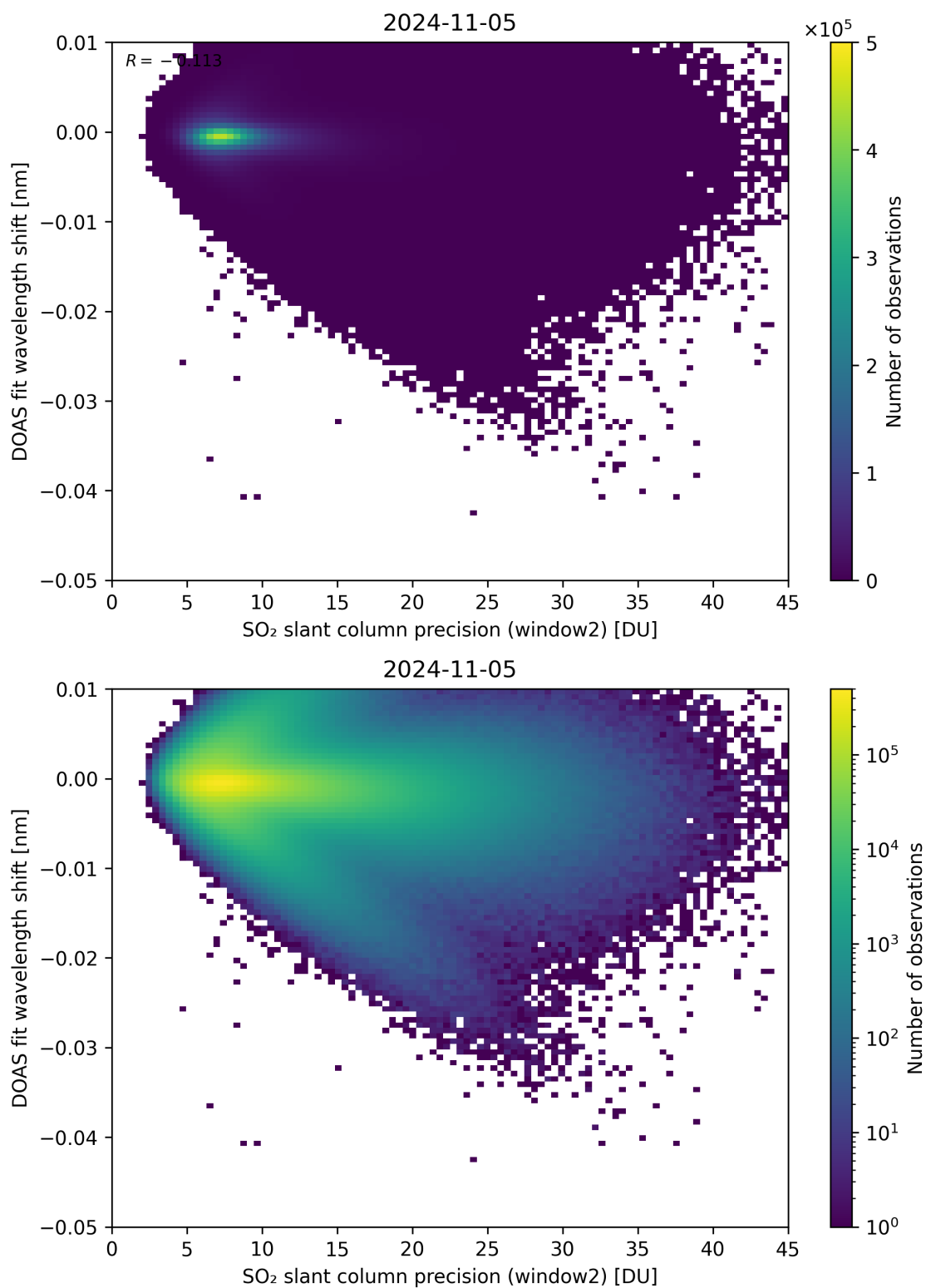
Figure 243: Scatter density plot of “SO 2 slant column precision (window2)” against “DOAS fit wavelength shift” for 2024-11-04 to 2024-11-06.
