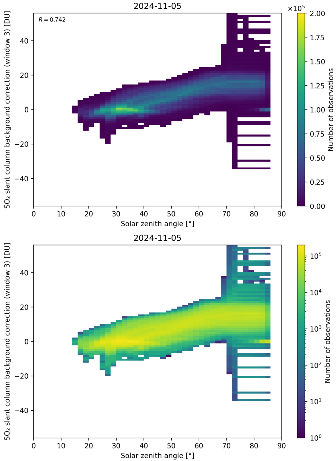
Figure 160: Scatter density plot of “Solar zenith angle” against “SO 2 slant column background correction (window 3)” for 2024-11-04 to 2024-11-06.
