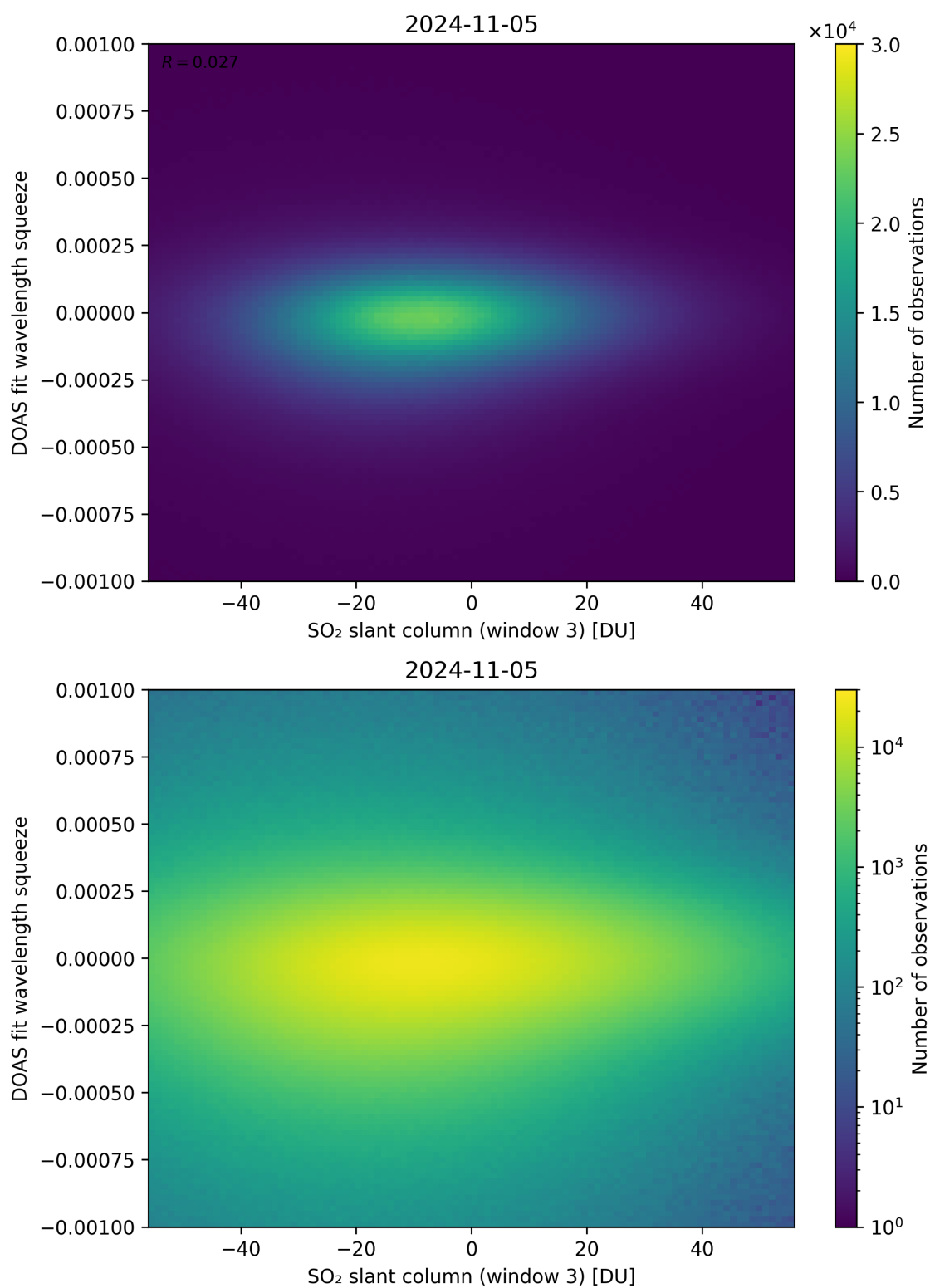
Figure 255: Scatter density plot of “SO 2 slant column (window 3)” against “DOAS fit wavelength squeeze” for 2024-11-04 to 2024-11-06.
