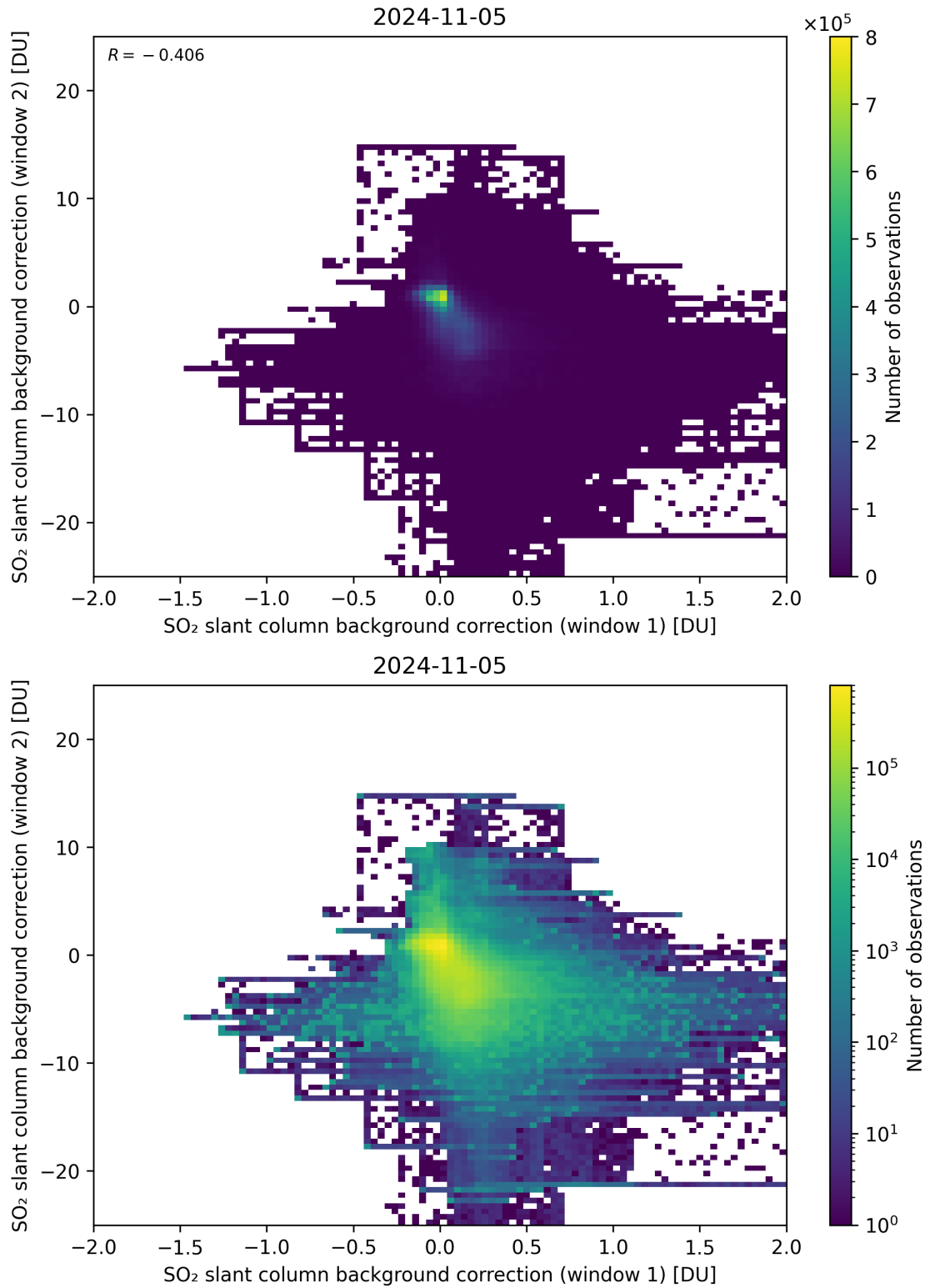
Figure 98: Scatter density plot of “SO 2 slant column background correction (window 1)” against “SO 2 slant column background correction (window 2)” for 2024-11-04 to 2024-11-06.
