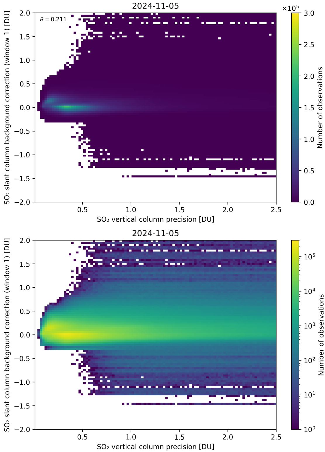
Figure 279: Scatter density plot of “SO 2 vertical column precision” against “SO 2 slant column background correction (window 1)” for 2024-11-04 to 2024-11-06.
