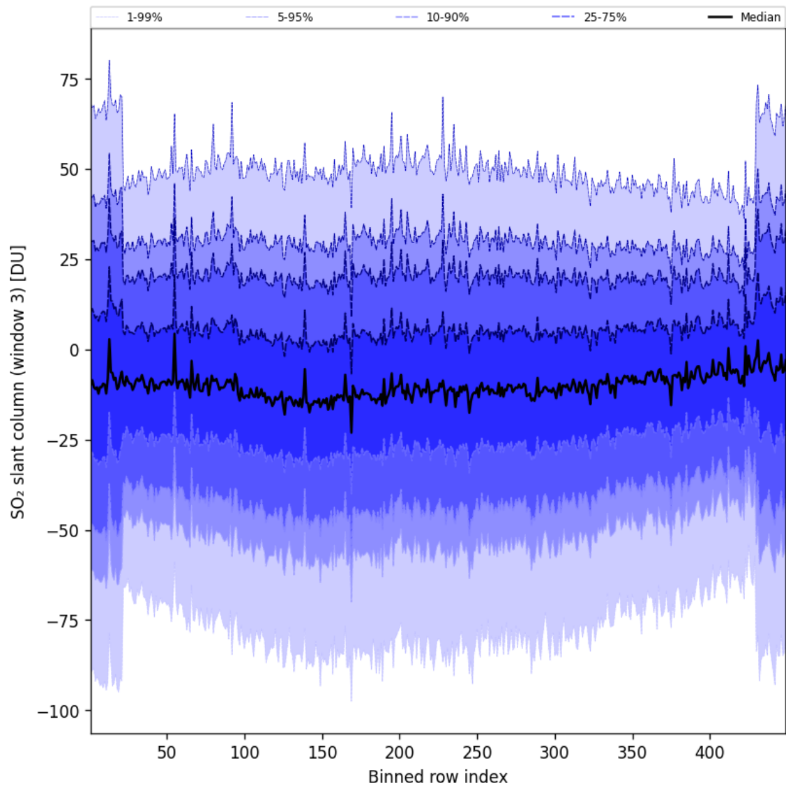
Figure 87: Along track statistics of “SO 2 slant column (window 3)” for 2024-11-04 to 2024-11-06
