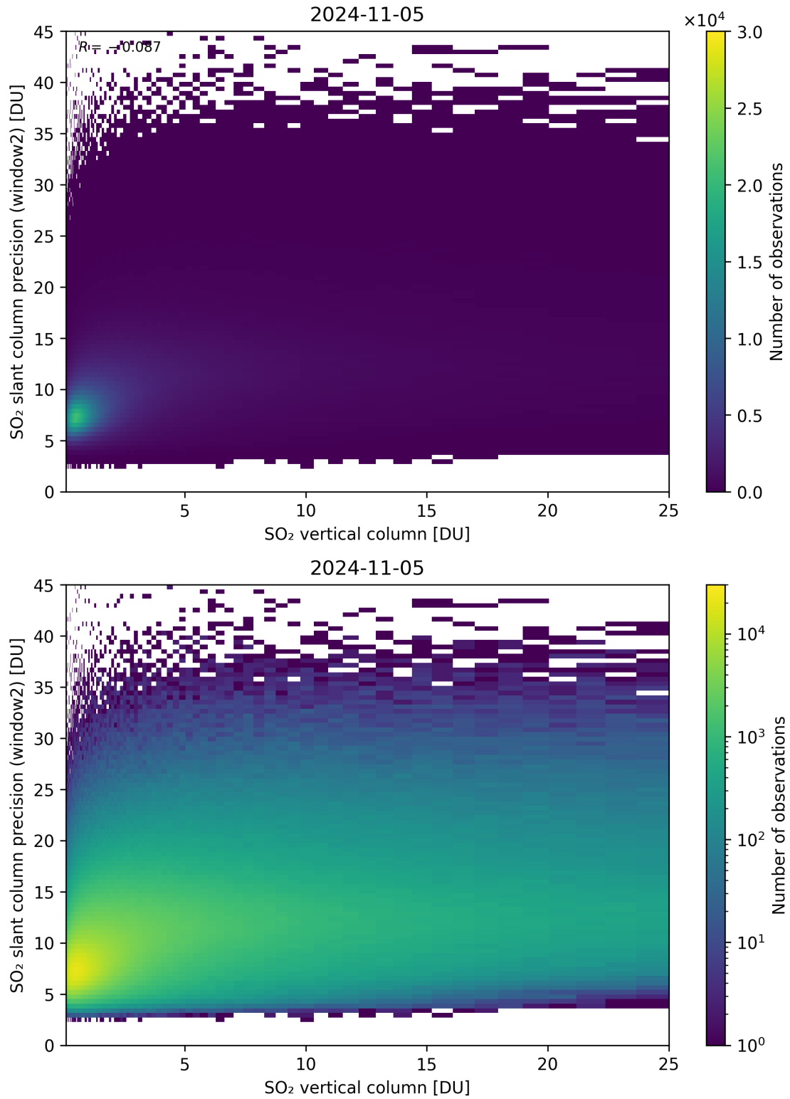
Figure 302: Scatter density plot of “SO 2 vertical column” against “SO 2 slant column precision (window2)” for 2024-11-04 to 2024-11-06.
