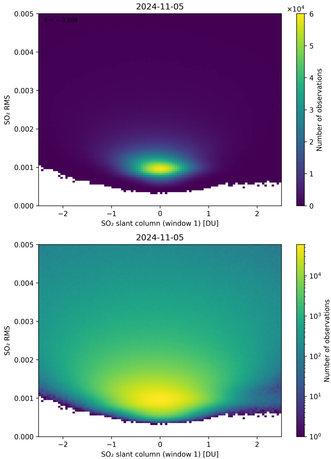
Figure 217: Scatter density plot of “SO 2 slant column (window 1)” against “SO 2 RMS” for 2024-11-04 to 2024-11-06.
