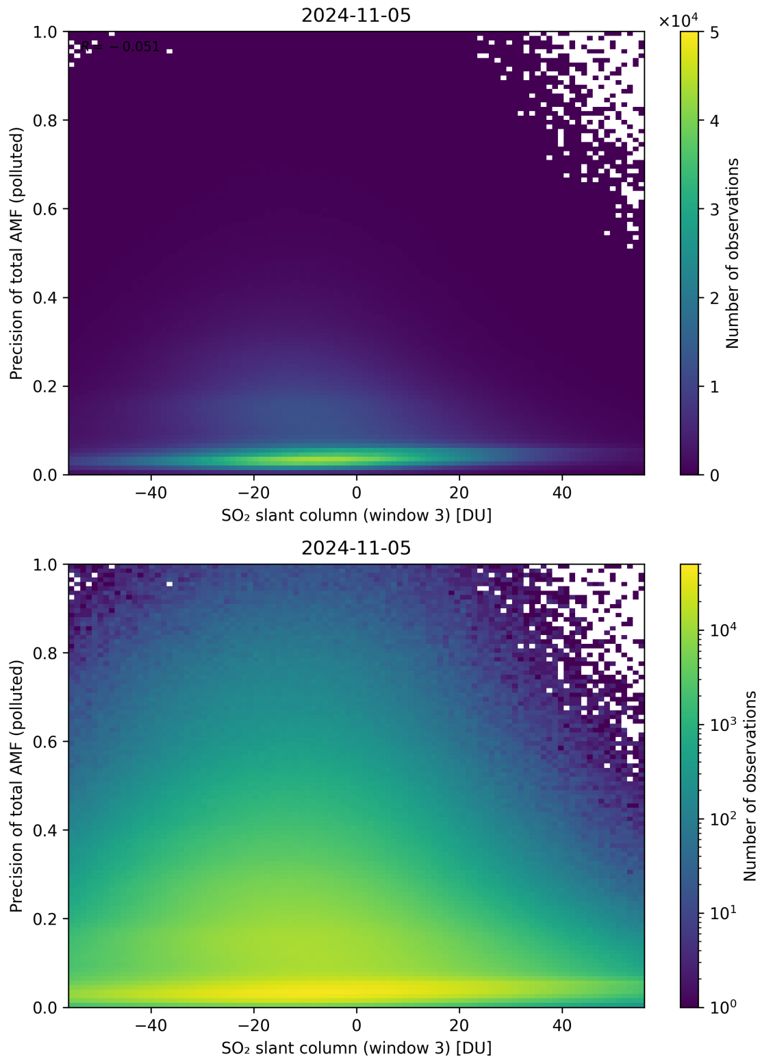
Figure 269: Scatter density plot of “SO 2 slant column (window 3)” against “Precision of total AMF (polluted)” for 2024-11-04 to 2024-11-06.
