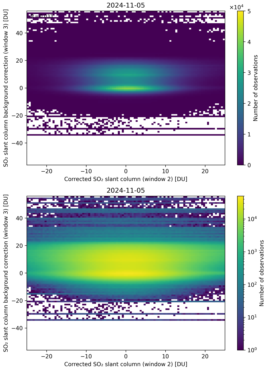
Figure 195: Scatter density plot of “Corrected SO 2 slant column (window 2)” against “SO 2 slant column background correction (window 3)” for 2024-11-04 to 2024-11-06.
