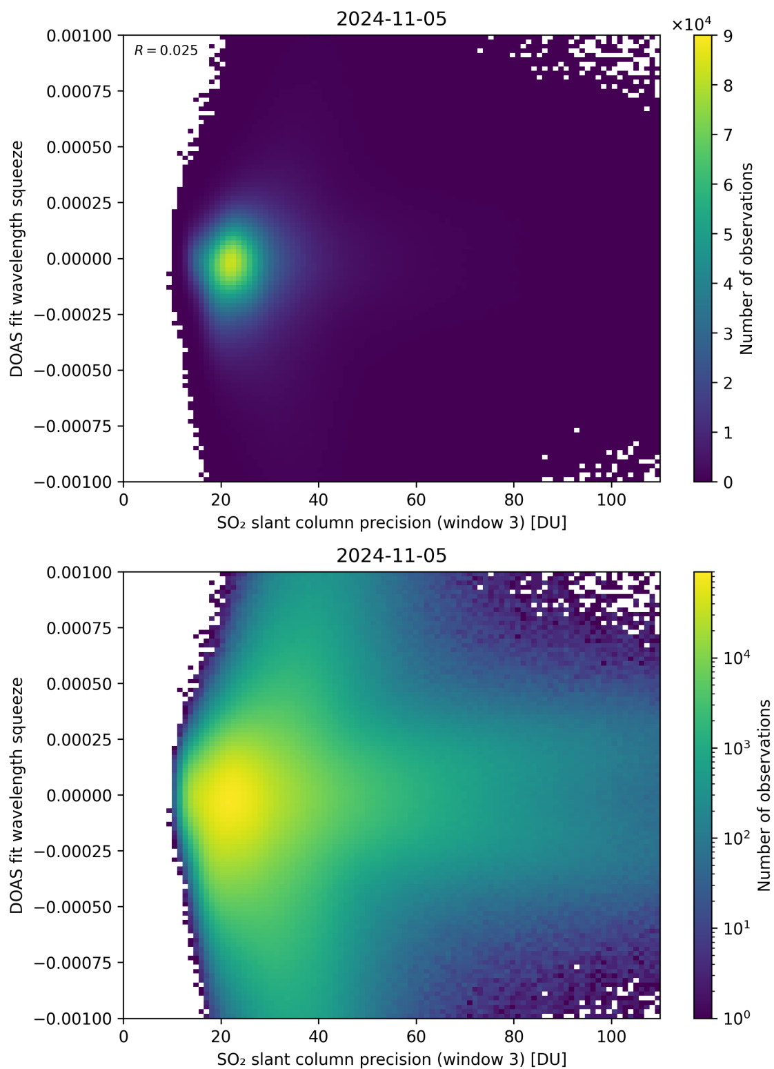
Figure 259: Scatter density plot of “SO 2 slant column precision (window 3)” against “DOAS fit wavelength squeeze” for 2024-11-04 to 2024-11-06.
