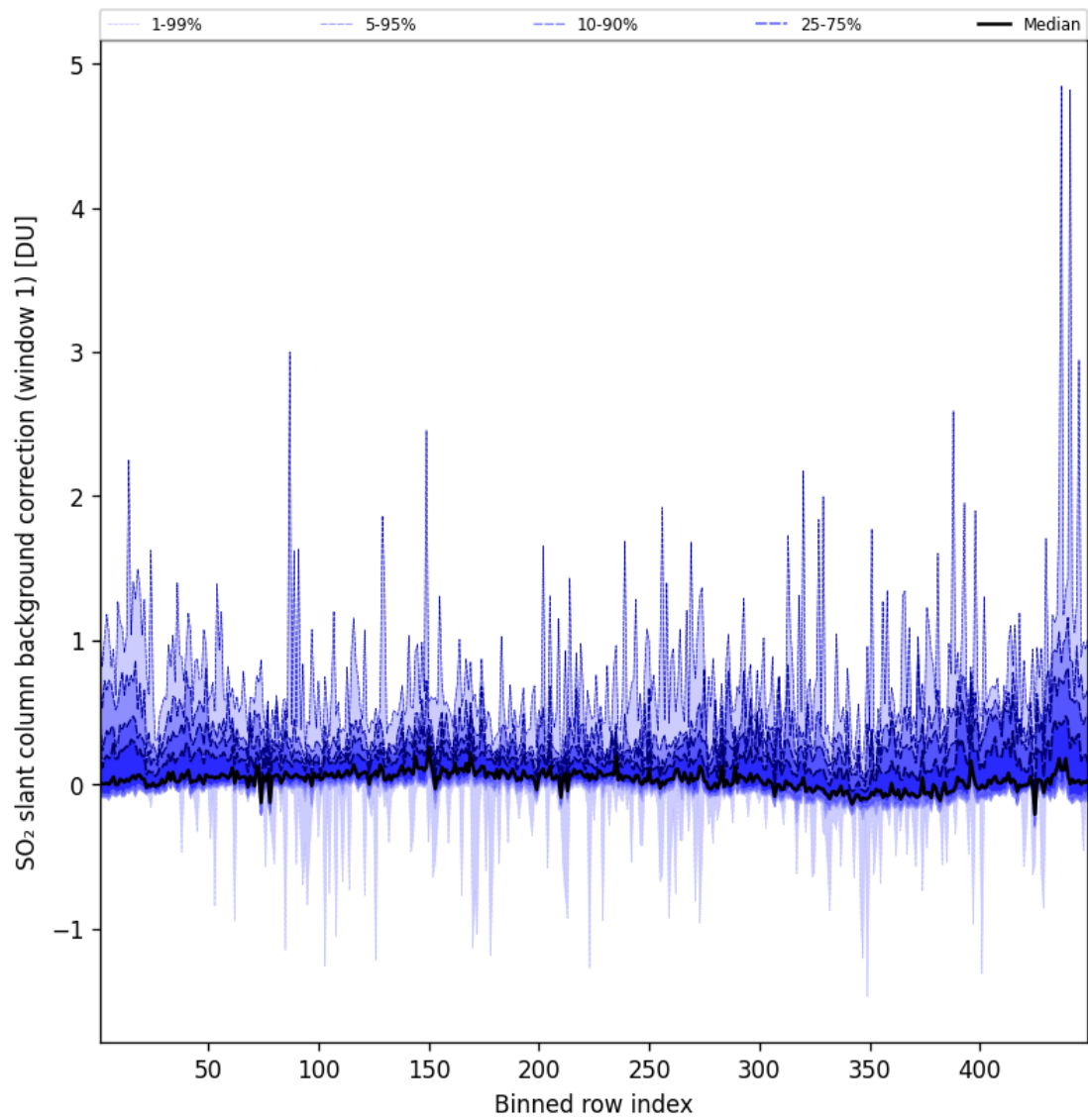
Figure 82: Along track statistics of “SO 2 slant column background correction (window 1)” for 2024-11-04 to 2024-11-06
