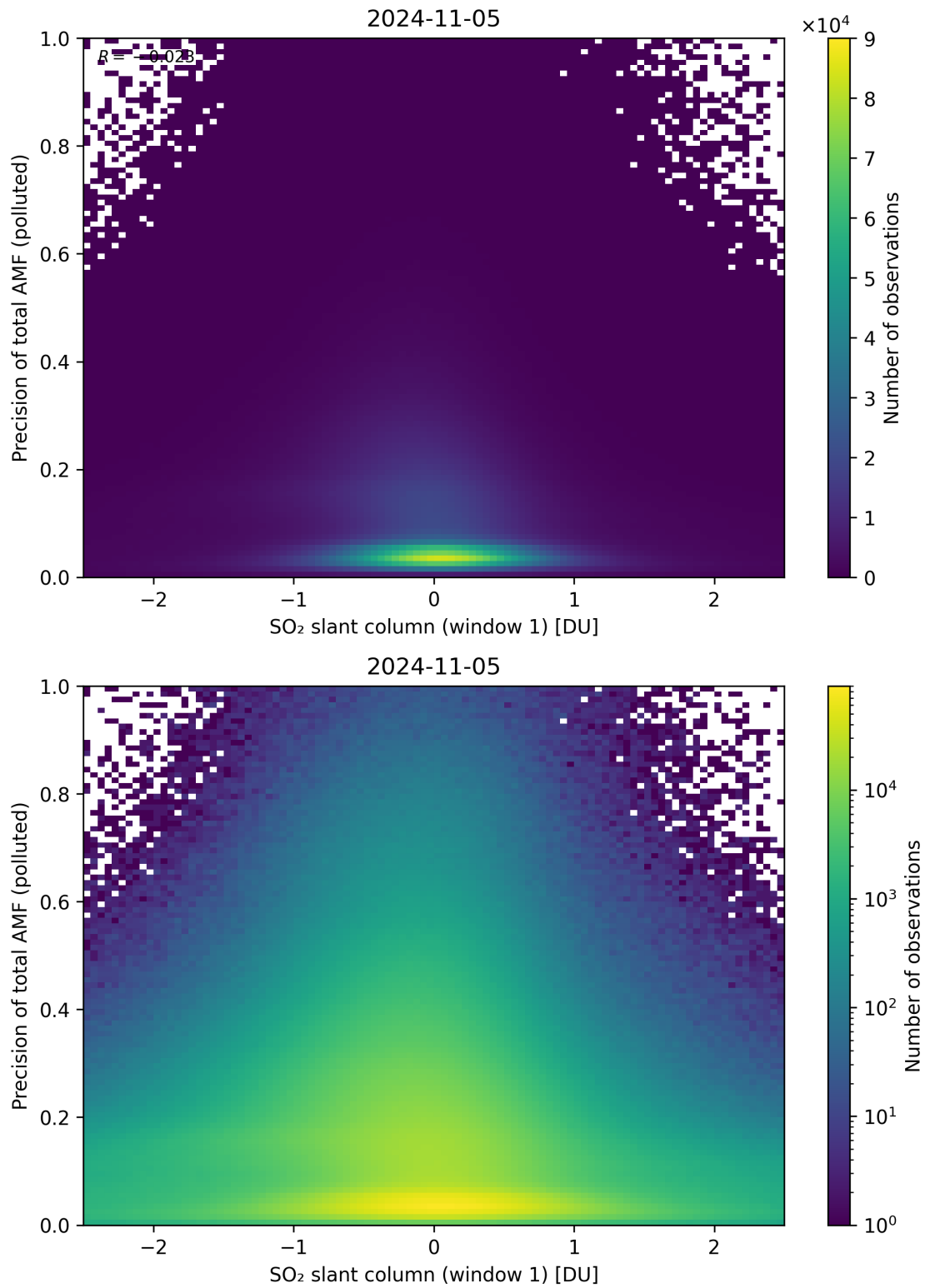
Figure 240: Scatter density plot of “SO 2 slant column (window 1)” against “Precision of total AMF (polluted)” for 2024-11-04 to 2024-11-06.
