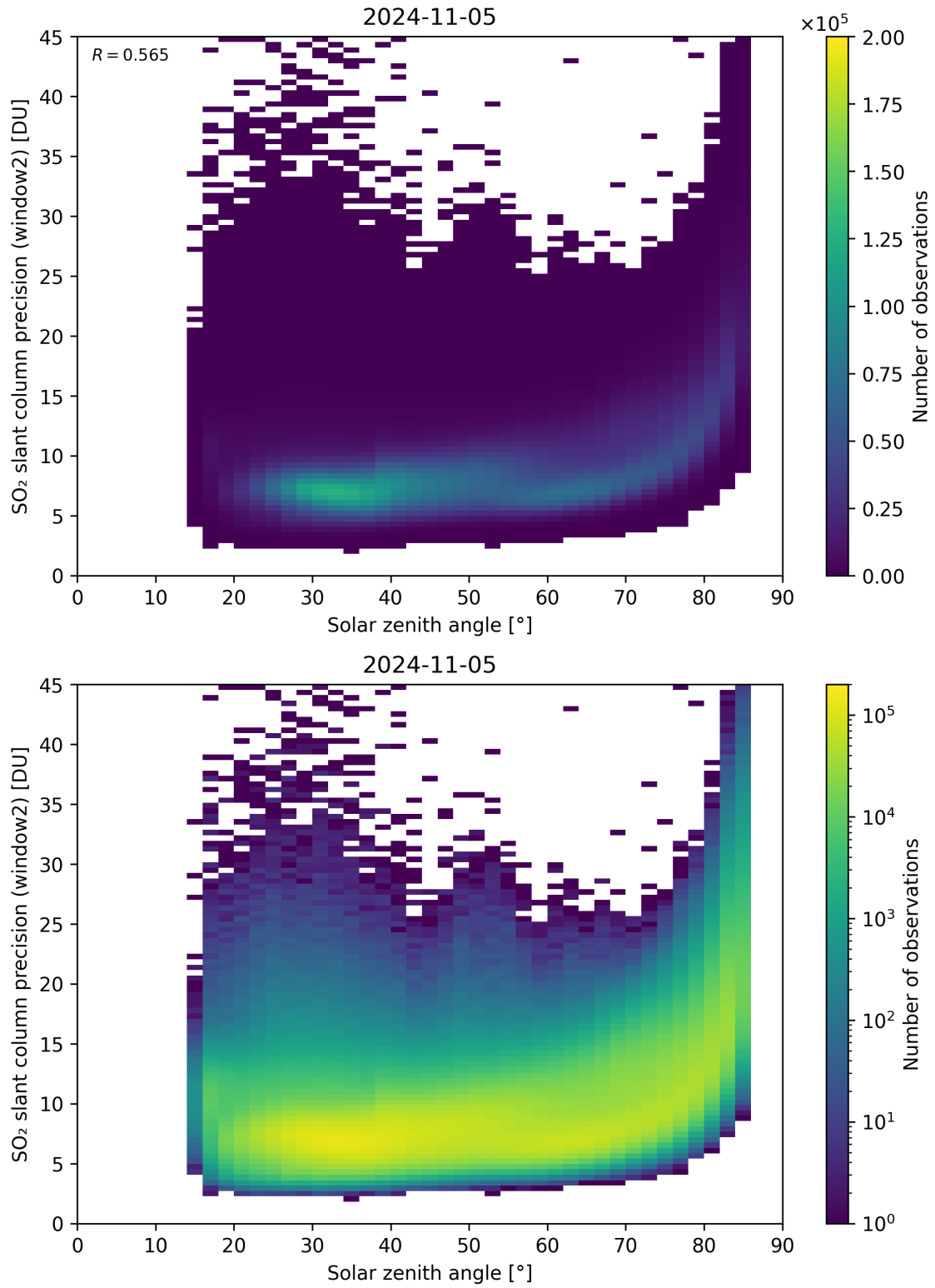
Figure 171: Scatter density plot of “Solar zenith angle” against “SO 2 slant column precision (window2)” for 2024-11-04 to 2024-11-06.
