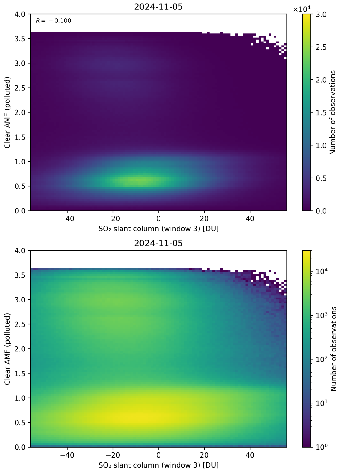
Figure 265: Scatter density plot of “SO 2 slant column (window 3)” against “Clear AMF (polluted)” for 2024-11-04 to 2024-11-06.
