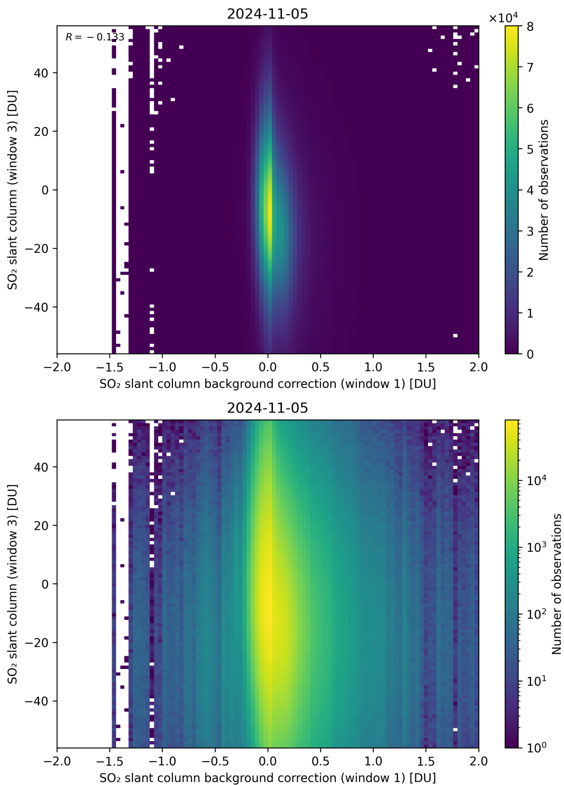
Figure 107: Scatter density plot of “SO 2 slant column background correction (window 1)” against “SO 2 slant column (window 3)” for 2024-11-04 to 2024-11-06.
