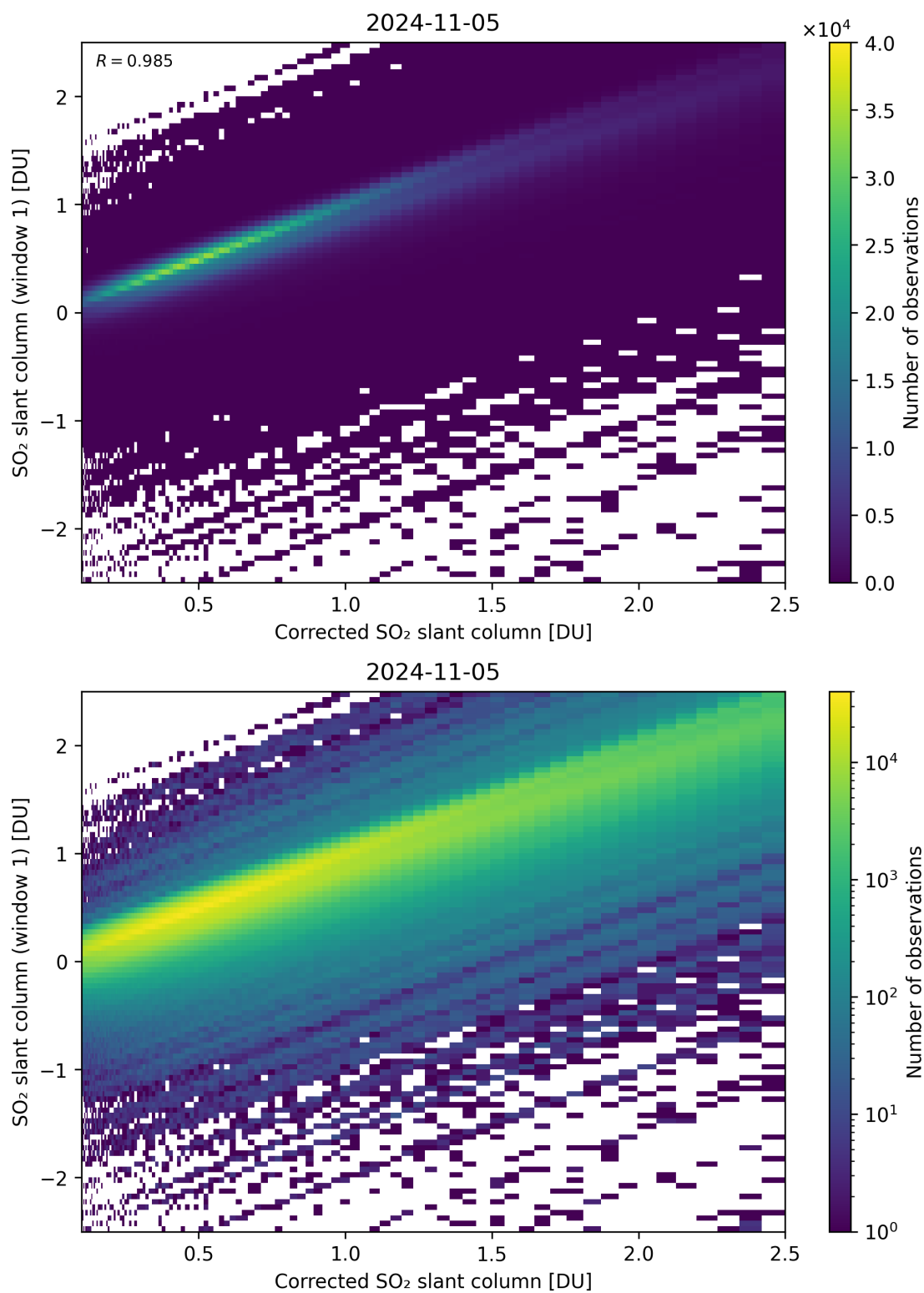
Figure 187: Scatter density plot of “Corrected SO 2 slant column” against “SO 2 slant column (window 1)” for 2024-11-04 to 2024-11-06.
