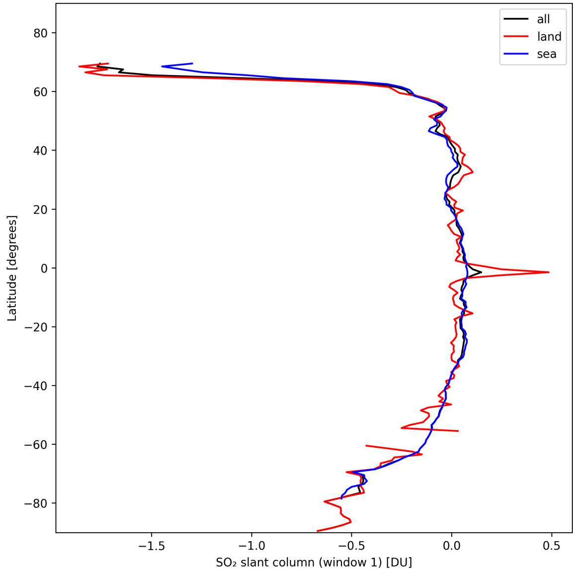
Figure 33: Zonal average of “SO 2 slant column (window 1)” for 2024-11-04 to 2024-11-06.
