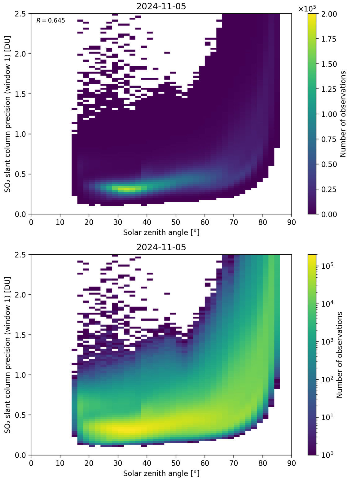
Figure 170: Scatter density plot of “Solar zenith angle” against “SO 2 slant column precision (window 1)” for 2024-11-04 to 2024-11-06.
