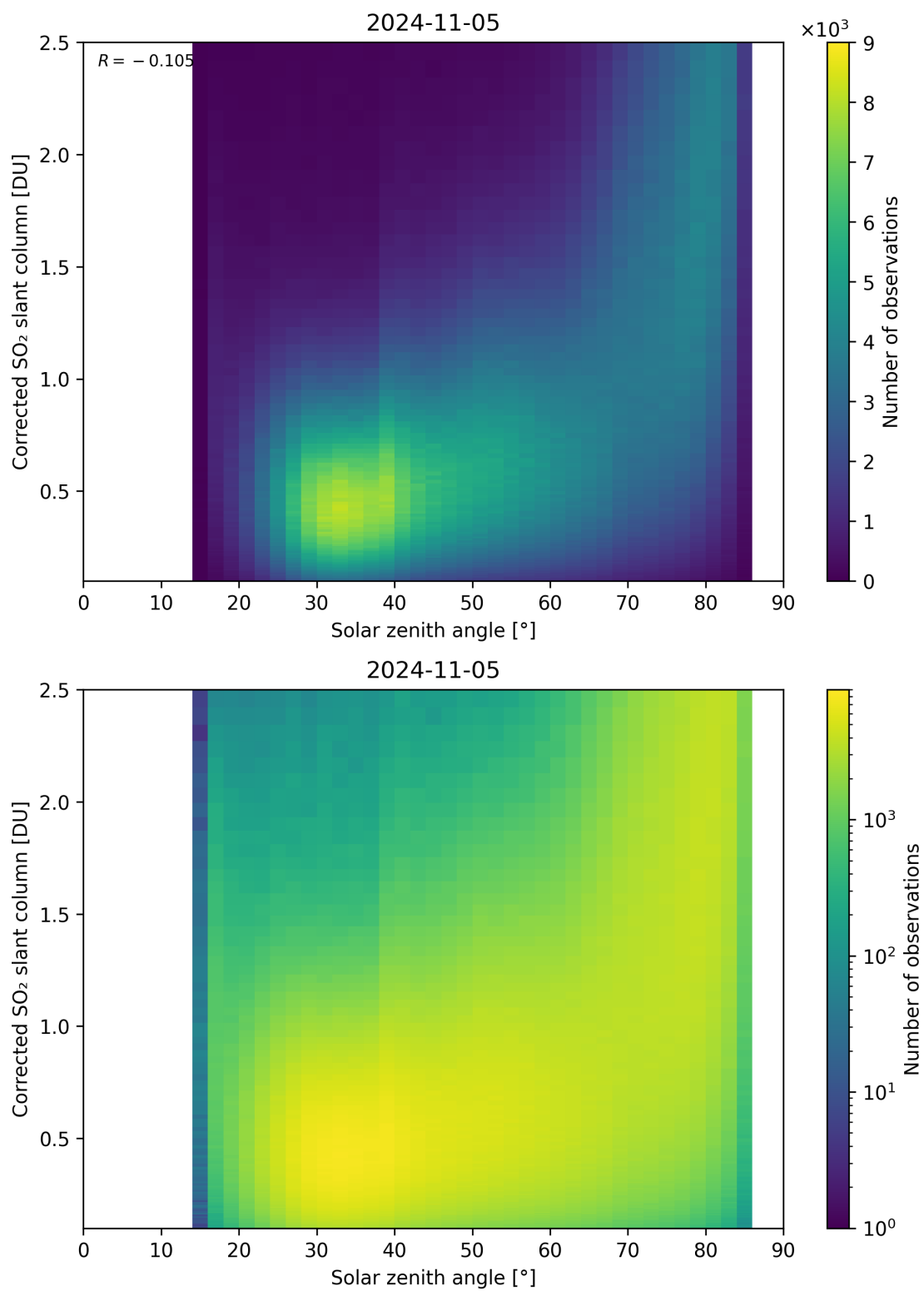
Figure 166: Scatter density plot of “Solar zenith angle” against “Corrected SO 2 slant column” for 2024-11-04 to 2024-11-06.
