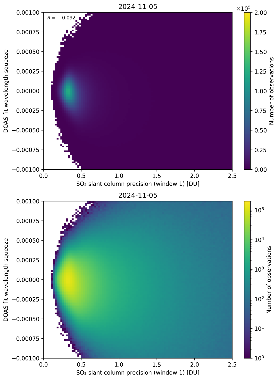
Figure 222: Scatter density plot of “SO 2 slant column precision (window 1)” against “DOAS fit wavelength squeeze” for 2024-11-04 to 2024-11-06.
