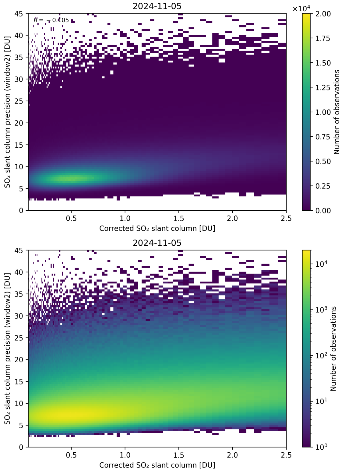
Figure 189: Scatter density plot of “Corrected SO 2 slant column” against “SO 2 slant column precision (window2)” for 2024-11-04 to 2024-11-06.
