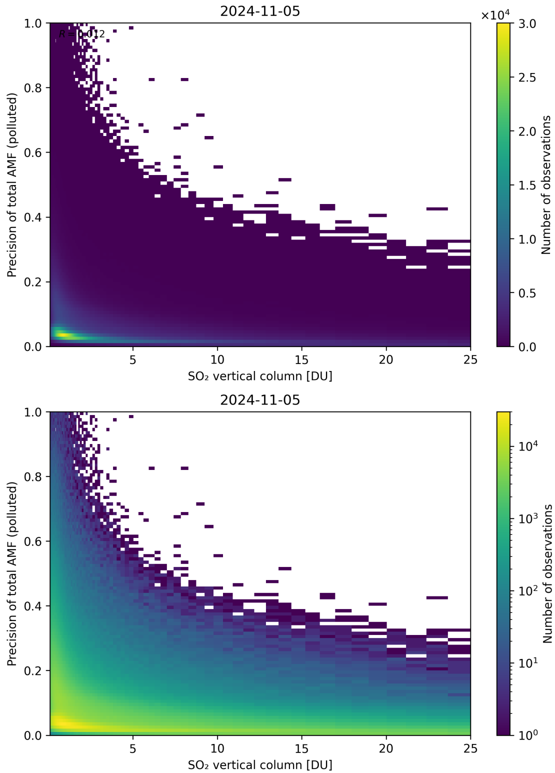
Figure 306: Scatter density plot of “SO 2 vertical column” against “Precision of total AMF (polluted)” for 2024-11-04 to 2024-11-06.
