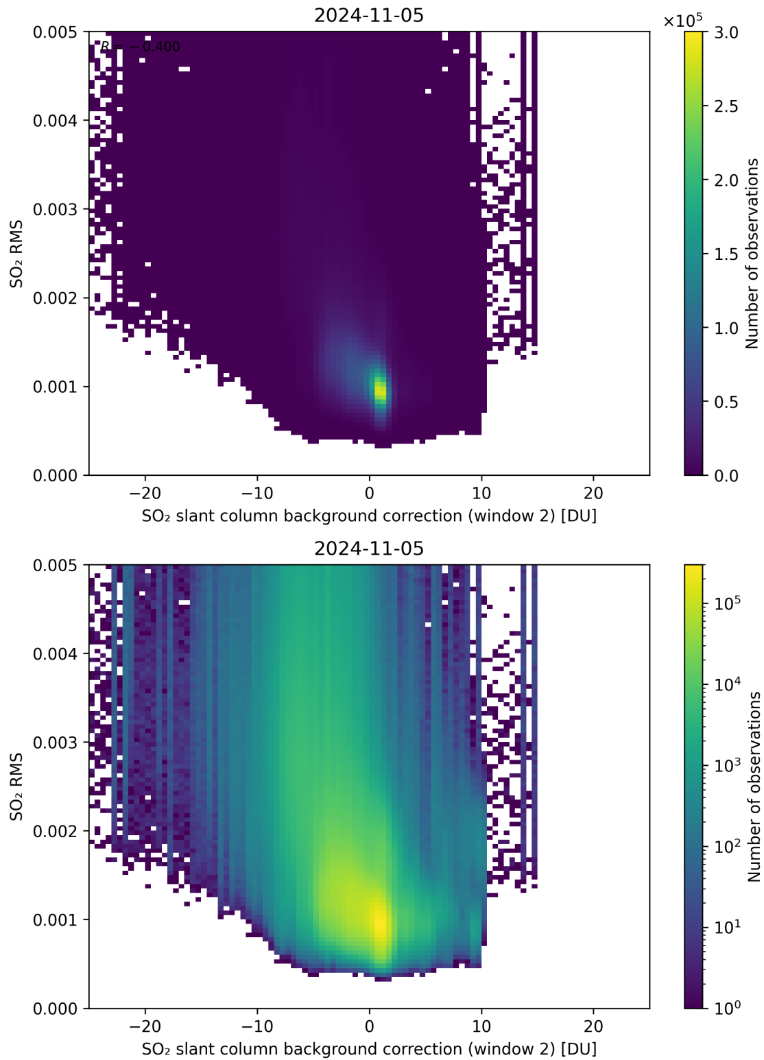
Figure 114: Scatter density plot of “SO 2 slant column background correction (window 2)” against “SO 2 RMS” for 2024-11-04 to 2024-11-06.
