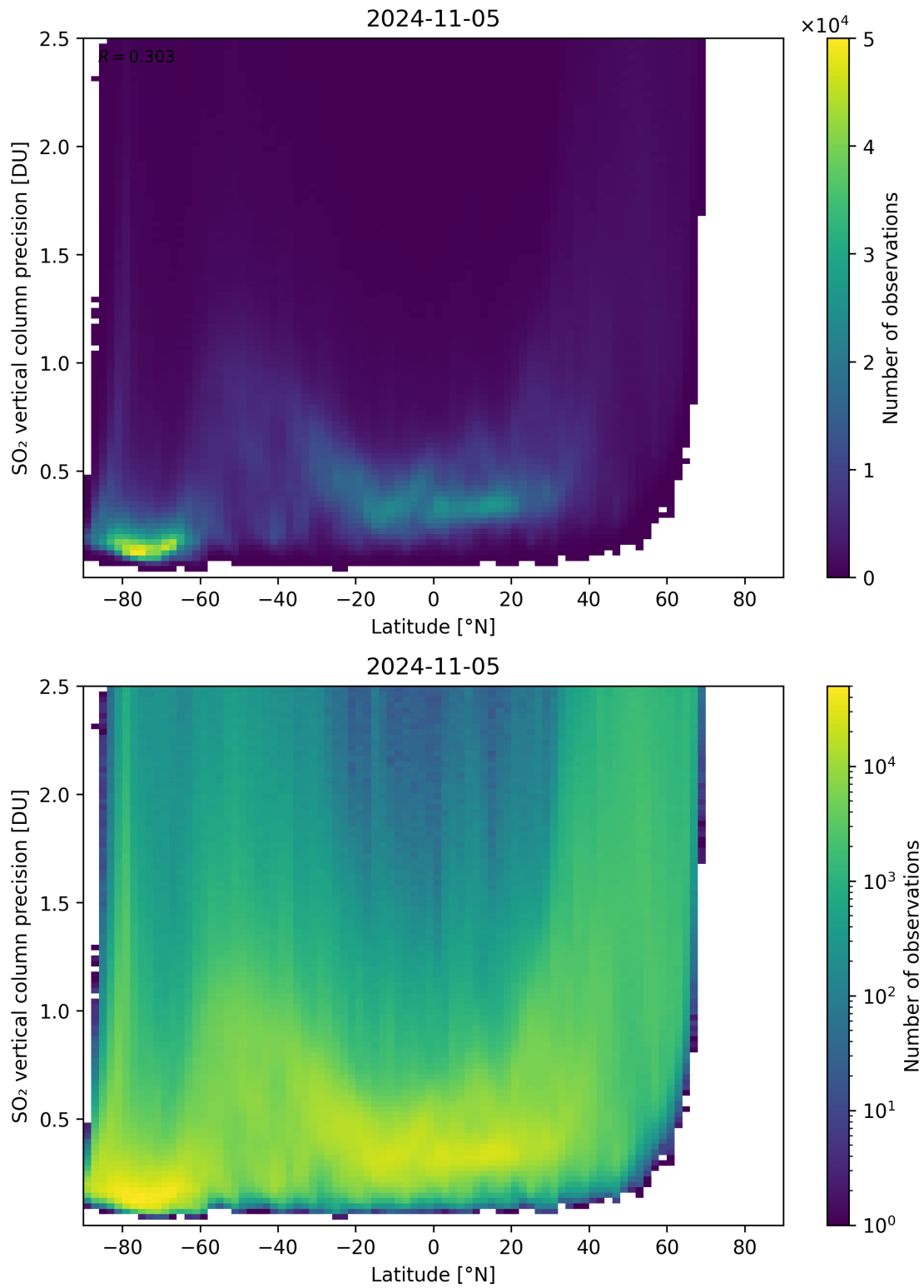
Figure 157: Scatter density plot of “Latitude” against “SO 2 vertical column precision” for 2024-11-04 to 2024-11-06.
