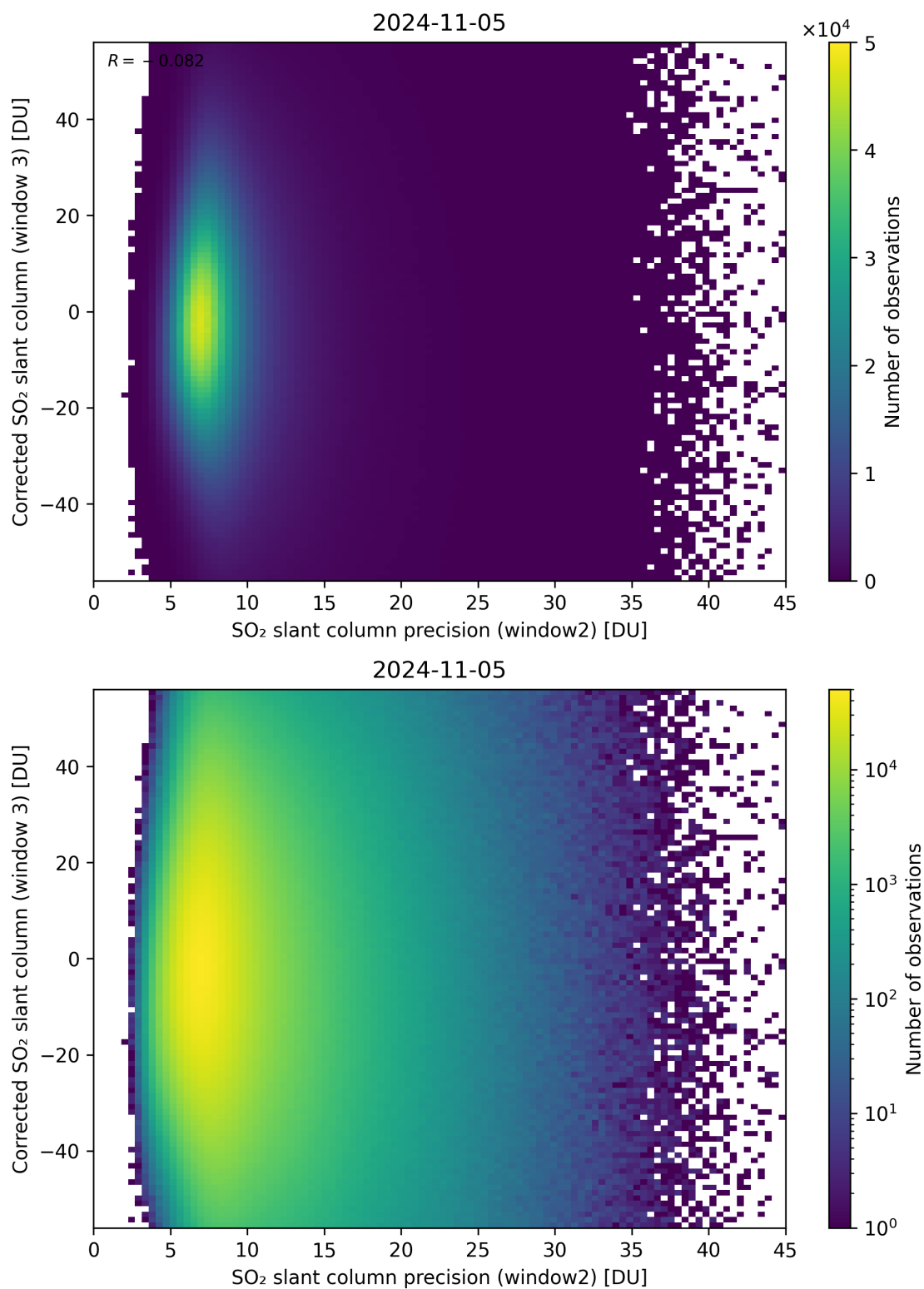
Figure 248: Scatter density plot of “SO 2 slant column precision (window2)” against “Corrected SO 2 slant column (window 3)” for 2024-11-04 to 2024-11-06.
