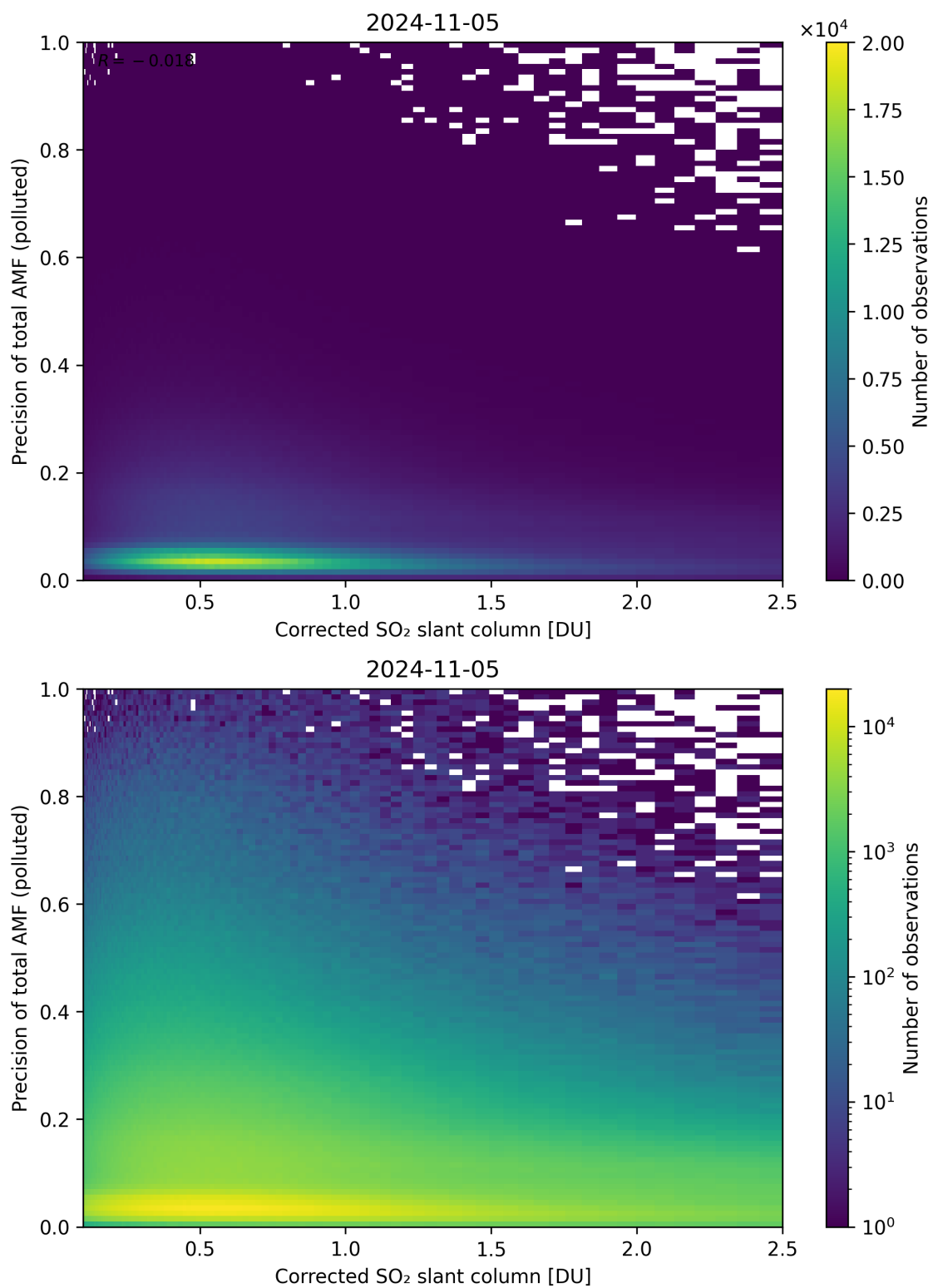
Figure 193: Scatter density plot of “Corrected SO 2 slant column” against “Precision of total AMF (polluted)” for 2024-11-04 to 2024-11-06.
