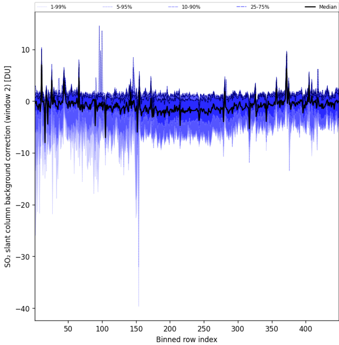
Figure 86: Along track statistics of “SO 2 slant column background correction (window 2)” for 2024-11-04 to 2024-11-06
