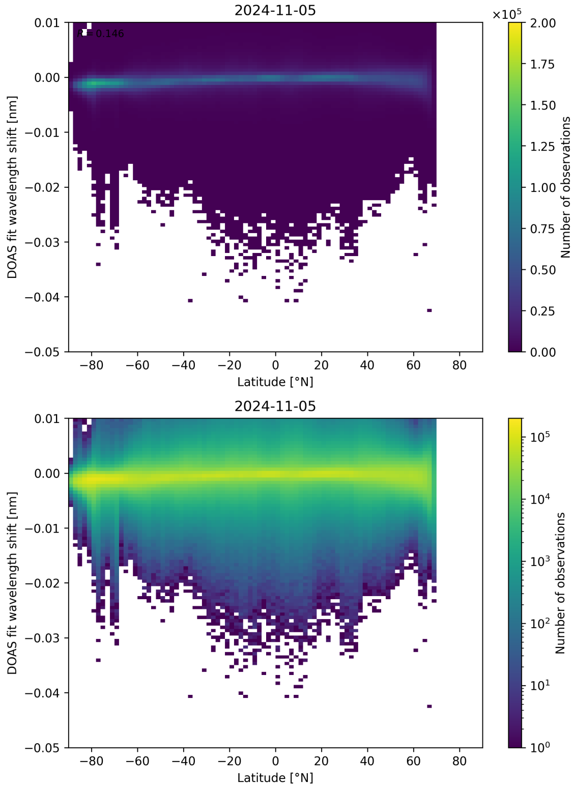
Figure 142: Scatter density plot of “Latitude” against “DOAS fit wavelength shift” for 2024-11-04 to 2024-11-06.
