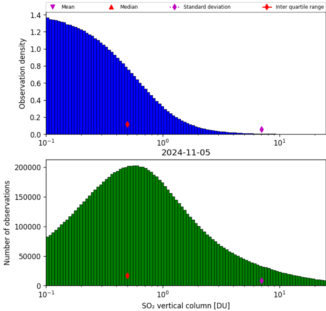
Figure 53: Histogram of “SO 2 vertical column” for 2024-11-04 to 2024-11-06
