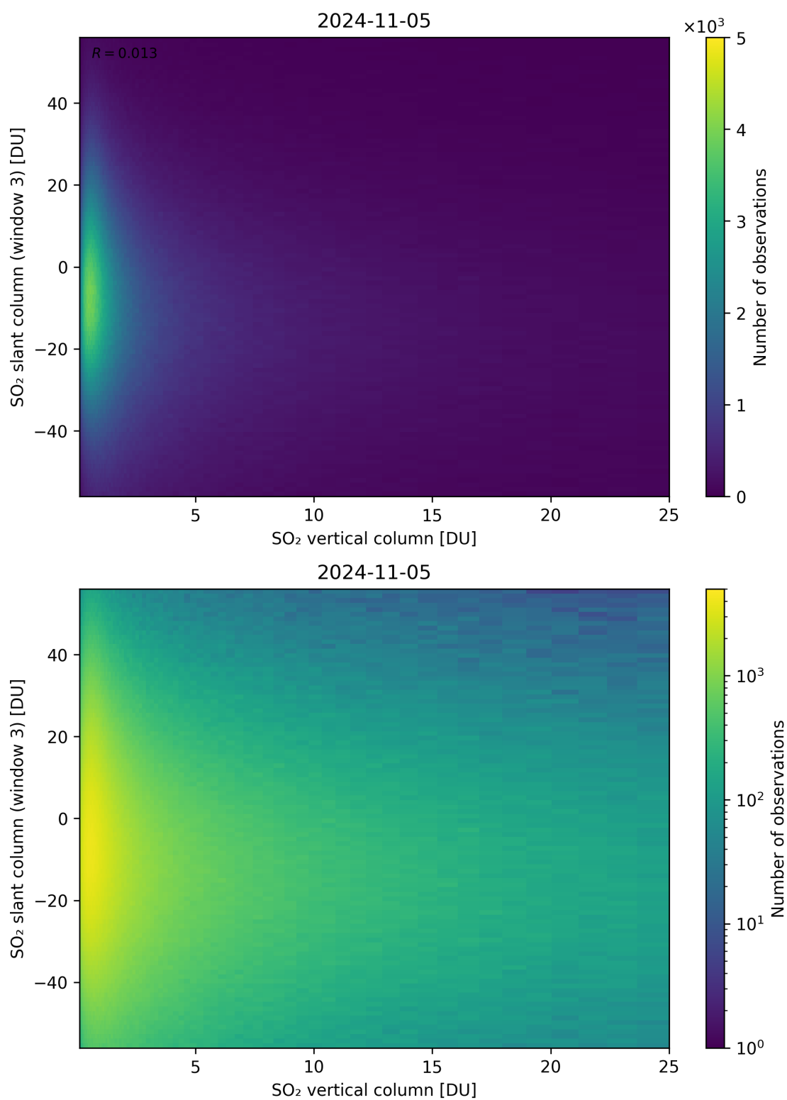
Figure 303: Scatter density plot of “SO 2 vertical column” against “SO 2 slant column (window 3)” for 2024-11-04 to 2024-11-06.
