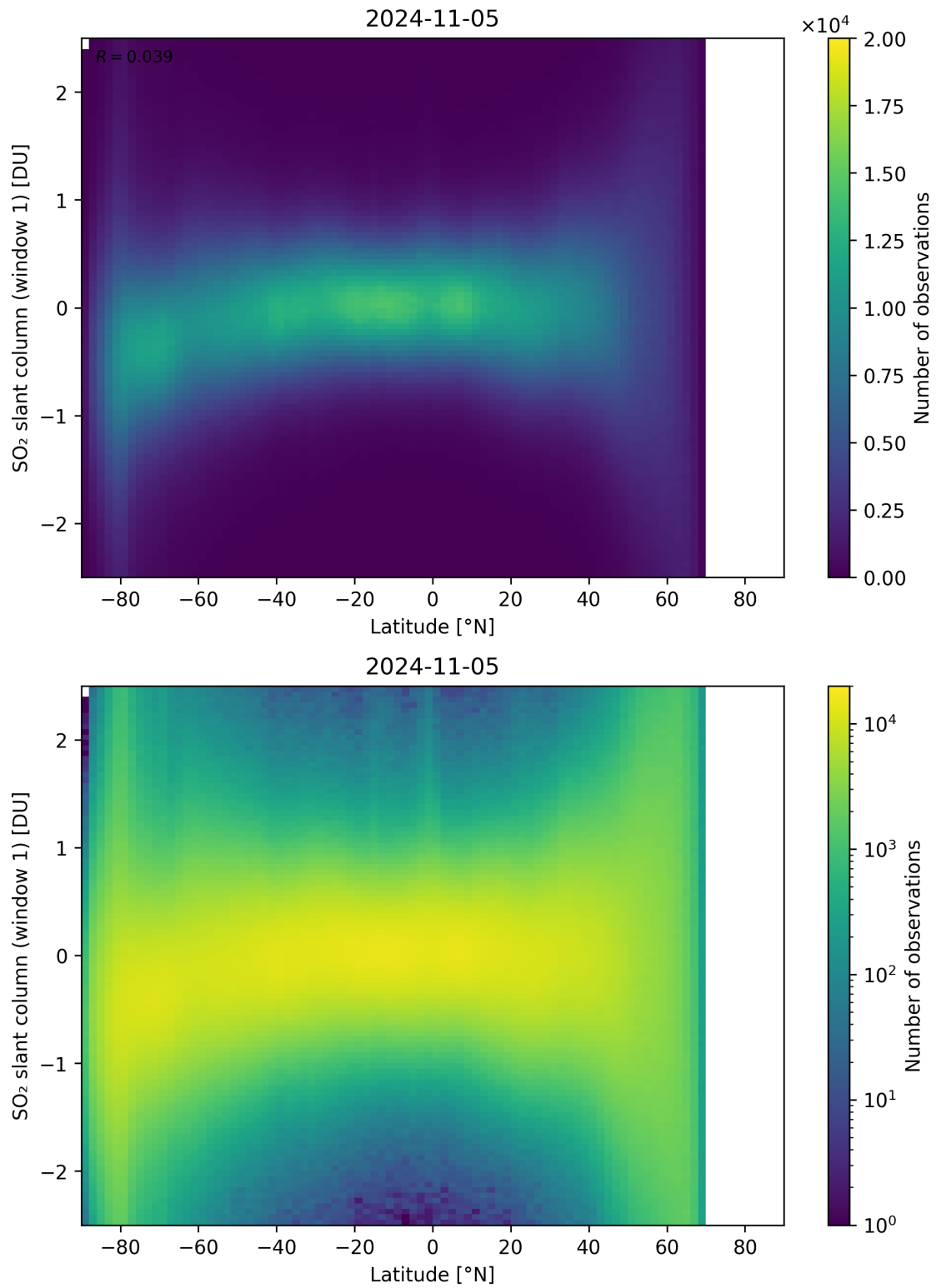
Figure 149: Scatter density plot of “Latitude” against “SO 2 slant column (window 1)” for 2024-11-04 to 2024-11-06.
