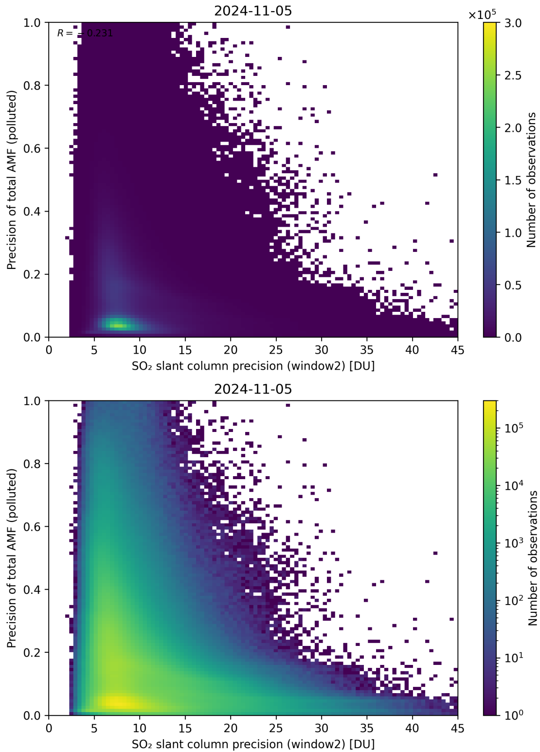
Figure 252: Scatter density plot of “SO 2 slant column precision (window2)” against “Precision of total AMF (polluted)” for 2024-11-04 to 2024-11-06.
