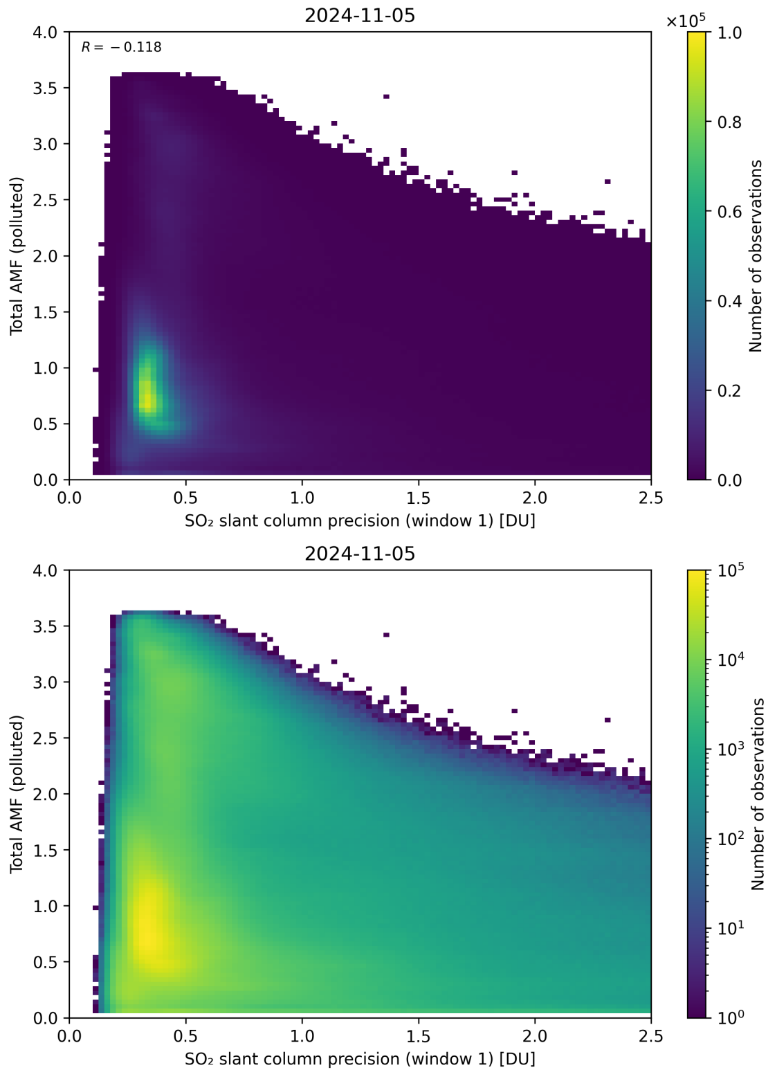
Figure 230: Scatter density plot of “SO 2 slant column precision (window 1)” against “Total AMF (polluted)” for 2024-11-04 to 2024-11-06.
