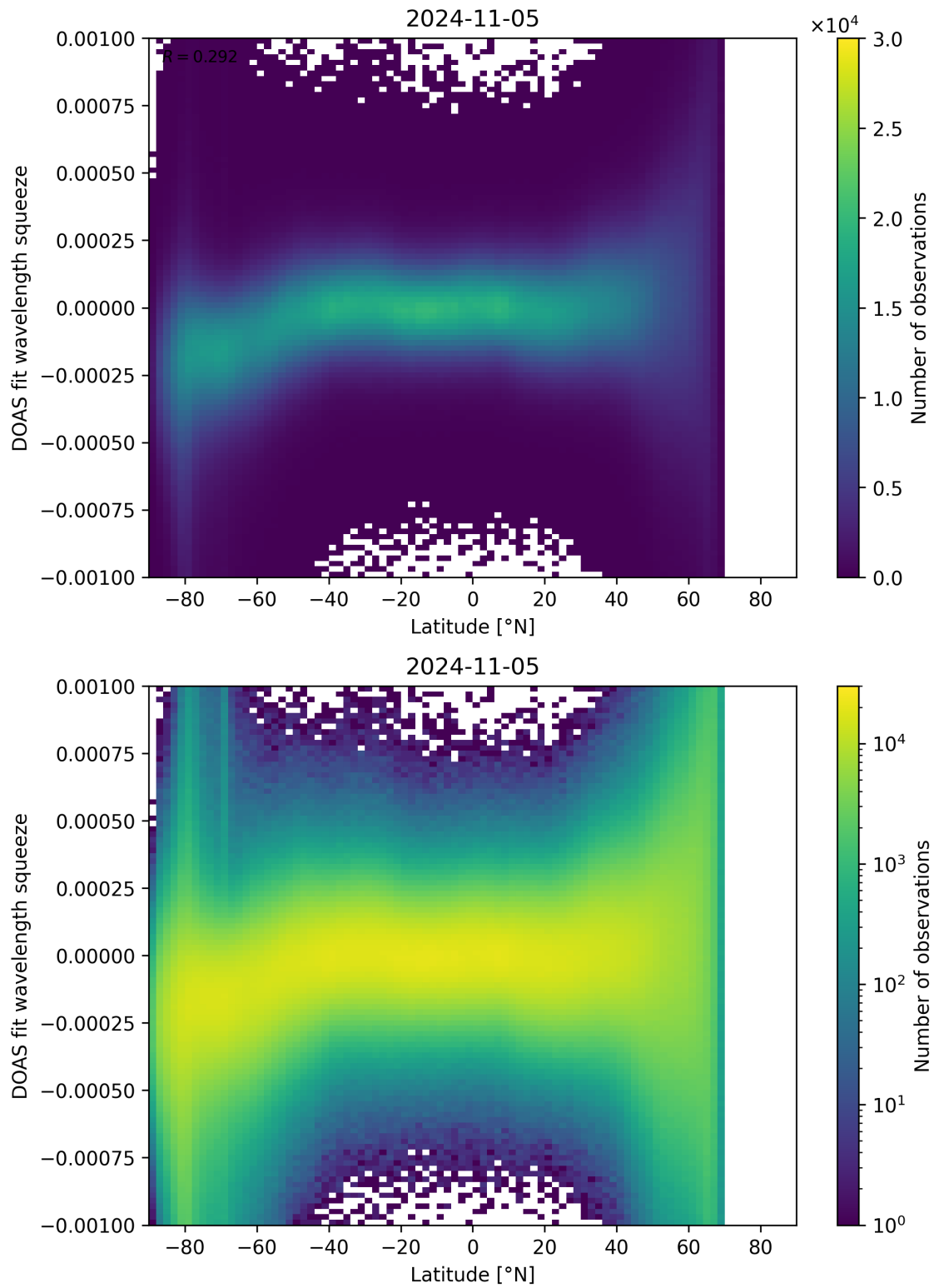
Figure 143: Scatter density plot of “Latitude” against “DOAS fit wavelength squeeze” for 2024-11-04 to 2024-11-06.
