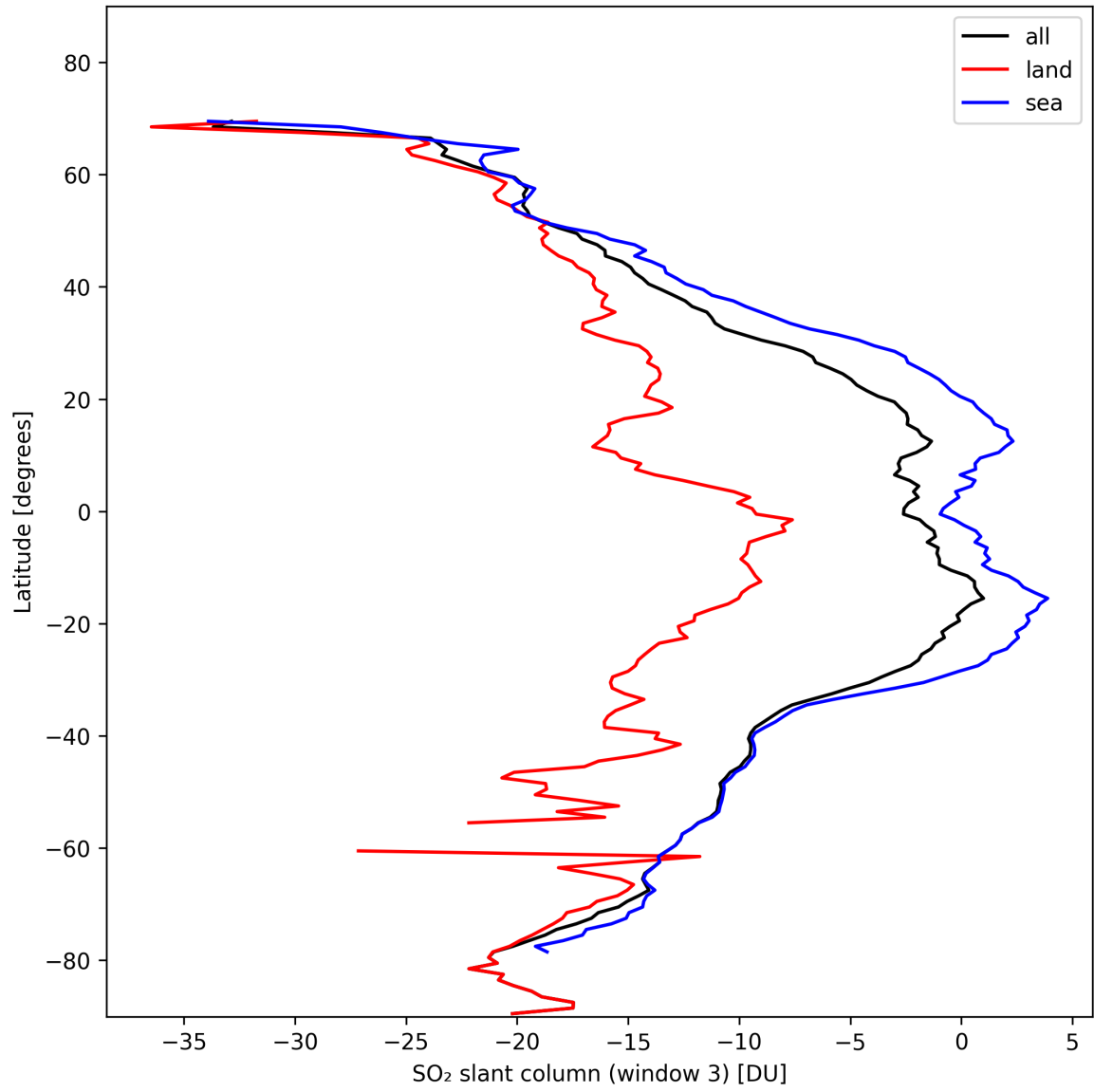
Figure 41: Zonal average of “SO 2 slant column (window 3)” for 2024-11-04 to 2024-11-06.
