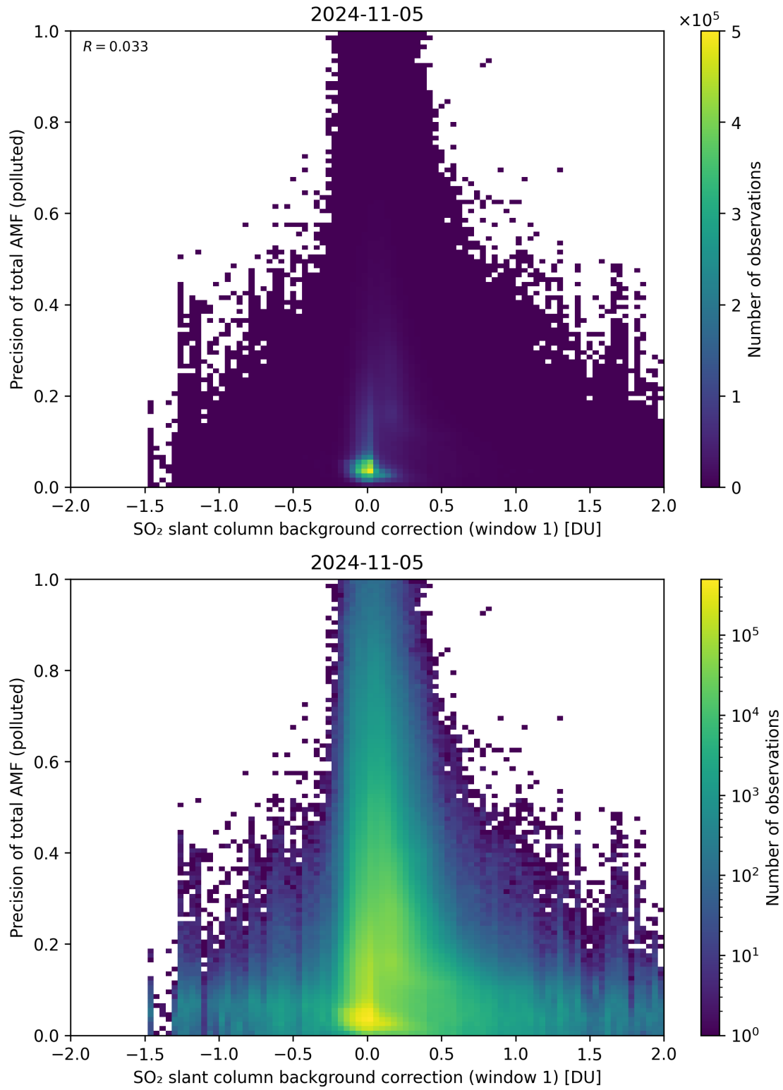
Figure 110: Scatter density plot of “SO 2 slant column background correction (window 1)” against “Precision of total AMF (polluted)” for 2024-11-04 to 2024-11-06.
