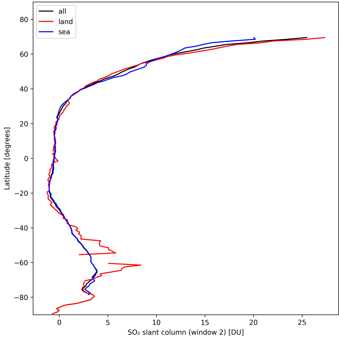
Figure 37: Zonal average of “SO 2 slant column (window 2)” for 2024-11-04 to 2024-11-06.
