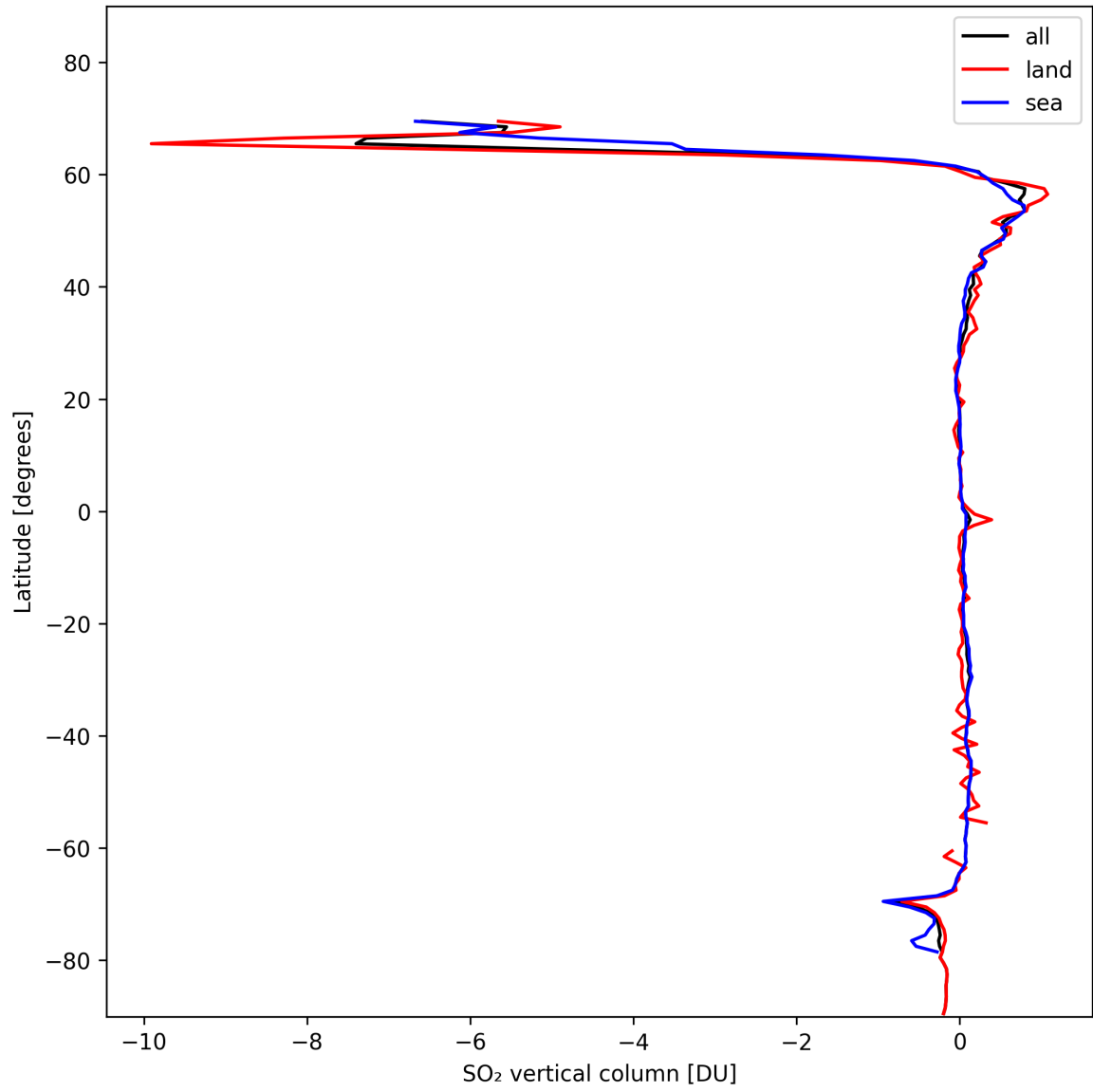
Figure 30: Zonal average of “SO 2 vertical column” for 2024-11-04 to 2024-11-06.
