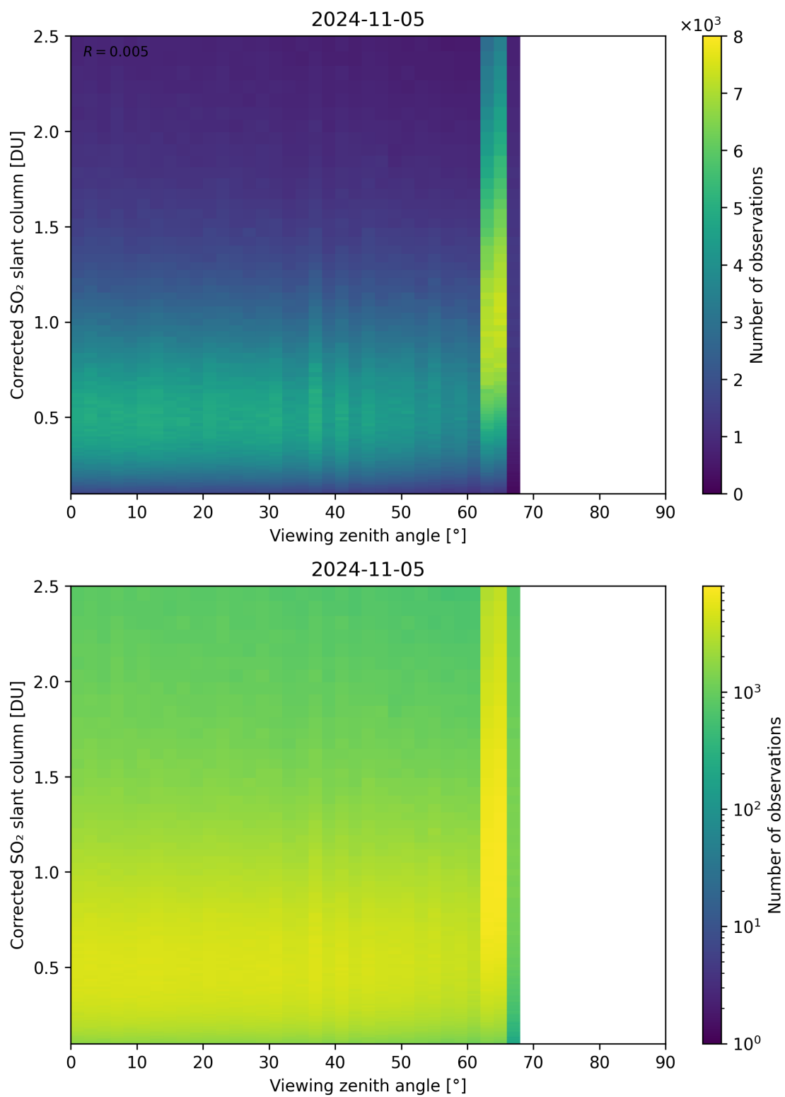
Figure 317: Scatter density plot of “Viewing zenith angle” against “Corrected SO 2 slant column” for 2024-11-04 to 2024-11-06.
