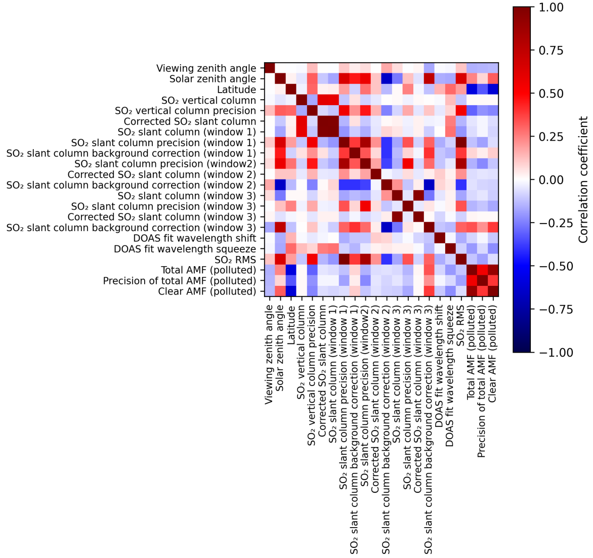
Figure 2: Map of correlation matrix for 2024-11-04 to 2024-11-06.
