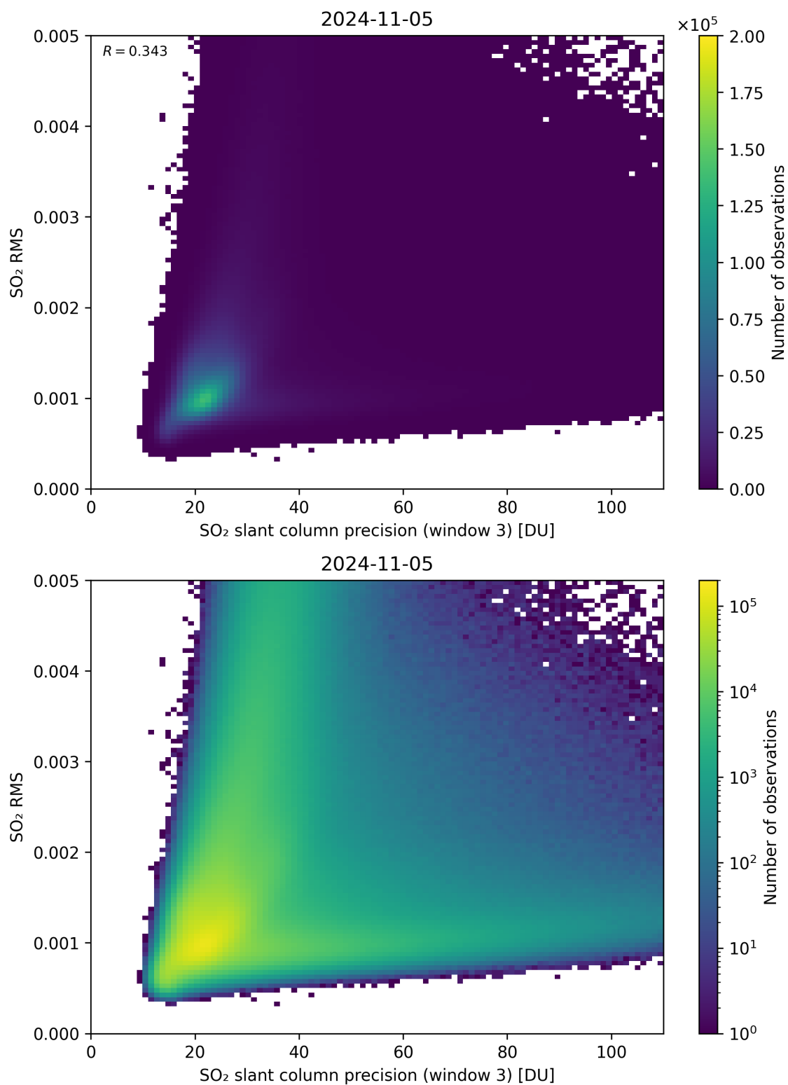
Figure 260: Scatter density plot of “SO 2 slant column precision (window 3)” against “SO 2 RMS” for 2024-11-04 to 2024-11-06.
