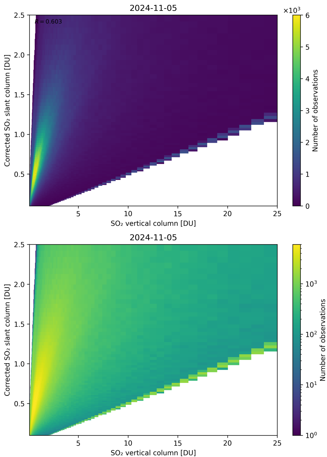
Figure 297: Scatter density plot of “SO 2 vertical column” against “Corrected SO 2 slant column” for 2024-11-04 to 2024-11-06.
