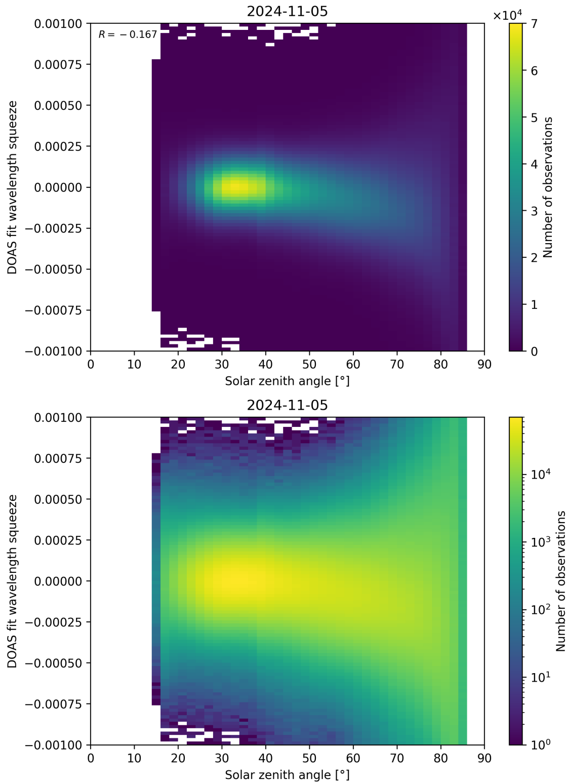
Figure 162: Scatter density plot of “Solar zenith angle” against “DOAS fit wavelength squeeze” for 2024-11-04 to 2024-11-06.
