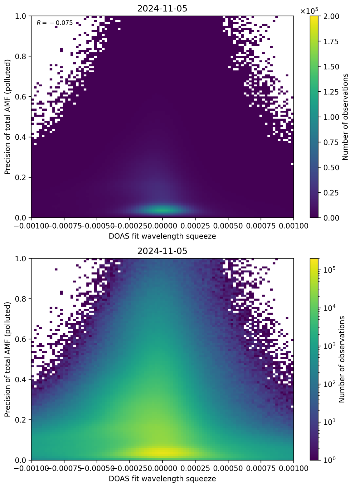
Figure 135: Scatter density plot of “DOAS fit wavelength squeeze” against “Precision of total AMF (polluted)” for 2024-11-04 to 2024-11-06.
