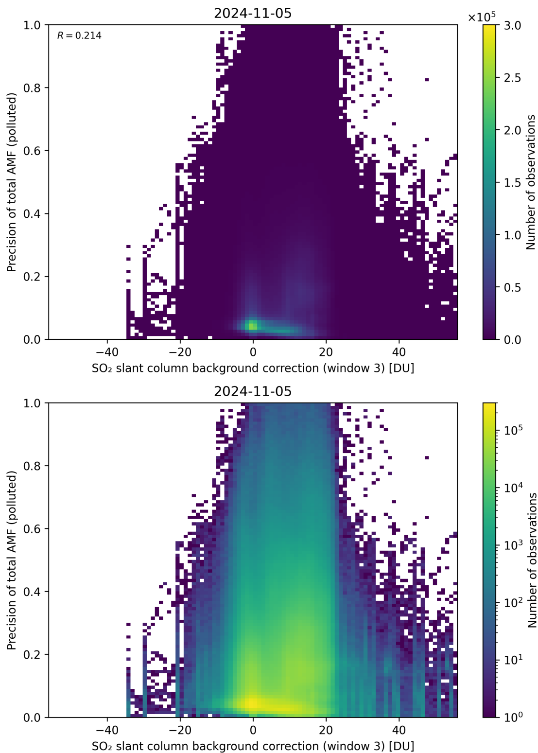
Figure 126: Scatter density plot of “SO 2 slant column background correction (window 3)” against “Precision of total AMF (polluted)” for 2024-11-04 to 2024-11-06.
