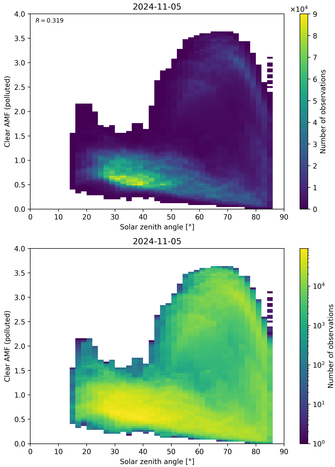
Figure 165: Scatter density plot of “Solar zenith angle” against “Clear AMF (polluted)” for 2024-11-04 to 2024-11-06.
