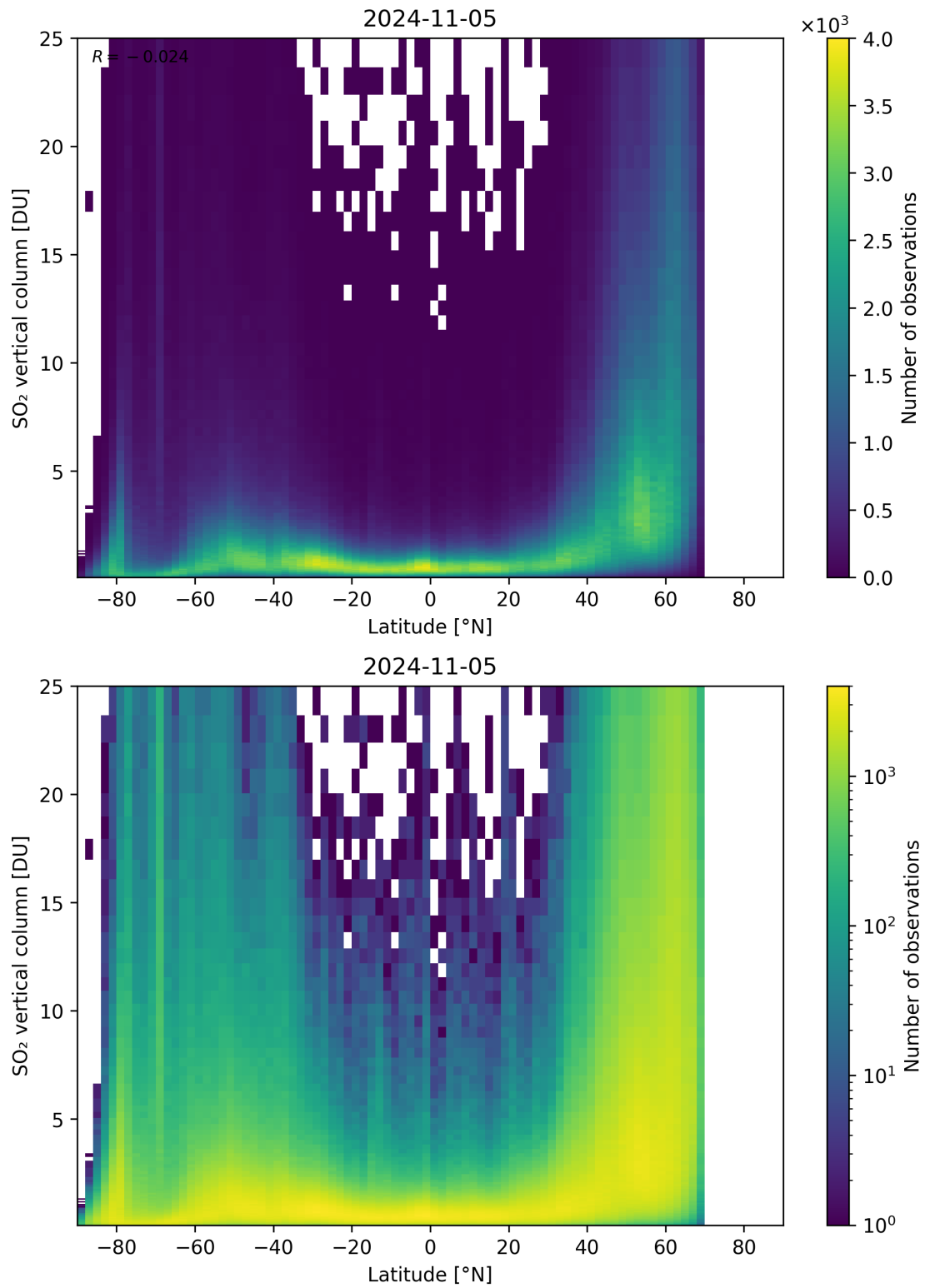
Figure 156: Scatter density plot of “Latitude” against “SO 2 vertical column” for 2024-11-04 to 2024-11-06.
