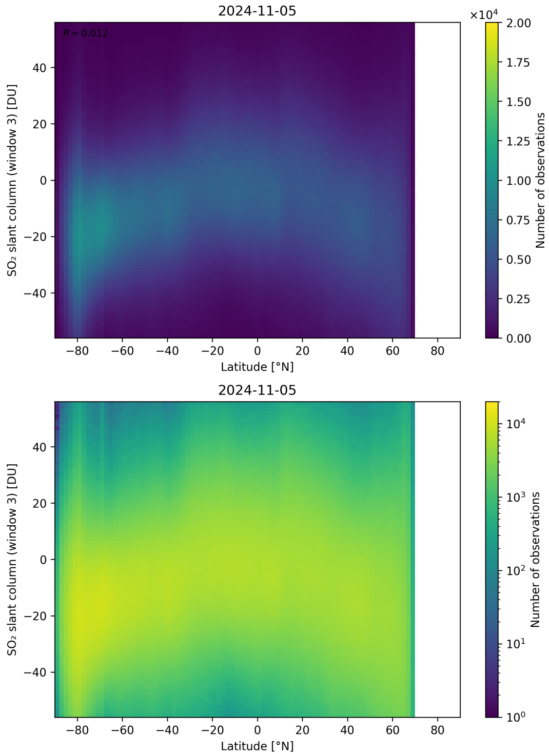
Figure 152: Scatter density plot of “Latitude” against “SO 2 slant column (window 3)” for 2024-11-04 to 2024-11-06.
