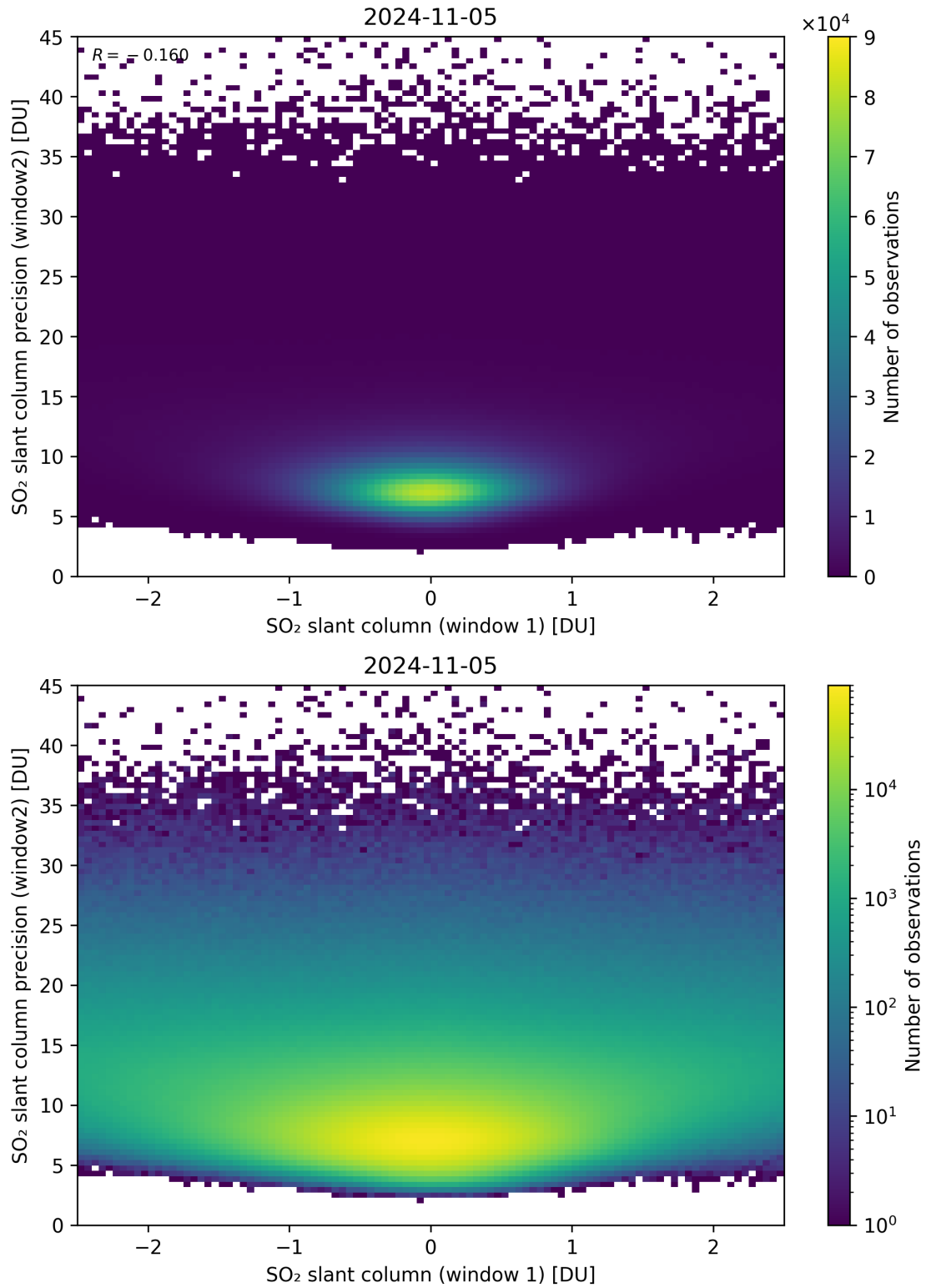
Figure 236: Scatter density plot of “SO 2 slant column (window 1)” against “SO 2 slant column precision (window2)” for 2024-11-04 to 2024-11-06.
