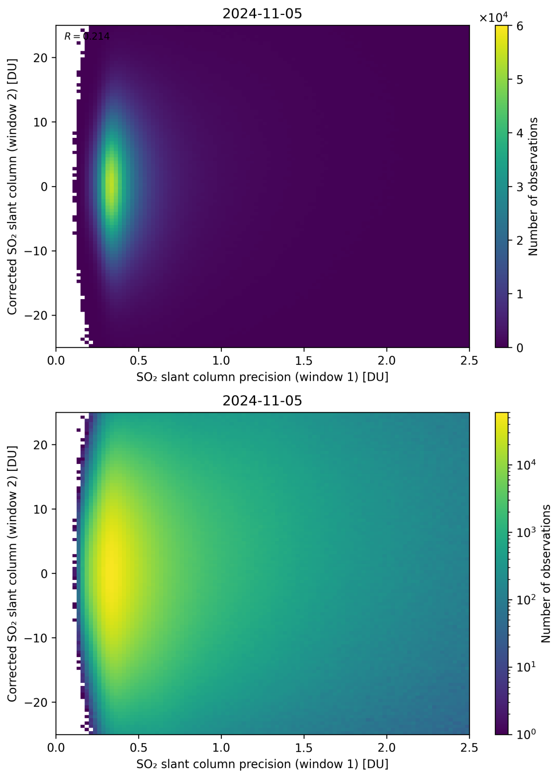
Figure 225: Scatter density plot of “SO 2 slant column precision (window 1)” against “Corrected SO 2 slant column (window 2)” for 2024-11-04 to 2024-11-06.
