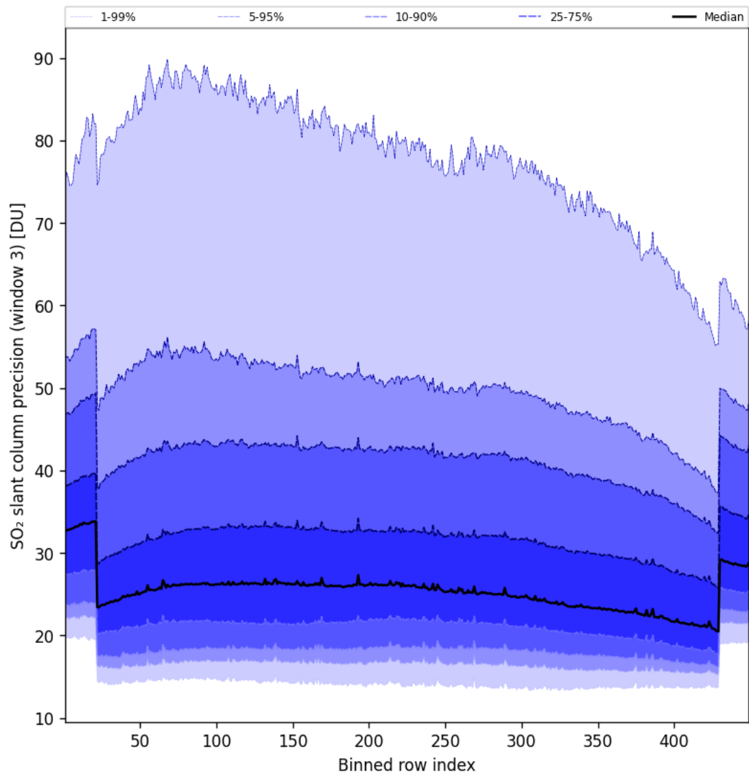
Figure 88: Along track statistics of “SO 2 slant column precision (window 3)” for 2024-11-04 to 2024-11-06
