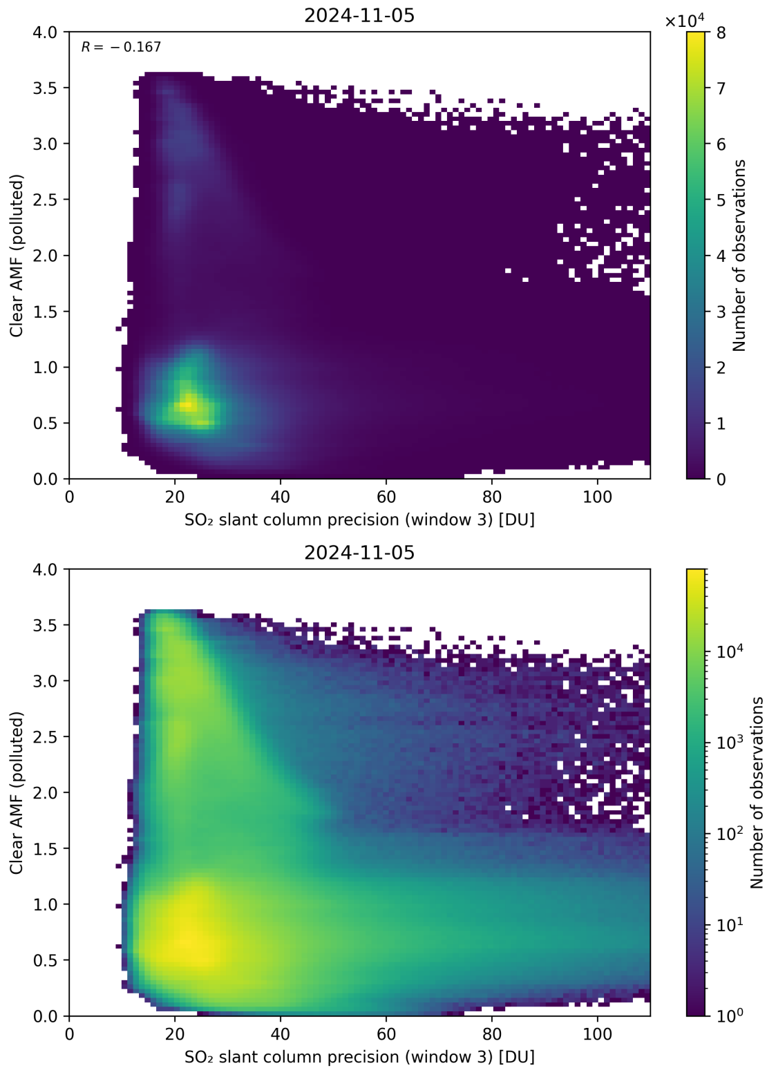
Figure 261: Scatter density plot of “SO 2 slant column precision (window 3)” against “Clear AMF (polluted)” for 2024-11-04 to 2024-11-06.
