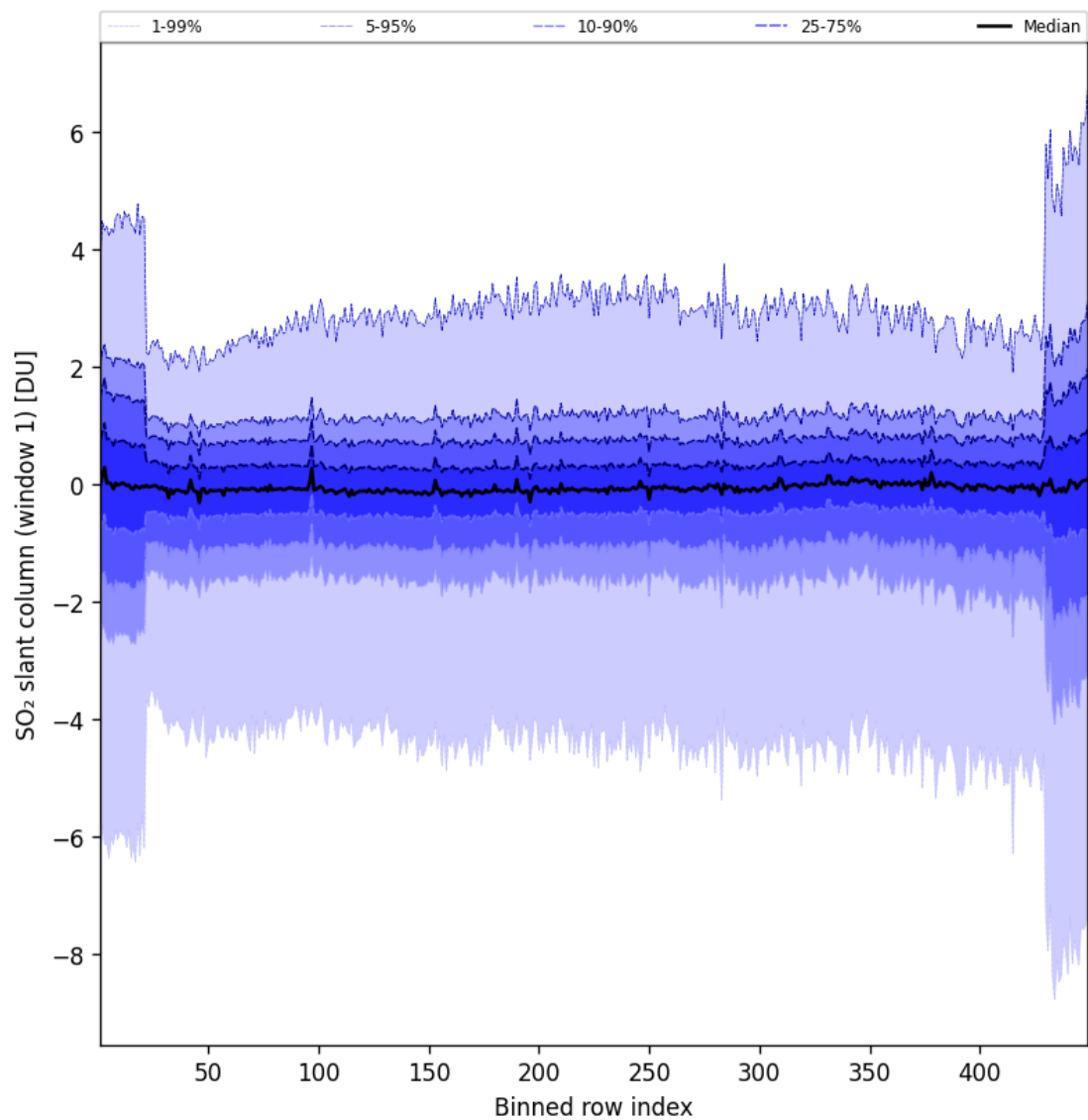
Figure 79: Along track statistics of “SO 2 slant column (window 1)” for 2024-11-04 to 2024-11-06
