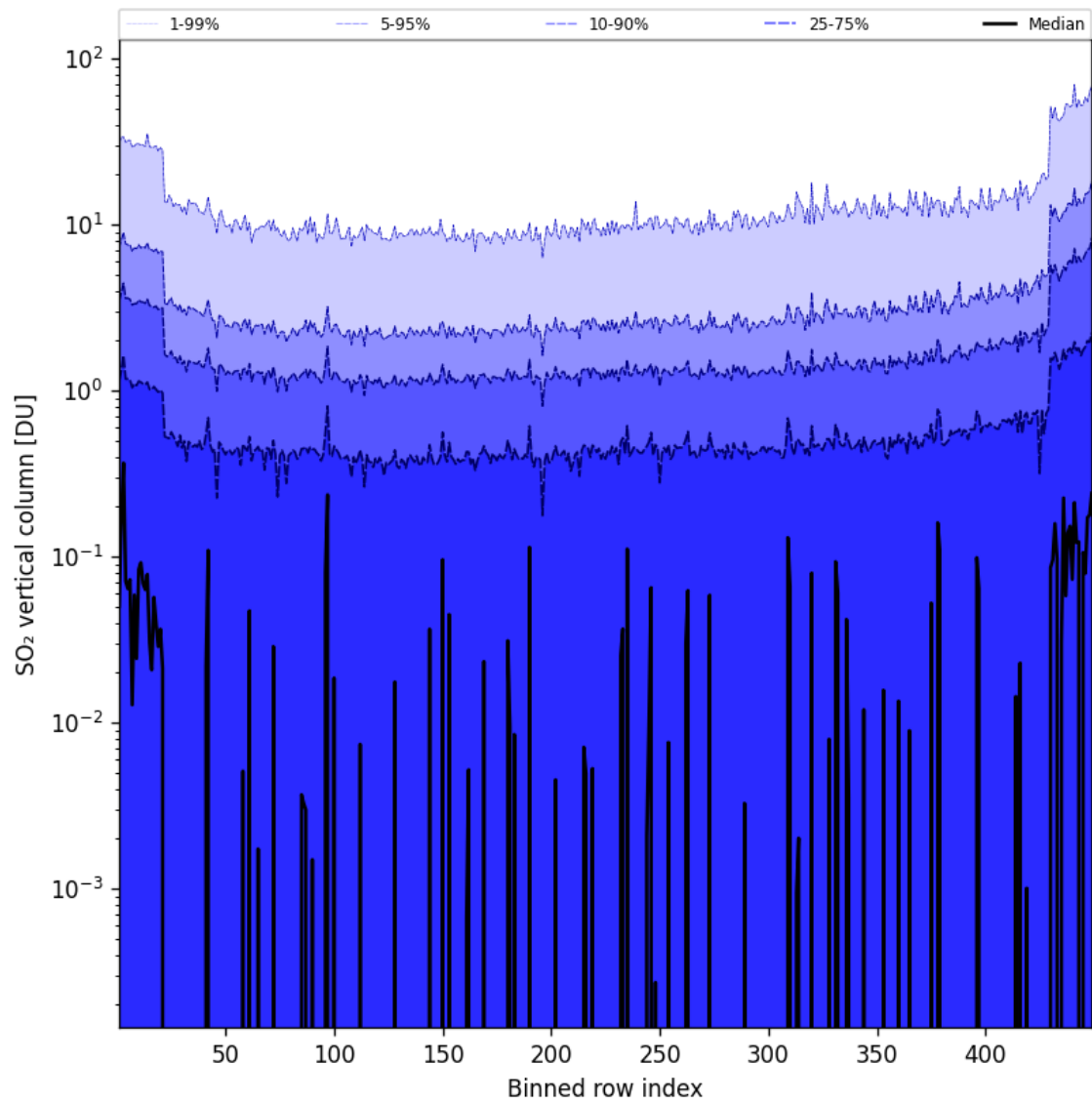
Figure 76: Along track statistics of “SO 2 vertical column” for 2024-11-04 to 2024-11-06
