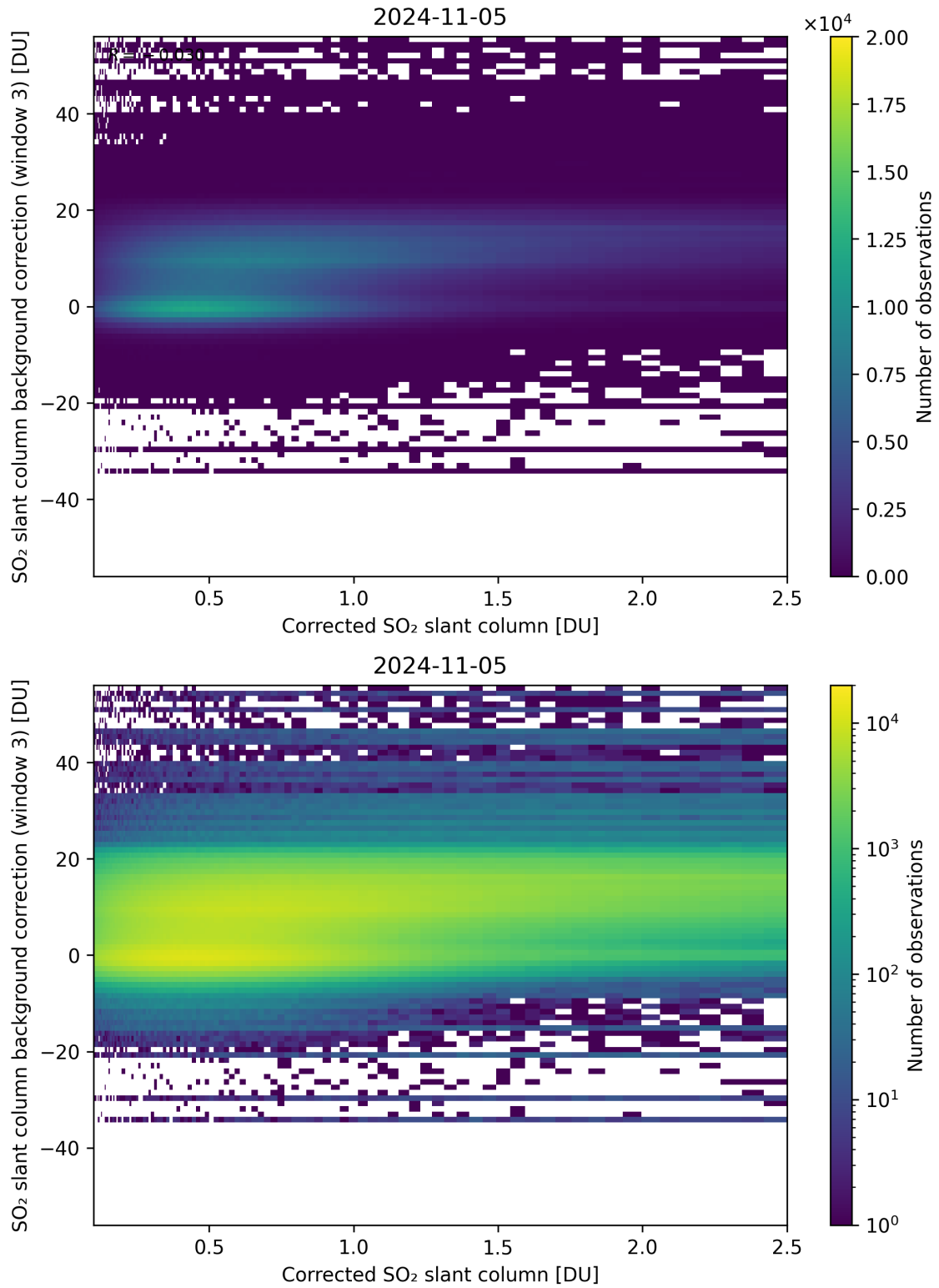
Figure 180: Scatter density plot of “Corrected SO 2 slant column” against “SO 2 slant column background correction (window 3)” for 2024-11-04 to 2024-11-06.
