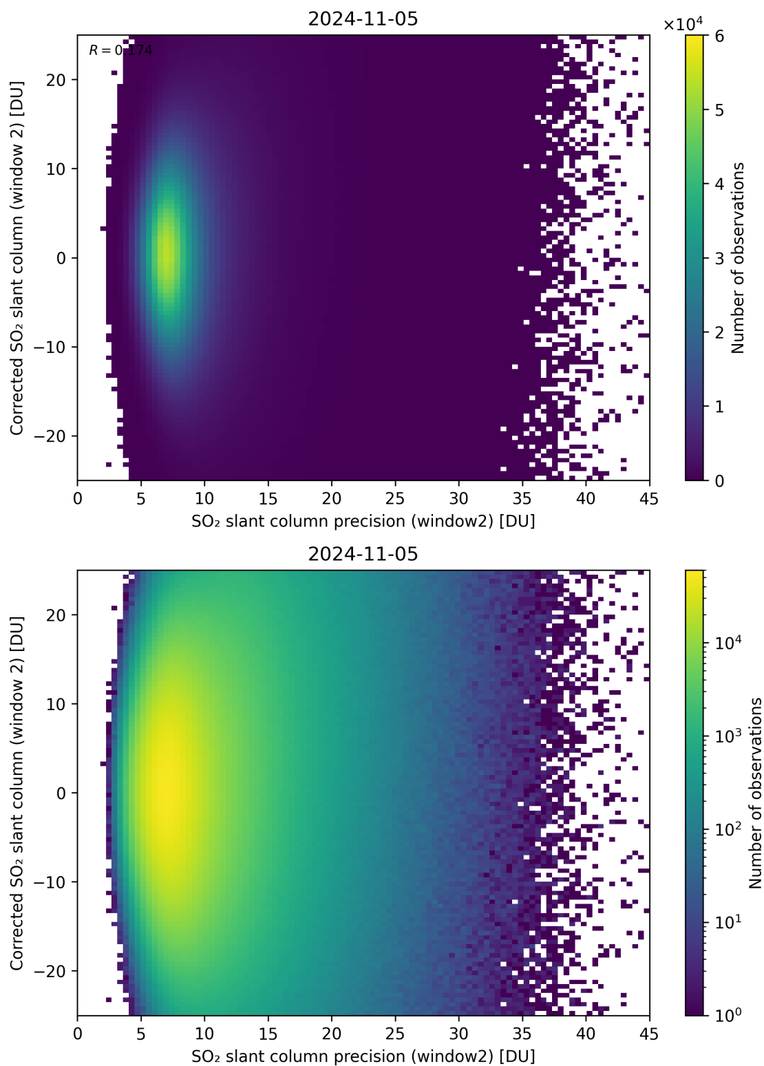
Figure 247: Scatter density plot of “SO 2 slant column precision (window2)” against “Corrected SO 2 slant column (window 2)” for 2024-11-04 to 2024-11-06.
