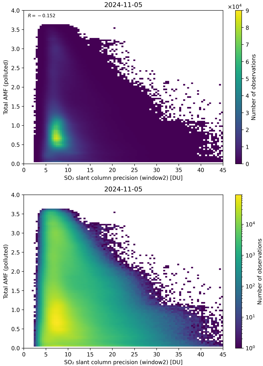
Figure 251: Scatter density plot of “SO 2 slant column precision (window2)” against “Total AMF (polluted)” for 2024-11-04 to 2024-11-06.
