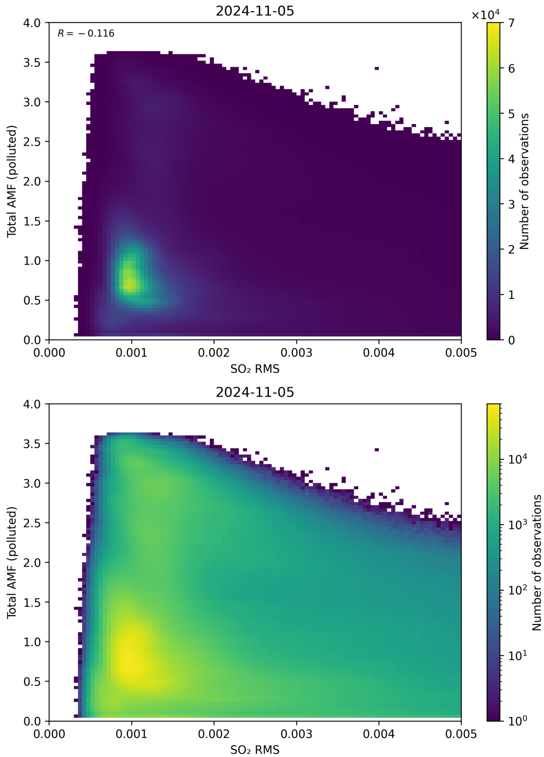
Figure 137: Scatter density plot of “SO 2 RMS” against “Total AMF (polluted)” for 2024-11-04 to 2024-11-06.
