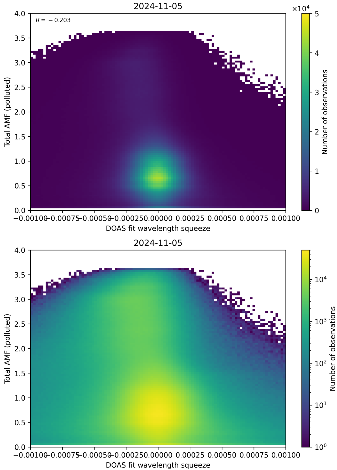
Figure 134: Scatter density plot of “DOAS fit wavelength squeeze” against “Total AMF (polluted)” for 2024-11-04 to 2024-11-06.
