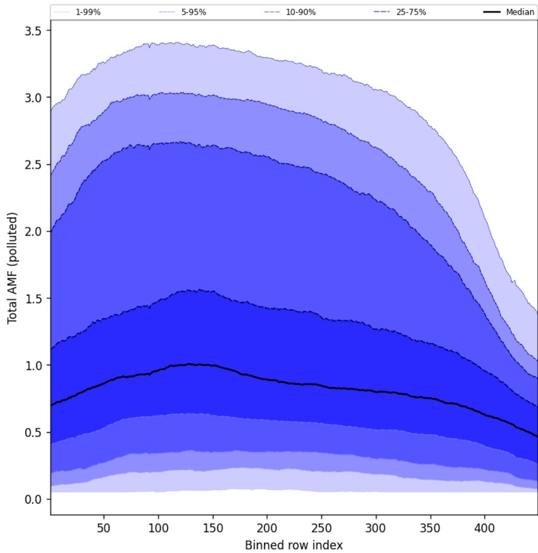
Figure 94: Along track statistics of “Total AMF (polluted)” for 2024-11-04 to 2024-11-06
