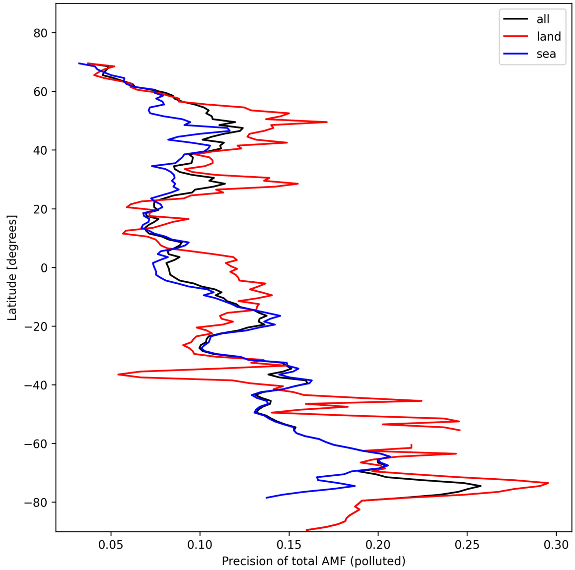
Figure 49: Zonal average of “Precision of total AMF (polluted)” for 2024-11-04 to 2024-11-06.
