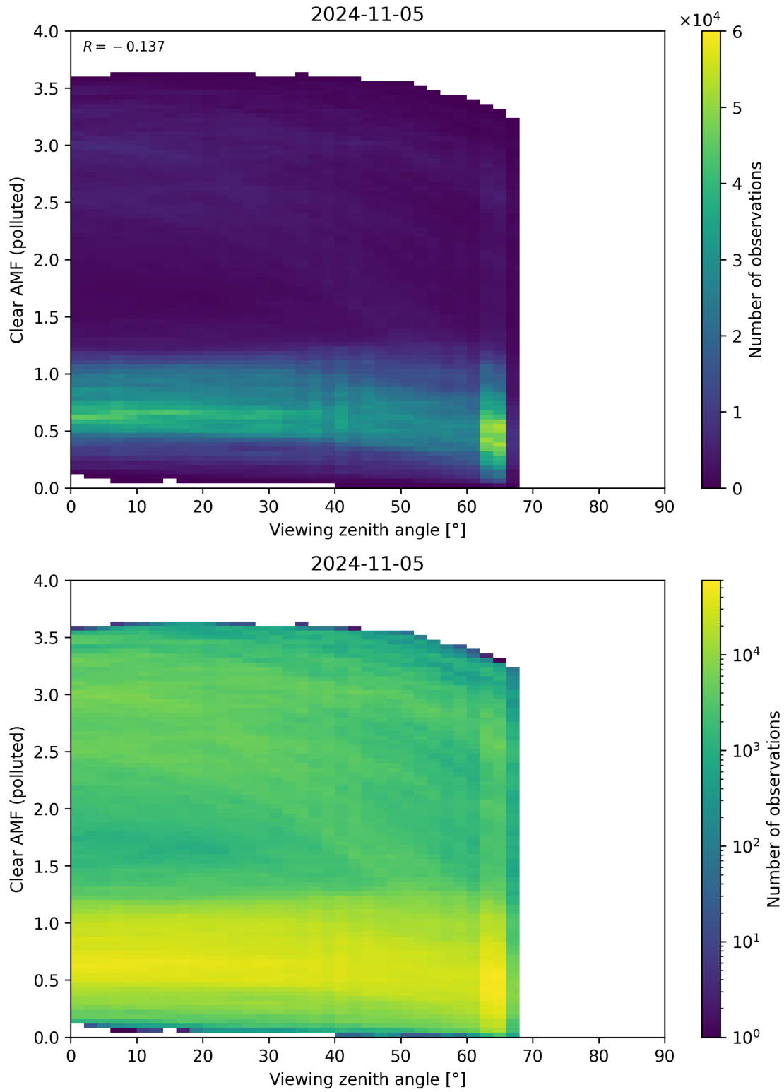
Figure 316: Scatter density plot of “Viewing zenith angle” against “Clear AMF (polluted)” for 2024-11-04 to 2024-11-06.
