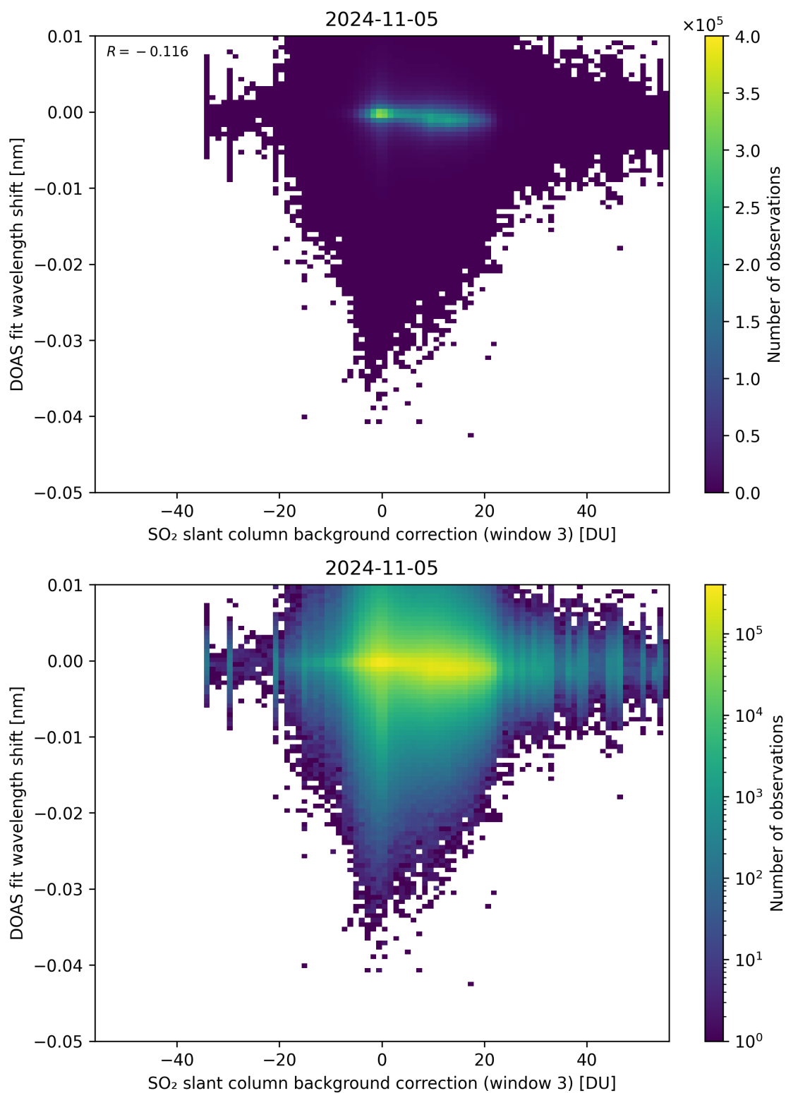
Figure 121: Scatter density plot of “SO 2 slant column background correction (window 3)” against “DOAS fit wavelength shift” for 2024-11-04 to 2024-11-06.
