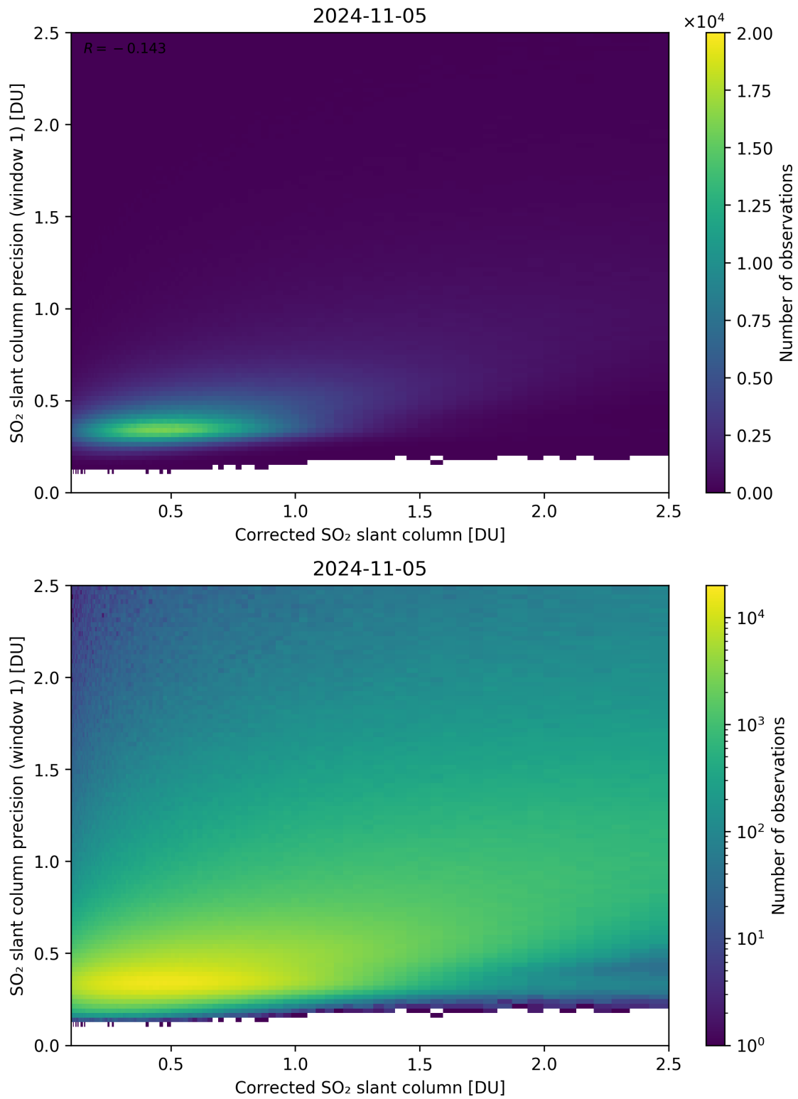
Figure 188: Scatter density plot of “Corrected SO 2 slant column” against “SO 2 slant column precision (window 1)” for 2024-11-04 to 2024-11-06.
