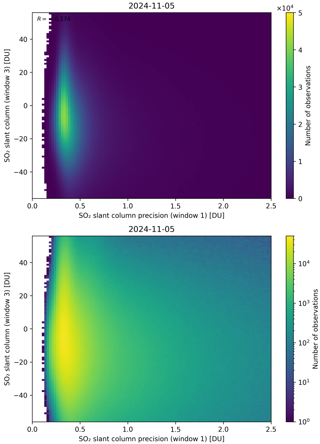
Figure 228: Scatter density plot of “SO 2 slant column precision (window 1)” against “SO 2 slant column (window 3)” for 2024-11-04 to 2024-11-06.
