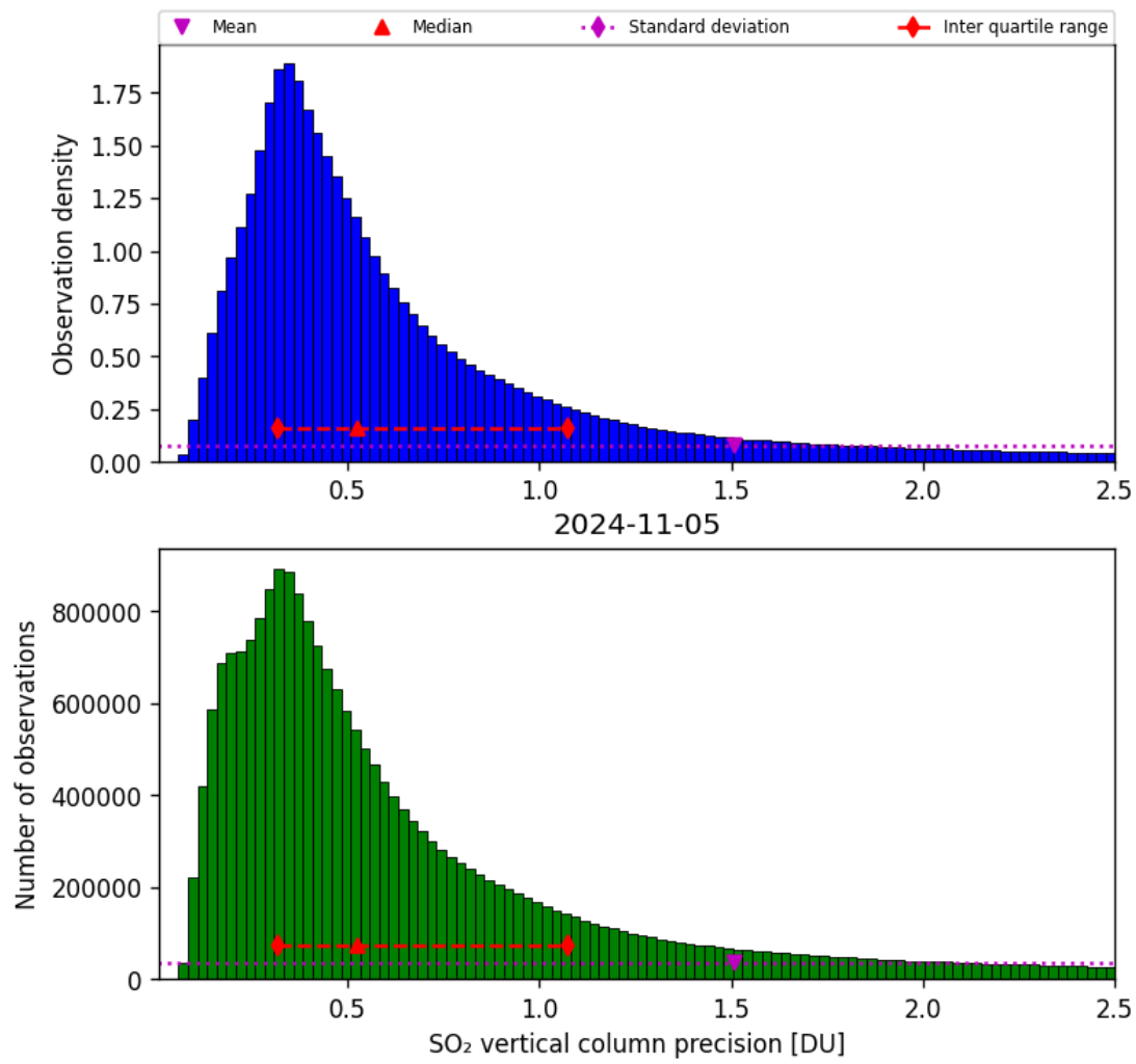
Figure 54: Histogram of “SO 2 vertical column precision” for 2024-11-04 to 2024-11-06
