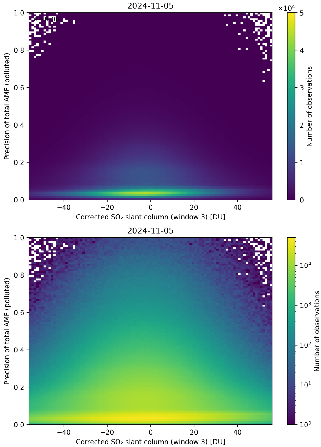
Figure 211: Scatter density plot of “Corrected SO 2 slant column (window 3)” against “Precision of total AMF (polluted)” for 2024-11-04 to 2024-11-06.
