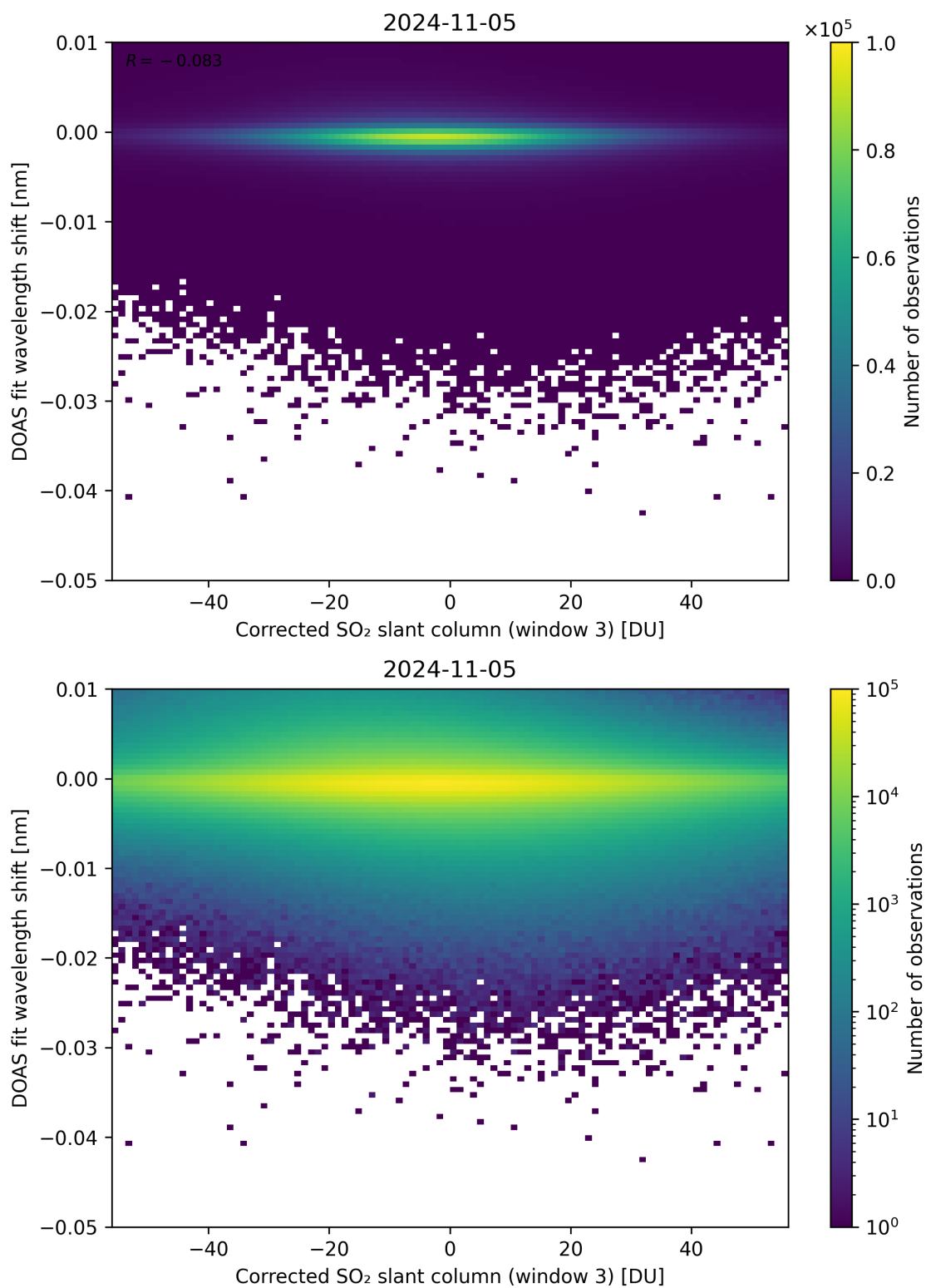
Figure 206: Scatter density plot of “Corrected SO 2 slant column (window 3)” against “DOAS fit wavelength shift” for 2024-11-04 to 2024-11-06.
