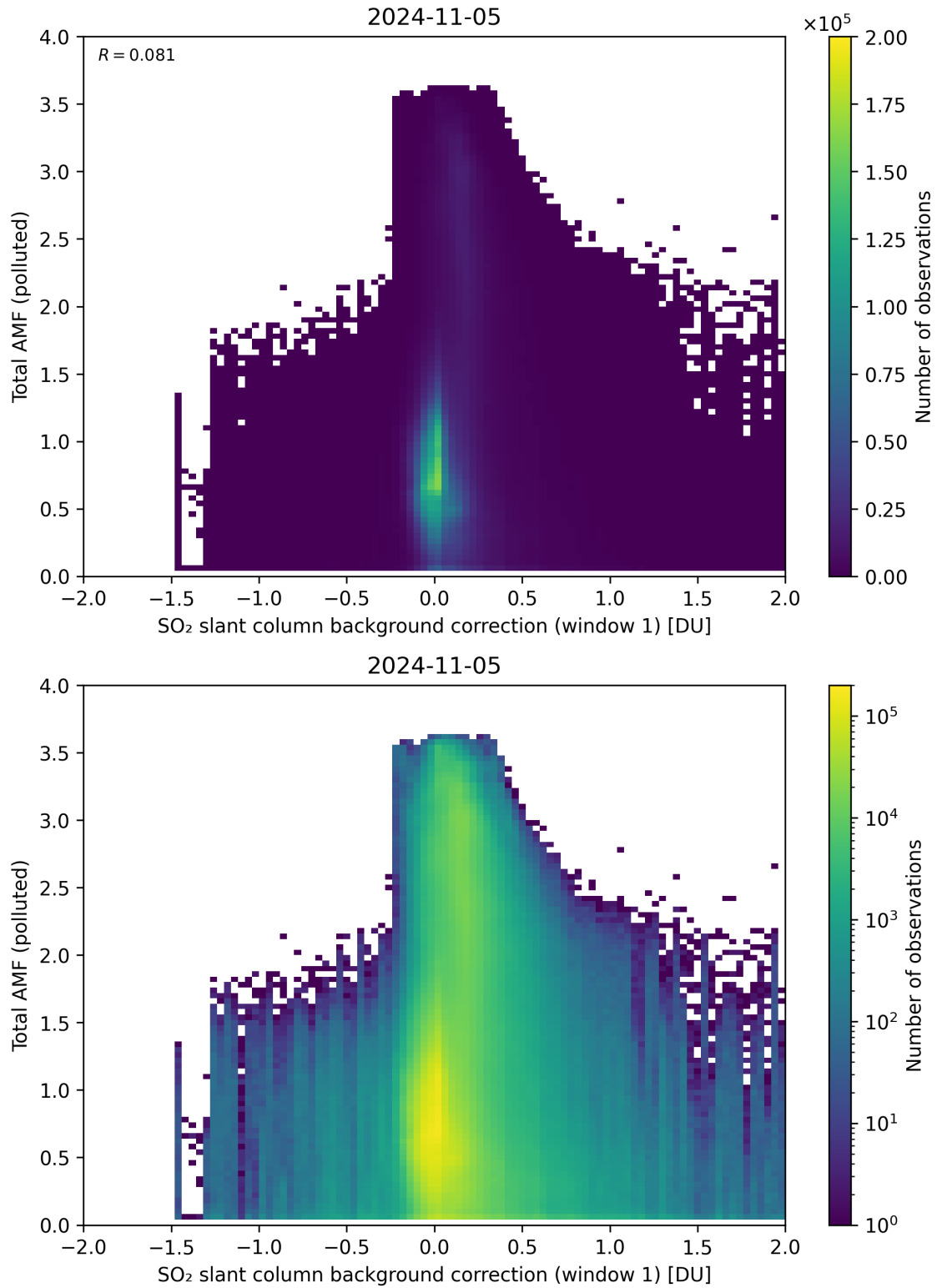
Figure 109: Scatter density plot of “SO 2 slant column background correction (window 1)” against “Total AMF (polluted)” for 2024-11-04 to 2024-11-06.
