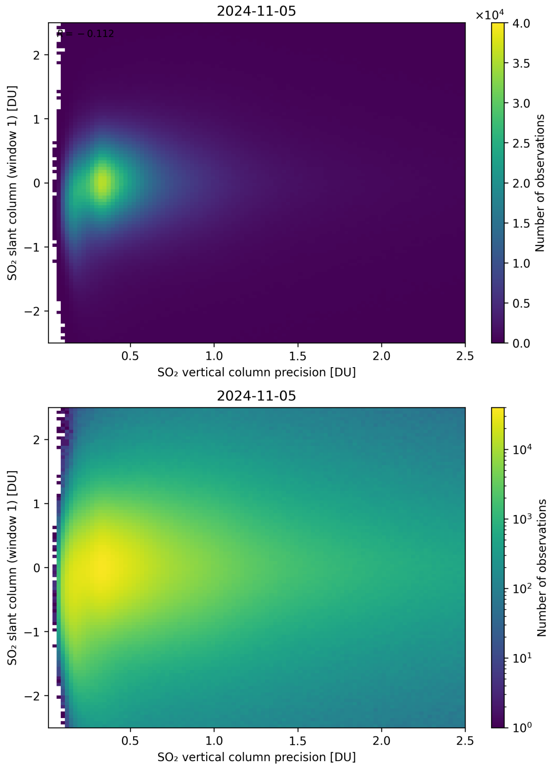
Figure 289: Scatter density plot of “SO 2 vertical column precision” against “SO 2 slant column (window 1)” for 2024-11-04 to 2024-11-06.
