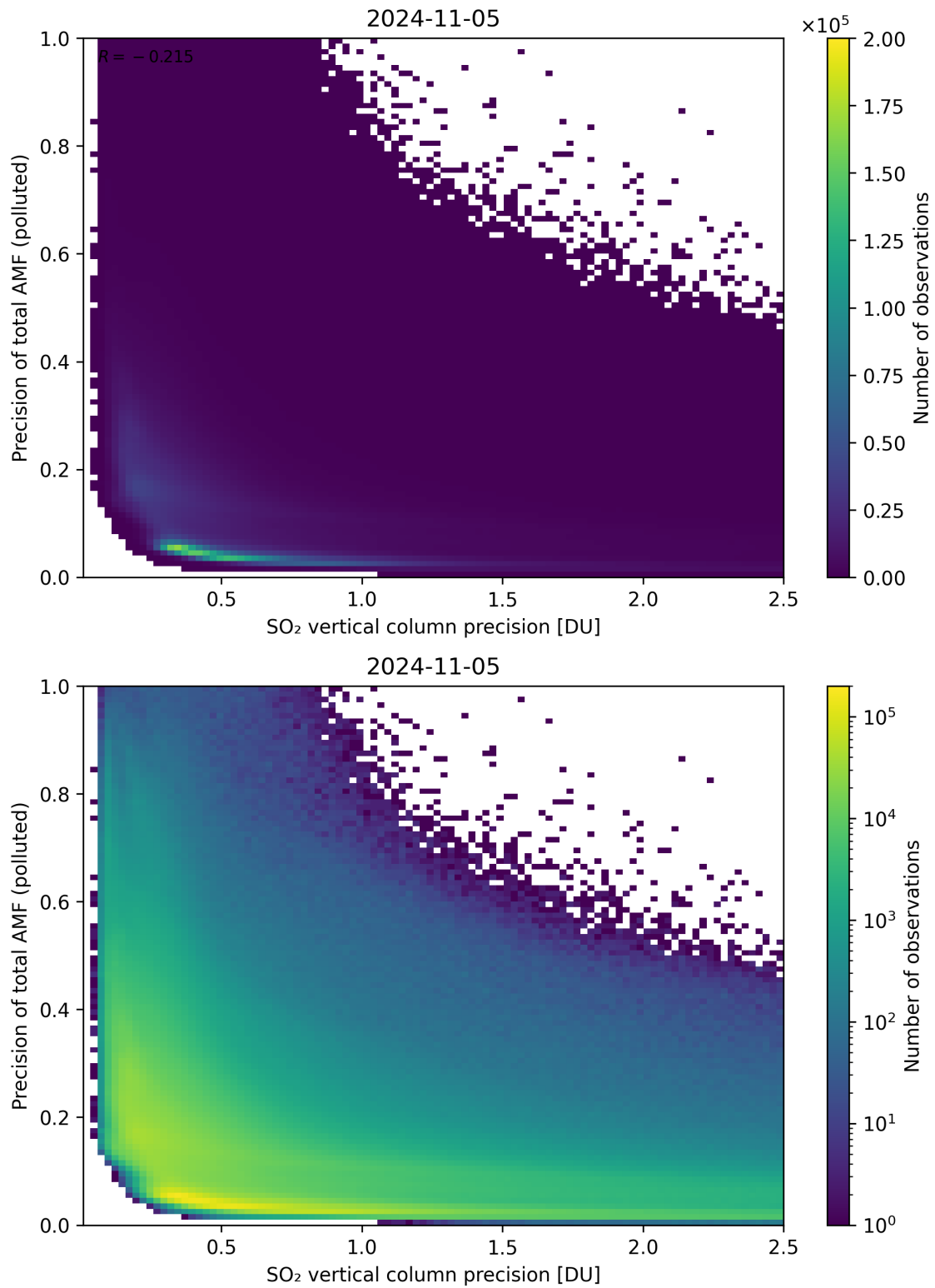
Figure 295: Scatter density plot of “SO 2 vertical column precision” against “Precision of total AMF (polluted)” for 2024-11-04 to 2024-11-06.
