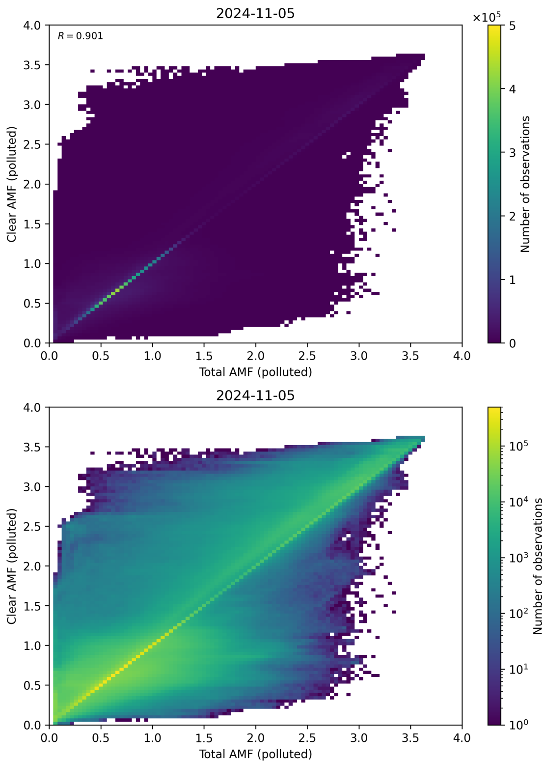
Figure 271: Scatter density plot of “Total AMF (polluted)” against “Clear AMF (polluted)” for 2024-11-04 to 2024-11-06.
