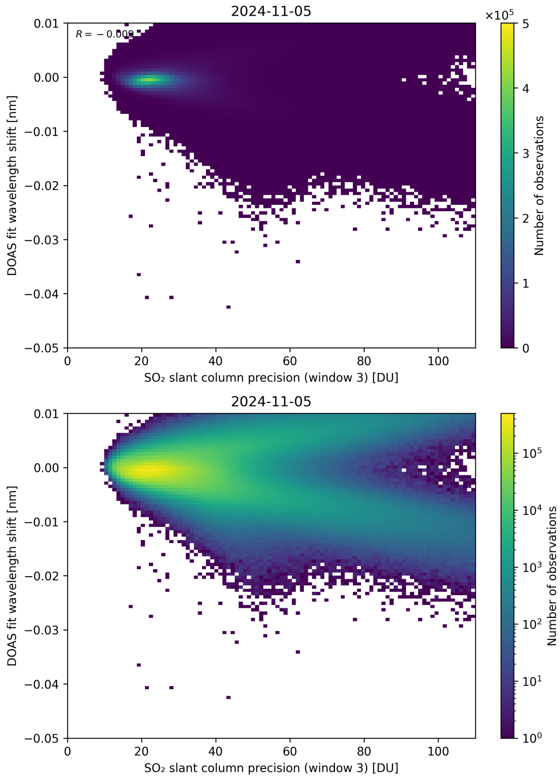
Figure 258: Scatter density plot of “SO 2 slant column precision (window 3)” against “DOAS fit wavelength shift” for 2024-11-04 to 2024-11-06.
