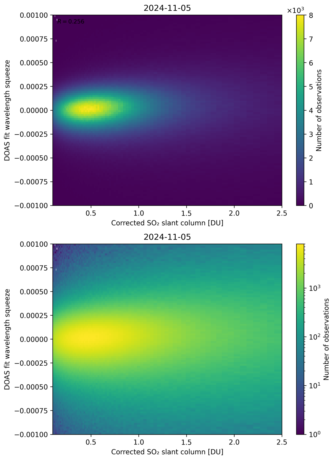
Figure 182: Scatter density plot of “Corrected SO 2 slant column” against “DOAS fit wavelength squeeze” for 2024-11-04 to 2024-11-06.
