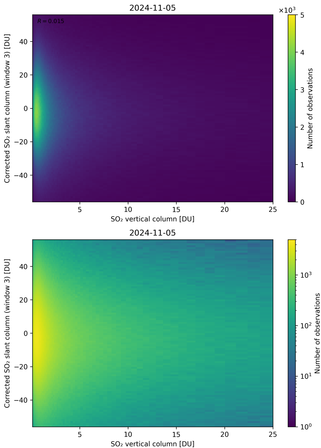
Figure 299: Scatter density plot of “SO 2 vertical column” against “Corrected SO 2 slant column (window 3)” for 2024-11-04 to 2024-11-06.
