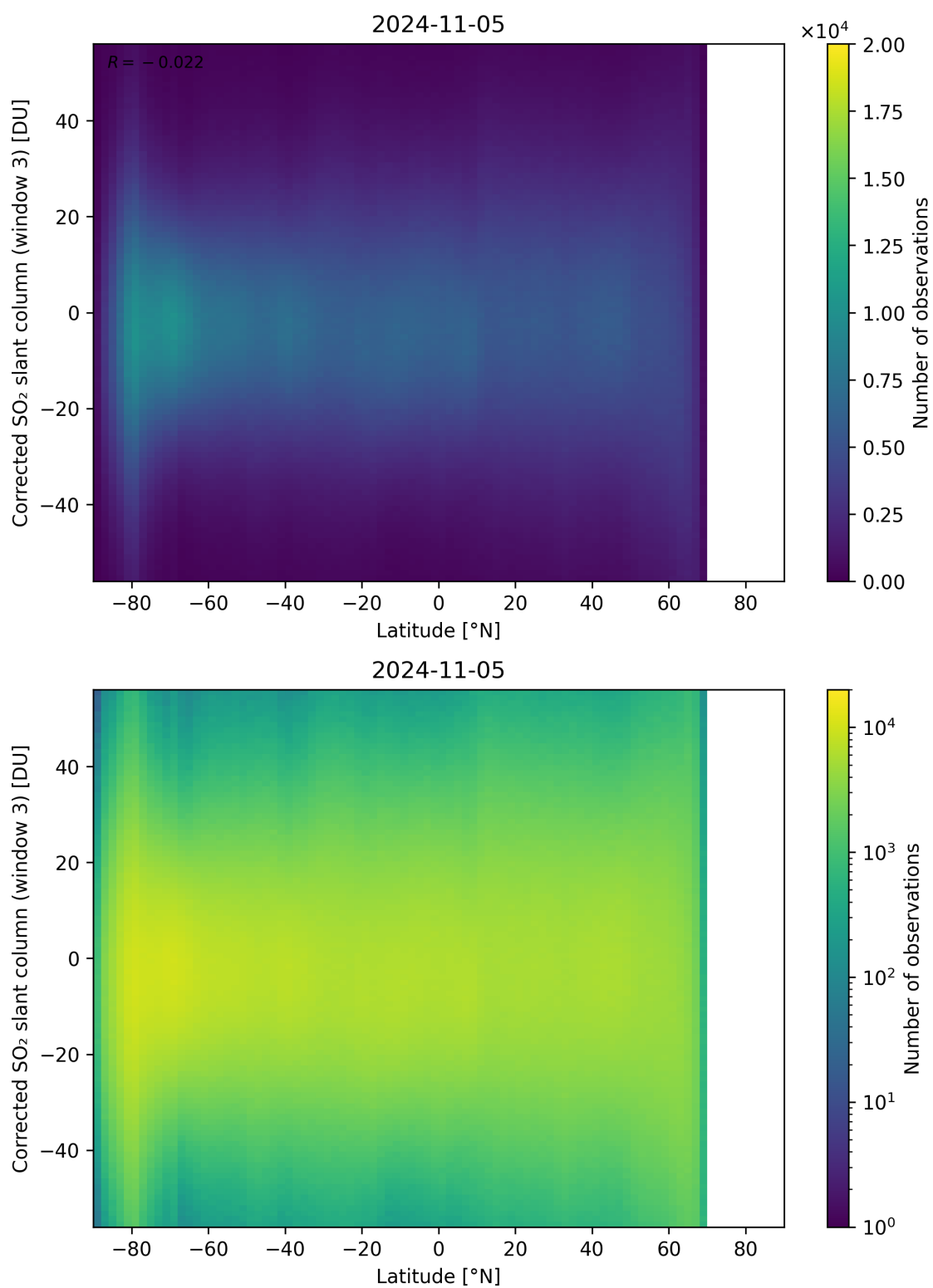
Figure 148: Scatter density plot of “Latitude” against “Corrected SO 2 slant column (window 3)” for 2024-11-04 to 2024-11-06.
