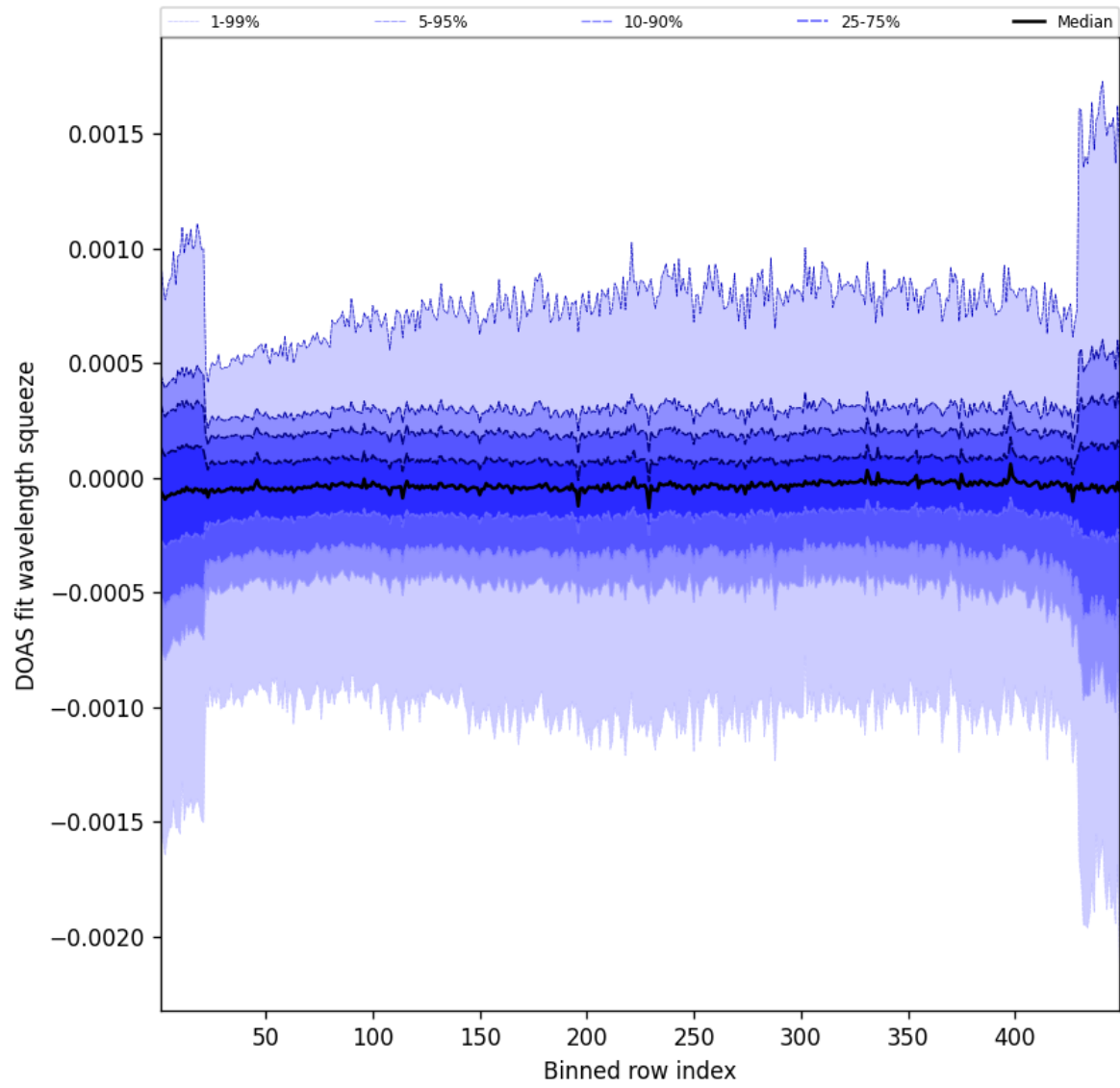
Figure 92: Along track statistics of “DOAS fit wavelength squeeze” for 2024-11-04 to 2024-11-06
