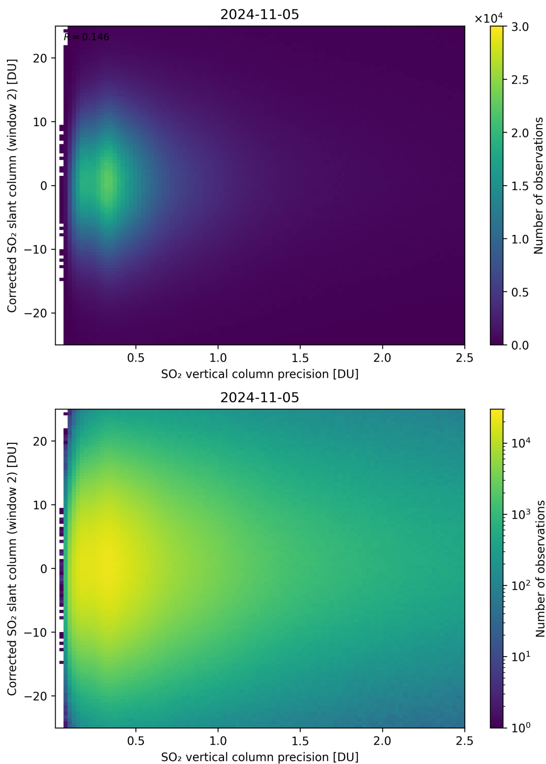
Figure 287: Scatter density plot of “SO 2 vertical column precision” against “Corrected SO 2 slant column (window 2)” for 2024-11-04 to 2024-11-06.
