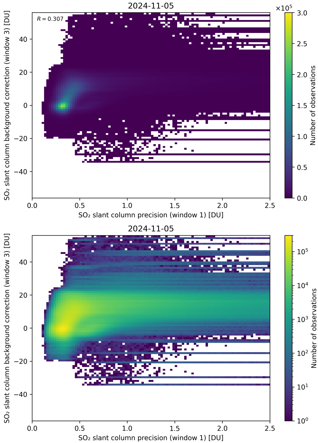
Figure 220: Scatter density plot of “SO 2 slant column precision (window 1)” against “SO 2 slant column background correction (window 3)” for 2024-11-04 to 2024-11-06.
