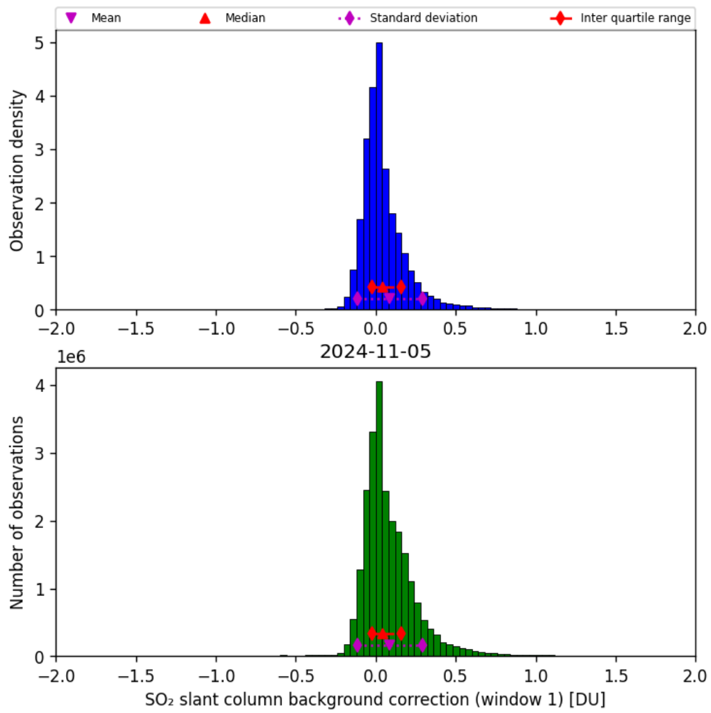
Figure 59: Histogram of “SO 2 slant column background correction (window 1)” for 2024-11-04 to 2024-11-06
