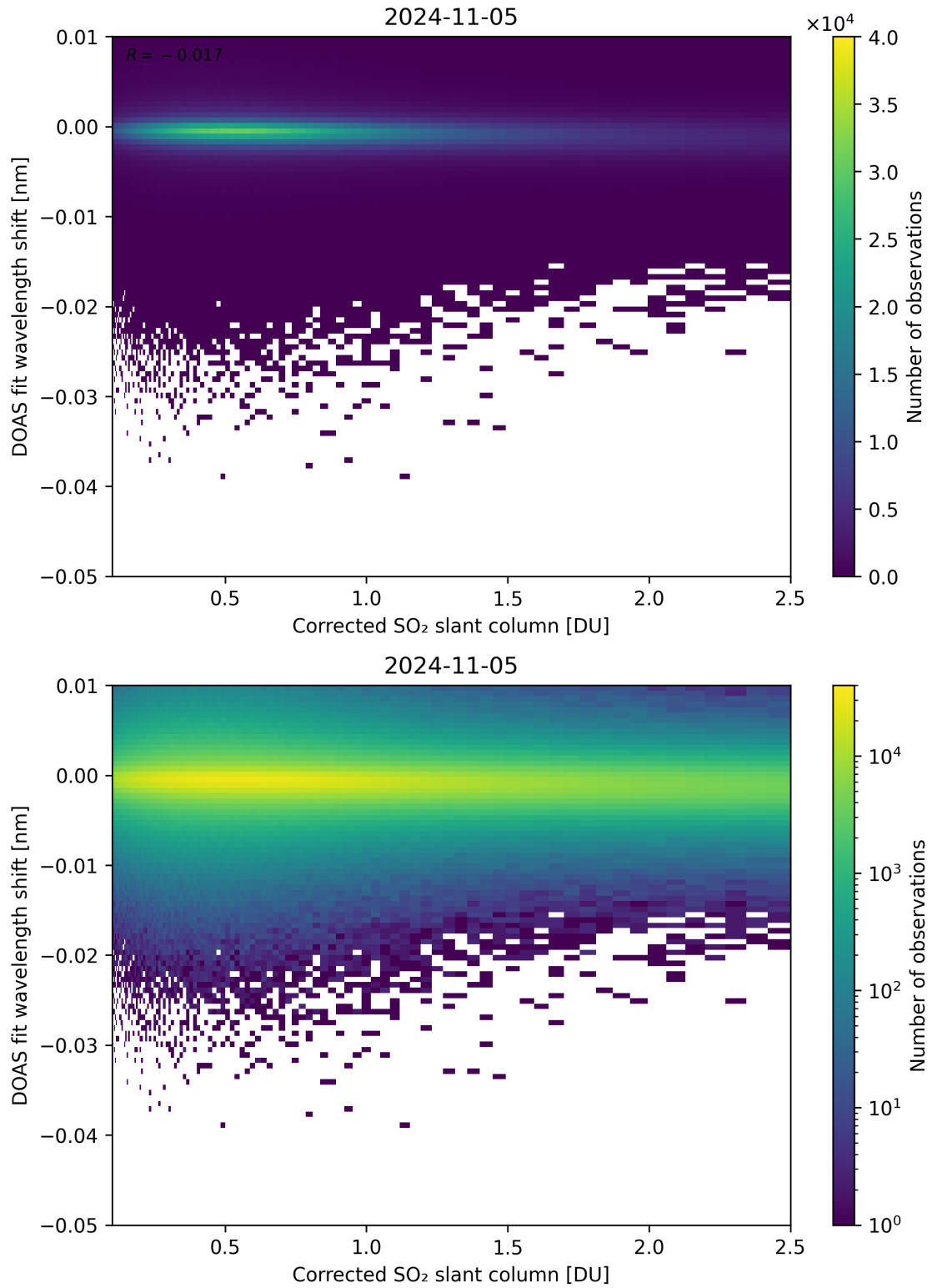
Figure 181: Scatter density plot of “Corrected SO 2 slant column” against “DOAS fit wavelength shift” for 2024-11-04 to 2024-11-06.
