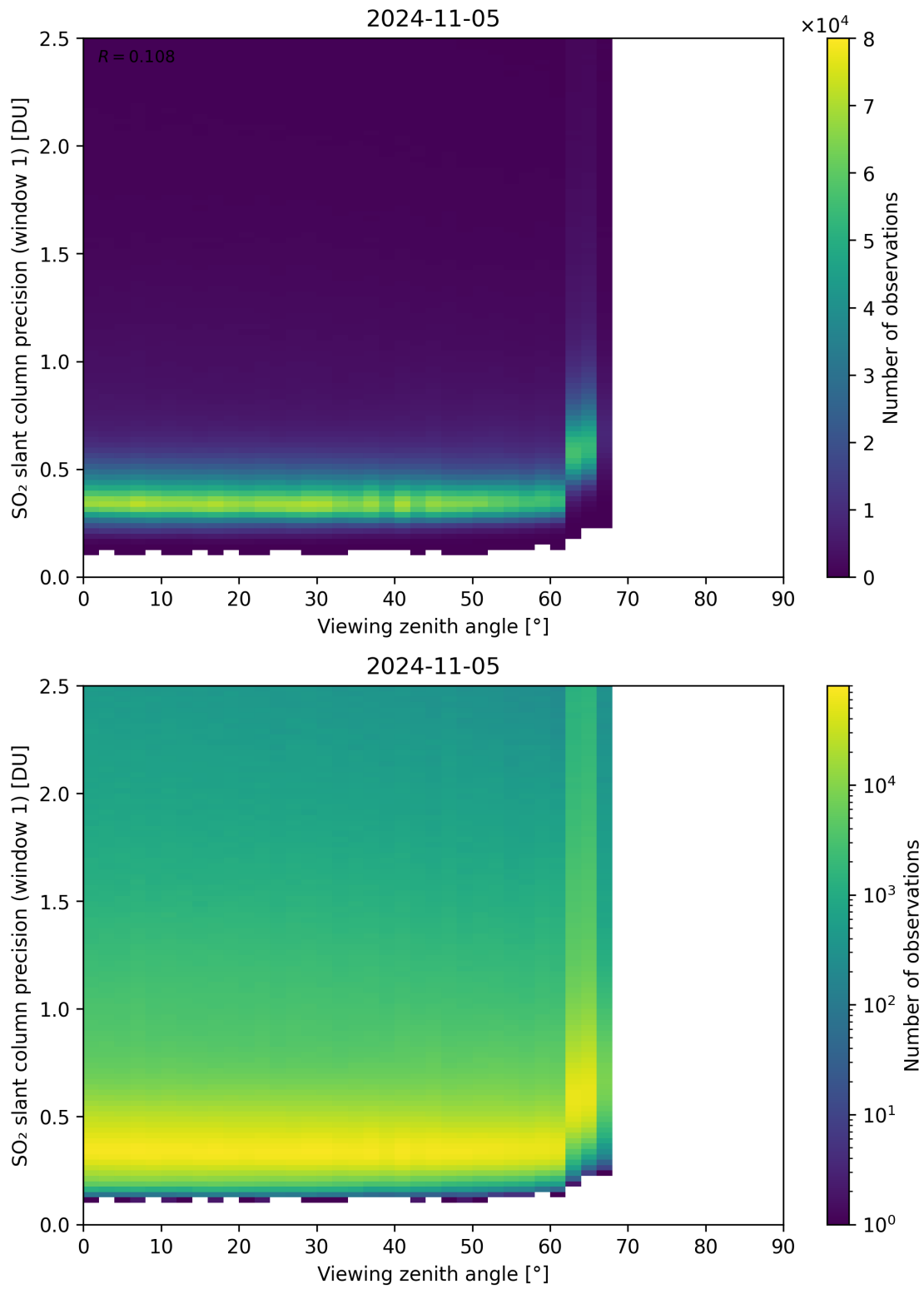
Figure 321: Scatter density plot of “Viewing zenith angle” against “SO 2 slant column precision (window 1)” for 2024-11-04 to 2024-11-06.
