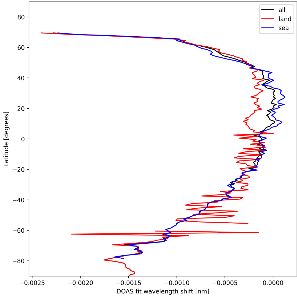
Figure 45: Zonal average of “DOAS fit wavelength shift” for 2024-11-04 to 2024-11-06.
