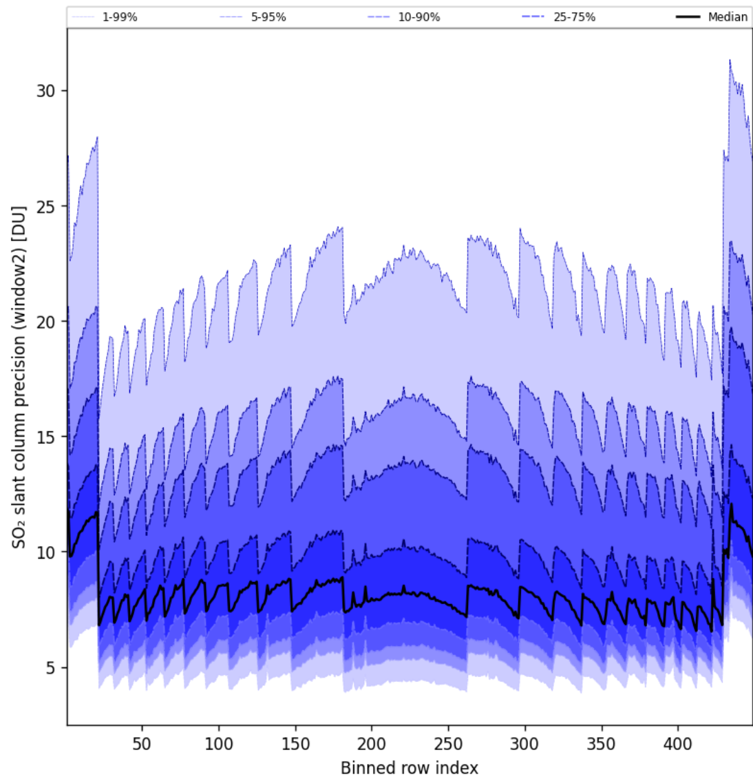
Figure 84: Along track statistics of “SO 2 slant column precision (window2)” for 2024-11-04 to 2024-11-06
