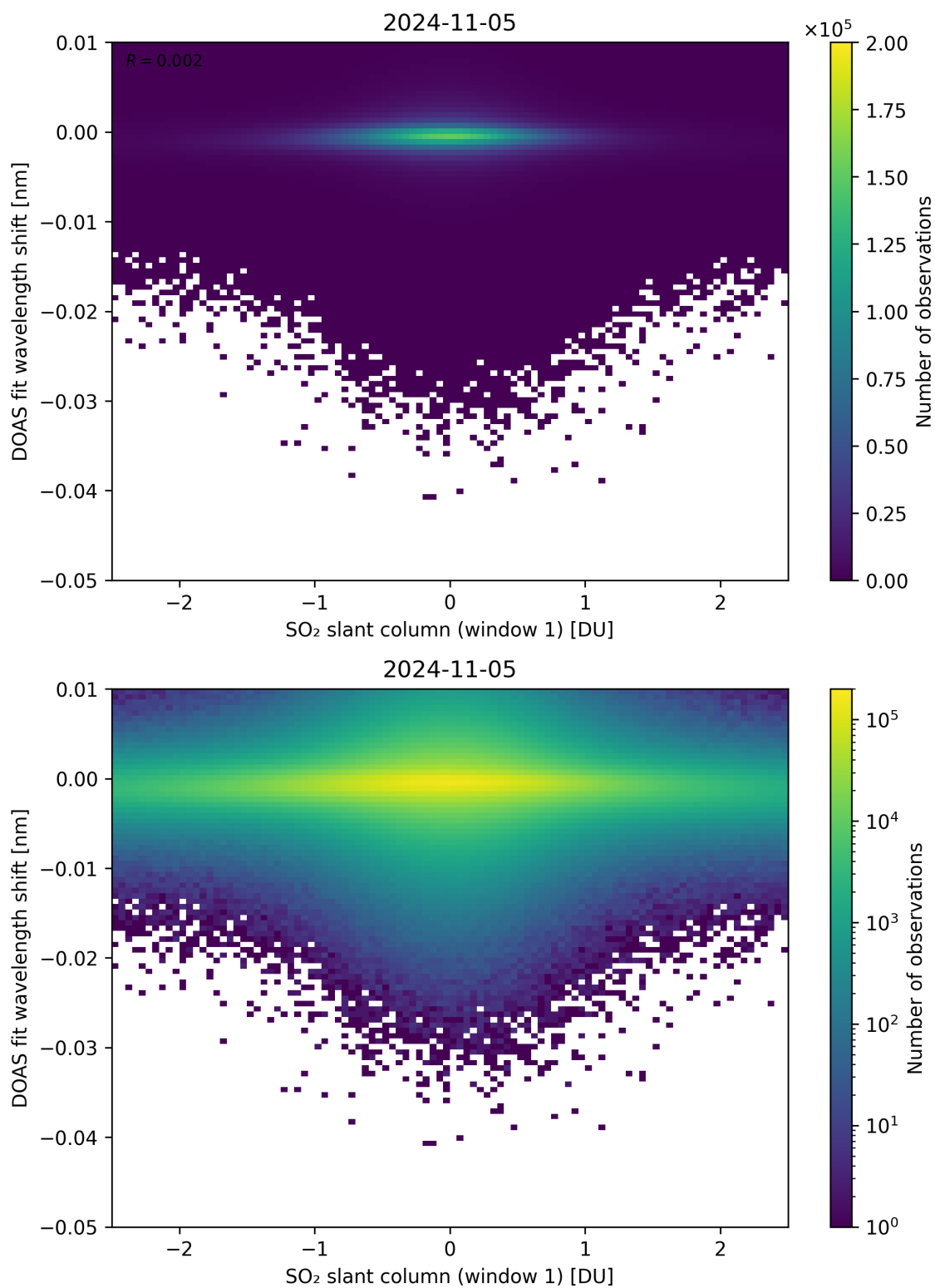
Figure 215: Scatter density plot of “SO 2 slant column (window 1)” against “DOAS fit wavelength shift” for 2024-11-04 to 2024-11-06.
