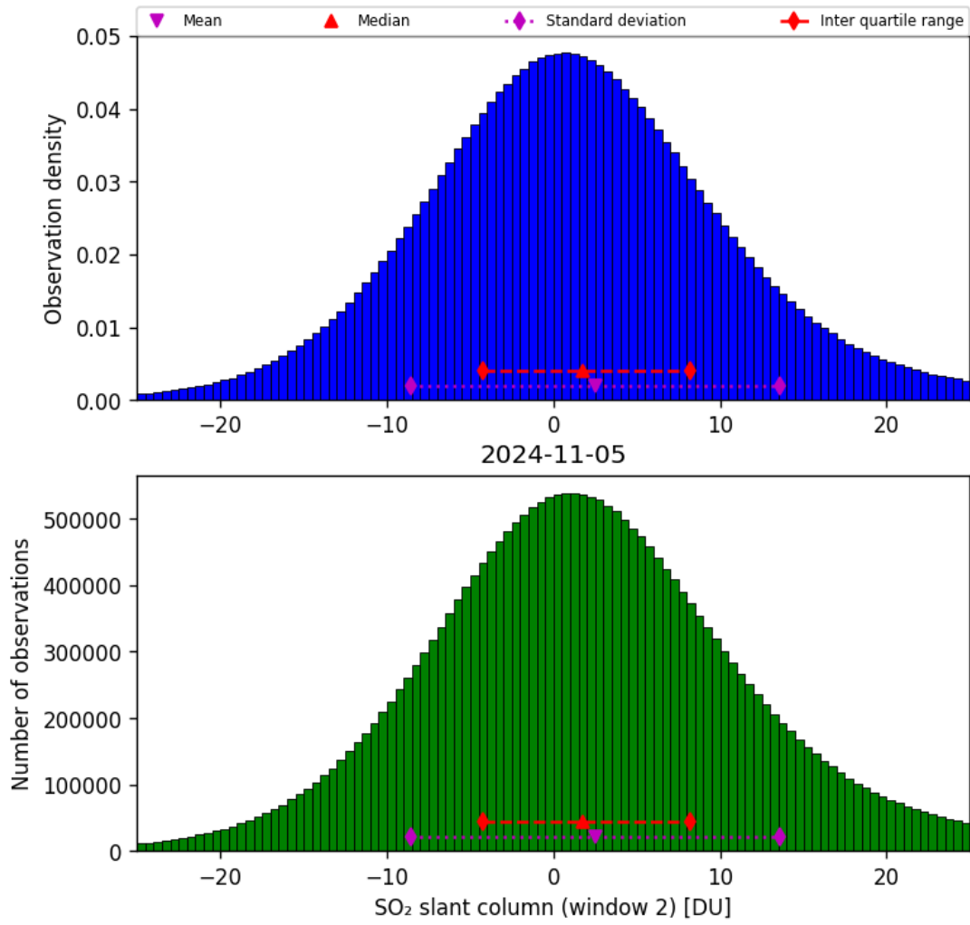
Figure 60: Histogram of “SO 2 slant column (window 2)” for 2024-11-04 to 2024-11-06
