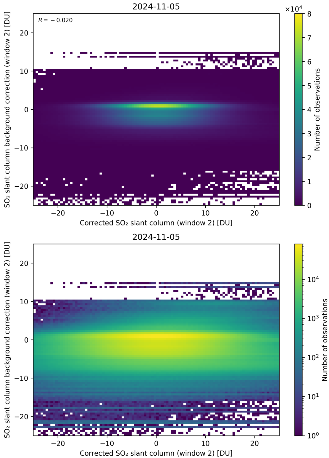
Figure 194: Scatter density plot of “Corrected SO 2 slant column (window 2)” against “SO 2 slant column background correction (window 2)” for 2024-11-04 to 2024-11-06.
