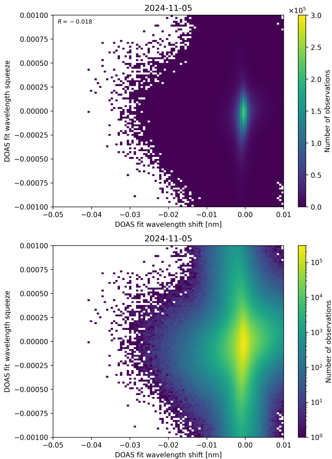
Figure 127: Scatter density plot of “DOAS fit wavelength shift” against “DOAS fit wavelength squeeze” for 2024-11-04 to 2024-11-06.
