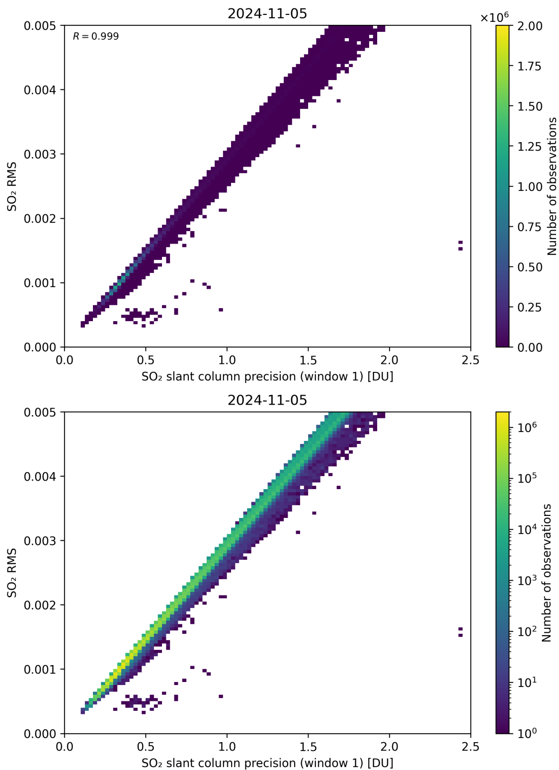
Figure 223: Scatter density plot of “SO 2 slant column precision (window 1)” against “SO 2 RMS” for 2024-11-04 to 2024-11-06.
