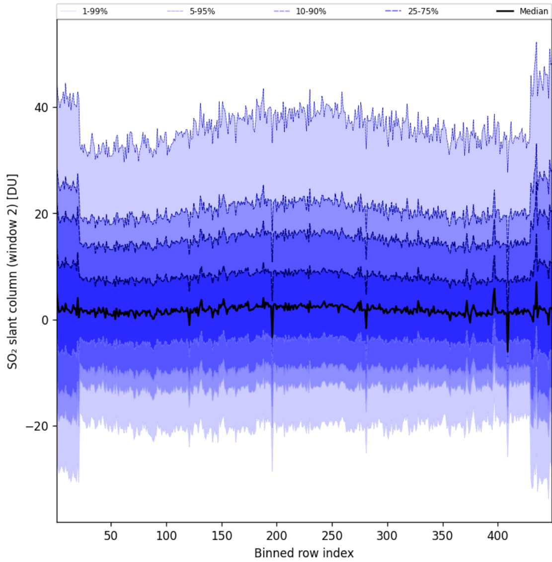
Figure 83: Along track statistics of “SO 2 slant column (window 2)” for 2024-11-04 to 2024-11-06
