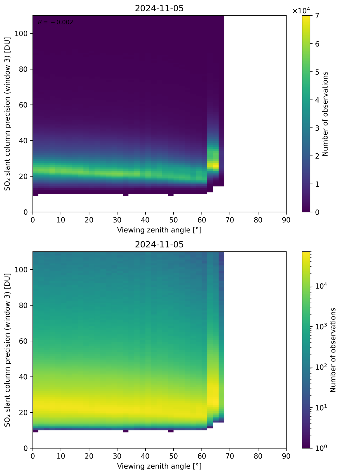
Figure 324: Scatter density plot of “Viewing zenith angle” against “SO 2 slant column precision (window 3)” for 2024-11-04 to 2024-11-06.
