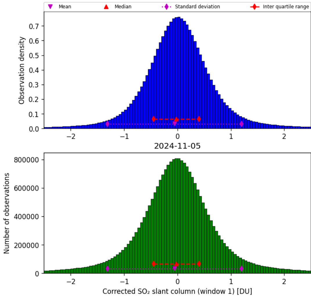
Figure 58: Histogram of “Corrected SO 2 slant column (window 1)” for 2024-11-04 to 2024-11-06
