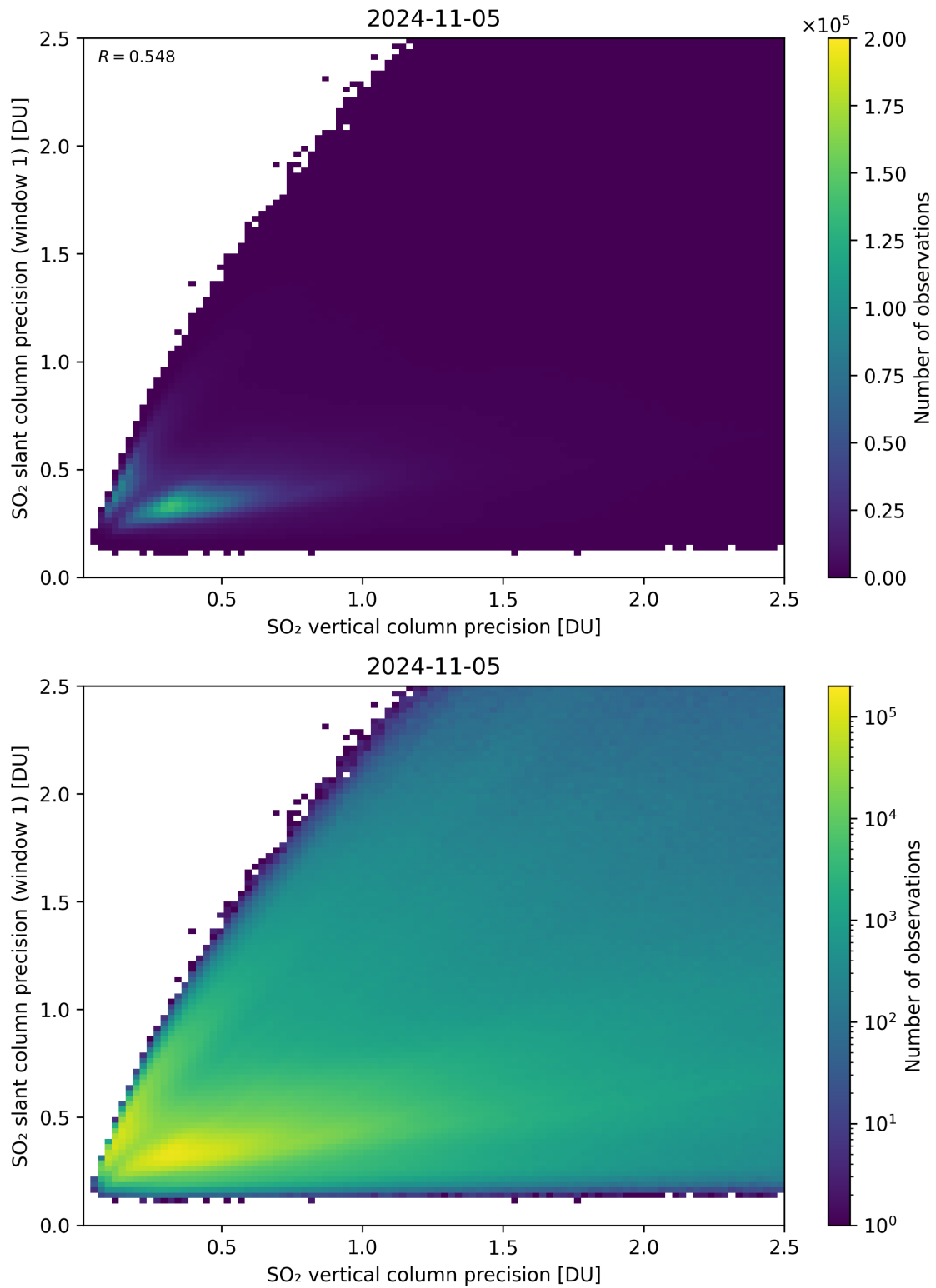
Figure 290: Scatter density plot of “SO 2 vertical column precision” against “SO 2 slant column precision (window 1)” for 2024-11-04 to 2024-11-06.
