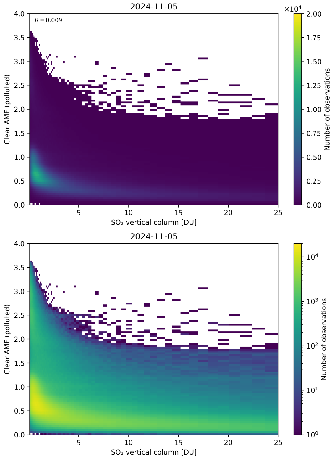
Figure 296: Scatter density plot of “SO 2 vertical column” against “Clear AMF (polluted)” for 2024-11-04 to 2024-11-06.
