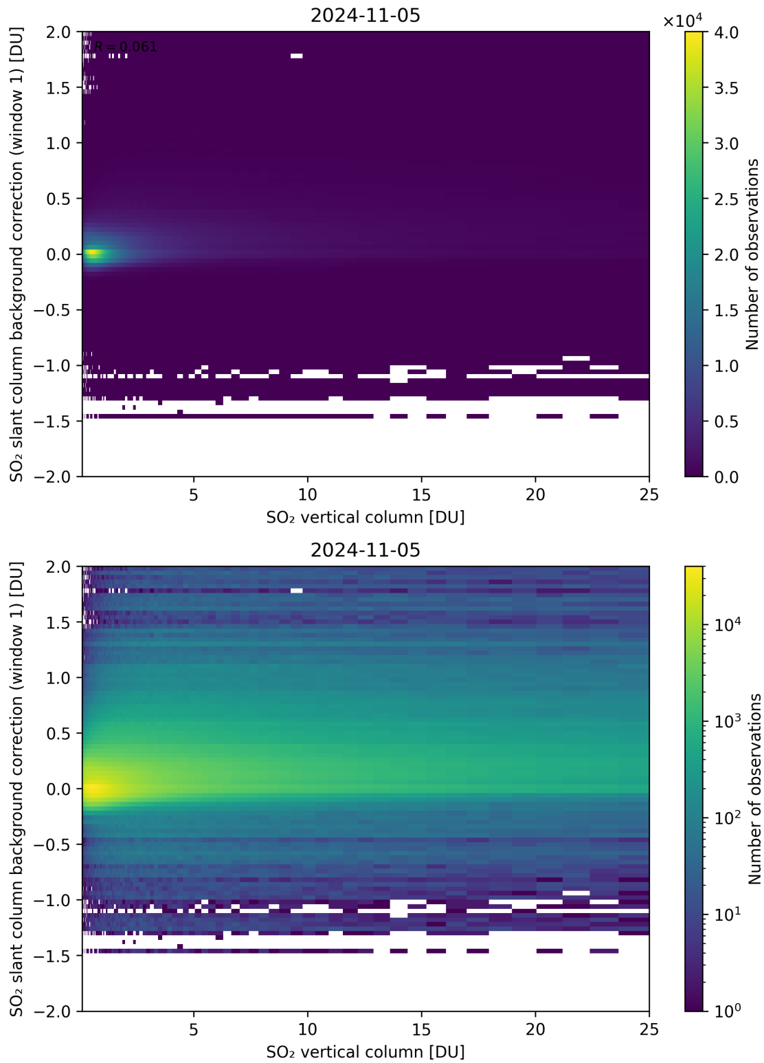
Figure 273: Scatter density plot of “SO 2 vertical column” against “SO 2 slant column background correction (window 1)” for 2024-11-04 to 2024-11-06.
