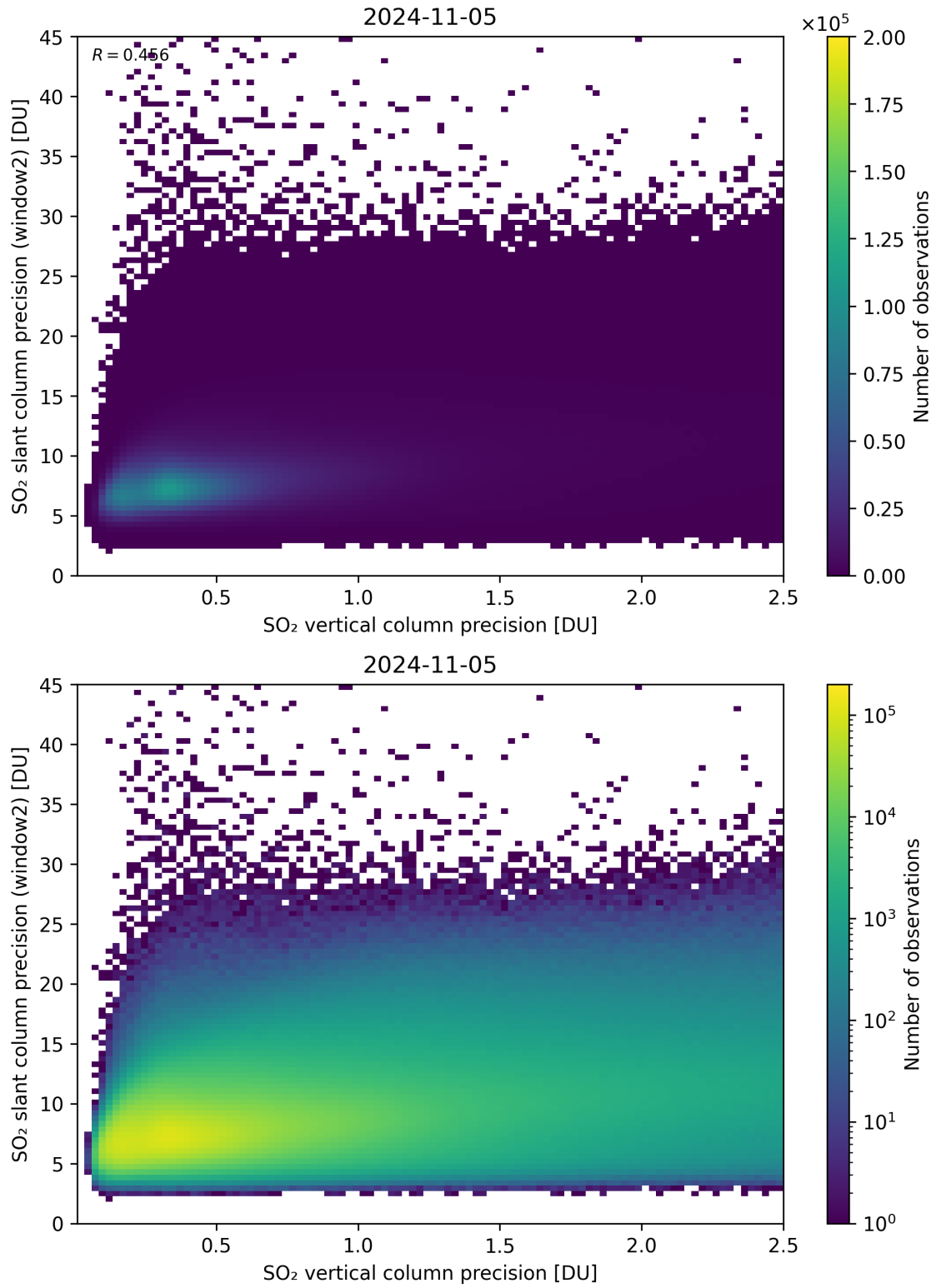
Figure 291: Scatter density plot of “SO 2 vertical column precision” against “SO 2 slant column precision (window2)” for 2024-11-04 to 2024-11-06.
