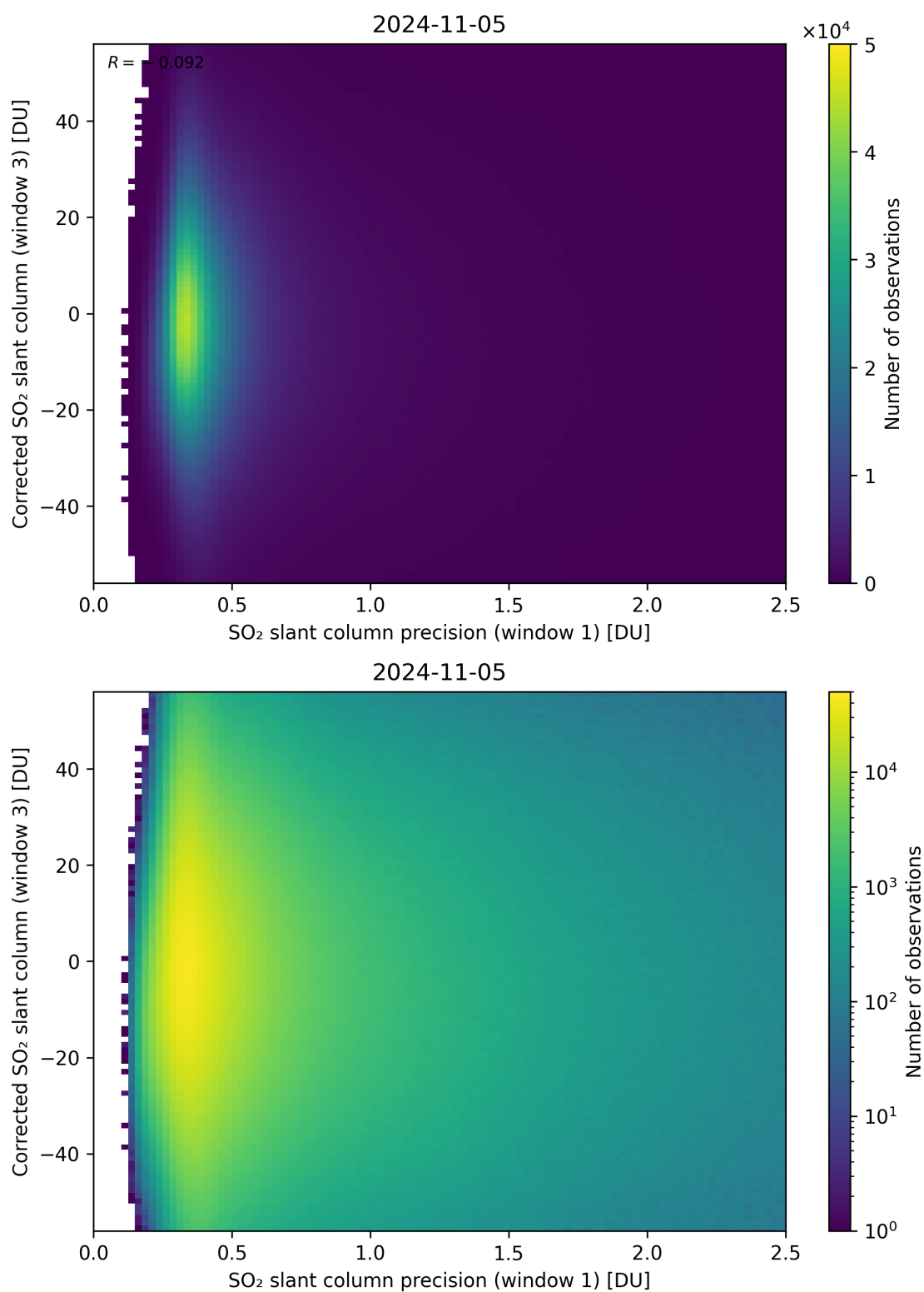
Figure 226: Scatter density plot of “SO 2 slant column precision (window 1)” against “Corrected SO 2 slant column (window 3)” for 2024-11-04 to 2024-11-06.
