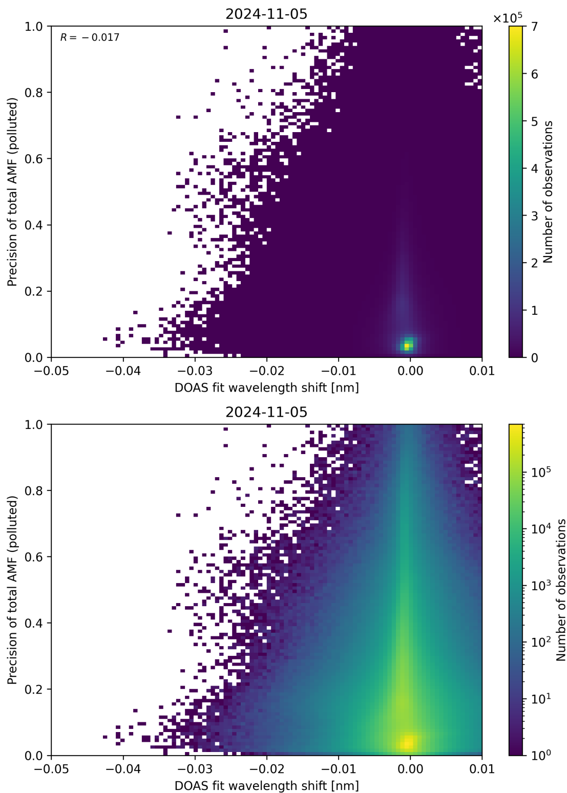
Figure 131: Scatter density plot of “DOAS fit wavelength shift” against “Precision of total AMF (polluted)” for 2024-11-04 to 2024-11-06.
