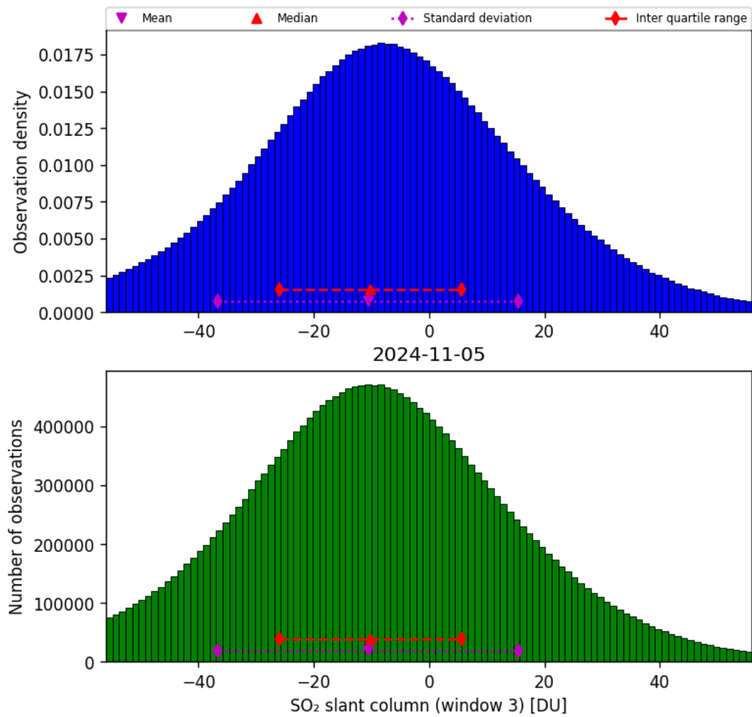
Figure 64: Histogram of “SO 2 slant column (window 3)” for 2024-11-04 to 2024-11-06
