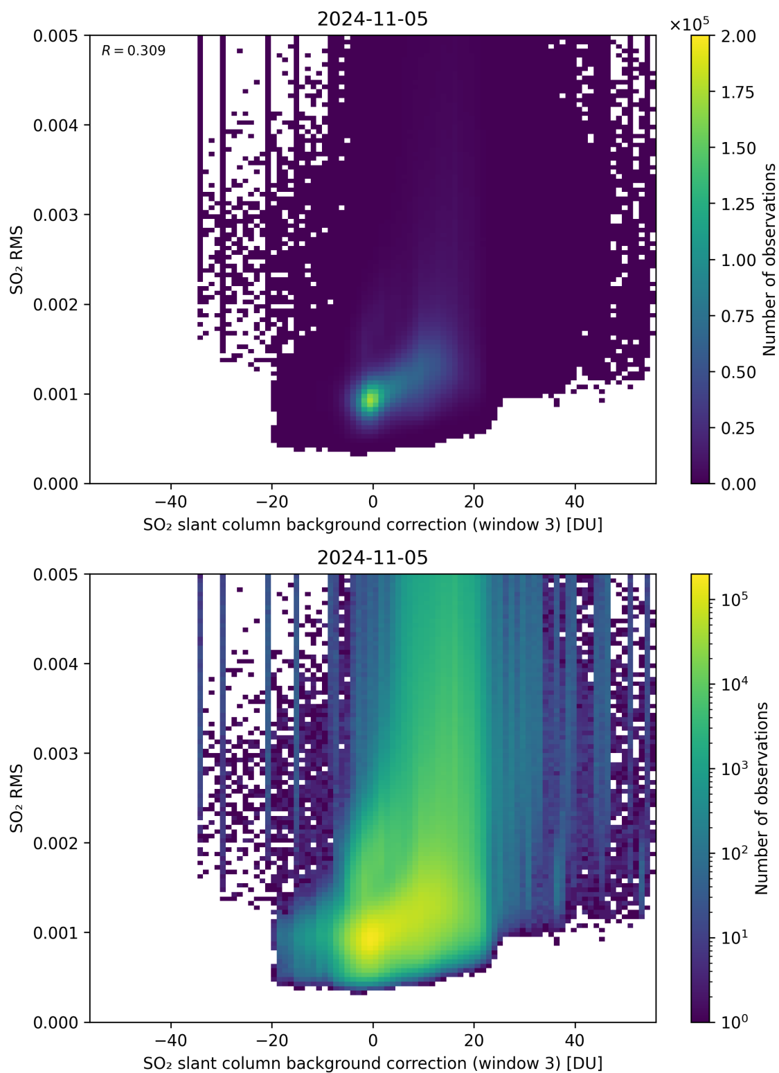
Figure 123: Scatter density plot of “SO 2 slant column background correction (window 3)” against “SO 2 RMS” for 2024-11-04 to 2024-11-06.
