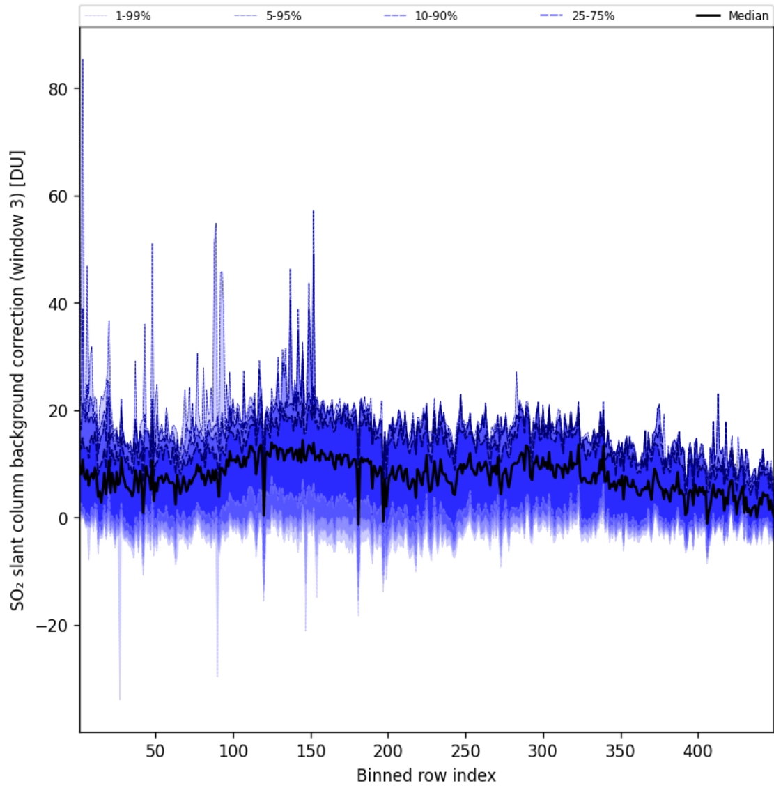
Figure 90: Along track statistics of “SO 2 slant column background correction (window 3)” for 2024-11-04 to 2024-11-06
