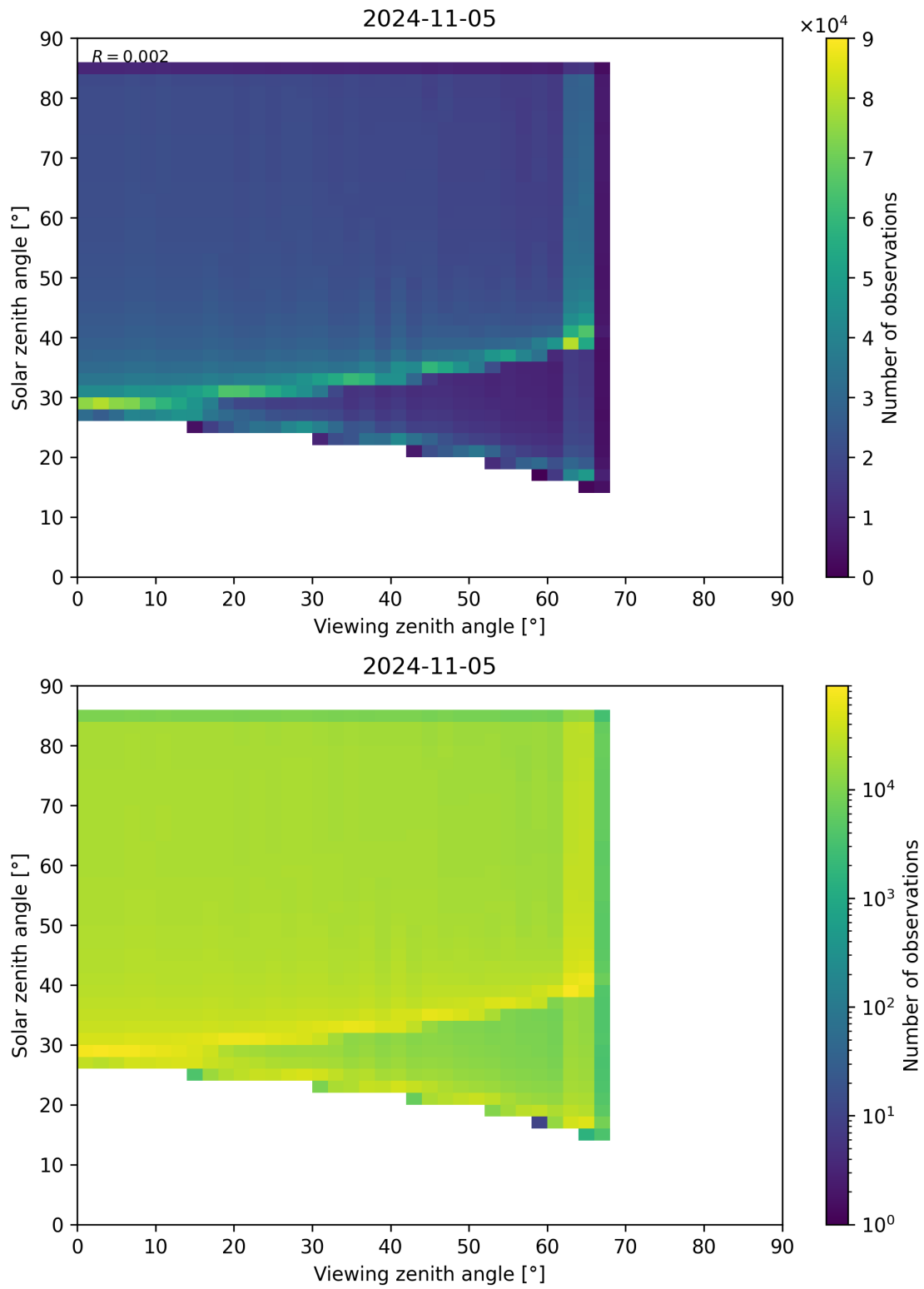
Figure 315: Scatter density plot of “Viewing zenith angle” against “Solar zenith angle” for 2024-11-04 to 2024-11-06.
