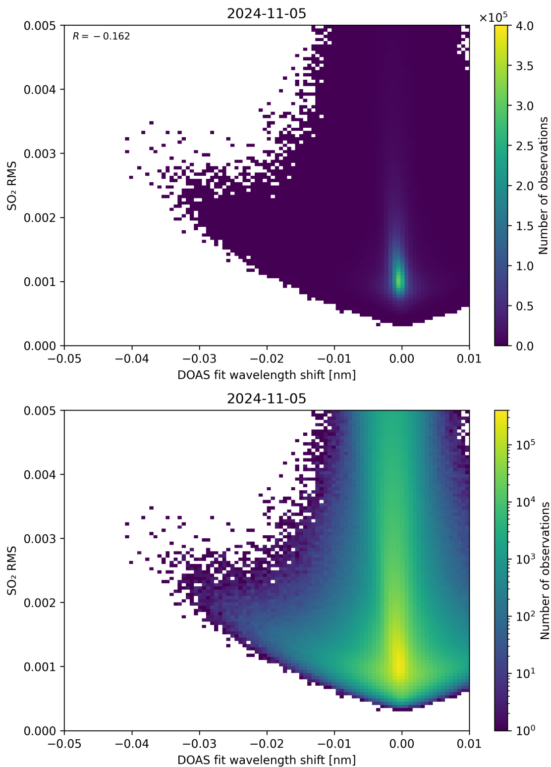
Figure 128: Scatter density plot of “DOAS fit wavelength shift” against “SO 2 RMS” for 2024-11-04 to 2024-11-06.
