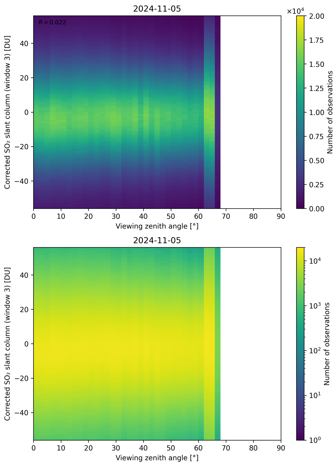
Figure 319: Scatter density plot of “Viewing zenith angle” against “Corrected SO 2 slant column (window 3)” for 2024-11-04 to 2024-11-06.
