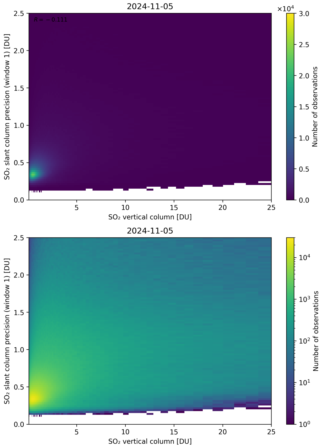
Figure 301: Scatter density plot of “SO 2 vertical column” against “SO 2 slant column precision (window 1)” for 2024-11-04 to 2024-11-06.
