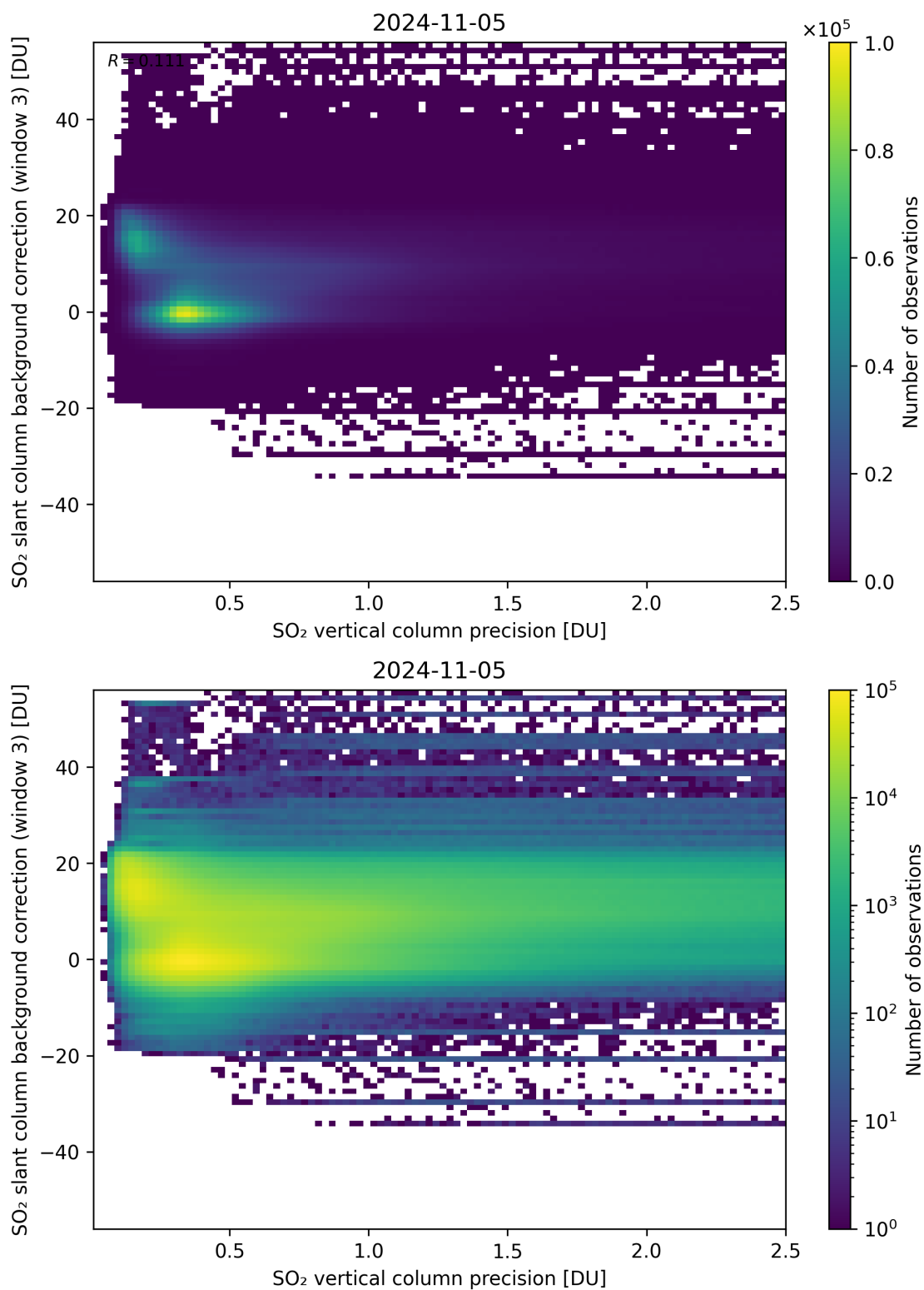
Figure 281: Scatter density plot of “SO 2 vertical column precision” against “SO 2 slant column background correction (window 3)” for 2024-11-04 to 2024-11-06.
