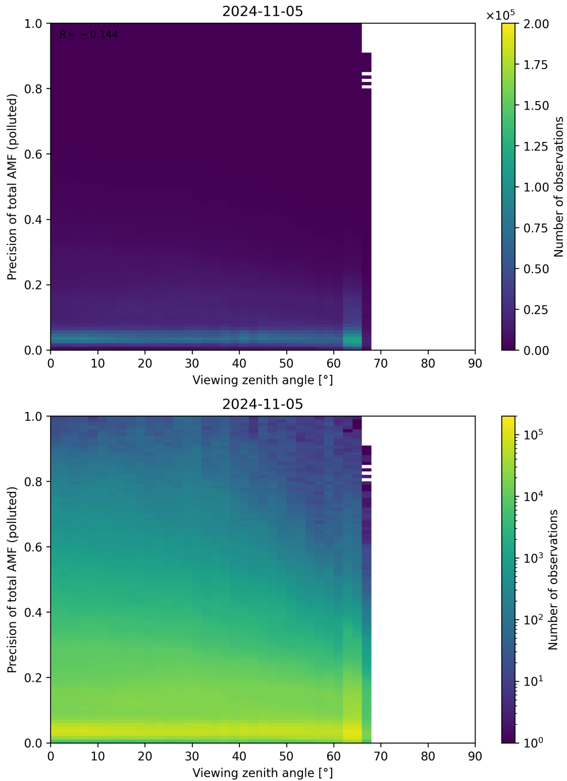
Figure 326: Scatter density plot of “Viewing zenith angle” against “Precision of total AMF (polluted)” for 2024-11-04 to 2024-11-06.
