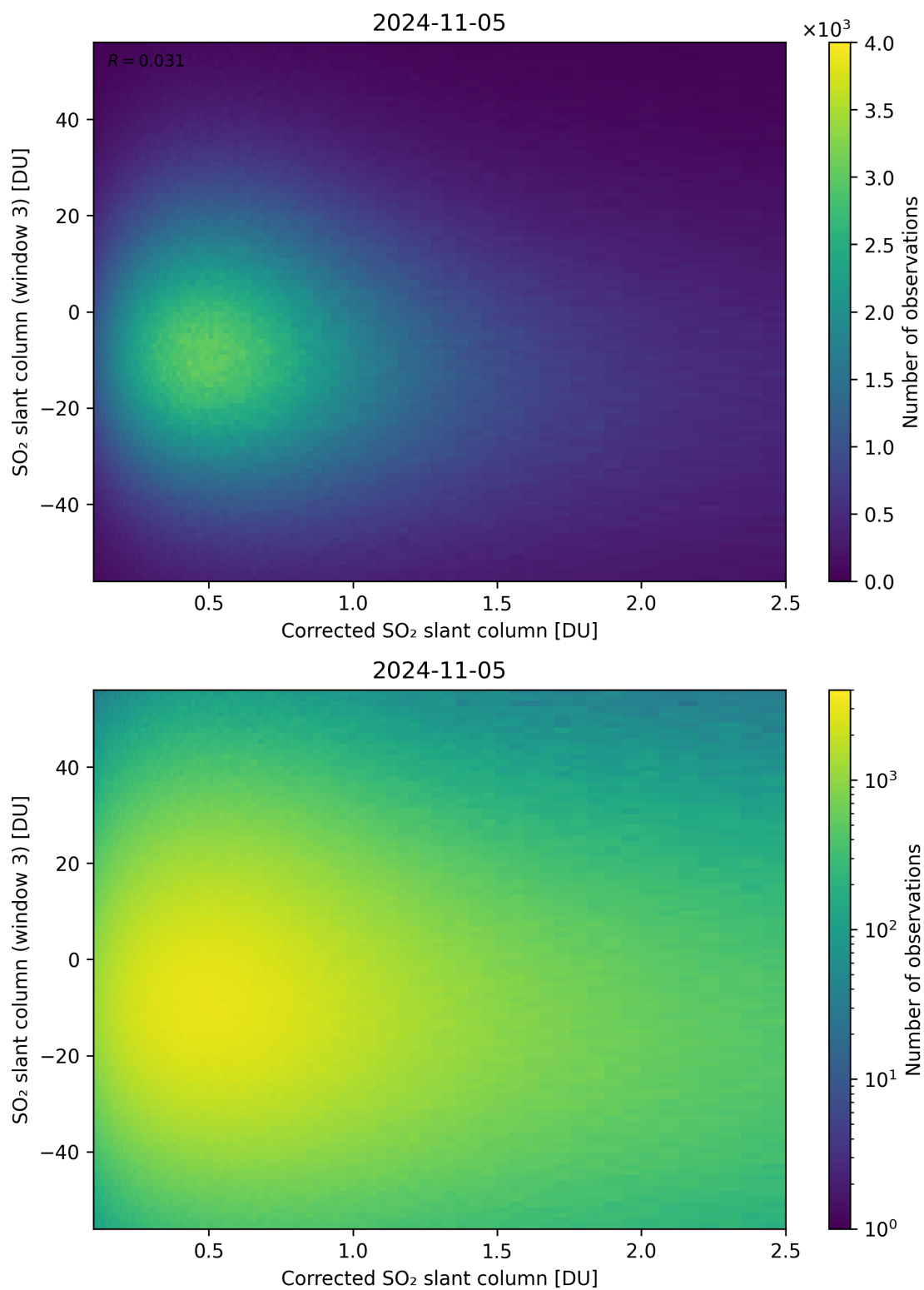
Figure 190: Scatter density plot of “Corrected SO 2 slant column” against “SO 2 slant column (window 3)” for 2024-11-04 to 2024-11-06.
