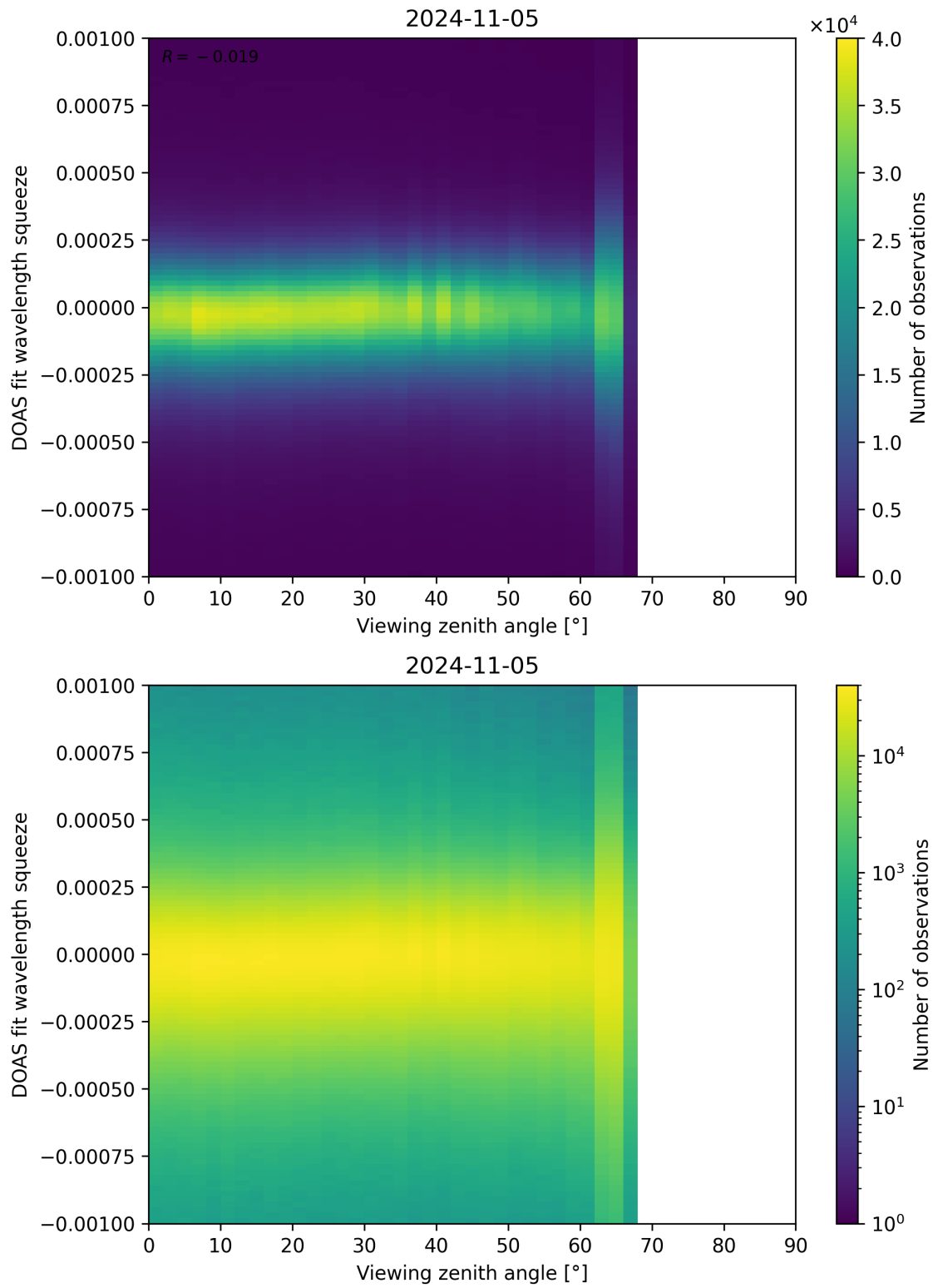
Figure 312: Scatter density plot of “Viewing zenith angle” against “DOAS fit wavelength squeeze” for 2024-11-04 to 2024-11-06.
