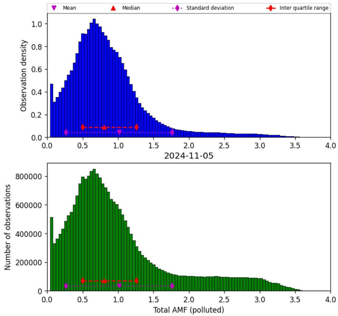
Figure 71: Histogram of “Total AMF (polluted)” for 2024-11-04 to 2024-11-06
