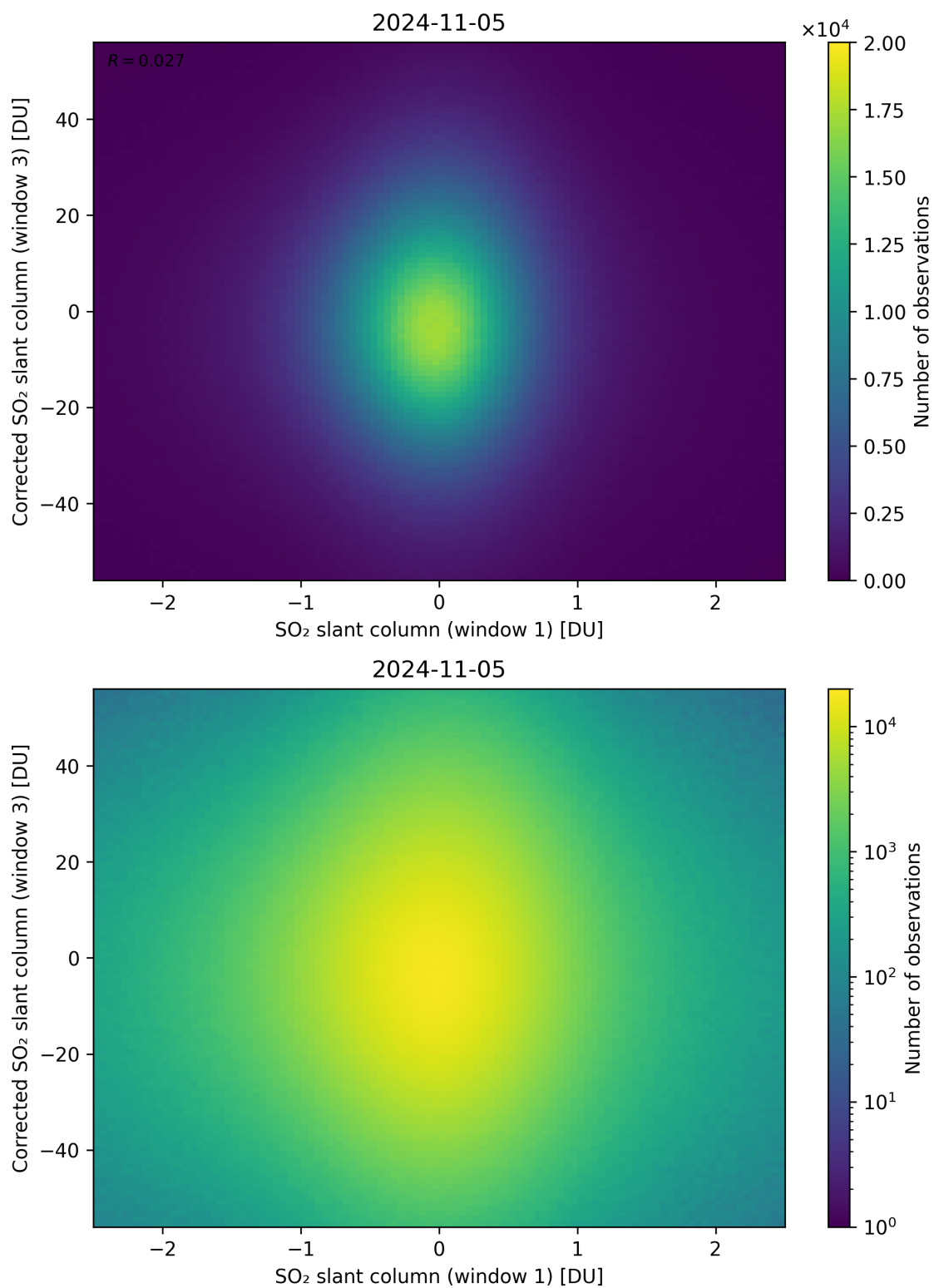
Figure 234: Scatter density plot of “SO 2 slant column (window 1)” against “Corrected SO 2 slant column (window 3)” for 2024-11-04 to 2024-11-06.
