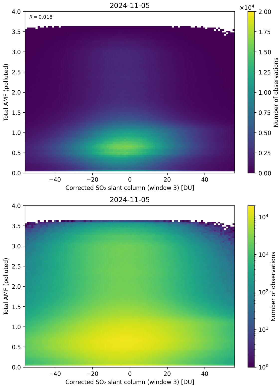
Figure 210: Scatter density plot of “Corrected SO 2 slant column (window 3)” against “Total AMF (polluted)” for 2024-11-04 to 2024-11-06.
