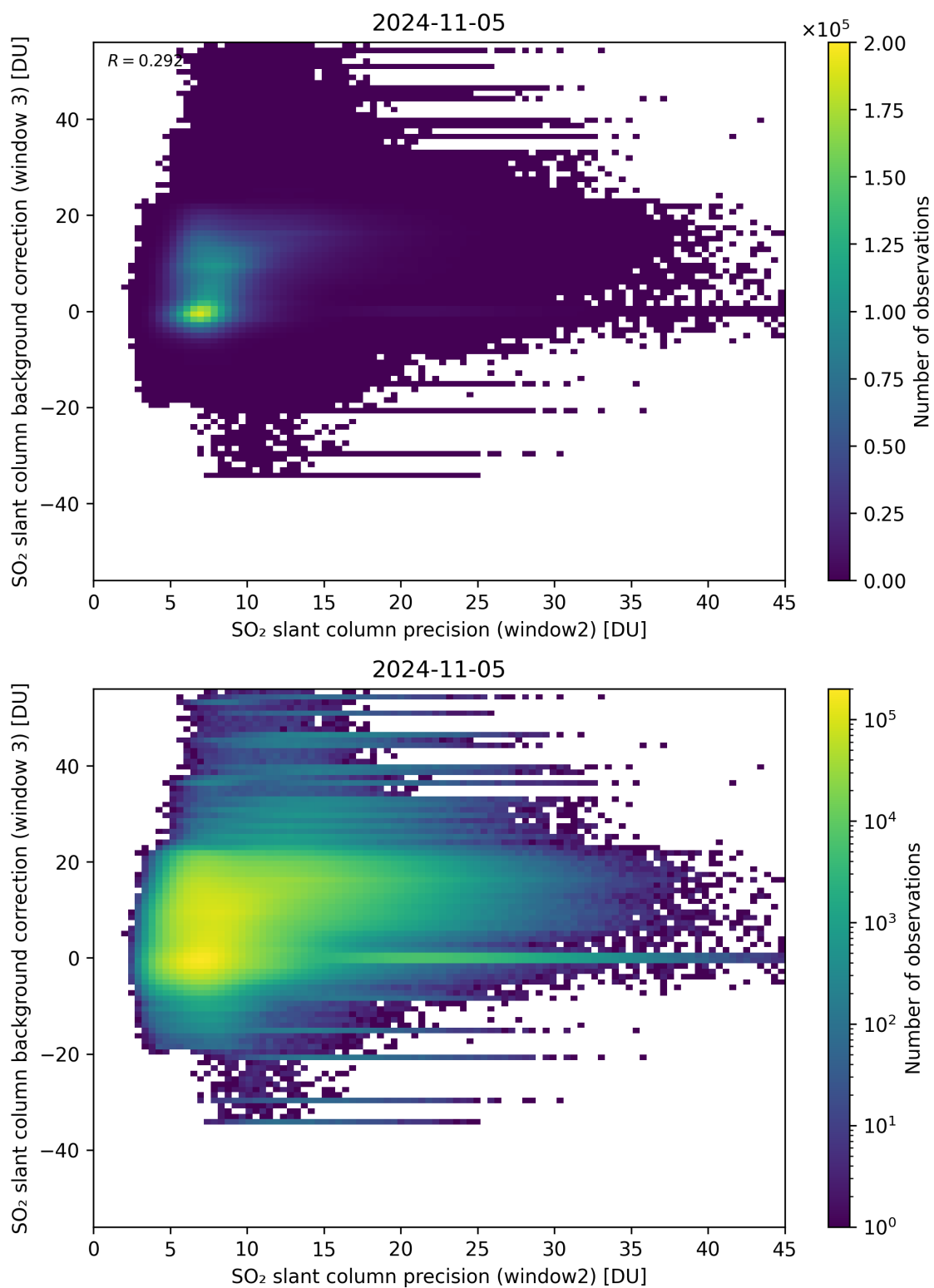
Figure 242: Scatter density plot of “SO 2 slant column precision (window2)” against “SO 2 slant column background correction (window 3)” for 2024-11-04 to 2024-11-06.
