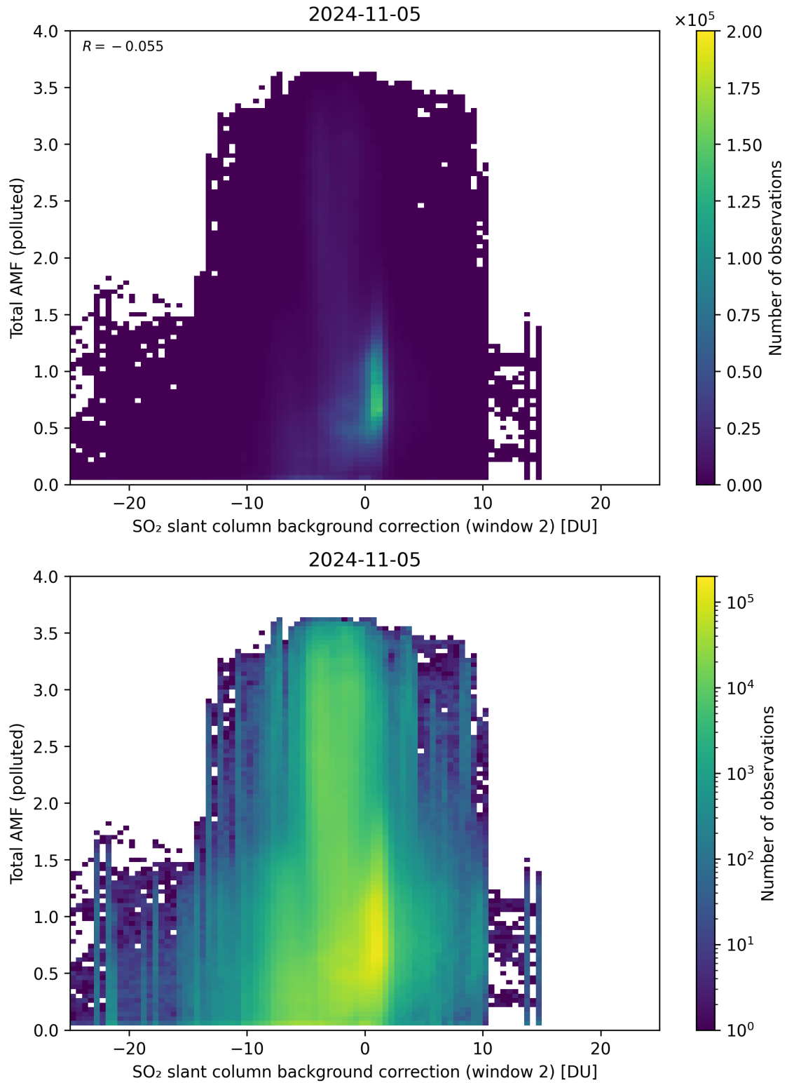
Figure 119: Scatter density plot of “SO 2 slant column background correction (window 2)” against “Total AMF (polluted)” for 2024-11-04 to 2024-11-06.
