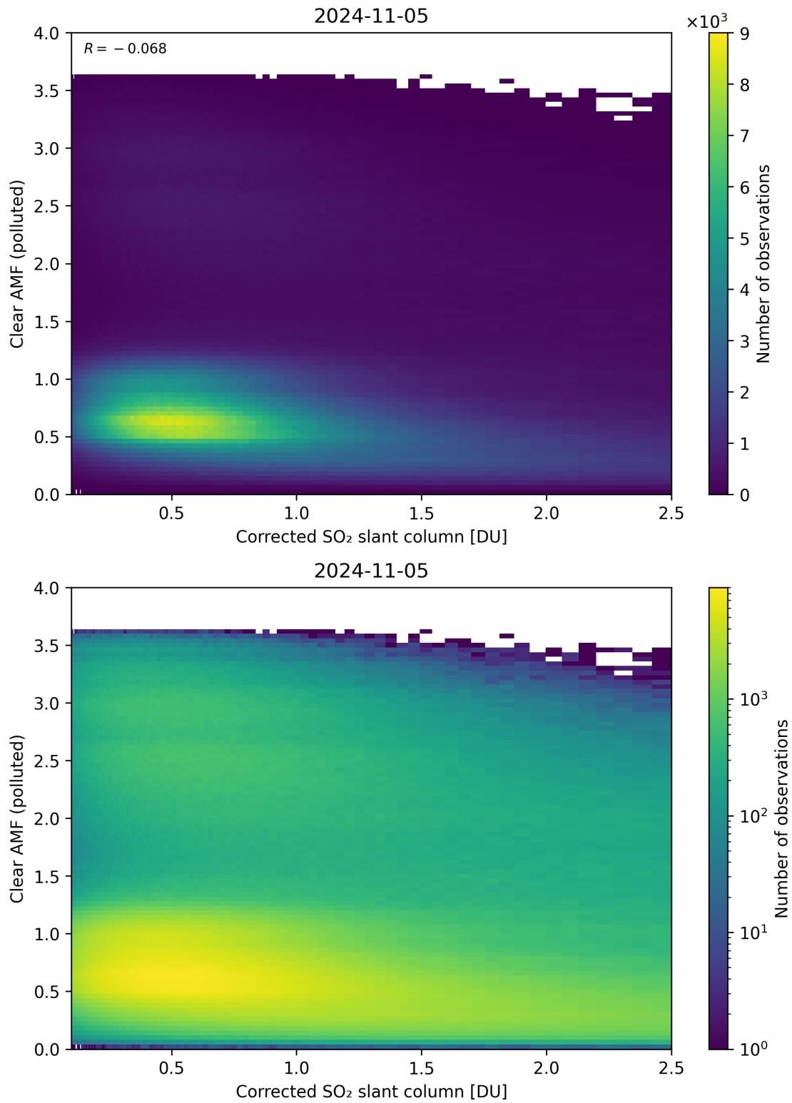
Figure 184: Scatter density plot of “Corrected SO 2 slant column” against “Clear AMF (polluted)” for 2024-11-04 to 2024-11-06.
