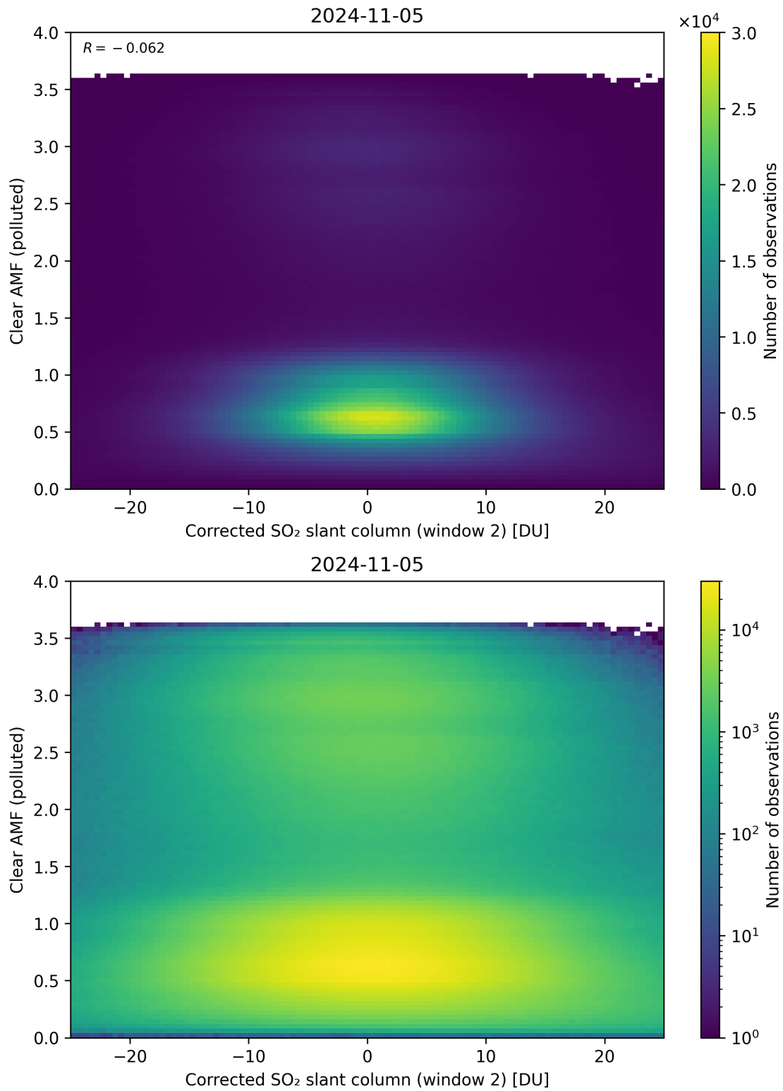
Figure 199: Scatter density plot of “Corrected SO 2 slant column (window 2)” against “Clear AMF (polluted)” for 2024-11-04 to 2024-11-06.
