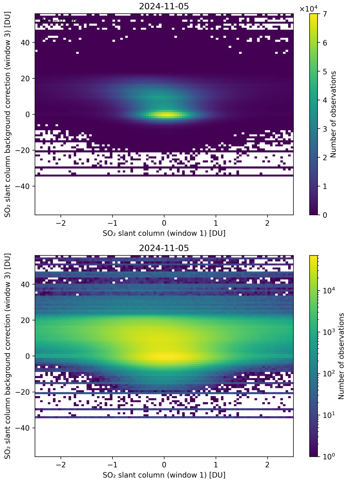
Figure 214: Scatter density plot of “SO 2 slant column (window 1)” against “SO 2 slant column background correction (window 3)” for 2024-11-04 to 2024-11-06.
