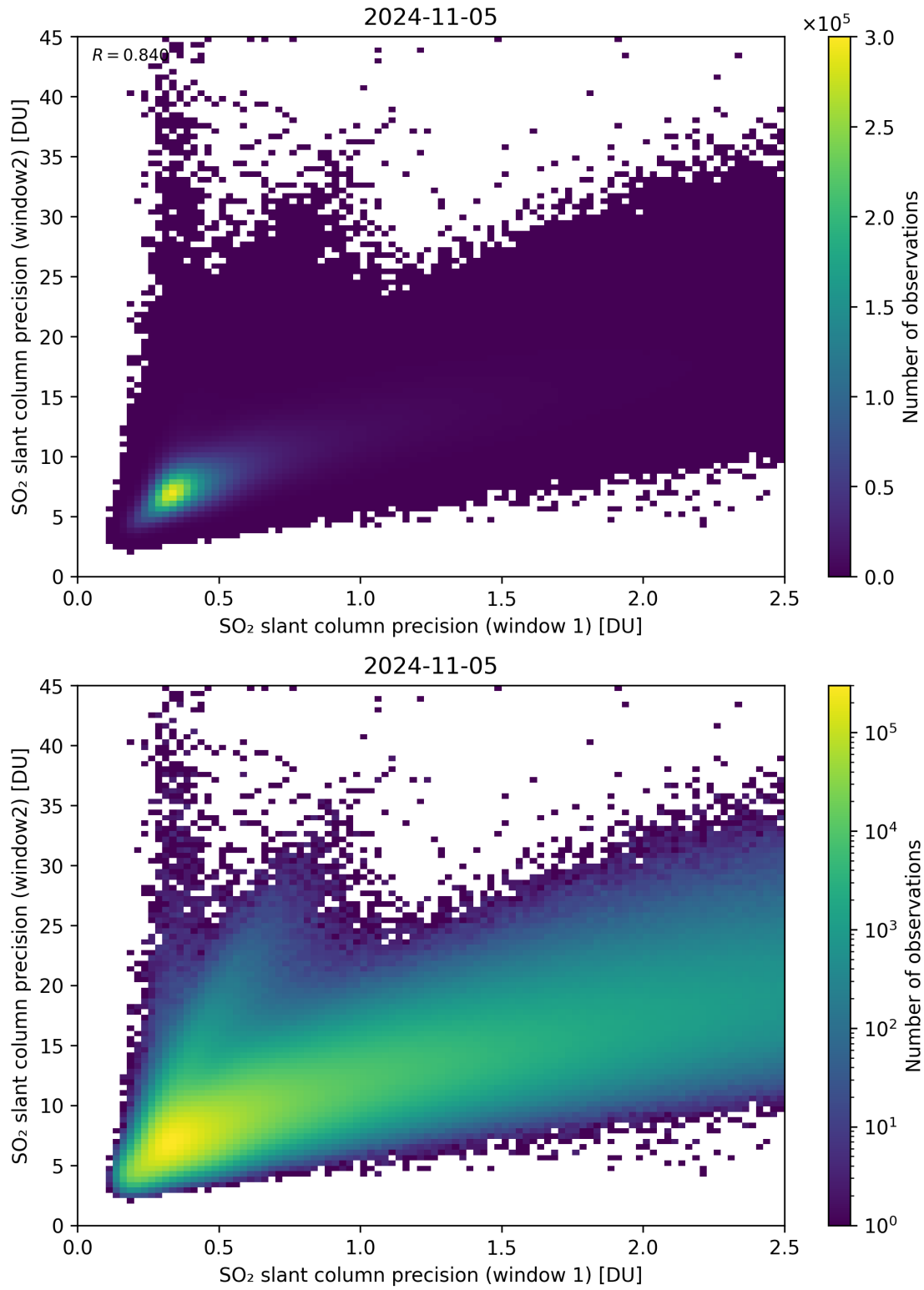
Figure 227: Scatter density plot of “SO 2 slant column precision (window 1)” against “SO 2 slant column precision (window2)” for 2024-11-04 to 2024-11-06.
