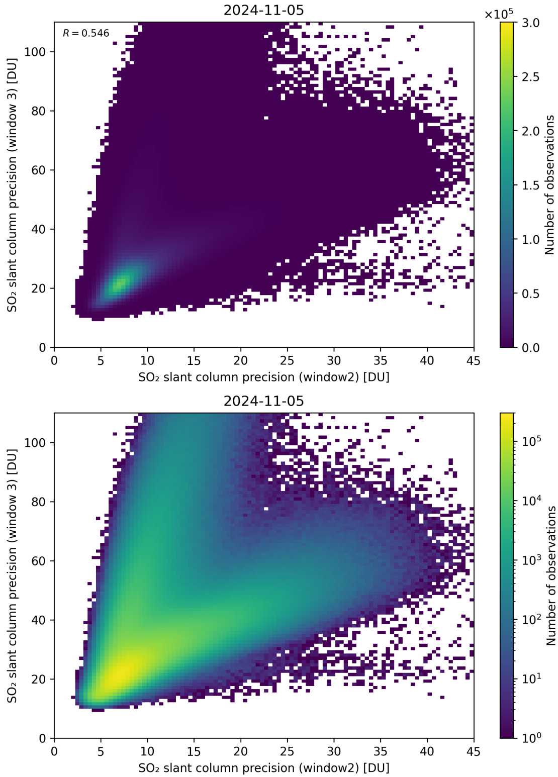
Figure 250: Scatter density plot of “SO 2 slant column precision (window2)” against “SO 2 slant column precision (window 3)” for 2024-11-04 to 2024-11-06.
