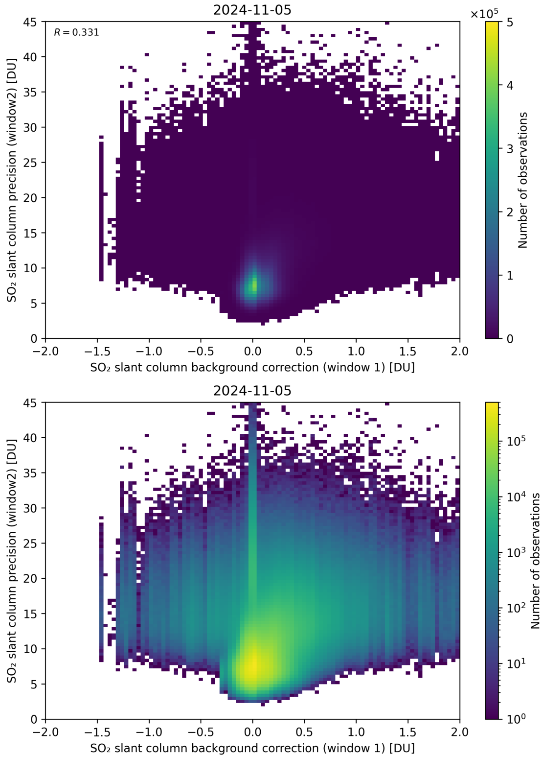
Figure 106: Scatter density plot of “SO 2 slant column background correction (window 1)” against “SO 2 slant column precision (window2)” for 2024-11-04 to 2024-11-06.
