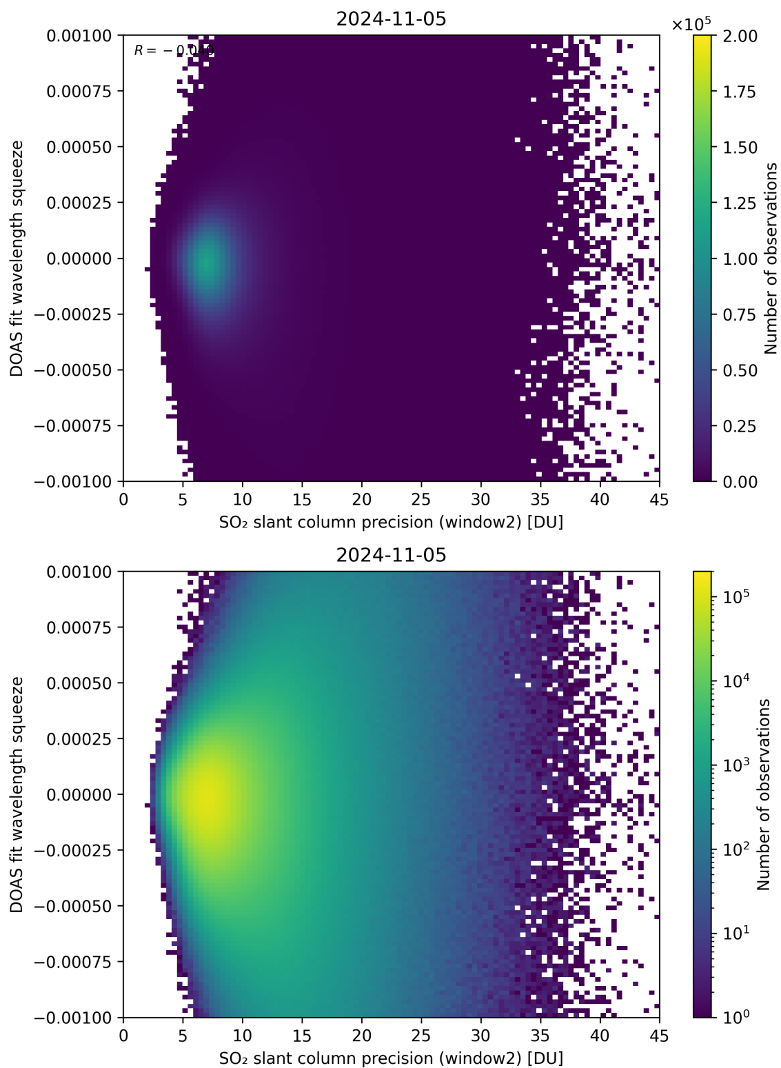
Figure 244: Scatter density plot of “SO 2 slant column precision (window2)” against “DOAS fit wavelength squeeze” for 2024-11-04 to 2024-11-06.
