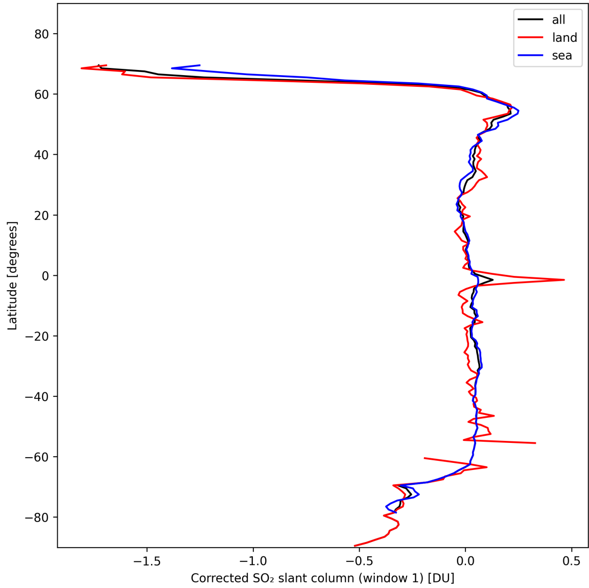
Figure 35: Zonal average of “Corrected SO 2 slant column (window 1)” for 2024-11-04 to 2024-11-06.
