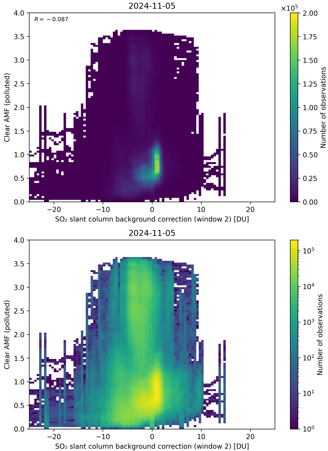
Figure 115: Scatter density plot of “SO 2 slant column background correction (window 2)” against “Clear AMF (polluted)” for 2024-11-04 to 2024-11-06.
