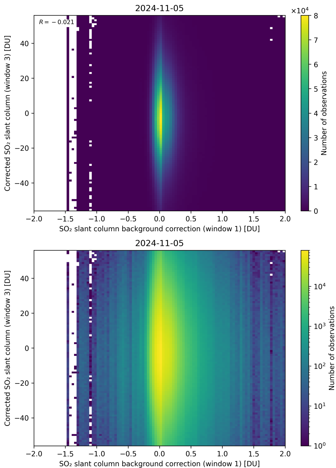
Figure 105: Scatter density plot of “SO 2 slant column background correction (window 1)” against “Corrected SO 2 slant column (window 3)” for 2024-11-04 to 2024-11-06.
