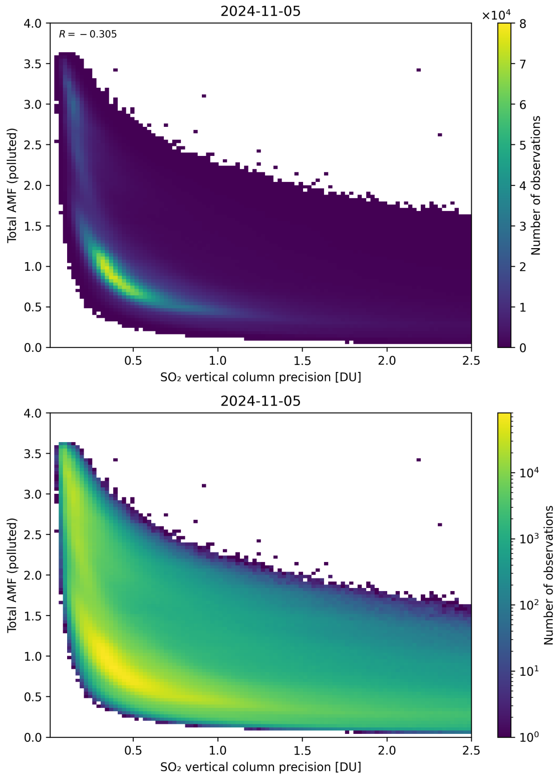
Figure 294: Scatter density plot of “SO 2 vertical column precision” against “Total AMF (polluted)” for 2024-11-04 to 2024-11-06.
