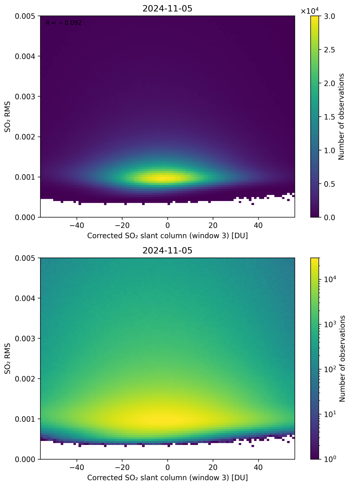
Figure 208: Scatter density plot of “Corrected SO 2 slant column (window 3)” against “SO 2 RMS” for 2024-11-04 to 2024-11-06.
