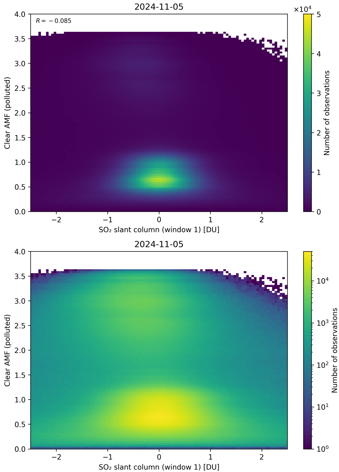
Figure 232: Scatter density plot of “SO 2 slant column (window 1)” against “Clear AMF (polluted)” for 2024-11-04 to 2024-11-06.
