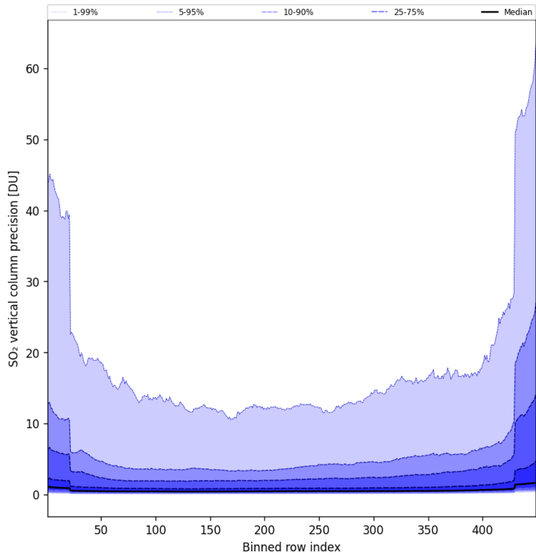
Figure 77: Along track statistics of “SO 2 vertical column precision” for 2024-11-04 to 2024-11-06
