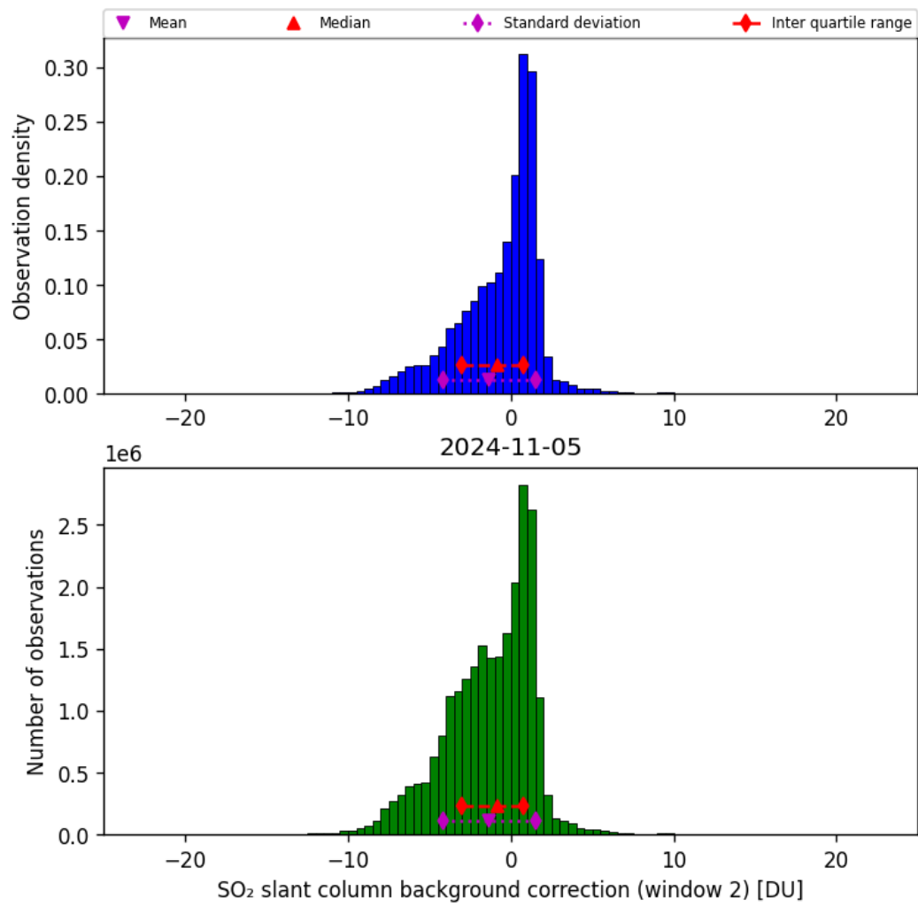
Figure 63: Histogram of “SO 2 slant column background correction (window 2)” for 2024-11-04 to 2024-11-06
