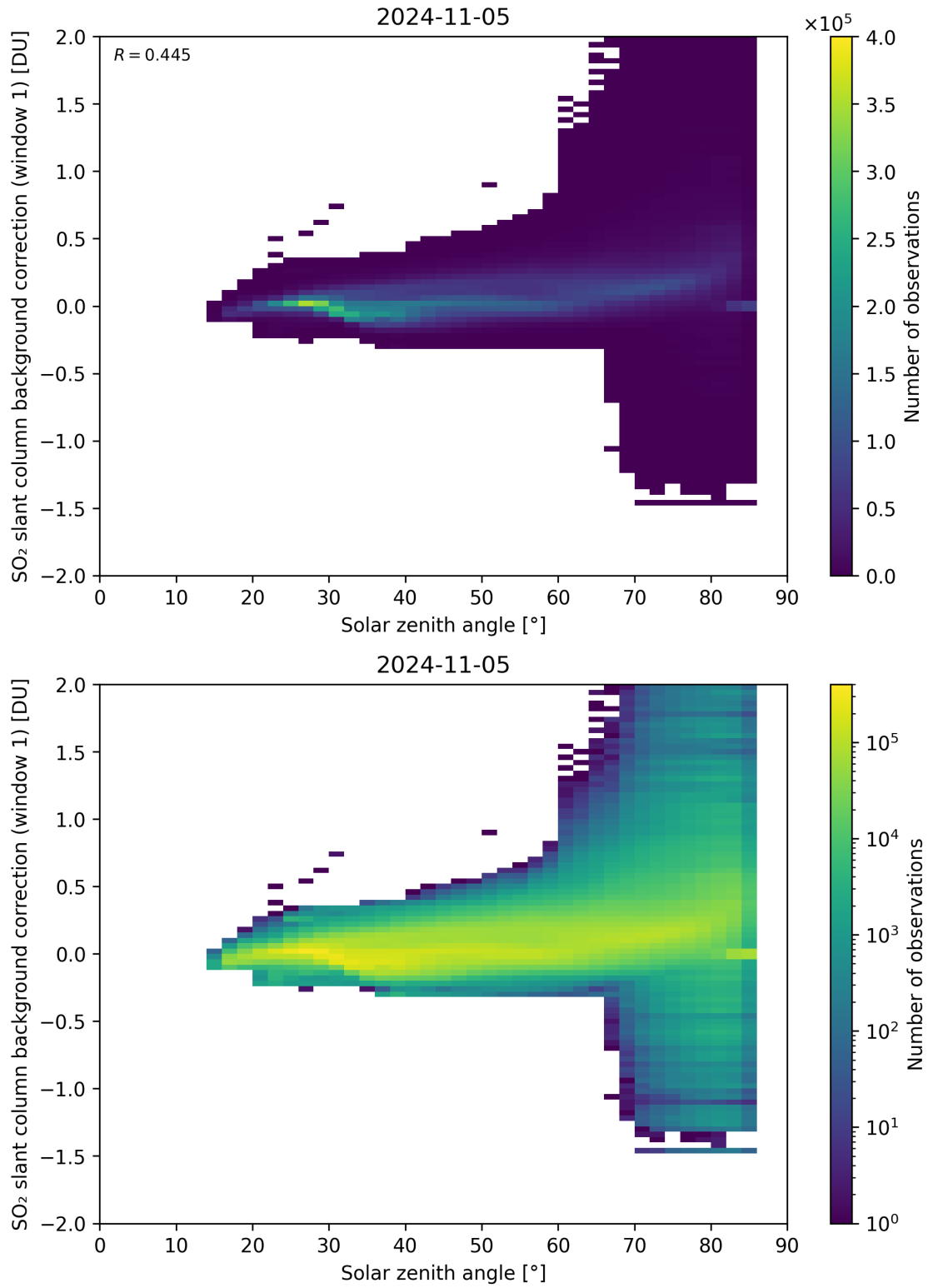
Figure 158: Scatter density plot of “Solar zenith angle” against “SO 2 slant column background correction (window 1)” for 2024-11-04 to 2024-11-06.
