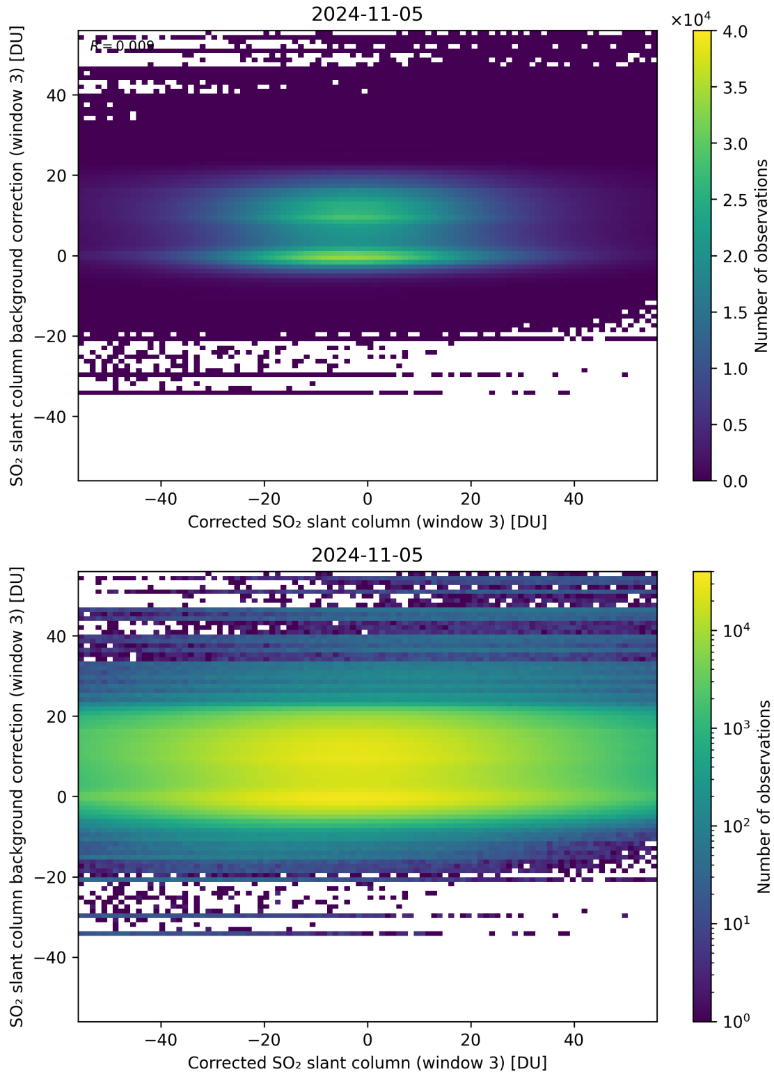
Figure 205: Scatter density plot of “Corrected SO 2 slant column (window 3)” against “SO 2 slant column background correction (window 3)” for 2024-11-04 to 2024-11-06.
