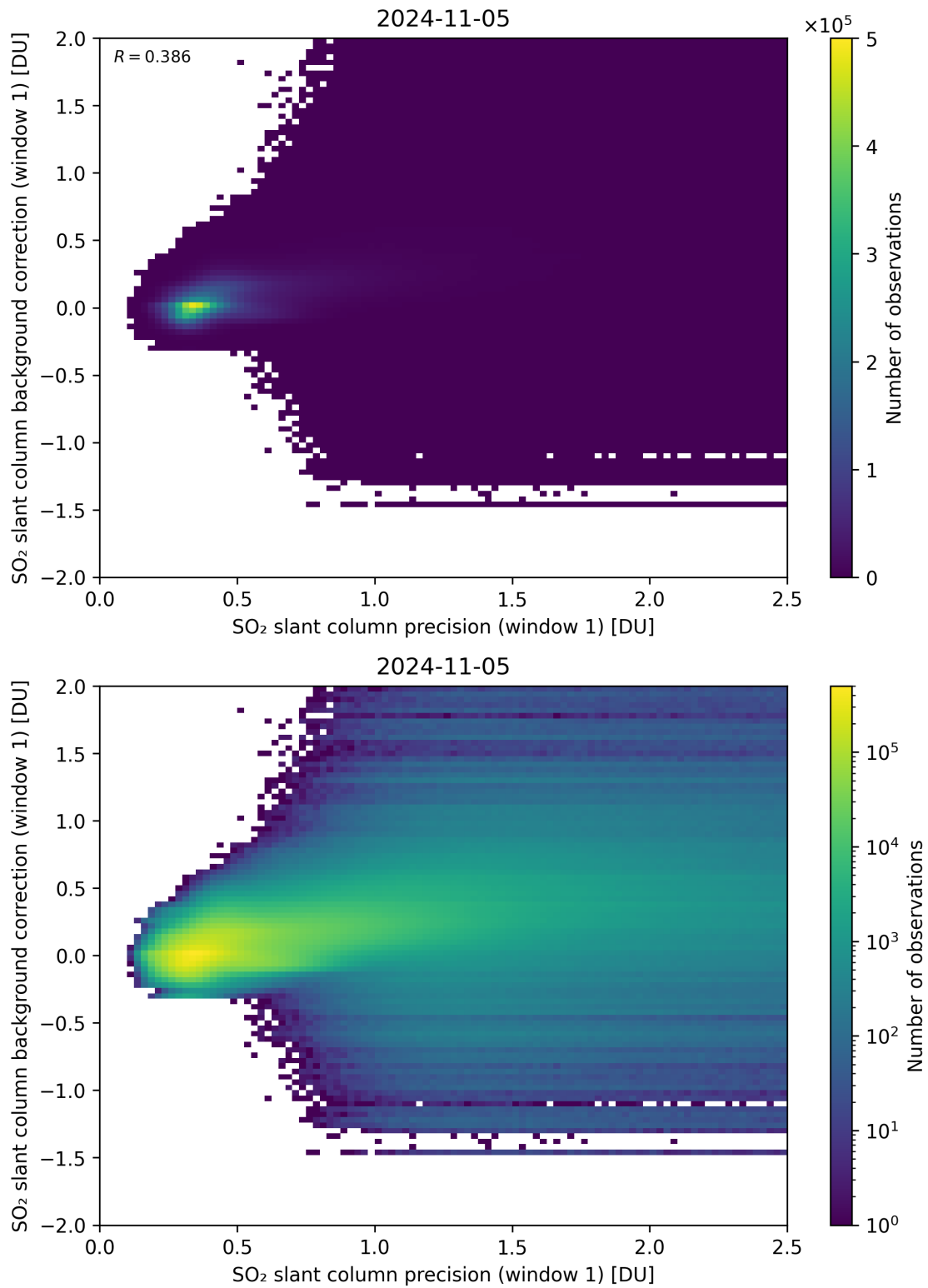
Figure 218: Scatter density plot of “SO 2 slant column precision (window 1)” against “SO 2 slant column background correction (window 1)” for 2024-11-04 to 2024-11-06.
