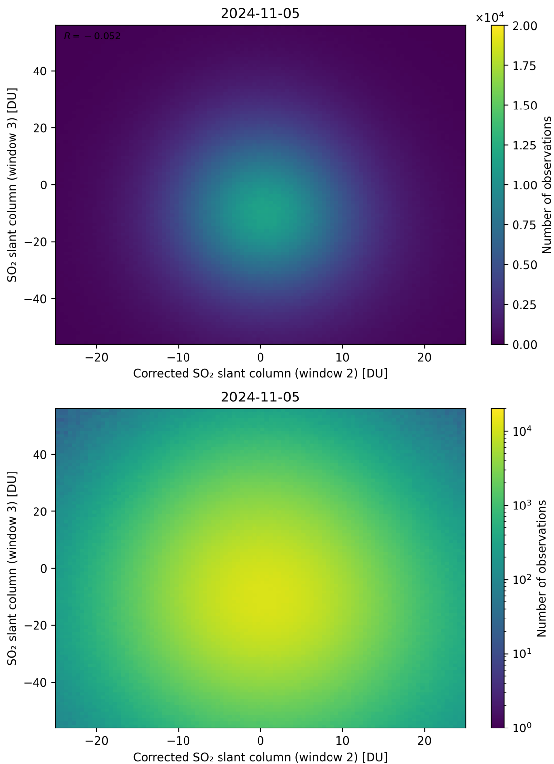
Figure 201: Scatter density plot of “Corrected SO 2 slant column (window 2)” against “SO 2 slant column (window 3)” for 2024-11-04 to 2024-11-06.
