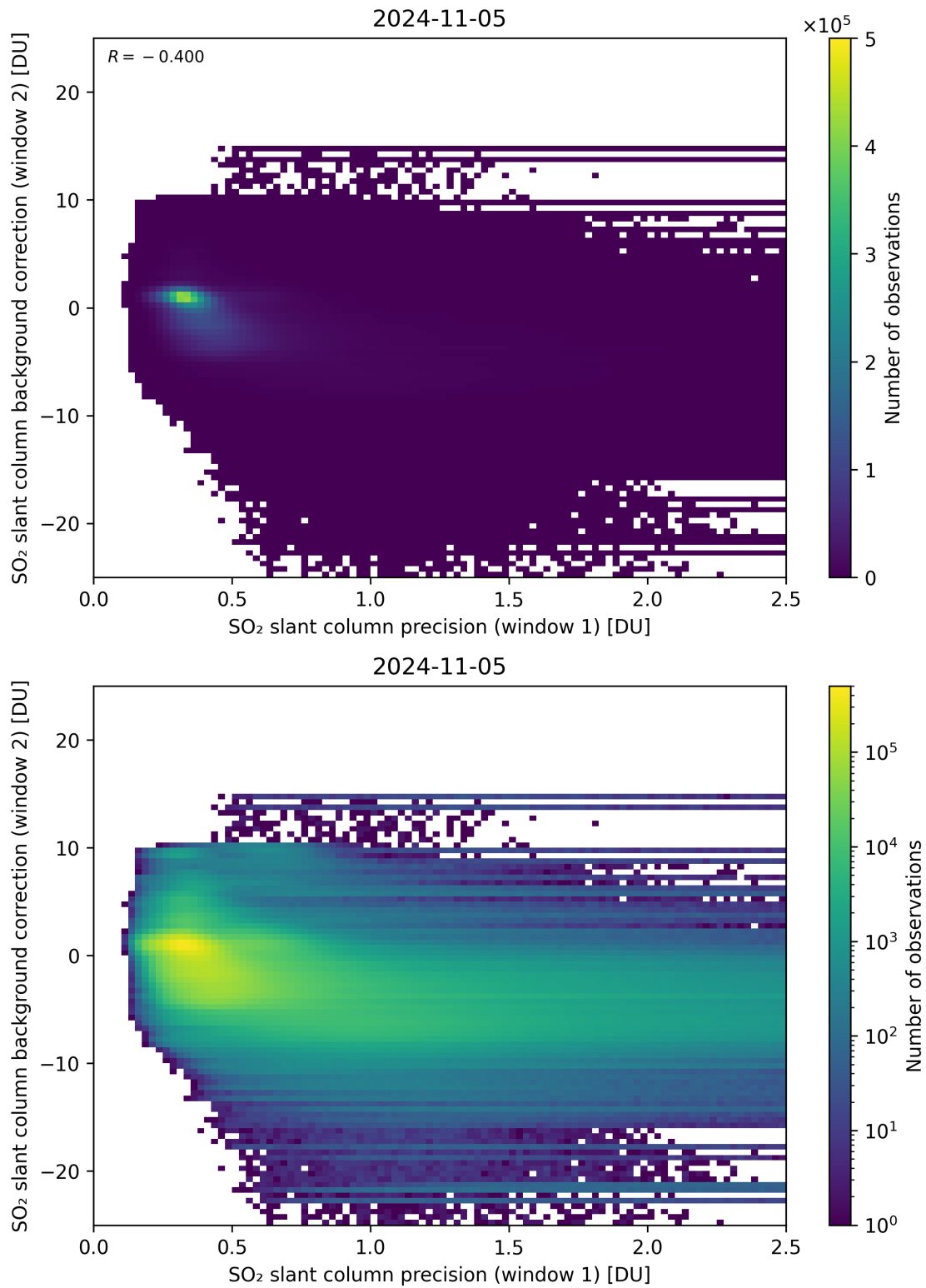
Figure 219: Scatter density plot of “SO 2 slant column precision (window 1)” against “SO 2 slant column background correction (window 2)” for 2024-11-04 to 2024-11-06.
