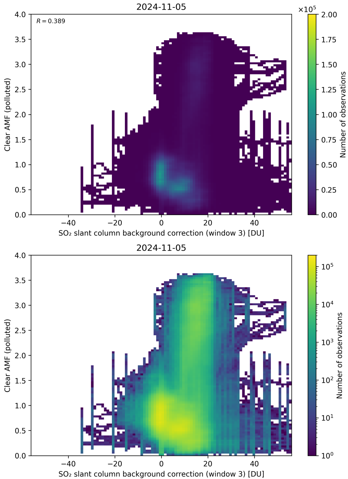
Figure 124: Scatter density plot of “SO 2 slant column background correction (window 3)” against “Clear AMF (polluted)” for 2024-11-04 to 2024-11-06.
