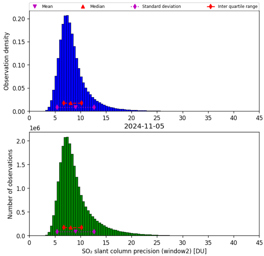
Figure 61: Histogram of “SO 2 slant column precision (window2)” for 2024-11-04 to 2024-11-06
