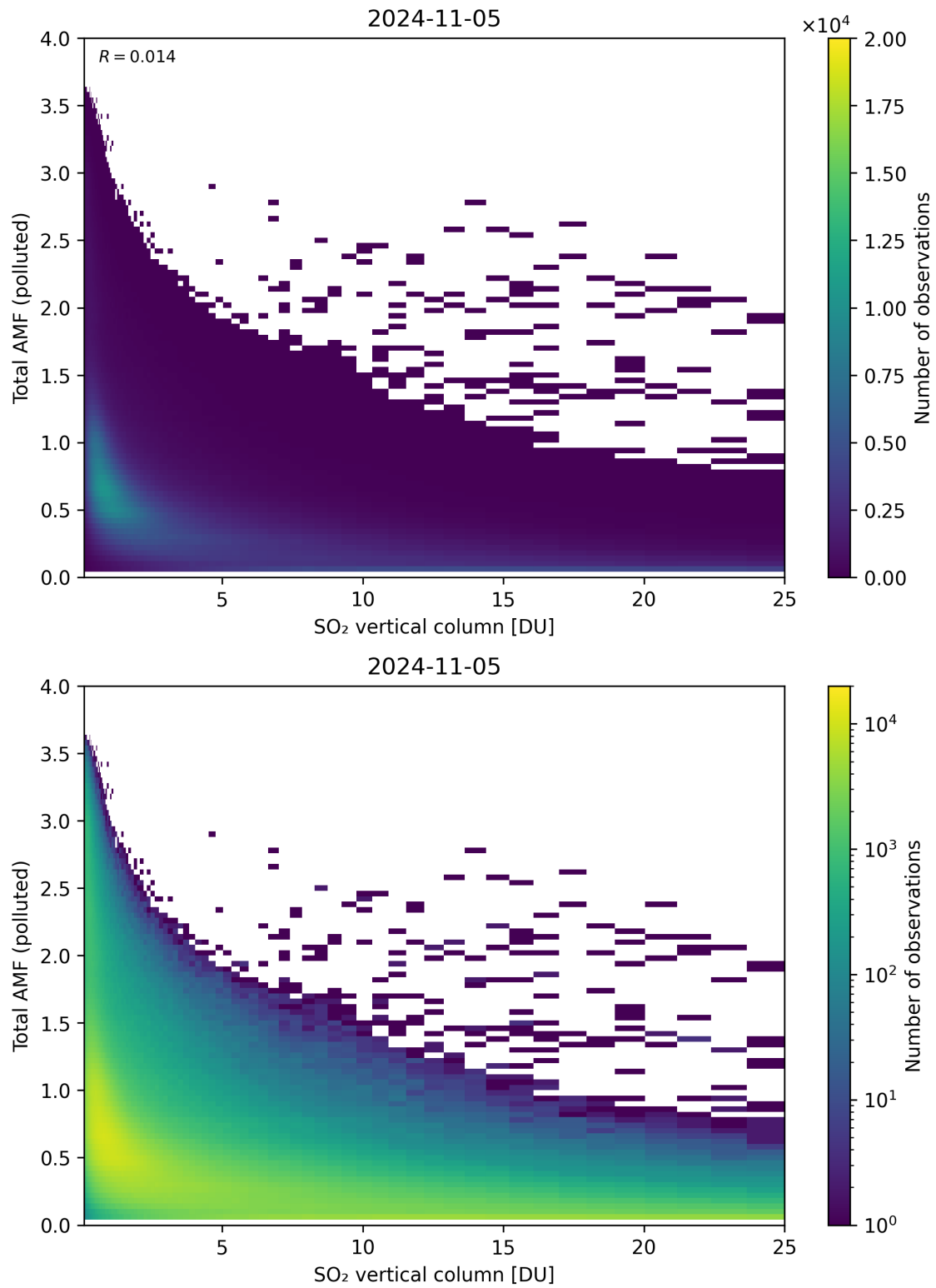
Figure 305: Scatter density plot of “SO 2 vertical column” against “Total AMF (polluted)” for 2024-11-04 to 2024-11-06.
