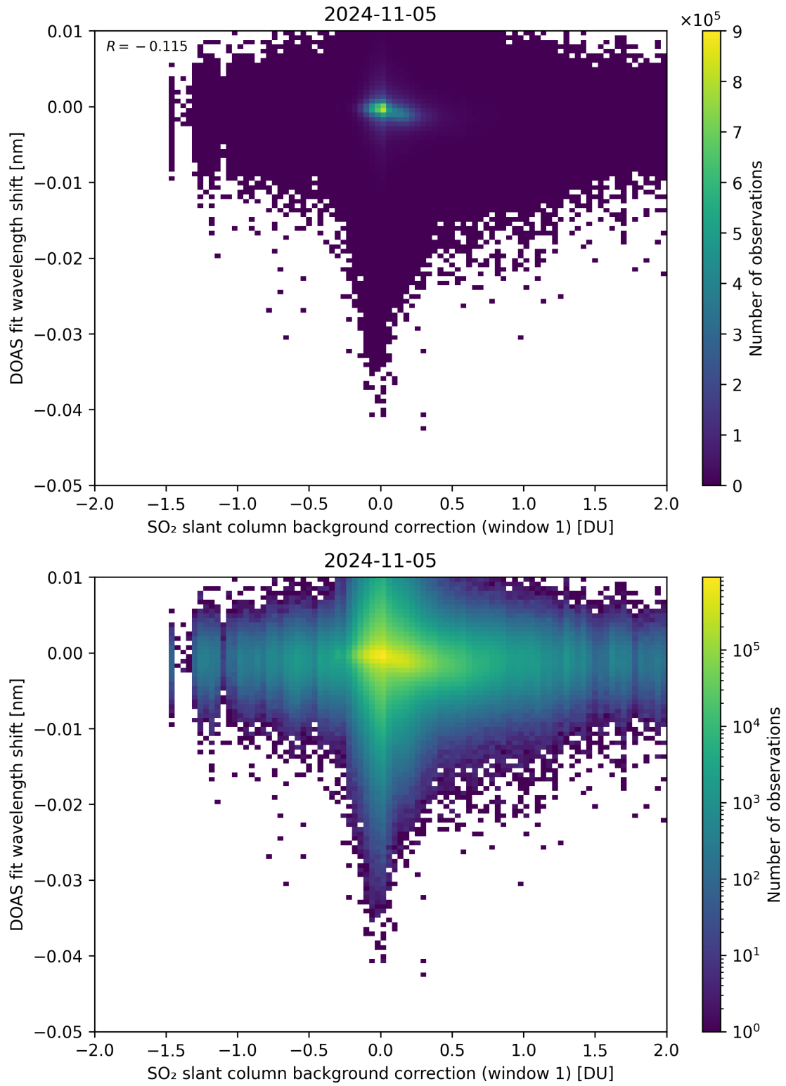
Figure 100: Scatter density plot of “SO 2 slant column background correction (window 1)” against “DOAS fit wavelength shift” for 2024-11-04 to 2024-11-06.
