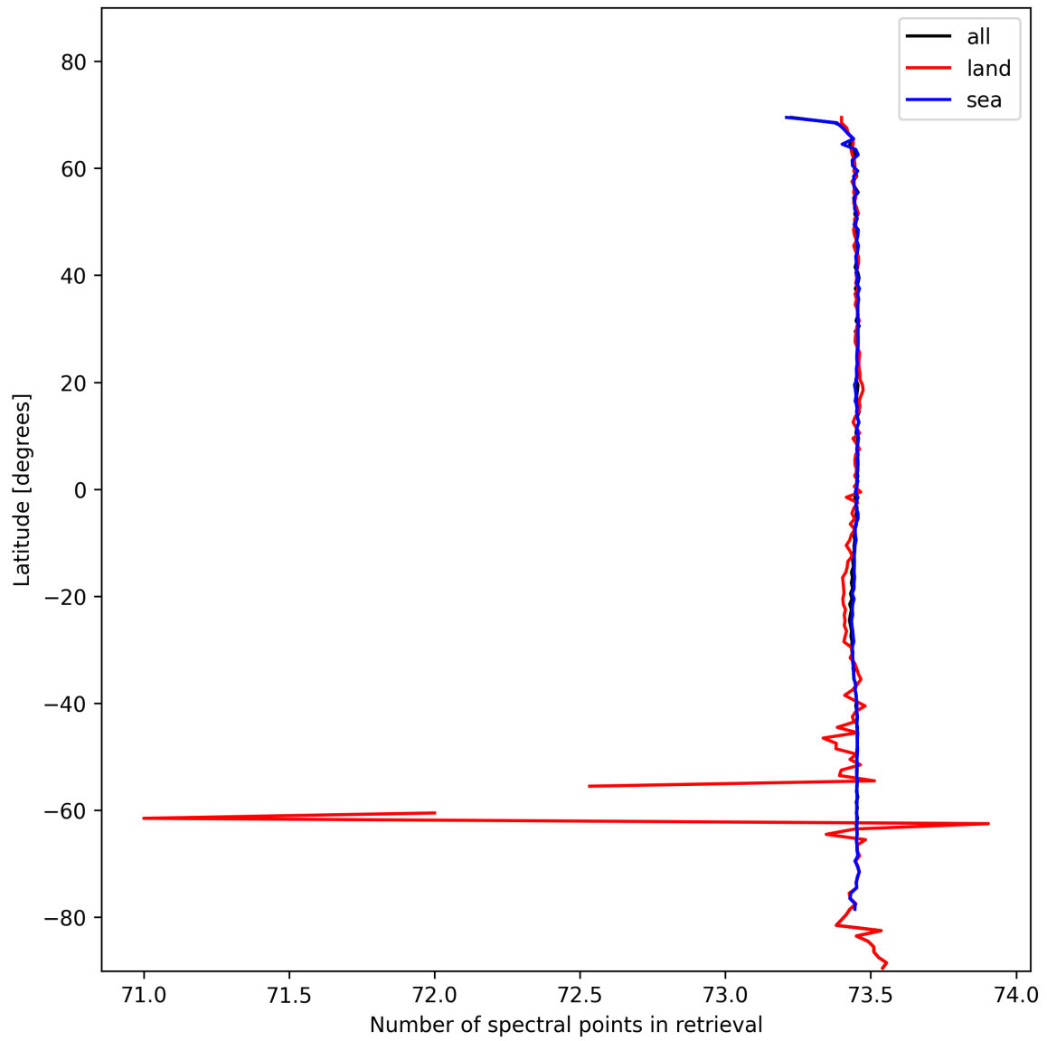
Figure 51: Zonal average of “Number of spectral points in retrieval” for 2024-11-04 to 2024-11-06.
