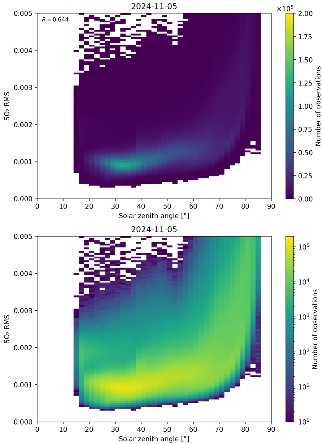
Figure 163: Scatter density plot of “Solar zenith angle” against “SO 2 RMS” for 2024-11-04 to 2024-11-06.
