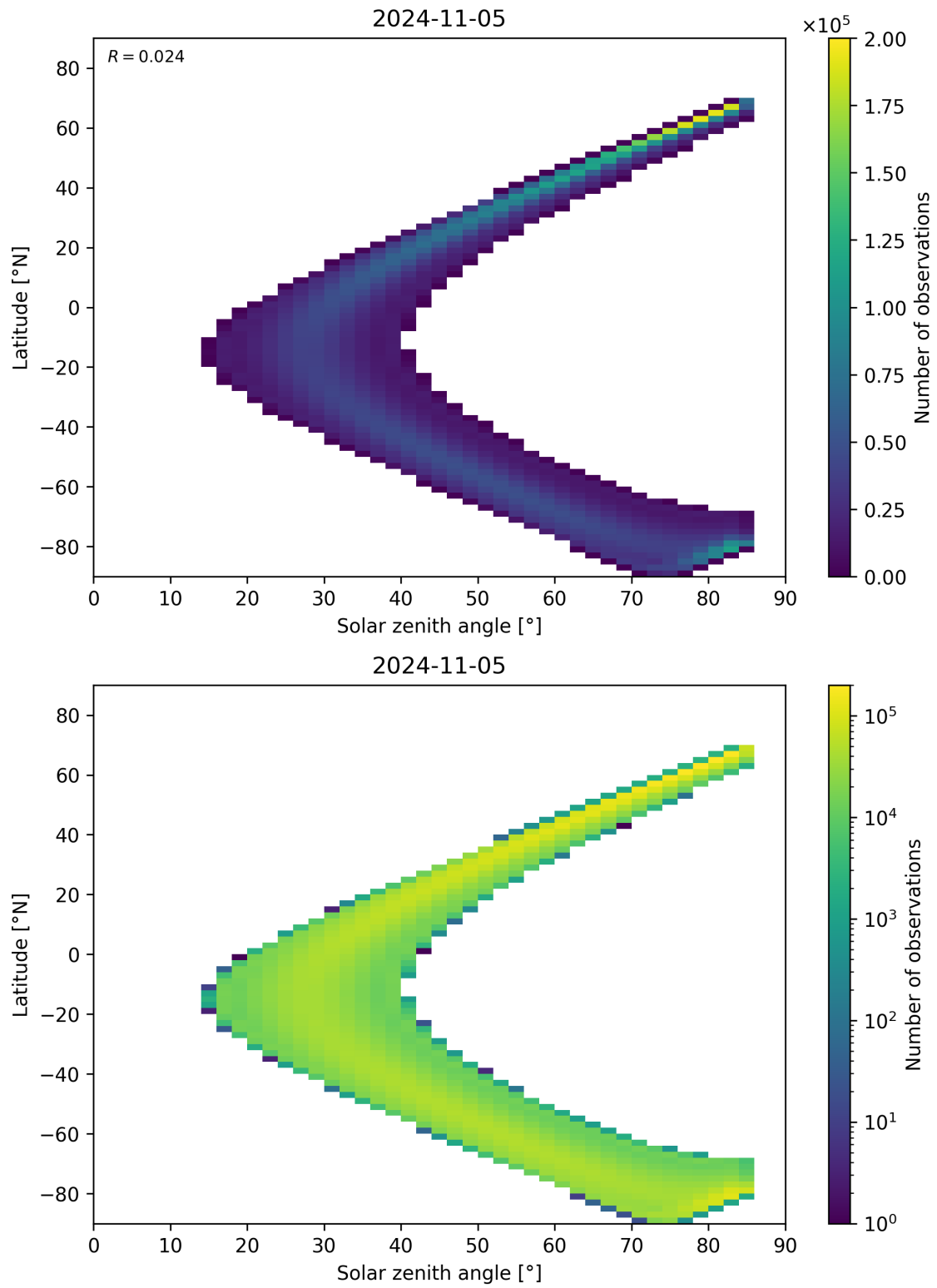
Figure 164: Scatter density plot of “Solar zenith angle” against “Latitude” for 2024-11-04 to 2024-11-06.
