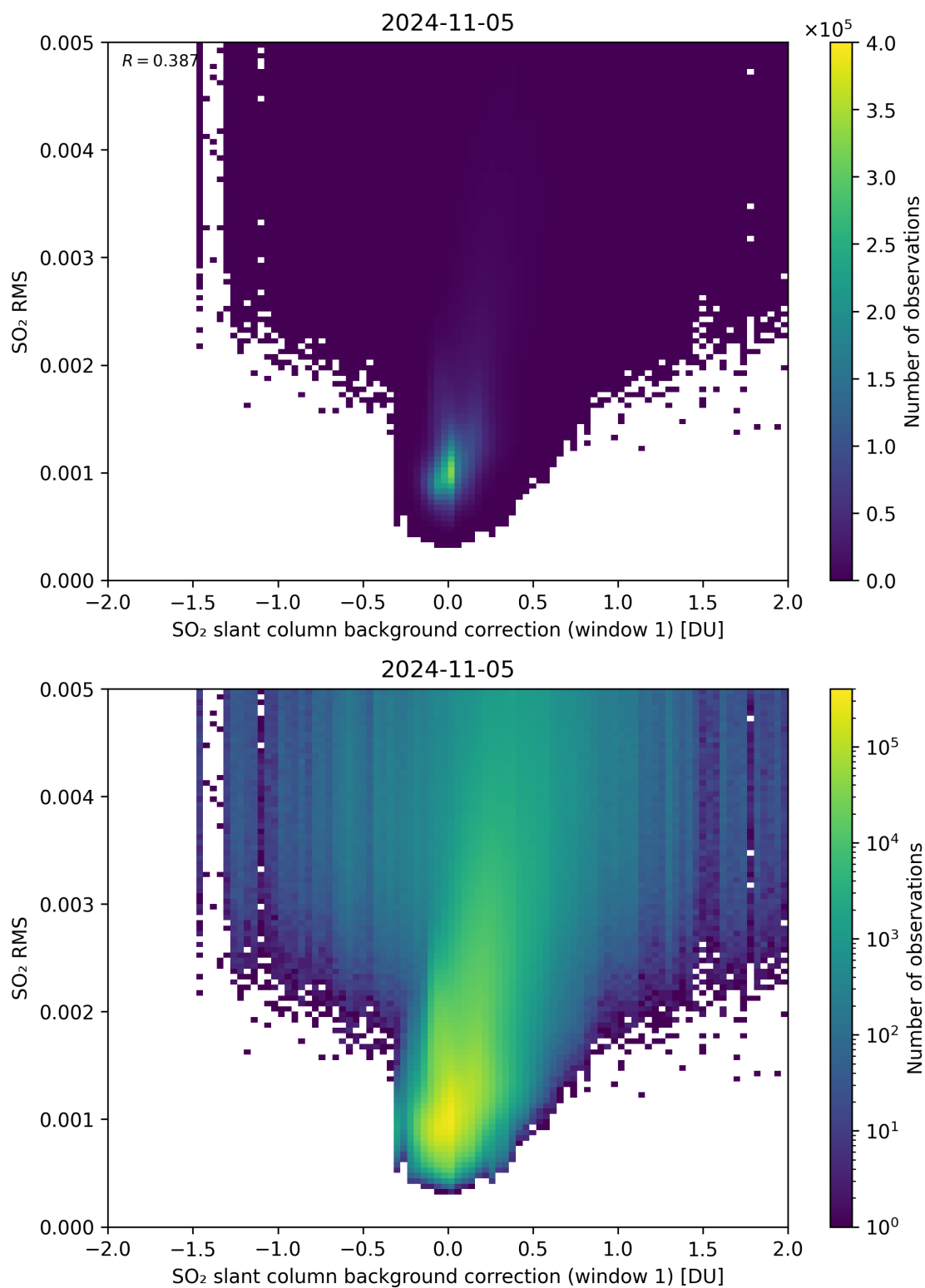
Figure 102: Scatter density plot of “SO 2 slant column background correction (window 1)” against “SO 2 RMS” for 2024-11-04 to 2024-11-06.
