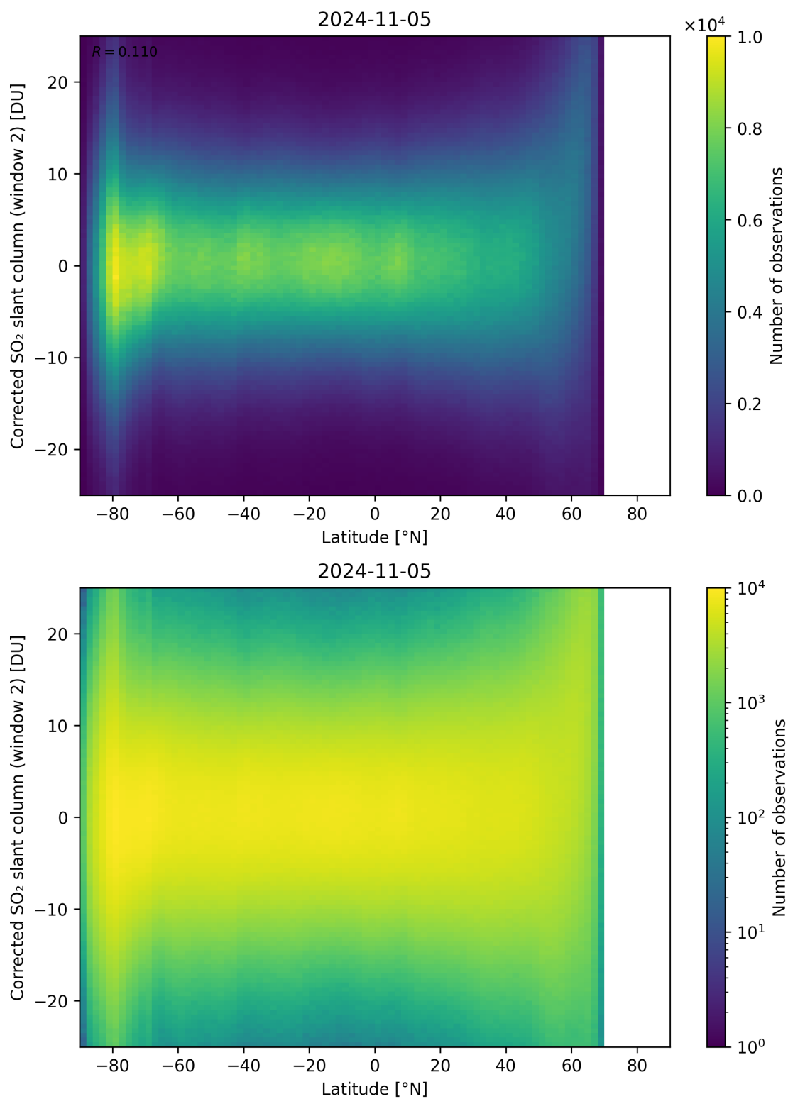
Figure 147: Scatter density plot of “Latitude” against “Corrected SO 2 slant column (window 2)” for 2024-11-04 to 2024-11-06.
