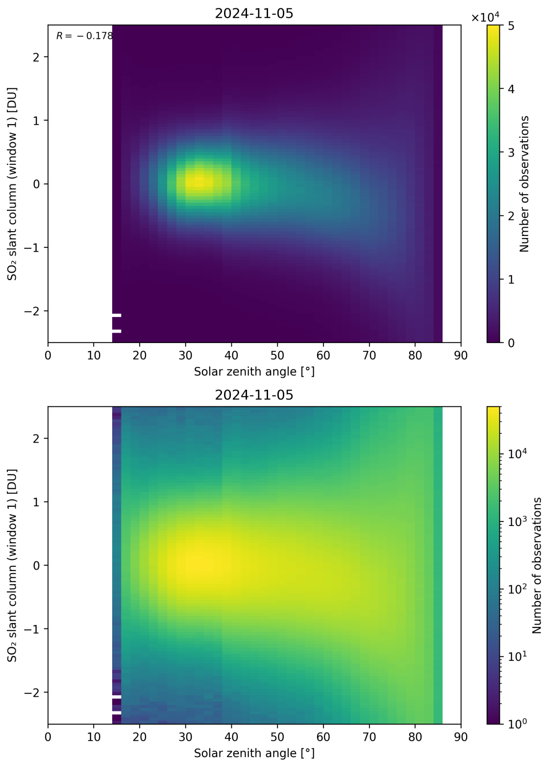
Figure 169: Scatter density plot of “Solar zenith angle” against “SO 2 slant column (window 1)” for 2024-11-04 to 2024-11-06.
