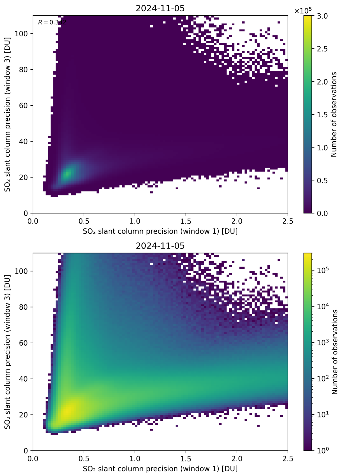
Figure 229: Scatter density plot of “SO 2 slant column precision (window 1)” against “SO 2 slant column precision (window 3)” for 2024-11-04 to 2024-11-06.
