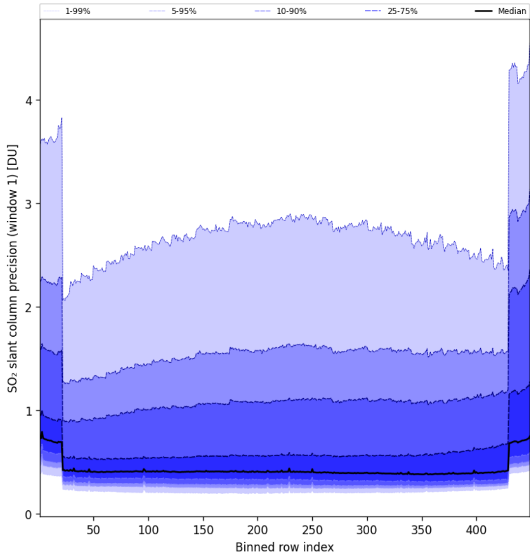
Figure 80: Along track statistics of “SO 2 slant column precision (window 1)” for 2024-11-04 to 2024-11-06
