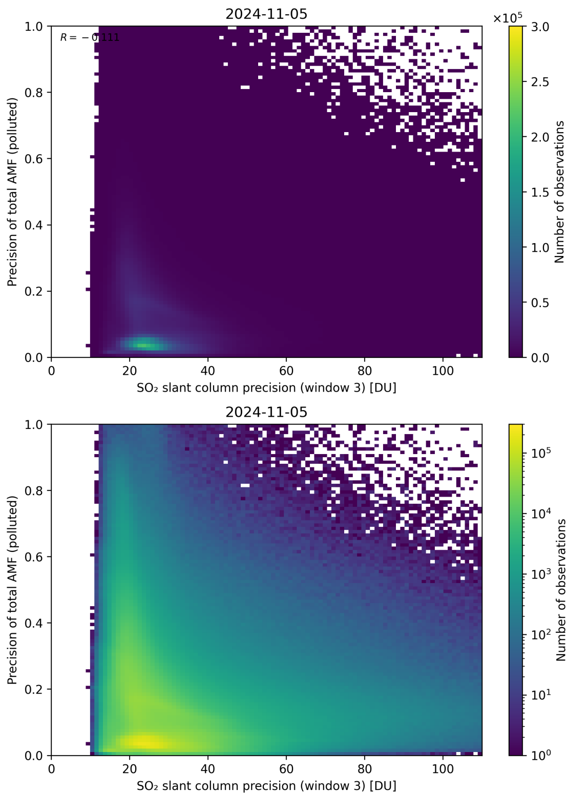
Figure 264: Scatter density plot of “SO 2 slant column precision (window 3)” against “Precision of total AMF (polluted)” for 2024-11-04 to 2024-11-06.
