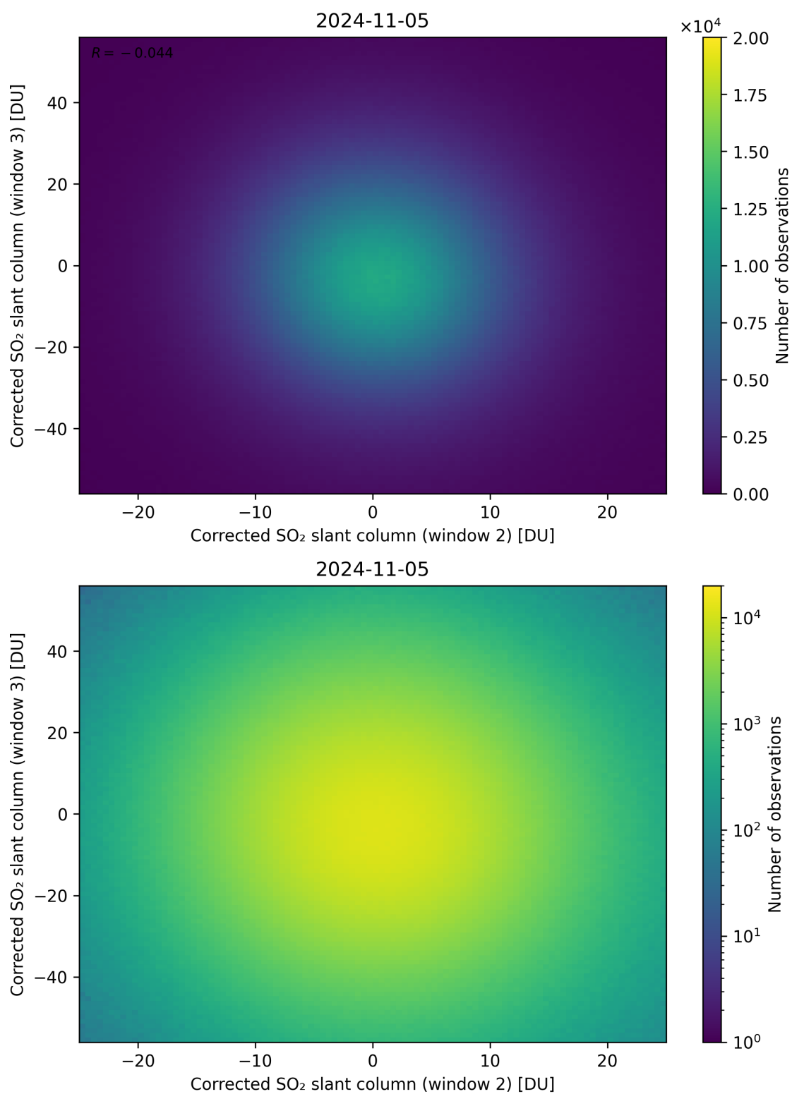
Figure 200: Scatter density plot of “Corrected SO 2 slant column (window 2)” against “Corrected SO 2 slant column (window 3)” for 2024-11-04 to 2024-11-06.
