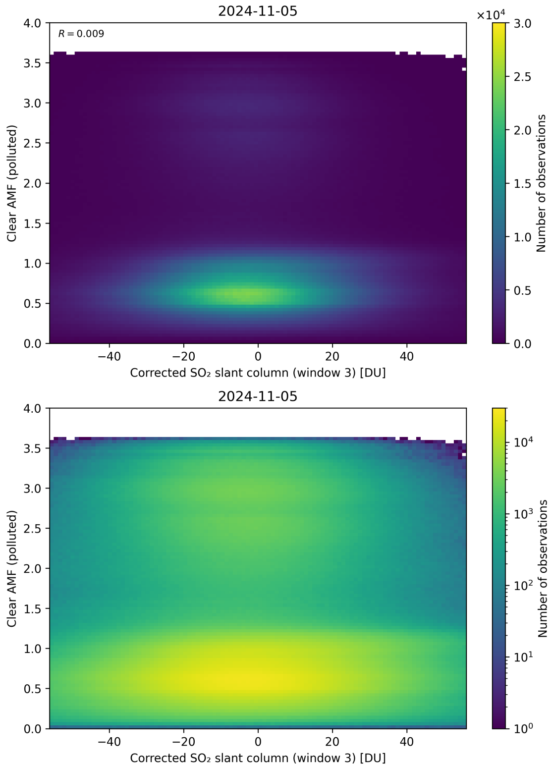
Figure 209: Scatter density plot of “Corrected SO 2 slant column (window 3)” against “Clear AMF (polluted)” for 2024-11-04 to 2024-11-06.
