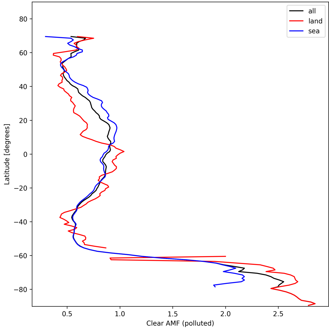
Figure 50: Zonal average of “Clear AMF (polluted)” for 2024-11-04 to 2024-11-06.
