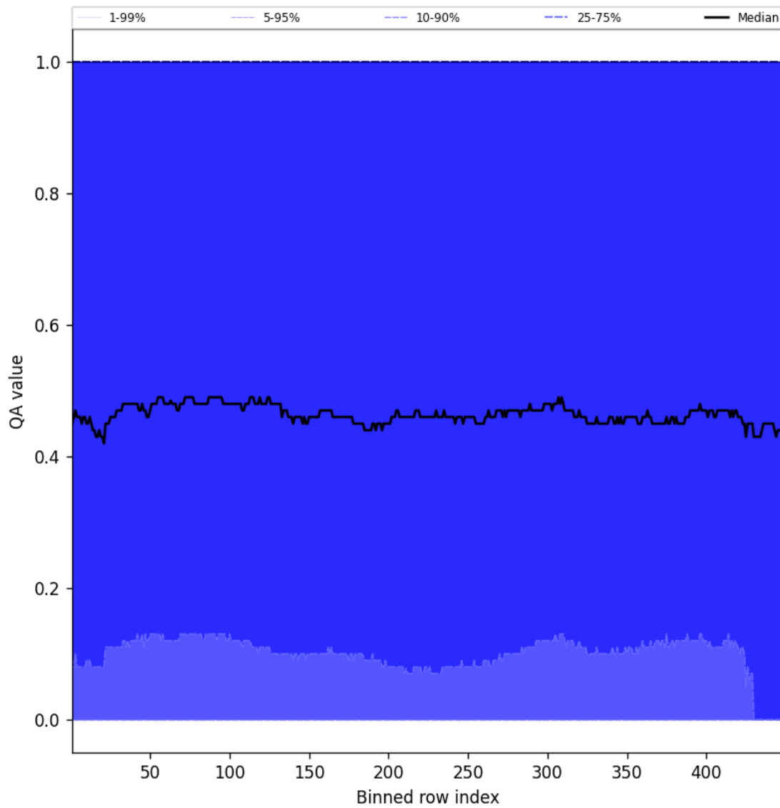
Figure 75: Along track statistics of “QA value” for 2024-11-04 to 2024-11-06
