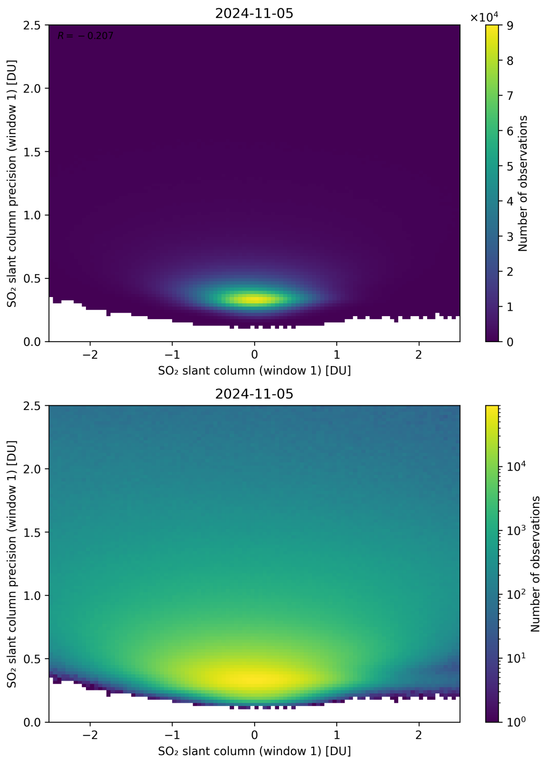
Figure 235: Scatter density plot of “SO 2 slant column (window 1)” against “SO 2 slant column precision (window 1)” for 2024-11-04 to 2024-11-06.
