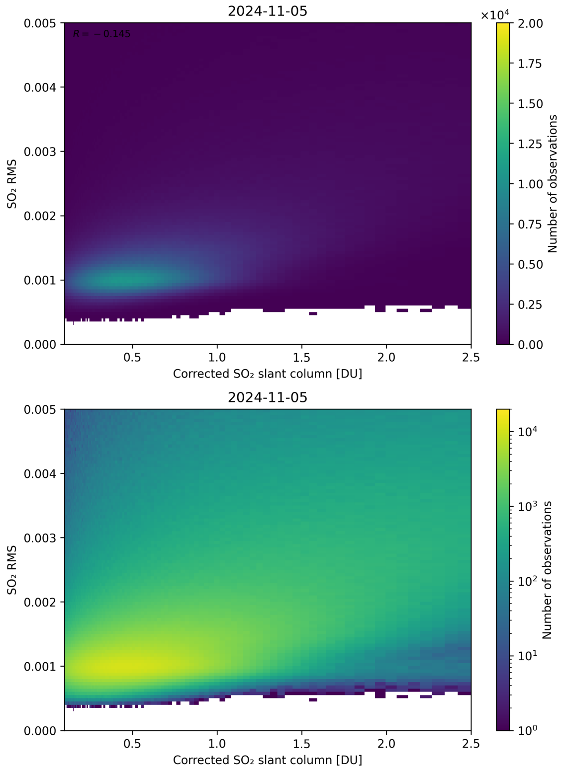
Figure 183: Scatter density plot of “Corrected SO 2 slant column” against “SO 2 RMS” for 2024-11-04 to 2024-11-06.
