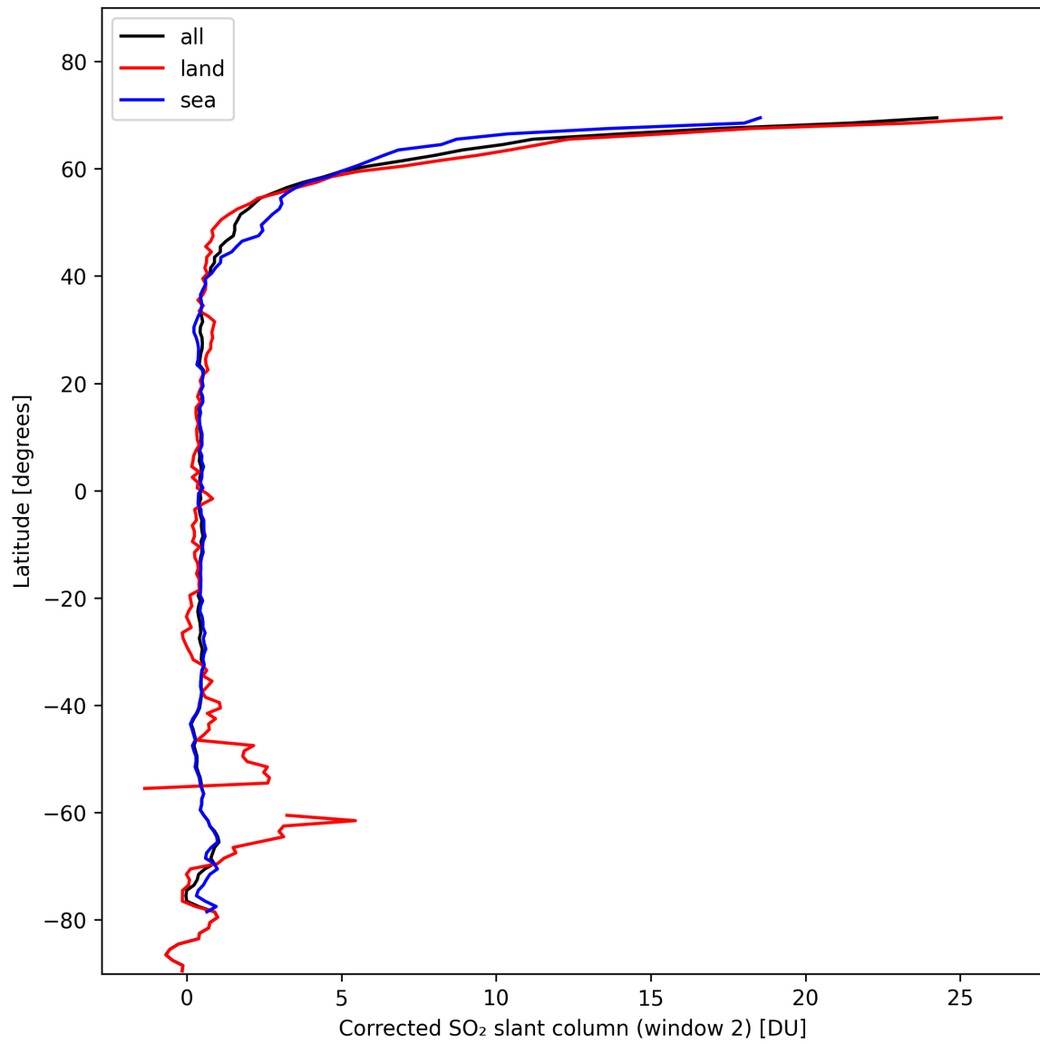
Figure 39: Zonal average of “Corrected SO 2 slant column (window 2)” for 2024-11-04 to 2024-11-06.
