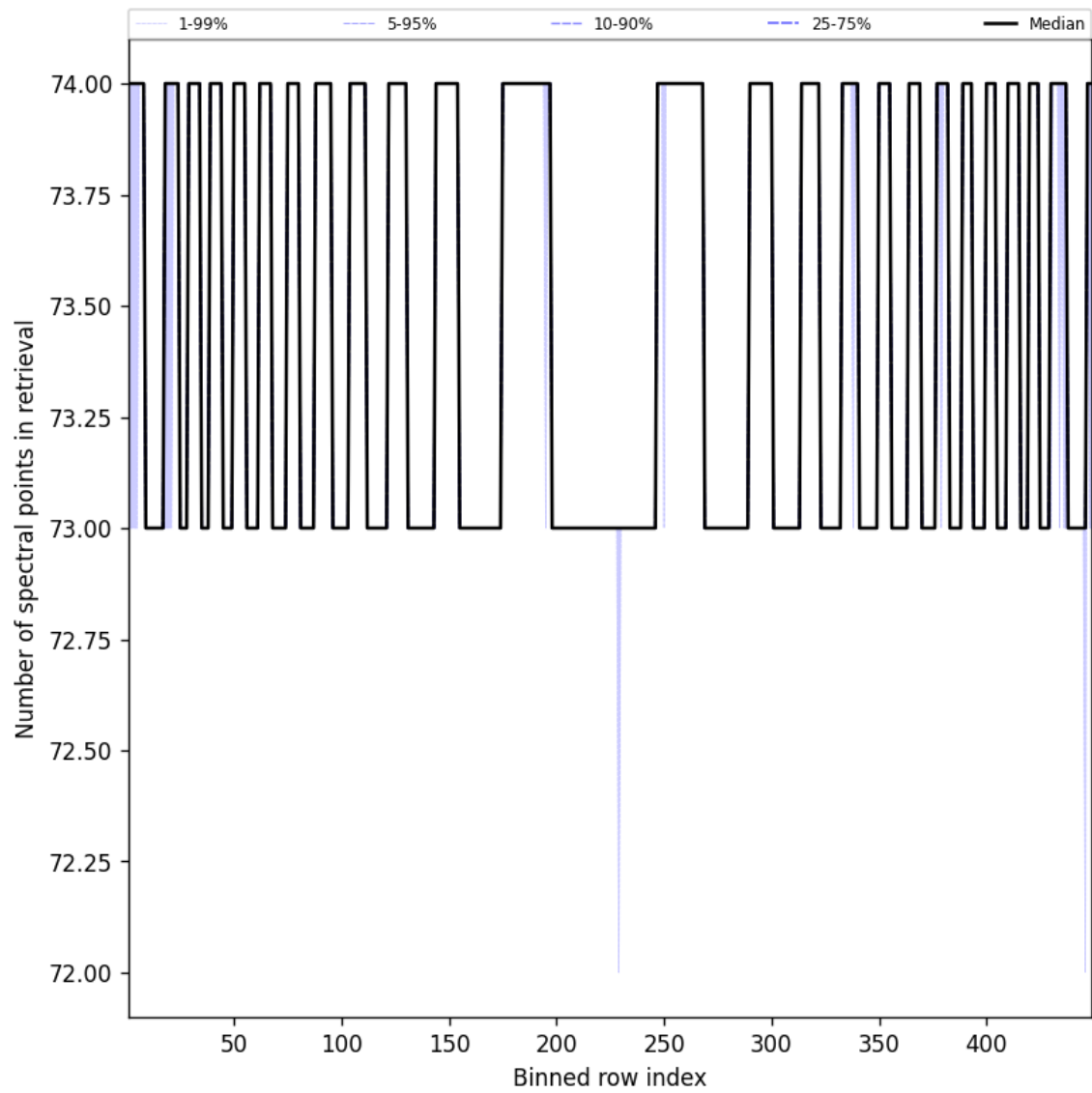
Figure 97: Along track statistics of “Number of spectral points in retrieval” for 2024-11-04 to 2024-11-06
