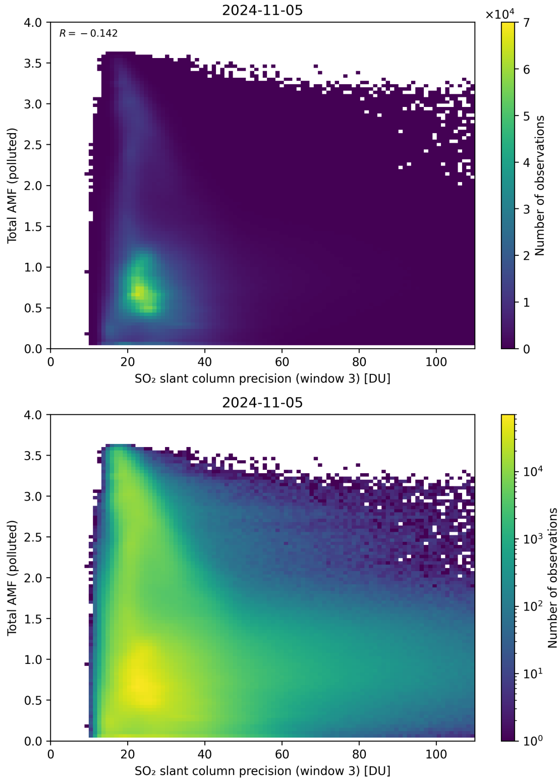
Figure 263: Scatter density plot of “SO 2 slant column precision (window 3)” against “Total AMF (polluted)” for 2024-11-04 to 2024-11-06.
