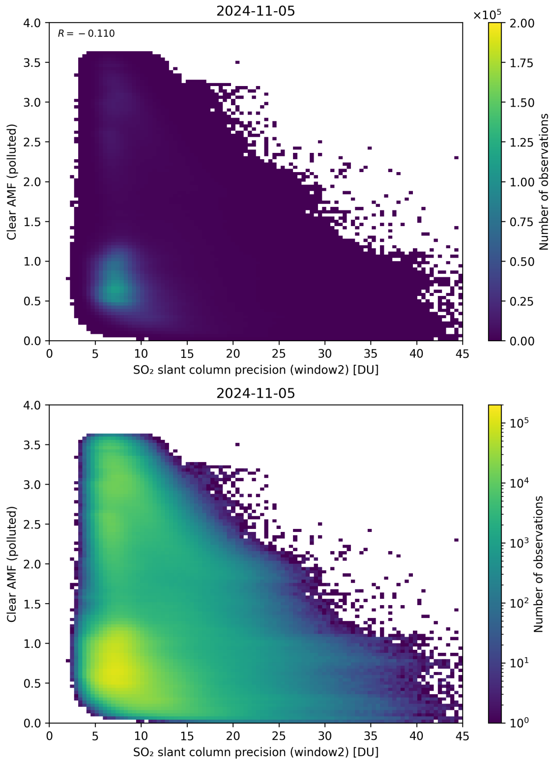
Figure 246: Scatter density plot of “SO 2 slant column precision (window2)” against “Clear AMF (polluted)” for 2024-11-04 to 2024-11-06.
