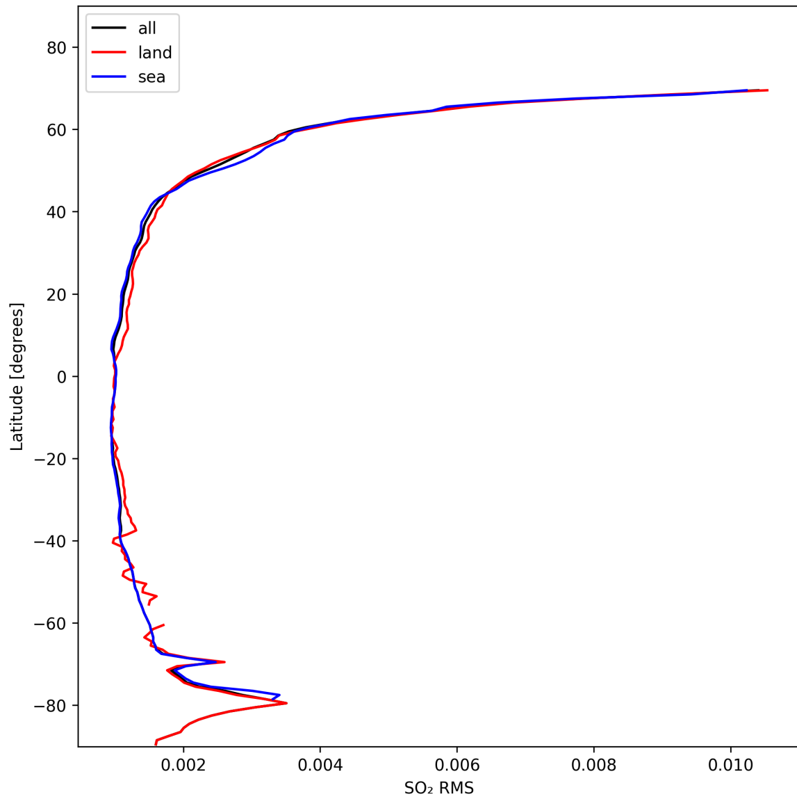
Figure 47: Zonal average of “SO 2 RMS” for 2024-11-04 to 2024-11-06.
