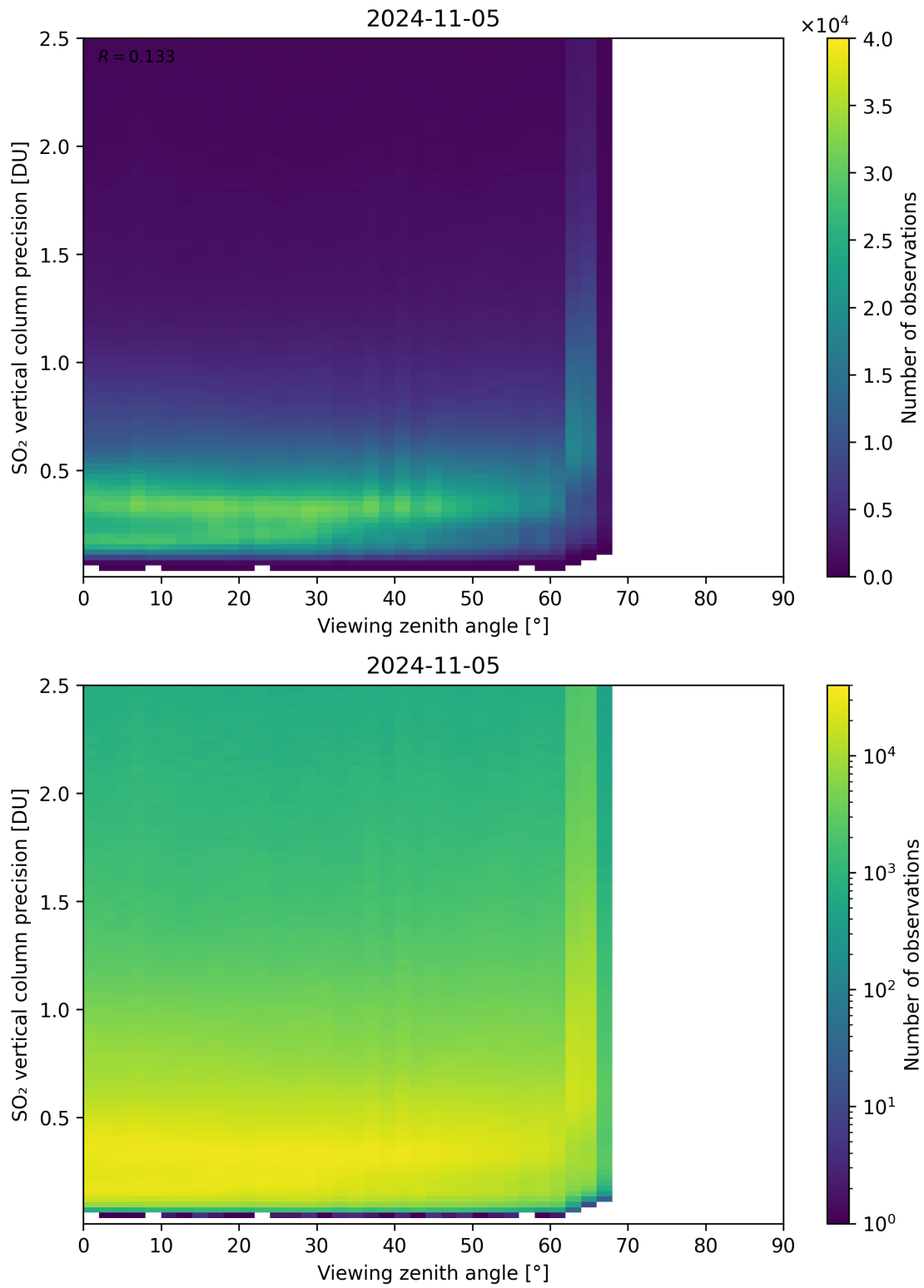
Figure 328: Scatter density plot of “Viewing zenith angle” against “SO 2 vertical column precision” for 2024-11-04 to 2024-11-06.
