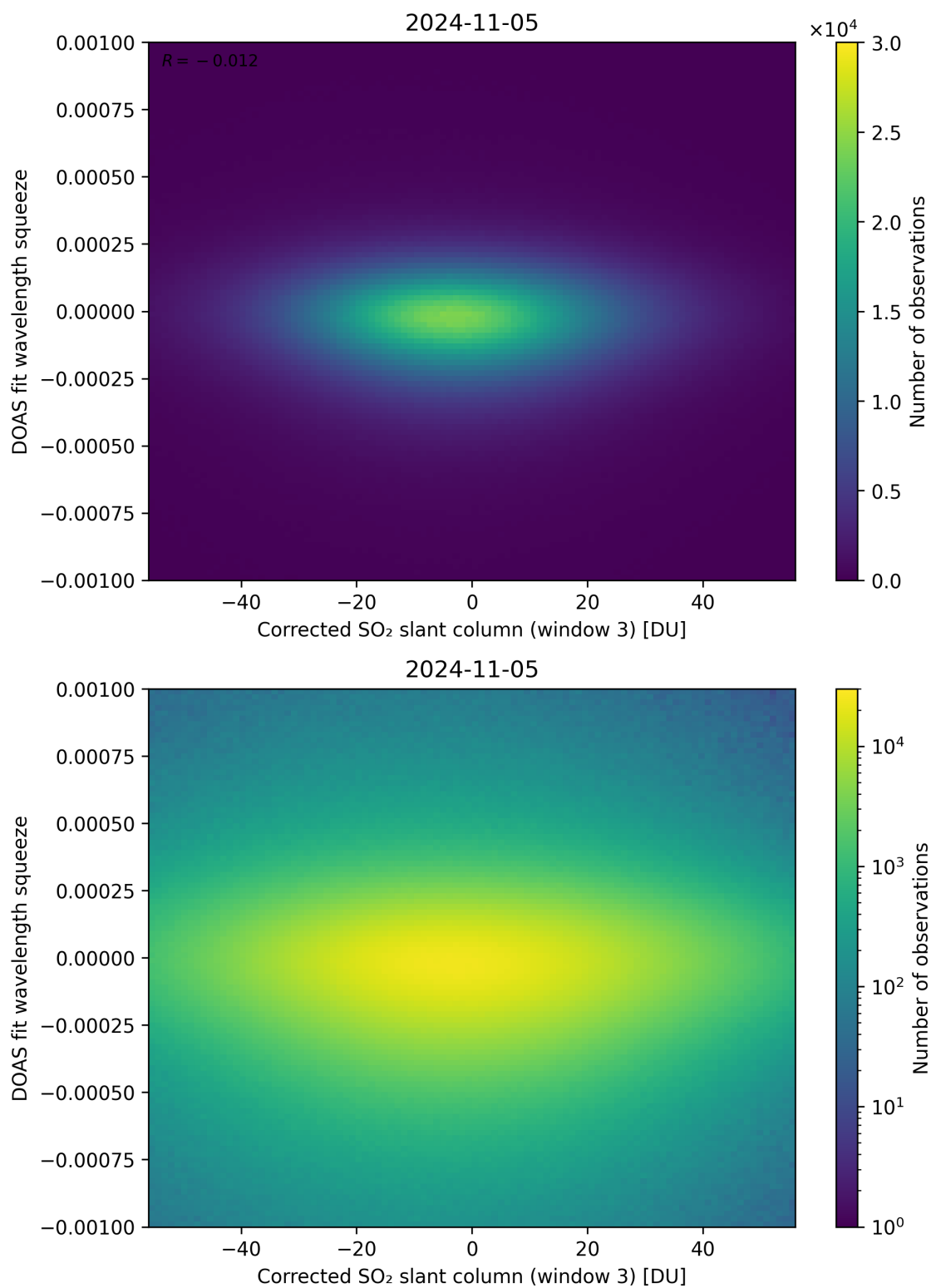
Figure 207: Scatter density plot of “Corrected SO 2 slant column (window 3)” against “DOAS fit wavelength squeeze” for 2024-11-04 to 2024-11-06.
