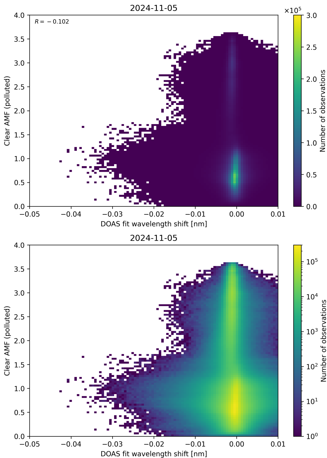
Figure 129: Scatter density plot of “DOAS fit wavelength shift” against “Clear AMF (polluted)” for 2024-11-04 to 2024-11-06.
