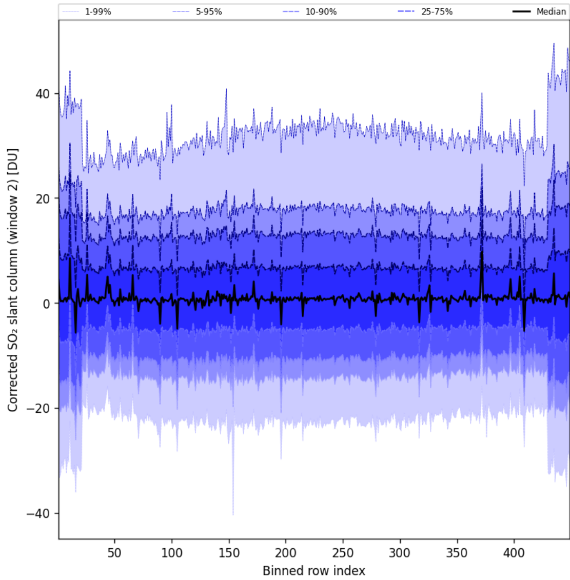
Figure 85: Along track statistics of “Corrected SO 2 slant column (window 2)” for 2024-11-04 to 2024-11-06
