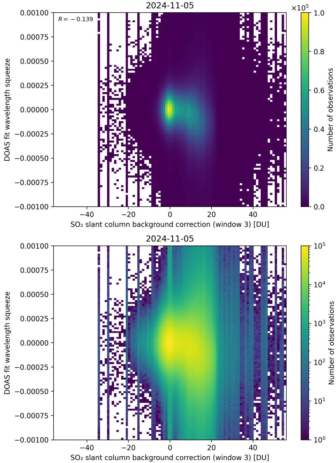
Figure 122: Scatter density plot of “SO 2 slant column background correction (window 3)” against “DOAS fit wavelength squeeze” for 2024-11-04 to 2024-11-06.
