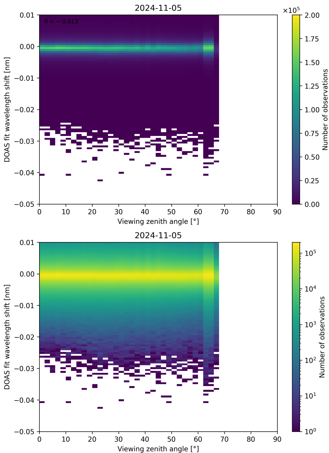
Figure 311: Scatter density plot of “Viewing zenith angle” against “DOAS fit wavelength shift” for 2024-11-04 to 2024-11-06.
