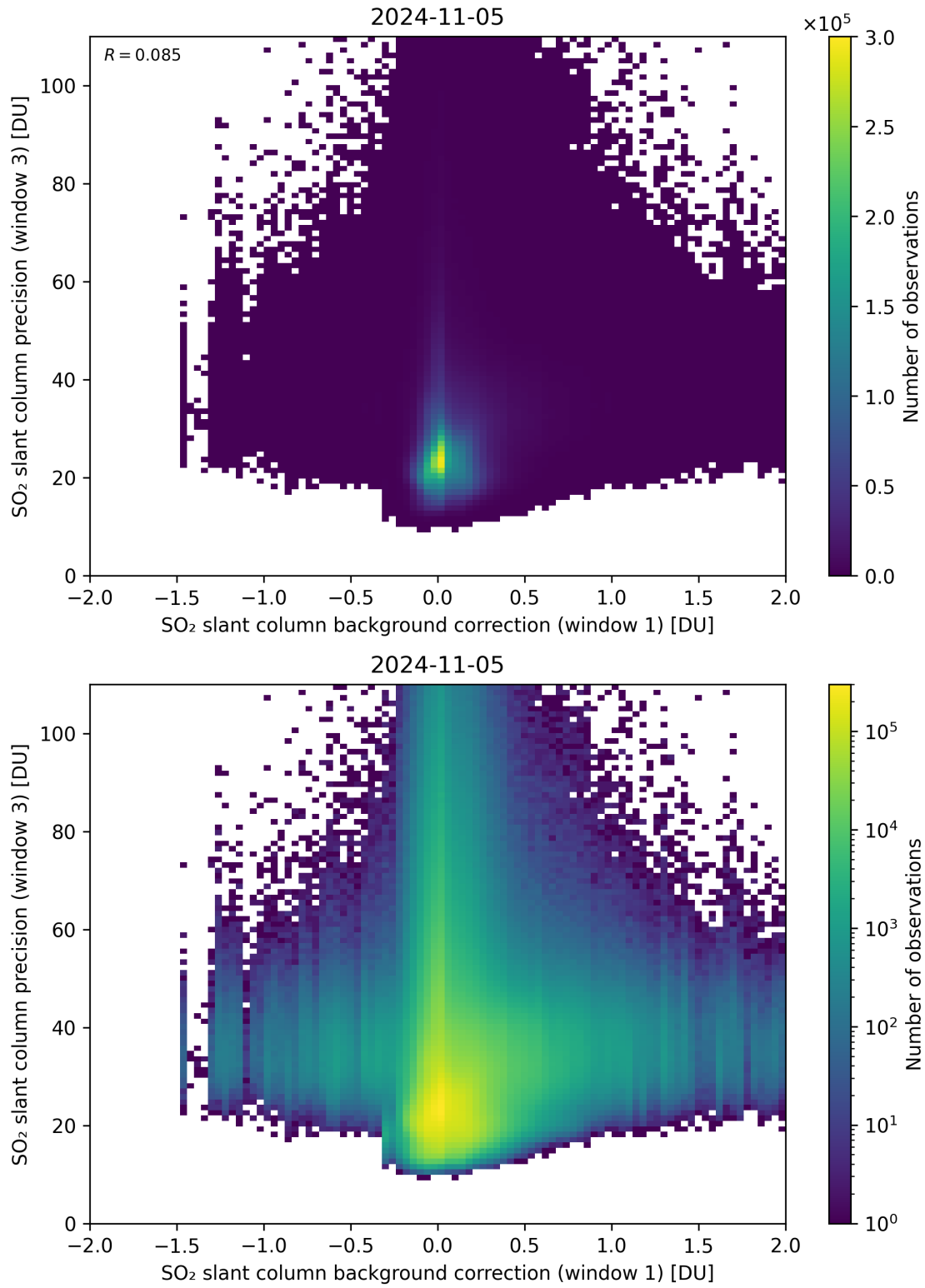
Figure 108: Scatter density plot of “SO 2 slant column background correction (window 1)” against “SO 2 slant column precision (window 3)” for 2024-11-04 to 2024-11-06.
