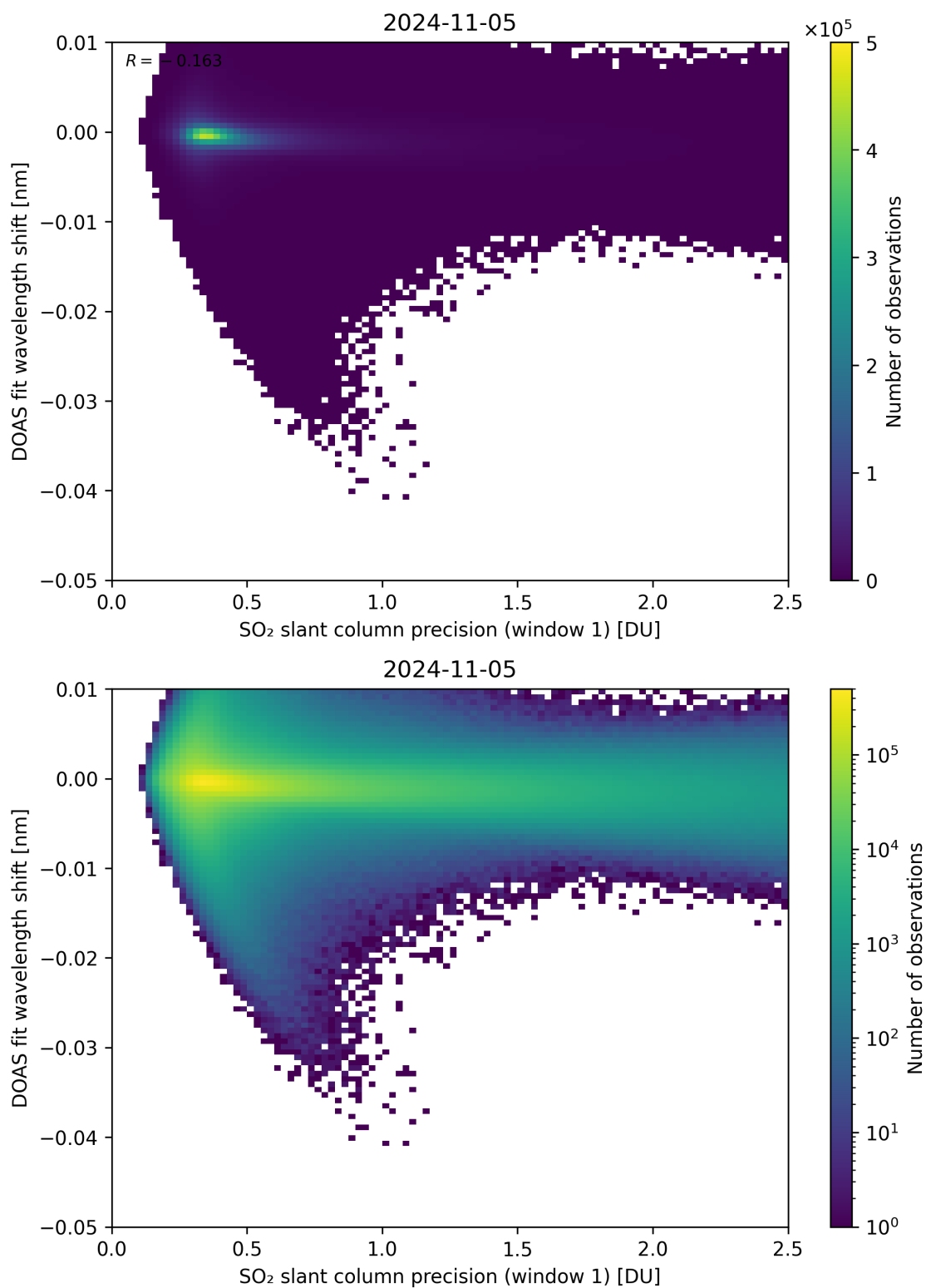
Figure 221: Scatter density plot of “SO 2 slant column precision (window 1)” against “DOAS fit wavelength shift” for 2024-11-04 to 2024-11-06.
