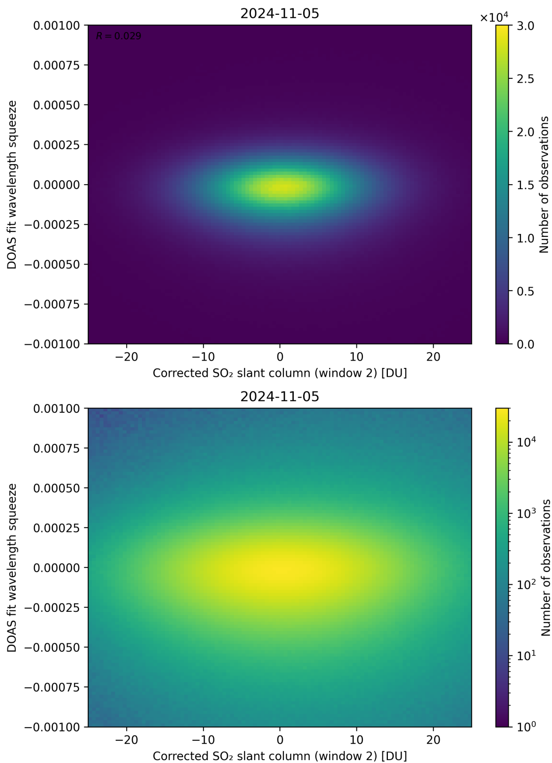
Figure 197: Scatter density plot of “Corrected SO 2 slant column (window 2)” against “DOAS fit wavelength squeeze” for 2024-11-04 to 2024-11-06.
