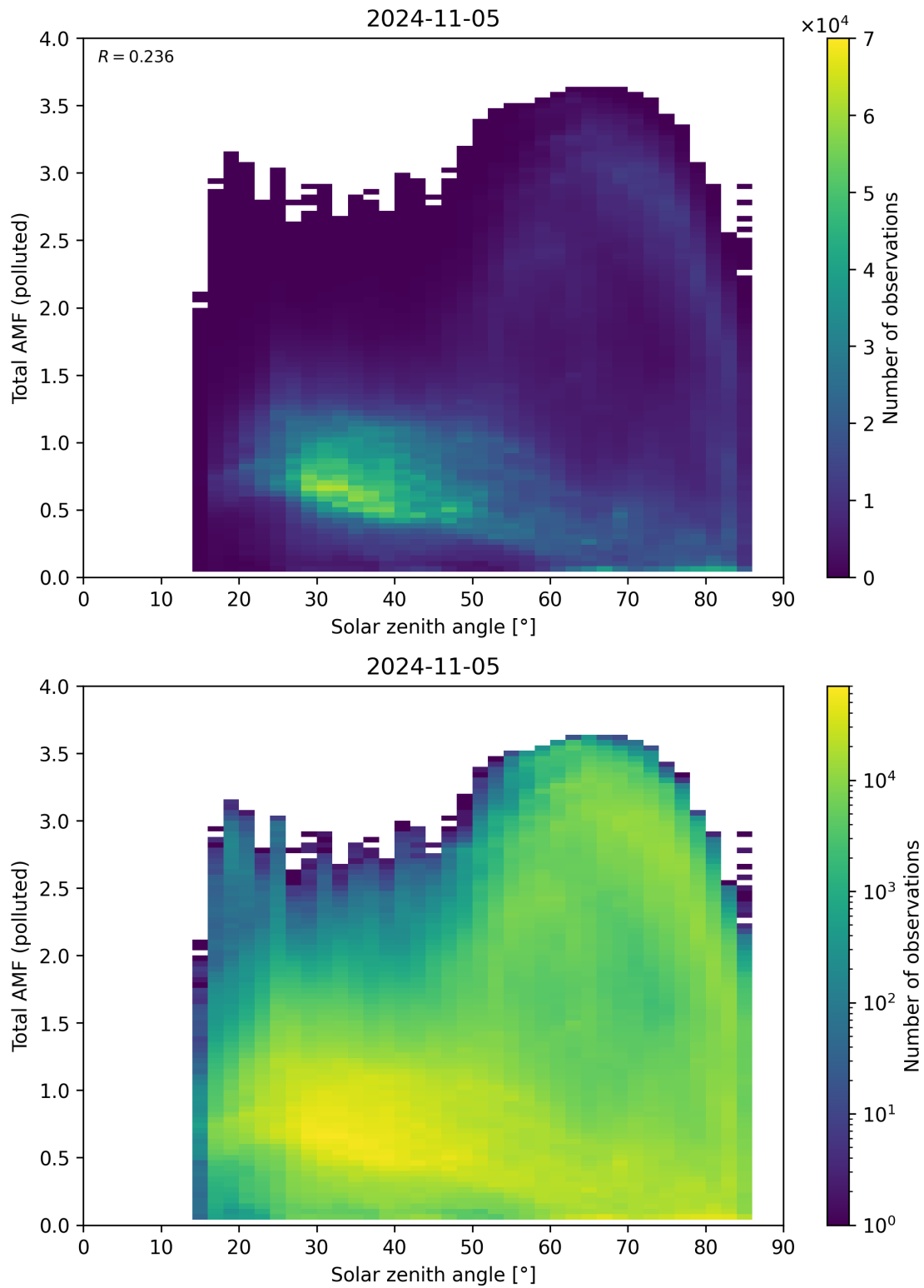
Figure 174: Scatter density plot of “Solar zenith angle” against “Total AMF (polluted)” for 2024-11-04 to 2024-11-06.
