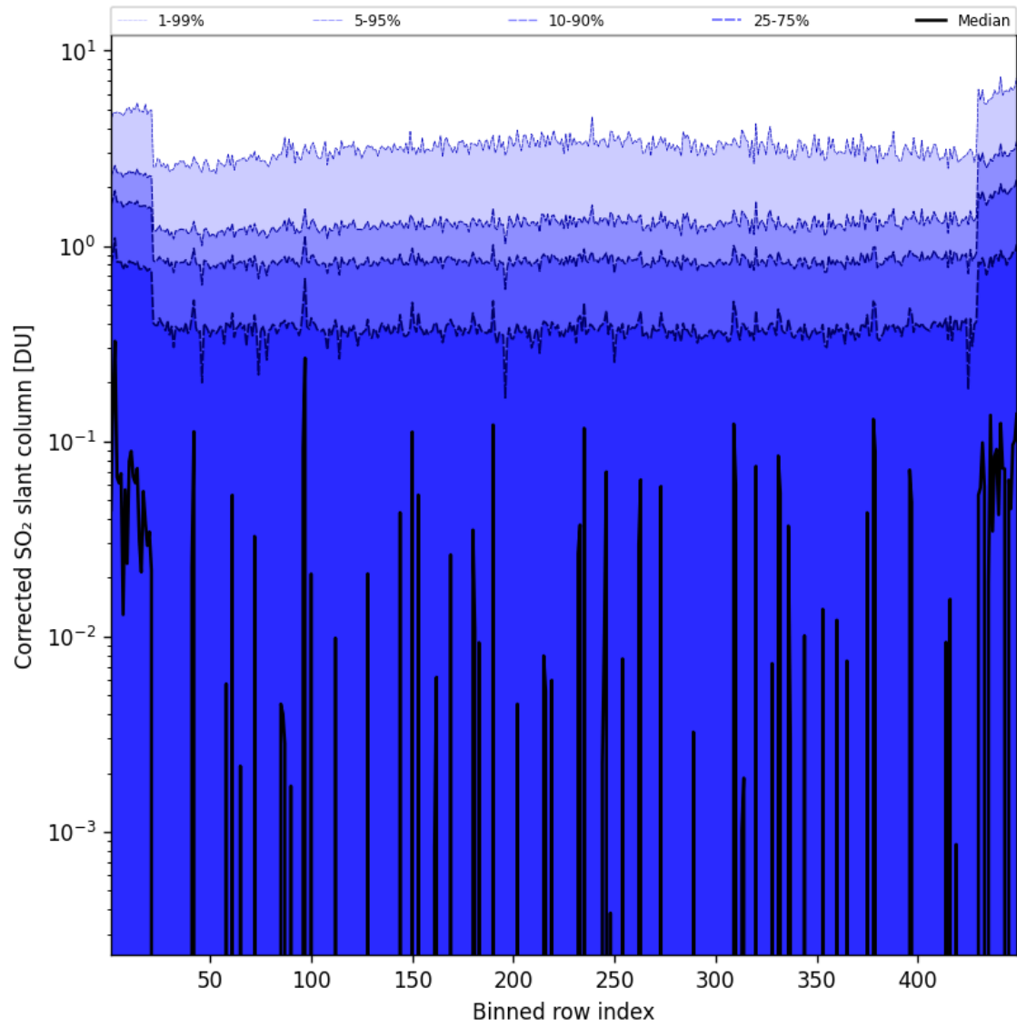
Figure 78: Along track statistics of “Corrected SO 2 slant column” for 2024-11-04 to 2024-11-06
