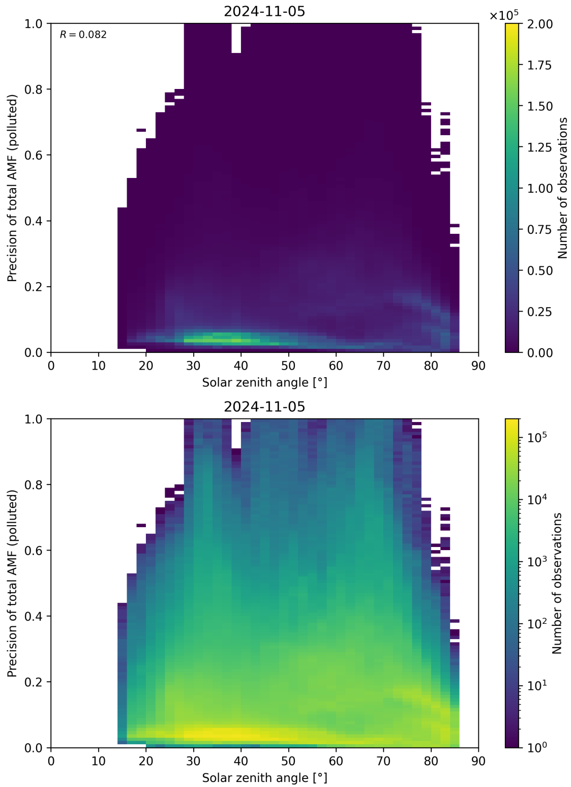
Figure 175: Scatter density plot of “Solar zenith angle” against “Precision of total AMF (polluted)” for 2024-11-04 to 2024-11-06.
