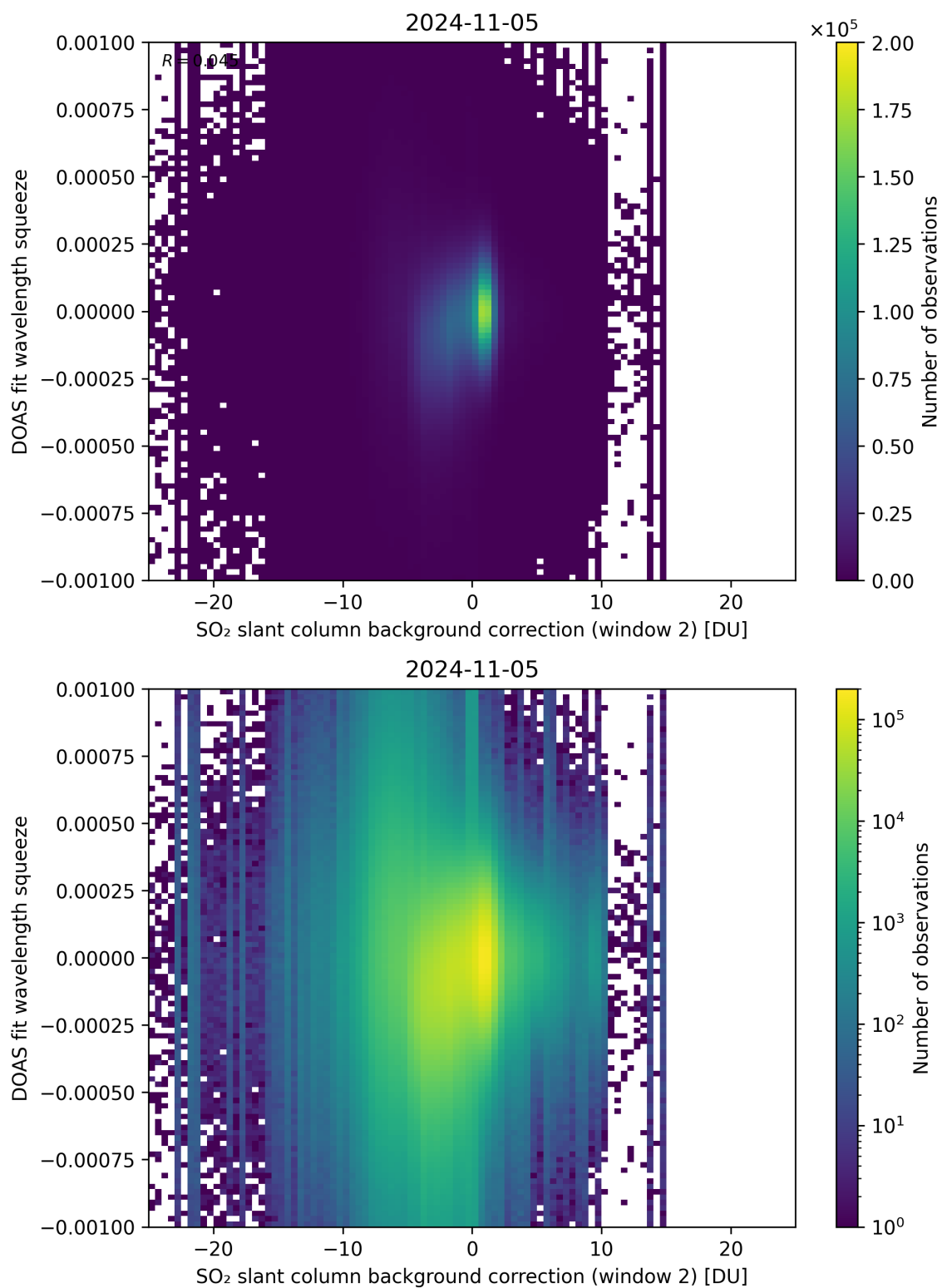
Figure 113: Scatter density plot of “SO 2 slant column background correction (window 2)” against “DOAS fit wavelength squeeze” for 2024-11-04 to 2024-11-06.
