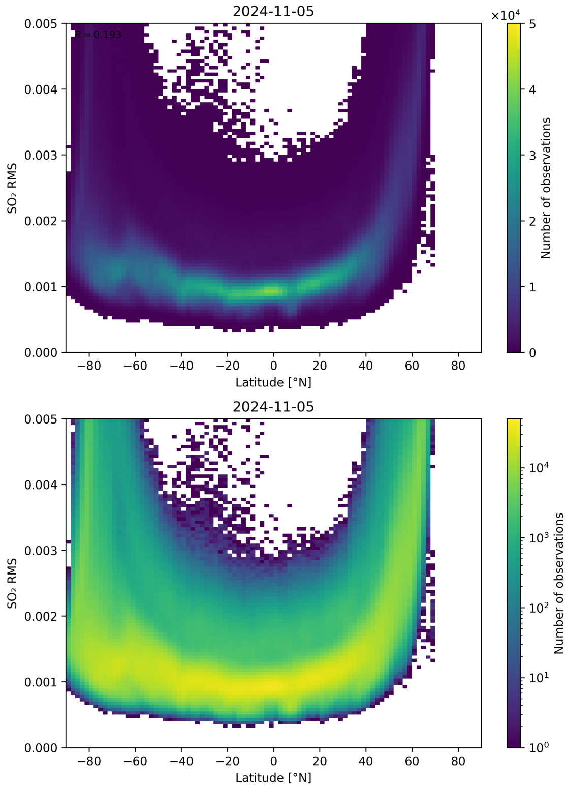
Figure 144: Scatter density plot of “Latitude” against “SO 2 RMS” for 2024-11-04 to 2024-11-06.
