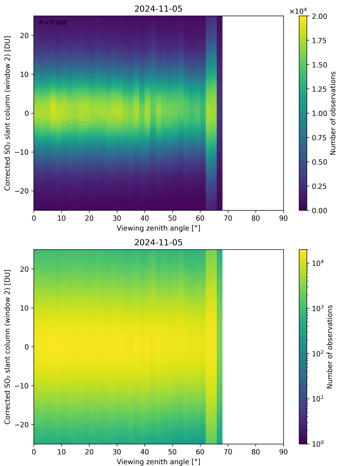
Figure 318: Scatter density plot of “Viewing zenith angle” against “Corrected SO 2 slant column (window 2)” for 2024-11-04 to 2024-11-06.
