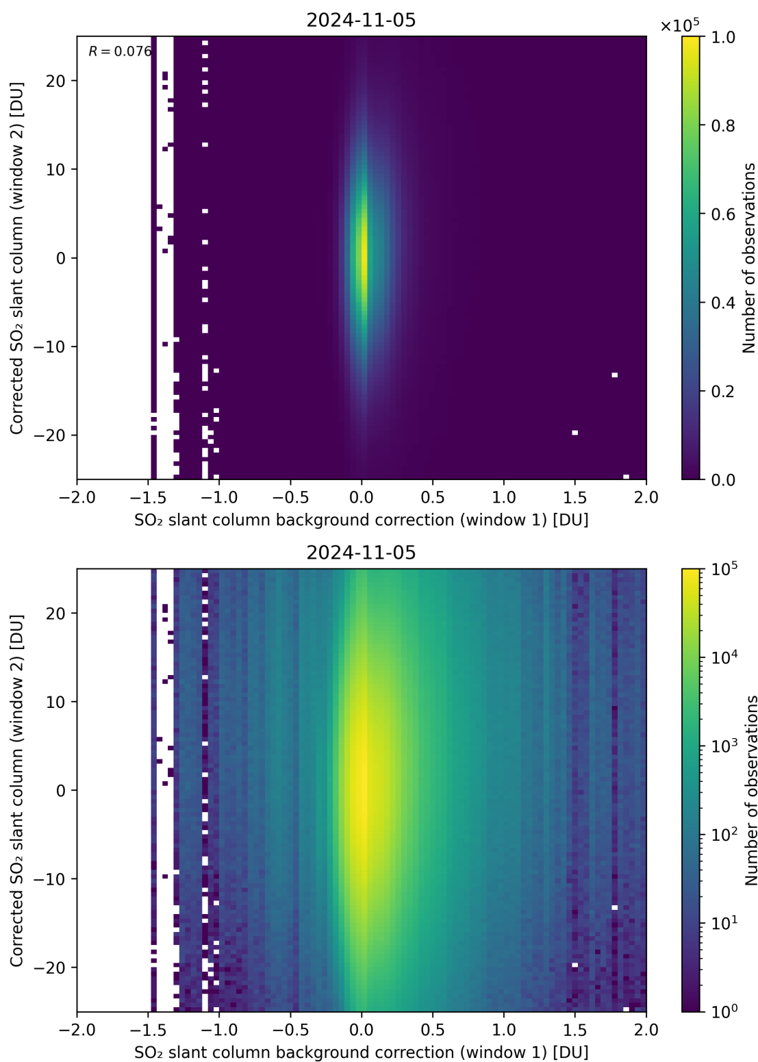
Figure 104: Scatter density plot of “SO 2 slant column background correction (window 1)” against “Corrected SO 2 slant column (window 2)” for 2024-11-04 to 2024-11-06.
