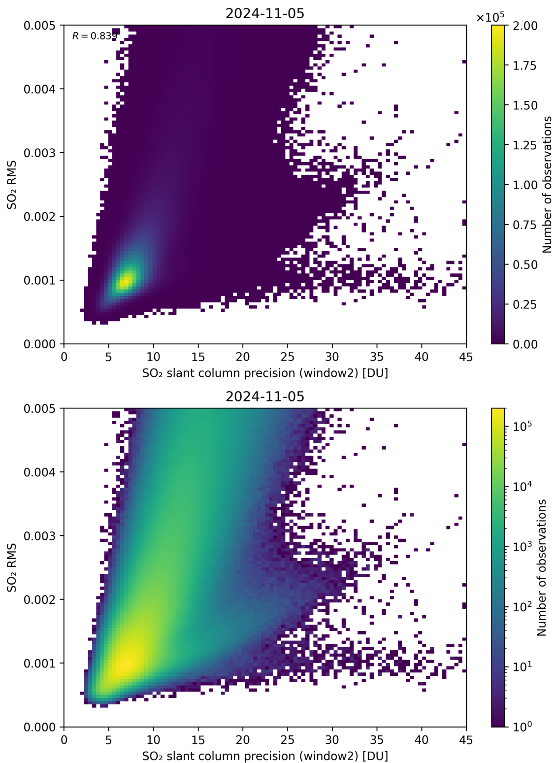
Figure 245: Scatter density plot of “SO 2 slant column precision (window2)” against “SO 2 RMS” for 2024-11-04 to 2024-11-06.
