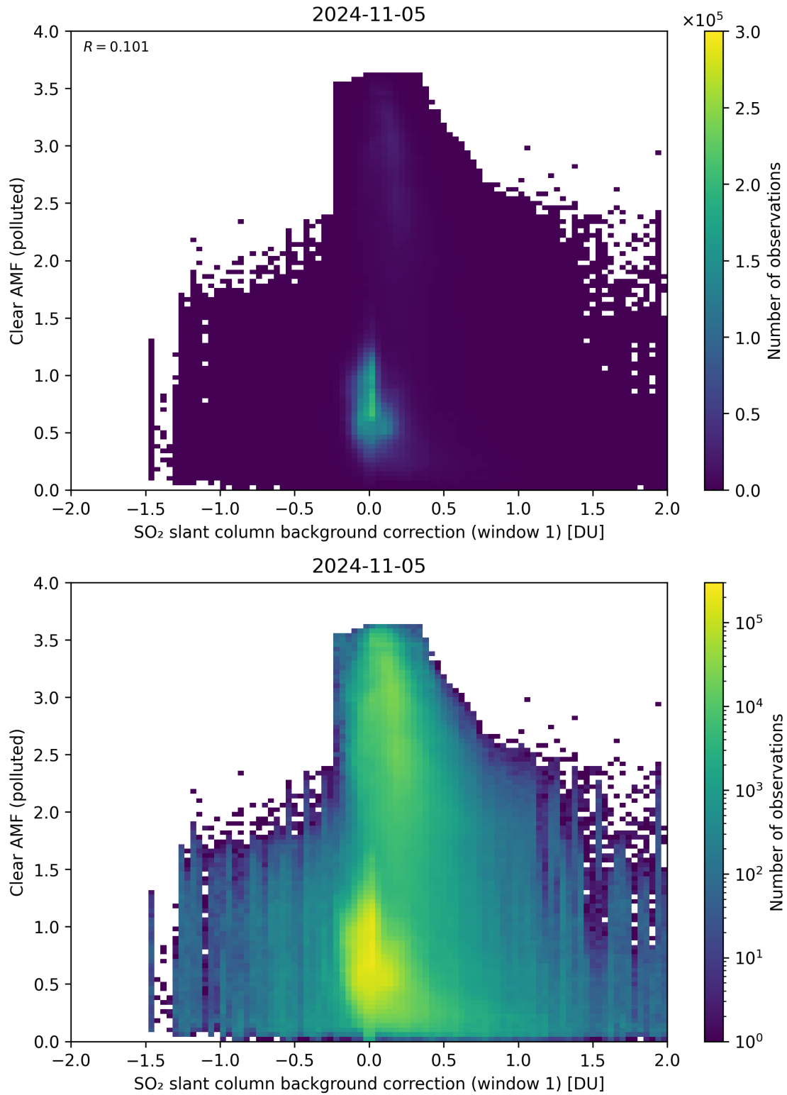
Figure 103: Scatter density plot of “SO 2 slant column background correction (window 1)” against “Clear AMF (polluted)” for 2024-11-04 to 2024-11-06.
