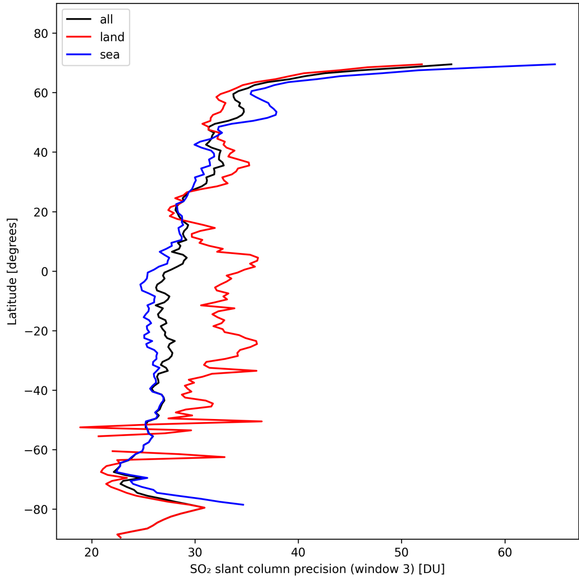
Figure 42: Zonal average of “SO 2 slant column precision (window 3)” for 2024-11-04 to 2024-11-06.
