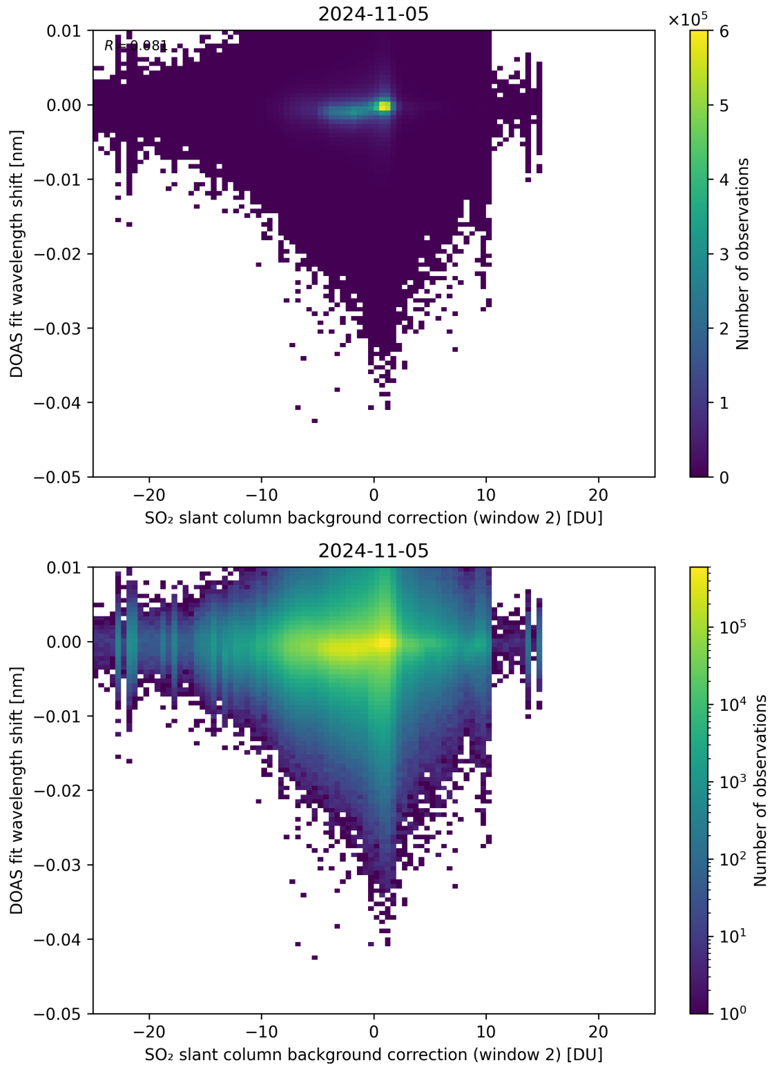
Figure 112: Scatter density plot of “SO 2 slant column background correction (window 2)” against “DOAS fit wavelength shift” for 2024-11-04 to 2024-11-06.
