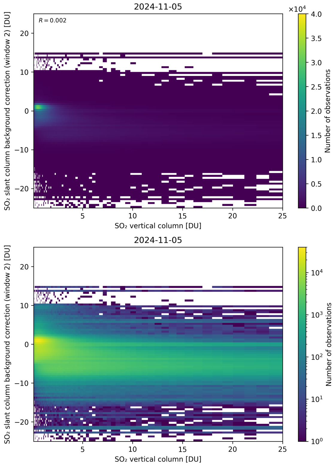
Figure 274: Scatter density plot of “SO 2 vertical column” against “SO 2 slant column background correction (window 2)” for 2024-11-04 to 2024-11-06.
