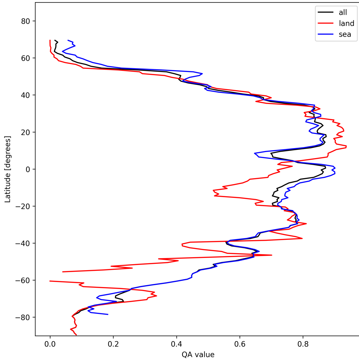
Figure 29: Zonal average of “QA value” for 2024-11-04 to 2024-11-06.
