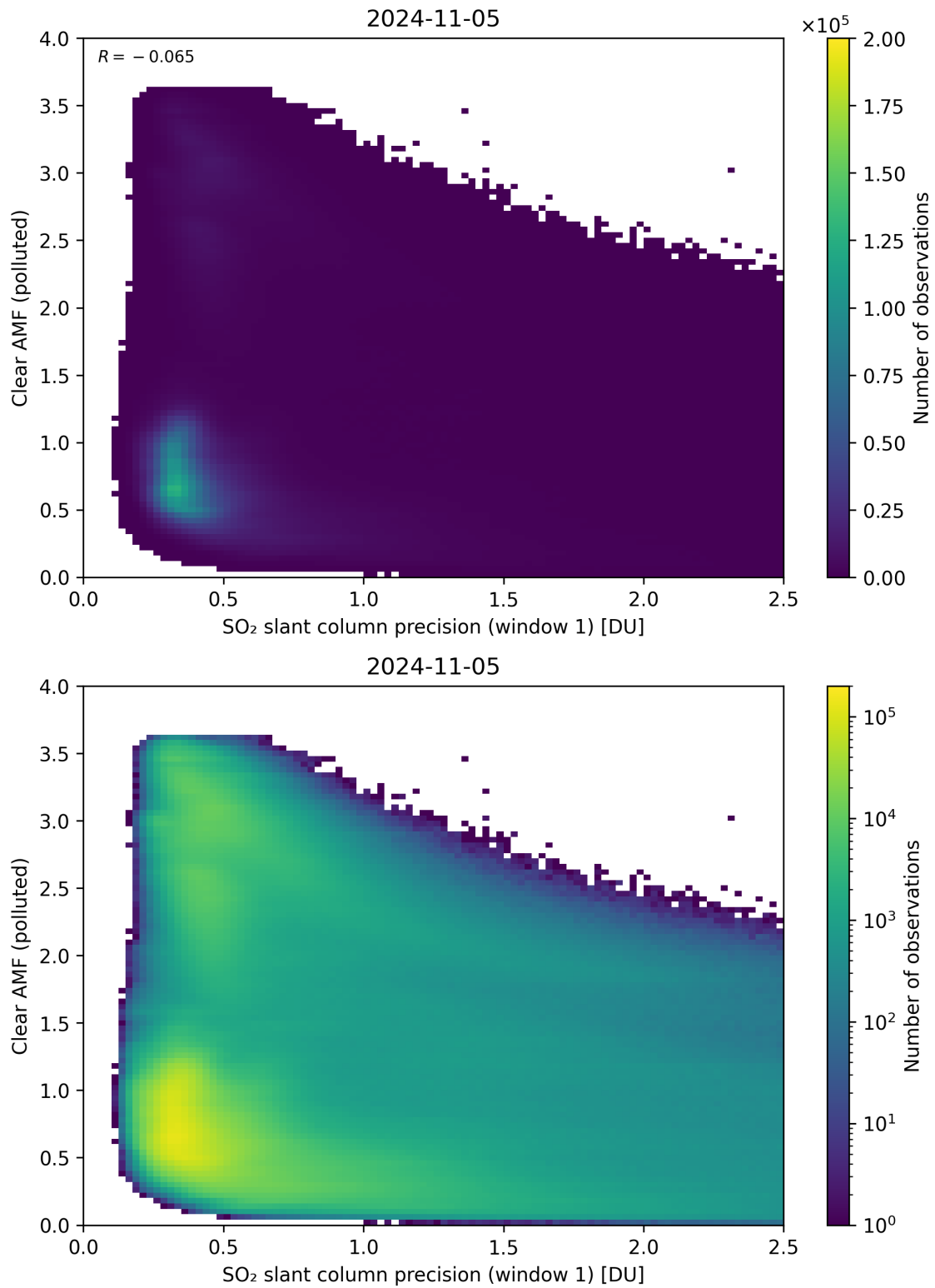
Figure 224: Scatter density plot of “SO 2 slant column precision (window 1)” against “Clear AMF (polluted)” for 2024-11-04 to 2024-11-06.
