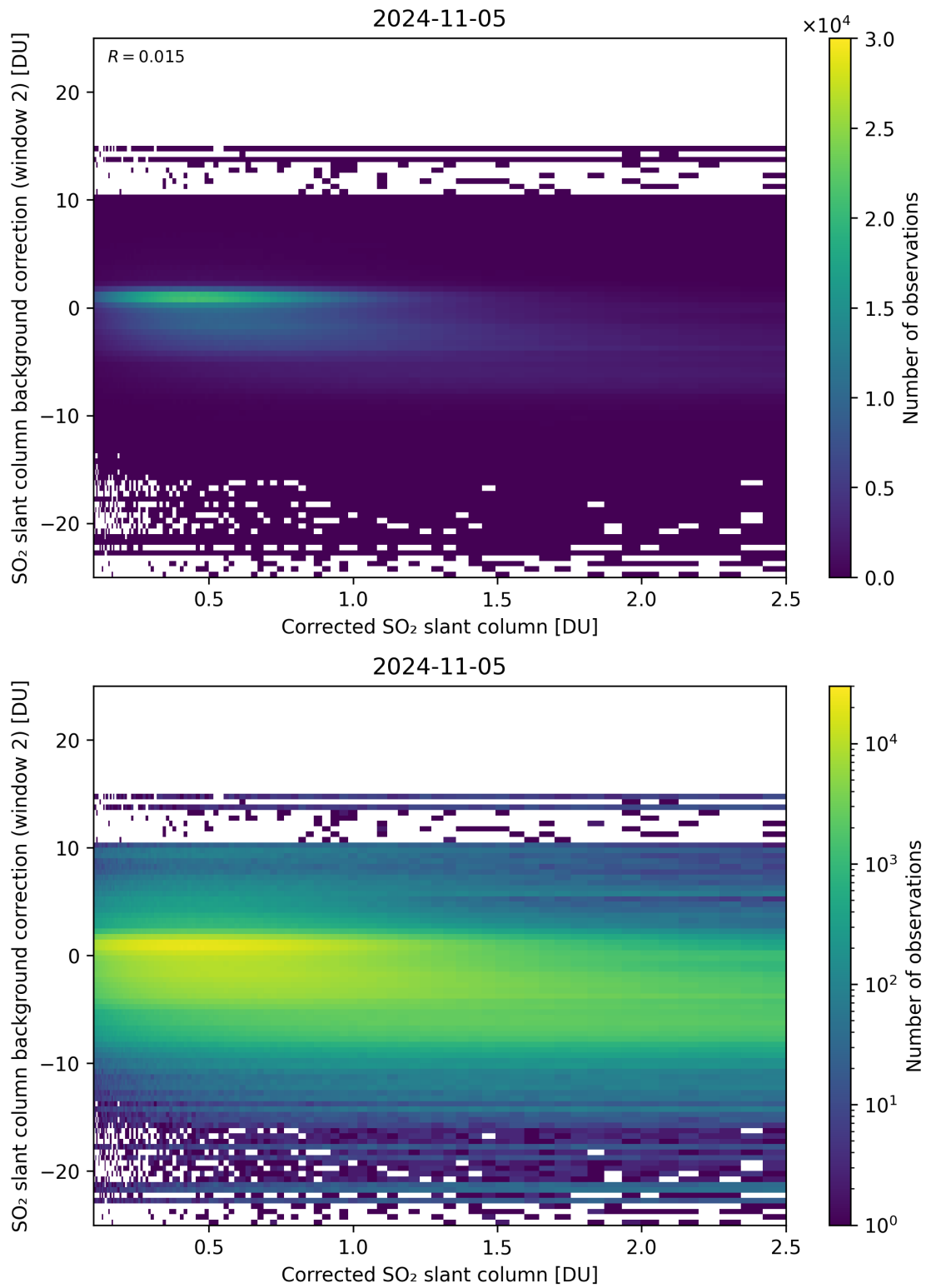
Figure 179: Scatter density plot of “Corrected SO 2 slant column” against “SO 2 slant column background correction (window 2)” for 2024-11-04 to 2024-11-06.
