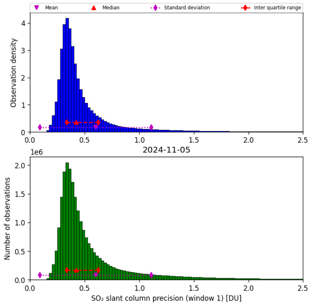
Figure 57: Histogram of “SO 2 slant column precision (window 1)” for 2024-11-04 to 2024-11-06
