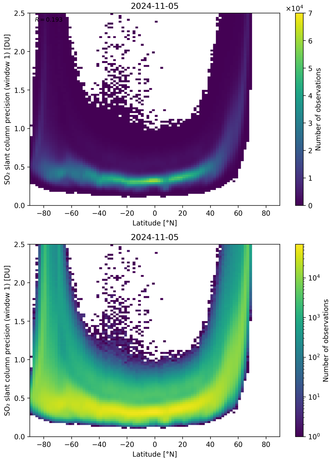
Figure 150: Scatter density plot of “Latitude” against “SO 2 slant column precision (window 1)” for 2024-11-04 to 2024-11-06.
