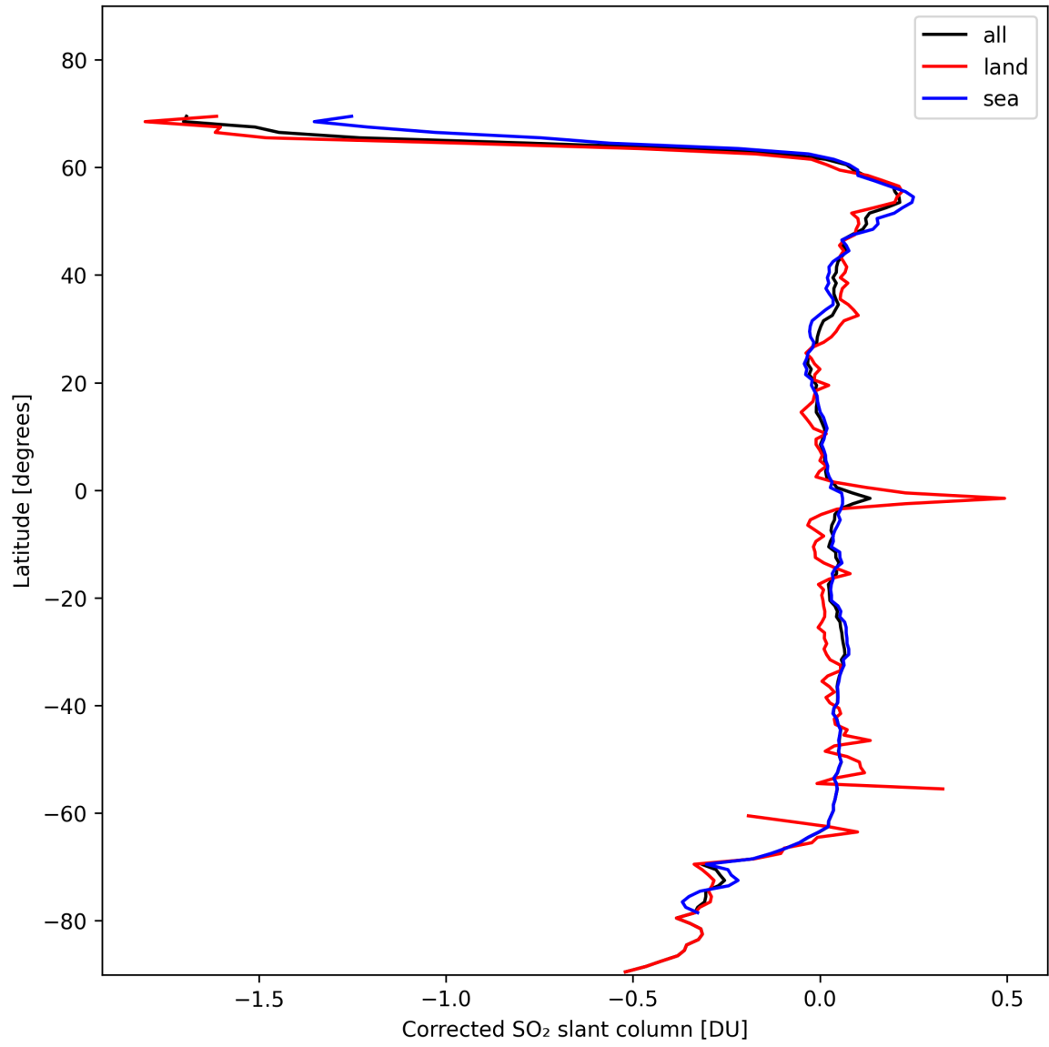
Figure 32: Zonal average of “Corrected SO 2 slant column” for 2024-11-04 to 2024-11-06.
