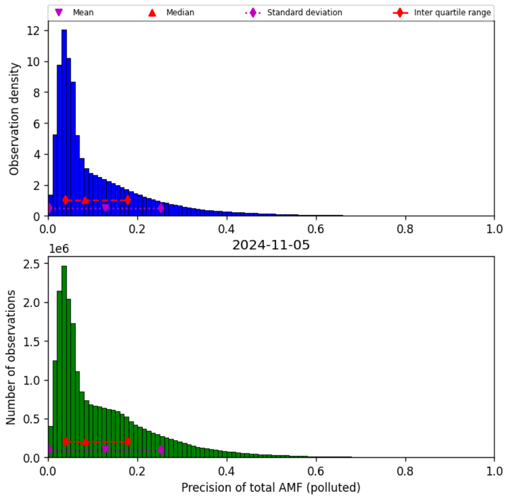
Figure 72: Histogram of “Precision of total AMF (polluted)” for 2024-11-04 to 2024-11-06
