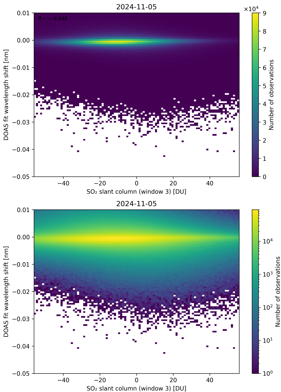
Figure 254: Scatter density plot of “SO 2 slant column (window 3)” against “DOAS fit wavelength shift” for 2024-11-04 to 2024-11-06.
