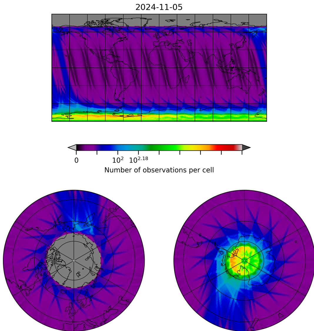
Figure 28: Map of the number of observations for 2024-11-04 to 2024-11-06
