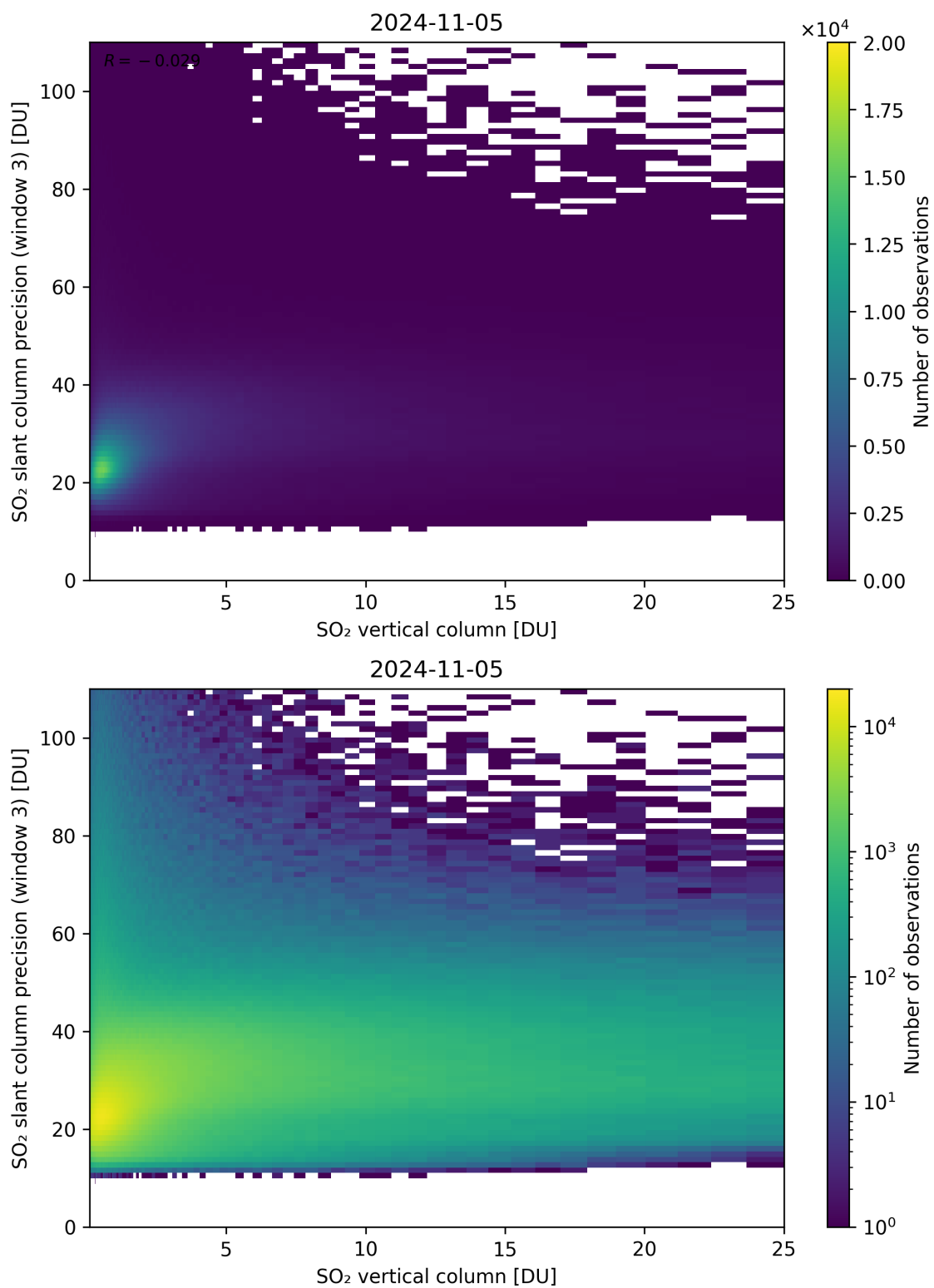
Figure 304: Scatter density plot of “SO 2 vertical column” against “SO 2 slant column precision (window 3)” for 2024-11-04 to 2024-11-06.
