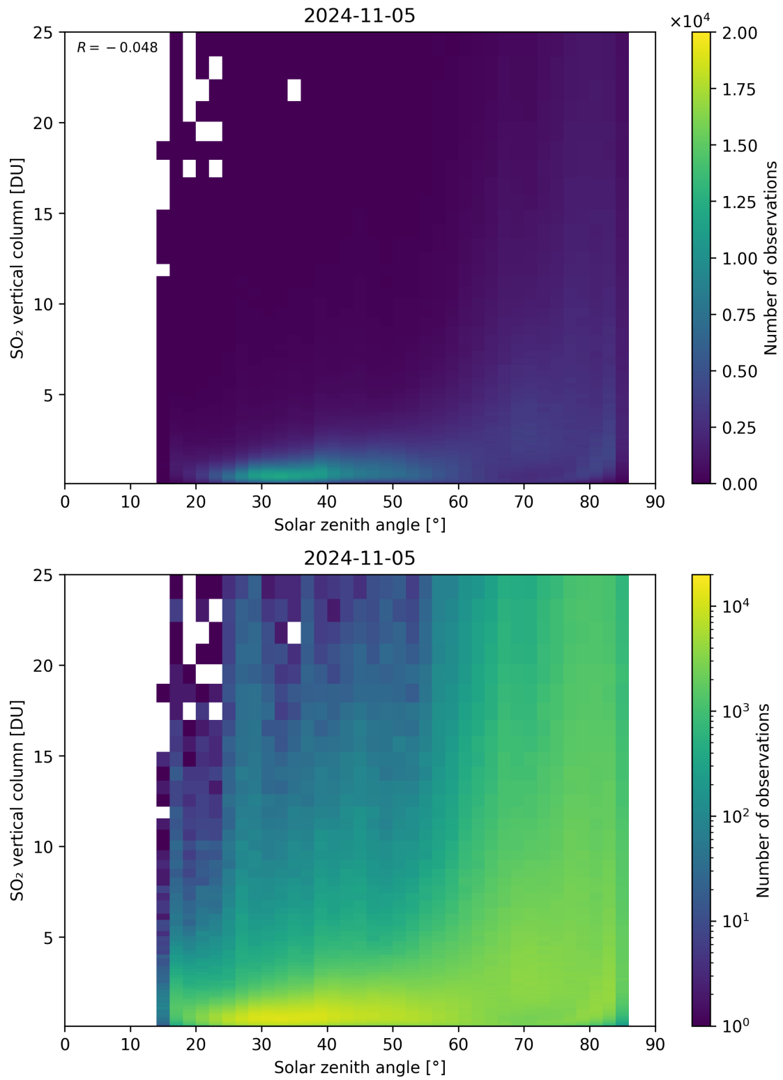
Figure 176: Scatter density plot of “Solar zenith angle” against “SO 2 vertical column” for 2024-11-04 to 2024-11-06.
