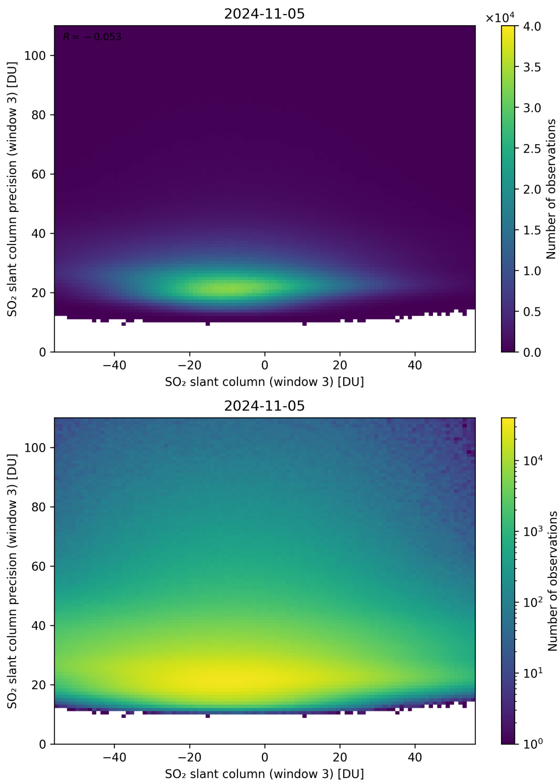
Figure 267: Scatter density plot of “SO 2 slant column (window 3)” against “SO 2 slant column precision (window 3)” for 2024-11-04 to 2024-11-06.
