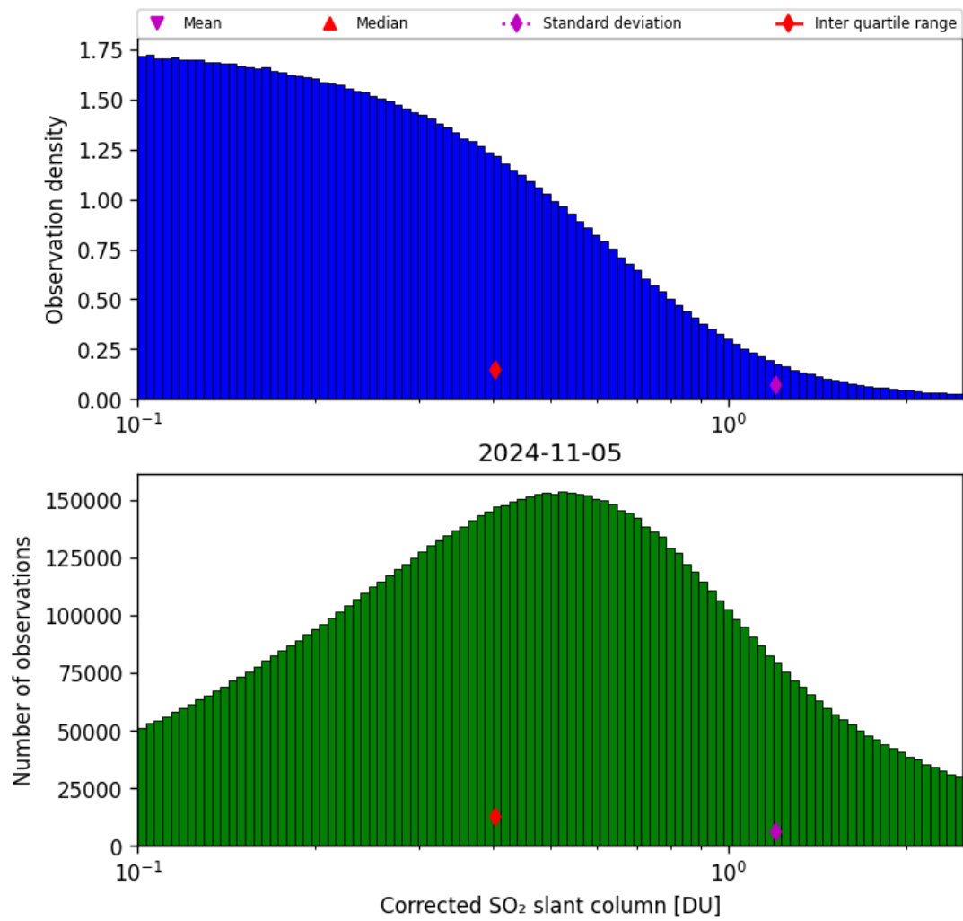
Figure 55: Histogram of “Corrected SO 2 slant column” for 2024-11-04 to 2024-11-06
