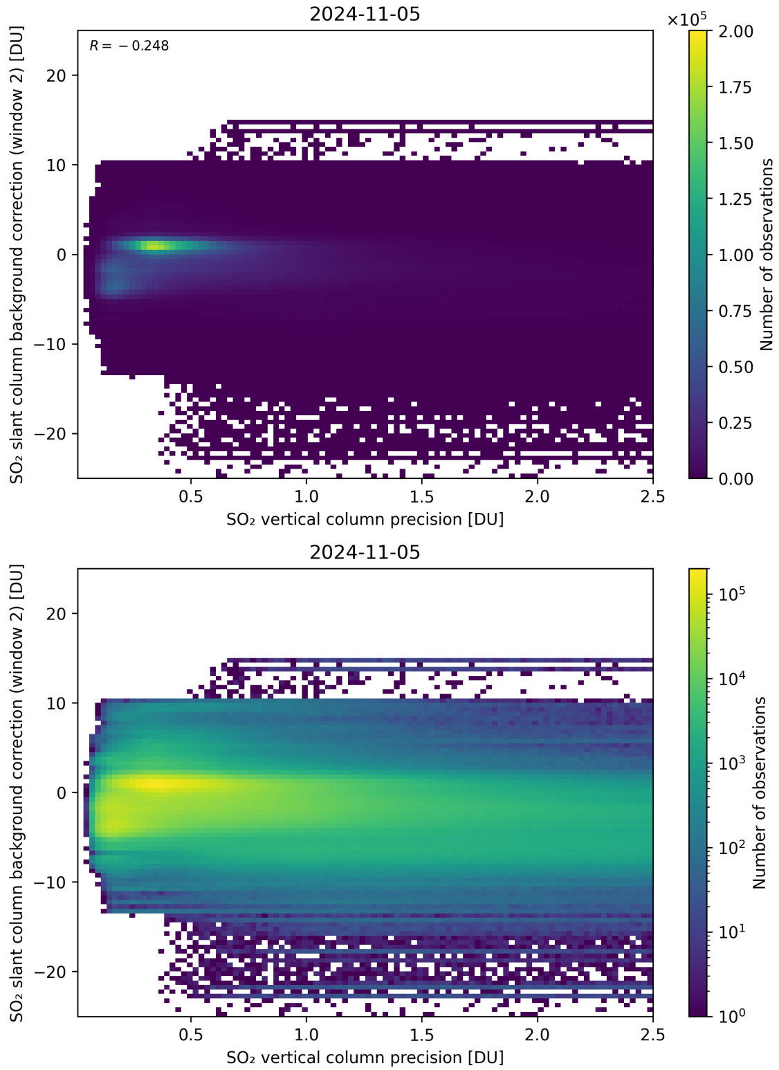
Figure 280: Scatter density plot of “SO 2 vertical column precision” against “SO 2 slant column background correction (window 2)” for 2024-11-04 to 2024-11-06.
