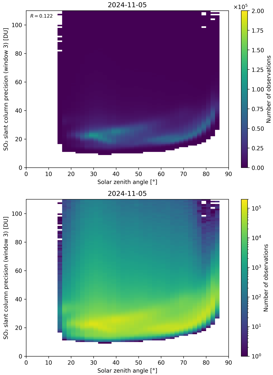
Figure 173: Scatter density plot of “Solar zenith angle” against “SO 2 slant column precision (window 3)” for 2024-11-04 to 2024-11-06.
