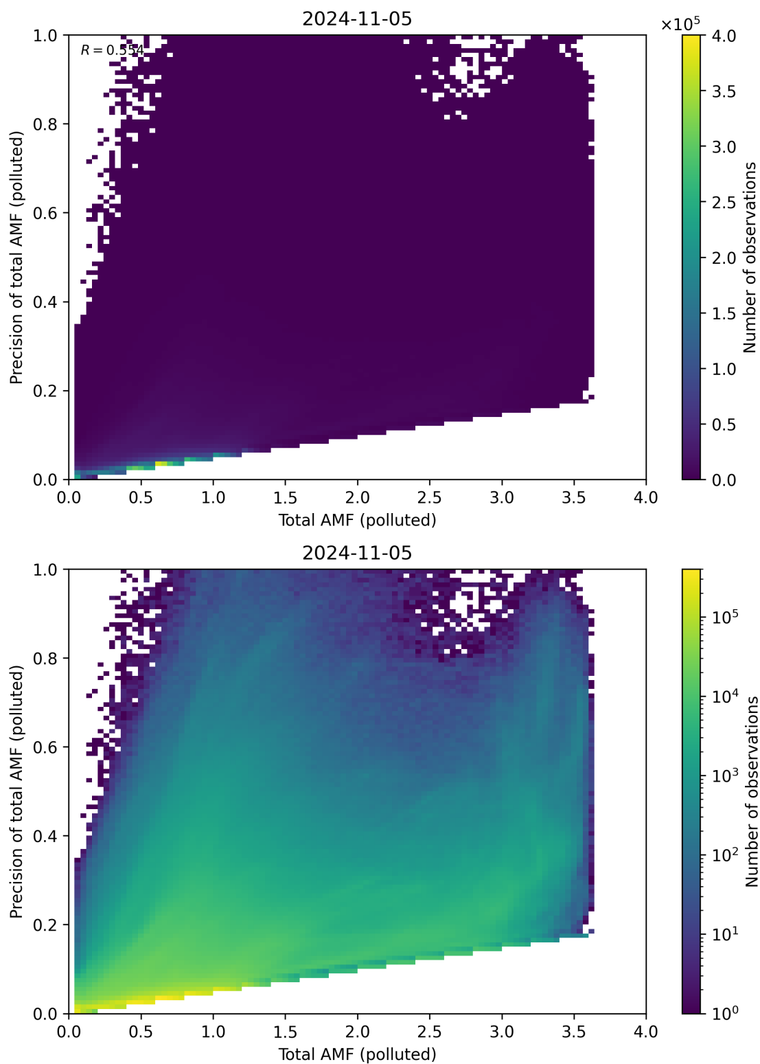
Figure 272: Scatter density plot of “Total AMF (polluted)” against “Precision of total AMF (polluted)” for 2024-11-04 to 2024-11-06.
