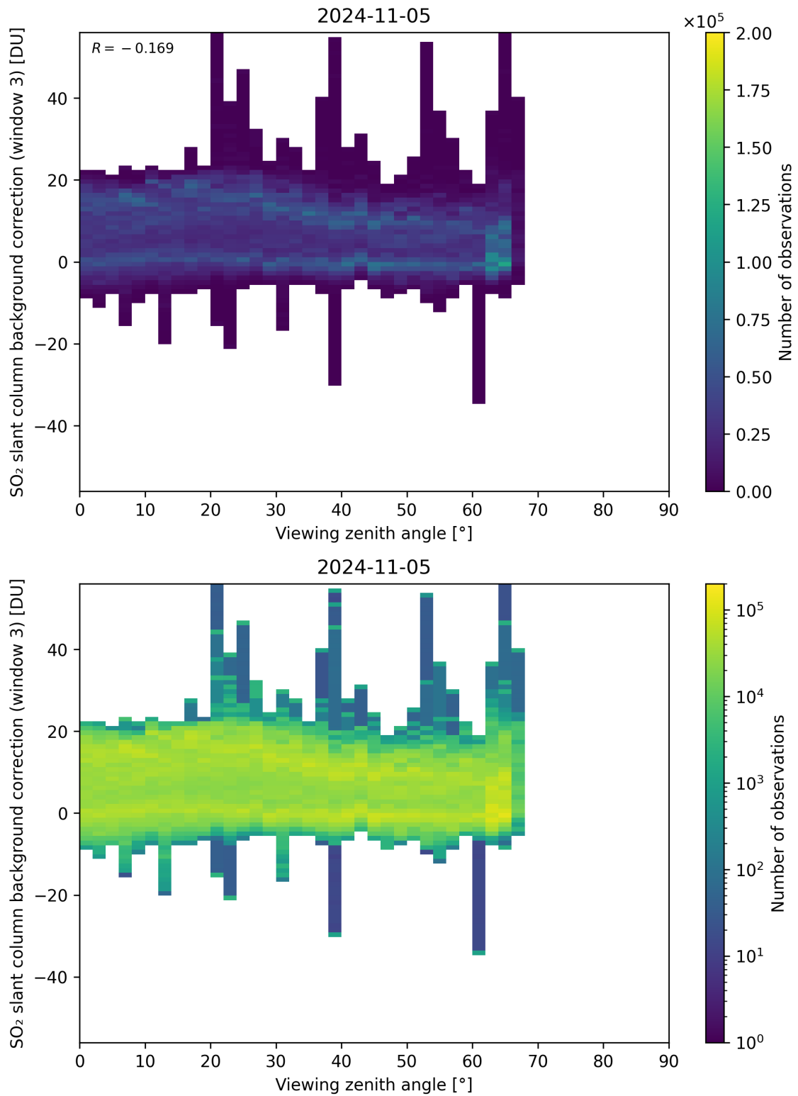
Figure 310: Scatter density plot of “Viewing zenith angle” against “SO 2 slant column background correction (window 3)” for 2024-11-04 to 2024-11-06.
