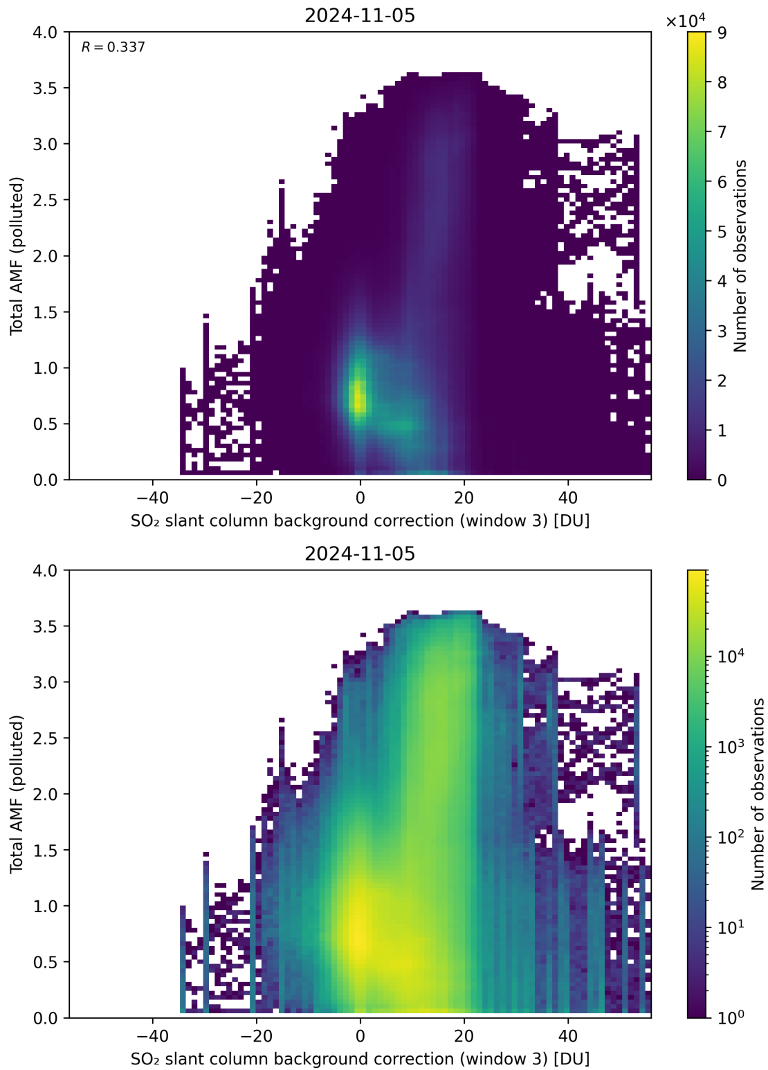
Figure 125: Scatter density plot of “SO 2 slant column background correction (window 3)” against “Total AMF (polluted)” for 2024-11-04 to 2024-11-06.
