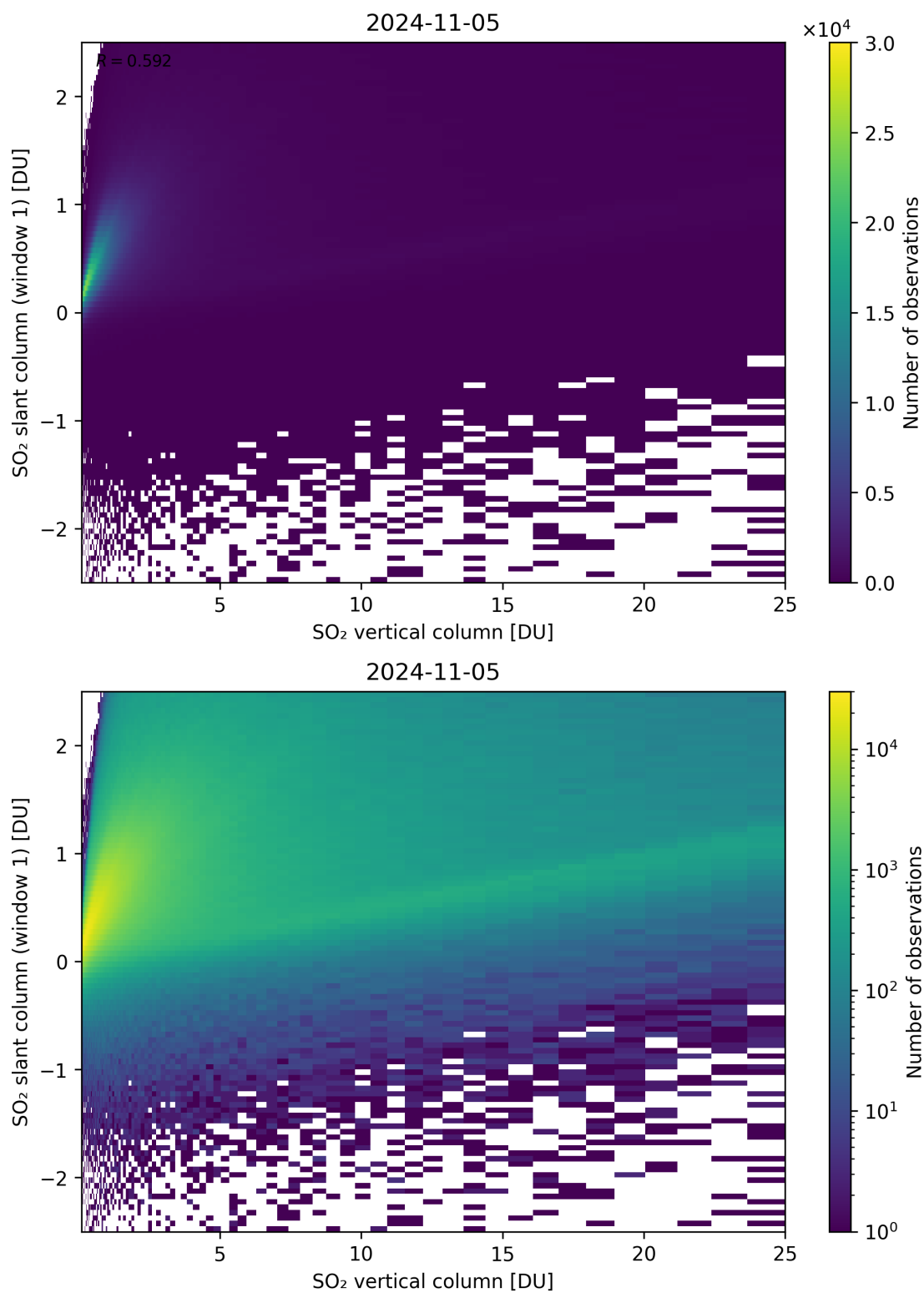
Figure 300: Scatter density plot of “SO 2 vertical column” against “SO 2 slant column (window 1)” for 2024-11-04 to 2024-11-06.
