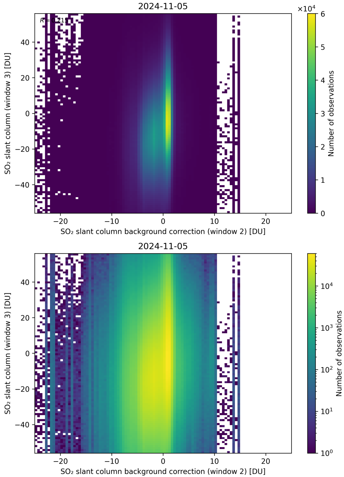
Figure 117: Scatter density plot of “SO 2 slant column background correction (window 2)” against “SO 2 slant column (window 3)” for 2024-11-04 to 2024-11-06.
