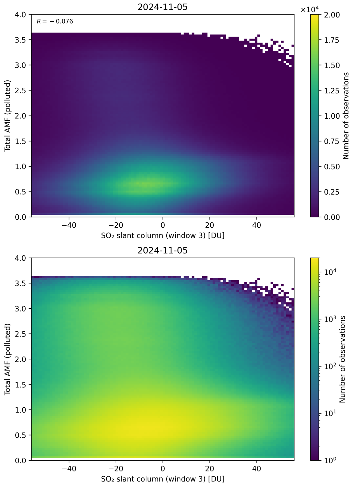
Figure 268: Scatter density plot of “SO 2 slant column (window 3)” against “Total AMF (polluted)” for 2024-11-04 to 2024-11-06.
