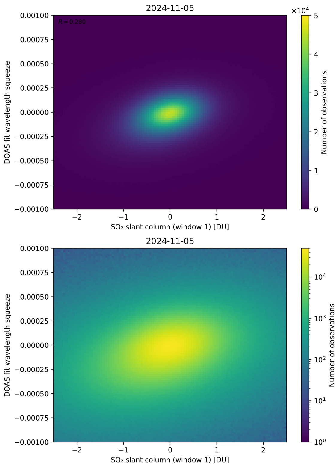
Figure 216: Scatter density plot of “SO 2 slant column (window 1)” against “DOAS fit wavelength squeeze” for 2024-11-04 to 2024-11-06.
