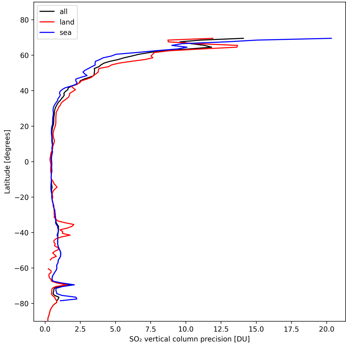
Figure 31: Zonal average of “SO 2 vertical column precision” for 2024-11-04 to 2024-11-06.
