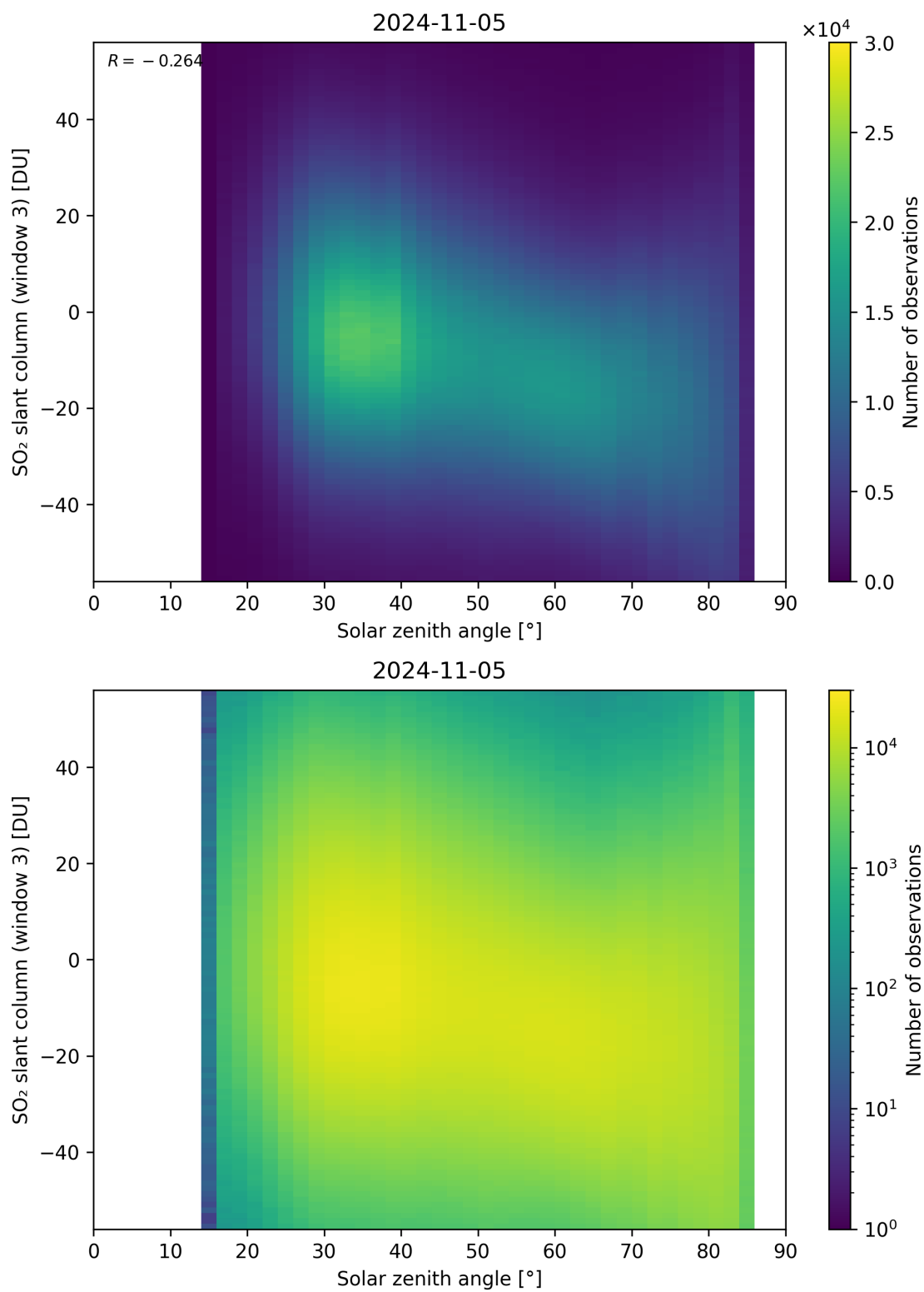
Figure 172: Scatter density plot of “Solar zenith angle” against “SO 2 slant column (window 3)” for 2024-11-04 to 2024-11-06.
