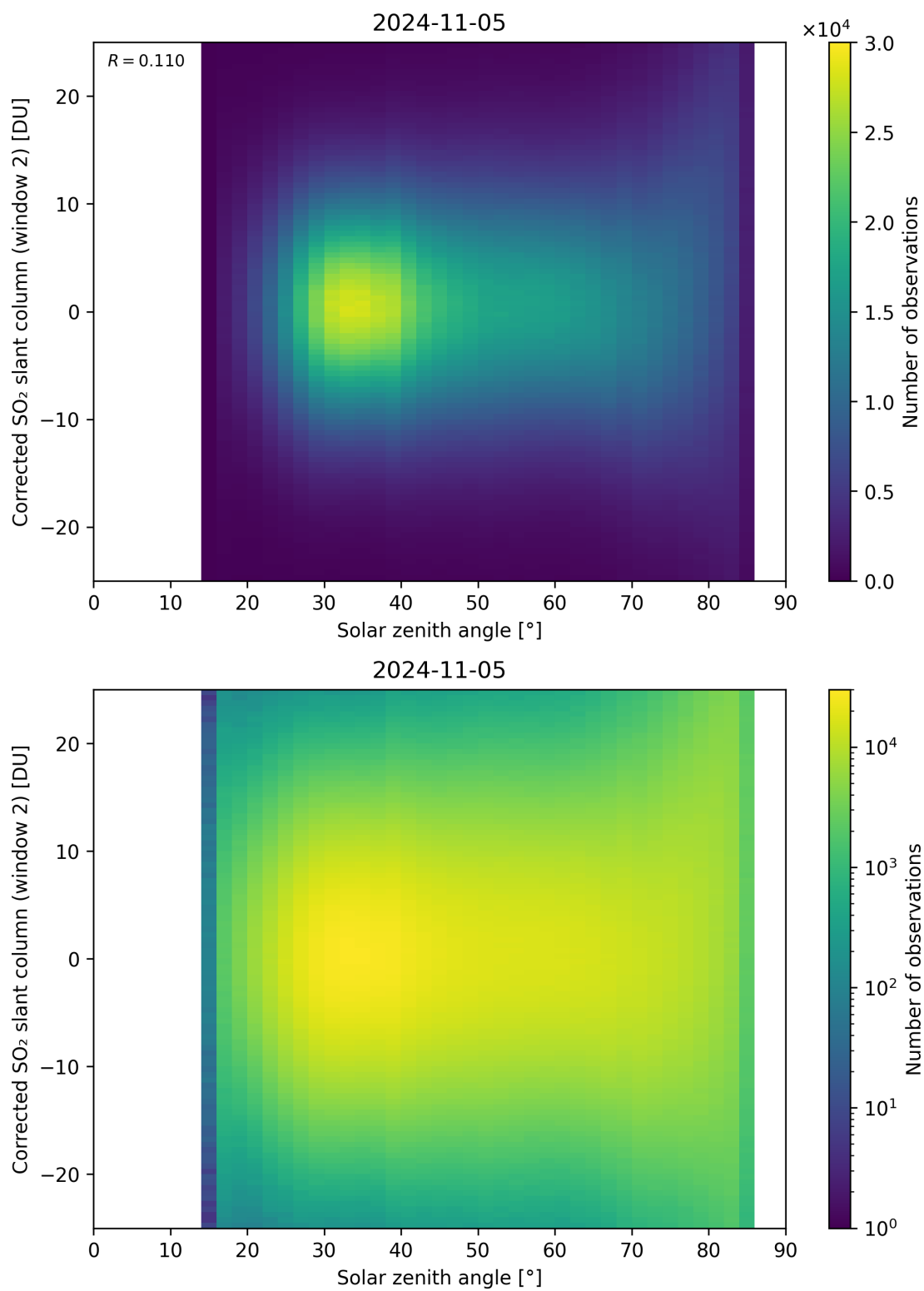
Figure 167: Scatter density plot of “Solar zenith angle” against “Corrected SO 2 slant column (window 2)” for 2024-11-04 to 2024-11-06.
