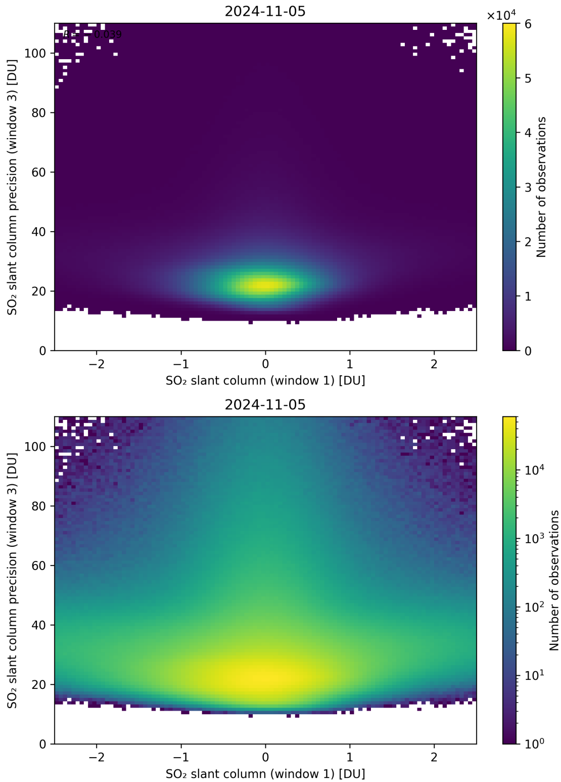
Figure 238: Scatter density plot of “SO 2 slant column (window 1)” against “SO 2 slant column precision (window 3)” for 2024-11-04 to 2024-11-06.
