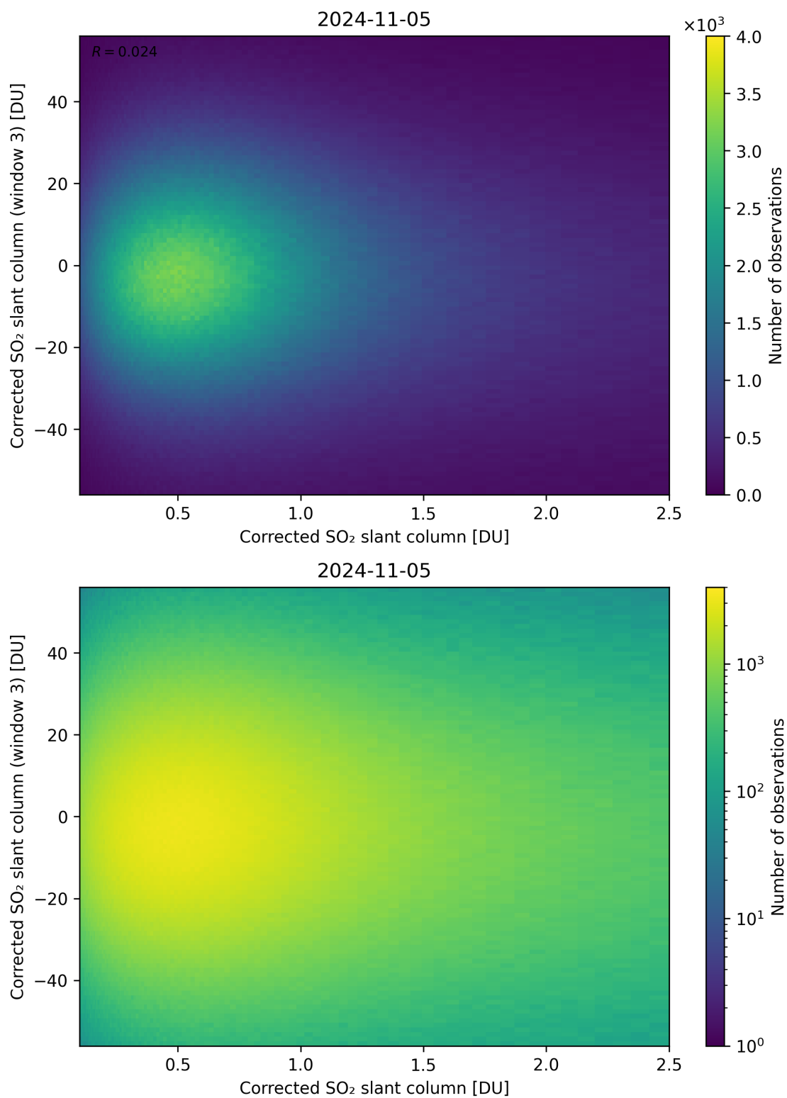
Figure 186: Scatter density plot of “Corrected SO 2 slant column” against “Corrected SO 2 slant column (window 3)” for 2024-11-04 to 2024-11-06.
