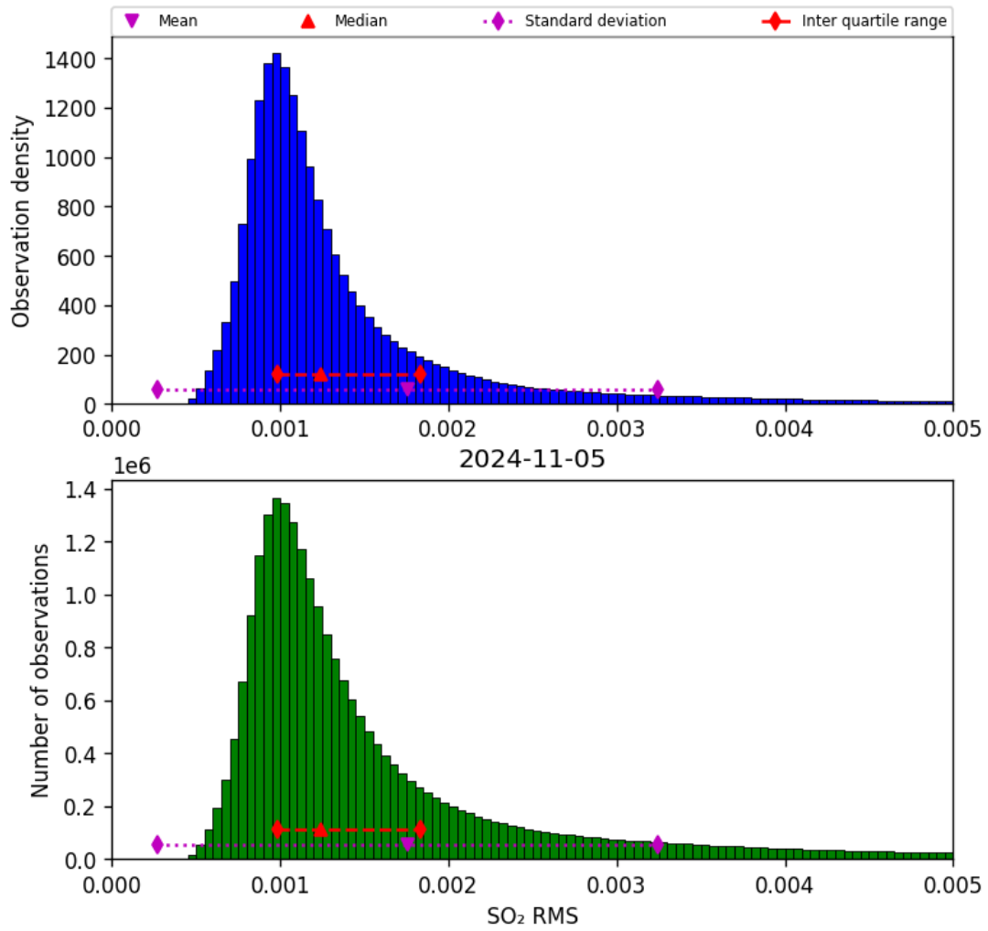
Figure 70: Histogram of “SO 2 RMS” for 2024-11-04 to 2024-11-06
