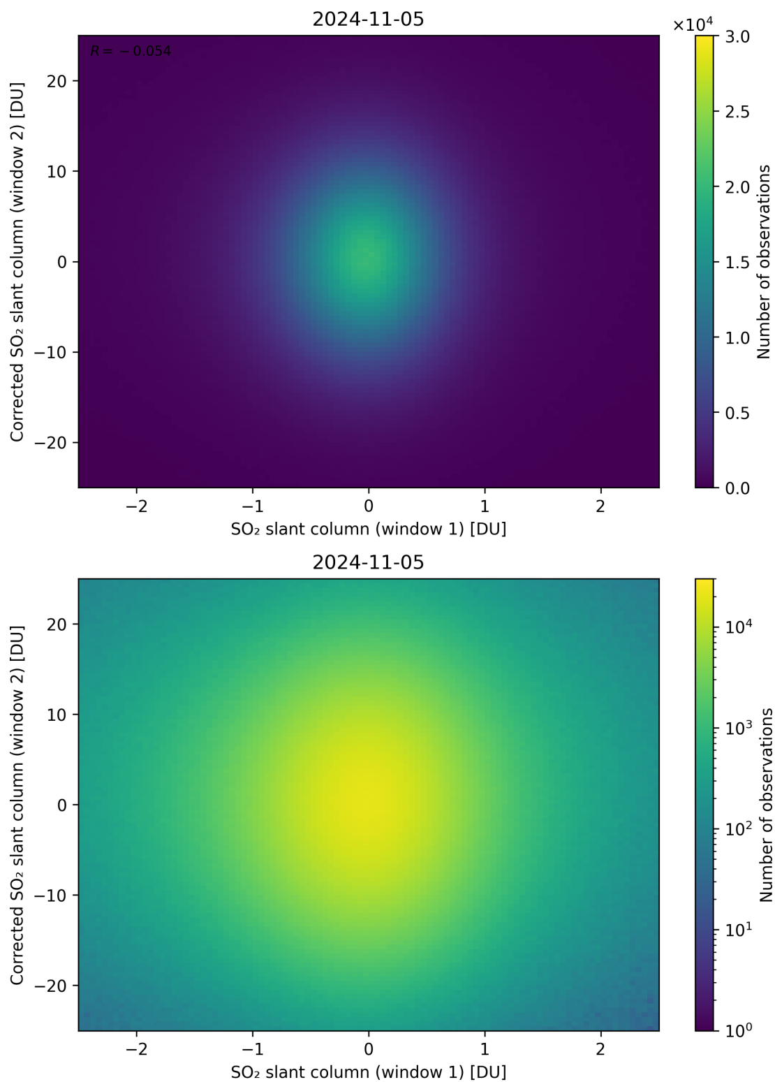
Figure 233: Scatter density plot of “SO 2 slant column (window 1)” against “Corrected SO 2 slant column (window 2)” for 2024-11-04 to 2024-11-06.
