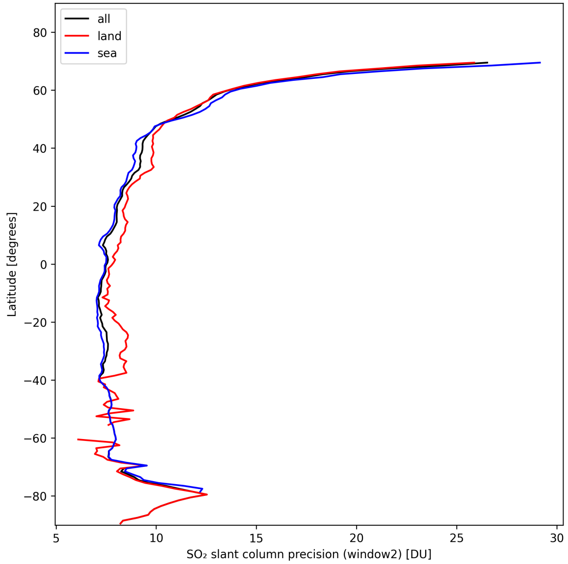
Figure 38: Zonal average of “SO 2 slant column precision (window2)” for 2024-11-04 to 2024-11-06.
