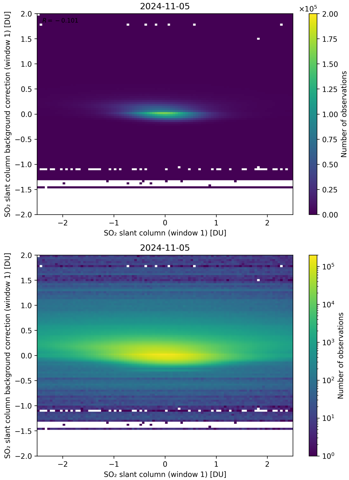
Figure 212: Scatter density plot of “SO 2 slant column (window 1)” against “SO 2 slant column background correction (window 1)” for 2024-11-04 to 2024-11-06.
