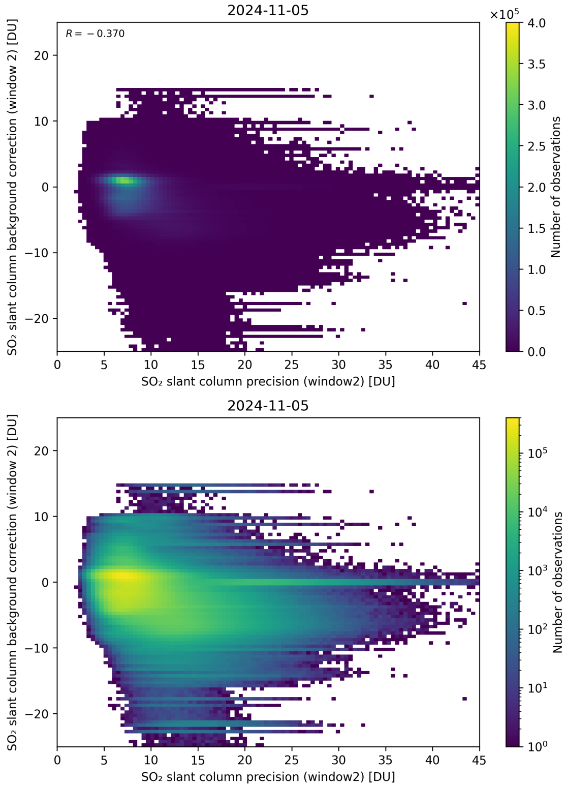
Figure 241: Scatter density plot of “SO 2 slant column precision (window2)” against “SO 2 slant column background correction (window 2)” for 2024-11-04 to 2024-11-06.
