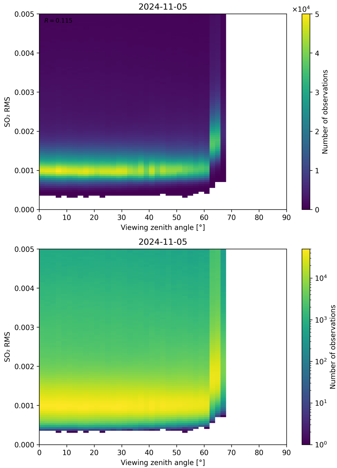
Figure 313: Scatter density plot of “Viewing zenith angle” against “SO 2 RMS” for 2024-11-04 to 2024-11-06.
