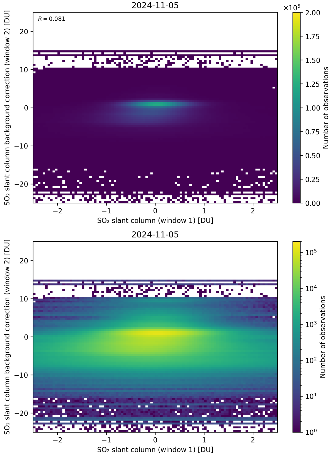
Figure 213: Scatter density plot of “SO 2 slant column (window 1)” against “SO 2 slant column background correction (window 2)” for 2024-11-04 to 2024-11-06.
