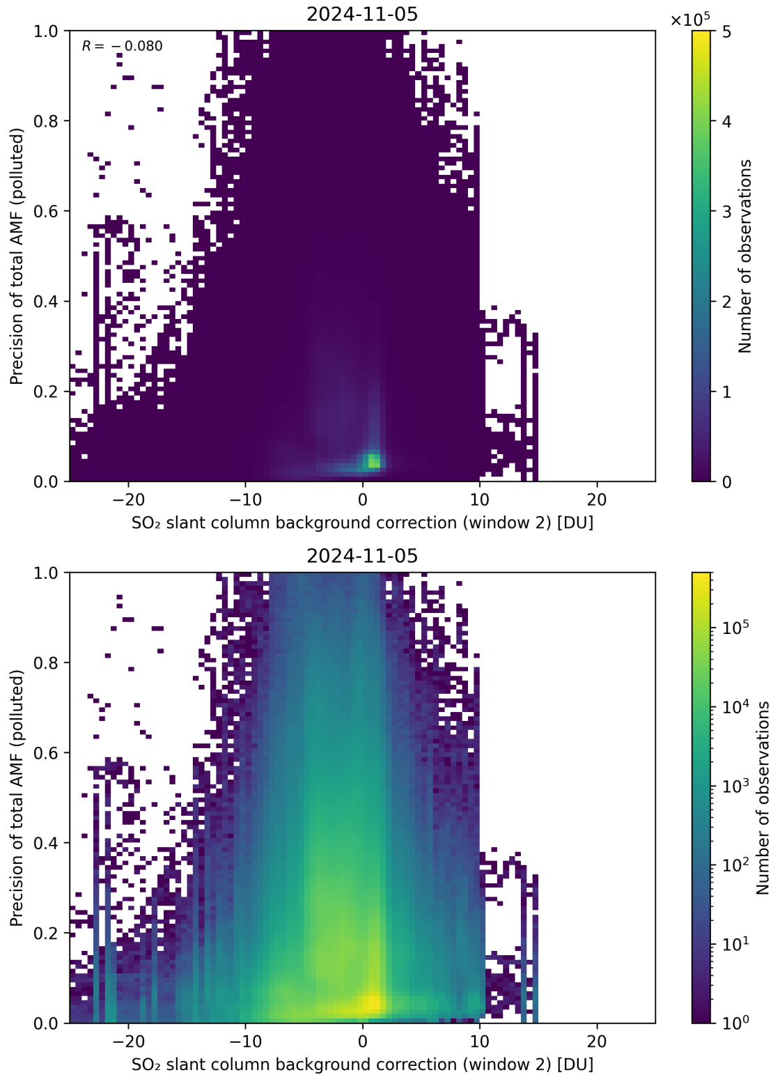
Figure 120: Scatter density plot of “SO 2 slant column background correction (window 2)” against “Precision of total AMF (polluted)” for 2024-11-04 to 2024-11-06.
