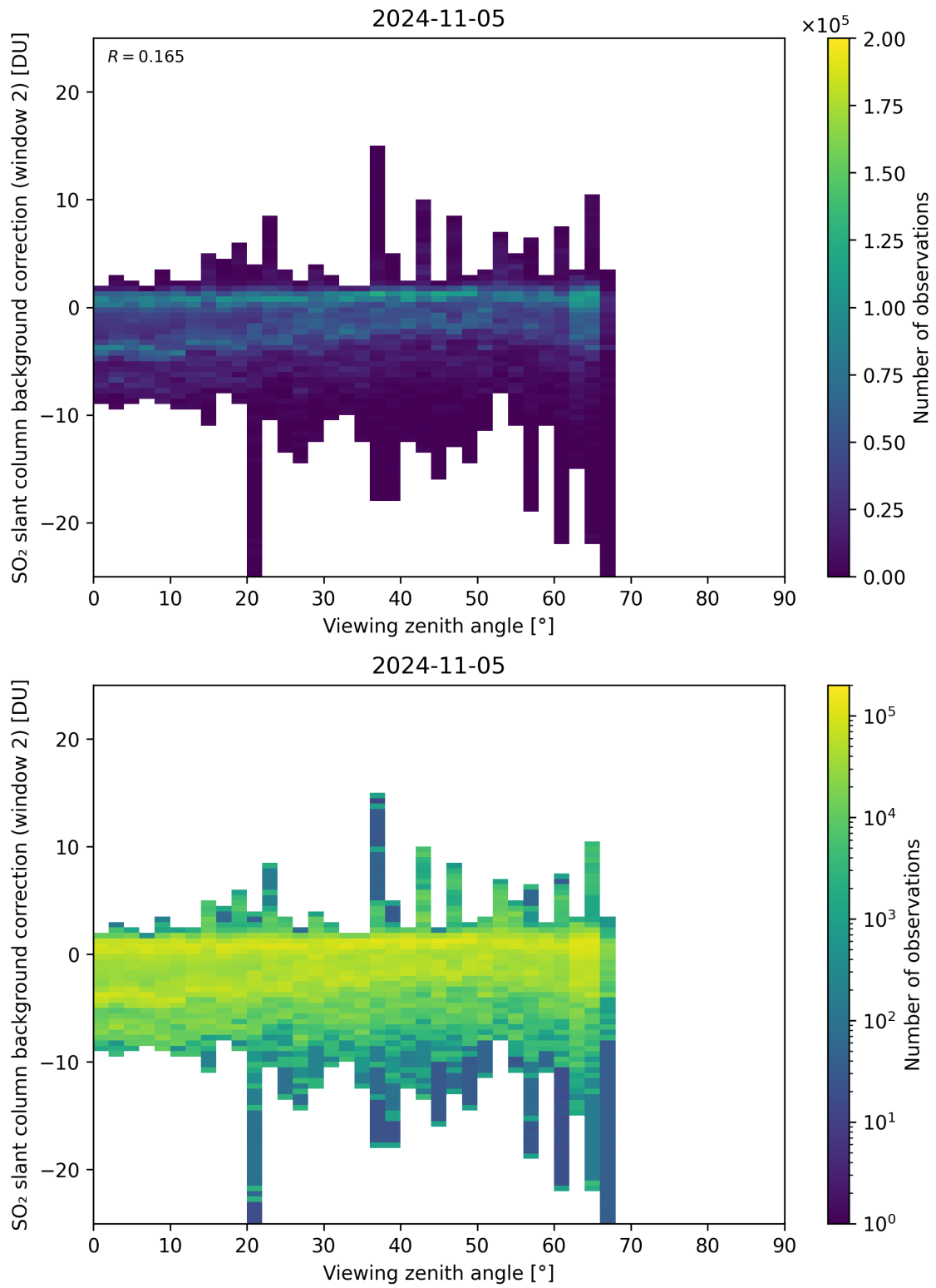
Figure 309: Scatter density plot of “Viewing zenith angle” against “SO 2 slant column background correction (window 2)” for 2024-11-04 to 2024-11-06.
