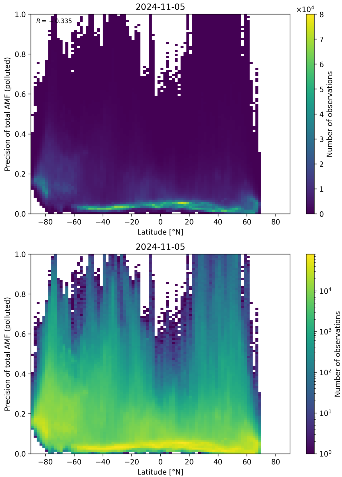
Figure 155: Scatter density plot of “Latitude” against “Precision of total AMF (polluted)” for 2024-11-04 to 2024-11-06.
