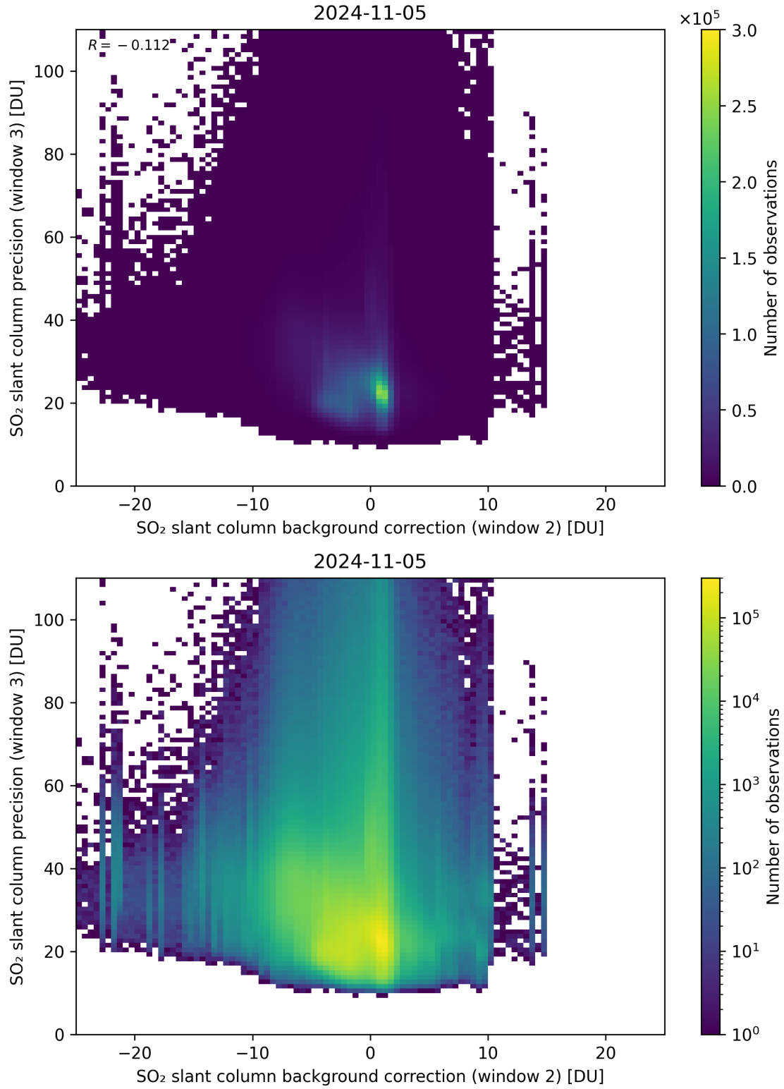
Figure 118: Scatter density plot of “SO 2 slant column background correction (window 2)” against “SO 2 slant column precision (window 3)” for 2024-11-04 to 2024-11-06.
