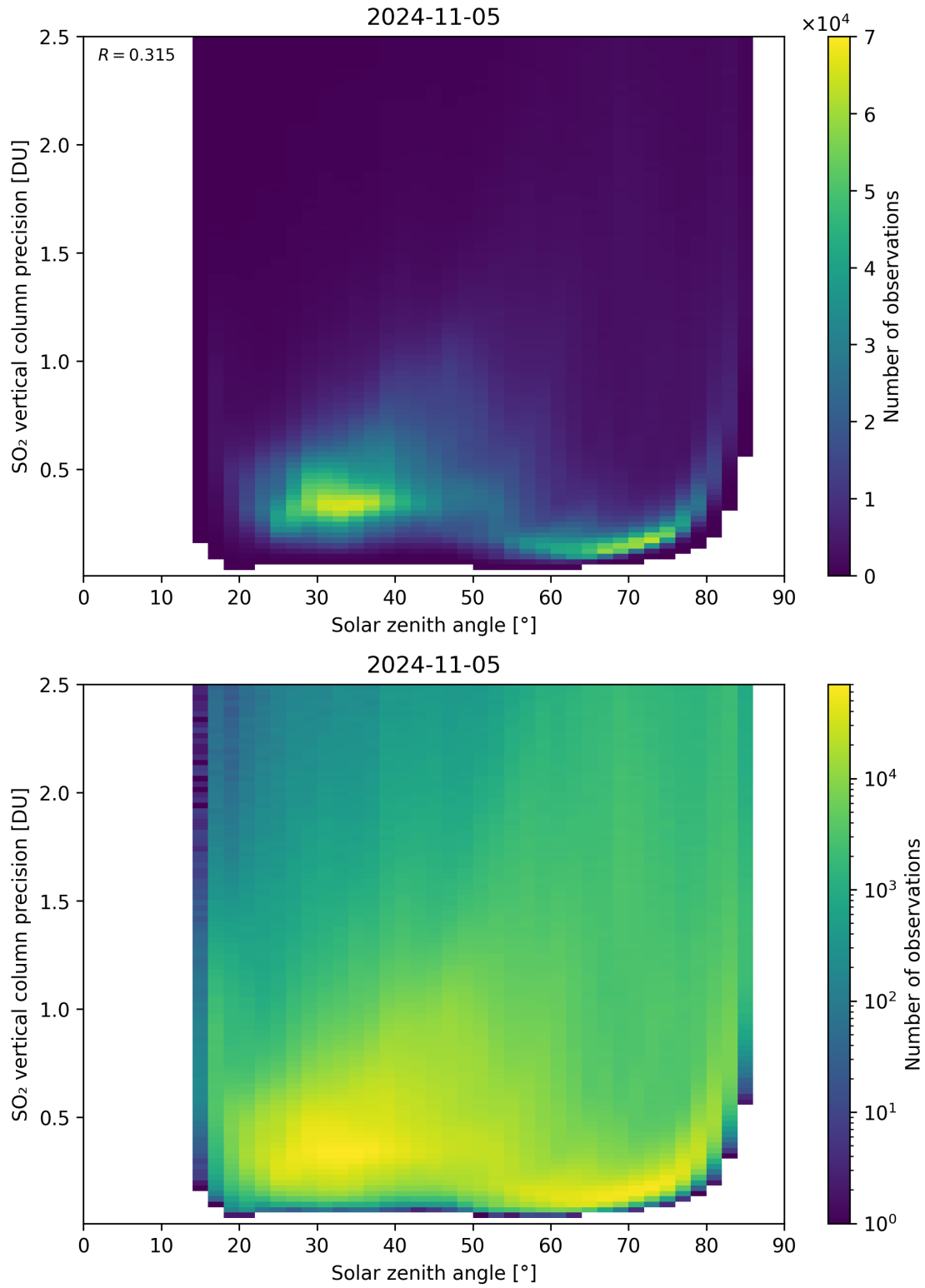
Figure 177: Scatter density plot of “Solar zenith angle” against “SO 2 vertical column precision” for 2024-11-04 to 2024-11-06.
