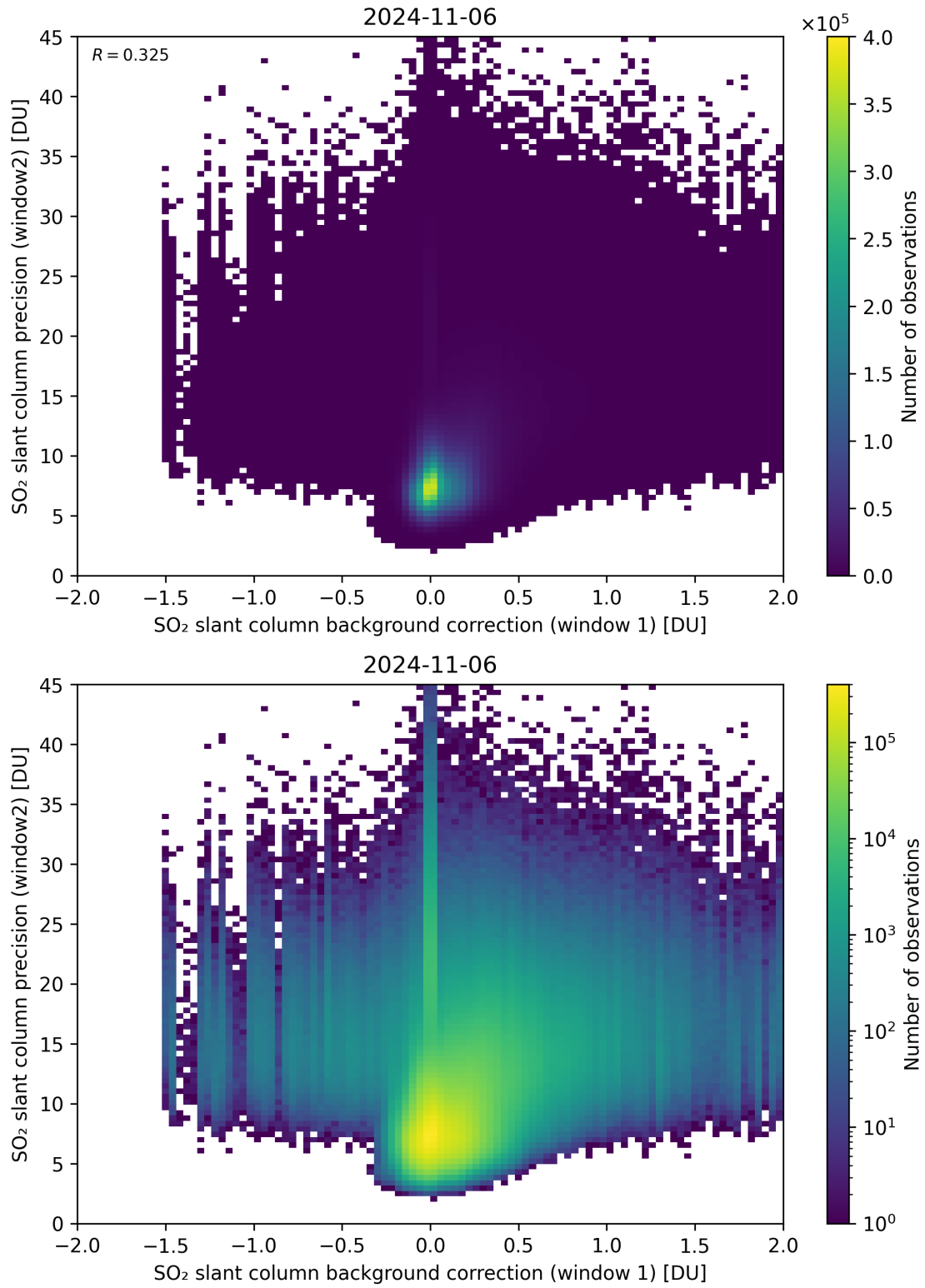
Figure 106: Scatter density plot of “SO 2 slant column background correction (window 1)” against “SO 2 slant column precision (window2)” for 2024-11-05 to 2024-11-07.
