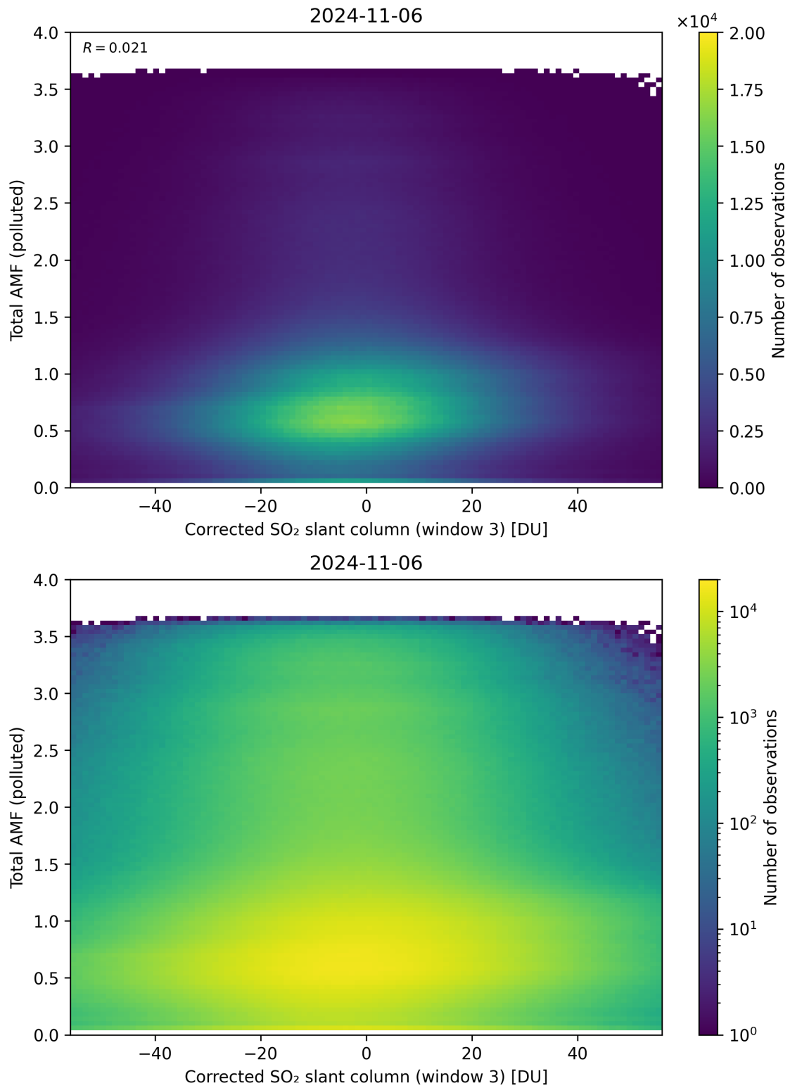
Figure 210: Scatter density plot of “Corrected SO 2 slant column (window 3)” against “Total AMF (polluted)” for 2024-11-05 to 2024-11-07.
