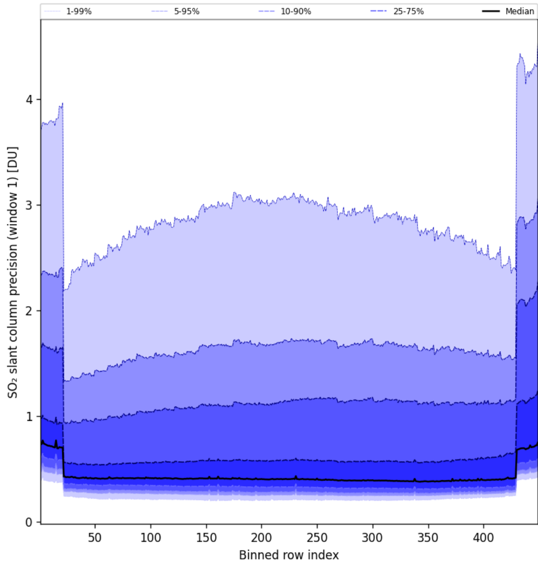
Figure 80: Along track statistics of “SO 2 slant column precision (window 1)” for 2024-11-05 to 2024-11-07
