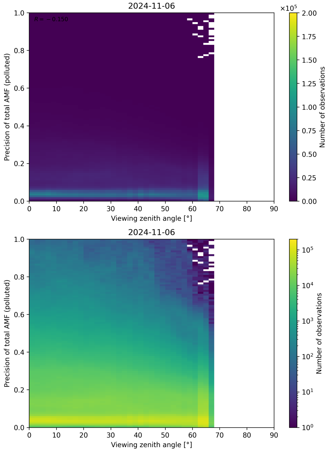
Figure 326: Scatter density plot of “Viewing zenith angle” against “Precision of total AMF (polluted)” for 2024-11-05 to 2024-11-07.
