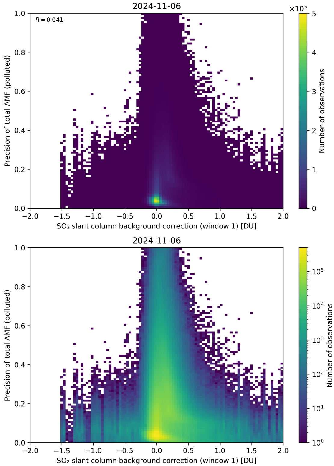
Figure 110: Scatter density plot of “SO 2 slant column background correction (window 1)” against “Precision of total AMF (polluted)” for 2024-11-05 to 2024-11-07.
