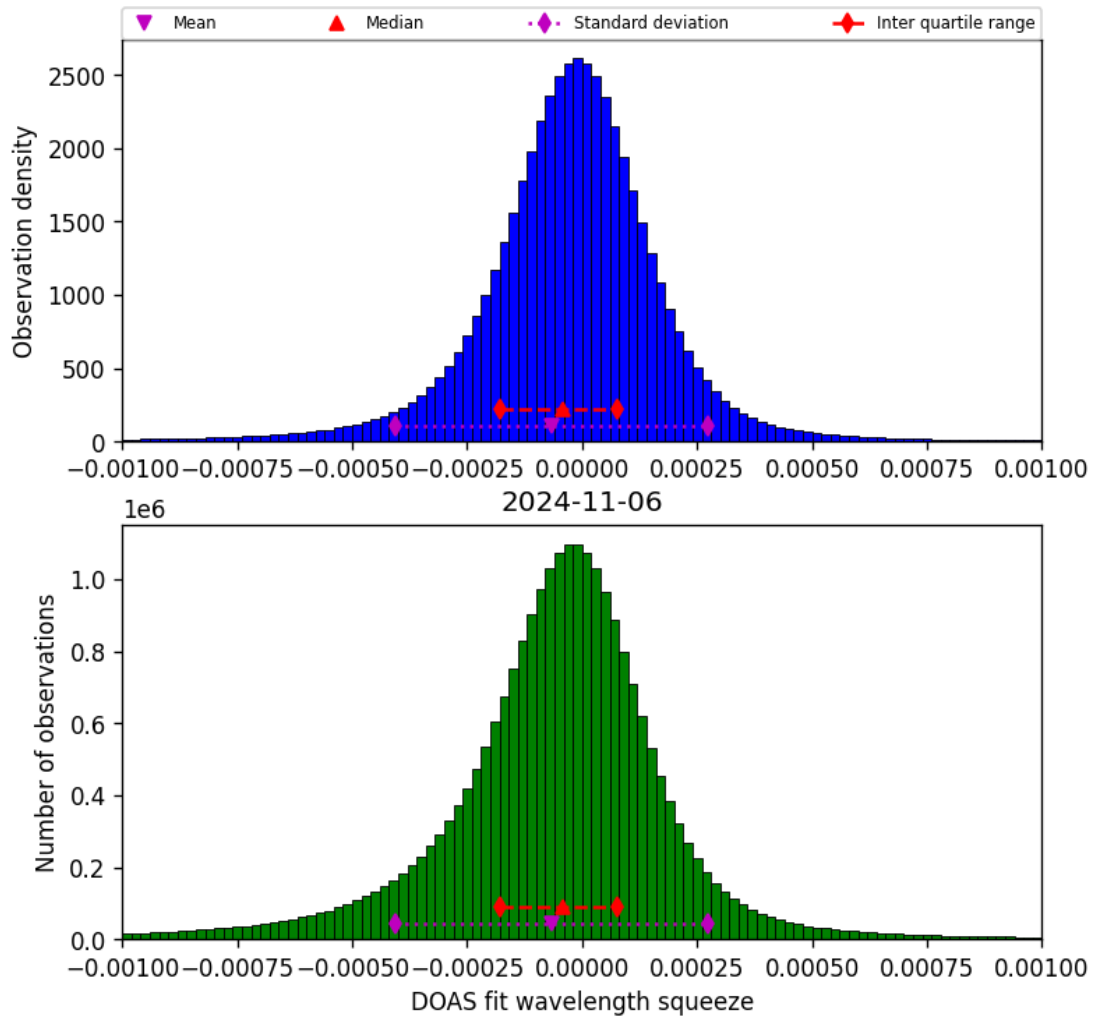
Figure 69: Histogram of “DOAS fit wavelength squeeze” for 2024-11-05 to 2024-11-07
