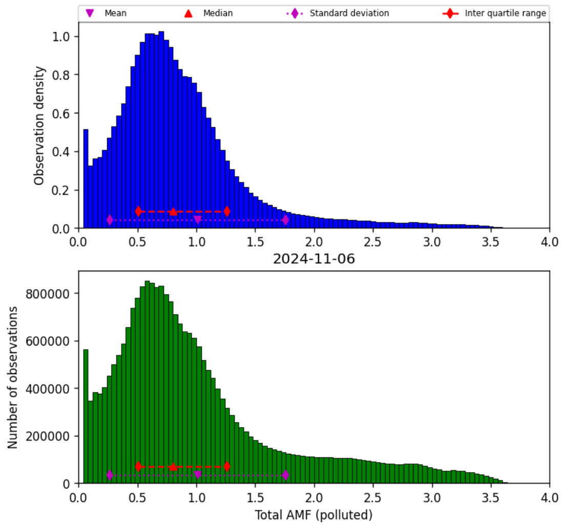
Figure 71: Histogram of “Total AMF (polluted)” for 2024-11-05 to 2024-11-07
