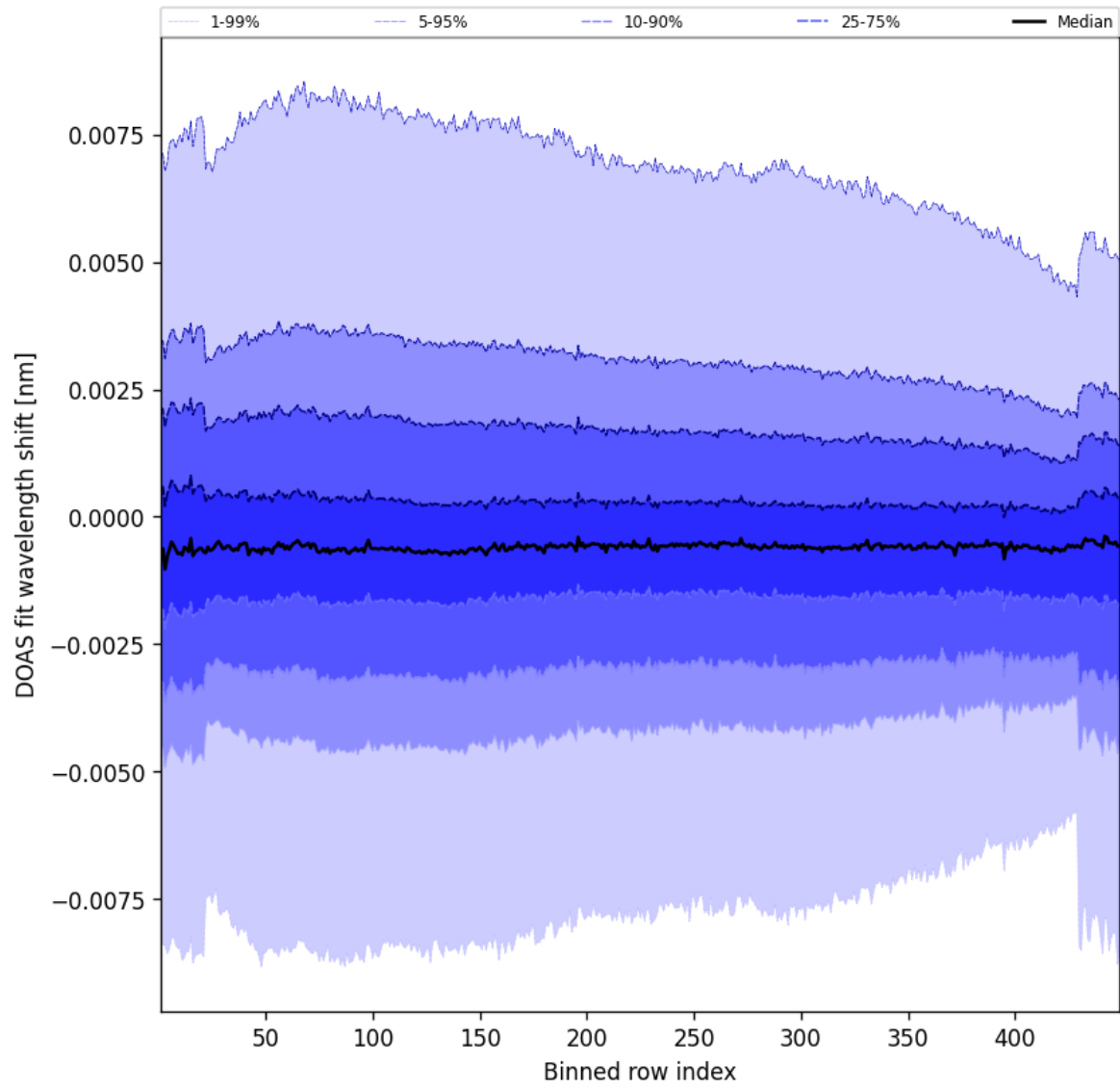
Figure 91: Along track statistics of “DOAS fit wavelength shift” for 2024-11-05 to 2024-11-07
