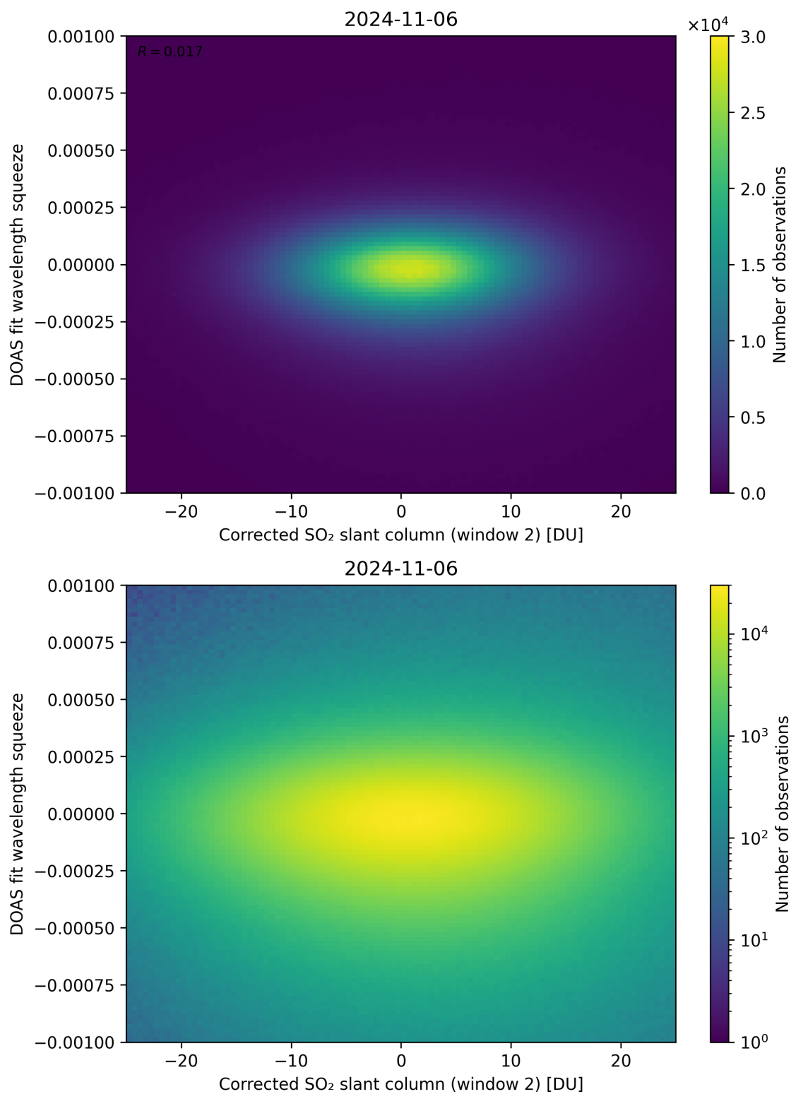
Figure 197: Scatter density plot of “Corrected SO 2 slant column (window 2)” against “DOAS fit wavelength squeeze” for 2024-11-05 to 2024-11-07.
