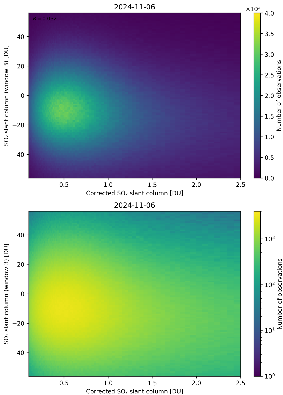
Figure 190: Scatter density plot of “Corrected SO 2 slant column” against “SO 2 slant column (window 3)” for 2024-11-05 to 2024-11-07.
