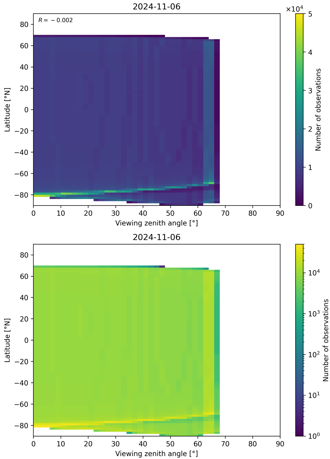
Figure 314: Scatter density plot of “Viewing zenith angle” against “Latitude” for 2024-11-05 to 2024-11-07.
