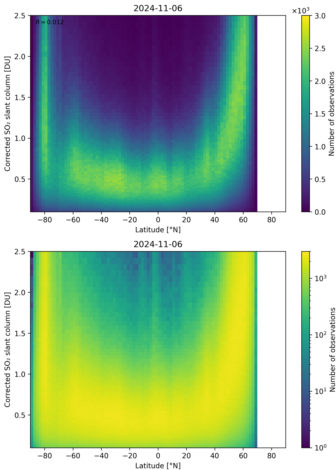
Figure 146: Scatter density plot of “Latitude” against “Corrected SO 2 slant column” for 2024-11-05 to 2024-11-07.
