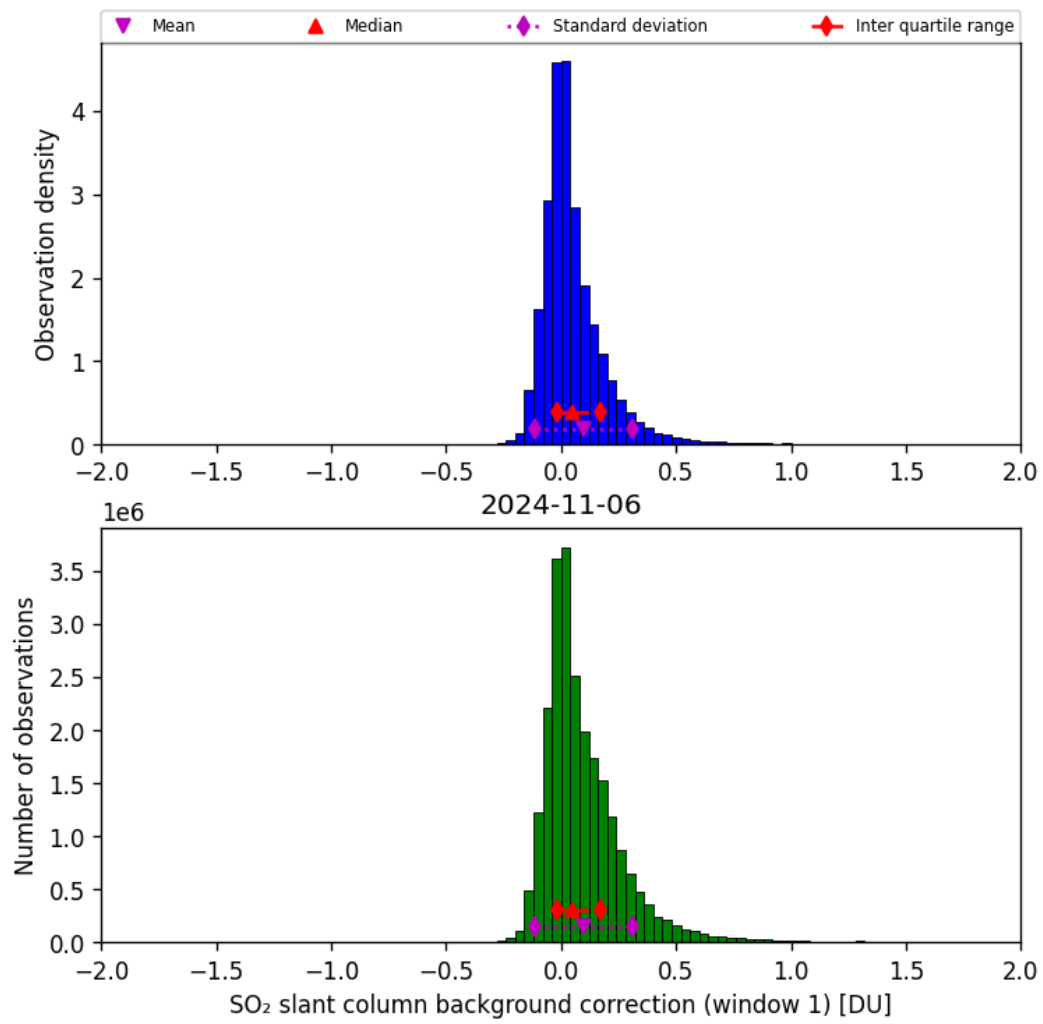
Figure 59: Histogram of “SO 2 slant column background correction (window 1)” for 2024-11-05 to 2024-11-07
