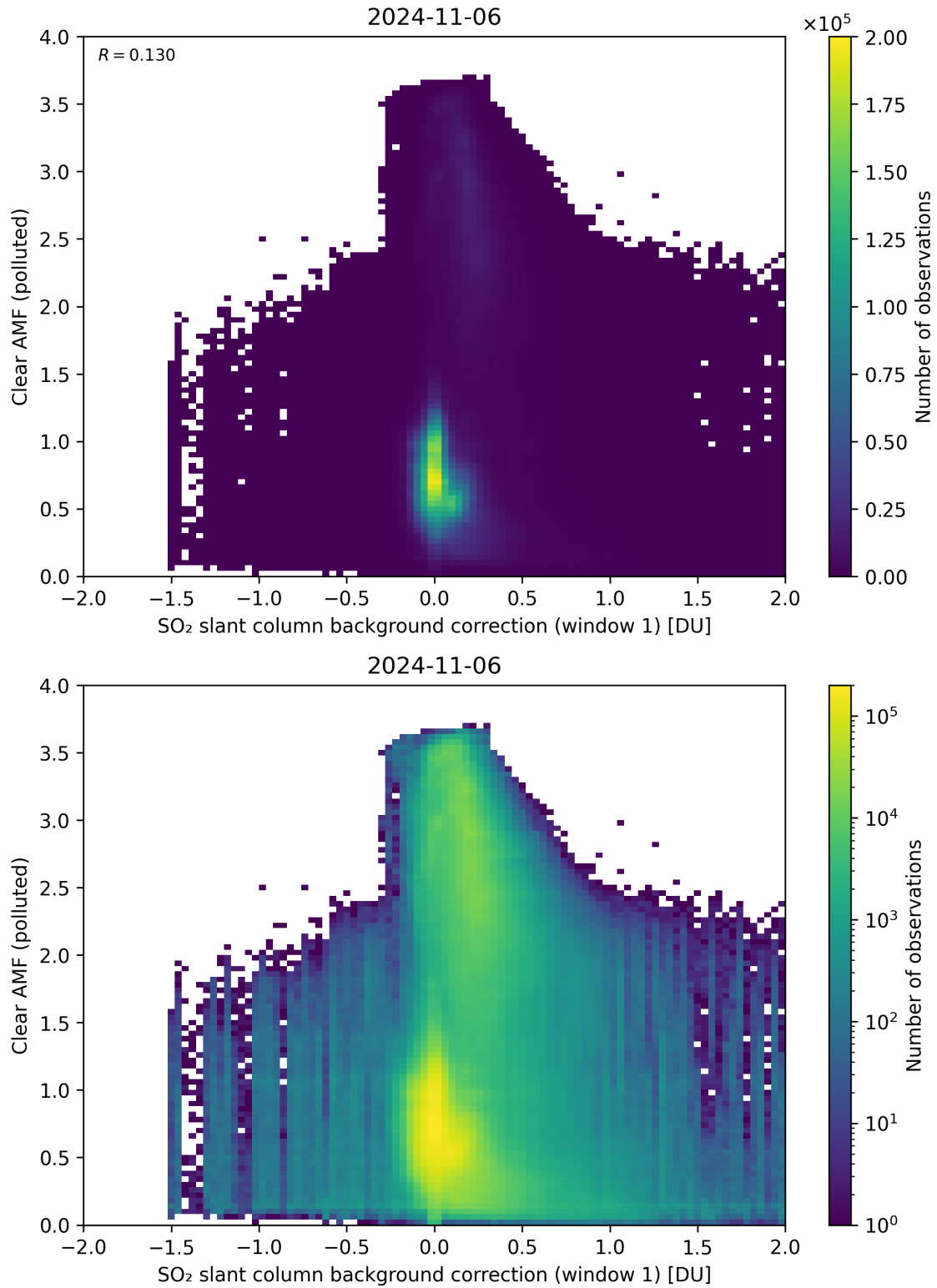
Figure 103: Scatter density plot of “SO 2 slant column background correction (window 1)” against “Clear AMF (polluted)” for 2024-11-05 to 2024-11-07.
