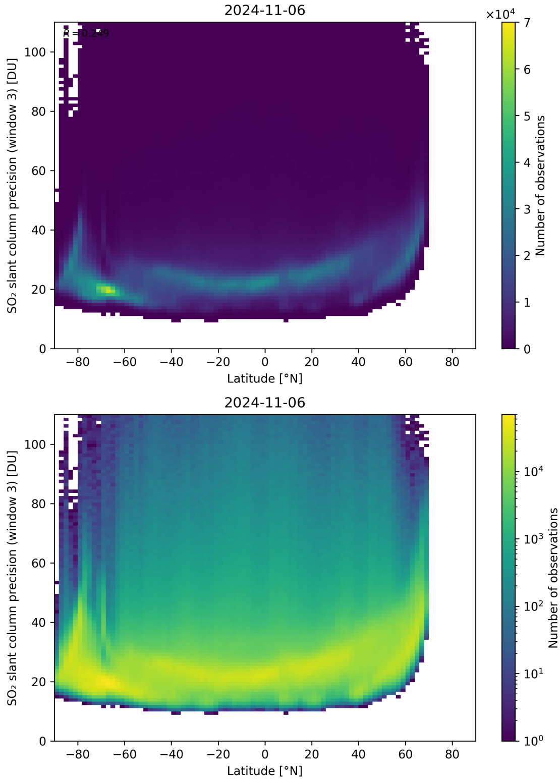
Figure 153: Scatter density plot of “Latitude” against “SO 2 slant column precision (window 3)” for 2024-11-05 to 2024-11-07.
