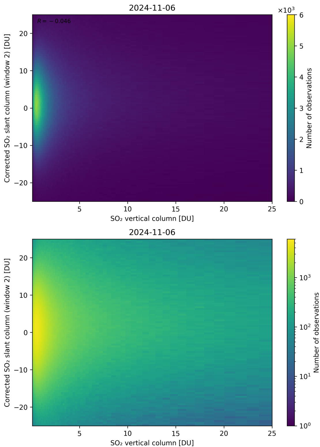
Figure 298: Scatter density plot of “SO 2 vertical column” against “Corrected SO 2 slant column (window 2)” for 2024-11-05 to 2024-11-07.
