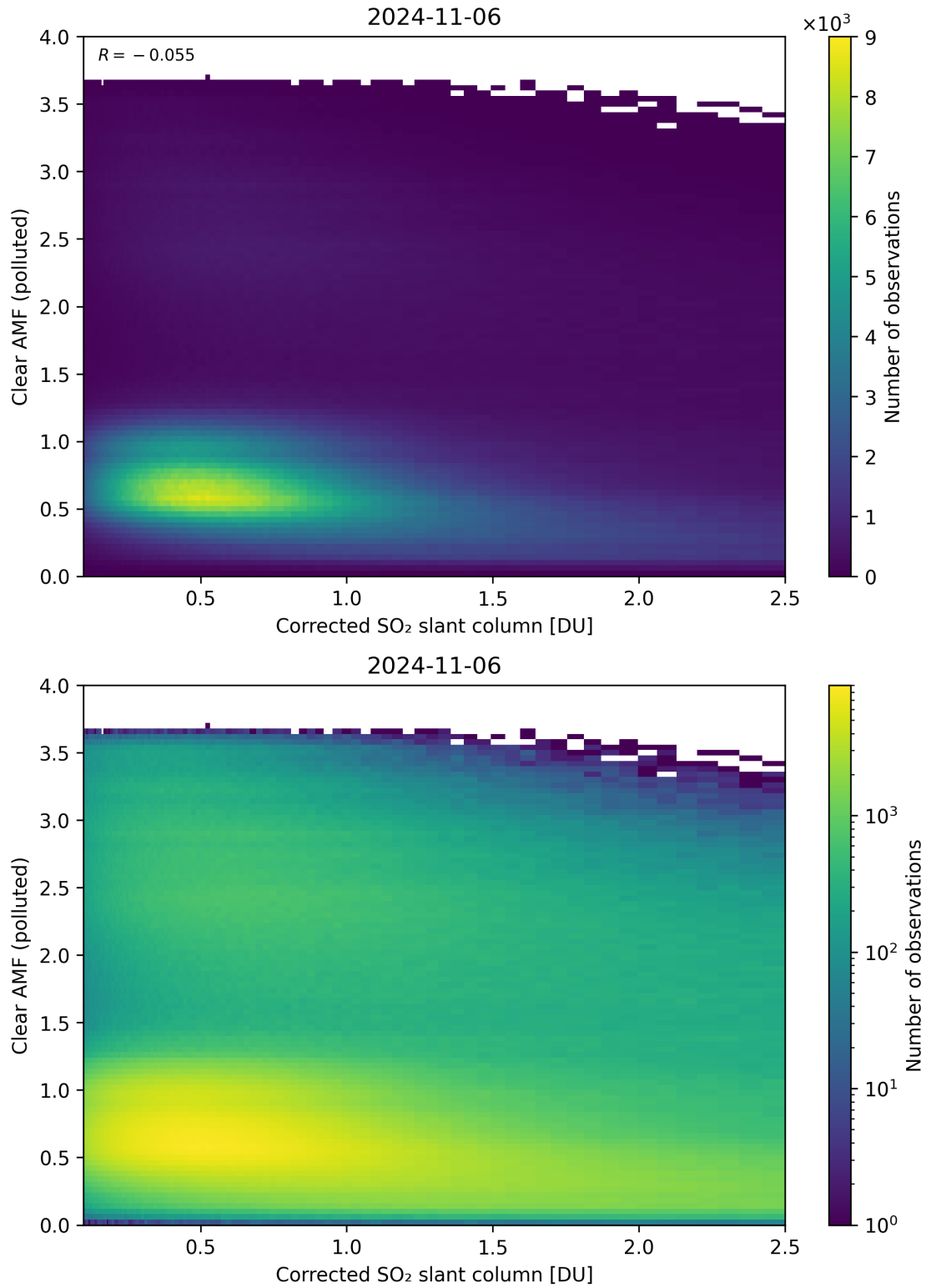
Figure 184: Scatter density plot of “Corrected SO 2 slant column” against “Clear AMF (polluted)” for 2024-11-05 to 2024-11-07.
