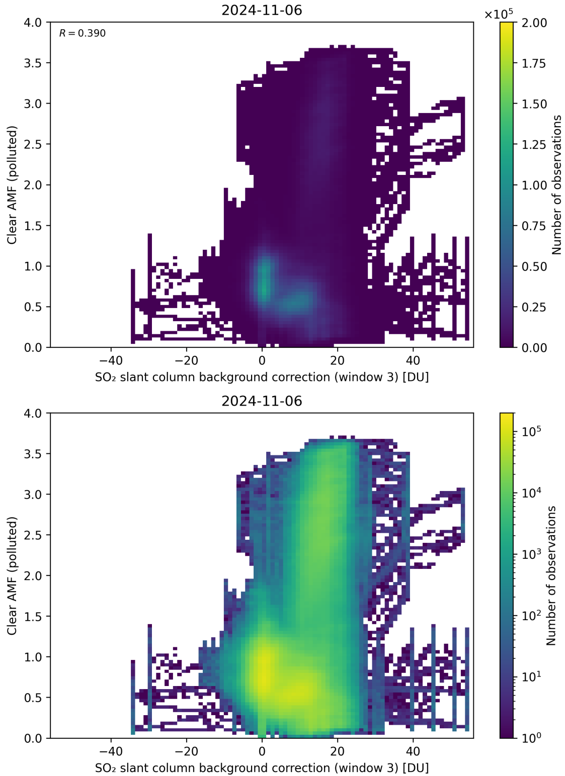
Figure 124: Scatter density plot of “SO 2 slant column background correction (window 3)” against “Clear AMF (polluted)” for 2024-11-05 to 2024-11-07.
