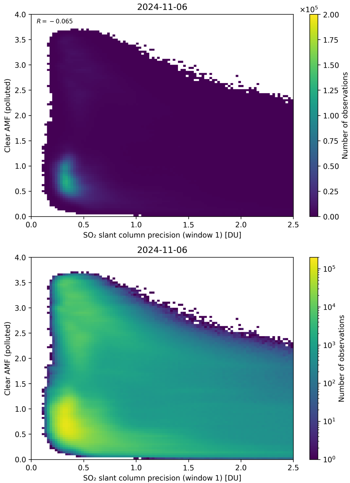
Figure 224: Scatter density plot of “SO 2 slant column precision (window 1)” against “Clear AMF (polluted)” for 2024-11-05 to 2024-11-07.
