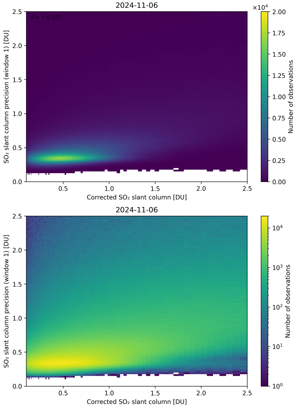
Figure 188: Scatter density plot of “Corrected SO 2 slant column” against “SO 2 slant column precision (window 1)” for 2024-11-05 to 2024-11-07.
