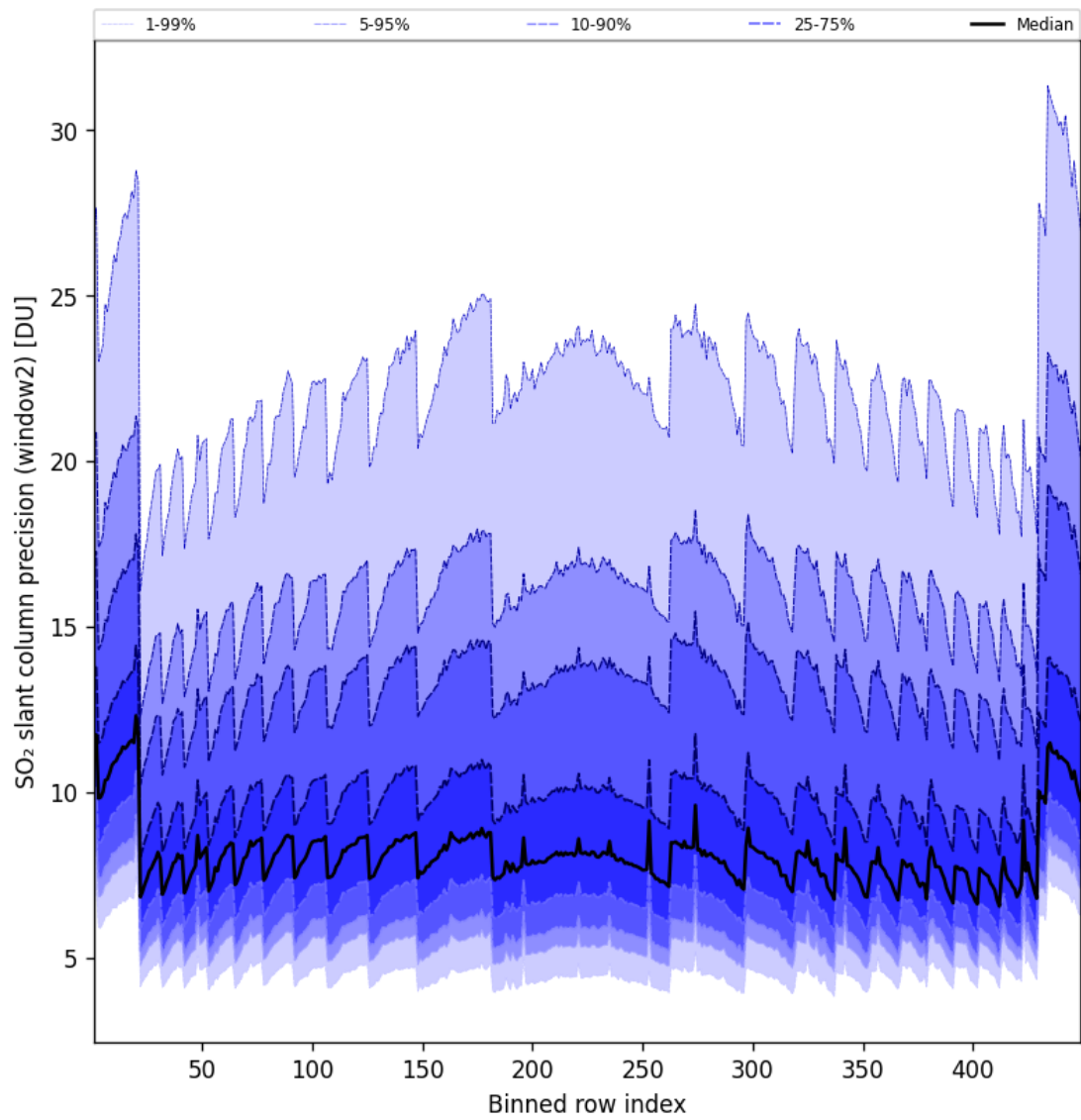
Figure 84: Along track statistics of “SO 2 slant column precision (window2)” for 2024-11-05 to 2024-11-07
