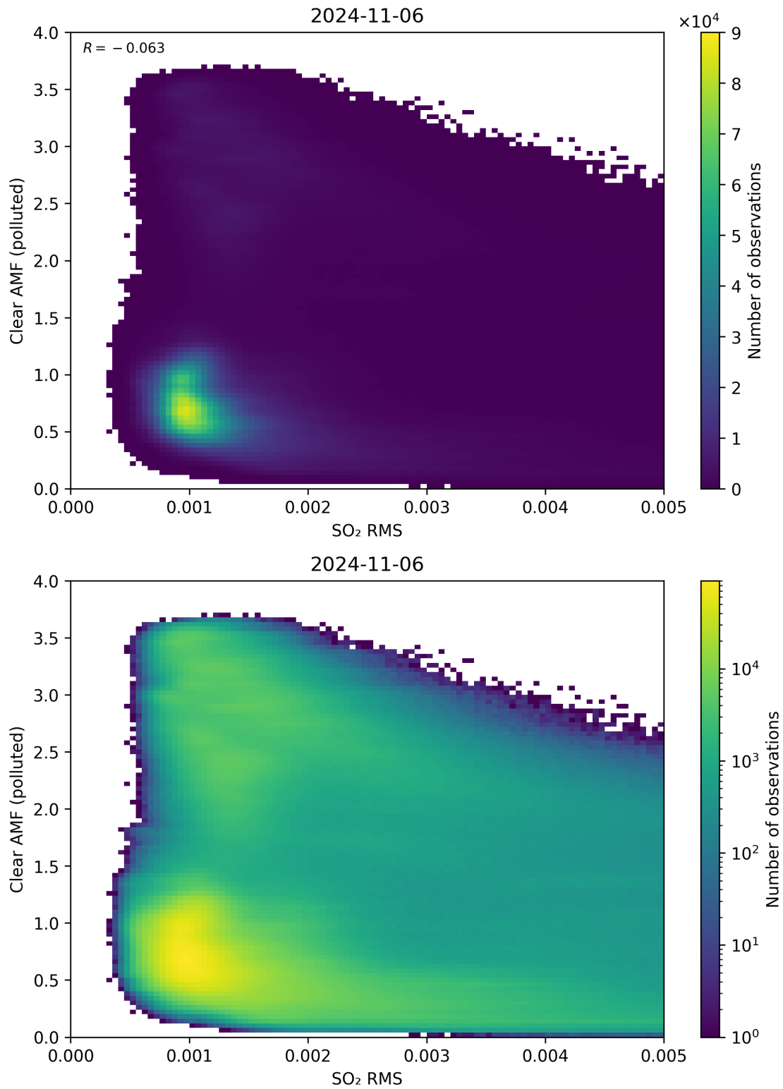
Figure 136: Scatter density plot of “SO 2 RMS” against “Clear AMF (polluted)” for 2024-11-05 to 2024-11-07.
