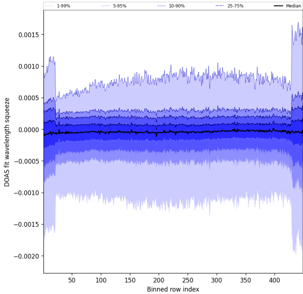
Figure 92: Along track statistics of “DOAS fit wavelength squeeze” for 2024-11-05 to 2024-11-07
