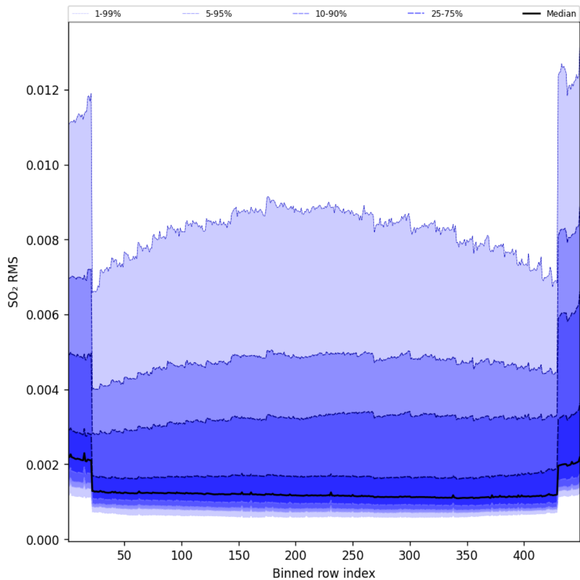
Figure 93: Along track statistics of “SO 2 RMS” for 2024-11-05 to 2024-11-07
