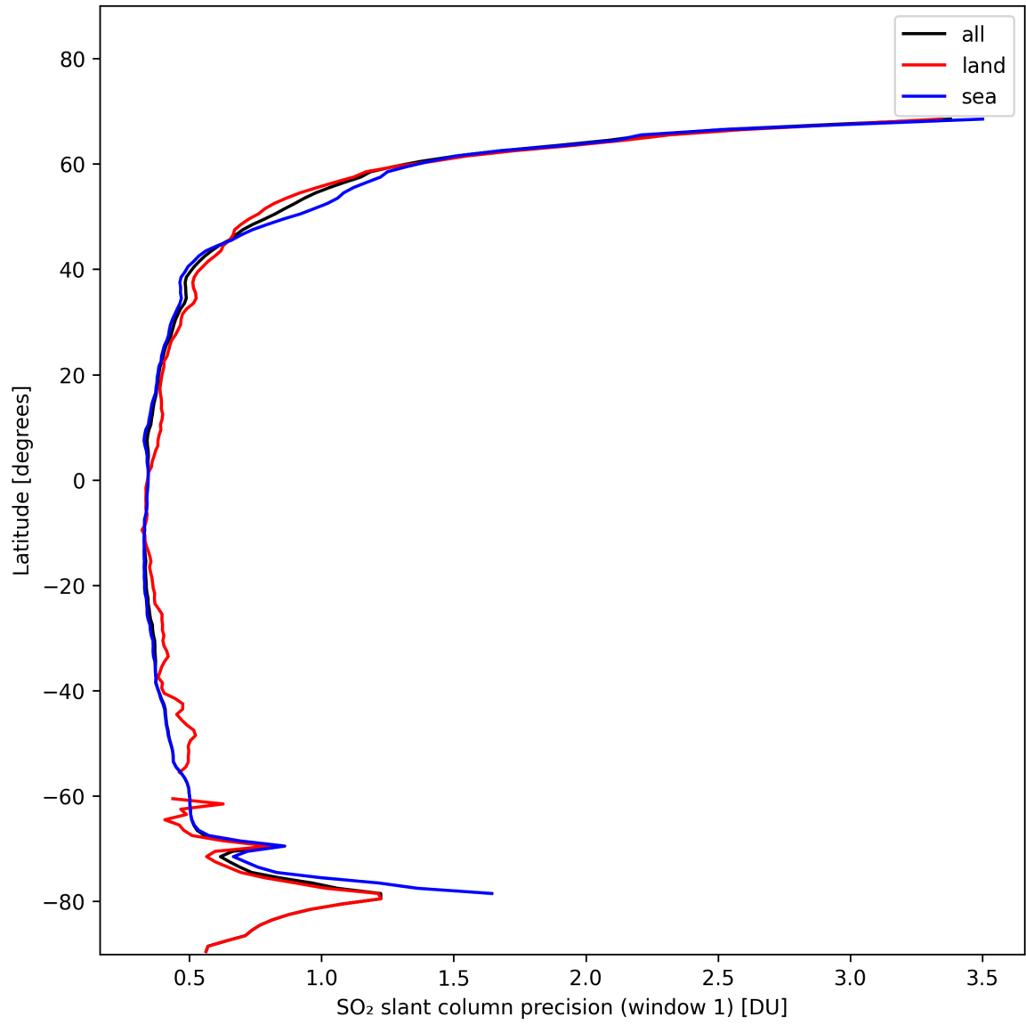
Figure 34: Zonal average of “SO 2 slant column precision (window 1)” for 2024-11-05 to 2024-11-07.
