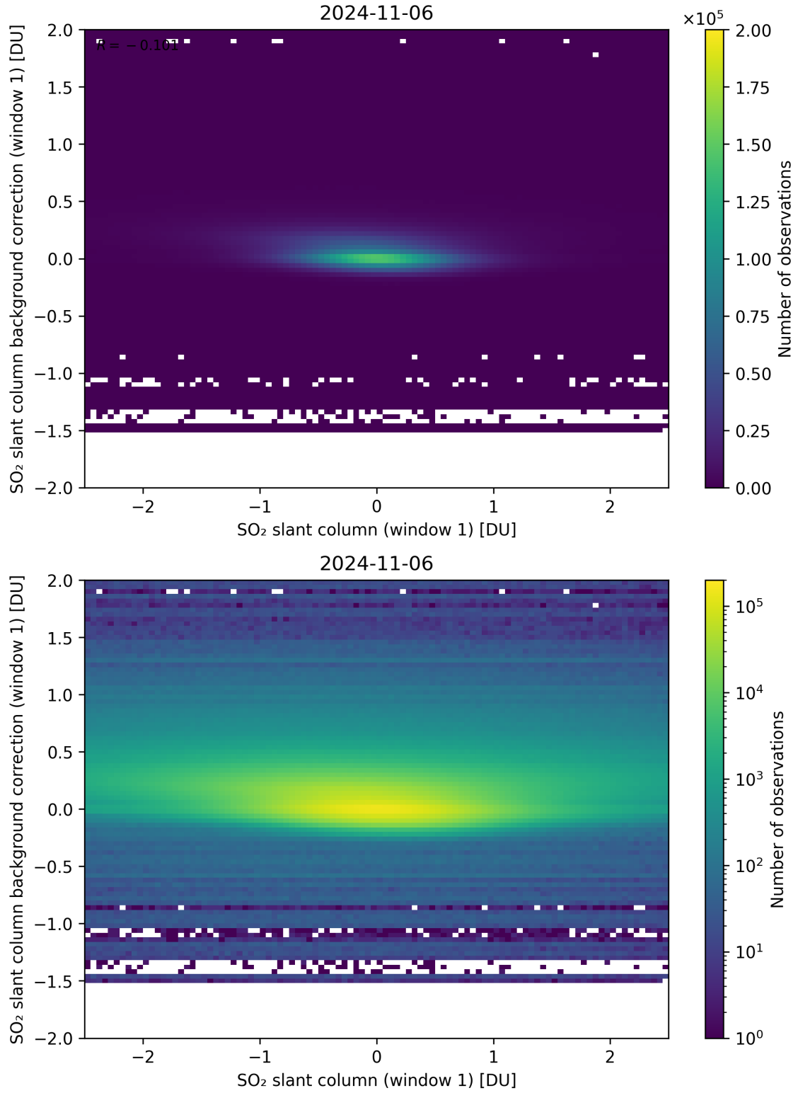
Figure 212: Scatter density plot of “SO 2 slant column (window 1)” against “SO 2 slant column background correction (window 1)” for 2024-11-05 to 2024-11-07.
