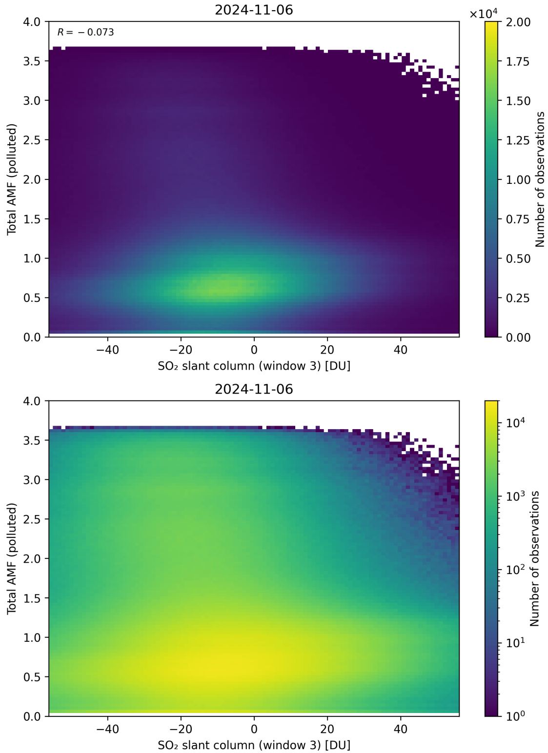
Figure 268: Scatter density plot of “SO 2 slant column (window 3)” against “Total AMF (polluted)” for 2024-11-05 to 2024-11-07.
