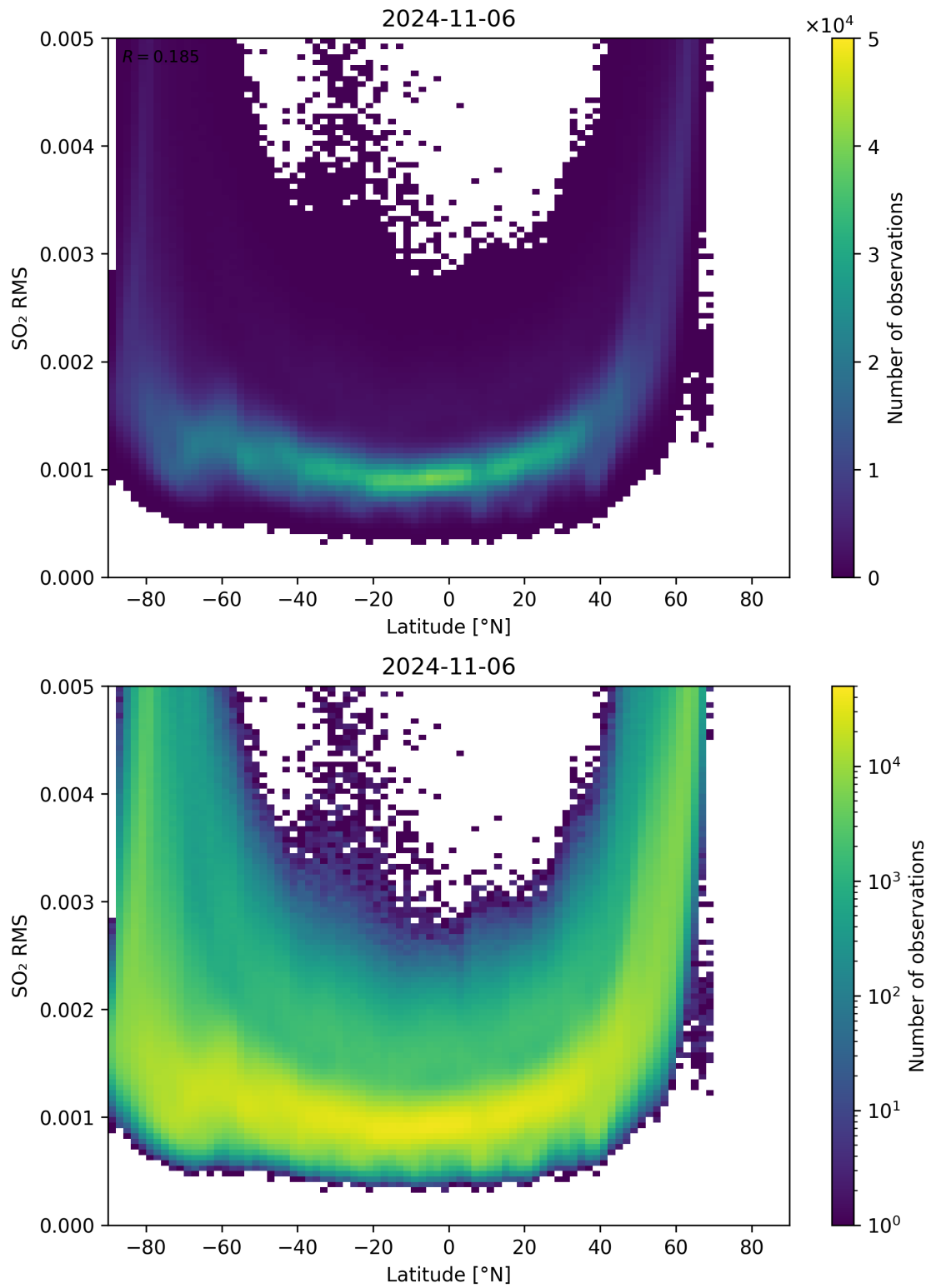
Figure 144: Scatter density plot of “Latitude” against “SO 2 RMS” for 2024-11-05 to 2024-11-07.
