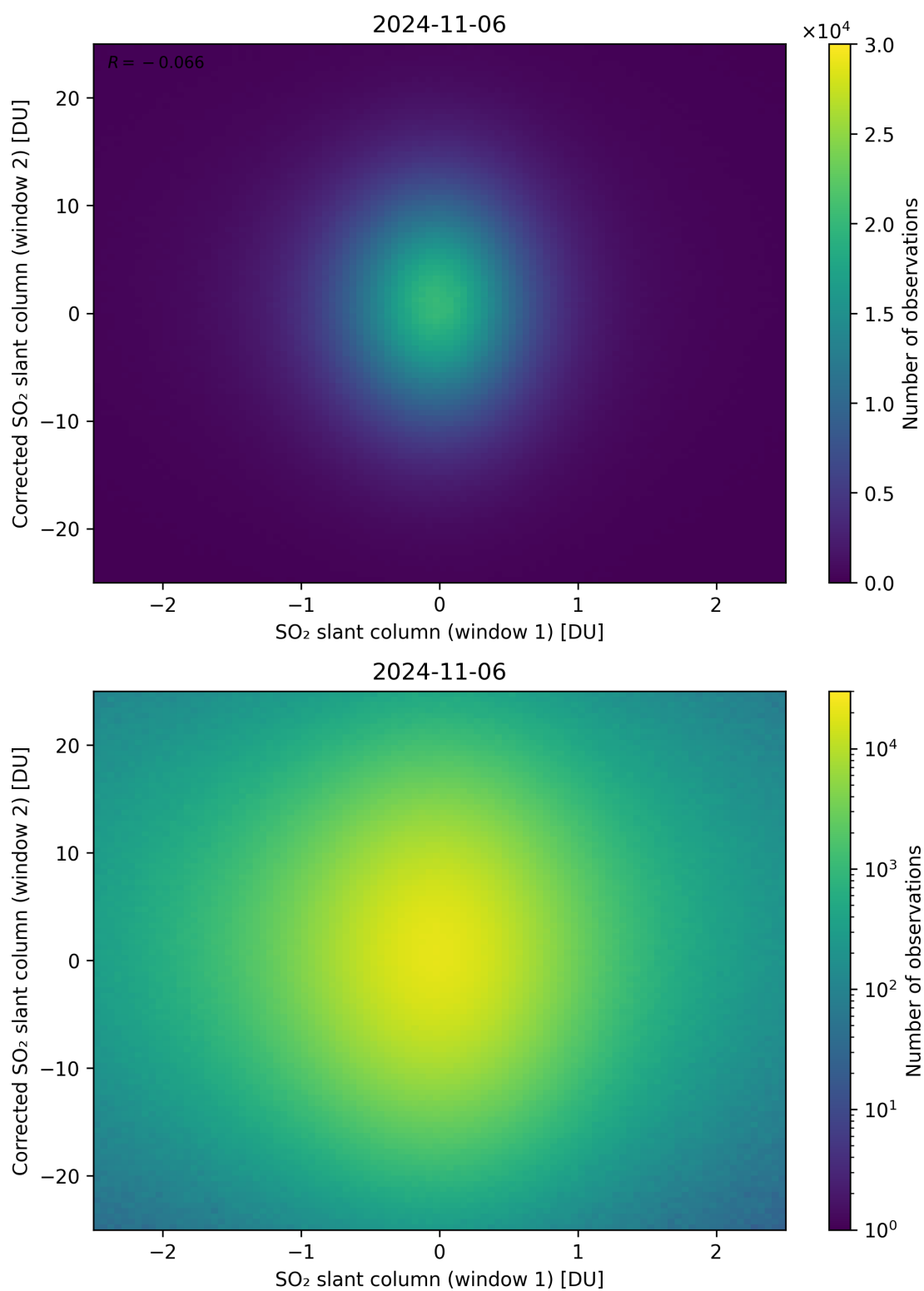
Figure 233: Scatter density plot of “SO 2 slant column (window 1)” against “Corrected SO 2 slant column (window 2)” for 2024-11-05 to 2024-11-07.
