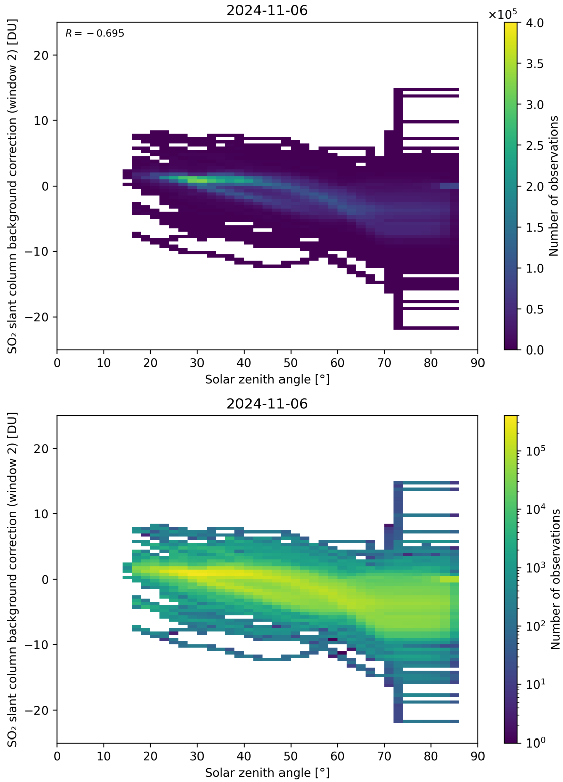
Figure 159: Scatter density plot of “Solar zenith angle” against “SO 2 slant column background correction (window 2)” for 2024-11-05 to 2024-11-07.
