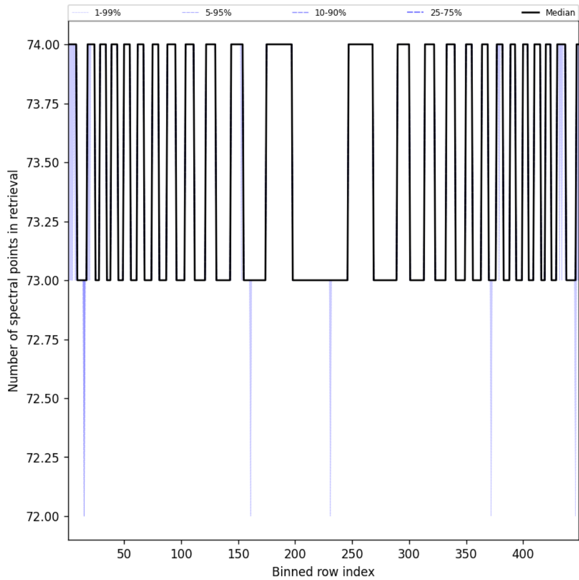
Figure 97: Along track statistics of “Number of spectral points in retrieval” for 2024-11-05 to 2024-11-07
