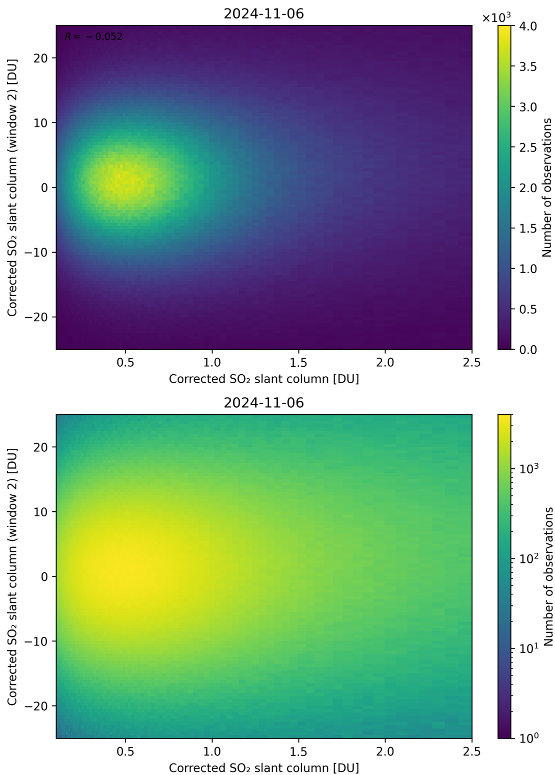
Figure 185: Scatter density plot of “Corrected SO 2 slant column” against “Corrected SO 2 slant column (window 2)” for 2024-11-05 to 2024-11-07.
