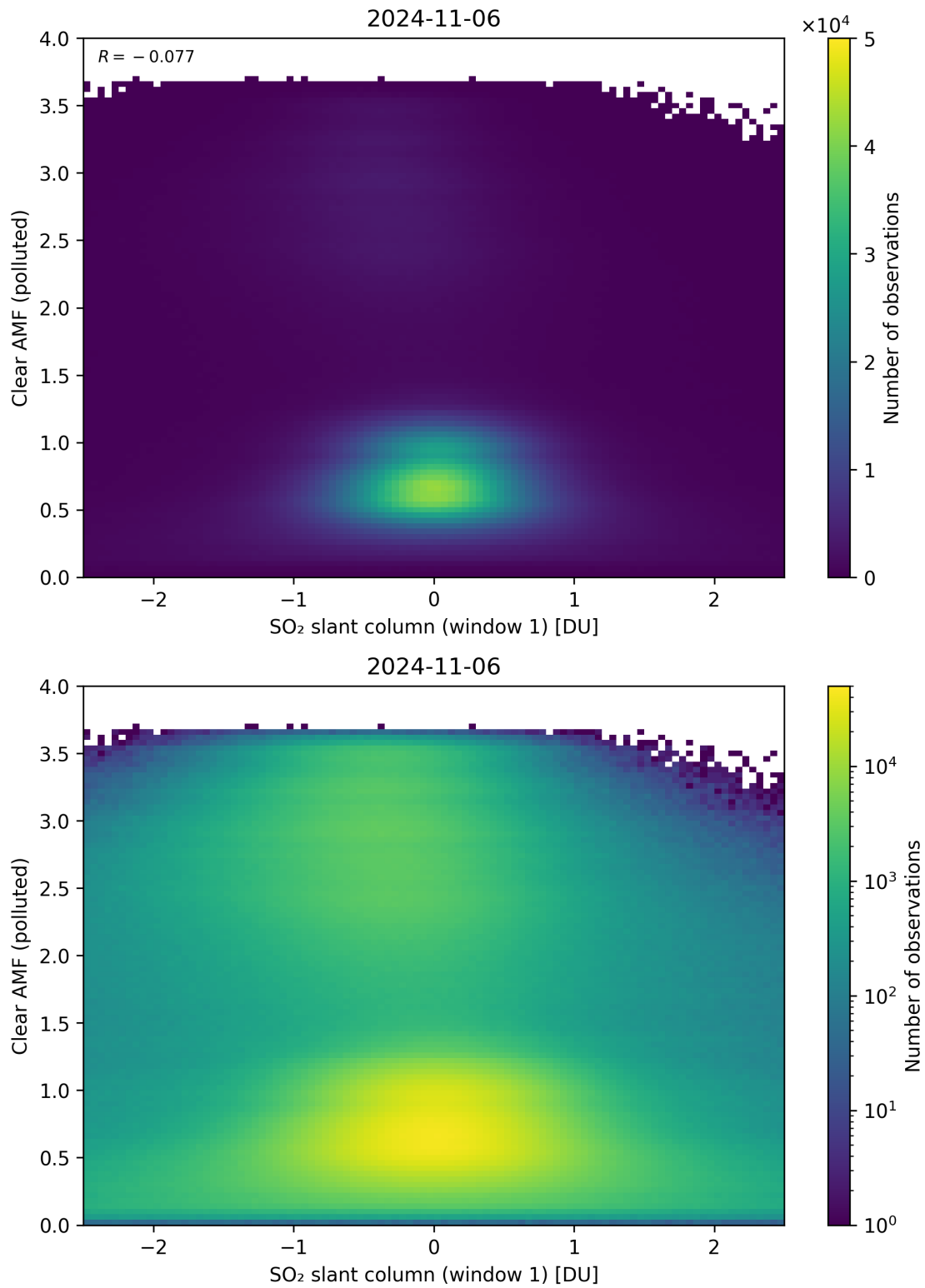
Figure 232: Scatter density plot of “SO 2 slant column (window 1)” against “Clear AMF (polluted)” for 2024-11-05 to 2024-11-07.
