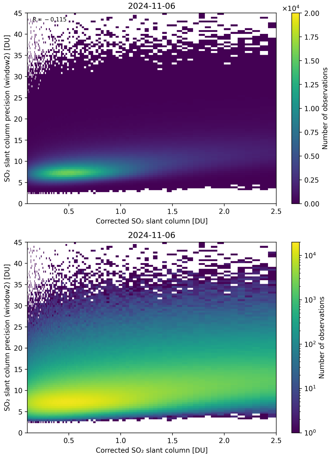
Figure 189: Scatter density plot of “Corrected SO 2 slant column” against “SO 2 slant column precision (window2)” for 2024-11-05 to 2024-11-07.
