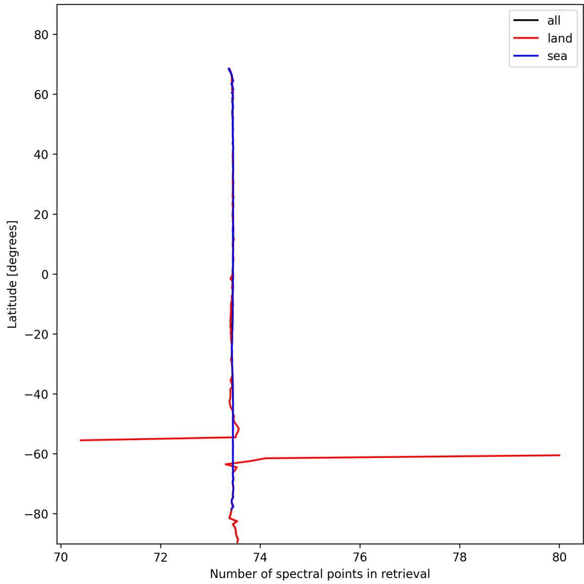
Figure 51: Zonal average of “Number of spectral points in retrieval” for 2024-11-05 to 2024-11-07.
