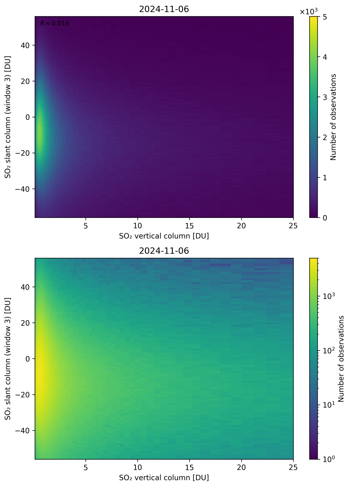
Figure 303: Scatter density plot of “SO 2 vertical column” against “SO 2 slant column (window 3)” for 2024-11-05 to 2024-11-07.
