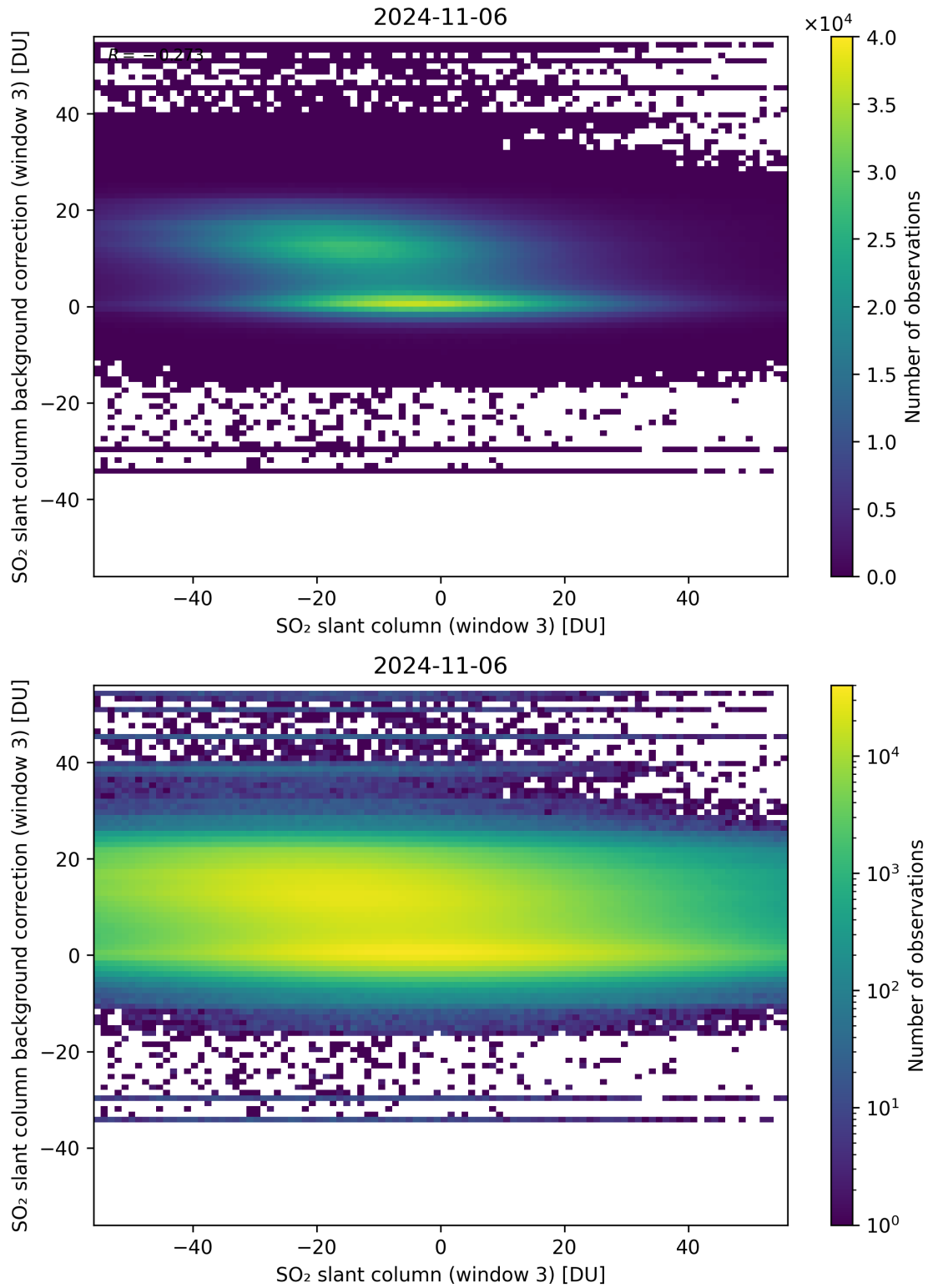
Figure 253: Scatter density plot of “SO 2 slant column (window 3)” against “SO 2 slant column background correction (window 3)” for 2024-11-05 to 2024-11-07.
