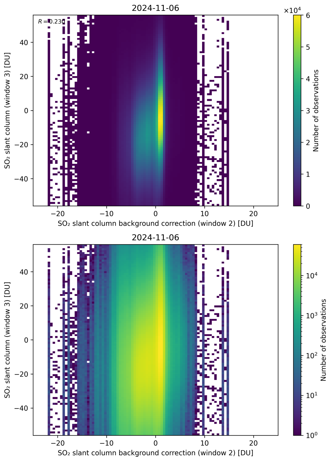
Figure 117: Scatter density plot of “SO 2 slant column background correction (window 2)” against “SO 2 slant column (window 3)” for 2024-11-05 to 2024-11-07.
