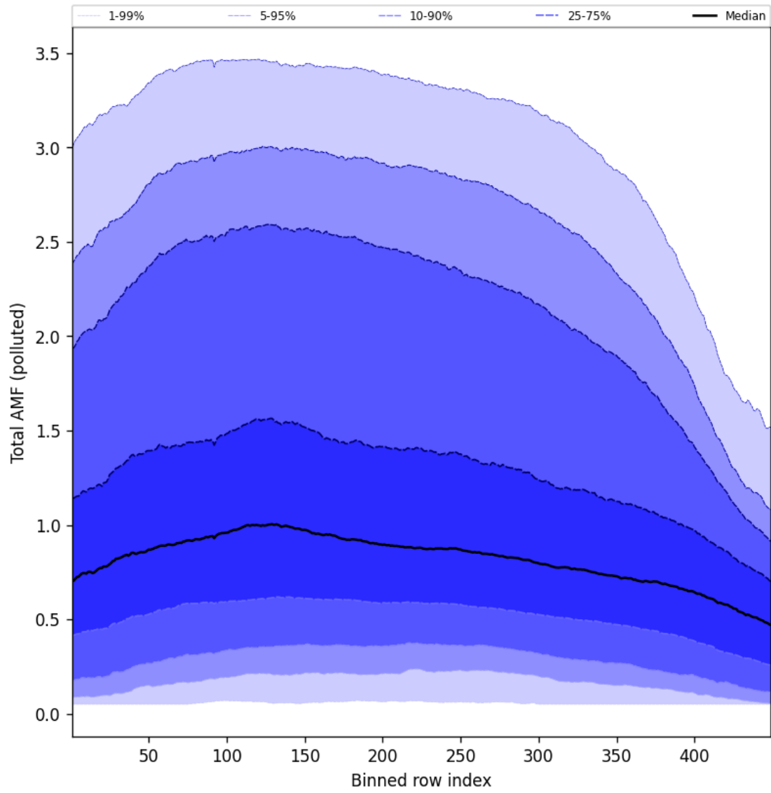
Figure 94: Along track statistics of “Total AMF (polluted)” for 2024-11-05 to 2024-11-07
