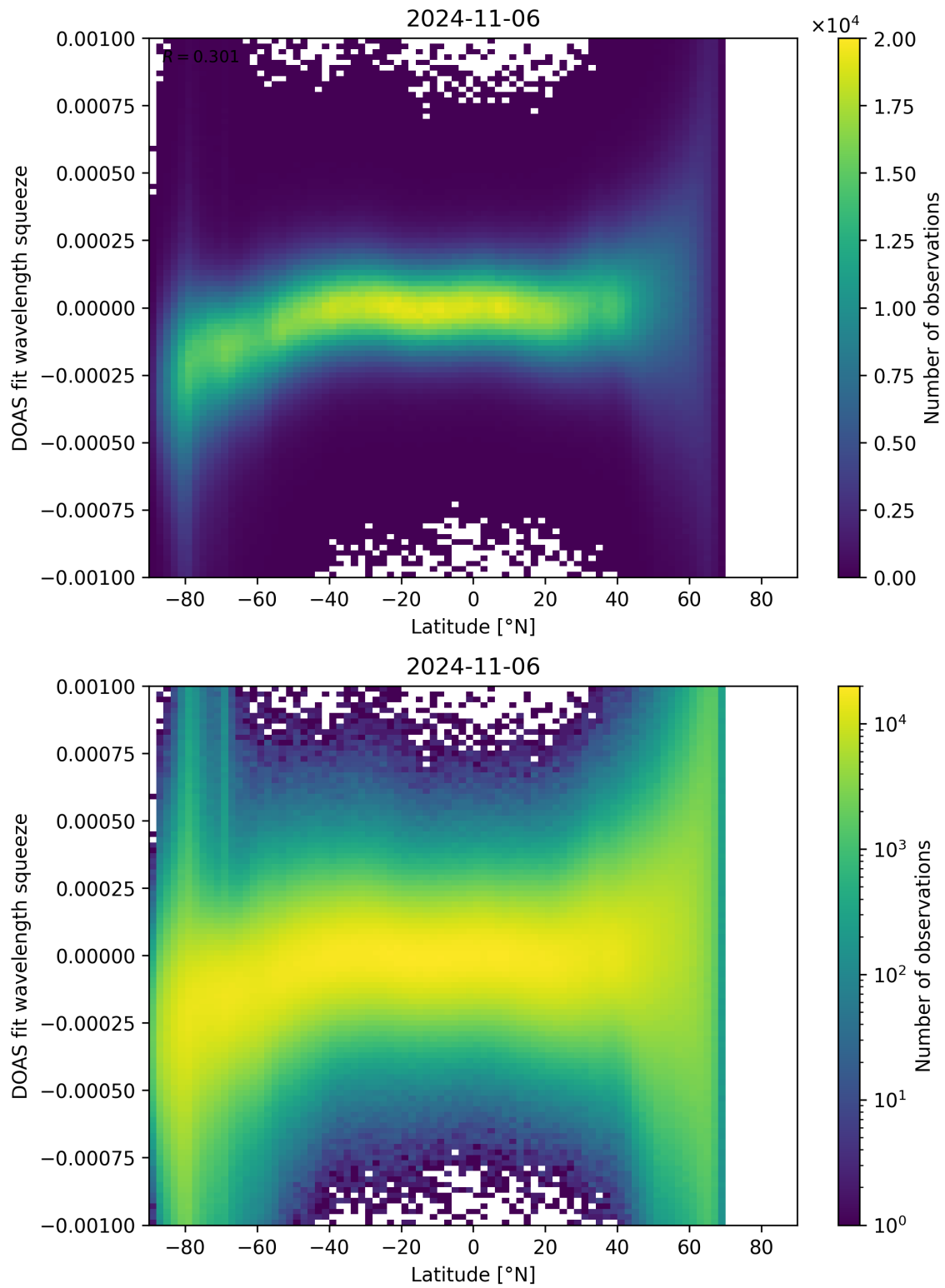
Figure 143: Scatter density plot of “Latitude” against “DOAS fit wavelength squeeze” for 2024-11-05 to 2024-11-07.
