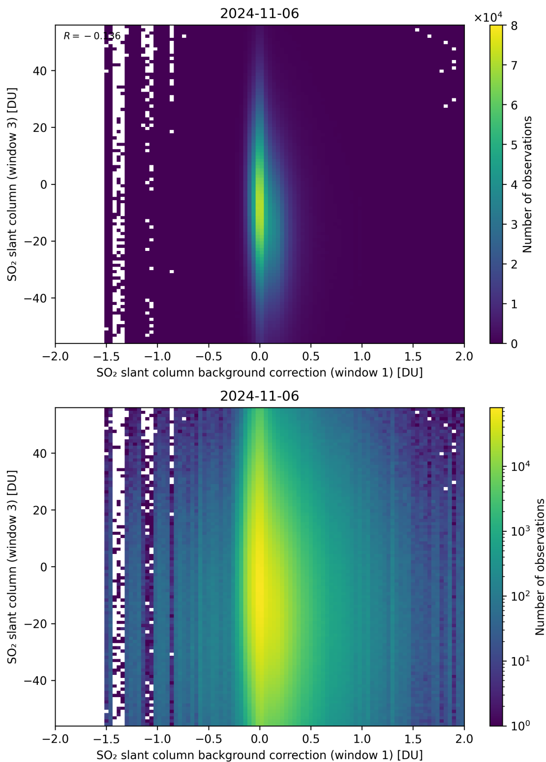
Figure 107: Scatter density plot of “SO 2 slant column background correction (window 1)” against “SO 2 slant column (window 3)” for 2024-11-05 to 2024-11-07.
