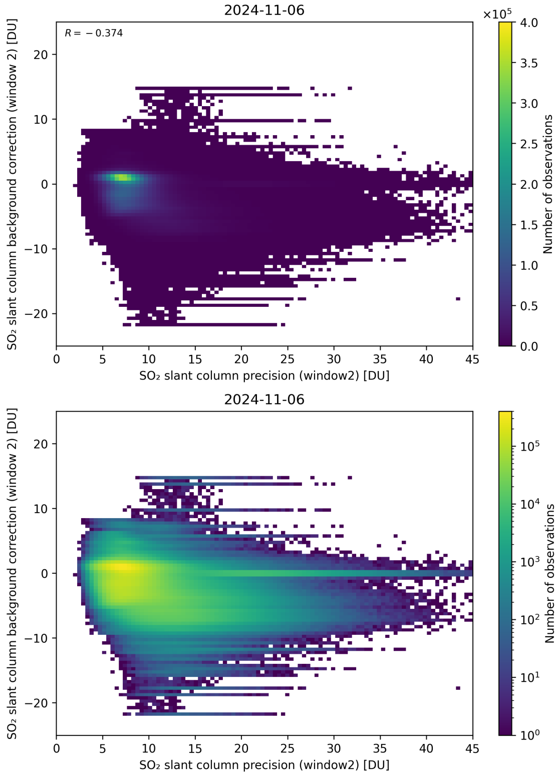
Figure 241: Scatter density plot of “SO 2 slant column precision (window2)” against “SO 2 slant column background correction (window 2)” for 2024-11-05 to 2024-11-07.
