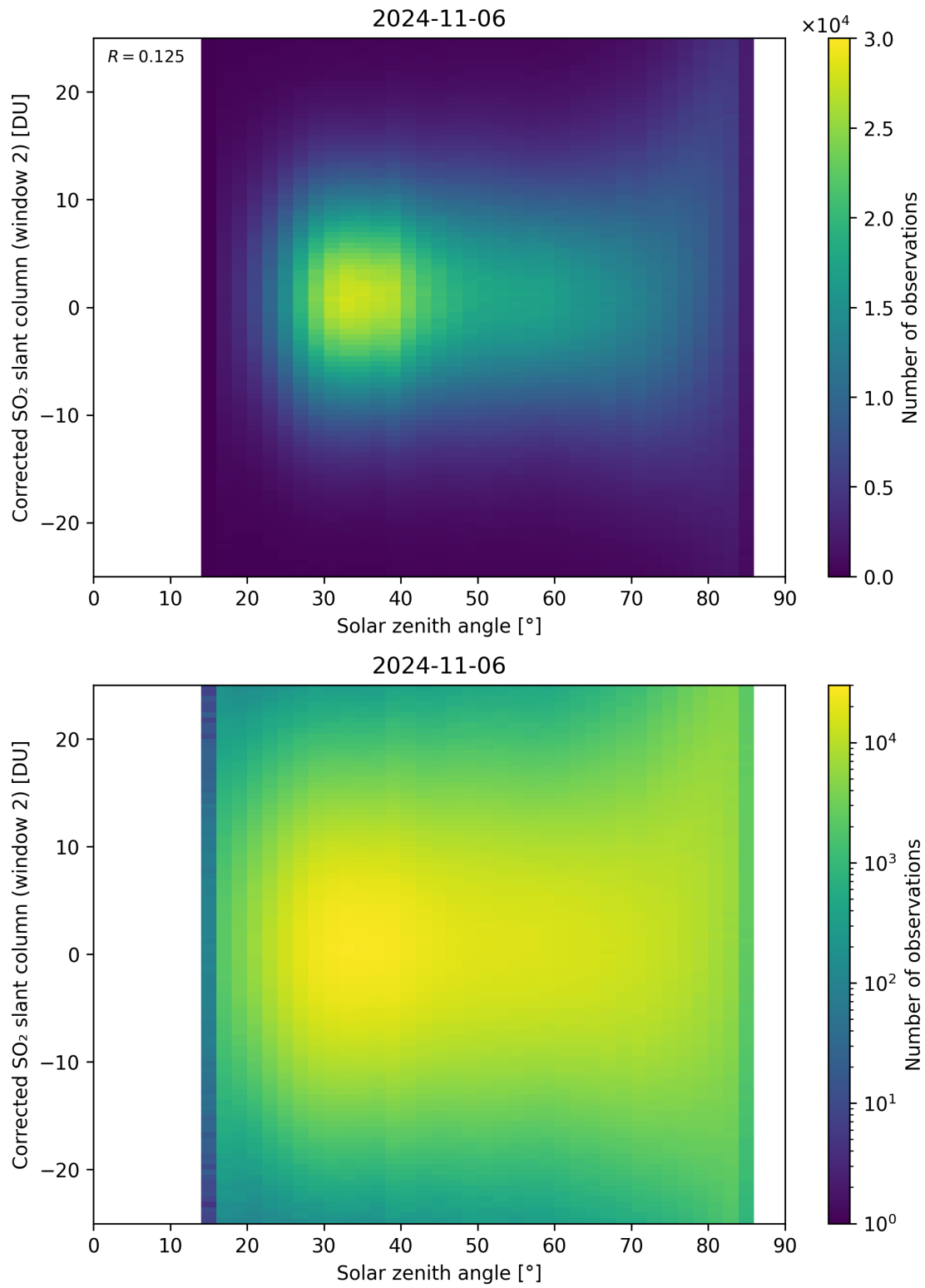
Figure 167: Scatter density plot of “Solar zenith angle” against “Corrected SO 2 slant column (window 2)” for 2024-11-05 to 2024-11-07.
