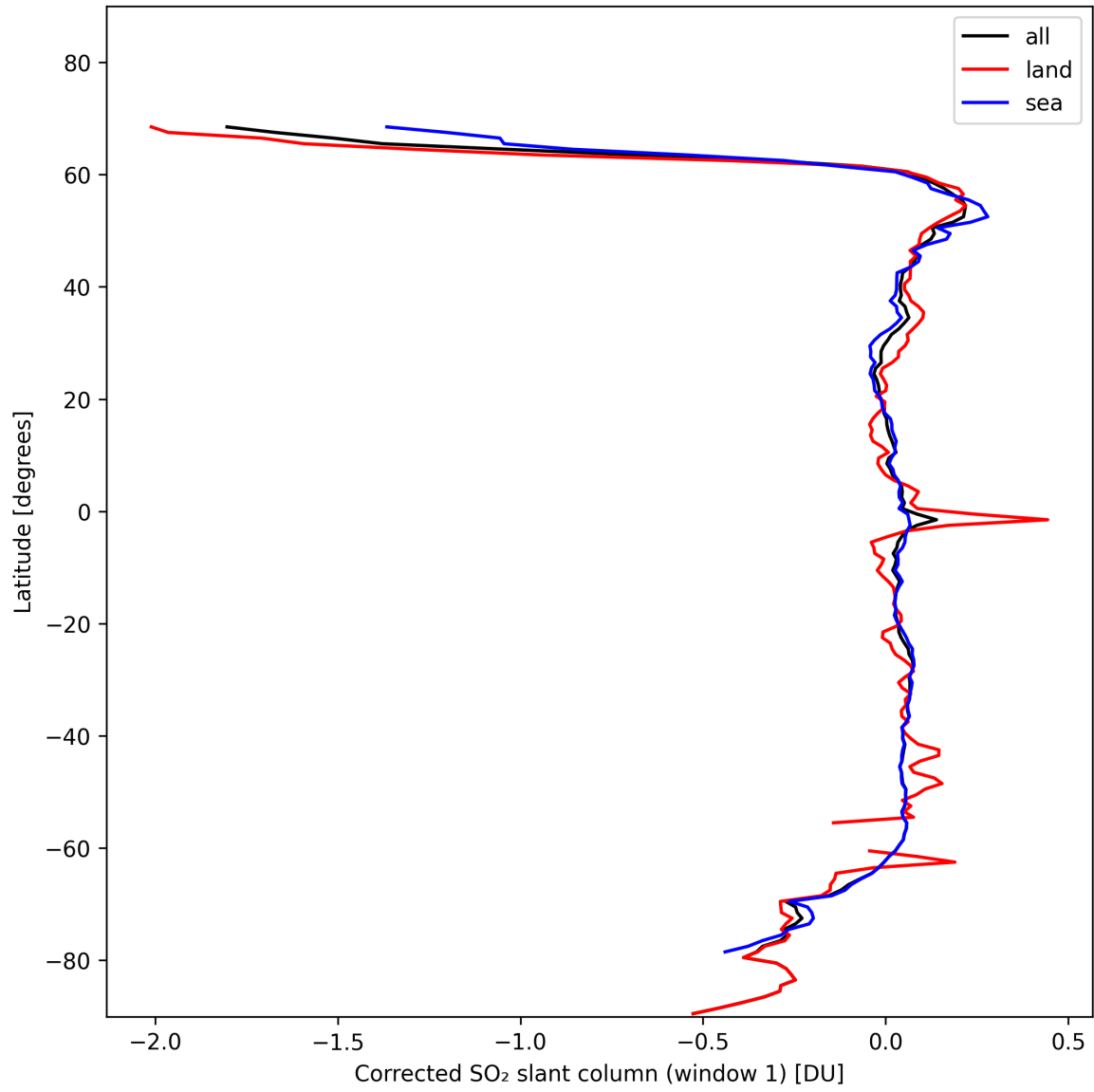
Figure 35: Zonal average of “Corrected SO 2 slant column (window 1)” for 2024-11-05 to 2024-11-07.
