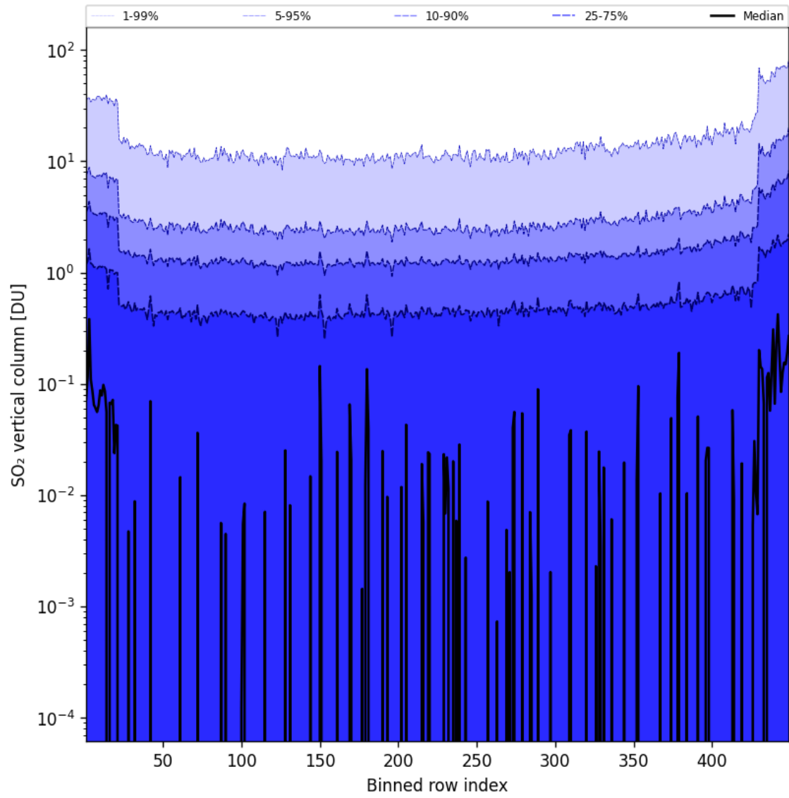
Figure 76: Along track statistics of “SO 2 vertical column” for 2024-11-05 to 2024-11-07
