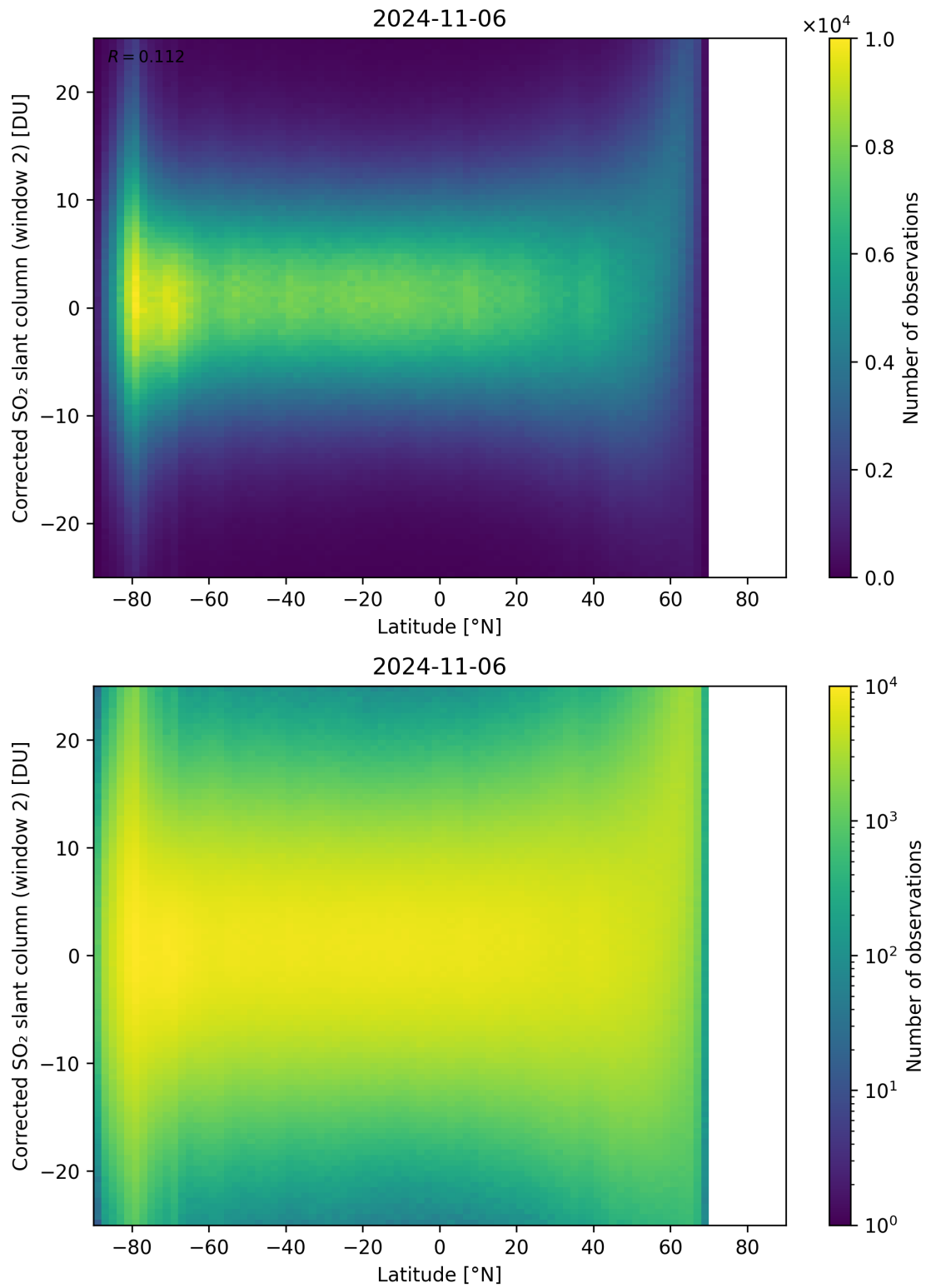
Figure 147: Scatter density plot of “Latitude” against “Corrected SO 2 slant column (window 2)” for 2024-11-05 to 2024-11-07.
