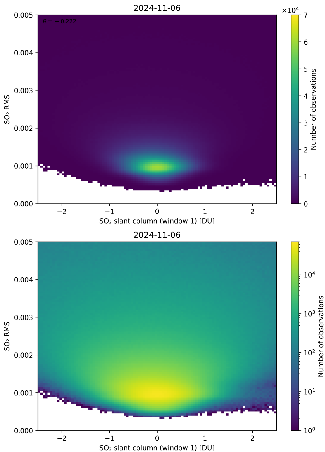
Figure 217: Scatter density plot of “SO 2 slant column (window 1)” against “SO 2 RMS” for 2024-11-05 to 2024-11-07.
