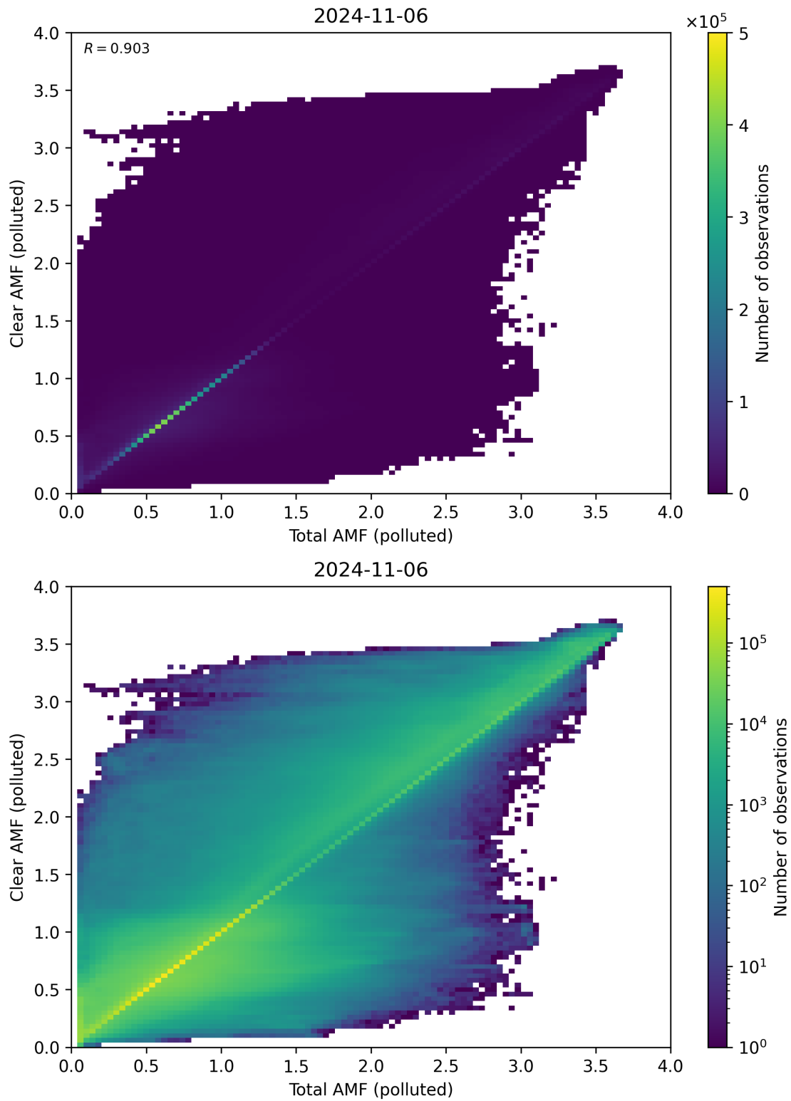
Figure 271: Scatter density plot of “Total AMF (polluted)” against “Clear AMF (polluted)” for 2024-11-05 to 2024-11-07.
