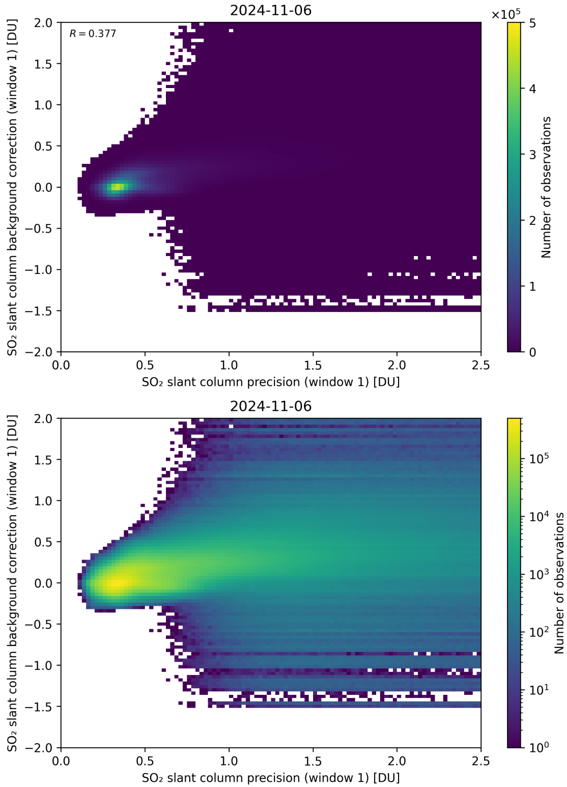
Figure 218: Scatter density plot of “SO 2 slant column precision (window 1)” against “SO 2 slant column background correction (window 1)” for 2024-11-05 to 2024-11-07.
