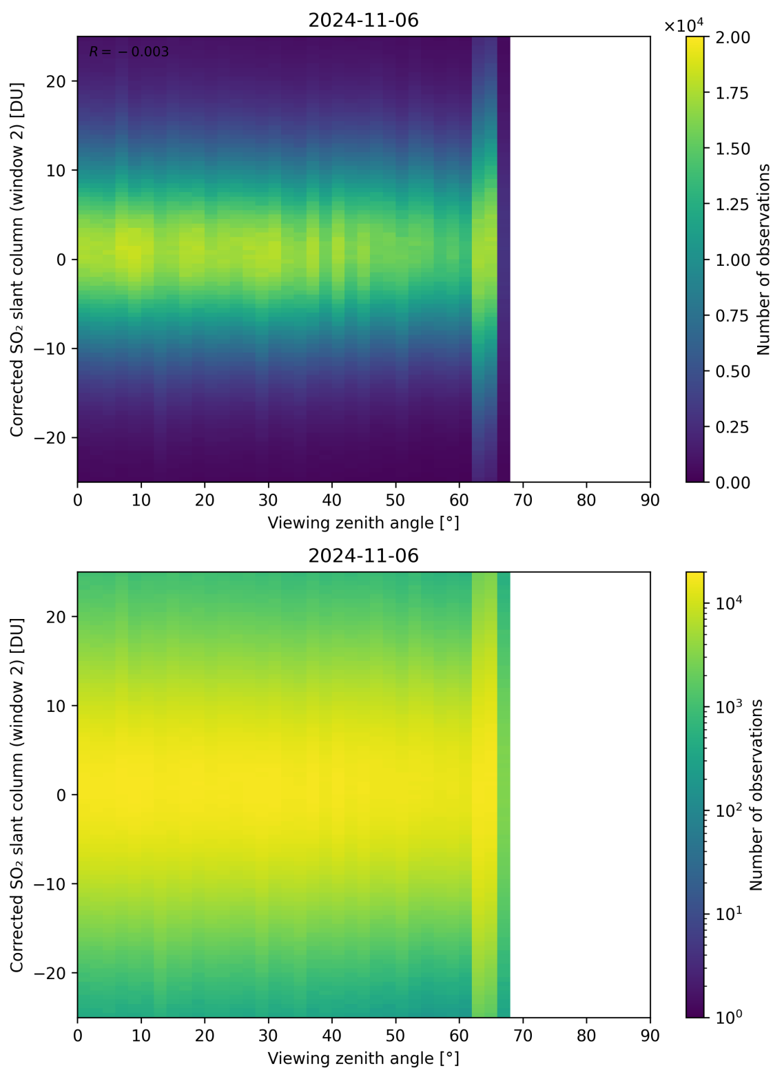
Figure 318: Scatter density plot of “Viewing zenith angle” against “Corrected SO 2 slant column (window 2)” for 2024-11-05 to 2024-11-07.
