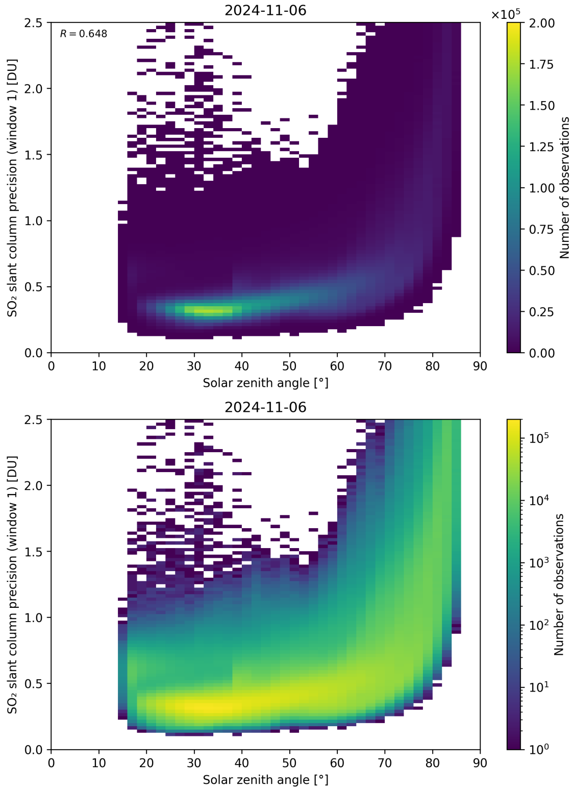
Figure 170: Scatter density plot of “Solar zenith angle” against “SO 2 slant column precision (window 1)” for 2024-11-05 to 2024-11-07.
