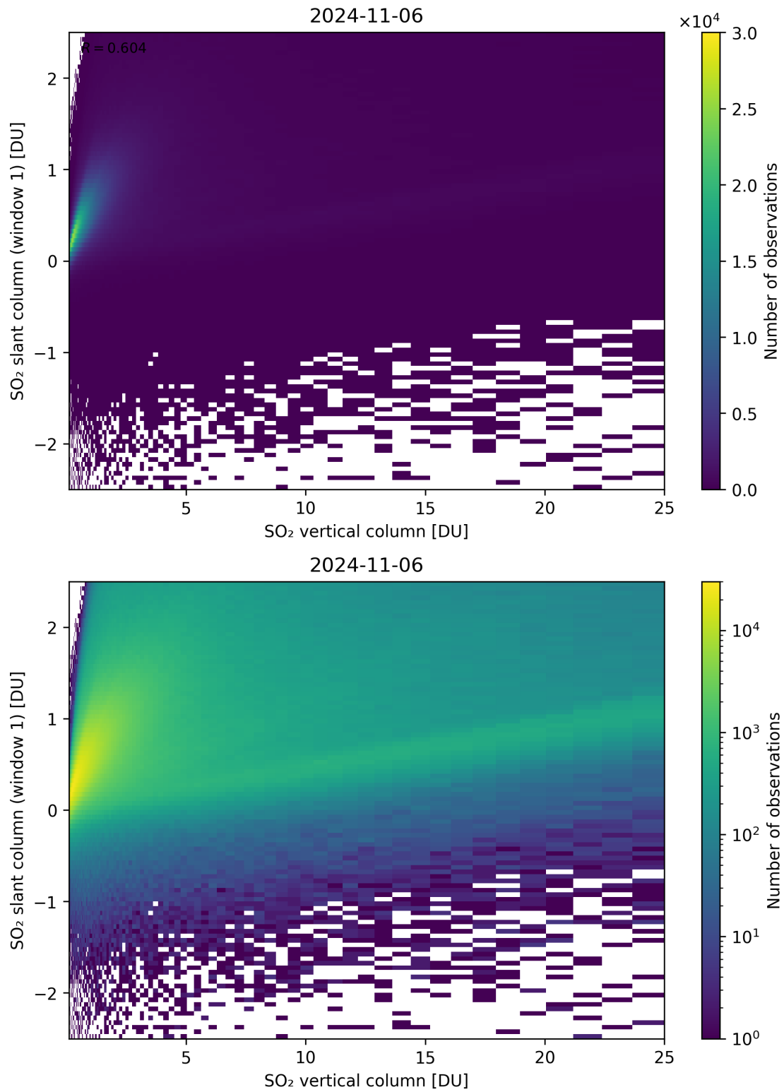
Figure 300: Scatter density plot of “SO 2 vertical column” against “SO 2 slant column (window 1)” for 2024-11-05 to 2024-11-07.
