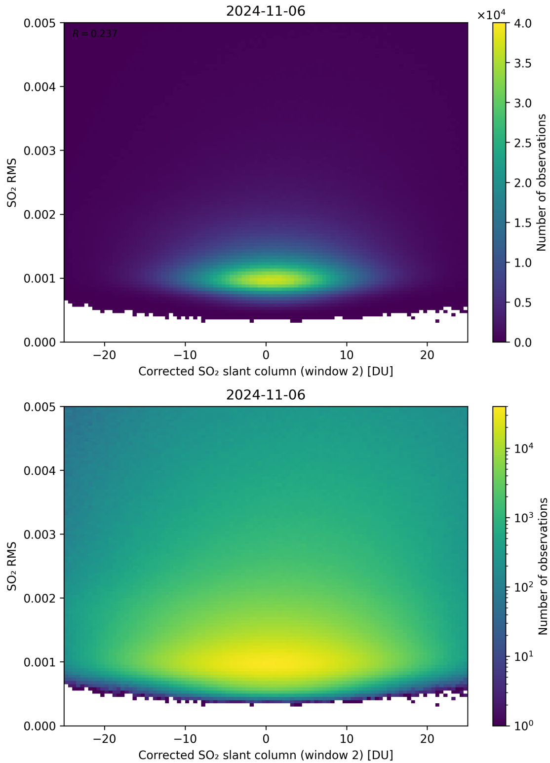
Figure 198: Scatter density plot of “Corrected SO 2 slant column (window 2)” against “SO 2 RMS” for 2024-11-05 to 2024-11-07.
