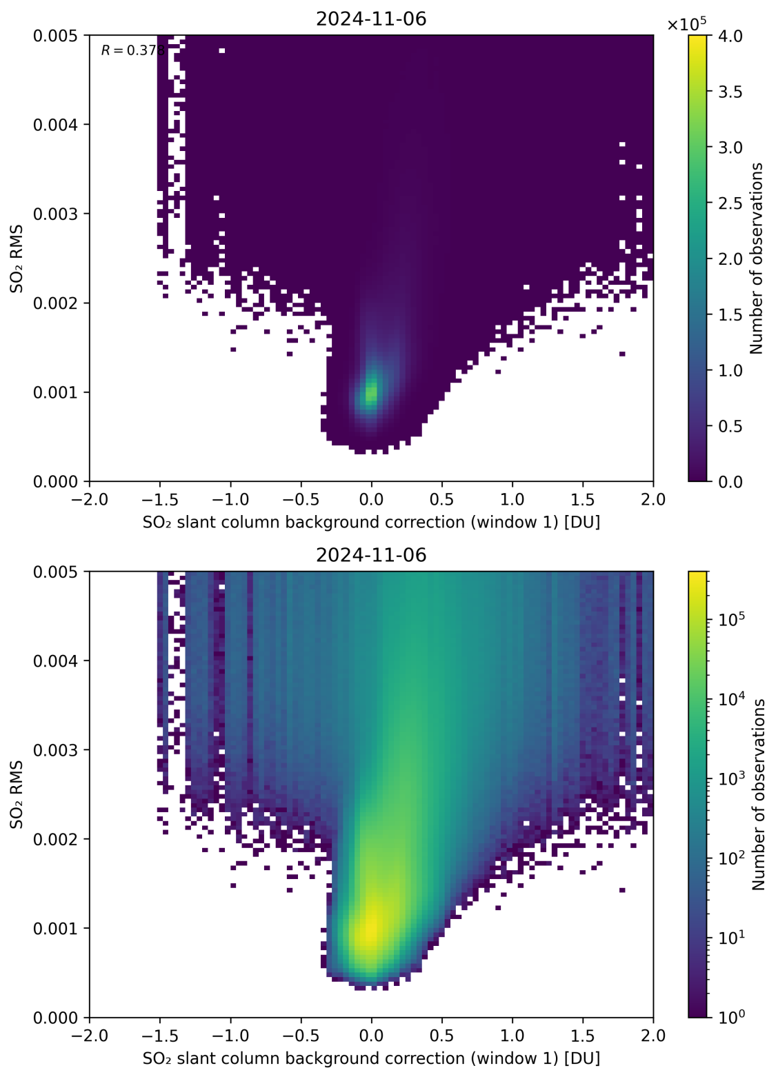
Figure 102: Scatter density plot of “SO 2 slant column background correction (window 1)” against “SO 2 RMS” for 2024-11-05 to 2024-11-07.
