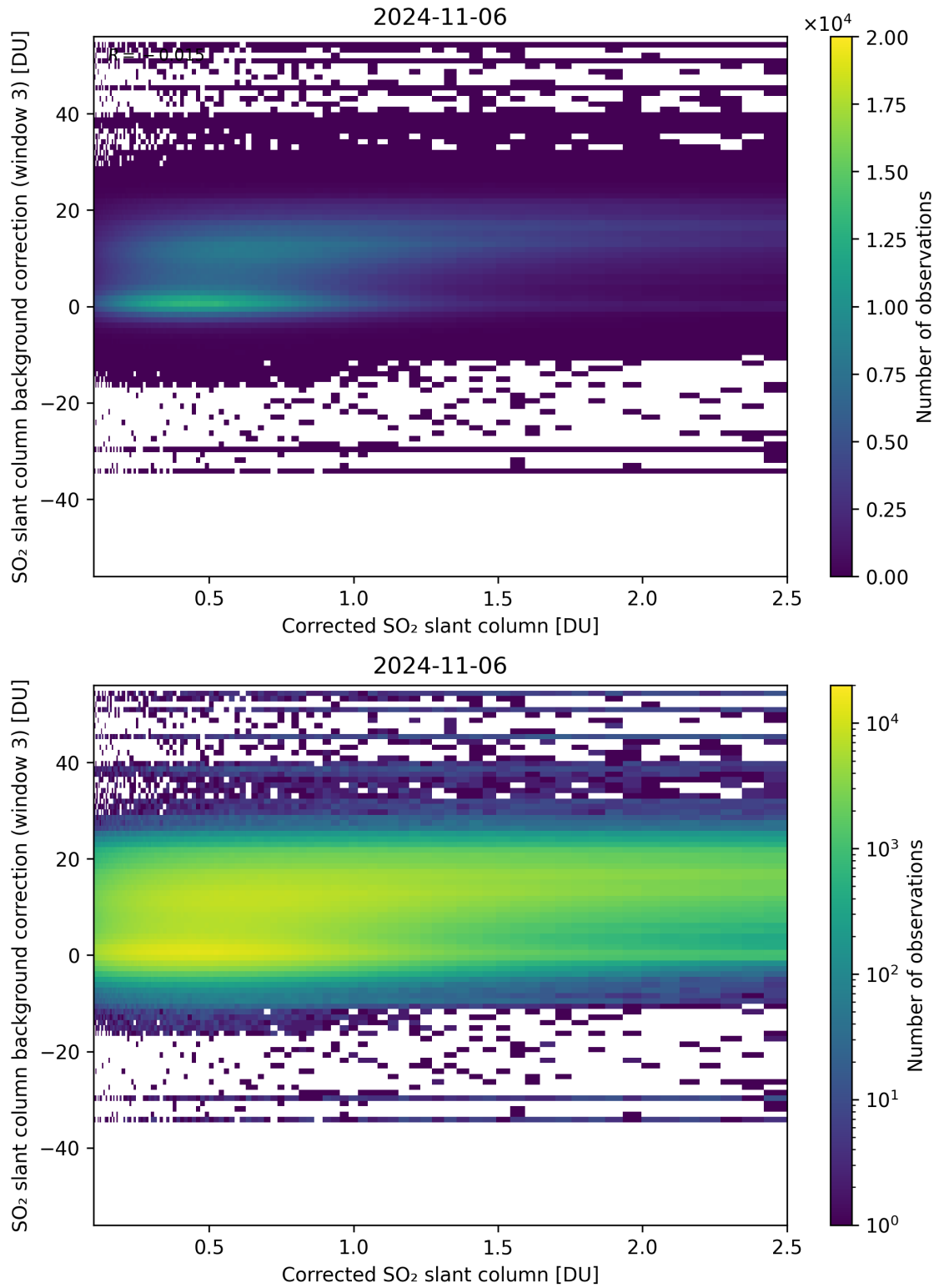
Figure 180: Scatter density plot of “Corrected SO 2 slant column” against “SO 2 slant column background correction (window 3)” for 2024-11-05 to 2024-11-07.
