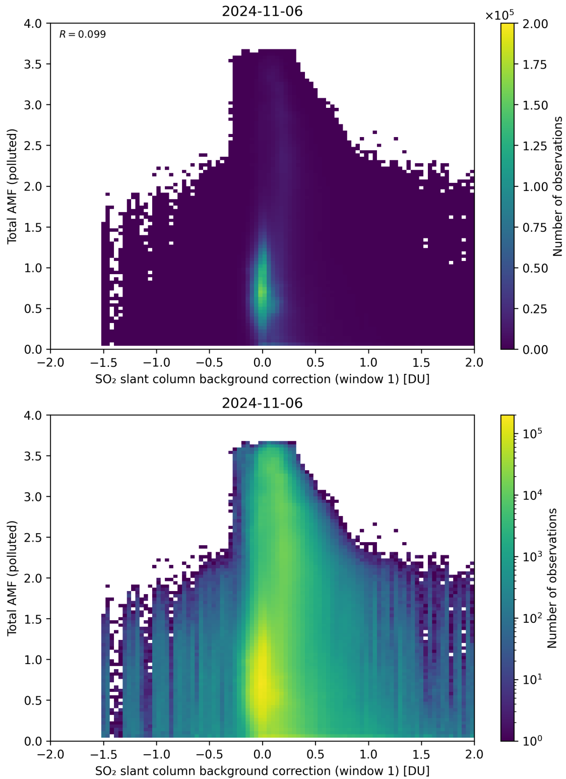
Figure 109: Scatter density plot of “SO 2 slant column background correction (window 1)” against “Total AMF (polluted)” for 2024-11-05 to 2024-11-07.
