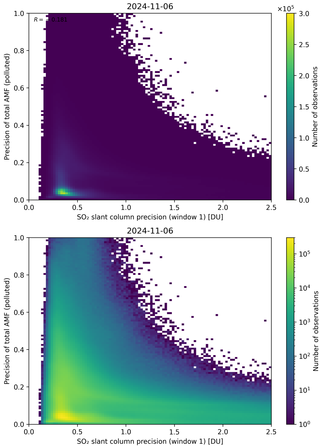
Figure 231: Scatter density plot of “SO 2 slant column precision (window 1)” against “Precision of total AMF (polluted)” for 2024-11-05 to 2024-11-07.
