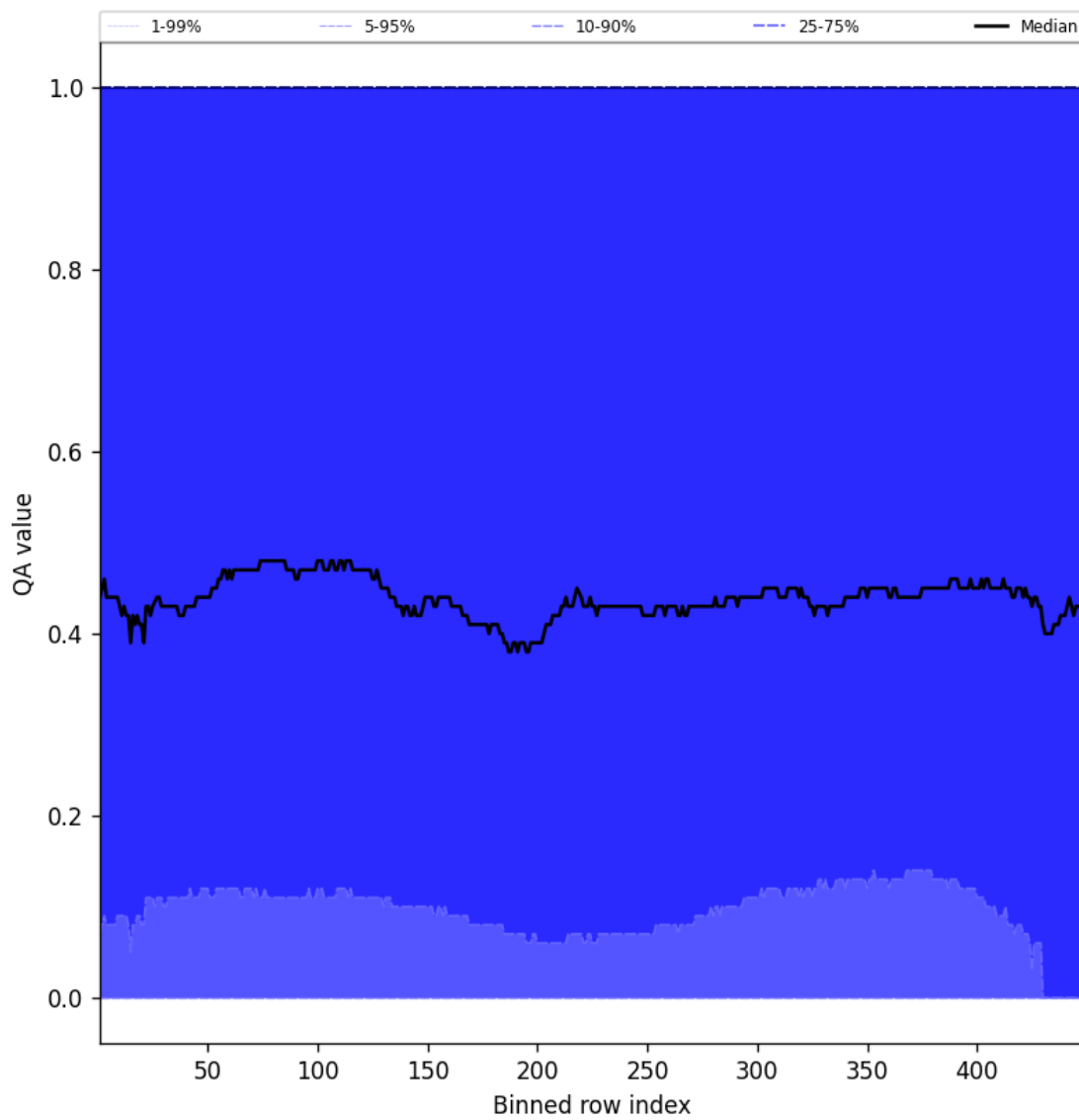
Figure 75: Along track statistics of “QA value” for 2024-11-05 to 2024-11-07
