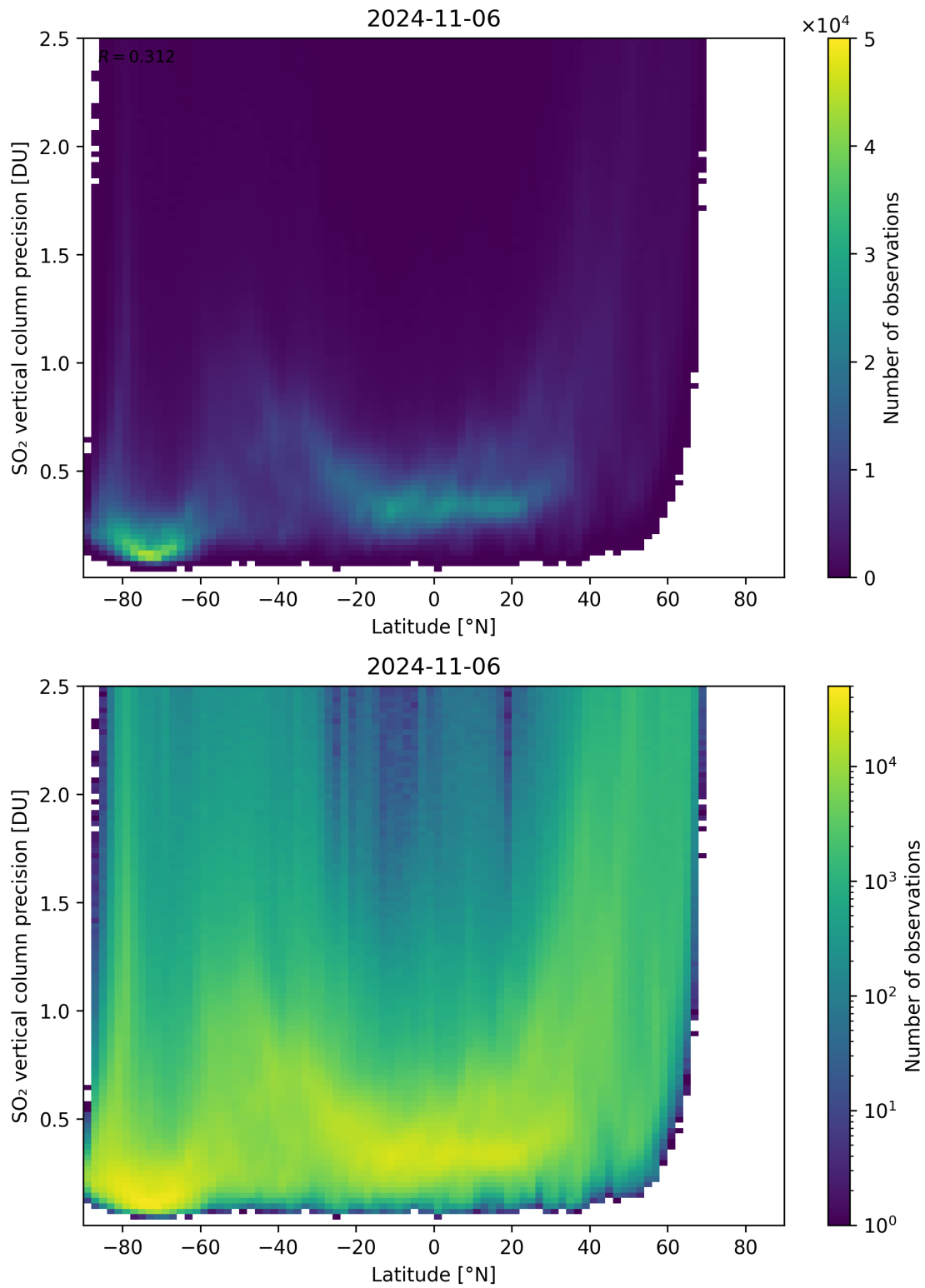
Figure 157: Scatter density plot of “Latitude” against “SO 2 vertical column precision” for 2024-11-05 to 2024-11-07.
