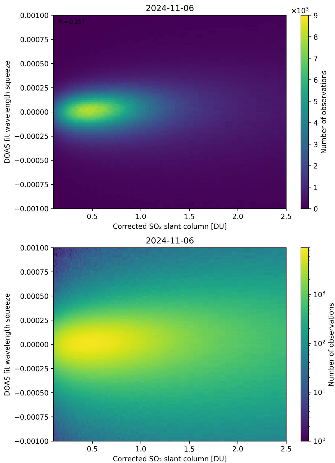
Figure 182: Scatter density plot of “Corrected SO 2 slant column” against “DOAS fit wavelength squeeze” for 2024-11-05 to 2024-11-07.
