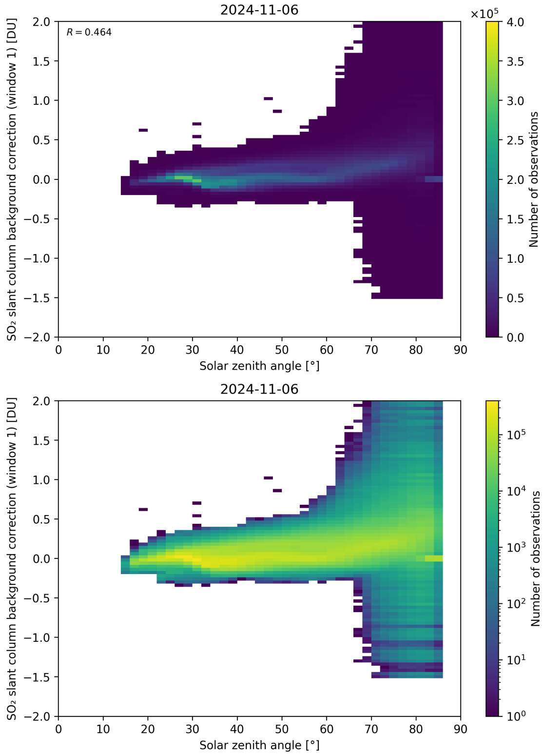
Figure 158: Scatter density plot of “Solar zenith angle” against “SO 2 slant column background correction (window 1)” for 2024-11-05 to 2024-11-07.
