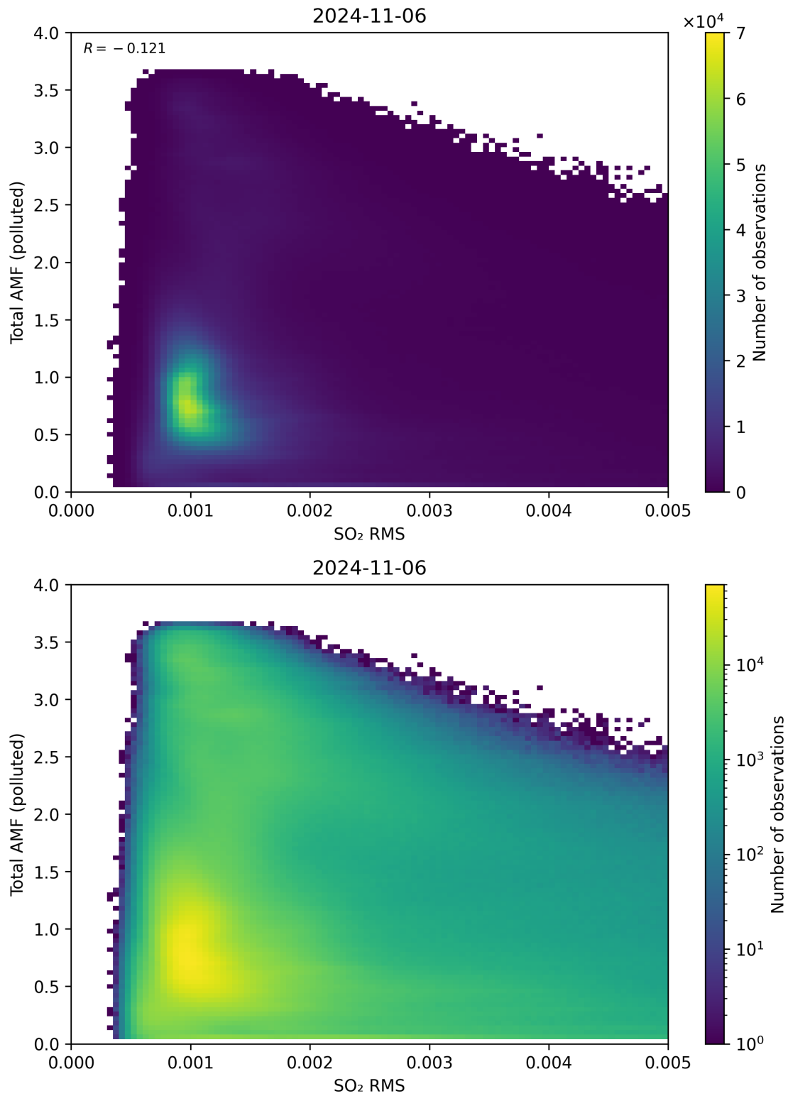
Figure 137: Scatter density plot of “SO 2 RMS” against “Total AMF (polluted)” for 2024-11-05 to 2024-11-07.
