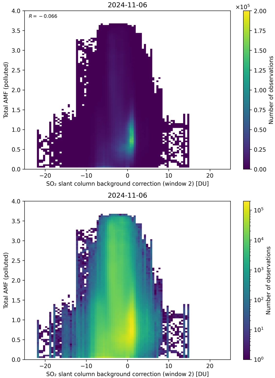
Figure 119: Scatter density plot of “SO 2 slant column background correction (window 2)” against “Total AMF (polluted)” for 2024-11-05 to 2024-11-07.
