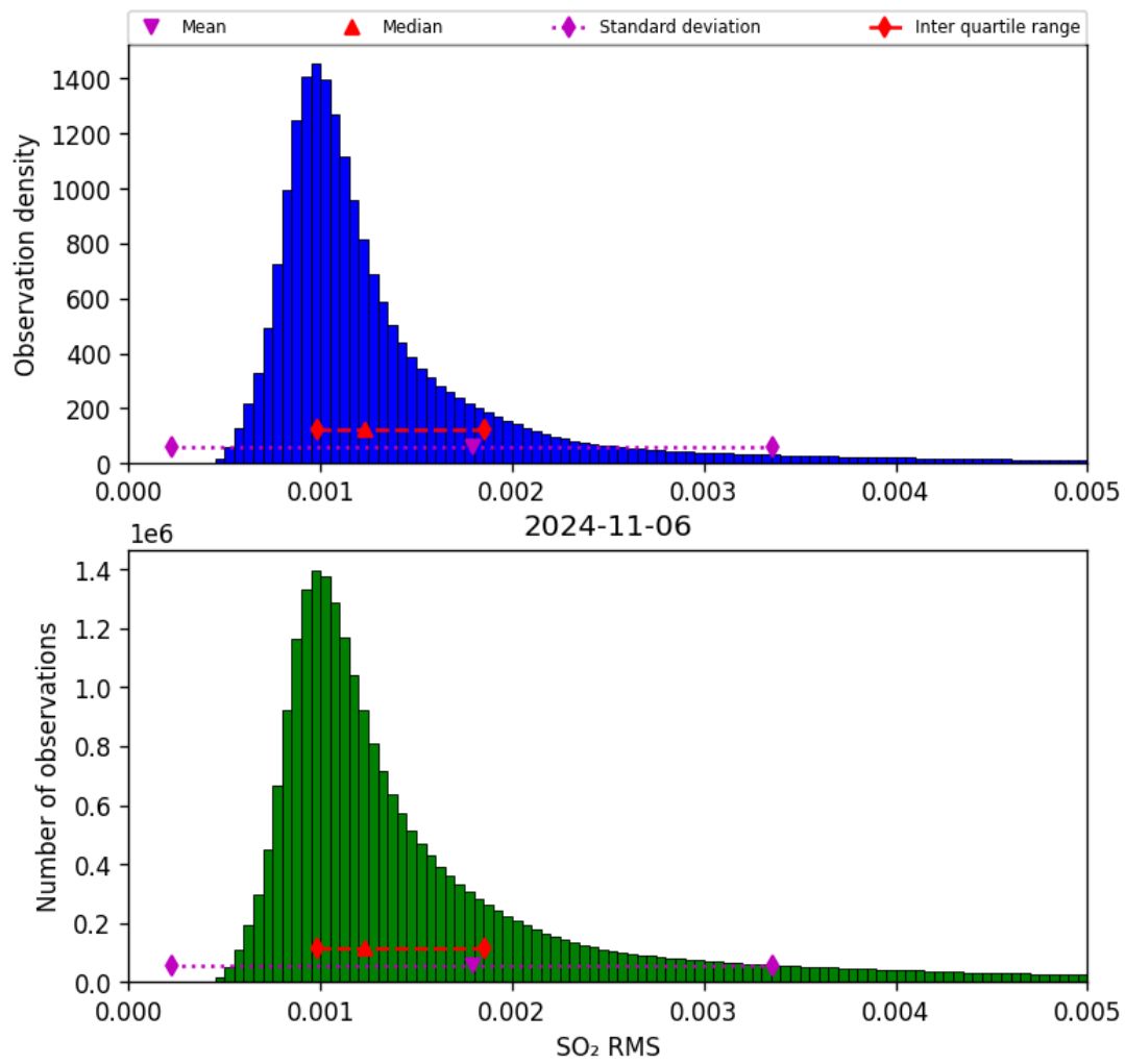
Figure 70: Histogram of “SO 2 RMS” for 2024-11-05 to 2024-11-07
