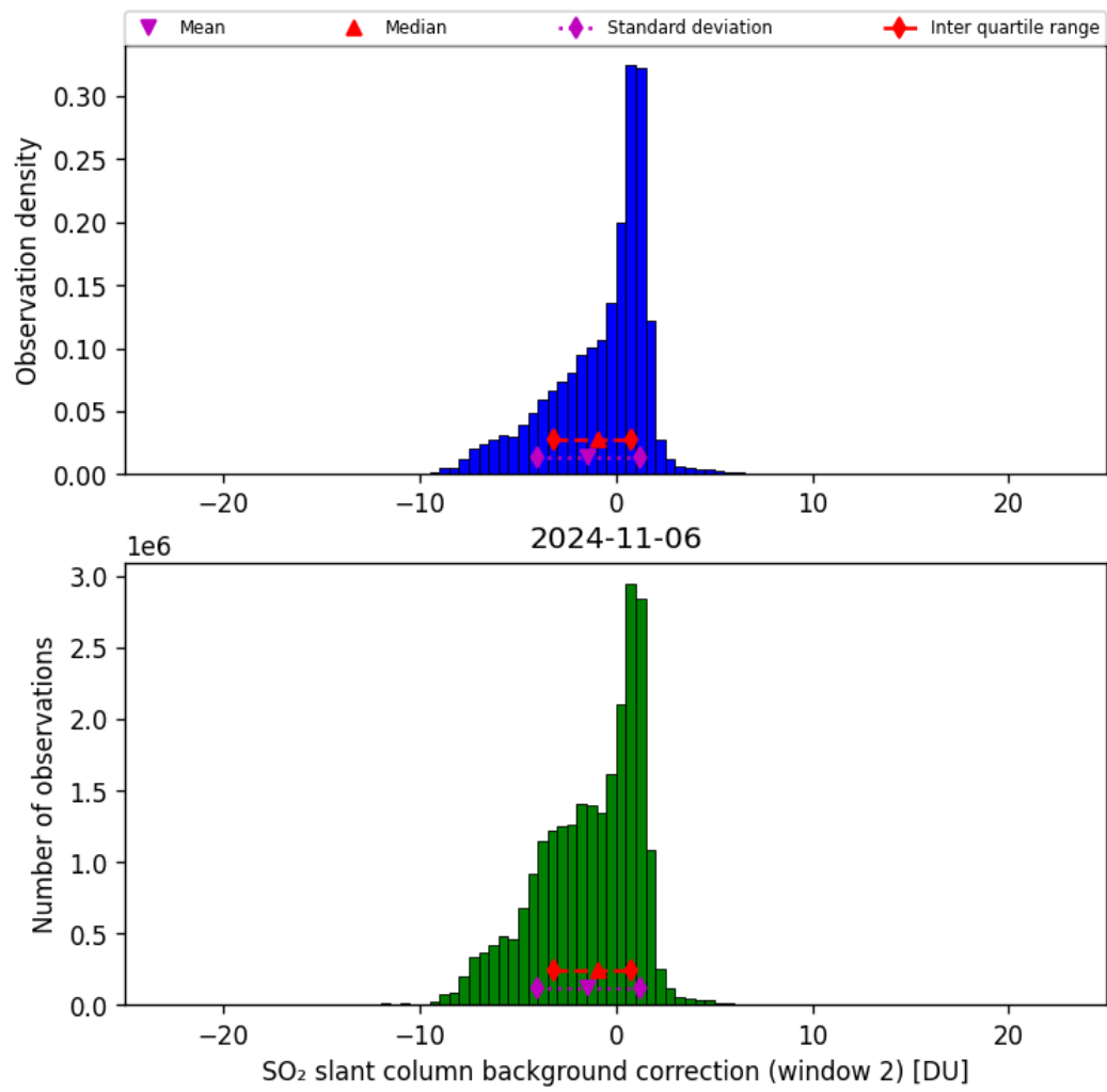
Figure 63: Histogram of “SO 2 slant column background correction (window 2)” for 2024-11-05 to 2024-11-07
