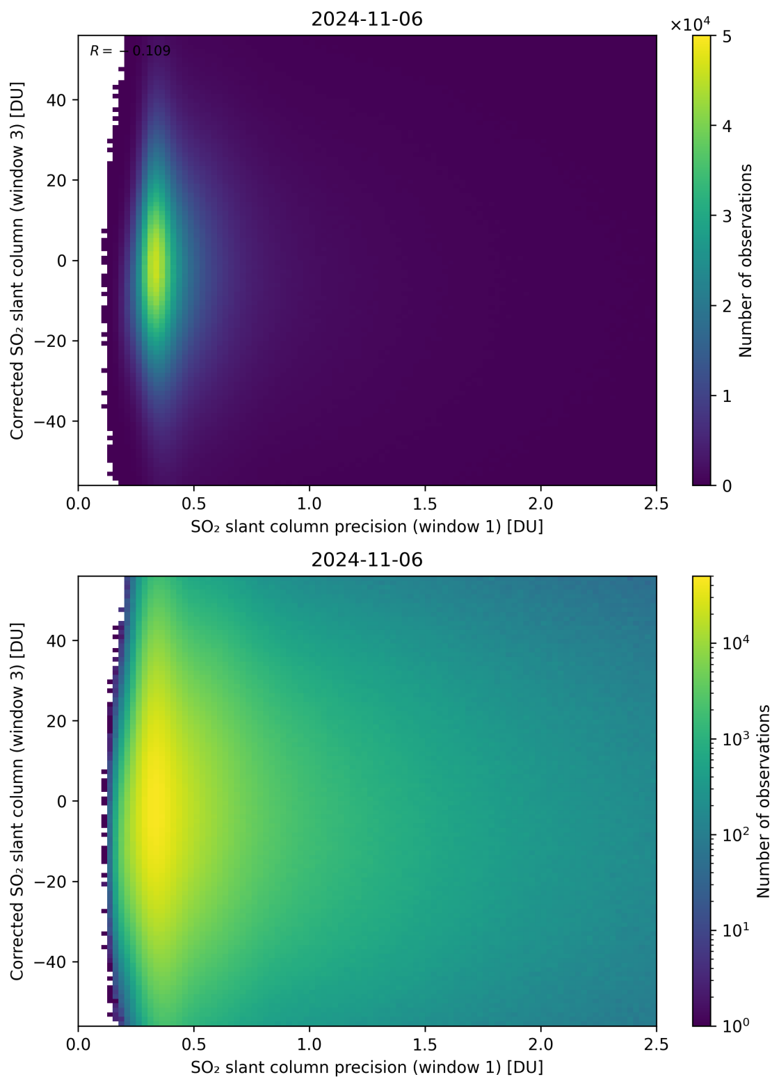
Figure 226: Scatter density plot of “SO 2 slant column precision (window 1)” against “Corrected SO 2 slant column (window 3)” for 2024-11-05 to 2024-11-07.
