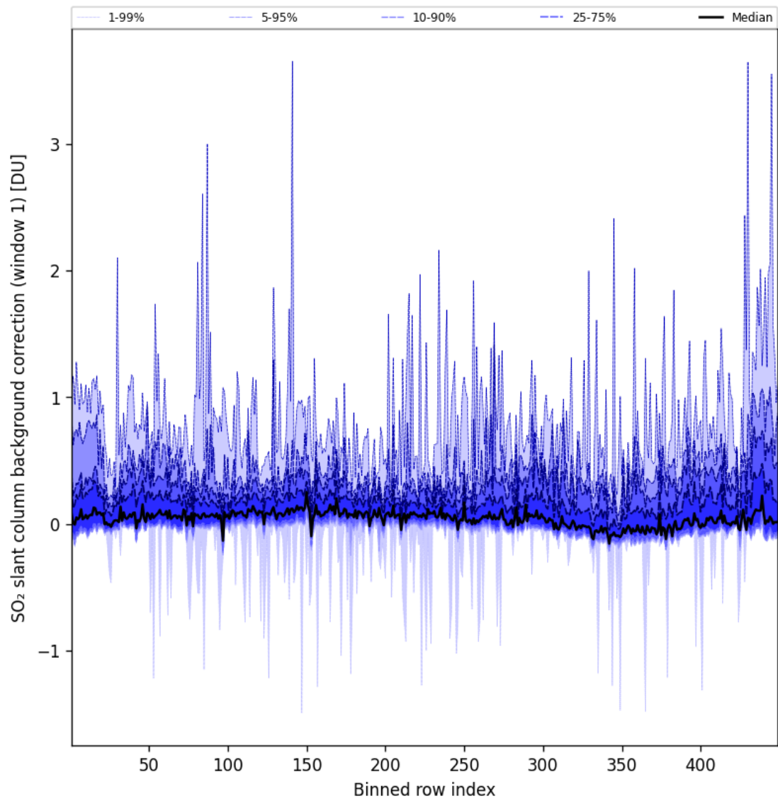
Figure 82: Along track statistics of “SO 2 slant column background correction (window 1)” for 2024-11-05 to 2024-11-07
