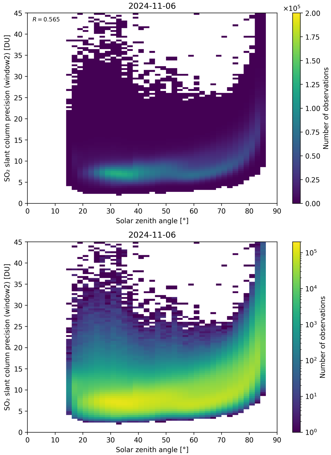
Figure 171: Scatter density plot of “Solar zenith angle” against “SO 2 slant column precision (window2)” for 2024-11-05 to 2024-11-07.
