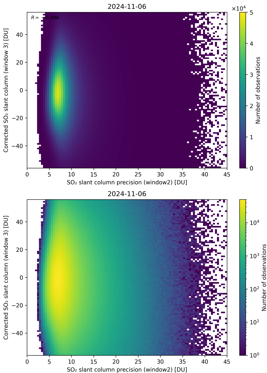
Figure 248: Scatter density plot of “SO 2 slant column precision (window2)” against “Corrected SO 2 slant column (window 3)” for 2024-11-05 to 2024-11-07.
