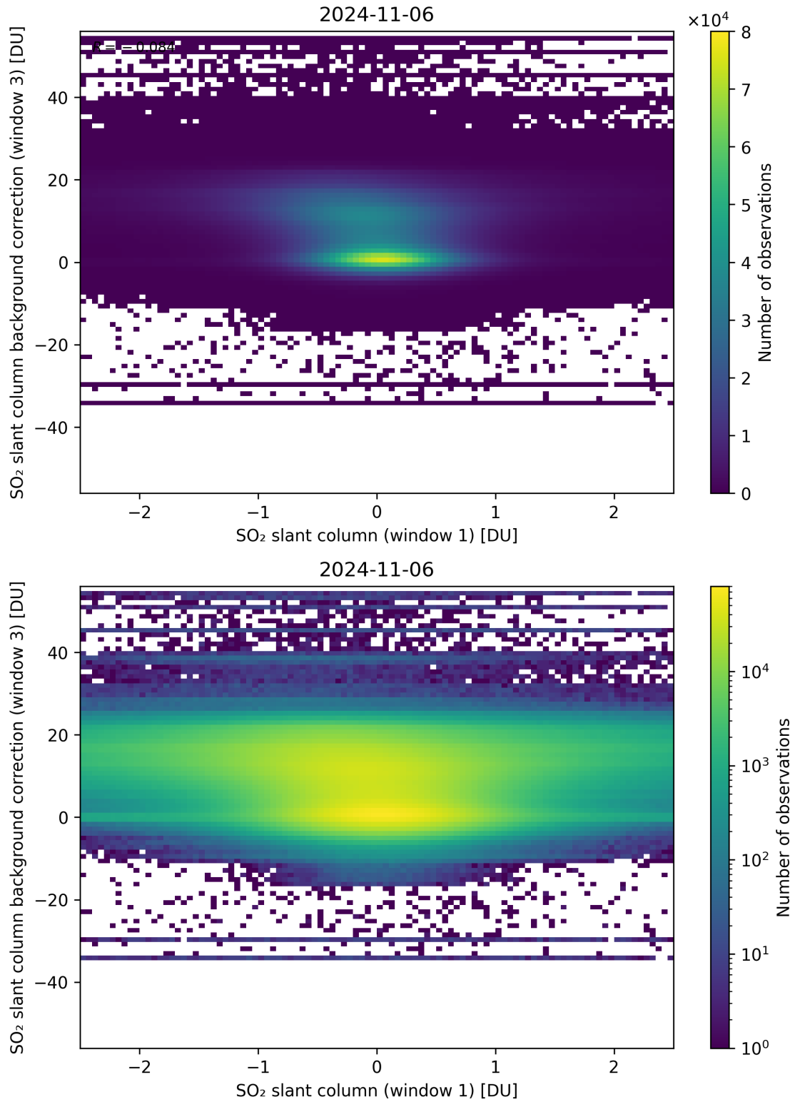
Figure 214: Scatter density plot of “SO 2 slant column (window 1)” against “SO 2 slant column background correction (window 3)” for 2024-11-05 to 2024-11-07.
