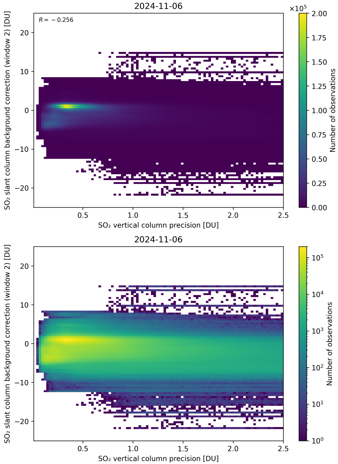
Figure 280: Scatter density plot of “SO 2 vertical column precision” against “SO 2 slant column background correction (window 2)” for 2024-11-05 to 2024-11-07.
