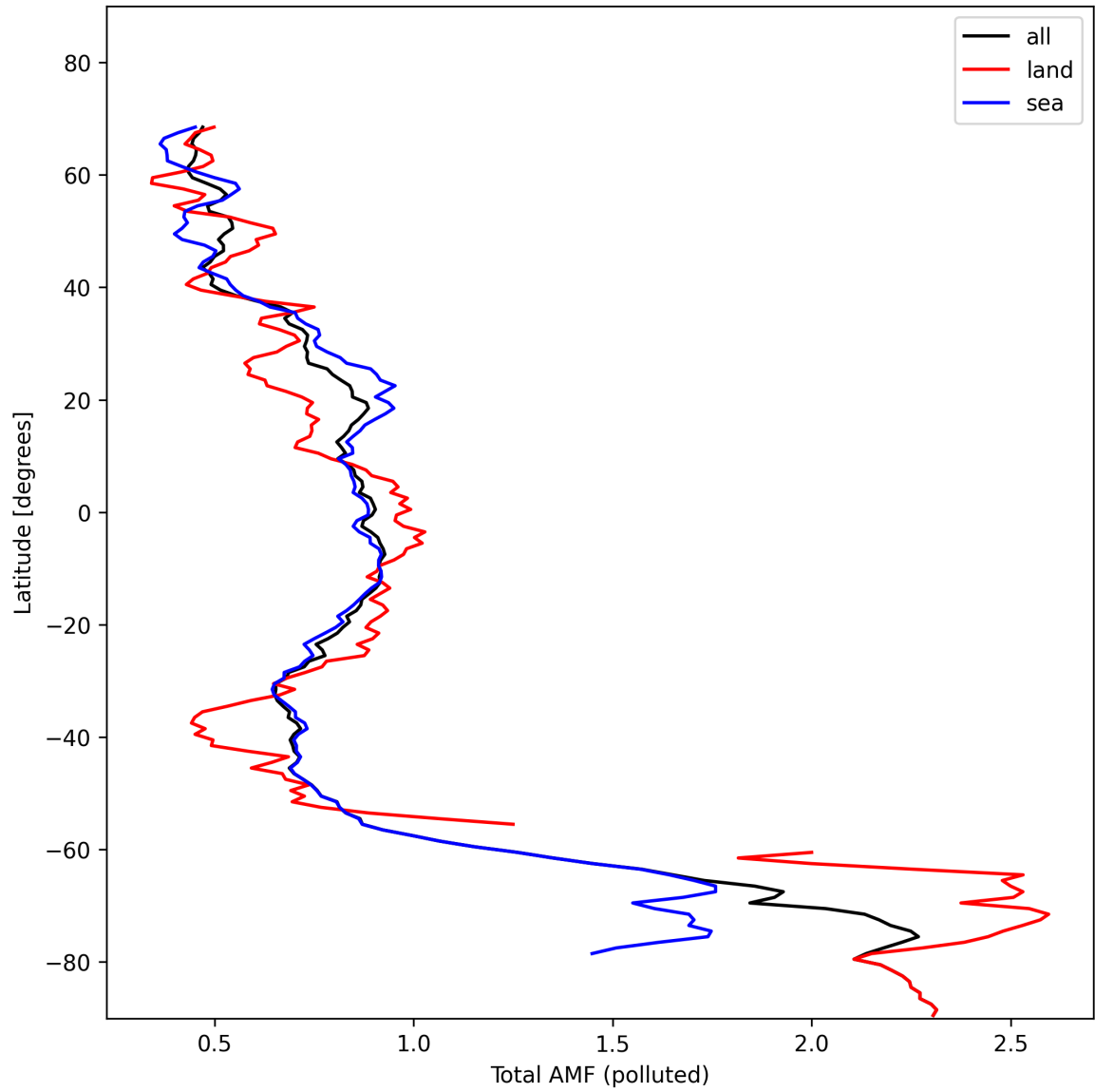
Figure 48: Zonal average of “Total AMF (polluted)” for 2024-11-05 to 2024-11-07.
