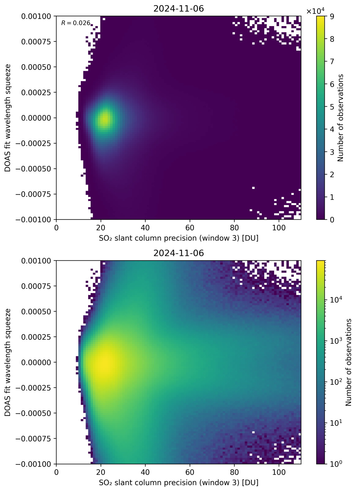
Figure 259: Scatter density plot of “SO 2 slant column precision (window 3)” against “DOAS fit wavelength squeeze” for 2024-11-05 to 2024-11-07.
