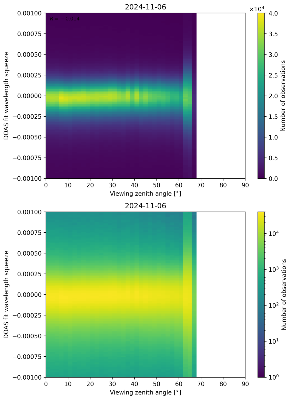
Figure 312: Scatter density plot of “Viewing zenith angle” against “DOAS fit wavelength squeeze” for 2024-11-05 to 2024-11-07.
