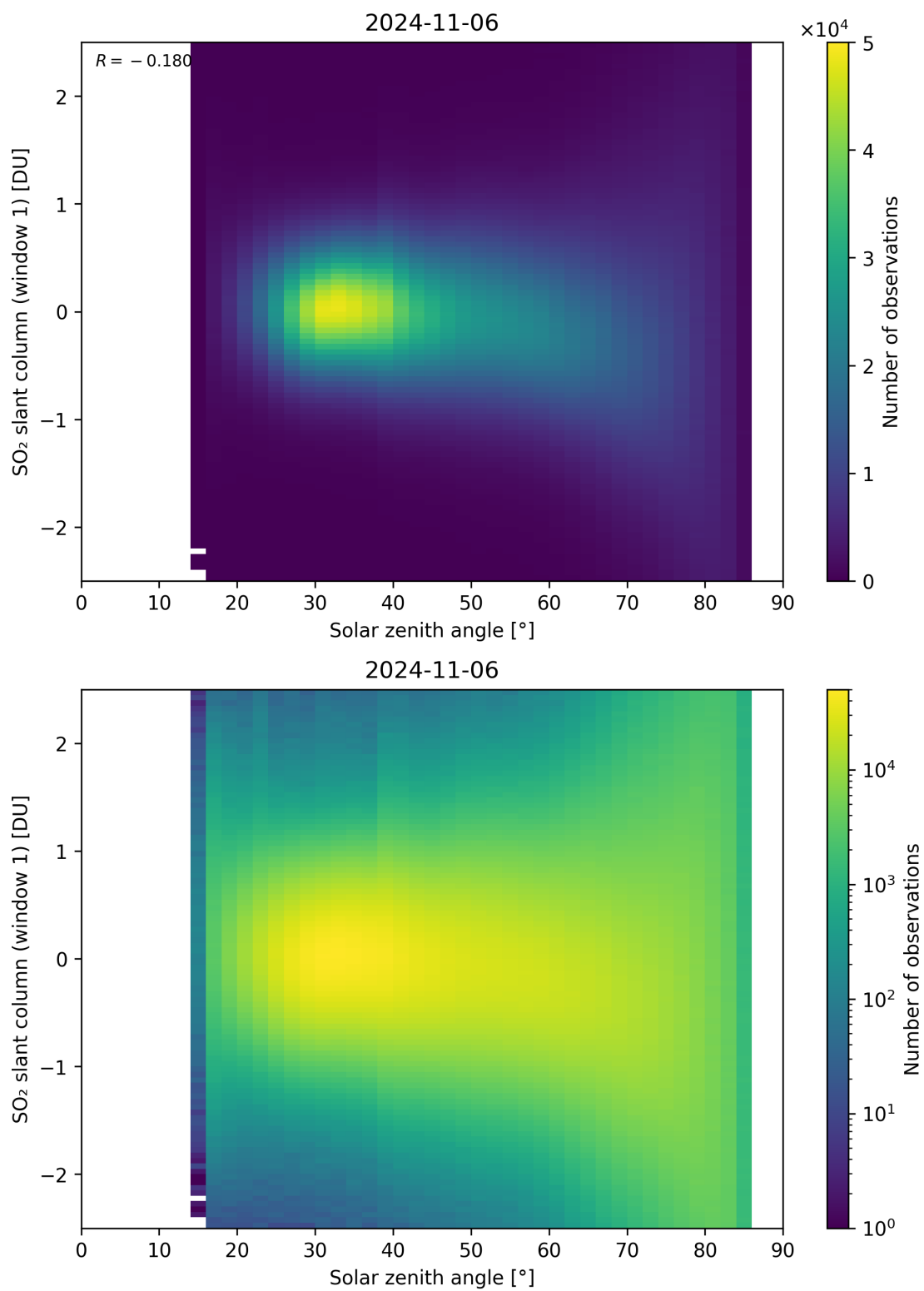
Figure 169: Scatter density plot of “Solar zenith angle” against “SO 2 slant column (window 1)” for 2024-11-05 to 2024-11-07.
