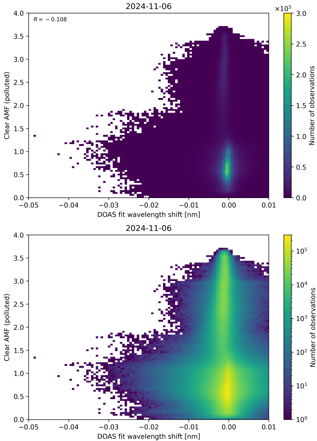
Figure 129: Scatter density plot of “DOAS fit wavelength shift” against “Clear AMF (polluted)” for 2024-11-05 to 2024-11-07.
