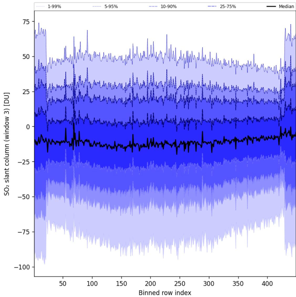
Figure 87: Along track statistics of “SO 2 slant column (window 3)” for 2024-11-05 to 2024-11-07
