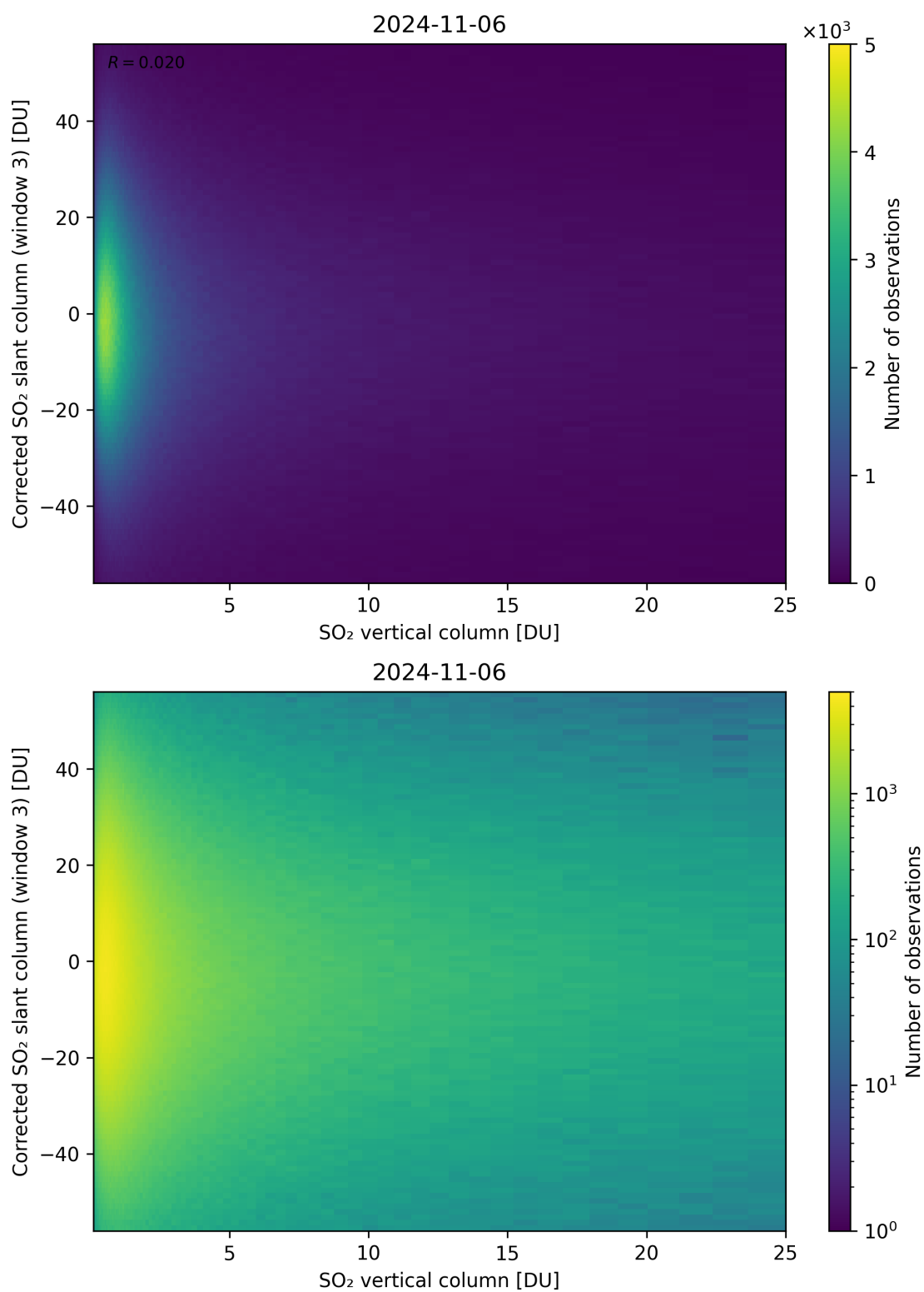
Figure 299: Scatter density plot of “SO 2 vertical column” against “Corrected SO 2 slant column (window 3)” for 2024-11-05 to 2024-11-07.
