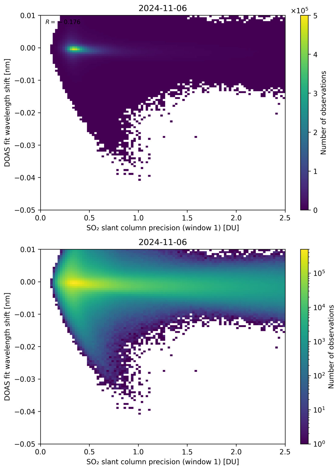
Figure 221: Scatter density plot of “SO 2 slant column precision (window 1)” against “DOAS fit wavelength shift” for 2024-11-05 to 2024-11-07.
