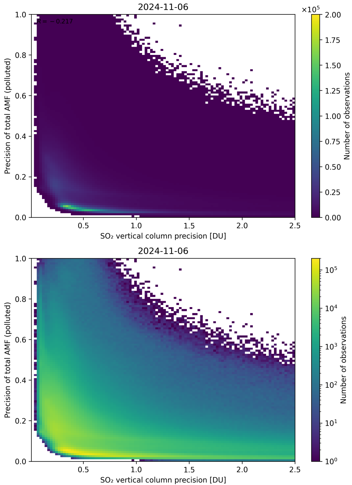
Figure 295: Scatter density plot of “SO 2 vertical column precision” against “Precision of total AMF (polluted)” for 2024-11-05 to 2024-11-07.
