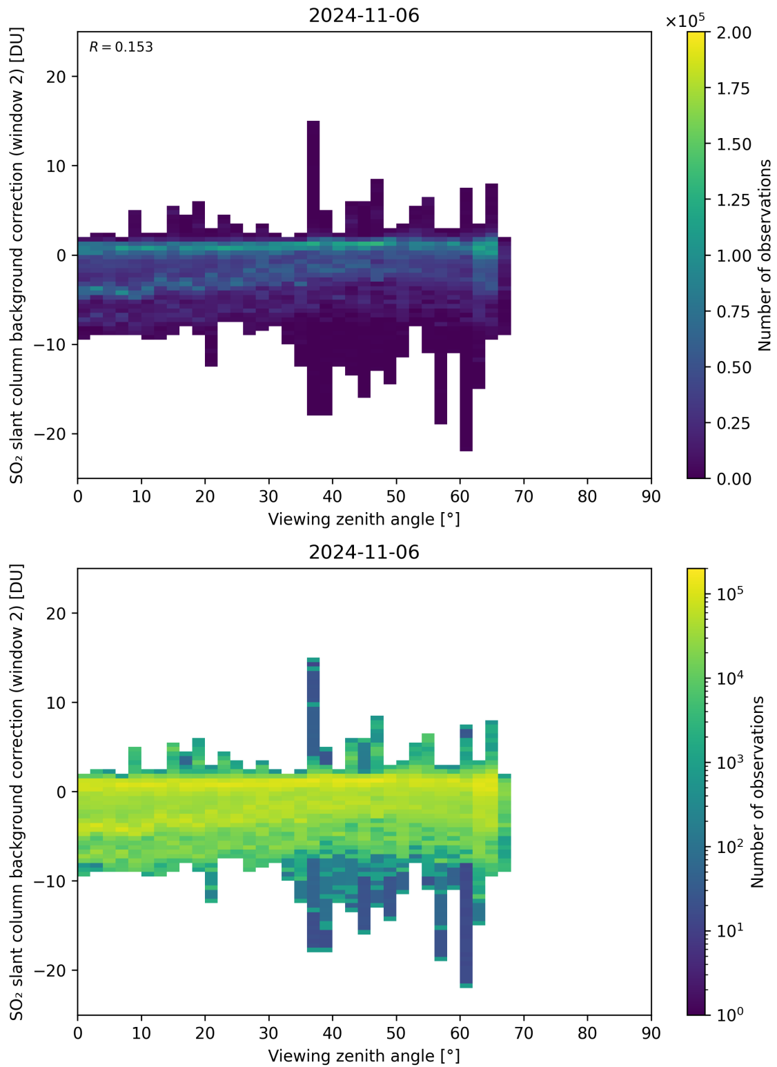
Figure 309: Scatter density plot of “Viewing zenith angle” against “SO 2 slant column background correction (window 2)” for 2024-11-05 to 2024-11-07.
