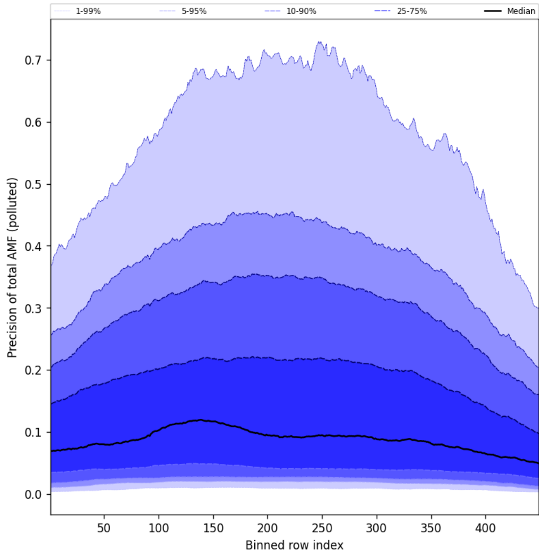
Figure 95: Along track statistics of “Precision of total AMF (polluted)” for 2024-11-05 to 2024-11-07
