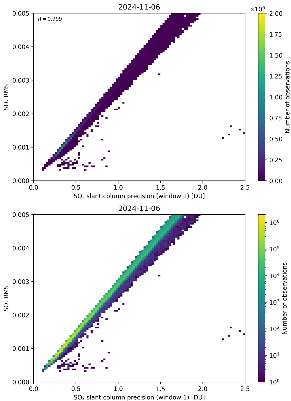
Figure 223: Scatter density plot of “SO 2 slant column precision (window 1)” against “SO 2 RMS” for 2024-11-05 to 2024-11-07.
