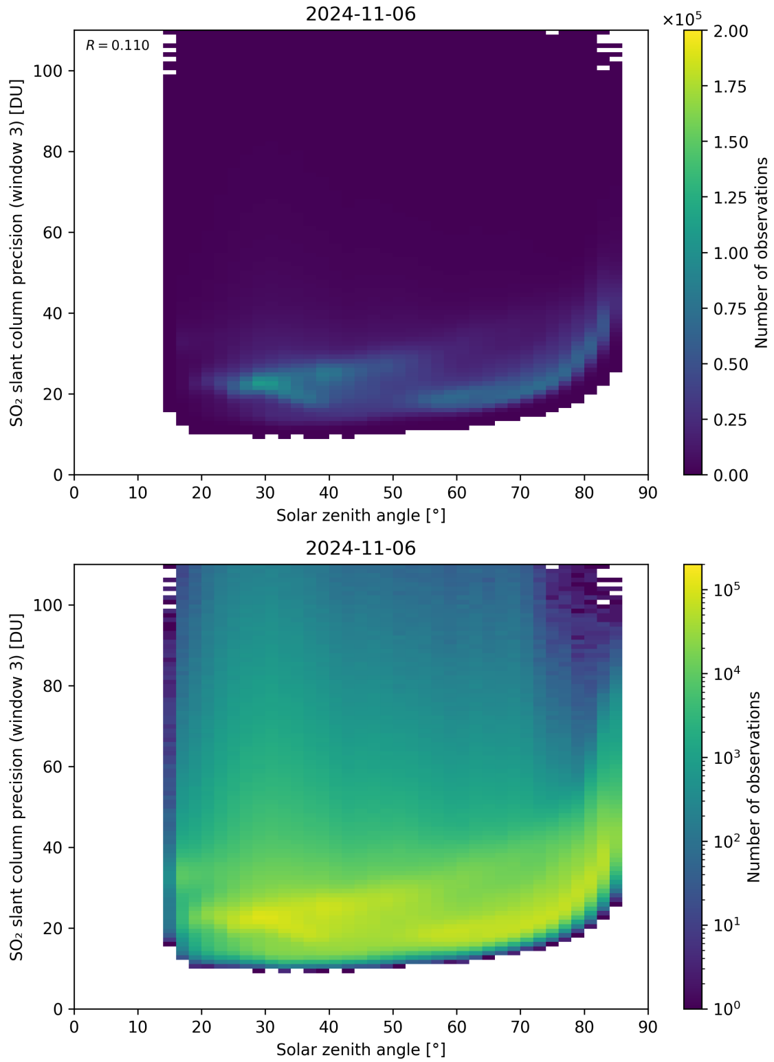
Figure 173: Scatter density plot of “Solar zenith angle” against “SO 2 slant column precision (window 3)” for 2024-11-05 to 2024-11-07.
