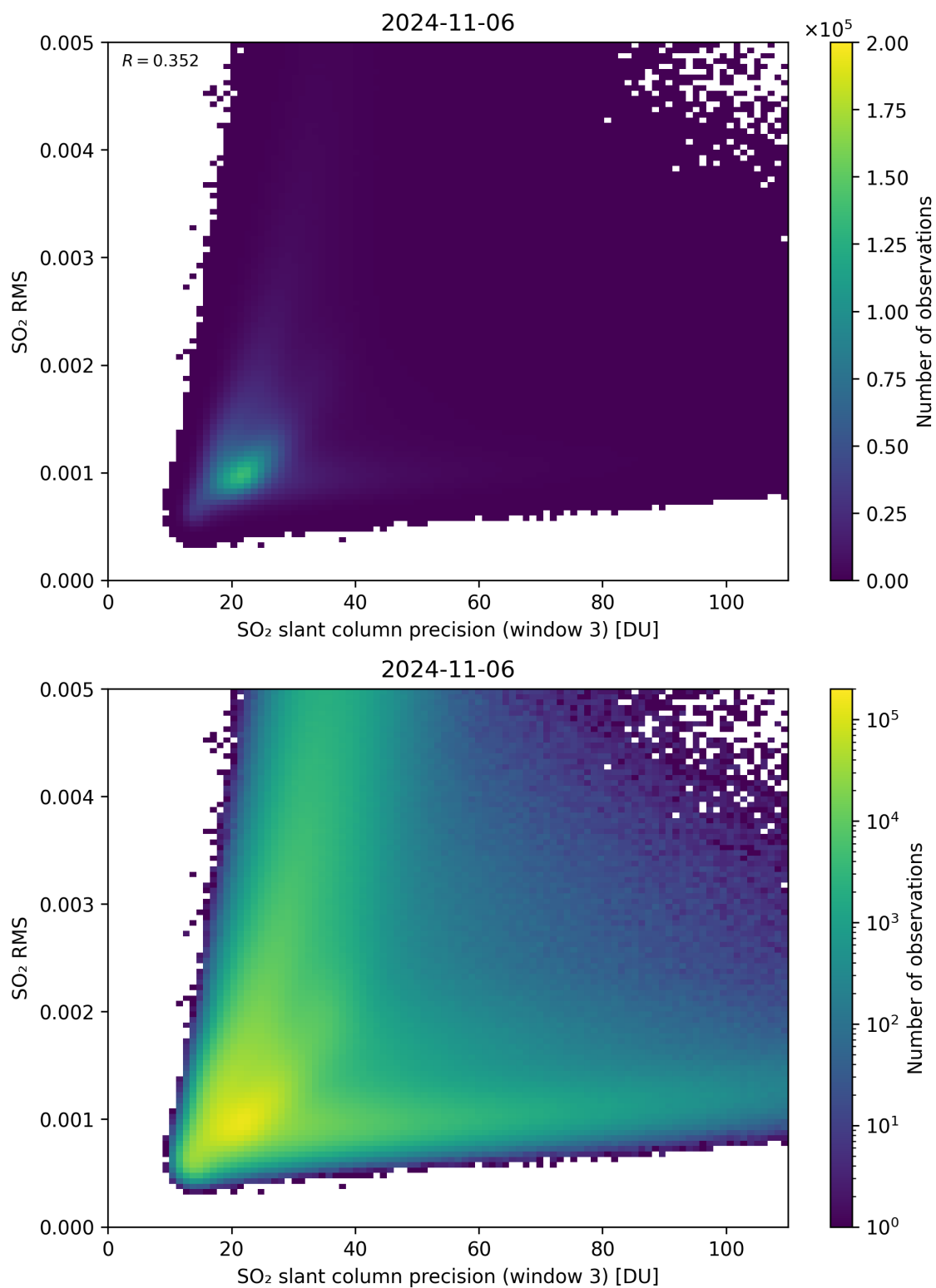
Figure 260: Scatter density plot of “SO 2 slant column precision (window 3)” against “SO 2 RMS” for 2024-11-05 to 2024-11-07.
