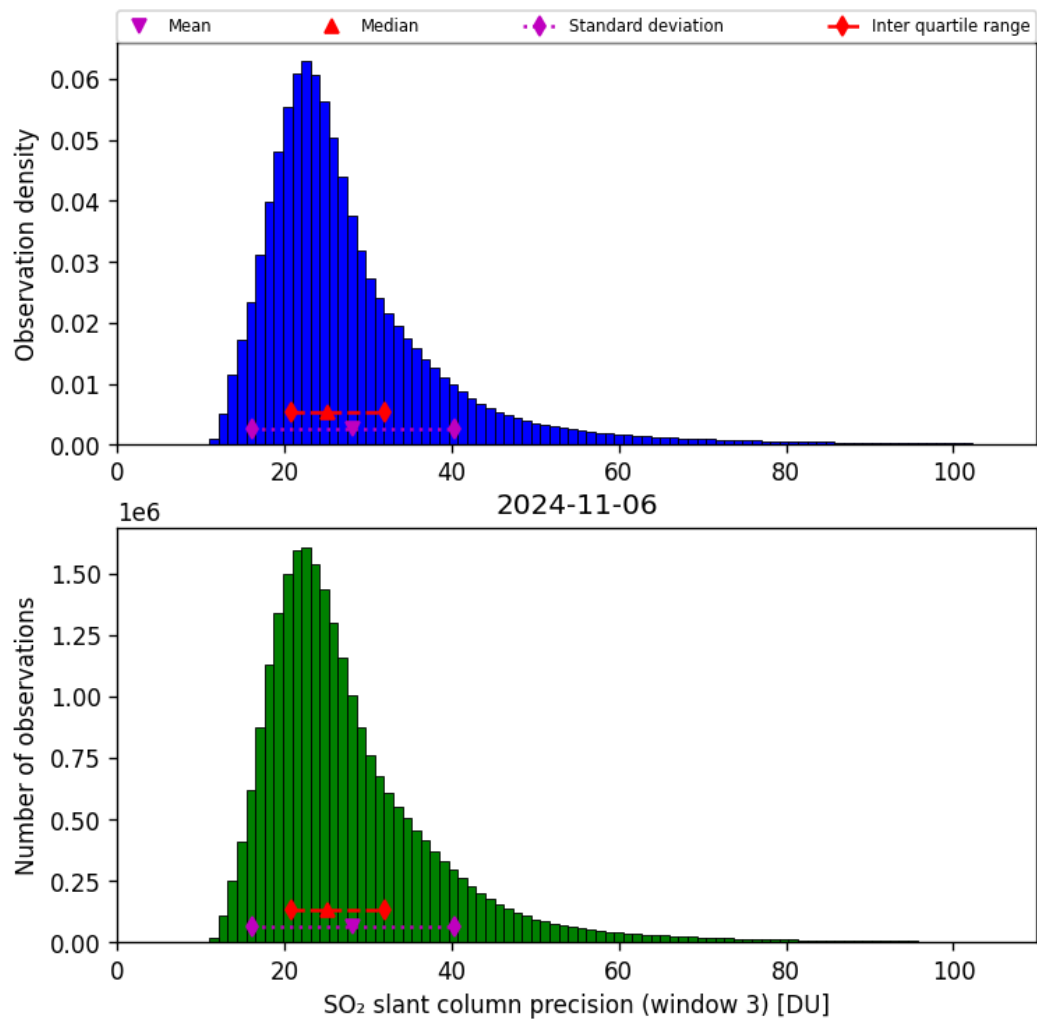
Figure 65: Histogram of “SO 2 slant column precision (window 3)” for 2024-11-05 to 2024-11-07
