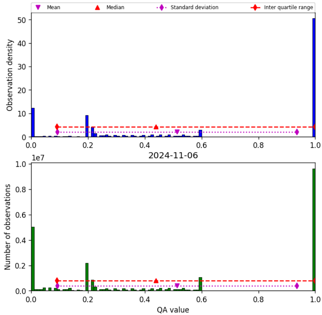
Figure 52: Histogram of “QA value” for 2024-11-05 to 2024-11-07
