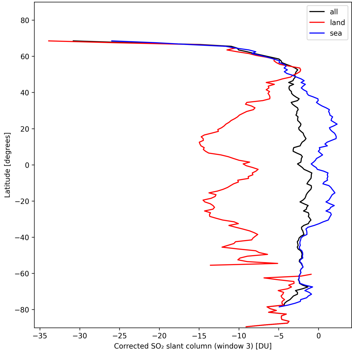
Figure 43: Zonal average of "Corrected SO 2 slant column (window 3)" for 2024-11-05 to 2024-11-07.
