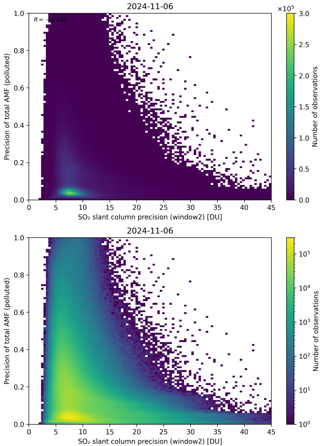
Figure 252: Scatter density plot of “SO 2 slant column precision (window2)” against “Precision of total AMF (polluted)” for 2024-11-05 to 2024-11-07.
