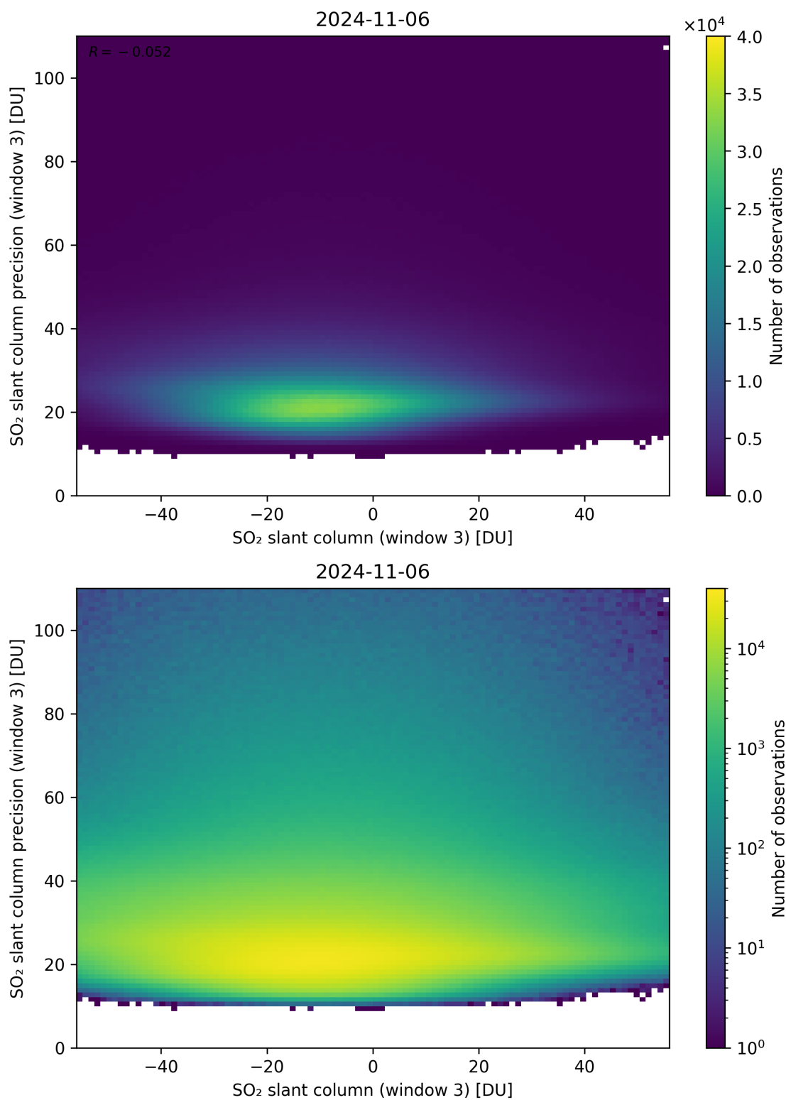
Figure 267: Scatter density plot of “SO 2 slant column (window 3)” against “SO 2 slant column precision (window 3)” for 2024-11-05 to 2024-11-07.
