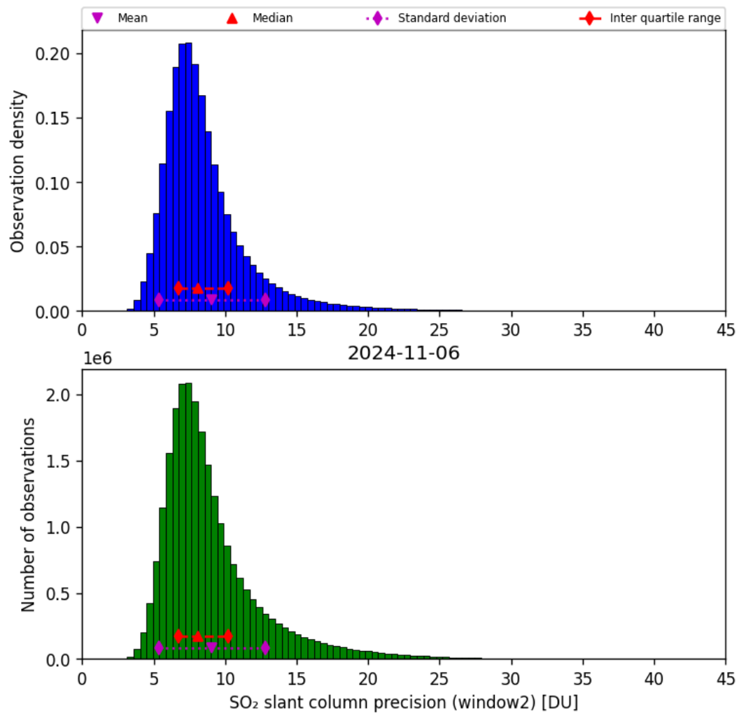
Figure 61: Histogram of “SO 2 slant column precision (window2)” for 2024-11-05 to 2024-11-07
