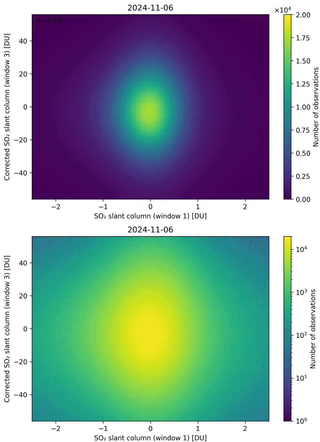
Figure 234: Scatter density plot of “SO 2 slant column (window 1)” against “Corrected SO 2 slant column (window 3)” for 2024-11-05 to 2024-11-07.
