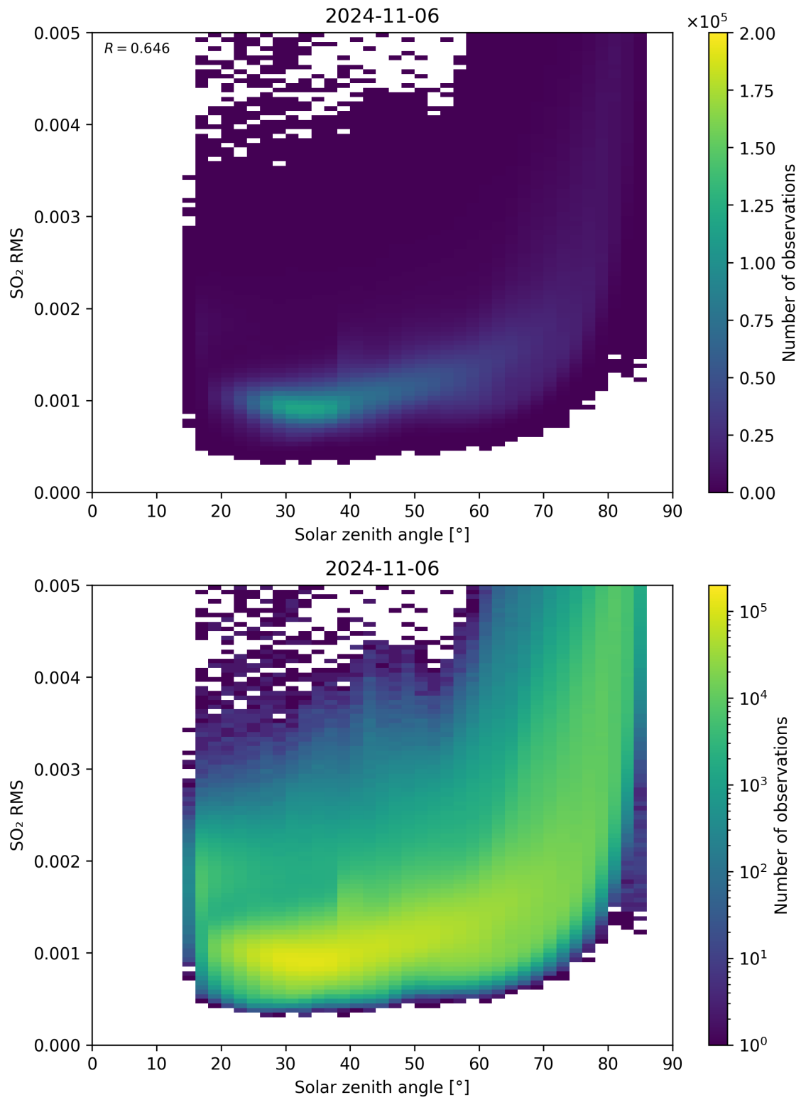
Figure 163: Scatter density plot of “Solar zenith angle” against “SO 2 RMS” for 2024-11-05 to 2024-11-07.
