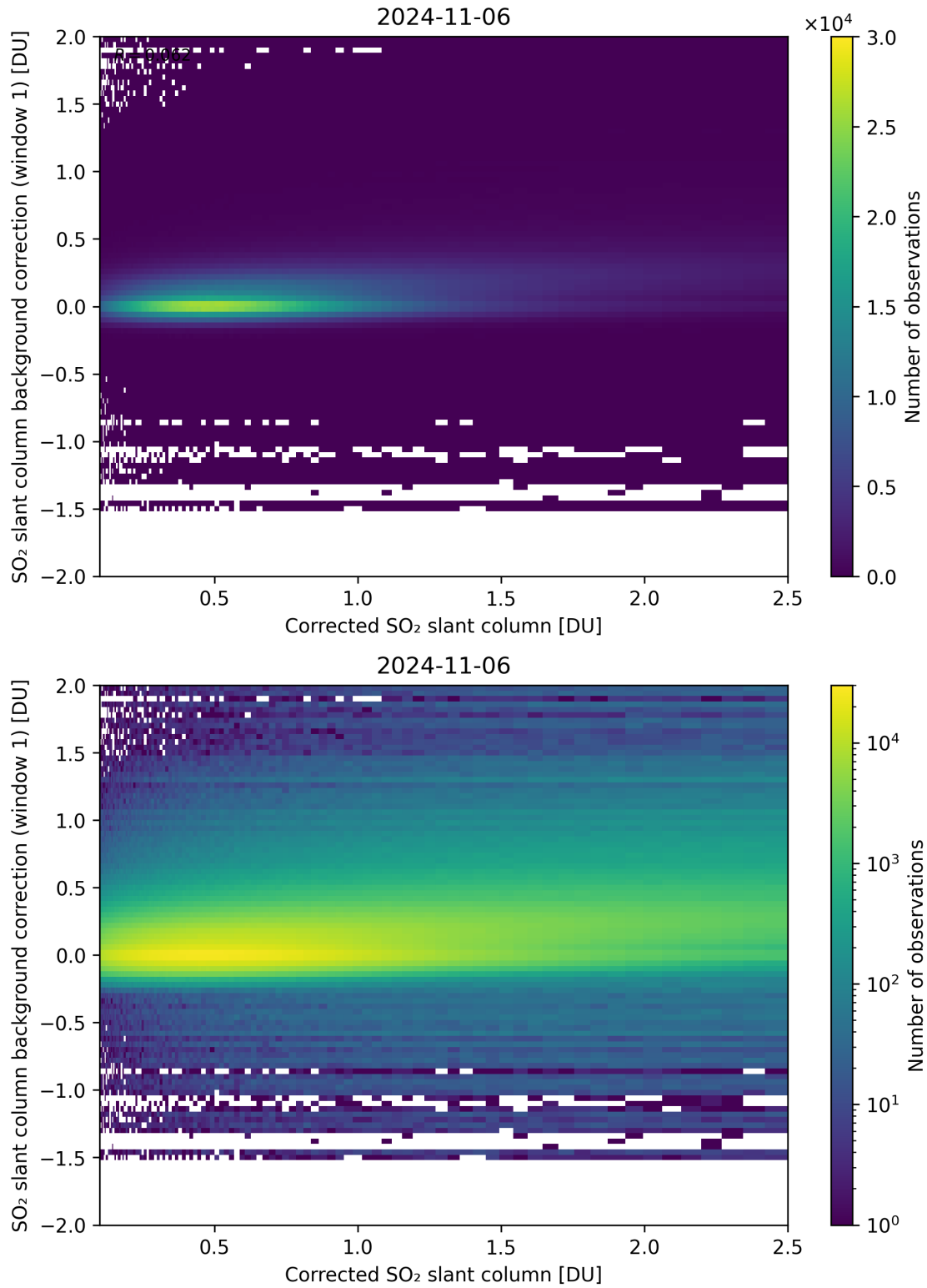
Figure 178: Scatter density plot of “Corrected SO 2 slant column” against “SO 2 slant column background correction (window 1)” for 2024-11-05 to 2024-11-07.
