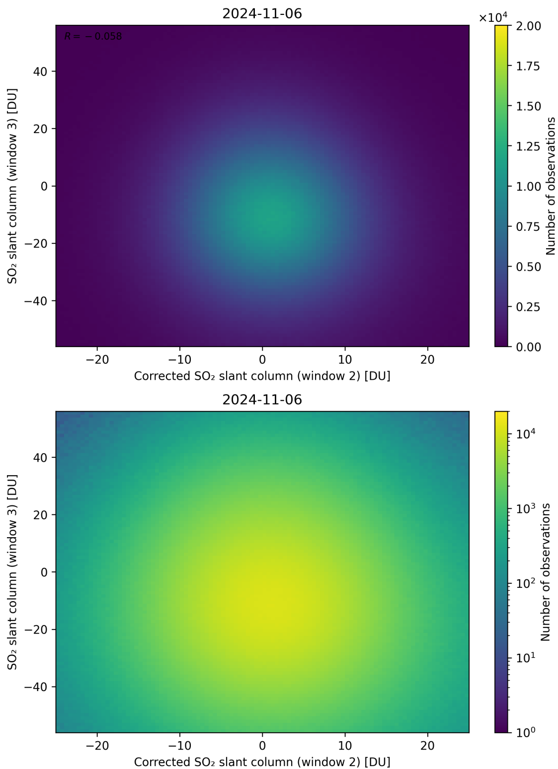
Figure 201: Scatter density plot of “Corrected SO 2 slant column (window 2)” against “SO 2 slant column (window 3)” for 2024-11-05 to 2024-11-07.
