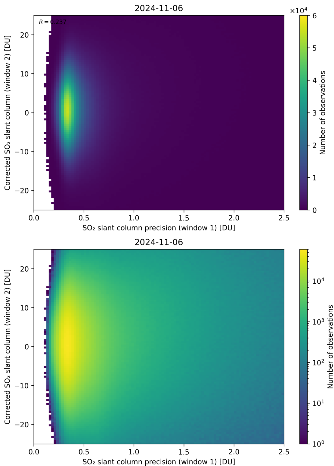
Figure 225: Scatter density plot of “SO 2 slant column precision (window 1)” against “Corrected SO 2 slant column (window 2)” for 2024-11-05 to 2024-11-07.
