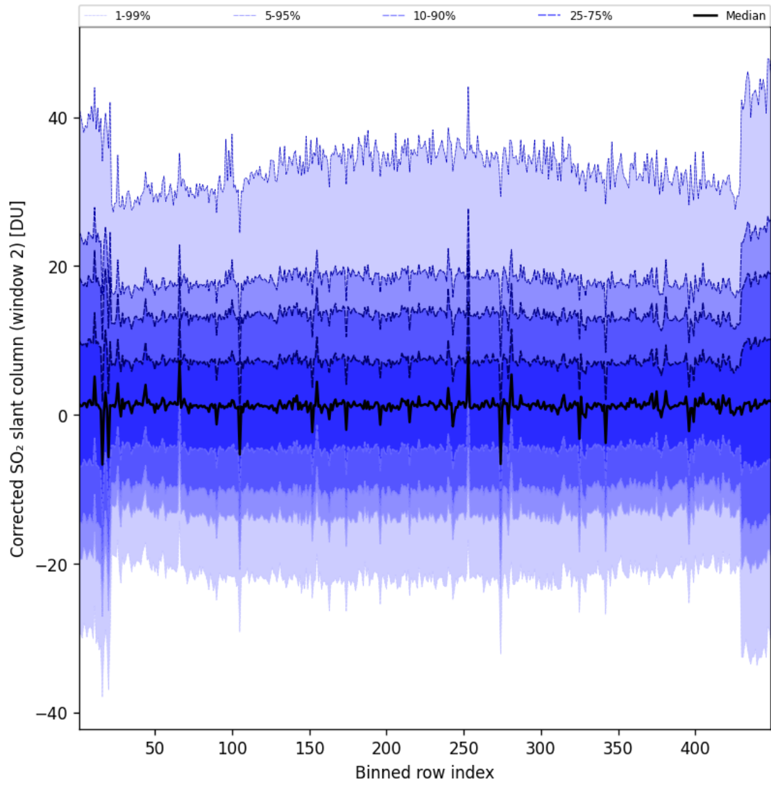
Figure 85: Along track statistics of “Corrected SO 2 slant column (window 2)” for 2024-11-05 to 2024-11-07
