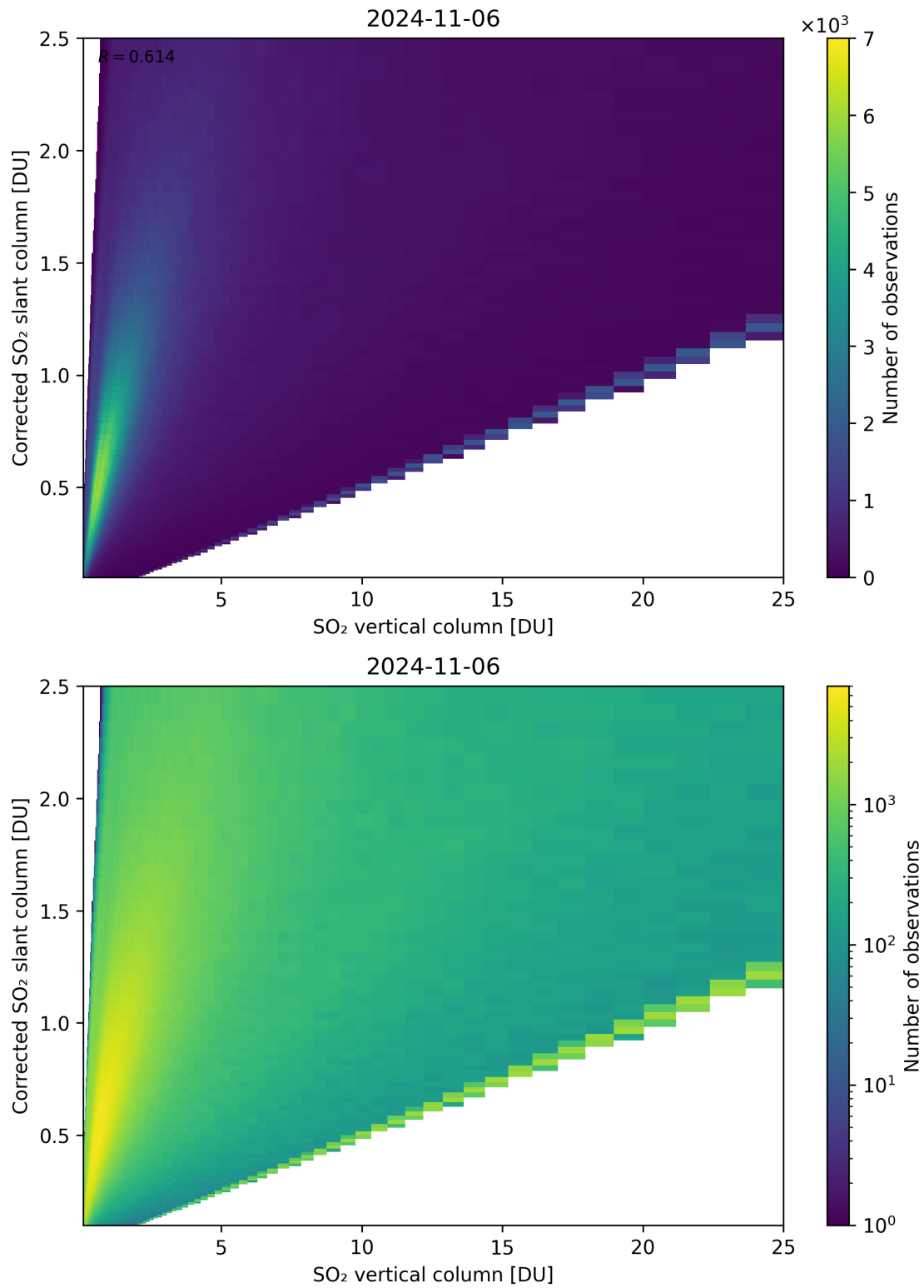
Figure 297: Scatter density plot of “SO 2 vertical column” against “Corrected SO 2 slant column” for 2024-11-05 to 2024-11-07.
