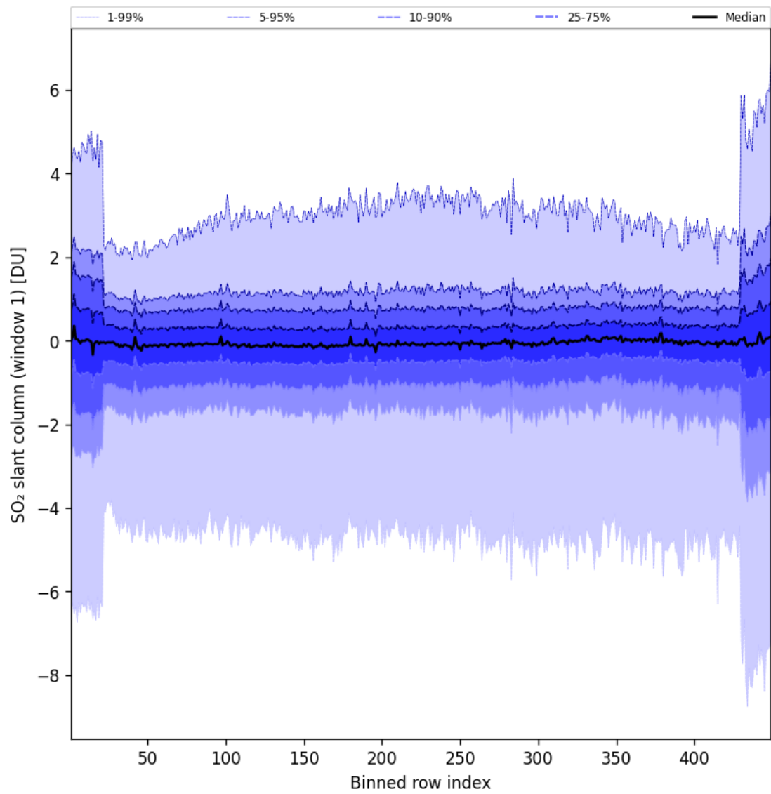
Figure 79: Along track statistics of “SO 2 slant column (window 1)” for 2024-11-05 to 2024-11-07
