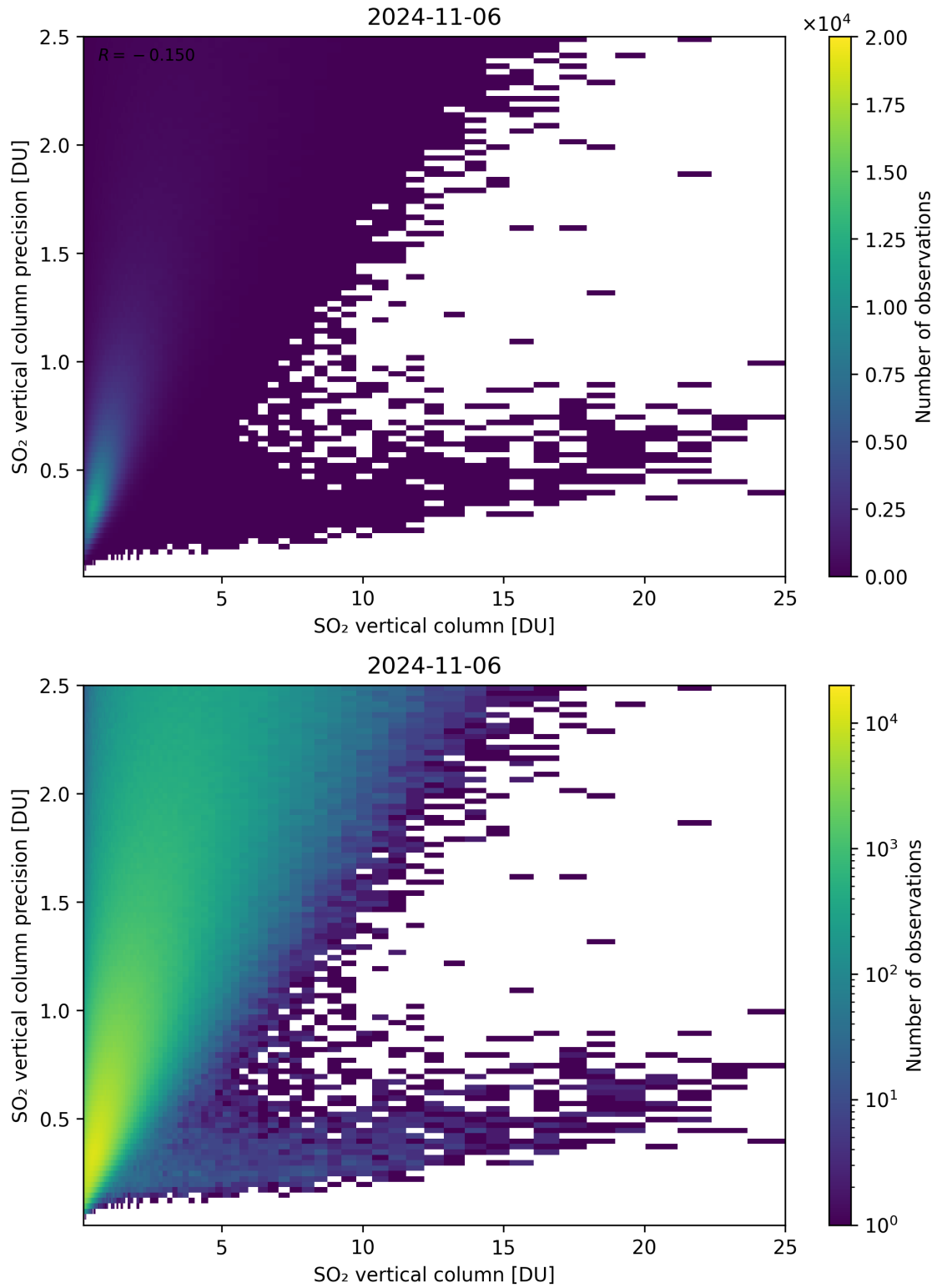
Figure 307: Scatter density plot of “SO 2 vertical column” against “SO 2 vertical column precision” for 2024-11-05 to 2024-11-07.
