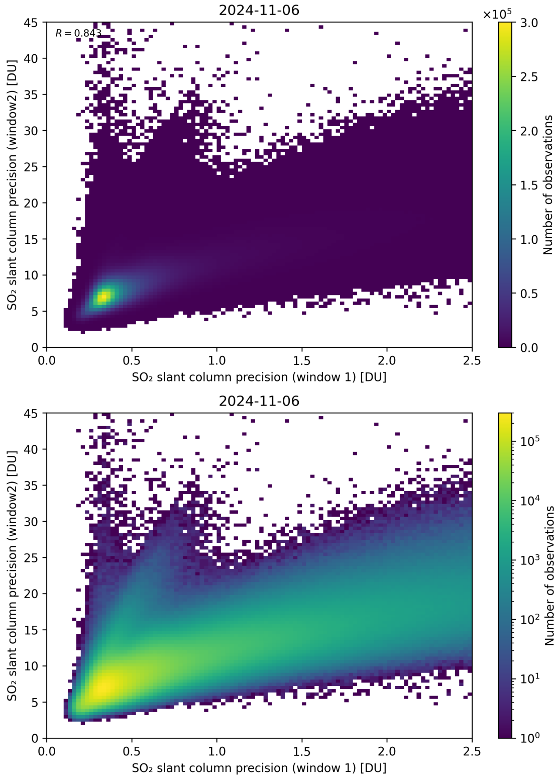
Figure 227: Scatter density plot of “SO 2 slant column precision (window 1)” against “SO 2 slant column precision (window2)” for 2024-11-05 to 2024-11-07.
