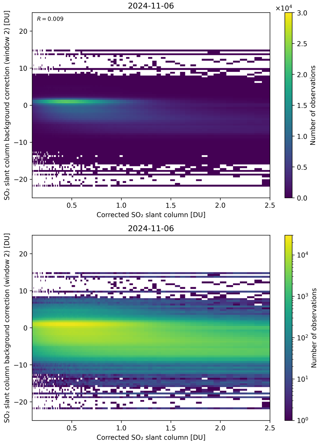
Figure 179: Scatter density plot of “Corrected SO 2 slant column” against “SO 2 slant column background correction (window 2)” for 2024-11-05 to 2024-11-07.
