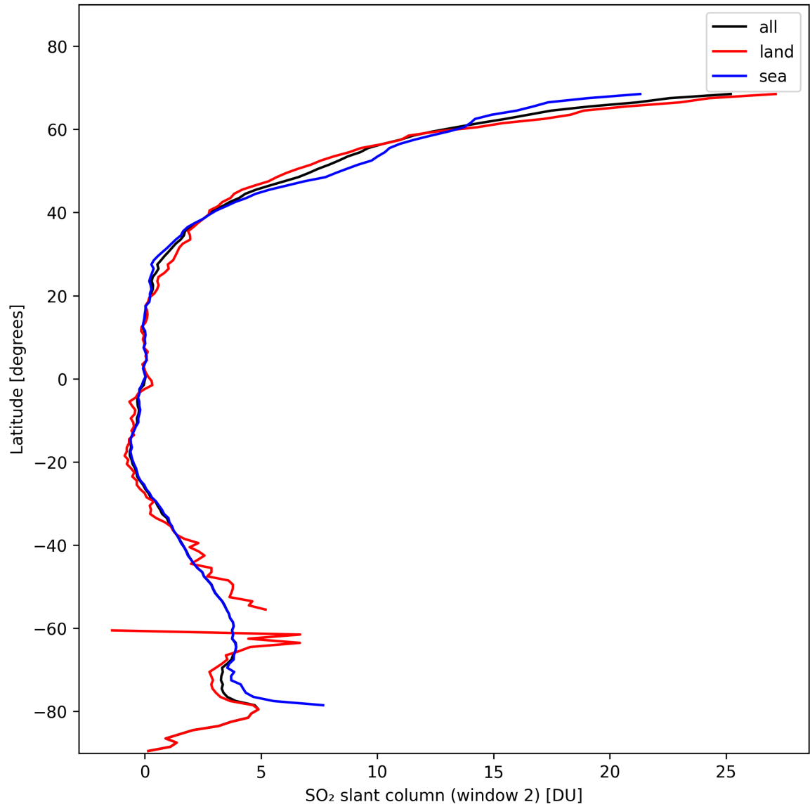
Figure 37: Zonal average of “SO 2 slant column (window 2)” for 2024-11-05 to 2024-11-07.
