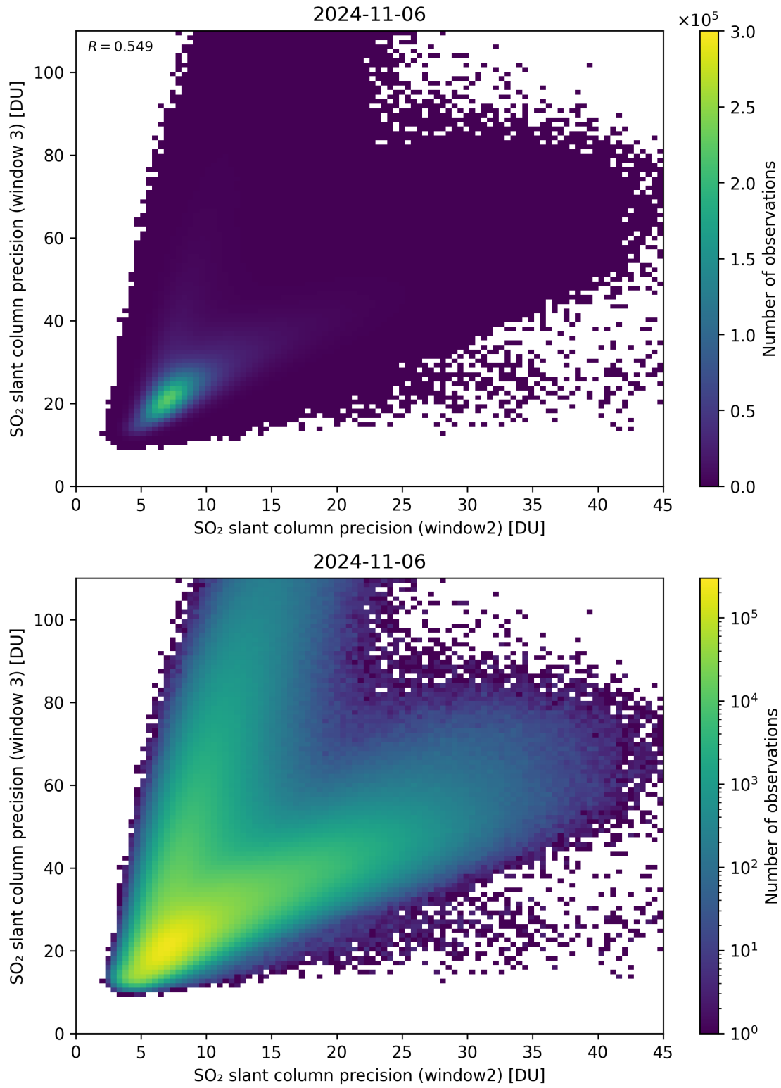
Figure 250: Scatter density plot of “SO 2 slant column precision (window2)” against “SO 2 slant column precision (window 3)” for 2024-11-05 to 2024-11-07.
