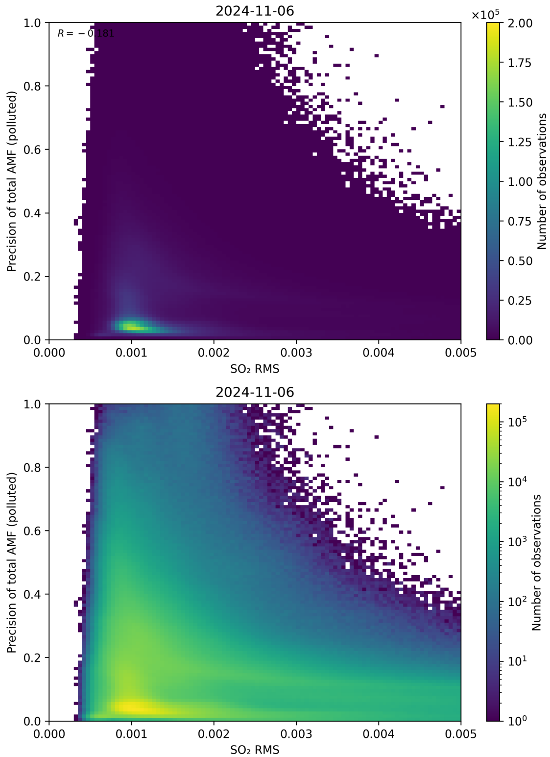
Figure 138: Scatter density plot of “SO 2 RMS” against “Precision of total AMF (polluted)” for 2024-11-05 to 2024-11-07.
