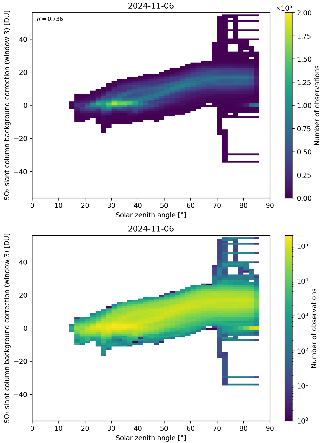
Figure 160: Scatter density plot of “Solar zenith angle” against “SO 2 slant column background correction (window 3)” for 2024-11-05 to 2024-11-07.
