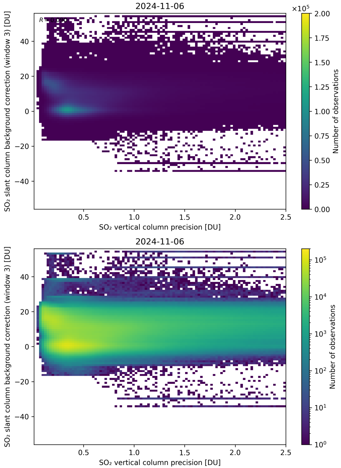
Figure 281: Scatter density plot of “SO 2 vertical column precision” against “SO 2 slant column background correction (window 3)” for 2024-11-05 to 2024-11-07.
