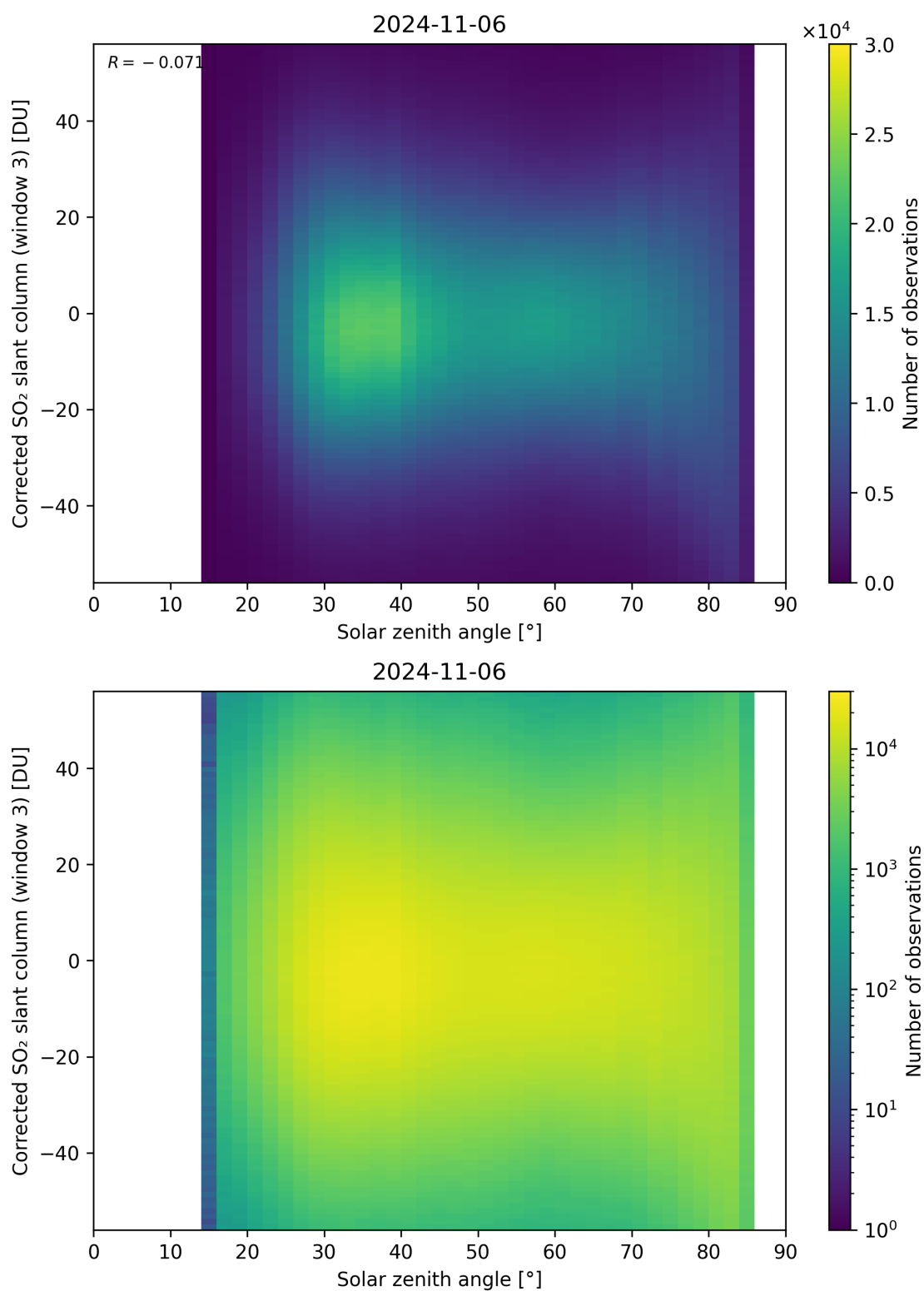
Figure 168: Scatter density plot of “Solar zenith angle” against “Corrected SO 2 slant column (window 3)” for 2024-11-05 to 2024-11-07.
