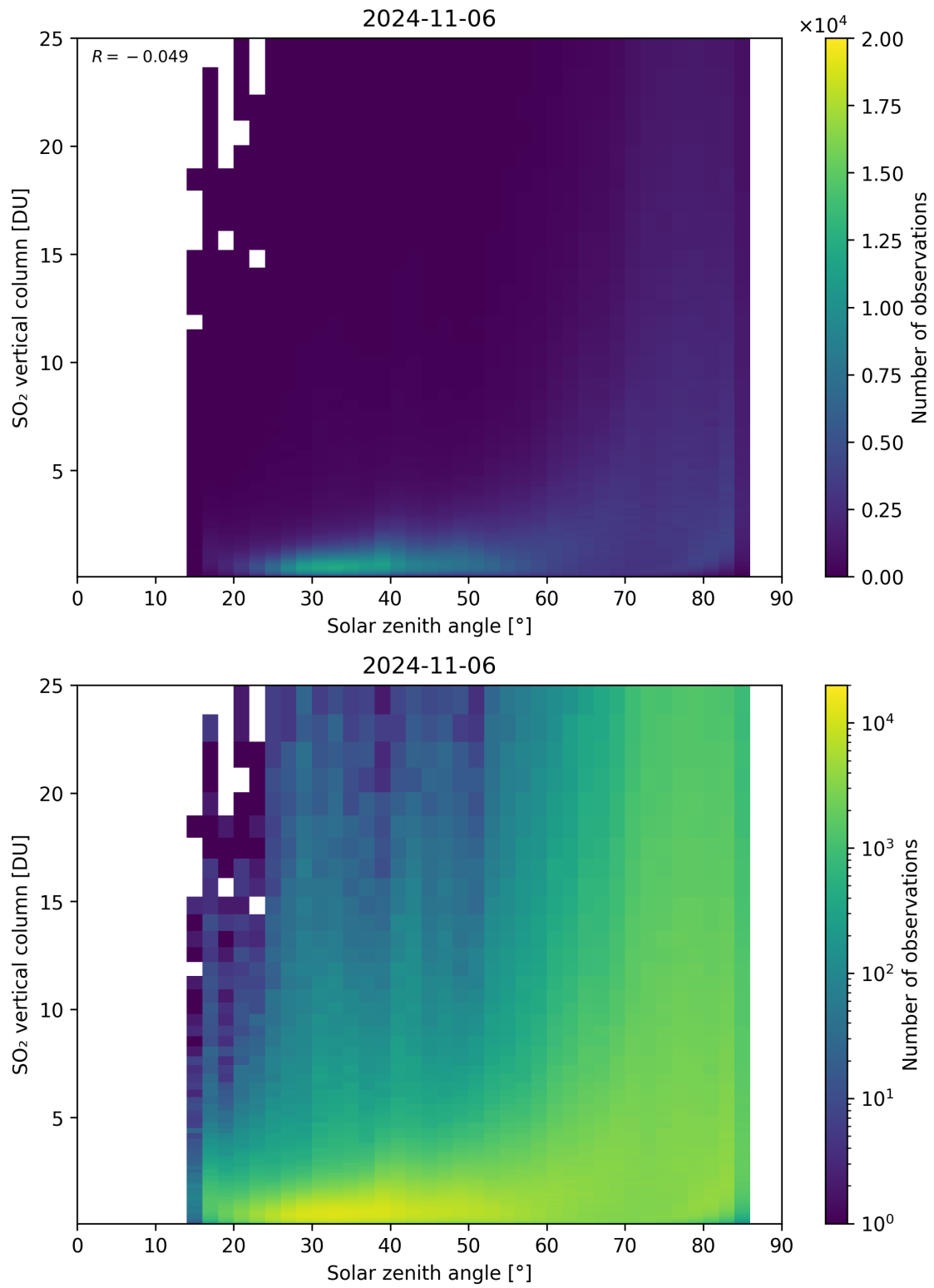
Figure 176: Scatter density plot of “Solar zenith angle” against “SO 2 vertical column” for 2024-11-05 to 2024-11-07.
