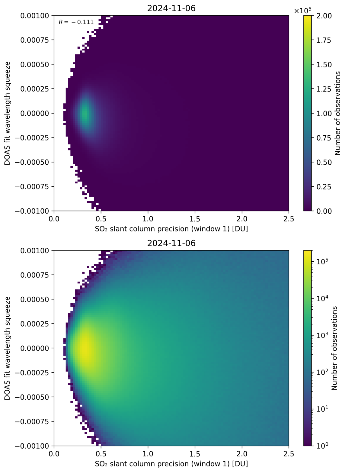
Figure 222: Scatter density plot of “SO 2 slant column precision (window 1)” against “DOAS fit wavelength squeeze” for 2024-11-05 to 2024-11-07.
