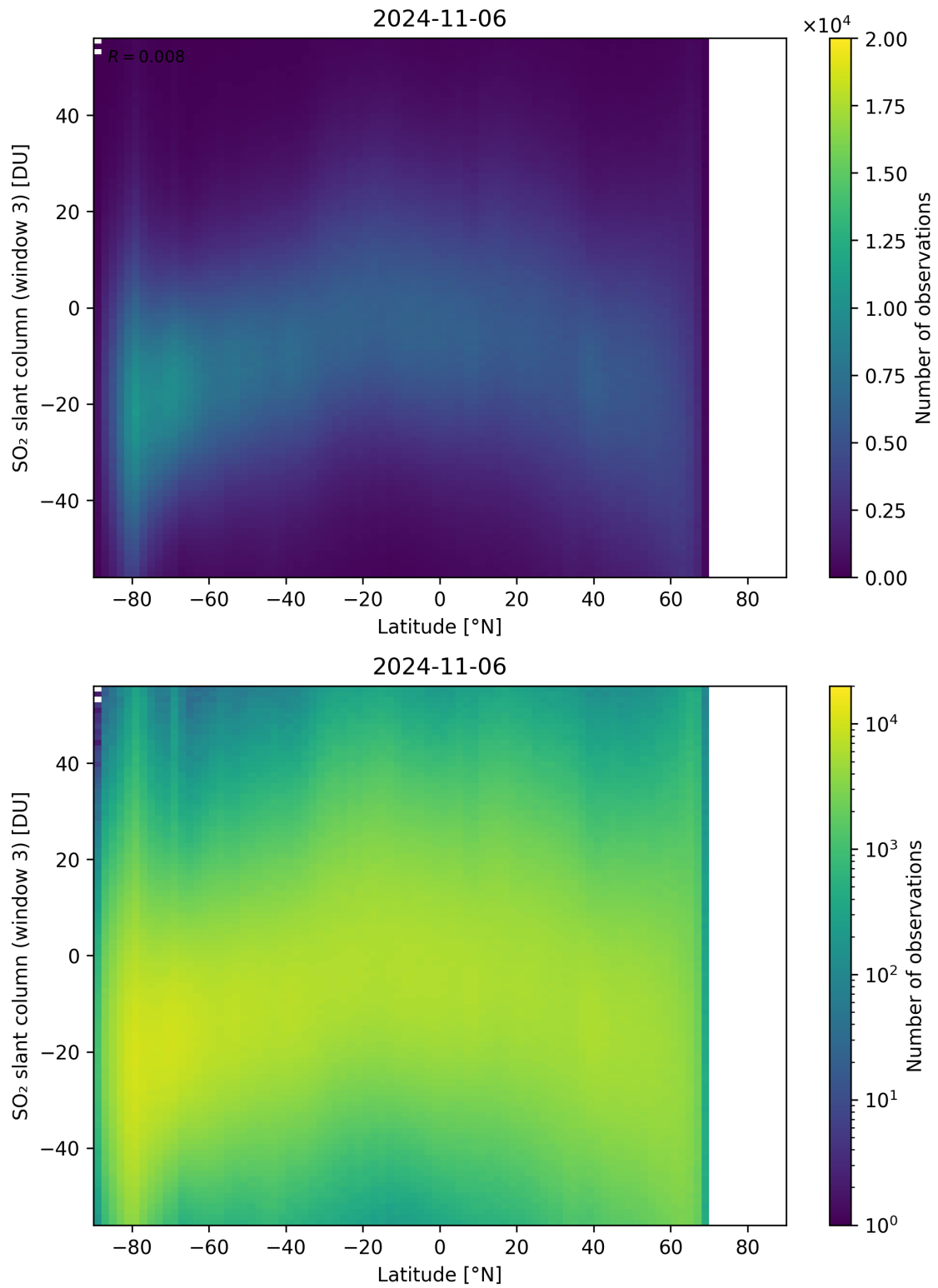
Figure 152: Scatter density plot of “Latitude” against “SO 2 slant column (window 3)” for 2024-11-05 to 2024-11-07.
