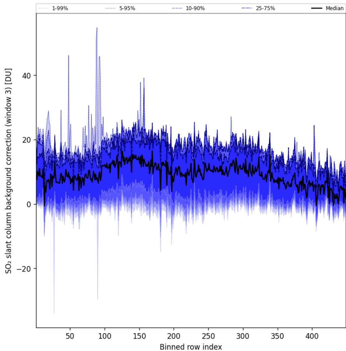
Figure 90: Along track statistics of “SO 2 slant column background correction (window 3)” for 2024-11-05 to 2024-11-07
