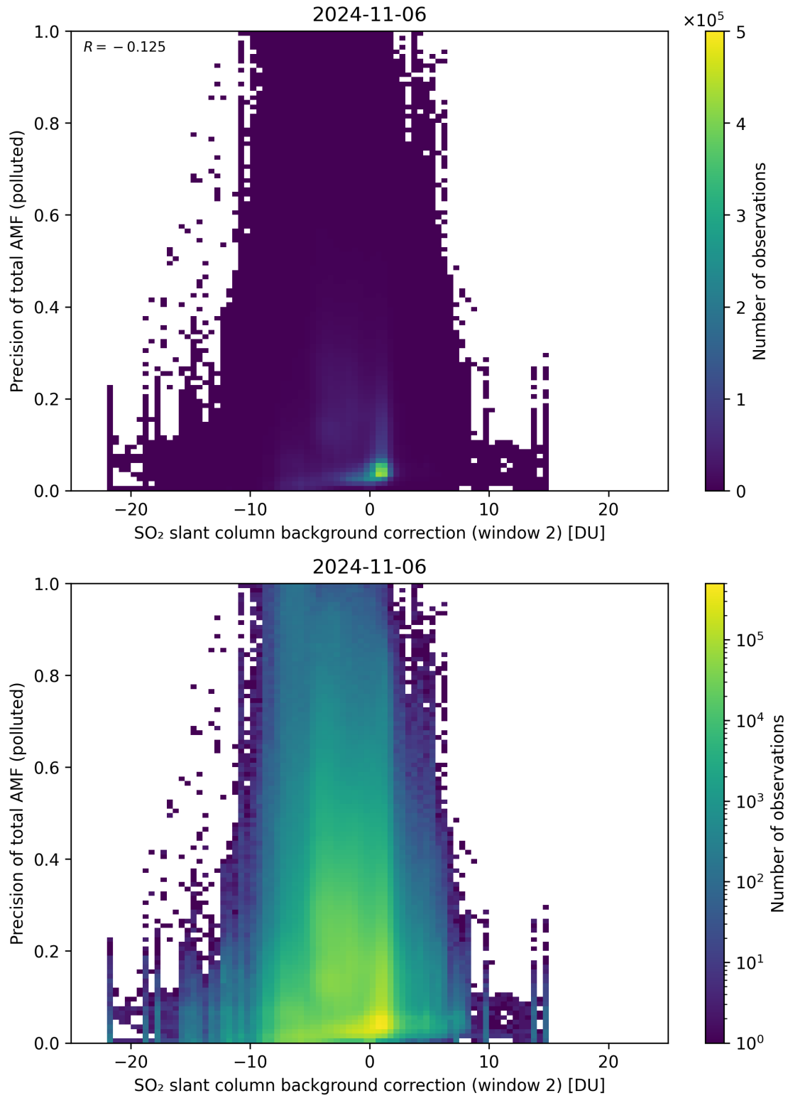
Figure 120: Scatter density plot of “SO 2 slant column background correction (window 2)” against “Precision of total AMF (polluted)” for 2024-11-05 to 2024-11-07.
