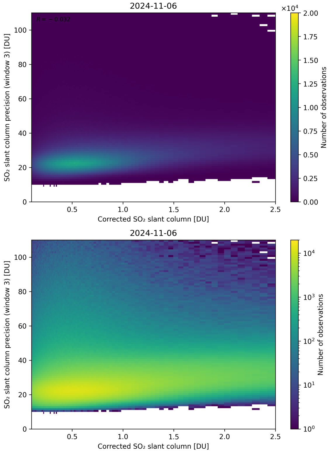
Figure 191: Scatter density plot of “Corrected SO 2 slant column” against “SO 2 slant column precision (window 3)” for 2024-11-05 to 2024-11-07.
