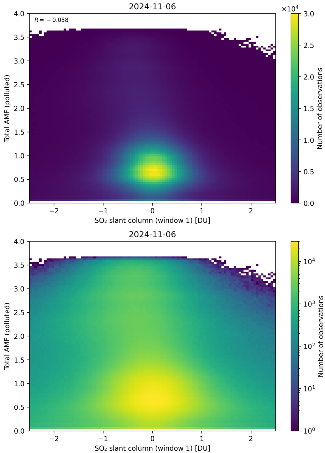
Figure 239: Scatter density plot of “SO 2 slant column (window 1)” against “Total AMF (polluted)” for 2024-11-05 to 2024-11-07.
