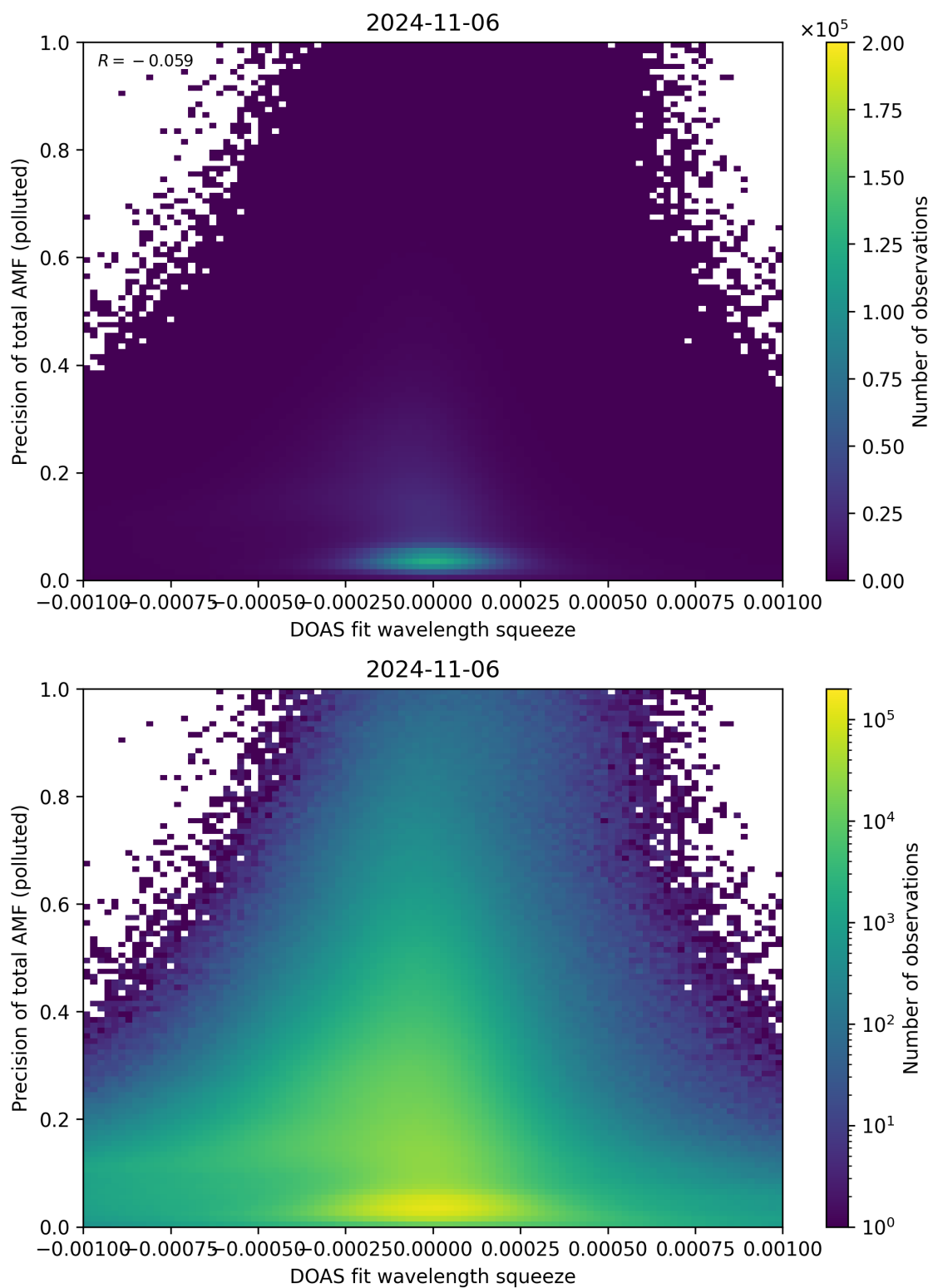
Figure 135: Scatter density plot of “DOAS fit wavelength squeeze” against “Precision of total AMF (polluted)” for 2024-11-05 to 2024-11-07.
