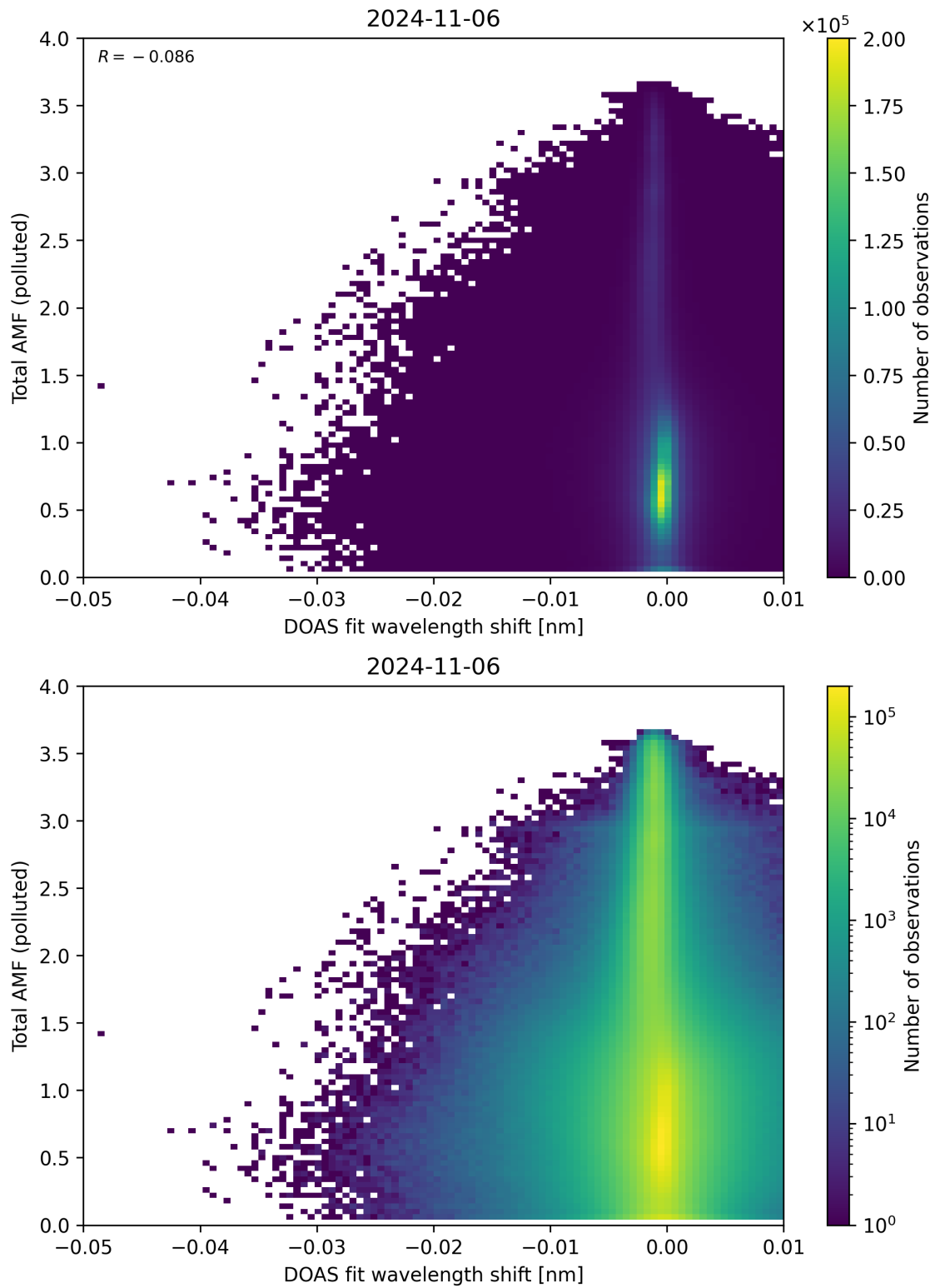
Figure 130: Scatter density plot of “DOAS fit wavelength shift” against “Total AMF (polluted)” for 2024-11-05 to 2024-11-07.
