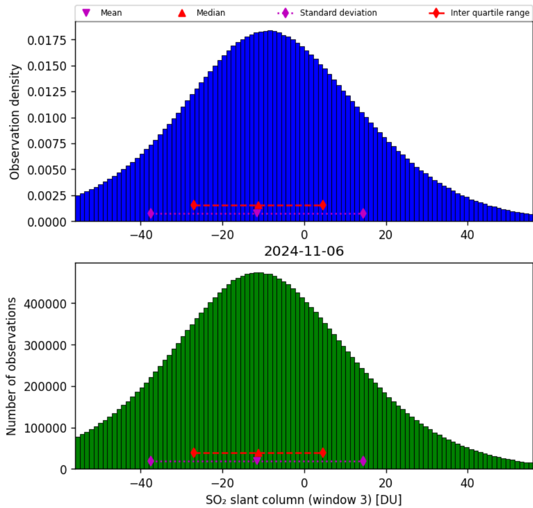
Figure 64: Histogram of “SO 2 slant column (window 3)” for 2024-11-05 to 2024-11-07
