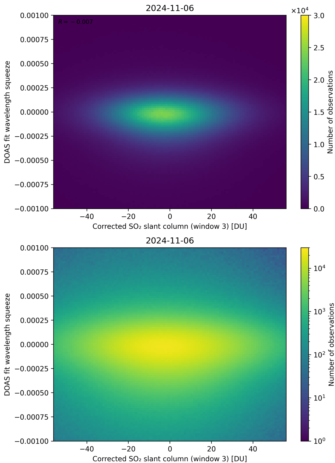
Figure 207: Scatter density plot of “Corrected SO 2 slant column (window 3)” against “DOAS fit wavelength squeeze” for 2024-11-05 to 2024-11-07.
