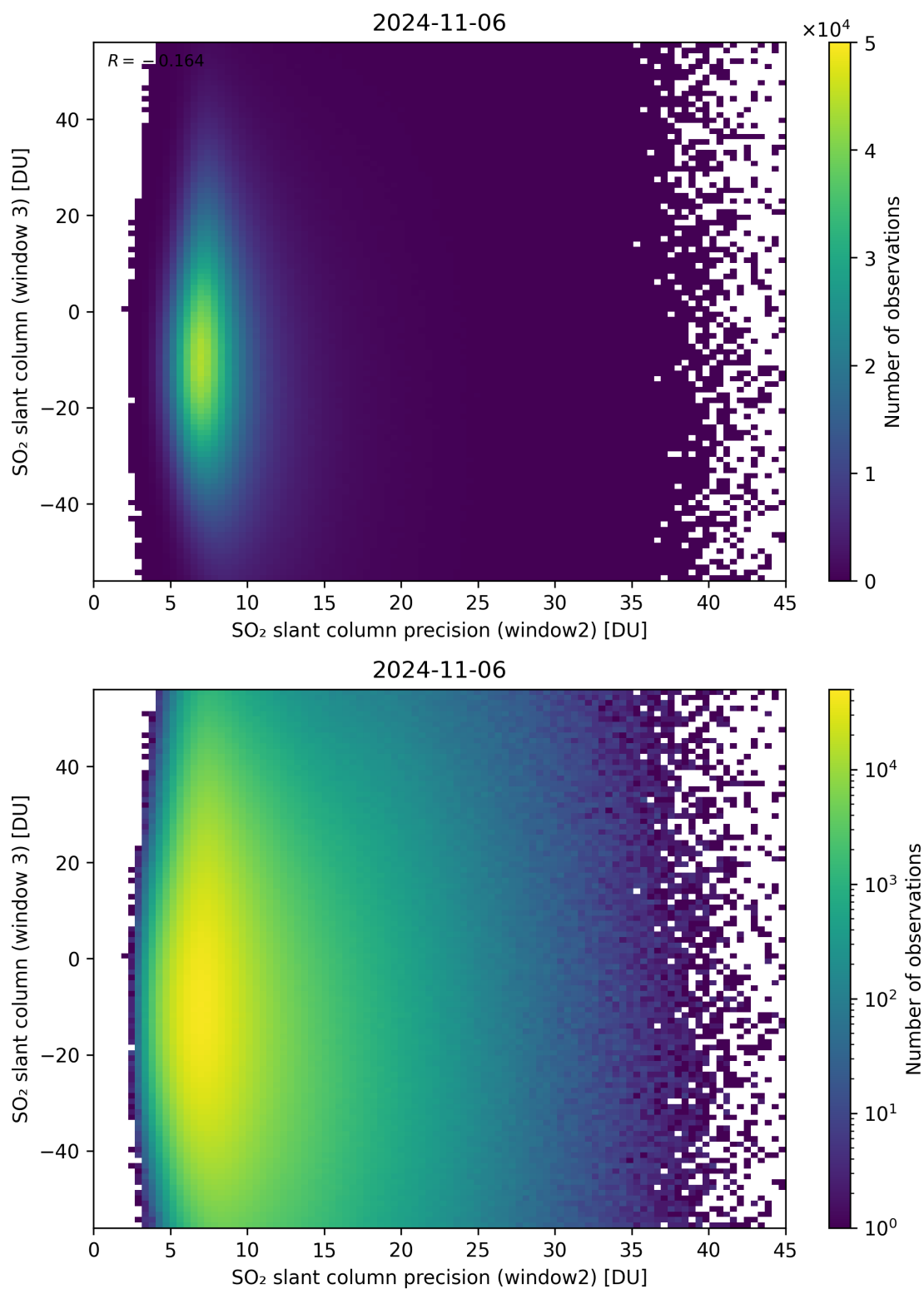
Figure 249: Scatter density plot of “SO 2 slant column precision (window2)” against “SO 2 slant column (window 3)” for 2024-11-05 to 2024-11-07.
