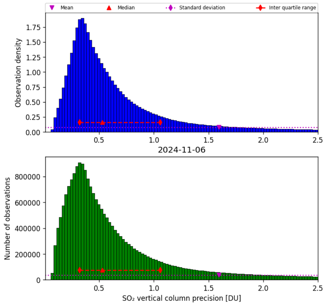
Figure 54: Histogram of “SO 2 vertical column precision” for 2024-11-05 to 2024-11-07
