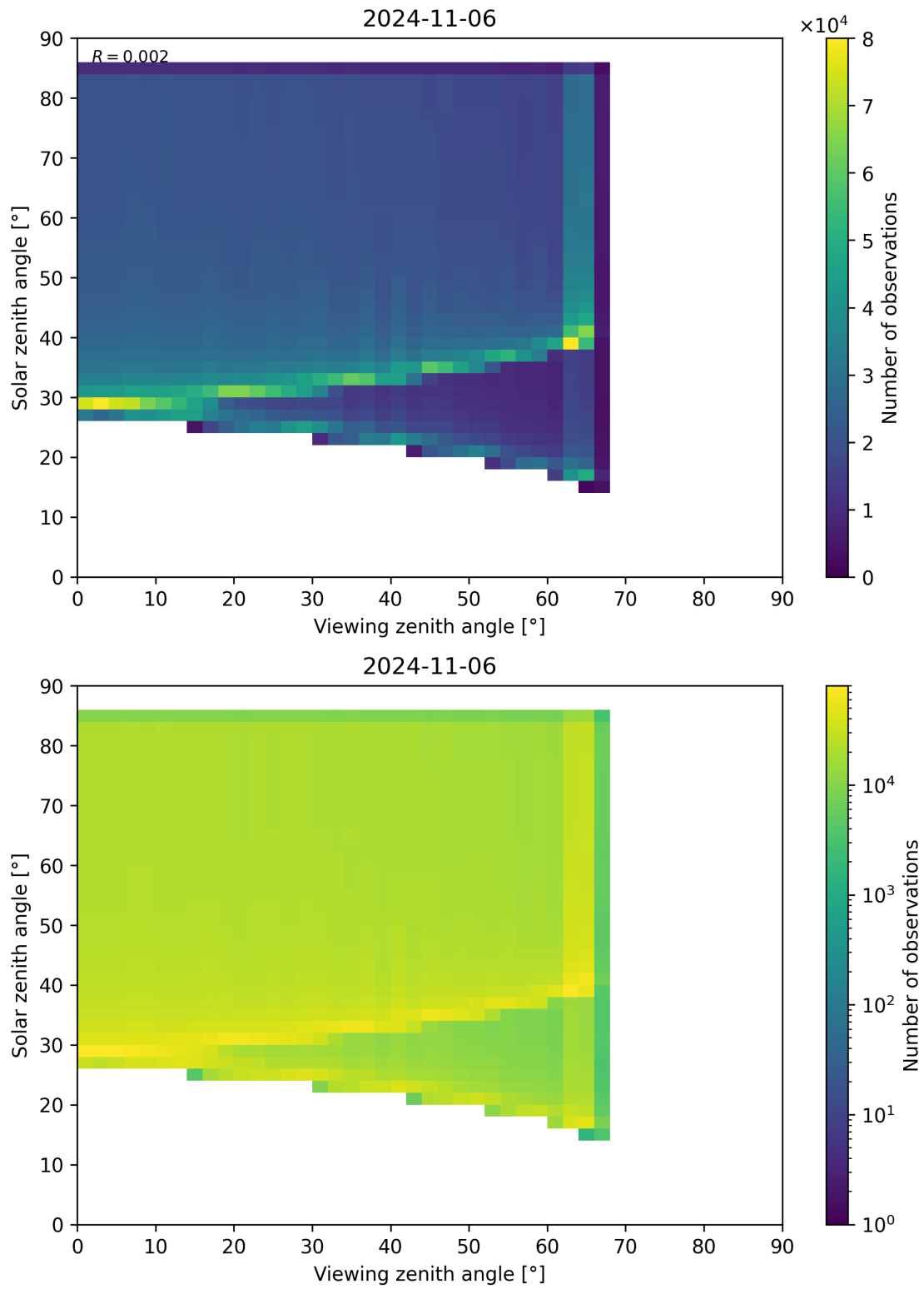
Figure 315: Scatter density plot of “Viewing zenith angle” against “Solar zenith angle” for 2024-11-05 to 2024-11-07.
