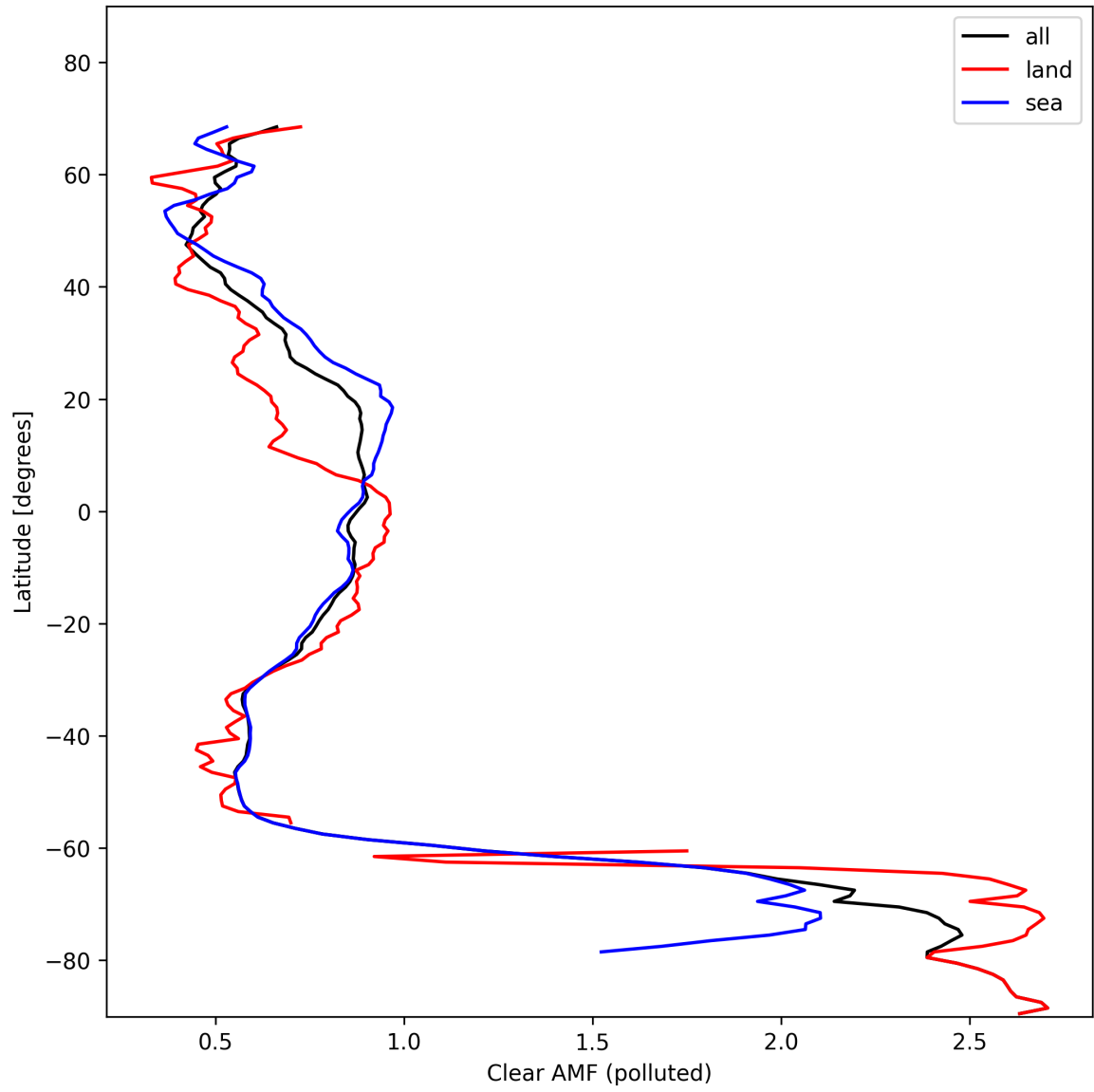
Figure 50: Zonal average of “Clear AMF (polluted)” for 2024-11-05 to 2024-11-07.
