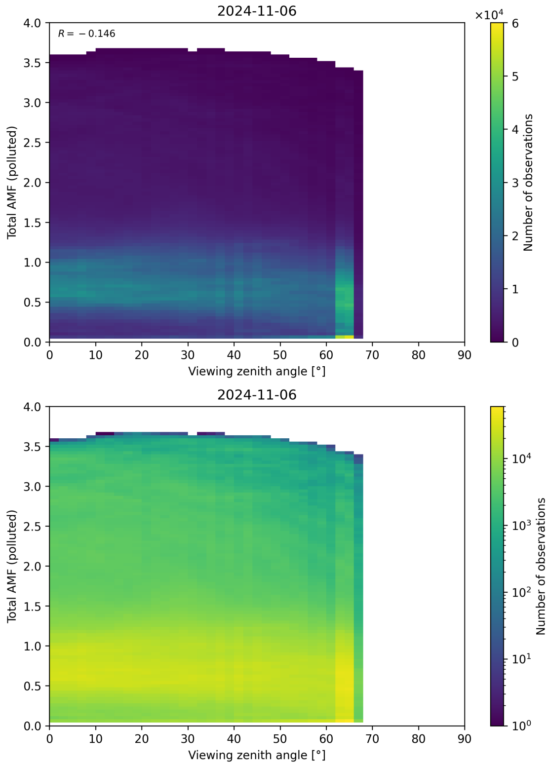
Figure 325: Scatter density plot of “Viewing zenith angle” against “Total AMF (polluted)” for 2024-11-05 to 2024-11-07.
