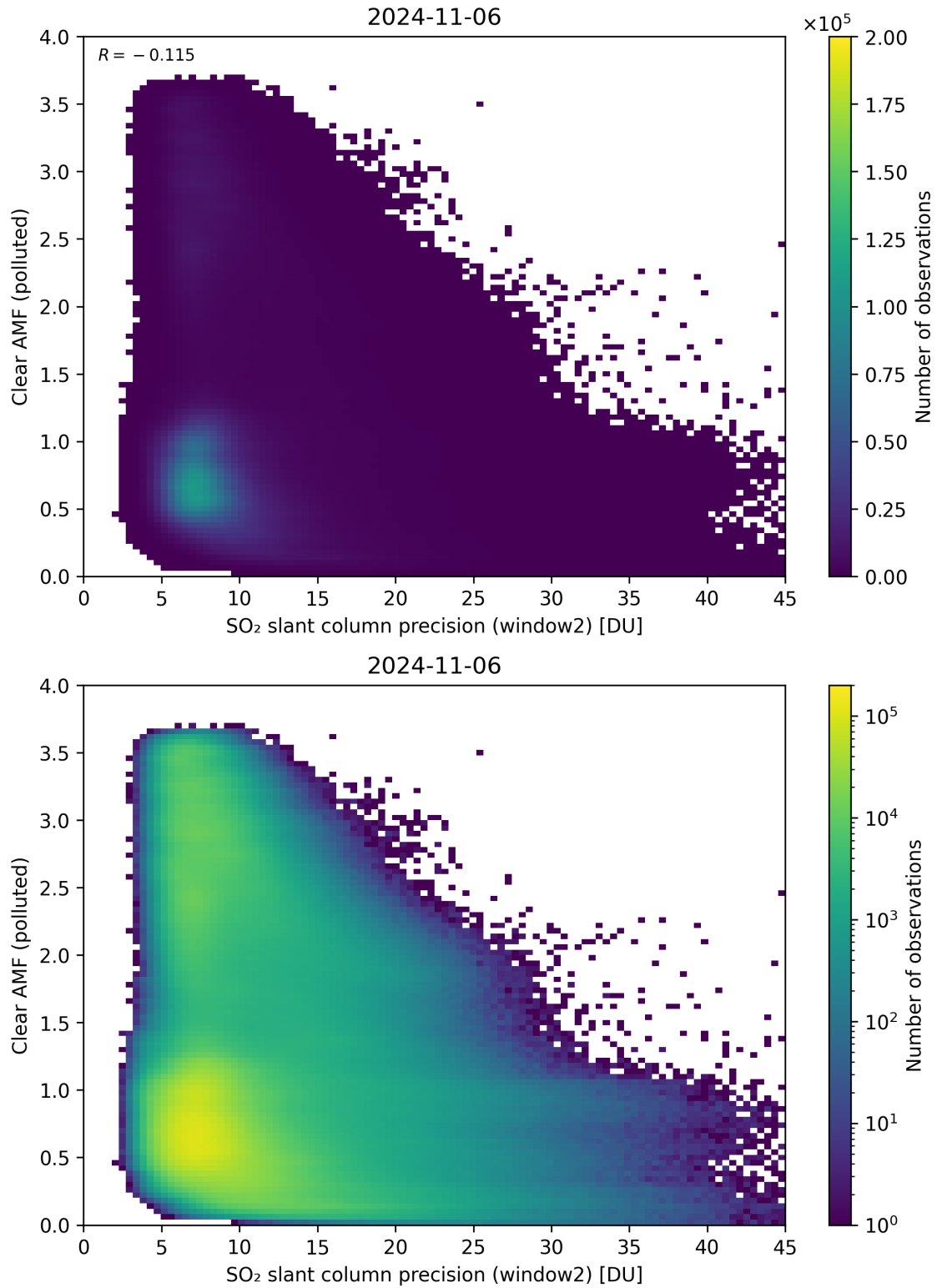
Figure 246: Scatter density plot of “SO 2 slant column precision (window2)” against “Clear AMF (polluted)” for 2024-11-05 to 2024-11-07.
