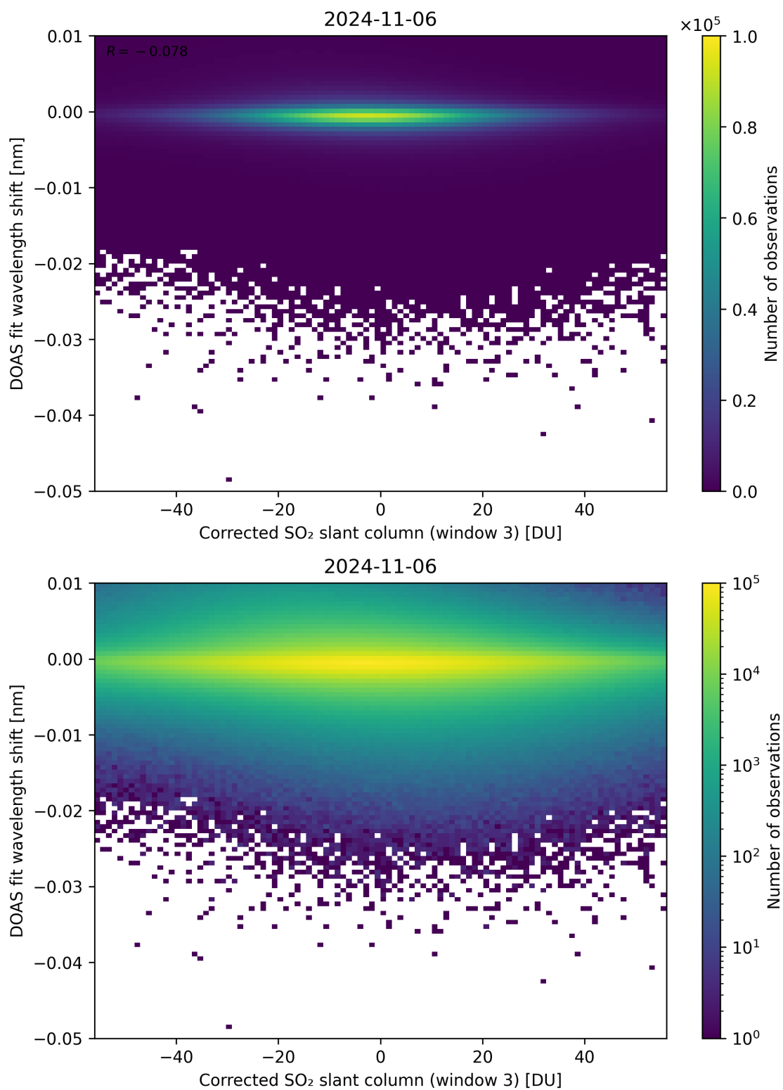
Figure 206: Scatter density plot of “Corrected SO 2 slant column (window 3)” against “DOAS fit wavelength shift” for 2024-11-05 to 2024-11-07.
