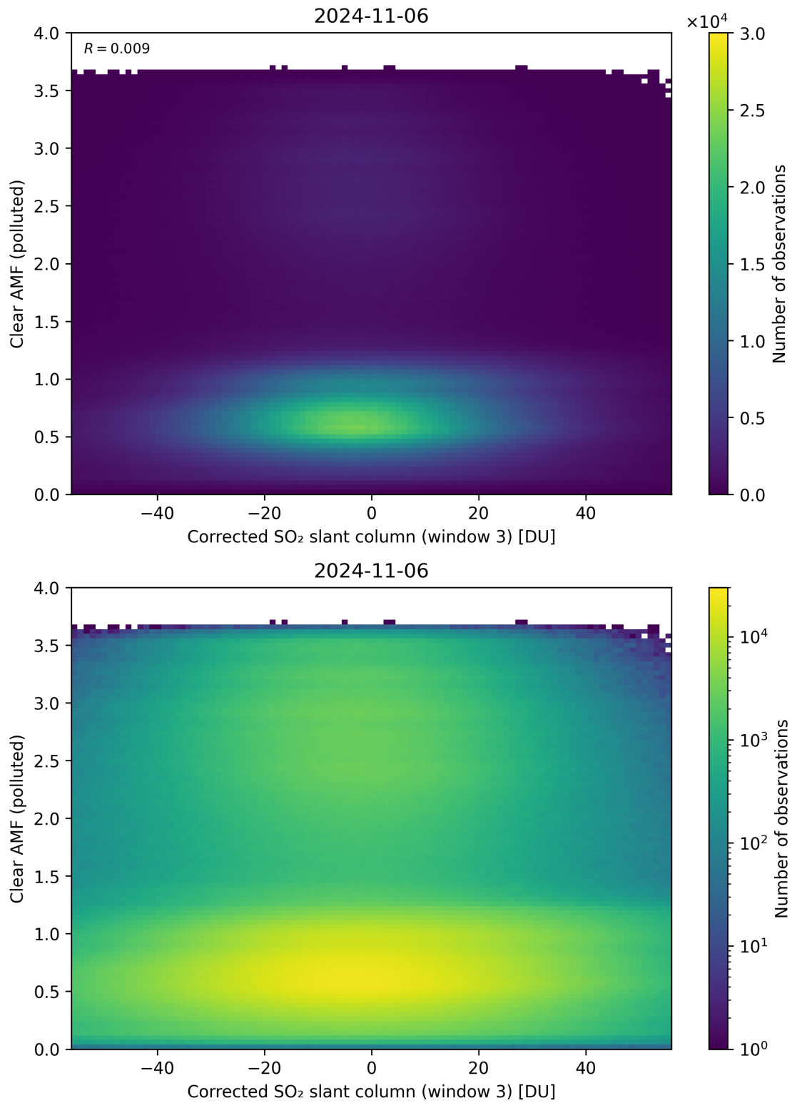
Figure 209: Scatter density plot of “Corrected SO 2 slant column (window 3)” against “Clear AMF (polluted)” for 2024-11-05 to 2024-11-07.
