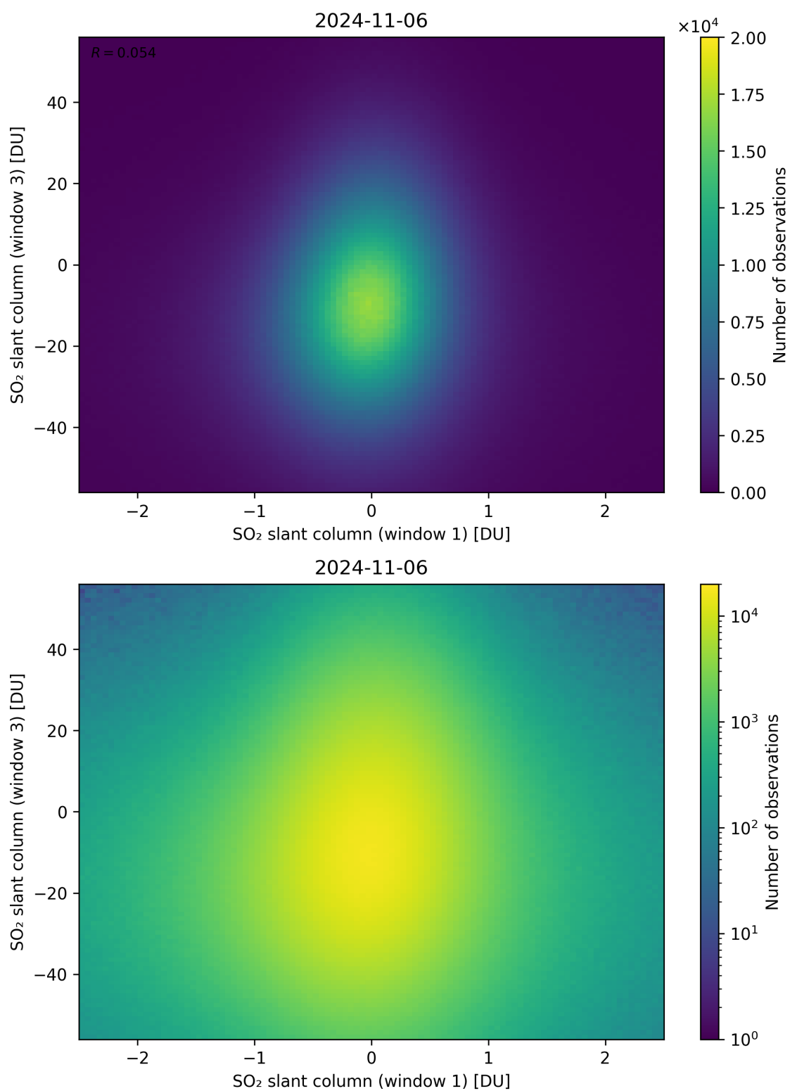
Figure 237: Scatter density plot of “SO 2 slant column (window 1)” against “SO 2 slant column (window 3)” for 2024-11-05 to 2024-11-07.
