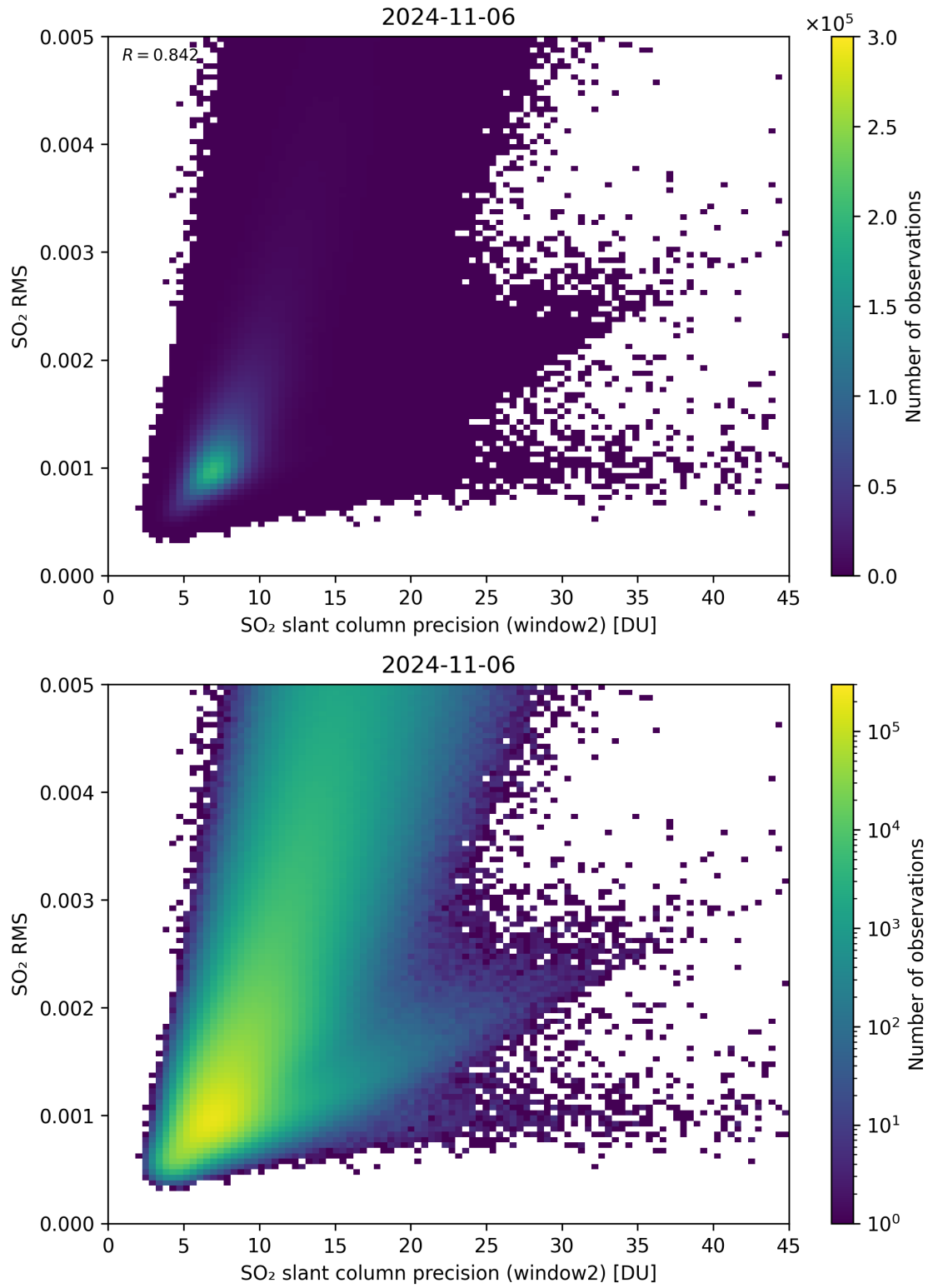
Figure 245: Scatter density plot of “SO 2 slant column precision (window2)” against “SO 2 RMS” for 2024-11-05 to 2024-11-07.
