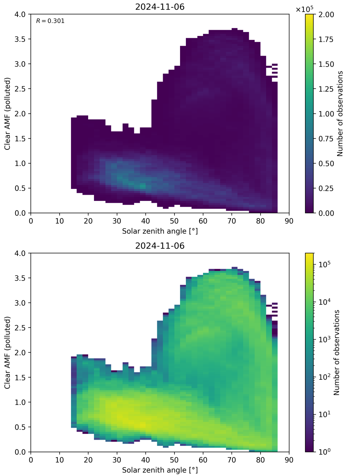
Figure 165: Scatter density plot of “Solar zenith angle” against “Clear AMF (polluted)” for 2024-11-05 to 2024-11-07.
