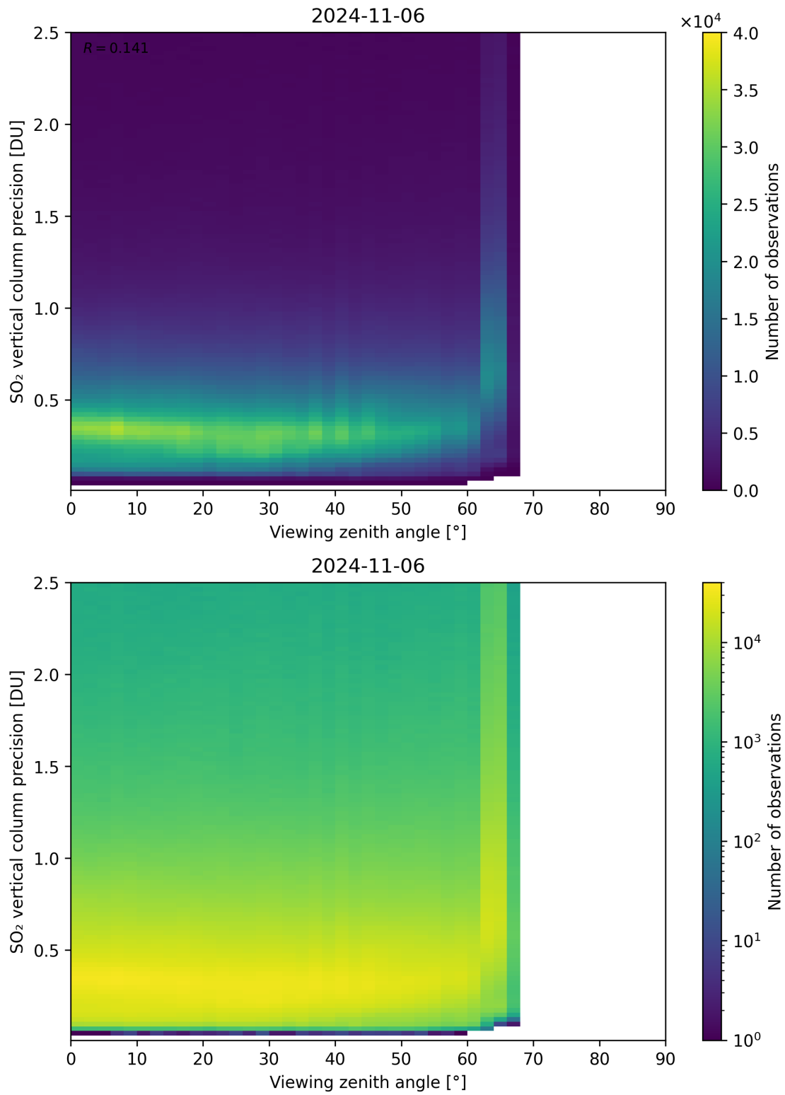
Figure 328: Scatter density plot of “Viewing zenith angle” against “SO 2 vertical column precision” for 2024-11-05 to 2024-11-07.
