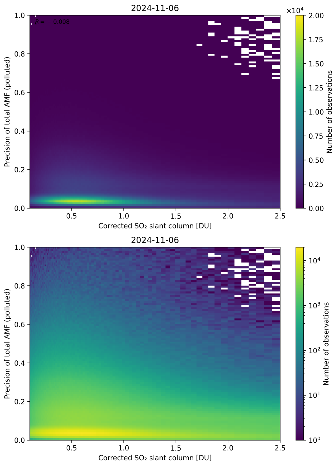
Figure 193: Scatter density plot of “Corrected SO 2 slant column” against “Precision of total AMF (polluted)” for 2024-11-05 to 2024-11-07.
