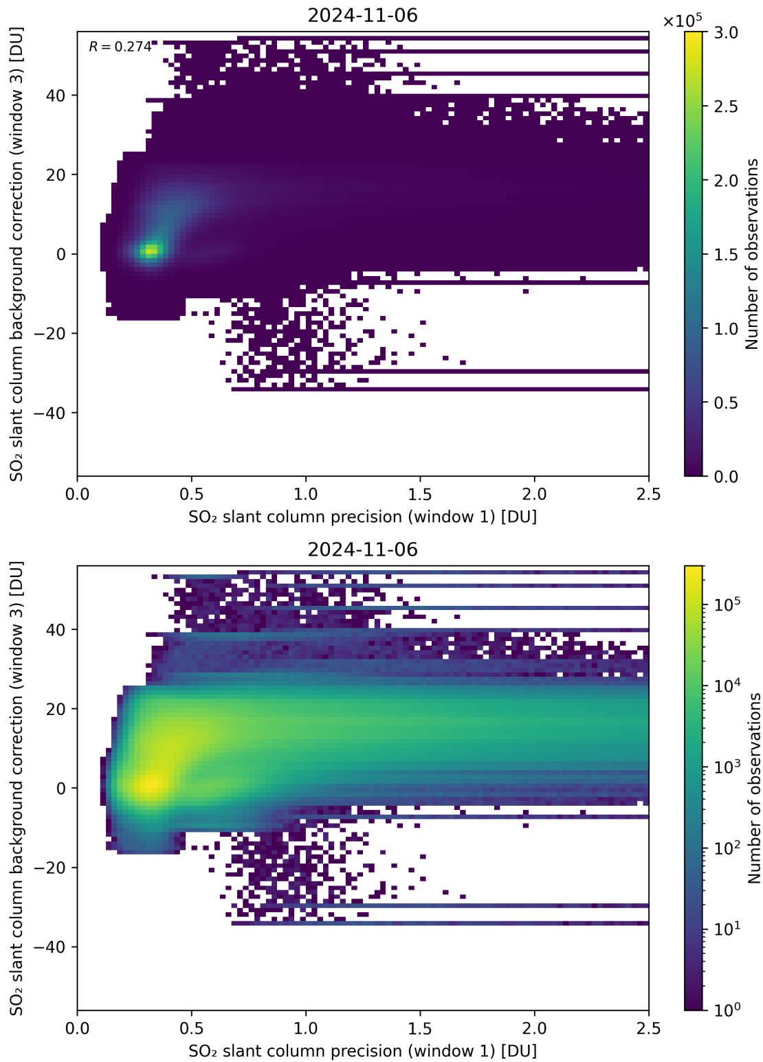
Figure 220: Scatter density plot of “SO 2 slant column precision (window 1)” against “SO 2 slant column background correction (window 3)” for 2024-11-05 to 2024-11-07.
