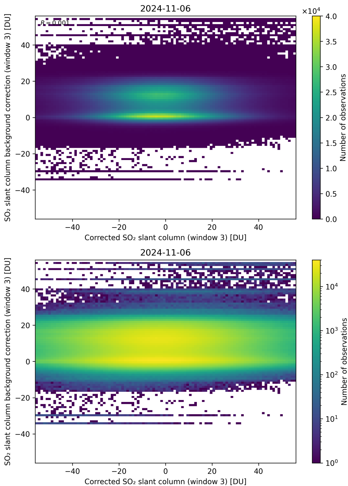
Figure 205: Scatter density plot of “Corrected SO 2 slant column (window 3)” against “SO 2 slant column background correction (window 3)” for 2024-11-05 to 2024-11-07.
