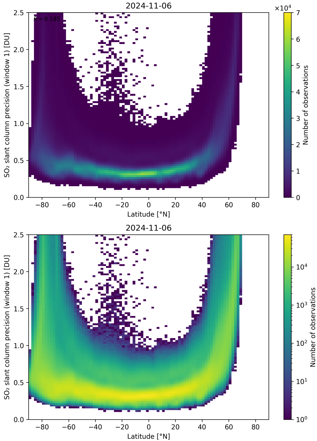
Figure 150: Scatter density plot of “Latitude” against “SO 2 slant column precision (window 1)” for 2024-11-05 to 2024-11-07.
