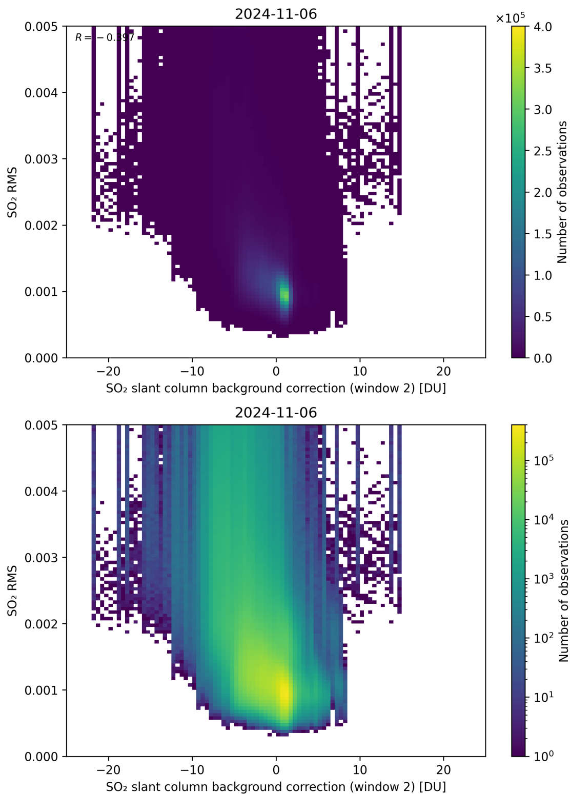
Figure 114: Scatter density plot of “SO 2 slant column background correction (window 2)” against “SO 2 RMS” for 2024-11-05 to 2024-11-07.
