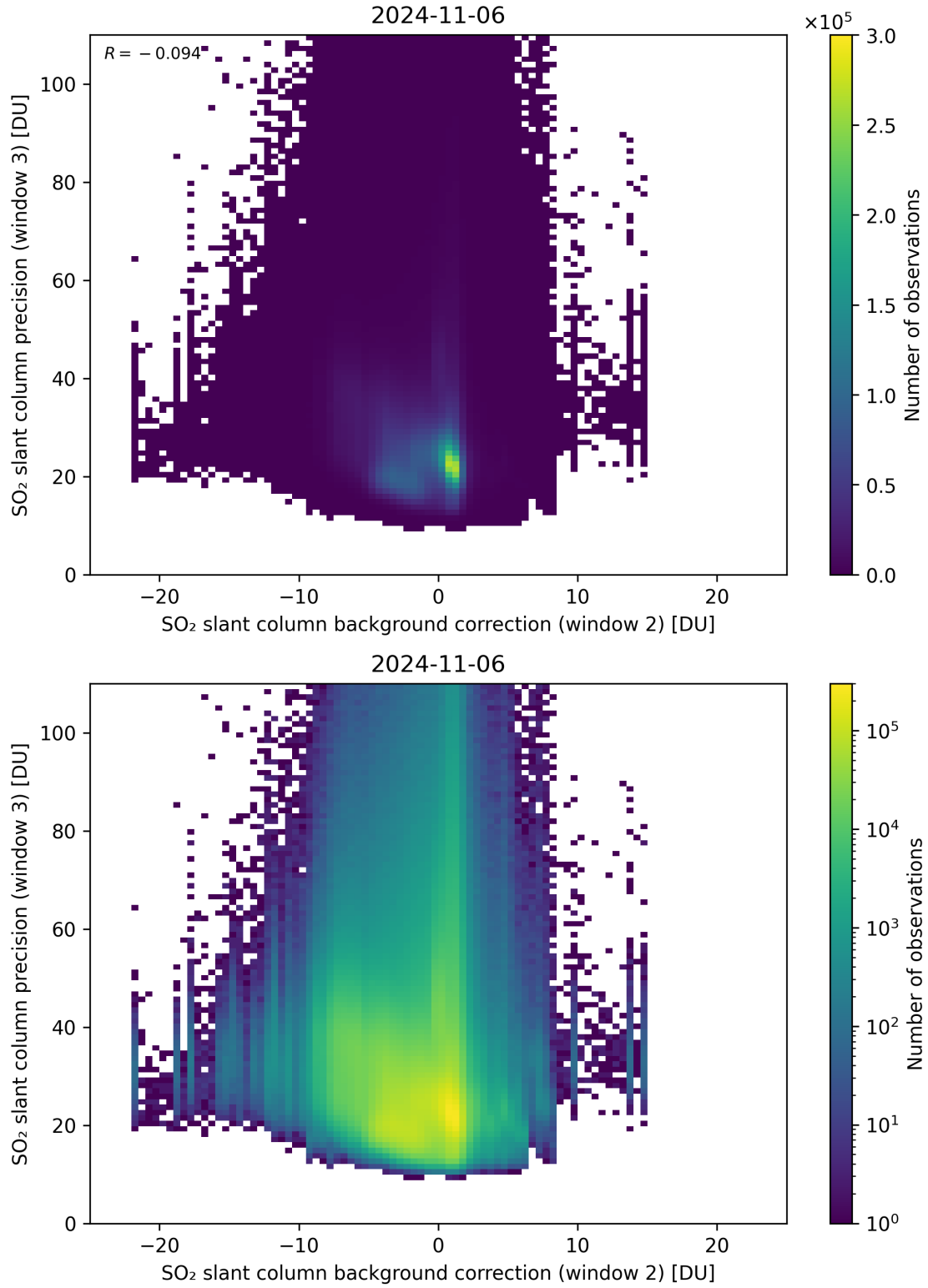
Figure 118: Scatter density plot of “SO 2 slant column background correction (window 2)” against “SO 2 slant column precision (window 3)” for 2024-11-05 to 2024-11-07.
