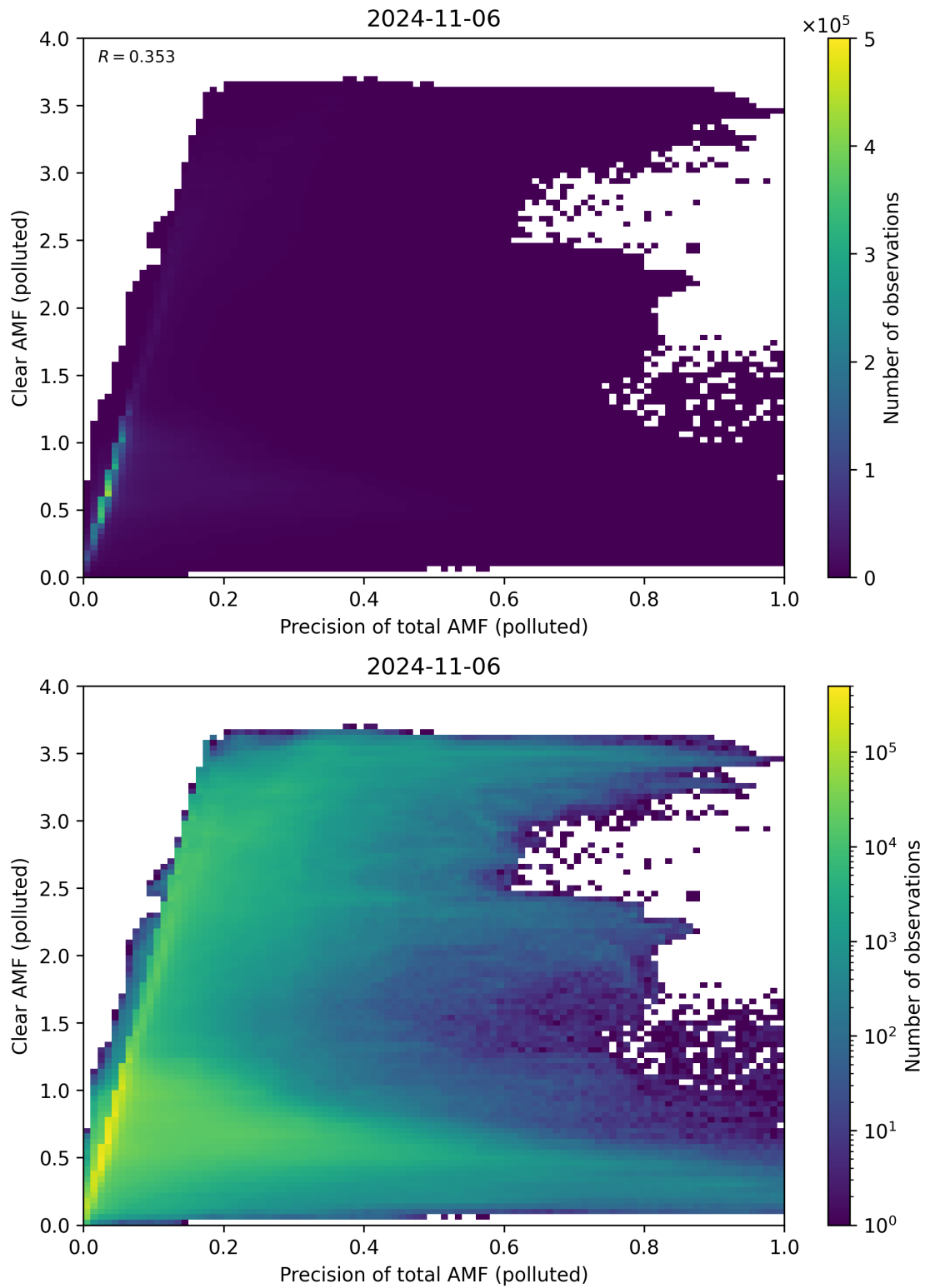
Figure 270: Scatter density plot of “Precision of total AMF (polluted)” against “Clear AMF (polluted)” for 2024-11-05 to 2024-11-07.
