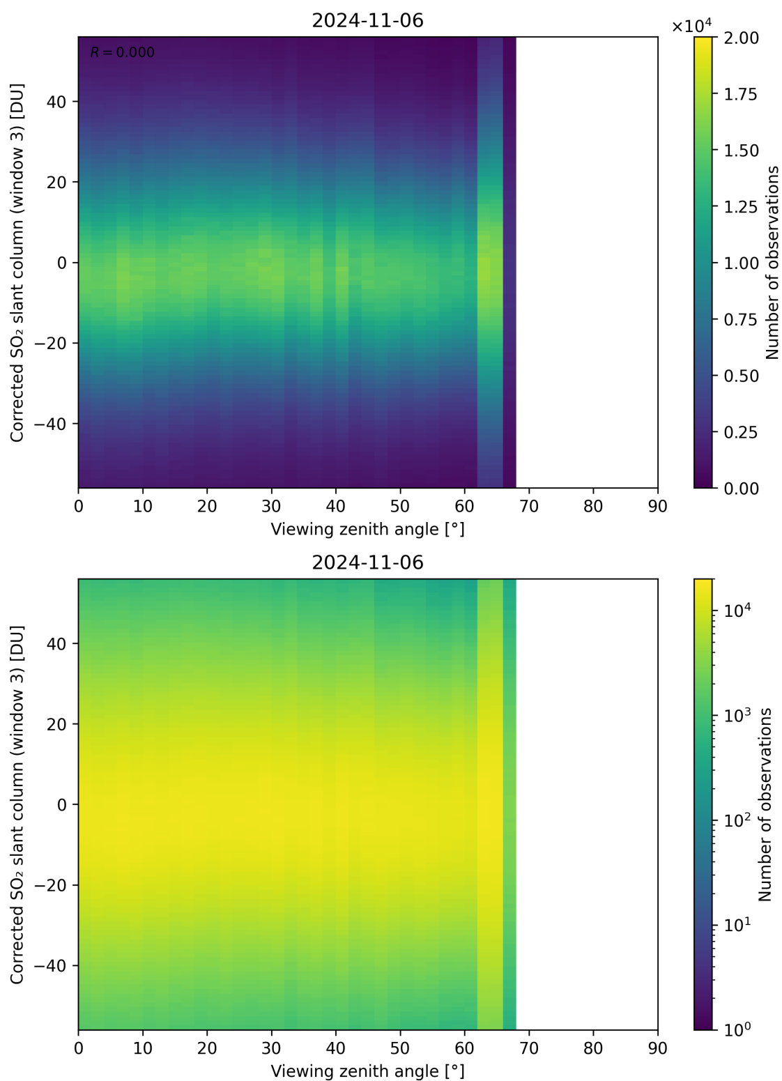
Figure 319: Scatter density plot of “Viewing zenith angle” against “Corrected SO 2 slant column (window 3)” for 2024-11-05 to 2024-11-07.
