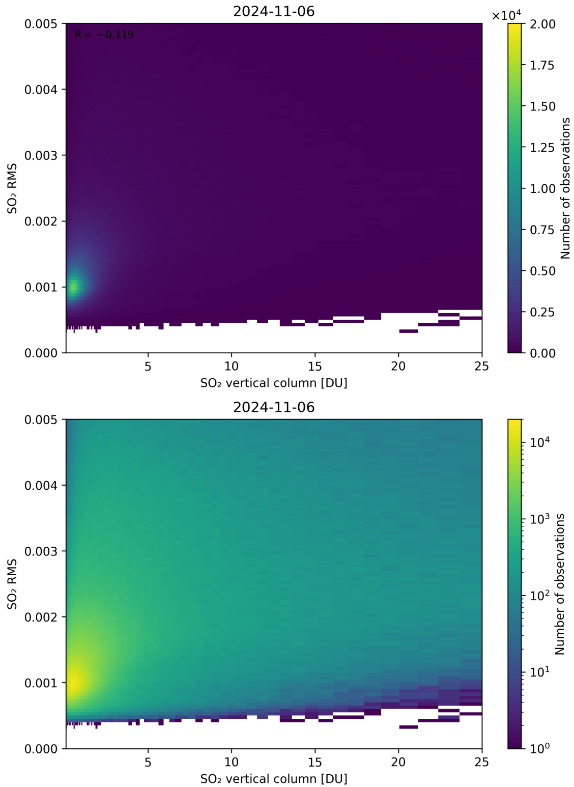
Figure 278: Scatter density plot of “SO 2 vertical column” against “SO 2 RMS” for 2024-11-05 to 2024-11-07.
