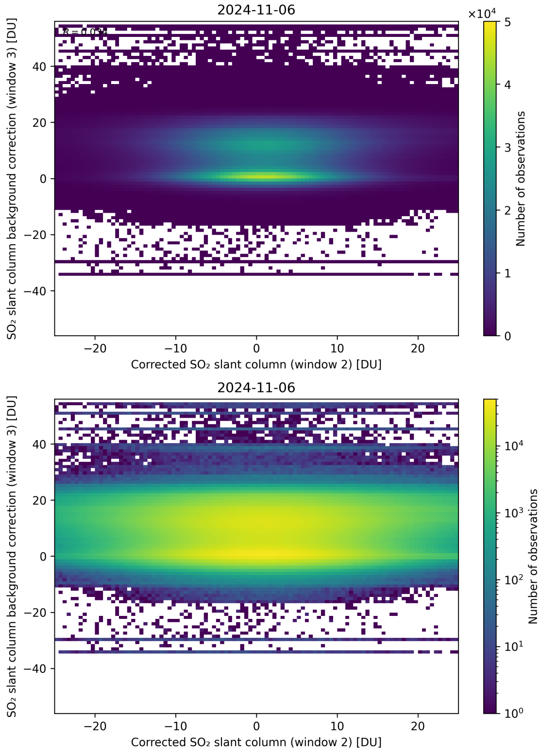
Figure 195: Scatter density plot of “Corrected SO 2 slant column (window 2)” against “SO 2 slant column background correction (window 3)” for 2024-11-05 to 2024-11-07.
