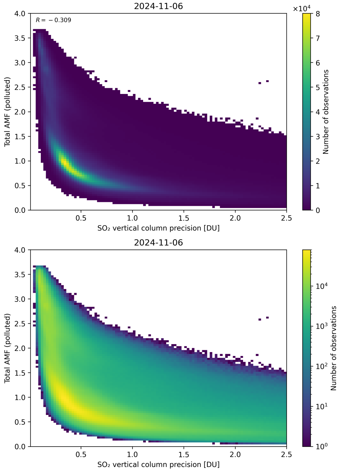
Figure 294: Scatter density plot of “SO 2 vertical column precision” against “Total AMF (polluted)” for 2024-11-05 to 2024-11-07.
