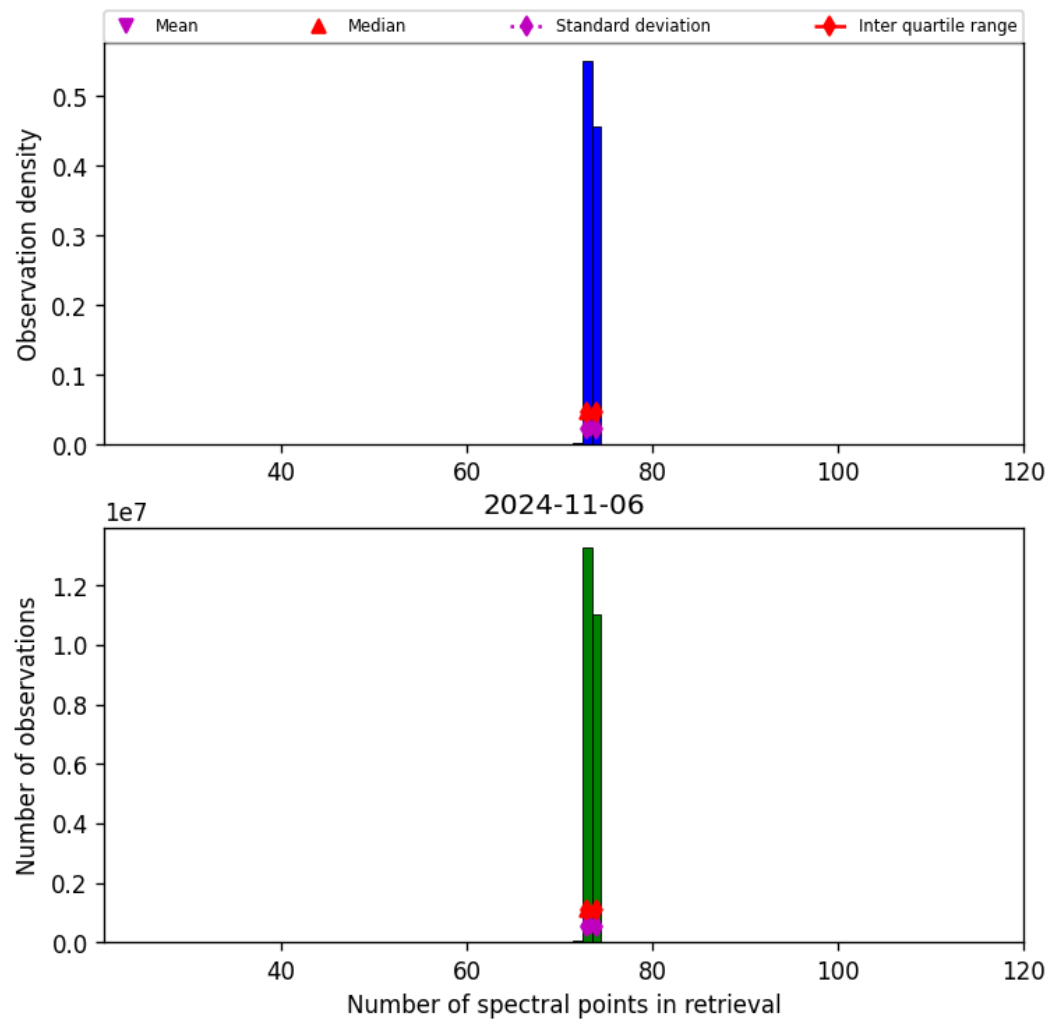
Figure 74: Histogram of “Number of spectral points in retrieval” for 2024-11-05 to 2024-11-07
