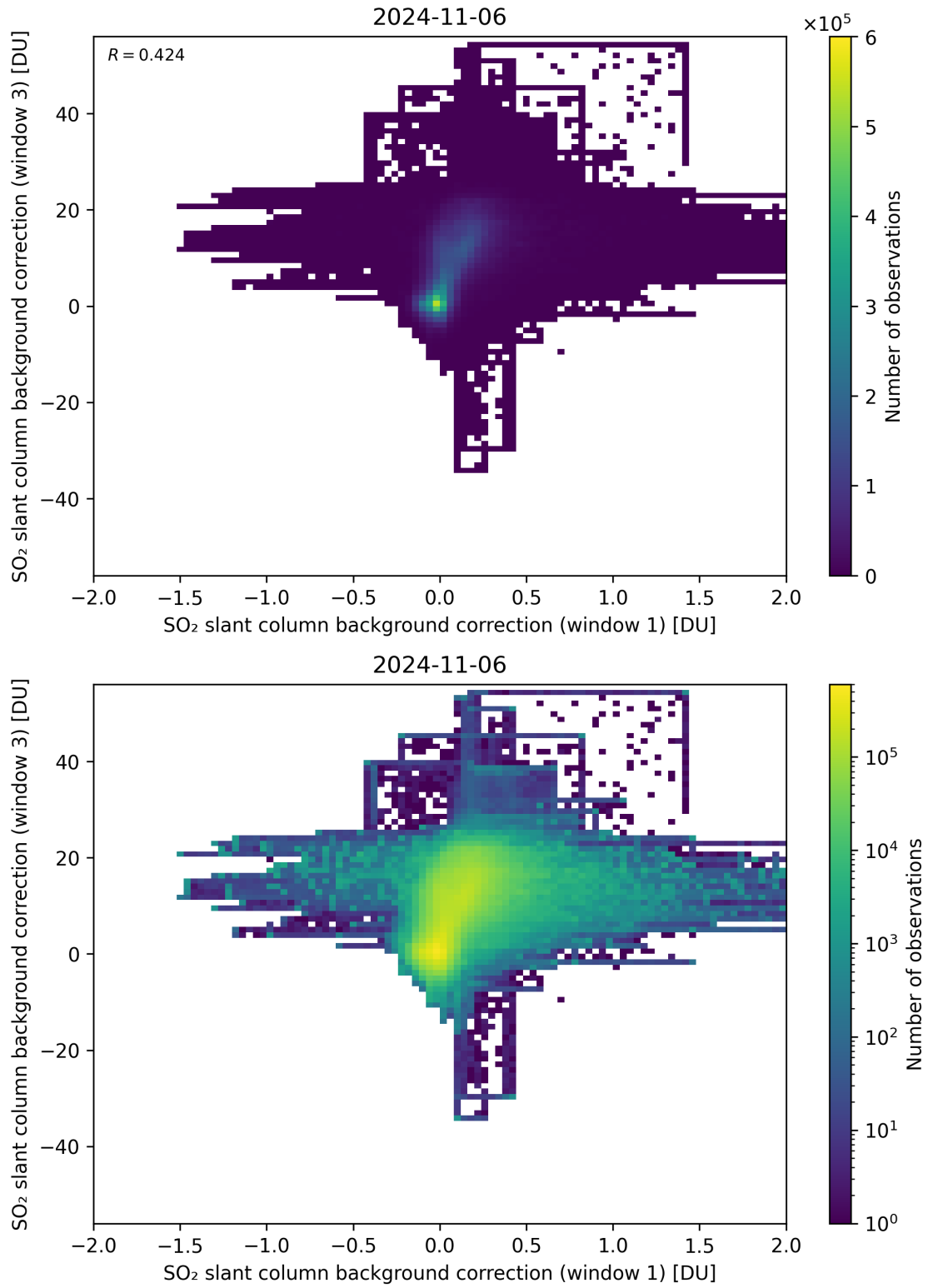
Figure 99: Scatter density plot of “SO 2 slant column background correction (window 1)” against “SO 2 slant column background correction (window 3)” for 2024-11-05 to 2024-11-07.
