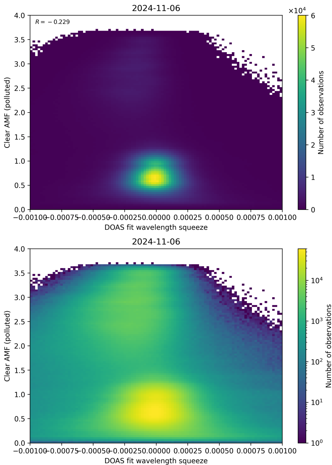
Figure 133: Scatter density plot of “DOAS fit wavelength squeeze” against “Clear AMF (polluted)” for 2024-11-05 to 2024-11-07.
