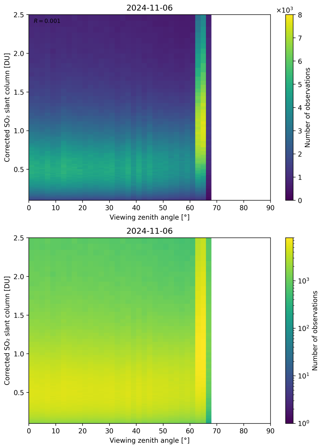
Figure 317: Scatter density plot of “Viewing zenith angle” against “Corrected SO 2 slant column” for 2024-11-05 to 2024-11-07.
