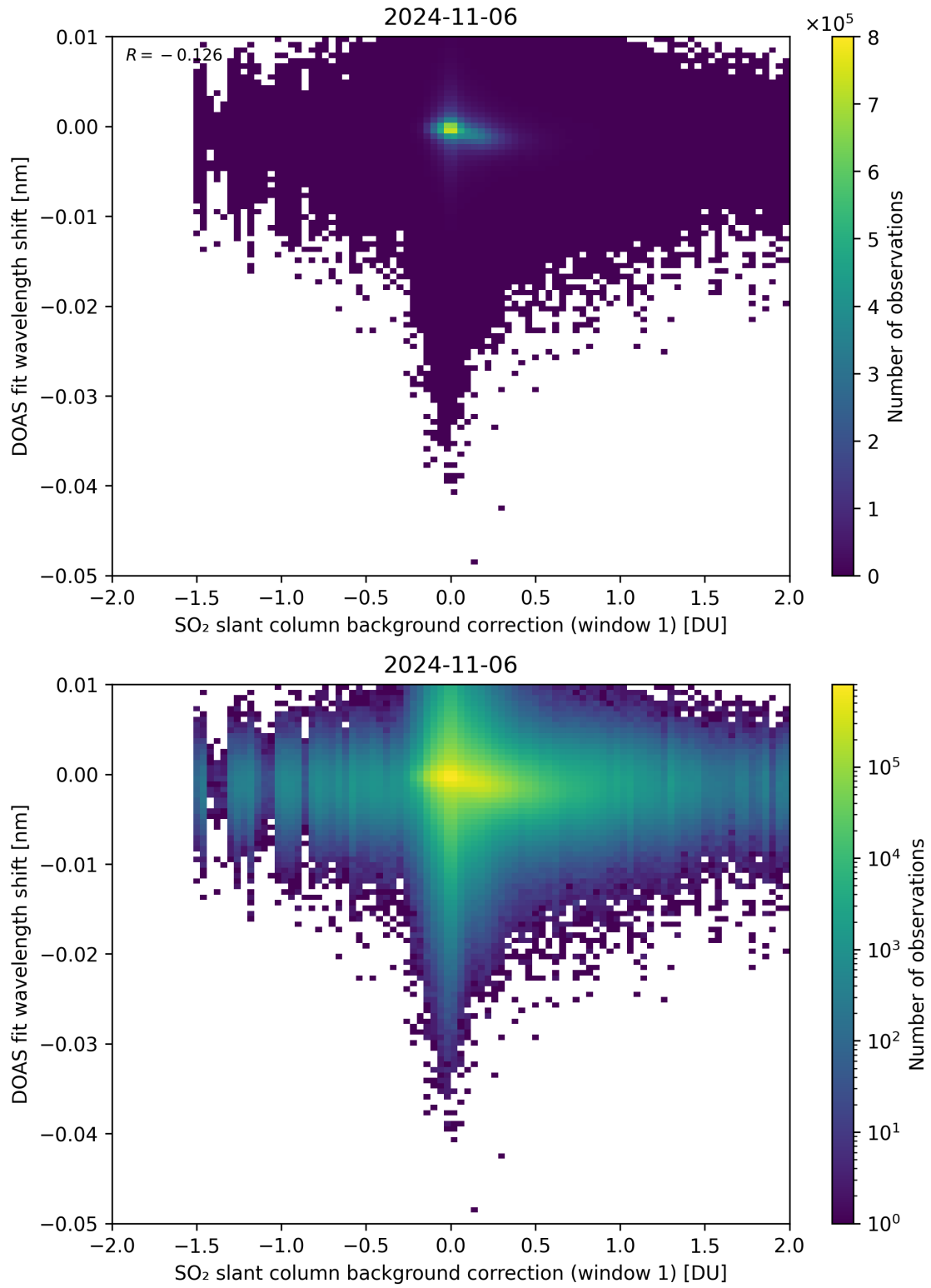
Figure 100: Scatter density plot of “SO 2 slant column background correction (window 1)” against “DOAS fit wavelength shift” for 2024-11-05 to 2024-11-07.
