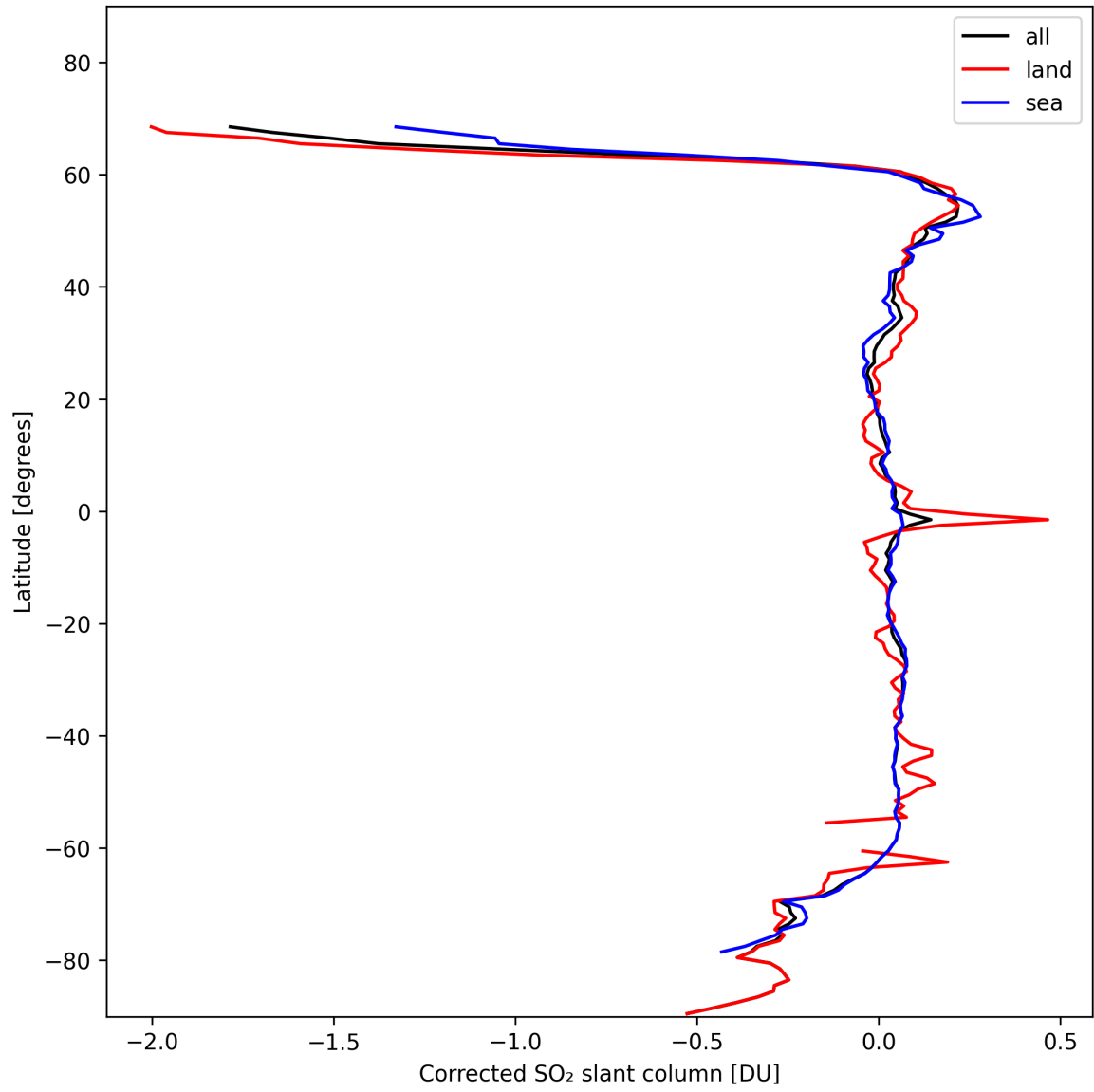
Figure 32: Zonal average of “Corrected SO 2 slant column” for 2024-11-05 to 2024-11-07.
