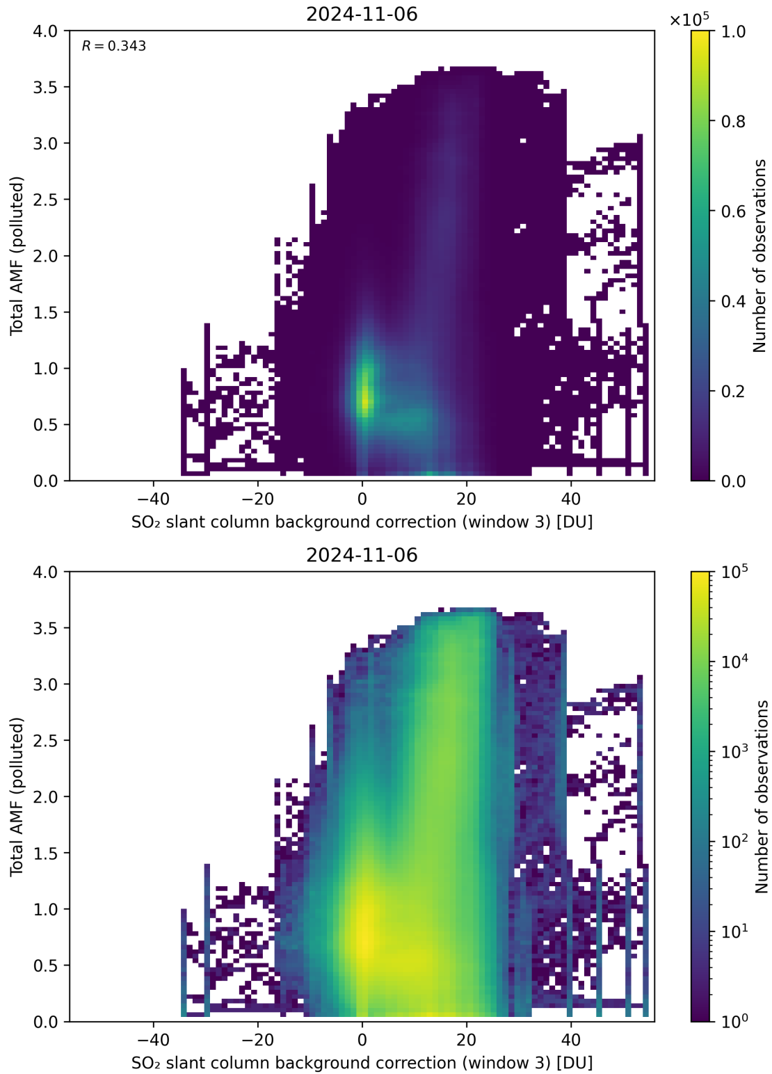
Figure 125: Scatter density plot of “SO 2 slant column background correction (window 3)” against “Total AMF (polluted)” for 2024-11-05 to 2024-11-07.
