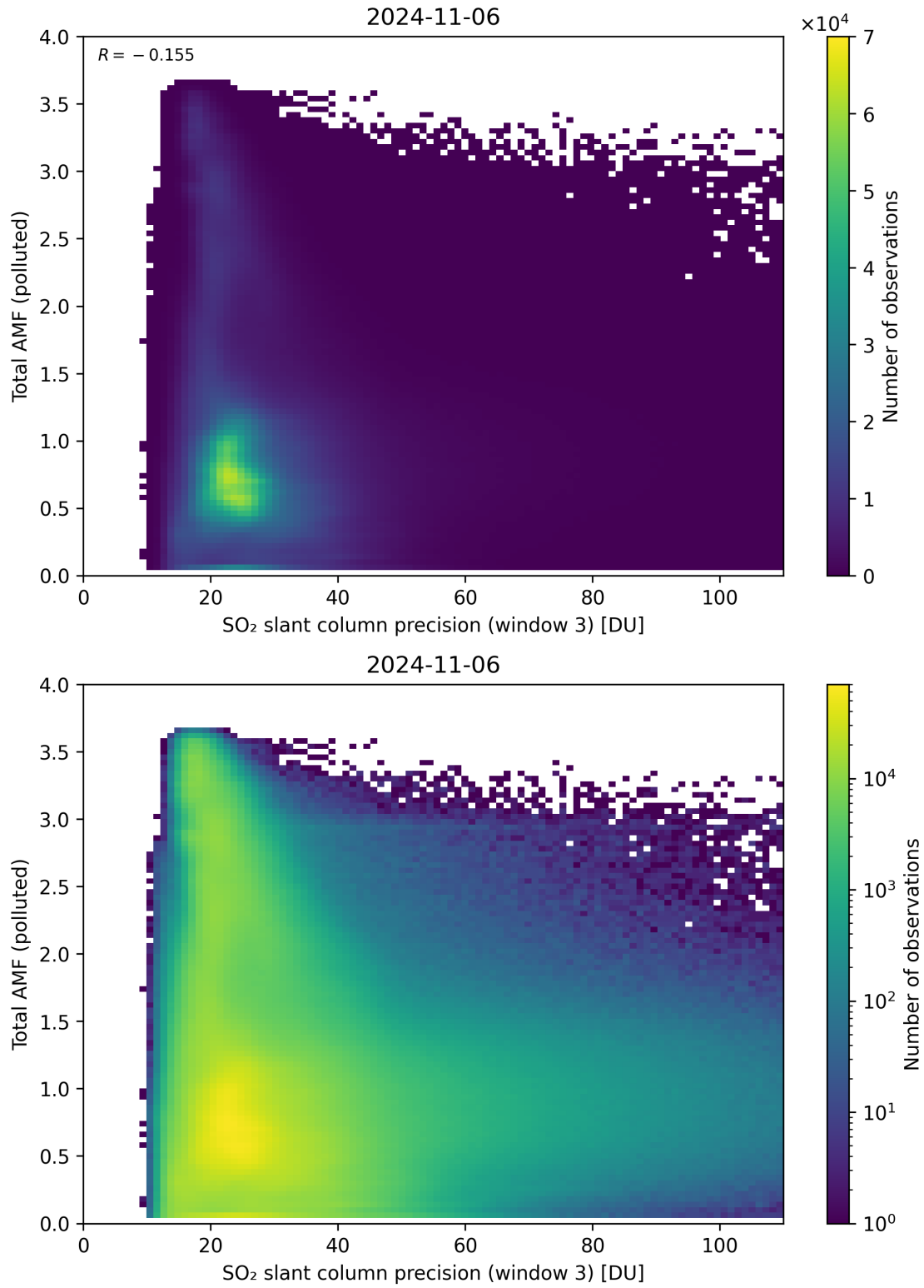
Figure 263: Scatter density plot of “SO 2 slant column precision (window 3)” against “Total AMF (polluted)” for 2024-11-05 to 2024-11-07.
