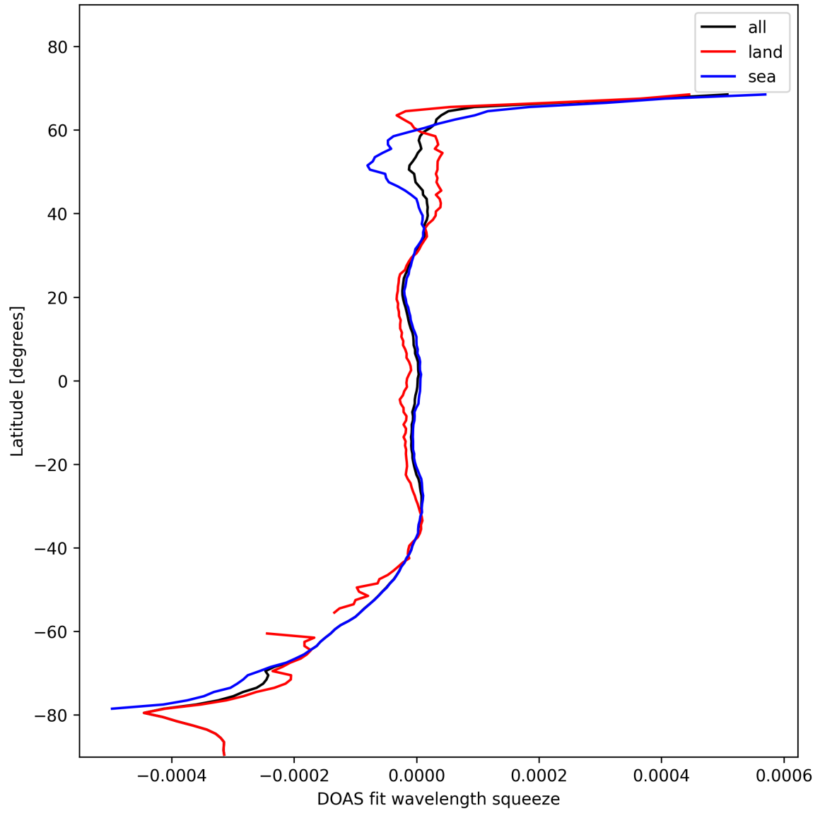
Figure 46: Zonal average of “DOAS fit wavelength squeeze” for 2024-11-05 to 2024-11-07.
