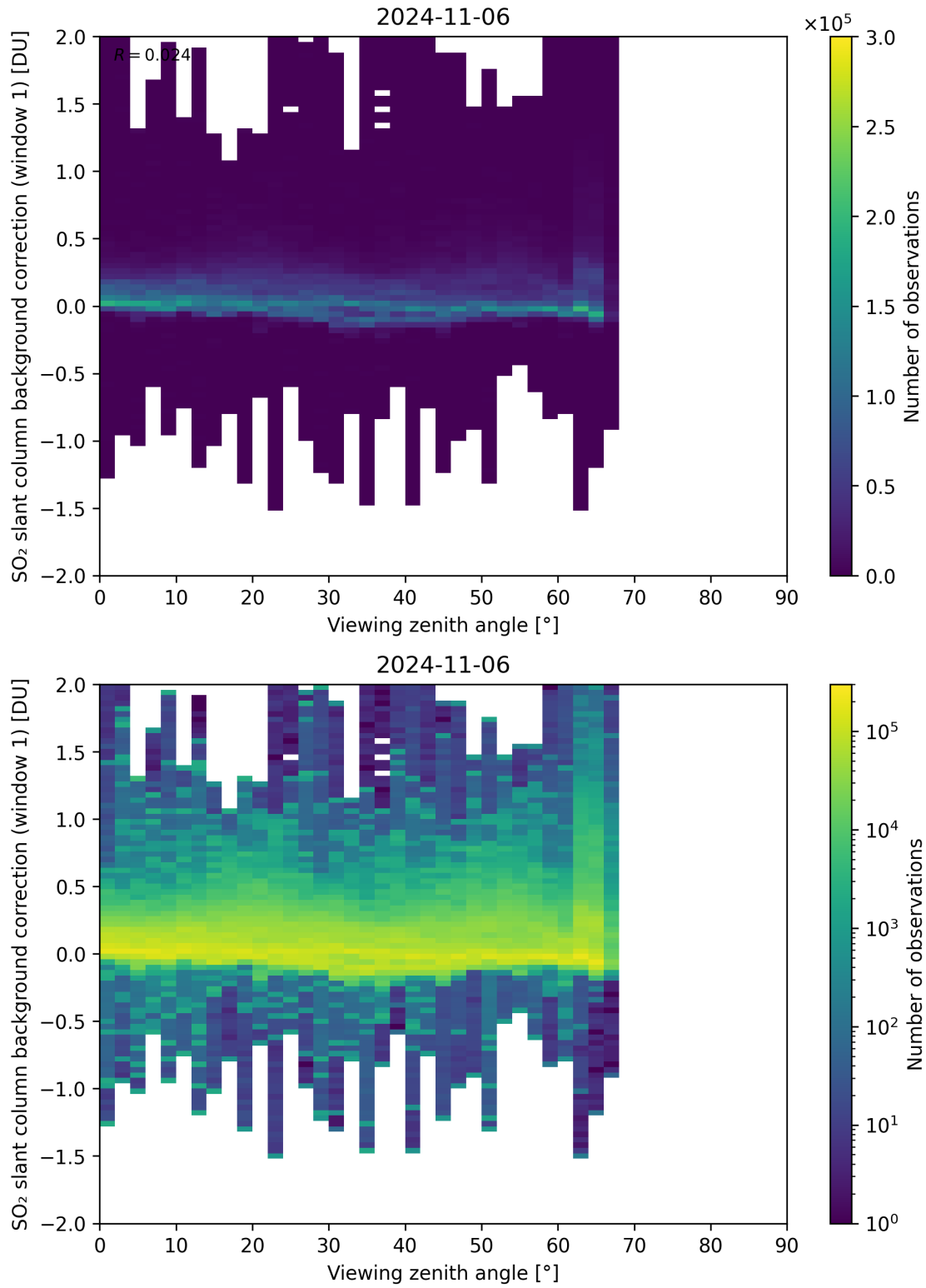
Figure 308: Scatter density plot of “Viewing zenith angle” against “SO 2 slant column background correction (window 1)” for 2024-11-05 to 2024-11-07.
