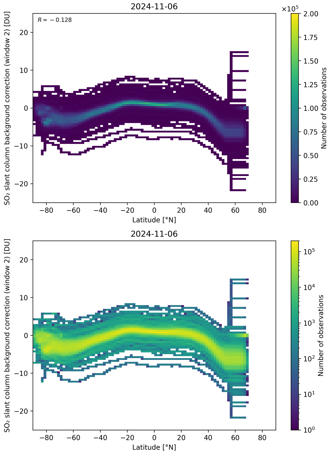
Figure 140: Scatter density plot of “Latitude” against “SO 2 slant column background correction (window 2)” for 2024-11-05 to 2024-11-07.
