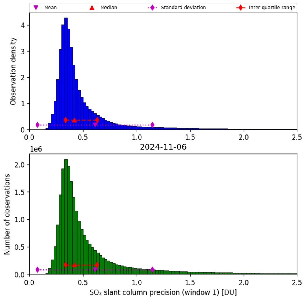
Figure 57: Histogram of “SO 2 slant column precision (window 1)” for 2024-11-05 to 2024-11-07
