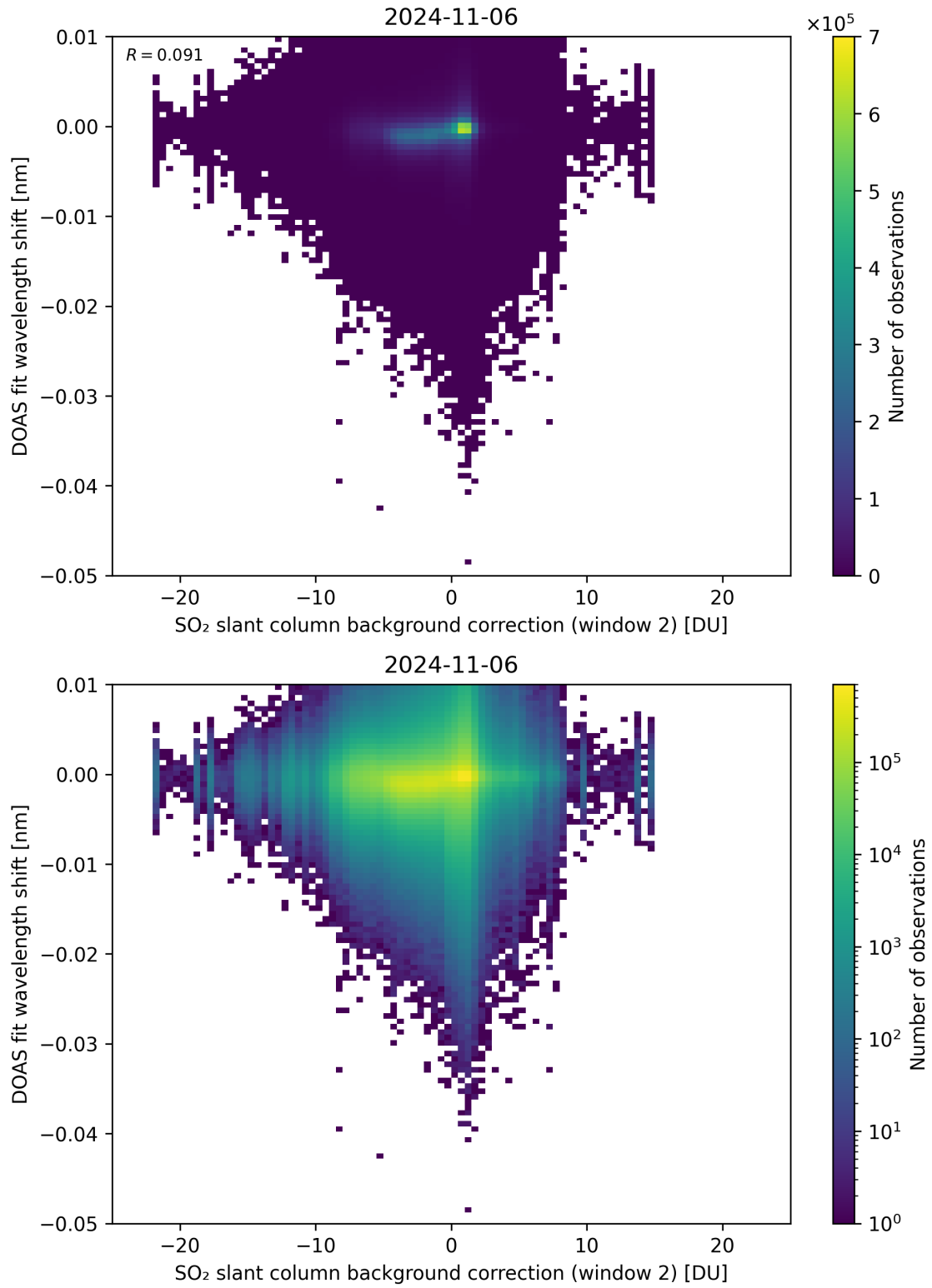
Figure 112: Scatter density plot of “SO 2 slant column background correction (window 2)” against “DOAS fit wavelength shift” for 2024-11-05 to 2024-11-07.
