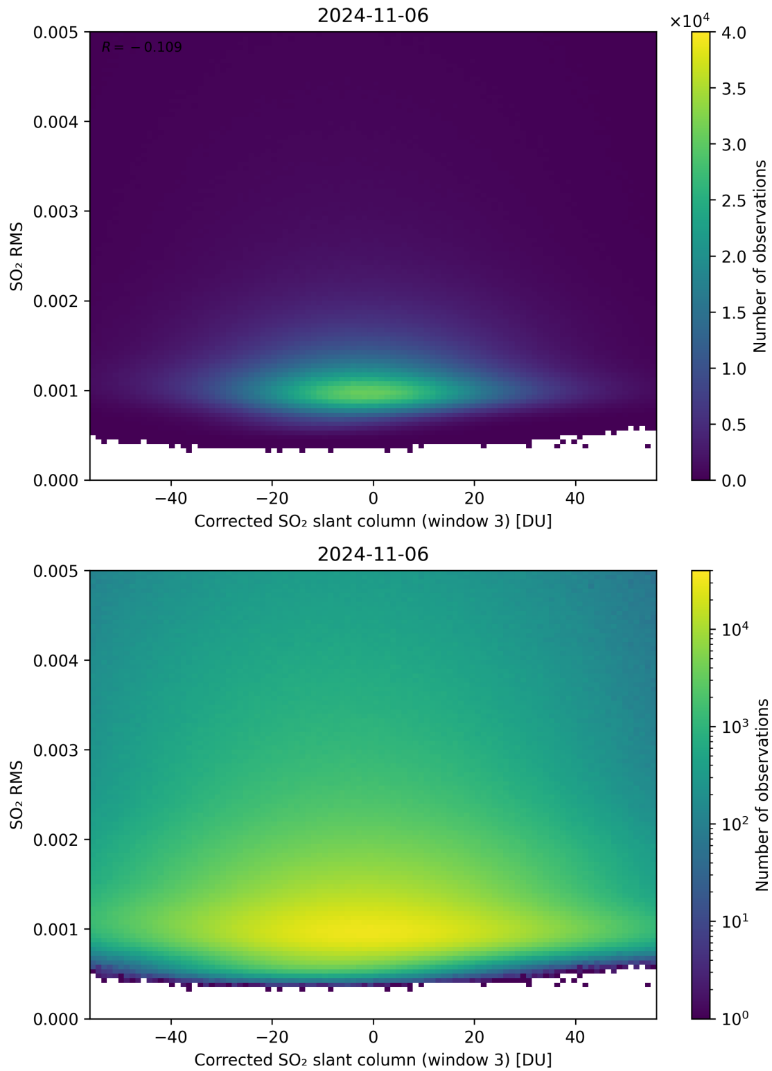
Figure 208: Scatter density plot of “Corrected SO 2 slant column (window 3)” against “SO 2 RMS” for 2024-11-05 to 2024-11-07.
