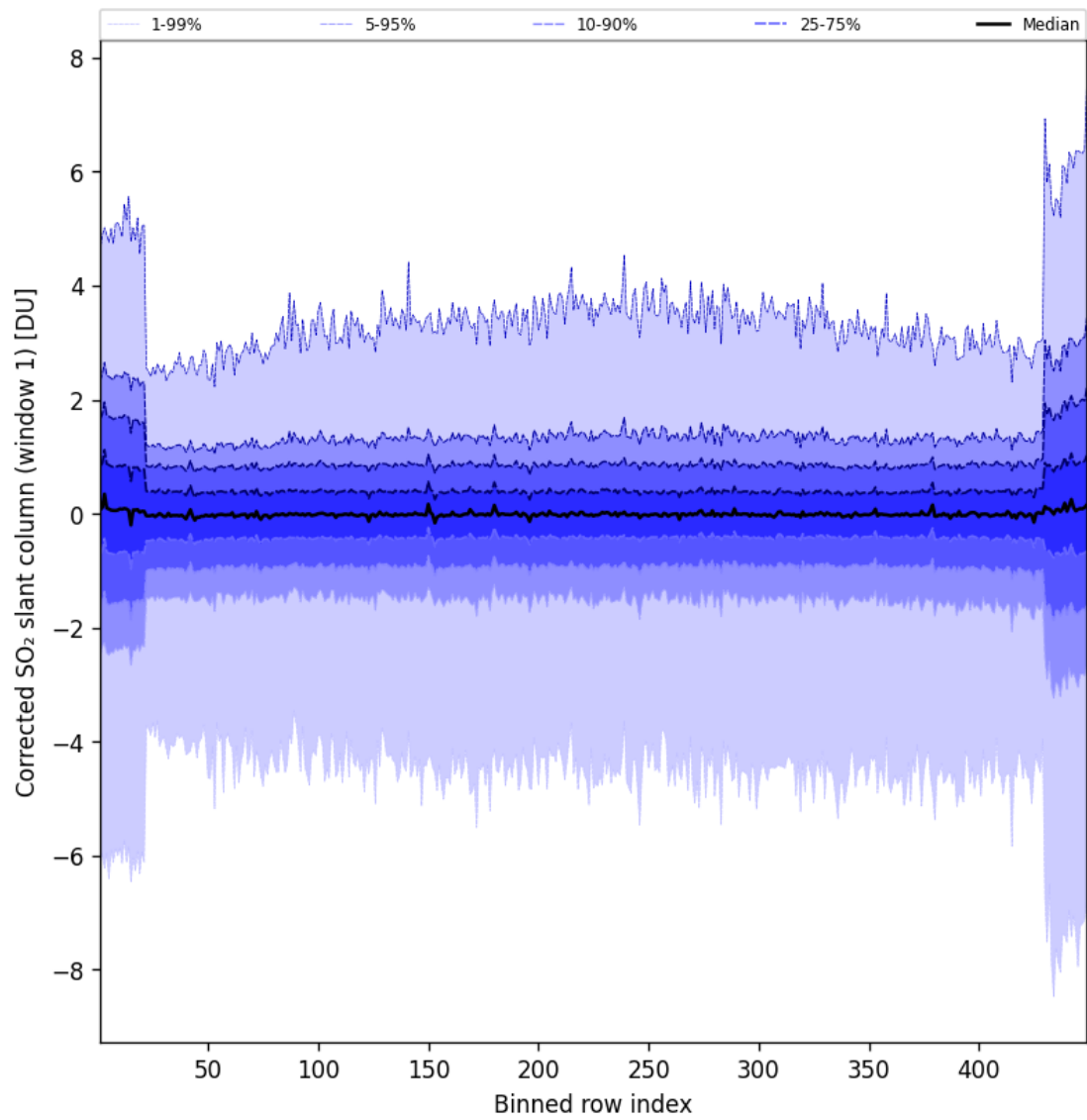
Figure 81: Along track statistics of “Corrected SO 2 slant column (window 1)” for 2024-11-05 to 2024-11-07
