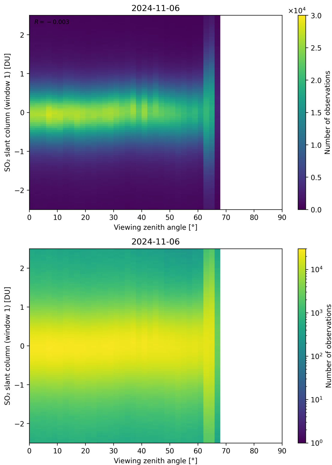
Figure 320: Scatter density plot of “Viewing zenith angle” against “SO 2 slant column (window 1)” for 2024-11-05 to 2024-11-07.
