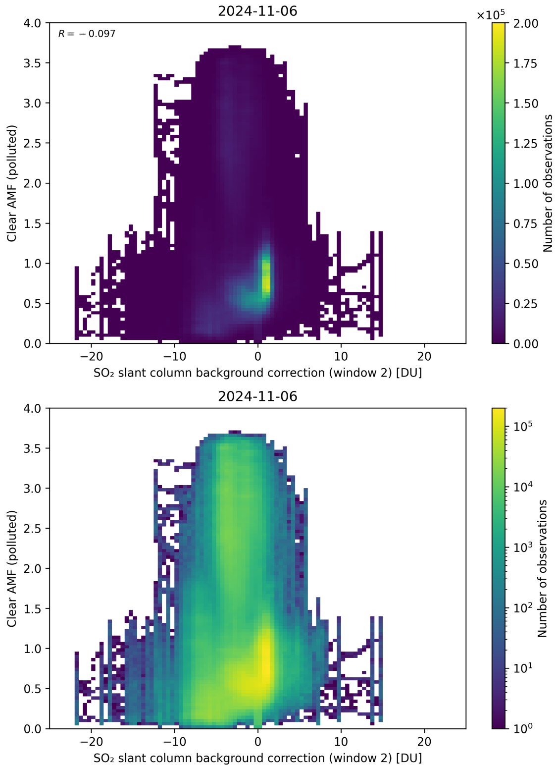
Figure 115: Scatter density plot of “SO 2 slant column background correction (window 2)” against “Clear AMF (polluted)” for 2024-11-05 to 2024-11-07.
