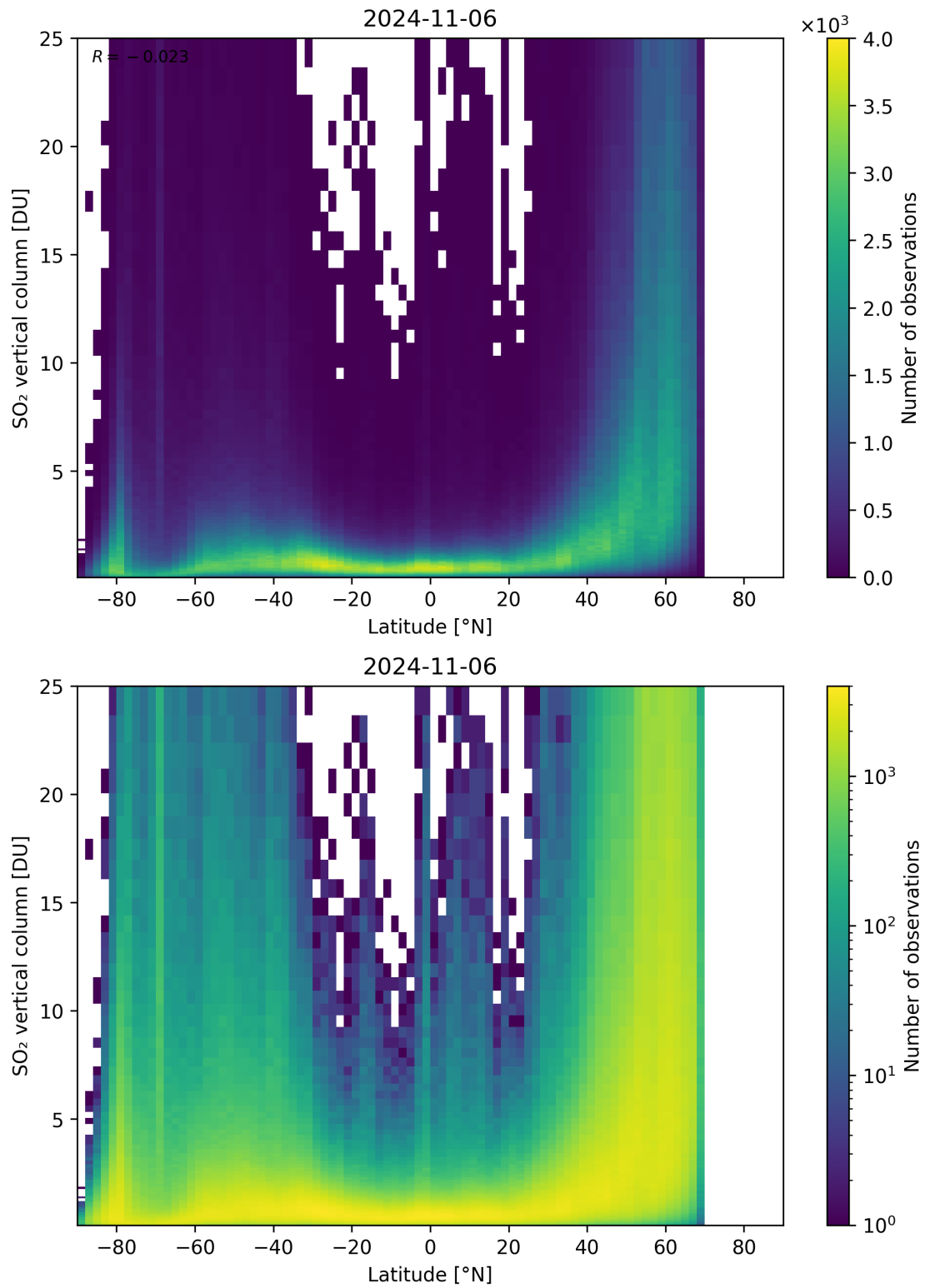
Figure 156: Scatter density plot of “Latitude” against “SO 2 vertical column” for 2024-11-05 to 2024-11-07.
