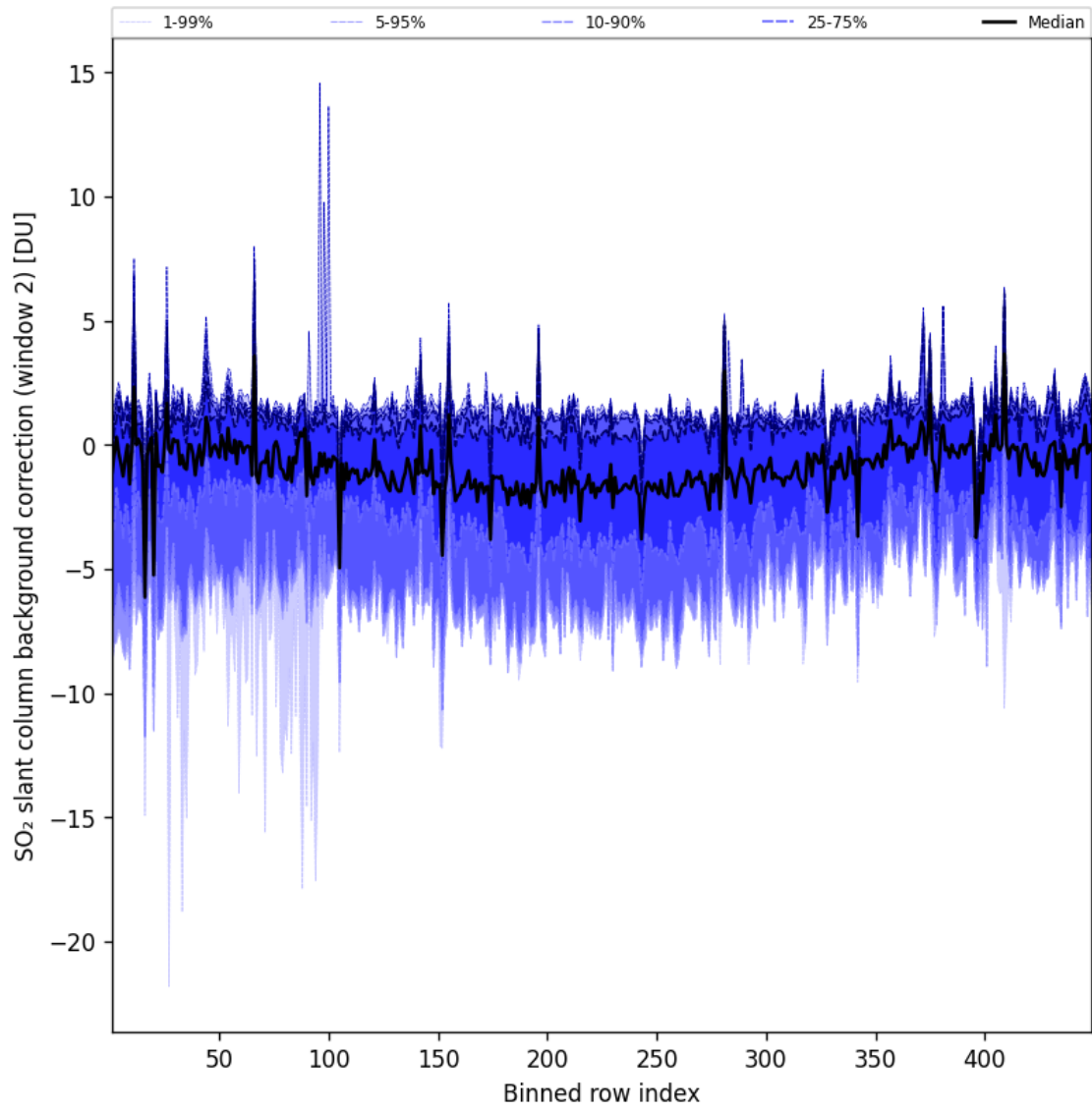
Figure 86: Along track statistics of “SO 2 slant column background correction (window 2)” for 2024-11-05 to 2024-11-07
