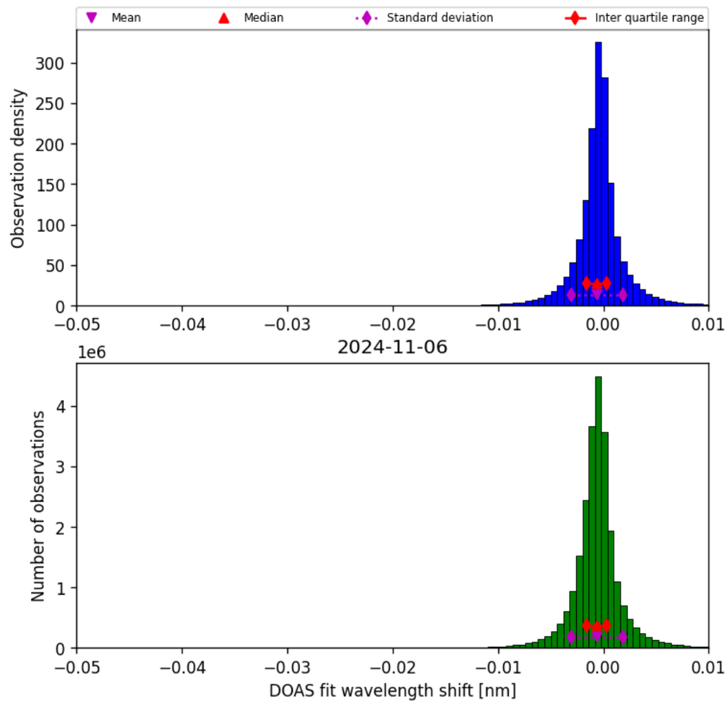
Figure 68: Histogram of “DOAS fit wavelength shift” for 2024-11-05 to 2024-11-07
