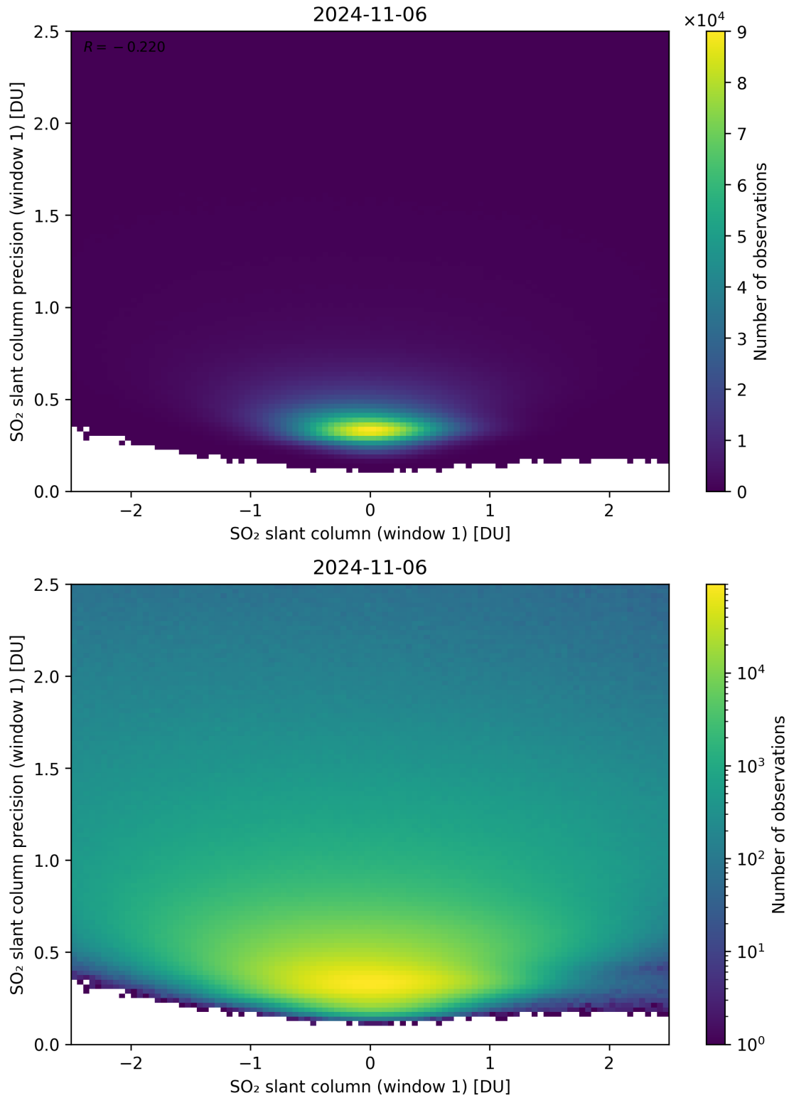
Figure 235: Scatter density plot of “SO 2 slant column (window 1)” against “SO 2 slant column precision (window 1)” for 2024-11-05 to 2024-11-07.
