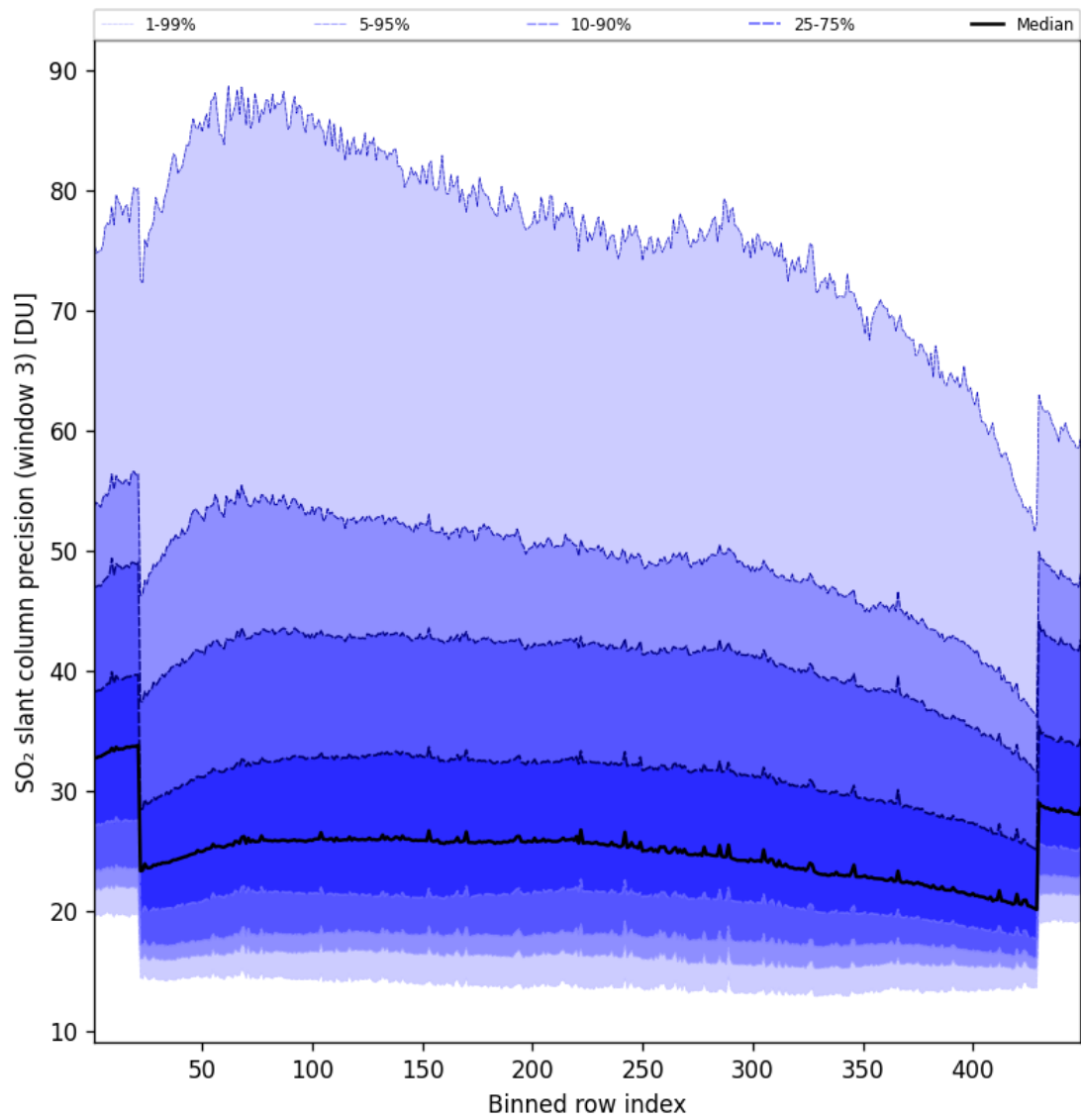
Figure 88: Along track statistics of “SO 2 slant column precision (window 3)” for 2024-11-05 to 2024-11-07
