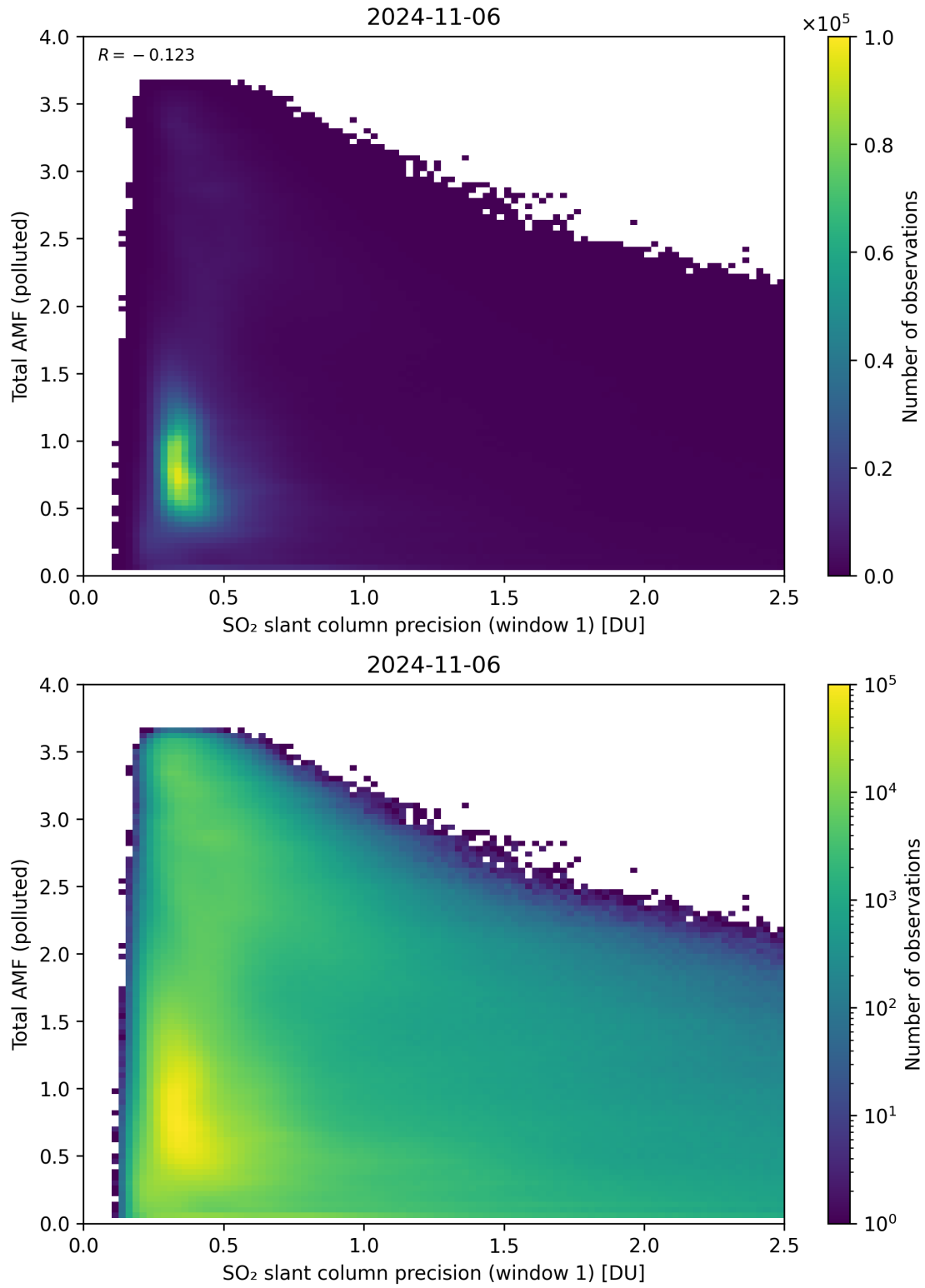
Figure 230: Scatter density plot of “SO 2 slant column precision (window 1)” against “Total AMF (polluted)” for 2024-11-05 to 2024-11-07.
