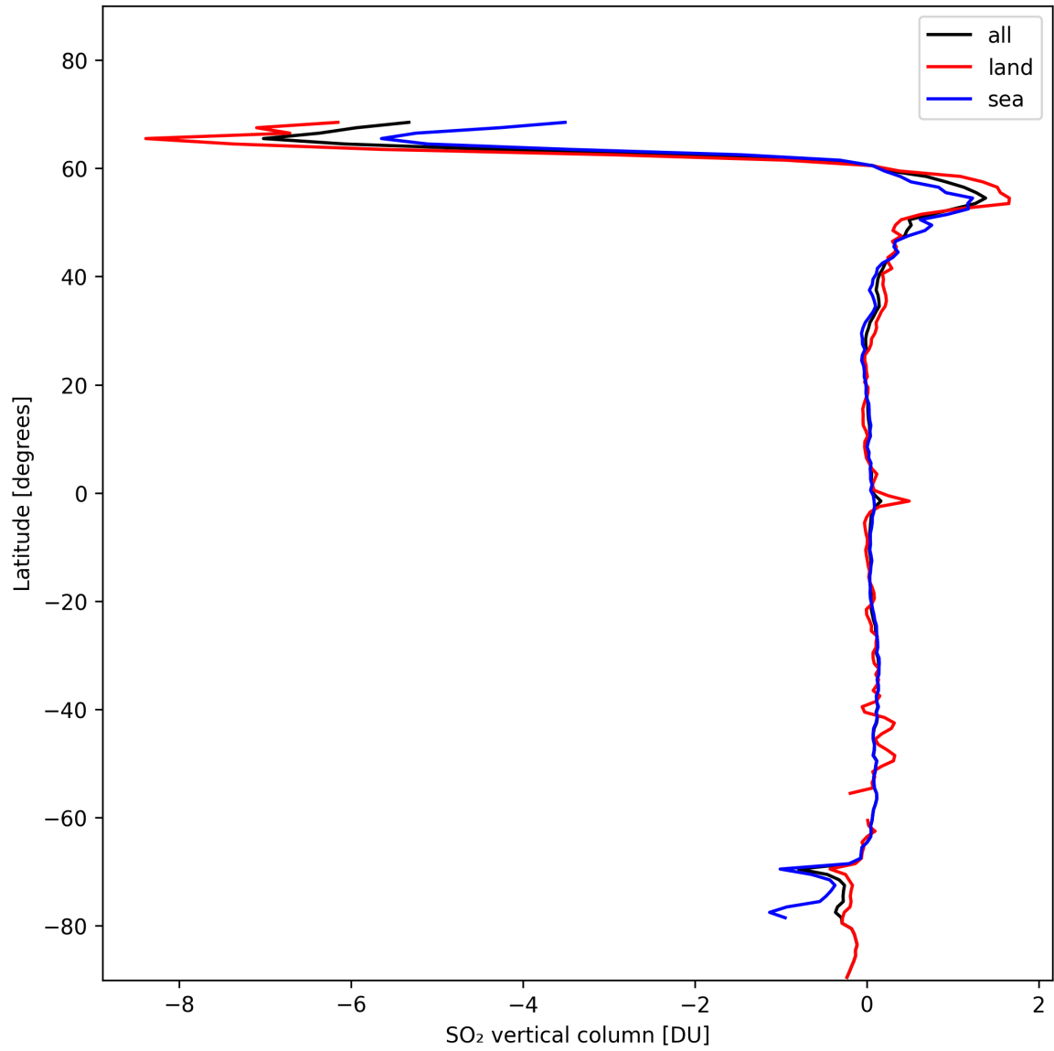
Figure 30: Zonal average of “SO 2 vertical column” for 2024-11-05 to 2024-11-07.
