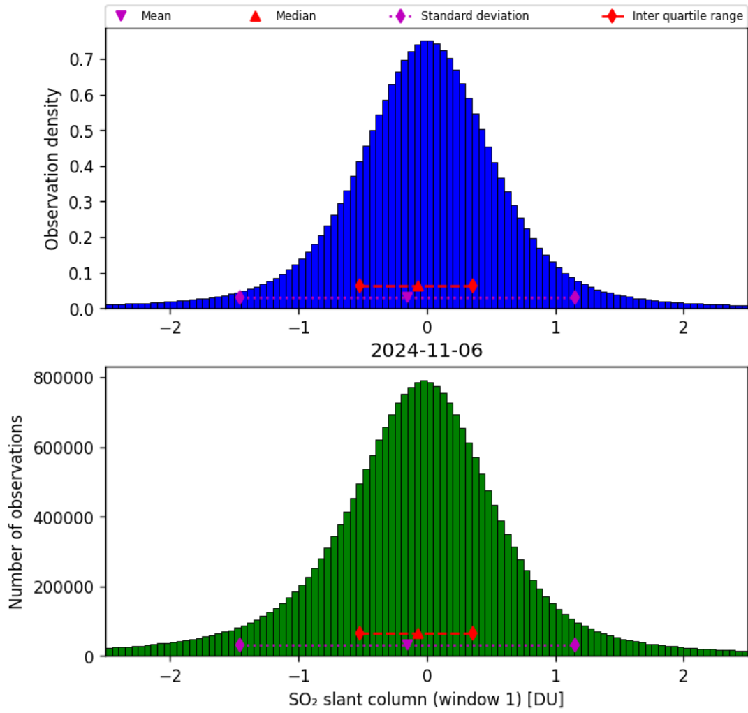
Figure 56: Histogram of “SO 2 slant column (window 1)” for 2024-11-05 to 2024-11-07
