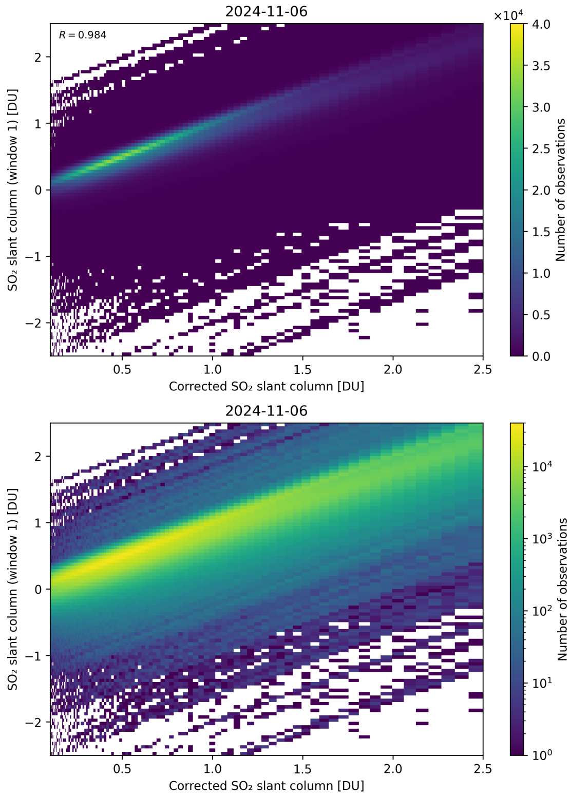
Figure 187: Scatter density plot of “Corrected SO 2 slant column” against “SO 2 slant column (window 1)” for 2024-11-05 to 2024-11-07.
