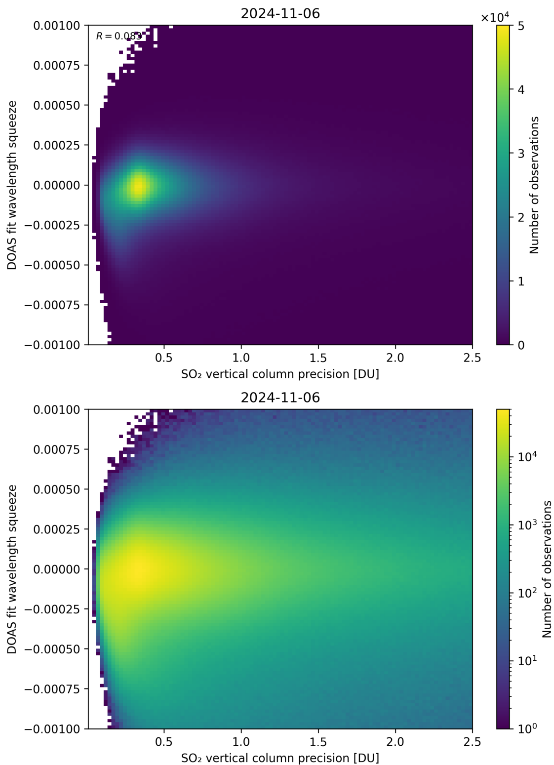
Figure 283: Scatter density plot of “SO 2 vertical column precision” against “DOAS fit wavelength squeeze” for 2024-11-05 to 2024-11-07.
