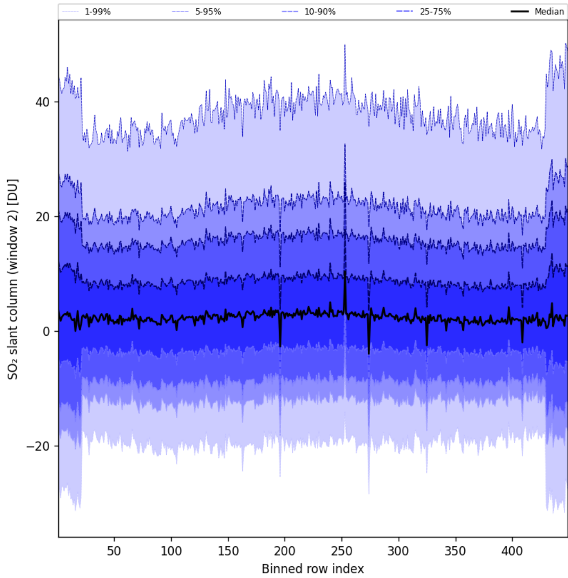
Figure 83: Along track statistics of “SO 2 slant column (window 2)” for 2024-11-05 to 2024-11-07
