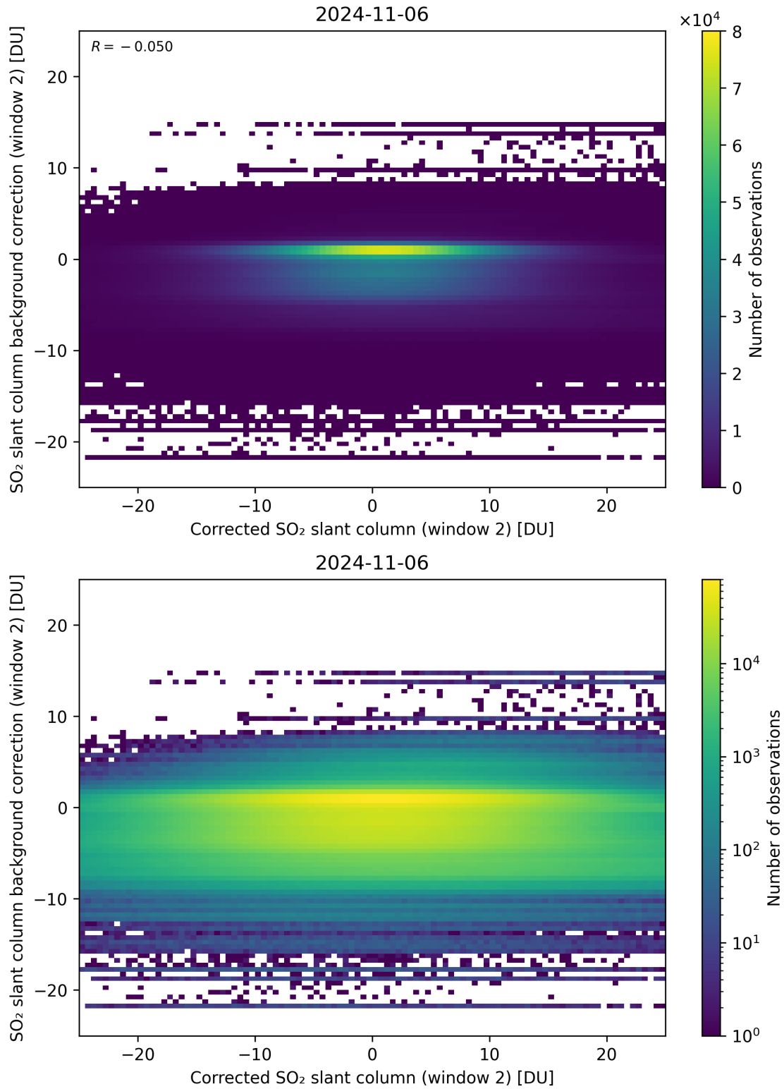
Figure 194: Scatter density plot of “Corrected SO 2 slant column (window 2)” against “SO 2 slant column background correction (window 2)” for 2024-11-05 to 2024-11-07.
