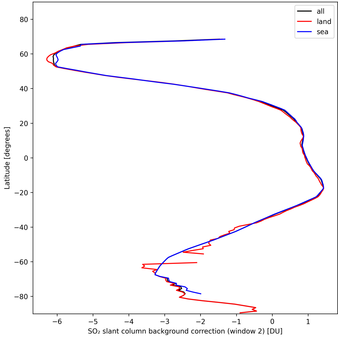
Figure 40: Zonal average of "SO 2 slant column background correction (window 2)" for 2024-11-05 to 2024-11-07.
