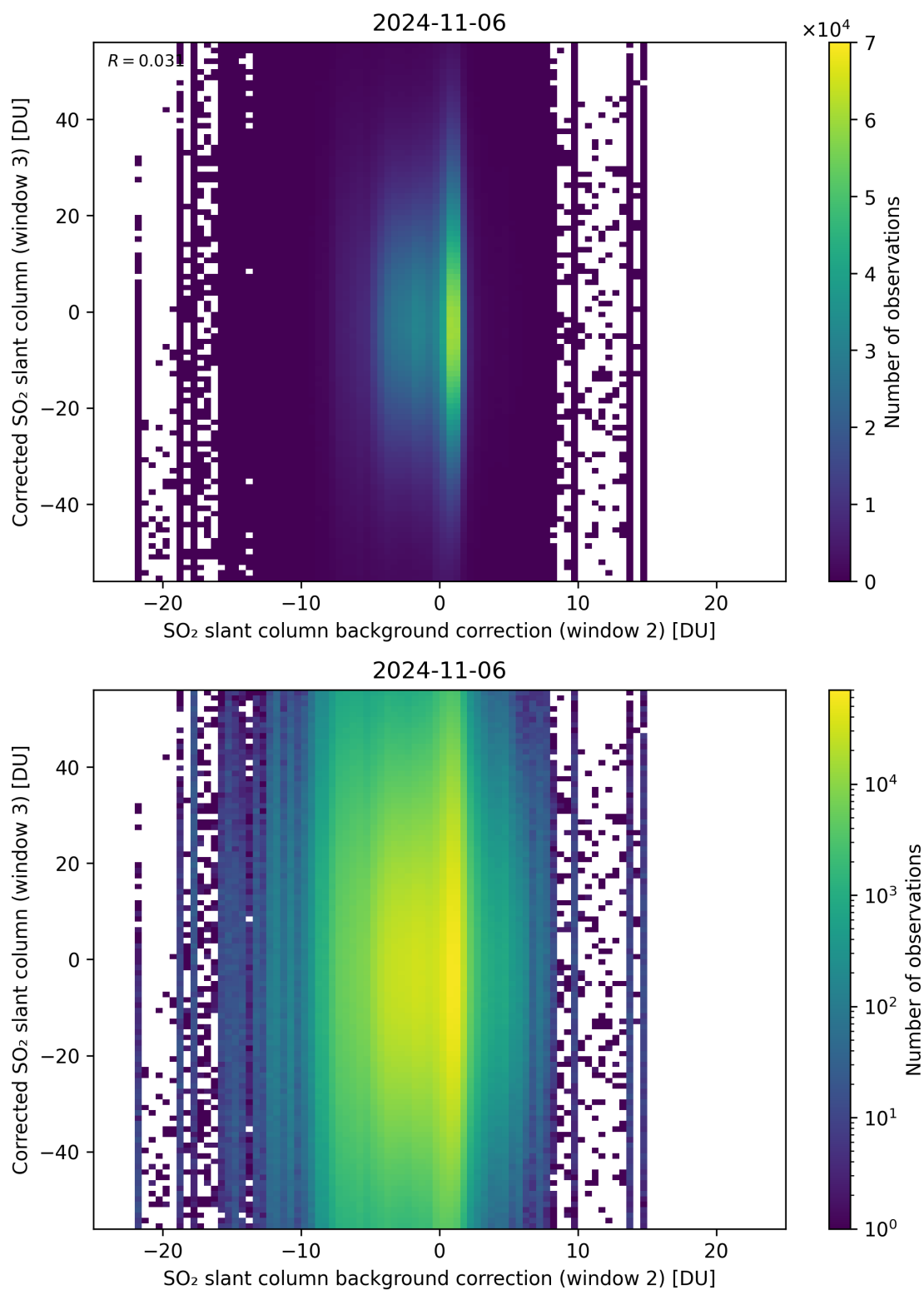
Figure 116: Scatter density plot of “SO 2 slant column background correction (window 2)” against “Corrected SO 2 slant column (window 3)” for 2024-11-05 to 2024-11-07.
