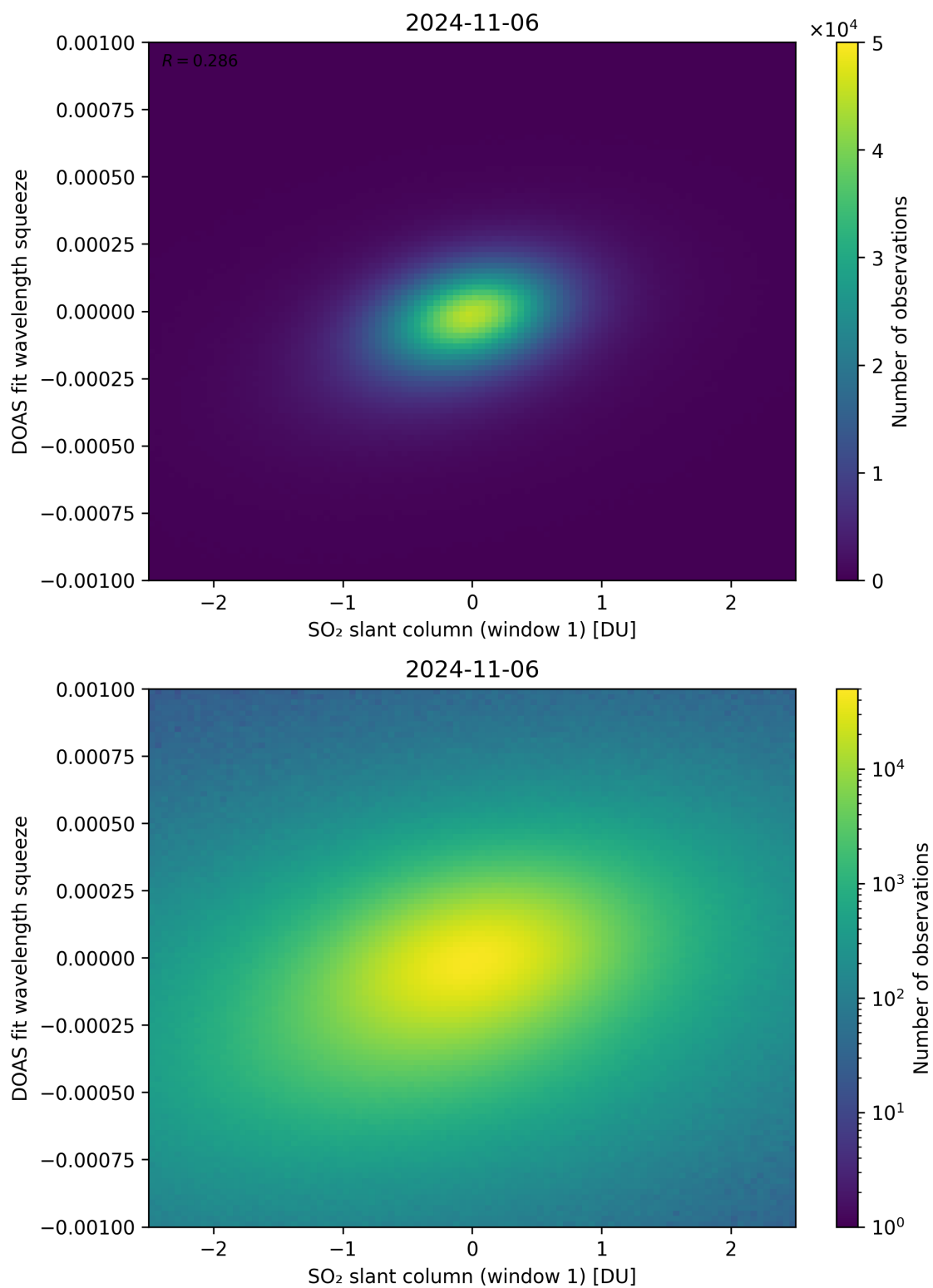
Figure 216: Scatter density plot of “SO 2 slant column (window 1)” against “DOAS fit wavelength squeeze” for 2024-11-05 to 2024-11-07.
