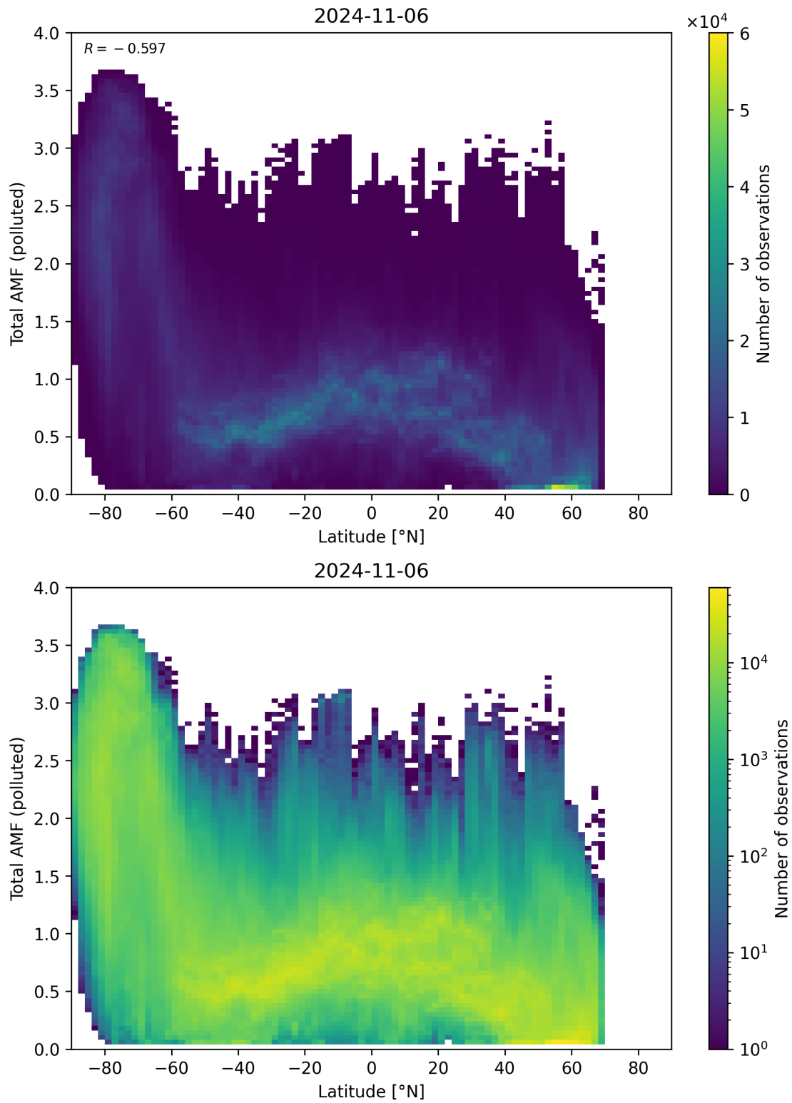
Figure 154: Scatter density plot of “Latitude” against “Total AMF (polluted)” for 2024-11-05 to 2024-11-07.
