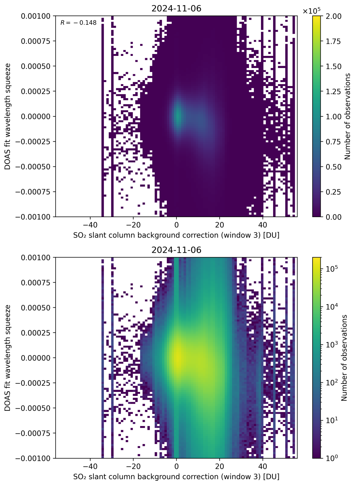
Figure 122: Scatter density plot of “SO 2 slant column background correction (window 3)” against “DOAS fit wavelength squeeze” for 2024-11-05 to 2024-11-07.
