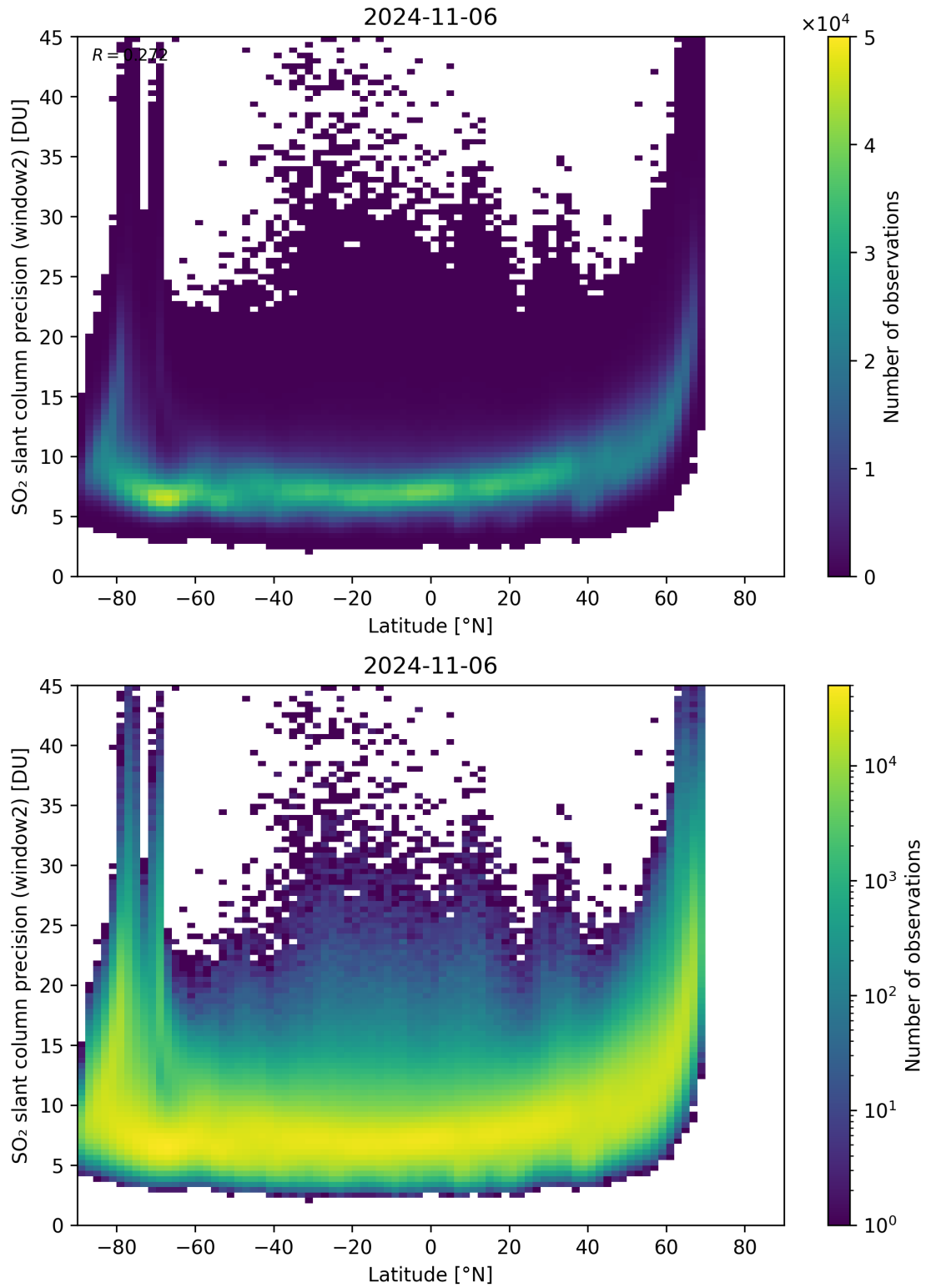
Figure 151: Scatter density plot of “Latitude” against “SO 2 slant column precision (window2)” for 2024-11-05 to 2024-11-07.
