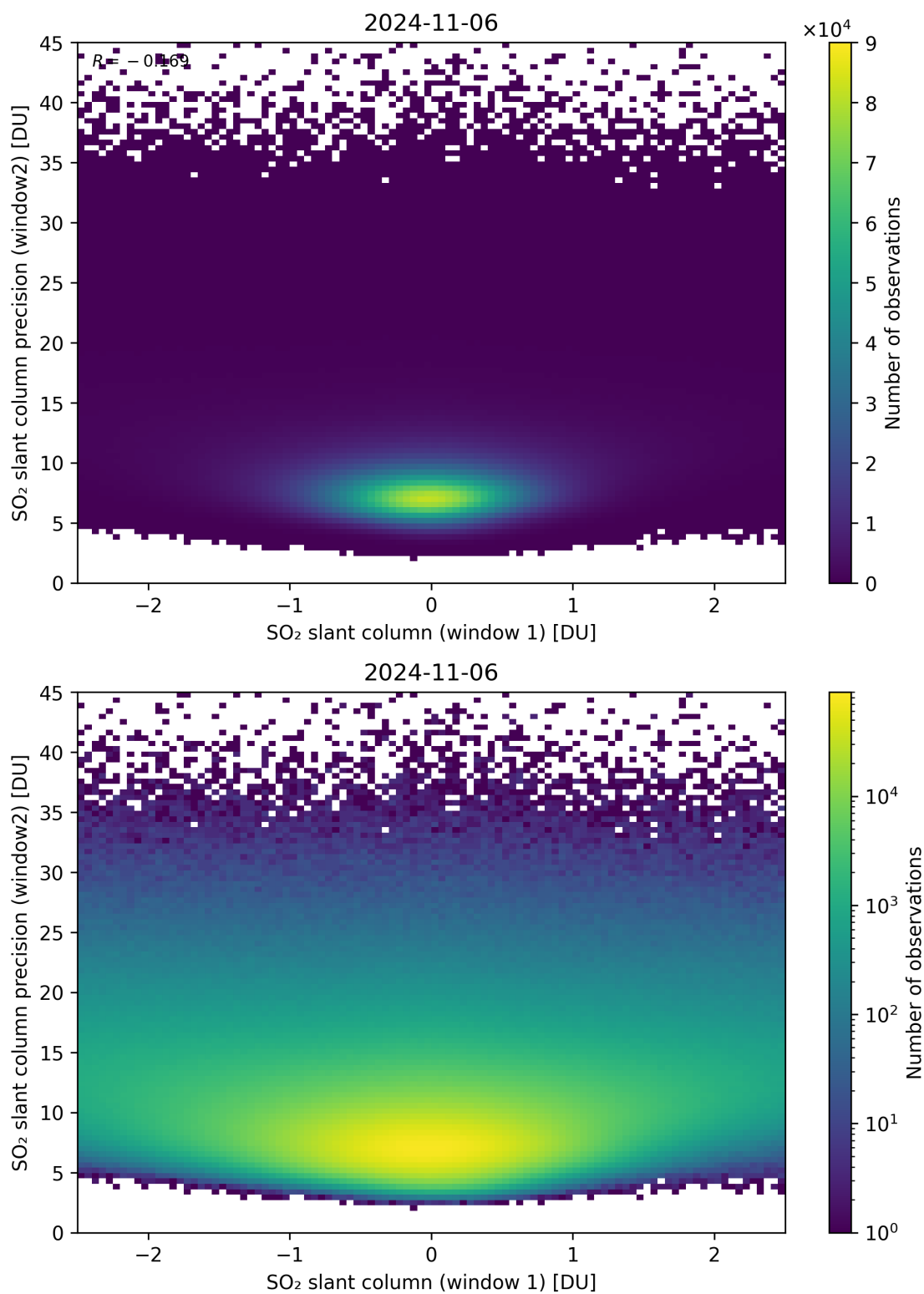
Figure 236: Scatter density plot of “SO 2 slant column (window 1)” against “SO 2 slant column precision (window2)” for 2024-11-05 to 2024-11-07.
