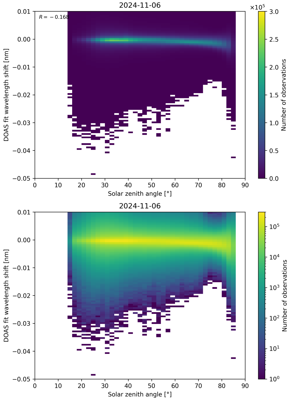
Figure 161: Scatter density plot of “Solar zenith angle” against “DOAS fit wavelength shift” for 2024-11-05 to 2024-11-07.
