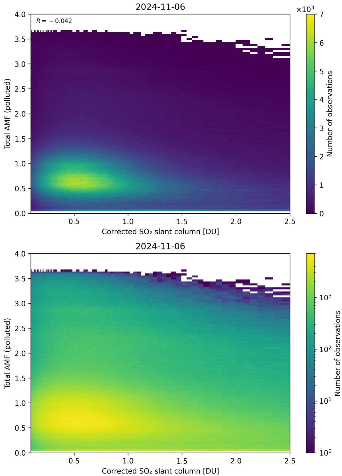
Figure 192: Scatter density plot of “Corrected SO 2 slant column” against “Total AMF (polluted)” for 2024-11-05 to 2024-11-07.
