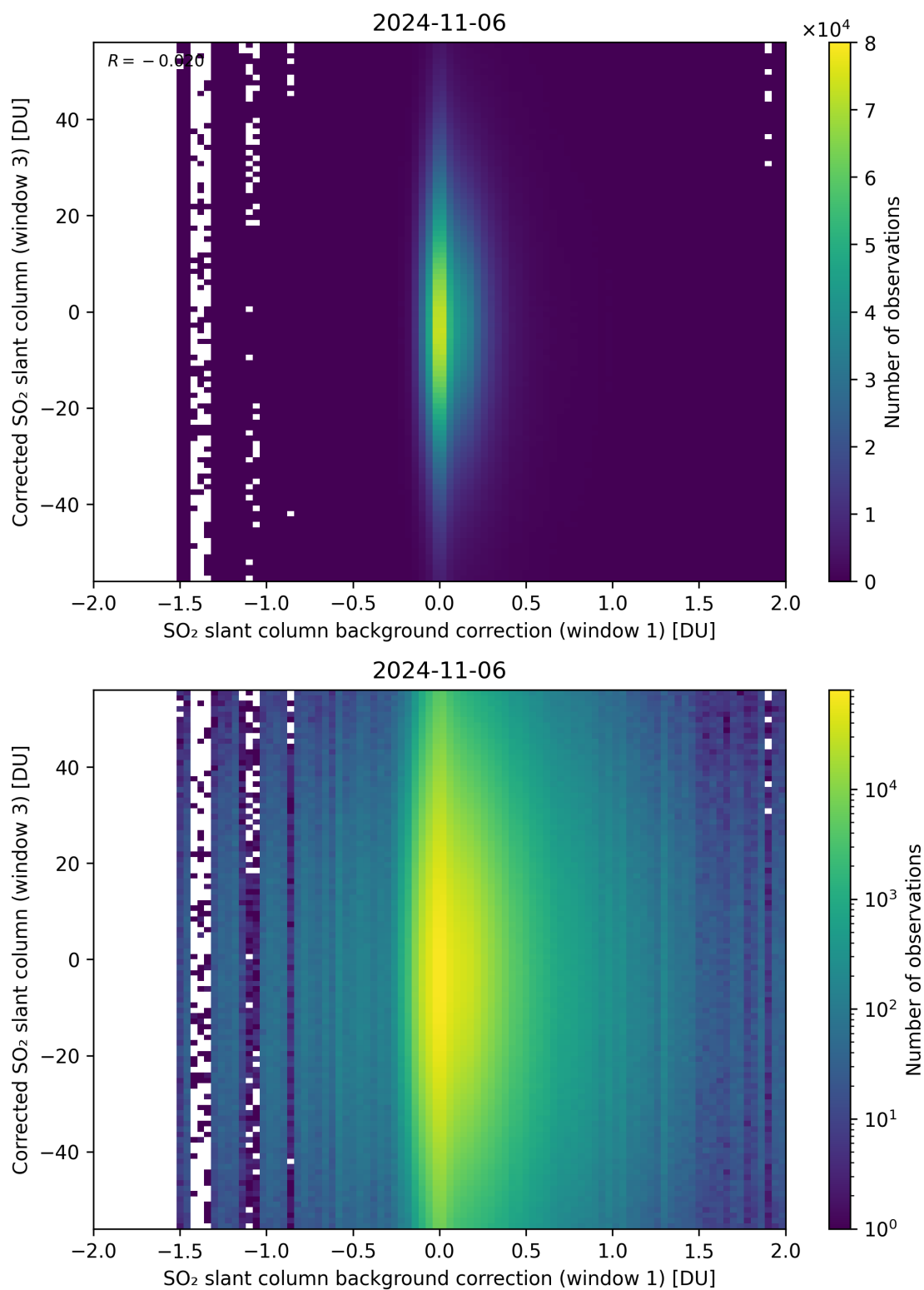
Figure 105: Scatter density plot of “SO 2 slant column background correction (window 1)” against “Corrected SO 2 slant column (window 3)” for 2024-11-05 to 2024-11-07.
