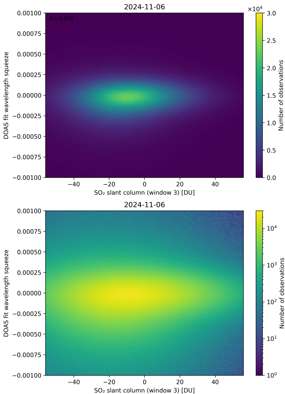
Figure 255: Scatter density plot of “SO 2 slant column (window 3)” against “DOAS fit wavelength squeeze” for 2024-11-05 to 2024-11-07.
