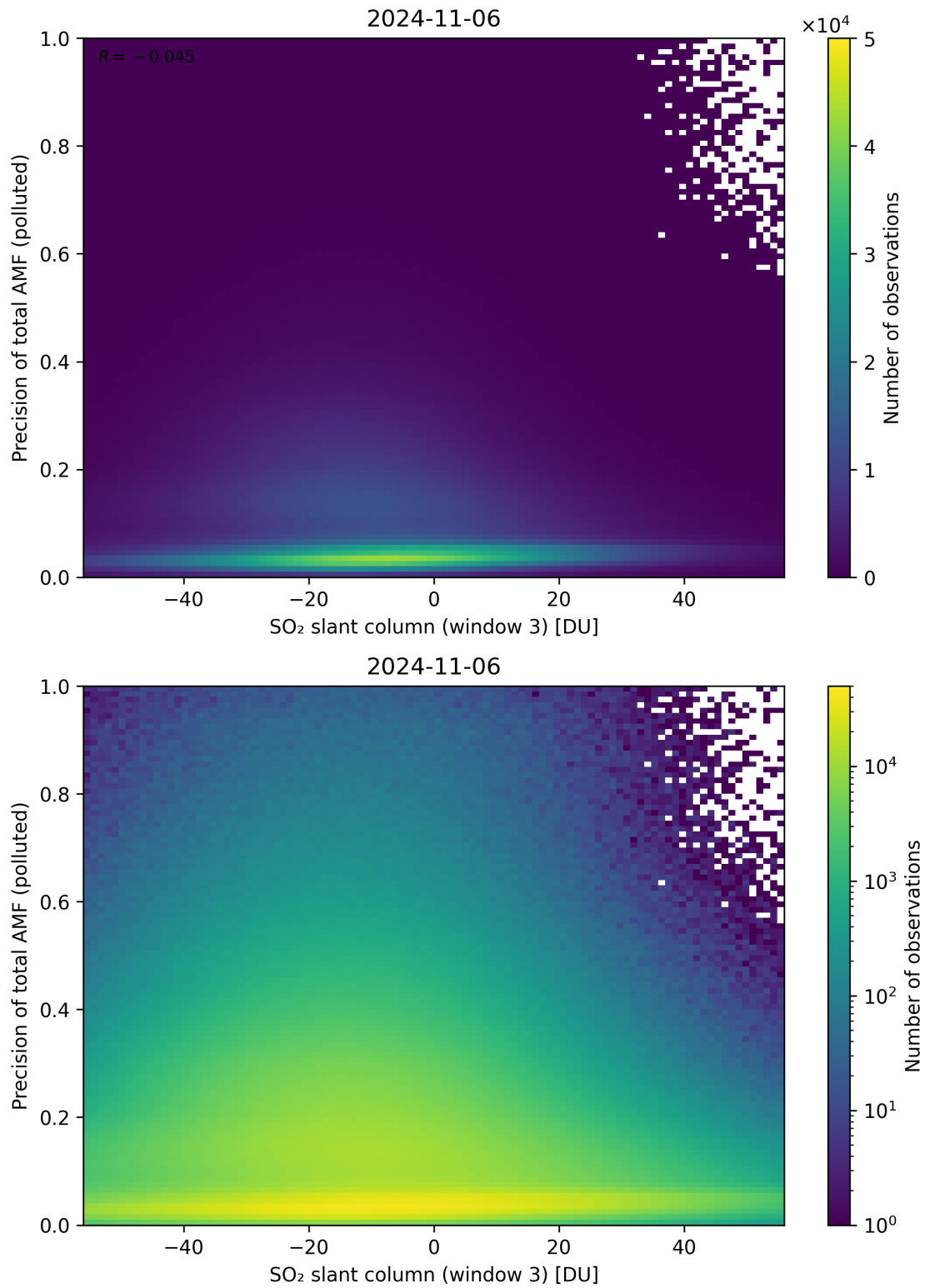
Figure 269: Scatter density plot of “SO 2 slant column (window 3)” against “Precision of total AMF (polluted)” for 2024-11-05 to 2024-11-07.
