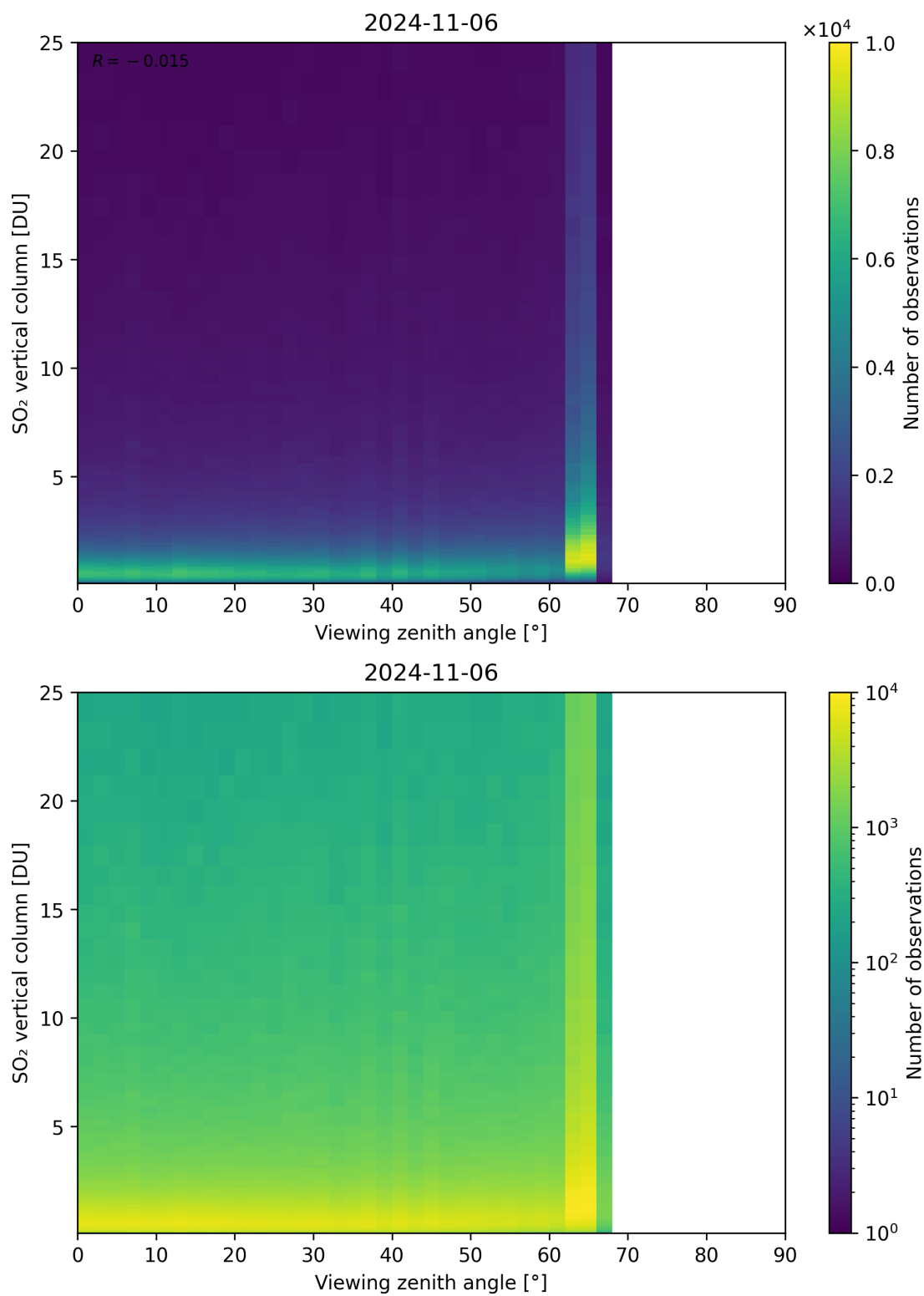
Figure 327: Scatter density plot of “Viewing zenith angle” against “SO 2 vertical column” for 2024-11-05 to 2024-11-07.
