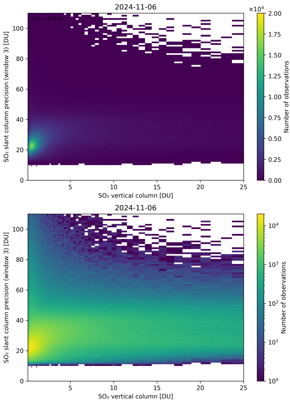
Figure 304: Scatter density plot of “SO 2 vertical column” against “SO 2 slant column precision (window 3)” for 2024-11-05 to 2024-11-07.
