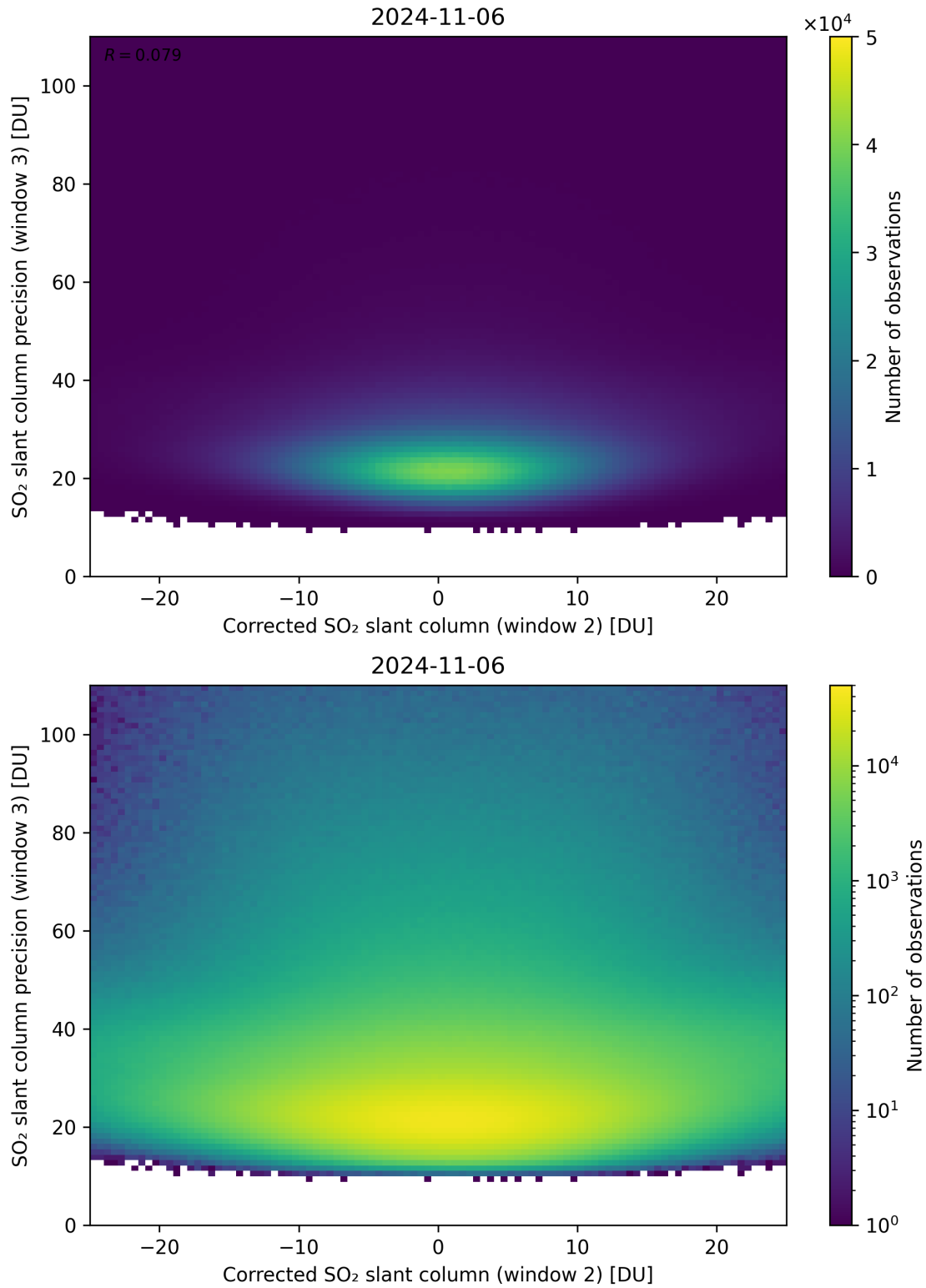
Figure 202: Scatter density plot of “Corrected SO 2 slant column (window 2)” against “SO 2 slant column precision (window 3)” for 2024-11-05 to 2024-11-07.
