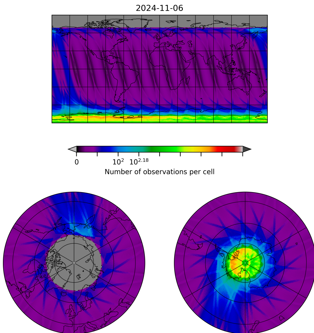
Figure 28: Map of the number of observations for 2024-11-05 to 2024-11-07
