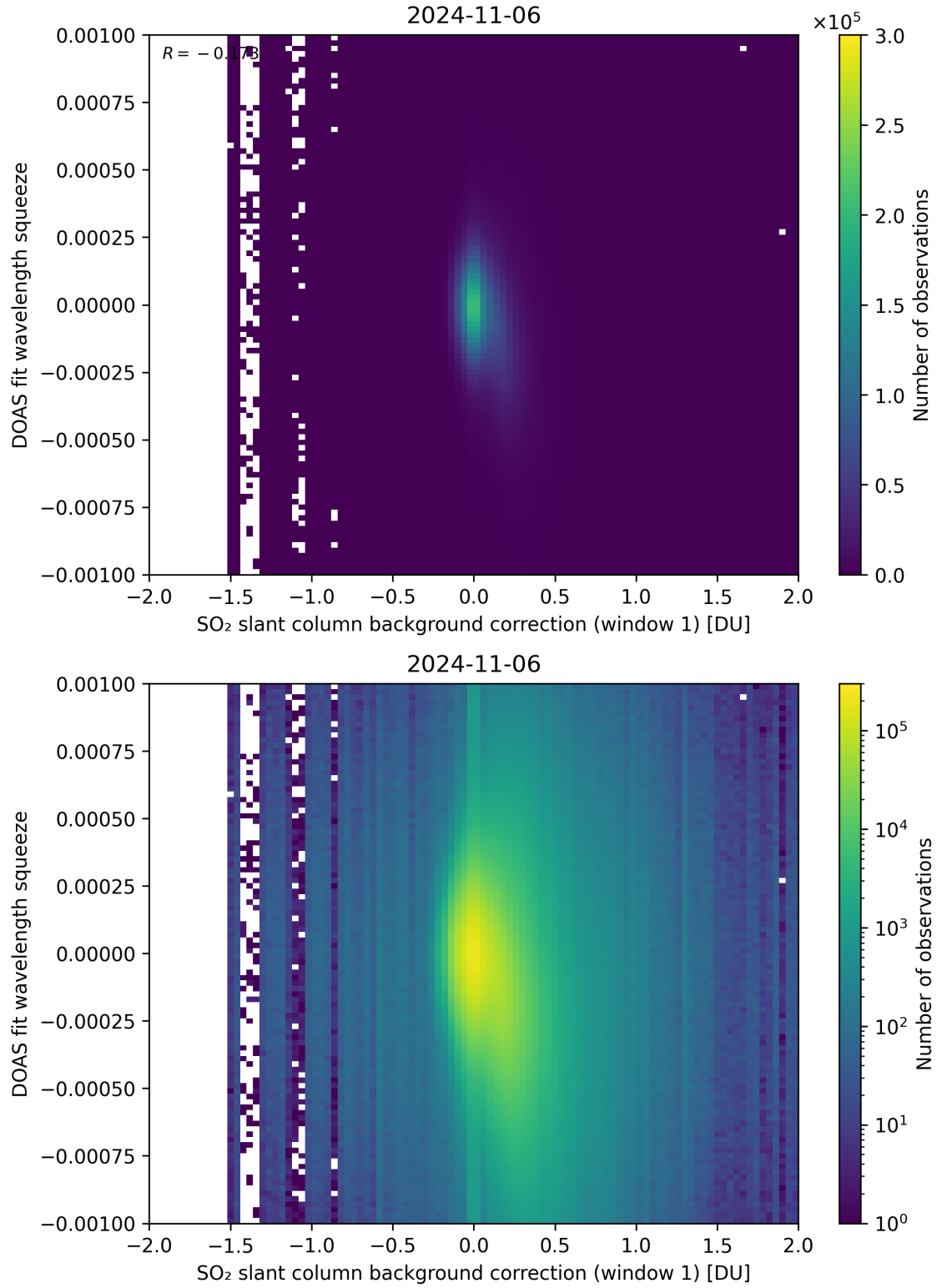
Figure 101: Scatter density plot of “SO 2 slant column background correction (window 1)” against “DOAS fit wavelength squeeze” for 2024-11-05 to 2024-11-07.
