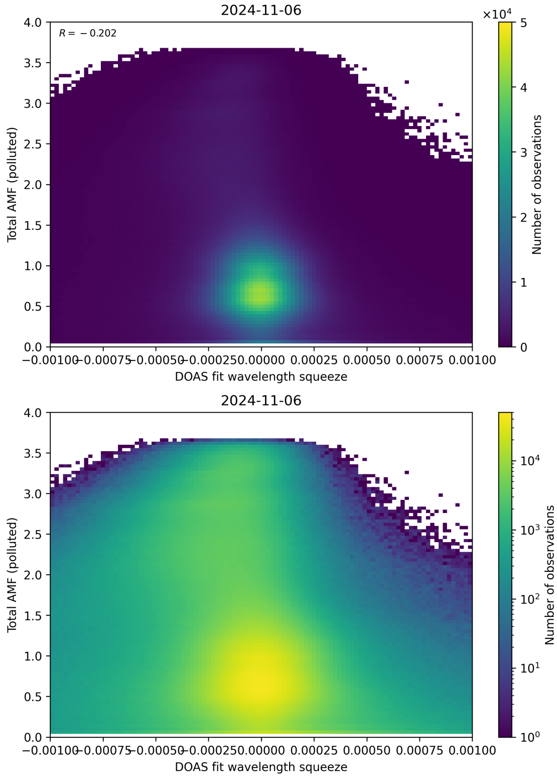
Figure 134: Scatter density plot of “DOAS fit wavelength squeeze” against “Total AMF (polluted)” for 2024-11-05 to 2024-11-07.
