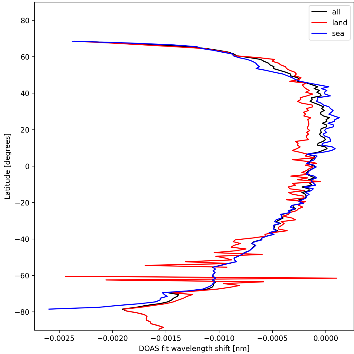
Figure 45: Zonal average of “DOAS fit wavelength shift” for 2024-11-05 to 2024-11-07.
