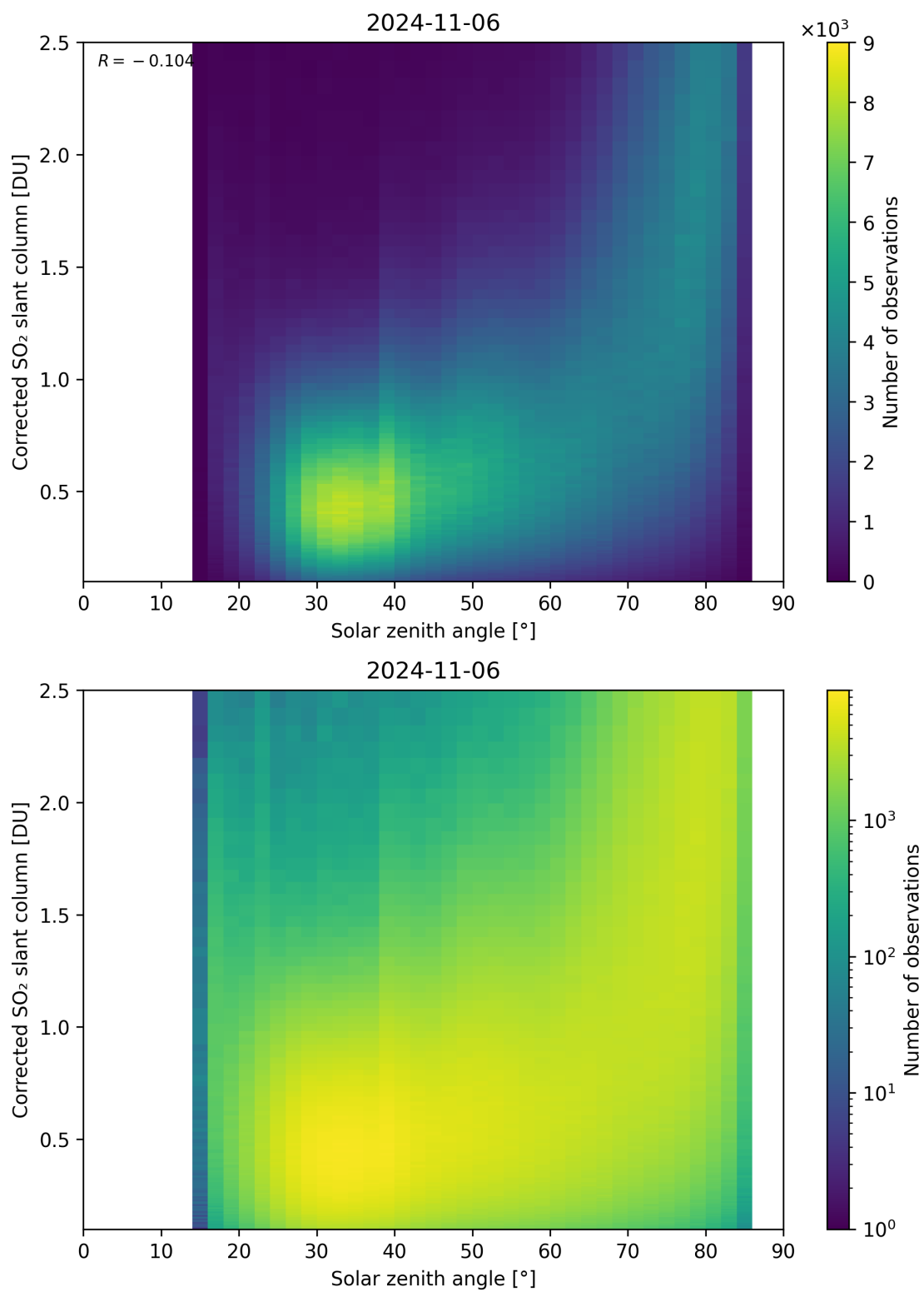
Figure 166: Scatter density plot of “Solar zenith angle” against “Corrected SO 2 slant column” for 2024-11-05 to 2024-11-07.
