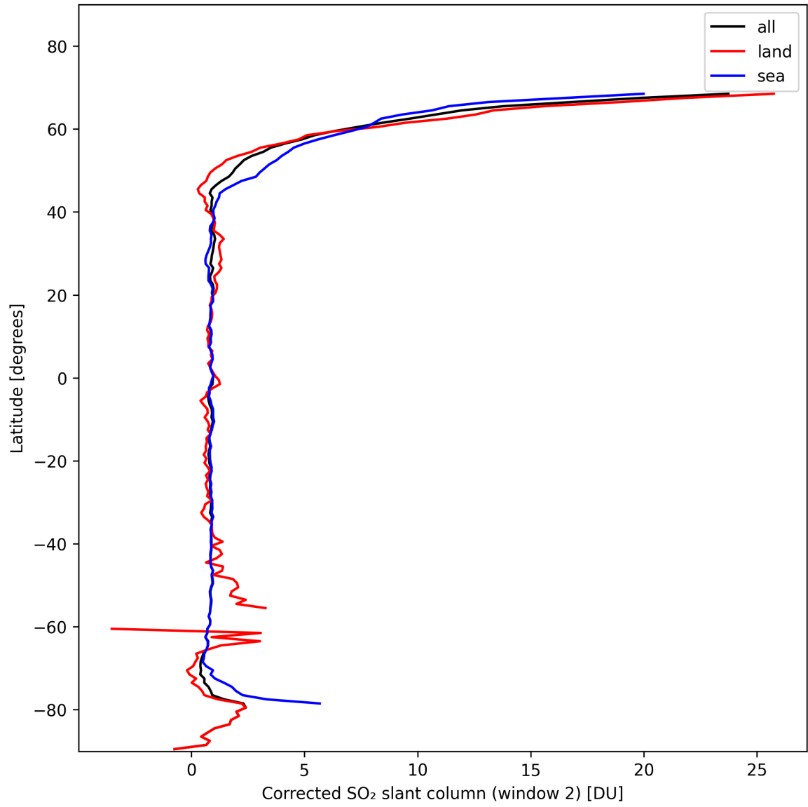
Figure 39: Zonal average of “Corrected SO 2 slant column (window 2)” for 2024-11-05 to 2024-11-07.
