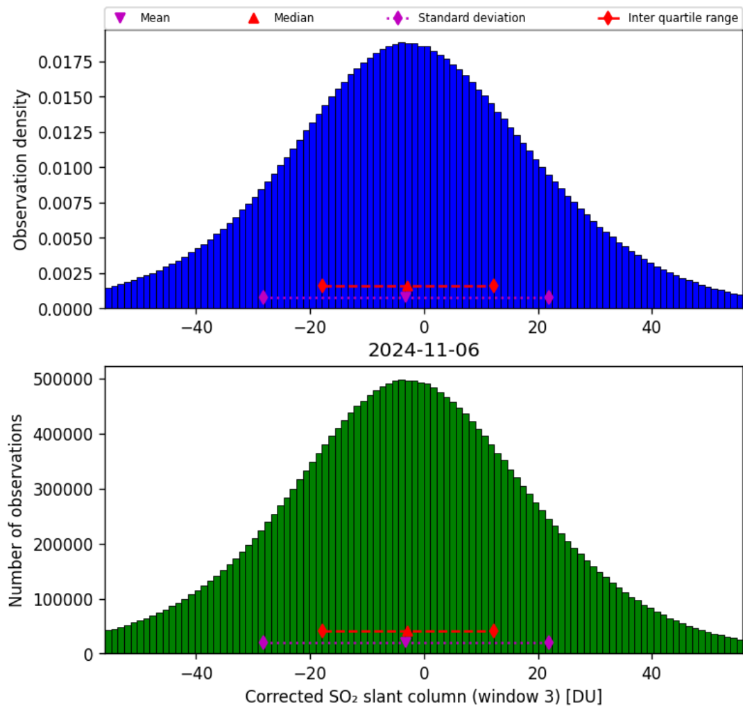
Figure 66: Histogram of “Corrected SO 2 slant column (window 3)” for 2024-11-05 to 2024-11-07
