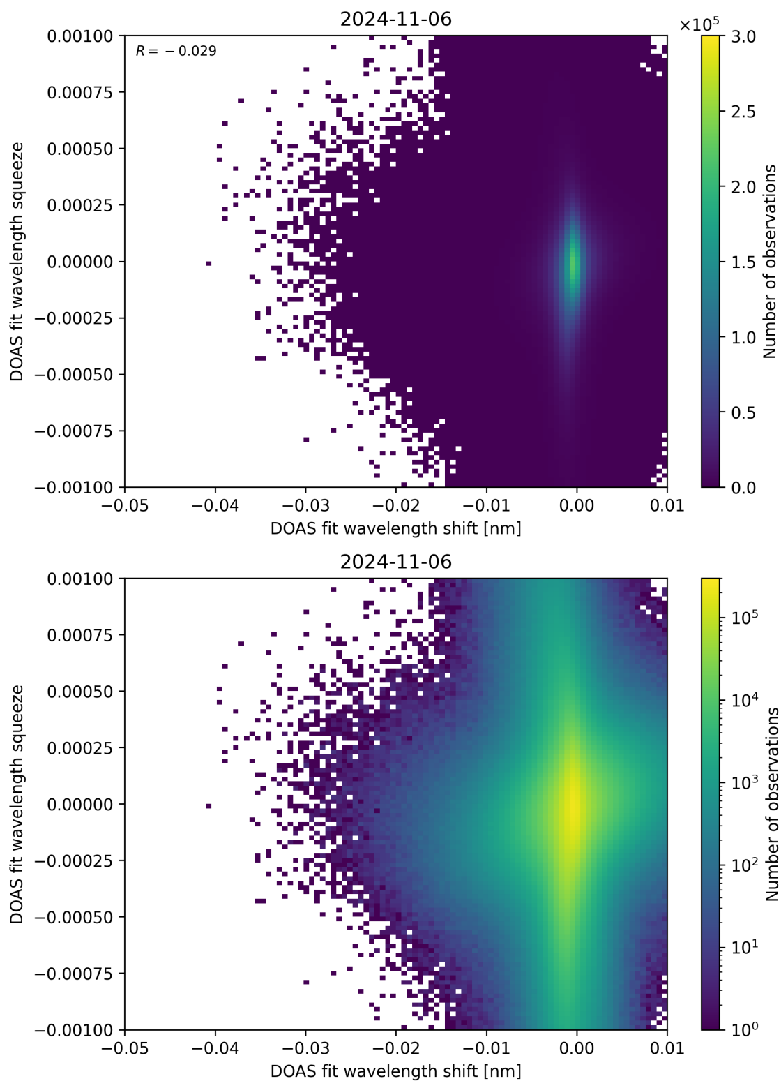
Figure 127: Scatter density plot of “DOAS fit wavelength shift” against “DOAS fit wavelength squeeze” for 2024-11-05 to 2024-11-07.
