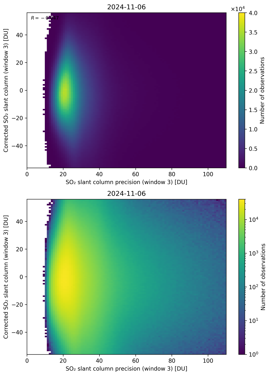
Figure 262: Scatter density plot of “SO 2 slant column precision (window 3)” against “Corrected SO 2 slant column (window 3)” for 2024-11-05 to 2024-11-07.
