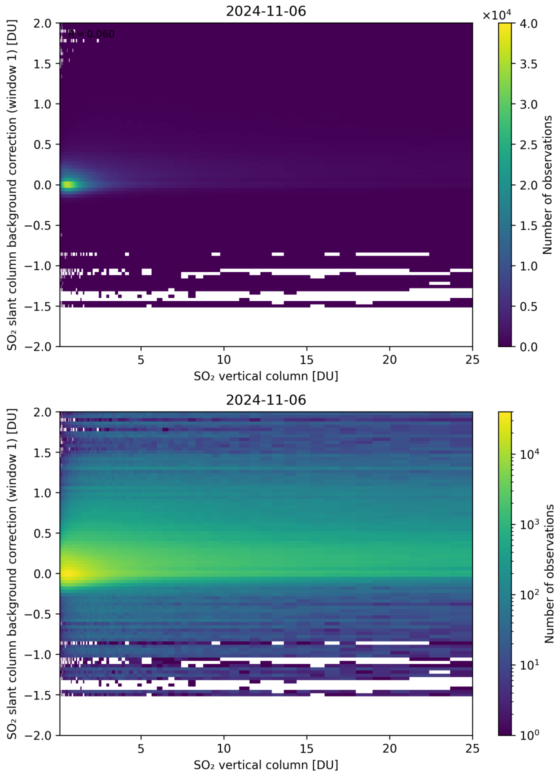
Figure 273: Scatter density plot of “SO 2 vertical column” against “SO 2 slant column background correction (window 1)” for 2024-11-05 to 2024-11-07.
