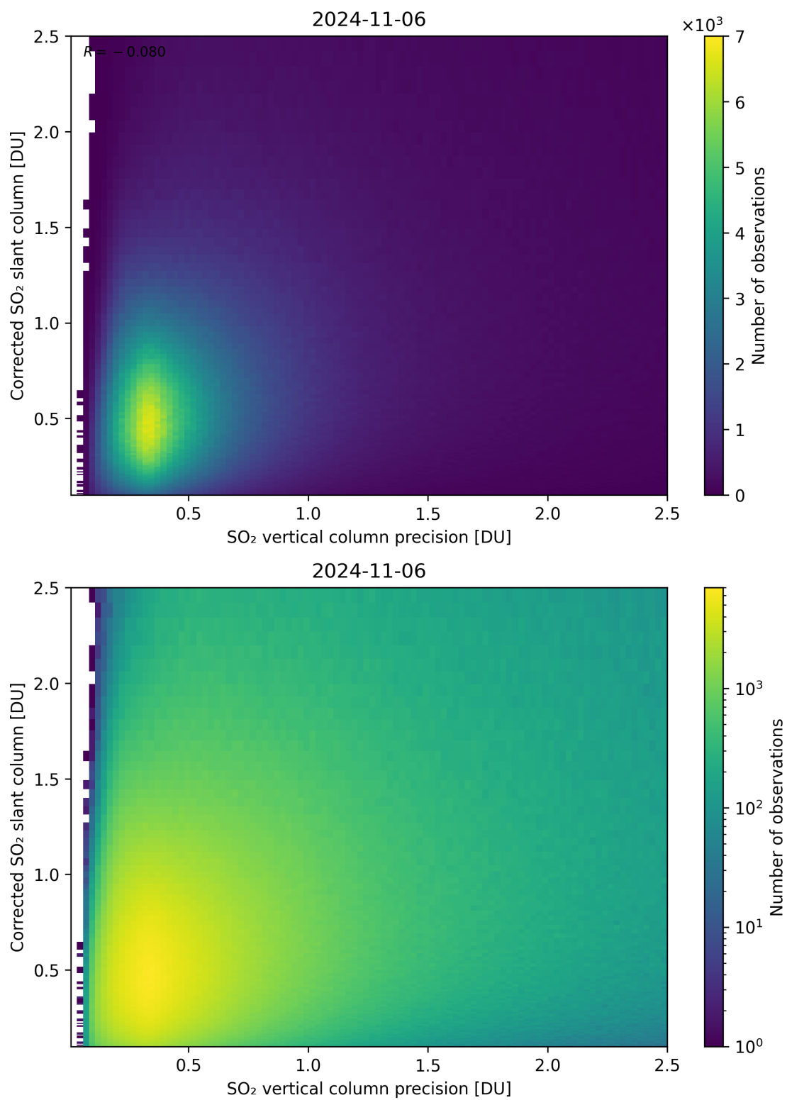
Figure 286: Scatter density plot of “SO 2 vertical column precision” against “Corrected SO 2 slant column” for 2024-11-05 to 2024-11-07.
