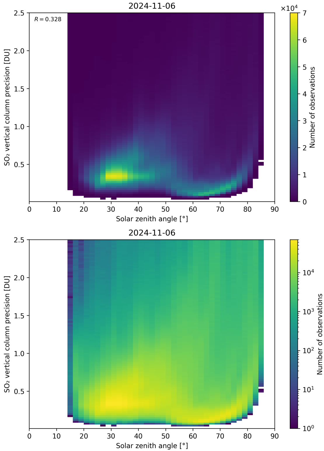
Figure 177: Scatter density plot of “Solar zenith angle” against “SO 2 vertical column precision” for 2024-11-05 to 2024-11-07.
