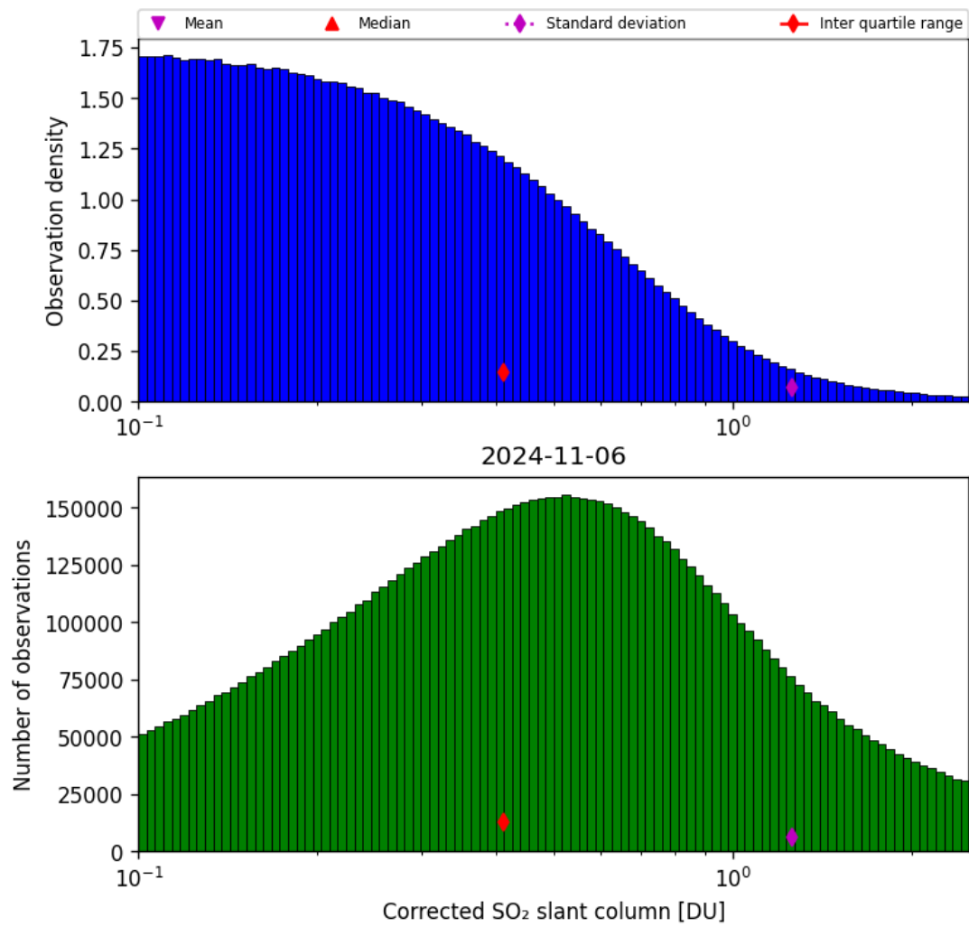
Figure 55: Histogram of “Corrected SO 2 slant column” for 2024-11-05 to 2024-11-07
