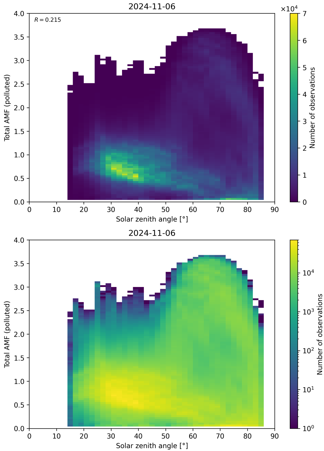
Figure 174: Scatter density plot of “Solar zenith angle” against “Total AMF (polluted)” for 2024-11-05 to 2024-11-07.
