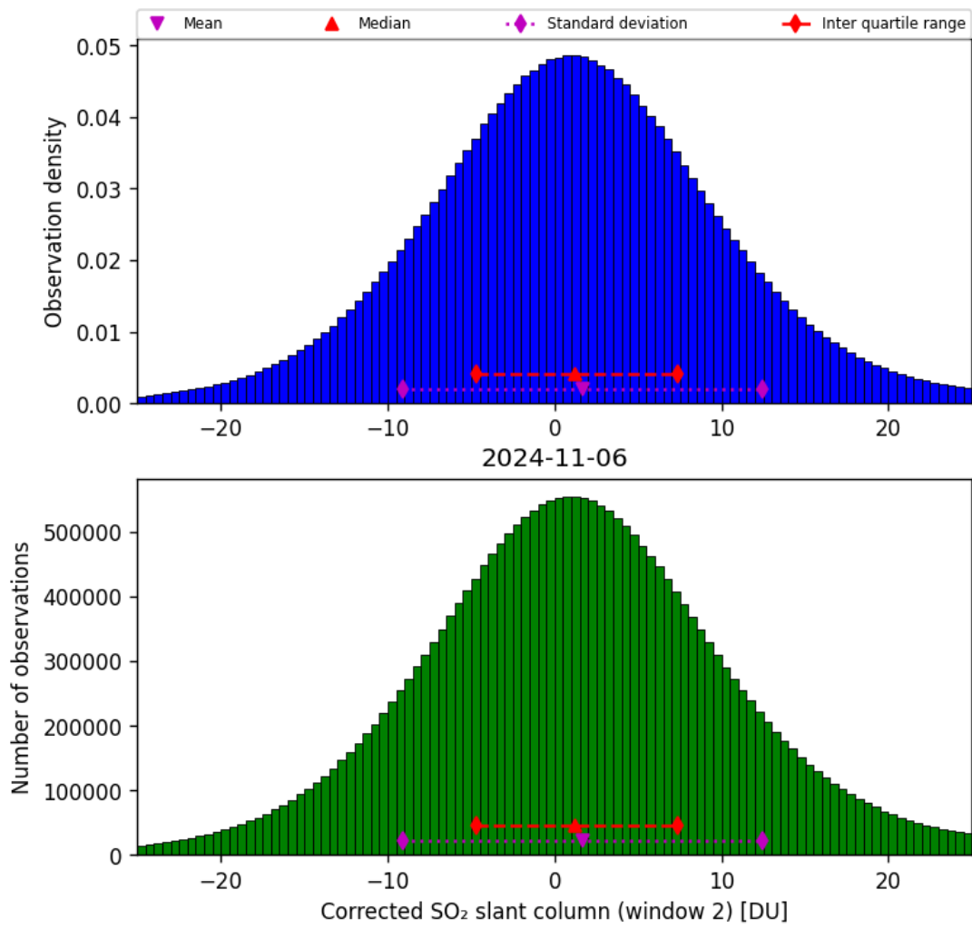
Figure 62: Histogram of “Corrected SO 2 slant column (window 2)” for 2024-11-05 to 2024-11-07
