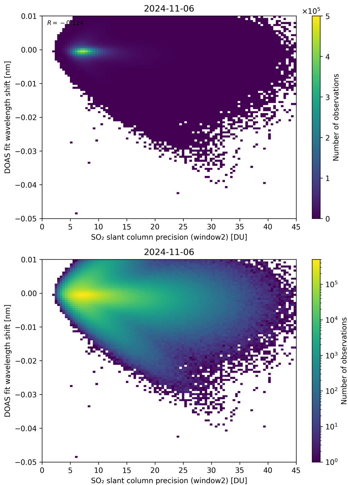
Figure 243: Scatter density plot of “SO 2 slant column precision (window2)” against “DOAS fit wavelength shift” for 2024-11-05 to 2024-11-07.
