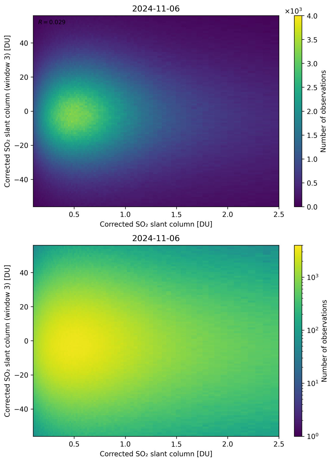
Figure 186: Scatter density plot of “Corrected SO 2 slant column” against “Corrected SO 2 slant column (window 3)” for 2024-11-05 to 2024-11-07.
