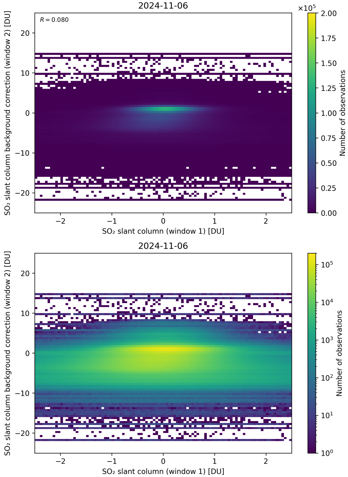
Figure 213: Scatter density plot of “SO 2 slant column (window 1)” against “SO 2 slant column background correction (window 2)” for 2024-11-05 to 2024-11-07.
