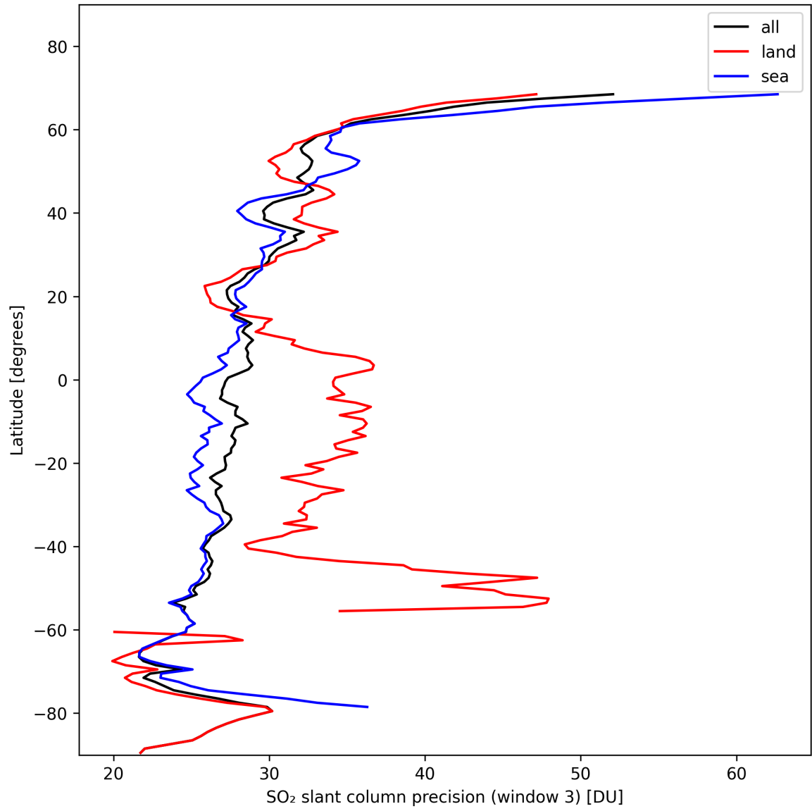
Figure 42: Zonal average of “SO 2 slant column precision (window 3)” for 2024-11-05 to 2024-11-07.
