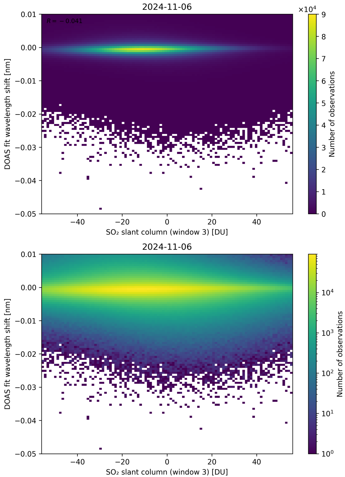
Figure 254: Scatter density plot of “SO 2 slant column (window 3)” against “DOAS fit wavelength shift” for 2024-11-05 to 2024-11-07.
