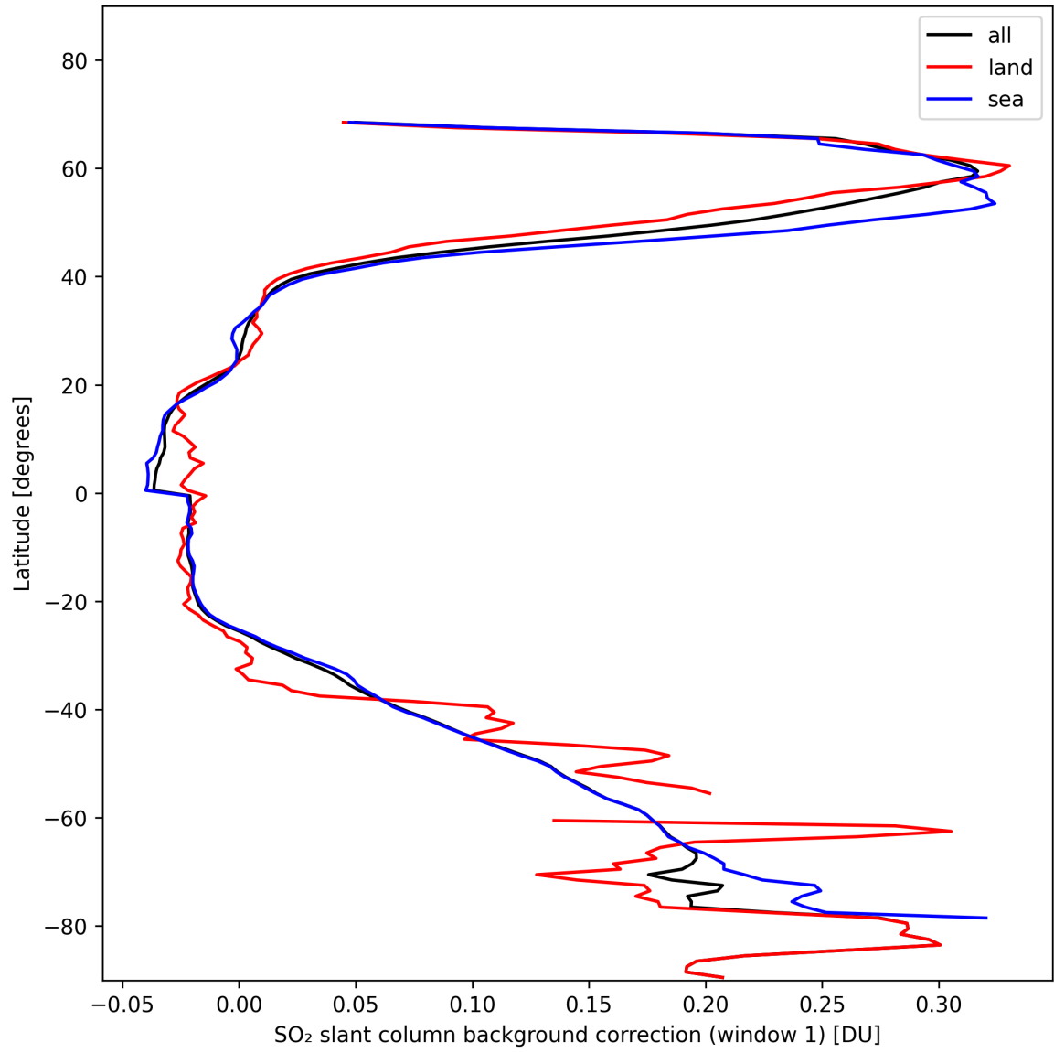
Figure 36: Zonal average of “SO 2 slant column background correction (window 1)” for 2024-11-05 to 2024-11-07.
