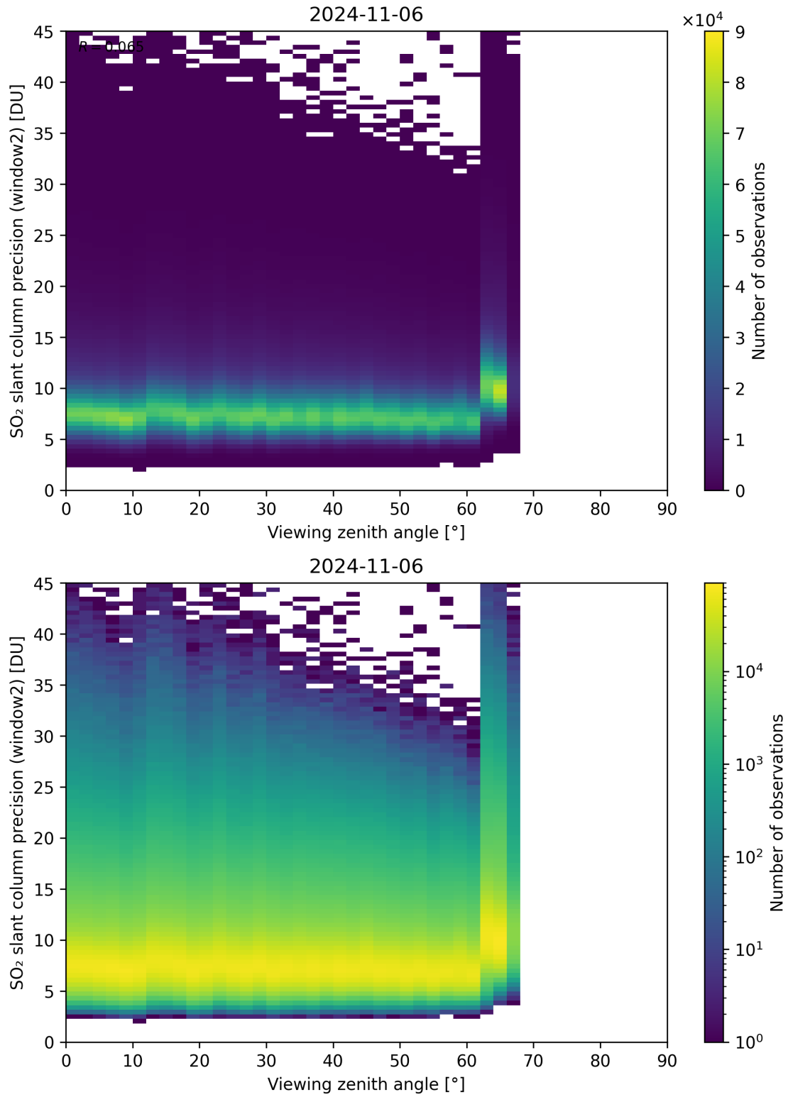
Figure 322: Scatter density plot of “Viewing zenith angle” against “SO 2 slant column precision (window2)” for 2024-11-05 to 2024-11-07.
