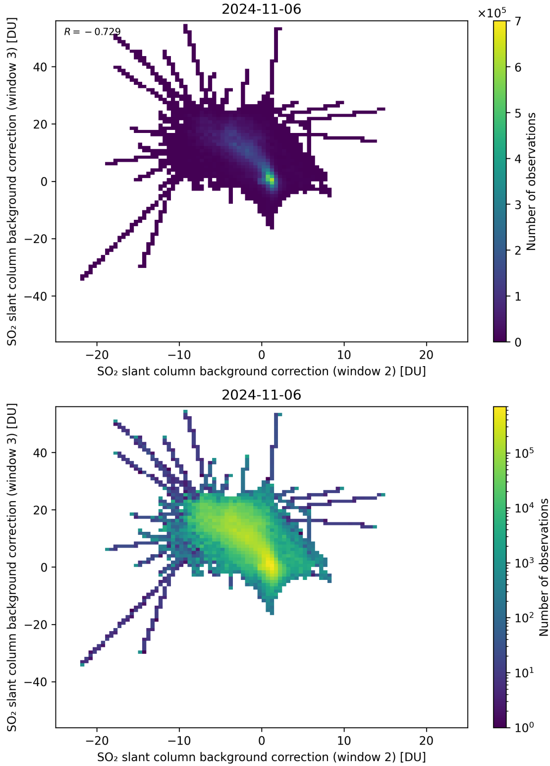
Figure 111: Scatter density plot of “SO 2 slant column background correction (window 2)” against “SO 2 slant column background correction (window 3)” for 2024-11-05 to 2024-11-07.
