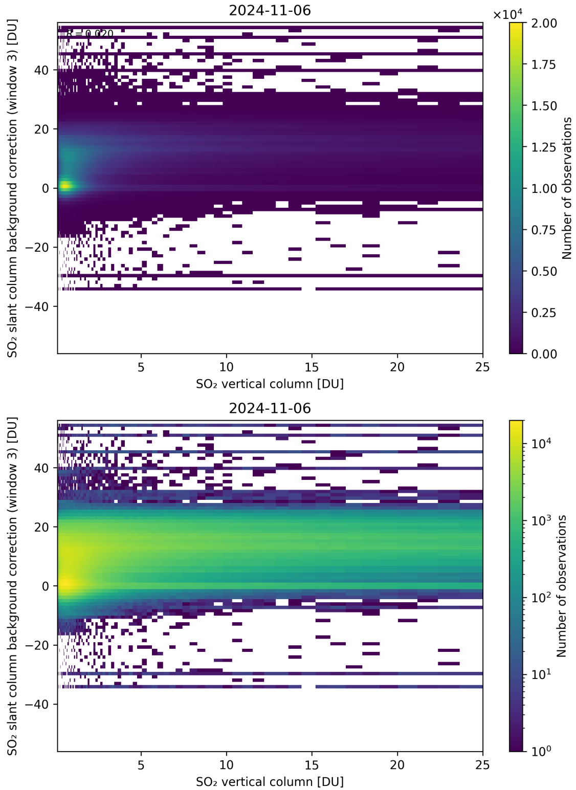
Figure 275: Scatter density plot of “SO 2 vertical column” against “SO 2 slant column background correction (window 3)” for 2024-11-05 to 2024-11-07.
