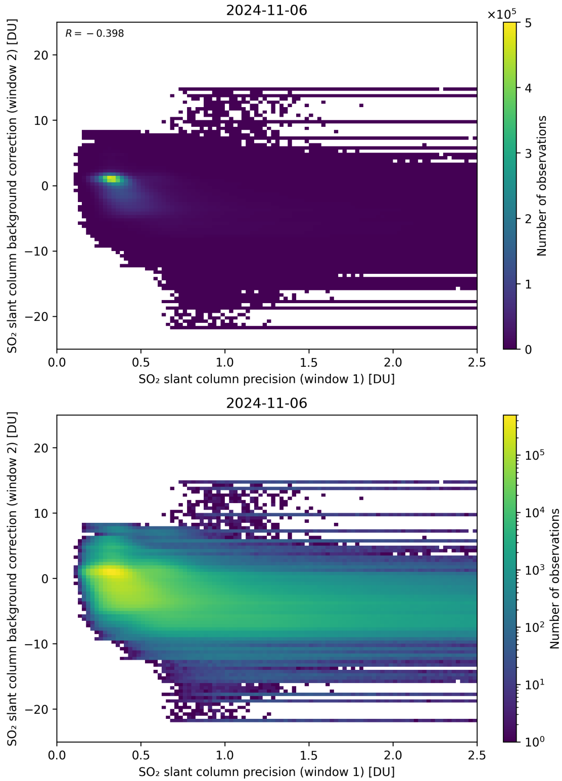
Figure 219: Scatter density plot of “SO 2 slant column precision (window 1)” against “SO 2 slant column background correction (window 2)” for 2024-11-05 to 2024-11-07.
