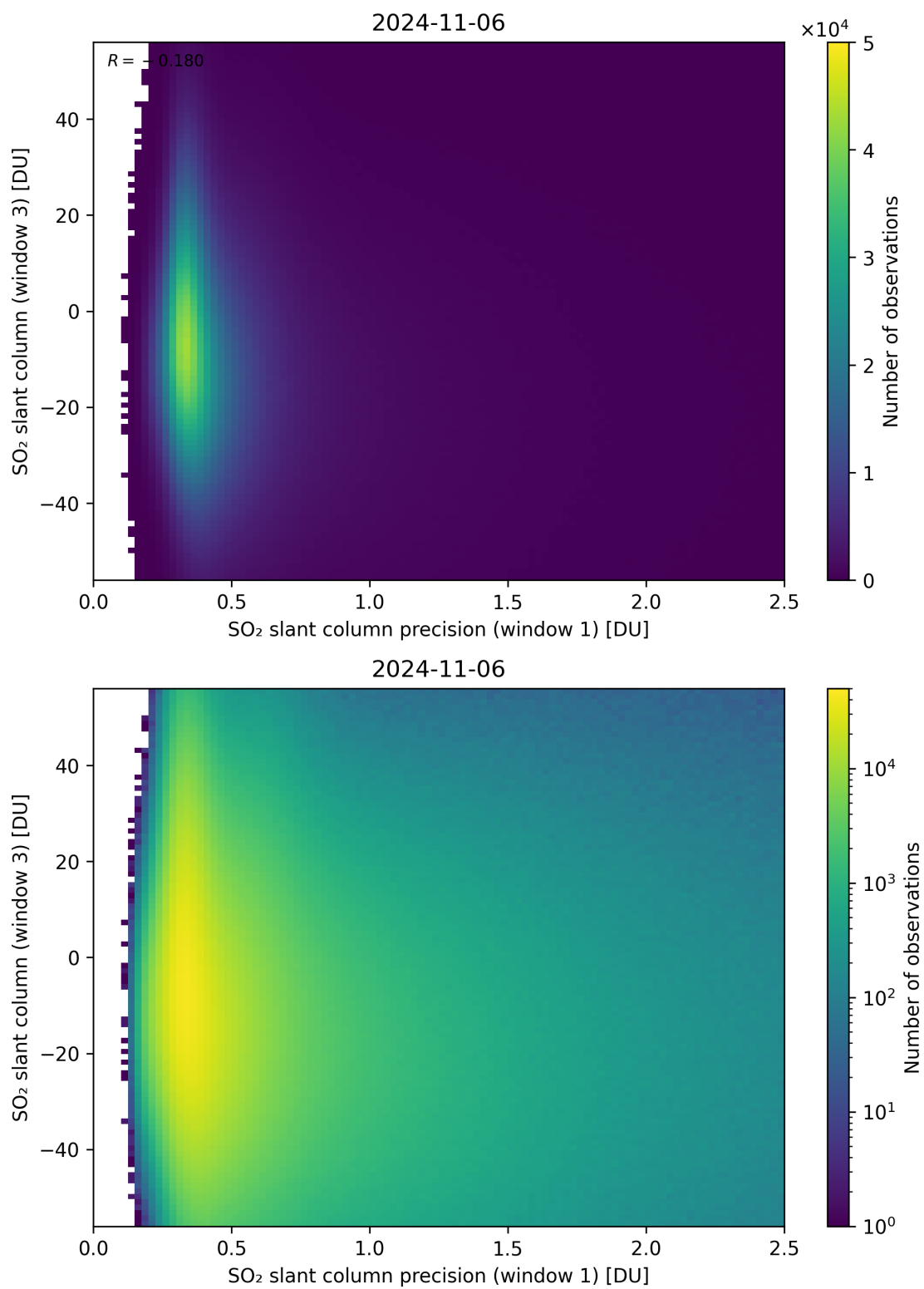
Figure 228: Scatter density plot of “SO 2 slant column precision (window 1)” against “SO 2 slant column (window 3)” for 2024-11-05 to 2024-11-07.
