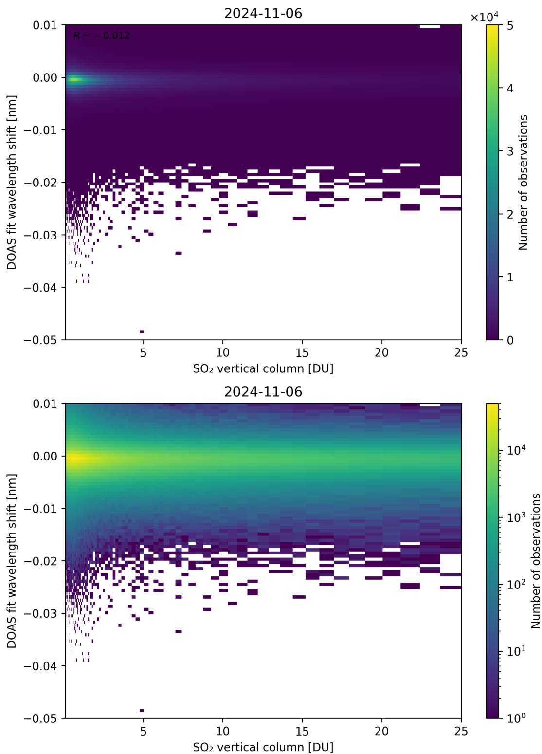
Figure 276: Scatter density plot of “SO 2 vertical column” against “DOAS fit wavelength shift” for 2024-11-05 to 2024-11-07.
