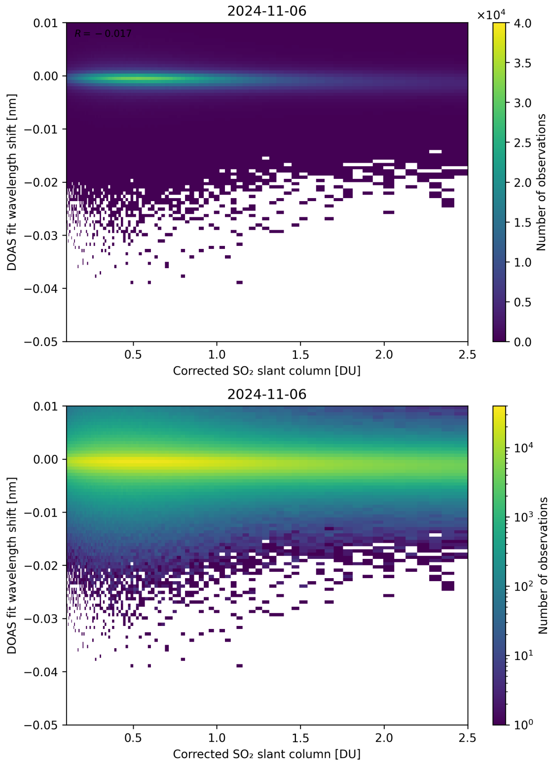
Figure 181: Scatter density plot of “Corrected SO 2 slant column” against “DOAS fit wavelength shift” for 2024-11-05 to 2024-11-07.
