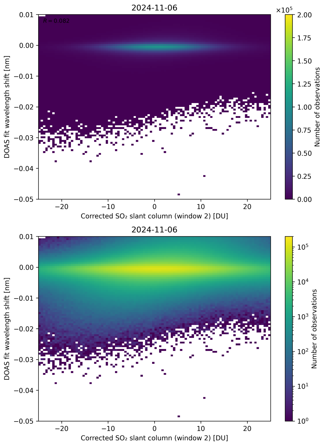
Figure 196: Scatter density plot of “Corrected SO 2 slant column (window 2)” against “DOAS fit wavelength shift” for 2024-11-05 to 2024-11-07.
