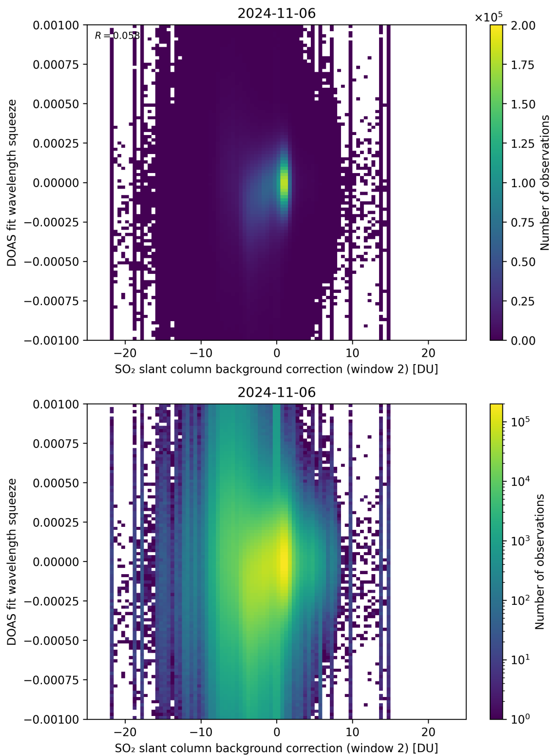
Figure 113: Scatter density plot of “SO 2 slant column background correction (window 2)” against “DOAS fit wavelength squeeze” for 2024-11-05 to 2024-11-07.
