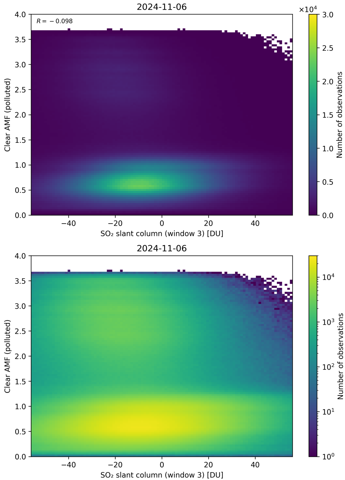
Figure 265: Scatter density plot of “SO 2 slant column (window 3)” against “Clear AMF (polluted)” for 2024-11-05 to 2024-11-07.
