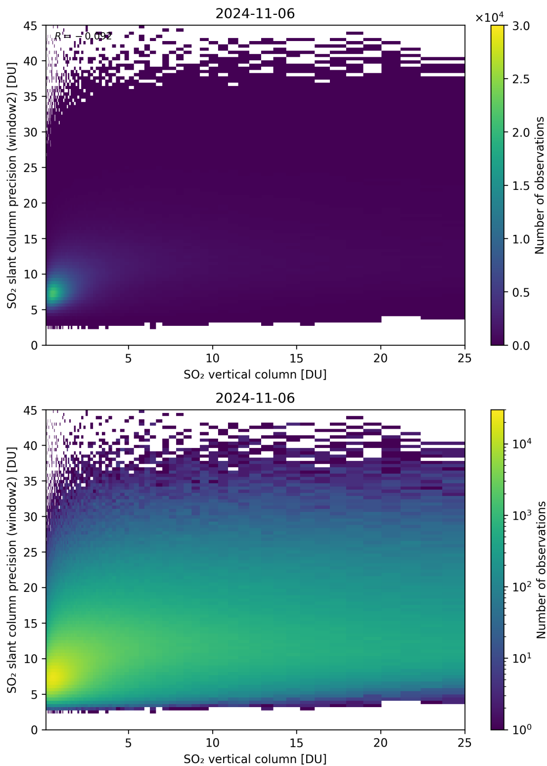
Figure 302: Scatter density plot of “SO 2 vertical column” against “SO 2 slant column precision (window2)” for 2024-11-05 to 2024-11-07.
