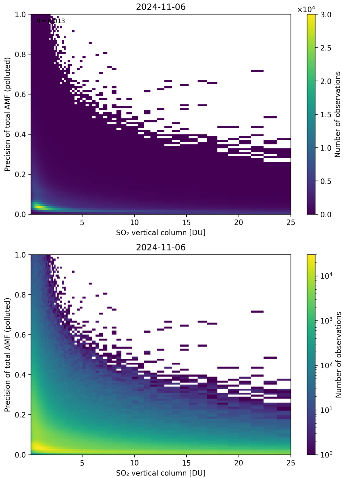
Figure 306: Scatter density plot of “SO 2 vertical column” against “Precision of total AMF (polluted)” for 2024-11-05 to 2024-11-07.
