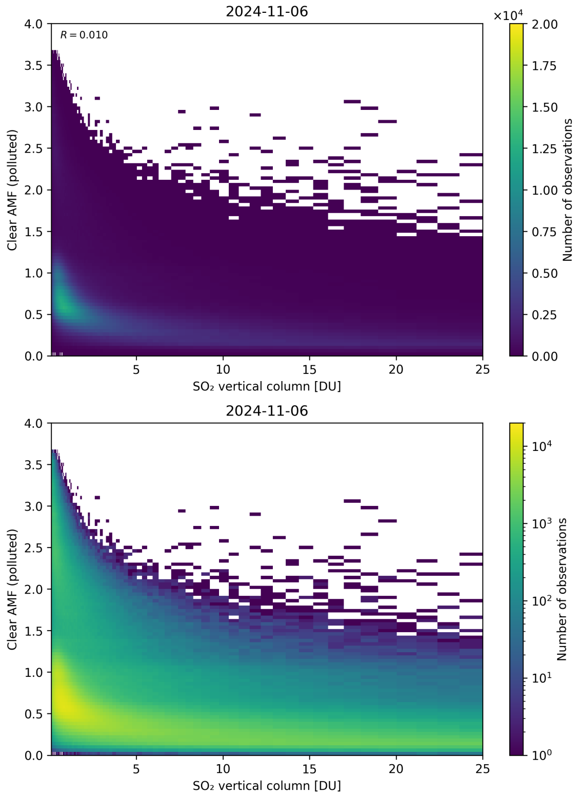
Figure 296: Scatter density plot of “SO 2 vertical column” against “Clear AMF (polluted)” for 2024-11-05 to 2024-11-07.
