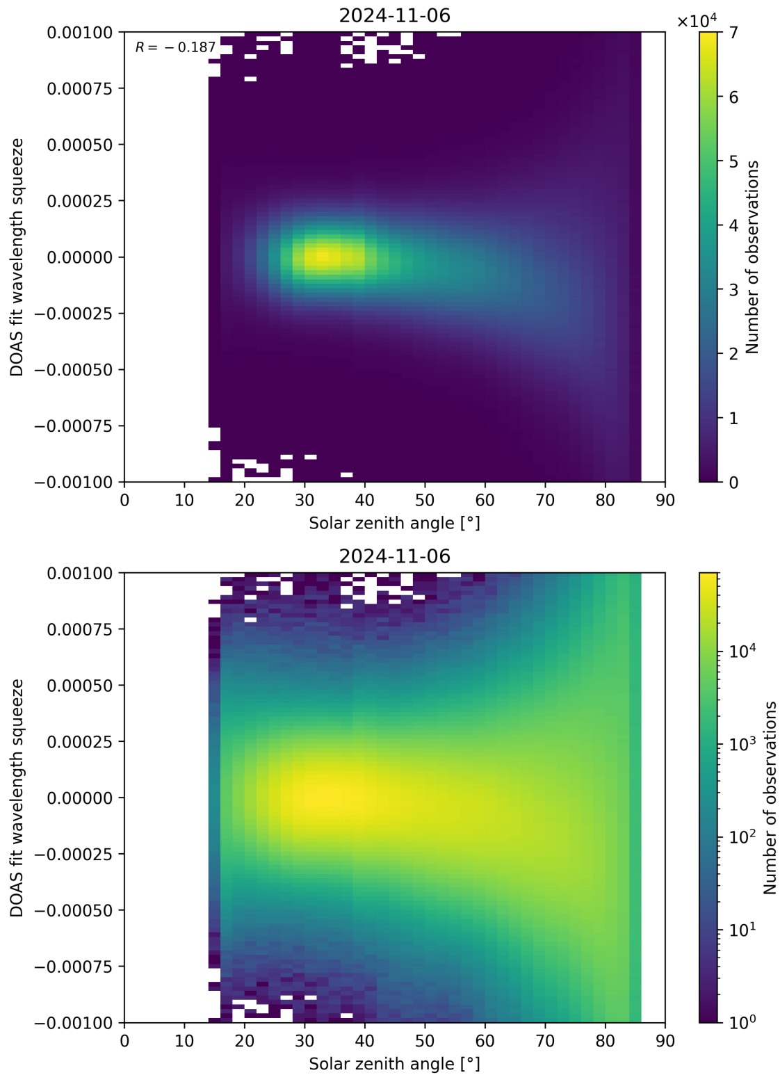
Figure 162: Scatter density plot of “Solar zenith angle” against “DOAS fit wavelength squeeze” for 2024-11-05 to 2024-11-07.
