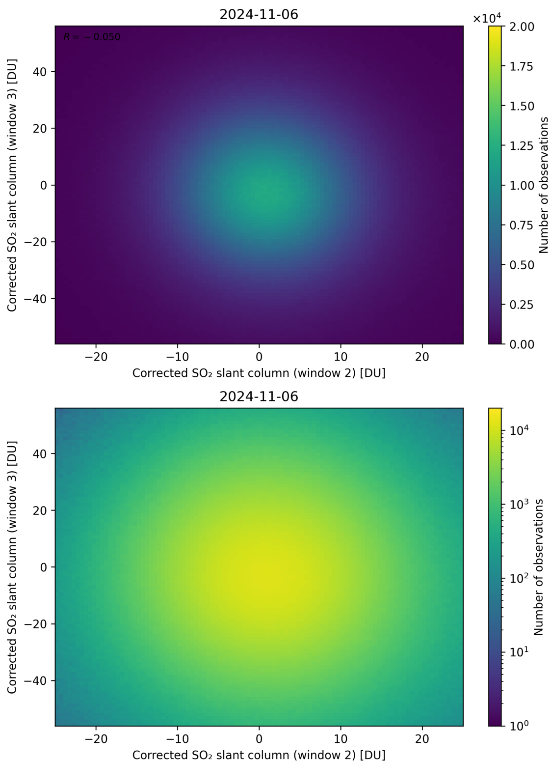
Figure 200: Scatter density plot of “Corrected SO 2 slant column (window 2)” against “Corrected SO 2 slant column (window 3)” for 2024-11-05 to 2024-11-07.
