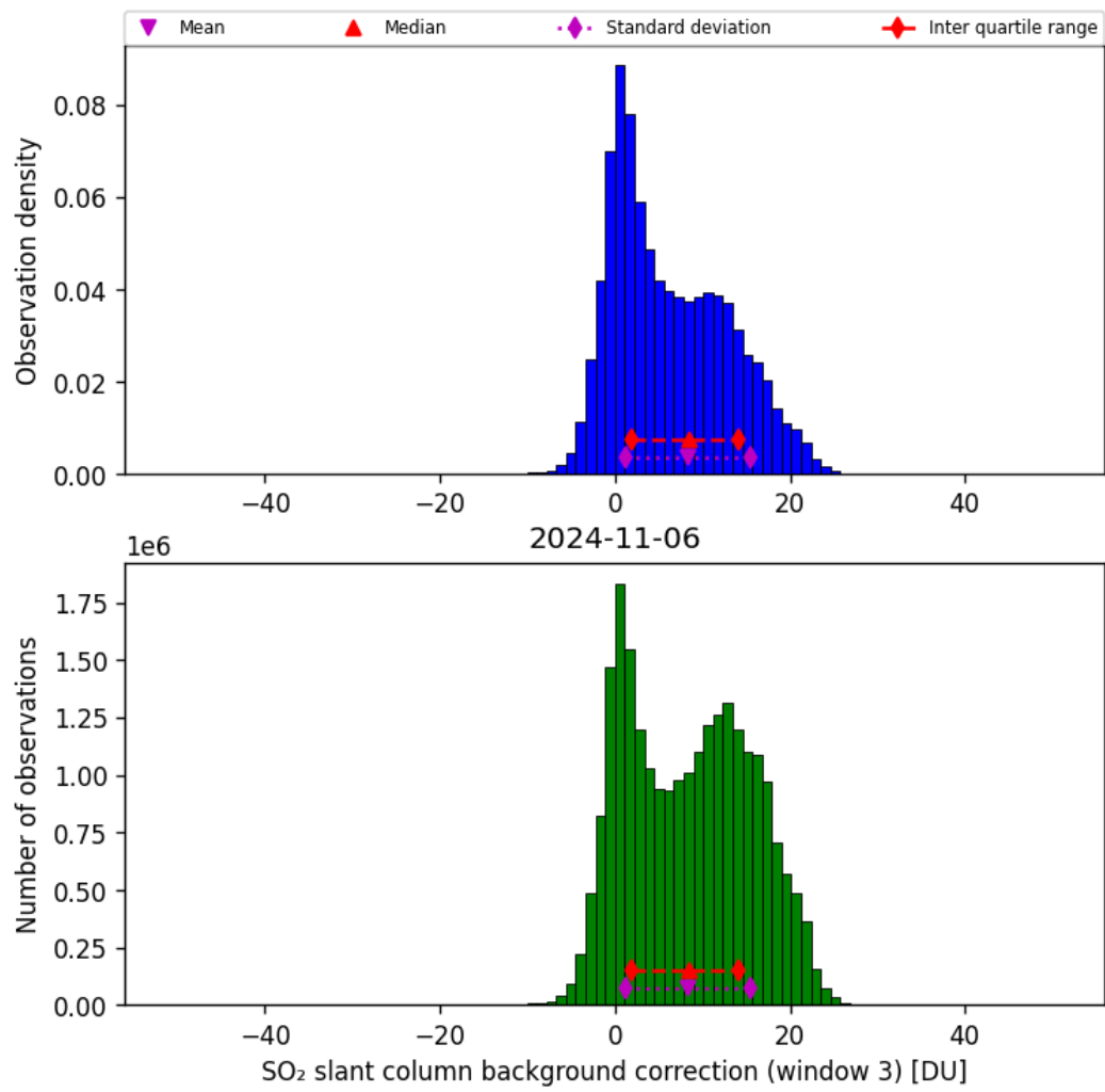
Figure 67: Histogram of “SO 2 slant column background correction (window 3)” for 2024-11-05 to 2024-11-07
