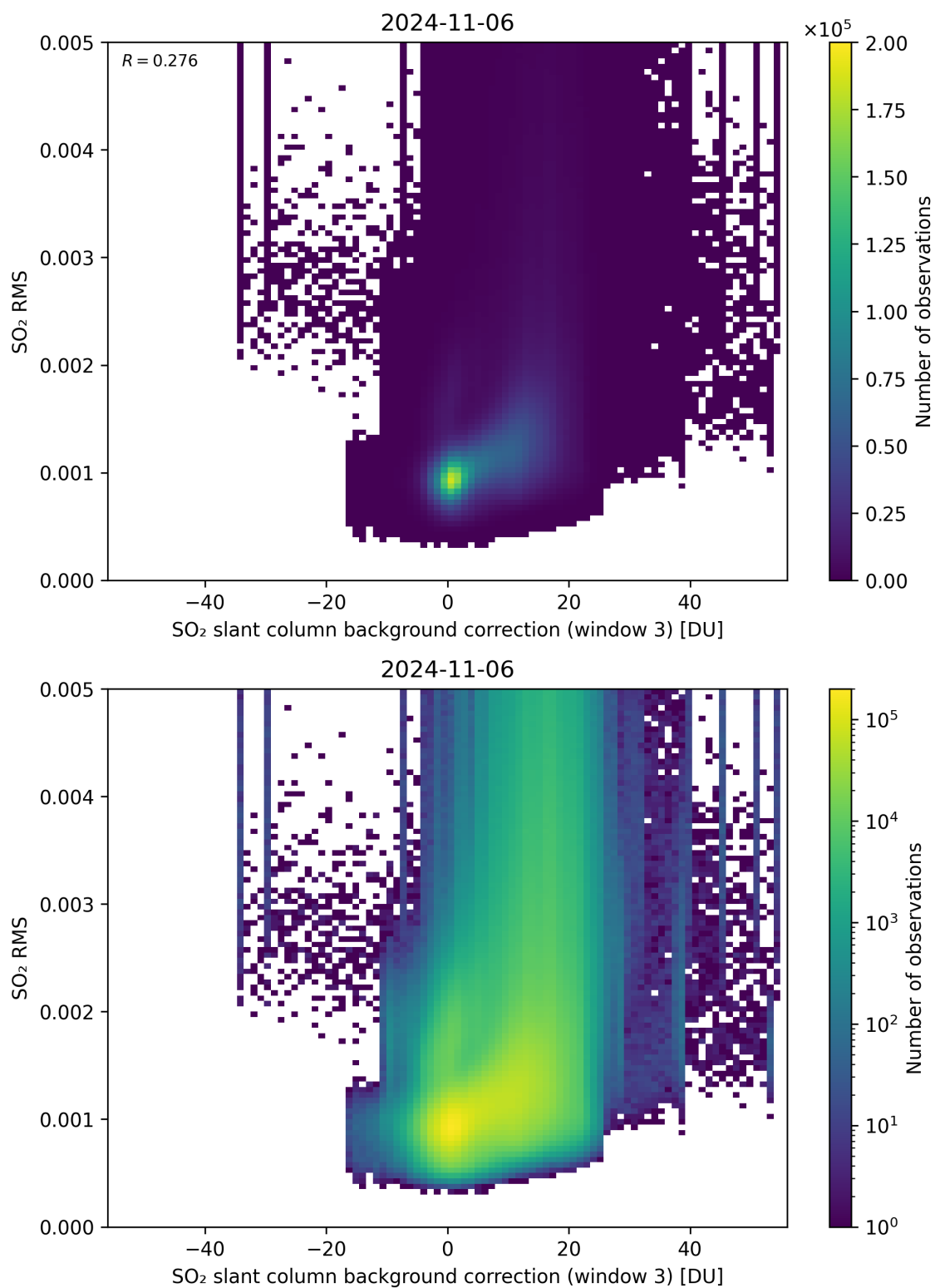
Figure 123: Scatter density plot of “SO 2 slant column background correction (window 3)” against “SO 2 RMS” for 2024-11-05 to 2024-11-07.
