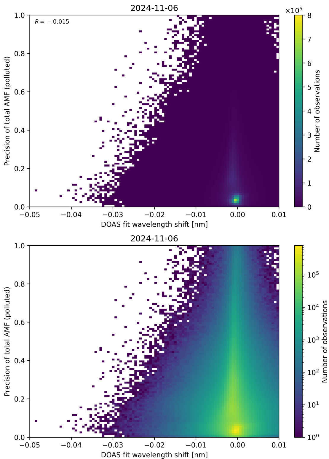
Figure 131: Scatter density plot of “DOAS fit wavelength shift” against “Precision of total AMF (polluted)” for 2024-11-05 to 2024-11-07.
