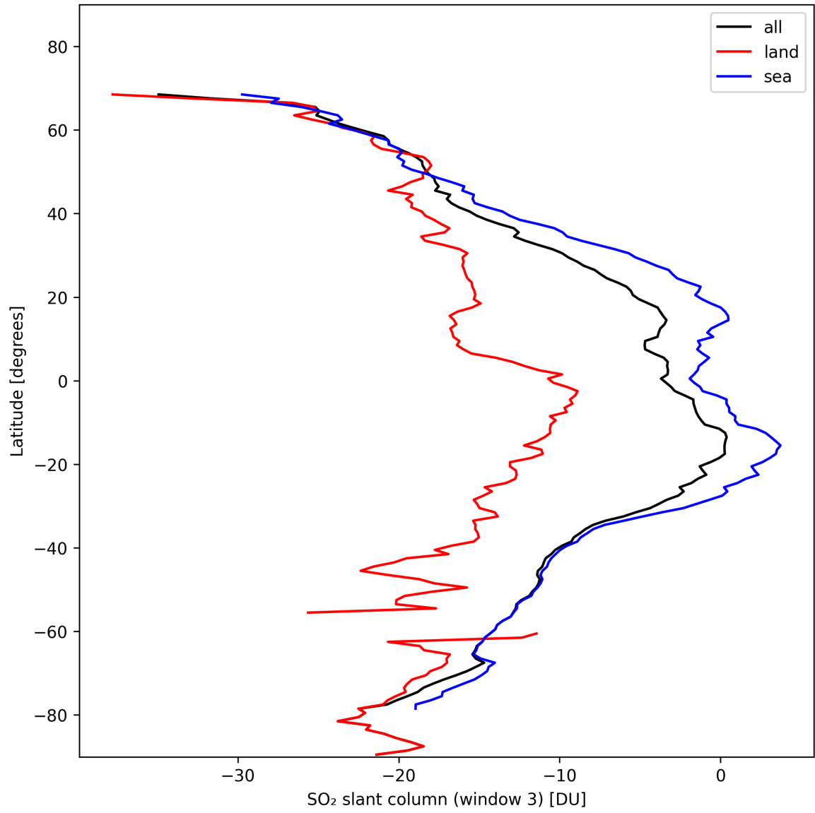
Figure 41: Zonal average of “SO 2 slant column (window 3)” for 2024-11-05 to 2024-11-07.
