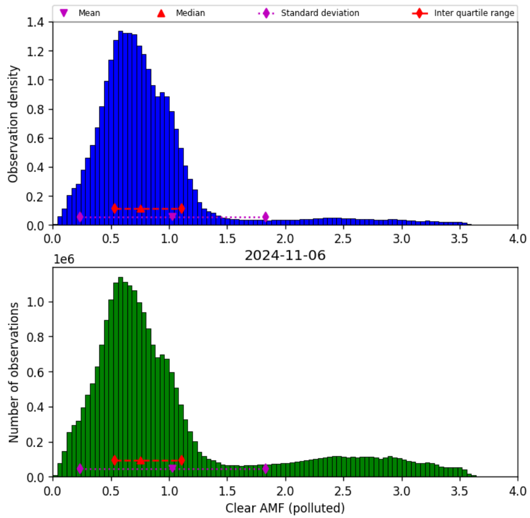
Figure 73: Histogram of “Clear AMF (polluted)” for 2024-11-05 to 2024-11-07
