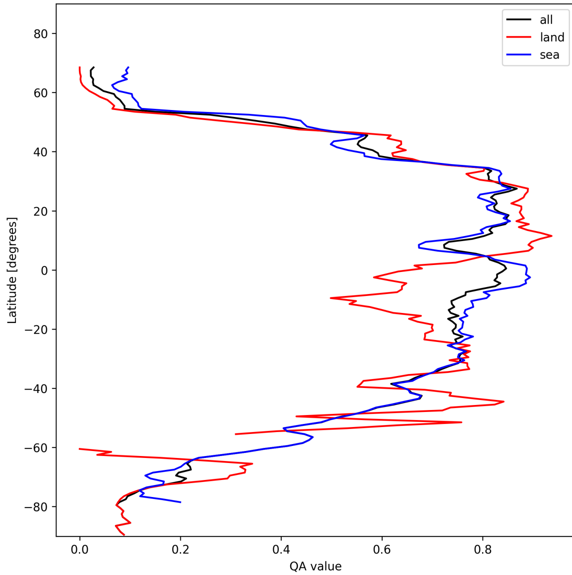
Figure 29: Zonal average of “QA value” for 2024-11-05 to 2024-11-07.
