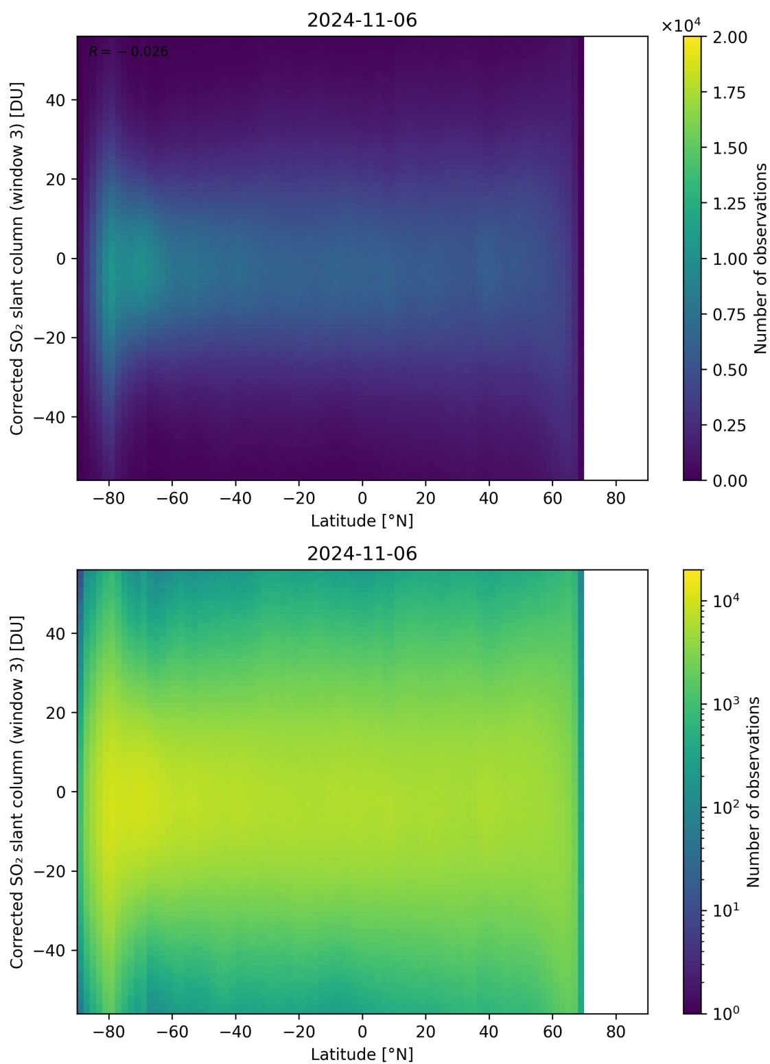
Figure 148: Scatter density plot of “Latitude” against “Corrected SO 2 slant column (window 3)” for 2024-11-05 to 2024-11-07.
