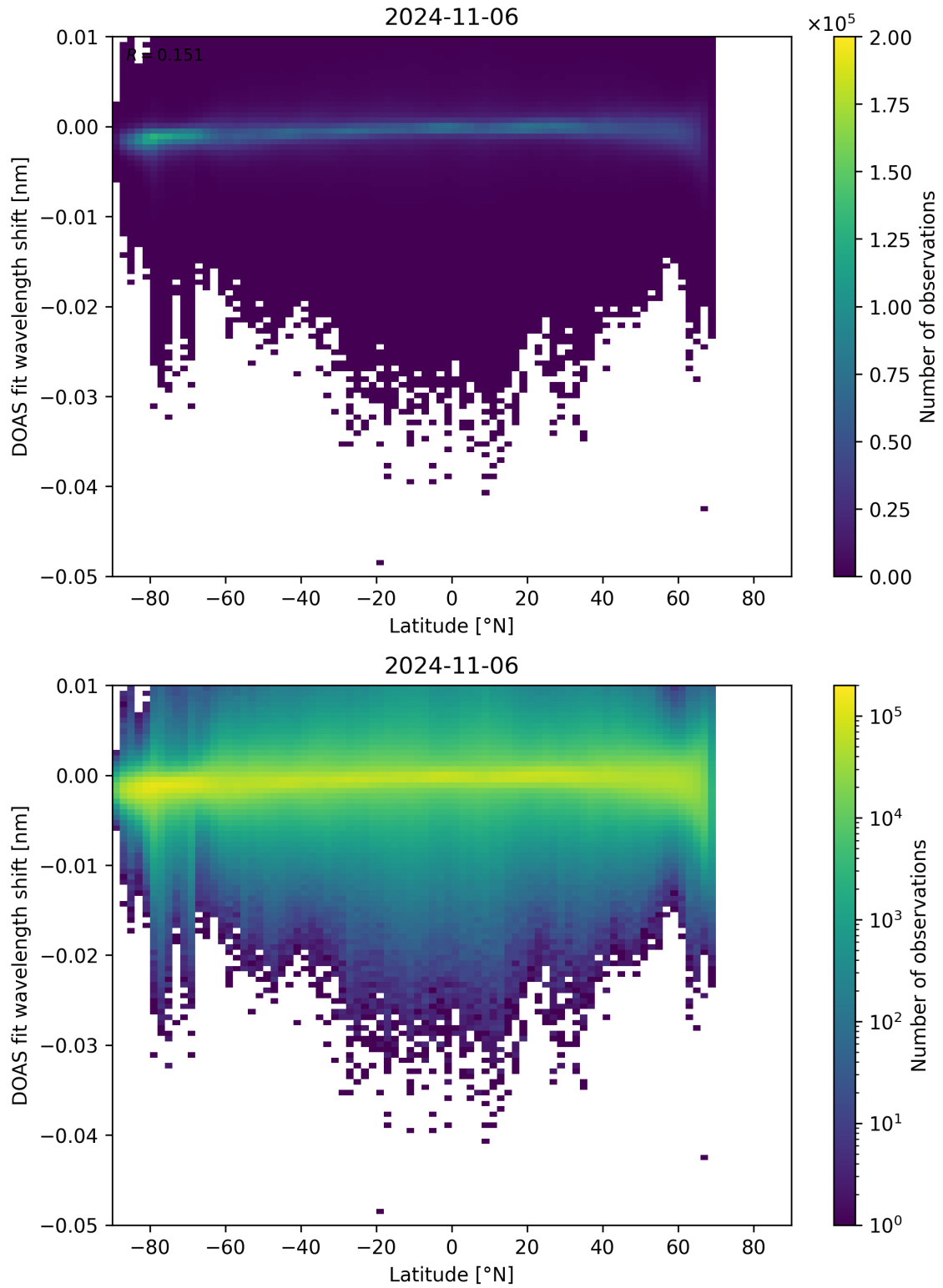
Figure 142: Scatter density plot of “Latitude” against “DOAS fit wavelength shift” for 2024-11-05 to 2024-11-07.
