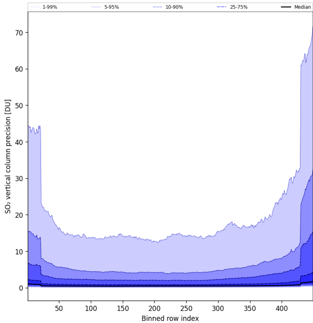
Figure 77: Along track statistics of “SO 2 vertical column precision” for 2024-11-05 to 2024-11-07
