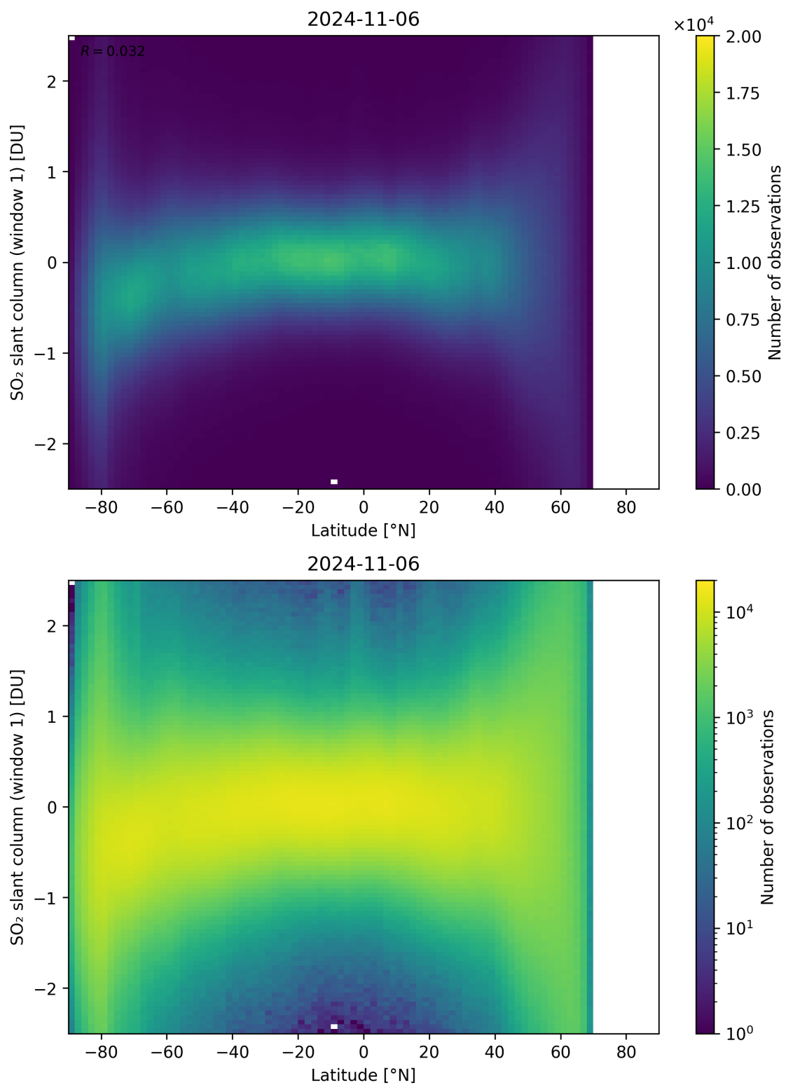
Figure 149: Scatter density plot of “Latitude” against “SO 2 slant column (window 1)” for 2024-11-05 to 2024-11-07.
