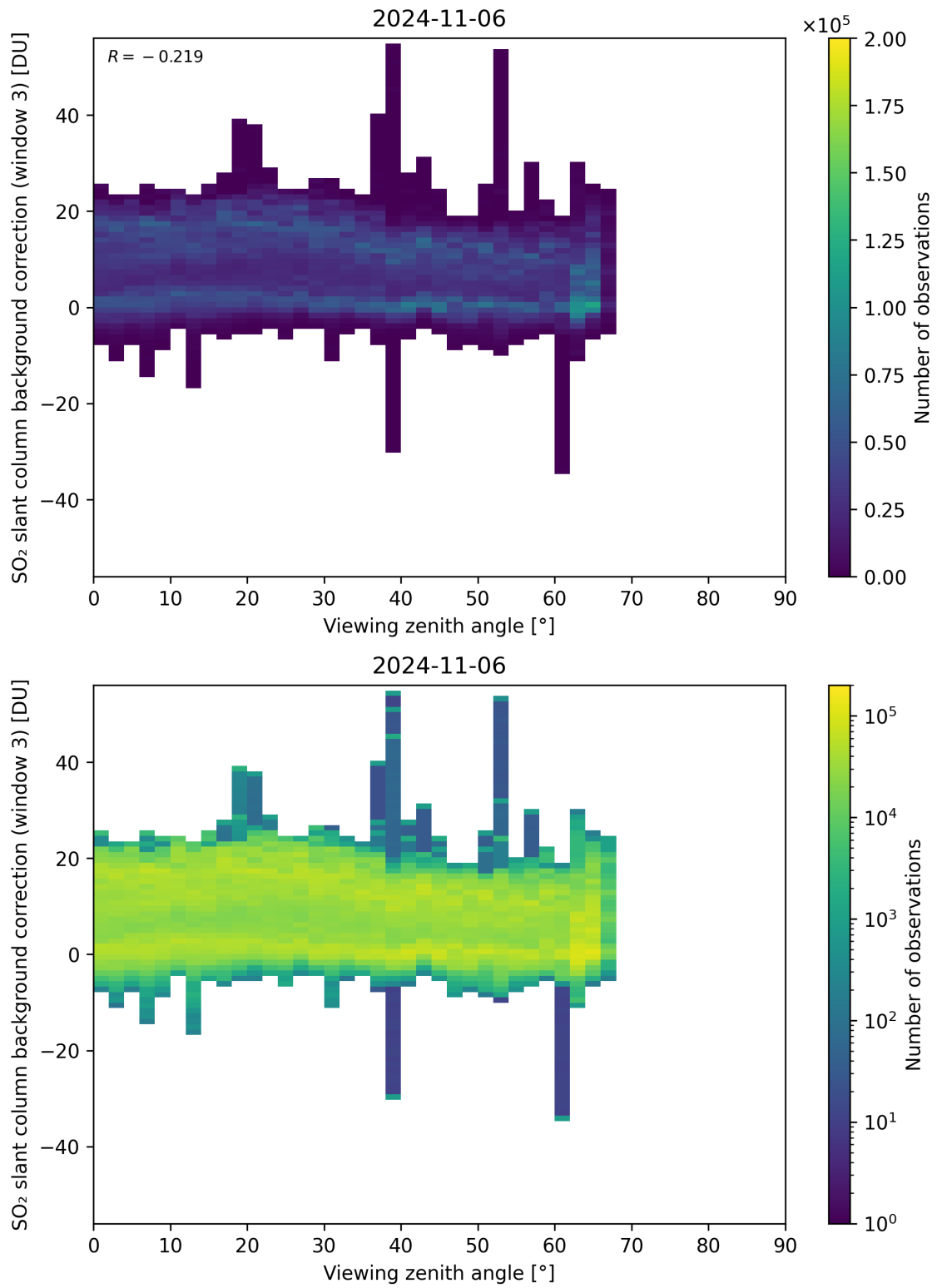
Figure 310: Scatter density plot of “Viewing zenith angle” against “SO 2 slant column background correction (window 3)” for 2024-11-05 to 2024-11-07.
