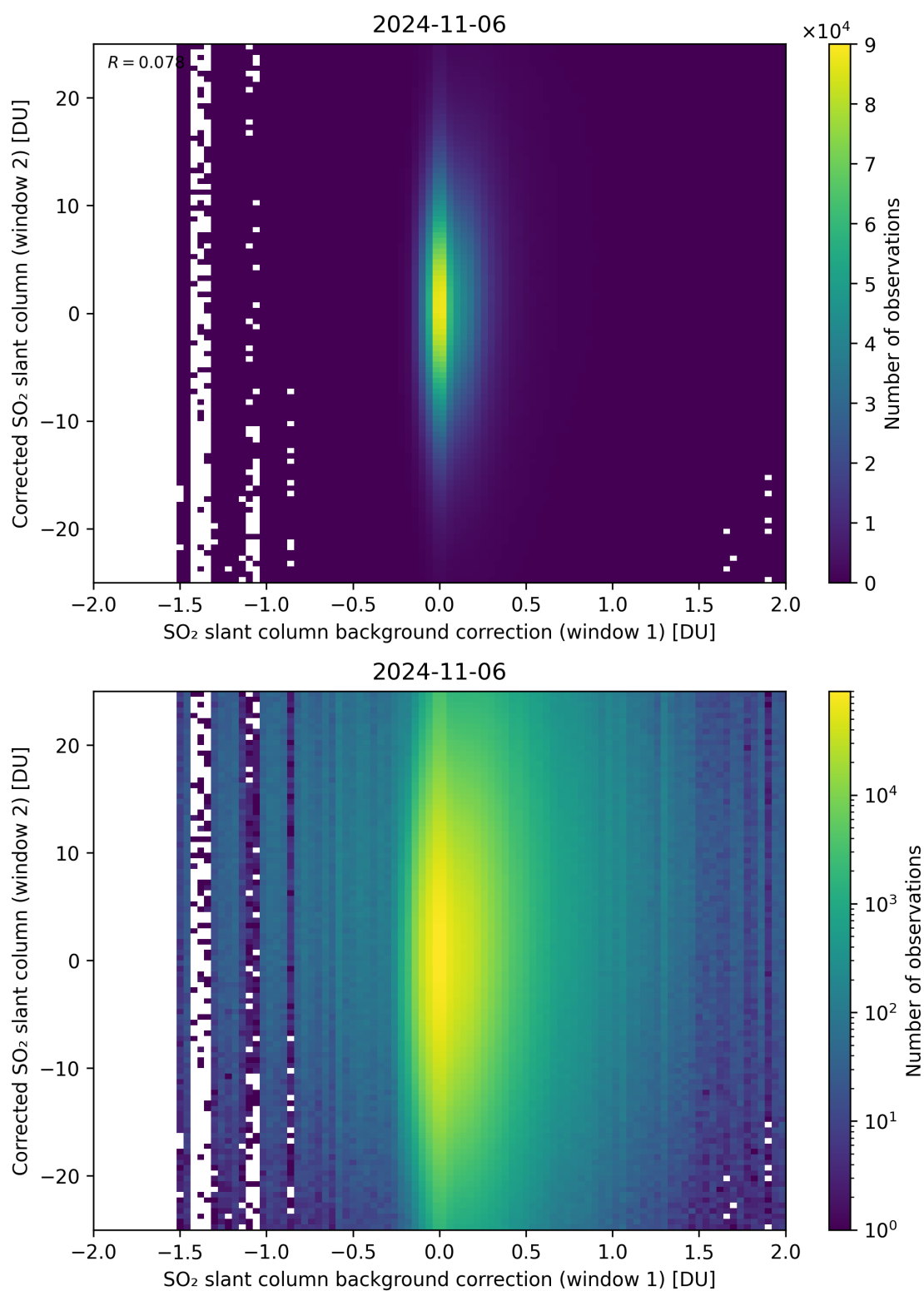
Figure 104: Scatter density plot of “SO 2 slant column background correction (window 1)” against “Corrected SO 2 slant column (window 2)” for 2024-11-05 to 2024-11-07.
