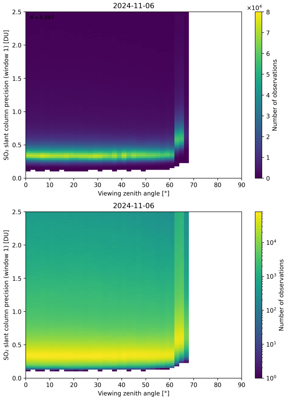
Figure 321: Scatter density plot of “Viewing zenith angle” against “SO 2 slant column precision (window 1)” for 2024-11-05 to 2024-11-07.
