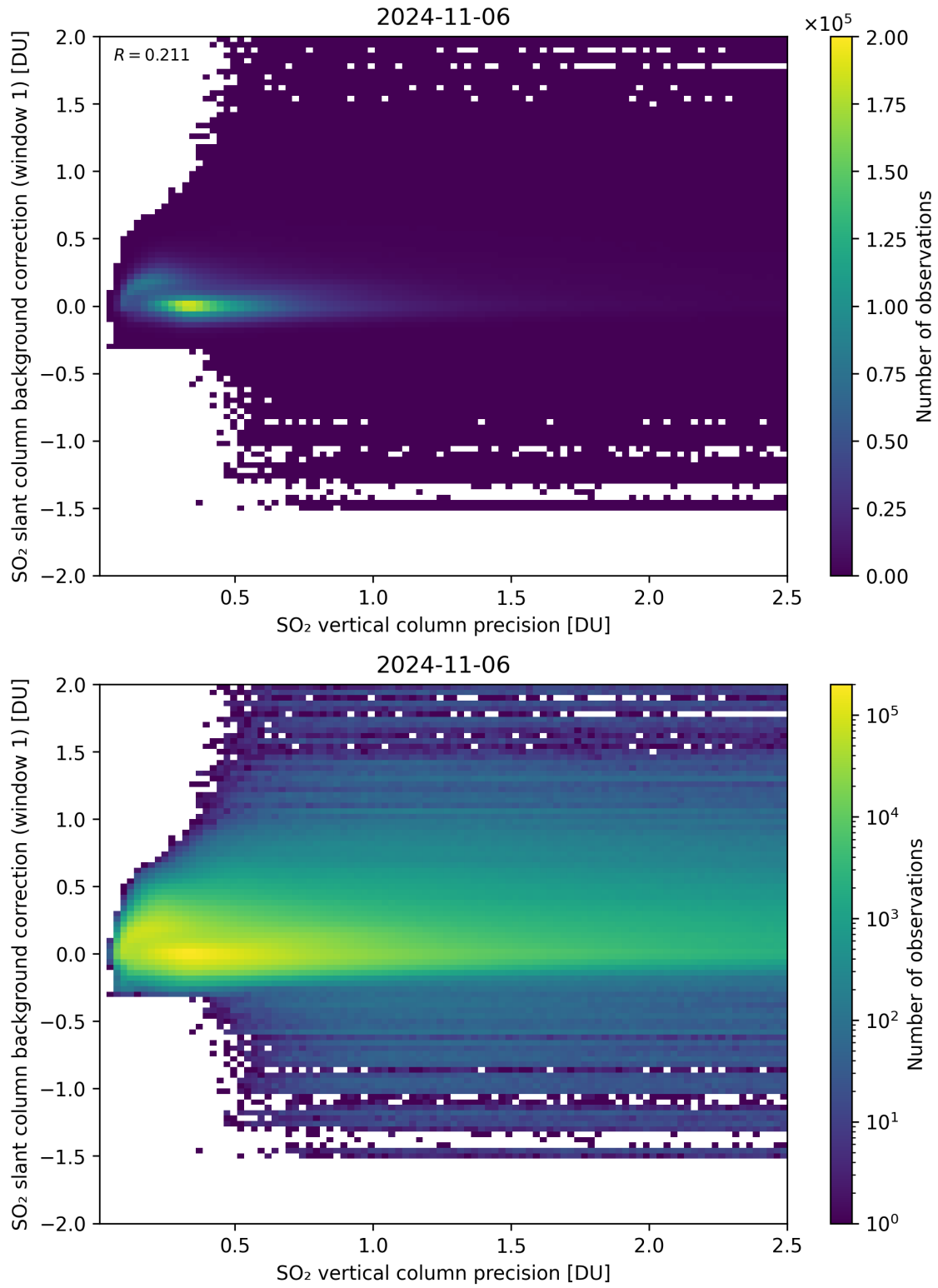
Figure 279: Scatter density plot of “SO 2 vertical column precision” against “SO 2 slant column background correction (window 1)” for 2024-11-05 to 2024-11-07.
