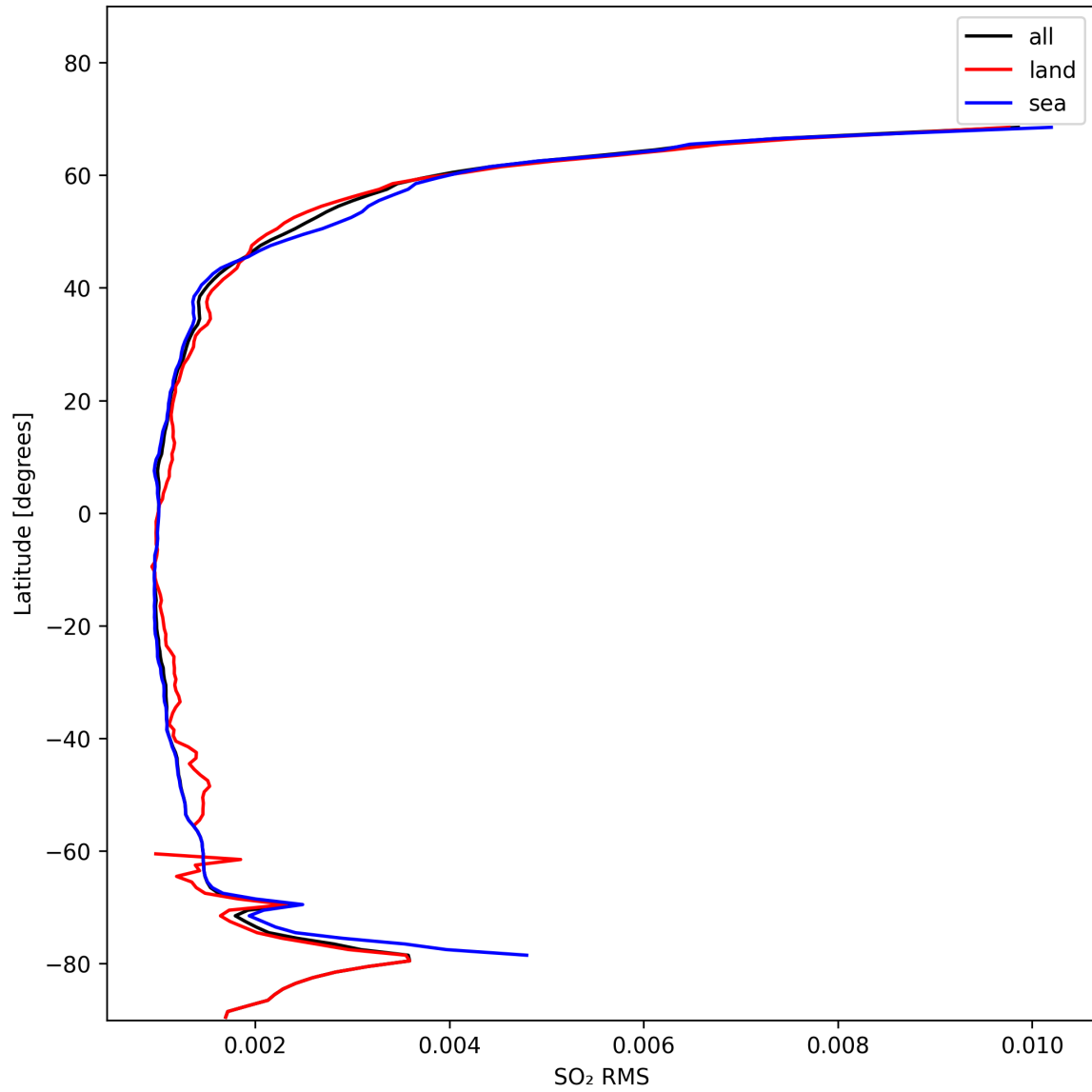
Figure 47: Zonal average of “SO 2 RMS” for 2024-11-05 to 2024-11-07.
