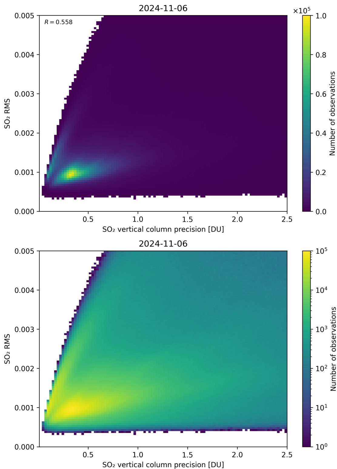
Figure 284: Scatter density plot of “SO 2 vertical column precision” against “SO 2 RMS” for 2024-11-05 to 2024-11-07.
