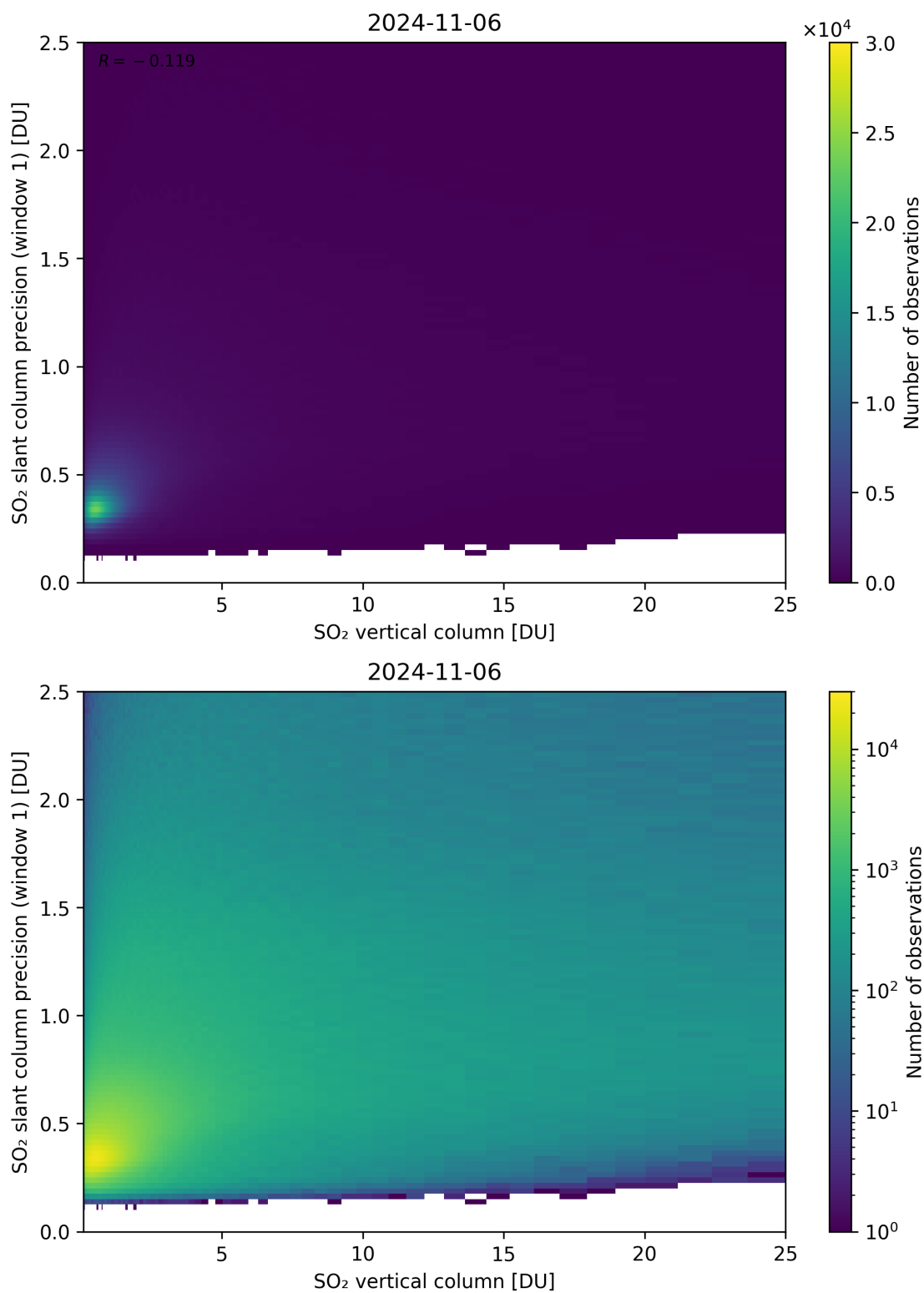
Figure 301: Scatter density plot of “SO 2 vertical column” against “SO 2 slant column precision (window 1)” for 2024-11-05 to 2024-11-07.
