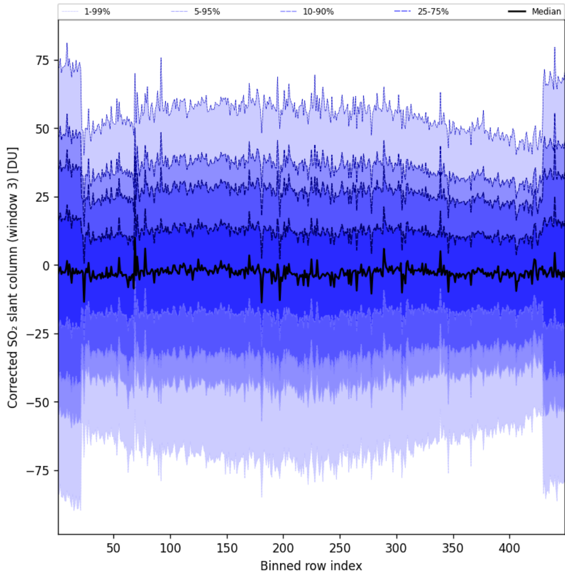
Figure 89: Along track statistics of “Corrected SO 2 slant column (window 3)” for 2024-11-05 to 2024-11-07
