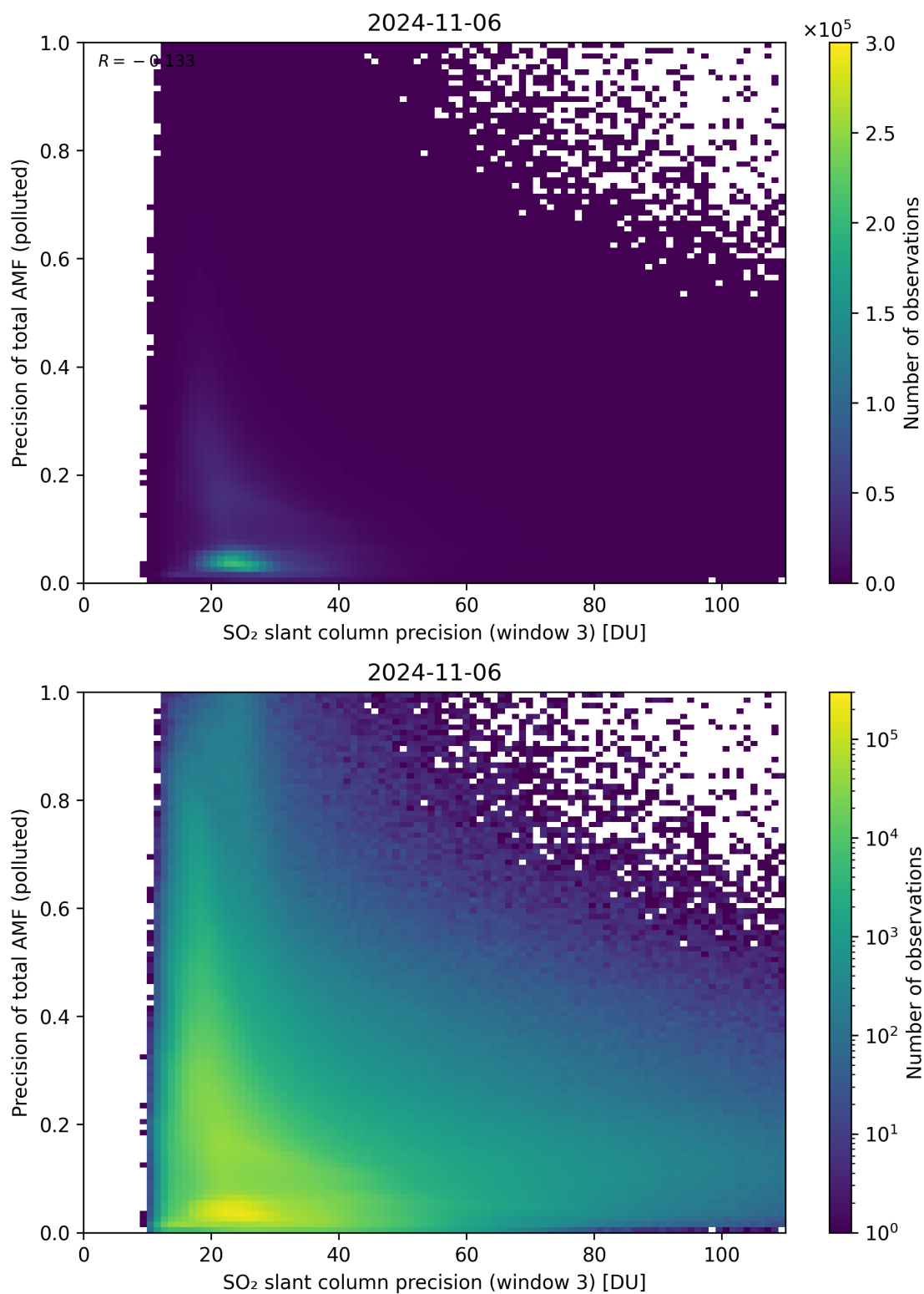
Figure 264: Scatter density plot of “SO 2 slant column precision (window 3)” against “Precision of total AMF (polluted)” for 2024-11-05 to 2024-11-07.
