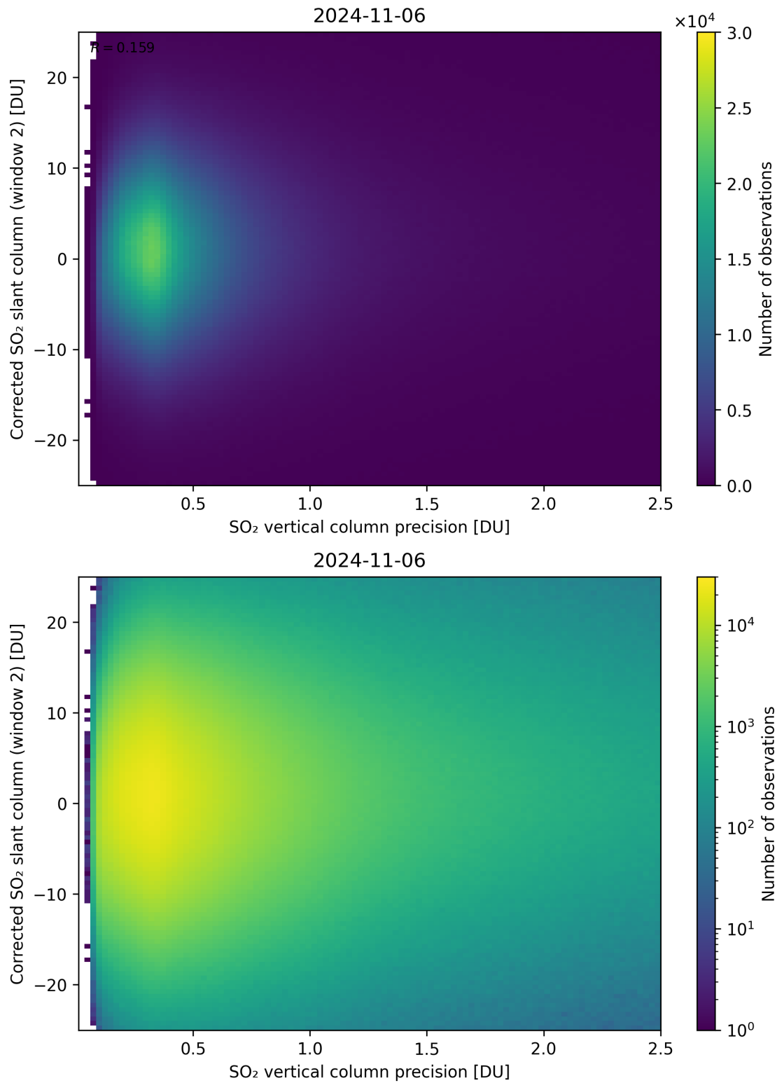
Figure 287: Scatter density plot of “SO 2 vertical column precision” against “Corrected SO 2 slant column (window 2)” for 2024-11-05 to 2024-11-07.
