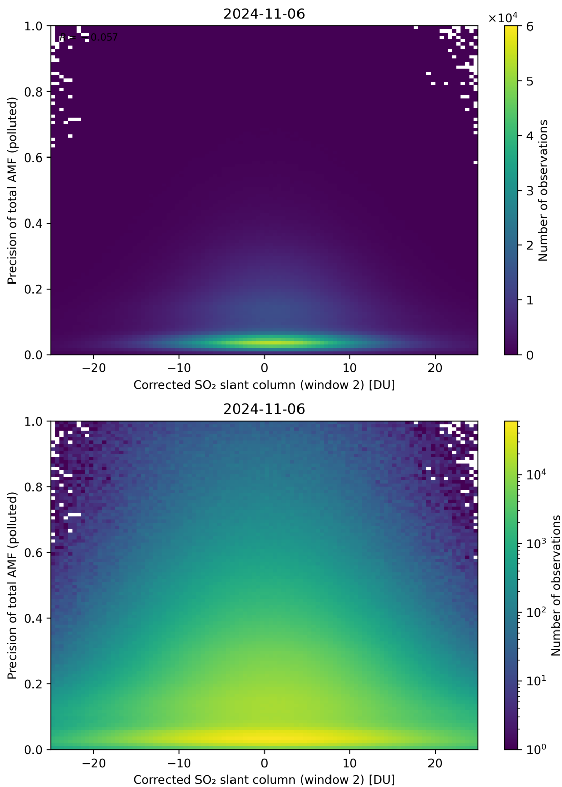
Figure 204: Scatter density plot of “Corrected SO 2 slant column (window 2)” against “Precision of total AMF (polluted)” for 2024-11-05 to 2024-11-07.
