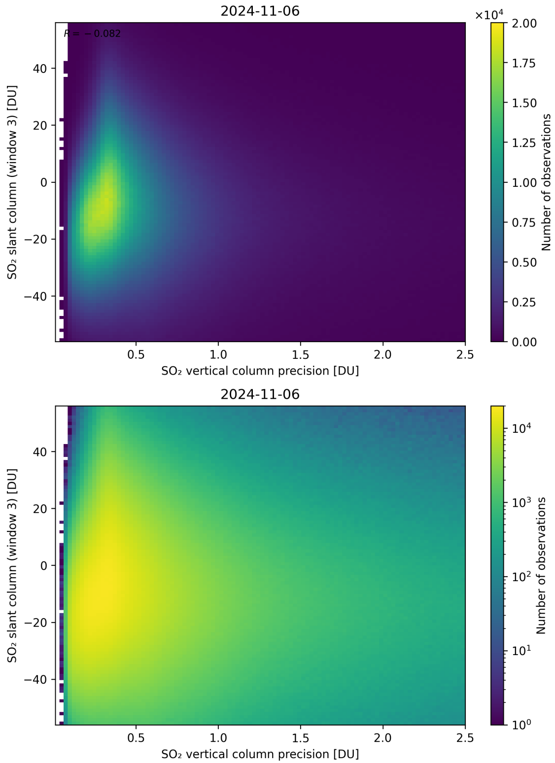
Figure 292: Scatter density plot of “SO 2 vertical column precision” against “SO 2 slant column (window 3)” for 2024-11-05 to 2024-11-07.
