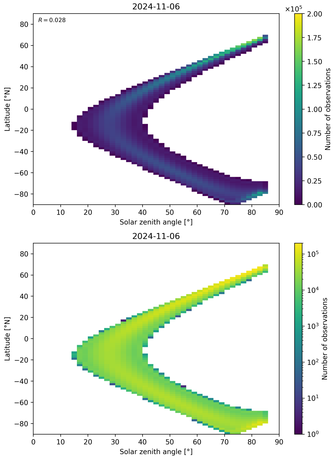
Figure 164: Scatter density plot of “Solar zenith angle” against “Latitude” for 2024-11-05 to 2024-11-07.
