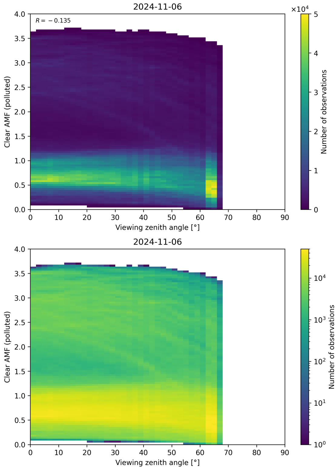
Figure 316: Scatter density plot of “Viewing zenith angle” against “Clear AMF (polluted)” for 2024-11-05 to 2024-11-07.
