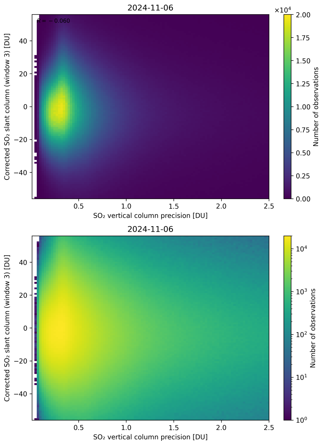
Figure 288: Scatter density plot of “SO 2 vertical column precision” against “Corrected SO 2 slant column (window 3)” for 2024-11-05 to 2024-11-07.
