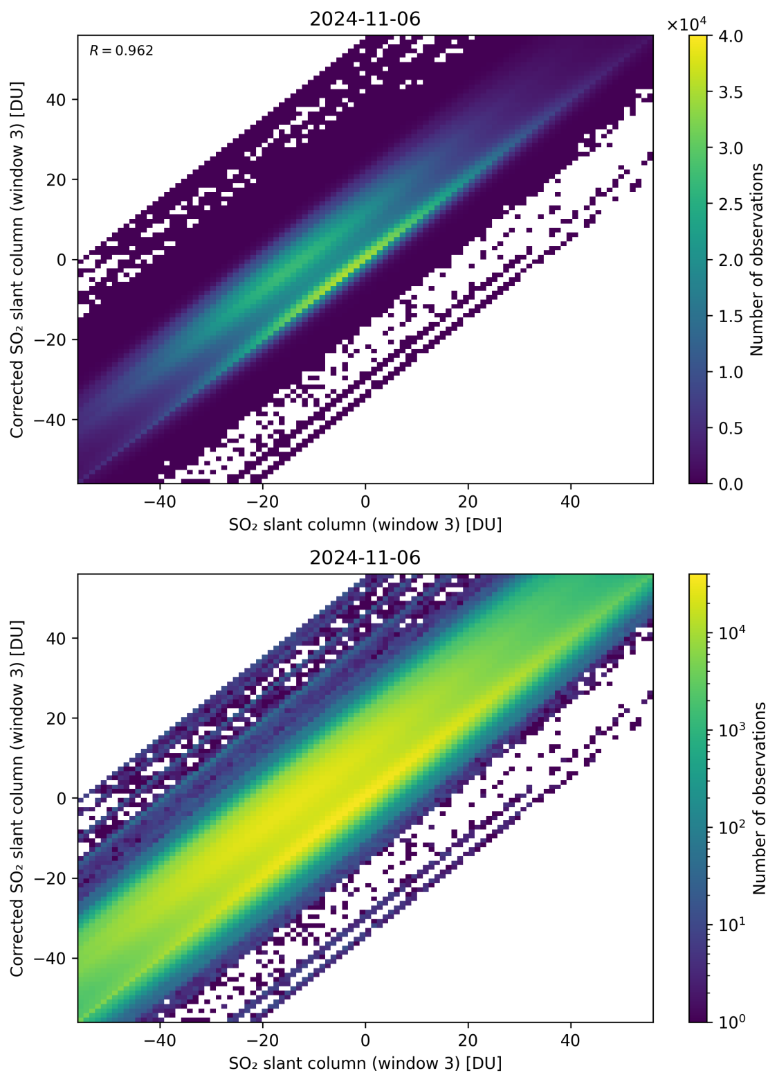
Figure 266: Scatter density plot of “SO 2 slant column (window 3)” against “Corrected SO 2 slant column (window 3)” for 2024-11-05 to 2024-11-07.
