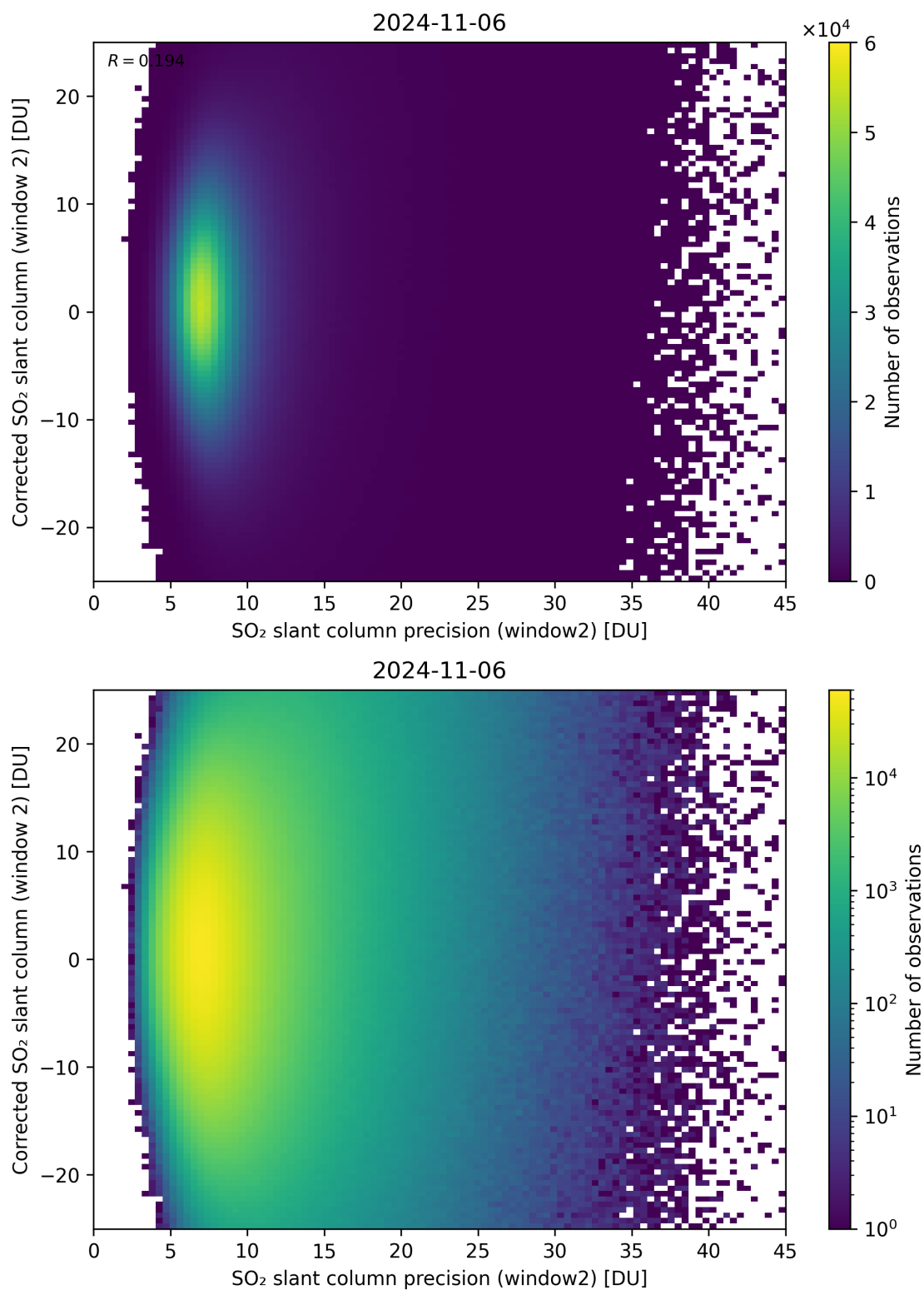
Figure 247: Scatter density plot of “SO 2 slant column precision (window2)” against “Corrected SO 2 slant column (window 2)” for 2024-11-05 to 2024-11-07.
