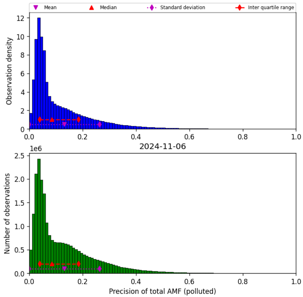
Figure 72: Histogram of “Precision of total AMF (polluted)” for 2024-11-05 to 2024-11-07
