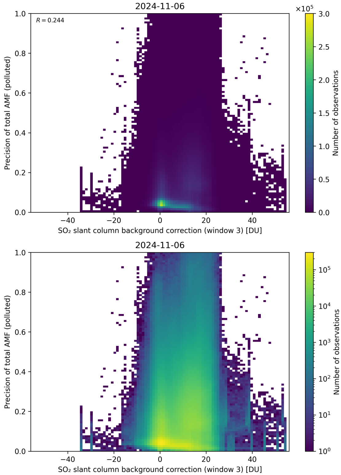
Figure 126: Scatter density plot of “SO 2 slant column background correction (window 3)” against “Precision of total AMF (polluted)” for 2024-11-05 to 2024-11-07.
