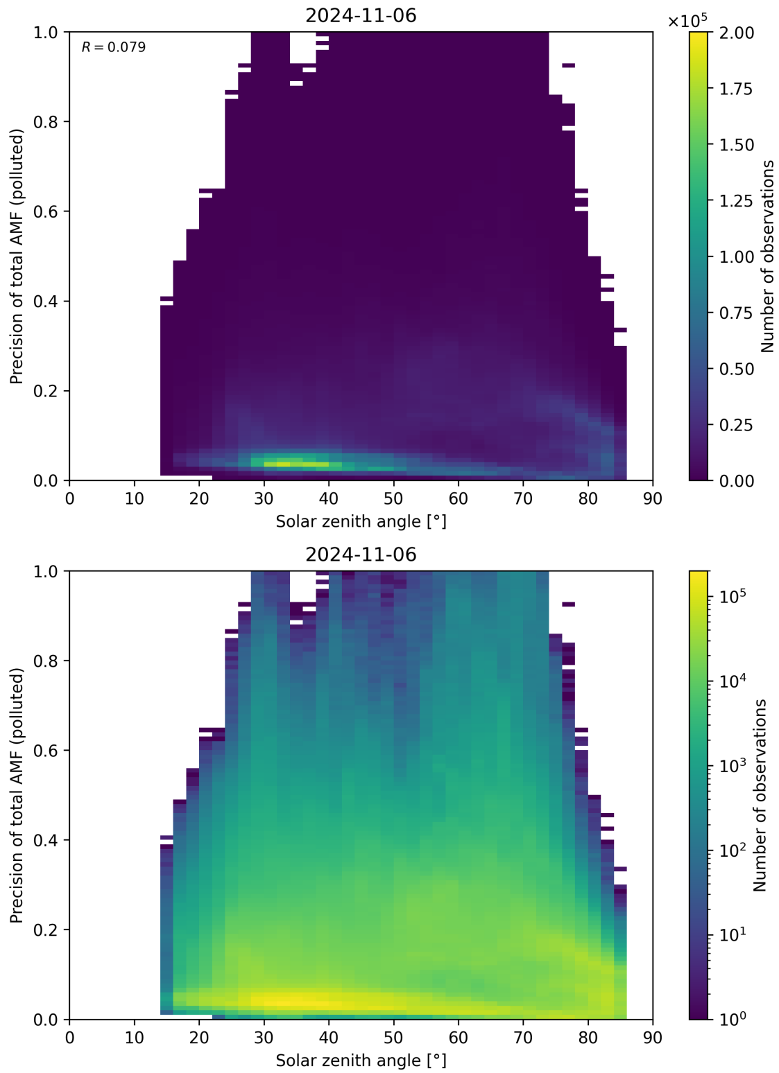
Figure 175: Scatter density plot of “Solar zenith angle” against “Precision of total AMF (polluted)” for 2024-11-05 to 2024-11-07.
