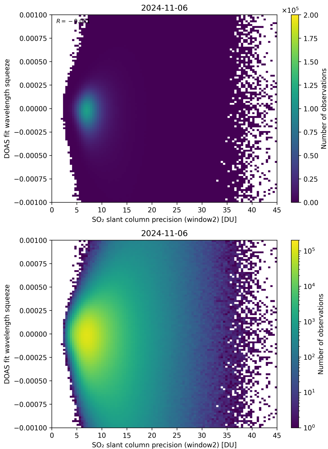
Figure 244: Scatter density plot of “SO 2 slant column precision (window2)” against “DOAS fit wavelength squeeze” for 2024-11-05 to 2024-11-07.
