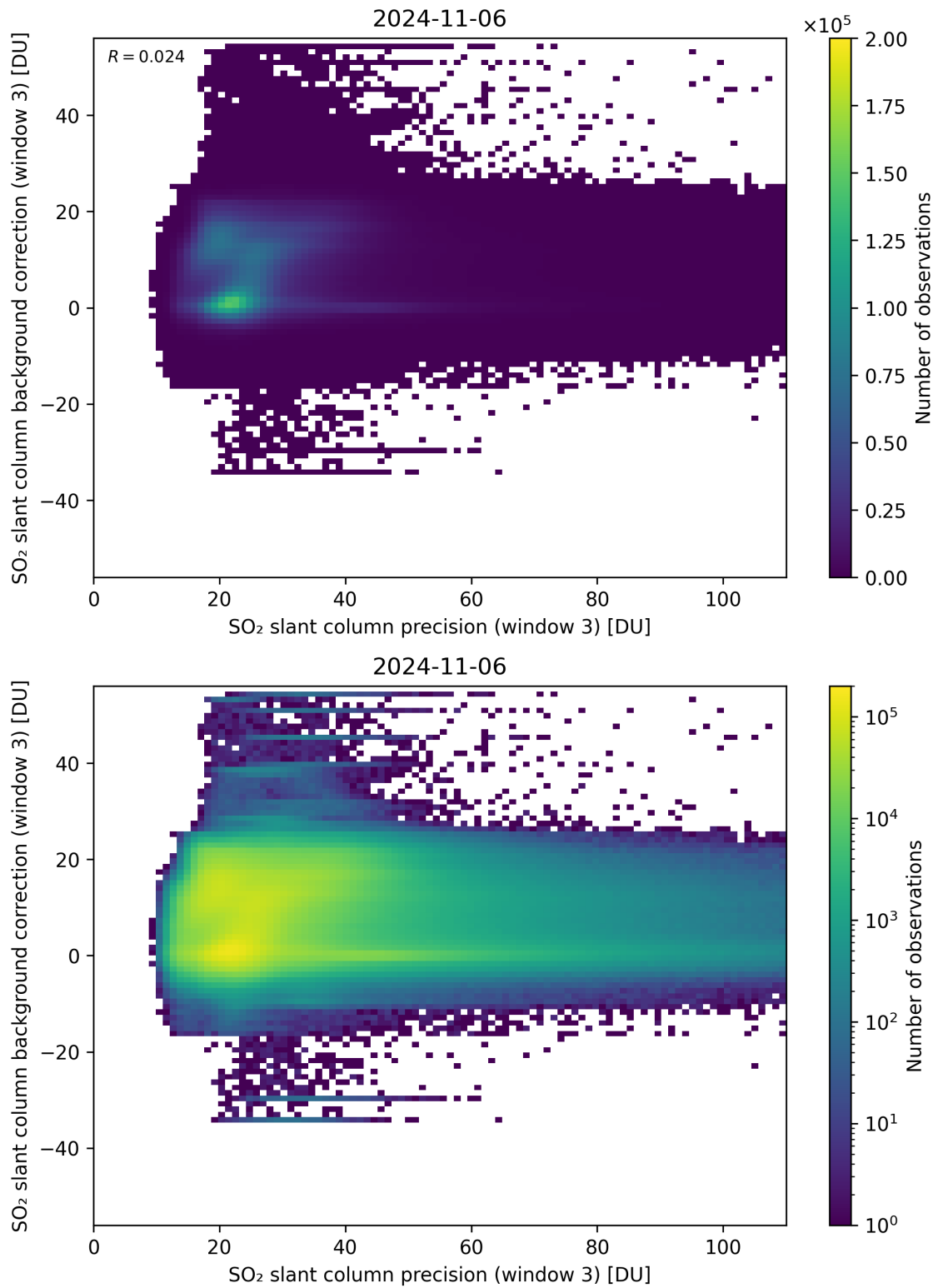
Figure 257: Scatter density plot of “SO 2 slant column precision (window 3)” against “SO 2 slant column background correction (window 3)” for 2024-11-05 to 2024-11-07.
