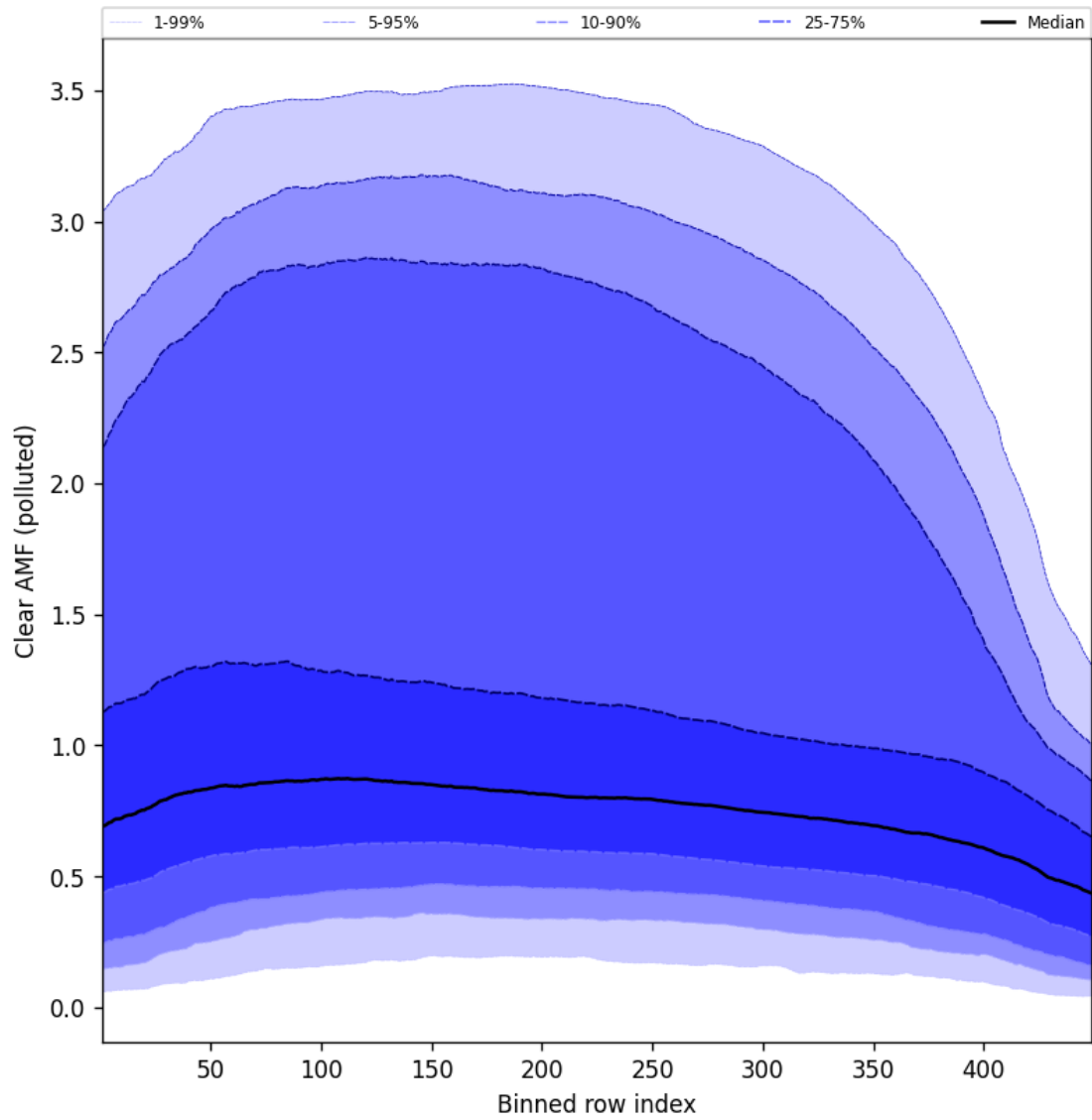
Figure 96: Along track statistics of “Clear AMF (polluted)” for 2024-11-05 to 2024-11-07
