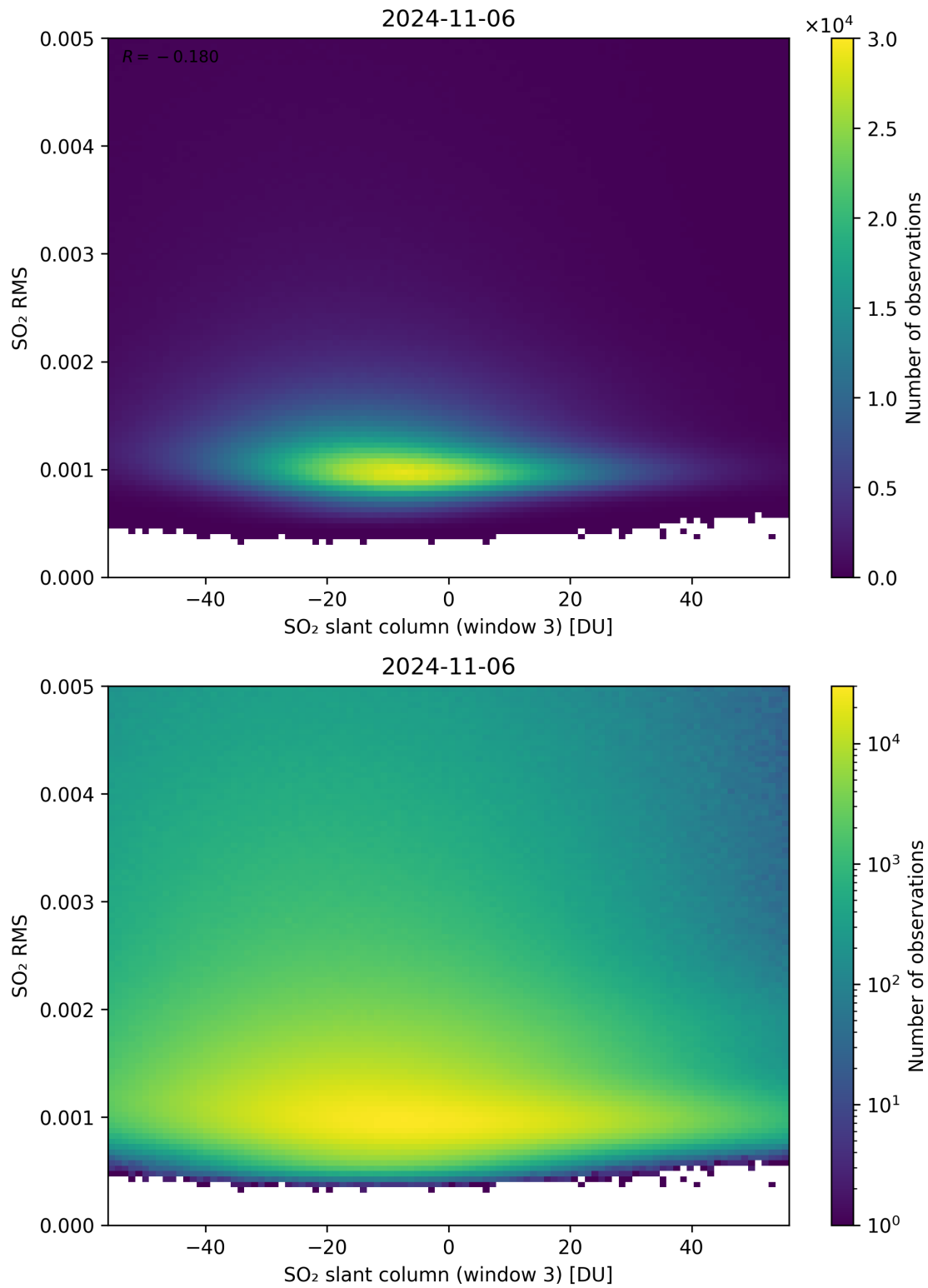
Figure 256: Scatter density plot of “SO 2 slant column (window 3)” against “SO 2 RMS” for 2024-11-05 to 2024-11-07.
