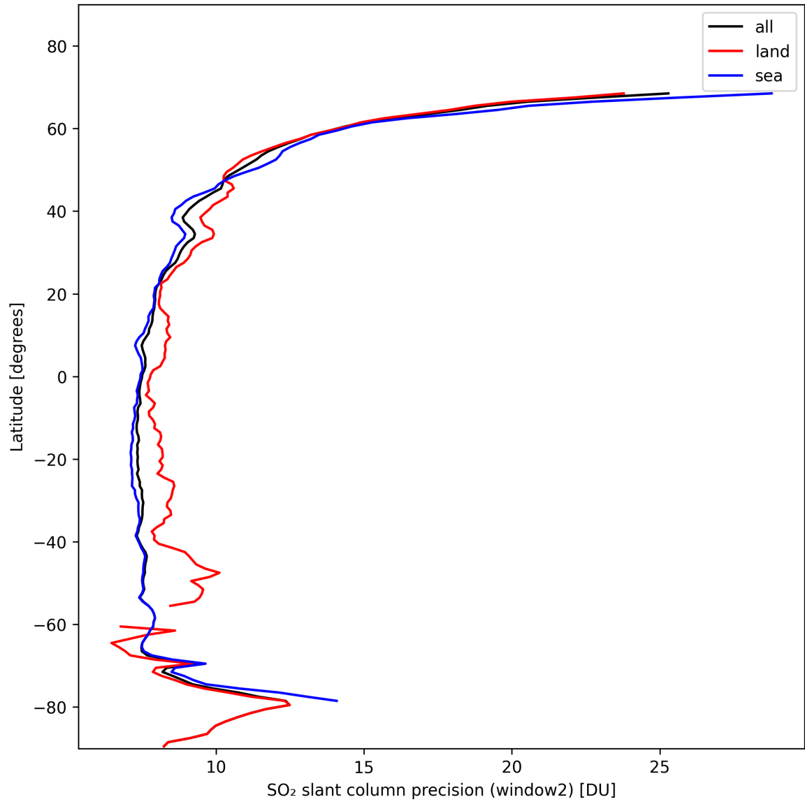
Figure 38: Zonal average of “SO 2 slant column precision (window2)” for 2024-11-05 to 2024-11-07.
