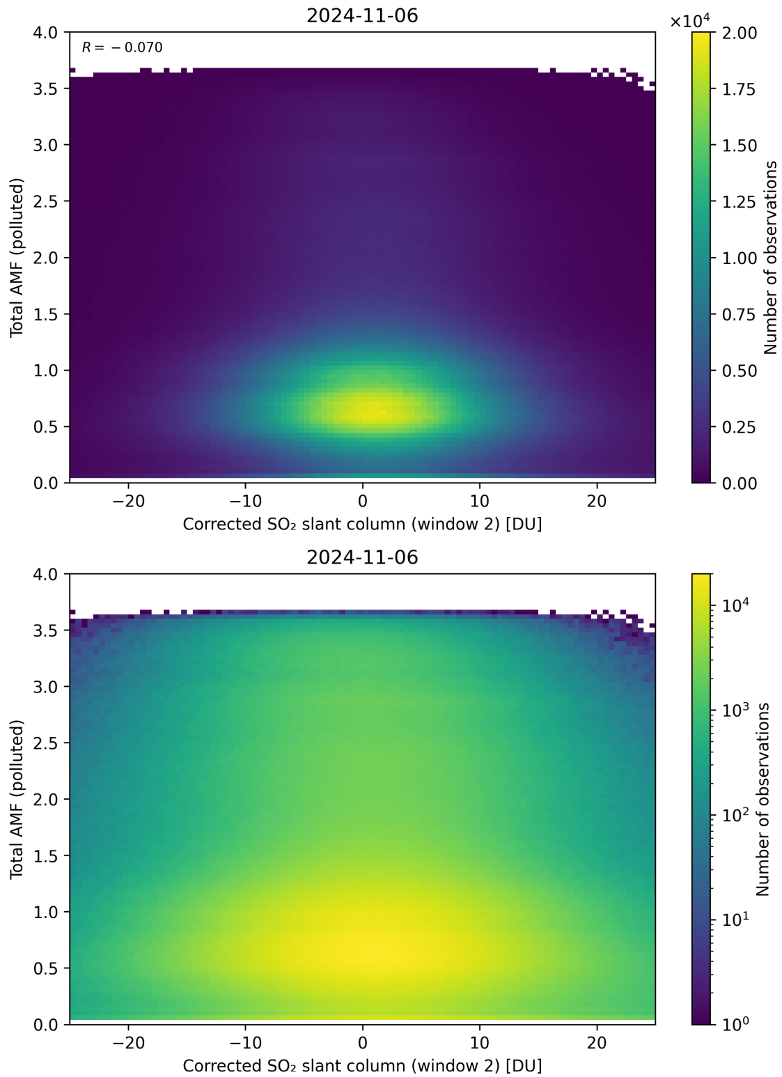
Figure 203: Scatter density plot of “Corrected SO 2 slant column (window 2)” against “Total AMF (polluted)” for 2024-11-05 to 2024-11-07.
