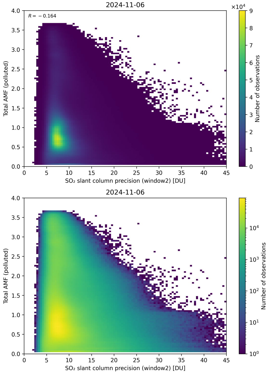
Figure 251: Scatter density plot of “SO 2 slant column precision (window2)” against “Total AMF (polluted)” for 2024-11-05 to 2024-11-07.
