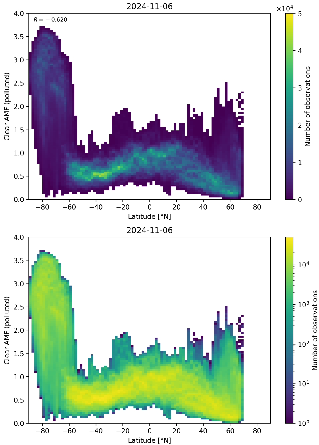
Figure 145: Scatter density plot of “Latitude” against “Clear AMF (polluted)” for 2024-11-05 to 2024-11-07.
