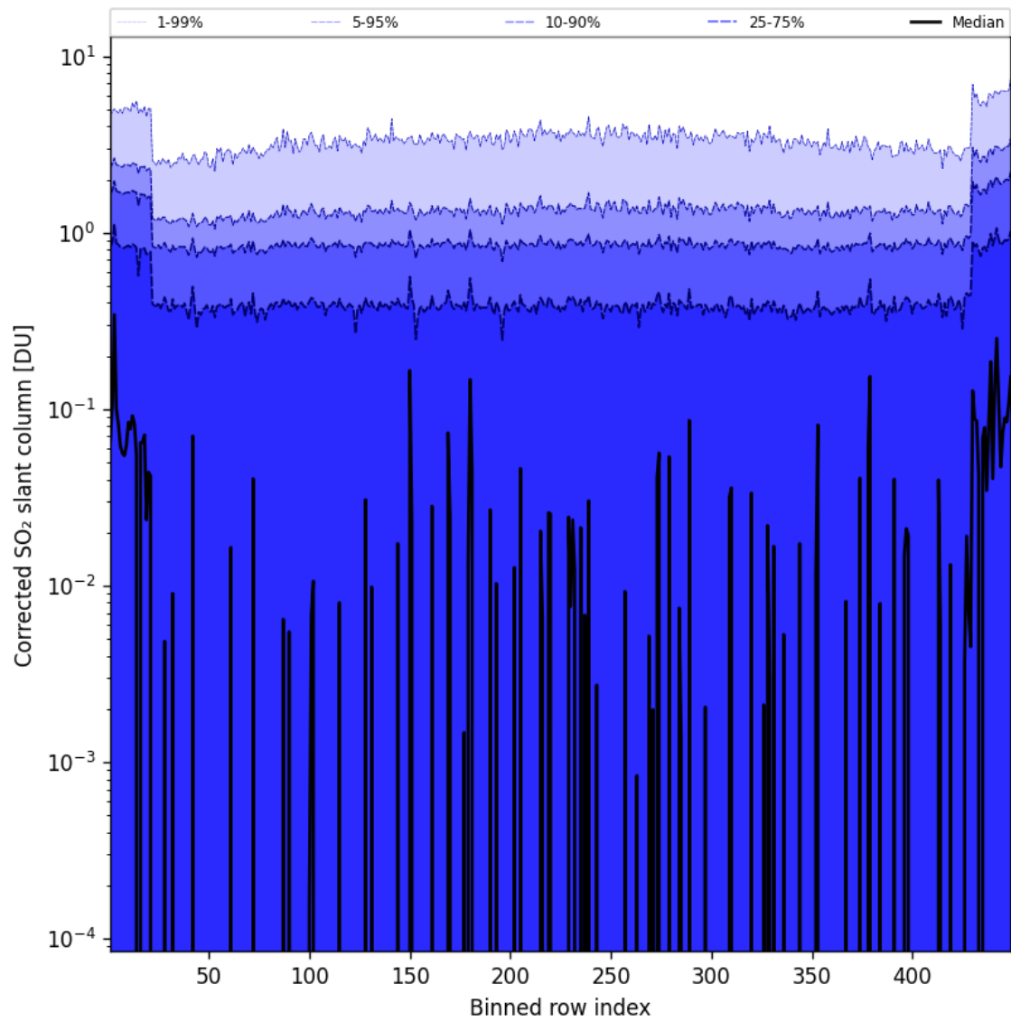
Figure 78: Along track statistics of “Corrected SO 2 slant column” for 2024-11-05 to 2024-11-07
