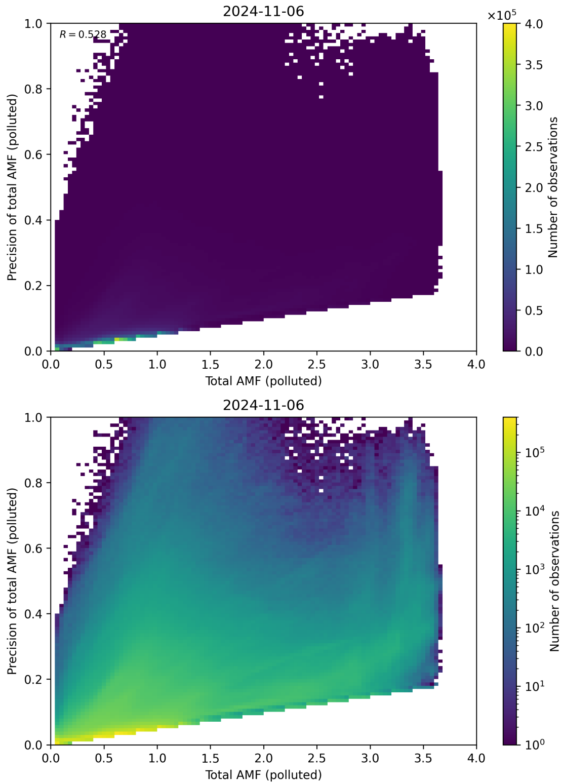
Figure 272: Scatter density plot of “Total AMF (polluted)” against “Precision of total AMF (polluted)” for 2024-11-05 to 2024-11-07.
