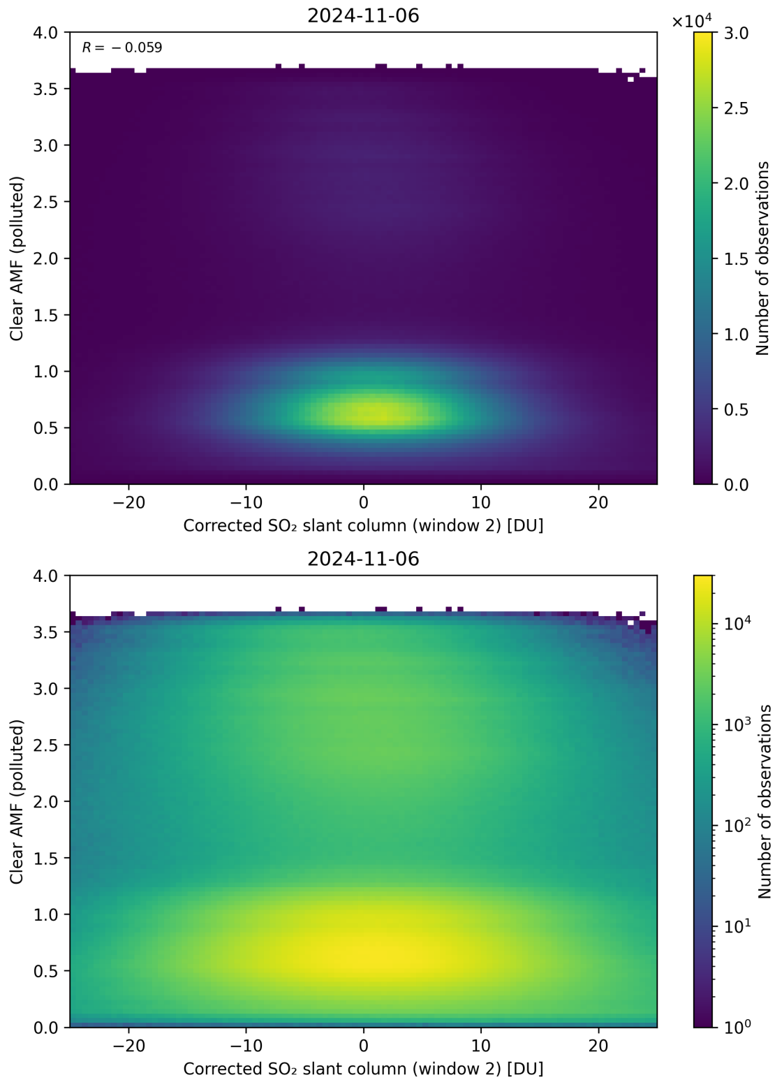
Figure 199: Scatter density plot of “Corrected SO 2 slant column (window 2)” against “Clear AMF (polluted)” for 2024-11-05 to 2024-11-07.
