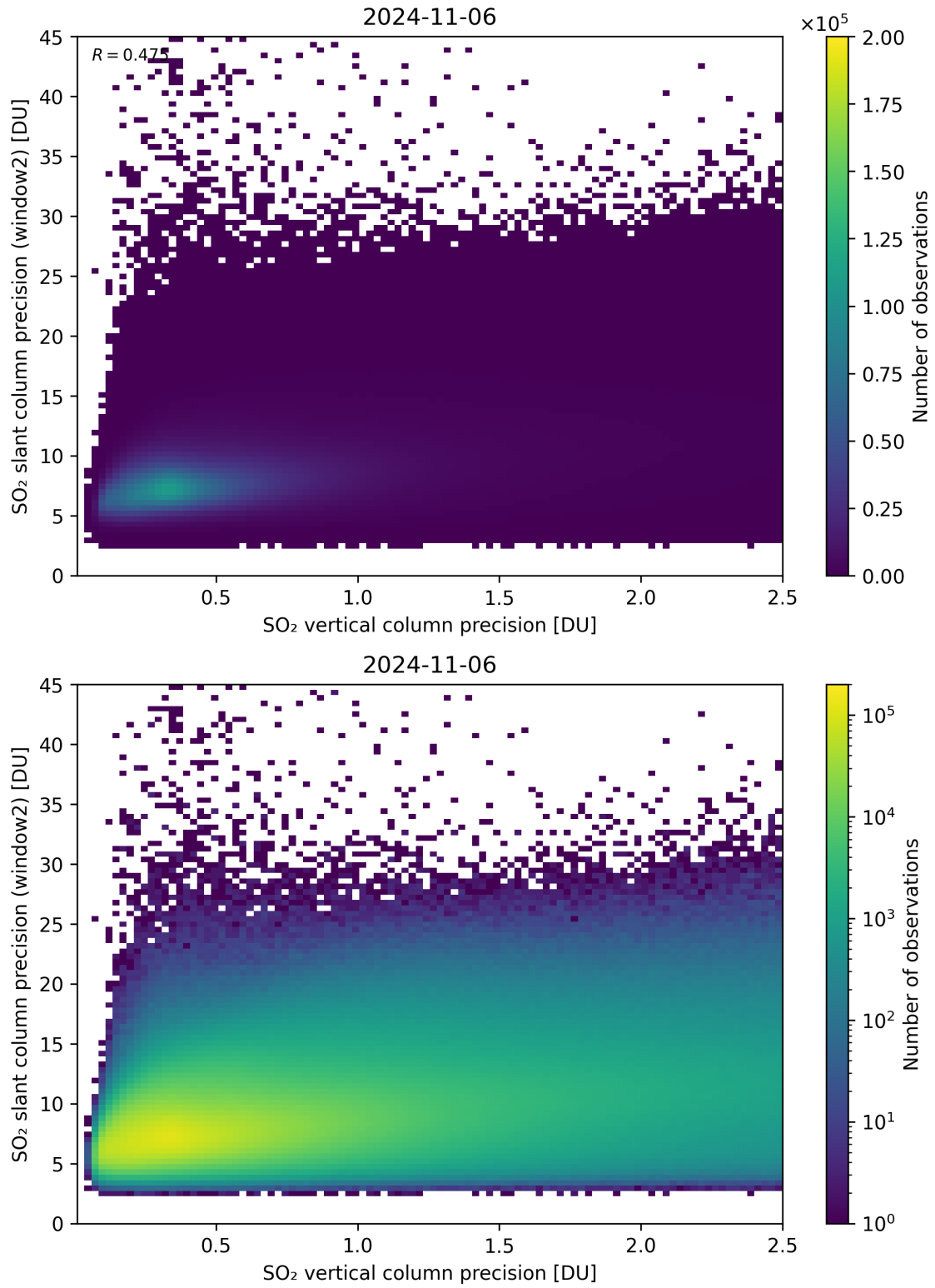
Figure 291: Scatter density plot of “SO 2 vertical column precision” against “SO 2 slant column precision (window2)” for 2024-11-05 to 2024-11-07.
