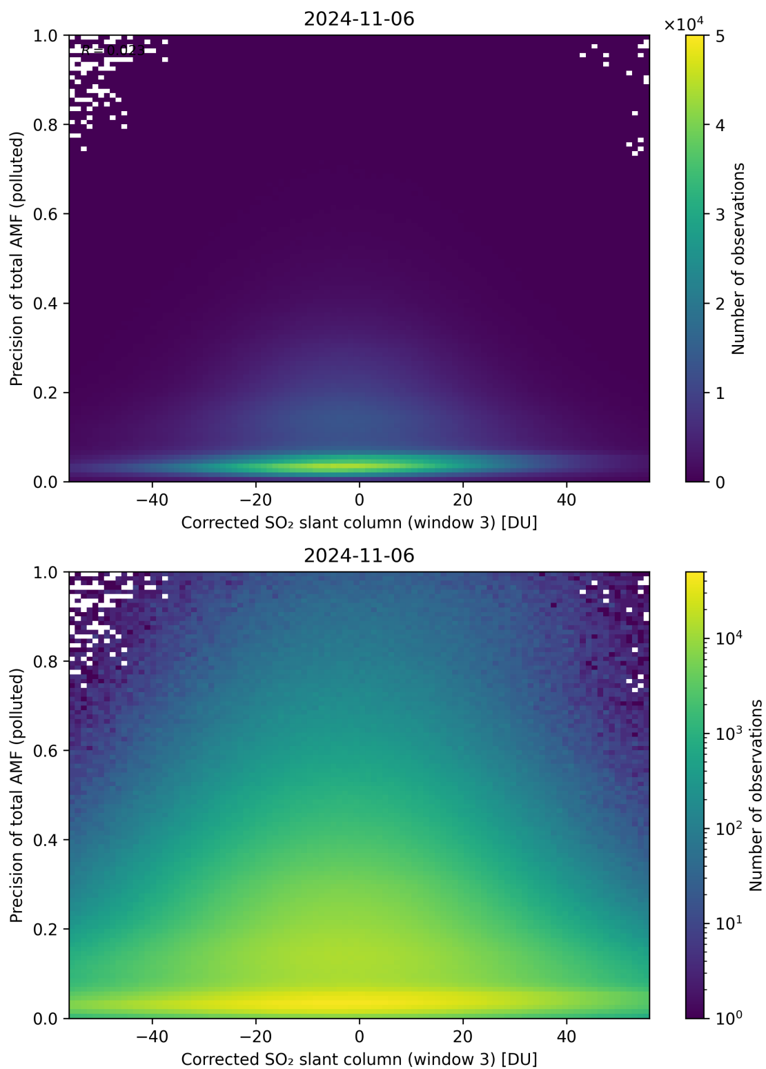
Figure 211: Scatter density plot of “Corrected SO 2 slant column (window 3)” against “Precision of total AMF (polluted)” for 2024-11-05 to 2024-11-07.
