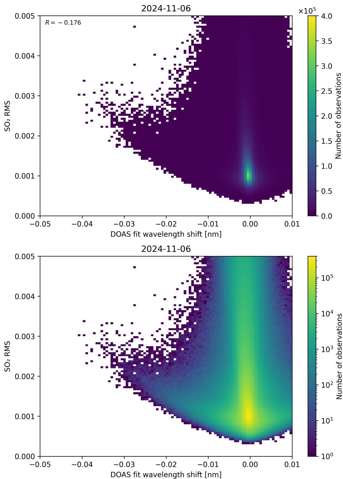
Figure 128: Scatter density plot of “DOAS fit wavelength shift” against “SO 2 RMS” for 2024-11-05 to 2024-11-07.
