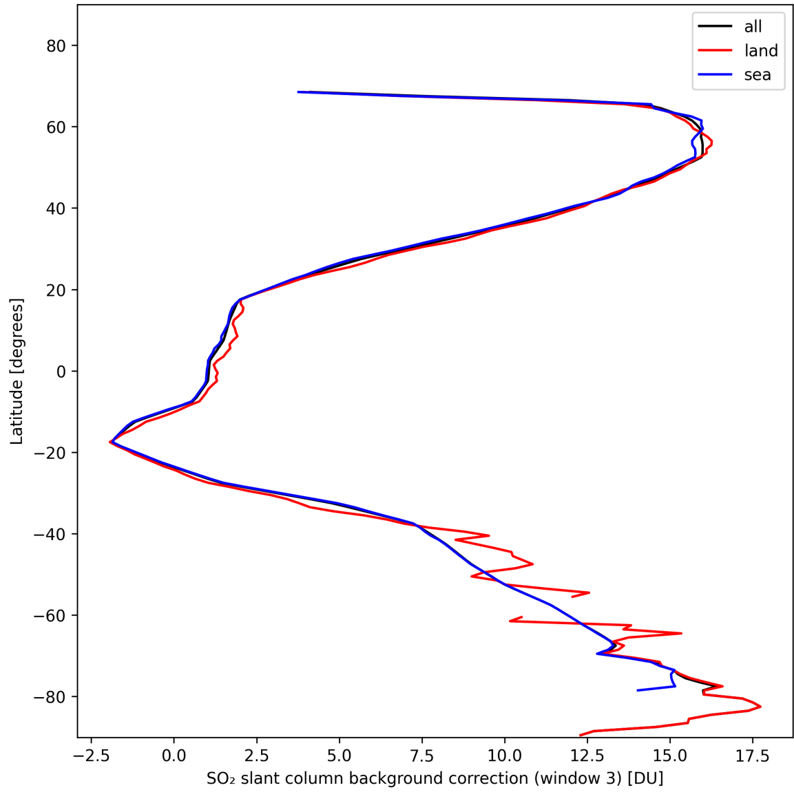
Figure 44: Zonal average of “SO 2 slant column background correction (window 3)” for 2024-11-05 to 2024-11-07.
