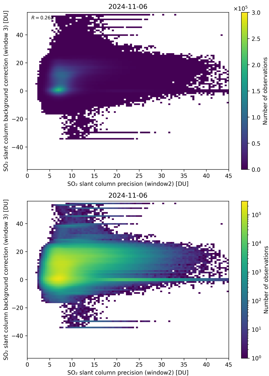
Figure 242: Scatter density plot of “SO 2 slant column precision (window2)” against “SO 2 slant column background correction (window 3)” for 2024-11-05 to 2024-11-07.
