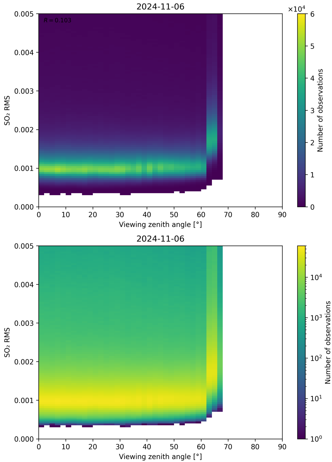
Figure 313: Scatter density plot of “Viewing zenith angle” against “SO 2 RMS” for 2024-11-05 to 2024-11-07.
