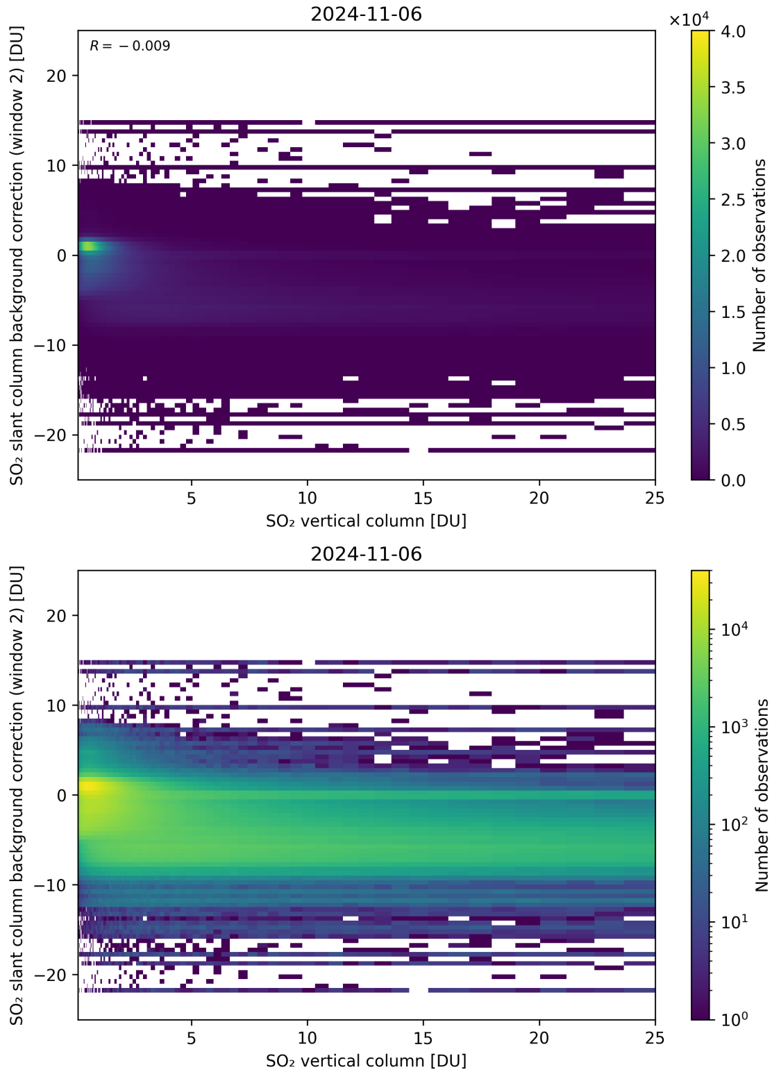
Figure 274: Scatter density plot of “SO 2 vertical column” against “SO 2 slant column background correction (window 2)” for 2024-11-05 to 2024-11-07.
