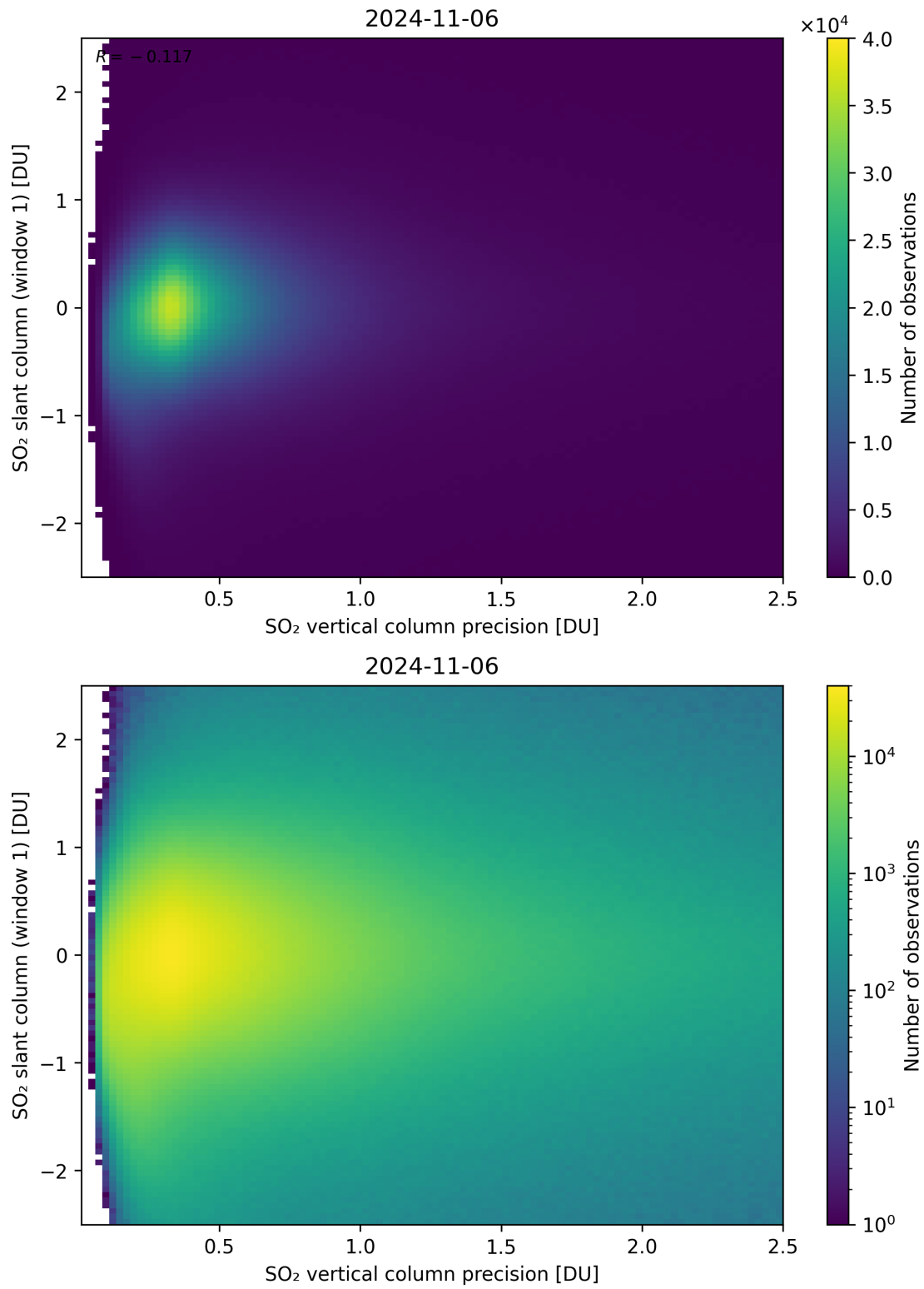
Figure 289: Scatter density plot of “SO 2 vertical column precision” against “SO 2 slant column (window 1)” for 2024-11-05 to 2024-11-07.
