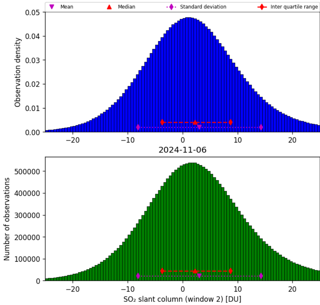
Figure 60: Histogram of “SO 2 slant column (window 2)” for 2024-11-05 to 2024-11-07
