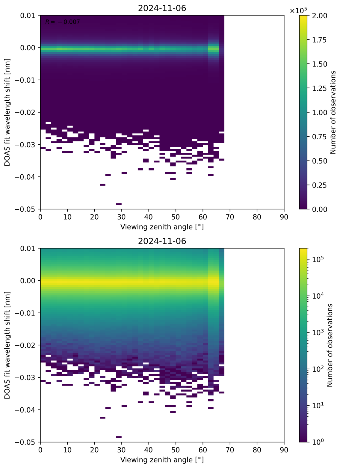
Figure 311: Scatter density plot of “Viewing zenith angle” against “DOAS fit wavelength shift” for 2024-11-05 to 2024-11-07.
