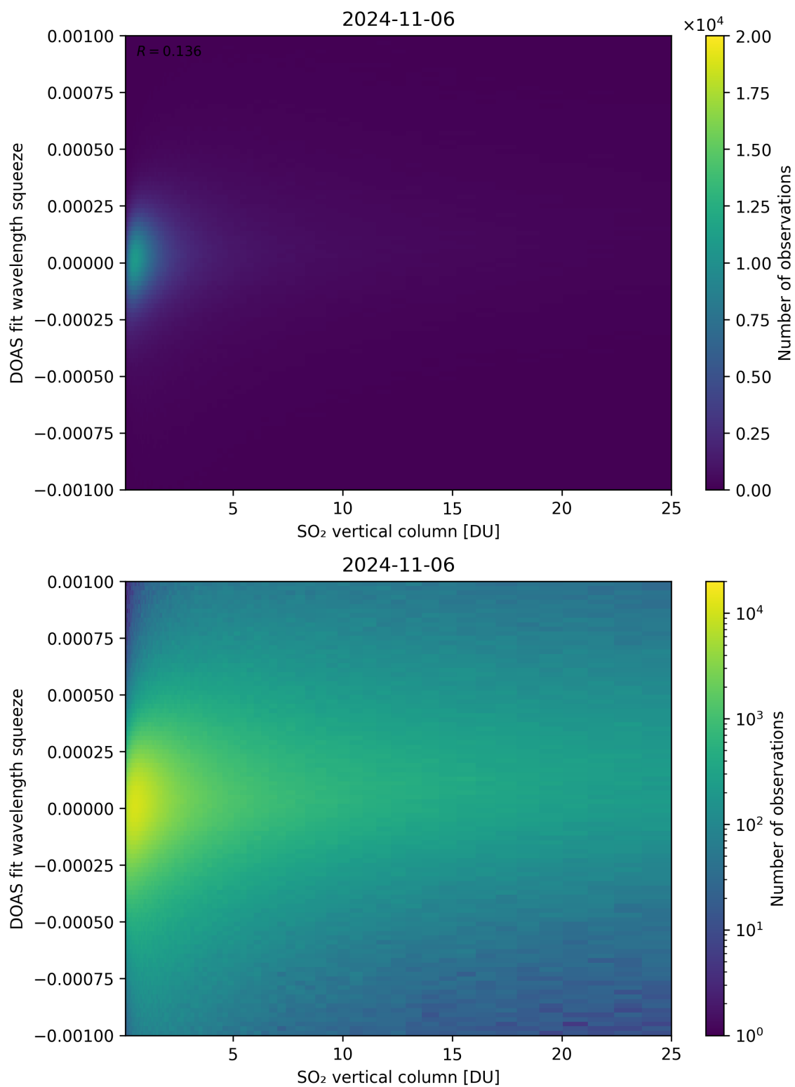
Figure 277: Scatter density plot of “SO 2 vertical column” against “DOAS fit wavelength squeeze” for 2024-11-05 to 2024-11-07.
