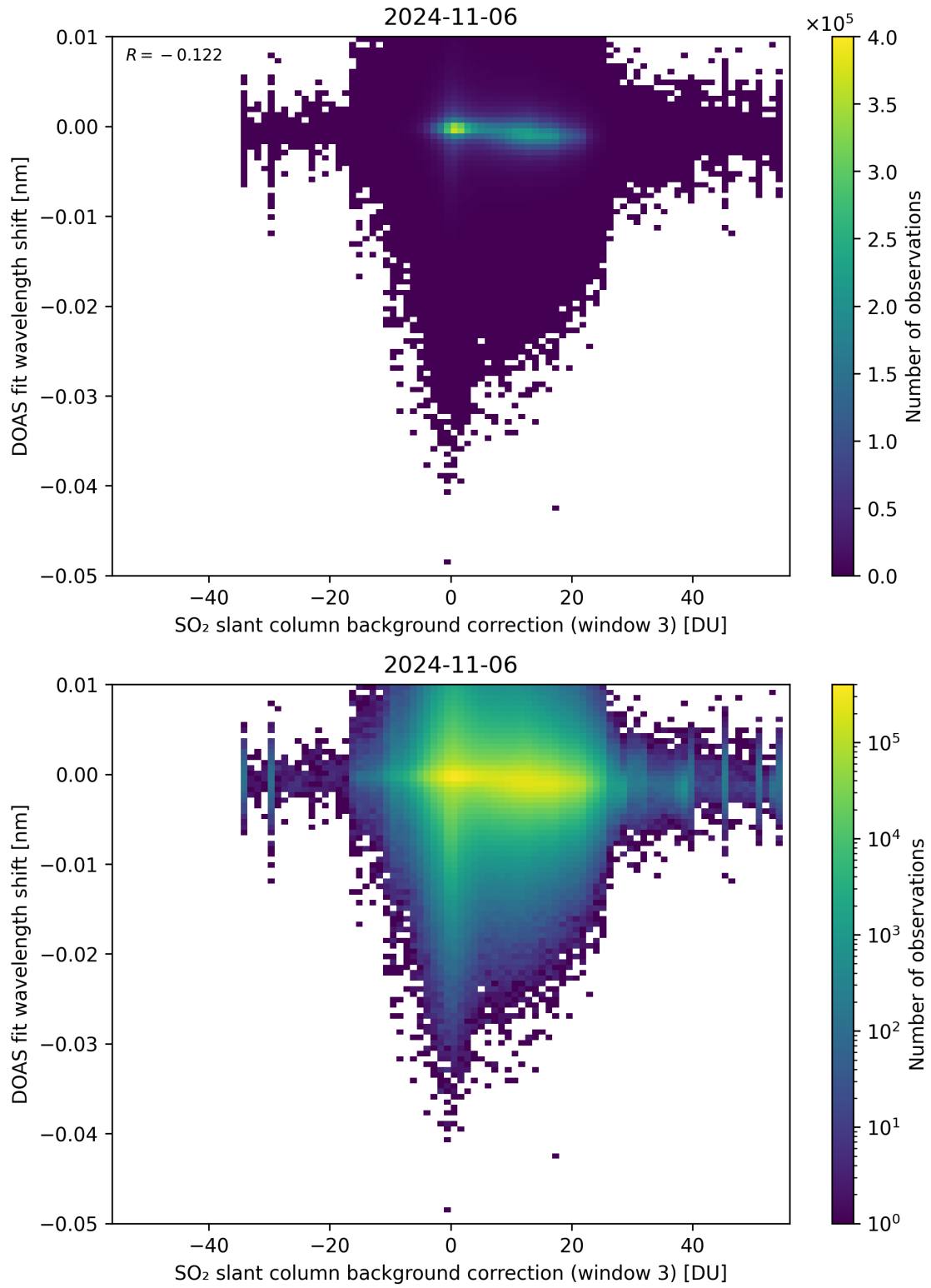
Figure 121: Scatter density plot of “SO 2 slant column background correction (window 3)” against “DOAS fit wavelength shift” for 2024-11-05 to 2024-11-07.
