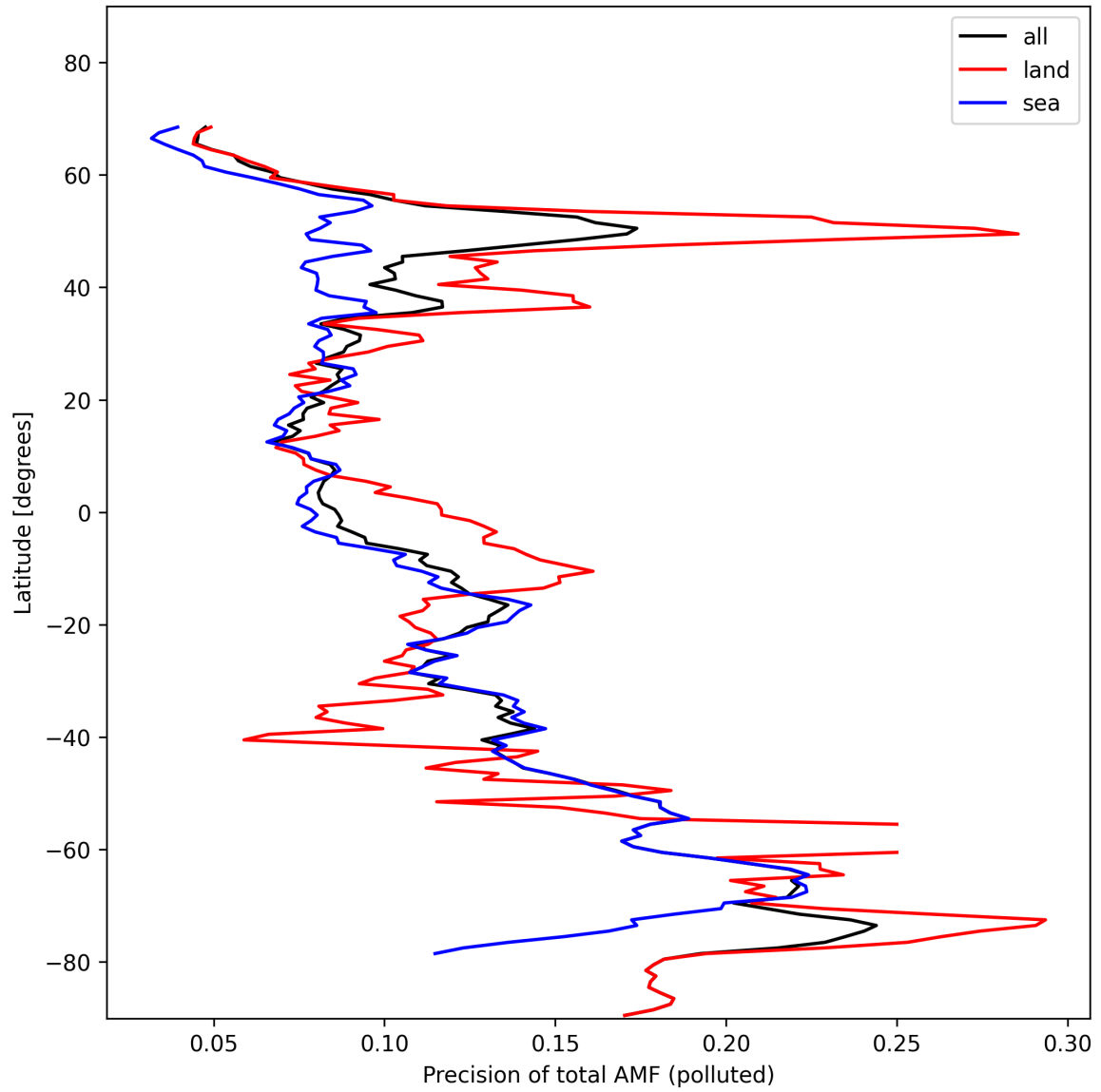
Figure 49: Zonal average of “Precision of total AMF (polluted)” for 2024-11-05 to 2024-11-07.
