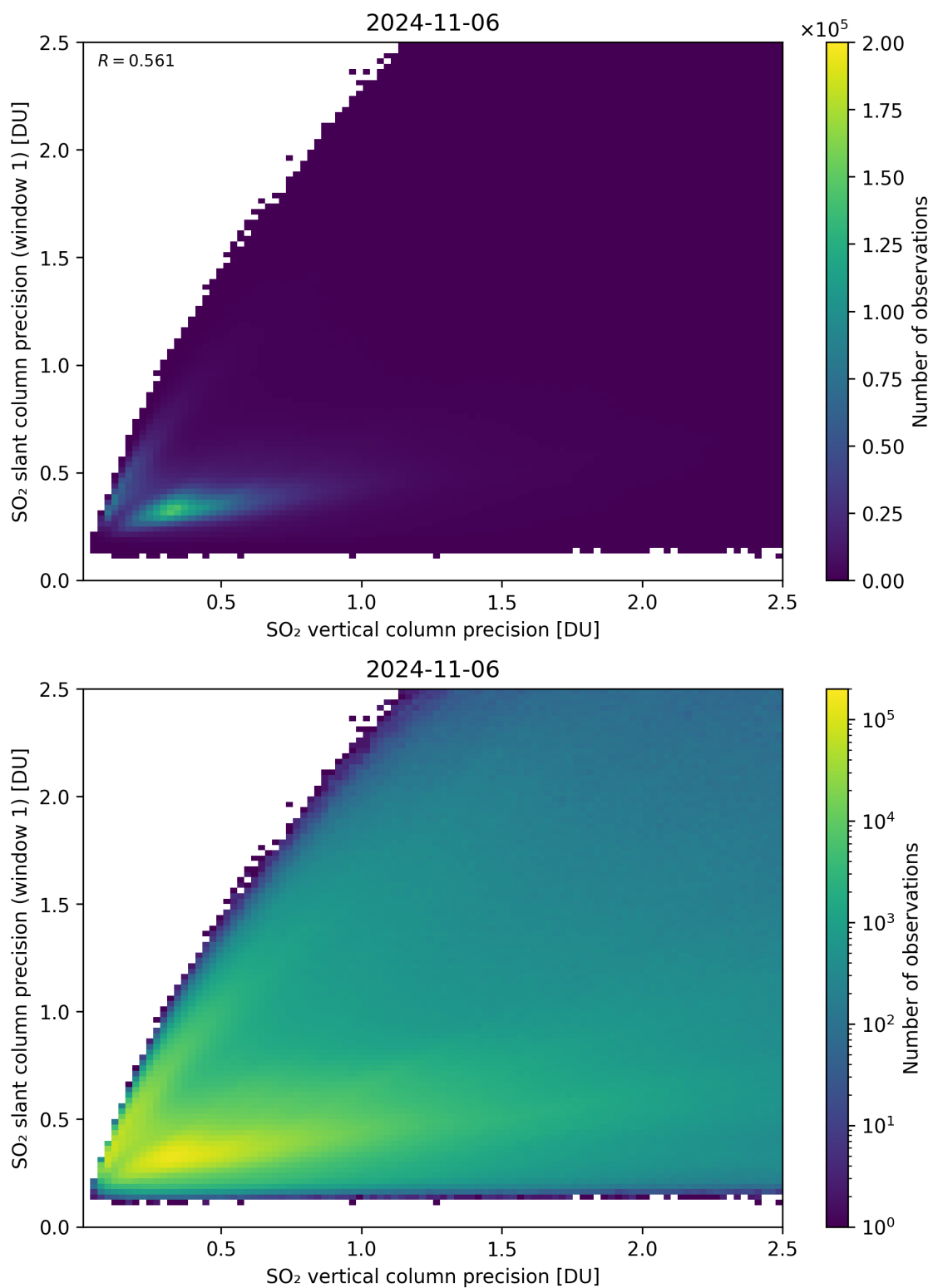
Figure 290: Scatter density plot of “SO 2 vertical column precision” against “SO 2 slant column precision (window 1)” for 2024-11-05 to 2024-11-07.
