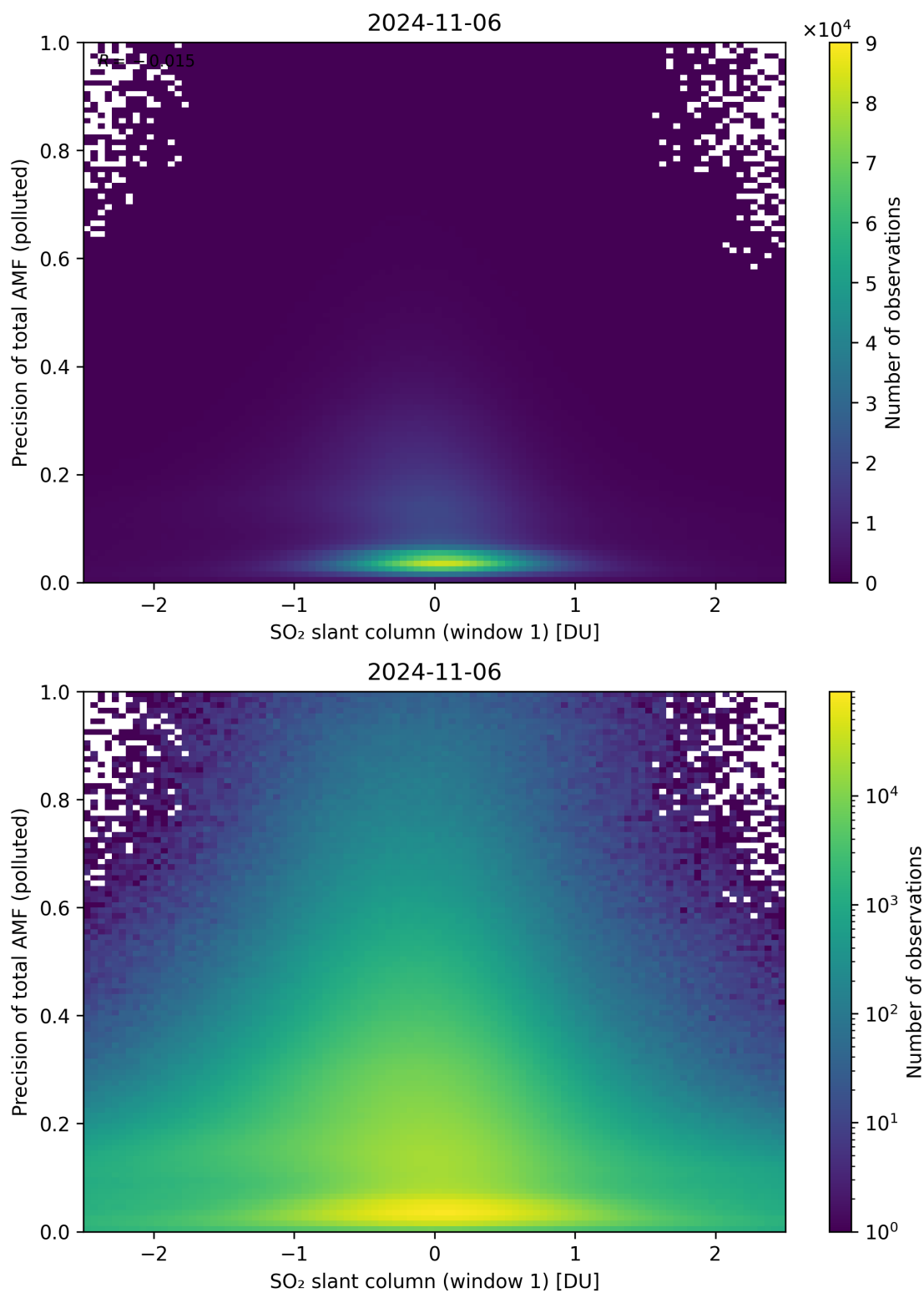
Figure 240: Scatter density plot of “SO 2 slant column (window 1)” against “Precision of total AMF (polluted)” for 2024-11-05 to 2024-11-07.
