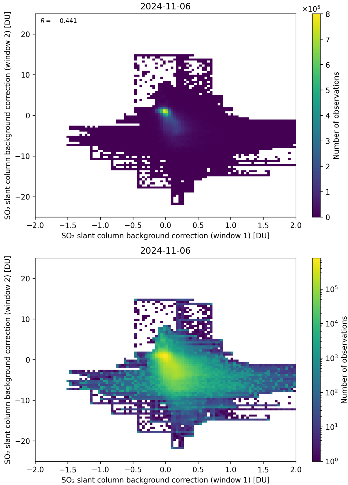
Figure 98: Scatter density plot of “SO 2 slant column background correction (window 1)” against “SO 2 slant column background correction (window 2)” for 2024-11-05 to 2024-11-07.
