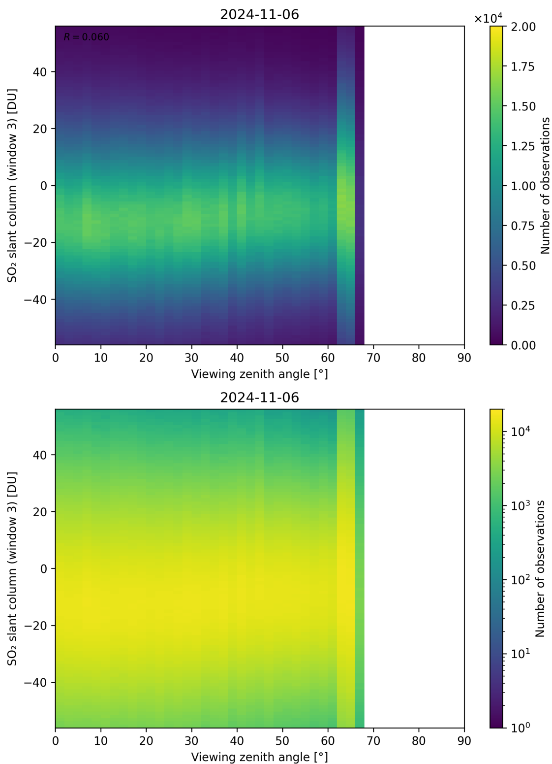
Figure 323: Scatter density plot of “Viewing zenith angle” against “SO 2 slant column (window 3)” for 2024-11-05 to 2024-11-07.
