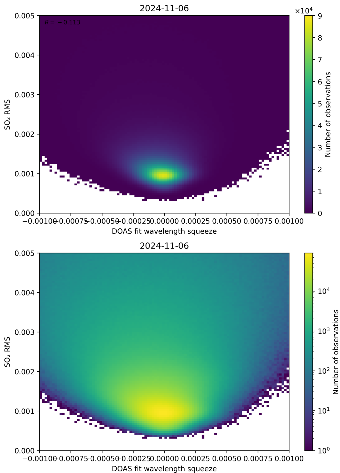
Figure 132: Scatter density plot of “DOAS fit wavelength squeeze” against “SO 2 RMS” for 2024-11-05 to 2024-11-07.
