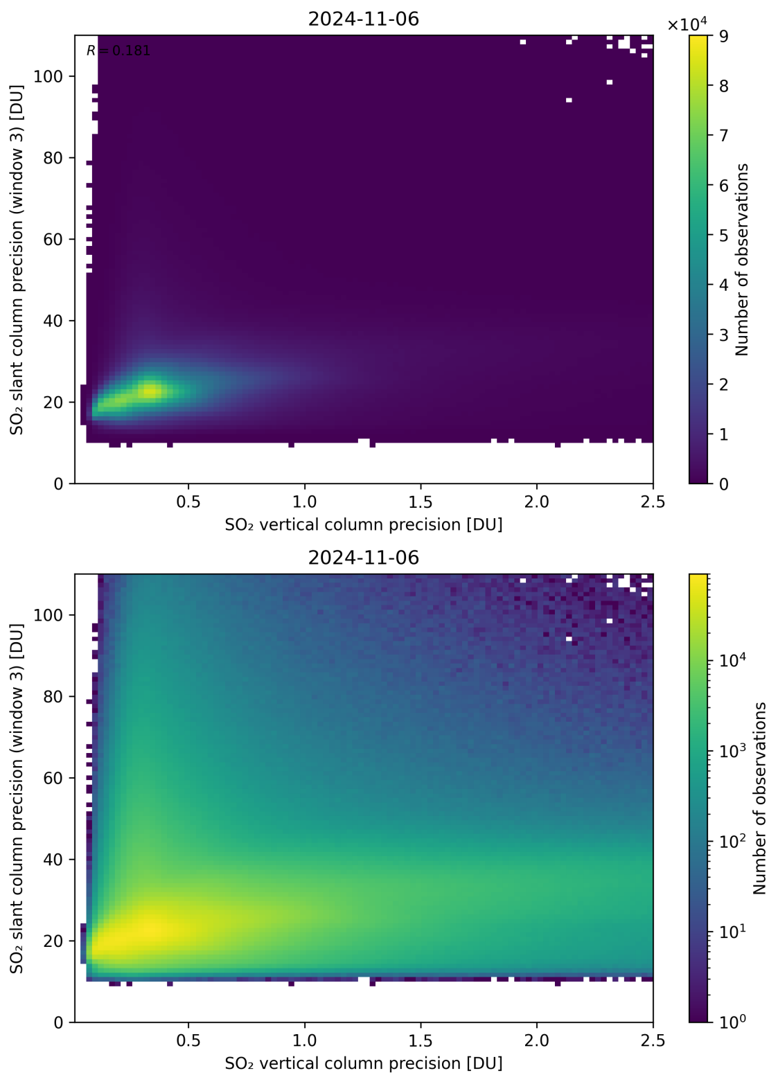
Figure 293: Scatter density plot of “SO 2 vertical column precision” against “SO 2 slant column precision (window 3)” for 2024-11-05 to 2024-11-07.
