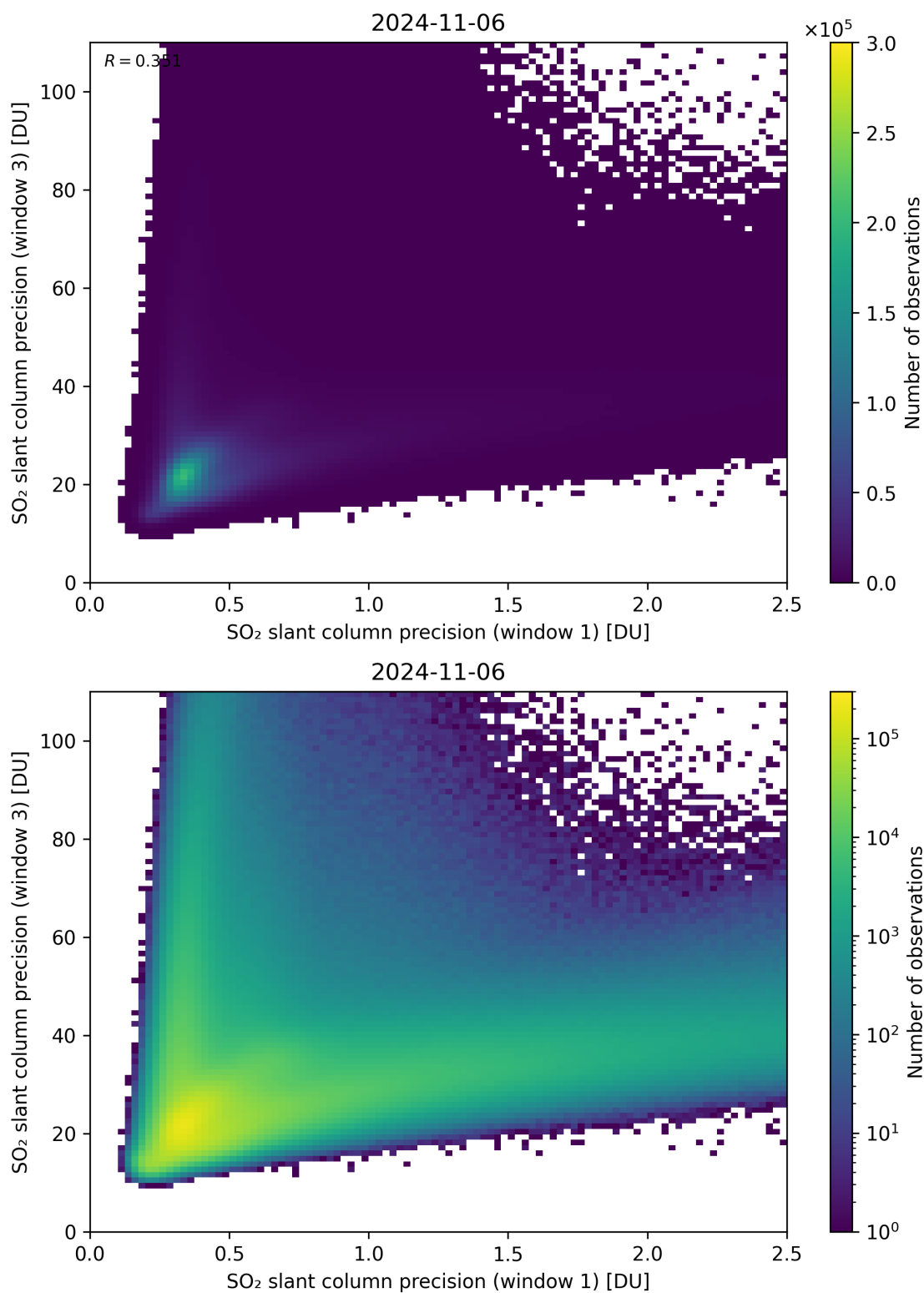
Figure 229: Scatter density plot of “SO 2 slant column precision (window 1)” against “SO 2 slant column precision (window 3)” for 2024-11-05 to 2024-11-07.
