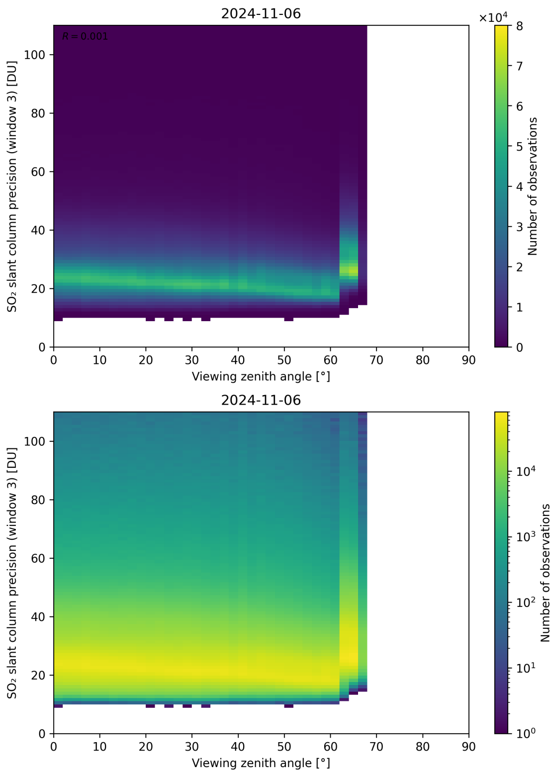
Figure 324: Scatter density plot of “Viewing zenith angle” against “SO 2 slant column precision (window 3)” for 2024-11-05 to 2024-11-07.
