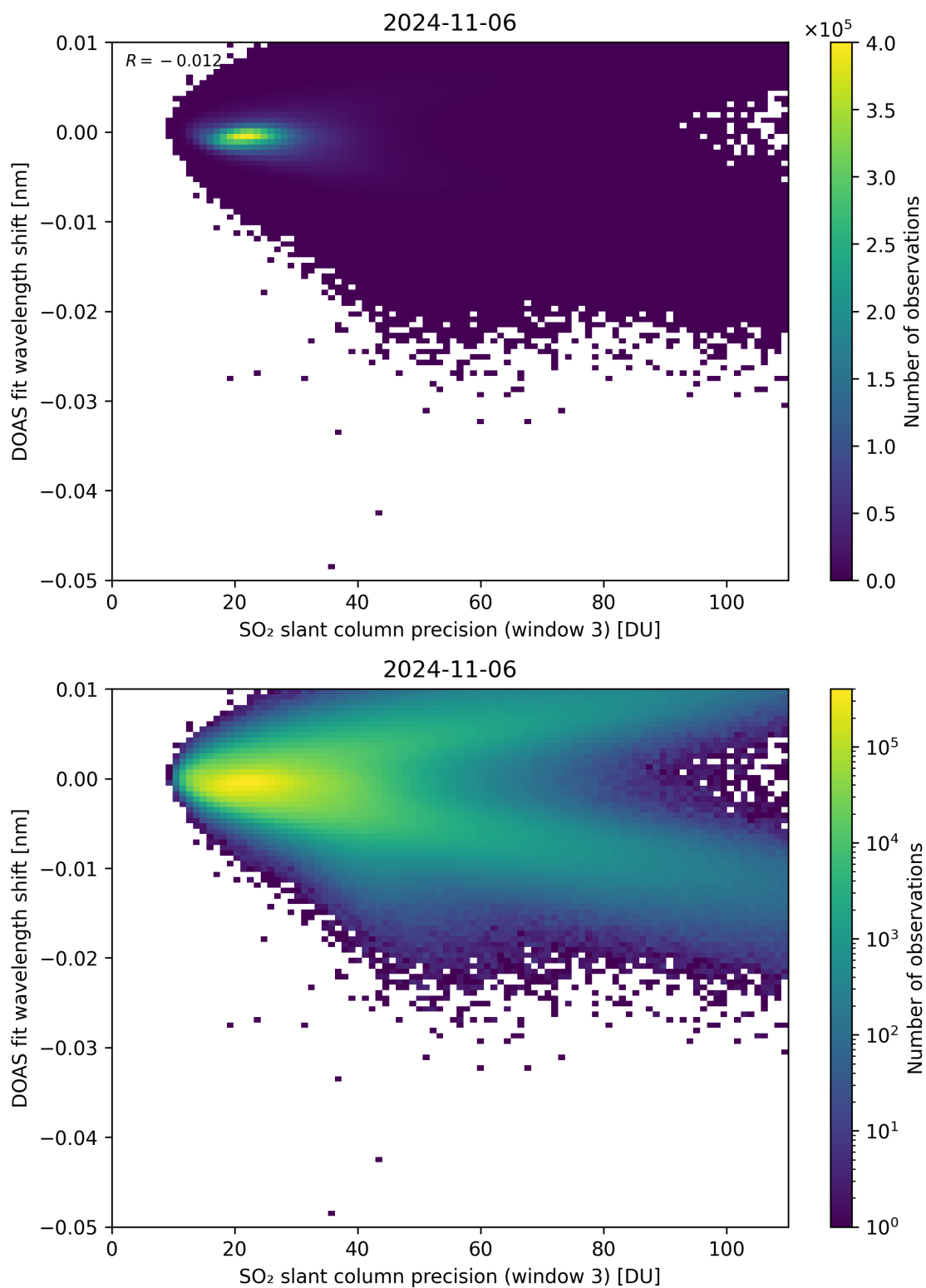
Figure 258: Scatter density plot of “SO 2 slant column precision (window 3)” against “DOAS fit wavelength shift” for 2024-11-05 to 2024-11-07.
