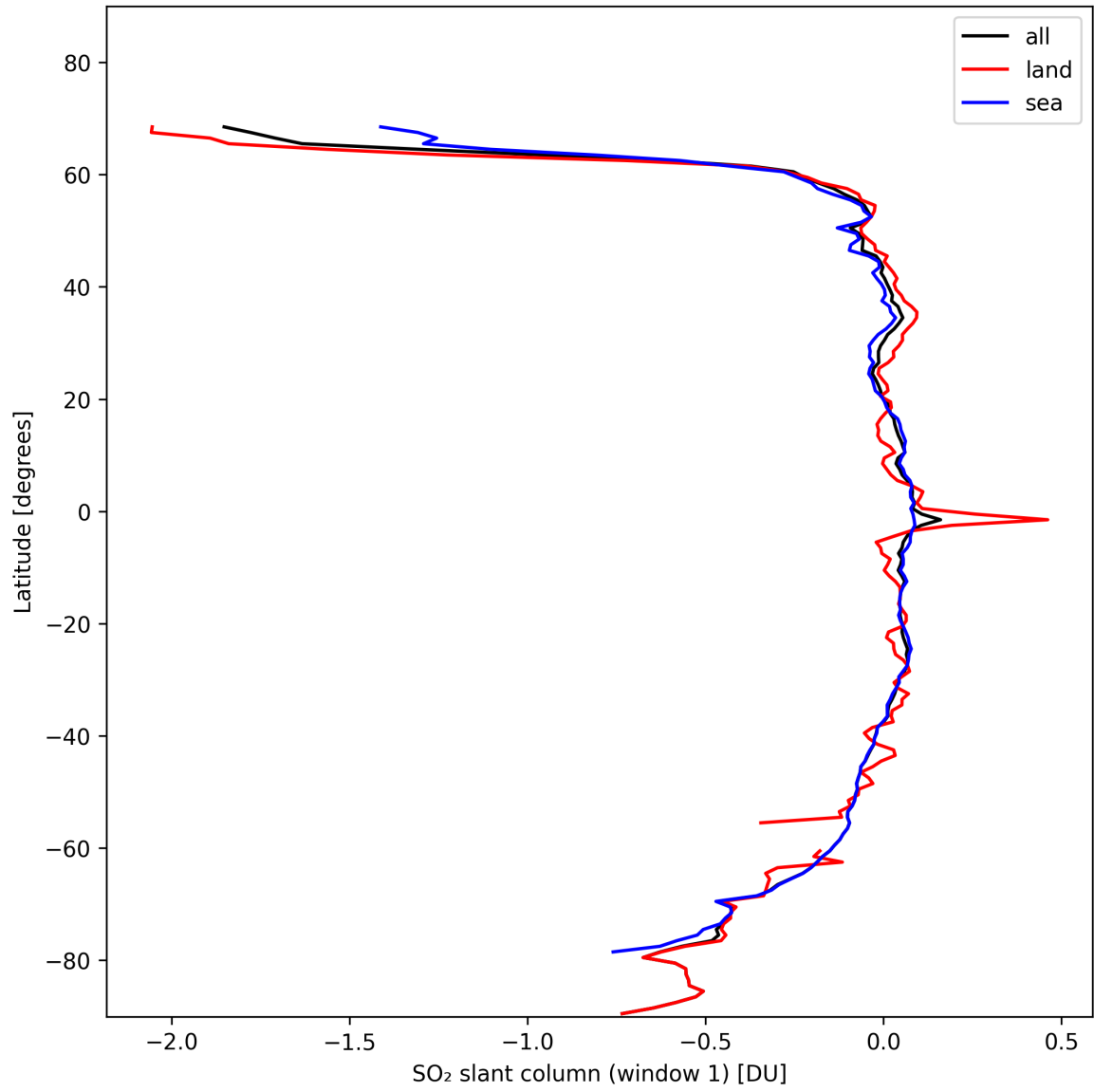
Figure 33: Zonal average of “SO 2 slant column (window 1)” for 2024-11-05 to 2024-11-07.
