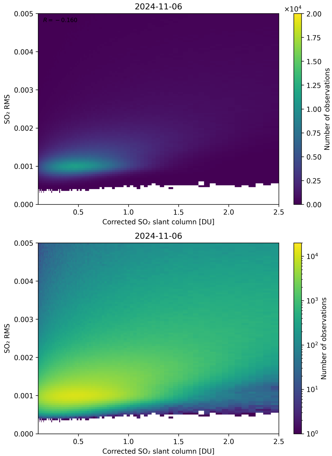
Figure 183: Scatter density plot of “Corrected SO 2 slant column” against “SO 2 RMS” for 2024-11-05 to 2024-11-07.
