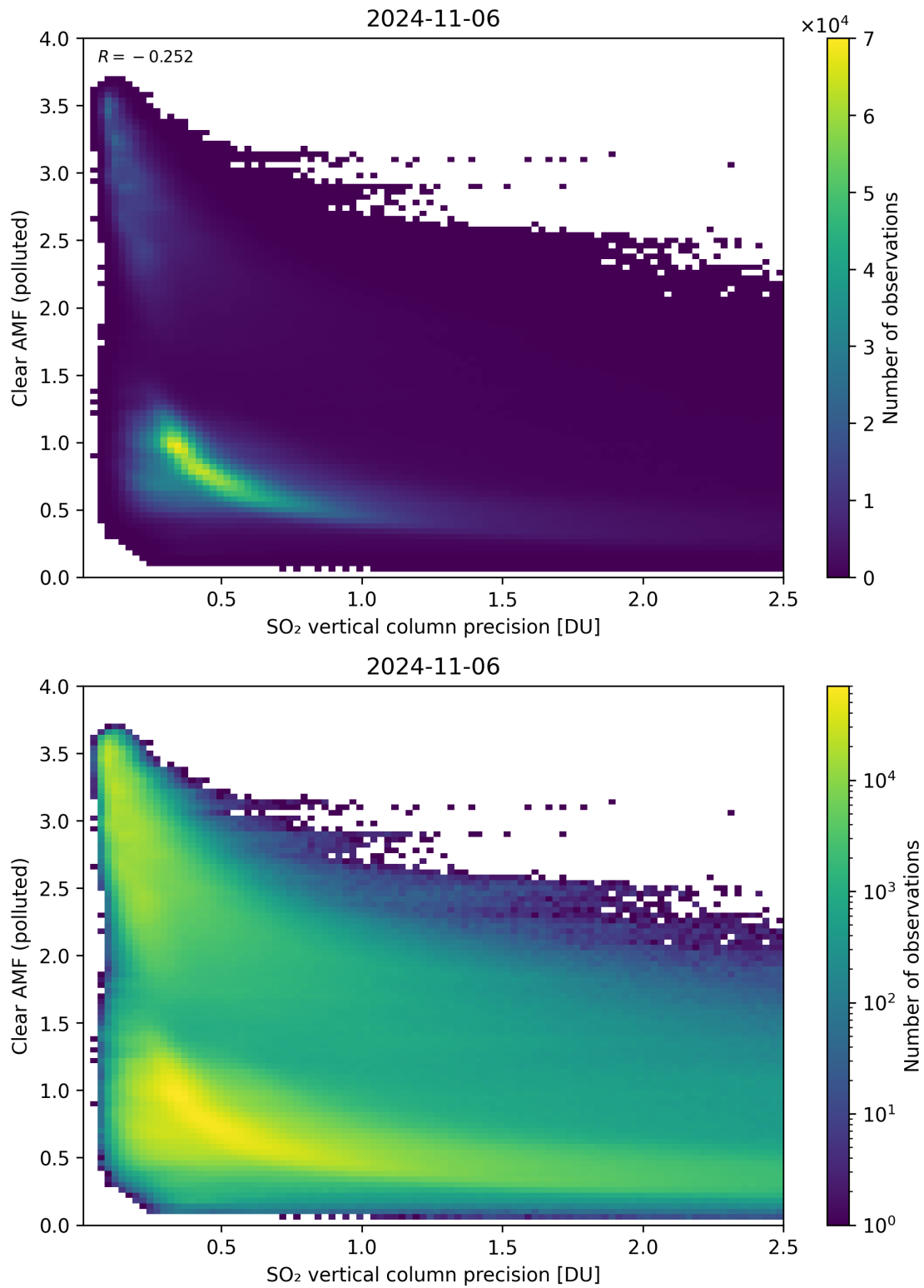
Figure 285: Scatter density plot of “SO 2 vertical column precision” against “Clear AMF (polluted)” for 2024-11-05 to 2024-11-07.
