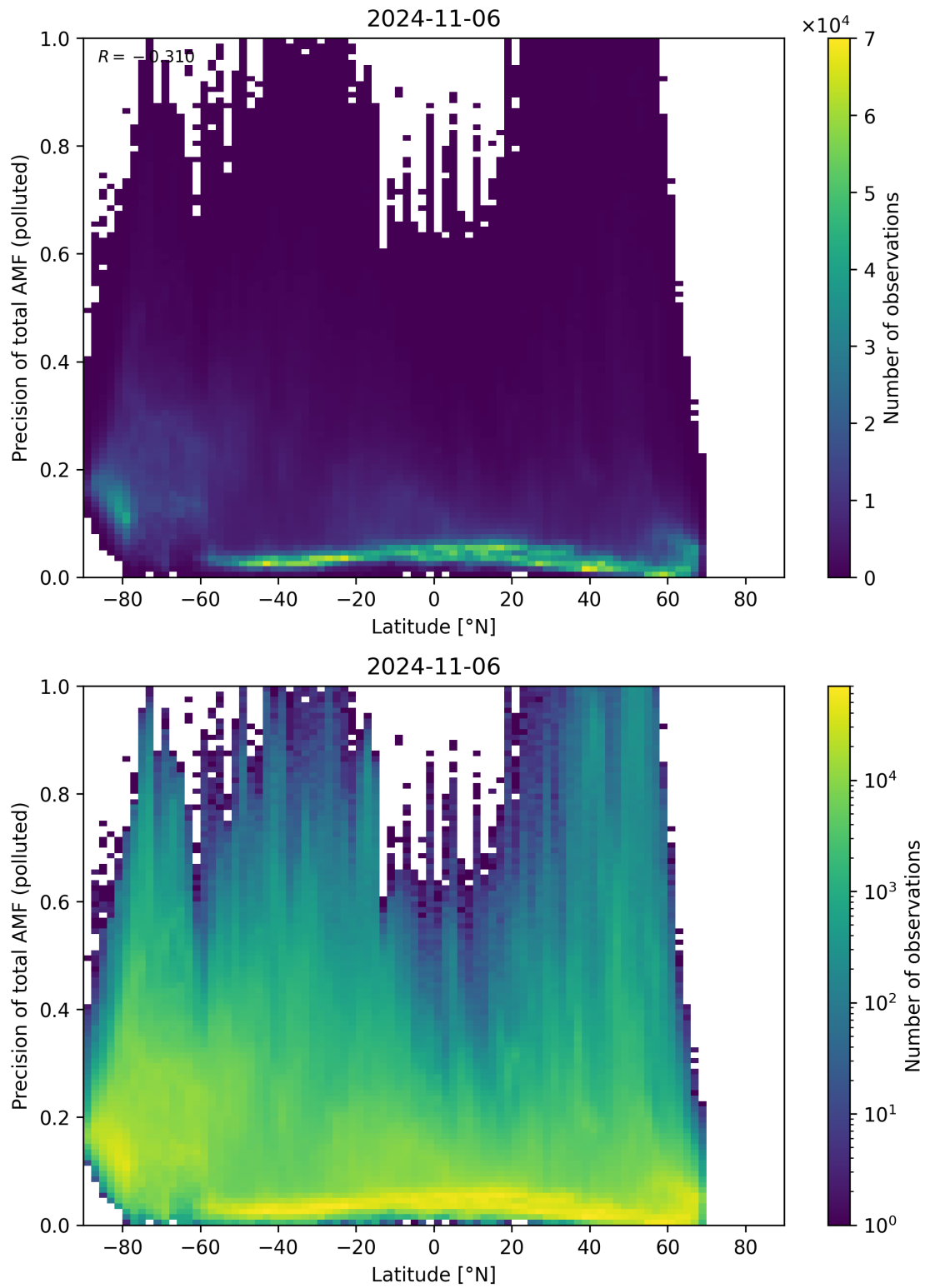
Figure 155: Scatter density plot of “Latitude” against “Precision of total AMF (polluted)” for 2024-11-05 to 2024-11-07.
