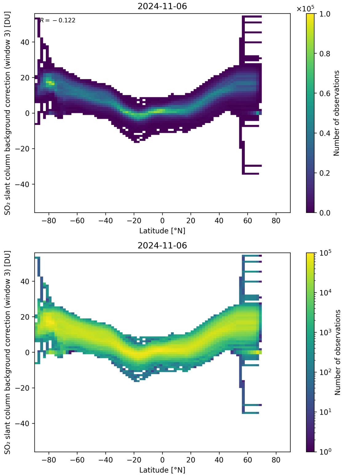
Figure 141: Scatter density plot of “Latitude” against “SO 2 slant column background correction (window 3)” for 2024-11-05 to 2024-11-07.
