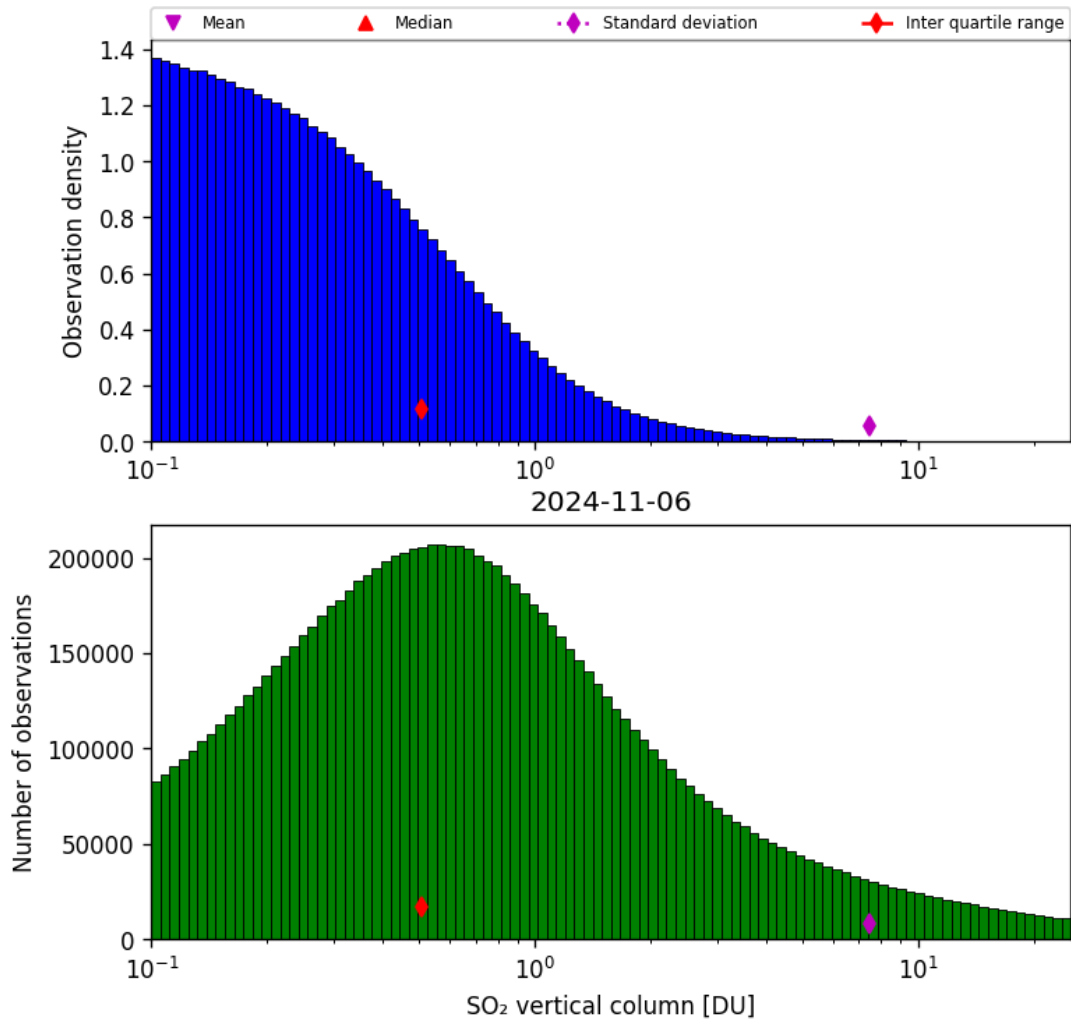
Figure 53: Histogram of “SO 2 vertical column” for 2024-11-05 to 2024-11-07
