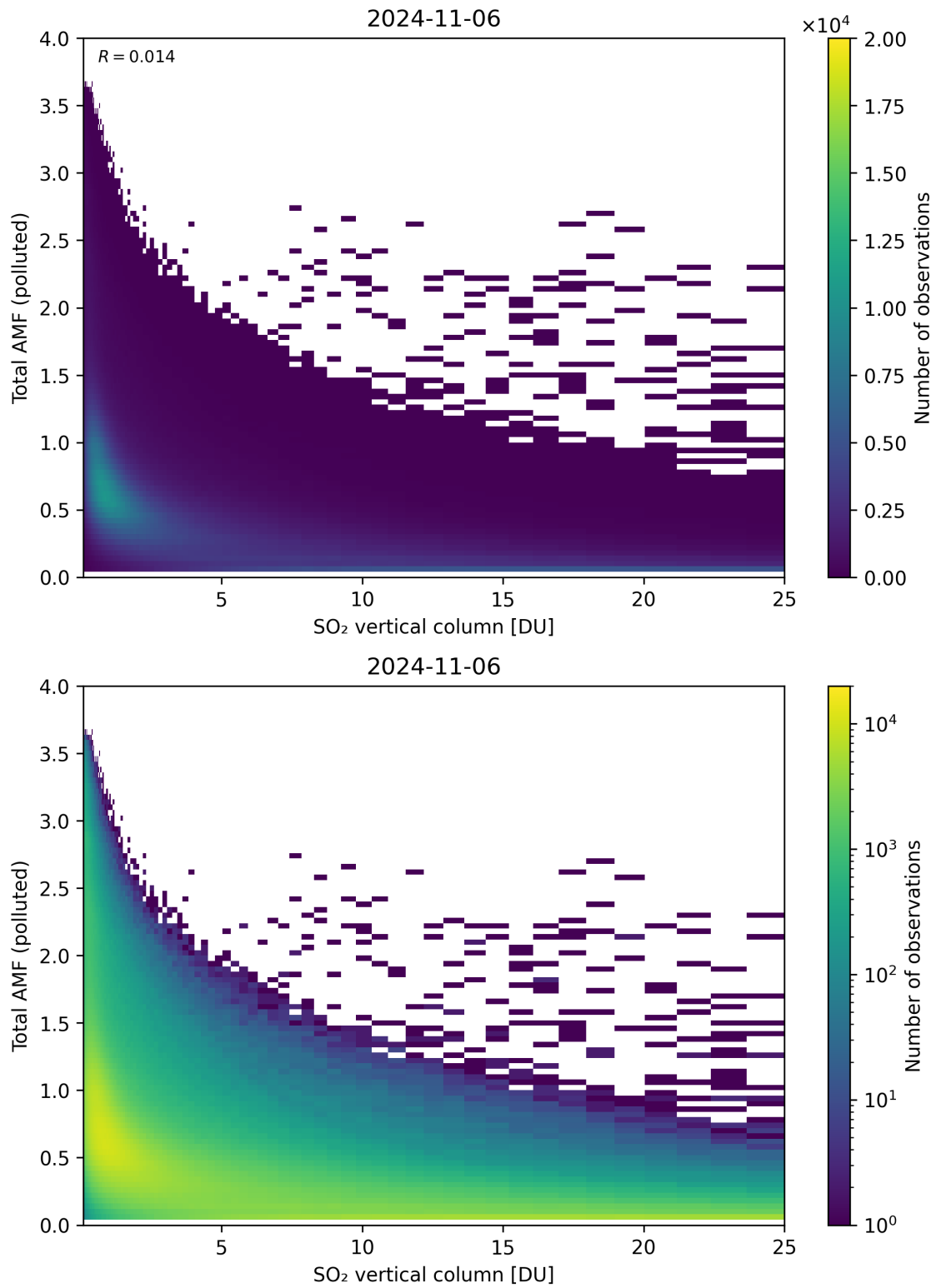
Figure 305: Scatter density plot of “SO 2 vertical column” against “Total AMF (polluted)” for 2024-11-05 to 2024-11-07.
