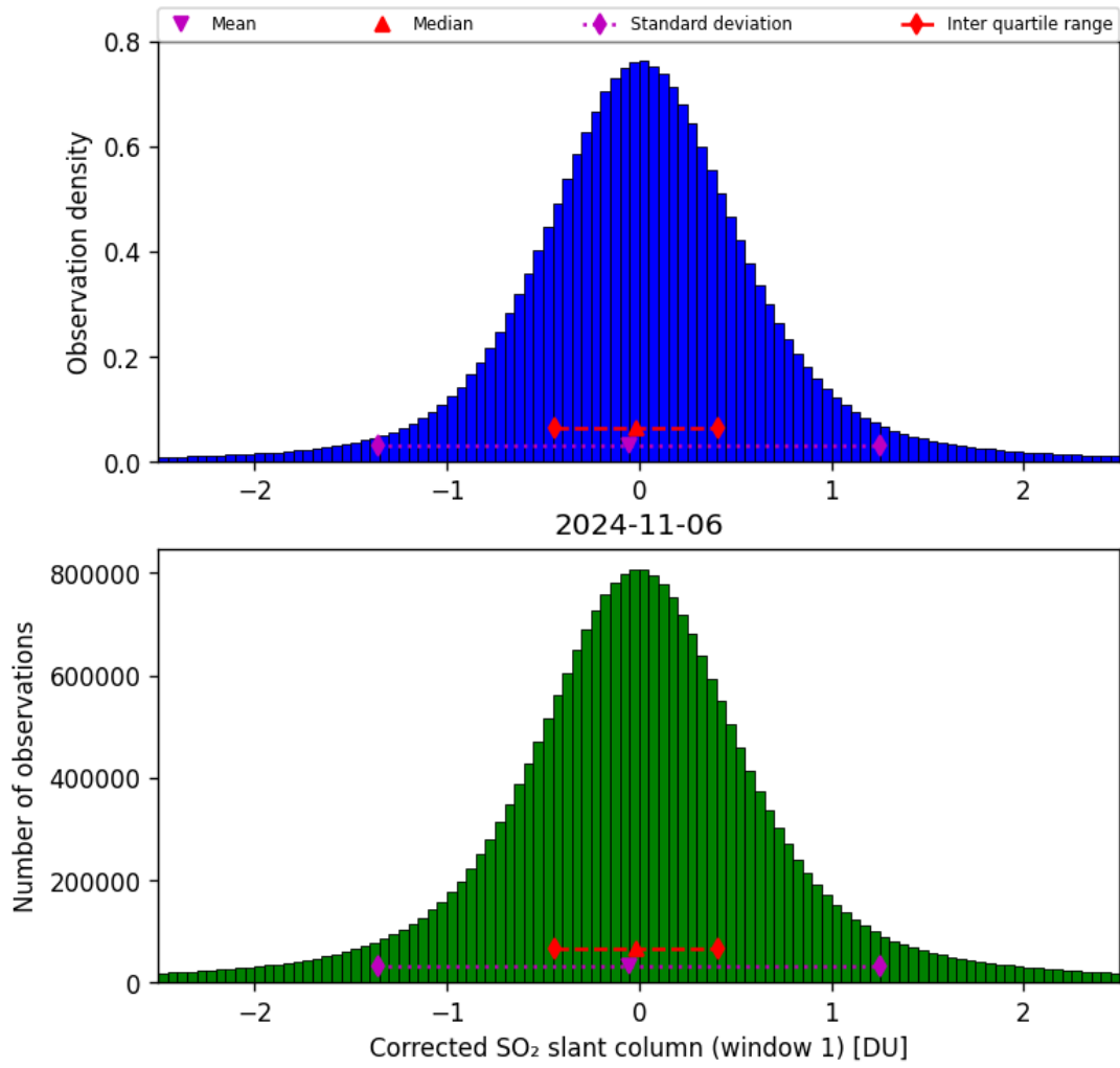
Figure 58: Histogram of “Corrected SO 2 slant column (window 1)” for 2024-11-05 to 2024-11-07
