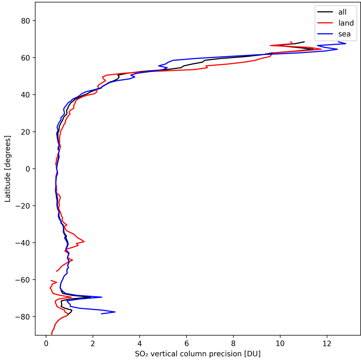
Figure 31: Zonal average of “SO 2 vertical column precision” for 2024-11-05 to 2024-11-07.
