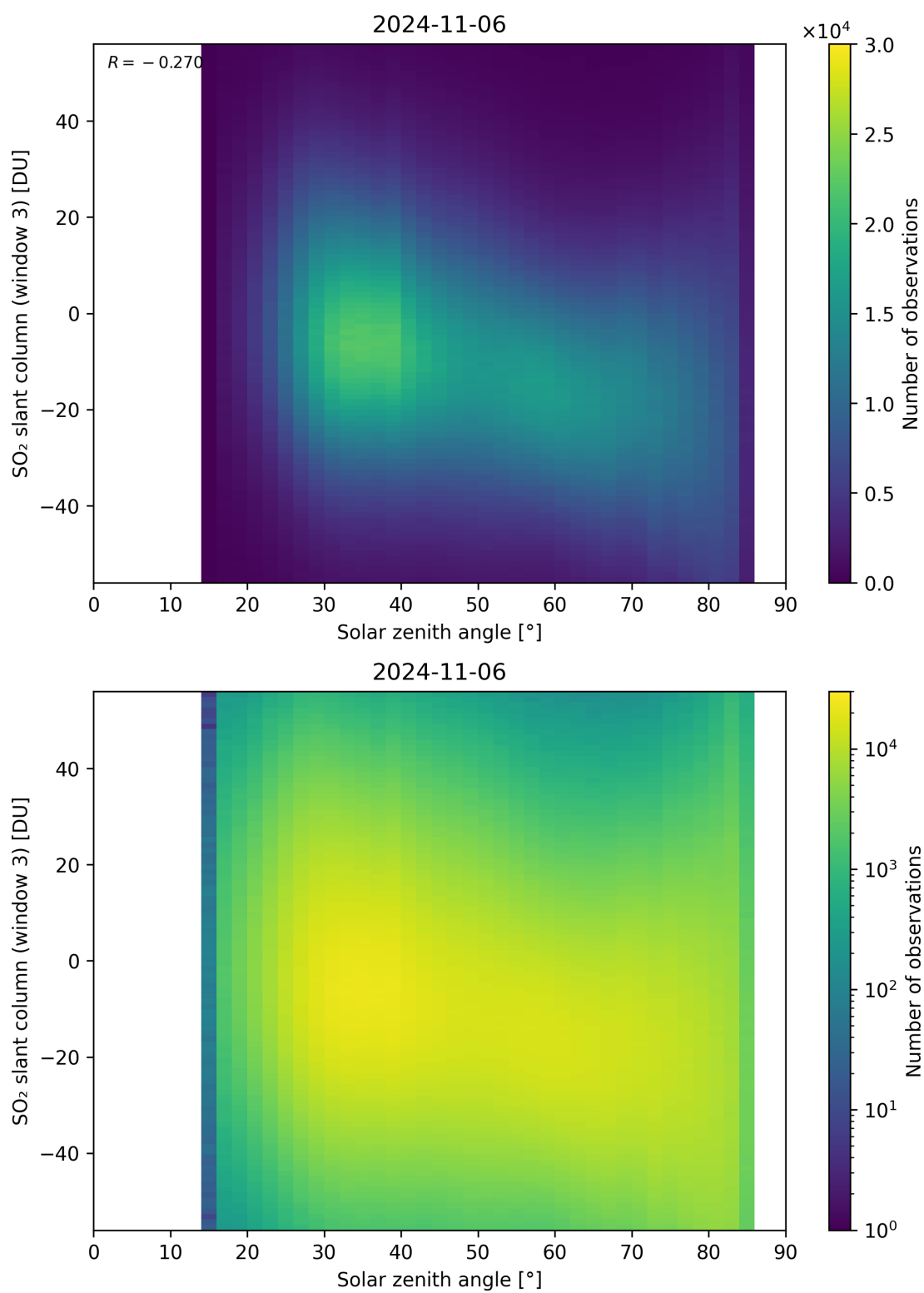
Figure 172: Scatter density plot of “Solar zenith angle” against “SO 2 slant column (window 3)” for 2024-11-05 to 2024-11-07.
