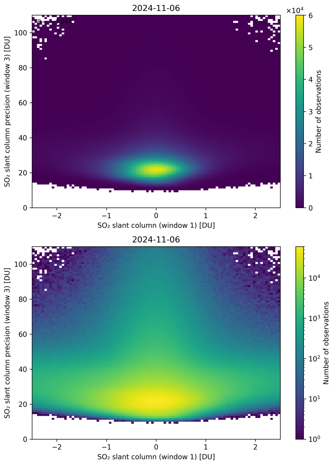
Figure 238: Scatter density plot of “SO 2 slant column (window 1)” against “SO 2 slant column precision (window 3)” for 2024-11-05 to 2024-11-07.
