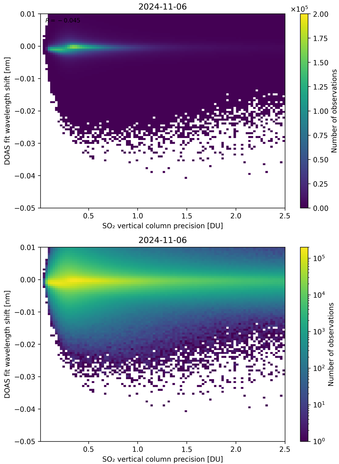
Figure 282: Scatter density plot of “SO 2 vertical column precision” against “DOAS fit wavelength shift” for 2024-11-05 to 2024-11-07.
