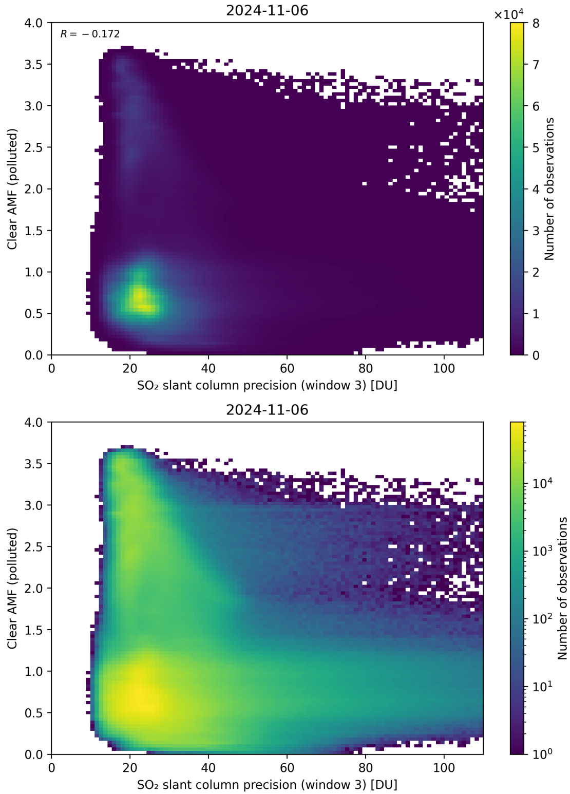
Figure 261: Scatter density plot of “SO 2 slant column precision (window 3)” against “Clear AMF (polluted)” for 2024-11-05 to 2024-11-07.
