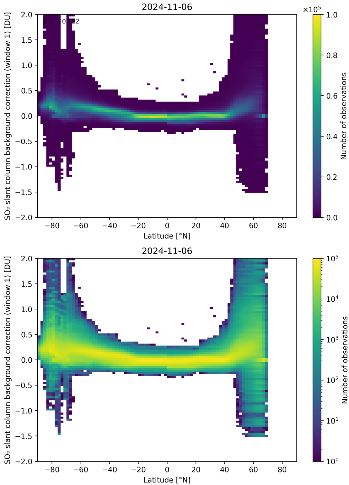
Figure 139: Scatter density plot of “Latitude” against “SO 2 slant column background correction (window 1)” for 2024-11-05 to 2024-11-07.
