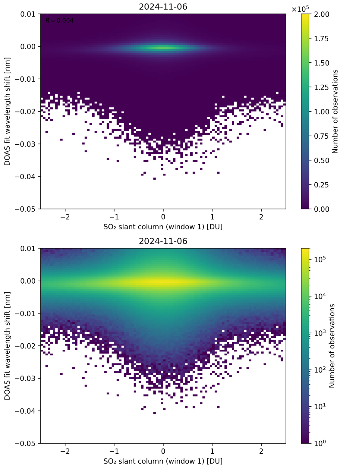
Figure 215: Scatter density plot of “SO 2 slant column (window 1)” against “DOAS fit wavelength shift” for 2024-11-05 to 2024-11-07.
