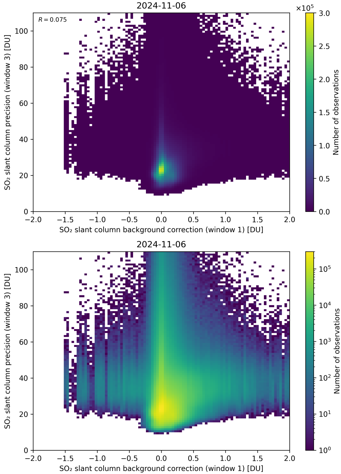
Figure 108: Scatter density plot of “SO 2 slant column background correction (window 1)” against “SO 2 slant column precision (window 3)” for 2024-11-05 to 2024-11-07.
