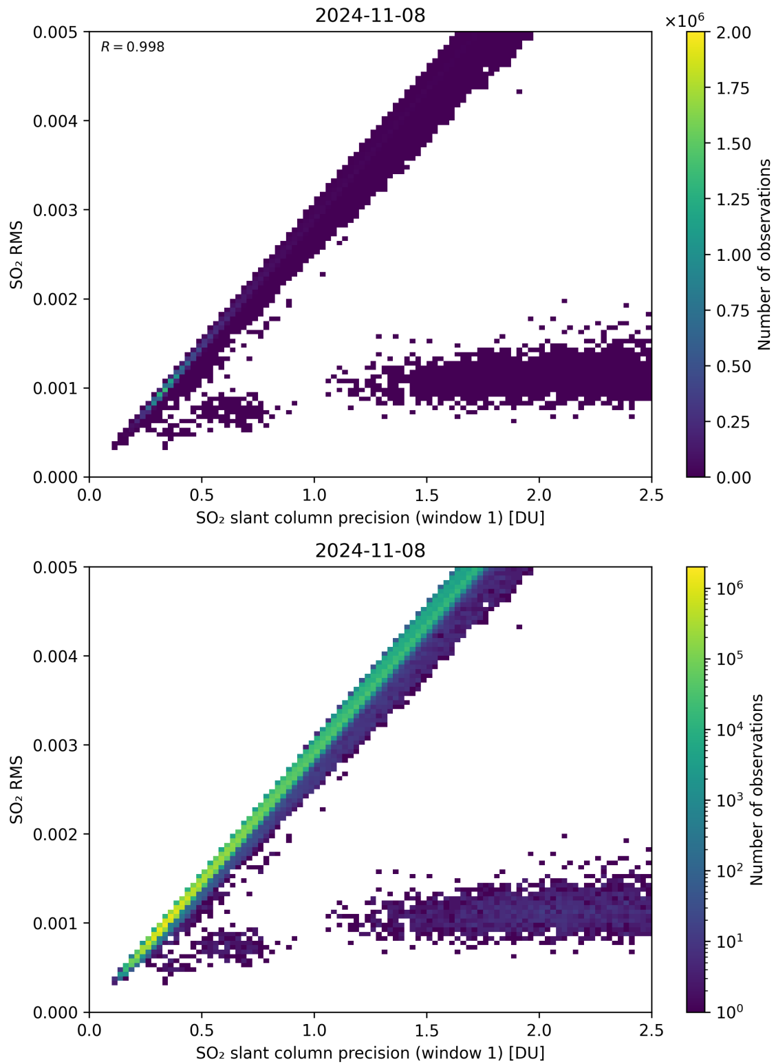
Figure 223: Scatter density plot of “SO 2 slant column precision (window 1)” against “SO 2 RMS” for 2024-11-07 to 2024-11-09.
