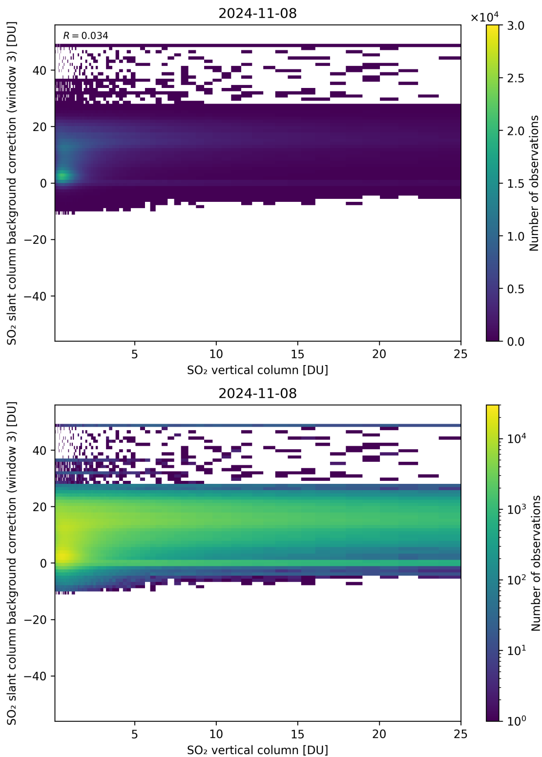
Figure 275: Scatter density plot of “SO 2 vertical column” against “SO 2 slant column background correction (window 3)” for 2024-11-07 to 2024-11-09.
