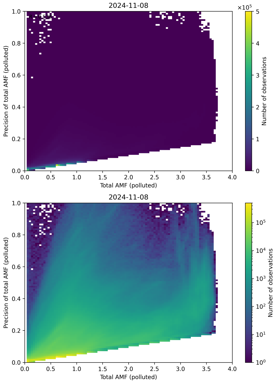
Figure 272: Scatter density plot of “Total AMF (polluted)” against “Precision of total AMF (polluted)” for 2024-11-07 to 2024-11-09.
