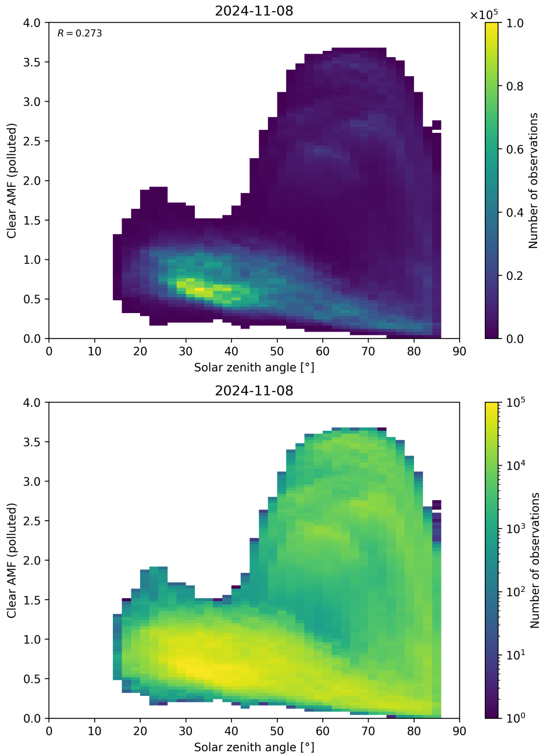
Figure 165: Scatter density plot of “Solar zenith angle” against “Clear AMF (polluted)” for 2024-11-07 to 2024-11-09.
