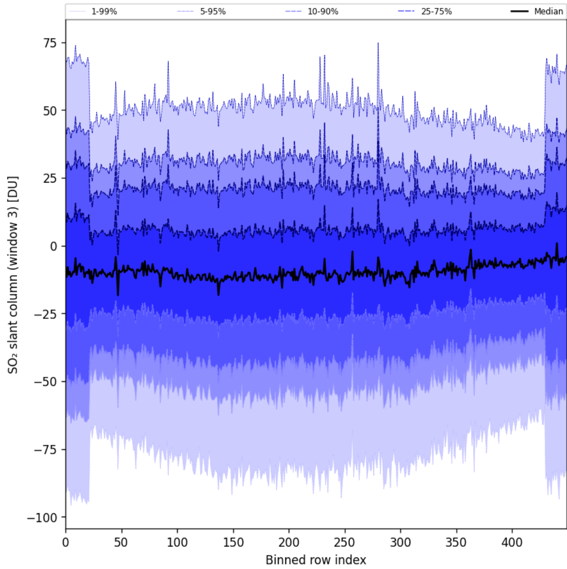
Figure 87: Along track statistics of “SO 2 slant column (window 3)” for 2024-11-07 to 2024-11-09
