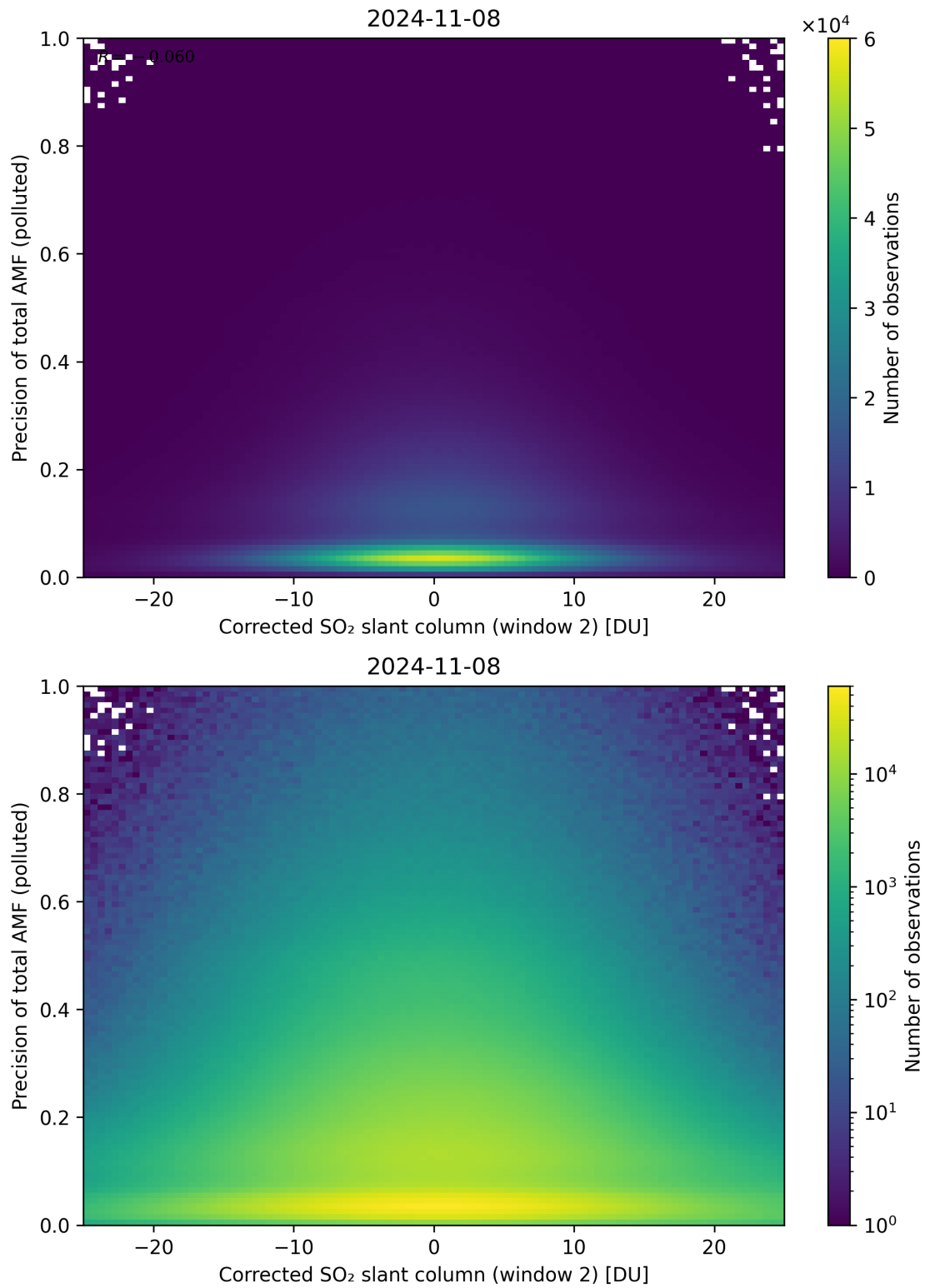
Figure 204: Scatter density plot of “Corrected SO 2 slant column (window 2)” against “Precision of total AMF (polluted)” for 2024-11-07 to 2024-11-09.
