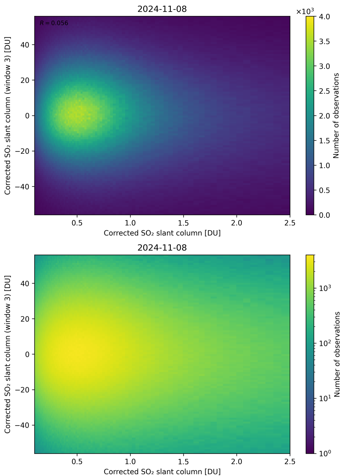
Figure 186: Scatter density plot of “Corrected SO 2 slant column” against “Corrected SO 2 slant column (window 3)” for 2024-11-07 to 2024-11-09.
