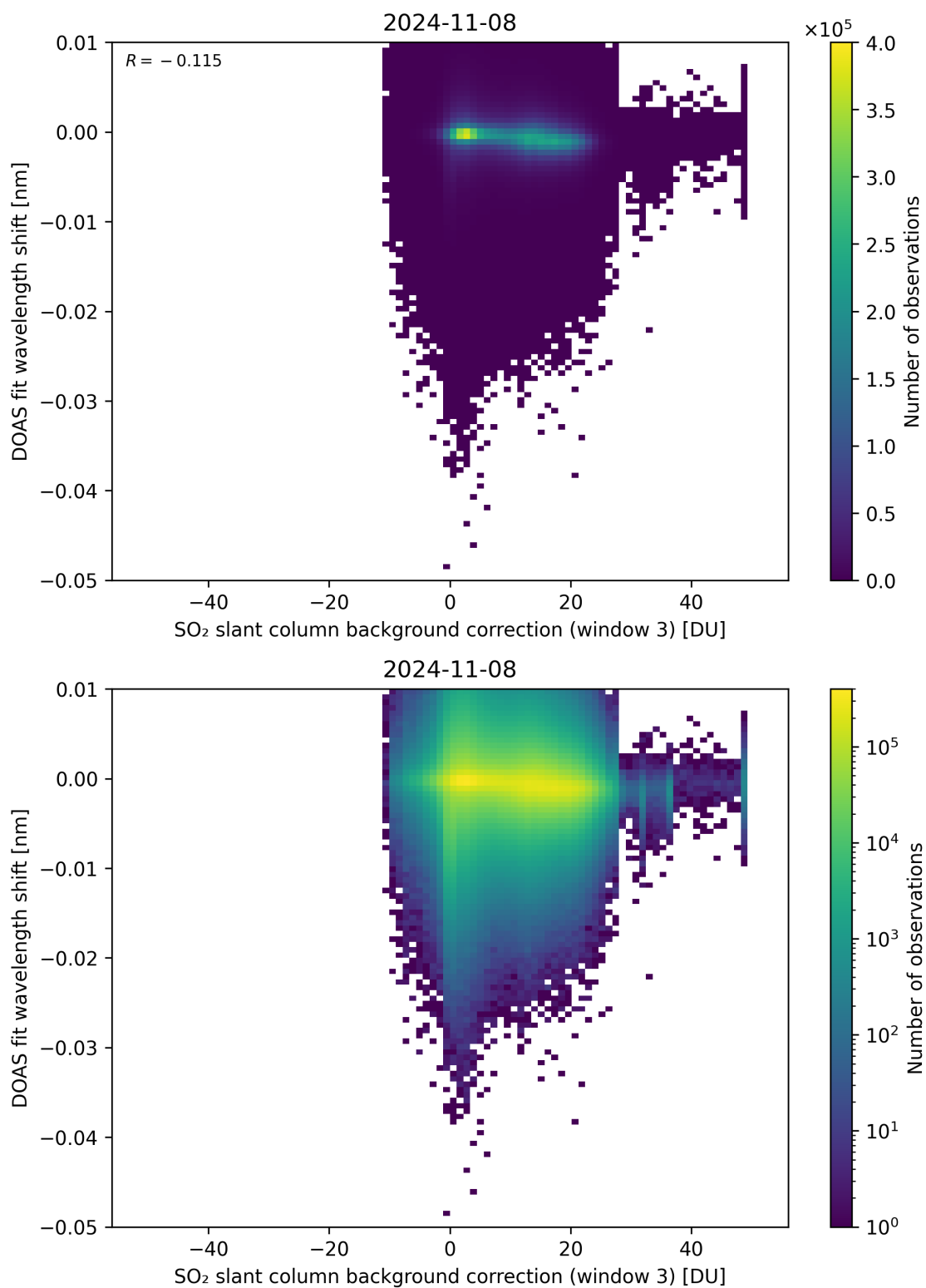
Figure 121: Scatter density plot of “SO 2 slant column background correction (window 3)” against “DOAS fit wavelength shift” for 2024-11-07 to 2024-11-09.
