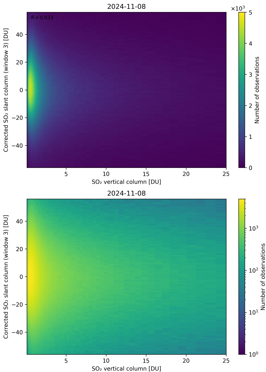
Figure 299: Scatter density plot of “SO 2 vertical column” against “Corrected SO 2 slant column (window 3)” for 2024-11-07 to 2024-11-09.
