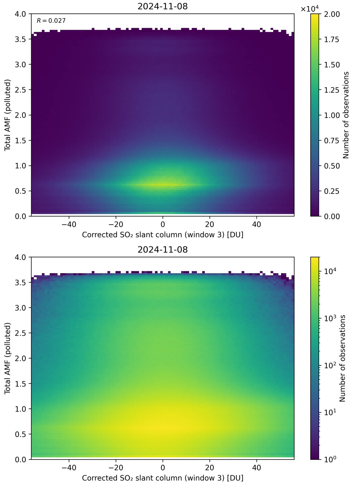
Figure 210: Scatter density plot of “Corrected SO 2 slant column (window 3)” against “Total AMF (polluted)” for 2024-11-07 to 2024-11-09.
