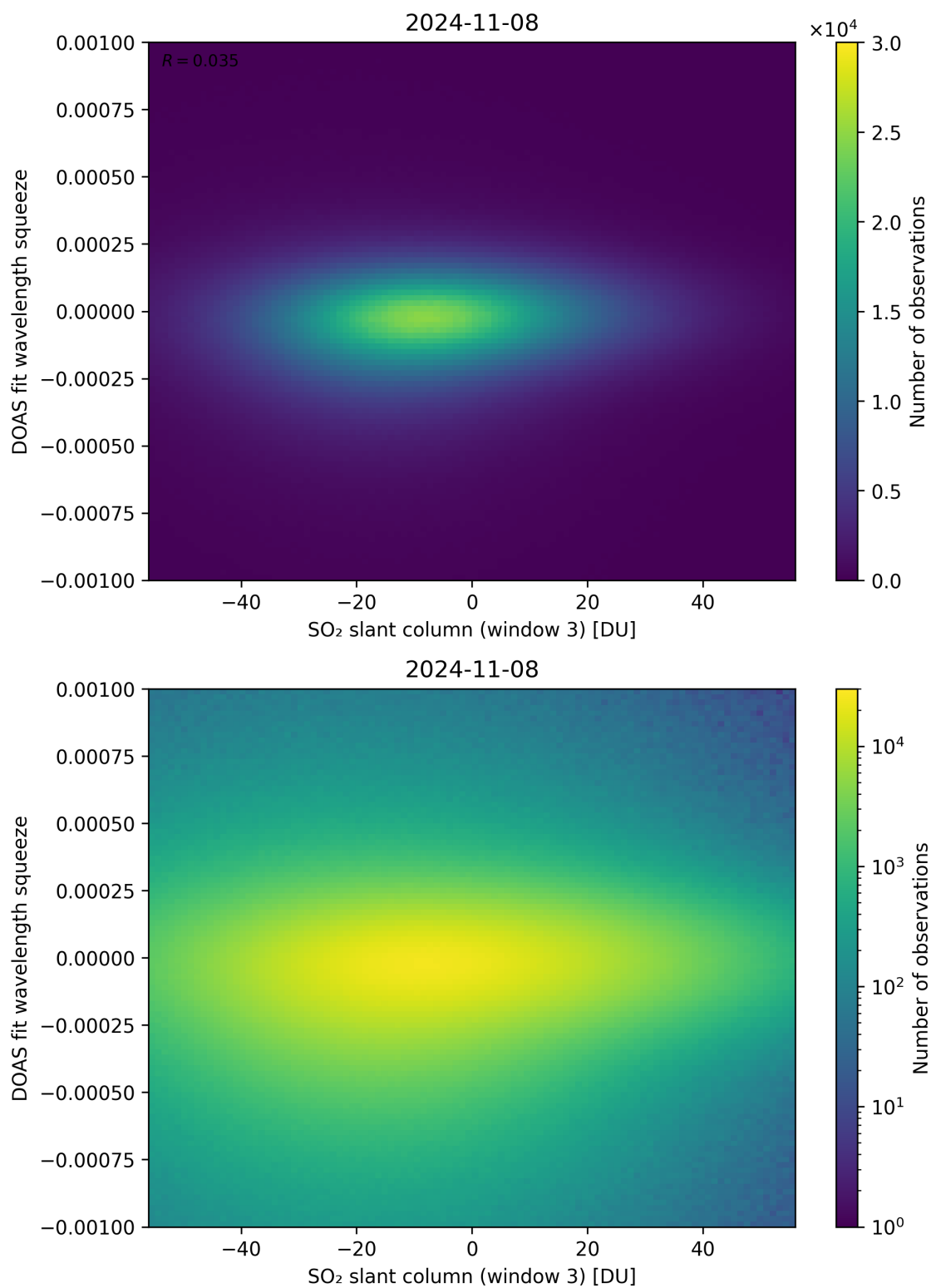
Figure 255: Scatter density plot of “SO 2 slant column (window 3)” against “DOAS fit wavelength squeeze” for 2024-11-07 to 2024-11-09.
