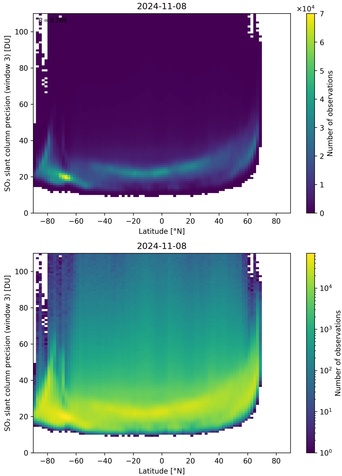
Figure 153: Scatter density plot of “Latitude” against “SO 2 slant column precision (window 3)” for 2024-11-07 to 2024-11-09.
