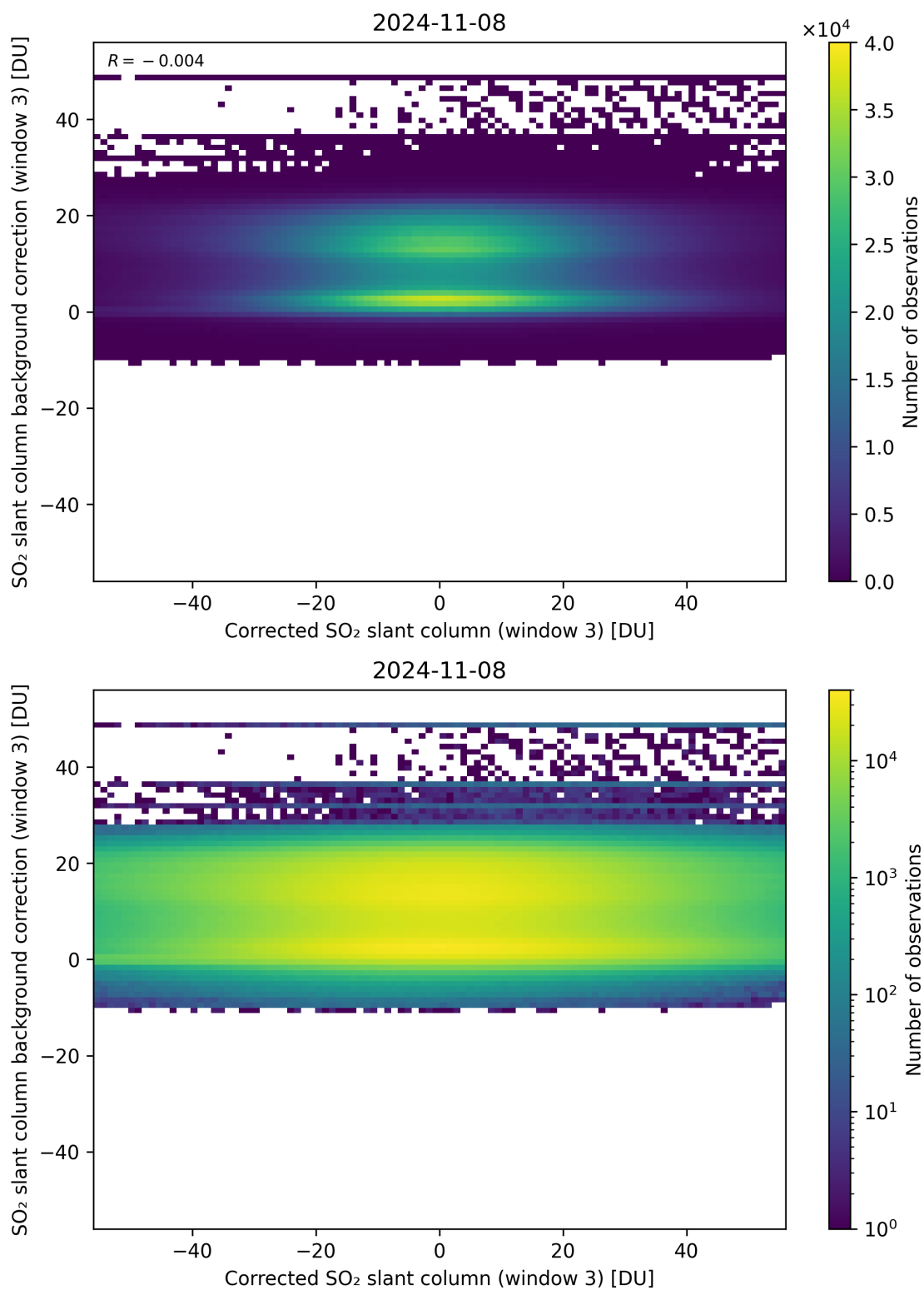
Figure 205: Scatter density plot of “Corrected SO 2 slant column (window 3)” against “SO 2 slant column background correction (window 3)” for 2024-11-07 to 2024-11-09.
