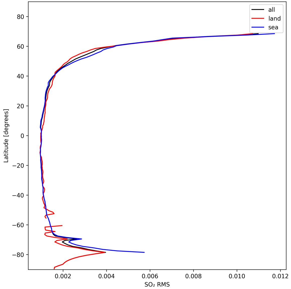
Figure 47: Zonal average of “SO 2 RMS” for 2024-11-07 to 2024-11-09.
