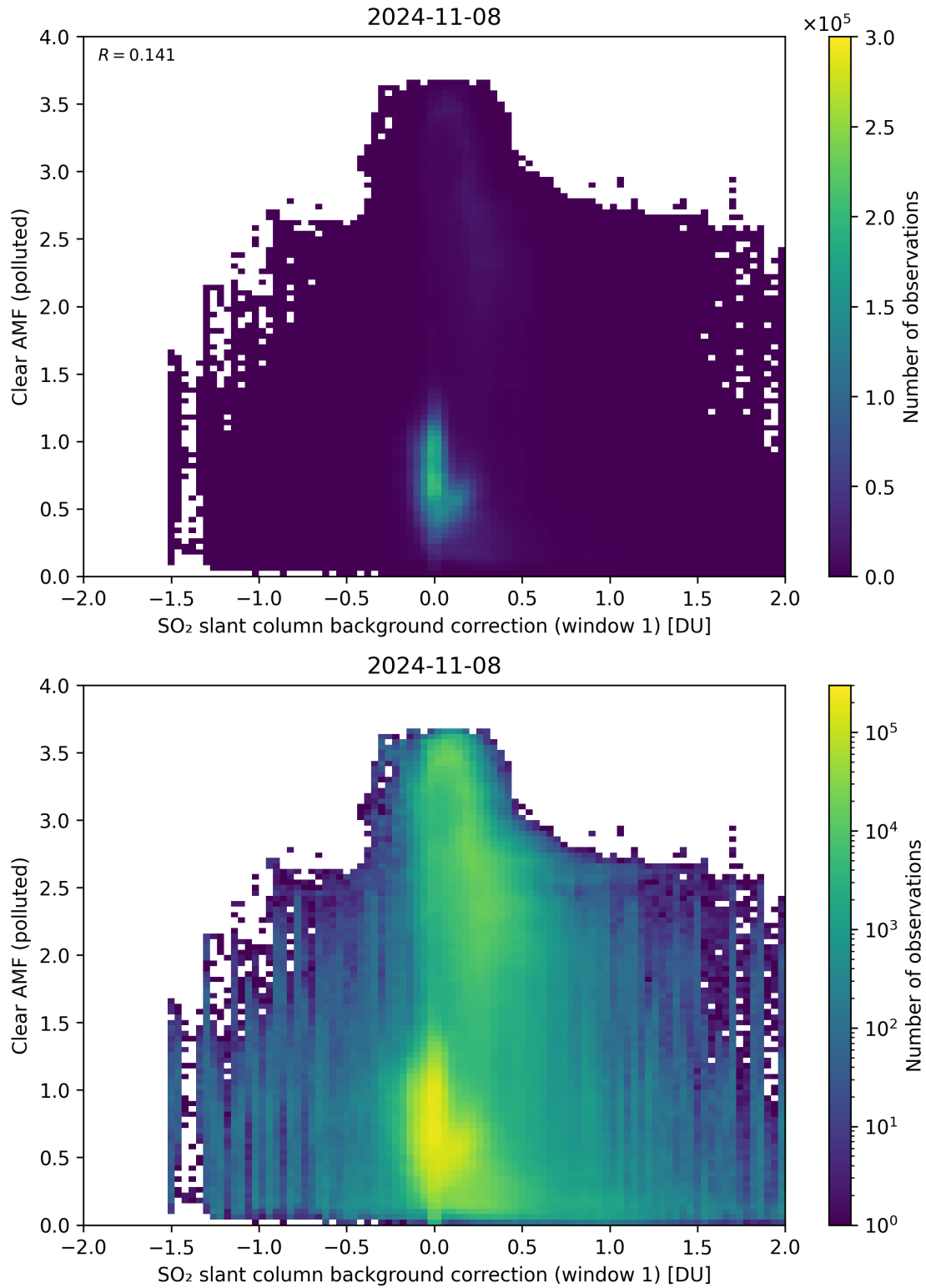
Figure 103: Scatter density plot of “SO 2 slant column background correction (window 1)” against “Clear AMF (polluted)” for 2024-11-07 to 2024-11-09.
