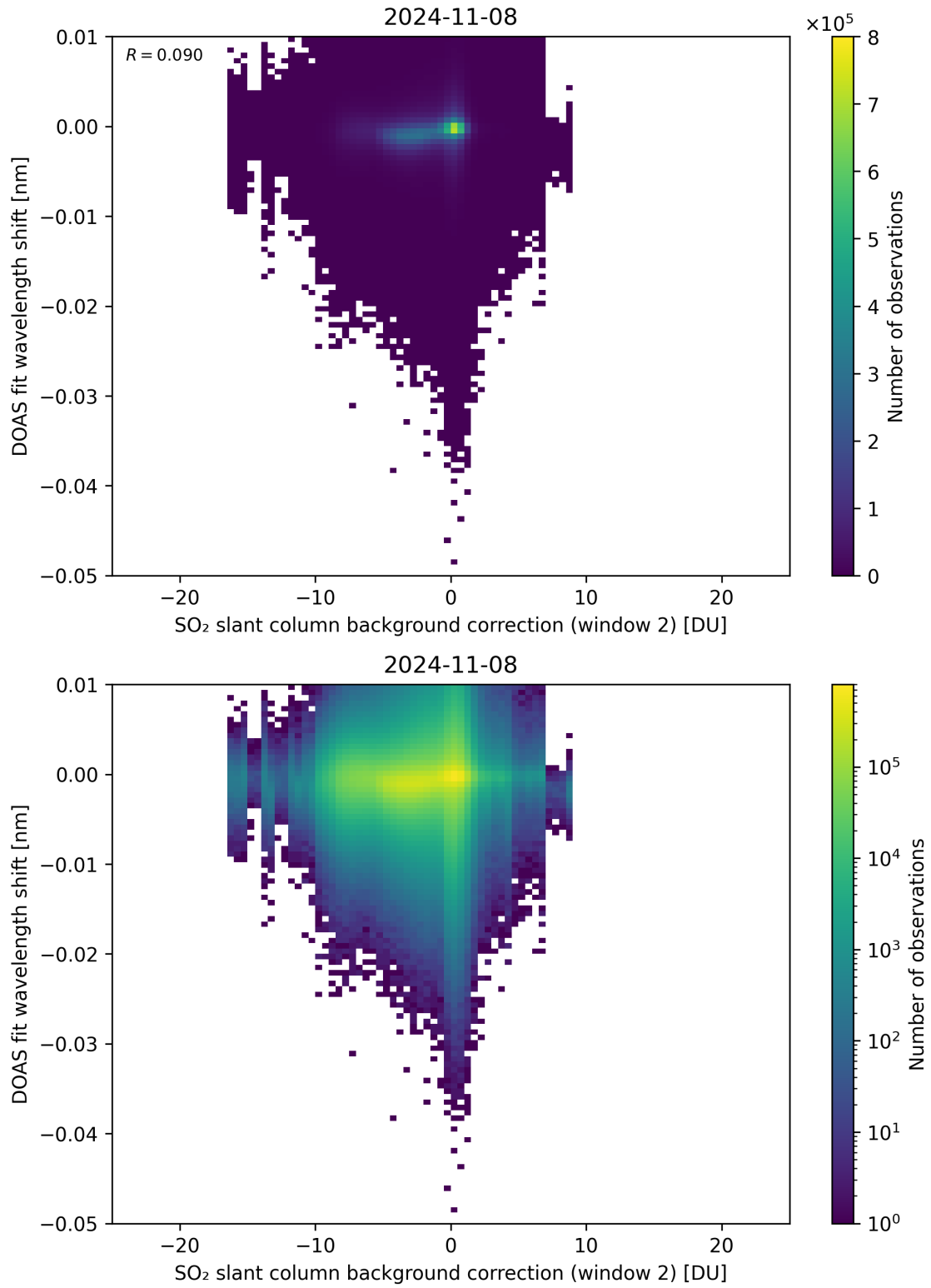
Figure 112: Scatter density plot of “SO 2 slant column background correction (window 2)” against “DOAS fit wavelength shift” for 2024-11-07 to 2024-11-09.
