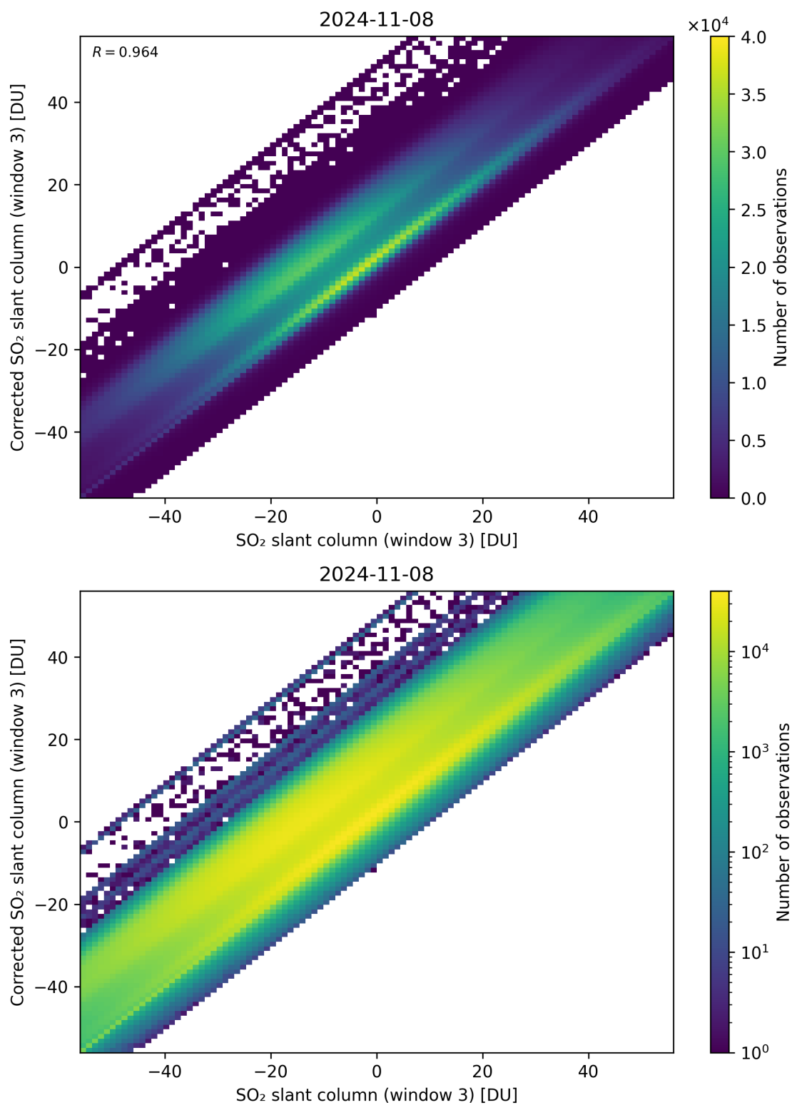
Figure 266: Scatter density plot of “SO 2 slant column (window 3)” against “Corrected SO 2 slant column (window 3)” for 2024-11-07 to 2024-11-09.
