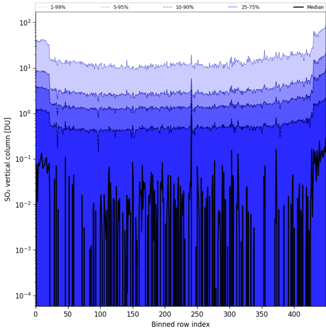
Figure 76: Along track statistics of “SO 2 vertical column” for 2024-11-07 to 2024-11-09
