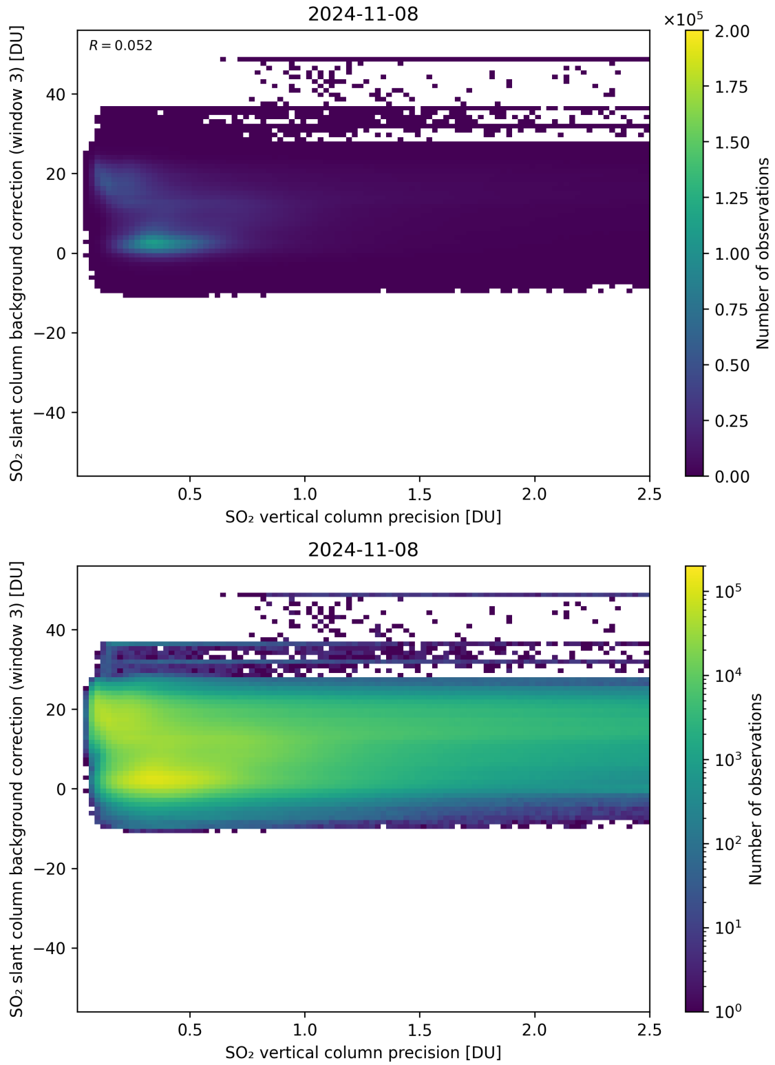
Figure 281: Scatter density plot of “SO 2 vertical column precision” against “SO 2 slant column background correction (window 3)” for 2024-11-07 to 2024-11-09.
