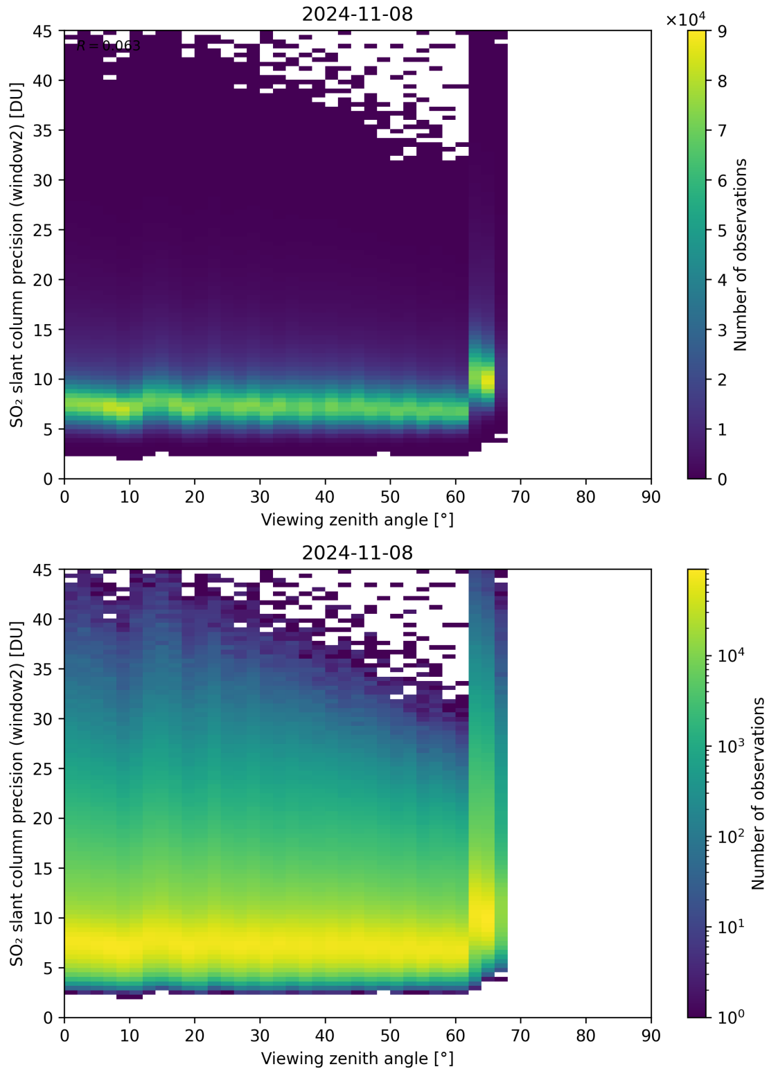
Figure 322: Scatter density plot of “Viewing zenith angle” against “SO 2 slant column precision (window2)” for 2024-11-07 to 2024-11-09.
