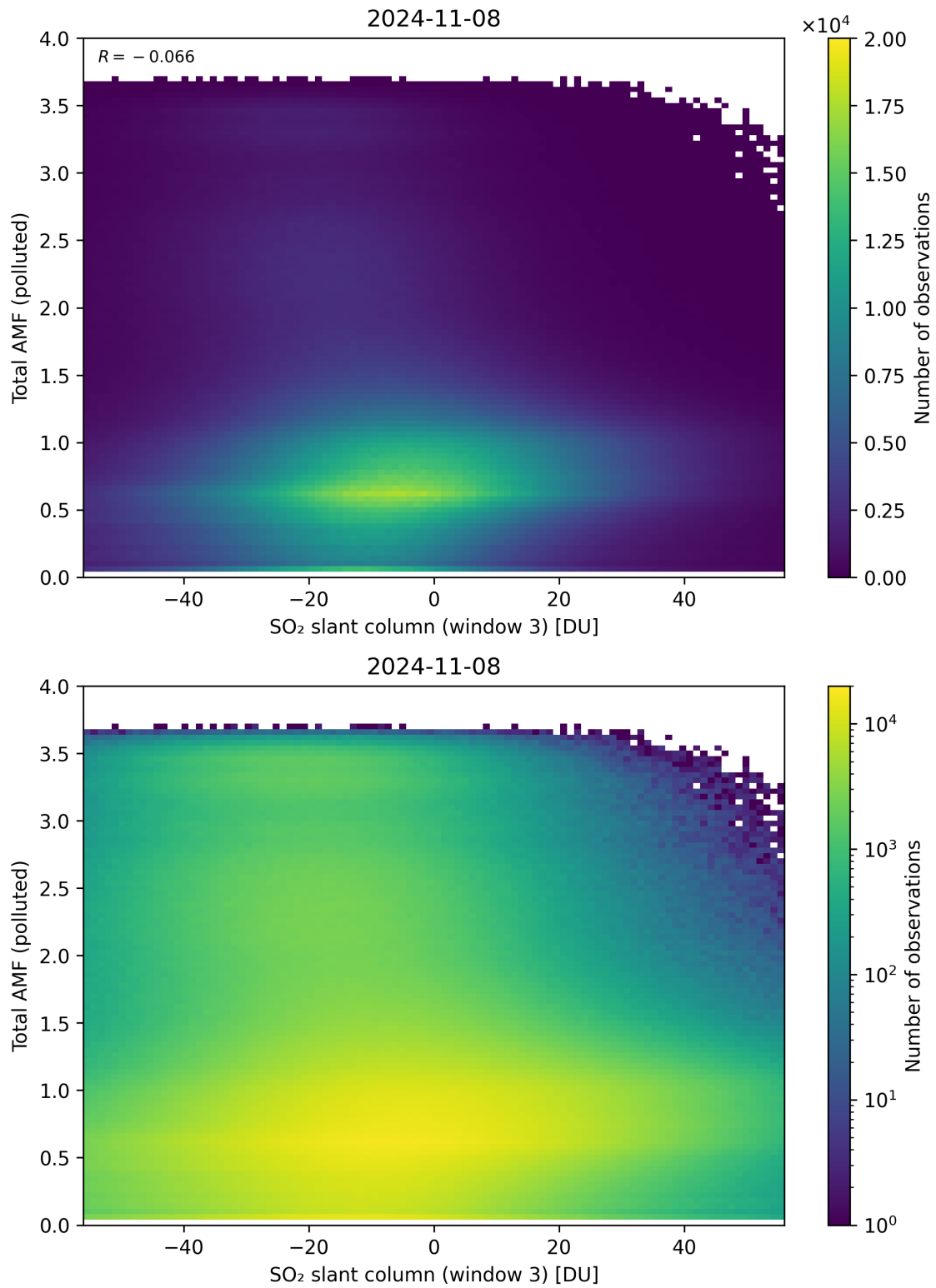
Figure 268: Scatter density plot of “SO 2 slant column (window 3)” against “Total AMF (polluted)” for 2024-11-07 to 2024-11-09.
