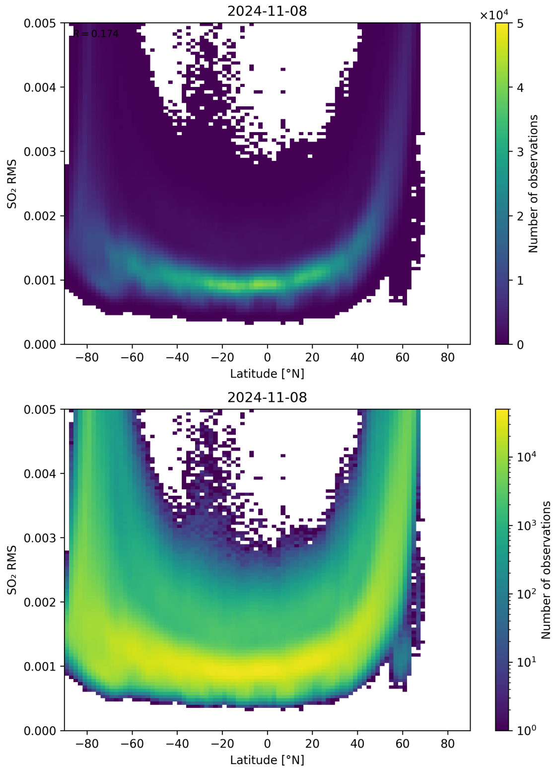
Figure 144: Scatter density plot of “Latitude” against “SO 2 RMS” for 2024-11-07 to 2024-11-09.
