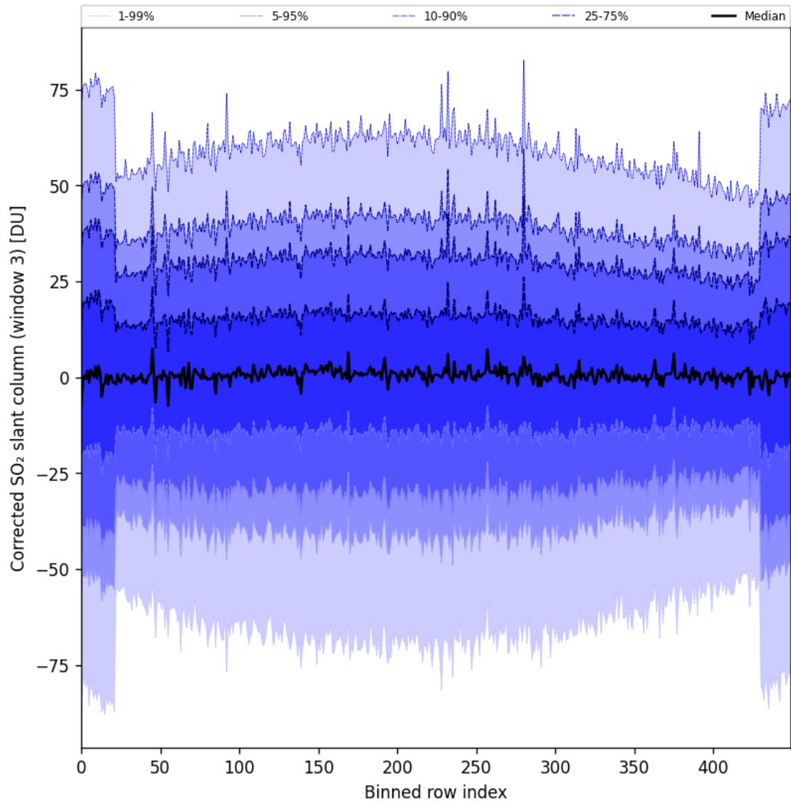
Figure 89: Along track statistics of “Corrected SO 2 slant column (window 3)” for 2024-11-07 to 2024-11-09
