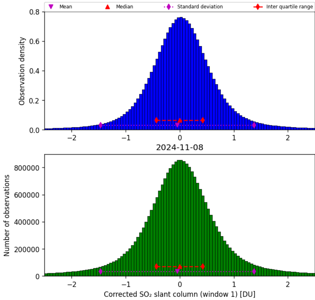
Figure 58: Histogram of “Corrected SO 2 slant column (window 1)” for 2024-11-07 to 2024-11-09
