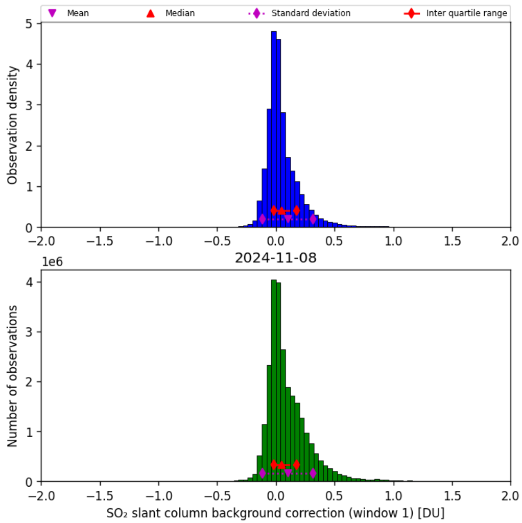
Figure 59: Histogram of “SO 2 slant column background correction (window 1)” for 2024-11-07 to 2024-11-09
