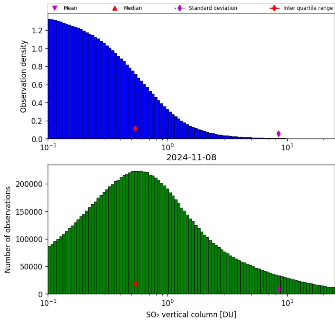
Figure 53: Histogram of “SO 2 vertical column” for 2024-11-07 to 2024-11-09
