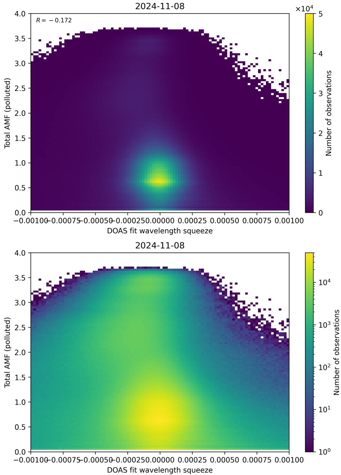
Figure 134: Scatter density plot of “DOAS fit wavelength squeeze” against “Total AMF (polluted)” for 2024-11-07 to 2024-11-09.
