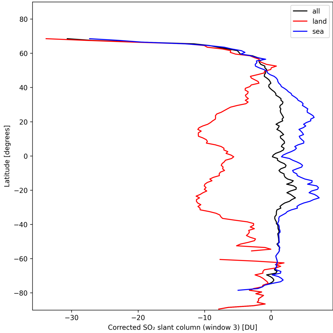
Figure 43: Zonal average of “Corrected SO 2 slant column (window 3)” for 2024-11-07 to 2024-11-09.
