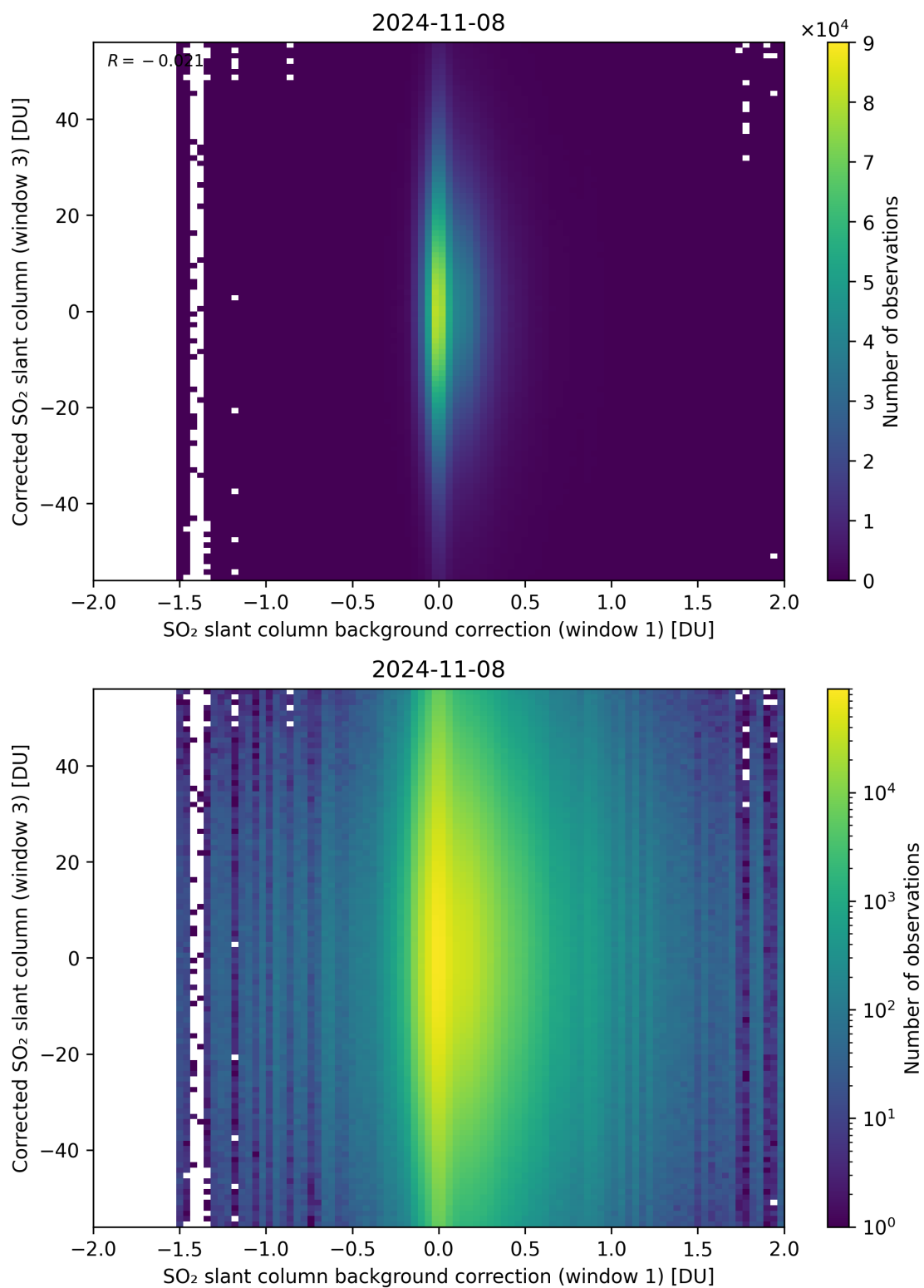
Figure 105: Scatter density plot of “SO 2 slant column background correction (window 1)” against “Corrected SO 2 slant column (window 3)” for 2024-11-07 to 2024-11-09.
