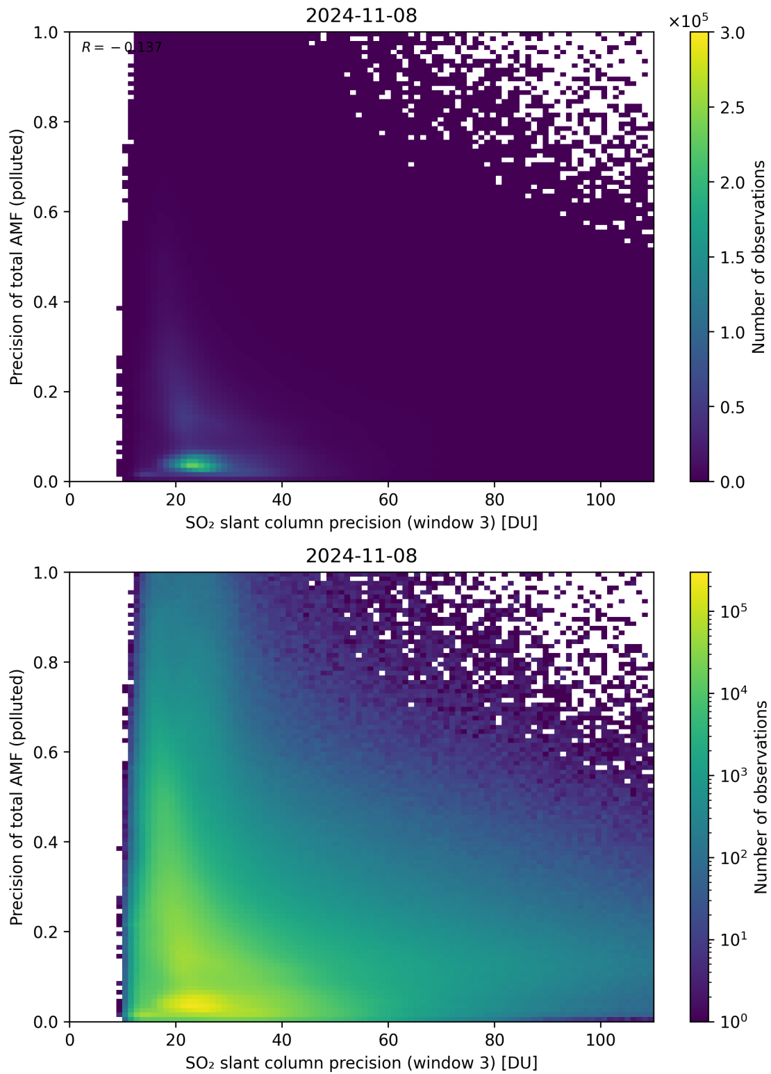
Figure 264: Scatter density plot of “SO 2 slant column precision (window 3)” against “Precision of total AMF (polluted)” for 2024-11-07 to 2024-11-09.
