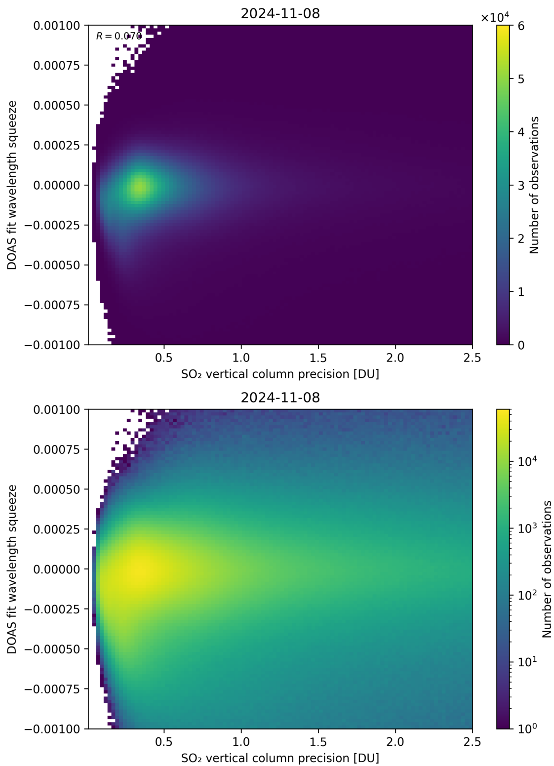
Figure 283: Scatter density plot of “SO 2 vertical column precision” against “DOAS fit wavelength squeeze” for 2024-11-07 to 2024-11-09.
