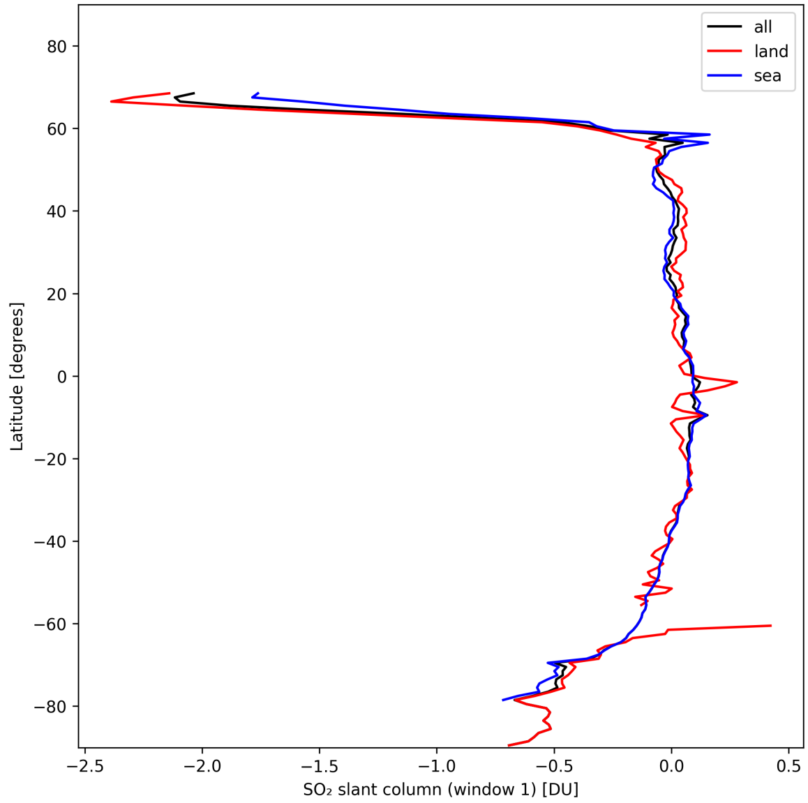
Figure 33: Zonal average of “SO 2 slant column (window 1)” for 2024-11-07 to 2024-11-09.
