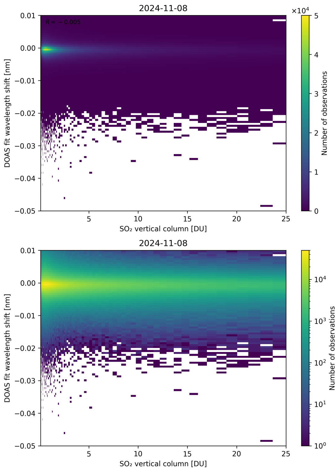
Figure 276: Scatter density plot of “SO 2 vertical column” against “DOAS fit wavelength shift” for 2024-11-07 to 2024-11-09.
