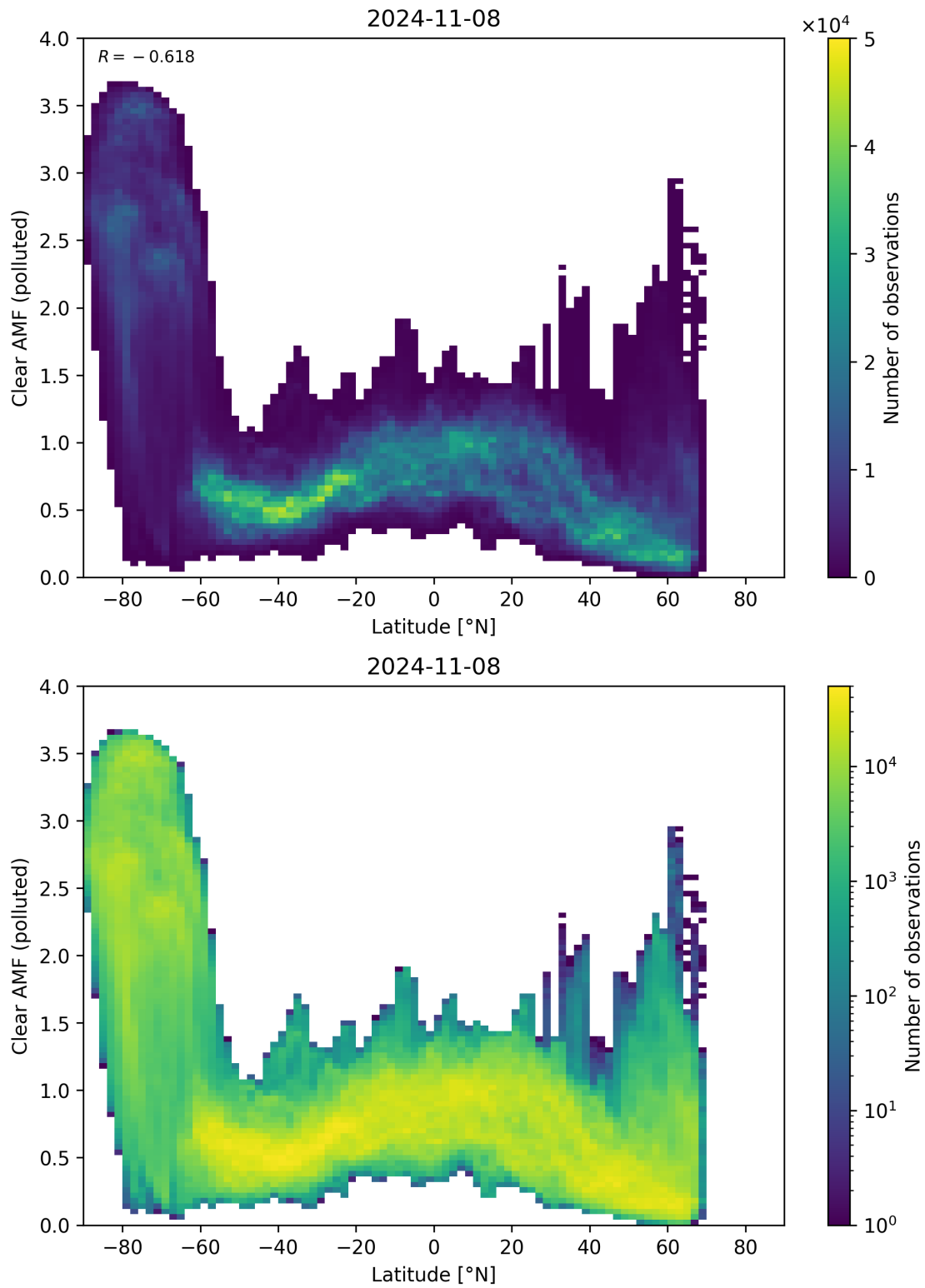
Figure 145: Scatter density plot of “Latitude” against “Clear AMF (polluted)” for 2024-11-07 to 2024-11-09.
