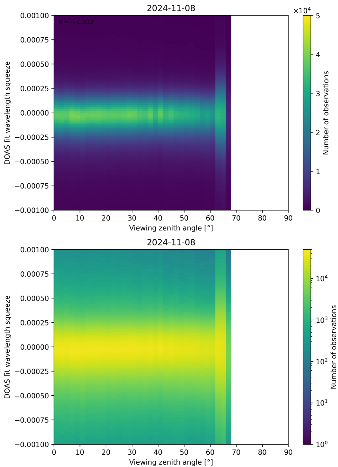
Figure 312: Scatter density plot of “Viewing zenith angle” against “DOAS fit wavelength squeeze” for 2024-11-07 to 2024-11-09.
