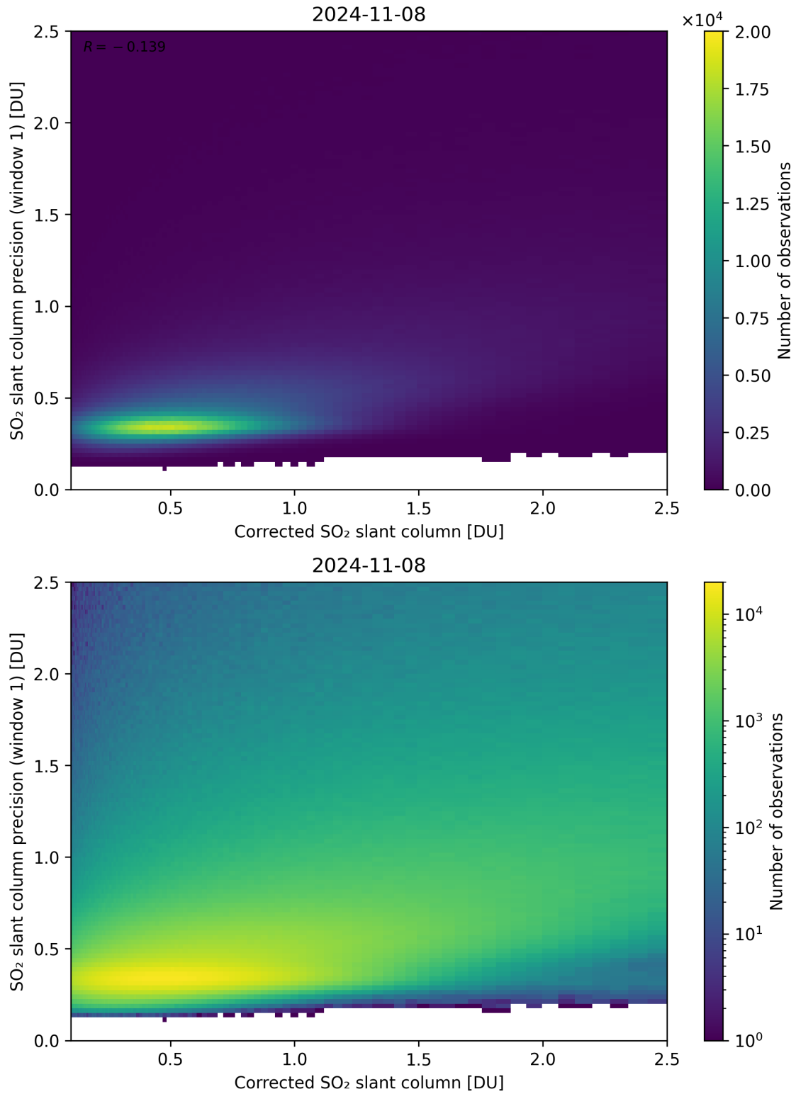
Figure 188: Scatter density plot of “Corrected SO 2 slant column” against “SO 2 slant column precision (window 1)” for 2024-11-07 to 2024-11-09.
