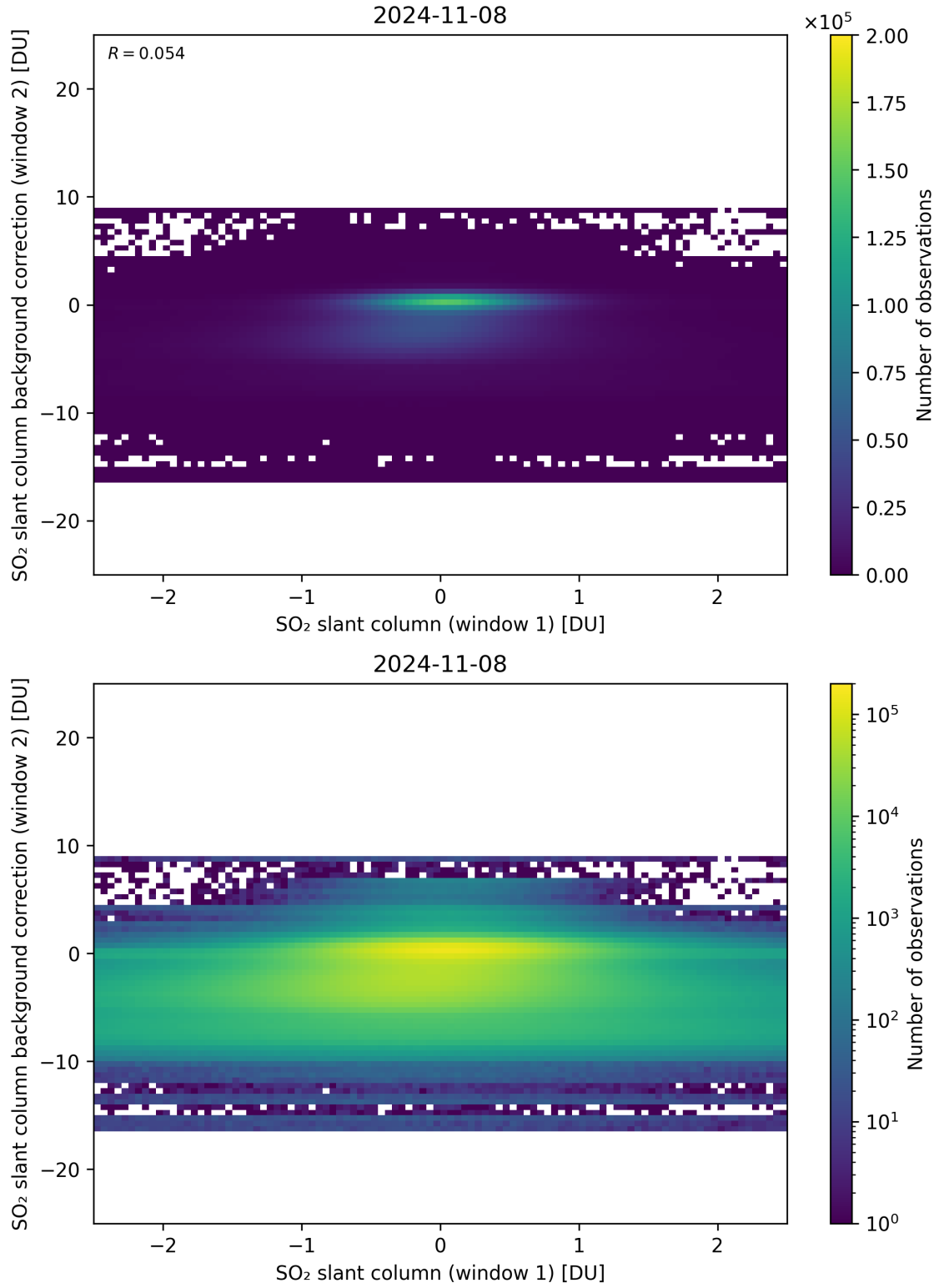
Figure 213: Scatter density plot of “SO 2 slant column (window 1)” against “SO 2 slant column background correction (window 2)” for 2024-11-07 to 2024-11-09.
