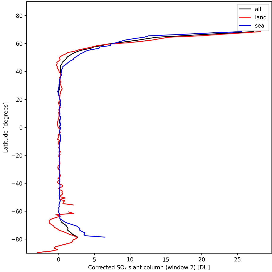
Figure 39: Zonal average of “Corrected SO 2 slant column (window 2)” for 2024-11-07 to 2024-11-09.
