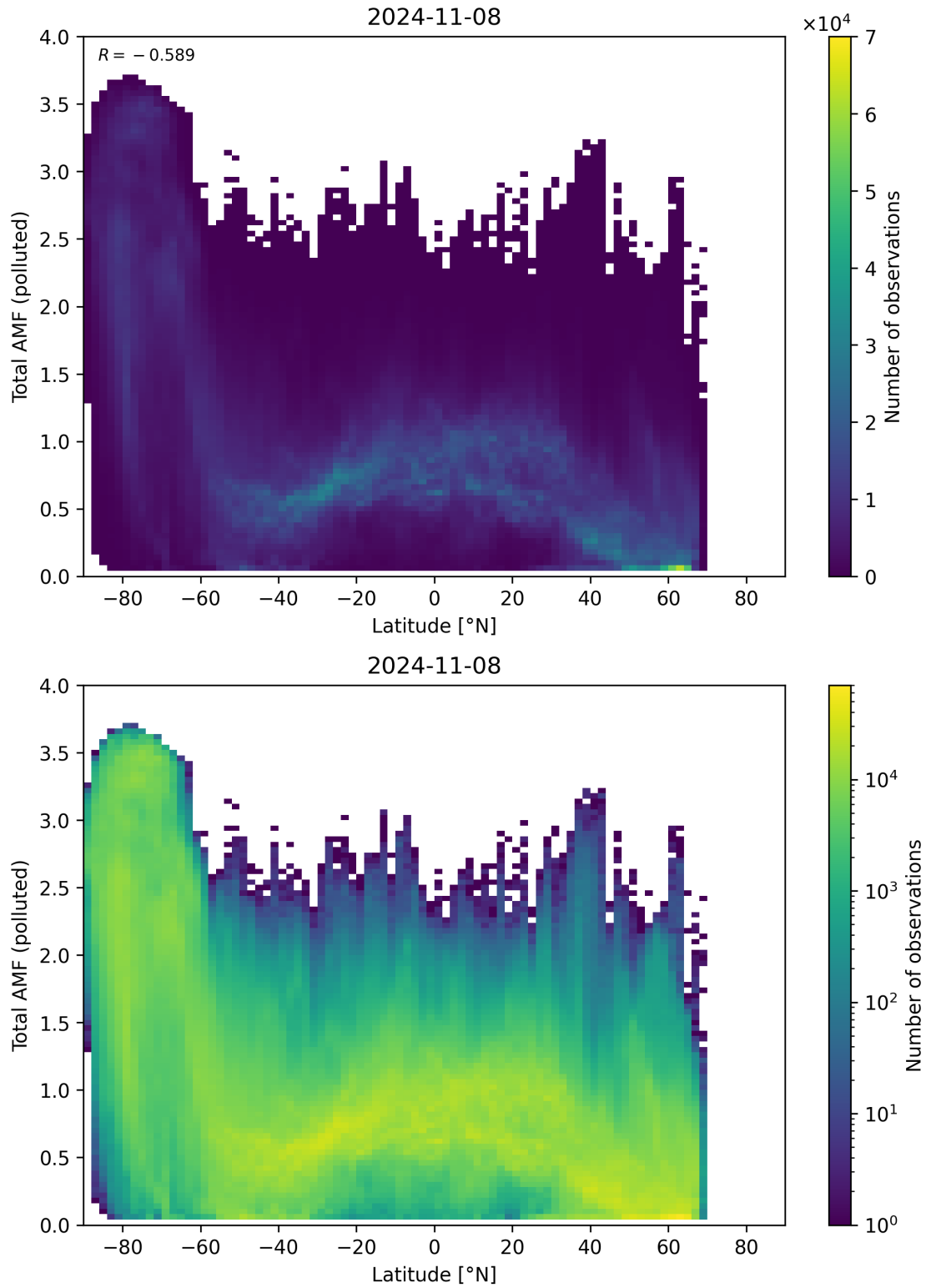
Figure 154: Scatter density plot of “Latitude” against “Total AMF (polluted)” for 2024-11-07 to 2024-11-09.
