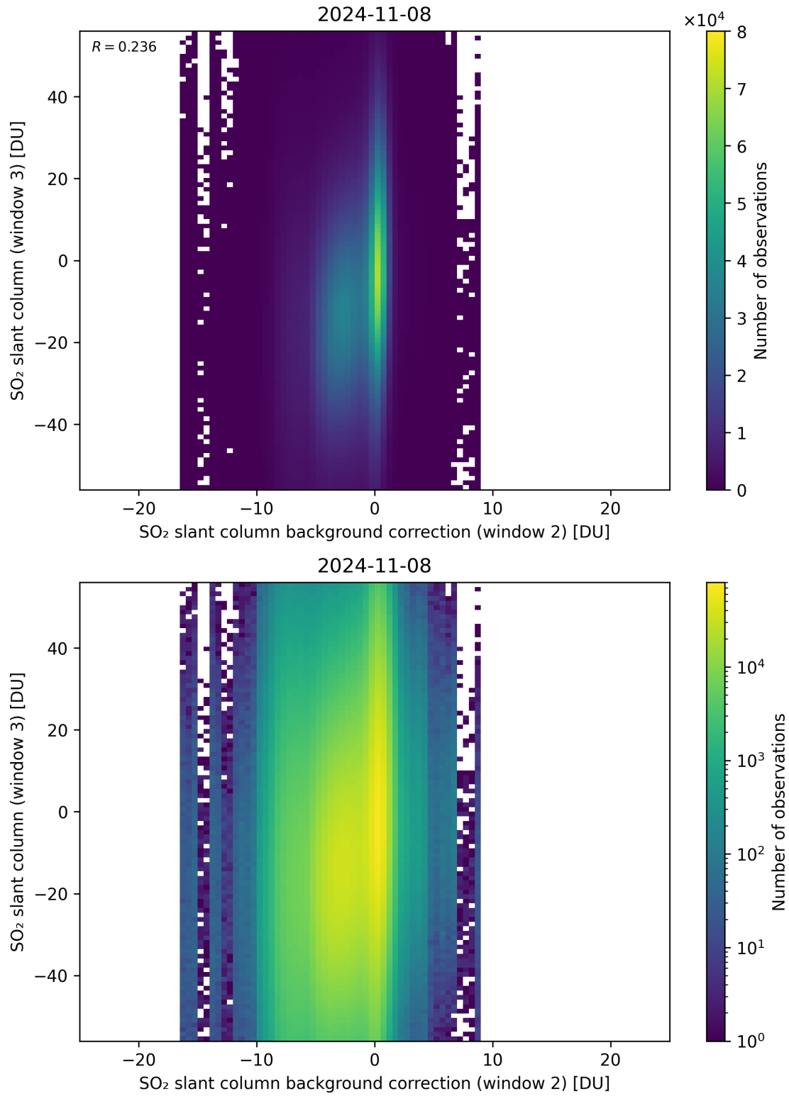
Figure 117: Scatter density plot of “SO 2 slant column background correction (window 2)” against “SO 2 slant column (window 3)” for 2024-11-07 to 2024-11-09.
