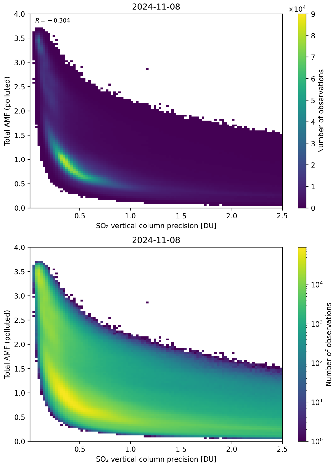
Figure 294: Scatter density plot of “SO 2 vertical column precision” against “Total AMF (polluted)” for 2024-11-07 to 2024-11-09.
