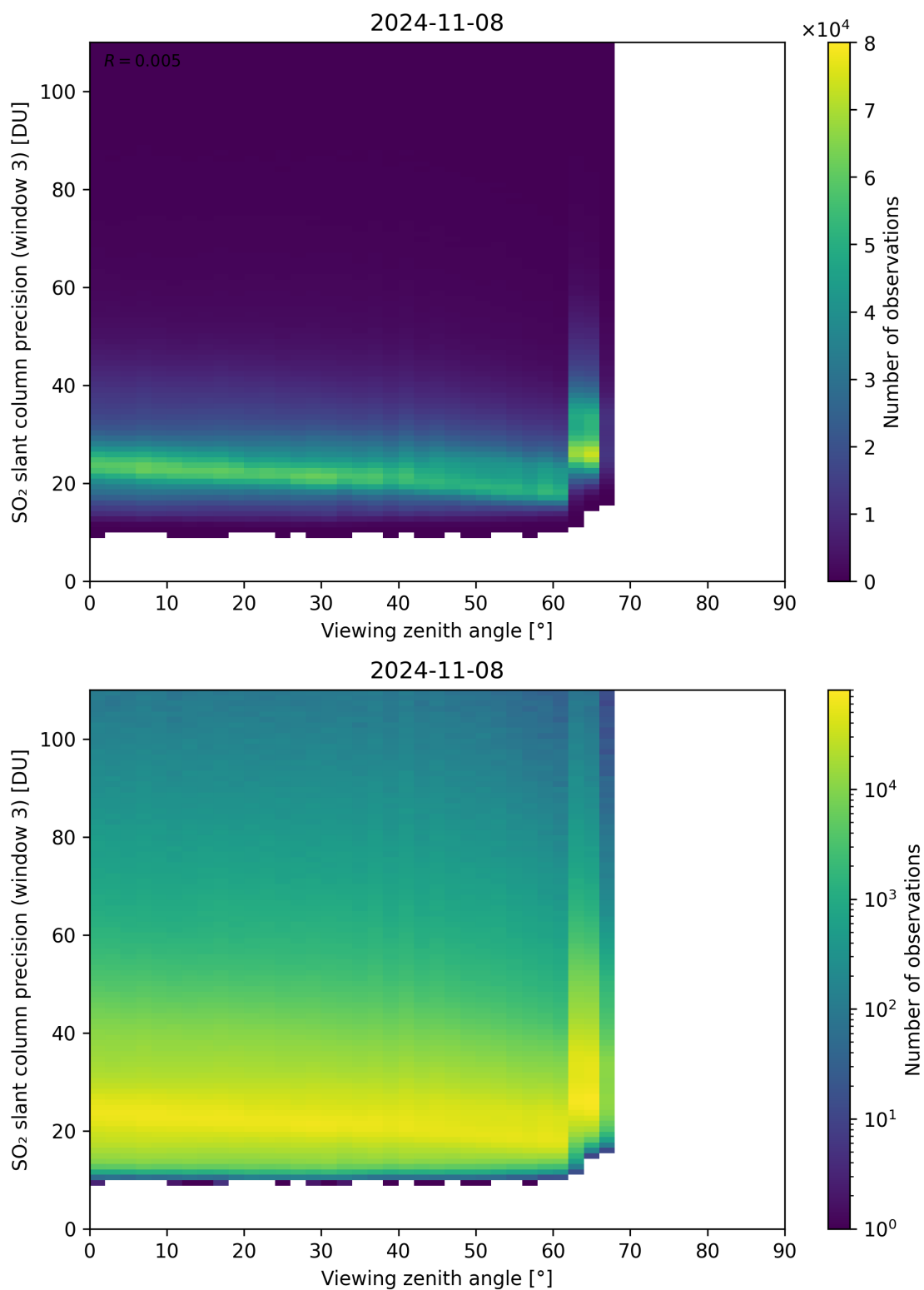
Figure 324: Scatter density plot of “Viewing zenith angle” against “SO 2 slant column precision (window 3)” for 2024-11-07 to 2024-11-09.
