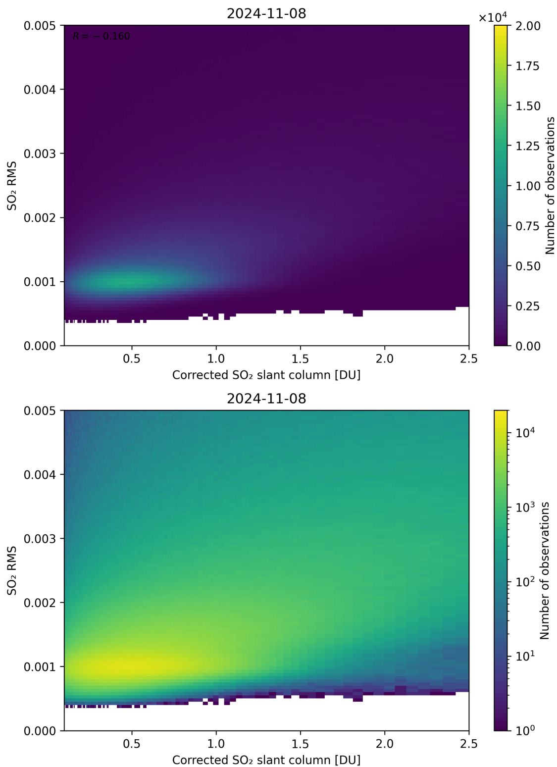
Figure 183: Scatter density plot of “Corrected SO 2 slant column” against “SO 2 RMS” for 2024-11-07 to 2024-11-09.
