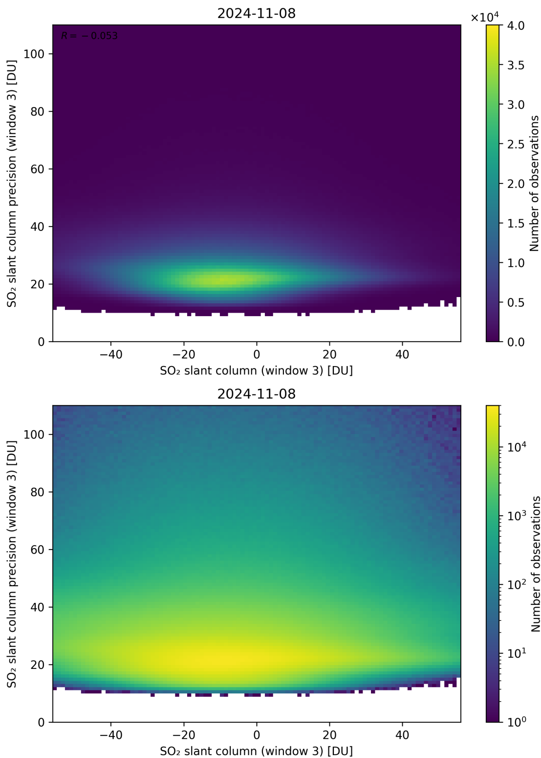
Figure 267: Scatter density plot of “SO 2 slant column (window 3)” against “SO 2 slant column precision (window 3)” for 2024-11-07 to 2024-11-09.
