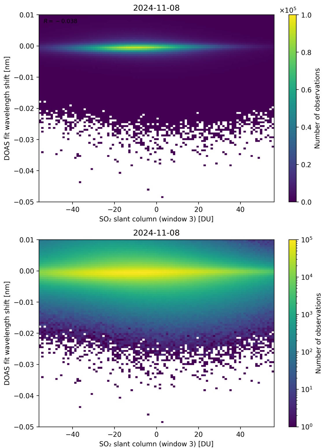
Figure 254: Scatter density plot of “SO 2 slant column (window 3)” against “DOAS fit wavelength shift” for 2024-11-07 to 2024-11-09.
