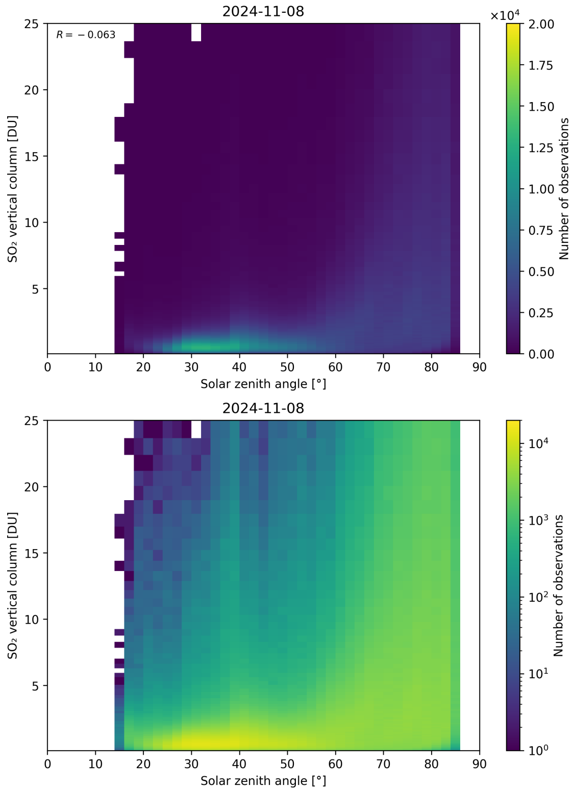
Figure 176: Scatter density plot of “Solar zenith angle” against “SO 2 vertical column” for 2024-11-07 to 2024-11-09.
