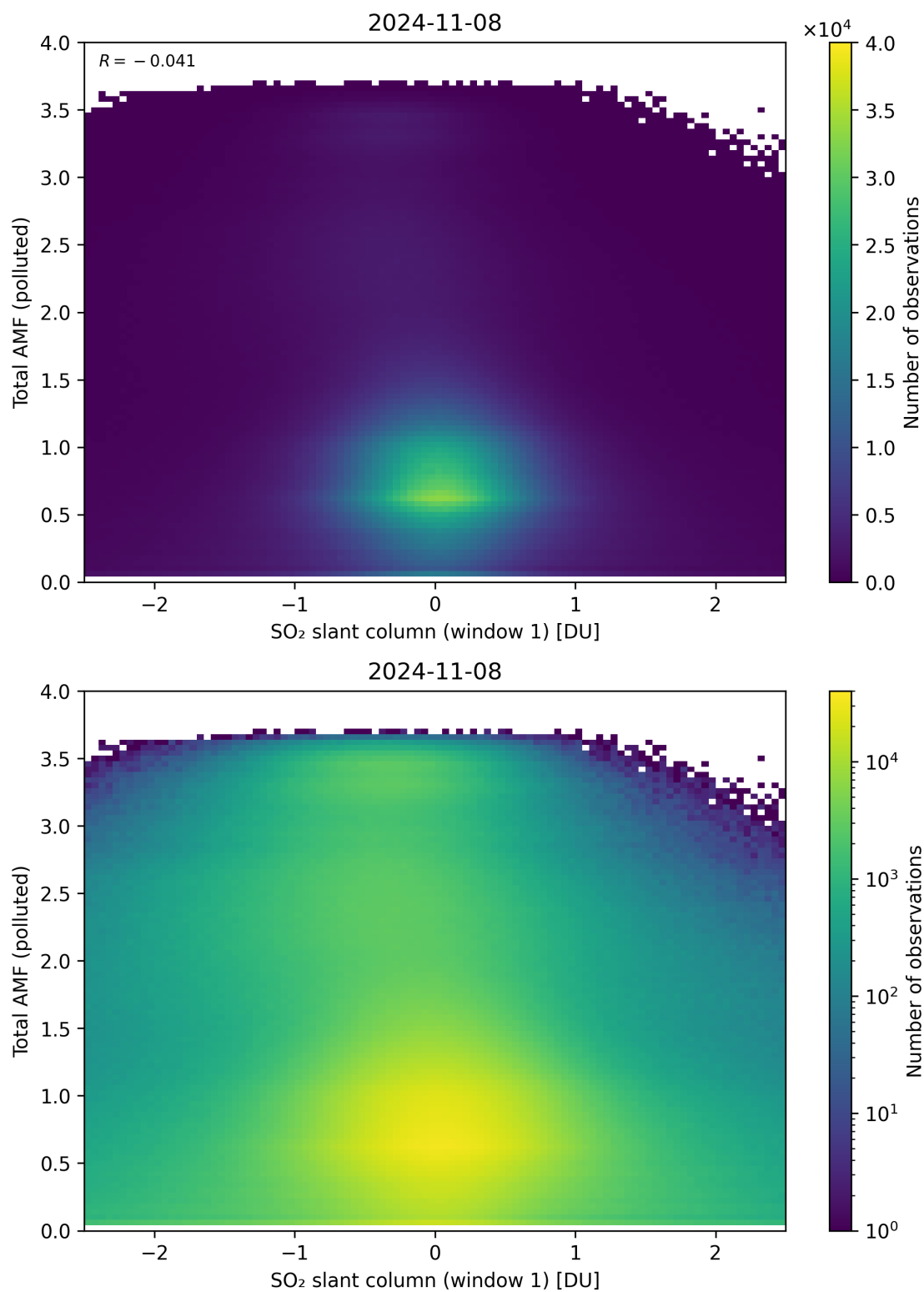
Figure 239: Scatter density plot of “SO 2 slant column (window 1)” against “Total AMF (polluted)” for 2024-11-07 to 2024-11-09.
