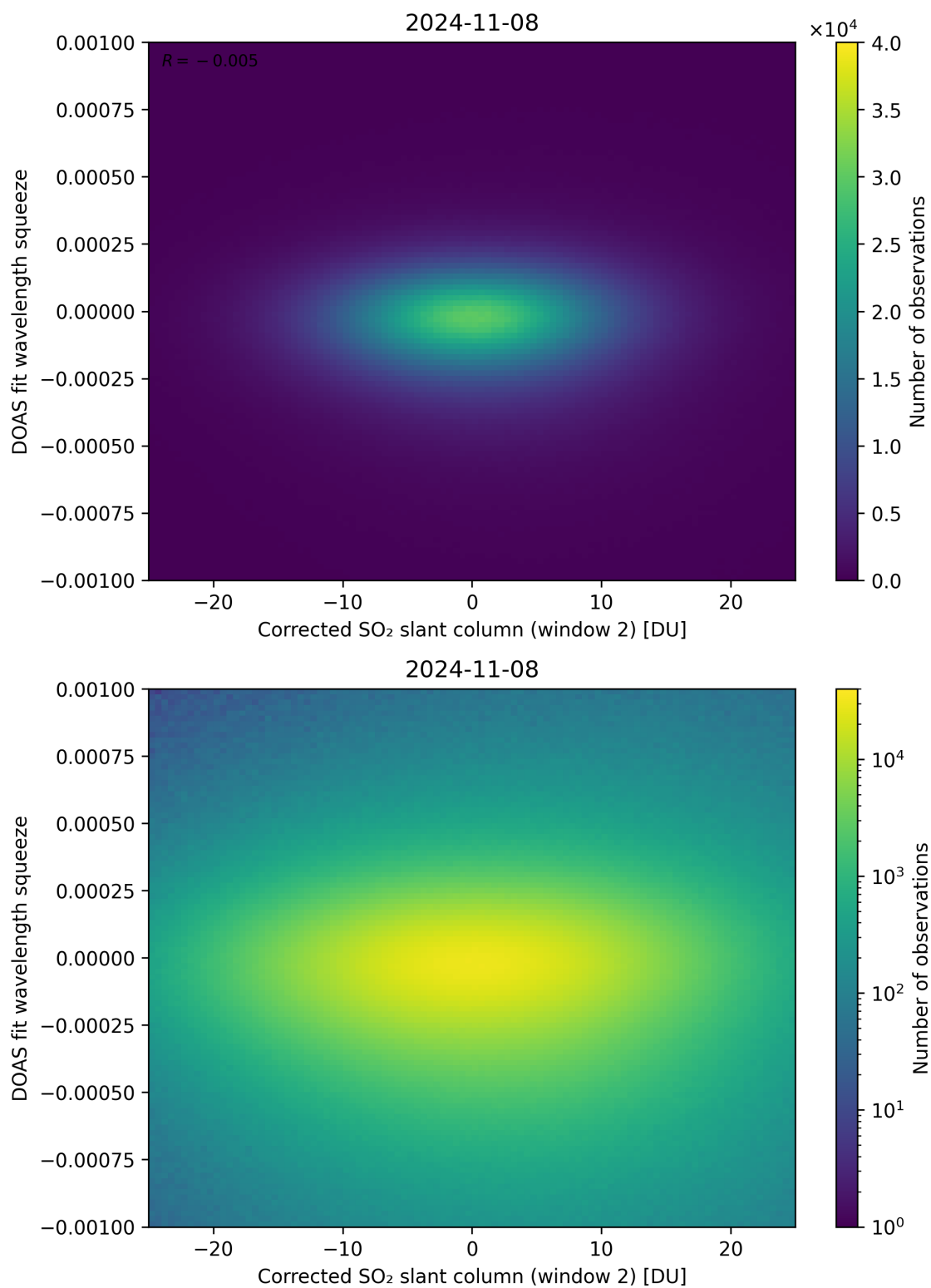
Figure 197: Scatter density plot of “Corrected SO 2 slant column (window 2)” against “DOAS fit wavelength squeeze” for 2024-11-07 to 2024-11-09.
