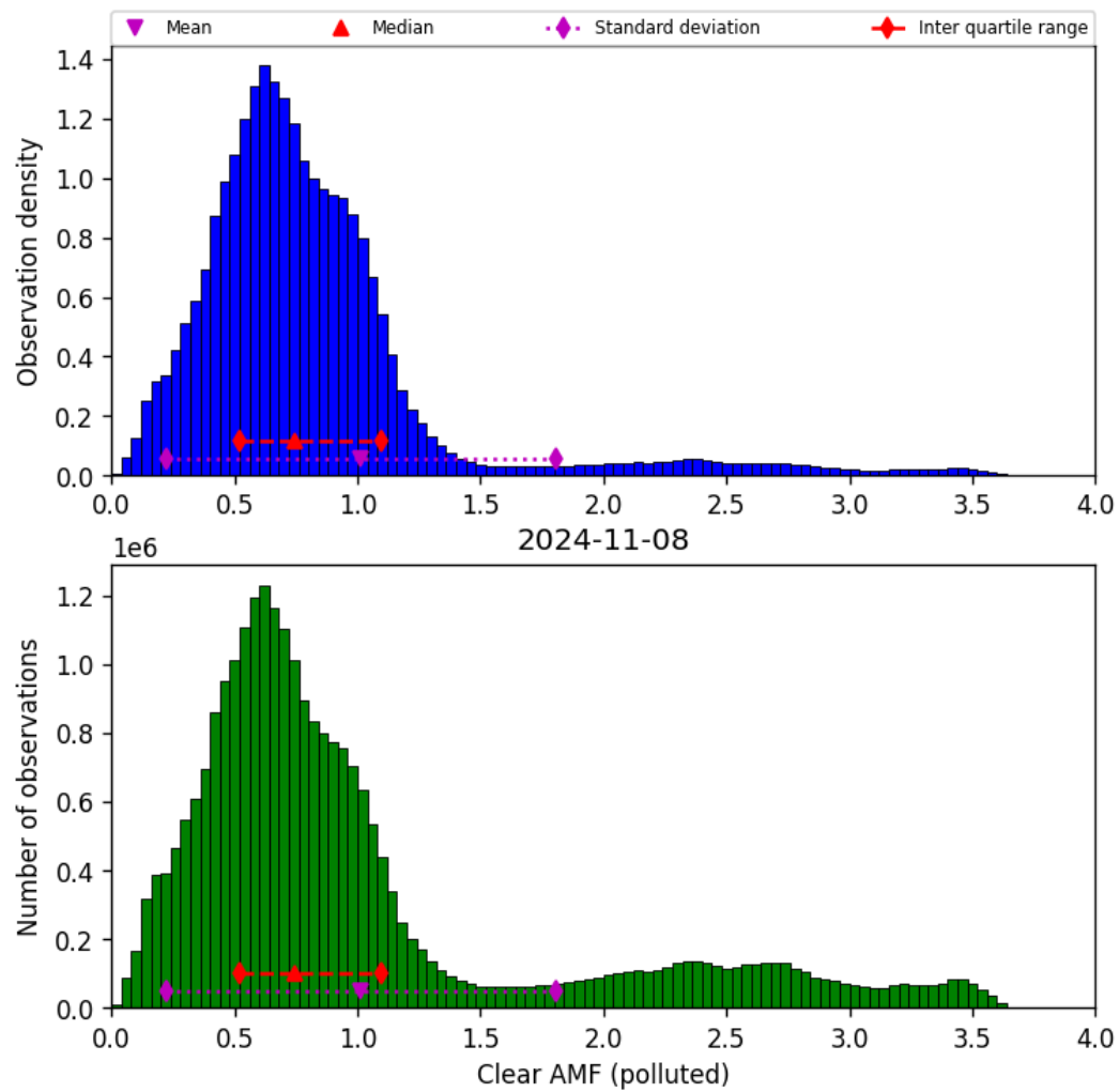
Figure 73: Histogram of “Clear AMF (polluted)” for 2024-11-07 to 2024-11-09
