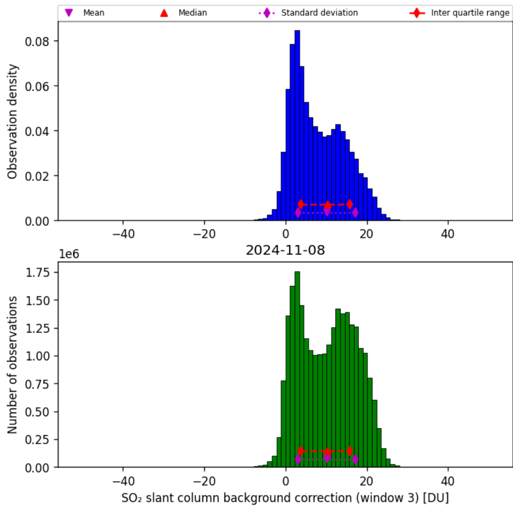
Figure 67: Histogram of “SO 2 slant column background correction (window 3)” for 2024-11-07 to 2024-11-09
