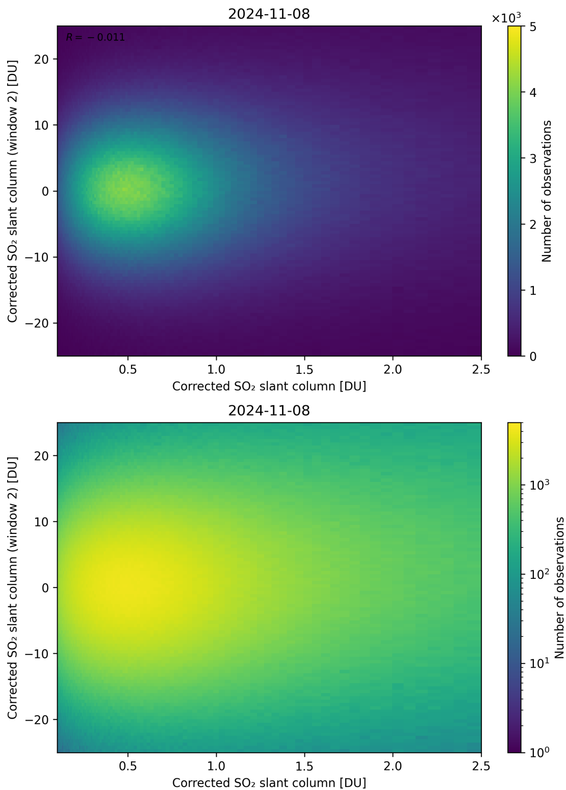
Figure 185: Scatter density plot of “Corrected SO 2 slant column” against “Corrected SO 2 slant column (window 2)” for 2024-11-07 to 2024-11-09.
