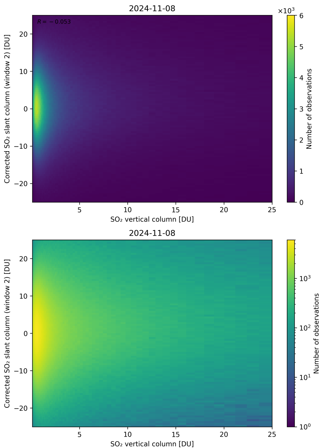
Figure 298: Scatter density plot of “SO 2 vertical column” against “Corrected SO 2 slant column (window 2)” for 2024-11-07 to 2024-11-09.
