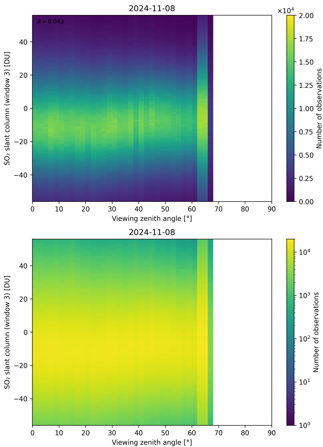
Figure 323: Scatter density plot of “Viewing zenith angle” against “SO 2 slant column (window 3)” for 2024-11-07 to 2024-11-09.
