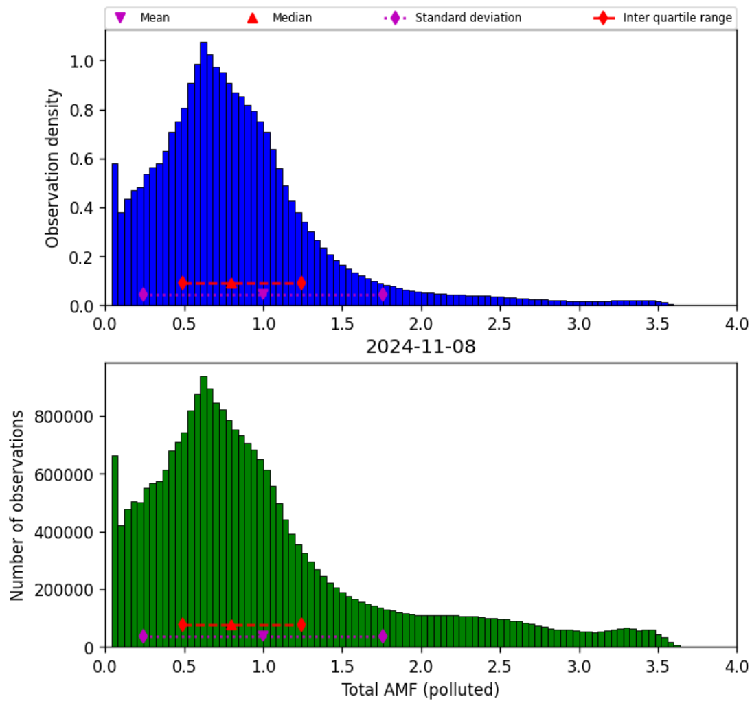
Figure 71: Histogram of “Total AMF (polluted)” for 2024-11-07 to 2024-11-09
