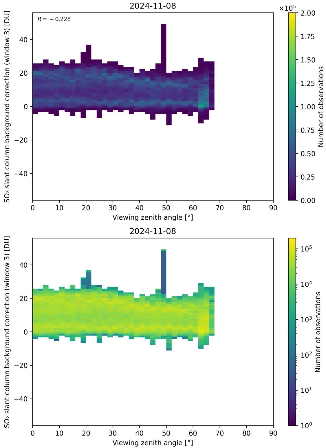
Figure 310: Scatter density plot of “Viewing zenith angle” against “SO 2 slant column background correction (window 3)” for 2024-11-07 to 2024-11-09.
