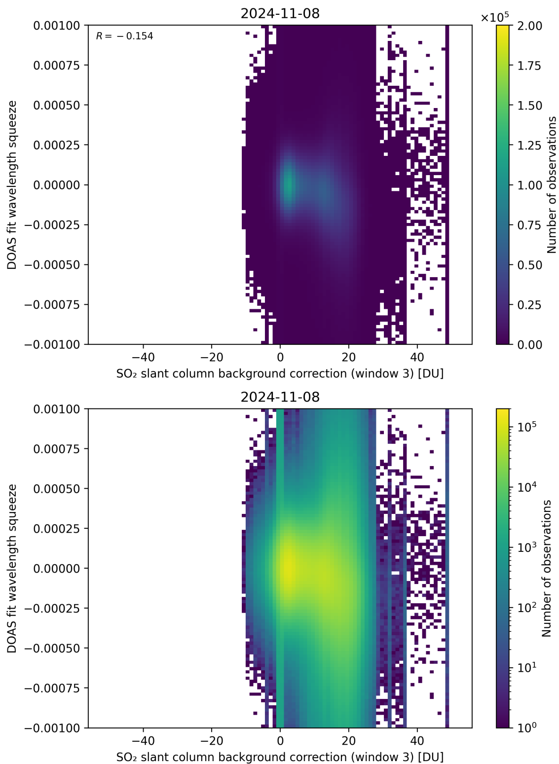
Figure 122: Scatter density plot of “SO 2 slant column background correction (window 3)” against “DOAS fit wavelength squeeze” for 2024-11-07 to 2024-11-09.
