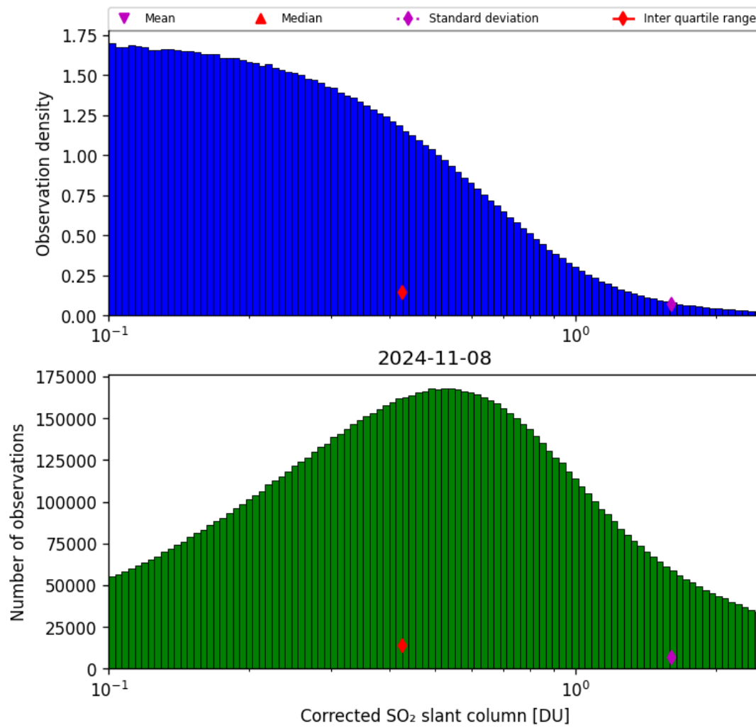
Figure 55: Histogram of “Corrected SO 2 slant column” for 2024-11-07 to 2024-11-09
