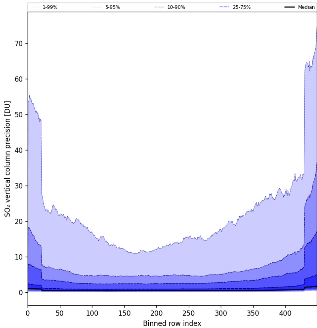
Figure 77: Along track statistics of “SO 2 vertical column precision” for 2024-11-07 to 2024-11-09
