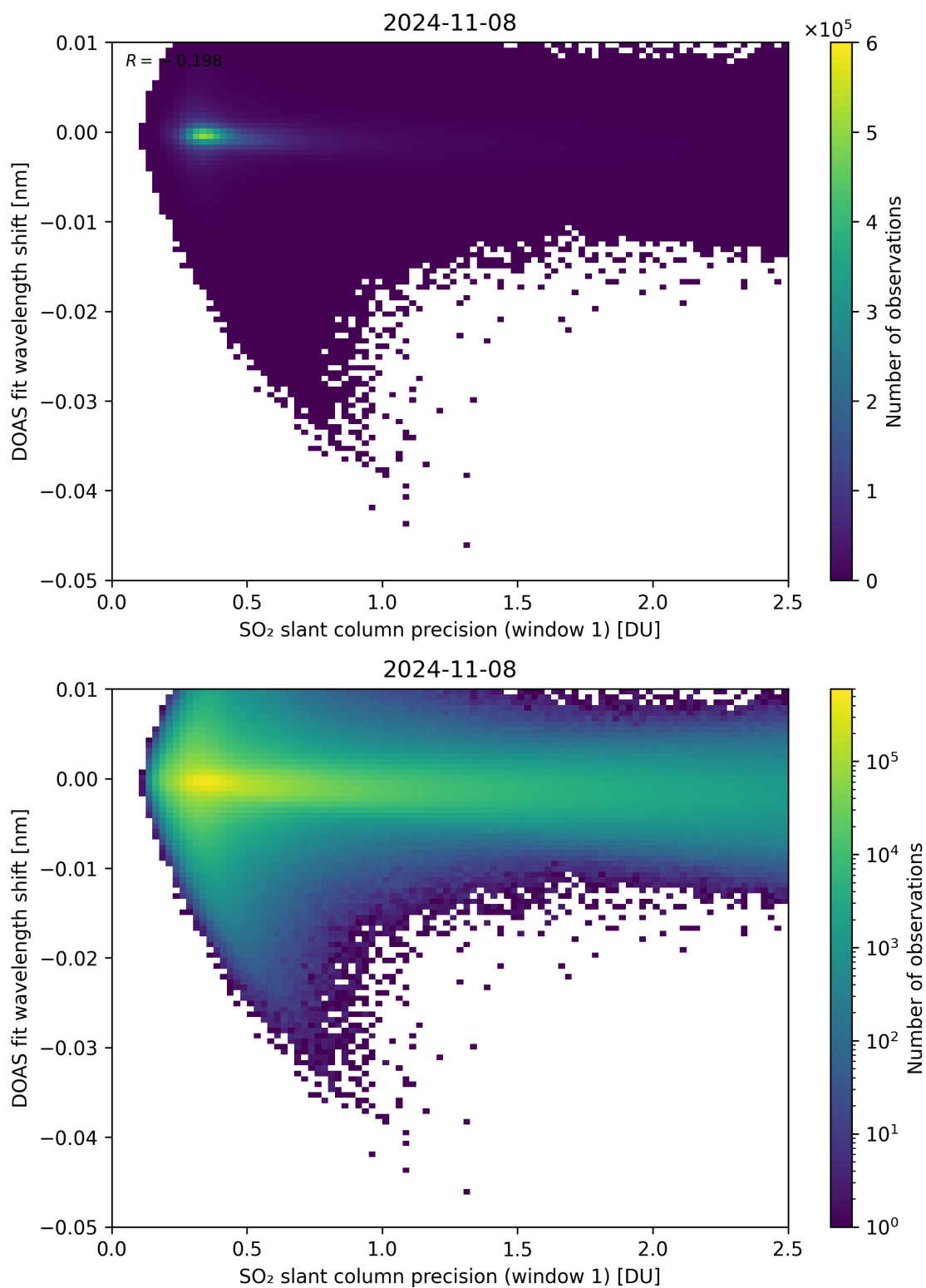
Figure 221: Scatter density plot of “SO 2 slant column precision (window 1)” against “DOAS fit wavelength shift” for 2024-11-07 to 2024-11-09.
