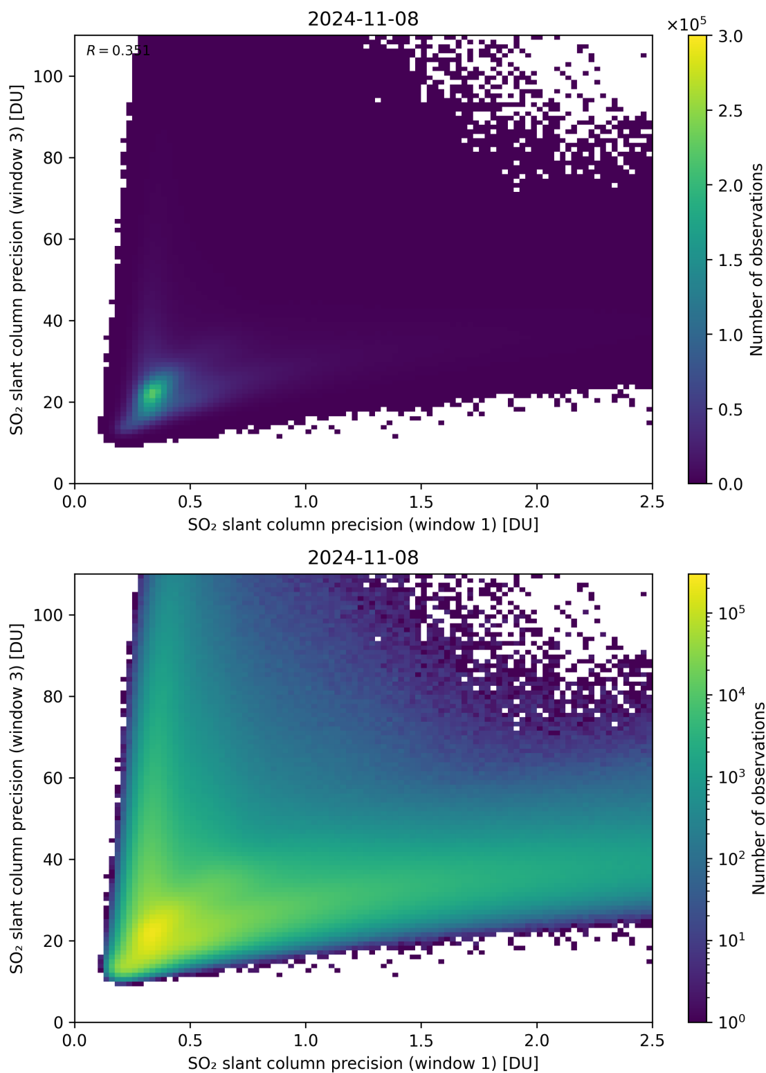
Figure 229: Scatter density plot of “SO 2 slant column precision (window 1)” against “SO 2 slant column precision (window 3)” for 2024-11-07 to 2024-11-09.
