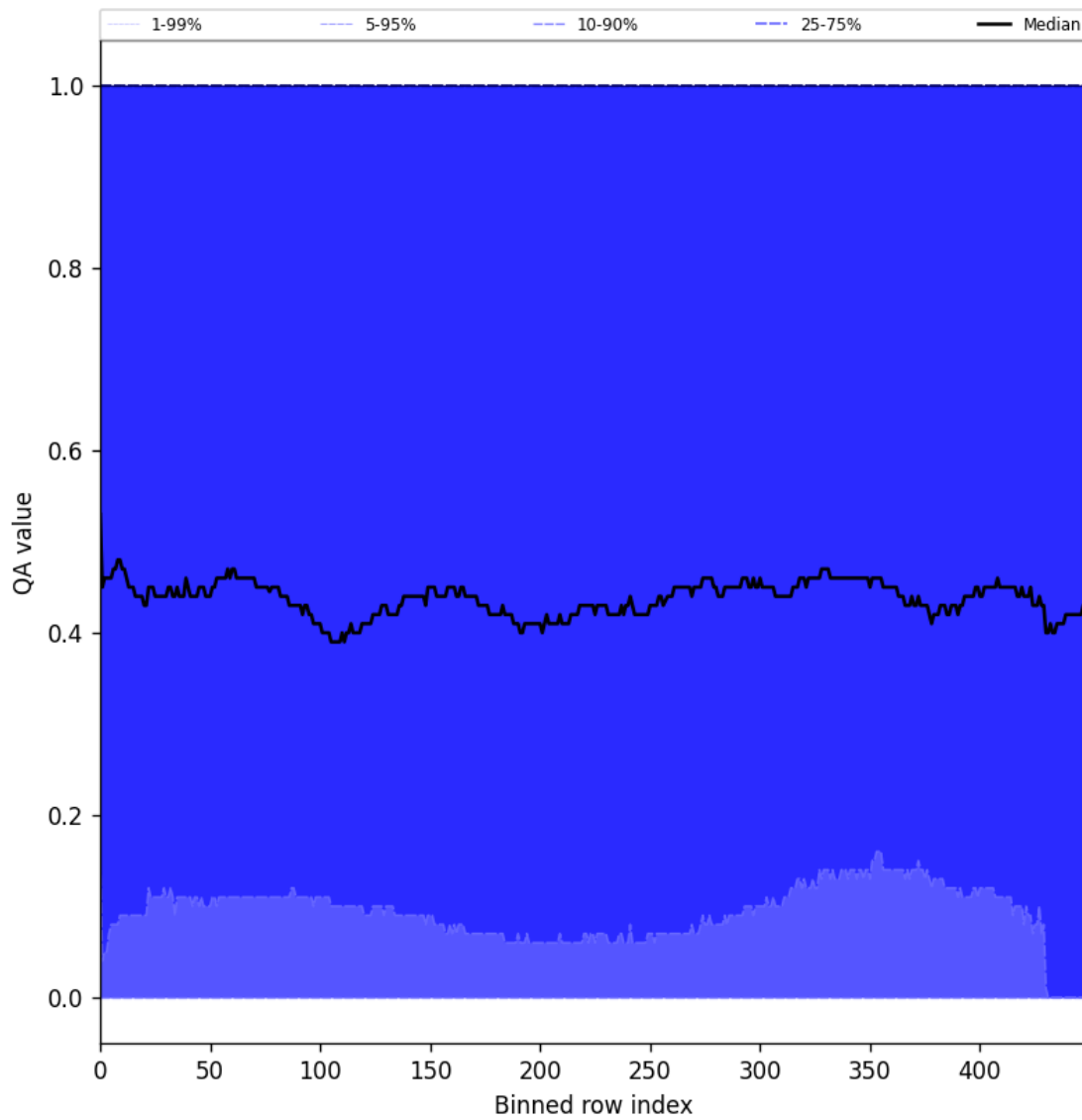
Figure 75: Along track statistics of “QA value” for 2024-11-07 to 2024-11-09
