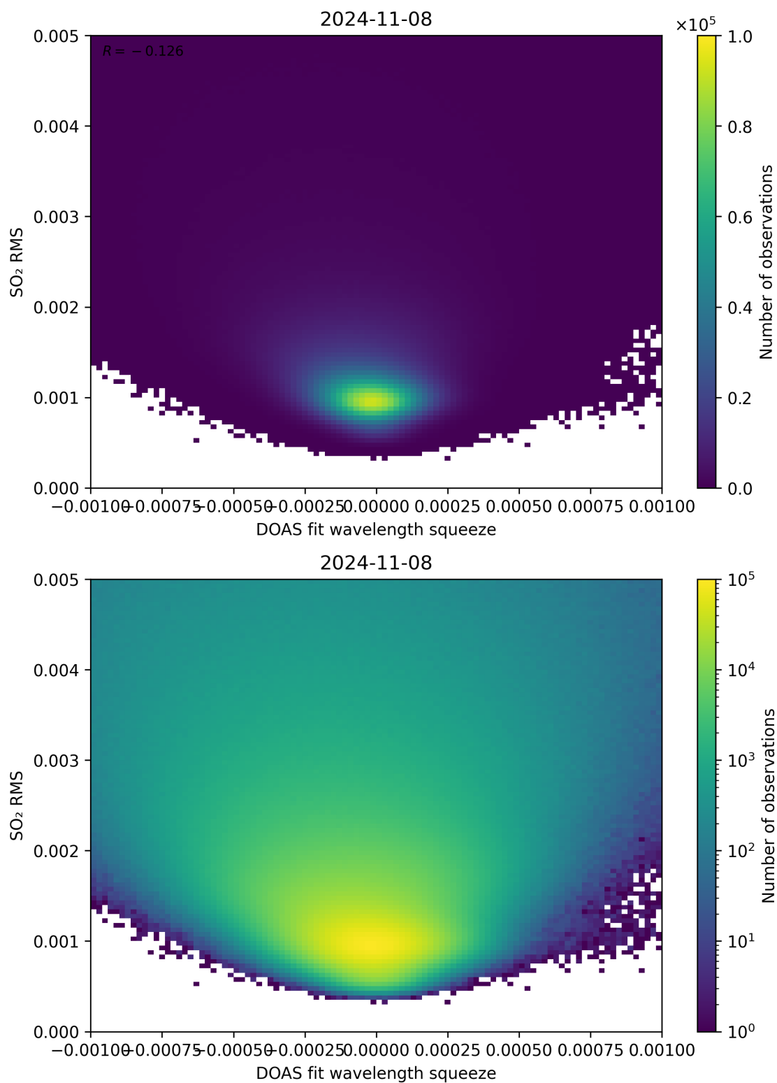
Figure 132: Scatter density plot of “DOAS fit wavelength squeeze” against “SO 2 RMS” for 2024-11-07 to 2024-11-09.
