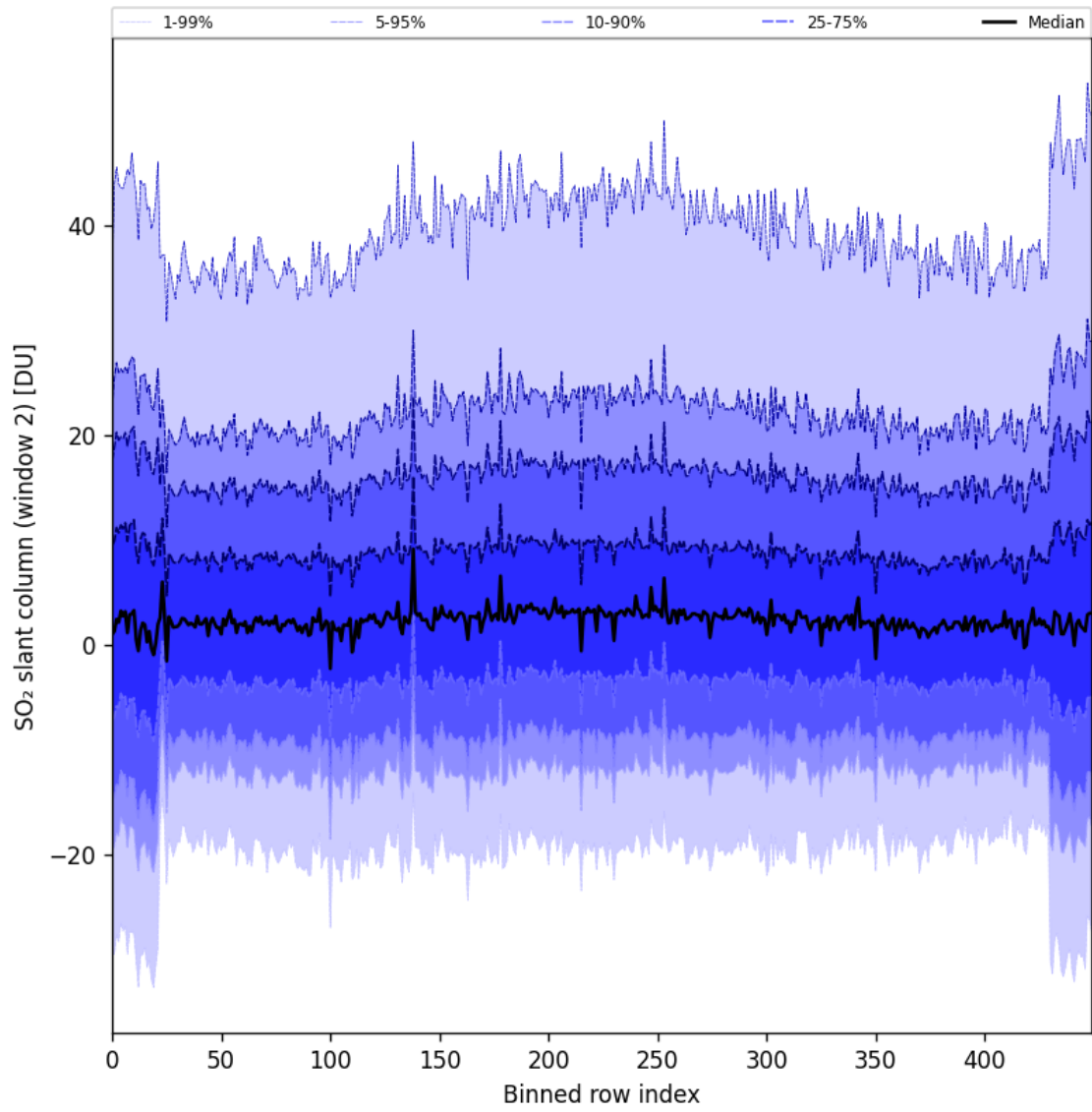
Figure 83: Along track statistics of “SO 2 slant column (window 2)” for 2024-11-07 to 2024-11-09
