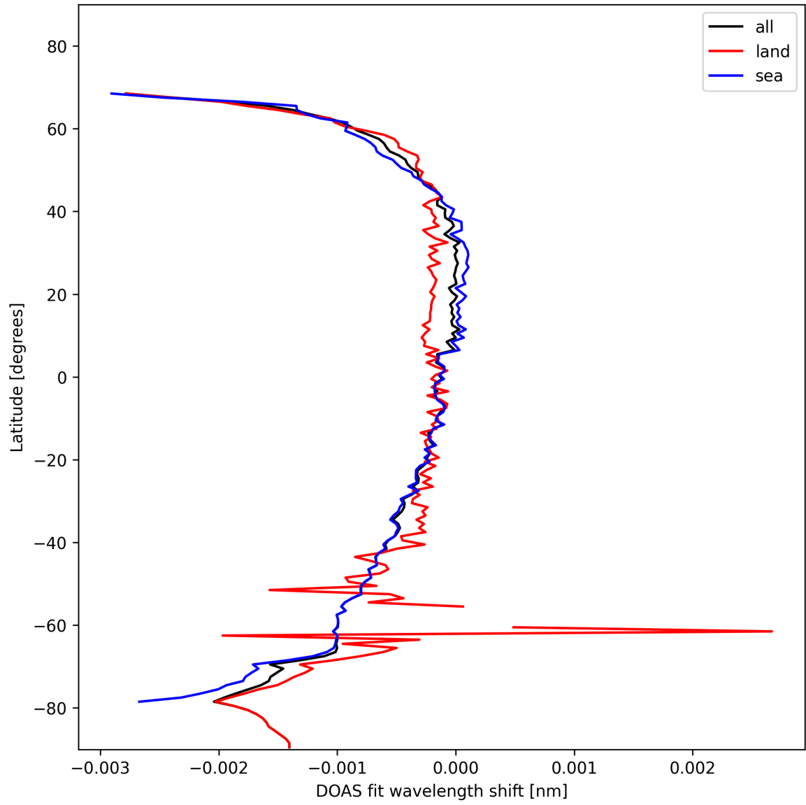
Figure 45: Zonal average of “DOAS fit wavelength shift” for 2024-11-07 to 2024-11-09.
