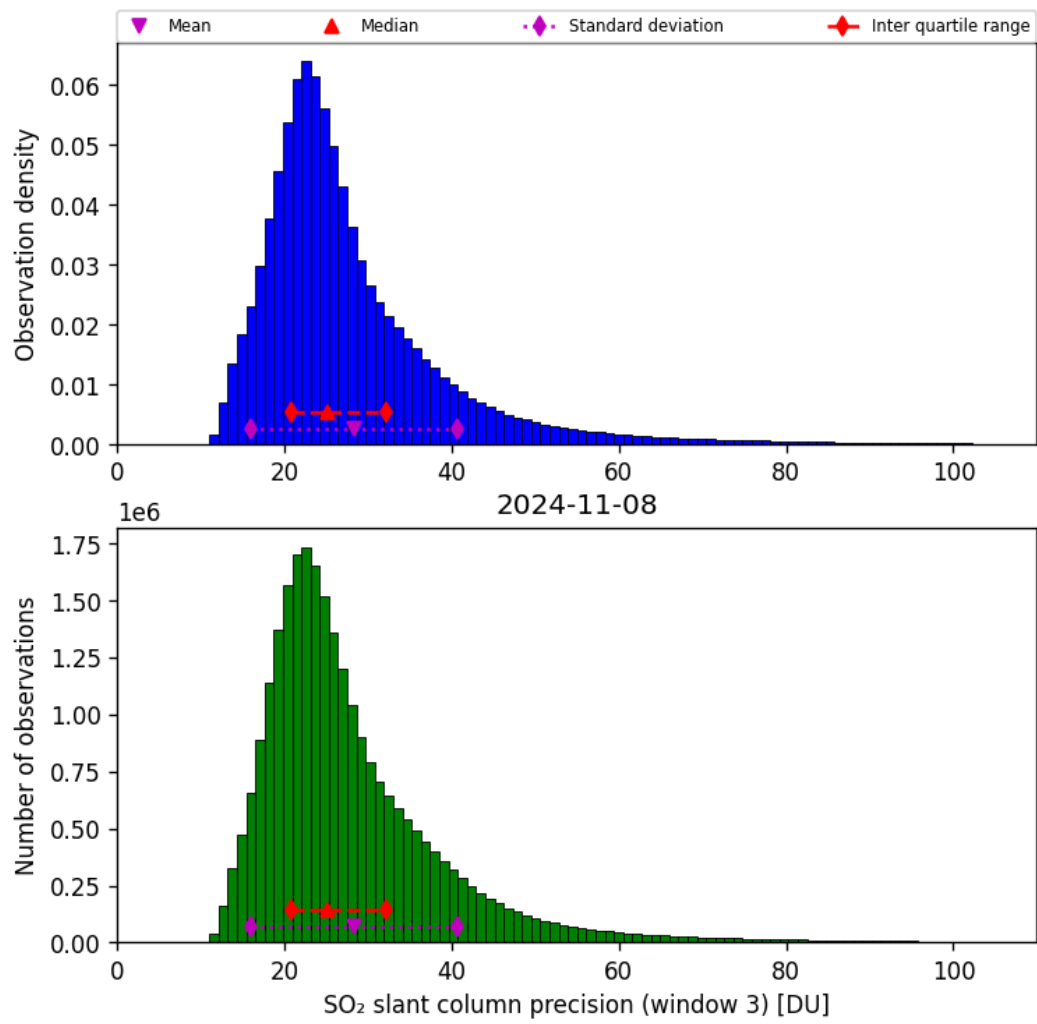
Figure 65: Histogram of “SO 2 slant column precision (window 3)” for 2024-11-07 to 2024-11-09
