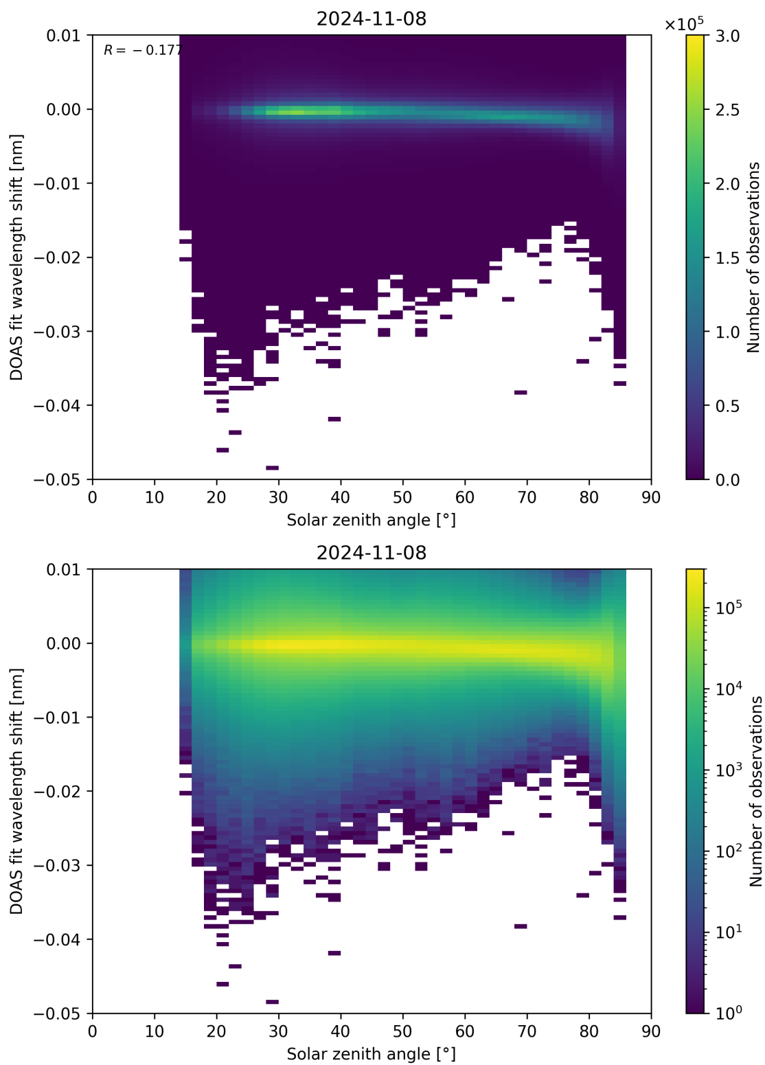
Figure 161: Scatter density plot of “Solar zenith angle” against “DOAS fit wavelength shift” for 2024-11-07 to 2024-11-09.
