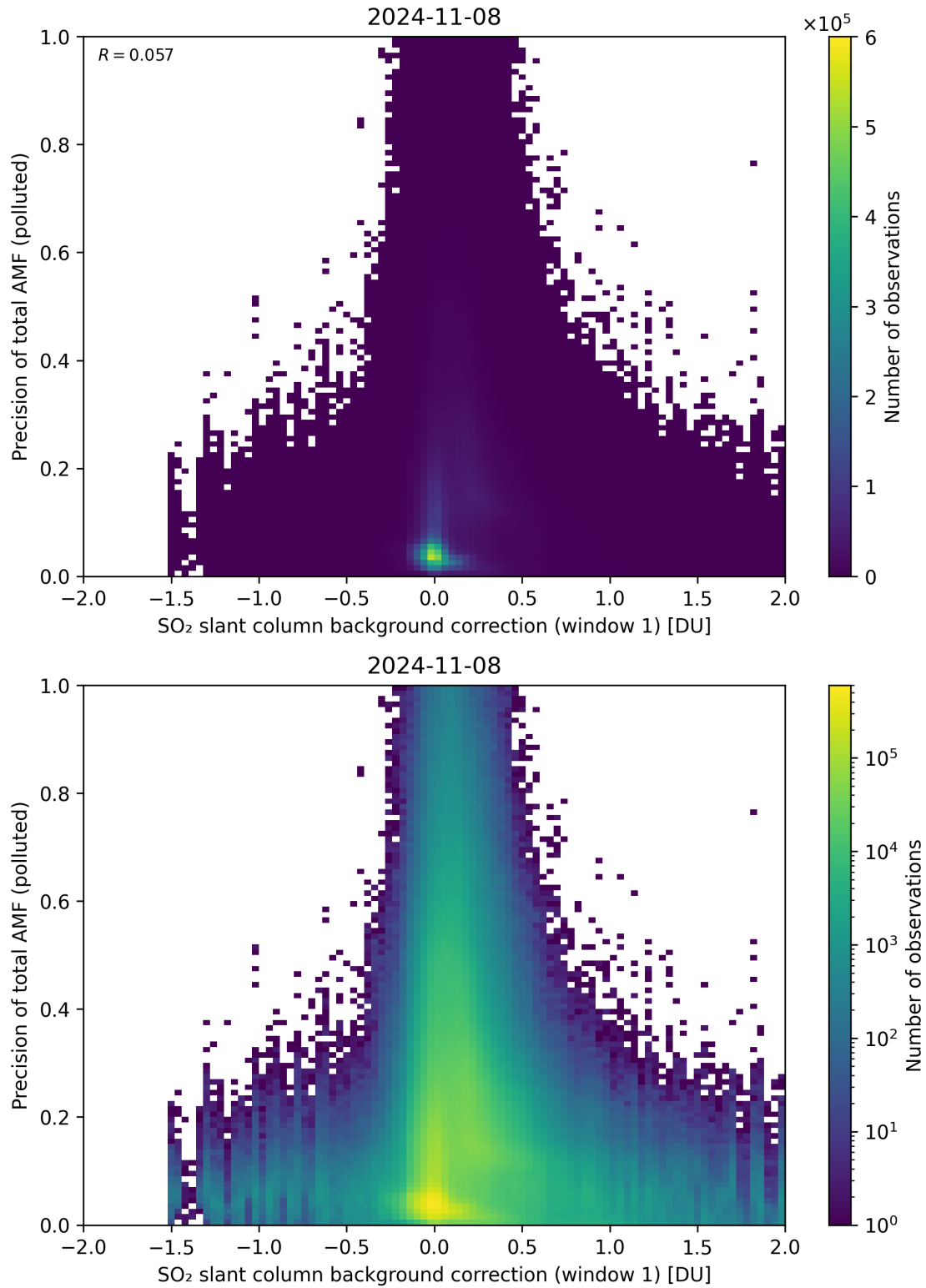
Figure 110: Scatter density plot of “SO 2 slant column background correction (window 1)” against “Precision of total AMF (polluted)” for 2024-11-07 to 2024-11-09.
