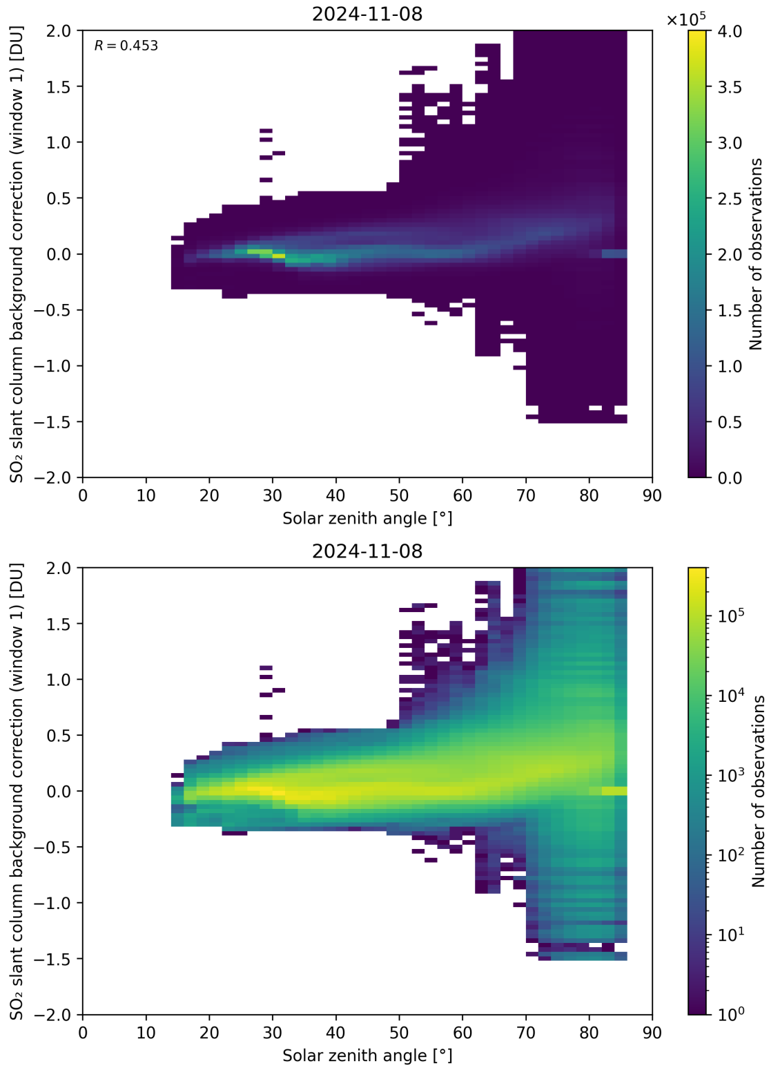
Figure 158: Scatter density plot of “Solar zenith angle” against “SO 2 slant column background correction (window 1)” for 2024-11-07 to 2024-11-09.
