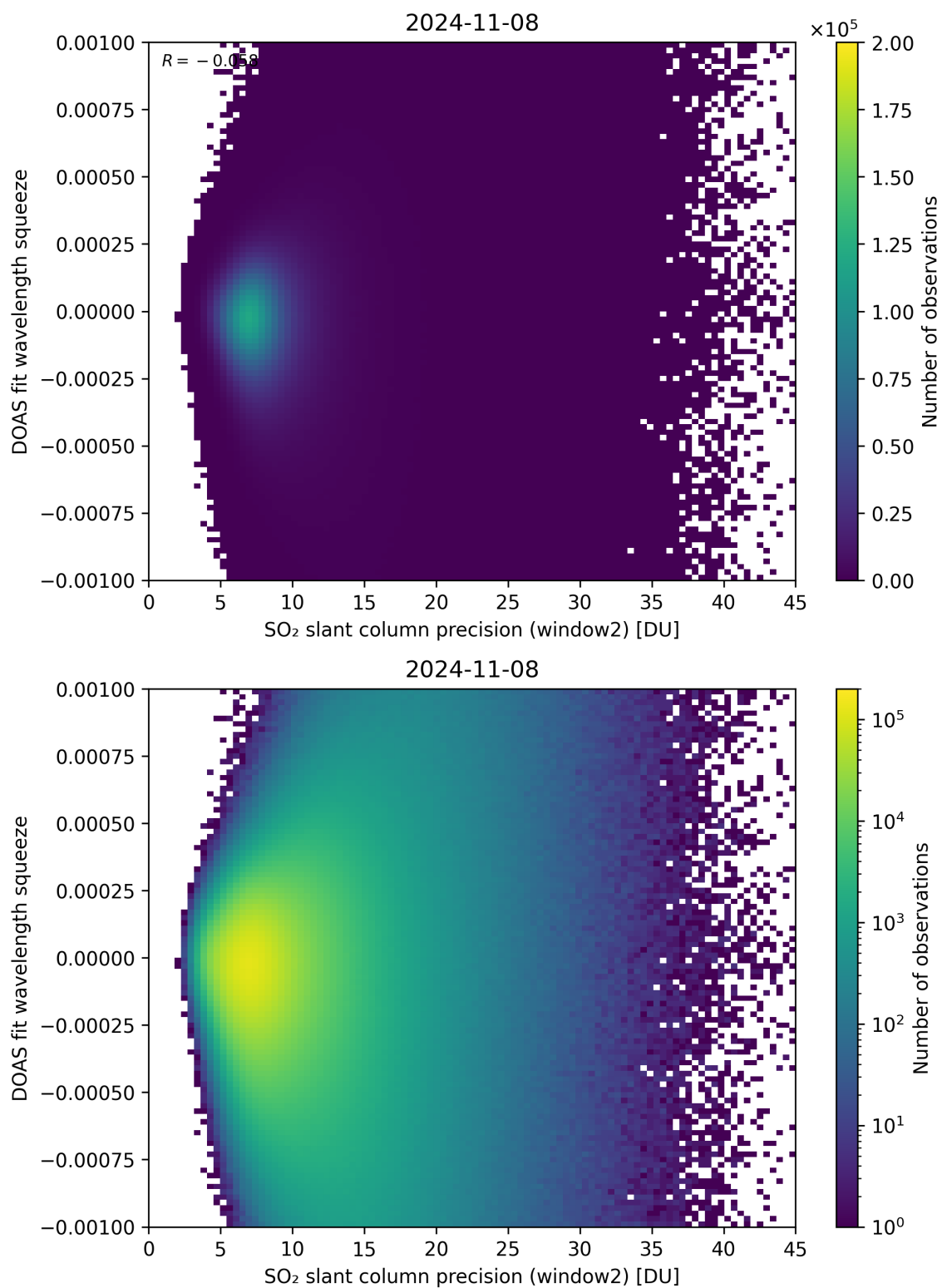
Figure 244: Scatter density plot of “SO 2 slant column precision (window2)” against “DOAS fit wavelength squeeze” for 2024-11-07 to 2024-11-09.
