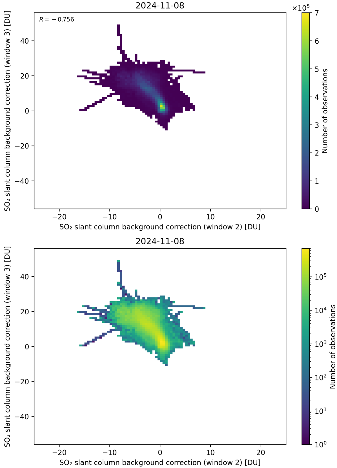
Figure 111: Scatter density plot of “SO 2 slant column background correction (window 2)” against “SO 2 slant column background correction (window 3)” for 2024-11-07 to 2024-11-09.
