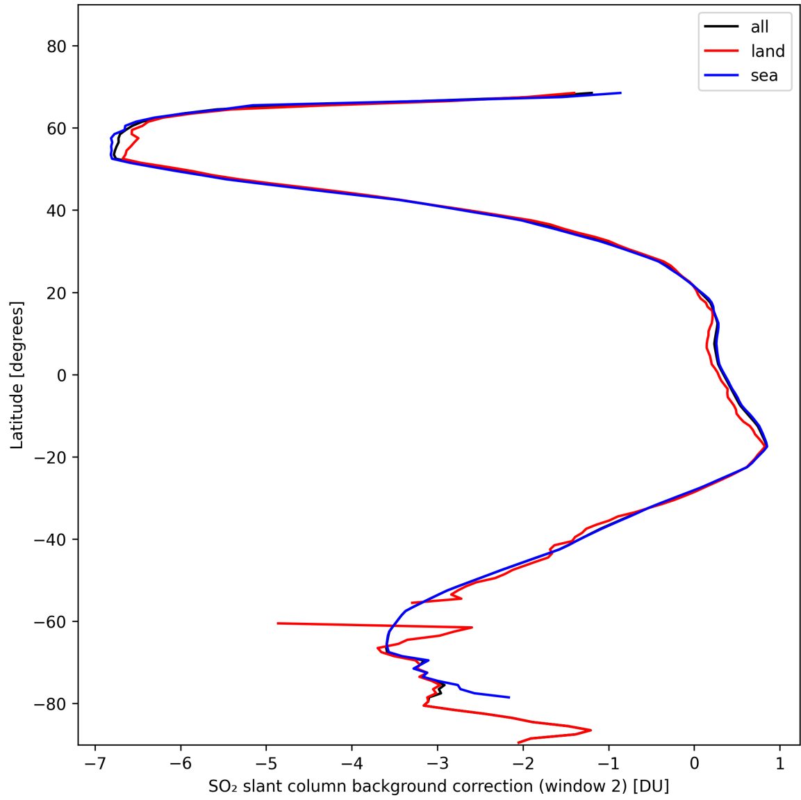
Figure 40: Zonal average of “SO 2 slant column background correction (window 2)” for 2024-11-07 to 2024-11-09.
