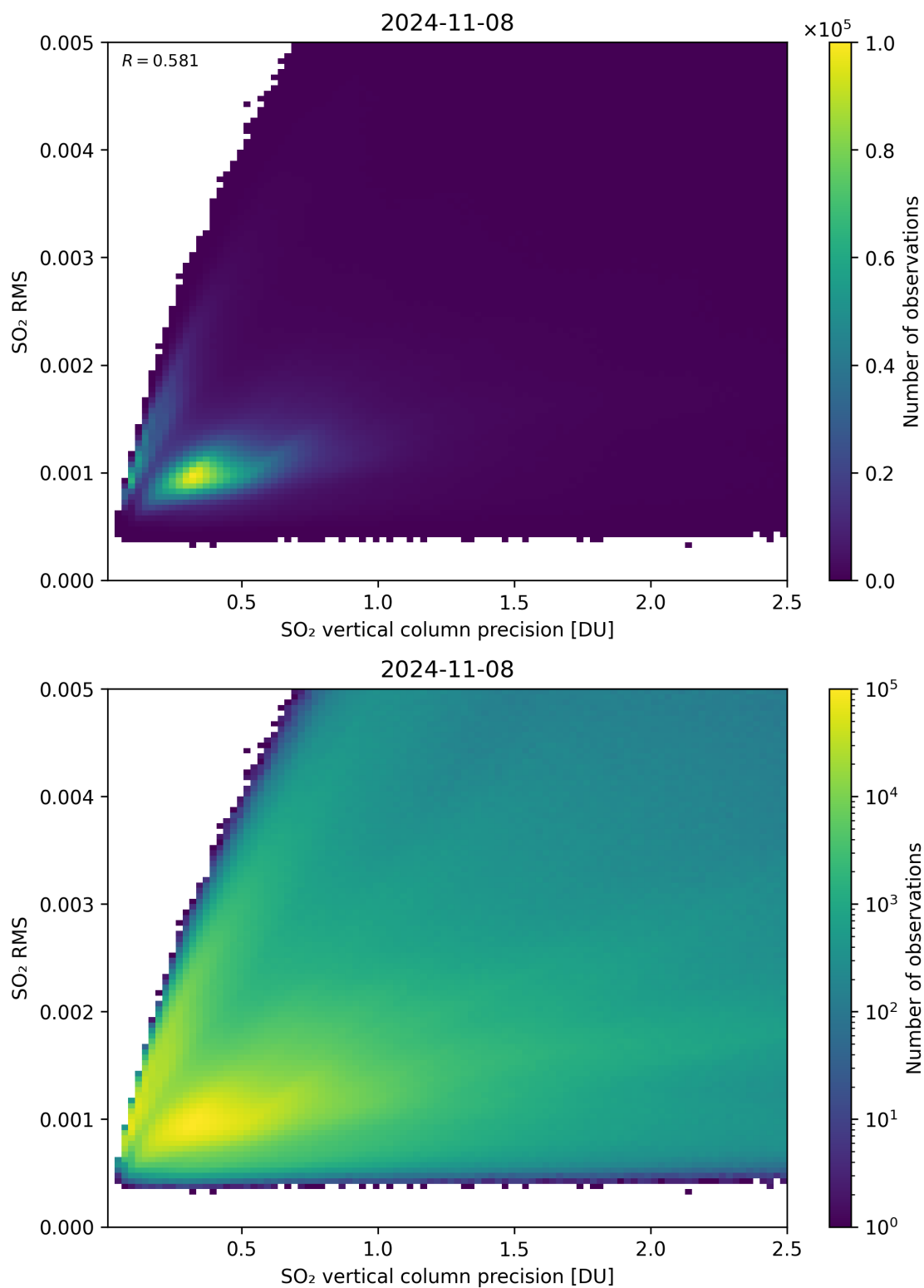
Figure 284: Scatter density plot of “SO 2 vertical column precision” against “SO 2 RMS” for 2024-11-07 to 2024-11-09.
