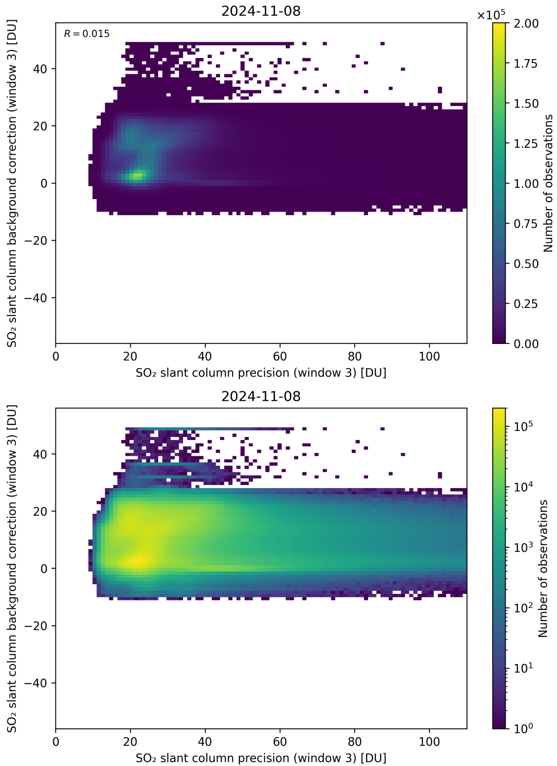
Figure 257: Scatter density plot of “SO 2 slant column precision (window 3)” against “SO 2 slant column background correction (window 3)” for 2024-11-07 to 2024-11-09.
