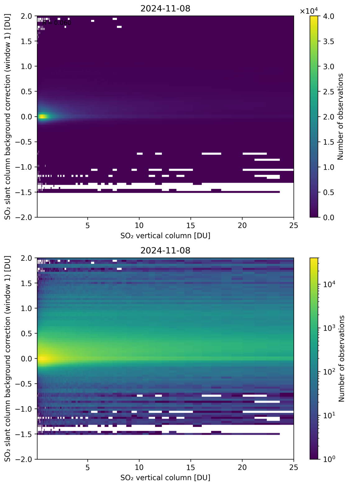
Figure 273: Scatter density plot of “SO 2 vertical column” against “SO 2 slant column background correction (window 1)” for 2024-11-07 to 2024-11-09.
