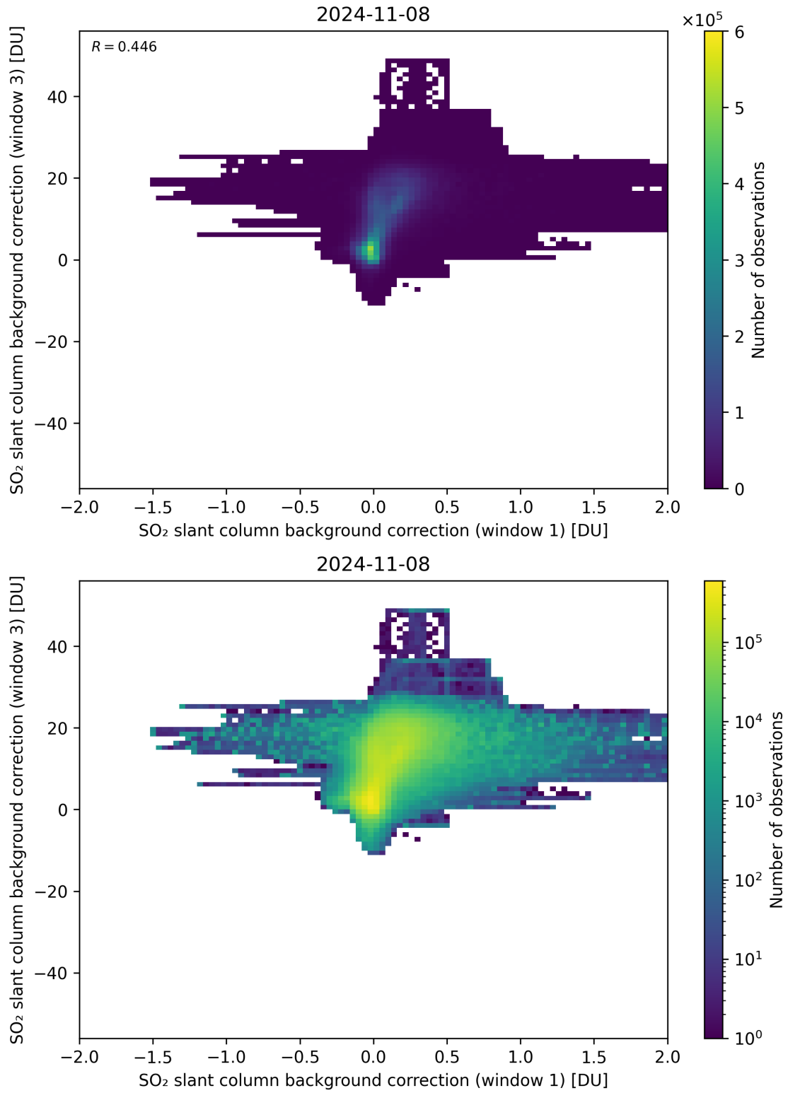
Figure 99: Scatter density plot of “SO 2 slant column background correction (window 1)” against “SO 2 slant column background correction (window 3)” for 2024-11-07 to 2024-11-09.
