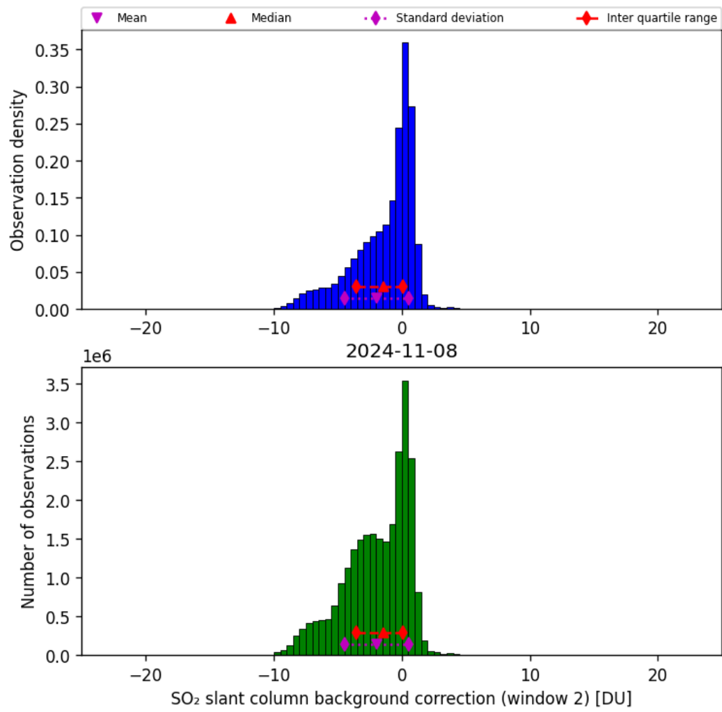
Figure 63: Histogram of “SO 2 slant column background correction (window 2)” for 2024-11-07 to 2024-11-09
