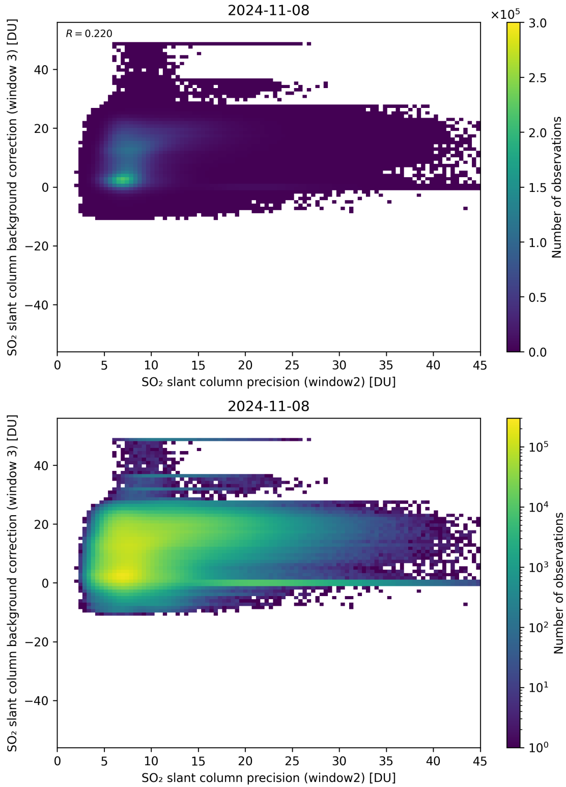
Figure 242: Scatter density plot of “SO 2 slant column precision (window2)” against “SO 2 slant column background correction (window 3)” for 2024-11-07 to 2024-11-09.
