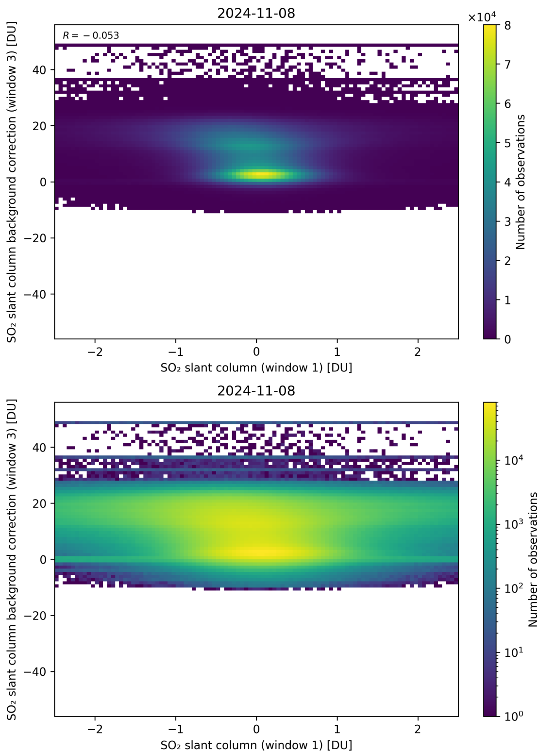
Figure 214: Scatter density plot of “SO 2 slant column (window 1)” against “SO 2 slant column background correction (window 3)” for 2024-11-07 to 2024-11-09.
