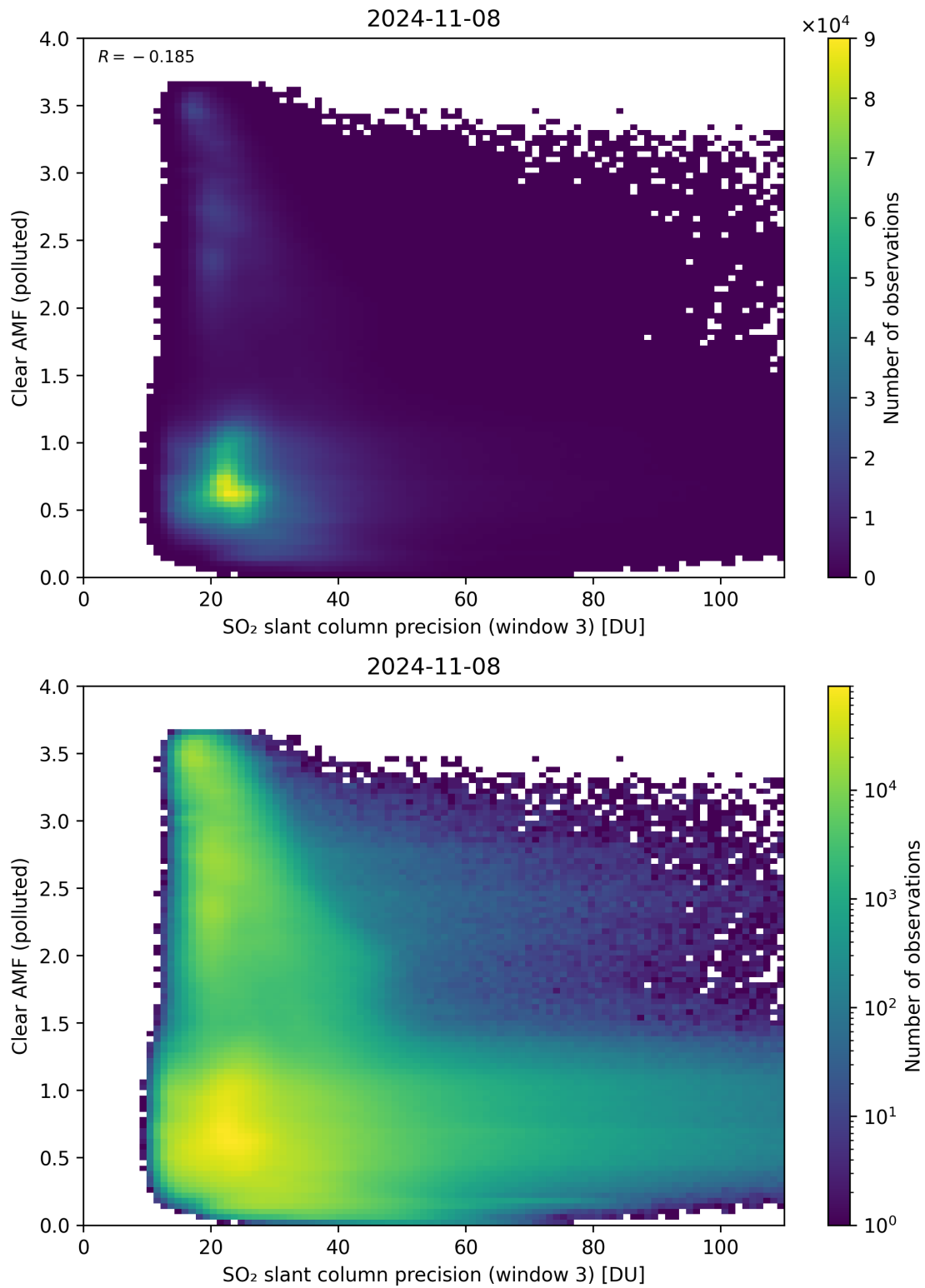
Figure 261: Scatter density plot of “SO 2 slant column precision (window 3)” against “Clear AMF (polluted)” for 2024-11-07 to 2024-11-09.
