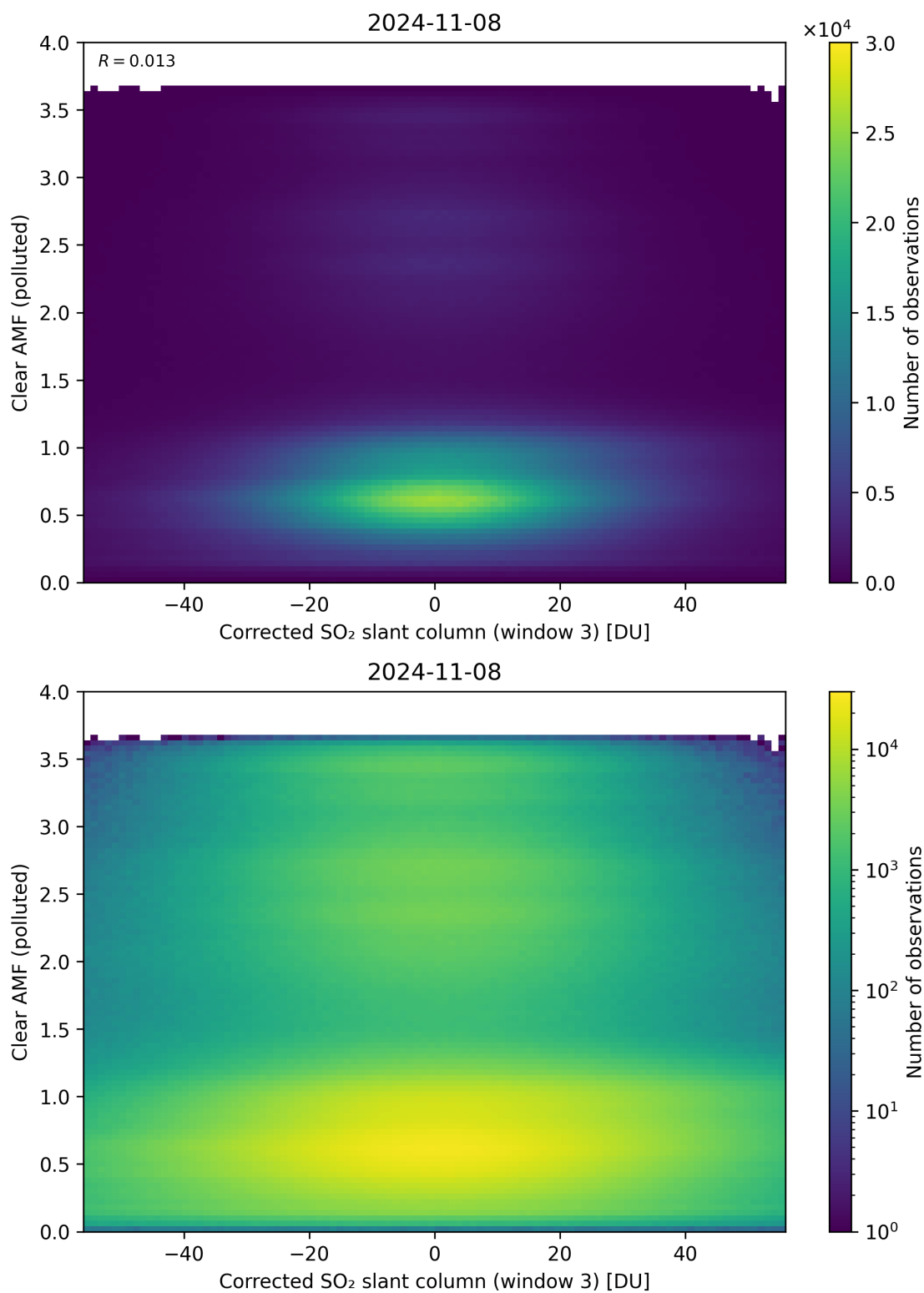
Figure 209: Scatter density plot of “Corrected SO 2 slant column (window 3)” against “Clear AMF (polluted)” for 2024-11-07 to 2024-11-09.
