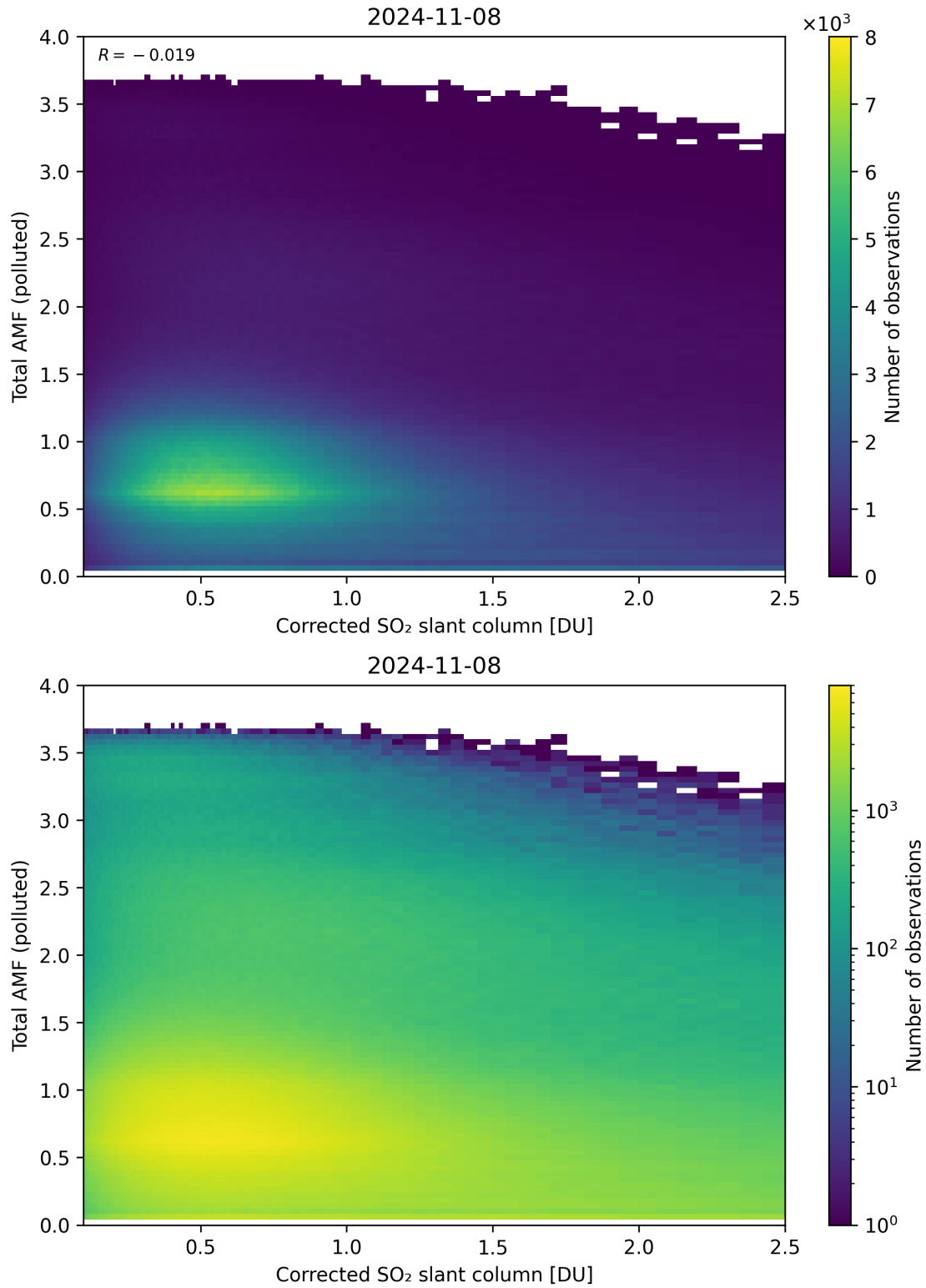
Figure 192: Scatter density plot of “Corrected SO 2 slant column” against “Total AMF (polluted)” for 2024-11-07 to 2024-11-09.
