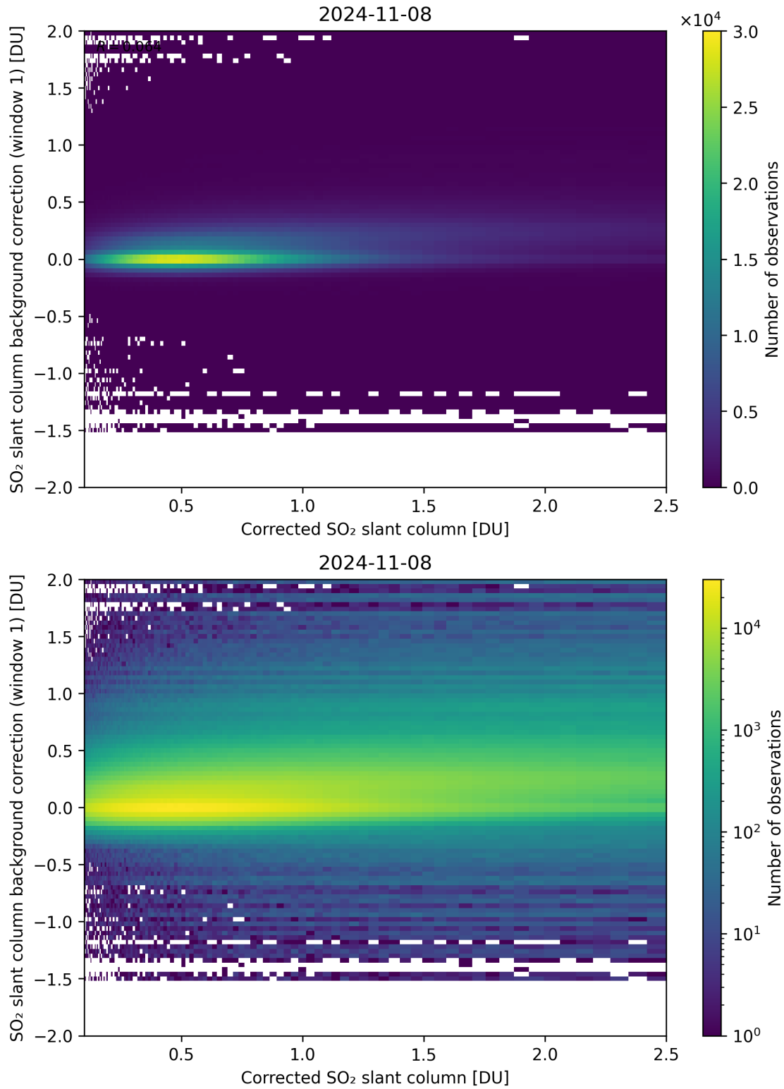
Figure 178: Scatter density plot of “Corrected SO 2 slant column” against “SO 2 slant column background correction (window 1)” for 2024-11-07 to 2024-11-09.
