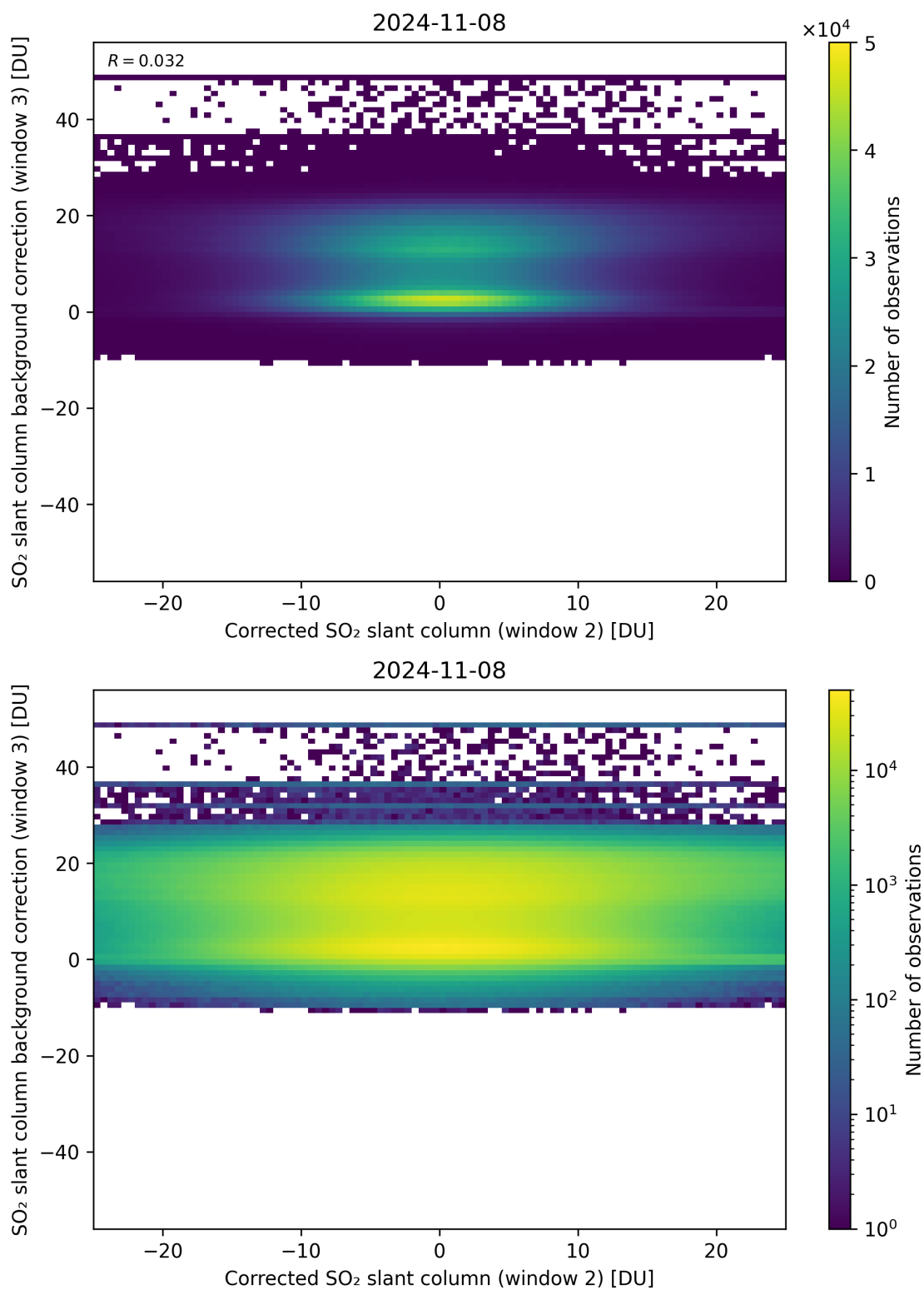
Figure 195: Scatter density plot of “Corrected SO 2 slant column (window 2)” against “SO 2 slant column background correction (window 3)” for 2024-11-07 to 2024-11-09.
