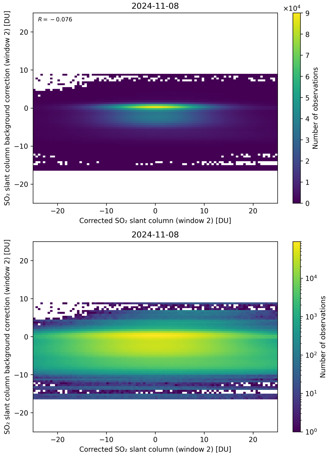
Figure 194: Scatter density plot of “Corrected SO 2 slant column (window 2)” against “SO 2 slant column background correction (window 2)” for 2024-11-07 to 2024-11-09.
