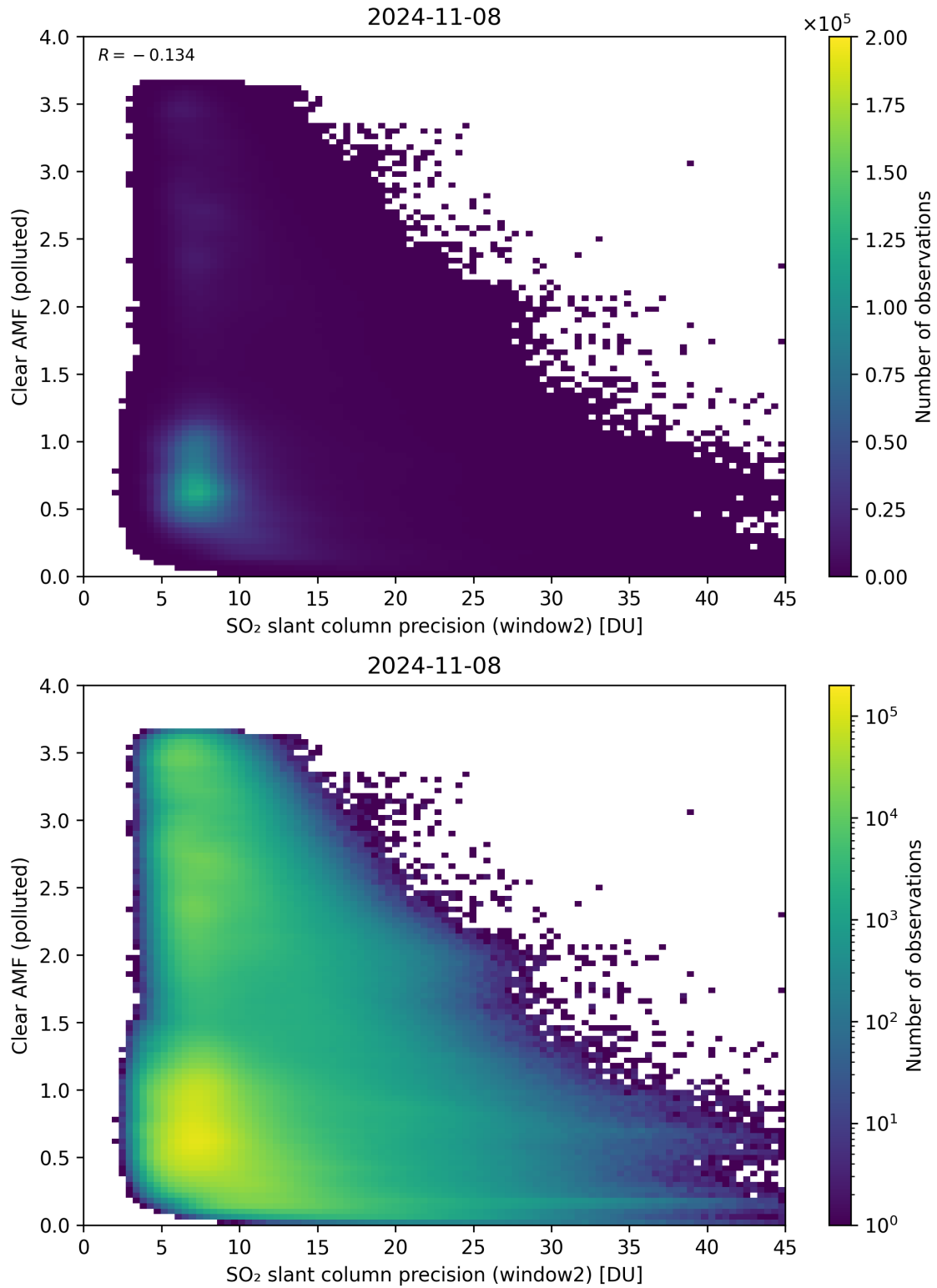
Figure 246: Scatter density plot of “SO 2 slant column precision (window2)” against “Clear AMF (polluted)” for 2024-11-07 to 2024-11-09.
