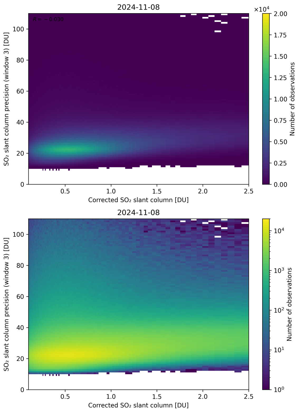
Figure 191: Scatter density plot of “Corrected SO 2 slant column” against “SO 2 slant column precision (window 3)” for 2024-11-07 to 2024-11-09.
