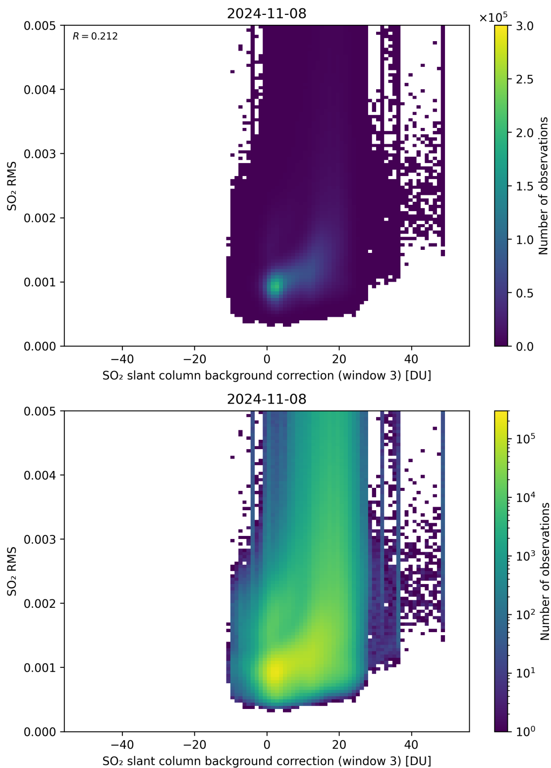
Figure 123: Scatter density plot of “SO 2 slant column background correction (window 3)” against “SO 2 RMS” for 2024-11-07 to 2024-11-09.
