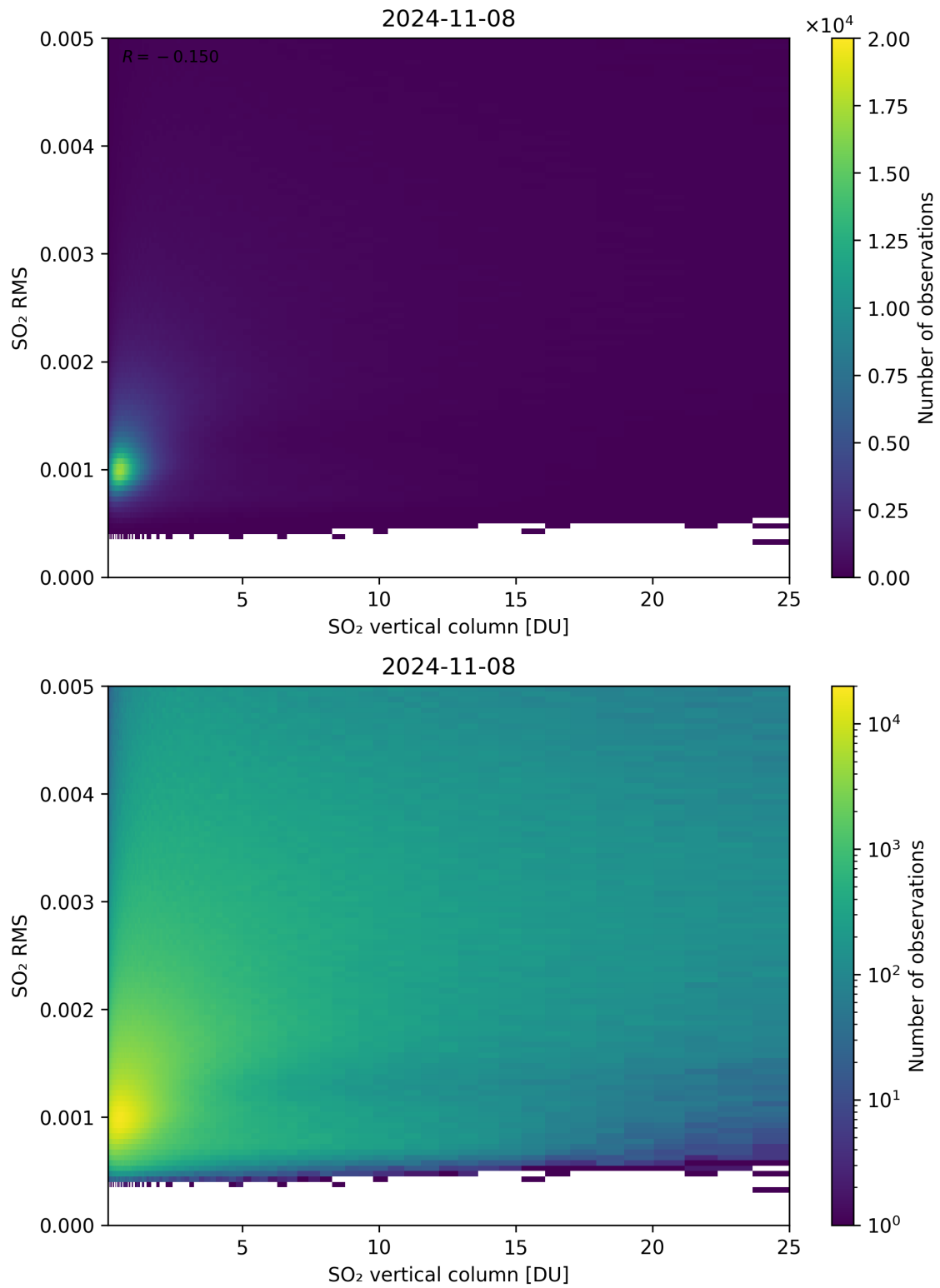
Figure 278: Scatter density plot of “SO 2 vertical column” against “SO 2 RMS” for 2024-11-07 to 2024-11-09.
