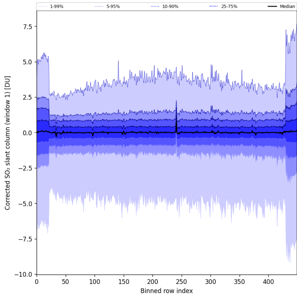
Figure 81: Along track statistics of “Corrected SO 2 slant column (window 1)” for 2024-11-07 to 2024-11-09
