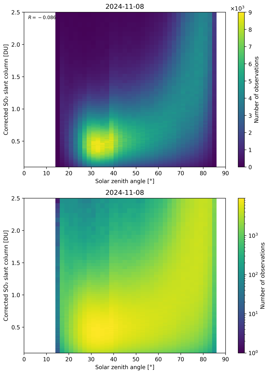
Figure 166: Scatter density plot of “Solar zenith angle” against “Corrected SO 2 slant column” for 2024-11-07 to 2024-11-09.
