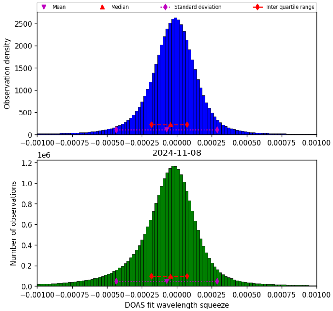
Figure 69: Histogram of “DOAS fit wavelength squeeze” for 2024-11-07 to 2024-11-09
