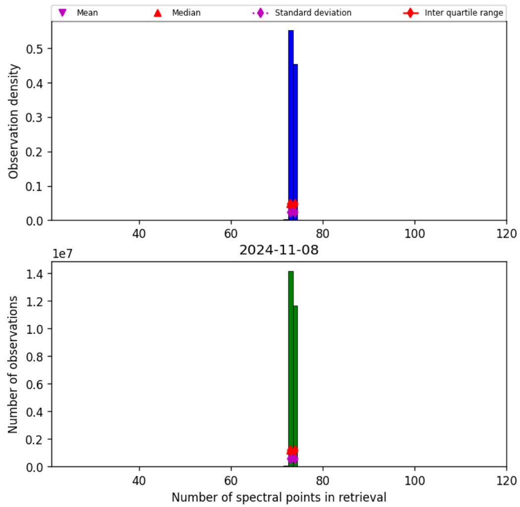
Figure 74: Histogram of “Number of spectral points in retrieval” for 2024-11-07 to 2024-11-09
