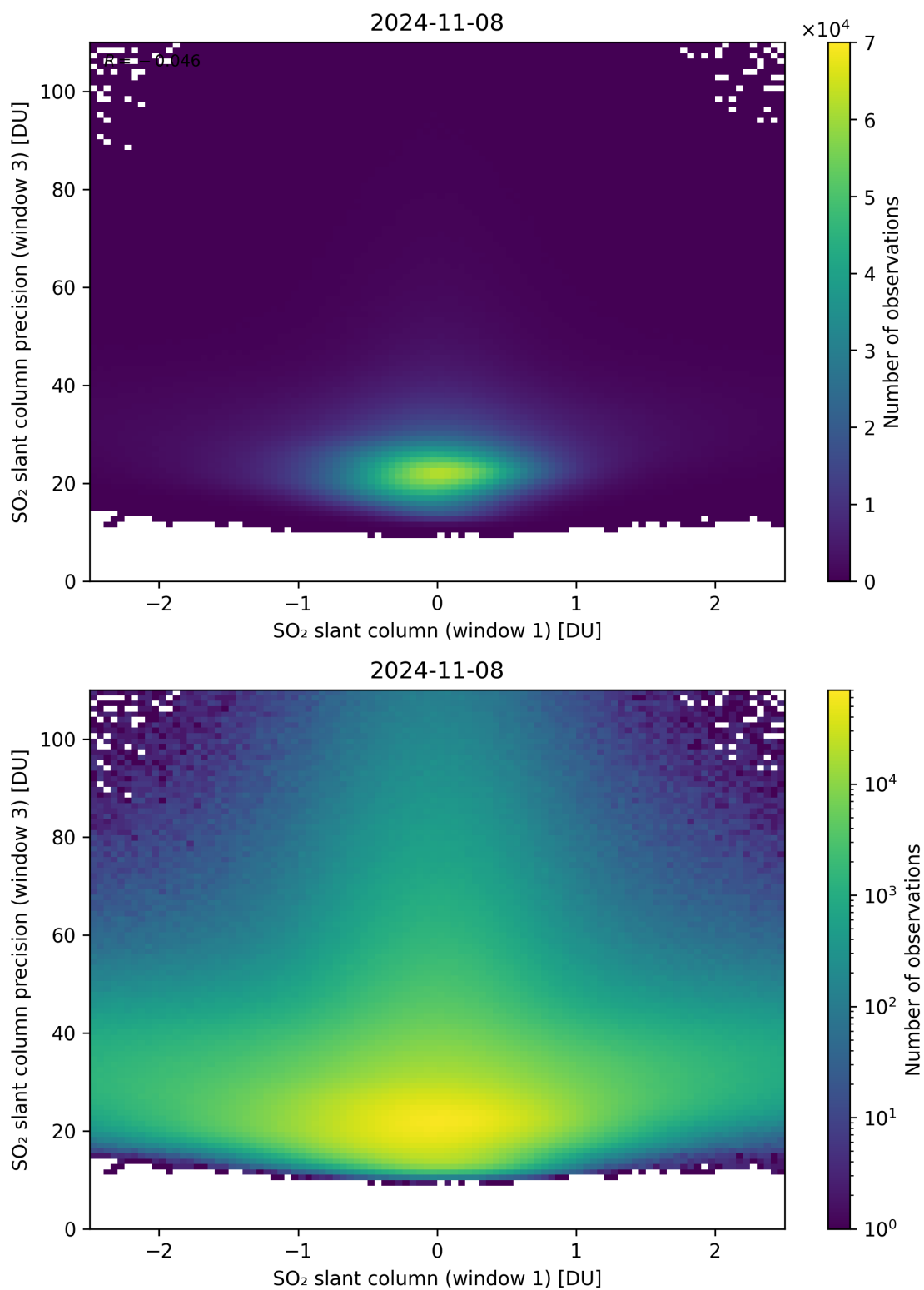
Figure 238: Scatter density plot of “SO 2 slant column (window 1)” against “SO 2 slant column precision (window 3)” for 2024-11-07 to 2024-11-09.
