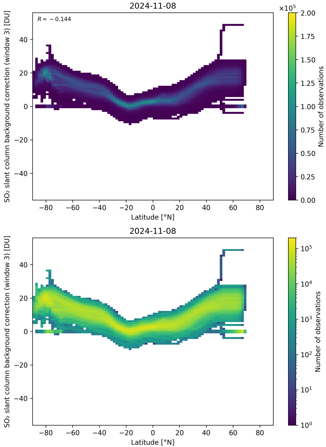
Figure 141: Scatter density plot of “Latitude” against “SO 2 slant column background correction (window 3)” for 2024-11-07 to 2024-11-09.
