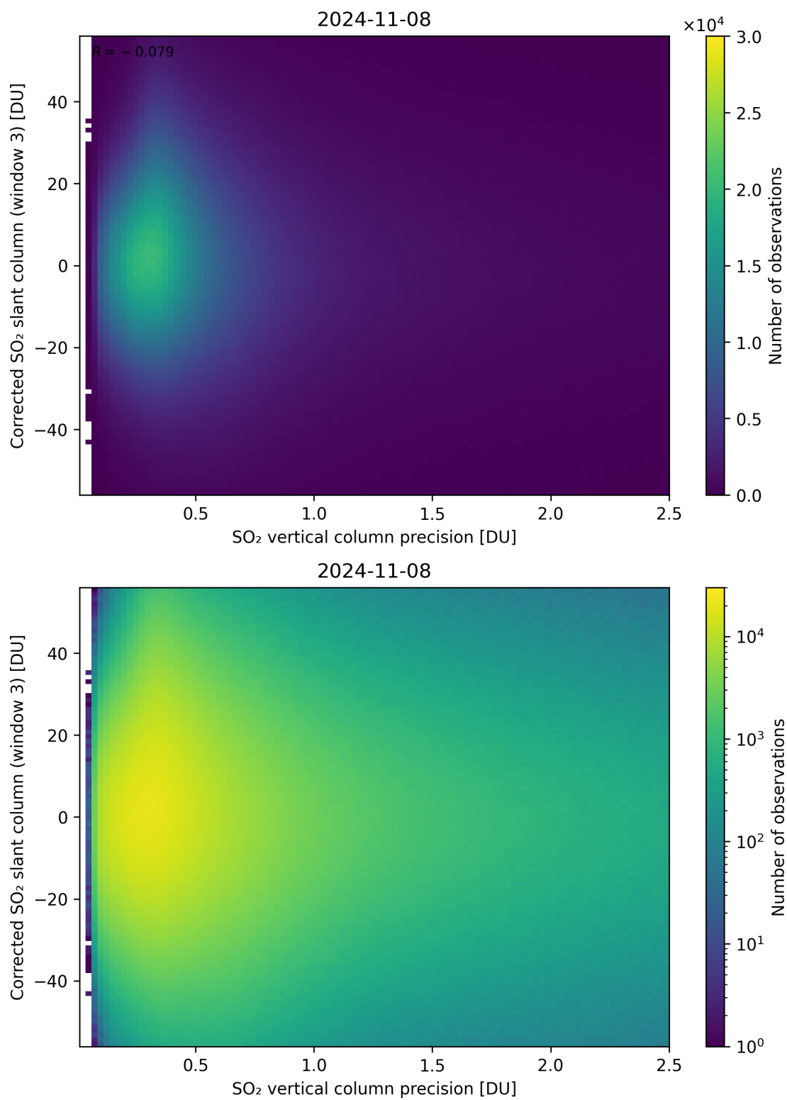
Figure 288: Scatter density plot of “SO 2 vertical column precision” against “Corrected SO 2 slant column (window 3)” for 2024-11-07 to 2024-11-09.
