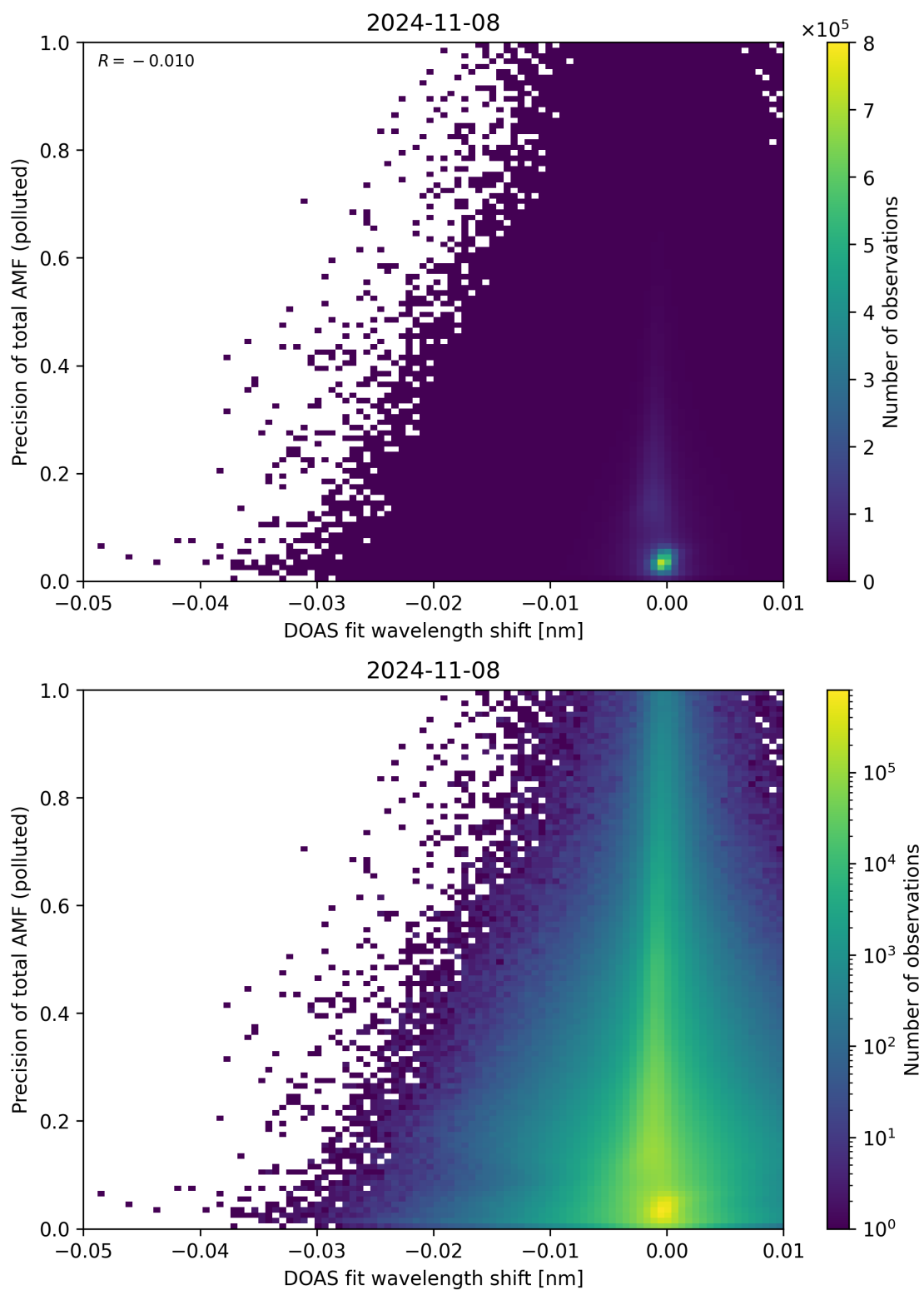
Figure 131: Scatter density plot of “DOAS fit wavelength shift” against “Precision of total AMF (polluted)” for 2024-11-07 to 2024-11-09.
