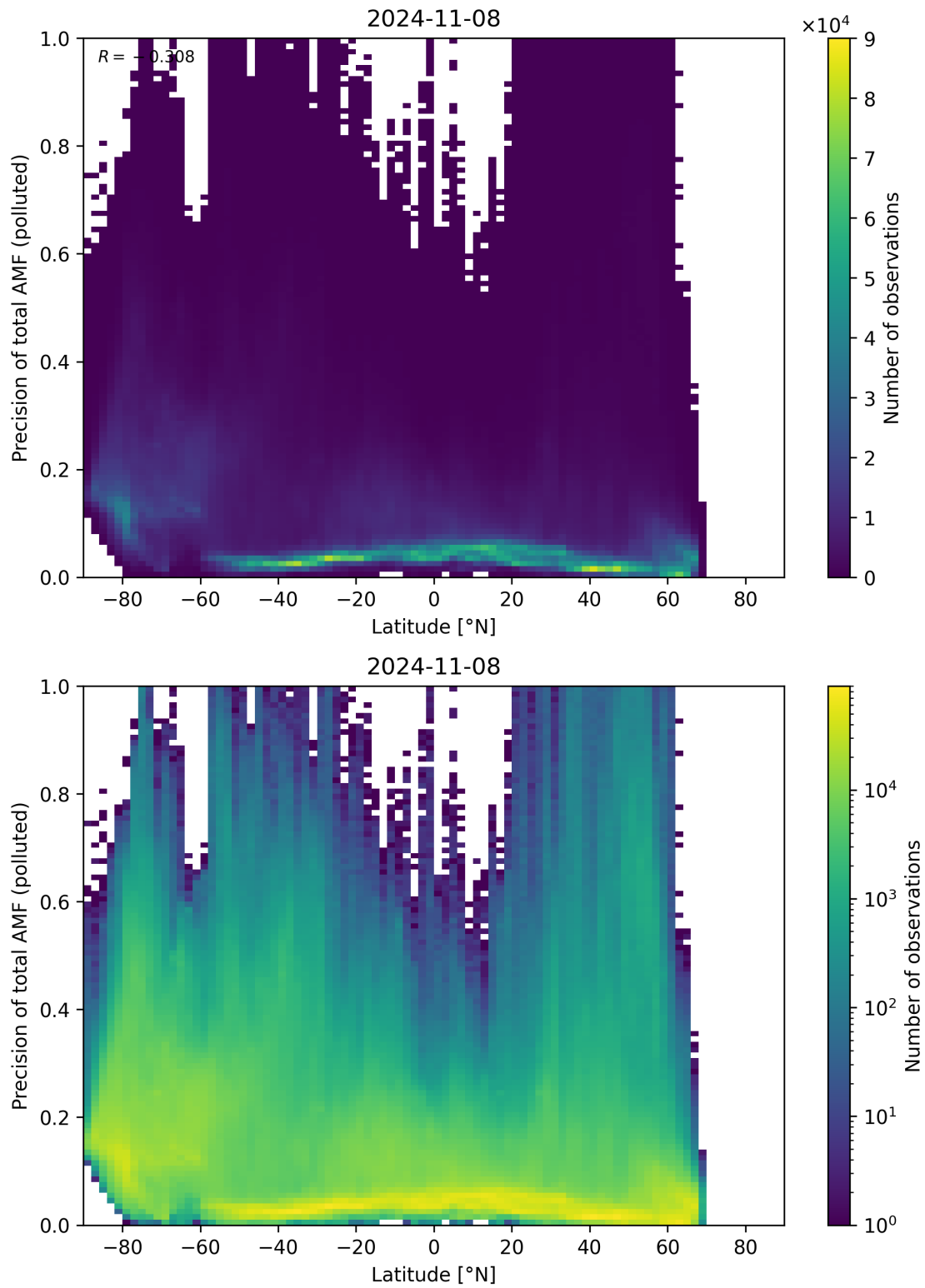
Figure 155: Scatter density plot of “Latitude” against “Precision of total AMF (polluted)” for 2024-11-07 to 2024-11-09.
