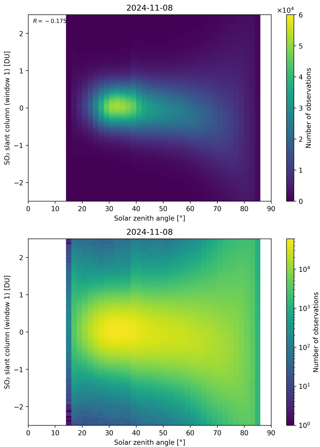
Figure 169: Scatter density plot of “Solar zenith angle” against “SO 2 slant column (window 1)” for 2024-11-07 to 2024-11-09.
