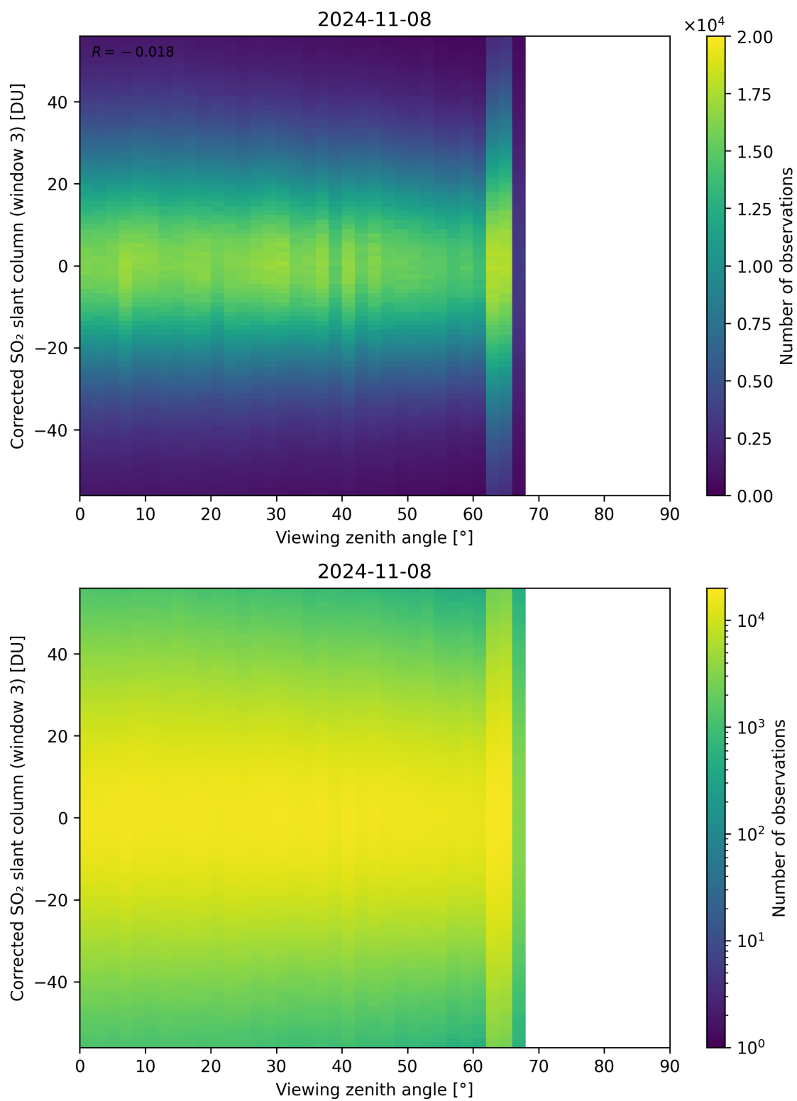
Figure 319: Scatter density plot of “Viewing zenith angle” against “Corrected SO 2 slant column (window 3)” for 2024-11-07 to 2024-11-09.
