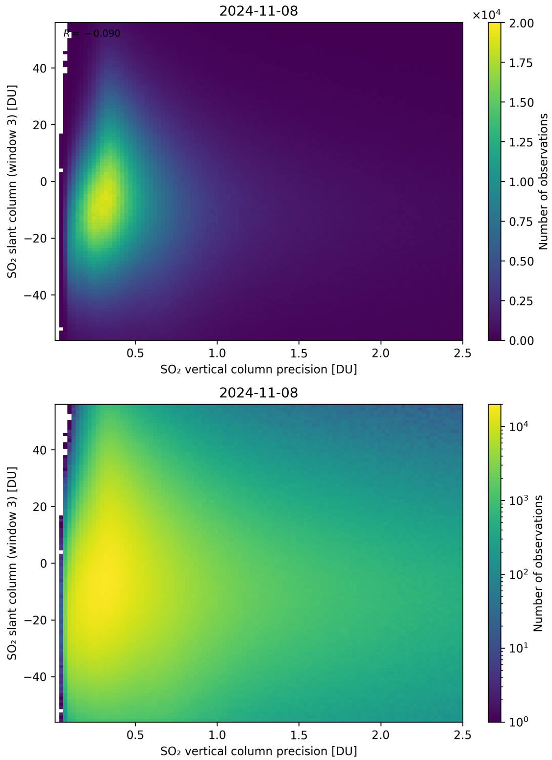
Figure 292: Scatter density plot of “SO 2 vertical column precision” against “SO 2 slant column (window 3)” for 2024-11-07 to 2024-11-09.
