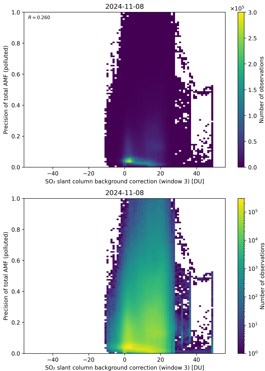
Figure 126: Scatter density plot of “SO 2 slant column background correction (window 3)” against “Precision of total AMF (polluted)” for 2024-11-07 to 2024-11-09.
