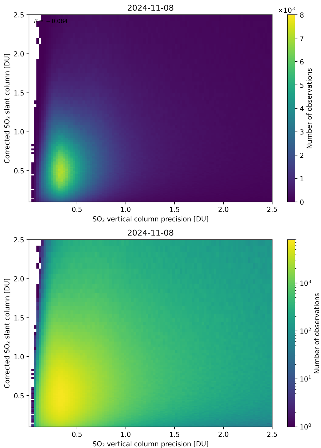
Figure 286: Scatter density plot of “SO 2 vertical column precision” against “Corrected SO 2 slant column” for 2024-11-07 to 2024-11-09.
