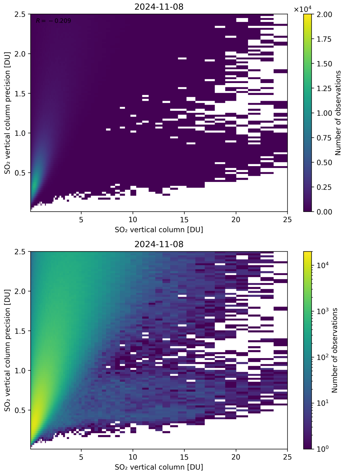
Figure 307: Scatter density plot of “SO 2 vertical column” against “SO 2 vertical column precision” for 2024-11-07 to 2024-11-09.
