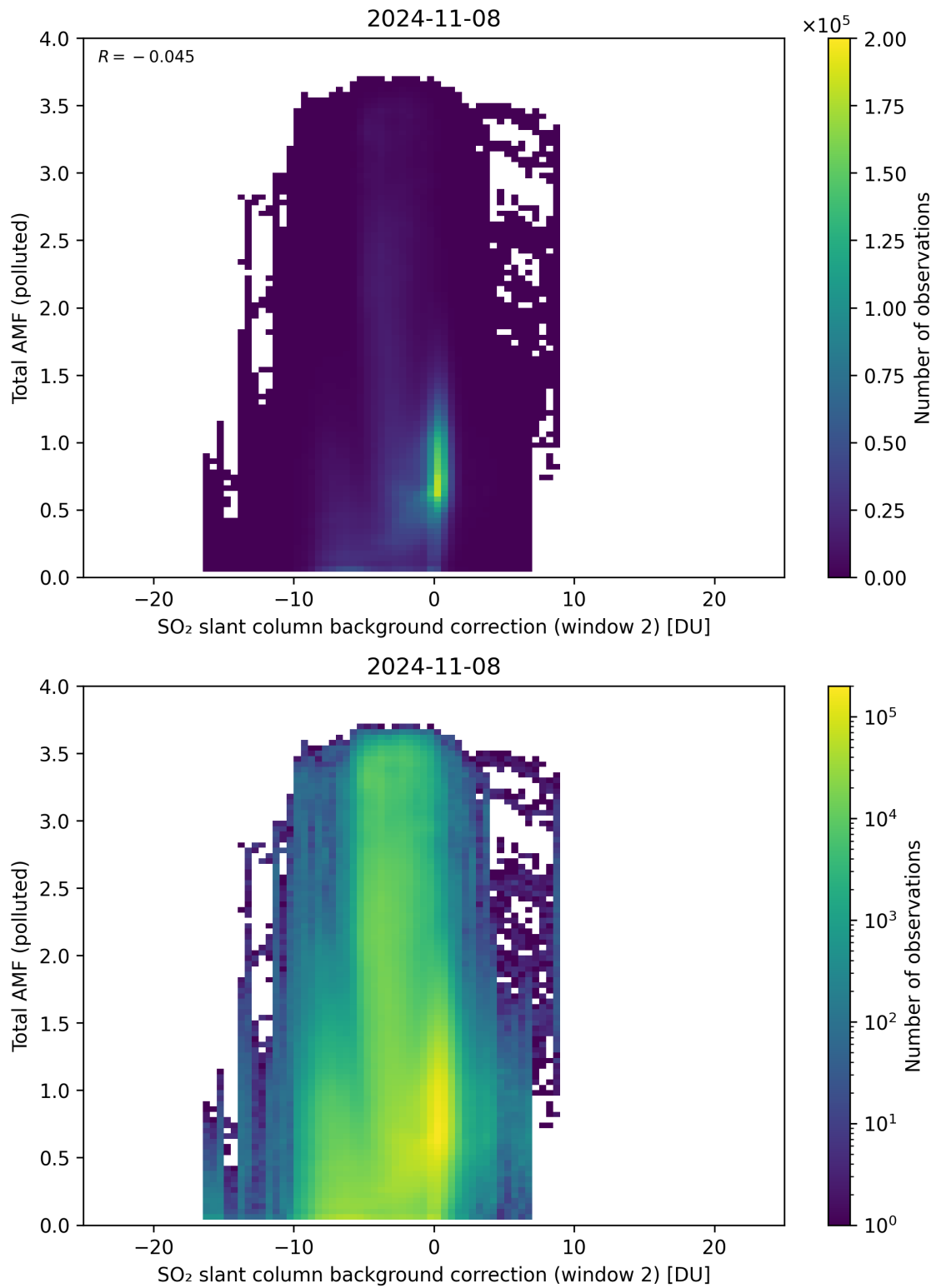
Figure 119: Scatter density plot of “SO 2 slant column background correction (window 2)” against “Total AMF (polluted)” for 2024-11-07 to 2024-11-09.
