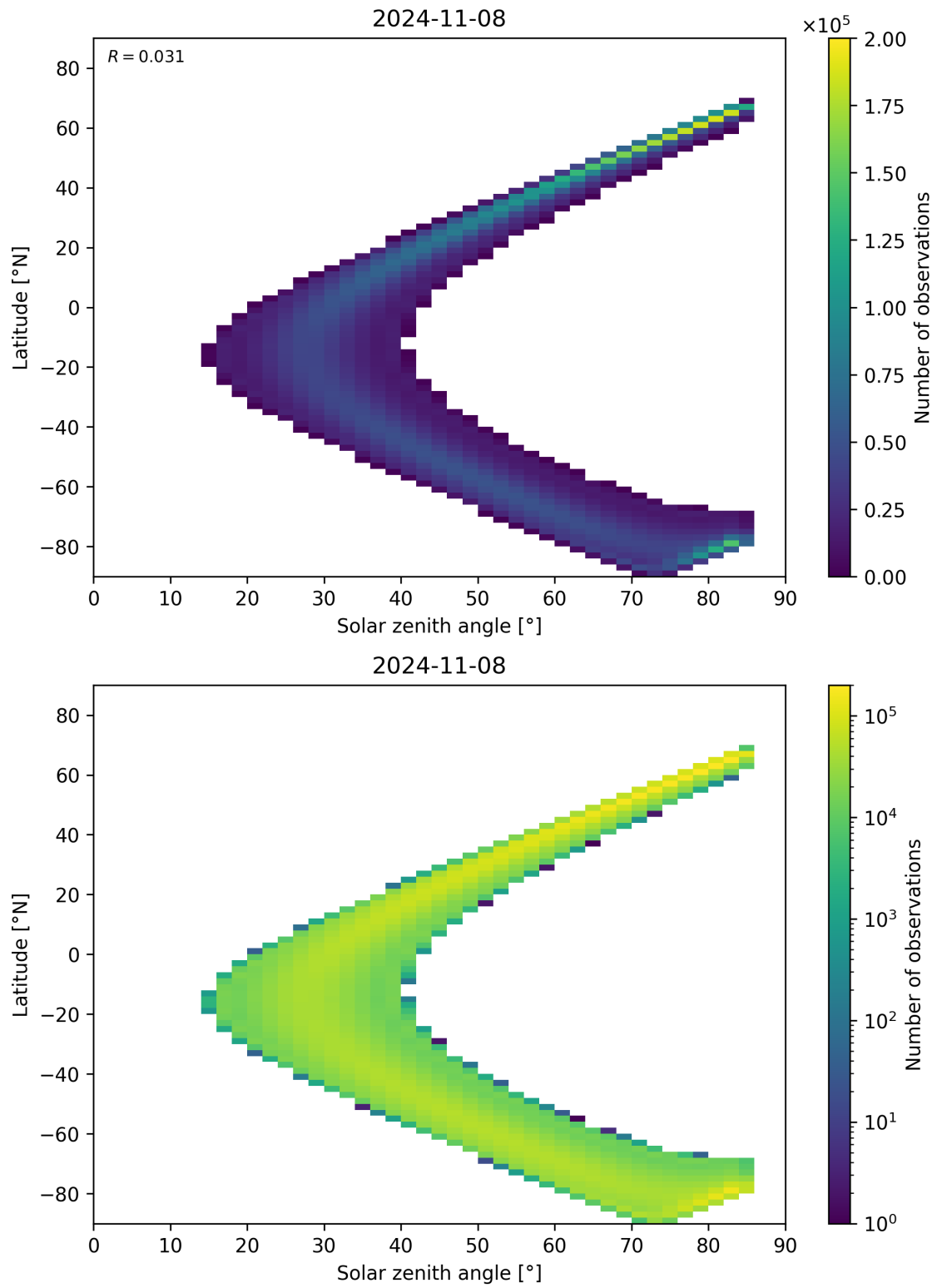
Figure 164: Scatter density plot of “Solar zenith angle” against “Latitude” for 2024-11-07 to 2024-11-09.
