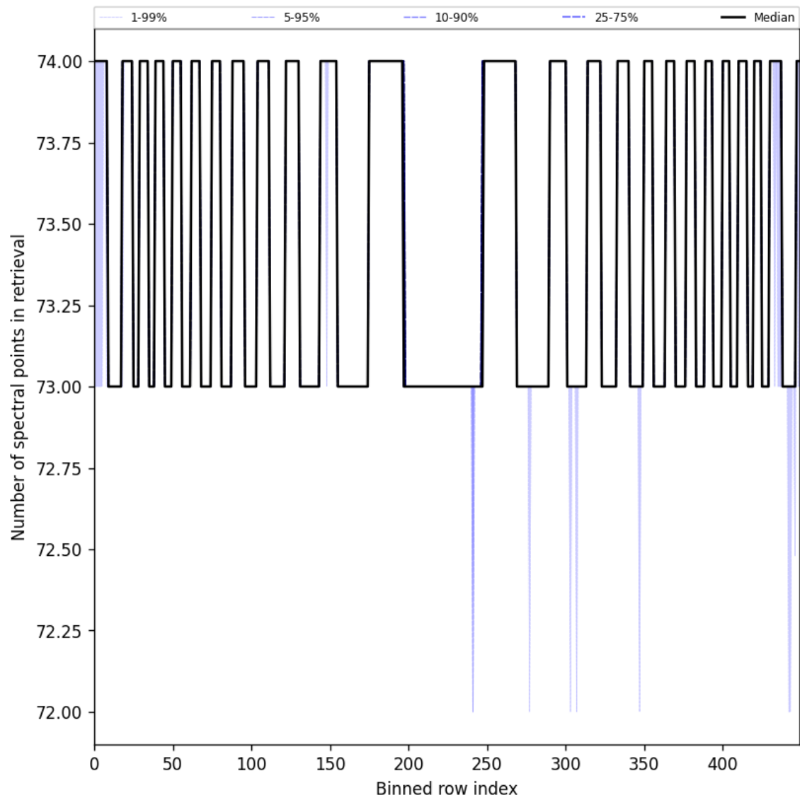
Figure 97: Along track statistics of “Number of spectral points in retrieval” for 2024-11-07 to 2024-11-09
