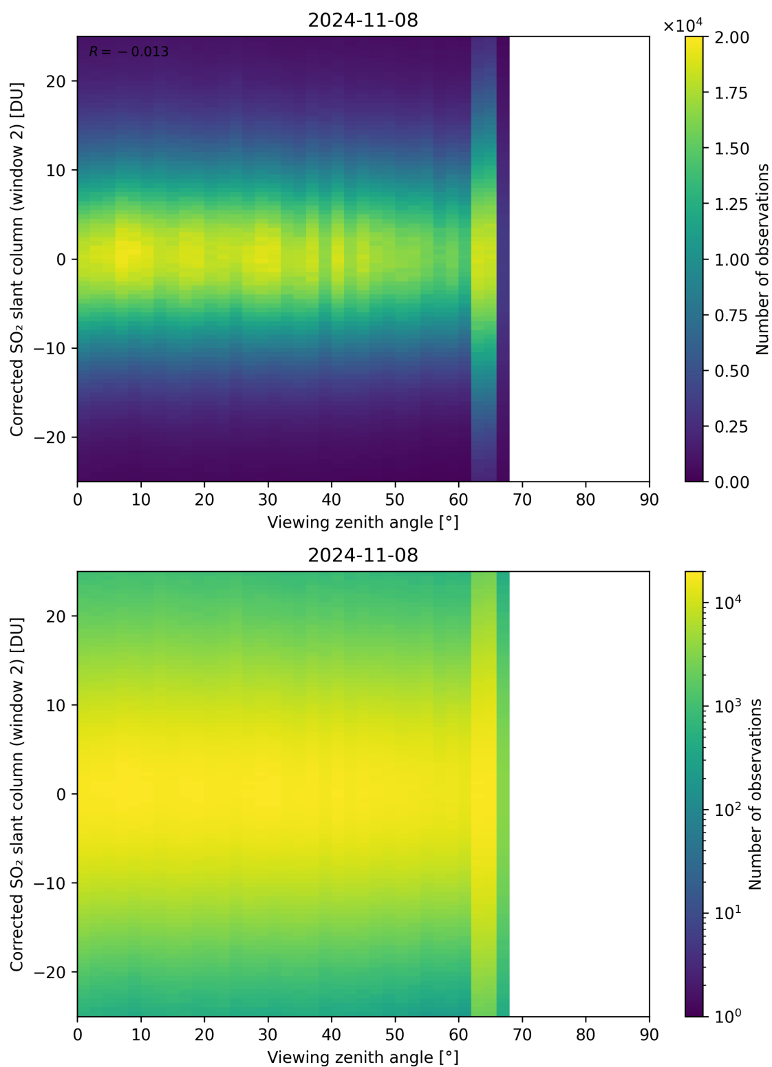
Figure 318: Scatter density plot of “Viewing zenith angle” against “Corrected SO 2 slant column (window 2)” for 2024-11-07 to 2024-11-09.
