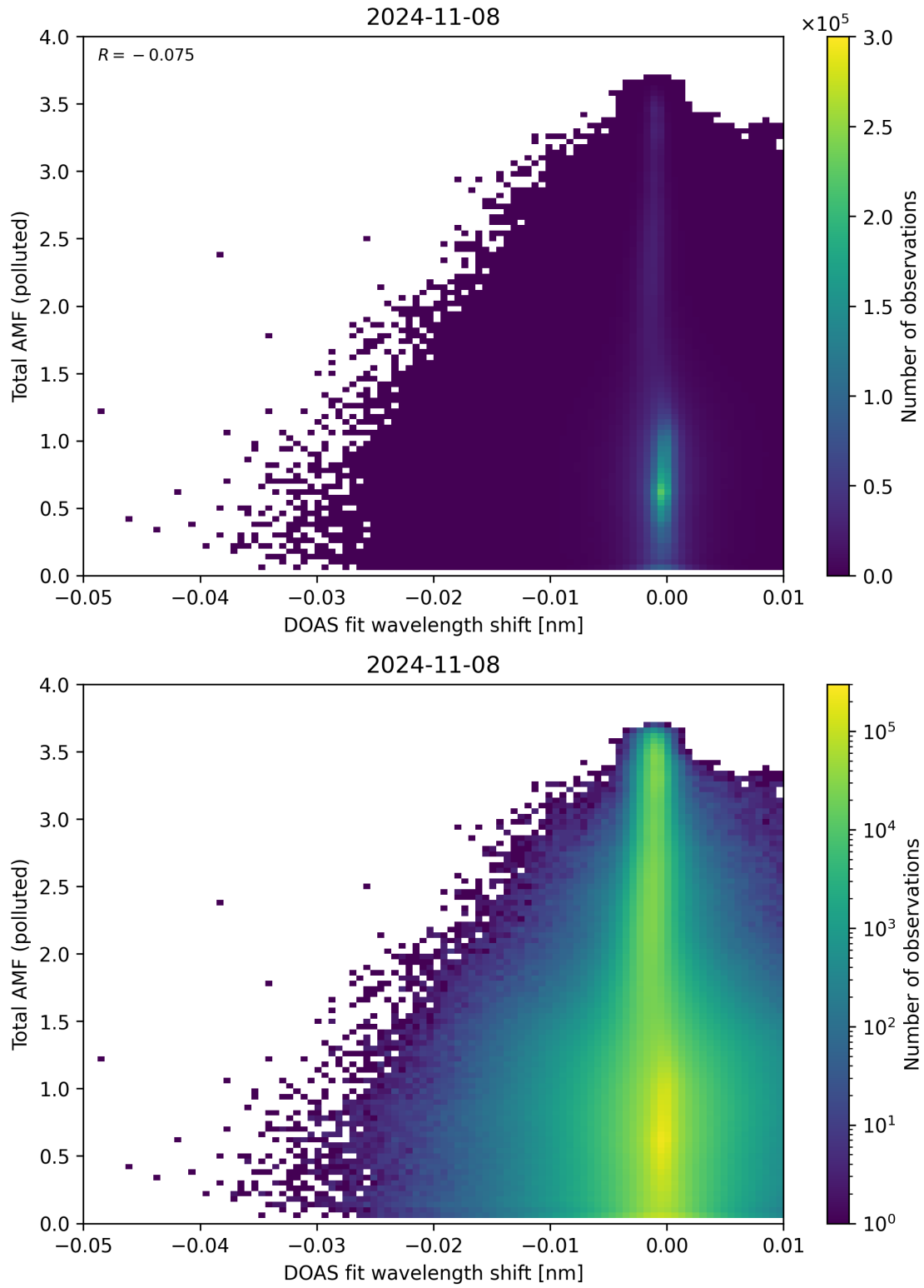
Figure 130: Scatter density plot of “DOAS fit wavelength shift” against “Total AMF (polluted)” for 2024-11-07 to 2024-11-09.
