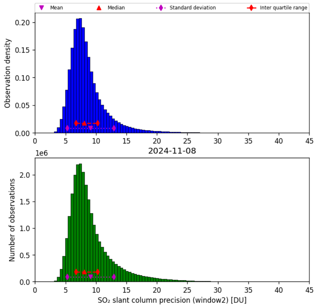
Figure 61: Histogram of “SO 2 slant column precision (window2)” for 2024-11-07 to 2024-11-09
