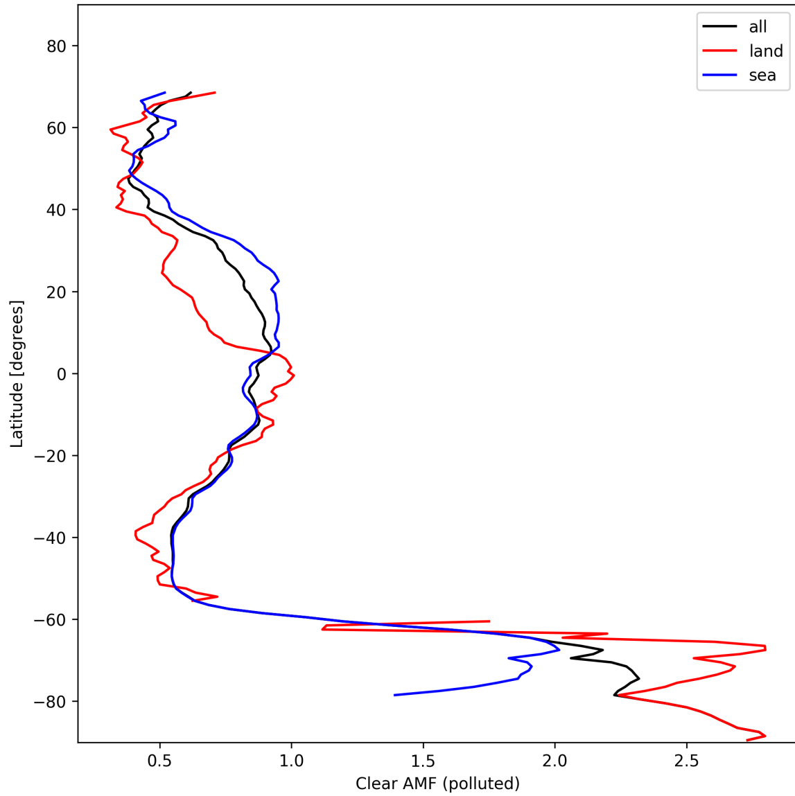
Figure 50: Zonal average of “Clear AMF (polluted)” for 2024-11-07 to 2024-11-09.
