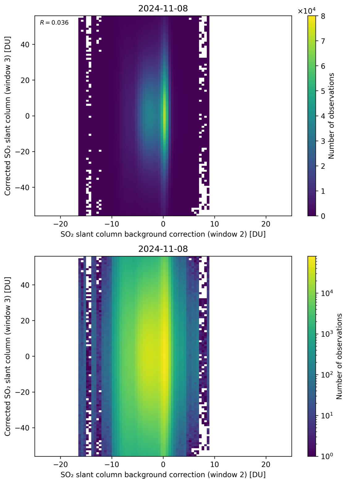
Figure 116: Scatter density plot of “SO 2 slant column background correction (window 2)” against “Corrected SO 2 slant column (window 3)” for 2024-11-07 to 2024-11-09.
