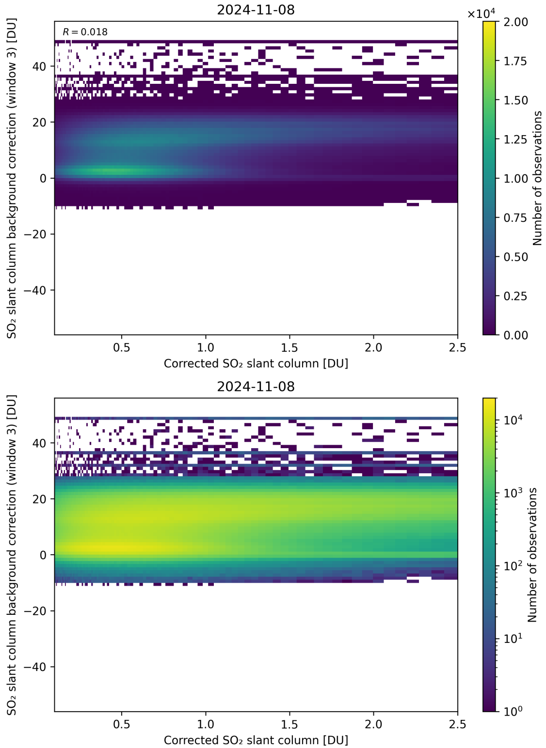
Figure 180: Scatter density plot of “Corrected SO 2 slant column” against “SO 2 slant column background correction (window 3)” for 2024-11-07 to 2024-11-09.
