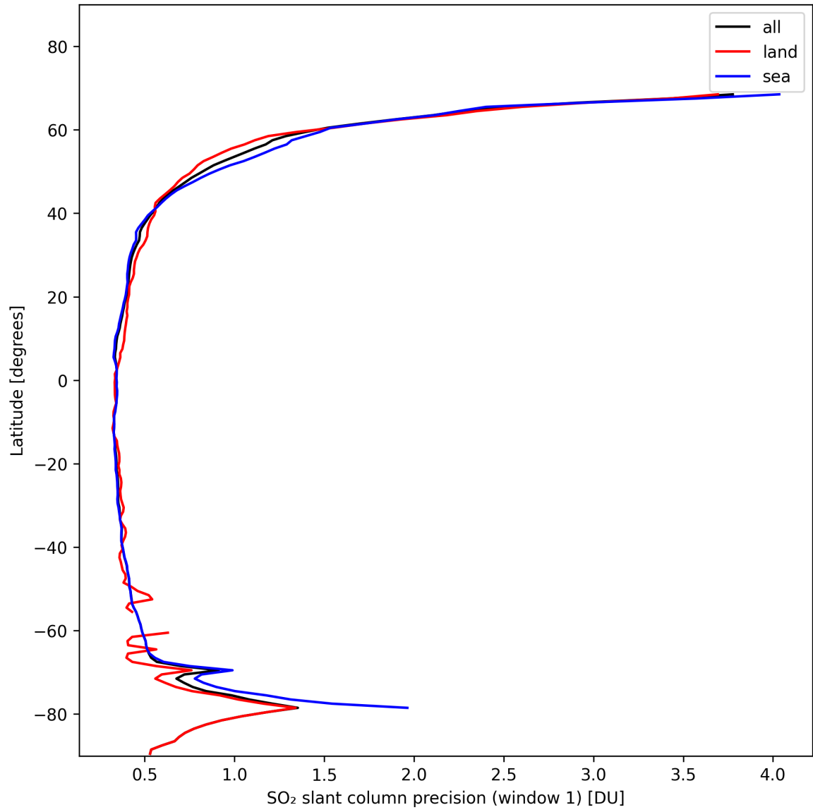
Figure 34: Zonal average of “SO 2 slant column precision (window 1)” for 2024-11-07 to 2024-11-09.
