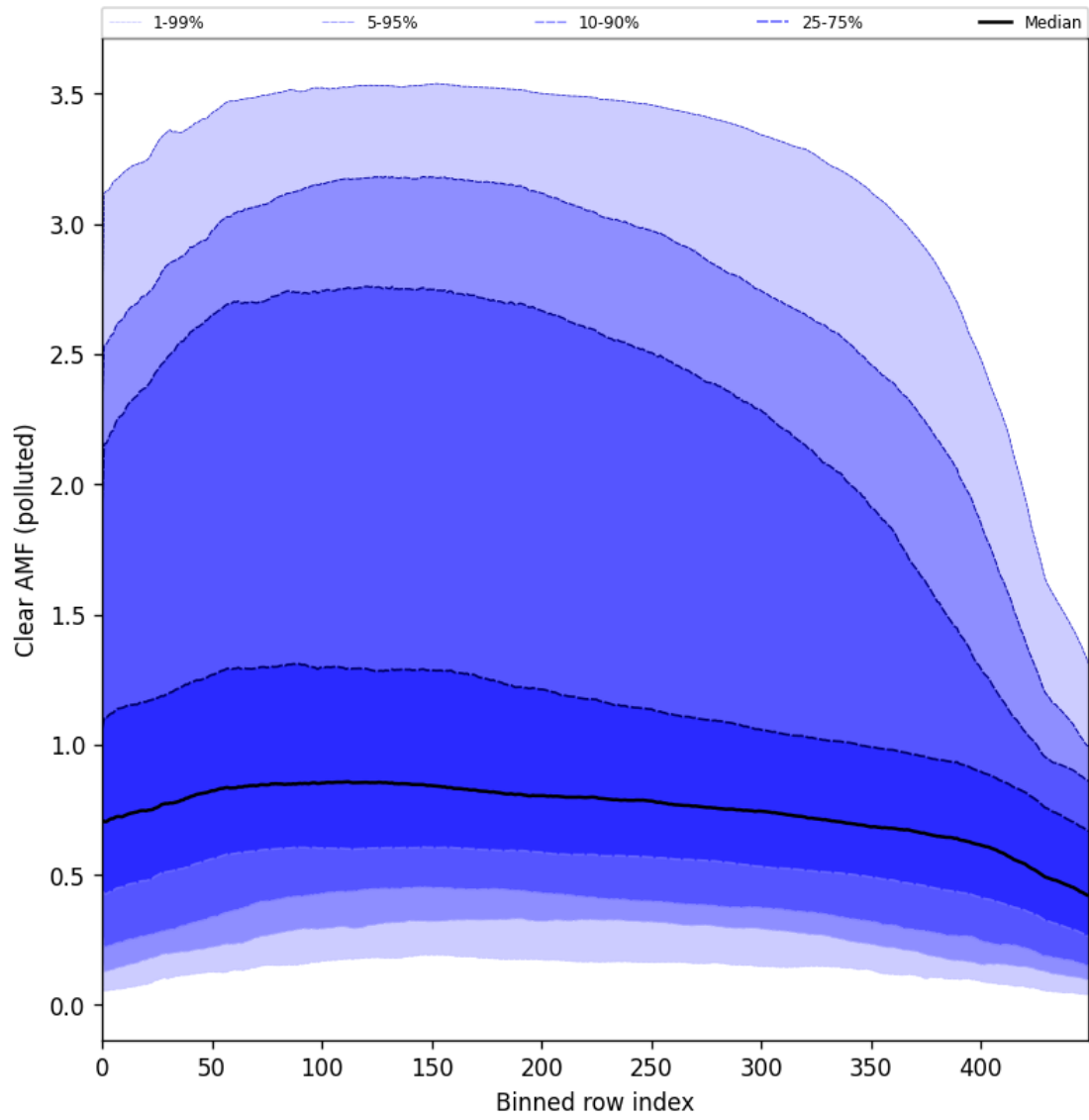
Figure 96: Along track statistics of “Clear AMF (polluted)” for 2024-11-07 to 2024-11-09
