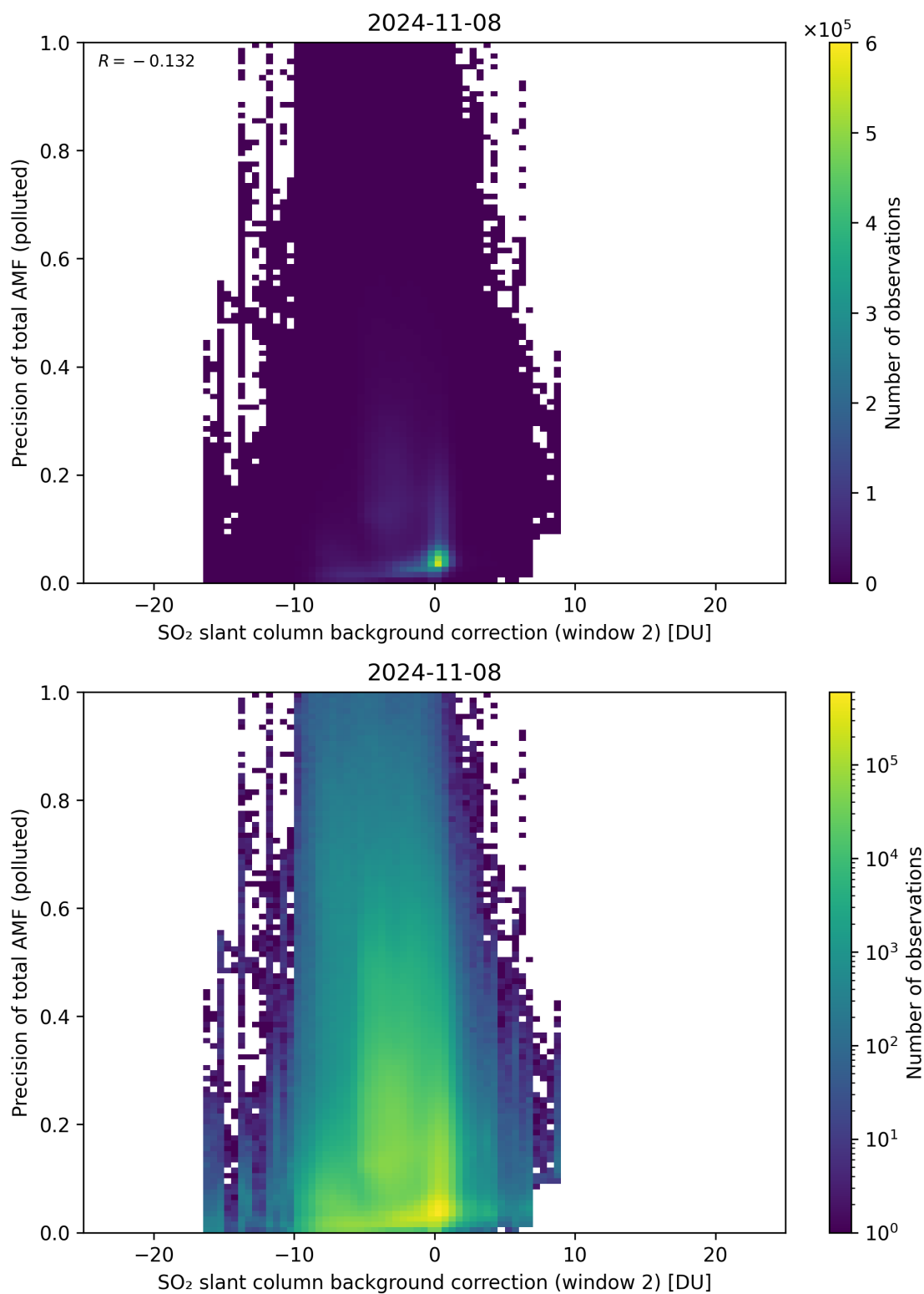
Figure 120: Scatter density plot of “SO 2 slant column background correction (window 2)” against “Precision of total AMF (polluted)” for 2024-11-07 to 2024-11-09.
