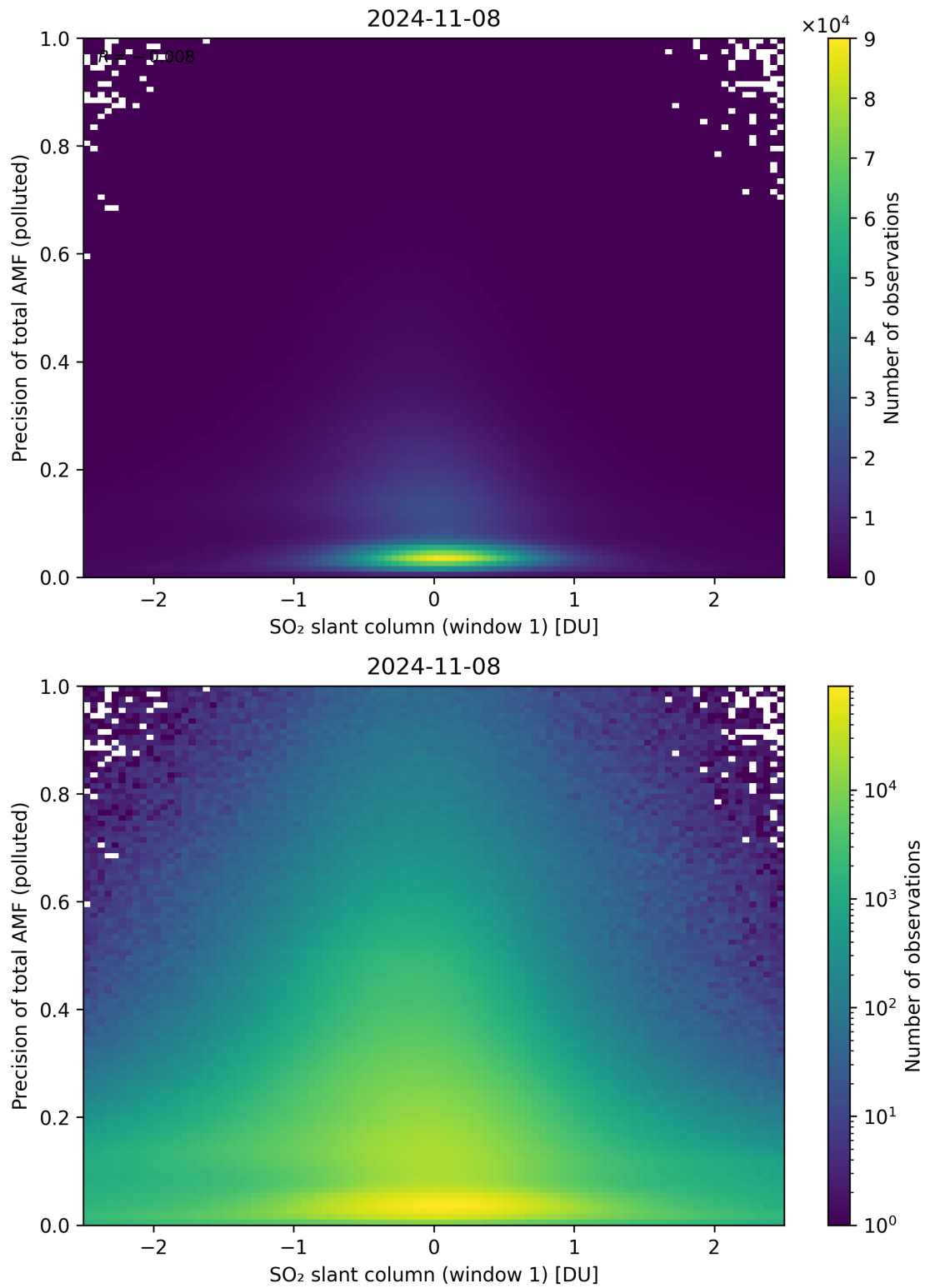
Figure 240: Scatter density plot of “SO 2 slant column (window 1)” against “Precision of total AMF (polluted)” for 2024-11-07 to 2024-11-09.
