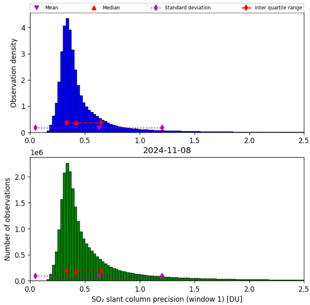
Figure 57: Histogram of “SO 2 slant column precision (window 1)” for 2024-11-07 to 2024-11-09
