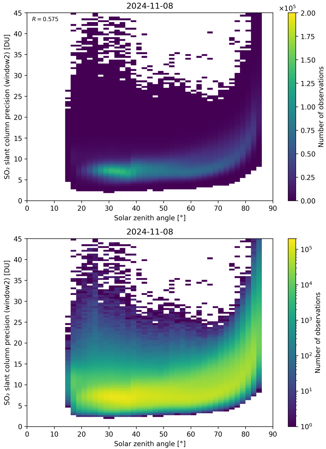
Figure 171: Scatter density plot of “Solar zenith angle” against “SO 2 slant column precision (window2)” for 2024-11-07 to 2024-11-09.
