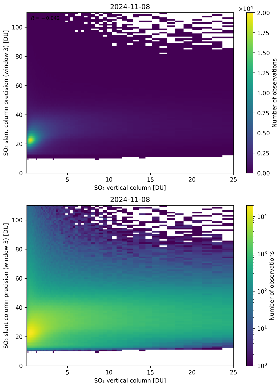
Figure 304: Scatter density plot of “SO 2 vertical column” against “SO 2 slant column precision (window 3)” for 2024-11-07 to 2024-11-09.
