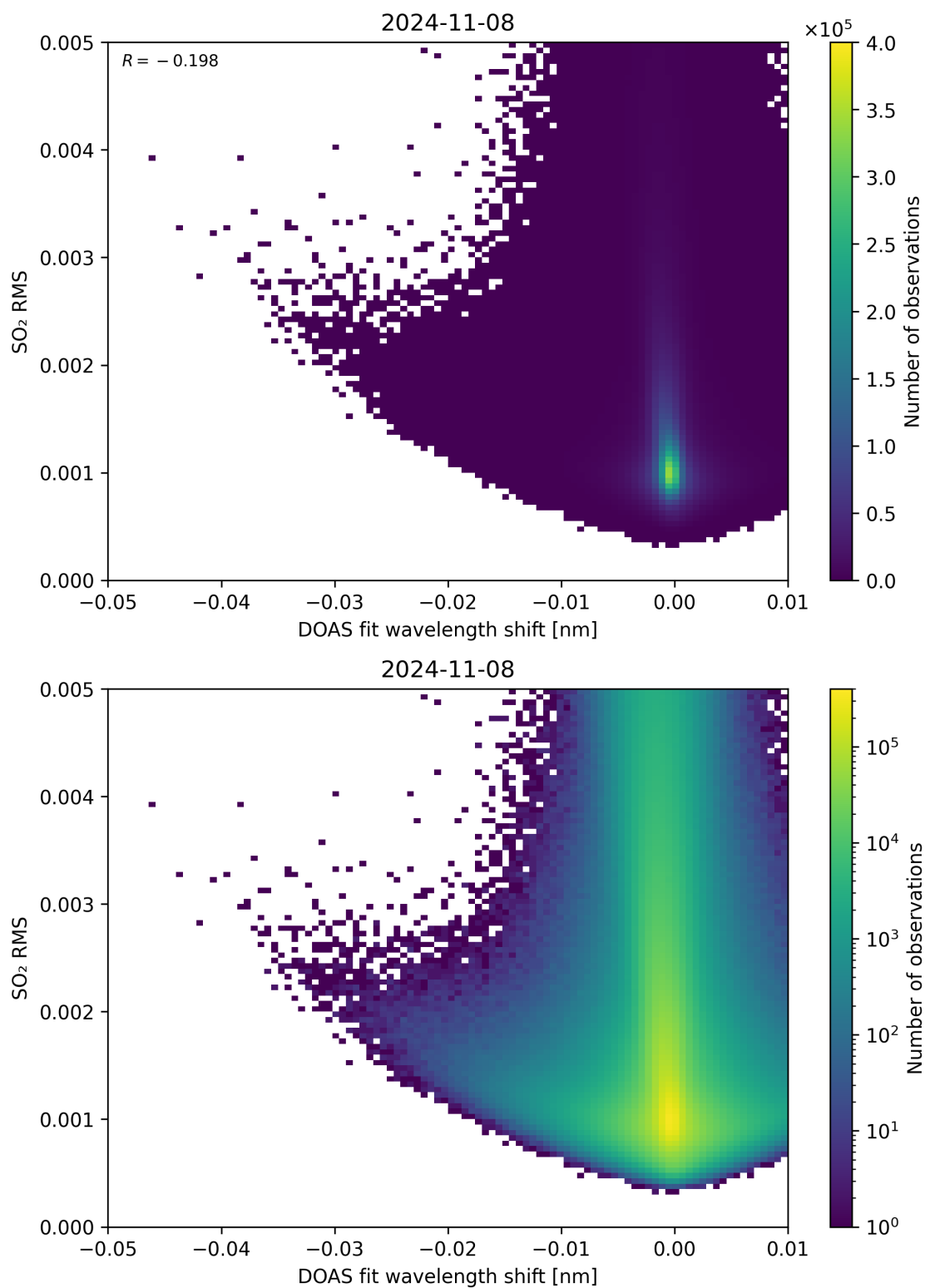
Figure 128: Scatter density plot of “DOAS fit wavelength shift” against “SO 2 RMS” for 2024-11-07 to 2024-11-09.
