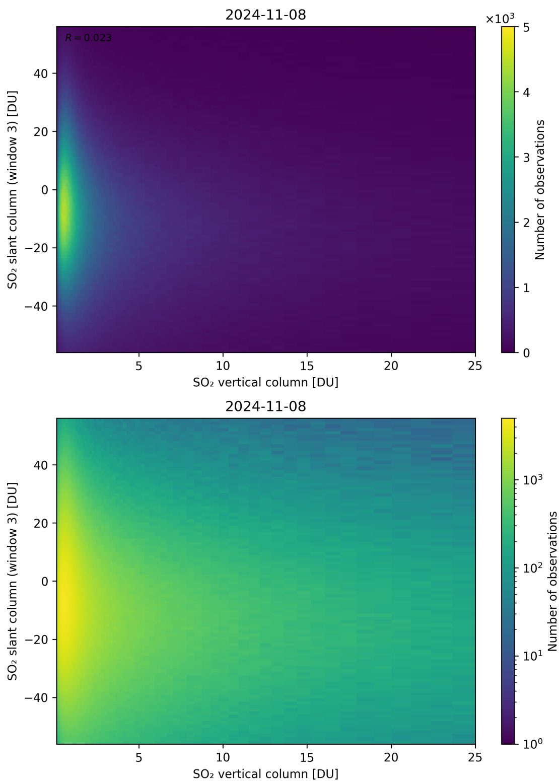
Figure 303: Scatter density plot of “SO 2 vertical column” against “SO 2 slant column (window 3)” for 2024-11-07 to 2024-11-09.
