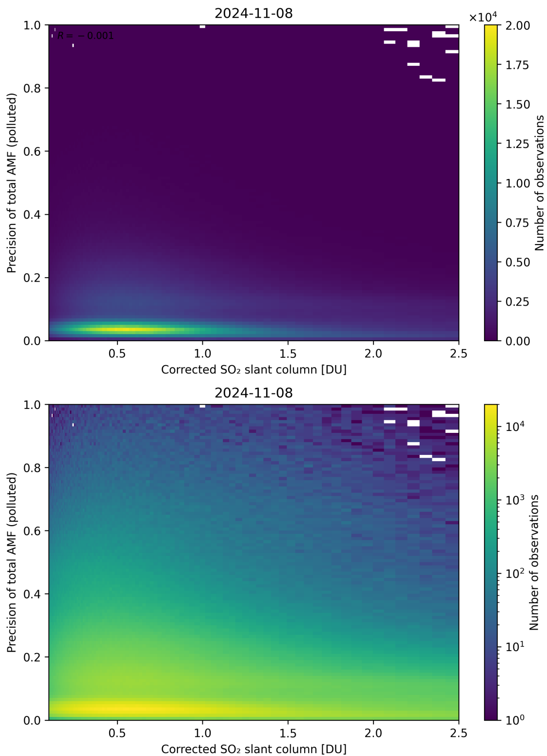
Figure 193: Scatter density plot of “Corrected SO 2 slant column” against “Precision of total AMF (polluted)” for 2024-11-07 to 2024-11-09.
