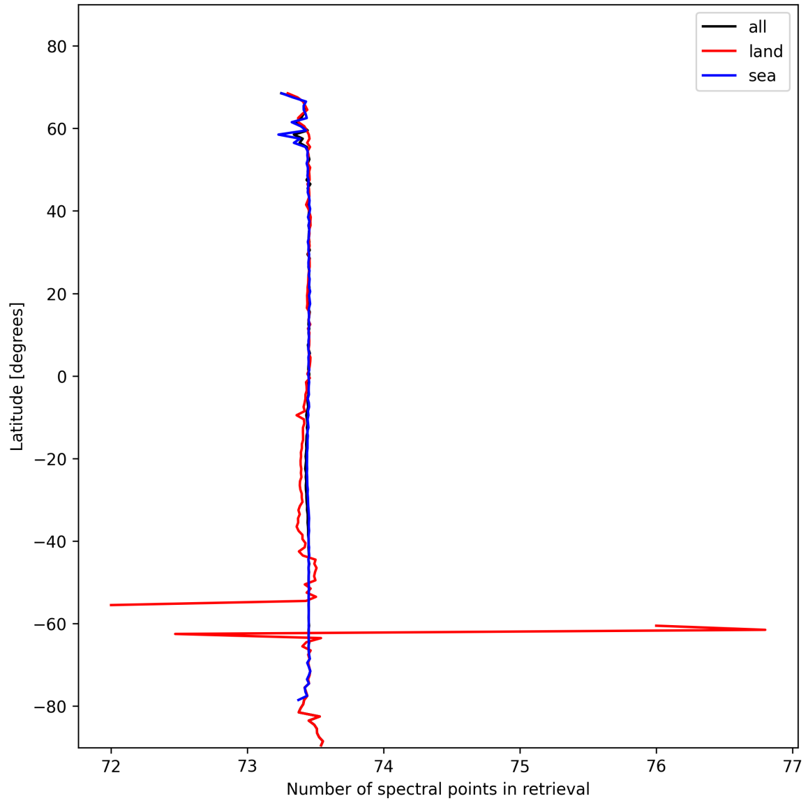
Figure 51: Zonal average of “Number of spectral points in retrieval” for 2024-11-07 to 2024-11-09.
