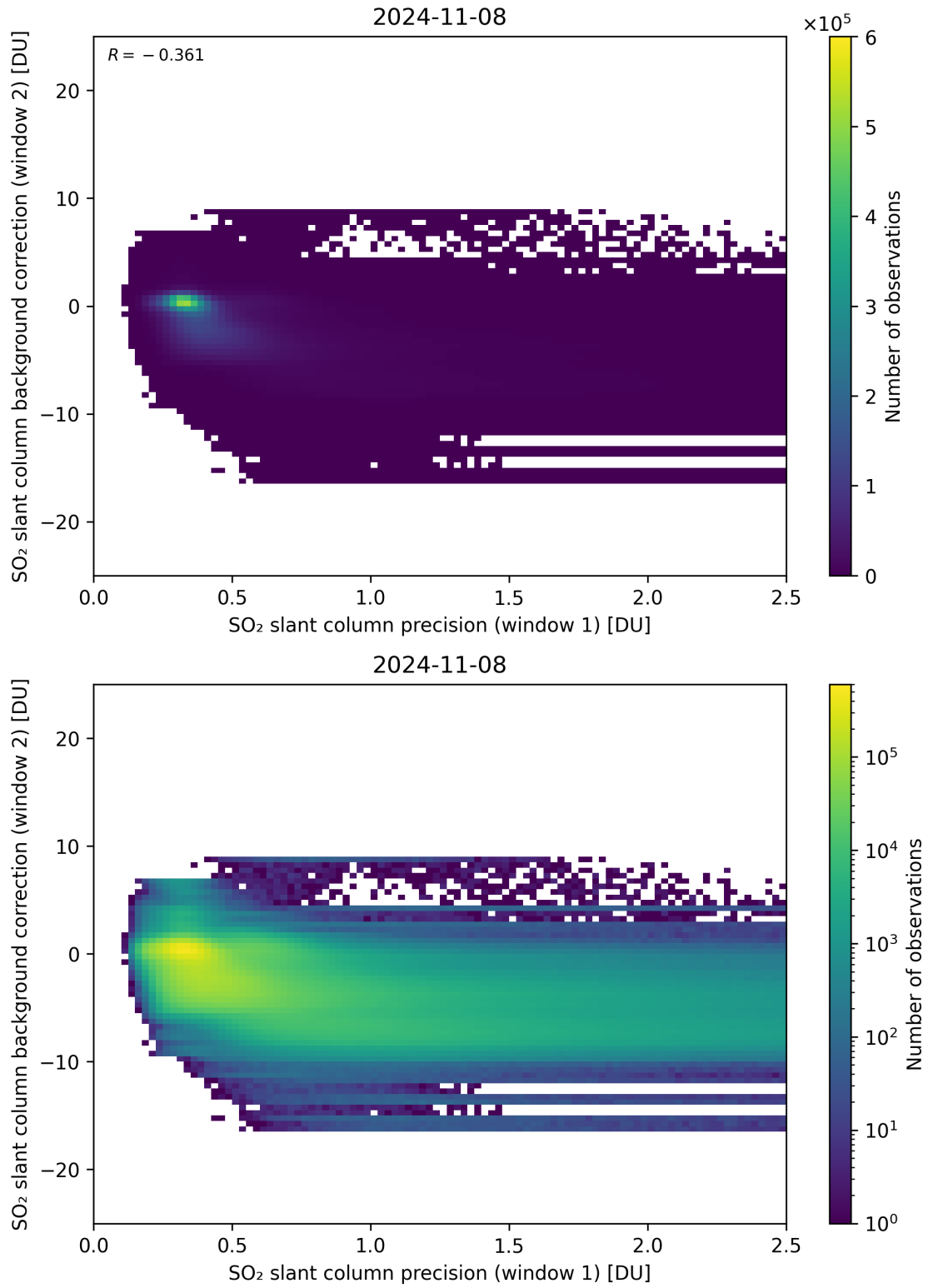
Figure 219: Scatter density plot of “SO 2 slant column precision (window 1)” against “SO 2 slant column background correction (window 2)” for 2024-11-07 to 2024-11-09.
