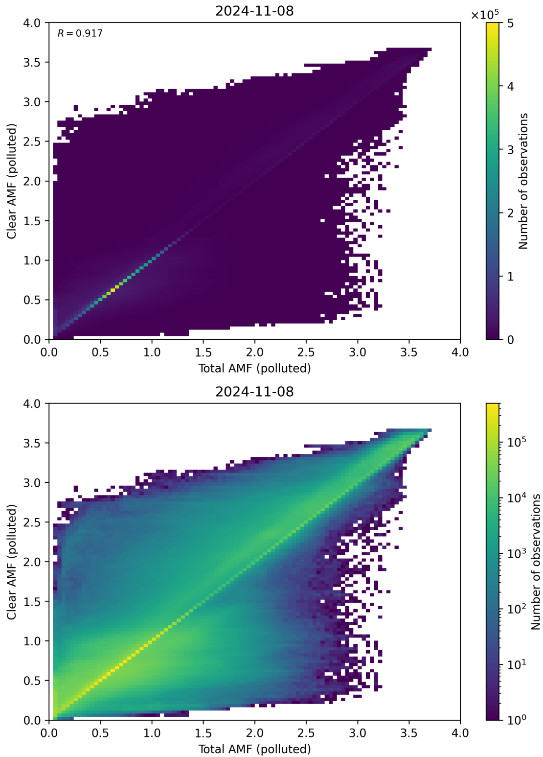
Figure 271: Scatter density plot of “Total AMF (polluted)” against “Clear AMF (polluted)” for 2024-11-07 to 2024-11-09.
