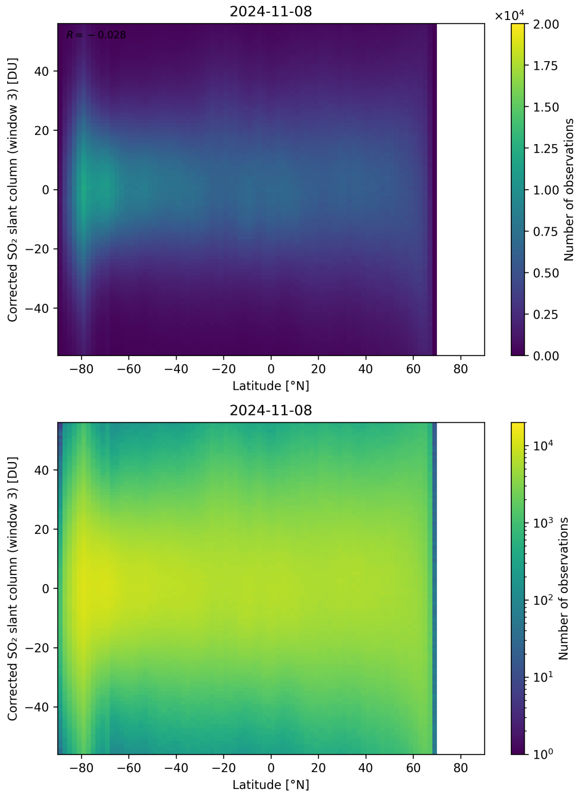
Figure 148: Scatter density plot of “Latitude” against “Corrected SO 2 slant column (window 3)” for 2024-11-07 to 2024-11-09.
