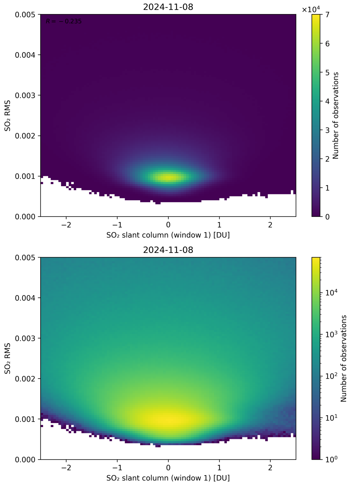
Figure 217: Scatter density plot of “SO 2 slant column (window 1)” against “SO 2 RMS” for 2024-11-07 to 2024-11-09.
