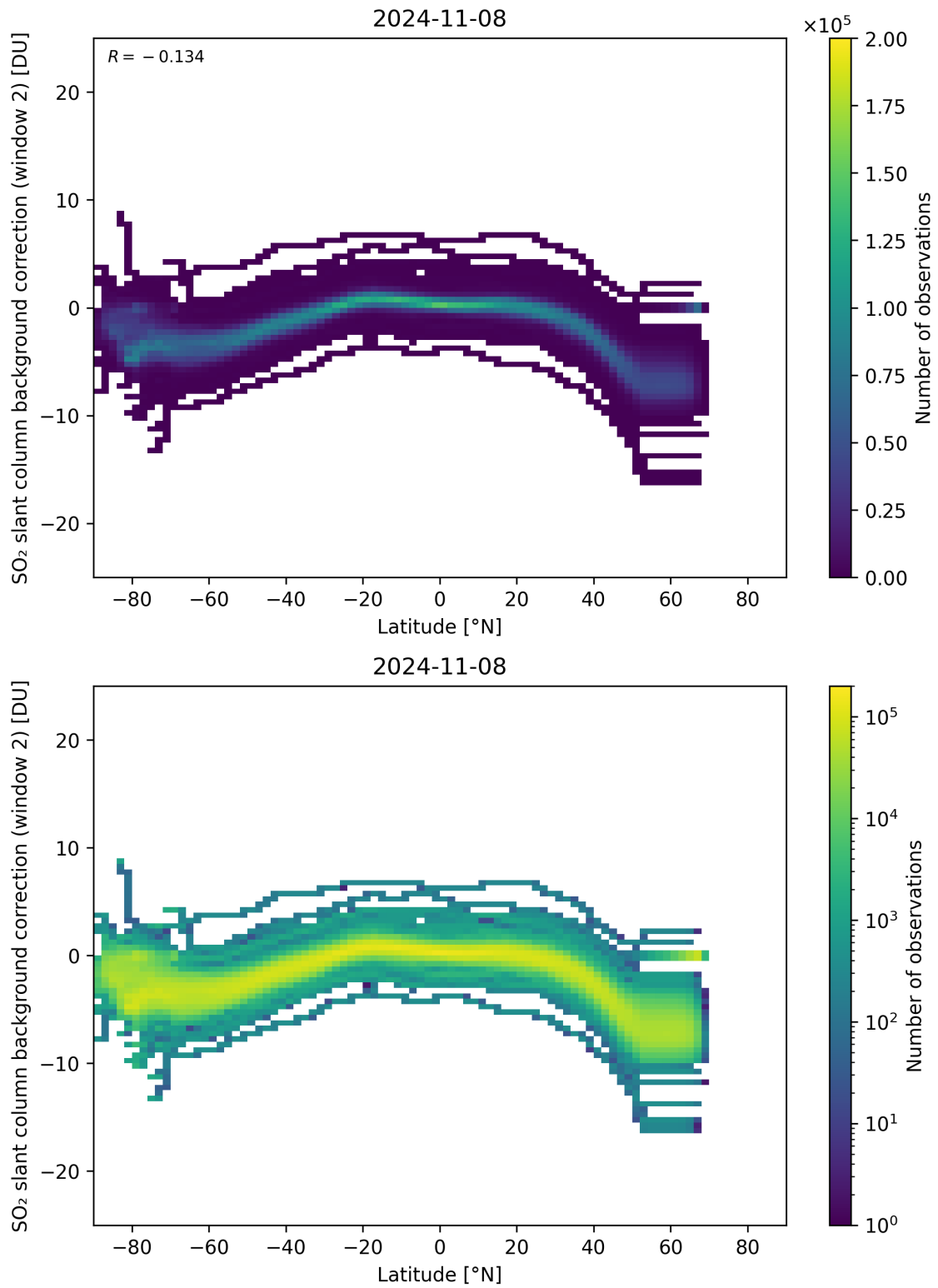
Figure 140: Scatter density plot of “Latitude” against “SO 2 slant column background correction (window 2)” for 2024-11-07 to 2024-11-09.
