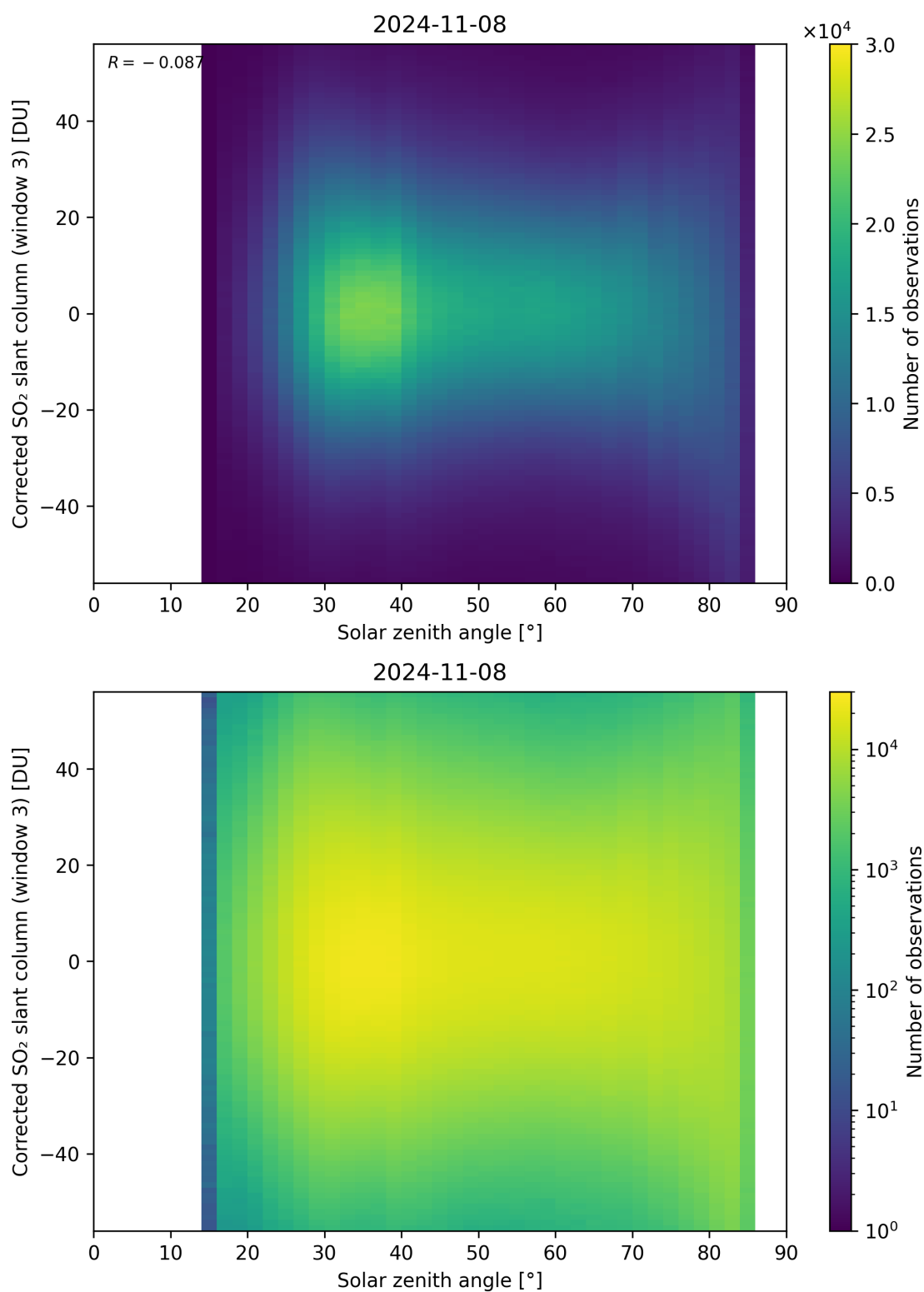
Figure 168: Scatter density plot of “Solar zenith angle” against “Corrected SO 2 slant column (window 3)” for 2024-11-07 to 2024-11-09.
