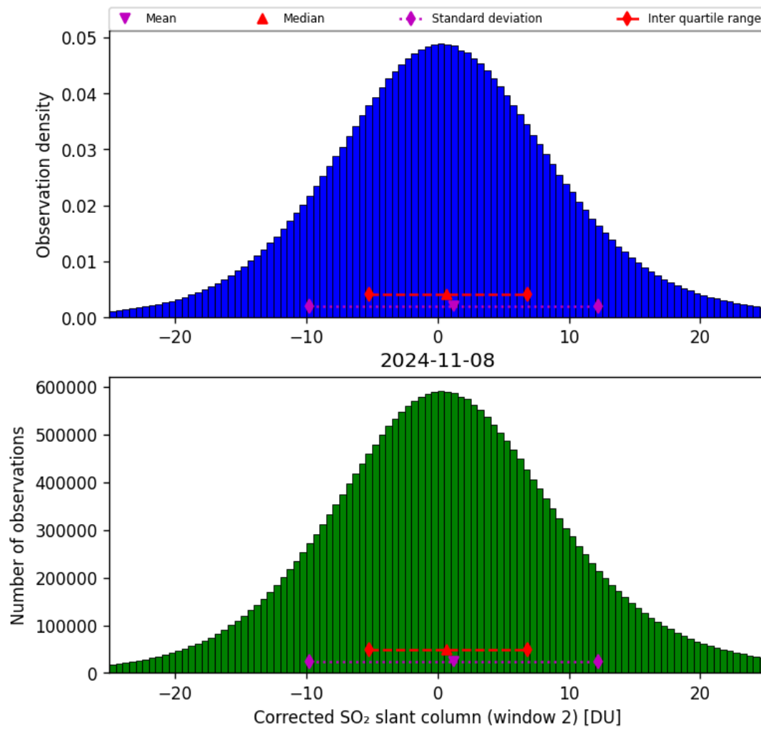
Figure 62: Histogram of “Corrected SO 2 slant column (window 2)” for 2024-11-07 to 2024-11-09
