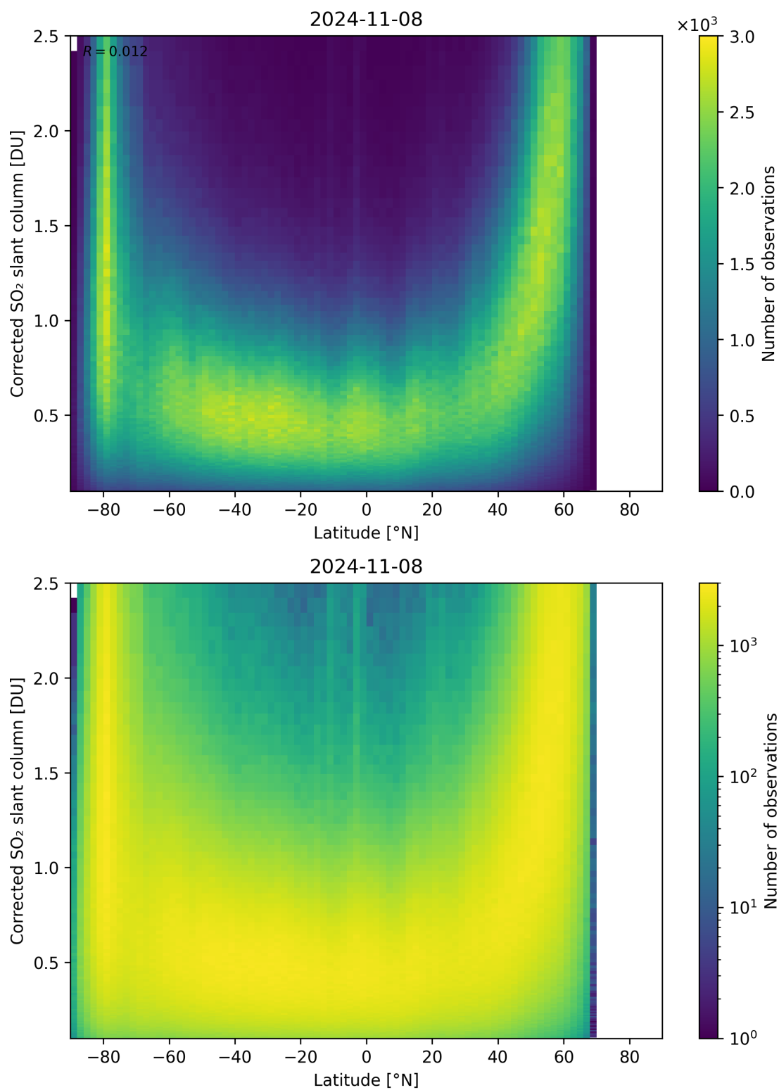
Figure 146: Scatter density plot of “Latitude” against “Corrected SO 2 slant column” for 2024-11-07 to 2024-11-09.
