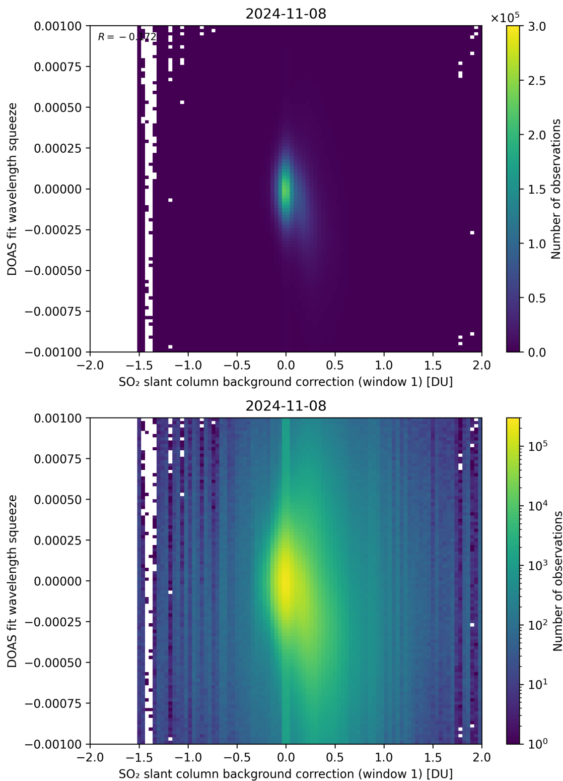
Figure 101: Scatter density plot of “SO 2 slant column background correction (window 1)” against “DOAS fit wavelength squeeze” for 2024-11-07 to 2024-11-09.
