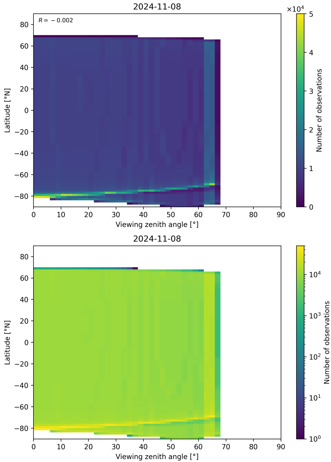
Figure 314: Scatter density plot of “Viewing zenith angle” against “Latitude” for 2024-11-07 to 2024-11-09.
