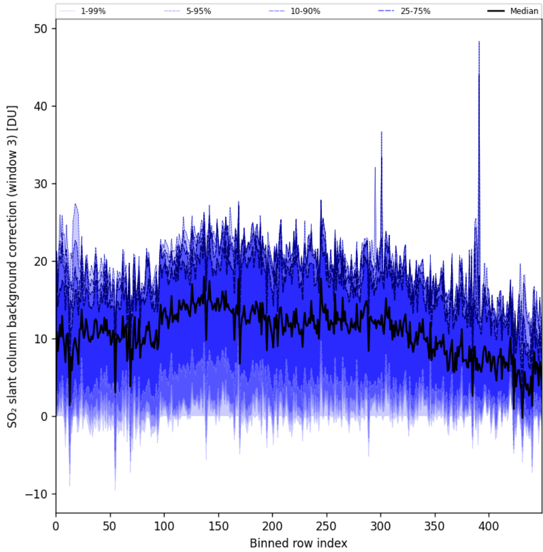
Figure 90: Along track statistics of “SO 2 slant column background correction (window 3)” for 2024-11-07 to 2024-11-09
