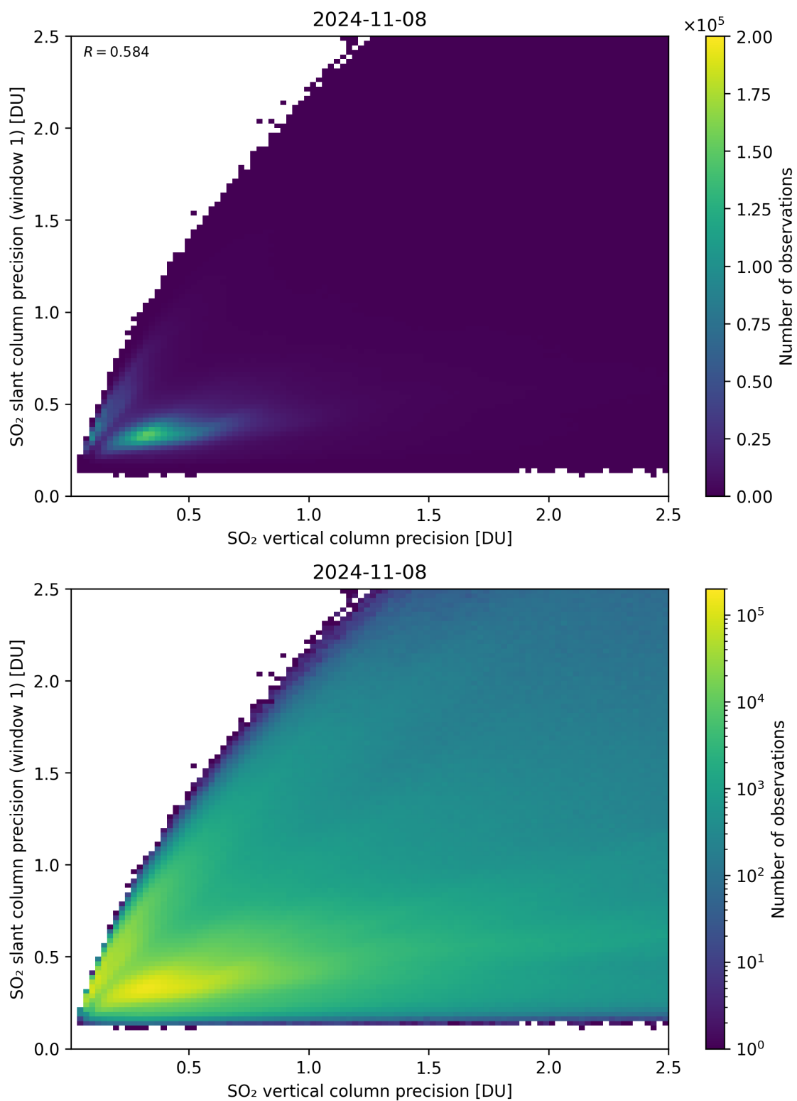
Figure 290: Scatter density plot of “SO 2 vertical column precision” against “SO 2 slant column precision (window 1)” for 2024-11-07 to 2024-11-09.
