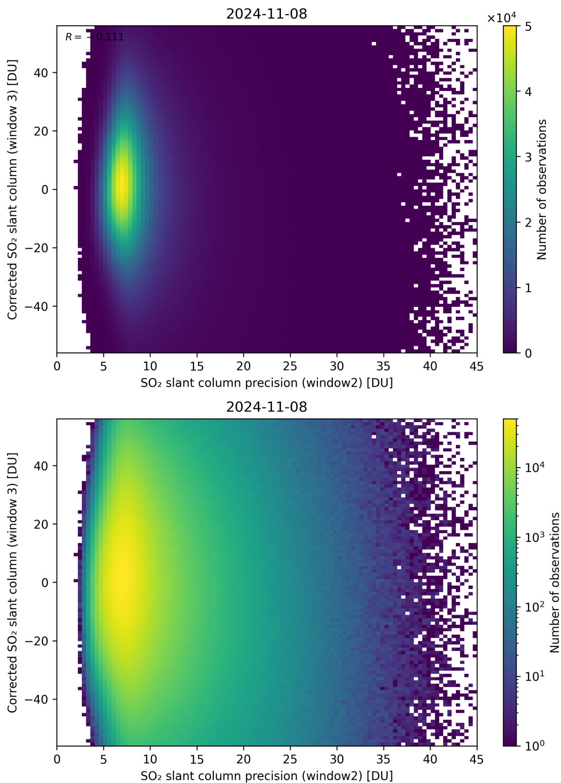
Figure 248: Scatter density plot of “SO 2 slant column precision (window2)” against “Corrected SO 2 slant column (window 3)” for 2024-11-07 to 2024-11-09.
