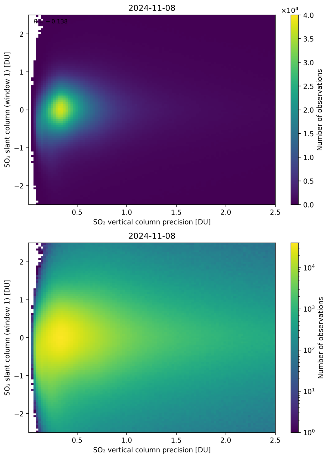
Figure 289: Scatter density plot of “SO 2 vertical column precision” against “SO 2 slant column (window 1)” for 2024-11-07 to 2024-11-09.
