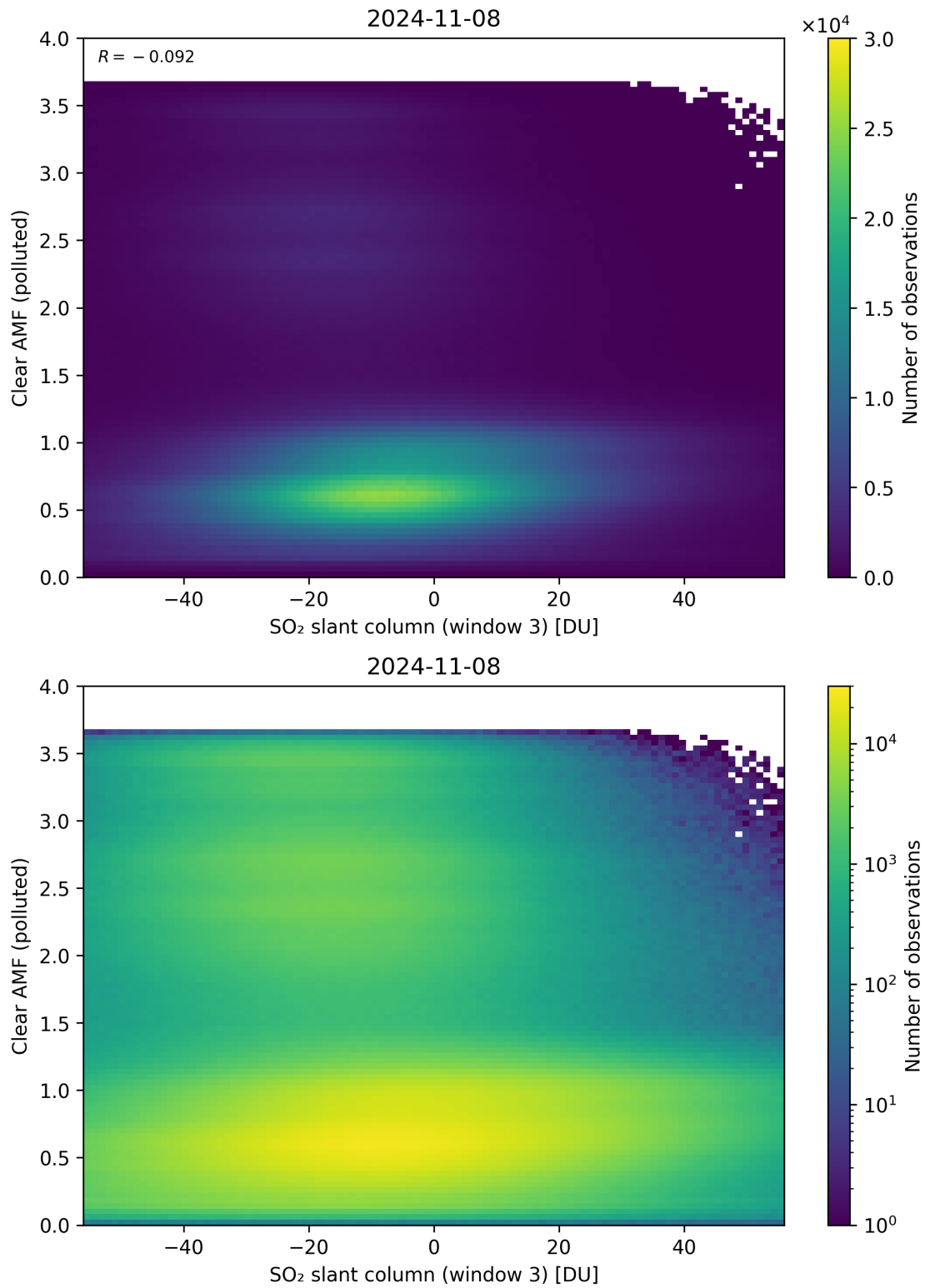
Figure 265: Scatter density plot of “SO 2 slant column (window 3)” against “Clear AMF (polluted)” for 2024-11-07 to 2024-11-09.
