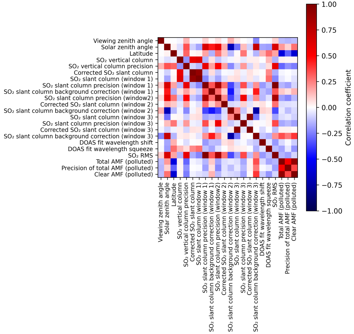
Figure 2: Map of correlation matrix for 2024-11-07 to 2024-11-09.
