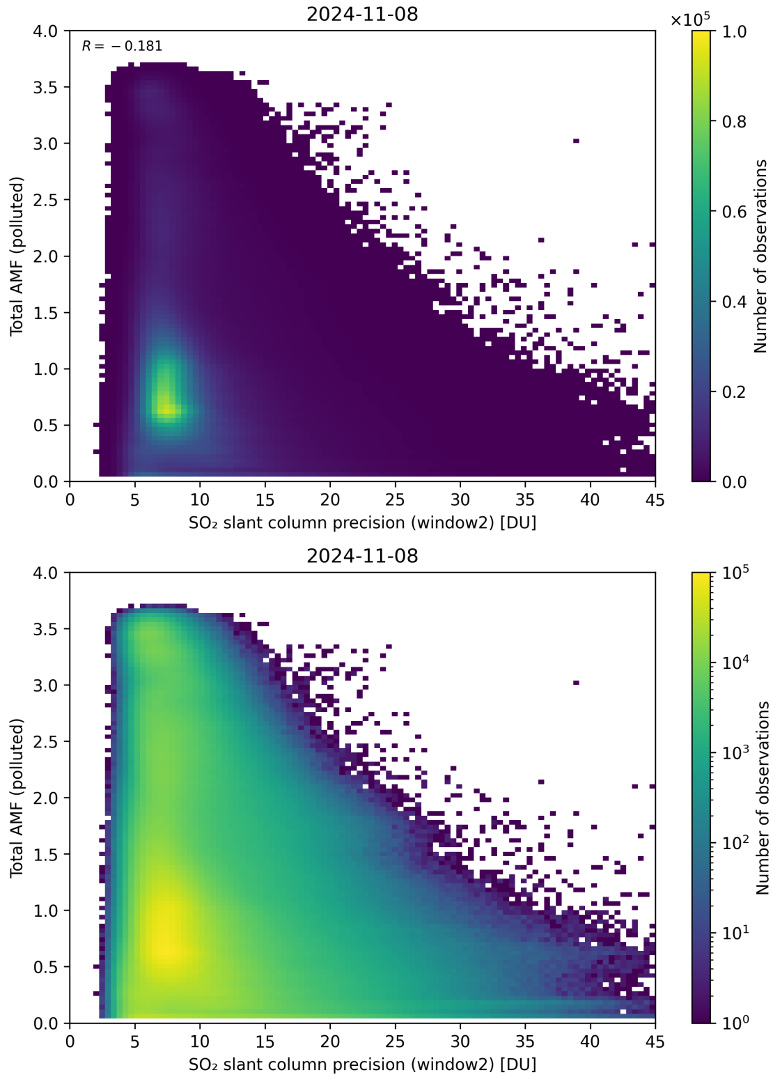
Figure 251: Scatter density plot of “SO 2 slant column precision (window2)” against “Total AMF (polluted)” for 2024-11-07 to 2024-11-09.
