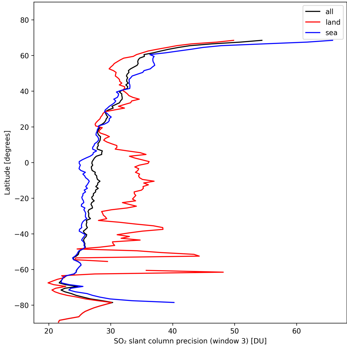
Figure 42: Zonal average of “SO 2 slant column precision (window 3)” for 2024-11-07 to 2024-11-09.
