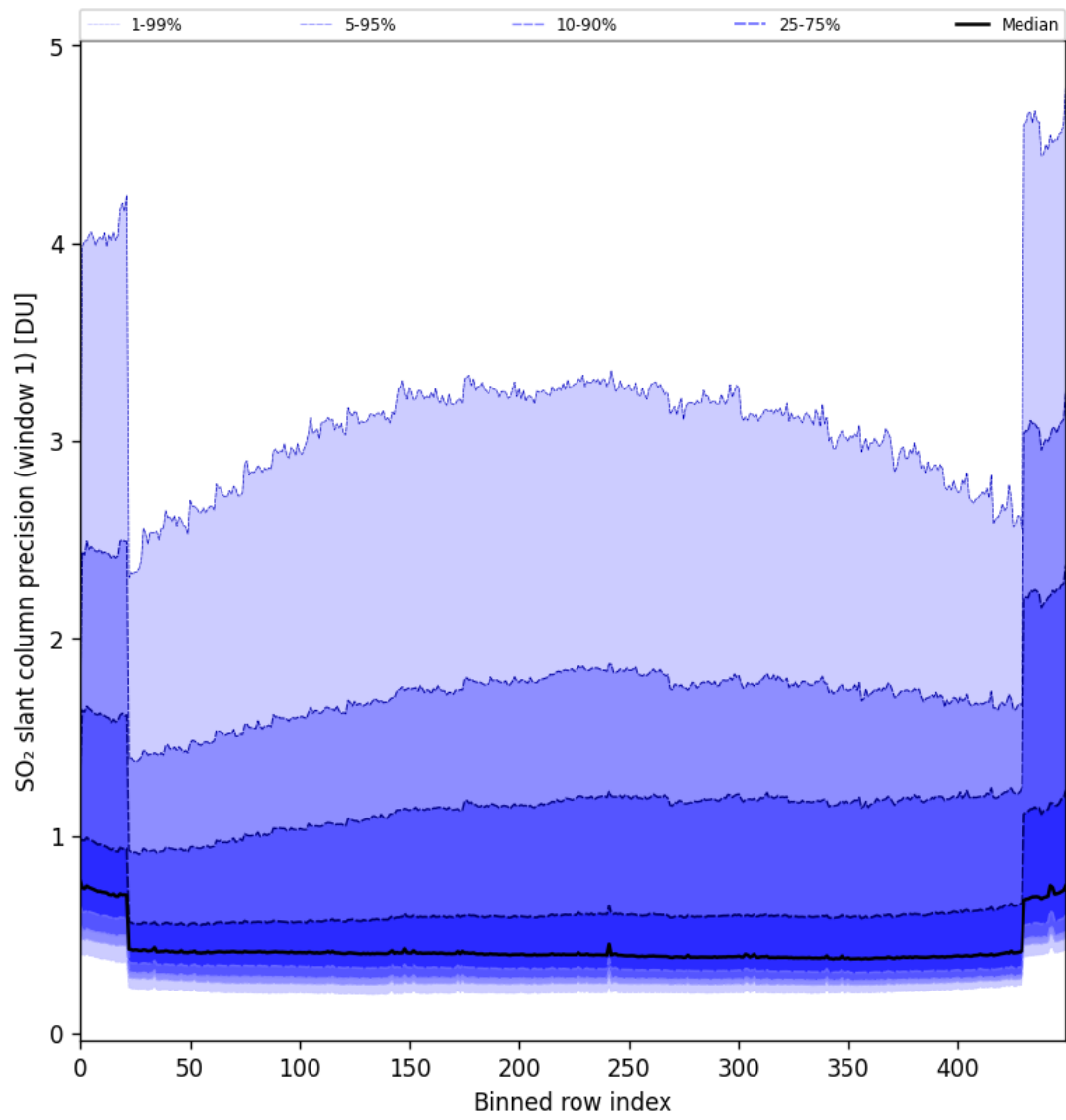
Figure 80: Along track statistics of “SO 2 slant column precision (window 1)” for 2024-11-07 to 2024-11-09
