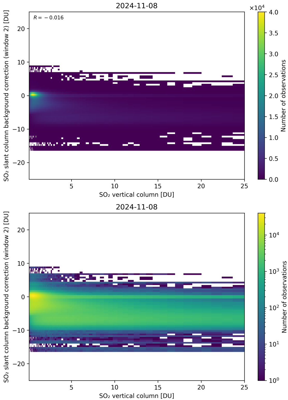
Figure 274: Scatter density plot of “SO 2 vertical column” against “SO 2 slant column background correction (window 2)” for 2024-11-07 to 2024-11-09.
