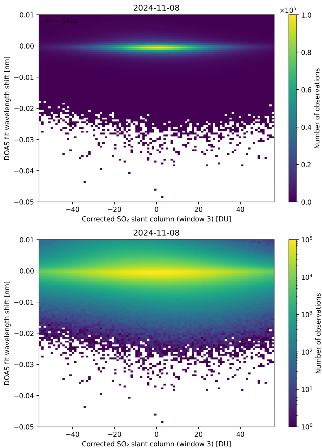
Figure 206: Scatter density plot of “Corrected SO 2 slant column (window 3)” against “DOAS fit wavelength shift” for 2024-11-07 to 2024-11-09.
