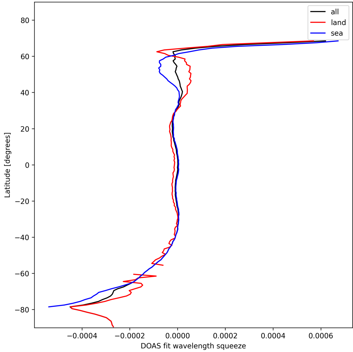
Figure 46: Zonal average of “DOAS fit wavelength squeeze” for 2024-11-07 to 2024-11-09.
