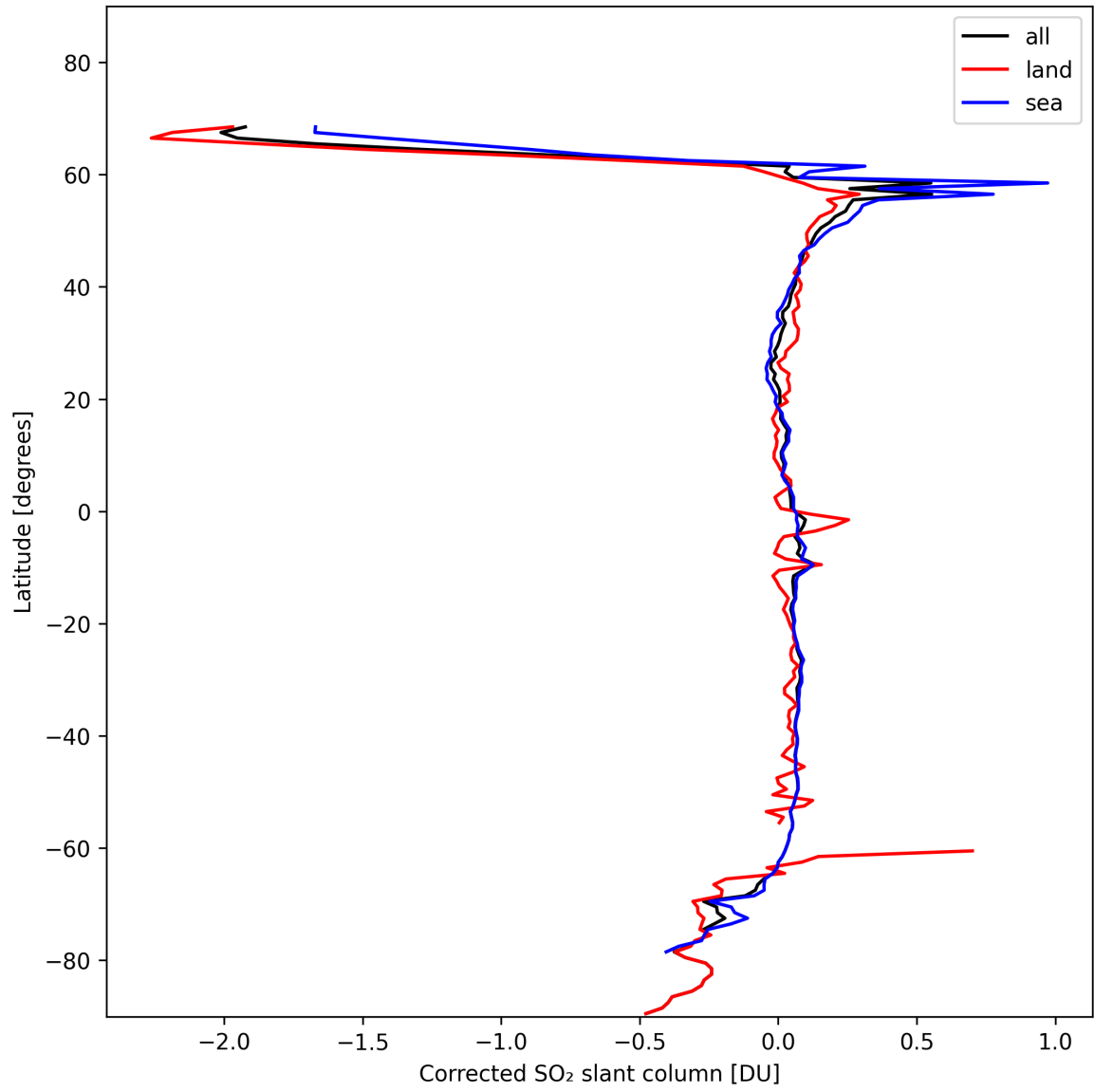
Figure 32: Zonal average of “Corrected SO 2 slant column” for 2024-11-07 to 2024-11-09.
