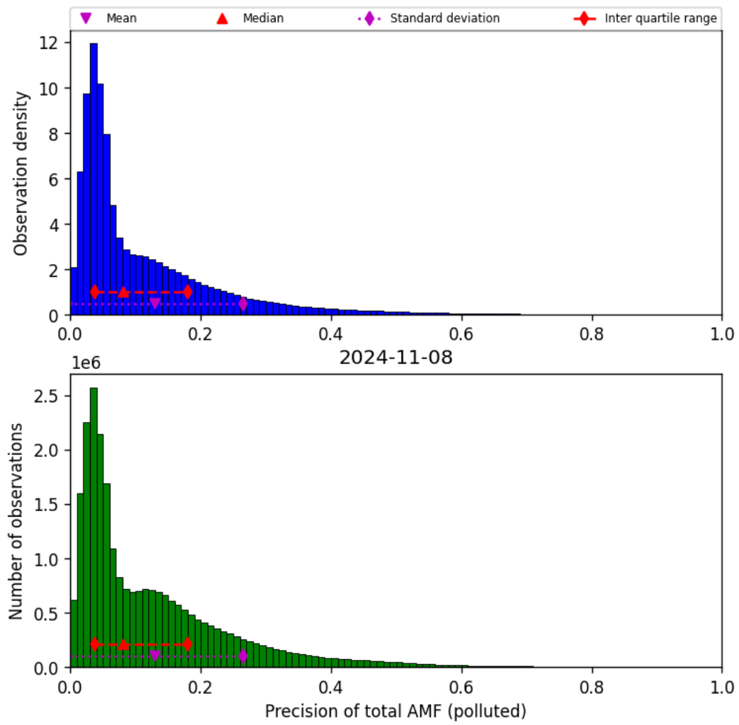
Figure 72: Histogram of “Precision of total AMF (polluted)” for 2024-11-07 to 2024-11-09
