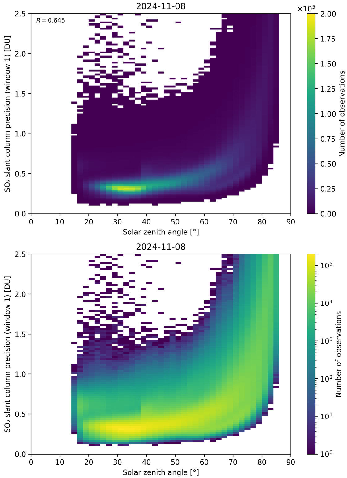
Figure 170: Scatter density plot of “Solar zenith angle” against “SO 2 slant column precision (window 1)” for 2024-11-07 to 2024-11-09.
