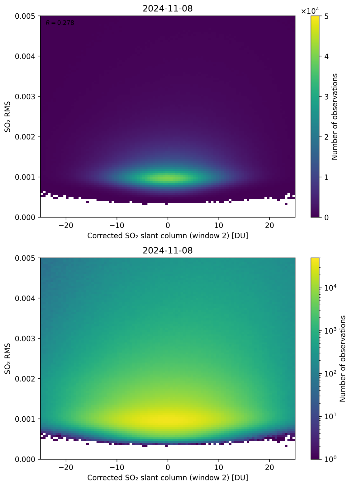
Figure 198: Scatter density plot of “Corrected SO 2 slant column (window 2)” against “SO 2 RMS” for 2024-11-07 to 2024-11-09.
