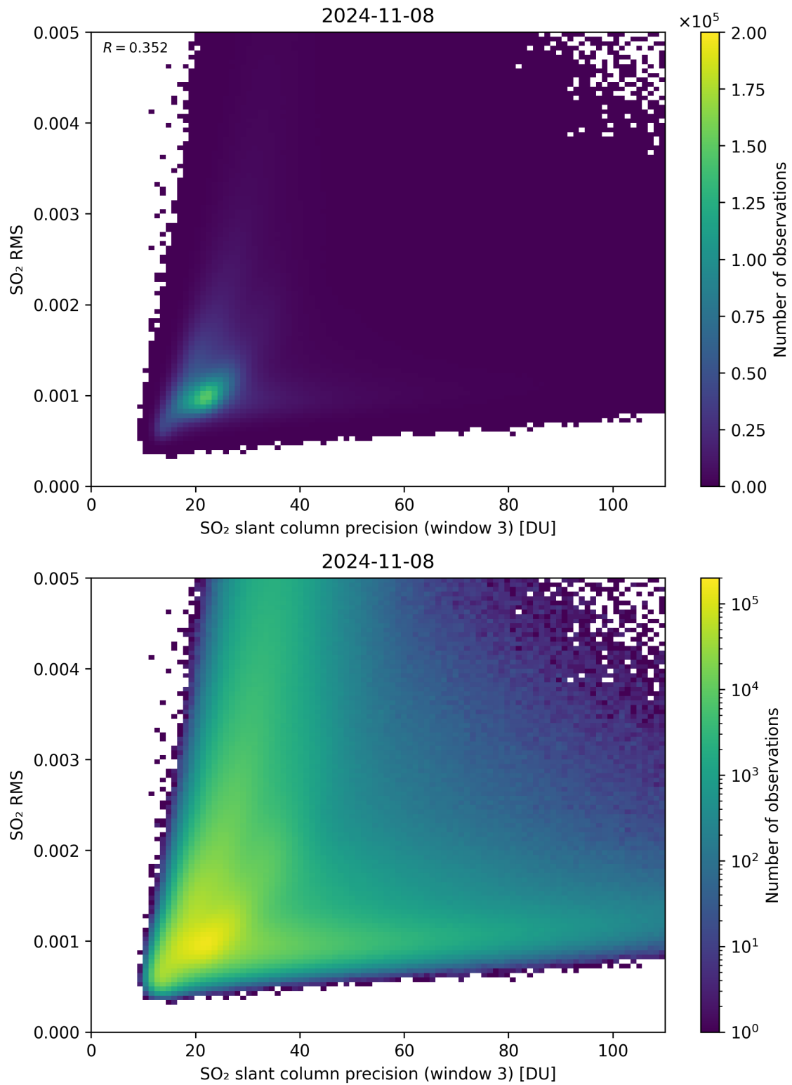
Figure 260: Scatter density plot of “SO 2 slant column precision (window 3)” against “SO 2 RMS” for 2024-11-07 to 2024-11-09.
