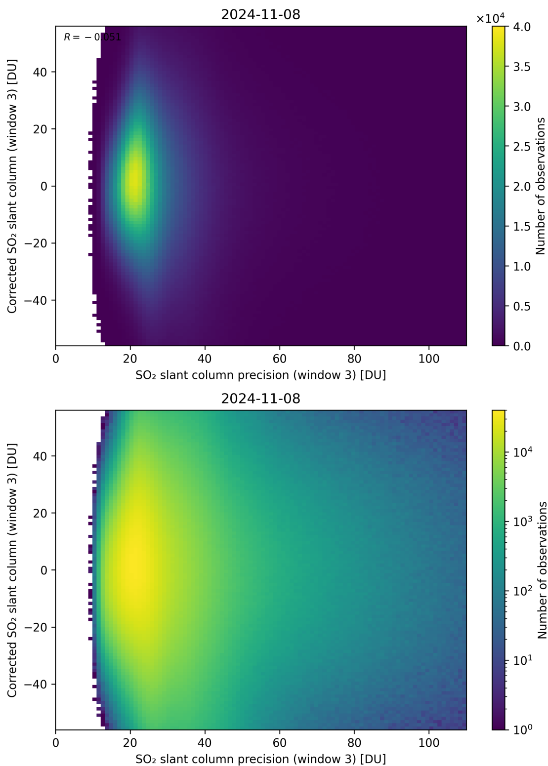
Figure 262: Scatter density plot of “SO 2 slant column precision (window 3)” against “Corrected SO 2 slant column (window 3)” for 2024-11-07 to 2024-11-09.
