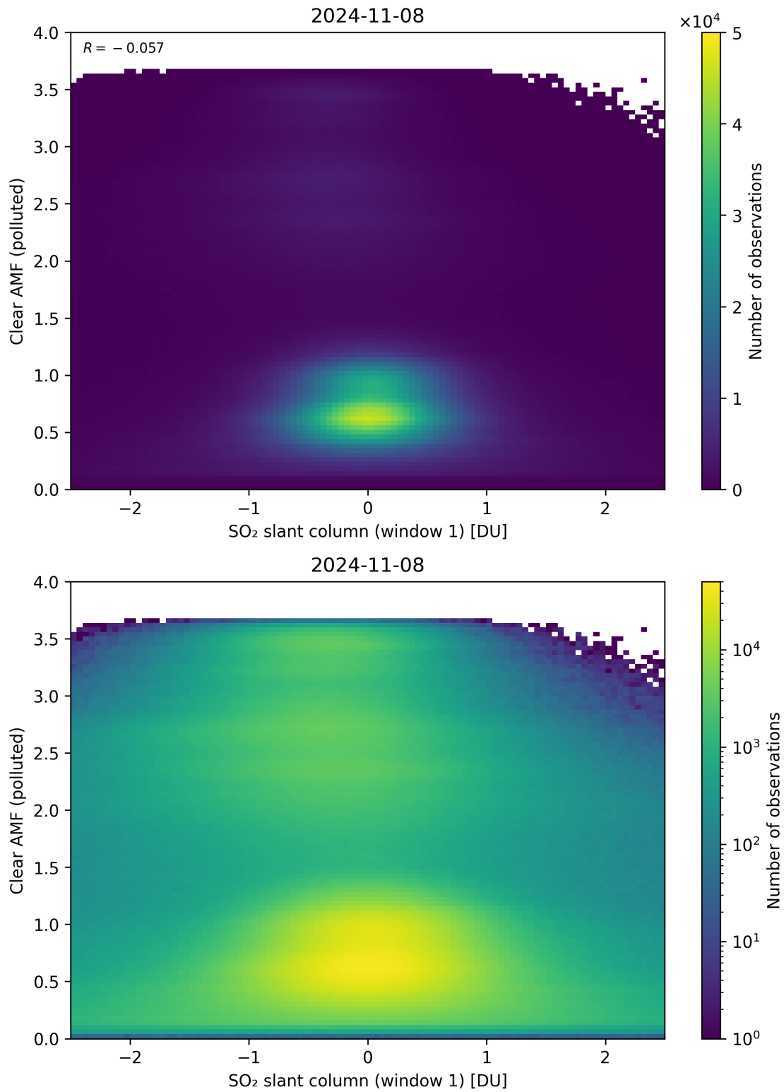
Figure 232: Scatter density plot of “SO 2 slant column (window 1)” against “Clear AMF (polluted)” for 2024-11-07 to 2024-11-09.
