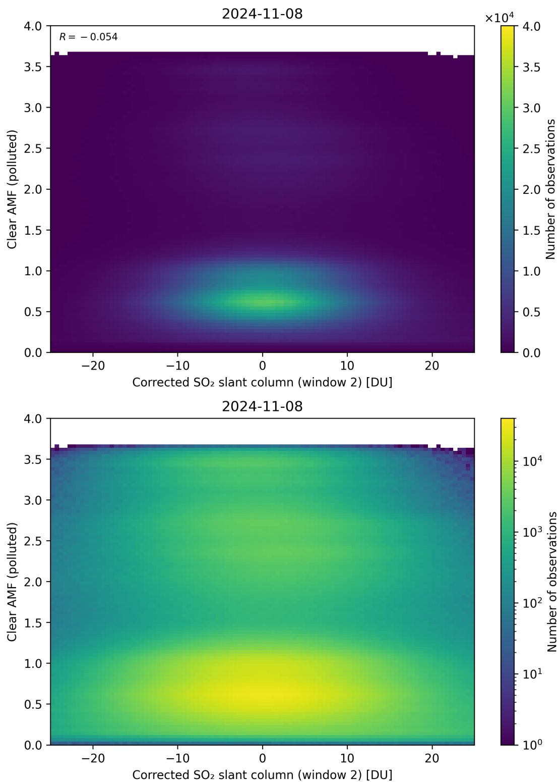
Figure 199: Scatter density plot of “Corrected SO 2 slant column (window 2)” against “Clear AMF (polluted)” for 2024-11-07 to 2024-11-09.
