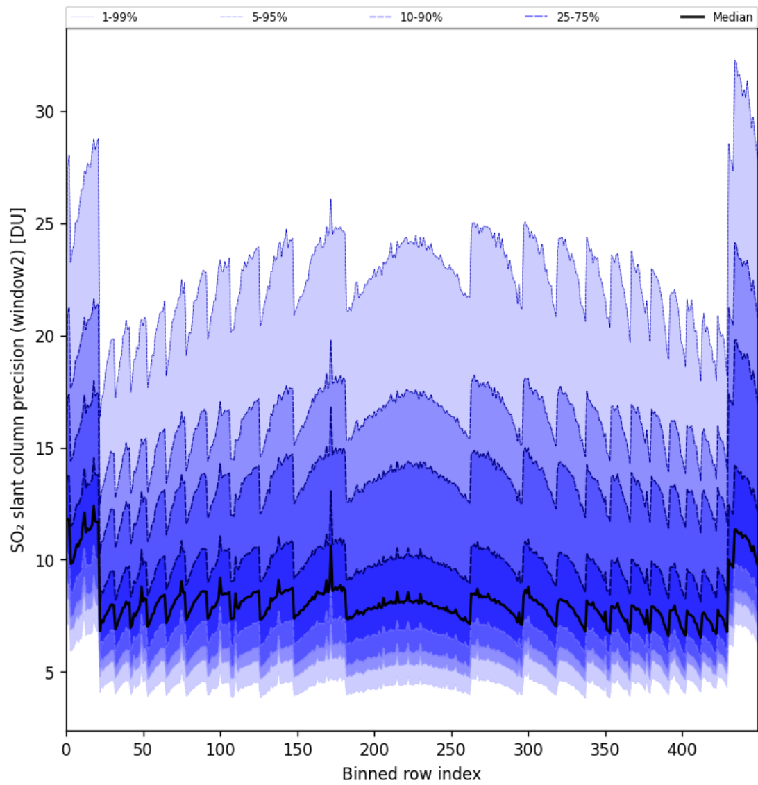
Figure 84: Along track statistics of “SO 2 slant column precision (window2)” for 2024-11-07 to 2024-11-09
