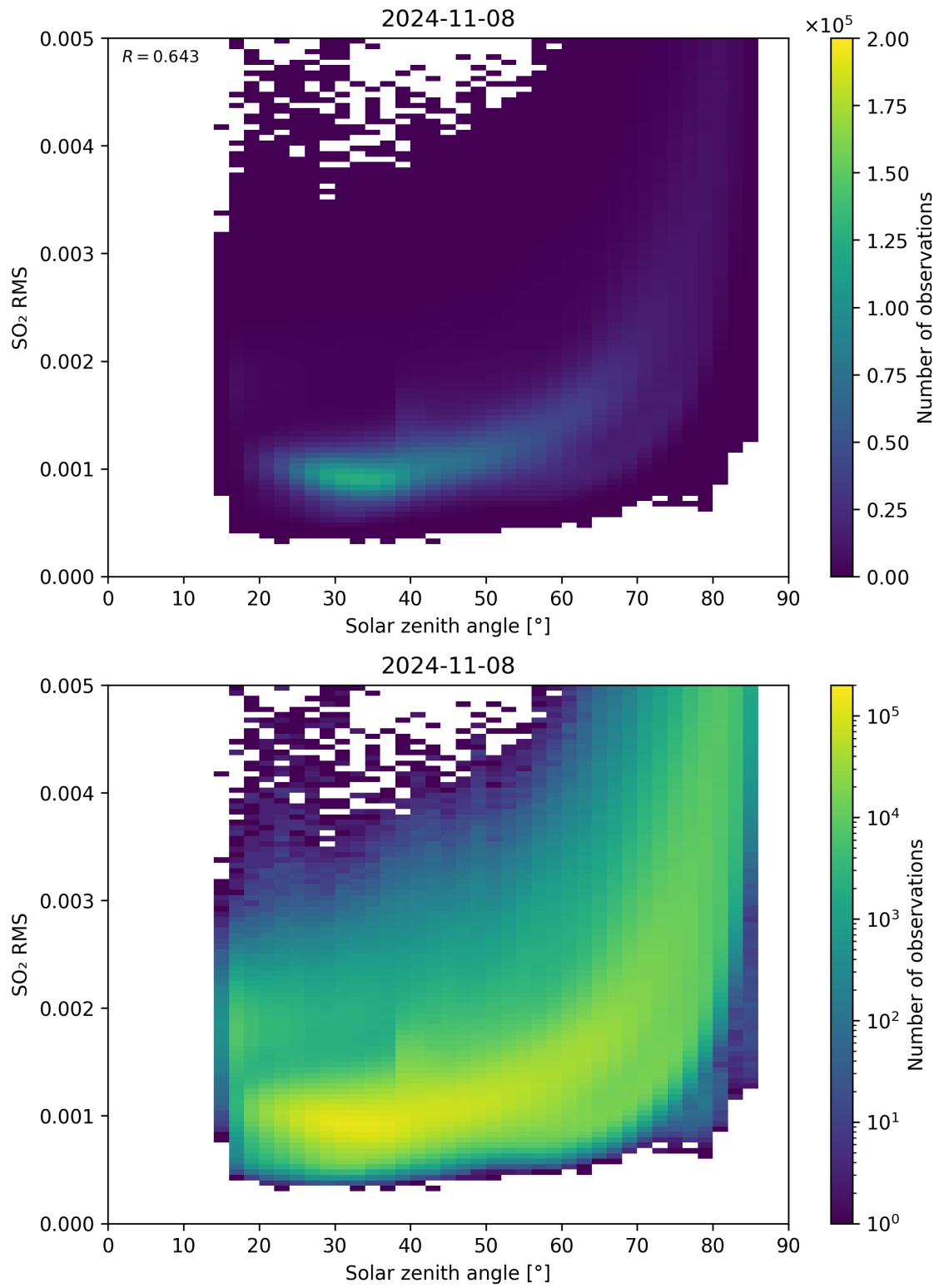
Figure 163: Scatter density plot of “Solar zenith angle” against “SO 2 RMS” for 2024-11-07 to 2024-11-09.
