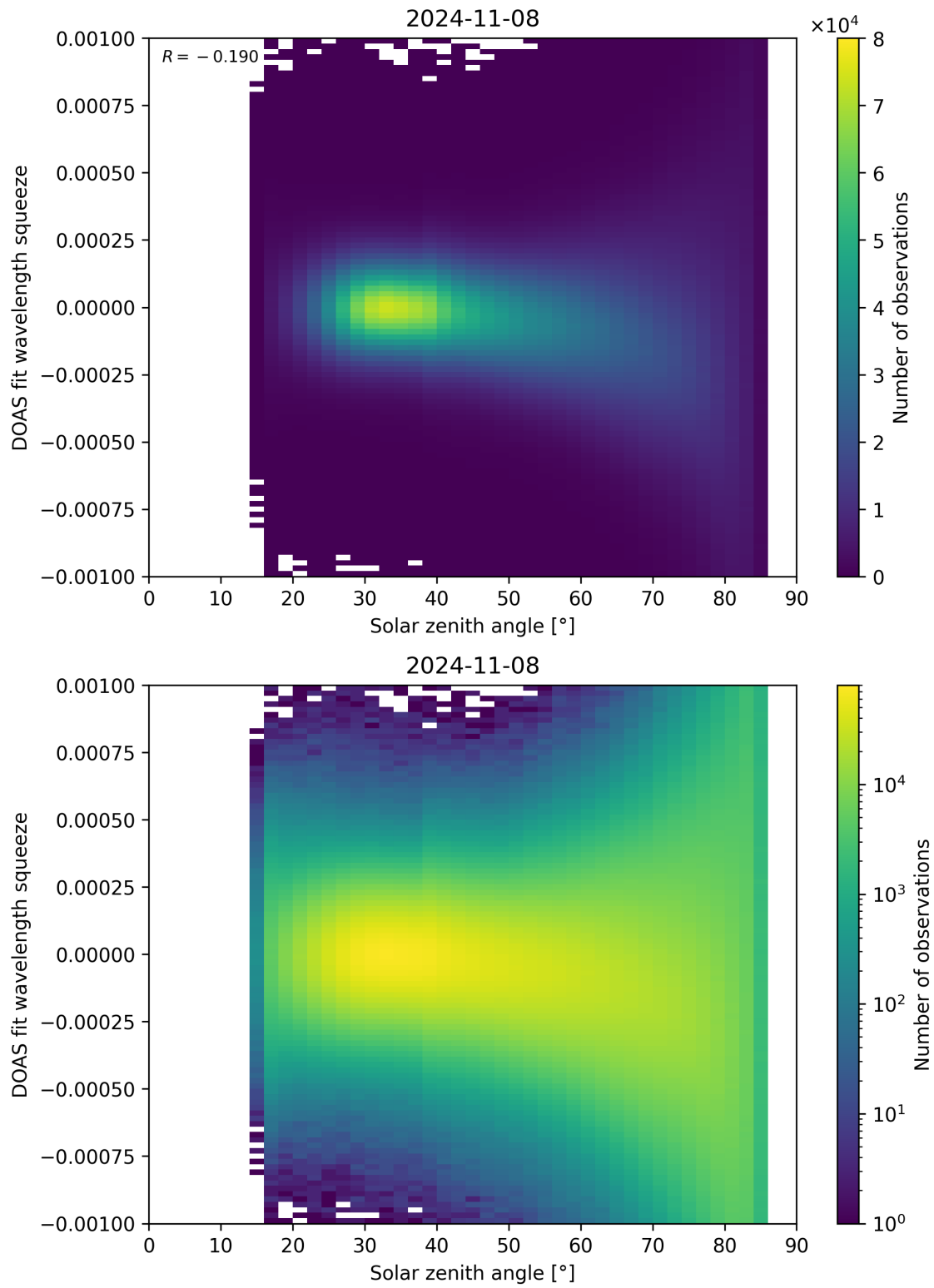
Figure 162: Scatter density plot of “Solar zenith angle” against “DOAS fit wavelength squeeze” for 2024-11-07 to 2024-11-09.
