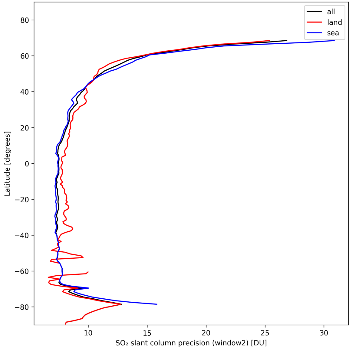
Figure 38: Zonal average of “SO 2 slant column precision (window2)” for 2024-11-07 to 2024-11-09.
