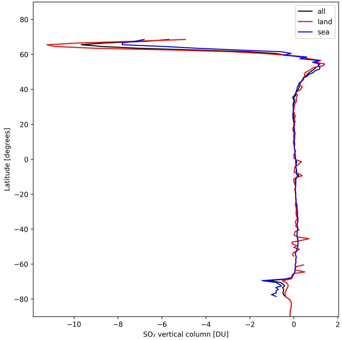
Figure 30: Zonal average of “SO 2 vertical column” for 2024-11-07 to 2024-11-09.
