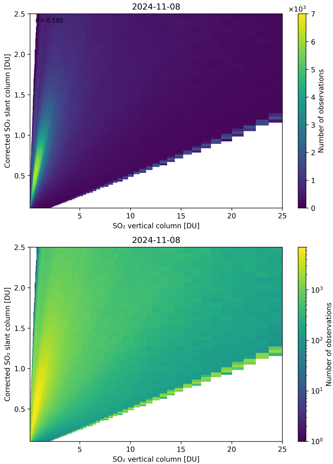
Figure 297: Scatter density plot of “SO 2 vertical column” against “Corrected SO 2 slant column” for 2024-11-07 to 2024-11-09.
