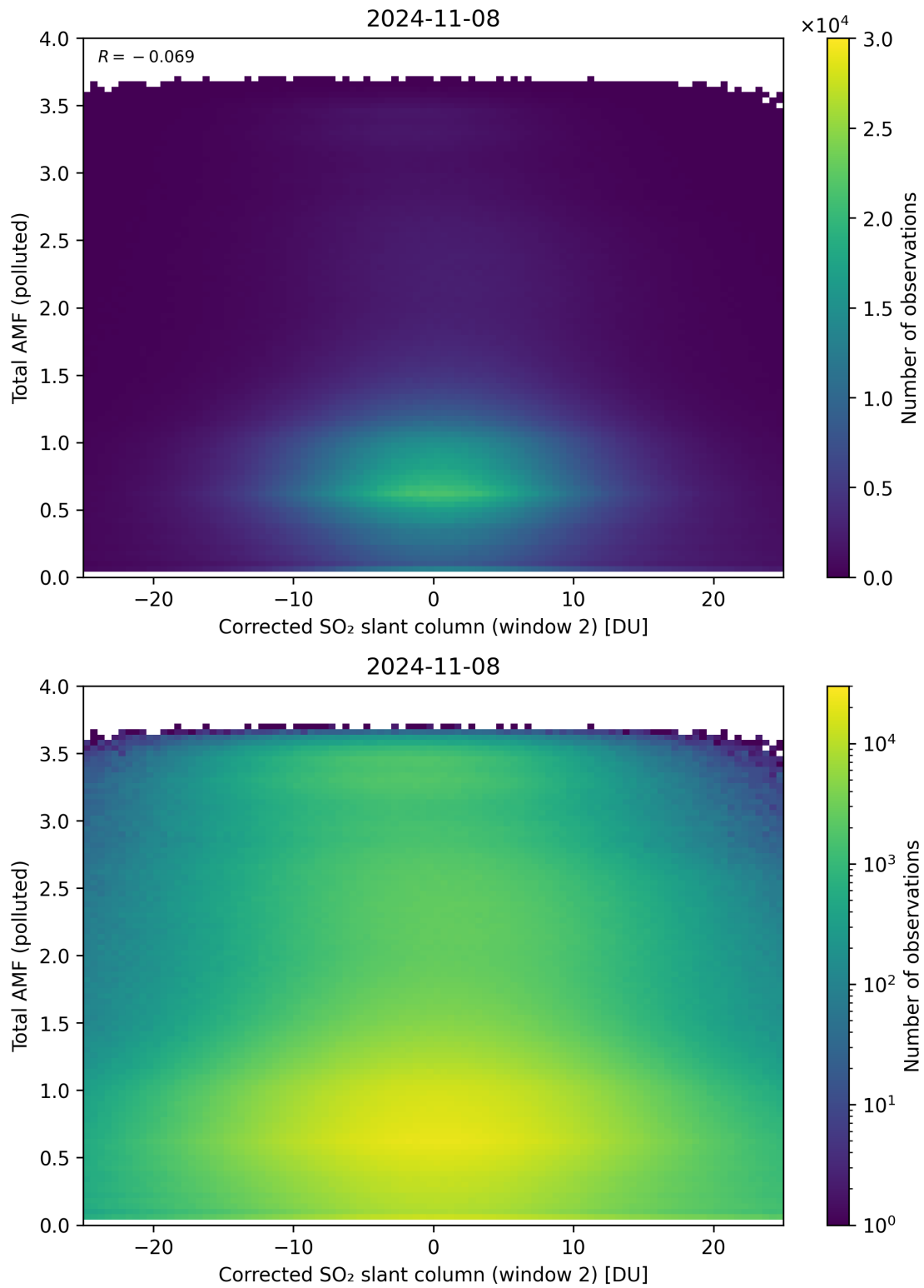
Figure 203: Scatter density plot of “Corrected SO 2 slant column (window 2)” against “Total AMF (polluted)” for 2024-11-07 to 2024-11-09.
