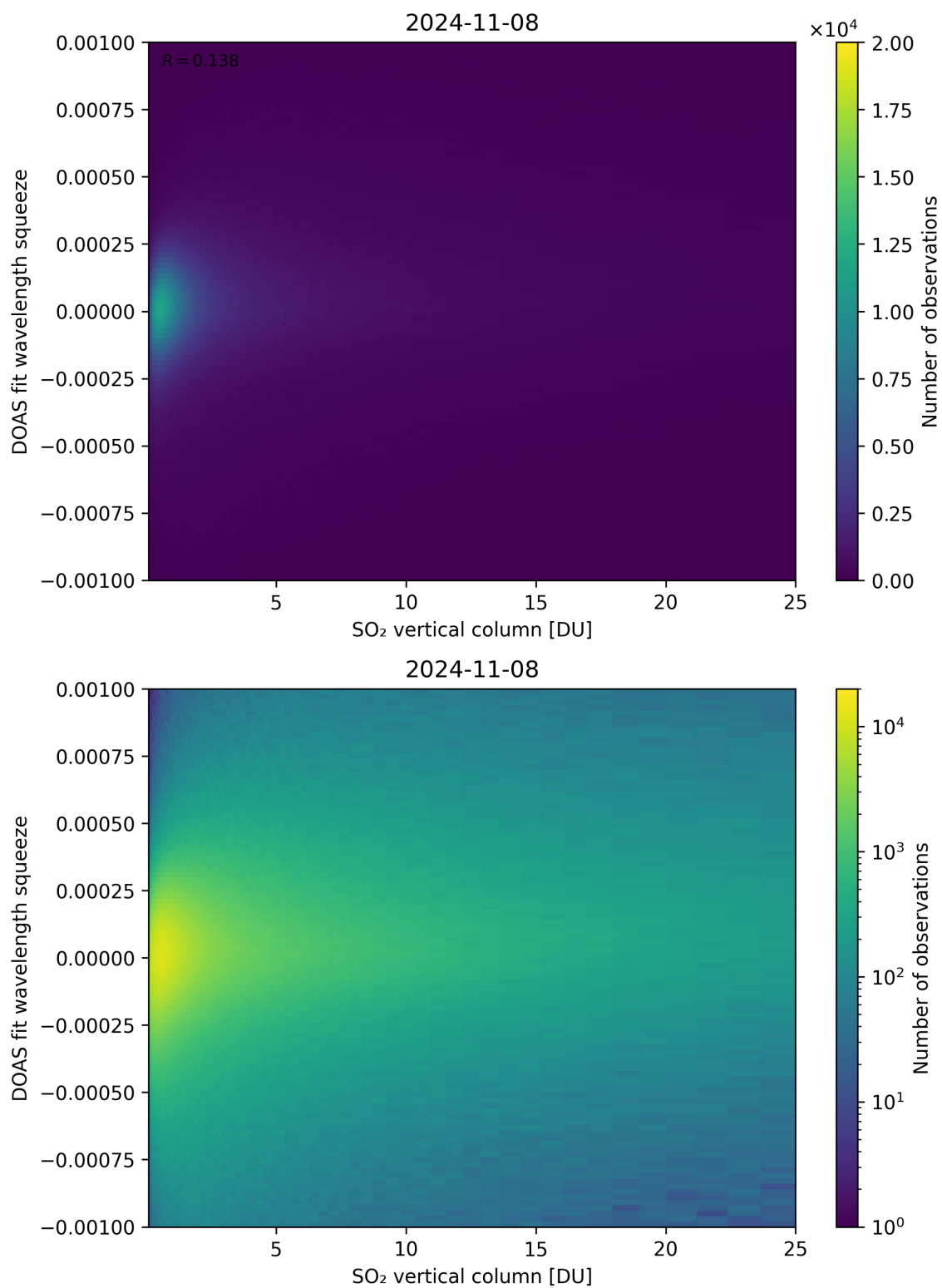
Figure 277: Scatter density plot of “SO 2 vertical column” against “DOAS fit wavelength squeeze” for 2024-11-07 to 2024-11-09.
