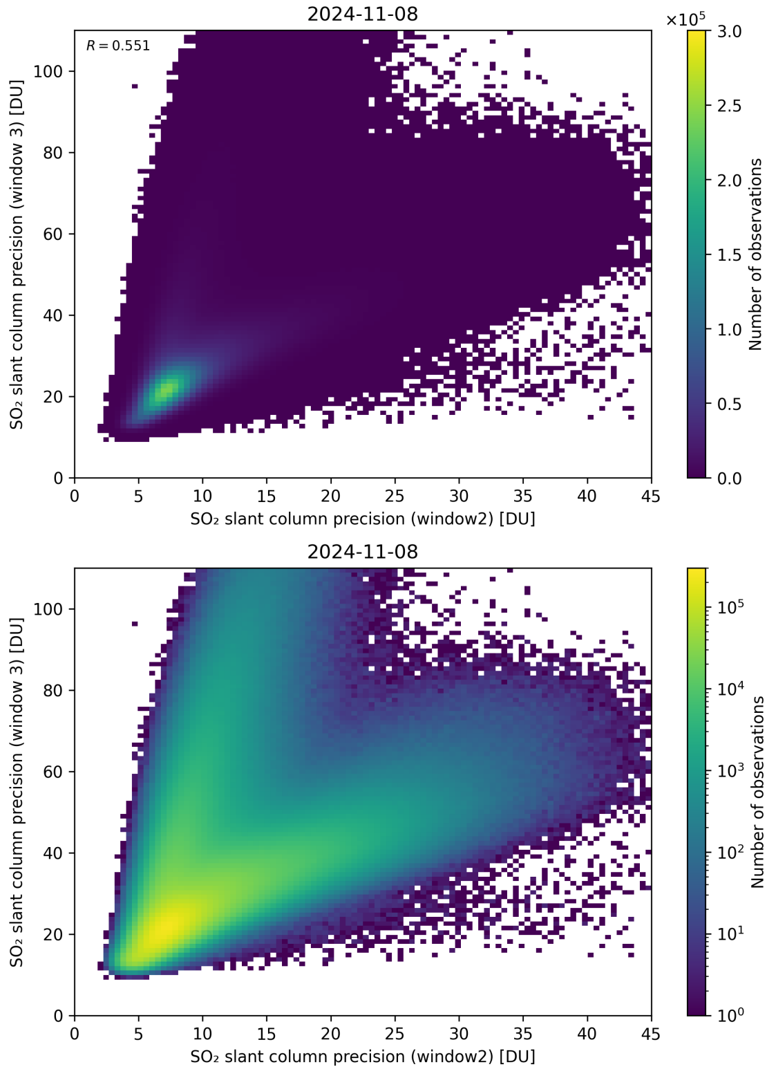
Figure 250: Scatter density plot of “SO 2 slant column precision (window2)” against “SO 2 slant column precision (window 3)” for 2024-11-07 to 2024-11-09.
