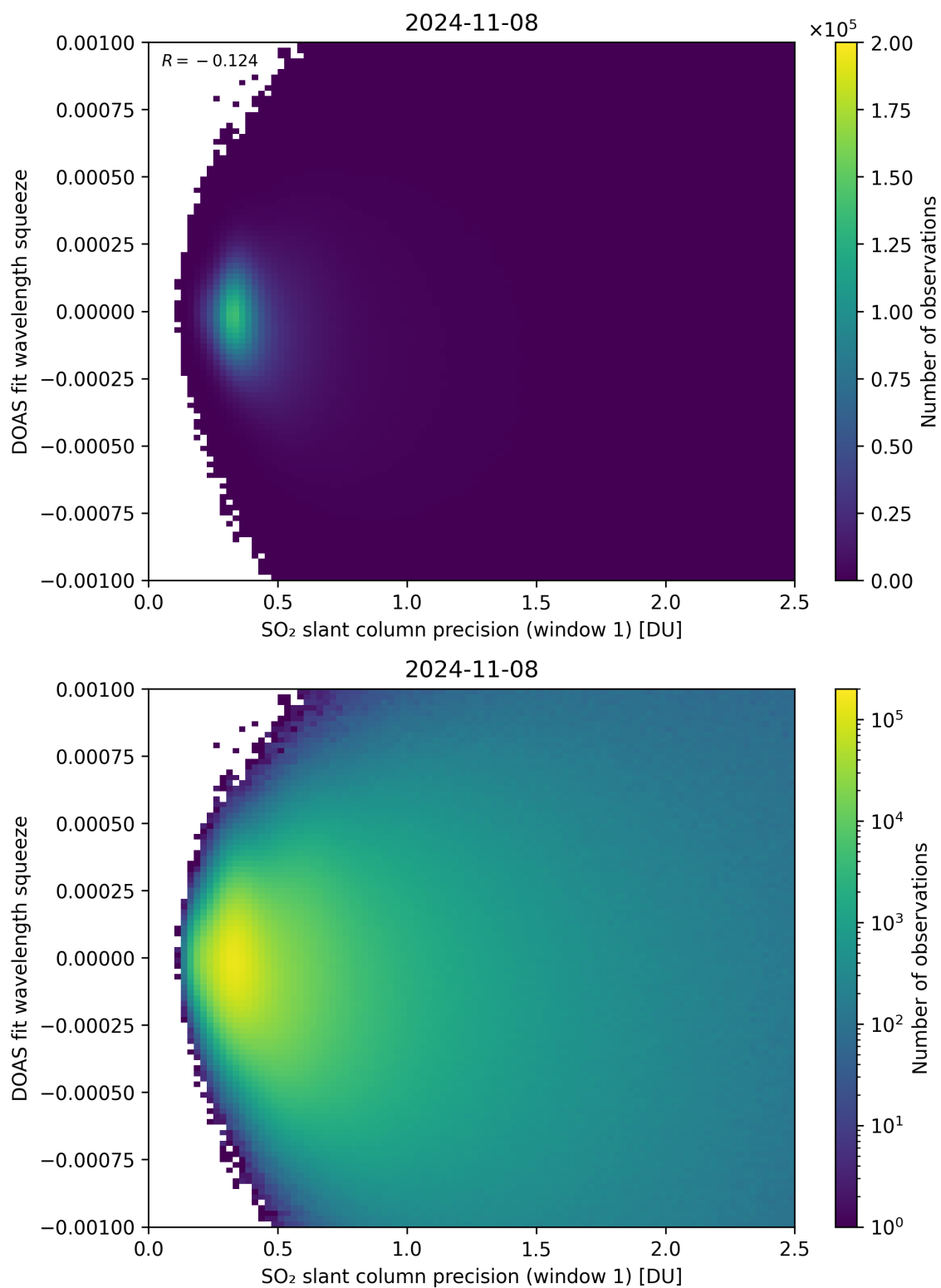
Figure 222: Scatter density plot of “SO 2 slant column precision (window 1)” against “DOAS fit wavelength squeeze” for 2024-11-07 to 2024-11-09.
