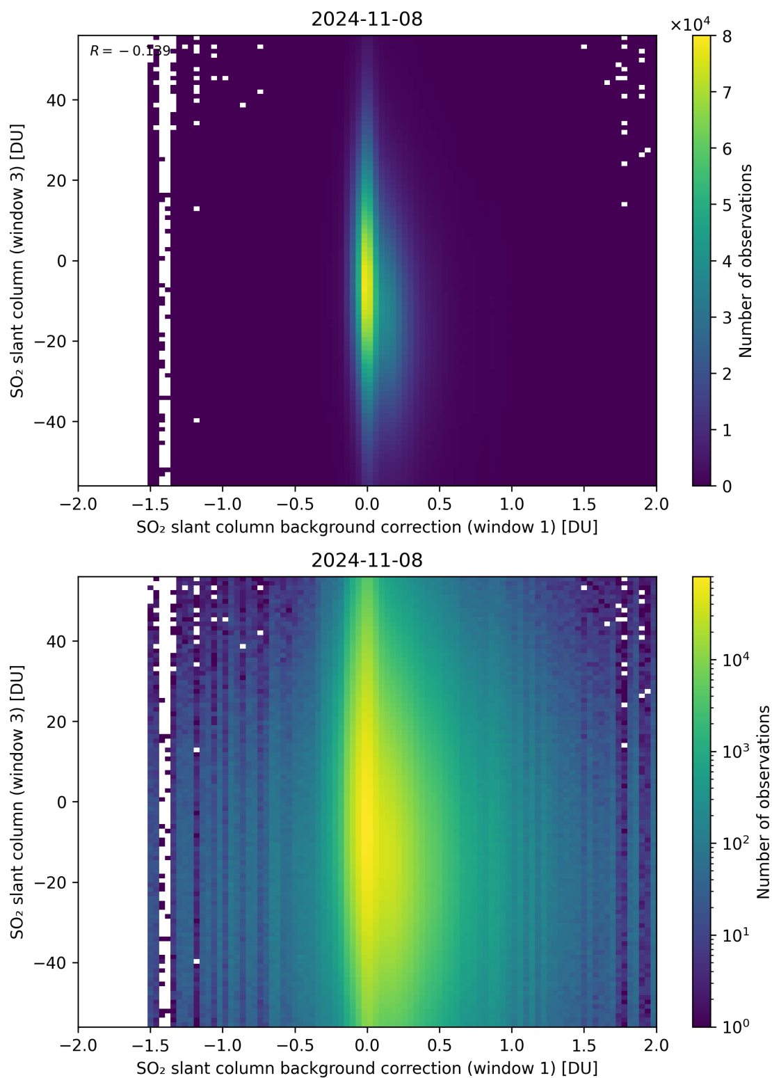
Figure 107: Scatter density plot of “SO 2 slant column background correction (window 1)” against “SO 2 slant column (window 3)” for 2024-11-07 to 2024-11-09.
