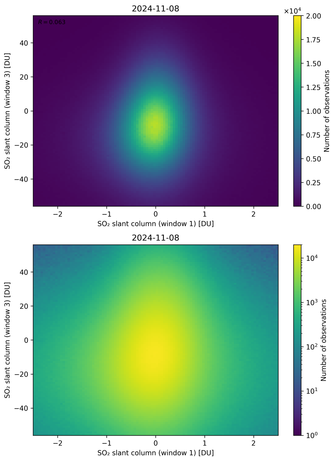
Figure 237: Scatter density plot of “SO 2 slant column (window 1)” against “SO 2 slant column (window 3)” for 2024-11-07 to 2024-11-09.
