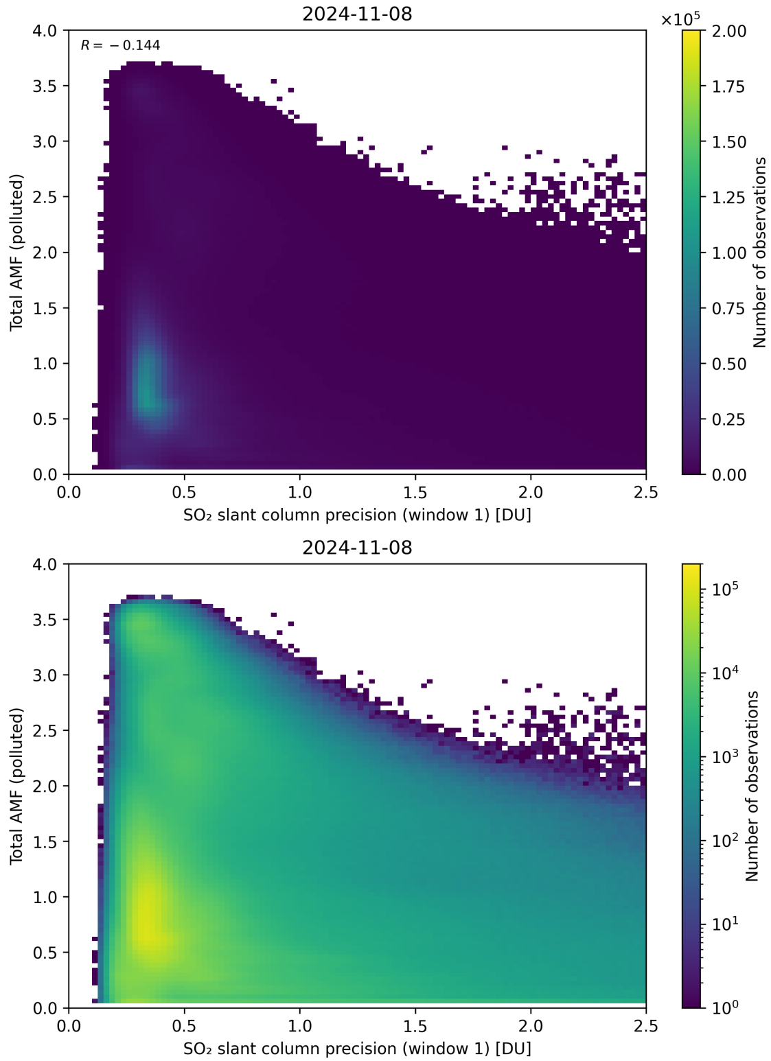
Figure 230: Scatter density plot of “SO 2 slant column precision (window 1)” against “Total AMF (polluted)” for 2024-11-07 to 2024-11-09.
