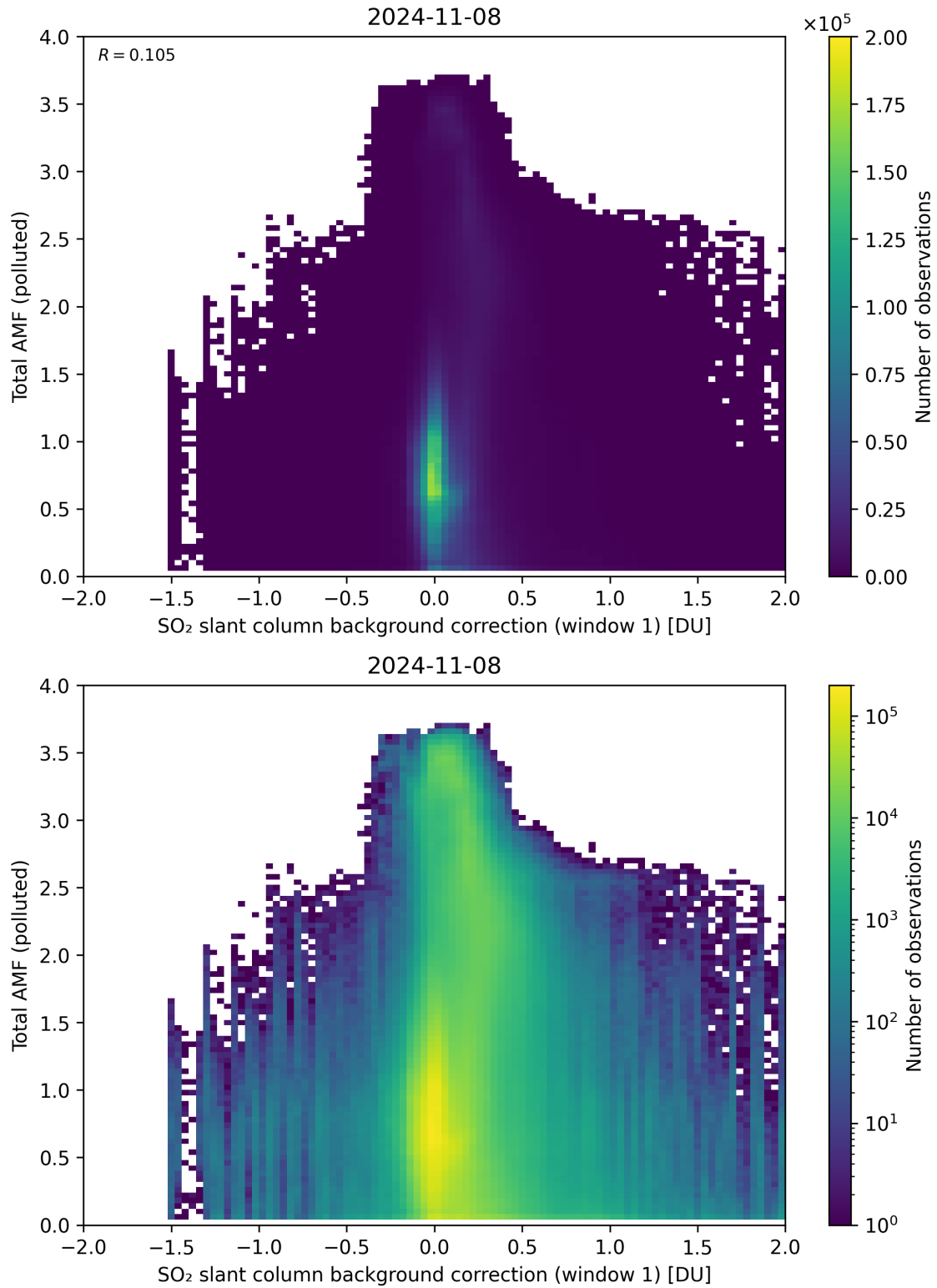
Figure 109: Scatter density plot of “SO 2 slant column background correction (window 1)” against “Total AMF (polluted)” for 2024-11-07 to 2024-11-09.
