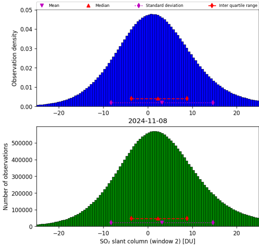
Figure 60: Histogram of “SO 2 slant column (window 2)” for 2024-11-07 to 2024-11-09
