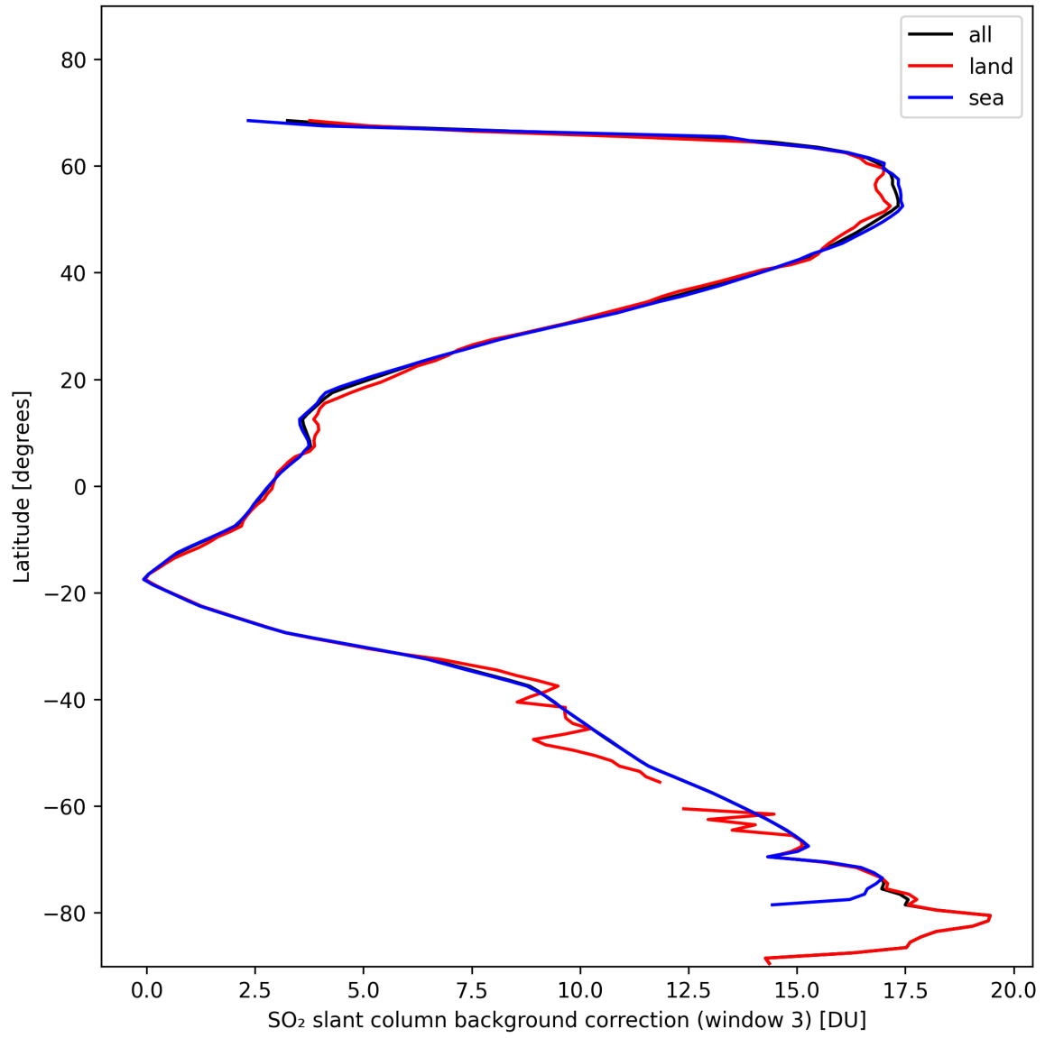
Figure 44: Zonal average of “SO 2 slant column background correction (window 3)” for 2024-11-07 to 2024-11-09.
