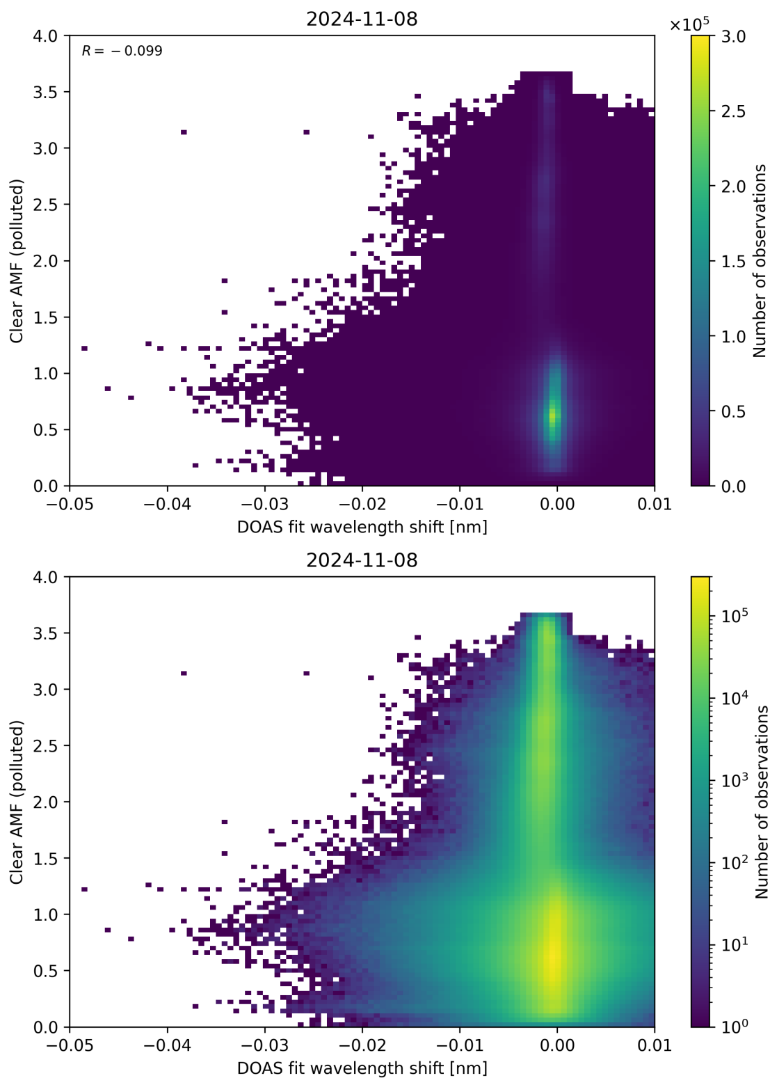
Figure 129: Scatter density plot of “DOAS fit wavelength shift” against “Clear AMF (polluted)” for 2024-11-07 to 2024-11-09.
