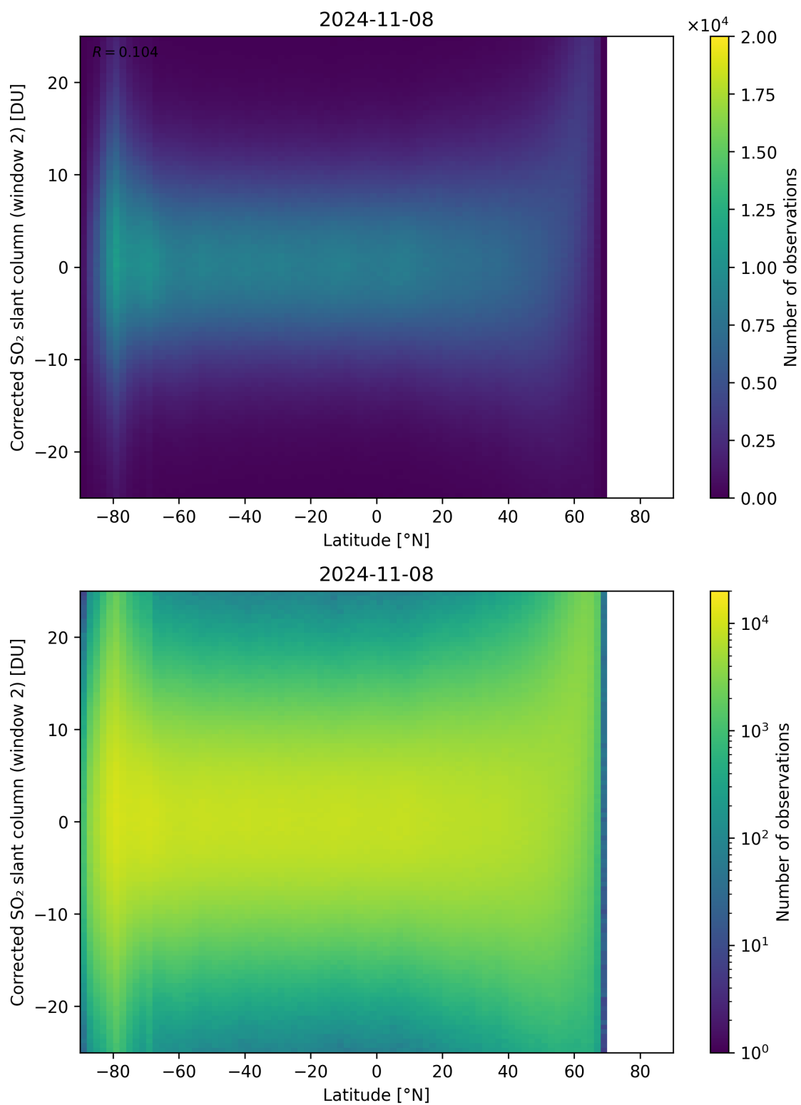
Figure 147: Scatter density plot of “Latitude” against “Corrected SO 2 slant column (window 2)” for 2024-11-07 to 2024-11-09.
