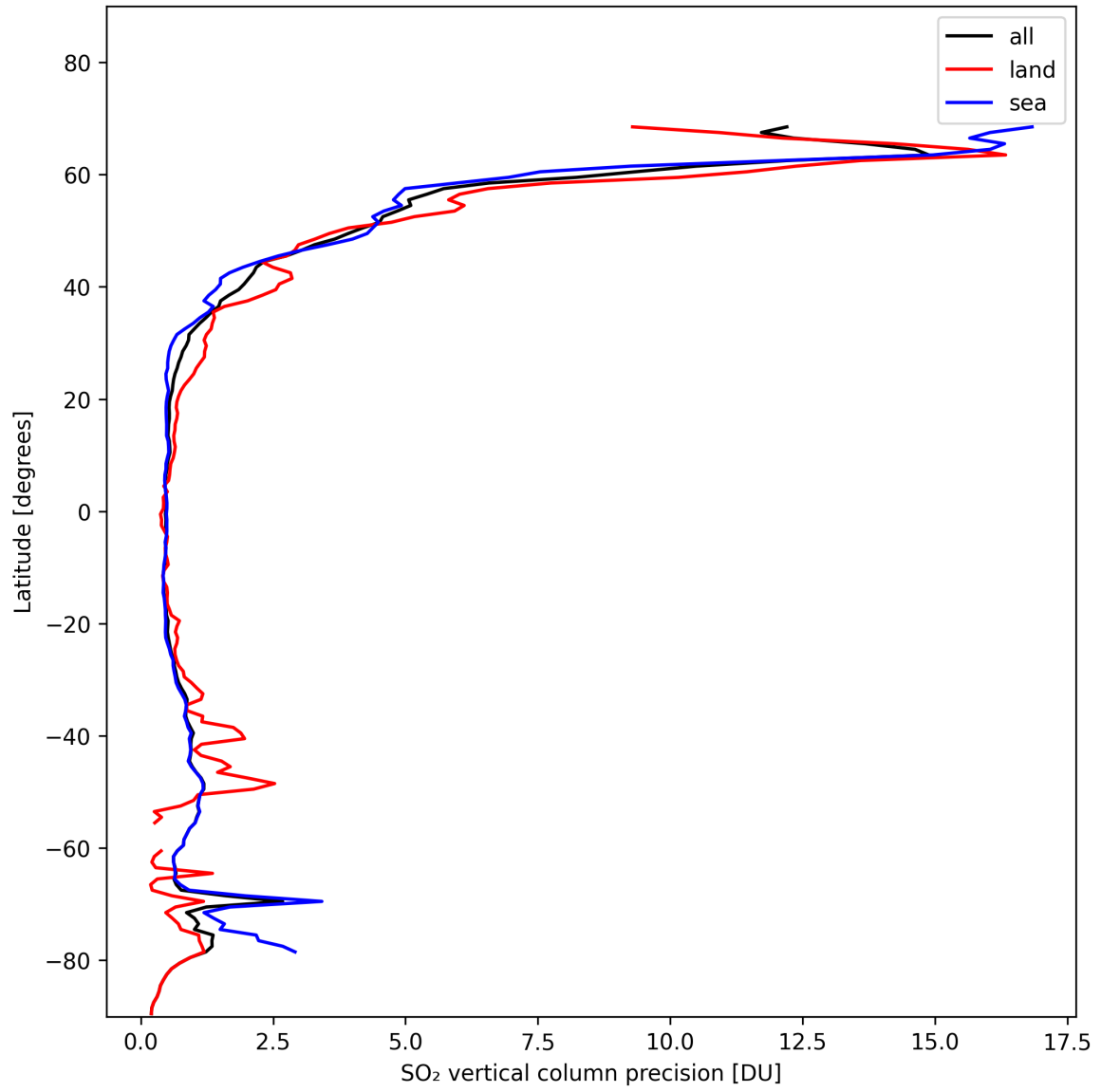
Figure 31: Zonal average of “SO 2 vertical column precision” for 2024-11-07 to 2024-11-09.
