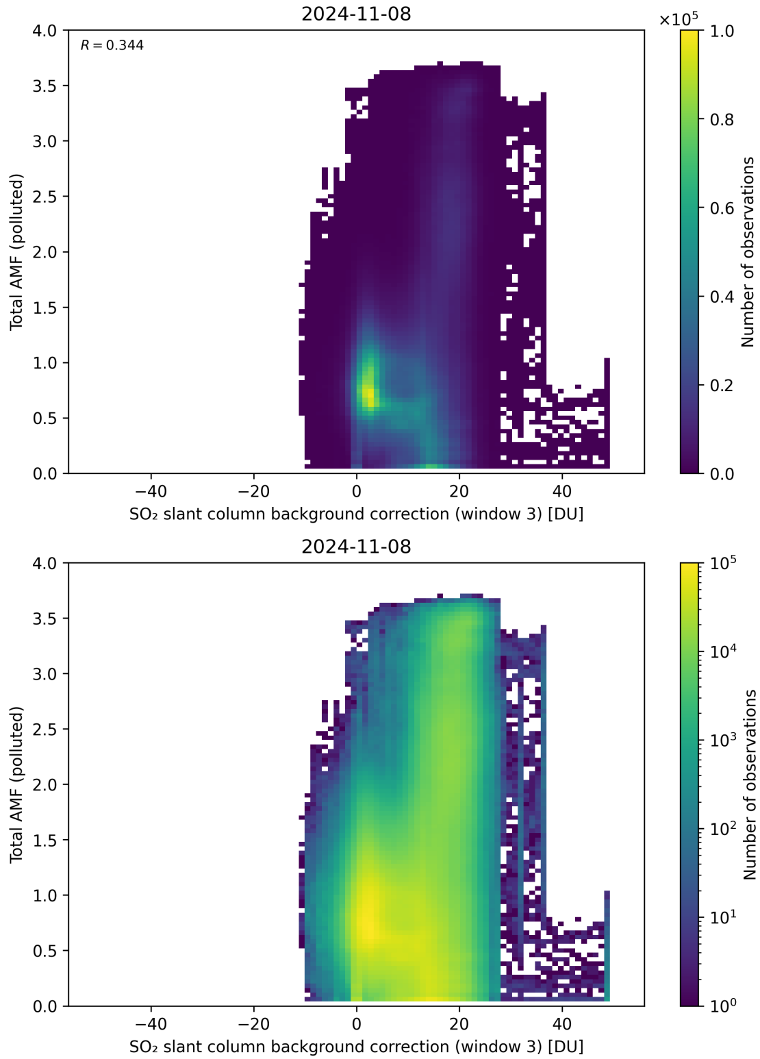
Figure 125: Scatter density plot of “SO 2 slant column background correction (window 3)” against “Total AMF (polluted)” for 2024-11-07 to 2024-11-09.
