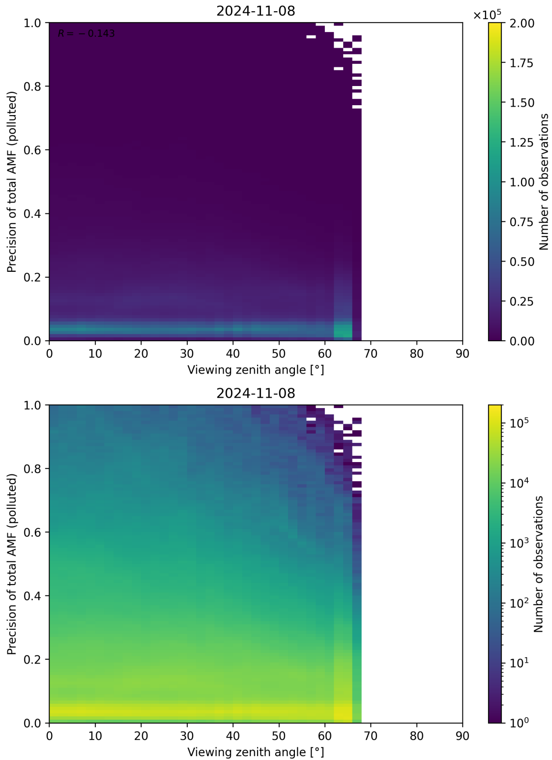
Figure 326: Scatter density plot of “Viewing zenith angle” against “Precision of total AMF (polluted)” for 2024-11-07 to 2024-11-09.
