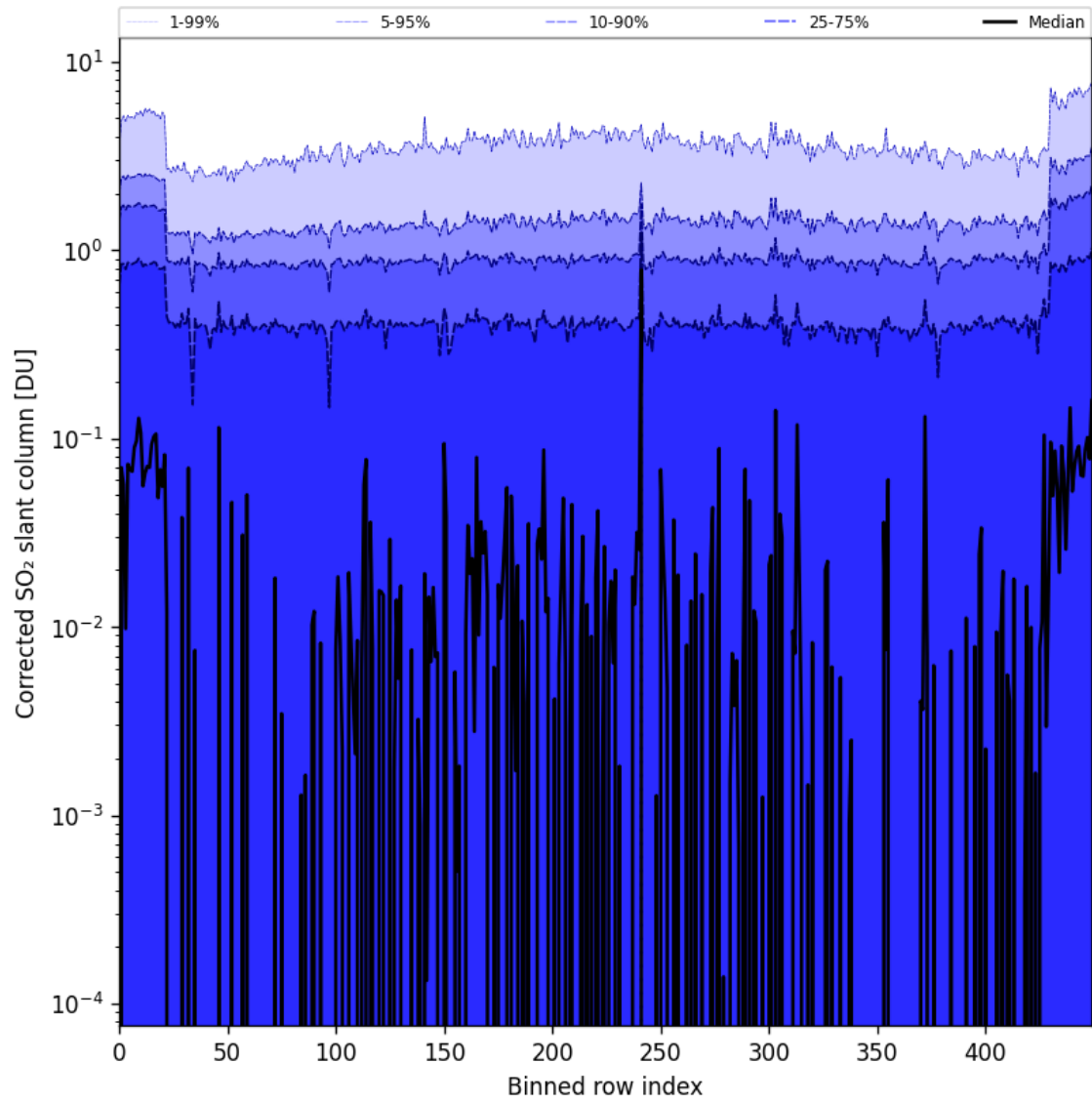
Figure 78: Along track statistics of “Corrected SO 2 slant column” for 2024-11-07 to 2024-11-09
