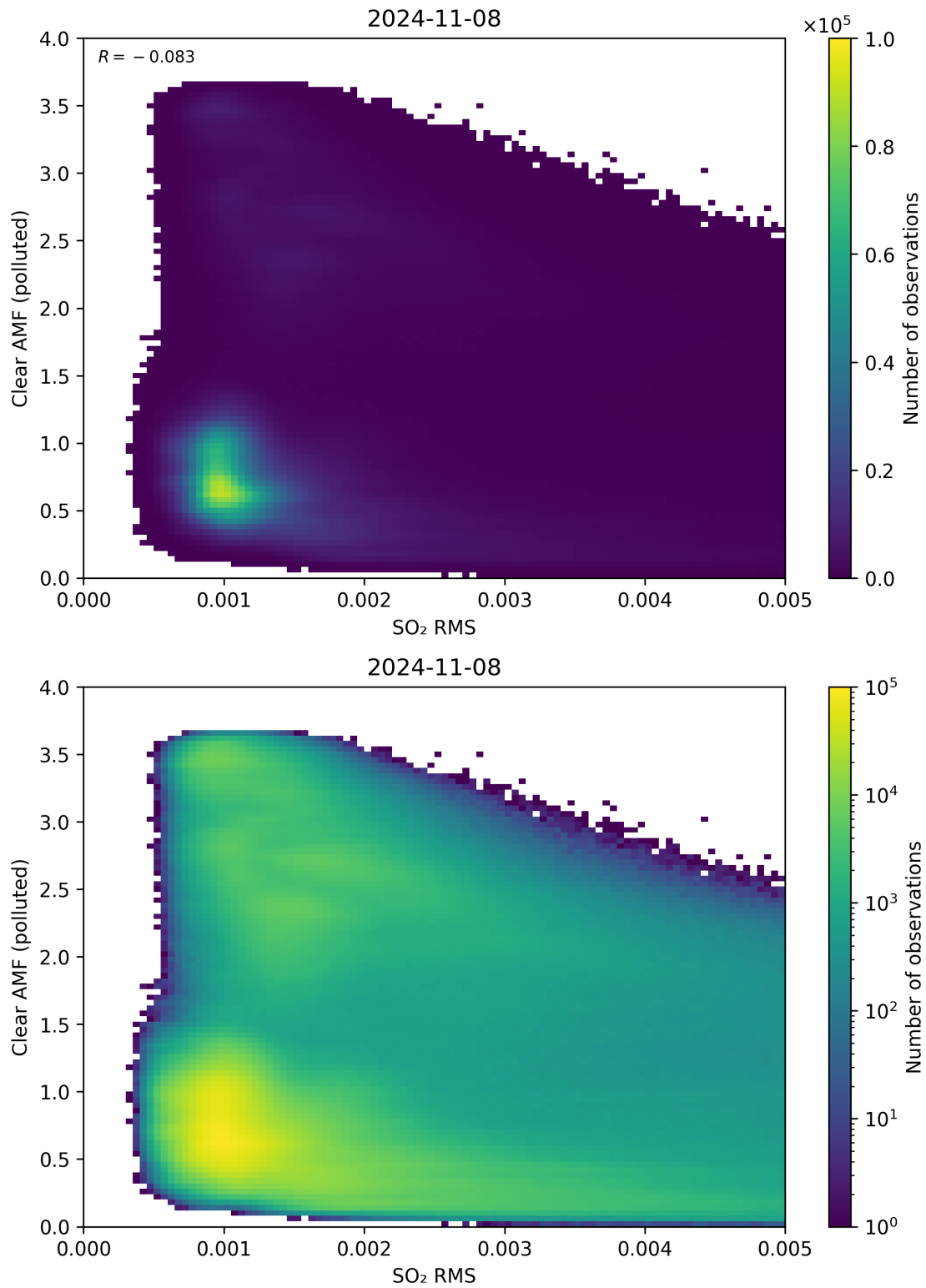
Figure 136: Scatter density plot of “SO 2 RMS” against “Clear AMF (polluted)” for 2024-11-07 to 2024-11-09.
