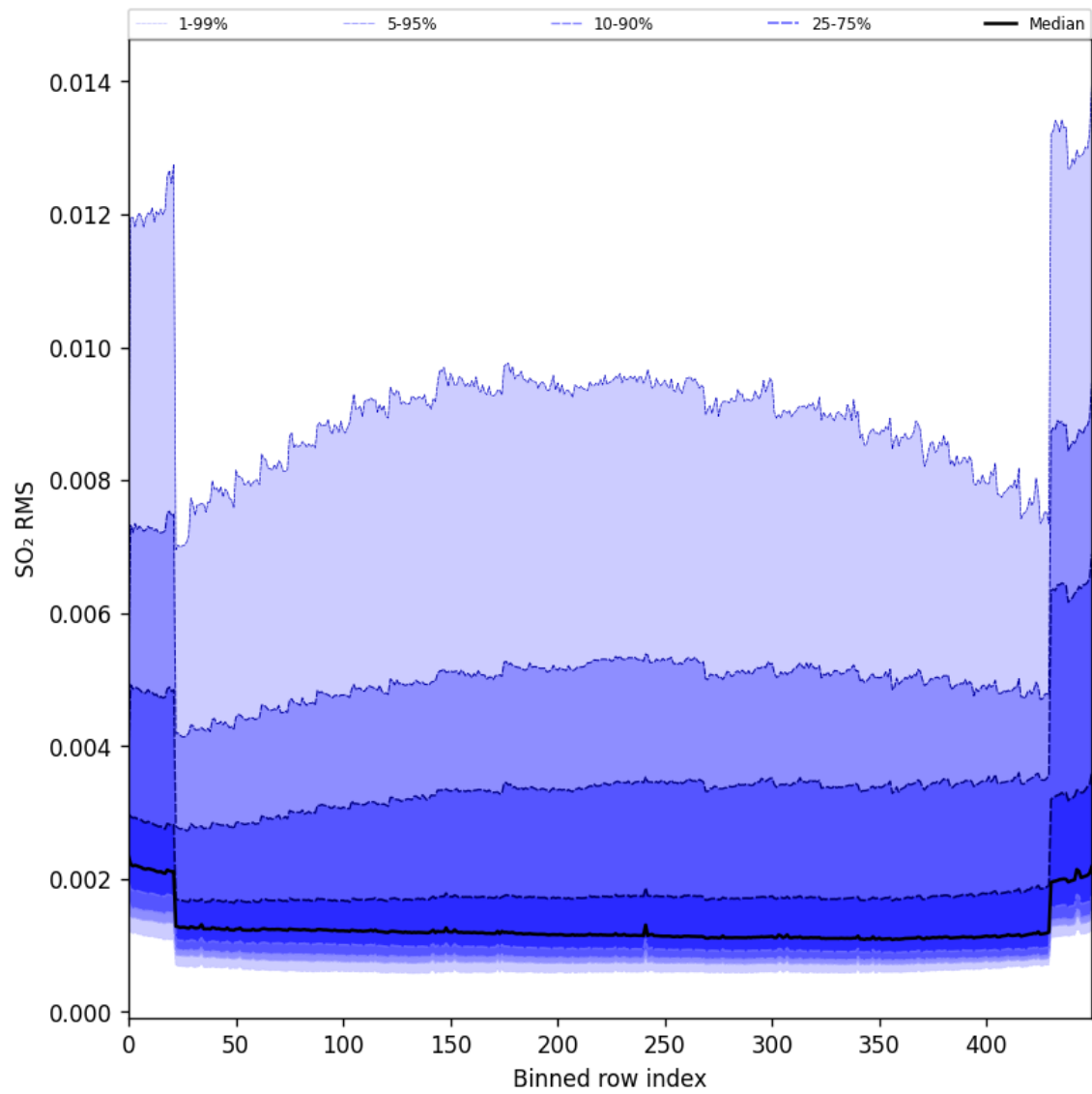
Figure 93: Along track statistics of “SO 2 RMS” for 2024-11-07 to 2024-11-09
