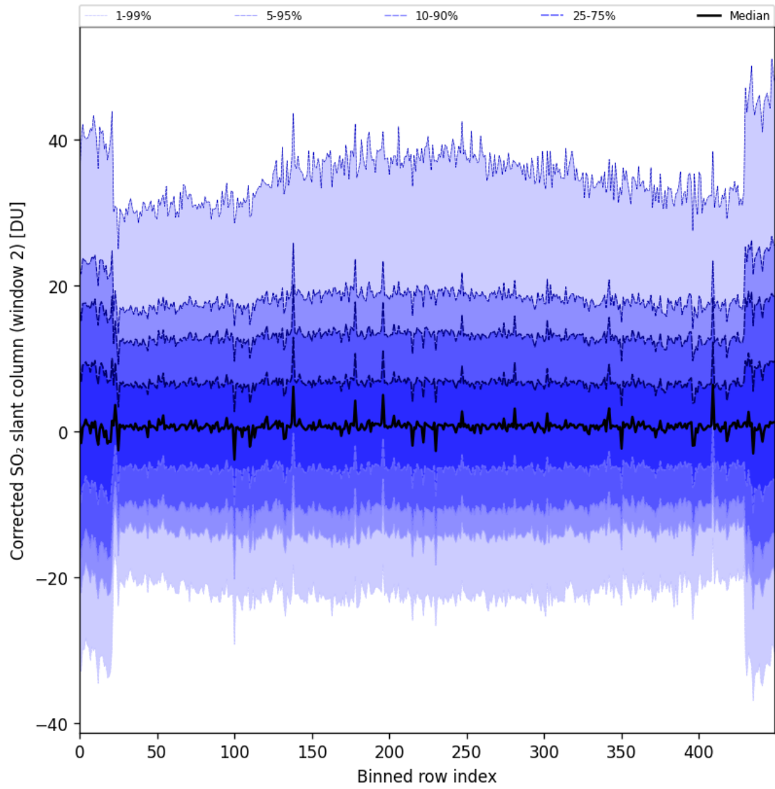
Figure 85: Along track statistics of “Corrected SO 2 slant column (window 2)” for 2024-11-07 to 2024-11-09
