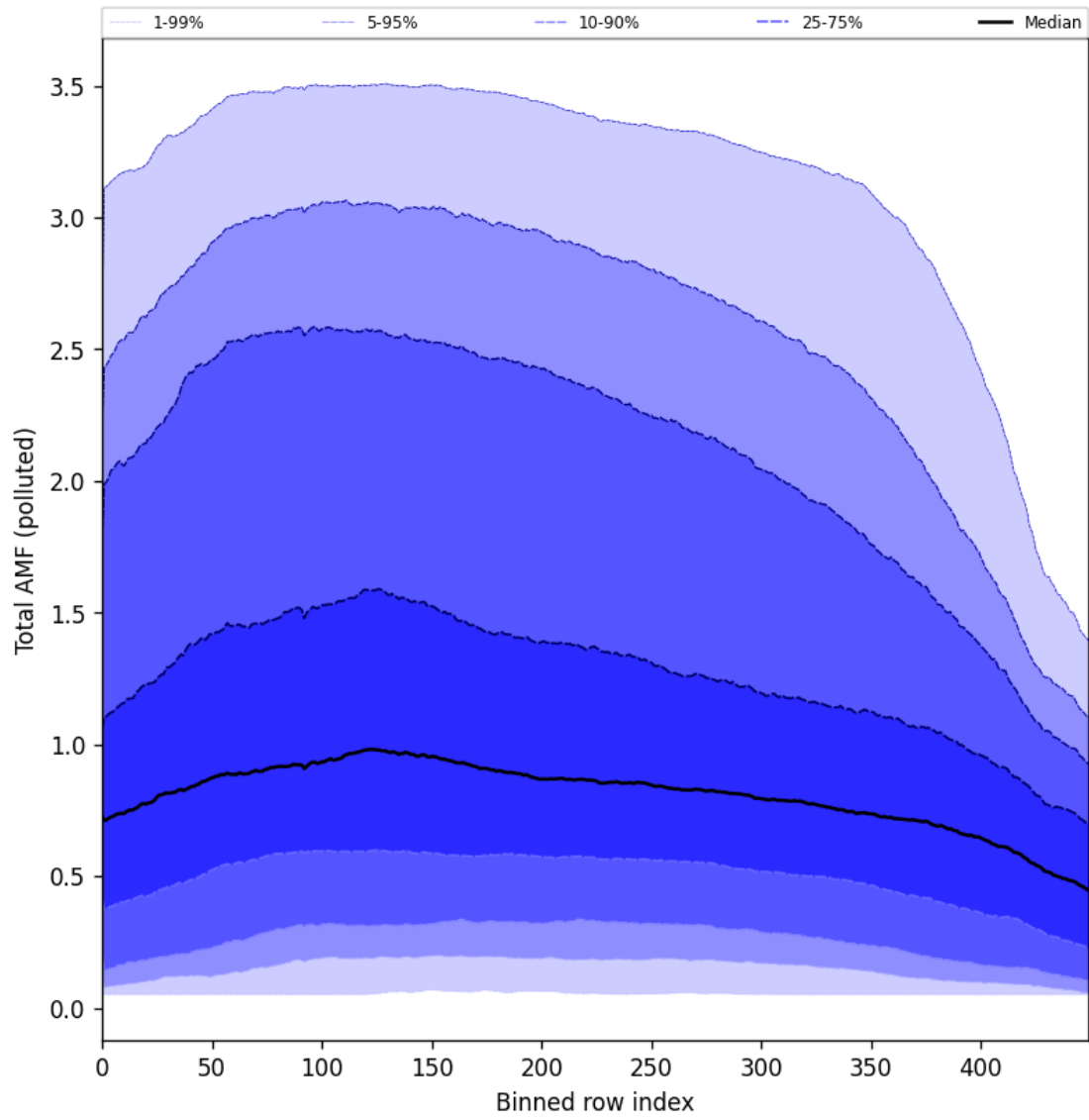
Figure 94: Along track statistics of “Total AMF (polluted)” for 2024-11-07 to 2024-11-09
