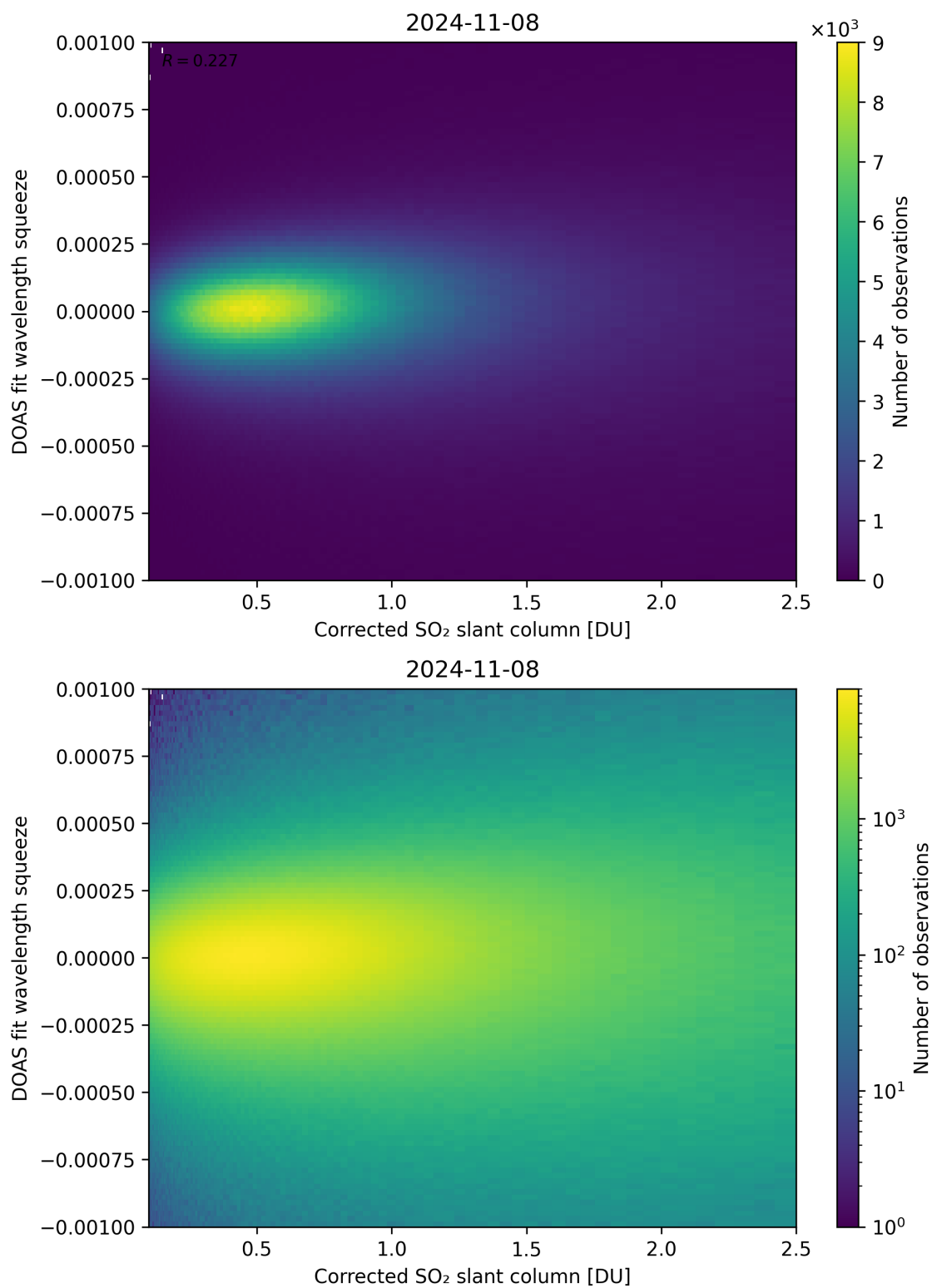
Figure 182: Scatter density plot of “Corrected SO 2 slant column” against “DOAS fit wavelength squeeze” for 2024-11-07 to 2024-11-09.
