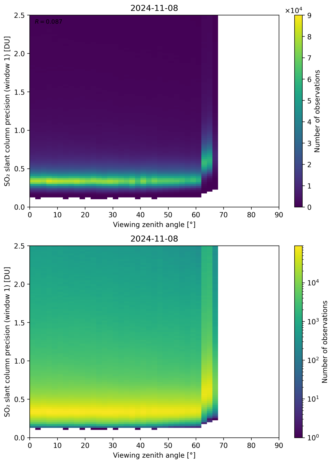
Figure 321: Scatter density plot of “Viewing zenith angle” against “SO 2 slant column precision (window 1)” for 2024-11-07 to 2024-11-09.
