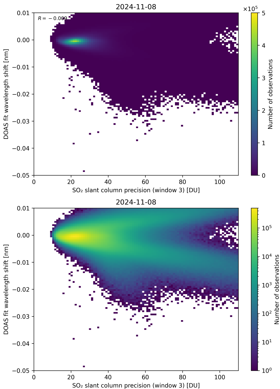
Figure 258: Scatter density plot of “SO 2 slant column precision (window 3)” against “DOAS fit wavelength shift” for 2024-11-07 to 2024-11-09.
