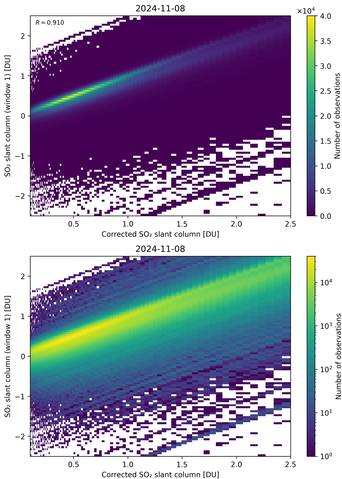
Figure 187: Scatter density plot of “Corrected SO 2 slant column” against “SO 2 slant column (window 1)” for 2024-11-07 to 2024-11-09.
