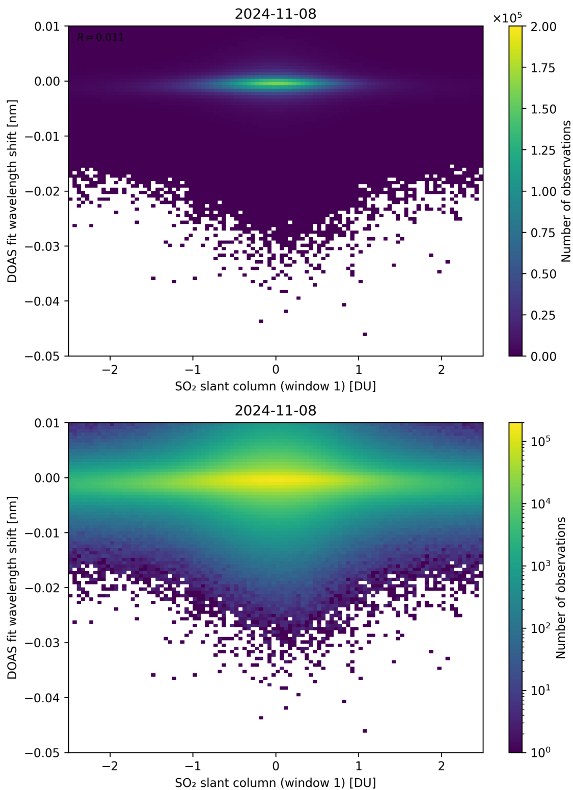
Figure 215: Scatter density plot of “SO 2 slant column (window 1)” against “DOAS fit wavelength shift” for 2024-11-07 to 2024-11-09.
