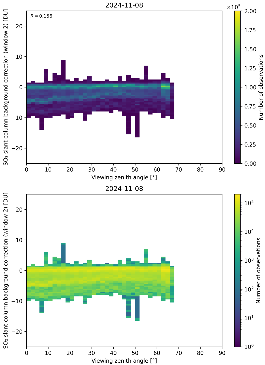
Figure 309: Scatter density plot of “Viewing zenith angle” against “SO 2 slant column background correction (window 2)” for 2024-11-07 to 2024-11-09.
