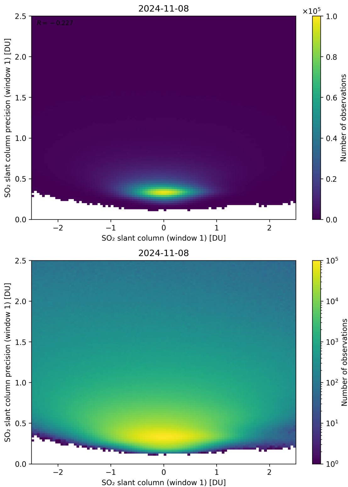
Figure 235: Scatter density plot of “SO 2 slant column (window 1)” against “SO 2 slant column precision (window 1)” for 2024-11-07 to 2024-11-09.
