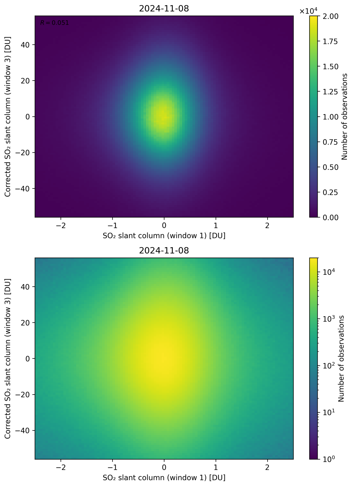
Figure 234: Scatter density plot of “SO 2 slant column (window 1)” against “Corrected SO 2 slant column (window 3)” for 2024-11-07 to 2024-11-09.
