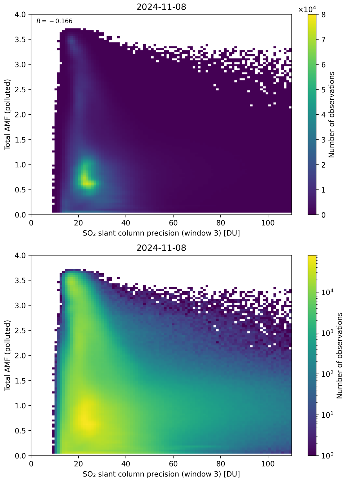
Figure 263: Scatter density plot of “SO 2 slant column precision (window 3)” against “Total AMF (polluted)” for 2024-11-07 to 2024-11-09.
