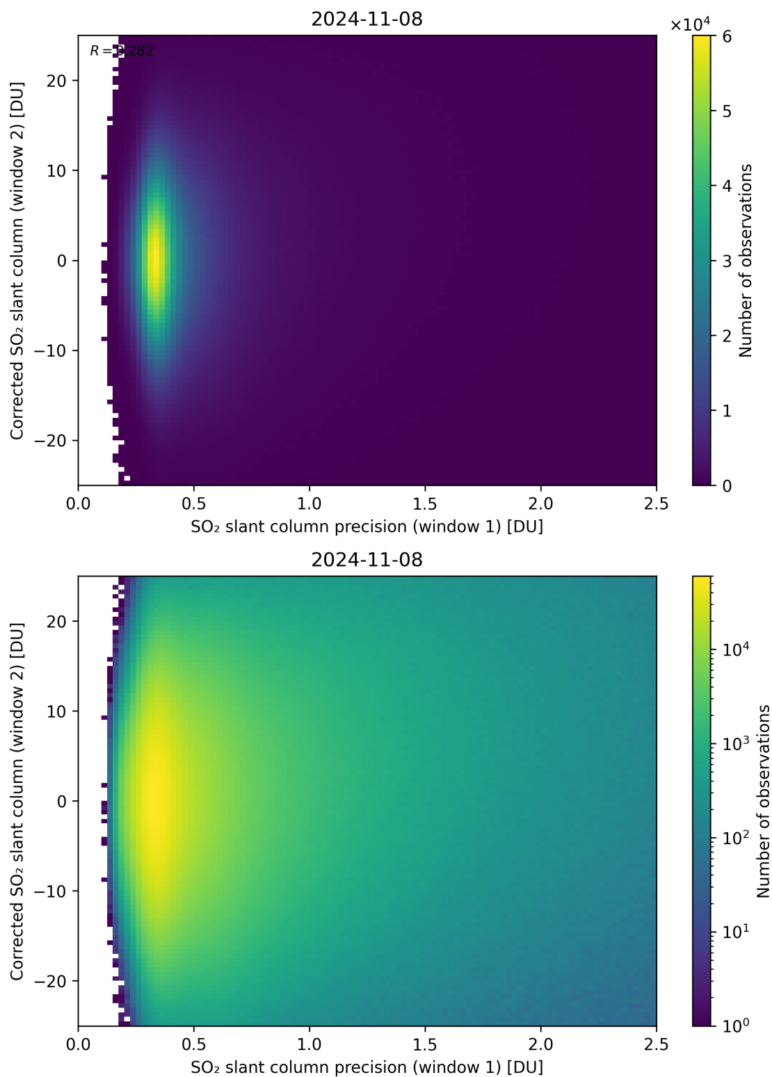
Figure 225: Scatter density plot of “SO 2 slant column precision (window 1)” against “Corrected SO 2 slant column (window 2)” for 2024-11-07 to 2024-11-09.
