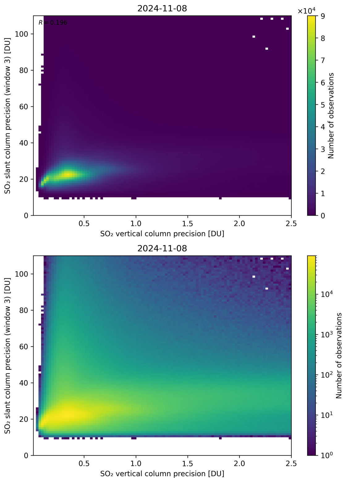
Figure 293: Scatter density plot of “SO 2 vertical column precision” against “SO 2 slant column precision (window 3)” for 2024-11-07 to 2024-11-09.
