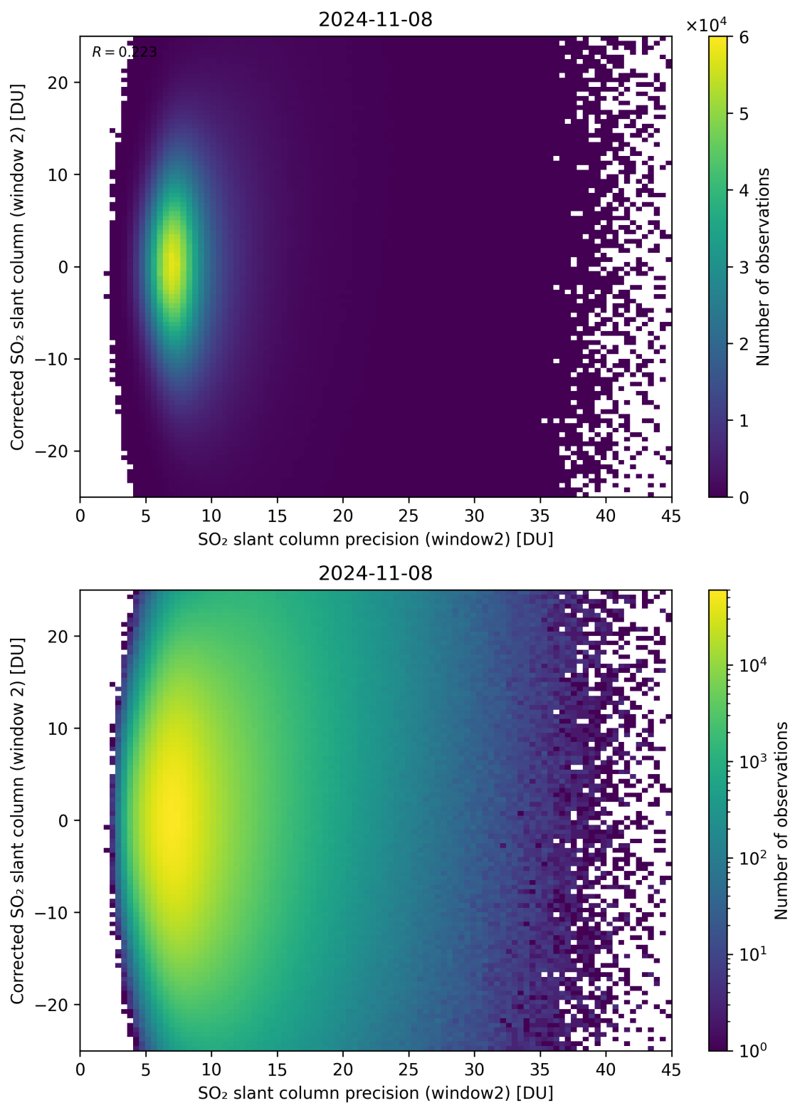
Figure 247: Scatter density plot of “SO 2 slant column precision (window2)” against “Corrected SO 2 slant column (window 2)” for 2024-11-07 to 2024-11-09.
