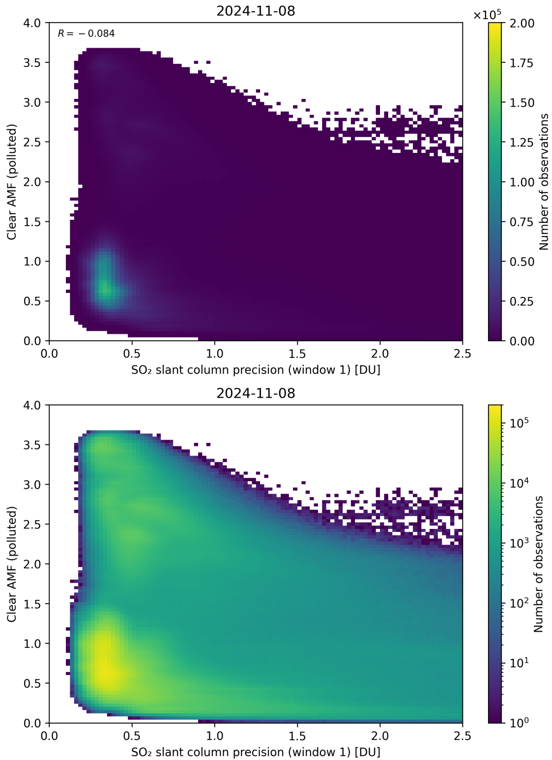
Figure 224: Scatter density plot of “SO 2 slant column precision (window 1)” against “Clear AMF (polluted)” for 2024-11-07 to 2024-11-09.
