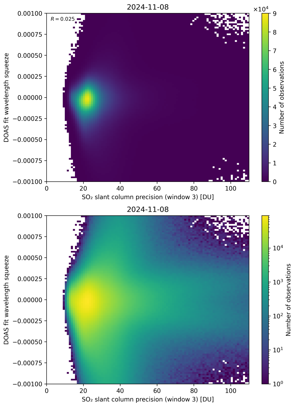
Figure 259: Scatter density plot of “SO 2 slant column precision (window 3)” against “DOAS fit wavelength squeeze” for 2024-11-07 to 2024-11-09.
