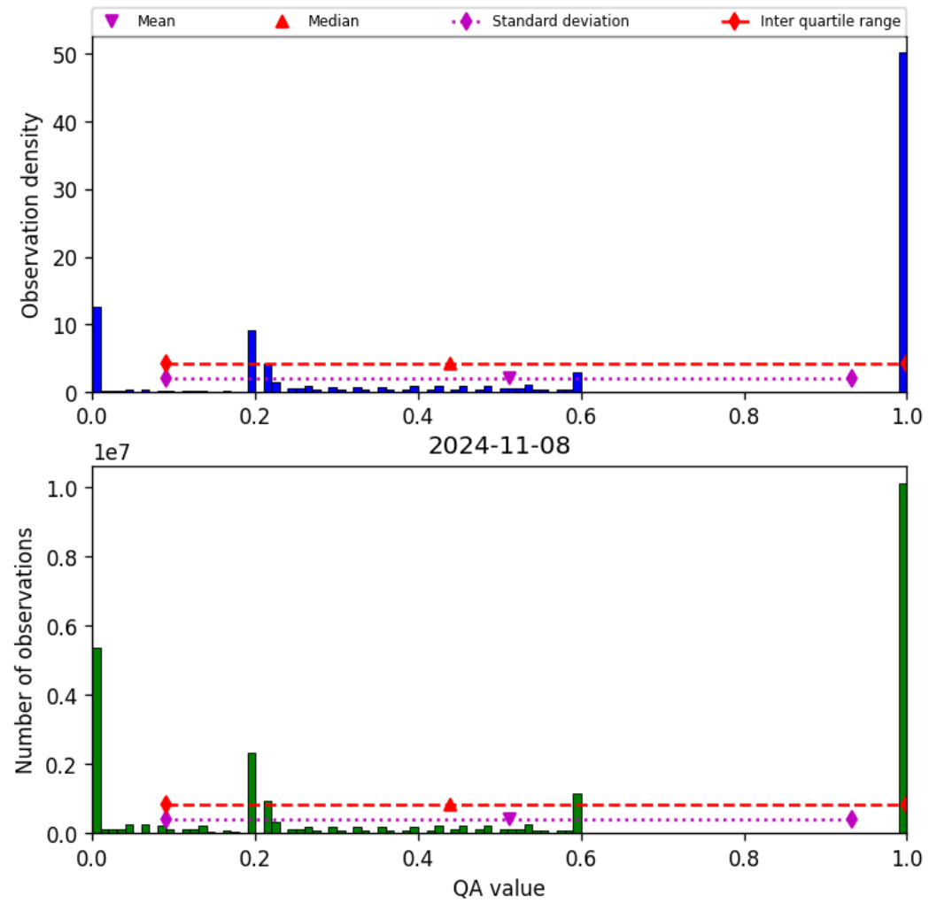
Figure 52: Histogram of “QA value” for 2024-11-07 to 2024-11-09
