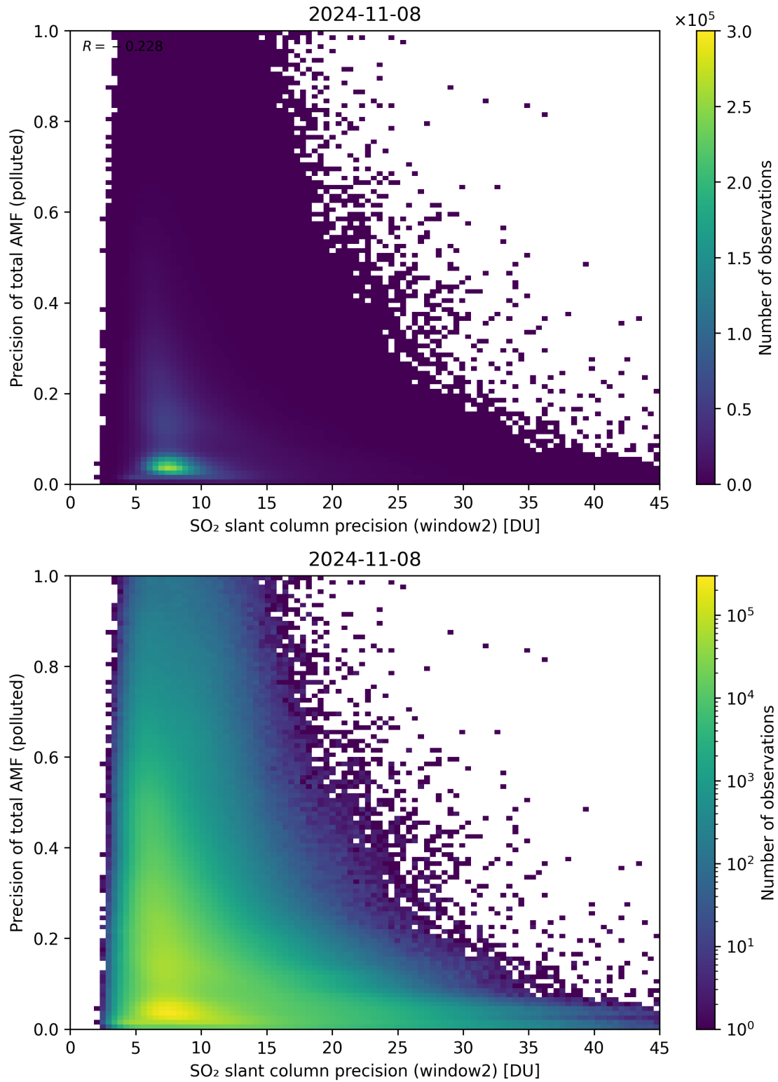
Figure 252: Scatter density plot of “SO 2 slant column precision (window2)” against “Precision of total AMF (polluted)” for 2024-11-07 to 2024-11-09.
