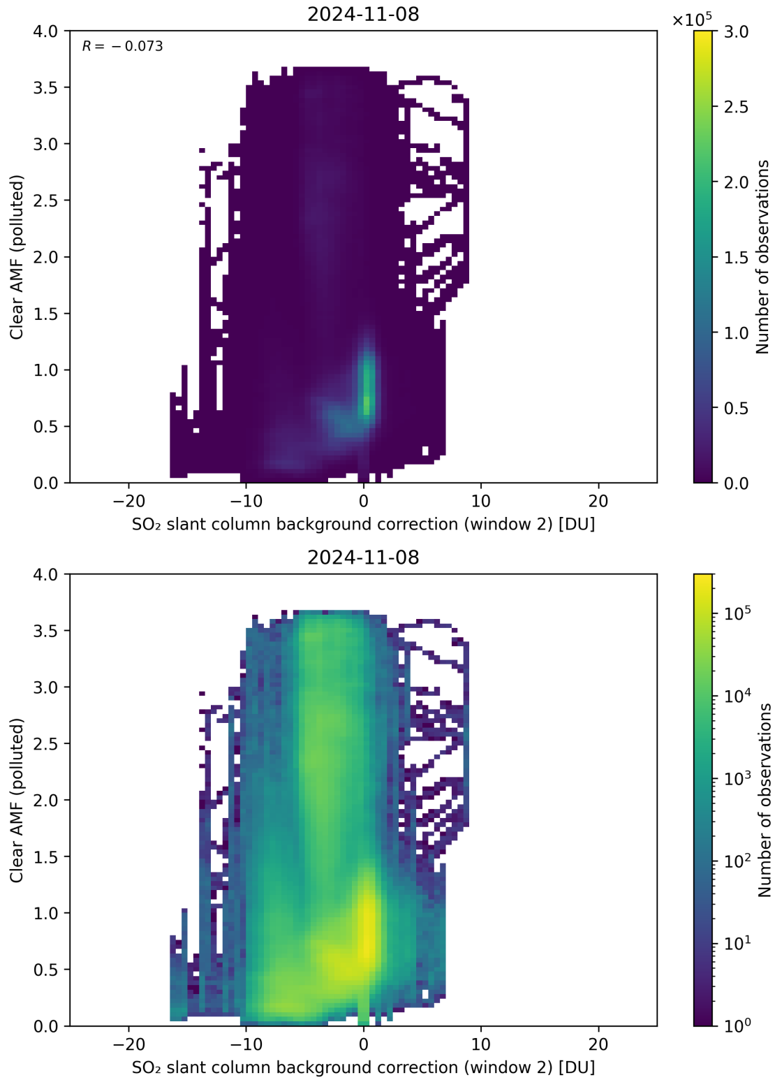
Figure 115: Scatter density plot of “SO 2 slant column background correction (window 2)” against “Clear AMF (polluted)” for 2024-11-07 to 2024-11-09.
