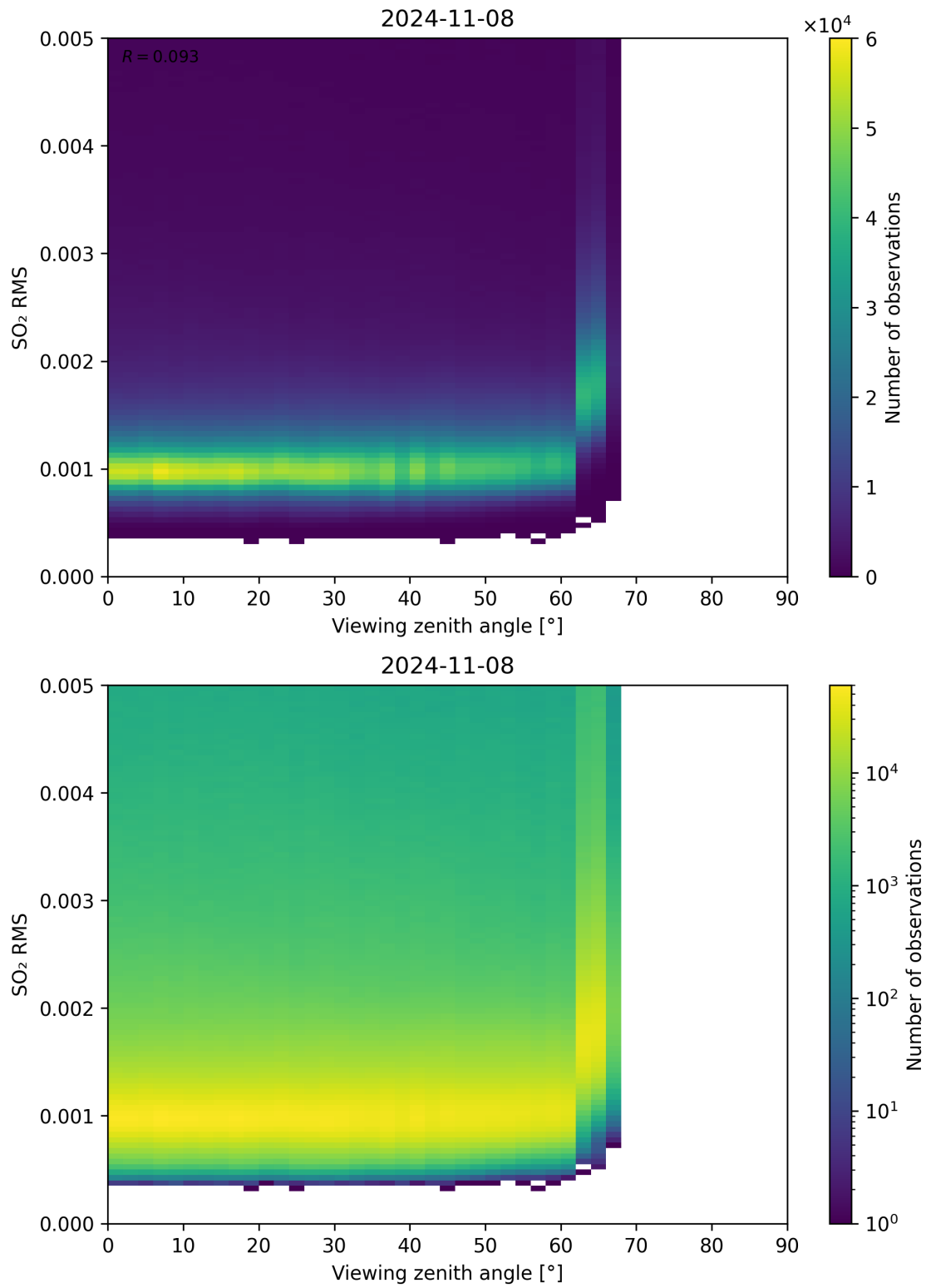
Figure 313: Scatter density plot of “Viewing zenith angle” against “SO 2 RMS” for 2024-11-07 to 2024-11-09.
