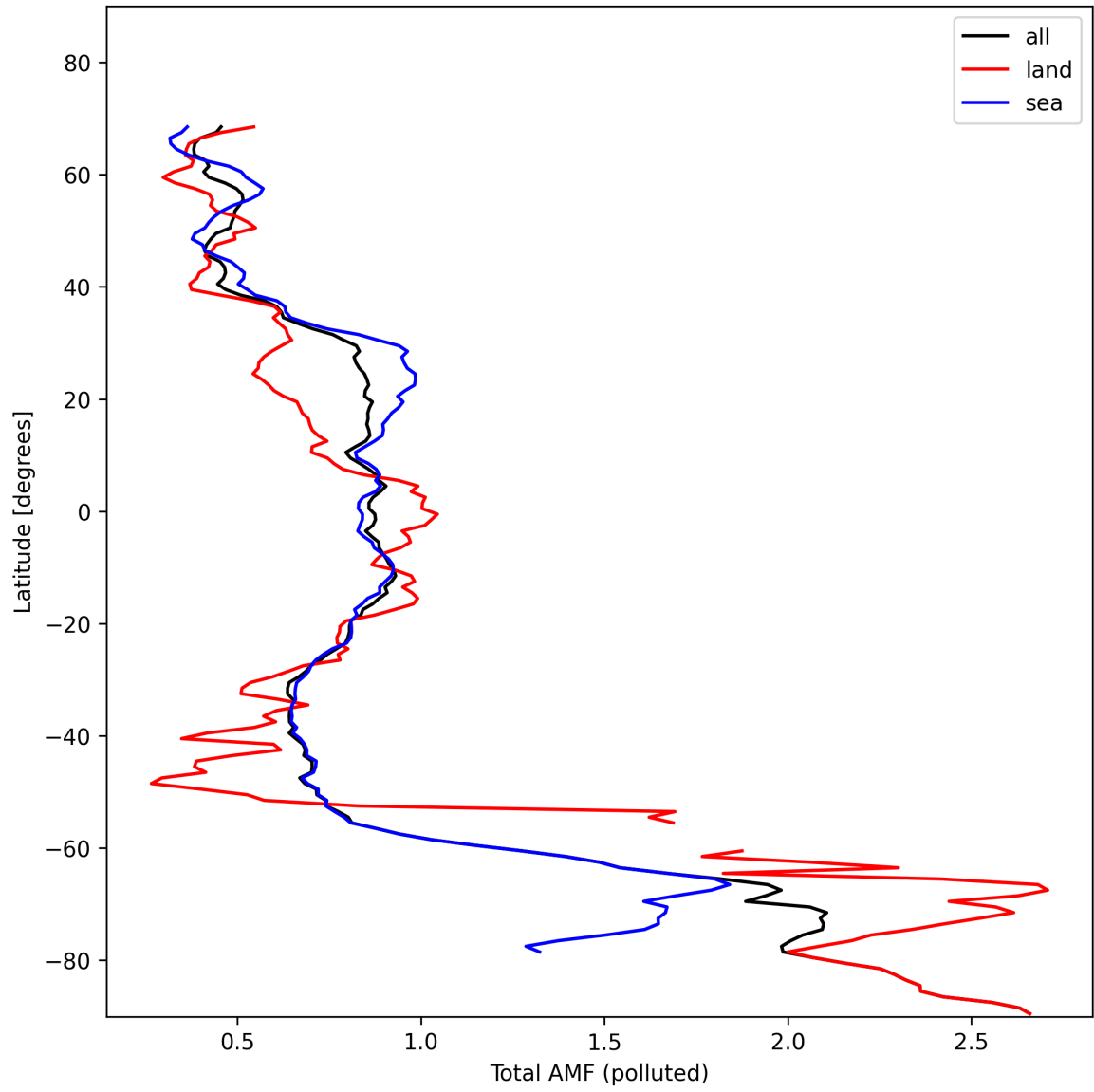
Figure 48: Zonal average of “Total AMF (polluted)” for 2024-11-07 to 2024-11-09.
