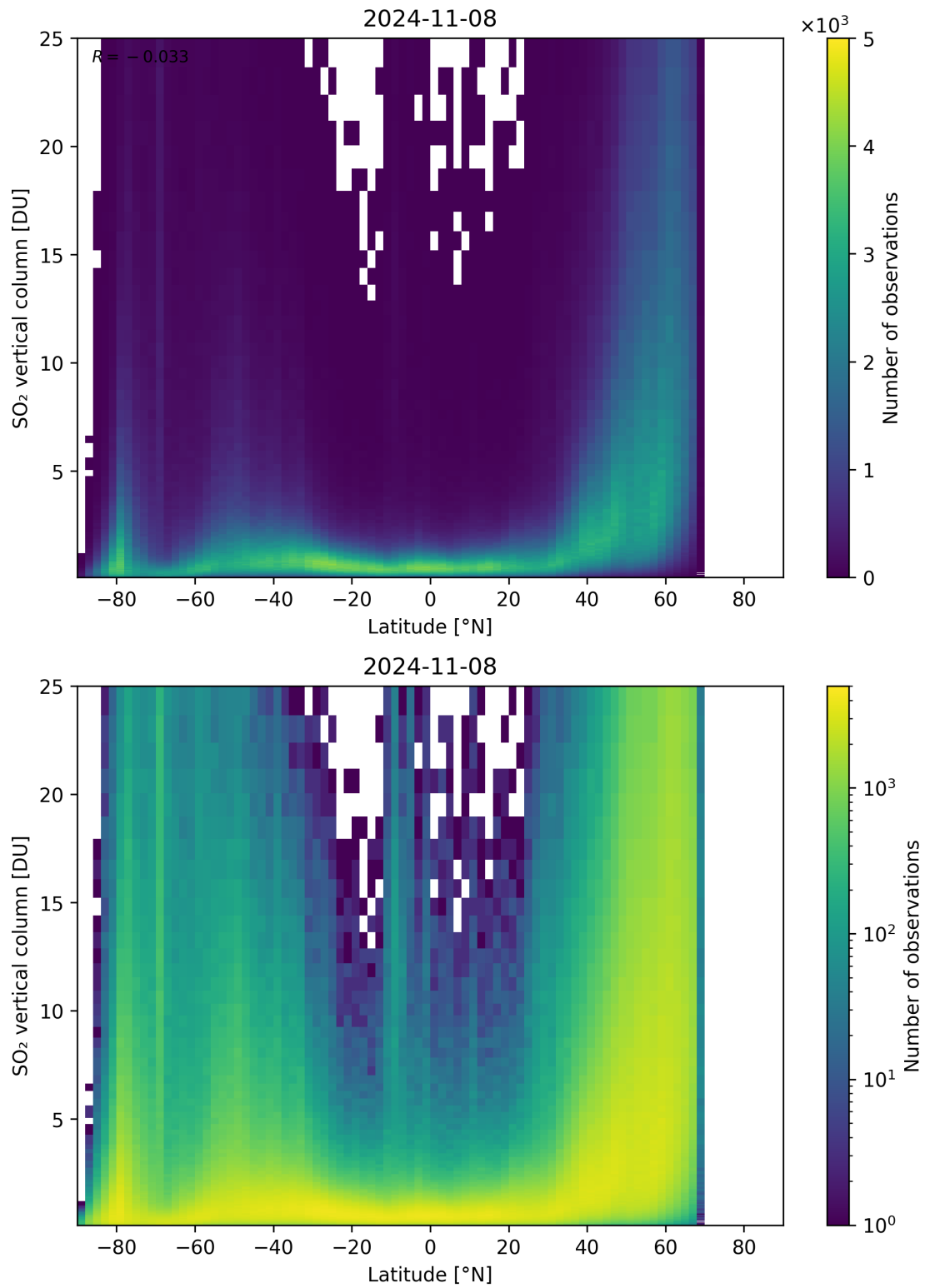
Figure 156: Scatter density plot of “Latitude” against “SO 2 vertical column” for 2024-11-07 to 2024-11-09.
