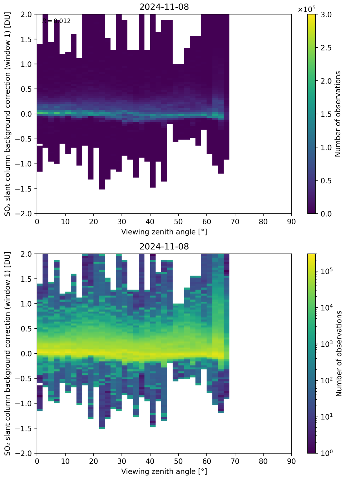
Figure 308: Scatter density plot of “Viewing zenith angle” against “SO 2 slant column background correction (window 1)” for 2024-11-07 to 2024-11-09.
