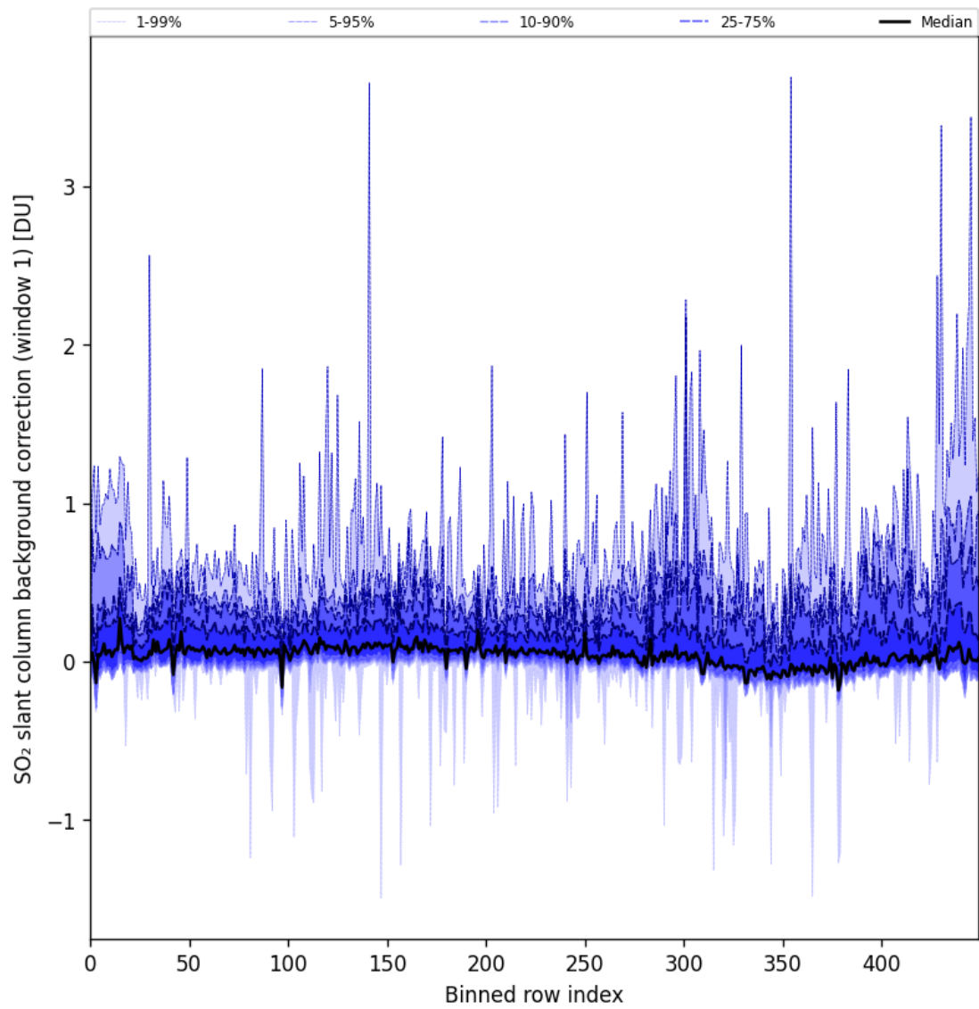
Figure 82: Along track statistics of "SO 2 slant column background correction (window 1)" for 2024-11-07 to 2024-11-09
