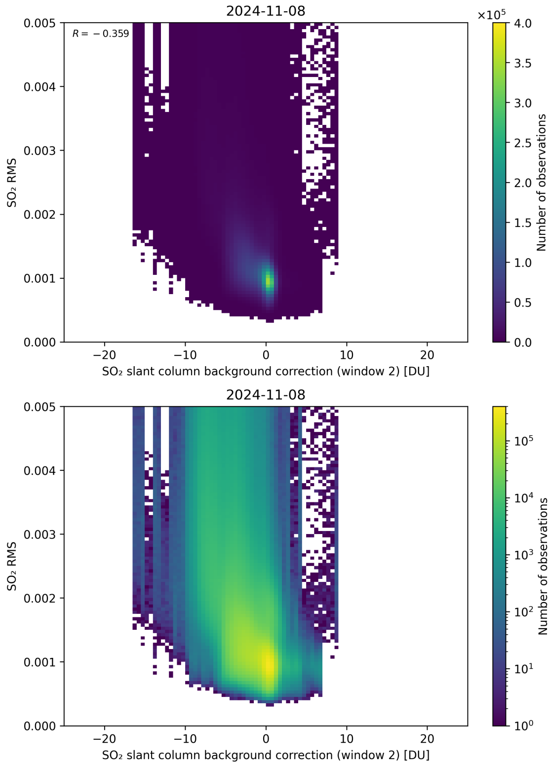
Figure 114: Scatter density plot of “SO 2 slant column background correction (window 2)” against “SO 2 RMS” for 2024-11-07 to 2024-11-09.
