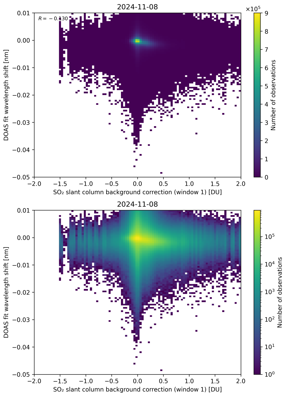
Figure 100: Scatter density plot of “SO 2 slant column background correction (window 1)” against “DOAS fit wavelength shift” for 2024-11-07 to 2024-11-09.
