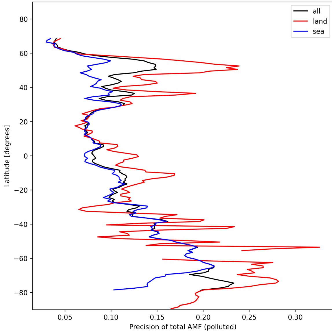
Figure 49: Zonal average of “Precision of total AMF (polluted)” for 2024-11-07 to 2024-11-09.
