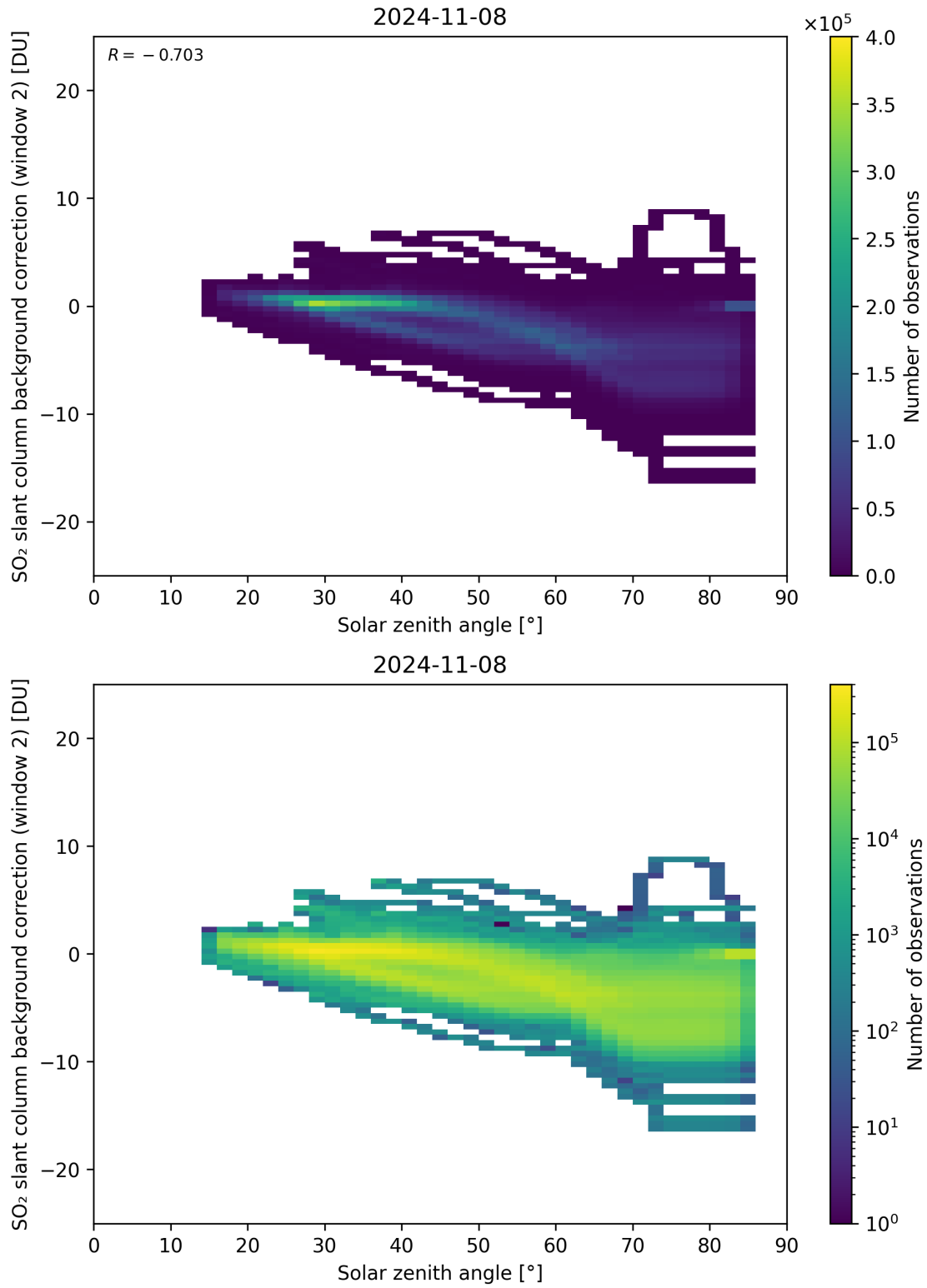
Figure 159: Scatter density plot of “Solar zenith angle” against “SO 2 slant column background correction (window 2)” for 2024-11-07 to 2024-11-09.
