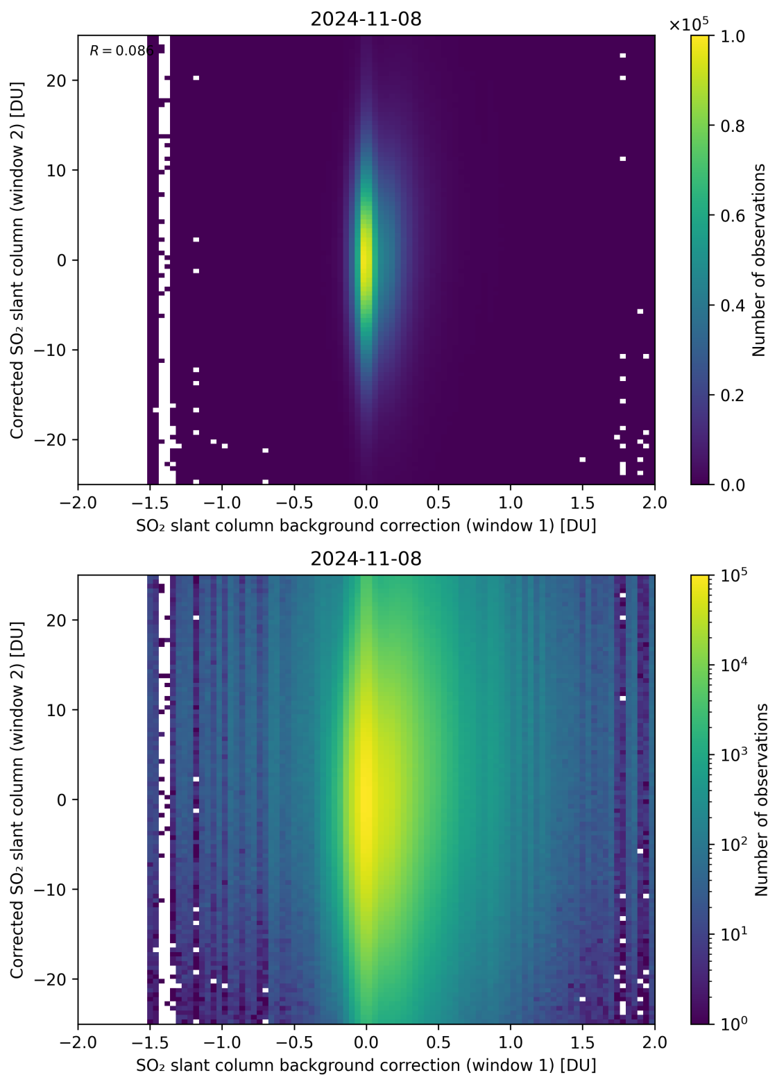
Figure 104: Scatter density plot of “SO 2 slant column background correction (window 1)” against “Corrected SO 2 slant column (window 2)” for 2024-11-07 to 2024-11-09.
