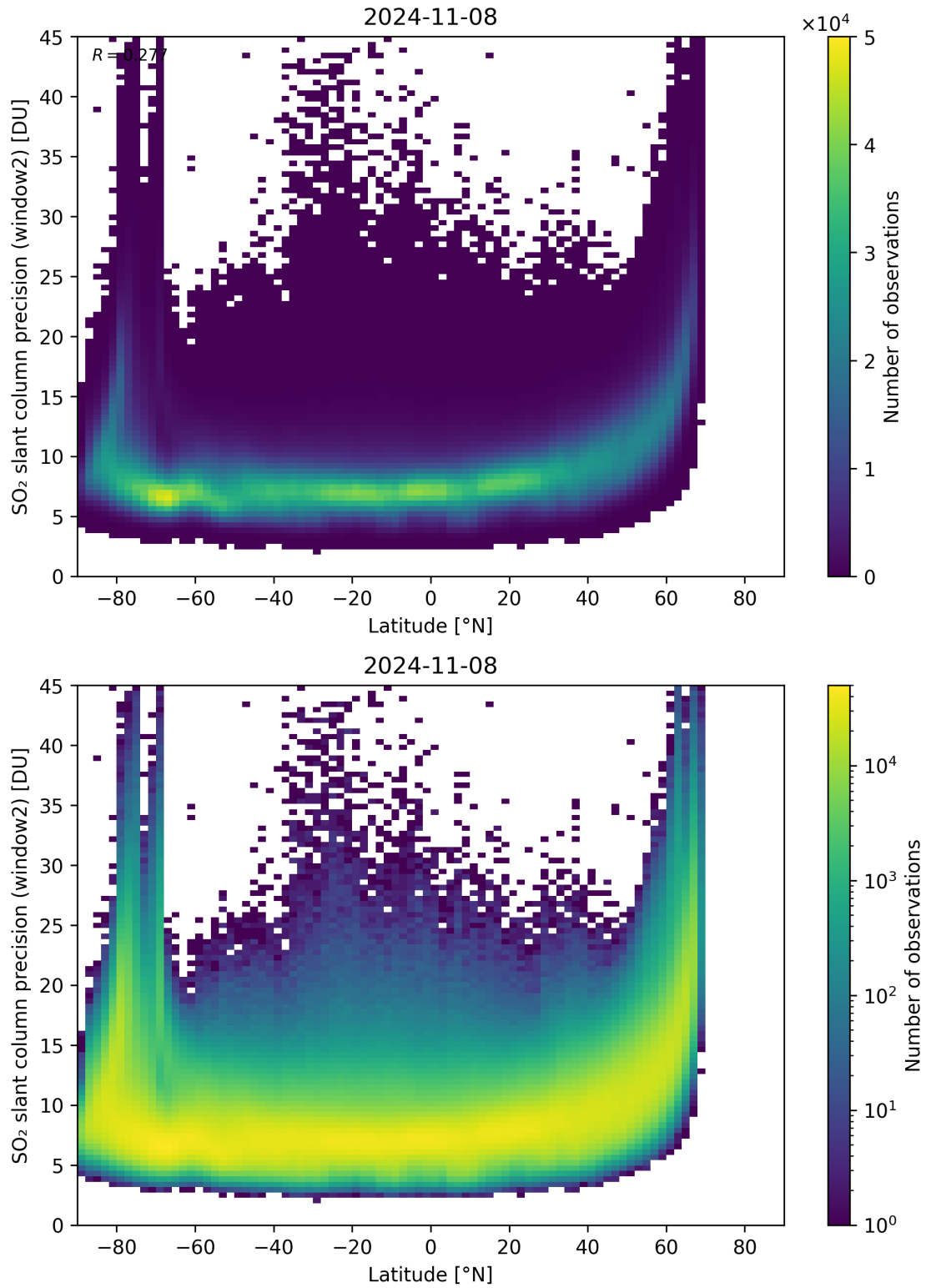
Figure 151: Scatter density plot of “Latitude” against “SO 2 slant column precision (window2)” for 2024-11-07 to 2024-11-09.
