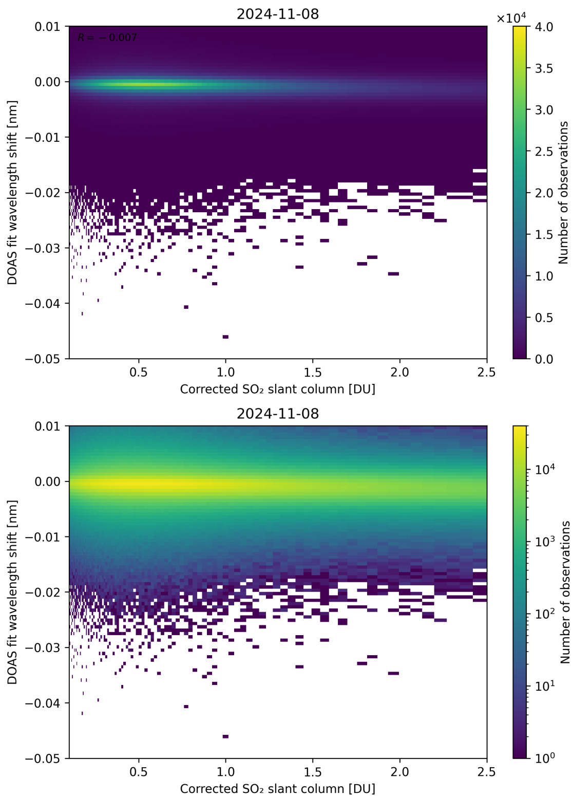
Figure 181: Scatter density plot of “Corrected SO 2 slant column” against “DOAS fit wavelength shift” for 2024-11-07 to 2024-11-09.
