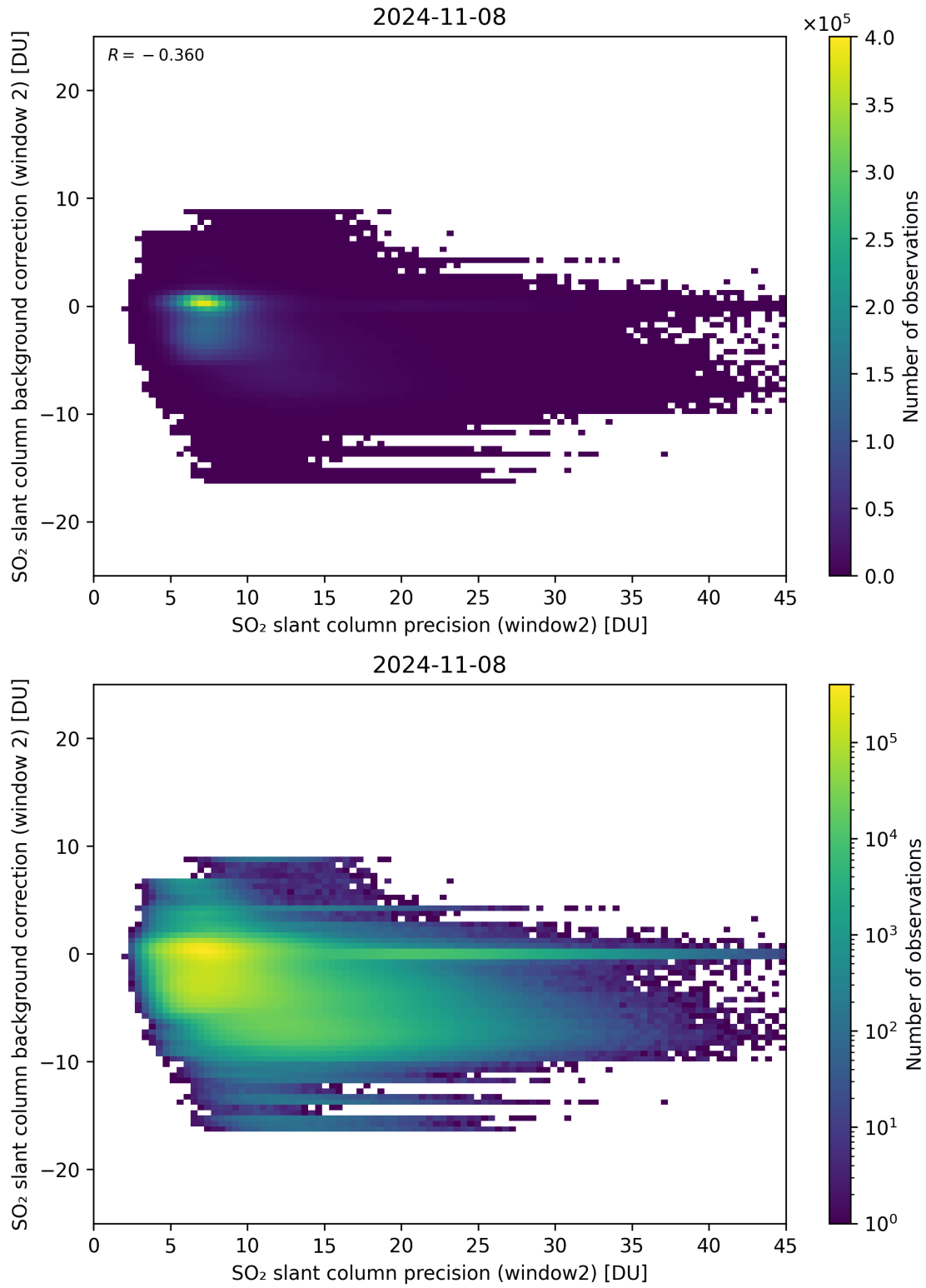
Figure 241: Scatter density plot of “SO 2 slant column precision (window2)” against “SO 2 slant column background correction (window 2)” for 2024-11-07 to 2024-11-09.
