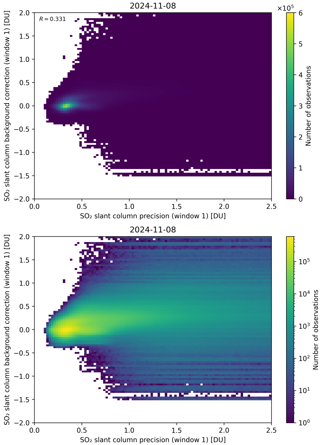
Figure 218: Scatter density plot of “SO 2 slant column precision (window 1)” against “SO 2 slant column background correction (window 1)” for 2024-11-07 to 2024-11-09.
