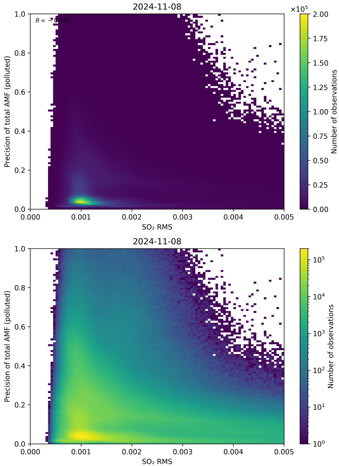
Figure 138: Scatter density plot of “SO 2 RMS” against “Precision of total AMF (polluted)” for 2024-11-07 to 2024-11-09.
