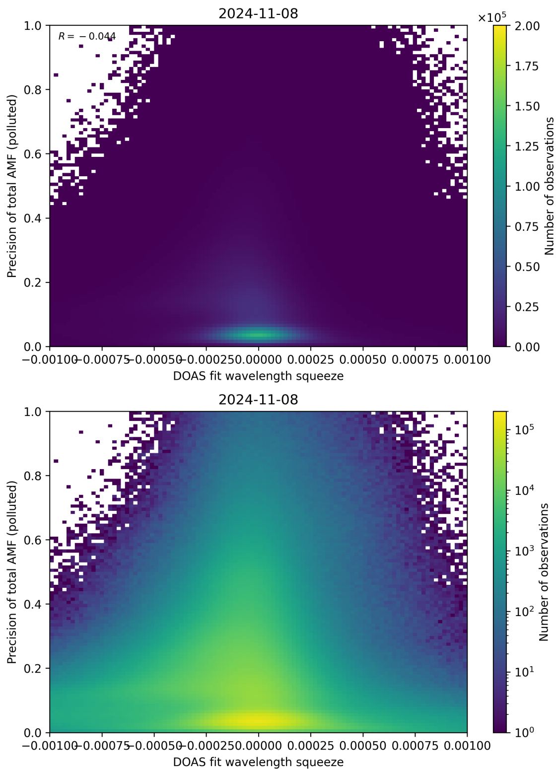
Figure 135: Scatter density plot of “DOAS fit wavelength squeeze” against “Precision of total AMF (polluted)” for 2024-11-07 to 2024-11-09.
