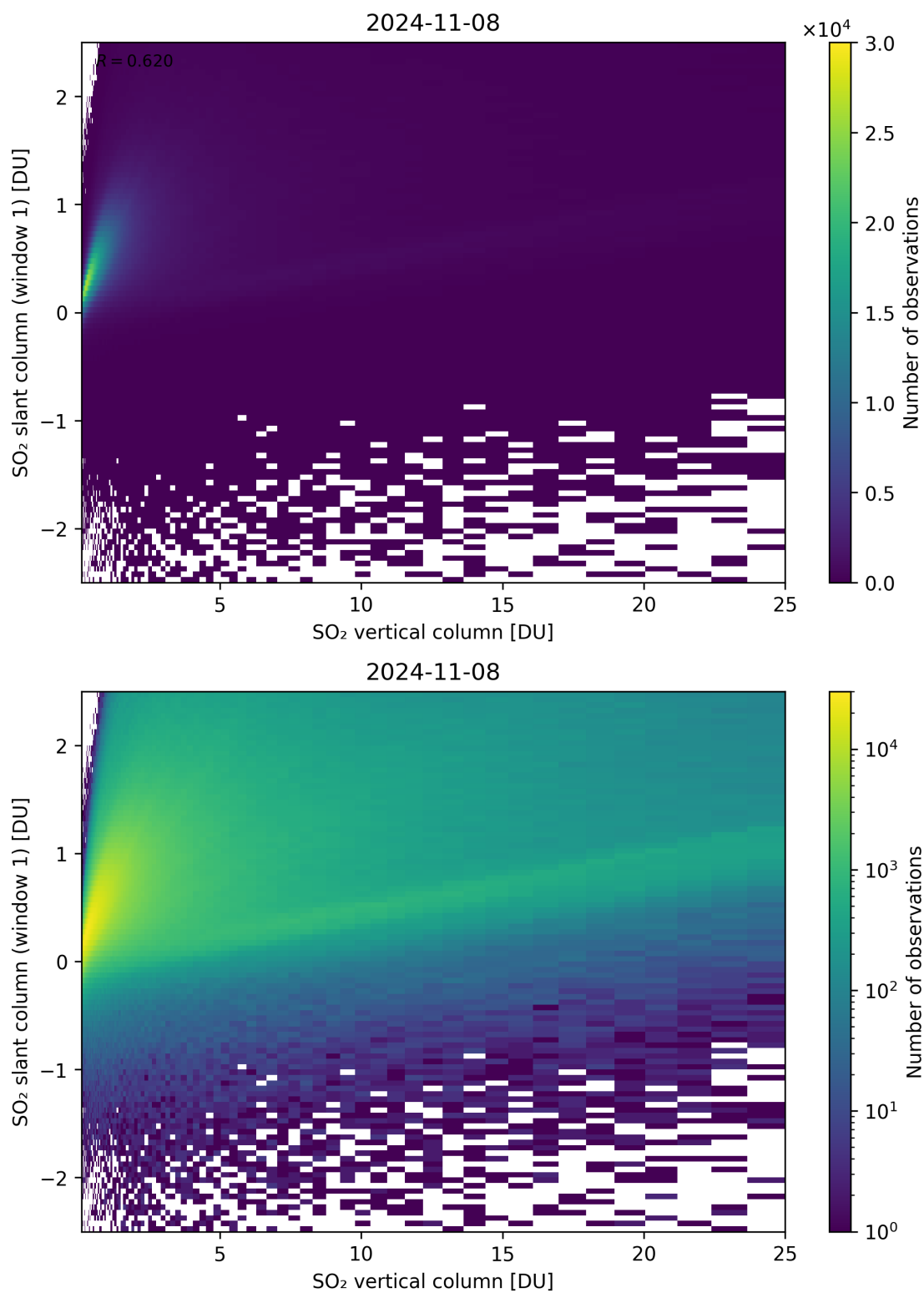
Figure 300: Scatter density plot of “SO 2 vertical column” against “SO 2 slant column (window 1)” for 2024-11-07 to 2024-11-09.
