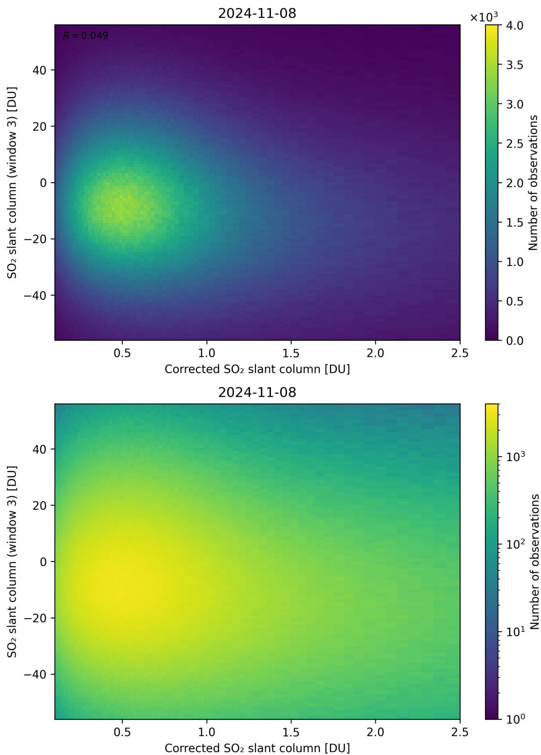
Figure 190: Scatter density plot of “Corrected SO 2 slant column” against “SO 2 slant column (window 3)” for 2024-11-07 to 2024-11-09.
