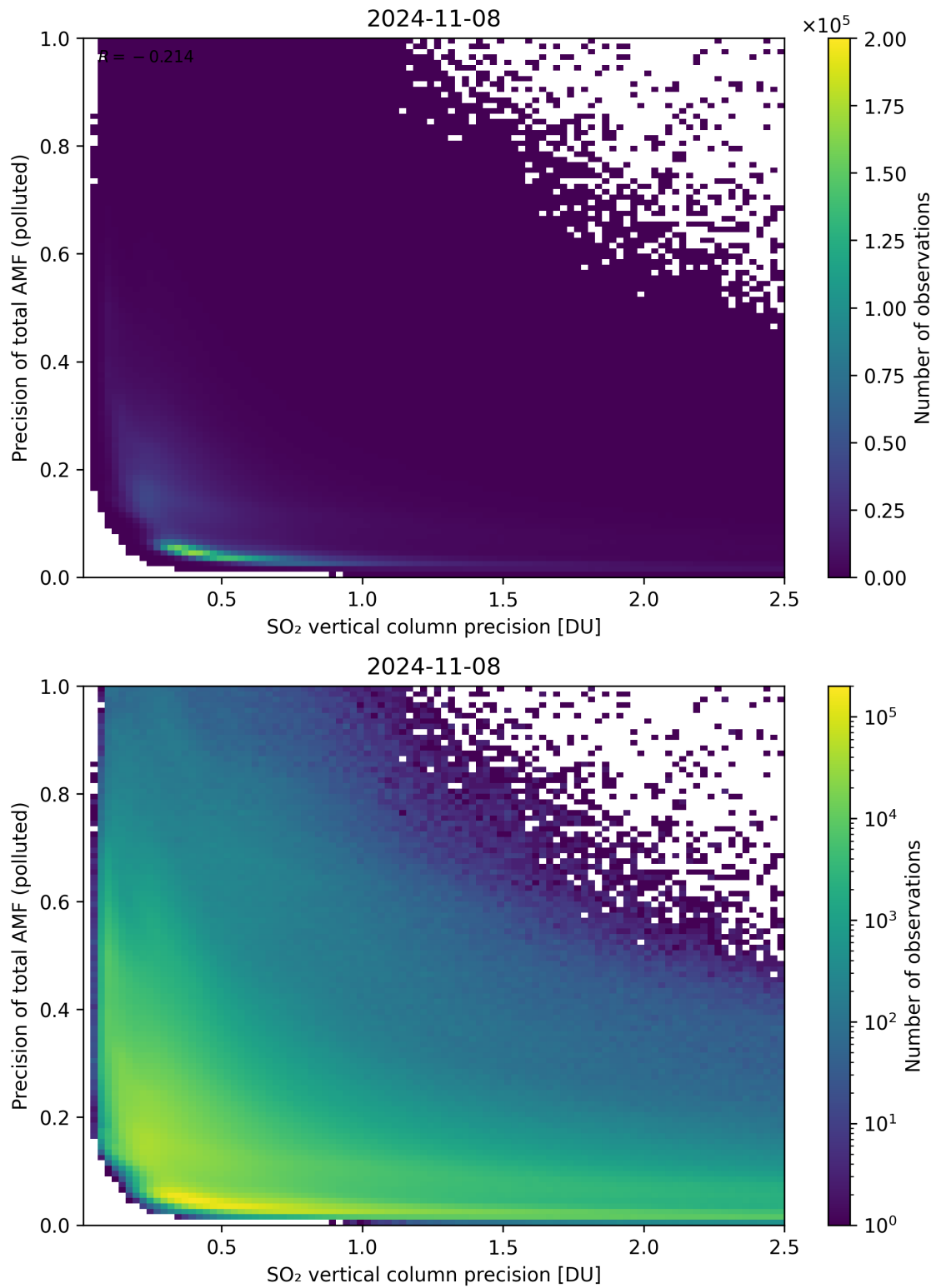
Figure 295: Scatter density plot of “SO 2 vertical column precision” against “Precision of total AMF (polluted)” for 2024-11-07 to 2024-11-09.
