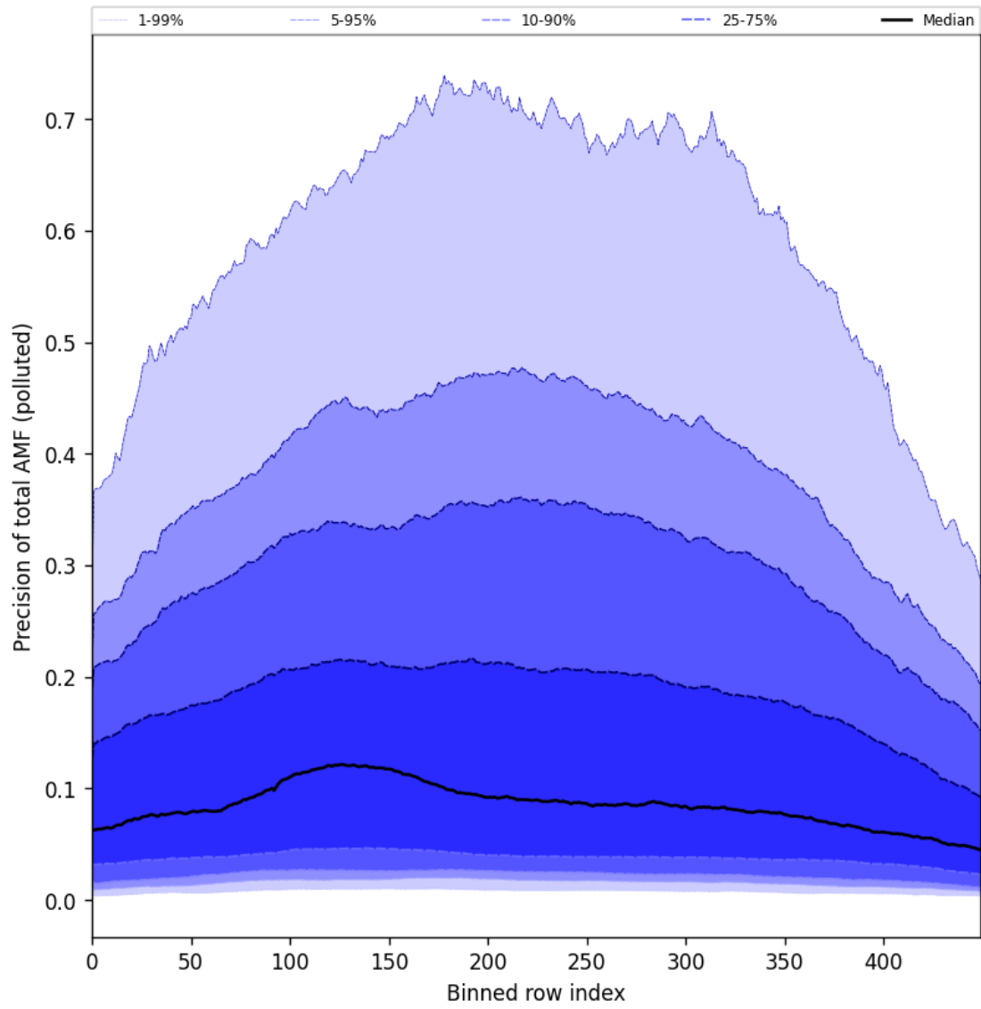
Figure 95: Along track statistics of “Precision of total AMF (polluted)” for 2024-11-07 to 2024-11-09
