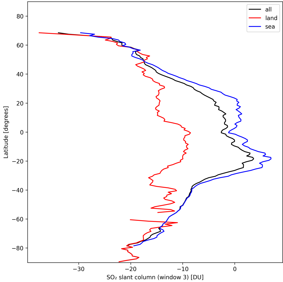
Figure 41: Zonal average of “SO 2 slant column (window 3)” for 2024-11-07 to 2024-11-09.
