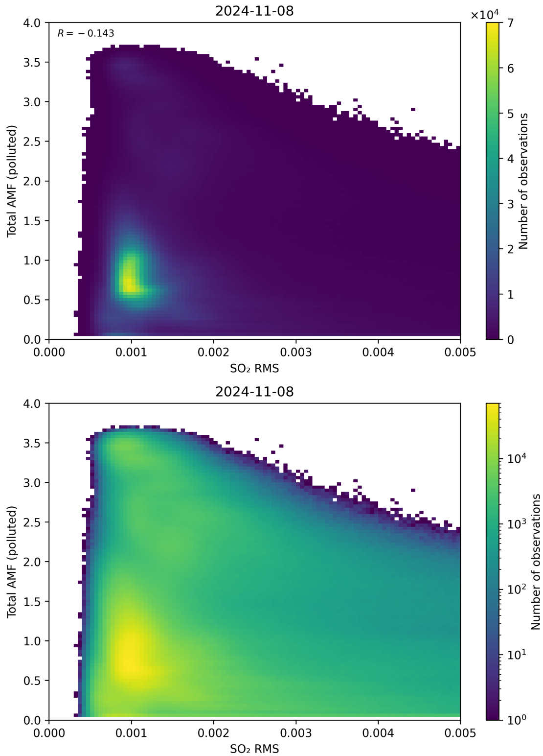
Figure 137: Scatter density plot of “SO 2 RMS” against “Total AMF (polluted)” for 2024-11-07 to 2024-11-09.
