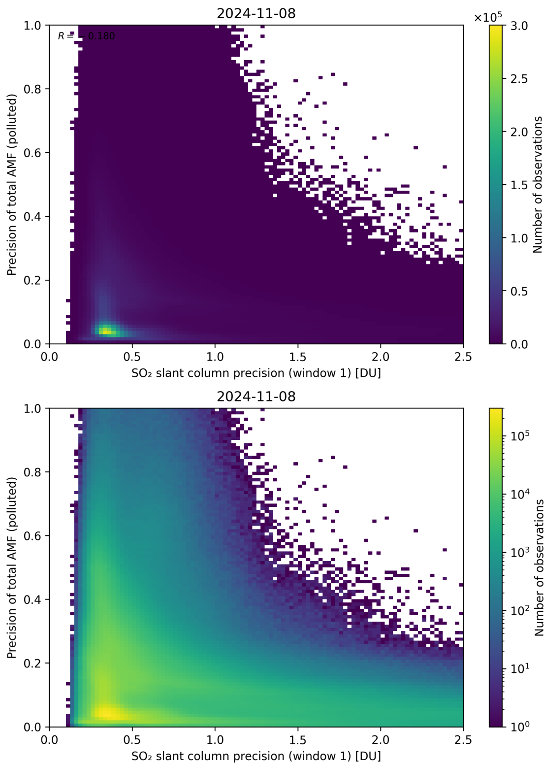
Figure 231: Scatter density plot of “SO 2 slant column precision (window 1)” against “Precision of total AMF (polluted)” for 2024-11-07 to 2024-11-09.
