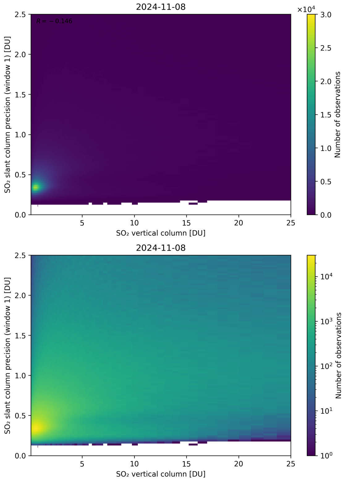
Figure 301: Scatter density plot of “SO 2 vertical column” against “SO 2 slant column precision (window 1)” for 2024-11-07 to 2024-11-09.
