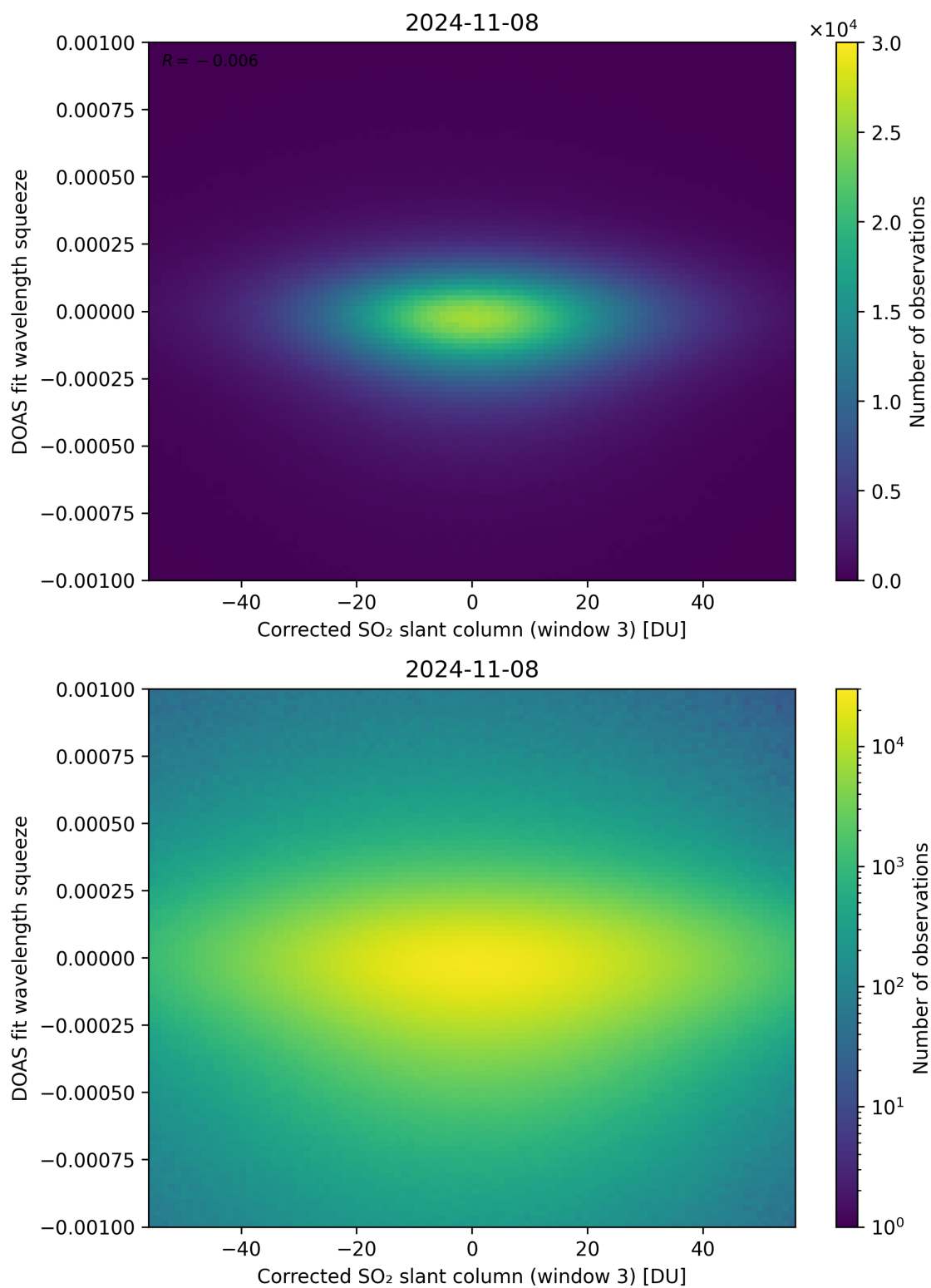
Figure 207: Scatter density plot of “Corrected SO 2 slant column (window 3)” against “DOAS fit wavelength squeeze” for 2024-11-07 to 2024-11-09.
