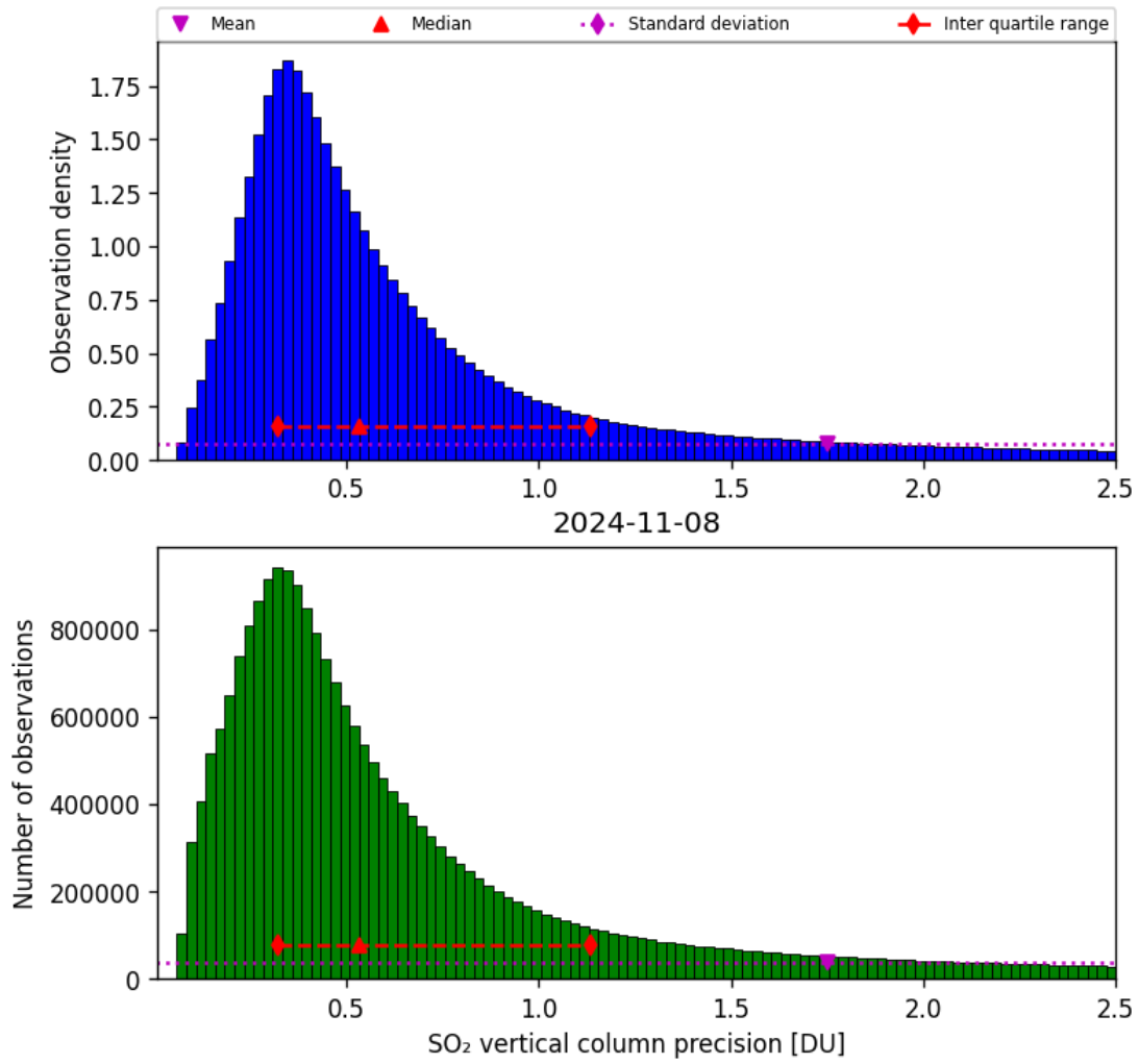
Figure 54: Histogram of “SO 2 vertical column precision” for 2024-11-07 to 2024-11-09
