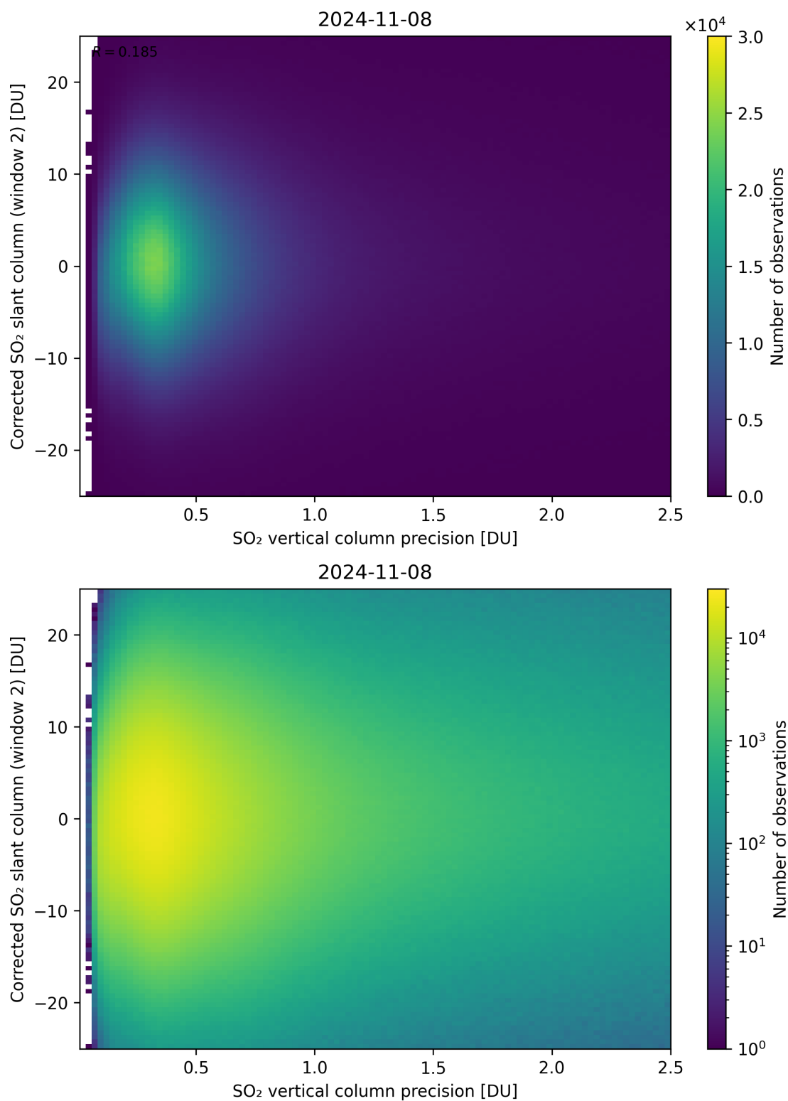
Figure 287: Scatter density plot of “SO 2 vertical column precision” against “Corrected SO 2 slant column (window 2)” for 2024-11-07 to 2024-11-09.
