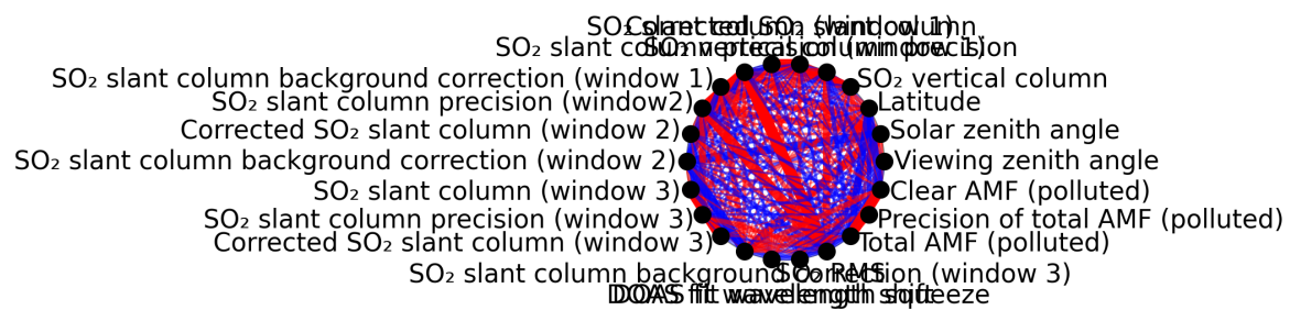
Figure 1: Map of correlation graph for 2024-11-07 to 2024-11-09.
