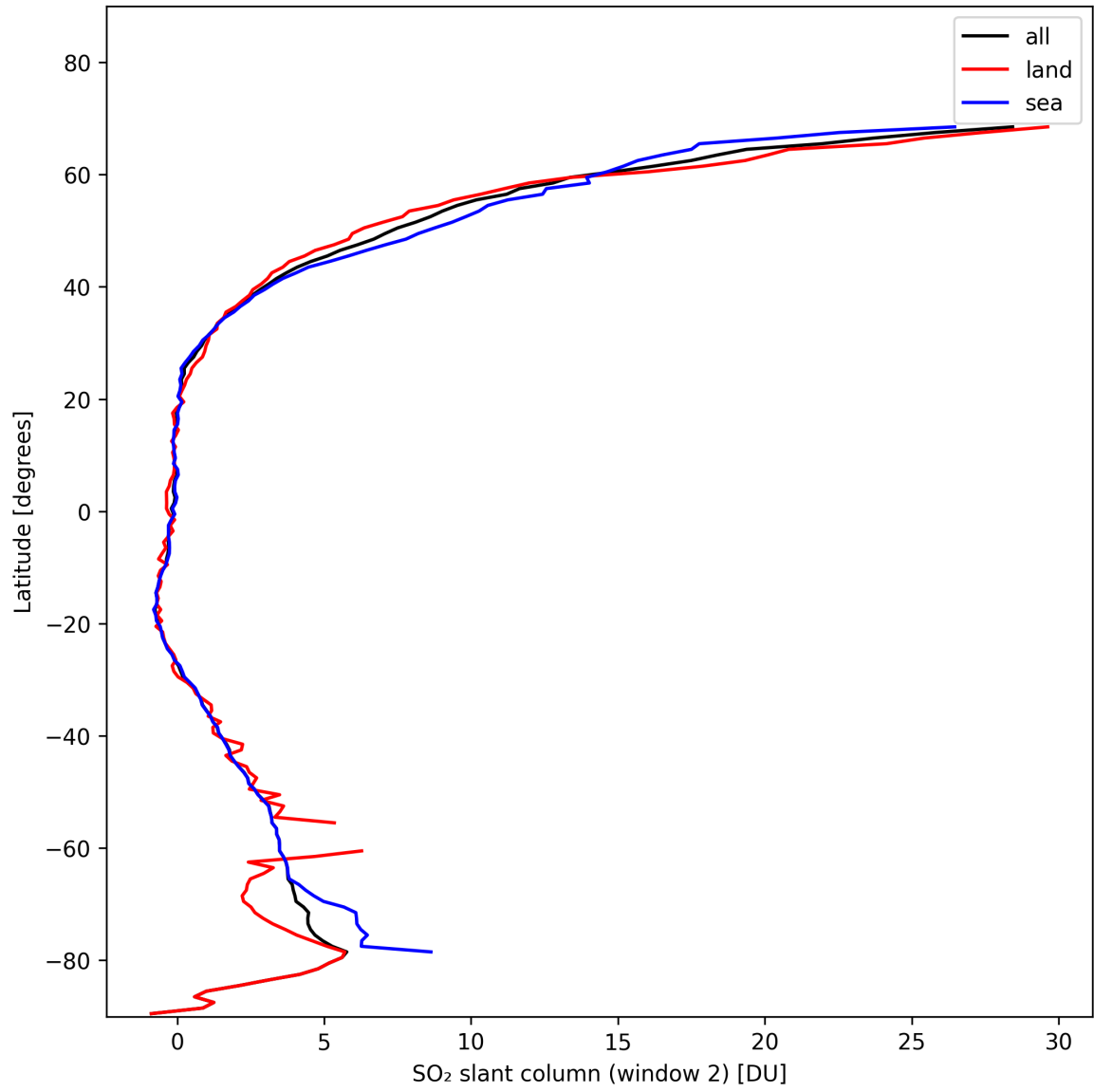
Figure 37: Zonal average of “SO 2 slant column (window 2)” for 2024-11-07 to 2024-11-09.
