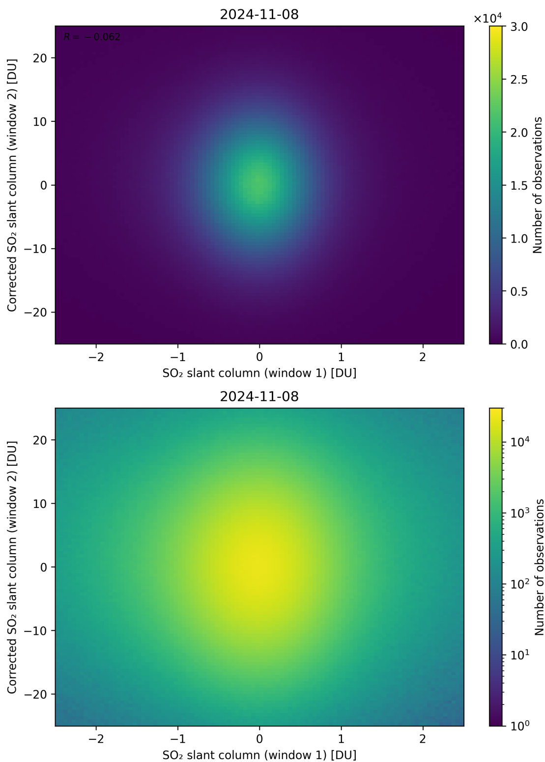
Figure 233: Scatter density plot of “SO 2 slant column (window 1)” against “Corrected SO 2 slant column (window 2)” for 2024-11-07 to 2024-11-09.
