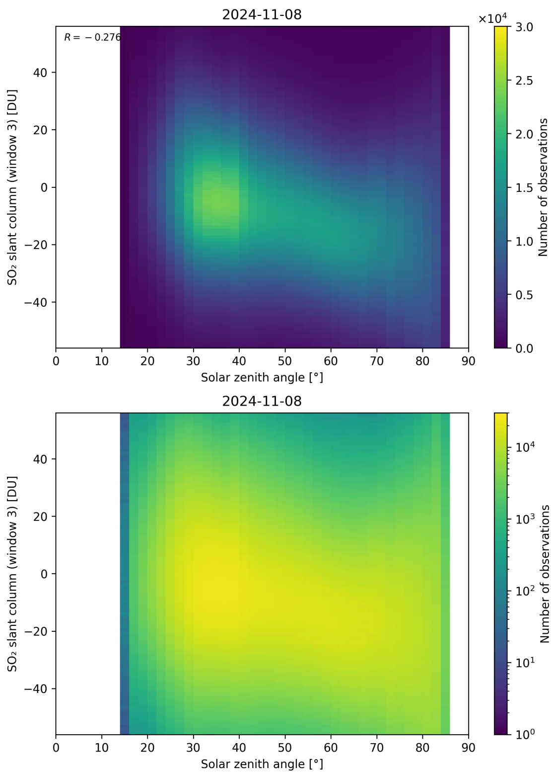
Figure 172: Scatter density plot of “Solar zenith angle” against “SO 2 slant column (window 3)” for 2024-11-07 to 2024-11-09.
