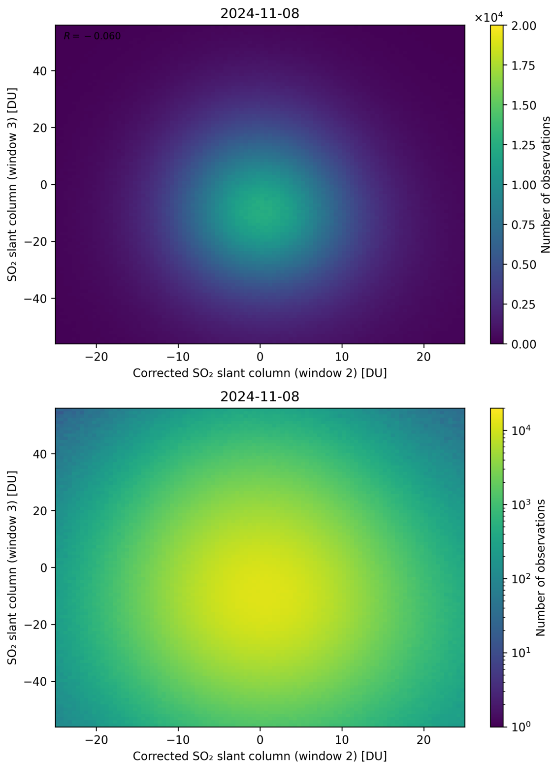
Figure 201: Scatter density plot of “Corrected SO 2 slant column (window 2)” against “SO 2 slant column (window 3)” for 2024-11-07 to 2024-11-09.
