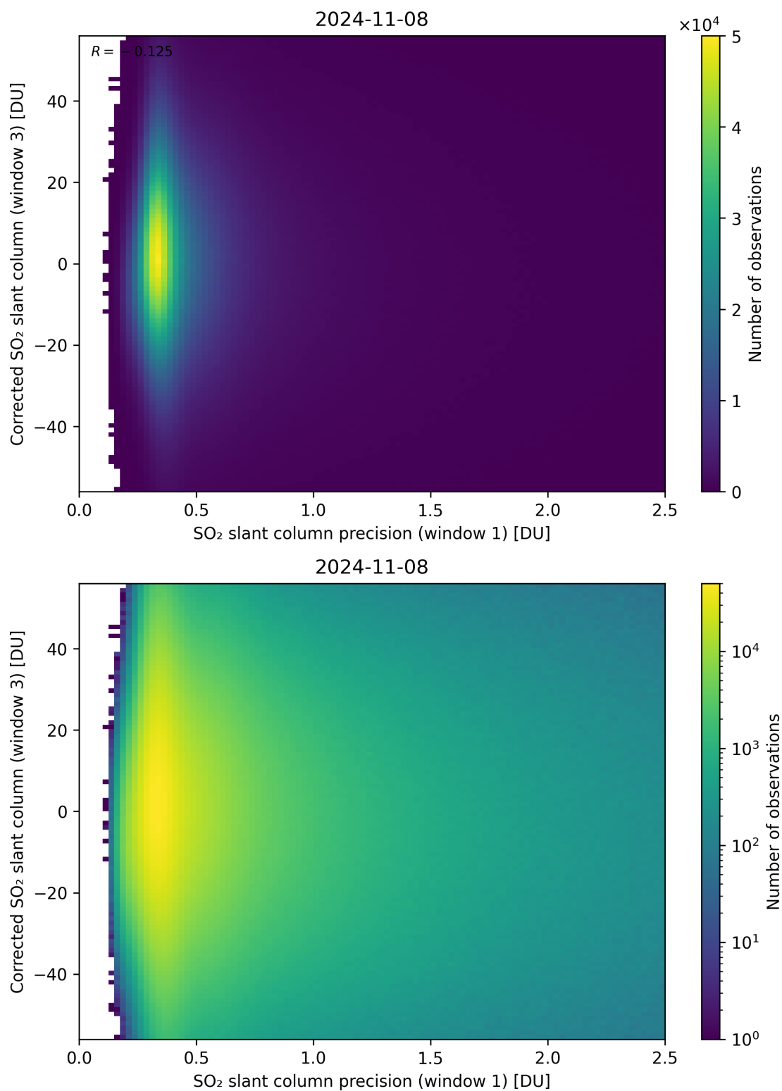
Figure 226: Scatter density plot of “SO 2 slant column precision (window 1)” against “Corrected SO 2 slant column (window 3)” for 2024-11-07 to 2024-11-09.
