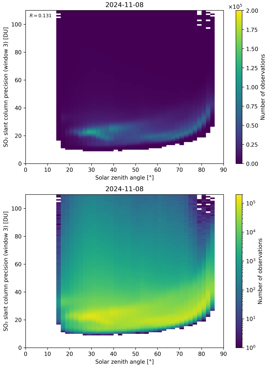
Figure 173: Scatter density plot of “Solar zenith angle” against “SO 2 slant column precision (window 3)” for 2024-11-07 to 2024-11-09.
