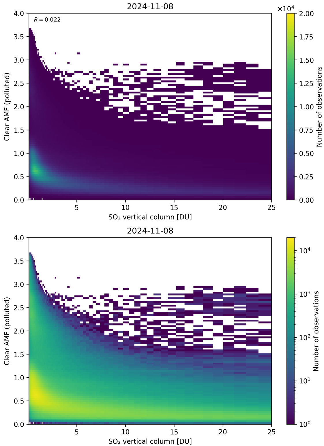
Figure 296: Scatter density plot of “SO 2 vertical column” against “Clear AMF (polluted)” for 2024-11-07 to 2024-11-09.
