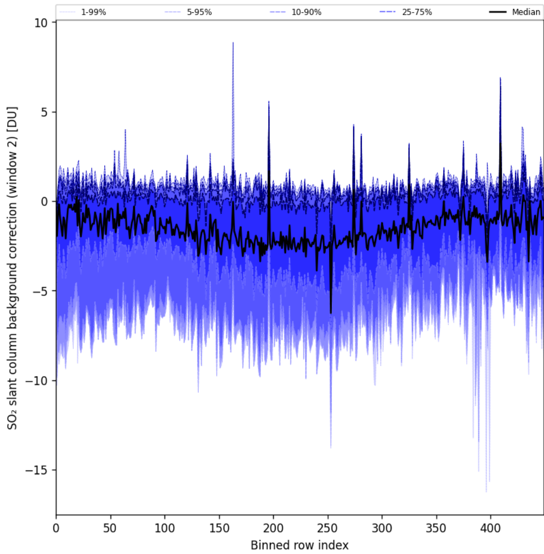
Figure 86: Along track statistics of “SO 2 slant column background correction (window 2)” for 2024-11-07 to 2024-11-09
