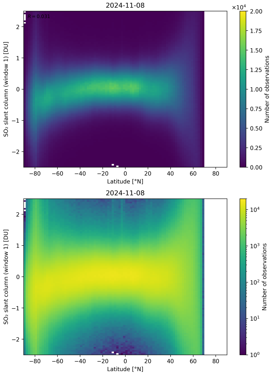
Figure 149: Scatter density plot of “Latitude” against “SO 2 slant column (window 1)” for 2024-11-07 to 2024-11-09.
