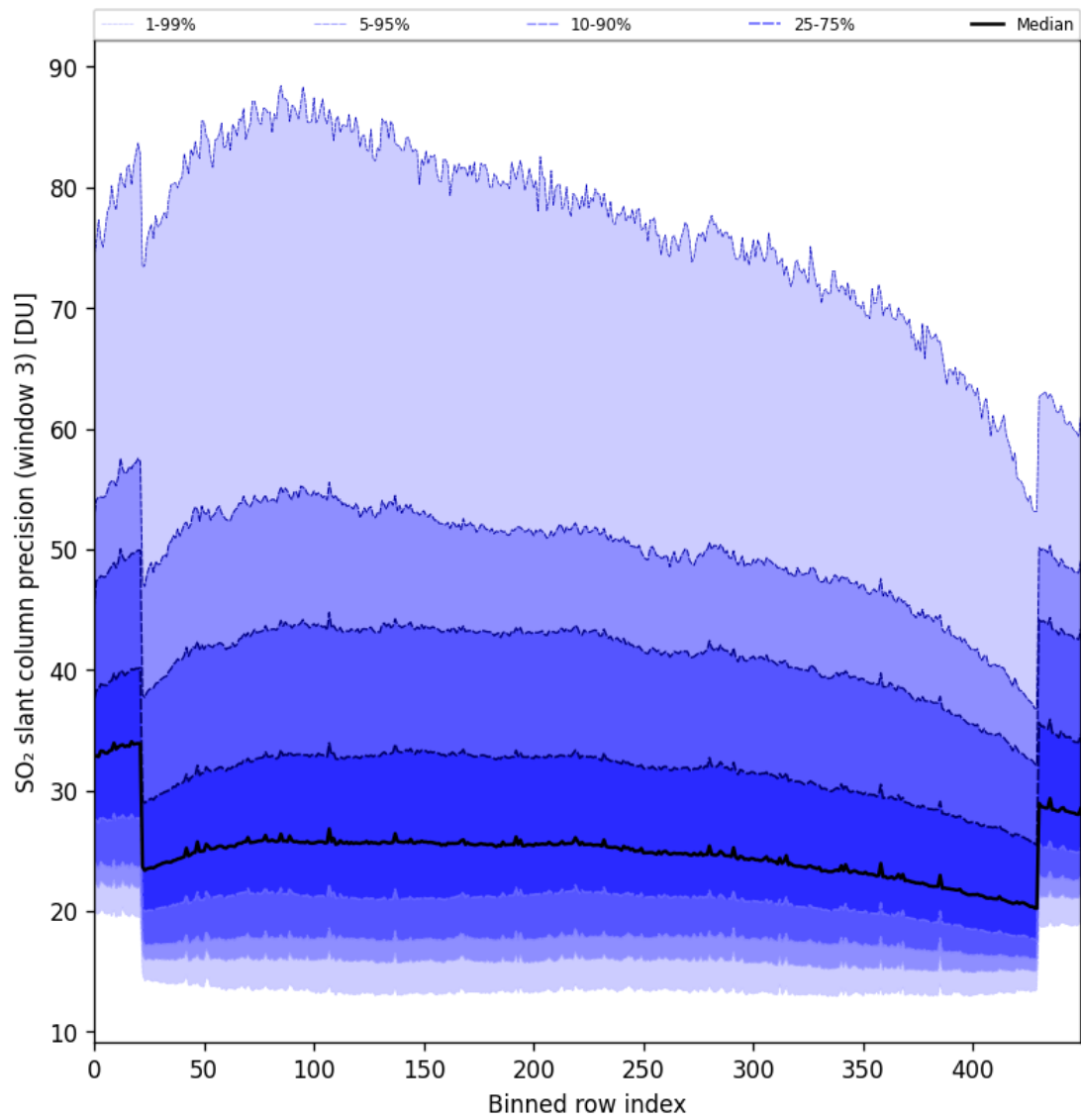
Figure 88: Along track statistics of “SO 2 slant column precision (window 3)” for 2024-11-07 to 2024-11-09
