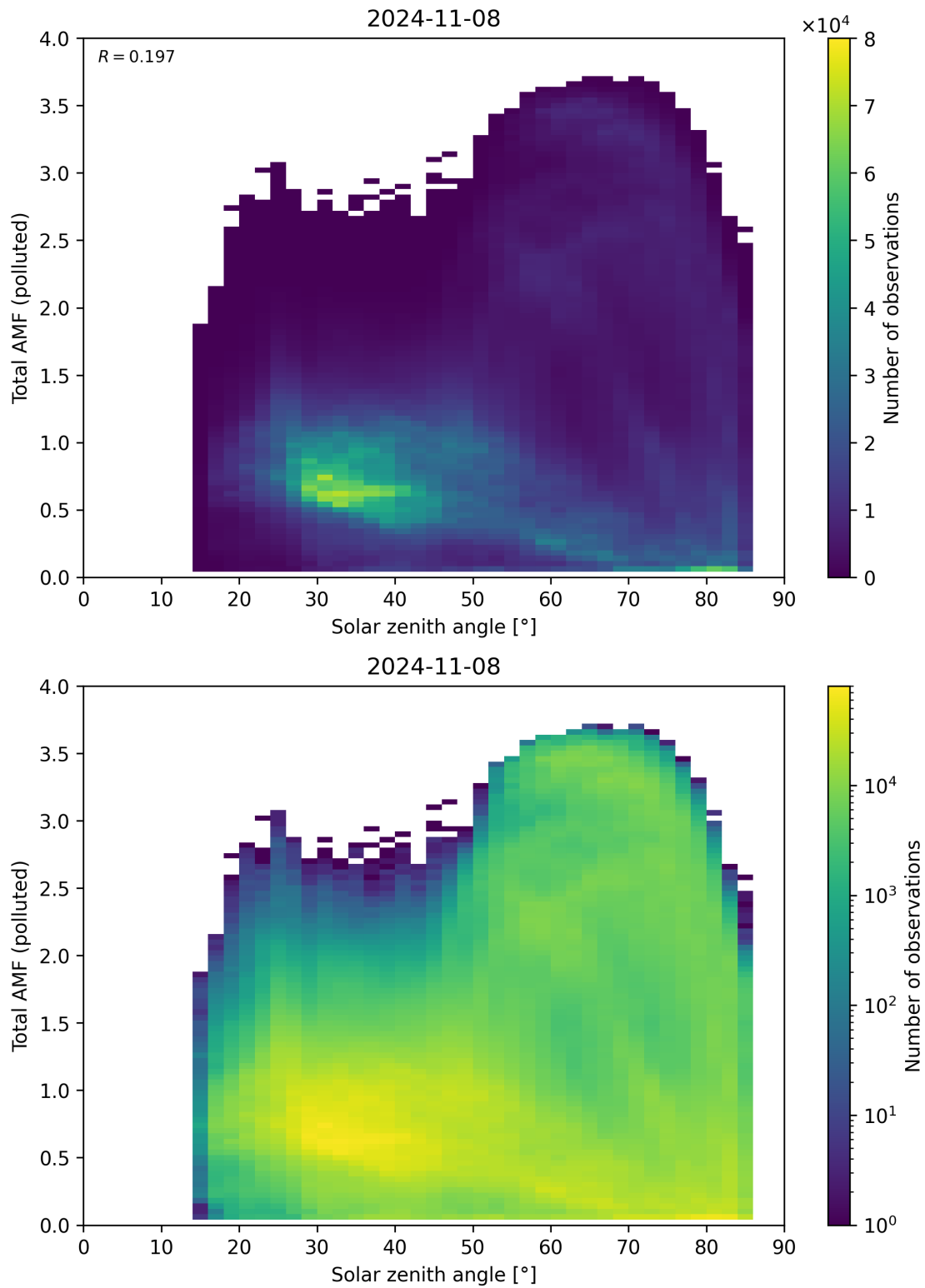
Figure 174: Scatter density plot of “Solar zenith angle” against “Total AMF (polluted)” for 2024-11-07 to 2024-11-09.
