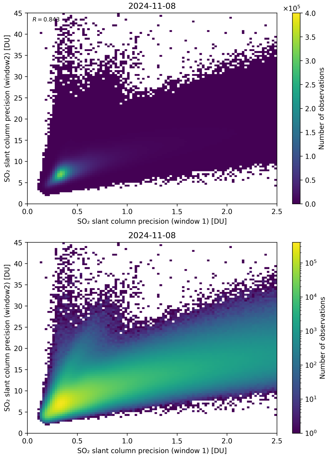
Figure 227: Scatter density plot of “SO 2 slant column precision (window 1)” against “SO 2 slant column precision (window 2)” for 2024-11-07 to 2024-11-09.
