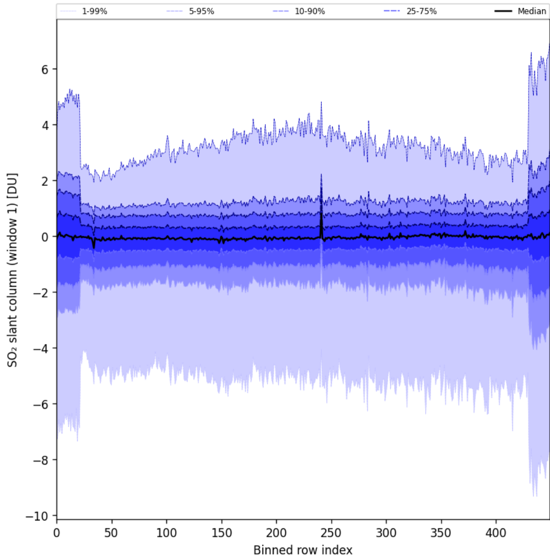
Figure 79: Along track statistics of “SO 2 slant column (window 1)” for 2024-11-07 to 2024-11-09
