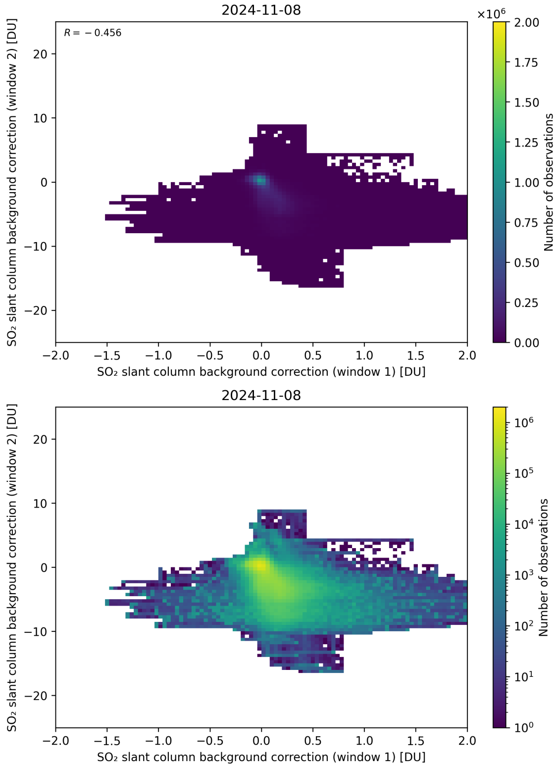
Figure 98: Scatter density plot of “SO 2 slant column background correction (window 1)” against “SO 2 slant column background correction (window 2)” for 2024-11-07 to 2024-11-09.
