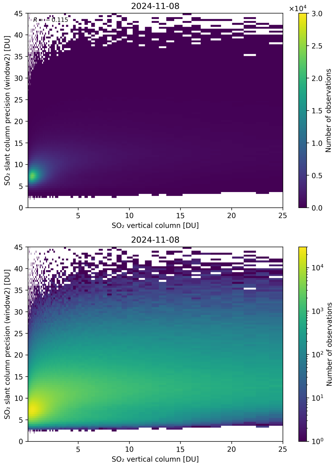
Figure 302: Scatter density plot of “SO 2 vertical column” against “SO 2 slant column precision (window2)” for 2024-11-07 to 2024-11-09.
