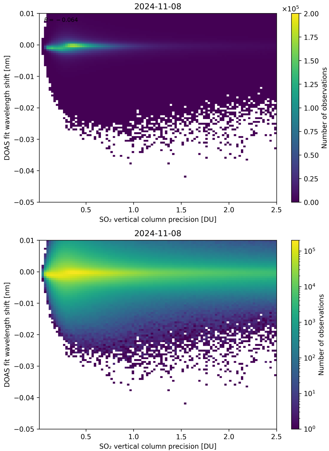
Figure 282: Scatter density plot of “SO 2 vertical column precision” against “DOAS fit wavelength shift” for 2024-11-07 to 2024-11-09.
