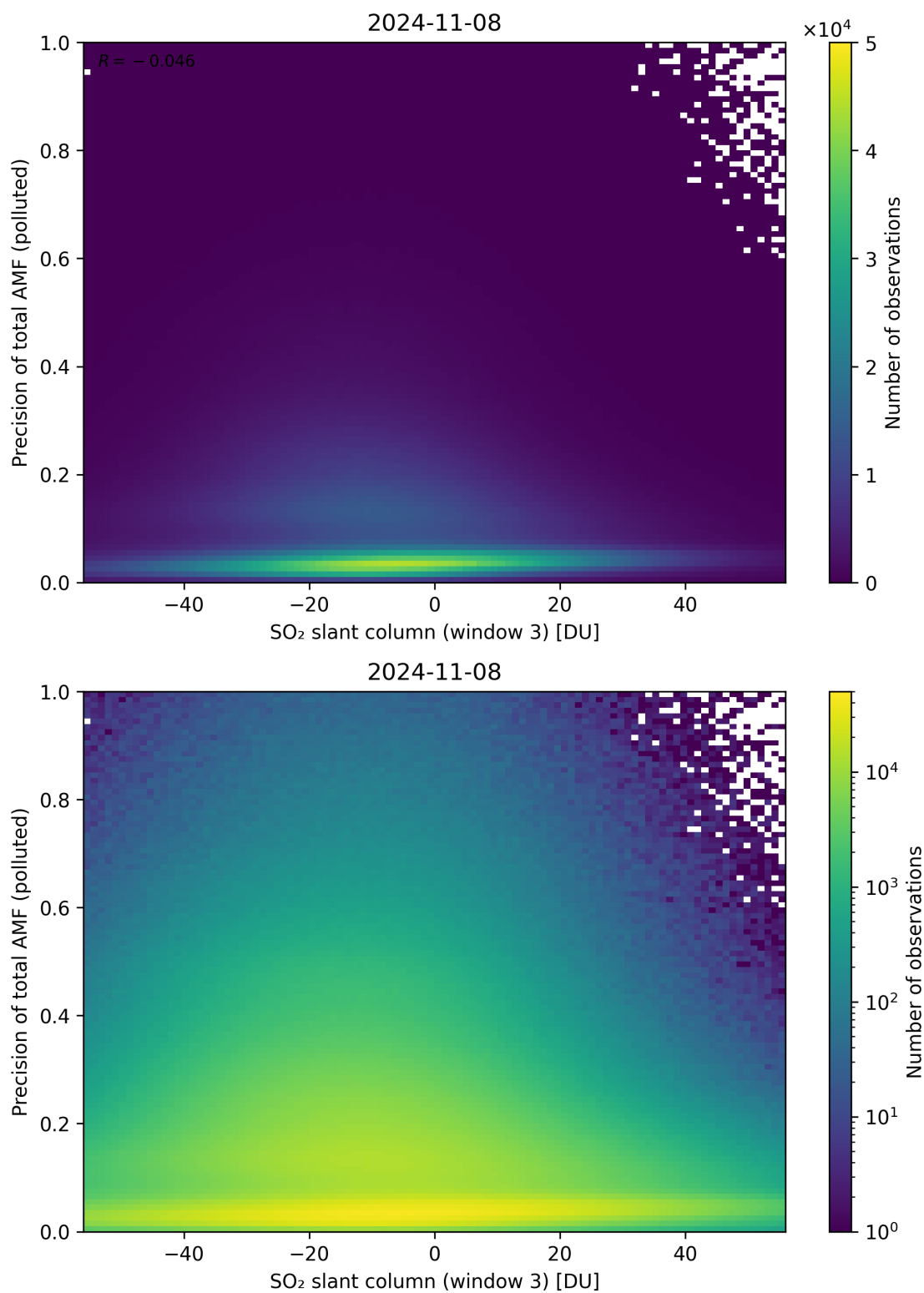
Figure 269: Scatter density plot of “SO 2 slant column (window 3)” against “Precision of total AMF (polluted)” for 2024-11-07 to 2024-11-09.
