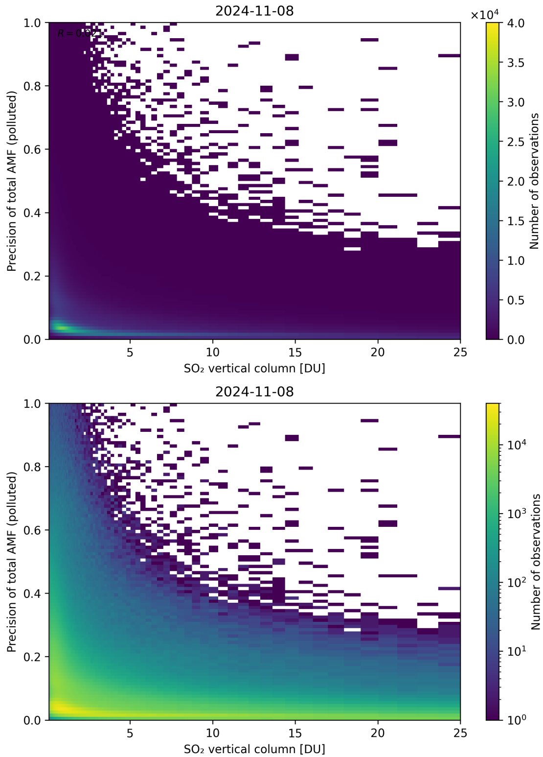
Figure 306: Scatter density plot of “SO 2 vertical column” against “Precision of total AMF (polluted)” for 2024-11-07 to 2024-11-09.
