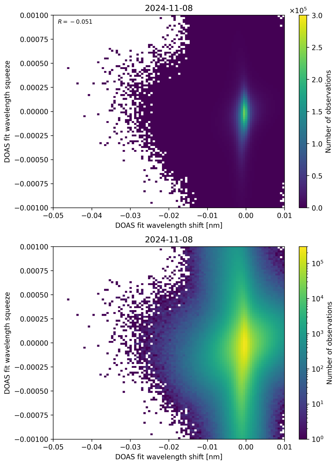
Figure 127: Scatter density plot of “DOAS fit wavelength shift” against “DOAS fit wavelength squeeze” for 2024-11-07 to 2024-11-09.
