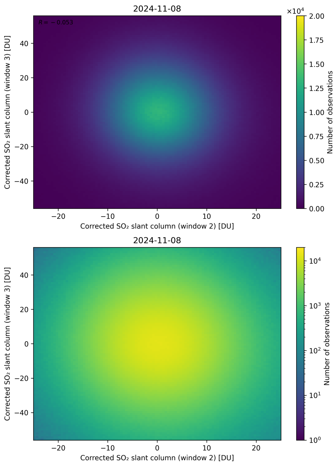
Figure 200: Scatter density plot of “Corrected SO 2 slant column (window 2)” against “Corrected SO 2 slant column (window 3)” for 2024-11-07 to 2024-11-09.
