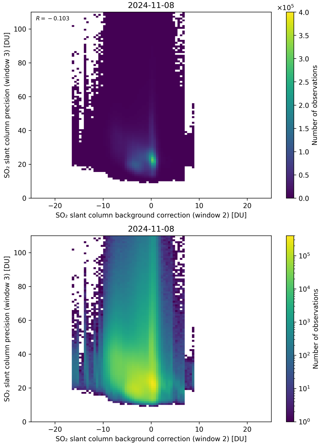
Figure 118: Scatter density plot of “SO 2 slant column background correction (window 2)” against “SO 2 slant column precision (window 3)” for 2024-11-07 to 2024-11-09.
