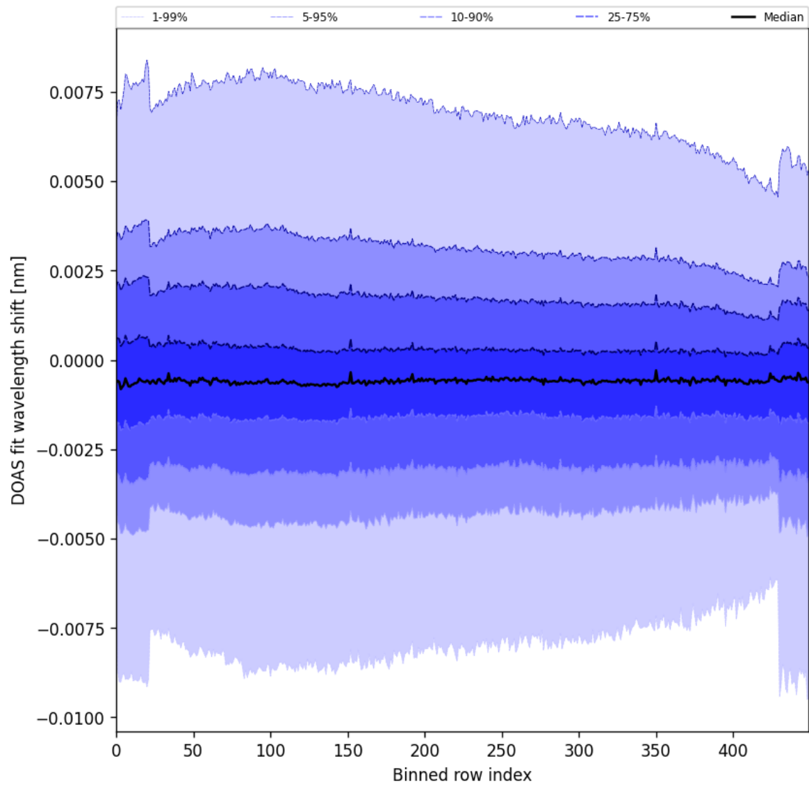
Figure 91: Along track statistics of “DOAS fit wavelength shift” for 2024-11-07 to 2024-11-09
