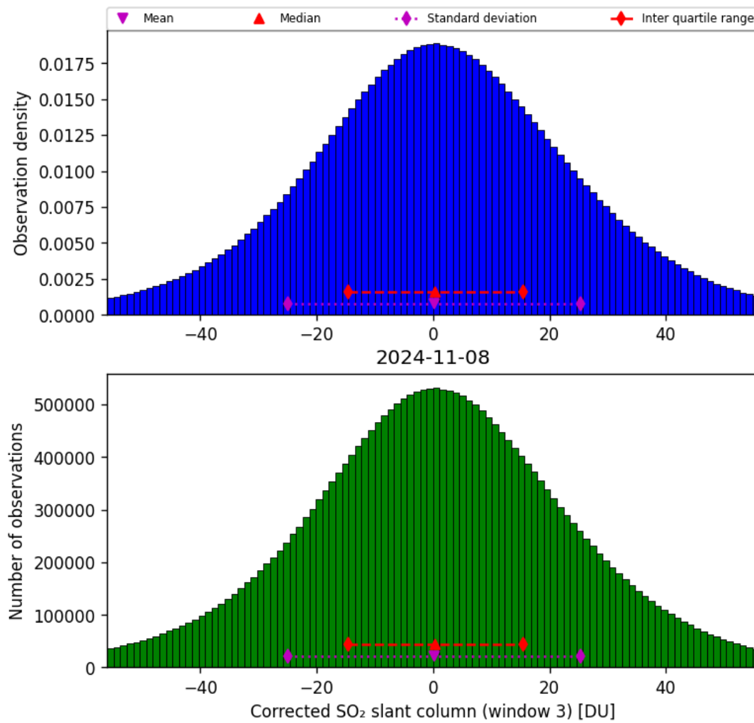
Figure 66: Histogram of “Corrected SO 2 slant column (window 3)” for 2024-11-07 to 2024-11-09
