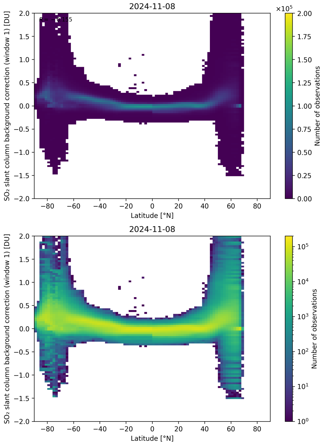
Figure 139: Scatter density plot of “Latitude” against “SO 2 slant column background correction (window 1)” for 2024-11-07 to 2024-11-09.
