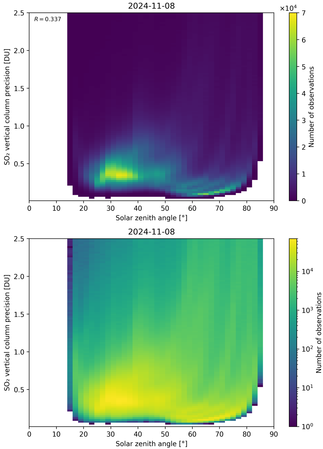
Figure 177: Scatter density plot of “Solar zenith angle” against “SO 2 vertical column precision” for 2024-11-07 to 2024-11-09.
