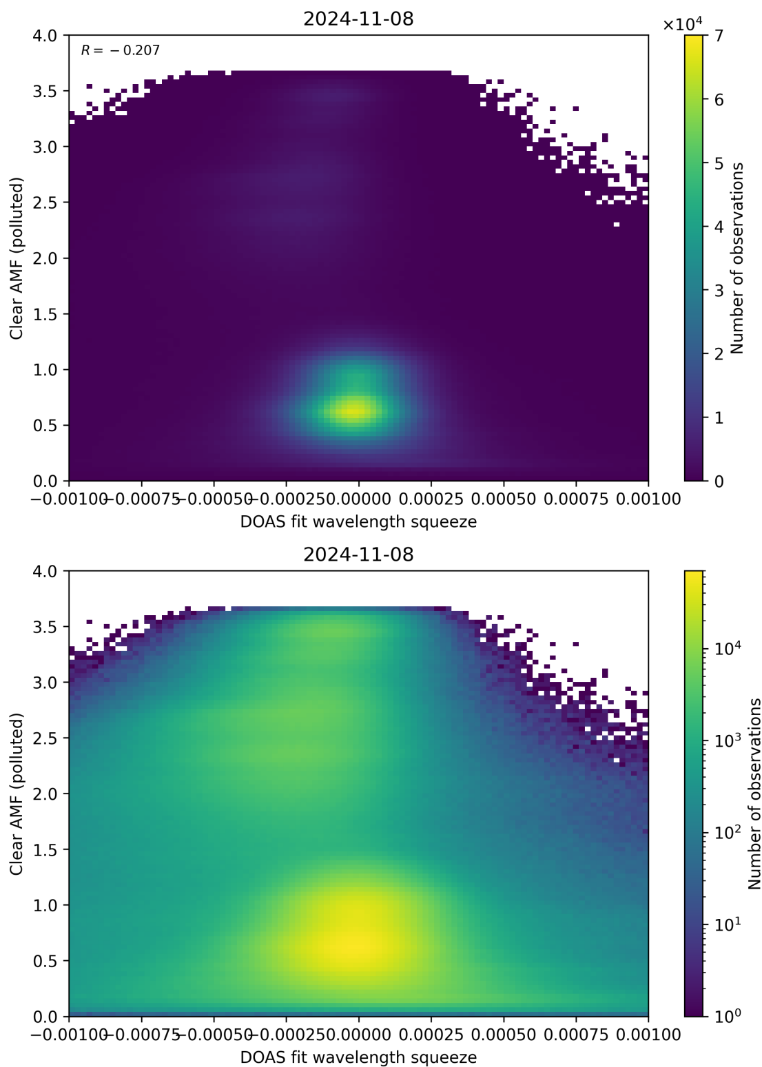
Figure 133: Scatter density plot of “DOAS fit wavelength squeeze” against “Clear AMF (polluted)” for 2024-11-07 to 2024-11-09.
