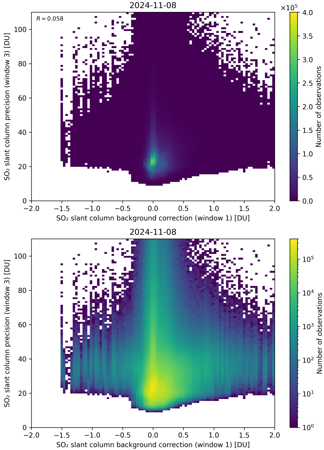
Figure 108: Scatter density plot of “SO 2 slant column background correction (window 1)” against “SO 2 slant column precision (window 3)” for 2024-11-07 to 2024-11-09.
