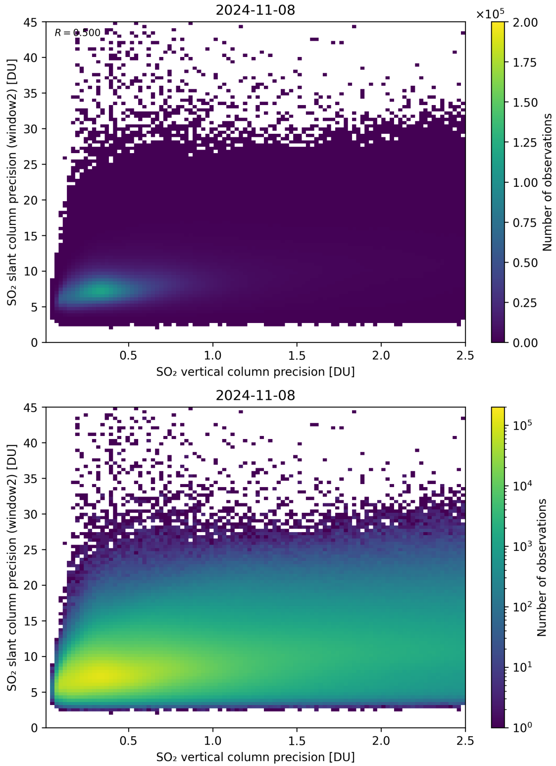
Figure 291: Scatter density plot of “SO 2 vertical column precision” against “SO 2 slant column precision (window2)” for 2024-11-07 to 2024-11-09.
