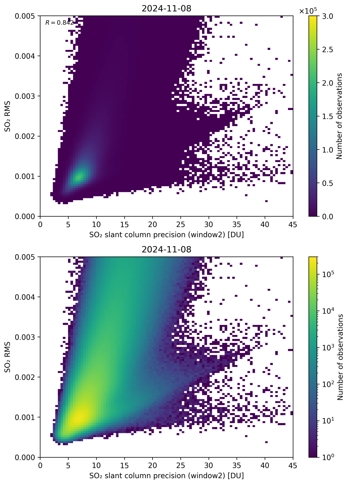
Figure 245: Scatter density plot of “SO 2 slant column precision (window2)” against “SO 2 RMS” for 2024-11-07 to 2024-11-09.
