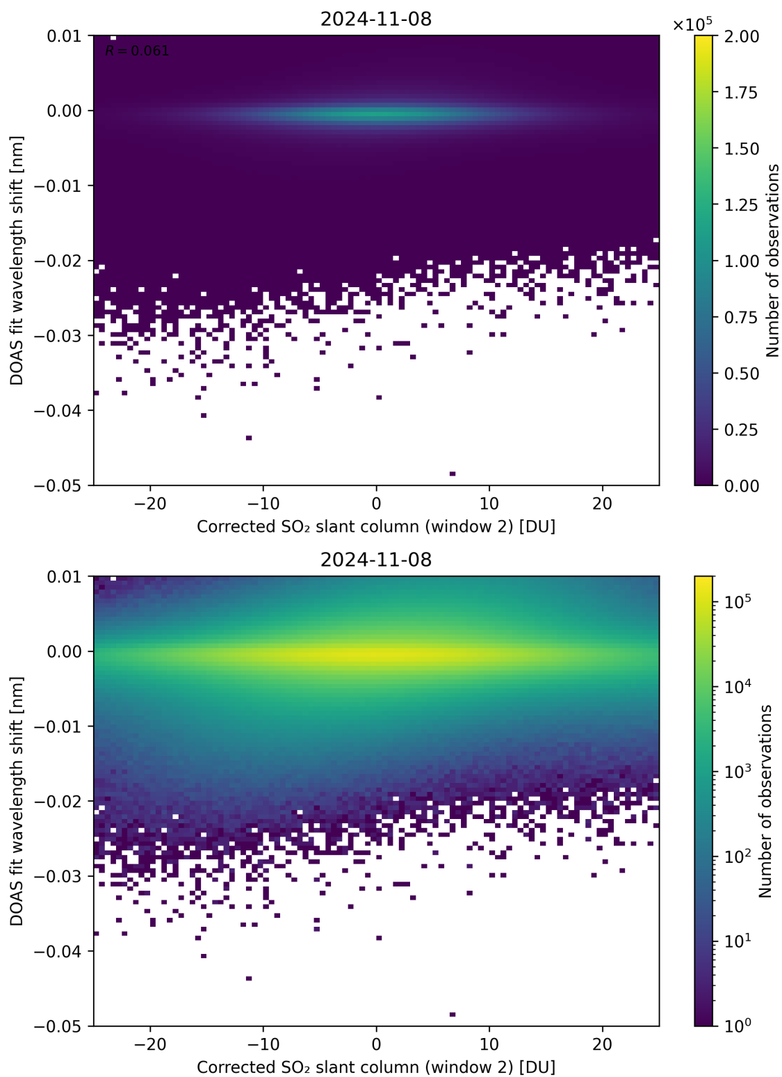
Figure 196: Scatter density plot of “Corrected SO 2 slant column (window 2)” against “DOAS fit wavelength shift” for 2024-11-07 to 2024-11-09.
