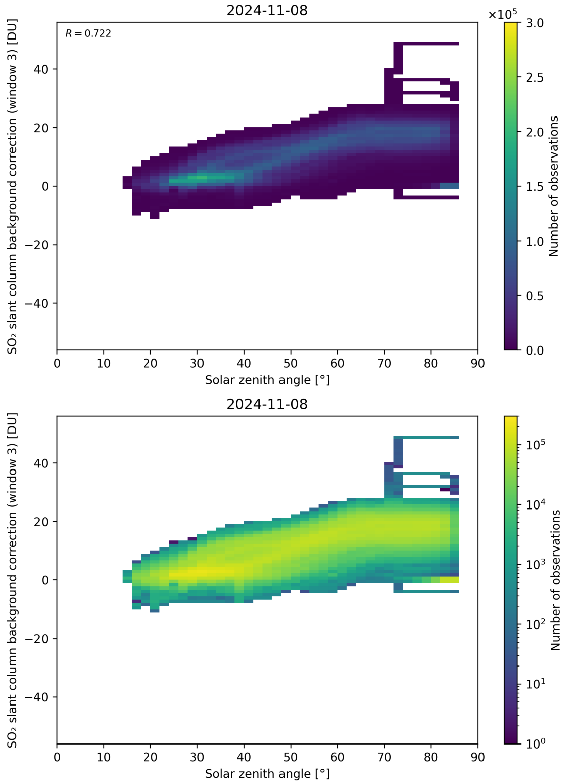
Figure 160: Scatter density plot of “Solar zenith angle” against “SO 2 slant column background correction (window 3)” for 2024-11-07 to 2024-11-09.
