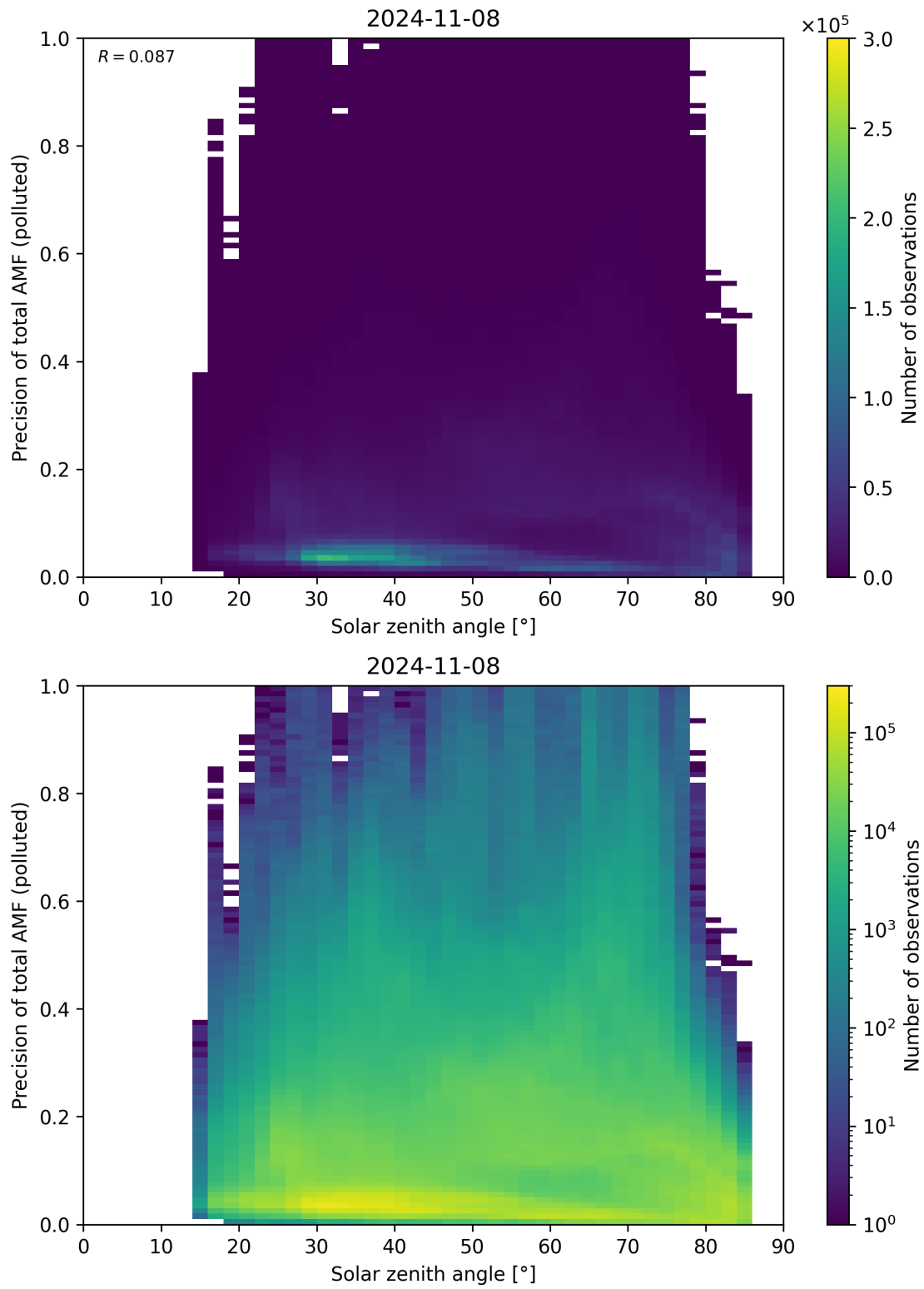
Figure 175: Scatter density plot of “Solar zenith angle” against “Precision of total AMF (polluted)” for 2024-11-07 to 2024-11-09.
