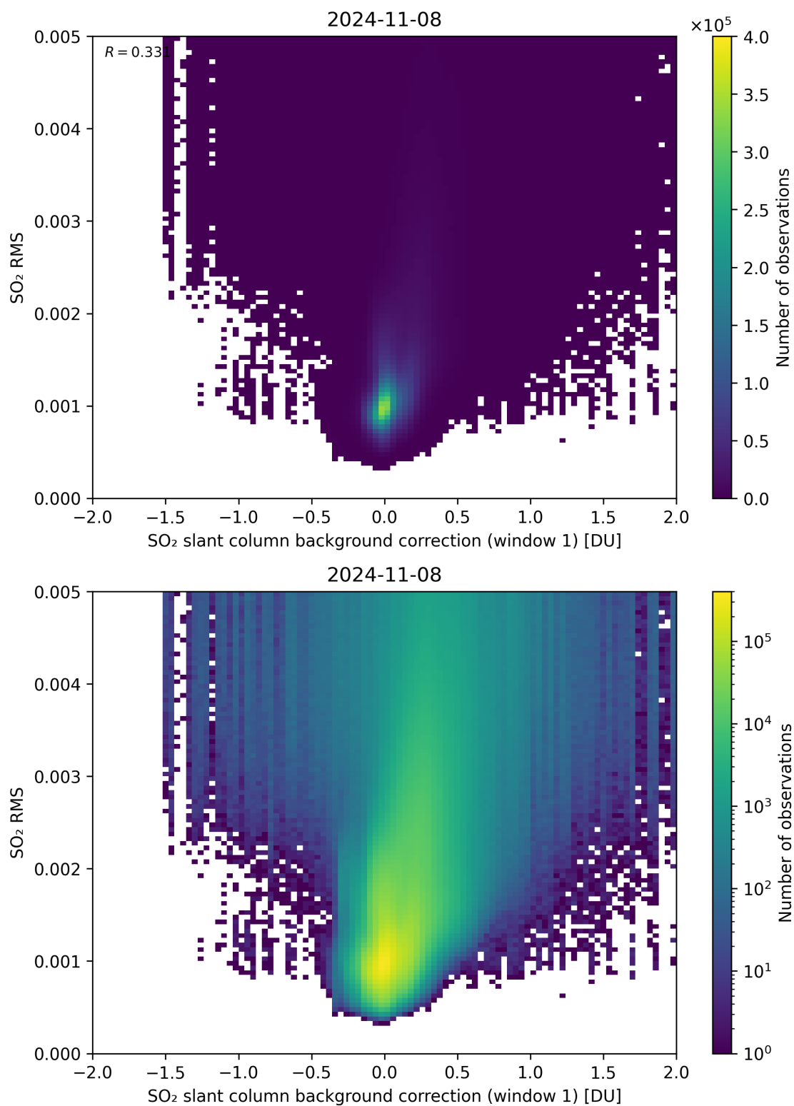
Figure 102: Scatter density plot of “SO 2 slant column background correction (window 1)” against “SO 2 RMS” for 2024-11-07 to 2024-11-09.
