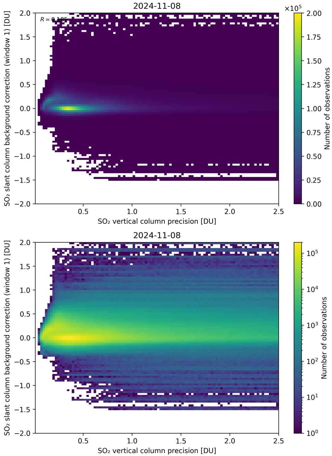
Figure 279: Scatter density plot of “SO 2 vertical column precision” against “SO 2 slant column background correction (window 1)” for 2024-11-07 to 2024-11-09.
