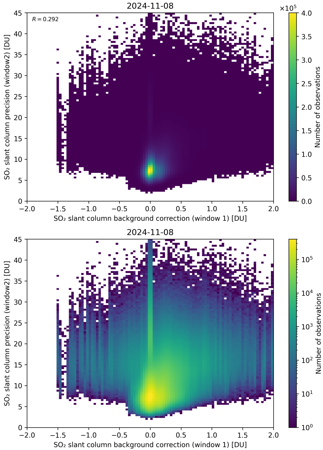
Figure 106: Scatter density plot of “SO 2 slant column background correction (window 1)” against “SO 2 slant column precision (window2)” for 2024-11-07 to 2024-11-09.
