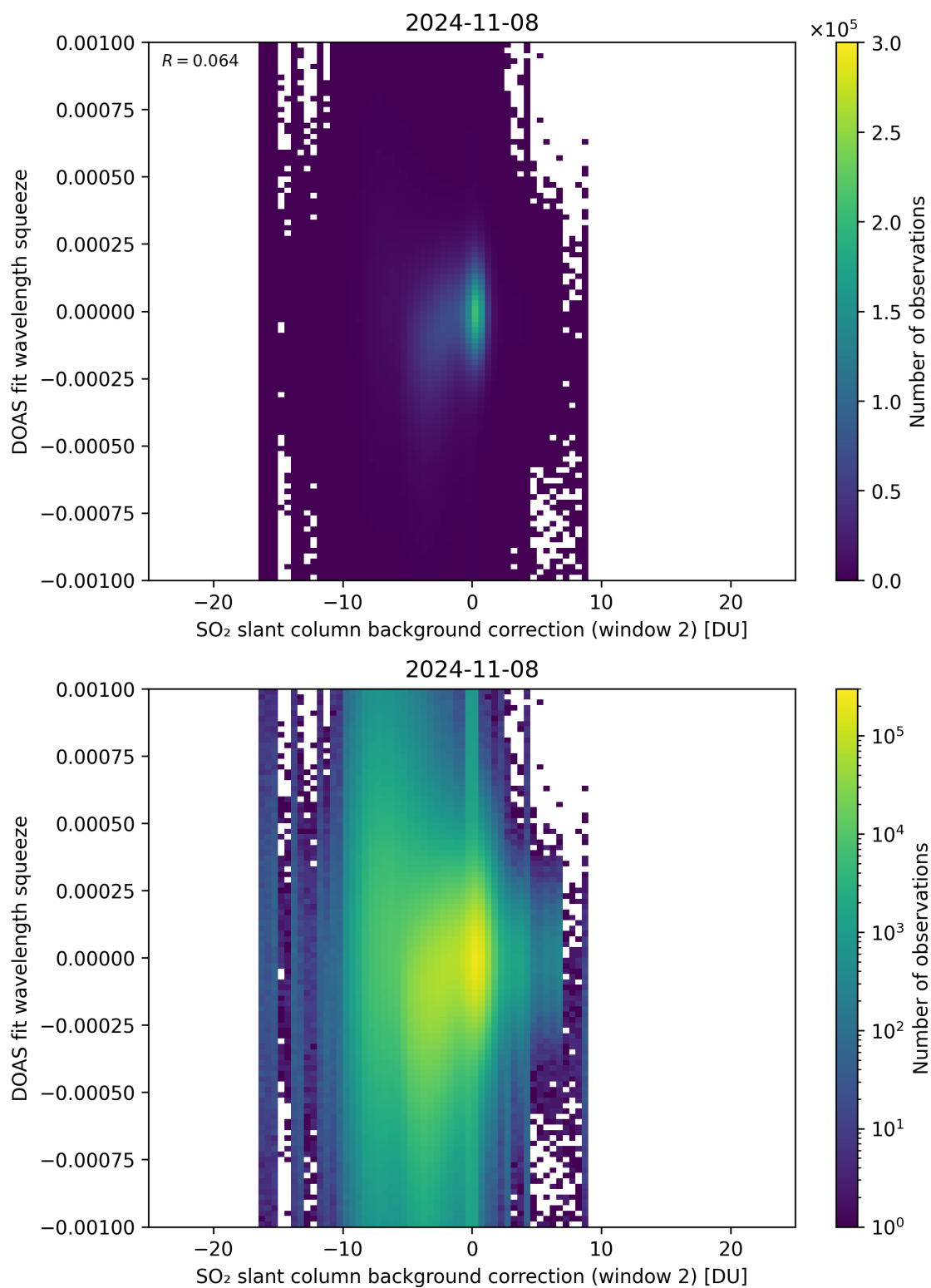
Figure 113: Scatter density plot of “SO 2 slant column background correction (window 2)” against “DOAS fit wavelength squeeze” for 2024-11-07 to 2024-11-09.
