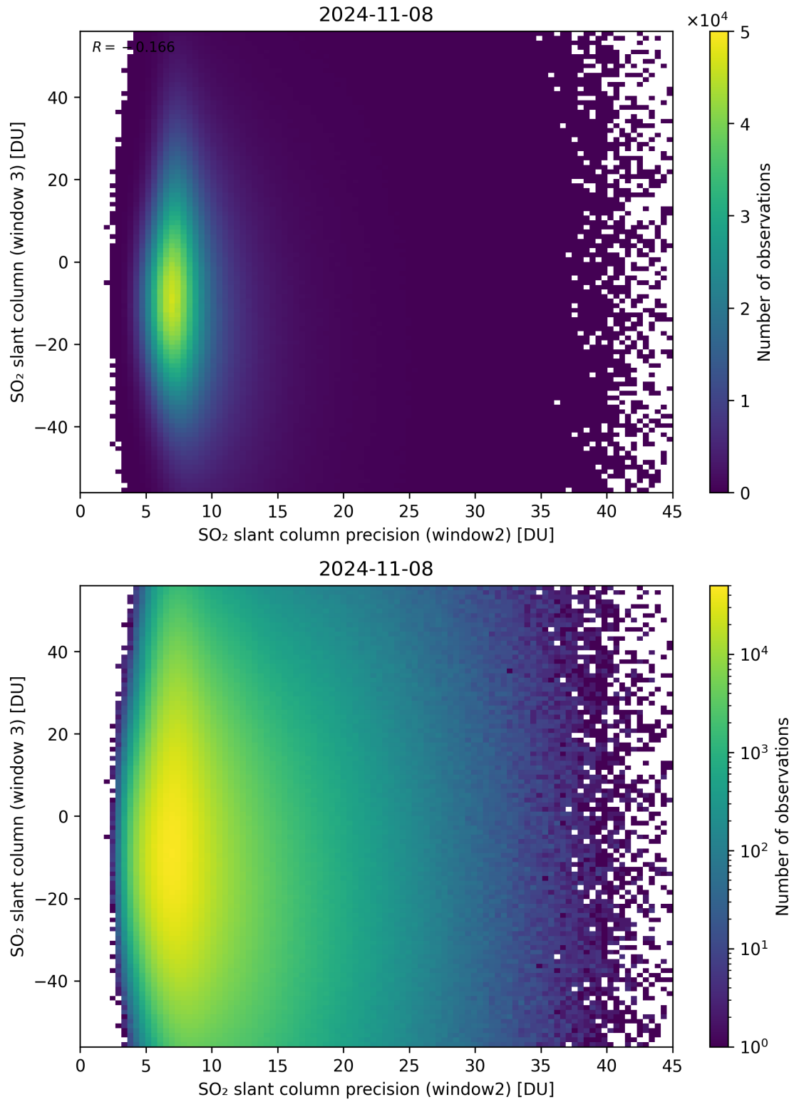
Figure 249: Scatter density plot of “SO 2 slant column precision (window2)” against “SO 2 slant column (window 3)” for 2024-11-07 to 2024-11-09.
