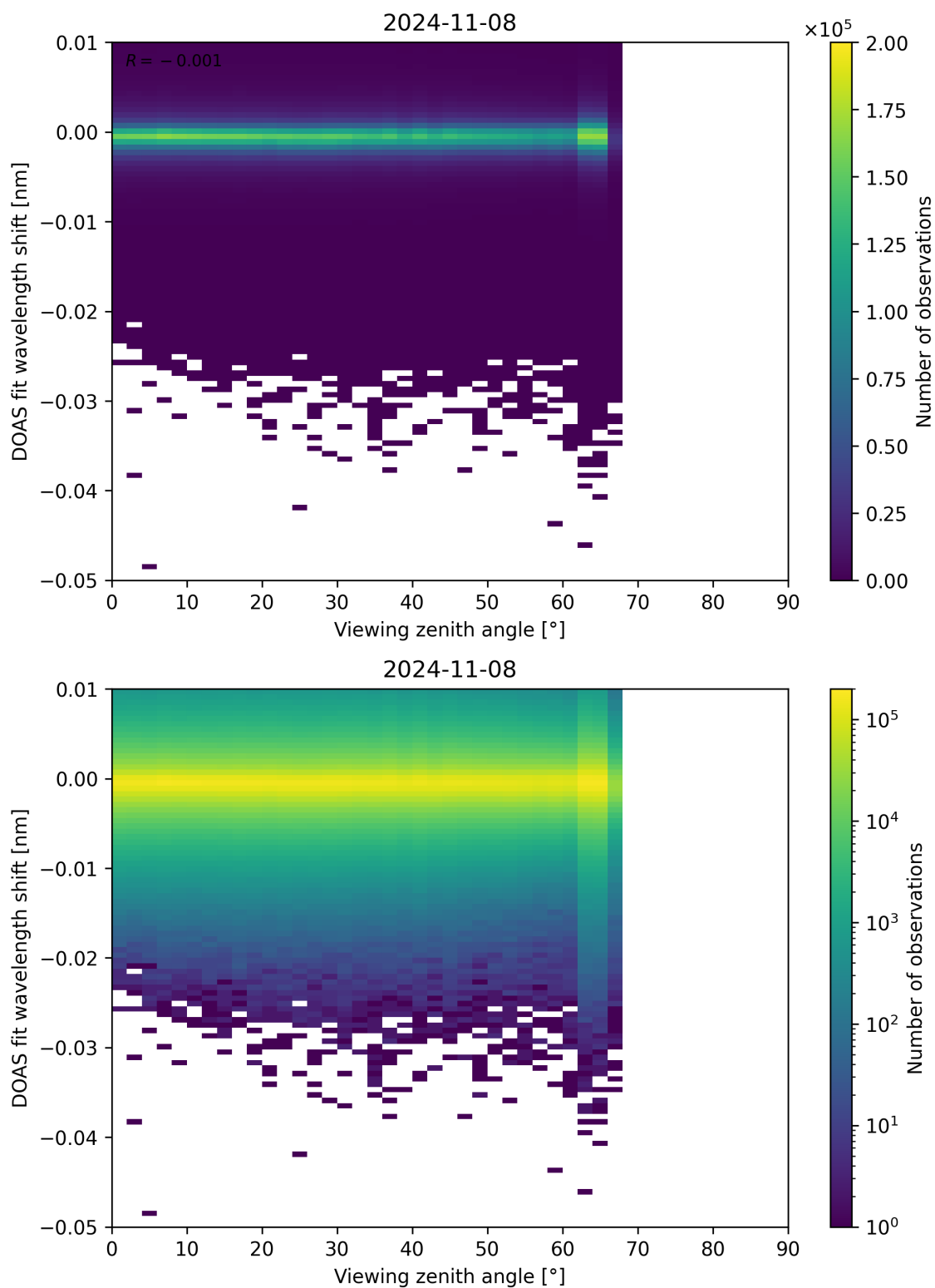
Figure 311: Scatter density plot of “Viewing zenith angle” against “DOAS fit wavelength shift” for 2024-11-07 to 2024-11-09.
