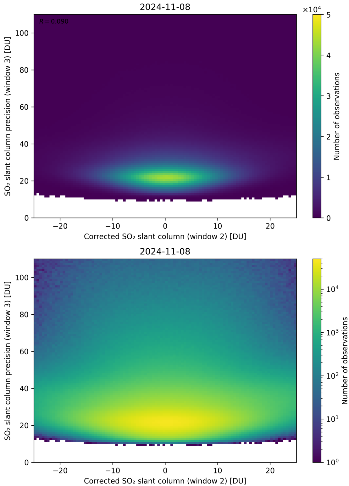
Figure 202: Scatter density plot of “Corrected SO 2 slant column (window 2)” against “SO 2 slant column precision (window 3)” for 2024-11-07 to 2024-11-09.
