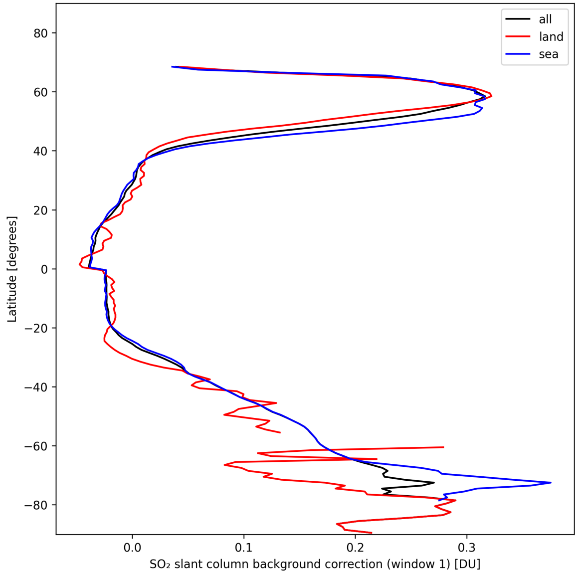
Figure 36: Zonal average of “SO 2 slant column background correction (window 1)” for 2024-11-07 to 2024-11-09.
