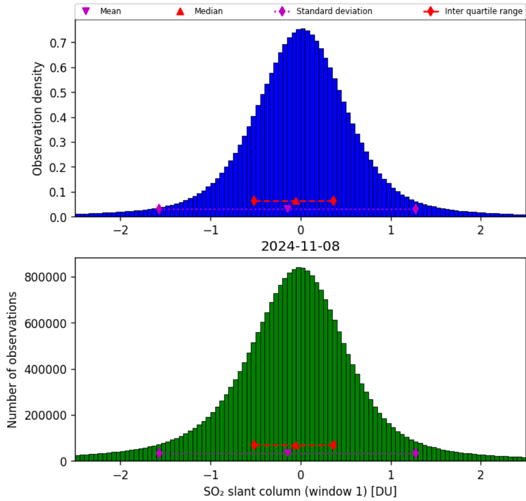
Figure 56: Histogram of “SO 2 slant column (window 1)” for 2024-11-07 to 2024-11-09
