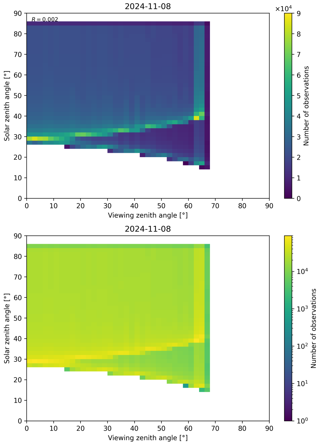
Figure 315: Scatter density plot of “Viewing zenith angle” against “Solar zenith angle” for 2024-11-07 to 2024-11-09.
