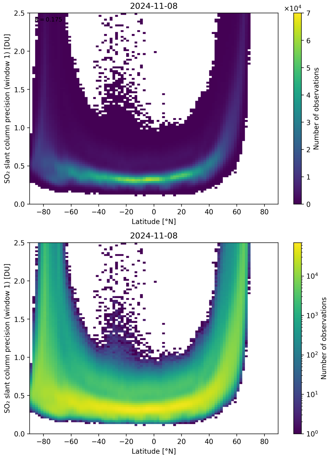
Figure 150: Scatter density plot of “Latitude” against “SO 2 slant column precision (window 1)” for 2024-11-07 to 2024-11-09.
