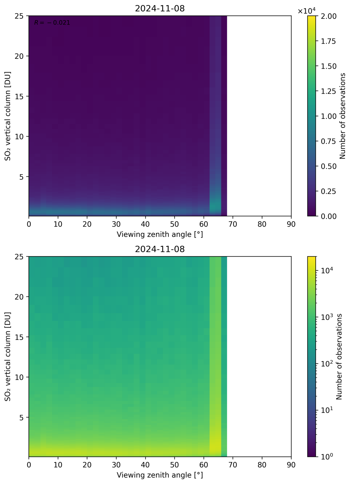
Figure 327: Scatter density plot of “Viewing zenith angle” against “SO 2 vertical column” for 2024-11-07 to 2024-11-09.
