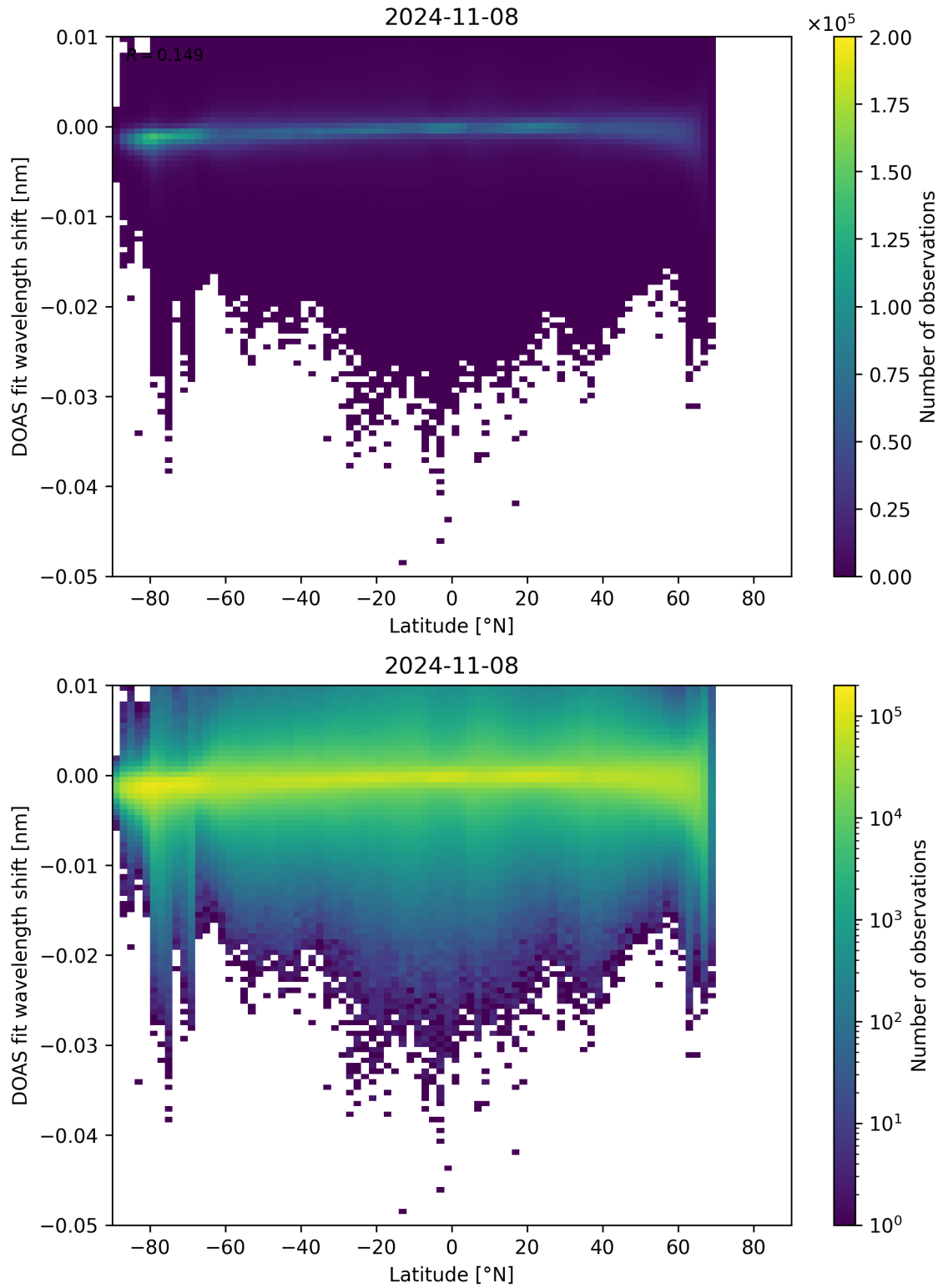
Figure 142: Scatter density plot of “Latitude” against “DOAS fit wavelength shift” for 2024-11-07 to 2024-11-09.
