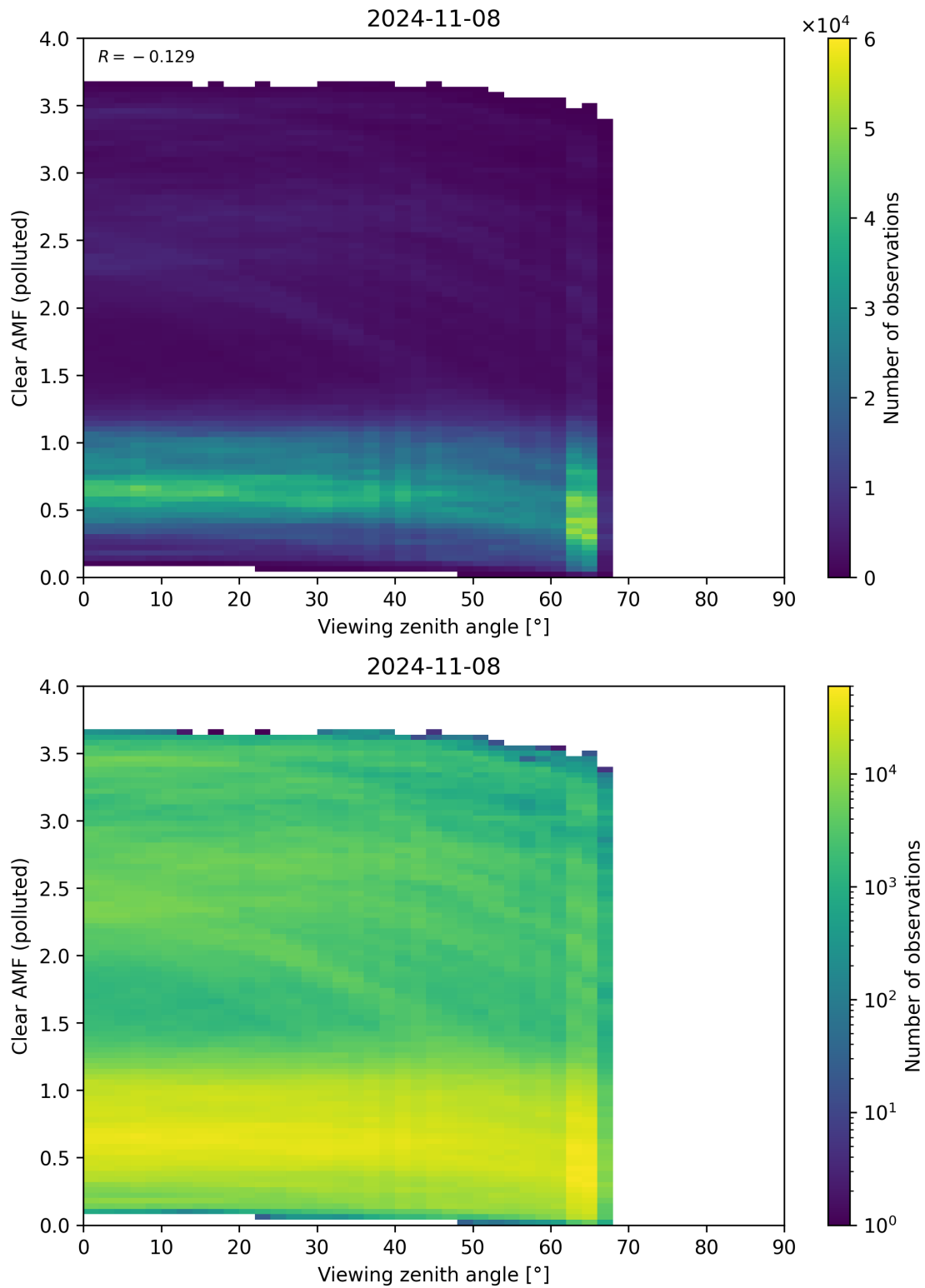
Figure 316: Scatter density plot of “Viewing zenith angle” against “Clear AMF (polluted)” for 2024-11-07 to 2024-11-09.
