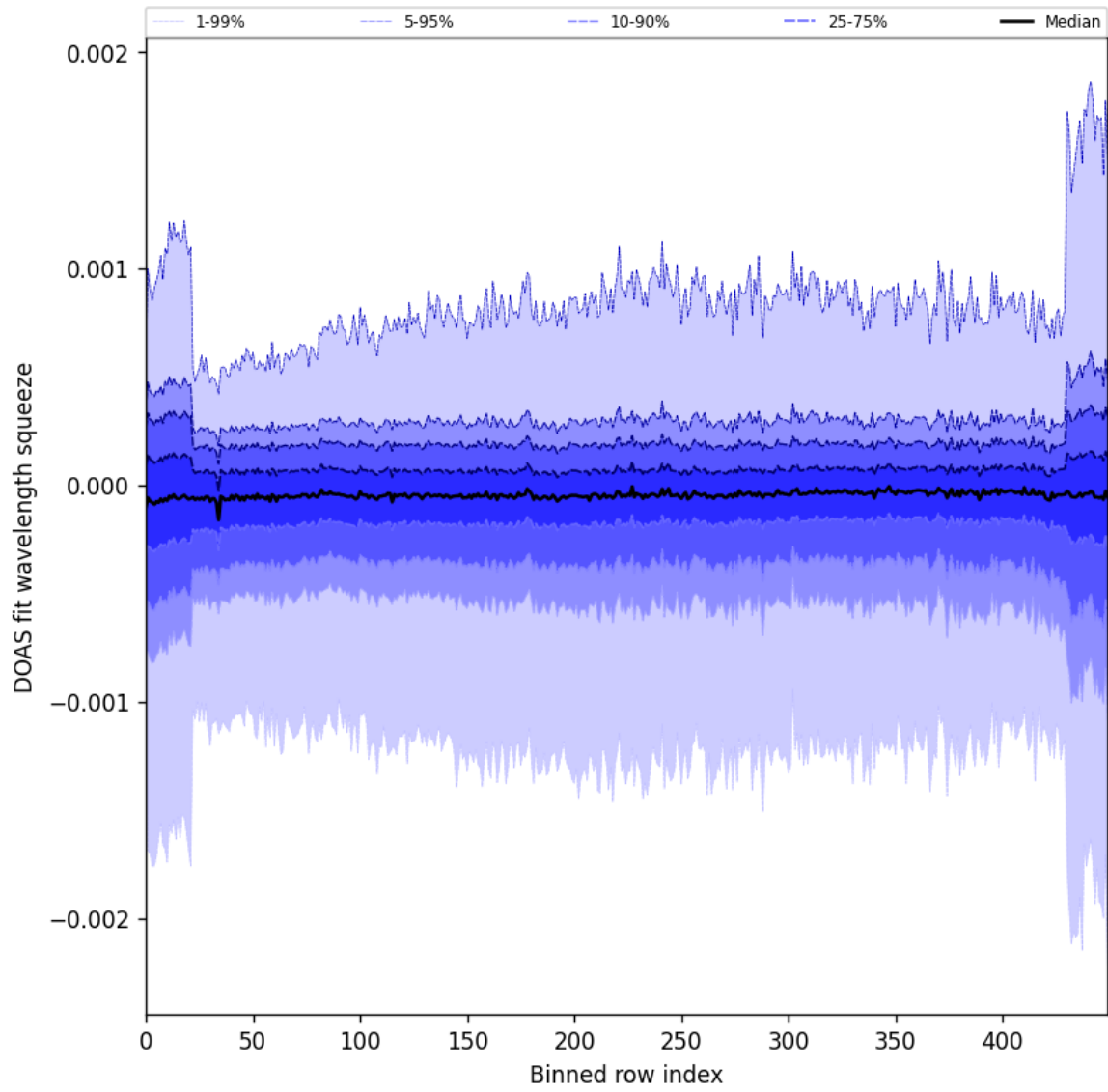
Figure 92: Along track statistics of “DOAS fit wavelength squeeze” for 2024-11-07 to 2024-11-09
