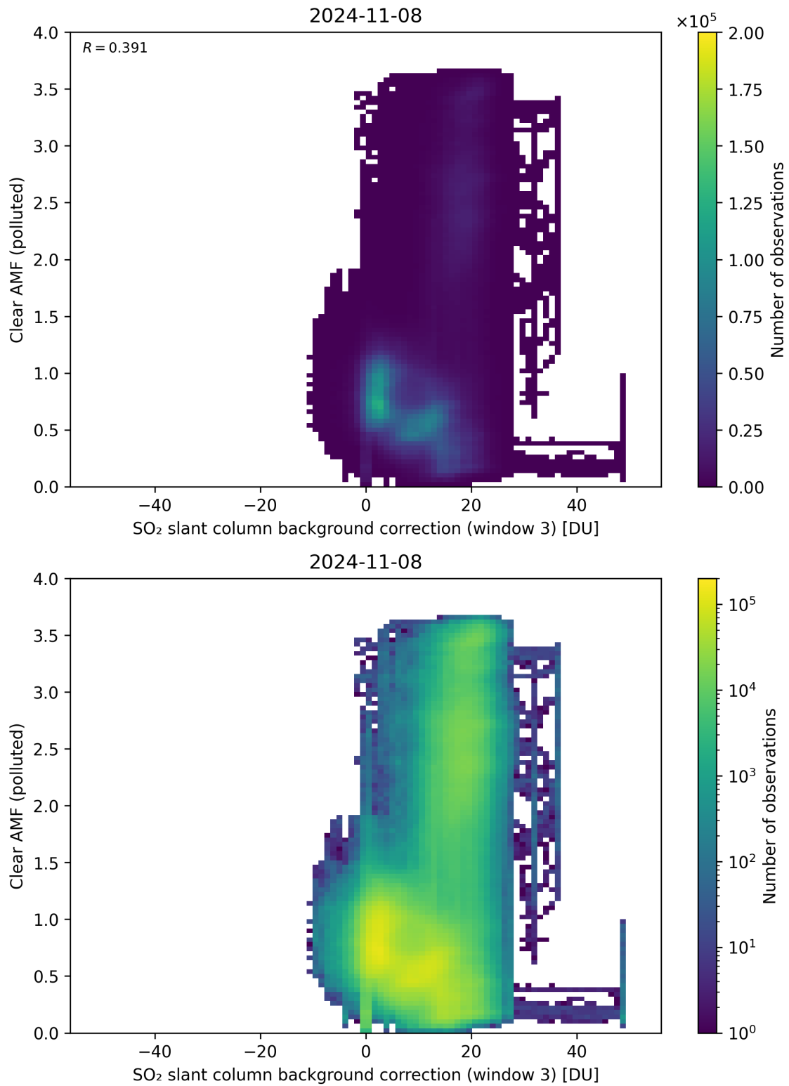
Figure 124: Scatter density plot of “SO 2 slant column background correction (window 3)” against “Clear AMF (polluted)” for 2024-11-07 to 2024-11-09.
