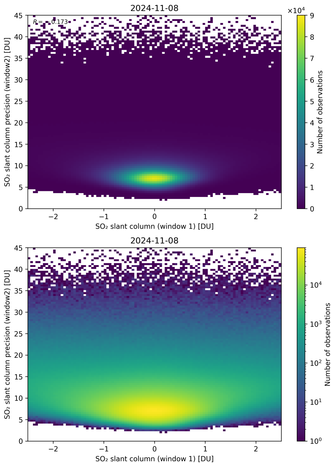
Figure 236: Scatter density plot of “SO 2 slant column (window 1)” against “SO 2 slant column precision (window2)” for 2024-11-07 to 2024-11-09.
