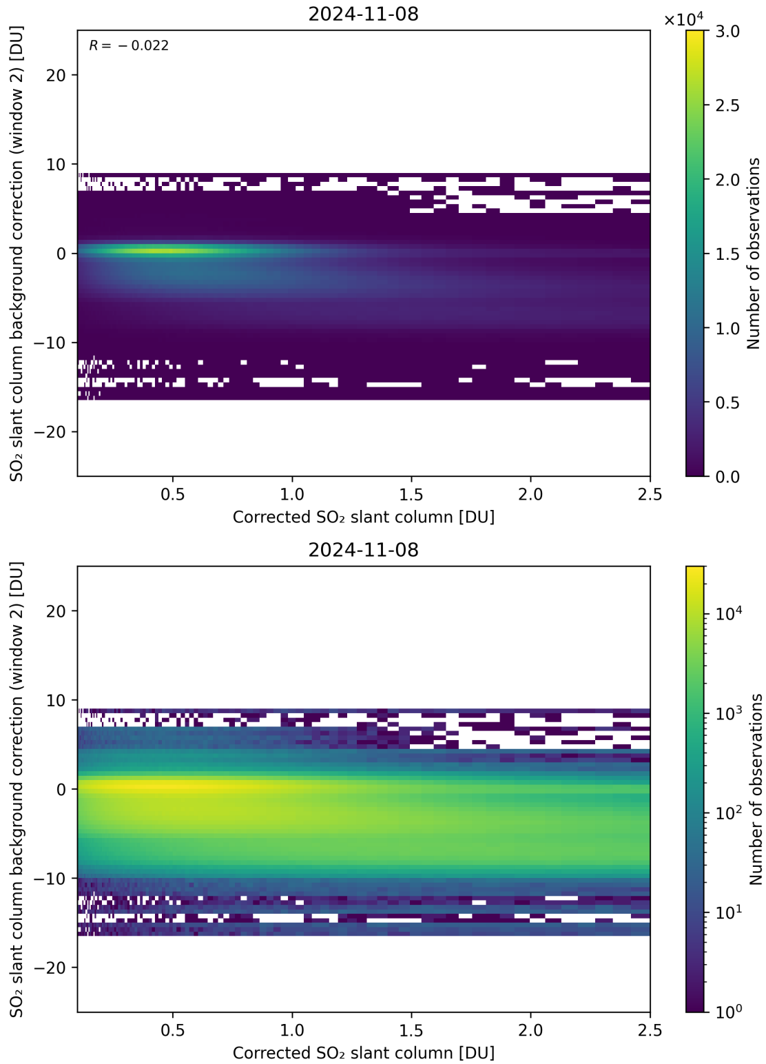
Figure 179: Scatter density plot of “Corrected SO 2 slant column” against “SO 2 slant column background correction (window 2)” for 2024-11-07 to 2024-11-09.
