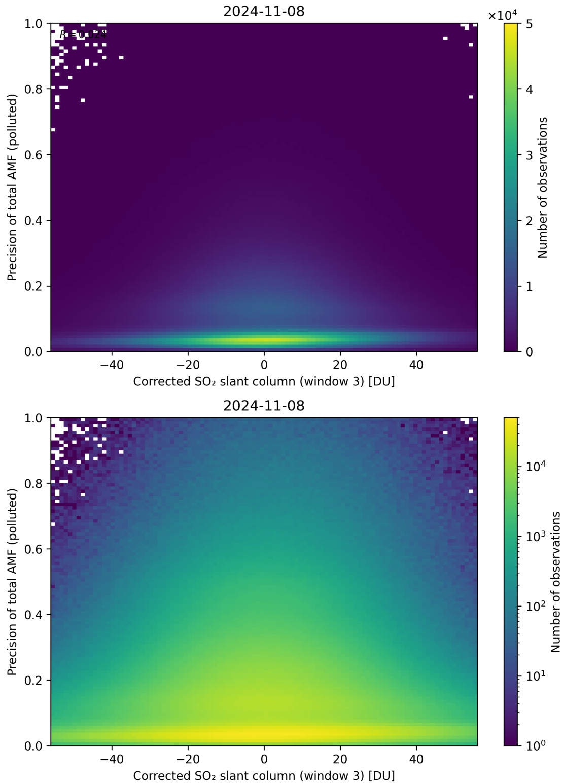
Figure 211: Scatter density plot of “Corrected SO 2 slant column (window 3)” against “Precision of total AMF (polluted)” for 2024-11-07 to 2024-11-09.
