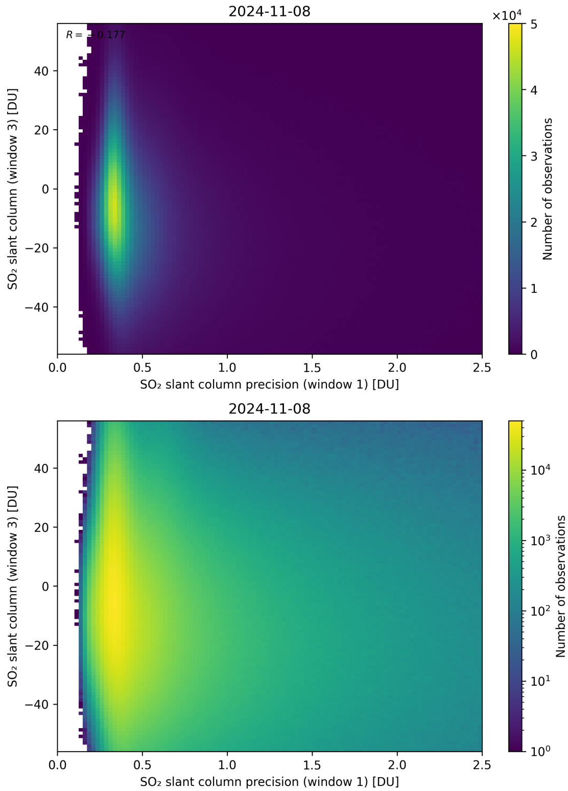
Figure 228: Scatter density plot of “SO 2 slant column precision (window 1)” against “SO 2 slant column (window 3)” for 2024-11-07 to 2024-11-09.
