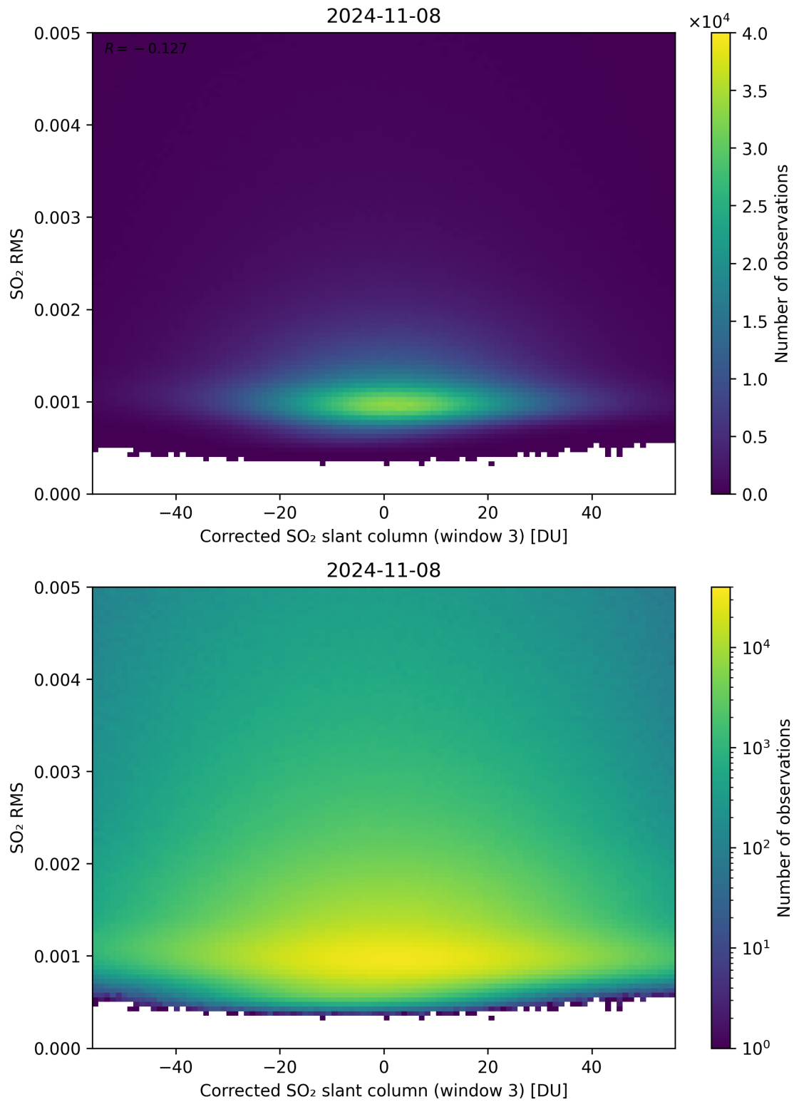
Figure 208: Scatter density plot of “Corrected SO 2 slant column (window 3)” against “SO 2 RMS” for 2024-11-07 to 2024-11-09.
