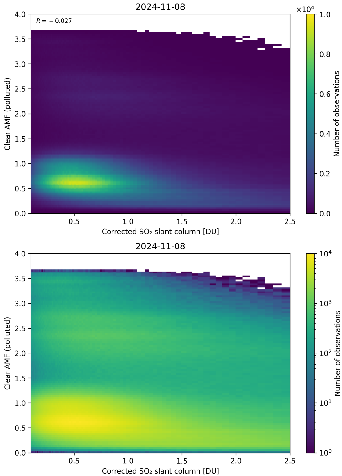
Figure 184: Scatter density plot of “Corrected SO 2 slant column” against “Clear AMF (polluted)” for 2024-11-07 to 2024-11-09.
