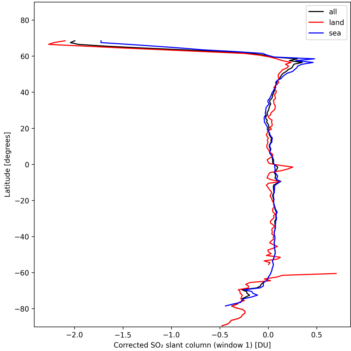
Figure 35: Zonal average of “Corrected SO 2 slant column (window 1)” for 2024-11-07 to 2024-11-09.
