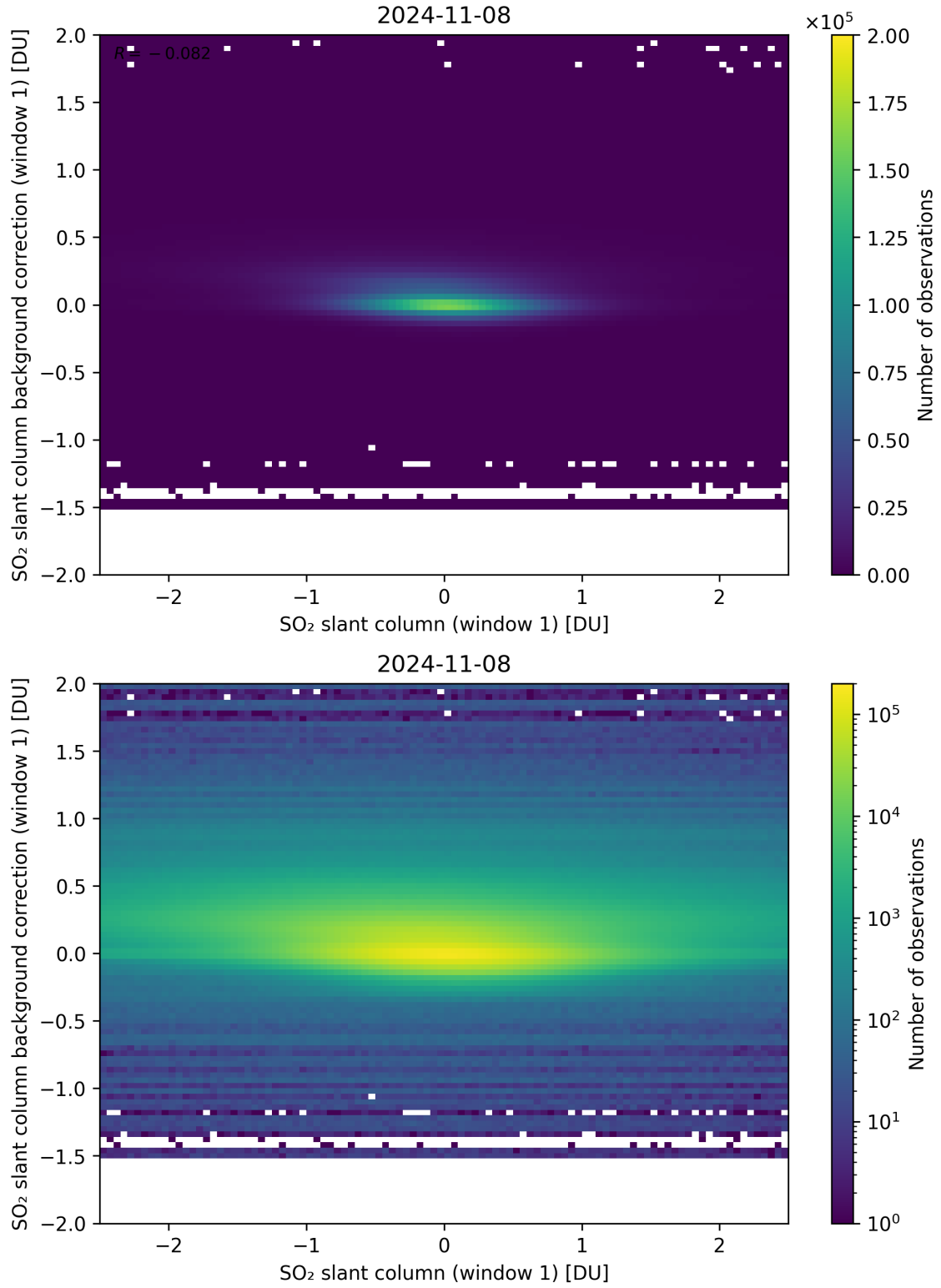
Figure 212: Scatter density plot of “SO 2 slant column (window 1)” against “SO 2 slant column background correction (window 1)” for 2024-11-07 to 2024-11-09.
