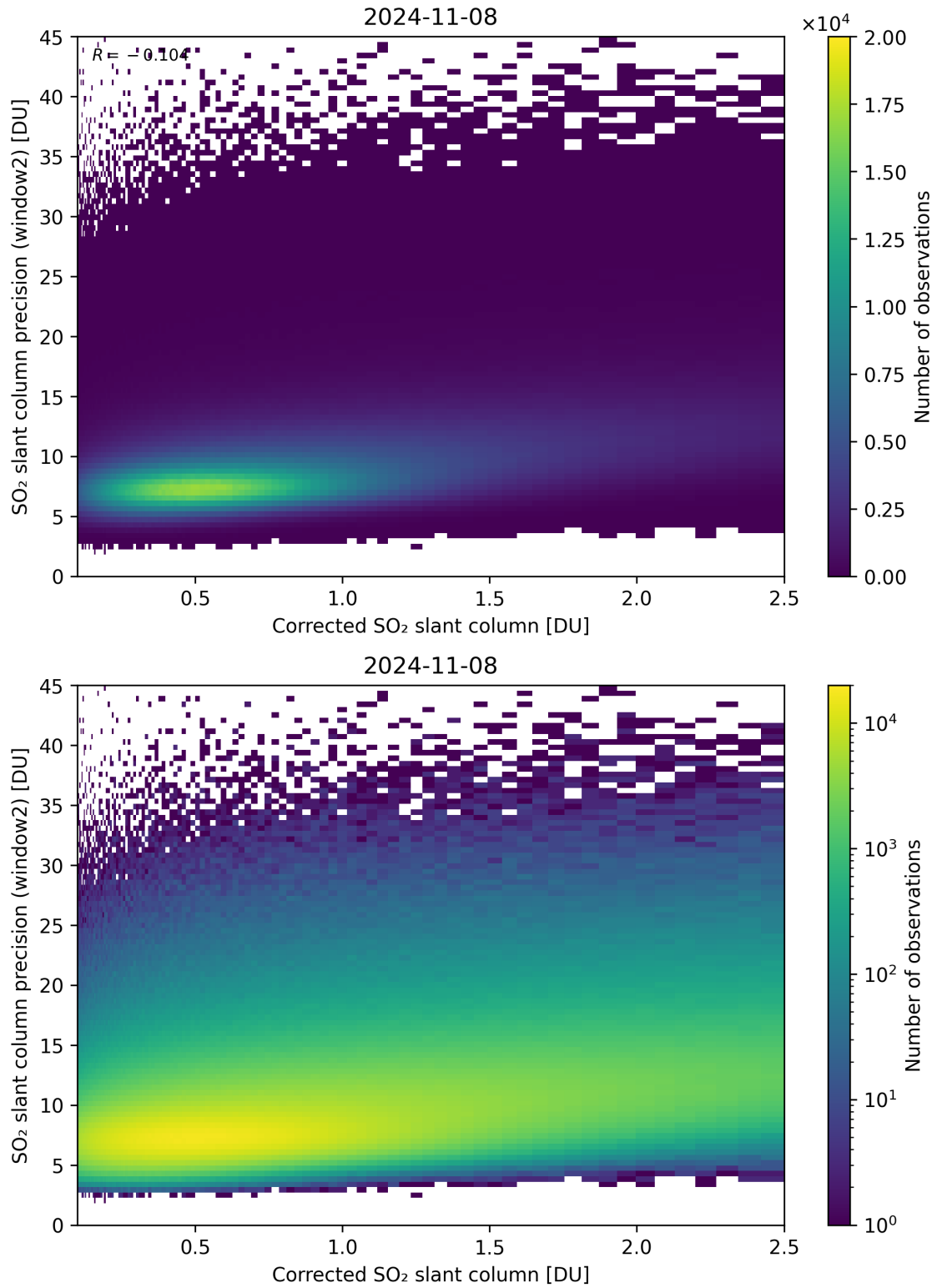
Figure 189: Scatter density plot of “Corrected SO 2 slant column” against “SO 2 slant column precision (window2)” for 2024-11-07 to 2024-11-09.
