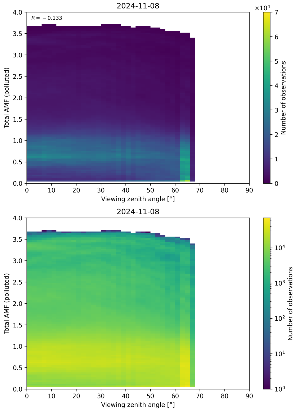
Figure 325: Scatter density plot of “Viewing zenith angle” against “Total AMF (polluted)” for 2024-11-07 to 2024-11-09.
