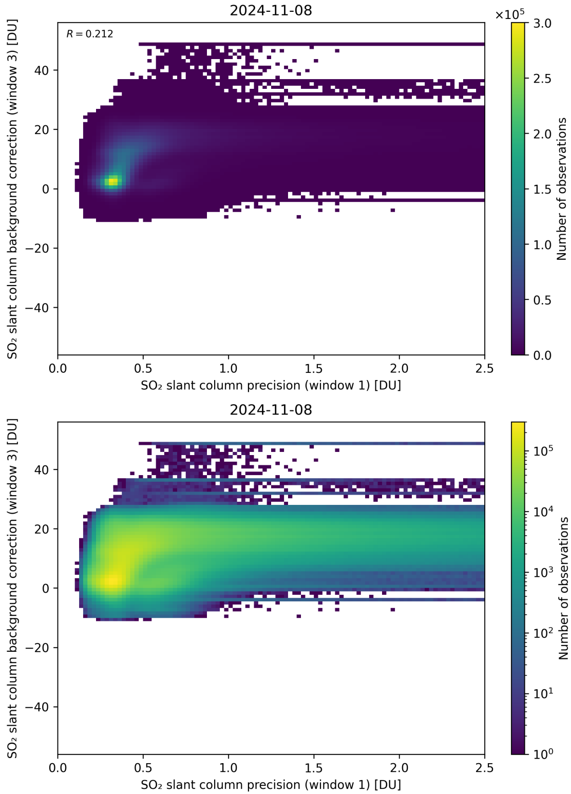
Figure 220: Scatter density plot of “SO 2 slant column precision (window 1)” against “SO 2 slant column background correction (window 3)” for 2024-11-07 to 2024-11-09.
