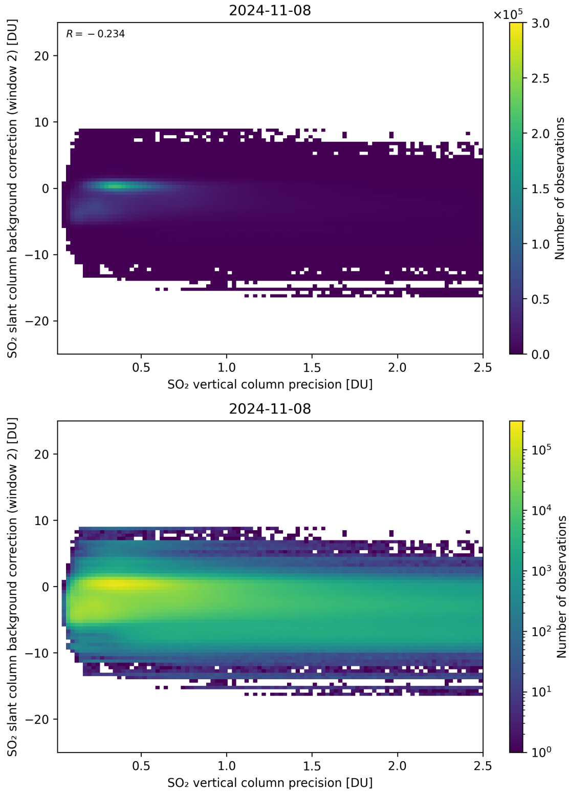
Figure 280: Scatter density plot of “SO 2 vertical column precision” against “SO 2 slant column background correction (window 2)” for 2024-11-07 to 2024-11-09.
