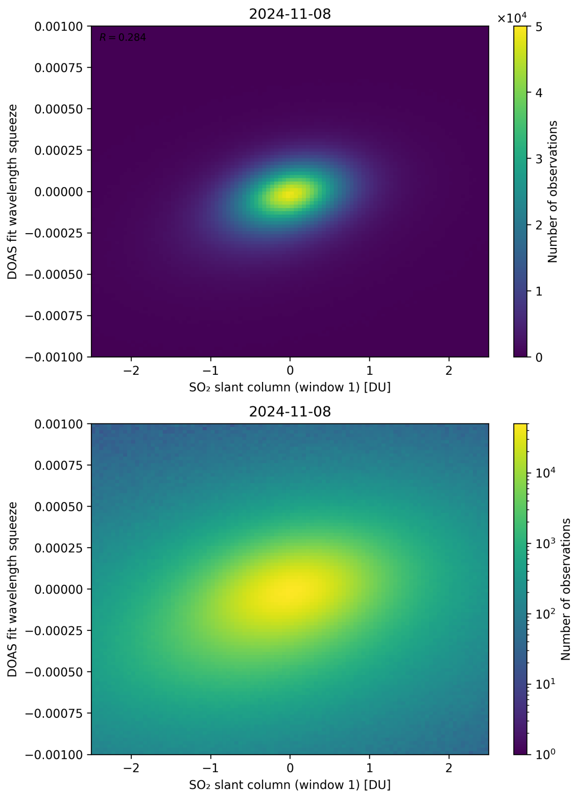
Figure 216: Scatter density plot of “SO 2 slant column (window 1)” against “DOAS fit wavelength squeeze” for 2024-11-07 to 2024-11-09.
