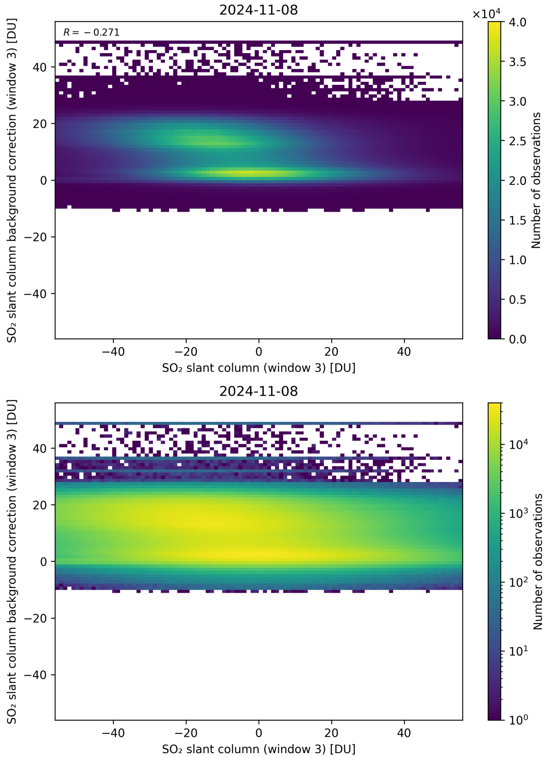
Figure 253: Scatter density plot of “SO 2 slant column (window 3)” against “SO 2 slant column background correction (window 3)” for 2024-11-07 to 2024-11-09.
