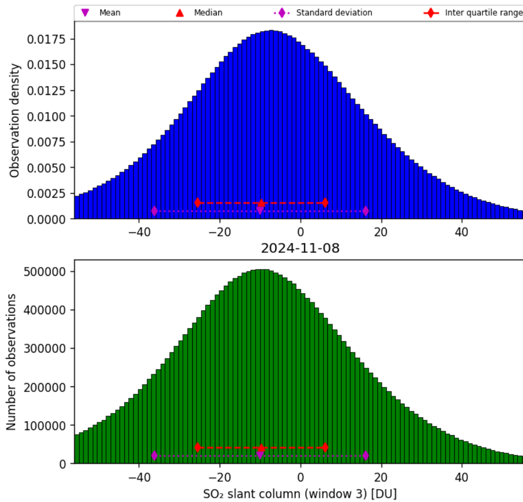
Figure 64: Histogram of “SO 2 slant column (window 3)” for 2024-11-07 to 2024-11-09
