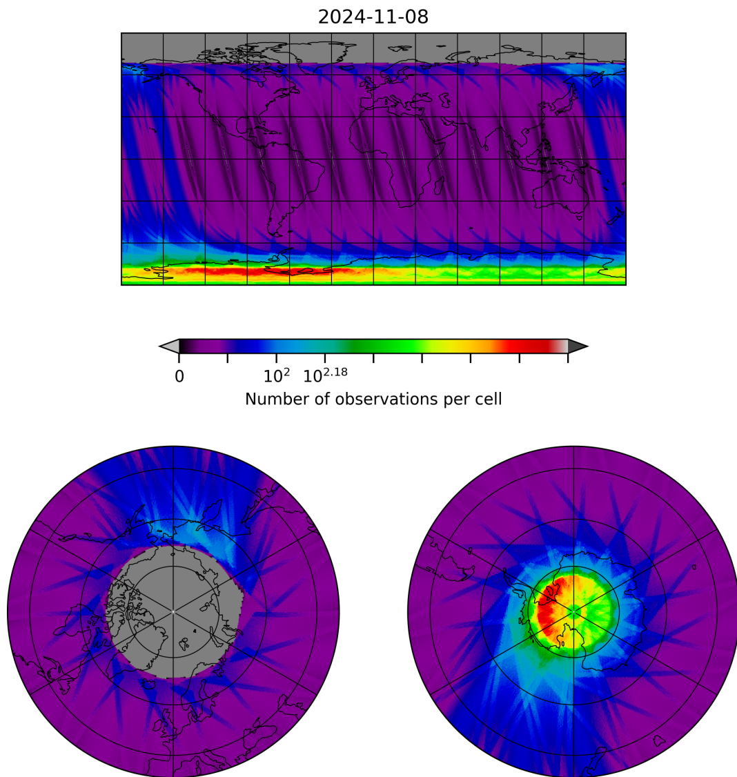
Figure 28: Map of the number of observations for 2024-11-07 to 2024-11-09
