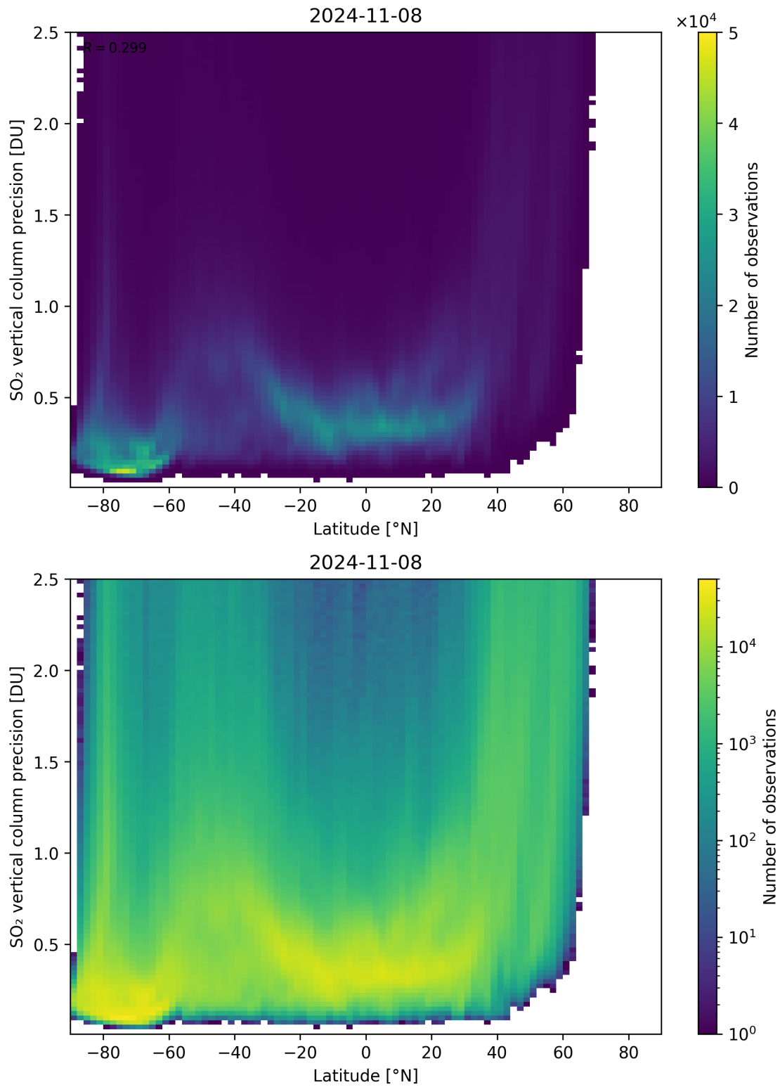
Figure 157: Scatter density plot of “Latitude” against “SO 2 vertical column precision” for 2024-11-07 to 2024-11-09.
