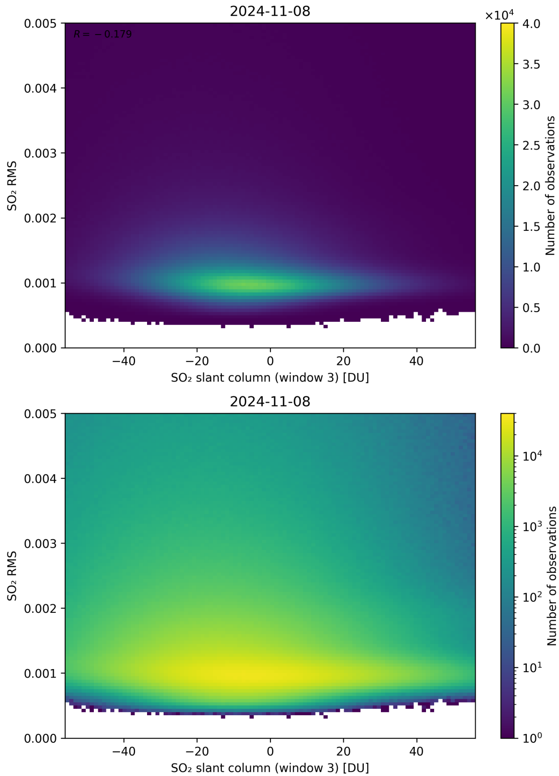
Figure 256: Scatter density plot of “SO 2 slant column (window 3)” against “SO 2 RMS” for 2024-11-07 to 2024-11-09.
