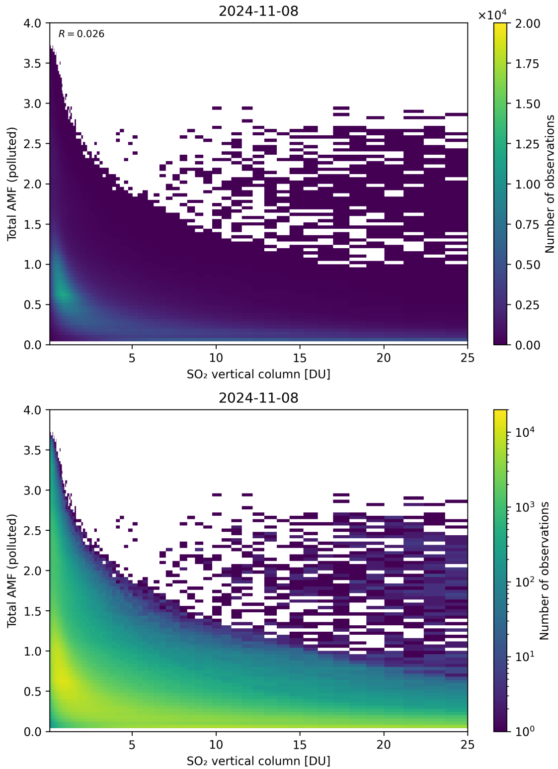
Figure 305: Scatter density plot of “SO 2 vertical column” against “Total AMF (polluted)” for 2024-11-07 to 2024-11-09.
