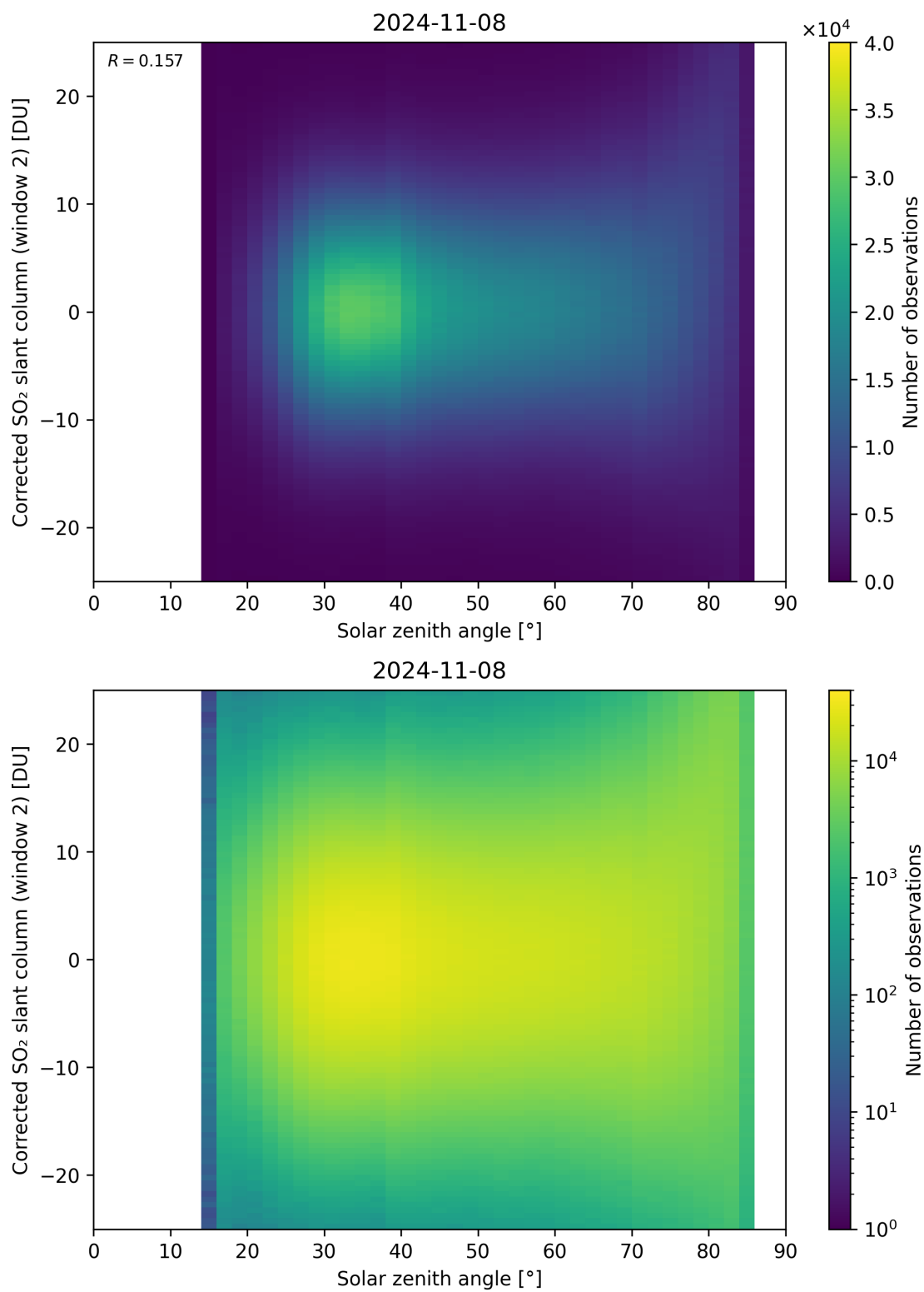
Figure 167: Scatter density plot of “Solar zenith angle” against “Corrected SO 2 slant column (window 2)” for 2024-11-07 to 2024-11-09.
