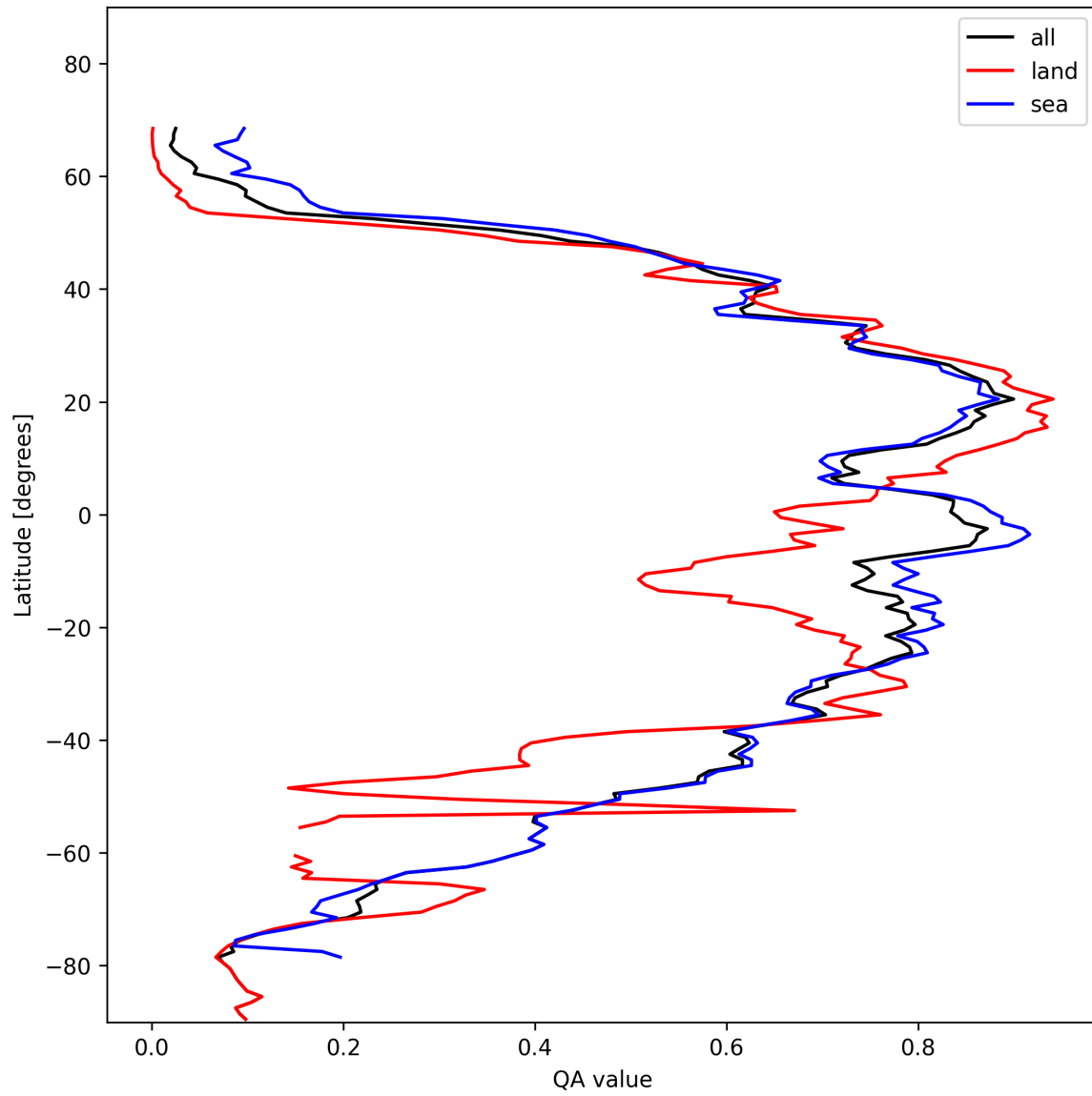
Figure 29: Zonal average of “QA value” for 2024-11-07 to 2024-11-09.
