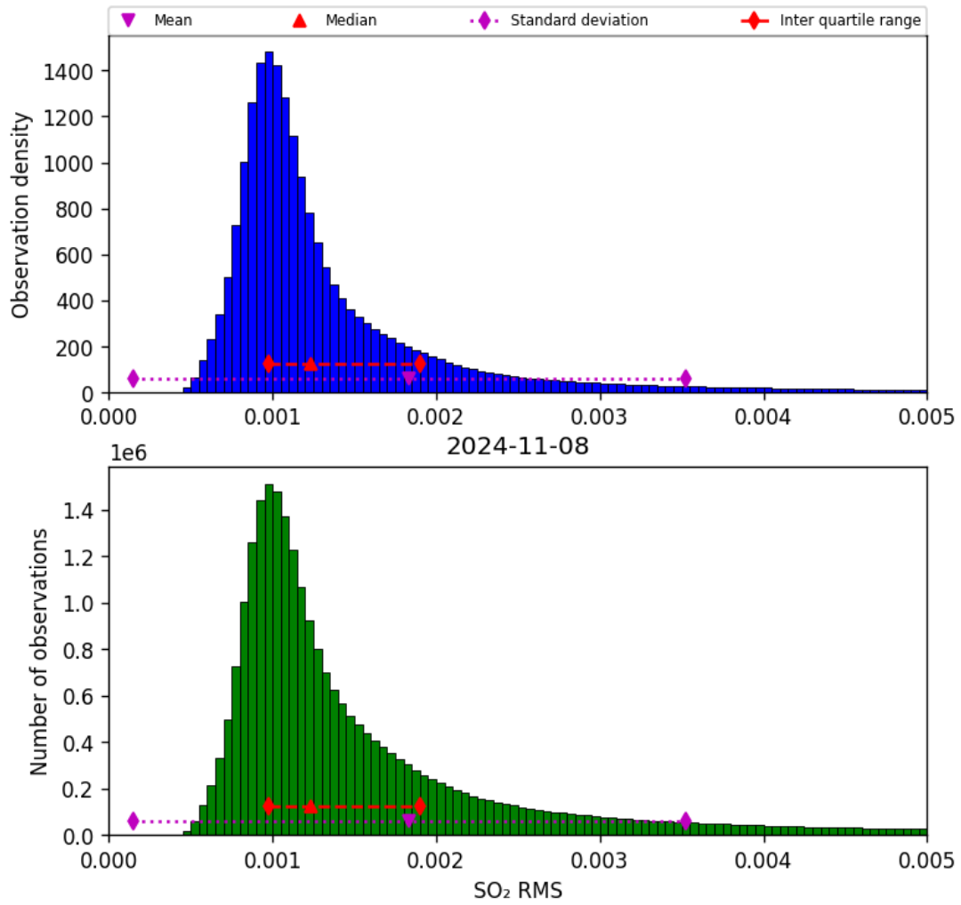
Figure 70: Histogram of “SO 2 RMS” for 2024-11-07 to 2024-11-09
