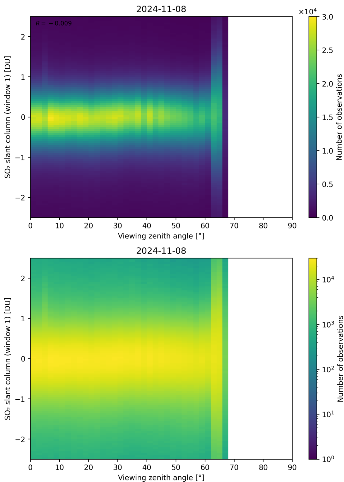
Figure 320: Scatter density plot of “Viewing zenith angle” against “SO 2 slant column (window 1)” for 2024-11-07 to 2024-11-09.
