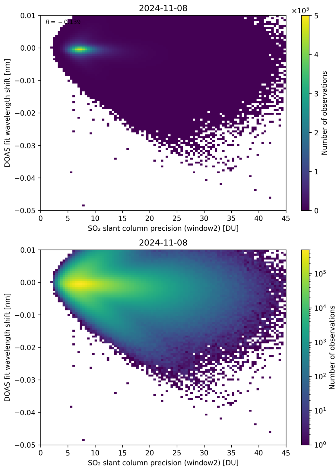
Figure 243: Scatter density plot of “SO 2 slant column precision (window2)” against “DOAS fit wavelength shift” for 2024-11-07 to 2024-11-09.
