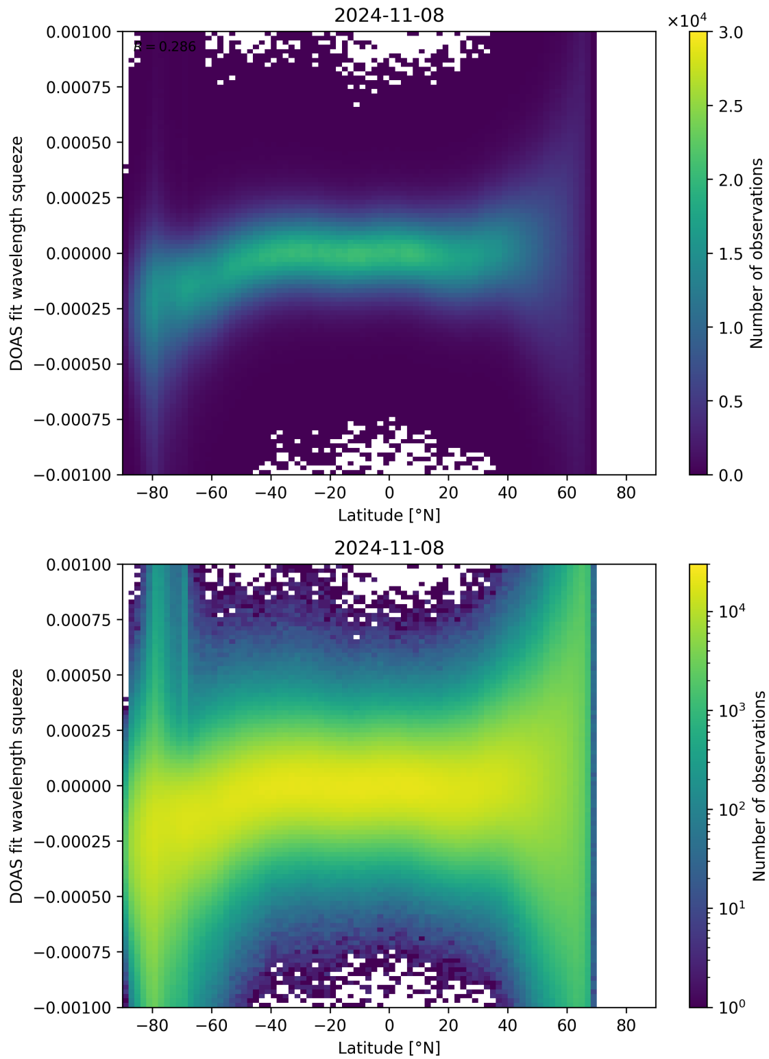
Figure 143: Scatter density plot of “Latitude” against “DOAS fit wavelength squeeze” for 2024-11-07 to 2024-11-09.
