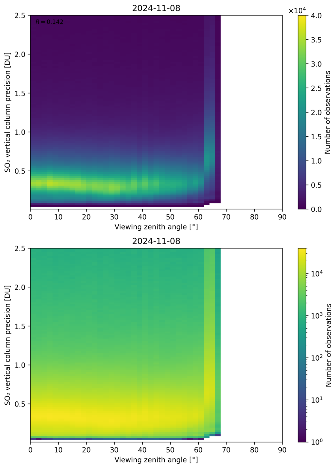
Figure 328: Scatter density plot of “Viewing zenith angle” against “SO 2 vertical column precision” for 2024-11-07 to 2024-11-09.
