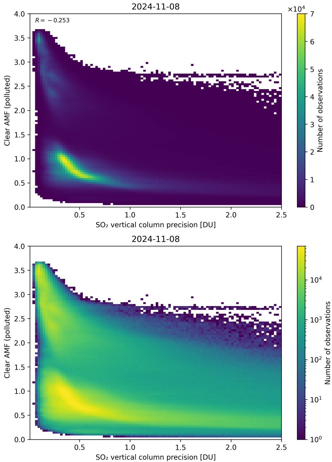
Figure 285: Scatter density plot of “SO 2 vertical column precision” against “Clear AMF (polluted)” for 2024-11-07 to 2024-11-09.
