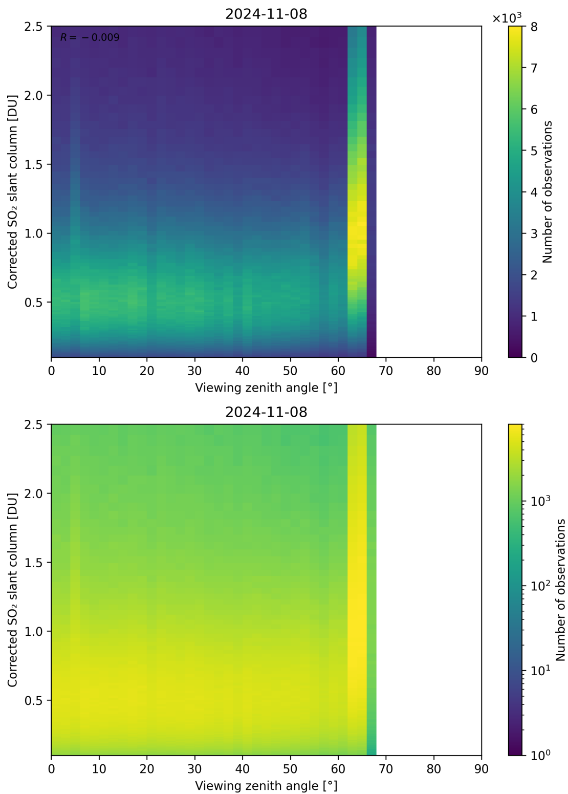
Figure 317: Scatter density plot of “Viewing zenith angle” against “Corrected SO 2 slant column” for 2024-11-07 to 2024-11-09.
