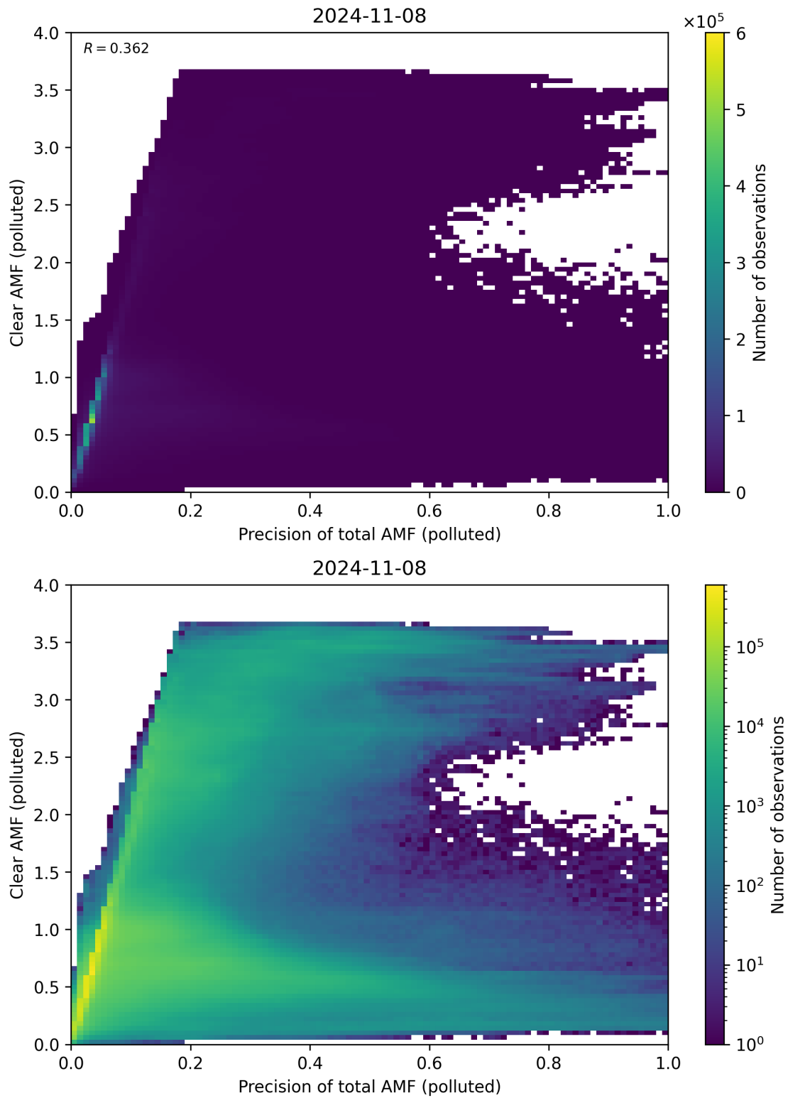
Figure 270: Scatter density plot of “Precision of total AMF (polluted)” against “Clear AMF (polluted)” for 2024-11-07 to 2024-11-09.
