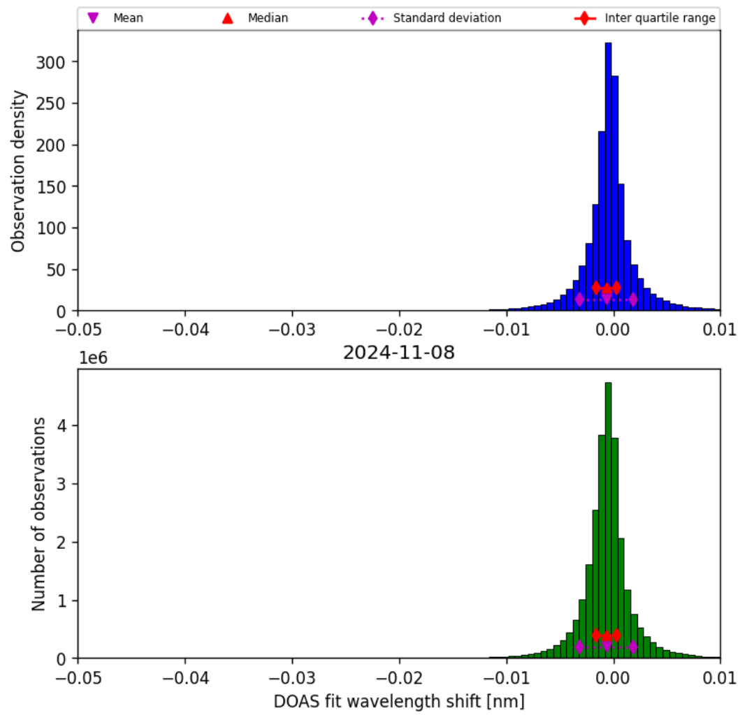
Figure 68: Histogram of “DOAS fit wavelength shift” for 2024-11-07 to 2024-11-09
