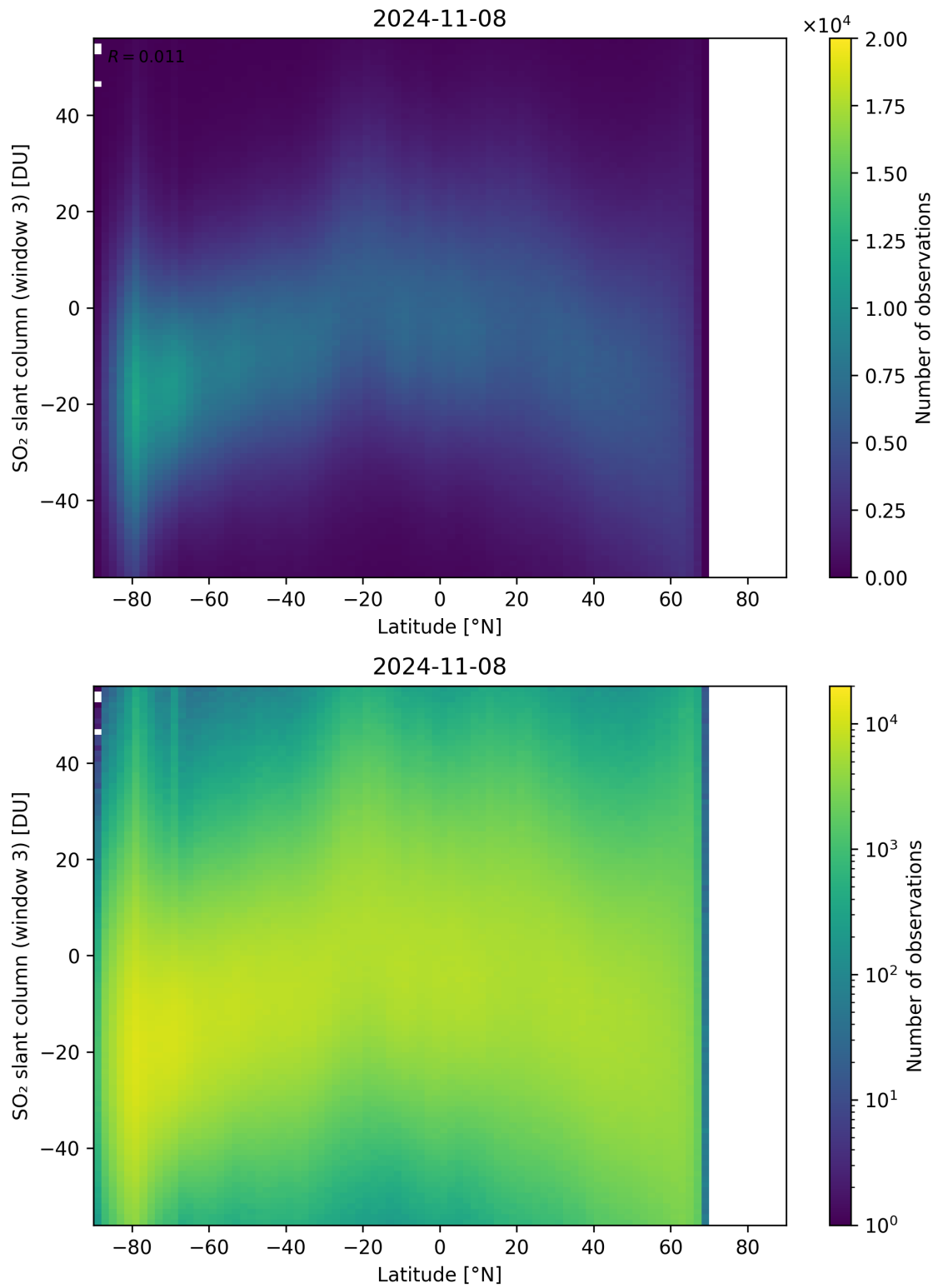
Figure 152: Scatter density plot of “Latitude” against “SO 2 slant column (window 3)” for 2024-11-07 to 2024-11-09.
