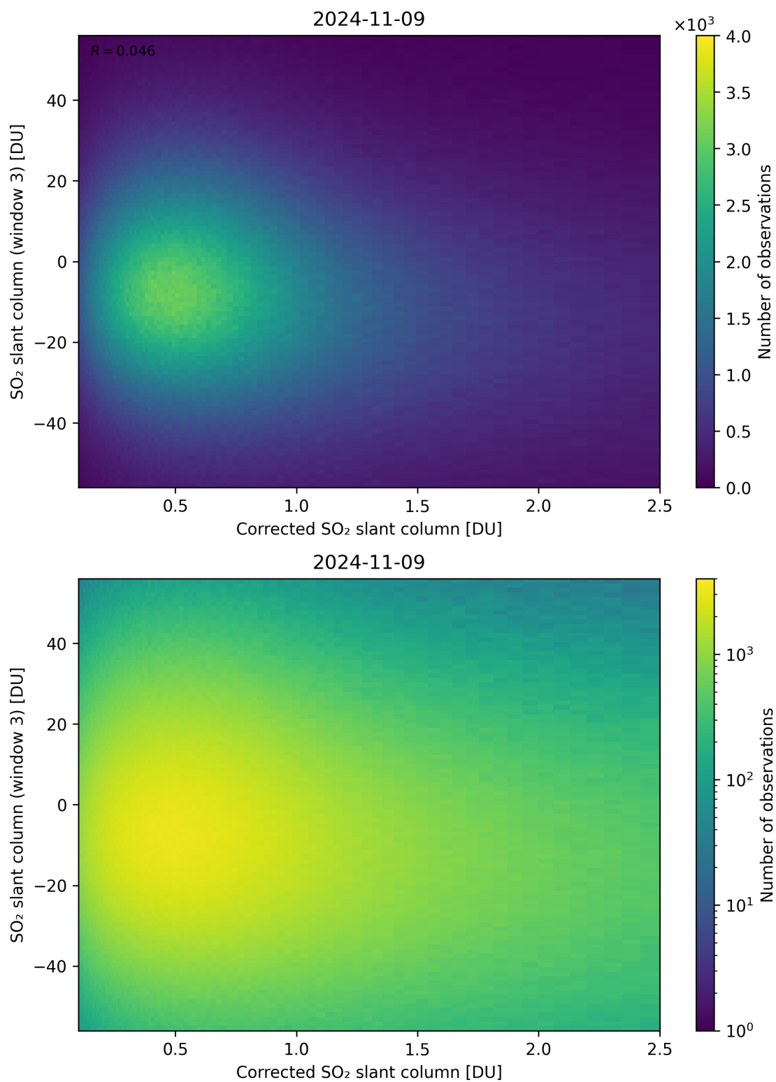
Figure 190: Scatter density plot of “Corrected SO 2 slant column” against “SO 2 slant column (window 3)” for 2024-11-09 to 2024-11-10.
