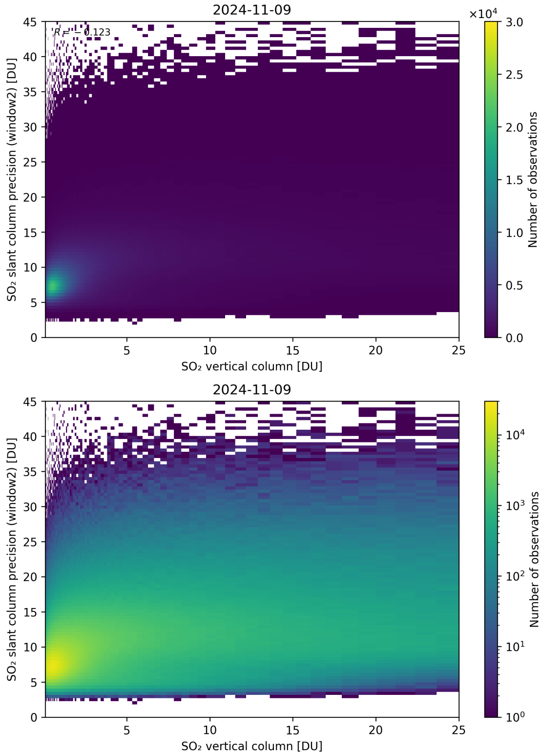
Figure 302: Scatter density plot of “SO 2 vertical column” against “SO 2 slant column precision (window2)” for 2024-11-09 to 2024-11-10.
