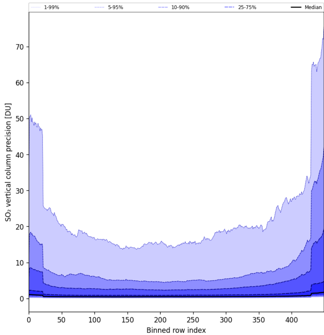
Figure 77: Along track statistics of “SO 2 vertical column precision” for 2024-11-09 to 2024-11-10
