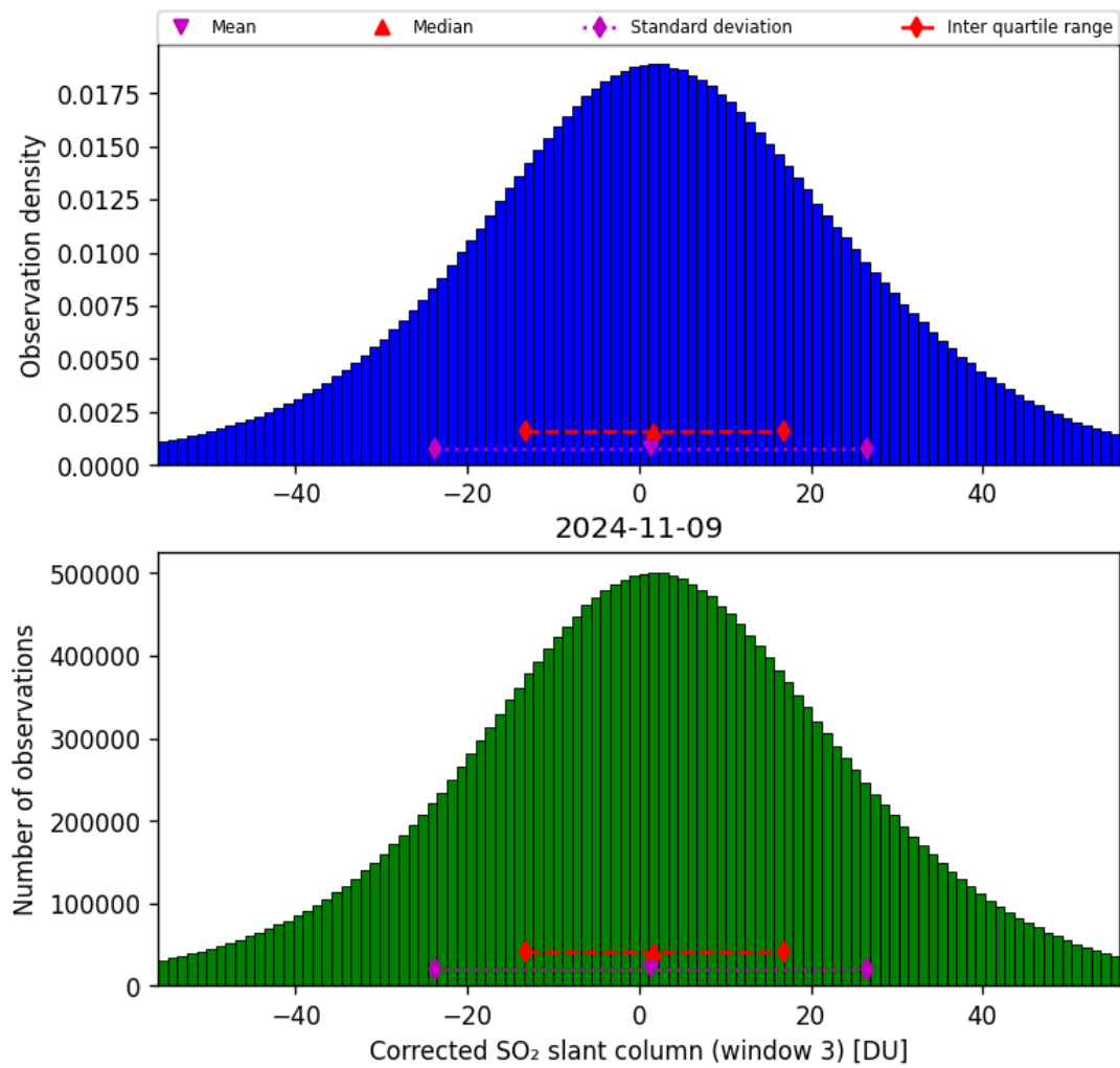
Figure 66: Histogram of “Corrected SO 2 slant column (window 3)” for 2024-11-09 to 2024-11-10
