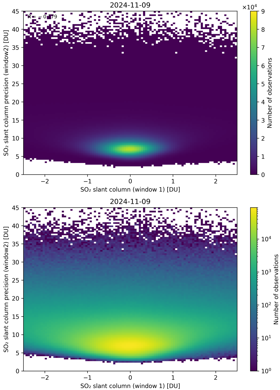
Figure 236: Scatter density plot of “SO 2 slant column (window 1)” against “SO 2 slant column precision (window2)” for 2024-11-09 to 2024-11-10.
