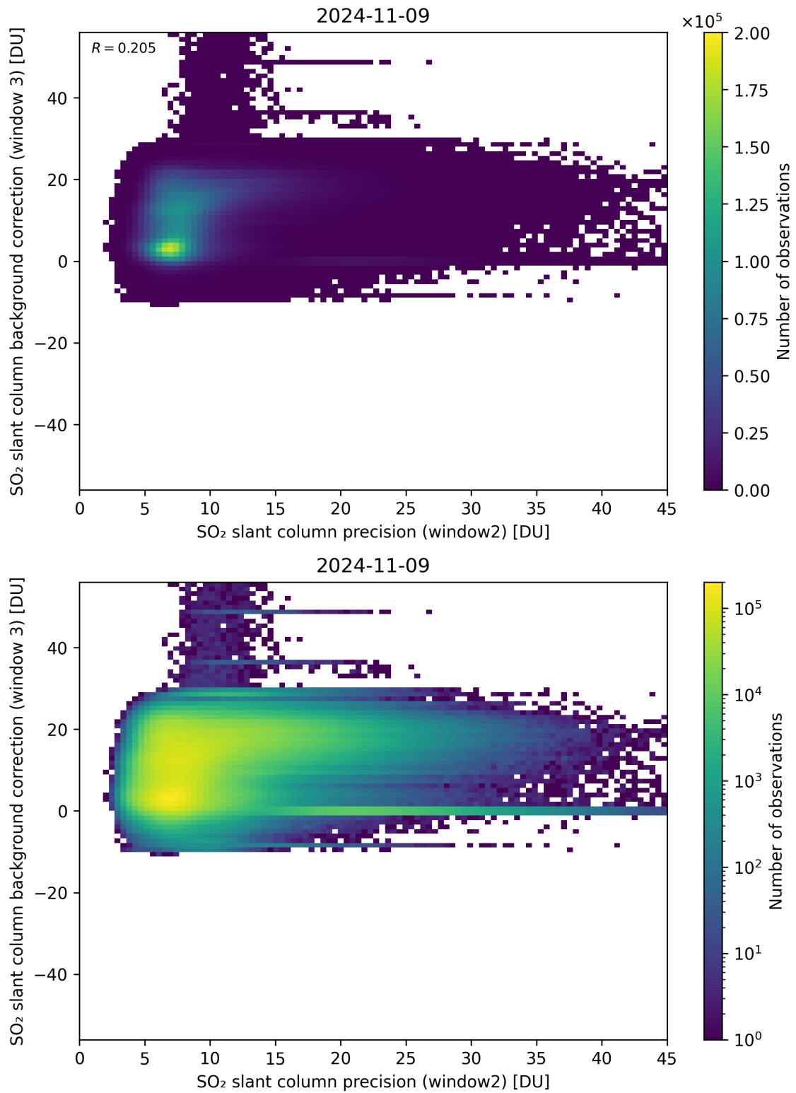
Figure 242: Scatter density plot of “SO 2 slant column precision (window2)” against “SO 2 slant column background correction (window 3)” for 2024-11-09 to 2024-11-10.
