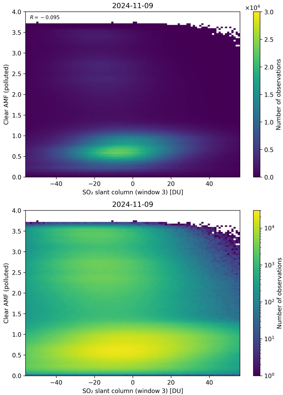
Figure 265: Scatter density plot of “SO 2 slant column (window 3)” against “Clear AMF (polluted)” for 2024-11-09 to 2024-11-10.
