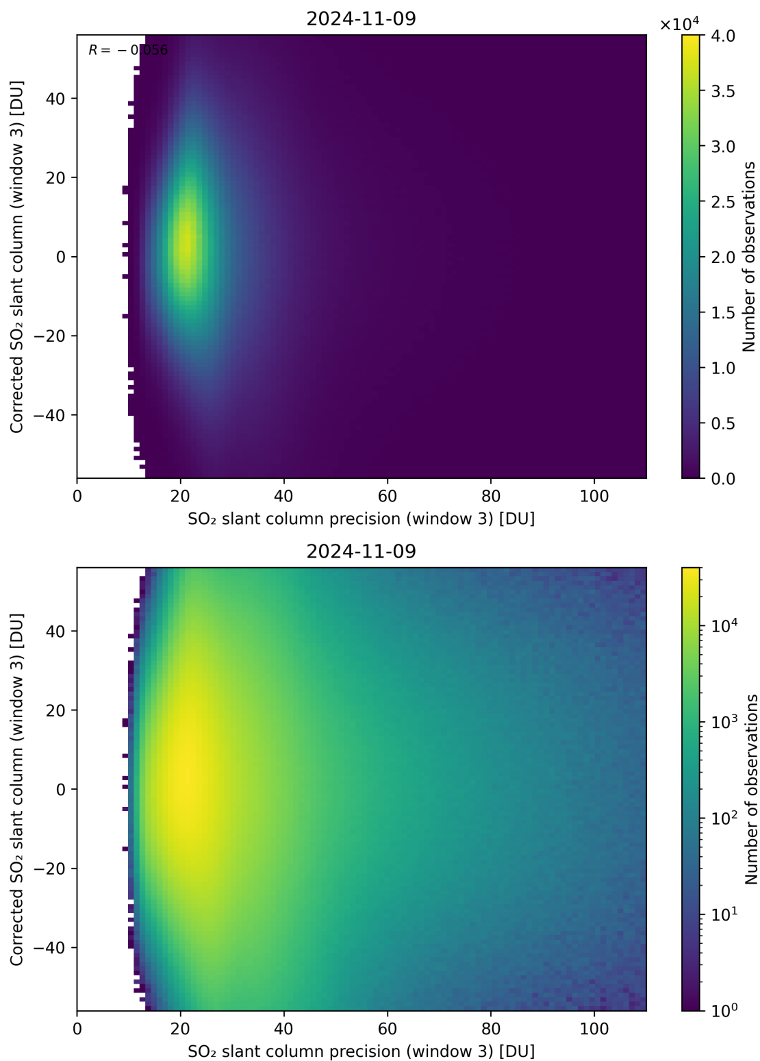
Figure 262: Scatter density plot of “SO 2 slant column precision (window 3)” against “Corrected SO 2 slant column (window 3)” for 2024-11-09 to 2024-11-10.
