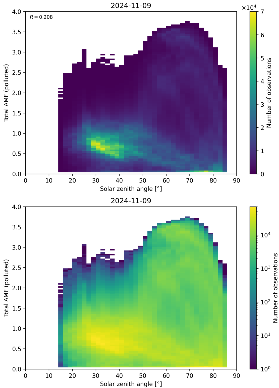
Figure 174: Scatter density plot of “Solar zenith angle” against “Total AMF (polluted)” for 2024-11-09 to 2024-11-10.
