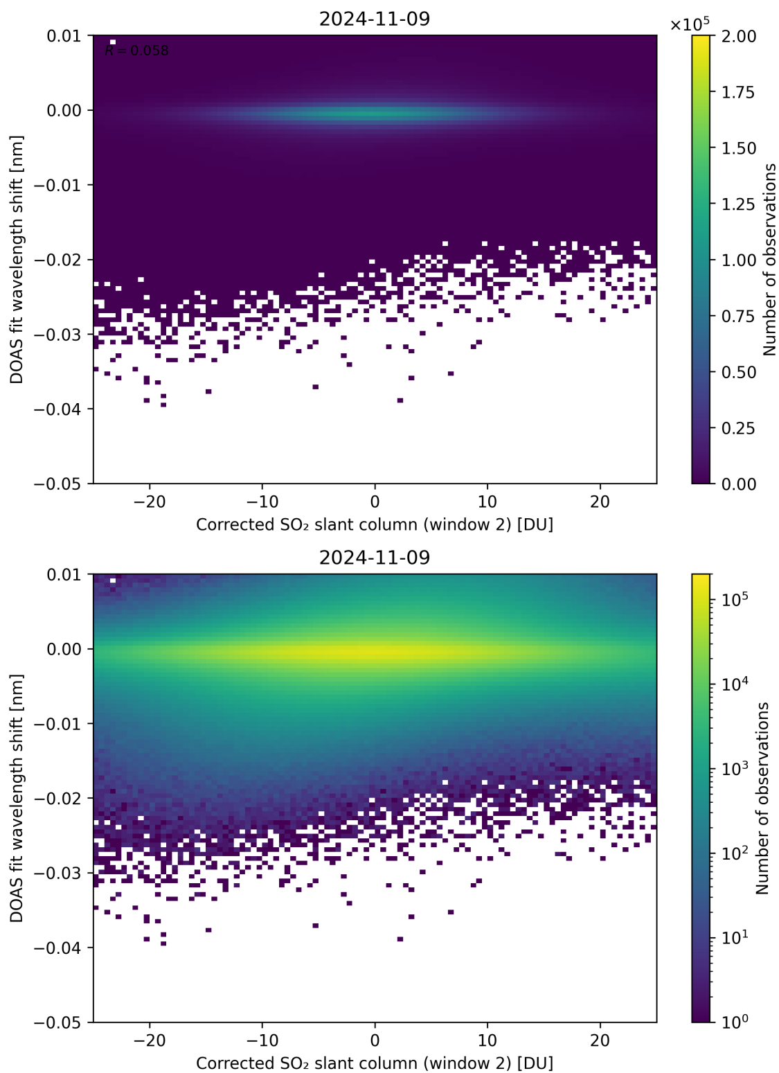
Figure 196: Scatter density plot of “Corrected SO 2 slant column (window 2)” against “DOAS fit wavelength shift” for 2024-11-09 to 2024-11-10.
