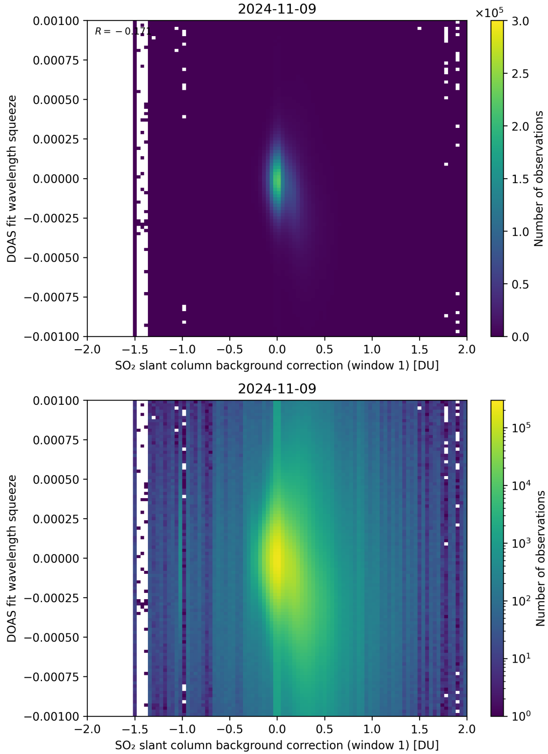
Figure 101: Scatter density plot of “SO 2 slant column background correction (window 1)” against “DOAS fit wavelength squeeze” for 2024-11-09 to 2024-11-10.
