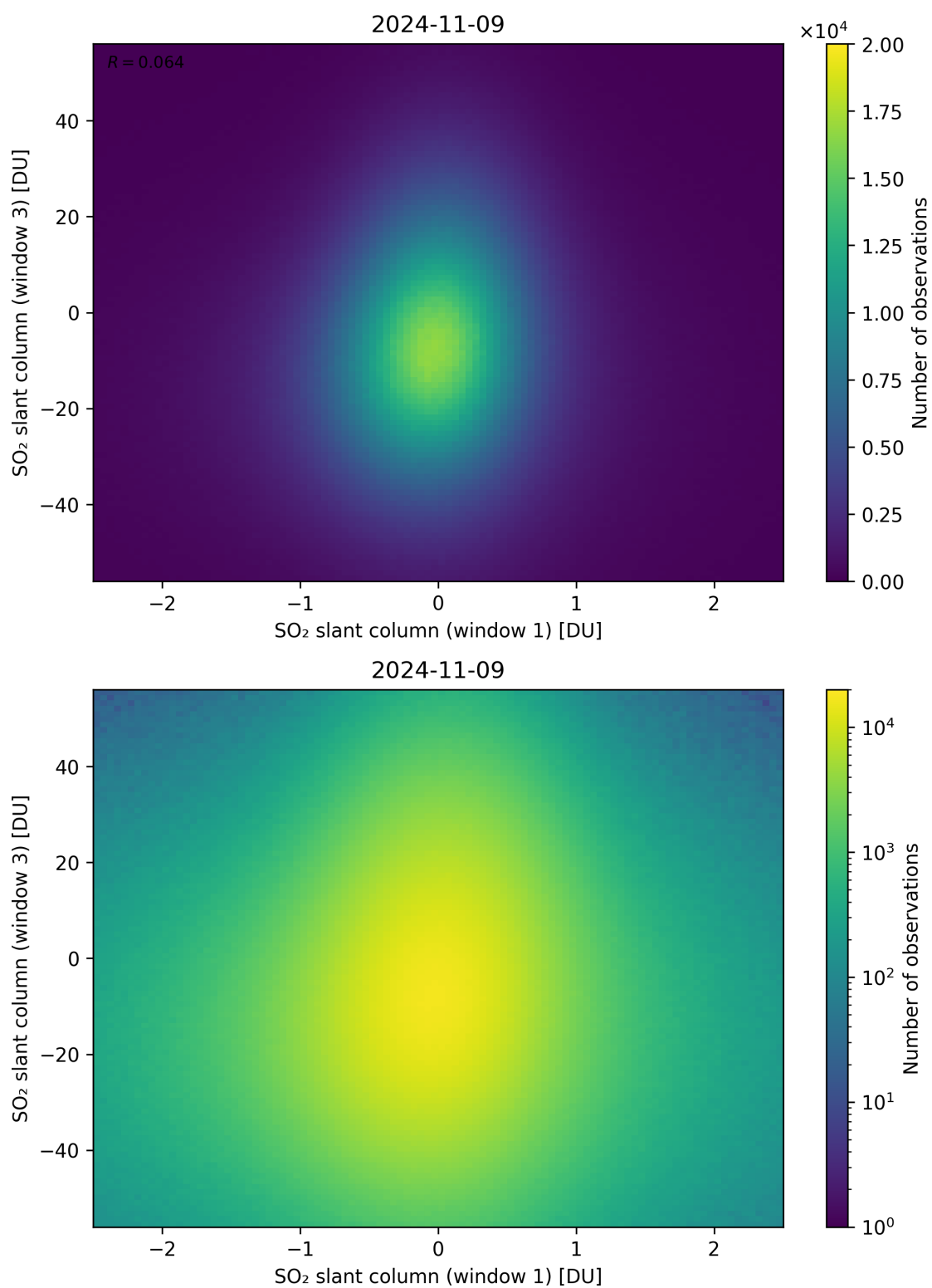
Figure 237: Scatter density plot of “SO 2 slant column (window 1)” against “SO 2 slant column (window 3)” for 2024-11-09 to 2024-11-10.
