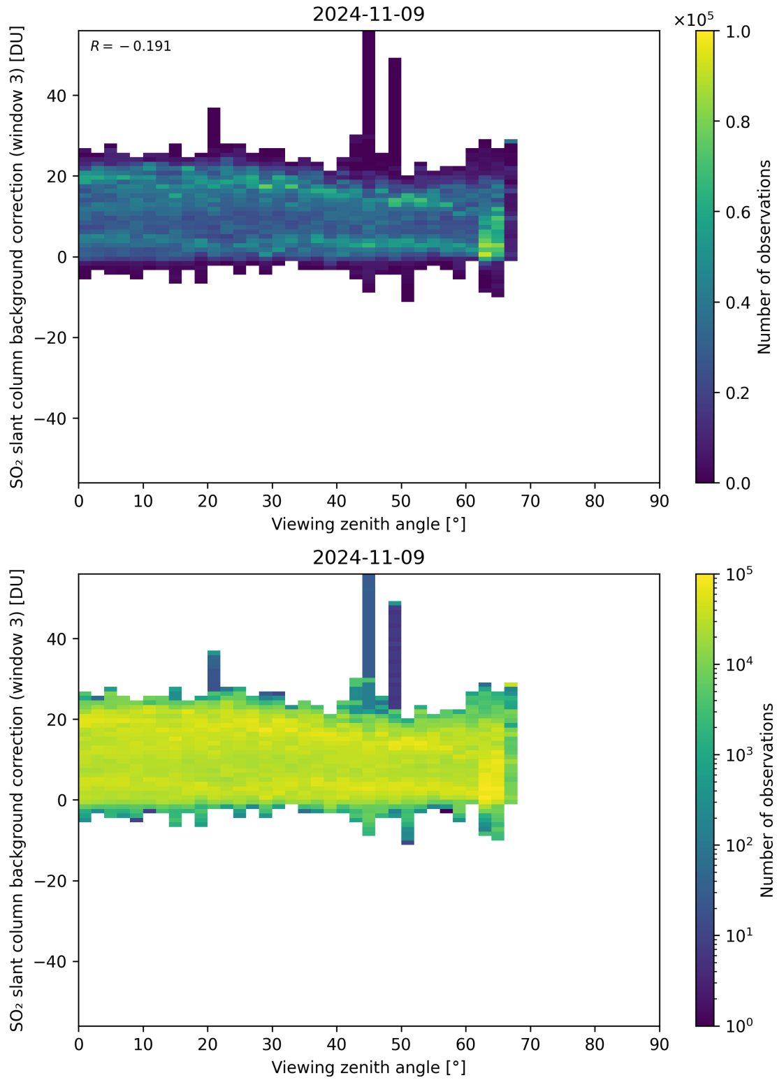
Figure 310: Scatter density plot of “Viewing zenith angle” against “SO 2 slant column background correction (window 3)” for 2024-11-09 to 2024-11-10.
