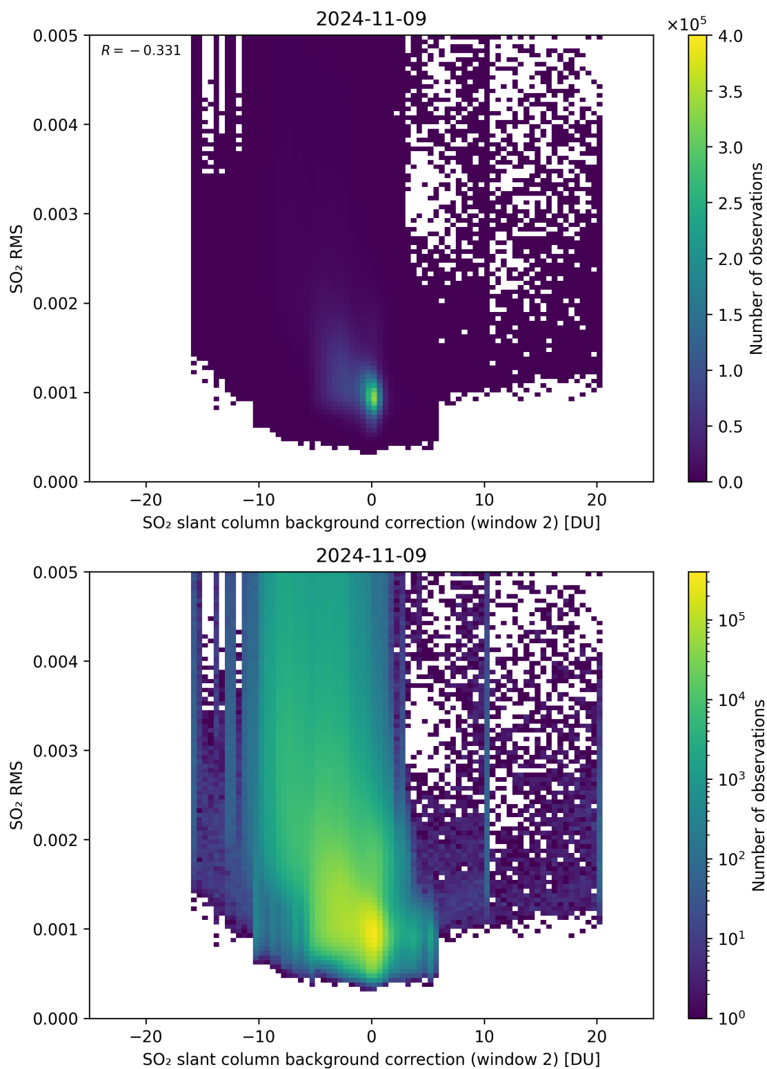
Figure 114: Scatter density plot of “SO 2 slant column background correction (window 2)” against “SO 2 RMS” for 2024-11-09 to 2024-11-10.
