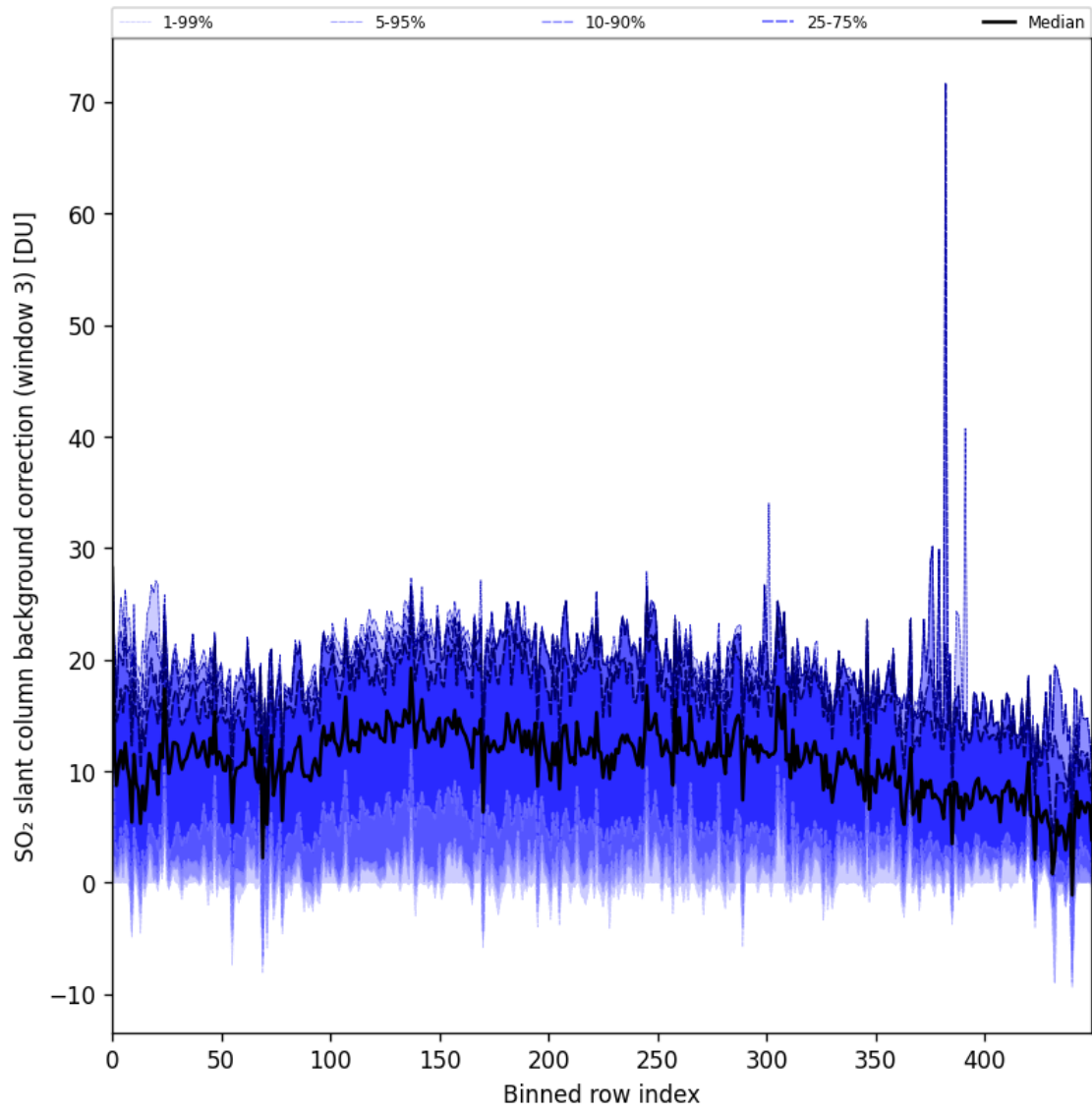
Figure 90: Along track statistics of “SO 2 slant column background correction (window 3)” for 2024-11-09 to 2024-11-10
