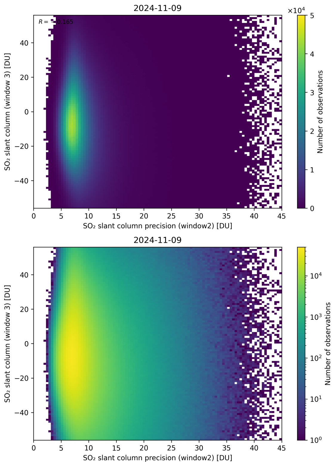
Figure 249: Scatter density plot of “SO 2 slant column precision (window2)” against “SO 2 slant column (window 3)” for 2024-11-09 to 2024-11-10.
