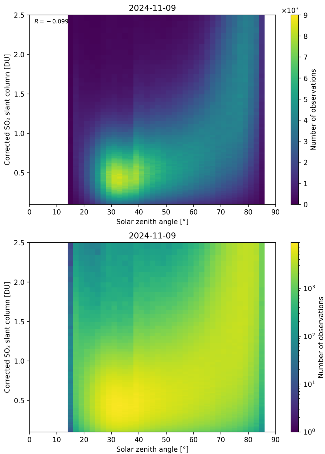
Figure 166: Scatter density plot of “Solar zenith angle” against “Corrected SO 2 slant column” for 2024-11-09 to 2024-11-10.
