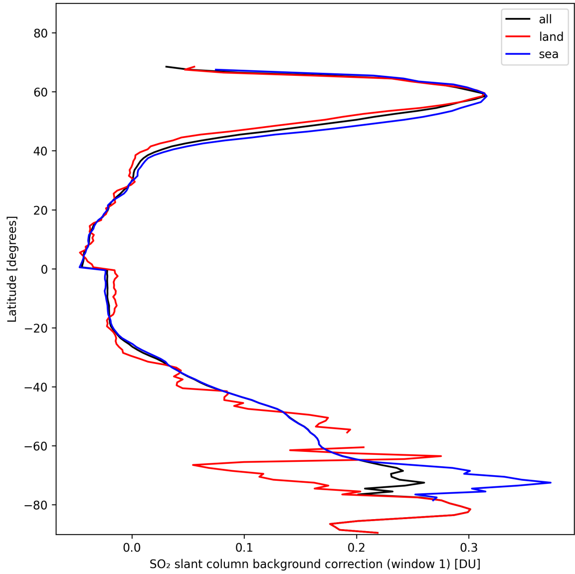
Figure 36: Zonal average of “SO 2 slant column background correction (window 1)” for 2024-11-09 to 2024-11-10.
