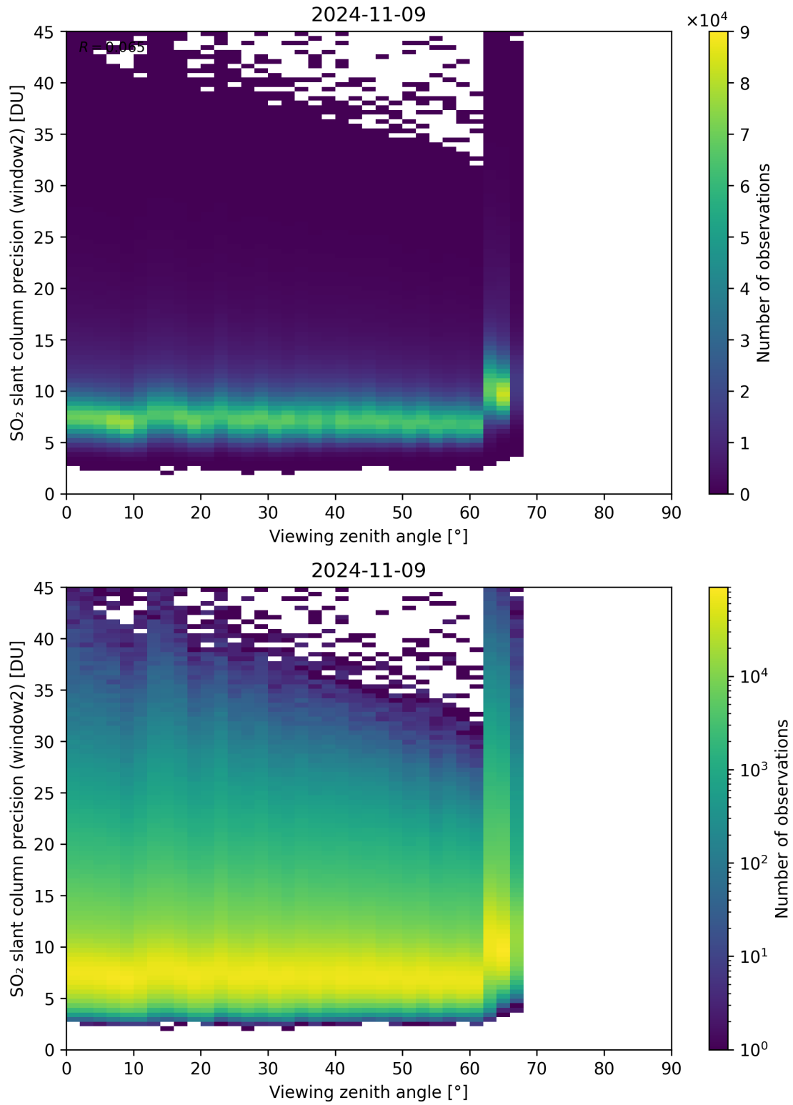
Figure 322: Scatter density plot of “Viewing zenith angle” against “SO 2 slant column precision (window2)” for 2024-11-09 to 2024-11-10.
