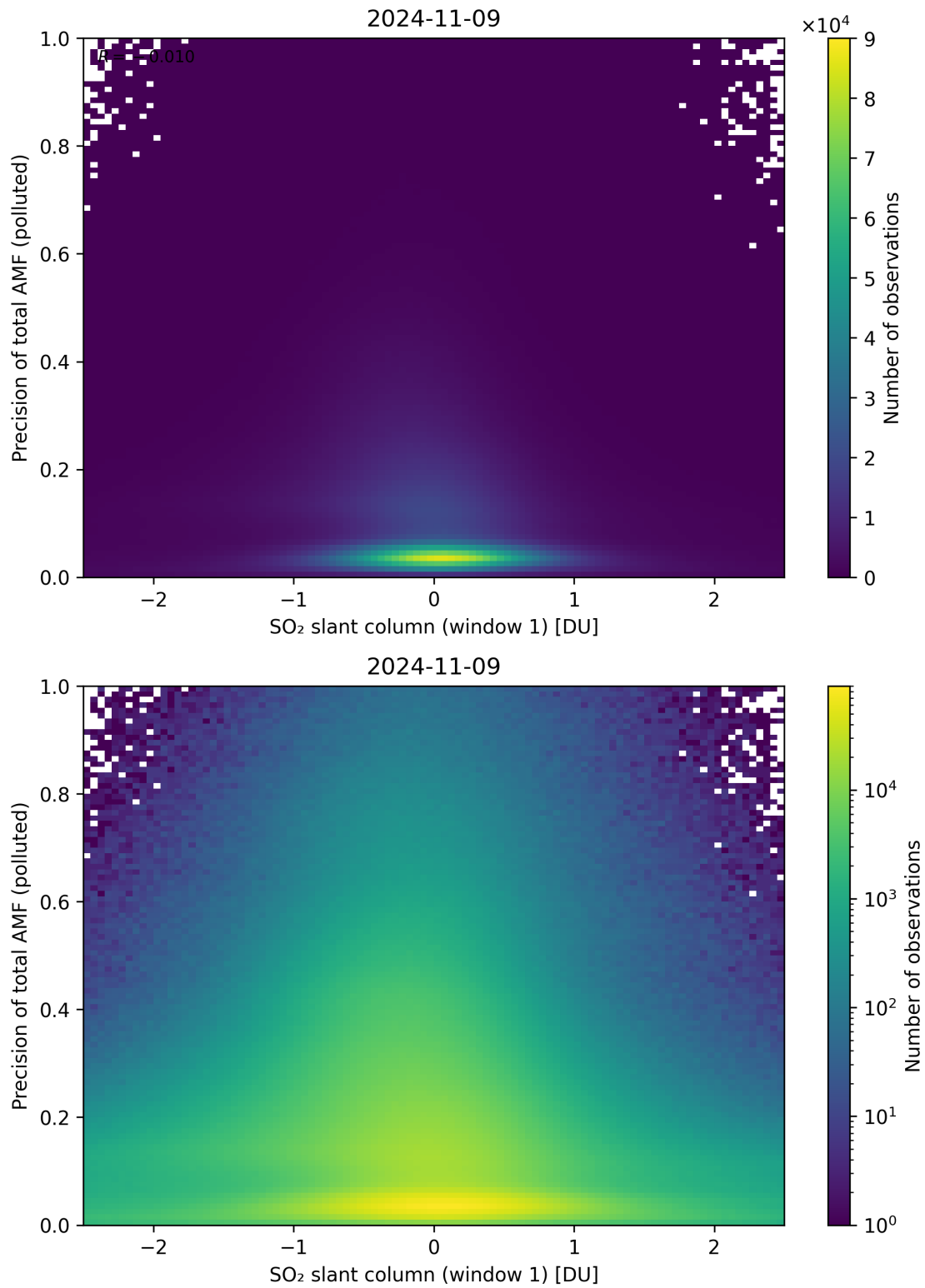
Figure 240: Scatter density plot of “SO 2 slant column (window 1)” against “Precision of total AMF (polluted)” for 2024-11-09 to 2024-11-10.
