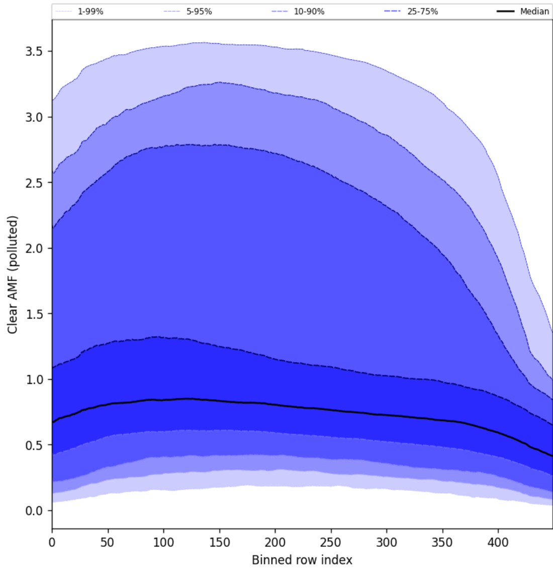
Figure 96: Along track statistics of “Clear AMF (polluted)” for 2024-11-09 to 2024-11-10
