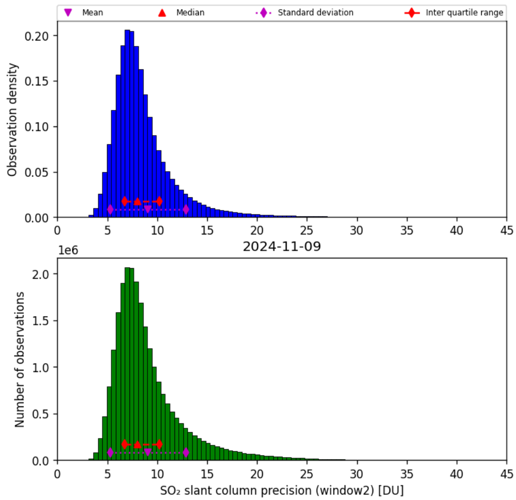
Figure 61: Histogram of “SO 2 slant column precision (window2)” for 2024-11-09 to 2024-11-10
