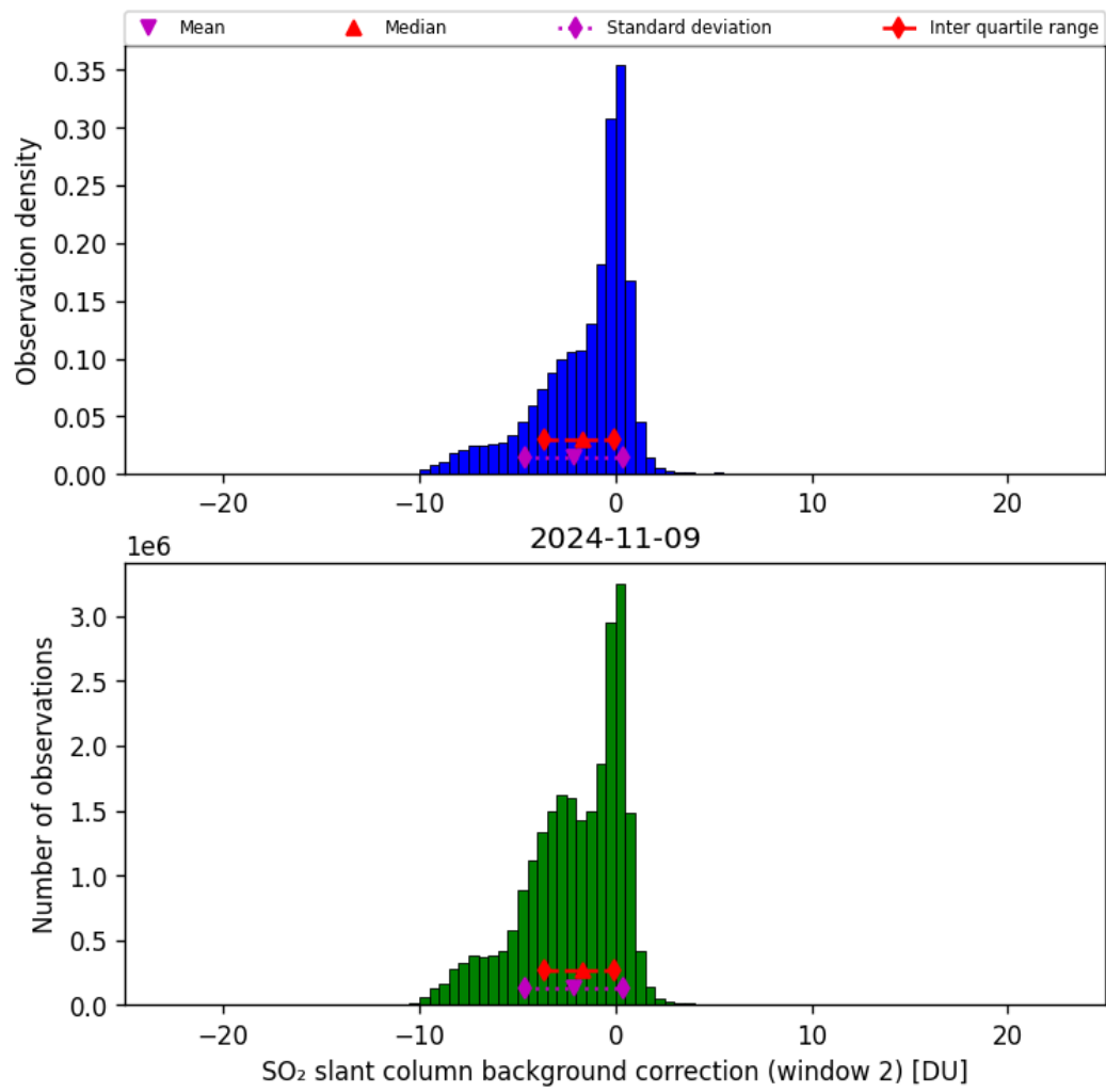
Figure 63: Histogram of “SO 2 slant column background correction (window 2)” for 2024-11-09 to 2024-11-10
