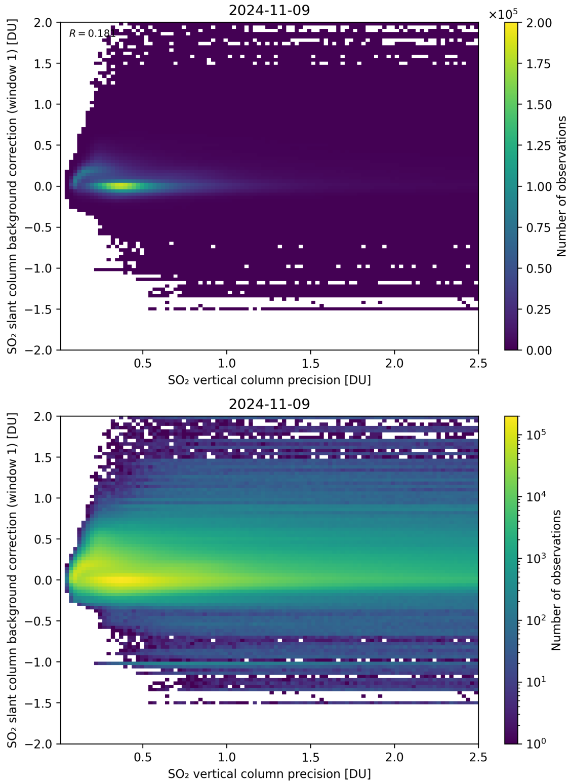
Figure 279: Scatter density plot of “SO 2 vertical column precision” against “SO 2 slant column background correction (window 1)” for 2024-11-09 to 2024-11-10.
