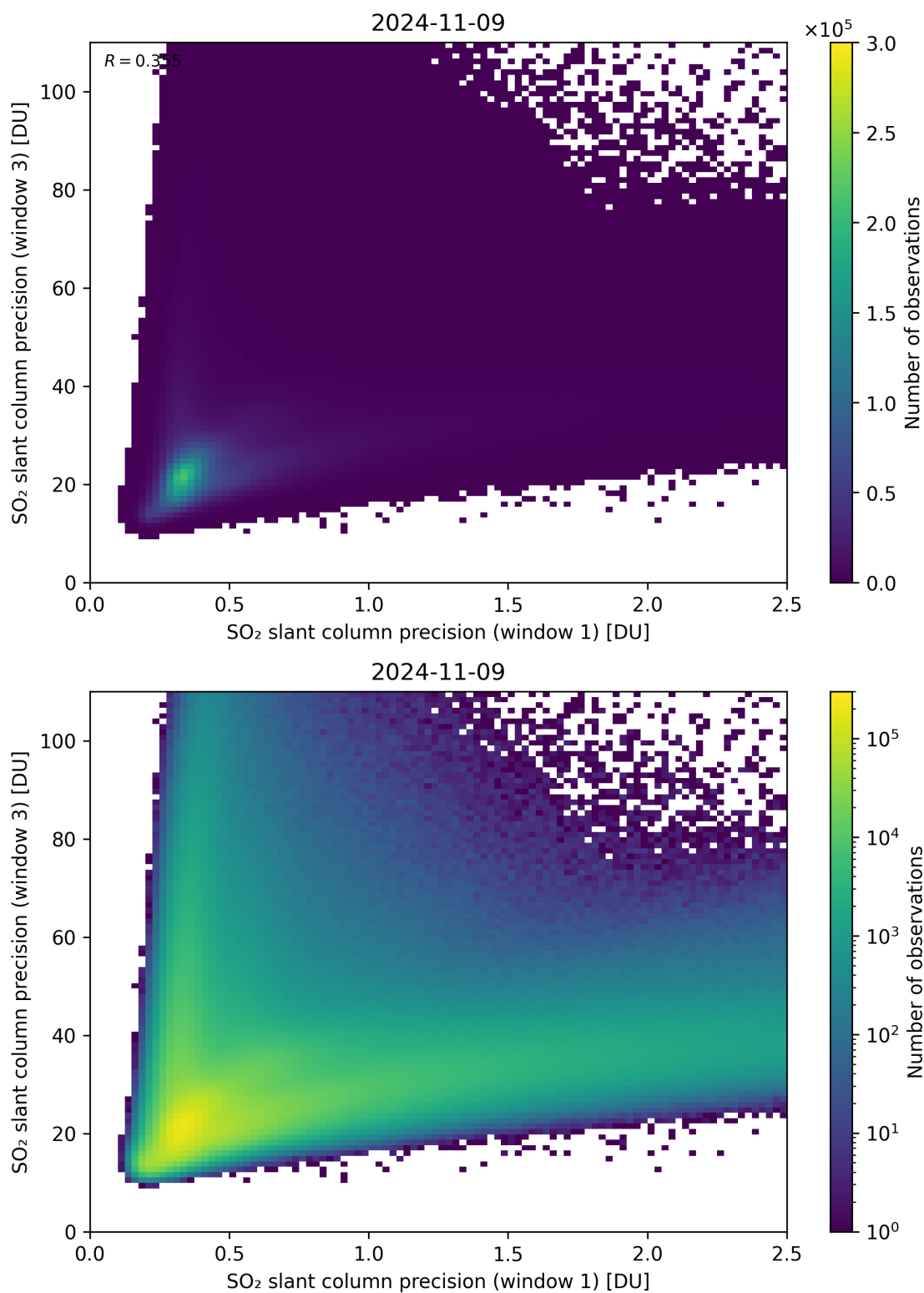
Figure 229: Scatter density plot of “SO 2 slant column precision (window 1)” against “SO 2 slant column precision (window 3)” for 2024-11-09 to 2024-11-10.
