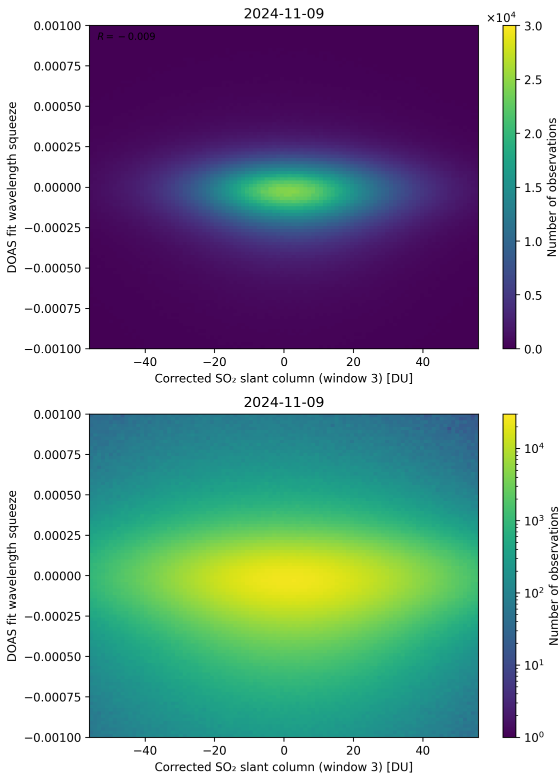
Figure 207: Scatter density plot of “Corrected SO 2 slant column (window 3)” against “DOAS fit wavelength squeeze” for 2024-11-09 to 2024-11-10.
