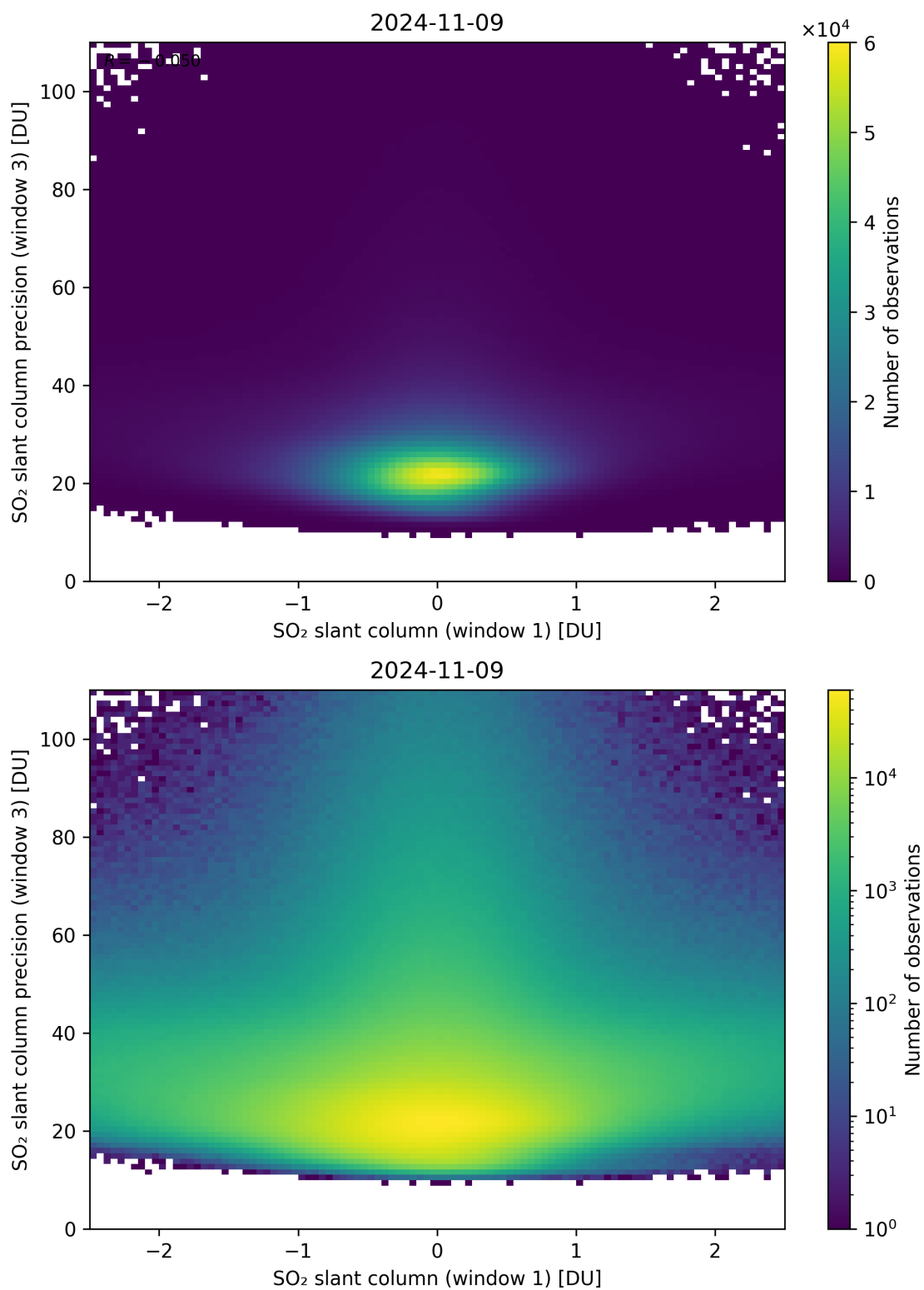
Figure 238: Scatter density plot of “SO 2 slant column (window 1)” against “SO 2 slant column precision (window 3)” for 2024-11-09 to 2024-11-10.
