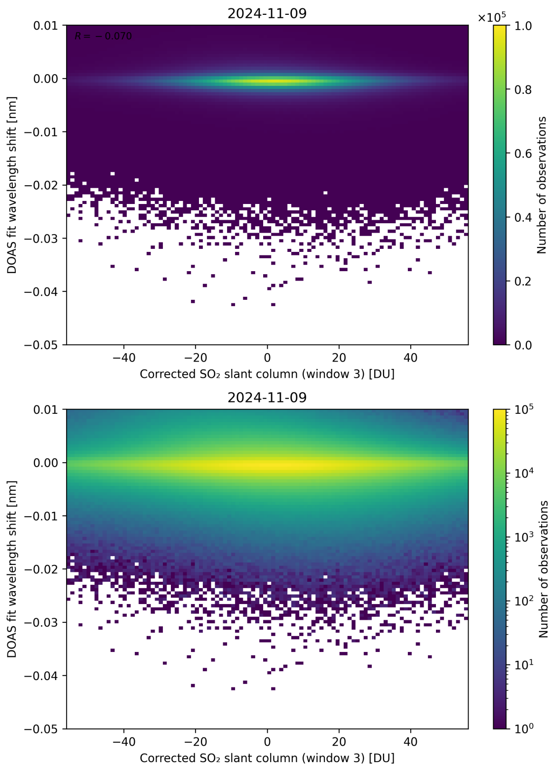
Figure 206: Scatter density plot of “Corrected SO 2 slant column (window 3)” against “DOAS fit wavelength shift” for 2024-11-09 to 2024-11-10.
