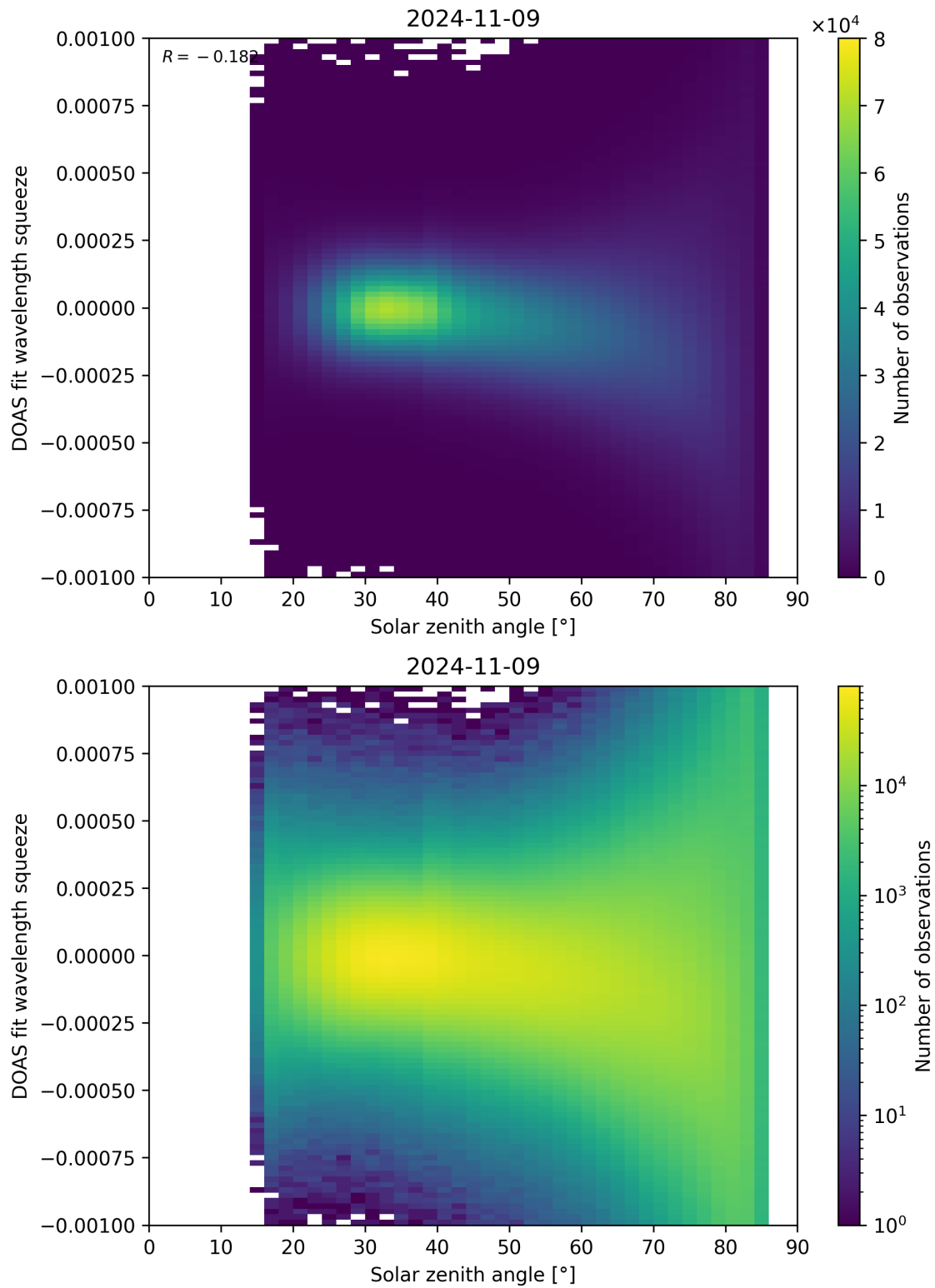
Figure 162: Scatter density plot of “Solar zenith angle” against “DOAS fit wavelength squeeze” for 2024-11-09 to 2024-11-10.
