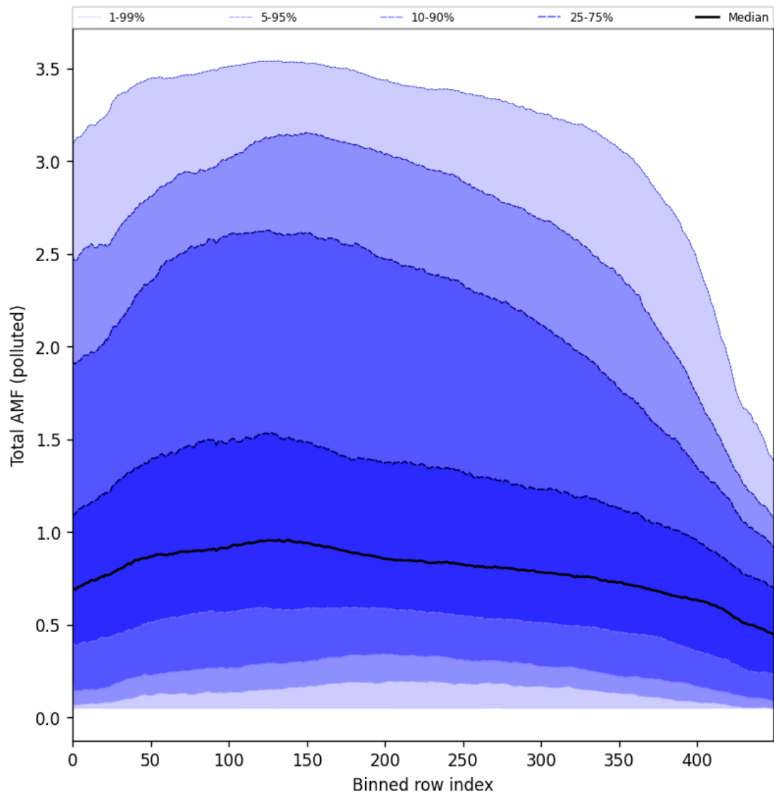
Figure 94: Along track statistics of “Total AMF (polluted)” for 2024-11-09 to 2024-11-10
