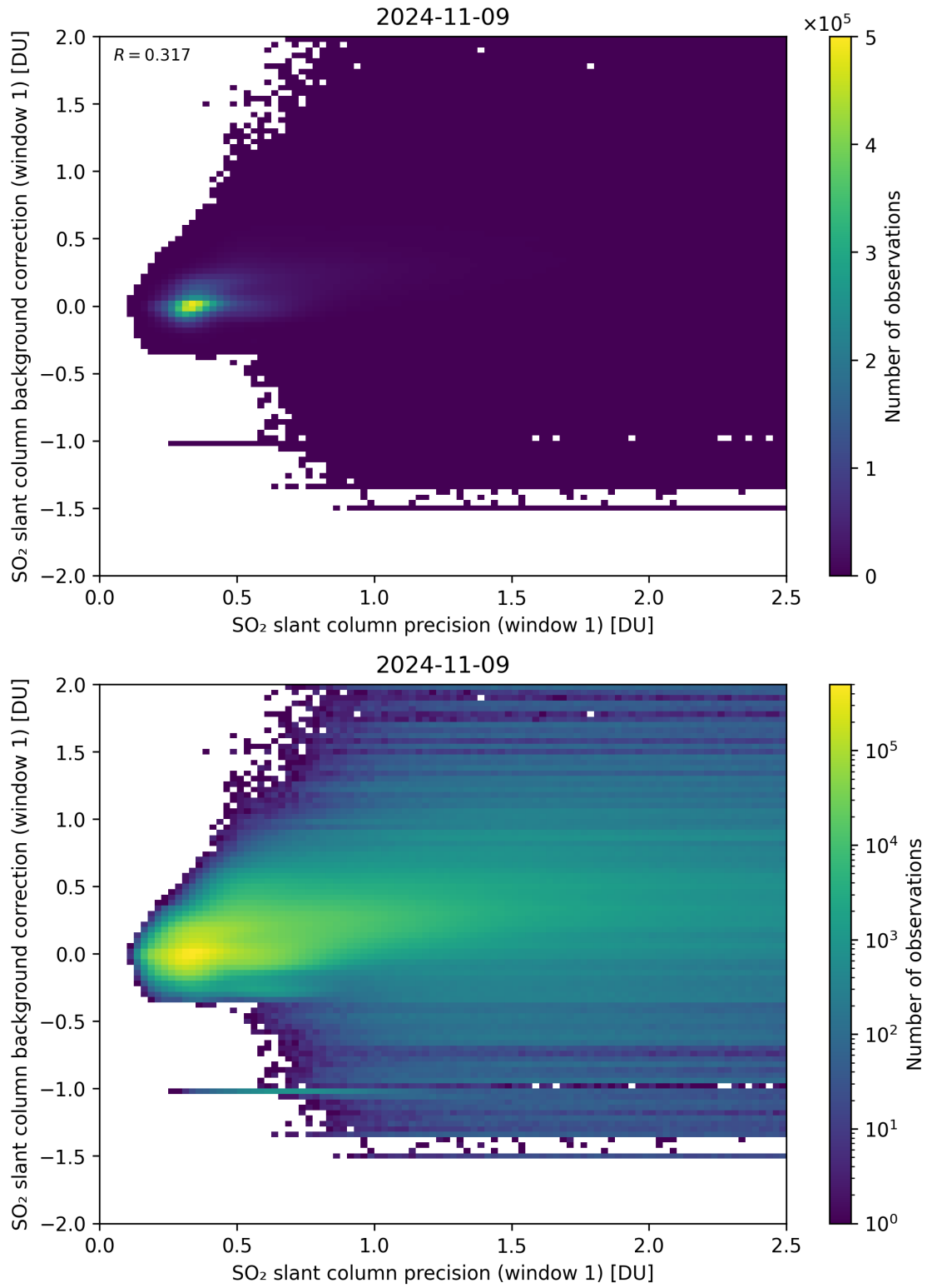
Figure 218: Scatter density plot of “SO 2 slant column precision (window 1)” against “SO 2 slant column background correction (window 1)” for 2024-11-09 to 2024-11-10.
