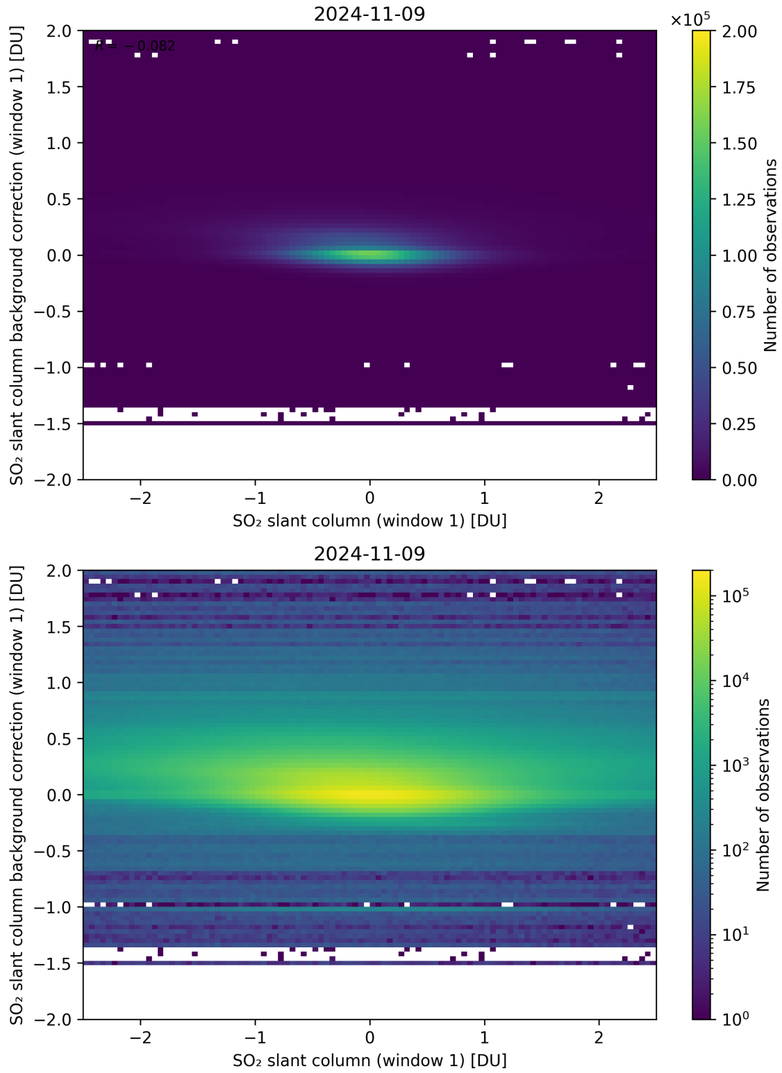
Figure 212: Scatter density plot of “SO 2 slant column (window 1)” against “SO 2 slant column background correction (window 1)” for 2024-11-09 to 2024-11-10.
