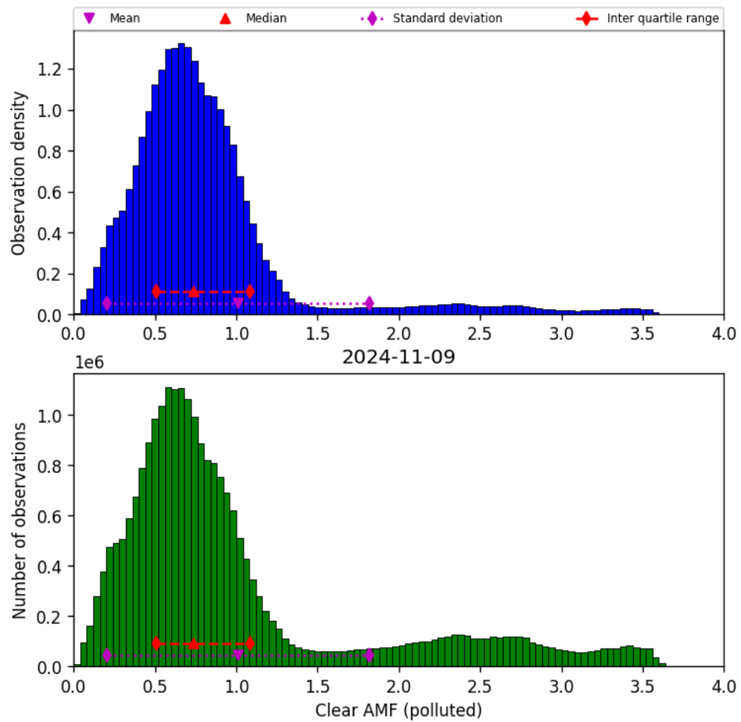
Figure 73: Histogram of “Clear AMF (polluted)” for 2024-11-09 to 2024-11-10
