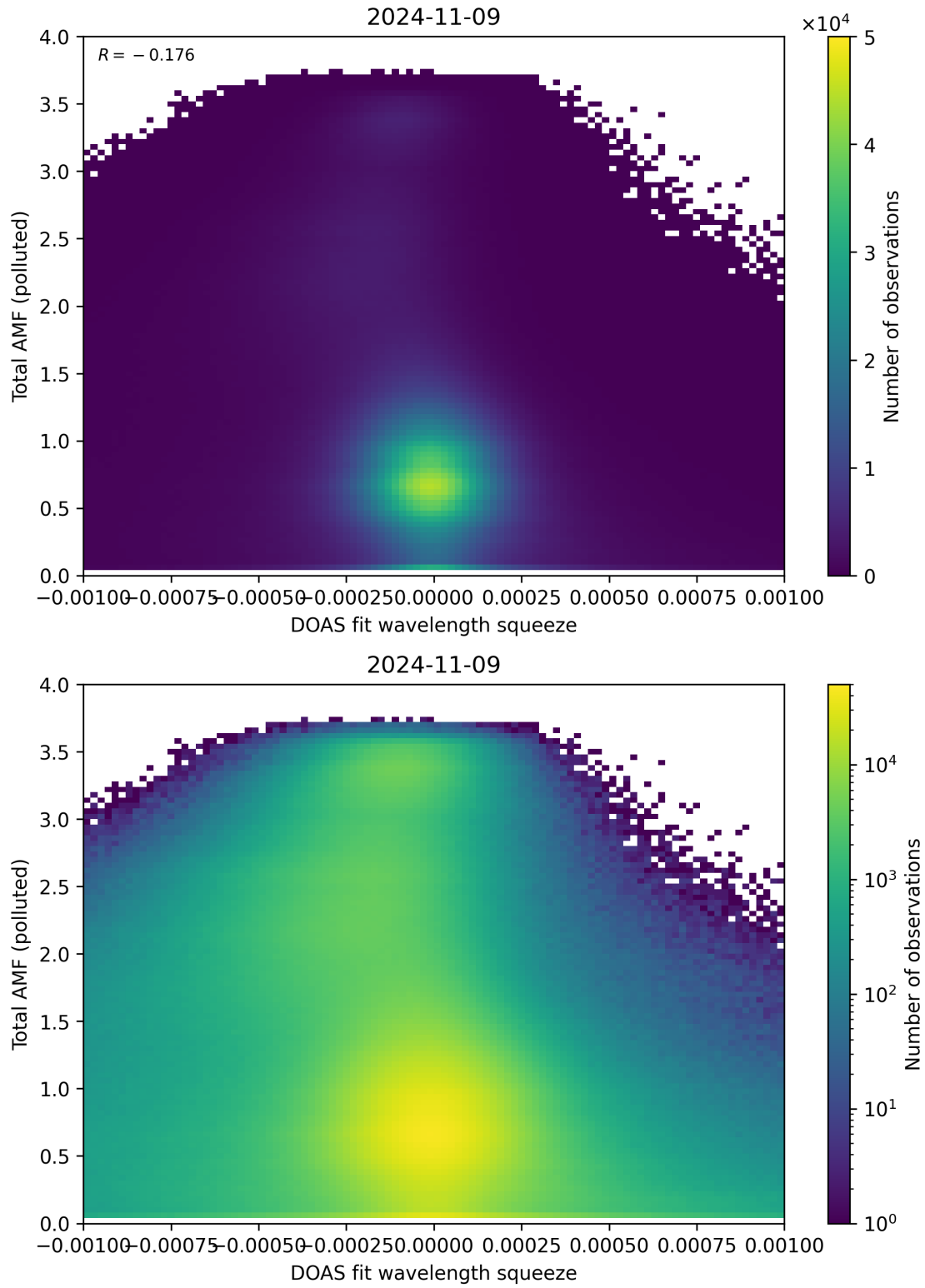
Figure 134: Scatter density plot of “DOAS fit wavelength squeeze” against “Total AMF (polluted)” for 2024-11-09 to 2024-11-10.
