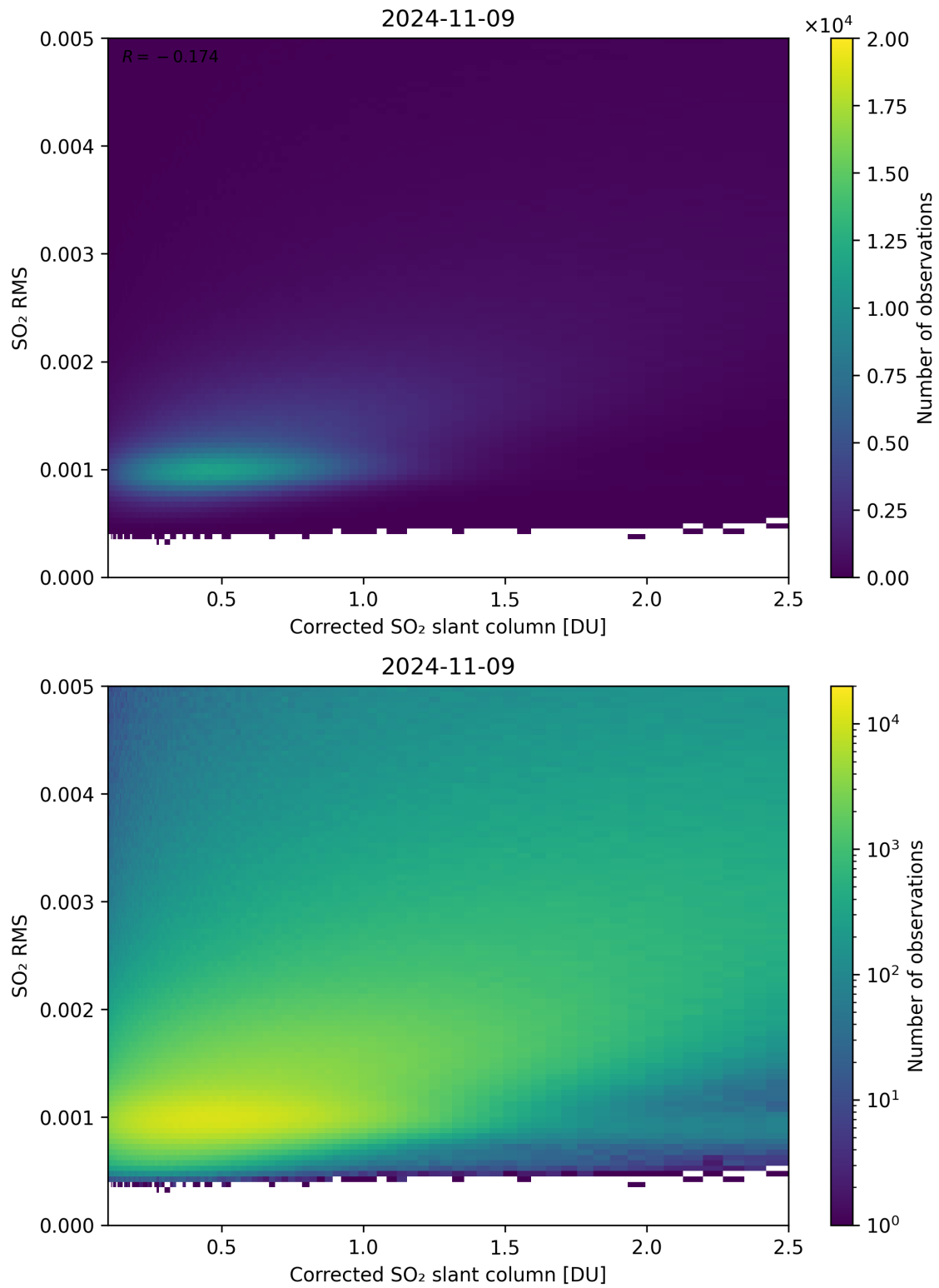
Figure 183: Scatter density plot of “Corrected SO 2 slant column” against “SO 2 RMS” for 2024-11-09 to 2024-11-10.
