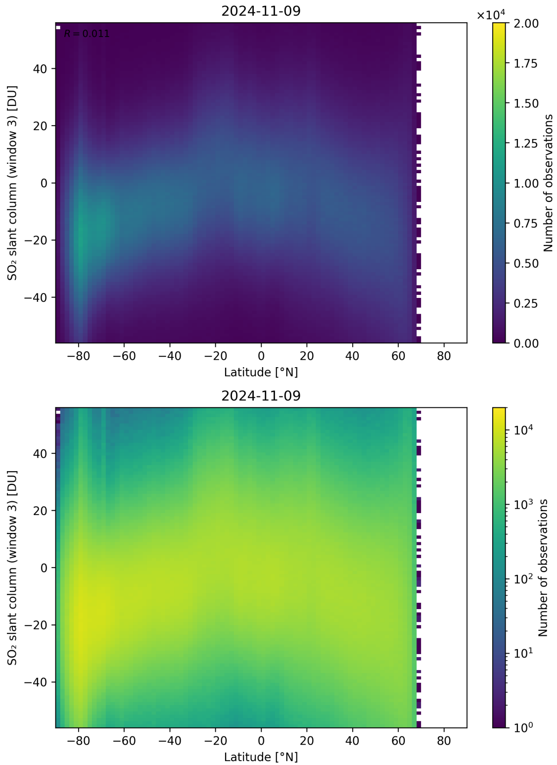
Figure 152: Scatter density plot of “Latitude” against “SO 2 slant column (window 3)” for 2024-11-09 to 2024-11-10.
