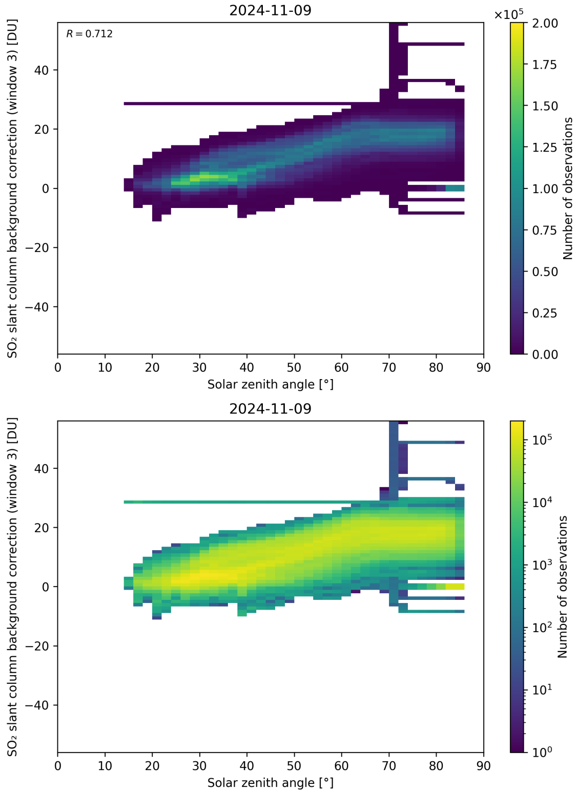
Figure 160: Scatter density plot of “Solar zenith angle” against “SO 2 slant column background correction (window 3)” for 2024-11-09 to 2024-11-10.
