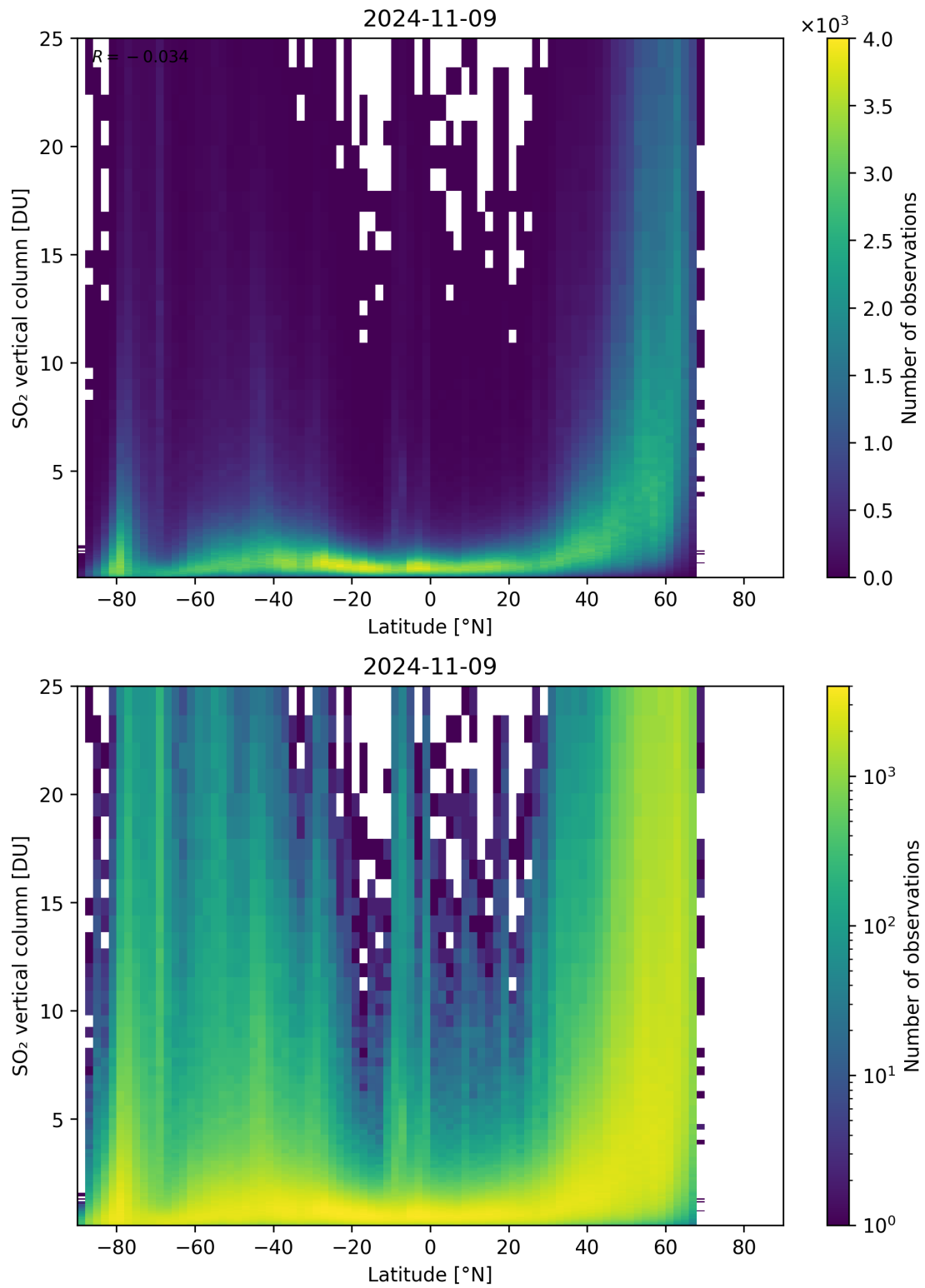
Figure 156: Scatter density plot of “Latitude” against “SO 2 vertical column” for 2024-11-09 to 2024-11-10.
