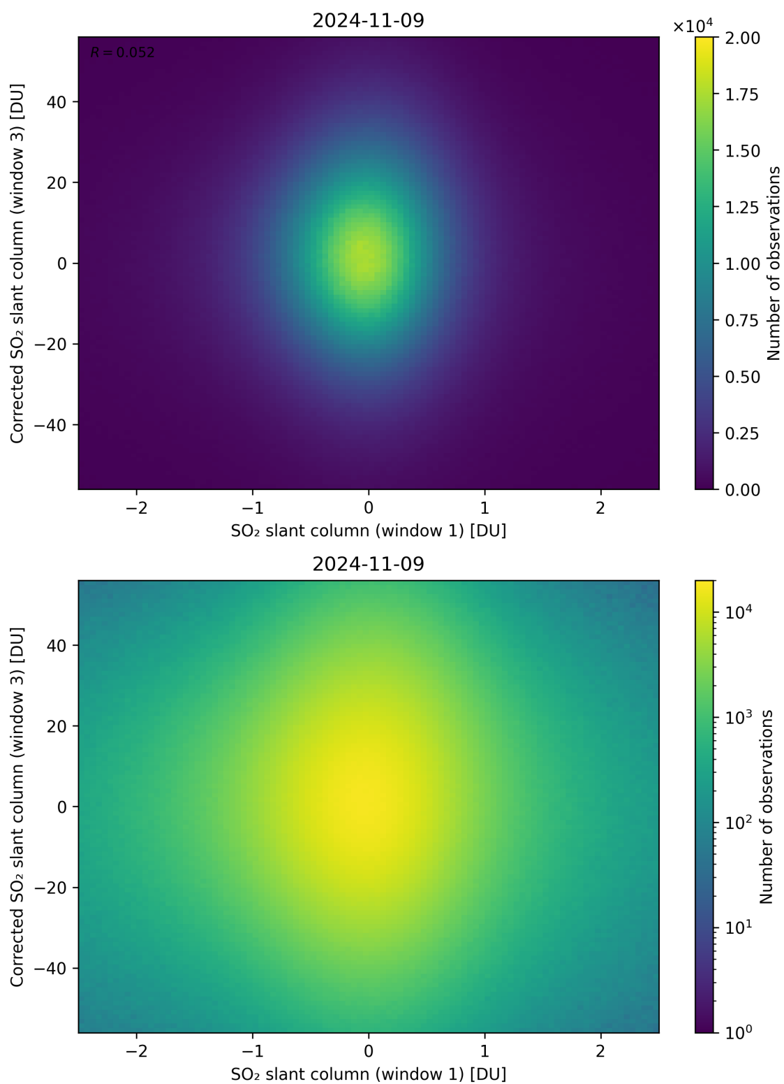
Figure 234: Scatter density plot of “SO 2 slant column (window 1)” against “Corrected SO 2 slant column (window 3)” for 2024-11-09 to 2024-11-10.
