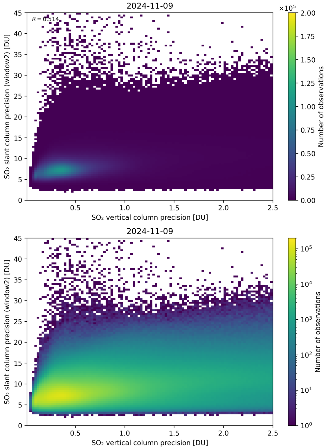
Figure 291: Scatter density plot of “SO 2 vertical column precision” against “SO 2 slant column precision (window2)” for 2024-11-09 to 2024-11-10.
