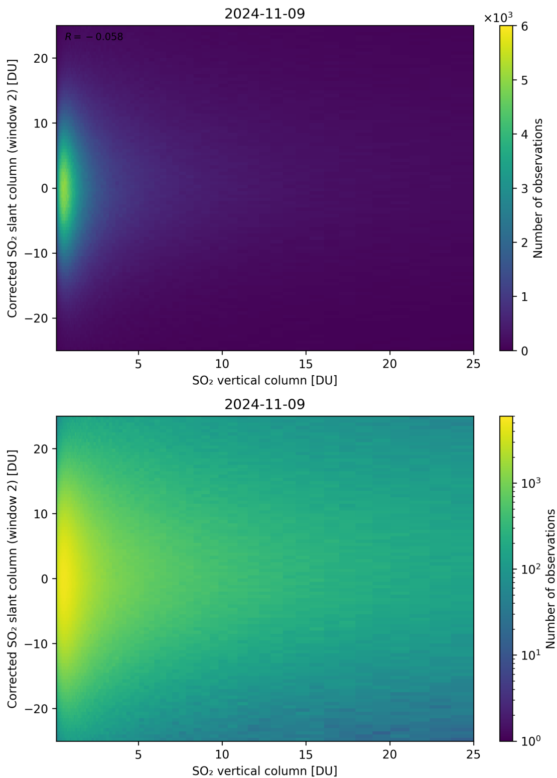
Figure 298: Scatter density plot of “SO 2 vertical column” against “Corrected SO 2 slant column (window 2)” for 2024-11-09 to 2024-11-10.
