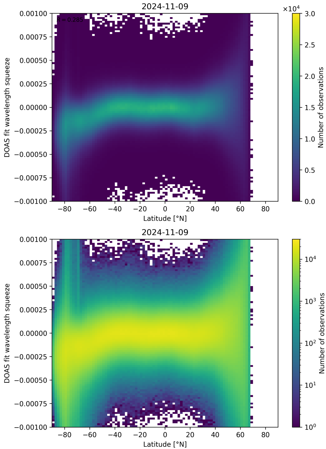
Figure 143: Scatter density plot of “Latitude” against “DOAS fit wavelength squeeze” for 2024-11-09 to 2024-11-10.
