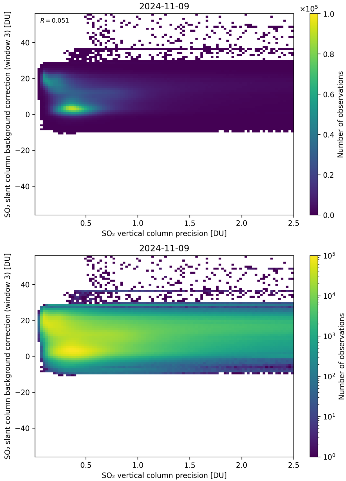
Figure 281: Scatter density plot of “SO 2 vertical column precision” against “SO 2 slant column background correction (window 3)” for 2024-11-09 to 2024-11-10.
