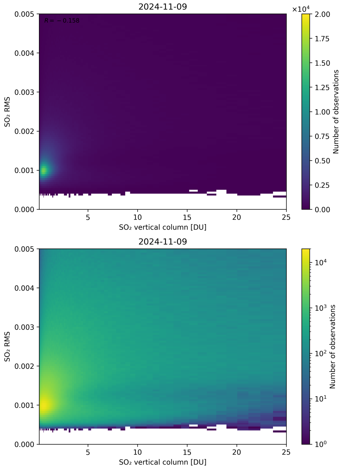
Figure 278: Scatter density plot of “SO 2 vertical column” against “SO 2 RMS” for 2024-11-09 to 2024-11-10.
