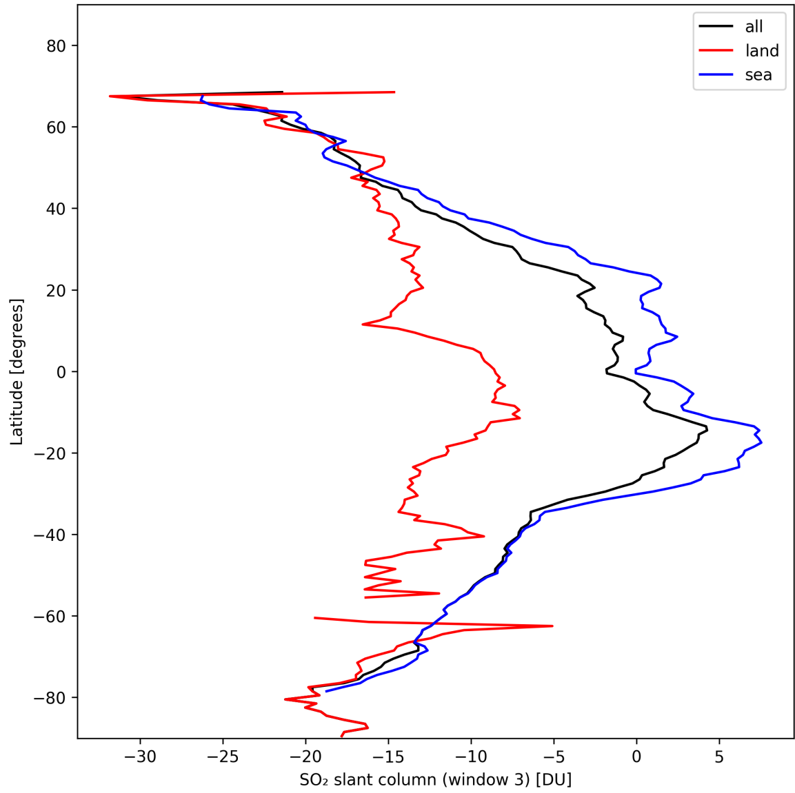
Figure 41: Zonal average of “SO 2 slant column (window 3)” for 2024-11-09 to 2024-11-10.
