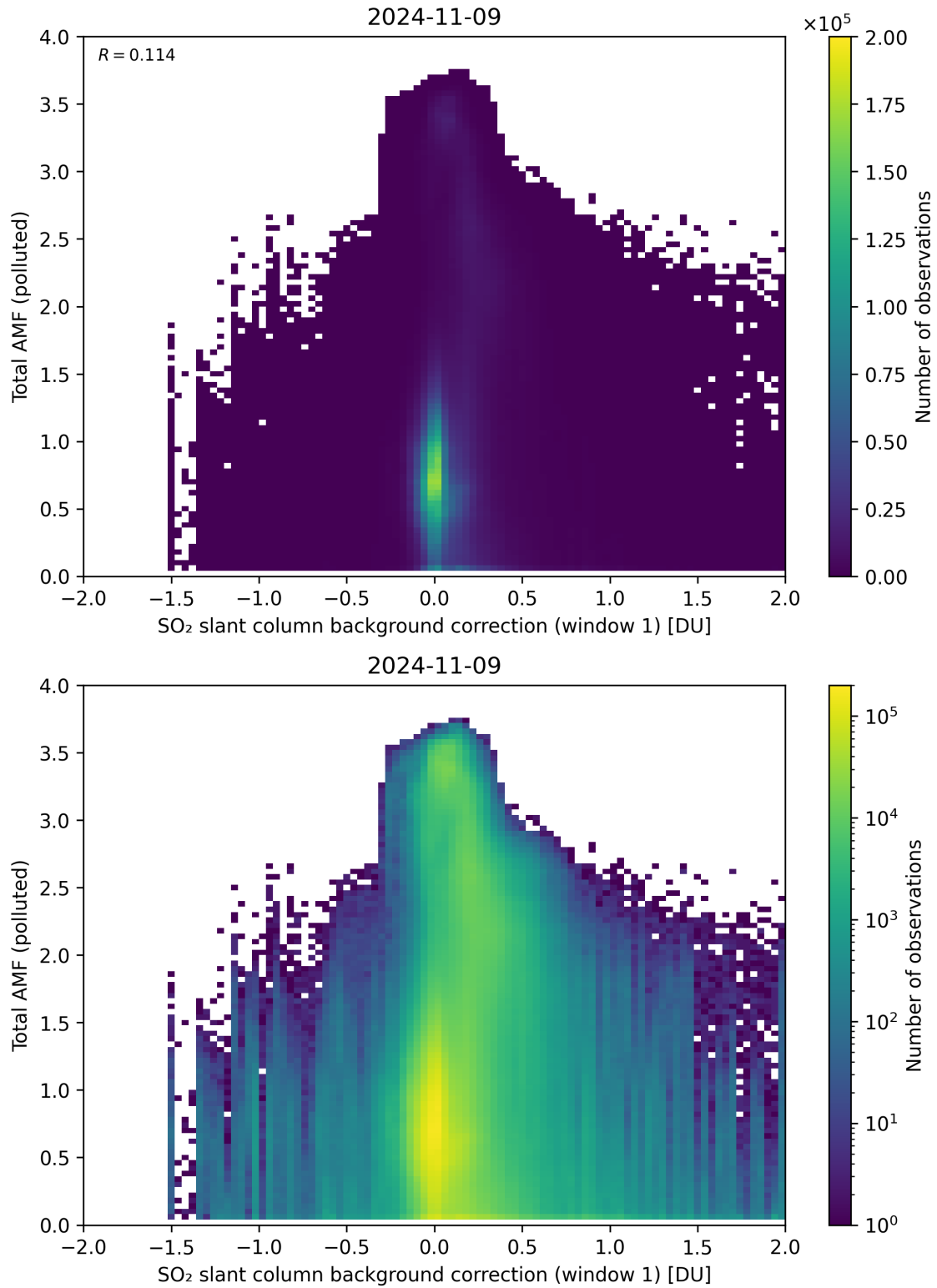
Figure 109: Scatter density plot of “SO 2 slant column background correction (window 1)” against “Total AMF (polluted)” for 2024-11-09 to 2024-11-10.
