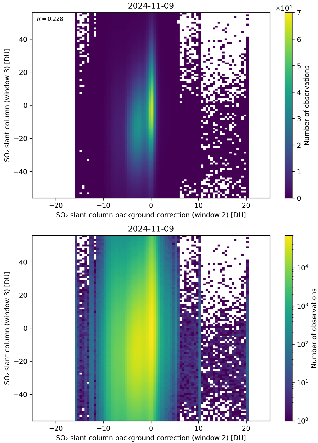
Figure 117: Scatter density plot of “SO 2 slant column background correction (window 2)” against “SO 2 slant column (window 3)” for 2024-11-09 to 2024-11-10.
