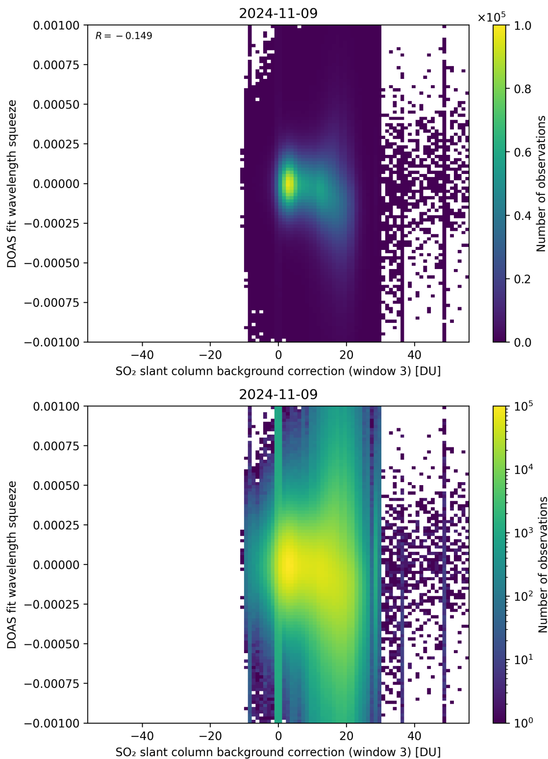
Figure 122: Scatter density plot of “SO 2 slant column background correction (window 3)” against “DOAS fit wavelength squeeze” for 2024-11-09 to 2024-11-10.
