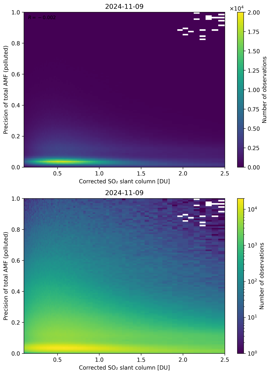
Figure 193: Scatter density plot of “Corrected SO 2 slant column” against “Precision of total AMF (polluted)” for 2024-11-09 to 2024-11-10.
