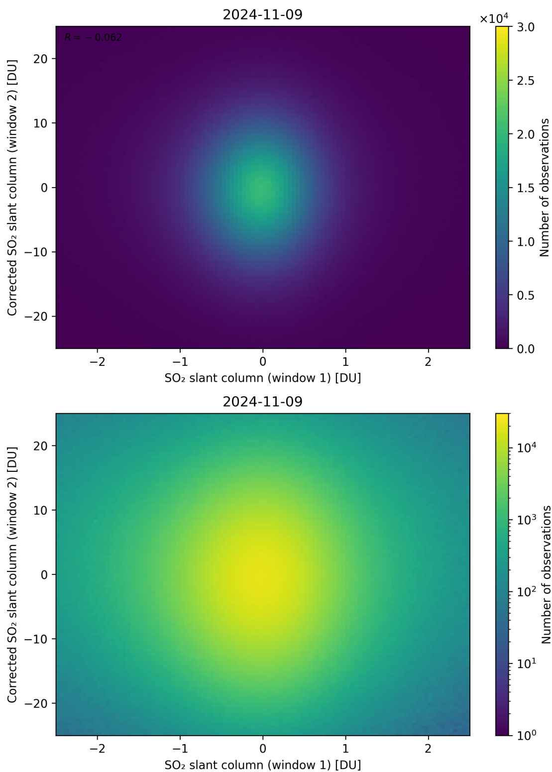
Figure 233: Scatter density plot of “SO 2 slant column (window 1)” against “Corrected SO 2 slant column (window 2)” for 2024-11-09 to 2024-11-10.
