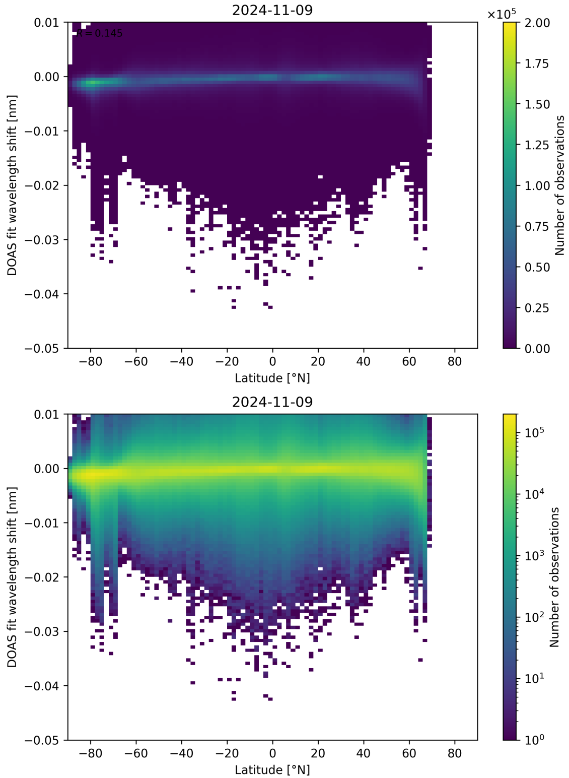
Figure 142: Scatter density plot of “Latitude” against “DOAS fit wavelength shift” for 2024-11-09 to 2024-11-10.
