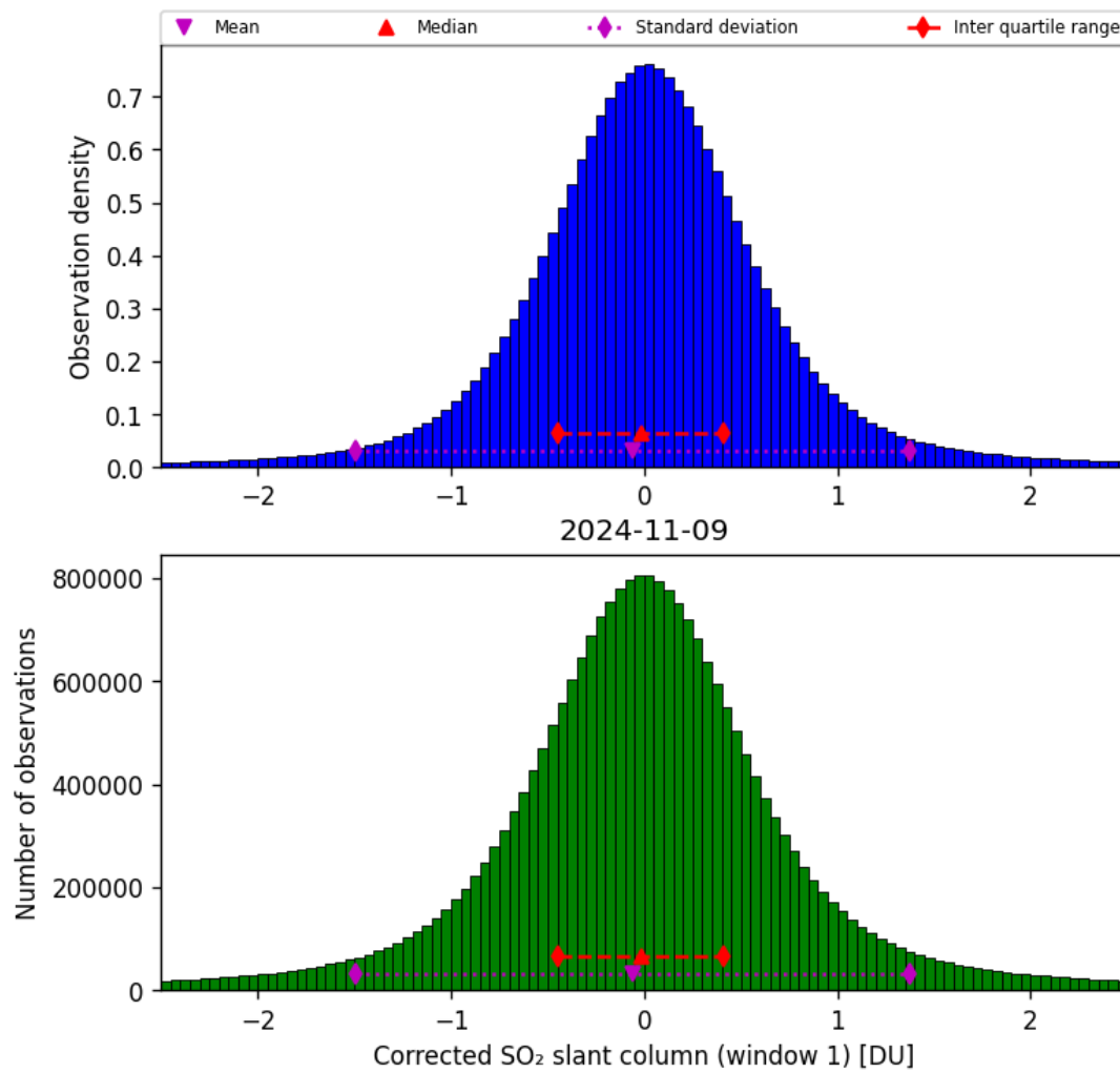
Figure 58: Histogram of “Corrected SO 2 slant column (window 1)” for 2024-11-09 to 2024-11-10
