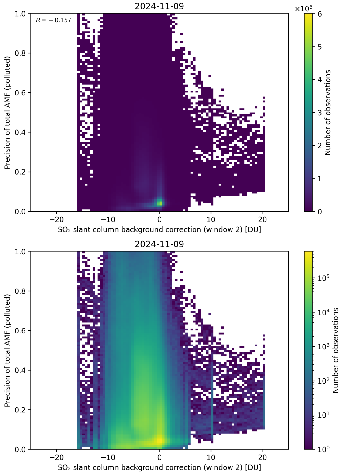
Figure 120: Scatter density plot of “SO 2 slant column background correction (window 2)” against “Precision of total AMF (polluted)” for 2024-11-09 to 2024-11-10.
