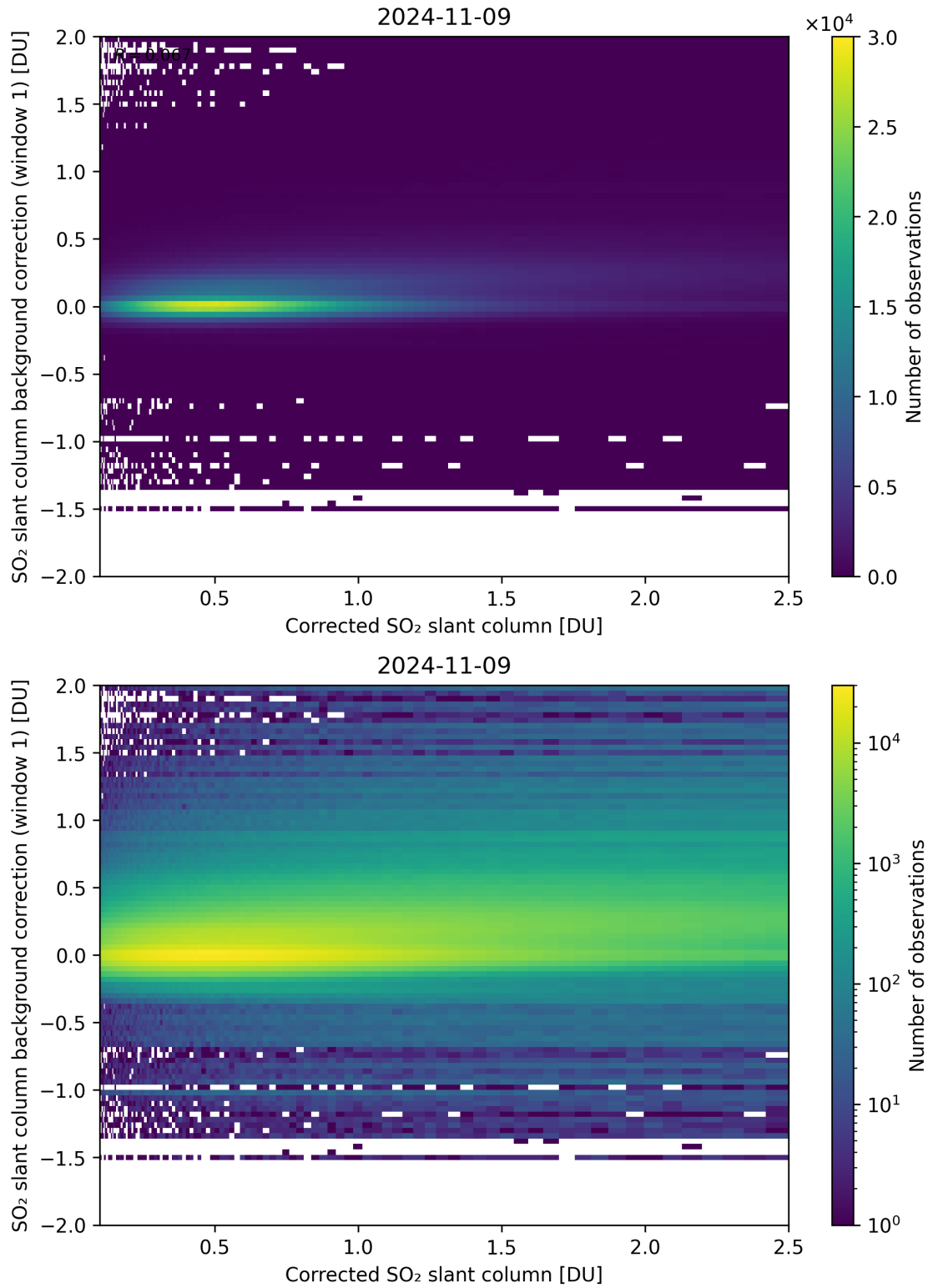
Figure 178: Scatter density plot of “Corrected SO 2 slant column” against “SO 2 slant column background correction (window 1)” for 2024-11-09 to 2024-11-10.
