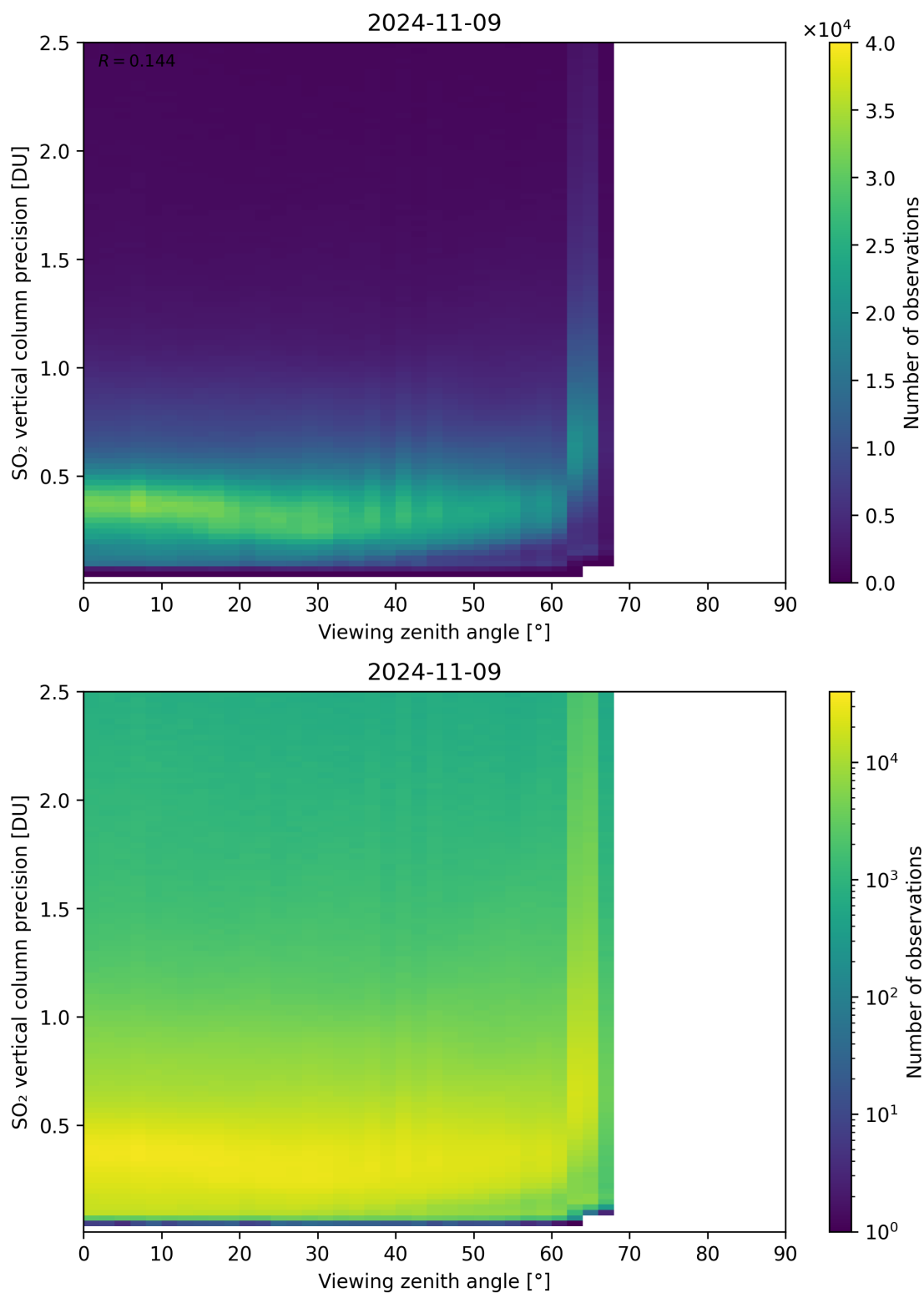
Figure 328: Scatter density plot of “Viewing zenith angle” against “SO 2 vertical column precision” for 2024-11-09 to 2024-11-10.
