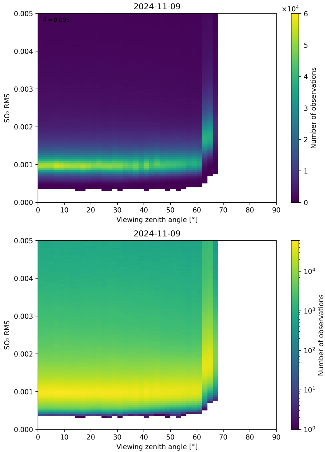
Figure 313: Scatter density plot of “Viewing zenith angle” against “SO 2 RMS” for 2024-11-09 to 2024-11-10.
