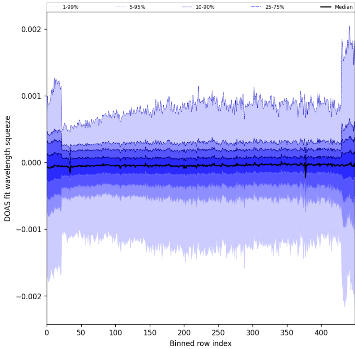
Figure 92: Along track statistics of “DOAS fit wavelength squeeze” for 2024-11-09 to 2024-11-10
