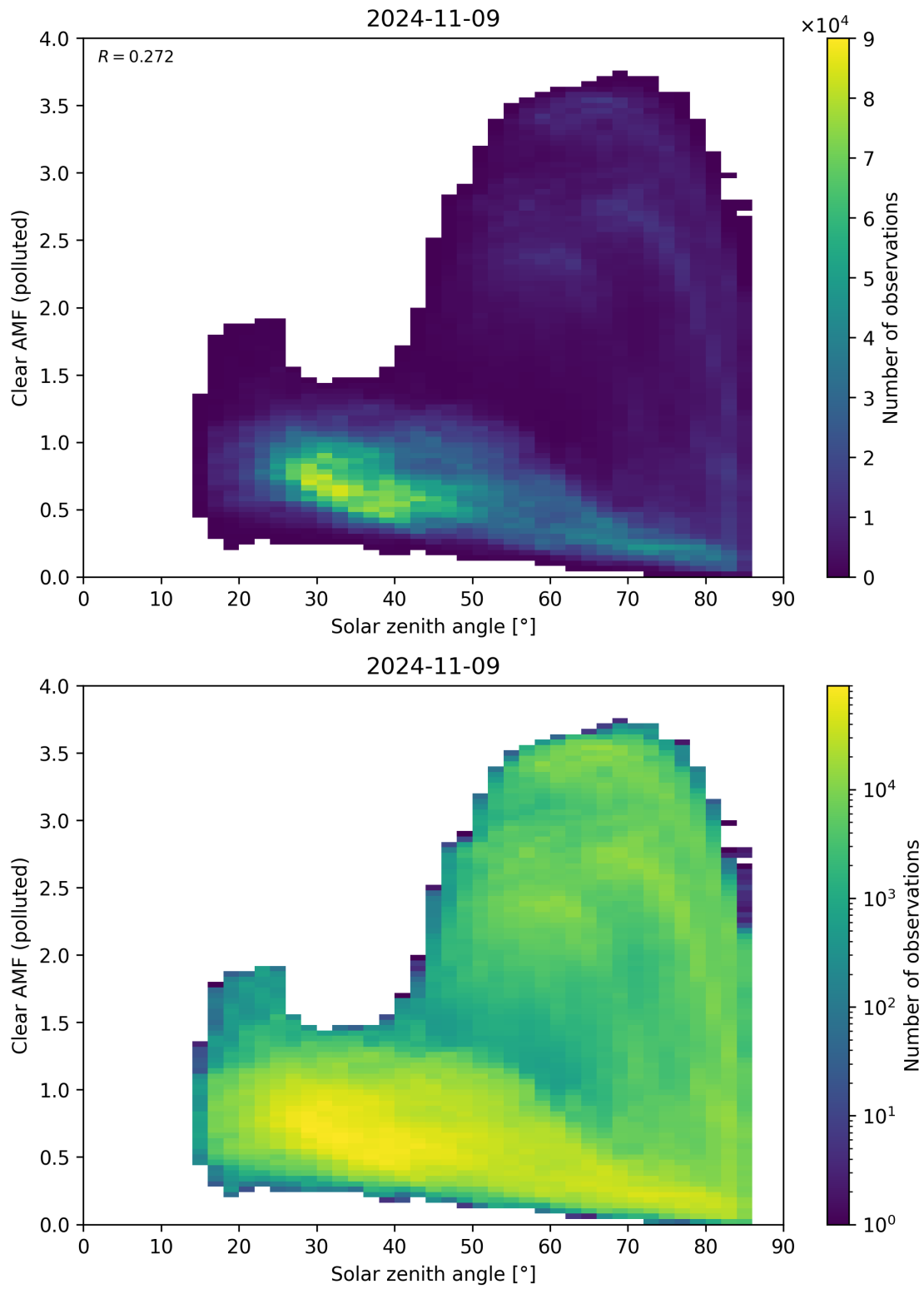
Figure 165: Scatter density plot of “Solar zenith angle” against “Clear AMF (polluted)” for 2024-11-09 to 2024-11-10.
