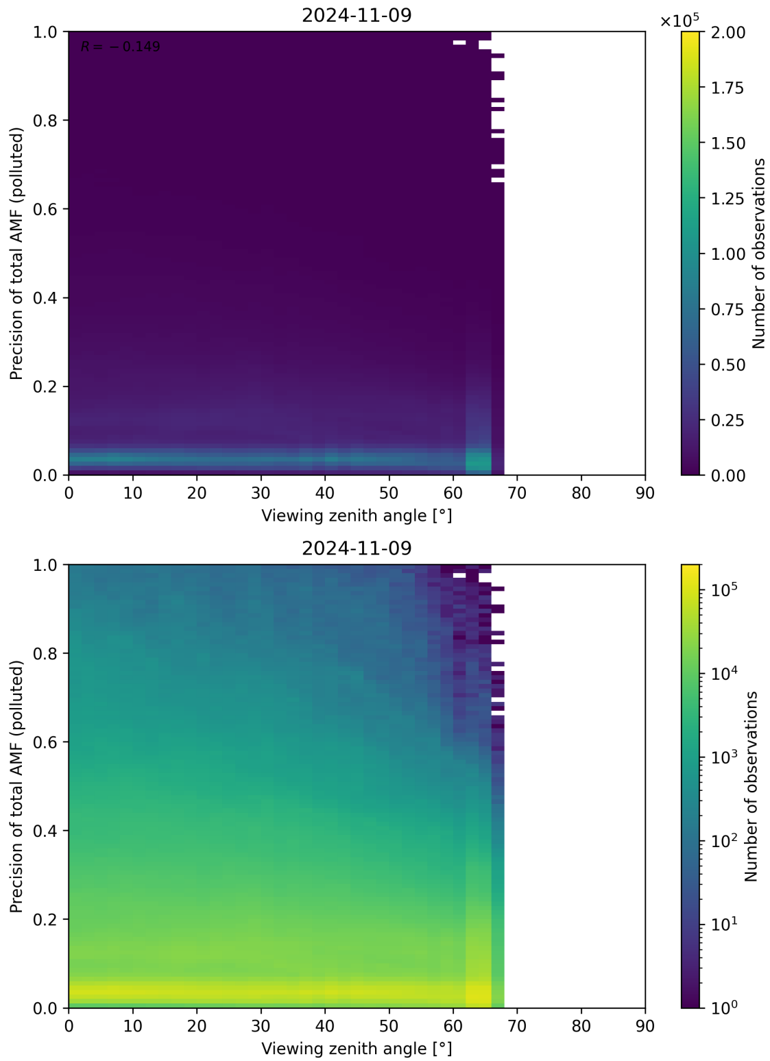
Figure 326: Scatter density plot of “Viewing zenith angle” against “Precision of total AMF (polluted)” for 2024-11-09 to 2024-11-10.
