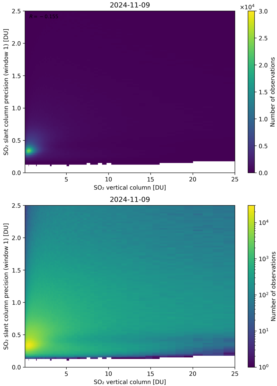
Figure 301: Scatter density plot of “SO 2 vertical column” against “SO 2 slant column precision (window 1)” for 2024-11-09 to 2024-11-10.
