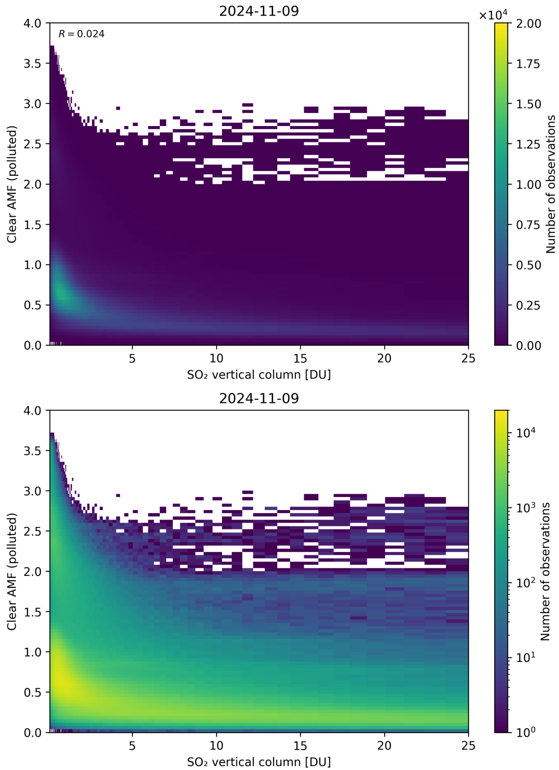
Figure 296: Scatter density plot of “SO 2 vertical column” against “Clear AMF (polluted)” for 2024-11-09 to 2024-11-10.
