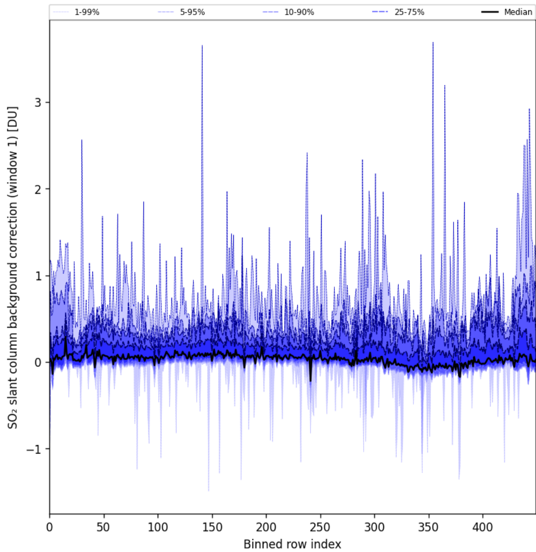
Figure 82: Along track statistics of “SO 2 slant column background correction (window 1)” for 2024-11-09 to 2024-11-10
