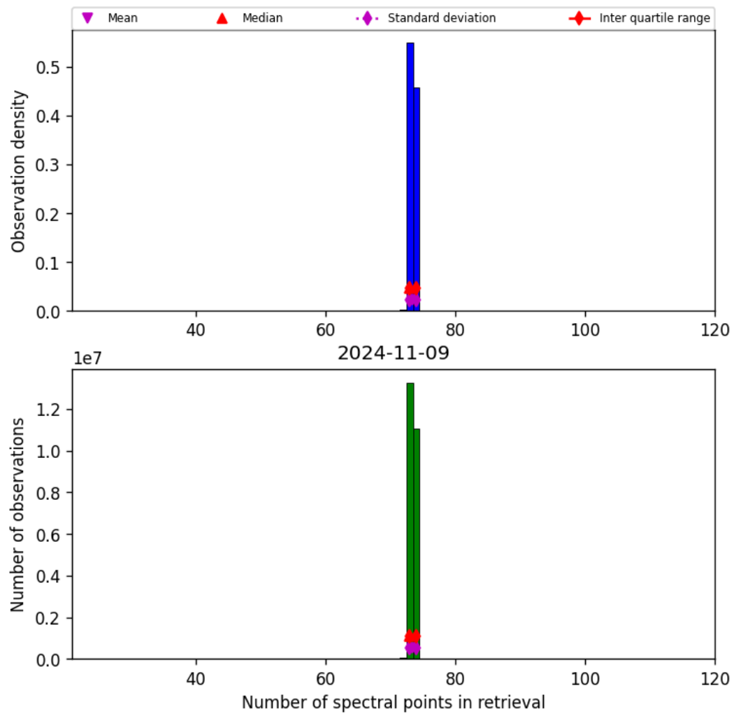
Figure 74: Histogram of “Number of spectral points in retrieval” for 2024-11-09 to 2024-11-10
