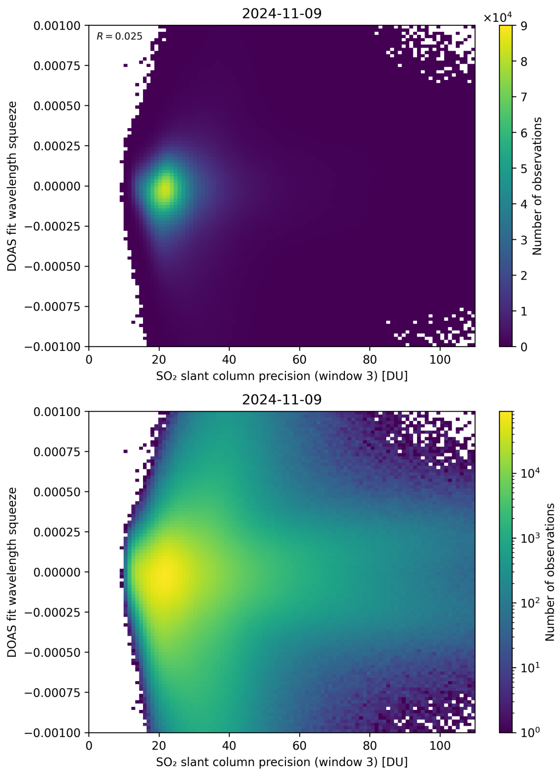
Figure 259: Scatter density plot of “SO 2 slant column precision (window 3)” against “DOAS fit wavelength squeeze” for 2024-11-09 to 2024-11-10.
