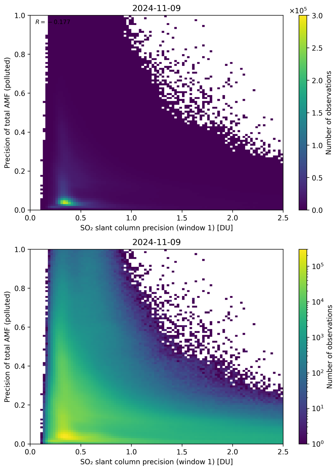
Figure 231: Scatter density plot of “SO 2 slant column precision (window 1)” against “Precision of total AMF (polluted)” for 2024-11-09 to 2024-11-10.
