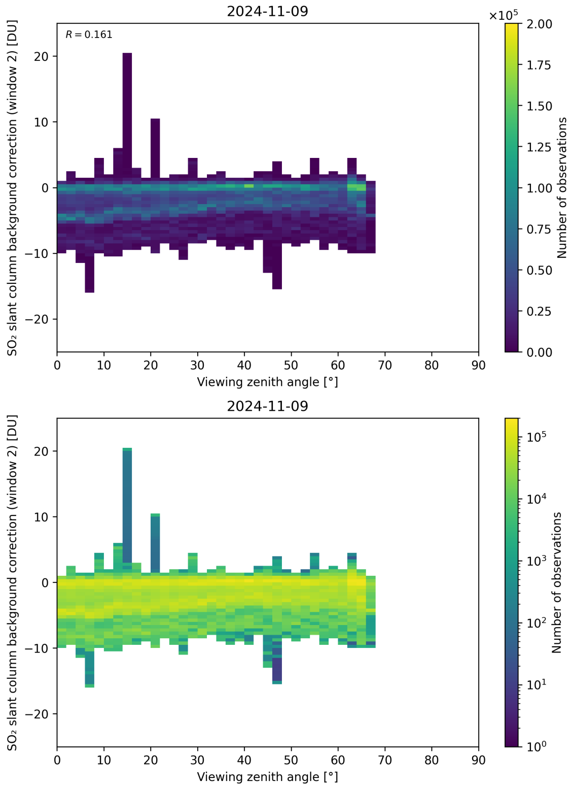
Figure 309: Scatter density plot of “Viewing zenith angle” against “SO 2 slant column background correction (window 2)” for 2024-11-09 to 2024-11-10.
