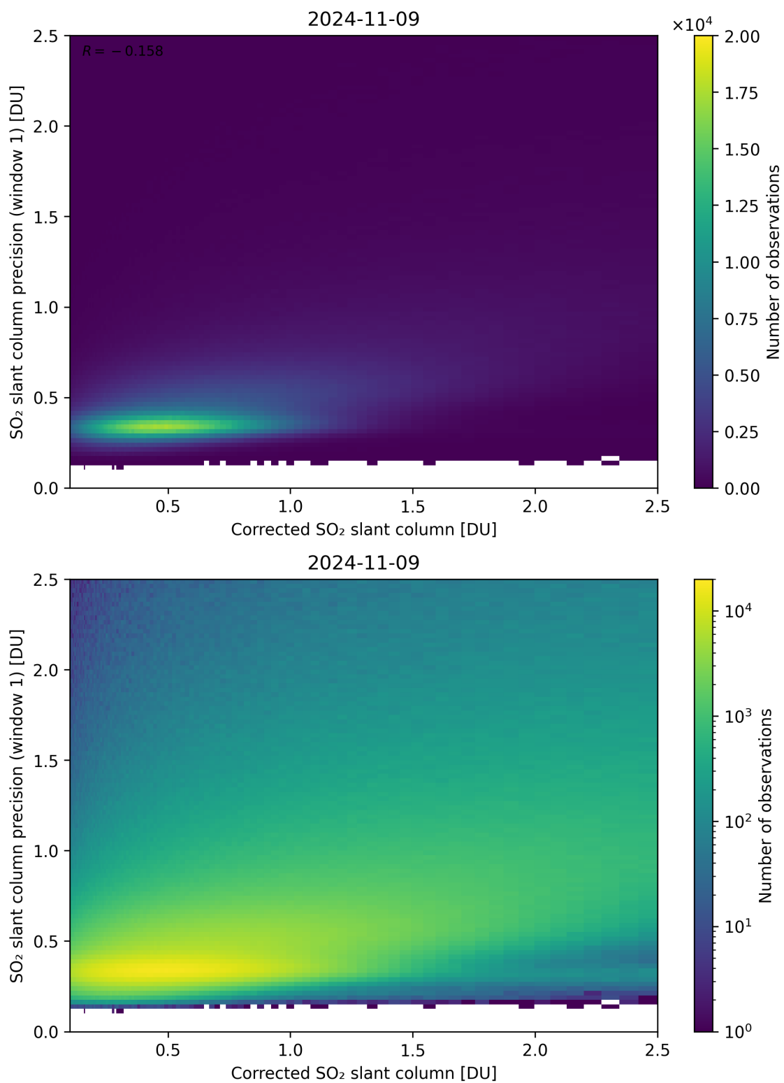
Figure 188: Scatter density plot of “Corrected SO 2 slant column” against “SO 2 slant column precision (window 1)” for 2024-11-09 to 2024-11-10.
