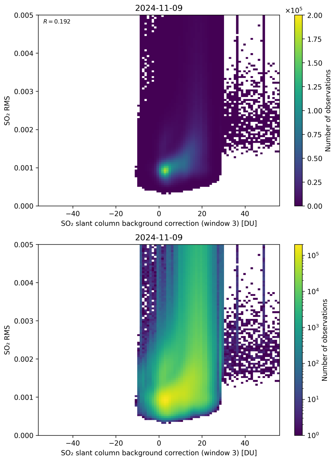
Figure 123: Scatter density plot of “SO 2 slant column background correction (window 3)” against “SO 2 RMS” for 2024-11-09 to 2024-11-10.
