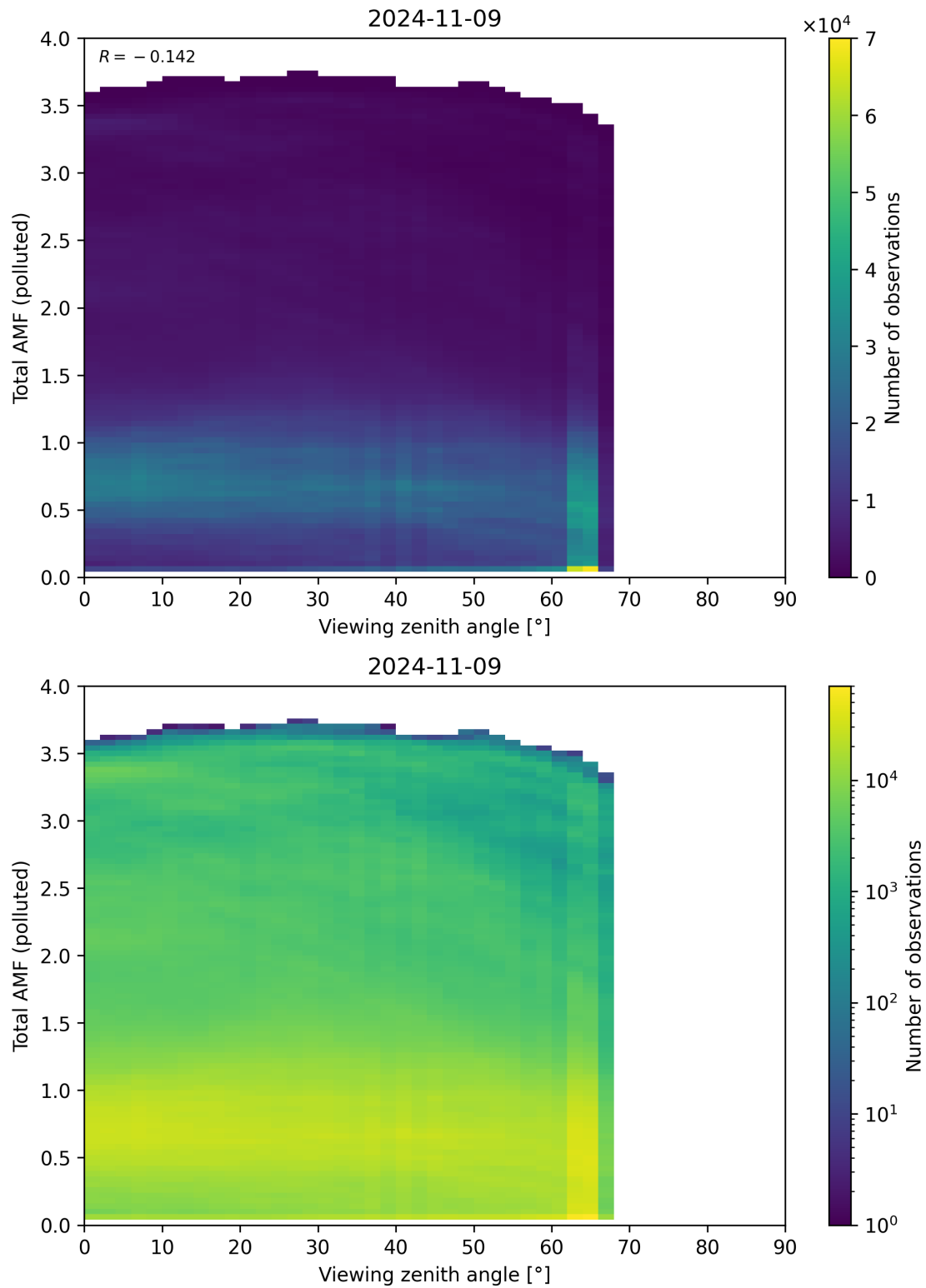
Figure 325: Scatter density plot of “Viewing zenith angle” against “Total AMF (polluted)” for 2024-11-09 to 2024-11-10.
