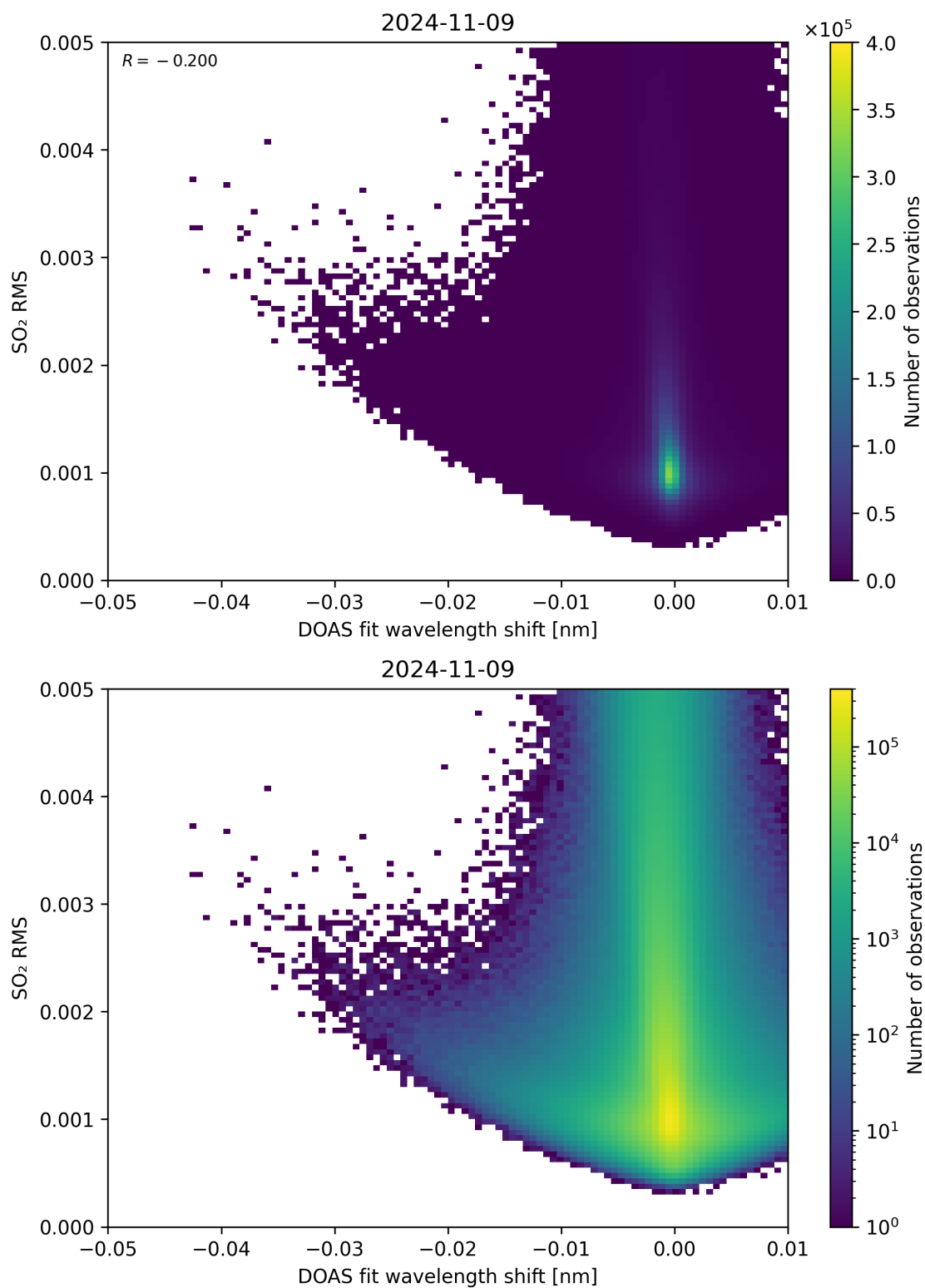
Figure 128: Scatter density plot of “DOAS fit wavelength shift” against “SO 2 RMS” for 2024-11-09 to 2024-11-10.
