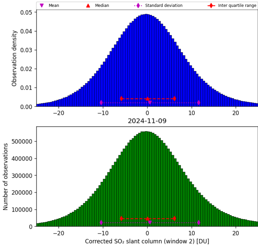
Figure 62: Histogram of “Corrected SO 2 slant column (window 2)” for 2024-11-09 to 2024-11-10
