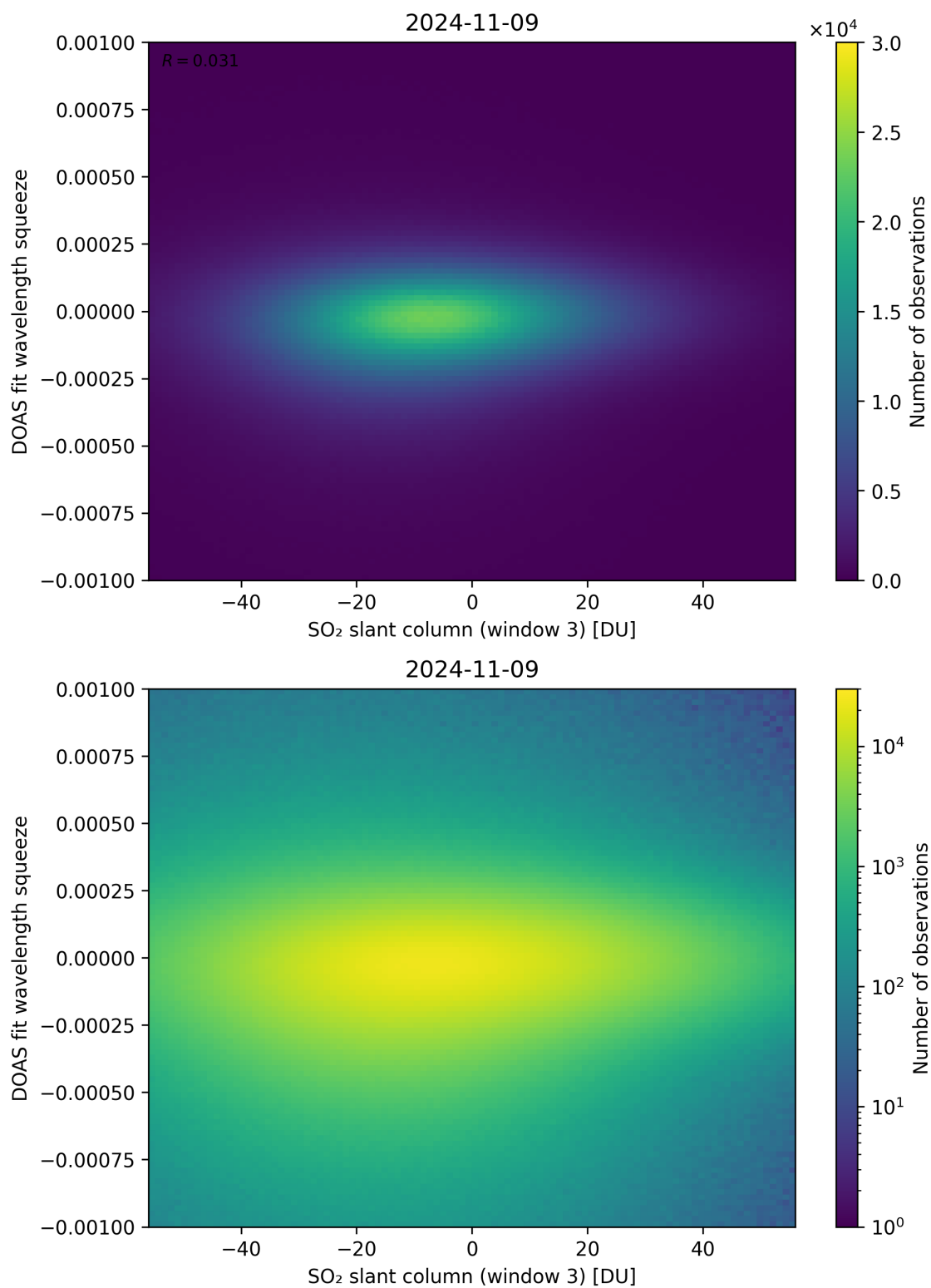
Figure 255: Scatter density plot of “SO 2 slant column (window 3)” against “DOAS fit wavelength squeeze” for 2024-11-09 to 2024-11-10.
