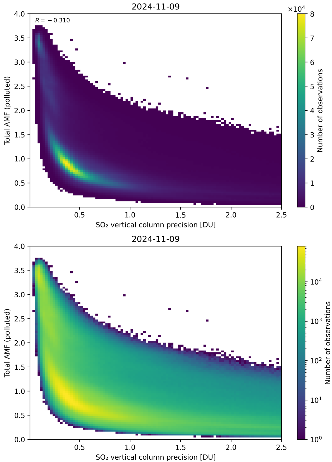
Figure 294: Scatter density plot of “SO 2 vertical column precision” against “Total AMF (polluted)” for 2024-11-09 to 2024-11-10.
