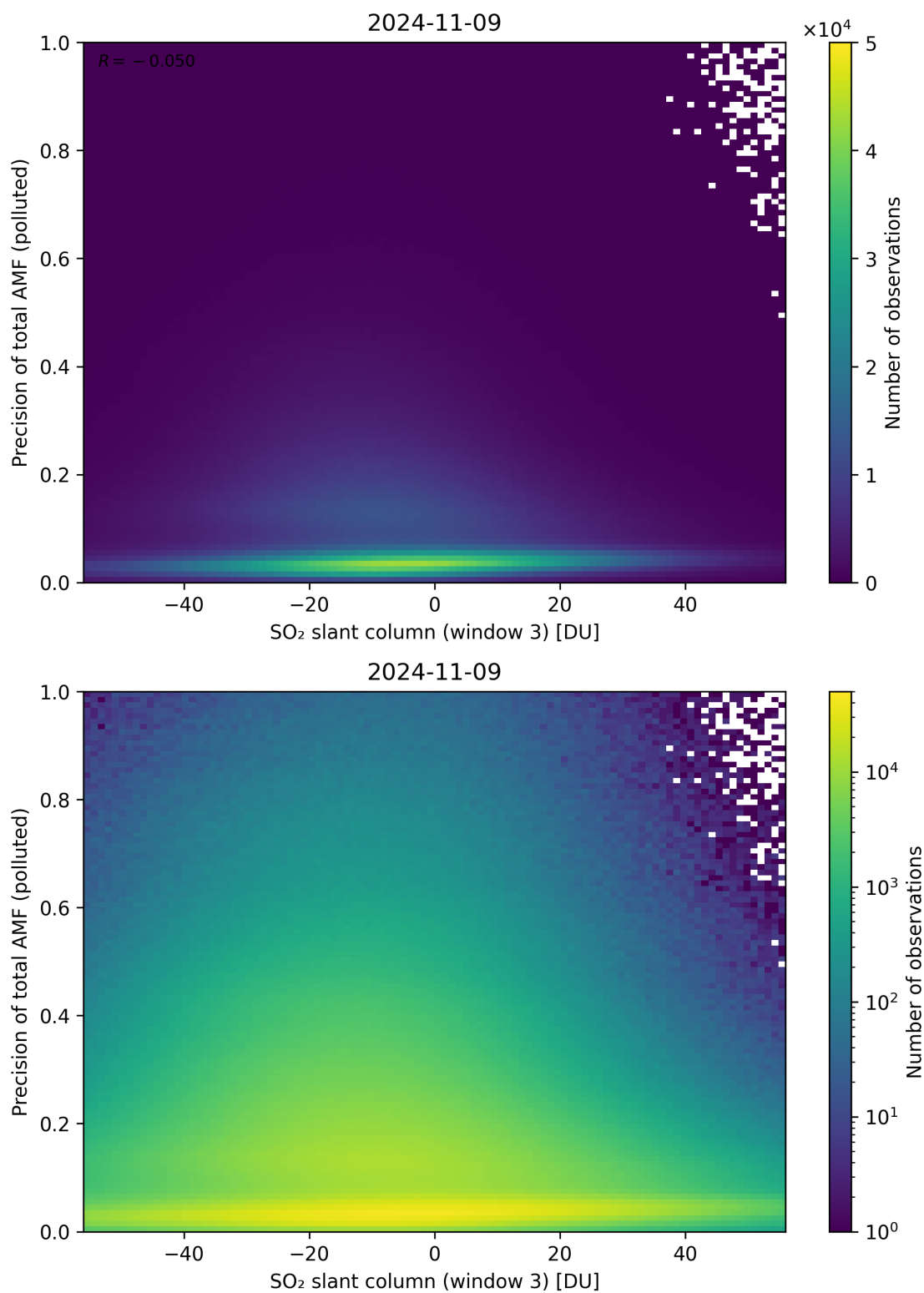
Figure 269: Scatter density plot of “SO 2 slant column (window 3)” against “Precision of total AMF (polluted)” for 2024-11-09 to 2024-11-10.
