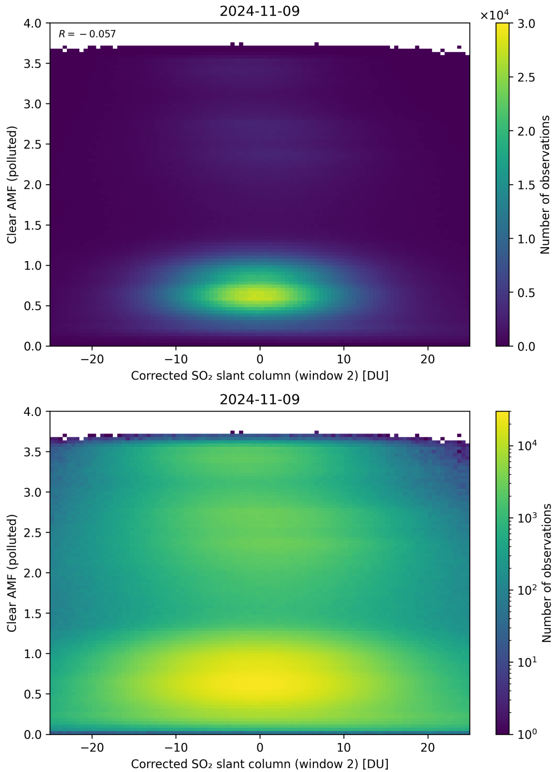
Figure 199: Scatter density plot of “Corrected SO 2 slant column (window 2)” against “Clear AMF (polluted)” for 2024-11-09 to 2024-11-10.
