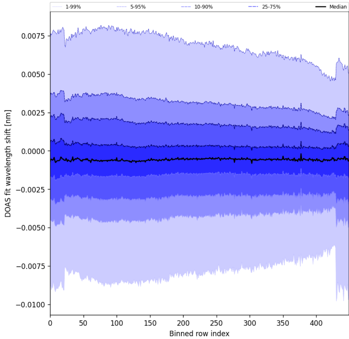
Figure 91: Along track statistics of “DOAS fit wavelength shift” for 2024-11-09 to 2024-11-10
