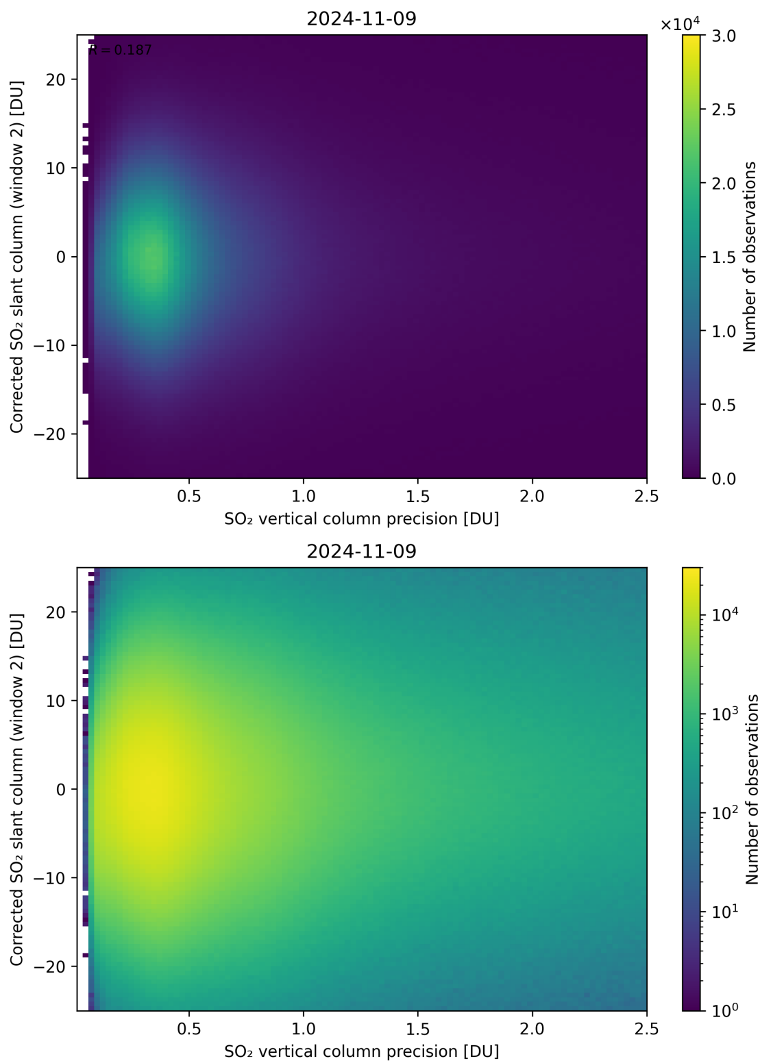
Figure 287: Scatter density plot of “SO 2 vertical column precision” against “Corrected SO 2 slant column (window 2)” for 2024-11-09 to 2024-11-10.
