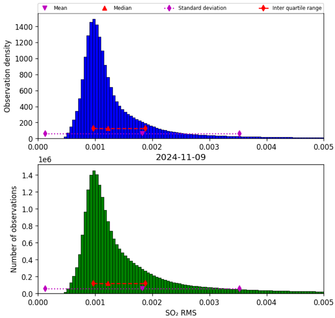
Figure 70: Histogram of “SO 2 RMS” for 2024-11-09 to 2024-11-10
