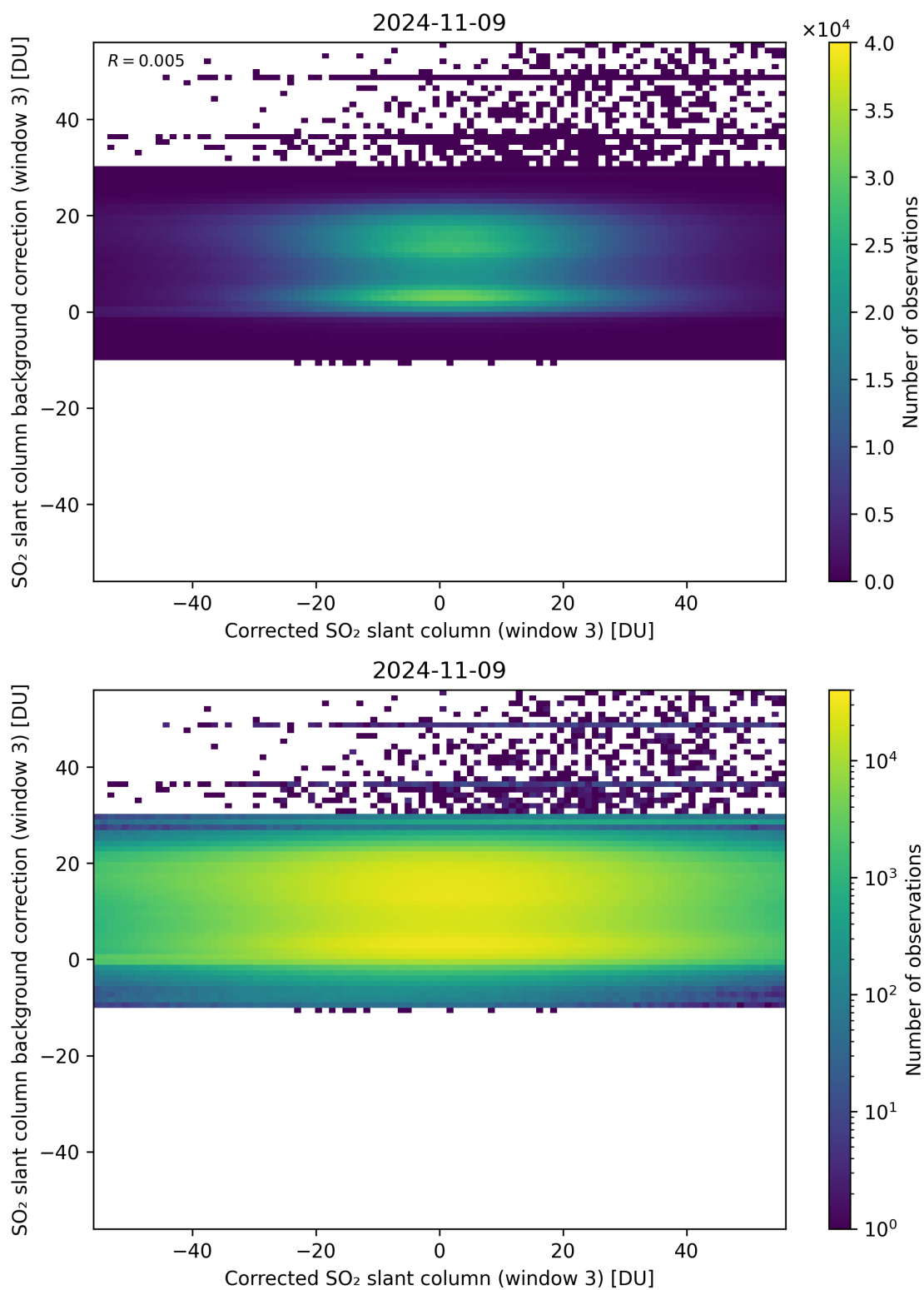
Figure 205: Scatter density plot of “Corrected SO 2 slant column (window 3)” against “SO 2 slant column background correction (window 3)” for 2024-11-09 to 2024-11-10.
