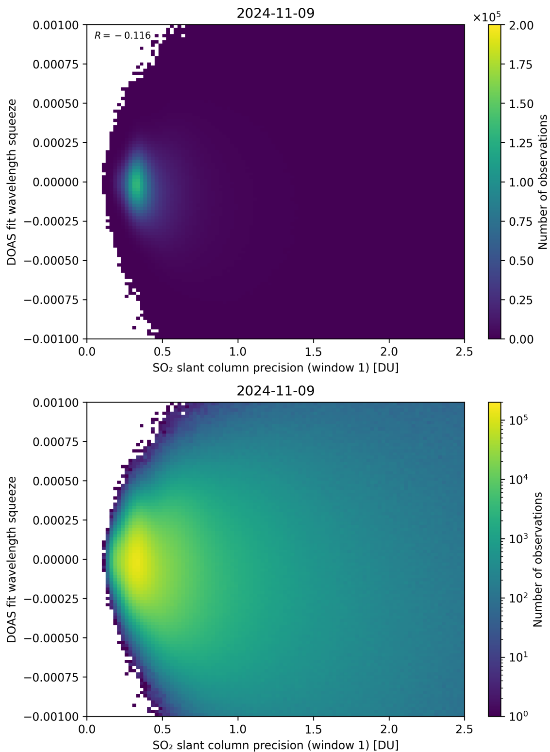
Figure 222: Scatter density plot of “SO 2 slant column precision (window 1)” against “DOAS fit wavelength squeeze” for 2024-11-09 to 2024-11-10.
