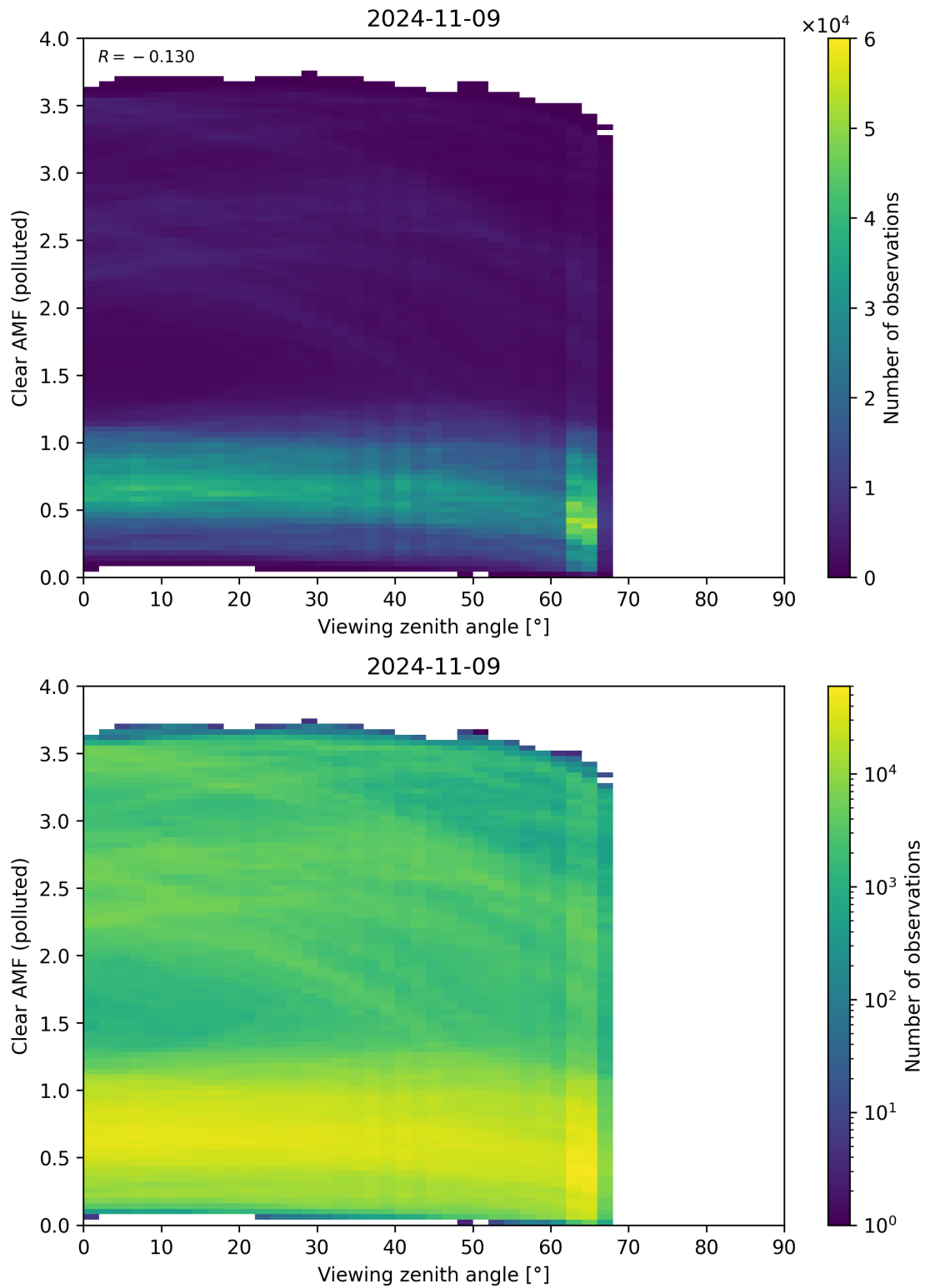
Figure 316: Scatter density plot of “Viewing zenith angle” against “Clear AMF (polluted)” for 2024-11-09 to 2024-11-10.
