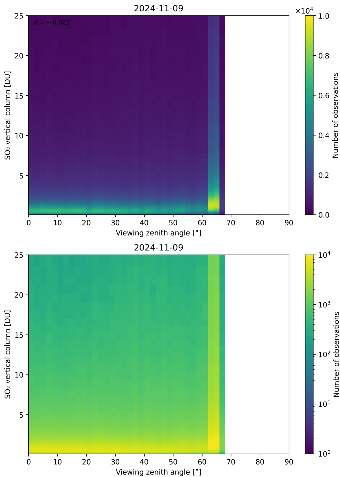
Figure 327: Scatter density plot of “Viewing zenith angle” against “SO 2 vertical column” for 2024-11-09 to 2024-11-10.
