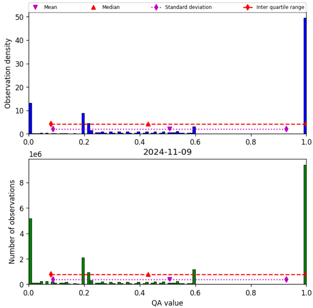
Figure 52: Histogram of “QA value” for 2024-11-09 to 2024-11-10
