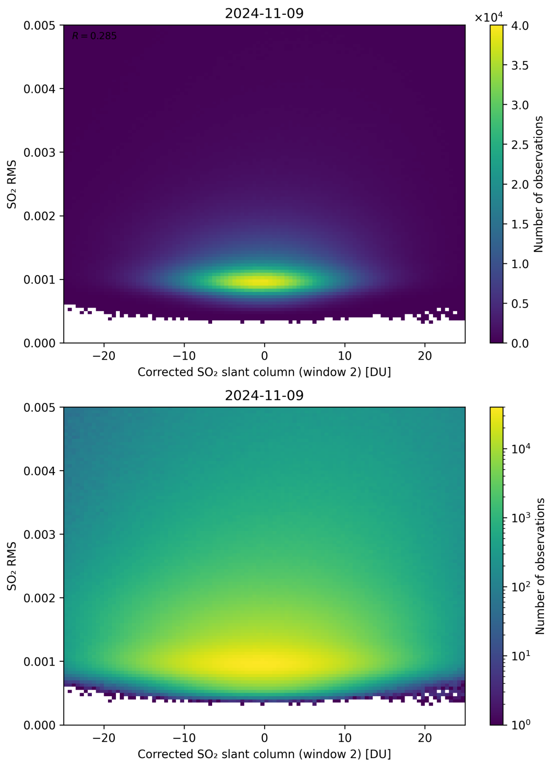
Figure 198: Scatter density plot of “Corrected SO 2 slant column (window 2)” against “SO 2 RMS” for 2024-11-09 to 2024-11-10.
