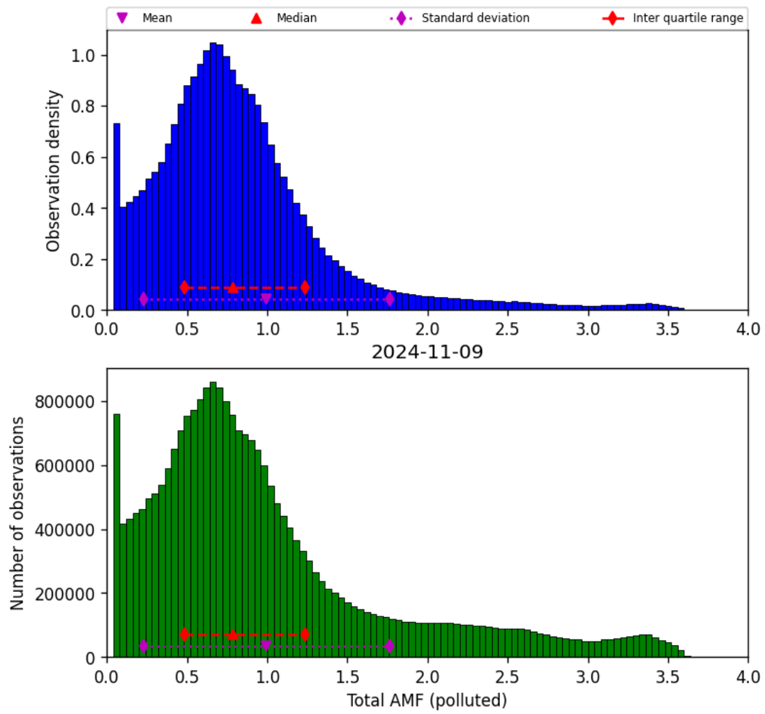
Figure 71: Histogram of “Total AMF (polluted)” for 2024-11-09 to 2024-11-10
