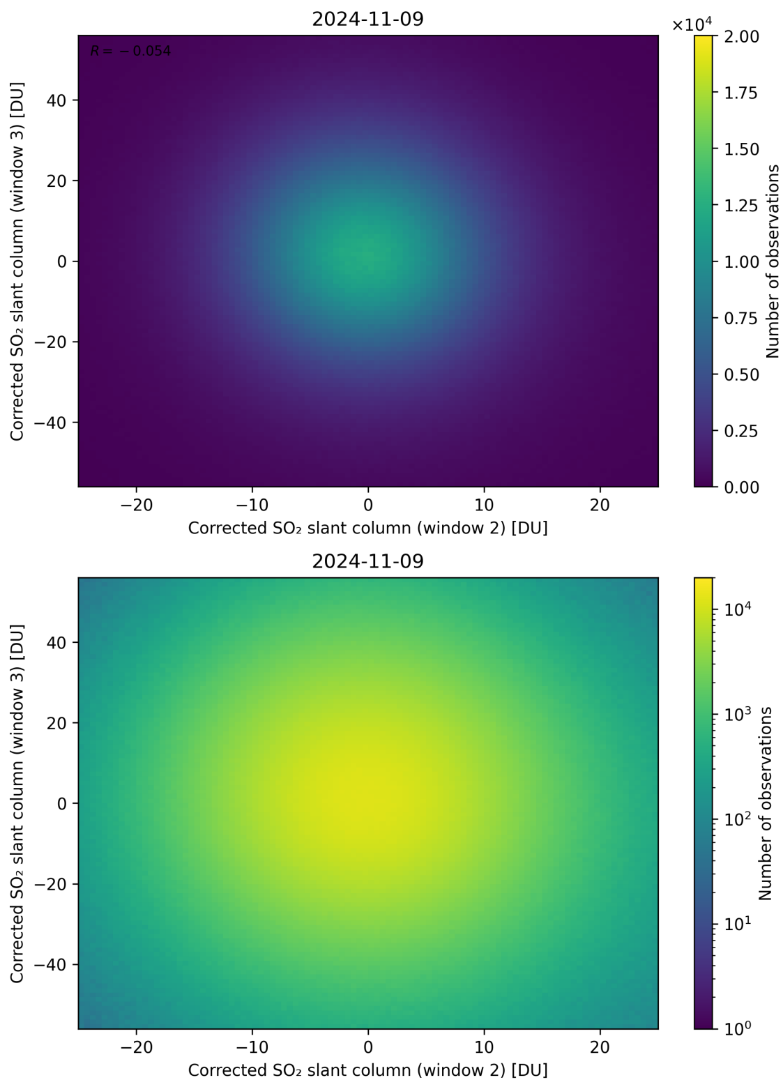
Figure 200: Scatter density plot of “Corrected SO 2 slant column (window 2)” against “Corrected SO 2 slant column (window 3)” for 2024-11-09 to 2024-11-10.
