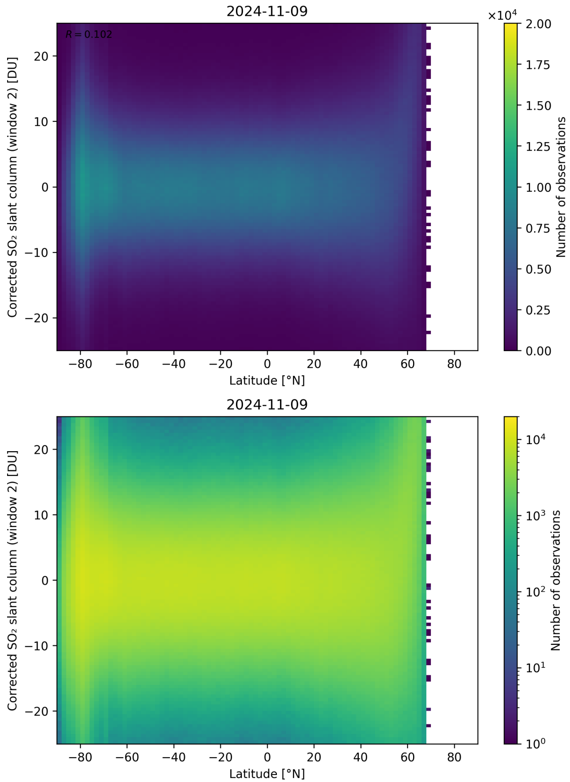
Figure 147: Scatter density plot of “Latitude” against “Corrected SO 2 slant column (window 2)” for 2024-11-09 to 2024-11-10.
