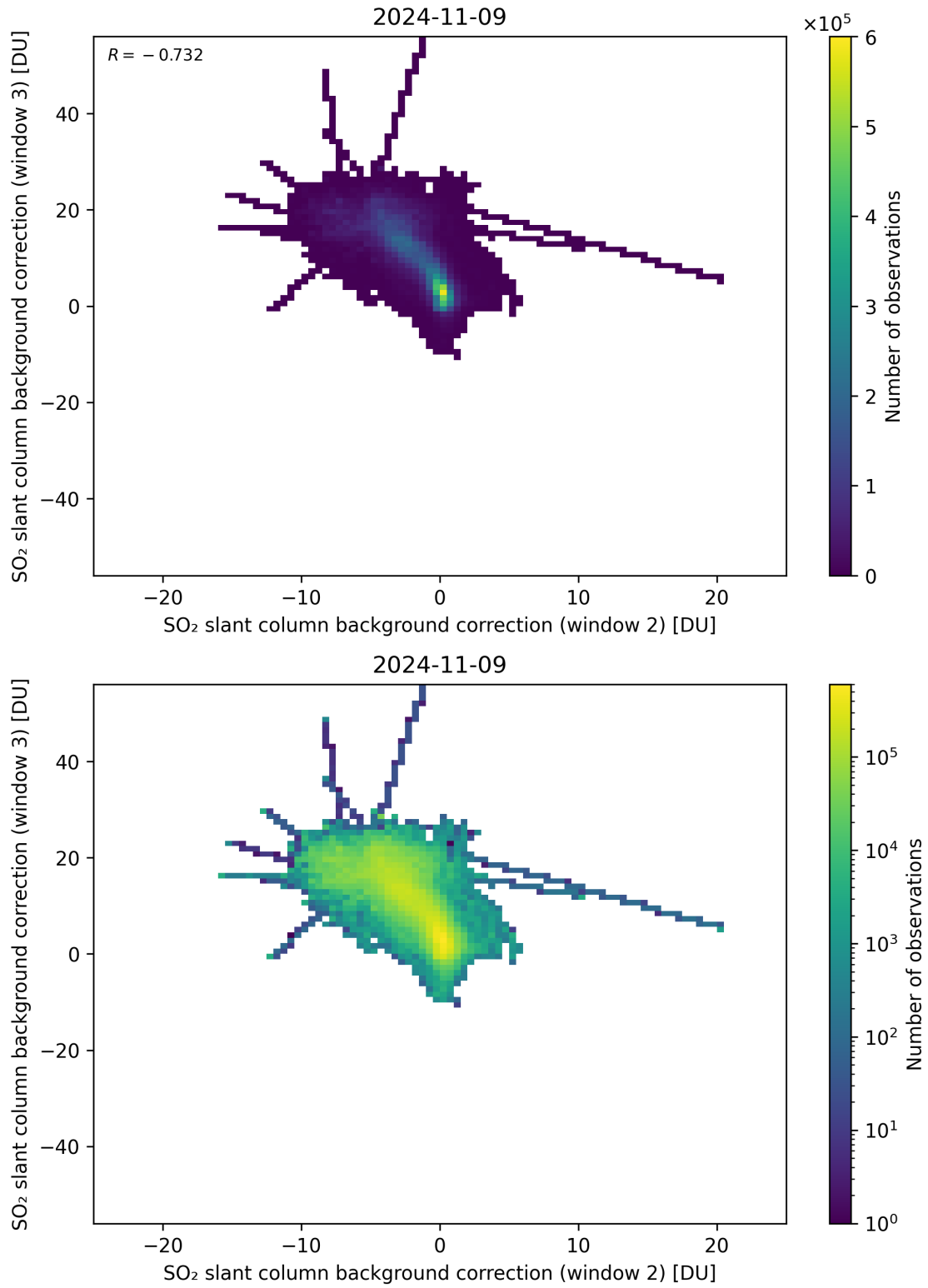
Figure 111: Scatter density plot of “SO 2 slant column background correction (window 2)” against “SO 2 slant column background correction (window 3)” for 2024-11-09 to 2024-11-10.
