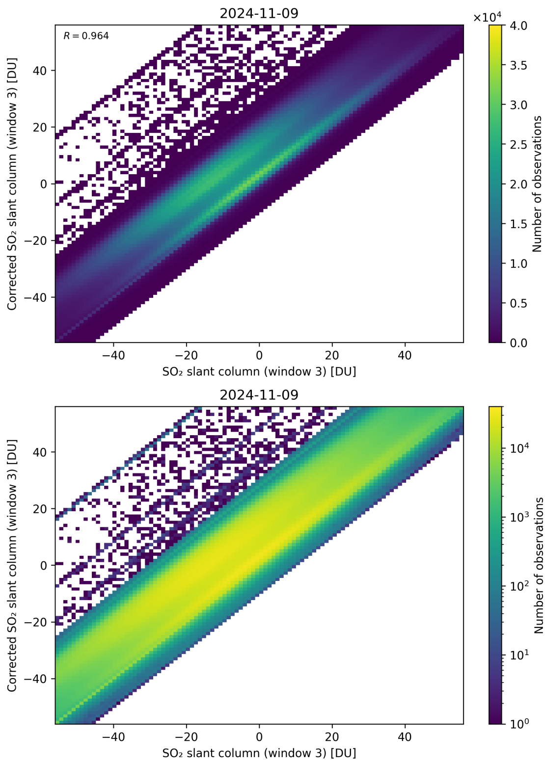
Figure 266: Scatter density plot of “SO 2 slant column (window 3)” against “Corrected SO 2 slant column (window 3)” for 2024-11-09 to 2024-11-10.
