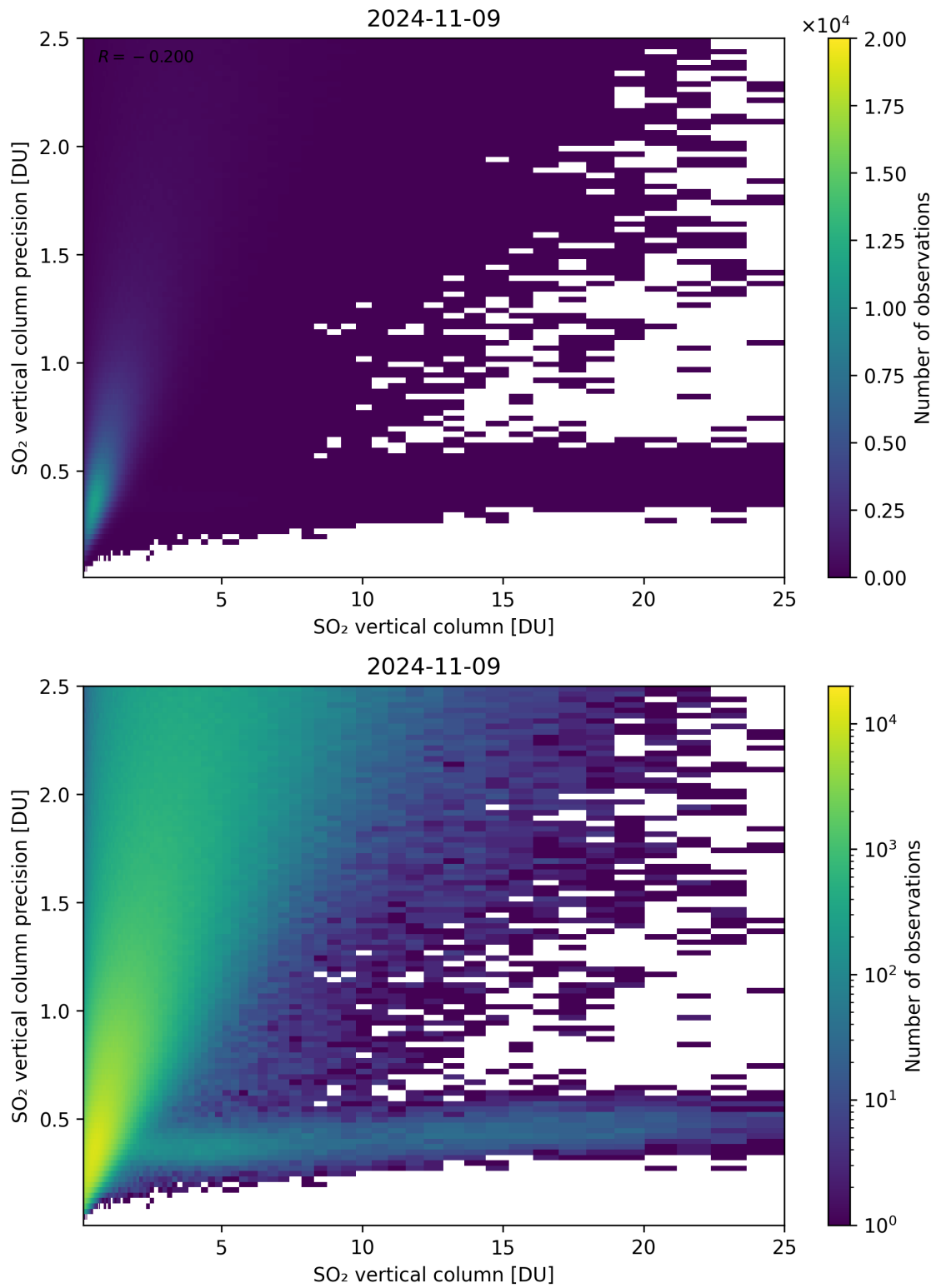
Figure 307: Scatter density plot of “SO 2 vertical column” against “SO 2 vertical column precision” for 2024-11-09 to 2024-11-10.
