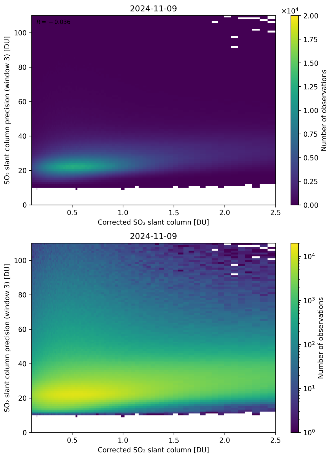
Figure 191: Scatter density plot of “Corrected SO 2 slant column” against “SO 2 slant column precision (window 3)” for 2024-11-09 to 2024-11-10.
