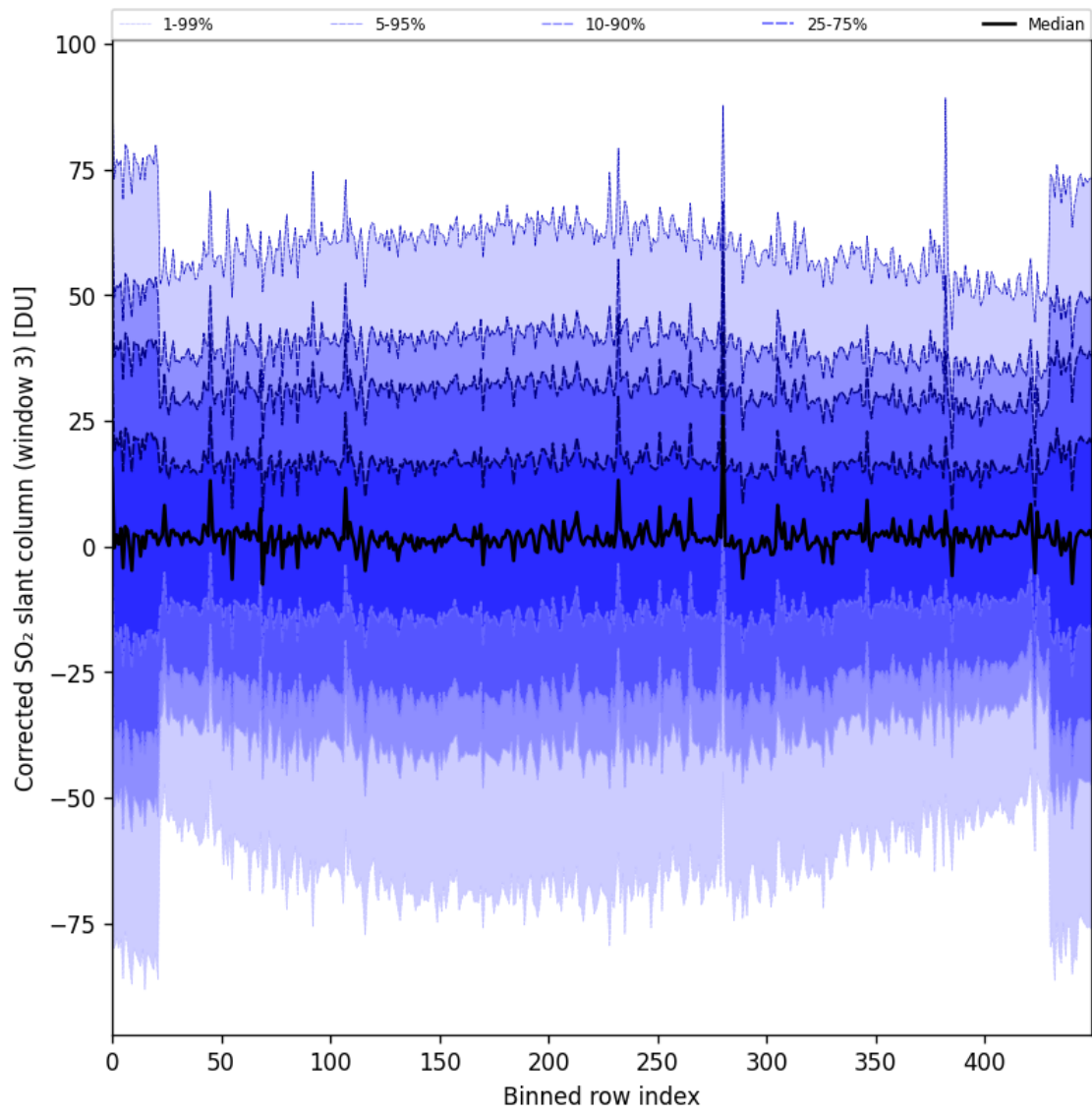
Figure 89: Along track statistics of “Corrected SO 2 slant column (window 3)” for 2024-11-09 to 2024-11-10
