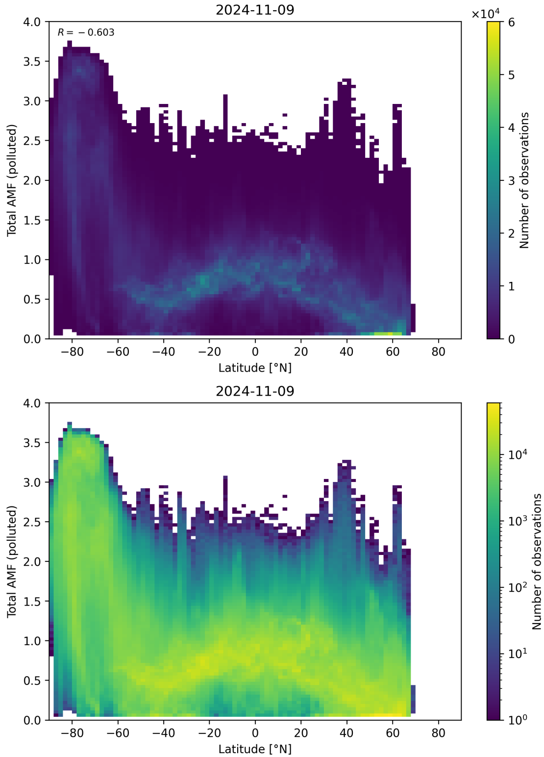
Figure 154: Scatter density plot of “Latitude” against “Total AMF (polluted)” for 2024-11-09 to 2024-11-10.
