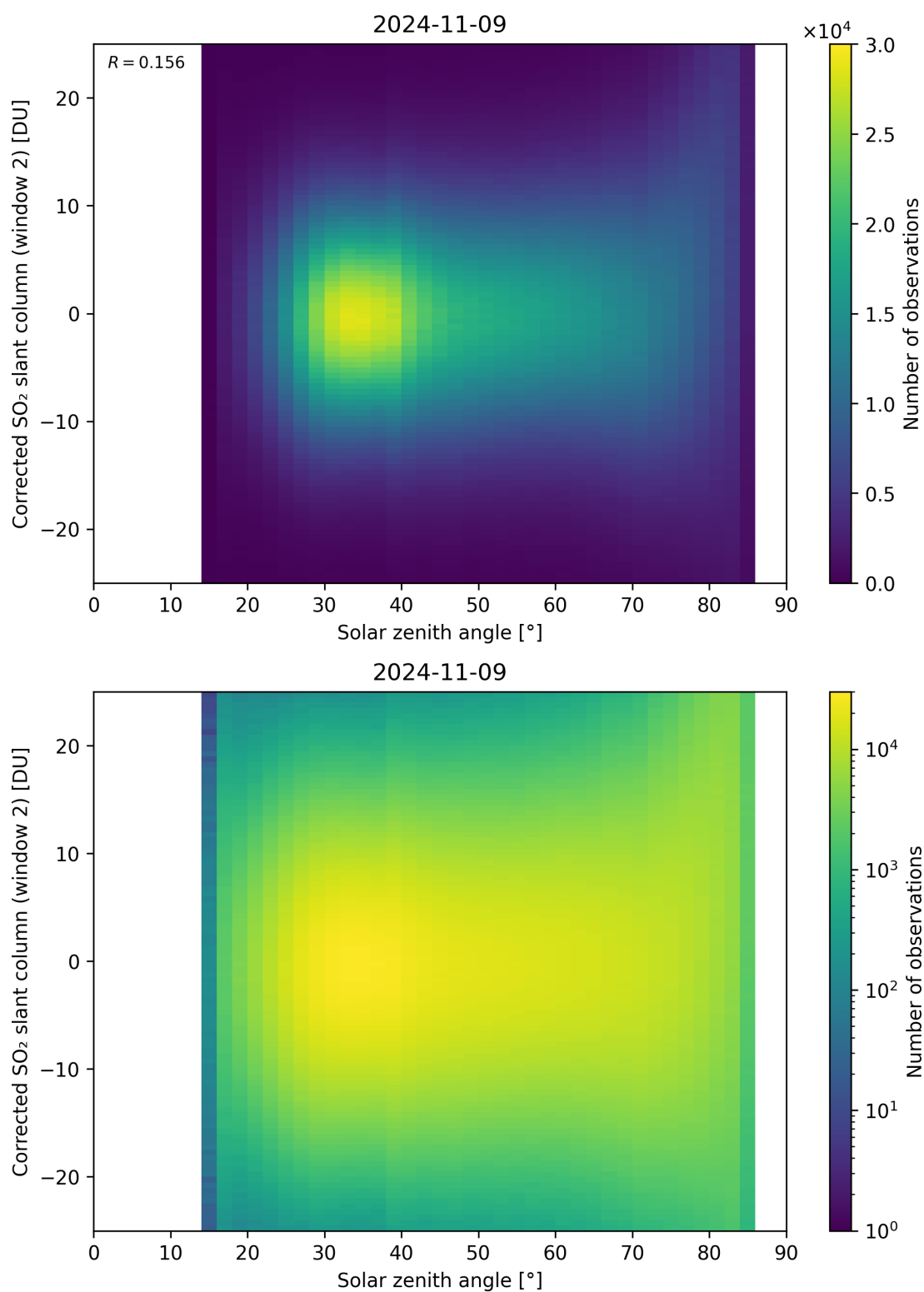
Figure 167: Scatter density plot of “Solar zenith angle” against “Corrected SO 2 slant column (window 2)” for 2024-11-09 to 2024-11-10.
