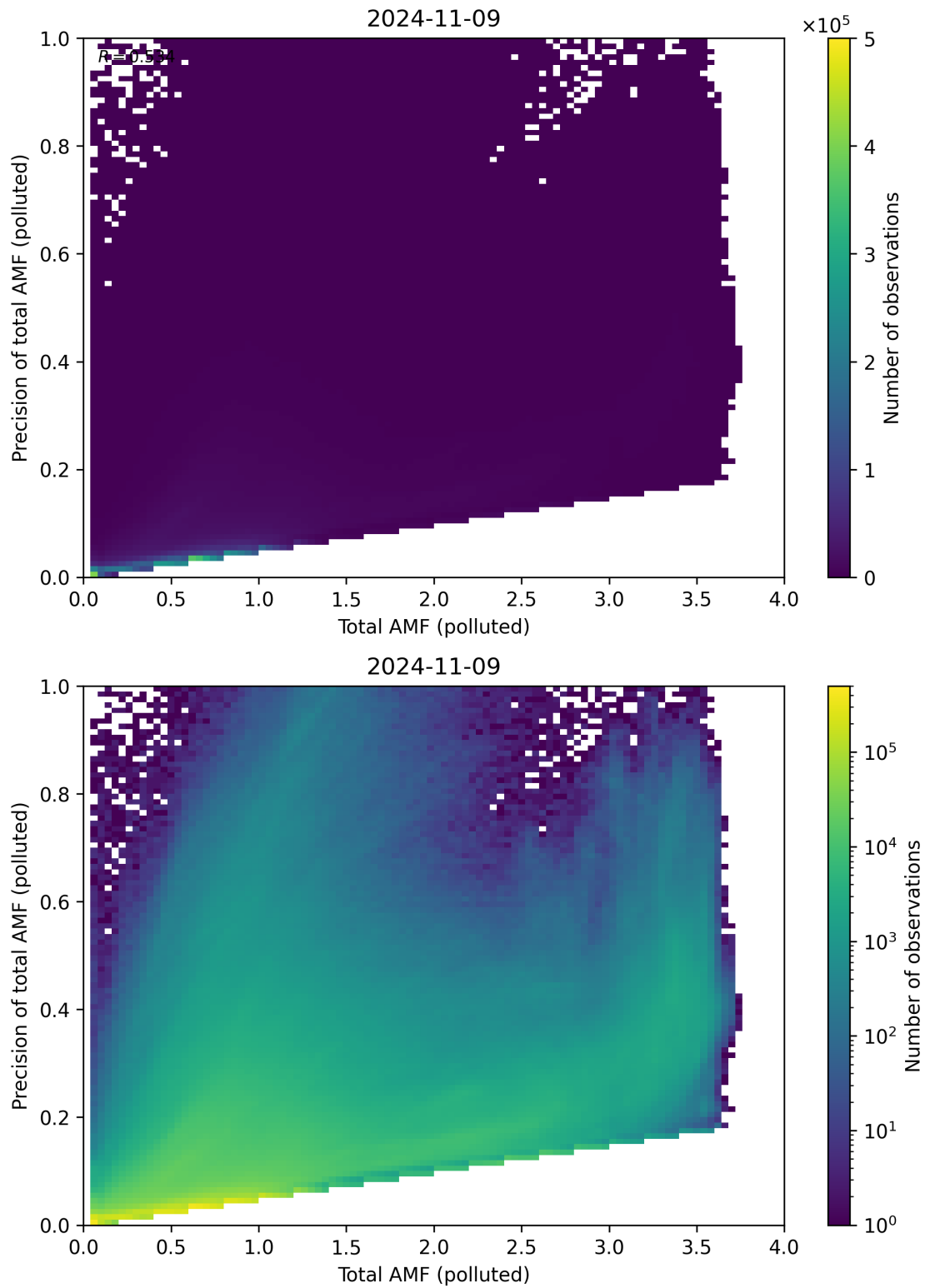
Figure 272: Scatter density plot of “Total AMF (polluted)” against “Precision of total AMF (polluted)” for 2024-11-09 to 2024-11-10.
