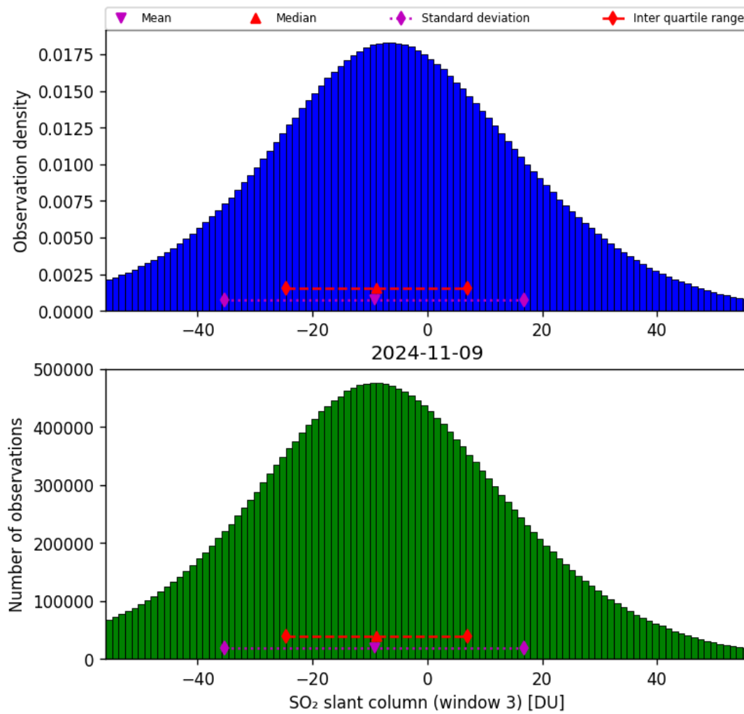
Figure 64: Histogram of “SO 2 slant column (window 3)” for 2024-11-09 to 2024-11-10
