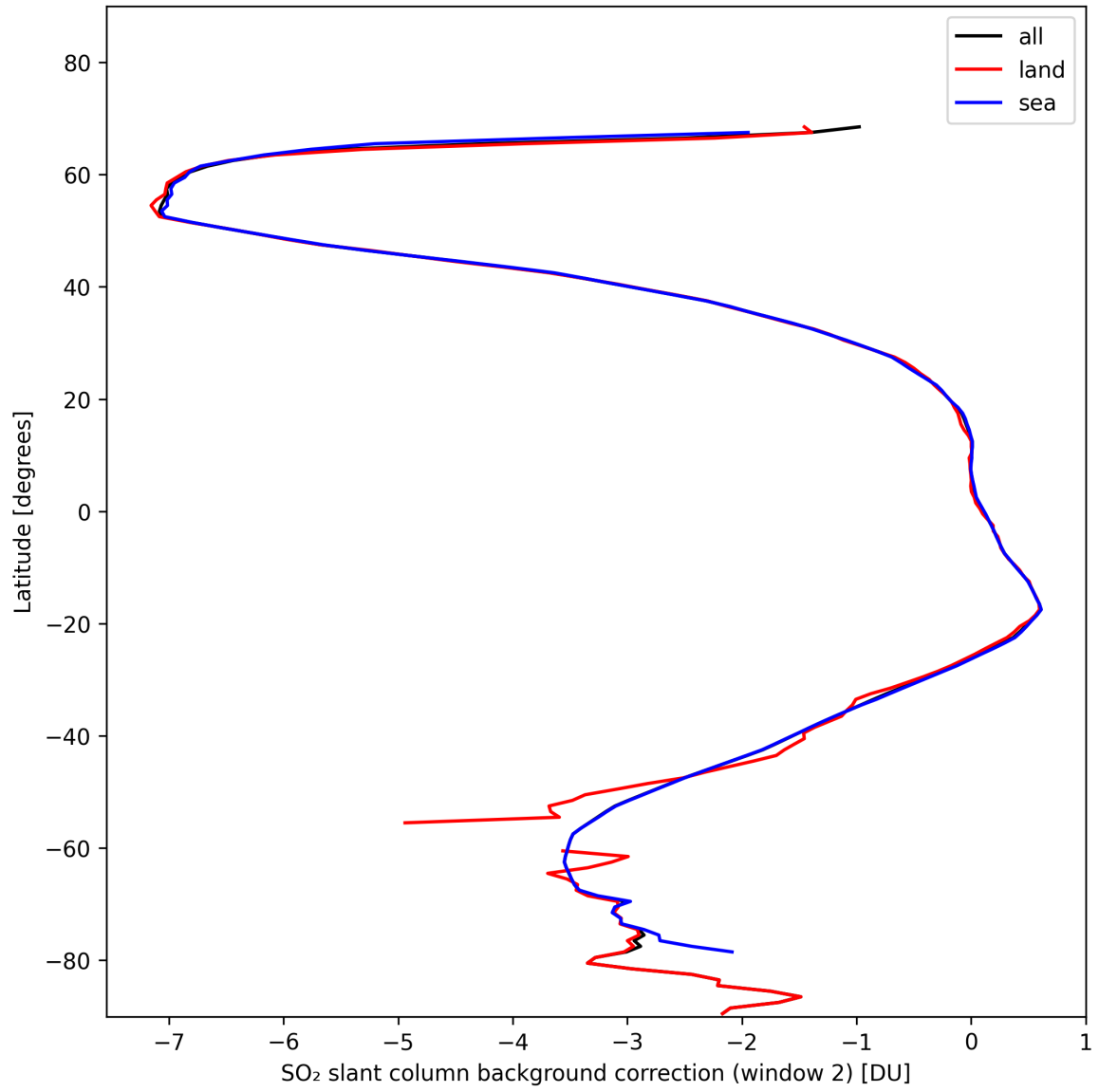
Figure 40: Zonal average of “SO 2 slant column background correction (window 2)” for 2024-11-09 to 2024-11-10.
