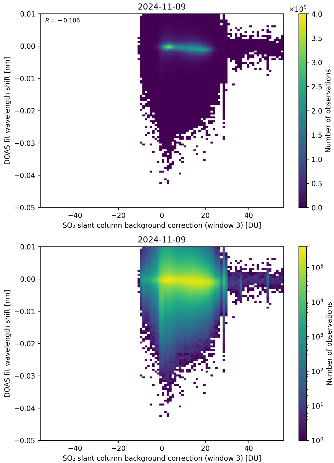
Figure 121: Scatter density plot of “SO 2 slant column background correction (window 3)” against “DOAS fit wavelength shift” for 2024-11-09 to 2024-11-10.
