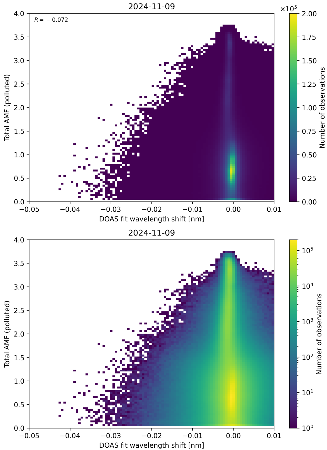
Figure 130: Scatter density plot of “DOAS fit wavelength shift” against “Total AMF (polluted)” for 2024-11-09 to 2024-11-10.
