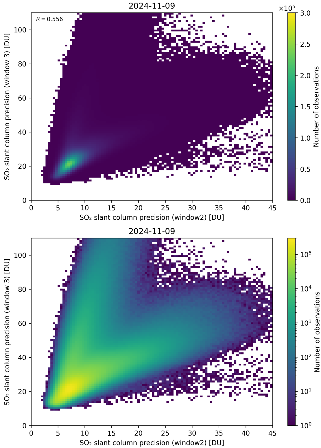
Figure 250: Scatter density plot of “SO 2 slant column precision (window2)” against “SO 2 slant column precision (window 3)” for 2024-11-09 to 2024-11-10.
