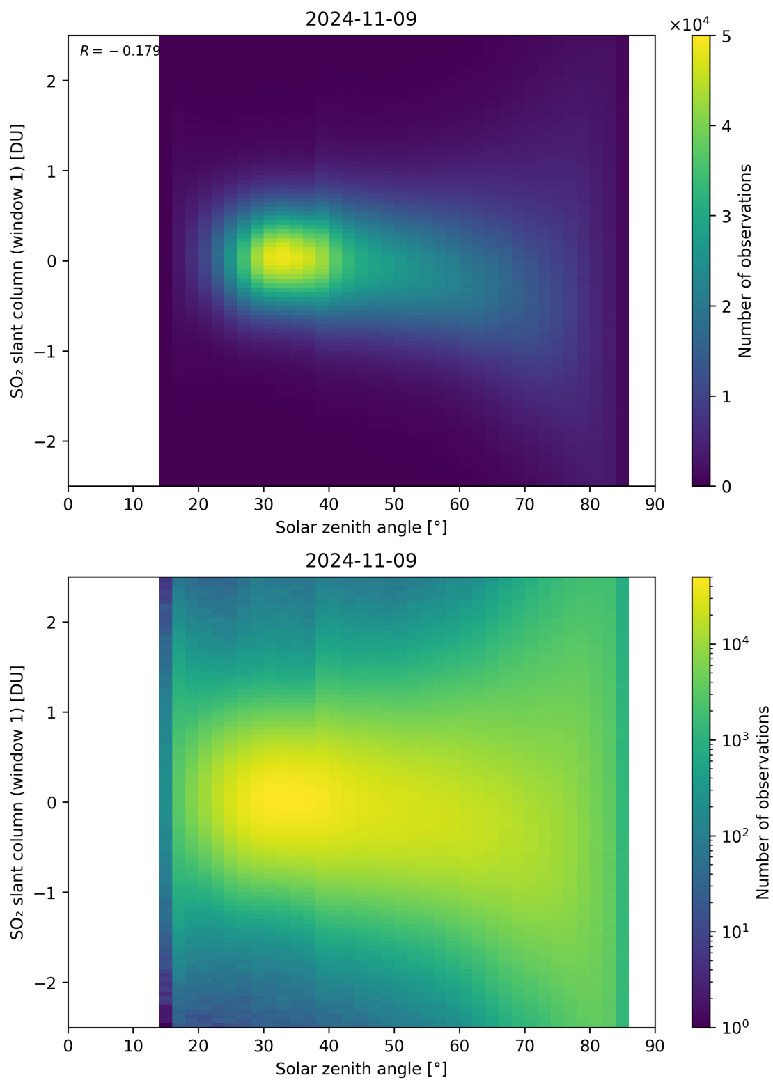
Figure 169: Scatter density plot of “Solar zenith angle” against “SO 2 slant column (window 1)” for 2024-11-09 to 2024-11-10.
