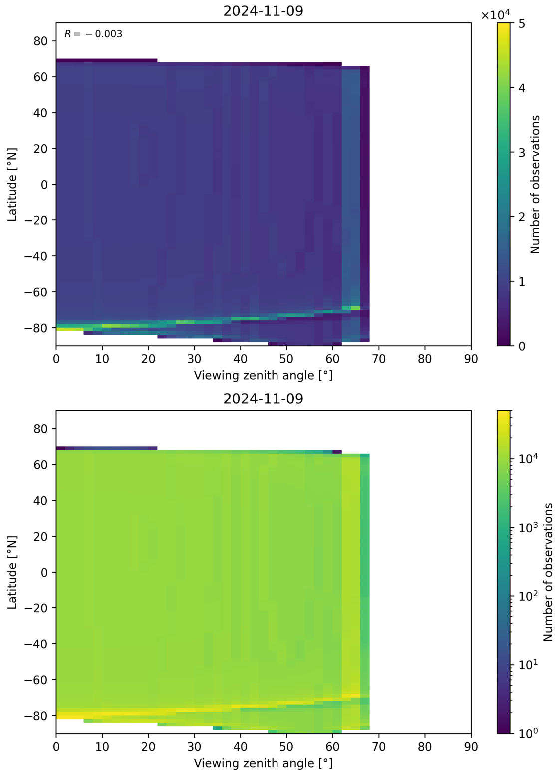
Figure 314: Scatter density plot of “Viewing zenith angle” against “Latitude” for 2024-11-09 to 2024-11-10.
