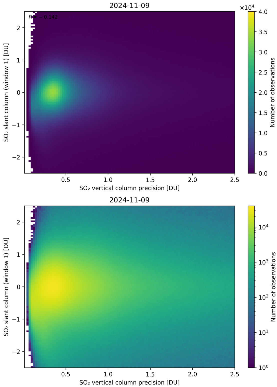
Figure 289: Scatter density plot of “SO 2 vertical column precision” against “SO 2 slant column (window 1)” for 2024-11-09 to 2024-11-10.
