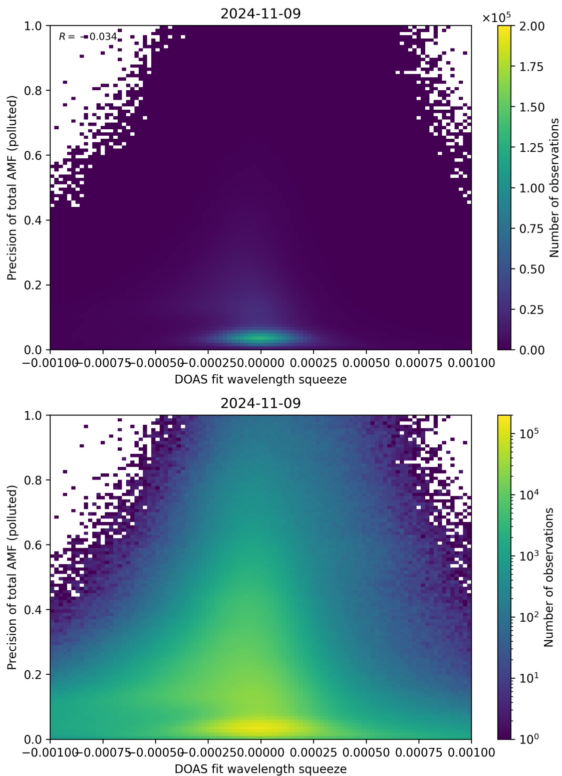
Figure 135: Scatter density plot of “DOAS fit wavelength squeeze” against “Precision of total AMF (polluted)” for 2024-11-09 to 2024-11-10.
