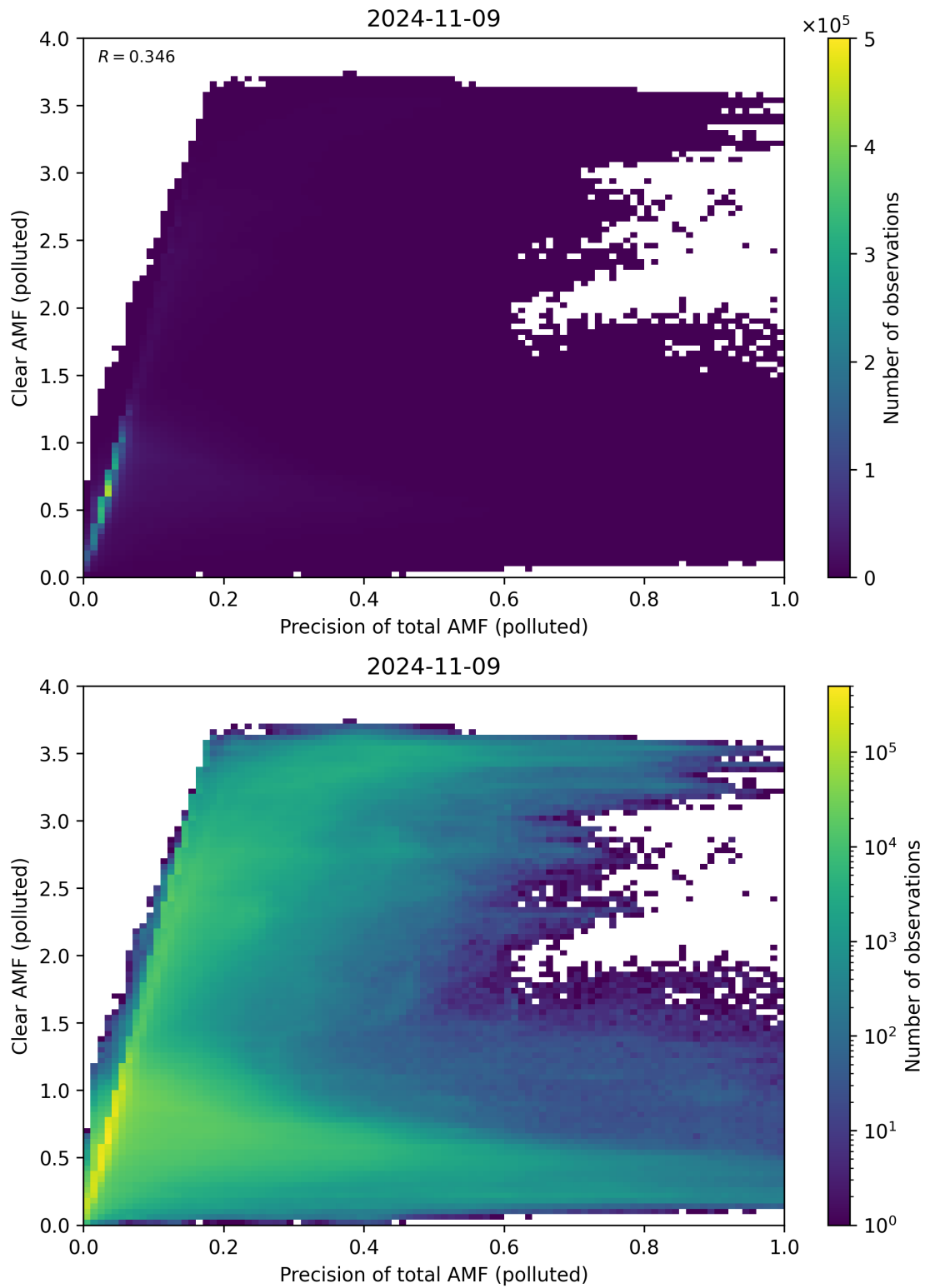
Figure 270: Scatter density plot of “Precision of total AMF (polluted)” against “Clear AMF (polluted)” for 2024-11-09 to 2024-11-10.
