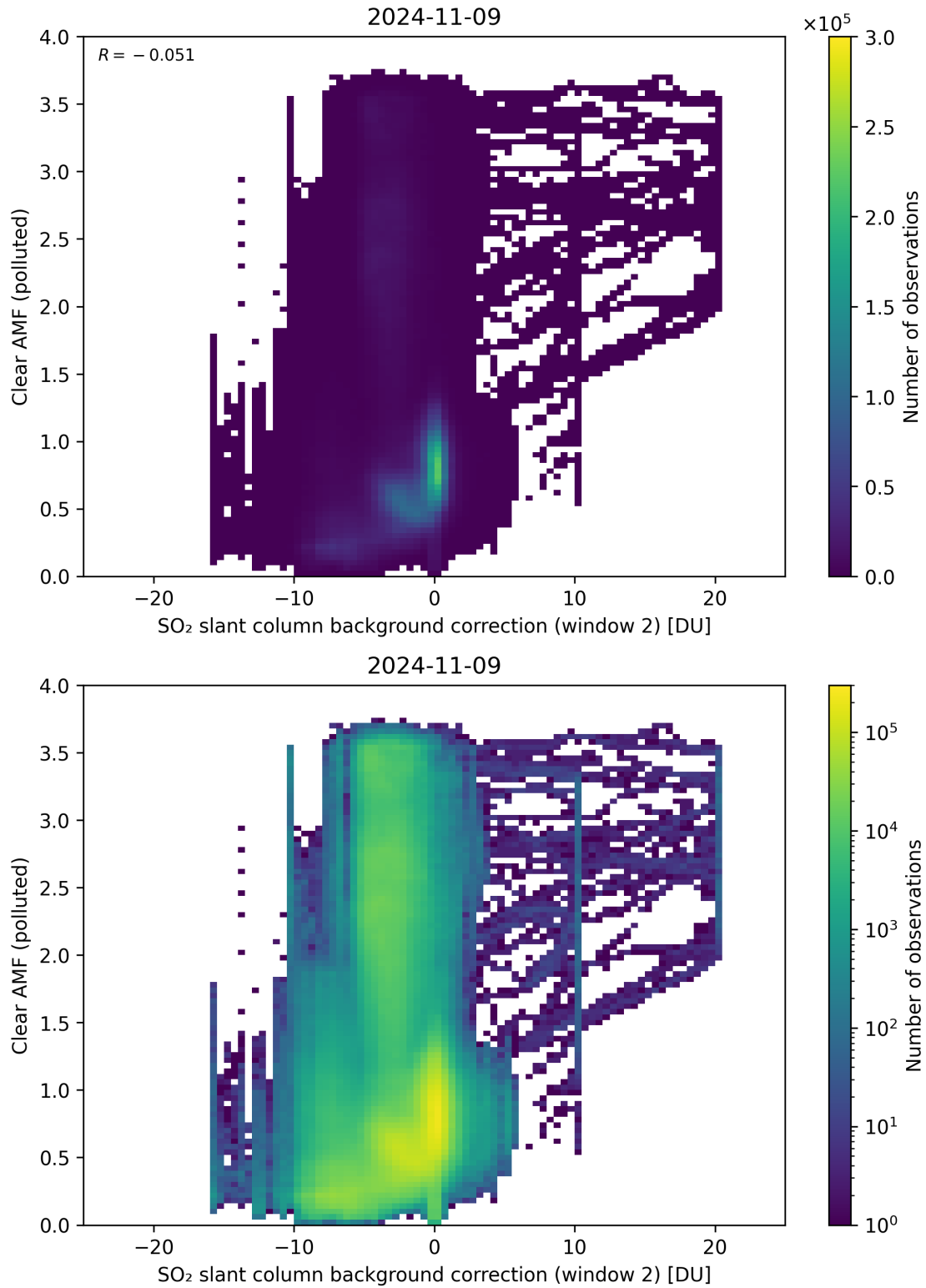
Figure 115: Scatter density plot of “SO 2 slant column background correction (window 2)” against “Clear AMF (polluted)” for 2024-11-09 to 2024-11-10.
