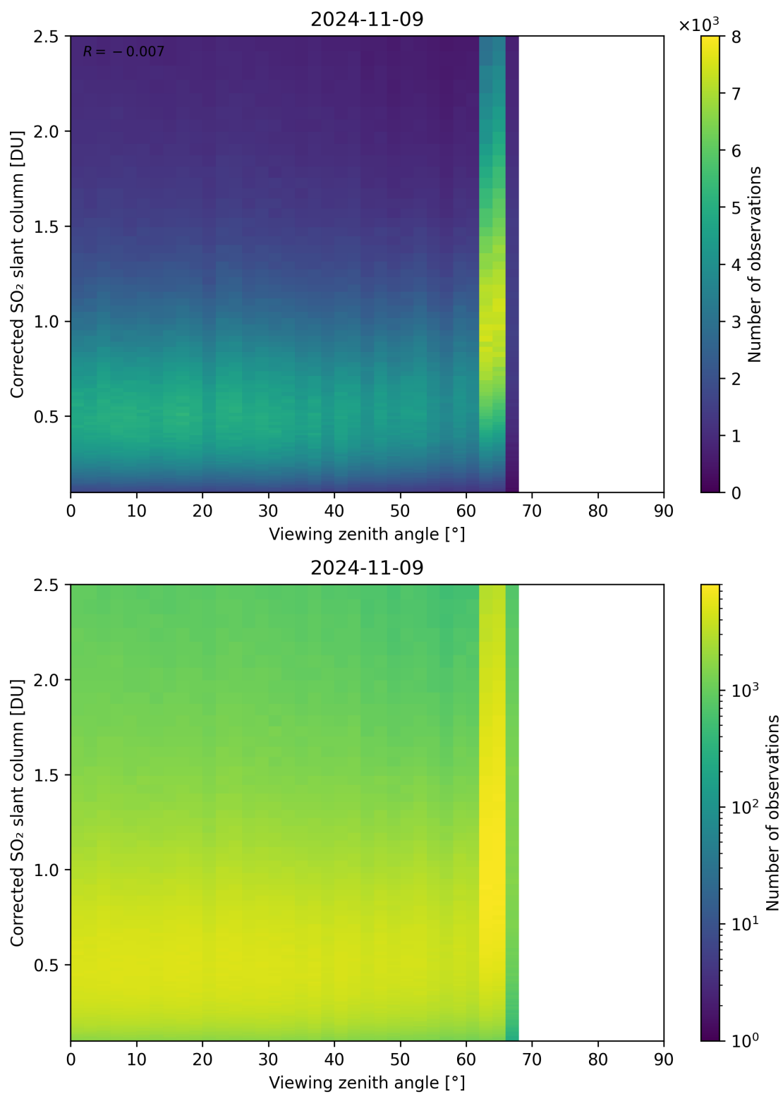
Figure 317: Scatter density plot of “Viewing zenith angle” against “Corrected SO 2 slant column” for 2024-11-09 to 2024-11-10.
