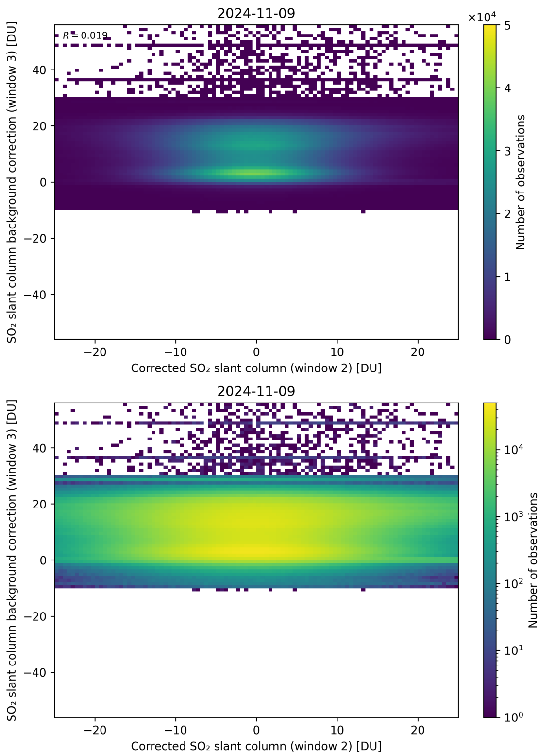
Figure 195: Scatter density plot of “Corrected SO 2 slant column (window 2)” against “SO 2 slant column background correction (window 3)” for 2024-11-09 to 2024-11-10.
