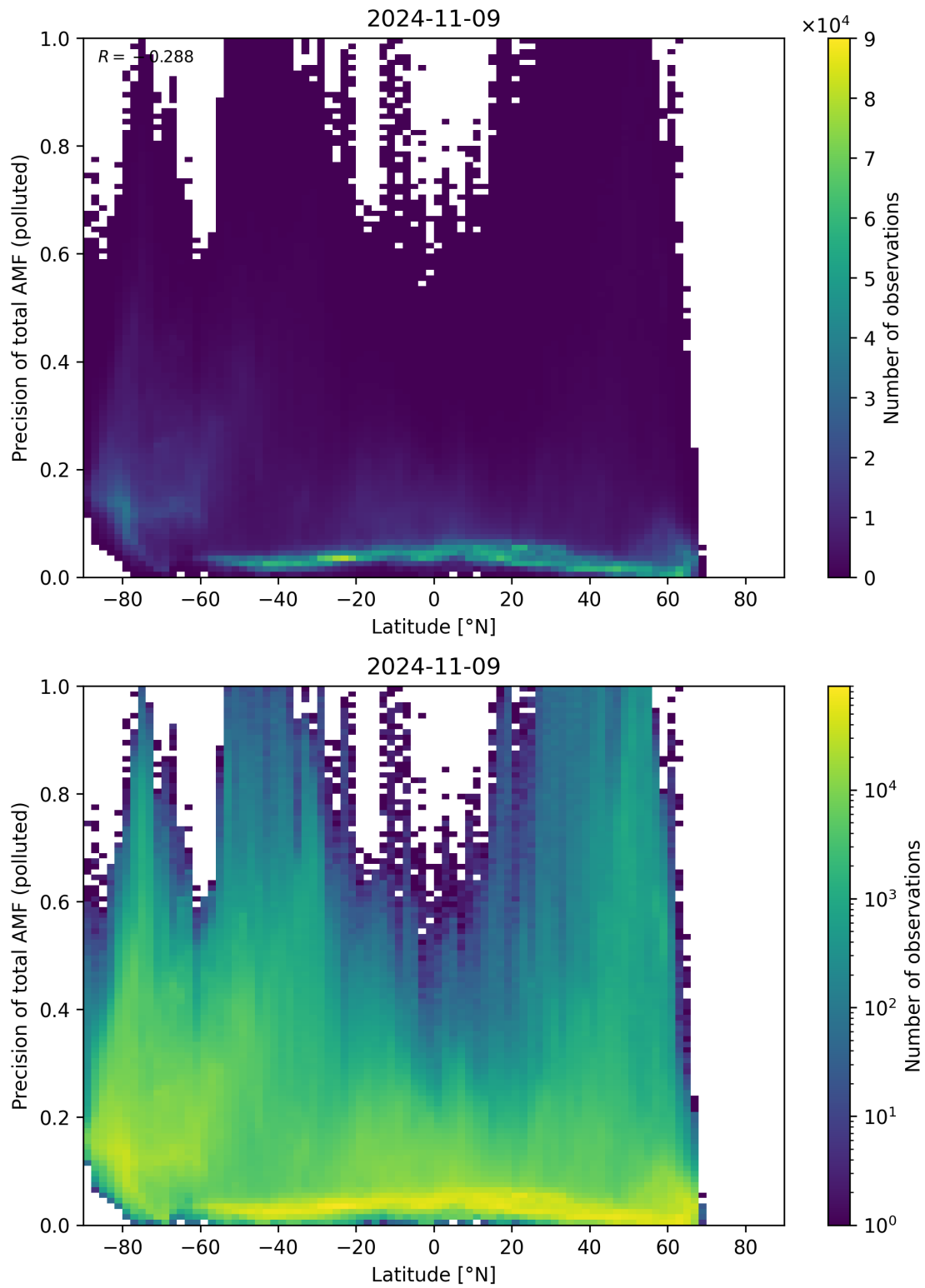
Figure 155: Scatter density plot of “Latitude” against “Precision of total AMF (polluted)” for 2024-11-09 to 2024-11-10.
