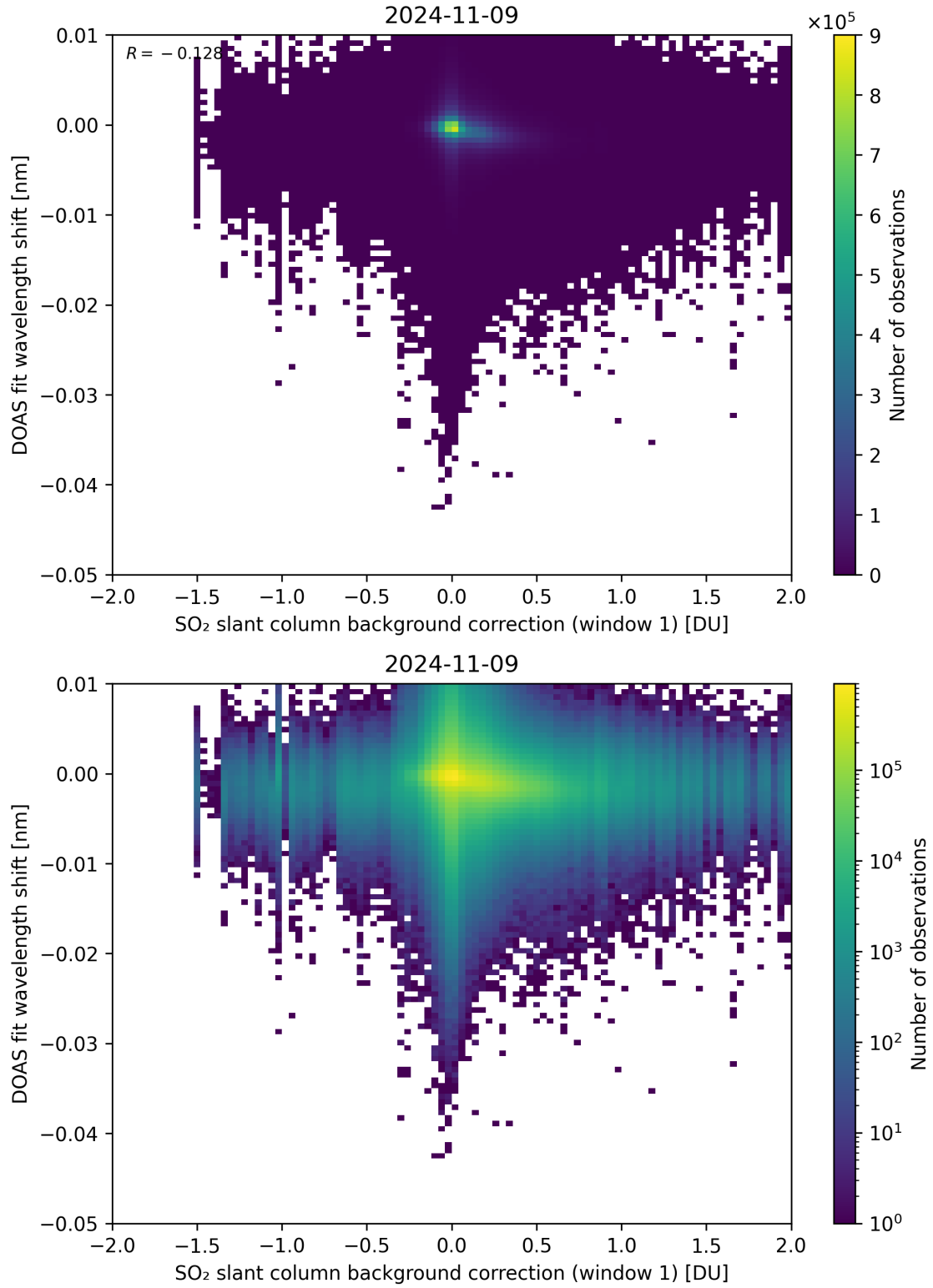
Figure 100: Scatter density plot of “SO 2 slant column background correction (window 1)” against “DOAS fit wavelength shift” for 2024-11-09 to 2024-11-10.
