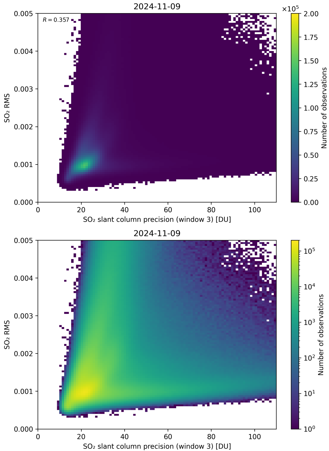
Figure 260: Scatter density plot of “SO 2 slant column precision (window 3)” against “SO 2 RMS” for 2024-11-09 to 2024-11-10.
