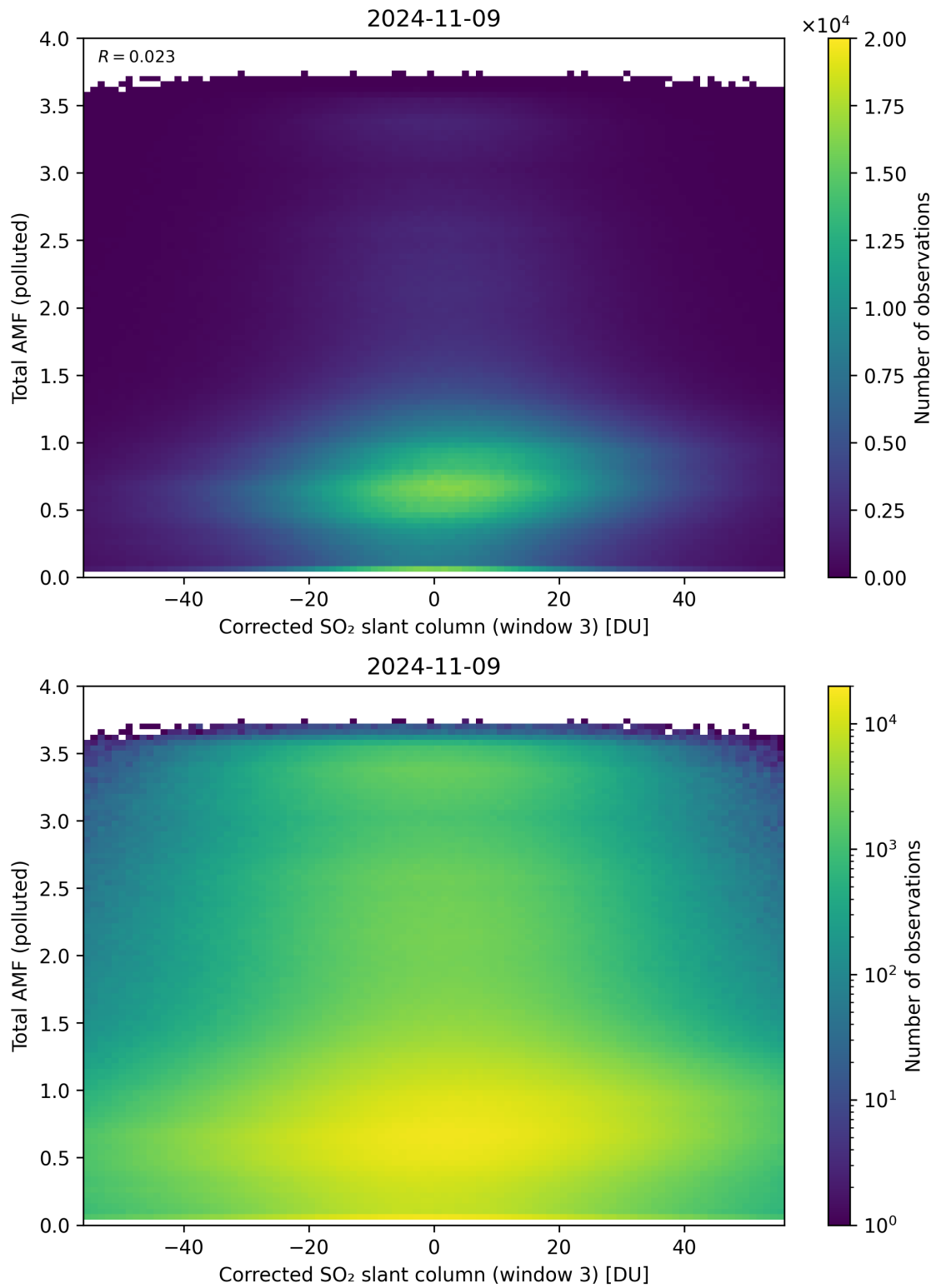
Figure 210: Scatter density plot of “Corrected SO 2 slant column (window 3)” against “Total AMF (polluted)” for 2024-11-09 to 2024-11-10.
