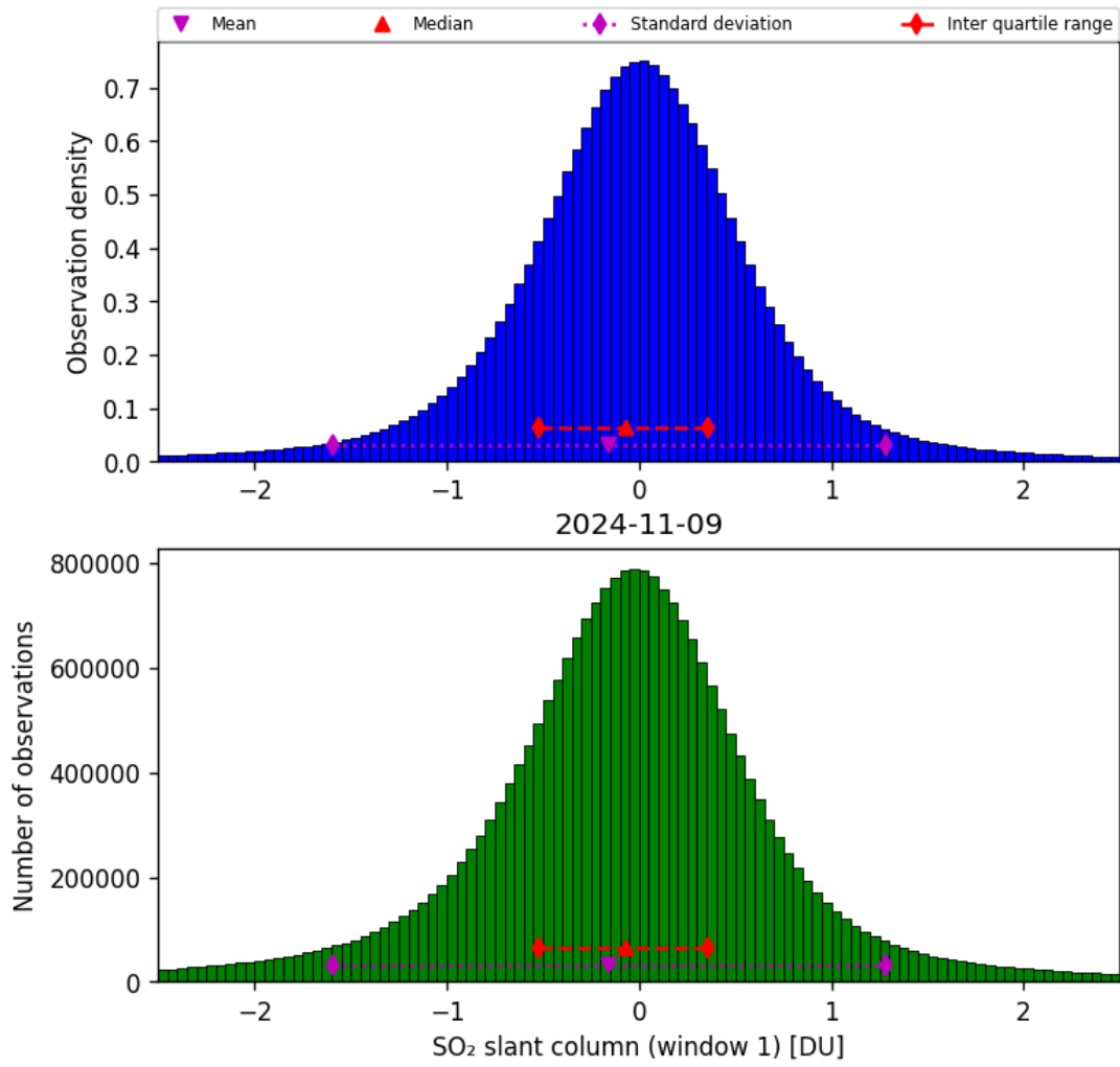
Figure 56: Histogram of “SO 2 slant column (window 1)” for 2024-11-09 to 2024-11-10
