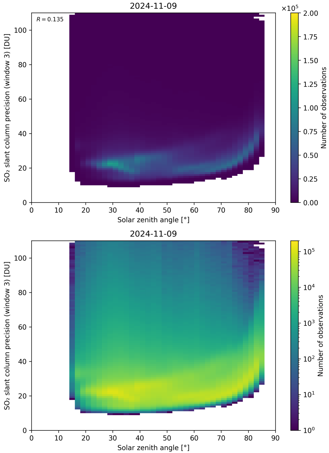
Figure 173: Scatter density plot of “Solar zenith angle” against “SO 2 slant column precision (window 3)” for 2024-11-09 to 2024-11-10.
