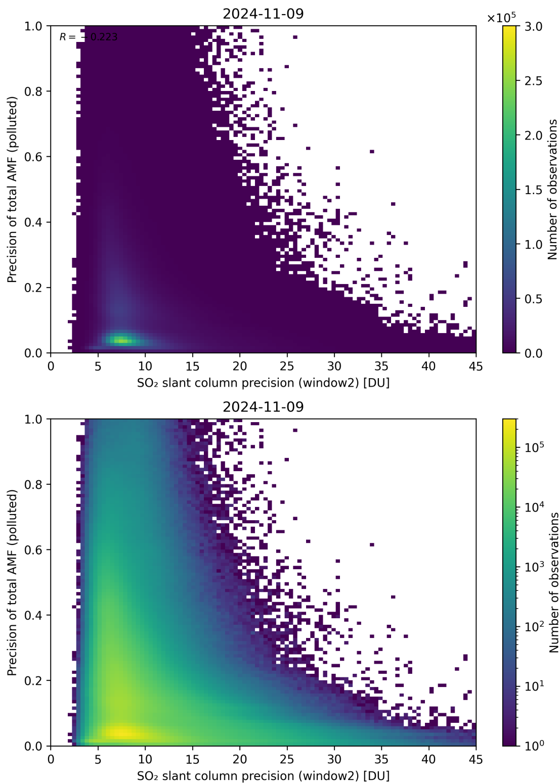
Figure 252: Scatter density plot of “SO 2 slant column precision (window2)” against “Precision of total AMF (polluted)” for 2024-11-09 to 2024-11-10.
