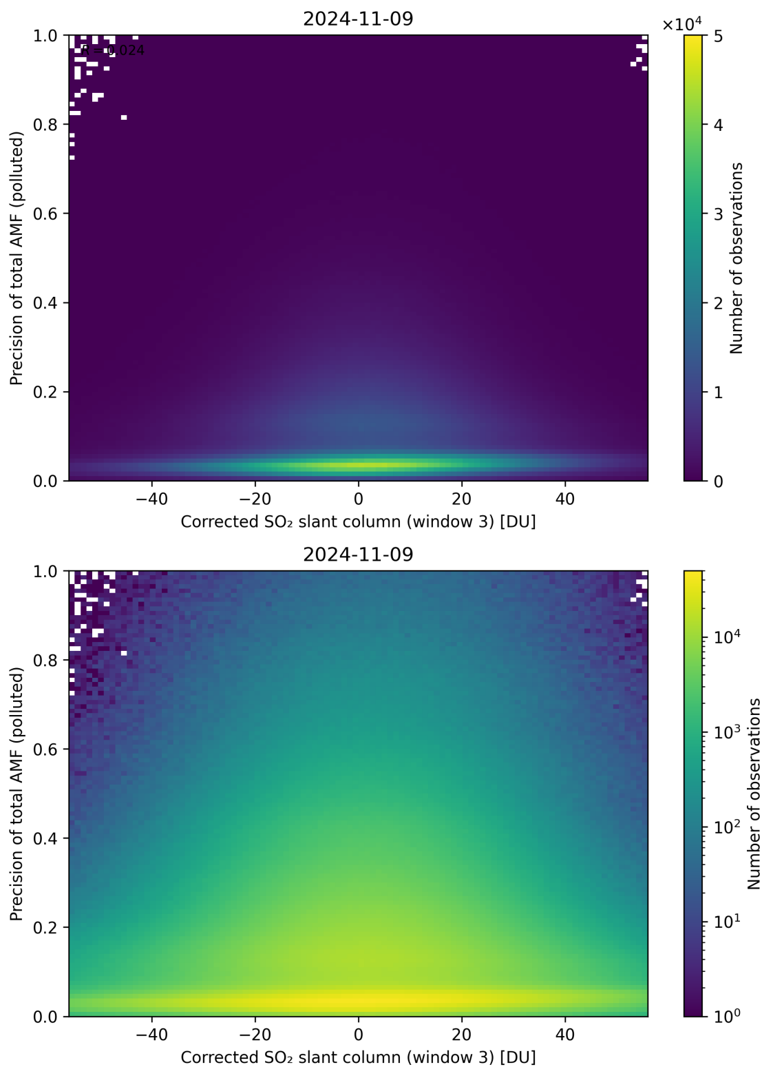
Figure 211: Scatter density plot of “Corrected SO 2 slant column (window 3)” against “Precision of total AMF (polluted)” for 2024-11-09 to 2024-11-10.
