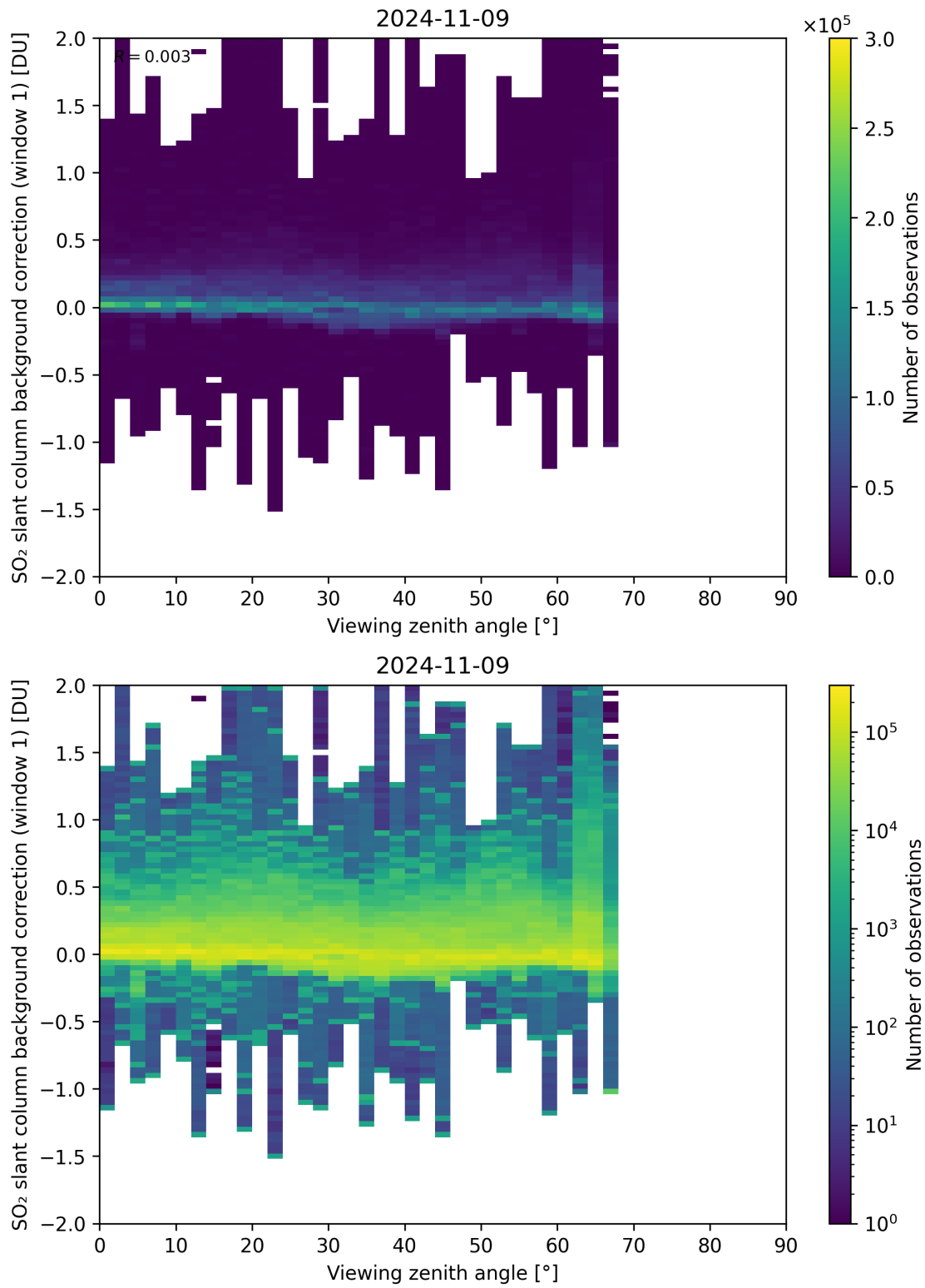
Figure 308: Scatter density plot of “Viewing zenith angle” against “SO 2 slant column background correction (window 1)” for 2024-11-09 to 2024-11-10.
