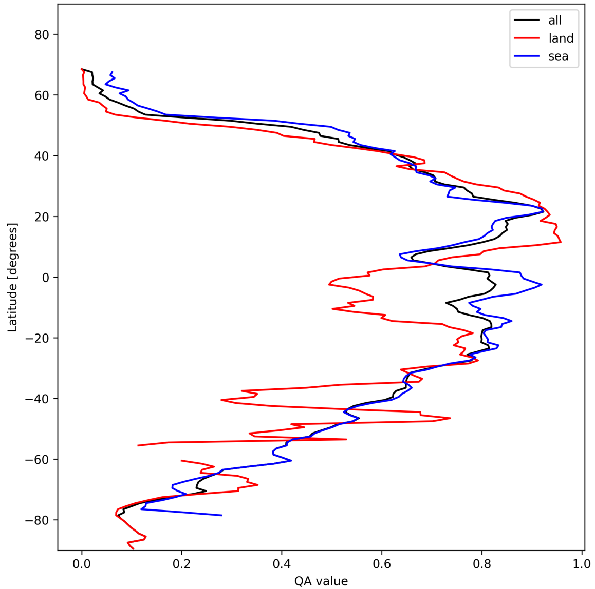
Figure 29: Zonal average of “QA value” for 2024-11-09 to 2024-11-10.
