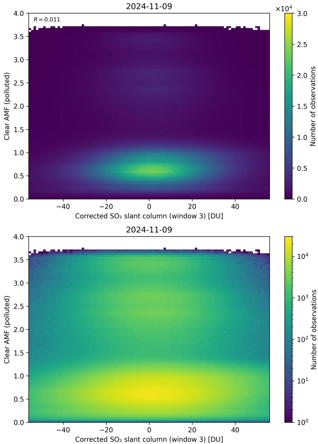
Figure 209: Scatter density plot of “Corrected SO 2 slant column (window 3)” against “Clear AMF (polluted)” for 2024-11-09 to 2024-11-10.
