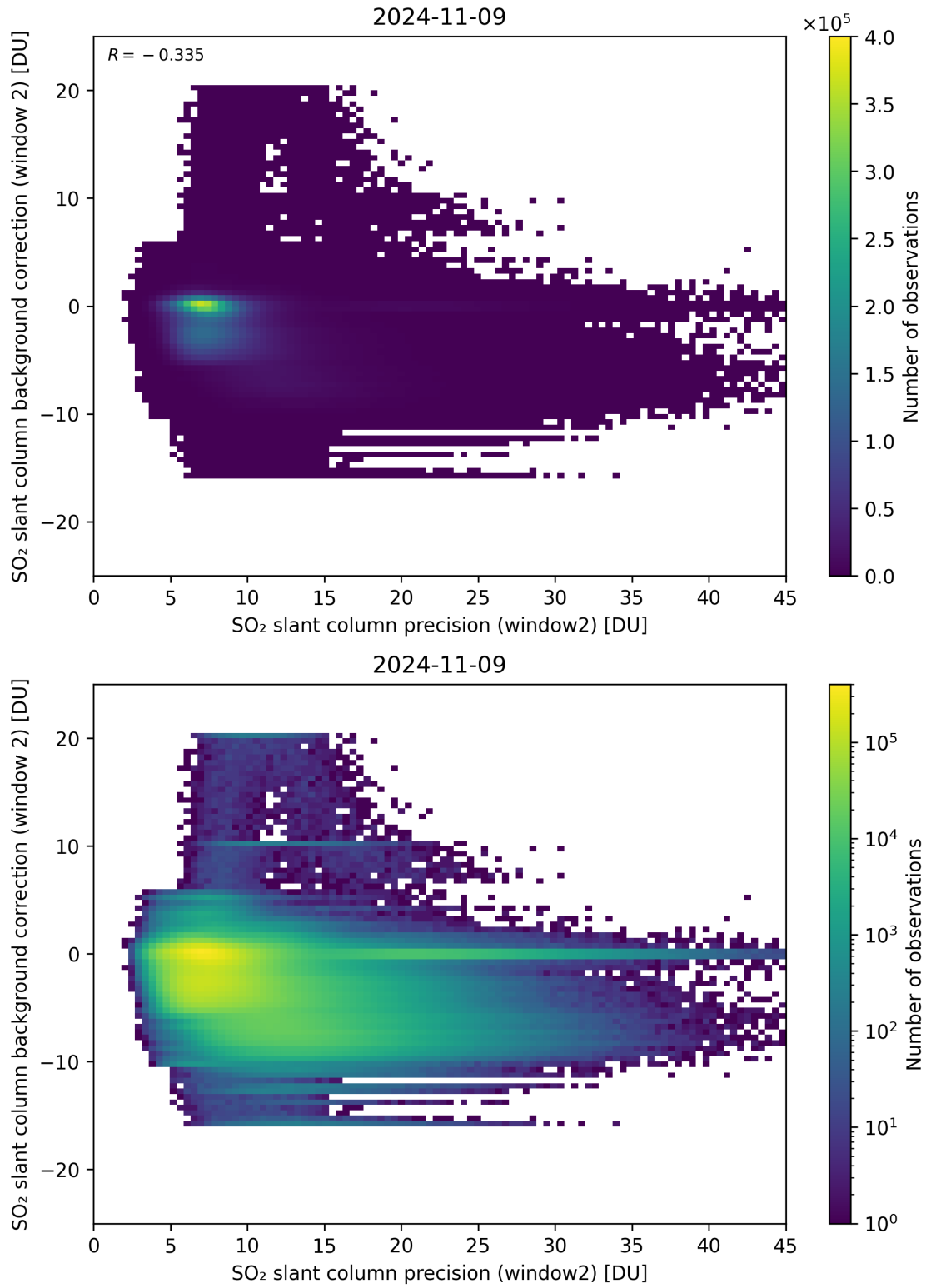
Figure 241: Scatter density plot of “SO 2 slant column precision (window2)” against “SO 2 slant column background correction (window 2)” for 2024-11-09 to 2024-11-10.
