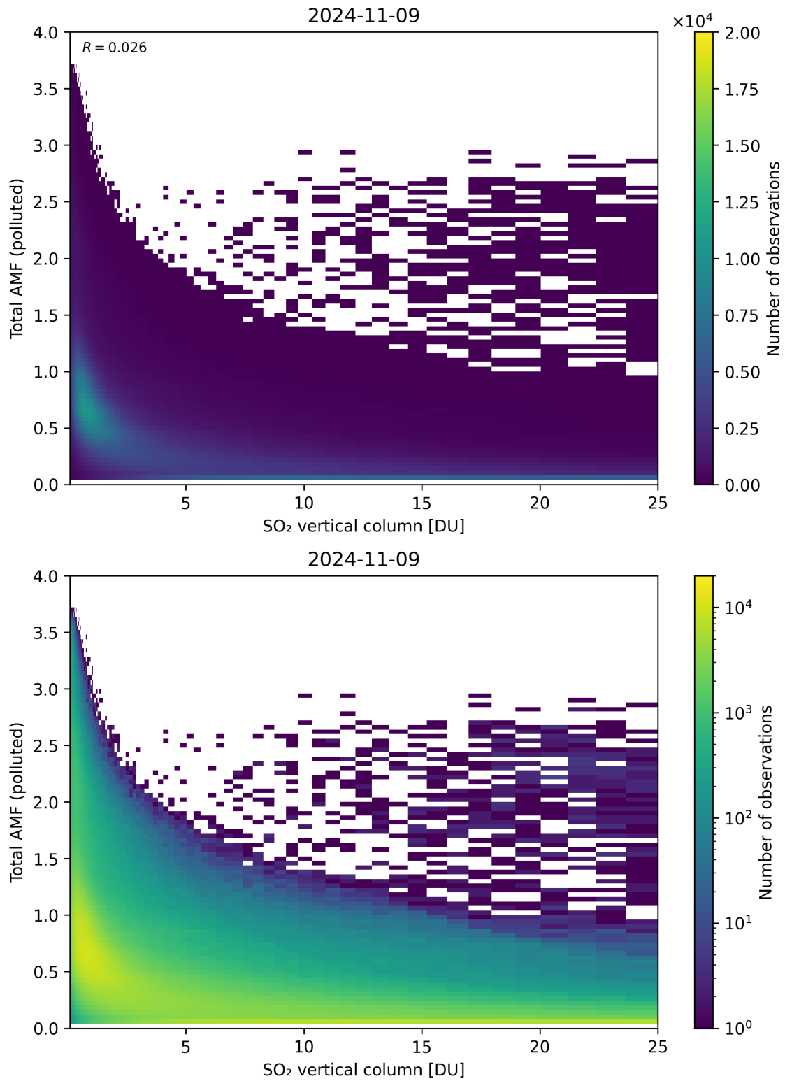
Figure 305: Scatter density plot of “SO 2 vertical column” against “Total AMF (polluted)” for 2024-11-09 to 2024-11-10.
