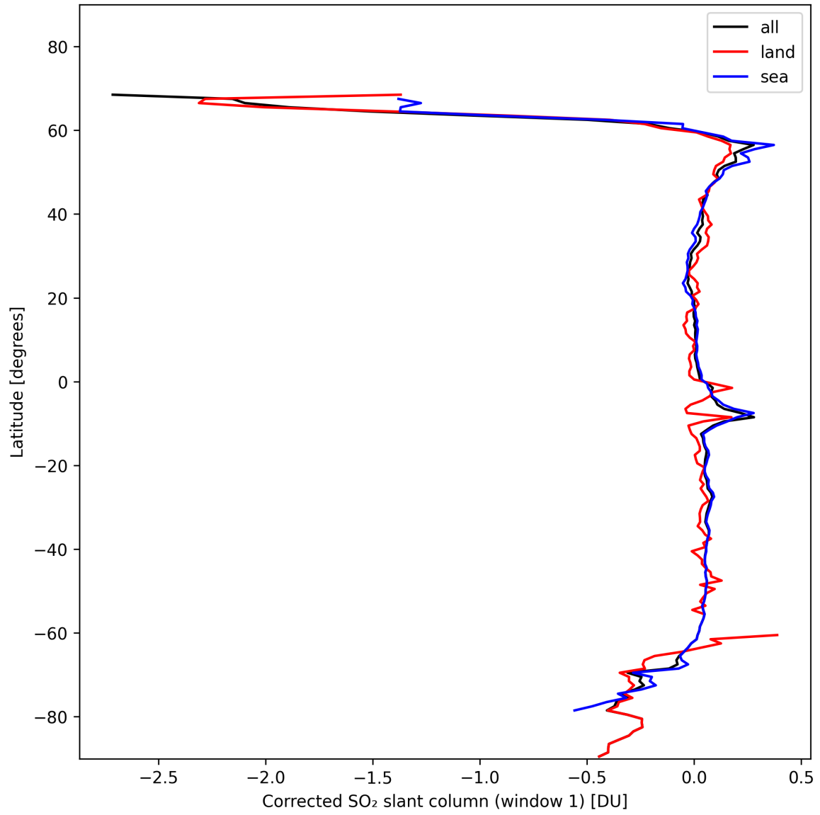
Figure 35: Zonal average of “Corrected SO 2 slant column (window 1)” for 2024-11-09 to 2024-11-10.
