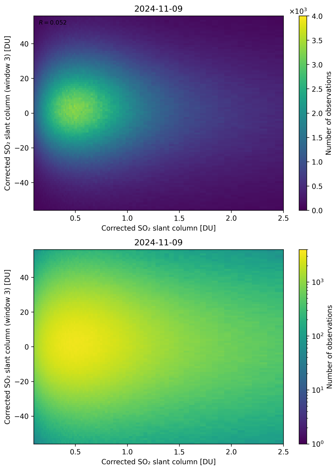
Figure 186: Scatter density plot of “Corrected SO 2 slant column” against “Corrected SO 2 slant column (window 3)” for 2024-11-09 to 2024-11-10.
