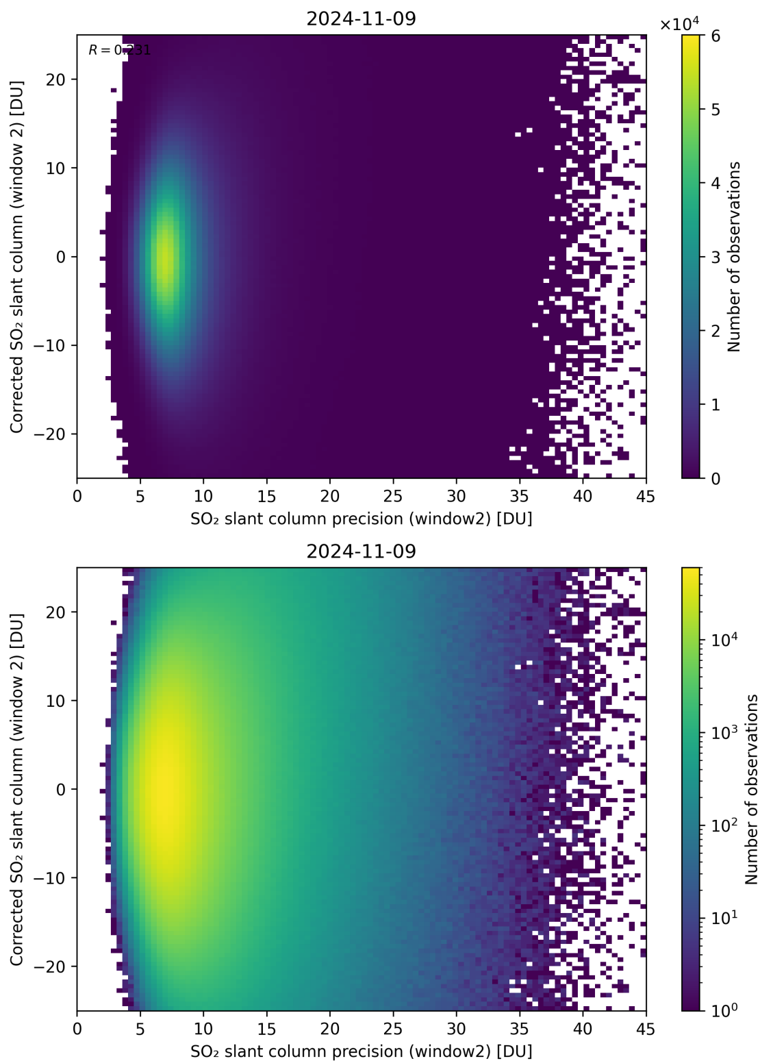
Figure 247: Scatter density plot of “SO 2 slant column precision (window2)” against “Corrected SO 2 slant column (window 2)” for 2024-11-09 to 2024-11-10.
