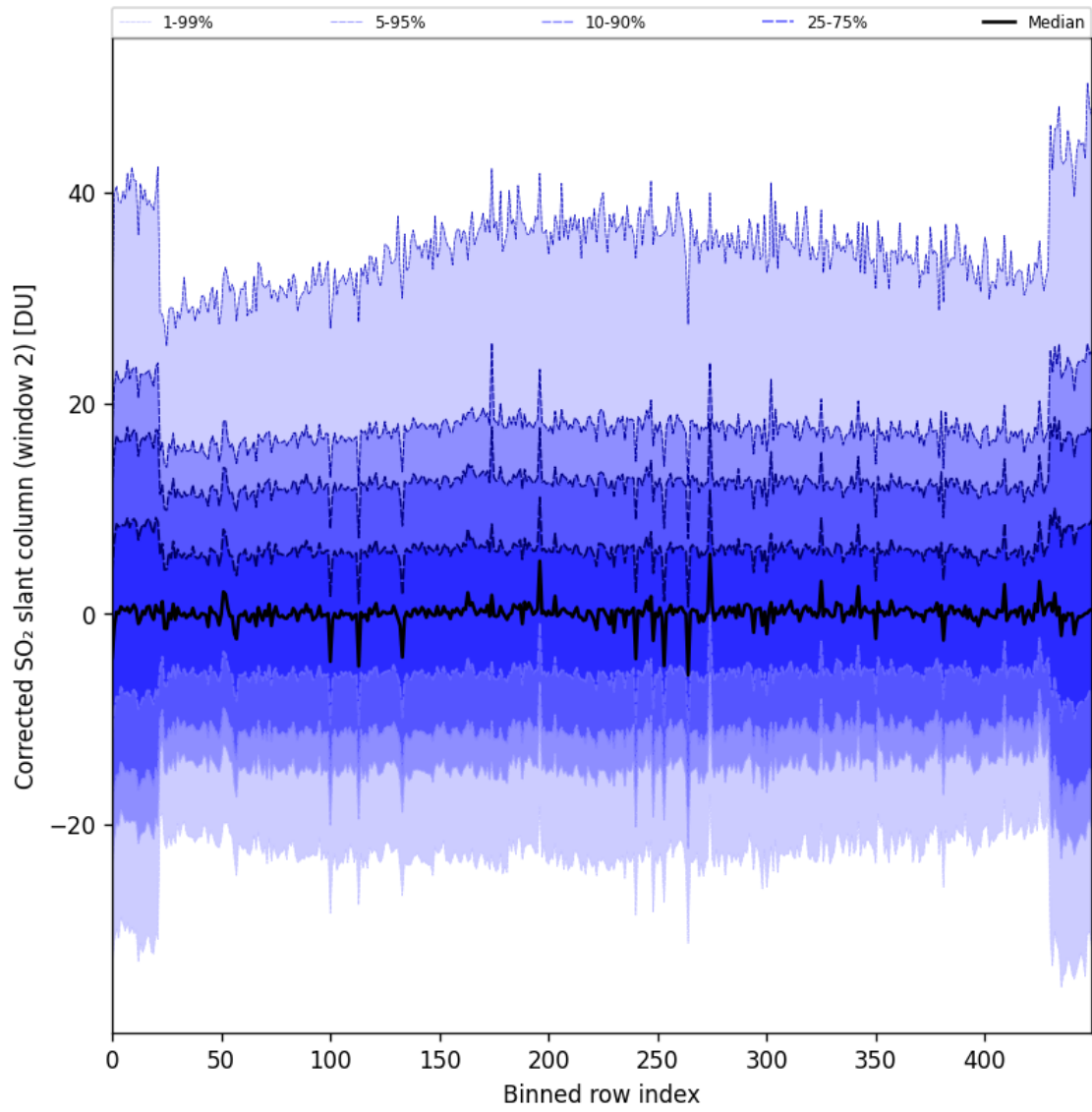
Figure 85: Along track statistics of “Corrected SO 2 slant column (window 2)” for 2024-11-09 to 2024-11-10
