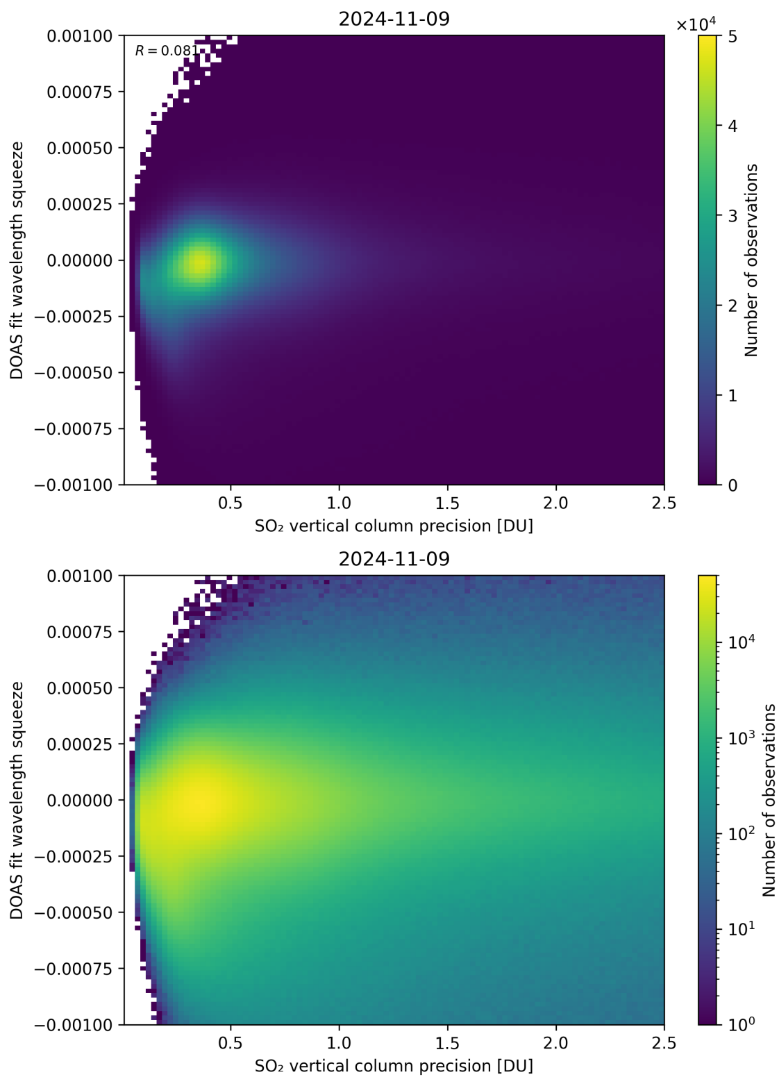
Figure 283: Scatter density plot of “SO 2 vertical column precision” against “DOAS fit wavelength squeeze” for 2024-11-09 to 2024-11-10.
