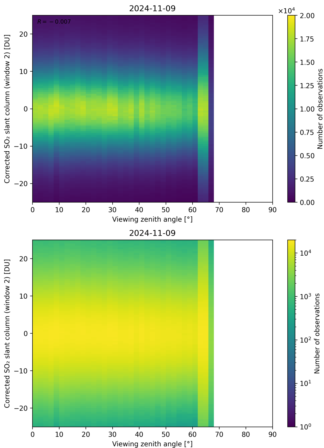
Figure 318: Scatter density plot of “Viewing zenith angle” against “Corrected SO 2 slant column (window 2)” for 2024-11-09 to 2024-11-10.
