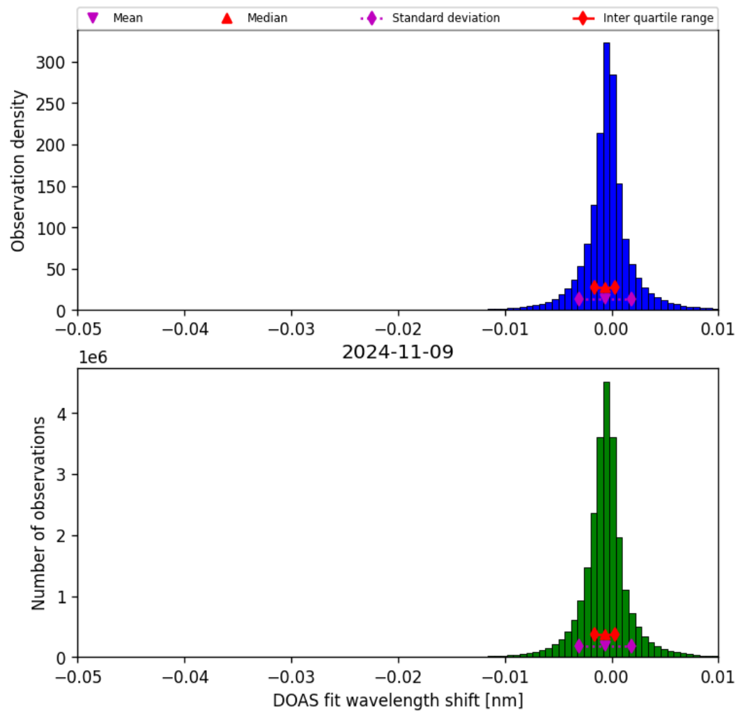
Figure 68: Histogram of “DOAS fit wavelength shift” for 2024-11-09 to 2024-11-10
