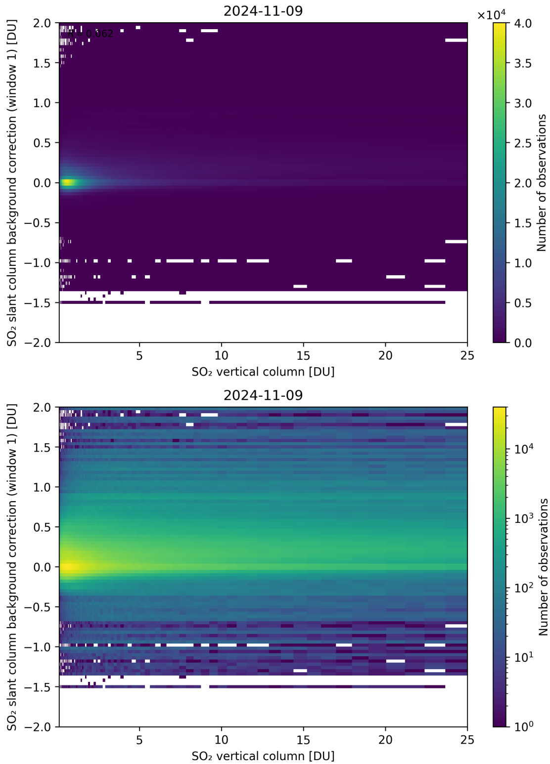
Figure 273: Scatter density plot of “SO 2 vertical column” against “SO 2 slant column background correction (window 1)” for 2024-11-09 to 2024-11-10.
