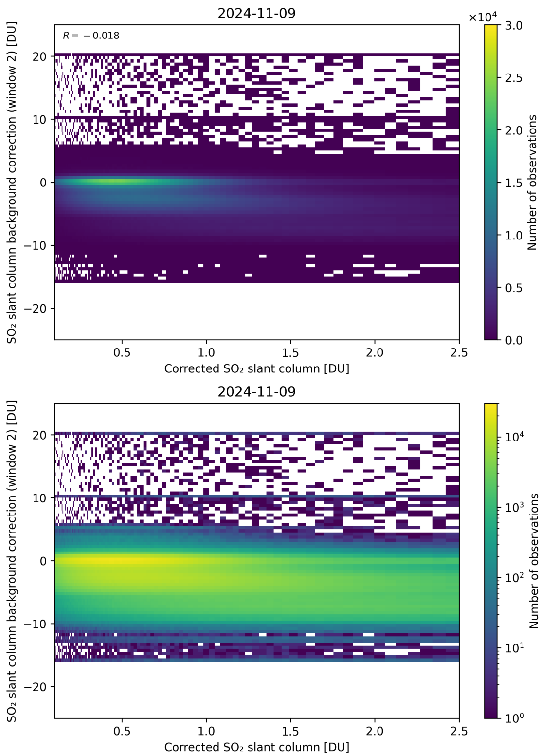
Figure 179: Scatter density plot of “Corrected SO 2 slant column” against “SO 2 slant column background correction (window 2)” for 2024-11-09 to 2024-11-10.
