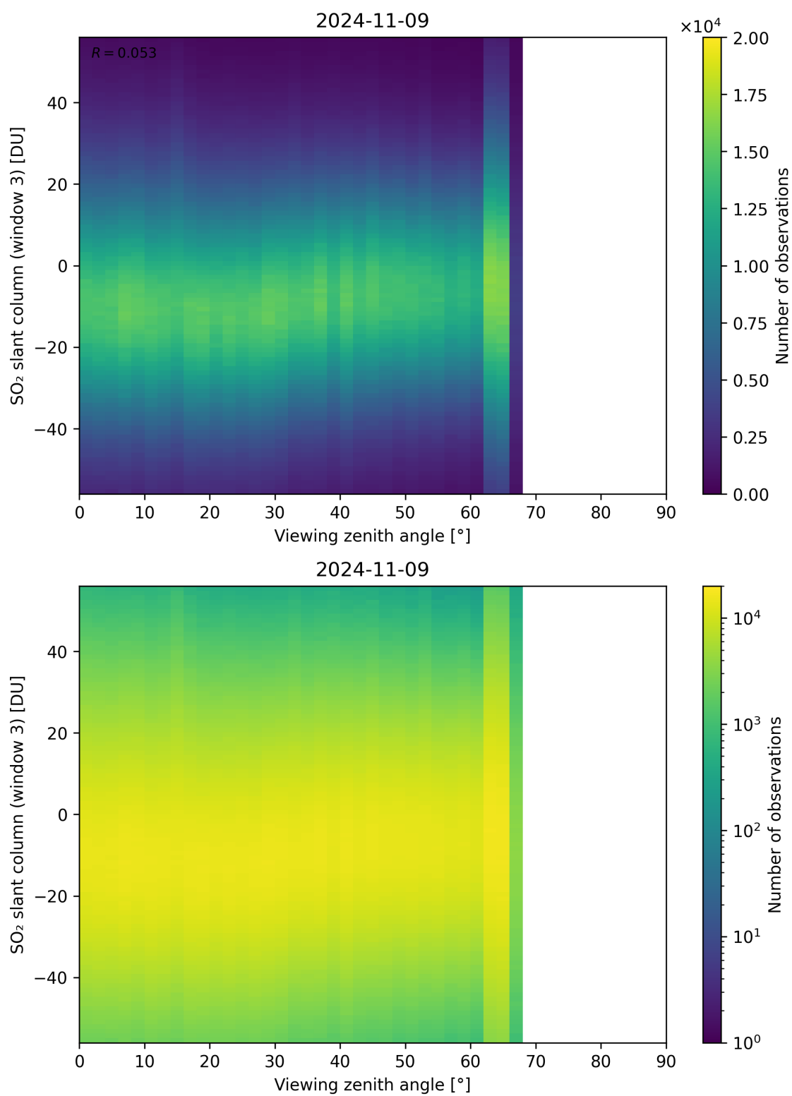
Figure 323: Scatter density plot of “Viewing zenith angle” against “SO 2 slant column (window 3)” for 2024-11-09 to 2024-11-10.
