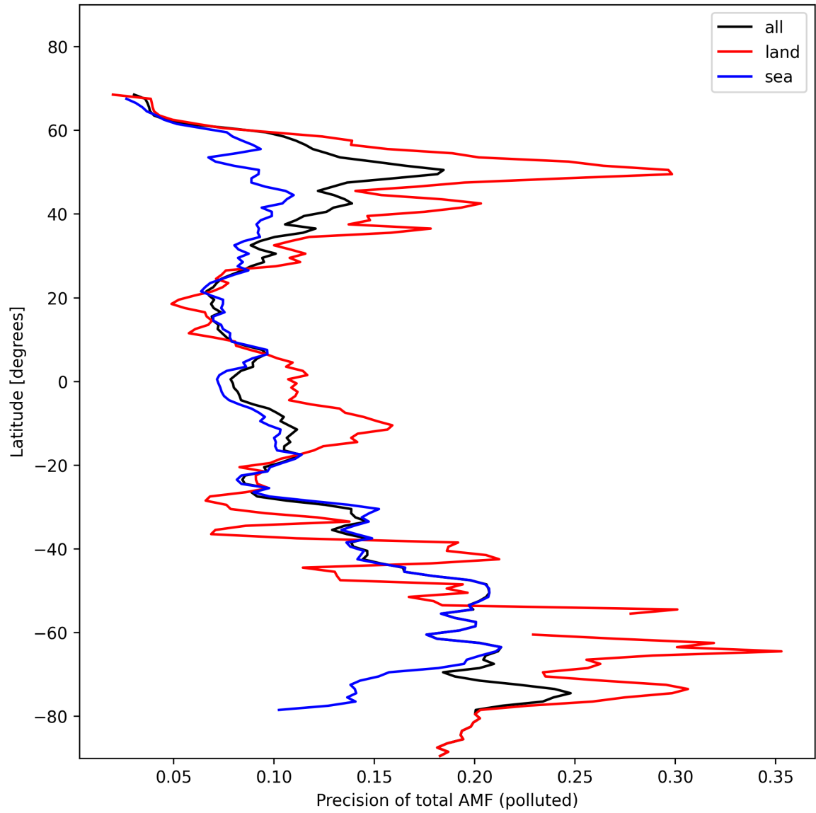
Figure 49: Zonal average of “Precision of total AMF (polluted)” for 2024-11-09 to 2024-11-10.
