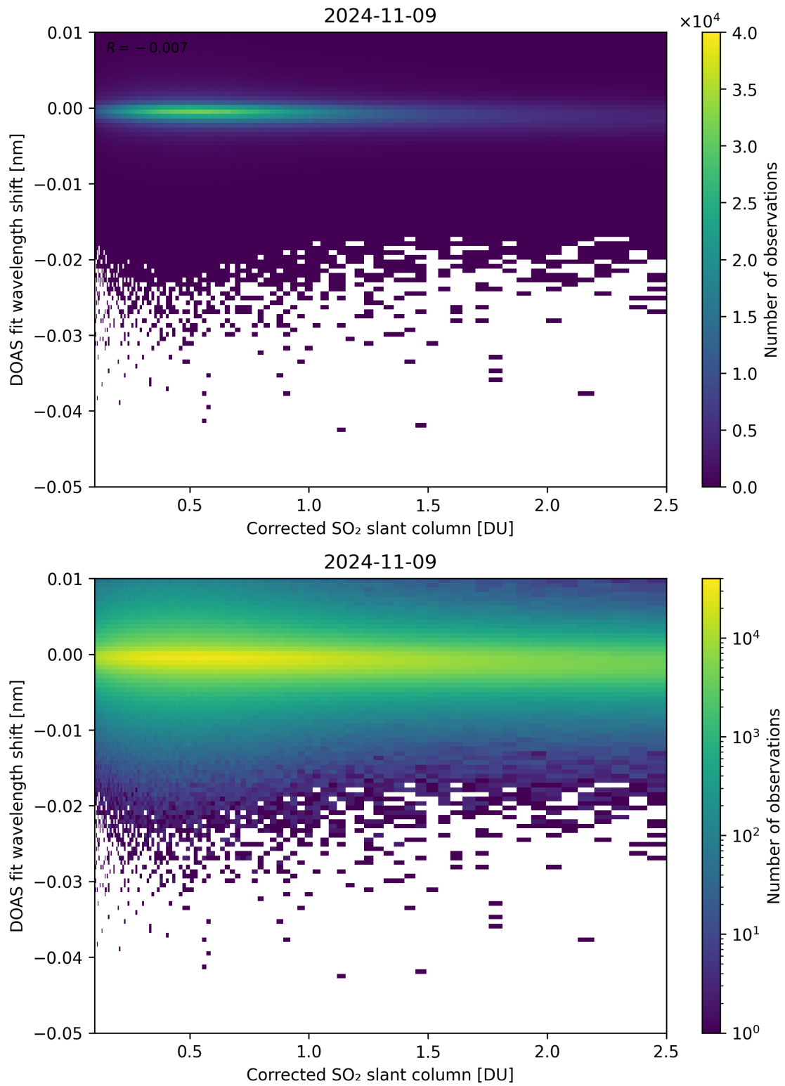
Figure 181: Scatter density plot of “Corrected SO 2 slant column” against “DOAS fit wavelength shift” for 2024-11-09 to 2024-11-10.
