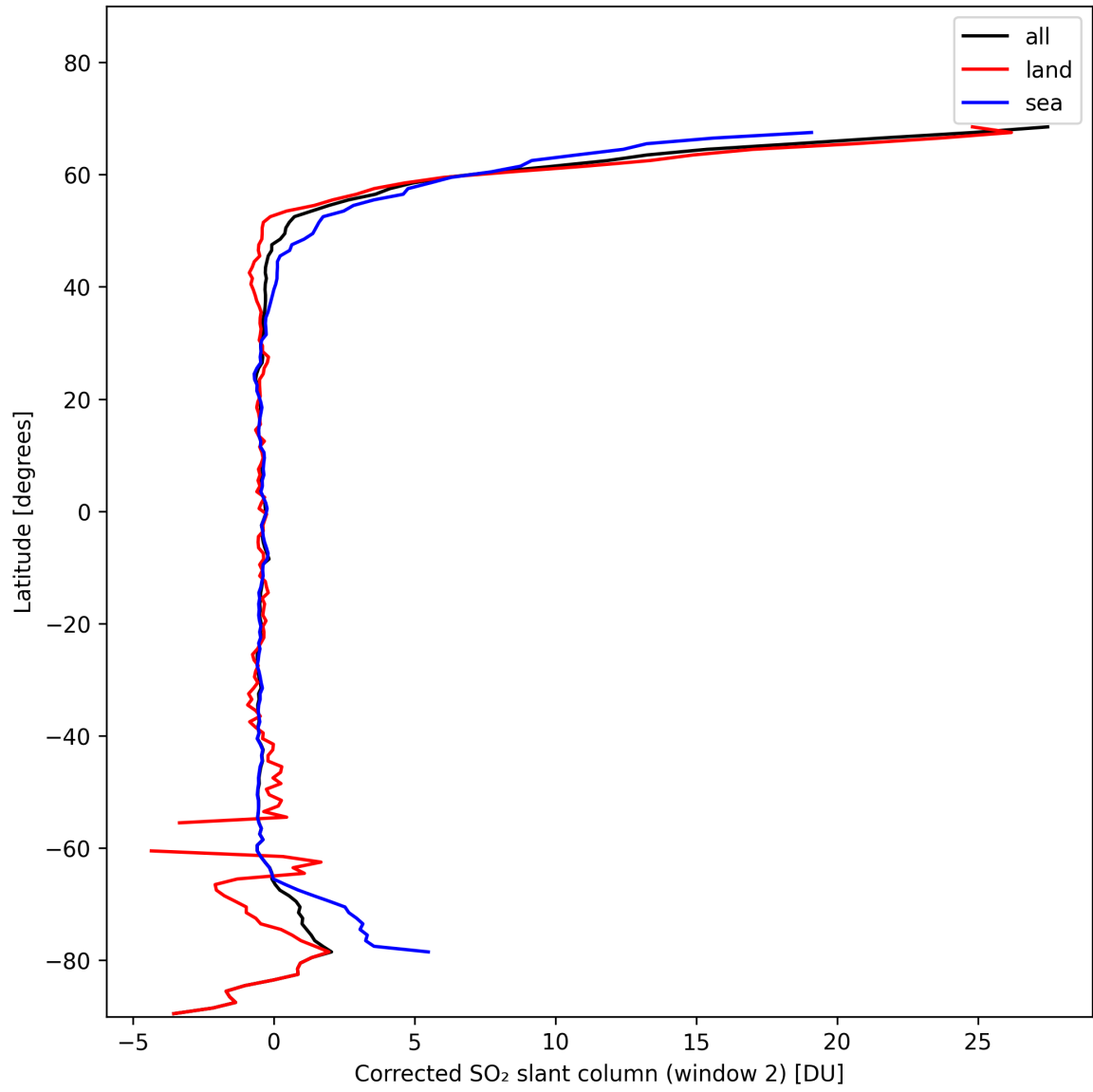
Figure 39: Zonal average of “Corrected SO 2 slant column (window 2)” for 2024-11-09 to 2024-11-10.
