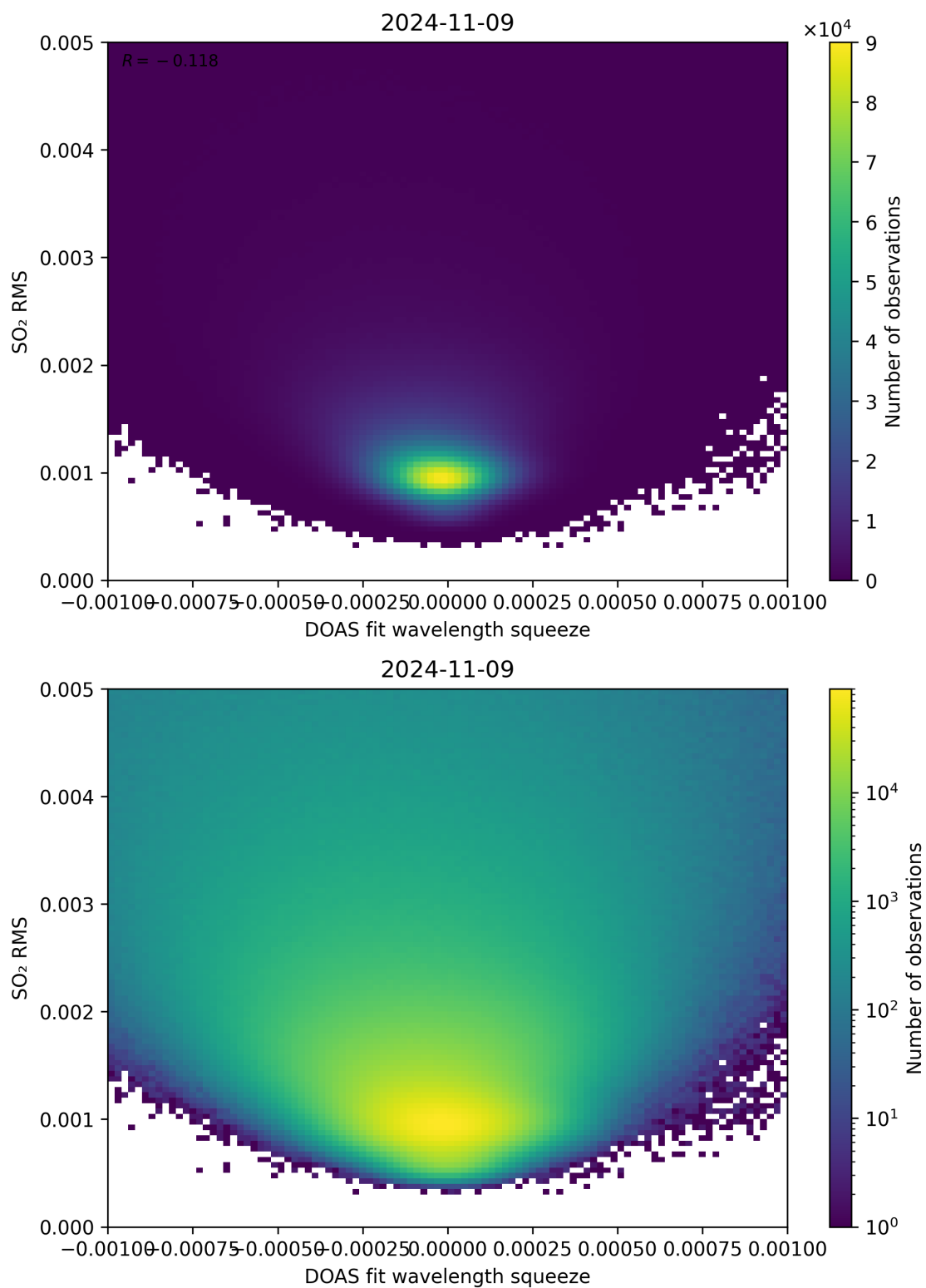
Figure 132: Scatter density plot of “DOAS fit wavelength squeeze” against “SO 2 RMS” for 2024-11-09 to 2024-11-10.
