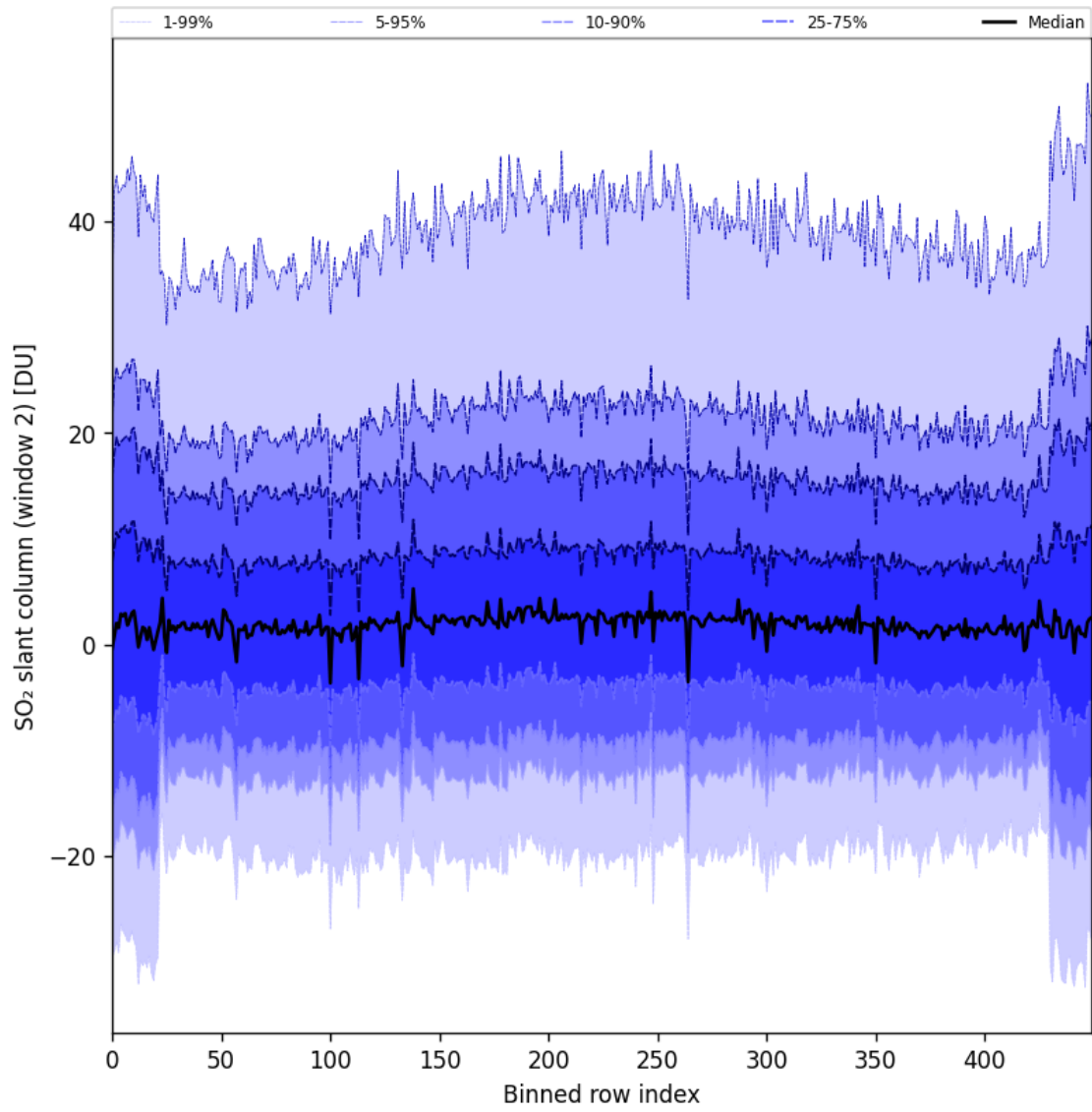
Figure 83: Along track statistics of “SO 2 slant column (window 2)” for 2024-11-09 to 2024-11-10
