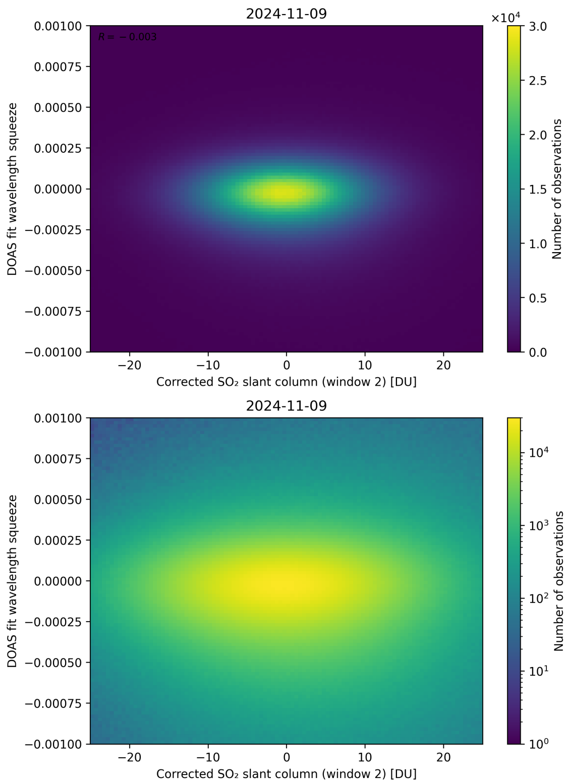
Figure 197: Scatter density plot of “Corrected SO 2 slant column (window 2)” against “DOAS fit wavelength squeeze” for 2024-11-09 to 2024-11-10.
