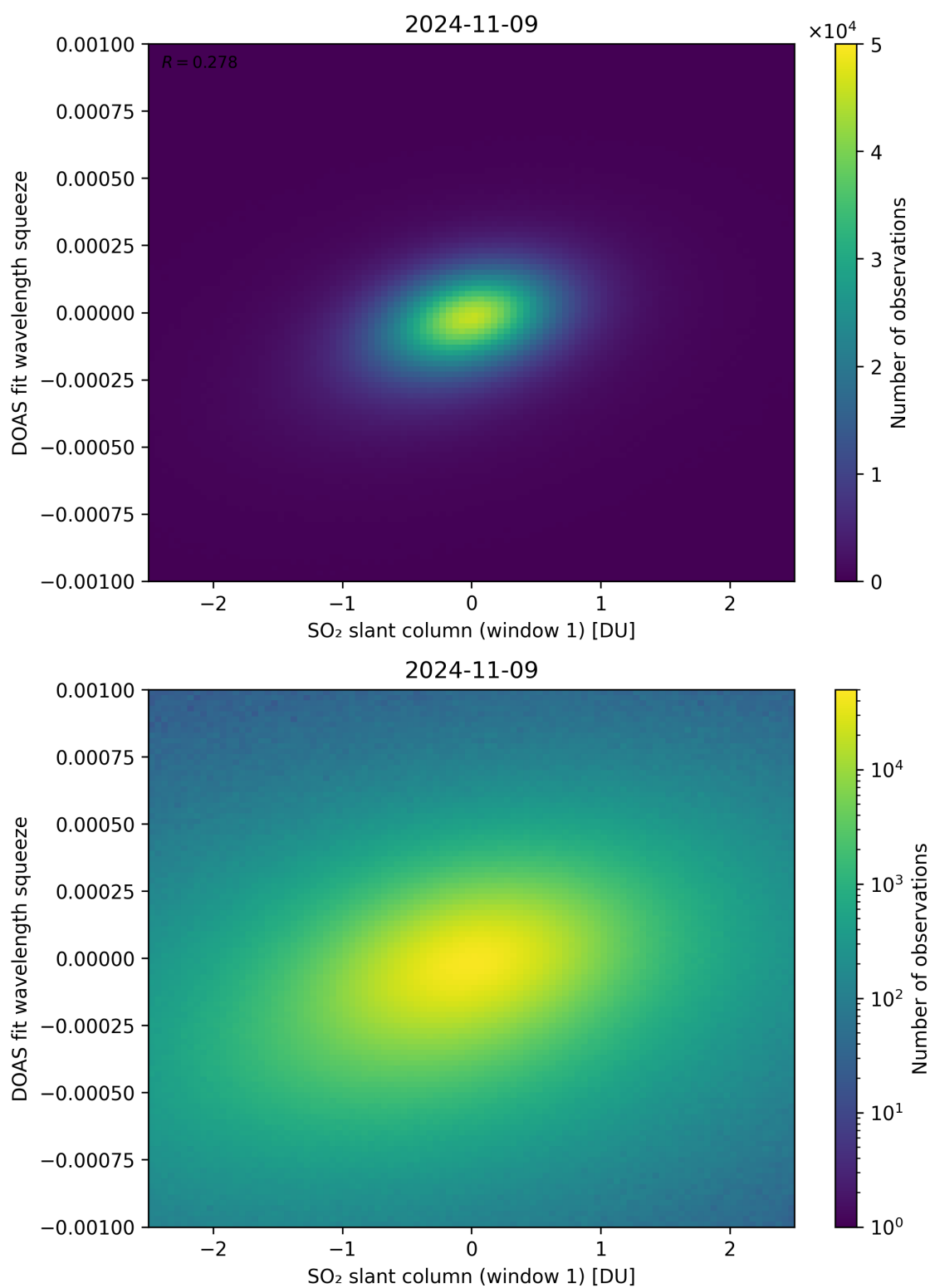
Figure 216: Scatter density plot of “SO 2 slant column (window 1)” against “DOAS fit wavelength squeeze” for 2024-11-09 to 2024-11-10.
