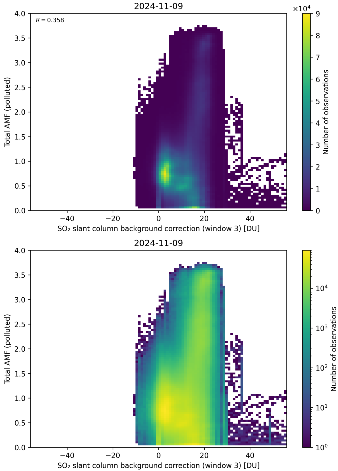
Figure 125: Scatter density plot of “SO 2 slant column background correction (window 3)” against “Total AMF (polluted)” for 2024-11-09 to 2024-11-10.
