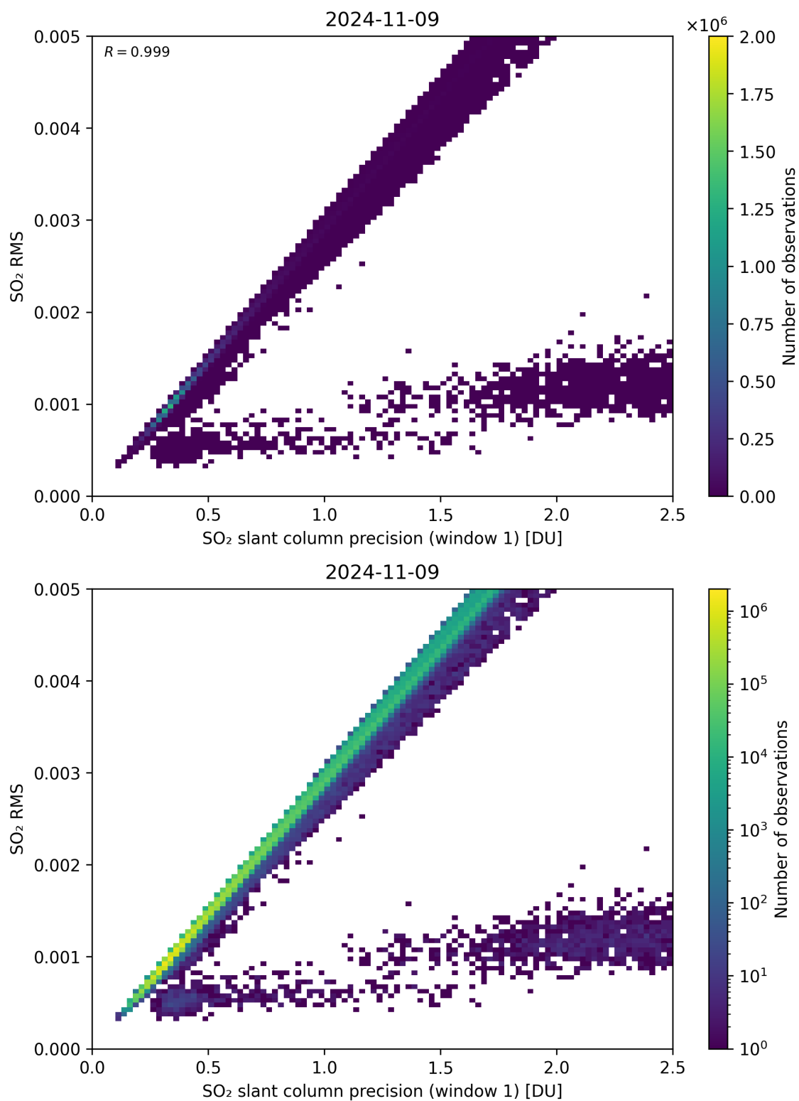
Figure 223: Scatter density plot of “SO 2 slant column precision (window 1)” against “SO 2 RMS” for 2024-11-09 to 2024-11-10.
