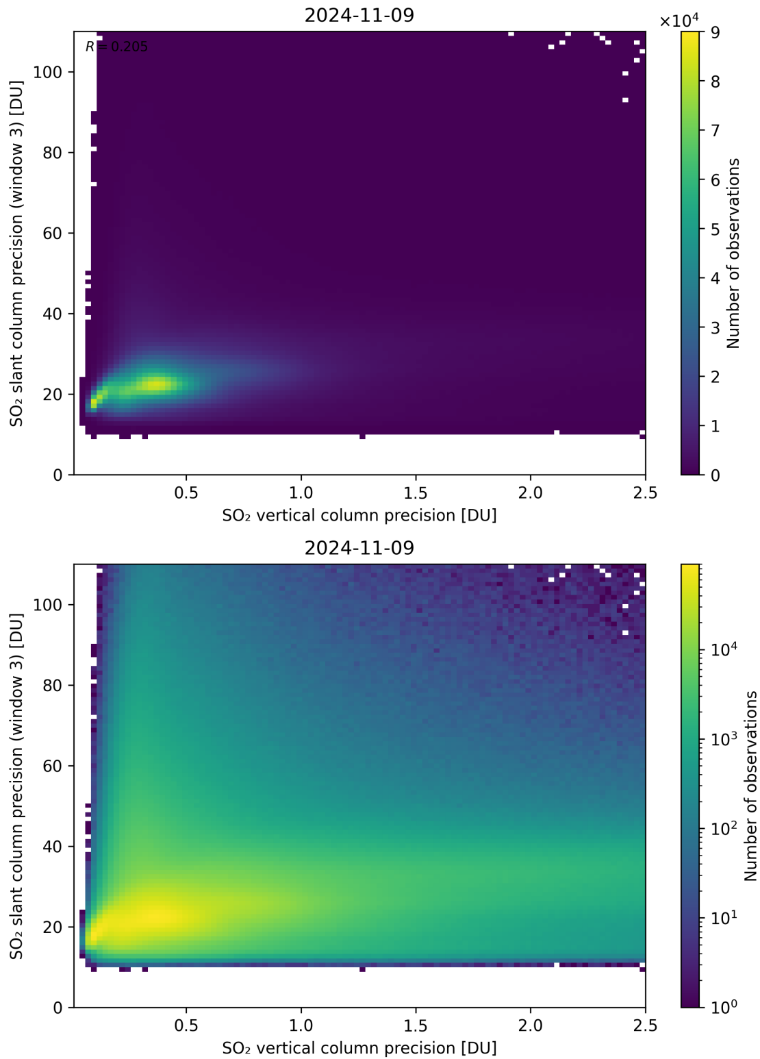
Figure 293: Scatter density plot of “SO 2 vertical column precision” against “SO 2 slant column precision (window 3)” for 2024-11-09 to 2024-11-10.
