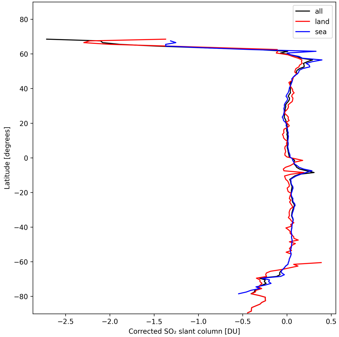
Figure 32: Zonal average of “Corrected SO 2 slant column” for 2024-11-09 to 2024-11-10.
