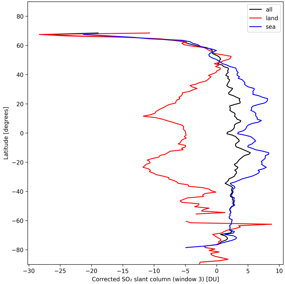
Figure 43: Zonal average of “Corrected SO 2 slant column (window 3)” for 2024-11-09 to 2024-11-10.
