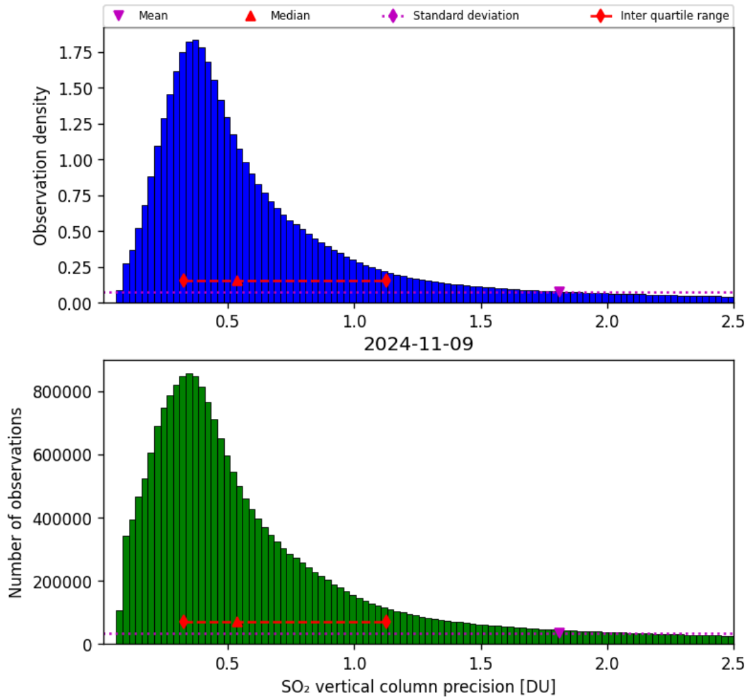
Figure 54: Histogram of “SO 2 vertical column precision” for 2024-11-09 to 2024-11-10
