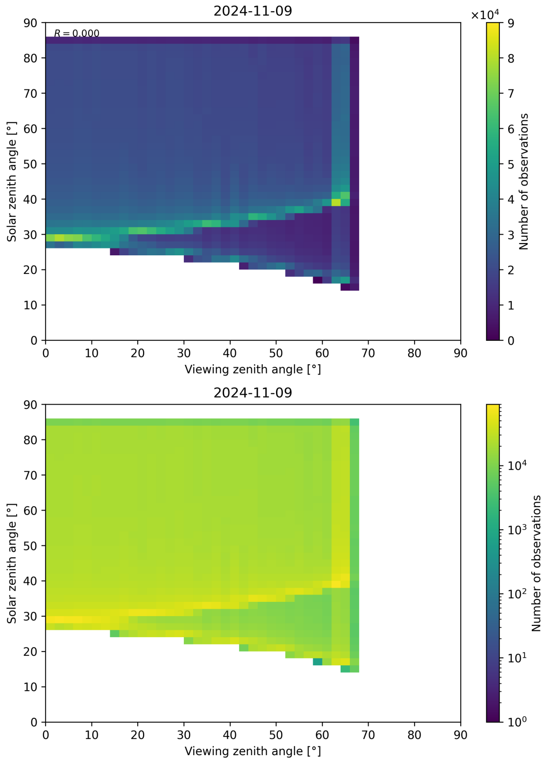
Figure 315: Scatter density plot of “Viewing zenith angle” against “Solar zenith angle” for 2024-11-09 to 2024-11-10.
