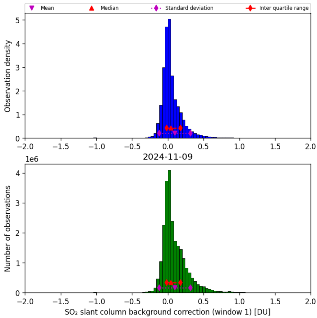
Figure 59: Histogram of “SO 2 slant column background correction (window 1)” for 2024-11-09 to 2024-11-10
