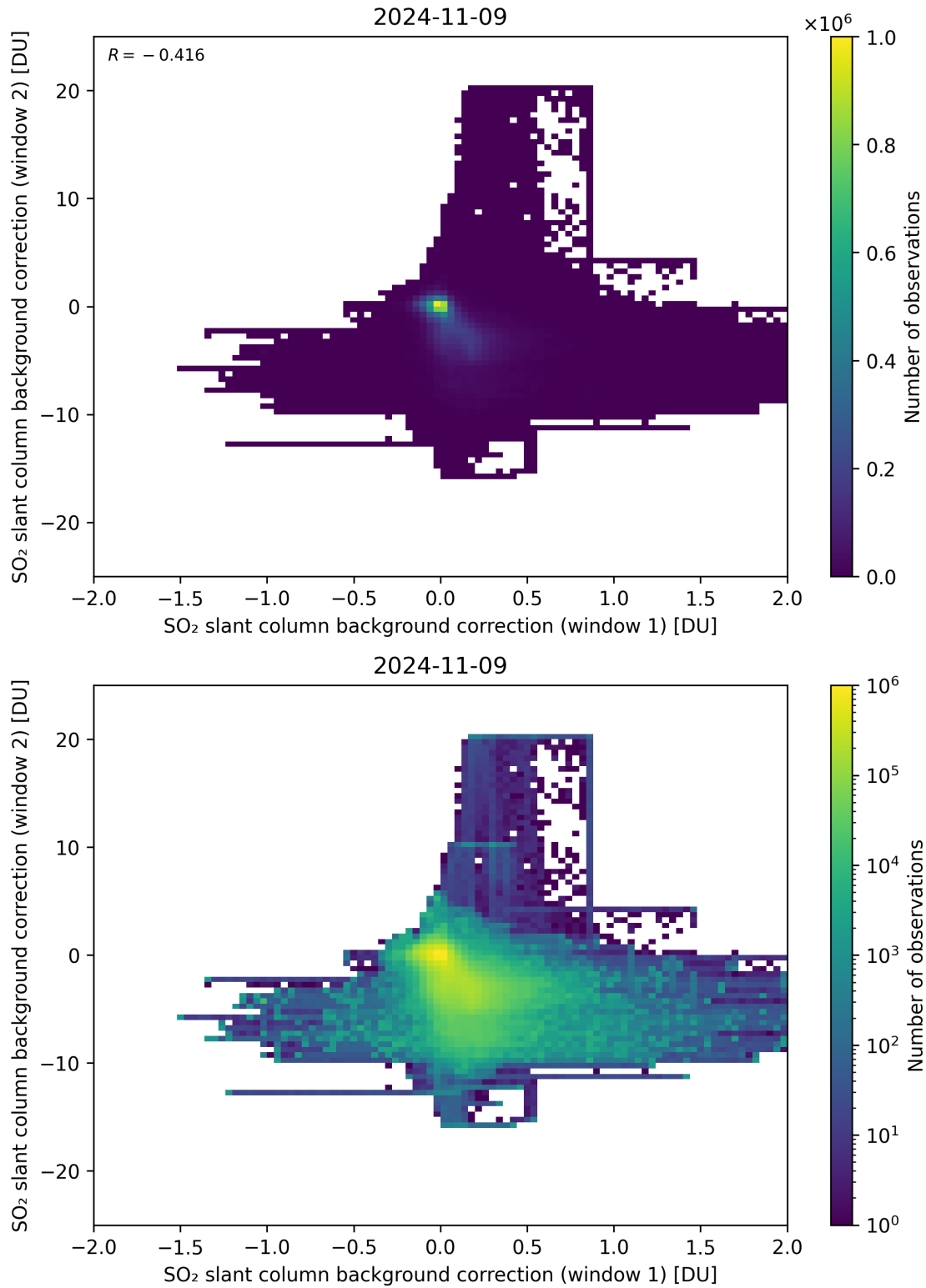
Figure 98: Scatter density plot of “SO 2 slant column background correction (window 1)” against “SO 2 slant column background correction (window 2)” for 2024-11-09 to 2024-11-10.
