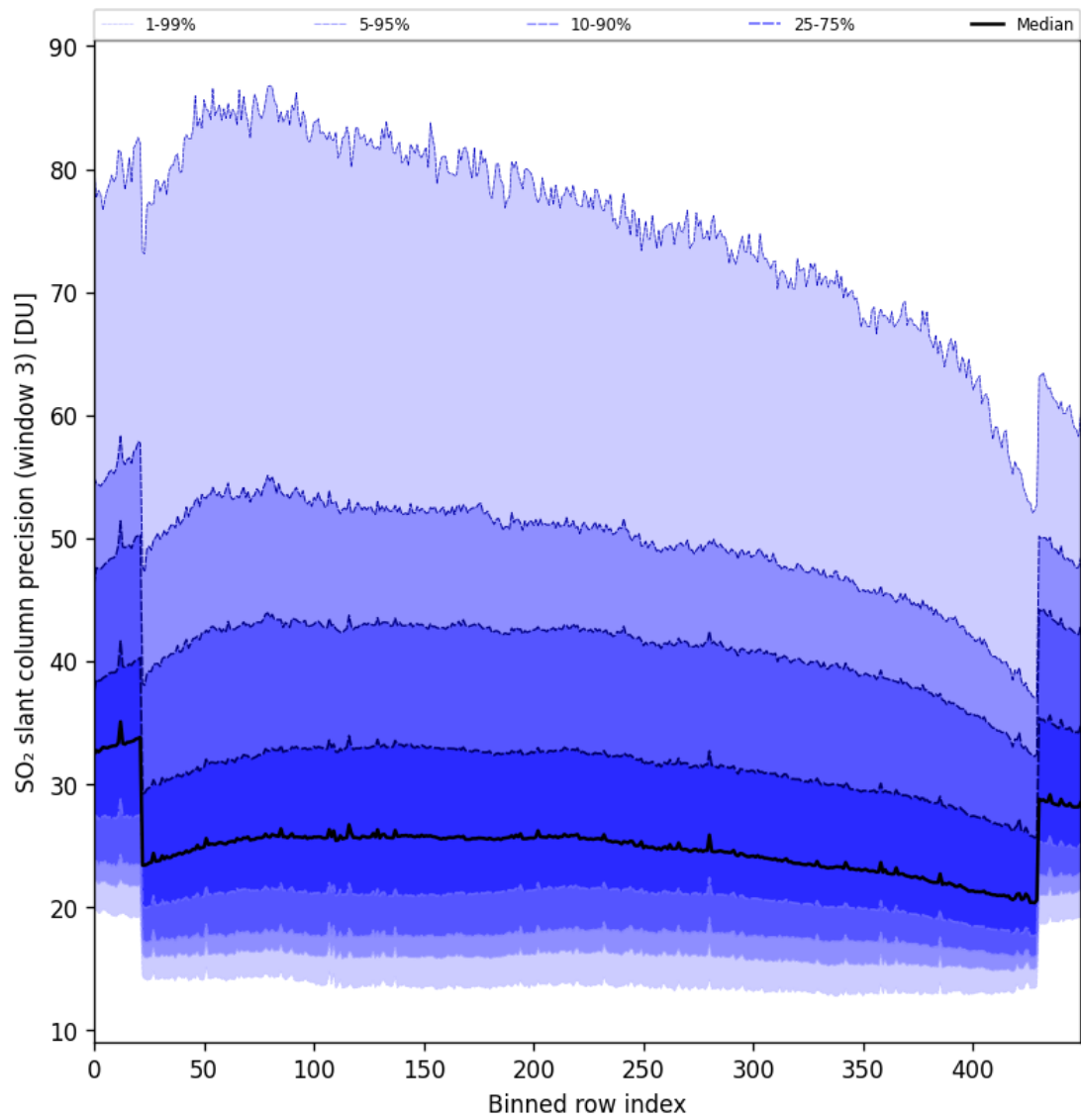
Figure 88: Along track statistics of “SO 2 slant column precision (window 3)” for 2024-11-09 to 2024-11-10
