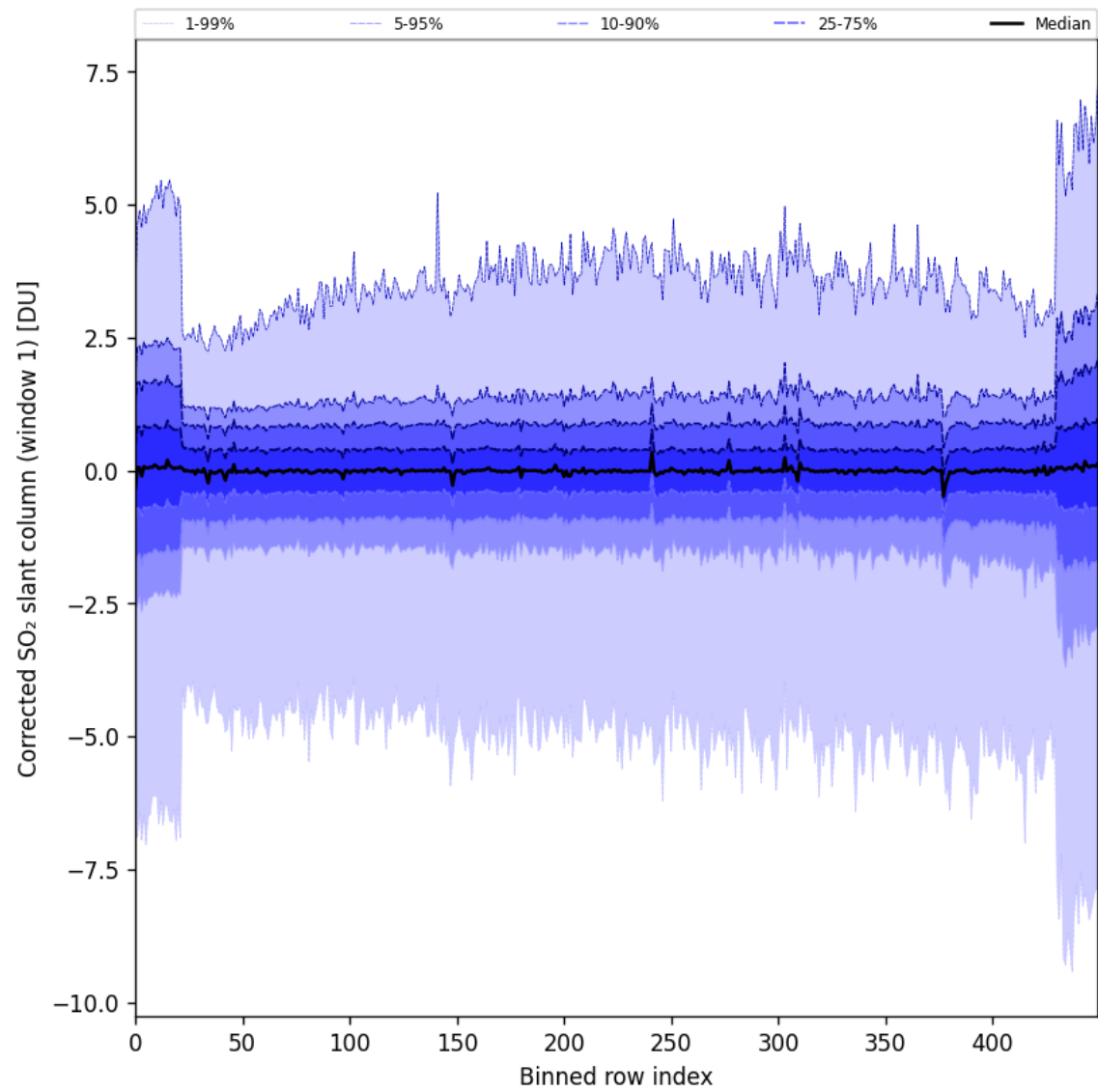
Figure 81: Along track statistics of “Corrected SO 2 slant column (window 1)” for 2024-11-09 to 2024-11-10
