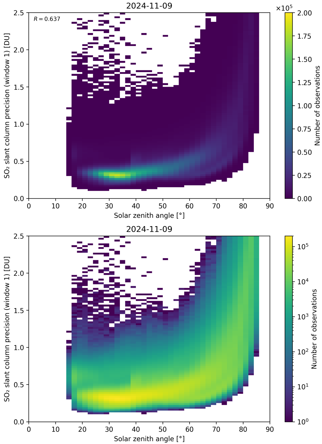
Figure 170: Scatter density plot of “Solar zenith angle” against “SO 2 slant column precision (window 1)” for 2024-11-09 to 2024-11-10.
