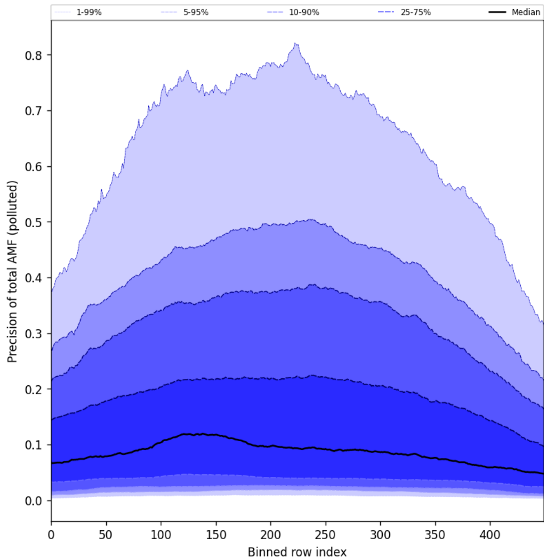
Figure 95: Along track statistics of “Precision of total AMF (polluted)” for 2024-11-09 to 2024-11-10
