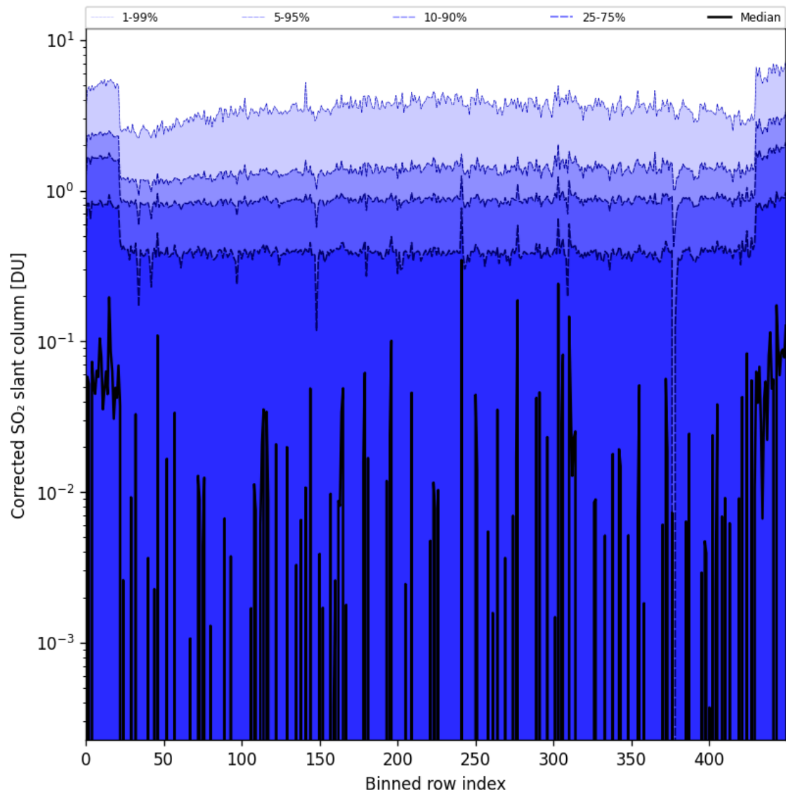
Figure 78: Along track statistics of “Corrected SO 2 slant column” for 2024-11-09 to 2024-11-10
