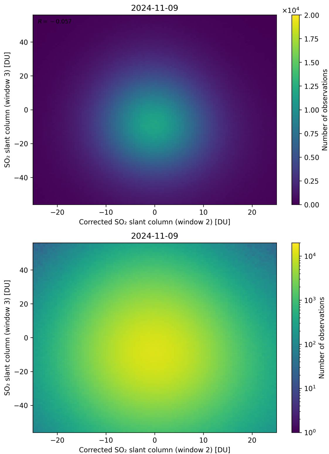
Figure 201: Scatter density plot of “Corrected SO 2 slant column (window 2)” against “SO 2 slant column (window 3)” for 2024-11-09 to 2024-11-10.
