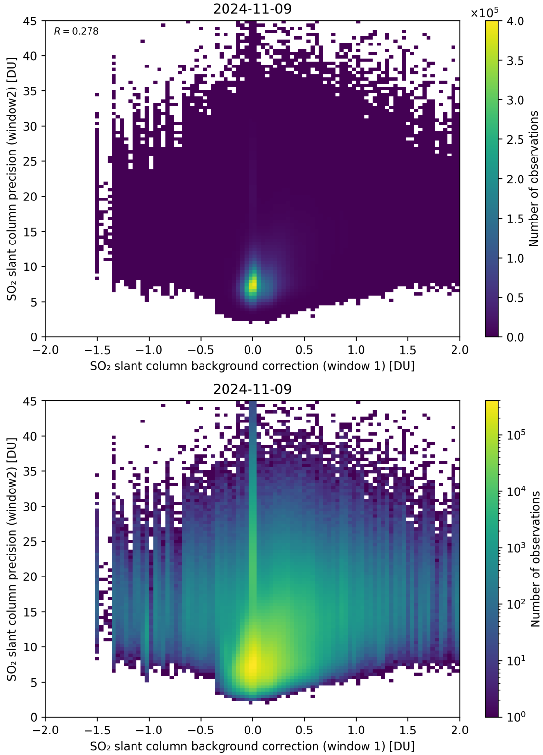
Figure 106: Scatter density plot of “SO 2 slant column background correction (window 1)” against “SO 2 slant column precision (window2)” for 2024-11-09 to 2024-11-10.
