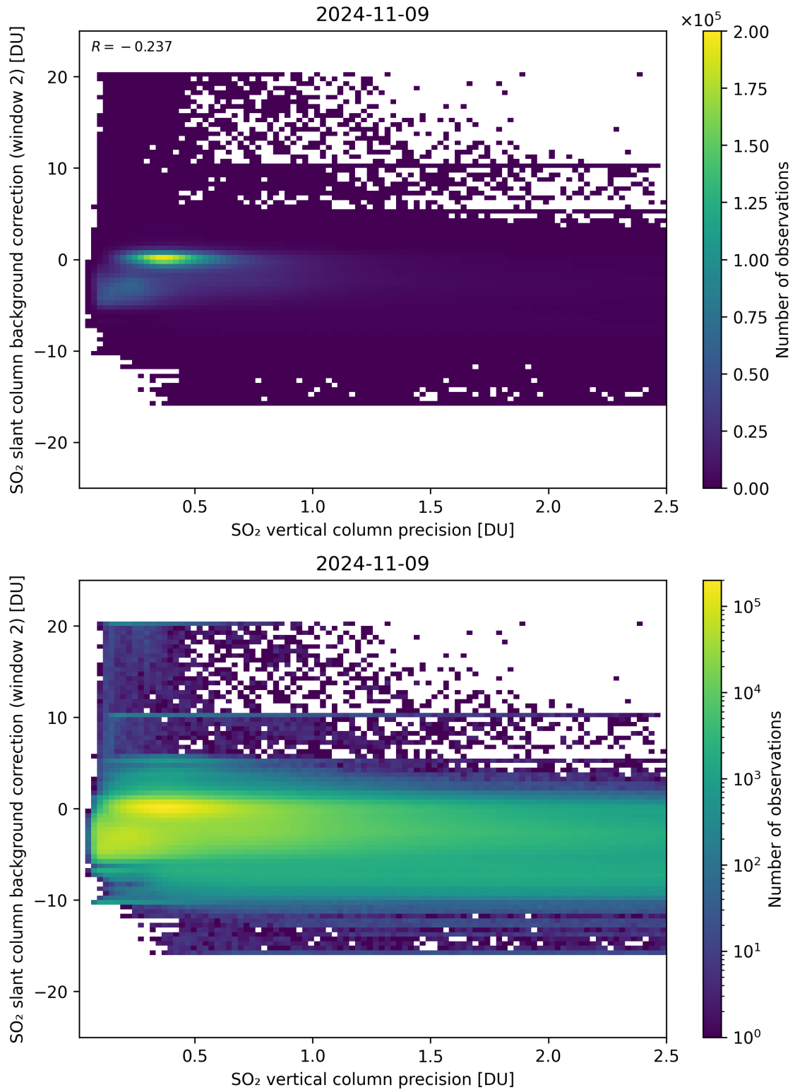
Figure 280: Scatter density plot of “SO 2 vertical column precision” against “SO 2 slant column background correction (window 2)” for 2024-11-09 to 2024-11-10.
