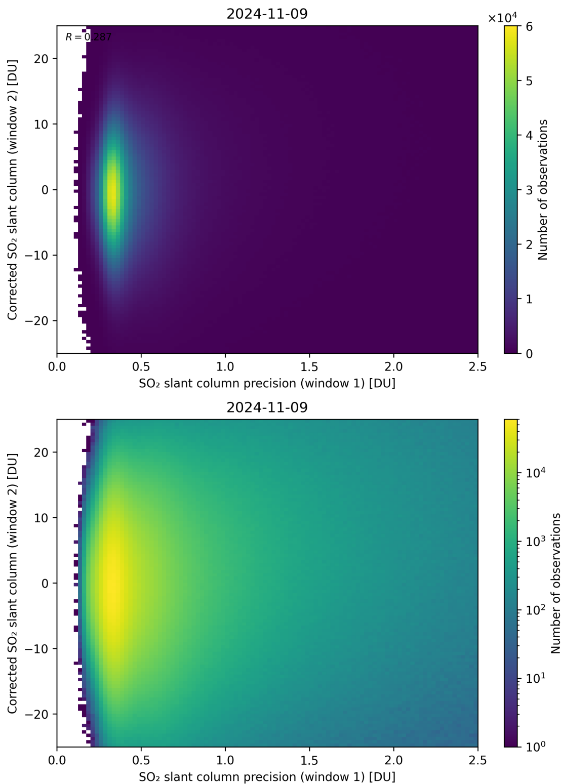
Figure 225: Scatter density plot of “SO 2 slant column precision (window 1)” against “Corrected SO 2 slant column (window 2)” for 2024-11-09 to 2024-11-10.
