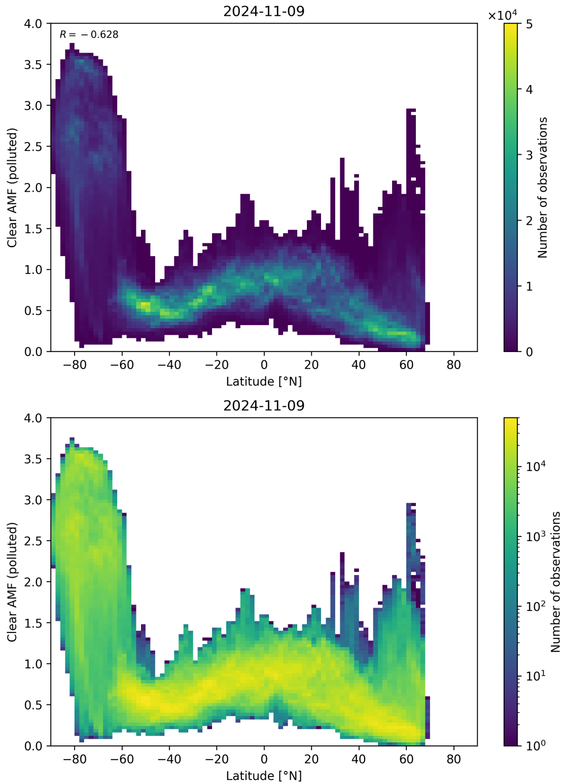
Figure 145: Scatter density plot of “Latitude” against “Clear AMF (polluted)” for 2024-11-09 to 2024-11-10.
