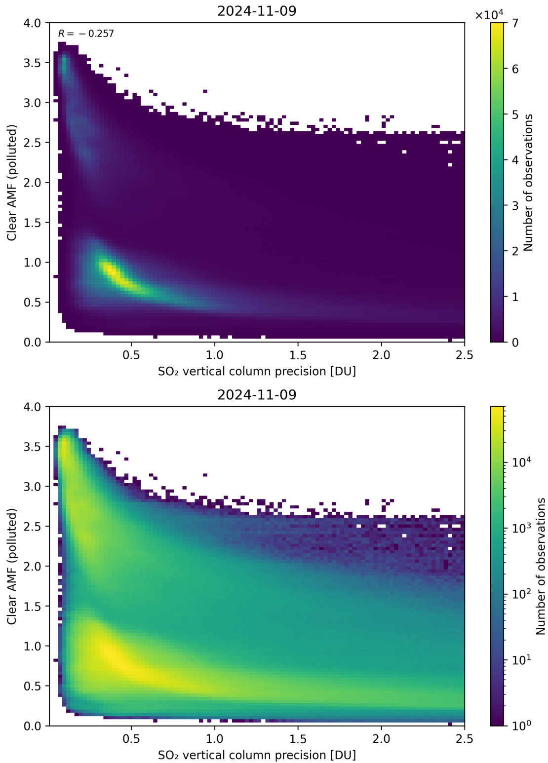
Figure 285: Scatter density plot of “SO 2 vertical column precision” against “Clear AMF (polluted)” for 2024-11-09 to 2024-11-10.
