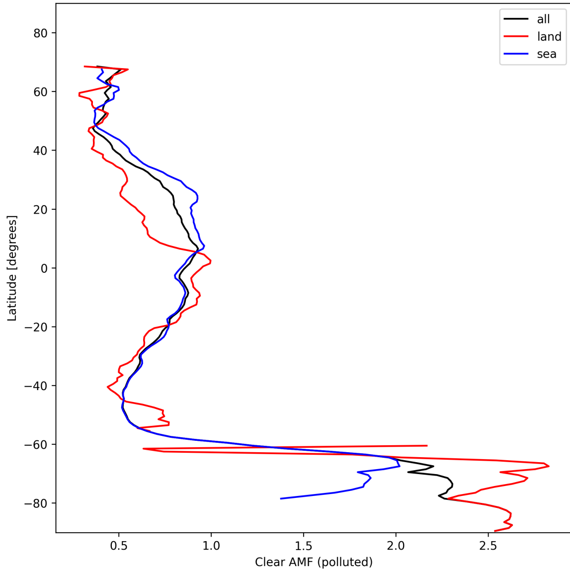
Figure 50: Zonal average of “Clear AMF (polluted)” for 2024-11-09 to 2024-11-10.
