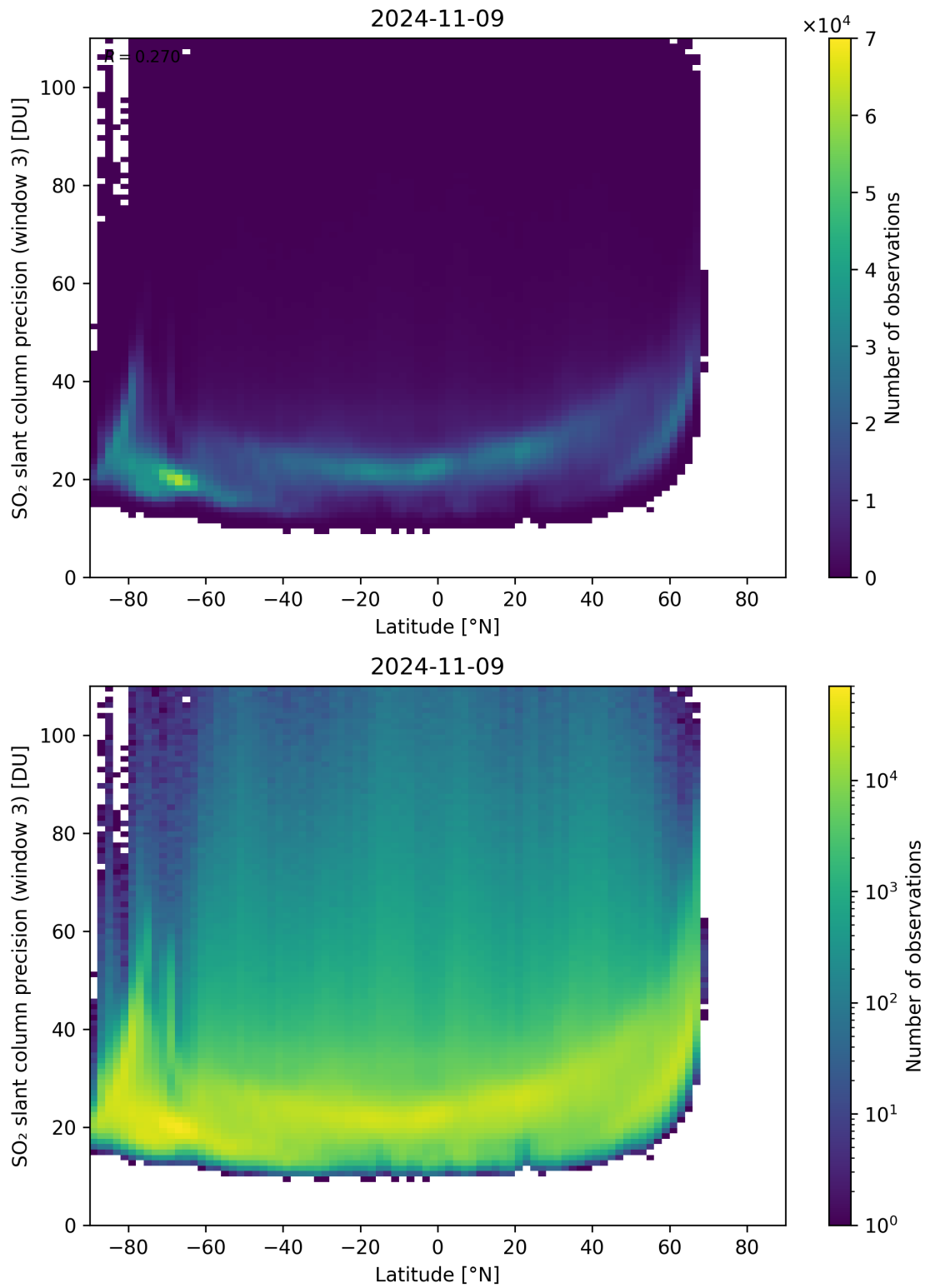
Figure 153: Scatter density plot of “Latitude” against “SO 2 slant column precision (window 3)” for 2024-11-09 to 2024-11-10.
