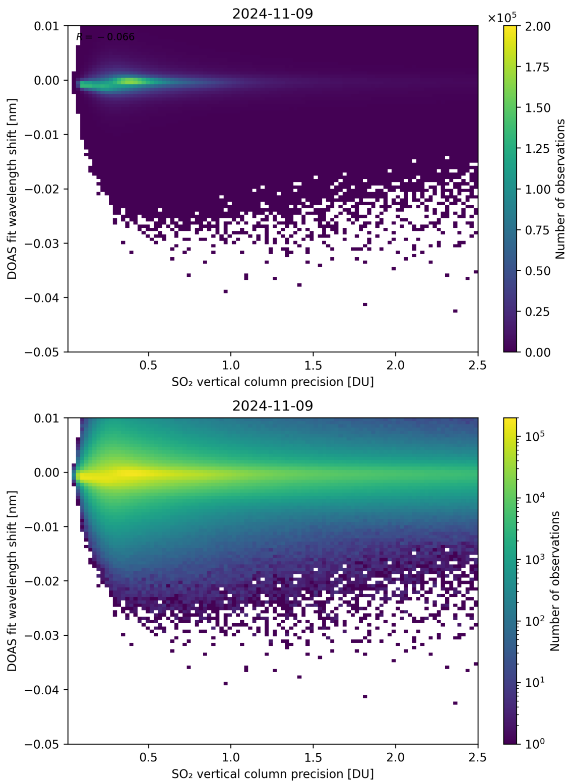
Figure 282: Scatter density plot of “SO 2 vertical column precision” against “DOAS fit wavelength shift” for 2024-11-09 to 2024-11-10.
