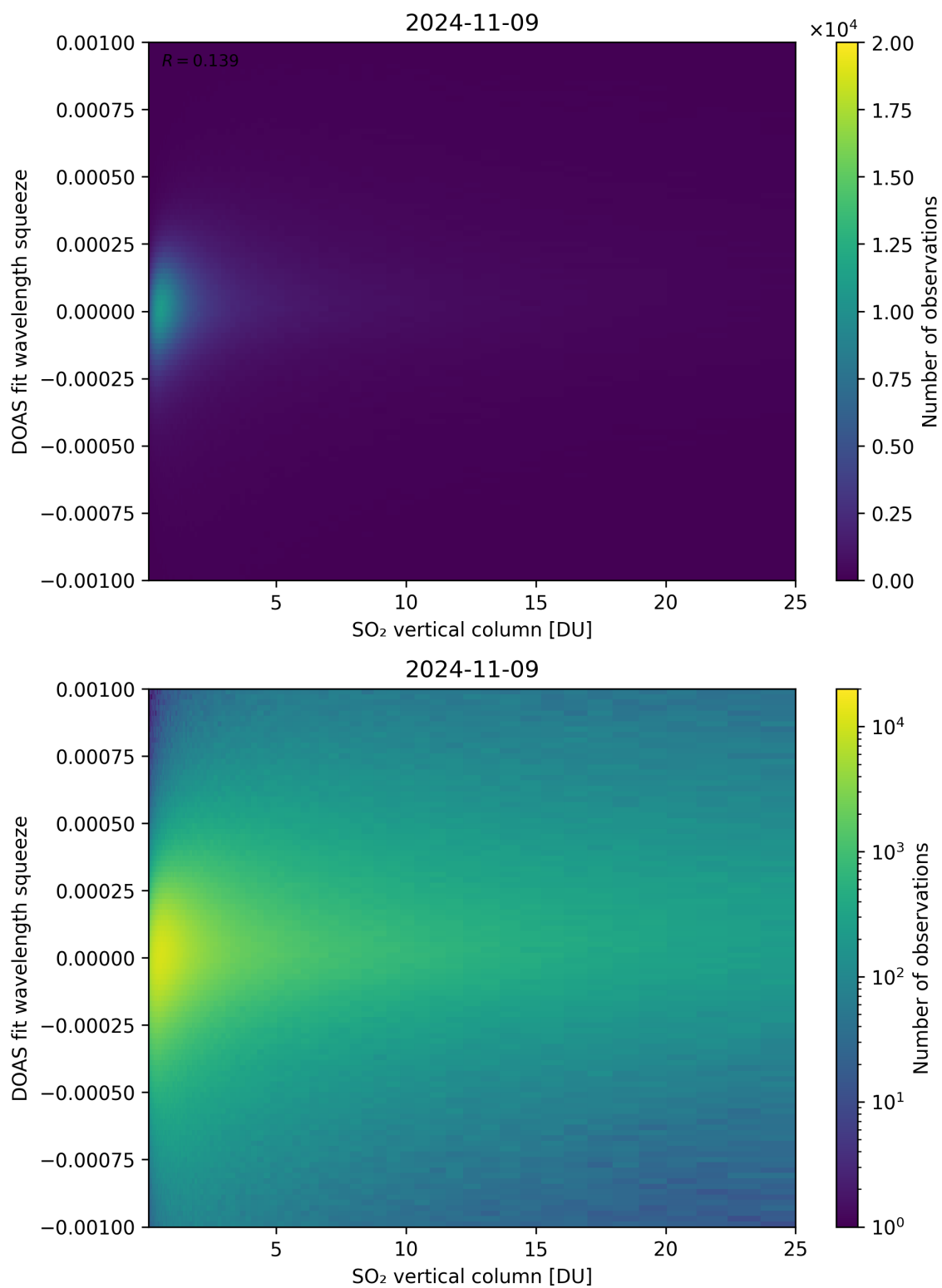
Figure 277: Scatter density plot of “SO 2 vertical column” against “DOAS fit wavelength squeeze” for 2024-11-09 to 2024-11-10.
