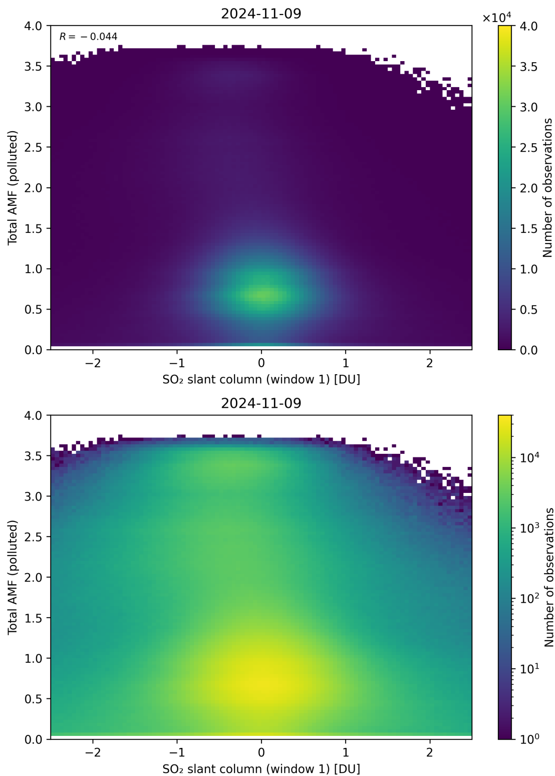
Figure 239: Scatter density plot of “SO 2 slant column (window 1)” against “Total AMF (polluted)” for 2024-11-09 to 2024-11-10.
