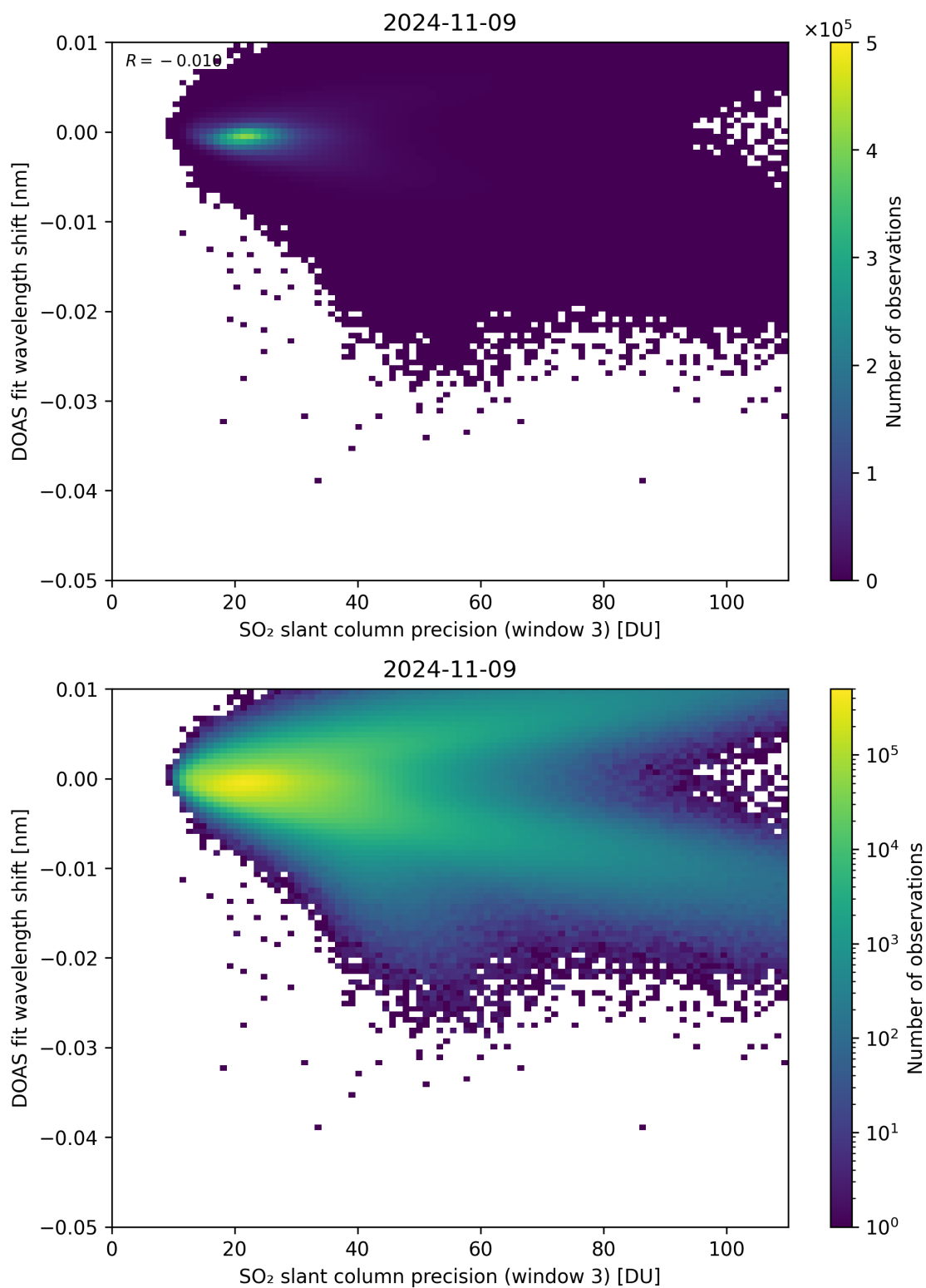
Figure 258: Scatter density plot of “SO 2 slant column precision (window 3)” against “DOAS fit wavelength shift” for 2024-11-09 to 2024-11-10.
