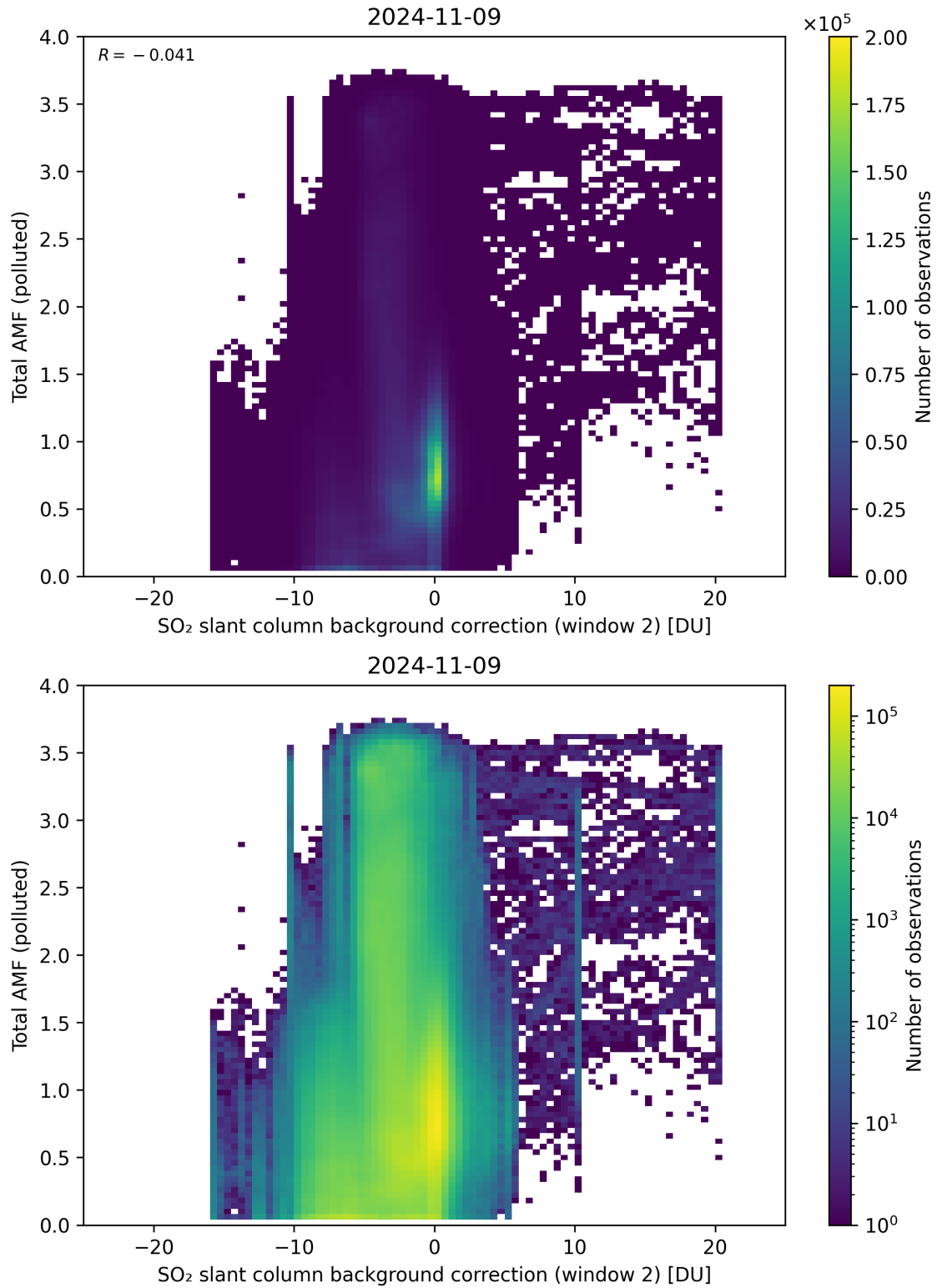
Figure 119: Scatter density plot of “SO 2 slant column background correction (window 2)” against “Total AMF (polluted)” for 2024-11-09 to 2024-11-10.
