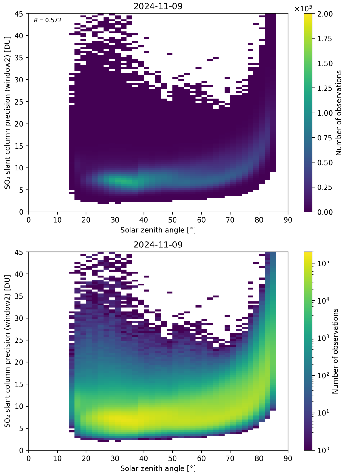
Figure 171: Scatter density plot of “Solar zenith angle” against “SO 2 slant column precision (window2)” for 2024-11-09 to 2024-11-10.
