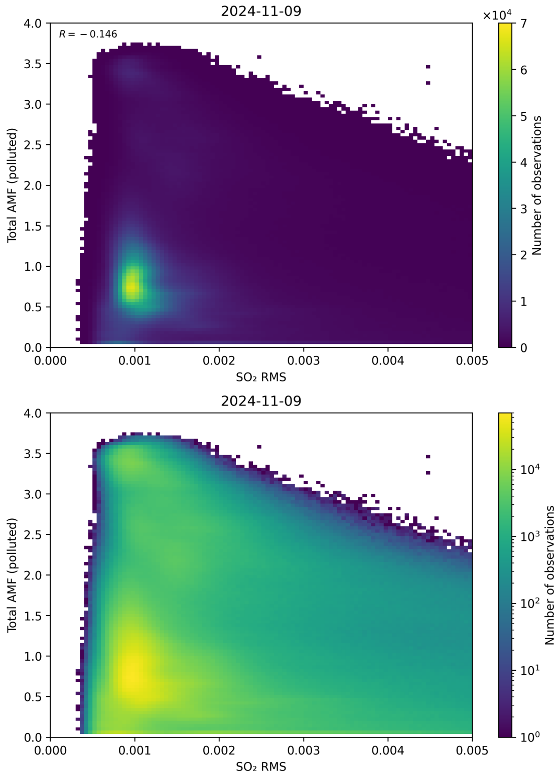
Figure 137: Scatter density plot of “SO 2 RMS” against “Total AMF (polluted)” for 2024-11-09 to 2024-11-10.
