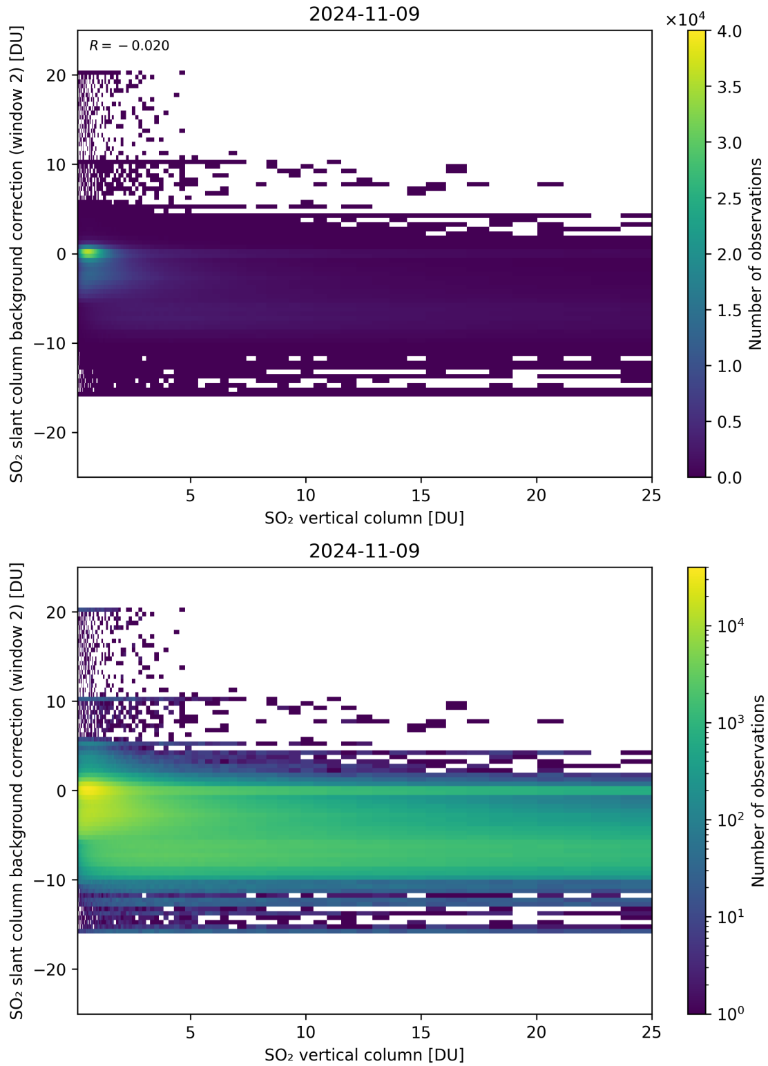
Figure 274: Scatter density plot of “SO 2 vertical column” against “SO 2 slant column background correction (window 2)” for 2024-11-09 to 2024-11-10.
