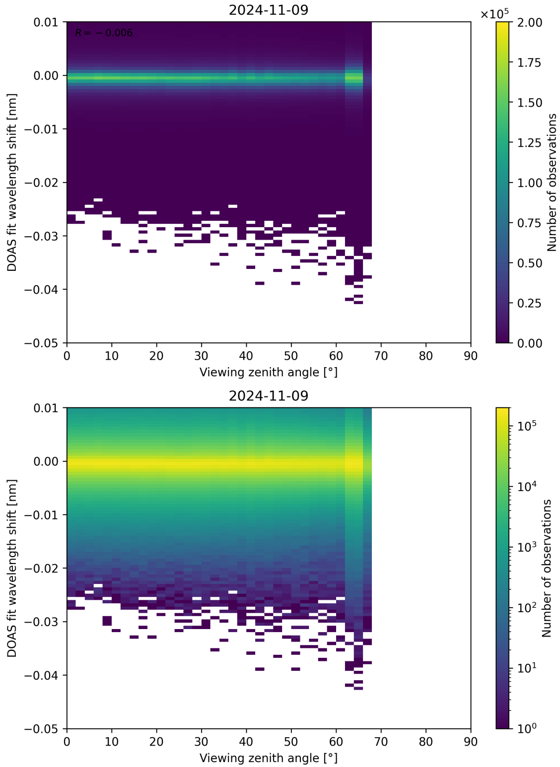
Figure 311: Scatter density plot of “Viewing zenith angle” against “DOAS fit wavelength shift” for 2024-11-09 to 2024-11-10.
