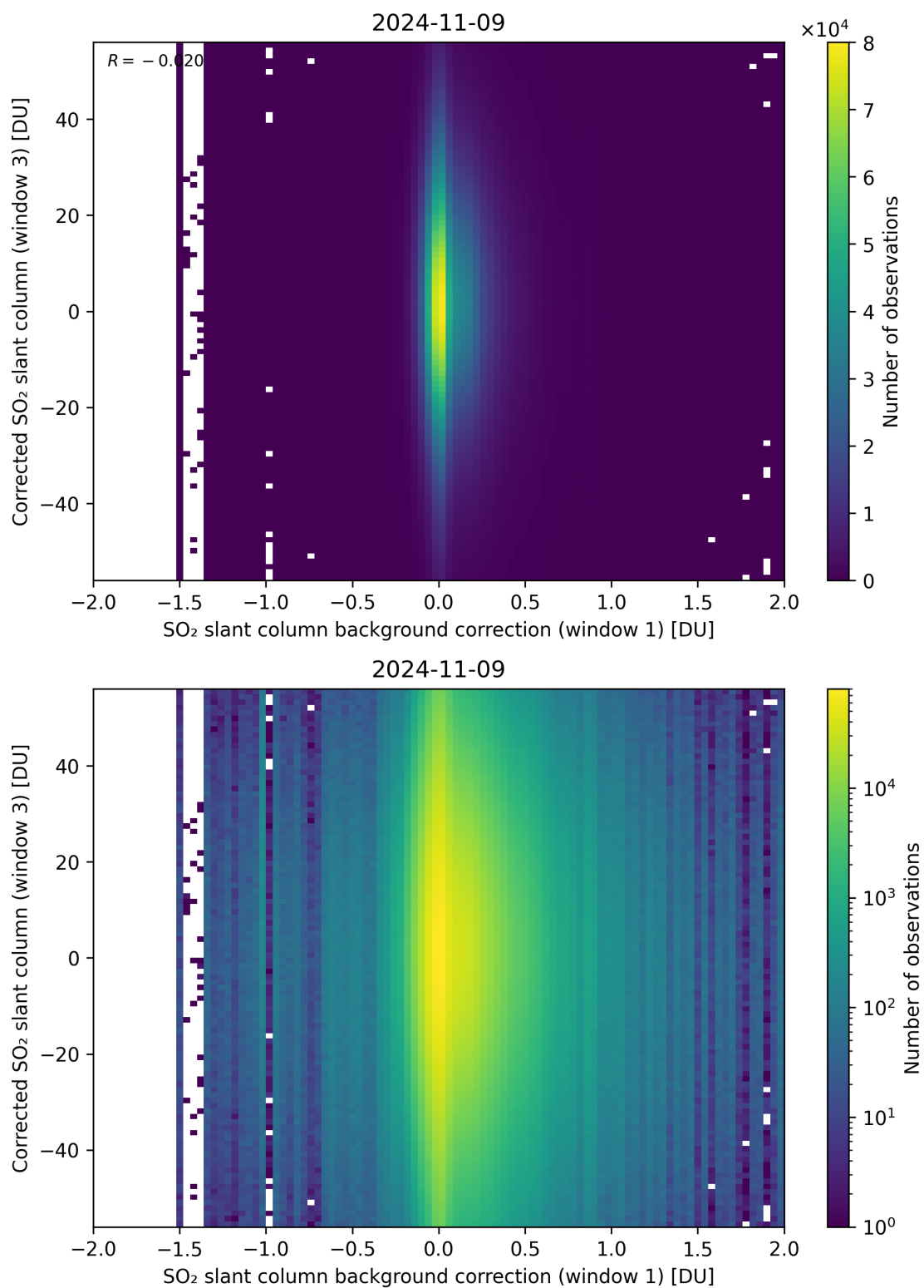
Figure 105: Scatter density plot of “SO 2 slant column background correction (window 1)” against “Corrected SO 2 slant column (window 3)” for 2024-11-09 to 2024-11-10.
