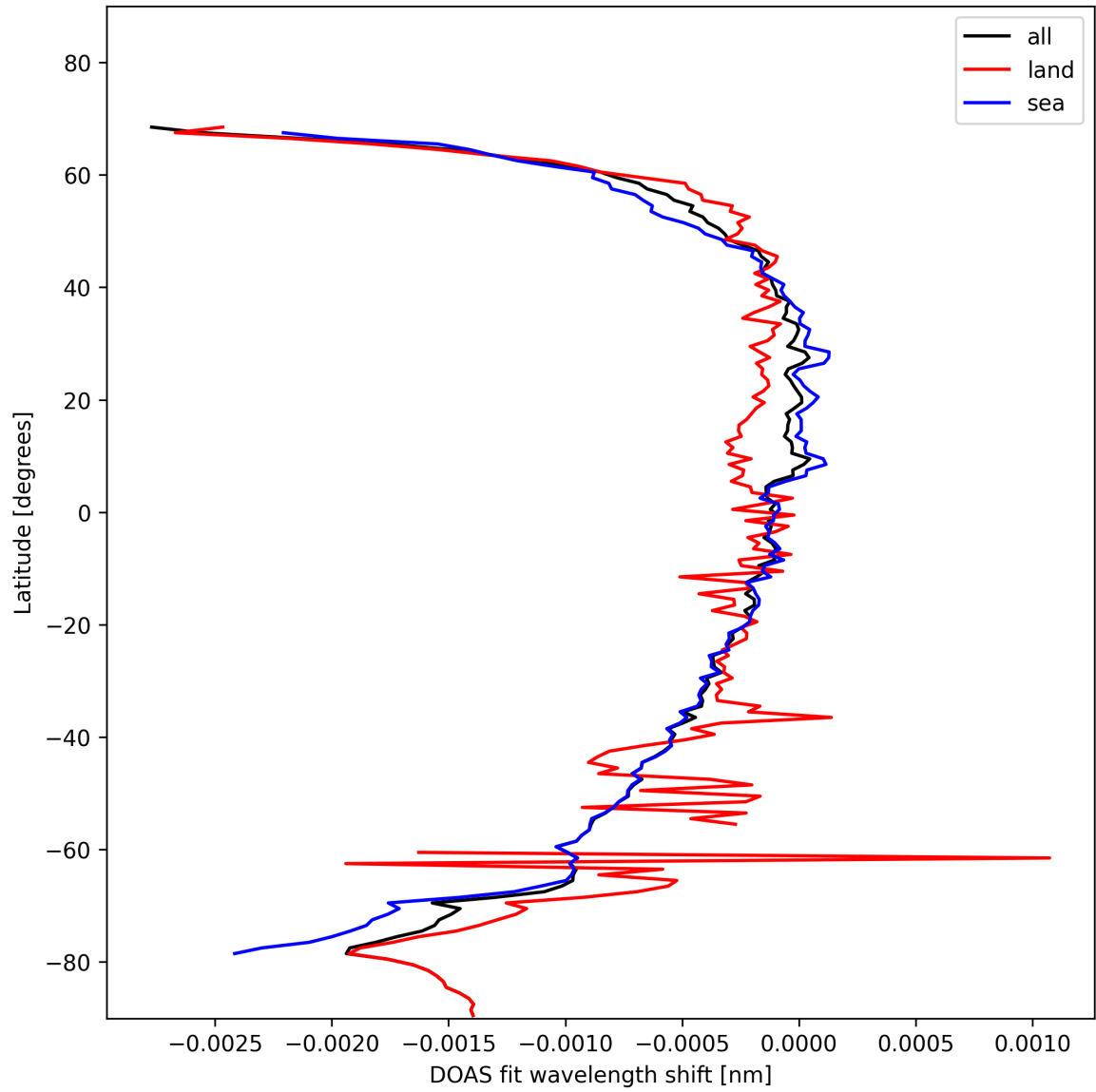
Figure 45: Zonal average of “DOAS fit wavelength shift” for 2024-11-09 to 2024-11-10.
