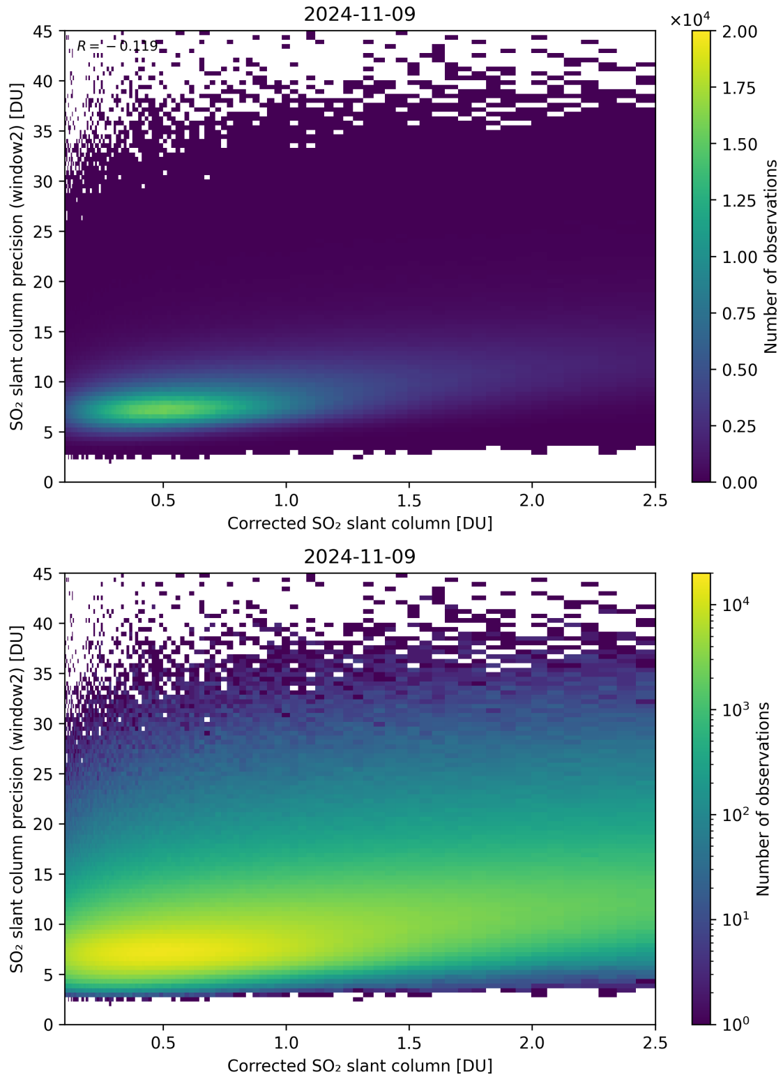
Figure 189: Scatter density plot of “Corrected SO 2 slant column” against “SO 2 slant column precision (window2)” for 2024-11-09 to 2024-11-10.
