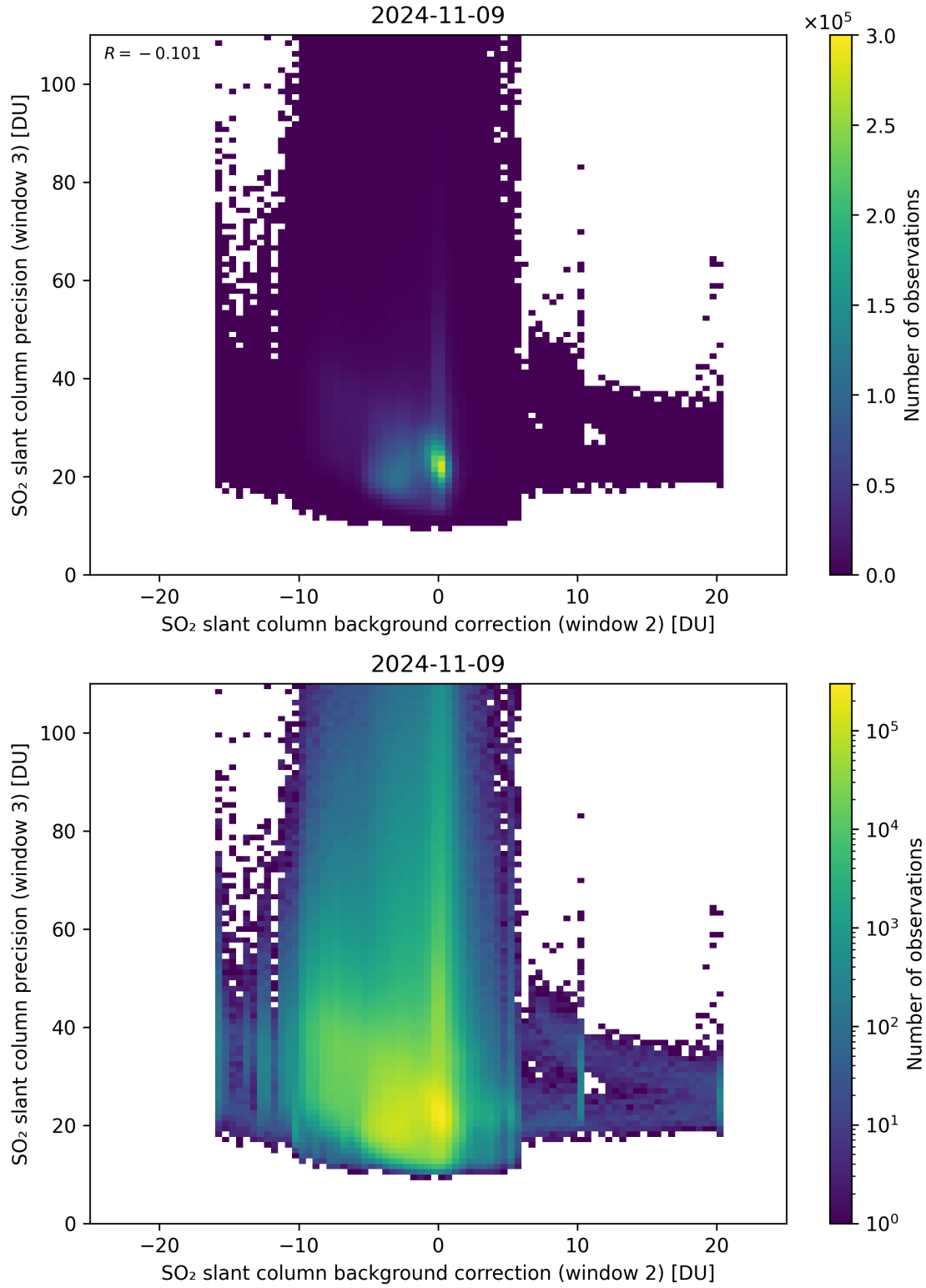
Figure 118: Scatter density plot of “SO 2 slant column background correction (window 2)” against “SO 2 slant column precision (window 3)” for 2024-11-09 to 2024-11-10.
