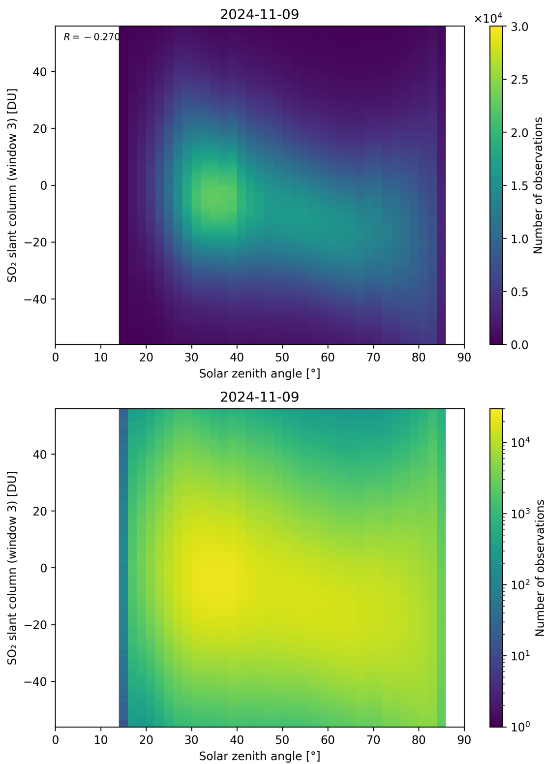
Figure 172: Scatter density plot of “Solar zenith angle” against “SO 2 slant column (window 3)” for 2024-11-09 to 2024-11-10.
