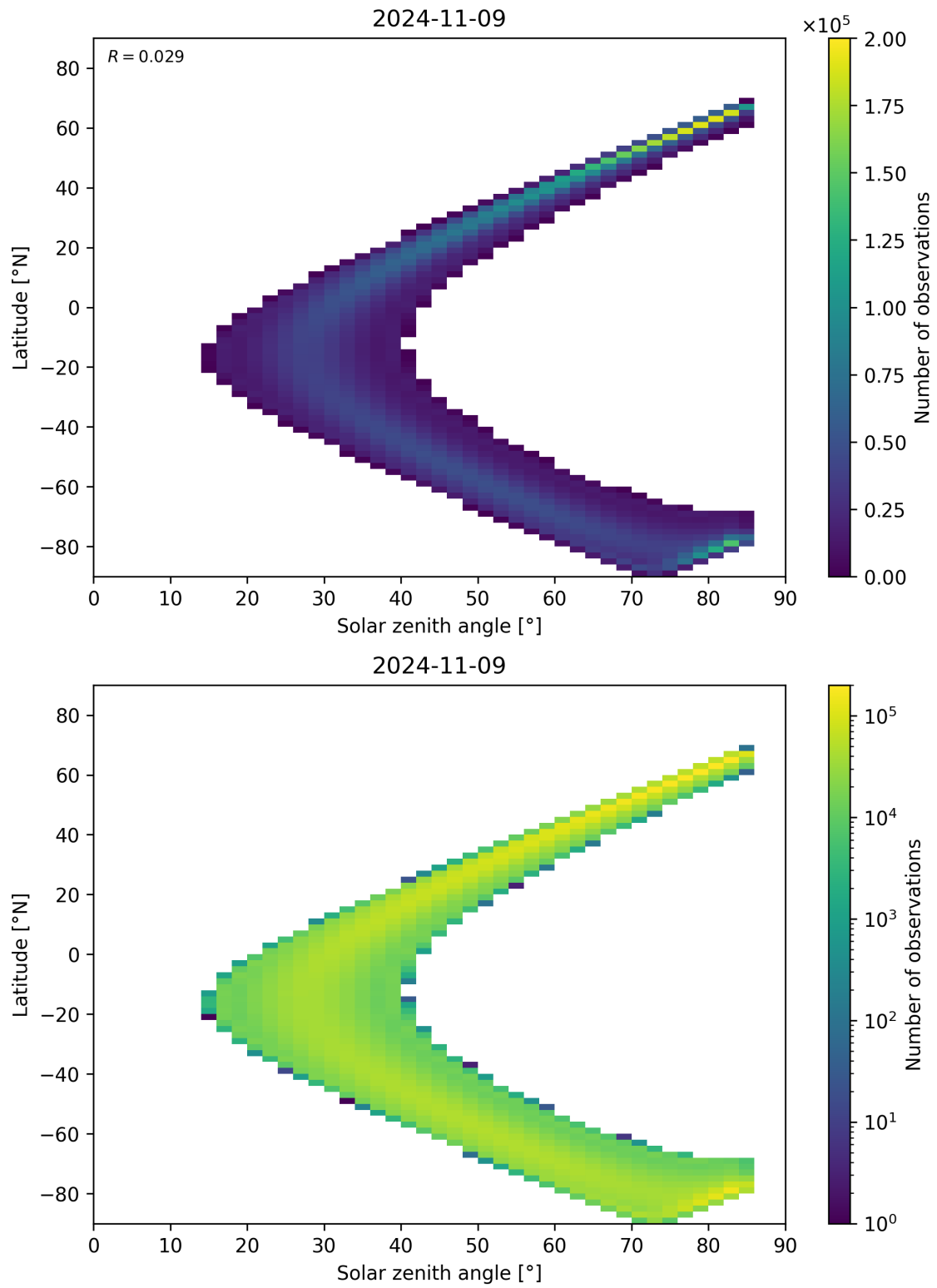
Figure 164: Scatter density plot of “Solar zenith angle” against “Latitude” for 2024-11-09 to 2024-11-10.
