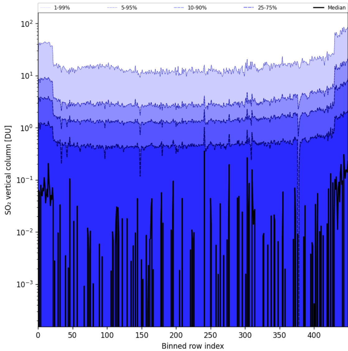
Figure 76: Along track statistics of “SO 2 vertical column” for 2024-11-09 to 2024-11-10
