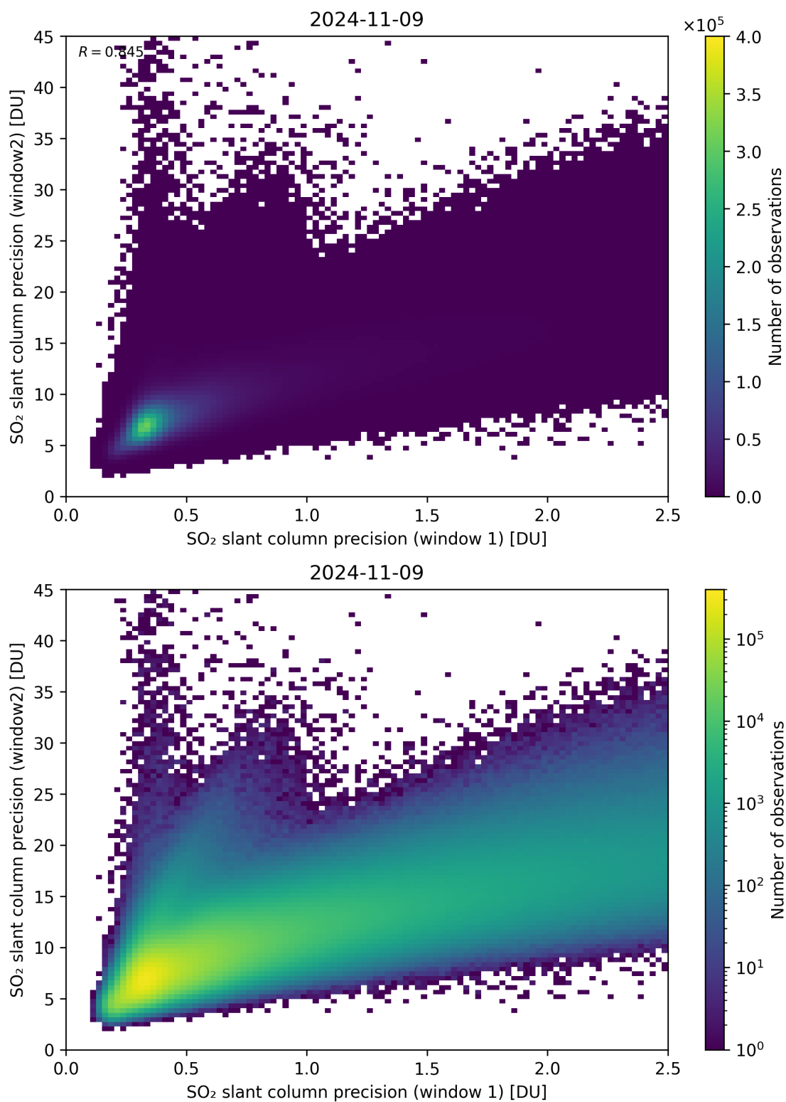
Figure 227: Scatter density plot of “SO 2 slant column precision (window 1)” against “SO 2 slant column precision (window2)” for 2024-11-09 to 2024-11-10.
