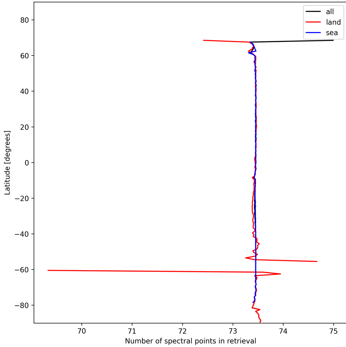
Figure 51: Zonal average of “Number of spectral points in retrieval” for 2024-11-09 to 2024-11-10.
