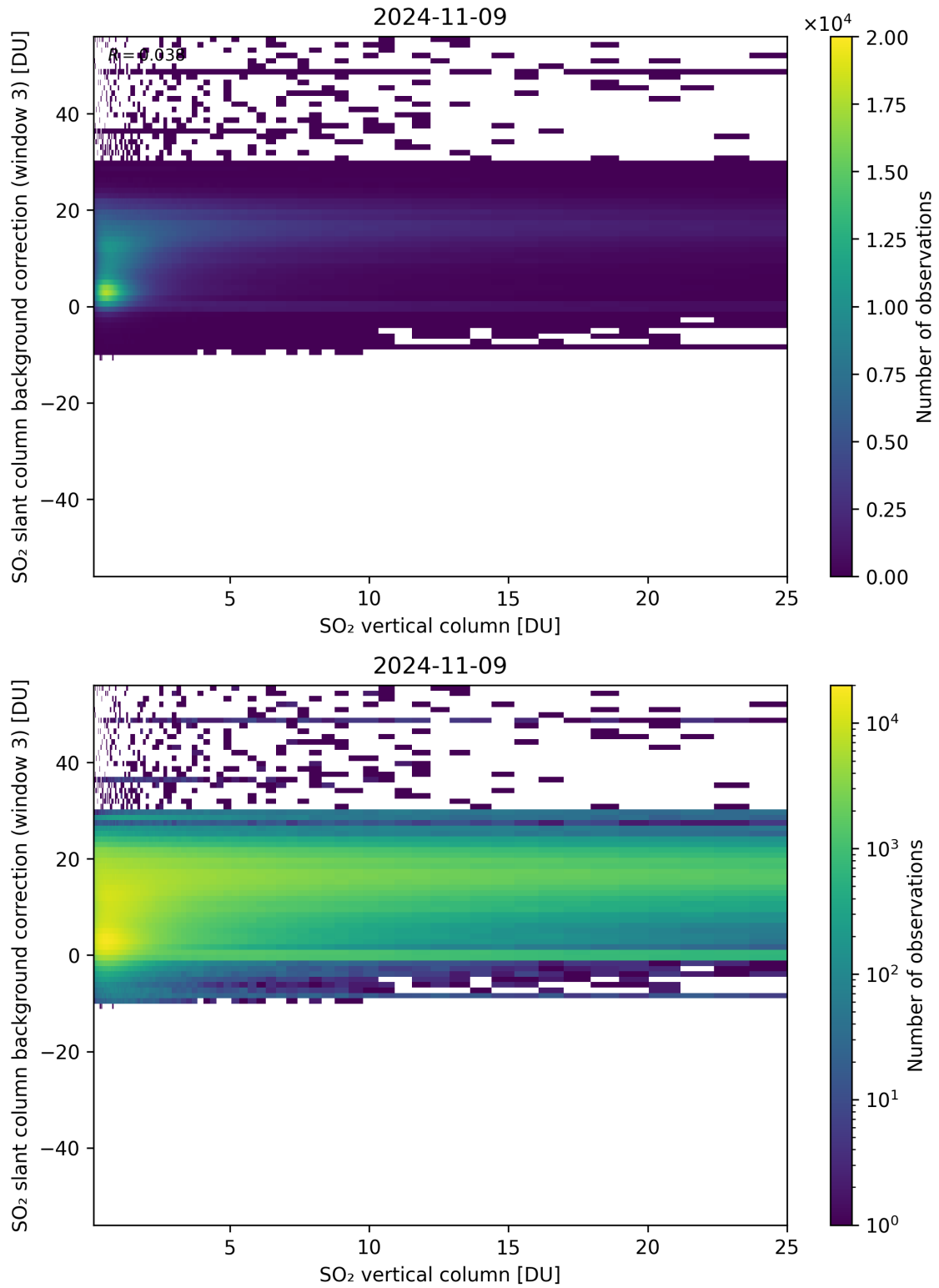
Figure 275: Scatter density plot of “SO 2 vertical column” against “SO 2 slant column background correction (window 3)” for 2024-11-09 to 2024-11-10.
