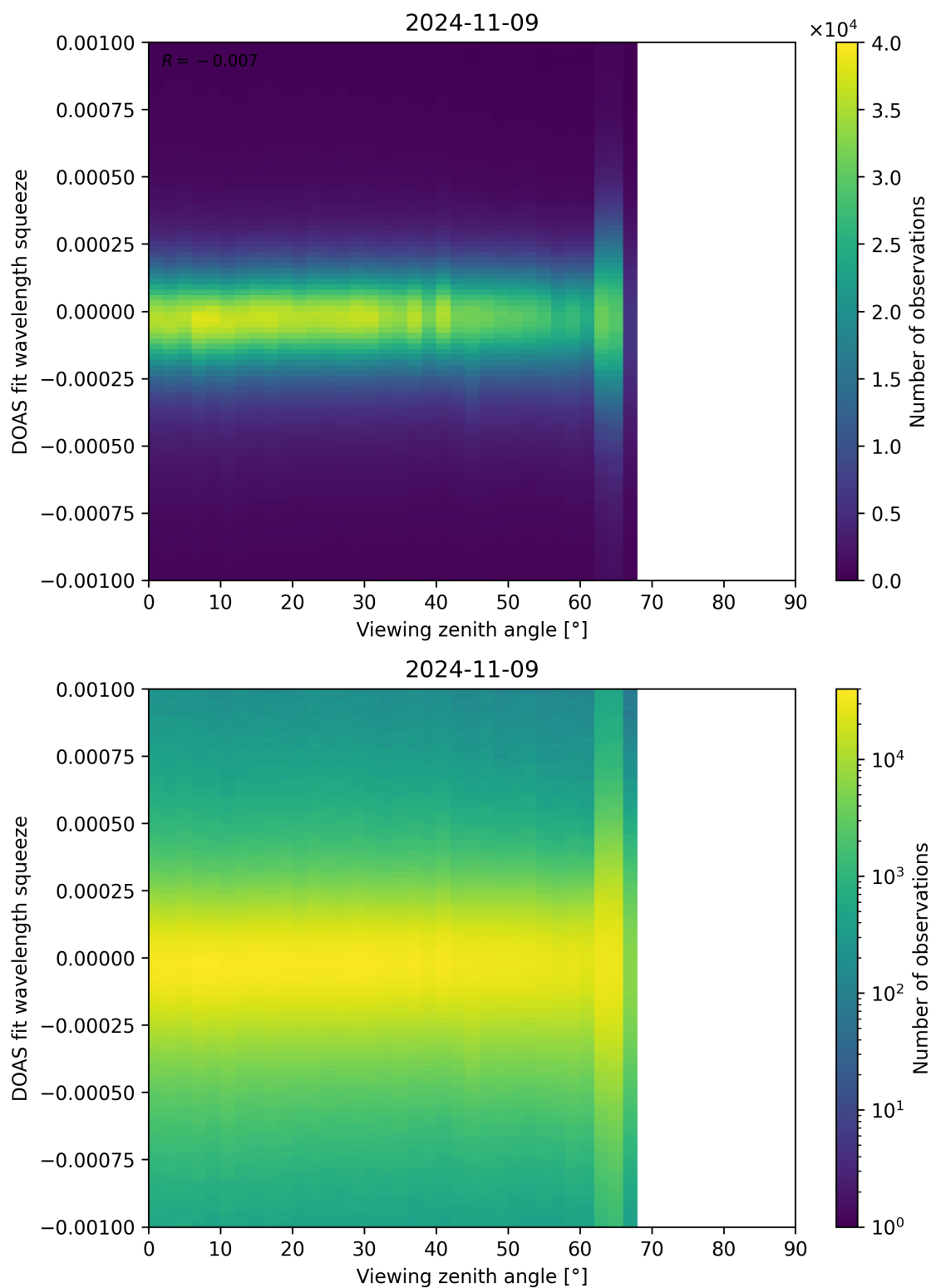
Figure 312: Scatter density plot of “Viewing zenith angle” against “DOAS fit wavelength squeeze” for 2024-11-09 to 2024-11-10.
