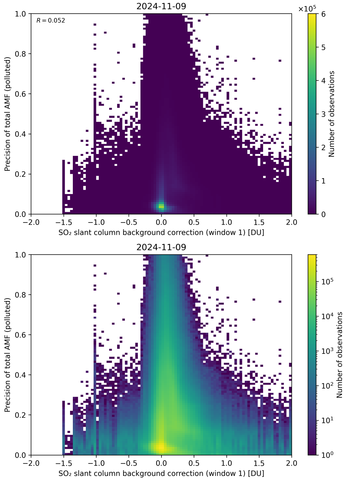
Figure 110: Scatter density plot of “SO 2 slant column background correction (window 1)” against “Precision of total AMF (polluted)” for 2024-11-09 to 2024-11-10.
