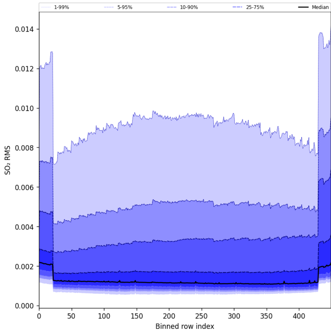
Figure 93: Along track statistics of “SO 2 RMS” for 2024-11-09 to 2024-11-10
