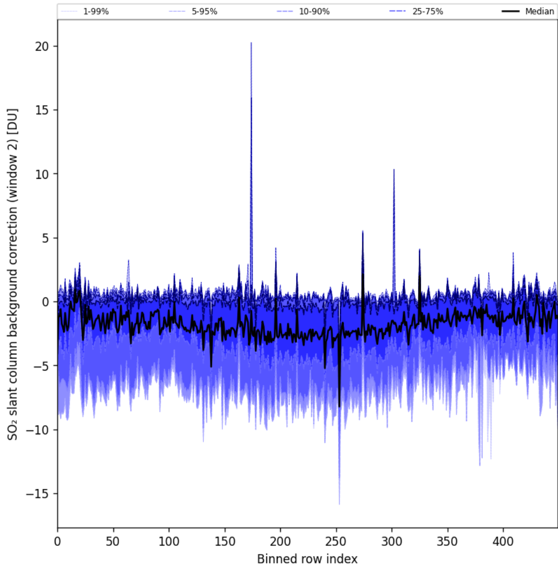
Figure 86: Along track statistics of “SO 2 slant column background correction (window 2)” for 2024-11-09 to 2024-11-10
