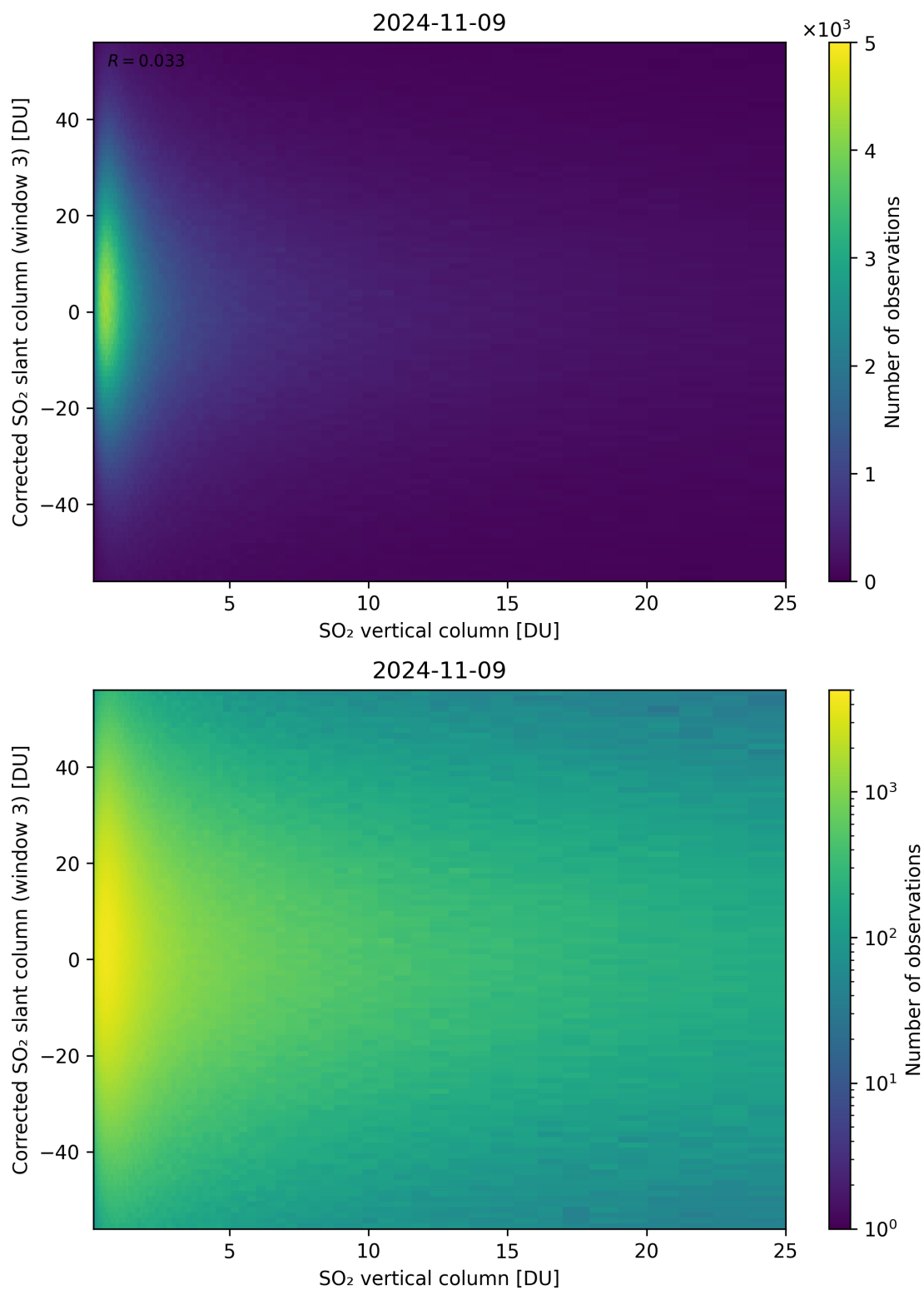
Figure 299: Scatter density plot of “SO 2 vertical column” against “Corrected SO 2 slant column (window 3)” for 2024-11-09 to 2024-11-10.
