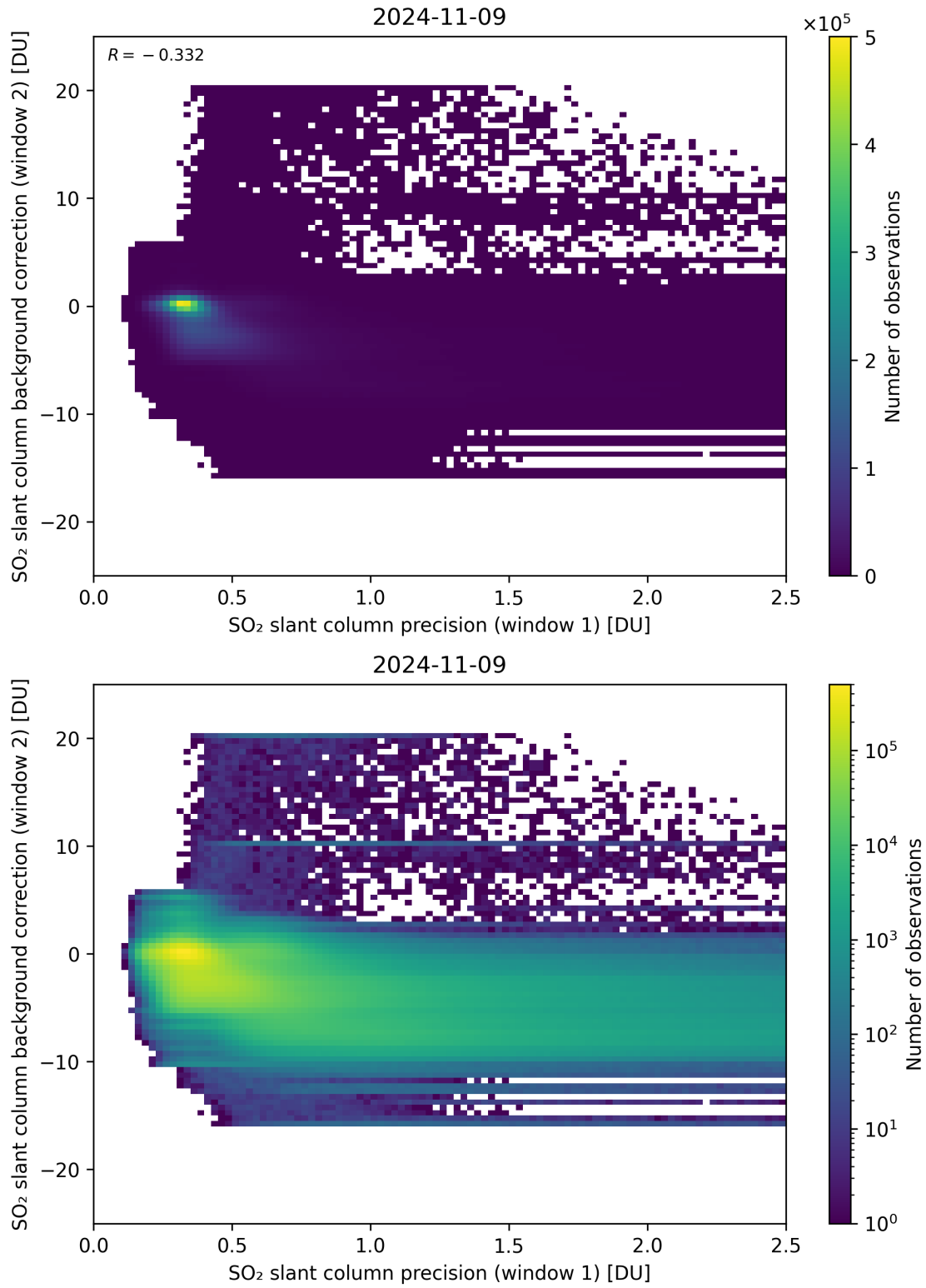
Figure 219: Scatter density plot of “SO 2 slant column precision (window 1)” against “SO 2 slant column background correction (window 2)” for 2024-11-09 to 2024-11-10.
