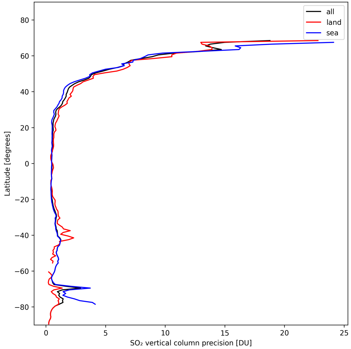
Figure 31: Zonal average of “SO 2 vertical column precision” for 2024-11-09 to 2024-11-10.
