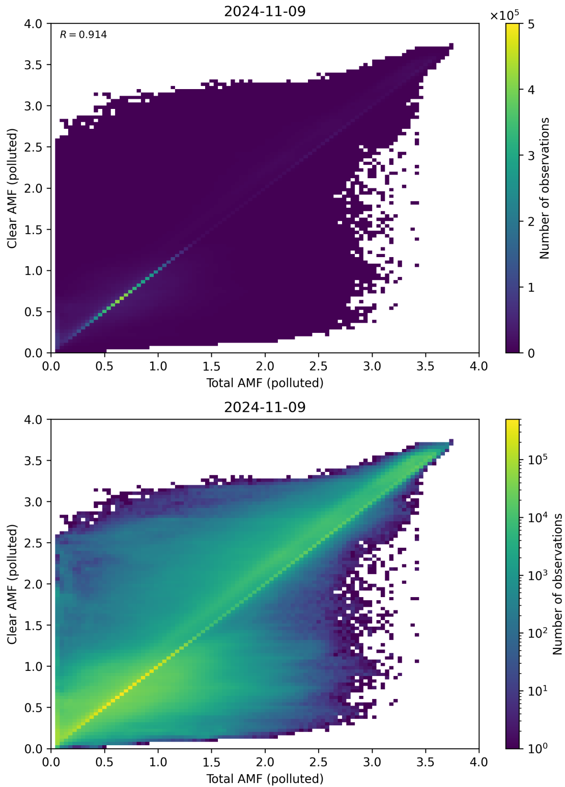
Figure 271: Scatter density plot of “Total AMF (polluted)” against “Clear AMF (polluted)” for 2024-11-09 to 2024-11-10.
