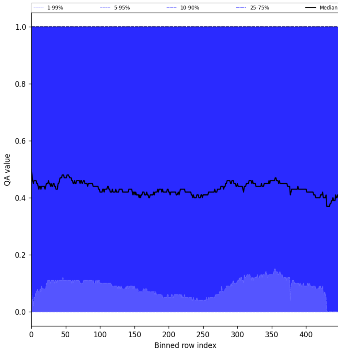
Figure 75: Along track statistics of “QA value” for 2024-11-09 to 2024-11-10
