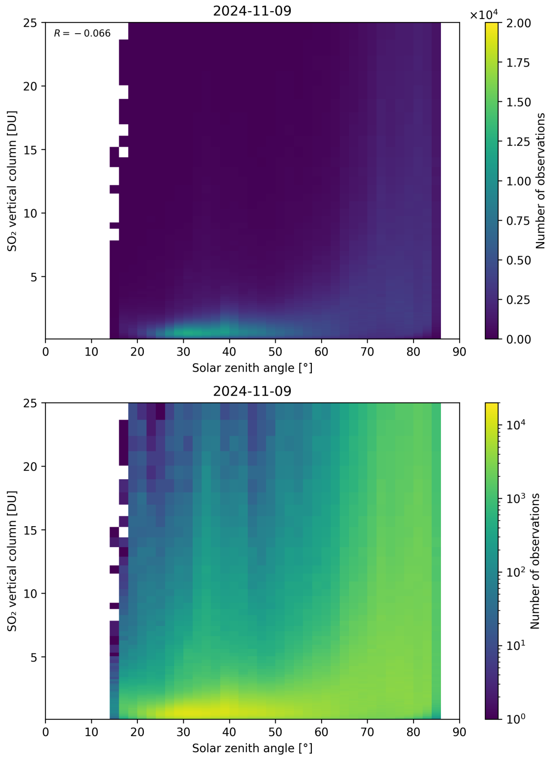
Figure 176: Scatter density plot of “Solar zenith angle” against “SO 2 vertical column” for 2024-11-09 to 2024-11-10.
