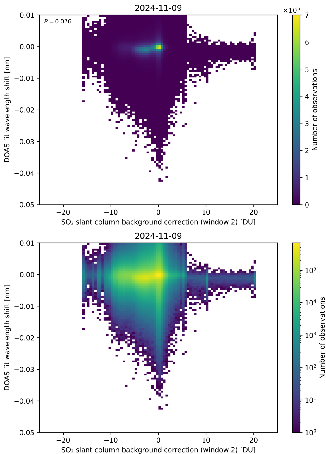
Figure 112: Scatter density plot of “SO 2 slant column background correction (window 2)” against “DOAS fit wavelength shift” for 2024-11-09 to 2024-11-10.
