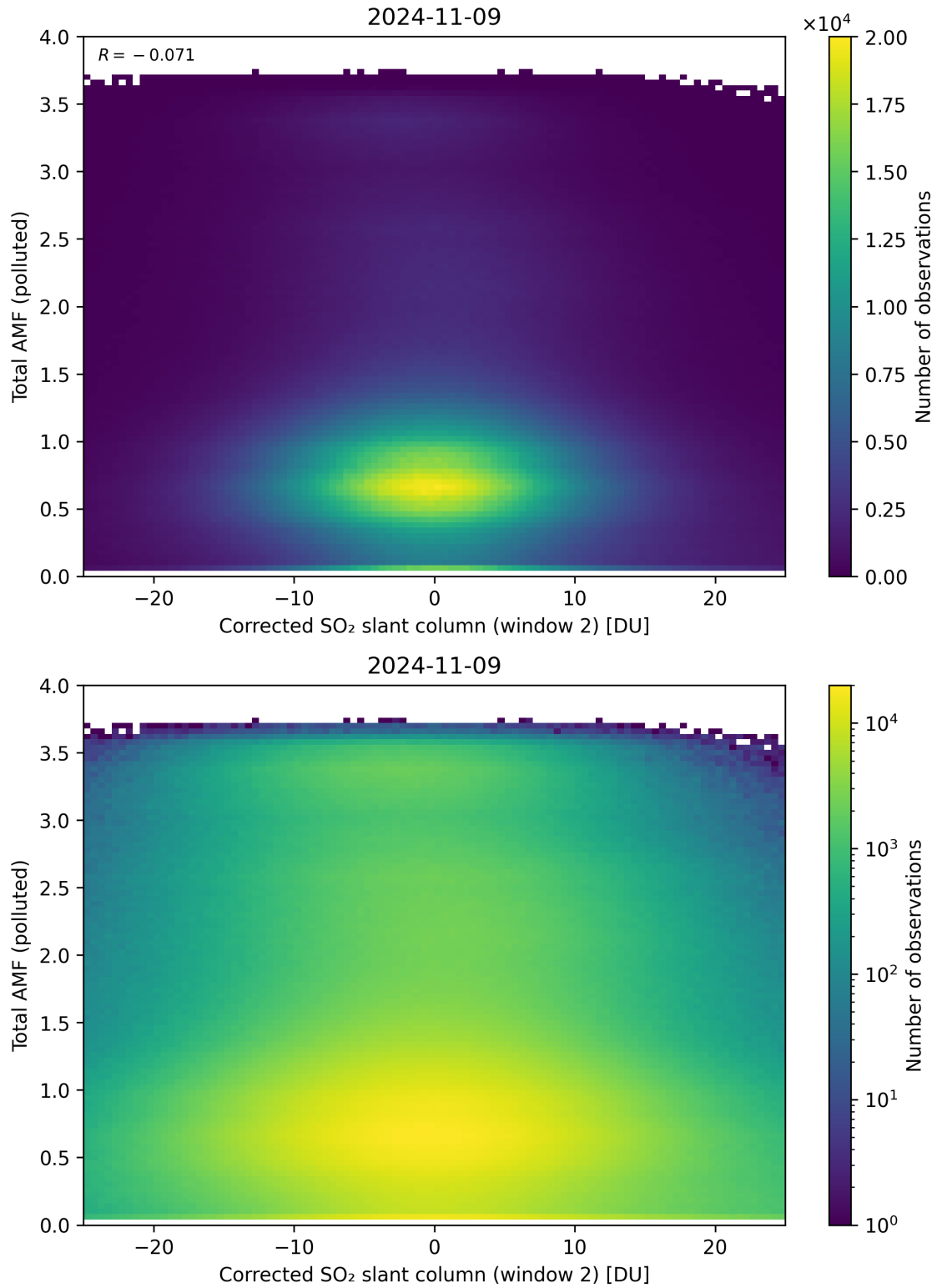
Figure 203: Scatter density plot of “Corrected SO 2 slant column (window 2)” against “Total AMF (polluted)” for 2024-11-09 to 2024-11-10.
