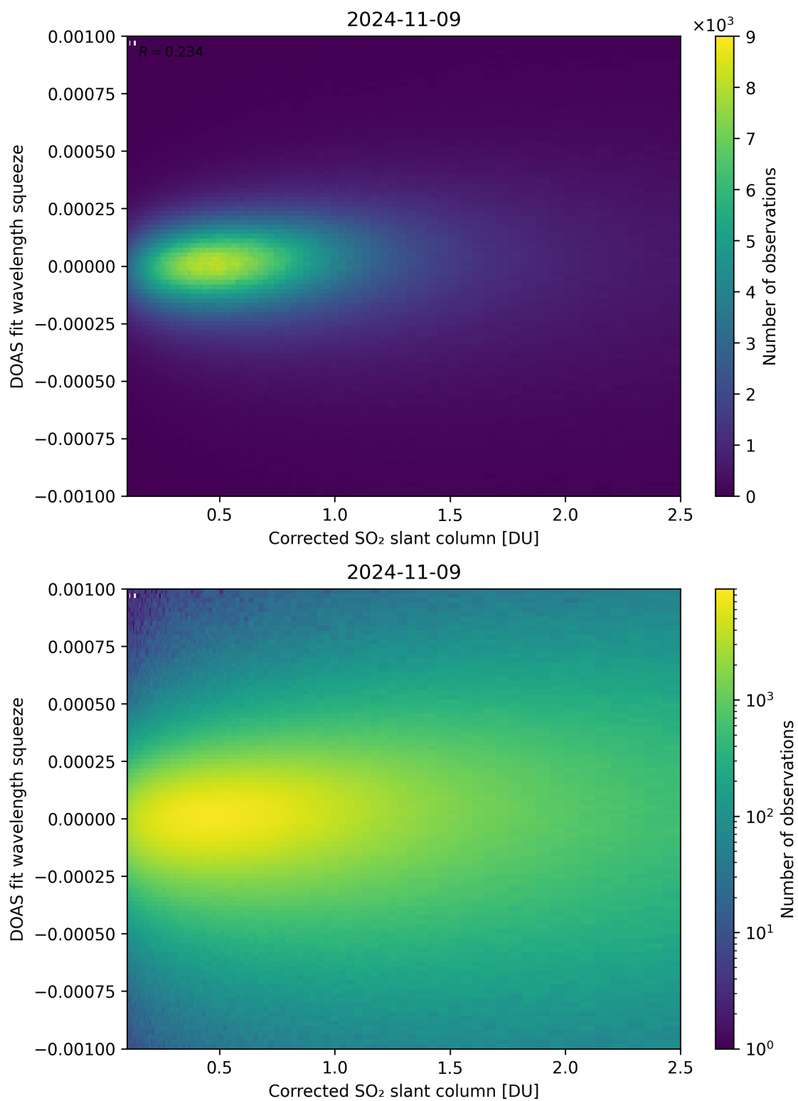
Figure 182: Scatter density plot of “Corrected SO 2 slant column” against “DOAS fit wavelength squeeze” for 2024-11-09 to 2024-11-10.
