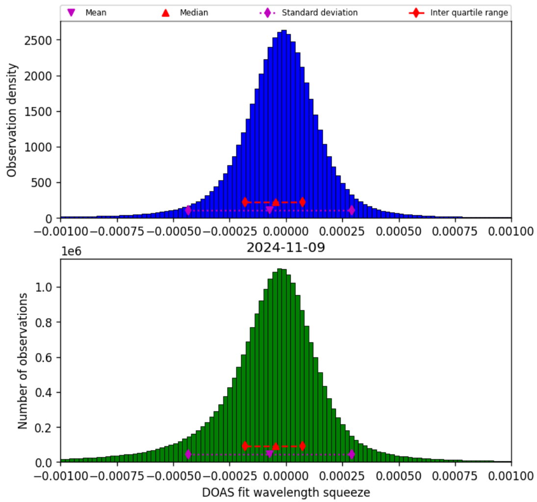
Figure 69: Histogram of “DOAS fit wavelength squeeze” for 2024-11-09 to 2024-11-10
