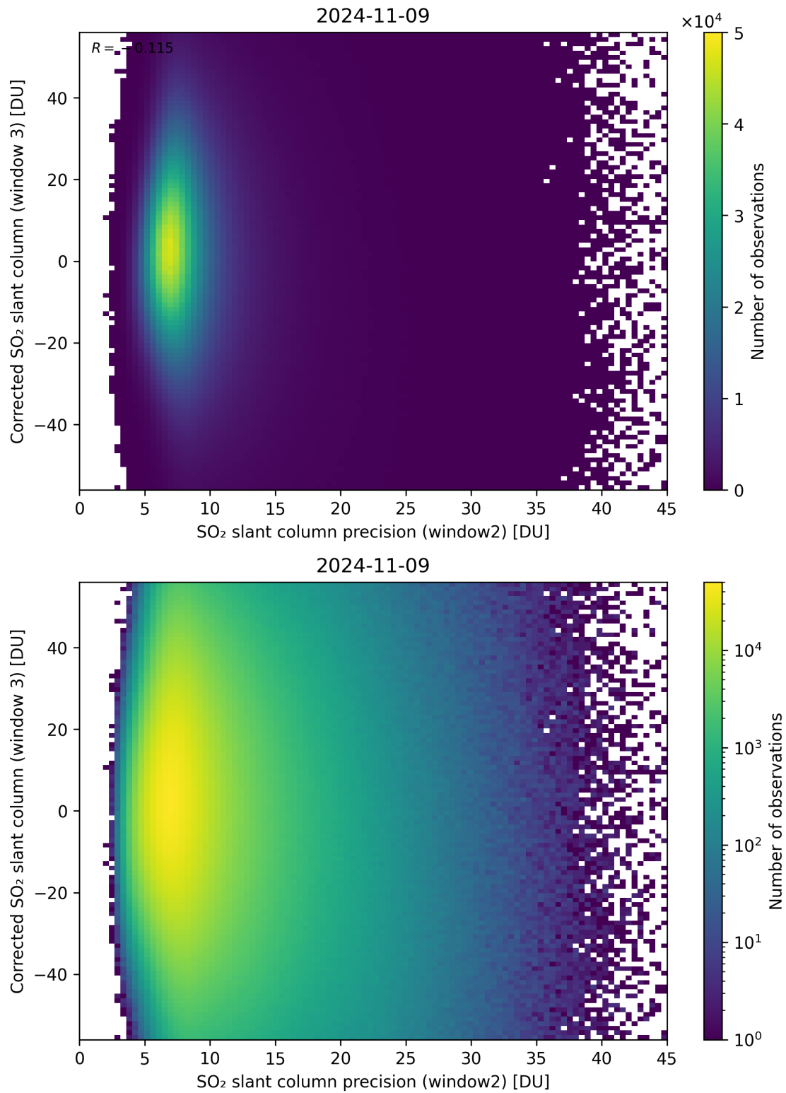
Figure 248: Scatter density plot of “SO 2 slant column precision (window2)” against “Corrected SO 2 slant column (window 3)” for 2024-11-09 to 2024-11-10.
