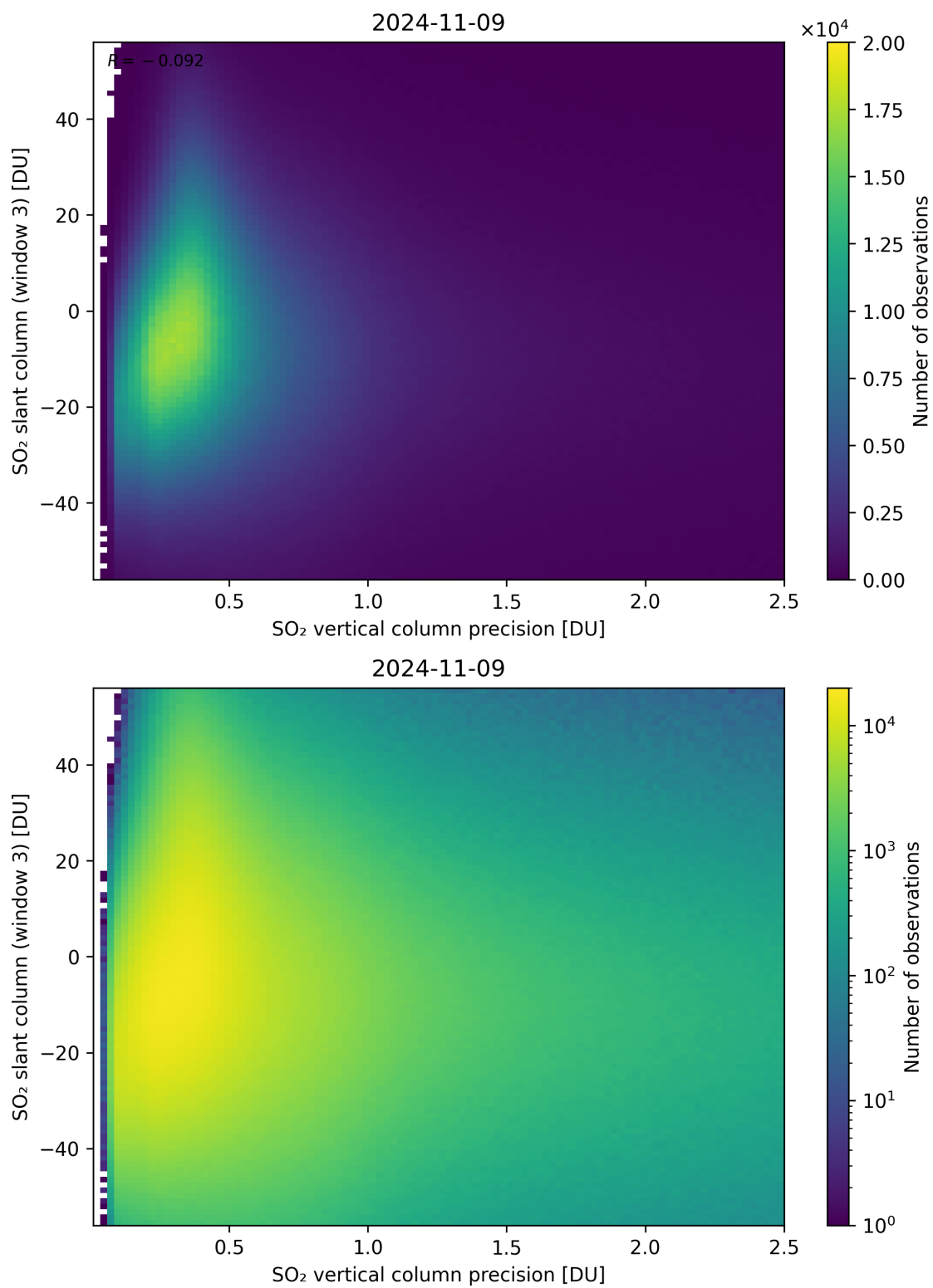
Figure 292: Scatter density plot of “SO 2 vertical column precision” against “SO 2 slant column (window 3)” for 2024-11-09 to 2024-11-10.
