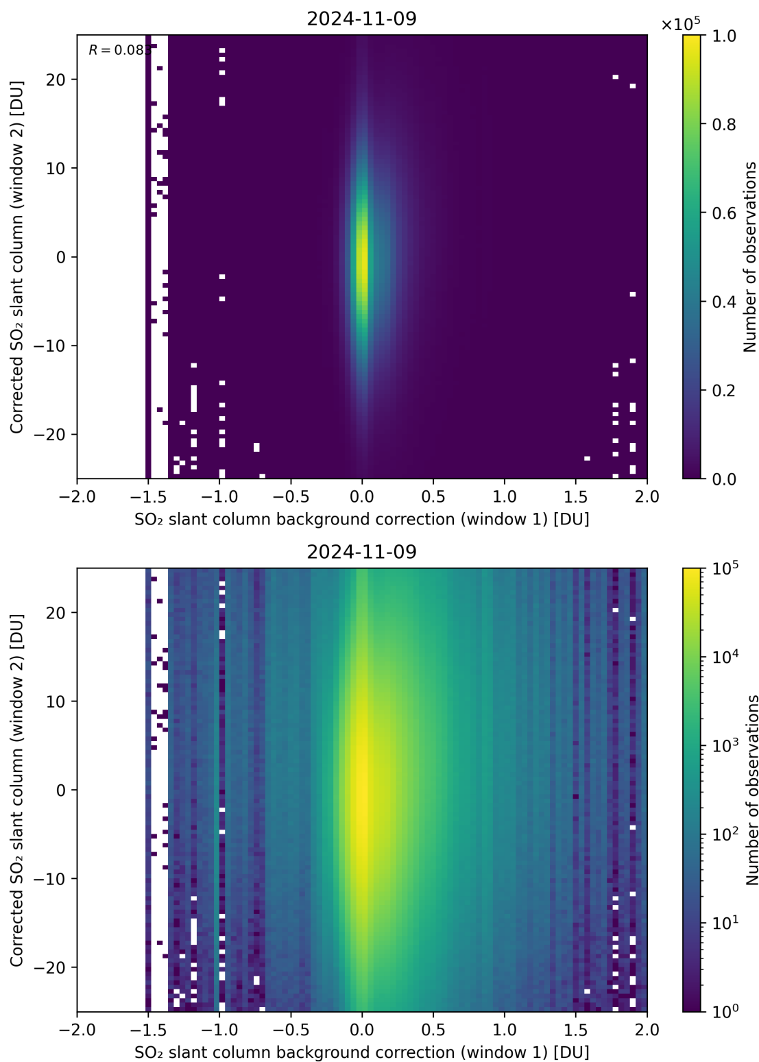
Figure 104: Scatter density plot of “SO 2 slant column background correction (window 1)” against “Corrected SO 2 slant column (window 2)” for 2024-11-09 to 2024-11-10.
