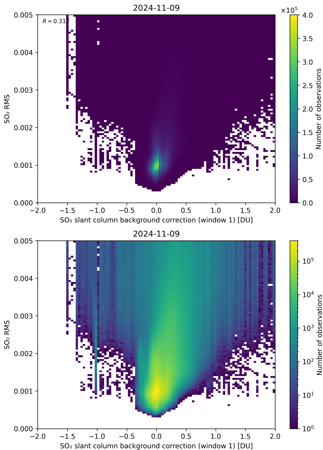
Figure 102: Scatter density plot of “SO 2 slant column background correction (window 1)” against “SO 2 RMS” for 2024-11-09 to 2024-11-10.
