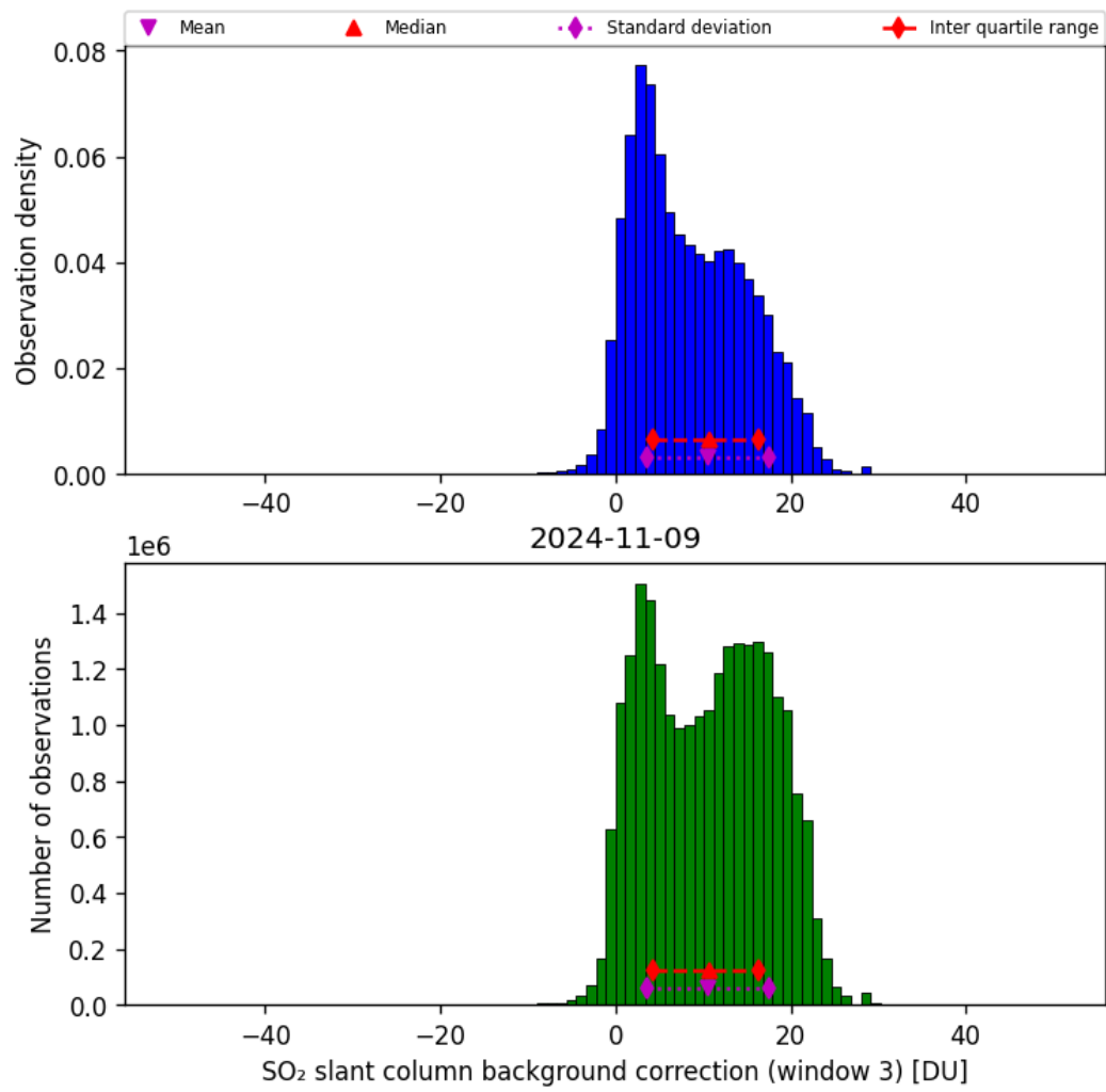
Figure 67: Histogram of “SO 2 slant column background correction (window 3)” for 2024-11-09 to 2024-11-10
