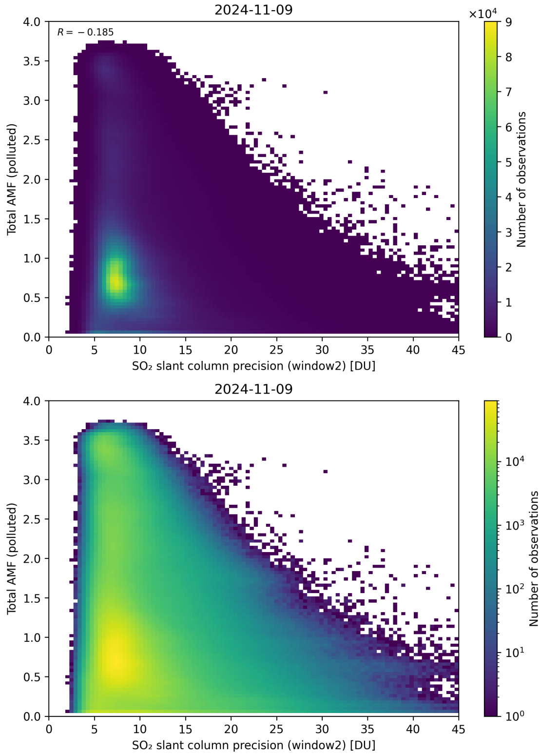
Figure 251: Scatter density plot of “SO 2 slant column precision (window2)” against “Total AMF (polluted)” for 2024-11-09 to 2024-11-10.
