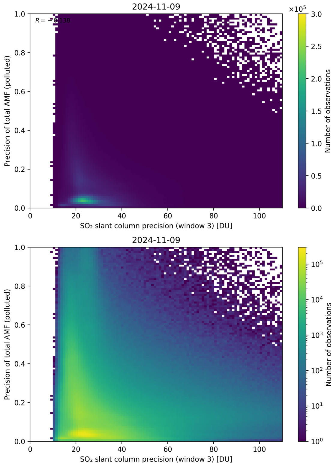
Figure 264: Scatter density plot of “SO 2 slant column precision (window 3)” against “Precision of total AMF (polluted)” for 2024-11-09 to 2024-11-10.
