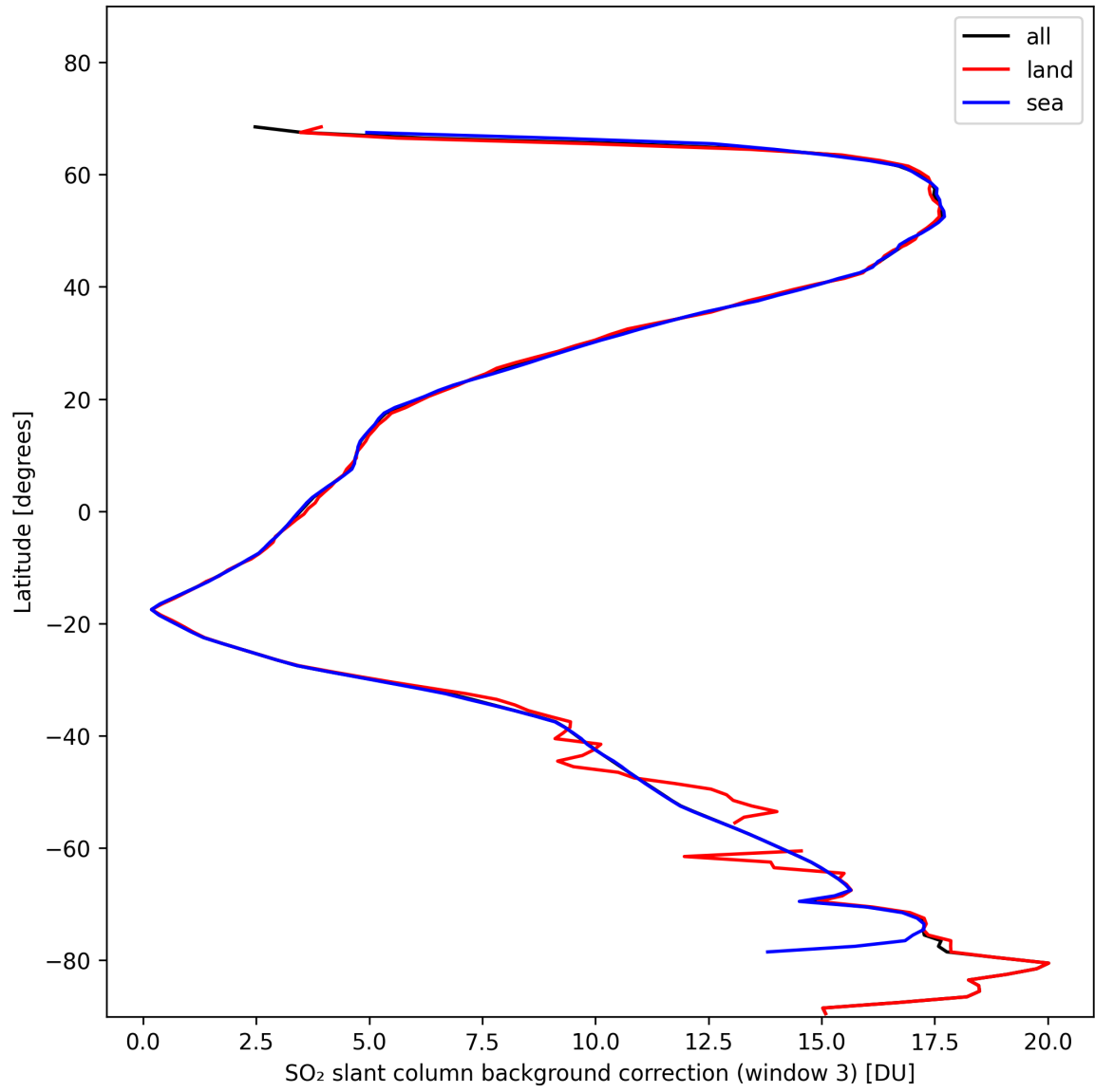
Figure 44: Zonal average of “SO 2 slant column background correction (window 3)” for 2024-11-09 to 2024-11-10.
