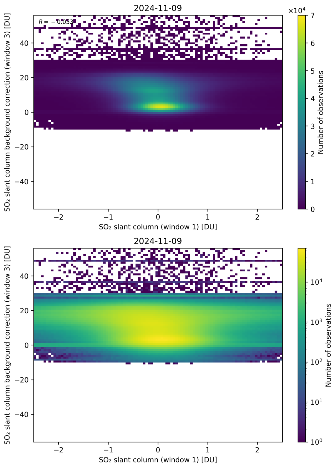
Figure 214: Scatter density plot of “SO 2 slant column (window 1)” against “SO 2 slant column background correction (window 3)” for 2024-11-09 to 2024-11-10.
