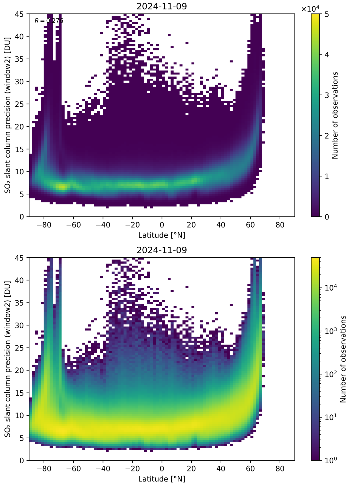
Figure 151: Scatter density plot of “Latitude” against “SO 2 slant column precision (window2)” for 2024-11-09 to 2024-11-10.
