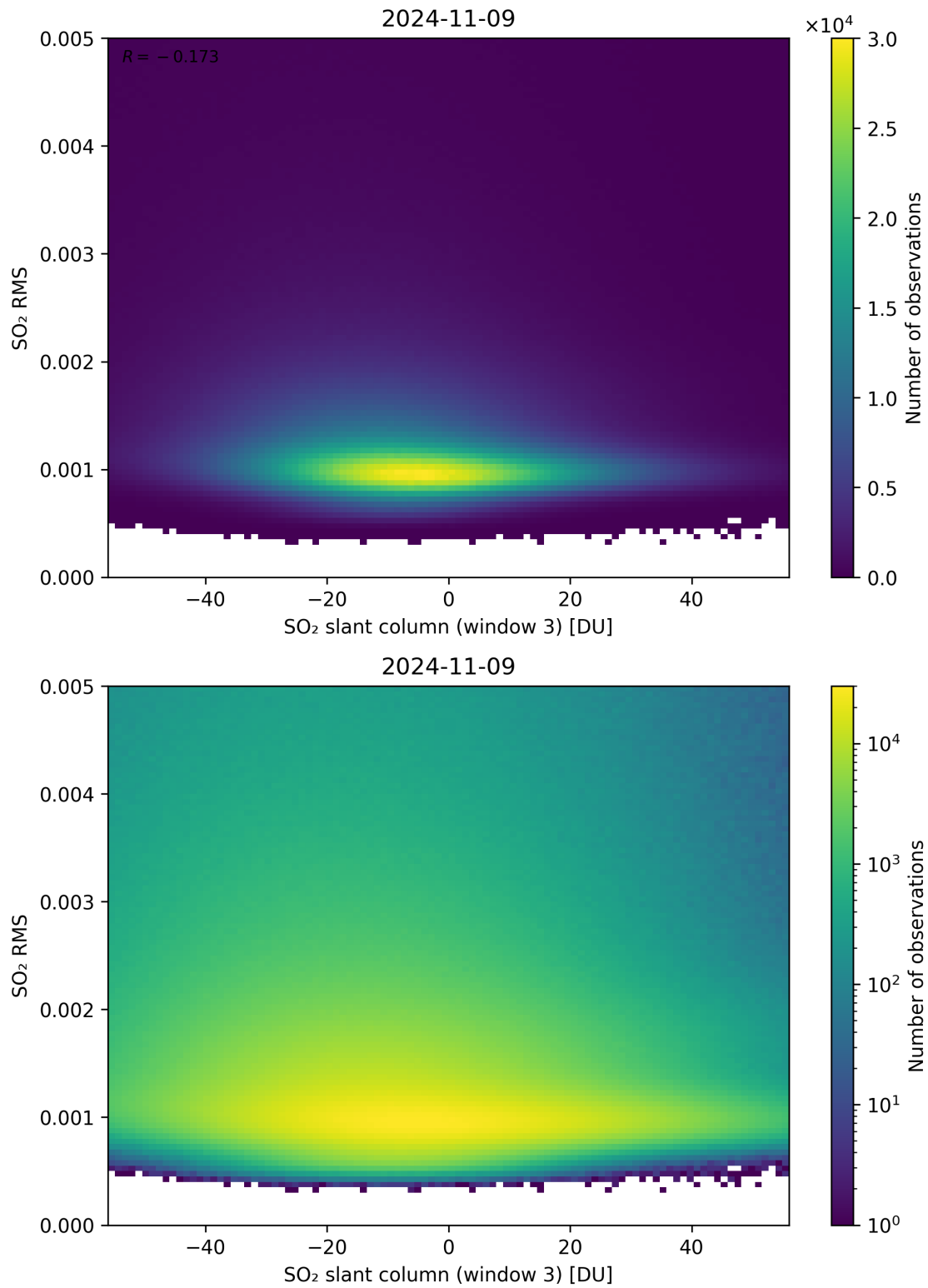
Figure 256: Scatter density plot of “SO 2 slant column (window 3)” against “SO 2 RMS” for 2024-11-09 to 2024-11-10.
