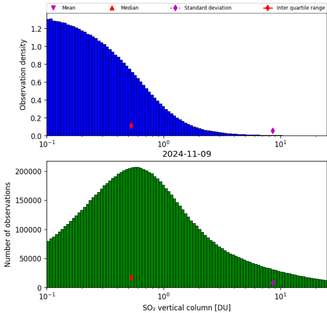
Figure 53: Histogram of “SO 2 vertical column” for 2024-11-09 to 2024-11-10
