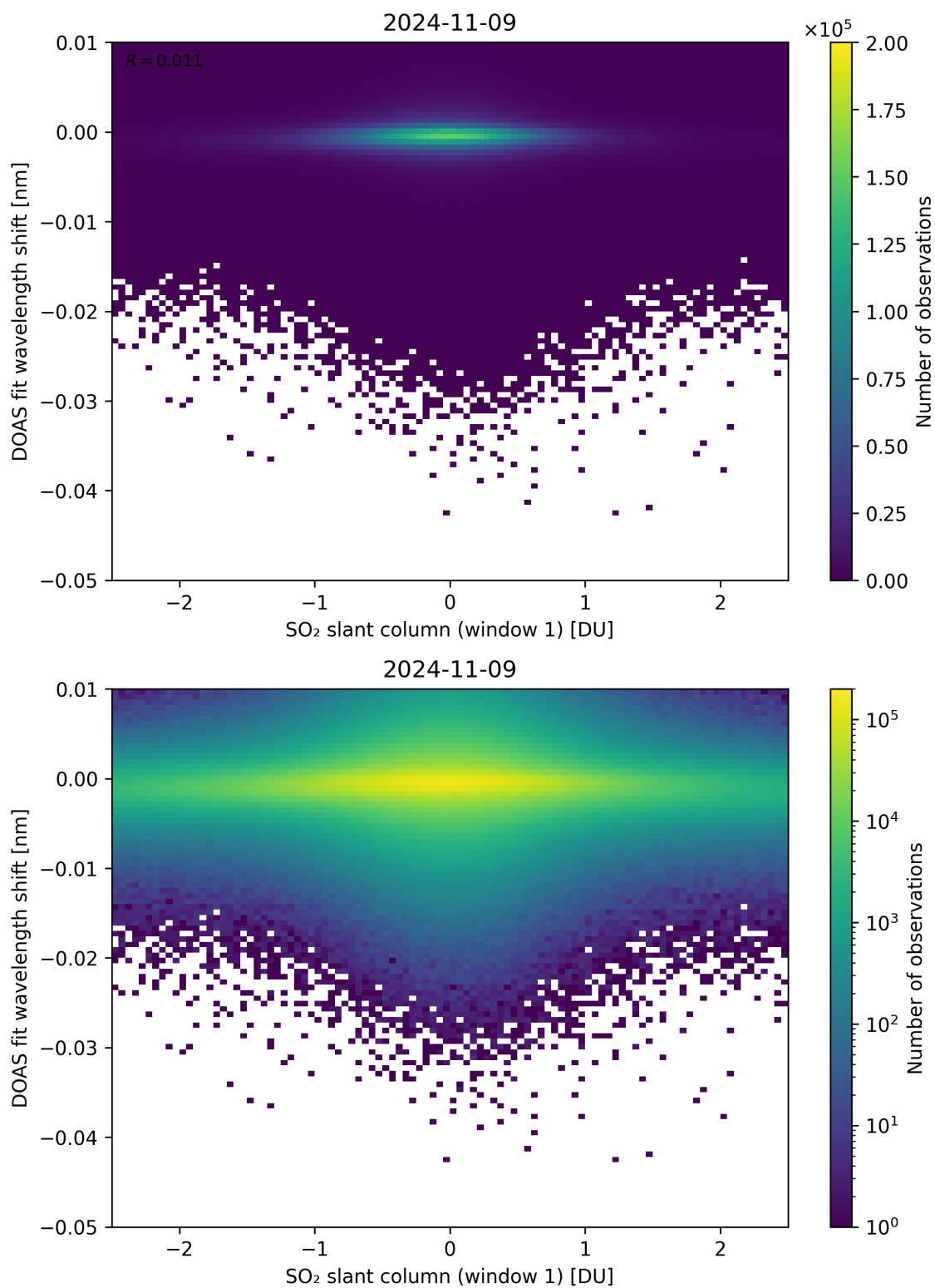
Figure 215: Scatter density plot of “SO 2 slant column (window 1)” against “DOAS fit wavelength shift” for 2024-11-09 to 2024-11-10.
