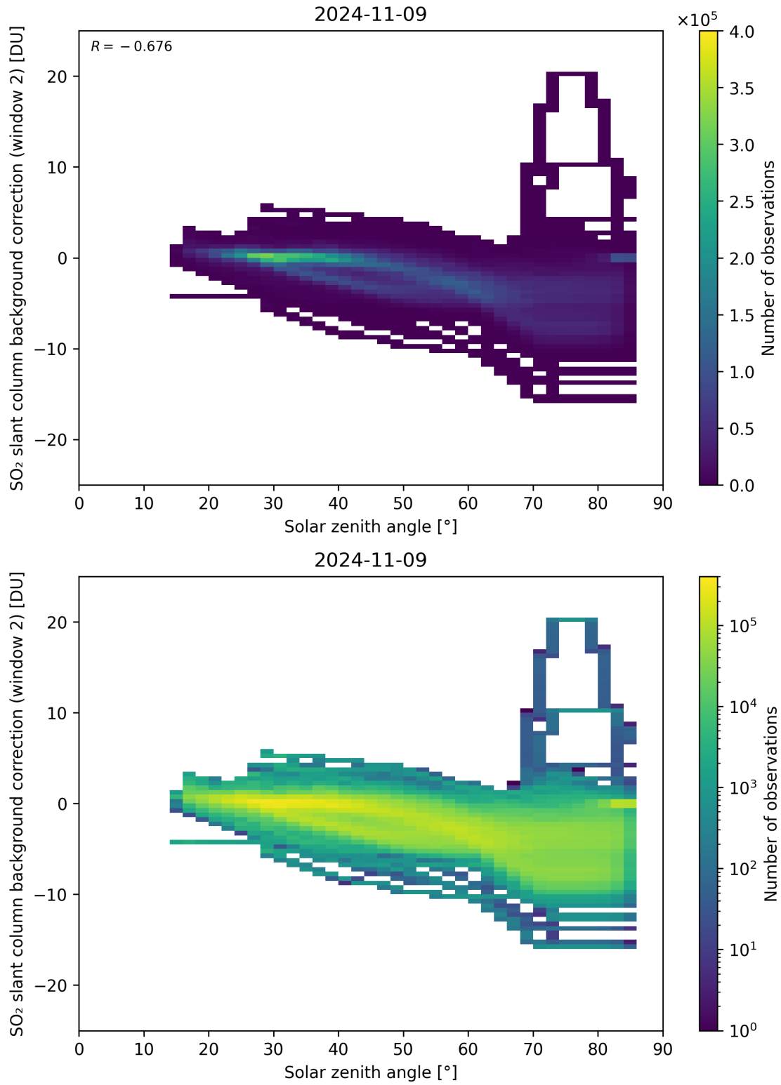
Figure 159: Scatter density plot of “Solar zenith angle” against “SO 2 slant column background correction (window 2)” for 2024-11-09 to 2024-11-10.
