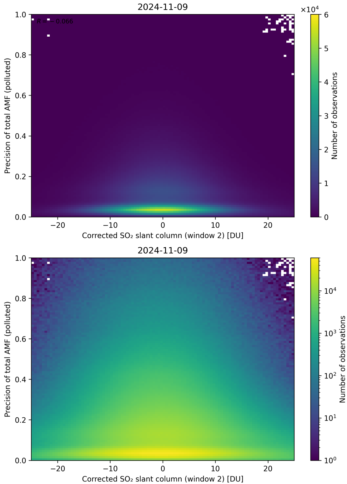
Figure 204: Scatter density plot of “Corrected SO 2 slant column (window 2)” against “Precision of total AMF (polluted)” for 2024-11-09 to 2024-11-10.
