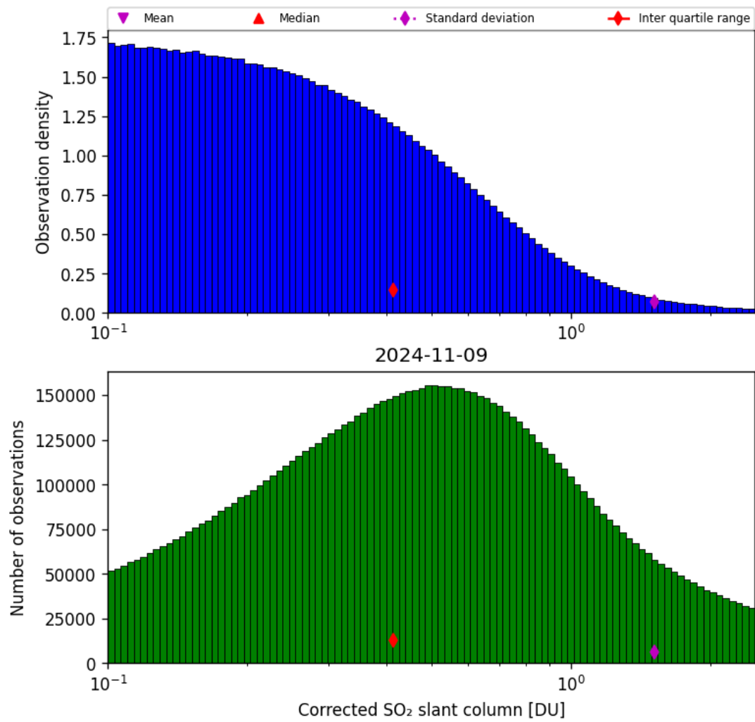
Figure 55: Histogram of "Corrected SO 2 slant column" for 2024-11-09 to 2024-11-10
