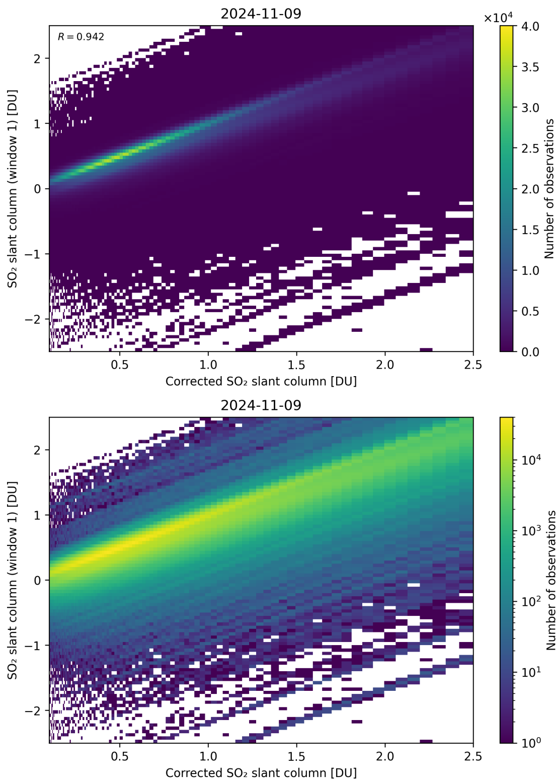
Figure 187: Scatter density plot of “Corrected SO 2 slant column” against “SO 2 slant column (window 1)” for 2024-11-09 to 2024-11-10.
