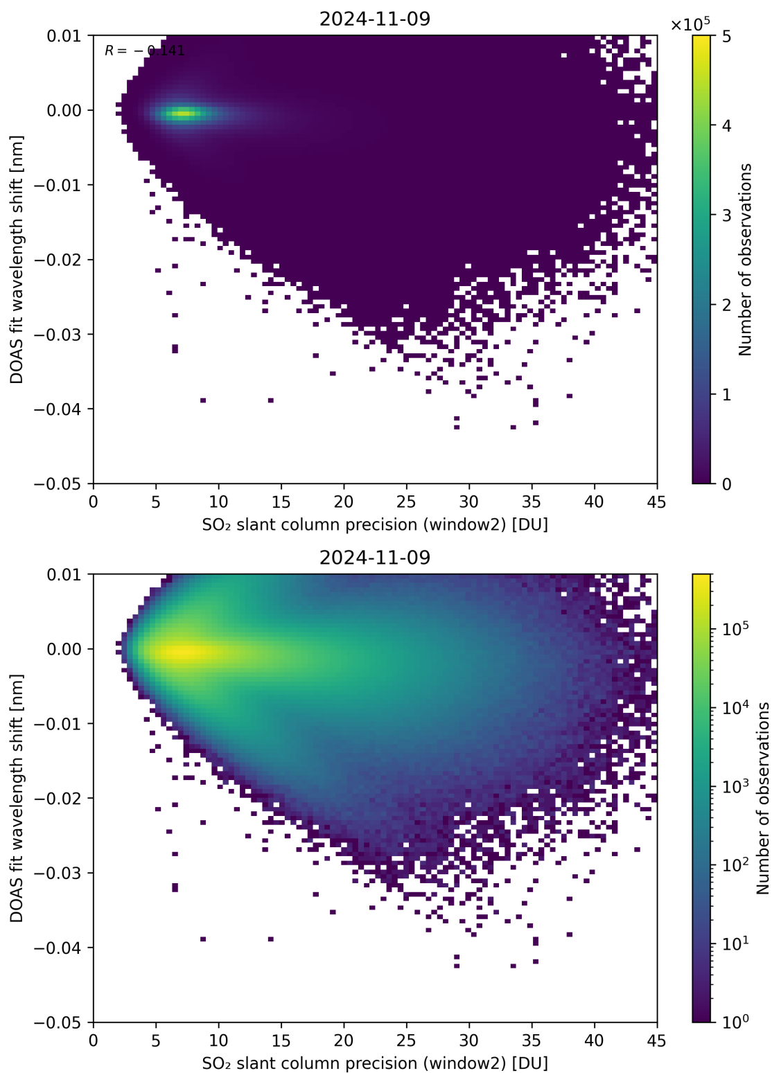
Figure 243: Scatter density plot of “SO 2 slant column precision (window2)” against “DOAS fit wavelength shift” for 2024-11-09 to 2024-11-10.
