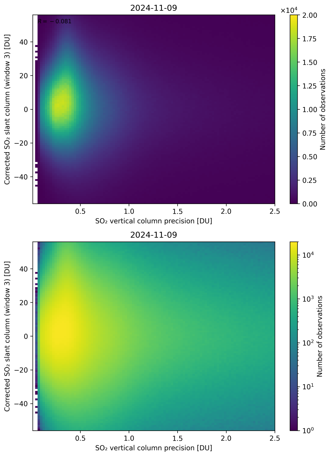
Figure 288: Scatter density plot of “SO 2 vertical column precision” against “Corrected SO 2 slant column (window 3)” for 2024-11-09 to 2024-11-10.
