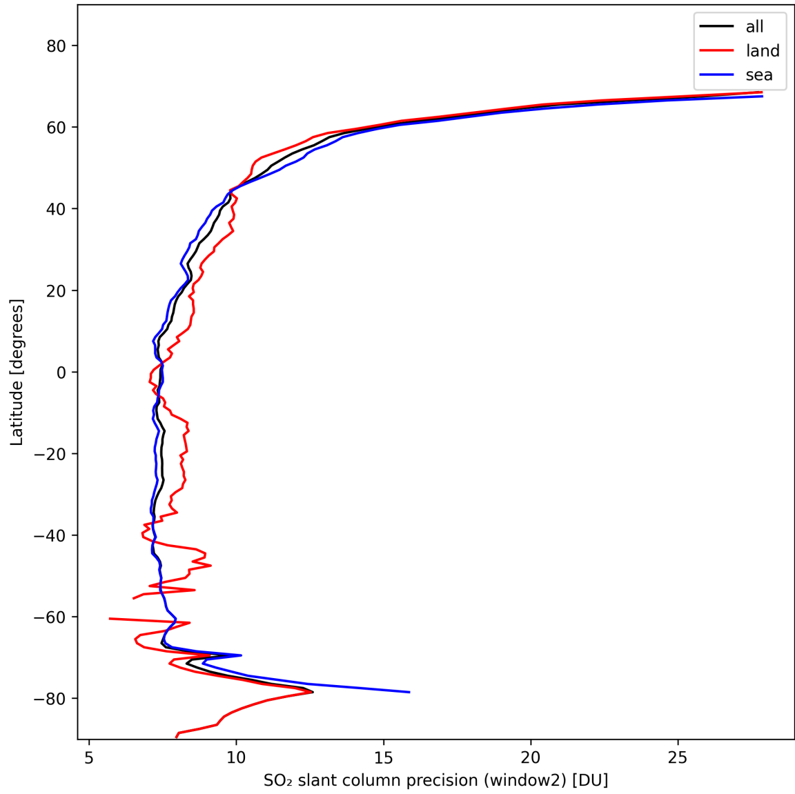
Figure 38: Zonal average of “SO 2 slant column precision (window2)” for 2024-11-09 to 2024-11-10.
