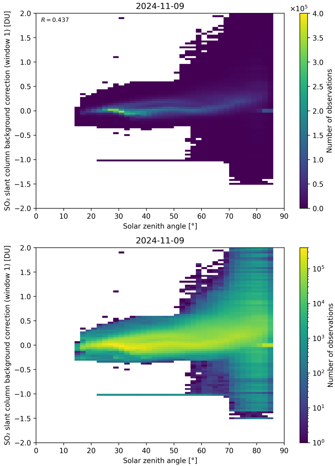
Figure 158: Scatter density plot of “Solar zenith angle” against “SO 2 slant column background correction (window 1)” for 2024-11-09 to 2024-11-10.
