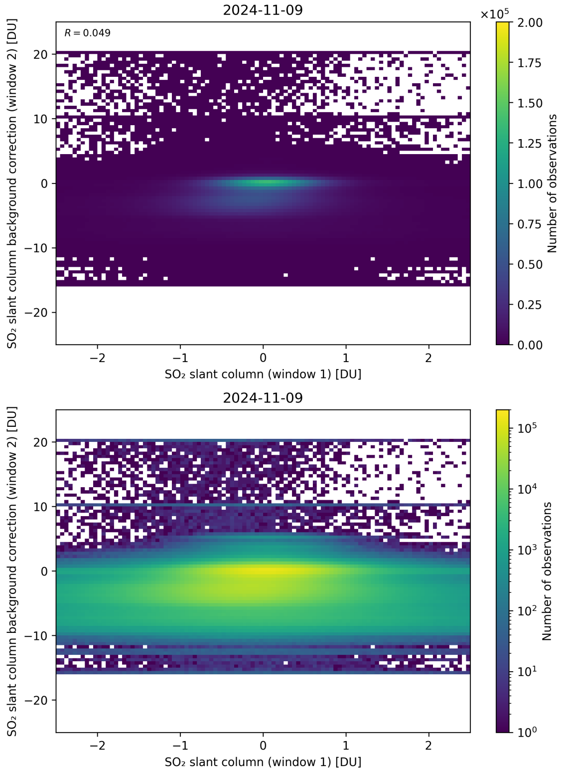
Figure 213: Scatter density plot of “SO 2 slant column (window 1)” against “SO 2 slant column background correction (window 2)” for 2024-11-09 to 2024-11-10.
