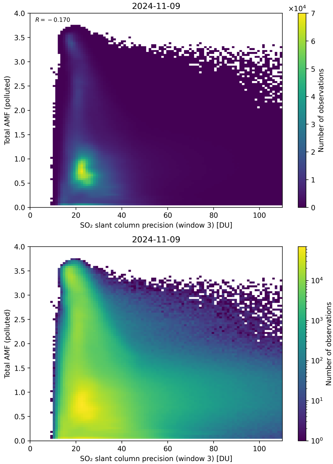
Figure 263: Scatter density plot of “SO 2 slant column precision (window 3)” against “Total AMF (polluted)” for 2024-11-09 to 2024-11-10.
