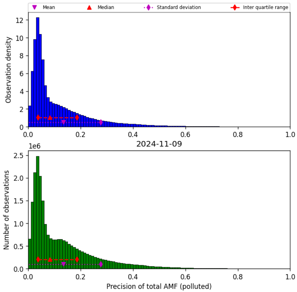
Figure 72: Histogram of “Precision of total AMF (polluted)” for 2024-11-09 to 2024-11-10
