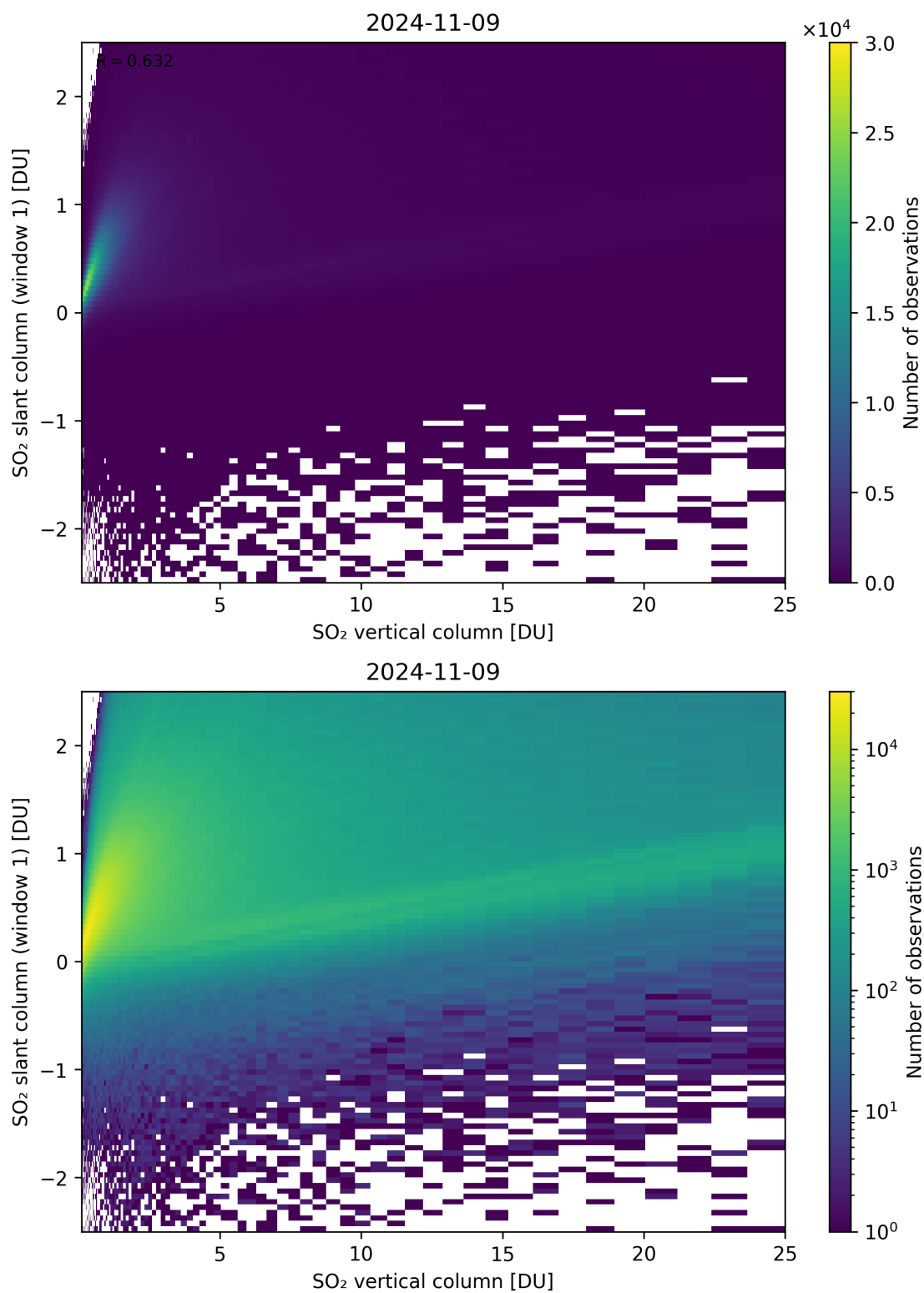
Figure 300: Scatter density plot of “SO 2 vertical column” against “SO 2 slant column (window 1)” for 2024-11-09 to 2024-11-10.
