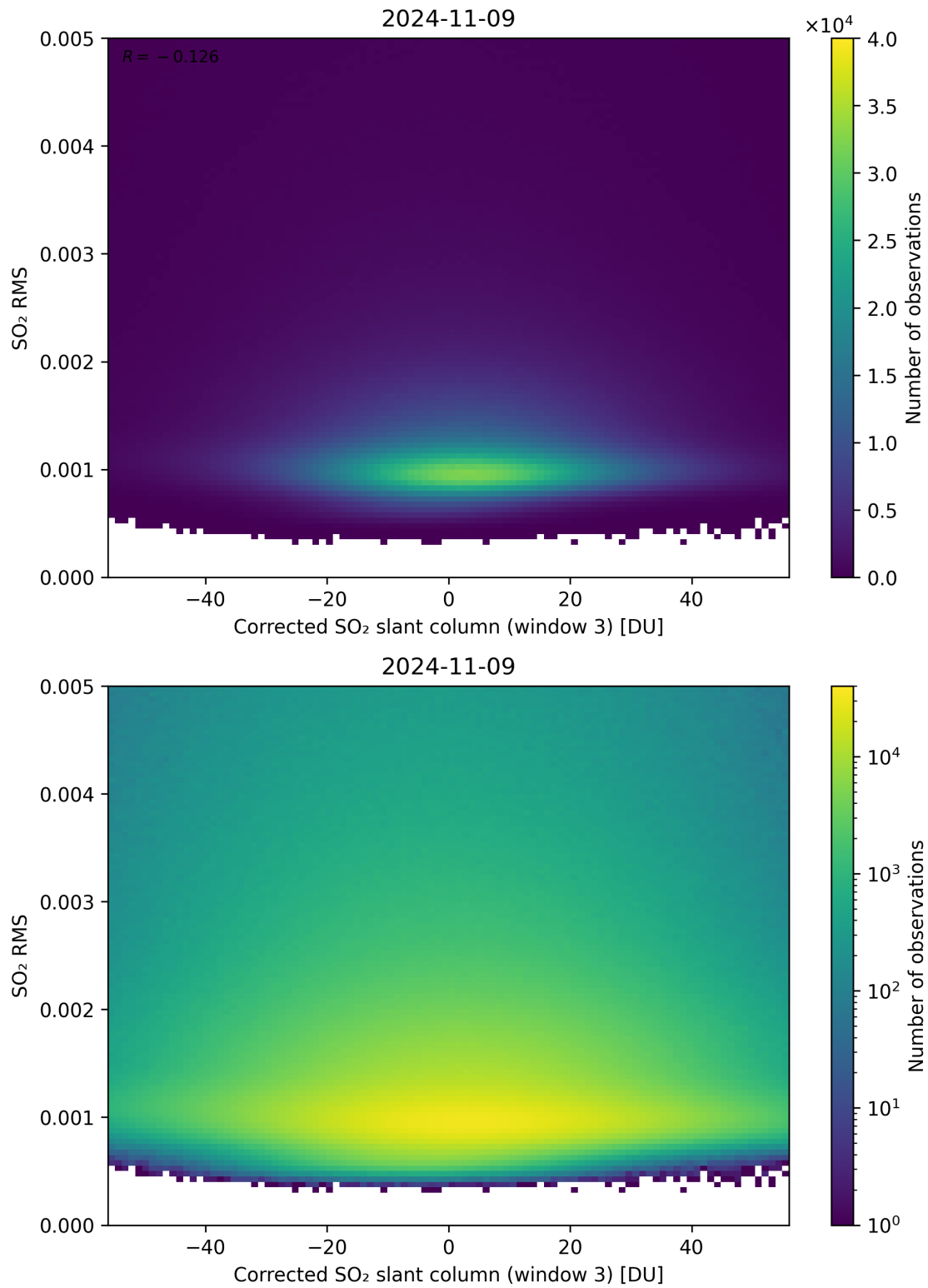
Figure 208: Scatter density plot of “Corrected SO 2 slant column (window 3)” against “SO 2 RMS” for 2024-11-09 to 2024-11-10.
