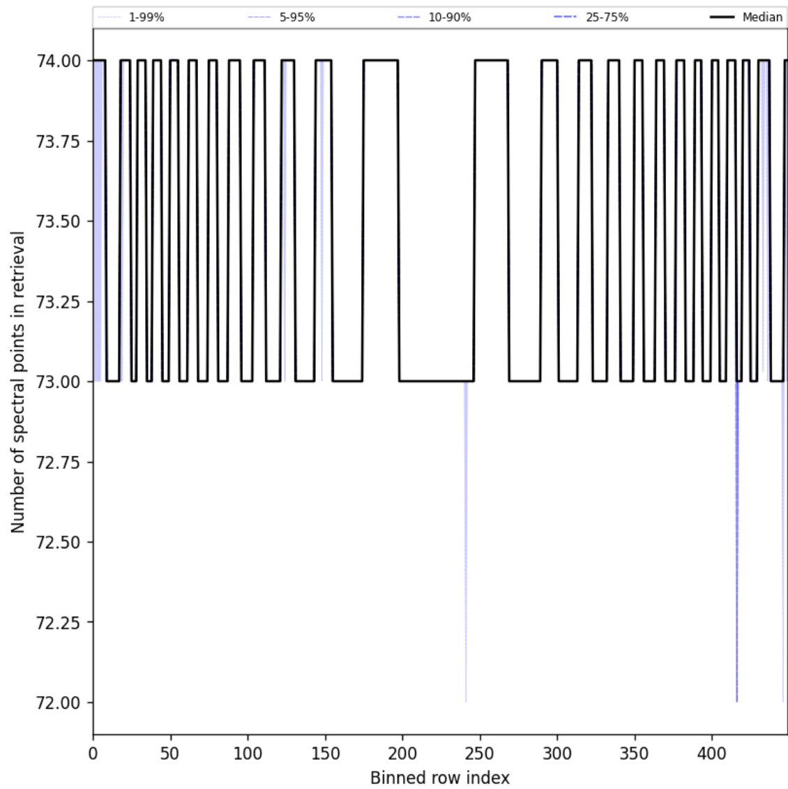
Figure 97: Along track statistics of “Number of spectral points in retrieval” for 2024-11-09 to 2024-11-10
