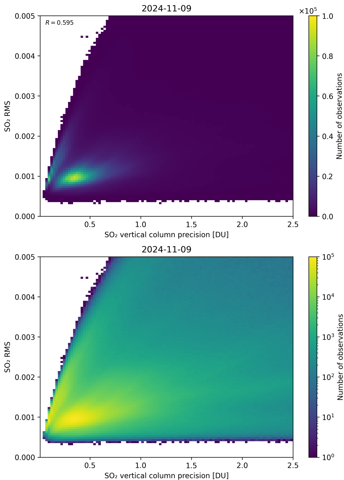
Figure 284: Scatter density plot of “SO 2 vertical column precision” against “SO 2 RMS” for 2024-11-09 to 2024-11-10.
