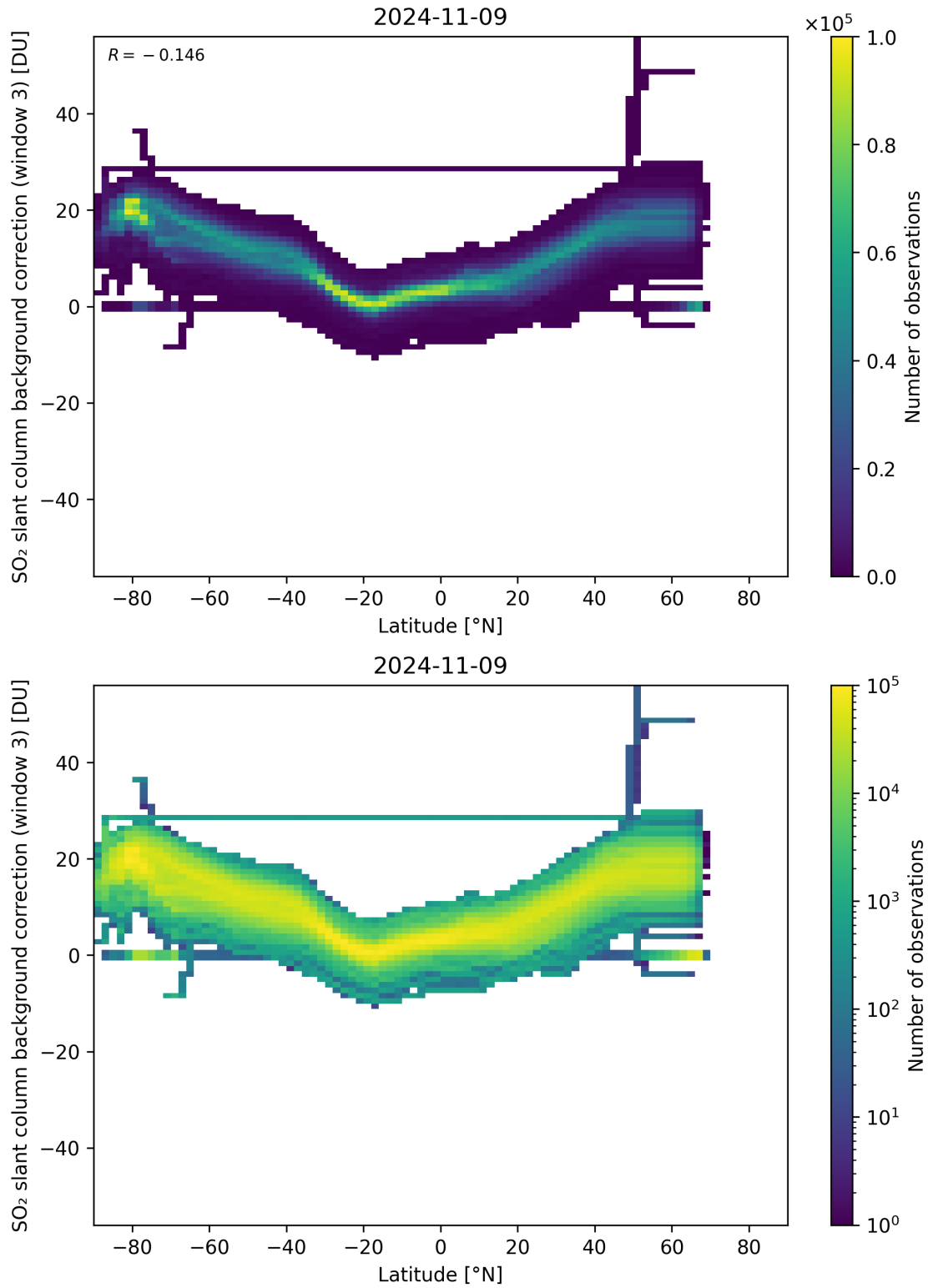
Figure 141: Scatter density plot of “Latitude” against “SO 2 slant column background correction (window 3)” for 2024-11-09 to 2024-11-10.
