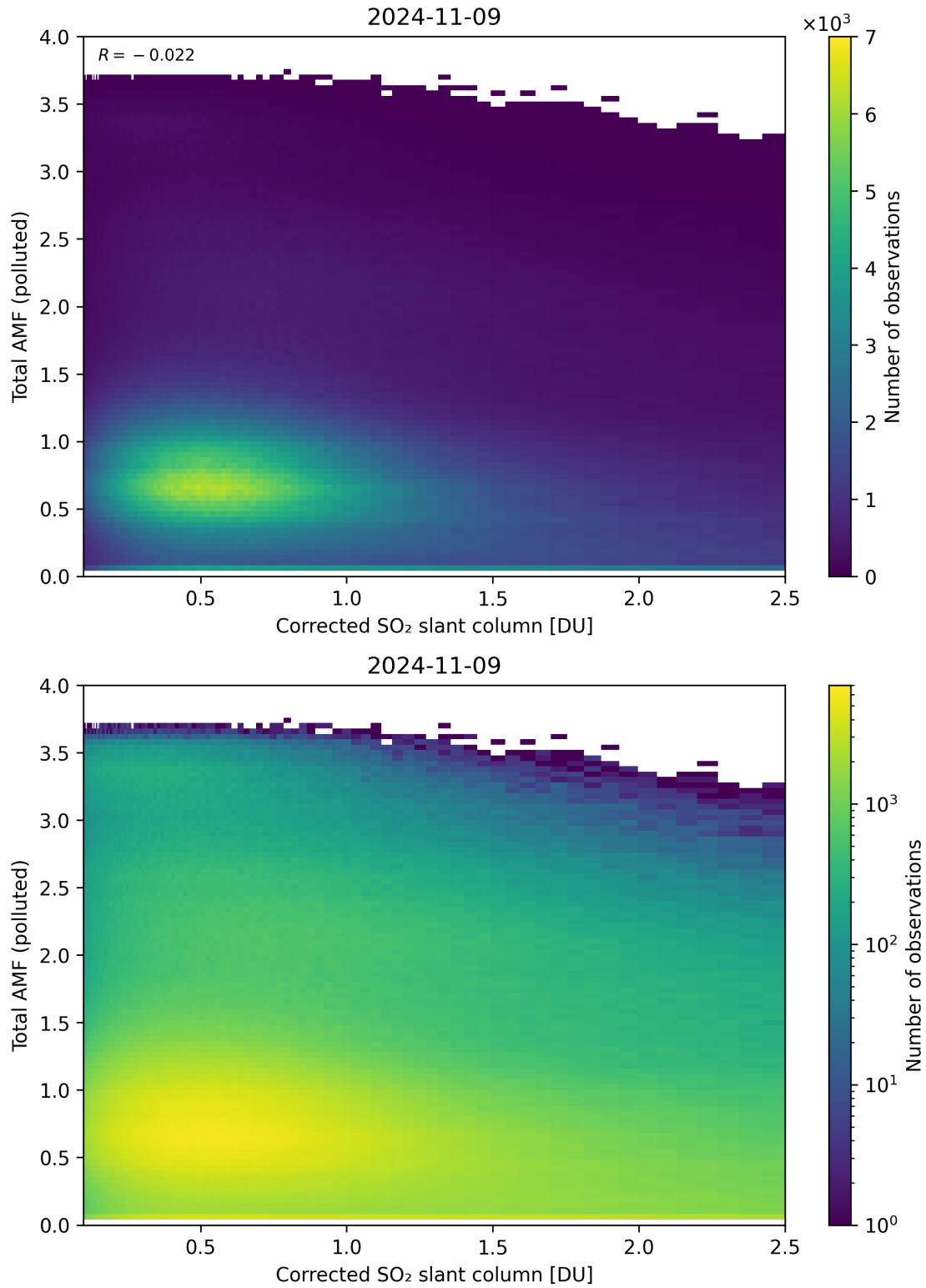
Figure 192: Scatter density plot of “Corrected SO 2 slant column” against “Total AMF (polluted)” for 2024-11-09 to 2024-11-10.
