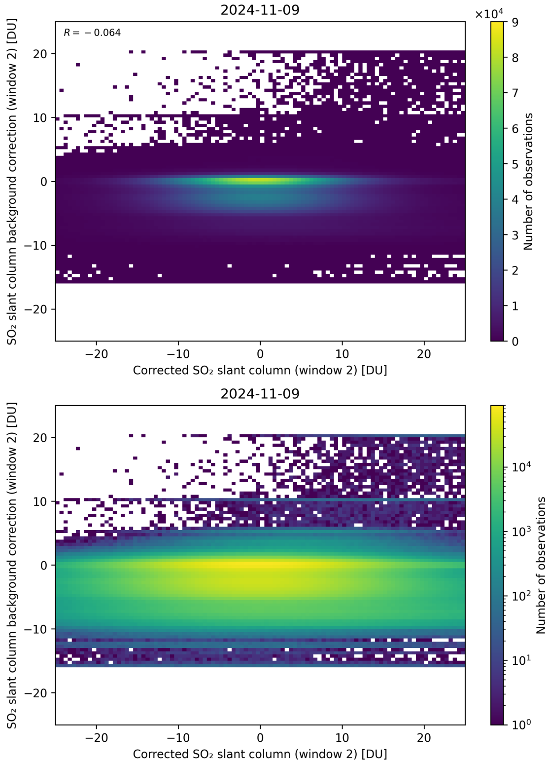
Figure 194: Scatter density plot of “Corrected SO 2 slant column (window 2)” against “SO 2 slant column background correction (window 2)” for 2024-11-09 to 2024-11-10.
