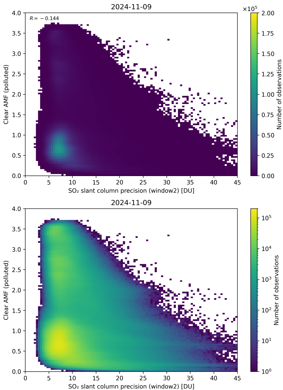
Figure 246: Scatter density plot of “SO 2 slant column precision (window2)” against “Clear AMF (polluted)” for 2024-11-09 to 2024-11-10.
