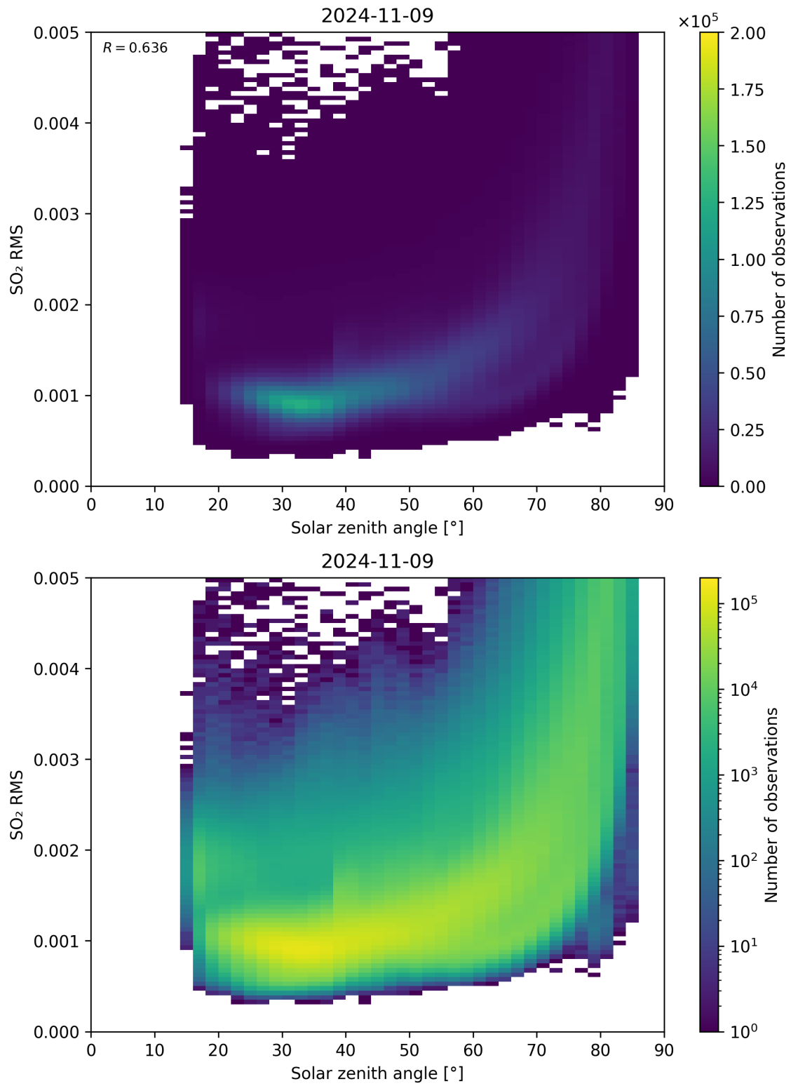
Figure 163: Scatter density plot of “Solar zenith angle” against “SO 2 RMS” for 2024-11-09 to 2024-11-10.
