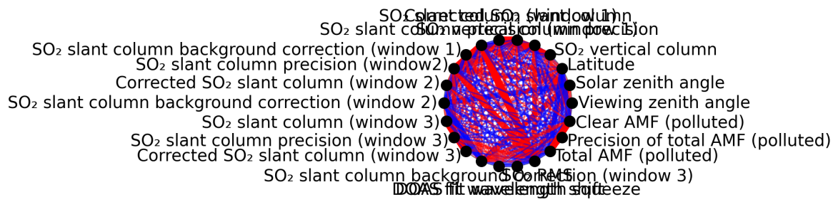
Figure 1: Map of correlation graph for 2024-11-09 to 2024-11-10.
