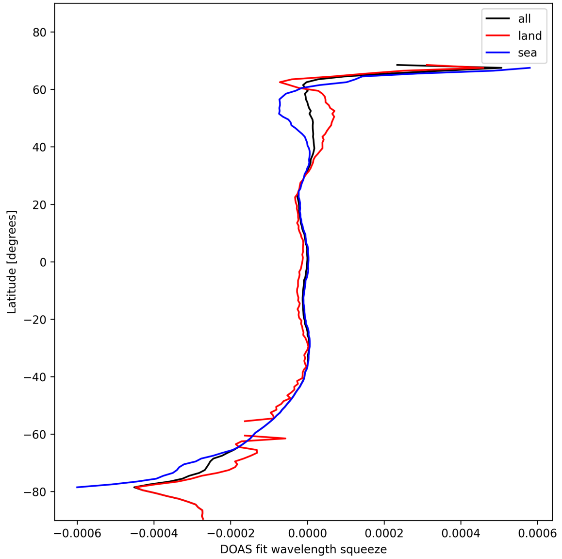
Figure 46: Zonal average of “DOAS fit wavelength squeeze” for 2024-11-09 to 2024-11-10.
