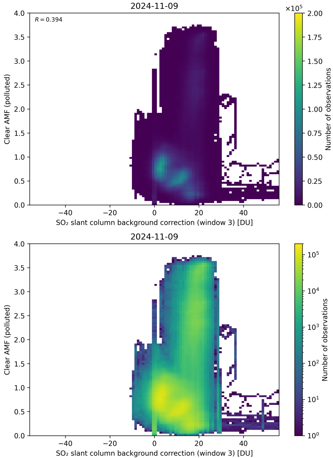
Figure 124: Scatter density plot of “SO 2 slant column background correction (window 3)” against “Clear AMF (polluted)” for 2024-11-09 to 2024-11-10.
