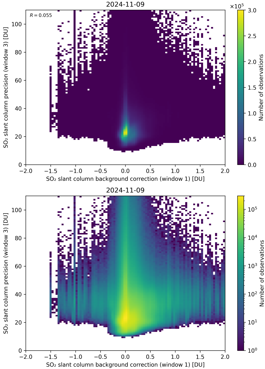
Figure 108: Scatter density plot of “SO 2 slant column background correction (window 1)” against “SO 2 slant column precision (window 3)” for 2024-11-09 to 2024-11-10.
