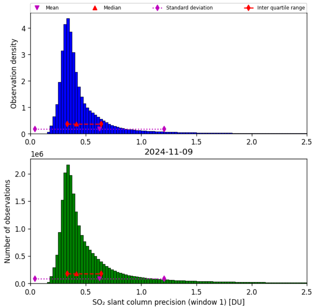
Figure 57: Histogram of “SO 2 slant column precision (window 1)” for 2024-11-09 to 2024-11-10
