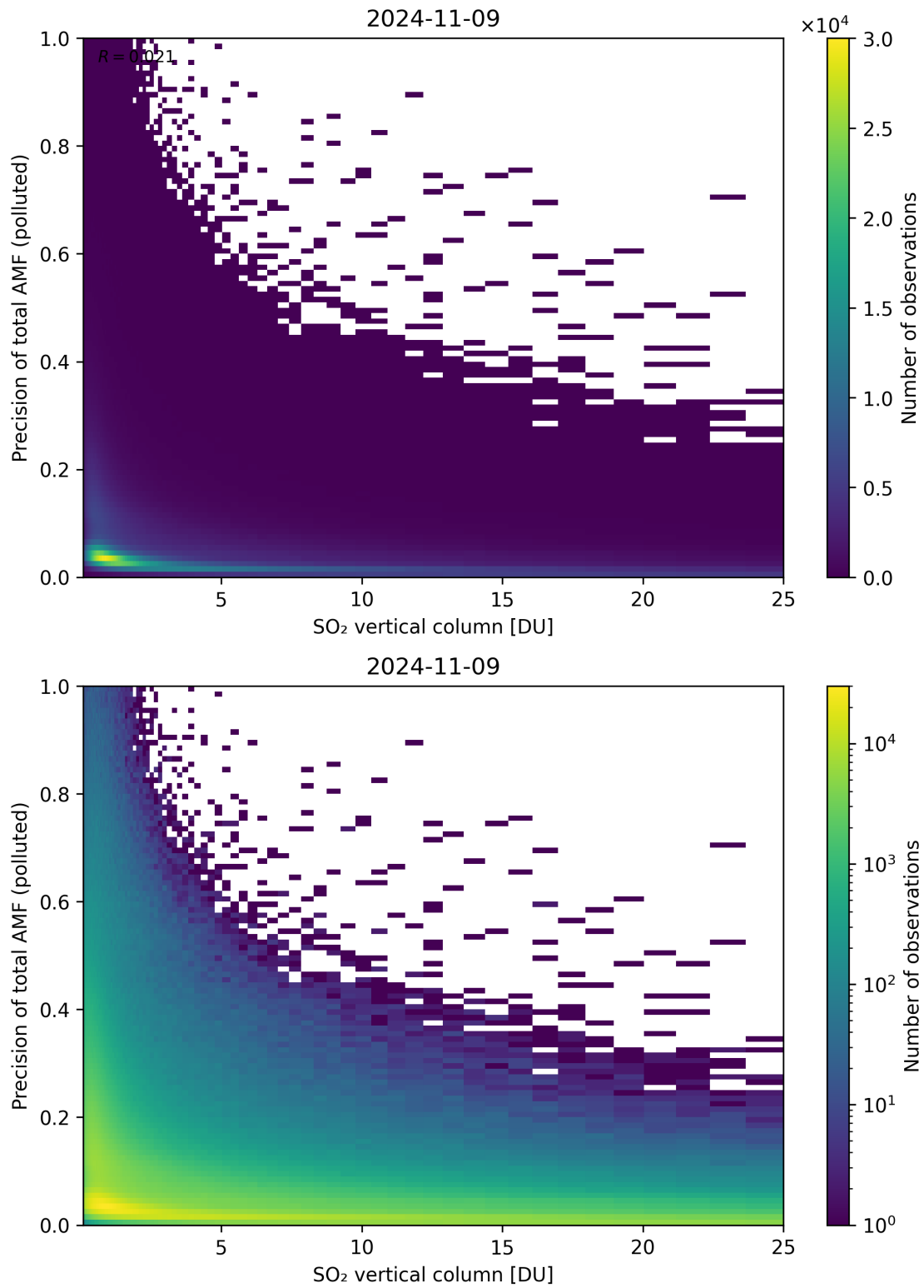
Figure 306: Scatter density plot of “SO 2 vertical column” against “Precision of total AMF (polluted)” for 2024-11-09 to 2024-11-10.
