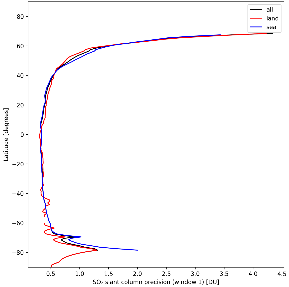
Figure 34: Zonal average of “SO 2 slant column precision (window 1)” for 2024-11-09 to 2024-11-10.
