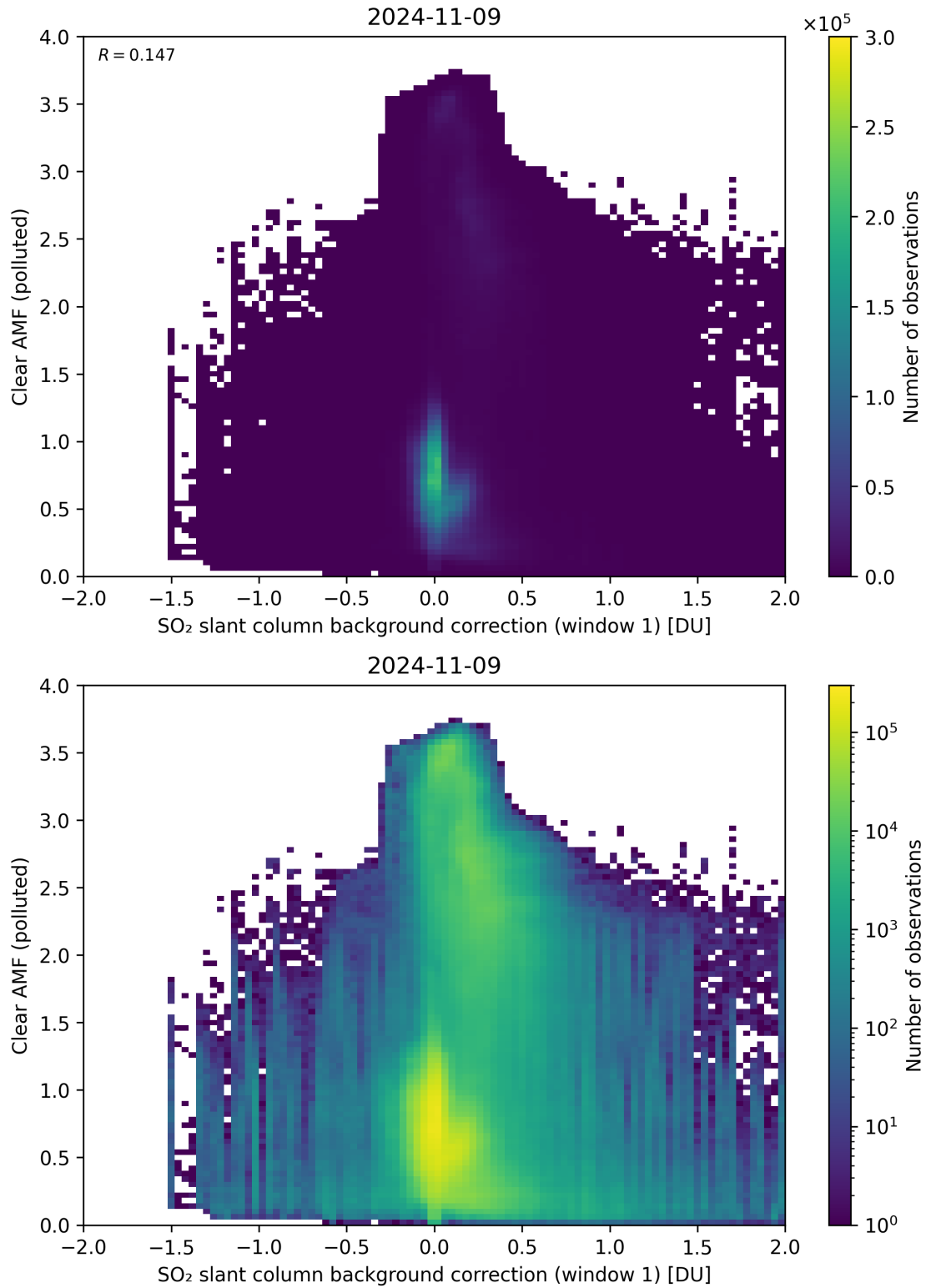
Figure 103: Scatter density plot of “SO 2 slant column background correction (window 1)” against “Clear AMF (polluted)” for 2024-11-09 to 2024-11-10.
