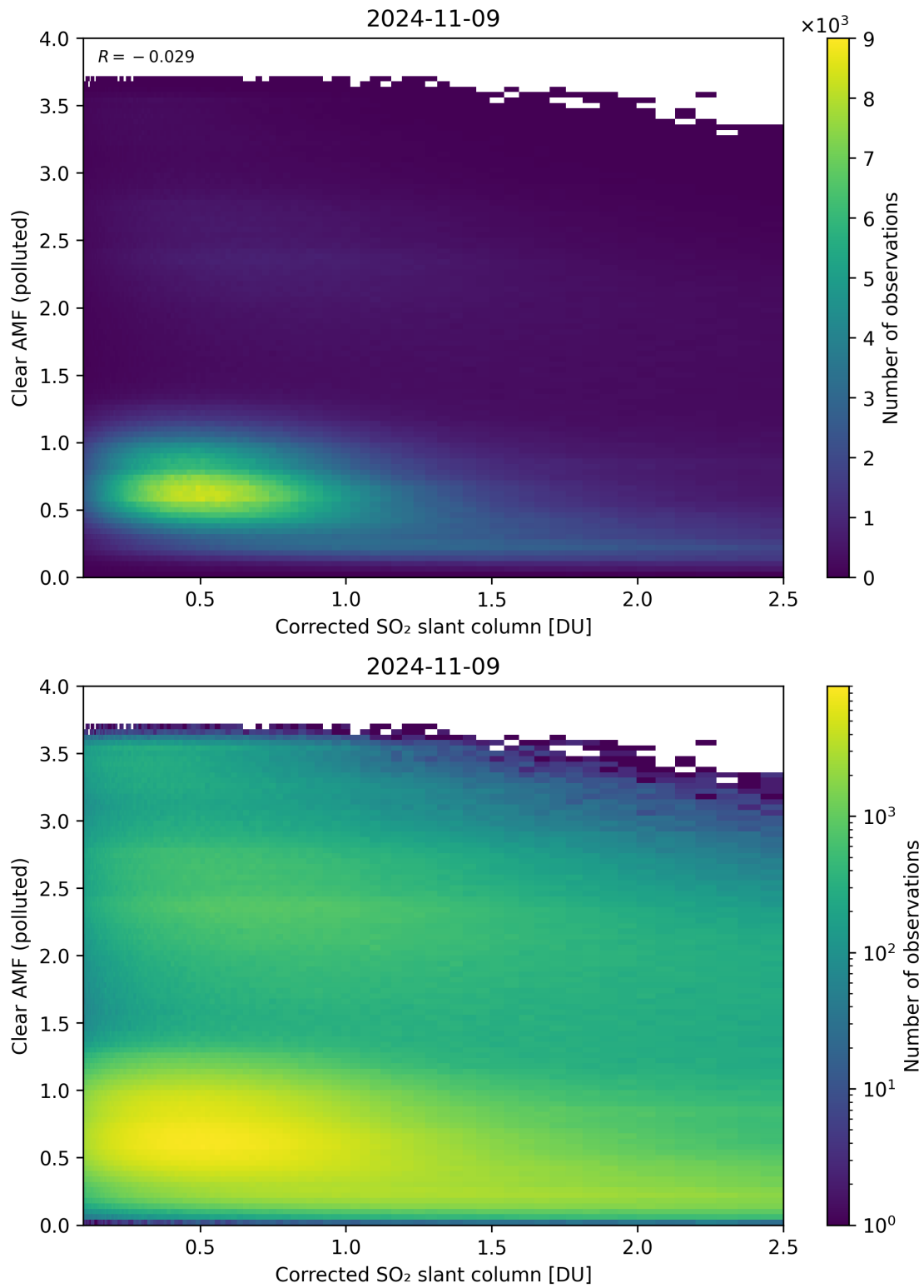
Figure 184: Scatter density plot of “Corrected SO 2 slant column” against “Clear AMF (polluted)” for 2024-11-09 to 2024-11-10.
