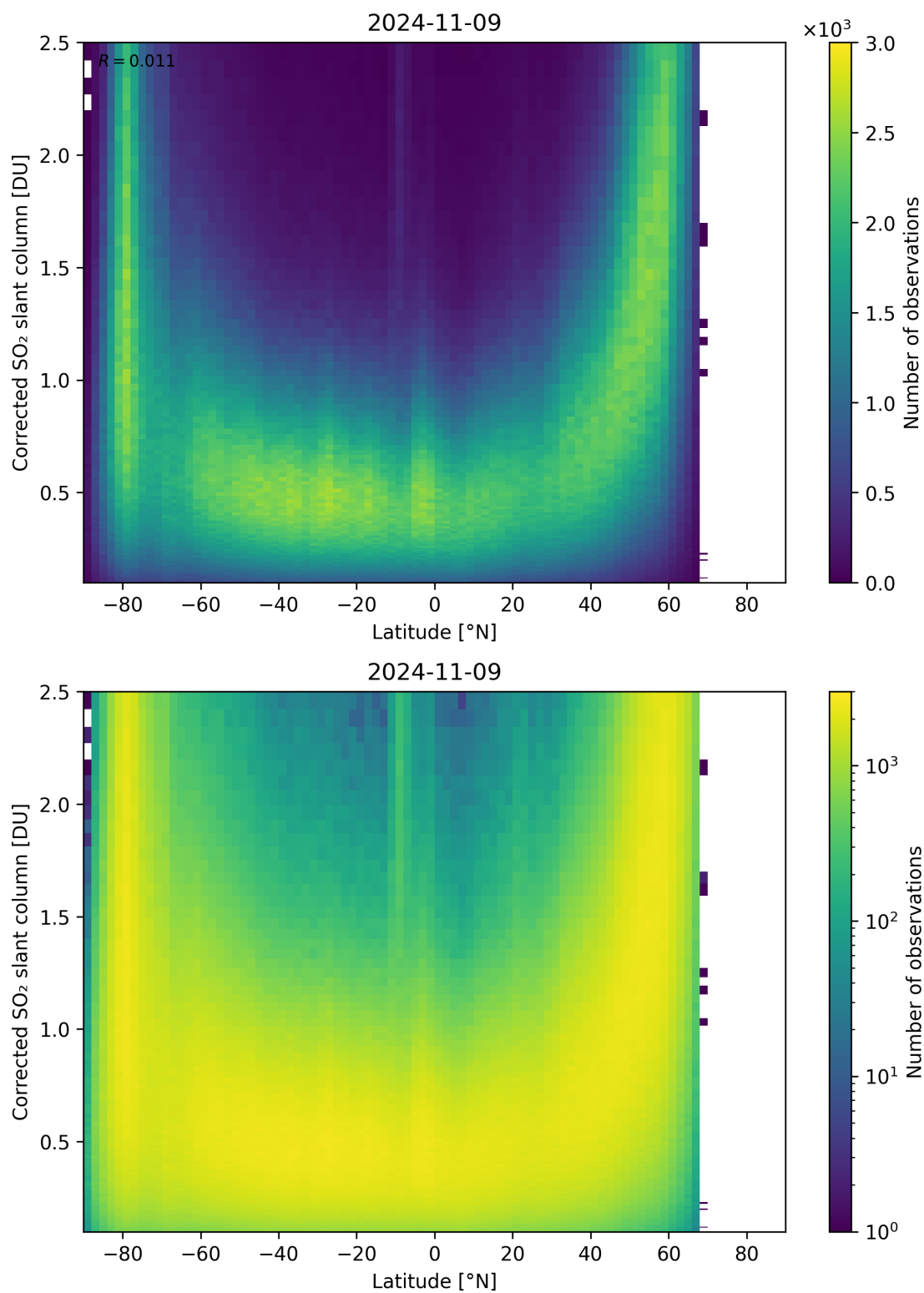
Figure 146: Scatter density plot of “Latitude” against “Corrected SO 2 slant column” for 2024-11-09 to 2024-11-10.
