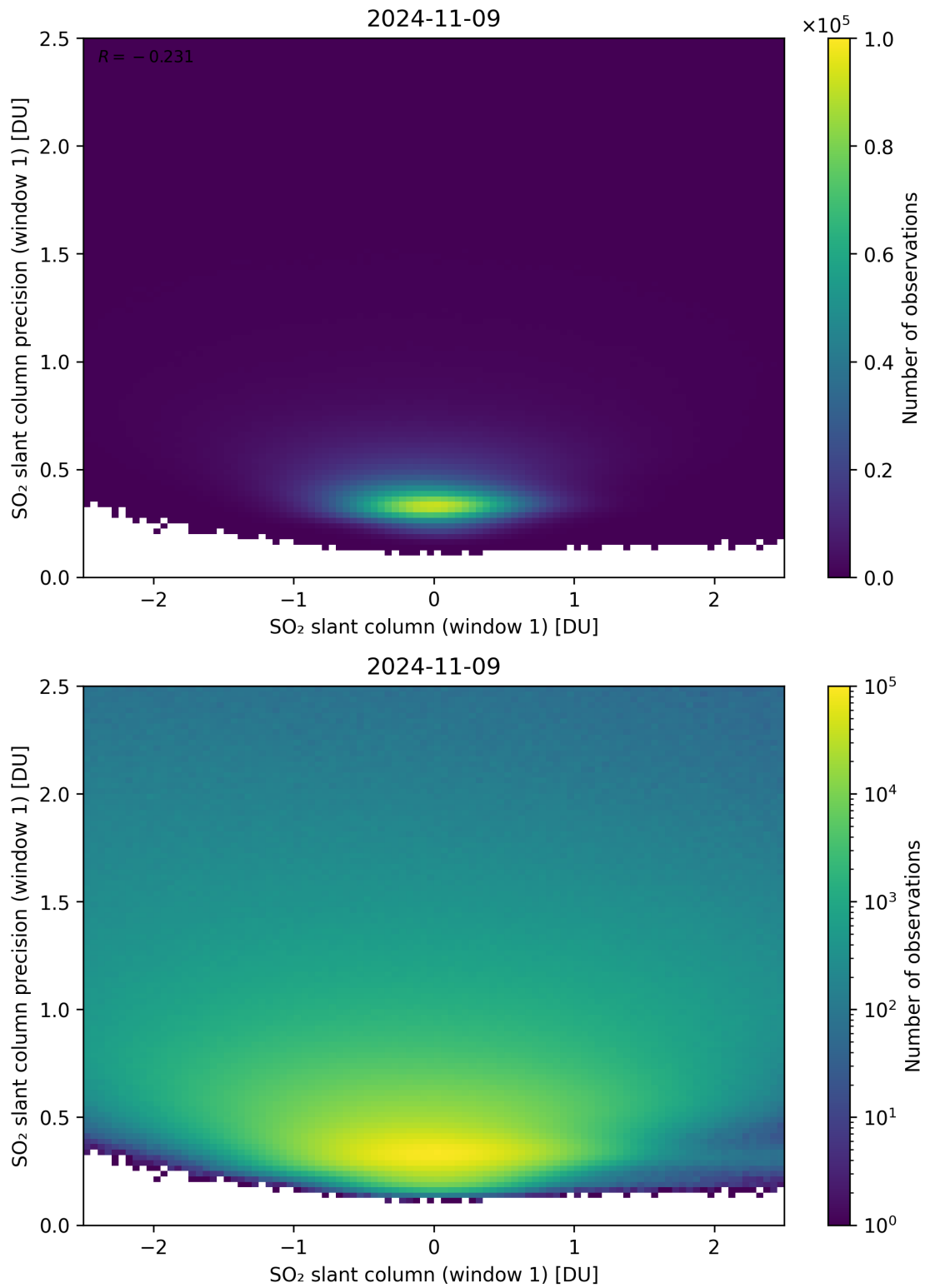
Figure 235: Scatter density plot of “SO 2 slant column (window 1)” against “SO 2 slant column precision (window 1)” for 2024-11-09 to 2024-11-10.
