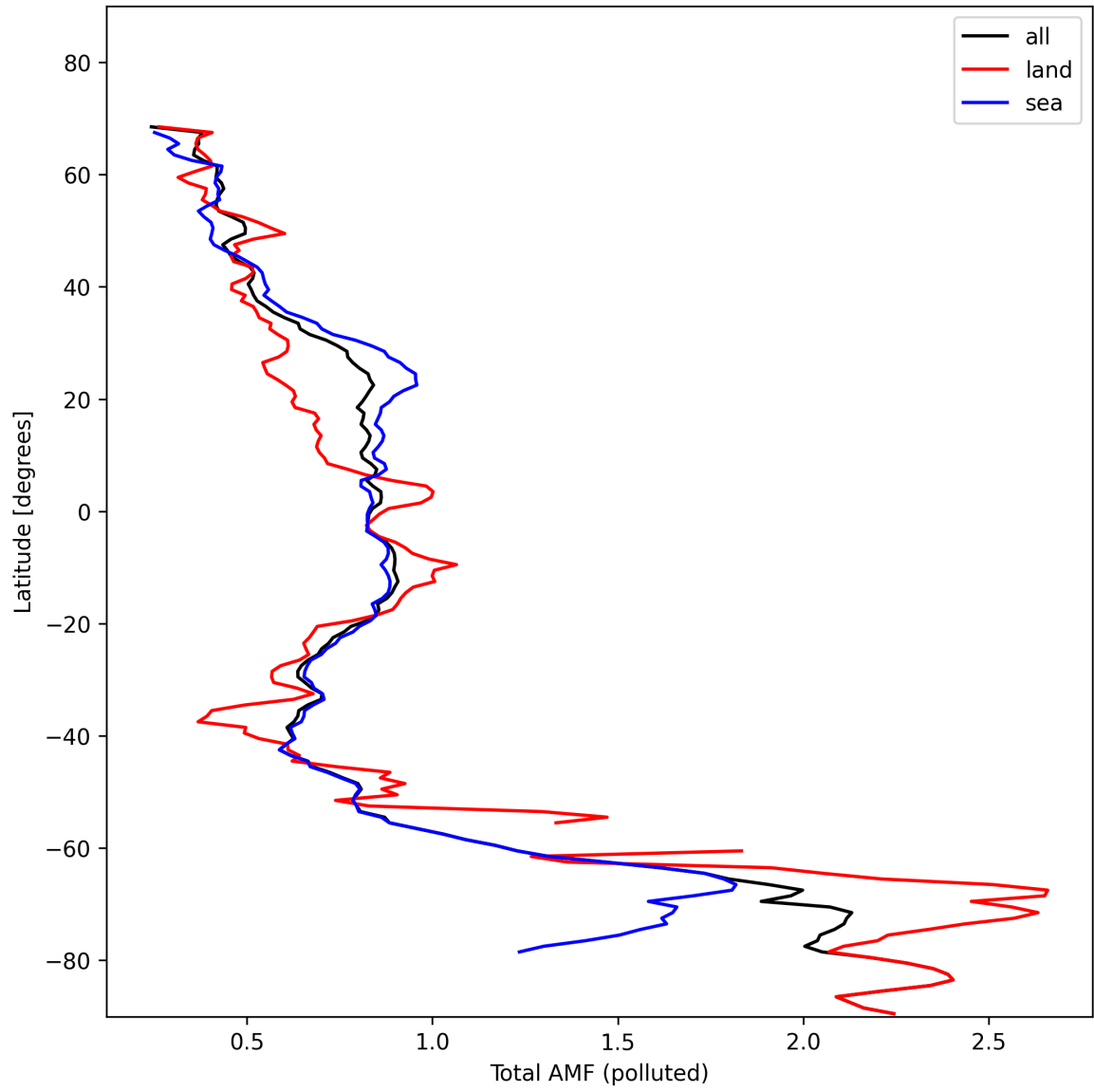
Figure 48: Zonal average of “Total AMF (polluted)” for 2024-11-09 to 2024-11-10.
