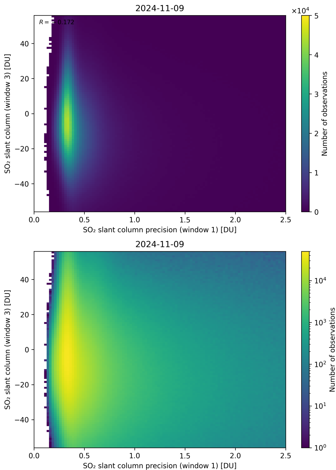
Figure 228: Scatter density plot of “SO 2 slant column precision (window 1)” against “SO 2 slant column (window 3)” for 2024-11-09 to 2024-11-10.
