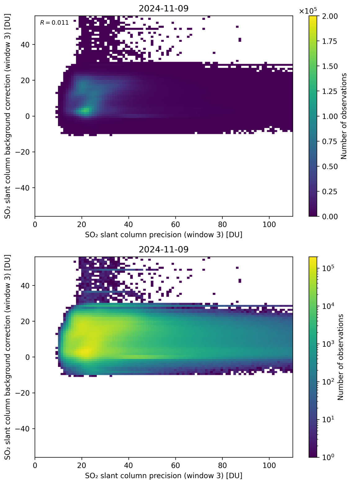
Figure 257: Scatter density plot of “SO 2 slant column precision (window 3)” against “SO 2 slant column background correction (window 3)” for 2024-11-09 to 2024-11-10.
