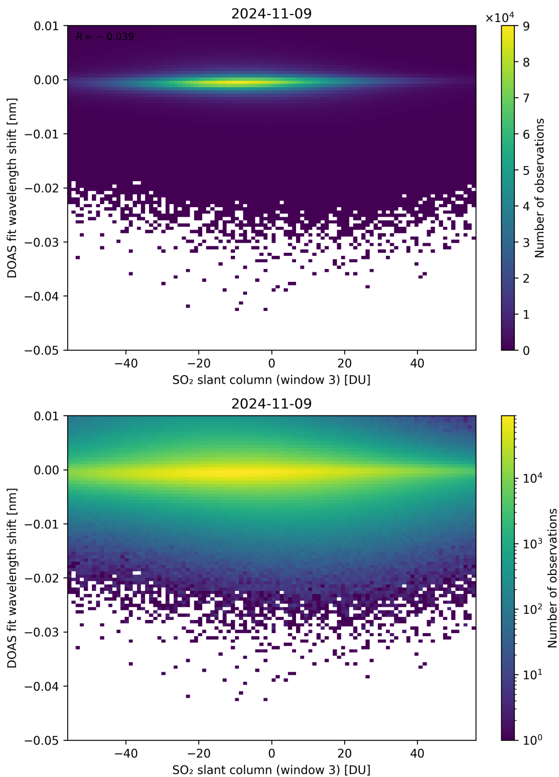
Figure 254: Scatter density plot of “SO 2 slant column (window 3)” against “DOAS fit wavelength shift” for 2024-11-09 to 2024-11-10.
