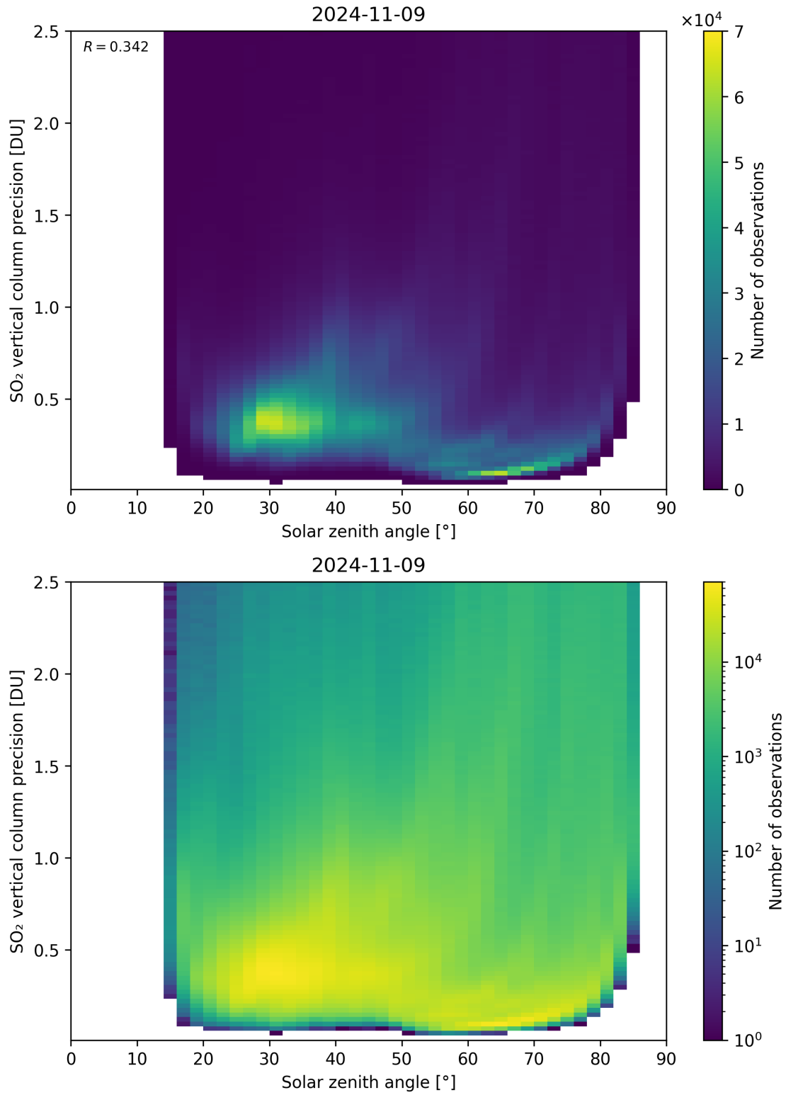
Figure 177: Scatter density plot of “Solar zenith angle” against “SO 2 vertical column precision” for 2024-11-09 to 2024-11-10.
