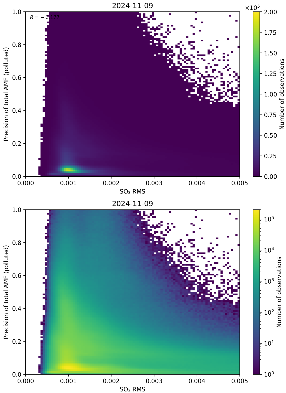
Figure 138: Scatter density plot of “SO 2 RMS” against “Precision of total AMF (polluted)” for 2024-11-09 to 2024-11-10.
