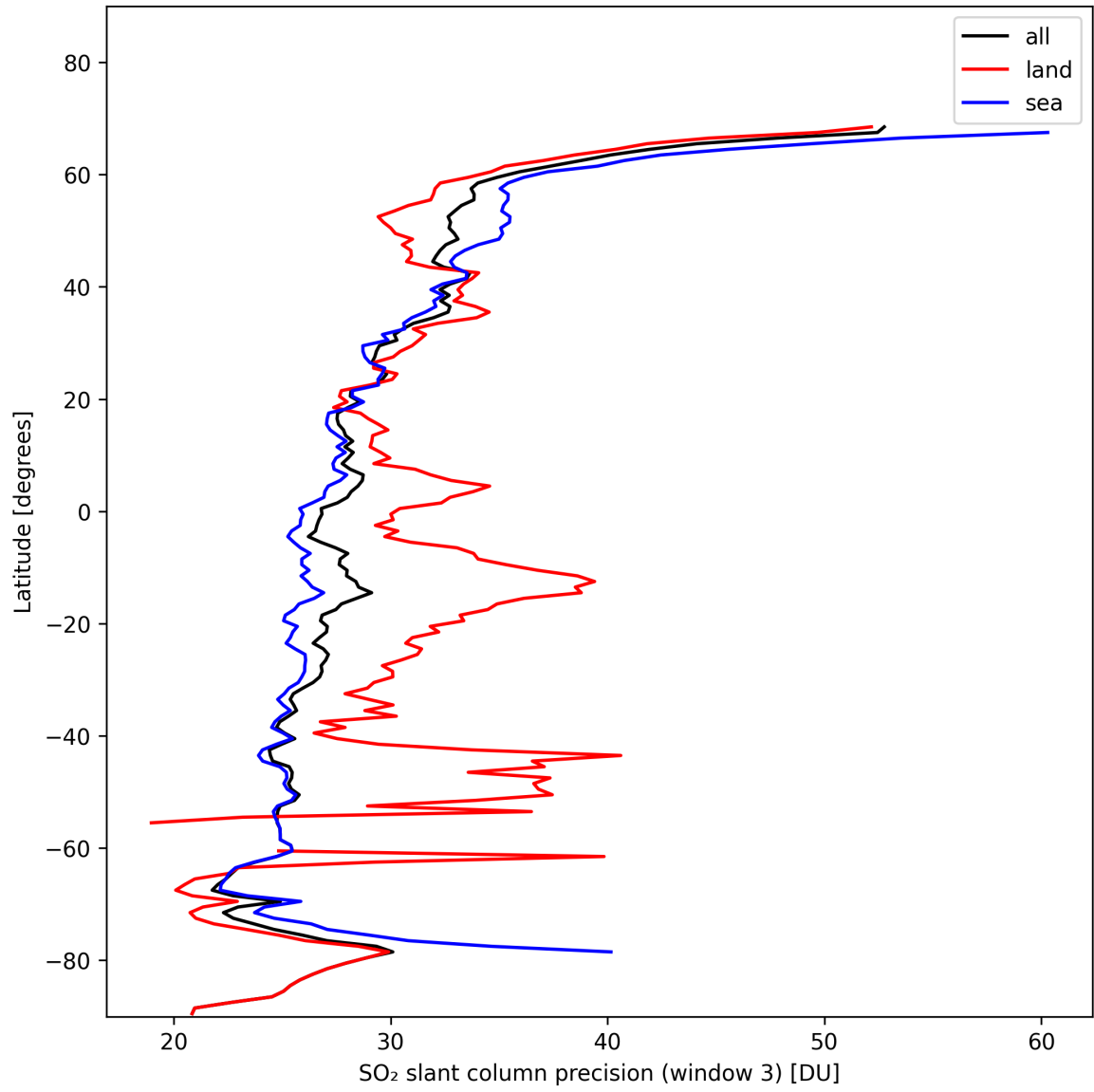
Figure 42: Zonal average of “SO 2 slant column precision (window 3)” for 2024-11-09 to 2024-11-10.
