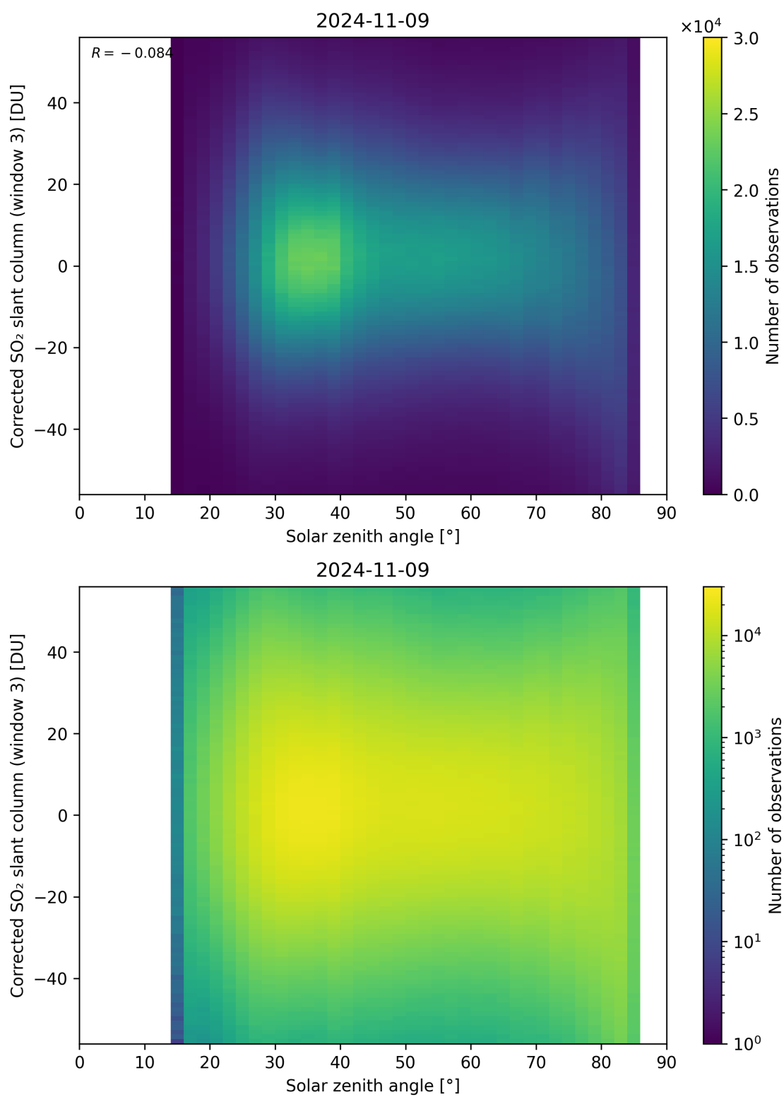
Figure 168: Scatter density plot of “Solar zenith angle” against “Corrected SO 2 slant column (window 3)” for 2024-11-09 to 2024-11-10.
