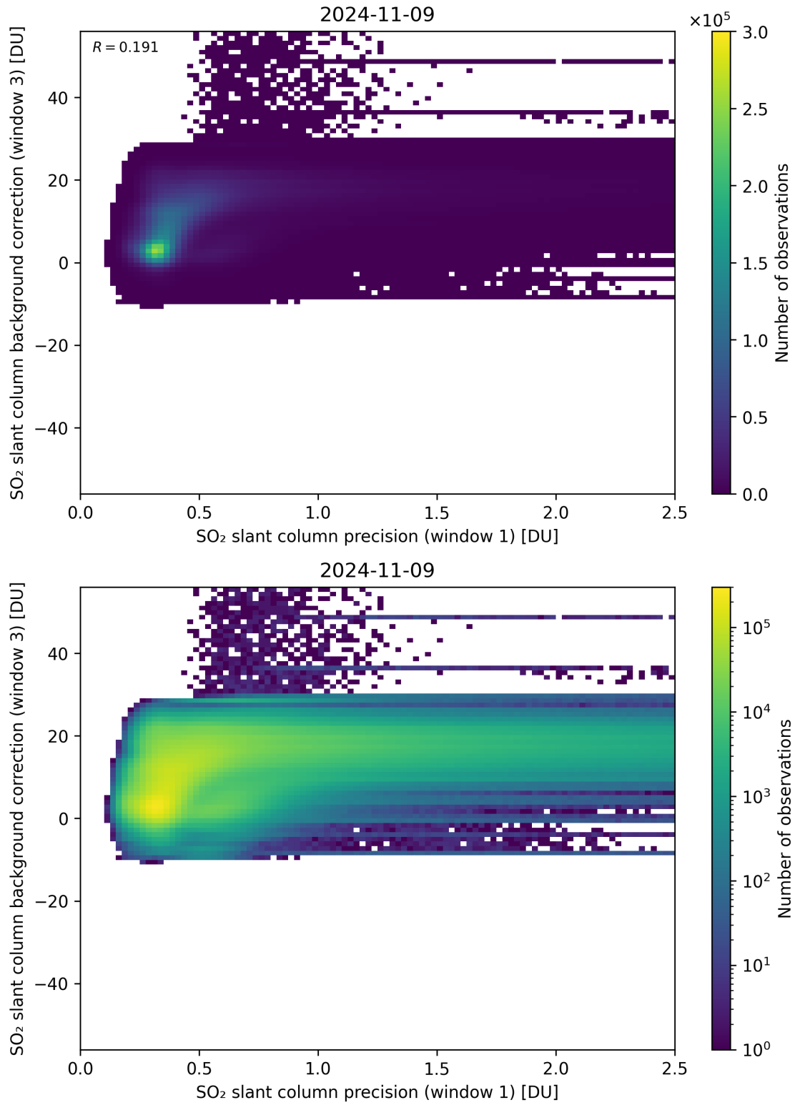
Figure 220: Scatter density plot of “SO 2 slant column precision (window 1)” against “SO 2 slant column background correction (window 3)” for 2024-11-09 to 2024-11-10.
