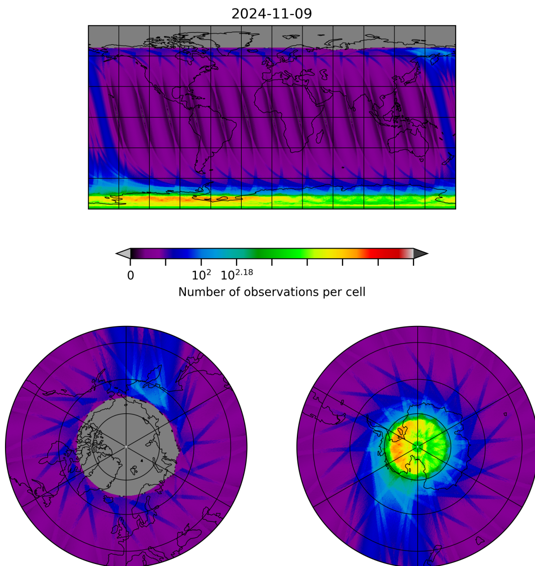
Figure 28: Map of the number of observations for 2024-11-09 to 2024-11-10
