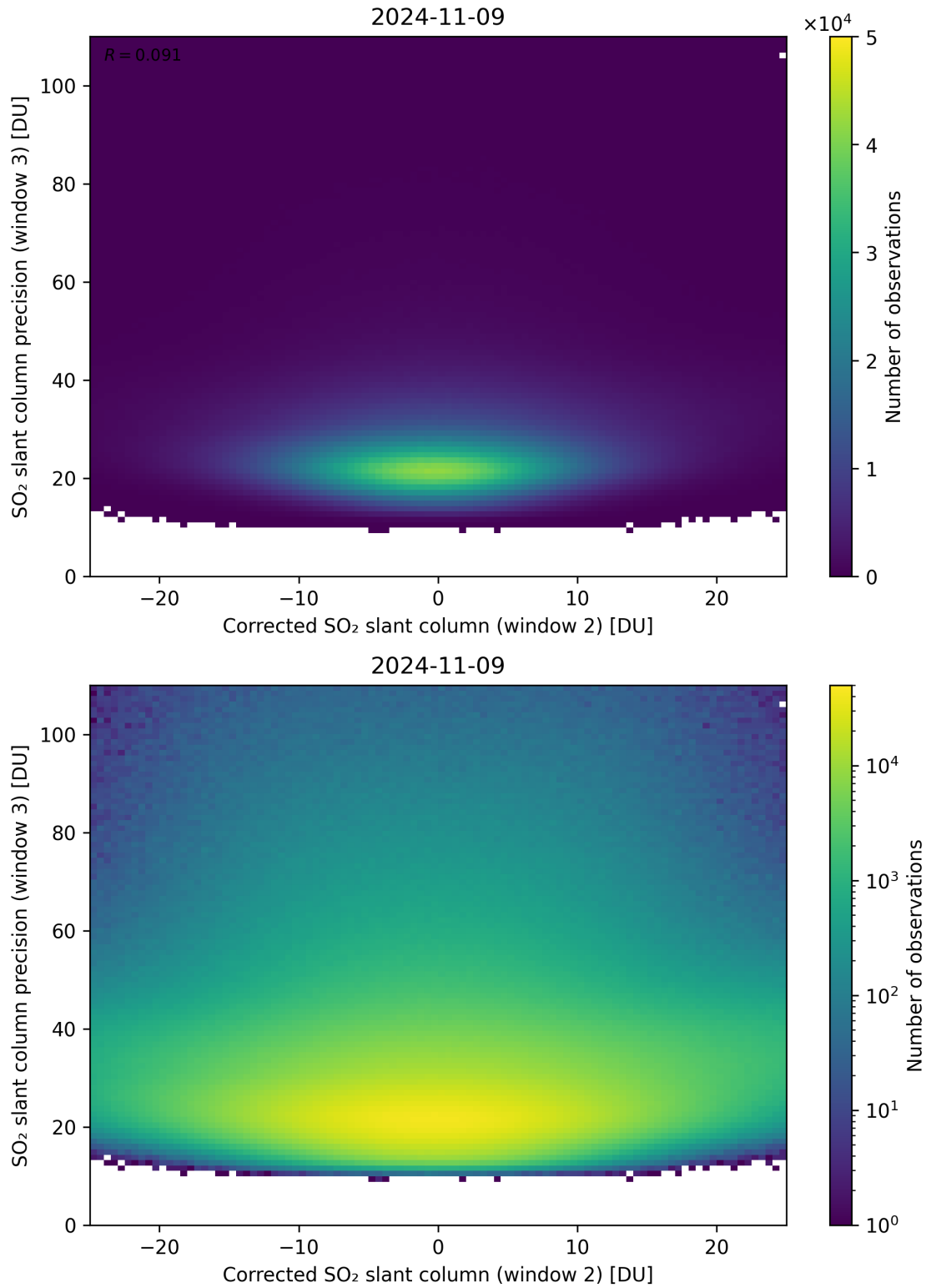
Figure 202: Scatter density plot of “Corrected SO 2 slant column (window 2)” against “SO 2 slant column precision (window 3)” for 2024-11-09 to 2024-11-10.
