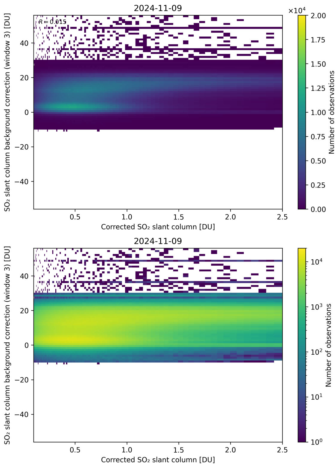
Figure 180: Scatter density plot of “Corrected SO 2 slant column” against “SO 2 slant column background correction (window 3)” for 2024-11-09 to 2024-11-10.
