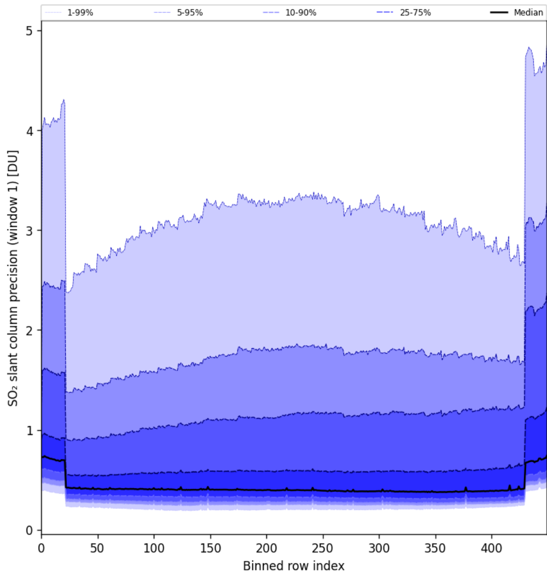
Figure 80: Along track statistics of “SO 2 slant column precision (window 1)” for 2024-11-09 to 2024-11-10
