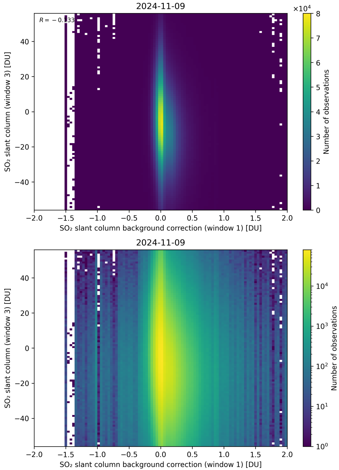
Figure 107: Scatter density plot of “SO 2 slant column background correction (window 1)” against “SO 2 slant column (window 3)” for 2024-11-09 to 2024-11-10.
