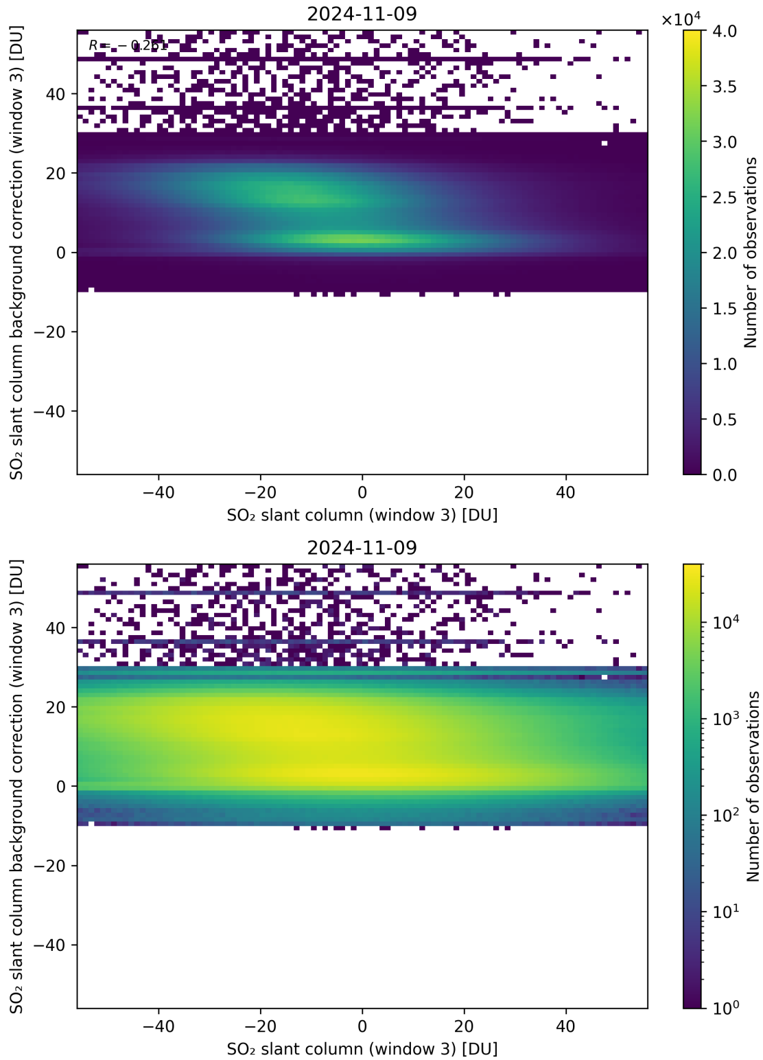
Figure 253: Scatter density plot of “SO 2 slant column (window 3)” against “SO 2 slant column background correction (window 3)” for 2024-11-09 to 2024-11-10.
