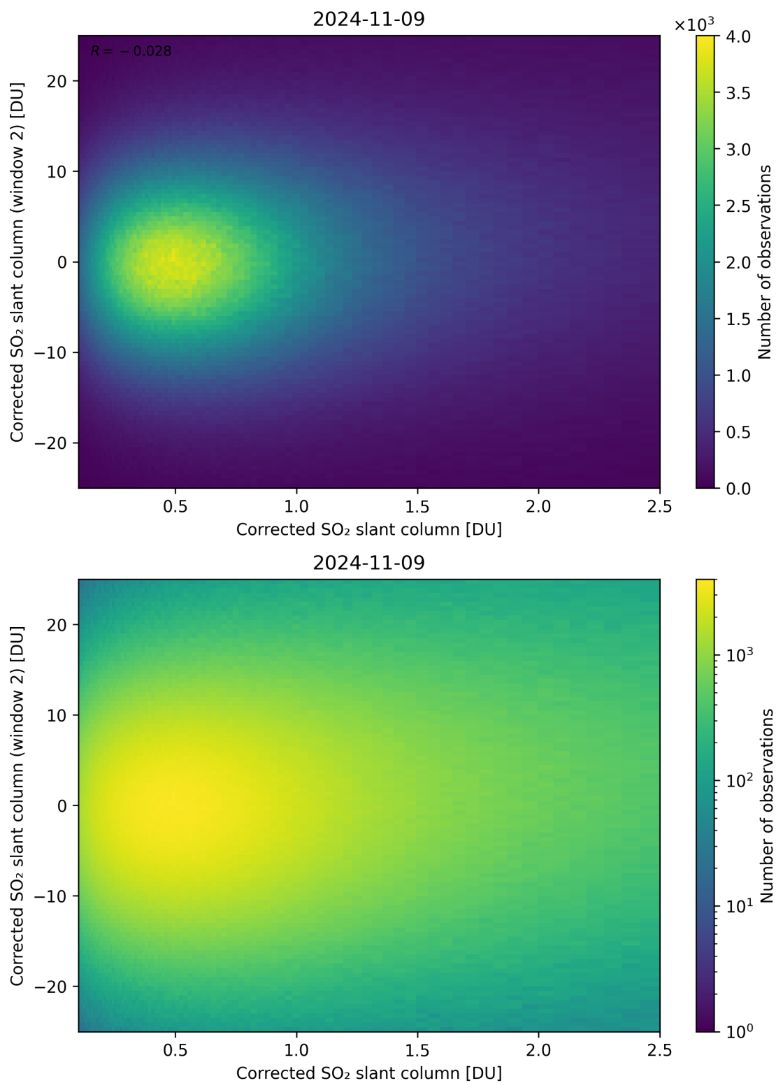
Figure 185: Scatter density plot of “Corrected SO 2 slant column” against “Corrected SO 2 slant column (window 2)” for 2024-11-09 to 2024-11-10.
