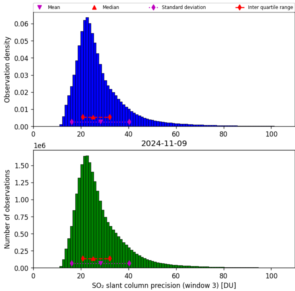
Figure 65: Histogram of “SO 2 slant column precision (window 3)” for 2024-11-09 to 2024-11-10
