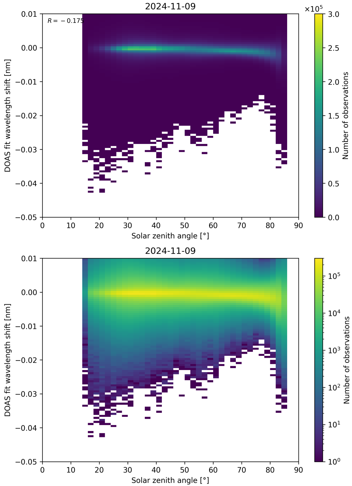
Figure 161: Scatter density plot of “Solar zenith angle” against “DOAS fit wavelength shift” for 2024-11-09 to 2024-11-10.
