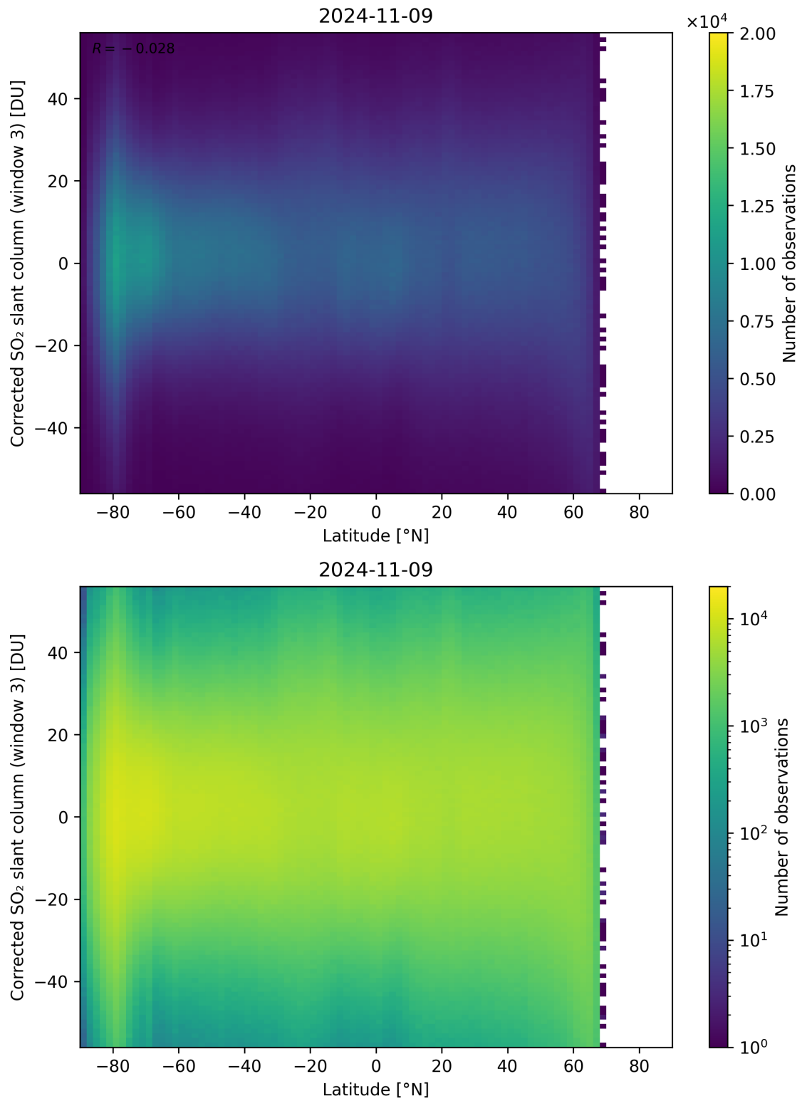
Figure 148: Scatter density plot of “Latitude” against “Corrected SO 2 slant column (window 3)” for 2024-11-09 to 2024-11-10.
