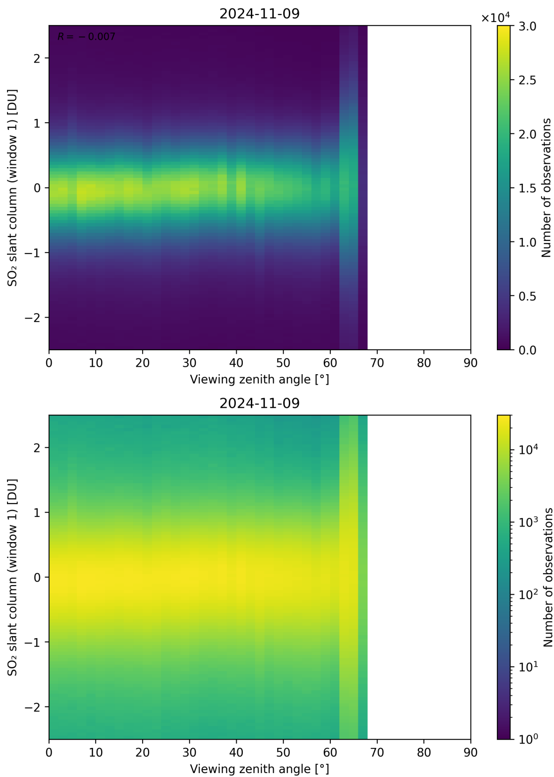
Figure 320: Scatter density plot of “Viewing zenith angle” against “SO 2 slant column (window 1)” for 2024-11-09 to 2024-11-10.
