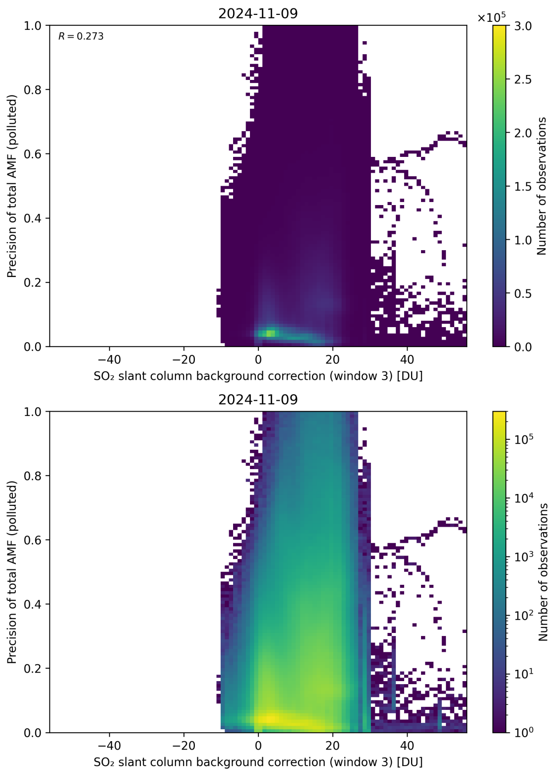
Figure 126: Scatter density plot of “SO 2 slant column background correction (window 3)” against “Precision of total AMF (polluted)” for 2024-11-09 to 2024-11-10.
