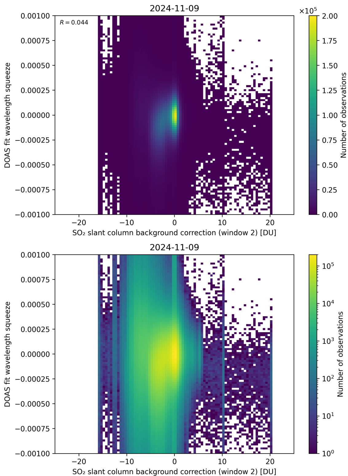
Figure 113: Scatter density plot of “SO 2 slant column background correction (window 2)” against “DOAS fit wavelength squeeze” for 2024-11-09 to 2024-11-10.
