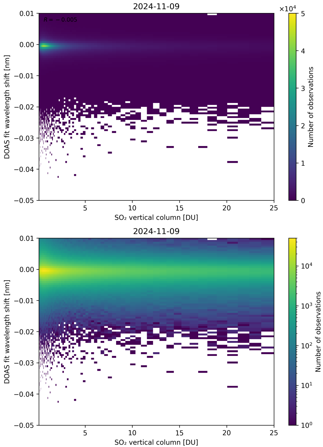
Figure 276: Scatter density plot of “SO 2 vertical column” against “DOAS fit wavelength shift” for 2024-11-09 to 2024-11-10.
