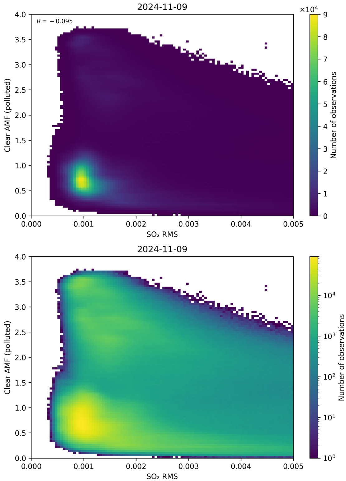
Figure 136: Scatter density plot of “SO 2 RMS” against “Clear AMF (polluted)” for 2024-11-09 to 2024-11-10.
