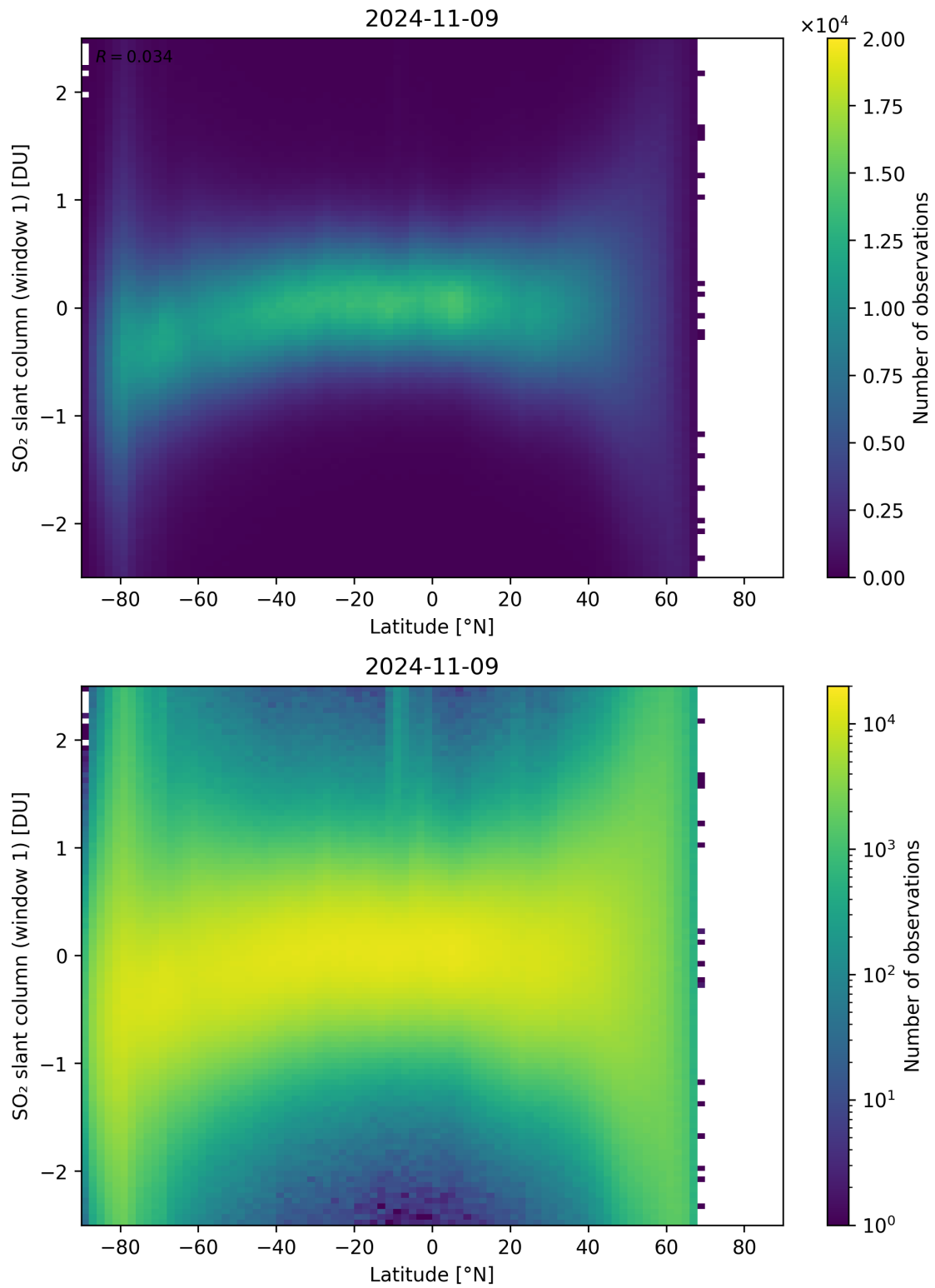
Figure 149: Scatter density plot of “Latitude” against “SO 2 slant column (window 1)” for 2024-11-09 to 2024-11-10.
