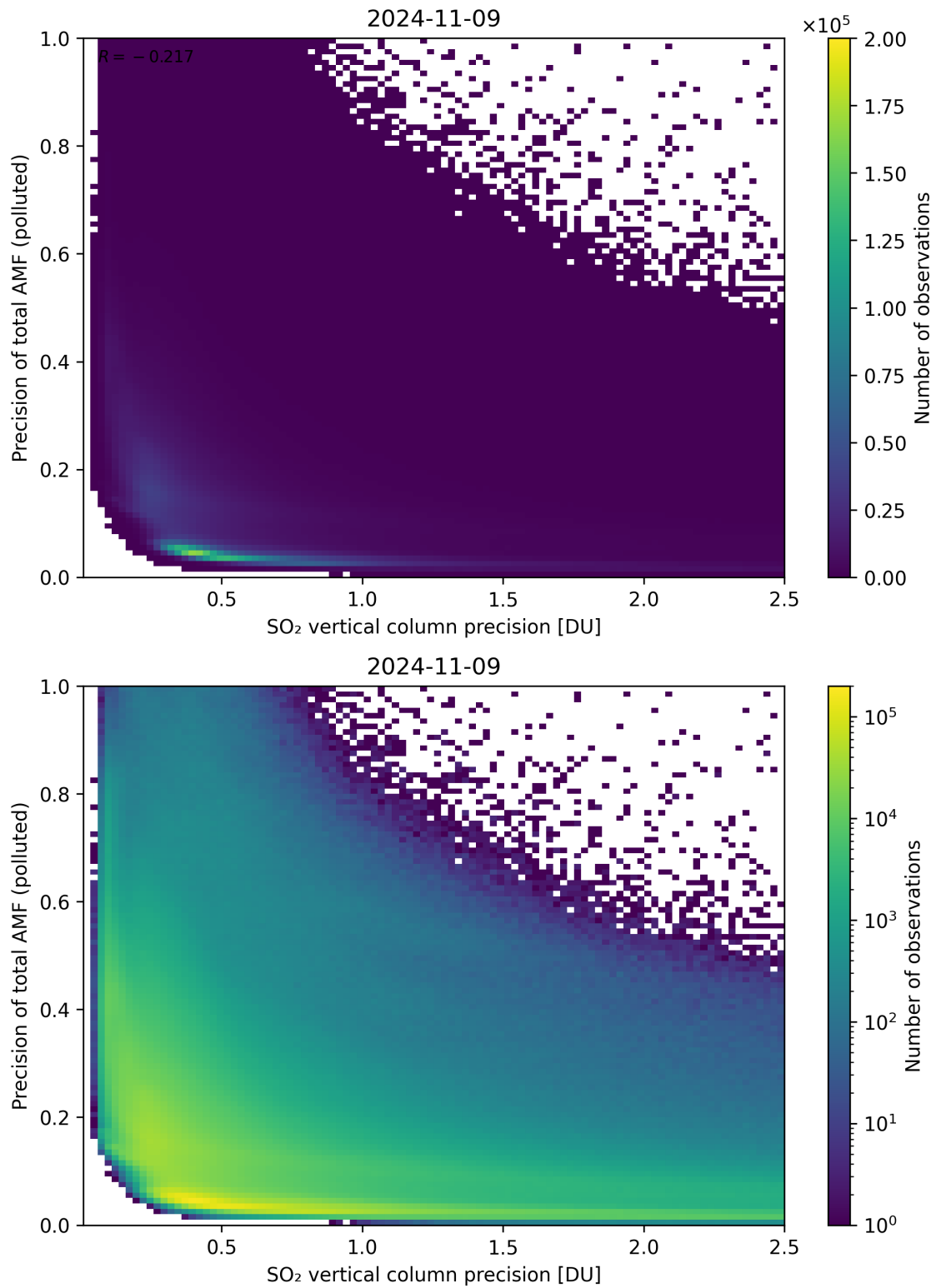
Figure 295: Scatter density plot of “SO 2 vertical column precision” against “Precision of total AMF (polluted)” for 2024-11-09 to 2024-11-10.
