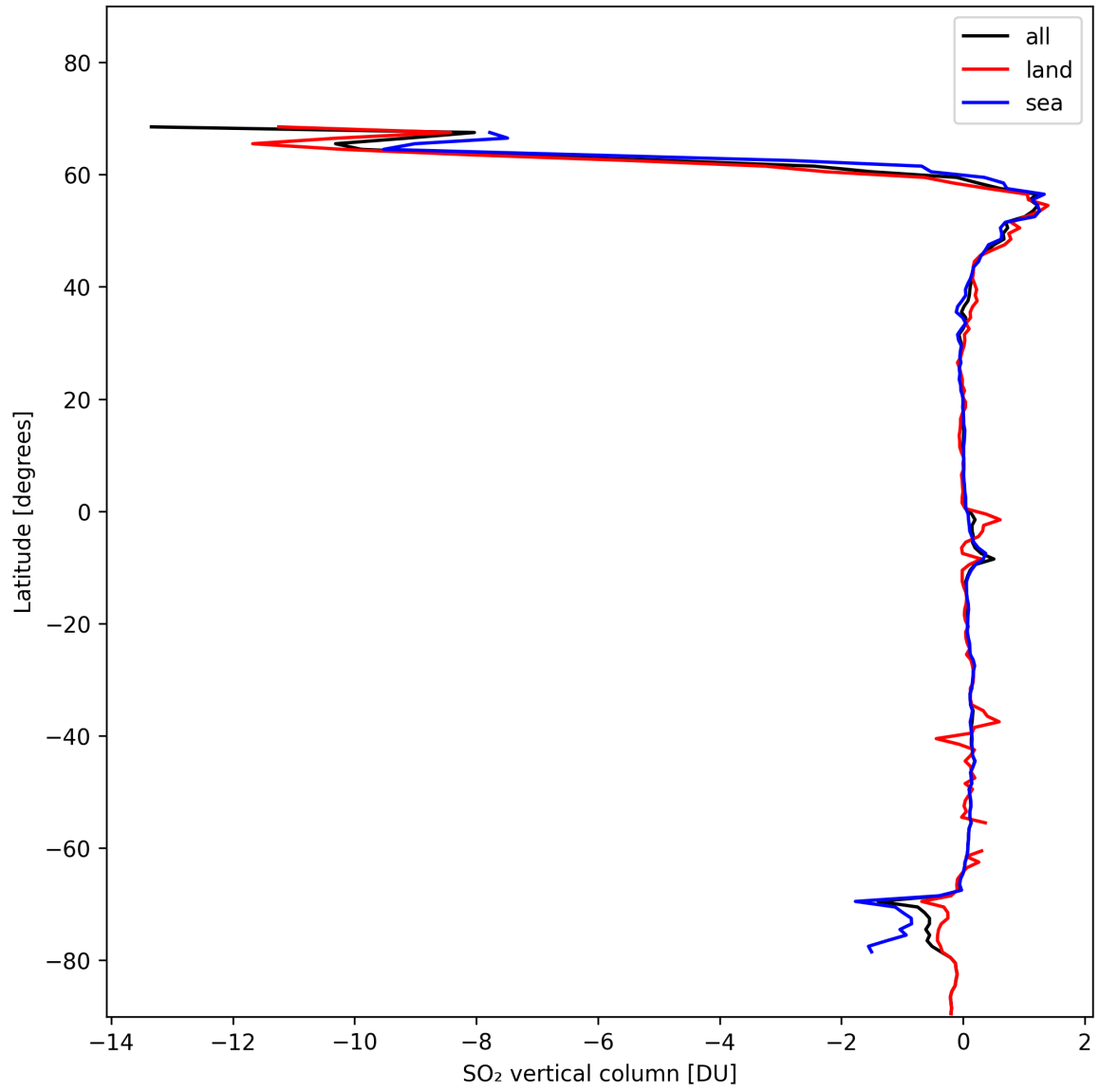
Figure 30: Zonal average of “SO 2 vertical column” for 2024-11-09 to 2024-11-10.
