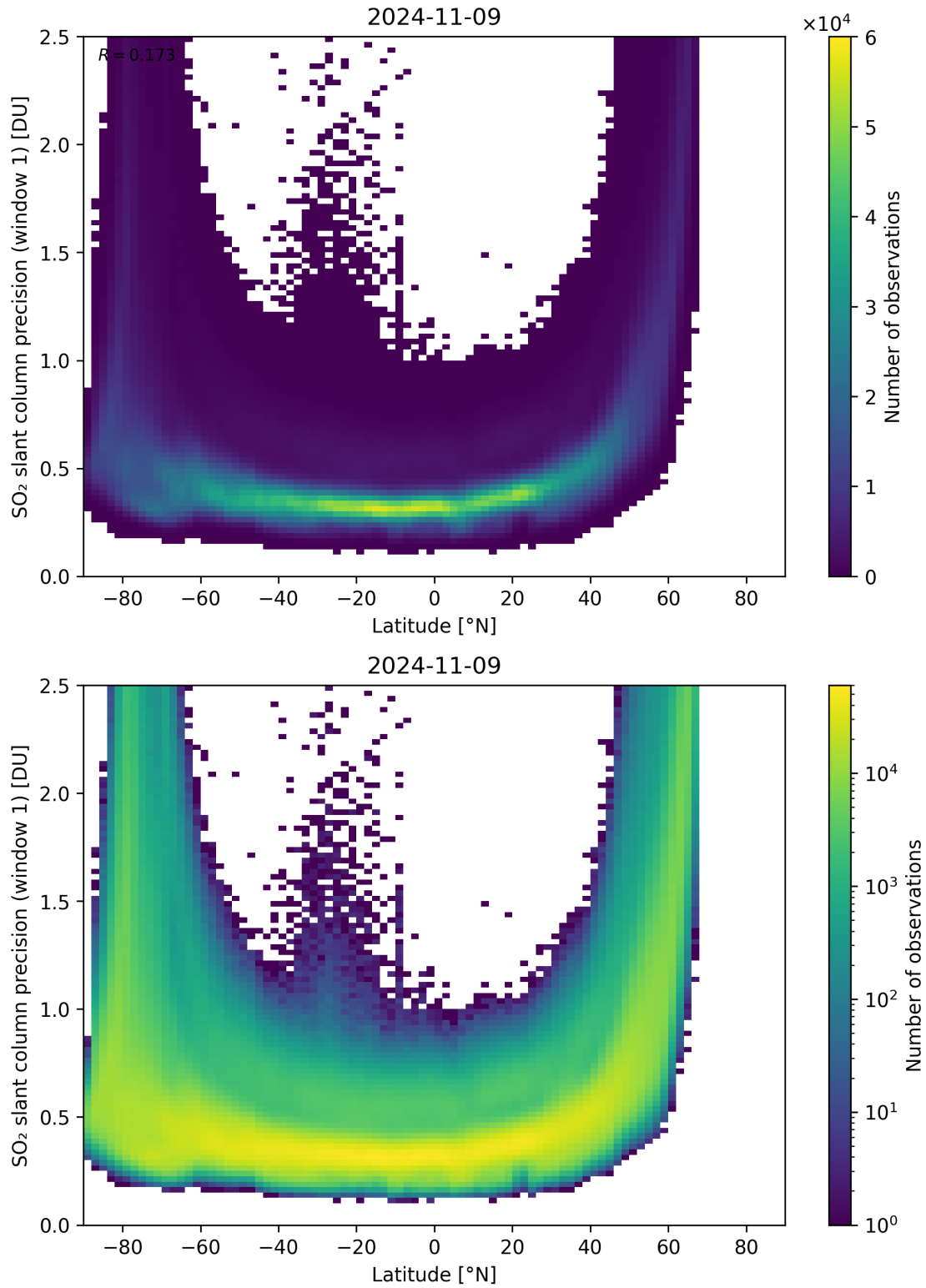
Figure 150: Scatter density plot of “Latitude” against “SO 2 slant column precision (window 1)” for 2024-11-09 to 2024-11-10.
