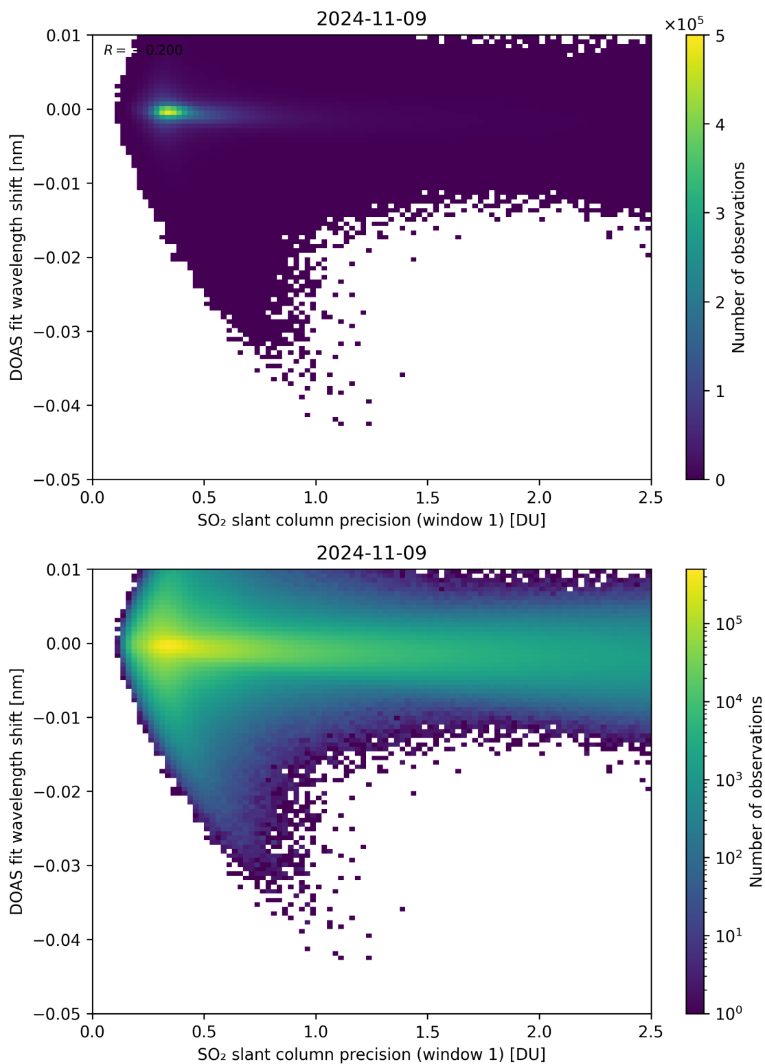
Figure 221: Scatter density plot of “SO 2 slant column precision (window 1)” against “DOAS fit wavelength shift” for 2024-11-09 to 2024-11-10.
