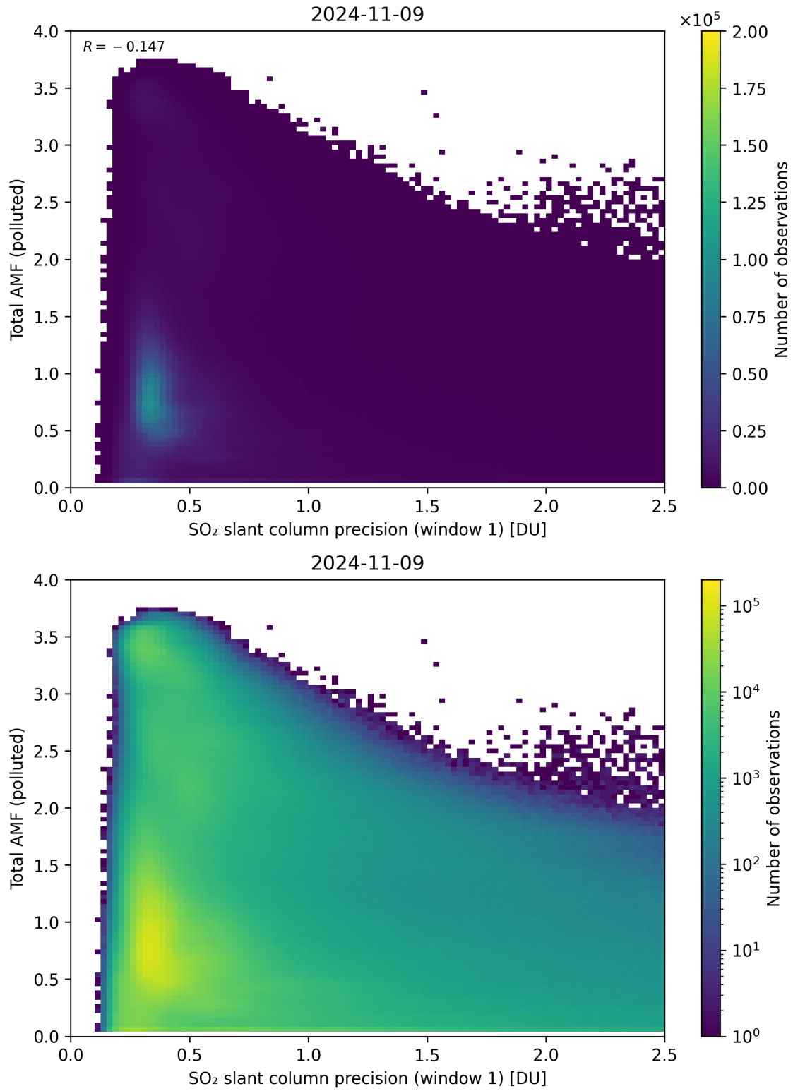
Figure 230: Scatter density plot of “SO 2 slant column precision (window 1)” against “Total AMF (polluted)” for 2024-11-09 to 2024-11-10.
