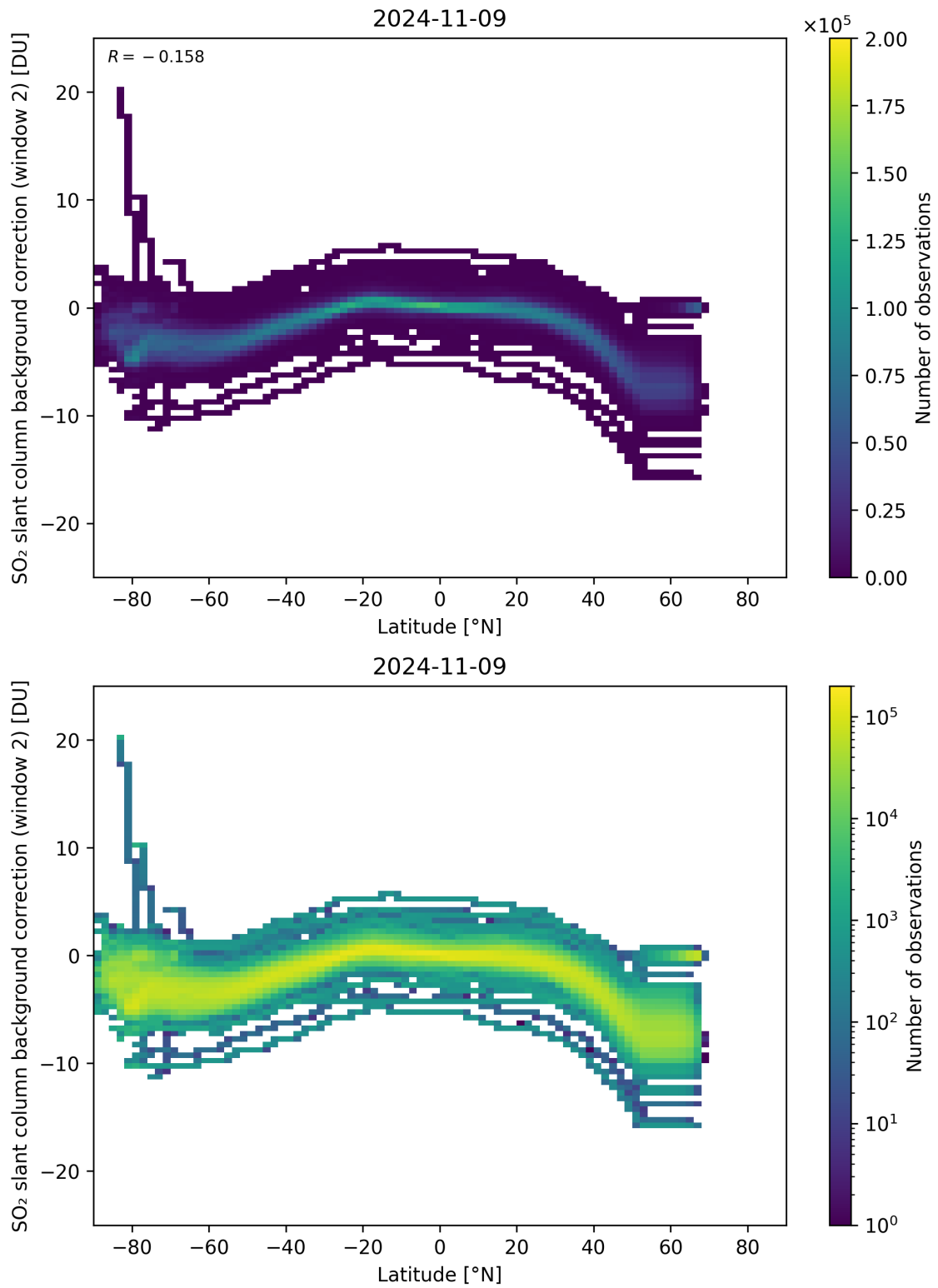
Figure 140: Scatter density plot of “Latitude” against “SO 2 slant column background correction (window 2)” for 2024-11-09 to 2024-11-10.
