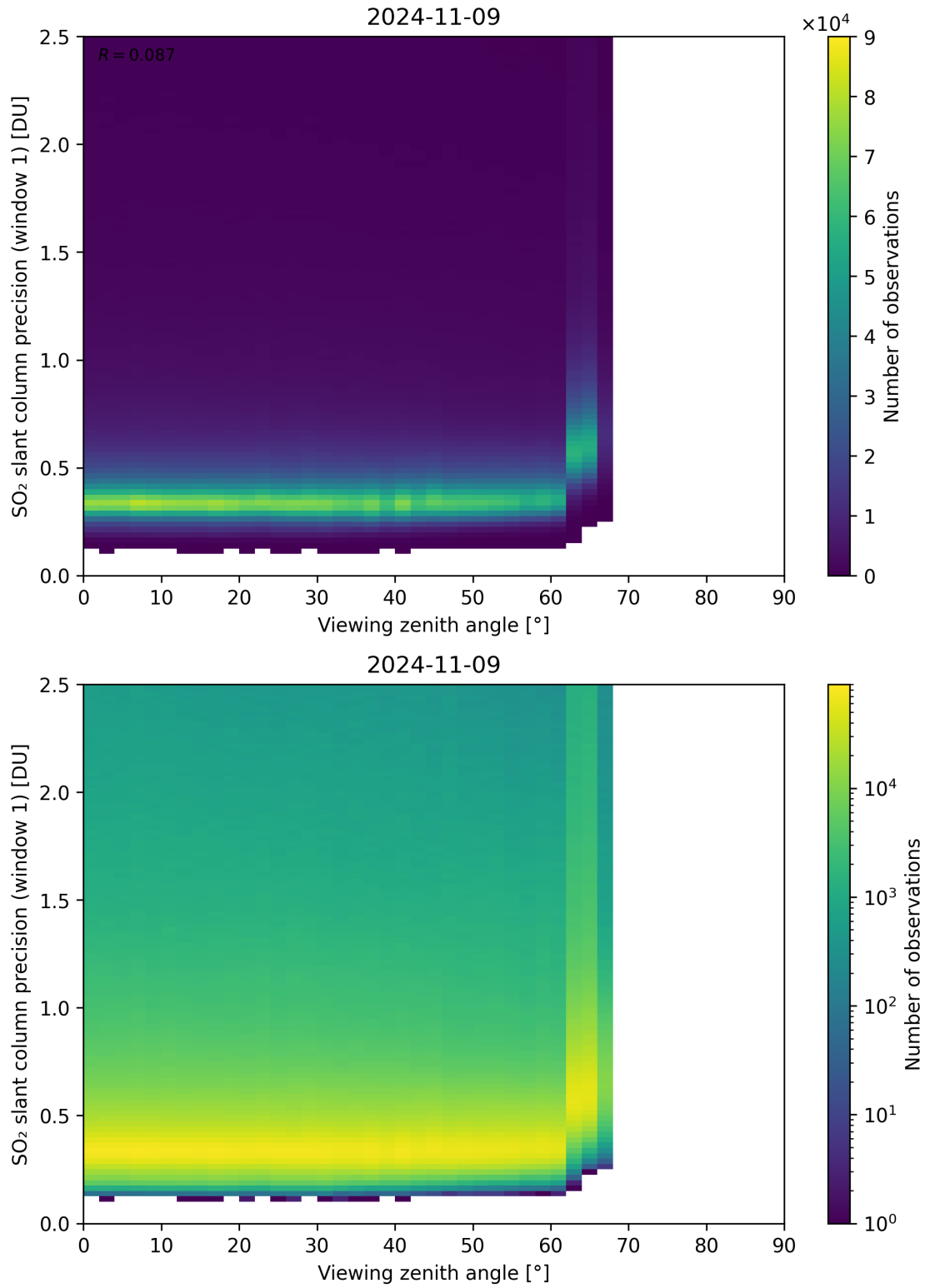
Figure 321: Scatter density plot of “Viewing zenith angle” against “SO 2 slant column precision (window 1)” for 2024-11-09 to 2024-11-10.
