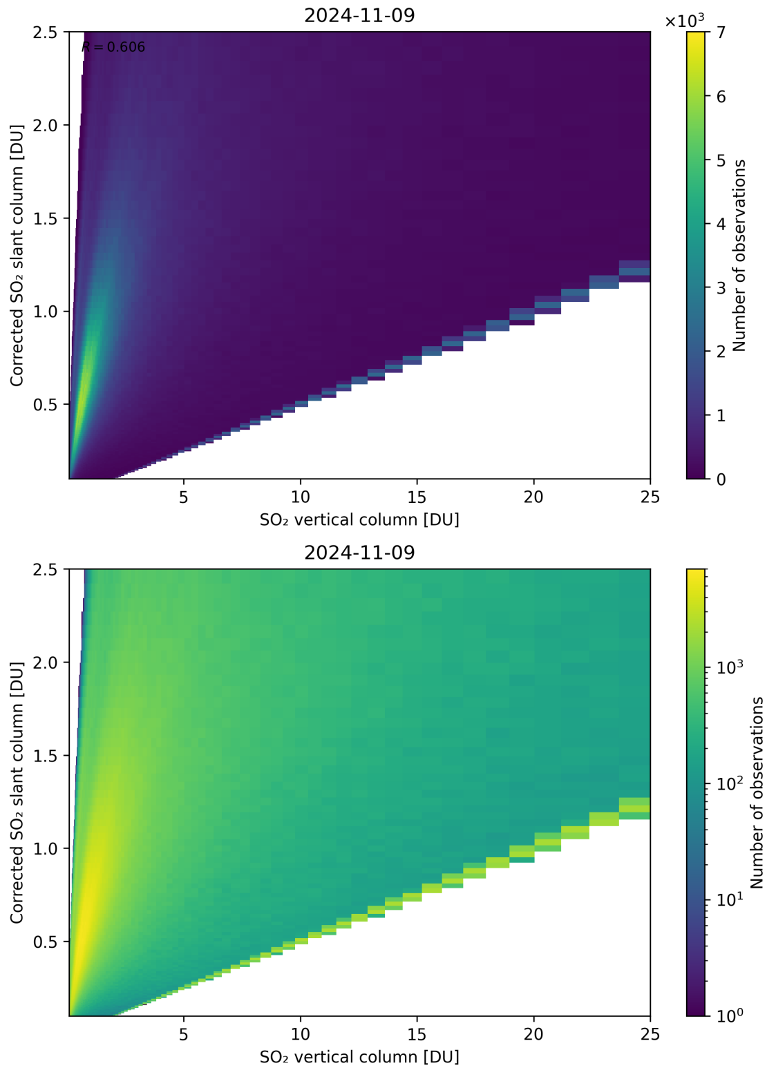
Figure 297: Scatter density plot of “SO 2 vertical column” against “Corrected SO 2 slant column” for 2024-11-09 to 2024-11-10.
