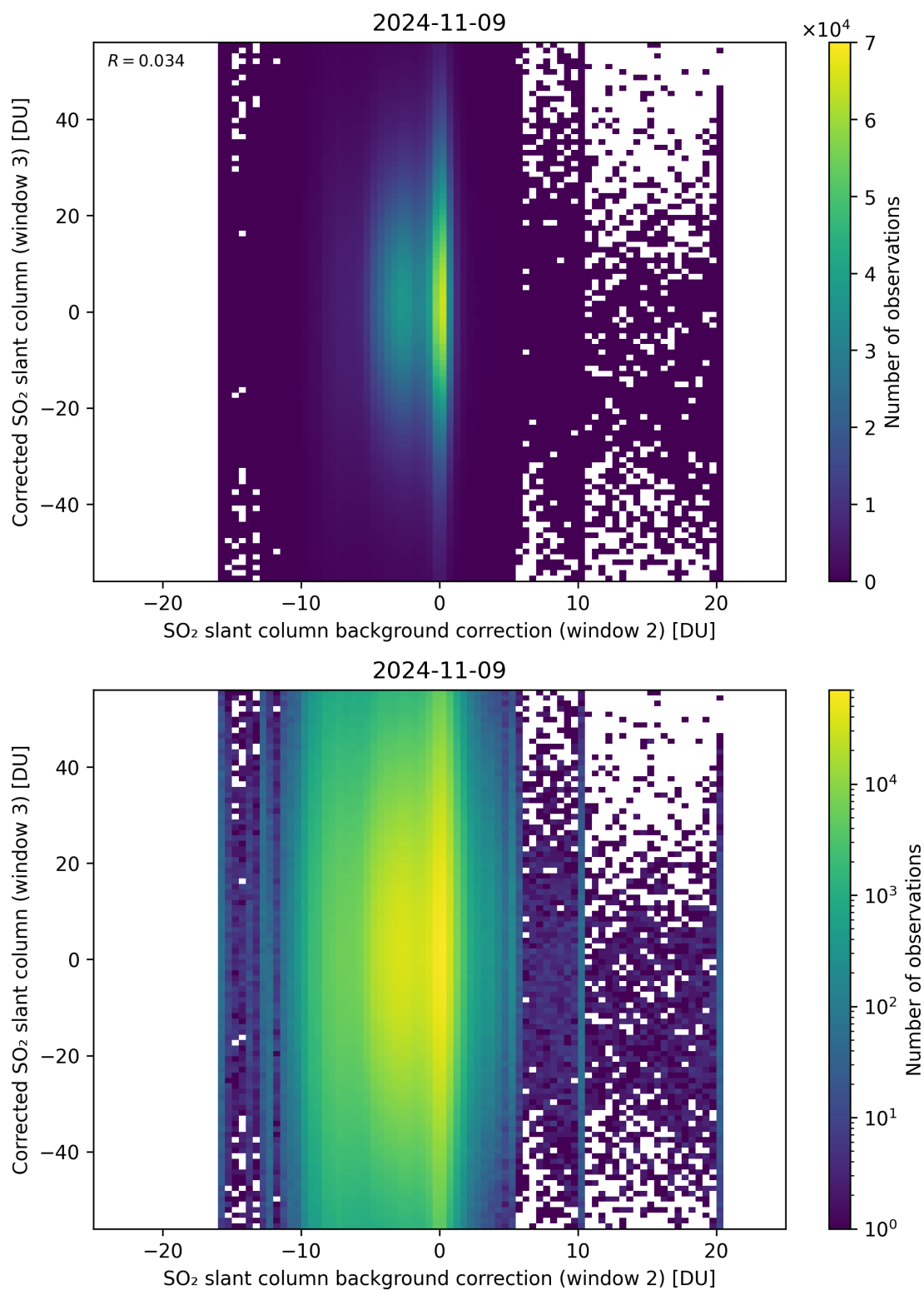
Figure 116: Scatter density plot of “SO 2 slant column background correction (window 2)” against “Corrected SO 2 slant column (window 3)” for 2024-11-09 to 2024-11-10.
