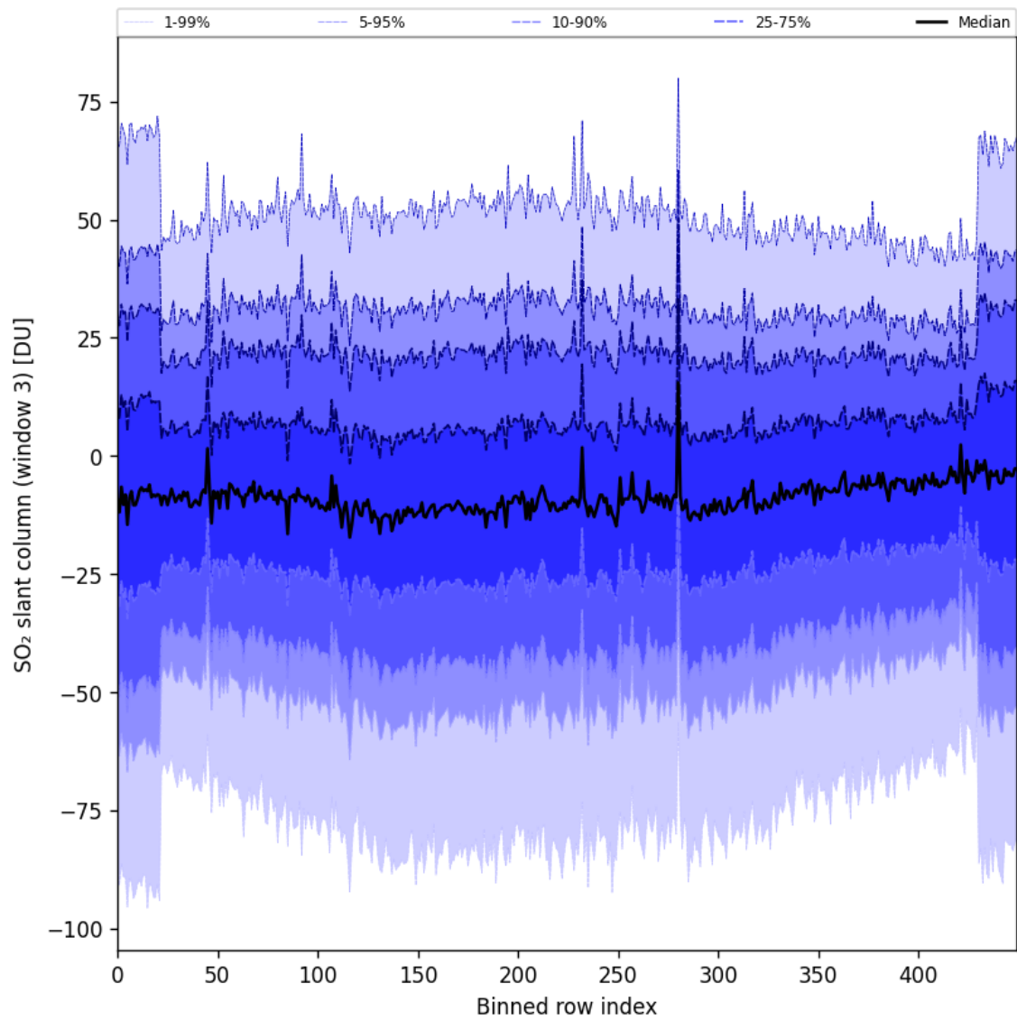
Figure 87: Along track statistics of “SO 2 slant column (window 3)” for 2024-11-09 to 2024-11-10
