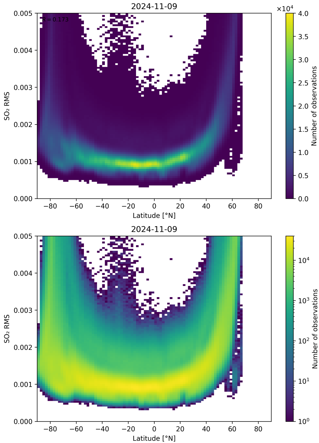
Figure 144: Scatter density plot of “Latitude” against “SO 2 RMS” for 2024-11-09 to 2024-11-10.
