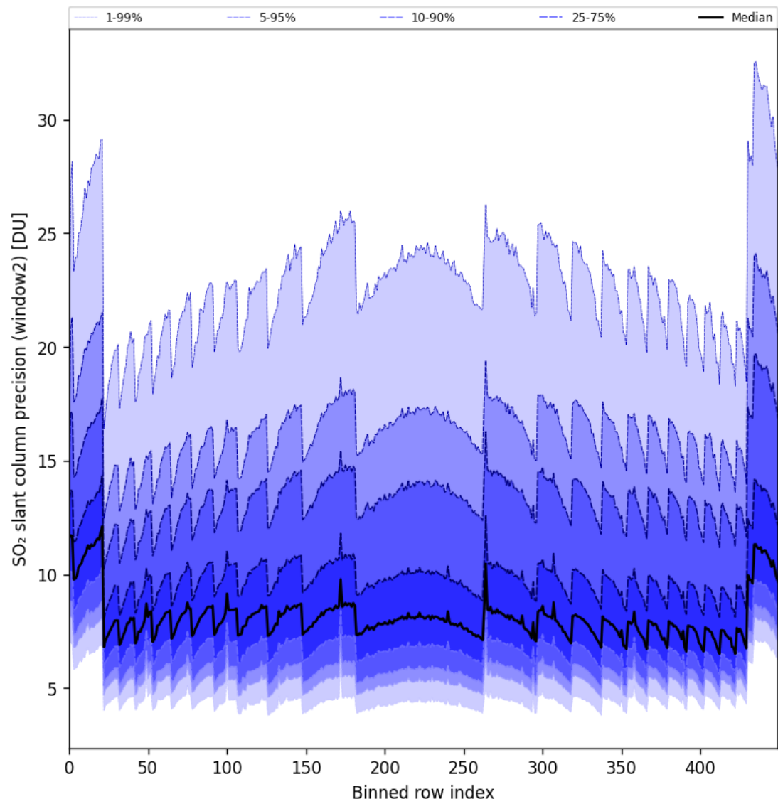
Figure 84: Along track statistics of “SO 2 slant column precision (window2)” for 2024-11-09 to 2024-11-10
