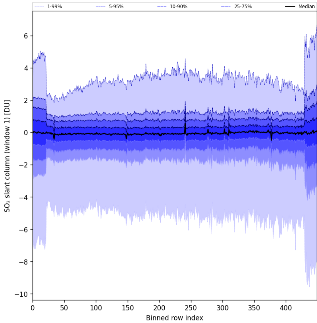
Figure 79: Along track statistics of “SO 2 slant column (window 1)” for 2024-11-09 to 2024-11-10
