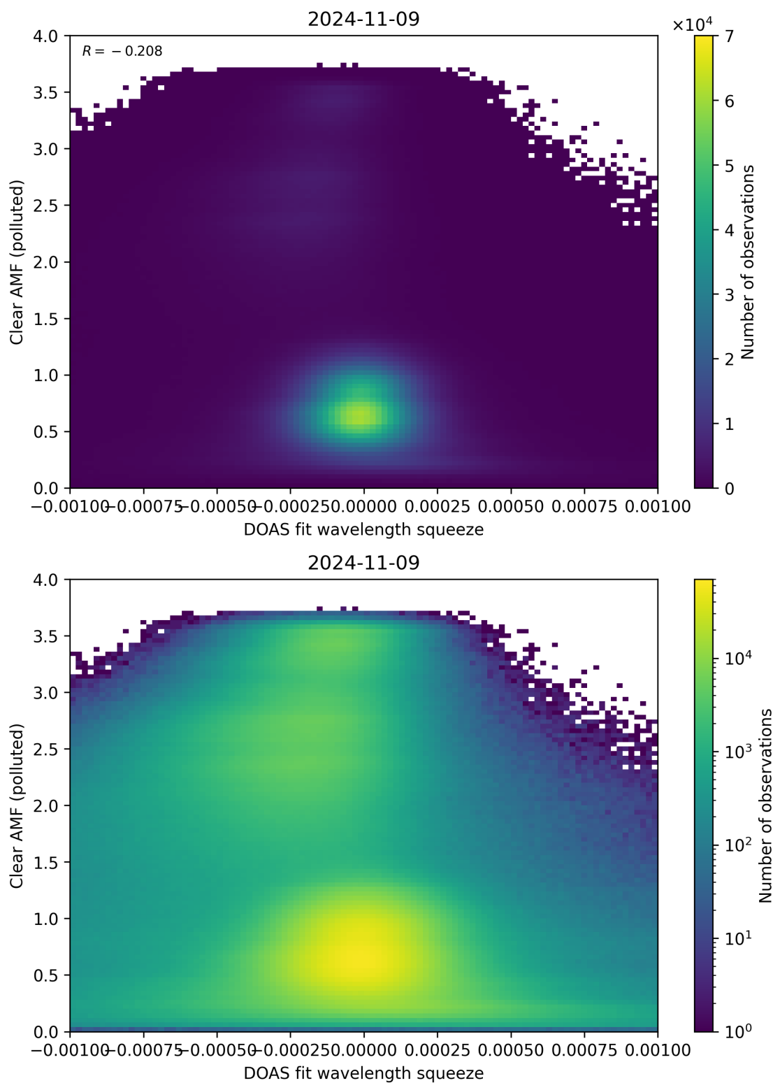
Figure 133: Scatter density plot of “DOAS fit wavelength squeeze” against “Clear AMF (polluted)” for 2024-11-09 to 2024-11-10.
