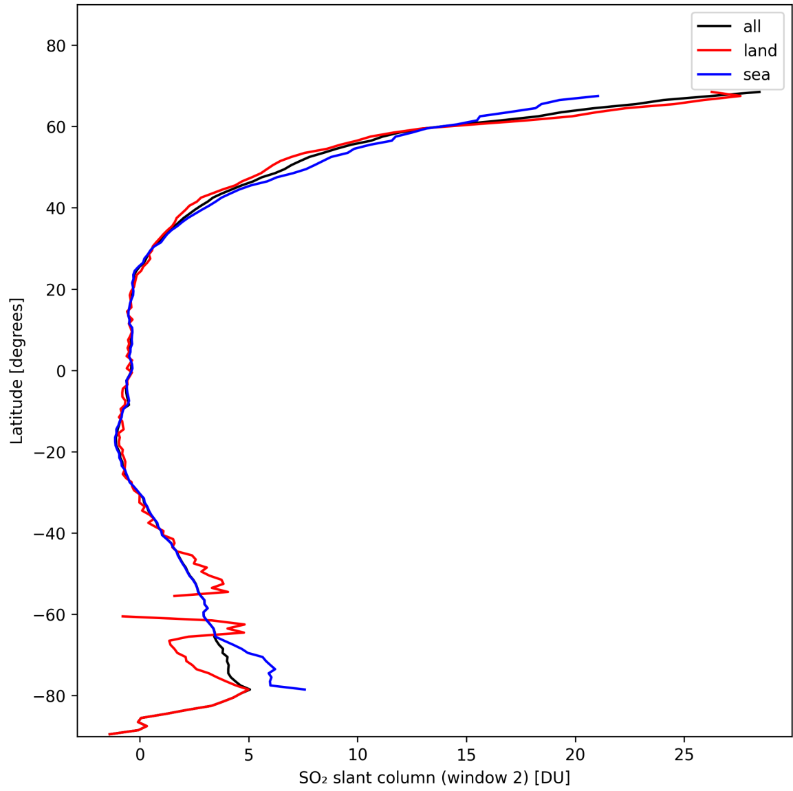
Figure 37: Zonal average of “SO 2 slant column (window 2)” for 2024-11-09 to 2024-11-10.
