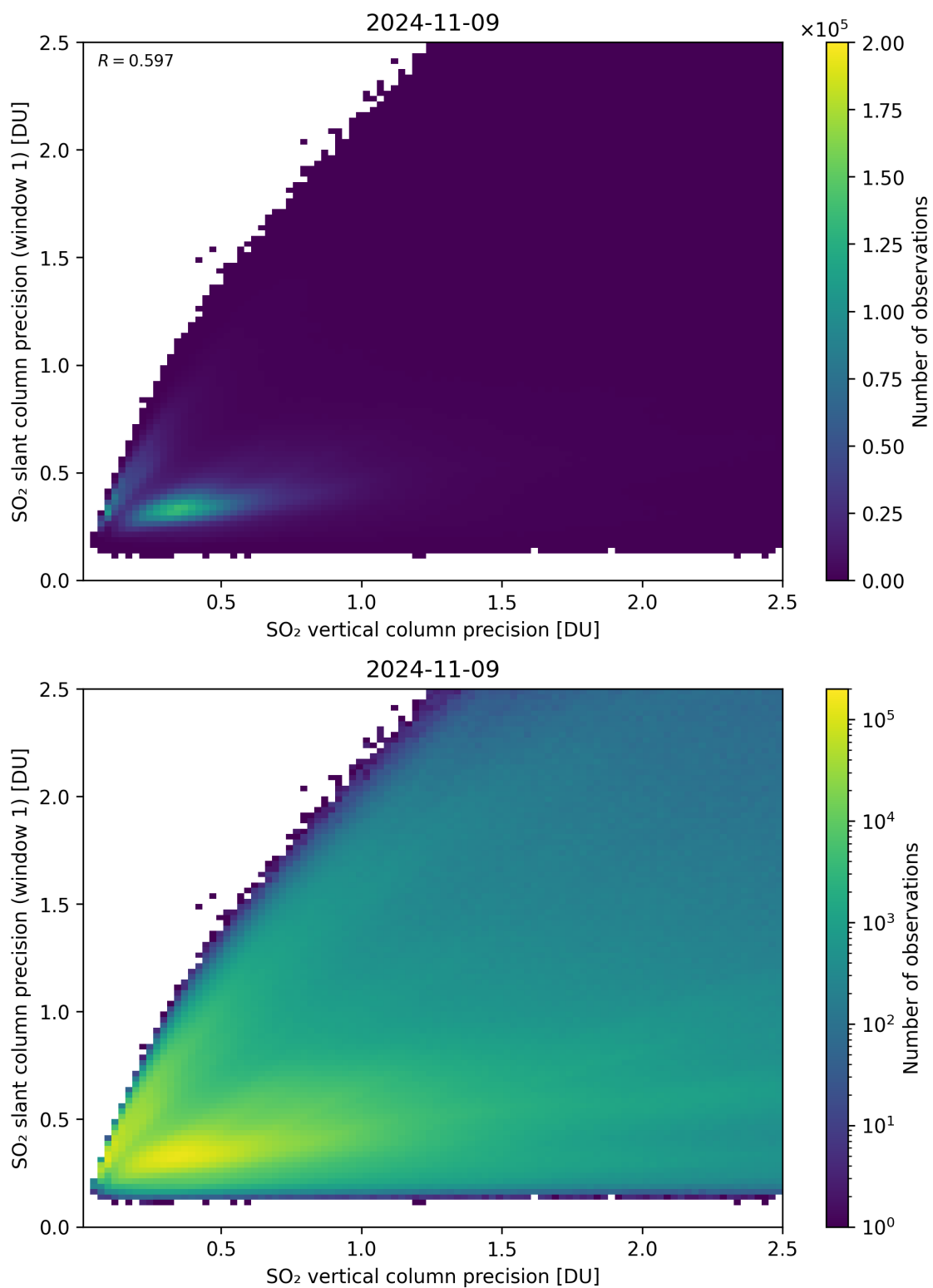
Figure 290: Scatter density plot of “SO 2 vertical column precision” against “SO 2 slant column precision (window 1)” for 2024-11-09 to 2024-11-10.
