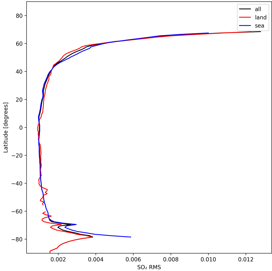
Figure 47: Zonal average of “SO 2 RMS” for 2024-11-09 to 2024-11-10.
