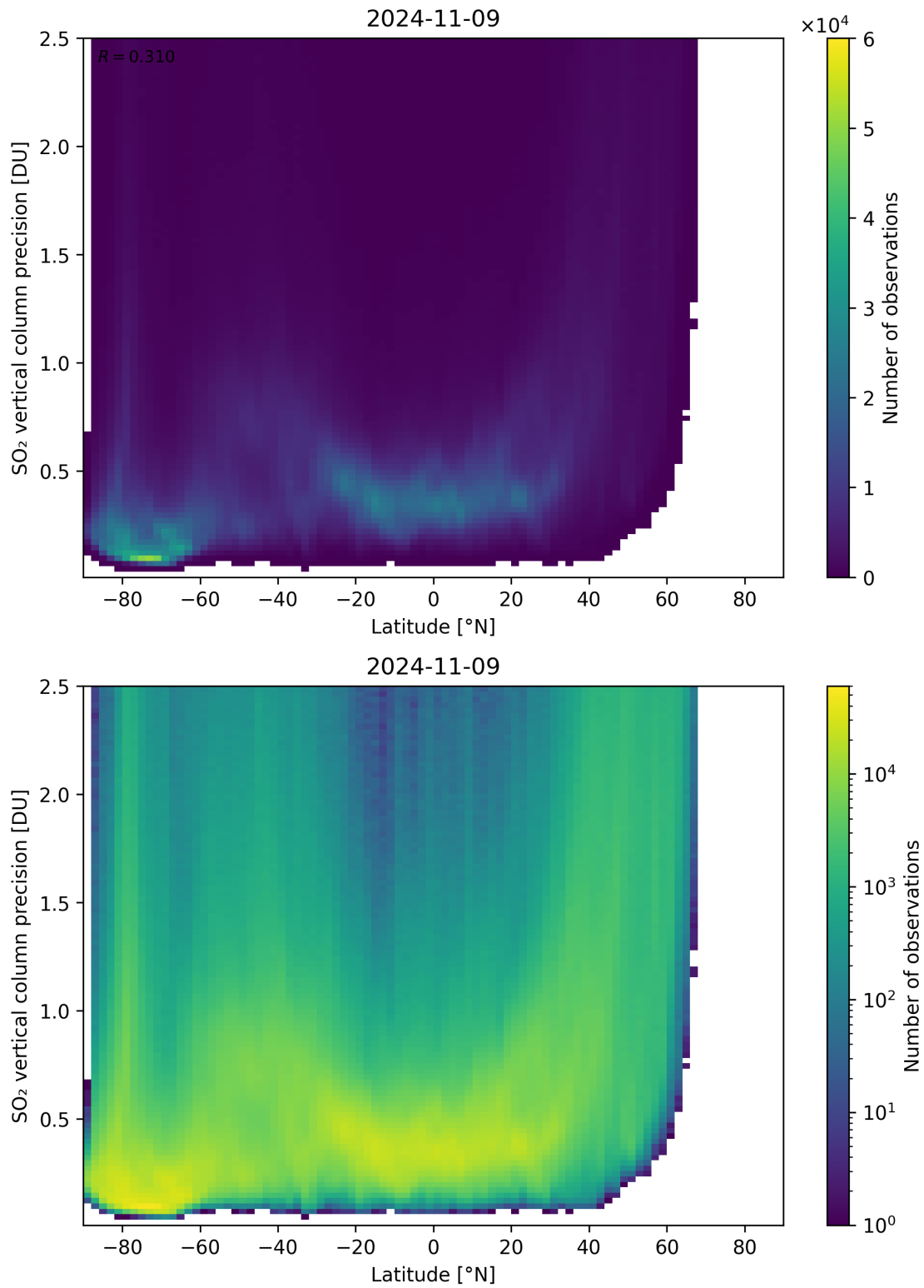
Figure 157: Scatter density plot of “Latitude” against “SO 2 vertical column precision” for 2024-11-09 to 2024-11-10.
