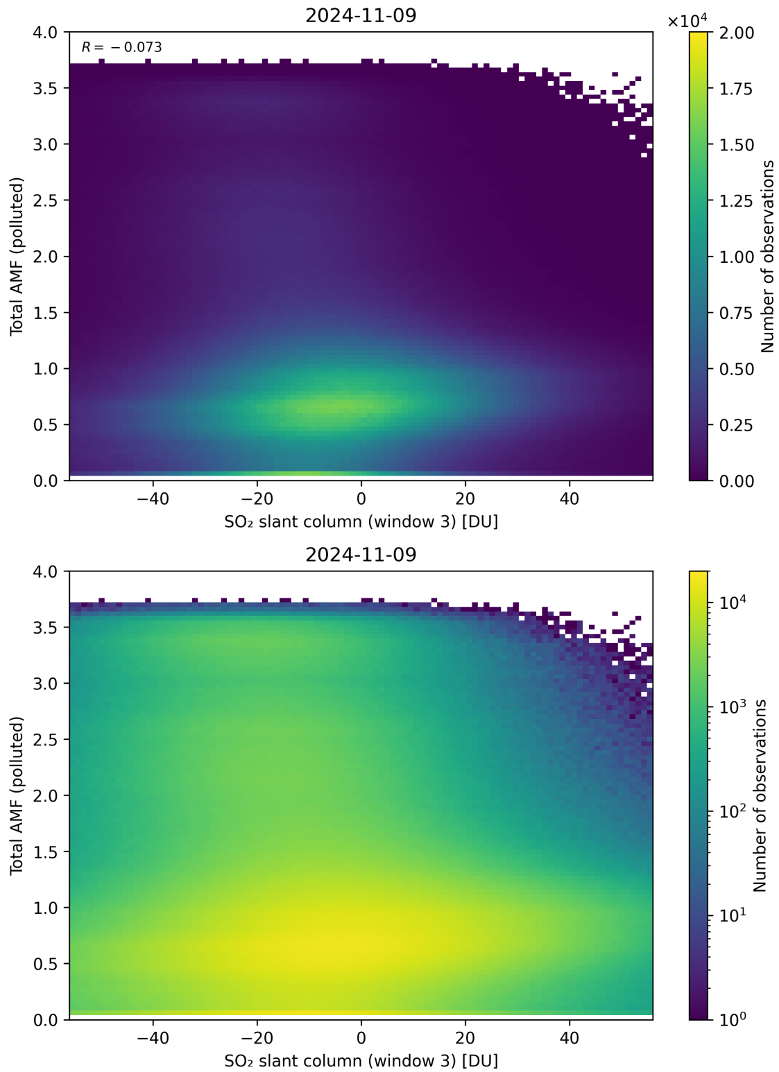
Figure 268: Scatter density plot of “SO 2 slant column (window 3)” against “Total AMF (polluted)” for 2024-11-09 to 2024-11-10.
