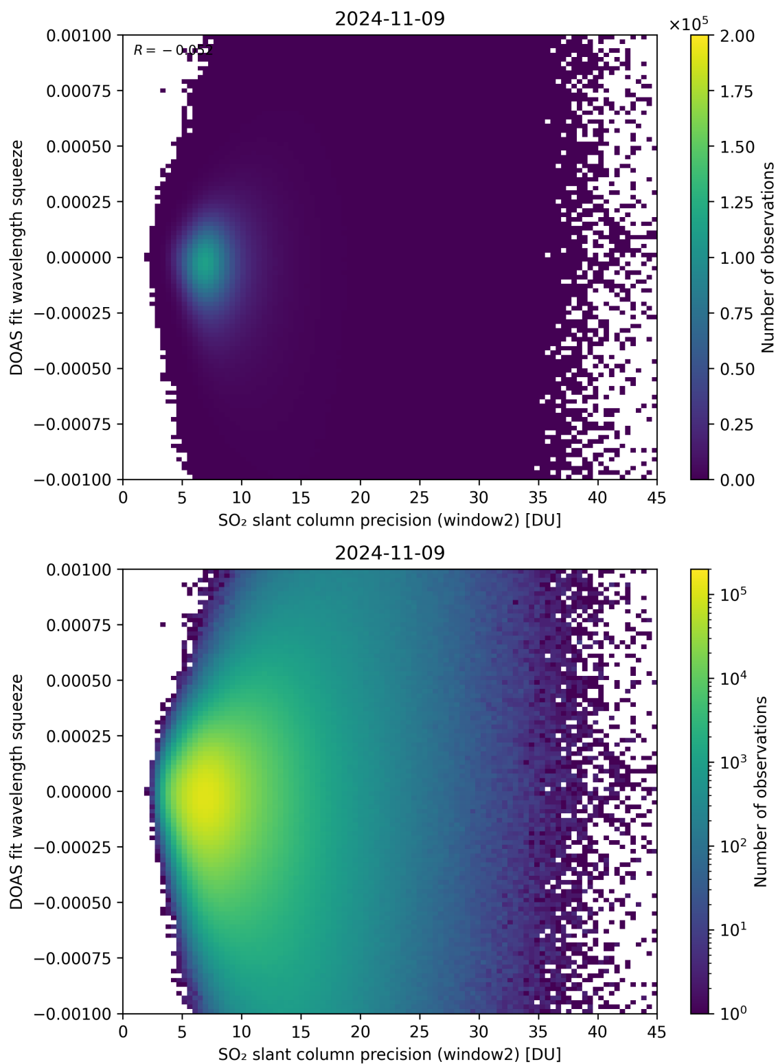
Figure 244: Scatter density plot of “SO 2 slant column precision (window2)” against “DOAS fit wavelength squeeze” for 2024-11-09 to 2024-11-10.
