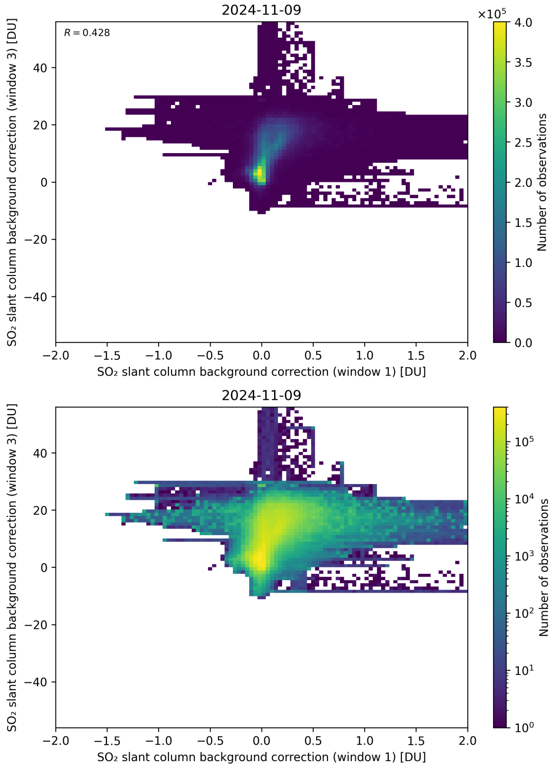
Figure 99: Scatter density plot of “SO 2 slant column background correction (window 1)” against “SO 2 slant column background correction (window 3)” for 2024-11-09 to 2024-11-10.
