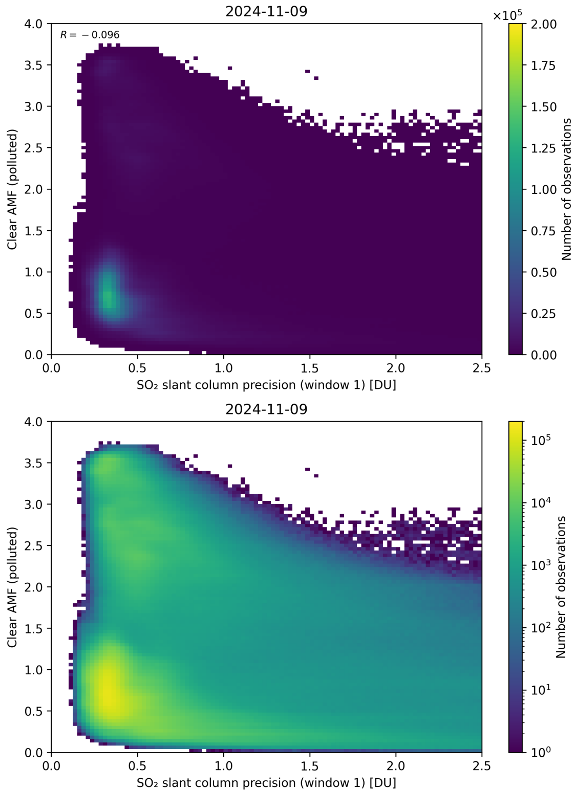
Figure 224: Scatter density plot of “SO 2 slant column precision (window 1)” against “Clear AMF (polluted)” for 2024-11-09 to 2024-11-10.
