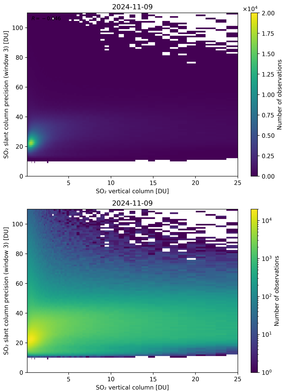
Figure 304: Scatter density plot of “SO 2 vertical column” against “SO 2 slant column precision (window 3)” for 2024-11-09 to 2024-11-10.
