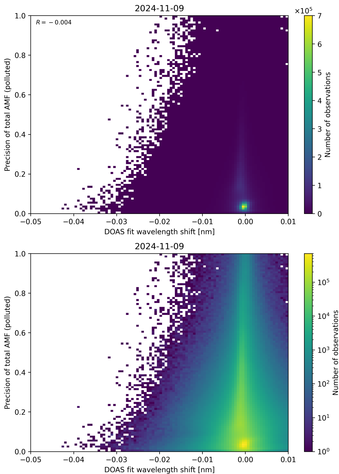
Figure 131: Scatter density plot of “DOAS fit wavelength shift” against “Precision of total AMF (polluted)” for 2024-11-09 to 2024-11-10.
