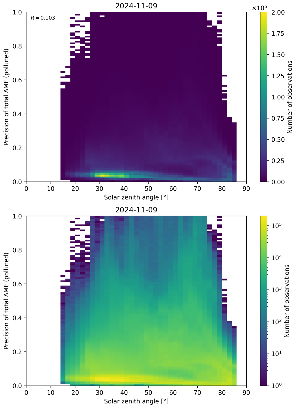
Figure 175: Scatter density plot of “Solar zenith angle” against “Precision of total AMF (polluted)” for 2024-11-09 to 2024-11-10.
