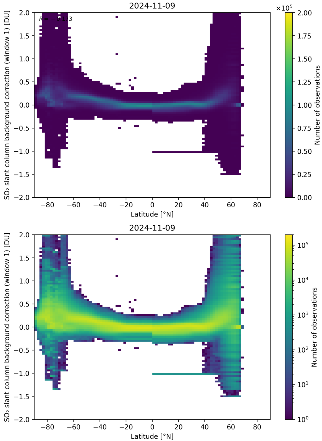
Figure 139: Scatter density plot of “Latitude” against “SO 2 slant column background correction (window 1)” for 2024-11-09 to 2024-11-10.
