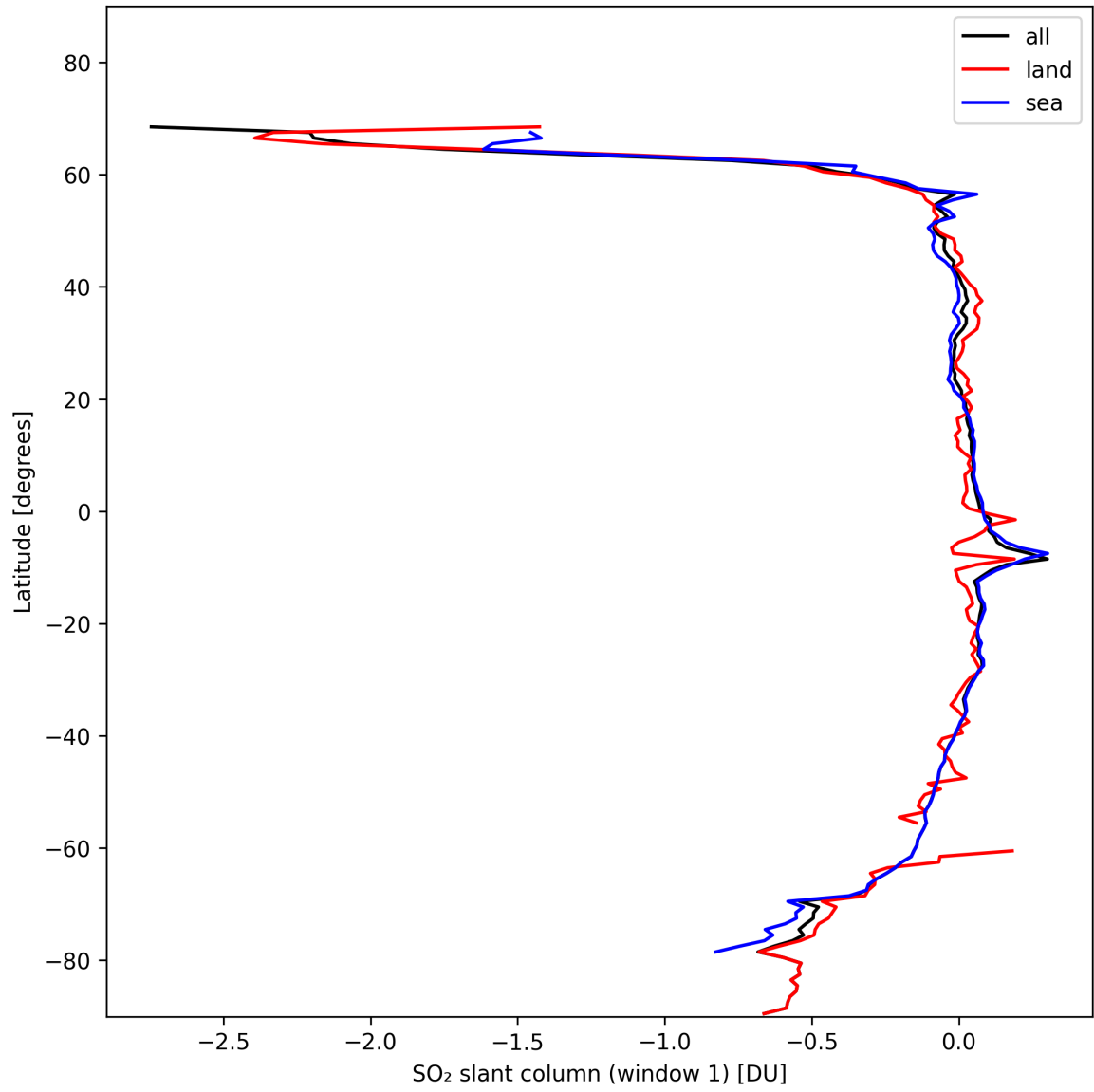
Figure 33: Zonal average of “SO 2 slant column (window 1)” for 2024-11-09 to 2024-11-10.
