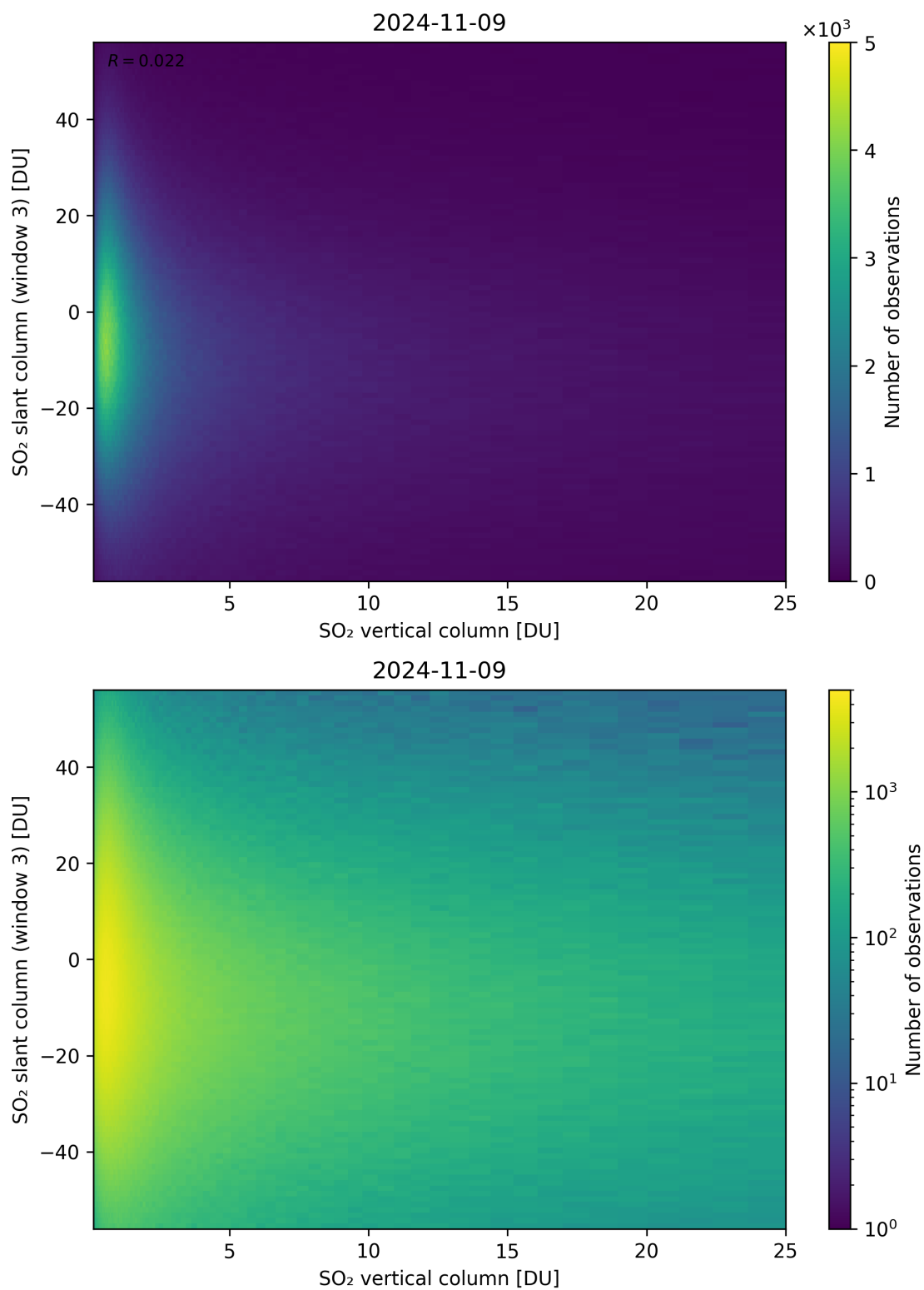
Figure 303: Scatter density plot of “SO 2 vertical column” against “SO 2 slant column (window 3)” for 2024-11-09 to 2024-11-10.
