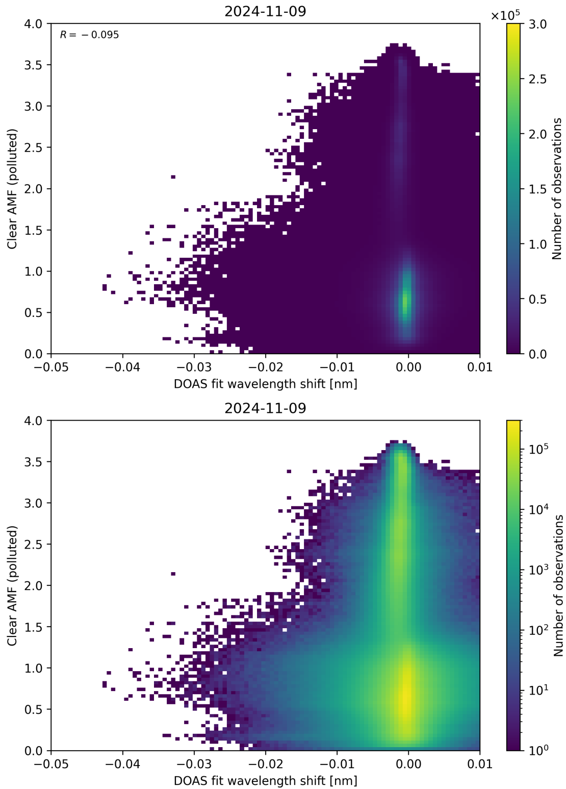
Figure 129: Scatter density plot of “DOAS fit wavelength shift” against “Clear AMF (polluted)” for 2024-11-09 to 2024-11-10.
