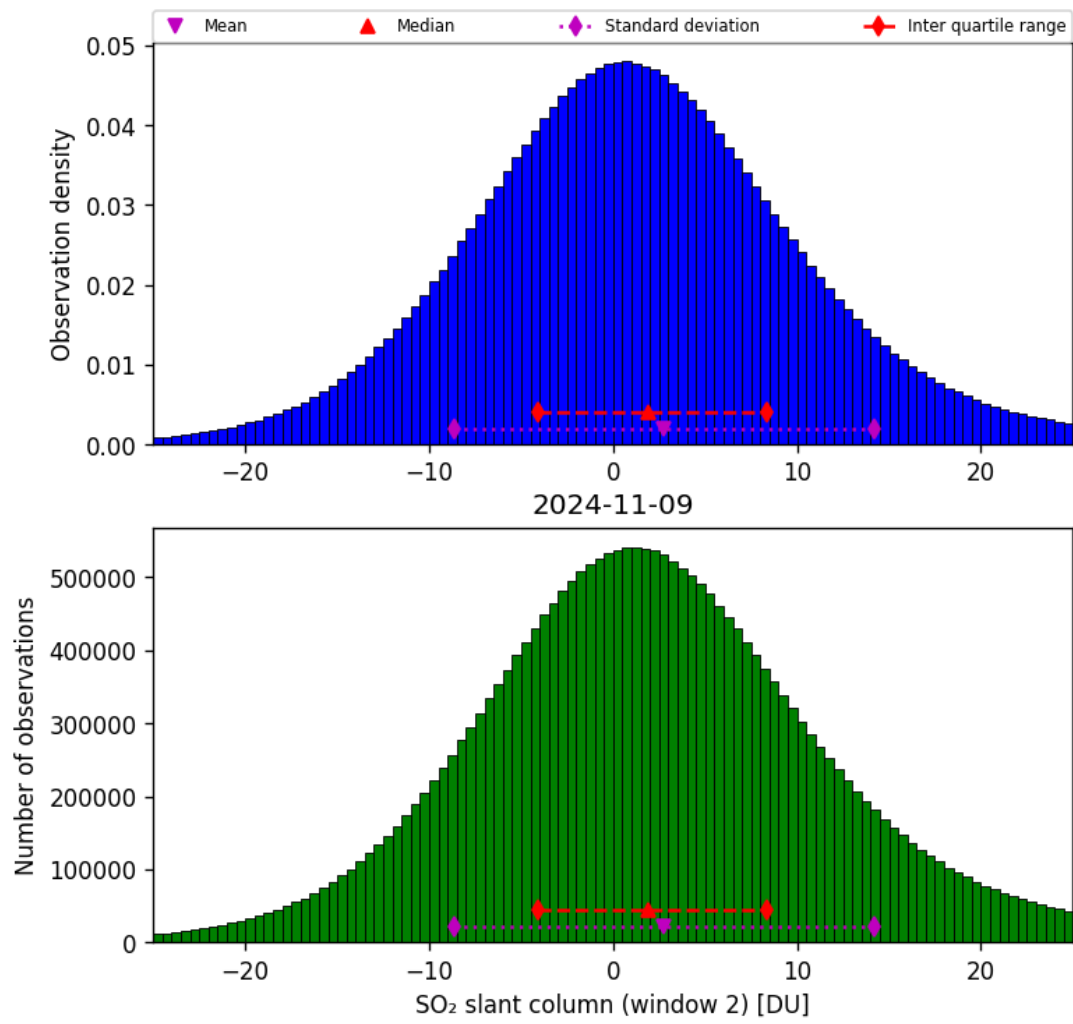
Figure 60: Histogram of “SO 2 slant column (window 2)” for 2024-11-09 to 2024-11-10
