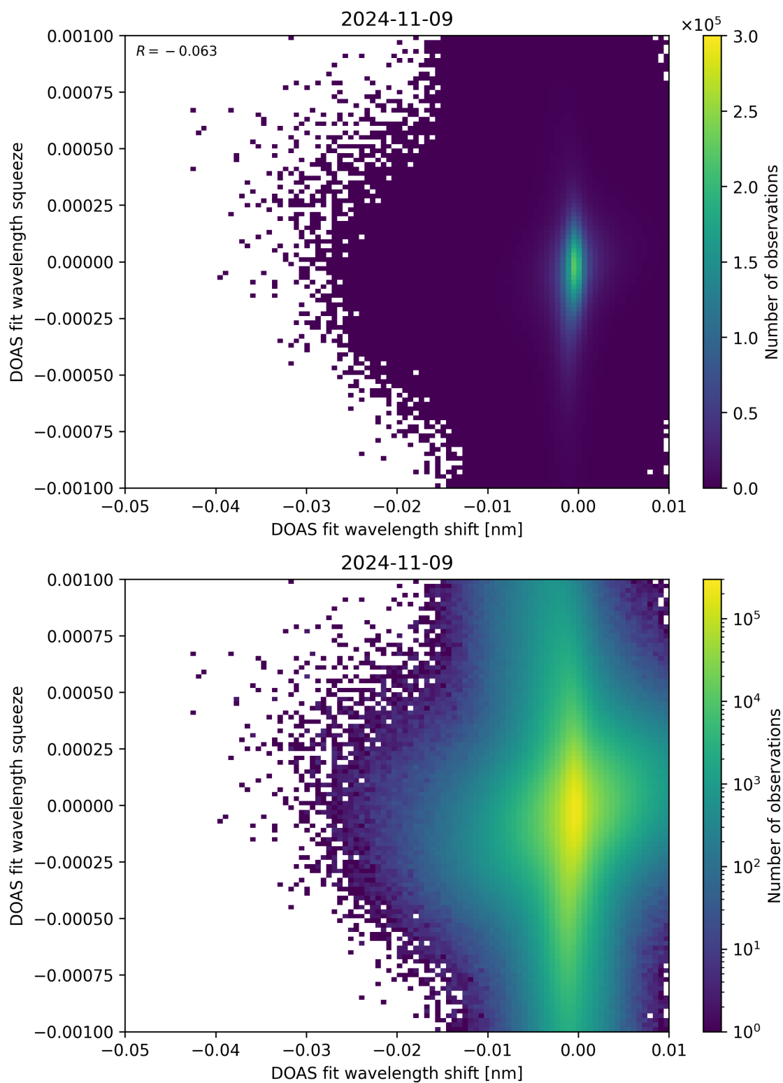
Figure 127: Scatter density plot of “DOAS fit wavelength shift” against “DOAS fit wavelength squeeze” for 2024-11-09 to 2024-11-10.
