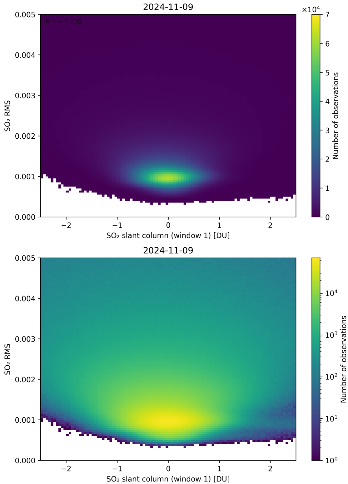
Figure 217: Scatter density plot of “SO 2 slant column (window 1)” against “SO 2 RMS” for 2024-11-09 to 2024-11-10.
