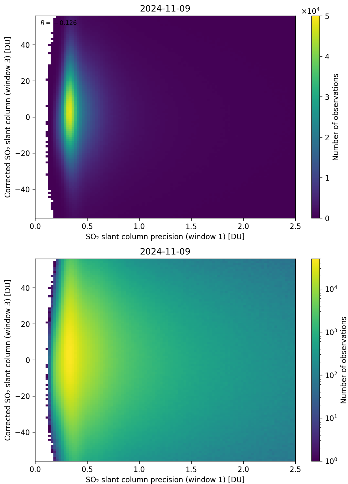
Figure 226: Scatter density plot of “SO 2 slant column precision (window 1)” against “Corrected SO 2 slant column (window 3)” for 2024-11-09 to 2024-11-10.
