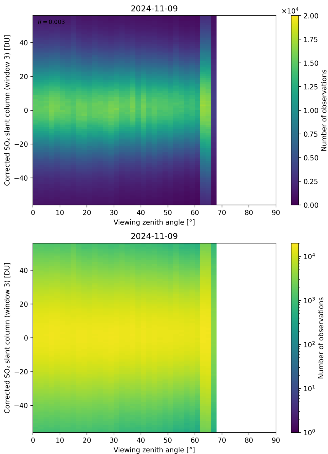
Figure 319: Scatter density plot of “Viewing zenith angle” against “Corrected SO 2 slant column (window 3)” for 2024-11-09 to 2024-11-10.
