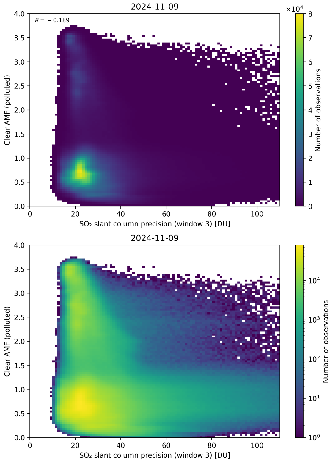
Figure 261: Scatter density plot of “SO 2 slant column precision (window 3)” against “Clear AMF (polluted)” for 2024-11-09 to 2024-11-10.
