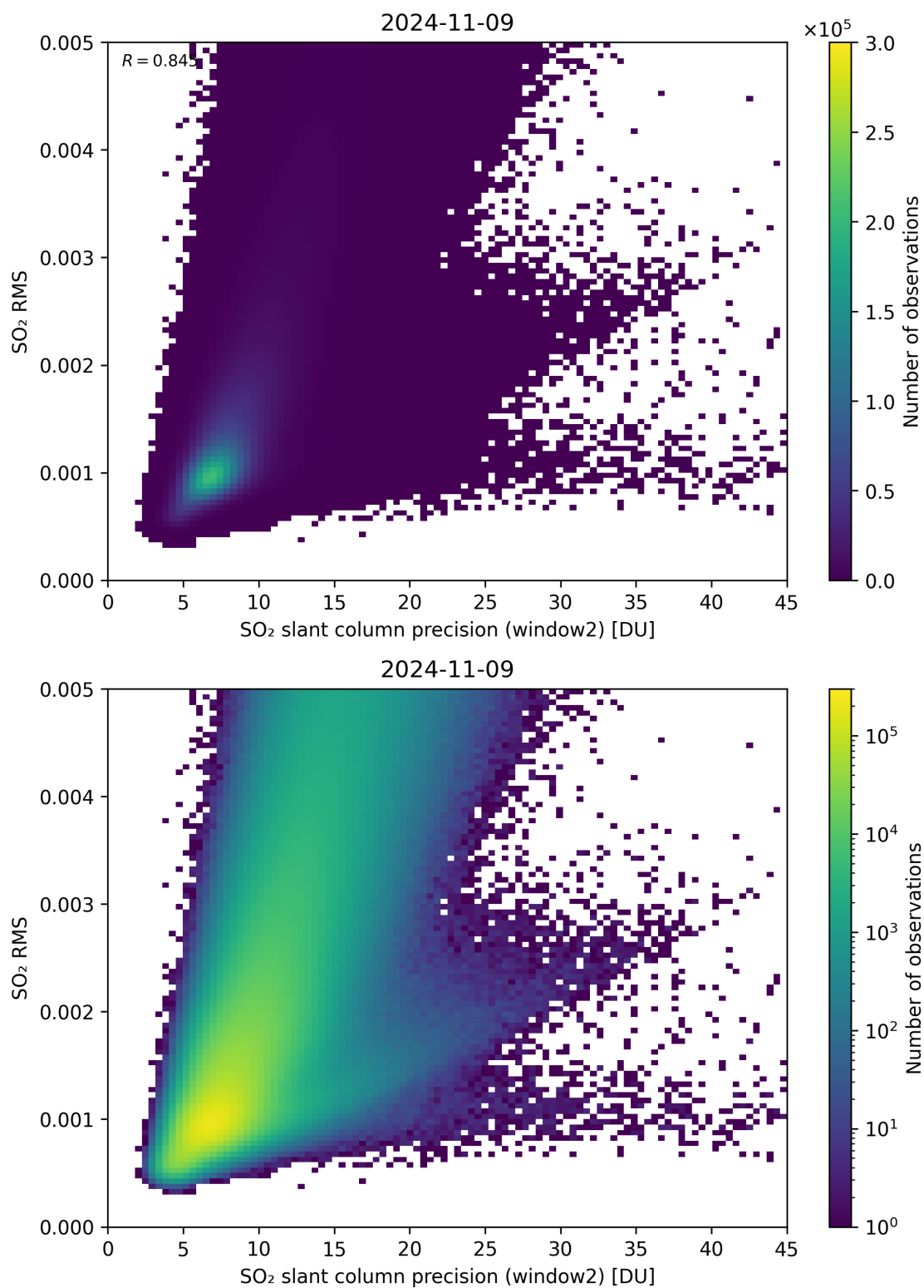
Figure 245: Scatter density plot of “SO 2 slant column precision (window2)” against “SO 2 RMS” for 2024-11-09 to 2024-11-10.
