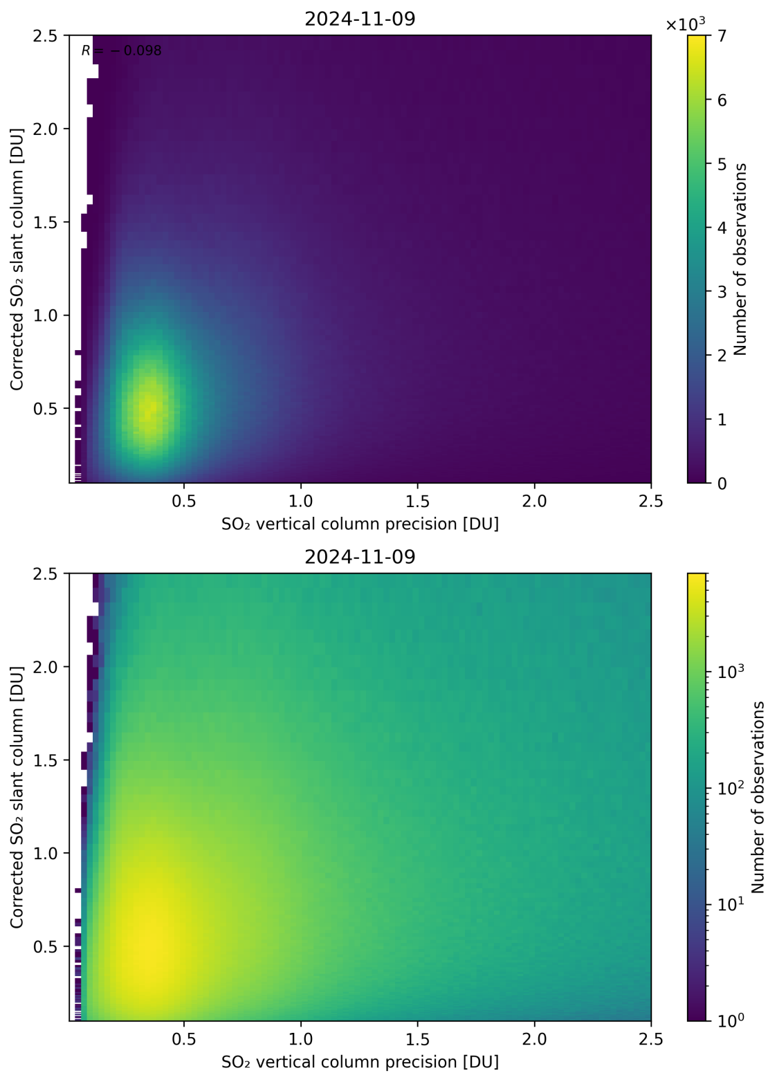
Figure 286: Scatter density plot of “SO 2 vertical column precision” against “Corrected SO 2 slant column” for 2024-11-09 to 2024-11-10.
