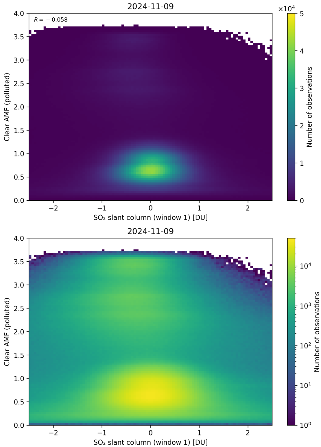
Figure 232: Scatter density plot of “SO 2 slant column (window 1)” against “Clear AMF (polluted)” for 2024-11-09 to 2024-11-10.
