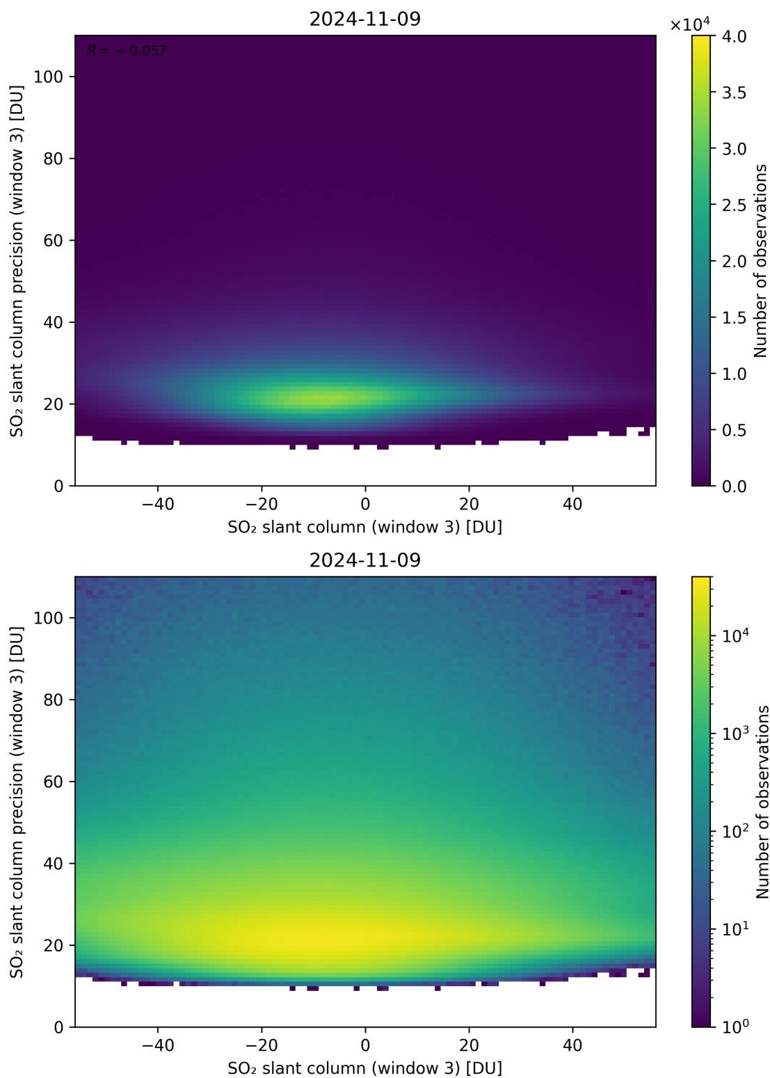
Figure 267: Scatter density plot of “SO 2 slant column (window 3)” against “SO 2 slant column precision (window 3)” for 2024-11-09 to 2024-11-10.
