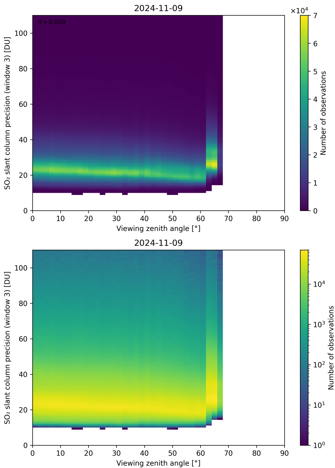
Figure 324: Scatter density plot of “Viewing zenith angle” against “SO 2 slant column precision (window 3)” for 2024-11-09 to 2024-11-10.
