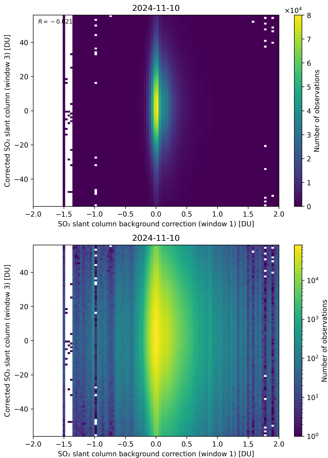
Figure 105: Scatter density plot of “SO 2 slant column background correction (window 1)” against “Corrected SO 2 slant column (window 3)” for 2024-11-09 to 2024-11-11.
