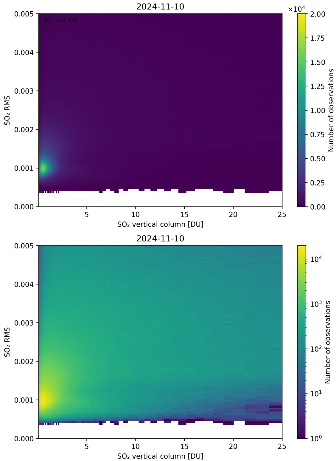
Figure 278: Scatter density plot of “SO 2 vertical column” against “SO 2 RMS” for 2024-11-09 to 2024-11-11.
