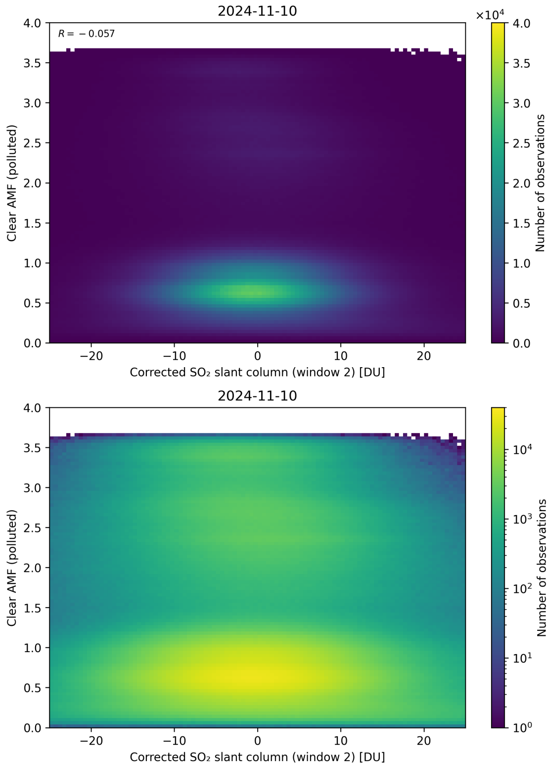
Figure 199: Scatter density plot of “Corrected SO 2 slant column (window 2)” against “Clear AMF (polluted)” for 2024-11-09 to 2024-11-11.
