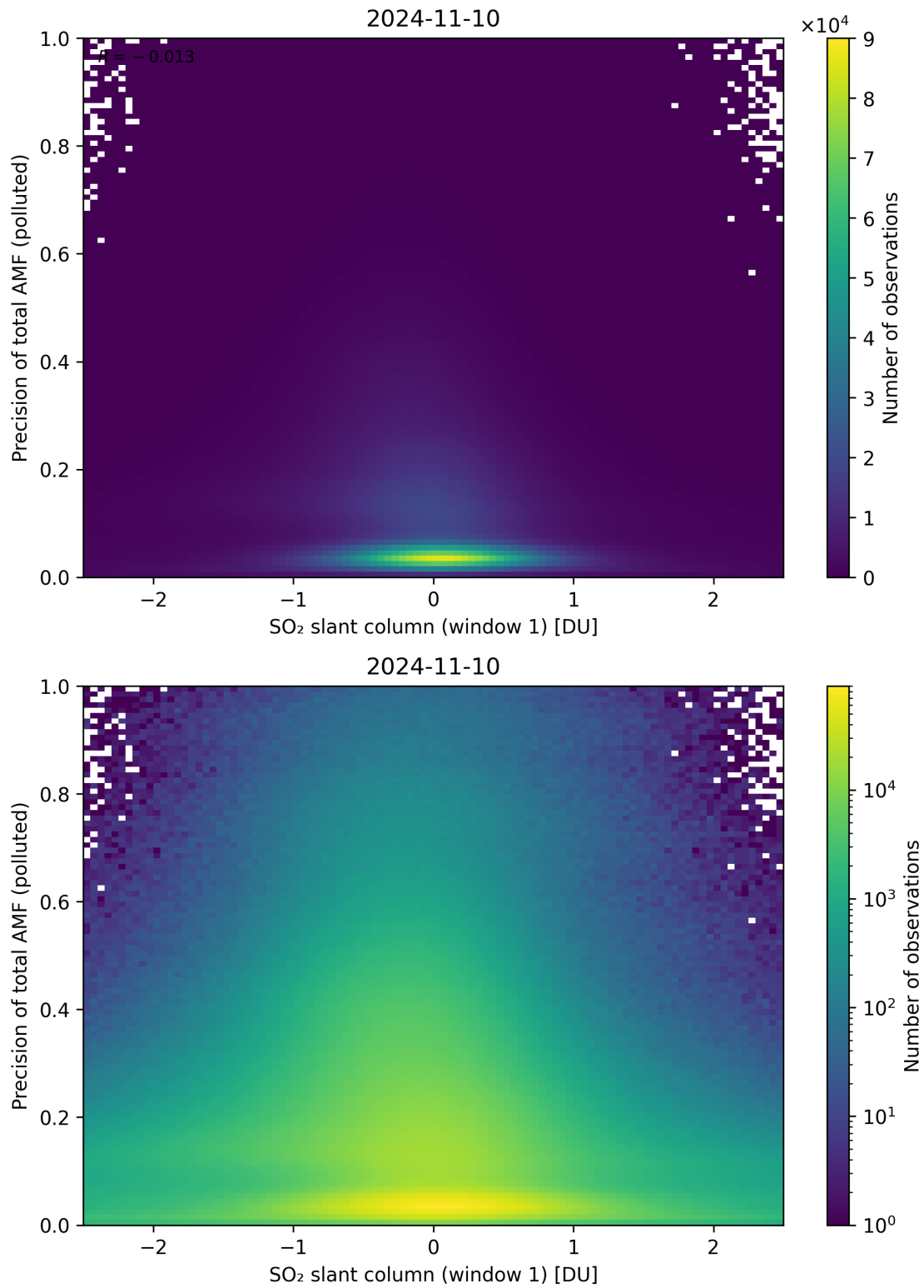
Figure 240: Scatter density plot of “SO 2 slant column (window 1)” against “Precision of total AMF (polluted)” for 2024-11-09 to 2024-11-11.
