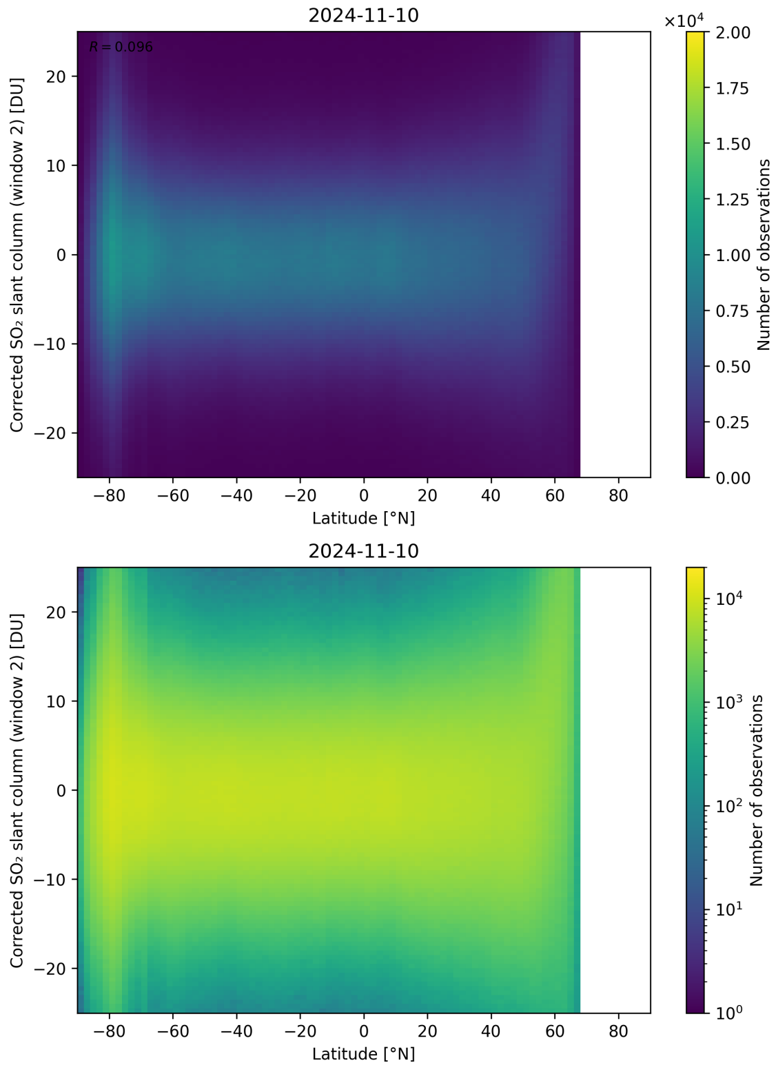
Figure 147: Scatter density plot of “Latitude” against “Corrected SO 2 slant column (window 2)” for 2024-11-09 to 2024-11-11.
