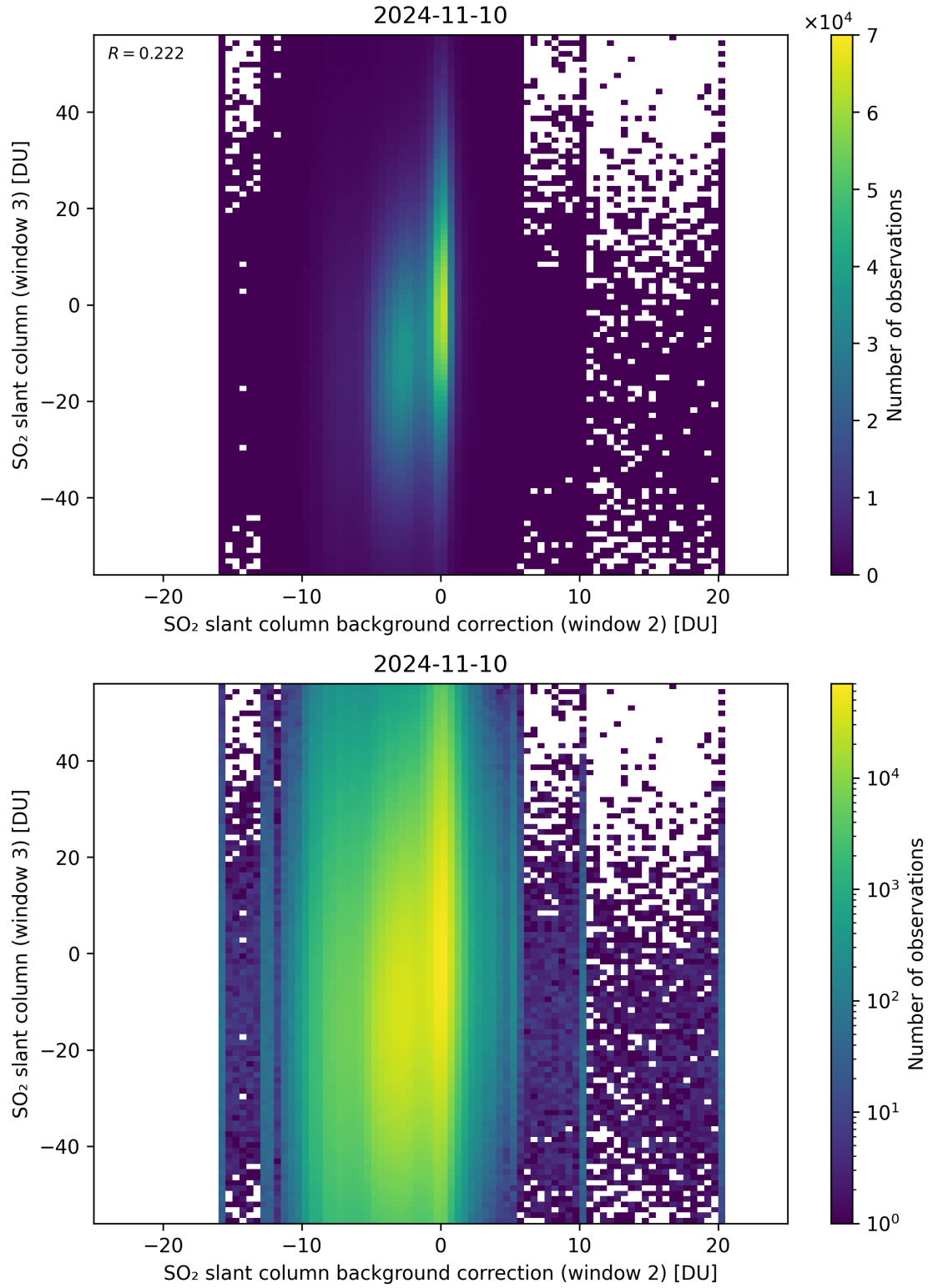
Figure 117: Scatter density plot of “SO 2 slant column background correction (window 2)” against “SO 2 slant column (window 3)” for 2024-11-09 to 2024-11-11.
