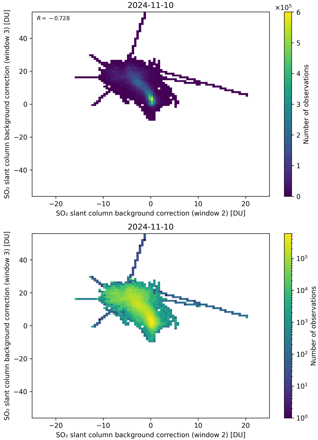
Figure 111: Scatter density plot of “SO 2 slant column background correction (window 2)” against “SO 2 slant column background correction (window 3)” for 2024-11-09 to 2024-11-11.
