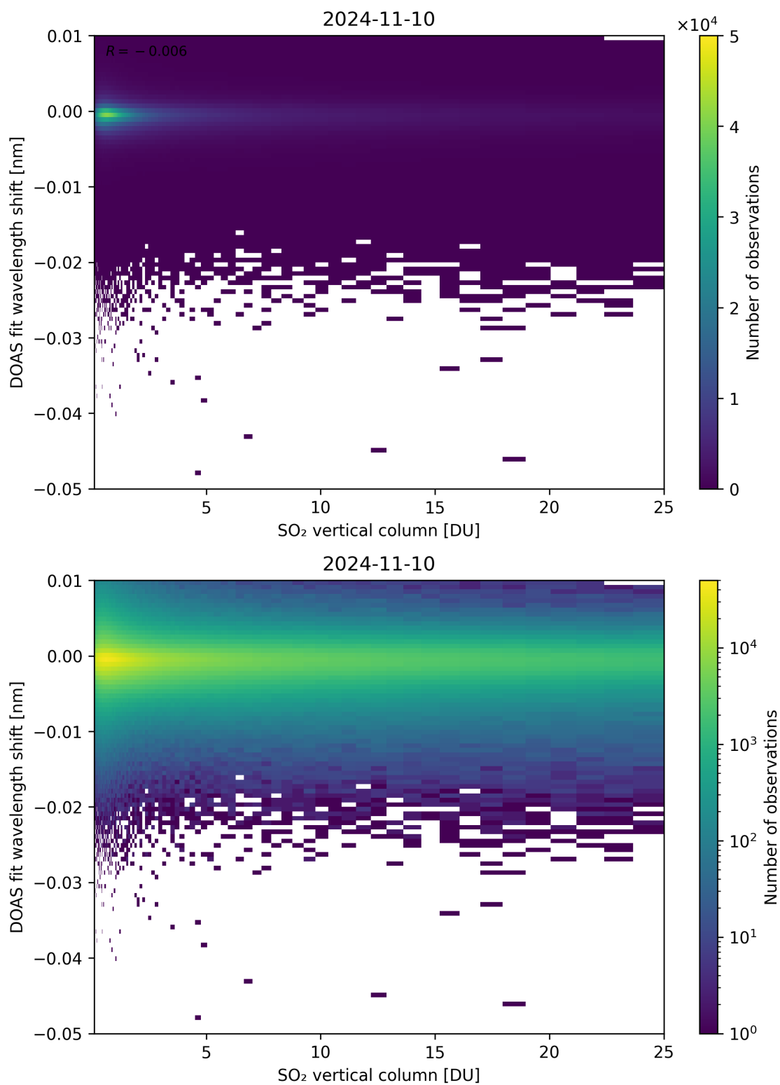
Figure 276: Scatter density plot of “SO 2 vertical column” against “DOAS fit wavelength shift” for 2024-11-09 to 2024-11-11.
