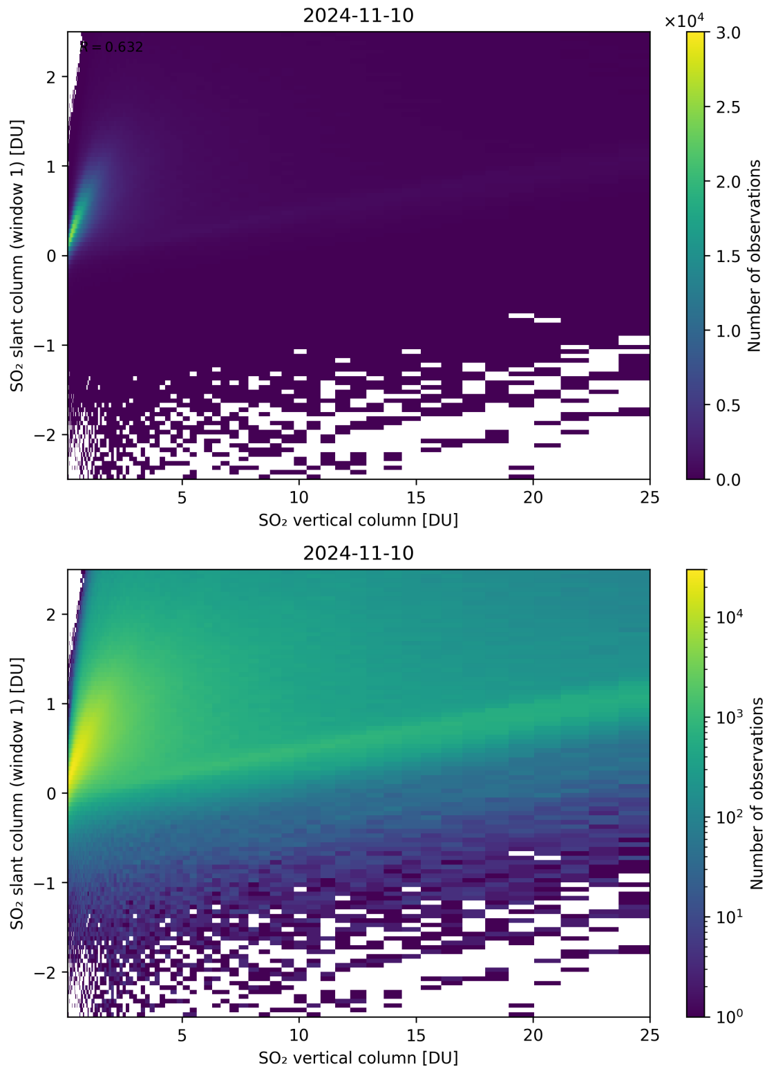
Figure 300: Scatter density plot of “SO 2 vertical column” against “SO 2 slant column (window 1)” for 2024-11-09 to 2024-11-11.
