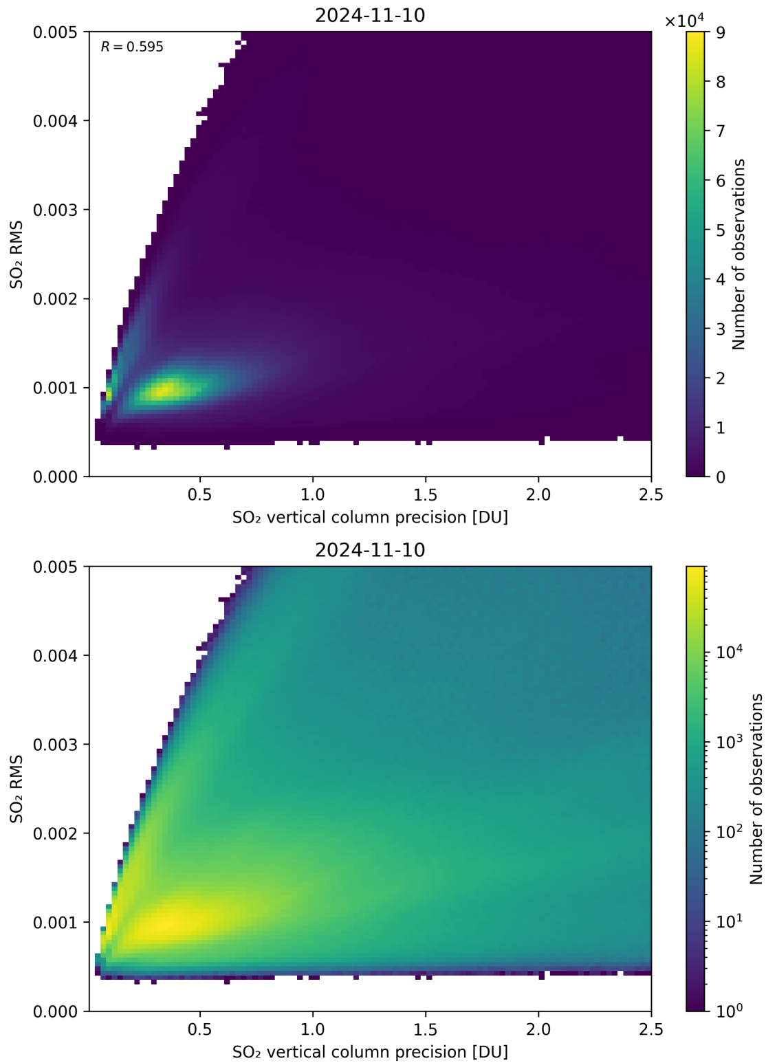
Figure 284: Scatter density plot of “SO 2 vertical column precision” against “SO 2 RMS” for 2024-11-09 to 2024-11-11.
