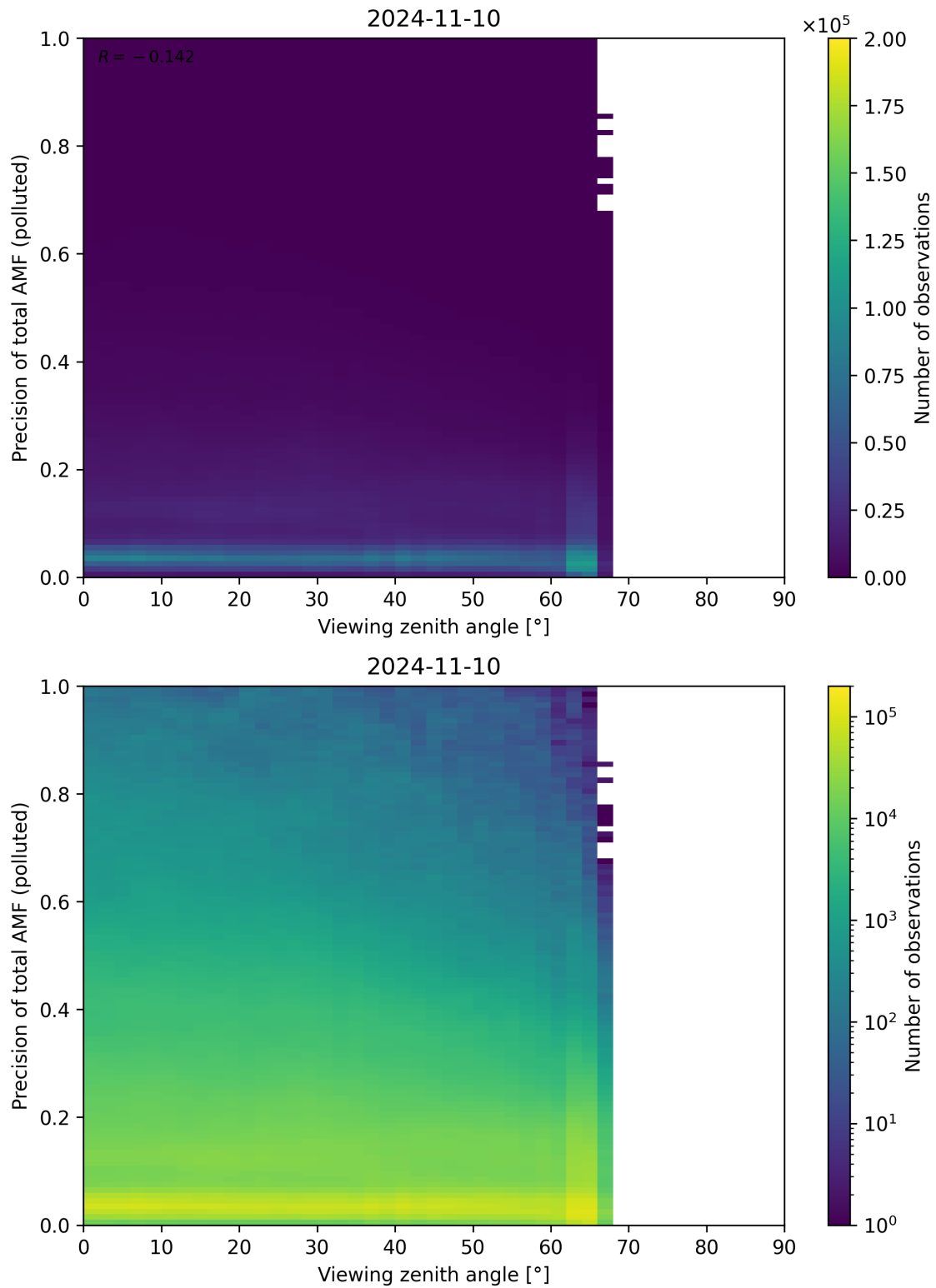
Figure 326: Scatter density plot of “Viewing zenith angle” against “Precision of total AMF (polluted)” for 2024-11-09 to 2024-11-11.
