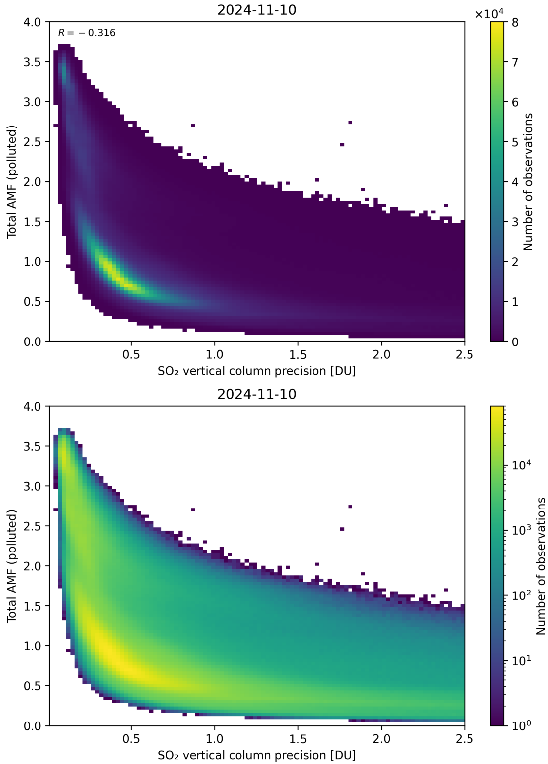
Figure 294: Scatter density plot of “SO 2 vertical column precision” against “Total AMF (polluted)” for 2024-11-09 to 2024-11-11.
