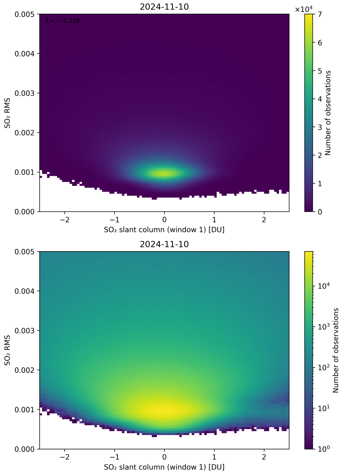
Figure 217: Scatter density plot of “SO 2 slant column (window 1)” against “SO 2 RMS” for 2024-11-09 to 2024-11-11.
