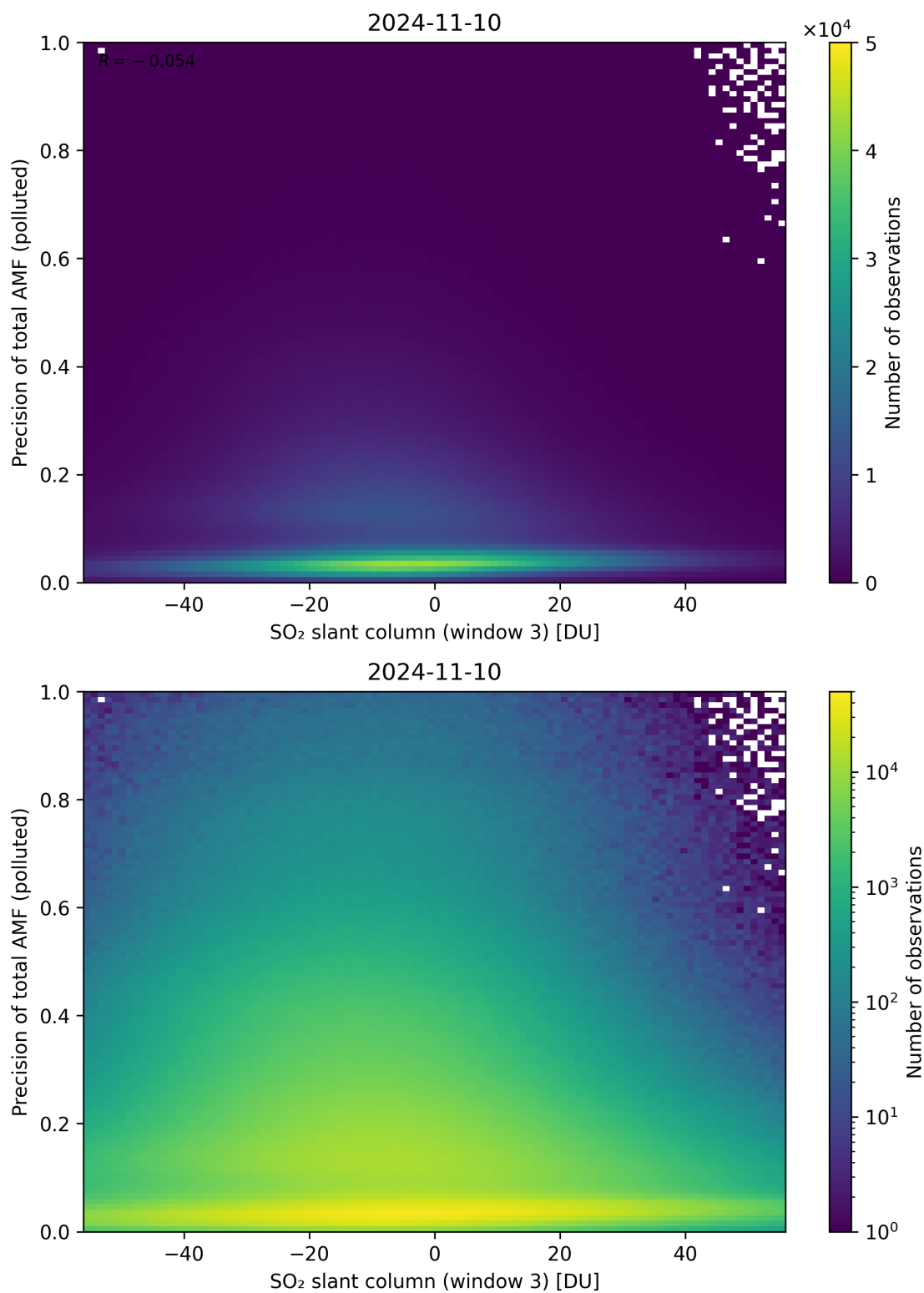
Figure 269: Scatter density plot of “SO 2 slant column (window 3)” against “Precision of total AMF (polluted)” for 2024-11-09 to 2024-11-11.
