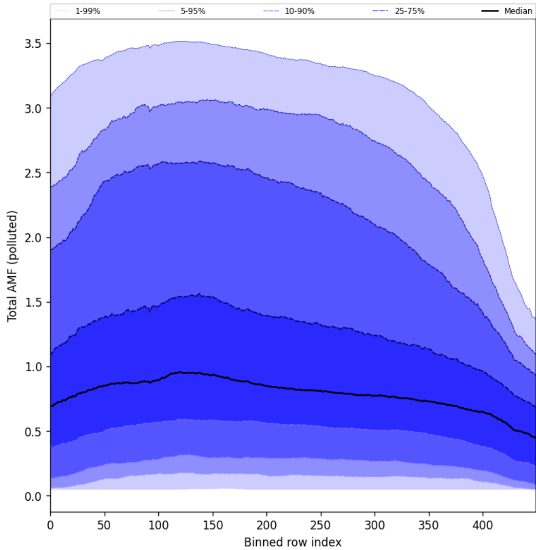
Figure 94: Along track statistics of “Total AMF (polluted)” for 2024-11-09 to 2024-11-11
