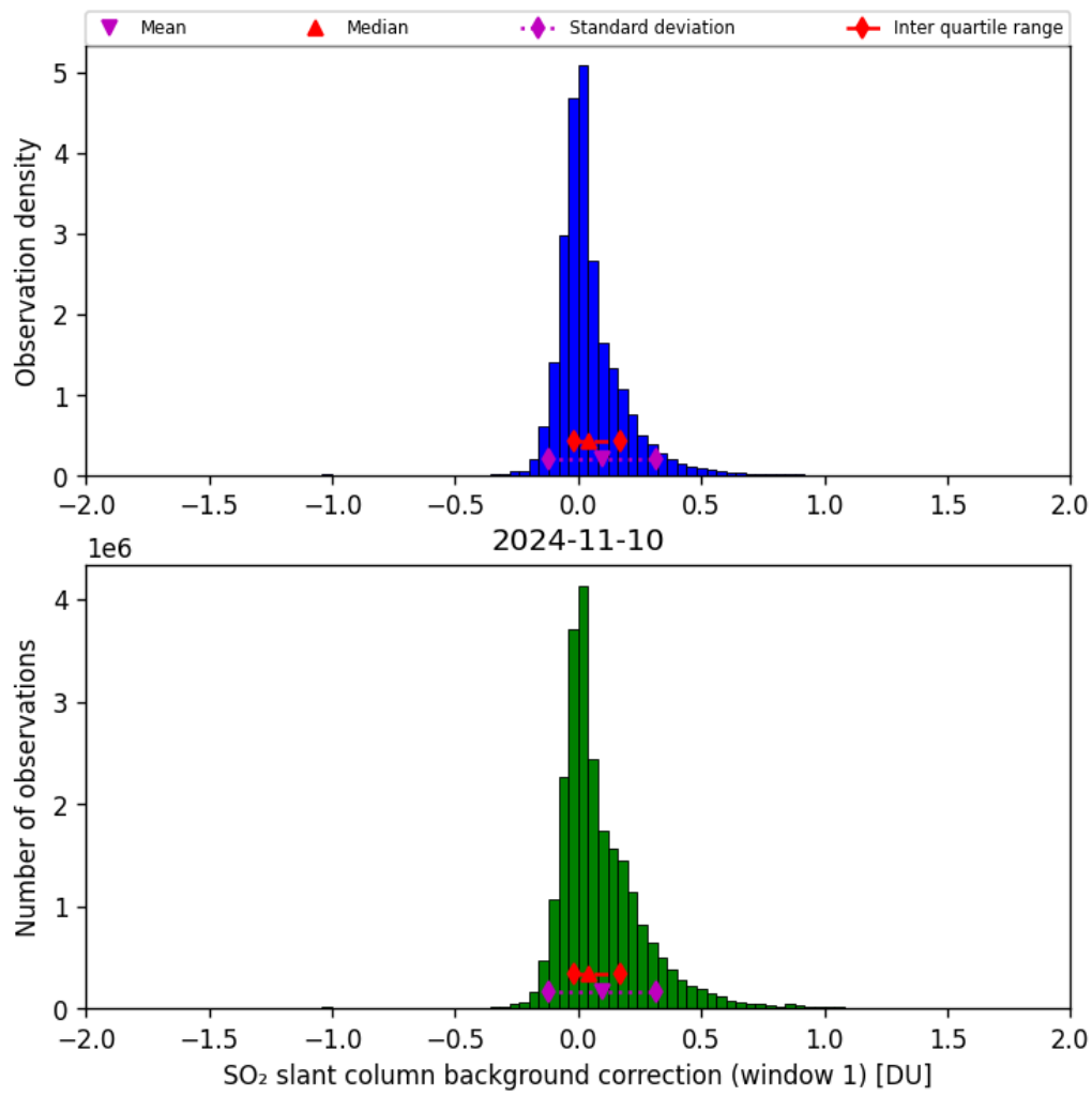
Figure 59: Histogram of “SO 2 slant column background correction (window 1)” for 2024-11-09 to 2024-11-11
