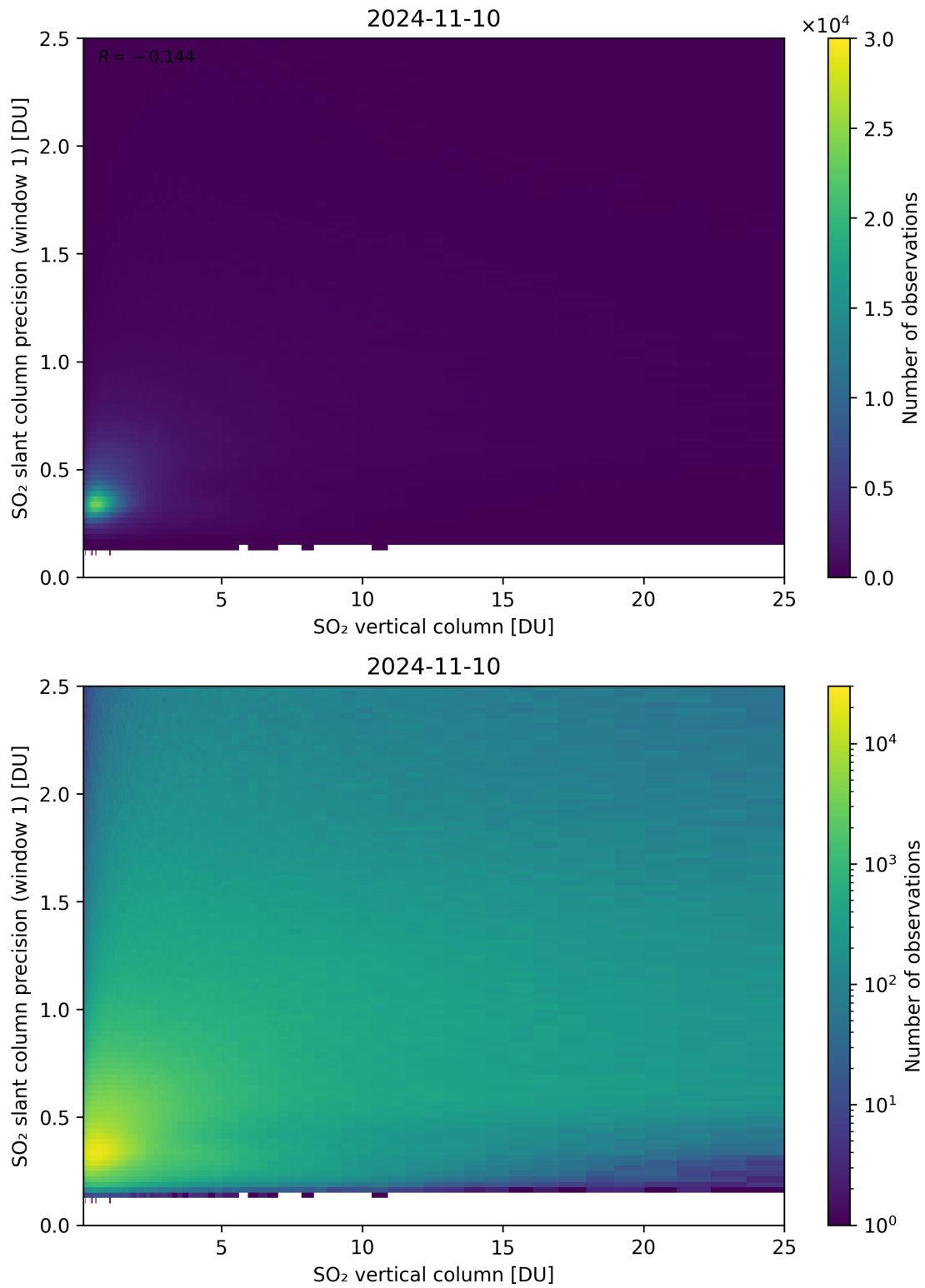
Figure 301: Scatter density plot of “SO 2 vertical column” against “SO 2 slant column precision (window 1)” for 2024-11-09 to 2024-11-11.
