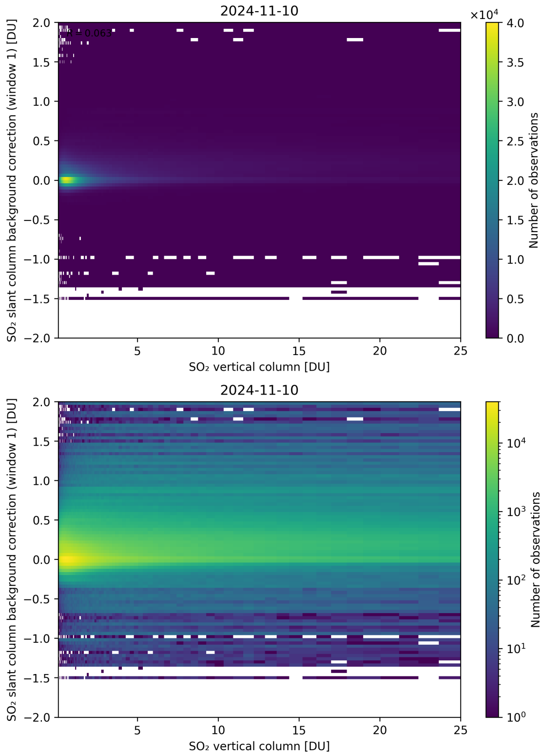
Figure 273: Scatter density plot of “SO 2 vertical column” against “SO 2 slant column background correction (window 1)” for 2024-11-09 to 2024-11-11.
