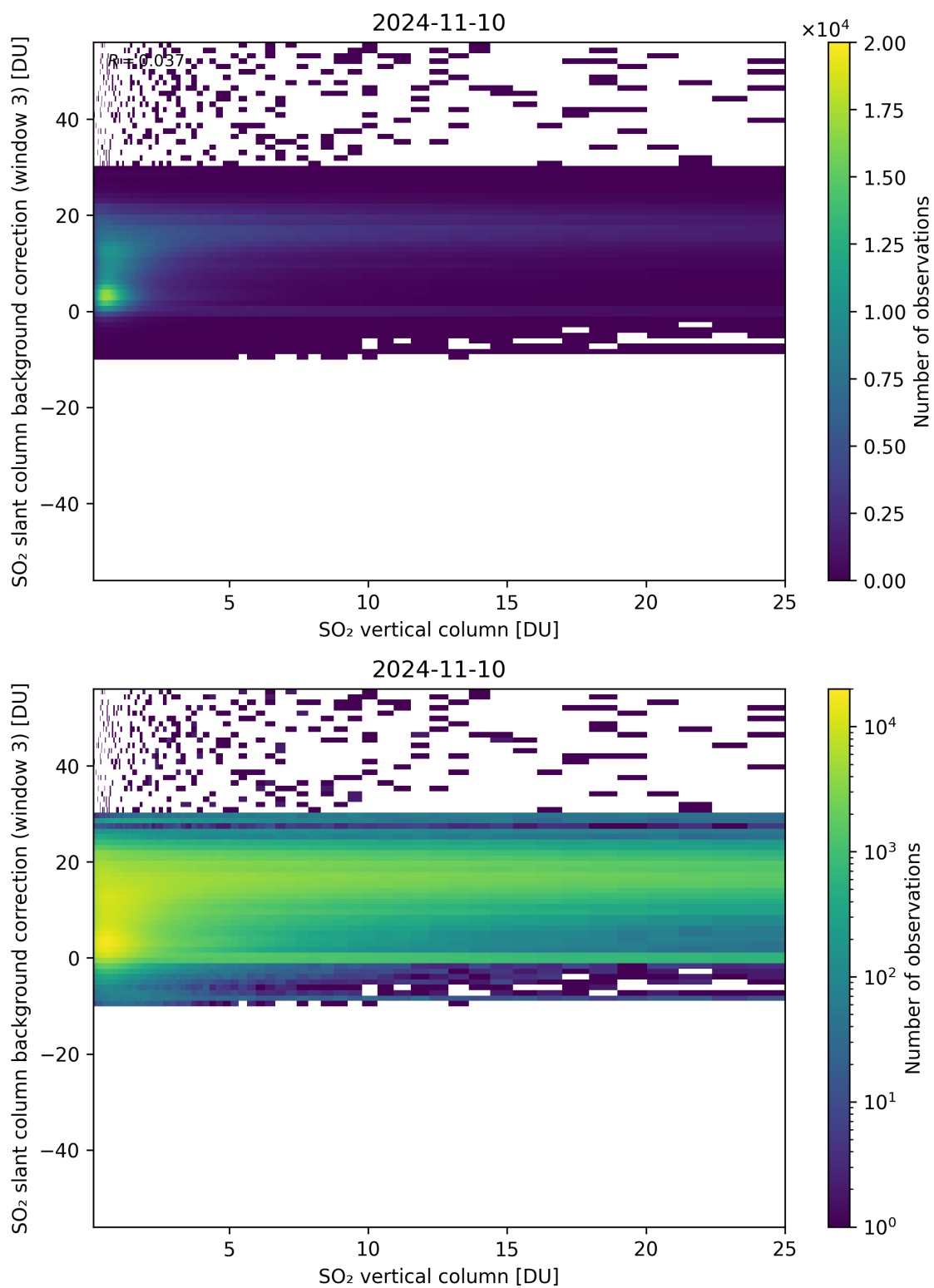
Figure 275: Scatter density plot of “SO 2 vertical column” against “SO 2 slant column background correction (window 3)” for 2024-11-09 to 2024-11-11.
