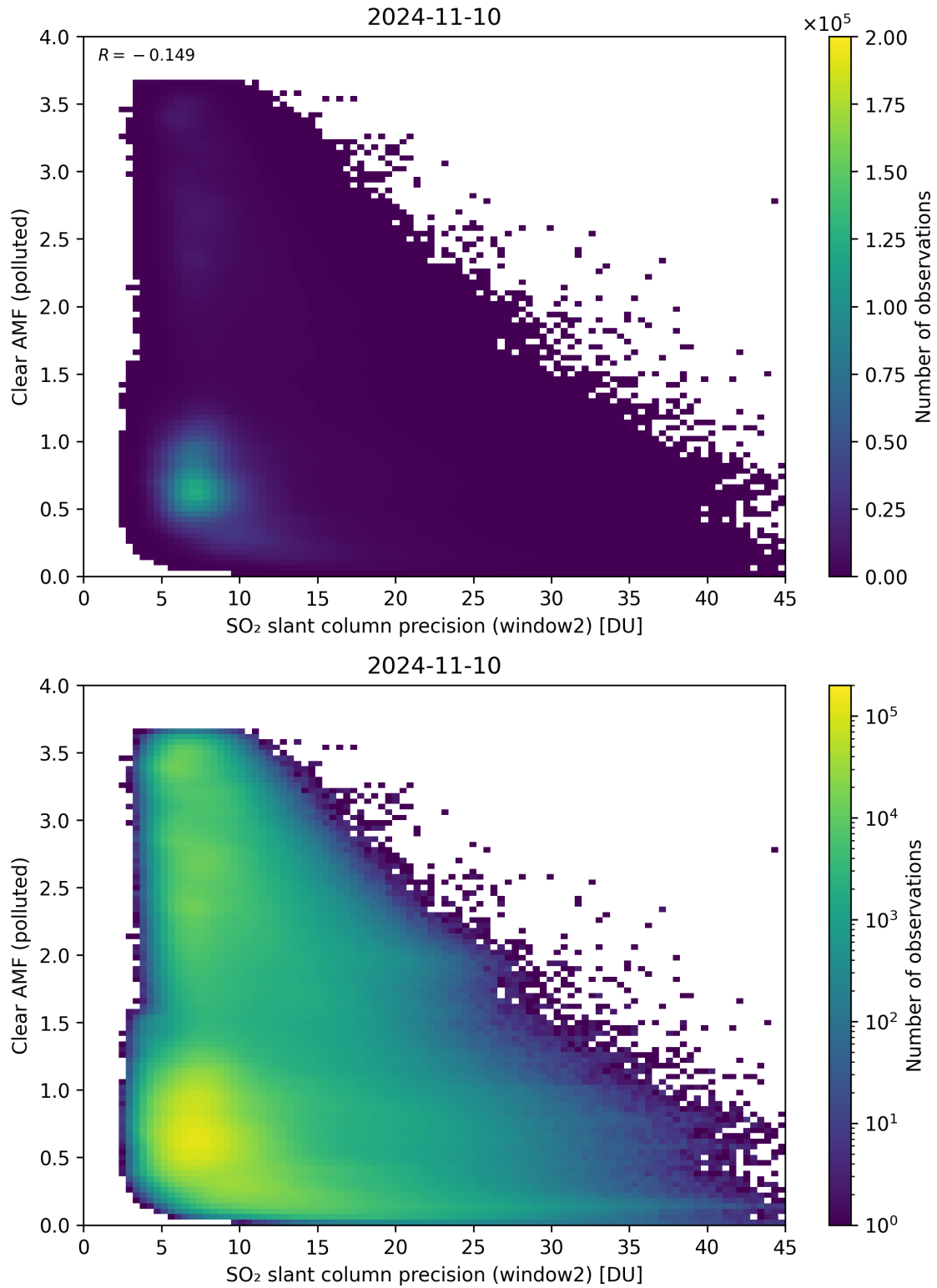
Figure 246: Scatter density plot of “SO 2 slant column precision (window2)” against “Clear AMF (polluted)” for 2024-11-09 to 2024-11-11.
