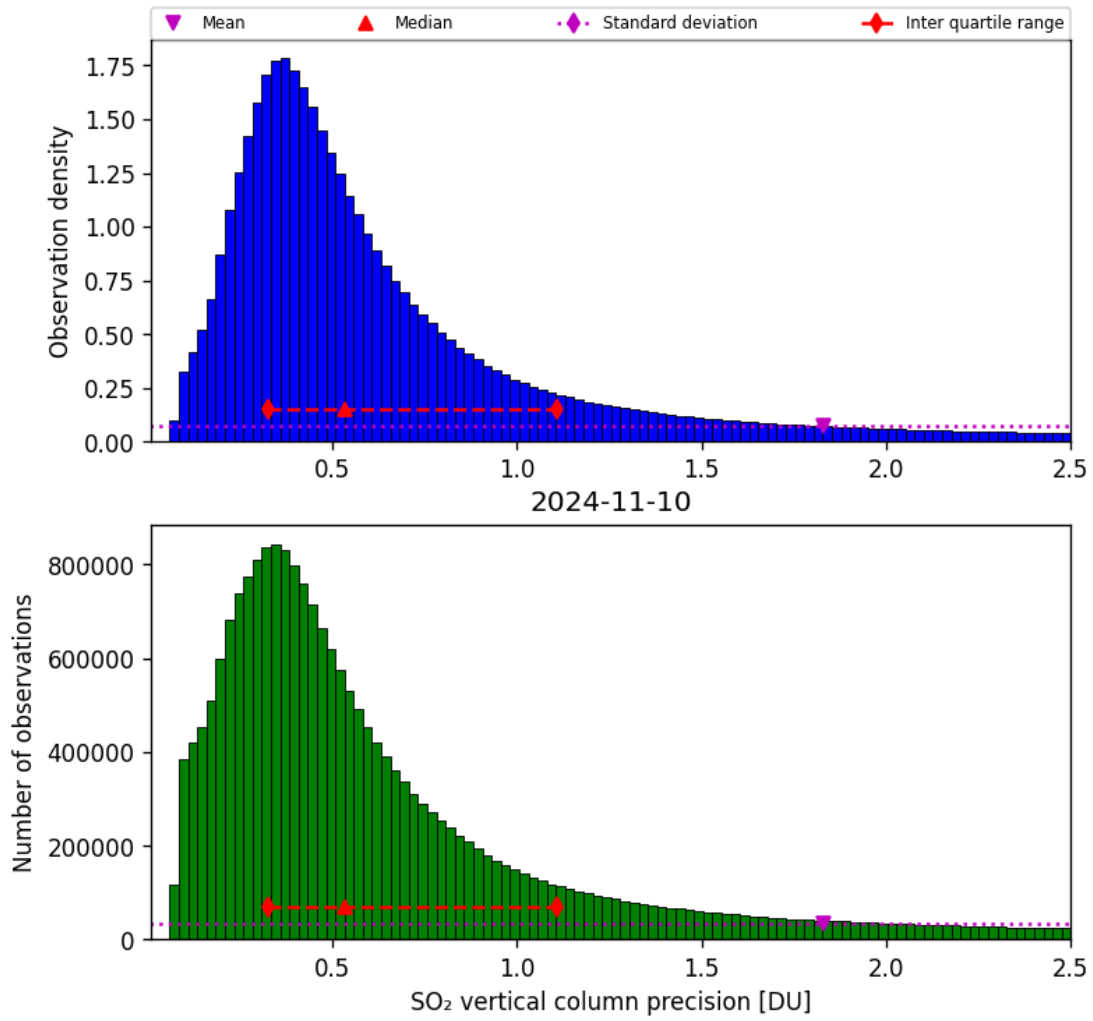
Figure 54: Histogram of “SO 2 vertical column precision” for 2024-11-09 to 2024-11-11
