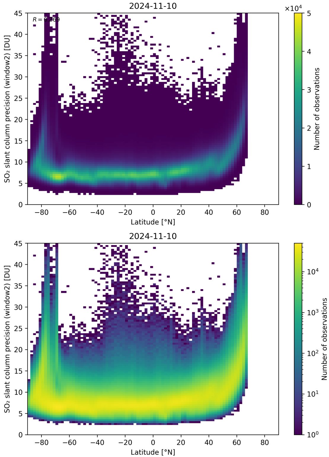
Figure 151: Scatter density plot of “Latitude” against “SO 2 slant column precision (window2)” for 2024-11-09 to 2024-11-11.
