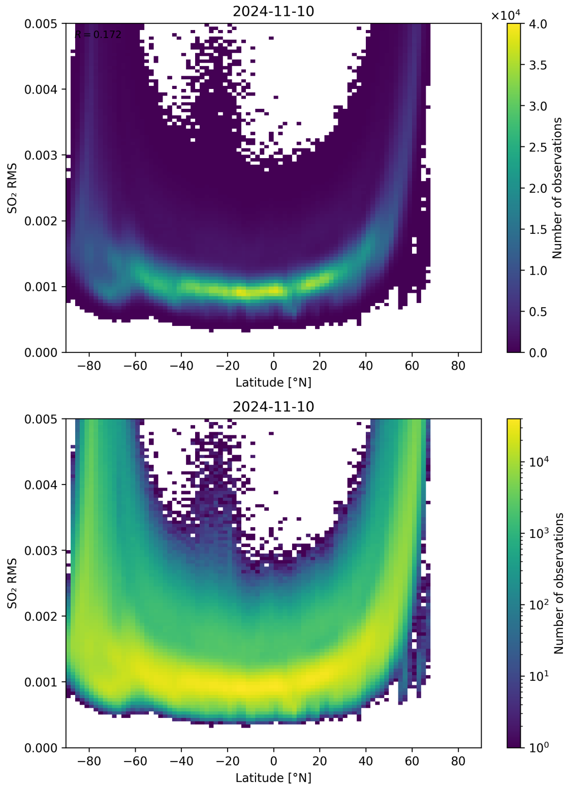
Figure 144: Scatter density plot of “Latitude” against “SO 2 RMS” for 2024-11-09 to 2024-11-11.
