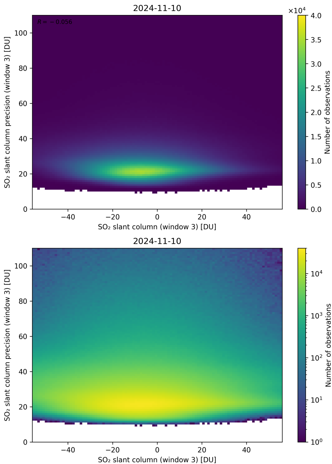
Figure 267: Scatter density plot of “SO 2 slant column (window 3)” against “SO 2 slant column precision (window 3)” for 2024-11-09 to 2024-11-11.
