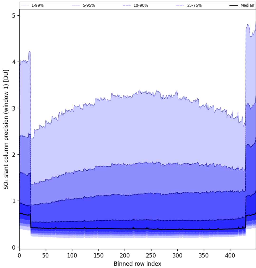
Figure 80: Along track statistics of “SO 2 slant column precision (window 1)” for 2024-11-09 to 2024-11-11
