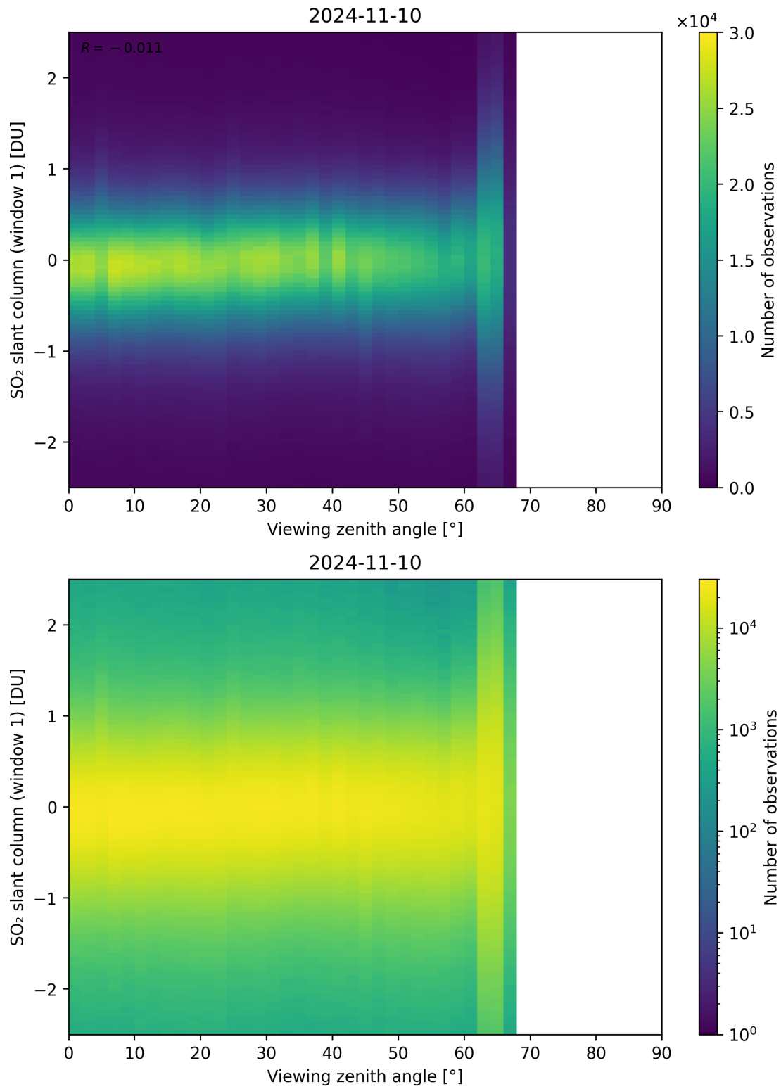
Figure 320: Scatter density plot of “Viewing zenith angle” against “SO 2 slant column (window 1)” for 2024-11-09 to 2024-11-11.
