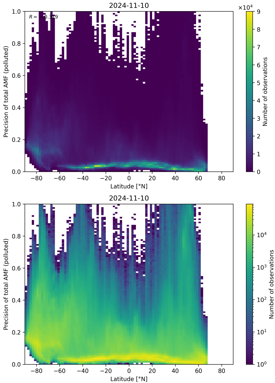
Figure 155: Scatter density plot of “Latitude” against “Precision of total AMF (polluted)” for 2024-11-09 to 2024-11-11.
