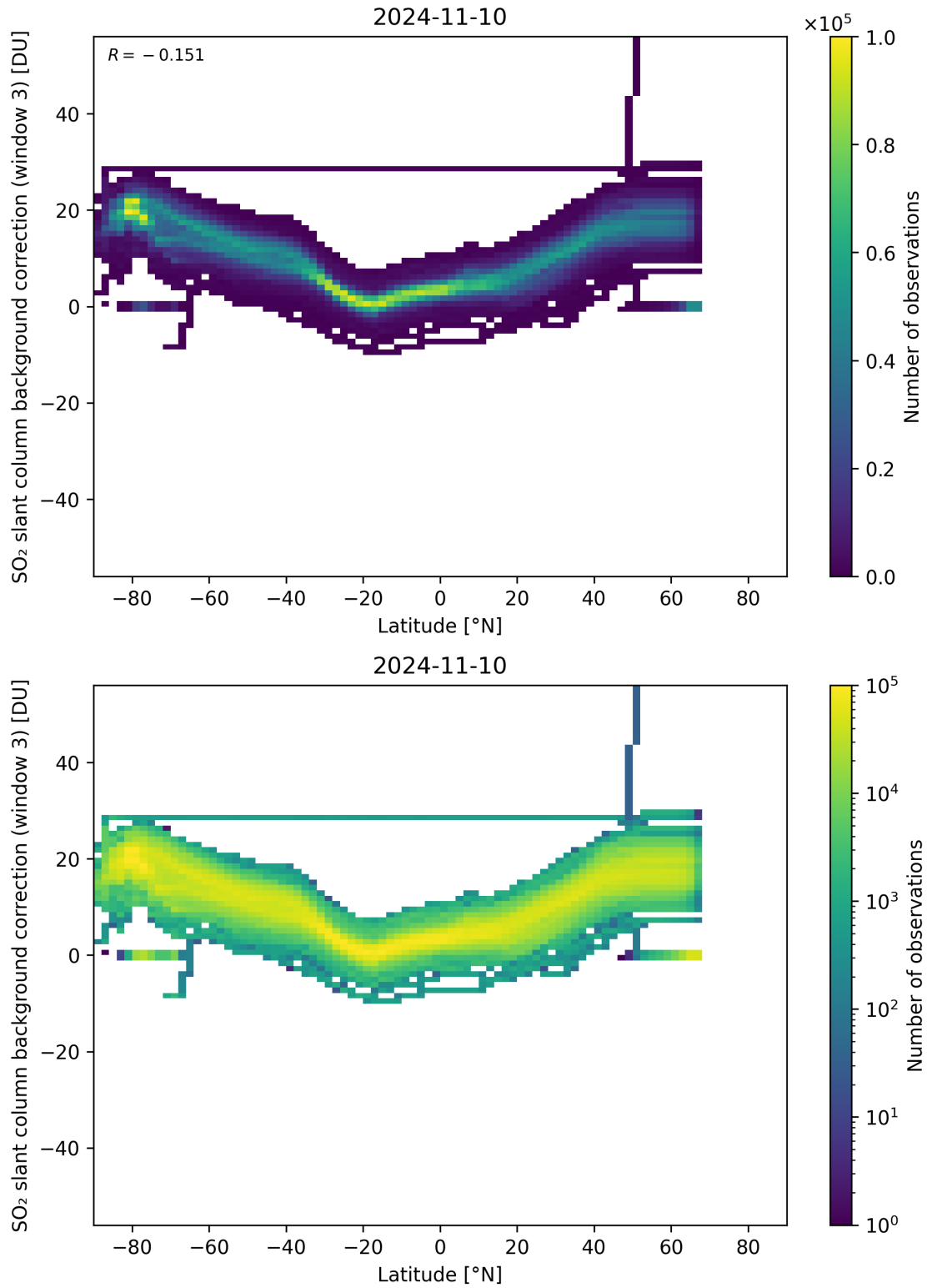
Figure 141: Scatter density plot of “Latitude” against “SO 2 slant column background correction (window 3)” for 2024-11-09 to 2024-11-11.
