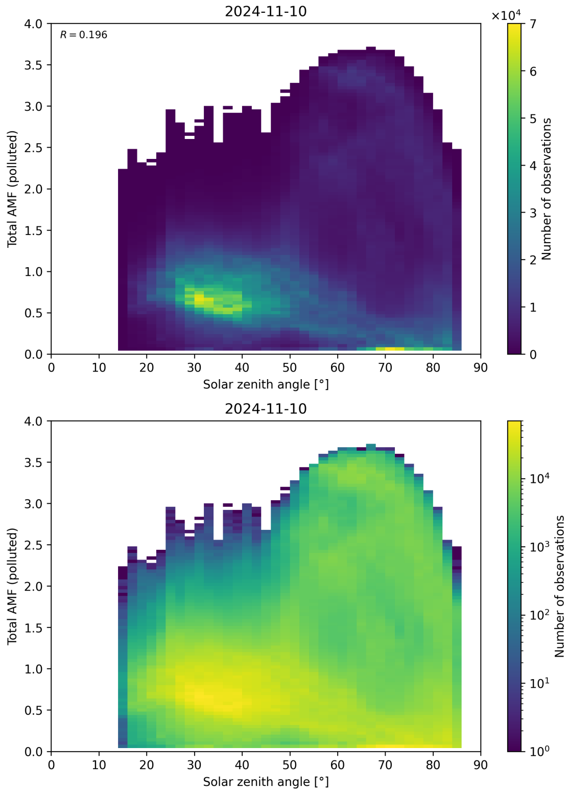
Figure 174: Scatter density plot of “Solar zenith angle” against “Total AMF (polluted)” for 2024-11-09 to 2024-11-11.
