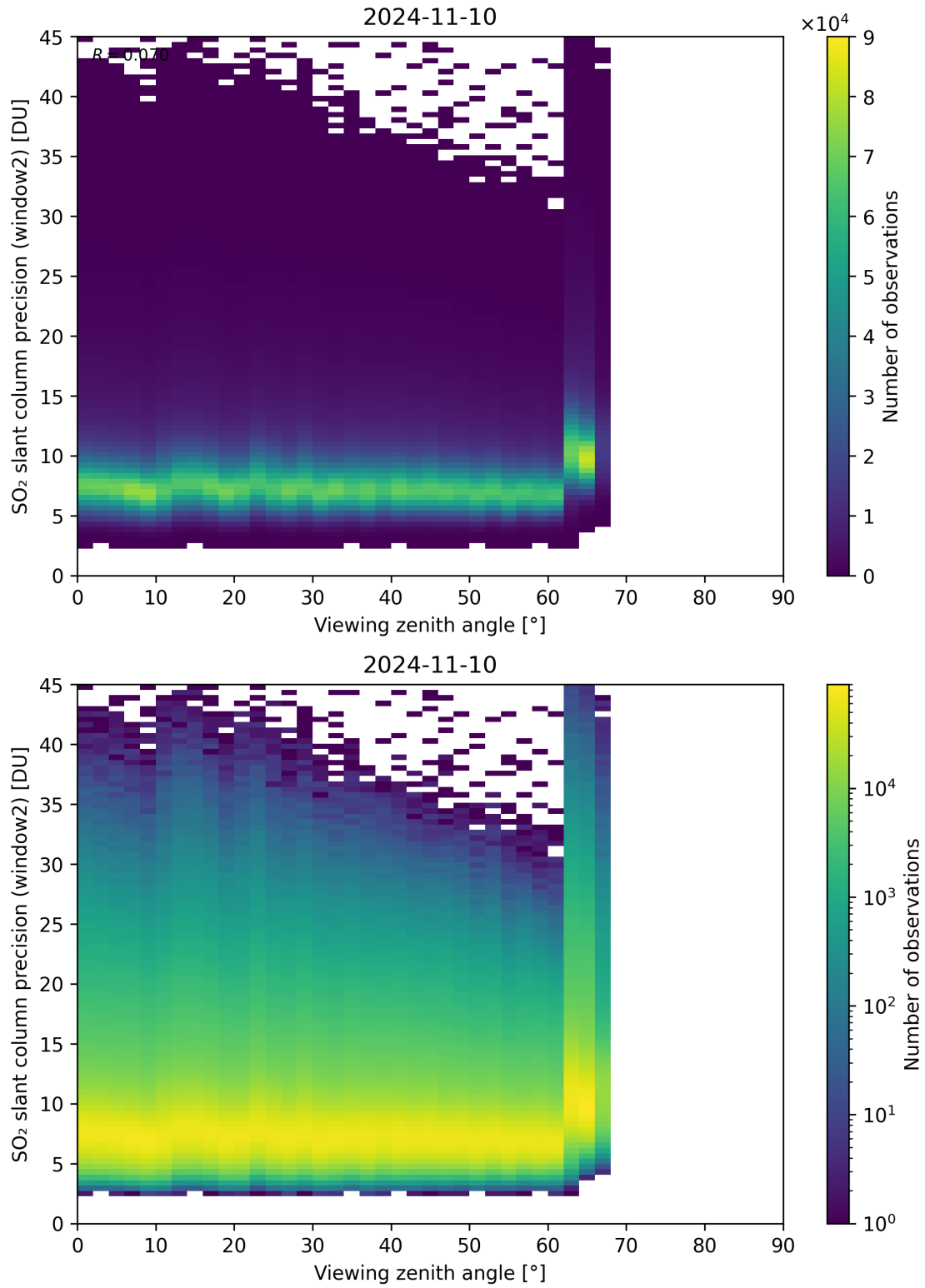
Figure 322: Scatter density plot of “Viewing zenith angle” against “SO 2 slant column precision (window2)” for 2024-11-09 to 2024-11-11.
