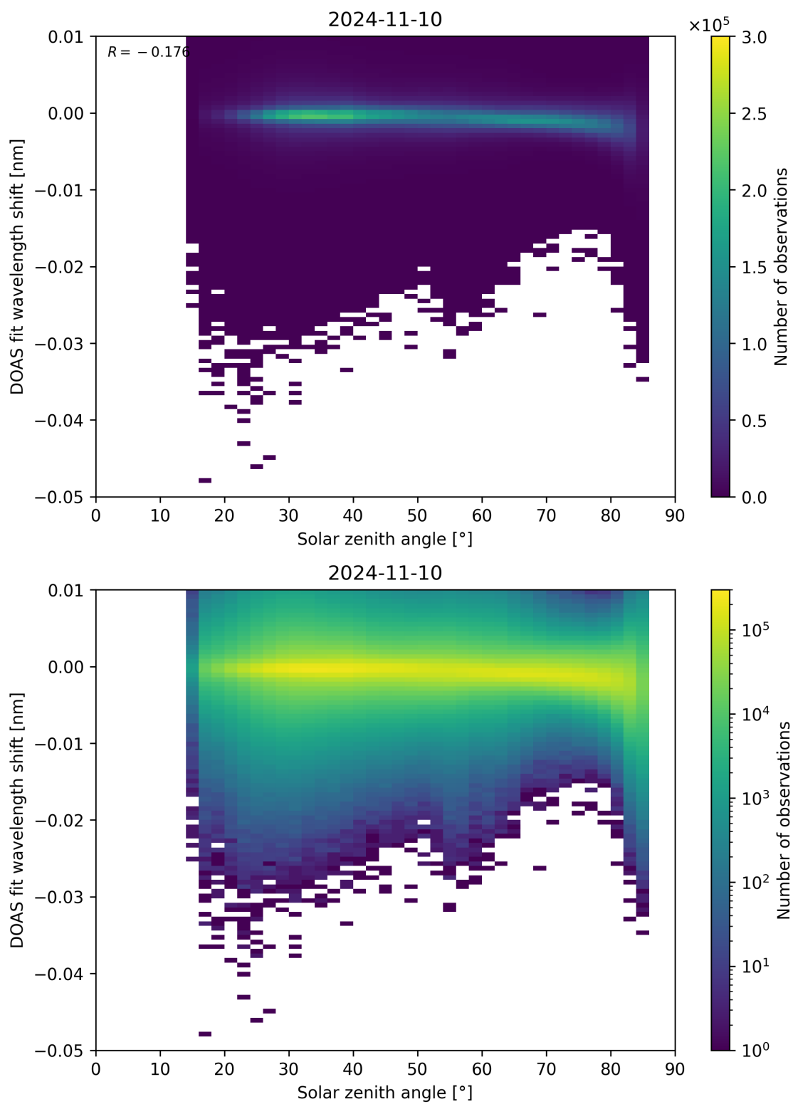
Figure 161: Scatter density plot of “Solar zenith angle” against “DOAS fit wavelength shift” for 2024-11-09 to 2024-11-11.
