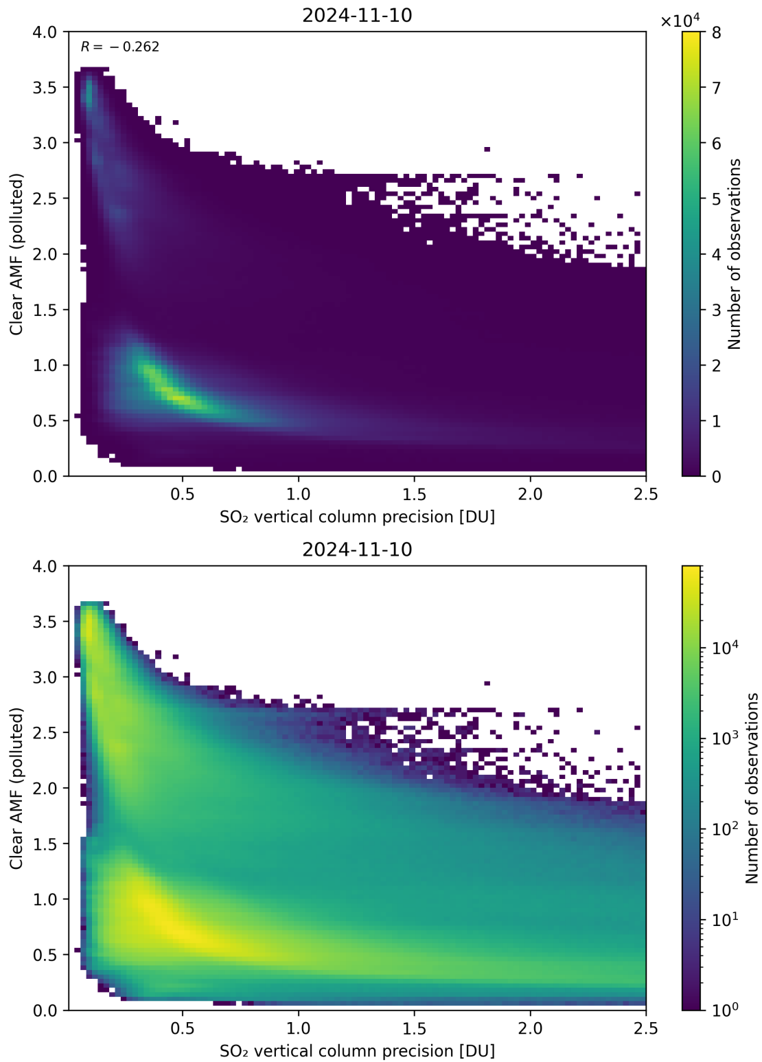
Figure 285: Scatter density plot of “SO 2 vertical column precision” against “Clear AMF (polluted)” for 2024-11-09 to 2024-11-11.
