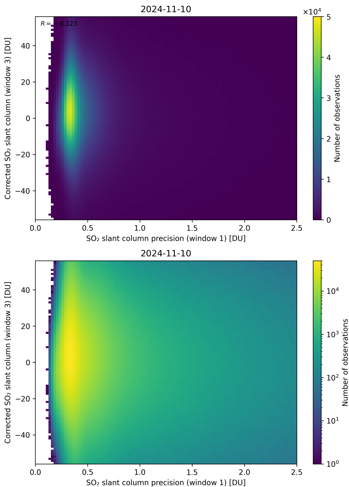
Figure 226: Scatter density plot of “SO 2 slant column precision (window 1)” against “Corrected SO 2 slant column (window 3)” for 2024-11-09 to 2024-11-11.
