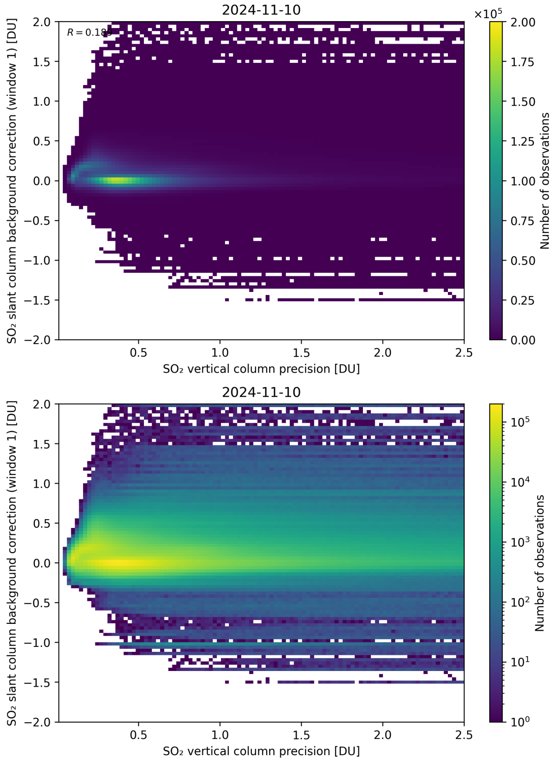
Figure 279: Scatter density plot of “SO 2 vertical column precision” against “SO 2 slant column background correction (window 1)” for 2024-11-09 to 2024-11-11.
