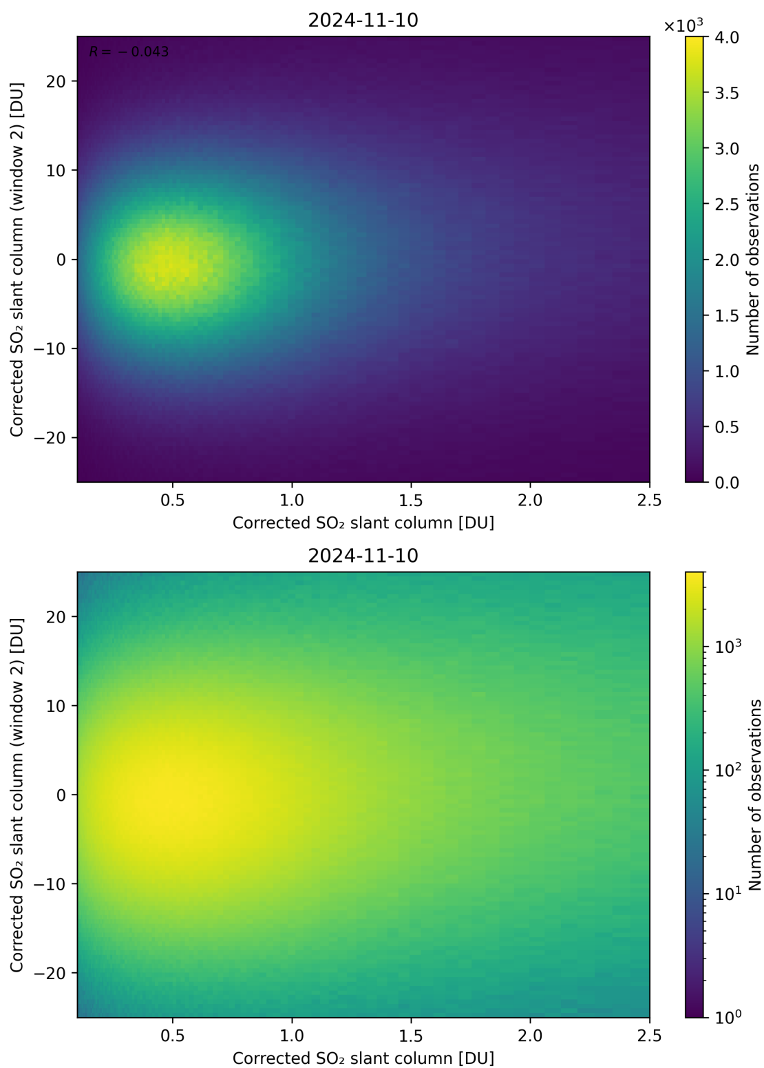
Figure 185: Scatter density plot of “Corrected SO 2 slant column” against “Corrected SO 2 slant column (window 2)” for 2024-11-09 to 2024-11-11.
