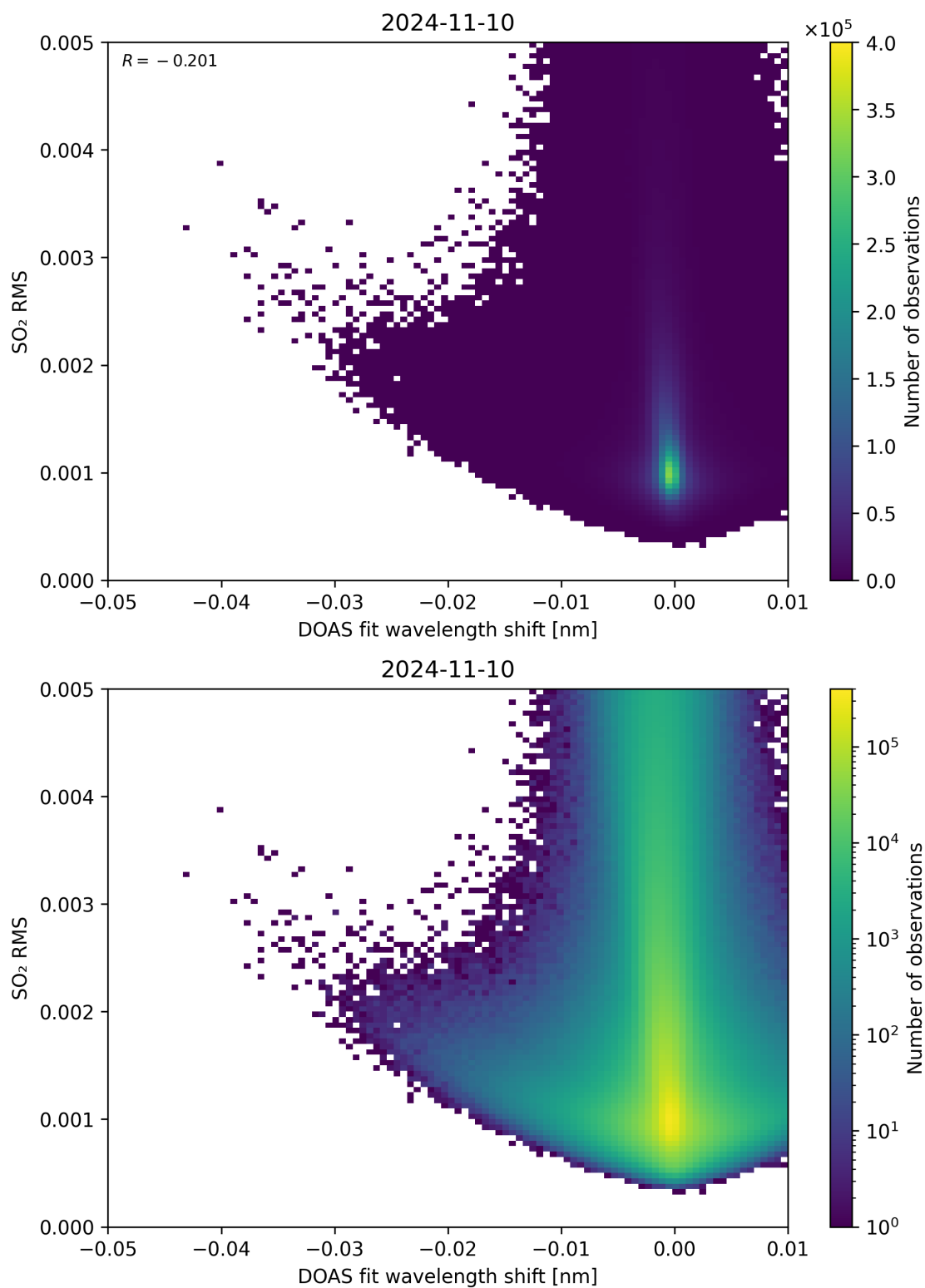
Figure 128: Scatter density plot of “DOAS fit wavelength shift” against “SO 2 RMS” for 2024-11-09 to 2024-11-11.
