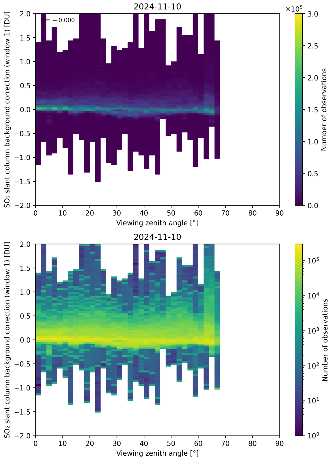
Figure 308: Scatter density plot of “Viewing zenith angle” against “SO 2 slant column background correction (window 1)” for 2024-11-09 to 2024-11-11.
