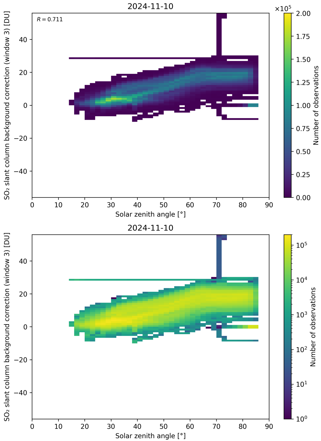
Figure 160: Scatter density plot of “Solar zenith angle” against “SO 2 slant column background correction (window 3)” for 2024-11-09 to 2024-11-11.
