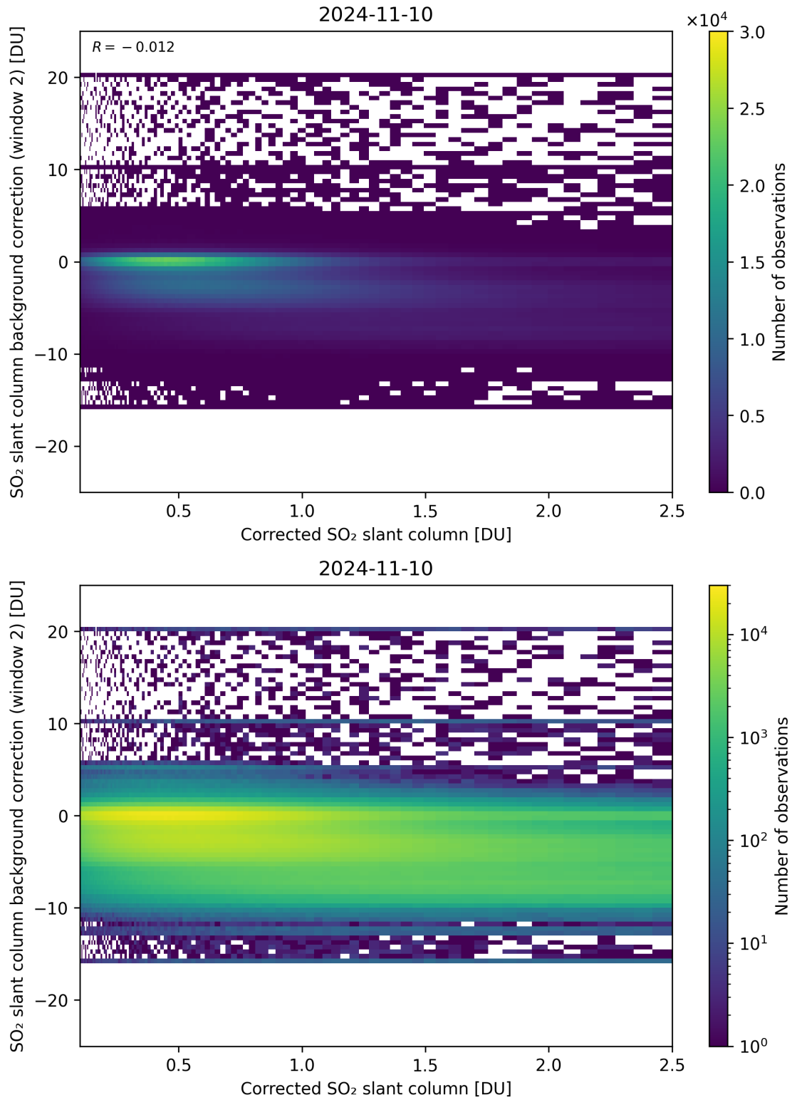
Figure 179: Scatter density plot of “Corrected SO 2 slant column” against “SO 2 slant column background correction (window 2)” for 2024-11-09 to 2024-11-11.
