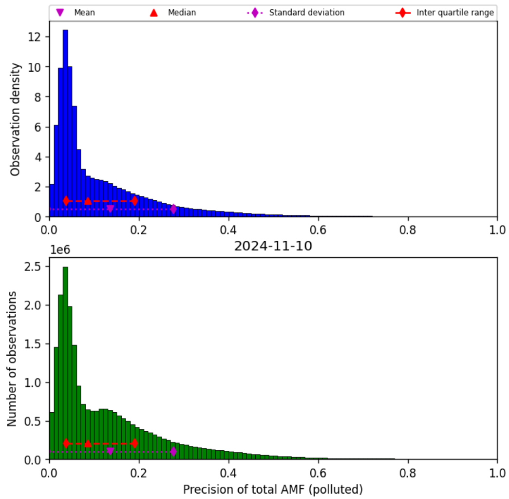
Figure 72: Histogram of “Precision of total AMF (polluted)” for 2024-11-09 to 2024-11-11
