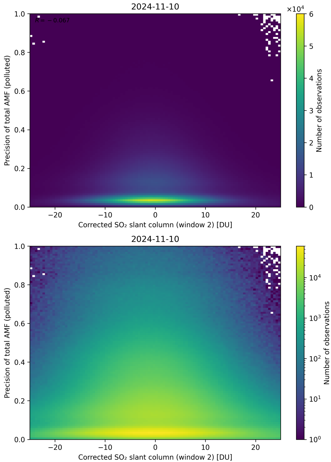
Figure 204: Scatter density plot of “Corrected SO 2 slant column (window 2)” against “Precision of total AMF (polluted)” for 2024-11-09 to 2024-11-11.
