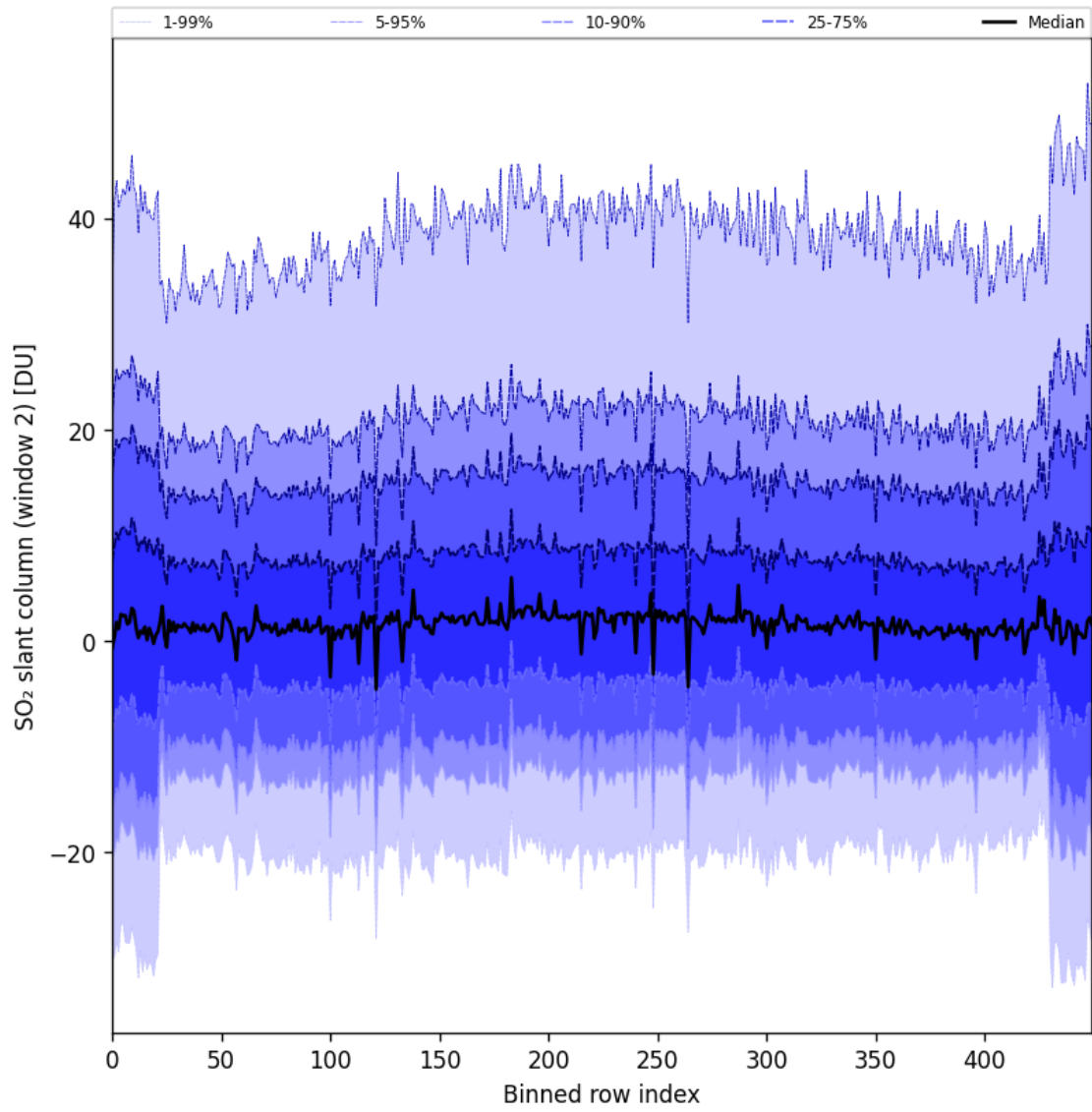
Figure 83: Along track statistics of “SO 2 slant column (window 2)” for 2024-11-09 to 2024-11-11
