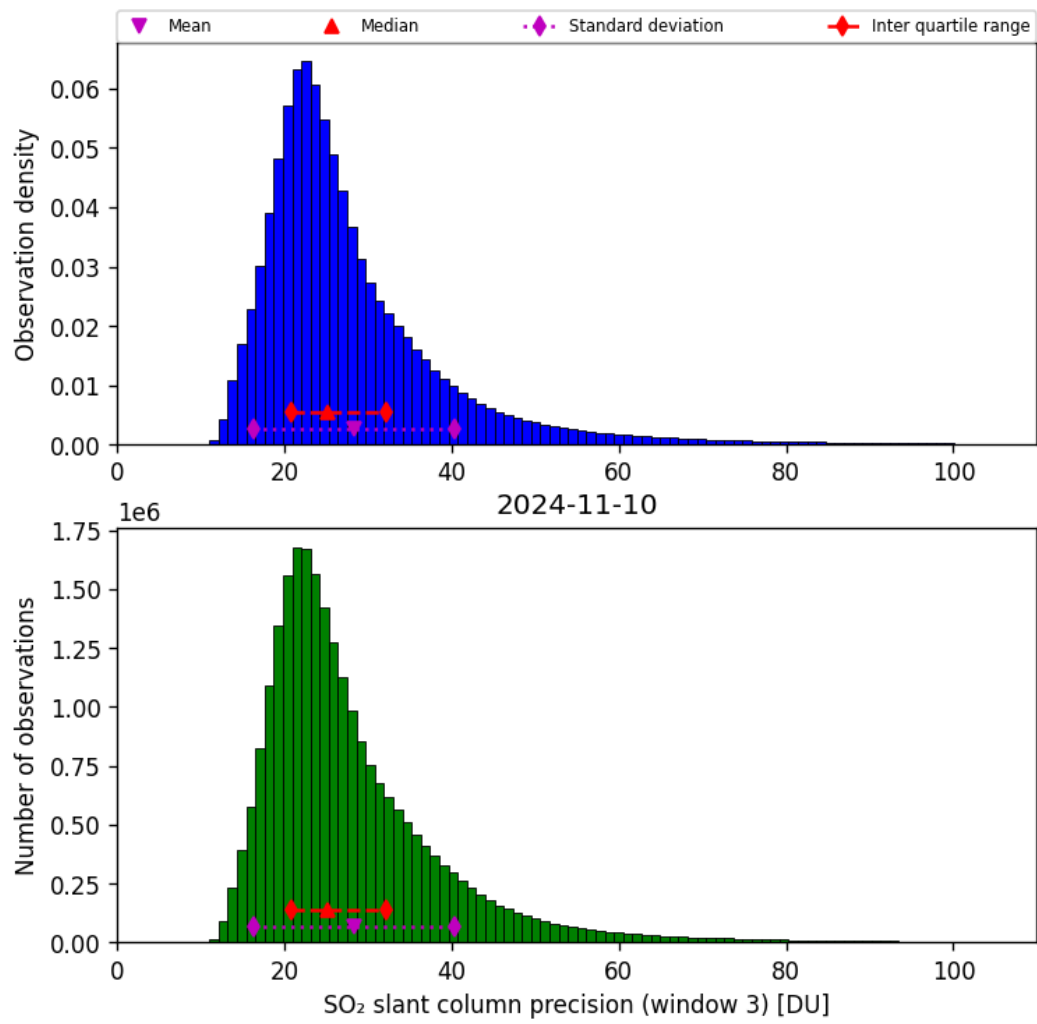
Figure 65: Histogram of “SO 2 slant column precision (window 3)” for 2024-11-09 to 2024-11-11
