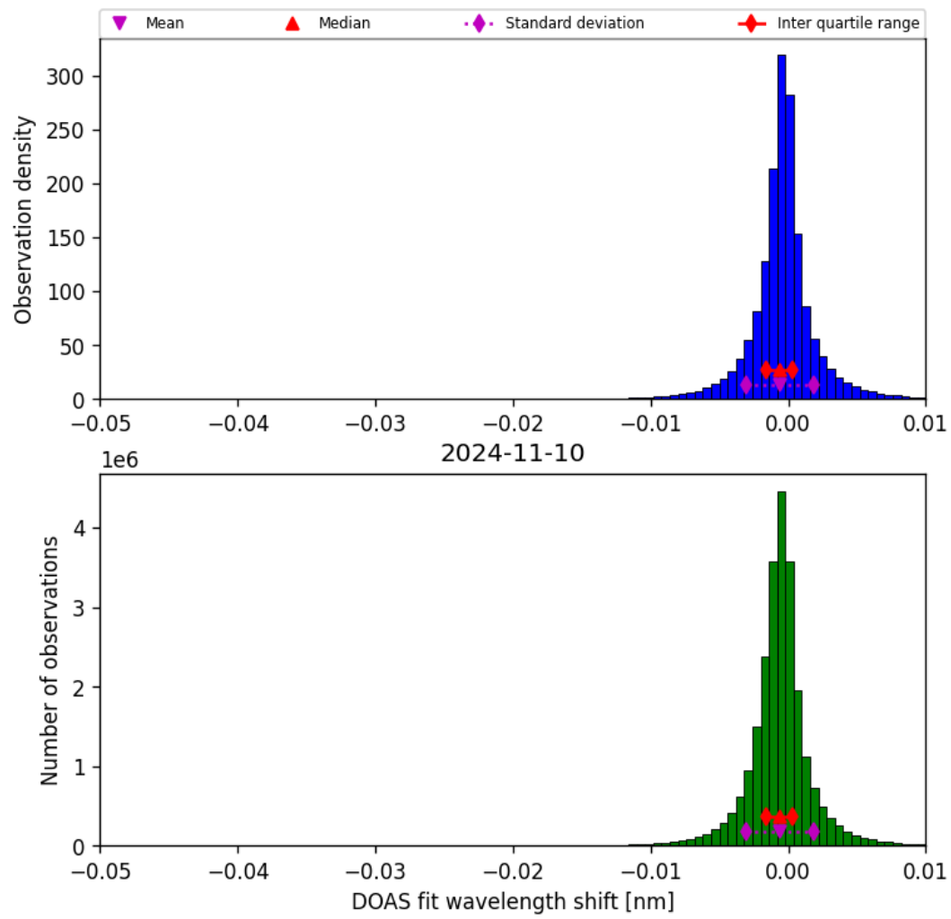
Figure 68: Histogram of “DOAS fit wavelength shift” for 2024-11-09 to 2024-11-11
