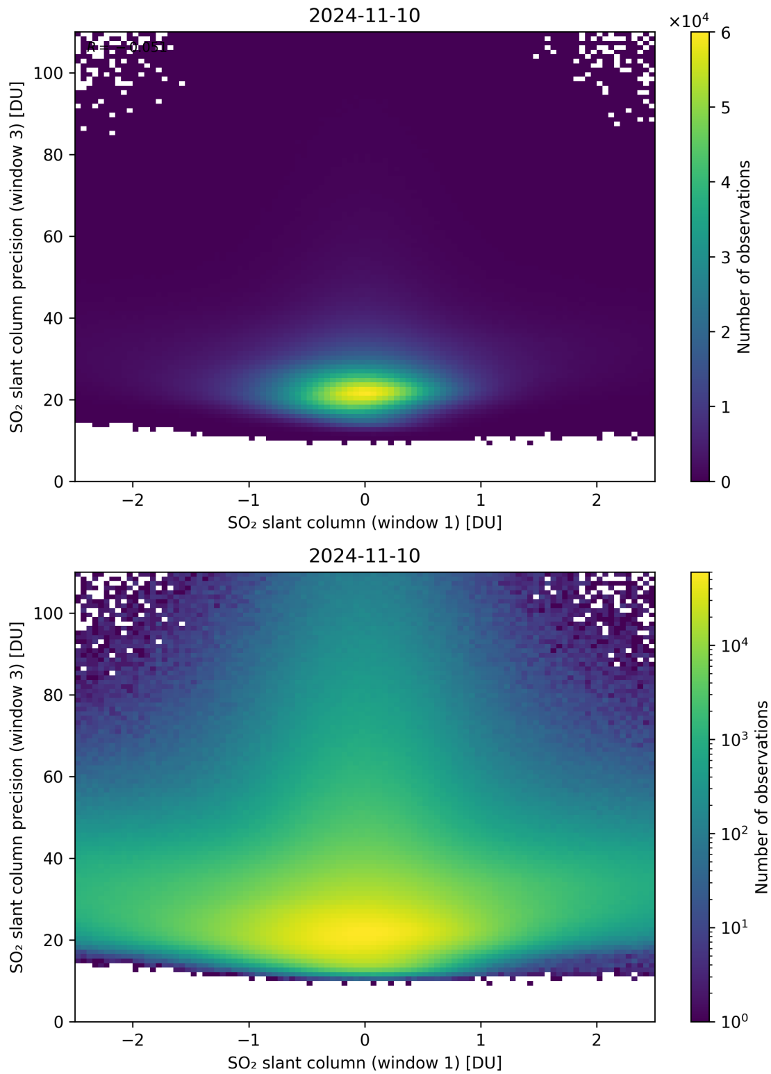
Figure 238: Scatter density plot of “SO 2 slant column (window 1)” against “SO 2 slant column precision (window 3)” for 2024-11-09 to 2024-11-11.
