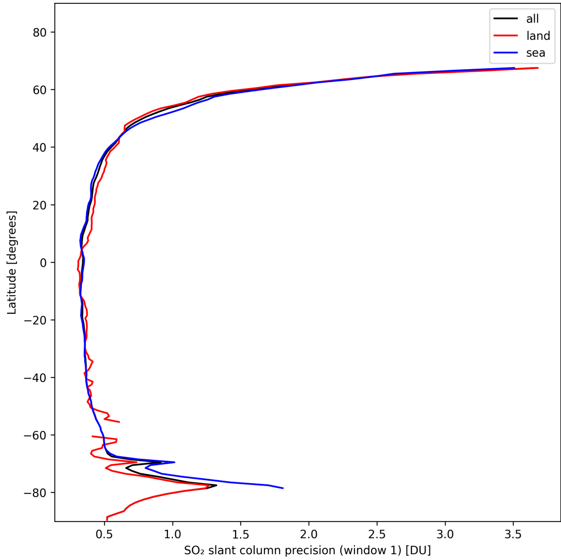
Figure 34: Zonal average of “SO 2 slant column precision (window 1)” for 2024-11-09 to 2024-11-11.
