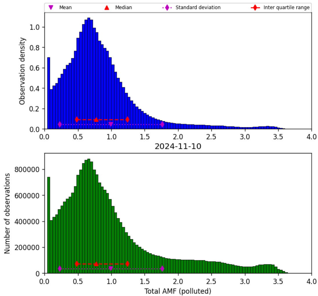
Figure 71: Histogram of “Total AMF (polluted)” for 2024-11-09 to 2024-11-11
