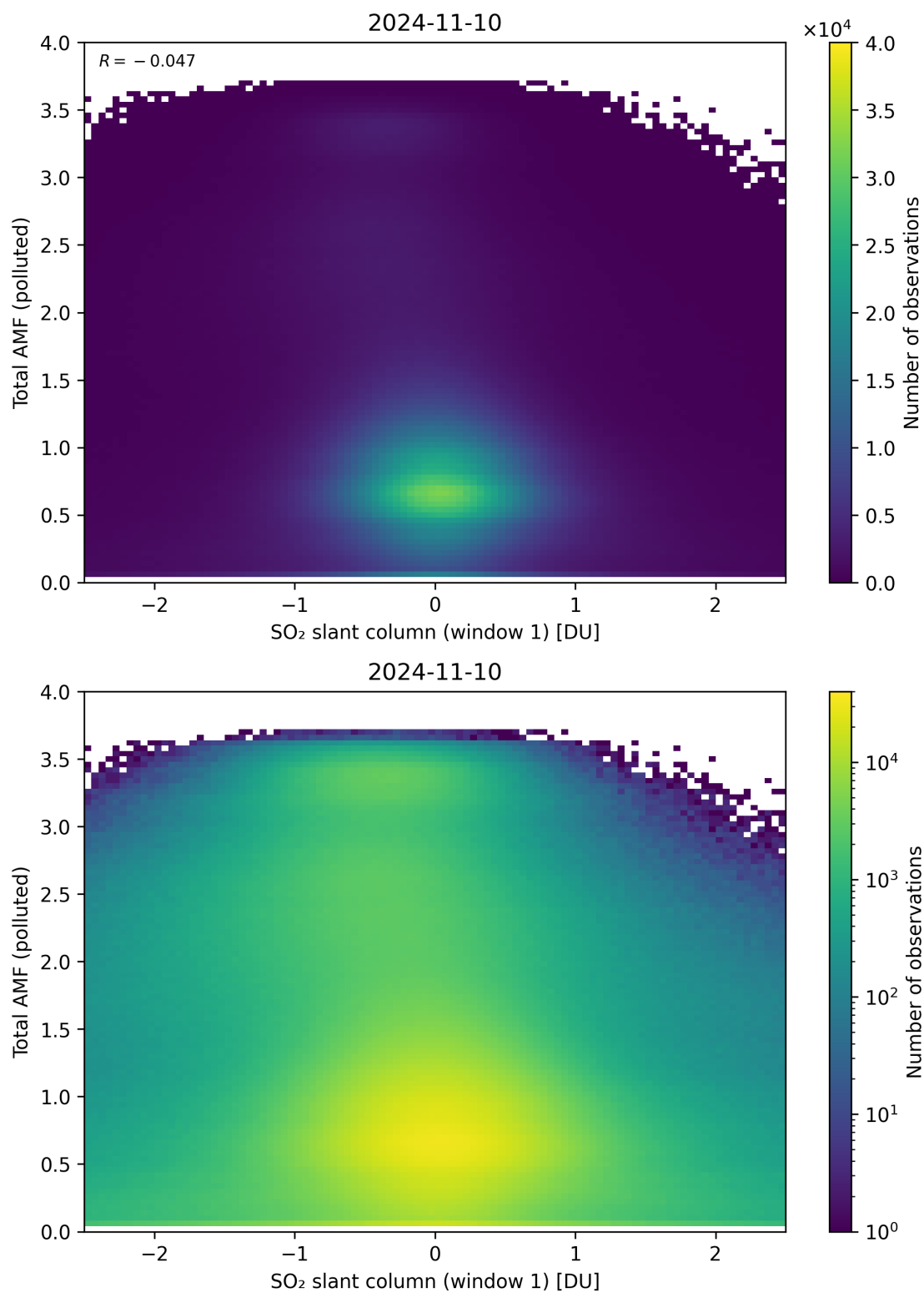
Figure 239: Scatter density plot of “SO 2 slant column (window 1)” against “Total AMF (polluted)” for 2024-11-09 to 2024-11-11.
