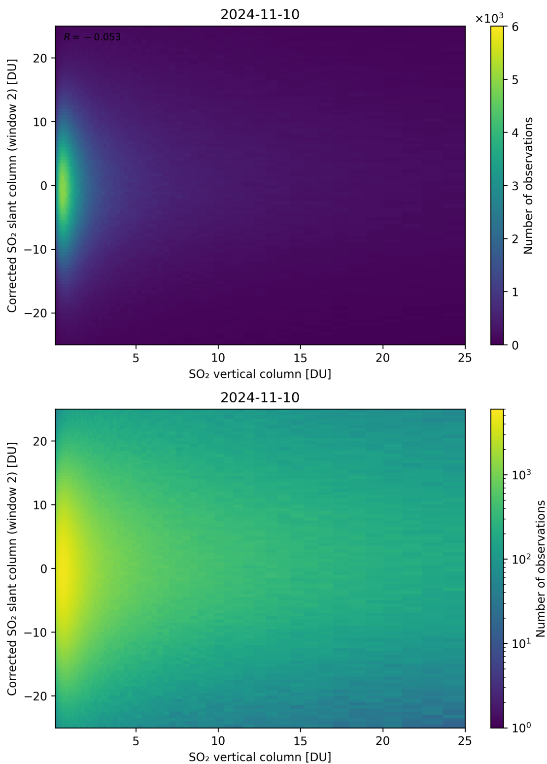
Figure 298: Scatter density plot of “SO 2 vertical column” against “Corrected SO 2 slant column (window 2)” for 2024-11-09 to 2024-11-11.
