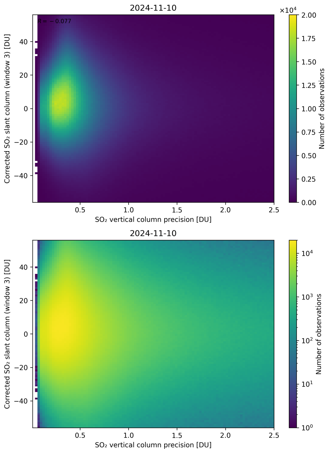
Figure 288: Scatter density plot of “SO 2 vertical column precision” against “Corrected SO 2 slant column (window 3)” for 2024-11-09 to 2024-11-11.
