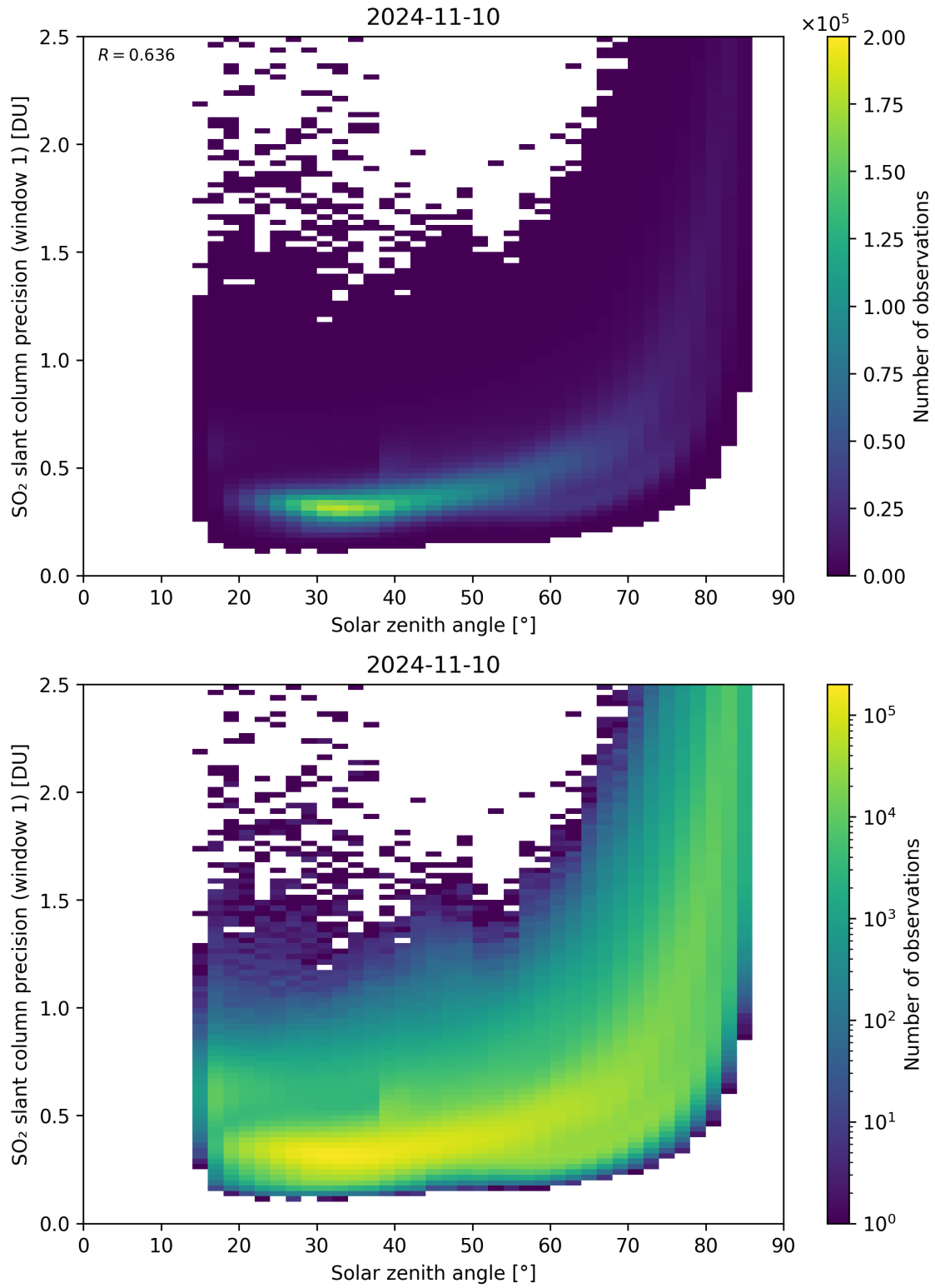
Figure 170: Scatter density plot of “Solar zenith angle” against “SO 2 slant column precision (window 1)” for 2024-11-09 to 2024-11-11.
