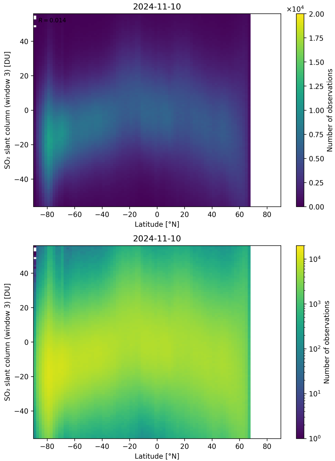
Figure 152: Scatter density plot of “Latitude” against “SO 2 slant column (window 3)” for 2024-11-09 to 2024-11-11.
