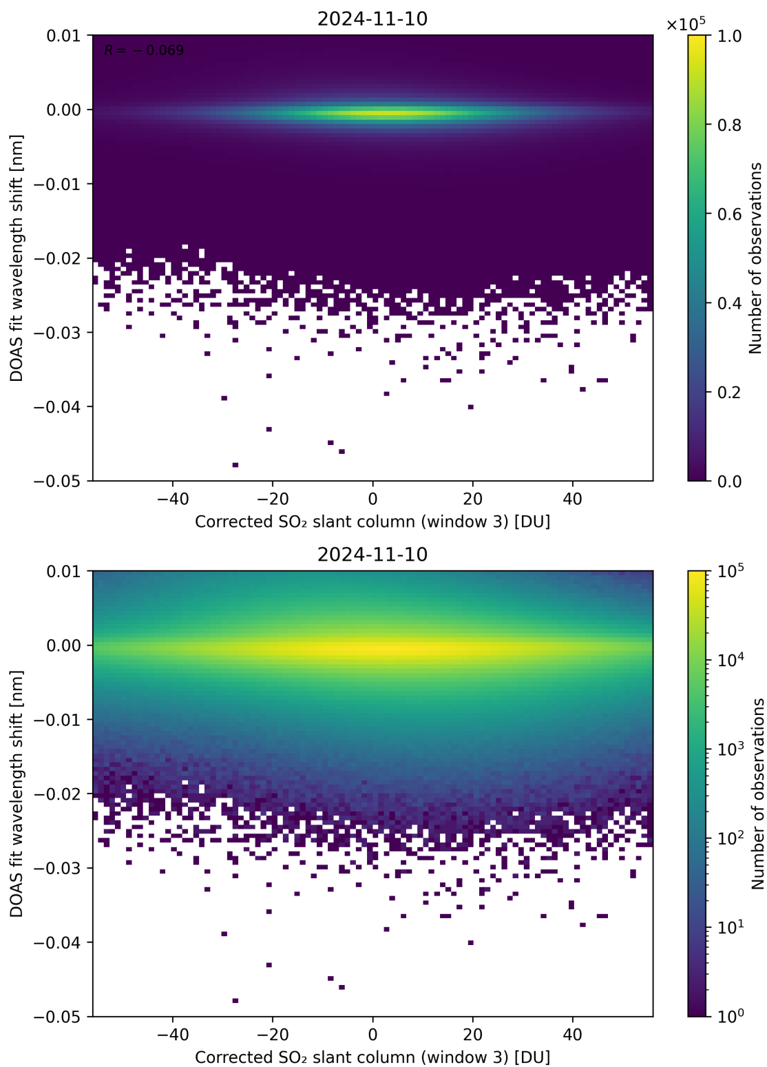
Figure 206: Scatter density plot of “Corrected SO 2 slant column (window 3)” against “DOAS fit wavelength shift” for 2024-11-09 to 2024-11-11.
