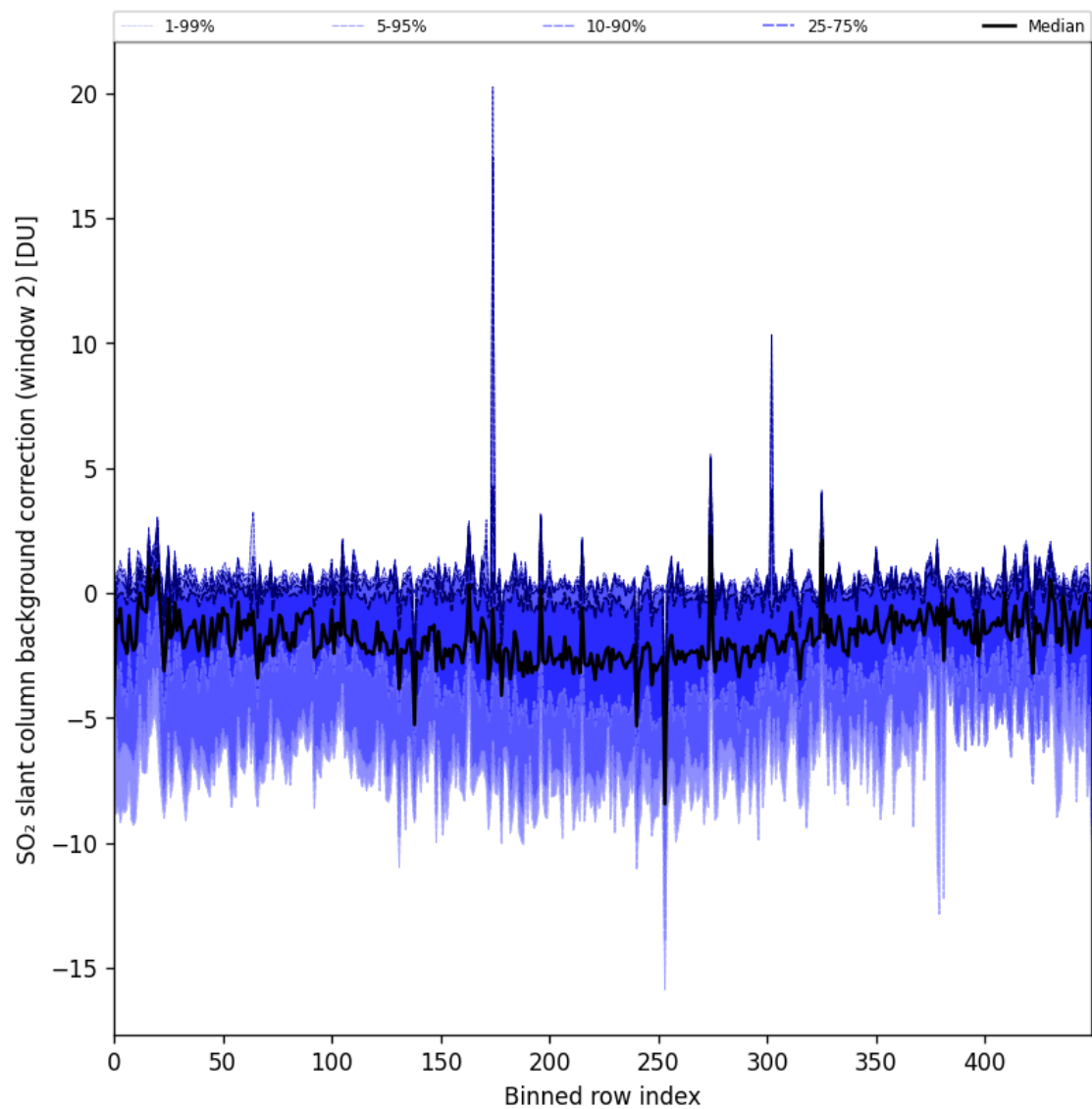
Figure 86: Along track statistics of “SO 2 slant column background correction (window 2)” for 2024-11-09 to 2024-11-11
