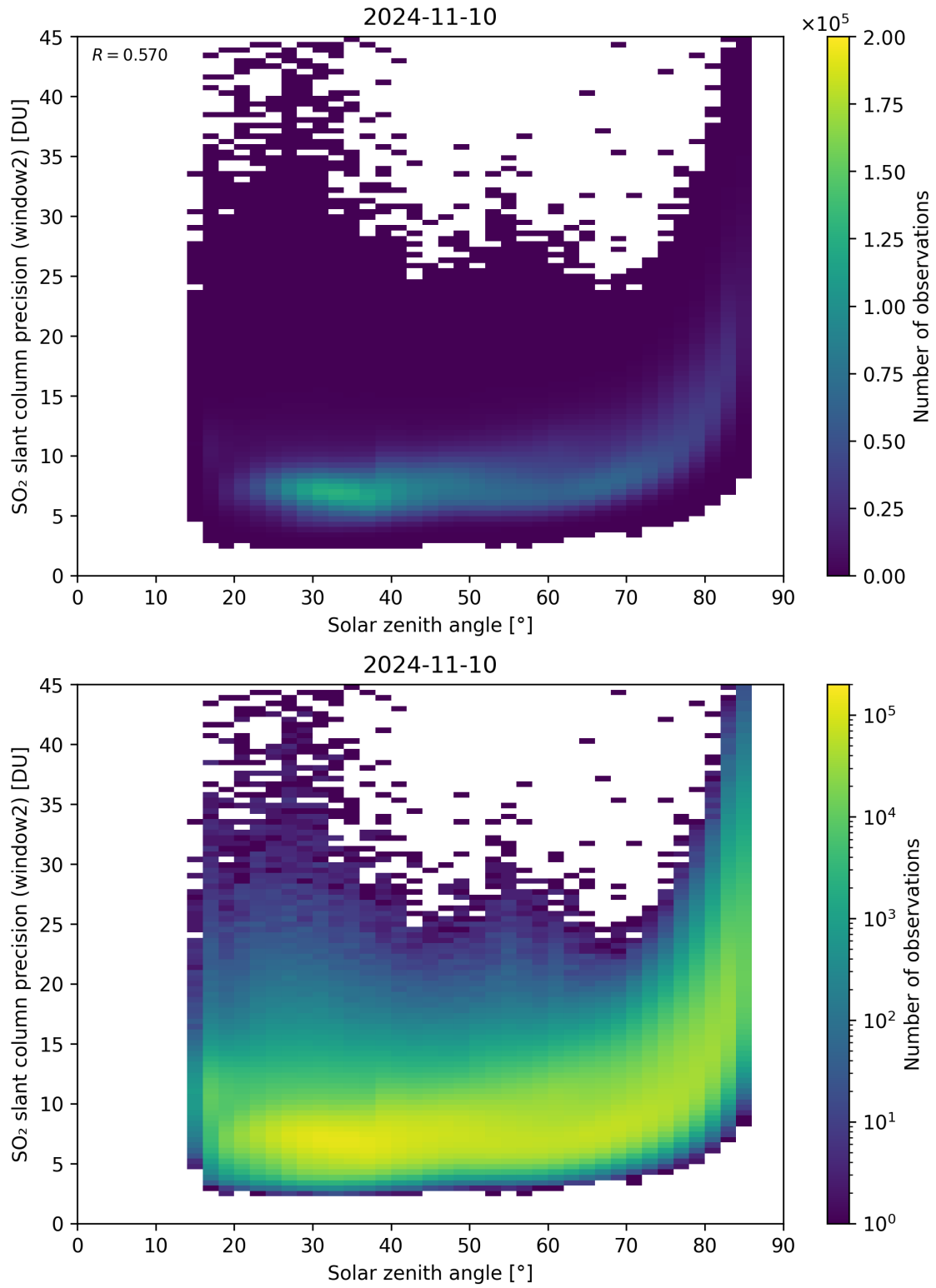
Figure 171: Scatter density plot of “Solar zenith angle” against “SO 2 slant column precision (window2)” for 2024-11-09 to 2024-11-11.
