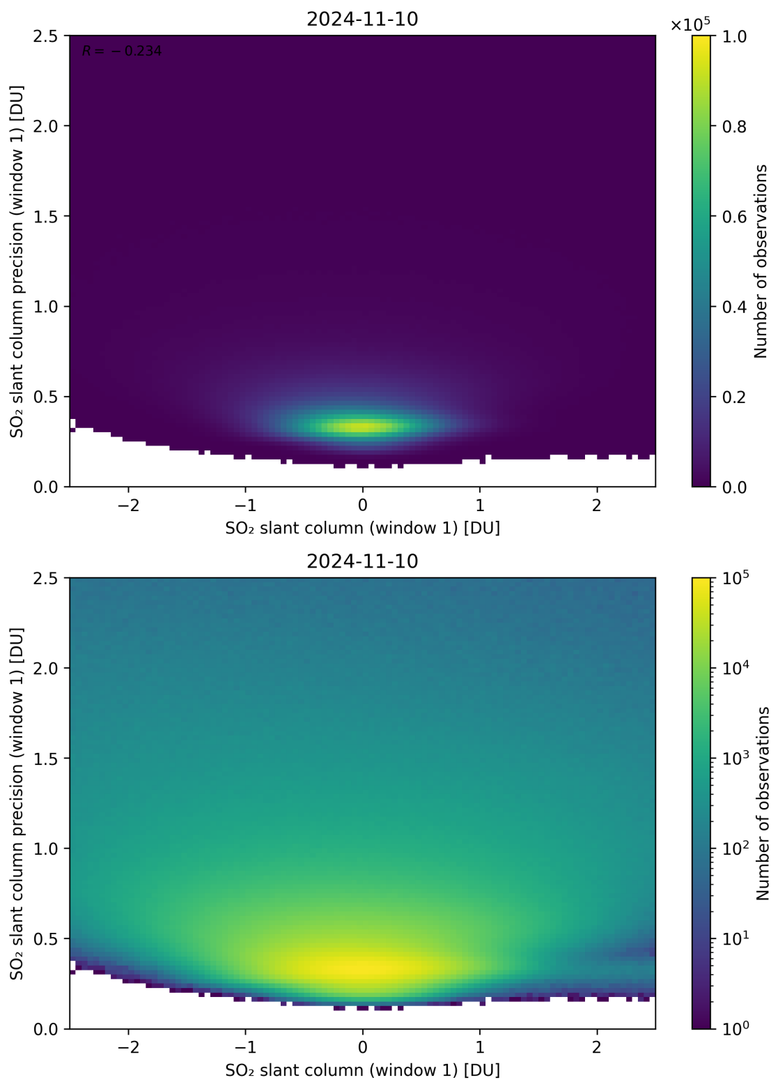
Figure 235: Scatter density plot of “SO 2 slant column (window 1)” against “SO 2 slant column precision (window 1)” for 2024-11-09 to 2024-11-11.
