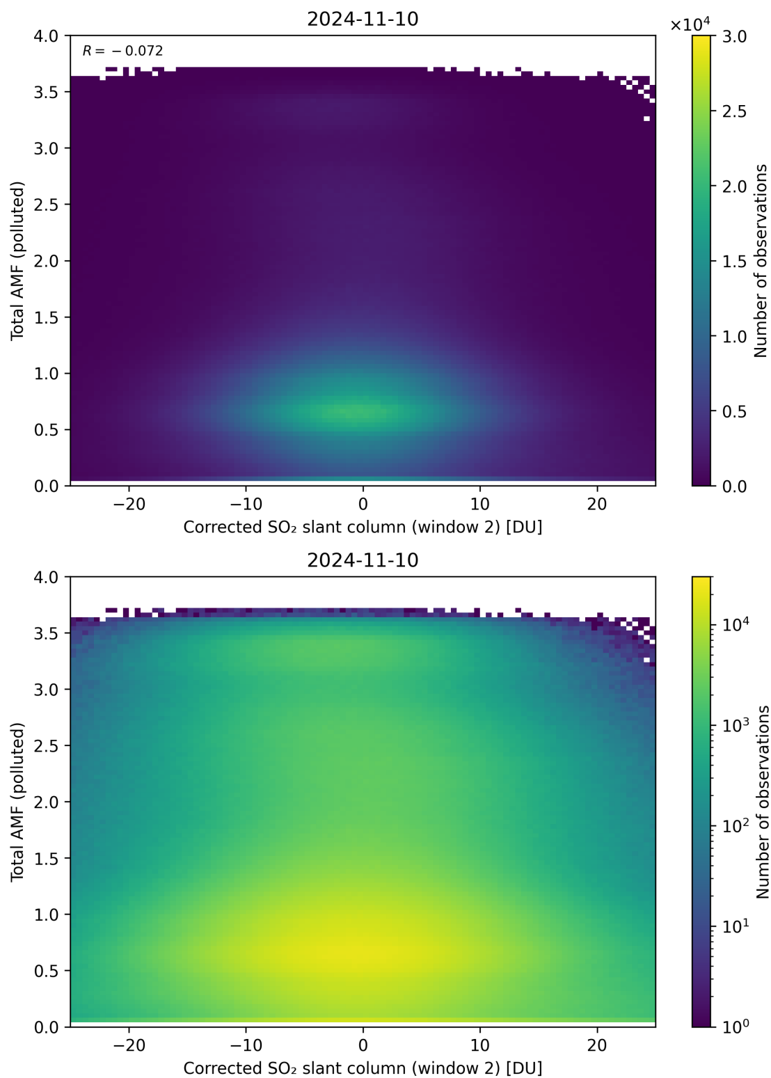
Figure 203: Scatter density plot of “Corrected SO 2 slant column (window 2)” against “Total AMF (polluted)” for 2024-11-09 to 2024-11-11.
