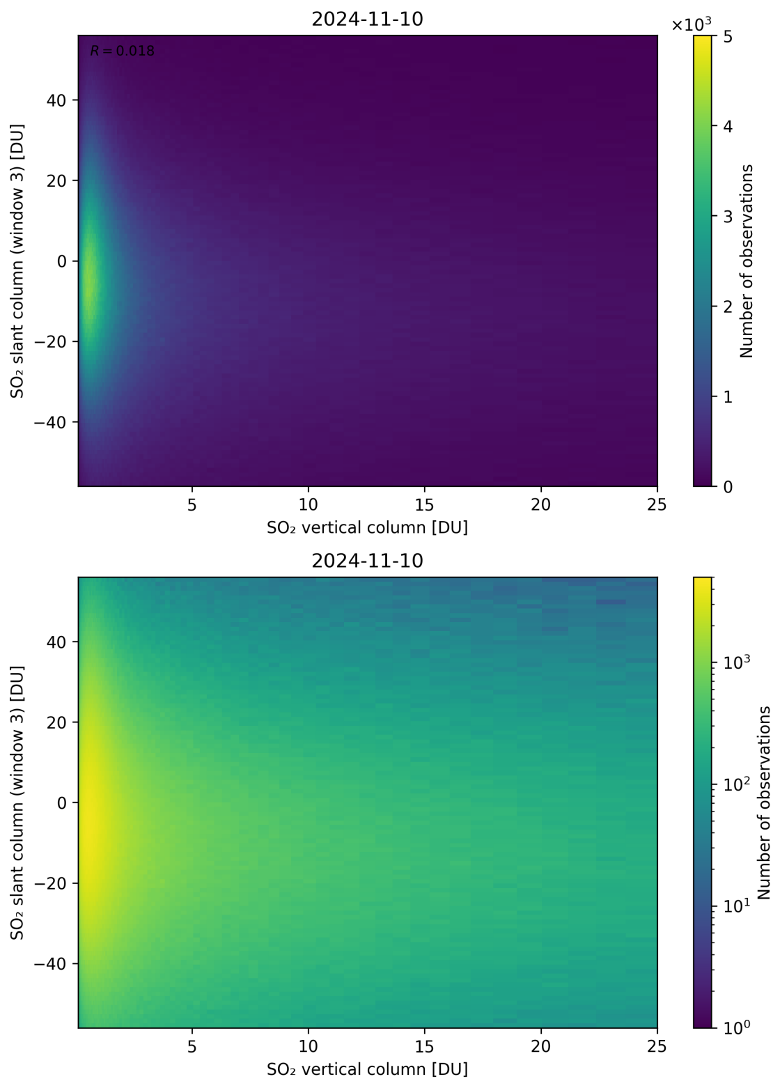
Figure 303: Scatter density plot of “SO 2 vertical column” against “SO 2 slant column (window 3)” for 2024-11-09 to 2024-11-11.
