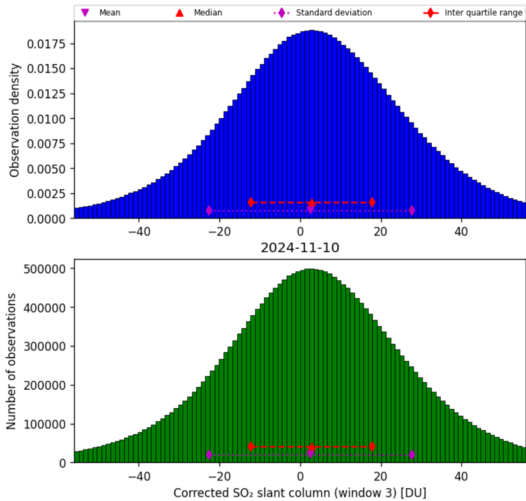
Figure 66: Histogram of “Corrected SO 2 slant column (window 3)” for 2024-11-09 to 2024-11-11
