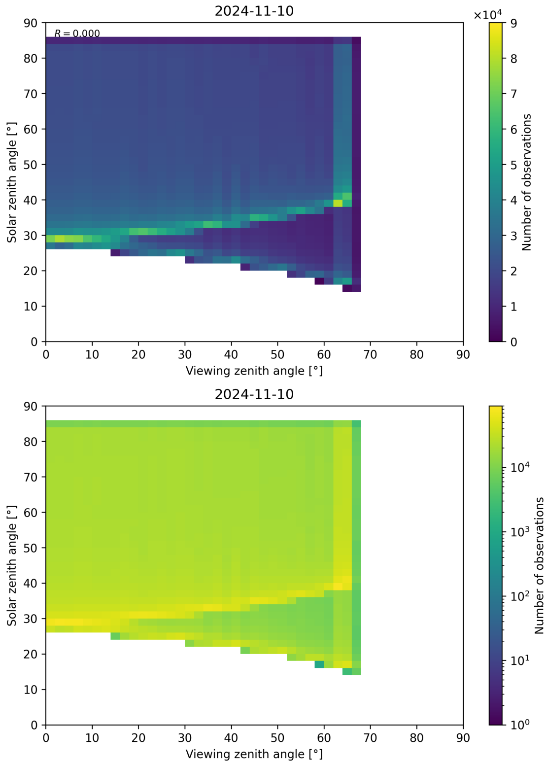
Figure 315: Scatter density plot of “Viewing zenith angle” against “Solar zenith angle” for 2024-11-09 to 2024-11-11.
