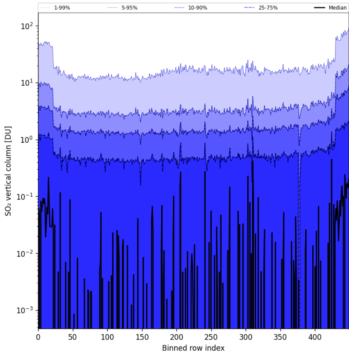
Figure 76: Along track statistics of “SO 2 vertical column” for 2024-11-09 to 2024-11-11
