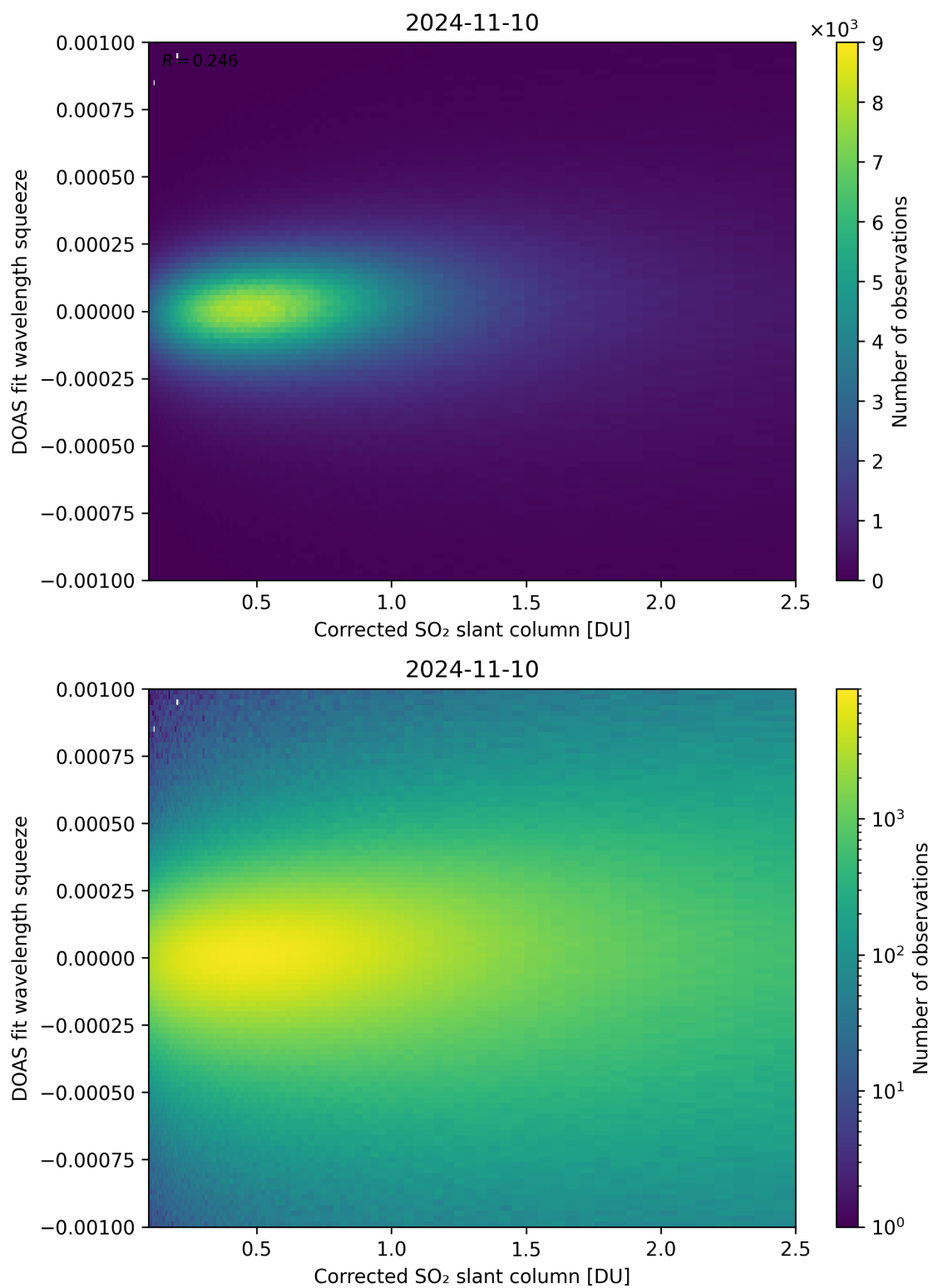
Figure 182: Scatter density plot of “Corrected SO 2 slant column” against “DOAS fit wavelength squeeze” for 2024-11-09 to 2024-11-11.
