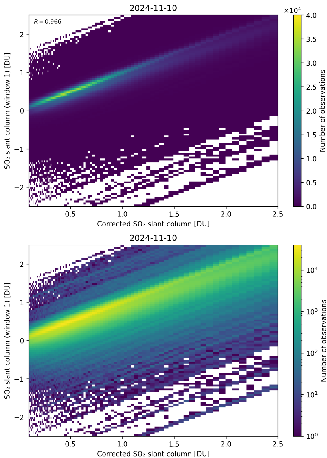
Figure 187: Scatter density plot of “Corrected SO 2 slant column” against “SO 2 slant column (window 1)” for 2024-11-09 to 2024-11-11.
