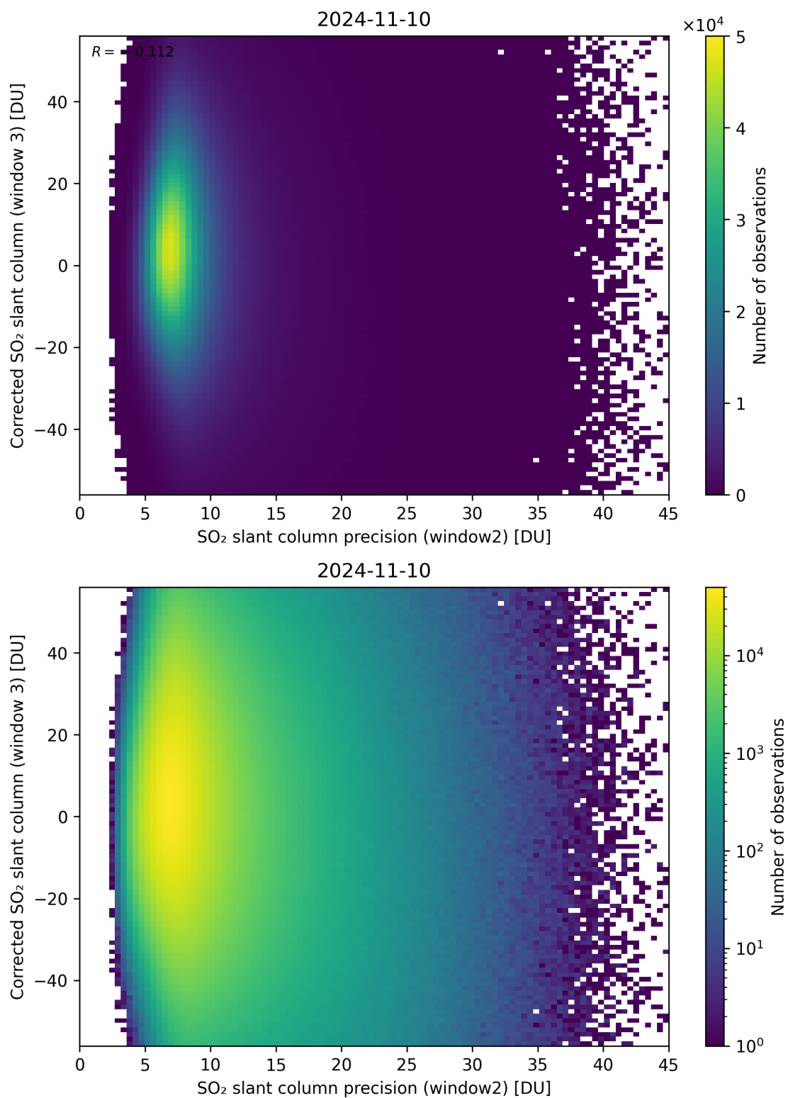
Figure 248: Scatter density plot of “SO 2 slant column precision (window2)” against “Corrected SO 2 slant column (window 3)” for 2024-11-09 to 2024-11-11.
