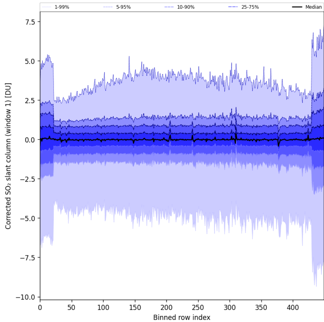
Figure 81: Along track statistics of “Corrected SO 2 slant column (window 1)” for 2024-11-09 to 2024-11-11
