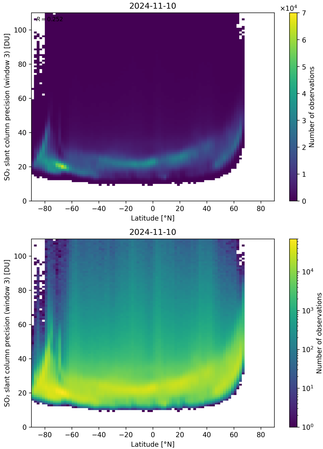
Figure 153: Scatter density plot of “Latitude” against “SO 2 slant column precision (window 3)” for 2024-11-09 to 2024-11-11.
