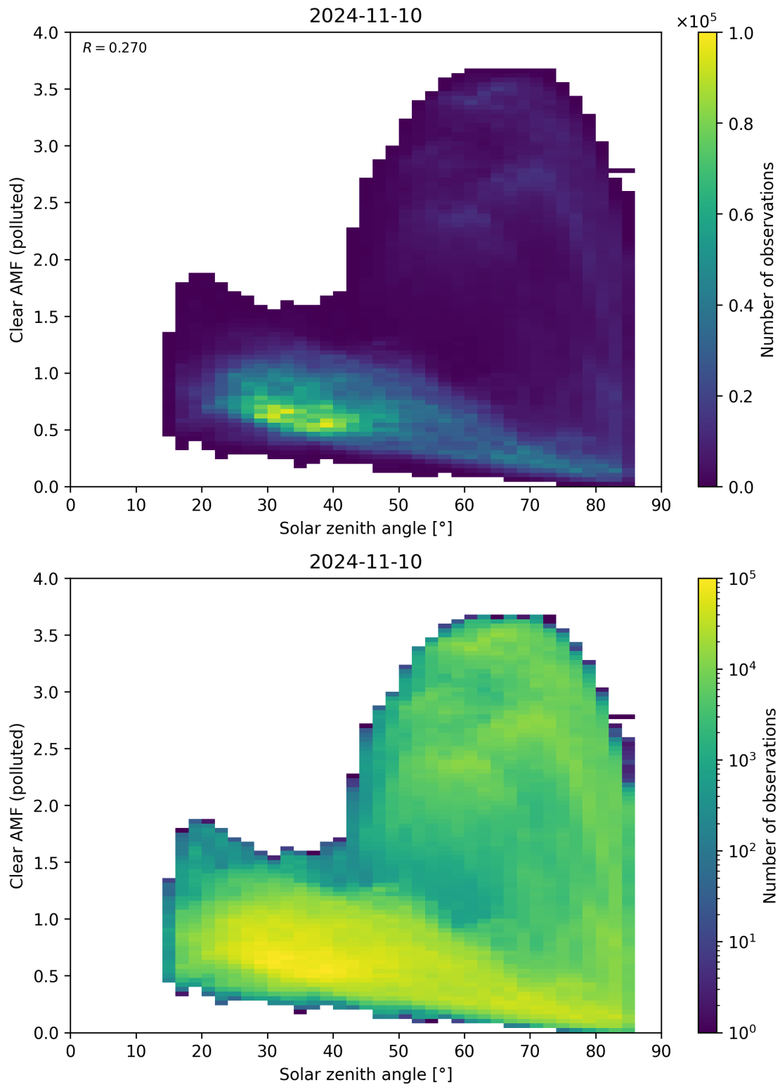
Figure 165: Scatter density plot of “Solar zenith angle” against “Clear AMF (polluted)” for 2024-11-09 to 2024-11-11.
