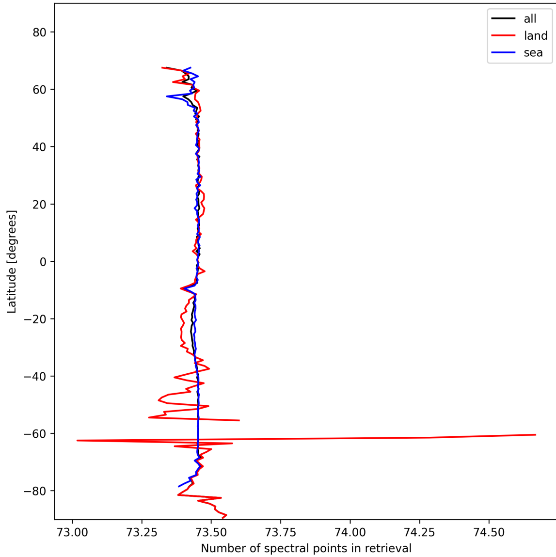
Figure 51: Zonal average of “Number of spectral points in retrieval” for 2024-11-09 to 2024-11-11.
