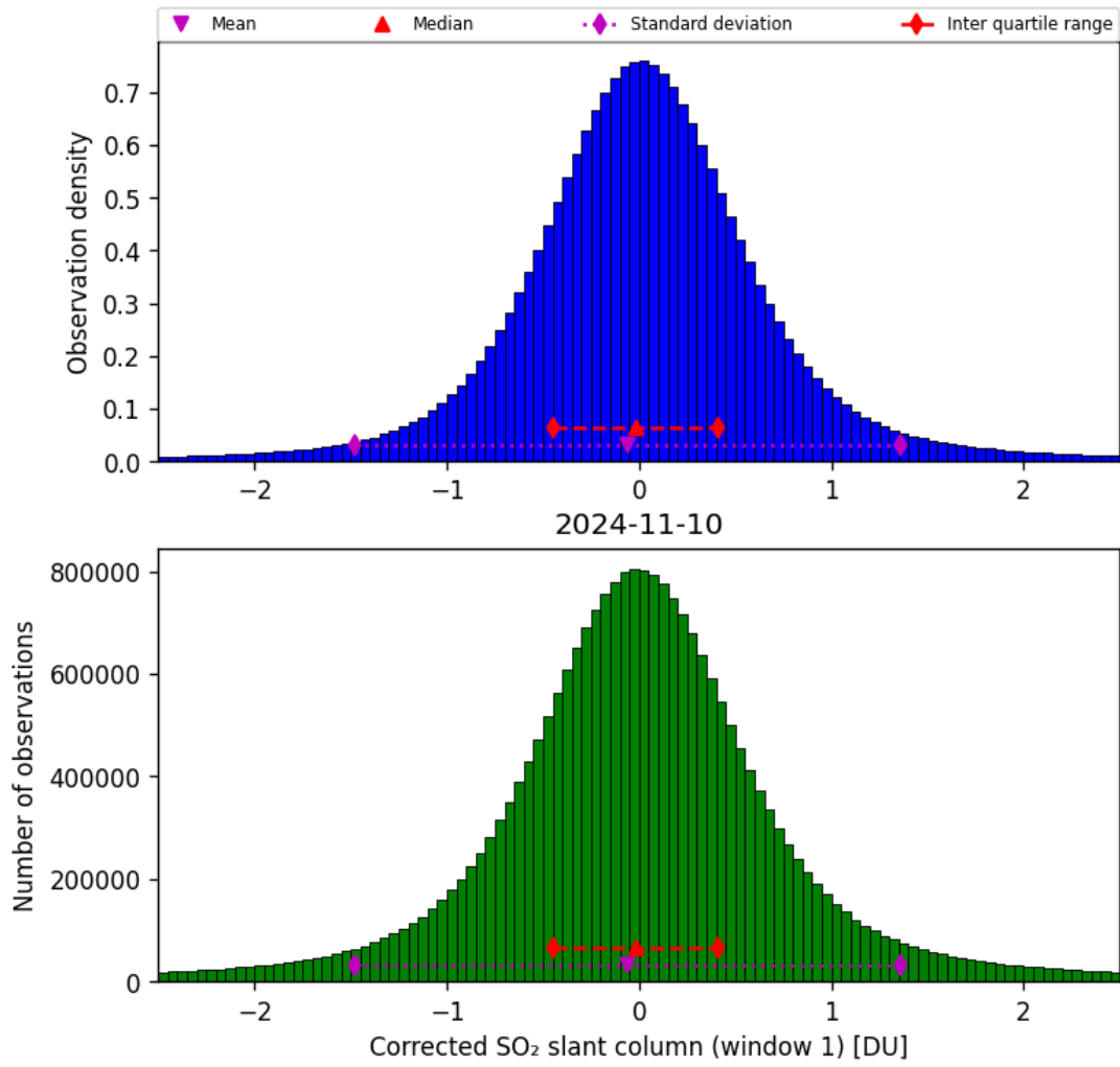
Figure 58: Histogram of “Corrected SO 2 slant column (window 1)” for 2024-11-09 to 2024-11-11
