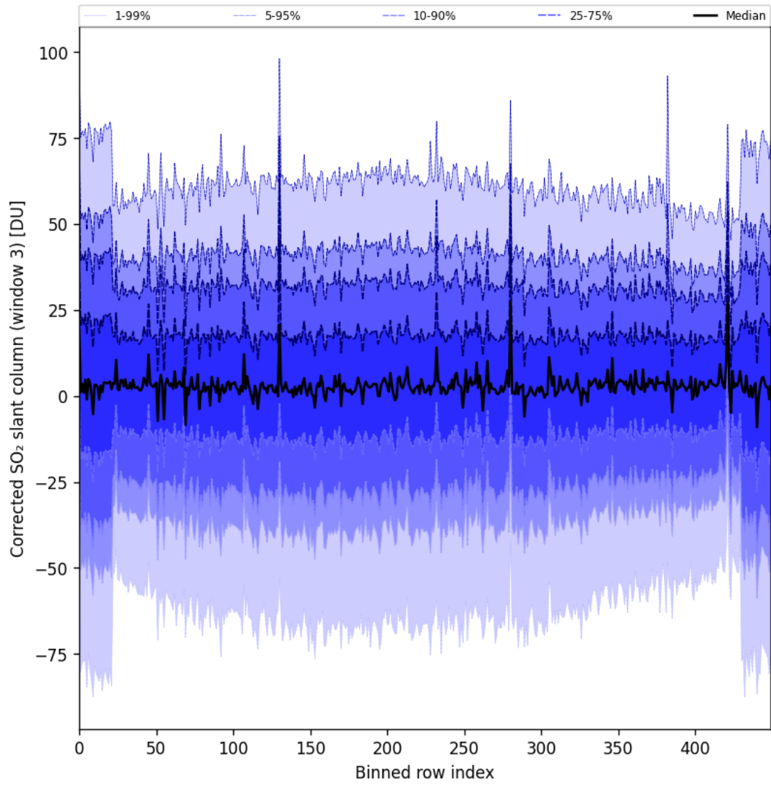
Figure 89: Along track statistics of “Corrected SO 2 slant column (window 3)” for 2024-11-09 to 2024-11-11
