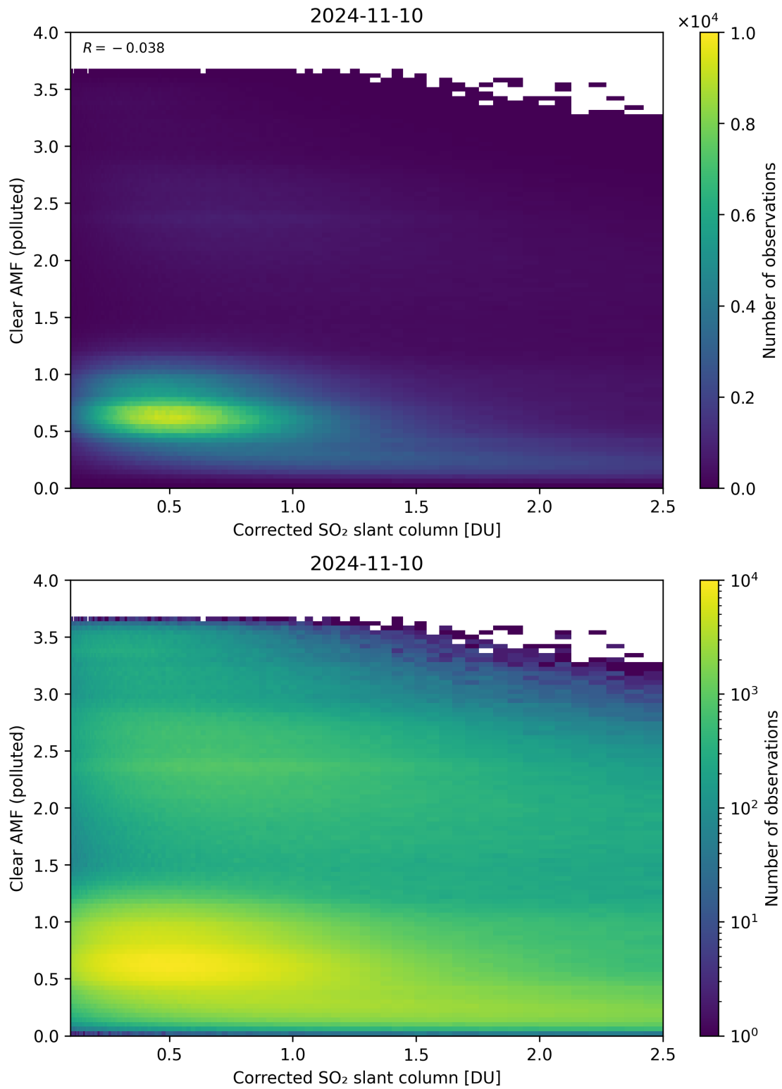
Figure 184: Scatter density plot of “Corrected SO 2 slant column” against “Clear AMF (polluted)” for 2024-11-09 to 2024-11-11.
