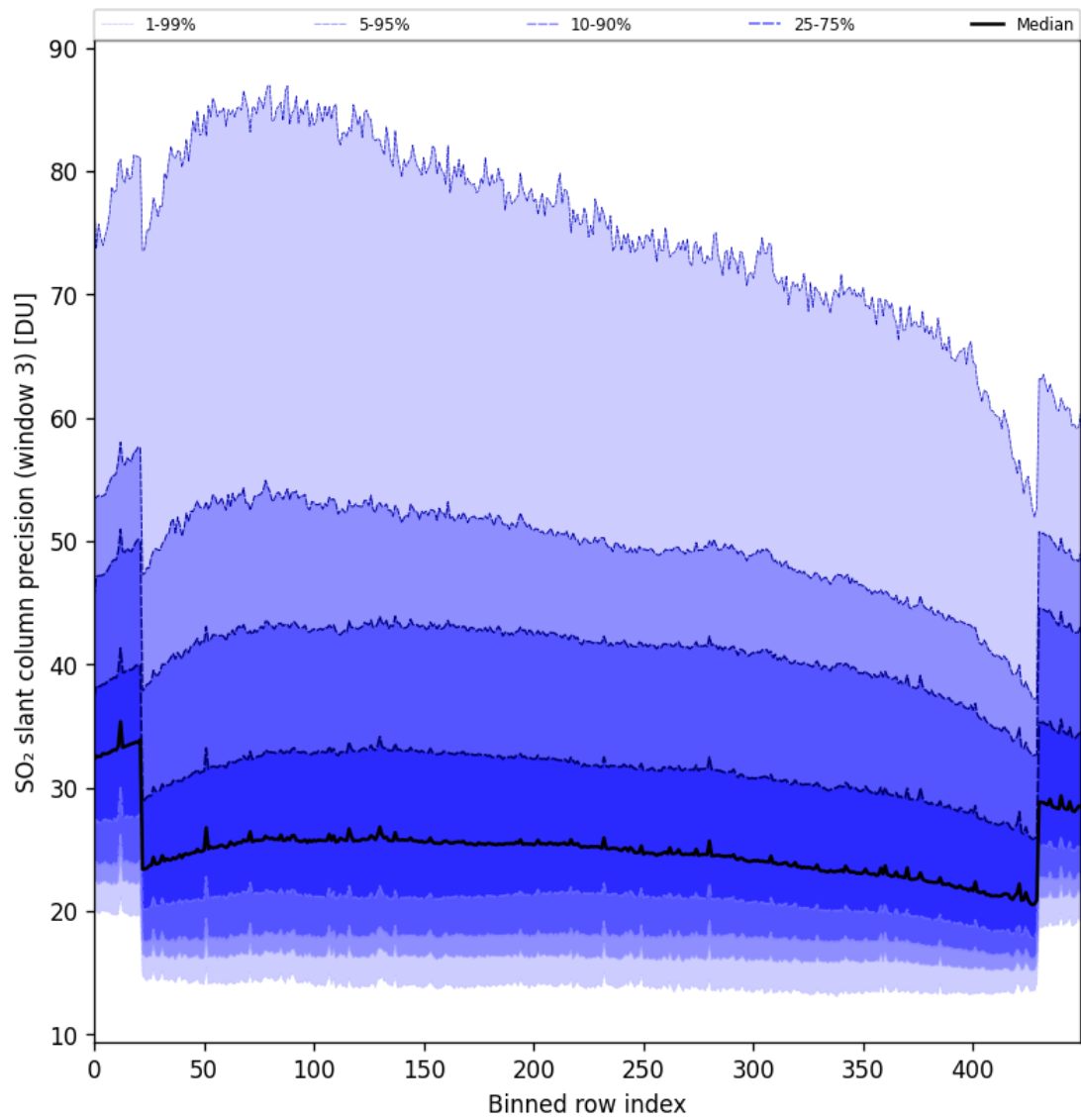
Figure 88: Along track statistics of “SO 2 slant column precision (window 3)” for 2024-11-09 to 2024-11-11
