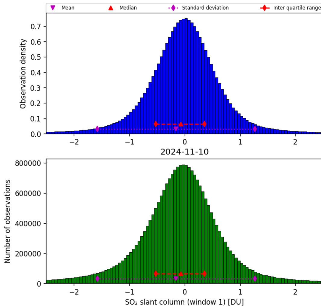
Figure 56: Histogram of “SO 2 slant column (window 1)” for 2024-11-09 to 2024-11-11
