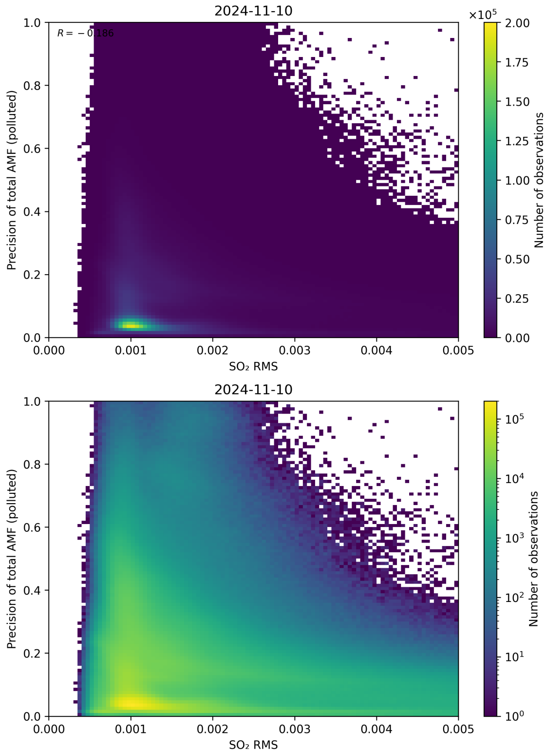
Figure 138: Scatter density plot of “SO 2 RMS” against “Precision of total AMF (polluted)” for 2024-11-09 to 2024-11-11.
