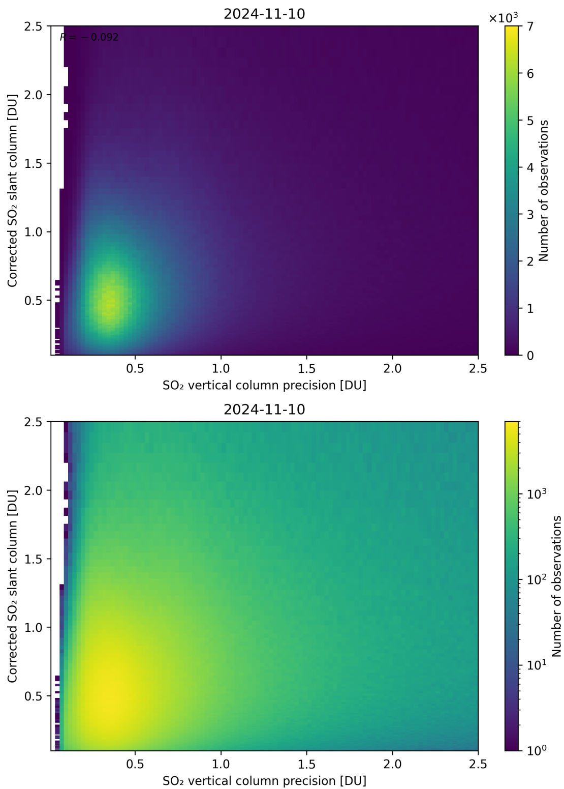
Figure 286: Scatter density plot of “SO 2 vertical column precision” against “Corrected SO 2 slant column” for 2024-11-09 to 2024-11-11.
