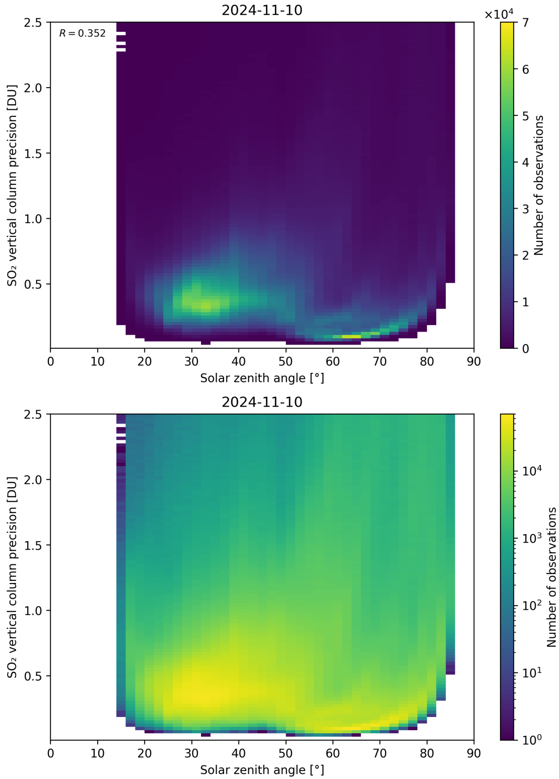
Figure 177: Scatter density plot of “Solar zenith angle” against “SO 2 vertical column precision” for 2024-11-09 to 2024-11-11.
