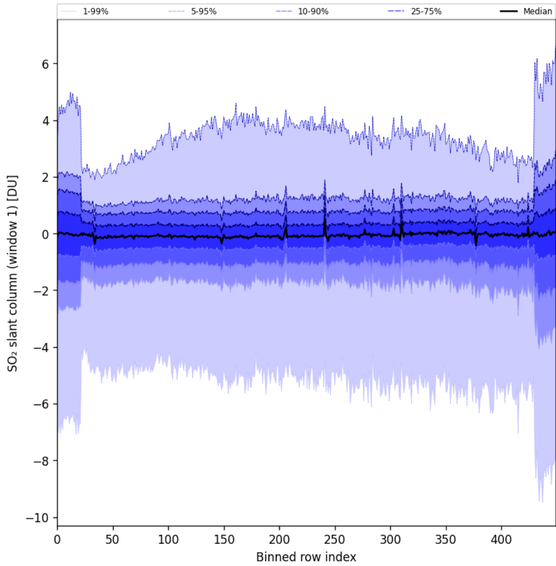
Figure 79: Along track statistics of “SO 2 slant column (window 1)” for 2024-11-09 to 2024-11-11
