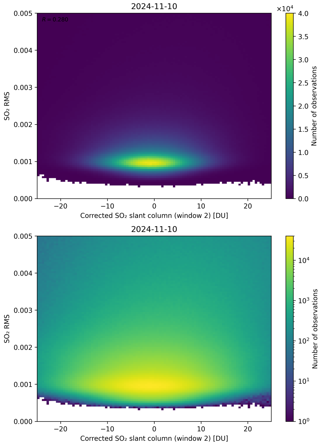
Figure 198: Scatter density plot of “Corrected SO 2 slant column (window 2)” against “SO 2 RMS” for 2024-11-09 to 2024-11-11.
