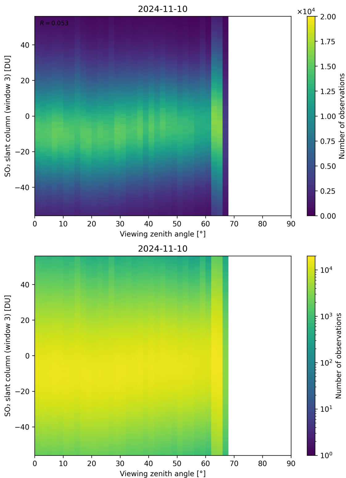
Figure 323: Scatter density plot of “Viewing zenith angle” against “SO 2 slant column (window 3)” for 2024-11-09 to 2024-11-11.
