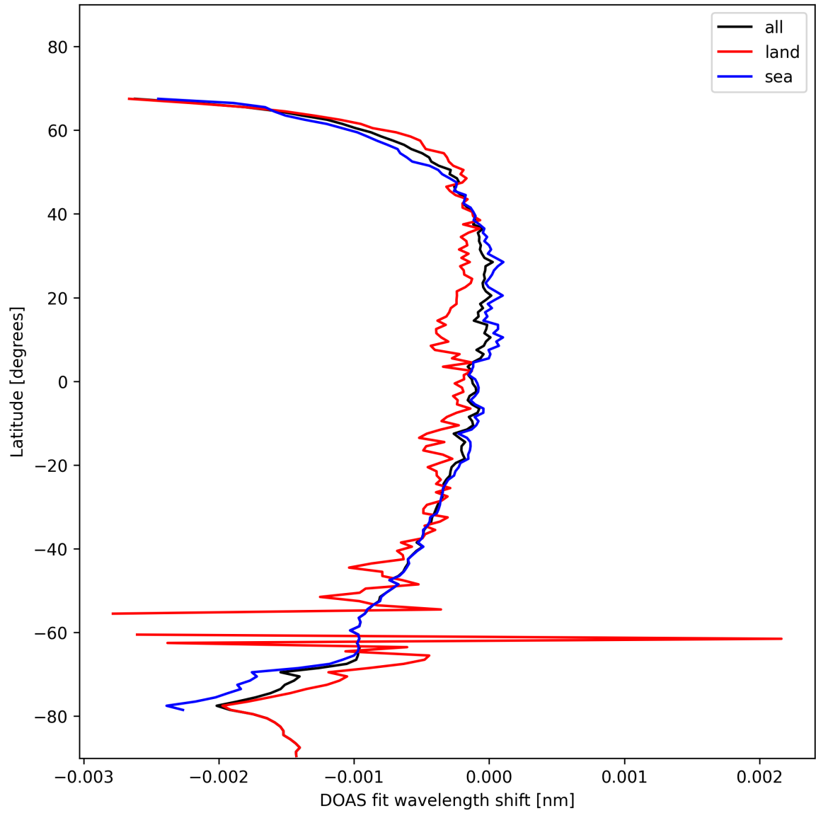
Figure 45: Zonal average of “DOAS fit wavelength shift” for 2024-11-09 to 2024-11-11.
