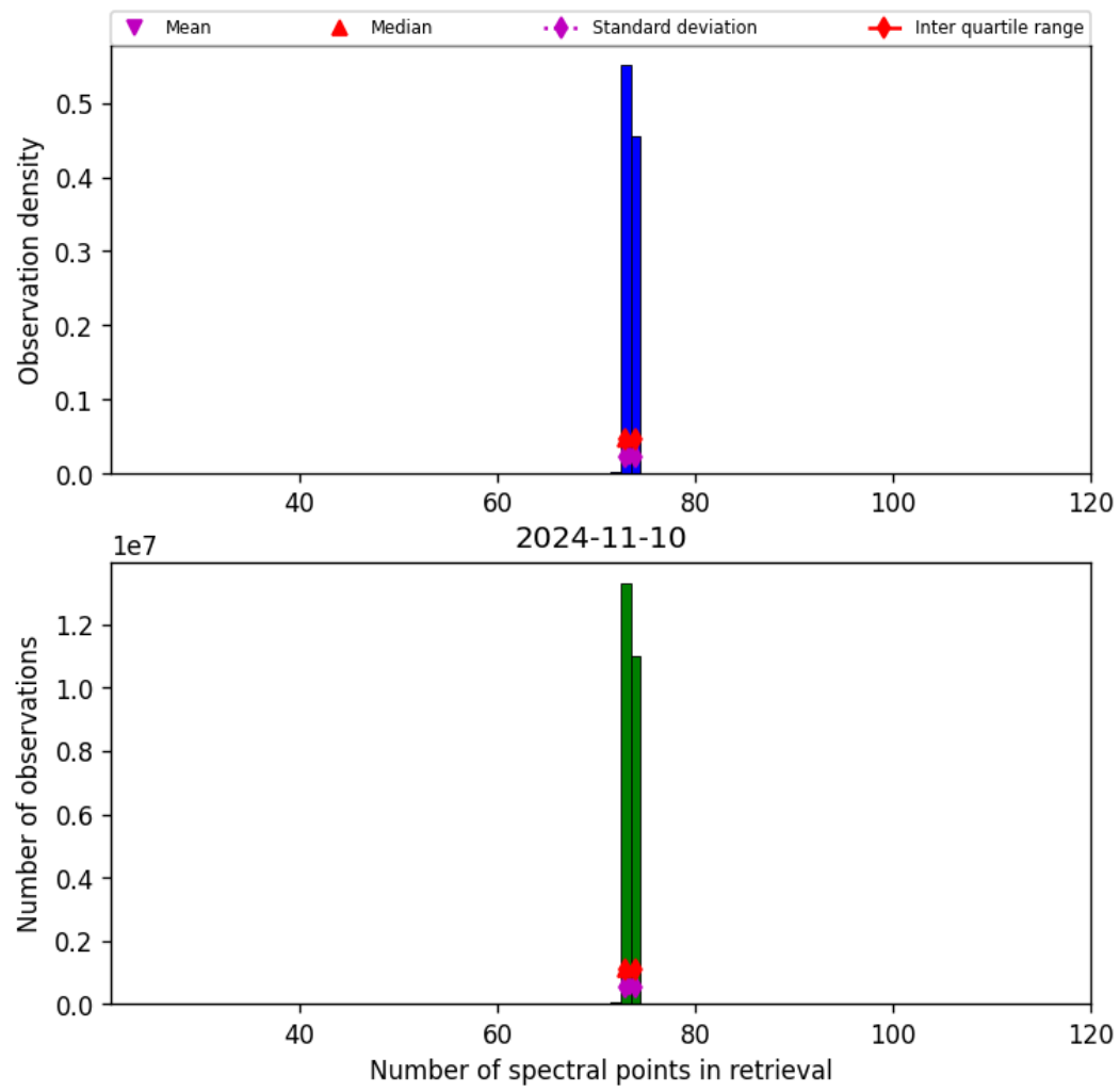
Figure 74: Histogram of “Number of spectral points in retrieval” for 2024-11-09 to 2024-11-11
