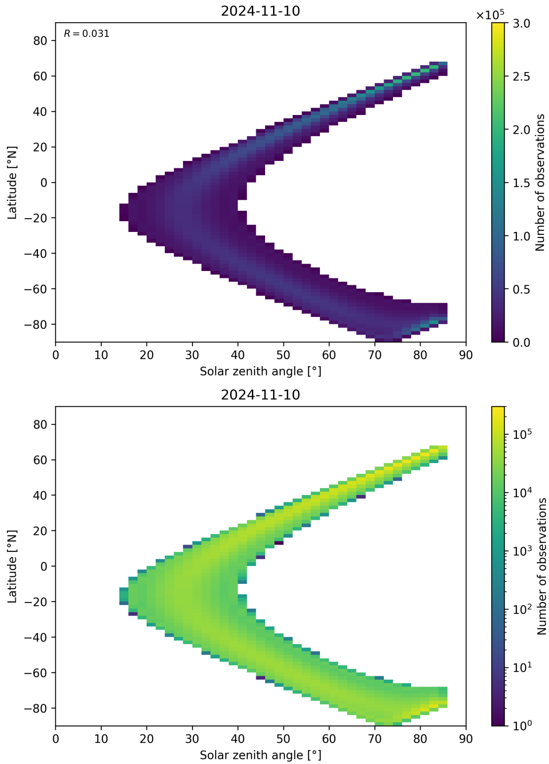
Figure 164: Scatter density plot of “Solar zenith angle” against “Latitude” for 2024-11-09 to 2024-11-11.
