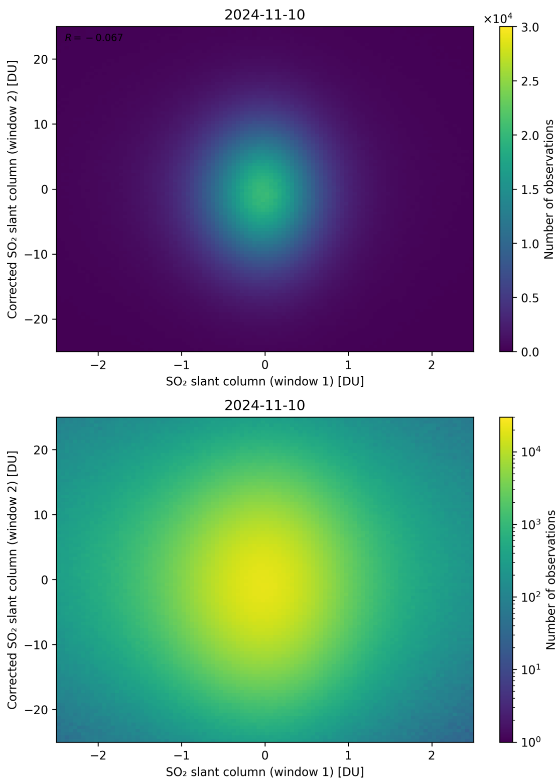
Figure 233: Scatter density plot of “SO 2 slant column (window 1)” against “Corrected SO 2 slant column (window 2)” for 2024-11-09 to 2024-11-11.
