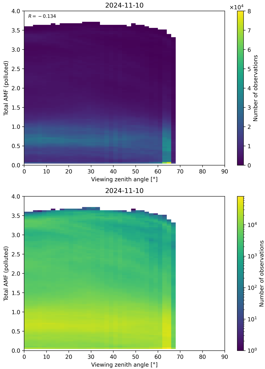
Figure 325: Scatter density plot of “Viewing zenith angle” against “Total AMF (polluted)” for 2024-11-09 to 2024-11-11.
