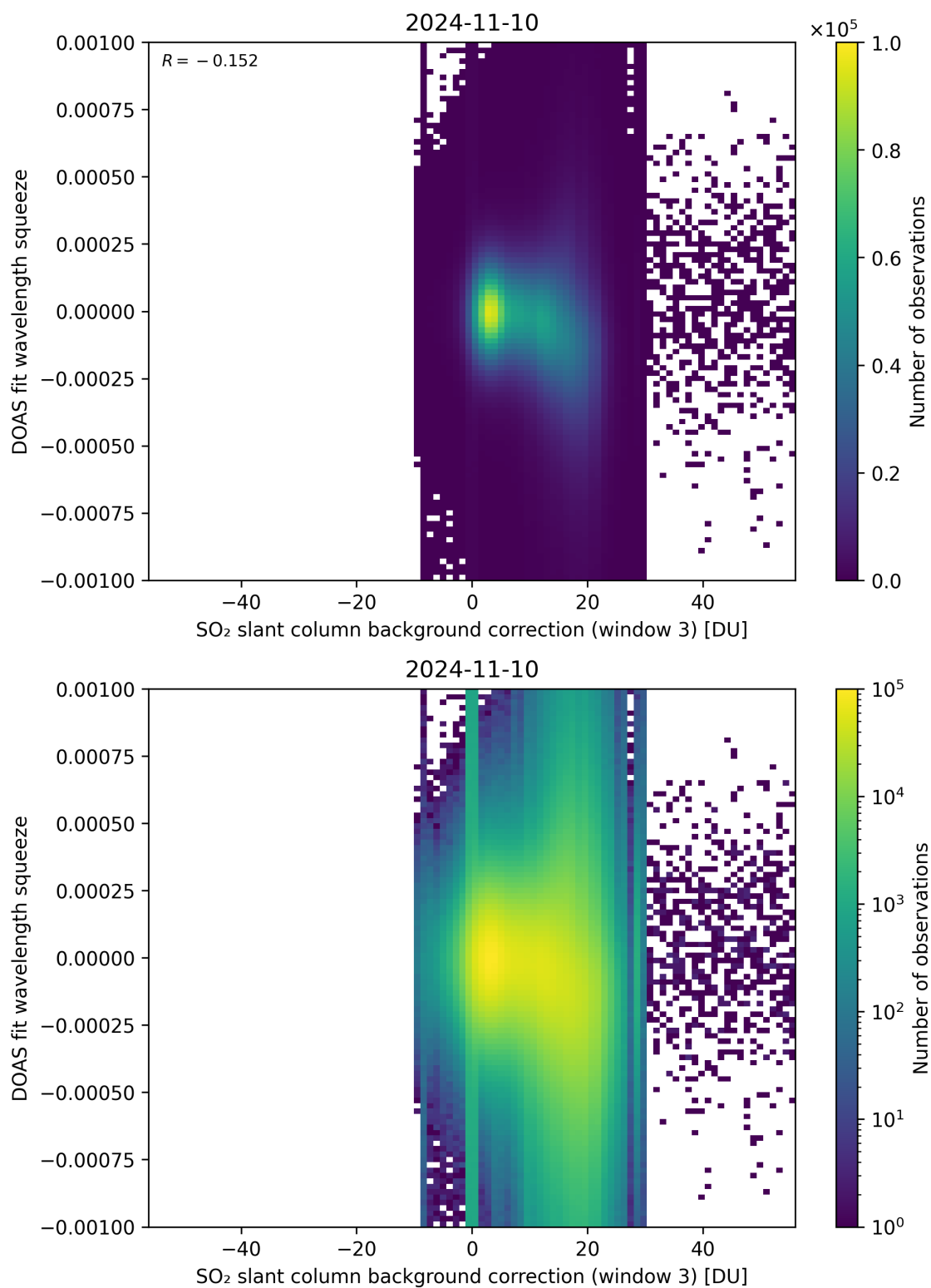
Figure 122: Scatter density plot of “SO 2 slant column background correction (window 3)” against “DOAS fit wavelength squeeze” for 2024-11-09 to 2024-11-11.
