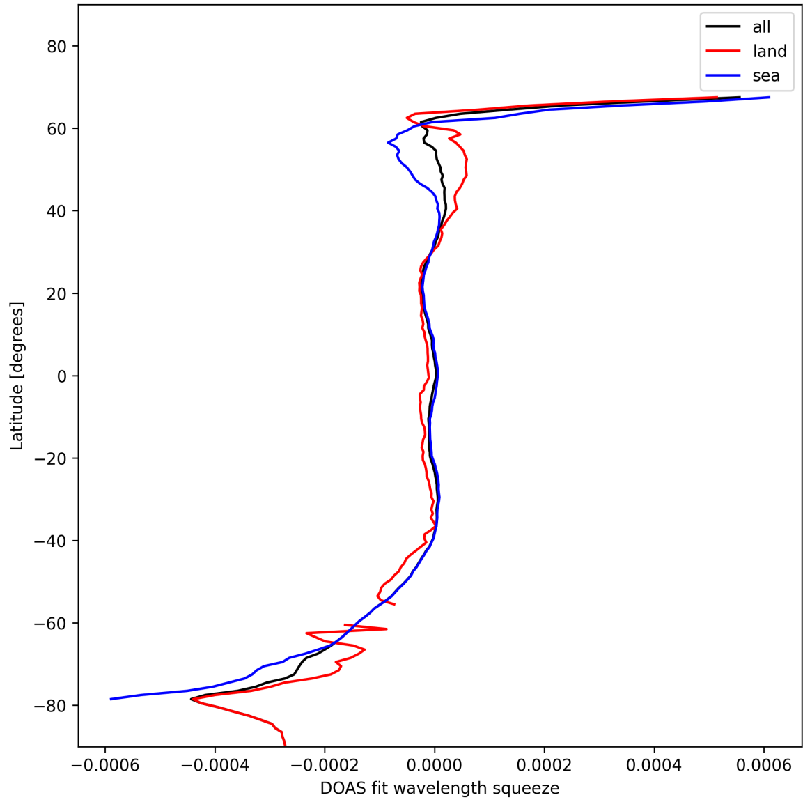
Figure 46: Zonal average of “DOAS fit wavelength squeeze” for 2024-11-09 to 2024-11-11.
