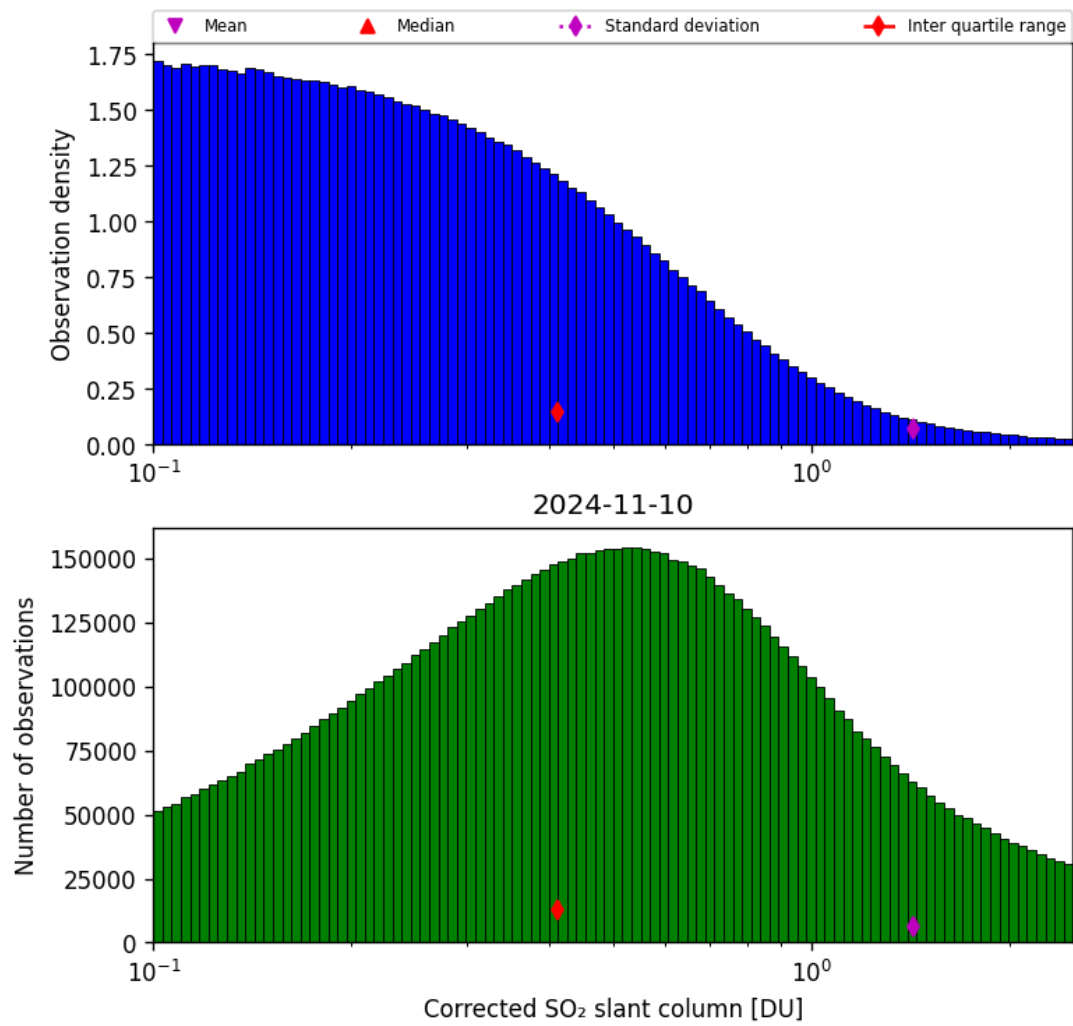
Figure 55: Histogram of “Corrected SO 2 slant column” for 2024-11-09 to 2024-11-11
