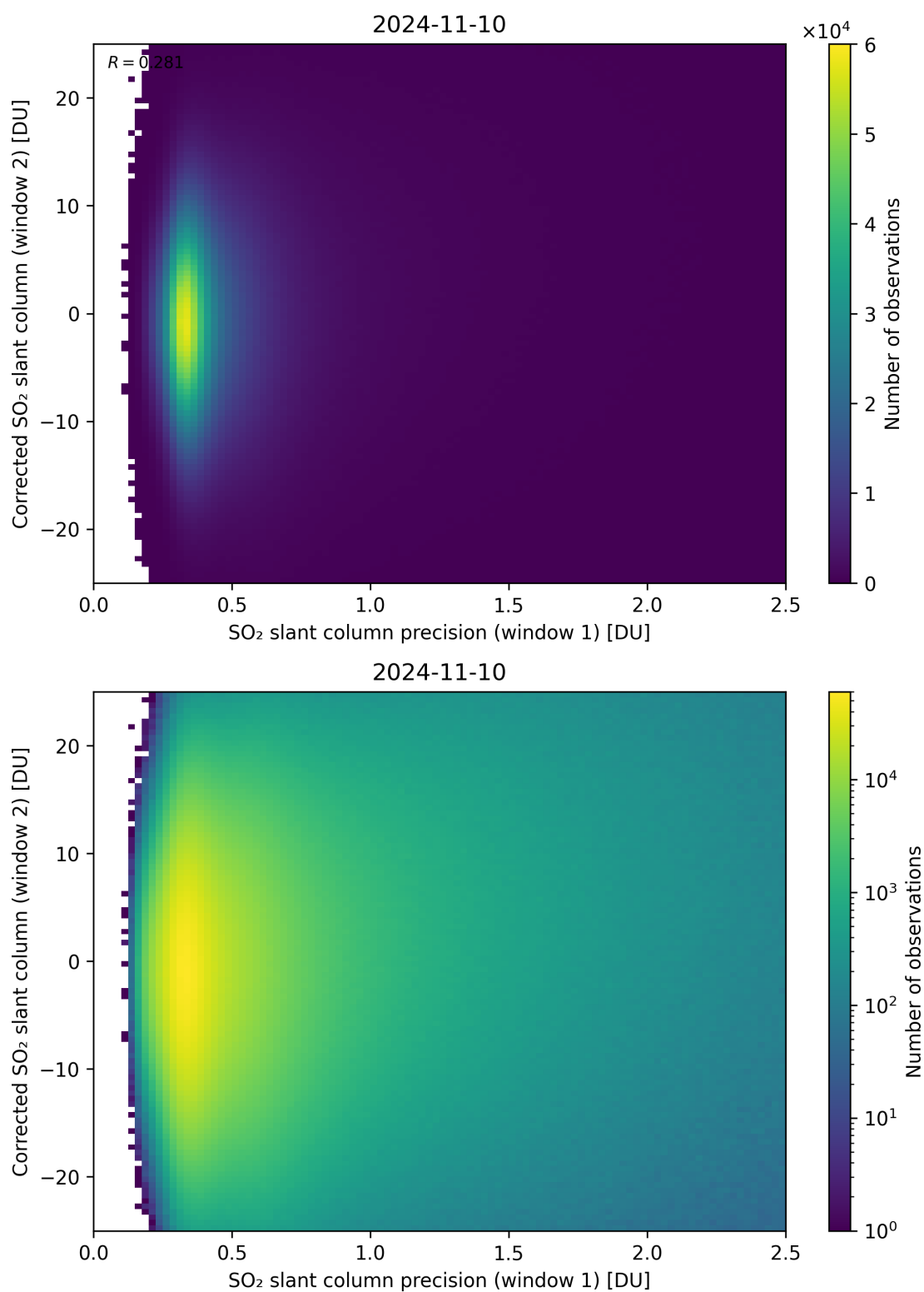
Figure 225: Scatter density plot of “SO 2 slant column precision (window 1)” against “Corrected SO 2 slant column (window 2)” for 2024-11-09 to 2024-11-11.
