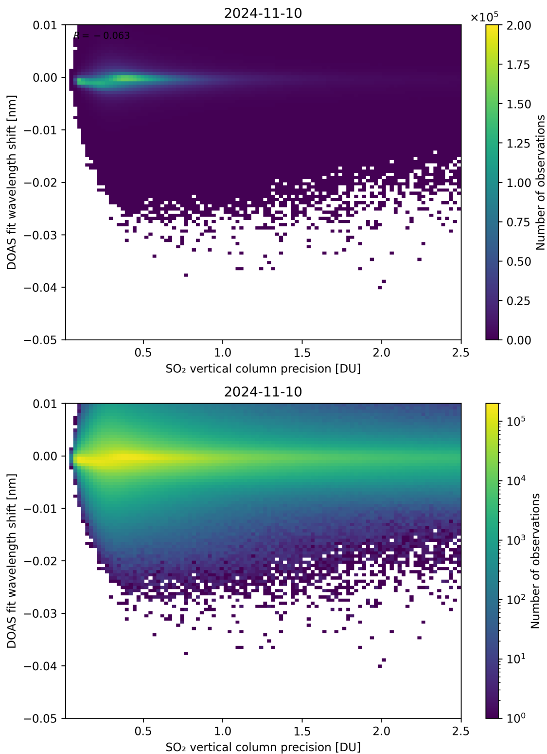
Figure 282: Scatter density plot of “SO 2 vertical column precision” against “DOAS fit wavelength shift” for 2024-11-09 to 2024-11-11.
