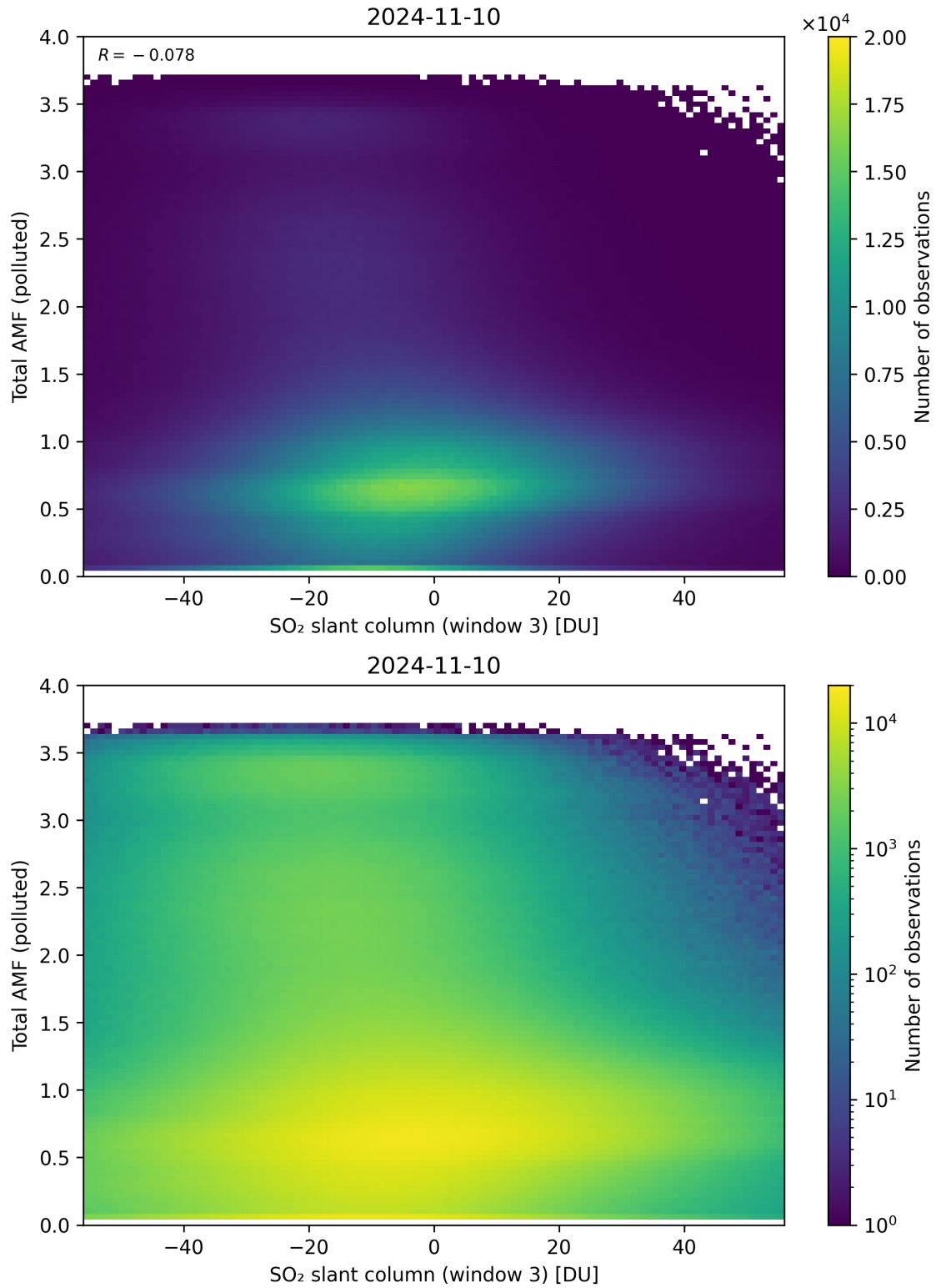
Figure 268: Scatter density plot of “SO 2 slant column (window 3)” against “Total AMF (polluted)” for 2024-11-09 to 2024-11-11.
