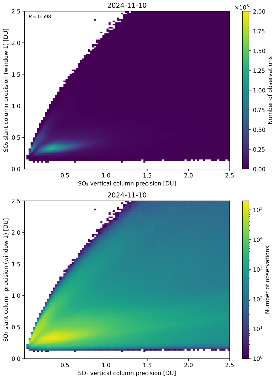
Figure 290: Scatter density plot of “SO 2 vertical column precision” against “SO 2 slant column precision (window 1)” for 2024-11-09 to 2024-11-11.
