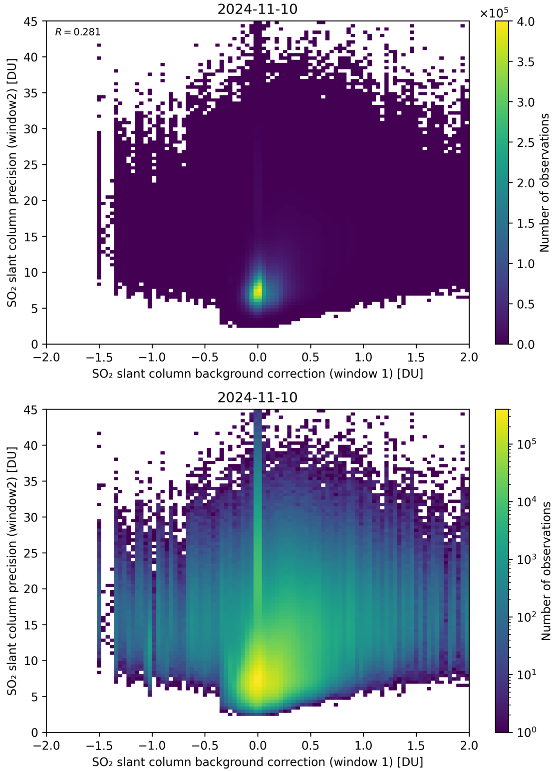
Figure 106: Scatter density plot of “SO 2 slant column background correction (window 1)” against “SO 2 slant column precision (window2)” for 2024-11-09 to 2024-11-11.
