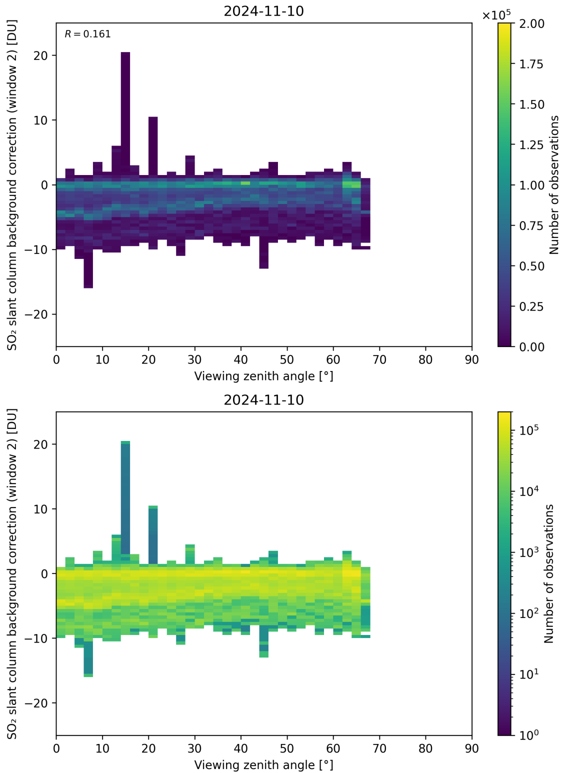
Figure 309: Scatter density plot of “Viewing zenith angle” against “SO 2 slant column background correction (window 2)” for 2024-11-09 to 2024-11-11.
