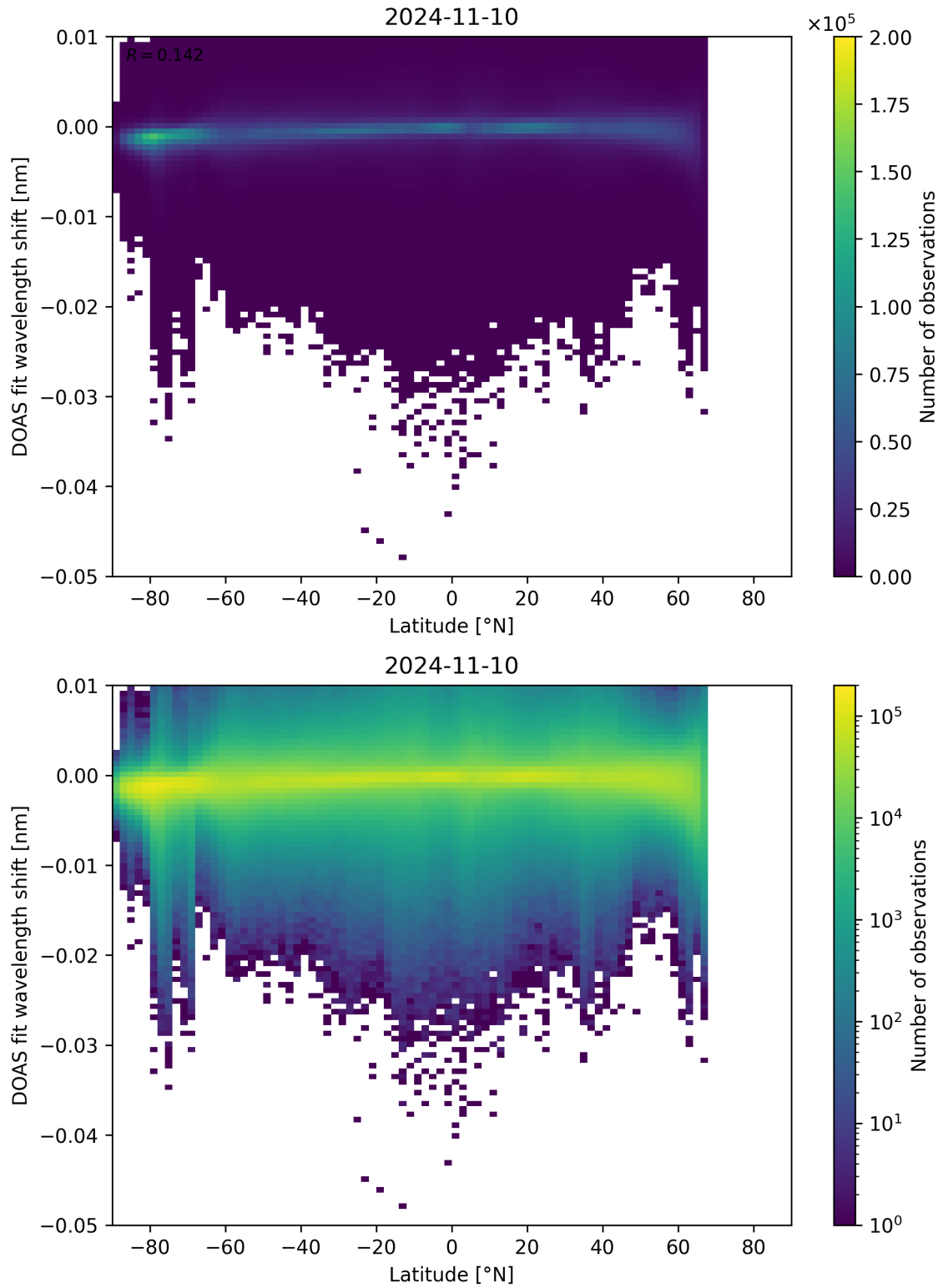
Figure 142: Scatter density plot of “Latitude” against “DOAS fit wavelength shift” for 2024-11-09 to 2024-11-11.
