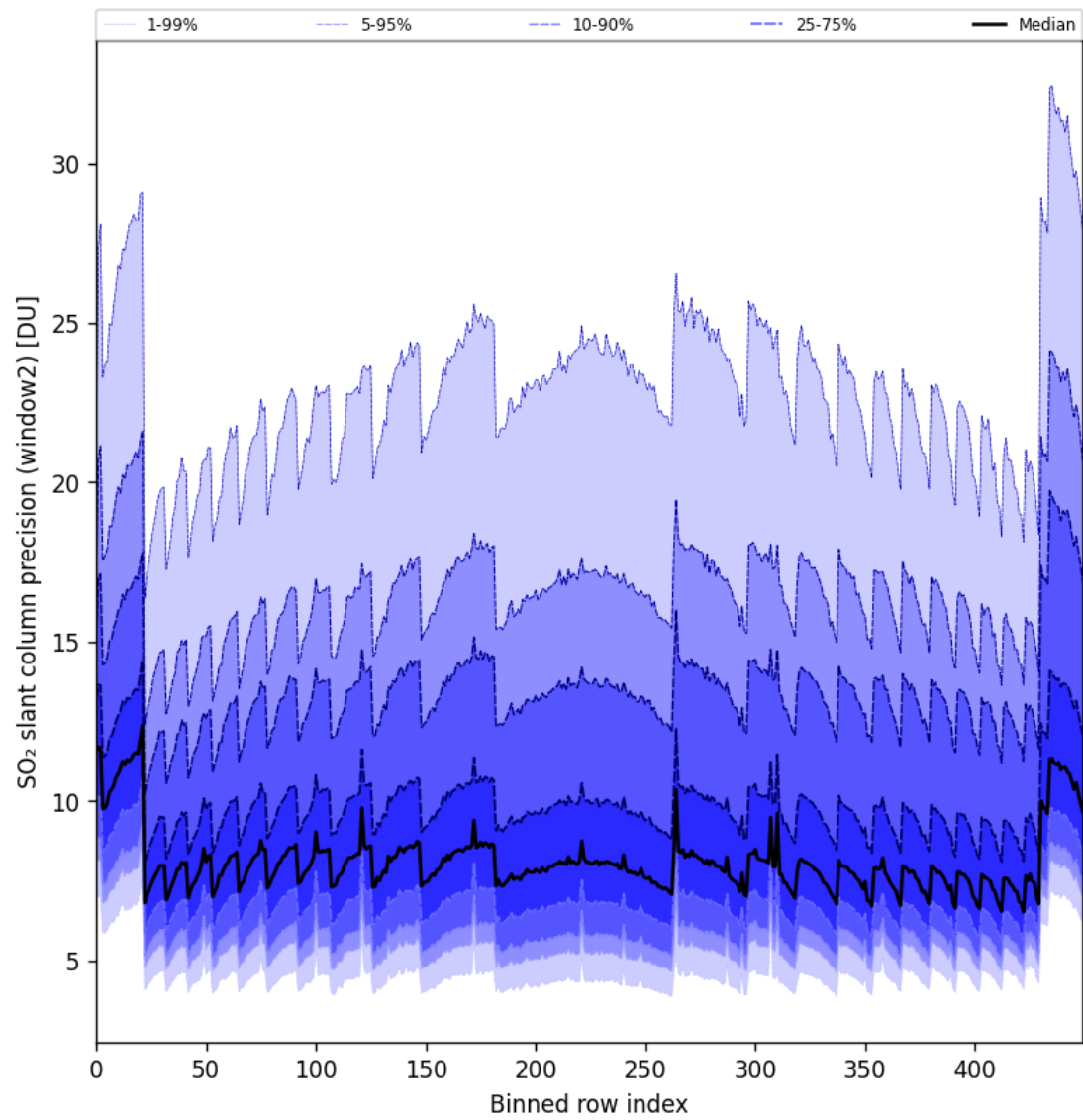
Figure 84: Along track statistics of “SO 2 slant column precision (window2)” for 2024-11-09 to 2024-11-11
