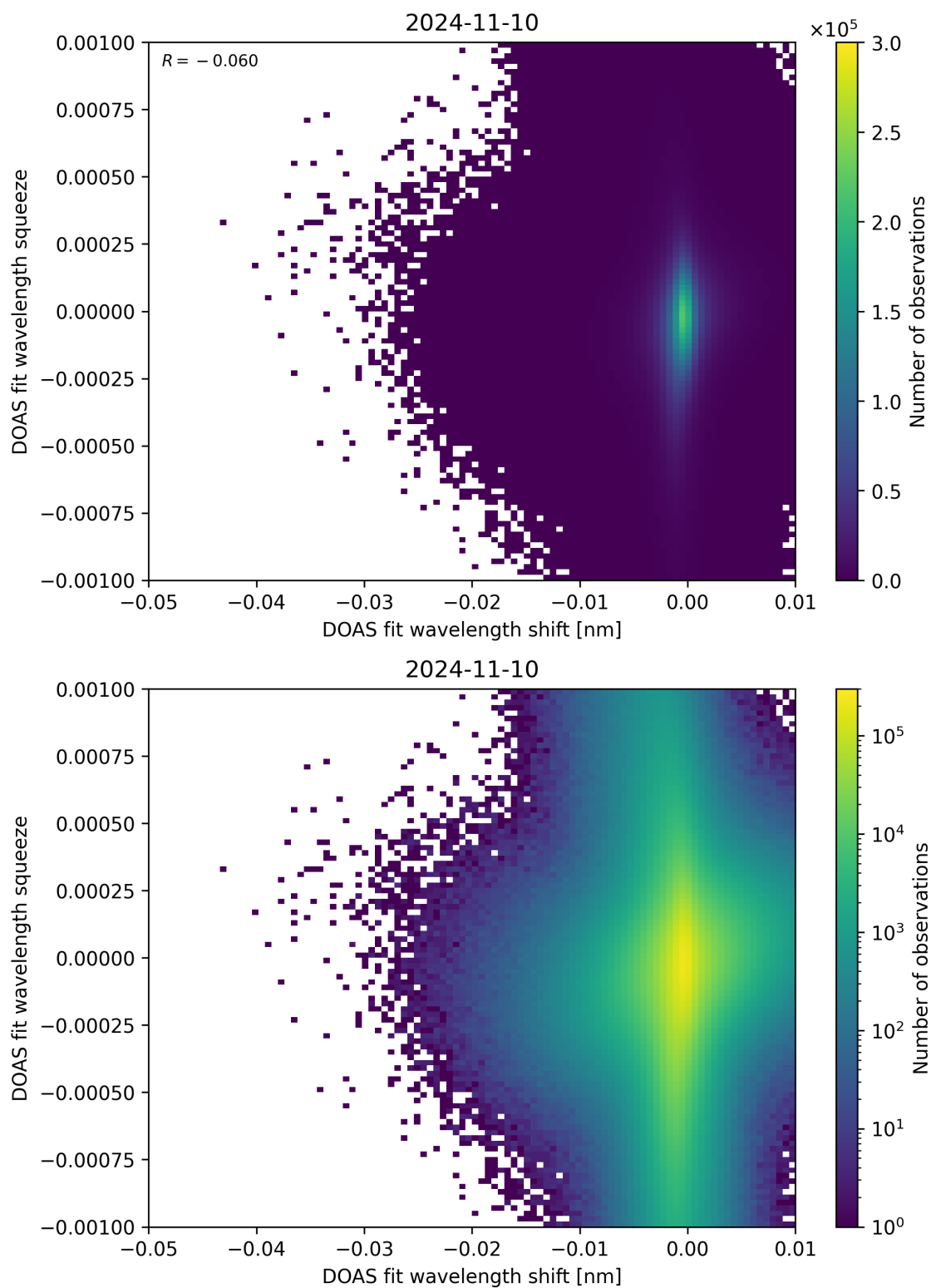
Figure 127: Scatter density plot of “DOAS fit wavelength shift” against “DOAS fit wavelength squeeze” for 2024-11-09 to 2024-11-11.
