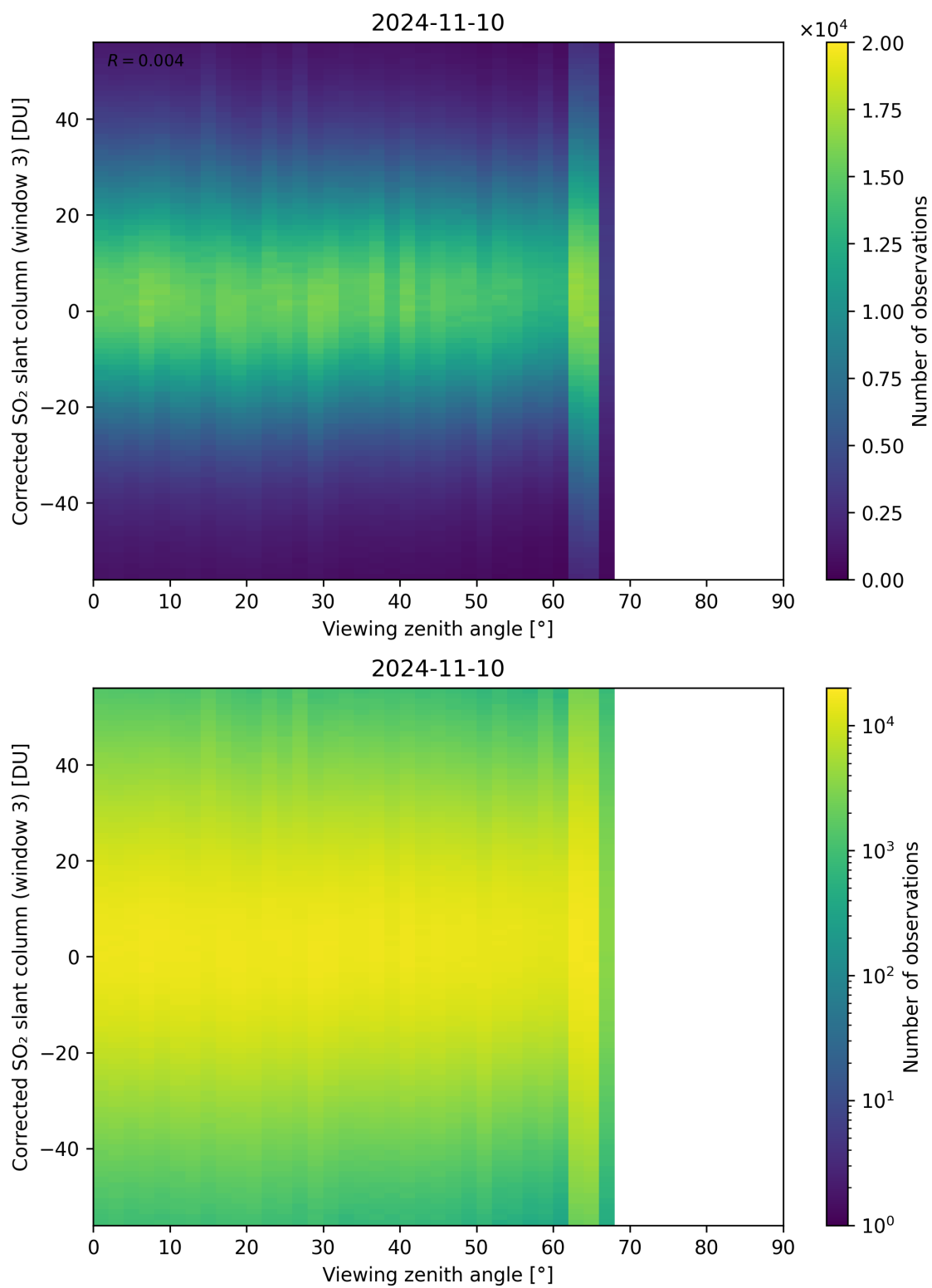
Figure 319: Scatter density plot of “Viewing zenith angle” against “Corrected SO 2 slant column (window 3)” for 2024-11-09 to 2024-11-11.
