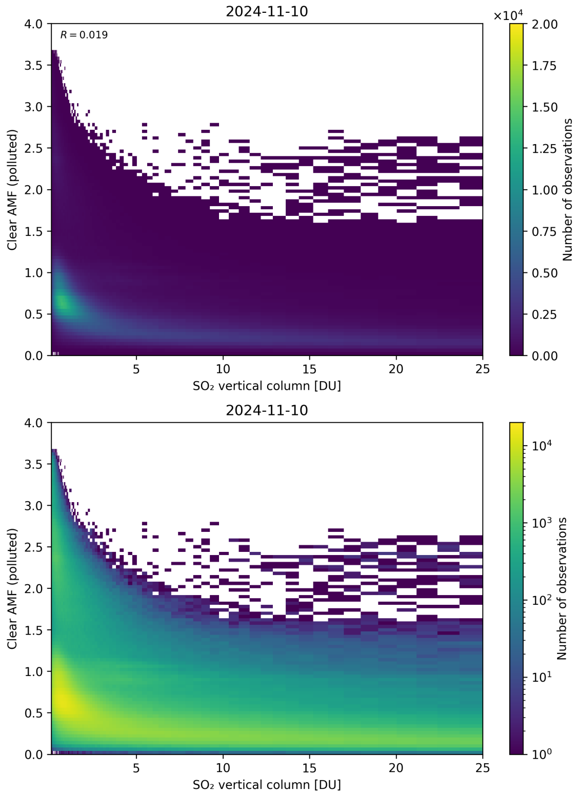
Figure 296: Scatter density plot of “SO 2 vertical column” against “Clear AMF (polluted)” for 2024-11-09 to 2024-11-11.
