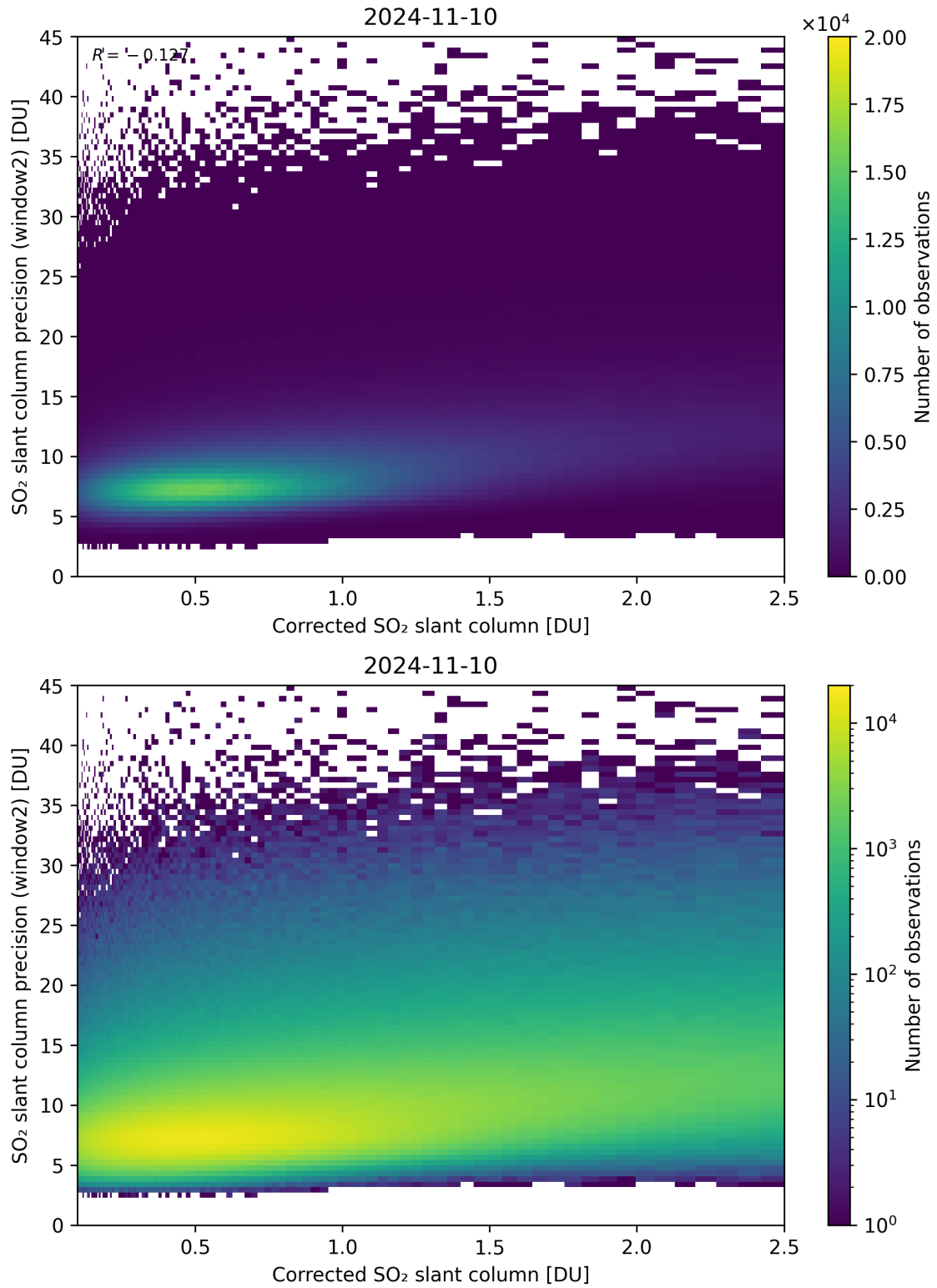
Figure 189: Scatter density plot of “Corrected SO 2 slant column” against “SO 2 slant column precision (window2)” for 2024-11-09 to 2024-11-11.
