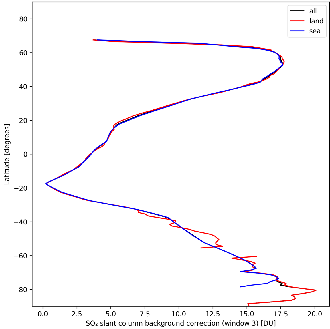
Figure 44: Zonal average of “SO 2 slant column background correction (window 3)” for 2024-11-09 to 2024-11-11.
