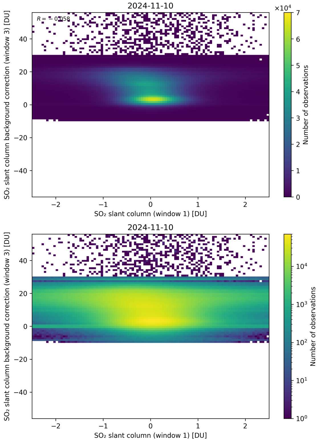
Figure 214: Scatter density plot of “SO 2 slant column (window 1)” against “SO 2 slant column background correction (window 3)” for 2024-11-09 to 2024-11-11.
