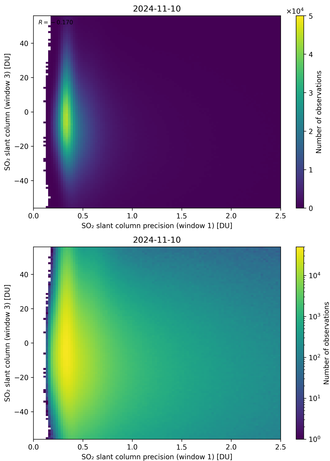
Figure 228: Scatter density plot of “SO 2 slant column precision (window 1)” against “SO 2 slant column (window 3)” for 2024-11-09 to 2024-11-11.
