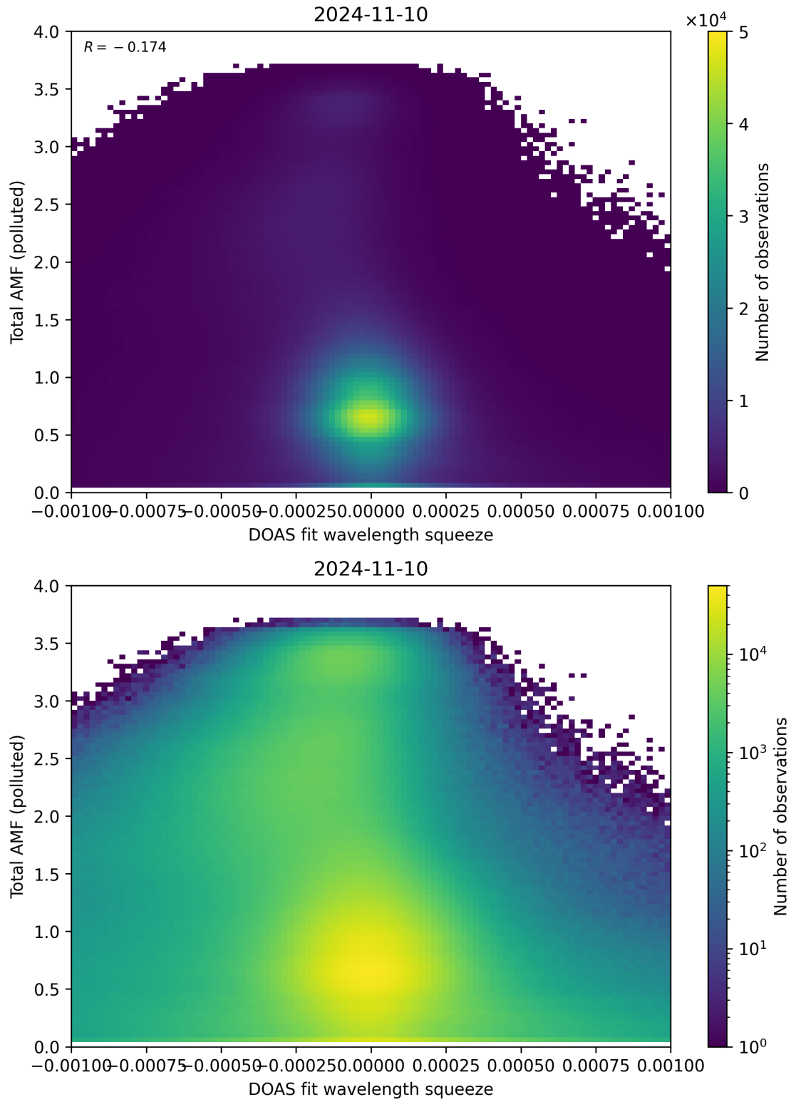
Figure 134: Scatter density plot of “DOAS fit wavelength squeeze” against “Total AMF (polluted)” for 2024-11-09 to 2024-11-11.
