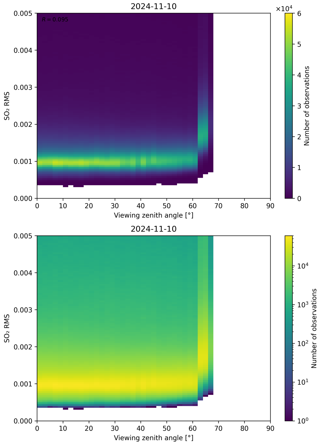
Figure 313: Scatter density plot of “Viewing zenith angle” against “SO 2 RMS” for 2024-11-09 to 2024-11-11.
