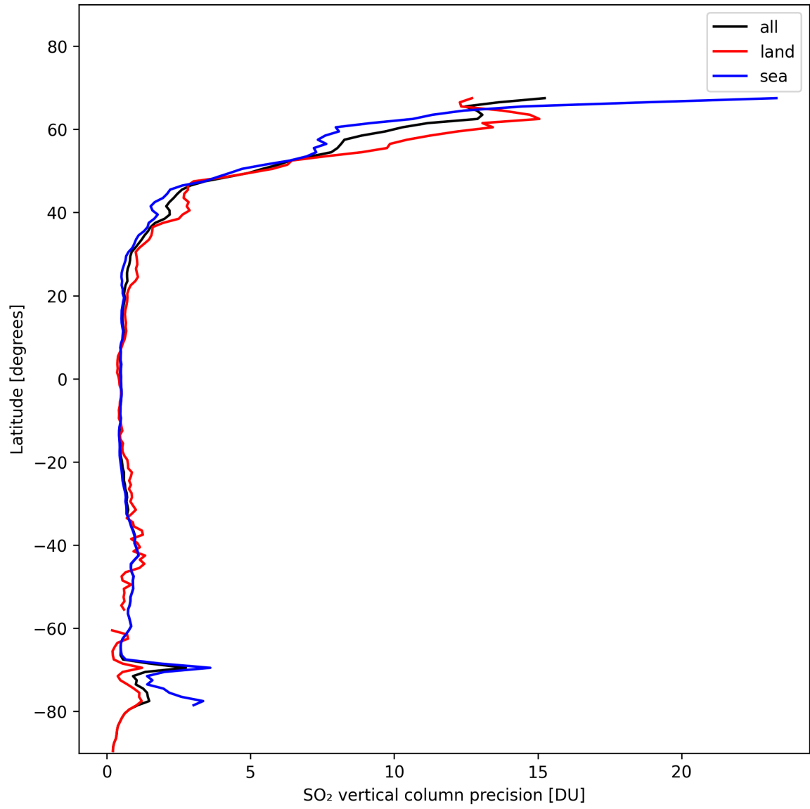
Figure 31: Zonal average of “SO 2 vertical column precision” for 2024-11-09 to 2024-11-11.
