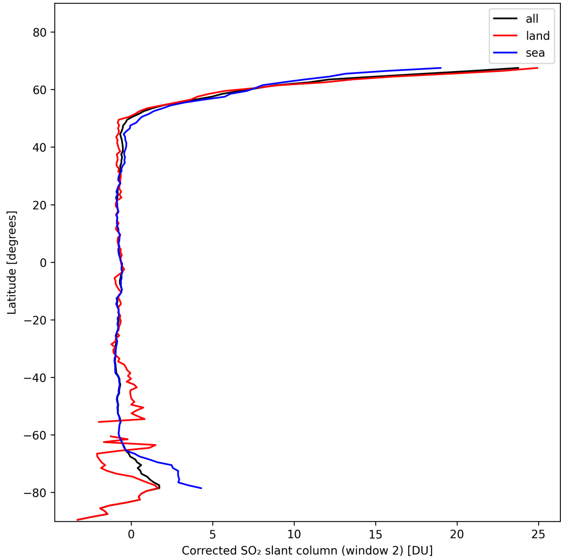
Figure 39: Zonal average of “Corrected SO 2 slant column (window 2)” for 2024-11-09 to 2024-11-11.
