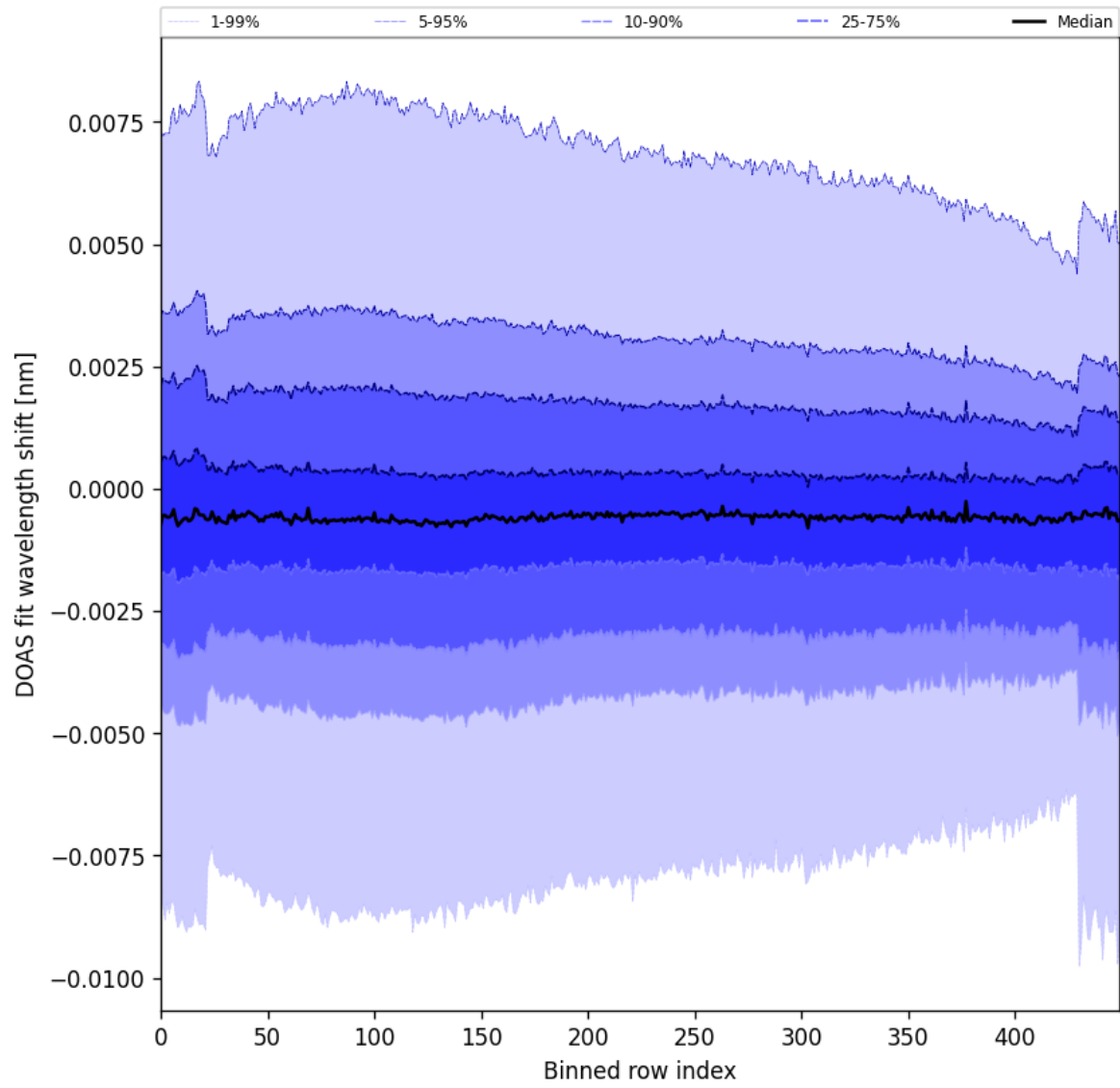
Figure 91: Along track statistics of “DOAS fit wavelength shift” for 2024-11-09 to 2024-11-11
