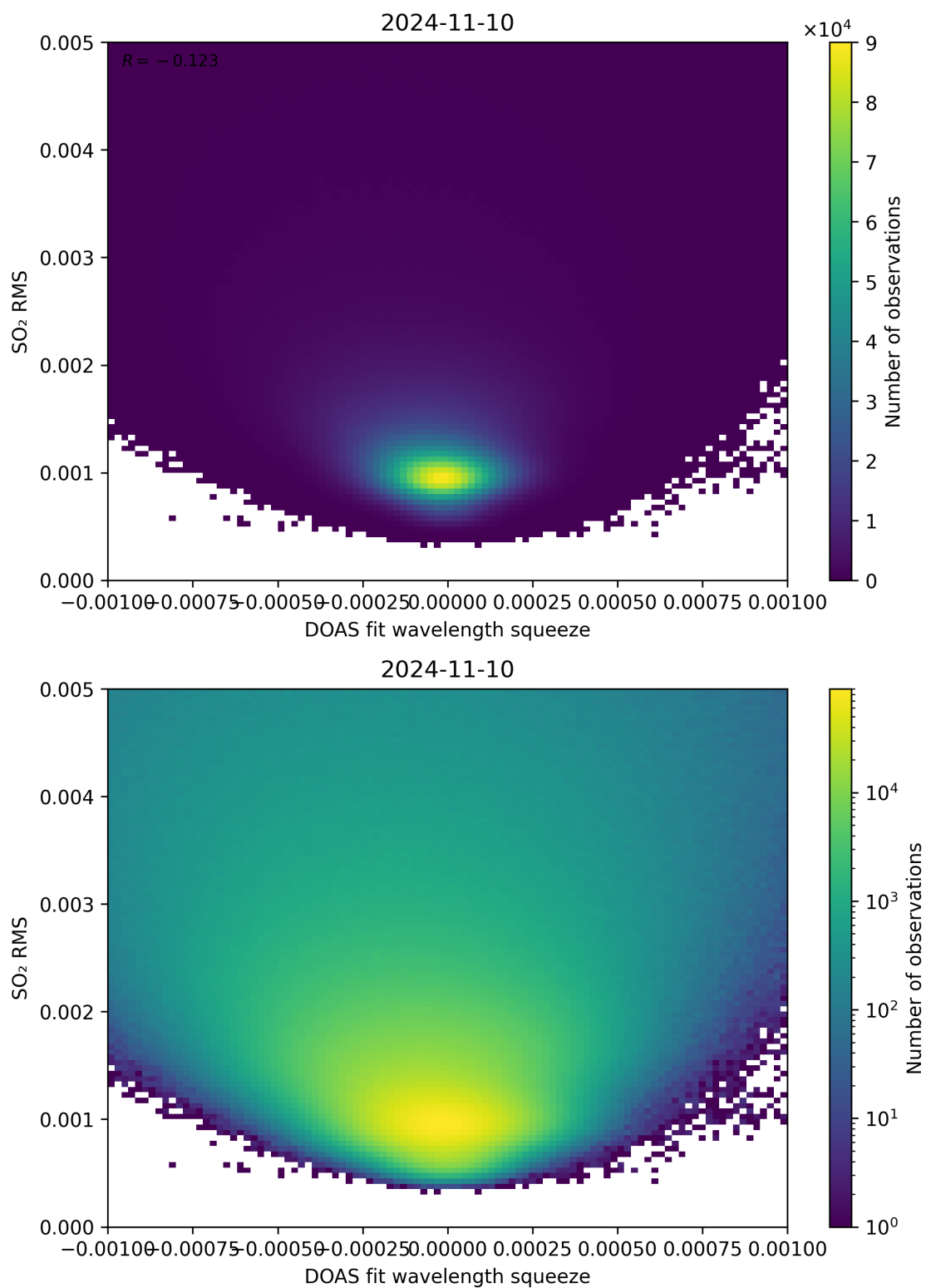
Figure 132: Scatter density plot of “DOAS fit wavelength squeeze” against “SO 2 RMS” for 2024-11-09 to 2024-11-11.
