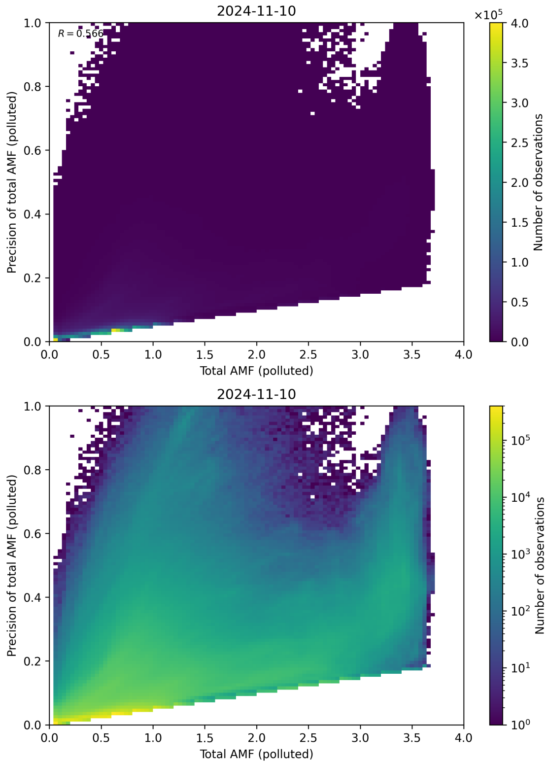
Figure 272: Scatter density plot of “Total AMF (polluted)” against “Precision of total AMF (polluted)” for 2024-11-09 to 2024-11-11.
