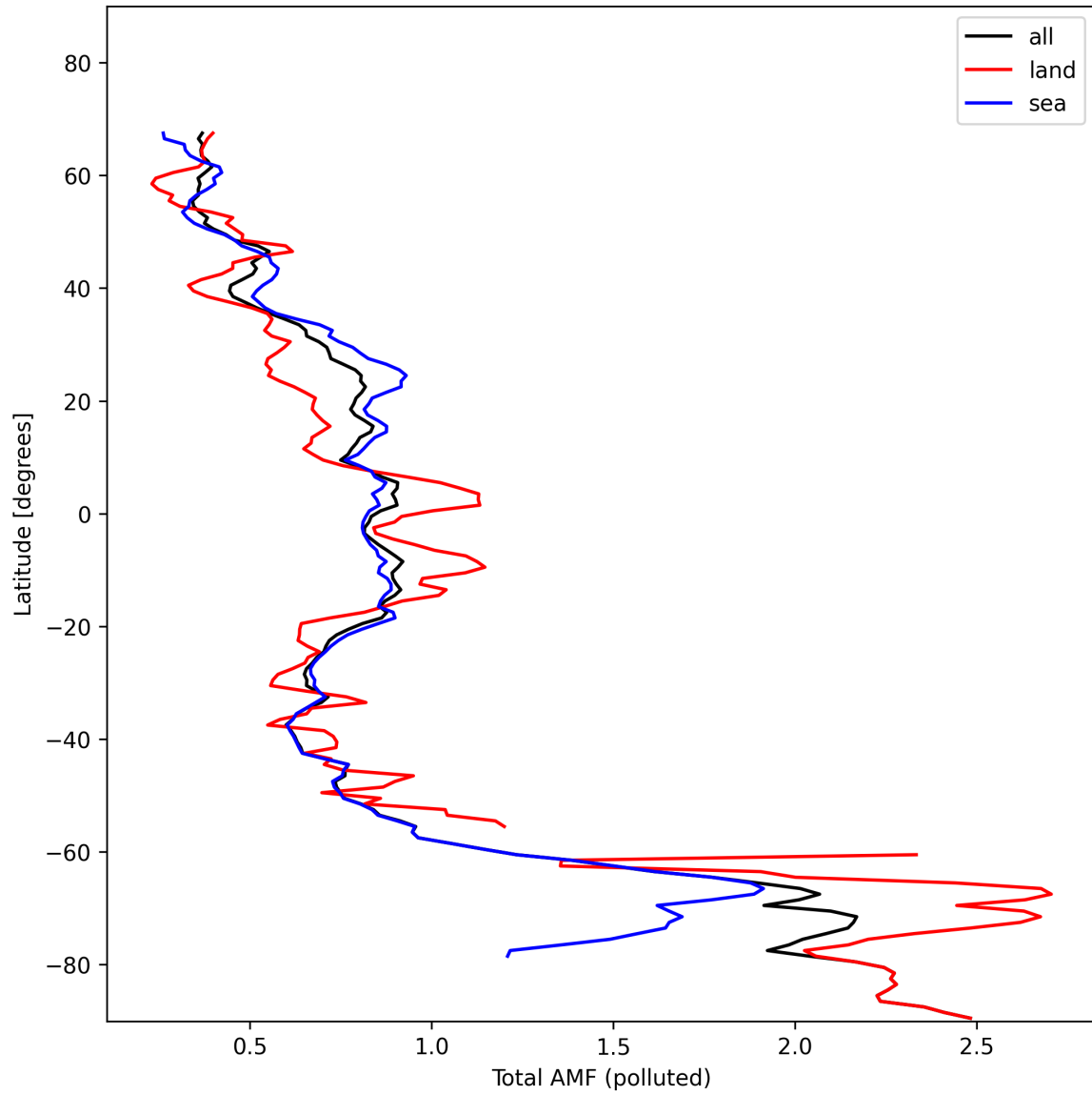
Figure 48: Zonal average of “Total AMF (polluted)” for 2024-11-09 to 2024-11-11.
