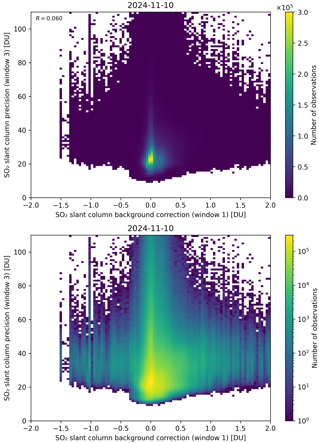
Figure 108: Scatter density plot of “SO 2 slant column background correction (window 1)” against “SO 2 slant column precision (window 3)” for 2024-11-09 to 2024-11-11.
