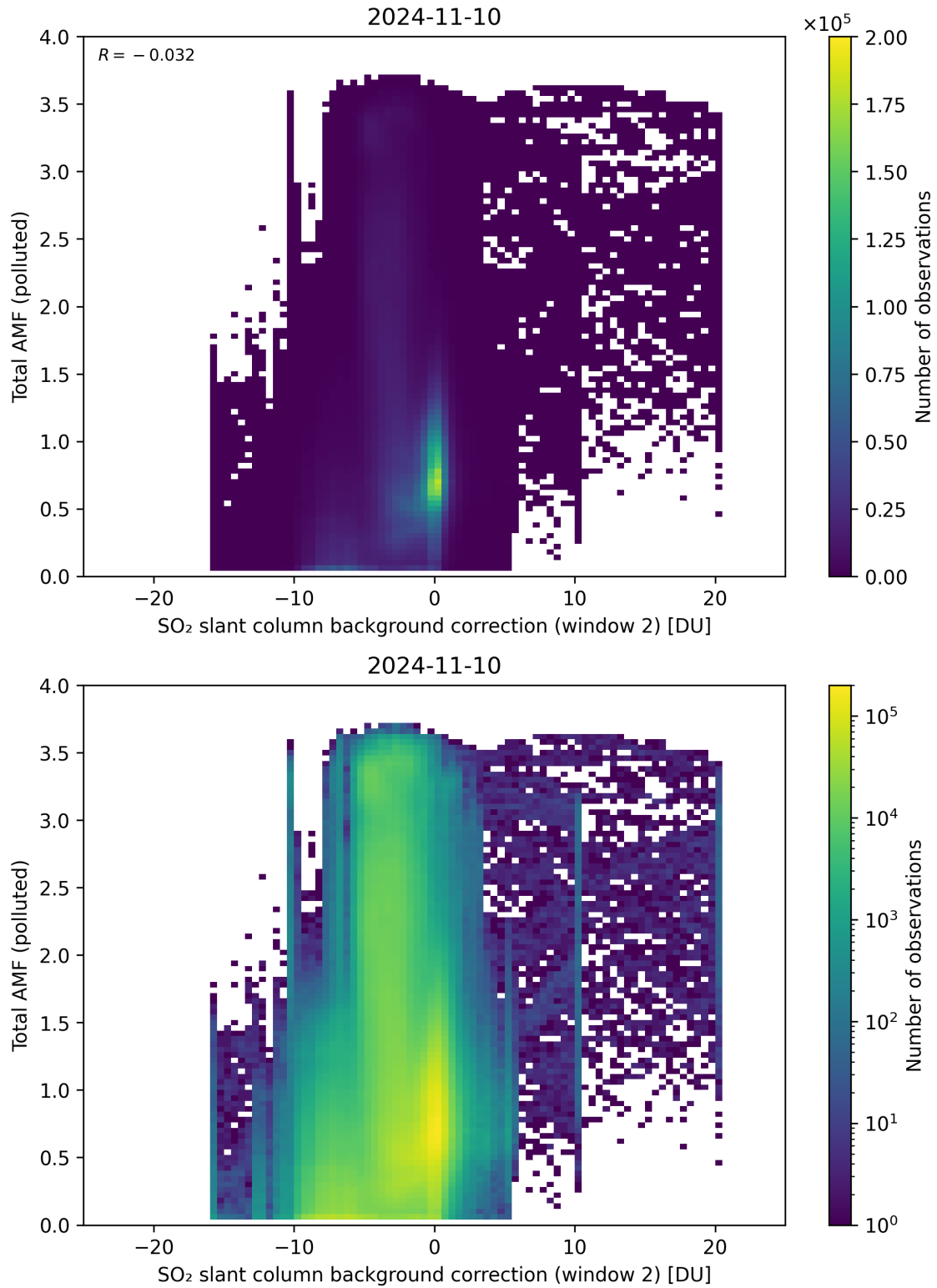
Figure 119: Scatter density plot of “SO 2 slant column background correction (window 2)” against “Total AMF (polluted)” for 2024-11-09 to 2024-11-11.
