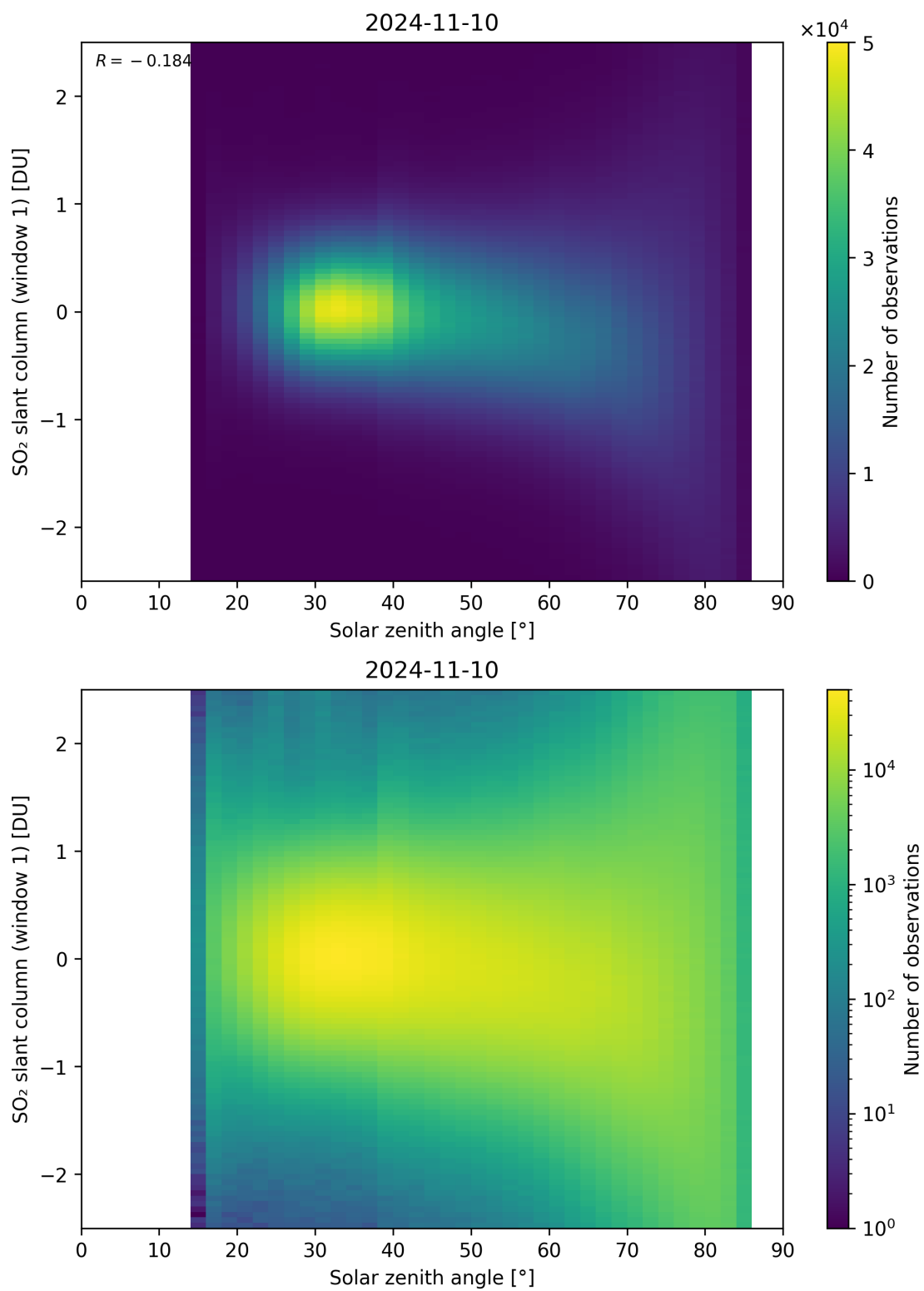
Figure 169: Scatter density plot of “Solar zenith angle” against “SO 2 slant column (window 1)” for 2024-11-09 to 2024-11-11.
