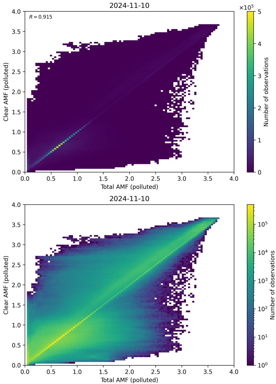
Figure 271: Scatter density plot of “Total AMF (polluted)” against “Clear AMF (polluted)” for 2024-11-09 to 2024-11-11.
