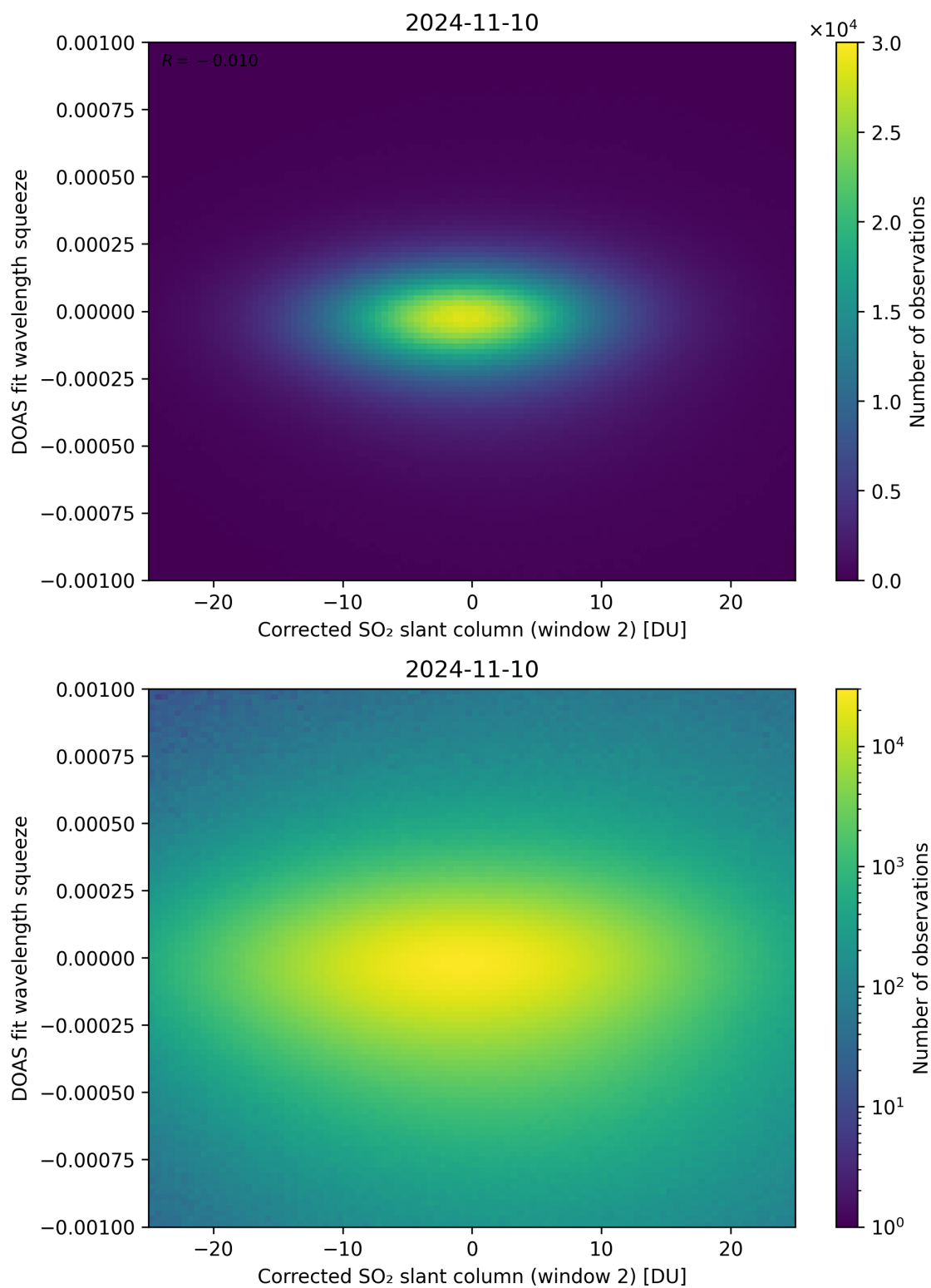
Figure 197: Scatter density plot of “Corrected SO 2 slant column (window 2)” against “DOAS fit wavelength squeeze” for 2024-11-09 to 2024-11-11.
