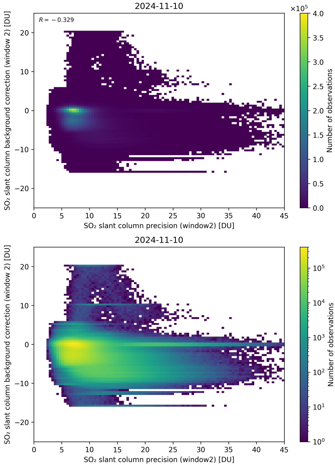
Figure 241: Scatter density plot of “SO 2 slant column precision (window2)” against “SO 2 slant column background correction (window 2)” for 2024-11-09 to 2024-11-11.
