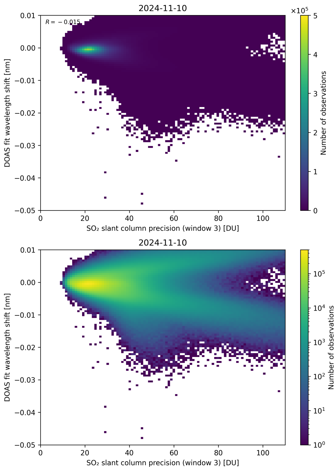
Figure 258: Scatter density plot of “SO 2 slant column precision (window 3)” against “DOAS fit wavelength shift” for 2024-11-09 to 2024-11-11.
