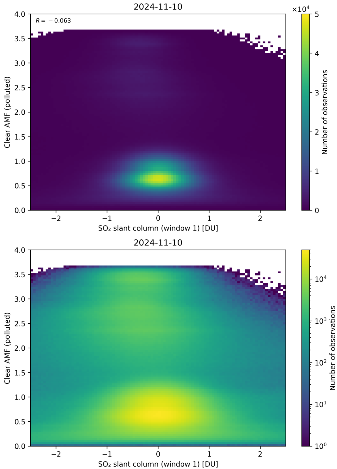
Figure 232: Scatter density plot of “SO 2 slant column (window 1)” against “Clear AMF (polluted)” for 2024-11-09 to 2024-11-11.
