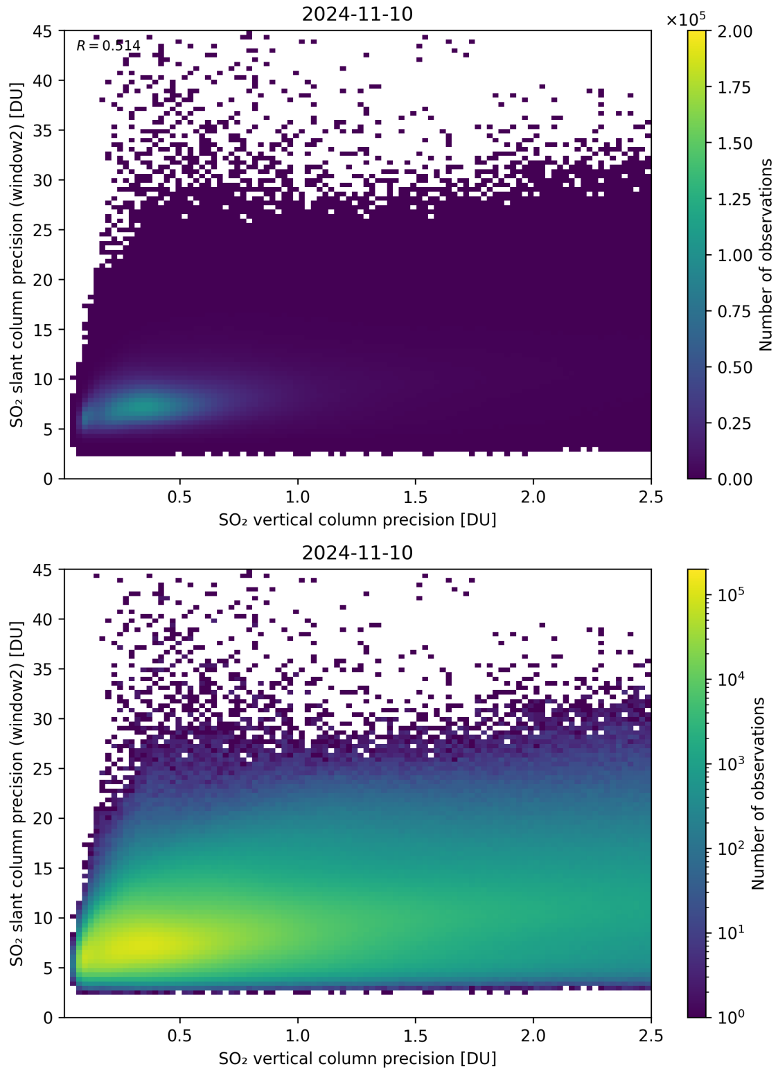
Figure 291: Scatter density plot of “SO 2 vertical column precision” against “SO 2 slant column precision (window2)” for 2024-11-09 to 2024-11-11.
