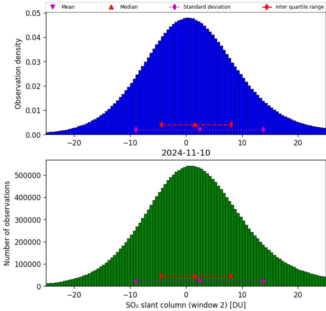
Figure 60: Histogram of “SO 2 slant column (window 2)” for 2024-11-09 to 2024-11-11
