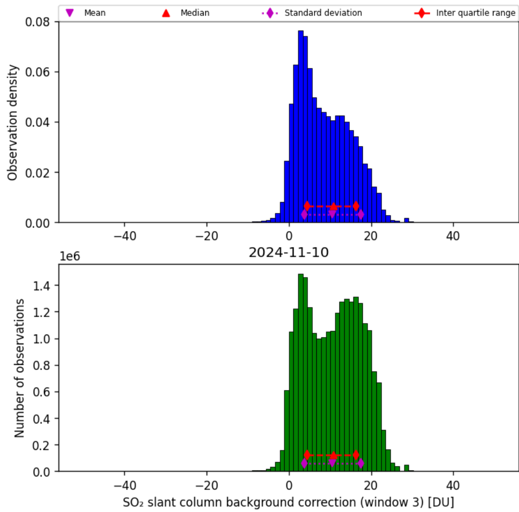
Figure 67: Histogram of “SO 2 slant column background correction (window 3)” for 2024-11-09 to 2024-11-11
