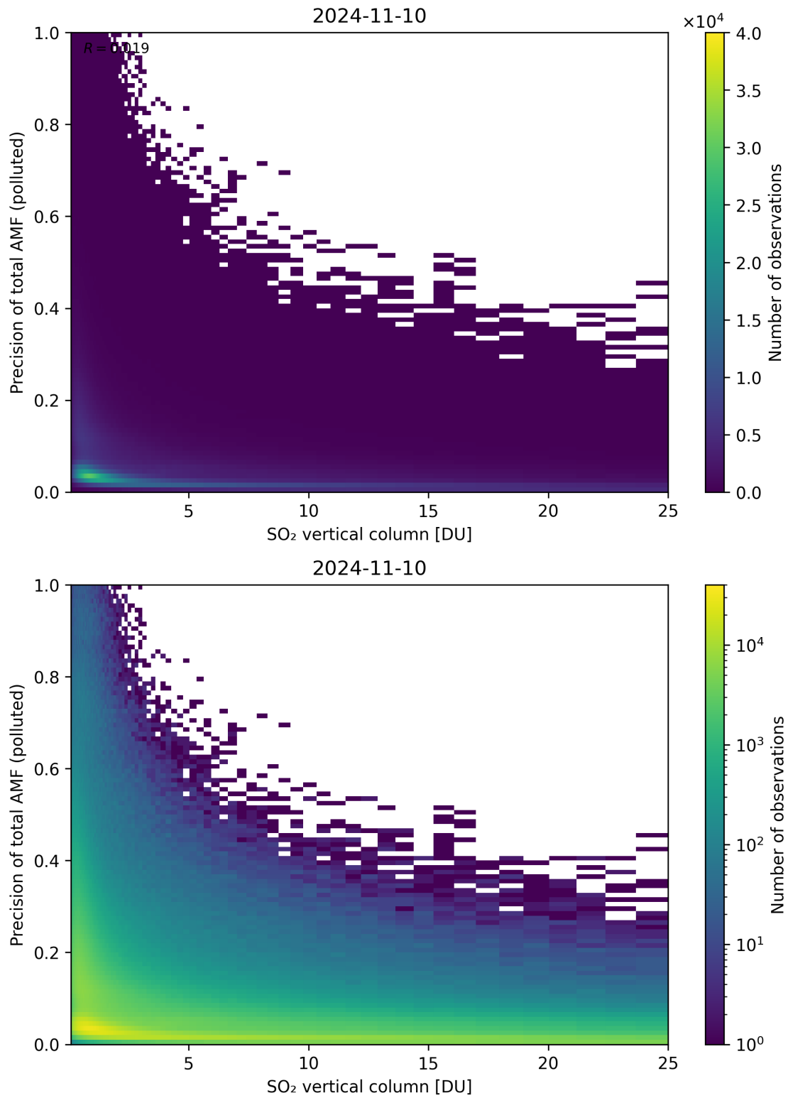
Figure 306: Scatter density plot of “SO 2 vertical column” against “Precision of total AMF (polluted)” for 2024-11-09 to 2024-11-11.
