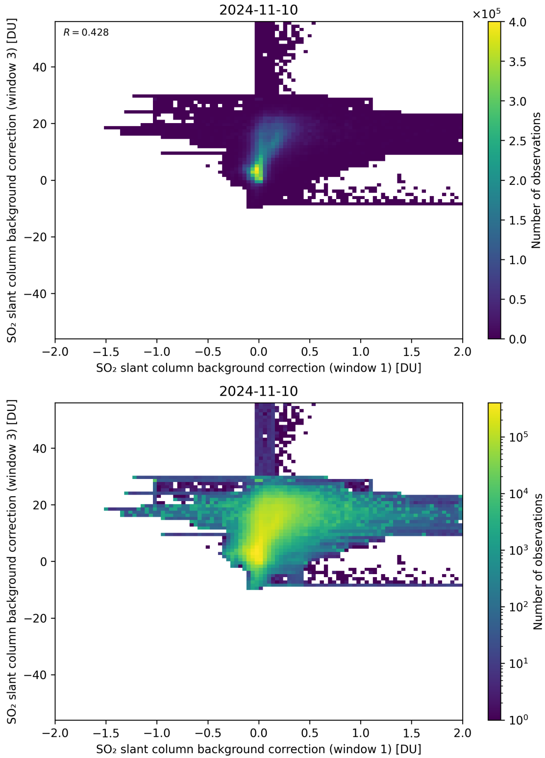
Figure 99: Scatter density plot of “SO 2 slant column background correction (window 1)” against “SO 2 slant column background correction (window 3)” for 2024-11-09 to 2024-11-11.
