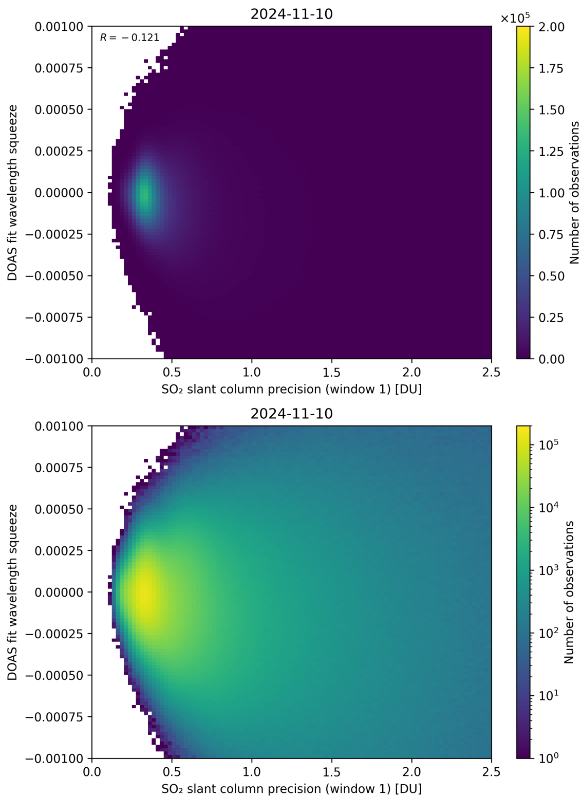
Figure 222: Scatter density plot of “SO 2 slant column precision (window 1)” against “DOAS fit wavelength squeeze” for 2024-11-09 to 2024-11-11.
