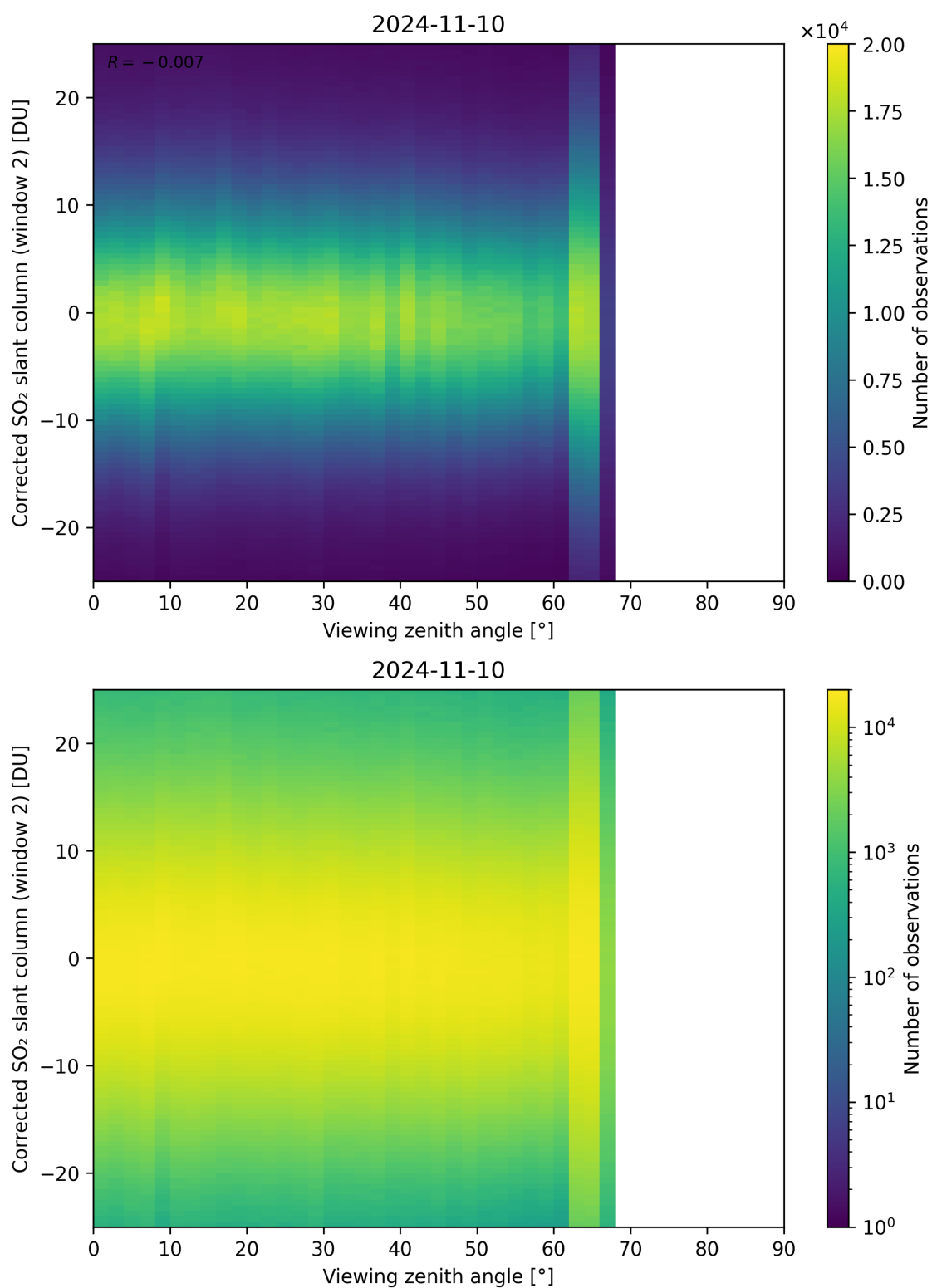
Figure 318: Scatter density plot of “Viewing zenith angle” against “Corrected SO 2 slant column (window 2)” for 2024-11-09 to 2024-11-11.
