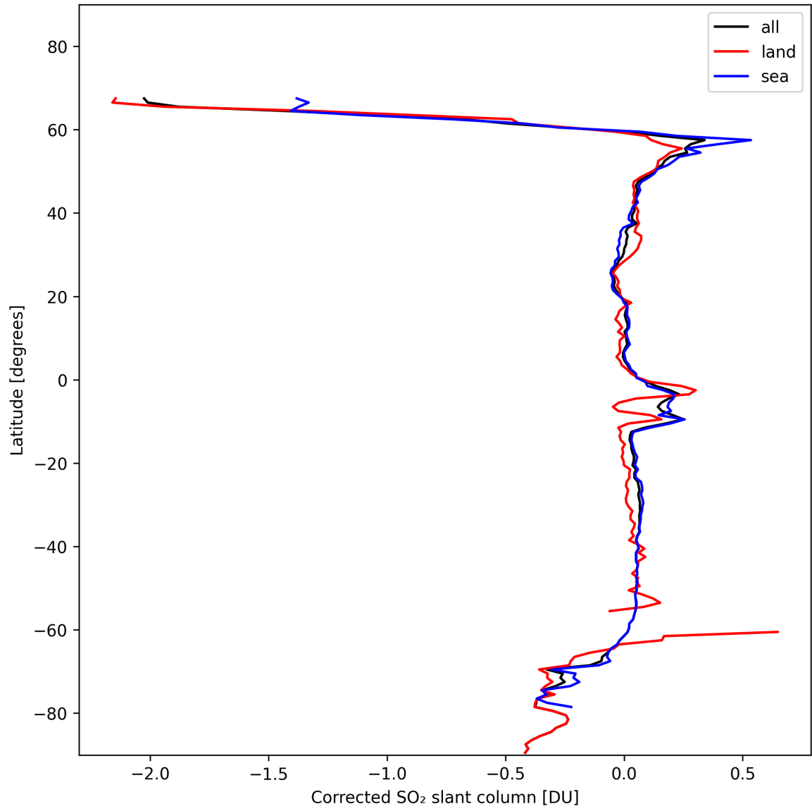
Figure 32: Zonal average of “Corrected SO 2 slant column” for 2024-11-09 to 2024-11-11.
