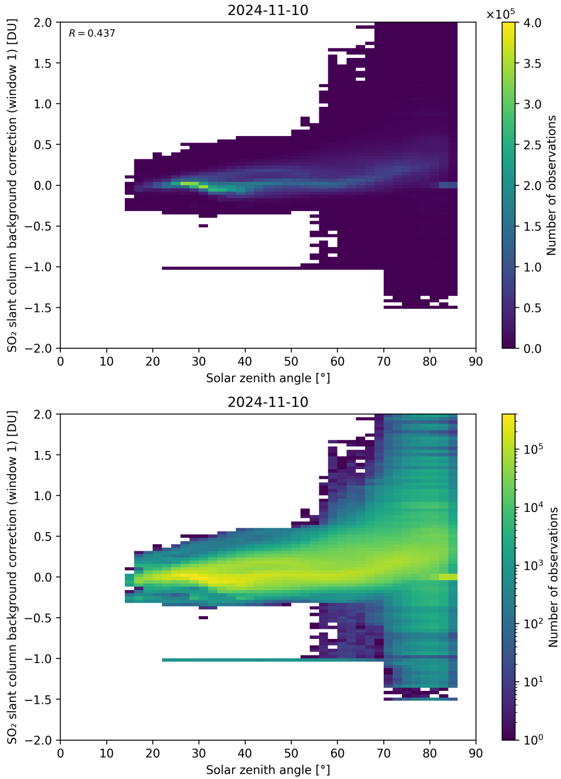
Figure 158: Scatter density plot of “Solar zenith angle” against “SO 2 slant column background correction (window 1)” for 2024-11-09 to 2024-11-11.
