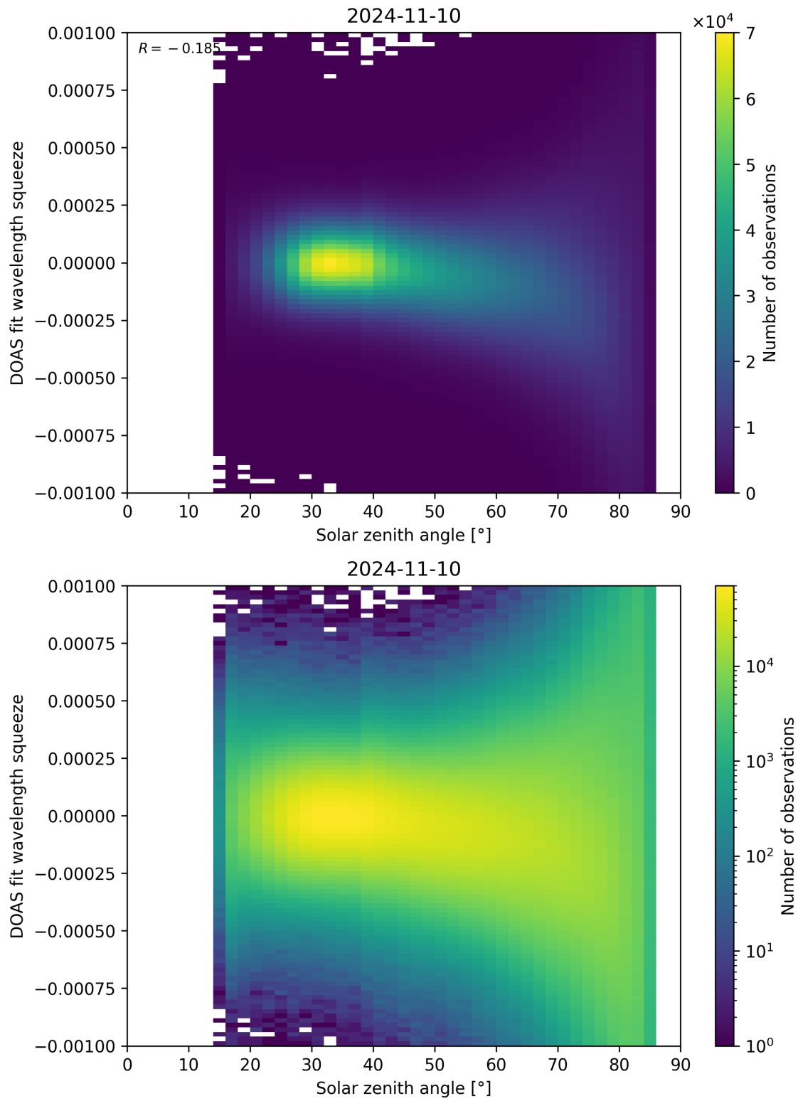
Figure 162: Scatter density plot of “Solar zenith angle” against “DOAS fit wavelength squeeze” for 2024-11-09 to 2024-11-11.
