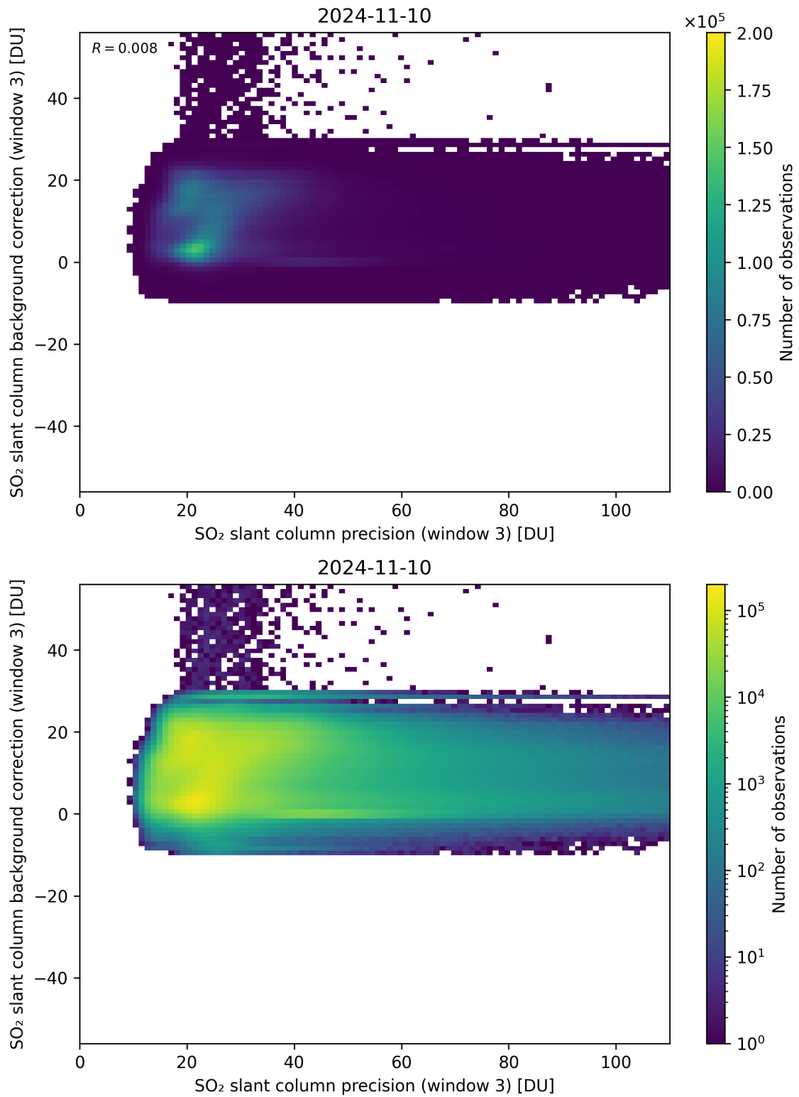
Figure 257: Scatter density plot of “SO 2 slant column precision (window 3)” against “SO 2 slant column background correction (window 3)” for 2024-11-09 to 2024-11-11.
