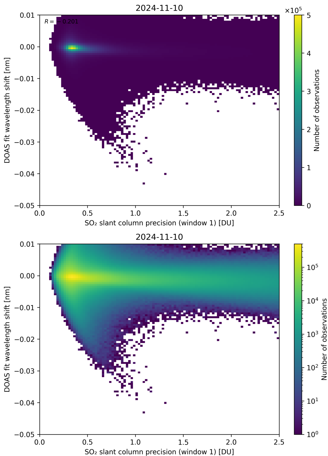
Figure 221: Scatter density plot of “SO 2 slant column precision (window 1)” against “DOAS fit wavelength shift” for 2024-11-09 to 2024-11-11.
