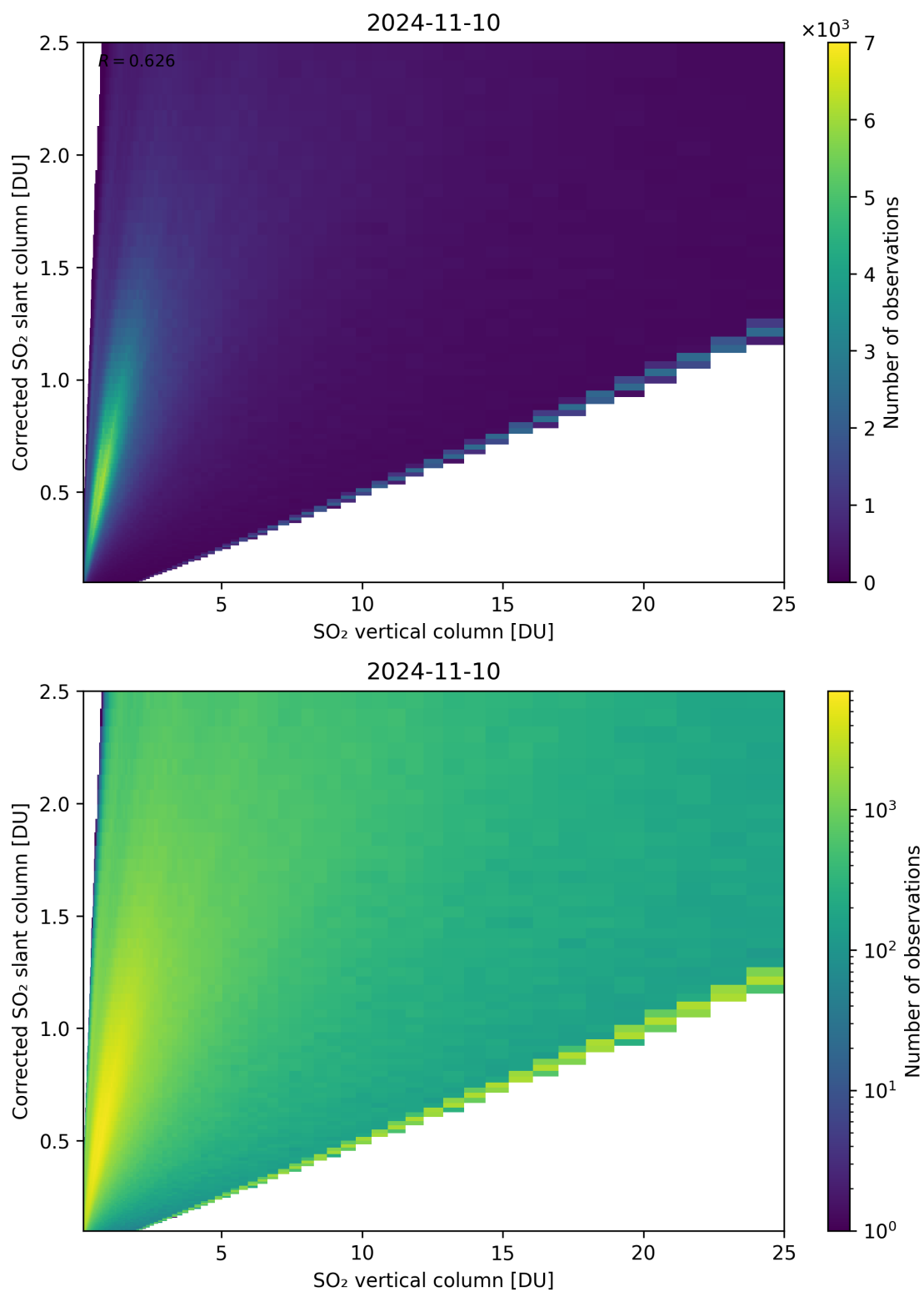
Figure 297: Scatter density plot of “SO 2 vertical column” against “Corrected SO 2 slant column” for 2024-11-09 to 2024-11-11.
