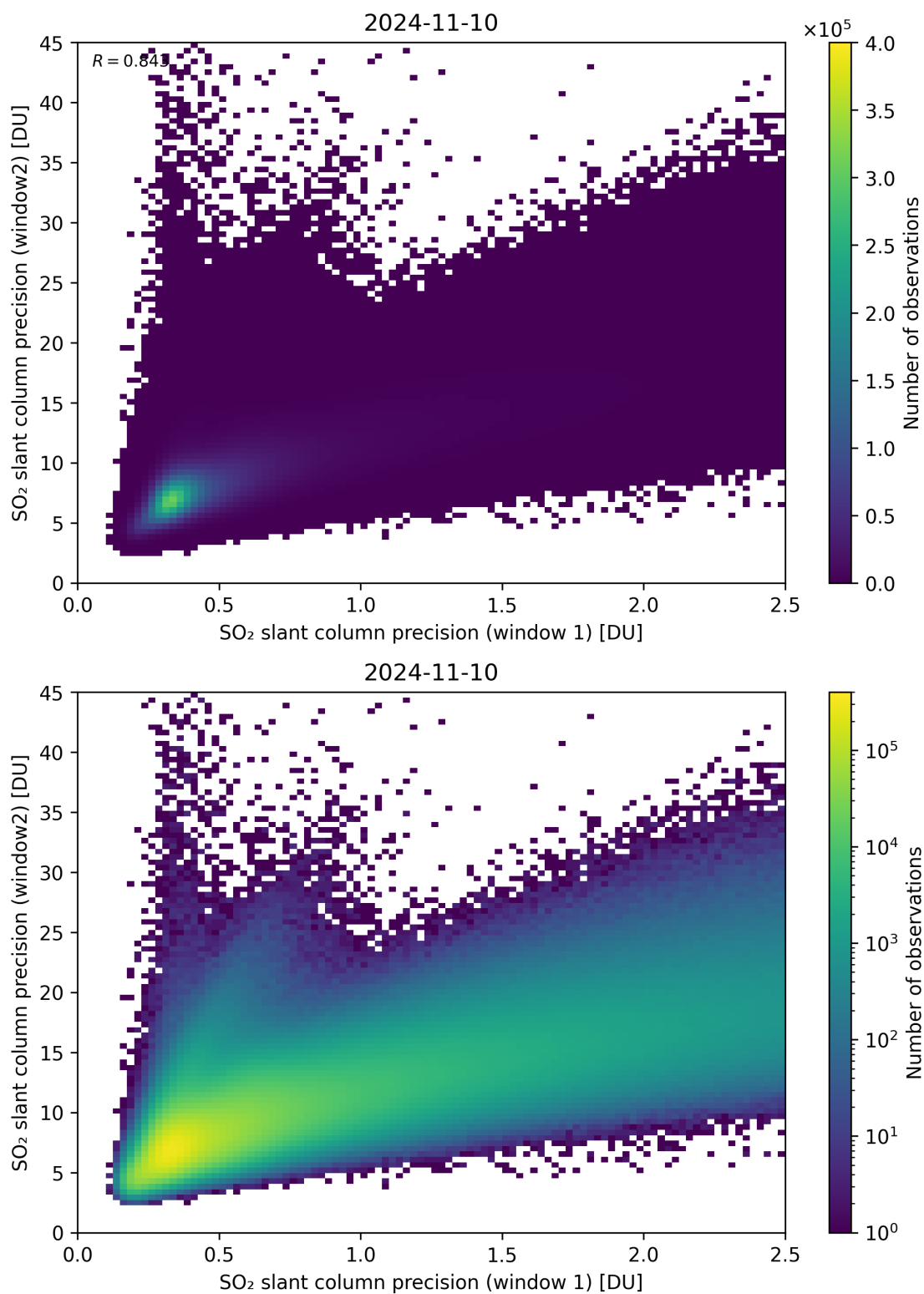
Figure 227: Scatter density plot of “SO 2 slant column precision (window 1)” against “SO 2 slant column precision (window2)” for 2024-11-09 to 2024-11-11.
