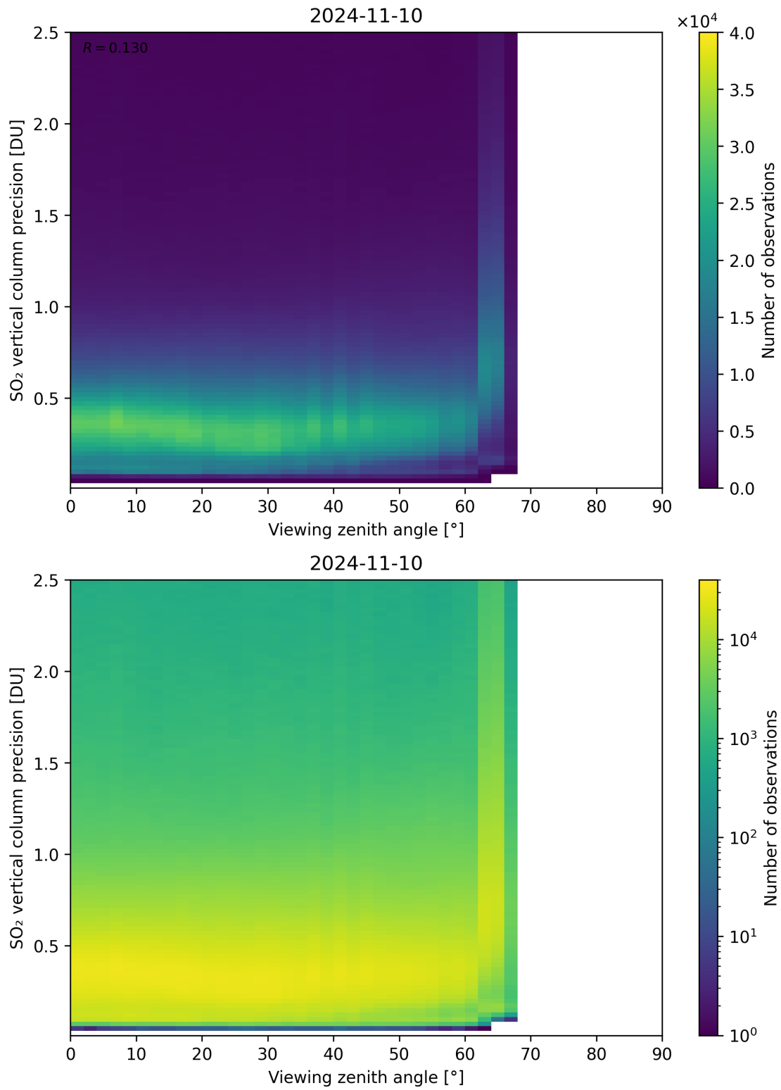
Figure 328: Scatter density plot of “Viewing zenith angle” against “SO 2 vertical column precision” for 2024-11-09 to 2024-11-11.
