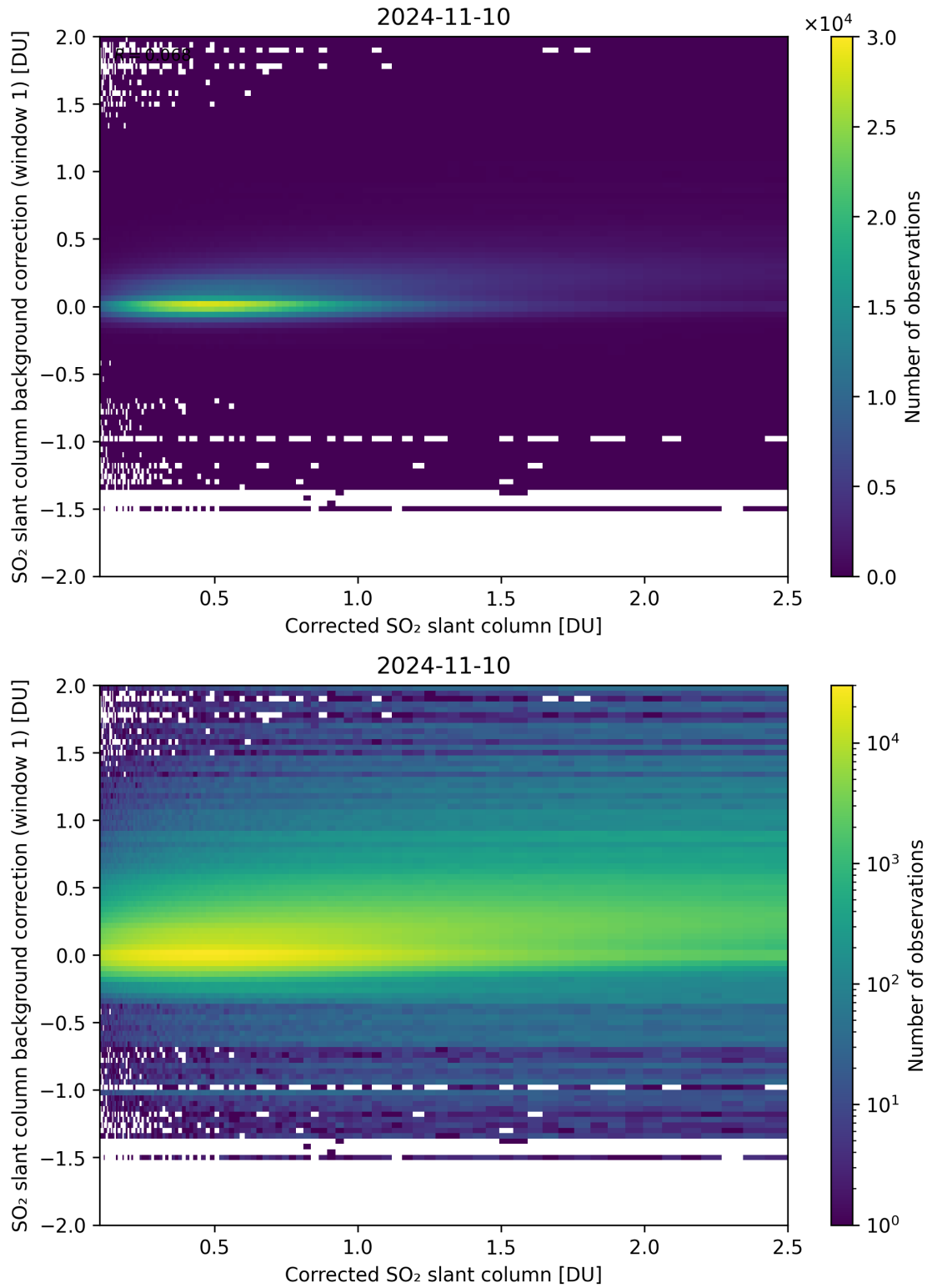
Figure 178: Scatter density plot of “Corrected SO 2 slant column” against “SO 2 slant column background correction (window 1)” for 2024-11-09 to 2024-11-11.
