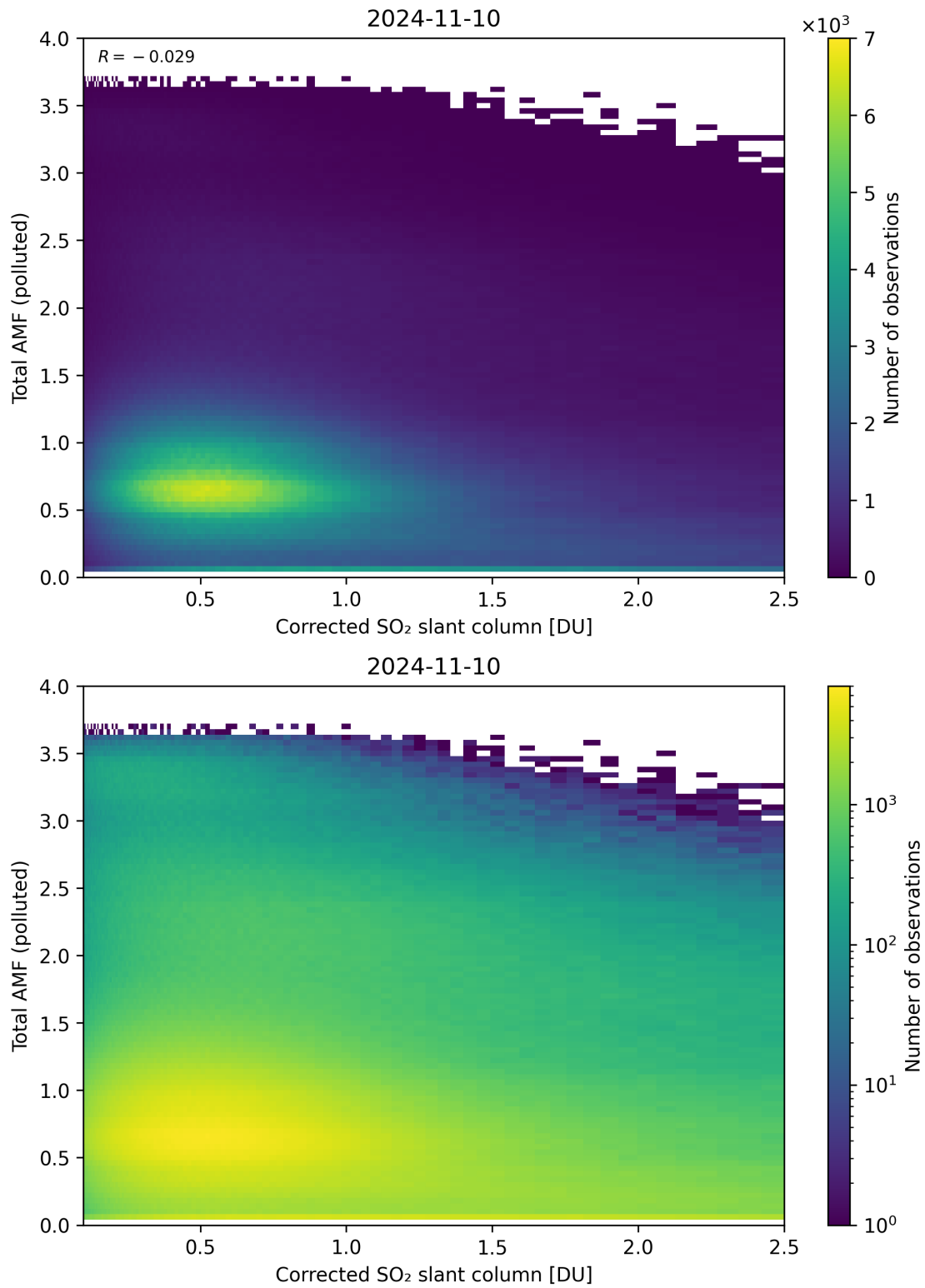
Figure 192: Scatter density plot of “Corrected SO 2 slant column” against “Total AMF (polluted)” for 2024-11-09 to 2024-11-11.
