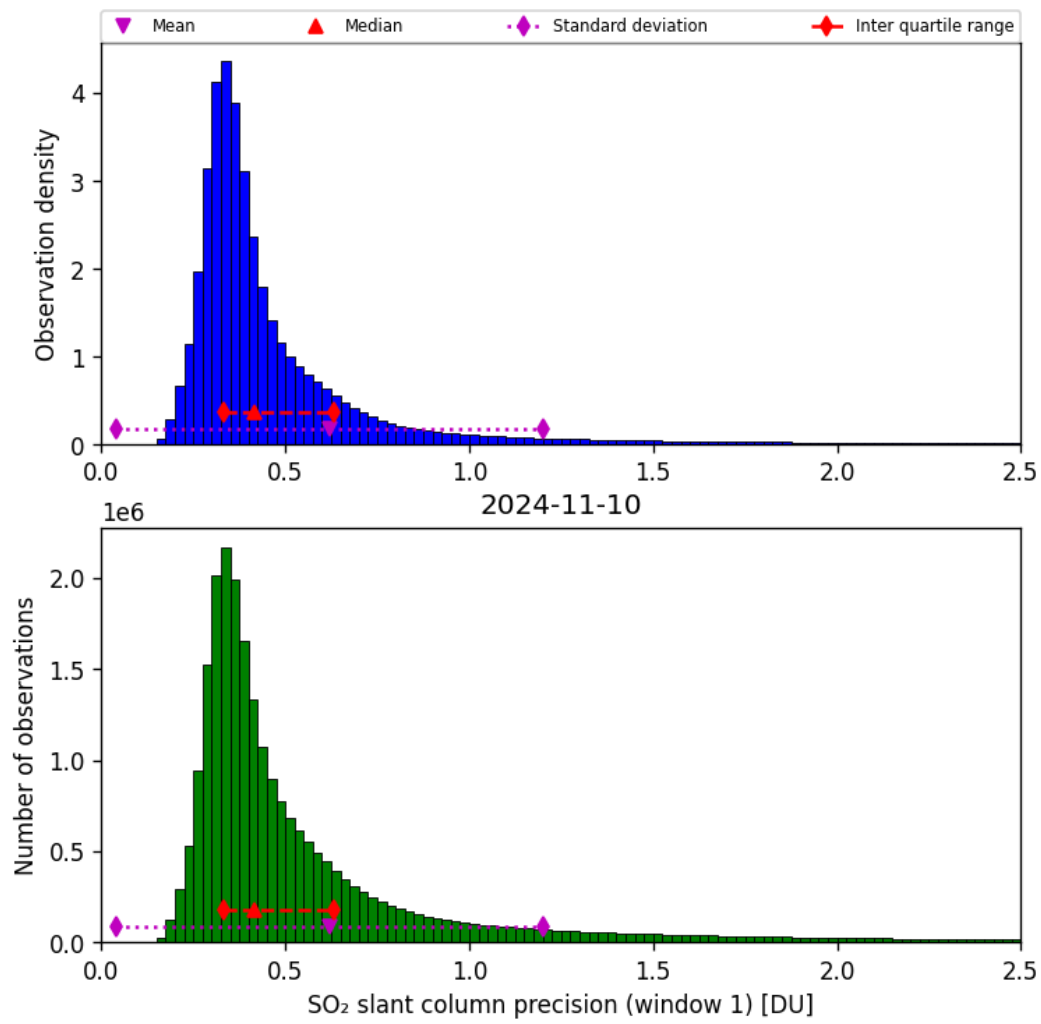
Figure 57: Histogram of “SO 2 slant column precision (window 1)” for 2024-11-09 to 2024-11-11
