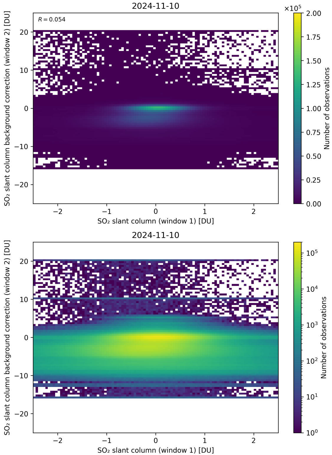
Figure 213: Scatter density plot of “SO 2 slant column (window 1)” against “SO 2 slant column background correction (window 2)” for 2024-11-09 to 2024-11-11.
