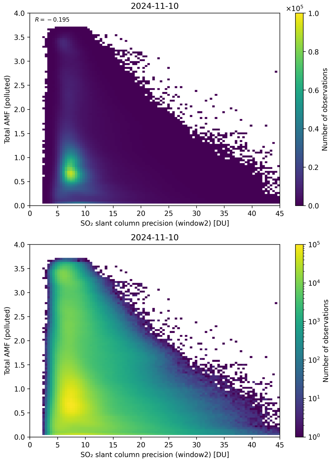
Figure 251: Scatter density plot of “SO 2 slant column precision (window2)” against “Total AMF (polluted)” for 2024-11-09 to 2024-11-11.
