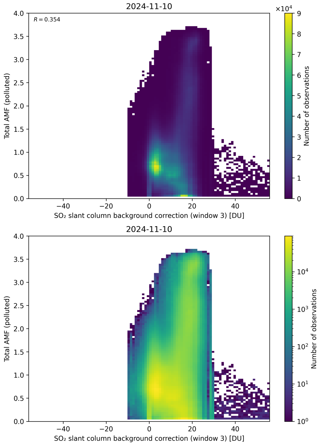
Figure 125: Scatter density plot of “SO 2 slant column background correction (window 3)” against “Total AMF (polluted)” for 2024-11-09 to 2024-11-11.
