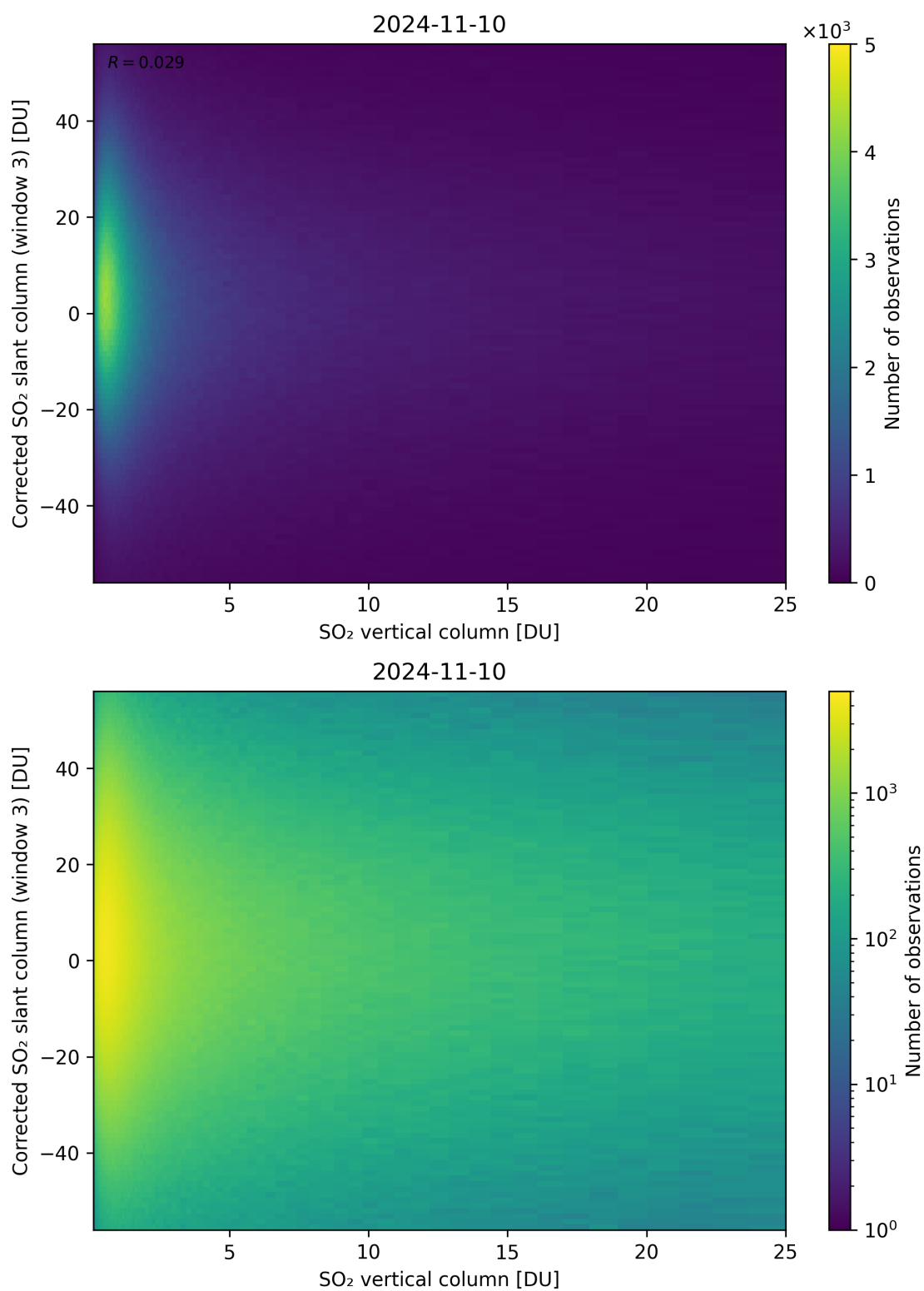
Figure 299: Scatter density plot of “SO 2 vertical column” against “Corrected SO 2 slant column (window 3)” for 2024-11-09 to 2024-11-11.
