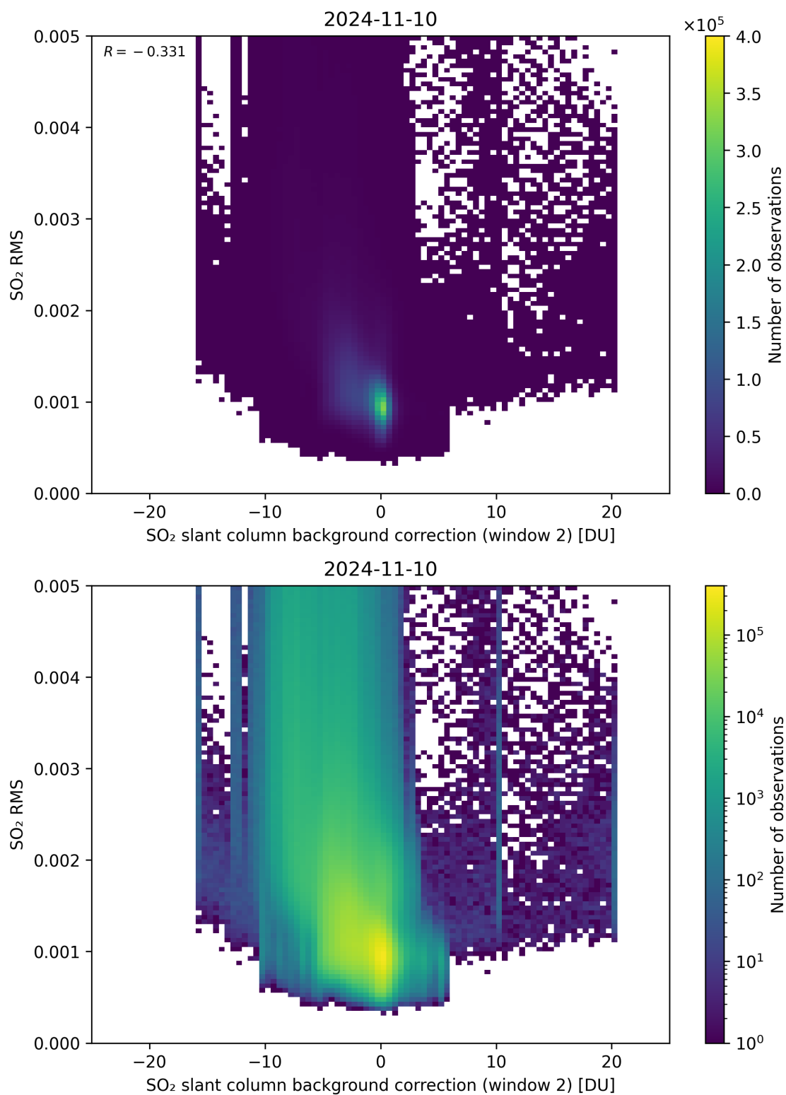
Figure 114: Scatter density plot of “SO 2 slant column background correction (window 2)” against “SO 2 RMS” for 2024-11-09 to 2024-11-11.
