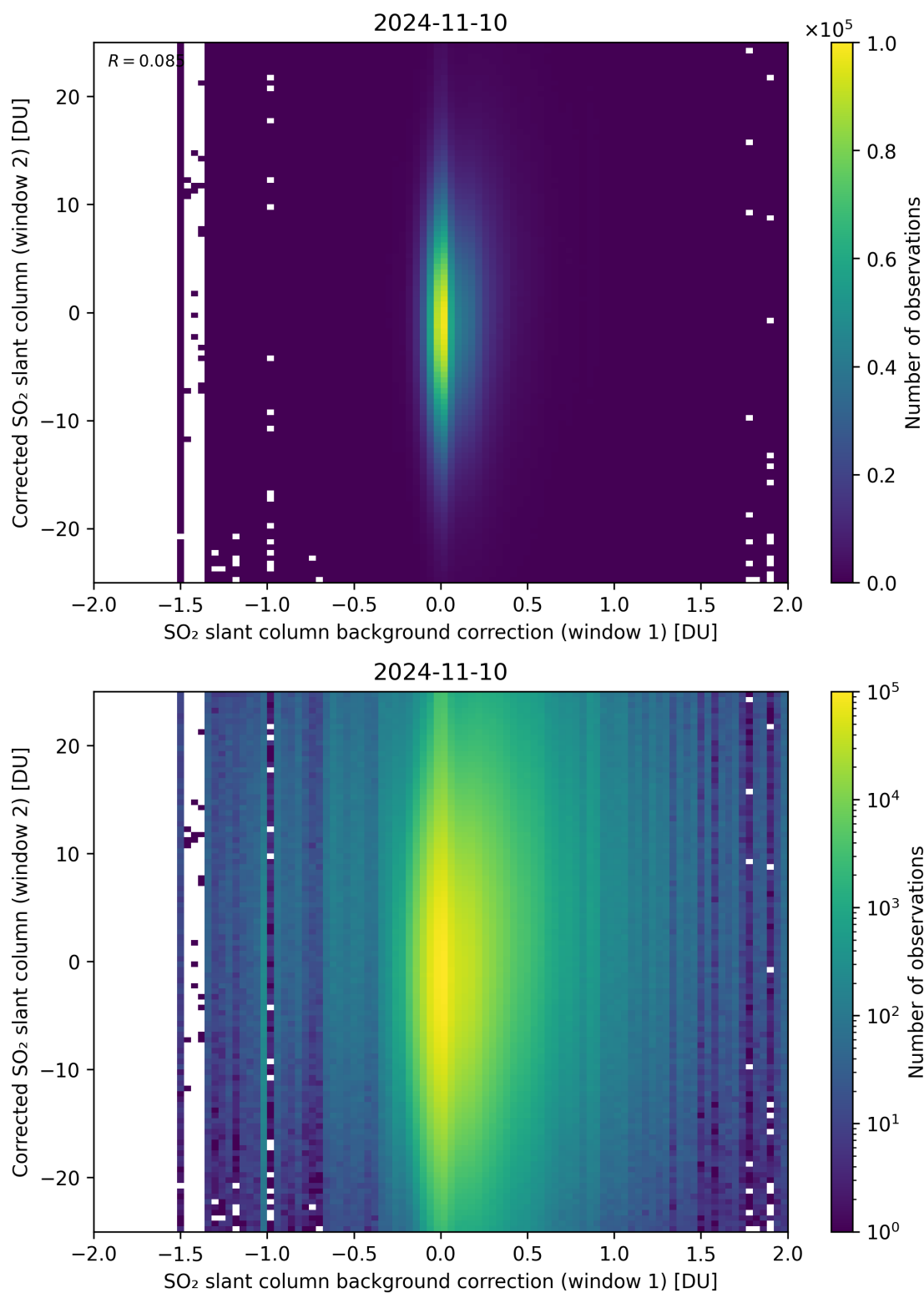
Figure 104: Scatter density plot of “SO 2 slant column background correction (window 1)” against “Corrected SO 2 slant column (window 2)” for 2024-11-09 to 2024-11-11.
