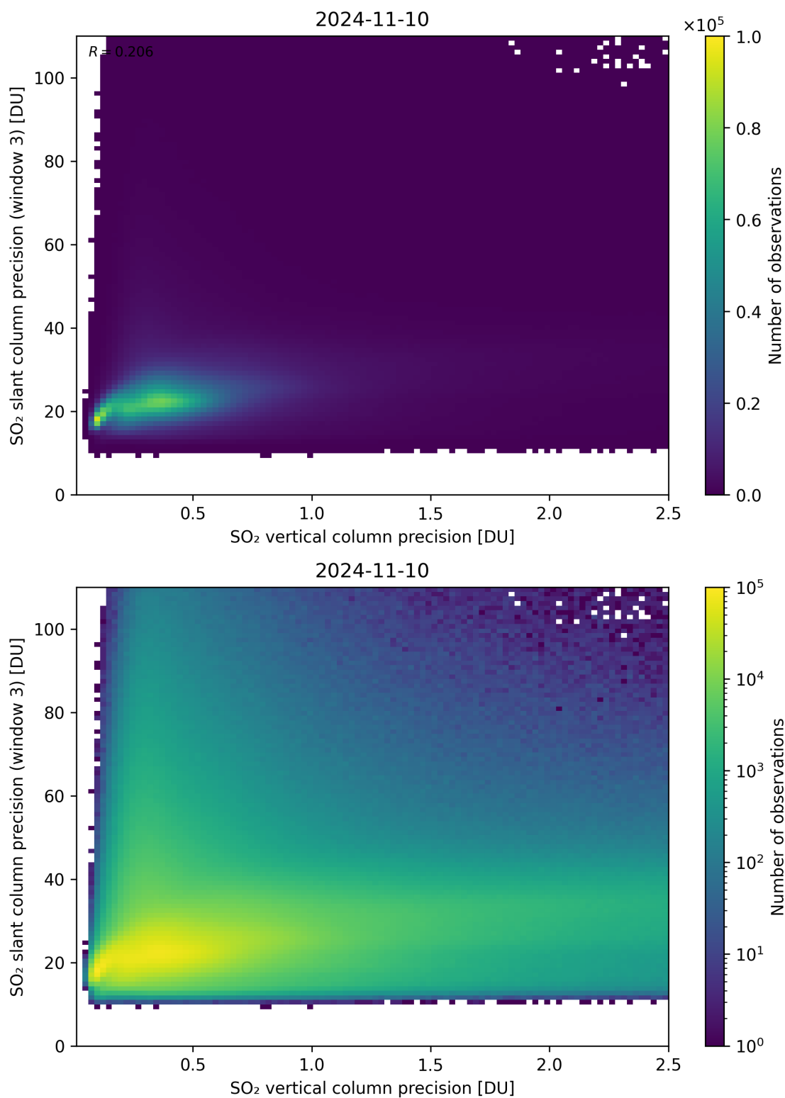
Figure 293: Scatter density plot of “SO 2 vertical column precision” against “SO 2 slant column precision (window 3)” for 2024-11-09 to 2024-11-11.
