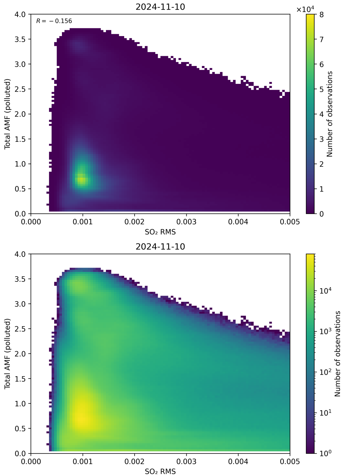
Figure 137: Scatter density plot of “SO 2 RMS” against “Total AMF (polluted)” for 2024-11-09 to 2024-11-11.
