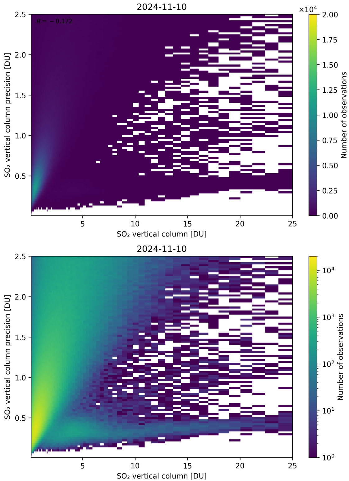
Figure 307: Scatter density plot of “SO 2 vertical column” against “SO 2 vertical column precision” for 2024-11-09 to 2024-11-11.
