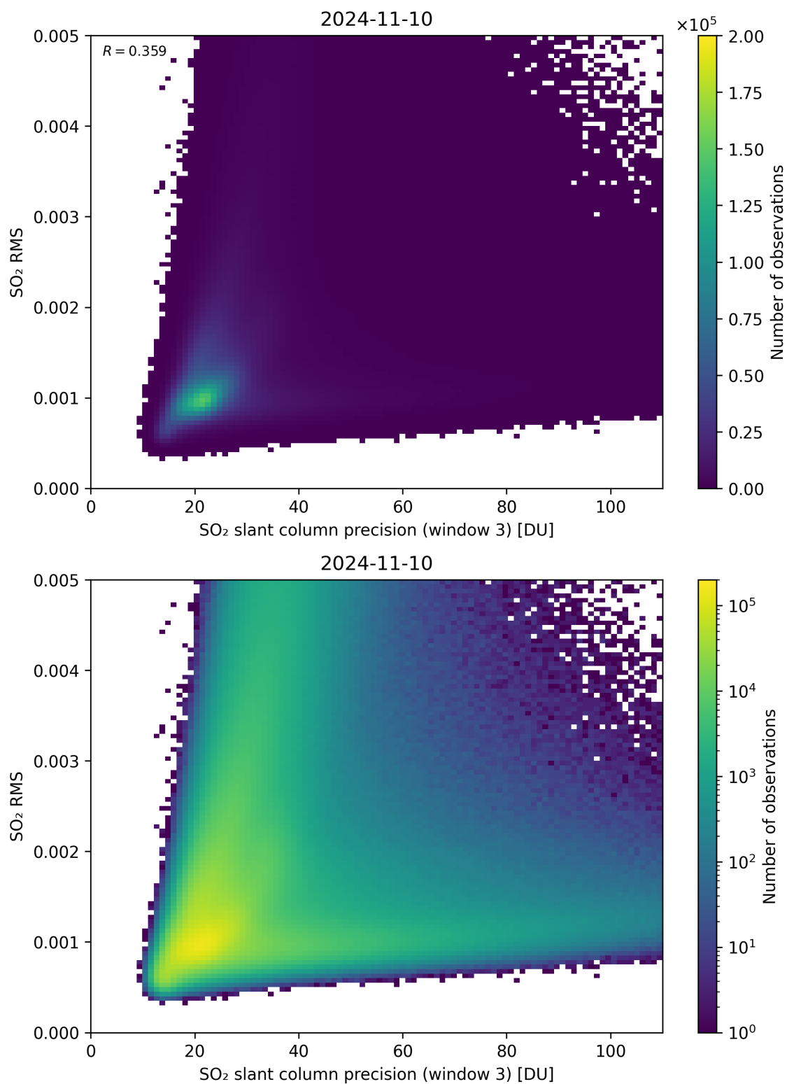
Figure 260: Scatter density plot of “SO 2 slant column precision (window 3)” against “SO 2 RMS” for 2024-11-09 to 2024-11-11.
