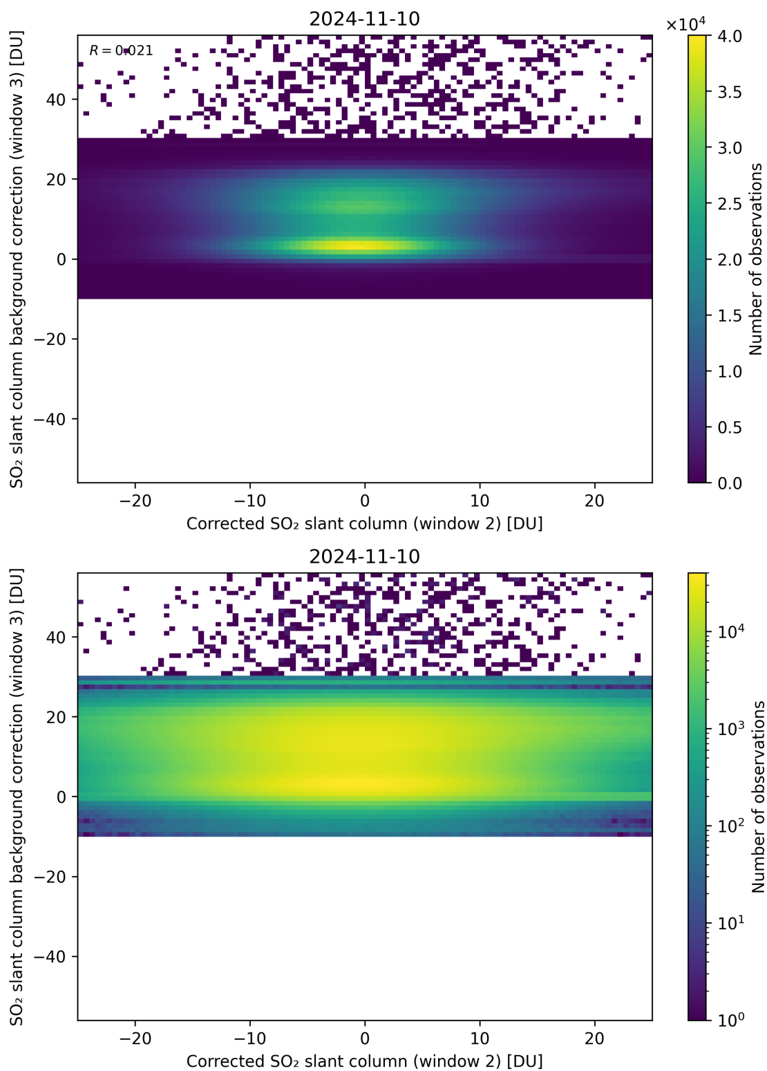
Figure 195: Scatter density plot of “Corrected SO 2 slant column (window 2)” against “SO 2 slant column background correction (window 3)” for 2024-11-09 to 2024-11-11.
