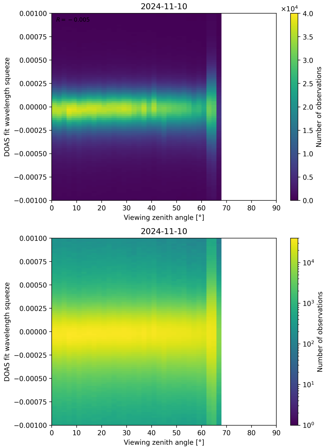
Figure 312: Scatter density plot of “Viewing zenith angle” against “DOAS fit wavelength squeeze” for 2024-11-09 to 2024-11-11.
