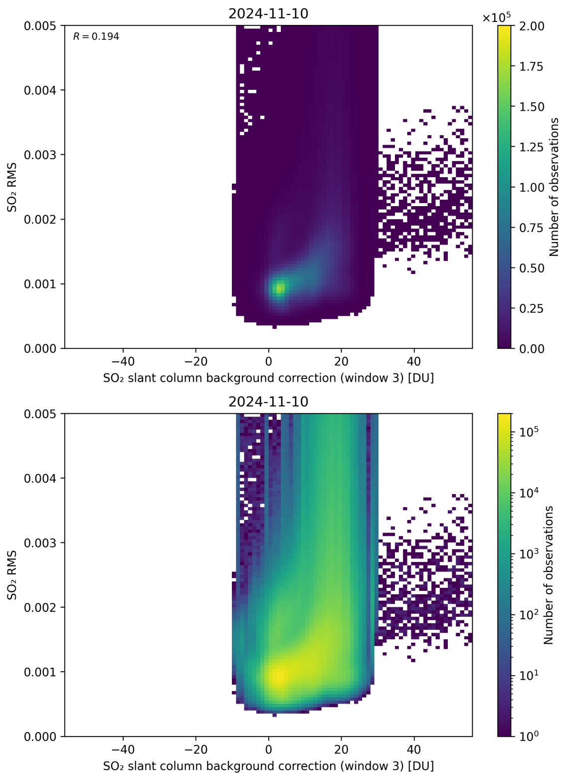
Figure 123: Scatter density plot of “SO 2 slant column background correction (window 3)” against “SO 2 RMS” for 2024-11-09 to 2024-11-11.
