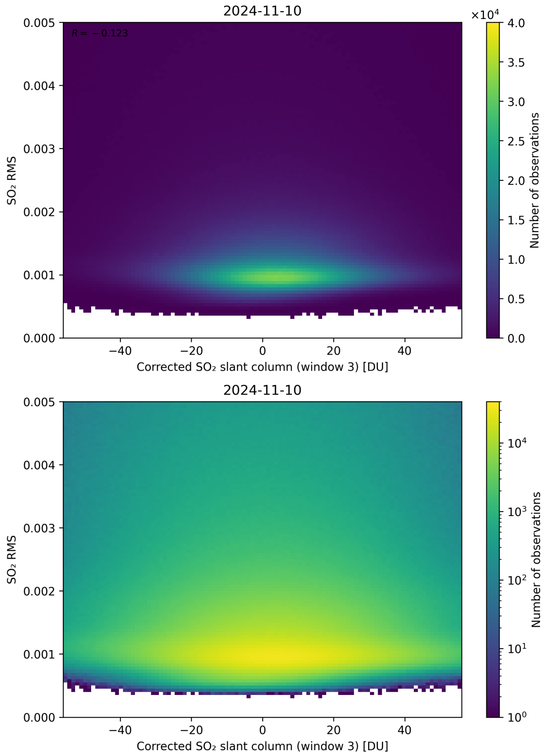
Figure 208: Scatter density plot of “Corrected SO 2 slant column (window 3)” against “SO 2 RMS” for 2024-11-09 to 2024-11-11.
