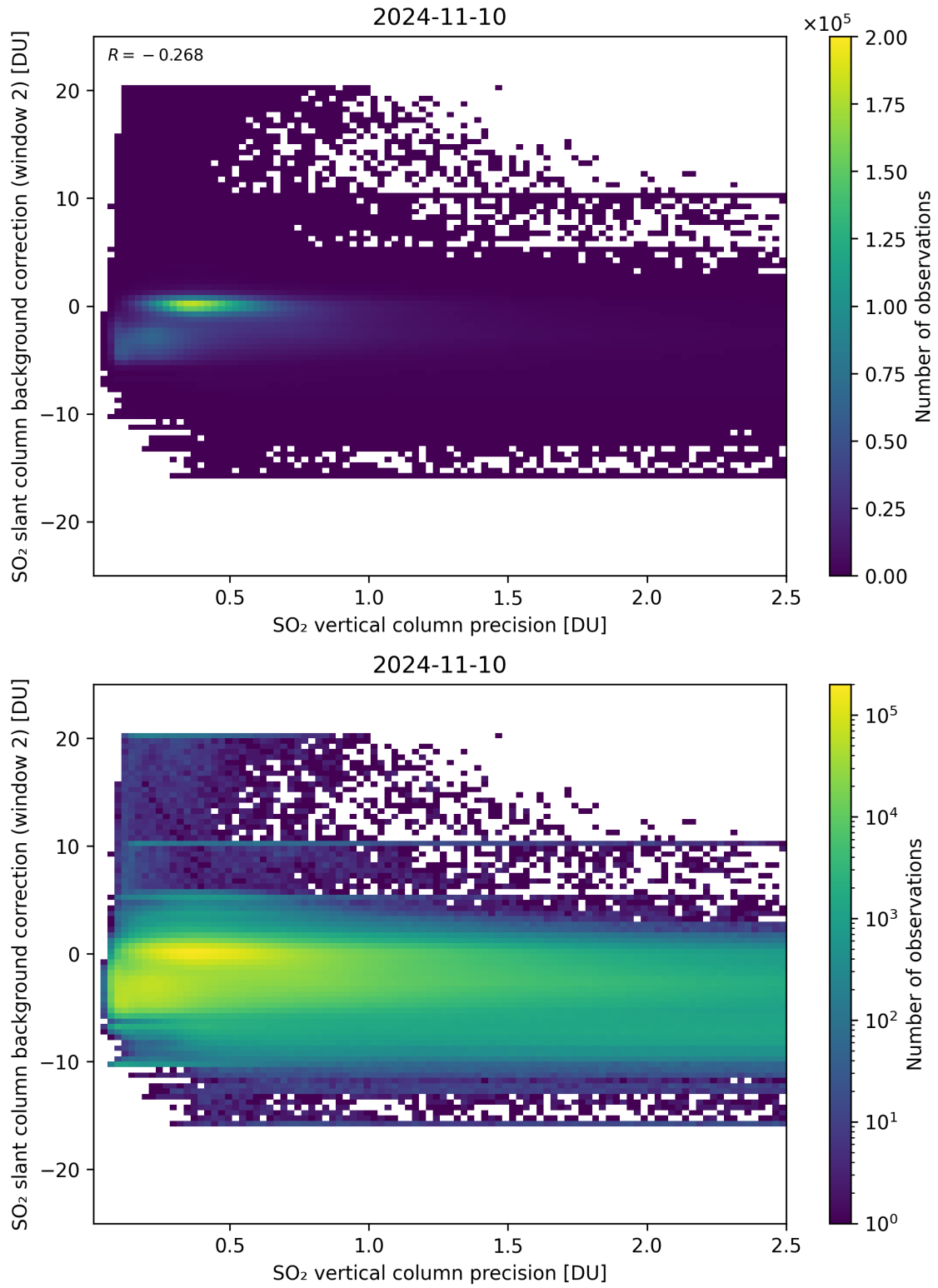
Figure 280: Scatter density plot of “SO 2 vertical column precision” against “SO 2 slant column background correction (window 2)” for 2024-11-09 to 2024-11-11.
