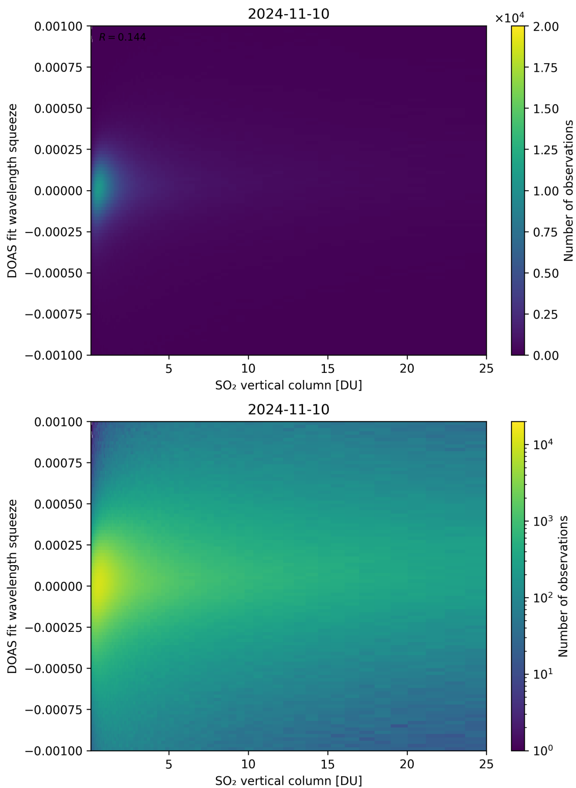
Figure 277: Scatter density plot of “SO 2 vertical column” against “DOAS fit wavelength squeeze” for 2024-11-09 to 2024-11-11.
