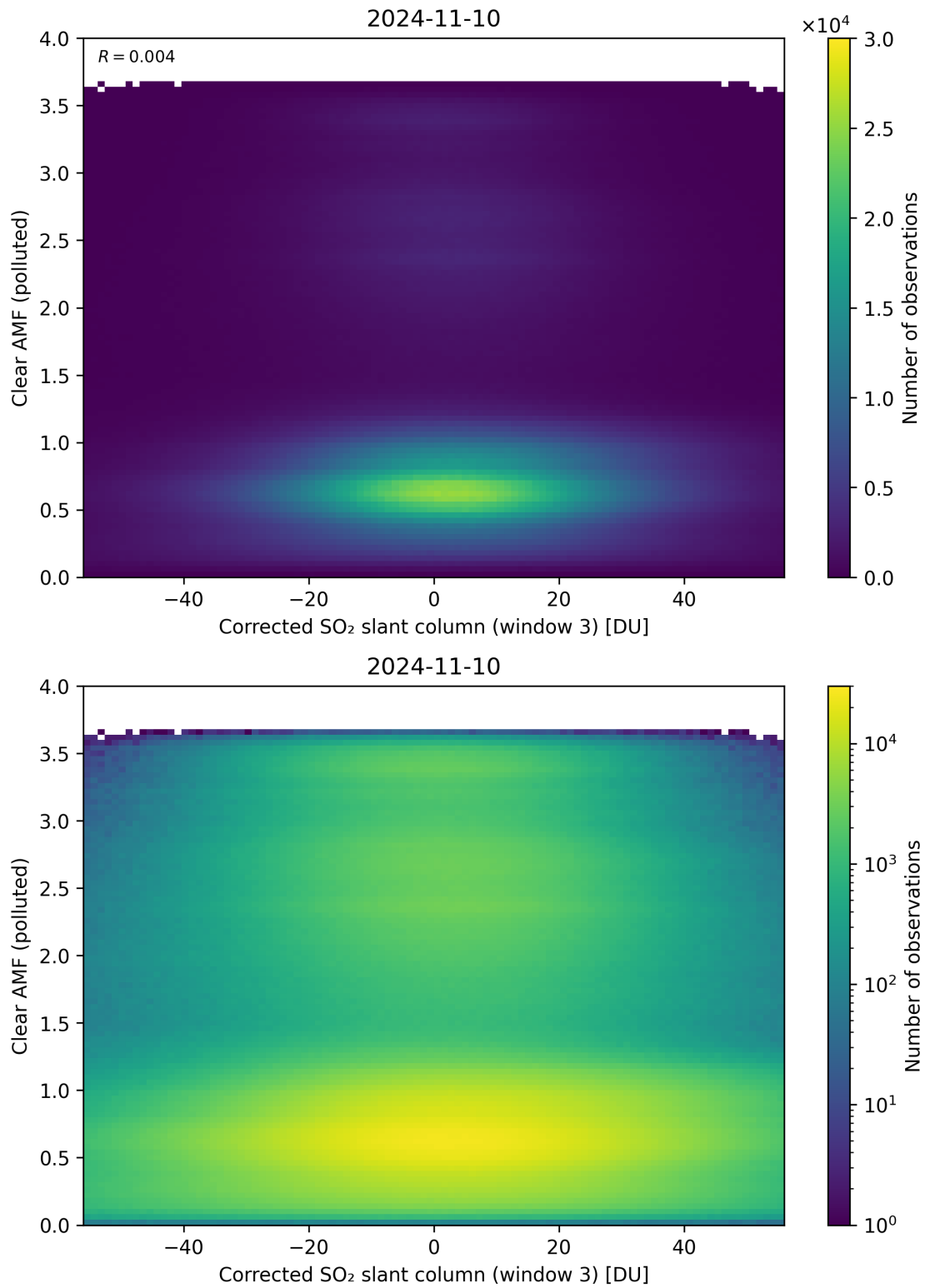
Figure 209: Scatter density plot of “Corrected SO 2 slant column (window 3)” against “Clear AMF (polluted)” for 2024-11-09 to 2024-11-11.
