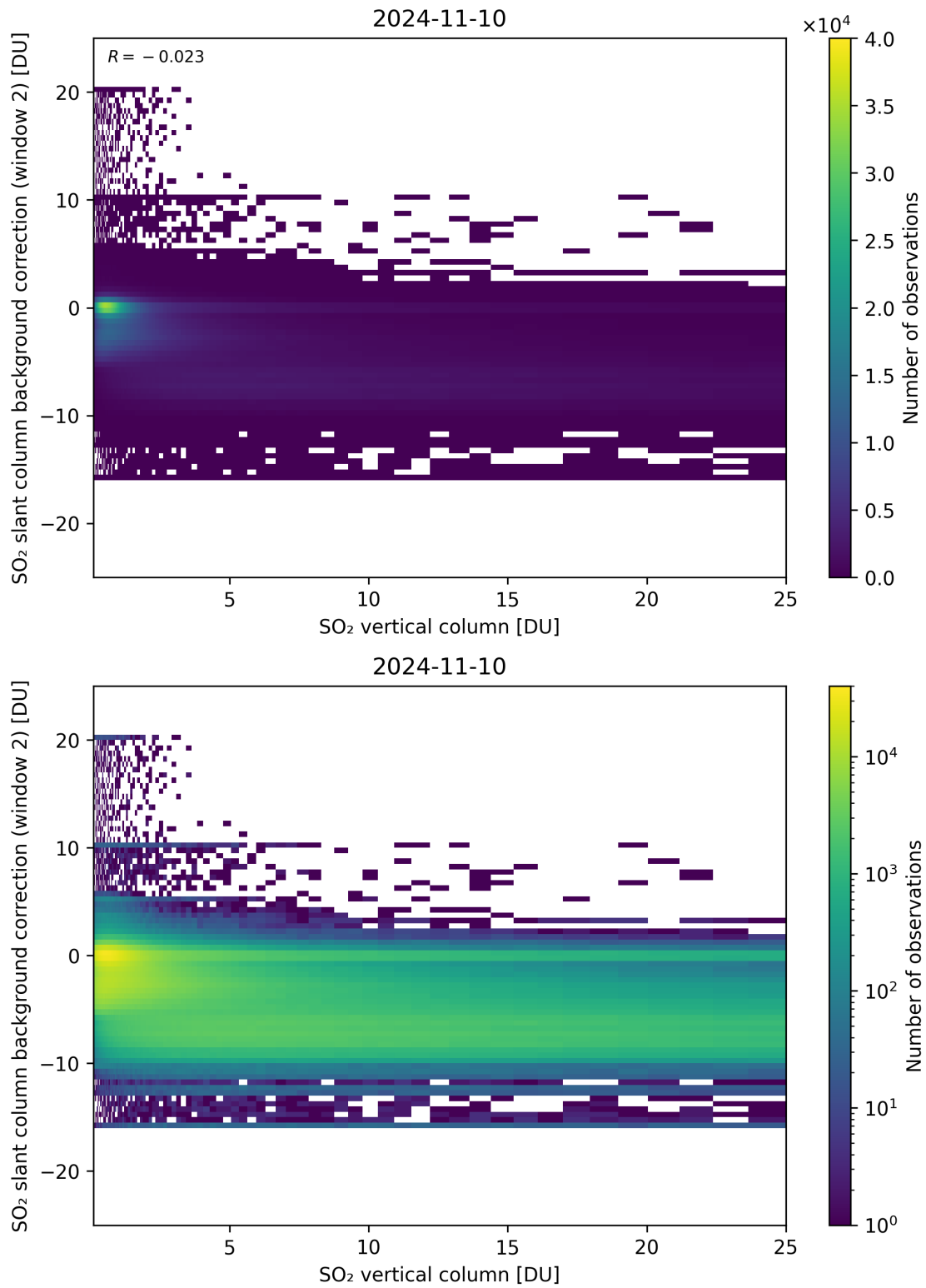
Figure 274: Scatter density plot of “SO 2 vertical column” against “SO 2 slant column background correction (window 2)” for 2024-11-09 to 2024-11-11.
