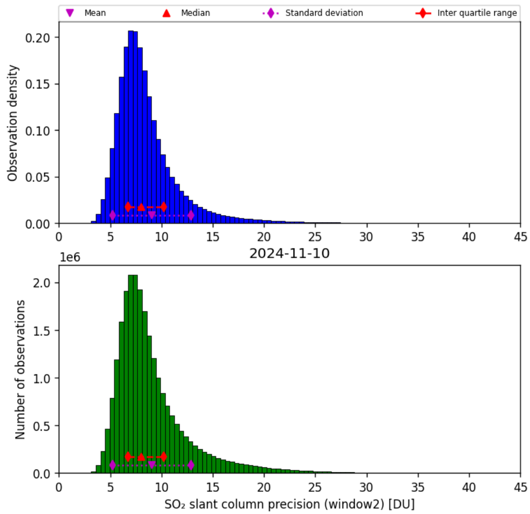
Figure 61: Histogram of “SO 2 slant column precision (window2)” for 2024-11-09 to 2024-11-11
