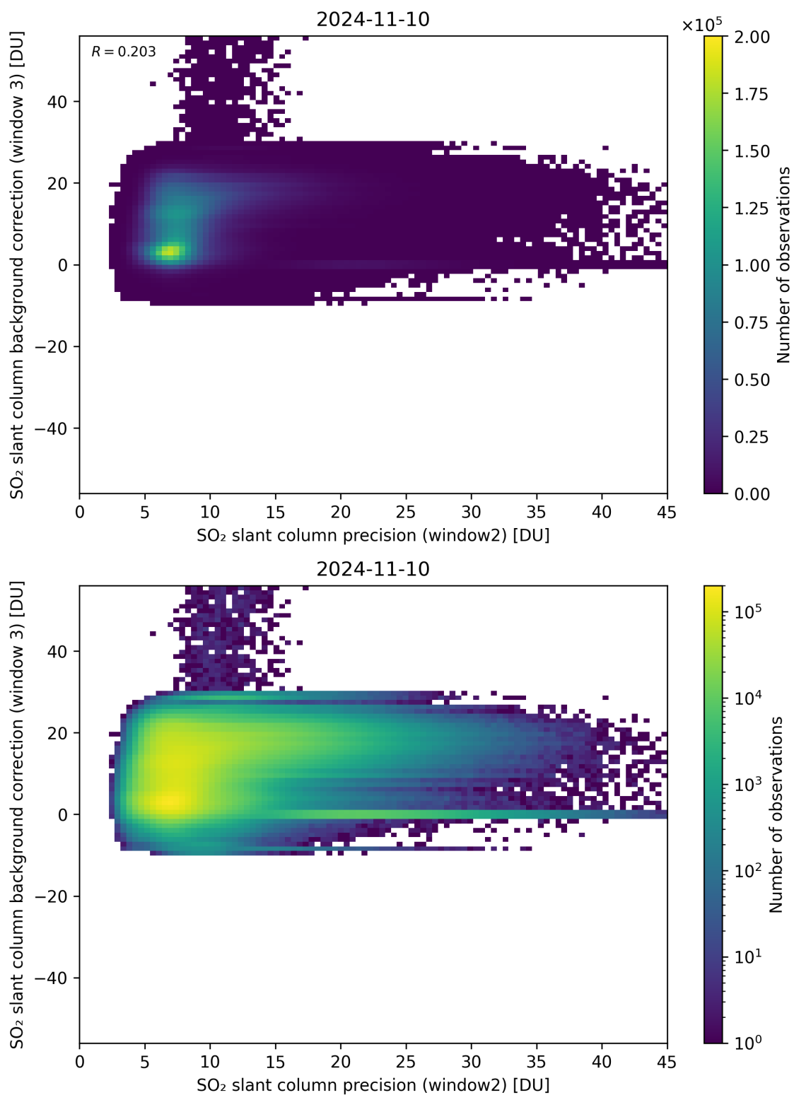
Figure 242: Scatter density plot of “SO 2 slant column precision (window2)” against “SO 2 slant column background correction (window 3)” for 2024-11-09 to 2024-11-11.
