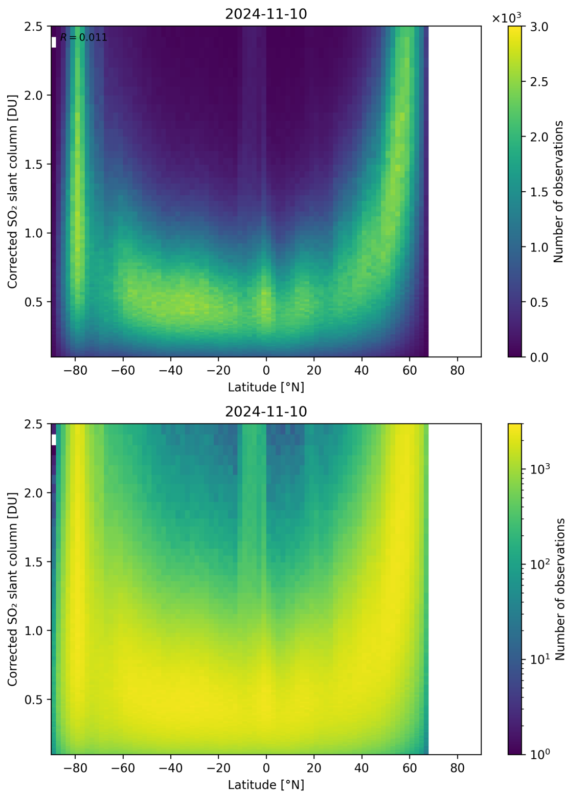
Figure 146: Scatter density plot of “Latitude” against “Corrected SO 2 slant column” for 2024-11-09 to 2024-11-11.
