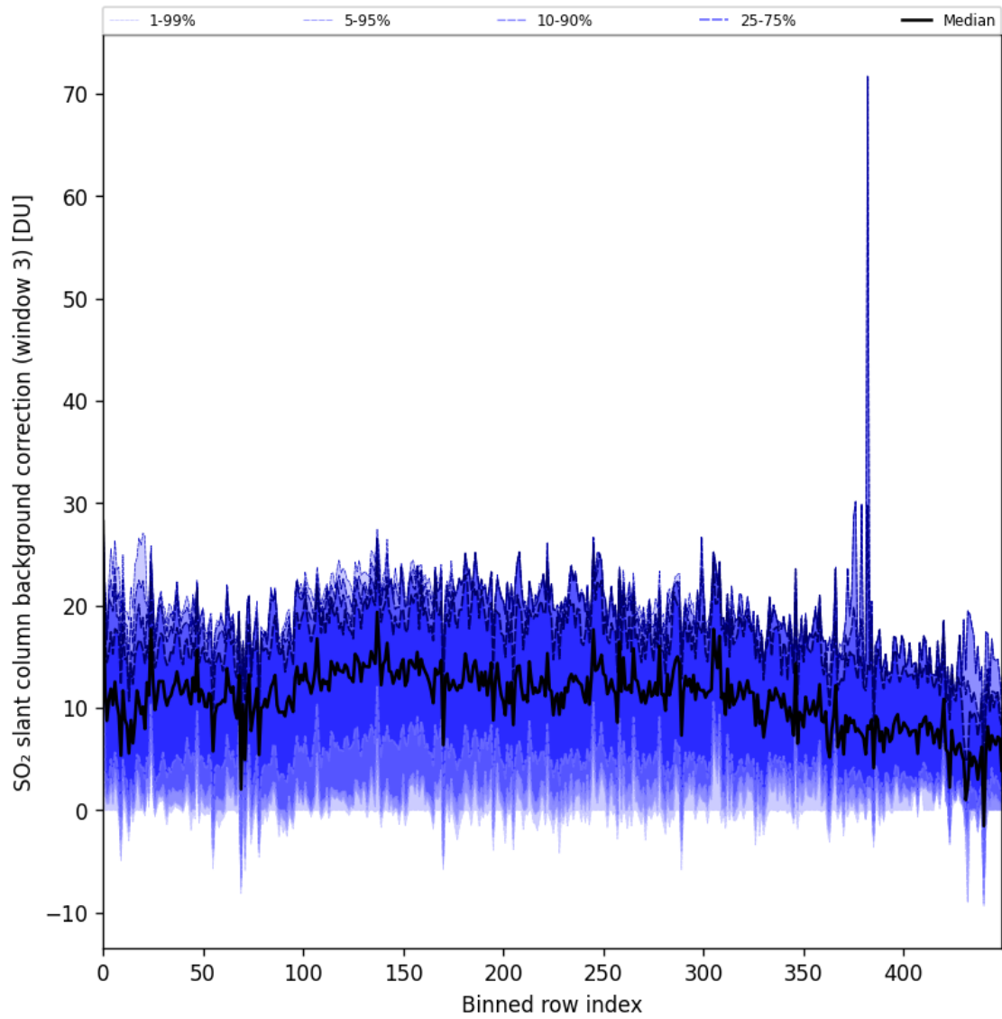
Figure 90: Along track statistics of “SO 2 slant column background correction (window 3)” for 2024-11-09 to 2024-11-11
