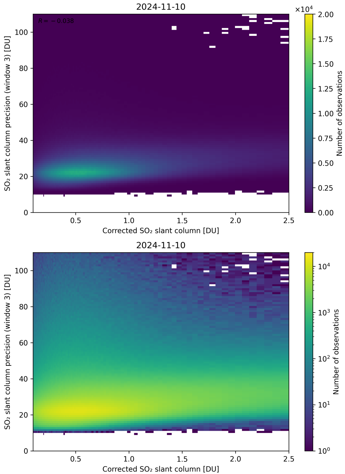
Figure 191: Scatter density plot of “Corrected SO 2 slant column” against “SO 2 slant column precision (window 3)” for 2024-11-09 to 2024-11-11.
