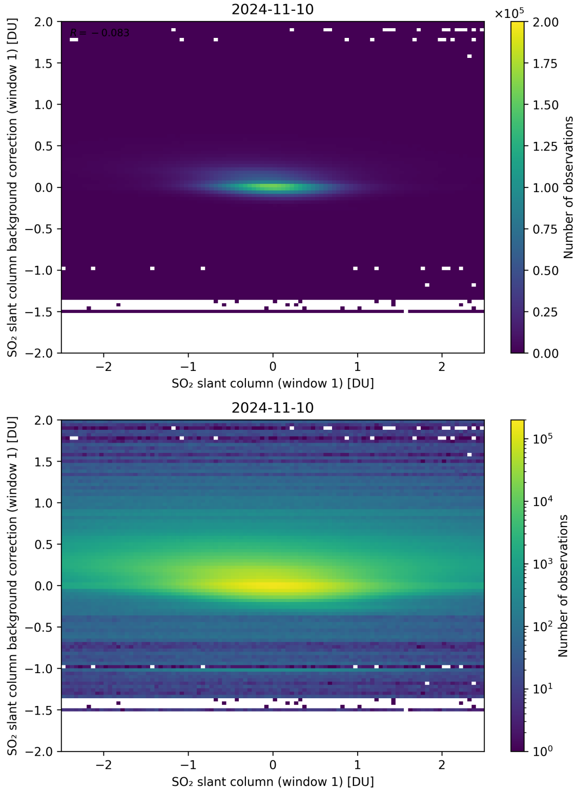
Figure 212: Scatter density plot of “SO 2 slant column (window 1)” against “SO 2 slant column background correction (window 1)” for 2024-11-09 to 2024-11-11.
