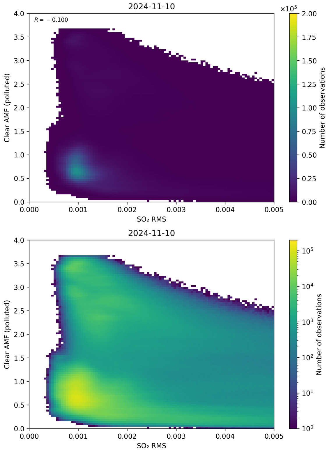
Figure 136: Scatter density plot of “SO 2 RMS” against “Clear AMF (polluted)” for 2024-11-09 to 2024-11-11.
