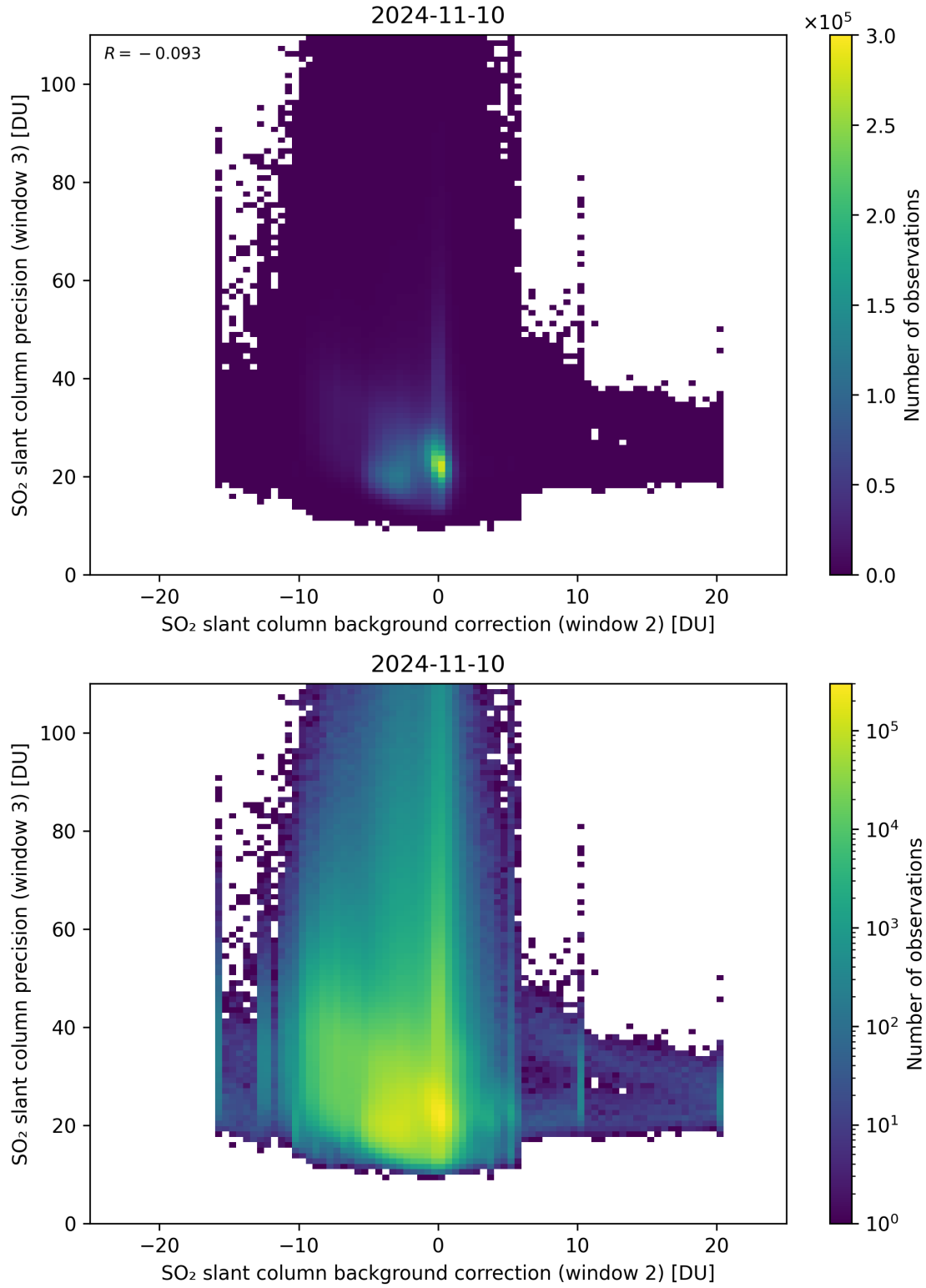
Figure 118: Scatter density plot of “SO 2 slant column background correction (window 2)” against “SO 2 slant column precision (window 3)” for 2024-11-09 to 2024-11-11.
