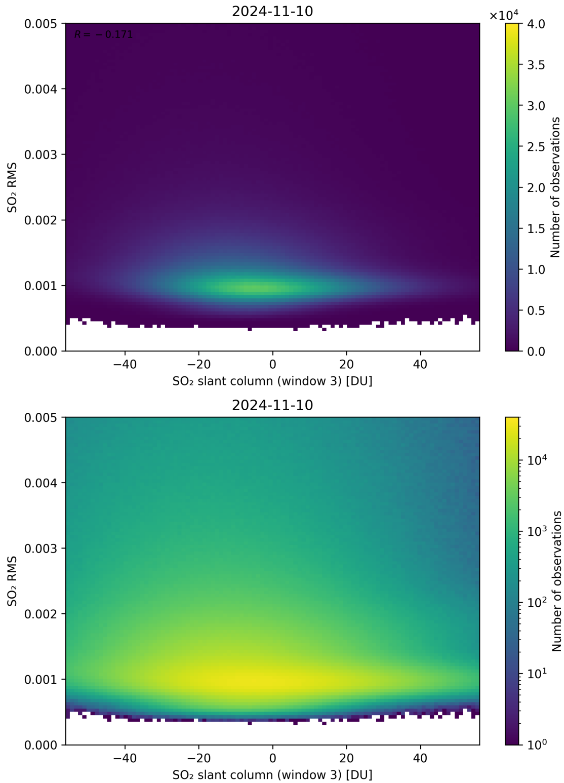
Figure 256: Scatter density plot of “SO 2 slant column (window 3)” against “SO 2 RMS” for 2024-11-09 to 2024-11-11.
