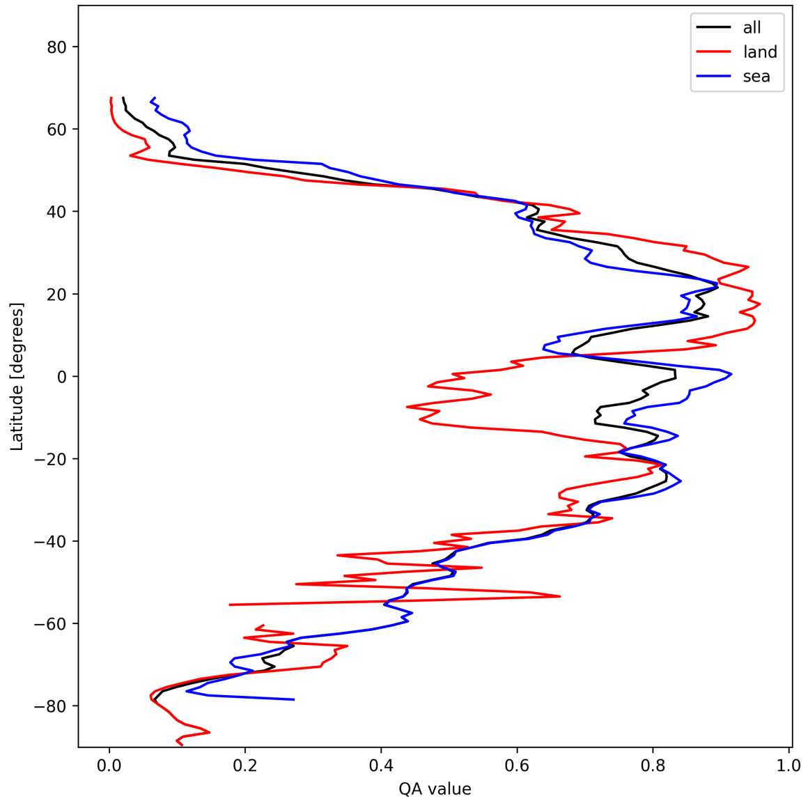
Figure 29: Zonal average of “QA value” for 2024-11-09 to 2024-11-11.
