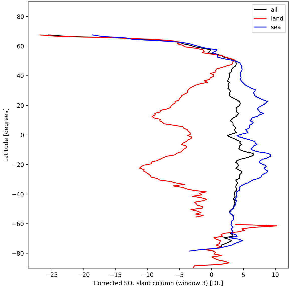
Figure 43: Zonal average of “Corrected SO 2 slant column (window 3)” for 2024-11-09 to 2024-11-11.
