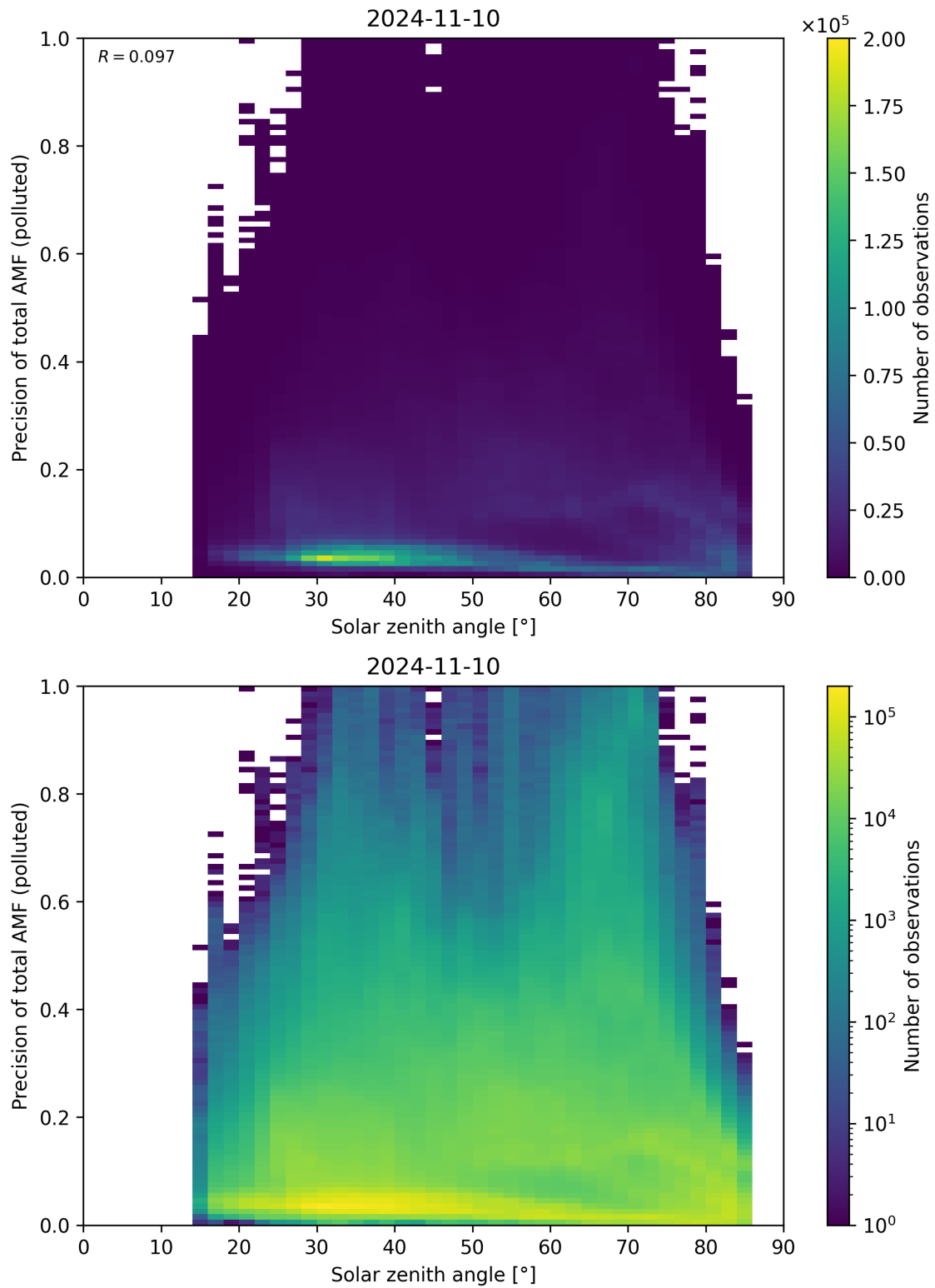
Figure 175: Scatter density plot of “Solar zenith angle” against “Precision of total AMF (polluted)” for 2024-11-09 to 2024-11-11.
