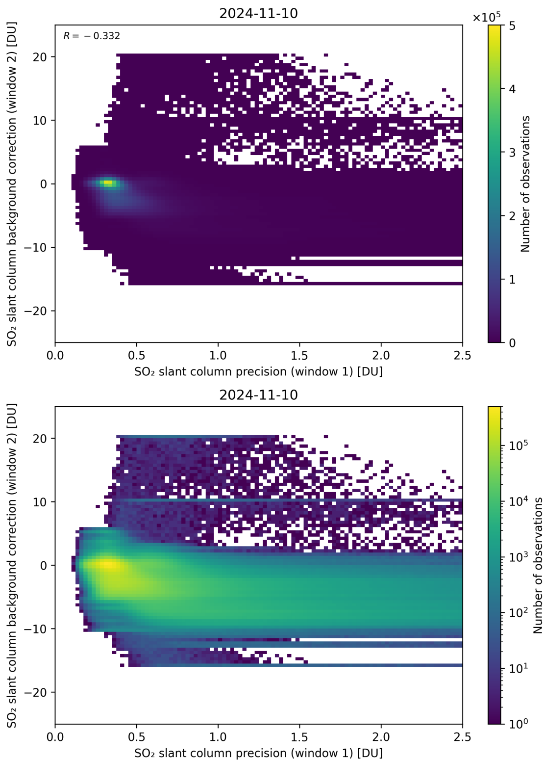
Figure 219: Scatter density plot of “SO 2 slant column precision (window 1)” against “SO 2 slant column background correction (window 2)” for 2024-11-09 to 2024-11-11.
