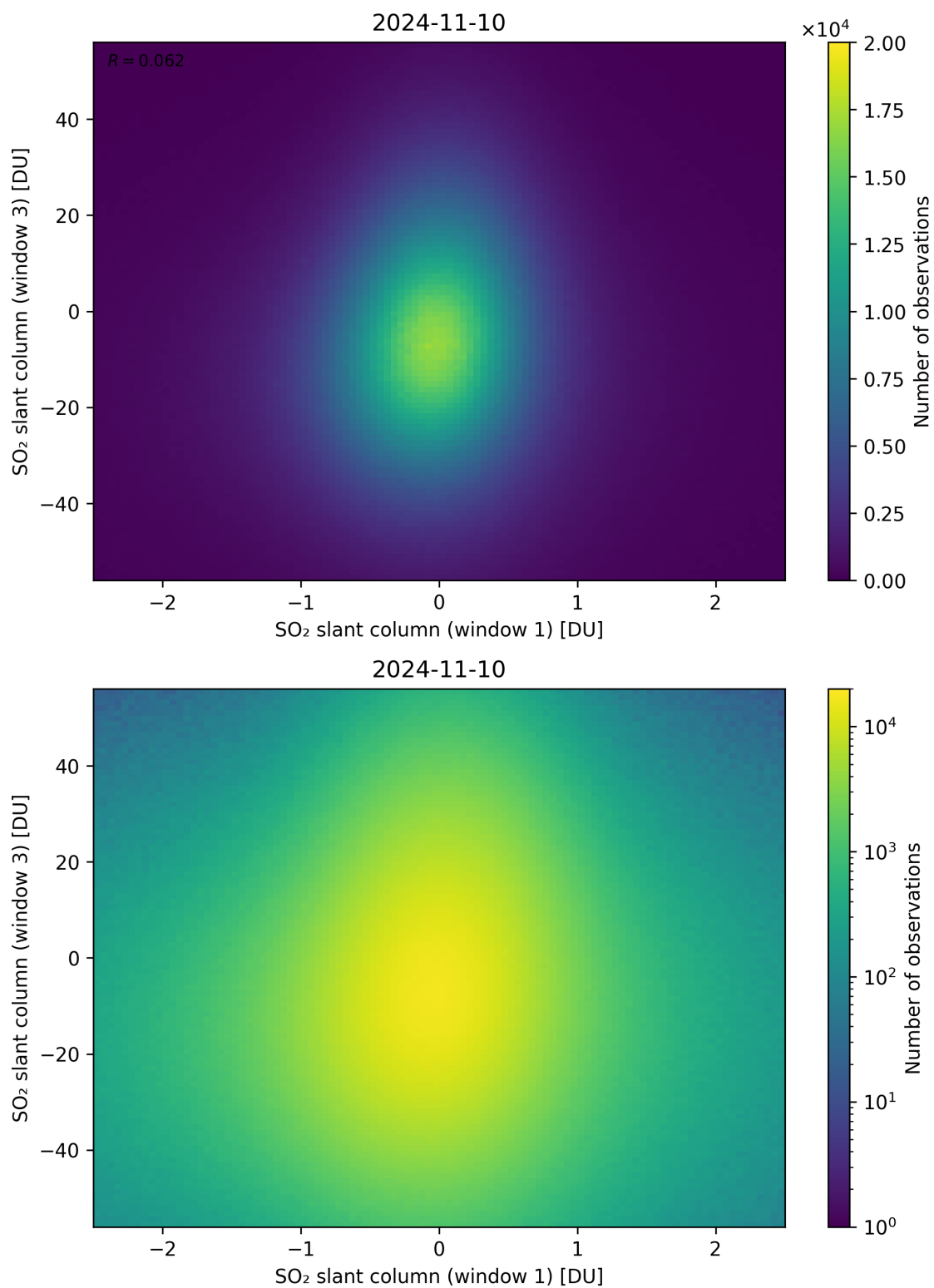
Figure 237: Scatter density plot of “SO 2 slant column (window 1)” against “SO 2 slant column (window 3)” for 2024-11-09 to 2024-11-11.
