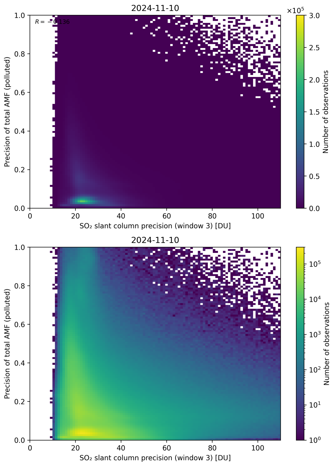
Figure 264: Scatter density plot of “SO 2 slant column precision (window 3)” against “Precision of total AMF (polluted)” for 2024-11-09 to 2024-11-11.
