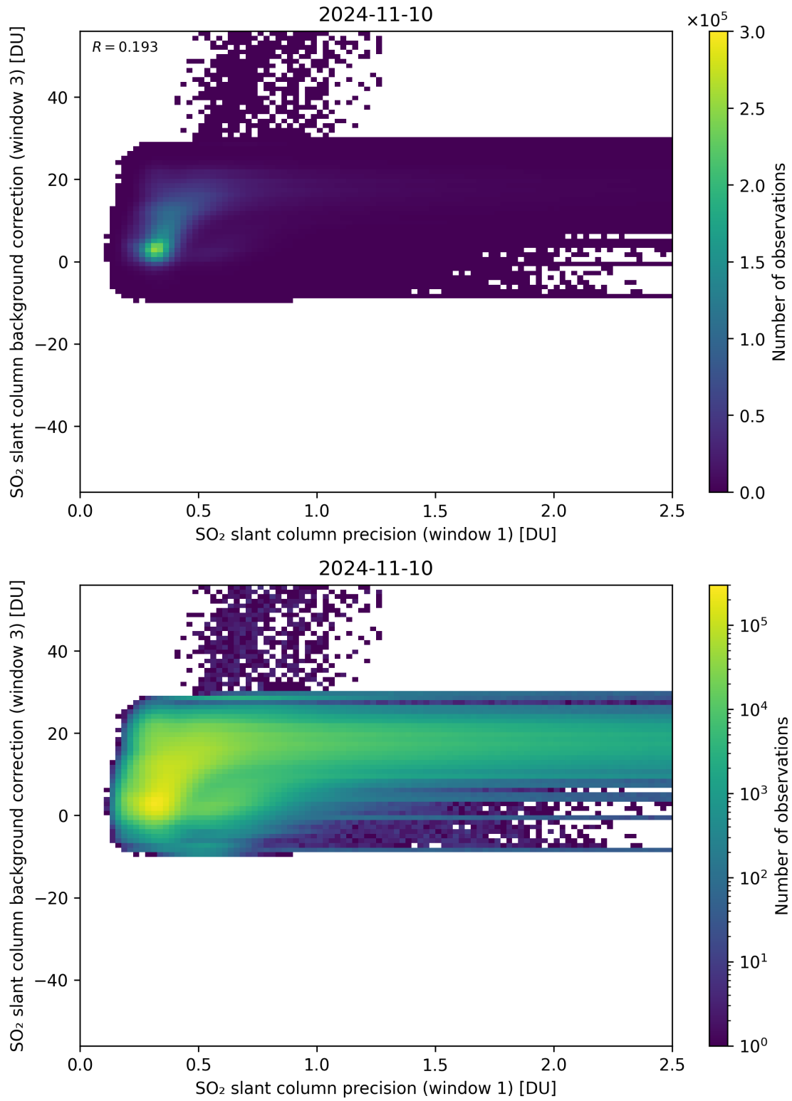
Figure 220: Scatter density plot of “SO 2 slant column precision (window 1)” against “SO 2 slant column background correction (window 3)” for 2024-11-09 to 2024-11-11.
