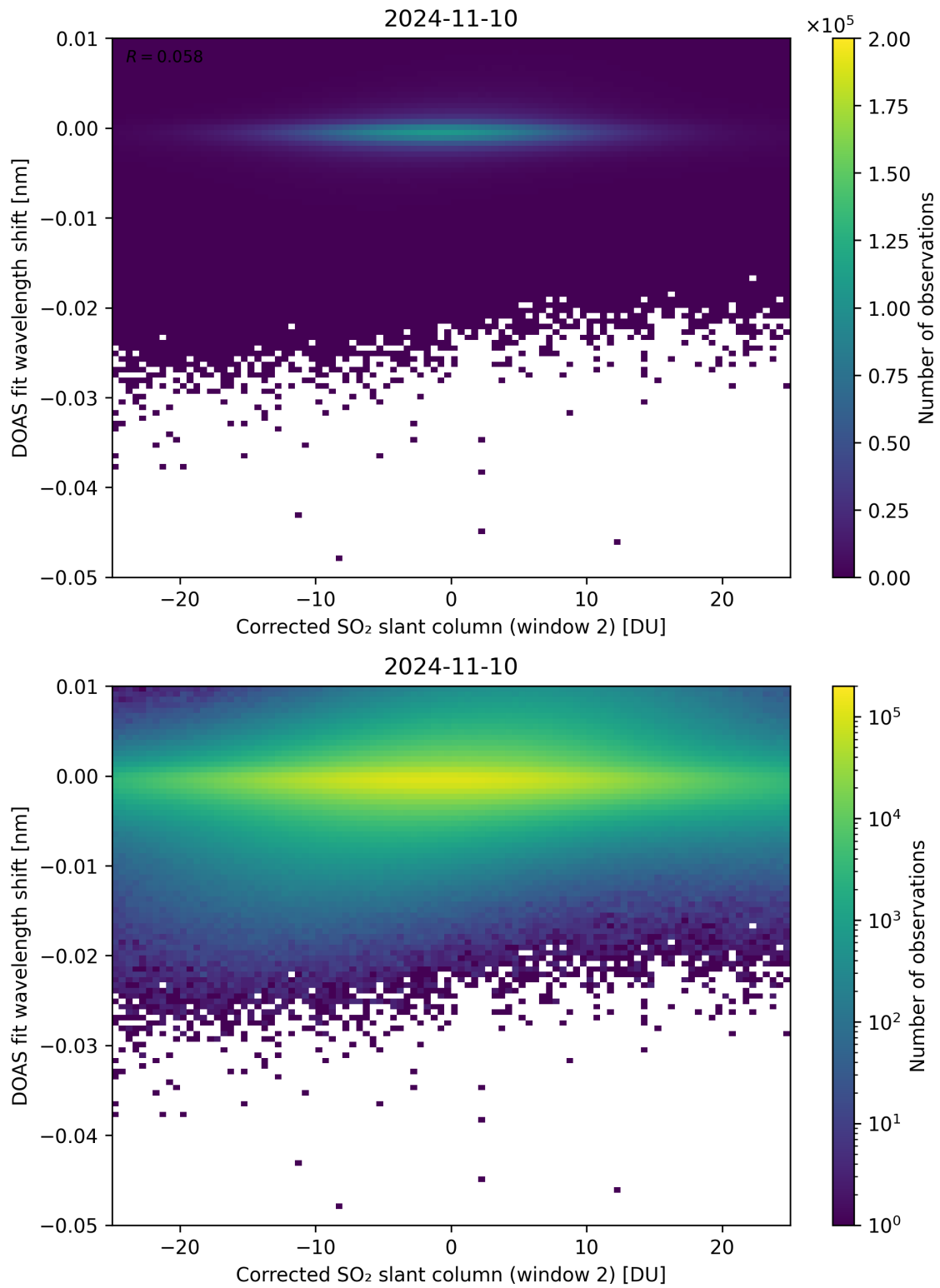
Figure 196: Scatter density plot of “Corrected SO 2 slant column (window 2)” against “DOAS fit wavelength shift” for 2024-11-09 to 2024-11-11.
