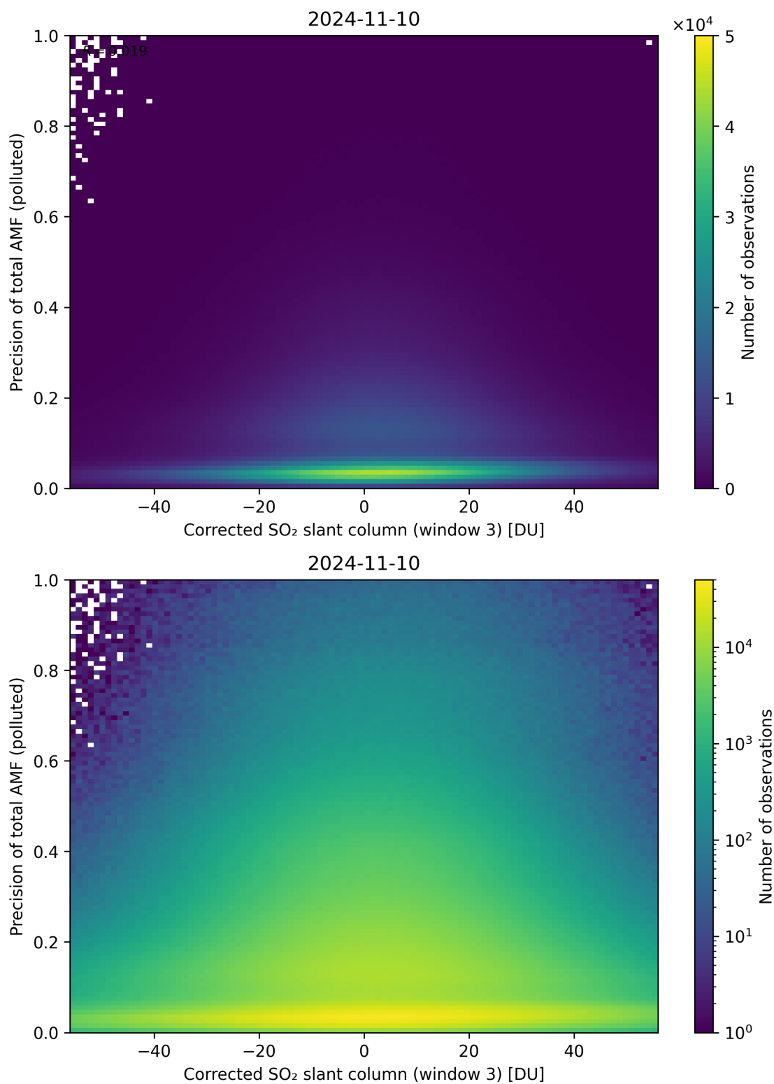
Figure 211: Scatter density plot of “Corrected SO 2 slant column (window 3)” against “Precision of total AMF (polluted)” for 2024-11-09 to 2024-11-11.
