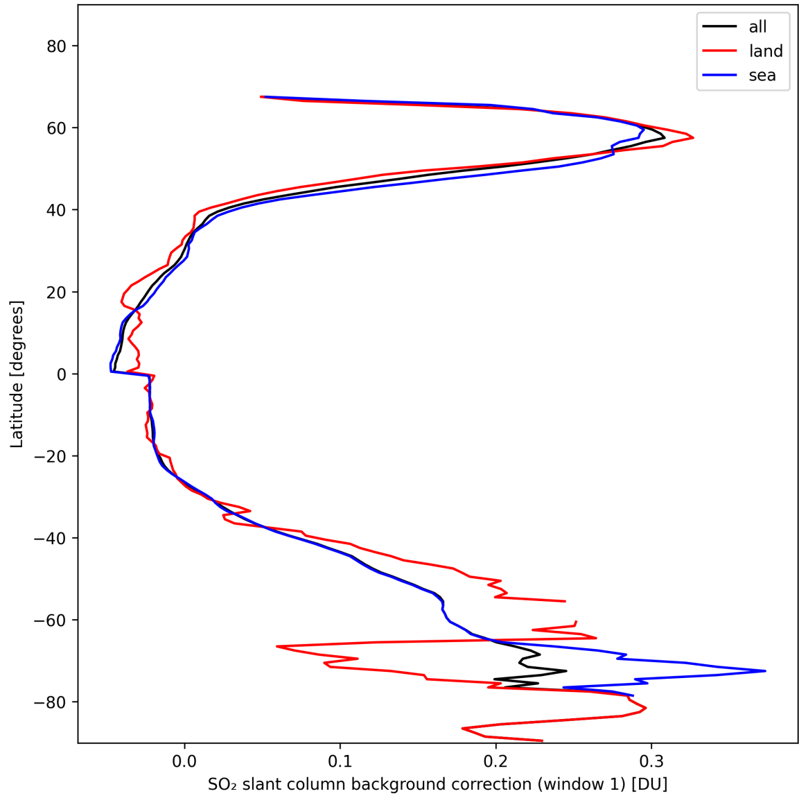
Figure 36: Zonal average of “SO 2 slant column background correction (window 1)” for 2024-11-09 to 2024-11-11.
