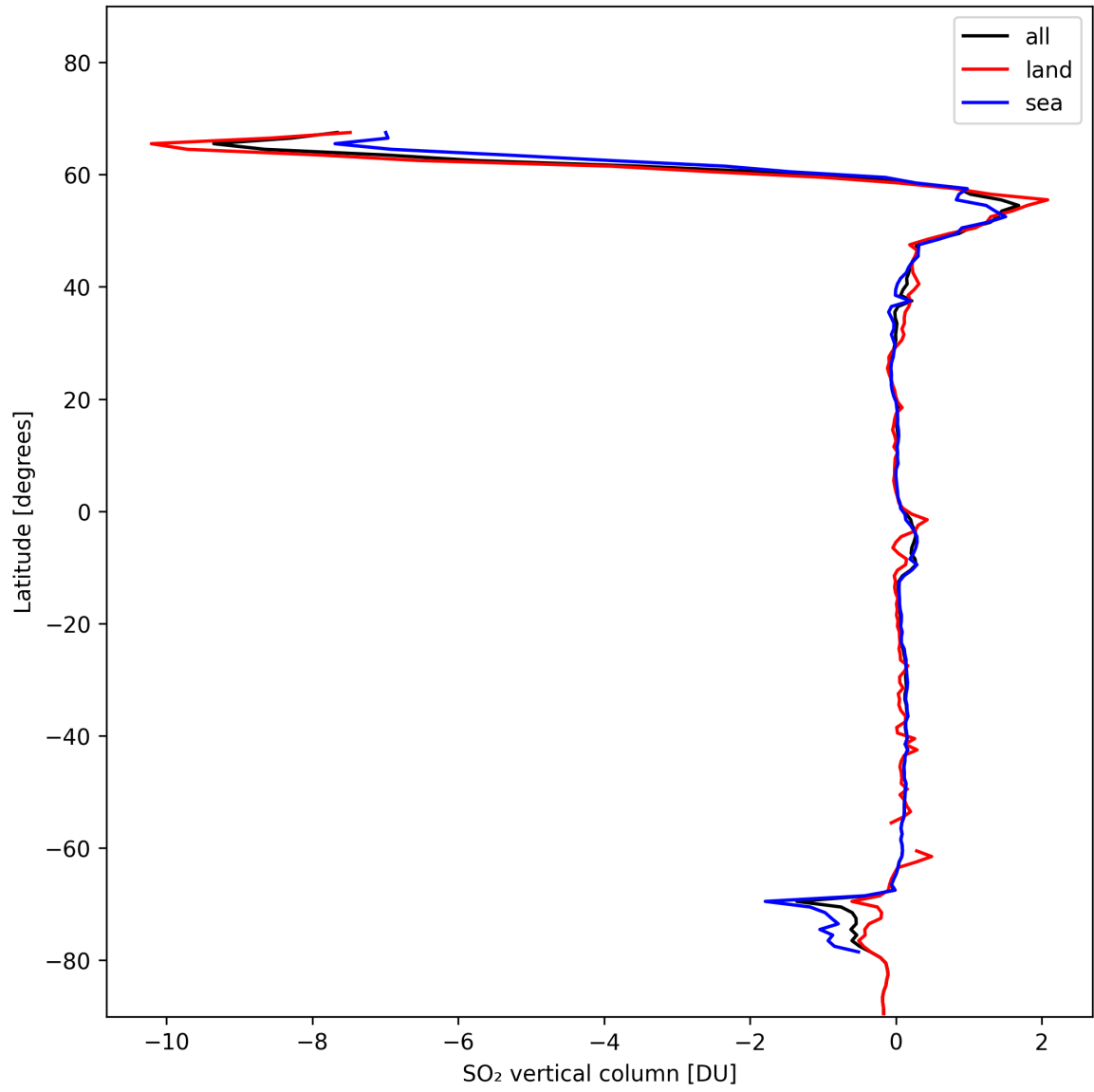
Figure 30: Zonal average of “SO 2 vertical column” for 2024-11-09 to 2024-11-11.
