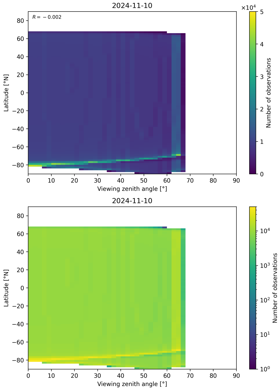
Figure 314: Scatter density plot of “Viewing zenith angle” against “Latitude” for 2024-11-09 to 2024-11-11.
