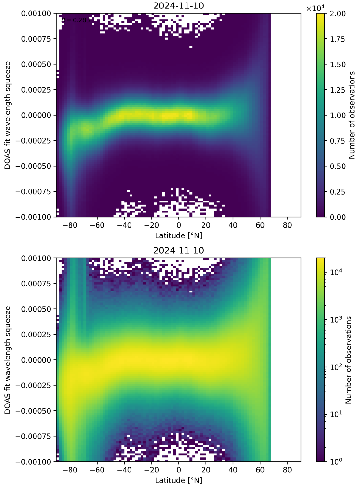
Figure 143: Scatter density plot of “Latitude” against “DOAS fit wavelength squeeze” for 2024-11-09 to 2024-11-11.
