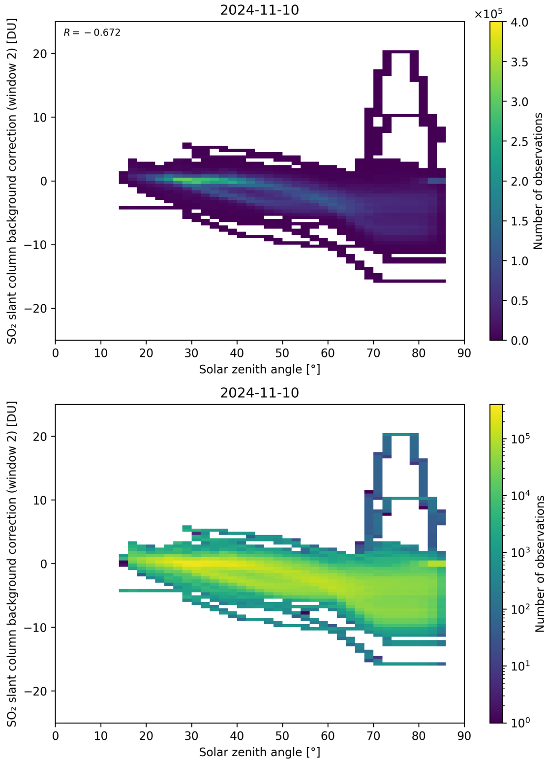
Figure 159: Scatter density plot of “Solar zenith angle” against “SO 2 slant column background correction (window 2)” for 2024-11-09 to 2024-11-11.
