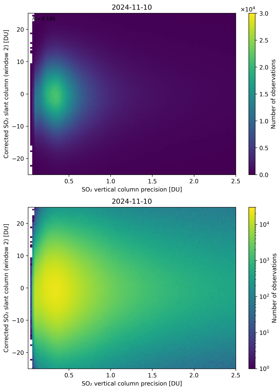
Figure 287: Scatter density plot of “SO 2 vertical column precision” against “Corrected SO 2 slant column (window 2)” for 2024-11-09 to 2024-11-11.
