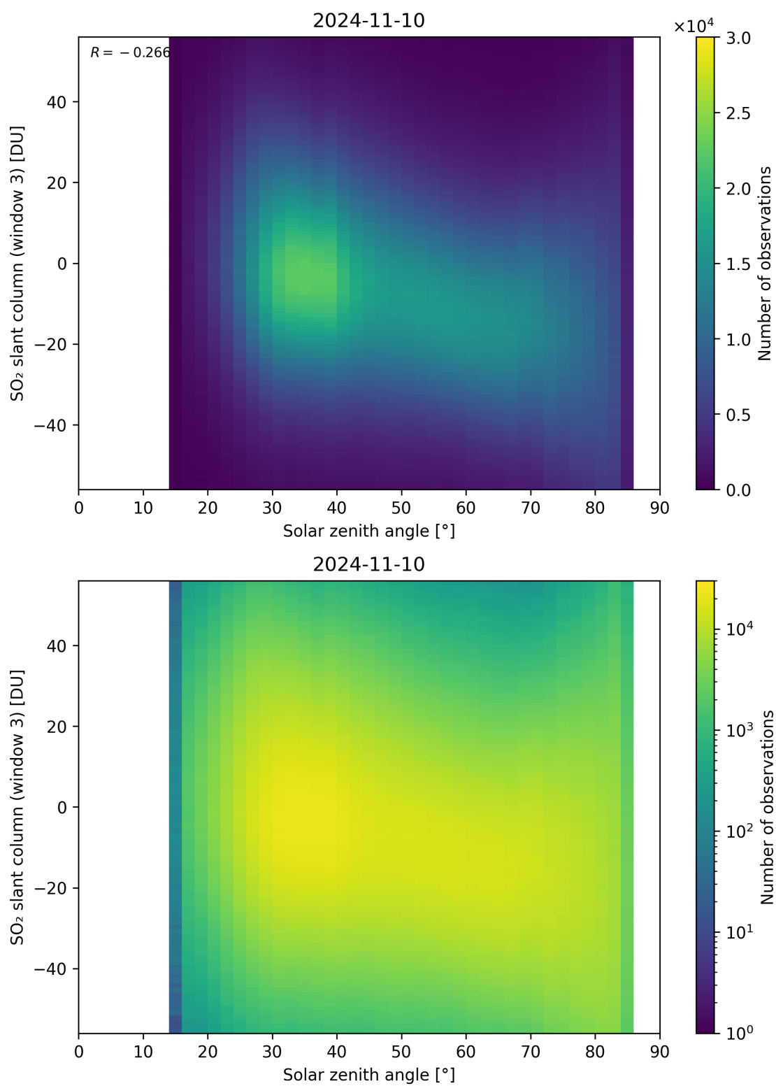
Figure 172: Scatter density plot of “Solar zenith angle” against “SO 2 slant column (window 3)” for 2024-11-09 to 2024-11-11.
