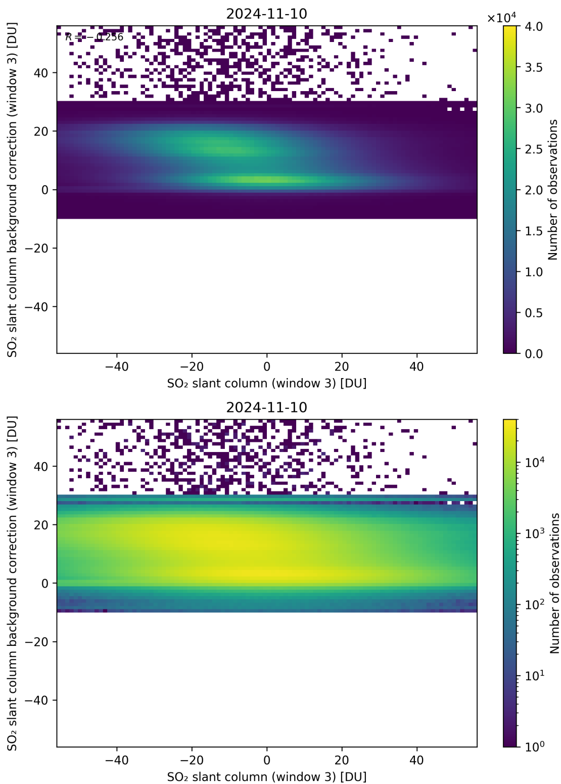
Figure 253: Scatter density plot of “SO 2 slant column (window 3)” against “SO 2 slant column background correction (window 3)” for 2024-11-09 to 2024-11-11.
