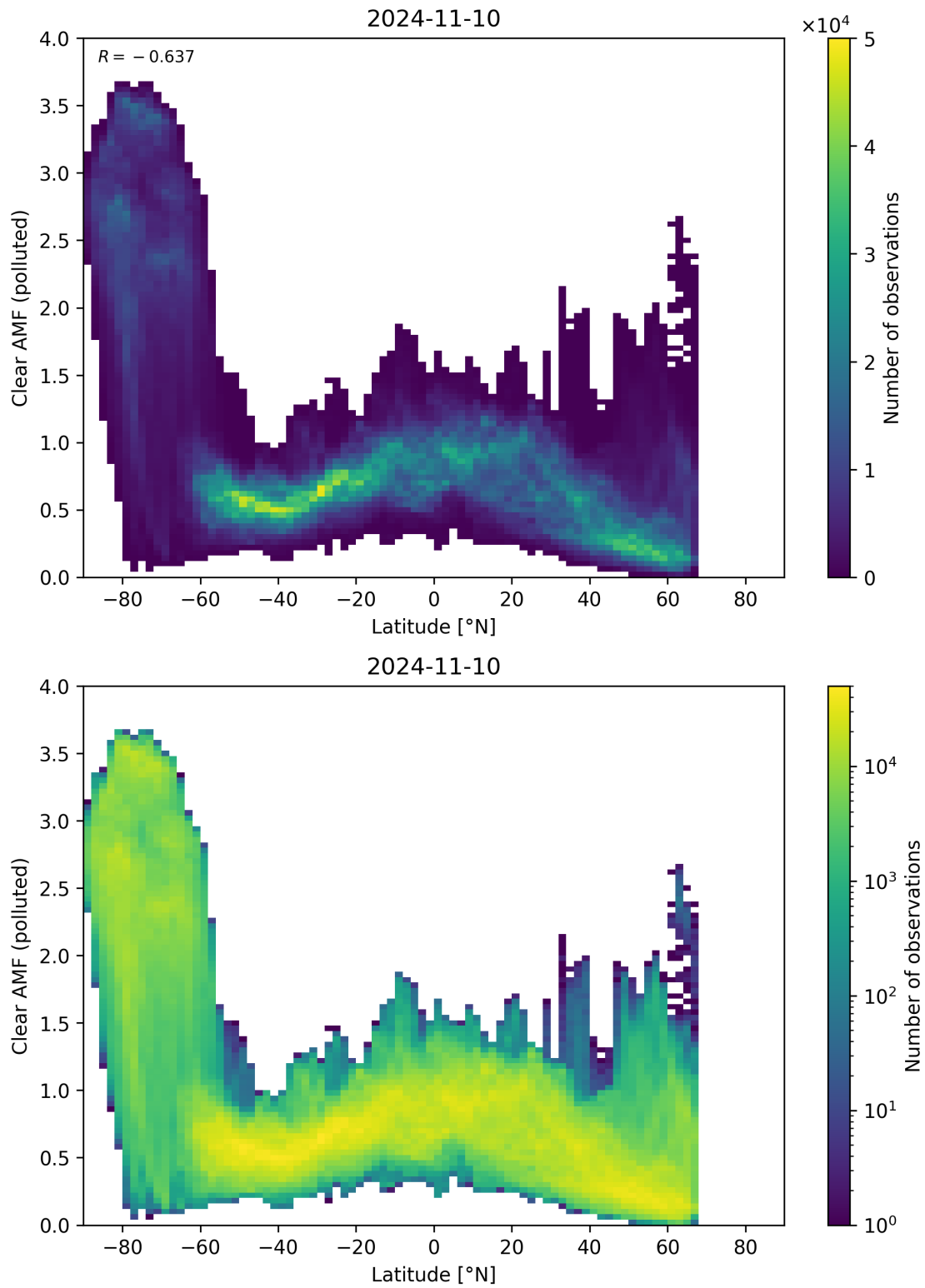
Figure 145: Scatter density plot of “Latitude” against “Clear AMF (polluted)” for 2024-11-09 to 2024-11-11.
