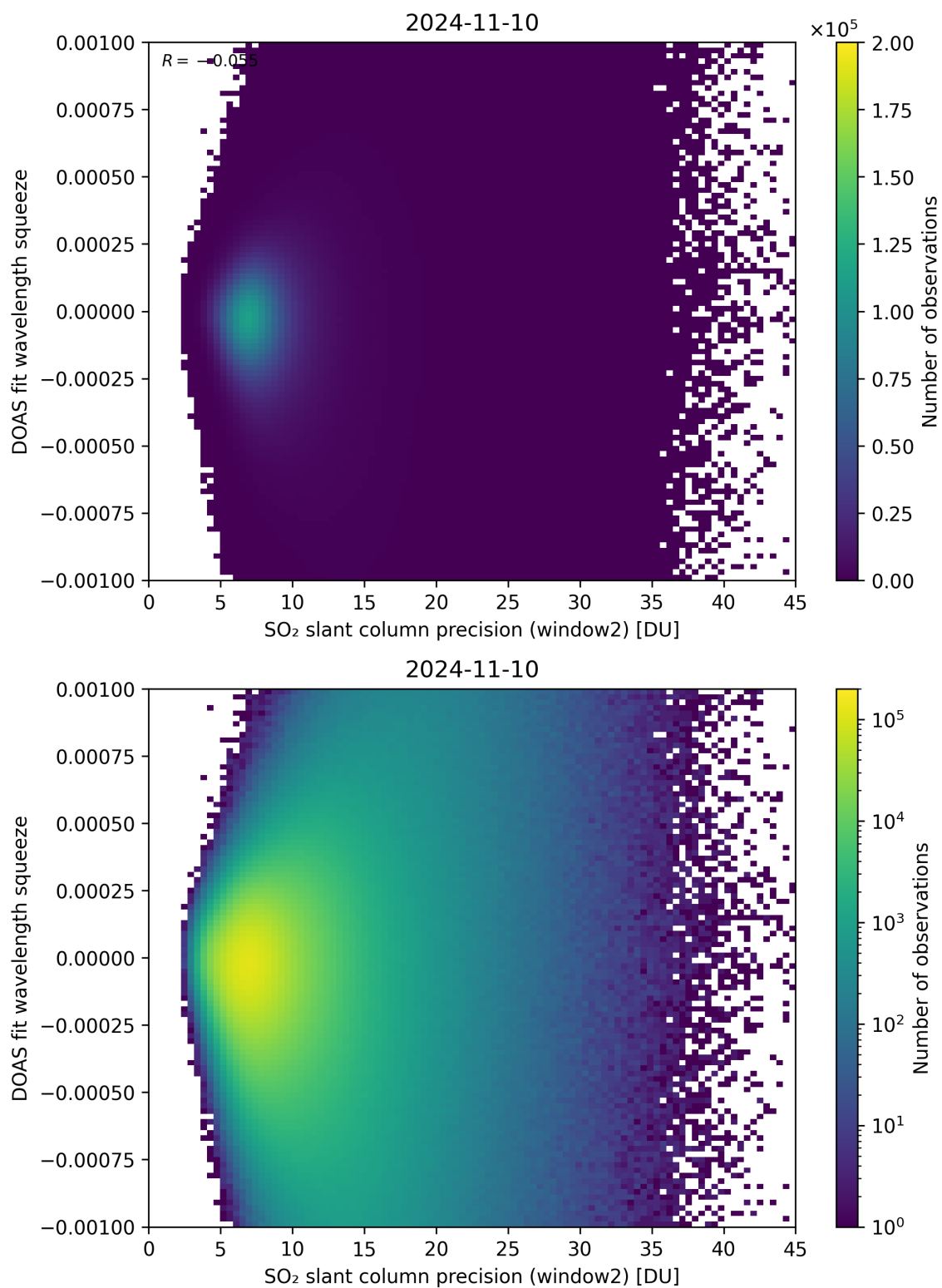
Figure 244: Scatter density plot of “SO 2 slant column precision (window2)” against “DOAS fit wavelength squeeze” for 2024-11-09 to 2024-11-11.
