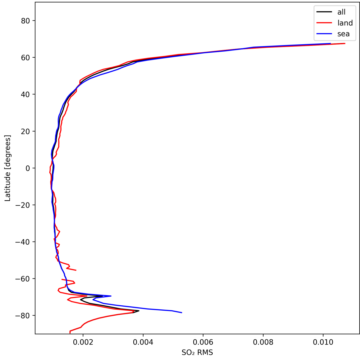
Figure 47: Zonal average of “SO 2 RMS” for 2024-11-09 to 2024-11-11.
