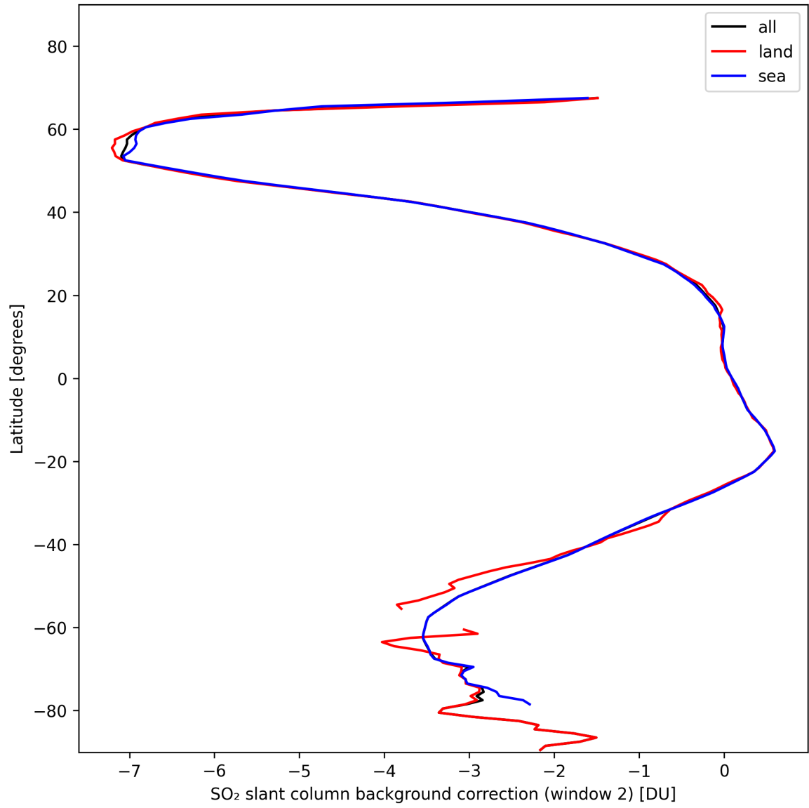
Figure 40: Zonal average of “SO 2 slant column background correction (window 2)” for 2024-11-09 to 2024-11-11.
