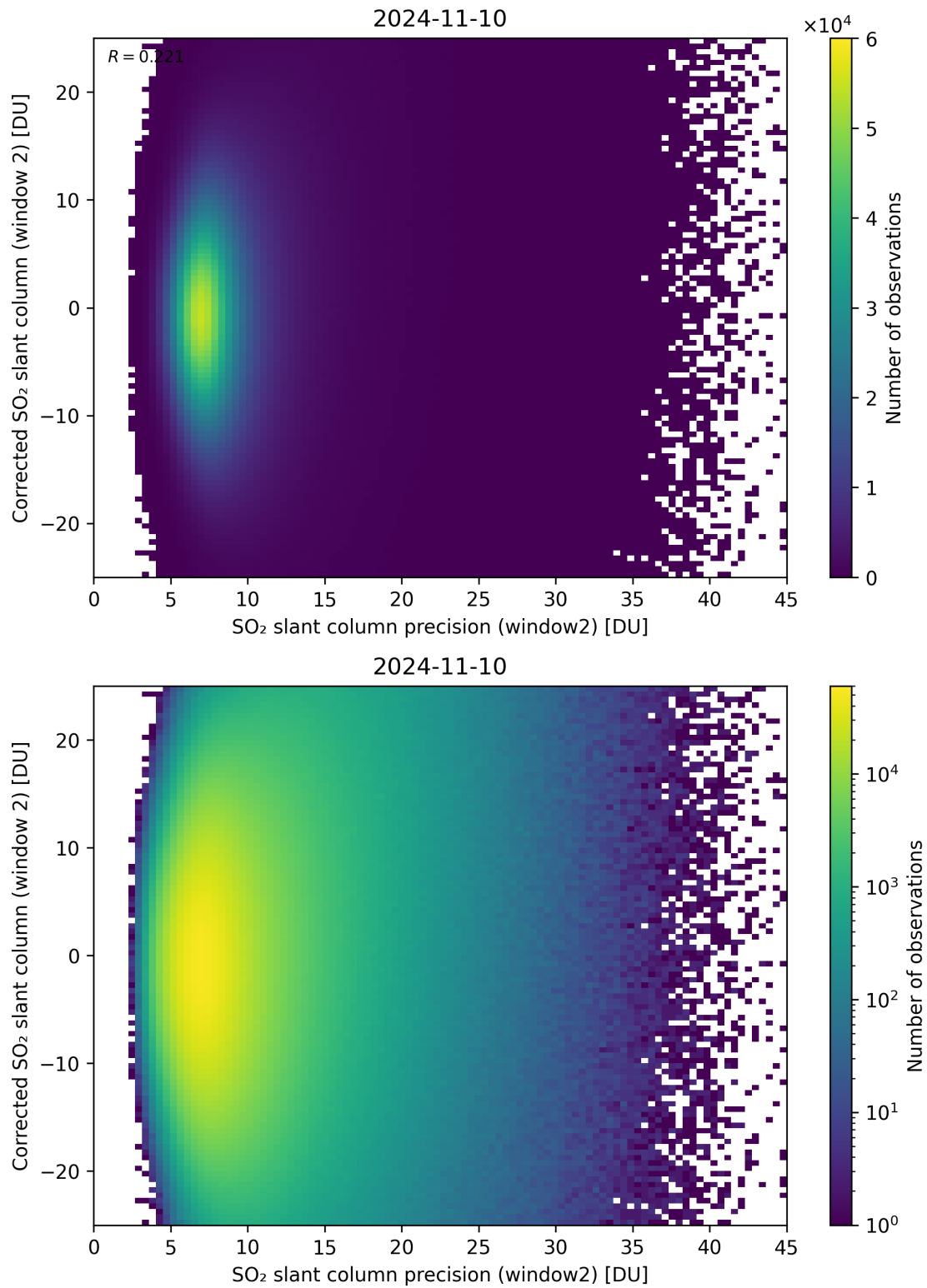
Figure 247: Scatter density plot of “SO 2 slant column precision (window2)” against “Corrected SO 2 slant column (window 2)” for 2024-11-09 to 2024-11-11.
