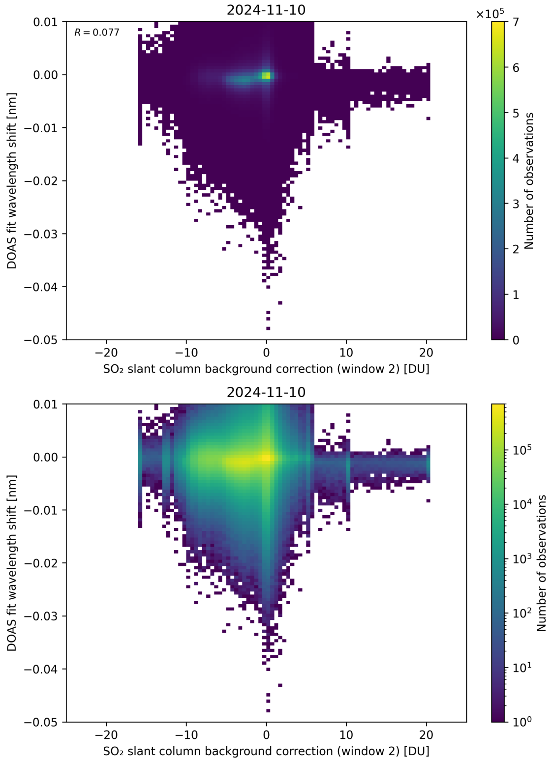
Figure 112: Scatter density plot of “SO 2 slant column background correction (window 2)” against “DOAS fit wavelength shift” for 2024-11-09 to 2024-11-11.
