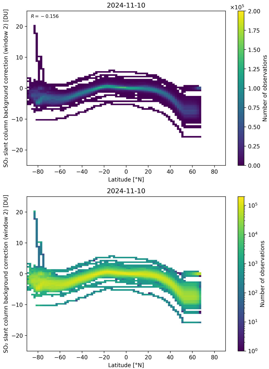
Figure 140: Scatter density plot of “Latitude” against “SO 2 slant column background correction (window 2)” for 2024-11-09 to 2024-11-11.
