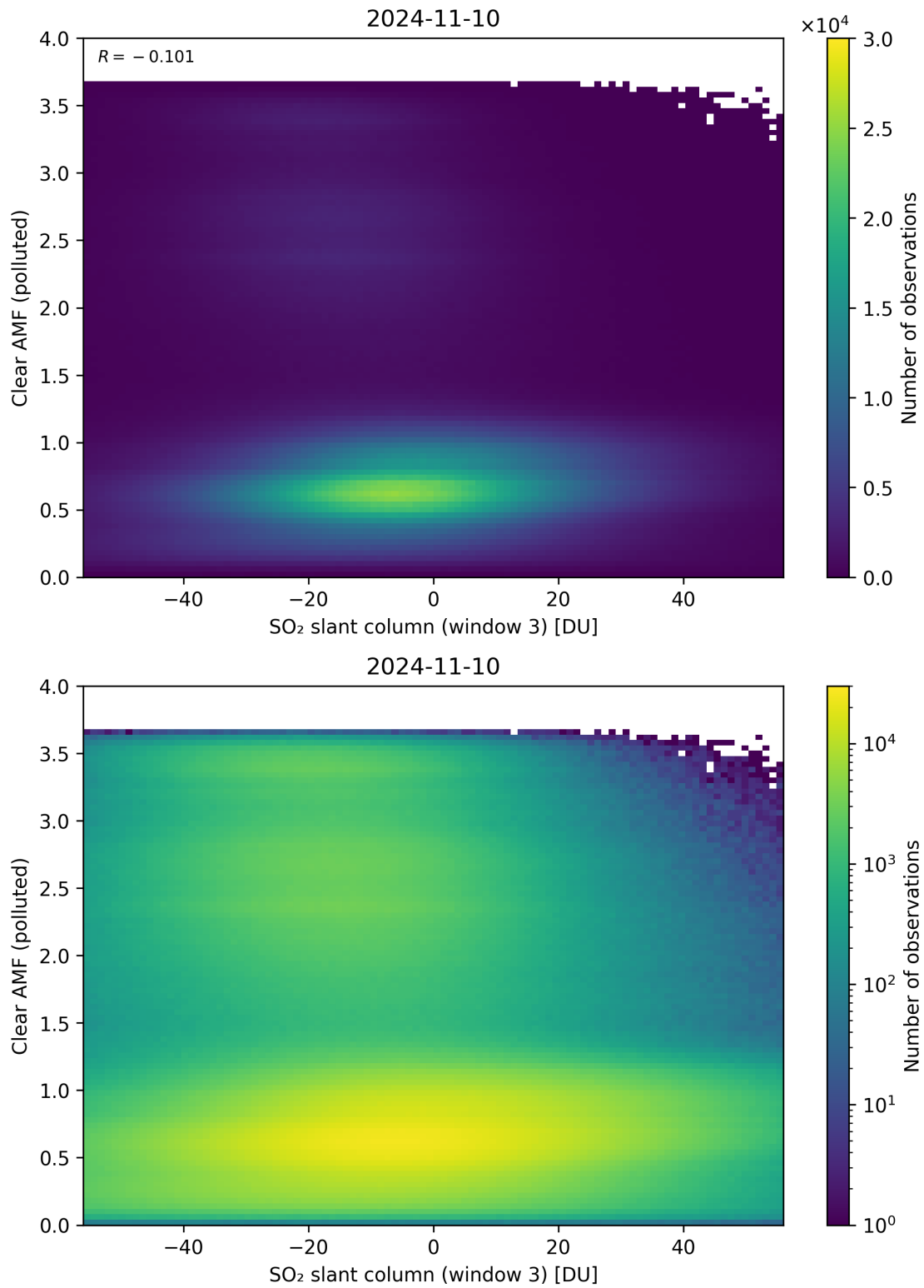
Figure 265: Scatter density plot of “SO 2 slant column (window 3)” against “Clear AMF (polluted)” for 2024-11-09 to 2024-11-11.
