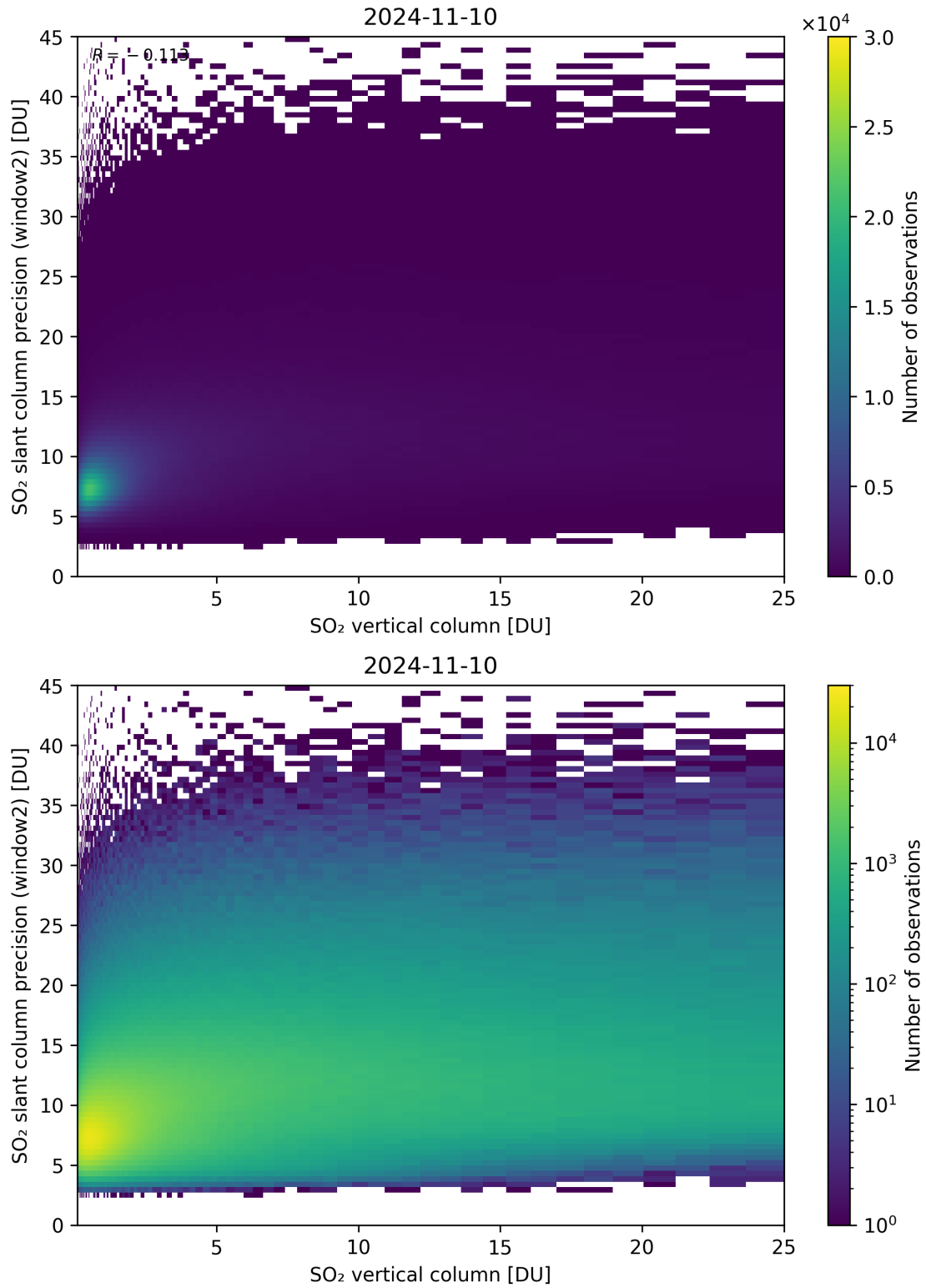
Figure 302: Scatter density plot of “SO 2 vertical column” against “SO 2 slant column precision (window2)” for 2024-11-09 to 2024-11-11.
