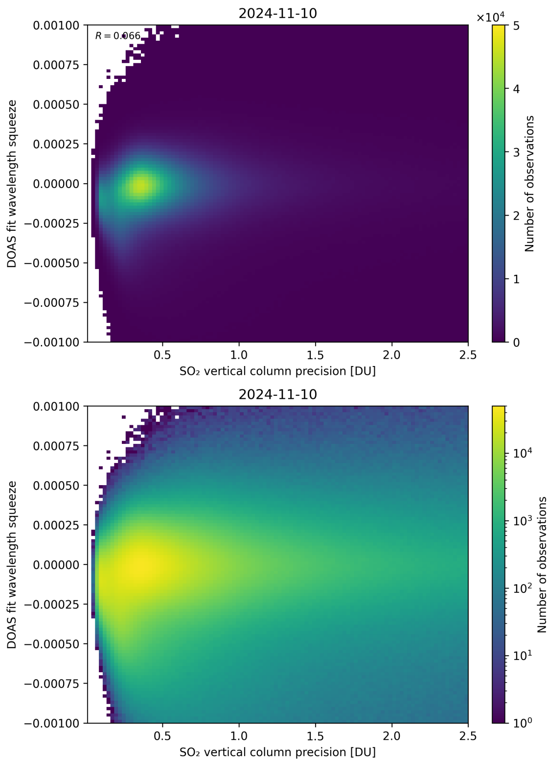
Figure 283: Scatter density plot of “SO 2 vertical column precision” against “DOAS fit wavelength squeeze” for 2024-11-09 to 2024-11-11.
