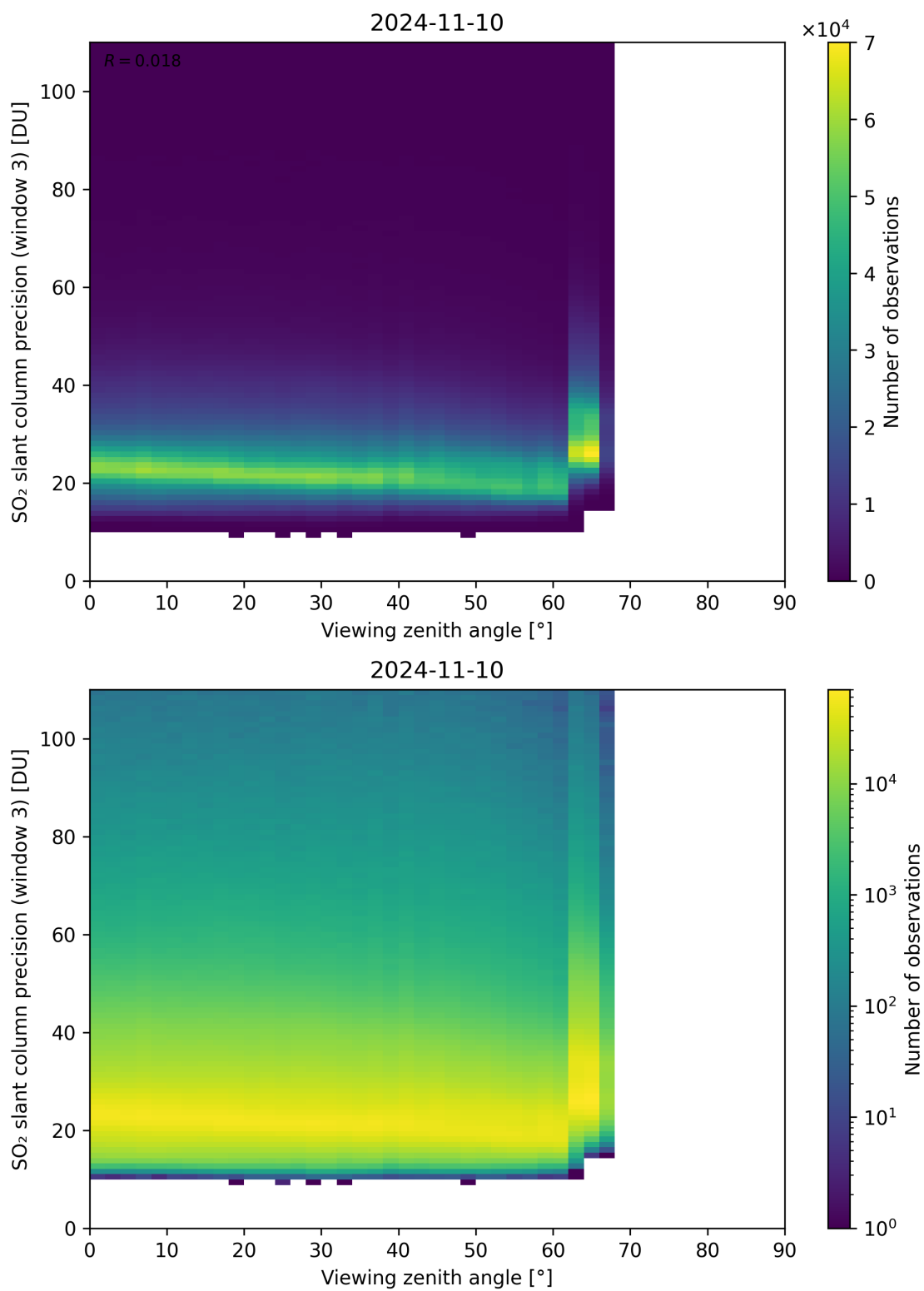
Figure 324: Scatter density plot of “Viewing zenith angle” against “SO 2 slant column precision (window 3)” for 2024-11-09 to 2024-11-11.
