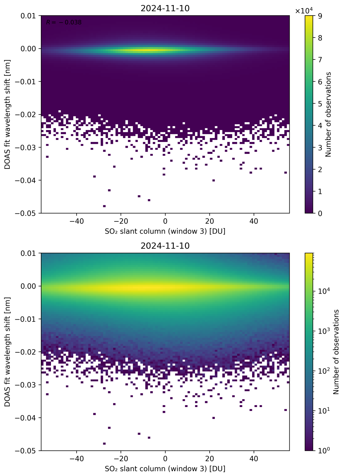
Figure 254: Scatter density plot of “SO 2 slant column (window 3)” against “DOAS fit wavelength shift” for 2024-11-09 to 2024-11-11.
