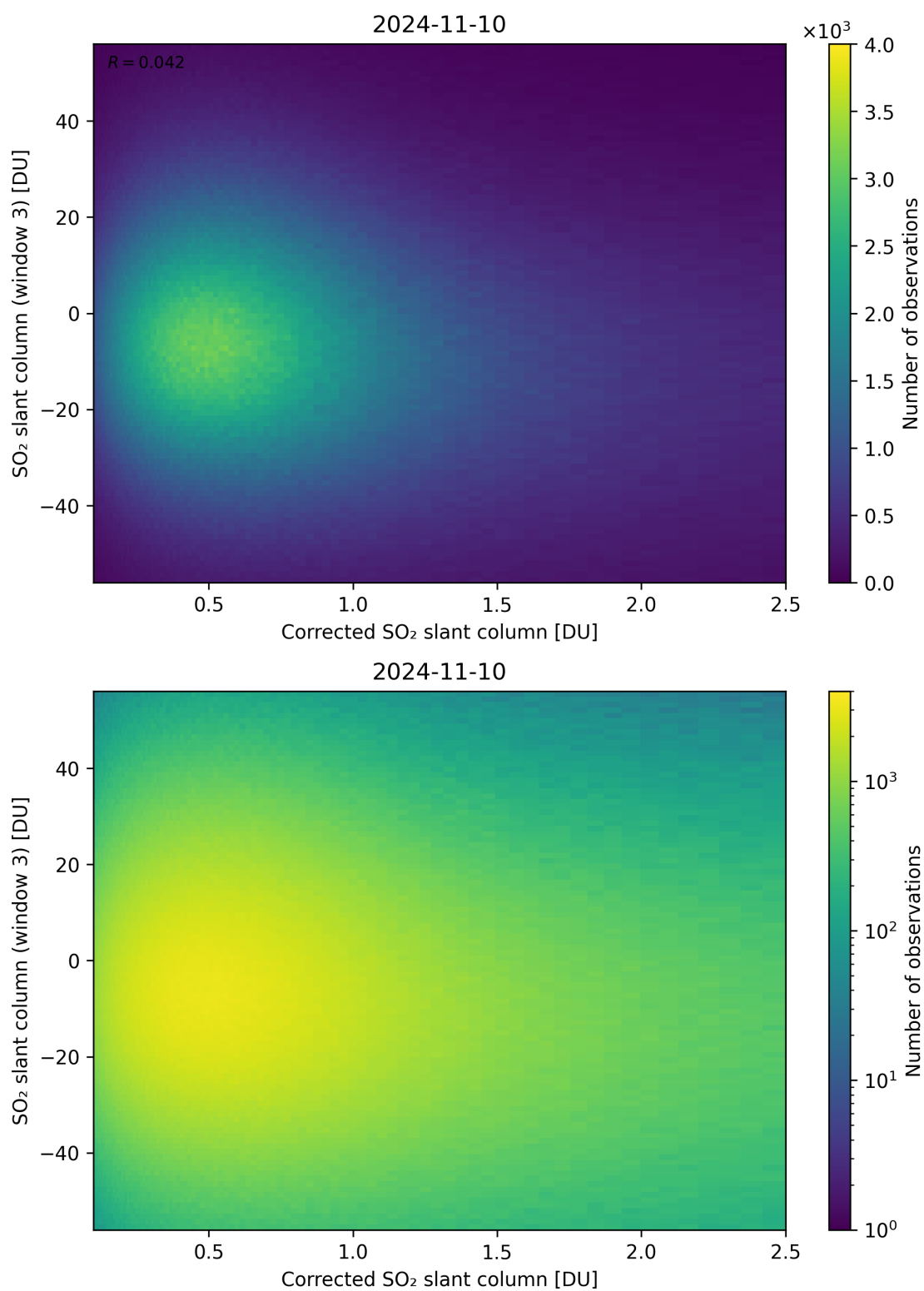
Figure 190: Scatter density plot of “Corrected SO 2 slant column” against “SO 2 slant column (window 3)” for 2024-11-09 to 2024-11-11.
