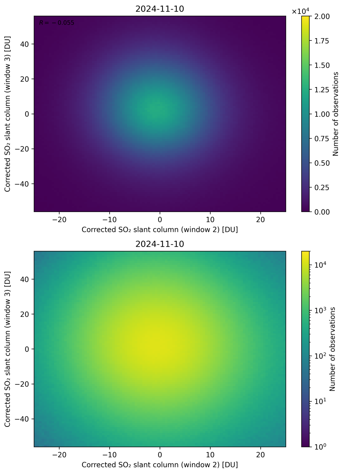
Figure 200: Scatter density plot of “Corrected SO 2 slant column (window 2)” against “Corrected SO 2 slant column (window 3)” for 2024-11-09 to 2024-11-11.
