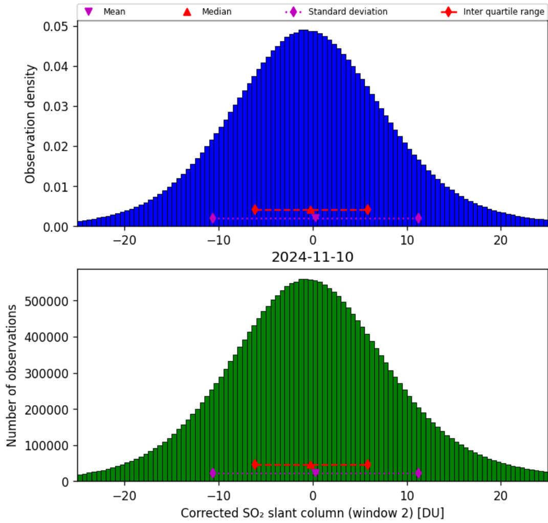
Figure 62: Histogram of “Corrected SO 2 slant column (window 2)” for 2024-11-09 to 2024-11-11
