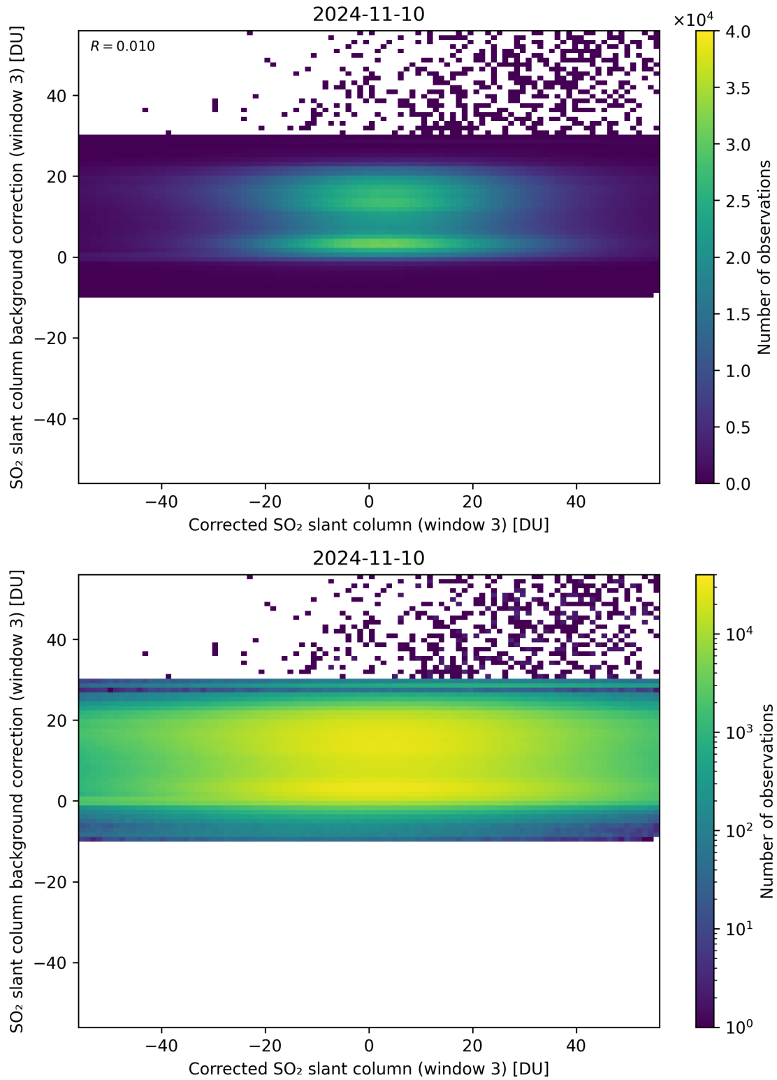
Figure 205: Scatter density plot of “Corrected SO 2 slant column (window 3)” against “SO 2 slant column background correction (window 3)” for 2024-11-09 to 2024-11-11.
