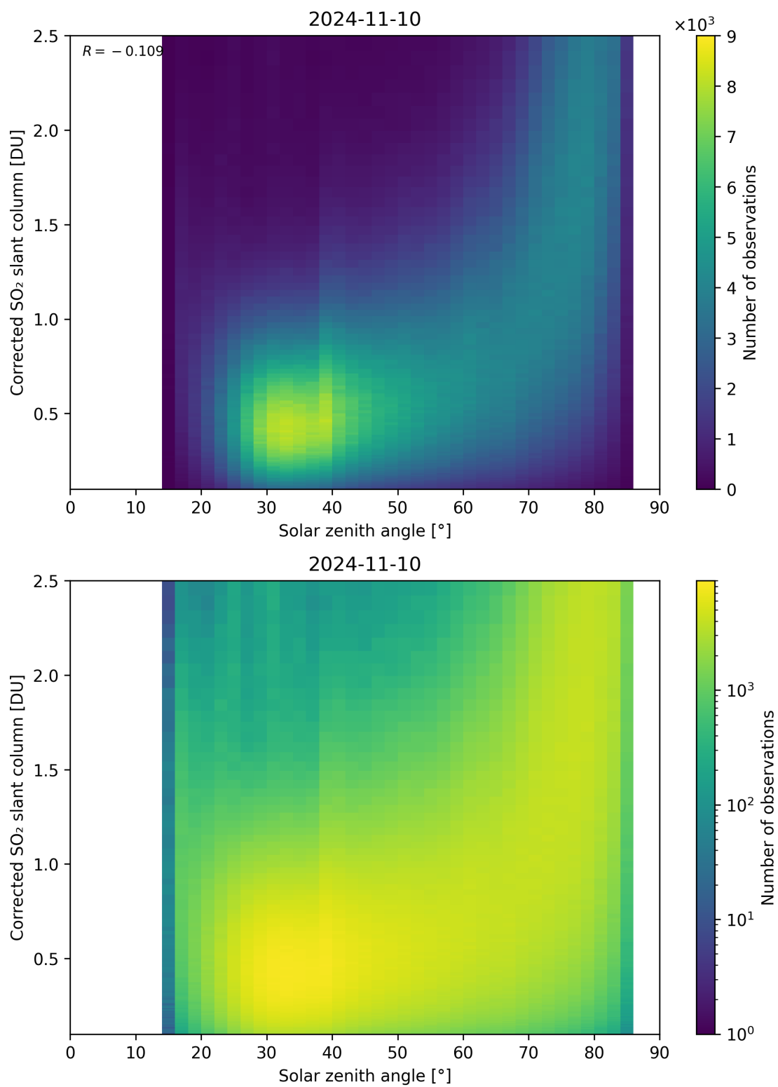
Figure 166: Scatter density plot of “Solar zenith angle” against “Corrected SO 2 slant column” for 2024-11-09 to 2024-11-11.
