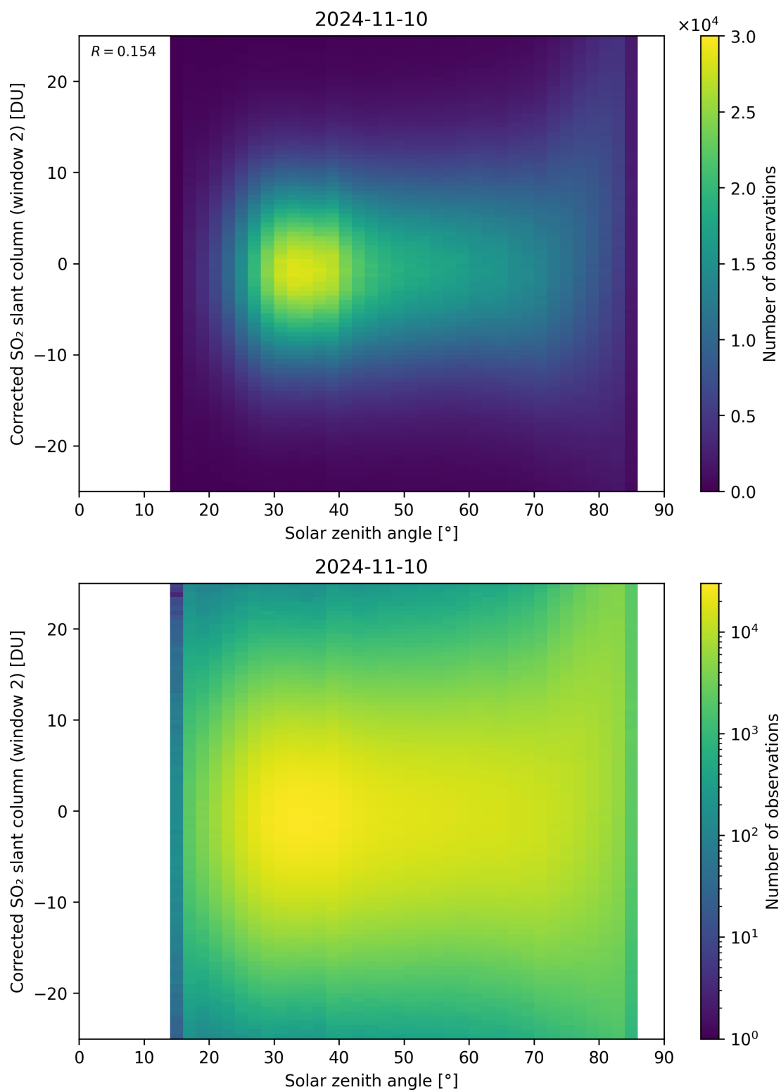
Figure 167: Scatter density plot of “Solar zenith angle” against “Corrected SO 2 slant column (window 2)” for 2024-11-09 to 2024-11-11.
