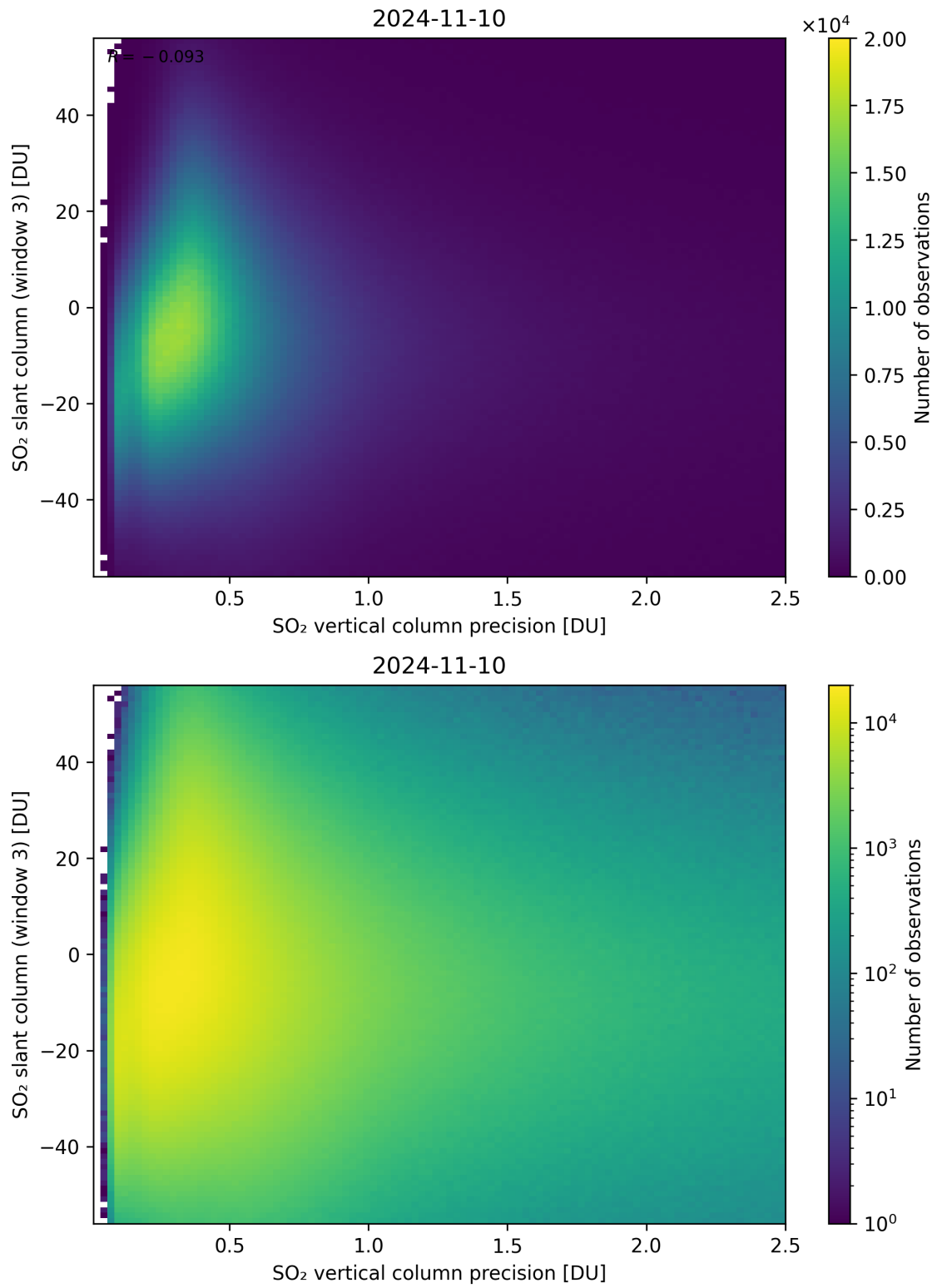
Figure 292: Scatter density plot of “SO 2 vertical column precision” against “SO 2 slant column (window 3)” for 2024-11-09 to 2024-11-11.
