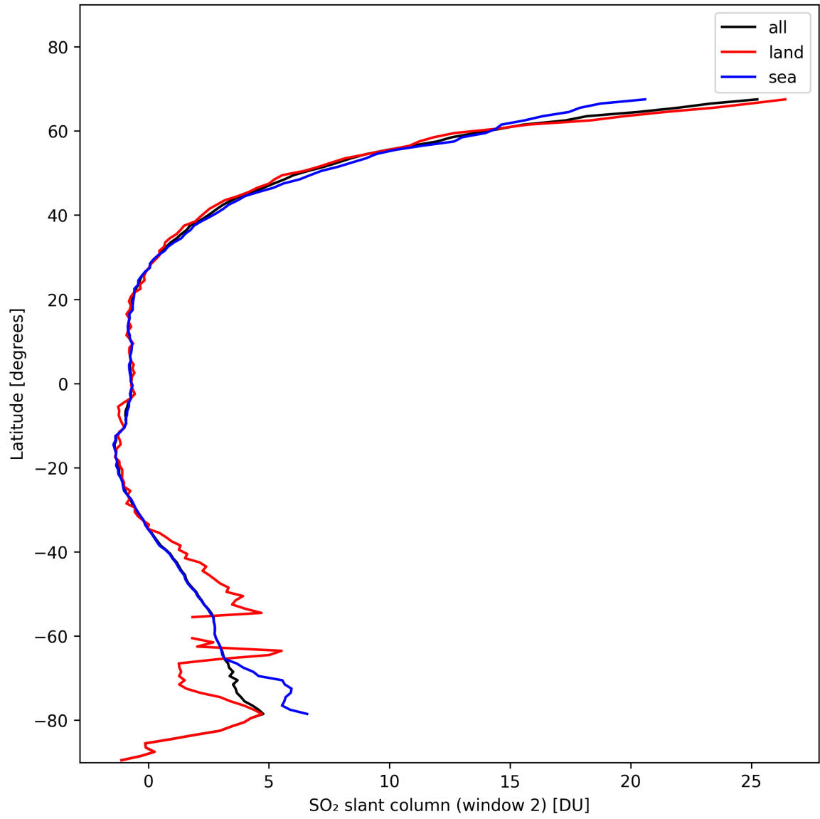
Figure 37: Zonal average of “SO 2 slant column (window 2)” for 2024-11-09 to 2024-11-11.
