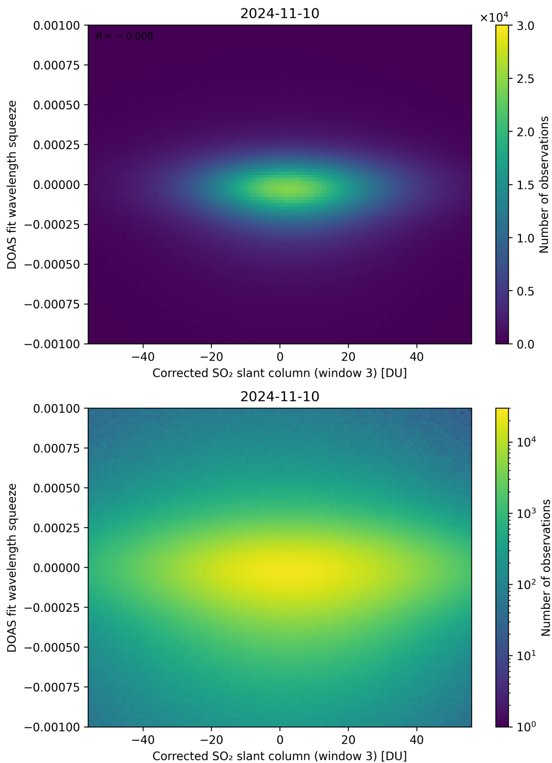
Figure 207: Scatter density plot of “Corrected SO 2 slant column (window 3)” against “DOAS fit wavelength squeeze” for 2024-11-09 to 2024-11-11.
