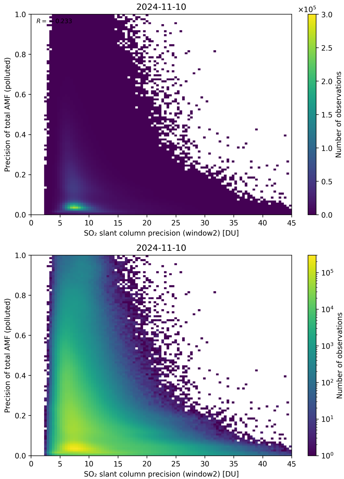
Figure 252: Scatter density plot of “SO 2 slant column precision (window2)” against “Precision of total AMF (polluted)” for 2024-11-09 to 2024-11-11.
