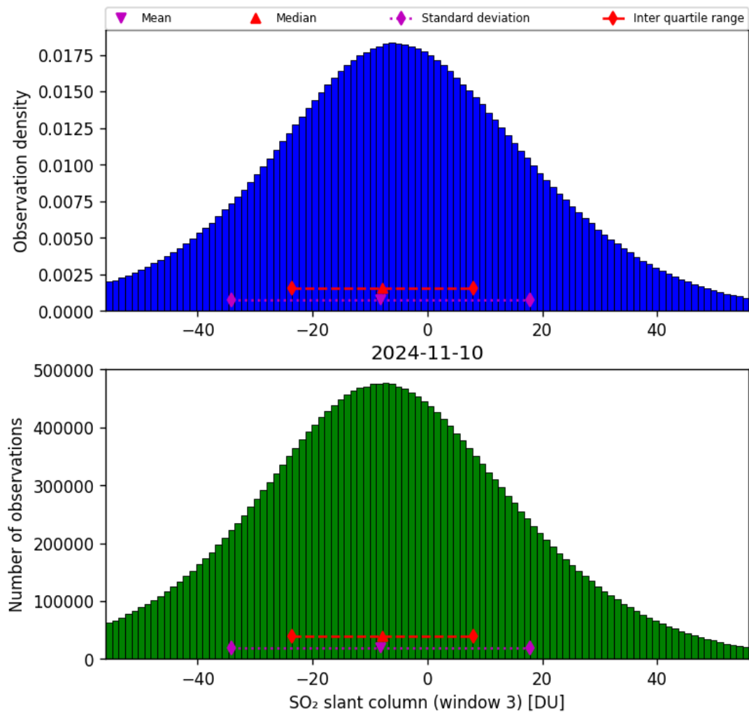
Figure 64: Histogram of “SO 2 slant column (window 3)” for 2024-11-09 to 2024-11-11
