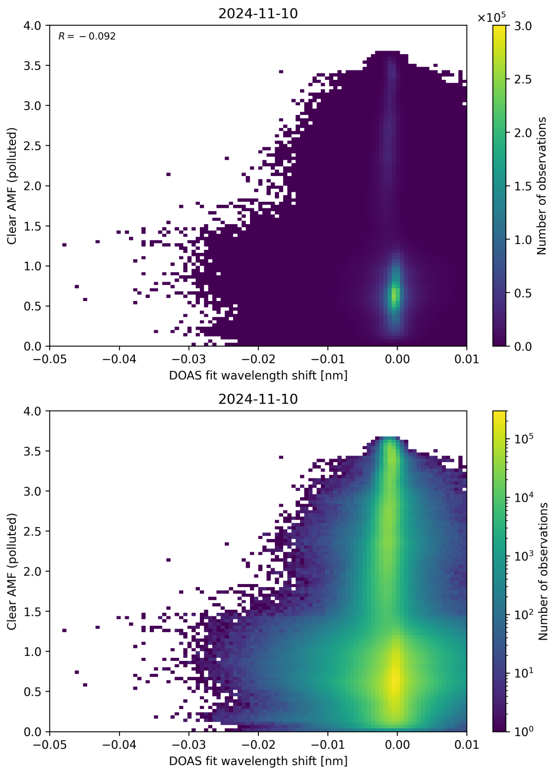
Figure 129: Scatter density plot of “DOAS fit wavelength shift” against “Clear AMF (polluted)” for 2024-11-09 to 2024-11-11.
