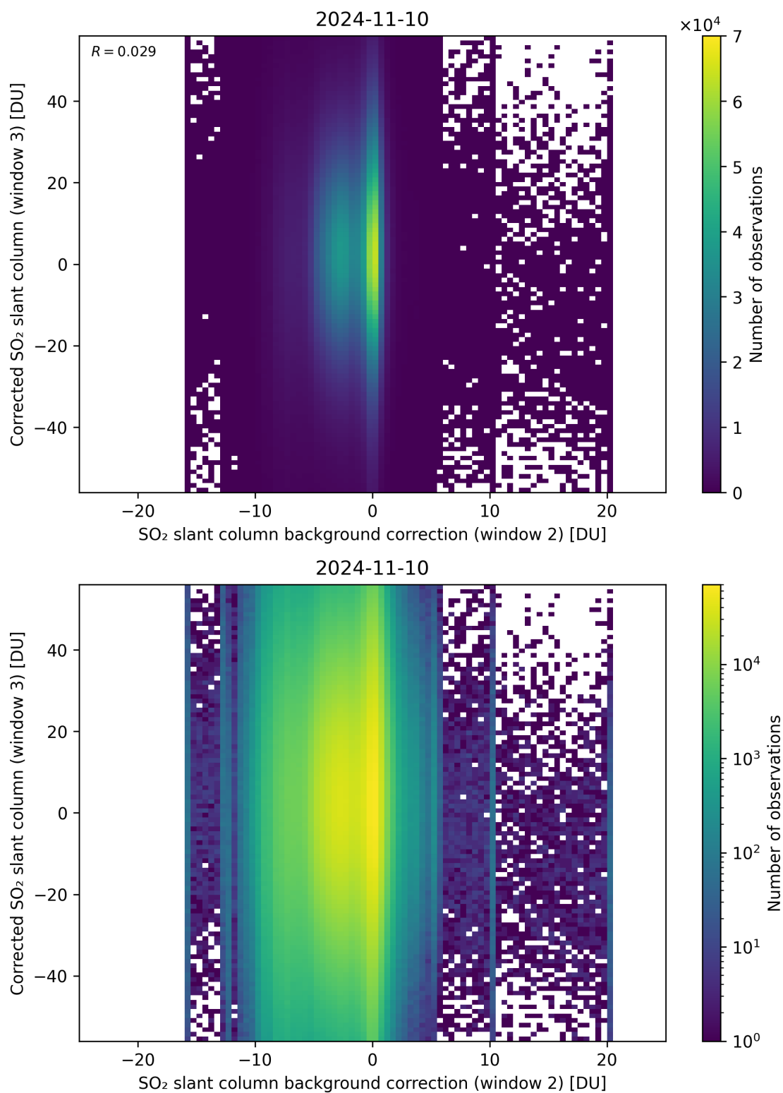
Figure 116: Scatter density plot of “SO 2 slant column background correction (window 2)” against “Corrected SO 2 slant column (window 3)” for 2024-11-09 to 2024-11-11.
