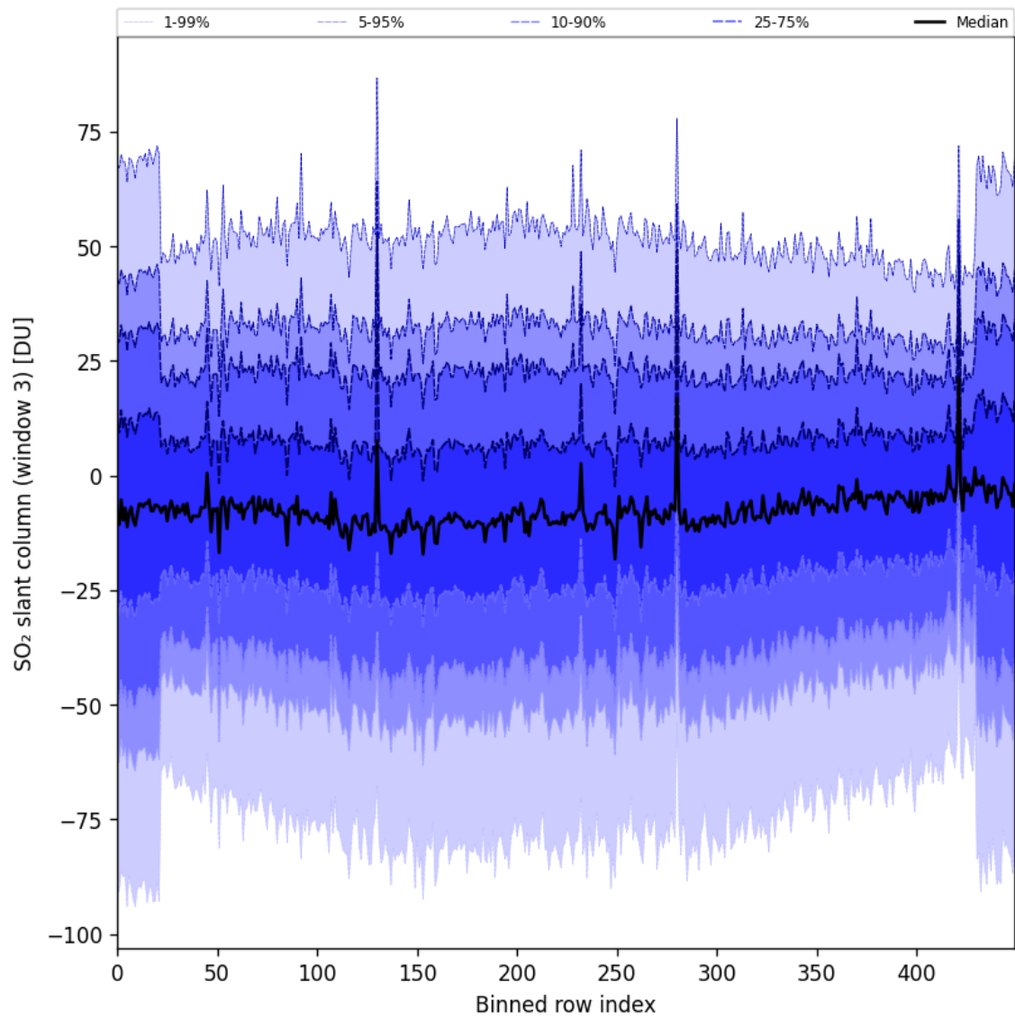
Figure 87: Along track statistics of “SO 2 slant column (window 3)” for 2024-11-09 to 2024-11-11
