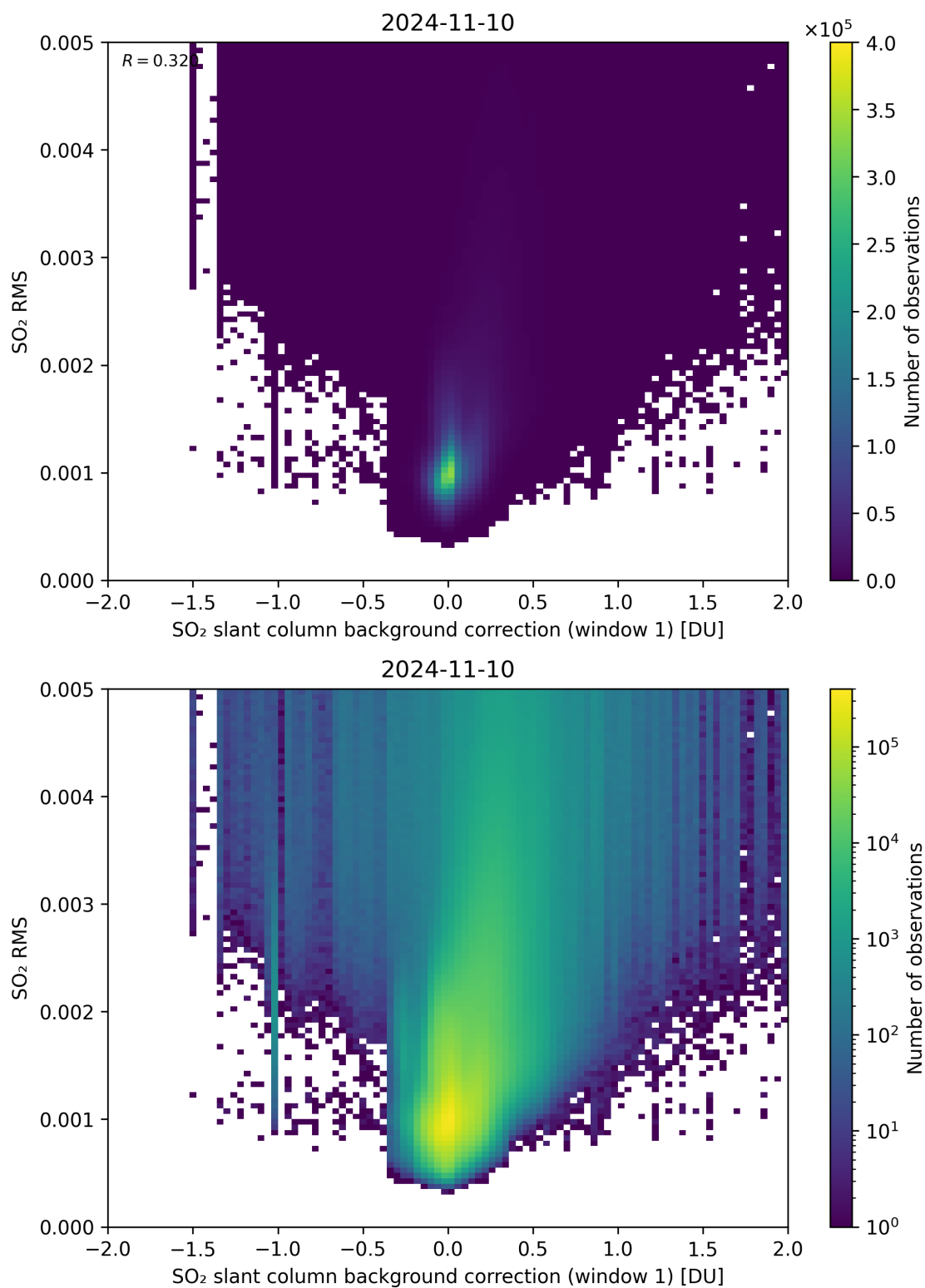
Figure 102: Scatter density plot of “SO 2 slant column background correction (window 1)” against “SO 2 RMS” for 2024-11-09 to 2024-11-11.
