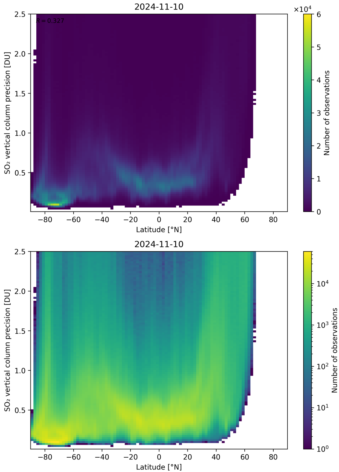
Figure 157: Scatter density plot of “Latitude” against “SO 2 vertical column precision” for 2024-11-09 to 2024-11-11.
