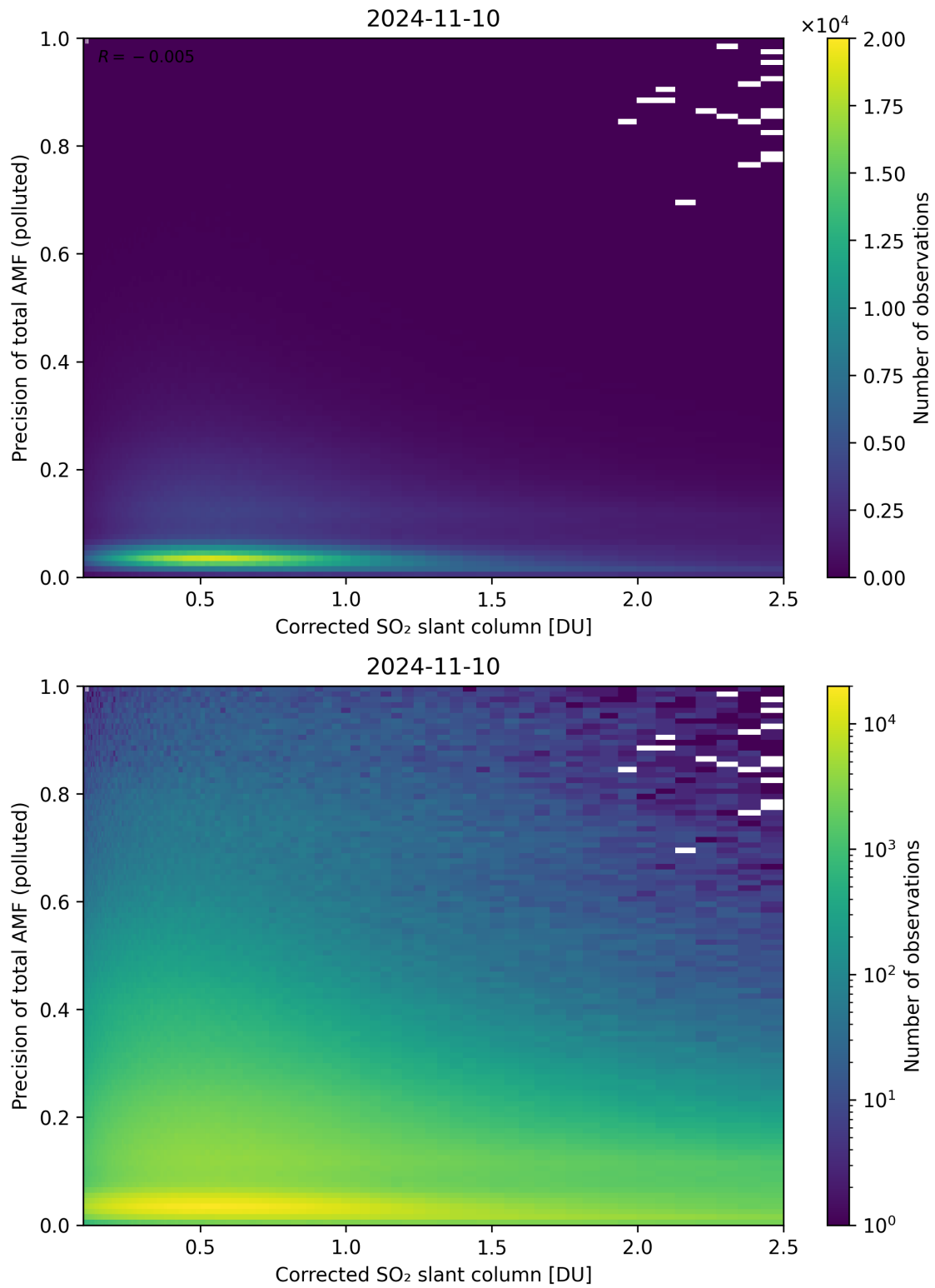
Figure 193: Scatter density plot of “Corrected SO 2 slant column” against “Precision of total AMF (polluted)” for 2024-11-09 to 2024-11-11.
