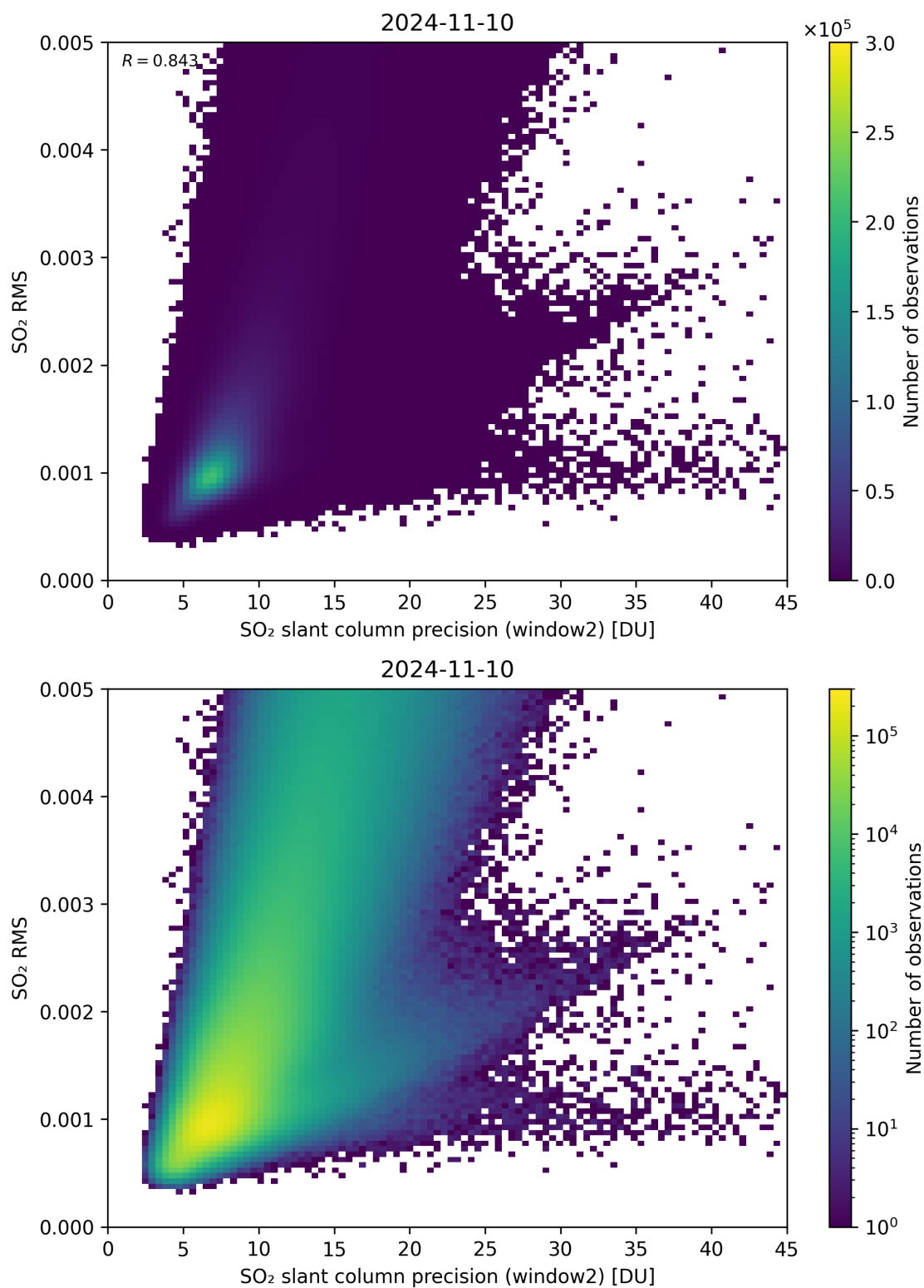
Figure 245: Scatter density plot of “SO 2 slant column precision (window2)” against “SO 2 RMS” for 2024-11-09 to 2024-11-11.
