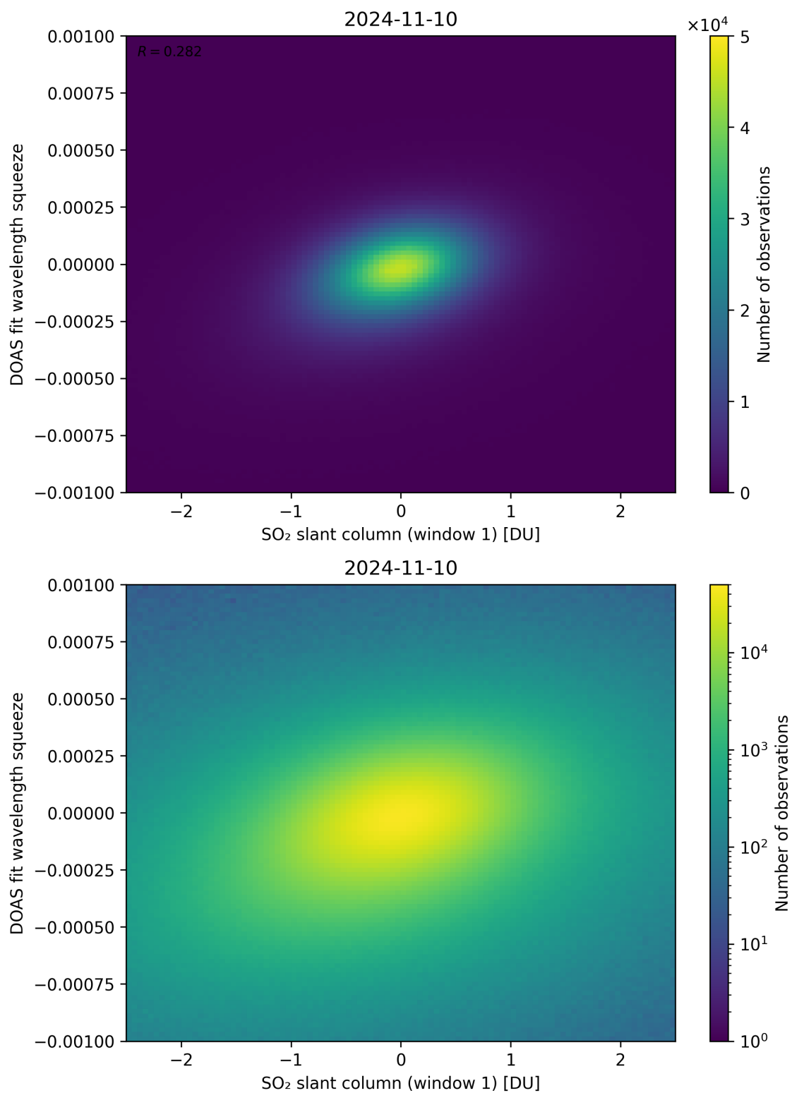
Figure 216: Scatter density plot of “SO 2 slant column (window 1)” against “DOAS fit wavelength squeeze” for 2024-11-09 to 2024-11-11.
