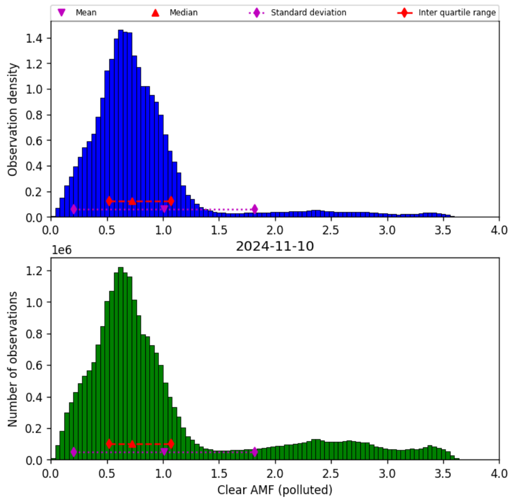
Figure 73: Histogram of “Clear AMF (polluted)” for 2024-11-09 to 2024-11-11
