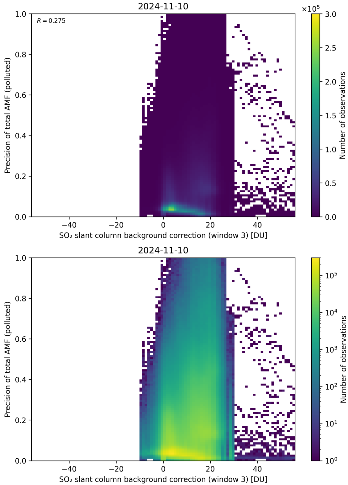
Figure 126: Scatter density plot of “SO 2 slant column background correction (window 3)” against “Precision of total AMF (polluted)” for 2024-11-09 to 2024-11-11.
