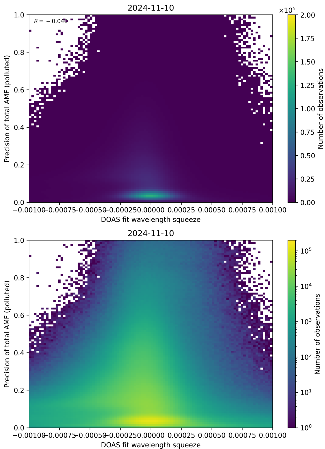
Figure 135: Scatter density plot of “DOAS fit wavelength squeeze” against “Precision of total AMF (polluted)” for 2024-11-09 to 2024-11-11.
