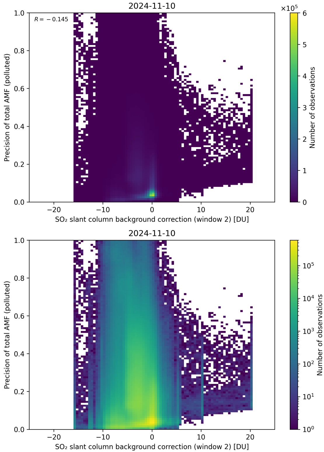
Figure 120: Scatter density plot of “SO 2 slant column background correction (window 2)” against “Precision of total AMF (polluted)” for 2024-11-09 to 2024-11-11.
