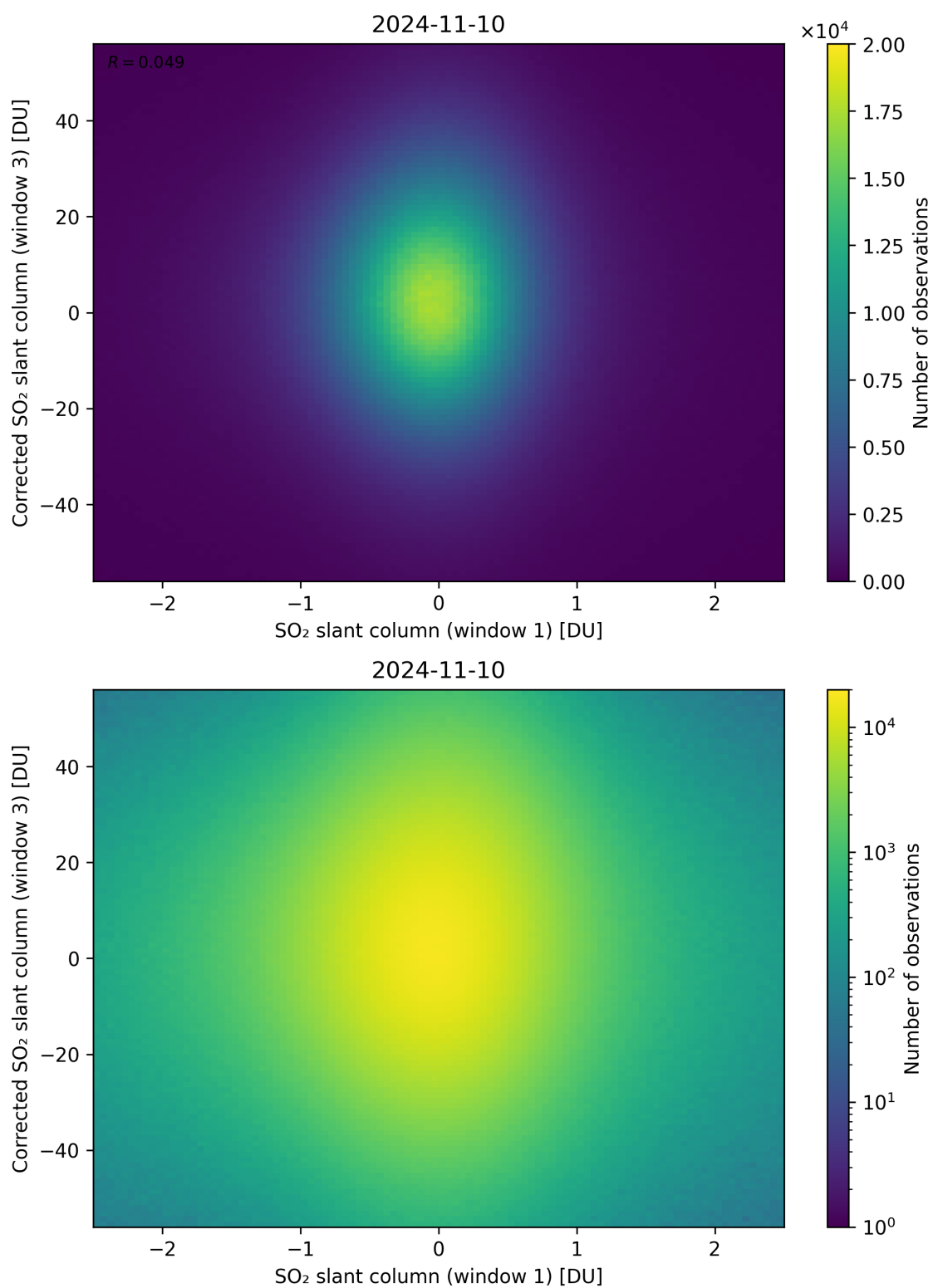
Figure 234: Scatter density plot of “SO 2 slant column (window 1)” against “Corrected SO 2 slant column (window 3)” for 2024-11-09 to 2024-11-11.
