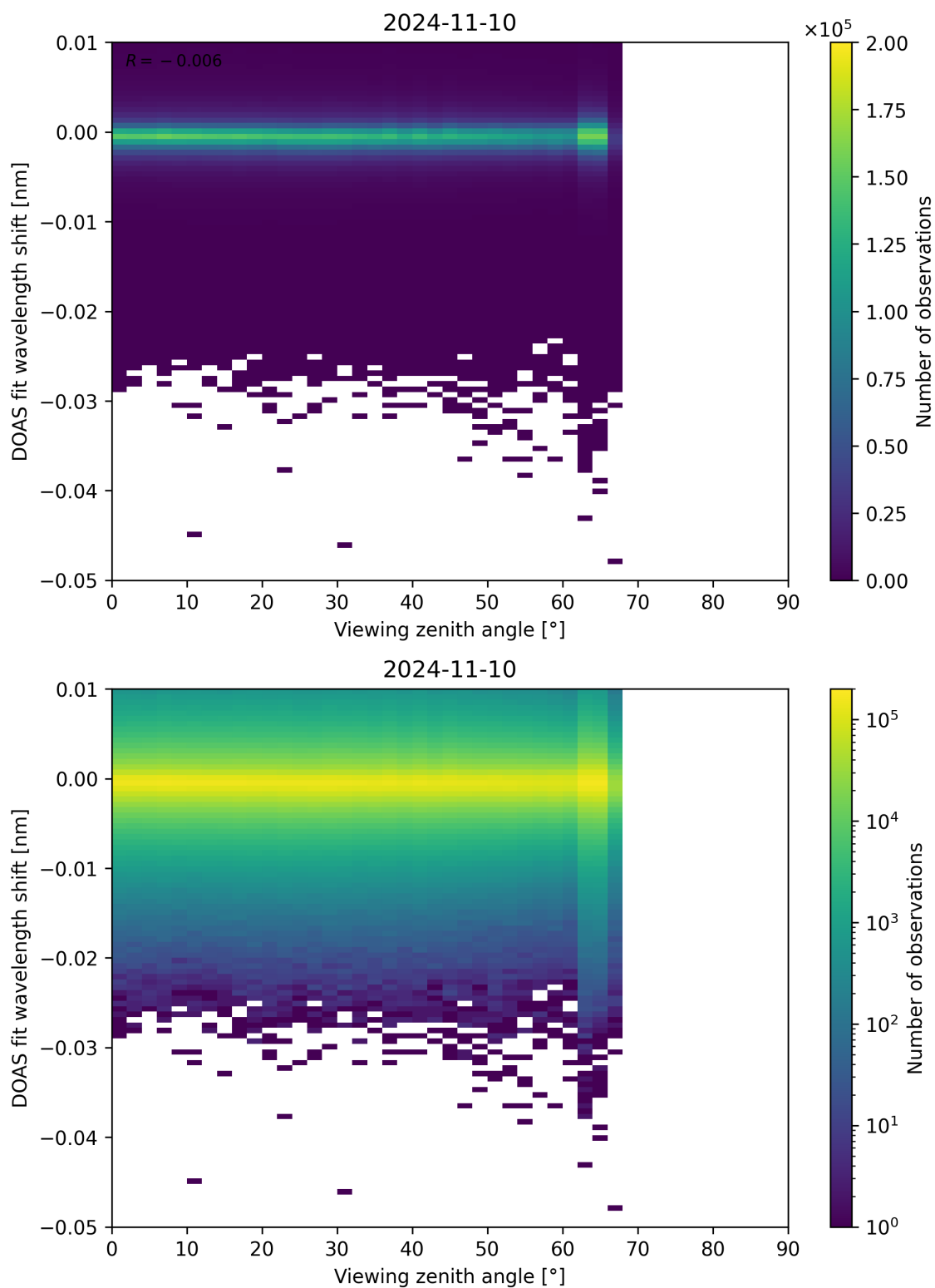
Figure 311: Scatter density plot of “Viewing zenith angle” against “DOAS fit wavelength shift” for 2024-11-09 to 2024-11-11.
