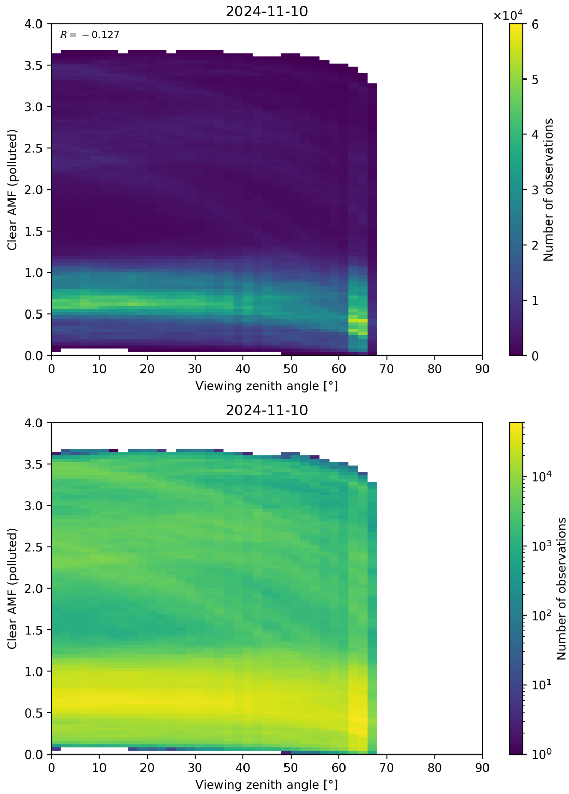
Figure 316: Scatter density plot of “Viewing zenith angle” against “Clear AMF (polluted)” for 2024-11-09 to 2024-11-11.
