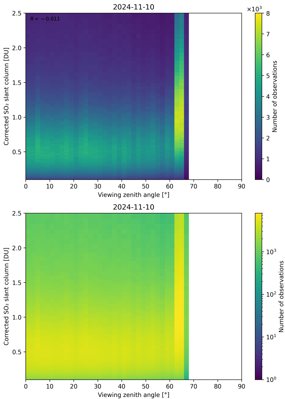
Figure 317: Scatter density plot of “Viewing zenith angle” against “Corrected SO 2 slant column” for 2024-11-09 to 2024-11-11.
