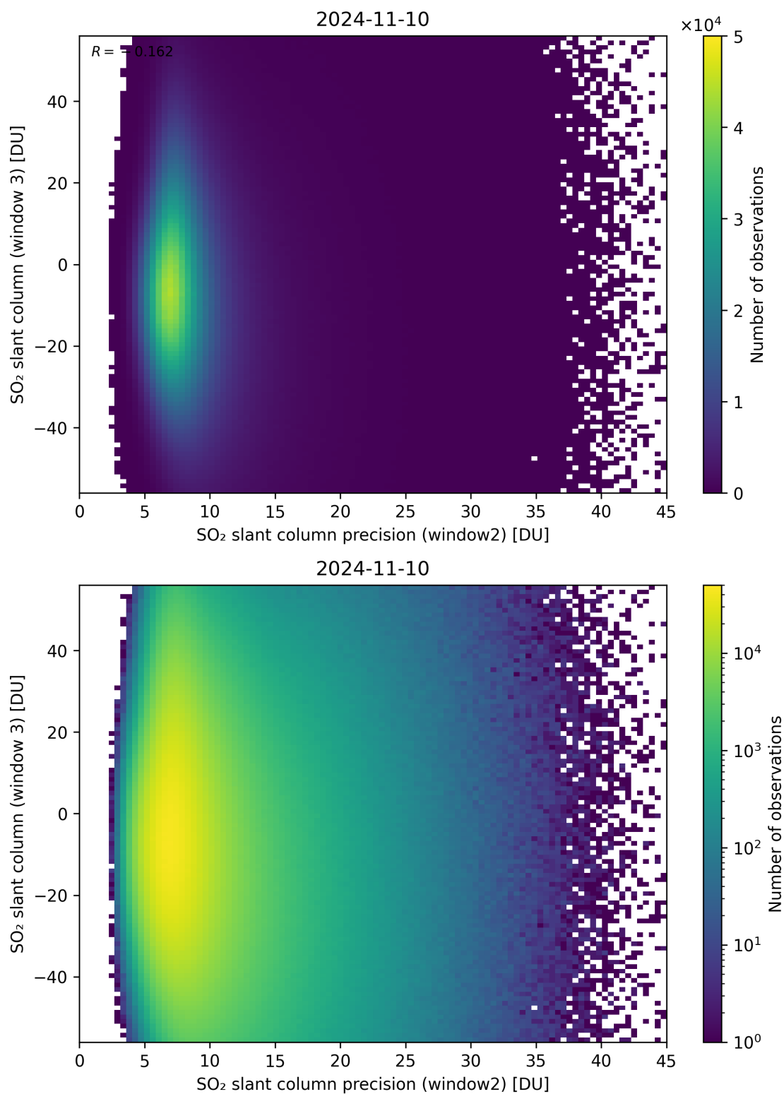
Figure 249: Scatter density plot of “SO 2 slant column precision (window2)” against “SO 2 slant column (window 3)” for 2024-11-09 to 2024-11-11.
