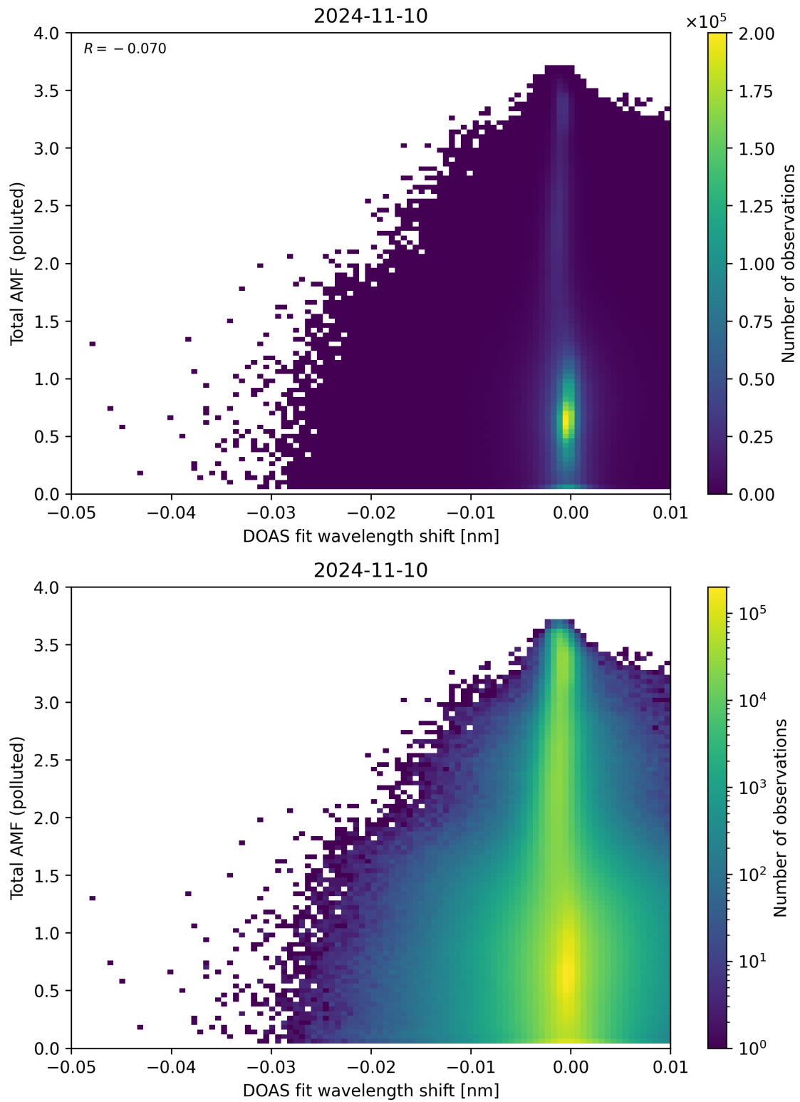
Figure 130: Scatter density plot of “DOAS fit wavelength shift” against “Total AMF (polluted)” for 2024-11-09 to 2024-11-11.
