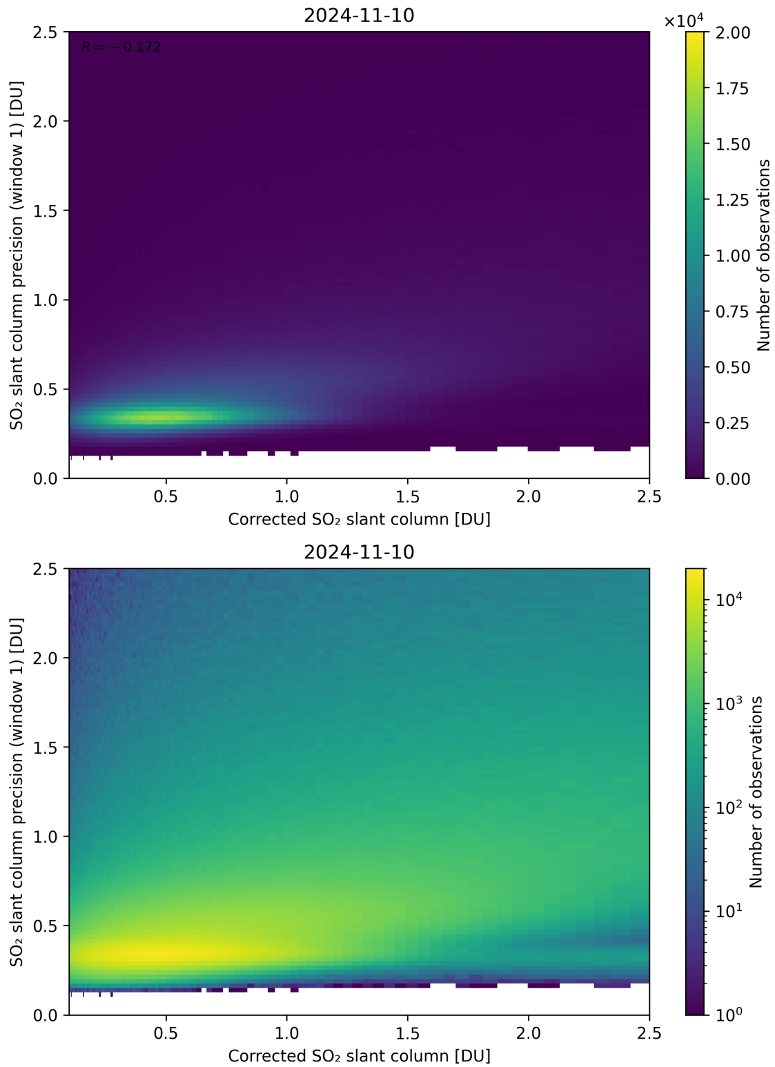
Figure 188: Scatter density plot of “Corrected SO 2 slant column” against “SO 2 slant column precision (window 1)” for 2024-11-09 to 2024-11-11.
