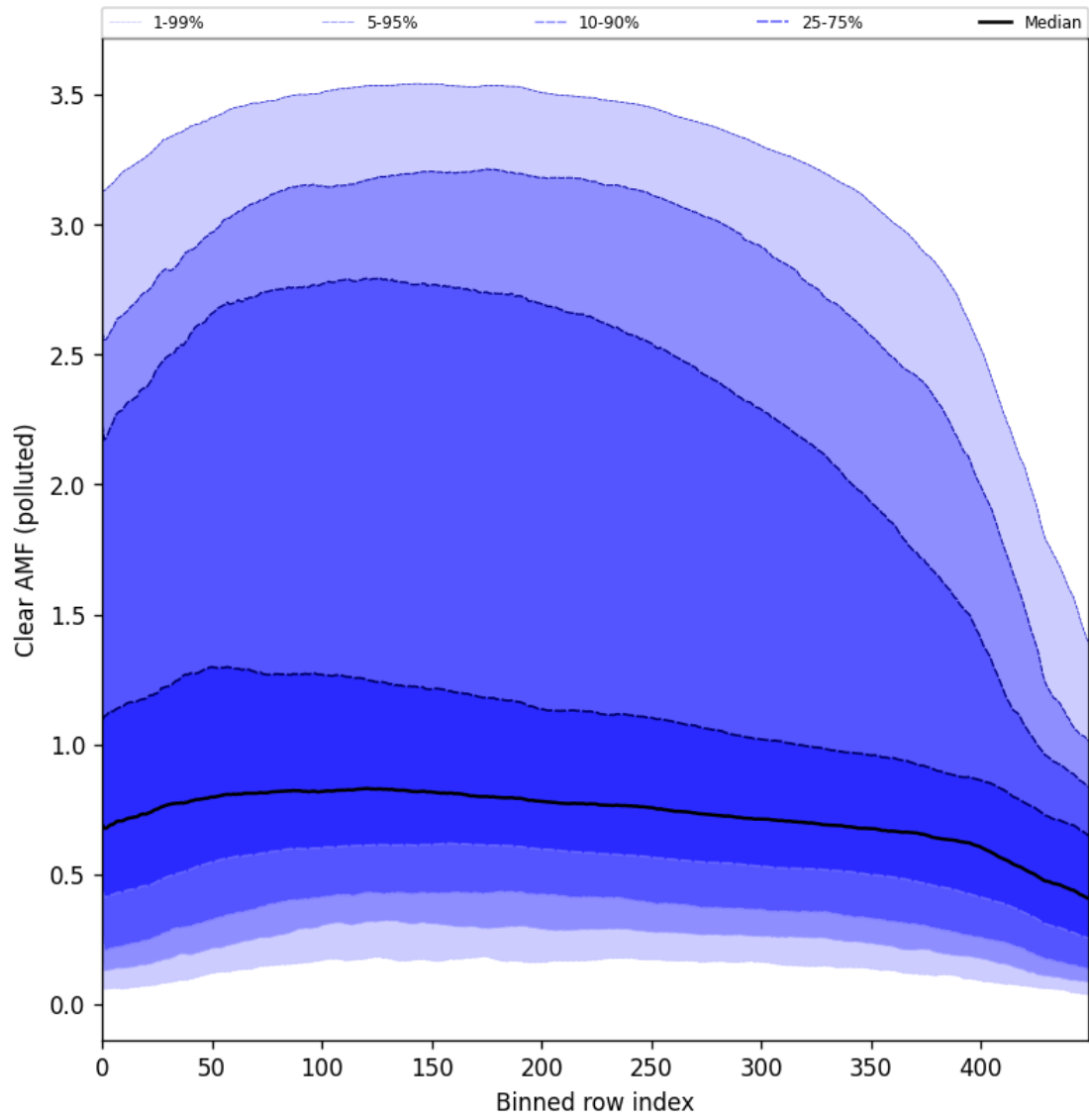
Figure 96: Along track statistics of “Clear AMF (polluted)” for 2024-11-09 to 2024-11-11
