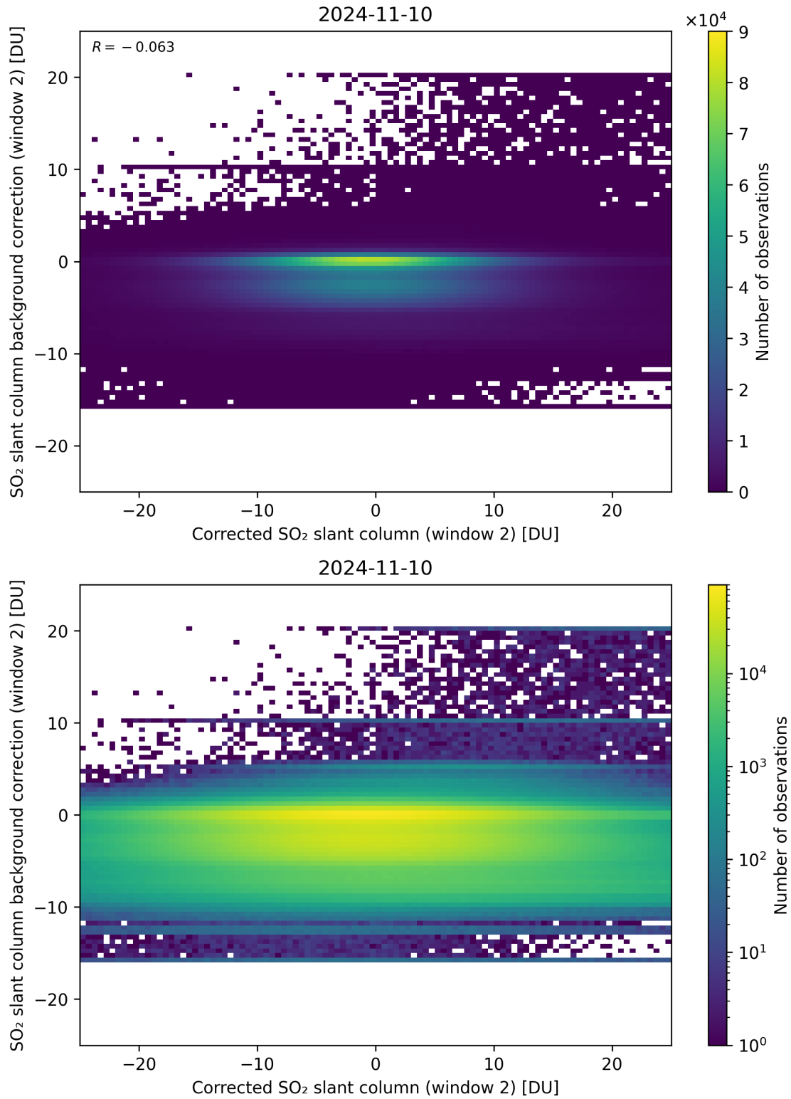
Figure 194: Scatter density plot of “Corrected SO 2 slant column (window 2)” against “SO 2 slant column background correction (window 2)” for 2024-11-09 to 2024-11-11.
