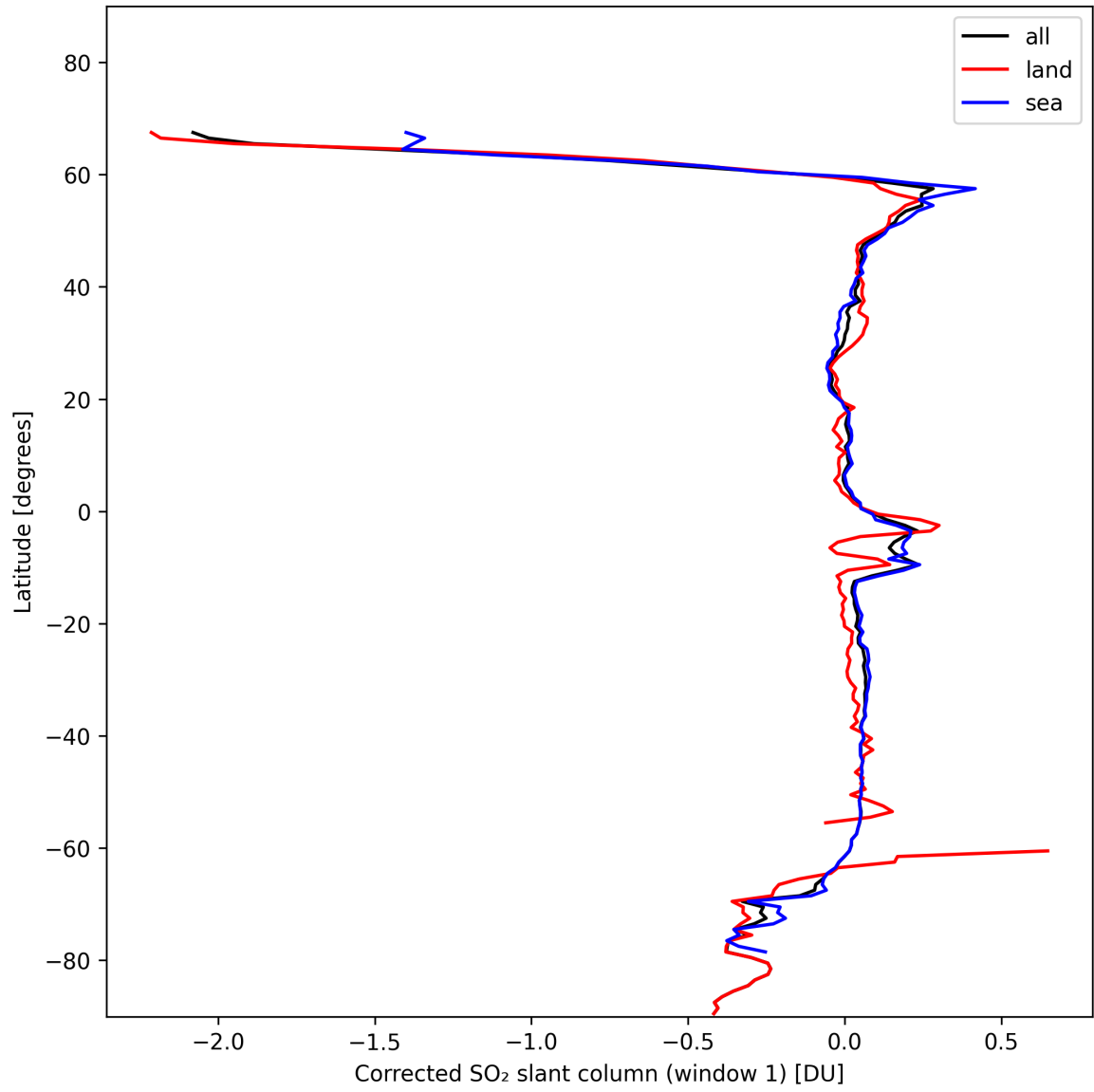
Figure 35: Zonal average of “Corrected SO 2 slant column (window 1)” for 2024-11-09 to 2024-11-11.
