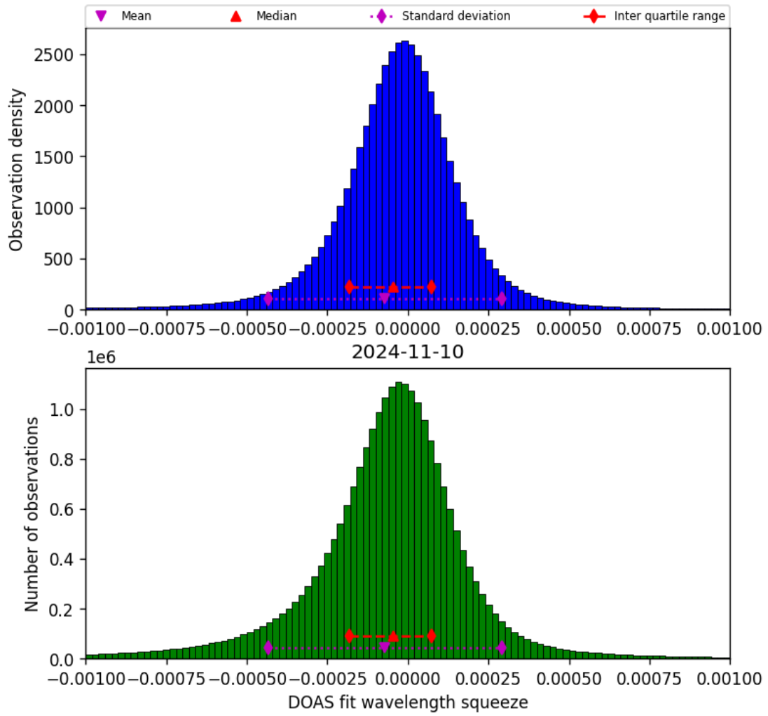
Figure 69: Histogram of “DOAS fit wavelength squeeze” for 2024-11-09 to 2024-11-11
