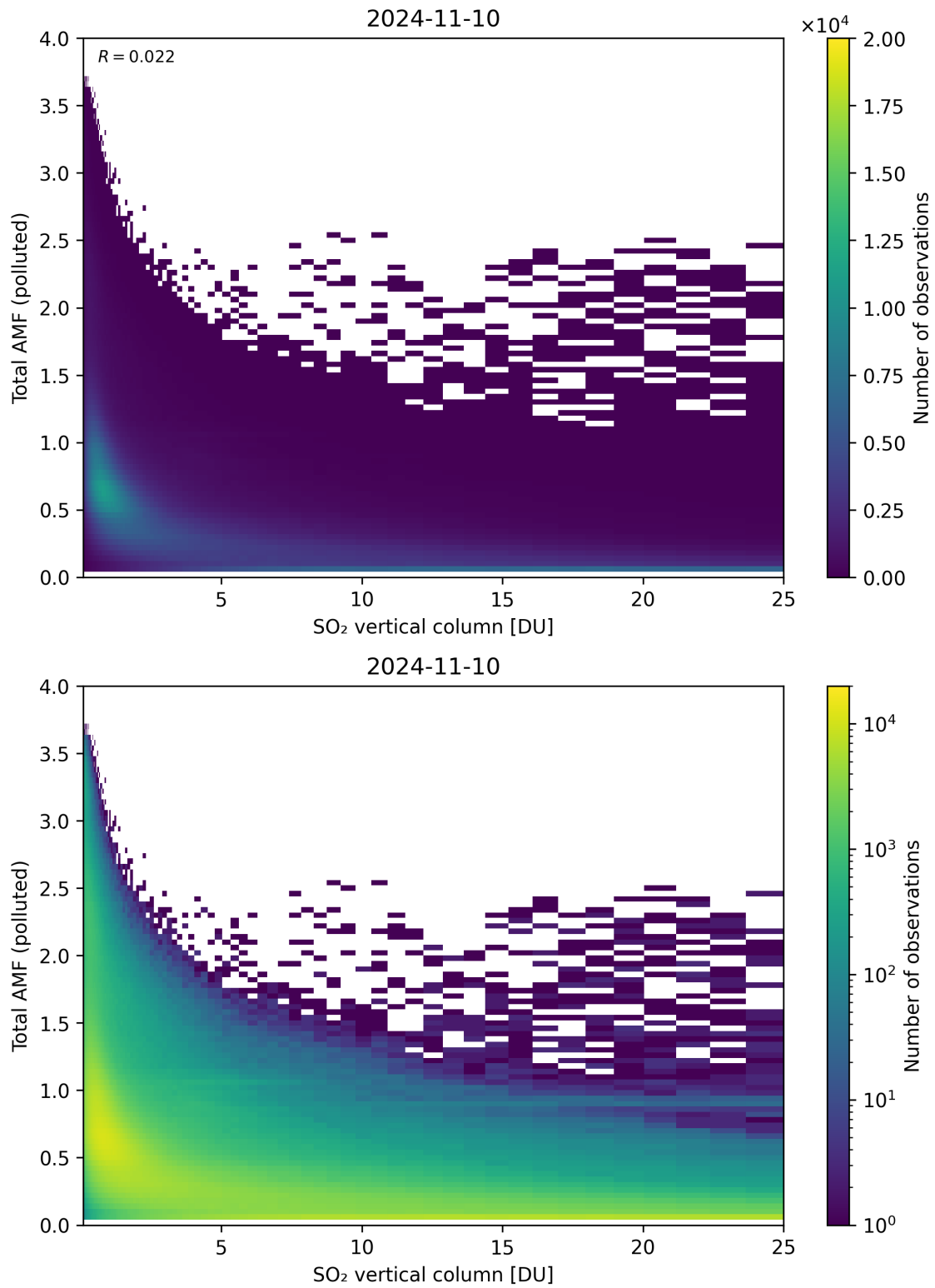
Figure 305: Scatter density plot of “SO 2 vertical column” against “Total AMF (polluted)” for 2024-11-09 to 2024-11-11.
