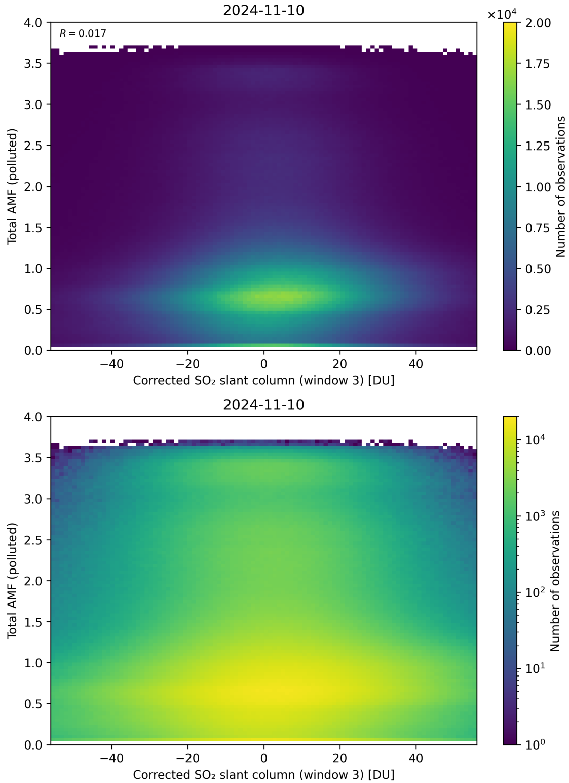
Figure 210: Scatter density plot of “Corrected SO 2 slant column (window 3)” against “Total AMF (polluted)” for 2024-11-09 to 2024-11-11.
