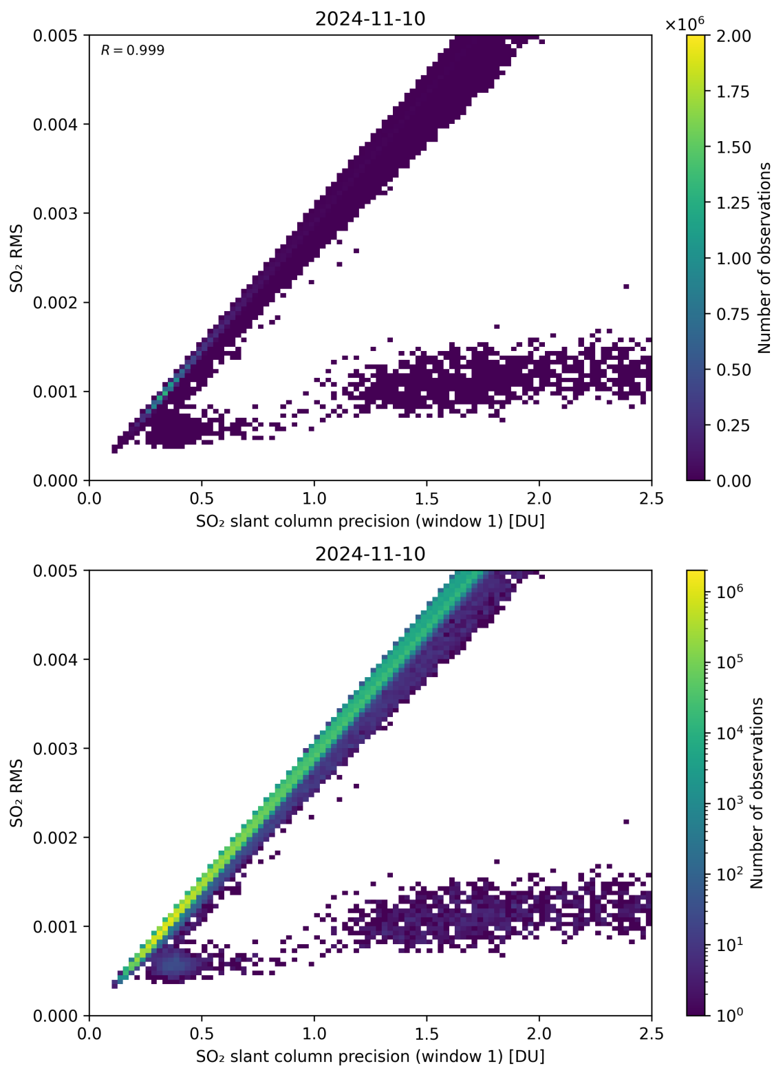
Figure 223: Scatter density plot of “SO 2 slant column precision (window 1)” against “SO 2 RMS” for 2024-11-09 to 2024-11-11.
