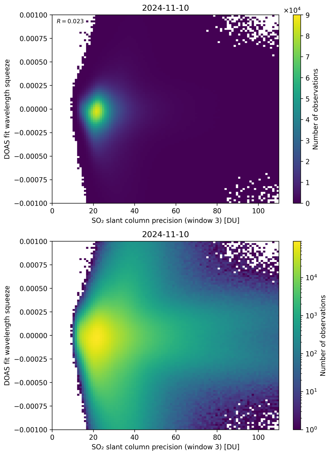
Figure 259: Scatter density plot of “SO 2 slant column precision (window 3)” against “DOAS fit wavelength squeeze” for 2024-11-09 to 2024-11-11.
