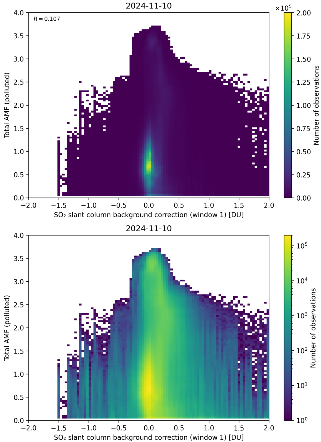
Figure 109: Scatter density plot of “SO 2 slant column background correction (window 1)” against “Total AMF (polluted)” for 2024-11-09 to 2024-11-11.
