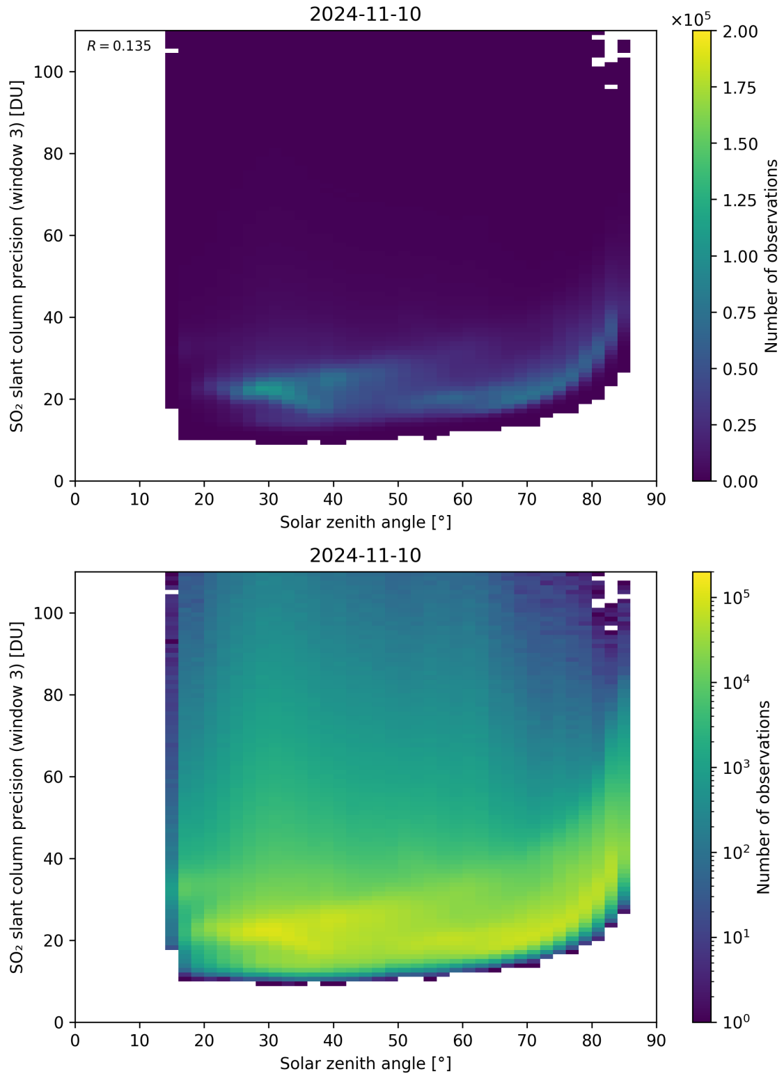
Figure 173: Scatter density plot of “Solar zenith angle” against “SO 2 slant column precision (window 3)” for 2024-11-09 to 2024-11-11.
