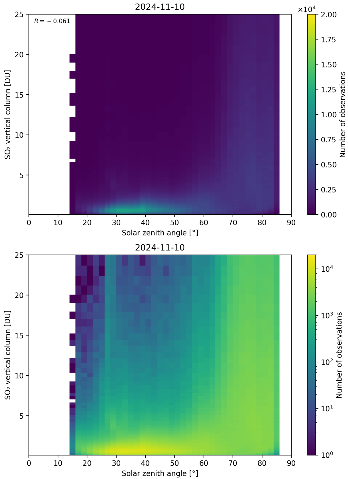
Figure 176: Scatter density plot of “Solar zenith angle” against “SO 2 vertical column” for 2024-11-09 to 2024-11-11.
