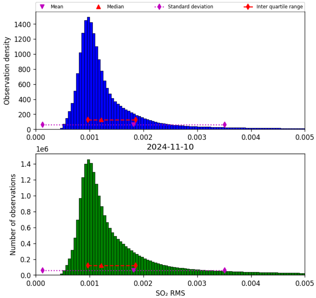
Figure 70: Histogram of “SO 2 RMS” for 2024-11-09 to 2024-11-11
