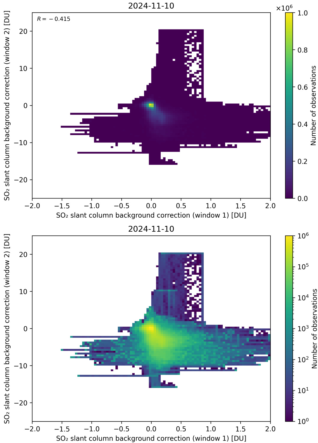
Figure 98: Scatter density plot of “SO 2 slant column background correction (window 1)” against “SO 2 slant column background correction (window 2)” for 2024-11-09 to 2024-11-11.
