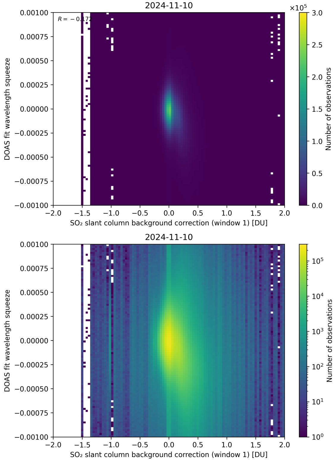
Figure 101: Scatter density plot of “SO 2 slant column background correction (window 1)” against “DOAS fit wavelength squeeze” for 2024-11-09 to 2024-11-11.
