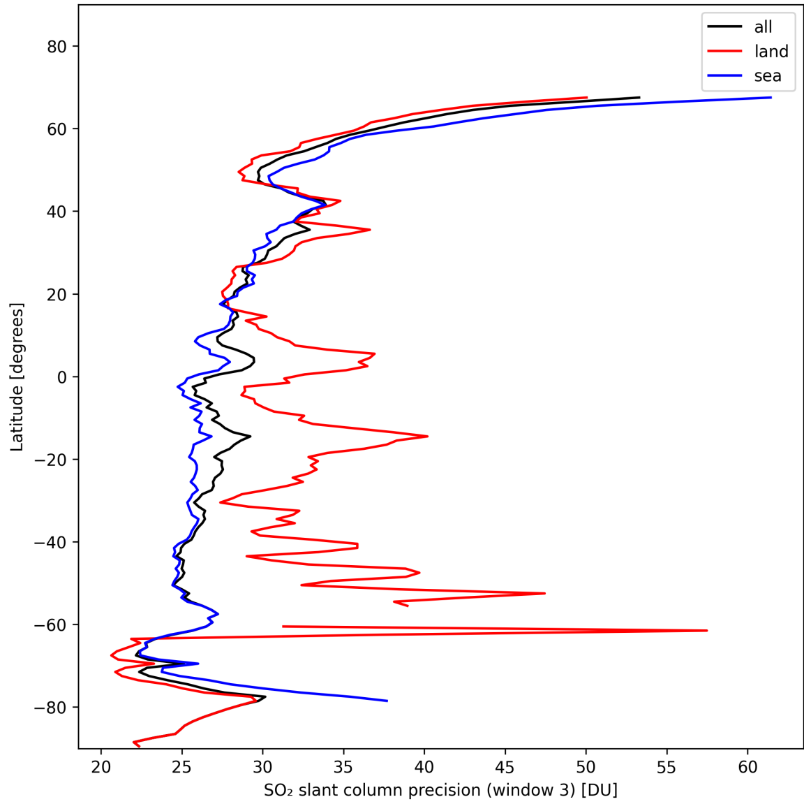
Figure 42: Zonal average of “SO 2 slant column precision (window 3)” for 2024-11-09 to 2024-11-11.
