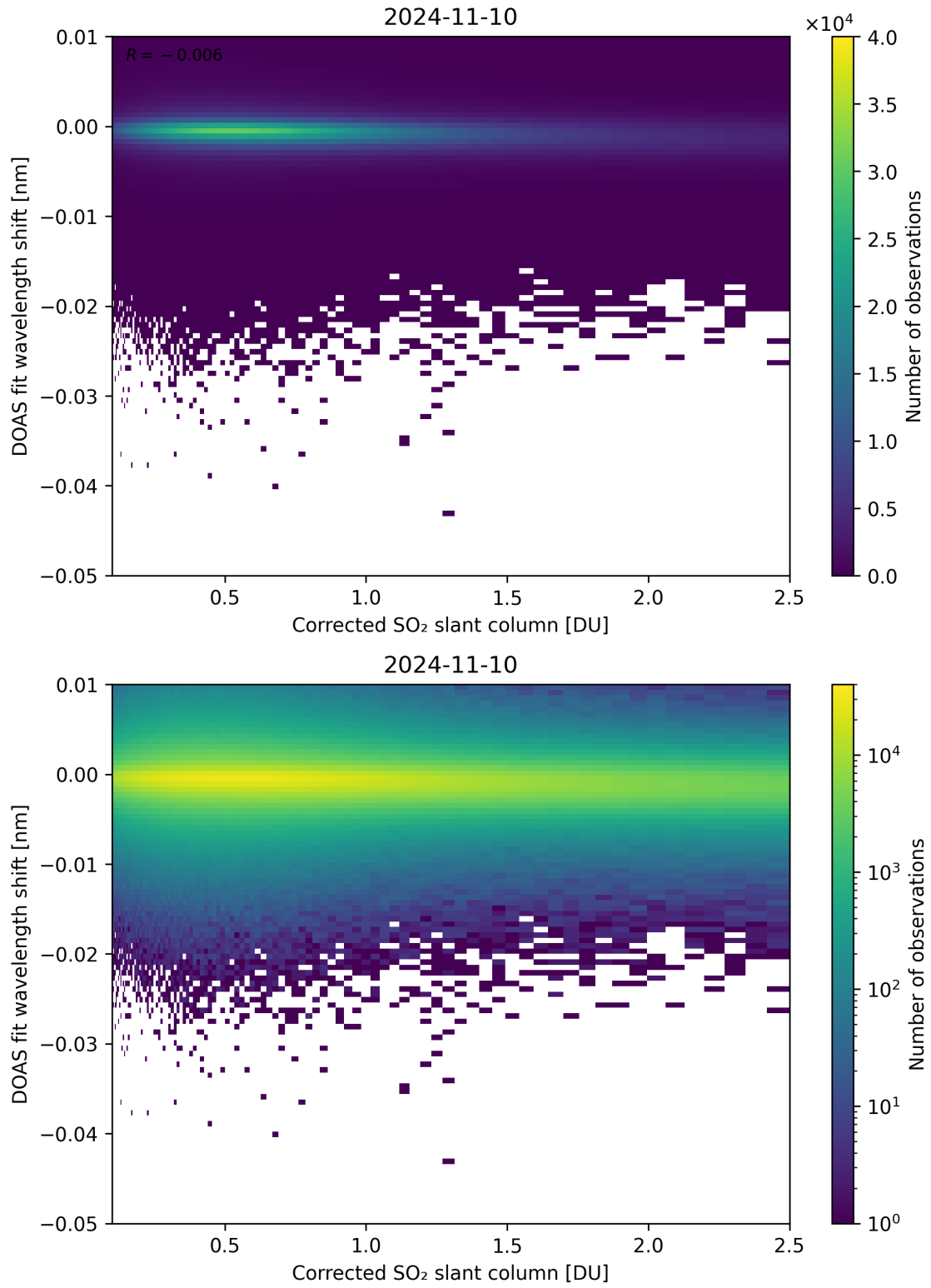
Figure 181: Scatter density plot of “Corrected SO 2 slant column” against “DOAS fit wavelength shift” for 2024-11-09 to 2024-11-11.
