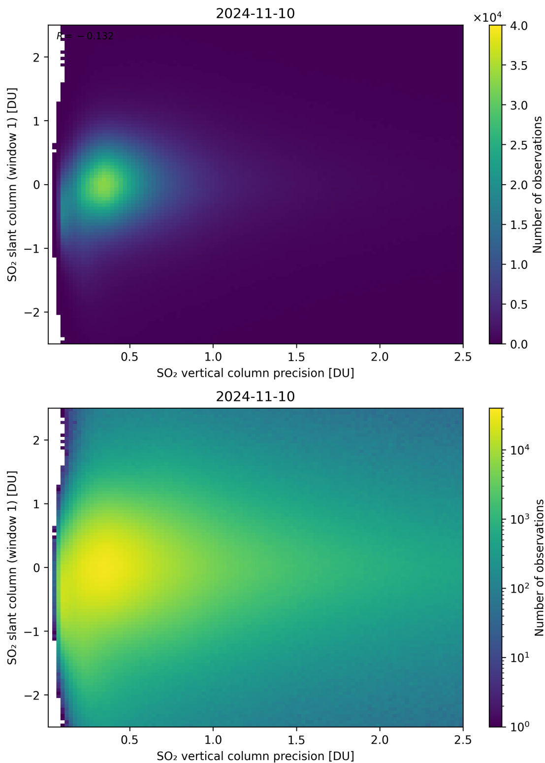
Figure 289: Scatter density plot of “SO 2 vertical column precision” against “SO 2 slant column (window 1)” for 2024-11-09 to 2024-11-11.
