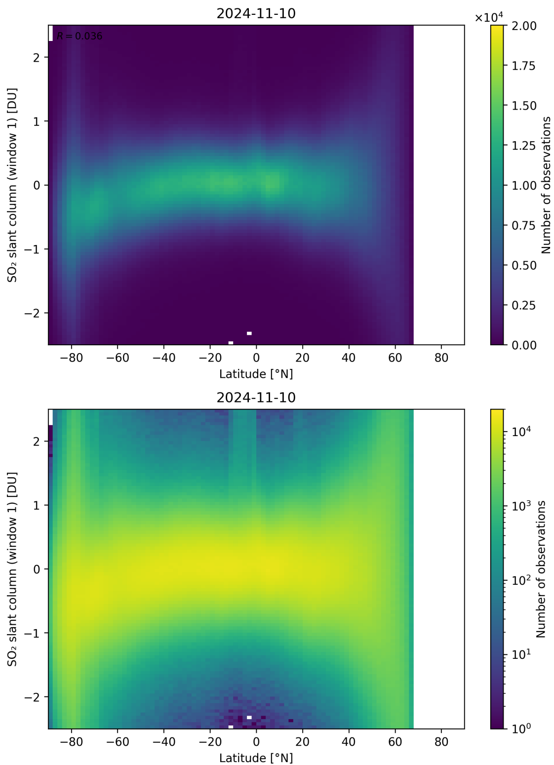
Figure 149: Scatter density plot of “Latitude” against “SO 2 slant column (window 1)” for 2024-11-09 to 2024-11-11.
