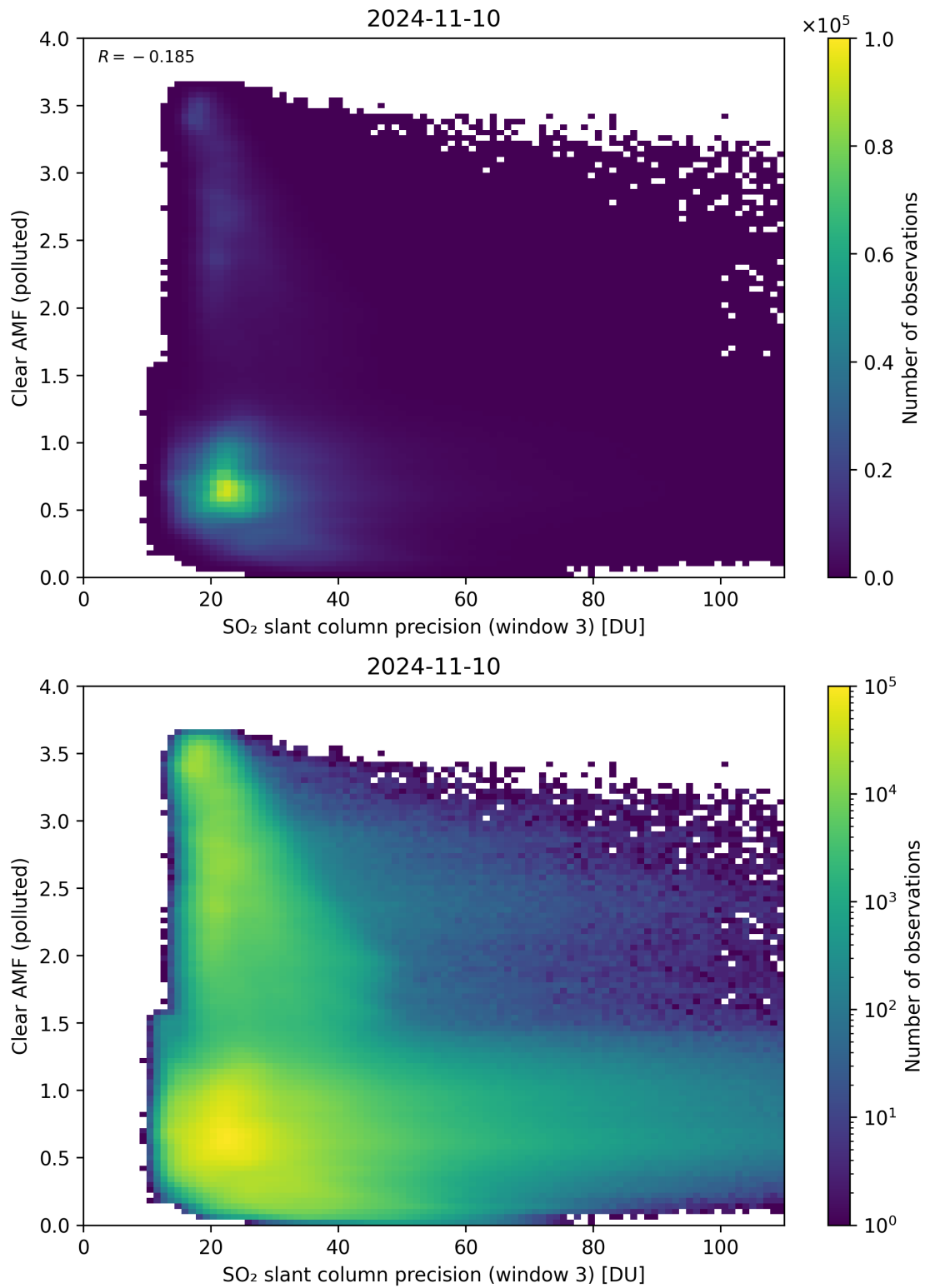
Figure 261: Scatter density plot of “SO 2 slant column precision (window 3)” against “Clear AMF (polluted)” for 2024-11-09 to 2024-11-11.
