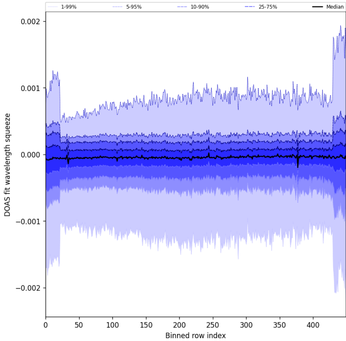
Figure 92: Along track statistics of “DOAS fit wavelength squeeze” for 2024-11-09 to 2024-11-11
