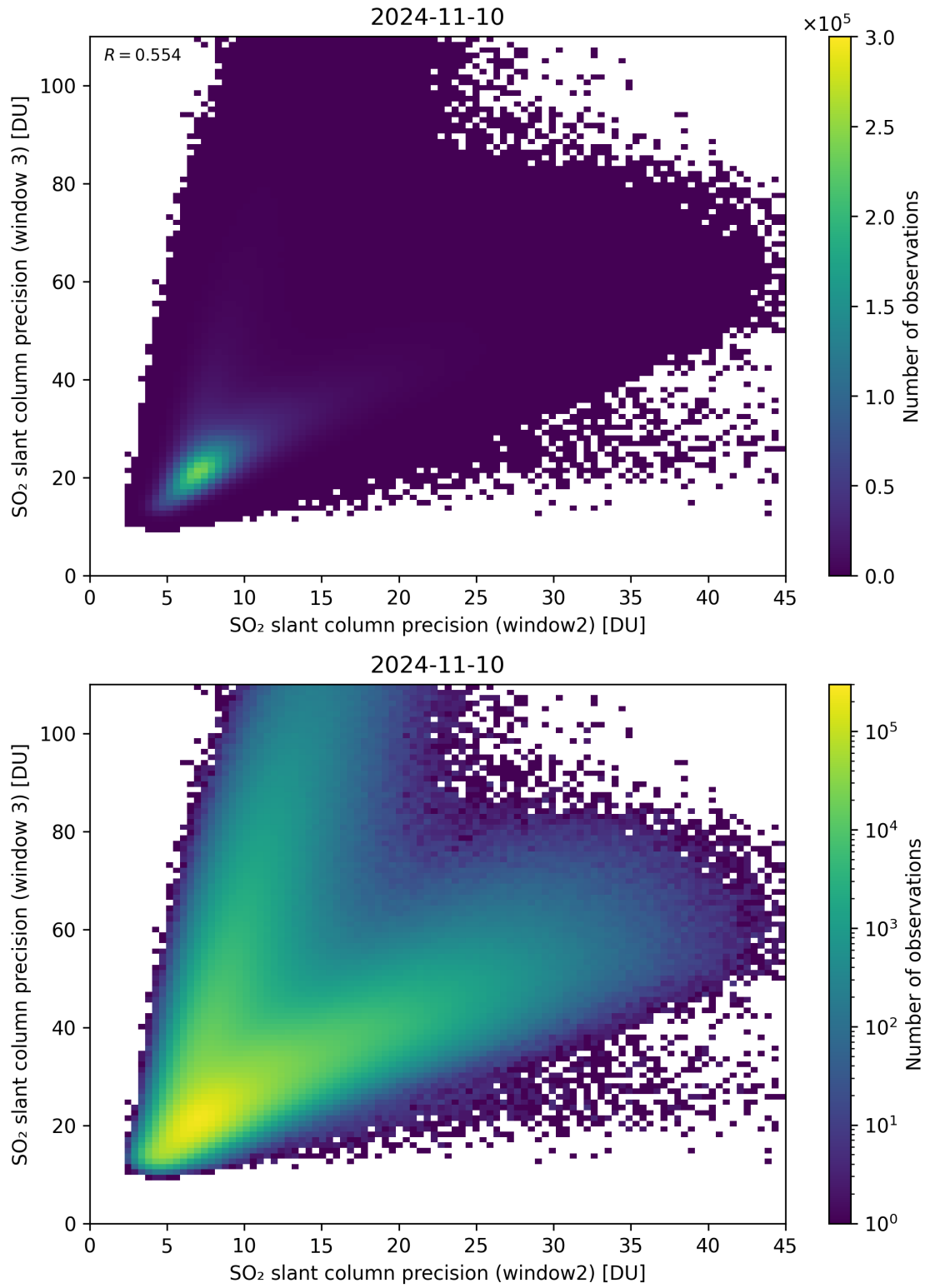
Figure 250: Scatter density plot of “SO 2 slant column precision (window2)” against “SO 2 slant column precision (window 3)” for 2024-11-09 to 2024-11-11.
