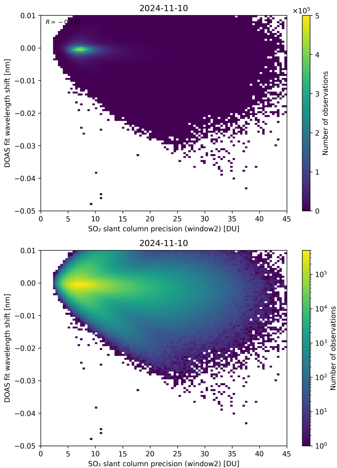
Figure 243: Scatter density plot of “SO 2 slant column precision (window2)” against “DOAS fit wavelength shift” for 2024-11-09 to 2024-11-11.
