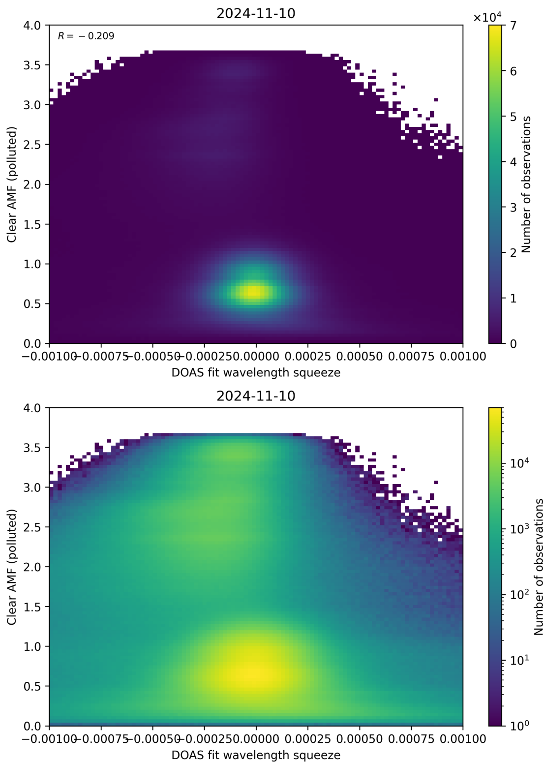
Figure 133: Scatter density plot of “DOAS fit wavelength squeeze” against “Clear AMF (polluted)” for 2024-11-09 to 2024-11-11.
