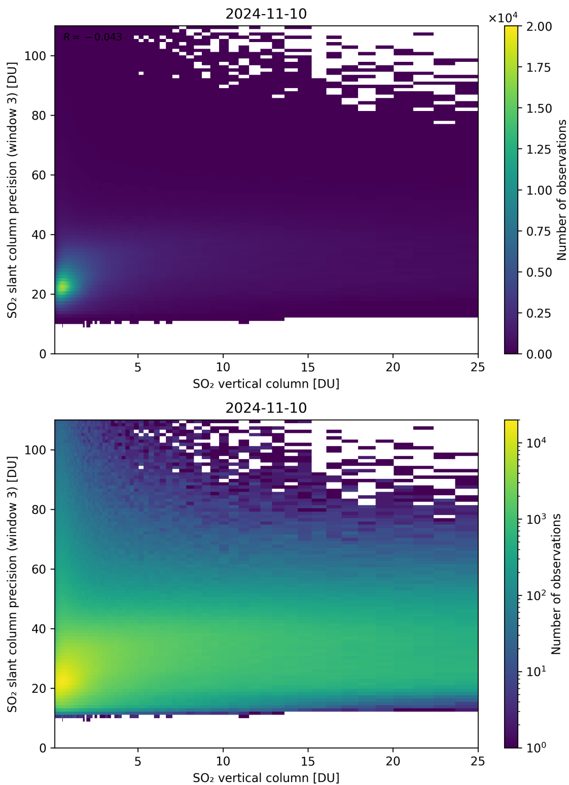
Figure 304: Scatter density plot of “SO 2 vertical column” against “SO 2 slant column precision (window 3)” for 2024-11-09 to 2024-11-11.
