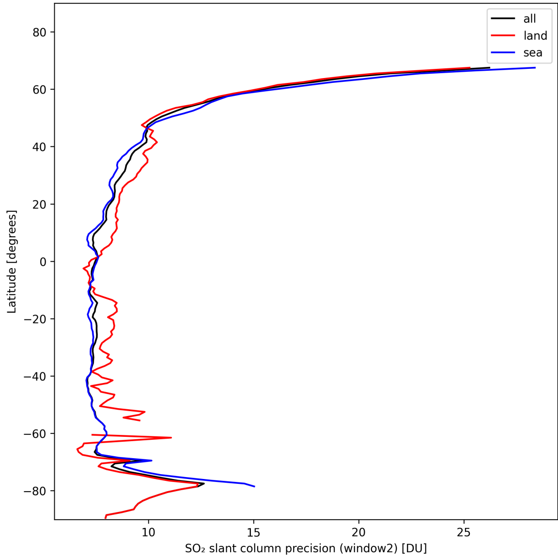
Figure 38: Zonal average of “SO 2 slant column precision (window2)” for 2024-11-09 to 2024-11-11.
