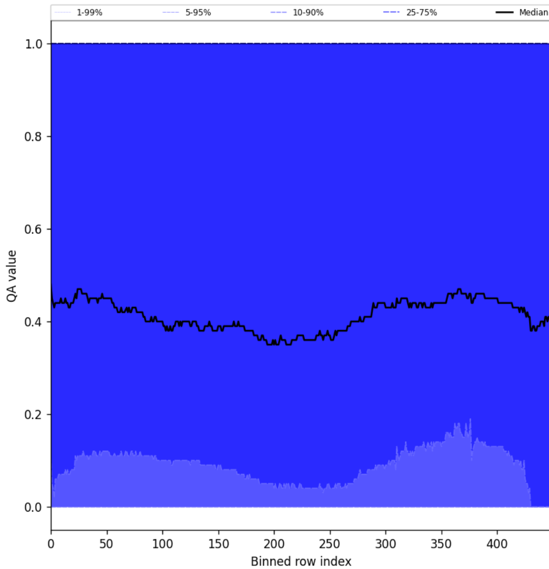
Figure 75: Along track statistics of “QA value” for 2024-11-09 to 2024-11-11
