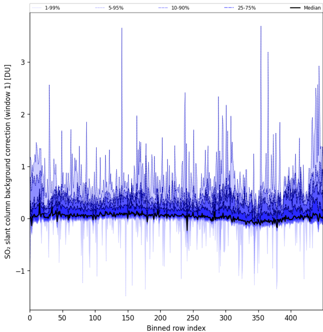
Figure 82: Along track statistics of “SO 2 slant column background correction (window 1)” for 2024-11-09 to 2024-11-11
