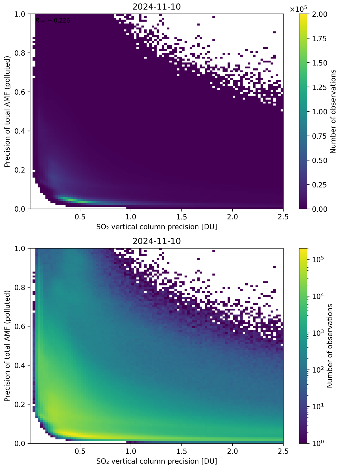
Figure 295: Scatter density plot of “SO 2 vertical column precision” against “Precision of total AMF (polluted)” for 2024-11-09 to 2024-11-11.
