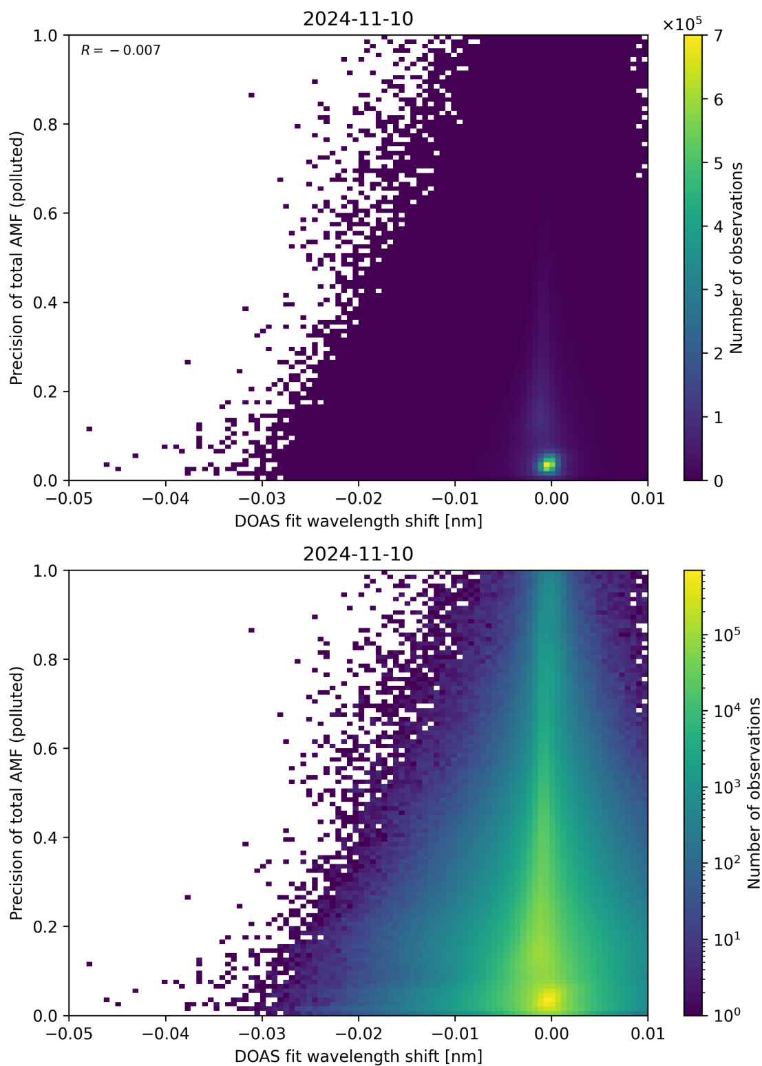
Figure 131: Scatter density plot of “DOAS fit wavelength shift” against “Precision of total AMF (polluted)” for 2024-11-09 to 2024-11-11.
