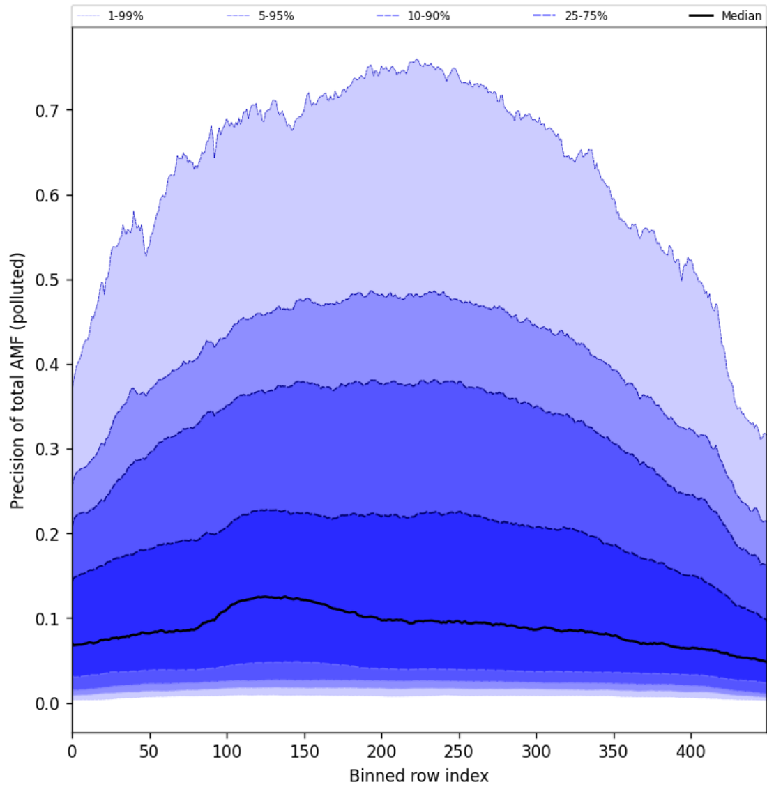
Figure 95: Along track statistics of “Precision of total AMF (polluted)” for 2024-11-09 to 2024-11-11
