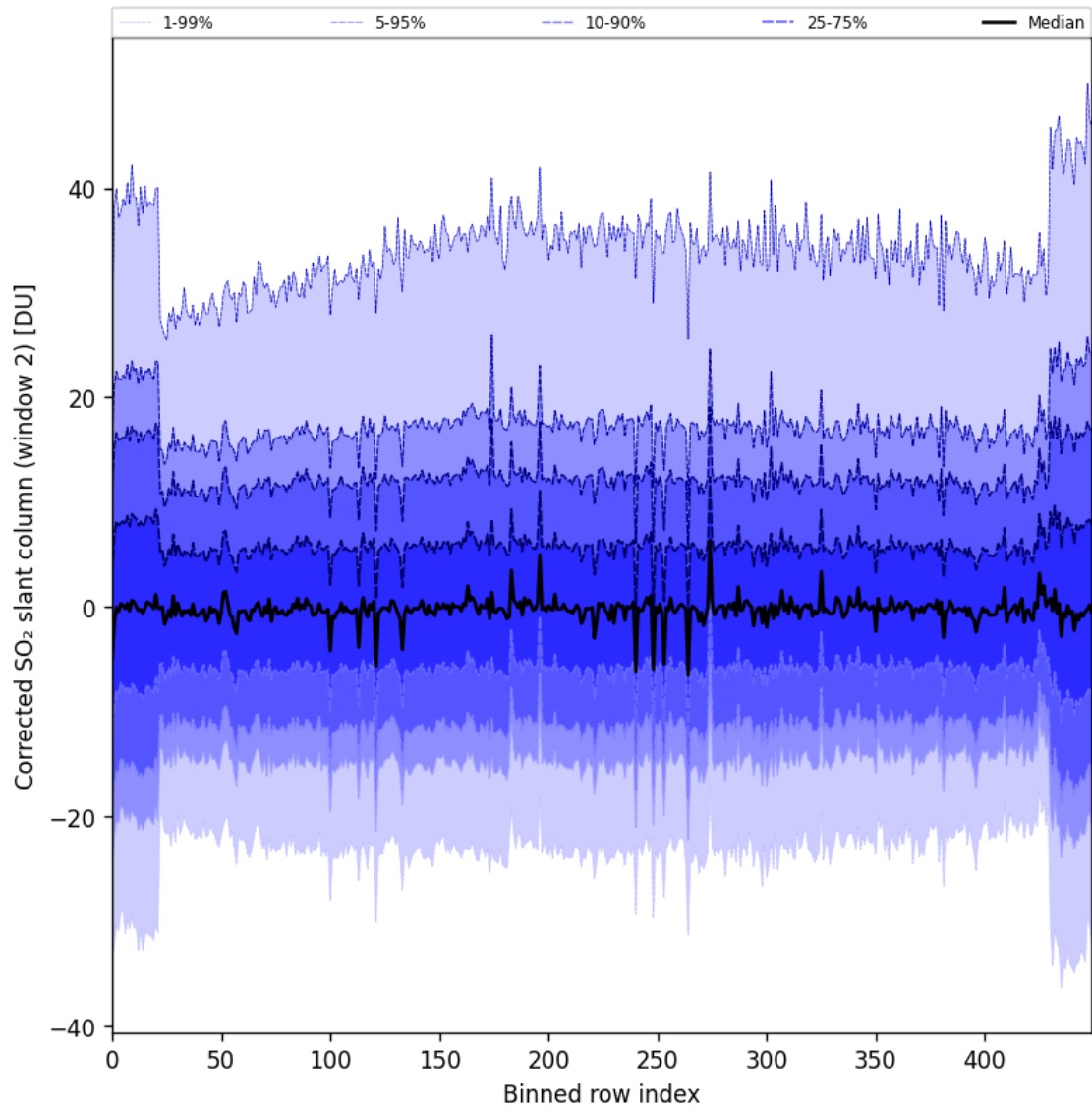
Figure 85: Along track statistics of “Corrected SO 2 slant column (window 2)” for 2024-11-09 to 2024-11-11
