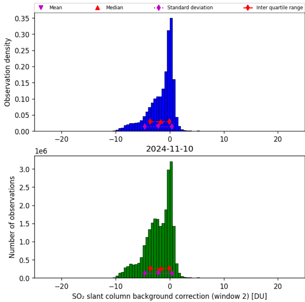
Figure 63: Histogram of “SO 2 slant column background correction (window 2)” for 2024-11-09 to 2024-11-11
