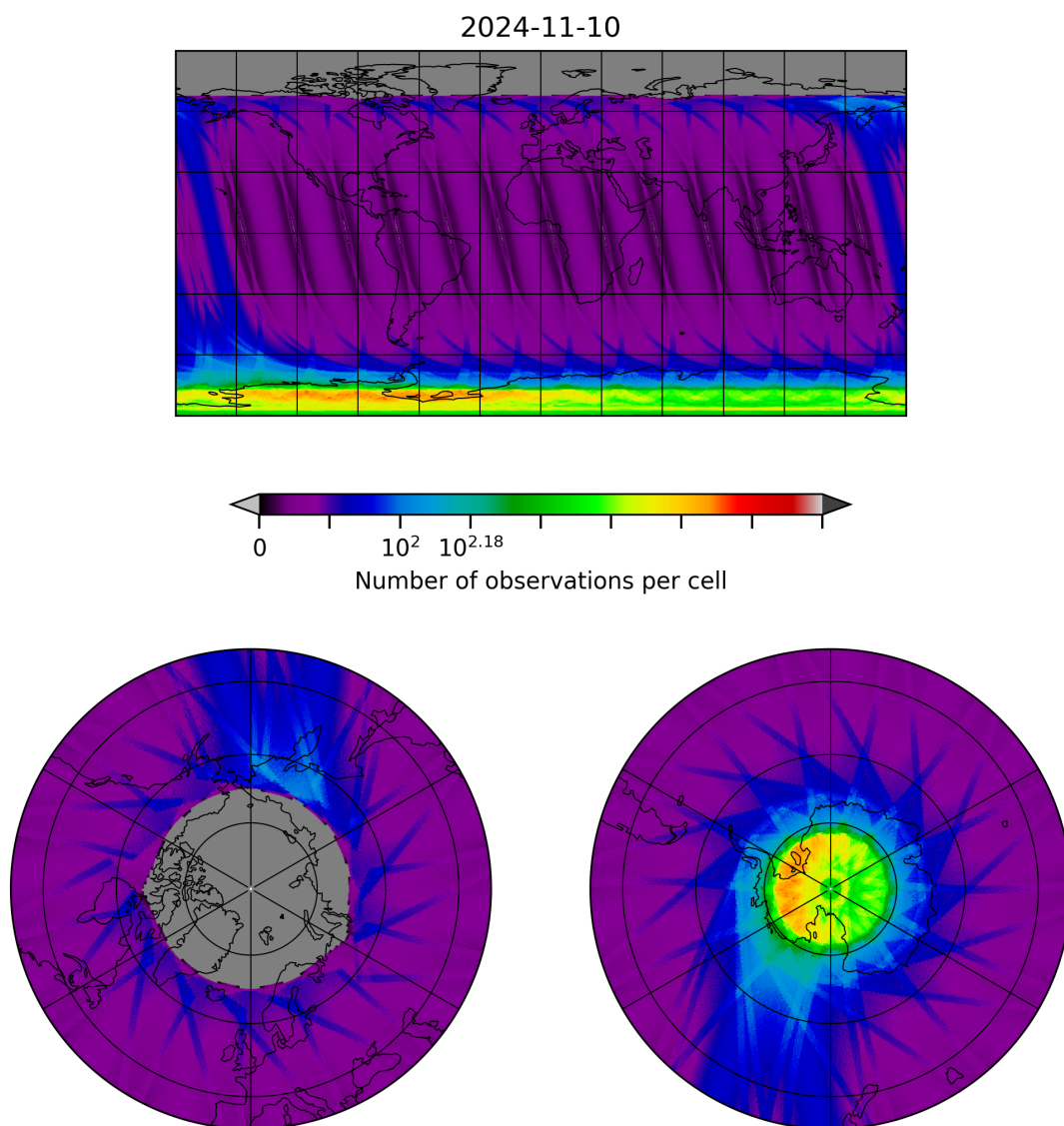
Figure 28: Map of the number of observations for 2024-11-09 to 2024-11-11
