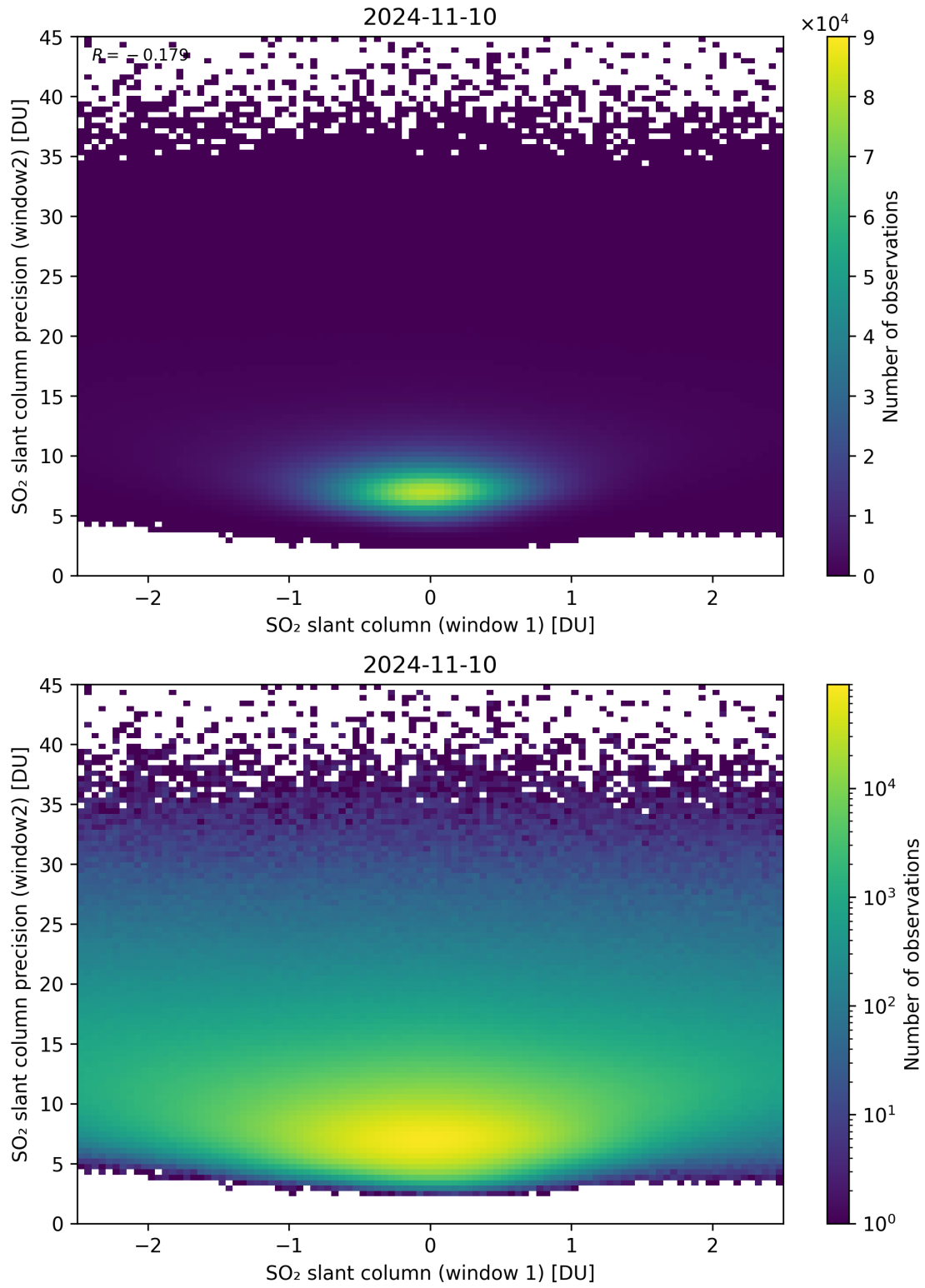
Figure 236: Scatter density plot of “SO 2 slant column (window 1)” against “SO 2 slant column precision (window2)” for 2024-11-09 to 2024-11-11.
