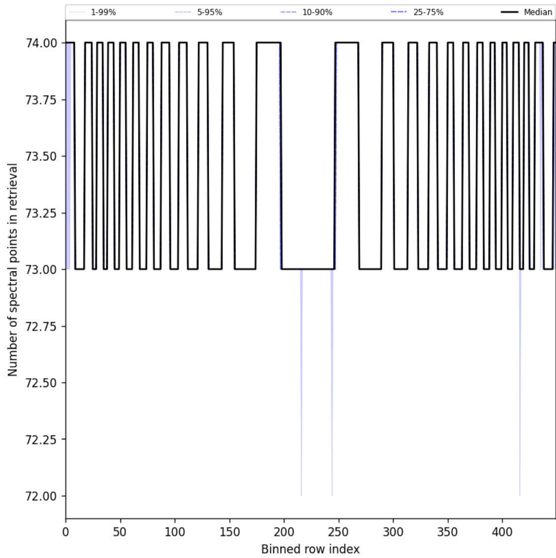
Figure 97: Along track statistics of “Number of spectral points in retrieval” for 2024-11-09 to 2024-11-11
