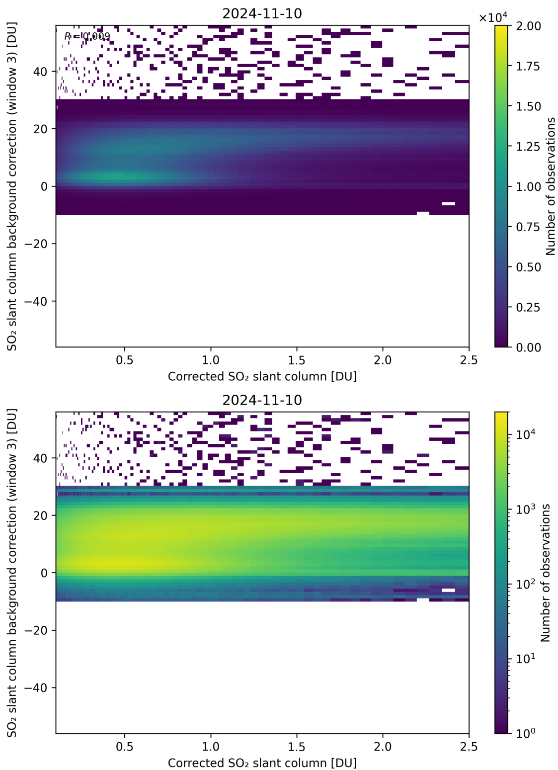
Figure 180: Scatter density plot of “Corrected SO 2 slant column” against “SO 2 slant column background correction (window 3)” for 2024-11-09 to 2024-11-11.
