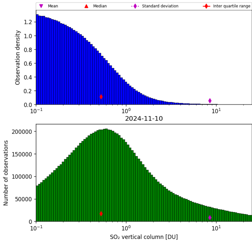
Figure 53: Histogram of “SO 2 vertical column” for 2024-11-09 to 2024-11-11
