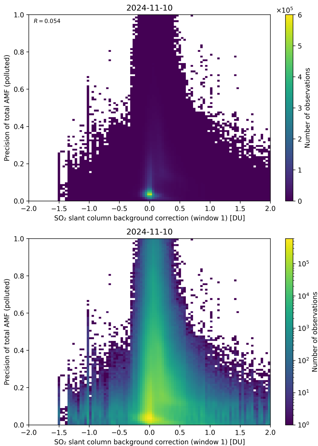
Figure 110: Scatter density plot of “SO 2 slant column background correction (window 1)” against “Precision of total AMF (polluted)” for 2024-11-09 to 2024-11-11.
