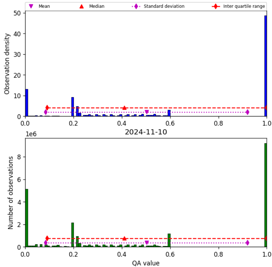
Figure 52: Histogram of “QA value” for 2024-11-09 to 2024-11-11
