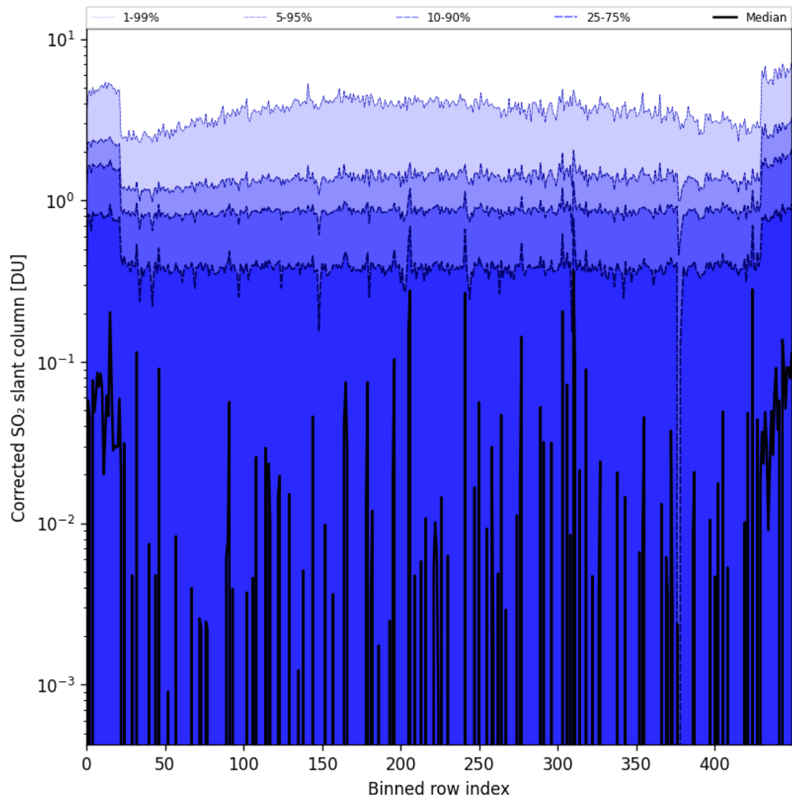
Figure 78: Along track statistics of “Corrected SO 2 slant column” for 2024-11-09 to 2024-11-11
