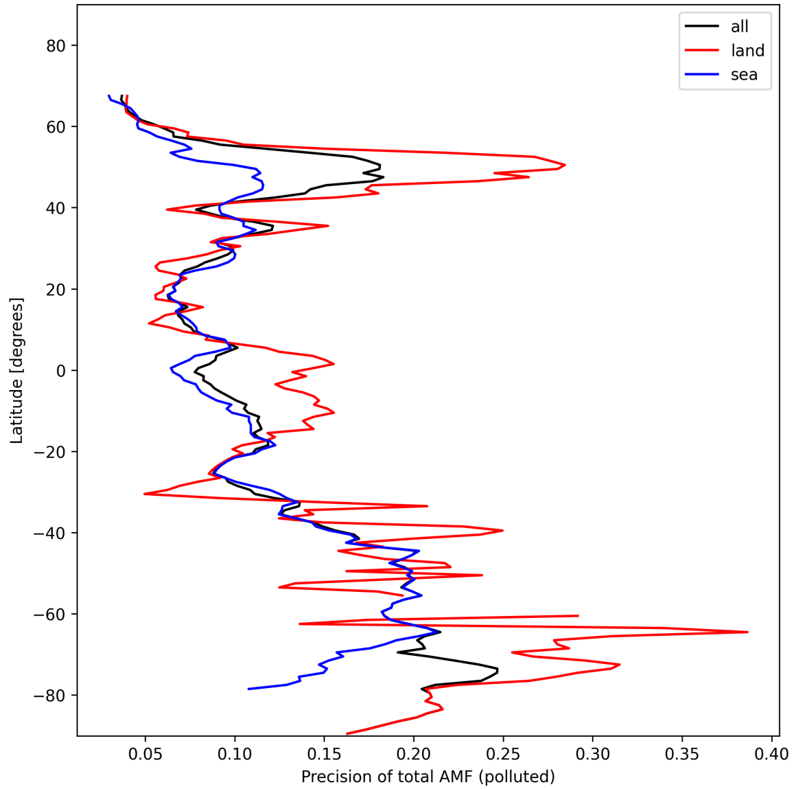
Figure 49: Zonal average of “Precision of total AMF (polluted)” for 2024-11-09 to 2024-11-11.
