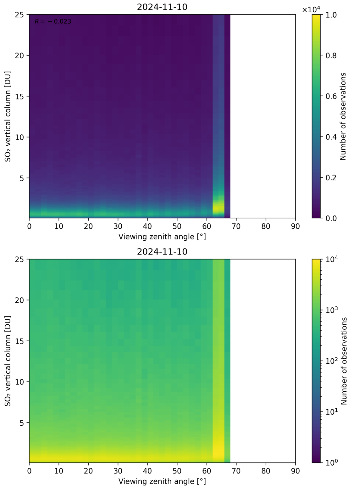
Figure 327: Scatter density plot of “Viewing zenith angle” against “SO 2 vertical column” for 2024-11-09 to 2024-11-11.
