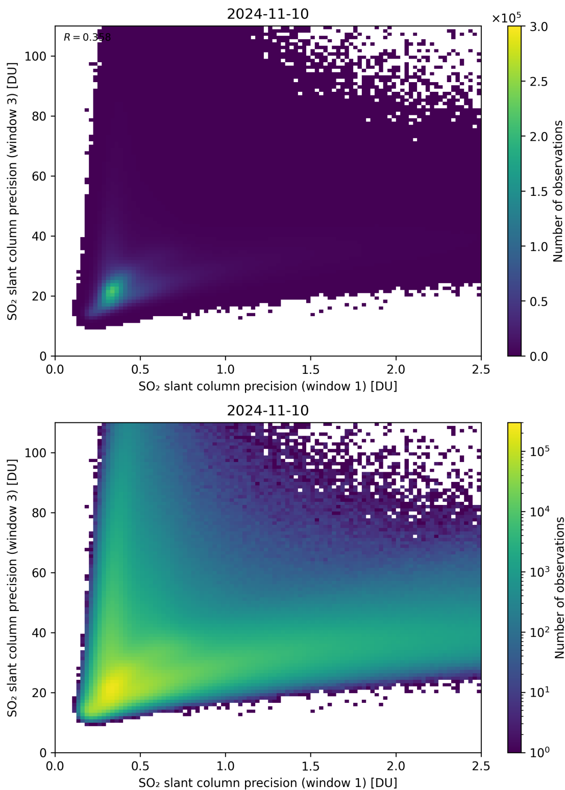
Figure 229: Scatter density plot of “SO 2 slant column precision (window 1)” against “SO 2 slant column precision (window 3)” for 2024-11-09 to 2024-11-11.
