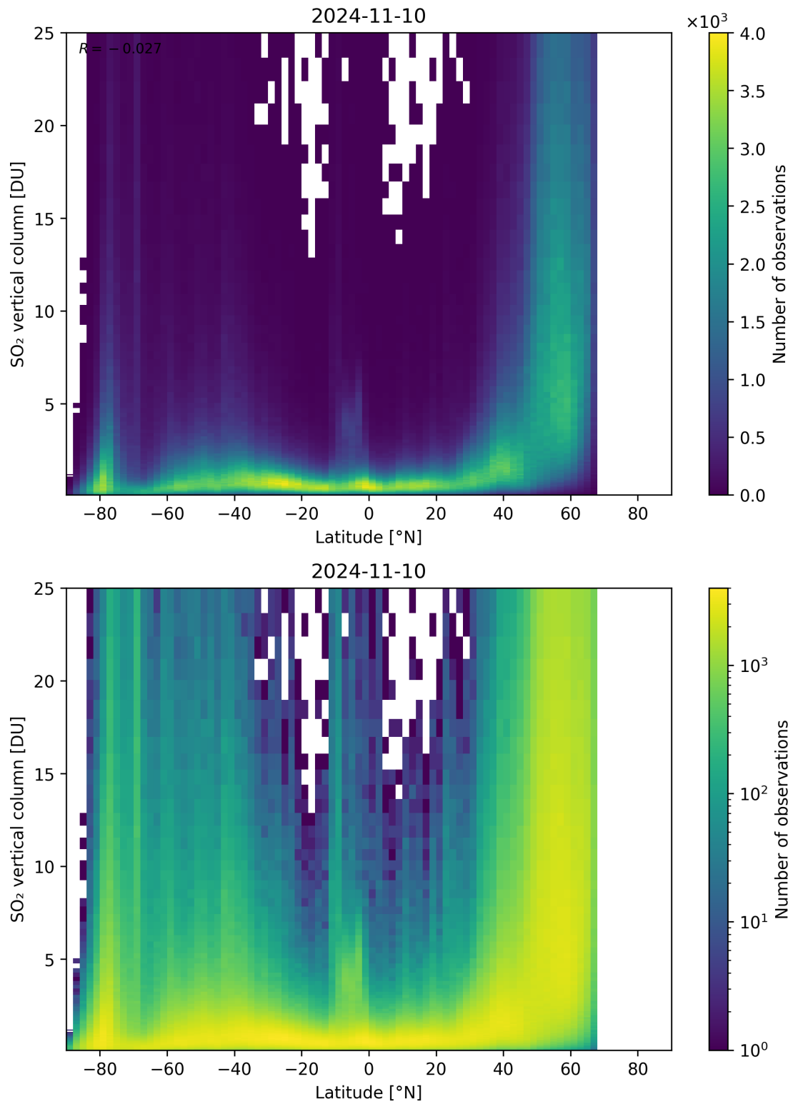
Figure 156: Scatter density plot of “Latitude” against “SO 2 vertical column” for 2024-11-09 to 2024-11-11.
