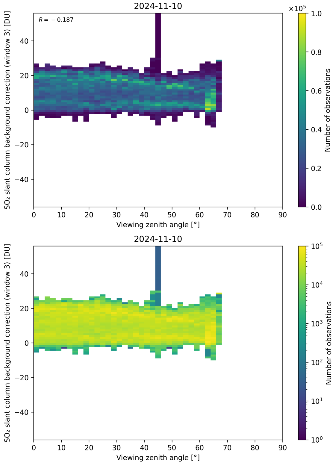
Figure 310: Scatter density plot of “Viewing zenith angle” against “SO 2 slant column background correction (window 3)” for 2024-11-09 to 2024-11-11.
