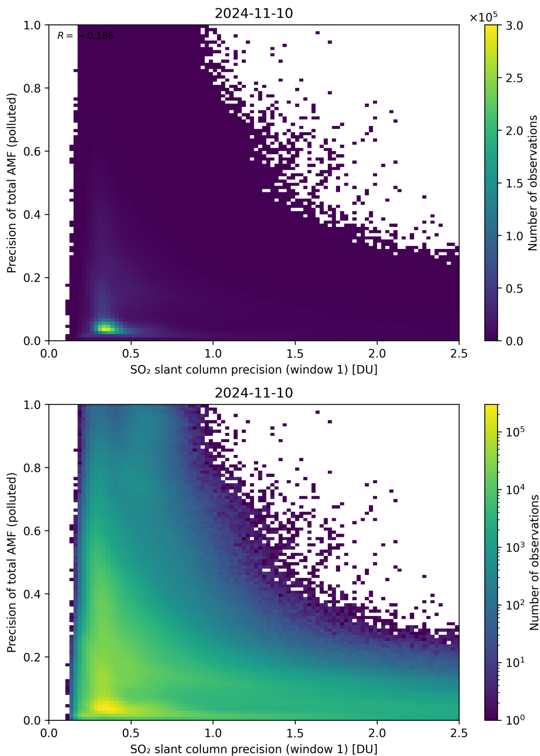
Figure 231: Scatter density plot of “SO 2 slant column precision (window 1)” against “Precision of total AMF (polluted)” for 2024-11-09 to 2024-11-11.
