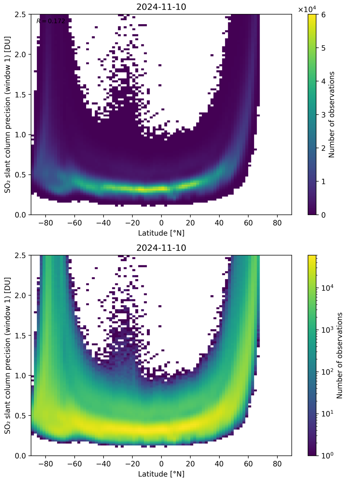
Figure 150: Scatter density plot of “Latitude” against “SO 2 slant column precision (window 1)” for 2024-11-09 to 2024-11-11.
