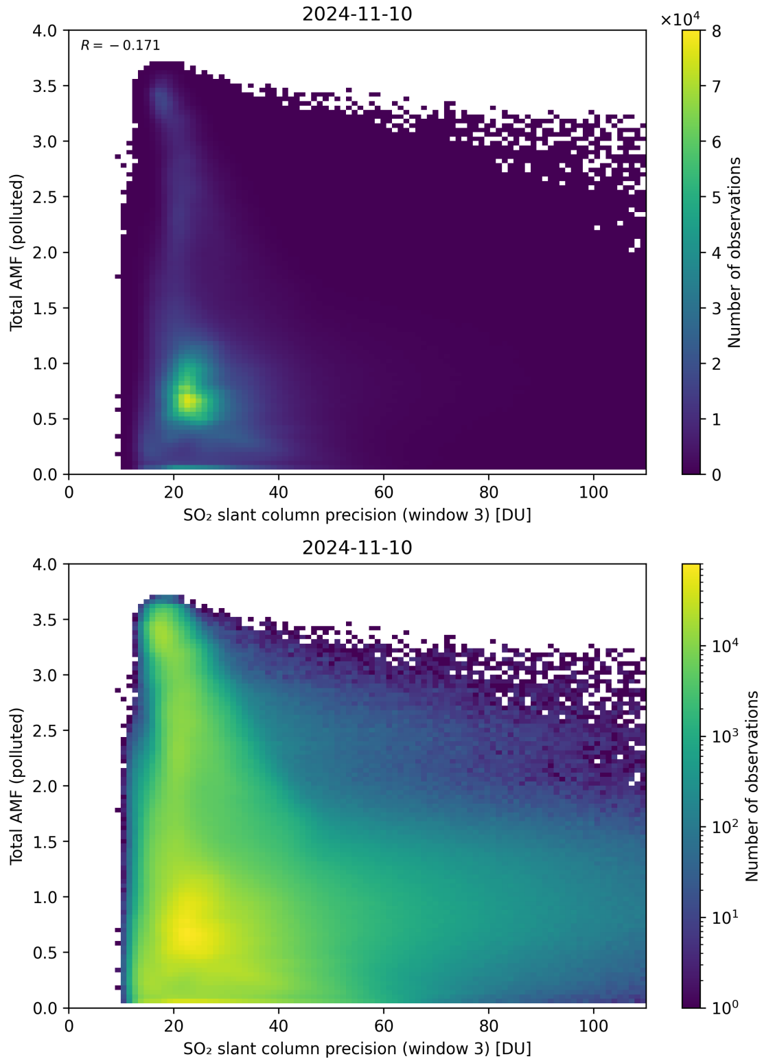
Figure 263: Scatter density plot of “SO 2 slant column precision (window 3)” against “Total AMF (polluted)” for 2024-11-09 to 2024-11-11.
