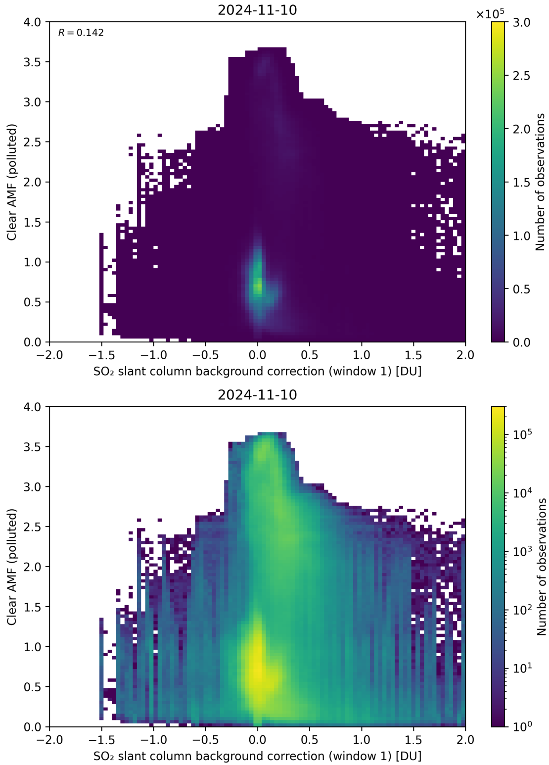
Figure 103: Scatter density plot of “SO 2 slant column background correction (window 1)” against “Clear AMF (polluted)” for 2024-11-09 to 2024-11-11.
