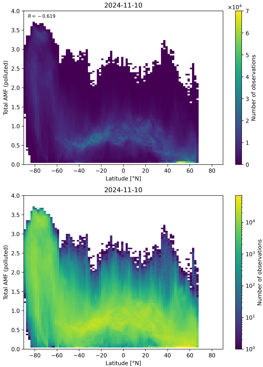
Figure 154: Scatter density plot of “Latitude” against “Total AMF (polluted)” for 2024-11-09 to 2024-11-11.
