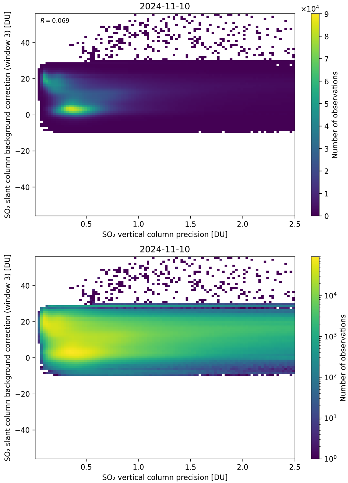
Figure 281: Scatter density plot of “SO 2 vertical column precision” against “SO 2 slant column background correction (window 3)” for 2024-11-09 to 2024-11-11.
