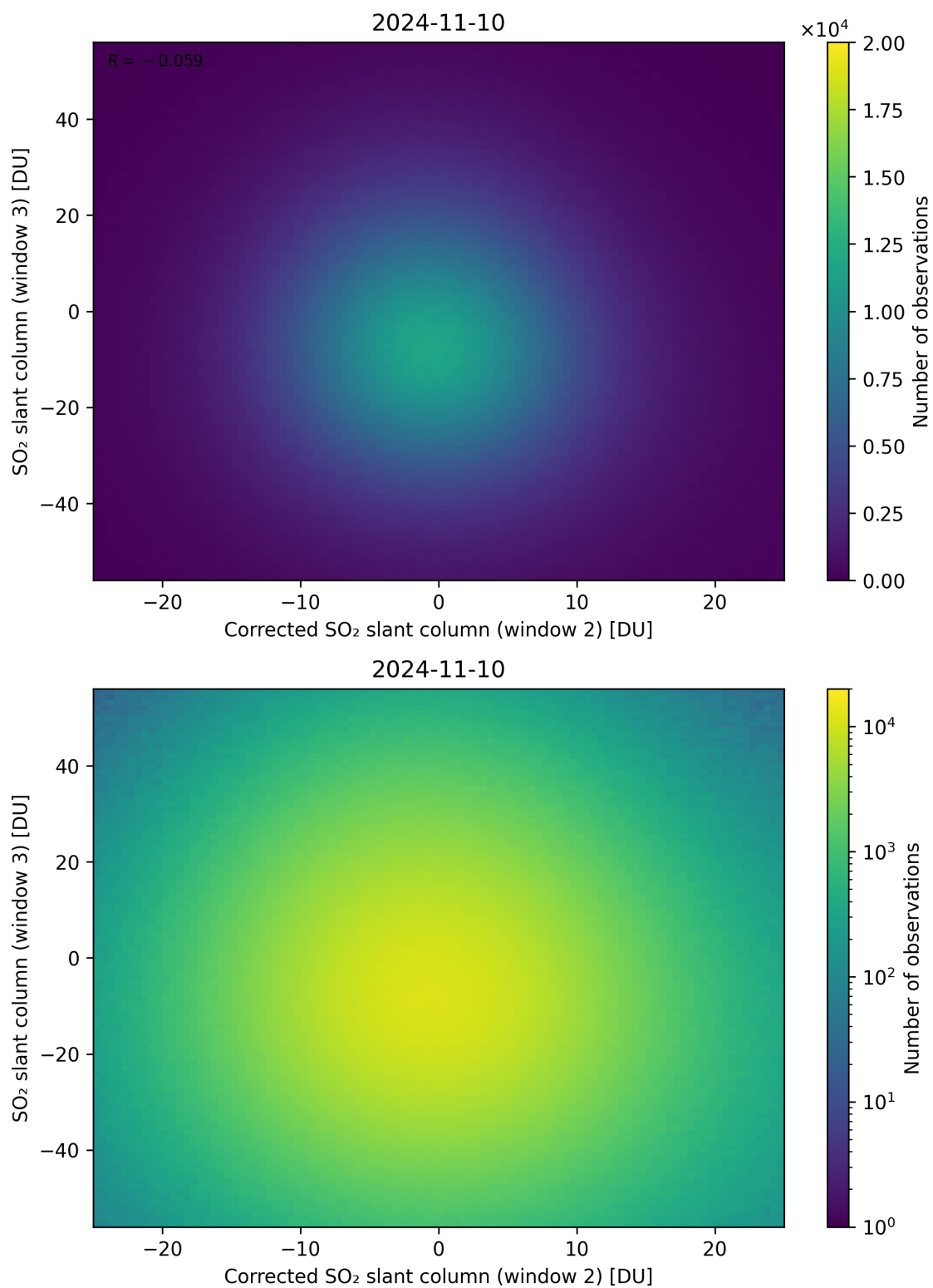
Figure 201: Scatter density plot of “Corrected SO 2 slant column (window 2)” against “SO 2 slant column (window 3)” for 2024-11-09 to 2024-11-11.
