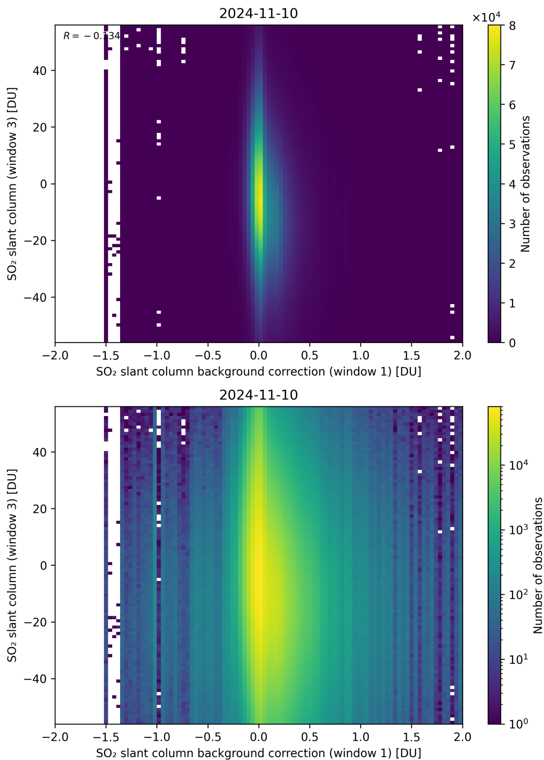
Figure 107: Scatter density plot of “SO 2 slant column background correction (window 1)” against “SO 2 slant column (window 3)” for 2024-11-09 to 2024-11-11.
