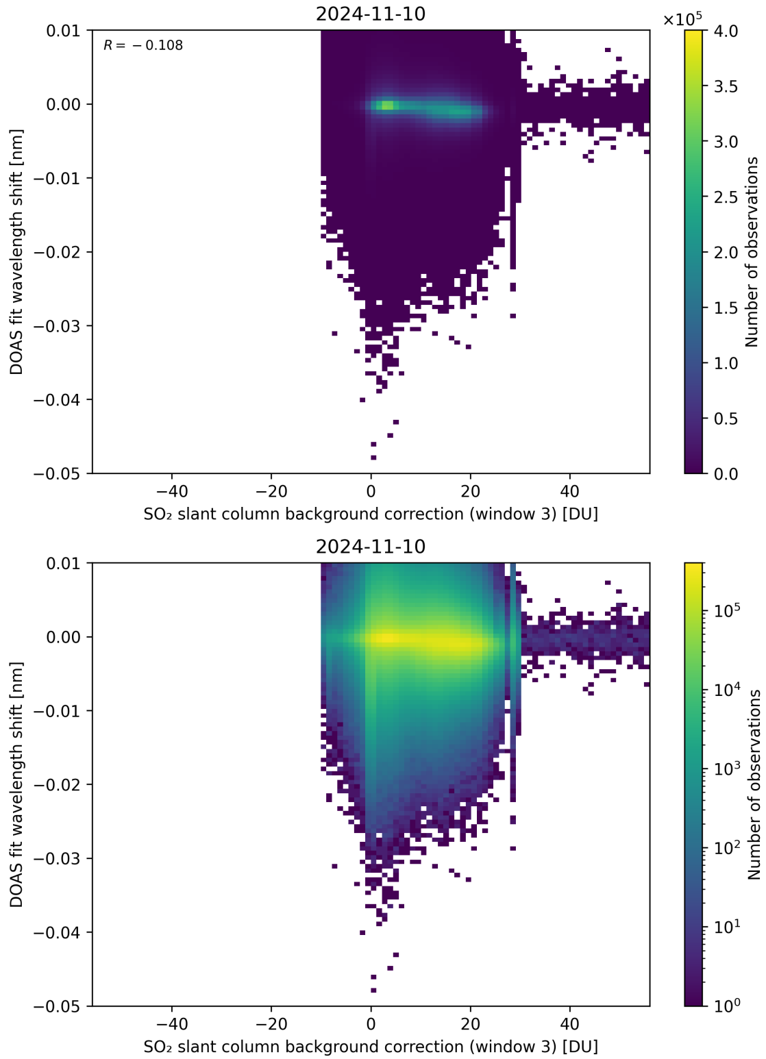
Figure 121: Scatter density plot of “SO 2 slant column background correction (window 3)” against “DOAS fit wavelength shift” for 2024-11-09 to 2024-11-11.
