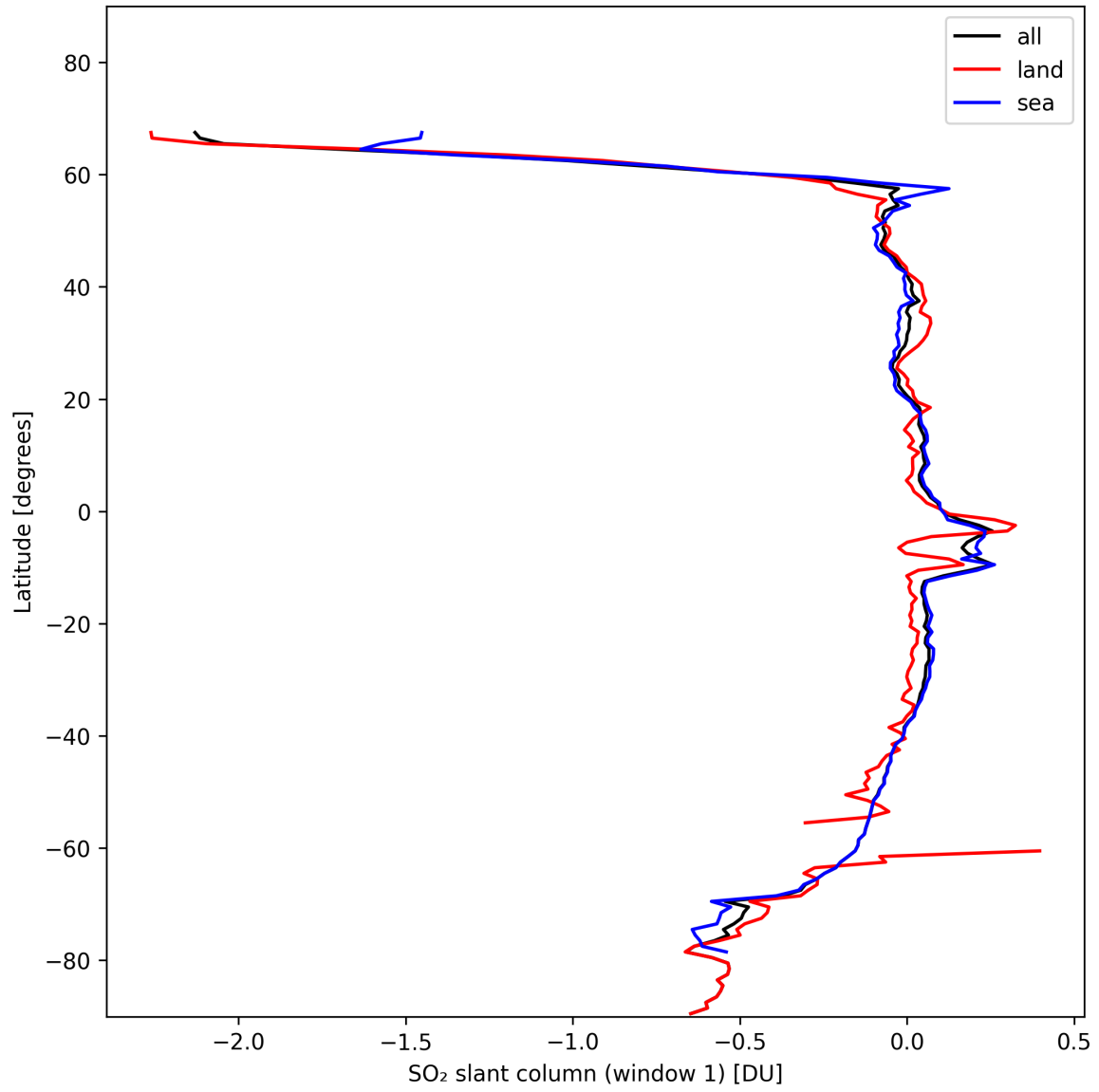
Figure 33: Zonal average of “SO 2 slant column (window 1)” for 2024-11-09 to 2024-11-11.
