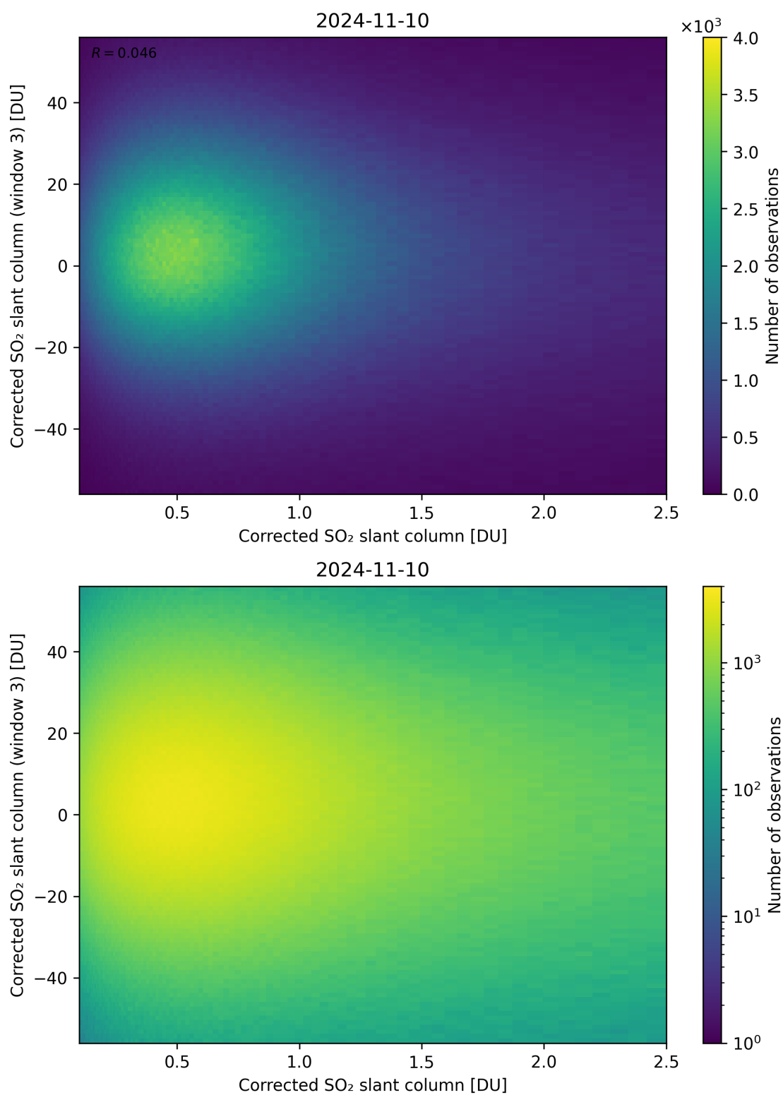
Figure 186: Scatter density plot of “Corrected SO 2 slant column” against “Corrected SO 2 slant column (window 3)” for 2024-11-09 to 2024-11-11.
