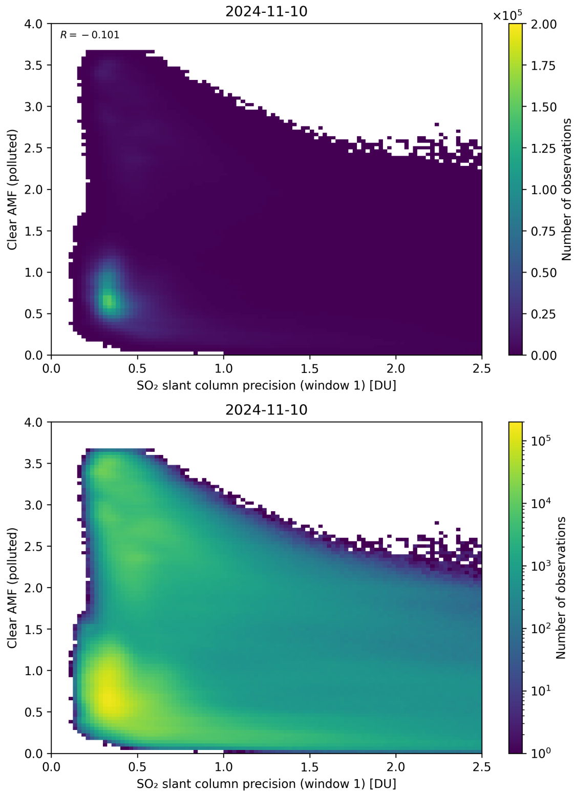
Figure 224: Scatter density plot of “SO 2 slant column precision (window 1)” against “Clear AMF (polluted)” for 2024-11-09 to 2024-11-11.
