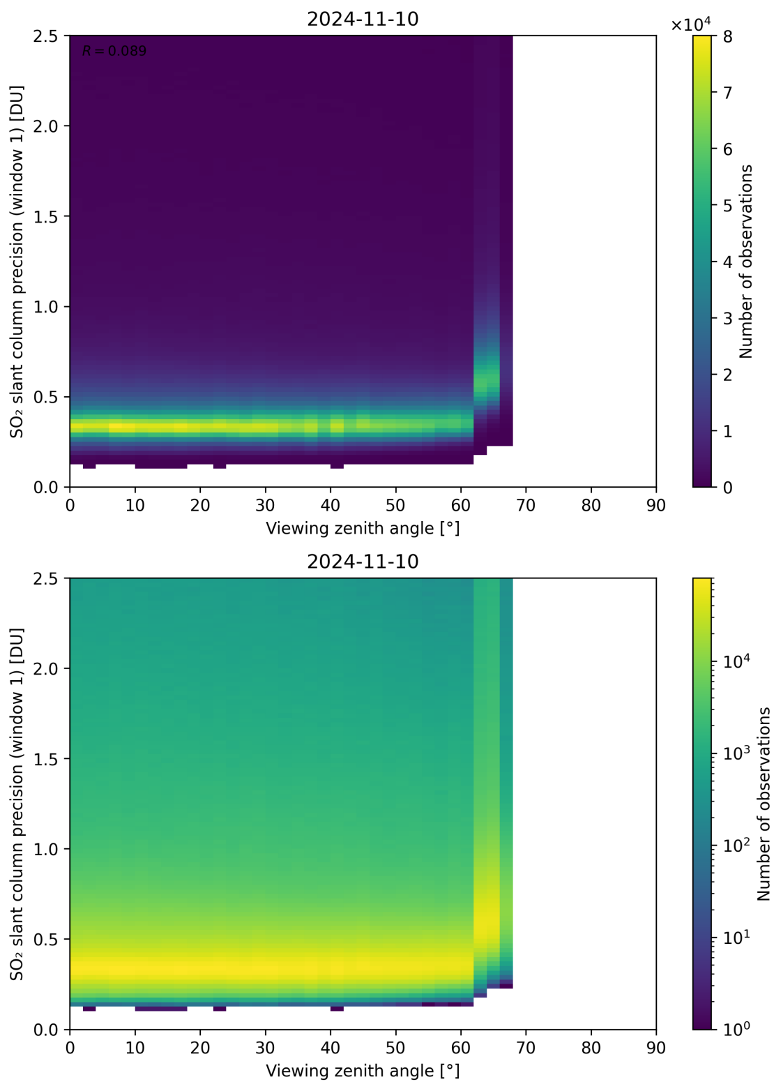
Figure 321: Scatter density plot of “Viewing zenith angle” against “SO 2 slant column precision (window 1)” for 2024-11-09 to 2024-11-11.
