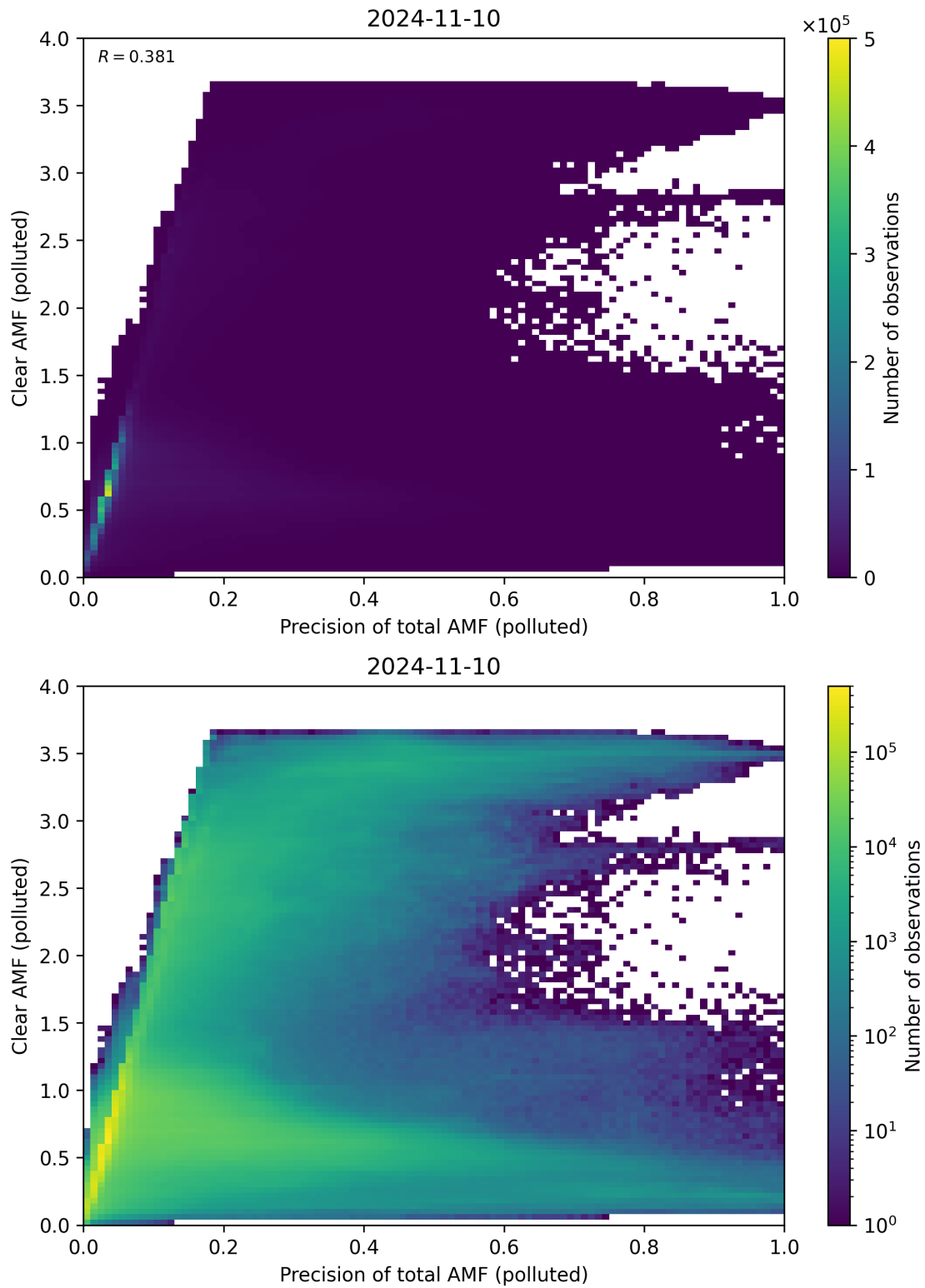
Figure 270: Scatter density plot of “Precision of total AMF (polluted)” against “Clear AMF (polluted)” for 2024-11-09 to 2024-11-11.
