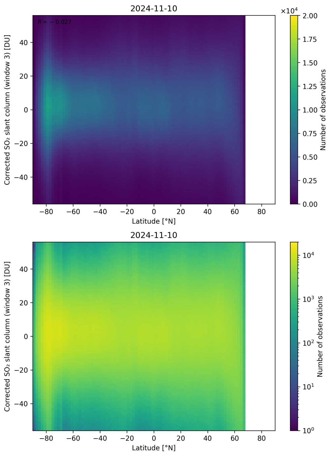
Figure 148: Scatter density plot of “Latitude” against “Corrected SO 2 slant column (window 3)” for 2024-11-09 to 2024-11-11.
