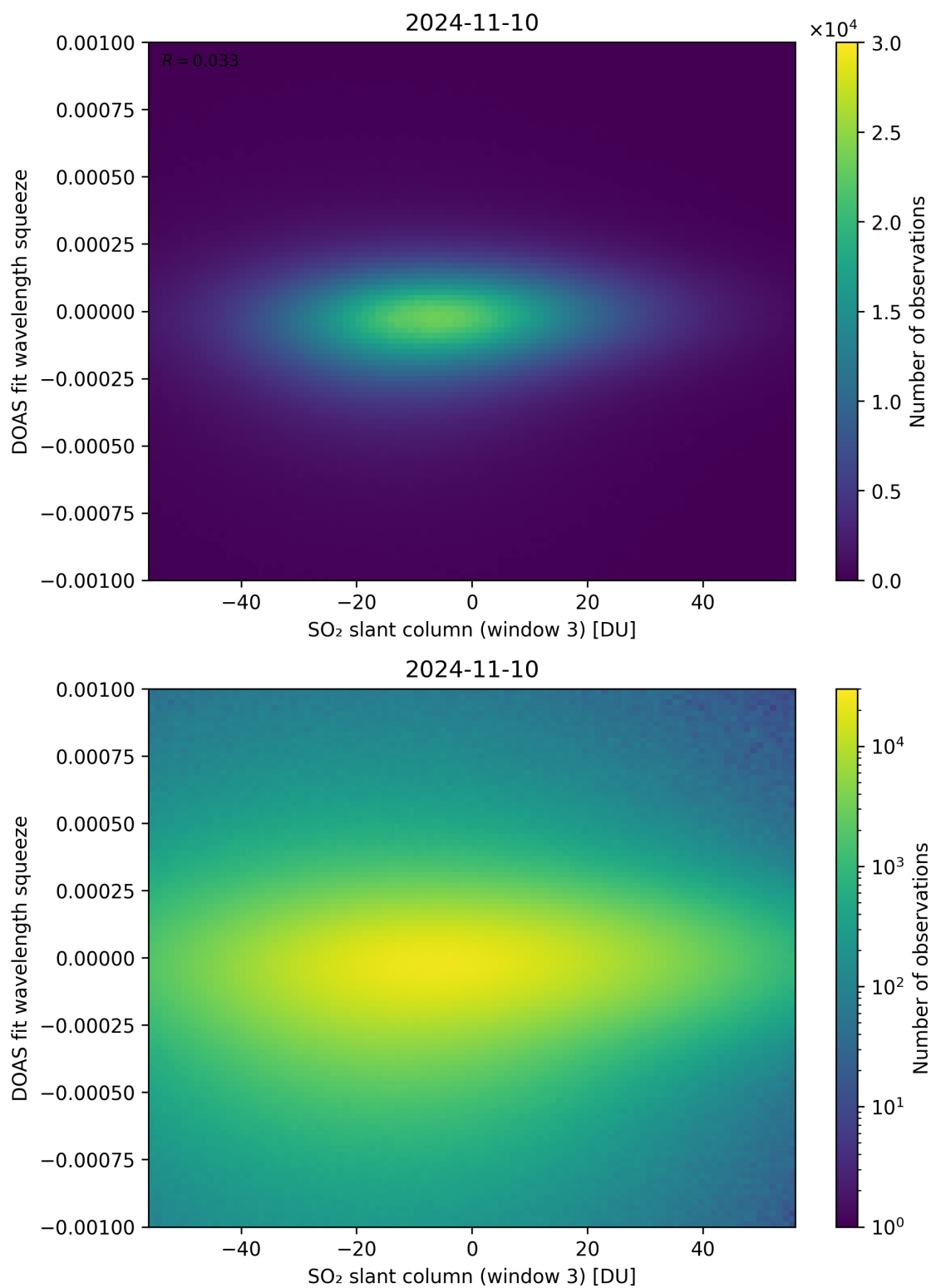
Figure 255: Scatter density plot of “SO 2 slant column (window 3)” against “DOAS fit wavelength squeeze” for 2024-11-09 to 2024-11-11.
