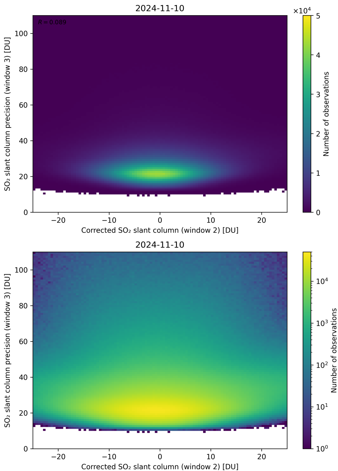
Figure 202: Scatter density plot of “Corrected SO 2 slant column (window 2)” against “SO 2 slant column precision (window 3)” for 2024-11-09 to 2024-11-11.
