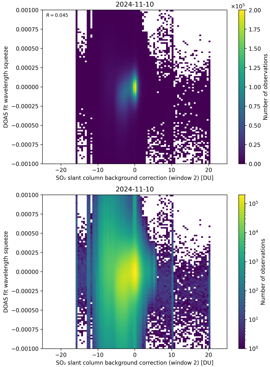
Figure 113: Scatter density plot of “SO 2 slant column background correction (window 2)” against “DOAS fit wavelength squeeze” for 2024-11-09 to 2024-11-11.
