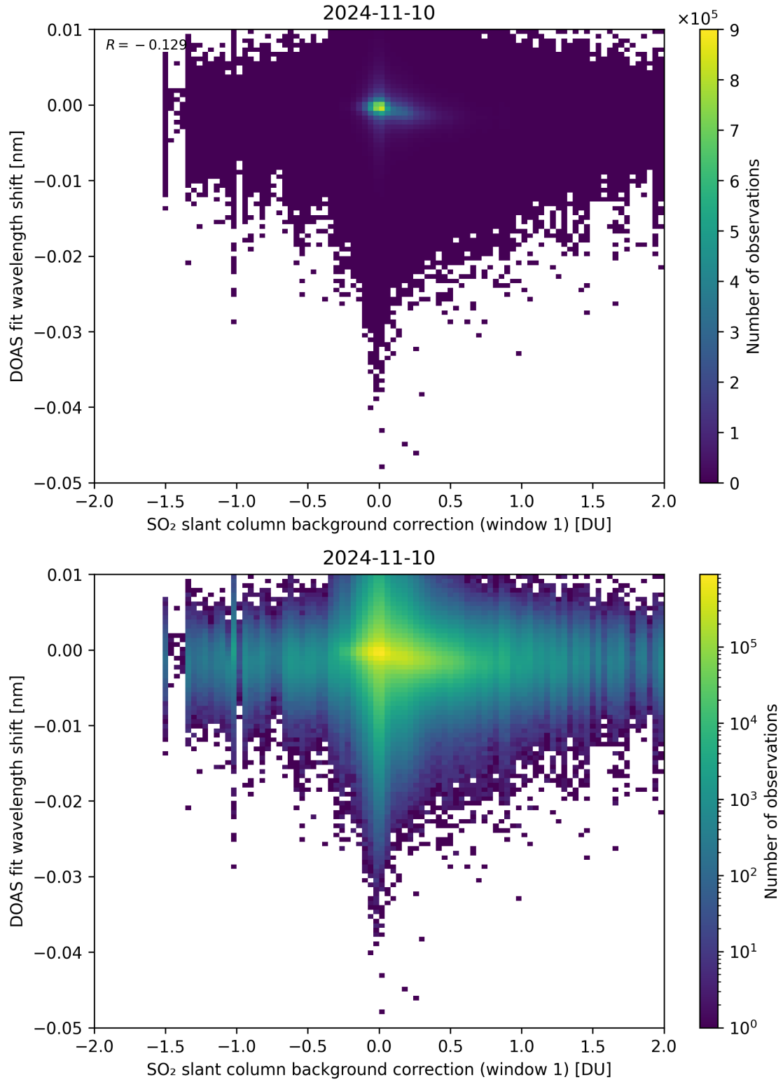
Figure 100: Scatter density plot of “SO 2 slant column background correction (window 1)” against “DOAS fit wavelength shift” for 2024-11-09 to 2024-11-11.
