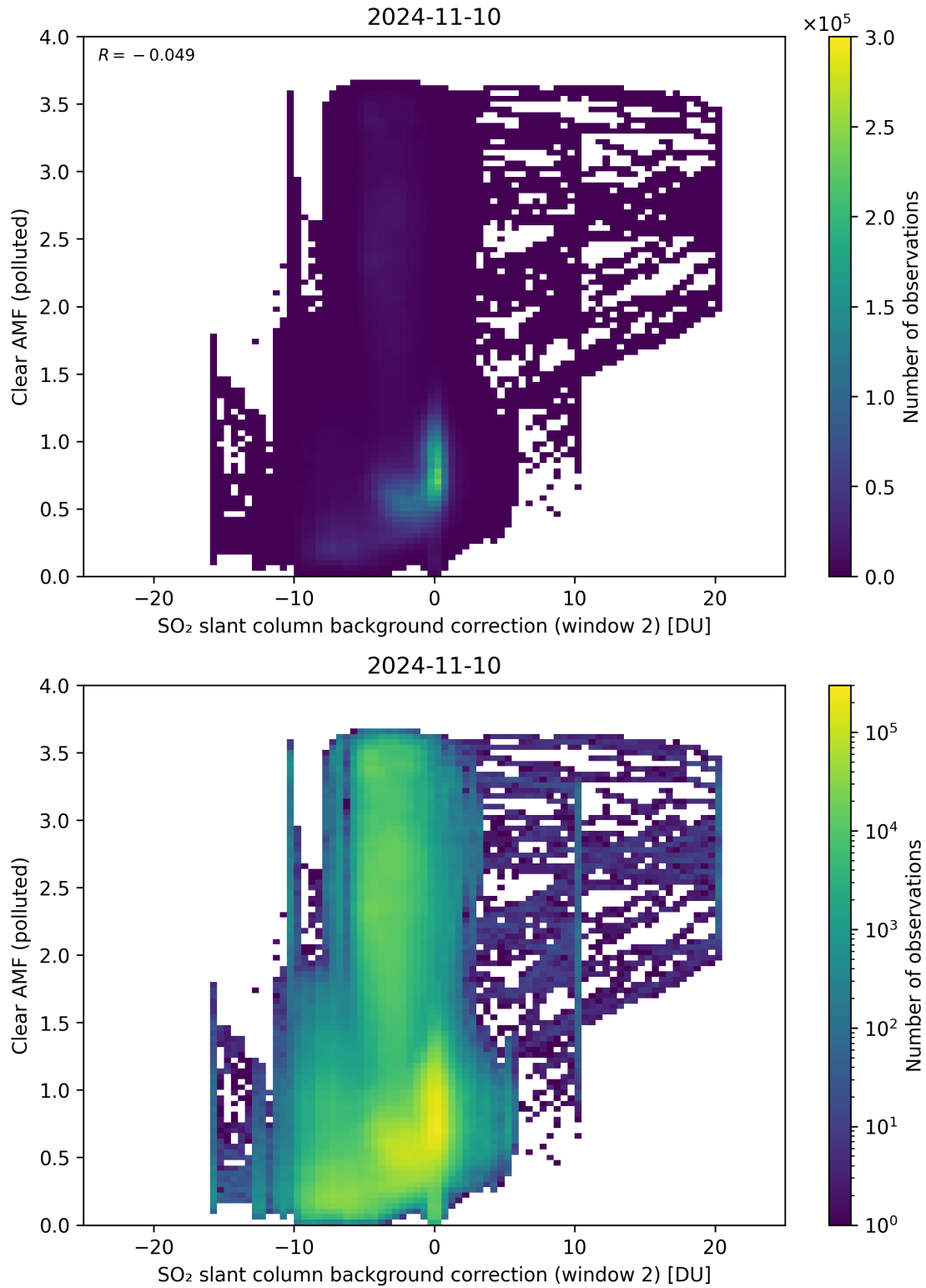
Figure 115: Scatter density plot of “SO 2 slant column background correction (window 2)” against “Clear AMF (polluted)” for 2024-11-09 to 2024-11-11.
