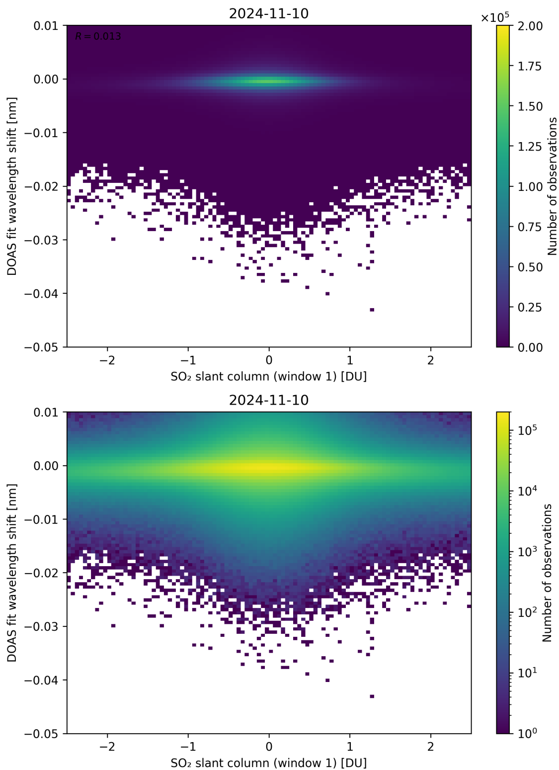
Figure 215: Scatter density plot of “SO 2 slant column (window 1)” against “DOAS fit wavelength shift” for 2024-11-09 to 2024-11-11.
