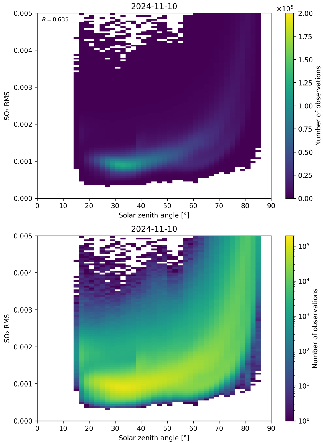
Figure 163: Scatter density plot of “Solar zenith angle” against “SO 2 RMS” for 2024-11-09 to 2024-11-11.
