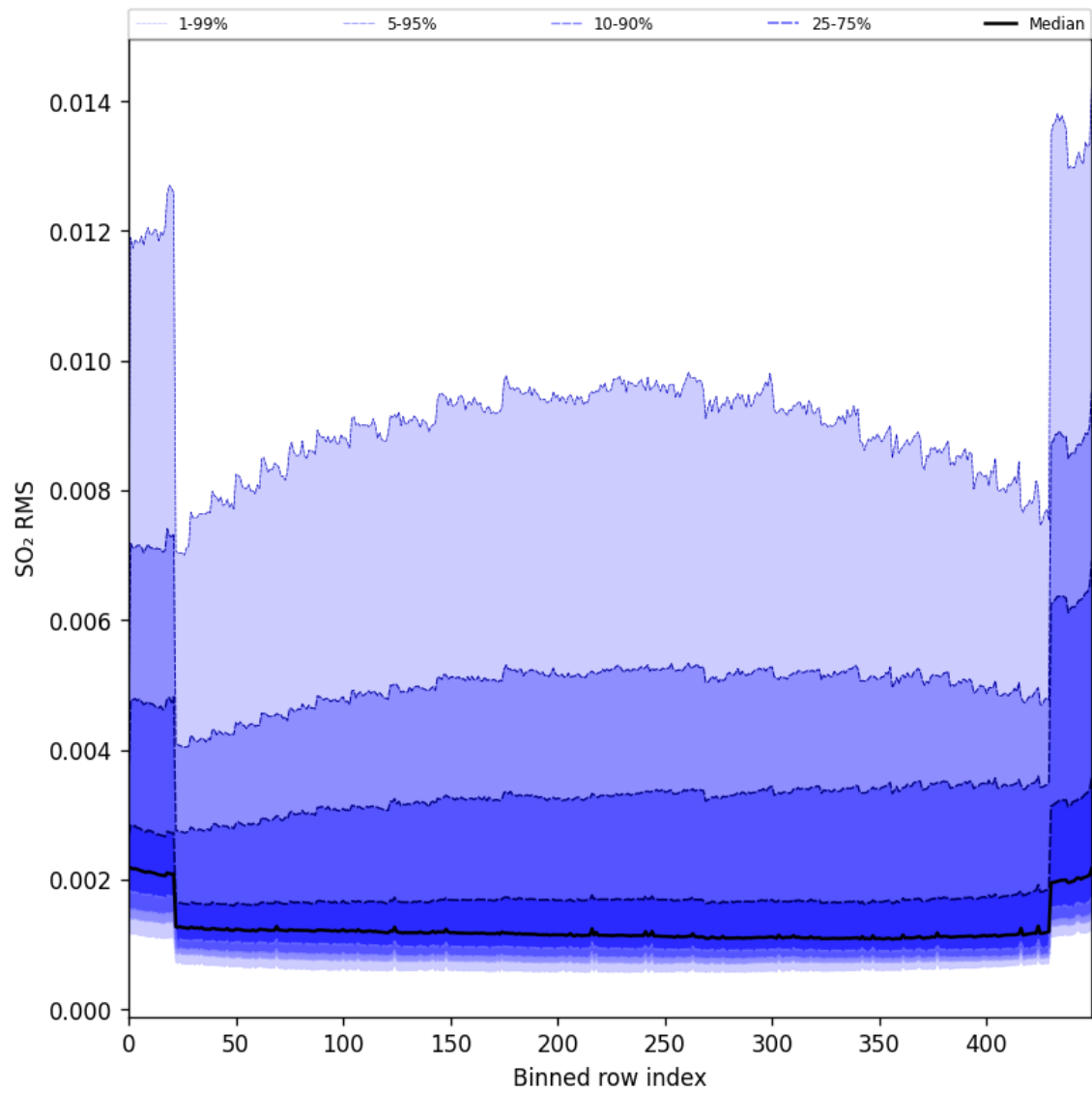
Figure 93: Along track statistics of “SO 2 RMS” for 2024-11-09 to 2024-11-11
