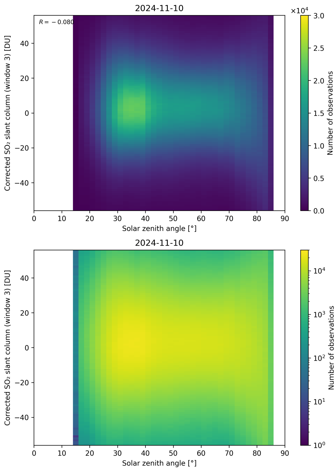
Figure 168: Scatter density plot of “Solar zenith angle” against “Corrected SO 2 slant column (window 3)” for 2024-11-09 to 2024-11-11.
