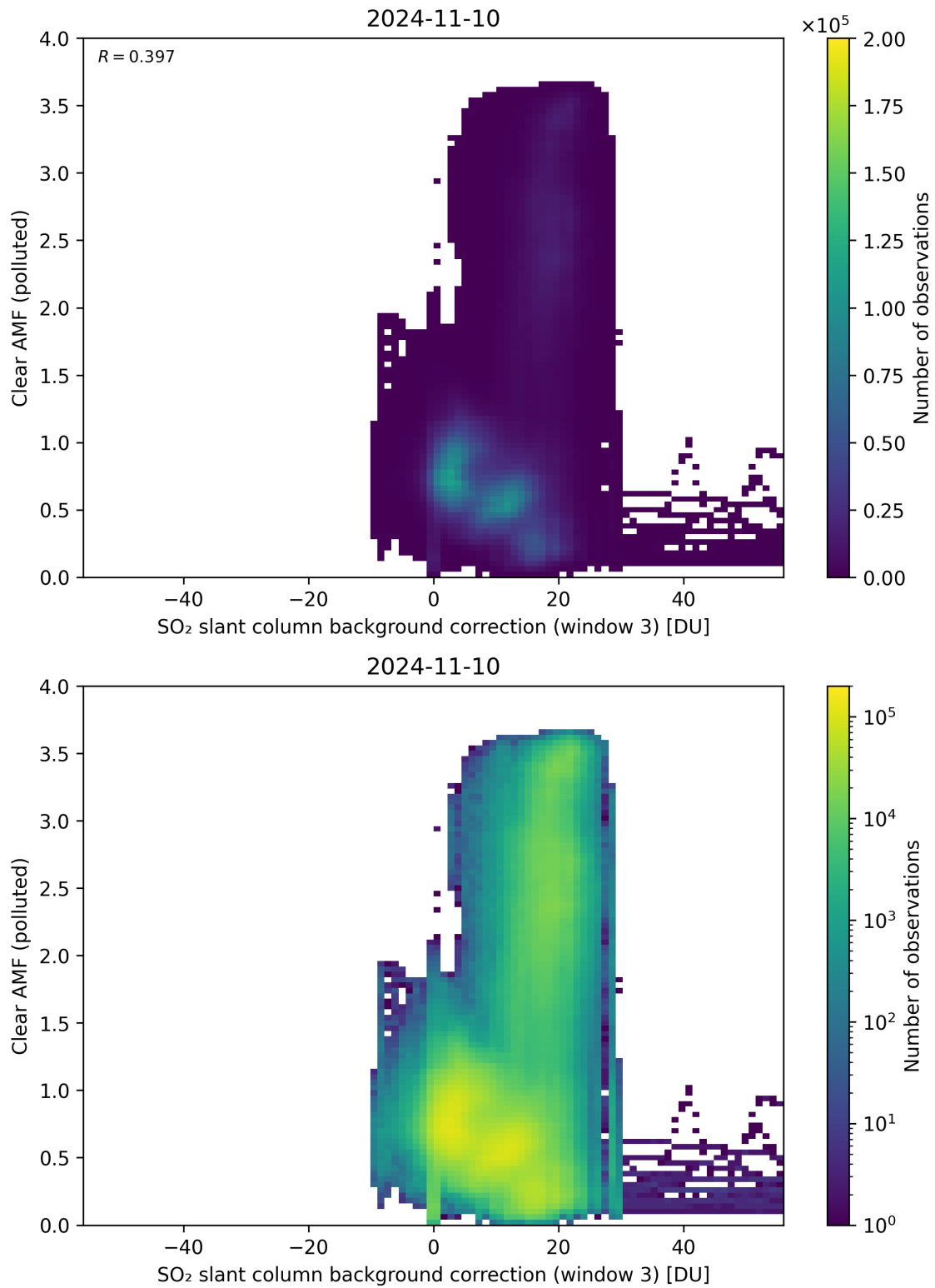
Figure 124: Scatter density plot of “SO 2 slant column background correction (window 3)” against “Clear AMF (polluted)” for 2024-11-09 to 2024-11-11.
