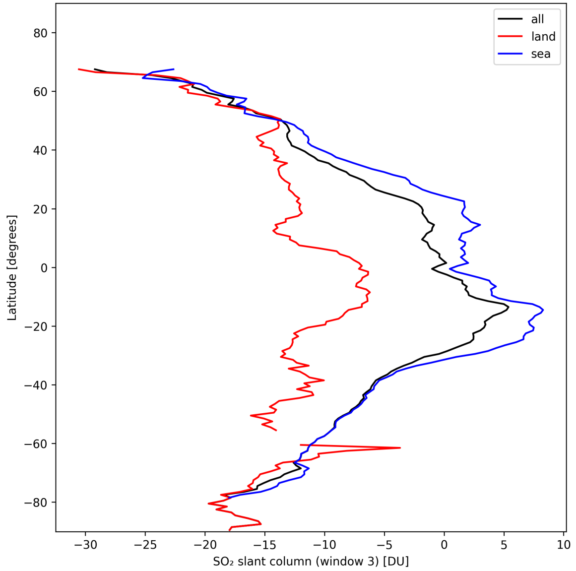
Figure 41: Zonal average of “SO 2 slant column (window 3)” for 2024-11-09 to 2024-11-11.
