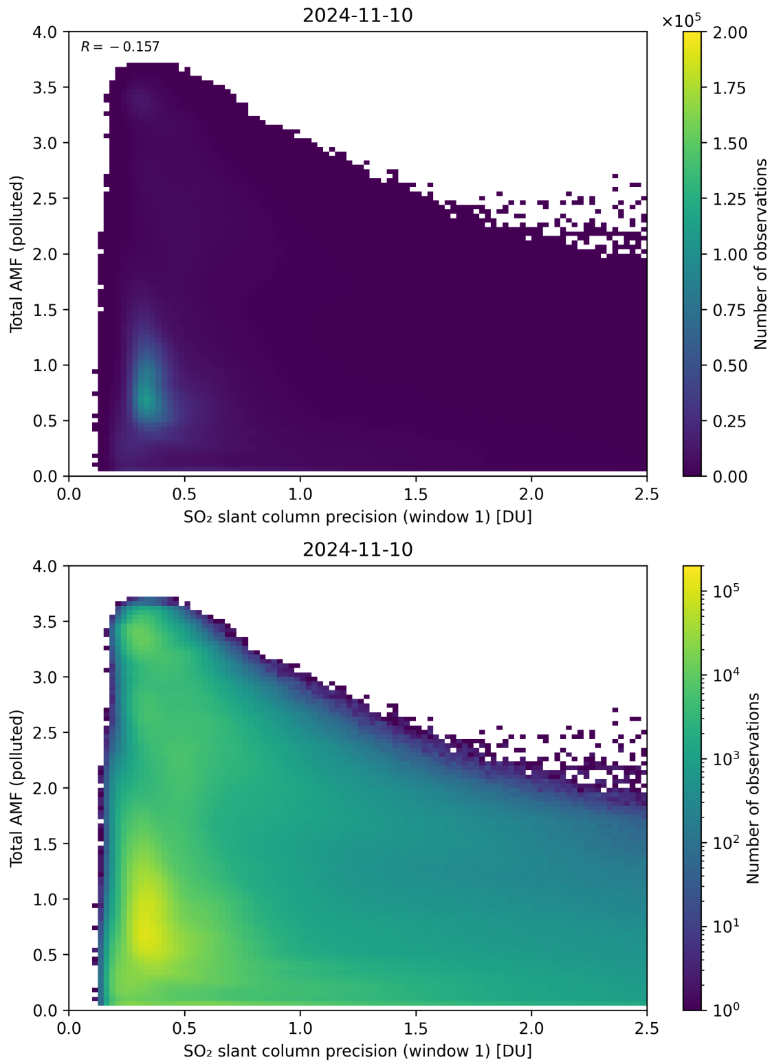
Figure 230: Scatter density plot of “SO 2 slant column precision (window 1)” against “Total AMF (polluted)” for 2024-11-09 to 2024-11-11.
