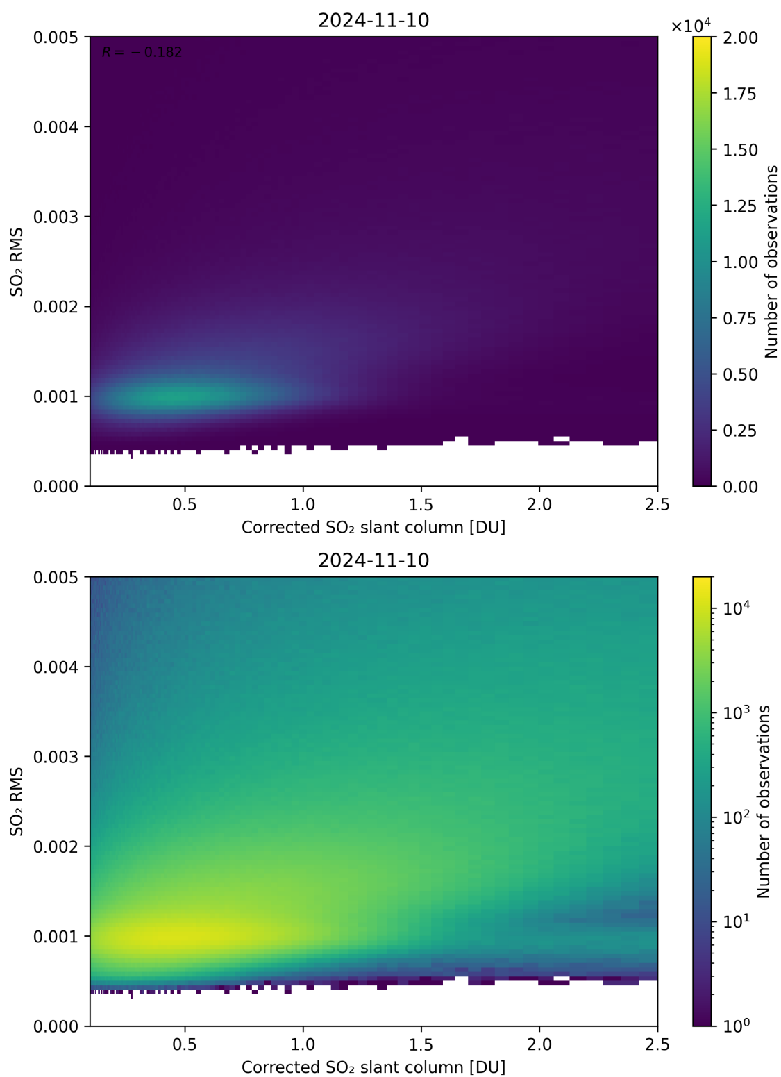
Figure 183: Scatter density plot of “Corrected SO 2 slant column” against “SO 2 RMS” for 2024-11-09 to 2024-11-11.
