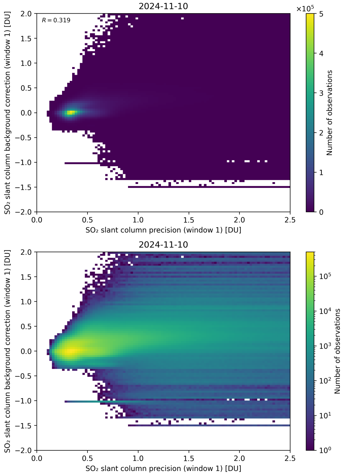
Figure 218: Scatter density plot of “SO 2 slant column precision (window 1)” against “SO 2 slant column background correction (window 1)” for 2024-11-09 to 2024-11-11.
