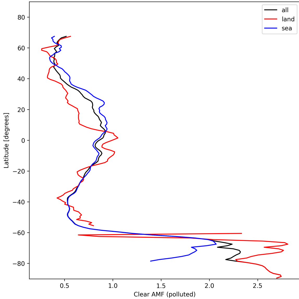
Figure 50: Zonal average of “Clear AMF (polluted)” for 2024-11-09 to 2024-11-11.
