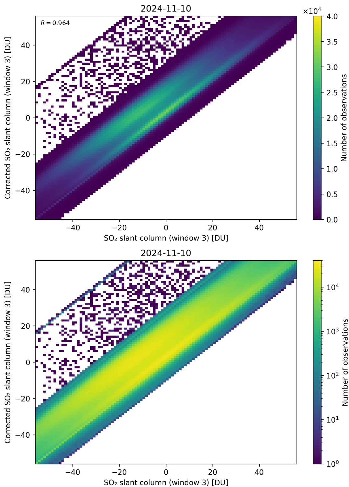
Figure 266: Scatter density plot of “SO 2 slant column (window 3)” against “Corrected SO 2 slant column (window 3)” for 2024-11-09 to 2024-11-11.
