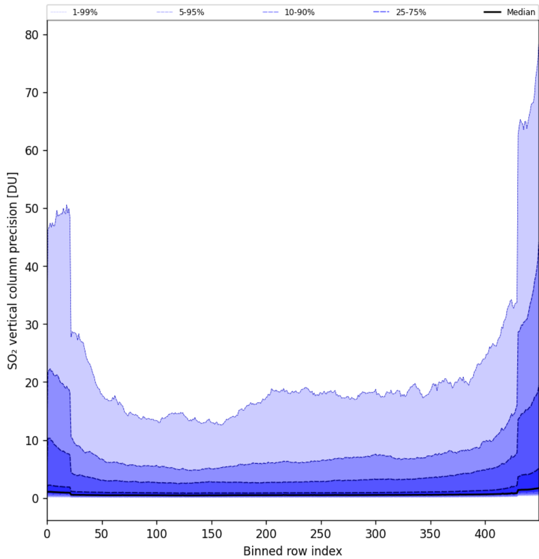
Figure 77: Along track statistics of “SO 2 vertical column precision” for 2024-11-09 to 2024-11-11
