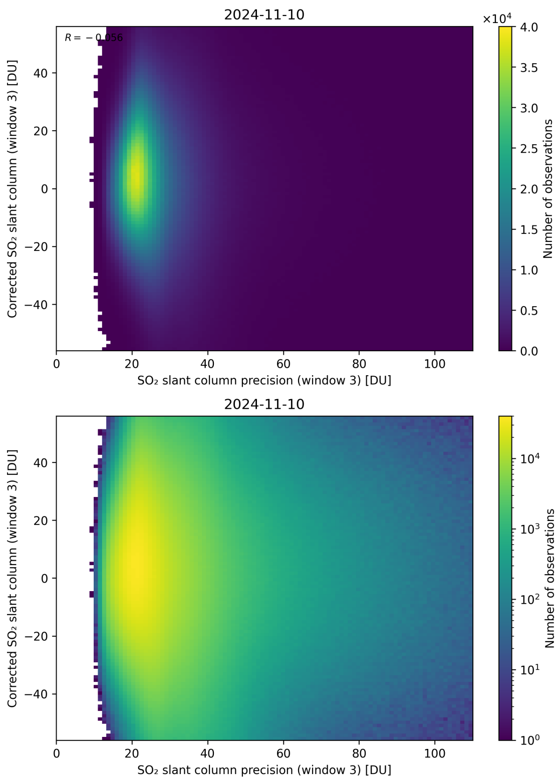
Figure 262: Scatter density plot of “SO 2 slant column precision (window 3)” against “Corrected SO 2 slant column (window 3)” for 2024-11-09 to 2024-11-11.
