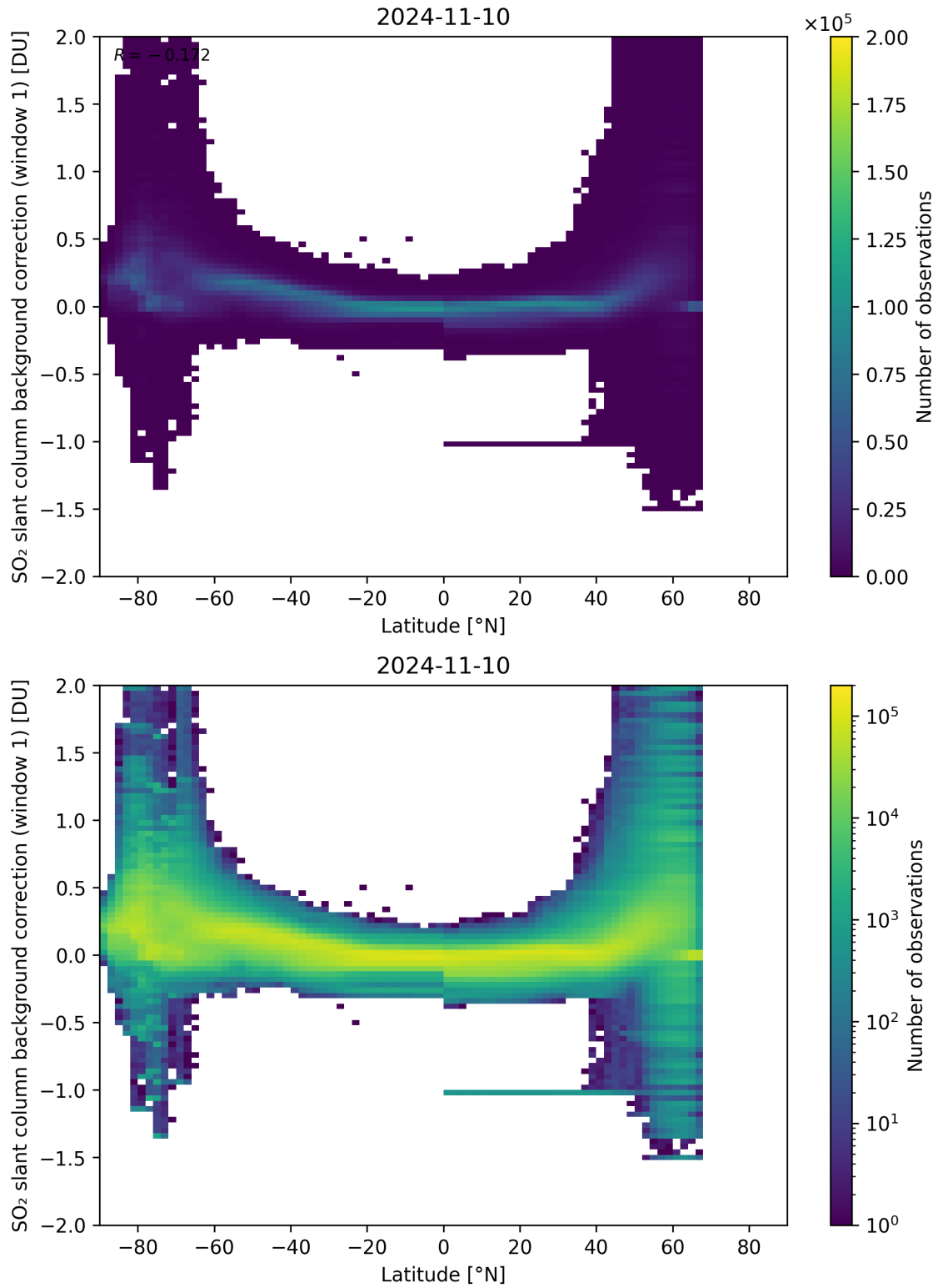
Figure 139: Scatter density plot of “Latitude” against “SO 2 slant column background correction (window 1)” for 2024-11-09 to 2024-11-11.
