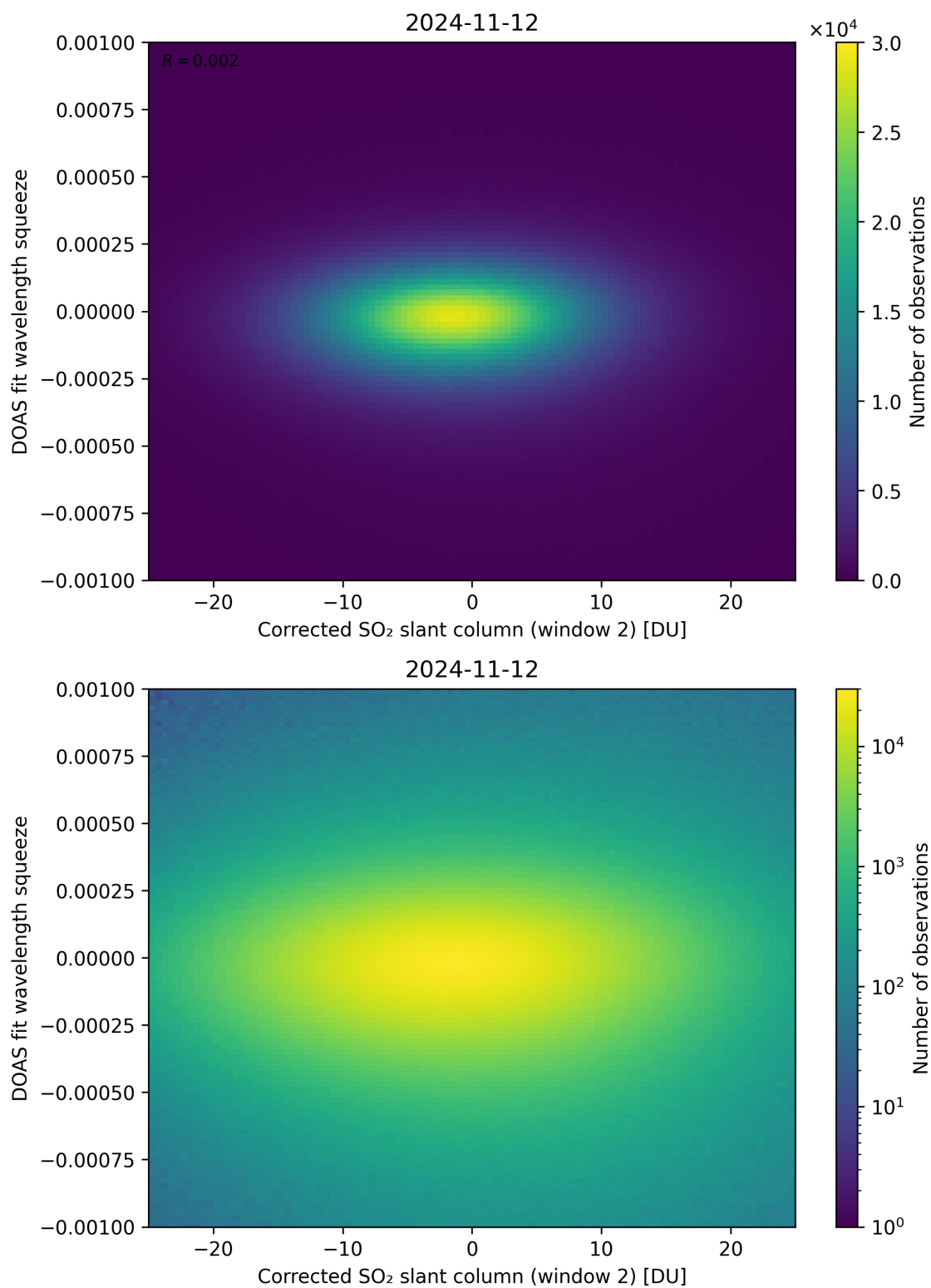
Figure 197: Scatter density plot of “Corrected SO 2 slant column (window 2)” against “DOAS fit wavelength squeeze” for 2024-11-11 to 2024-11-13.
