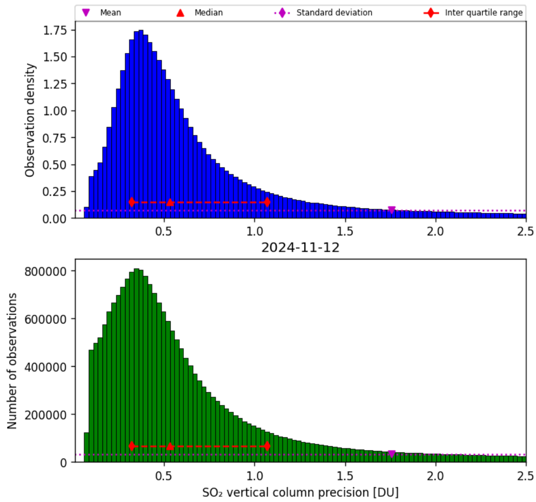
Figure 54: Histogram of “SO 2 vertical column precision” for 2024-11-11 to 2024-11-13
