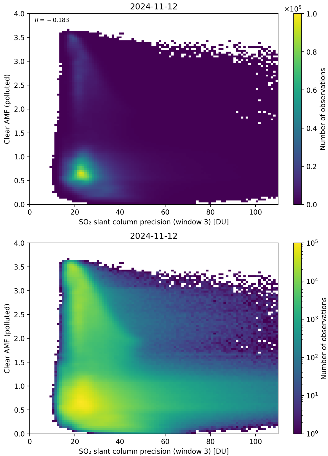
Figure 261: Scatter density plot of “SO 2 slant column precision (window 3)” against “Clear AMF (polluted)” for 2024-11-11 to 2024-11-13.
