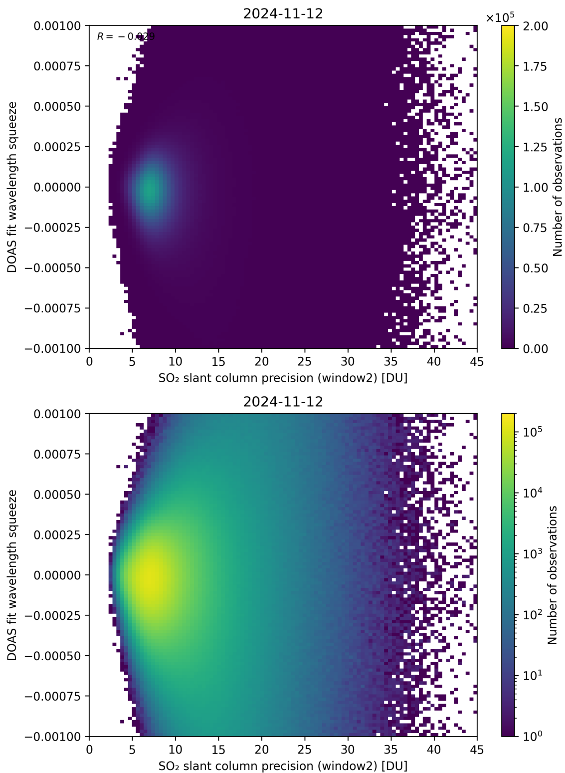
Figure 244: Scatter density plot of “SO 2 slant column precision (window2)” against “DOAS fit wavelength squeeze” for 2024-11-11 to 2024-11-13.
