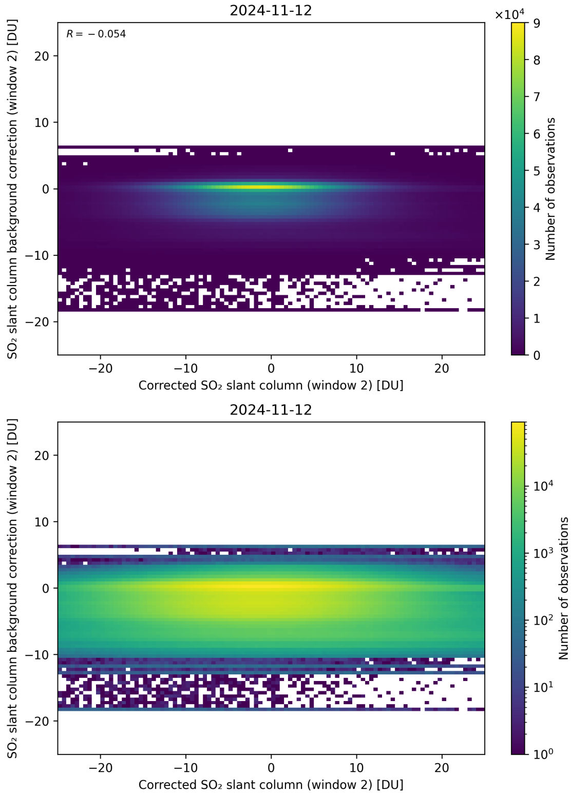
Figure 194: Scatter density plot of “Corrected SO 2 slant column (window 2)” against “SO 2 slant column background correction (window 2)” for 2024-11-11 to 2024-11-13.
