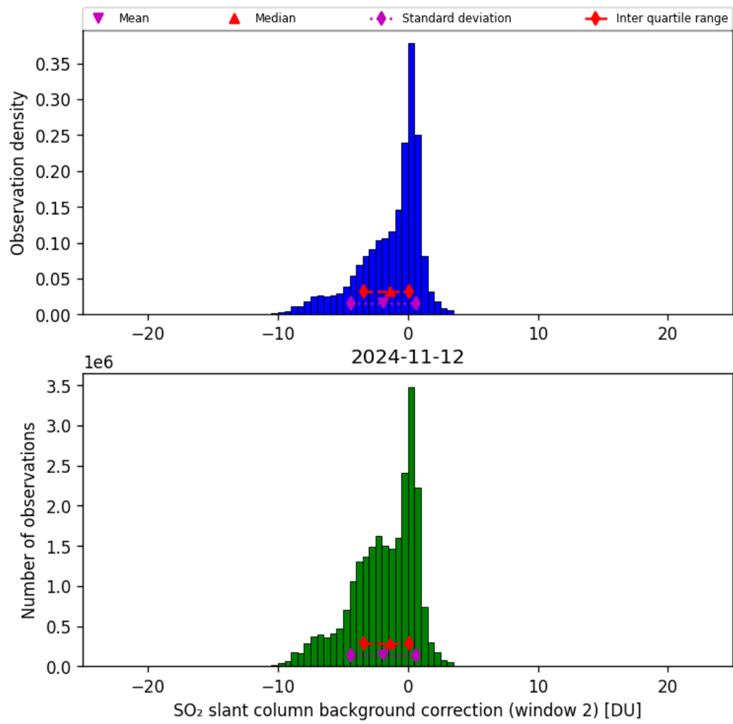
Figure 63: Histogram of “SO 2 slant column background correction (window 2)” for 2024-11-11 to 2024-11-13
