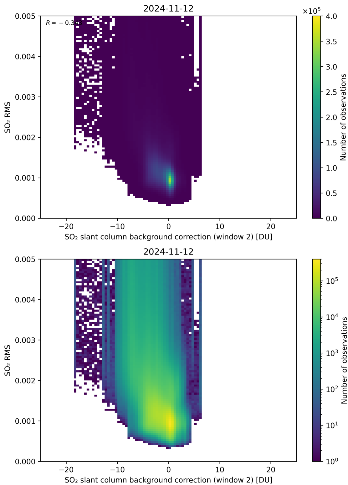
Figure 114: Scatter density plot of “SO 2 slant column background correction (window 2)” against “SO 2 RMS” for 2024-11-11 to 2024-11-13.
