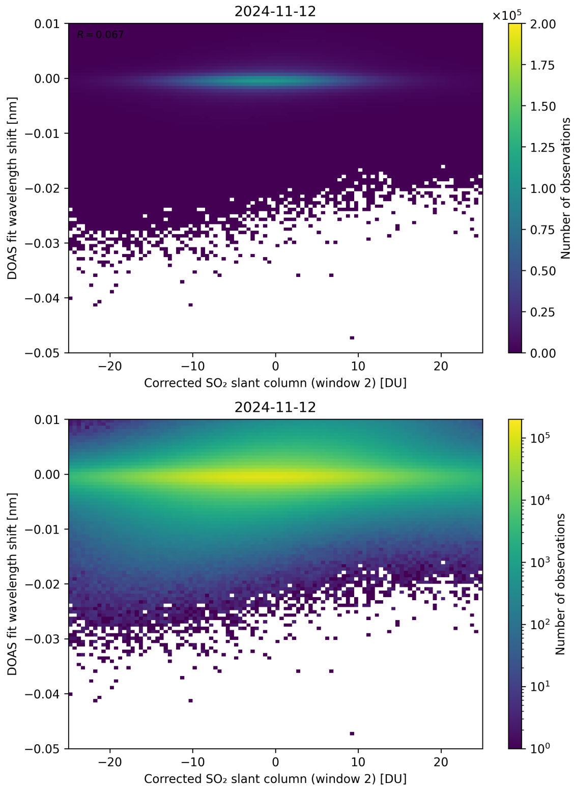
Figure 196: Scatter density plot of “Corrected SO 2 slant column (window 2)” against “DOAS fit wavelength shift” for 2024-11-11 to 2024-11-13.
