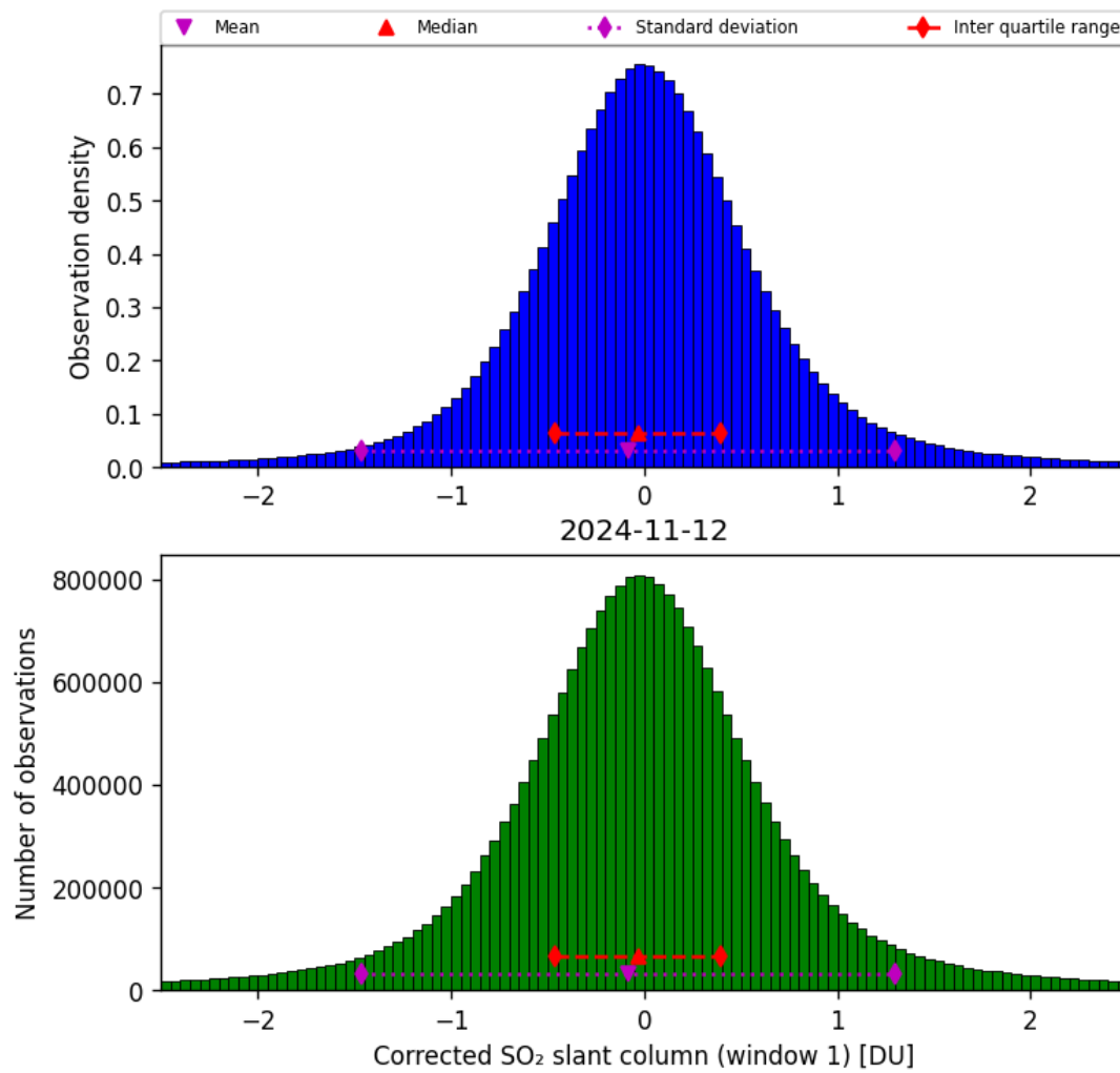
Figure 58: Histogram of “Corrected SO 2 slant column (window 1)” for 2024-11-11 to 2024-11-13
