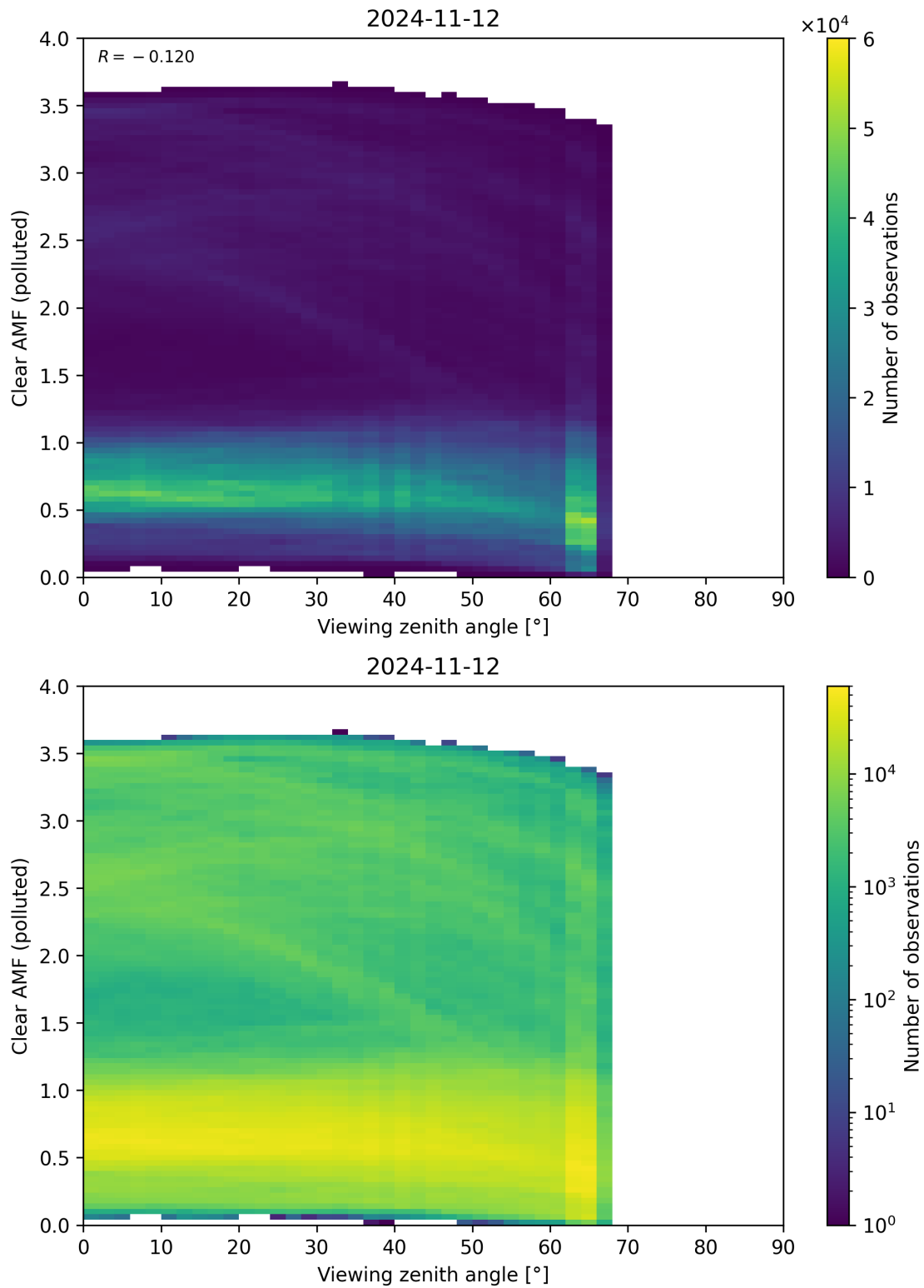
Figure 316: Scatter density plot of “Viewing zenith angle” against “Clear AMF (polluted)” for 2024-11-11 to 2024-11-13.
