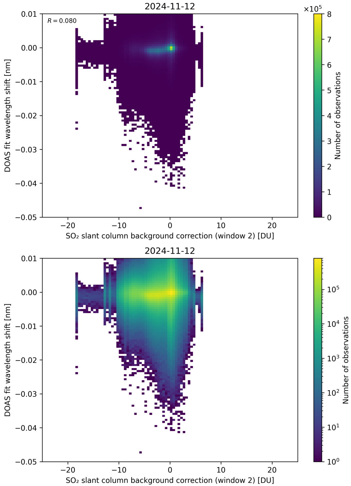
Figure 112: Scatter density plot of “SO 2 slant column background correction (window 2)” against “DOAS fit wavelength shift” for 2024-11-11 to 2024-11-13.
