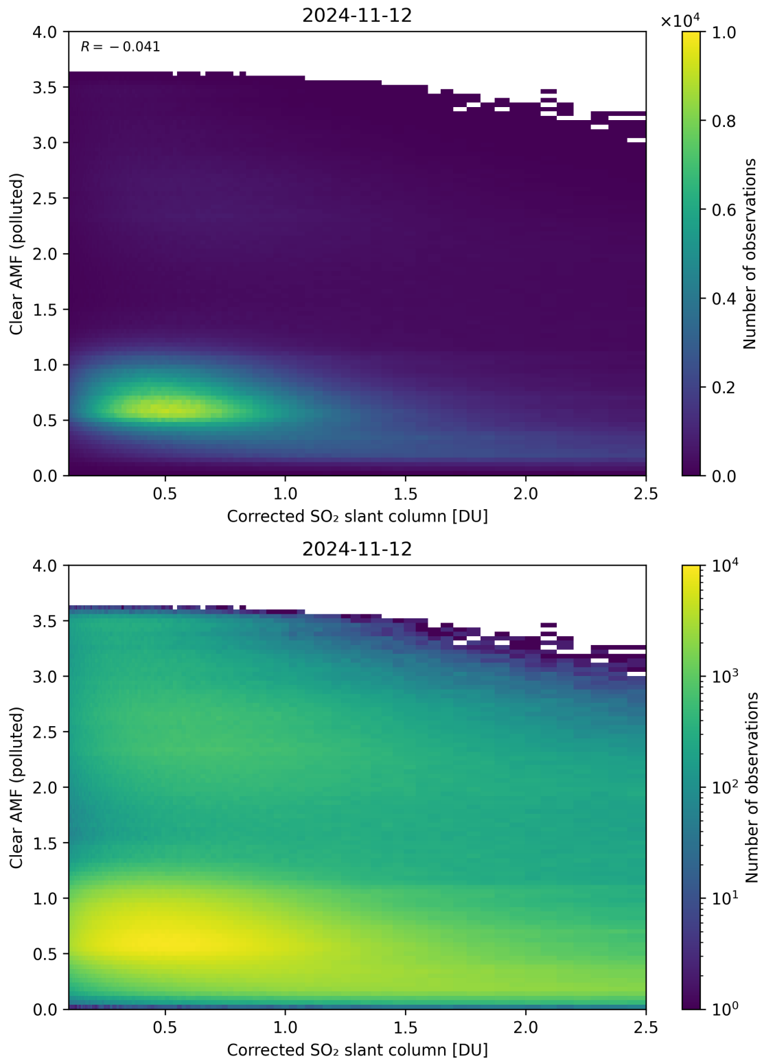
Figure 184: Scatter density plot of “Corrected SO 2 slant column” against “Clear AMF (polluted)” for 2024-11-11 to 2024-11-13.
