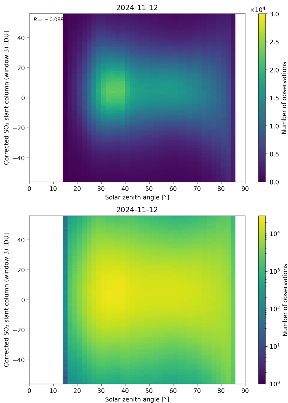
Figure 168: Scatter density plot of “Solar zenith angle” against “Corrected SO 2 slant column (window 3)” for 2024-11-11 to 2024-11-13.
