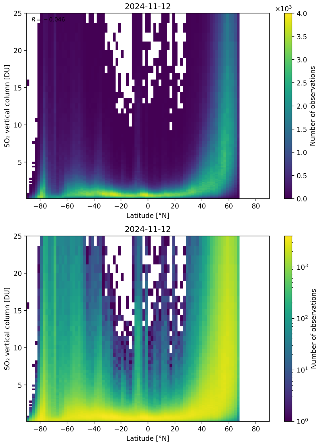
Figure 156: Scatter density plot of “Latitude” against “SO 2 vertical column” for 2024-11-11 to 2024-11-13.
