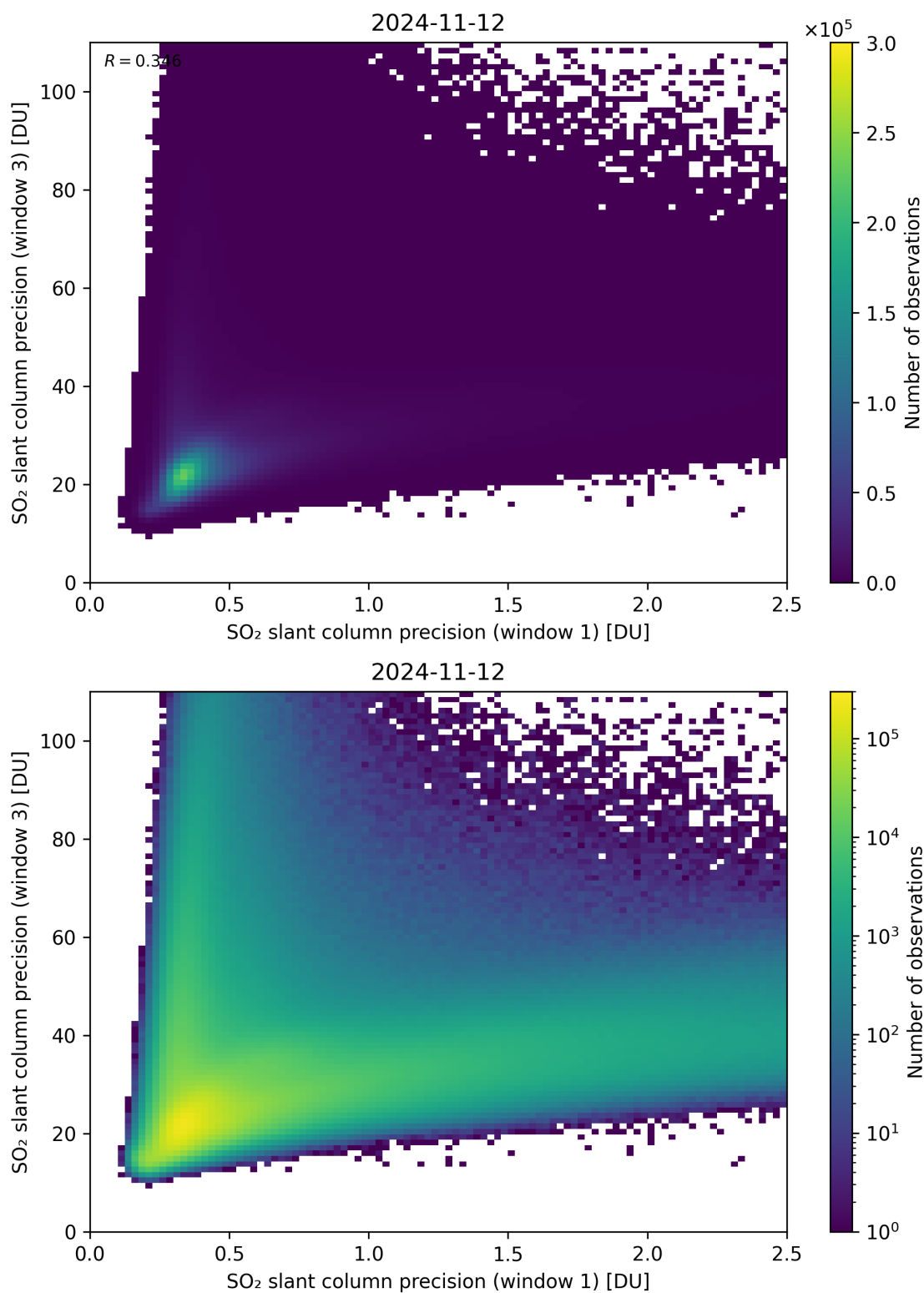
Figure 229: Scatter density plot of “SO 2 slant column precision (window 1)” against “SO 2 slant column precision (window 3)” for 2024-11-11 to 2024-11-13.
