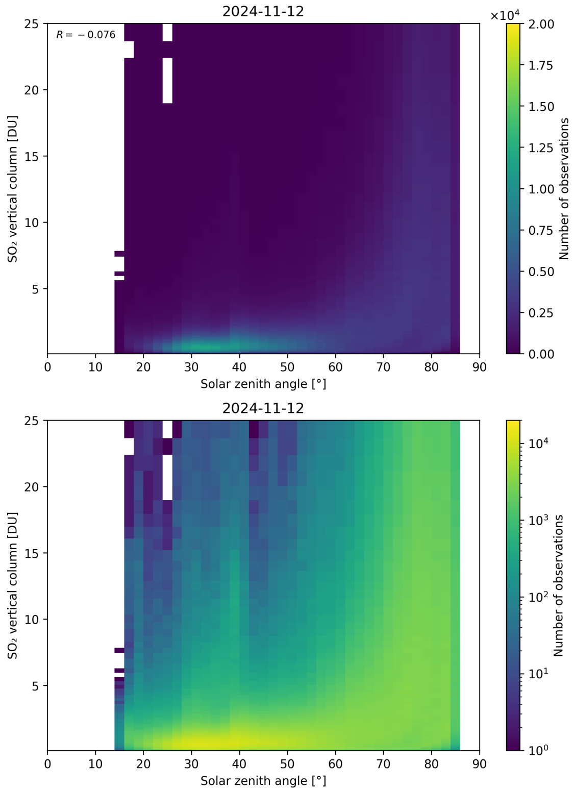
Figure 176: Scatter density plot of “Solar zenith angle” against “SO 2 vertical column” for 2024-11-11 to 2024-11-13.
