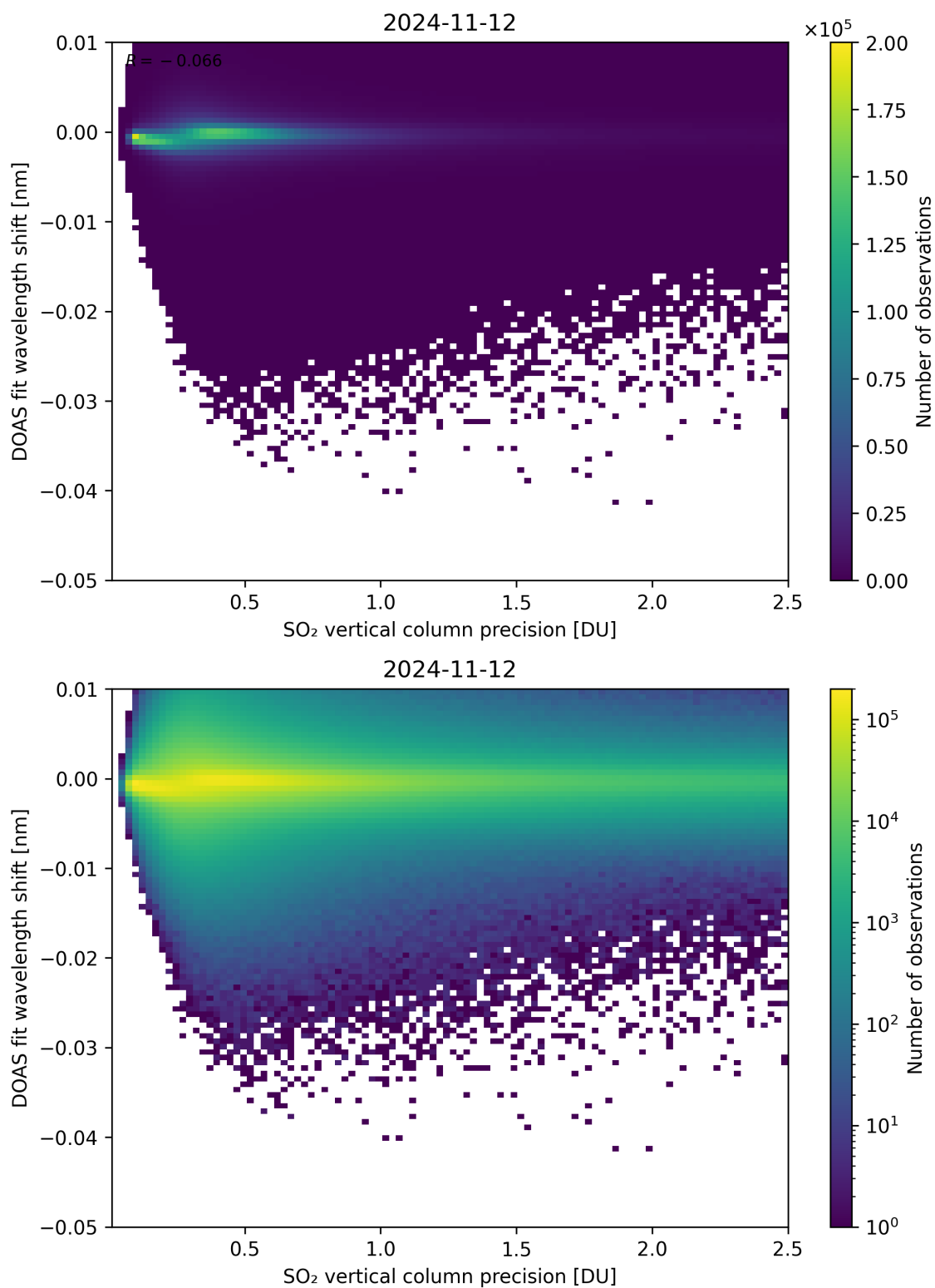
Figure 282: Scatter density plot of “SO 2 vertical column precision” against “DOAS fit wavelength shift” for 2024-11-11 to 2024-11-13.
