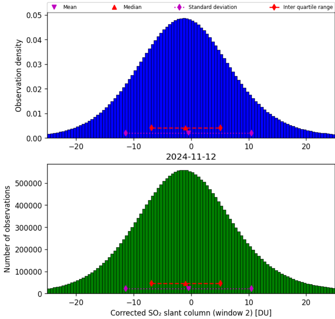
Figure 62: Histogram of “Corrected SO 2 slant column (window 2)” for 2024-11-11 to 2024-11-13
