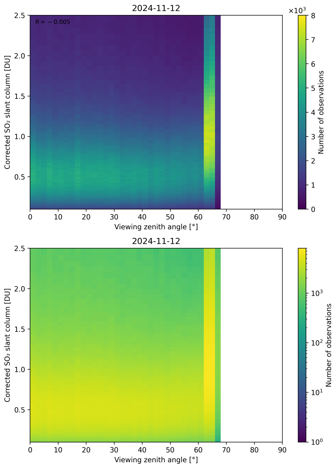
Figure 317: Scatter density plot of “Viewing zenith angle” against “Corrected SO 2 slant column” for 2024-11-11 to 2024-11-13.
