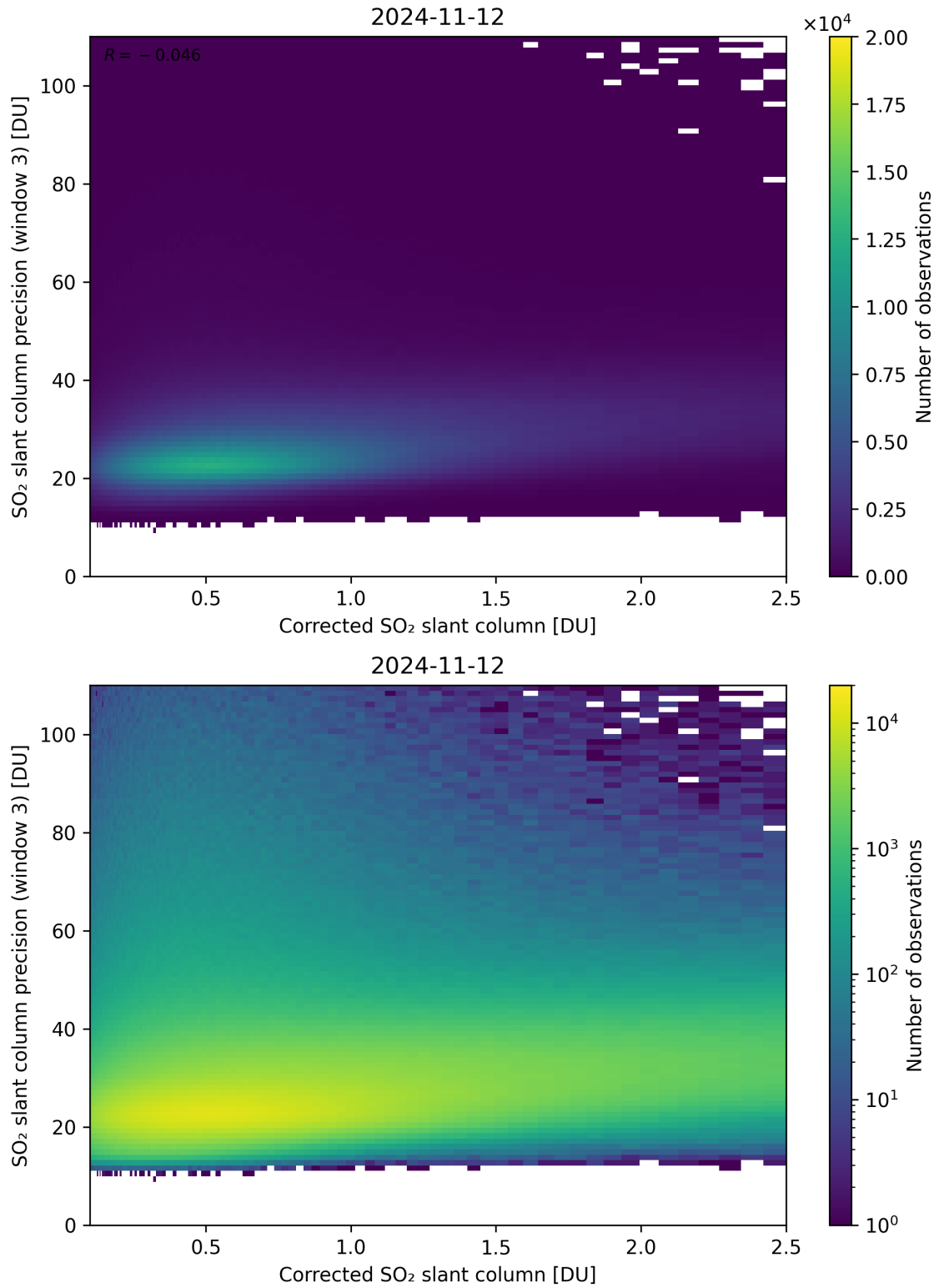
Figure 191: Scatter density plot of “Corrected SO 2 slant column” against “SO 2 slant column precision (window 3)” for 2024-11-11 to 2024-11-13.
