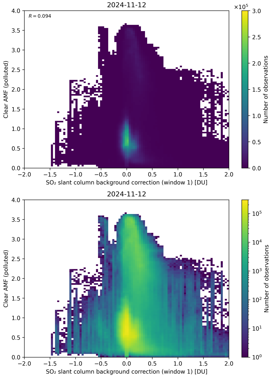
Figure 103: Scatter density plot of “SO 2 slant column background correction (window 1)” against “Clear AMF (polluted)” for 2024-11-11 to 2024-11-13.
