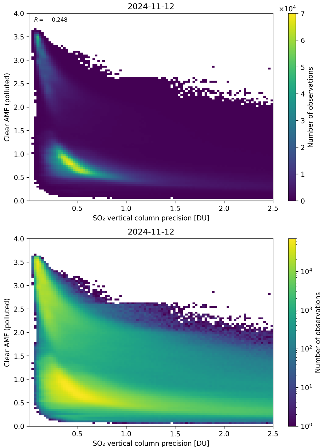
Figure 285: Scatter density plot of “SO 2 vertical column precision” against “Clear AMF (polluted)” for 2024-11-11 to 2024-11-13.
