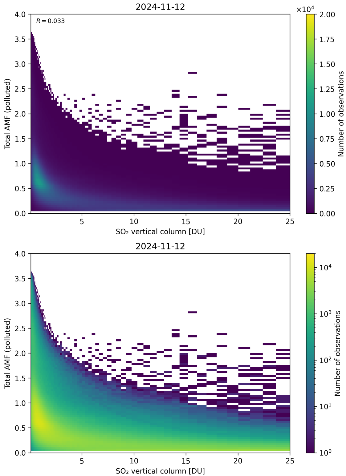
Figure 305: Scatter density plot of “SO 2 vertical column” against “Total AMF (polluted)” for 2024-11-11 to 2024-11-13.
