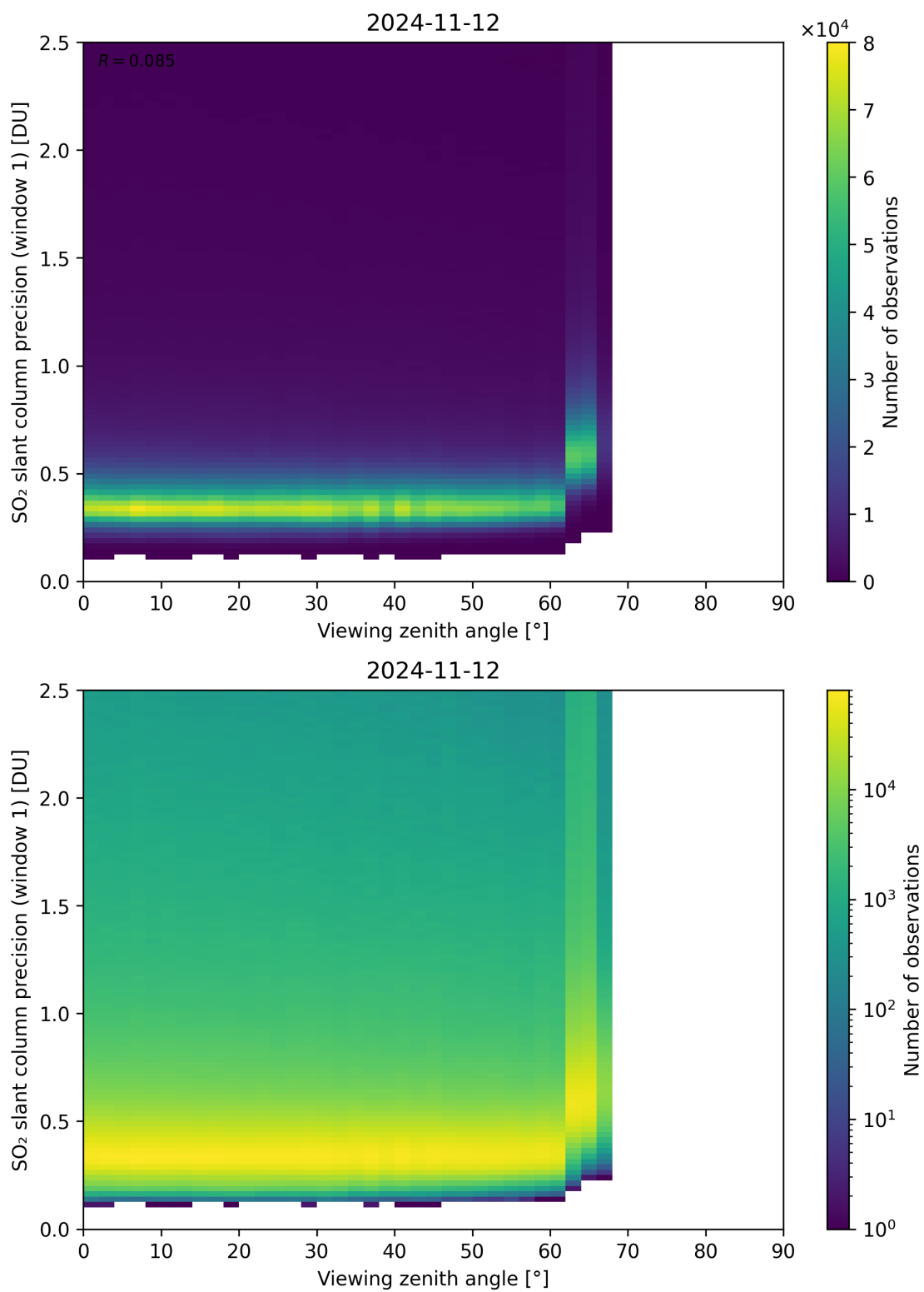
Figure 321: Scatter density plot of “Viewing zenith angle” against “SO 2 slant column precision (window 1)” for 2024-11-11 to 2024-11-13.
