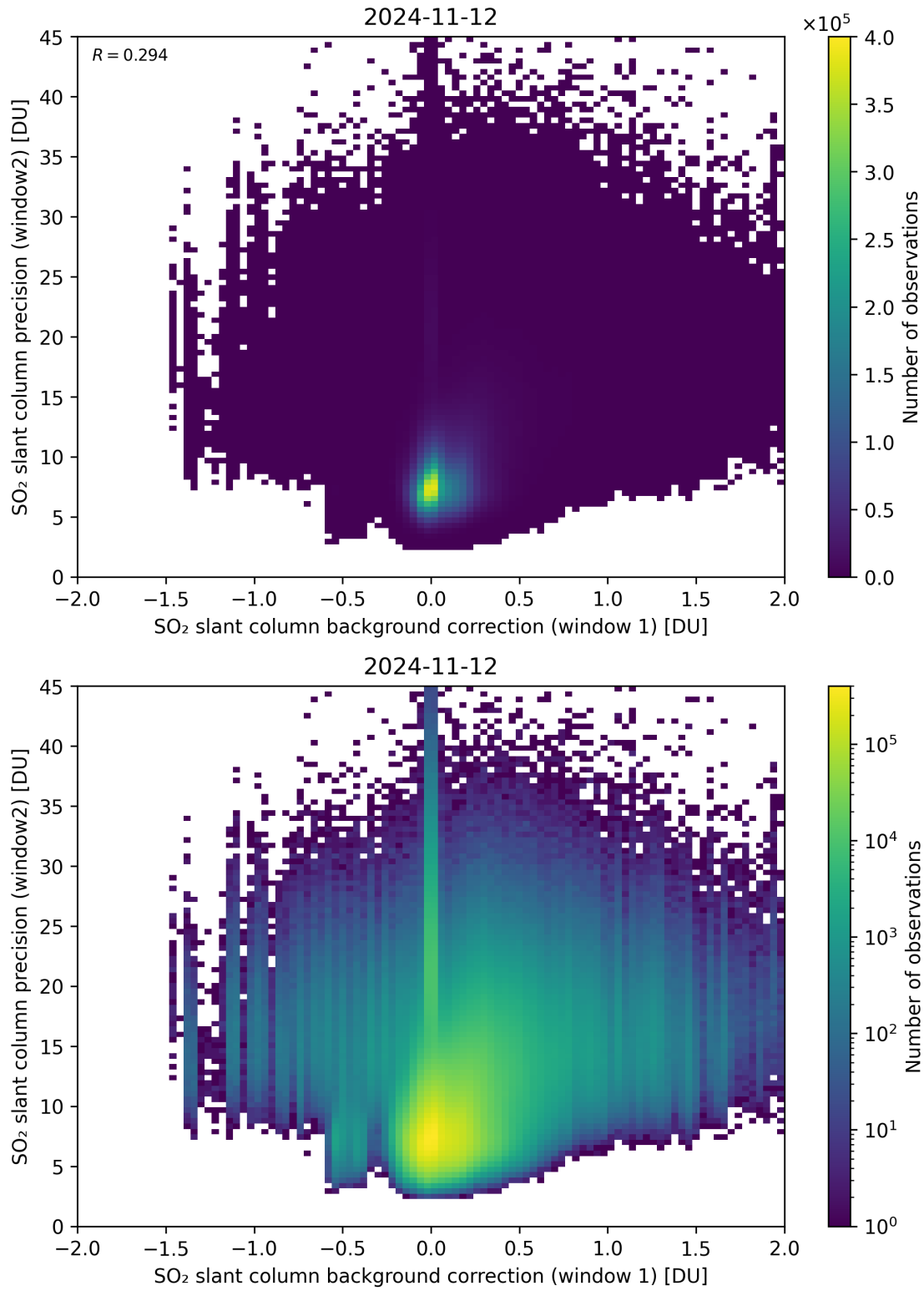
Figure 106: Scatter density plot of “SO 2 slant column background correction (window 1)” against “SO 2 slant column precision (window2)” for 2024-11-11 to 2024-11-13.
