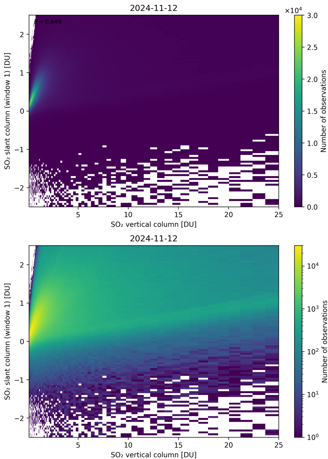
Figure 300: Scatter density plot of “SO 2 vertical column” against “SO 2 slant column (window 1)” for 2024-11-11 to 2024-11-13.
