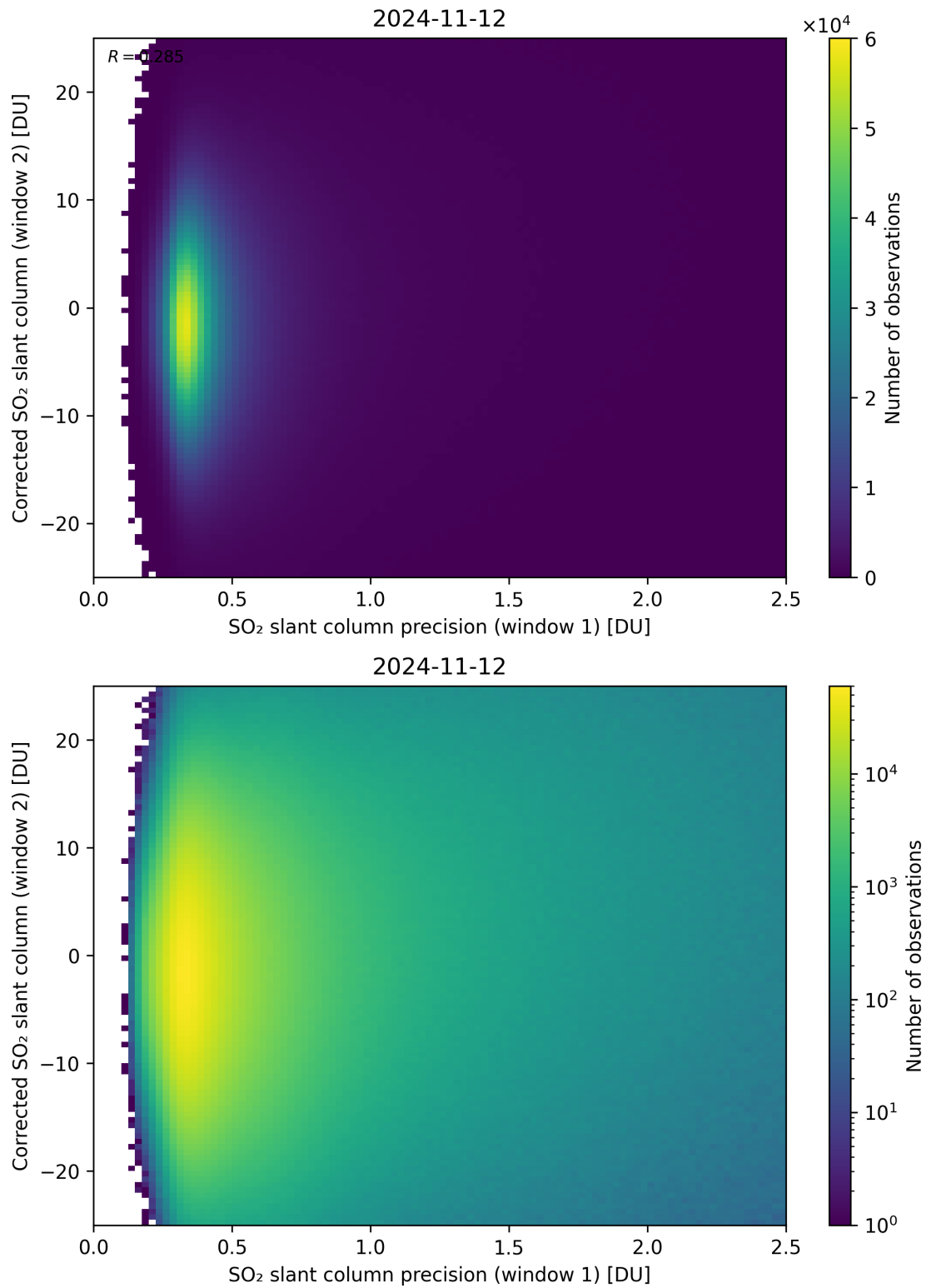
Figure 225: Scatter density plot of “SO 2 slant column precision (window 1)” against “Corrected SO 2 slant column (window 2)” for 2024-11-11 to 2024-11-13.
