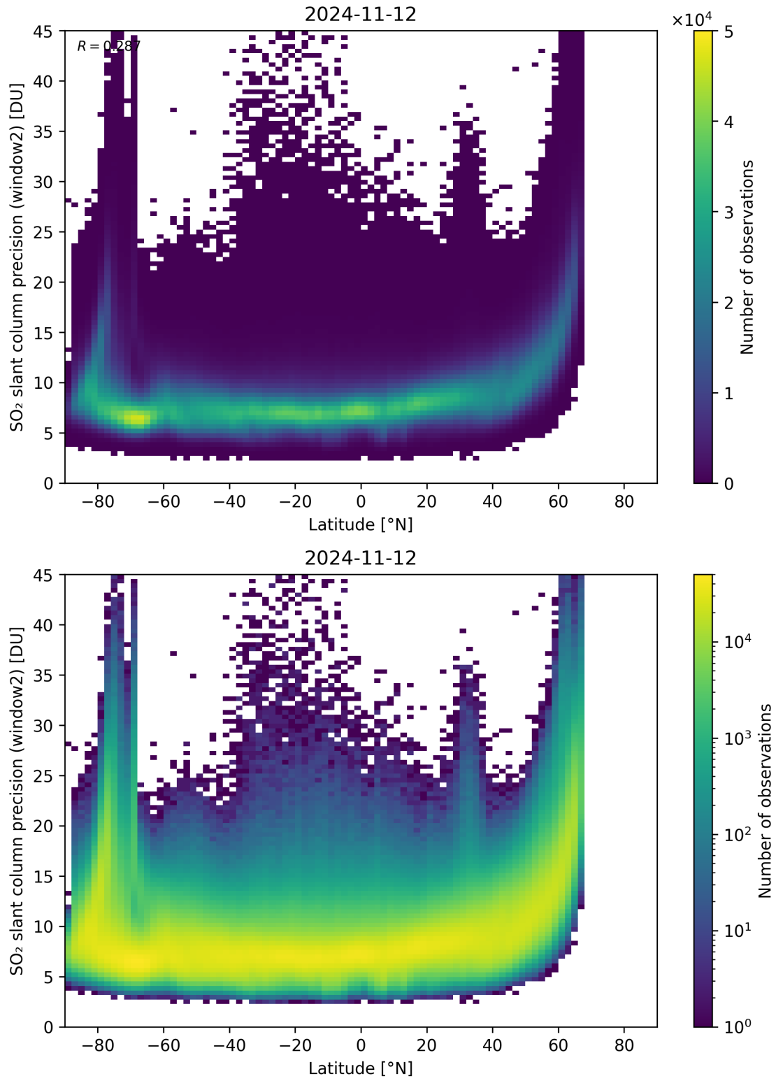
Figure 151: Scatter density plot of “Latitude” against “SO 2 slant column precision (window2)” for 2024-11-11 to 2024-11-13.
