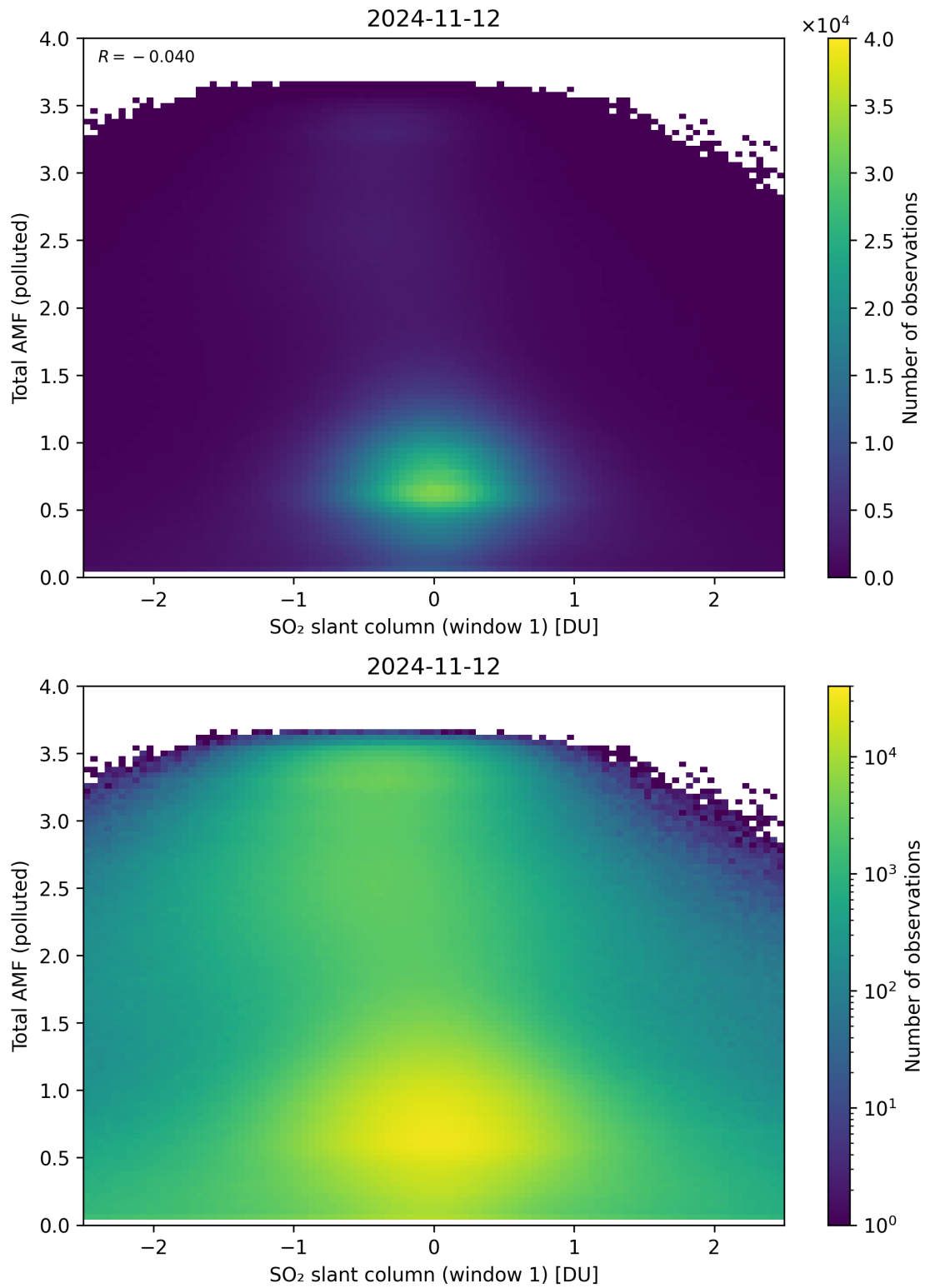
Figure 239: Scatter density plot of “SO 2 slant column (window 1)” against “Total AMF (polluted)” for 2024-11-11 to 2024-11-13.
