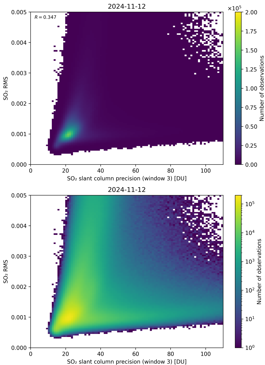
Figure 260: Scatter density plot of “SO 2 slant column precision (window 3)” against “SO 2 RMS” for 2024-11-11 to 2024-11-13.
