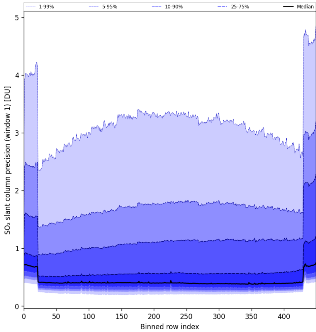
Figure 80: Along track statistics of “SO 2 slant column precision (window 1)” for 2024-11-11 to 2024-11-13
