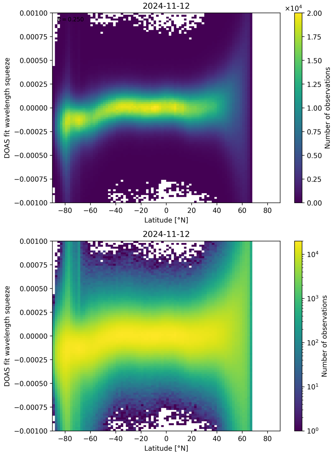
Figure 143: Scatter density plot of “Latitude” against “DOAS fit wavelength squeeze” for 2024-11-11 to 2024-11-13.
