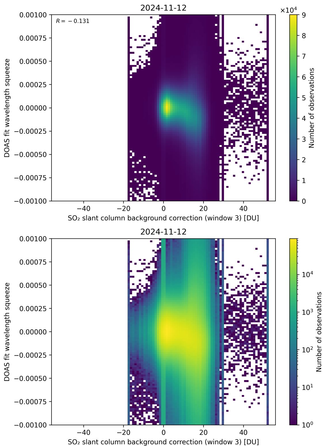
Figure 122: Scatter density plot of “SO 2 slant column background correction (window 3)” against “DOAS fit wavelength squeeze” for 2024-11-11 to 2024-11-13.
