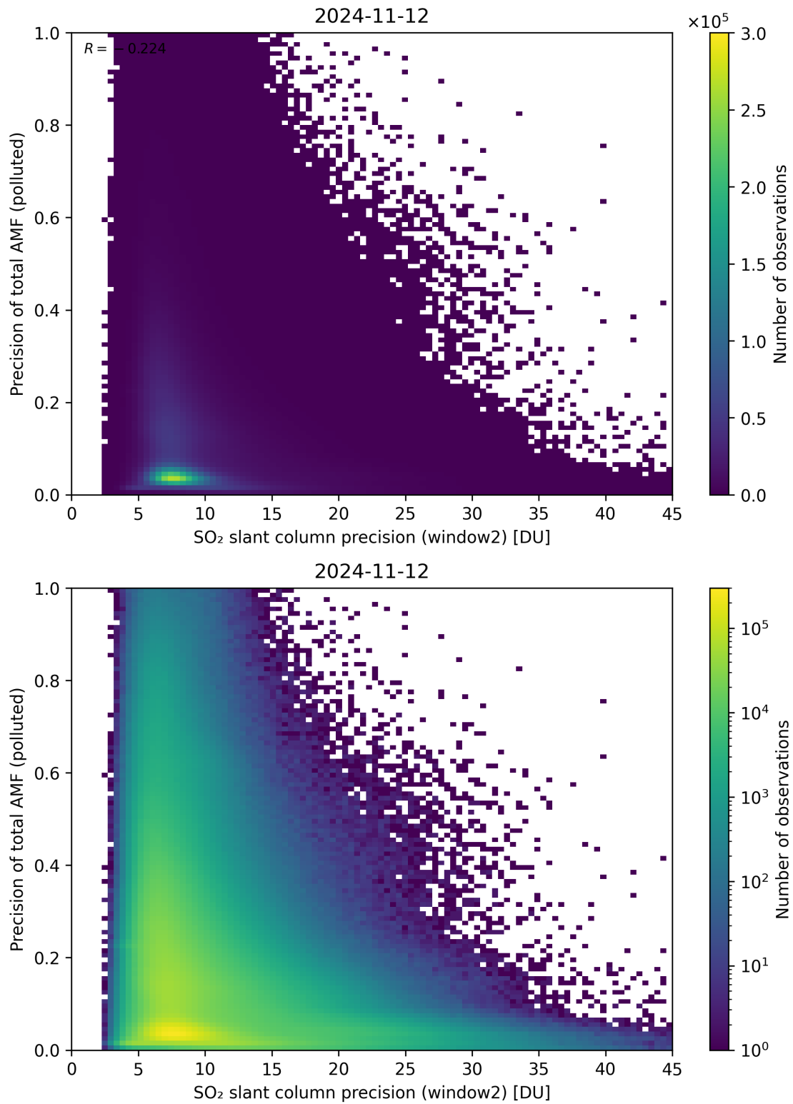
Figure 252: Scatter density plot of “SO 2 slant column precision (window2)” against “Precision of total AMF (polluted)” for 2024-11-11 to 2024-11-13.
