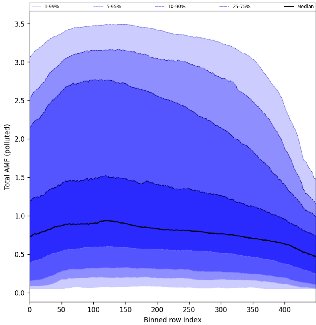
Figure 94: Along track statistics of “Total AMF (polluted)” for 2024-11-11 to 2024-11-13
