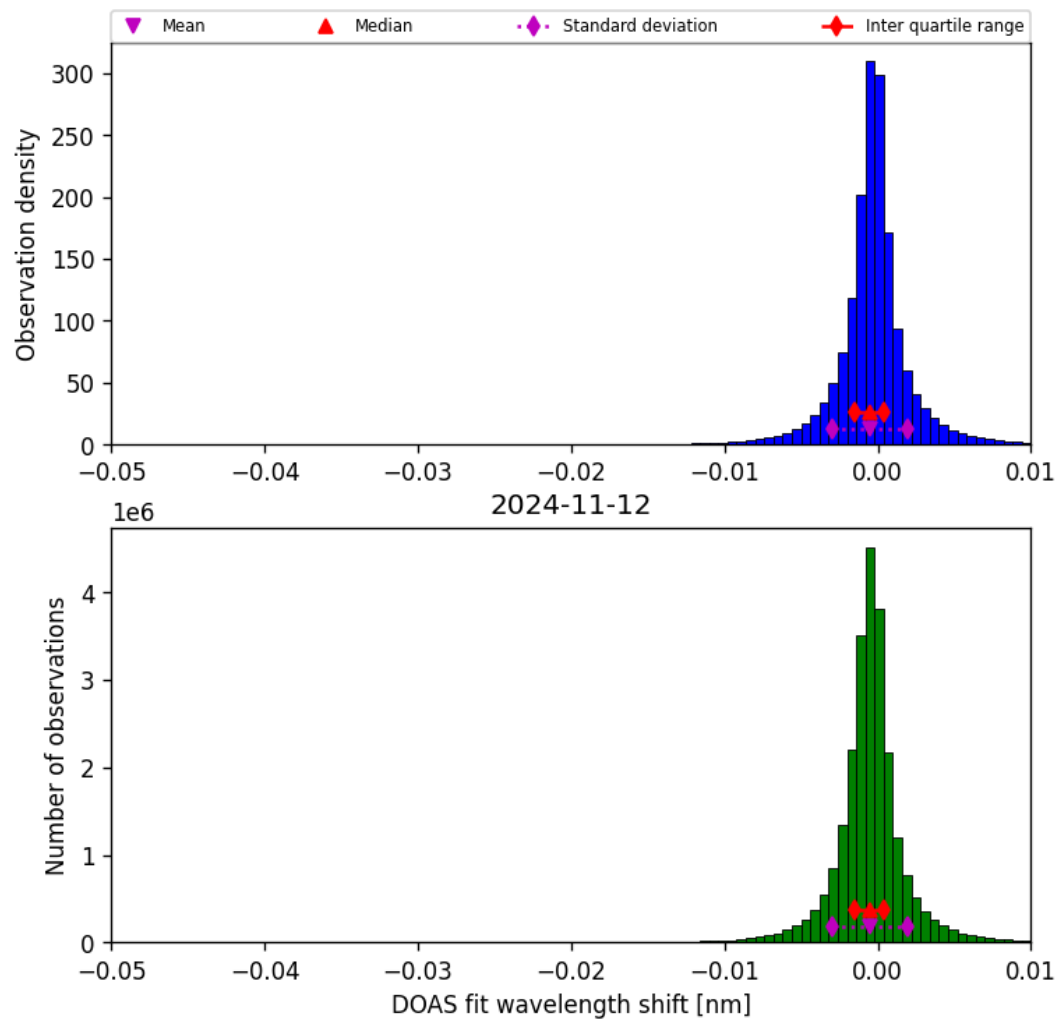
Figure 68: Histogram of “DOAS fit wavelength shift” for 2024-11-11 to 2024-11-13
