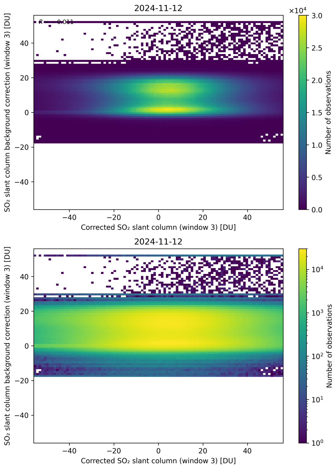
Figure 205: Scatter density plot of “Corrected SO 2 slant column (window 3)” against “SO 2 slant column background correction (window 3)” for 2024-11-11 to 2024-11-13.
