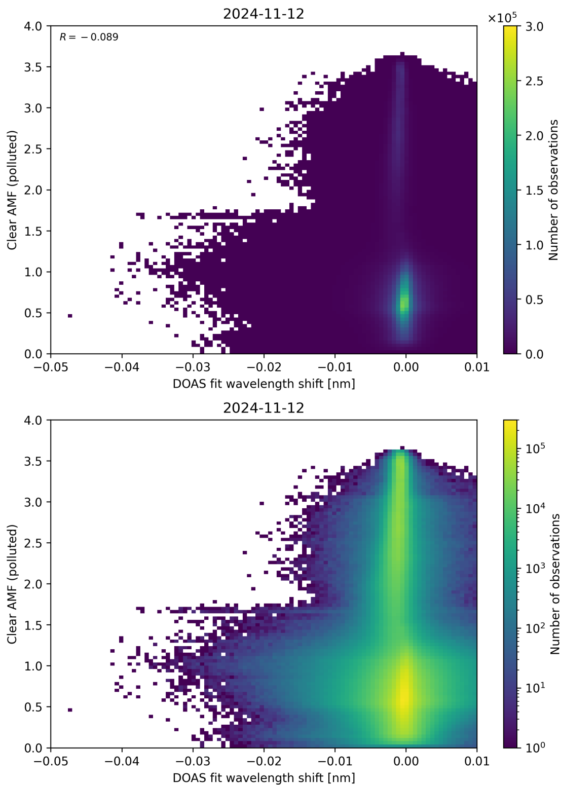
Figure 129: Scatter density plot of “DOAS fit wavelength shift” against “Clear AMF (polluted)” for 2024-11-11 to 2024-11-13.
