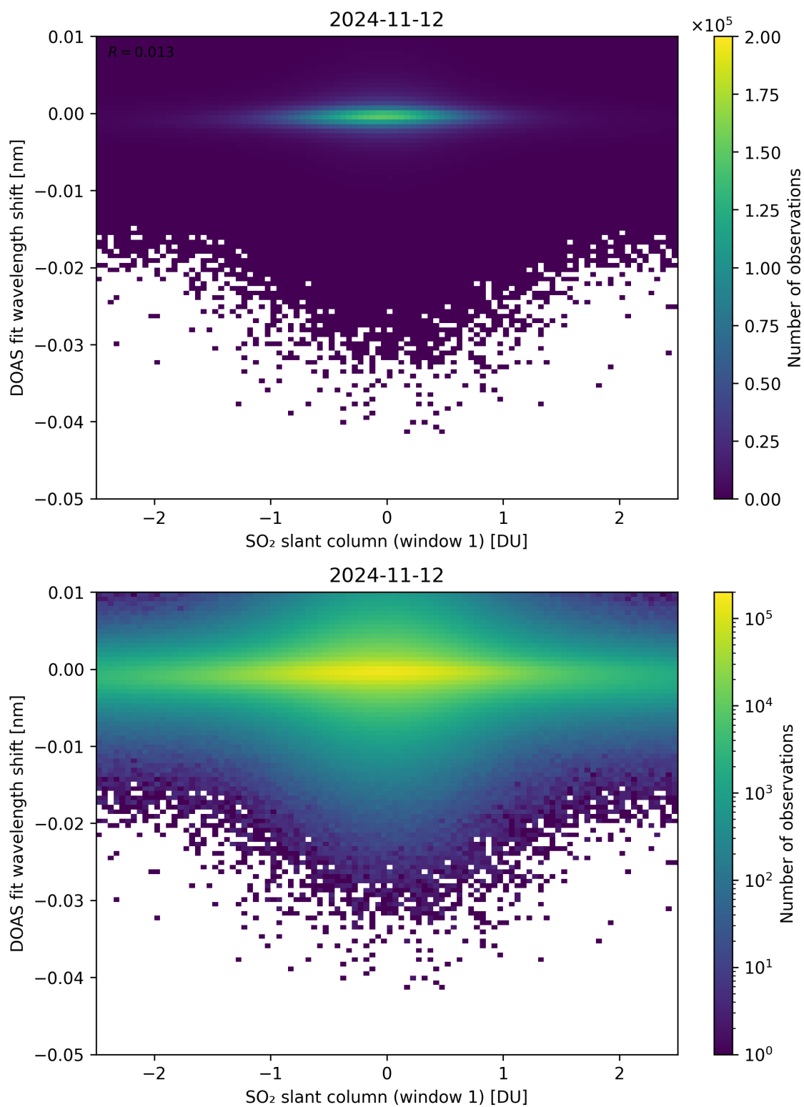
Figure 215: Scatter density plot of “SO 2 slant column (window 1)” against “DOAS fit wavelength shift” for 2024-11-11 to 2024-11-13.
