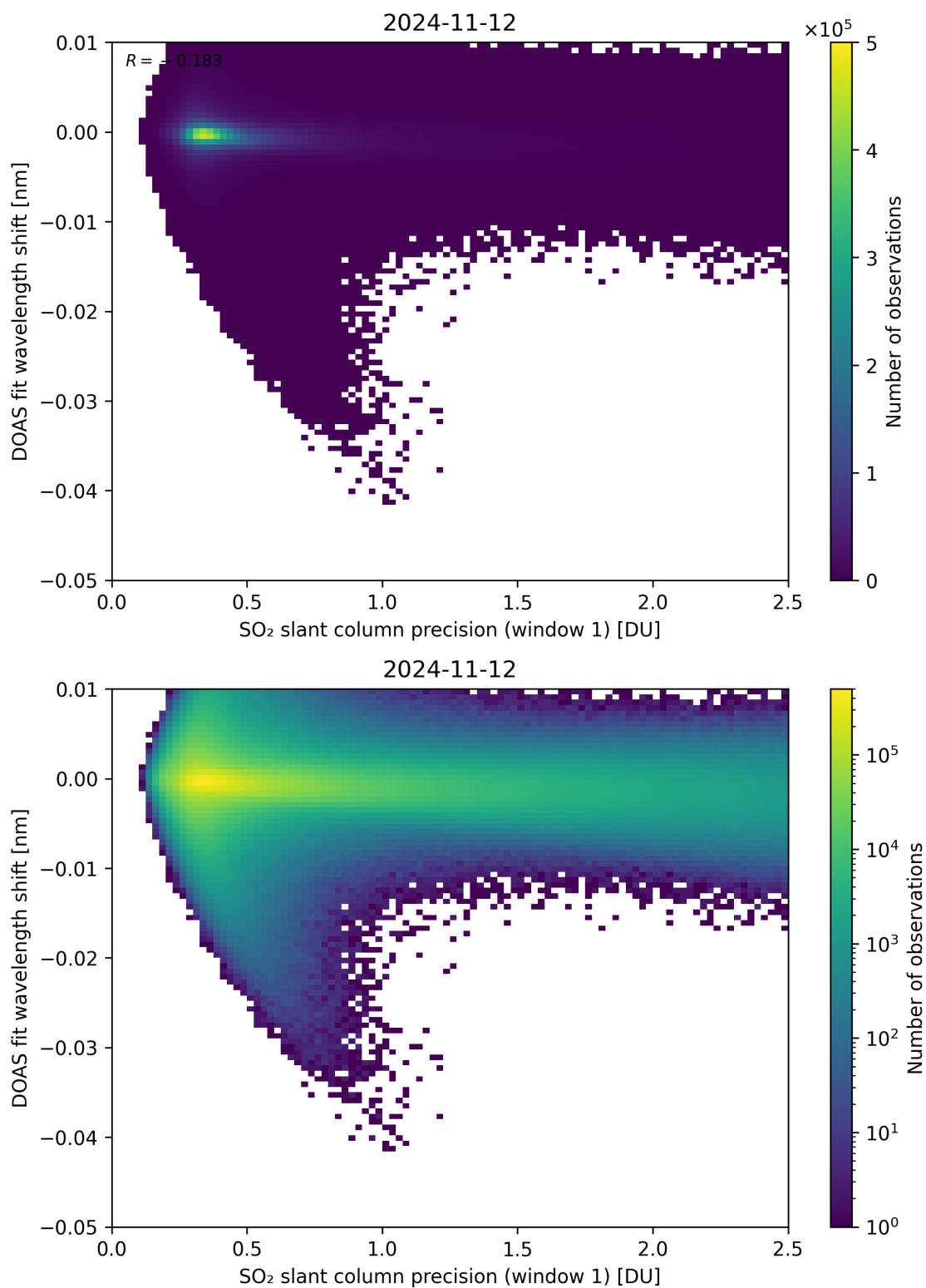
Figure 221: Scatter density plot of “SO 2 slant column precision (window 1)” against “DOAS fit wavelength shift” for 2024-11-11 to 2024-11-13.
