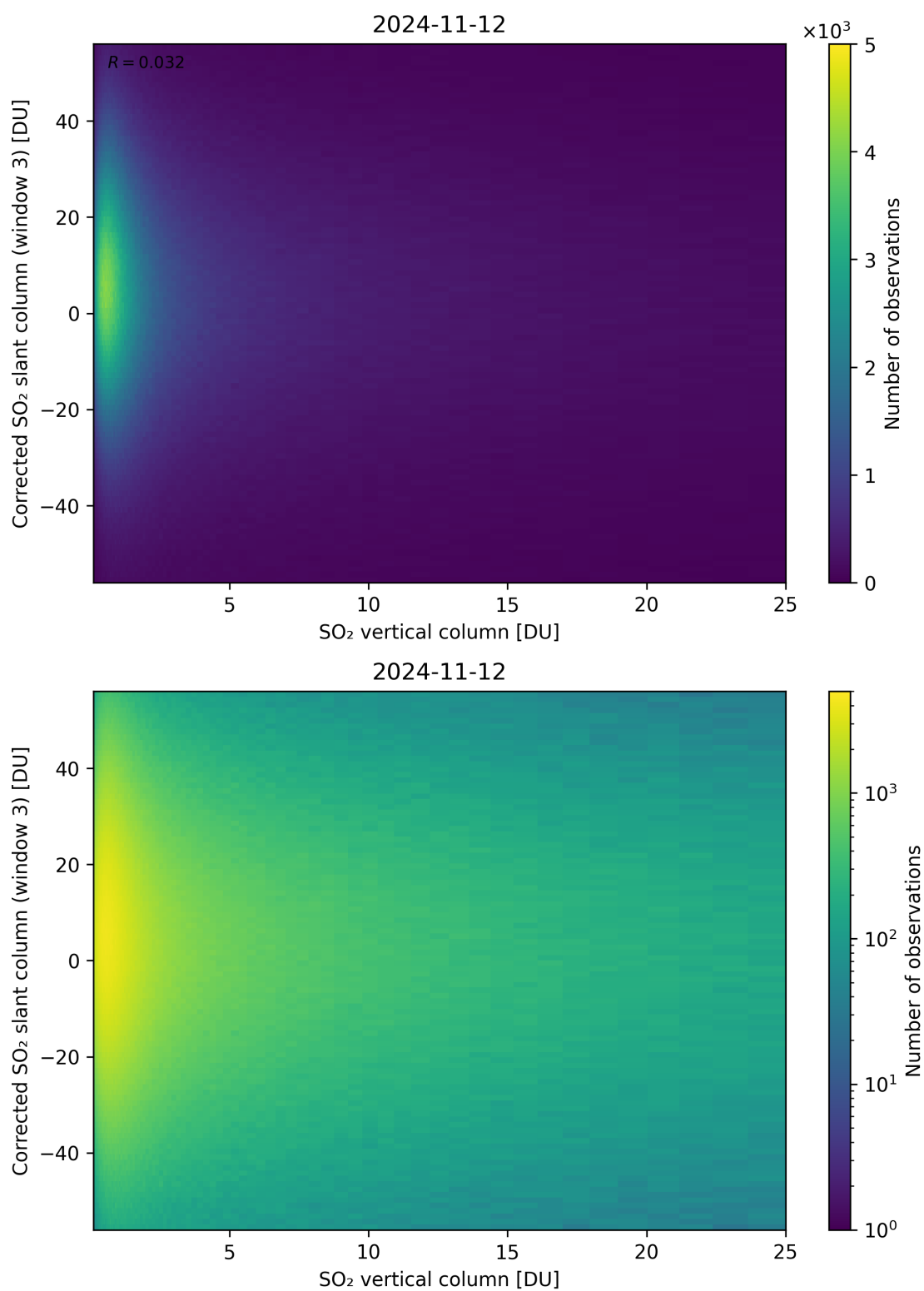
Figure 299: Scatter density plot of “SO 2 vertical column” against “Corrected SO 2 slant column (window 3)” for 2024-11-11 to 2024-11-13.
