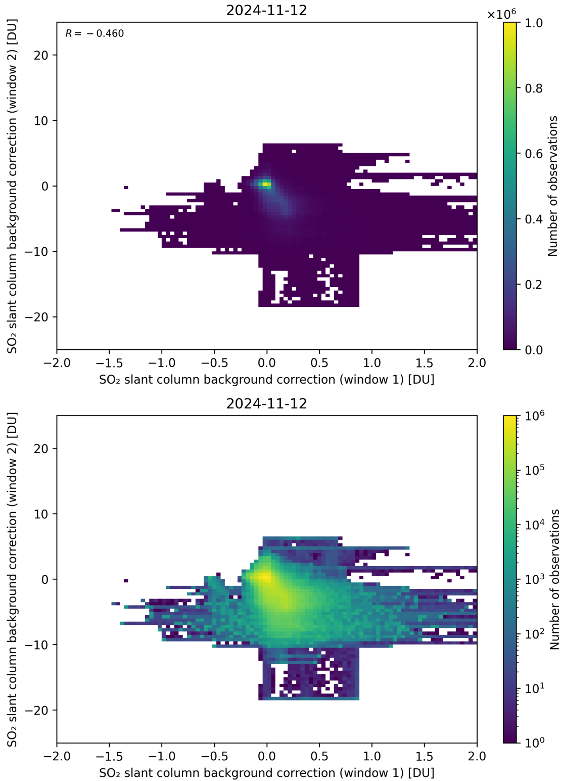
Figure 98: Scatter density plot of “SO 2 slant column background correction (window 1)” against “SO 2 slant column background correction (window 2)” for 2024-11-11 to 2024-11-13.
