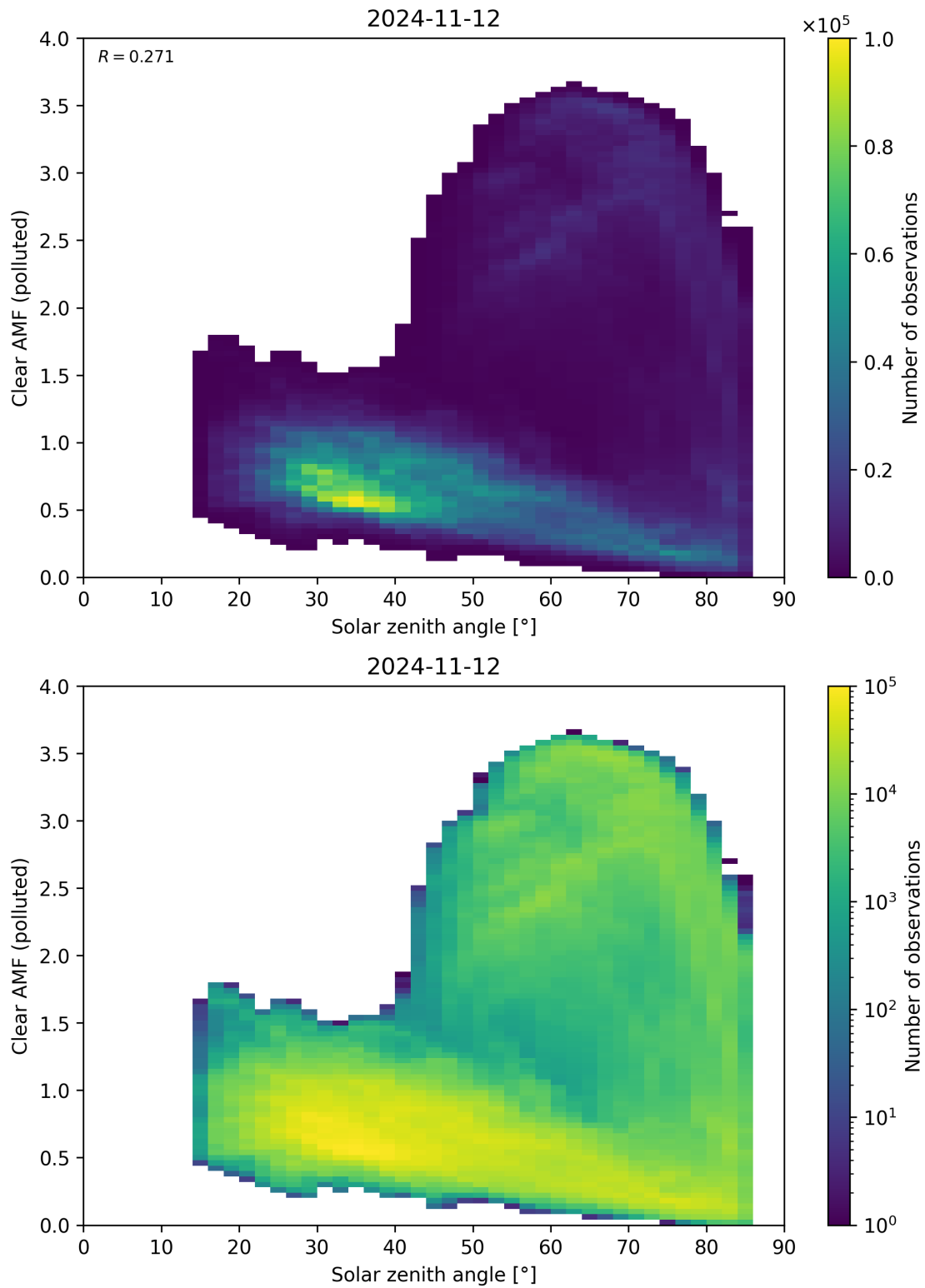
Figure 165: Scatter density plot of “Solar zenith angle” against “Clear AMF (polluted)” for 2024-11-11 to 2024-11-13.
