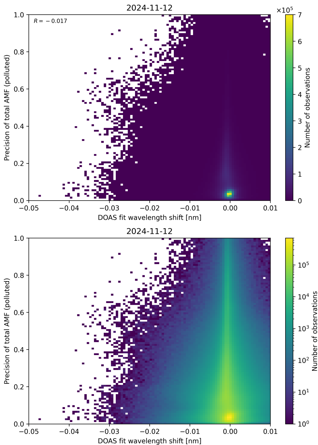
Figure 131: Scatter density plot of “DOAS fit wavelength shift” against “Precision of total AMF (polluted)” for 2024-11-11 to 2024-11-13.
