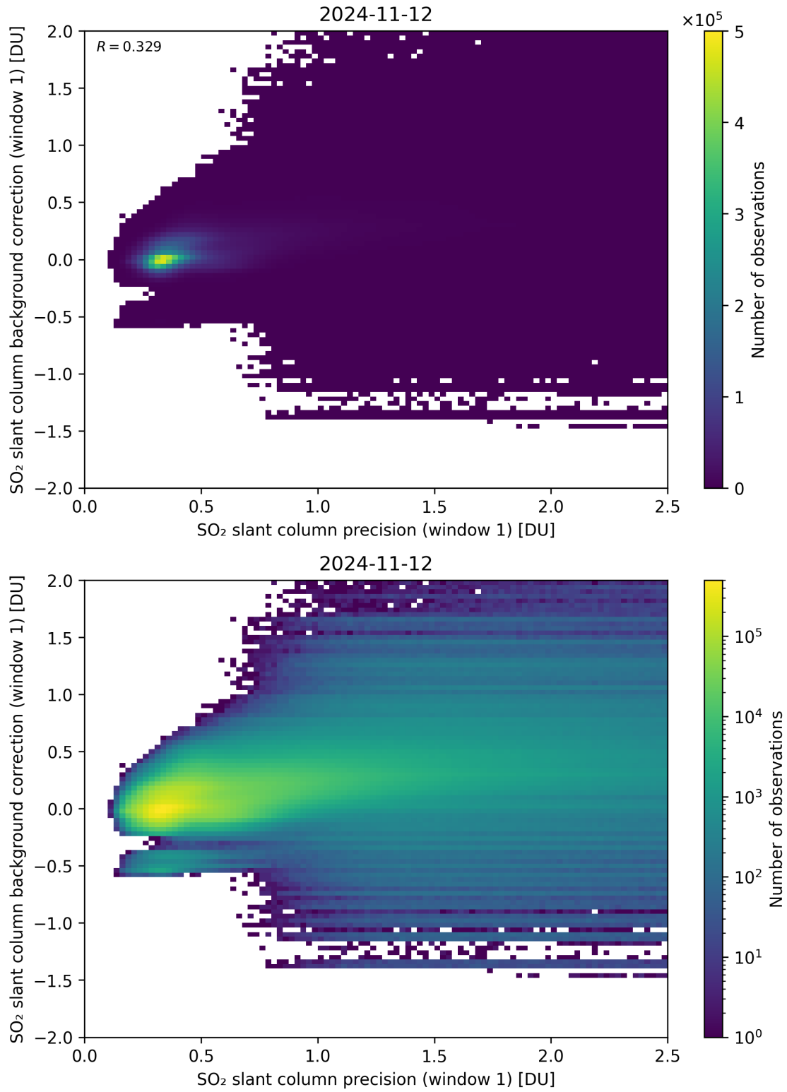
Figure 218: Scatter density plot of “SO 2 slant column precision (window 1)” against “SO 2 slant column background correction (window 1)” for 2024-11-11 to 2024-11-13.
