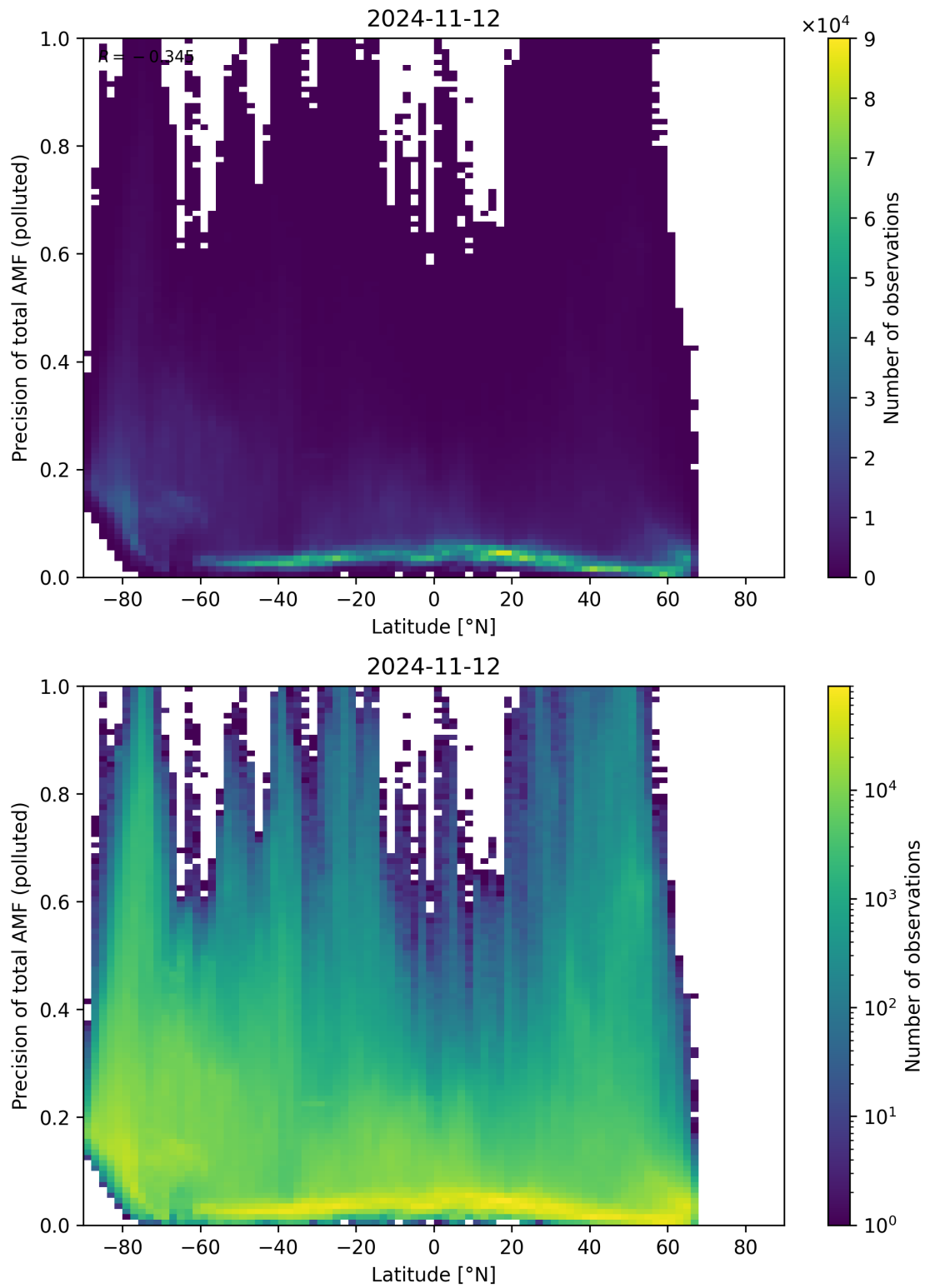
Figure 155: Scatter density plot of “Latitude” against “Precision of total AMF (polluted)” for 2024-11-11 to 2024-11-13.
