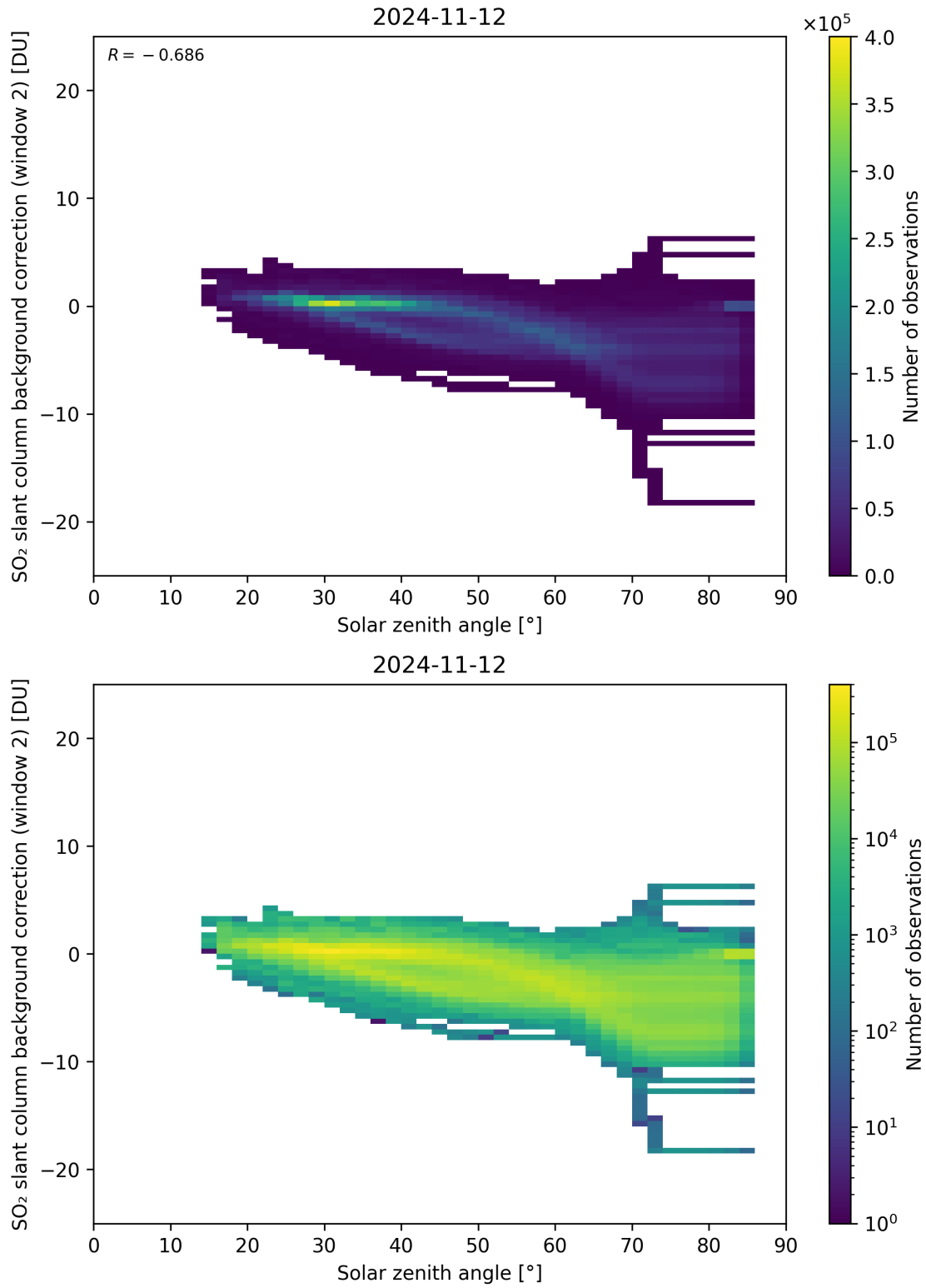
Figure 159: Scatter density plot of “Solar zenith angle” against “SO 2 slant column background correction (window 2)” for 2024-11-11 to 2024-11-13.
