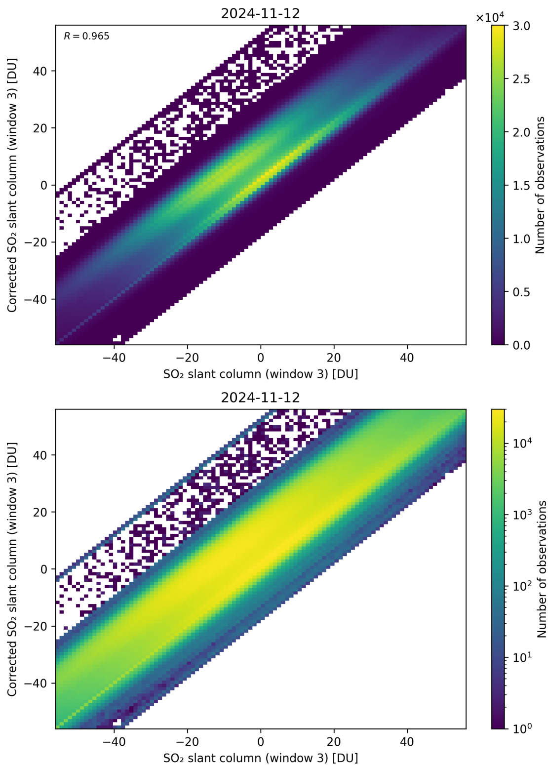
Figure 266: Scatter density plot of “SO 2 slant column (window 3)” against “Corrected SO 2 slant column (window 3)” for 2024-11-11 to 2024-11-13.
