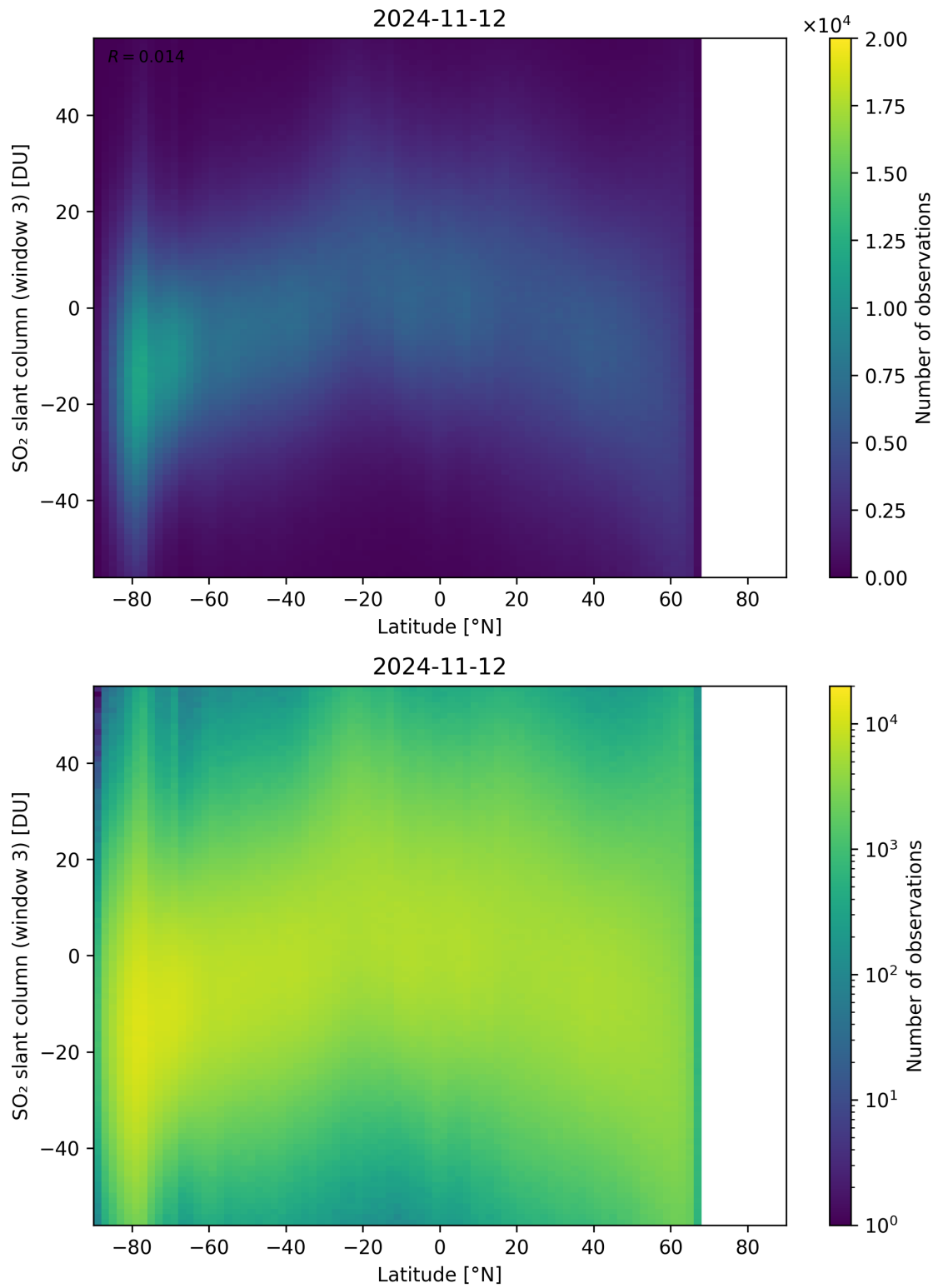
Figure 152: Scatter density plot of “Latitude” against “SO 2 slant column (window 3)” for 2024-11-11 to 2024-11-13.
