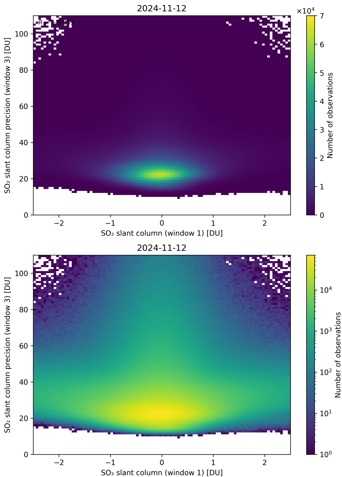
Figure 238: Scatter density plot of “SO 2 slant column (window 1)” against “SO 2 slant column precision (window 3)” for 2024-11-11 to 2024-11-13.
