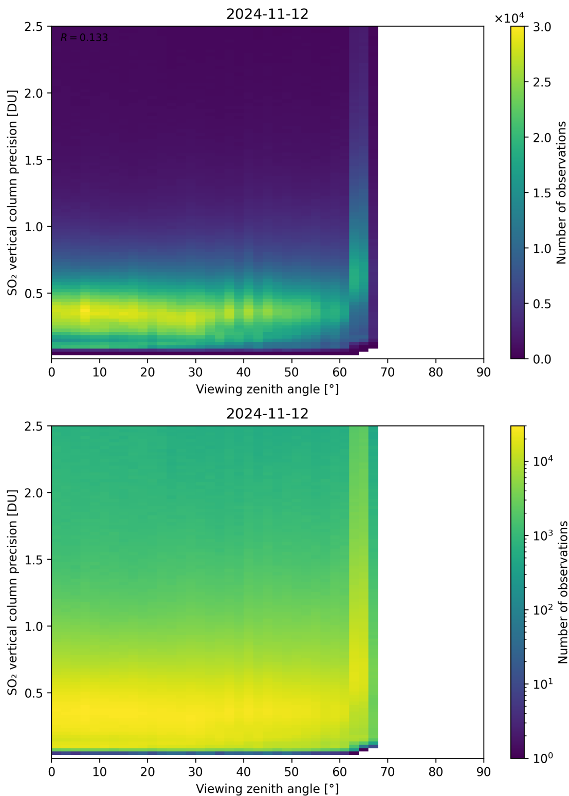
Figure 328: Scatter density plot of “Viewing zenith angle” against “SO 2 vertical column precision” for 2024-11-11 to 2024-11-13.
