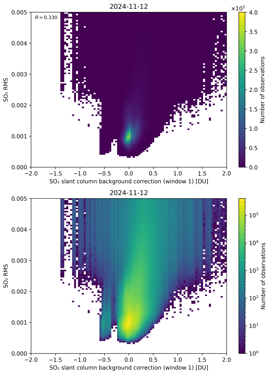
Figure 102: Scatter density plot of “SO 2 slant column background correction (window 1)” against “SO 2 RMS” for 2024-11-11 to 2024-11-13.
