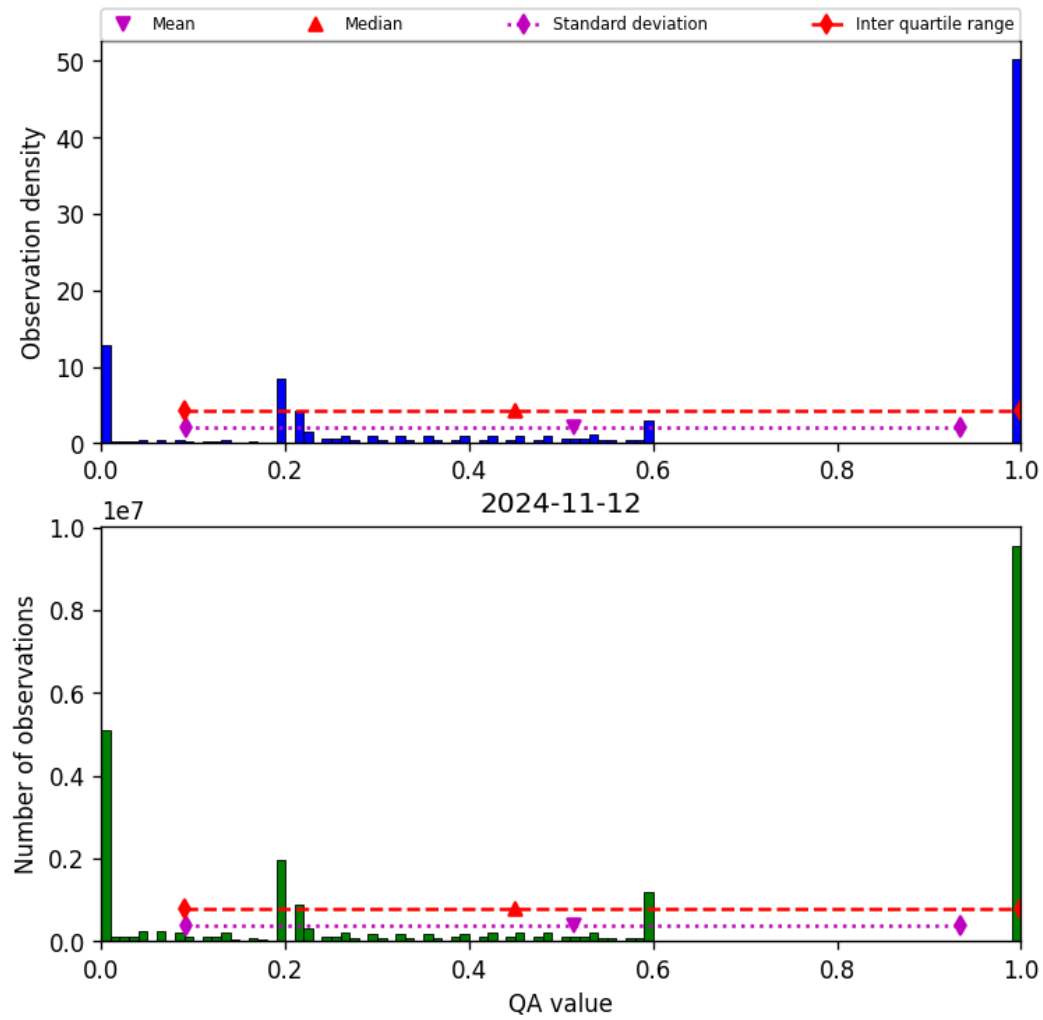
Figure 52: Histogram of “QA value” for 2024-11-11 to 2024-11-13
