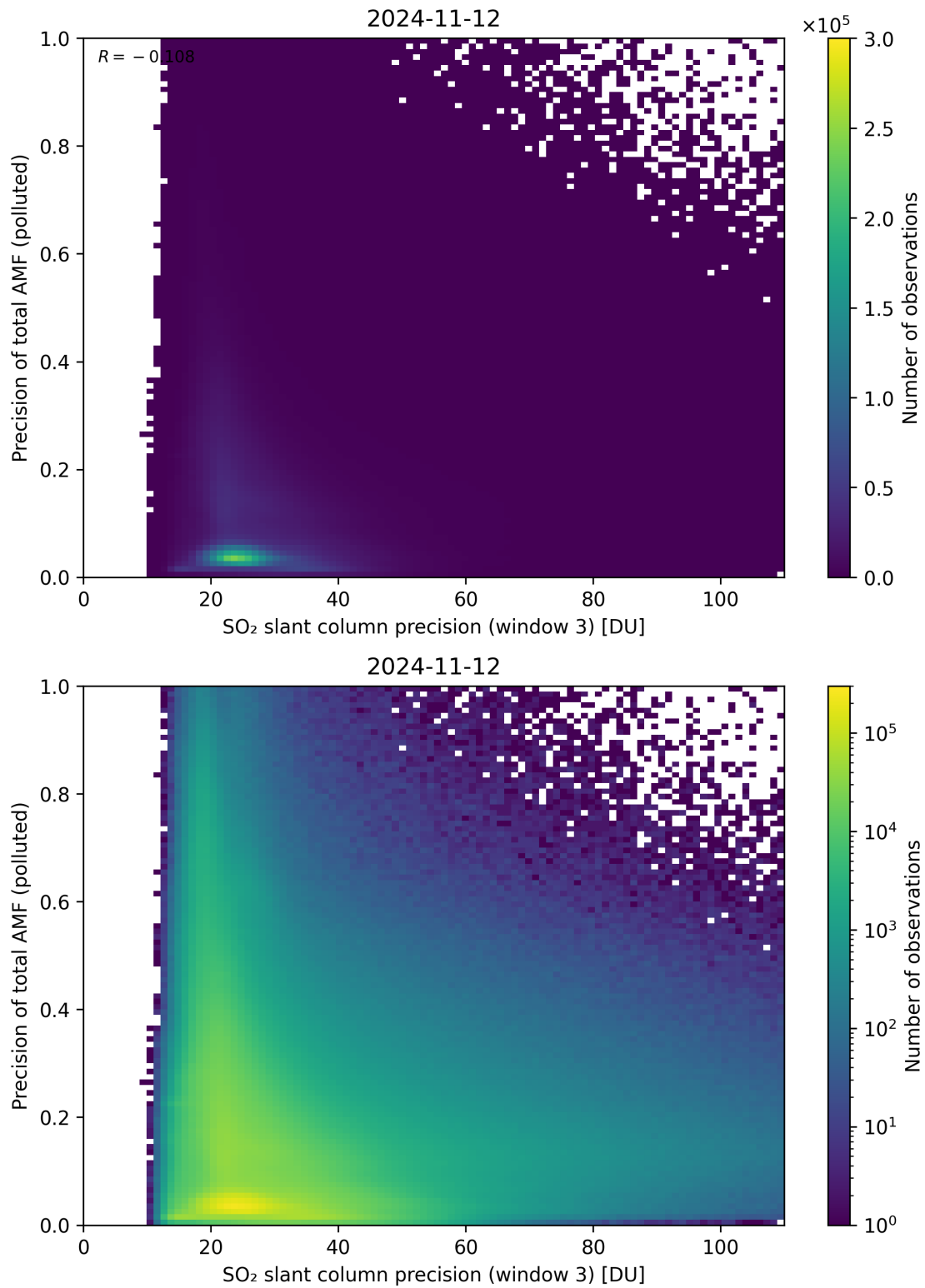
Figure 264: Scatter density plot of “SO 2 slant column precision (window 3)” against “Precision of total AMF (polluted)” for 2024-11-11 to 2024-11-13.
