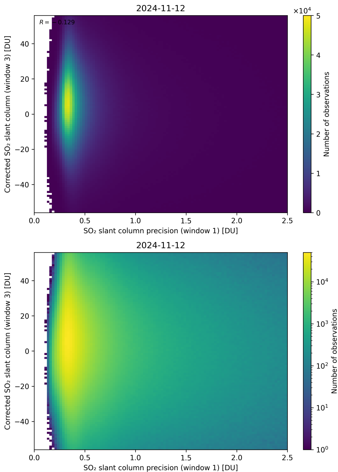
Figure 226: Scatter density plot of “SO 2 slant column precision (window 1)” against “Corrected SO 2 slant column (window 3)” for 2024-11-11 to 2024-11-13.
