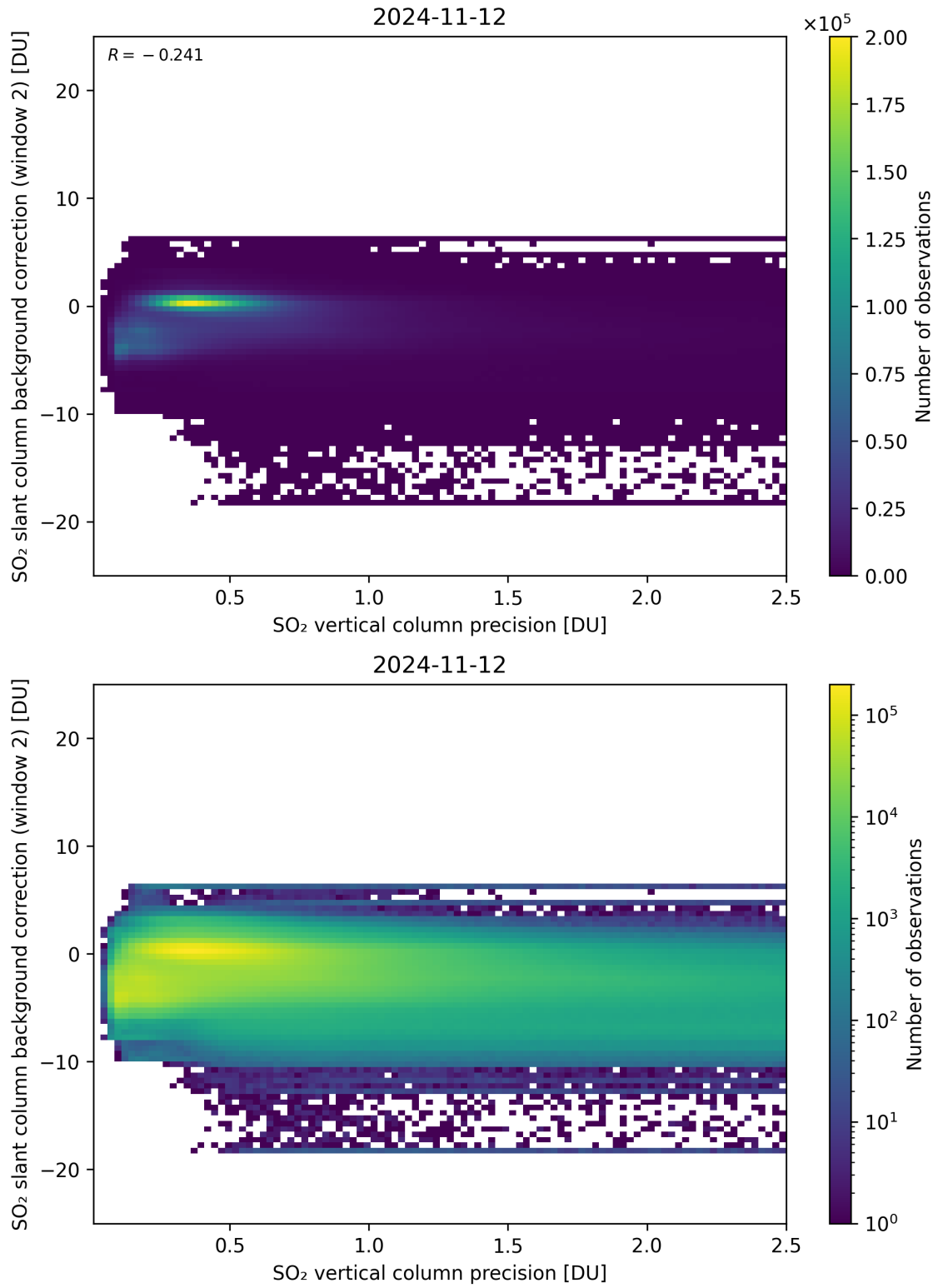
Figure 280: Scatter density plot of “SO 2 vertical column precision” against “SO 2 slant column background correction (window 2)” for 2024-11-11 to 2024-11-13.
