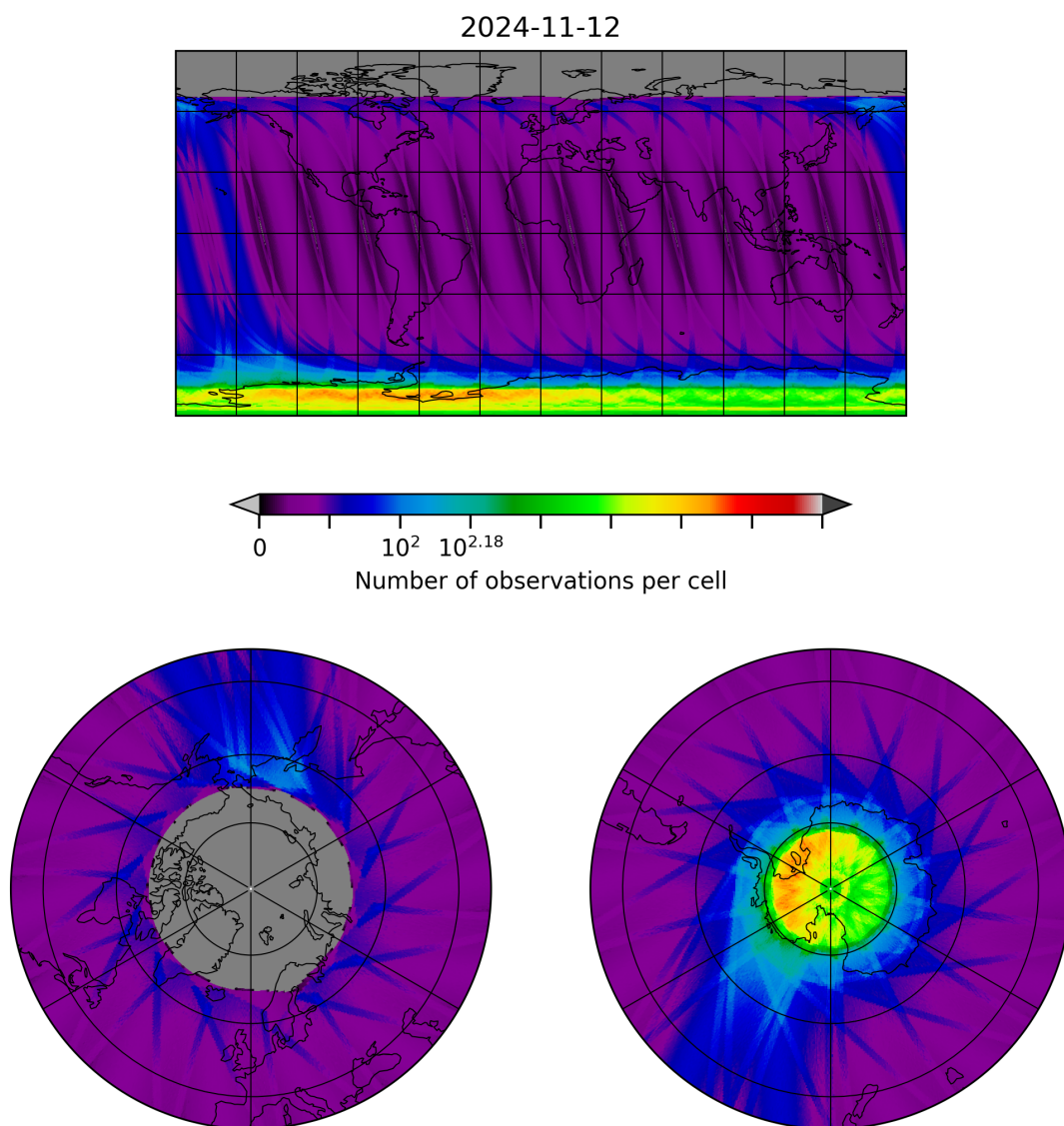
Figure 28: Map of the number of observations for 2024-11-11 to 2024-11-13
