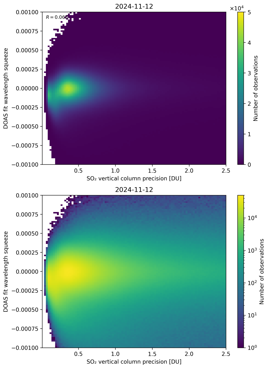
Figure 283: Scatter density plot of “SO 2 vertical column precision” against “DOAS fit wavelength squeeze” for 2024-11-11 to 2024-11-13.
