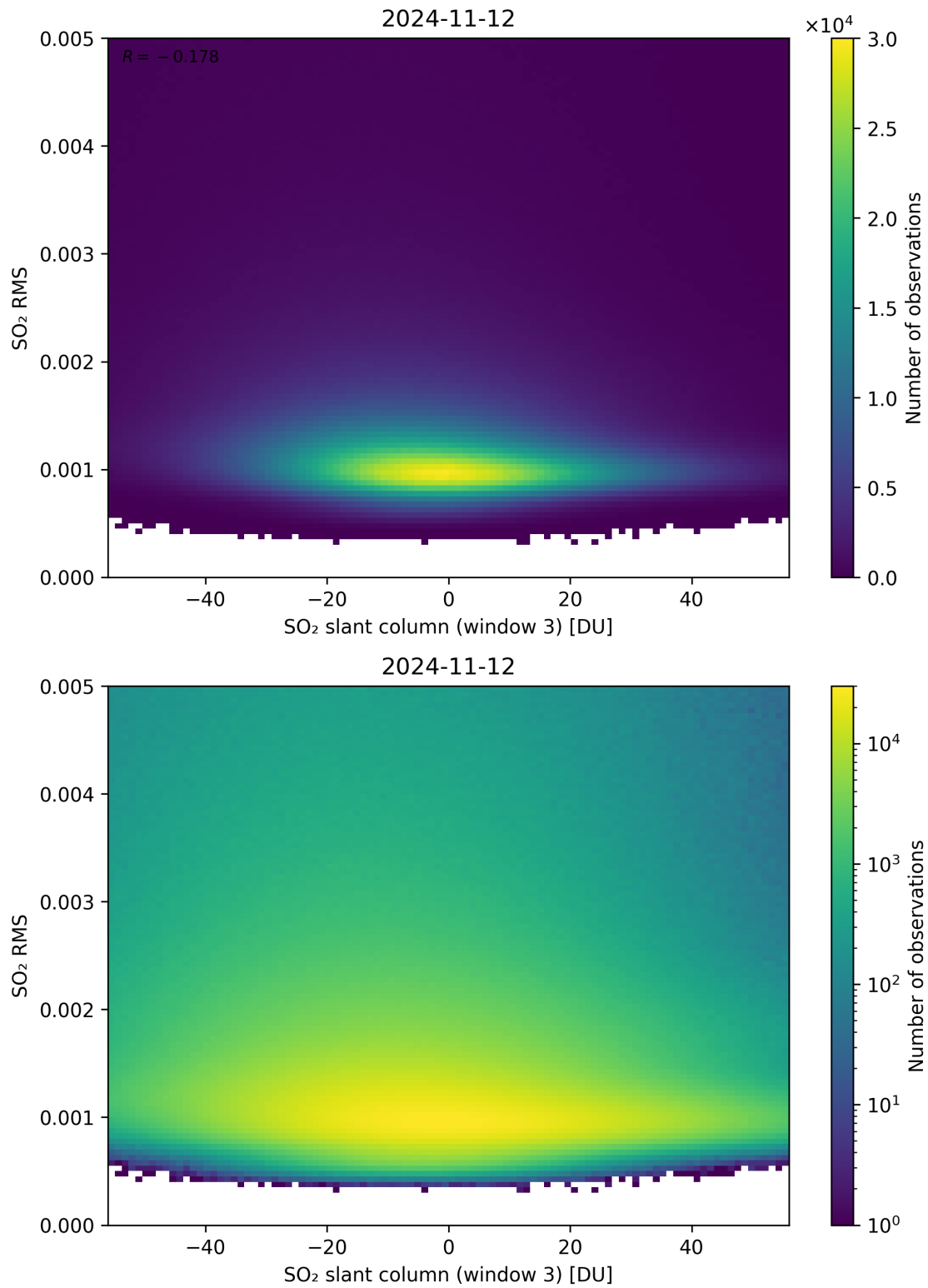
Figure 256: Scatter density plot of “SO 2 slant column (window 3)” against “SO 2 RMS” for 2024-11-11 to 2024-11-13.
