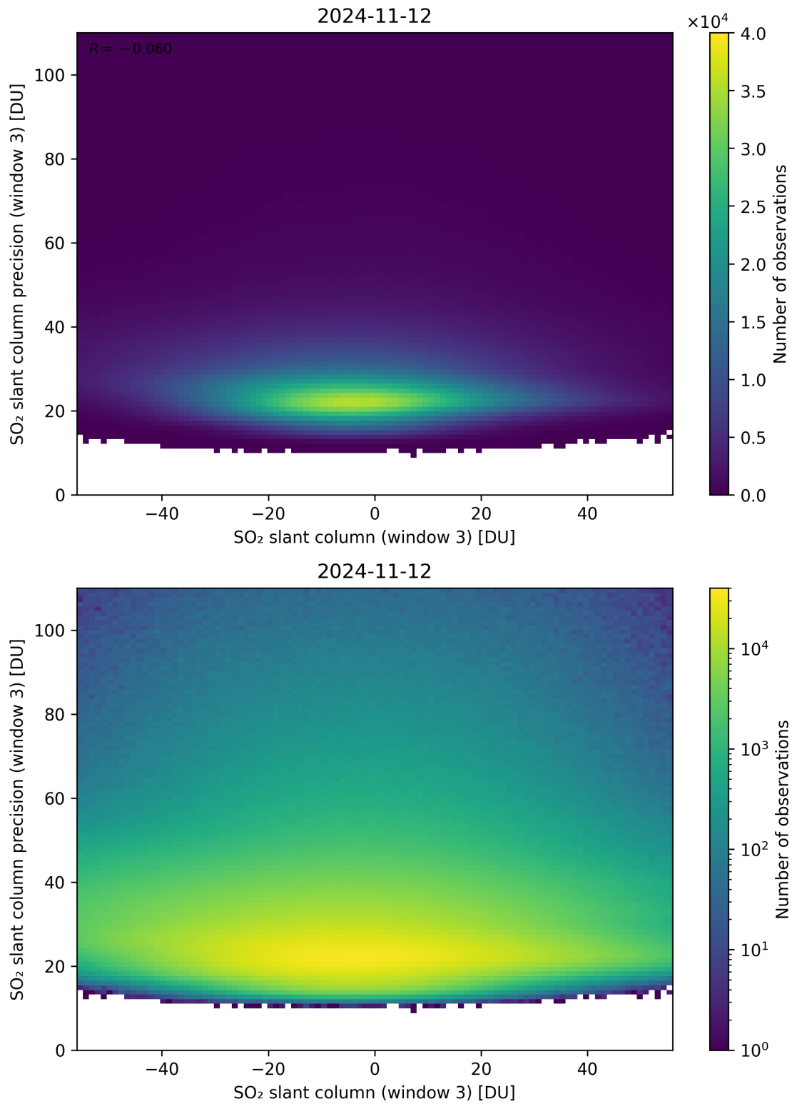
Figure 267: Scatter density plot of “SO 2 slant column (window 3)” against “SO 2 slant column precision (window 3)” for 2024-11-11 to 2024-11-13.
