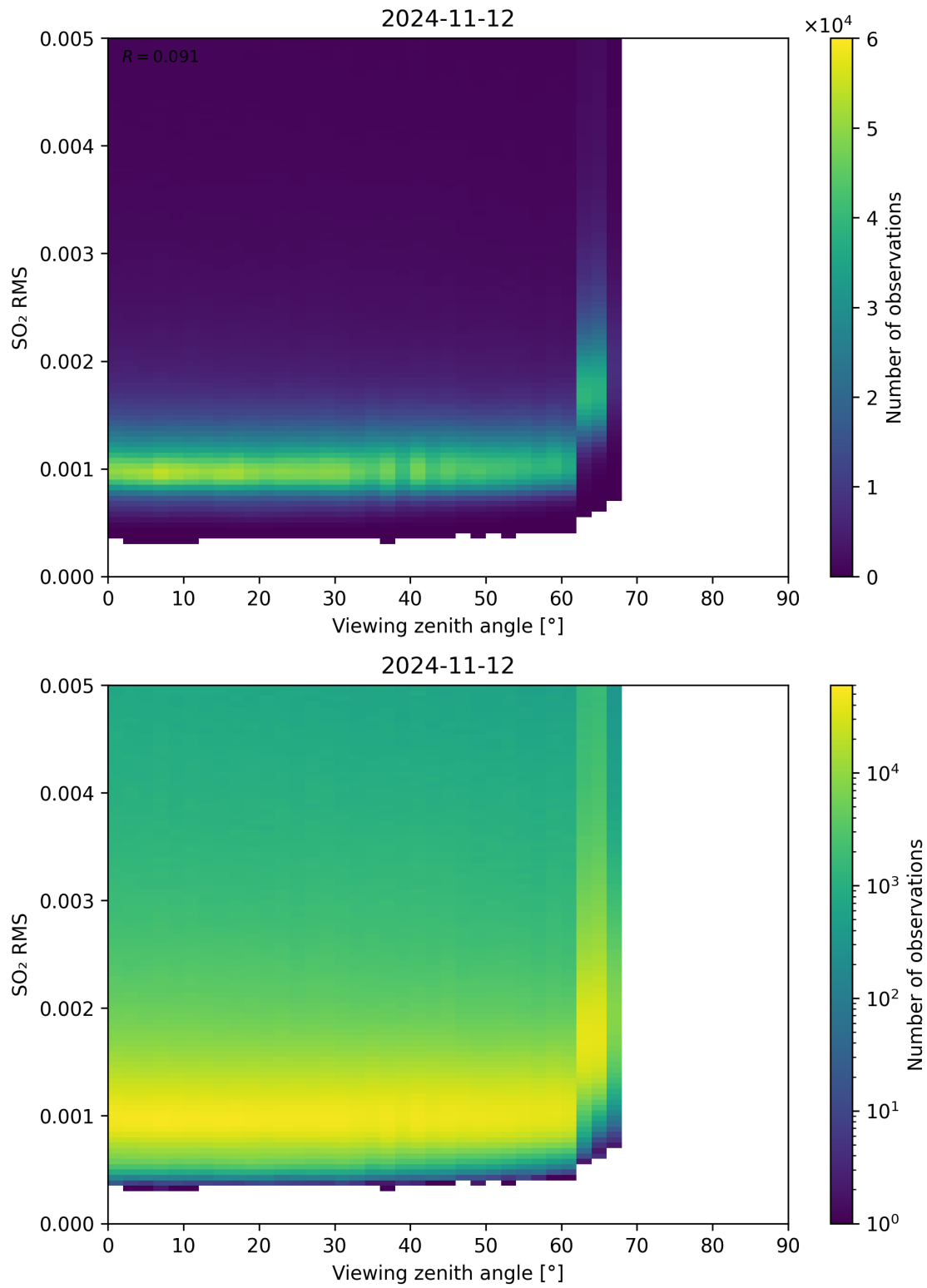
Figure 313: Scatter density plot of “Viewing zenith angle” against “SO 2 RMS” for 2024-11-11 to 2024-11-13.
