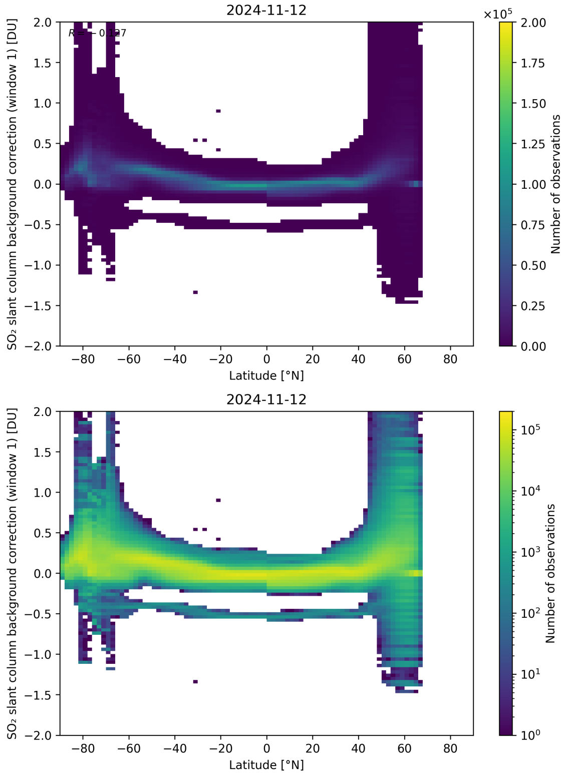
Figure 139: Scatter density plot of “Latitude” against “SO 2 slant column background correction (window 1)” for 2024-11-11 to 2024-11-13.
