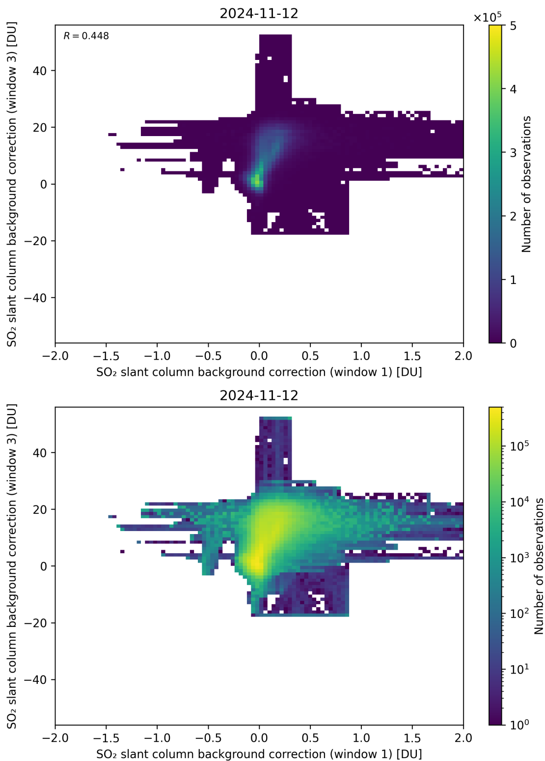
Figure 99: Scatter density plot of “SO 2 slant column background correction (window 1)” against “SO 2 slant column background correction (window 3)” for 2024-11-11 to 2024-11-13.
