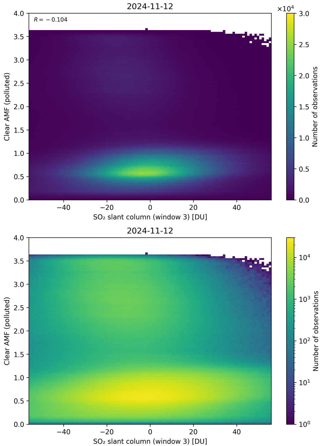
Figure 265: Scatter density plot of “SO 2 slant column (window 3)” against “Clear AMF (polluted)” for 2024-11-11 to 2024-11-13.
