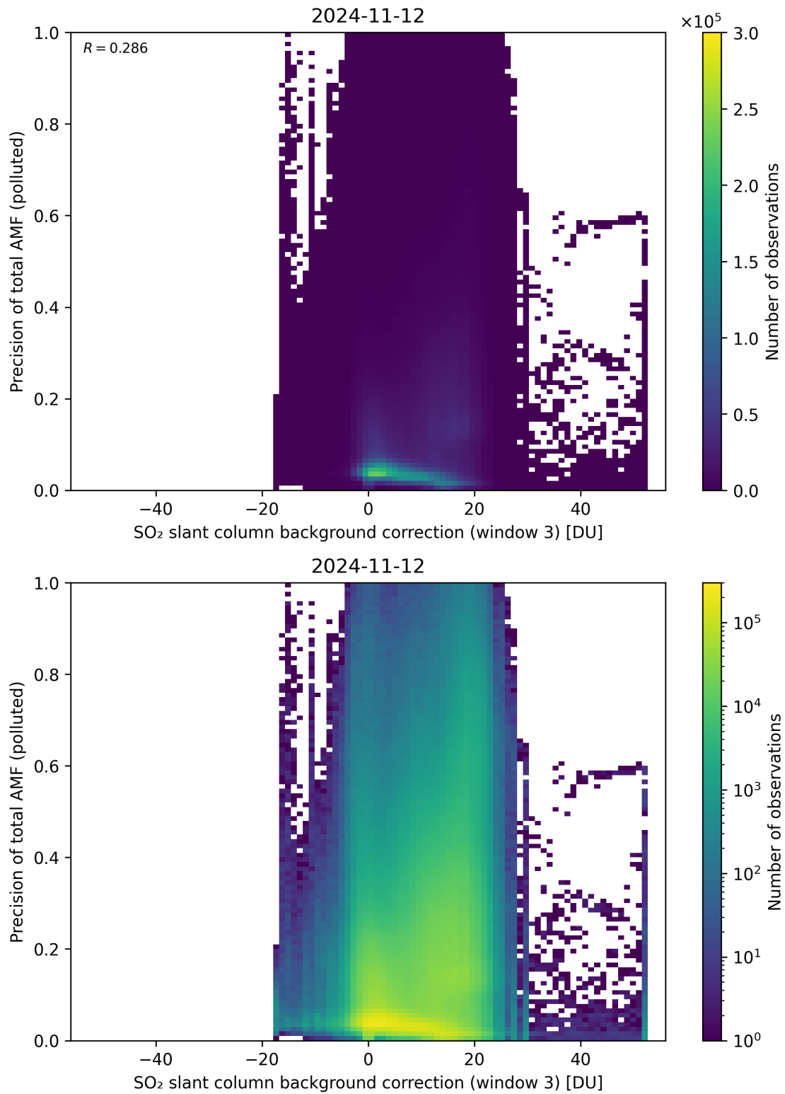
Figure 126: Scatter density plot of “SO 2 slant column background correction (window 3)” against “Precision of total AMF (polluted)” for 2024-11-11 to 2024-11-13.
