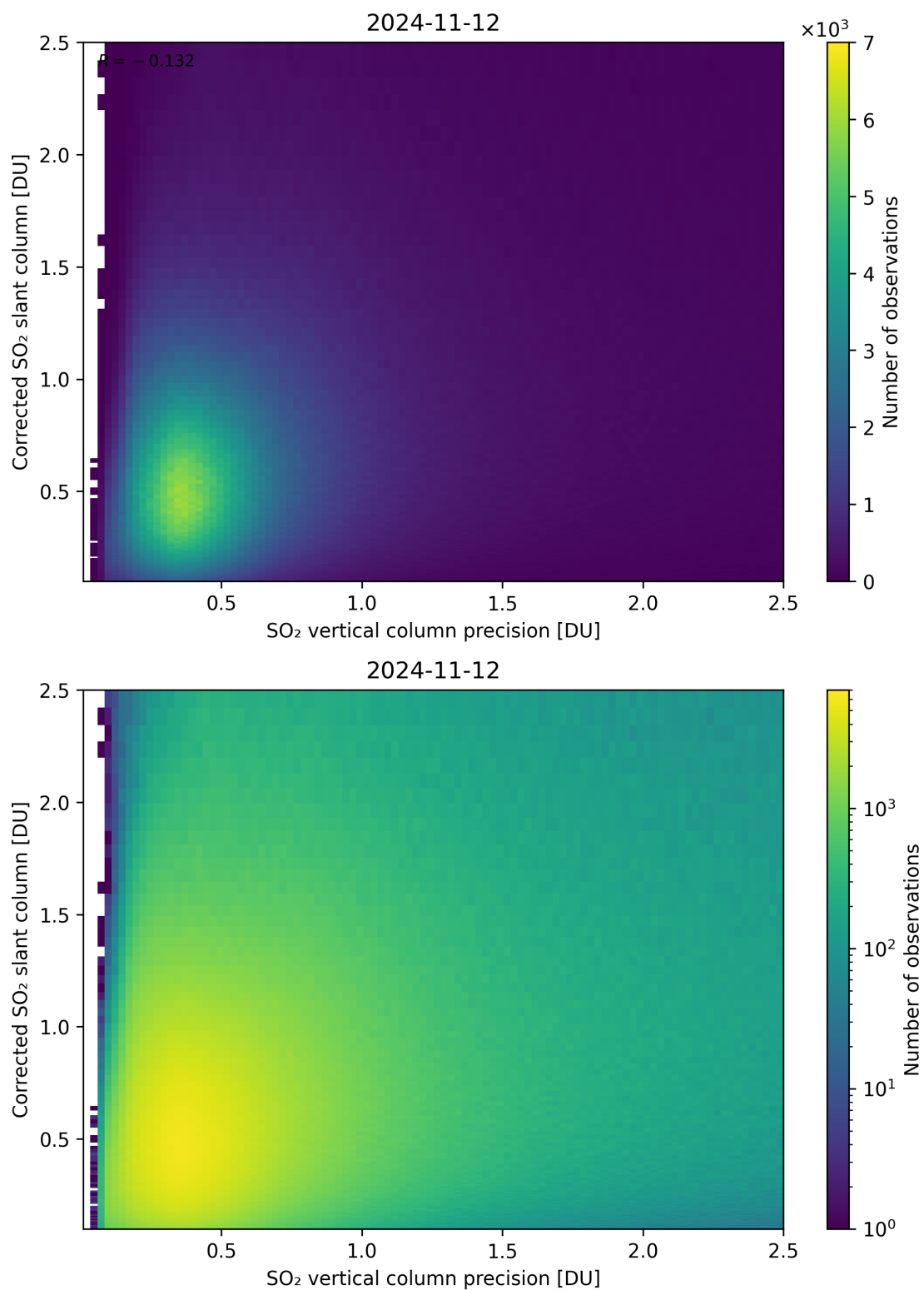
Figure 286: Scatter density plot of “SO 2 vertical column precision” against “Corrected SO 2 slant column” for 2024-11-11 to 2024-11-13.
