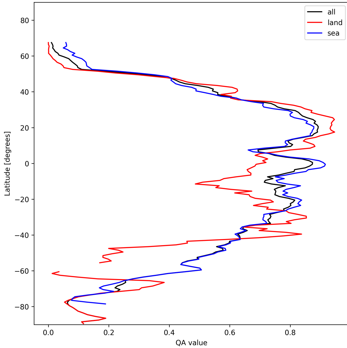
Figure 29: Zonal average of “QA value” for 2024-11-11 to 2024-11-13.
