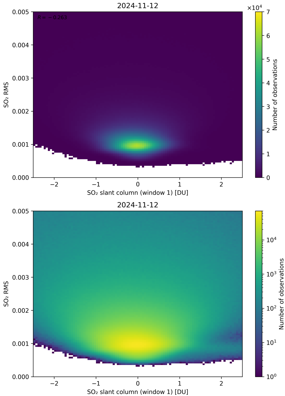
Figure 217: Scatter density plot of “SO 2 slant column (window 1)” against “SO 2 RMS” for 2024-11-11 to 2024-11-13.
