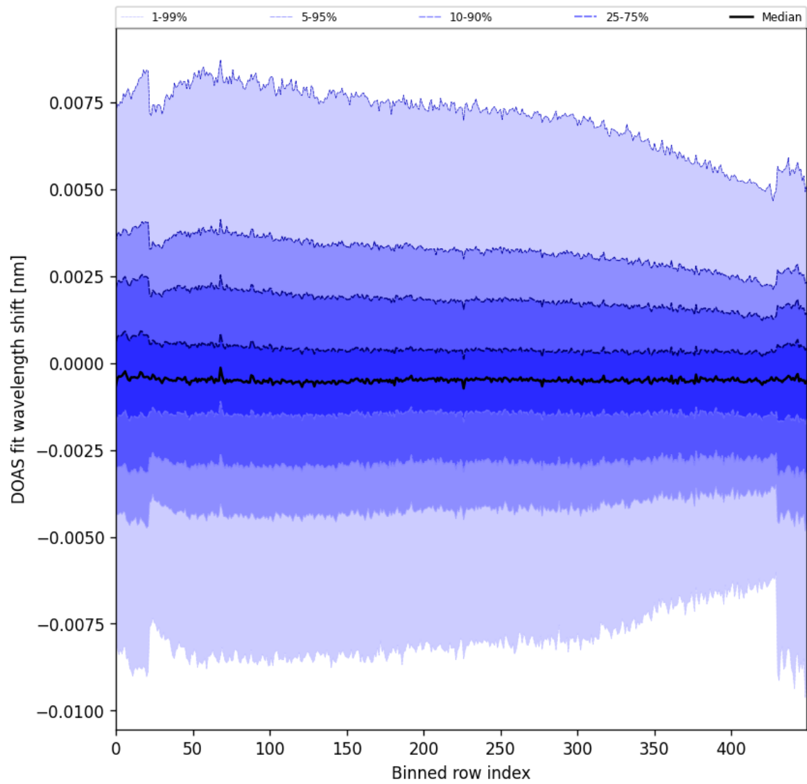
Figure 91: Along track statistics of “DOAS fit wavelength shift” for 2024-11-11 to 2024-11-13
