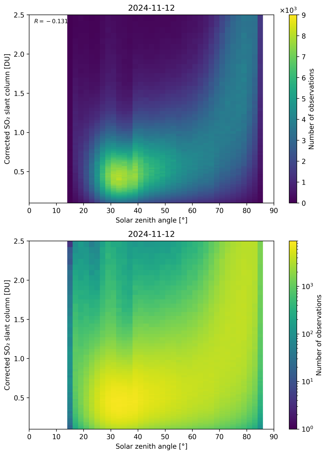
Figure 166: Scatter density plot of “Solar zenith angle” against “Corrected SO 2 slant column” for 2024-11-11 to 2024-11-13.
