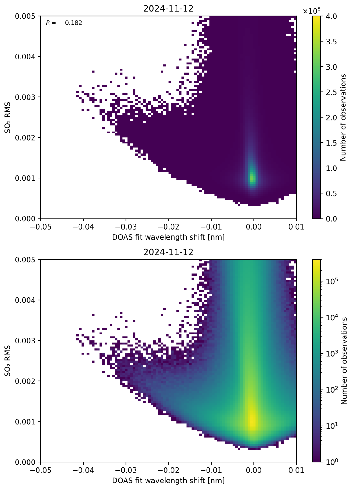
Figure 128: Scatter density plot of “DOAS fit wavelength shift” against “SO 2 RMS” for 2024-11-11 to 2024-11-13.
