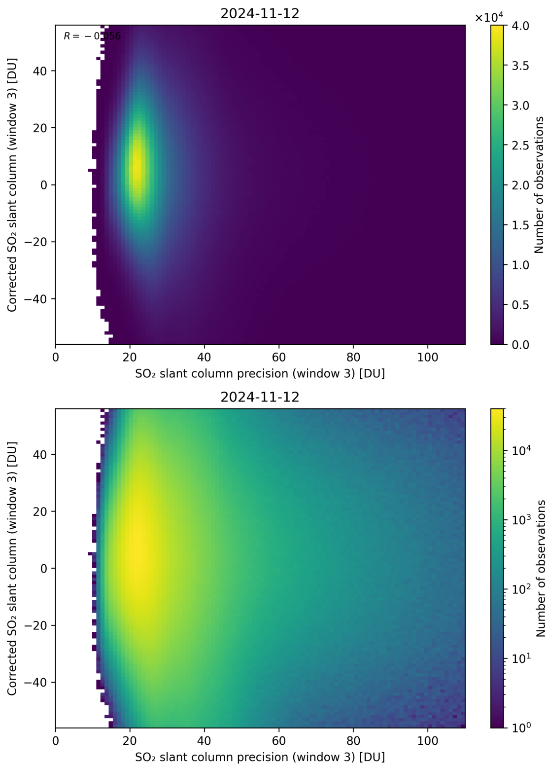
Figure 262: Scatter density plot of “SO 2 slant column precision (window 3)” against “Corrected SO 2 slant column (window 3)” for 2024-11-11 to 2024-11-13.
