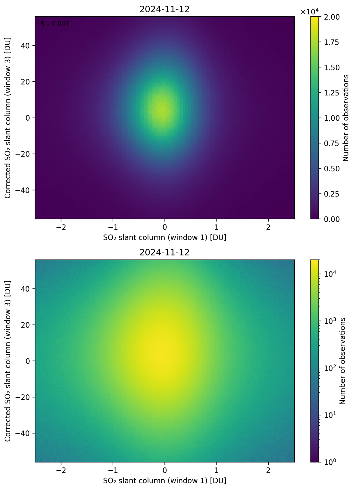
Figure 234: Scatter density plot of “SO 2 slant column (window 1)” against “Corrected SO 2 slant column (window 3)” for 2024-11-11 to 2024-11-13.
