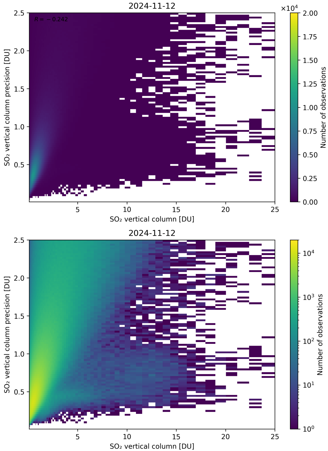
Figure 307: Scatter density plot of “SO 2 vertical column” against “SO 2 vertical column precision” for 2024-11-11 to 2024-11-13.
