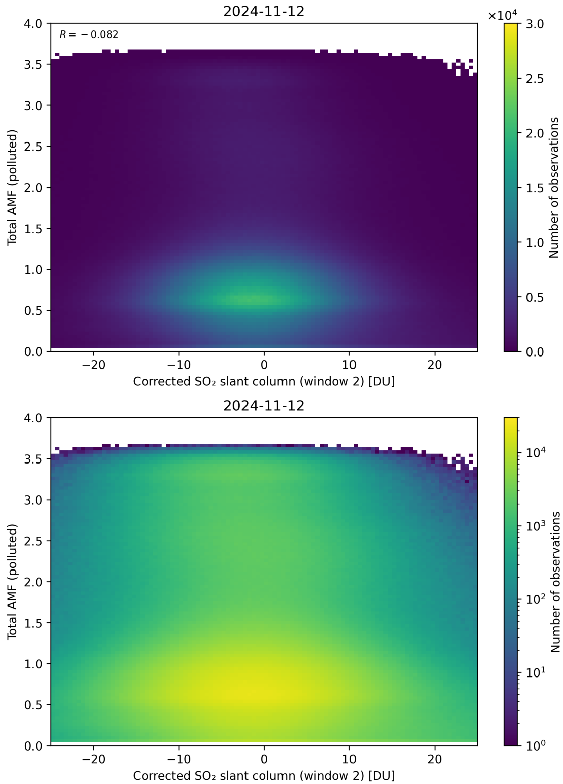
Figure 203: Scatter density plot of “Corrected SO 2 slant column (window 2)” against “Total AMF (polluted)” for 2024-11-11 to 2024-11-13.
