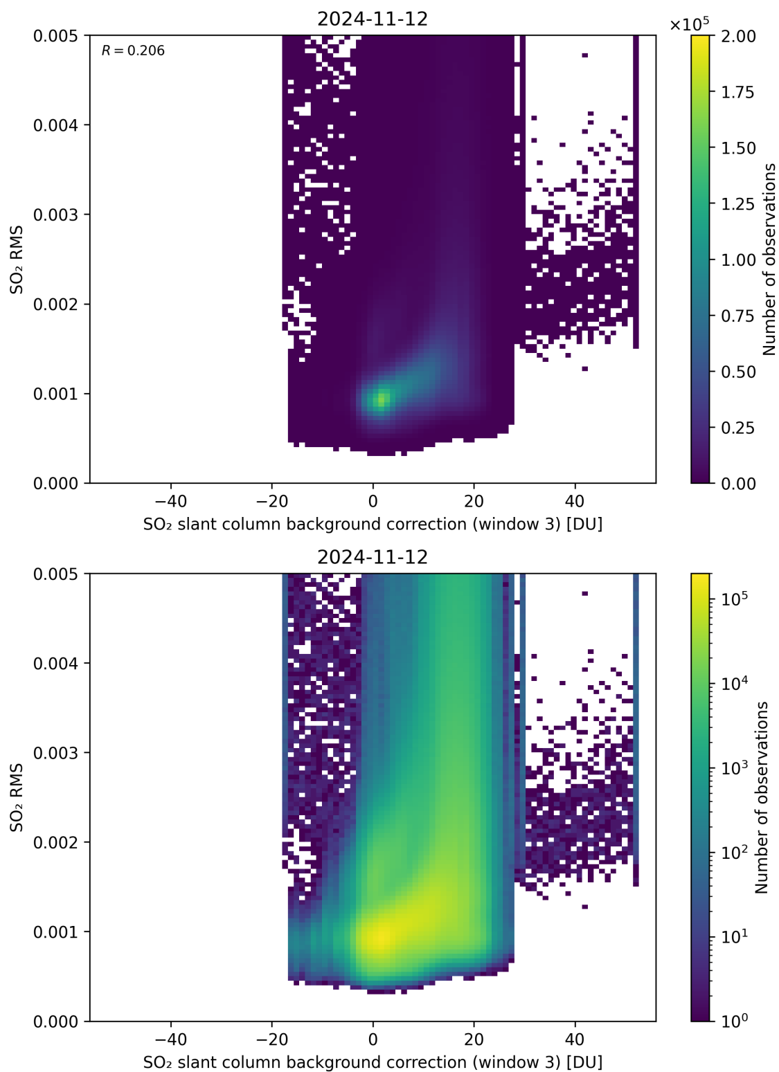
Figure 123: Scatter density plot of “SO 2 slant column background correction (window 3)” against “SO 2 RMS” for 2024-11-11 to 2024-11-13.
