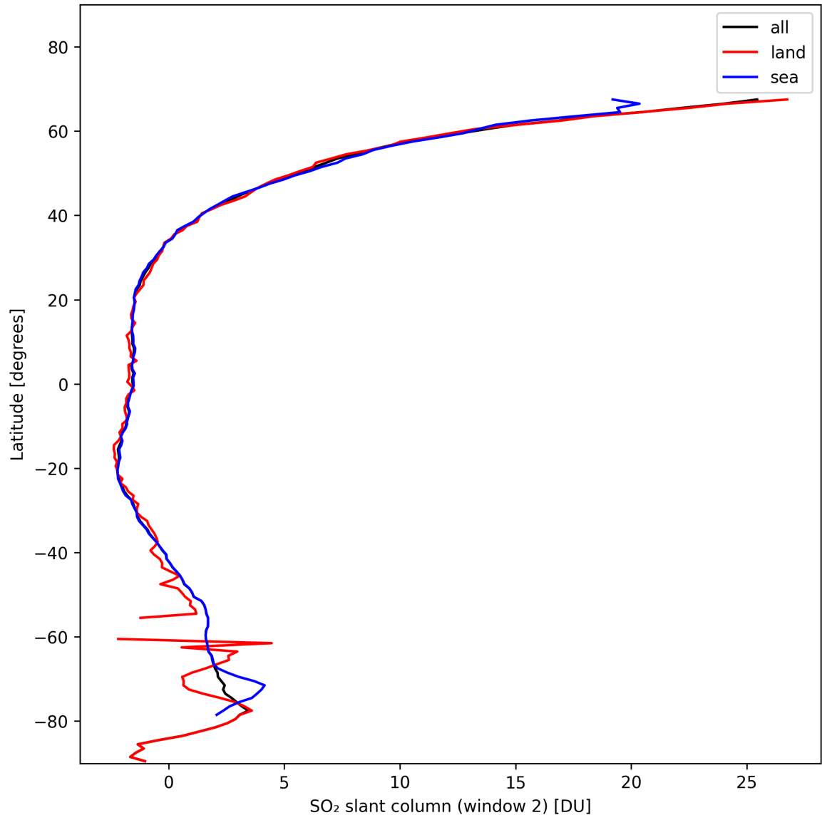
Figure 37: Zonal average of “SO 2 slant column (window 2)” for 2024-11-11 to 2024-11-13.
