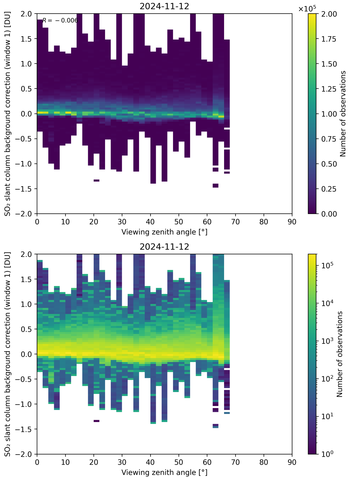
Figure 308: Scatter density plot of “Viewing zenith angle” against “SO 2 slant column background correction (window 1)” for 2024-11-11 to 2024-11-13.
