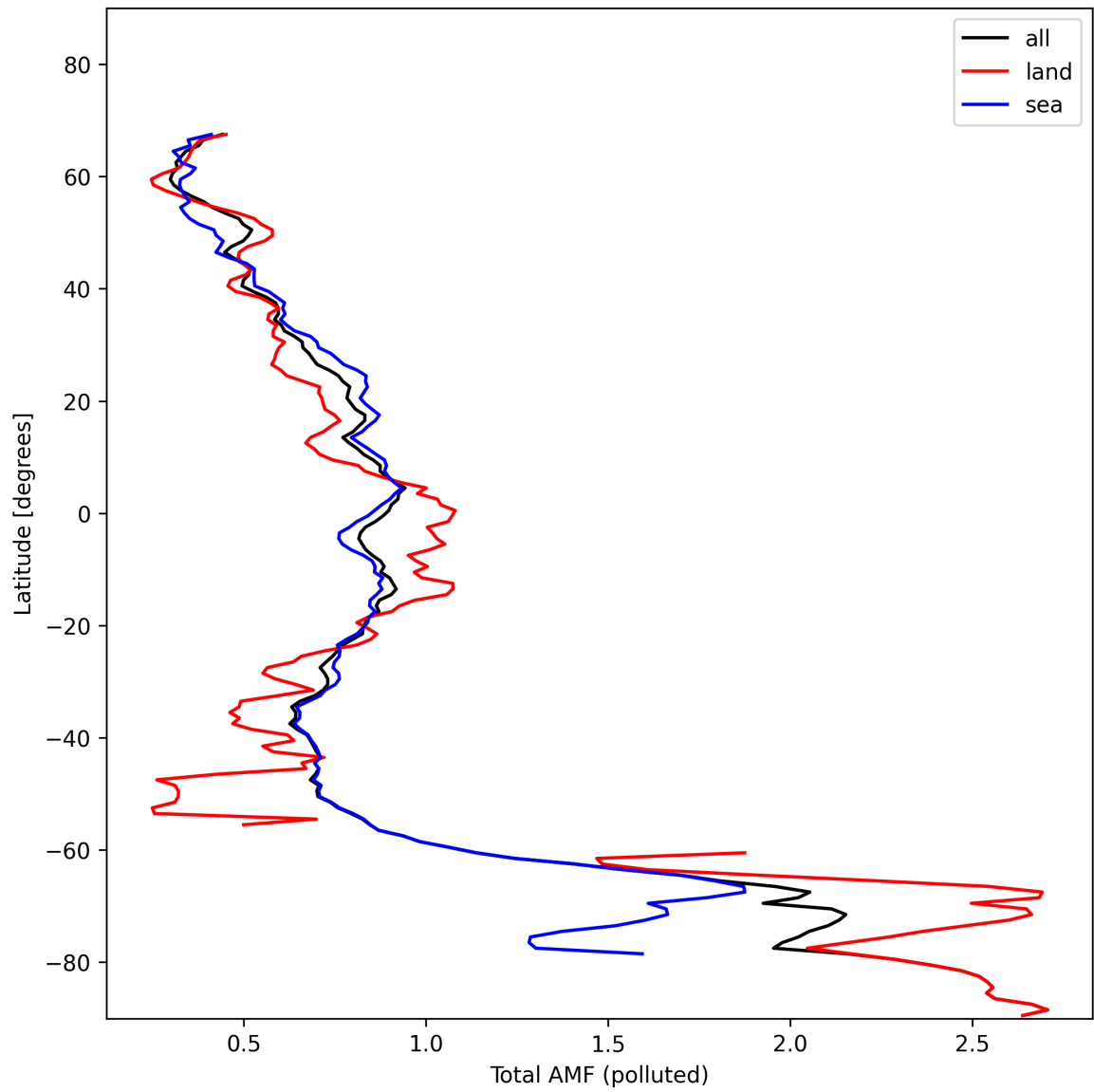
Figure 48: Zonal average of “Total AMF (polluted)” for 2024-11-11 to 2024-11-13.
