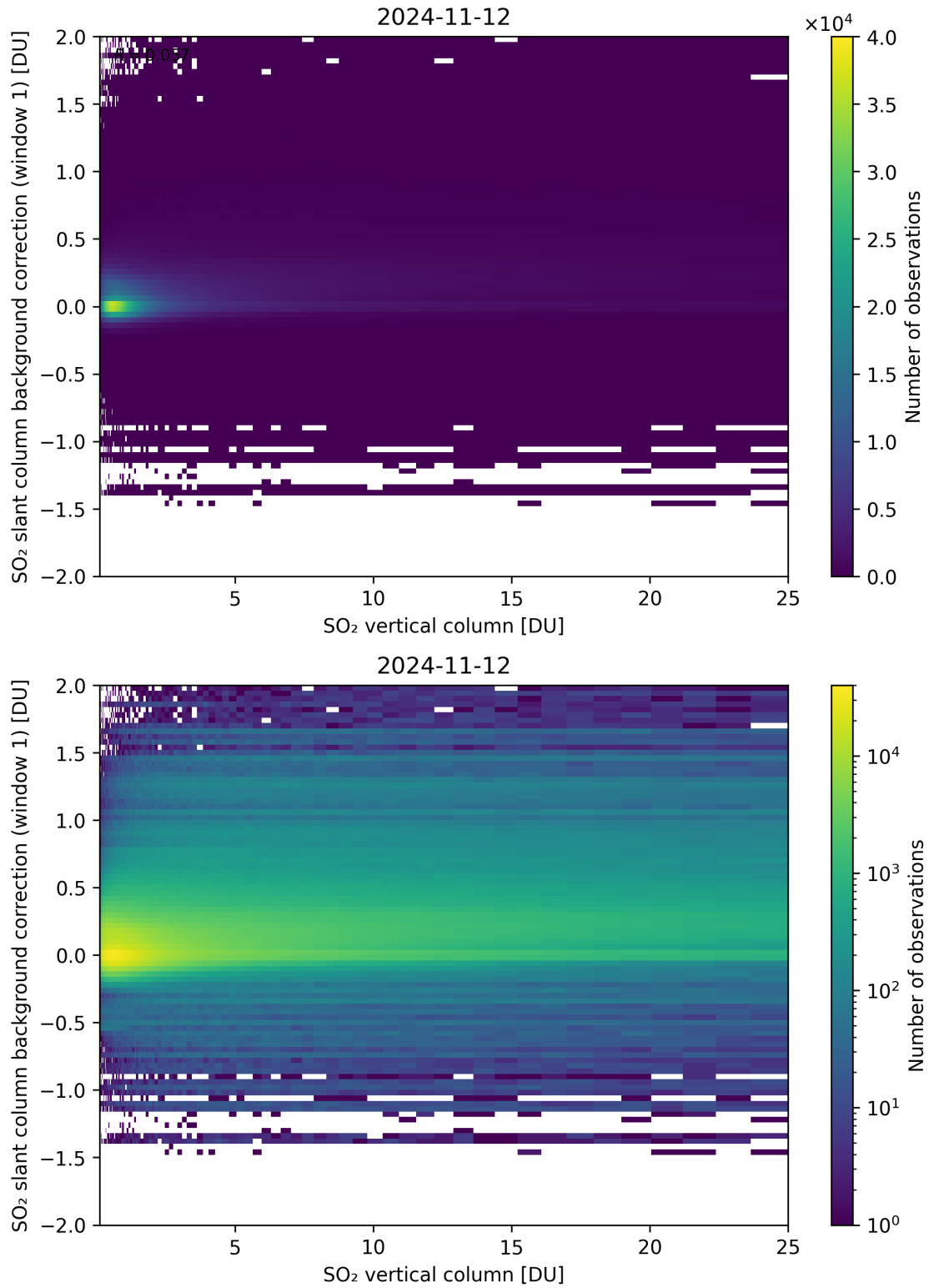
Figure 273: Scatter density plot of “SO 2 vertical column” against “SO 2 slant column background correction (window 1)” for 2024-11-11 to 2024-11-13.
