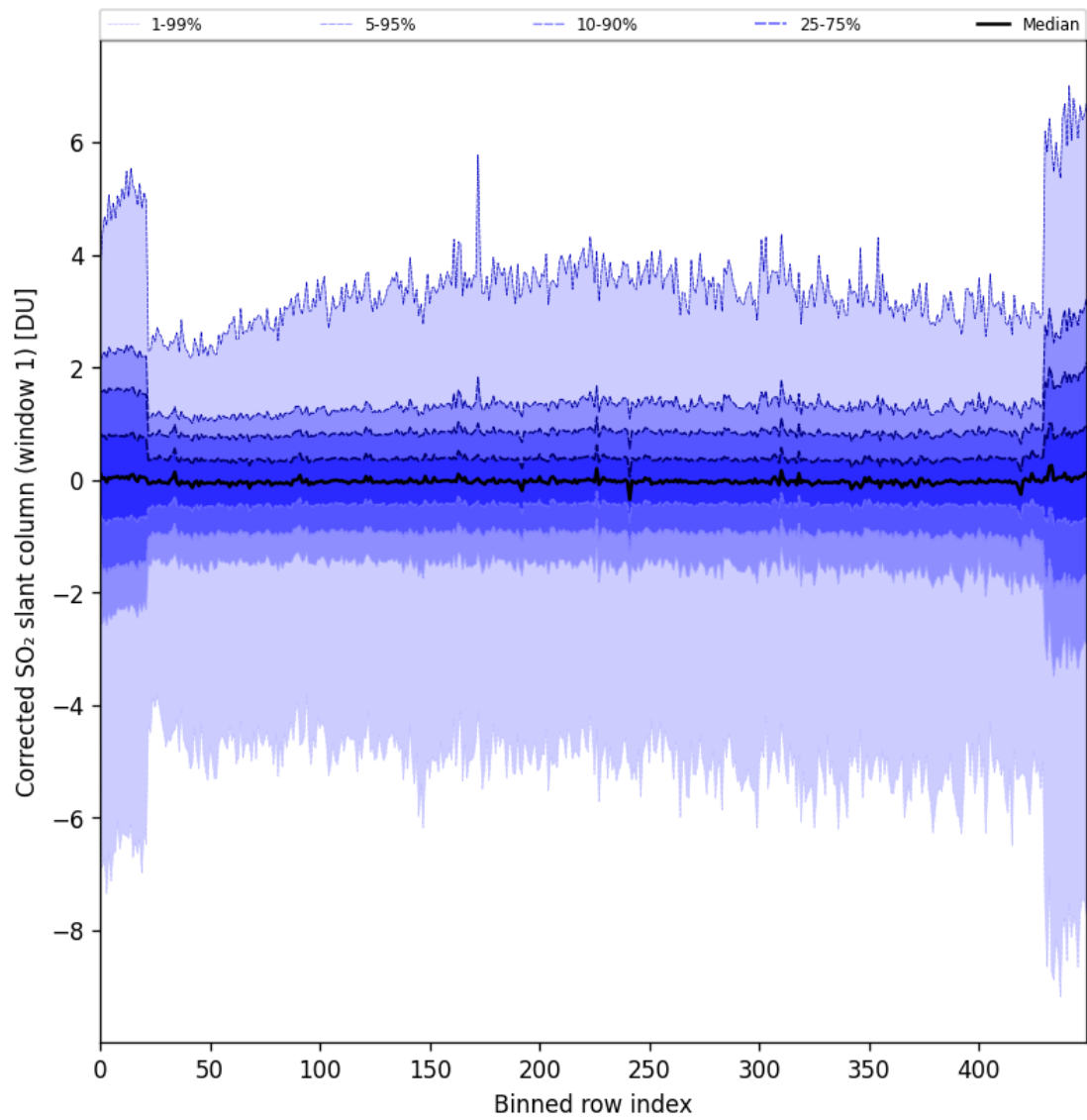
Figure 81: Along track statistics of “Corrected SO 2 slant column (window 1)” for 2024-11-11 to 2024-11-13
