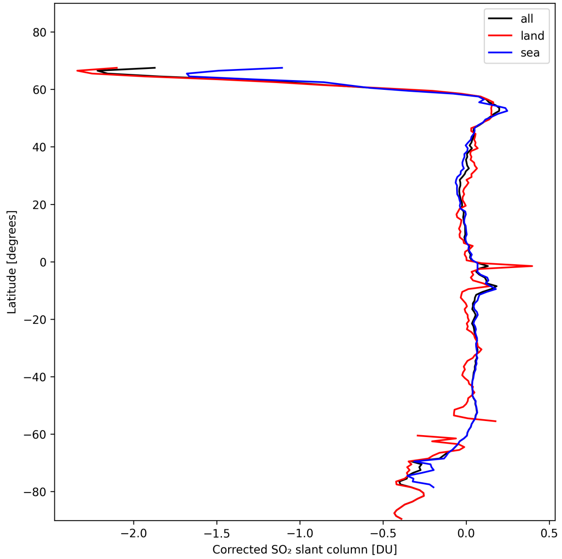
Figure 32: Zonal average of “Corrected SO 2 slant column” for 2024-11-11 to 2024-11-13.
