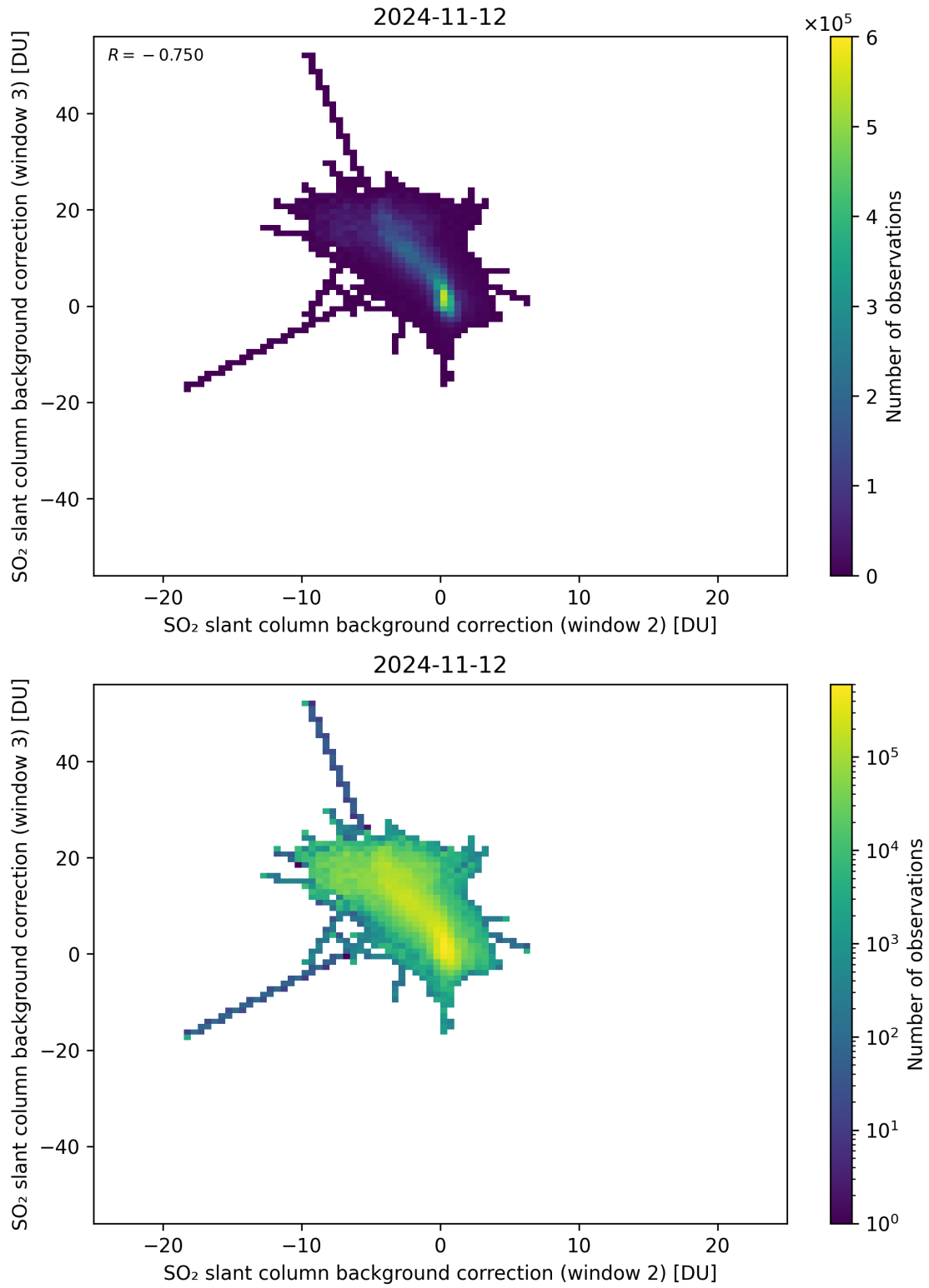
Figure 111: Scatter density plot of “SO 2 slant column background correction (window 2)” against “SO 2 slant column background correction (window 3)” for 2024-11-11 to 2024-11-13.
