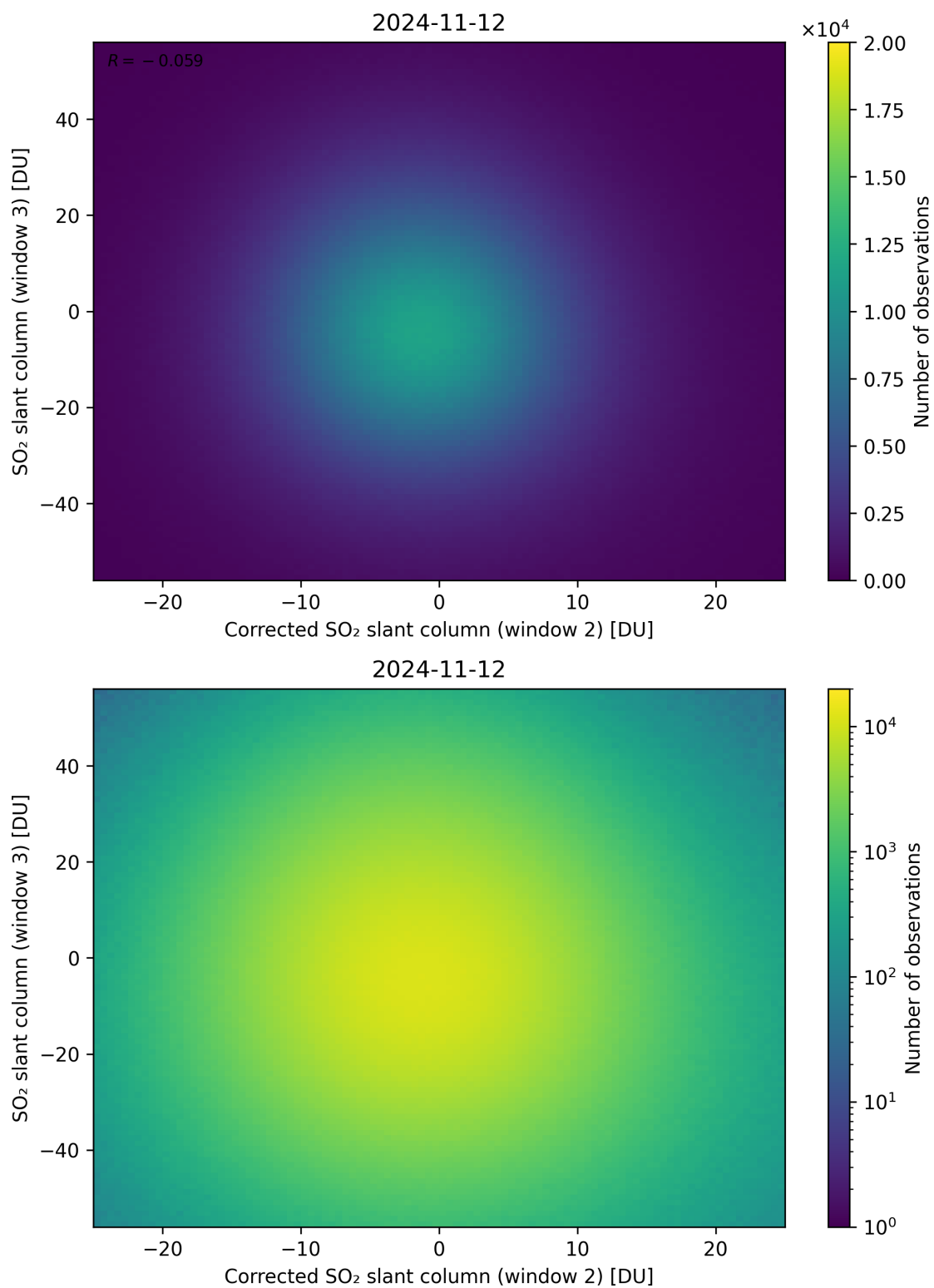
Figure 201: Scatter density plot of “Corrected SO 2 slant column (window 2)” against “SO 2 slant column (window 3)” for 2024-11-11 to 2024-11-13.
