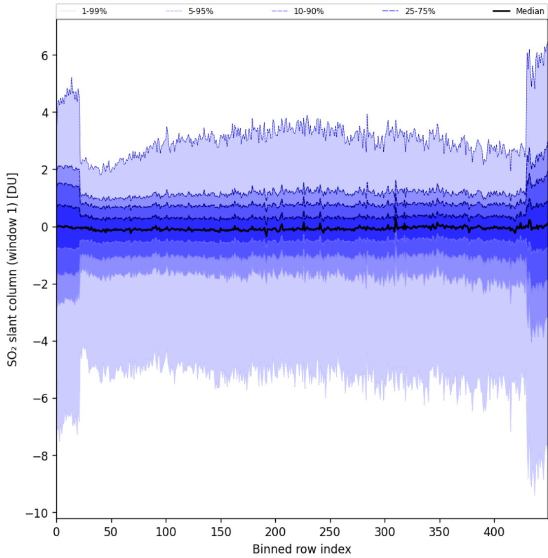
Figure 79: Along track statistics of “SO 2 slant column (window 1)” for 2024-11-11 to 2024-11-13
