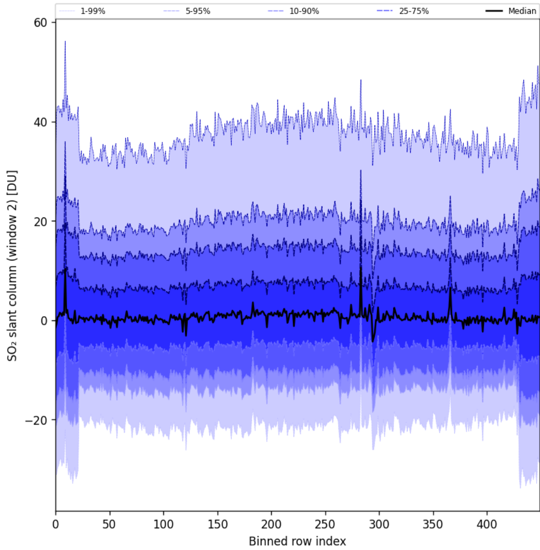
Figure 83: Along track statistics of “SO 2 slant column (window 2)” for 2024-11-11 to 2024-11-13
