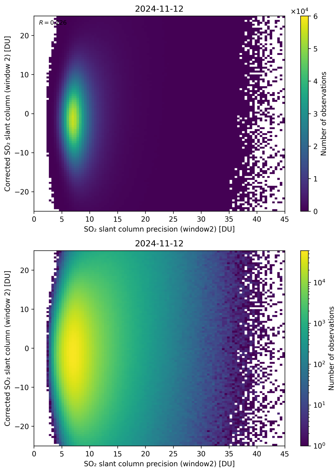
Figure 247: Scatter density plot of “SO 2 slant column precision (window2)” against “Corrected SO 2 slant column (window 2)” for 2024-11-11 to 2024-11-13.
