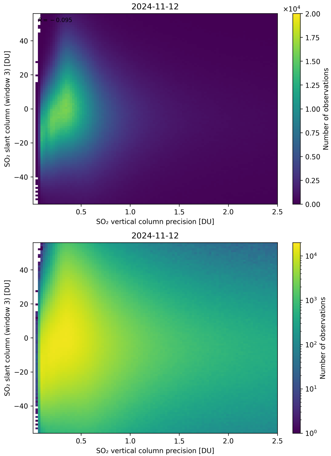
Figure 292: Scatter density plot of “SO 2 vertical column precision” against “SO 2 slant column (window 3)” for 2024-11-11 to 2024-11-13.
