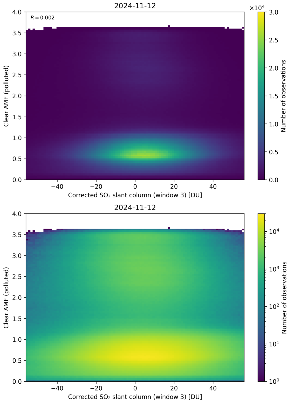
Figure 209: Scatter density plot of “Corrected SO 2 slant column (window 3)” against “Clear AMF (polluted)” for 2024-11-11 to 2024-11-13.
