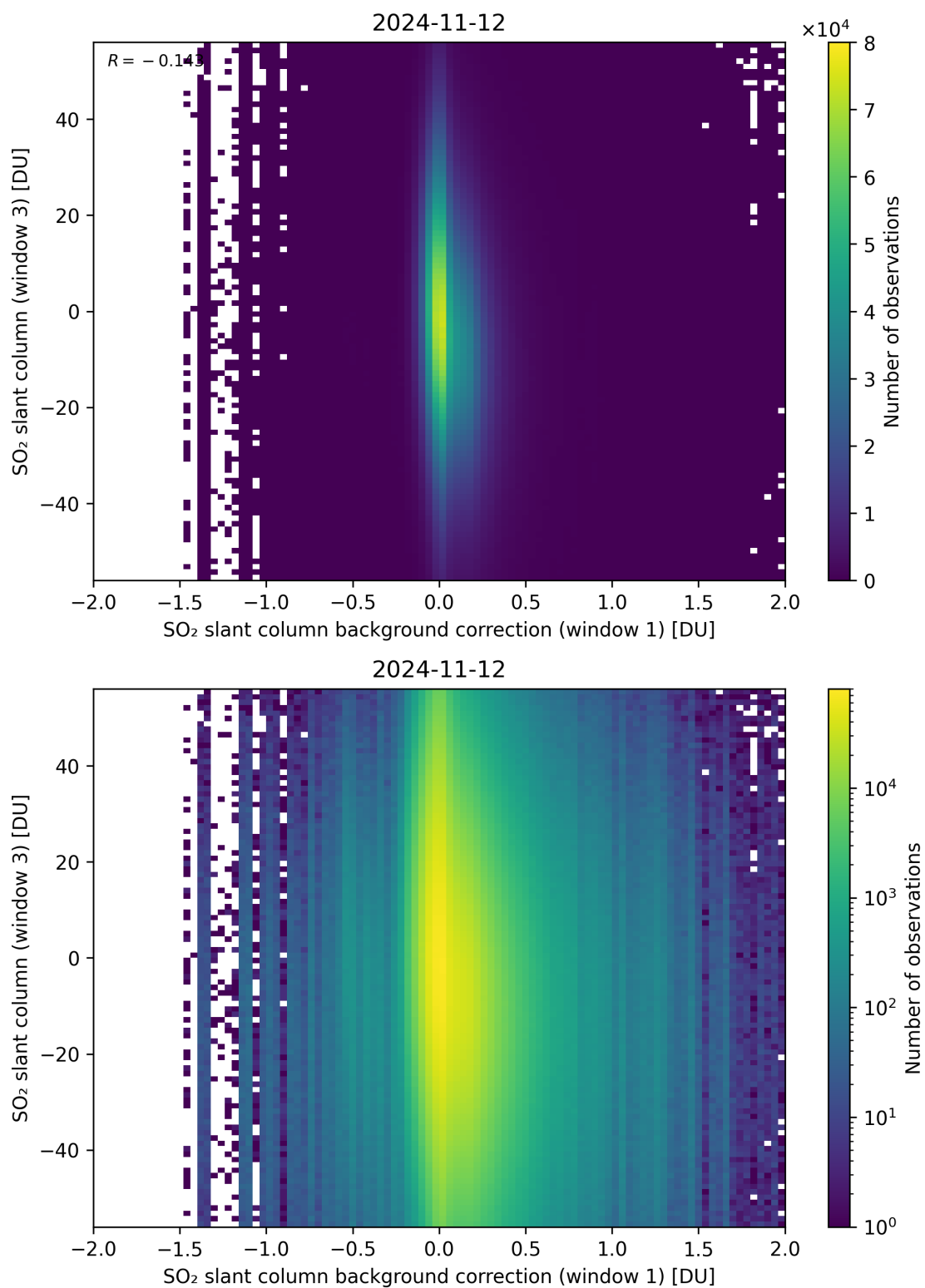
Figure 107: Scatter density plot of “SO 2 slant column background correction (window 1)” against “SO 2 slant column (window 3)” for 2024-11-11 to 2024-11-13.
