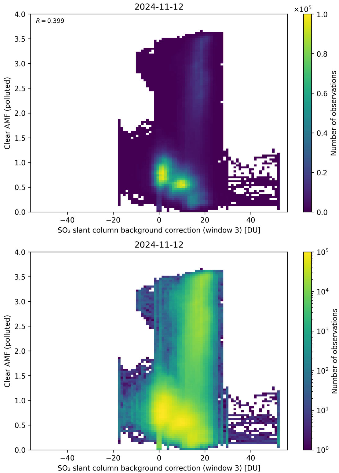
Figure 124: Scatter density plot of “SO 2 slant column background correction (window 3)” against “Clear AMF (polluted)” for 2024-11-11 to 2024-11-13.
