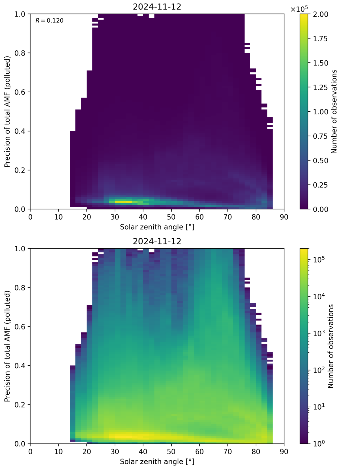
Figure 175: Scatter density plot of “Solar zenith angle” against “Precision of total AMF (polluted)” for 2024-11-11 to 2024-11-13.
