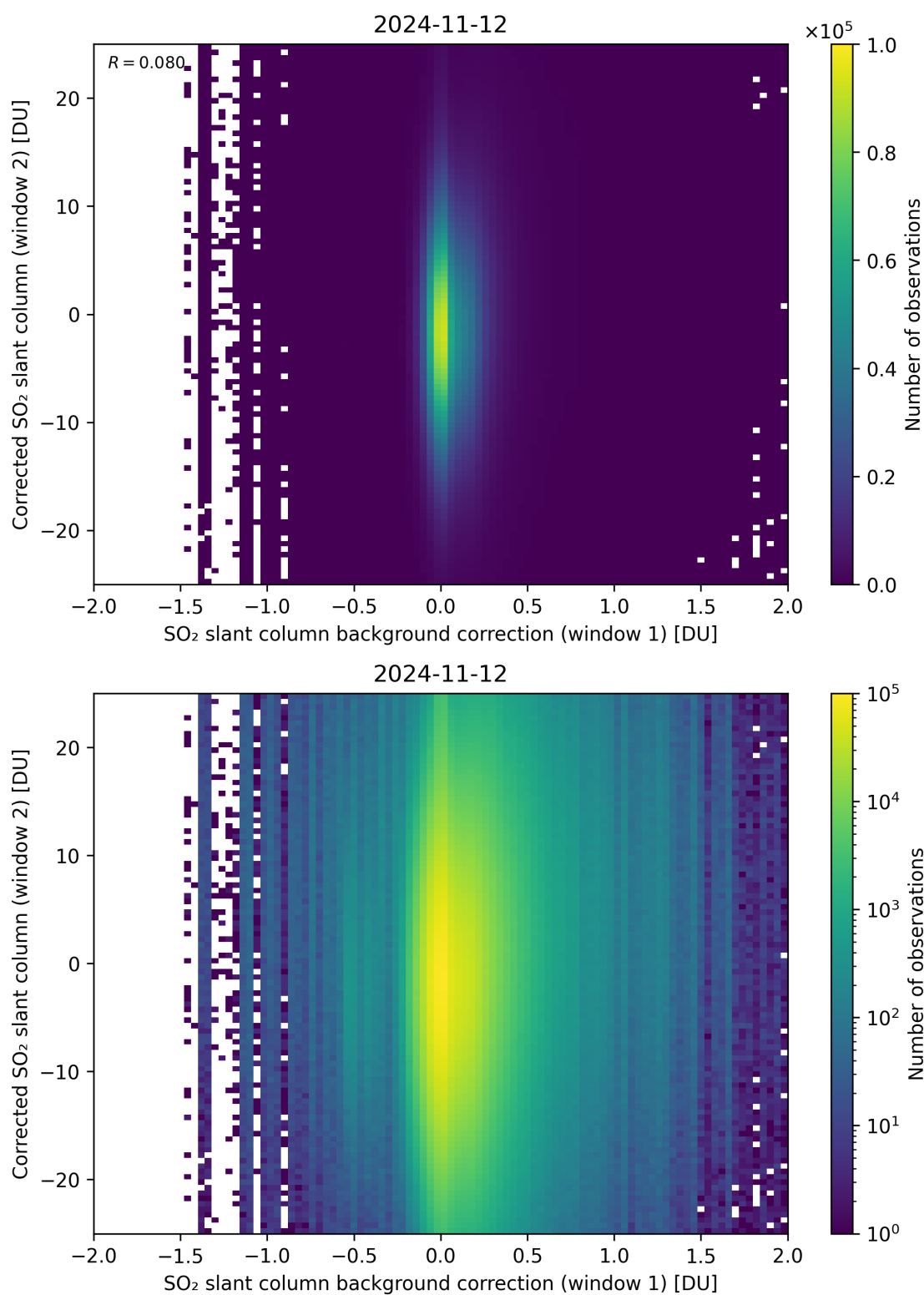
Figure 104: Scatter density plot of “SO 2 slant column background correction (window 1)” against “Corrected SO 2 slant column (window 2)” for 2024-11-11 to 2024-11-13.
