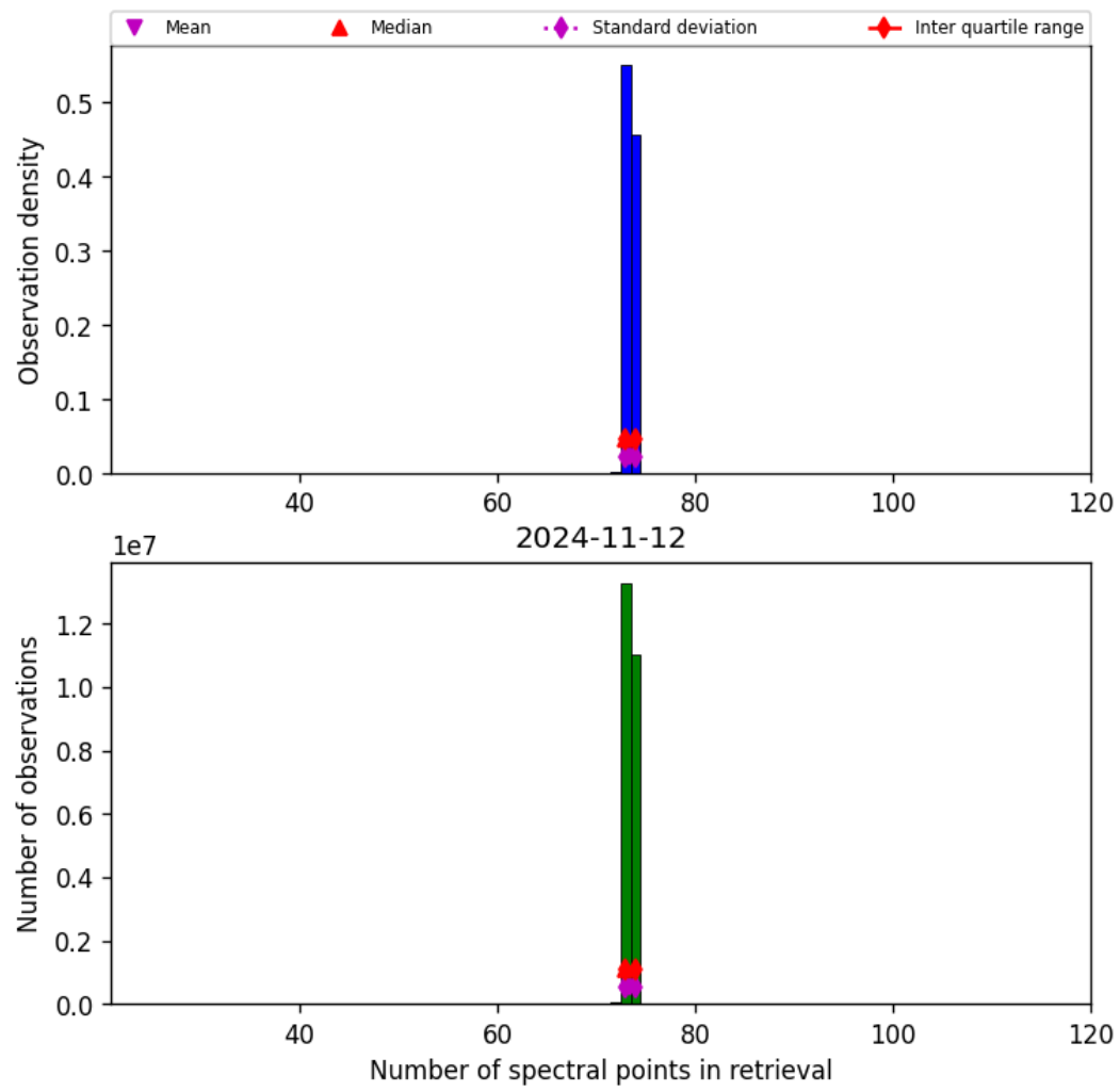
Figure 74: Histogram of “Number of spectral points in retrieval” for 2024-11-11 to 2024-11-13
