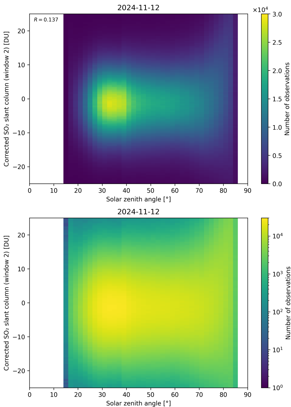
Figure 167: Scatter density plot of “Solar zenith angle” against “Corrected SO 2 slant column (window 2)” for 2024-11-11 to 2024-11-13.
