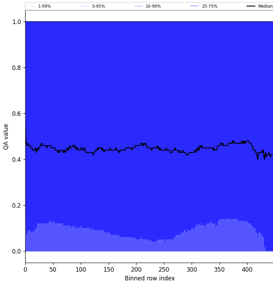
Figure 75: Along track statistics of “QA value” for 2024-11-11 to 2024-11-13
