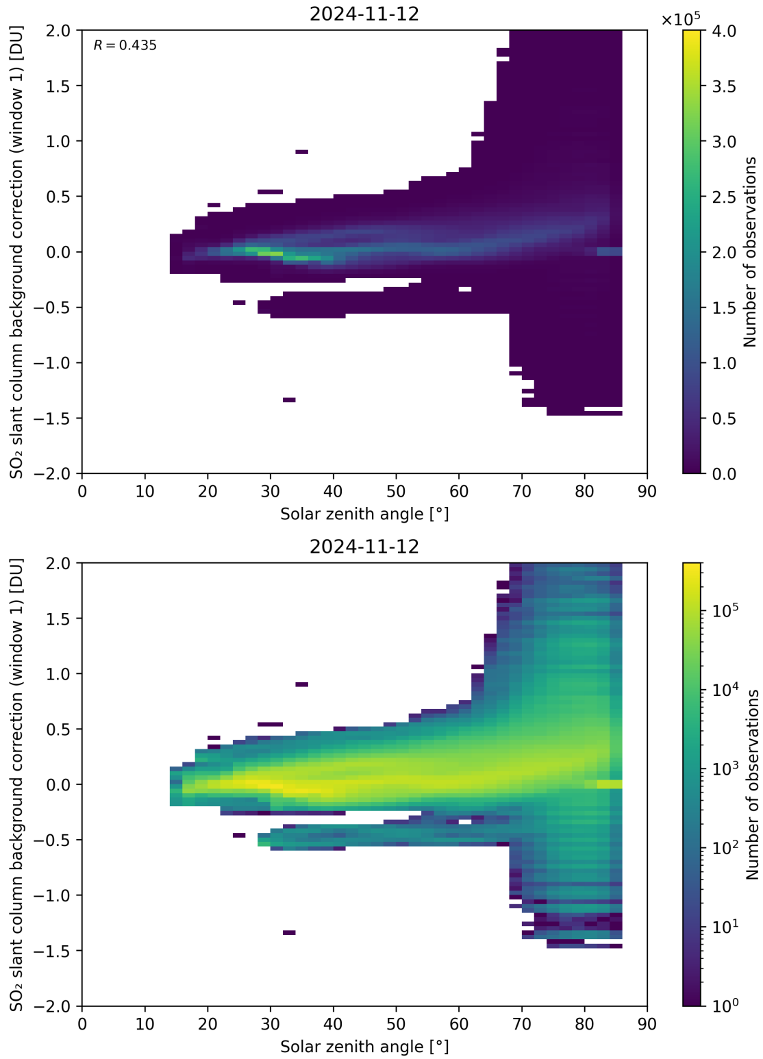
Figure 158: Scatter density plot of “Solar zenith angle” against “SO 2 slant column background correction (window 1)” for 2024-11-11 to 2024-11-13.
