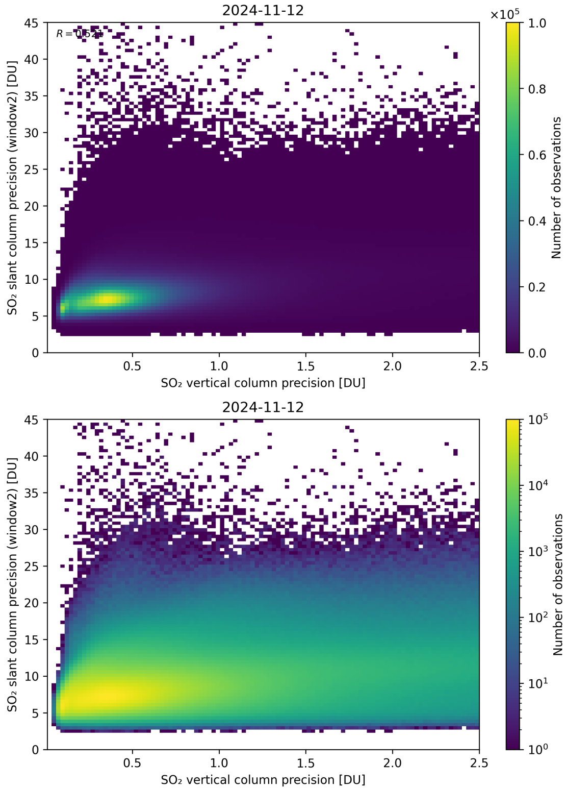
Figure 291: Scatter density plot of “SO 2 vertical column precision” against “SO 2 slant column precision (window2)” for 2024-11-11 to 2024-11-13.
