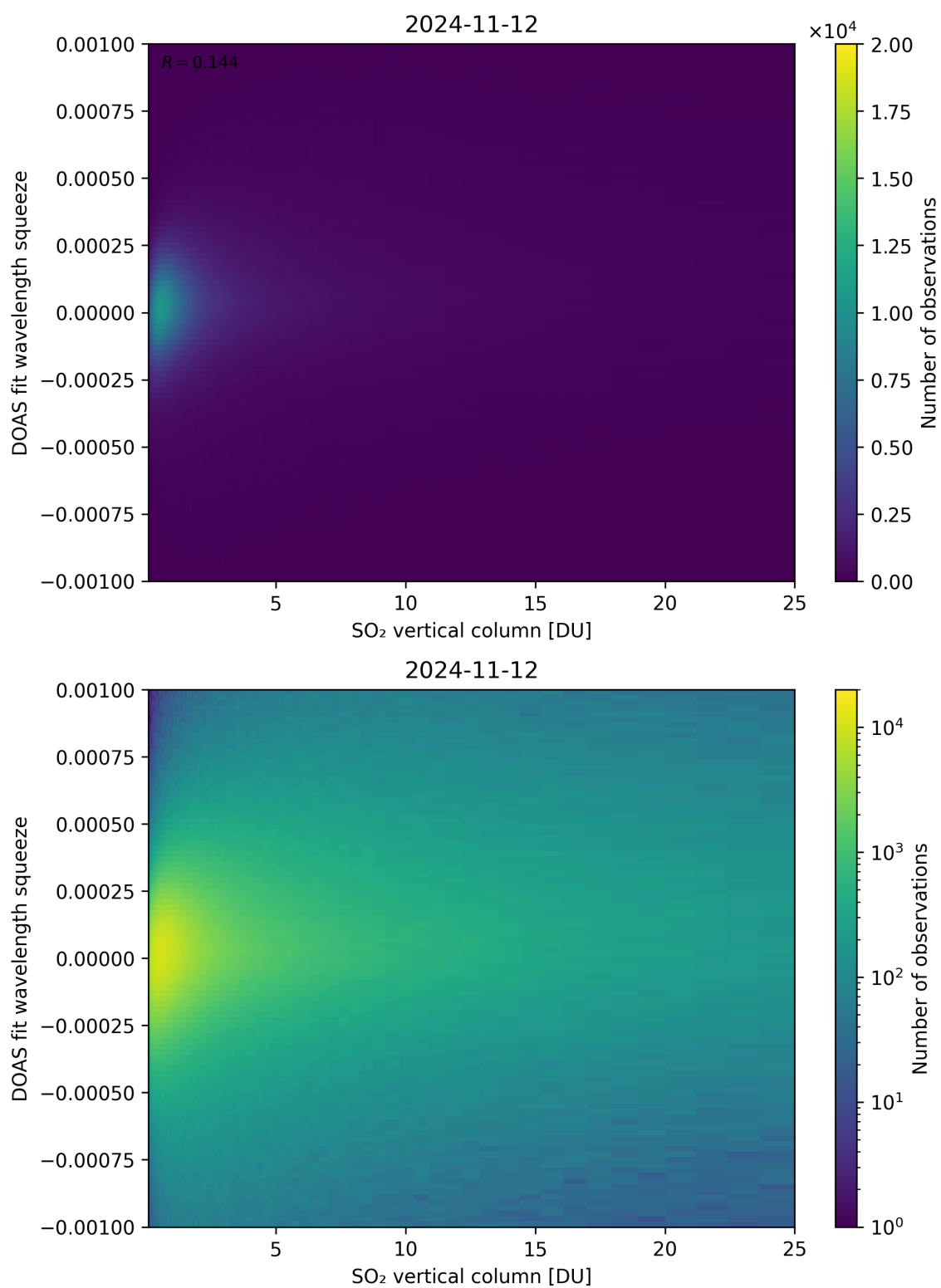
Figure 277: Scatter density plot of “SO 2 vertical column” against “DOAS fit wavelength squeeze” for 2024-11-11 to 2024-11-13.
