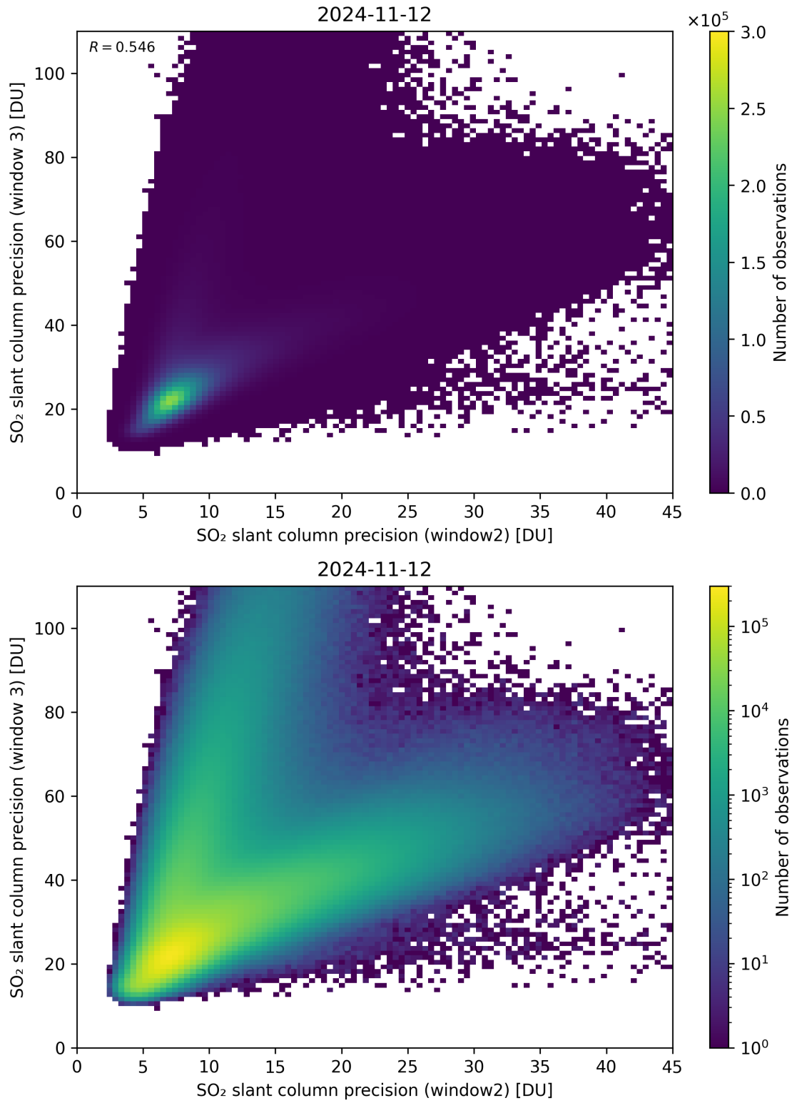
Figure 250: Scatter density plot of “SO 2 slant column precision (window2)” against “SO 2 slant column precision (window 3)” for 2024-11-11 to 2024-11-13.
