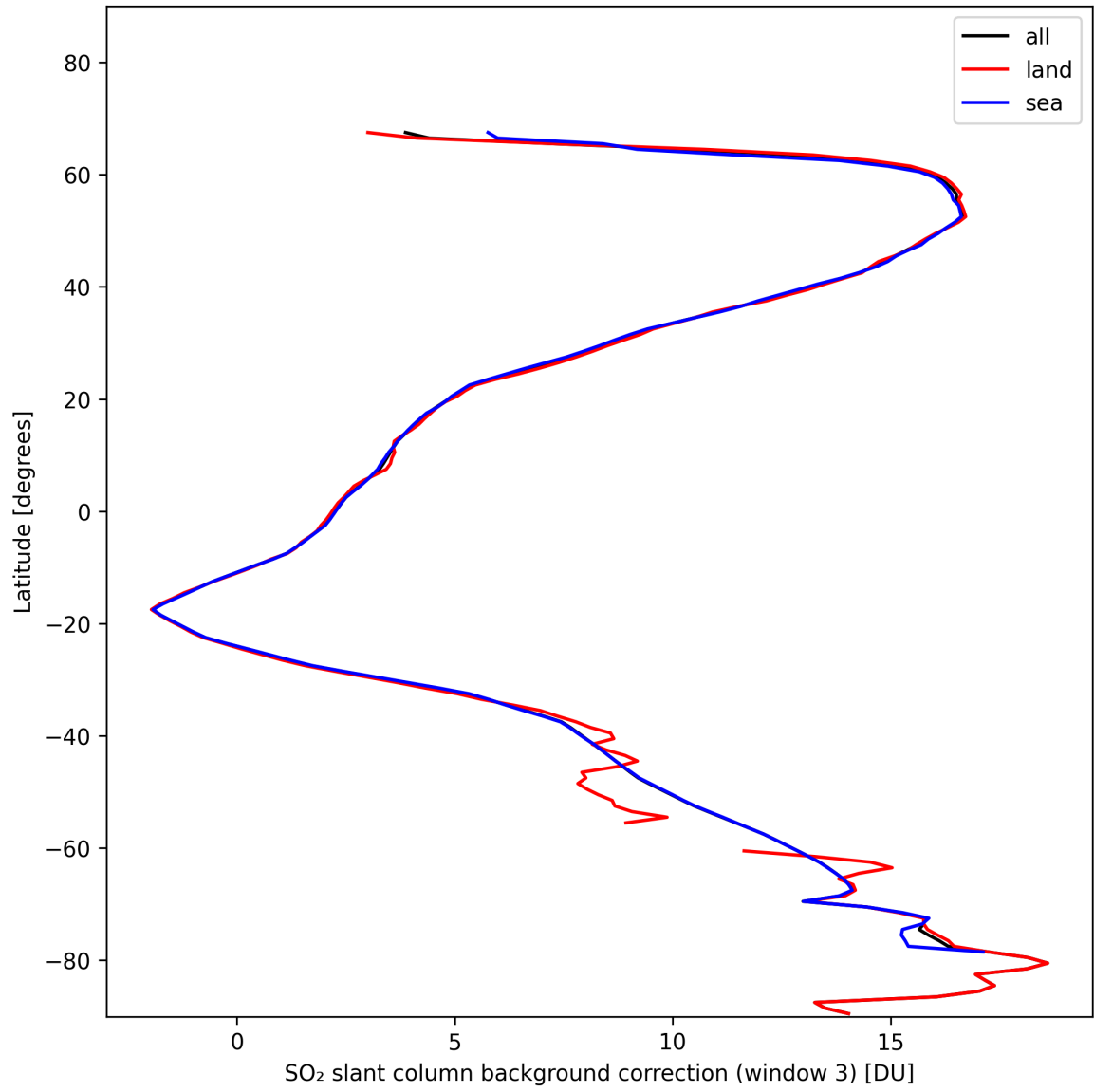
Figure 44: Zonal average of “SO 2 slant column background correction (window 3)” for 2024-11-11 to 2024-11-13.
