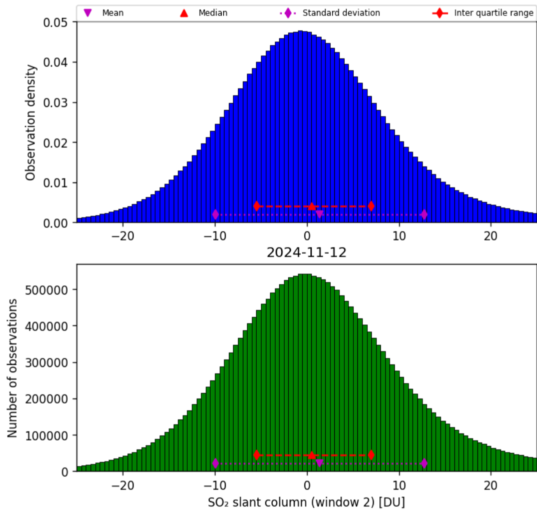
Figure 60: Histogram of “SO 2 slant column (window 2)” for 2024-11-11 to 2024-11-13
