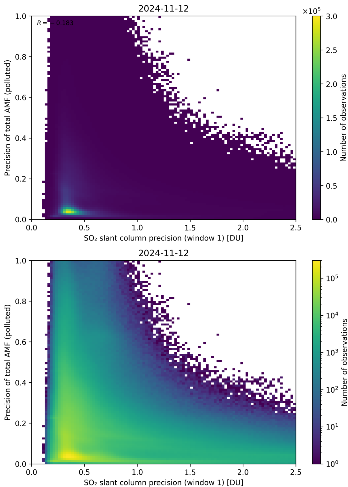
Figure 231: Scatter density plot of “SO 2 slant column precision (window 1)” against “Precision of total AMF (polluted)” for 2024-11-11 to 2024-11-13.
