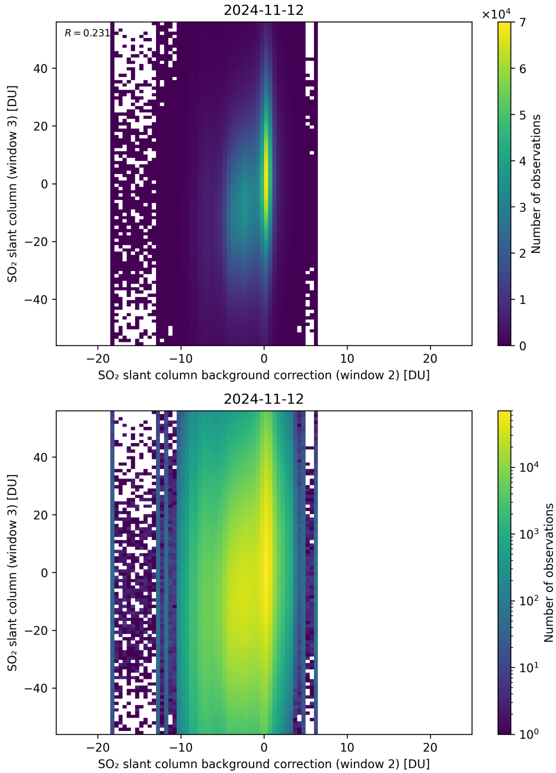
Figure 117: Scatter density plot of “SO 2 slant column background correction (window 2)” against “SO 2 slant column (window 3)” for 2024-11-11 to 2024-11-13.
