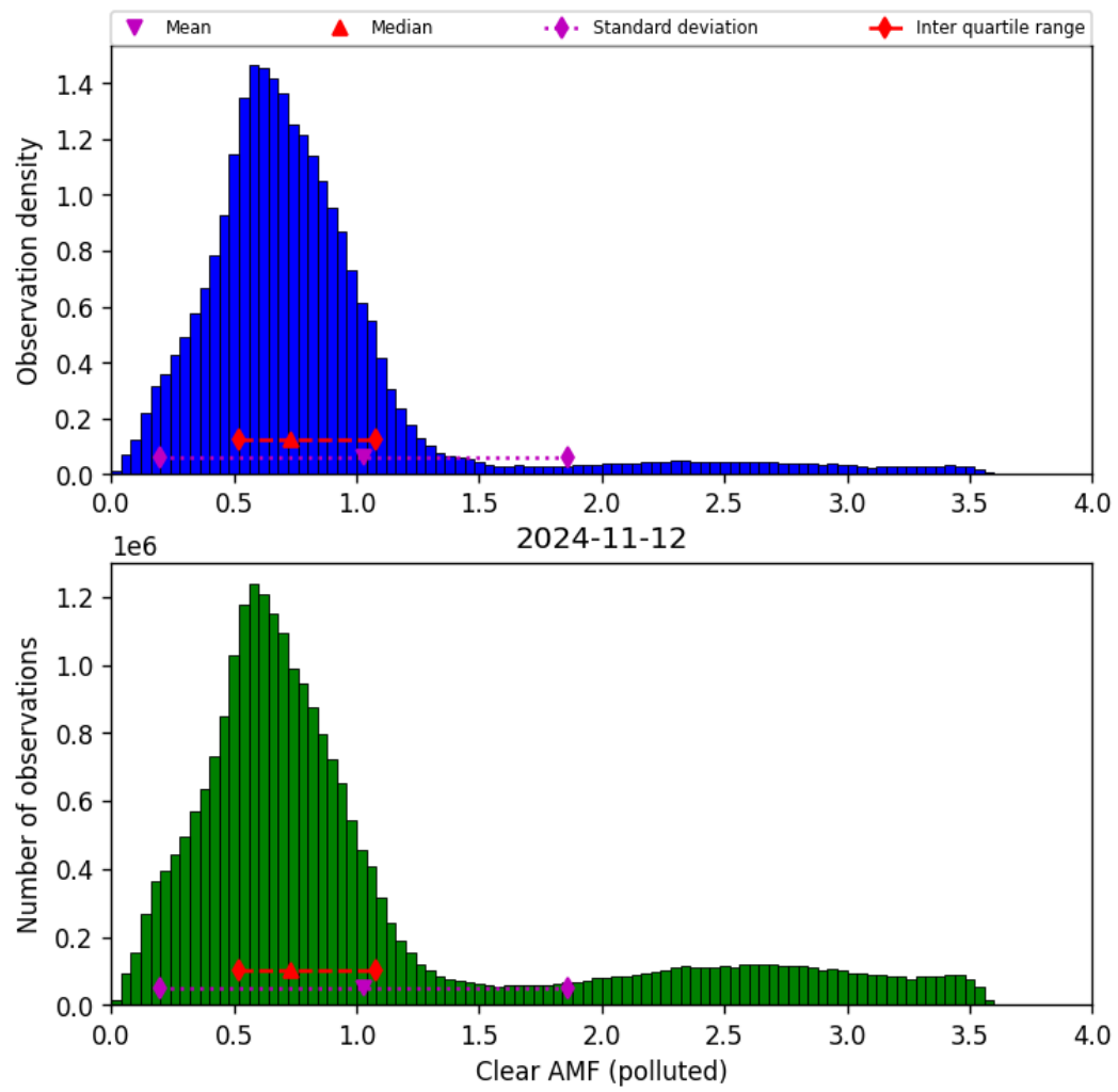
Figure 73: Histogram of “Clear AMF (polluted)” for 2024-11-11 to 2024-11-13
