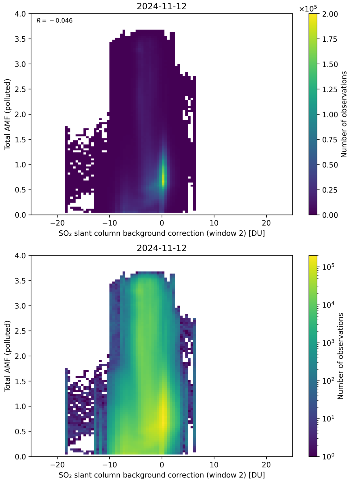
Figure 119: Scatter density plot of “SO 2 slant column background correction (window 2)” against “Total AMF (polluted)” for 2024-11-11 to 2024-11-13.
