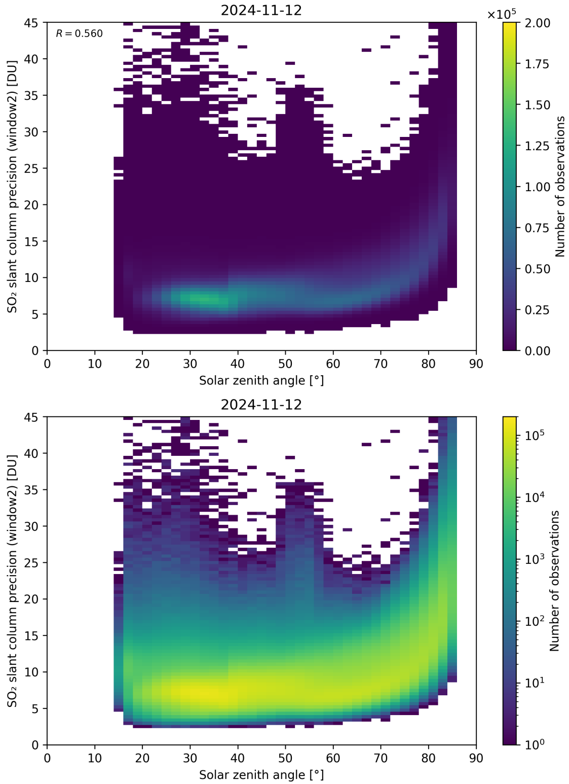
Figure 171: Scatter density plot of “Solar zenith angle” against “SO 2 slant column precision (window2)” for 2024-11-11 to 2024-11-13.
