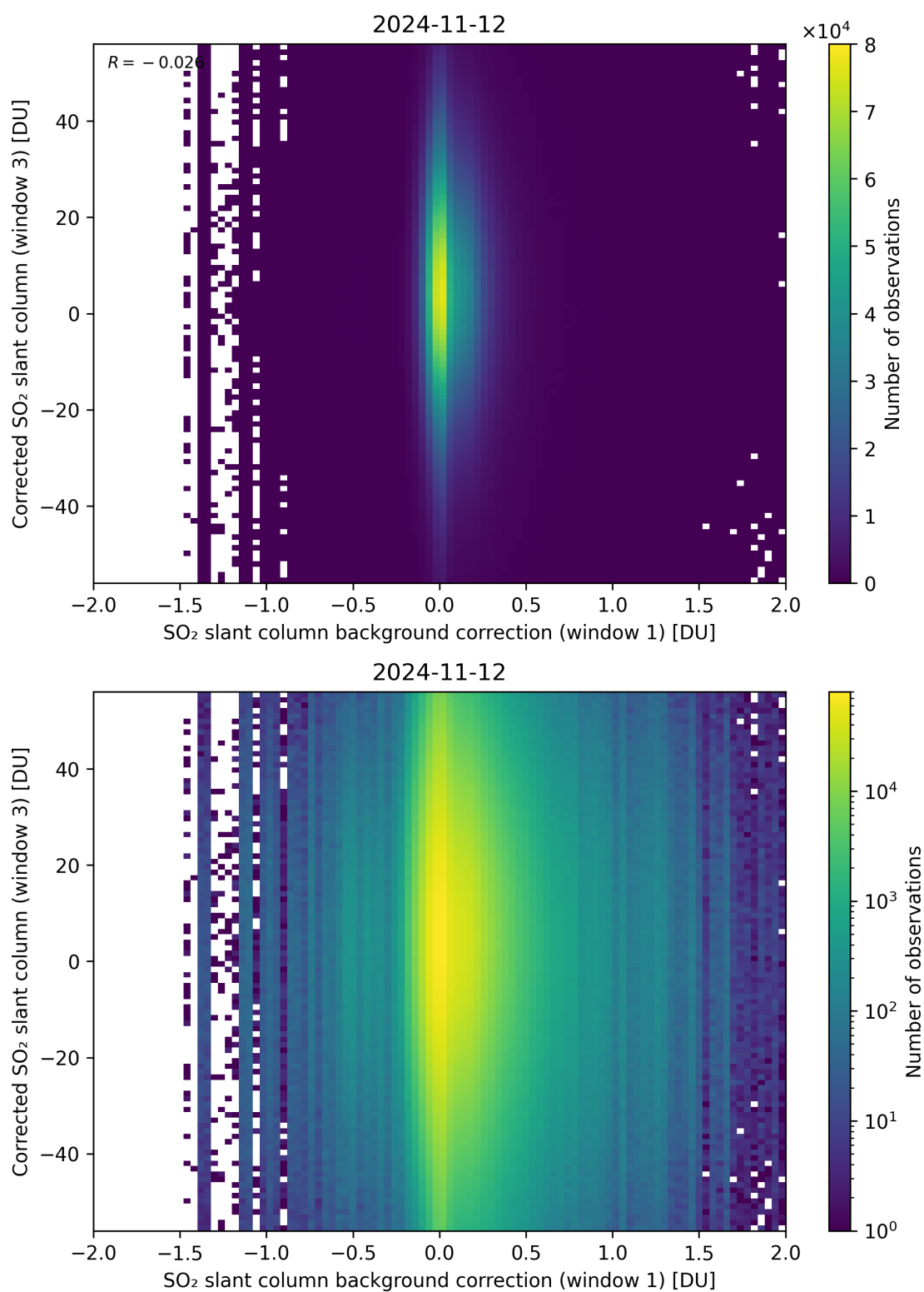
Figure 105: Scatter density plot of “SO 2 slant column background correction (window 1)” against “Corrected SO 2 slant column (window 3)” for 2024-11-11 to 2024-11-13.
