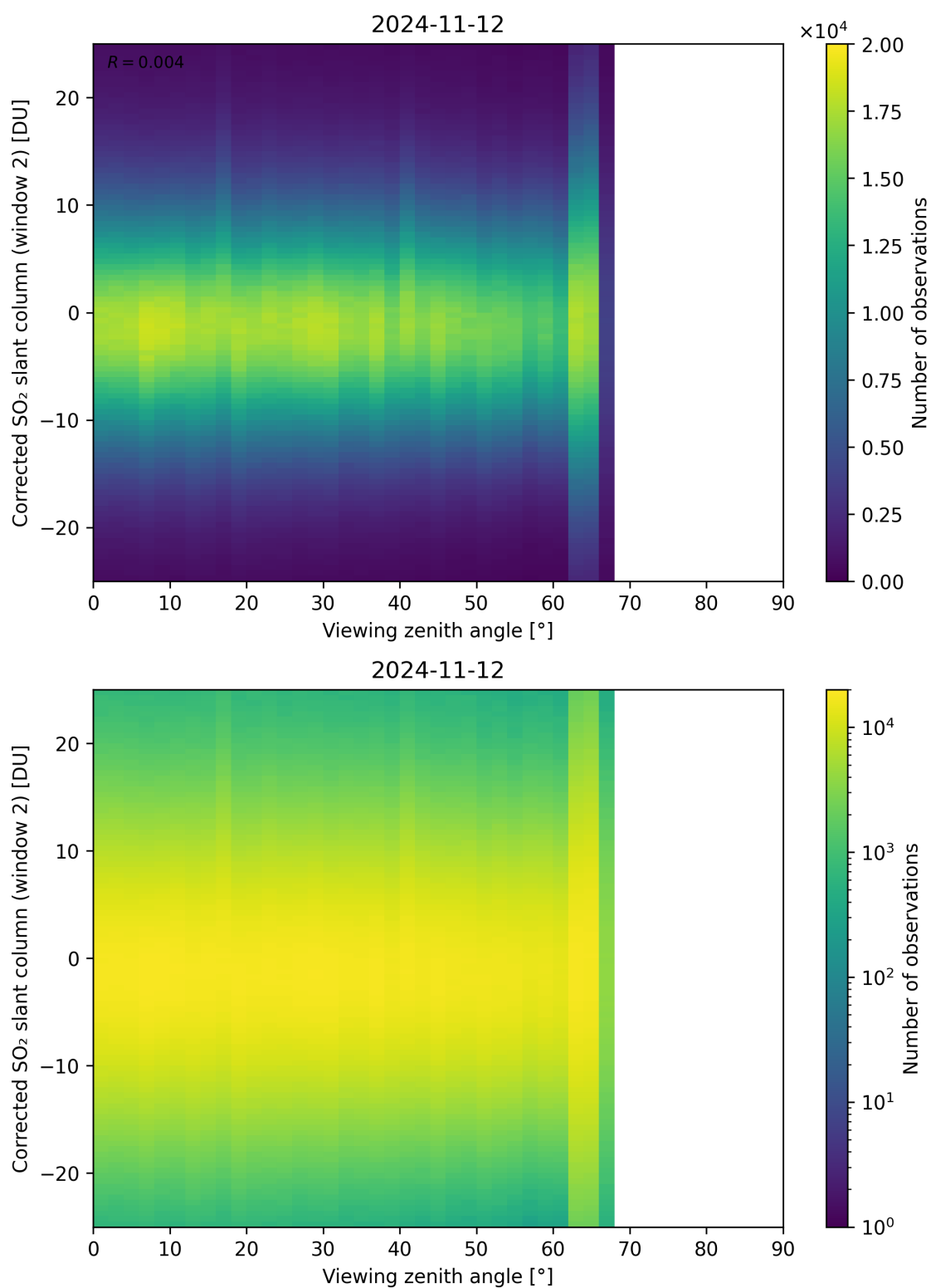
Figure 318: Scatter density plot of “Viewing zenith angle” against “Corrected SO 2 slant column (window 2)” for 2024-11-11 to 2024-11-13.
