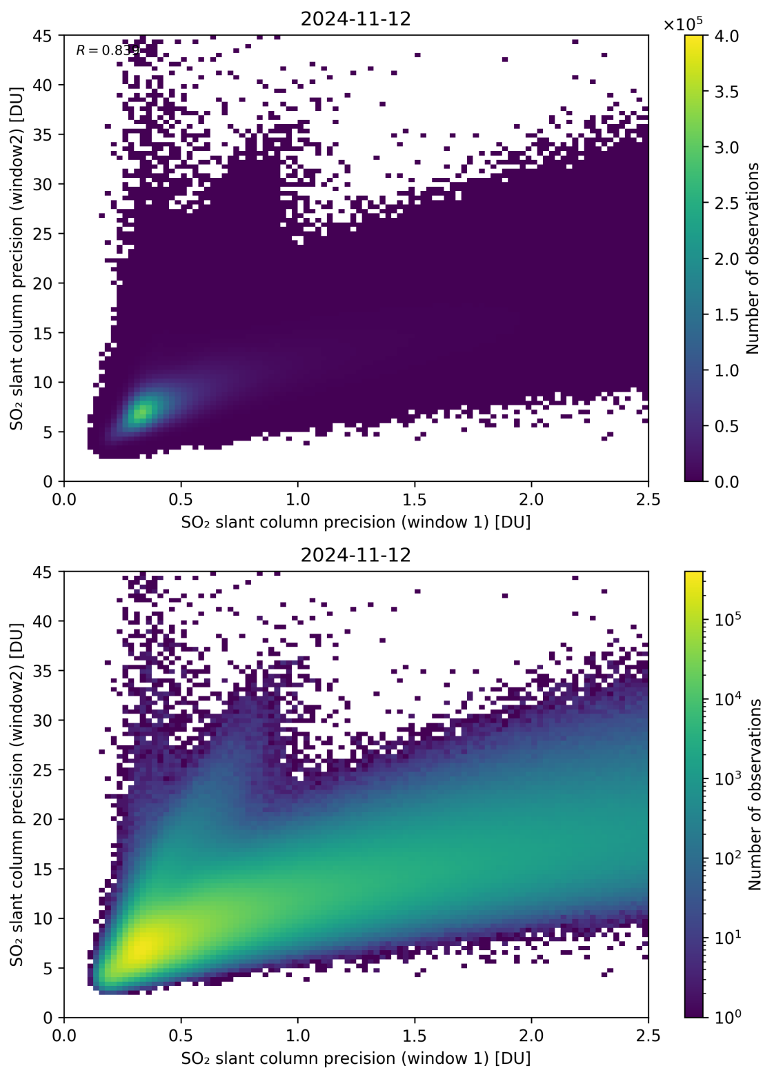
Figure 227: Scatter density plot of “SO 2 slant column precision (window 1)” against “SO 2 slant column precision (window2)” for 2024-11-11 to 2024-11-13.
