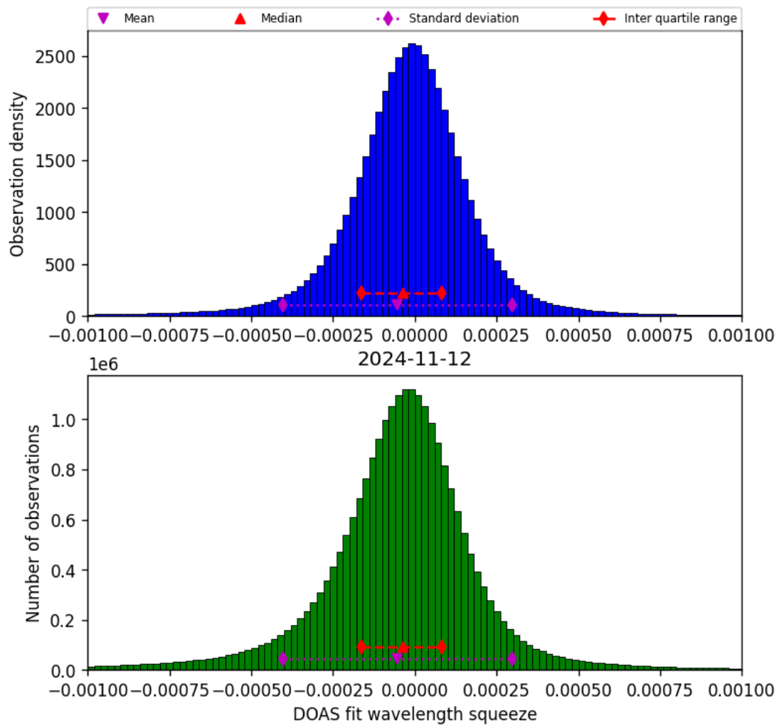
Figure 69: Histogram of “DOAS fit wavelength squeeze” for 2024-11-11 to 2024-11-13
