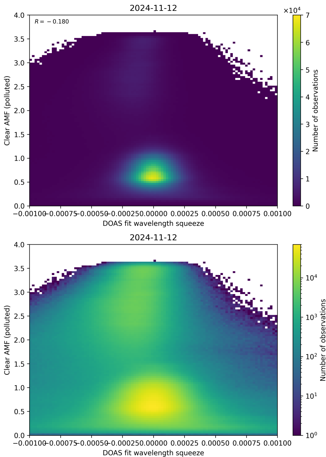
Figure 133: Scatter density plot of “DOAS fit wavelength squeeze” against “Clear AMF (polluted)” for 2024-11-11 to 2024-11-13.
