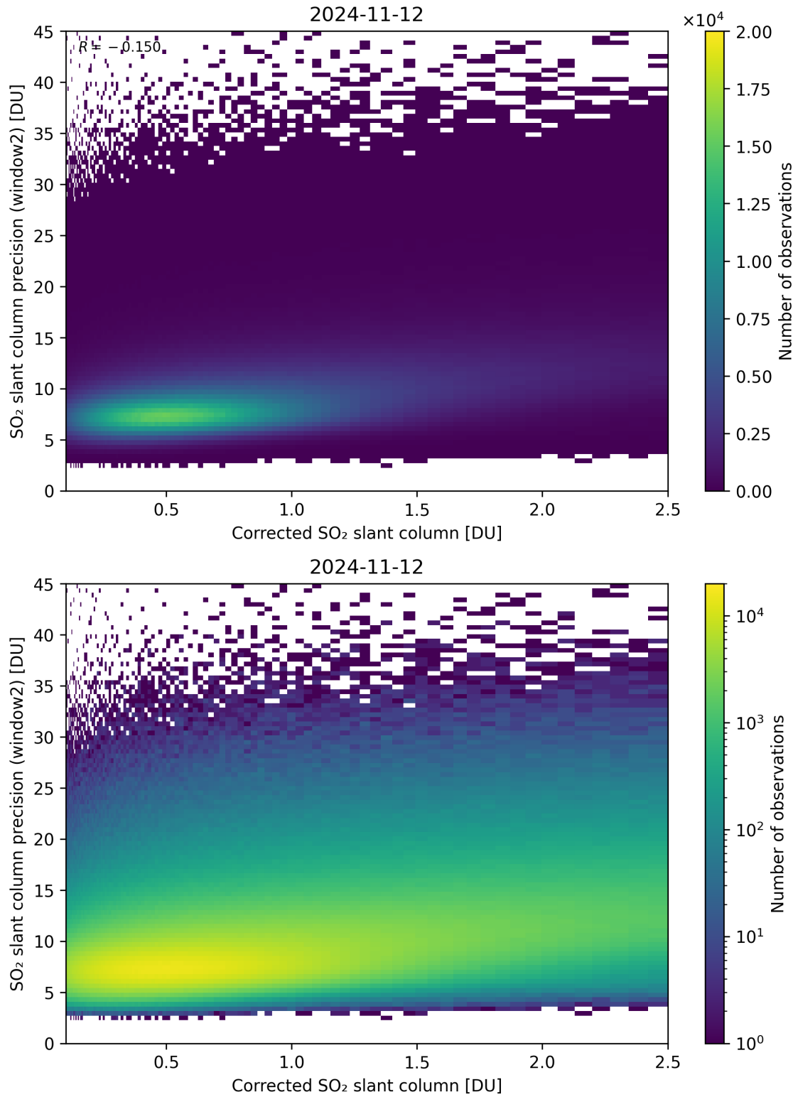
Figure 189: Scatter density plot of “Corrected SO 2 slant column” against “SO 2 slant column precision (window2)” for 2024-11-11 to 2024-11-13.
