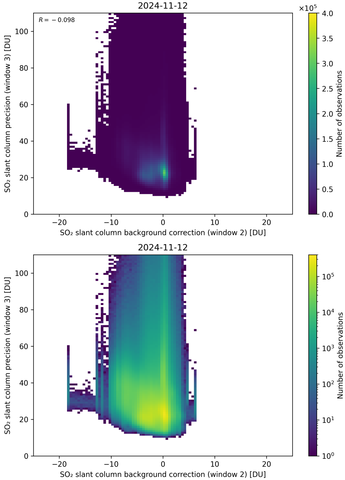
Figure 118: Scatter density plot of “SO 2 slant column background correction (window 2)” against “SO 2 slant column precision (window 3)” for 2024-11-11 to 2024-11-13.
