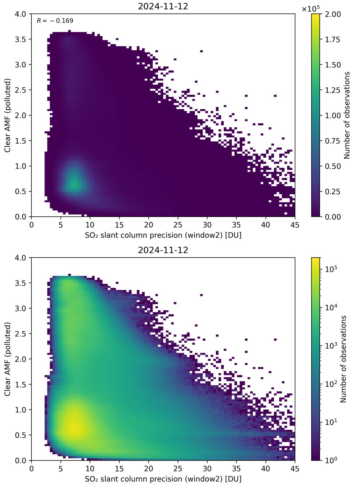
Figure 246: Scatter density plot of “SO 2 slant column precision (window2)” against “Clear AMF (polluted)” for 2024-11-11 to 2024-11-13.
