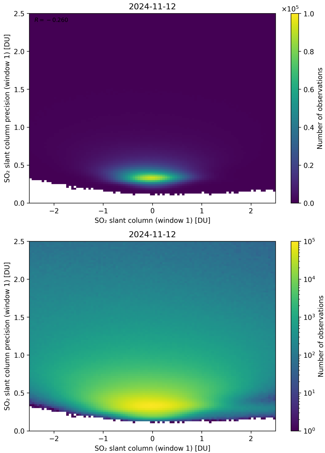
Figure 235: Scatter density plot of “SO 2 slant column (window 1)” against “SO 2 slant column precision (window 1)” for 2024-11-11 to 2024-11-13.
