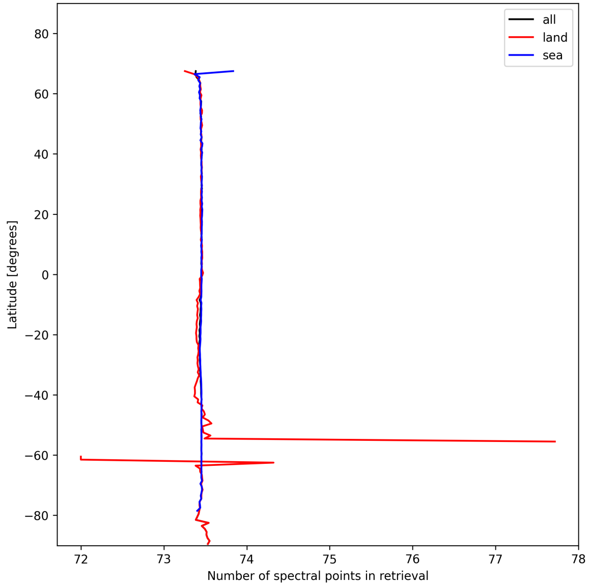
Figure 51: Zonal average of “Number of spectral points in retrieval” for 2024-11-11 to 2024-11-13.
