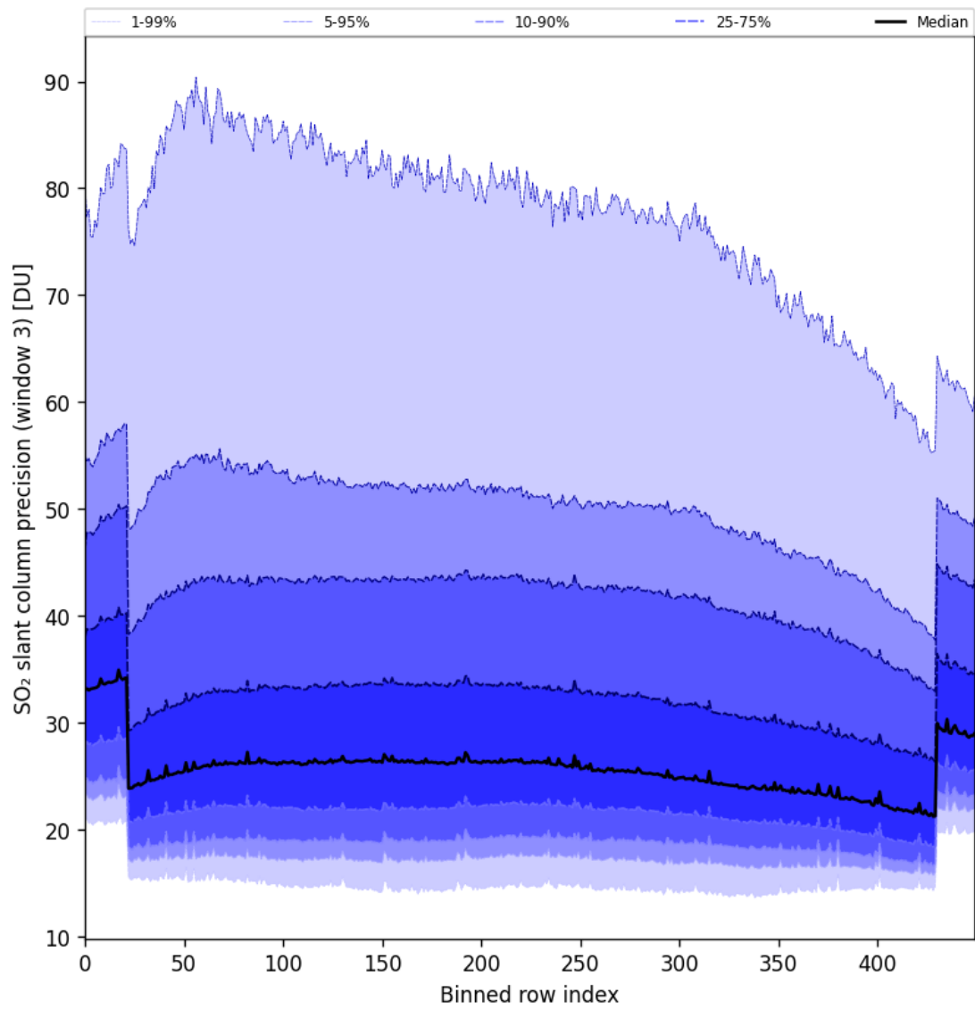
Figure 88: Along track statistics of “SO 2 slant column precision (window 3)” for 2024-11-11 to 2024-11-13
