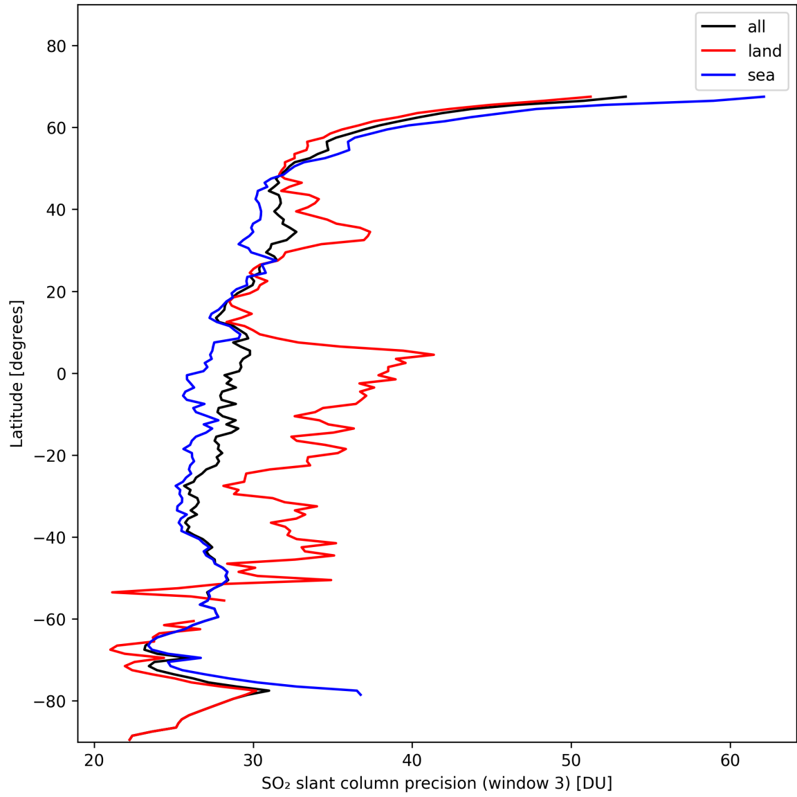
Figure 42: Zonal average of “SO 2 slant column precision (window 3)” for 2024-11-11 to 2024-11-13.
