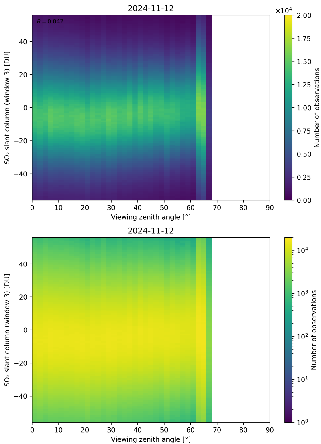
Figure 323: Scatter density plot of “Viewing zenith angle” against “SO 2 slant column (window 3)” for 2024-11-11 to 2024-11-13.
