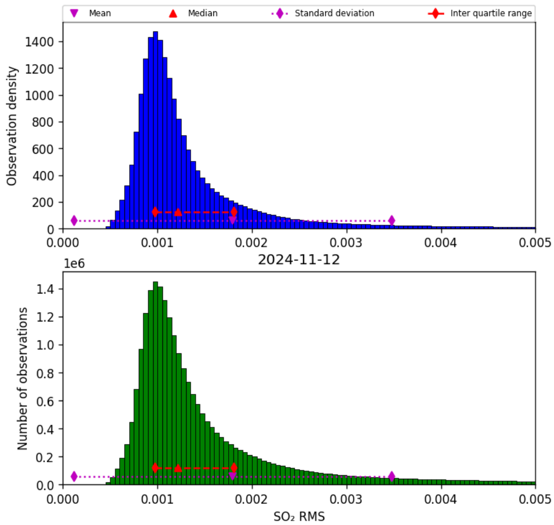
Figure 70: Histogram of “SO 2 RMS” for 2024-11-11 to 2024-11-13
