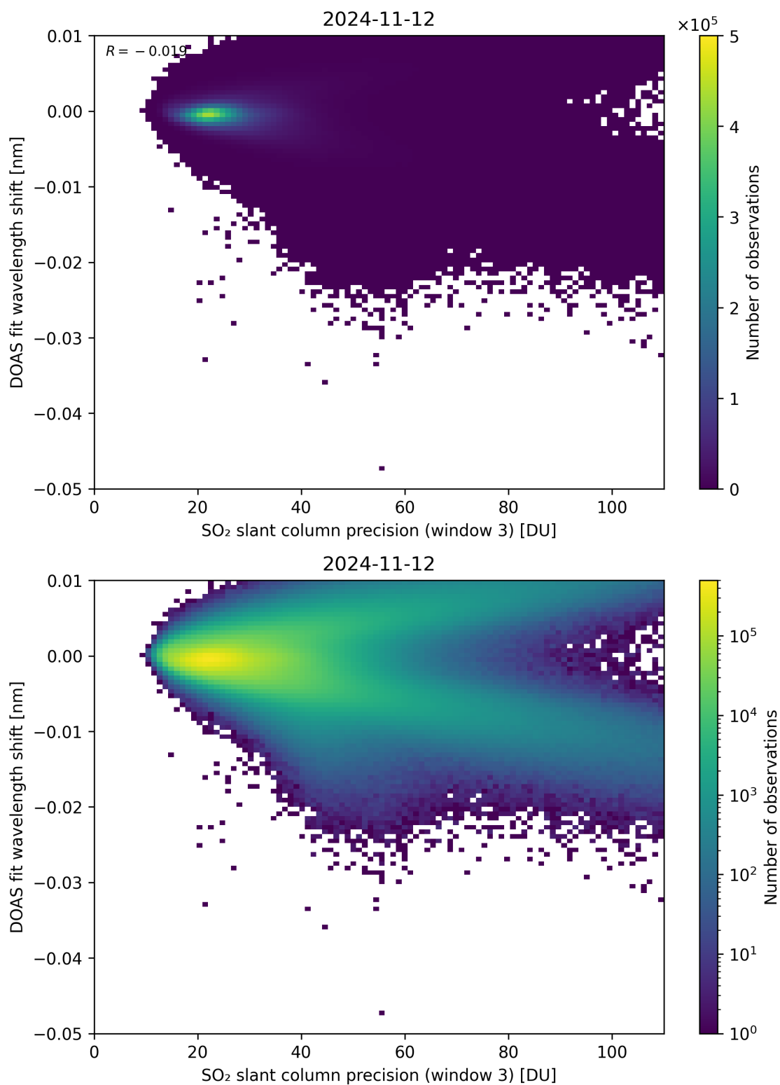
Figure 258: Scatter density plot of “SO 2 slant column precision (window 3)” against “DOAS fit wavelength shift” for 2024-11-11 to 2024-11-13.
