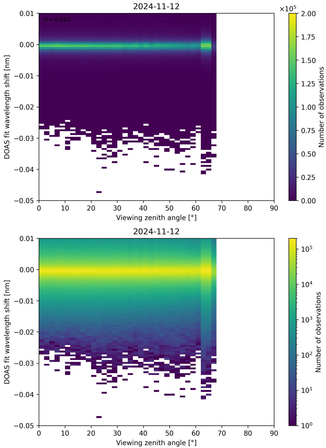
Figure 311: Scatter density plot of “Viewing zenith angle” against “DOAS fit wavelength shift” for 2024-11-11 to 2024-11-13.
