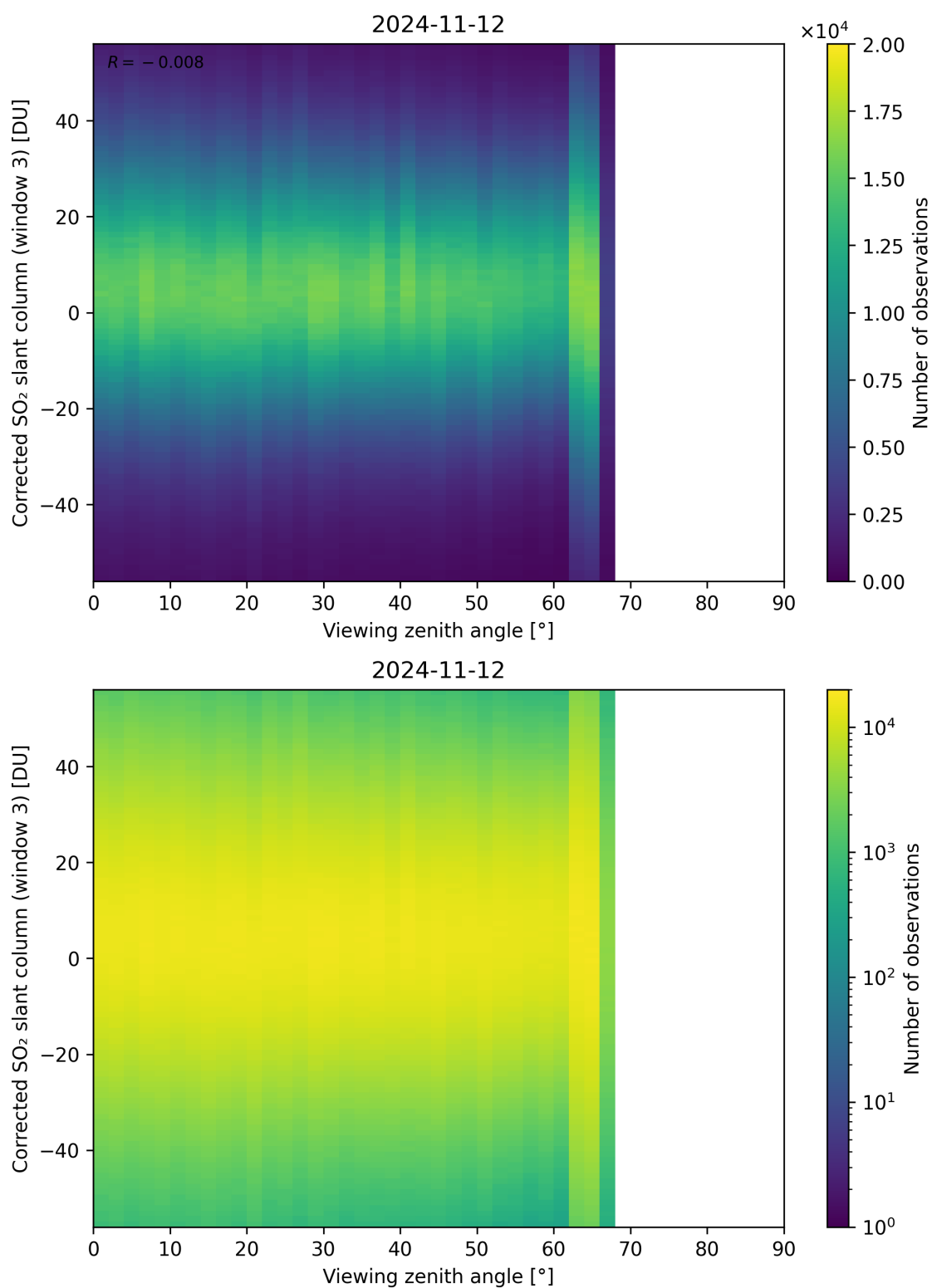
Figure 319: Scatter density plot of “Viewing zenith angle” against “Corrected SO 2 slant column (window 3)” for 2024-11-11 to 2024-11-13.
