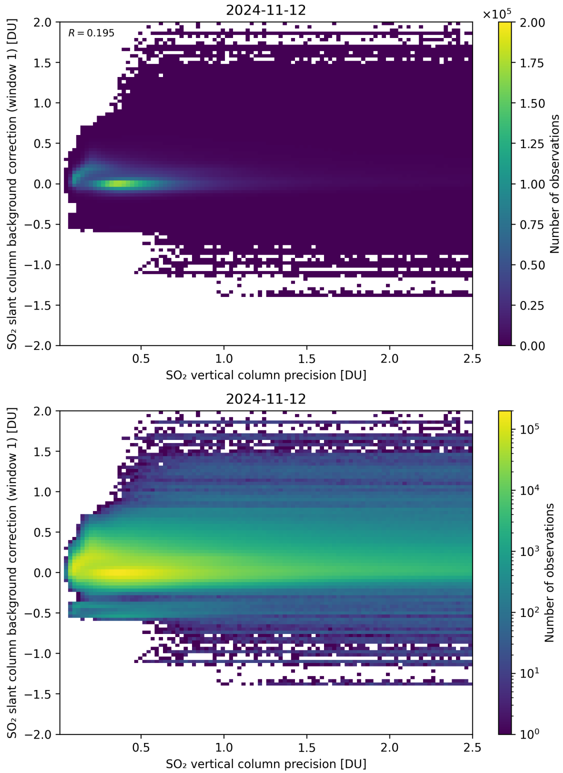
Figure 279: Scatter density plot of “SO 2 vertical column precision” against “SO 2 slant column background correction (window 1)” for 2024-11-11 to 2024-11-13.
