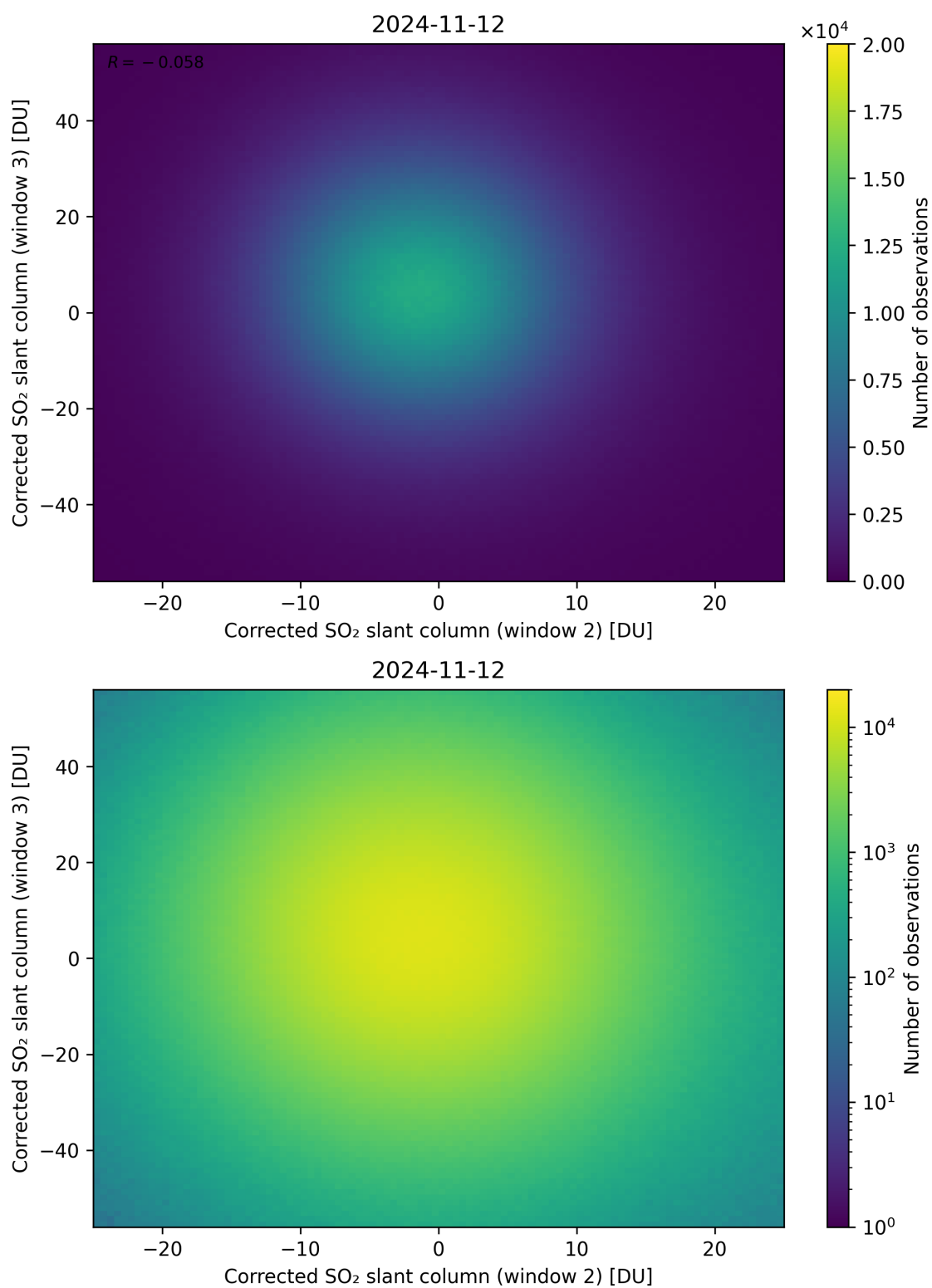
Figure 200: Scatter density plot of “Corrected SO 2 slant column (window 2)” against “Corrected SO 2 slant column (window 3)” for 2024-11-11 to 2024-11-13.
