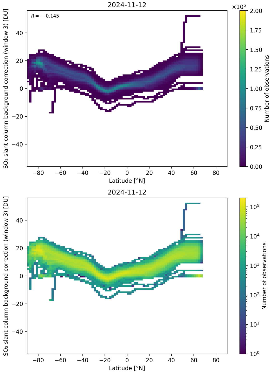
Figure 141: Scatter density plot of “Latitude” against “SO 2 slant column background correction (window 3)” for 2024-11-11 to 2024-11-13.
