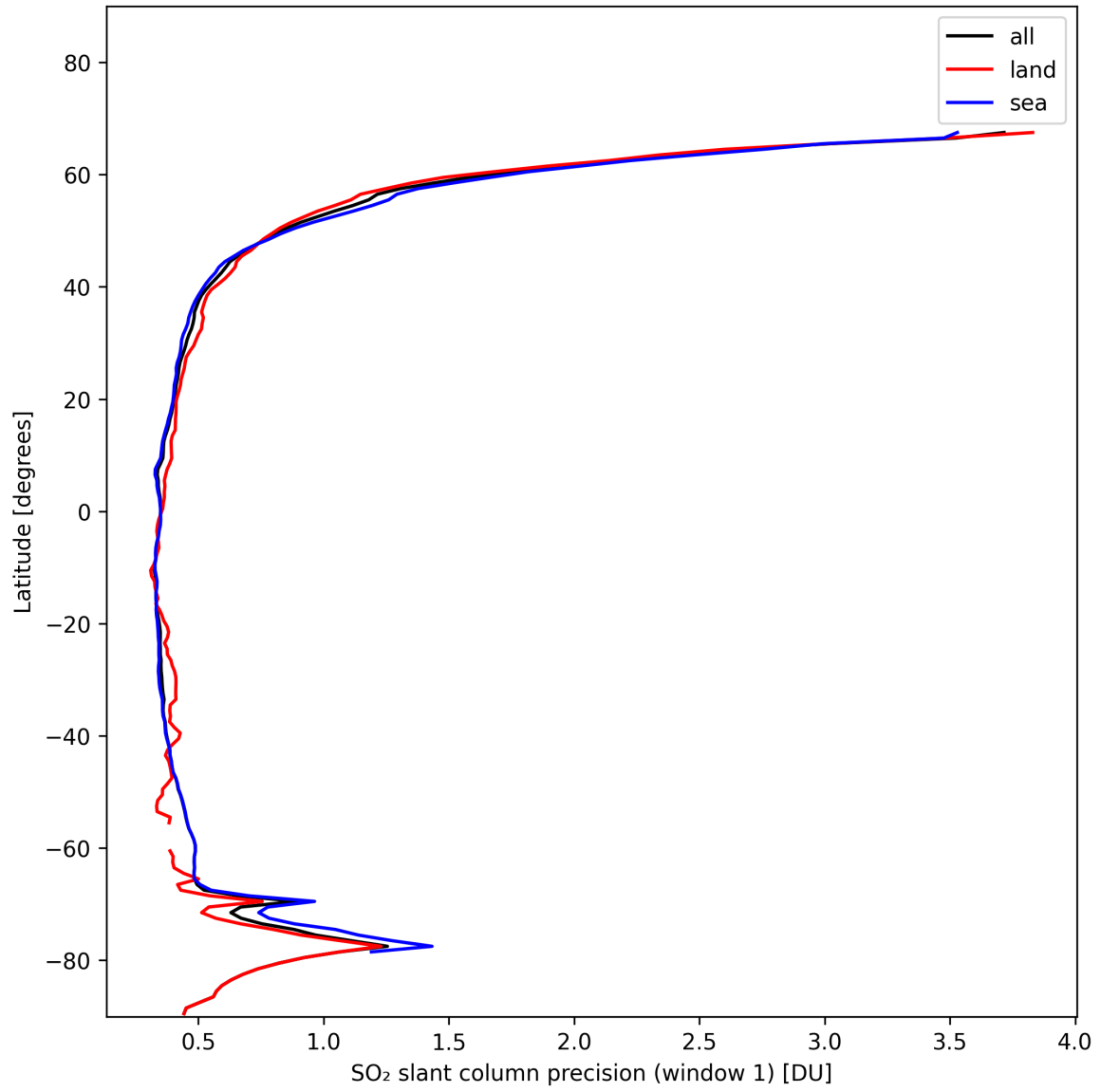
Figure 34: Zonal average of “SO 2 slant column precision (window 1)” for 2024-11-11 to 2024-11-13.
