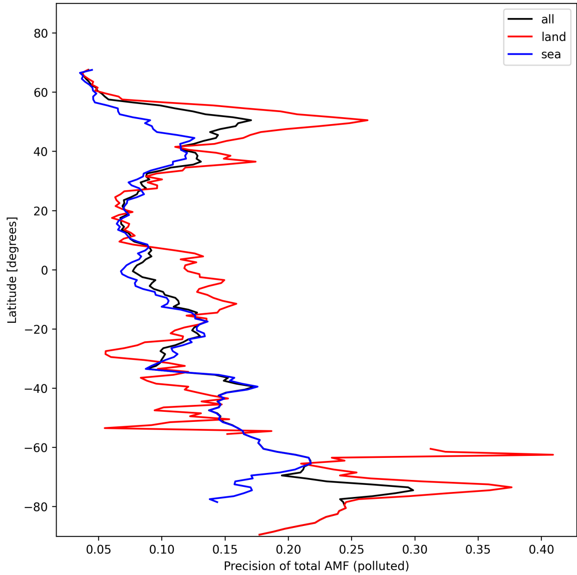
Figure 49: Zonal average of “Precision of total AMF (polluted)” for 2024-11-11 to 2024-11-13.
