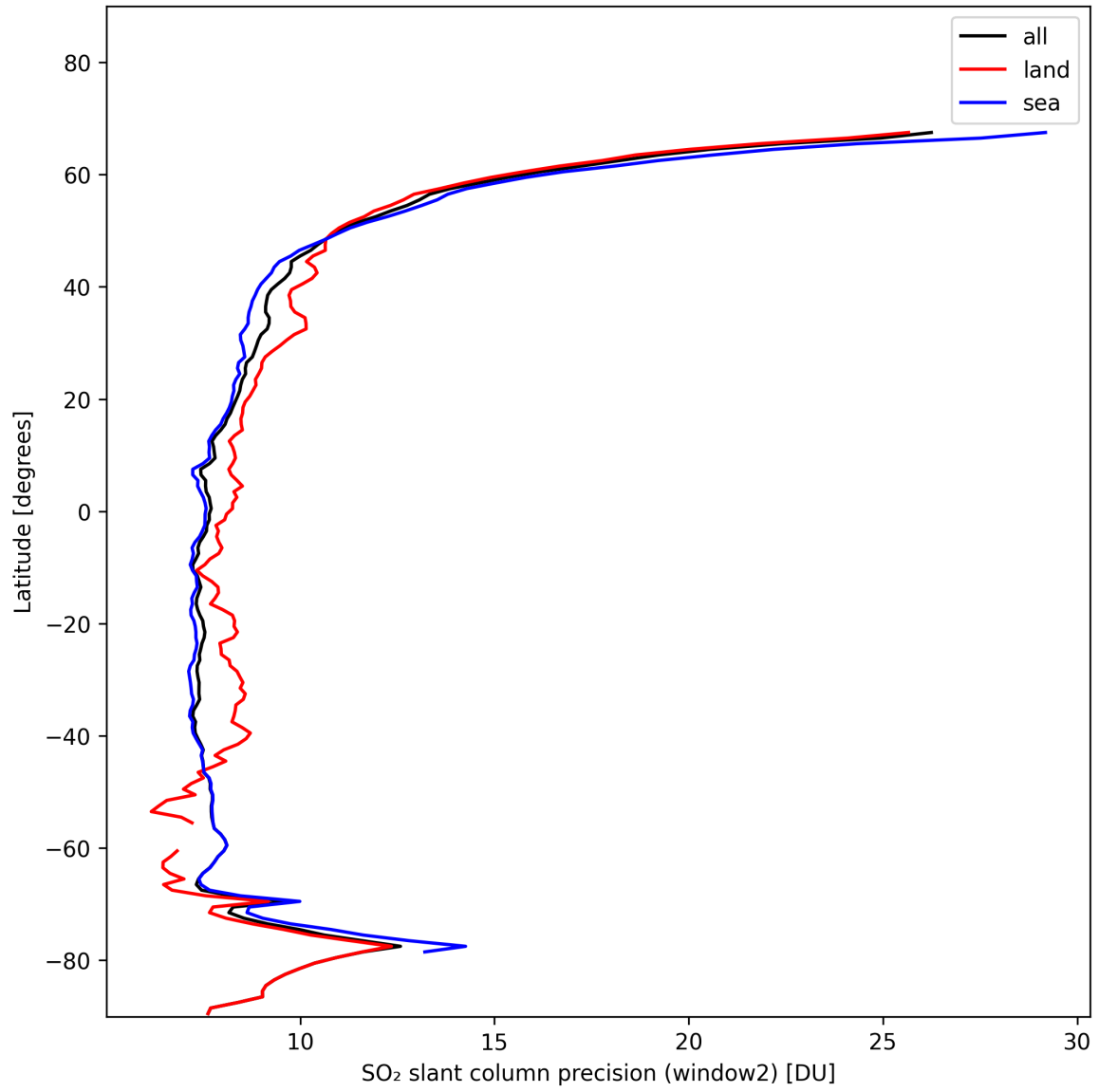
Figure 38: Zonal average of “SO 2 slant column precision (window2)” for 2024-11-11 to 2024-11-13.
