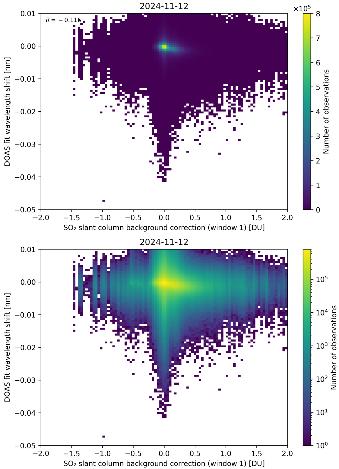
Figure 100: Scatter density plot of “SO 2 slant column background correction (window 1)” against “DOAS fit wavelength shift” for 2024-11-11 to 2024-11-13.
