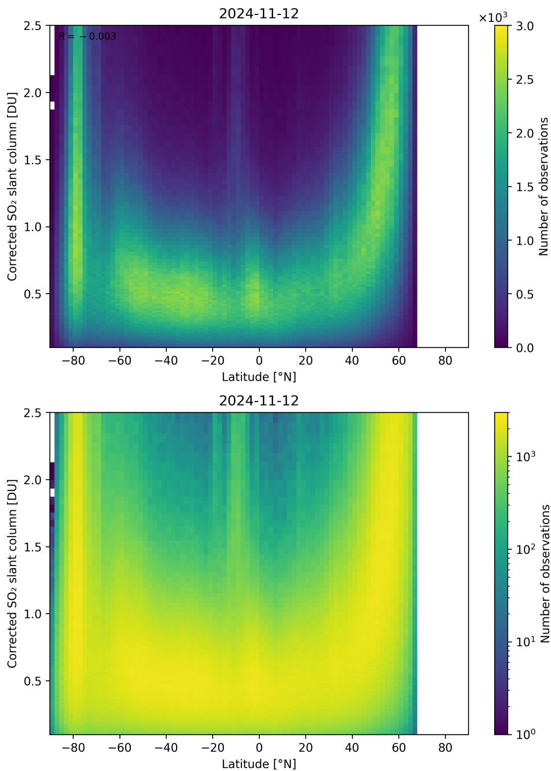
Figure 146: Scatter density plot of “Latitude” against “Corrected SO 2 slant column” for 2024-11-11 to 2024-11-13.
