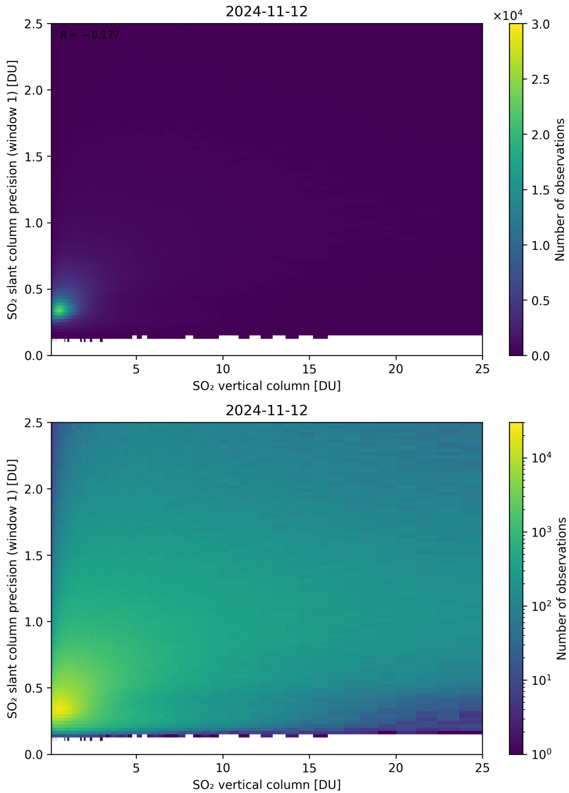
Figure 301: Scatter density plot of “SO 2 vertical column” against “SO 2 slant column precision (window 1)” for 2024-11-11 to 2024-11-13.
