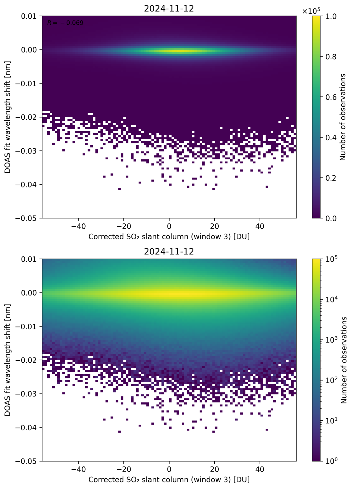
Figure 206: Scatter density plot of “Corrected SO 2 slant column (window 3)” against “DOAS fit wavelength shift” for 2024-11-11 to 2024-11-13.
