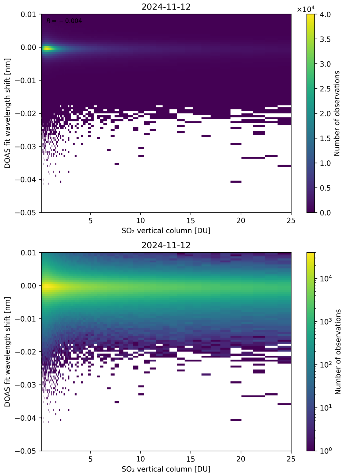
Figure 276: Scatter density plot of “SO 2 vertical column” against “DOAS fit wavelength shift” for 2024-11-11 to 2024-11-13.
