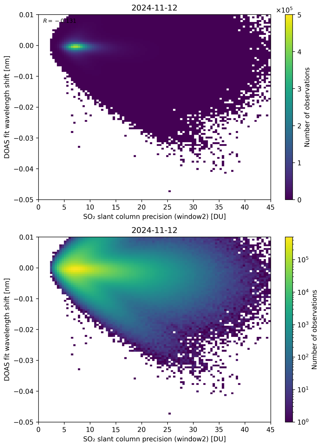
Figure 243: Scatter density plot of “SO 2 slant column precision (window2)” against “DOAS fit wavelength shift” for 2024-11-11 to 2024-11-13.
