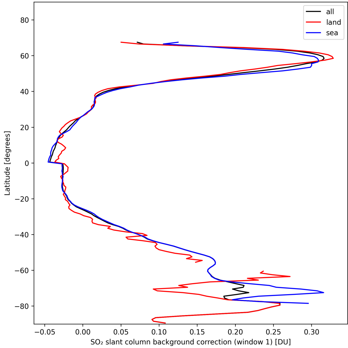
Figure 36: Zonal average of “SO 2 slant column background correction (window 1)” for 2024-11-11 to 2024-11-13.
