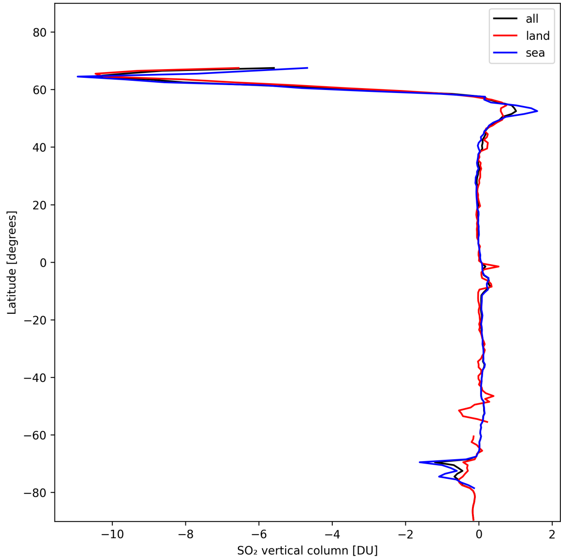
Figure 30: Zonal average of “SO 2 vertical column” for 2024-11-11 to 2024-11-13.
