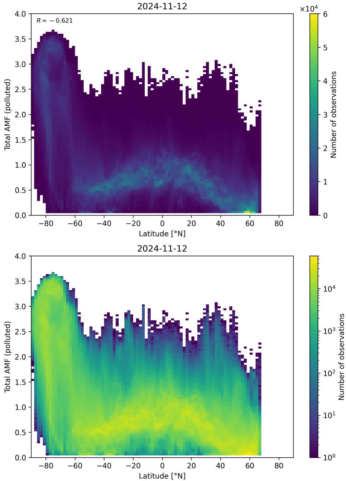
Figure 154: Scatter density plot of “Latitude” against “Total AMF (polluted)” for 2024-11-11 to 2024-11-13.
