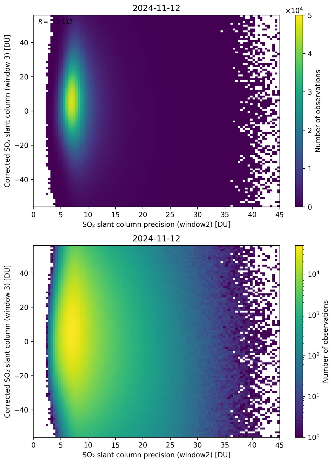
Figure 248: Scatter density plot of “SO 2 slant column precision (window2)” against “Corrected SO 2 slant column (window 3)” for 2024-11-11 to 2024-11-13.
