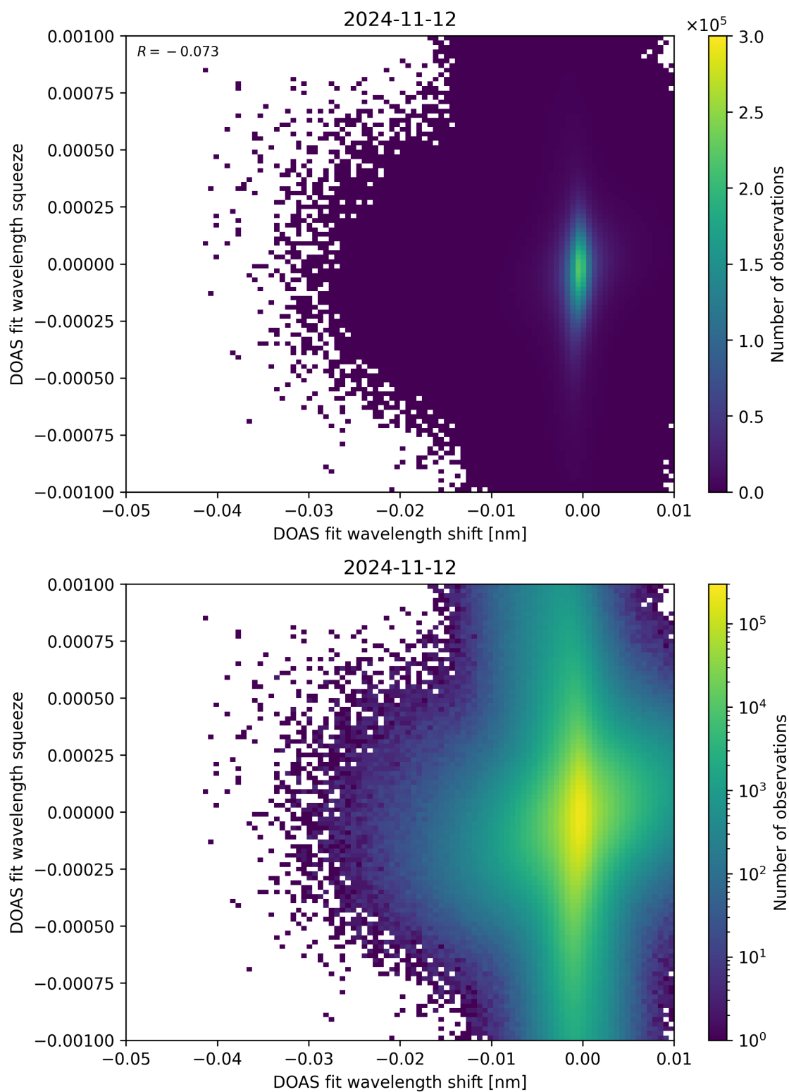
Figure 127: Scatter density plot of “DOAS fit wavelength shift” against “DOAS fit wavelength squeeze” for 2024-11-11 to 2024-11-13.
