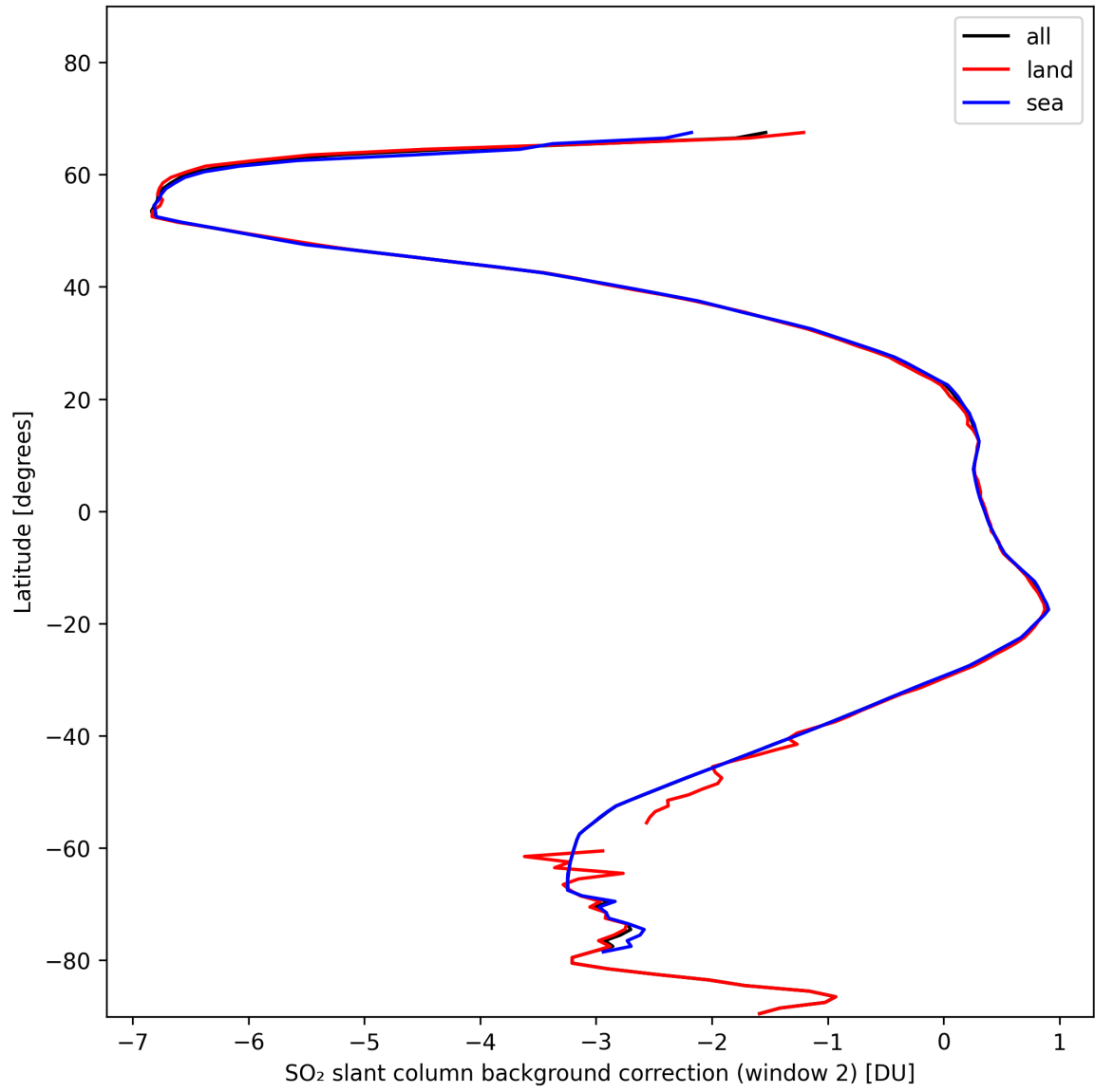
Figure 40: Zonal average of “SO 2 slant column background correction (window 2)” for 2024-11-11 to 2024-11-13.
