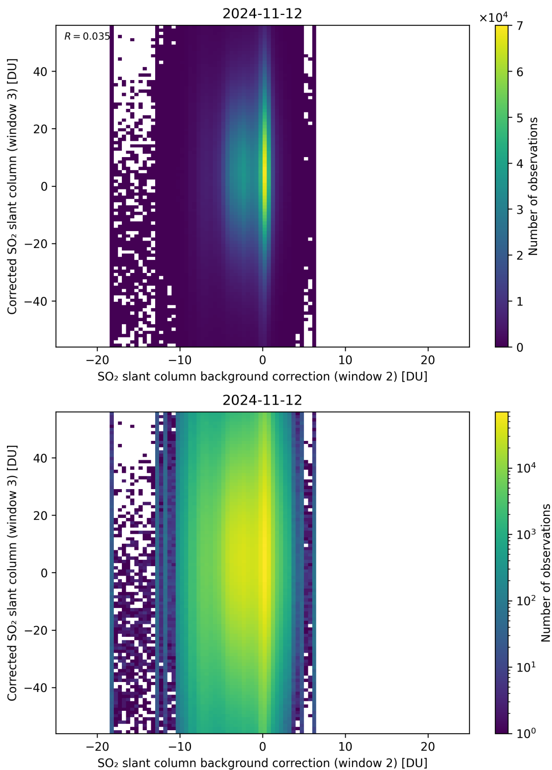
Figure 116: Scatter density plot of “SO 2 slant column background correction (window 2)” against “Corrected SO 2 slant column (window 3)” for 2024-11-11 to 2024-11-13.
