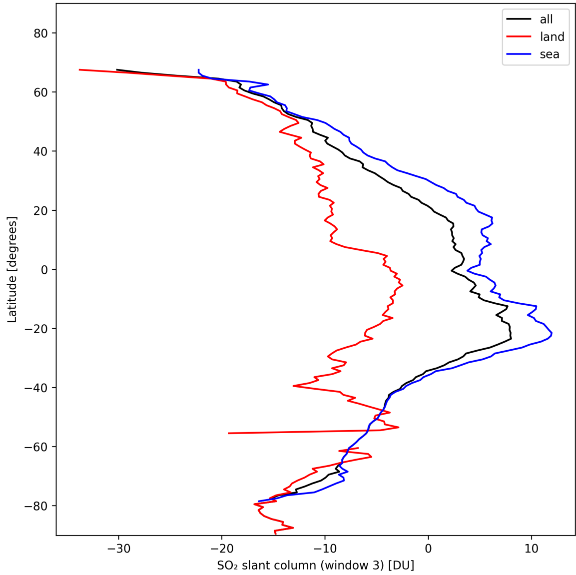
Figure 41: Zonal average of “SO 2 slant column (window 3)” for 2024-11-11 to 2024-11-13.
