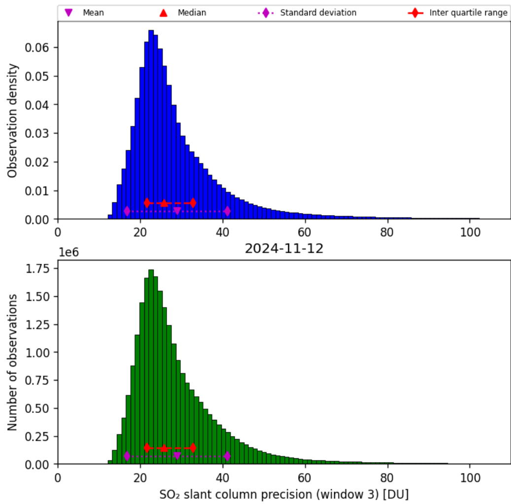
Figure 65: Histogram of “SO 2 slant column precision (window 3)” for 2024-11-11 to 2024-11-13
