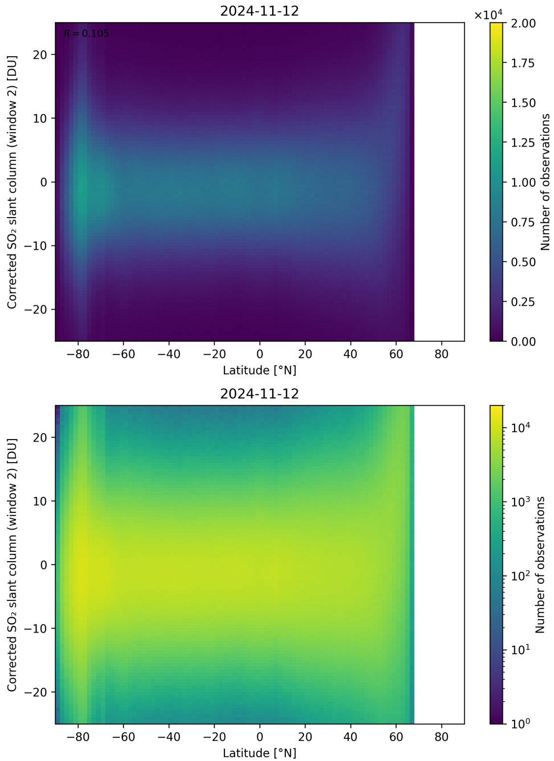
Figure 147: Scatter density plot of “Latitude” against “Corrected SO 2 slant column (window 2)” for 2024-11-11 to 2024-11-13.
