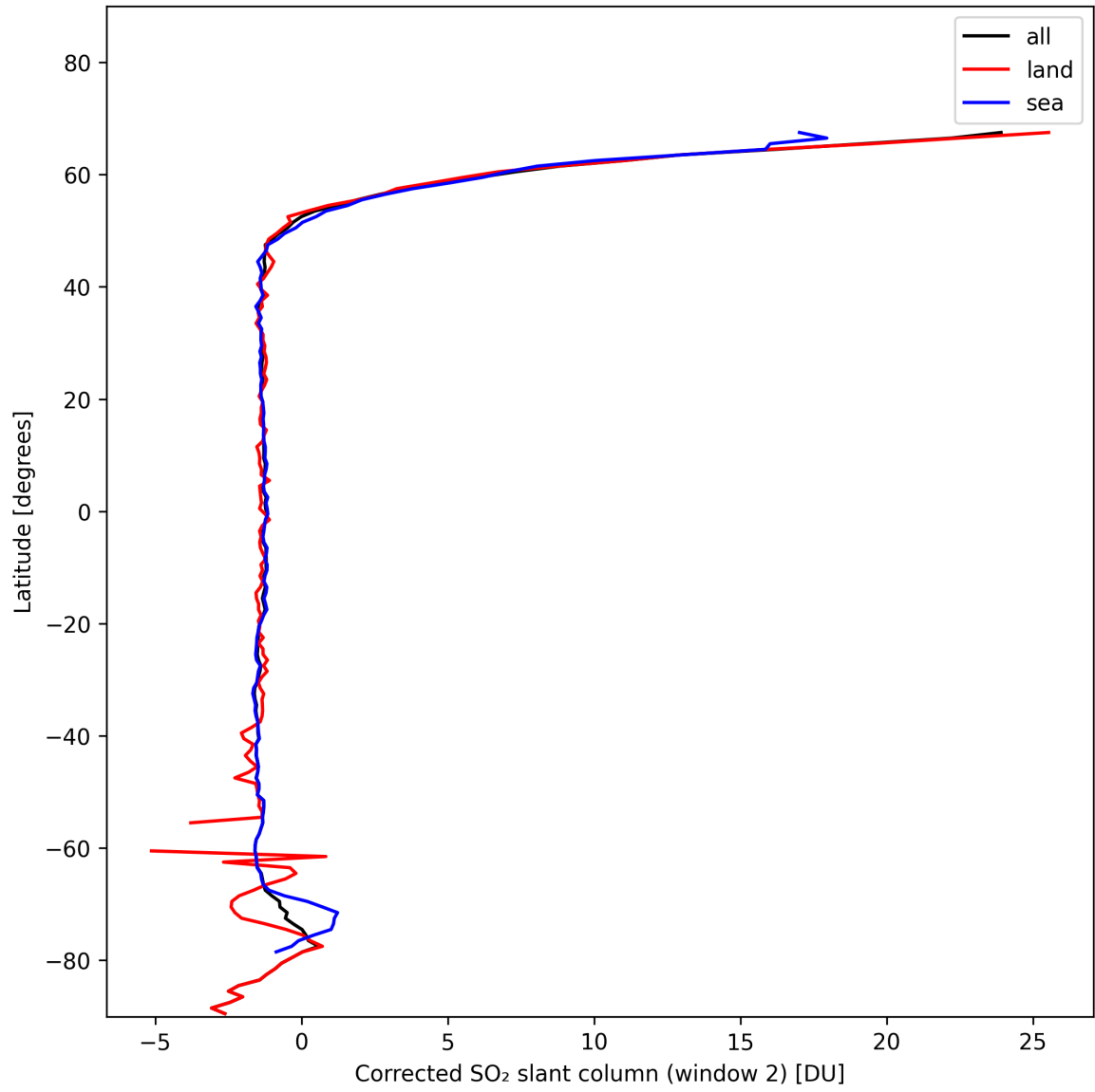
Figure 39: Zonal average of “Corrected SO 2 slant column (window 2)” for 2024-11-11 to 2024-11-13.
