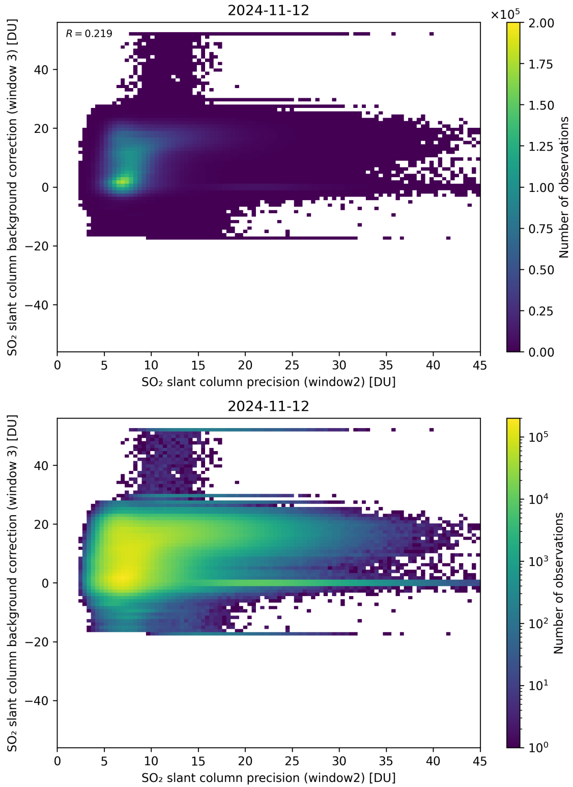
Figure 242: Scatter density plot of “SO 2 slant column precision (window2)” against “SO 2 slant column background correction (window 3)” for 2024-11-11 to 2024-11-13.
