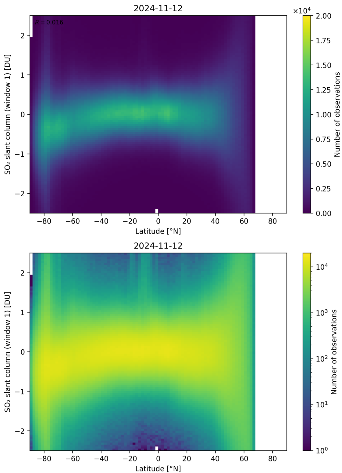
Figure 149: Scatter density plot of “Latitude” against “SO 2 slant column (window 1)” for 2024-11-11 to 2024-11-13.
