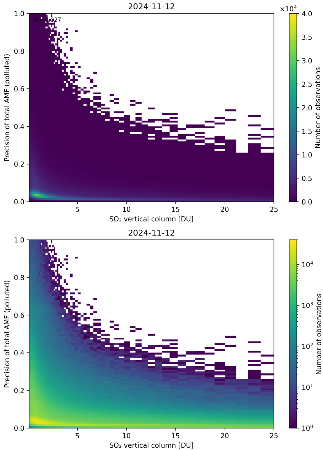
Figure 306: Scatter density plot of “SO 2 vertical column” against “Precision of total AMF (polluted)” for 2024-11-11 to 2024-11-13.
