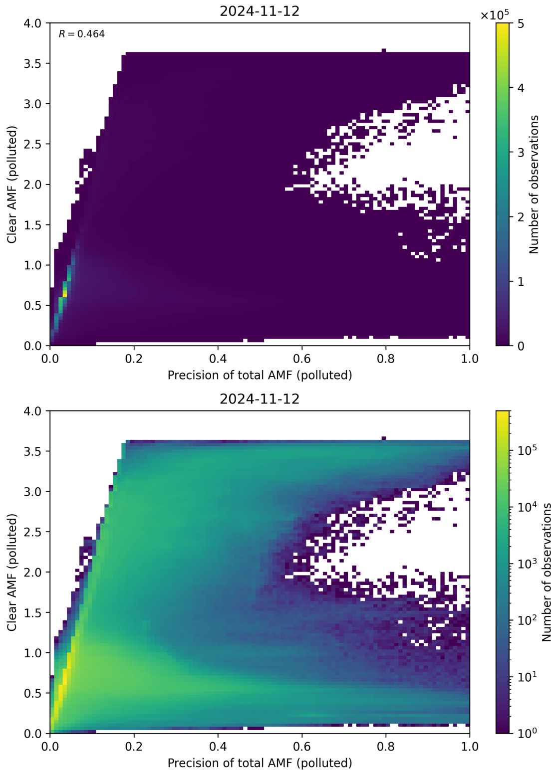
Figure 270: Scatter density plot of “Precision of total AMF (polluted)” against “Clear AMF (polluted)” for 2024-11-11 to 2024-11-13.
