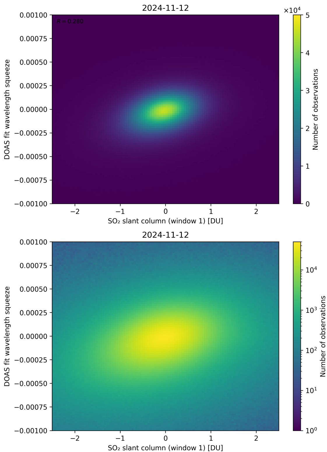
Figure 216: Scatter density plot of “SO 2 slant column (window 1)” against “DOAS fit wavelength squeeze” for 2024-11-11 to 2024-11-13.
