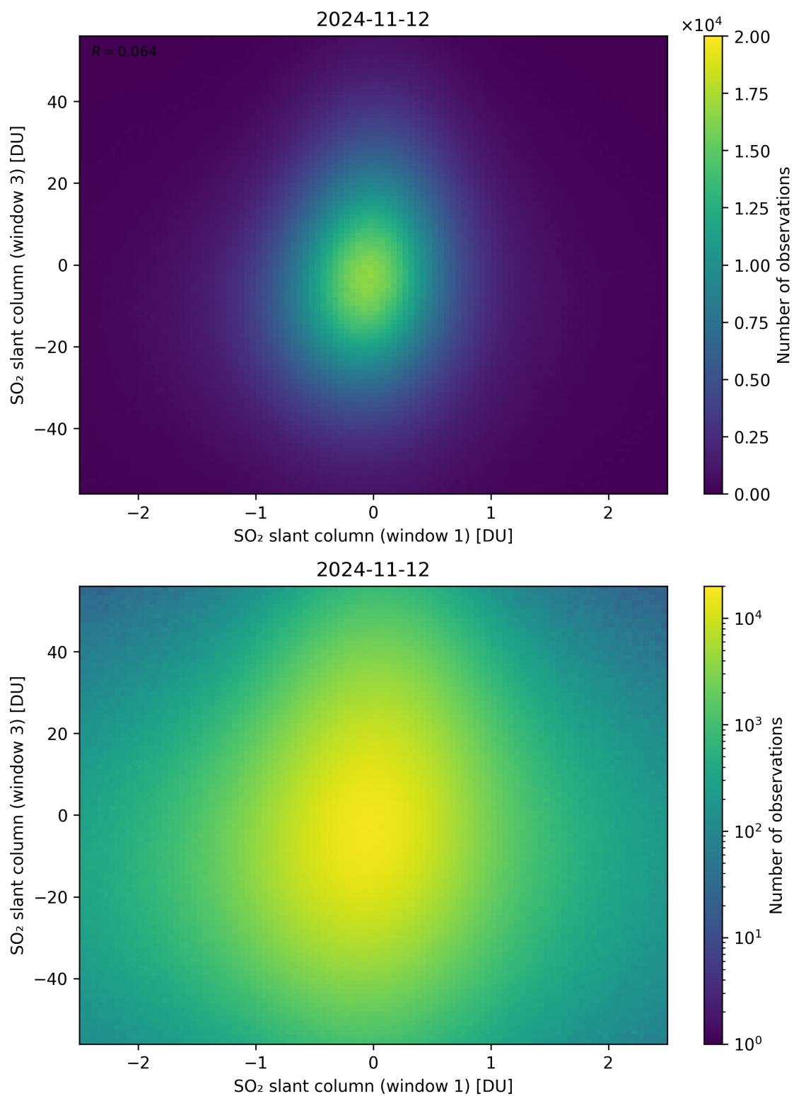
Figure 237: Scatter density plot of “SO 2 slant column (window 1)” against “SO 2 slant column (window 3)” for 2024-11-11 to 2024-11-13.
