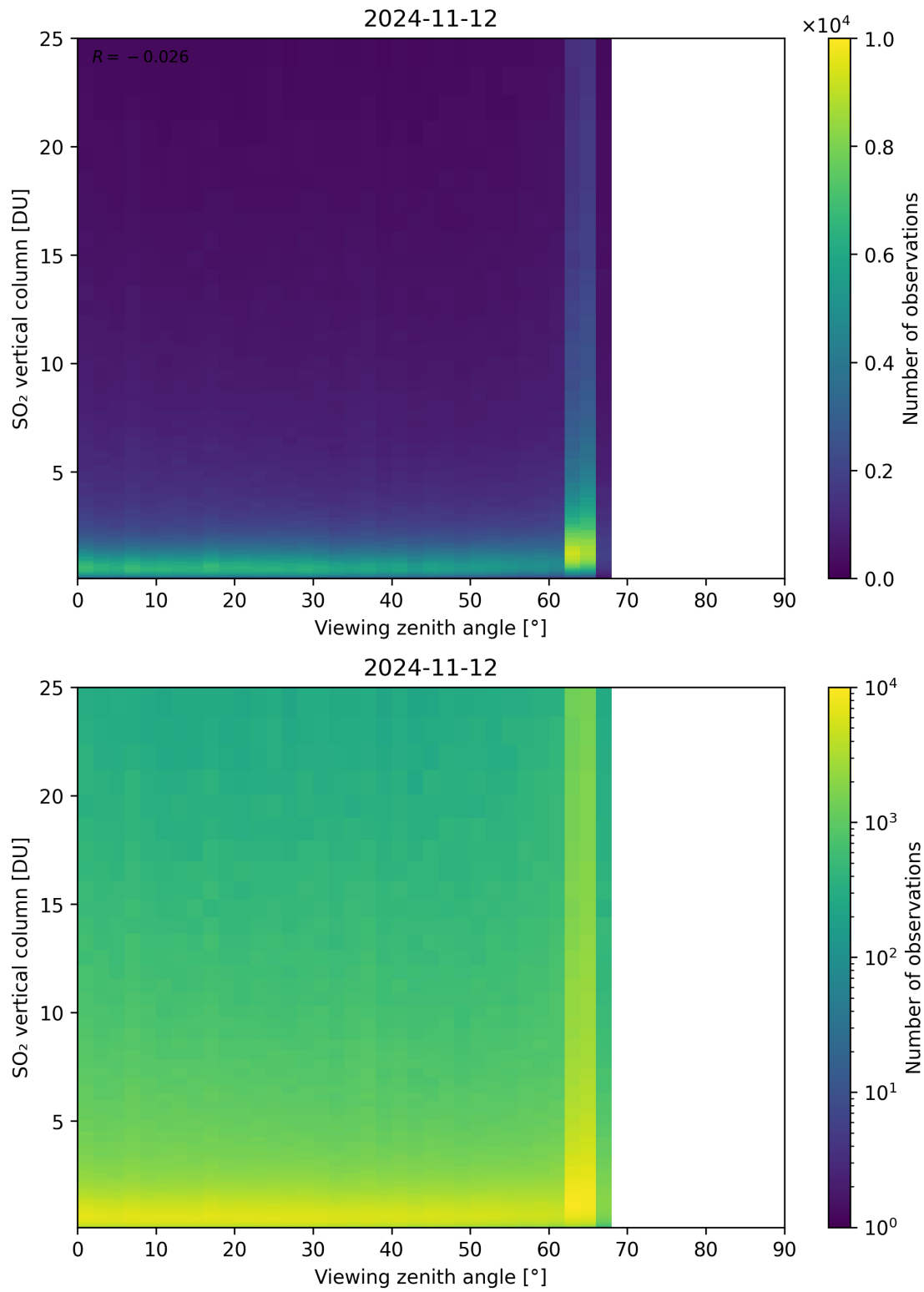
Figure 327: Scatter density plot of “Viewing zenith angle” against “SO 2 vertical column” for 2024-11-11 to 2024-11-13.
