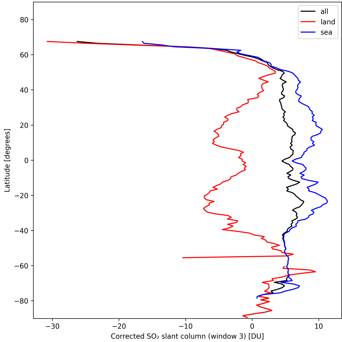
Figure 43: Zonal average of “Corrected SO 2 slant column (window 3)” for 2024-11-11 to 2024-11-13.
