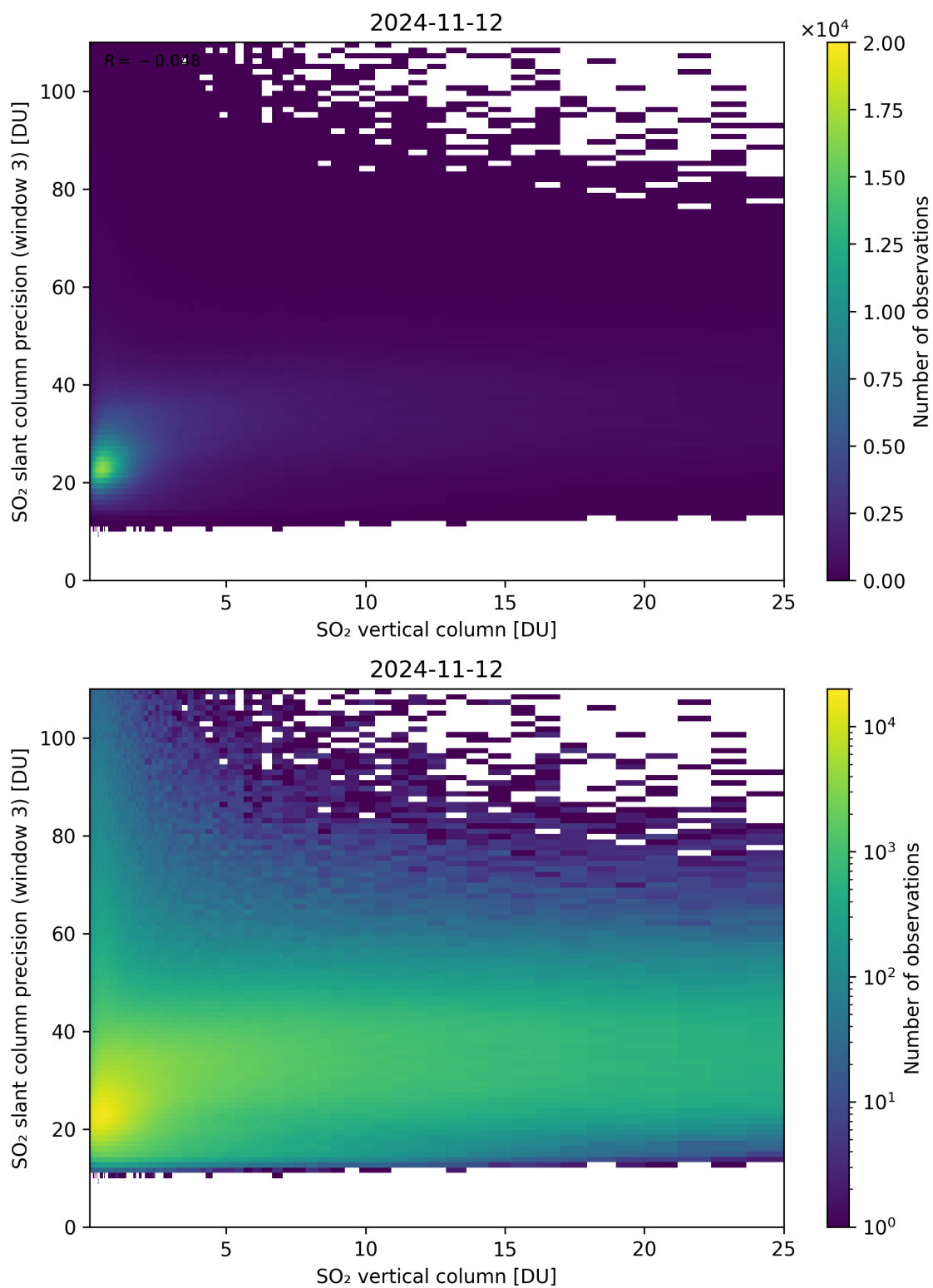
Figure 304: Scatter density plot of “SO 2 vertical column” against “SO 2 slant column precision (window 3)” for 2024-11-11 to 2024-11-13.
