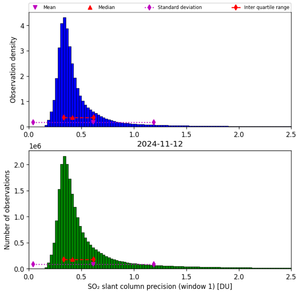
Figure 57: Histogram of “SO 2 slant column precision (window 1)” for 2024-11-11 to 2024-11-13
