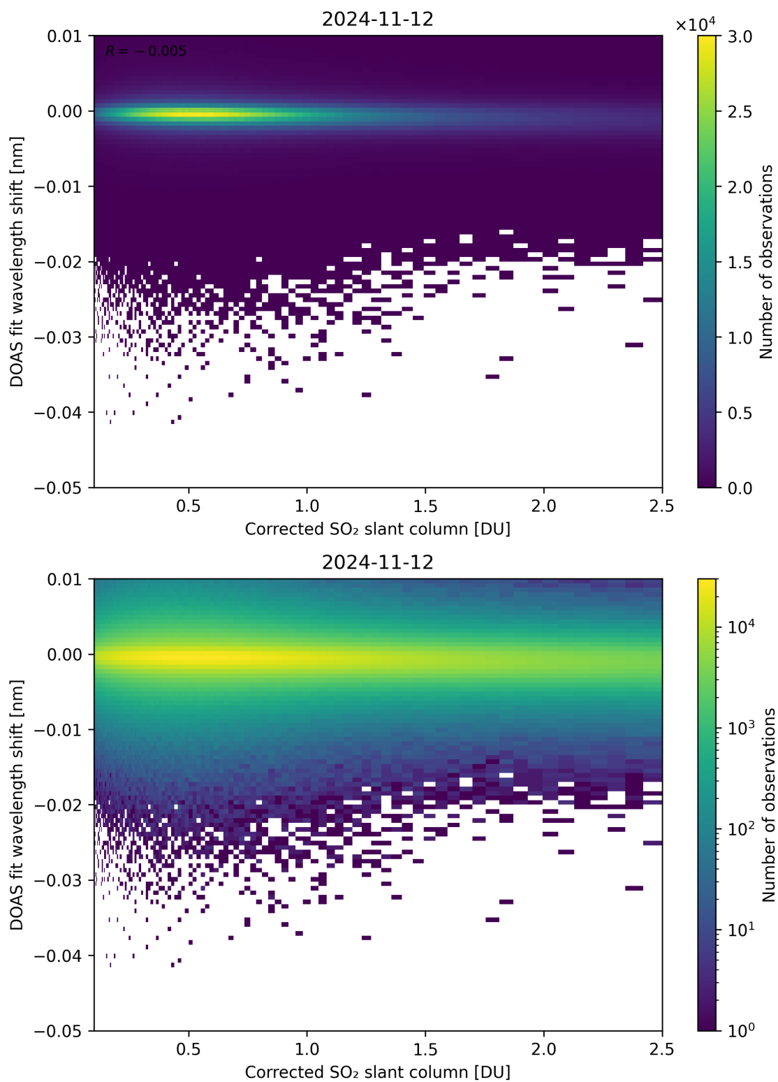
Figure 181: Scatter density plot of “Corrected SO 2 slant column” against “DOAS fit wavelength shift” for 2024-11-11 to 2024-11-13.
