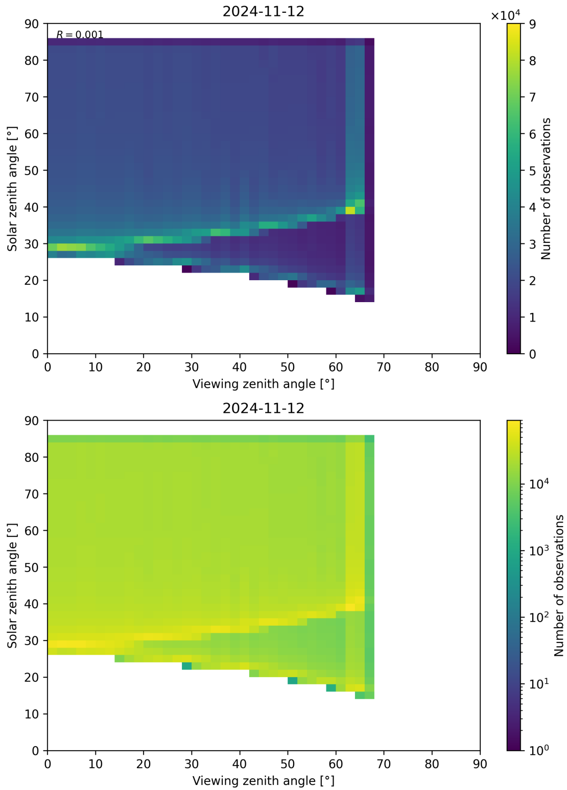
Figure 315: Scatter density plot of “Viewing zenith angle” against “Solar zenith angle” for 2024-11-11 to 2024-11-13.
