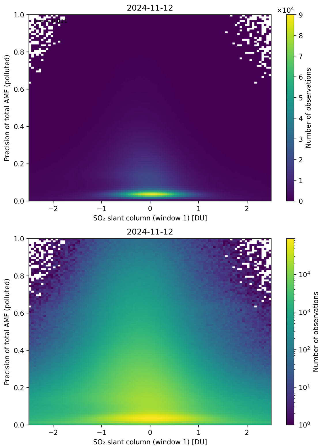
Figure 240: Scatter density plot of “SO 2 slant column (window 1)” against “Precision of total AMF (polluted)” for 2024-11-11 to 2024-11-13.
