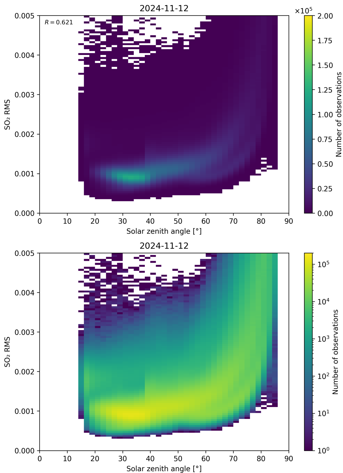
Figure 163: Scatter density plot of “Solar zenith angle” against “SO 2 RMS” for 2024-11-11 to 2024-11-13.
