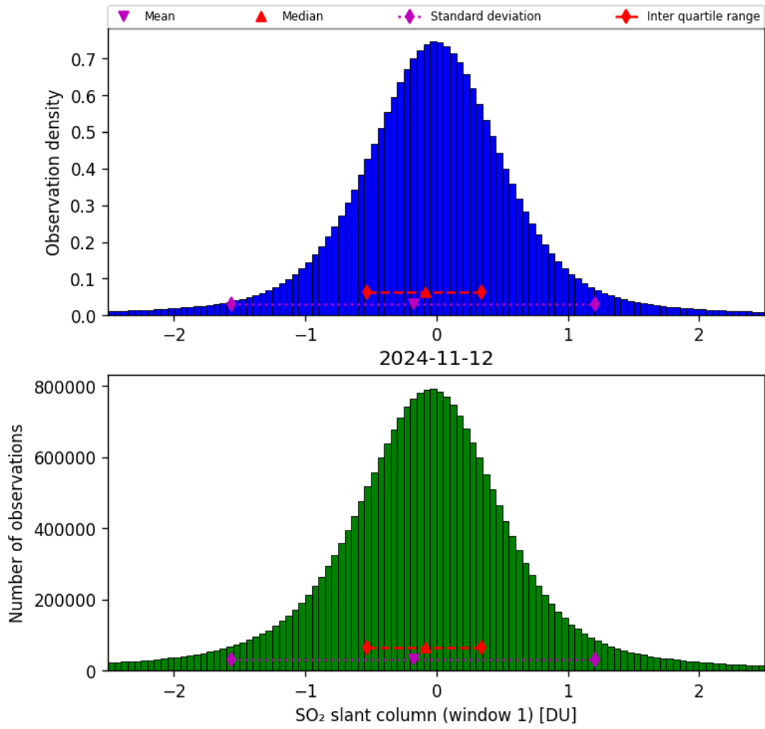
Figure 56: Histogram of “SO 2 slant column (window 1)” for 2024-11-11 to 2024-11-13
