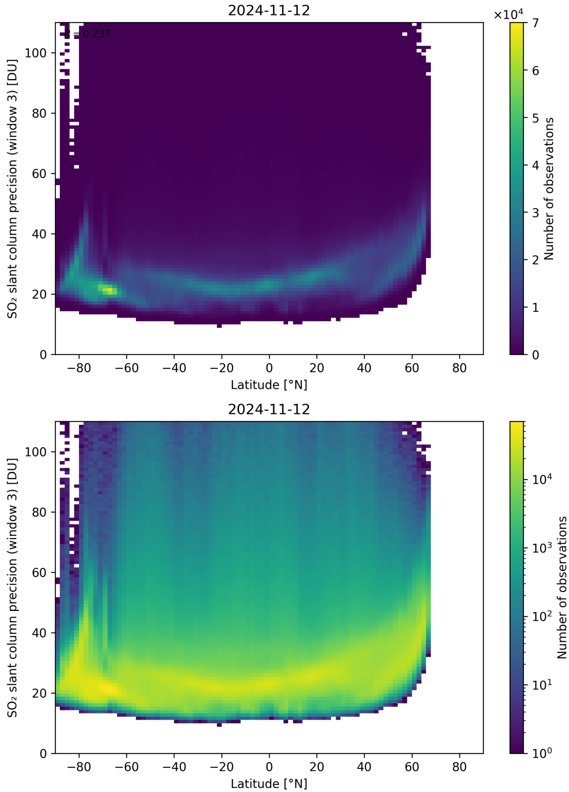
Figure 153: Scatter density plot of “Latitude” against “SO 2 slant column precision (window 3)” for 2024-11-11 to 2024-11-13.
