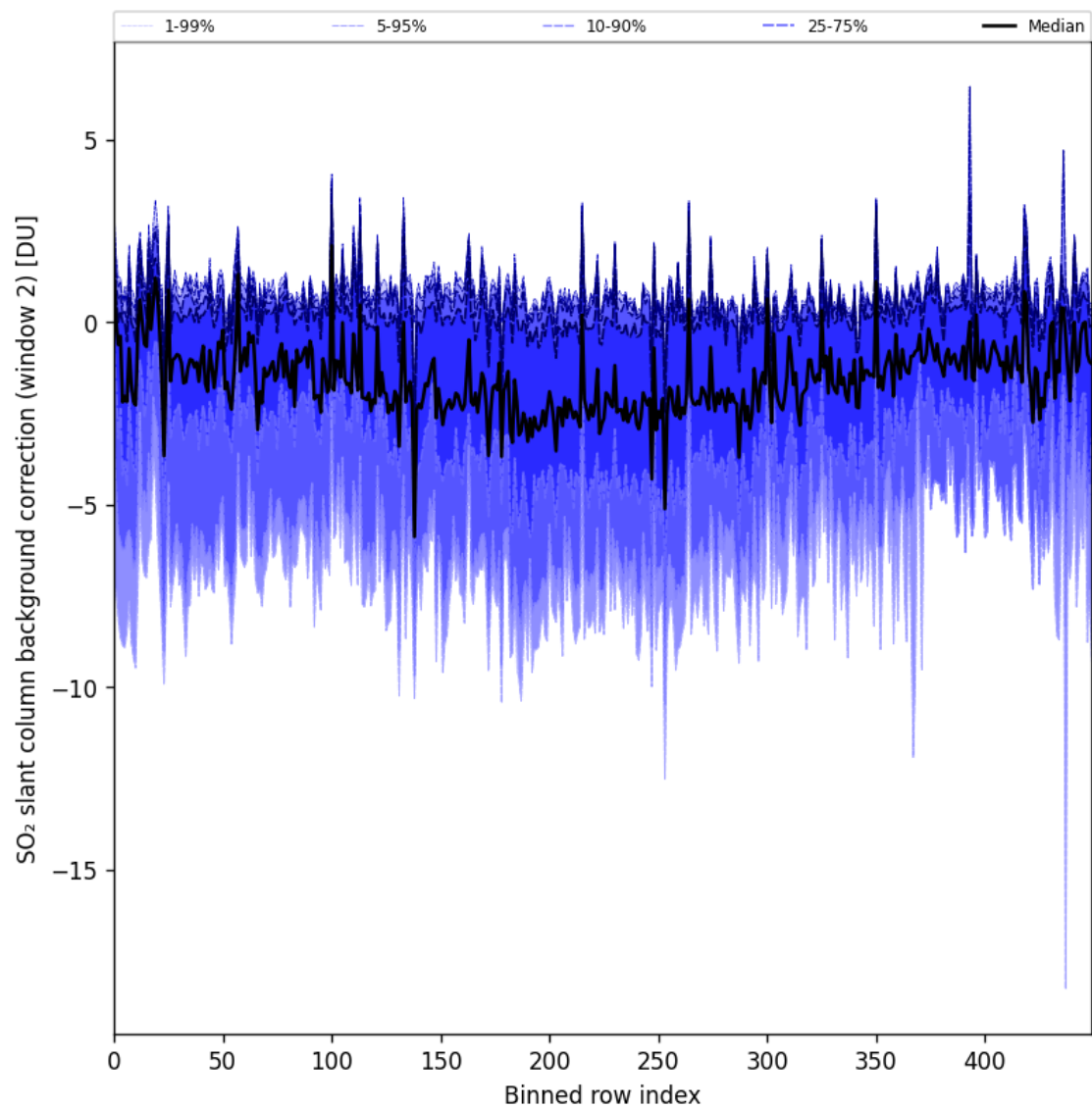
Figure 86: Along track statistics of “SO 2 slant column background correction (window 2)” for 2024-11-11 to 2024-11-13
