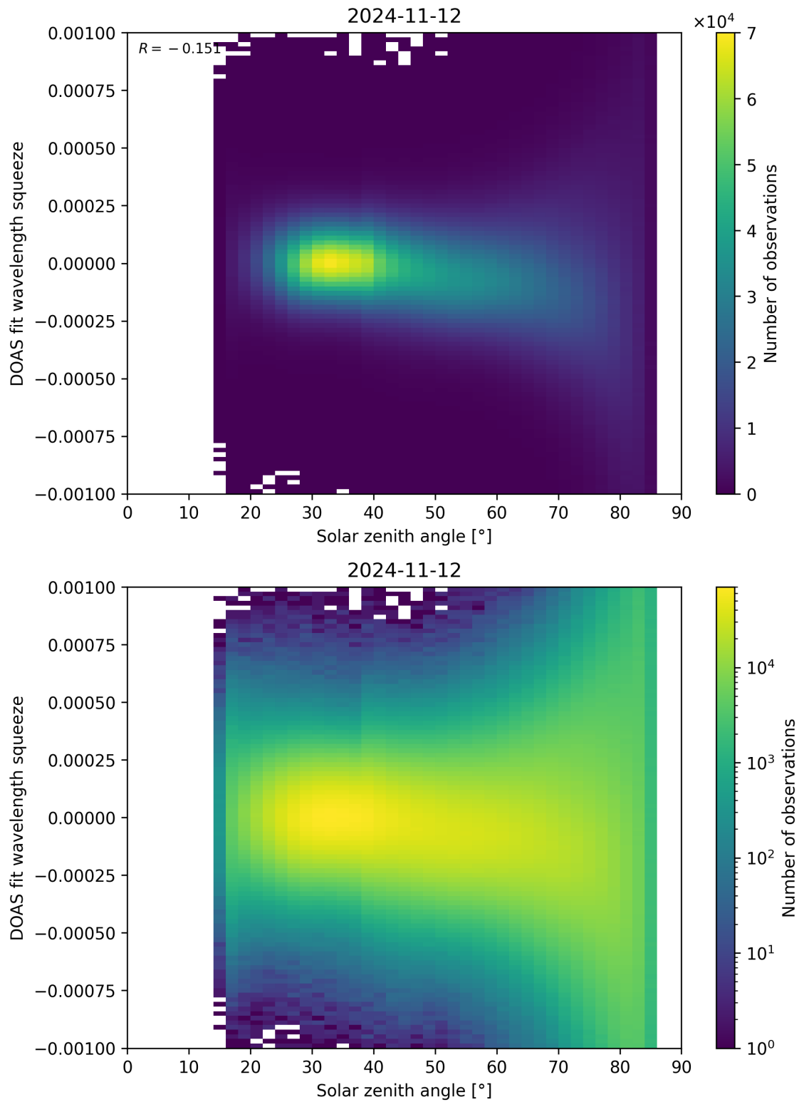
Figure 162: Scatter density plot of “Solar zenith angle” against “DOAS fit wavelength squeeze” for 2024-11-11 to 2024-11-13.
