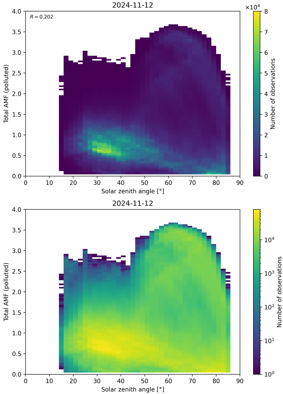
Figure 174: Scatter density plot of “Solar zenith angle” against “Total AMF (polluted)” for 2024-11-11 to 2024-11-13.
