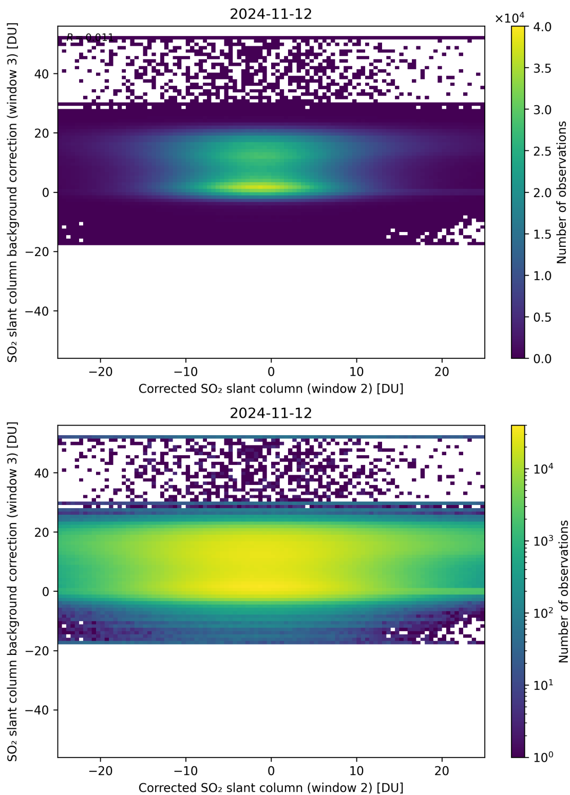
Figure 195: Scatter density plot of “Corrected SO 2 slant column (window 2)” against “SO 2 slant column background correction (window 3)” for 2024-11-11 to 2024-11-13.
