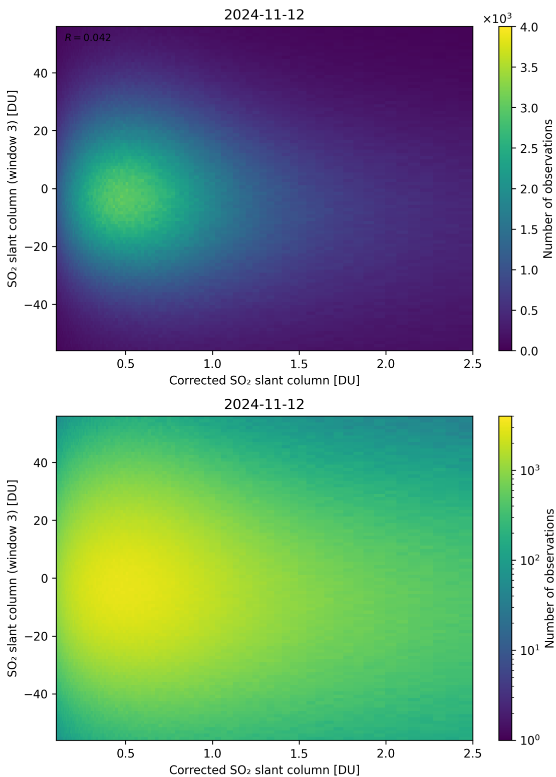
Figure 190: Scatter density plot of “Corrected SO 2 slant column” against “SO 2 slant column (window 3)” for 2024-11-11 to 2024-11-13.
