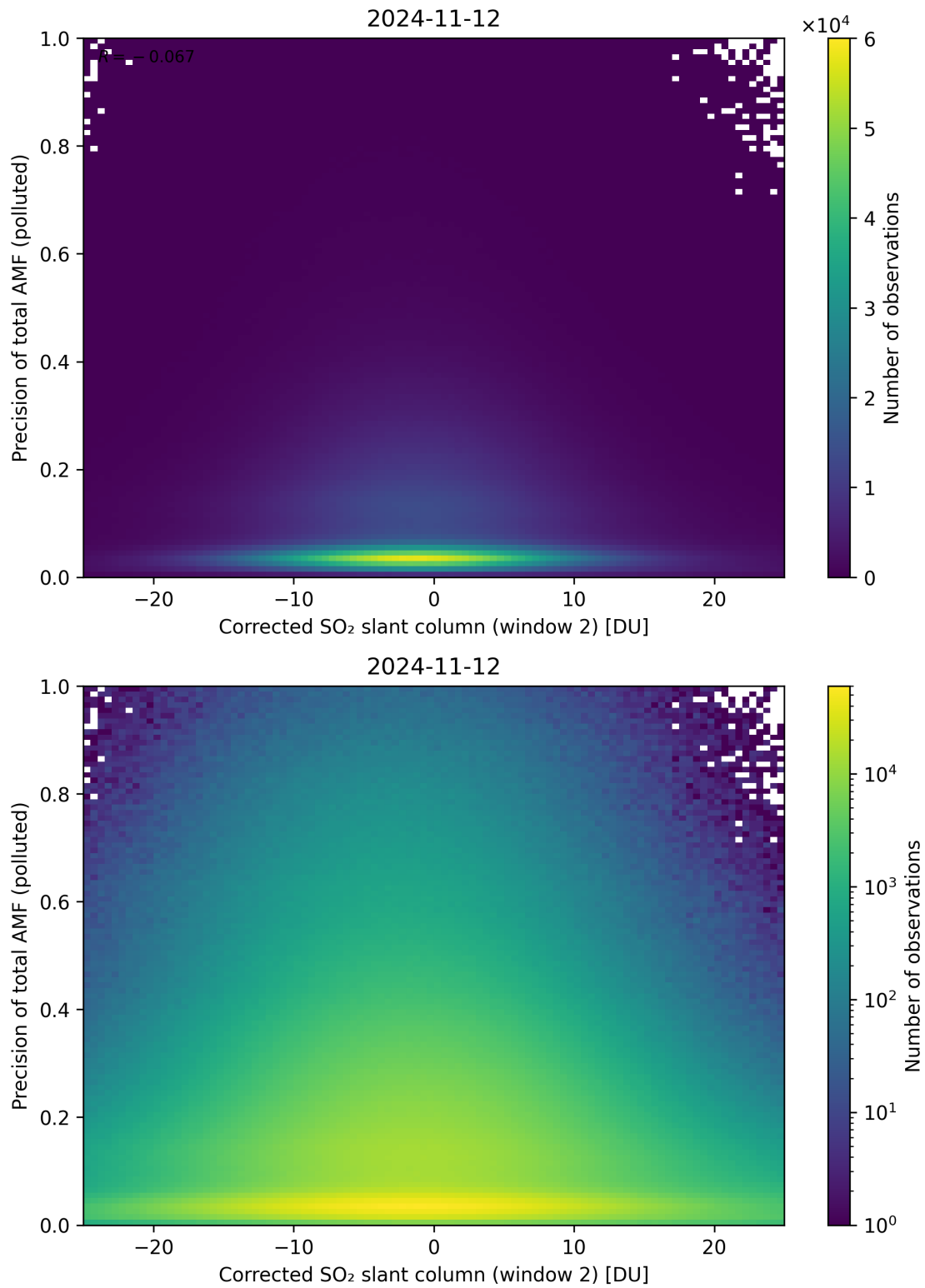
Figure 204: Scatter density plot of “Corrected SO 2 slant column (window 2)” against “Precision of total AMF (polluted)” for 2024-11-11 to 2024-11-13.
