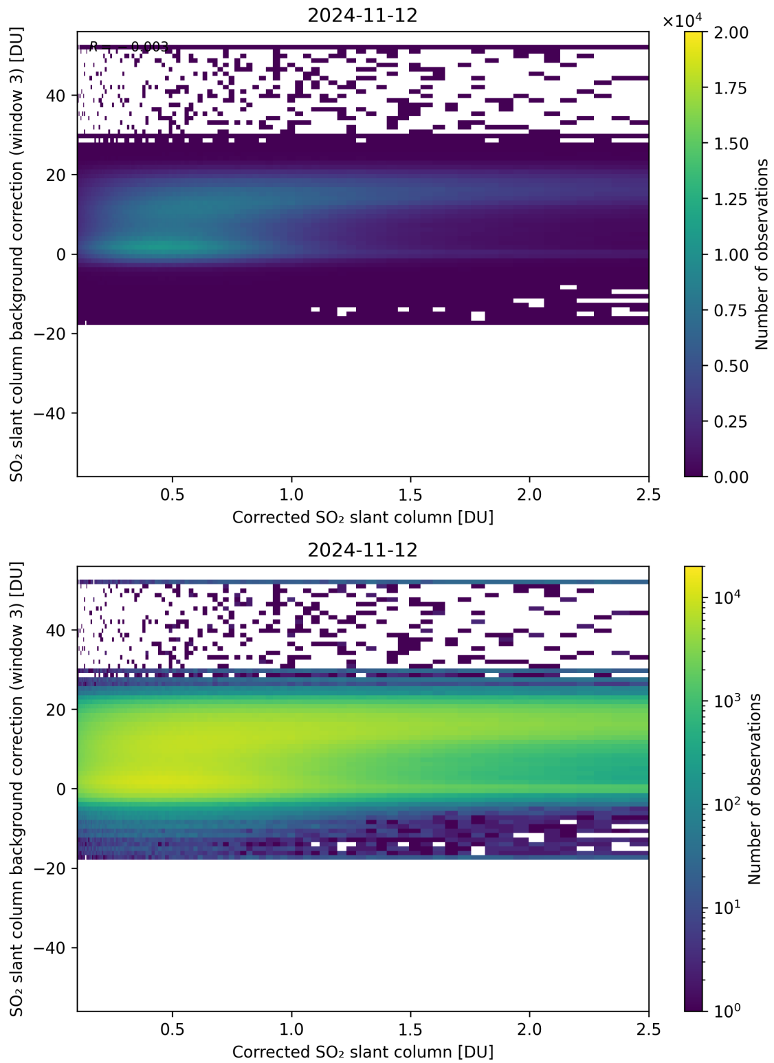
Figure 180: Scatter density plot of “Corrected SO 2 slant column” against “SO 2 slant column background correction (window 3)” for 2024-11-11 to 2024-11-13.
