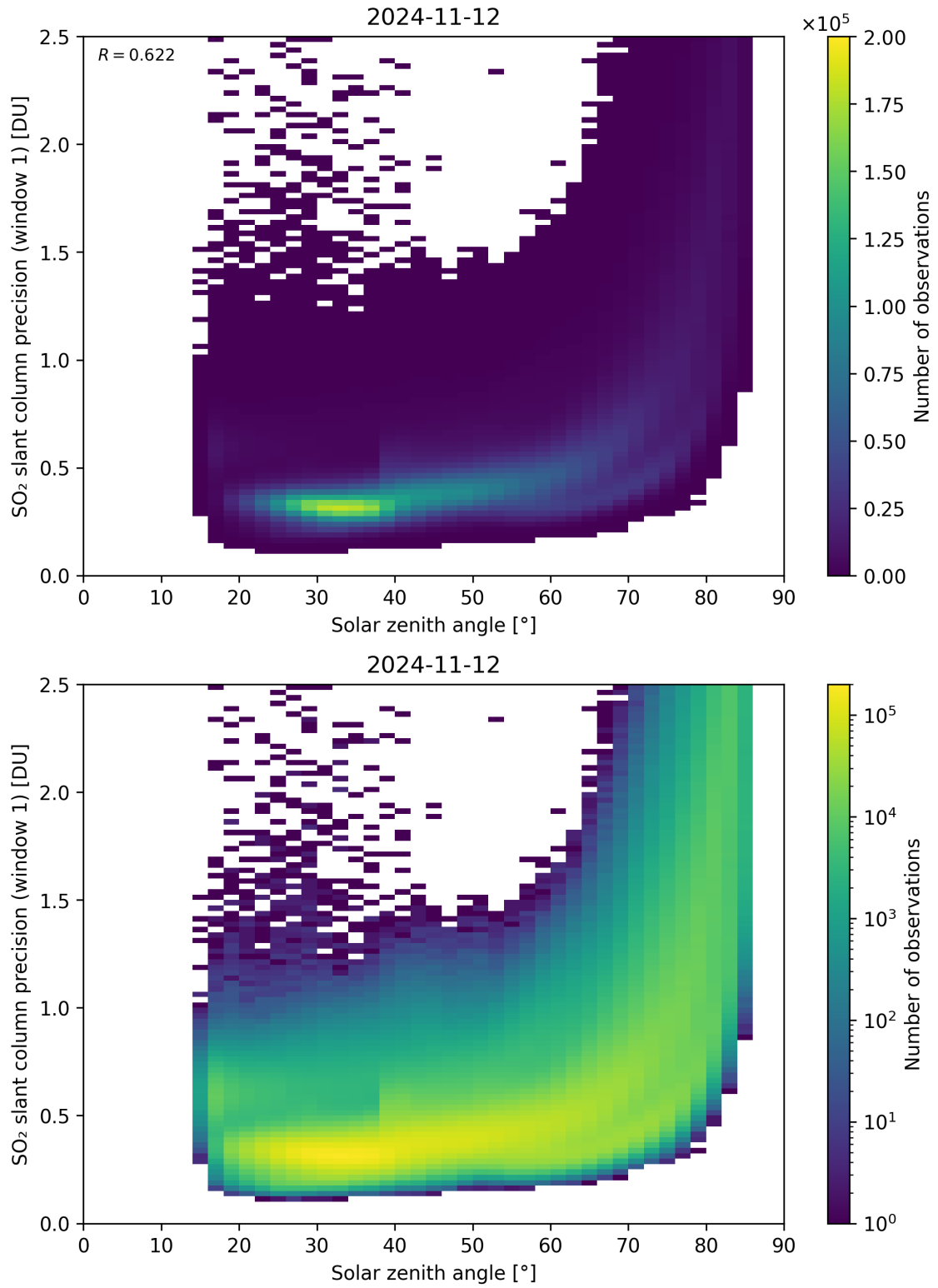
Figure 170: Scatter density plot of “Solar zenith angle” against “SO 2 slant column precision (window 1)” for 2024-11-11 to 2024-11-13.
