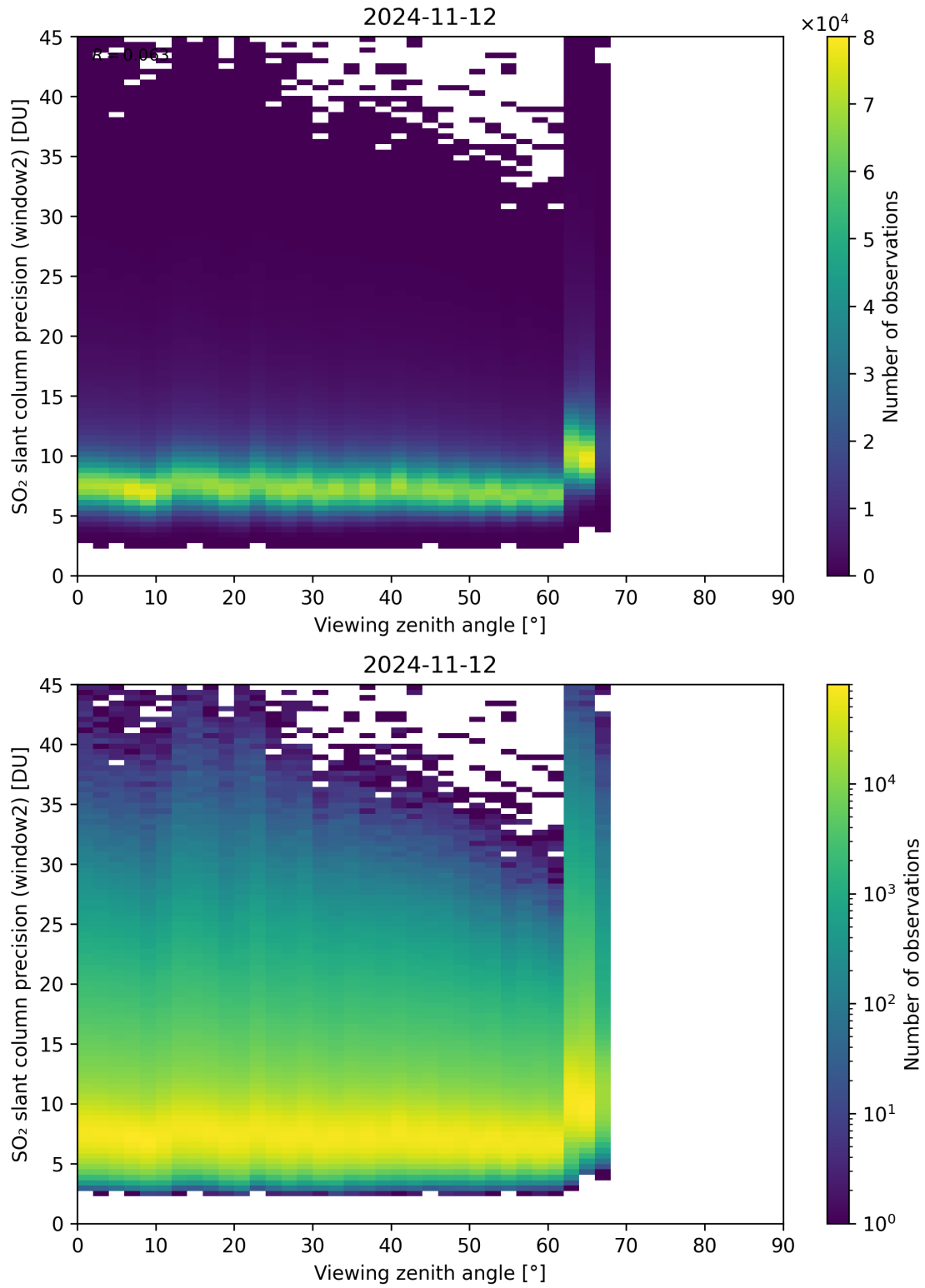
Figure 322: Scatter density plot of “Viewing zenith angle” against “SO 2 slant column precision (window2)” for 2024-11-11 to 2024-11-13.
