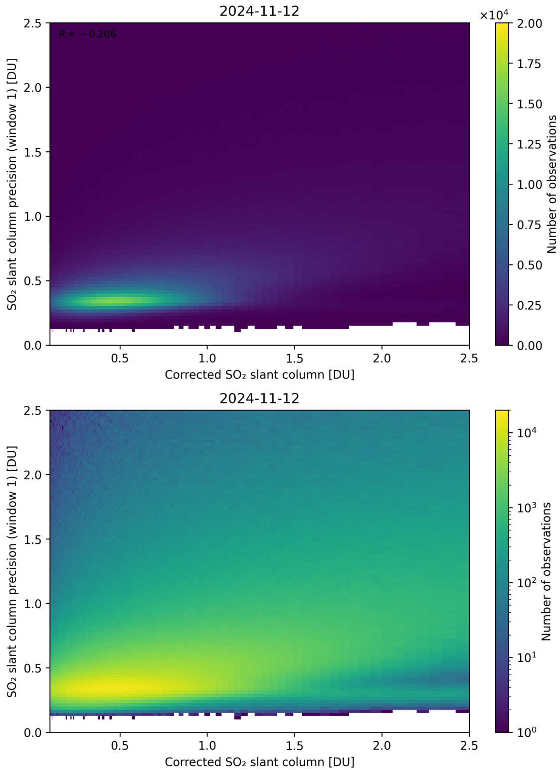
Figure 188: Scatter density plot of “Corrected SO 2 slant column” against “SO 2 slant column precision (window 1)” for 2024-11-11 to 2024-11-13.
