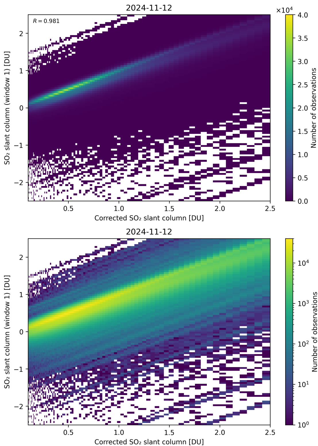
Figure 187: Scatter density plot of “Corrected SO 2 slant column” against “SO 2 slant column (window 1)” for 2024-11-11 to 2024-11-13.
