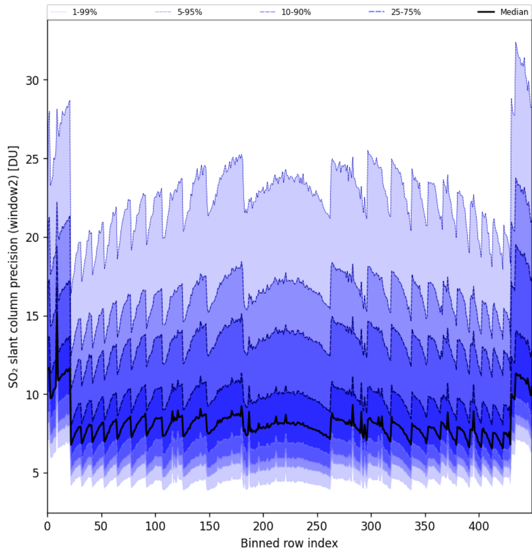
Figure 84: Along track statistics of “SO 2 slant column precision (window2)” for 2024-11-11 to 2024-11-13
