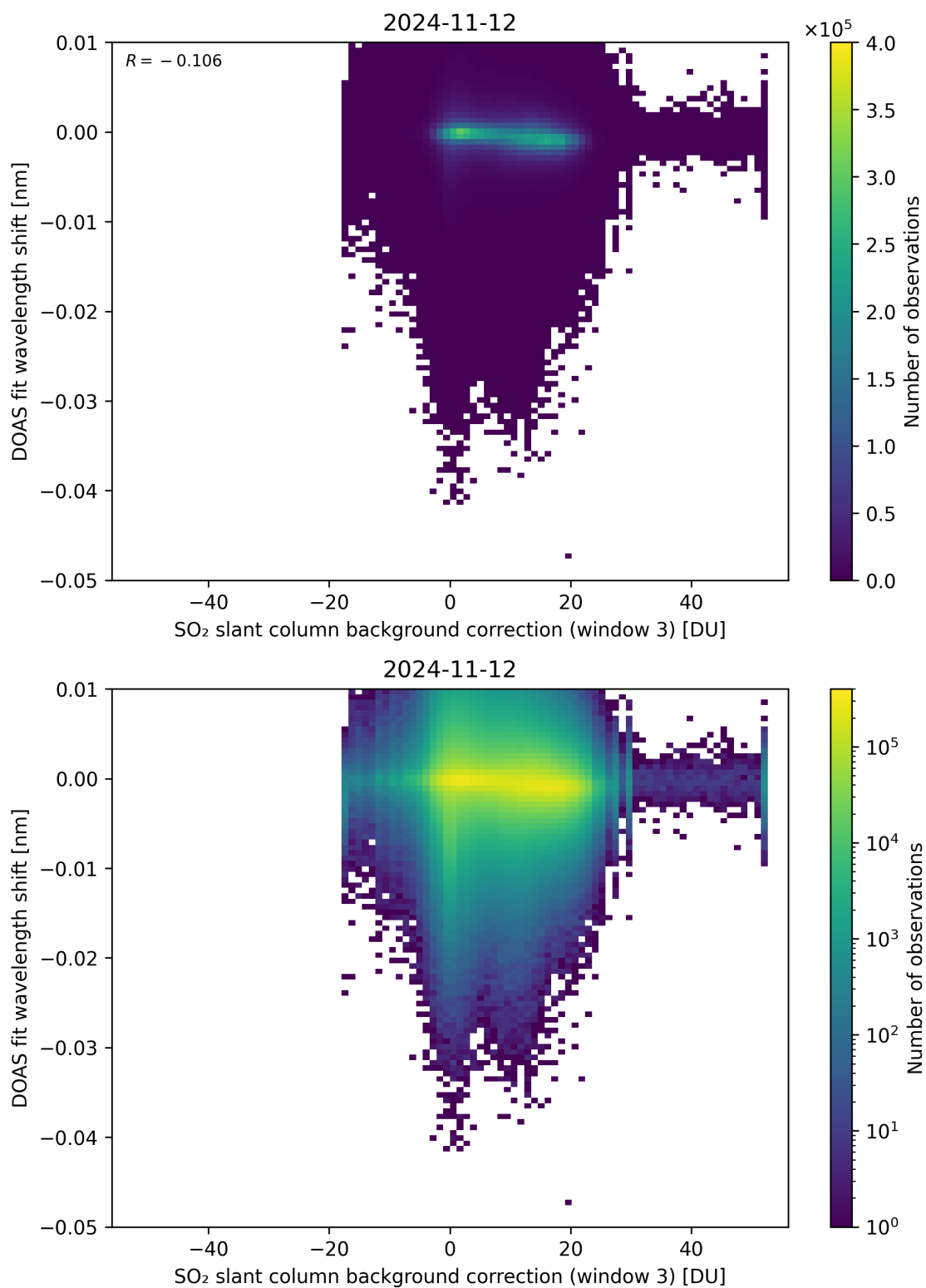
Figure 121: Scatter density plot of “SO 2 slant column background correction (window 3)” against “DOAS fit wavelength shift” for 2024-11-11 to 2024-11-13.
