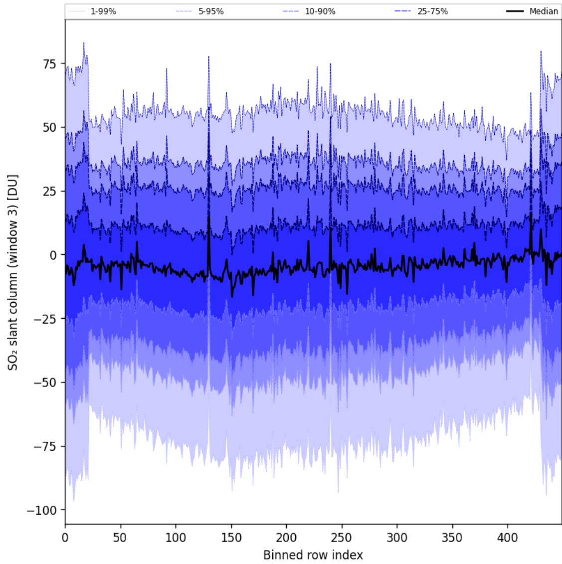
Figure 87: Along track statistics of “SO 2 slant column (window 3)” for 2024-11-11 to 2024-11-13
