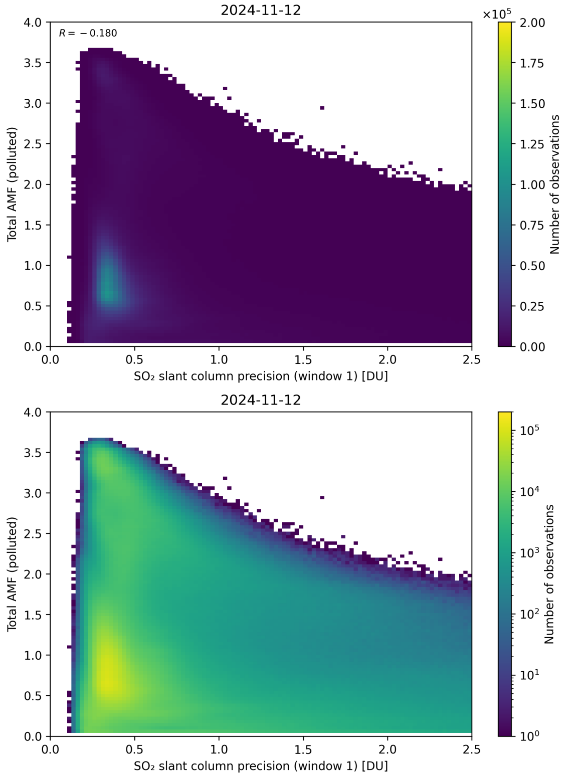
Figure 230: Scatter density plot of “SO 2 slant column precision (window 1)” against “Total AMF (polluted)” for 2024-11-11 to 2024-11-13.
