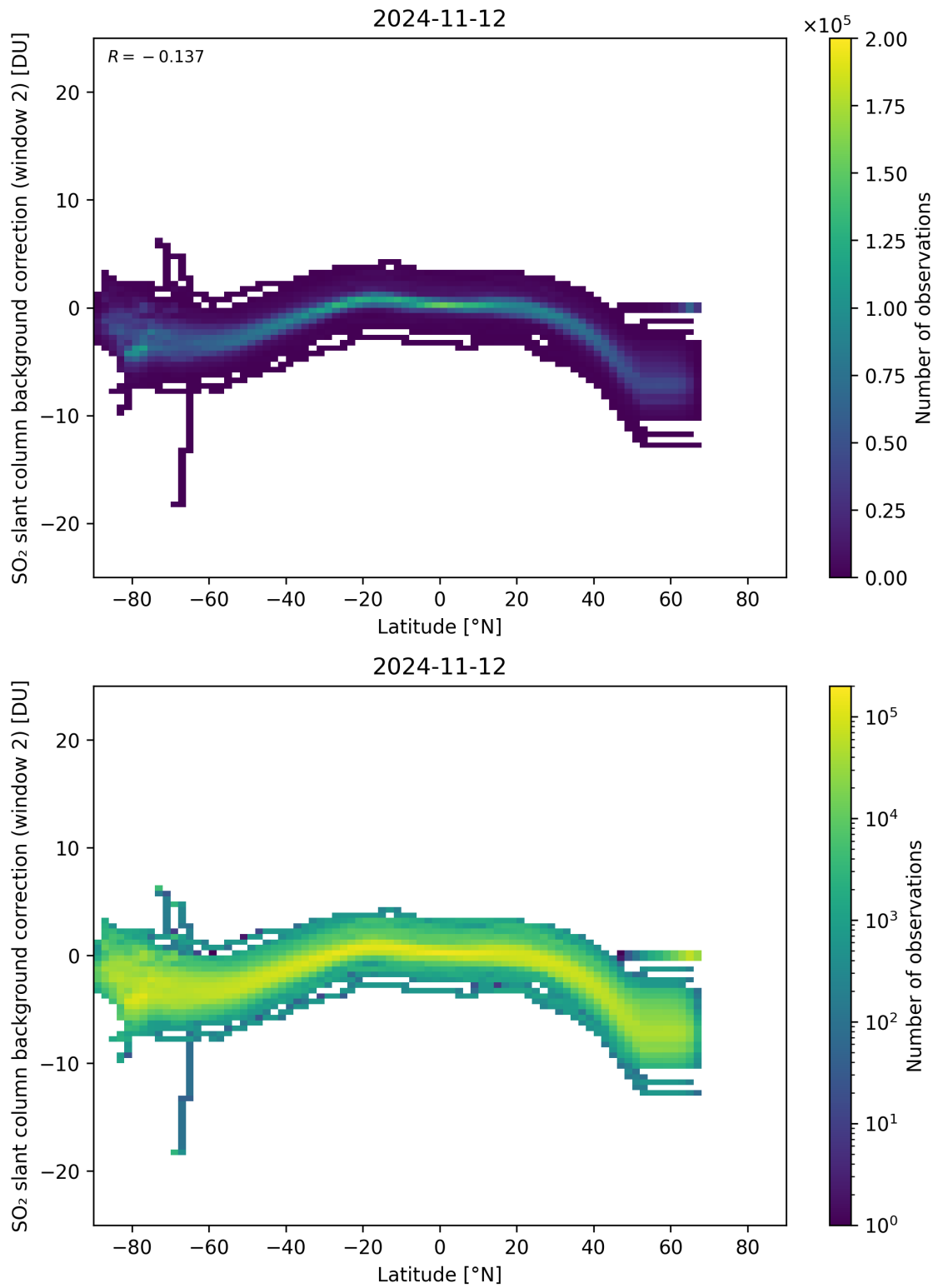
Figure 140: Scatter density plot of “Latitude” against “SO 2 slant column background correction (window 2)” for 2024-11-11 to 2024-11-13.
