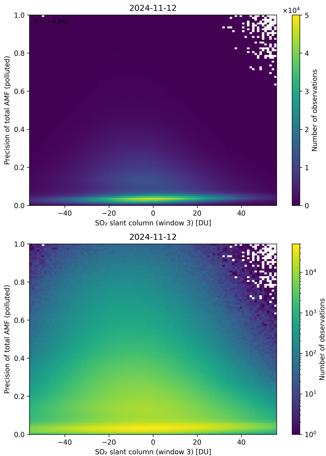
Figure 269: Scatter density plot of “SO 2 slant column (window 3)” against “Precision of total AMF (polluted)” for 2024-11-11 to 2024-11-13.
