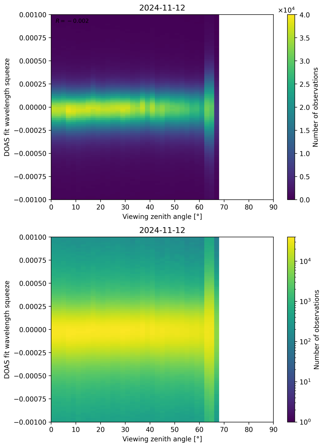
Figure 312: Scatter density plot of “Viewing zenith angle” against “DOAS fit wavelength squeeze” for 2024-11-11 to 2024-11-13.
