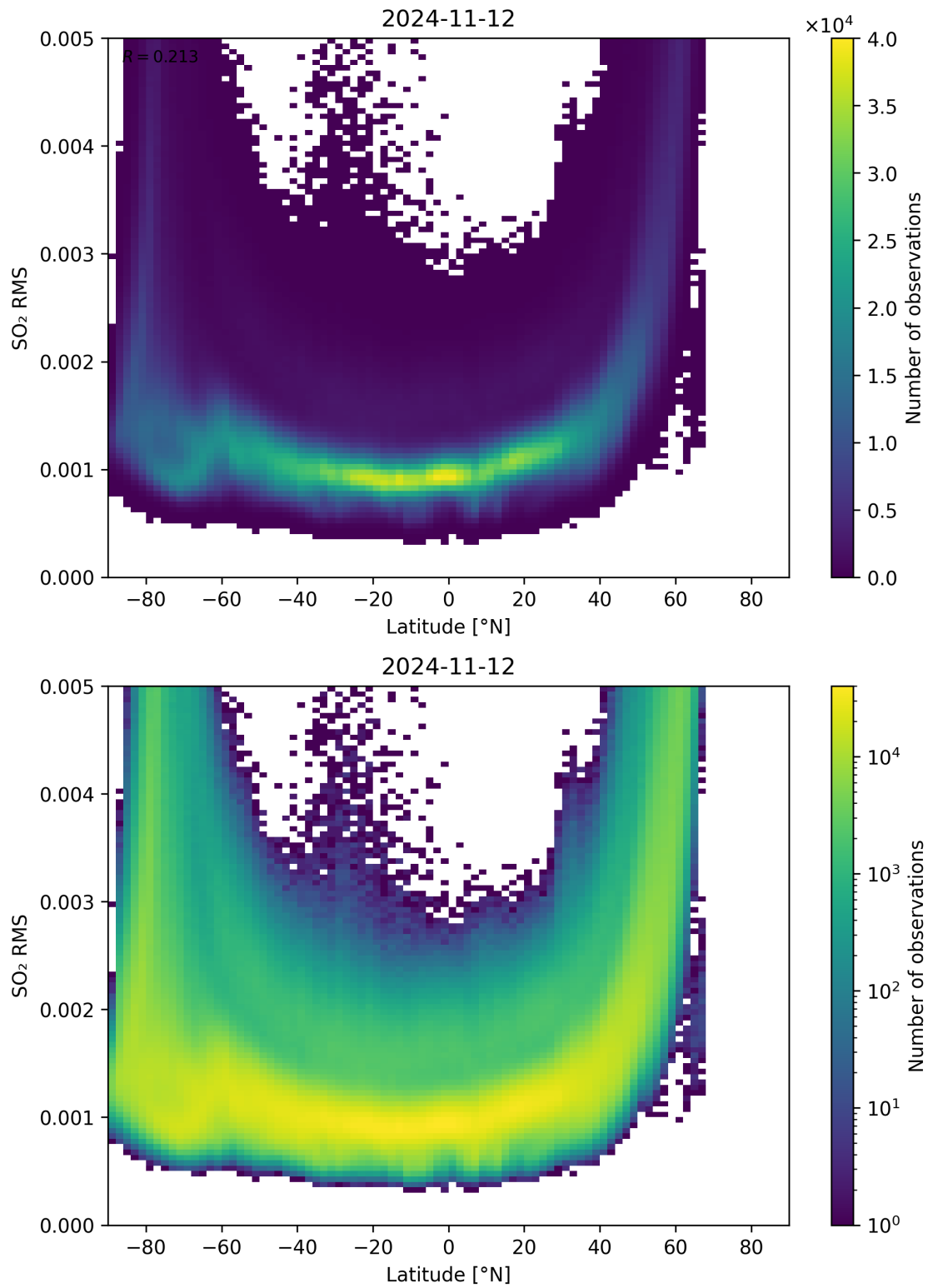
Figure 144: Scatter density plot of “Latitude” against “SO 2 RMS” for 2024-11-11 to 2024-11-13.
