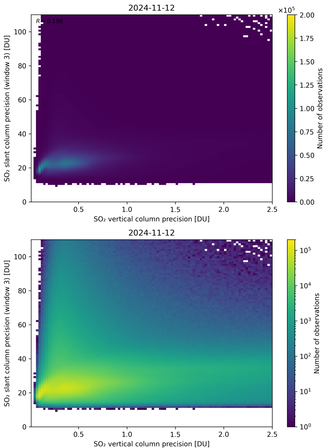
Figure 293: Scatter density plot of “SO 2 vertical column precision” against “SO 2 slant column precision (window 3)” for 2024-11-11 to 2024-11-13.
