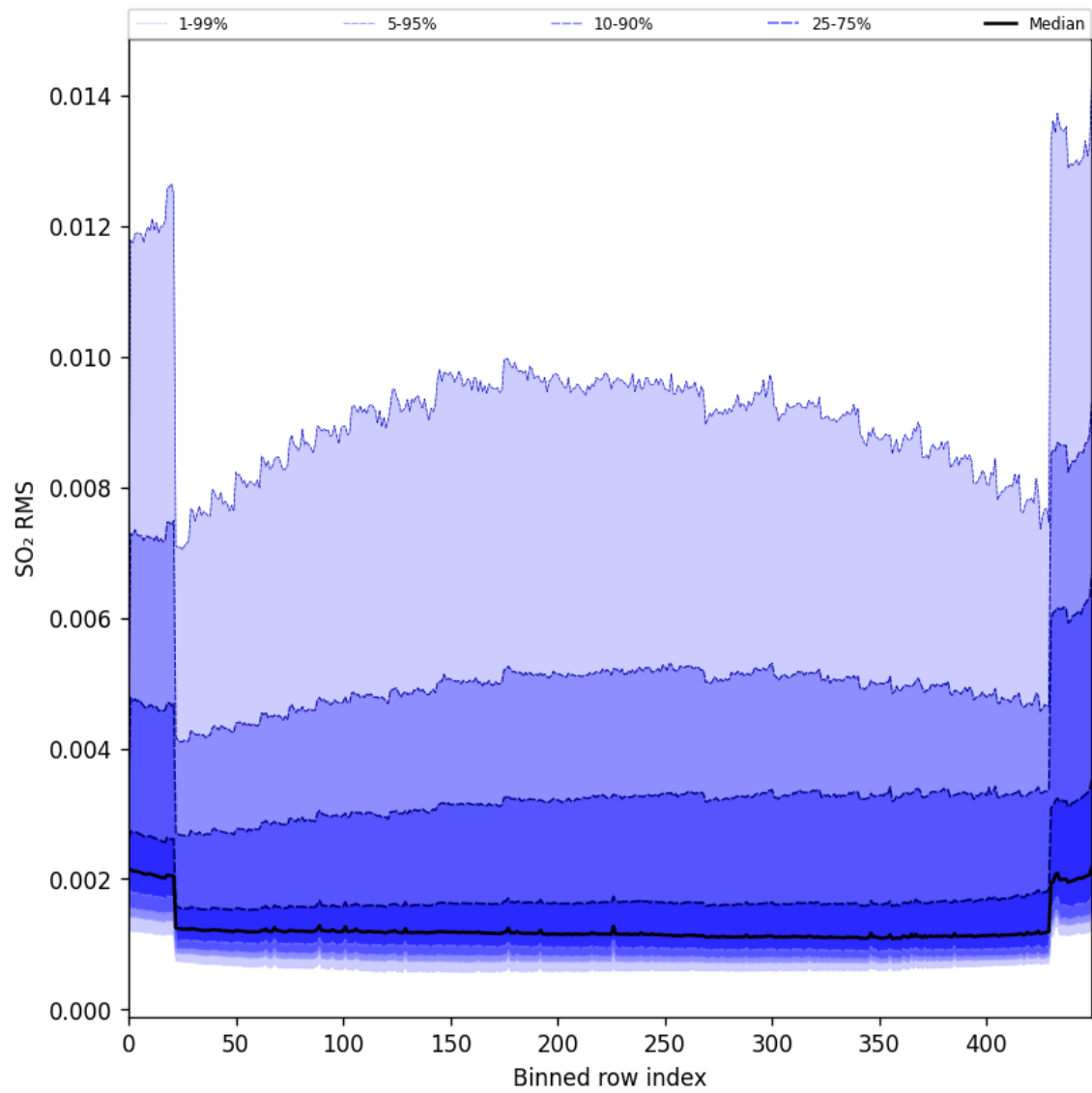
Figure 93: Along track statistics of “SO 2 RMS” for 2024-11-11 to 2024-11-13
