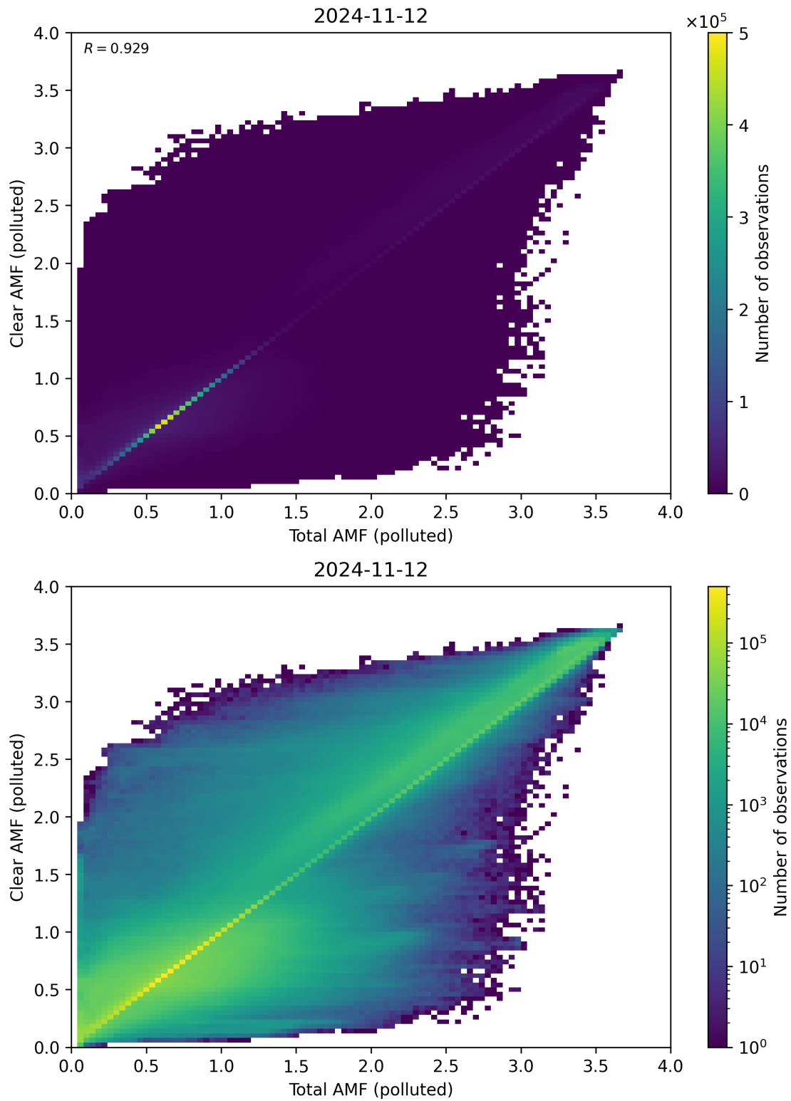
Figure 271: Scatter density plot of “Total AMF (polluted)” against “Clear AMF (polluted)” for 2024-11-11 to 2024-11-13.
