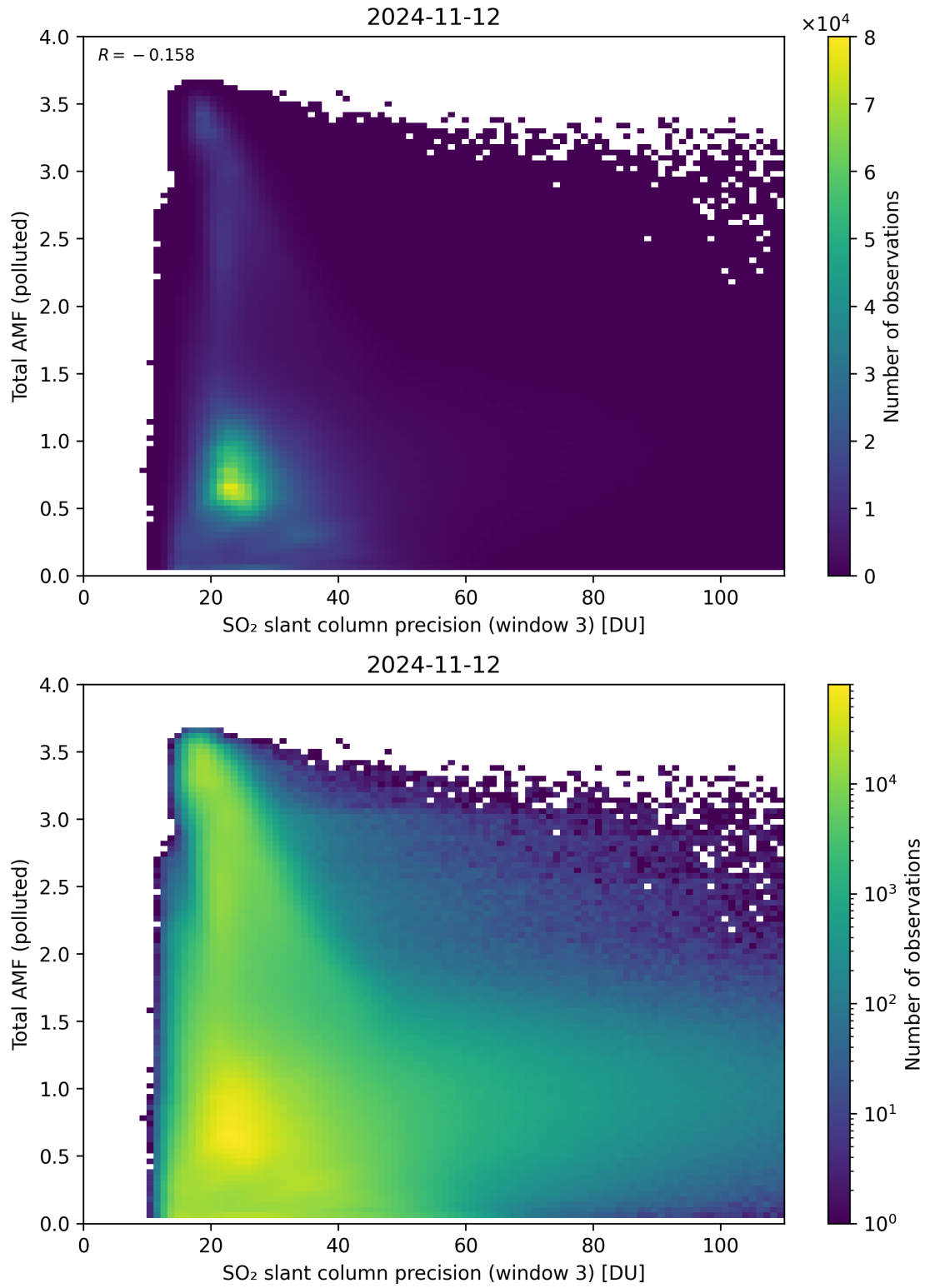
Figure 263: Scatter density plot of “SO 2 slant column precision (window 3)” against “Total AMF (polluted)” for 2024-11-11 to 2024-11-13.
