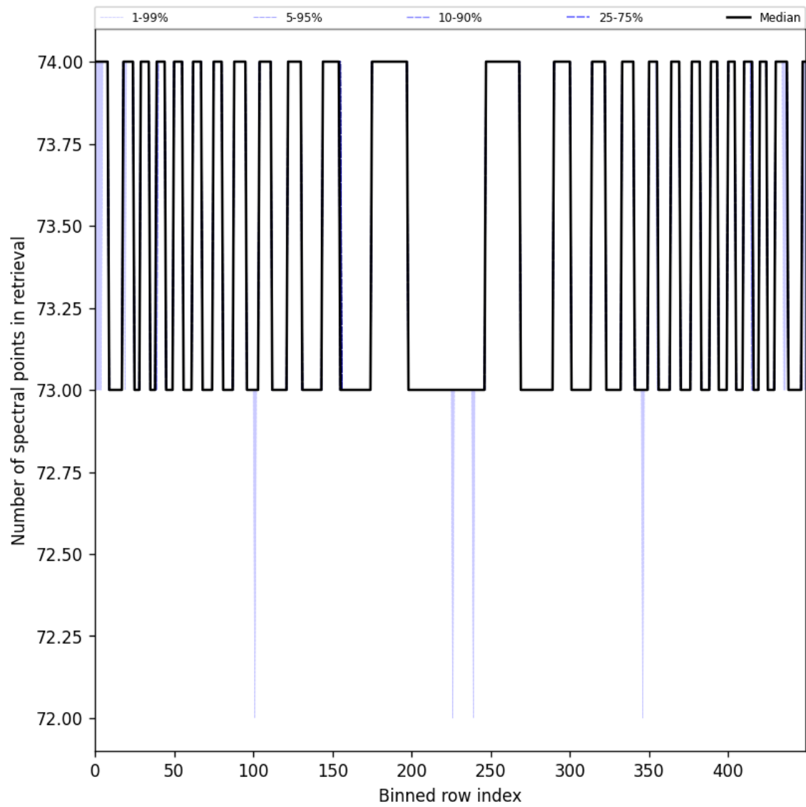
Figure 97: Along track statistics of “Number of spectral points in retrieval” for 2024-11-11 to 2024-11-13
