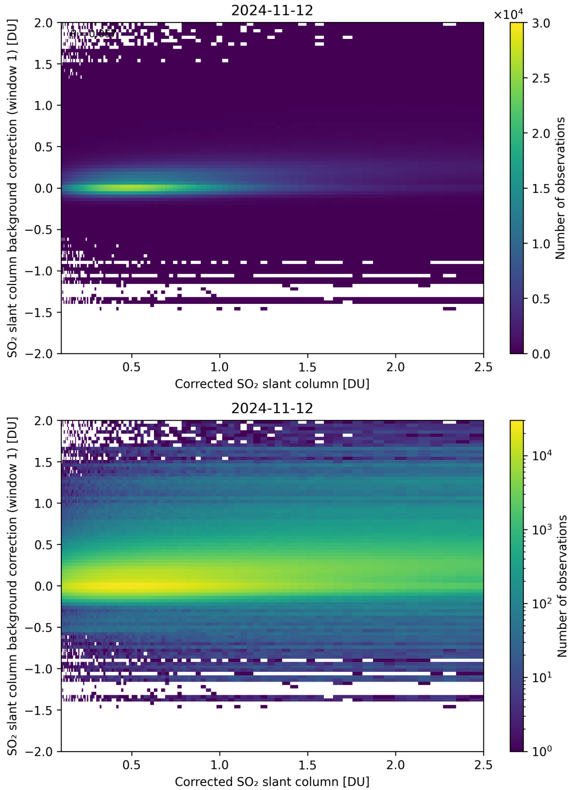
Figure 178: Scatter density plot of “Corrected SO 2 slant column” against “SO 2 slant column background correction (window 1)” for 2024-11-11 to 2024-11-13.
