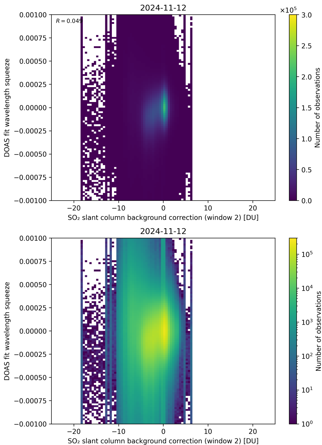
Figure 113: Scatter density plot of “SO 2 slant column background correction (window 2)” against “DOAS fit wavelength squeeze” for 2024-11-11 to 2024-11-13.
