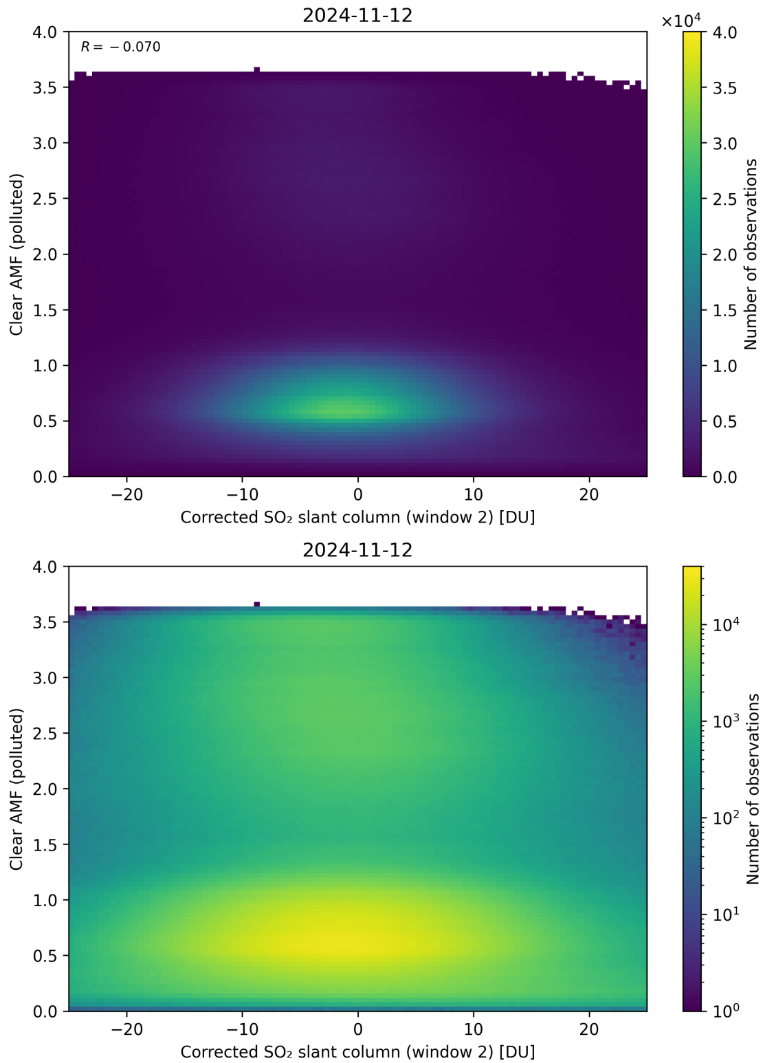
Figure 199: Scatter density plot of “Corrected SO 2 slant column (window 2)” against “Clear AMF (polluted)” for 2024-11-11 to 2024-11-13.
