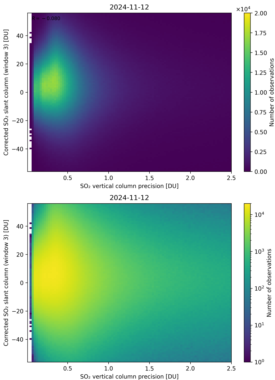
Figure 288: Scatter density plot of “SO 2 vertical column precision” against “Corrected SO 2 slant column (window 3)” for 2024-11-11 to 2024-11-13.
