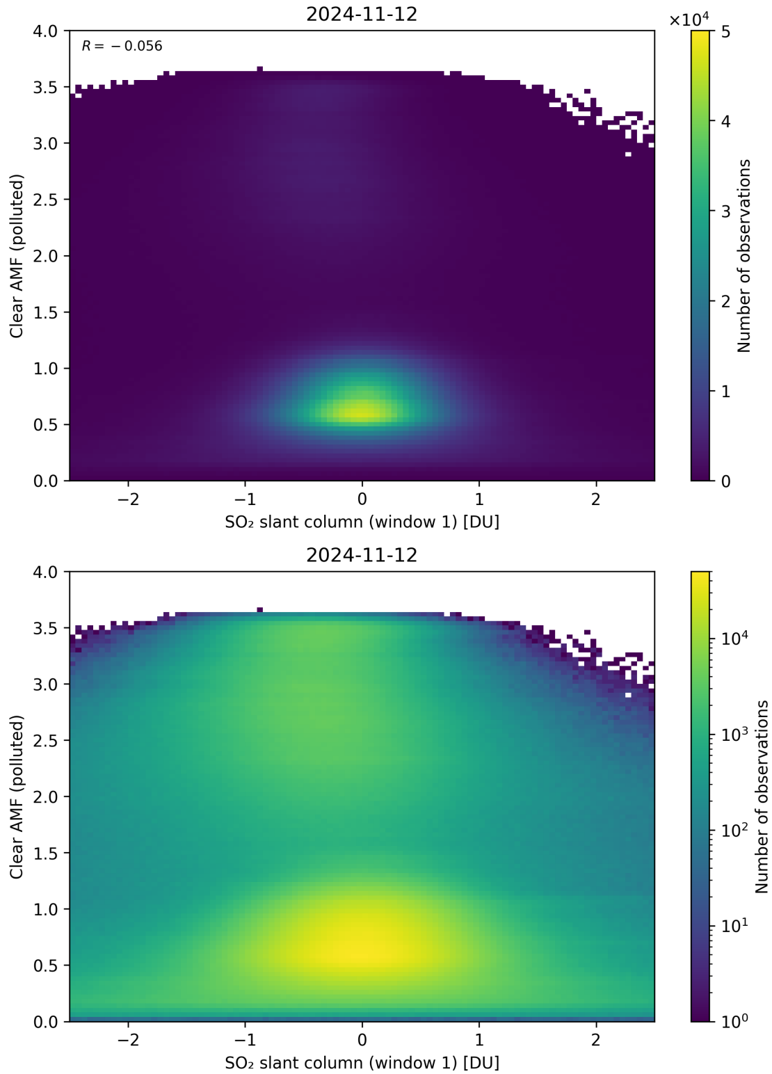
Figure 232: Scatter density plot of “SO 2 slant column (window 1)” against “Clear AMF (polluted)” for 2024-11-11 to 2024-11-13.
