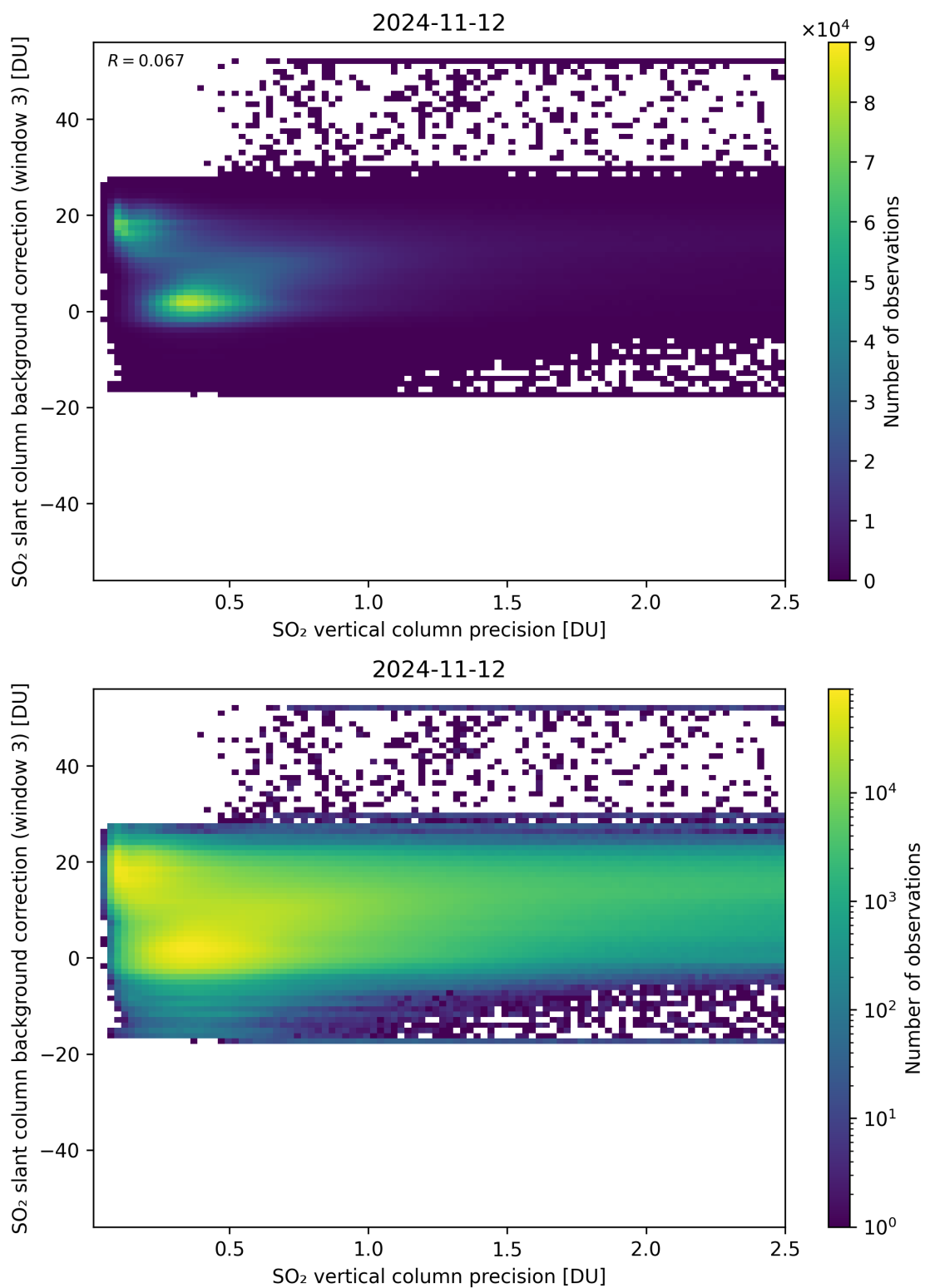
Figure 281: Scatter density plot of “SO 2 vertical column precision” against “SO 2 slant column background correction (window 3)” for 2024-11-11 to 2024-11-13.
