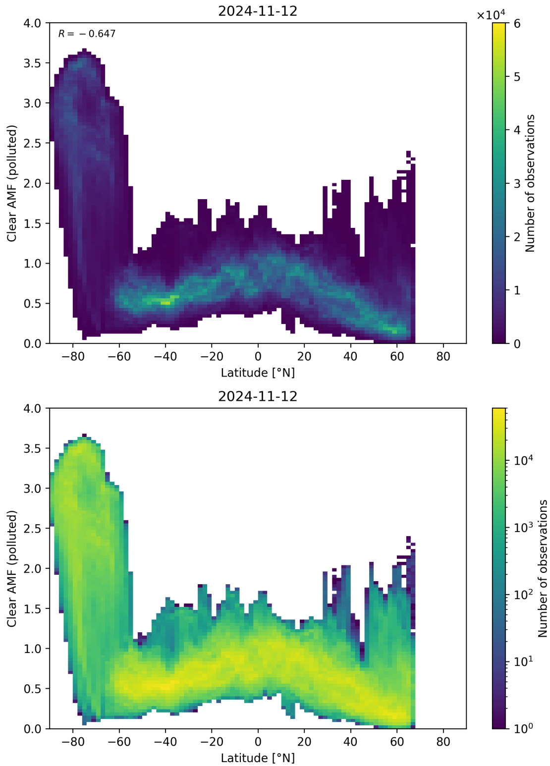
Figure 145: Scatter density plot of “Latitude” against “Clear AMF (polluted)” for 2024-11-11 to 2024-11-13.
