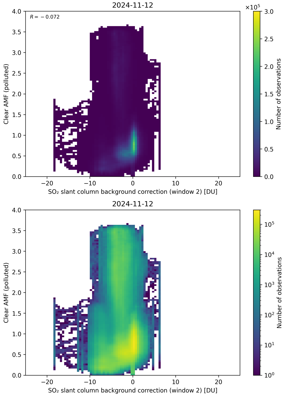
Figure 115: Scatter density plot of “SO 2 slant column background correction (window 2)” against “Clear AMF (polluted)” for 2024-11-11 to 2024-11-13.
