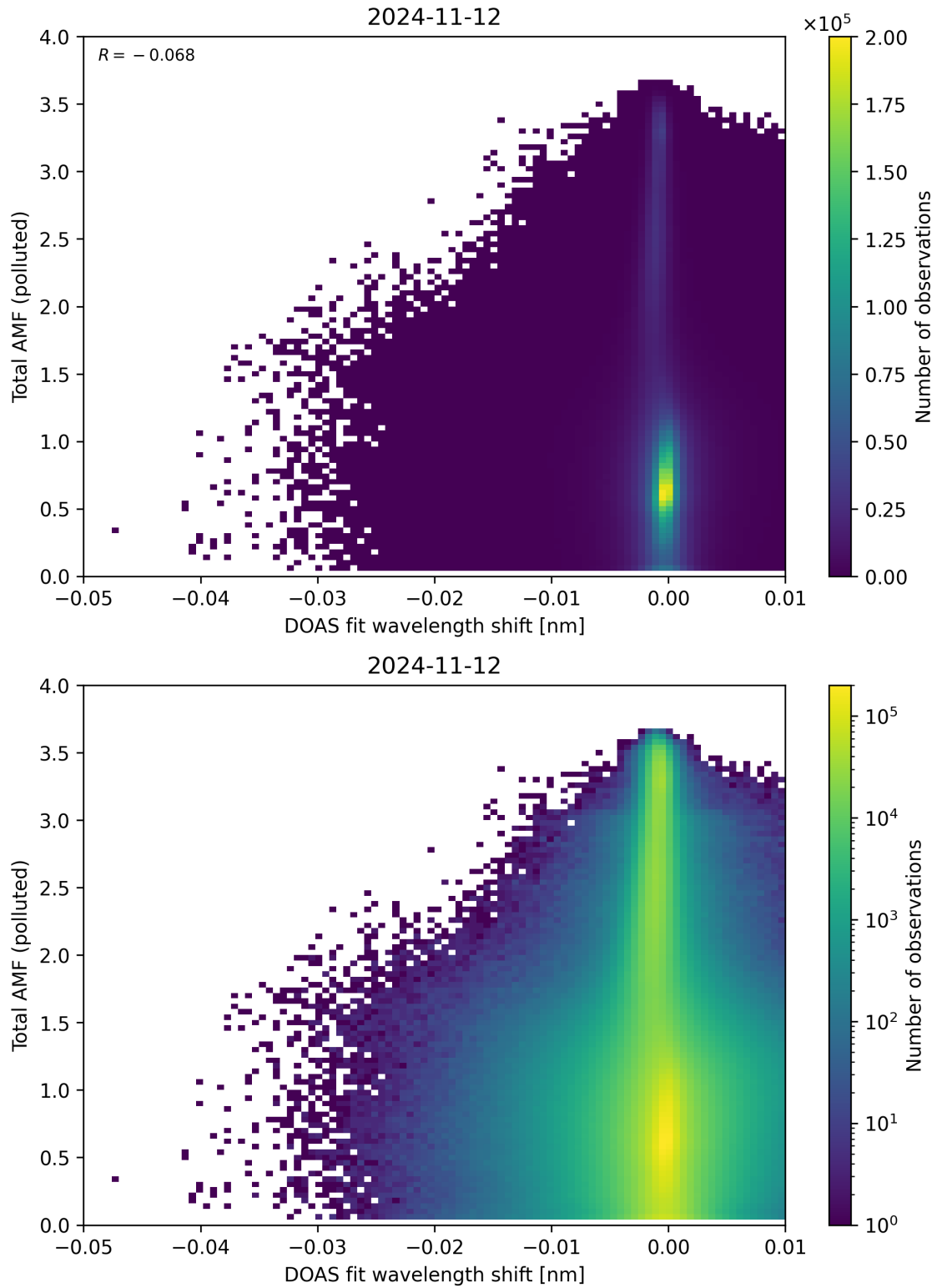
Figure 130: Scatter density plot of “DOAS fit wavelength shift” against “Total AMF (polluted)” for 2024-11-11 to 2024-11-13.
