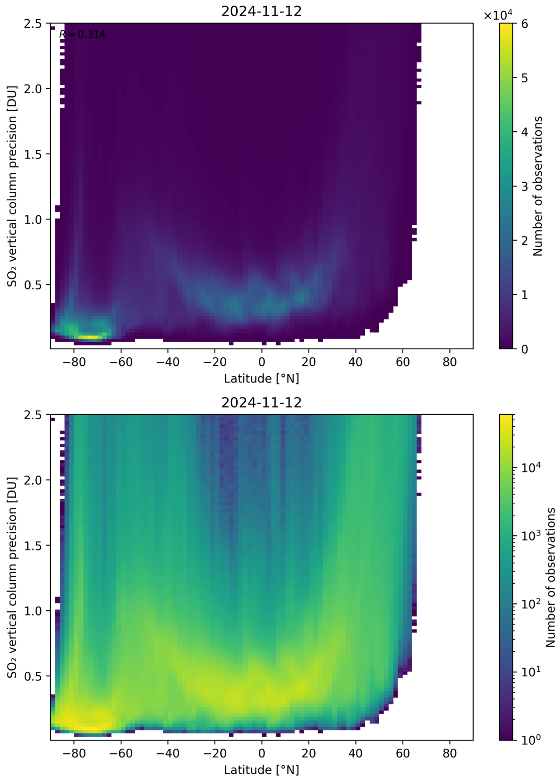
Figure 157: Scatter density plot of “Latitude” against “SO 2 vertical column precision” for 2024-11-11 to 2024-11-13.
