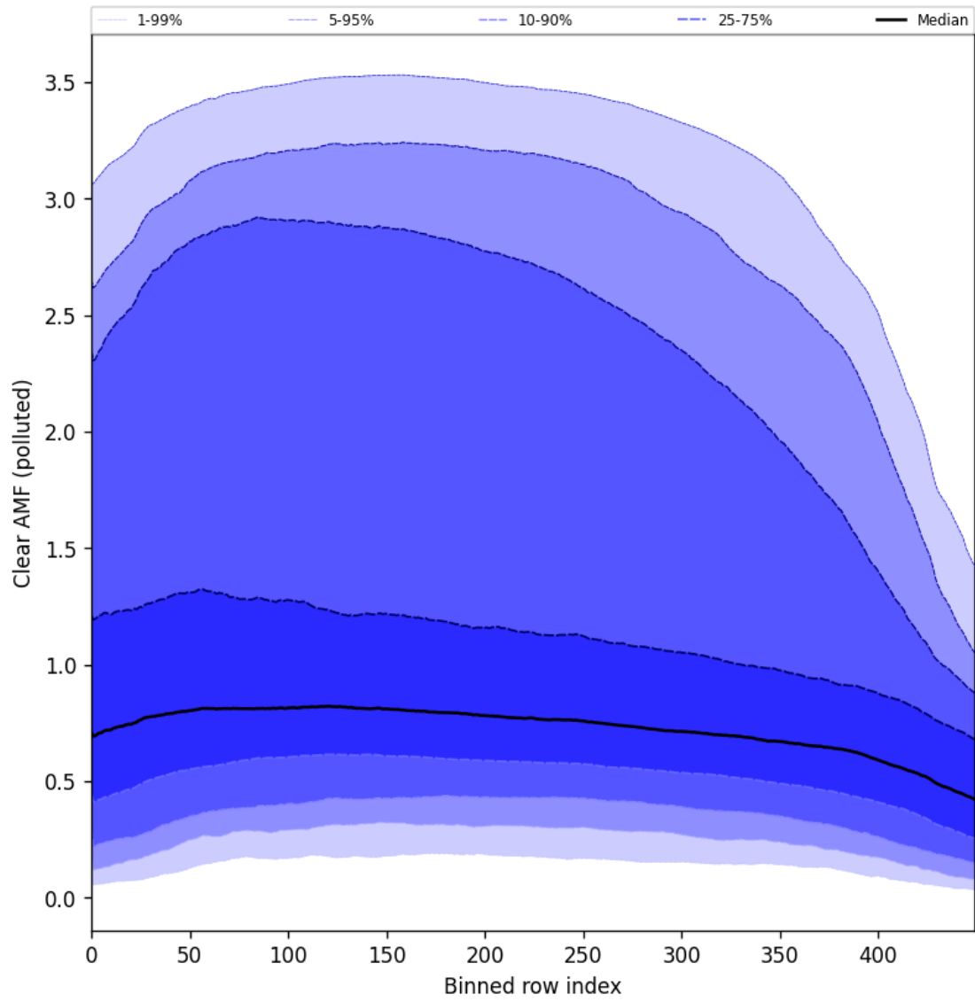
Figure 96: Along track statistics of “Clear AMF (polluted)” for 2024-11-11 to 2024-11-13
