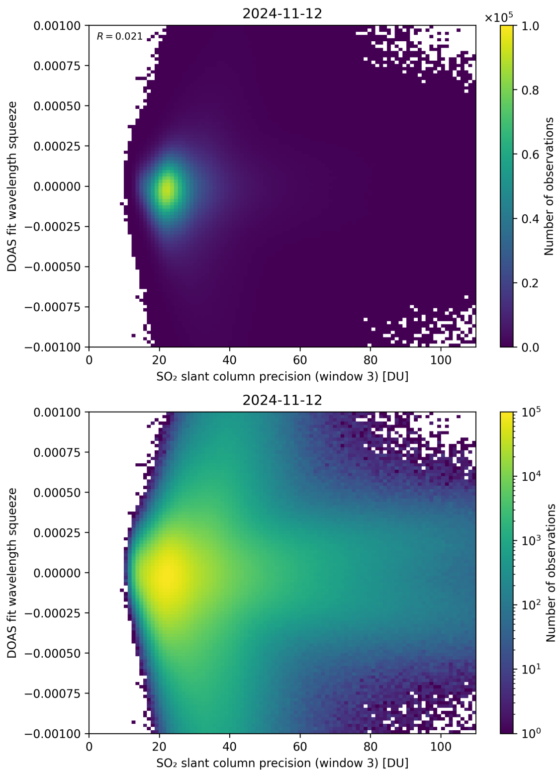
Figure 259: Scatter density plot of “SO 2 slant column precision (window 3)” against “DOAS fit wavelength squeeze” for 2024-11-11 to 2024-11-13.
