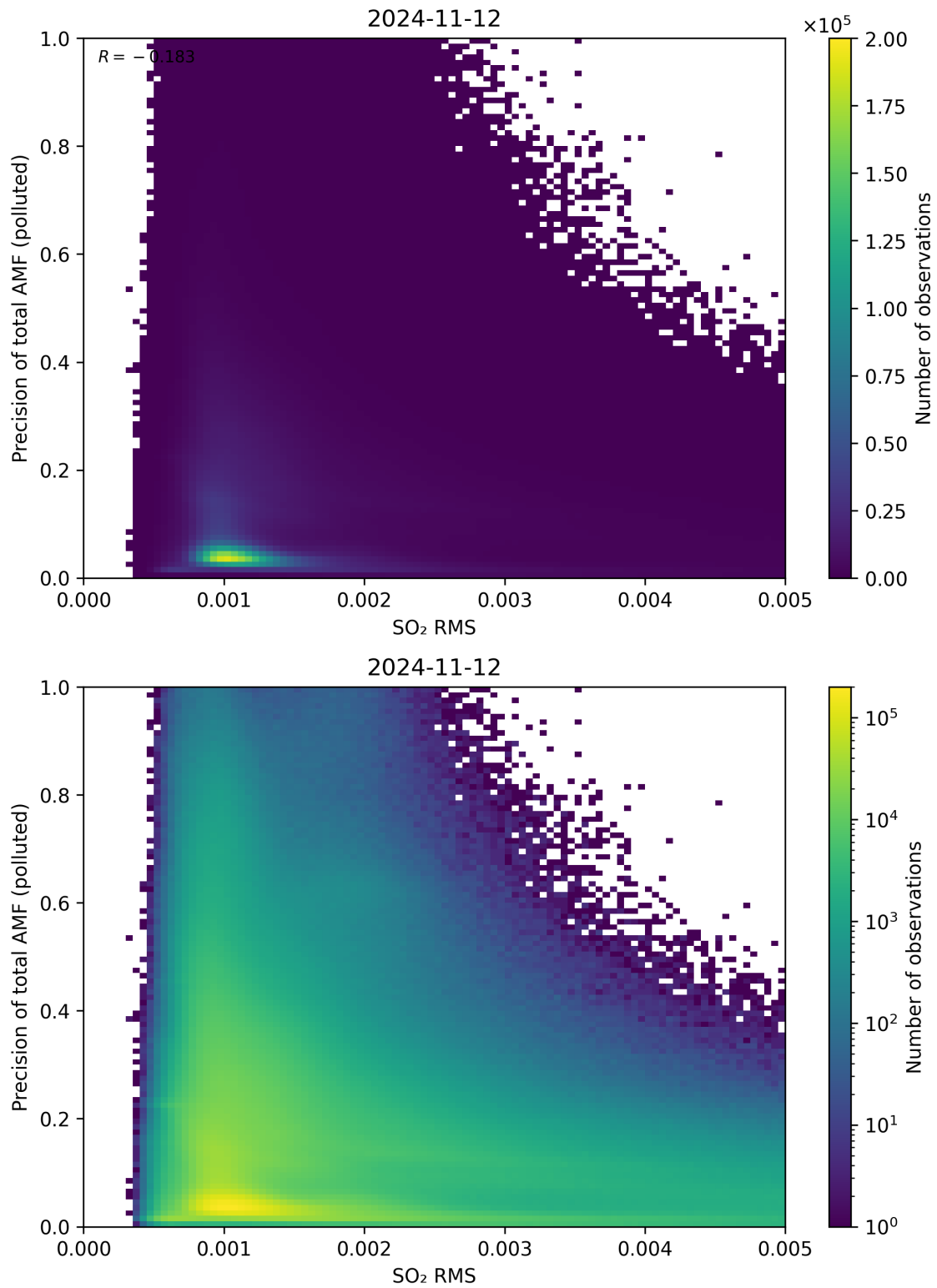
Figure 138: Scatter density plot of “SO 2 RMS” against “Precision of total AMF (polluted)” for 2024-11-11 to 2024-11-13.
