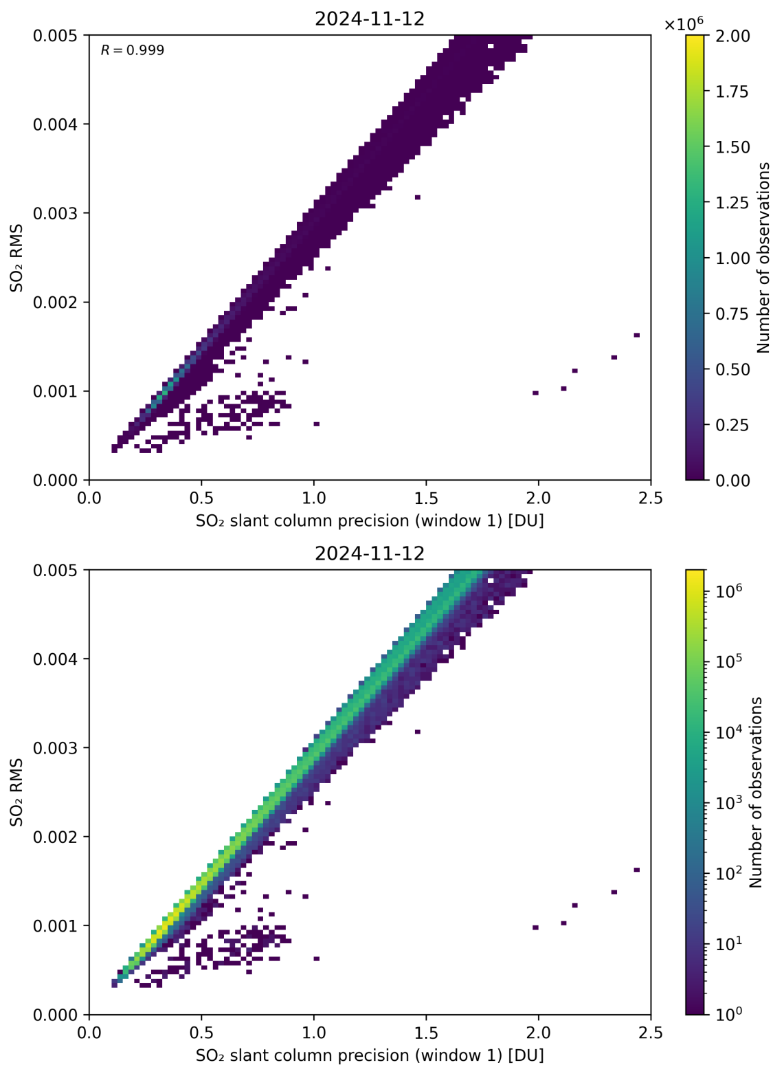
Figure 223: Scatter density plot of “SO 2 slant column precision (window 1)” against “SO 2 RMS” for 2024-11-11 to 2024-11-13.
