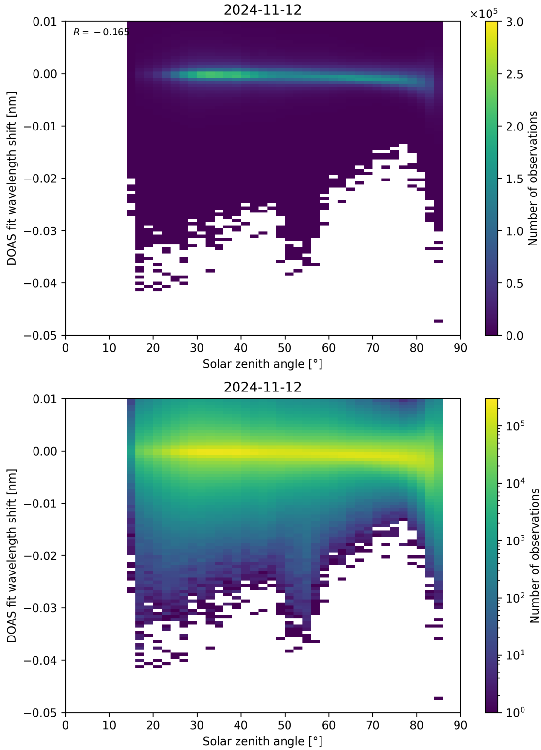
Figure 161: Scatter density plot of “Solar zenith angle” against “DOAS fit wavelength shift” for 2024-11-11 to 2024-11-13.
