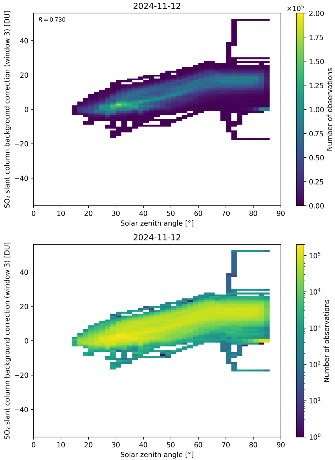
Figure 160: Scatter density plot of “Solar zenith angle” against “SO 2 slant column background correction (window 3)” for 2024-11-11 to 2024-11-13.
