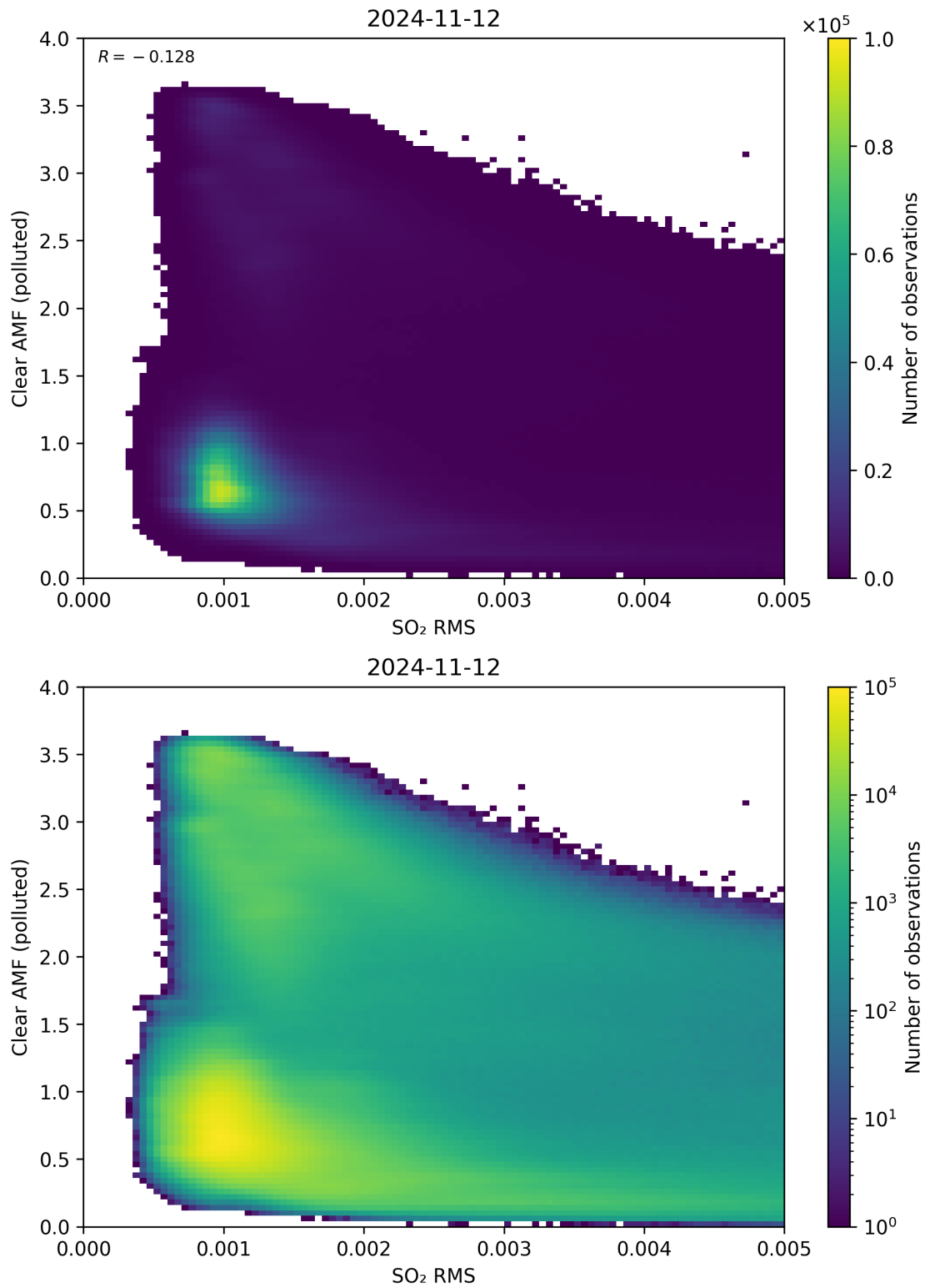
Figure 136: Scatter density plot of “SO 2 RMS” against “Clear AMF (polluted)” for 2024-11-11 to 2024-11-13.
