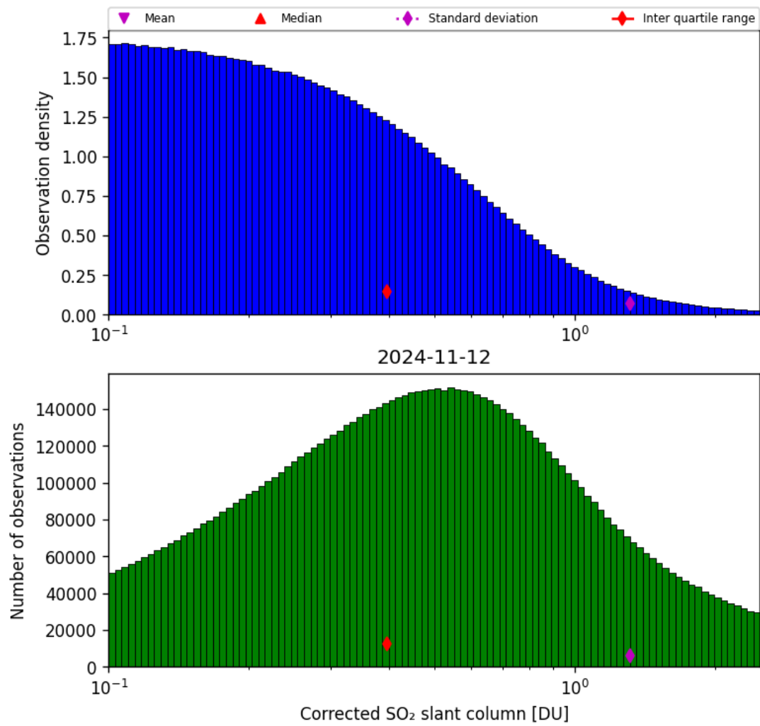
Figure 55: Histogram of “Corrected SO 2 slant column” for 2024-11-11 to 2024-11-13
