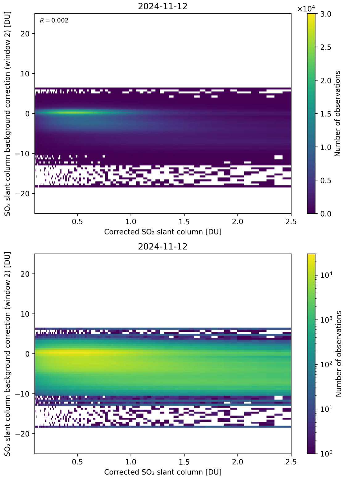
Figure 179: Scatter density plot of “Corrected SO 2 slant column” against “SO 2 slant column background correction (window 2)” for 2024-11-11 to 2024-11-13.
