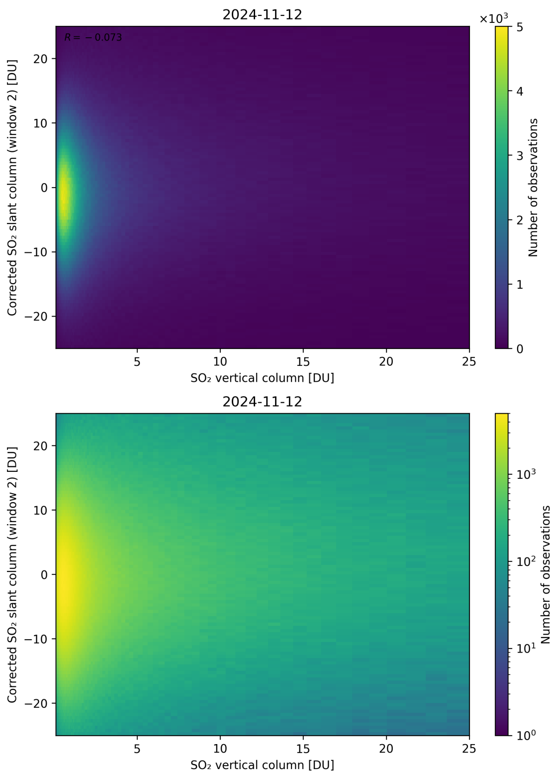
Figure 298: Scatter density plot of “SO 2 vertical column” against “Corrected SO 2 slant column (window 2)” for 2024-11-11 to 2024-11-13.
