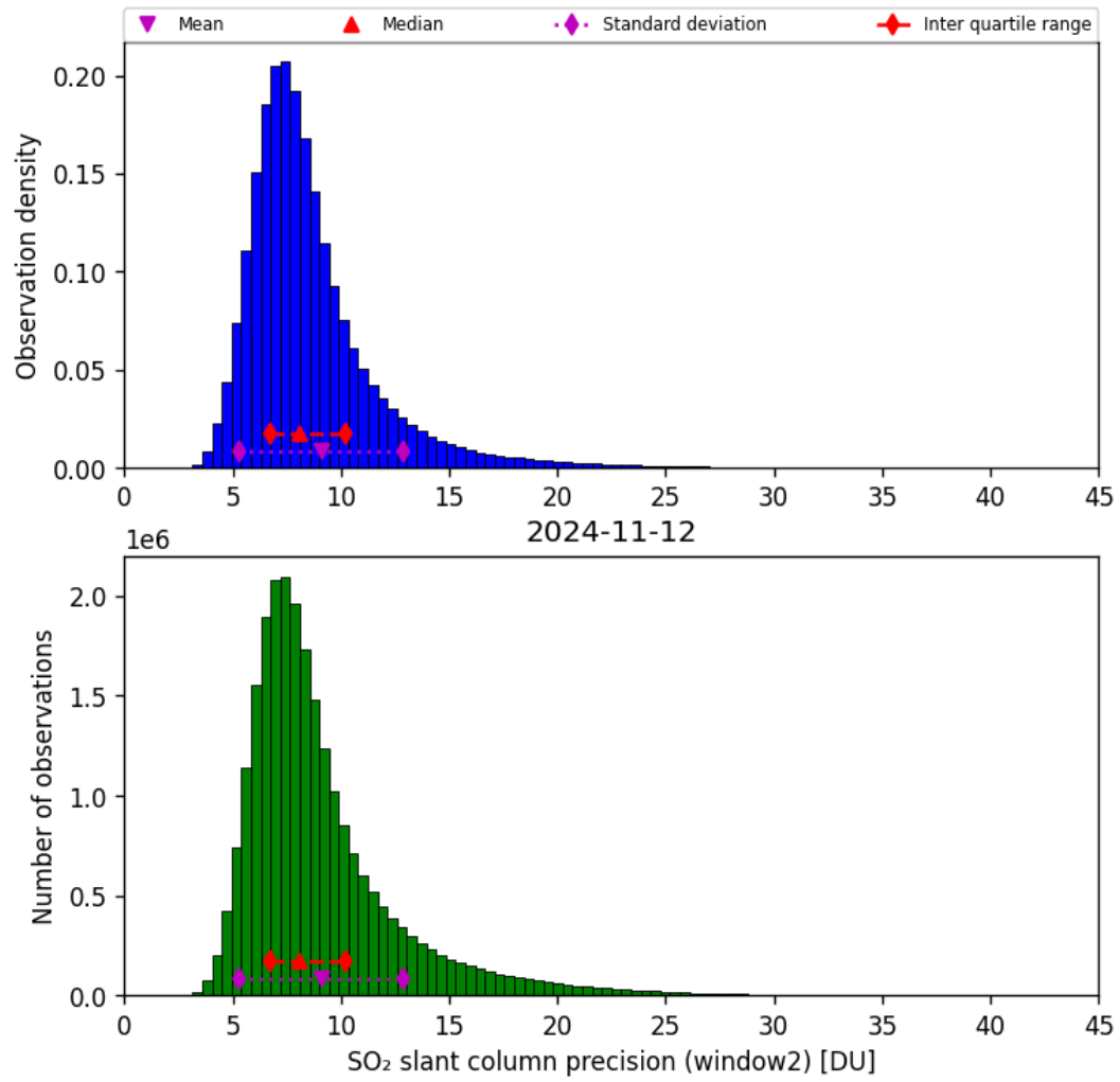
Figure 61: Histogram of “SO 2 slant column precision (window2)” for 2024-11-11 to 2024-11-13
