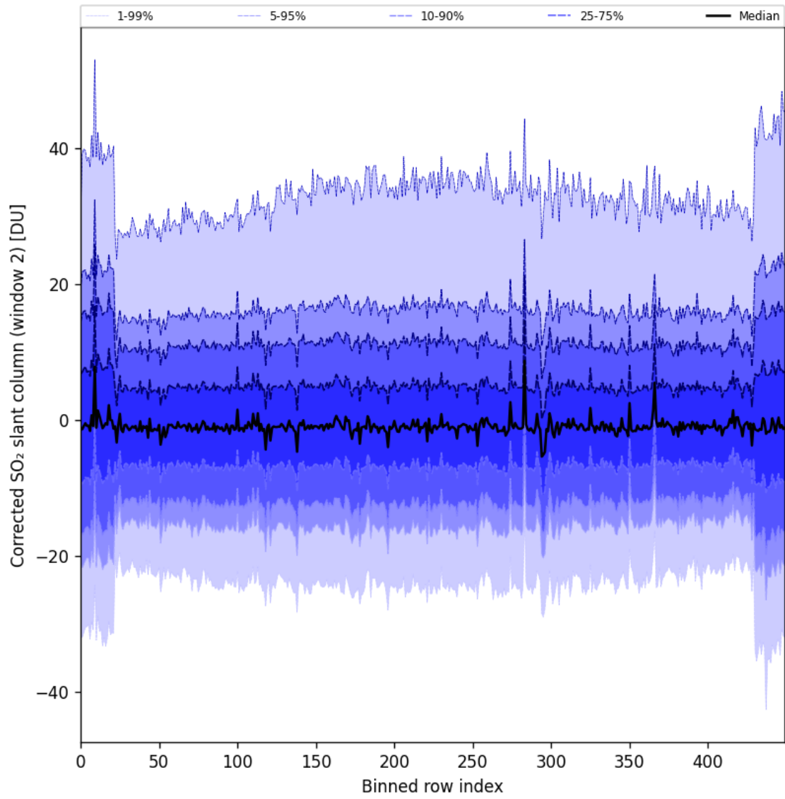
Figure 85: Along track statistics of “Corrected SO 2 slant column (window 2)” for 2024-11-11 to 2024-11-13
