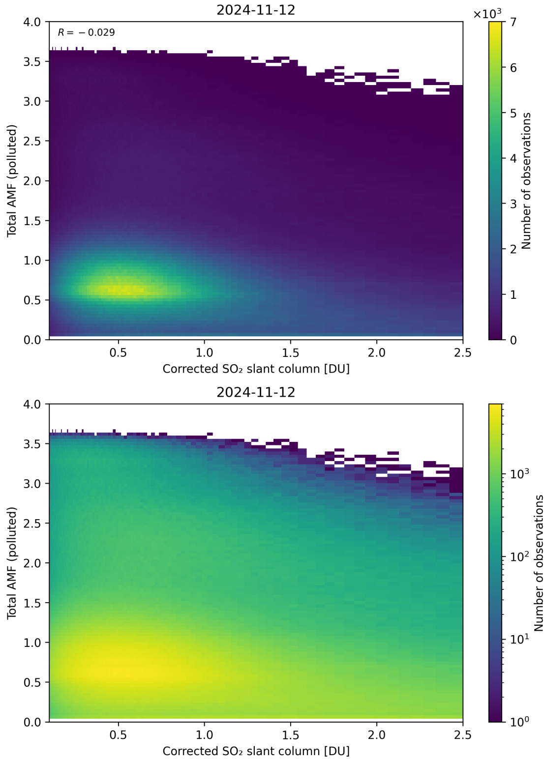
Figure 192: Scatter density plot of “Corrected SO 2 slant column” against “Total AMF (polluted)” for 2024-11-11 to 2024-11-13.
