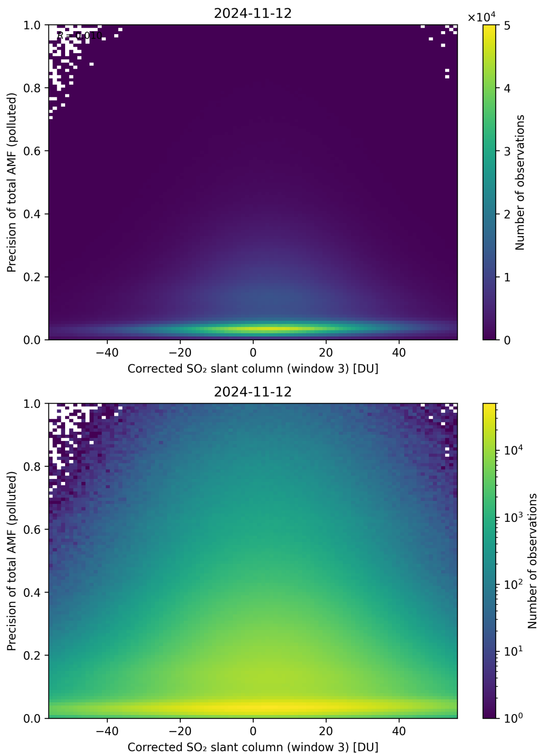
Figure 211: Scatter density plot of “Corrected SO 2 slant column (window 3)” against “Precision of total AMF (polluted)” for 2024-11-11 to 2024-11-13.
