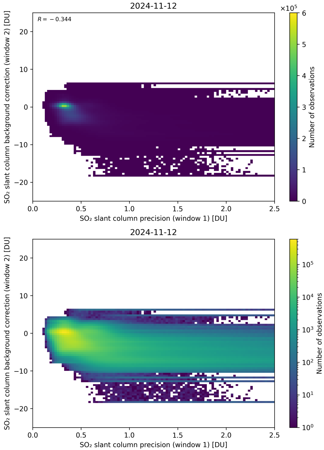
Figure 219: Scatter density plot of “SO 2 slant column precision (window 1)” against “SO 2 slant column background correction (window 2)” for 2024-11-11 to 2024-11-13.
