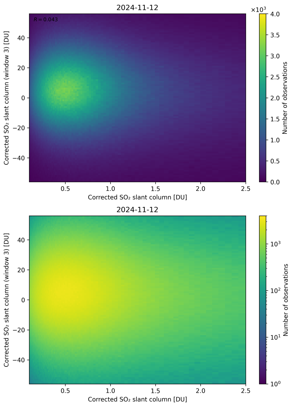
Figure 186: Scatter density plot of “Corrected SO 2 slant column” against “Corrected SO 2 slant column (window 3)” for 2024-11-11 to 2024-11-13.
