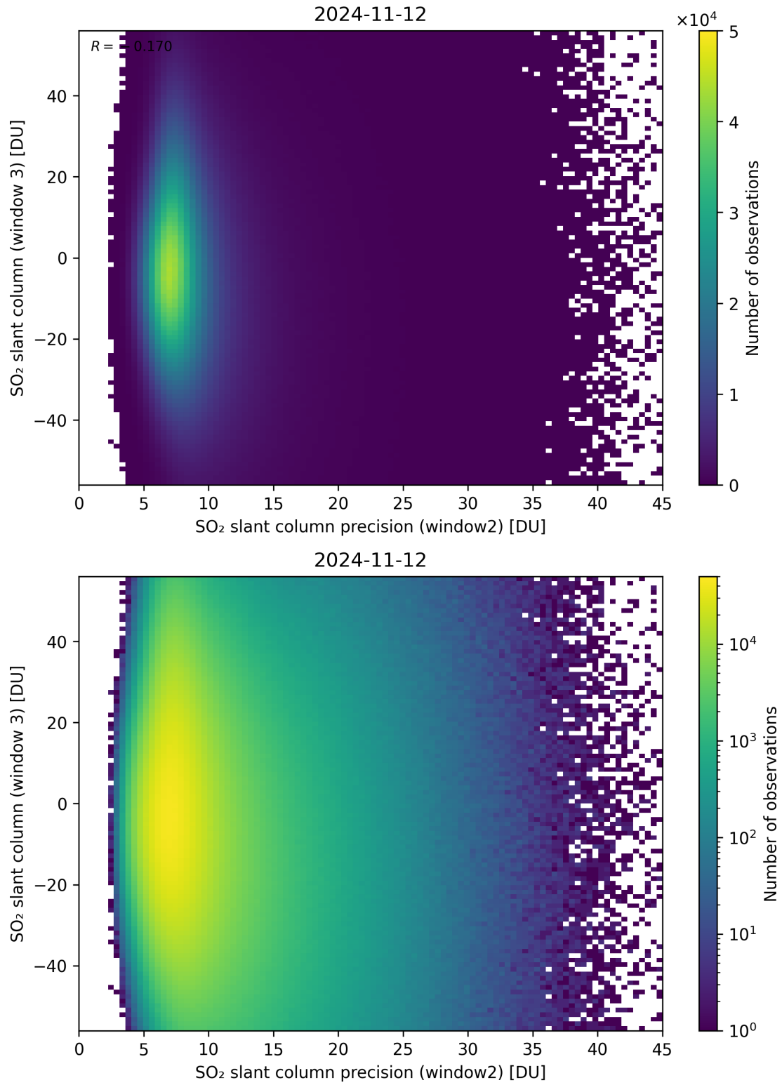
Figure 249: Scatter density plot of “SO 2 slant column precision (window2)” against “SO 2 slant column (window 3)” for 2024-11-11 to 2024-11-13.
