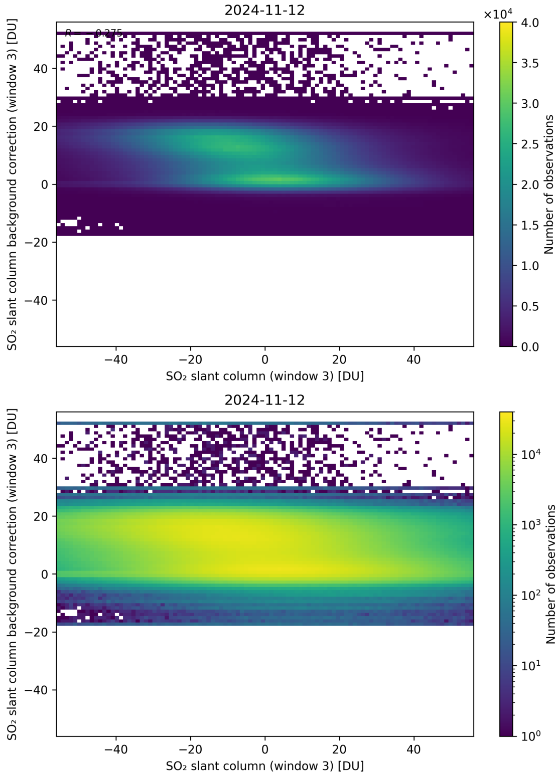
Figure 253: Scatter density plot of “SO 2 slant column (window 3)” against “SO 2 slant column background correction (window 3)” for 2024-11-11 to 2024-11-13.
