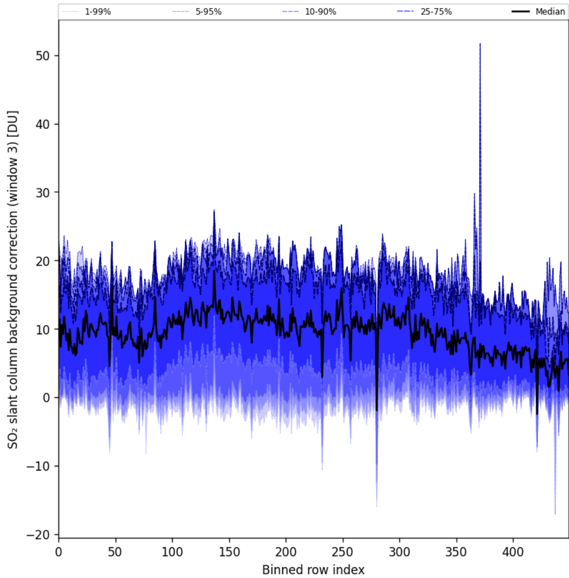
Figure 90: Along track statistics of “SO 2 slant column background correction (window 3)” for 2024-11-11 to 2024-11-13
