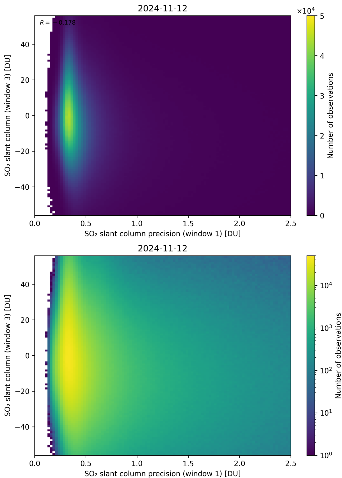
Figure 228: Scatter density plot of “SO 2 slant column precision (window 1)” against “SO 2 slant column (window 3)” for 2024-11-11 to 2024-11-13.
