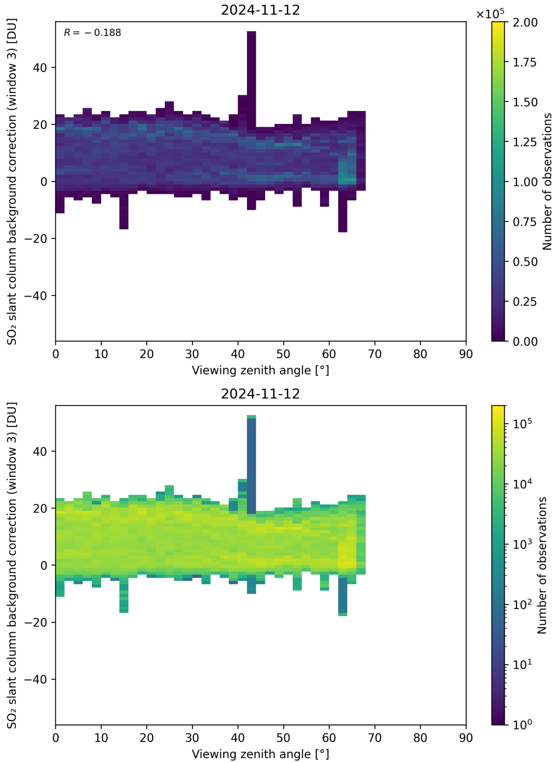
Figure 310: Scatter density plot of “Viewing zenith angle” against “SO 2 slant column background correction (window 3)” for 2024-11-11 to 2024-11-13.
