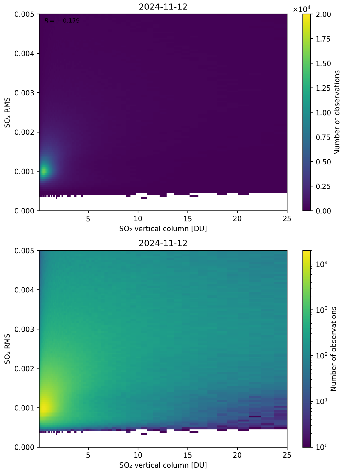
Figure 278: Scatter density plot of “SO 2 vertical column” against “SO 2 RMS” for 2024-11-11 to 2024-11-13.
