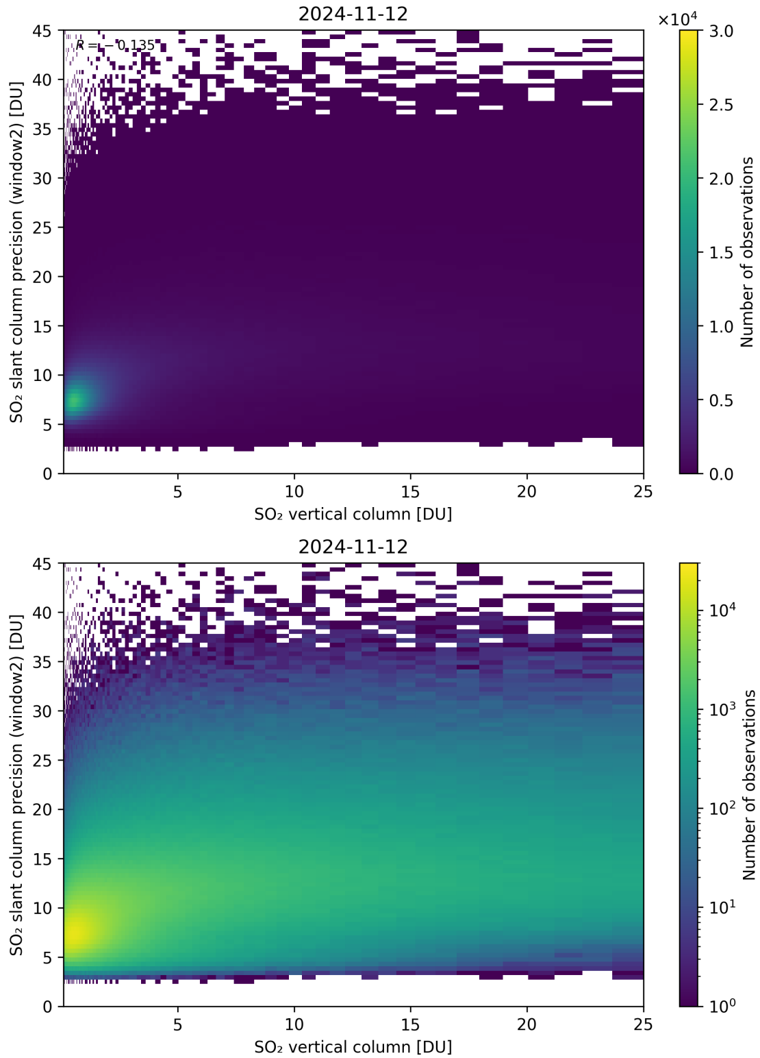
Figure 302: Scatter density plot of “SO 2 vertical column” against “SO 2 slant column precision (window2)” for 2024-11-11 to 2024-11-13.
