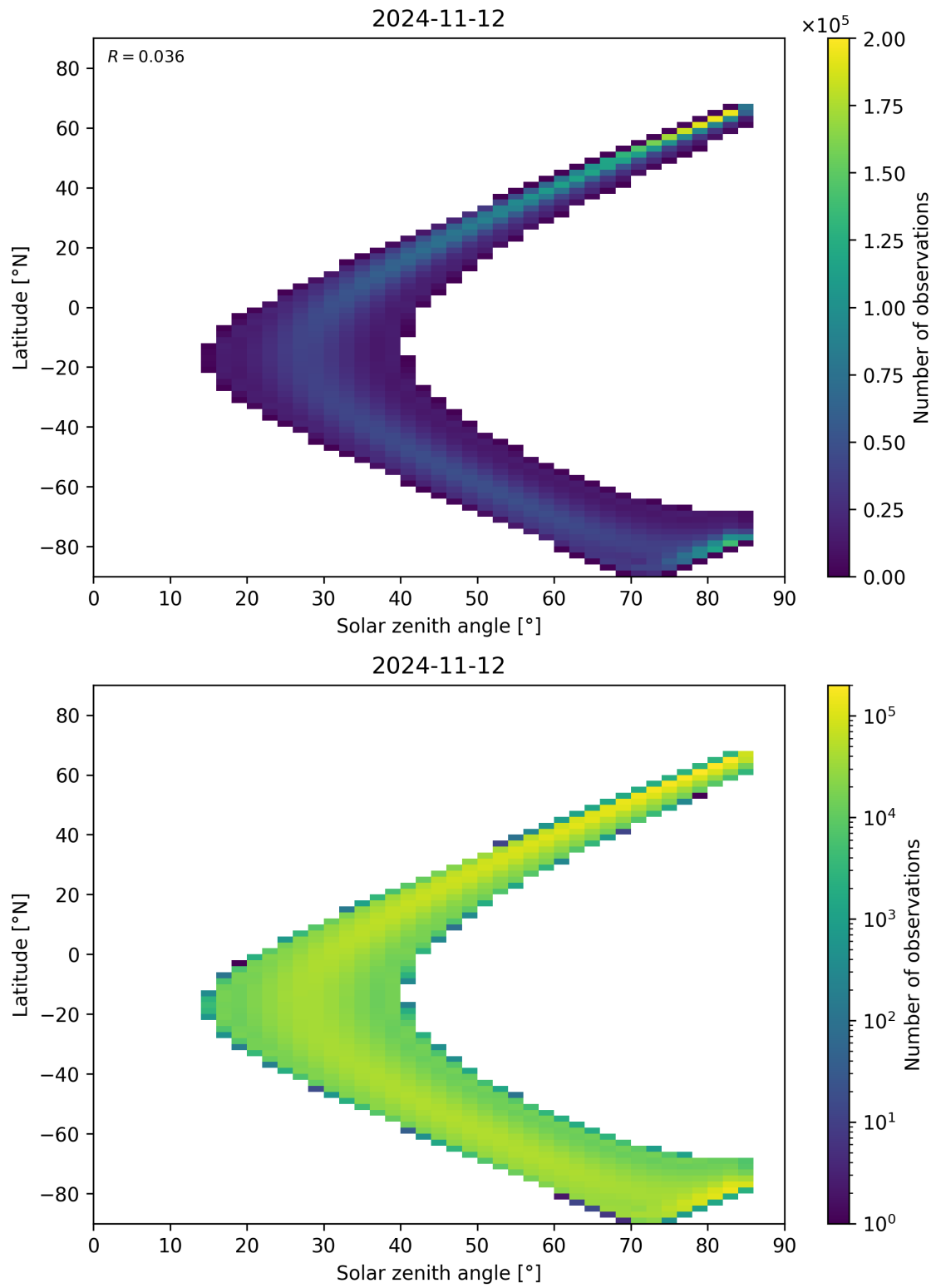
Figure 164: Scatter density plot of “Solar zenith angle” against “Latitude” for 2024-11-11 to 2024-11-13.
