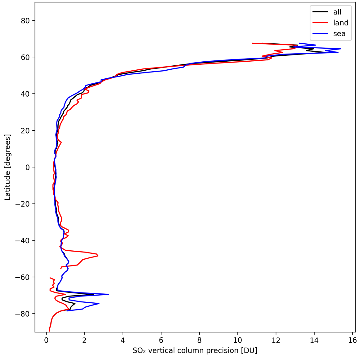
Figure 31: Zonal average of “SO 2 vertical column precision” for 2024-11-11 to 2024-11-13.
