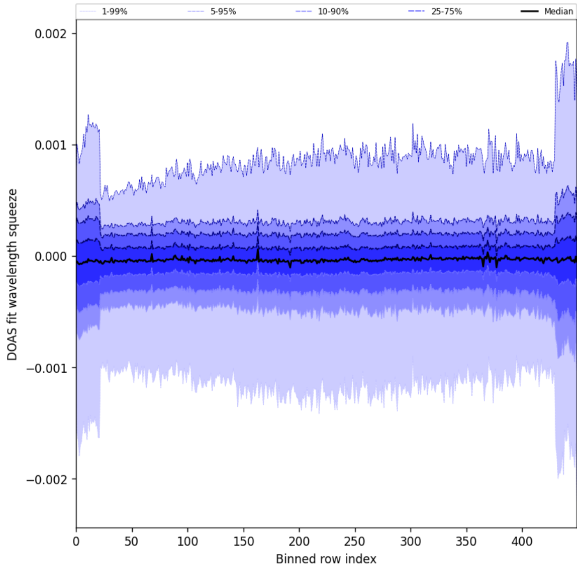
Figure 92: Along track statistics of “DOAS fit wavelength squeeze” for 2024-11-11 to 2024-11-13
