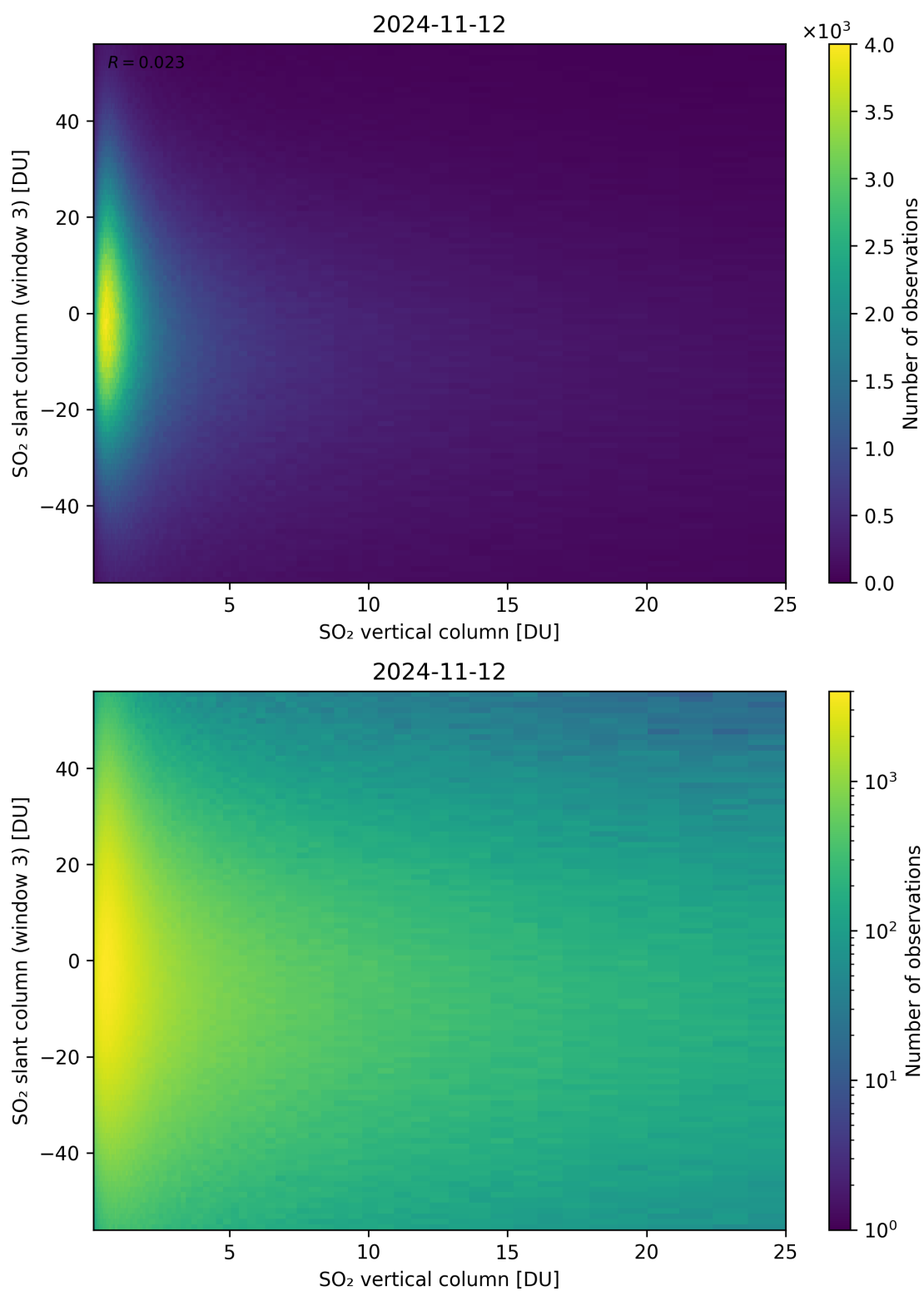
Figure 303: Scatter density plot of “SO 2 vertical column” against “SO 2 slant column (window 3)” for 2024-11-11 to 2024-11-13.
