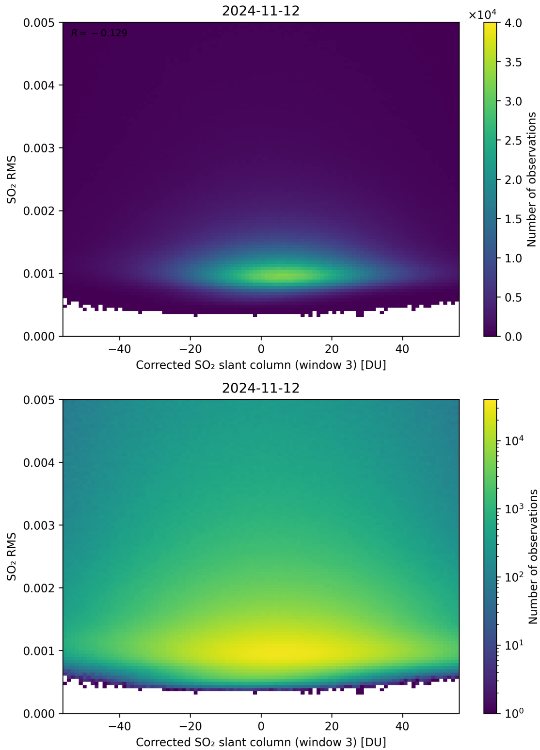
Figure 208: Scatter density plot of “Corrected SO 2 slant column (window 3)” against “SO 2 RMS” for 2024-11-11 to 2024-11-13.
