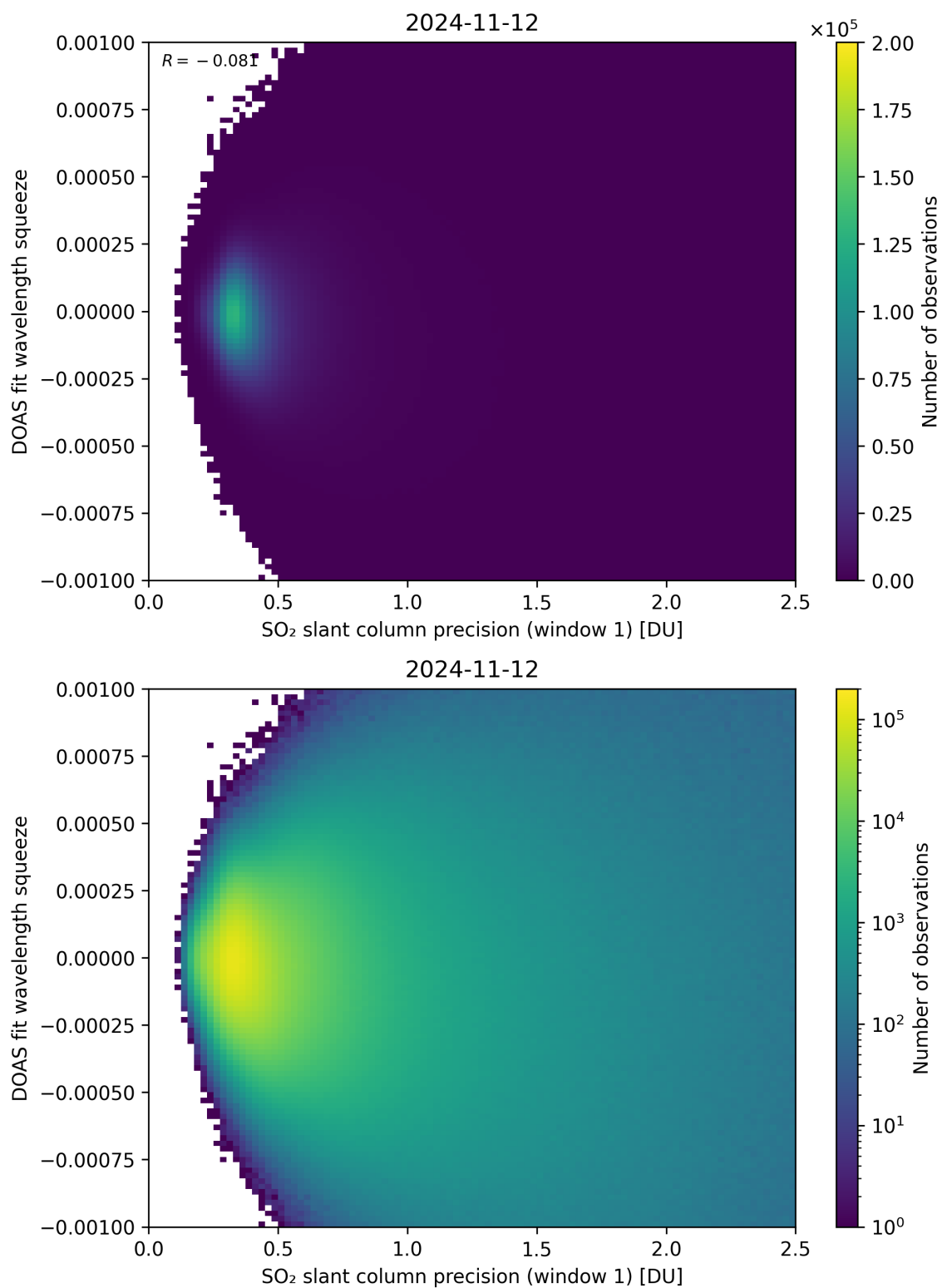
Figure 222: Scatter density plot of “SO 2 slant column precision (window 1)” against “DOAS fit wavelength squeeze” for 2024-11-11 to 2024-11-13.
