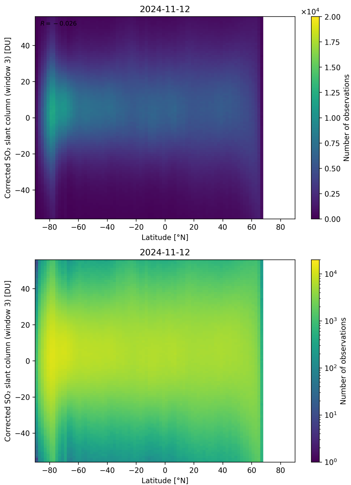
Figure 148: Scatter density plot of “Latitude” against “Corrected SO 2 slant column (window 3)” for 2024-11-11 to 2024-11-13.
