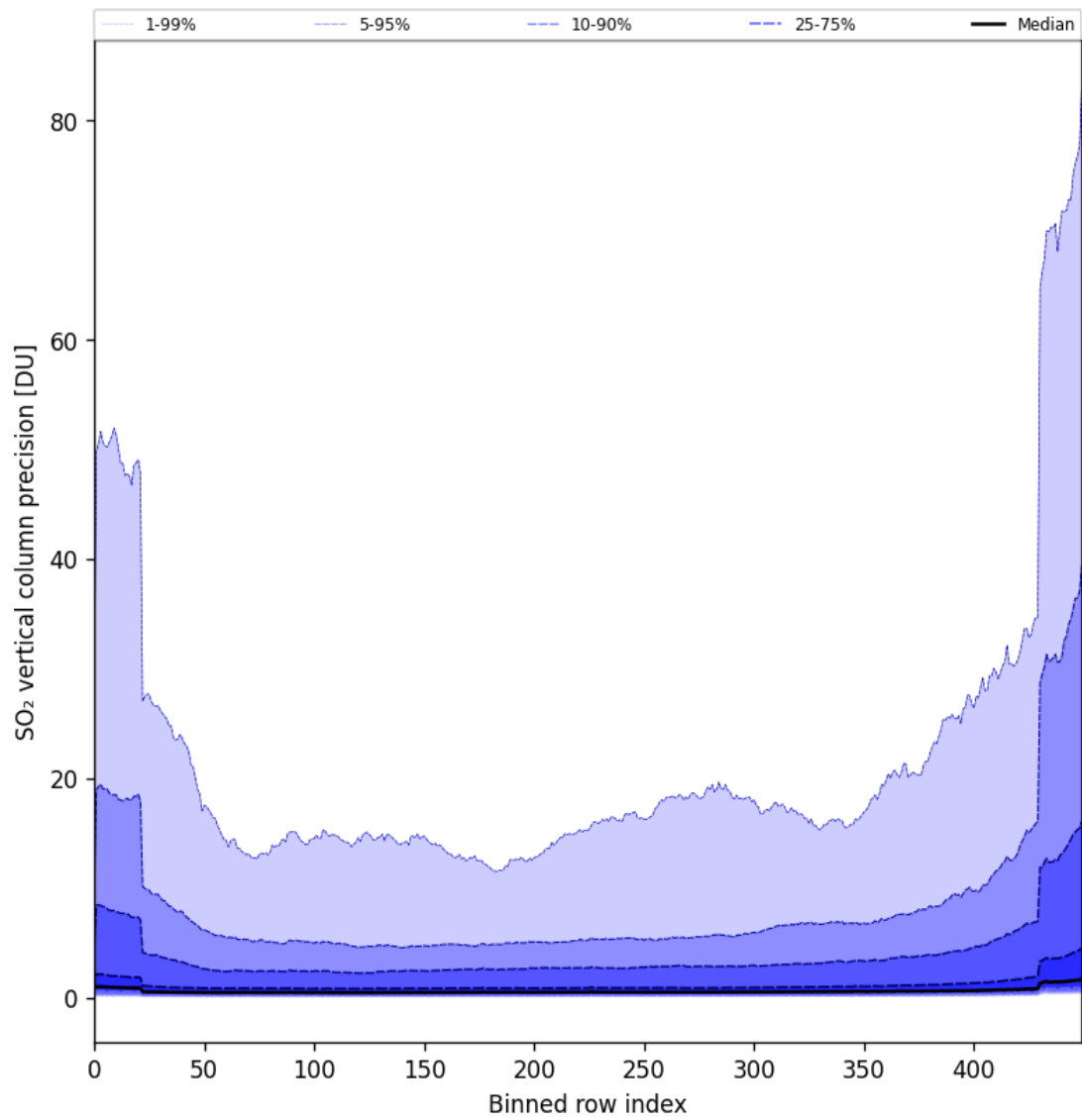
Figure 77: Along track statistics of “SO 2 vertical column precision” for 2024-11-11 to 2024-11-13
