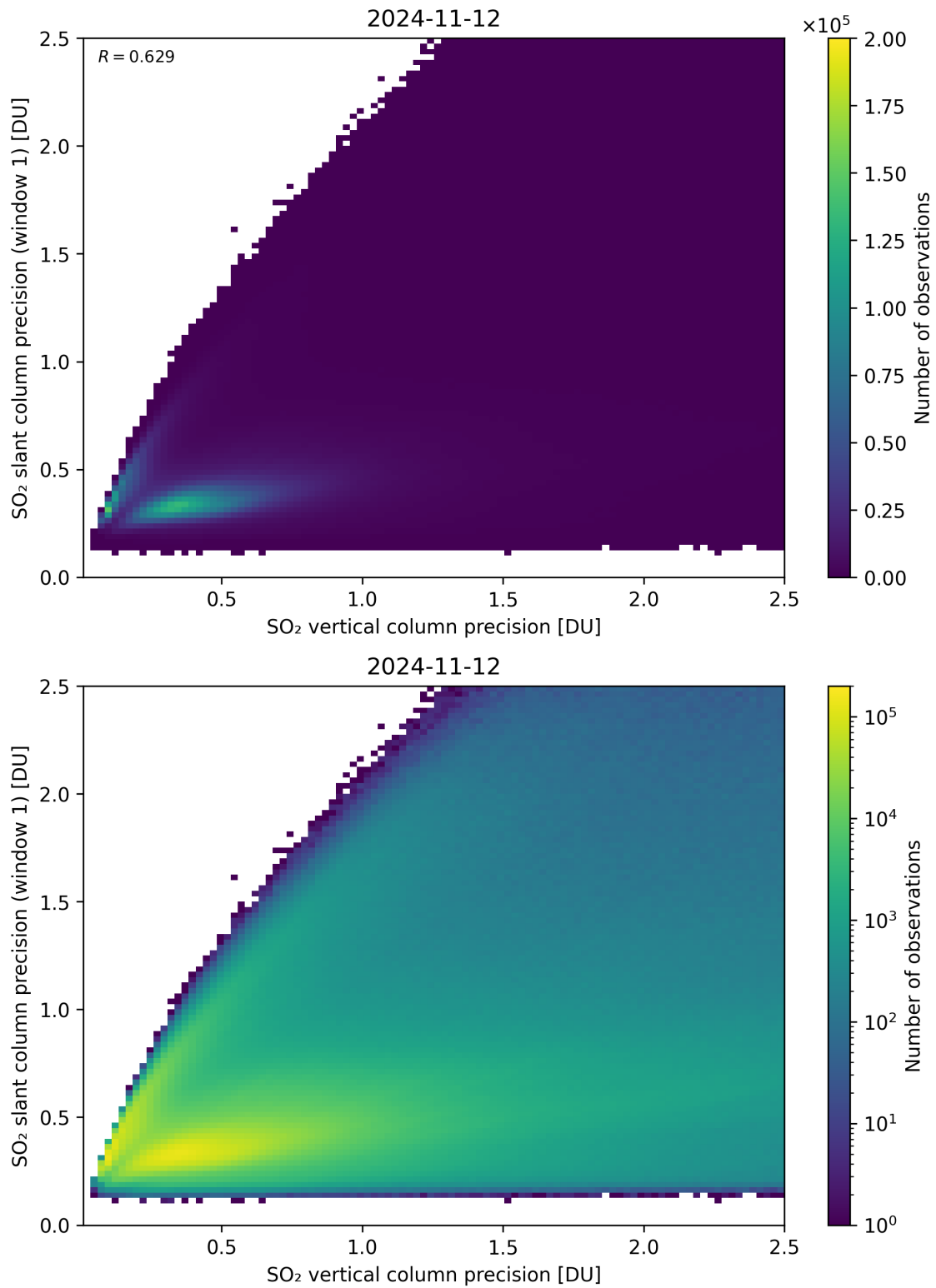
Figure 290: Scatter density plot of “SO 2 vertical column precision” against “SO 2 slant column precision (window 1)” for 2024-11-11 to 2024-11-13.
