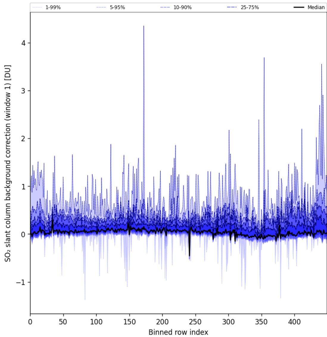
Figure 82: Along track statistics of “SO 2 slant column background correction (window 1)” for 2024-11-11 to 2024-11-13
