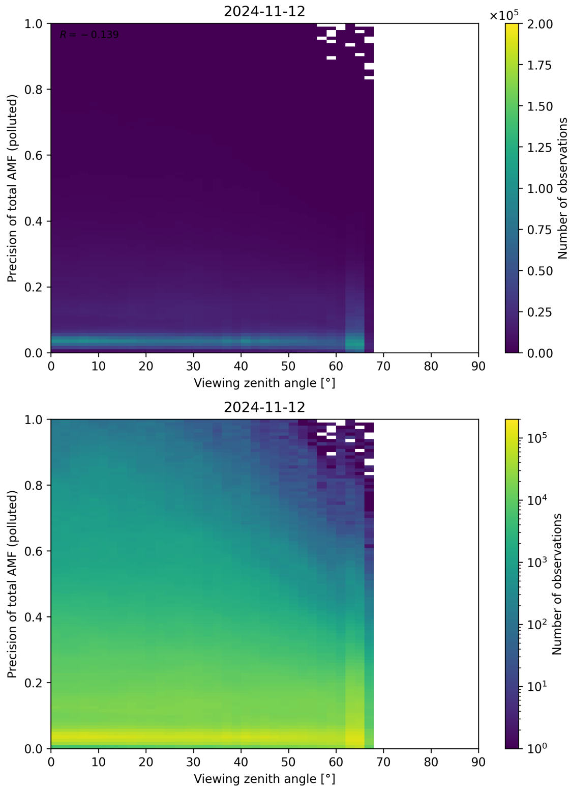
Figure 326: Scatter density plot of “Viewing zenith angle” against “Precision of total AMF (polluted)” for 2024-11-11 to 2024-11-13.
