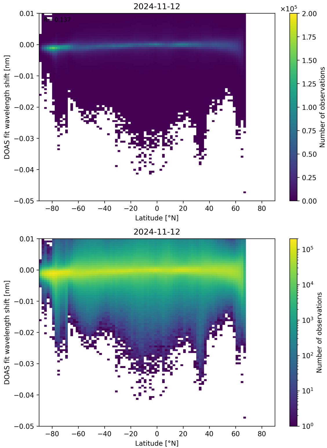
Figure 142: Scatter density plot of “Latitude” against “DOAS fit wavelength shift” for 2024-11-11 to 2024-11-13.
