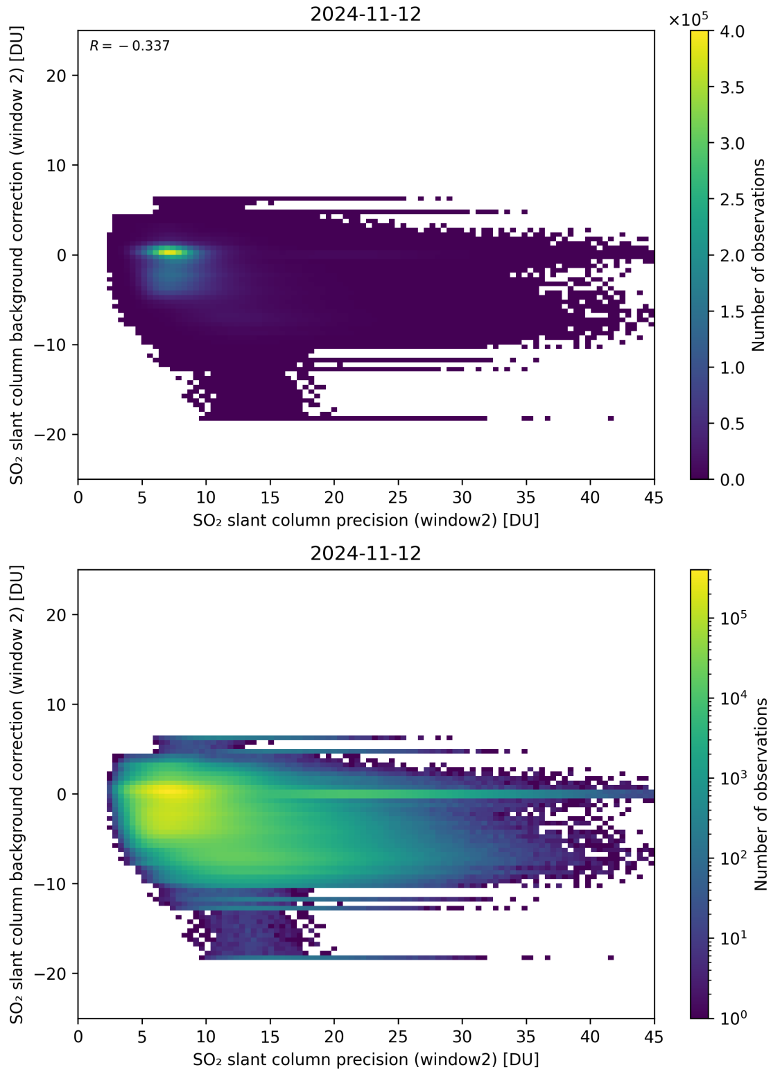
Figure 241: Scatter density plot of “SO 2 slant column precision (window2)” against “SO 2 slant column background correction (window 2)” for 2024-11-11 to 2024-11-13.
