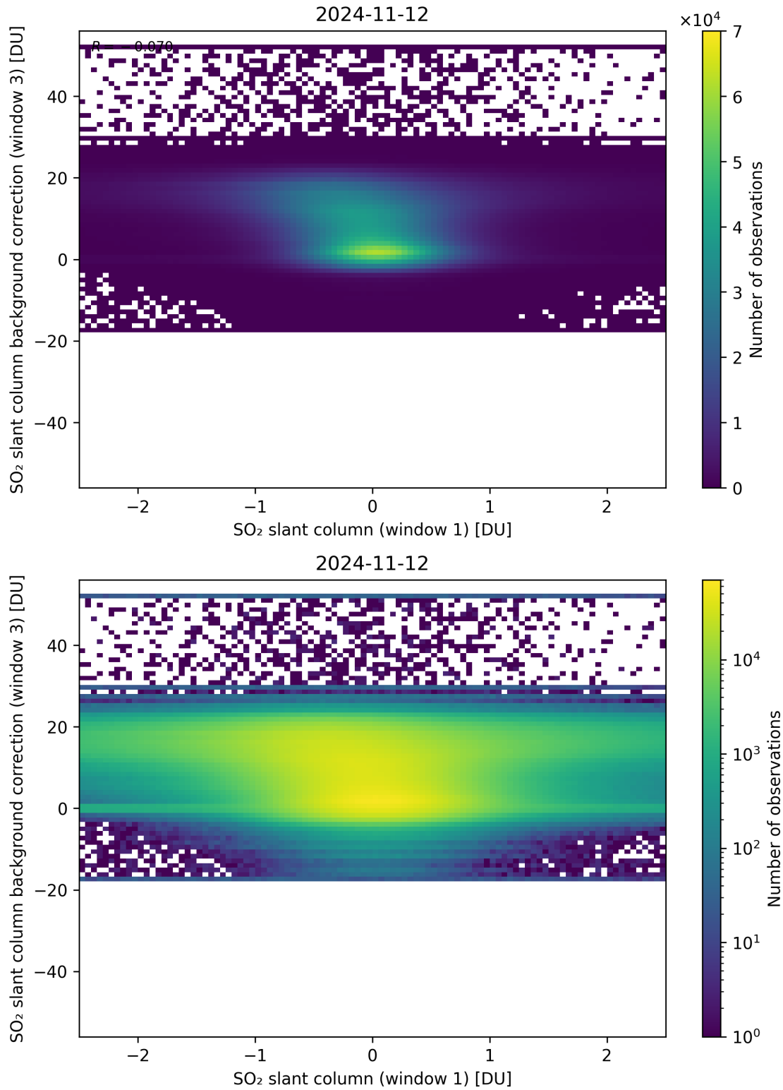
Figure 214: Scatter density plot of “SO 2 slant column (window 1)” against “SO 2 slant column background correction (window 3)” for 2024-11-11 to 2024-11-13.
