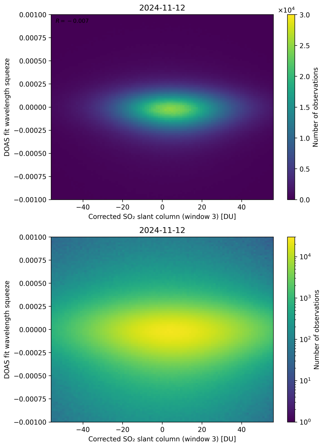
Figure 207: Scatter density plot of “Corrected SO 2 slant column (window 3)” against “DOAS fit wavelength squeeze” for 2024-11-11 to 2024-11-13.
