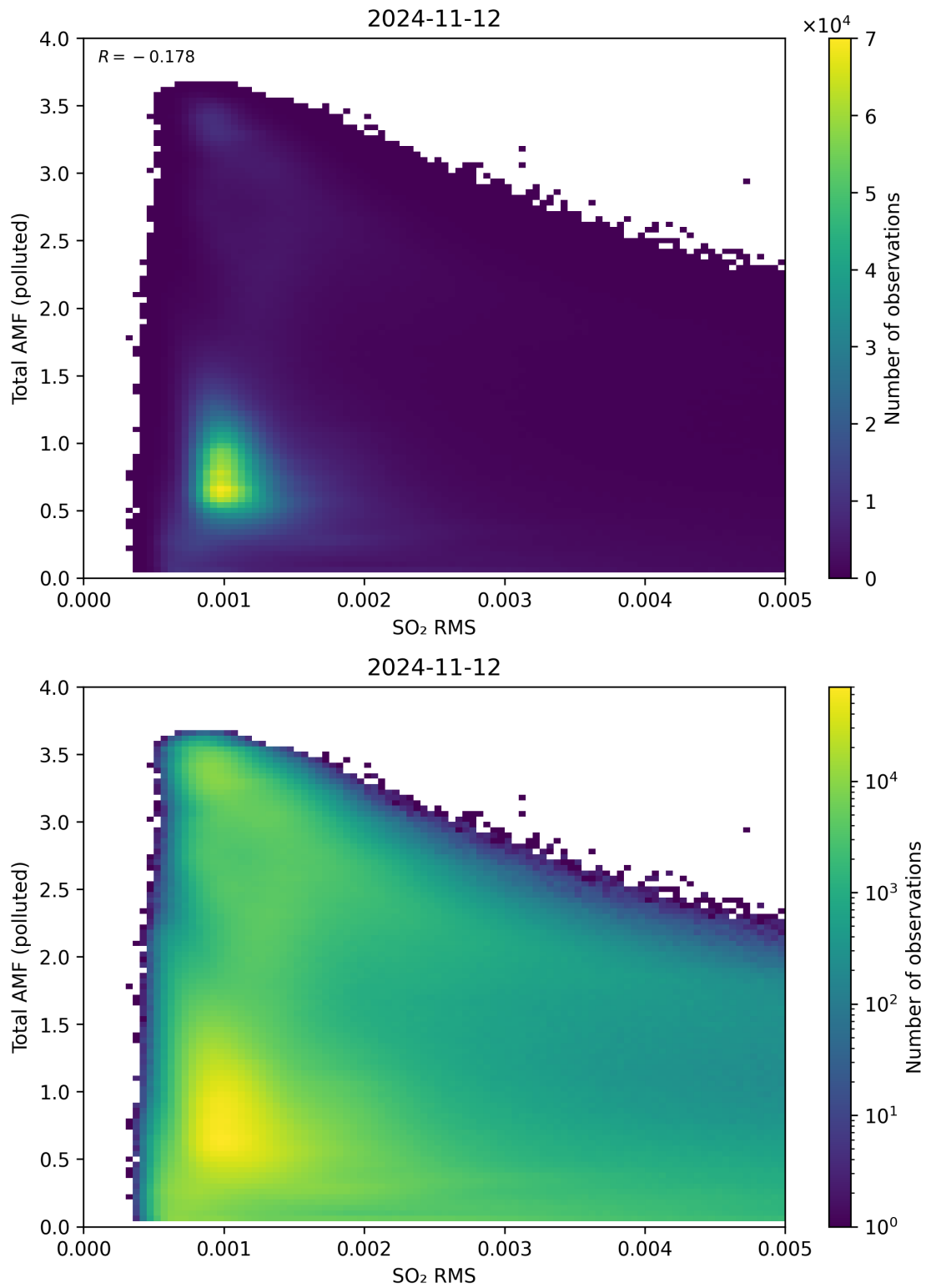
Figure 137: Scatter density plot of “SO 2 RMS” against “Total AMF (polluted)” for 2024-11-11 to 2024-11-13.
