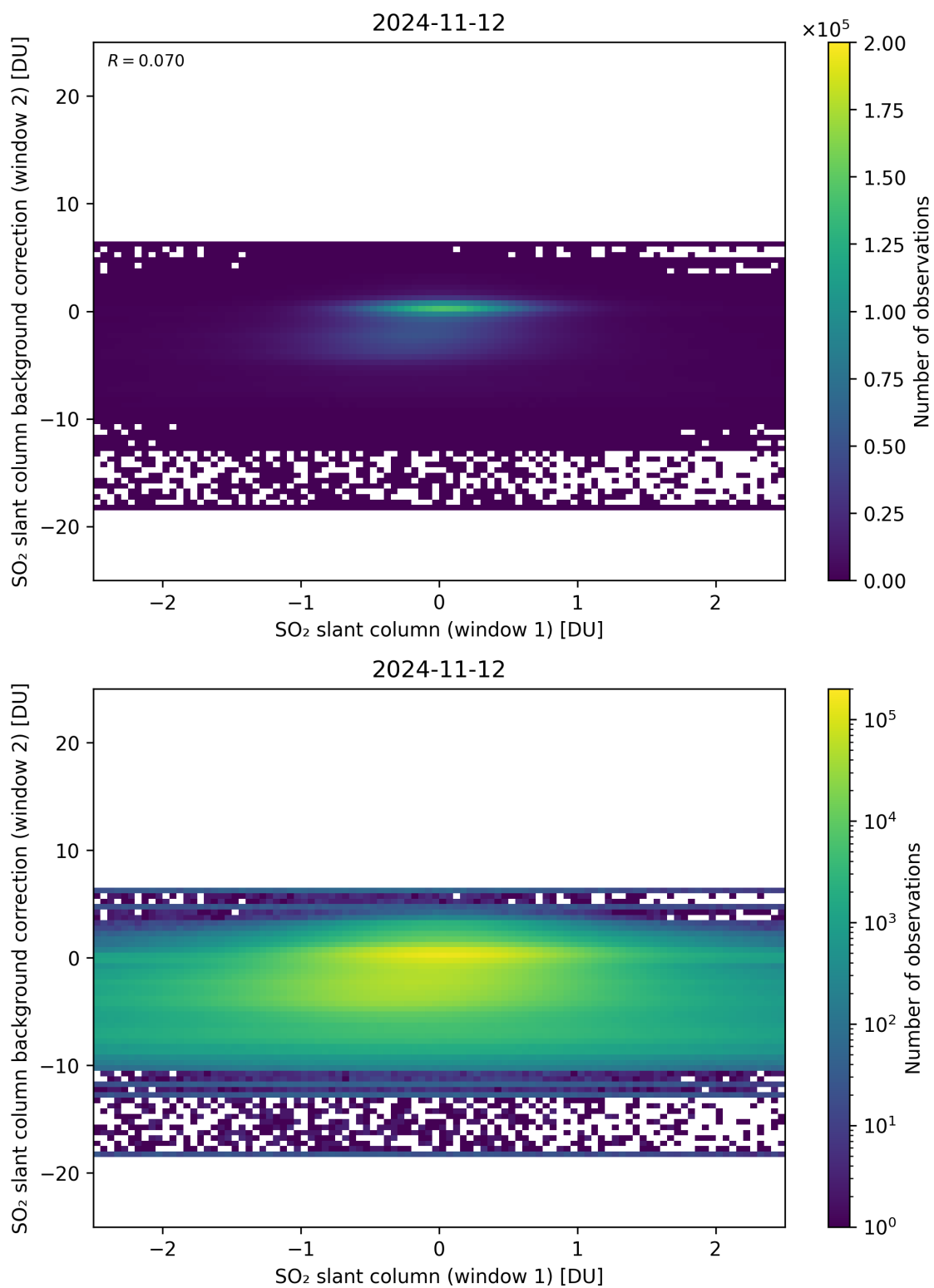
Figure 213: Scatter density plot of “SO 2 slant column (window 1)” against “SO 2 slant column background correction (window 2)” for 2024-11-11 to 2024-11-13.
