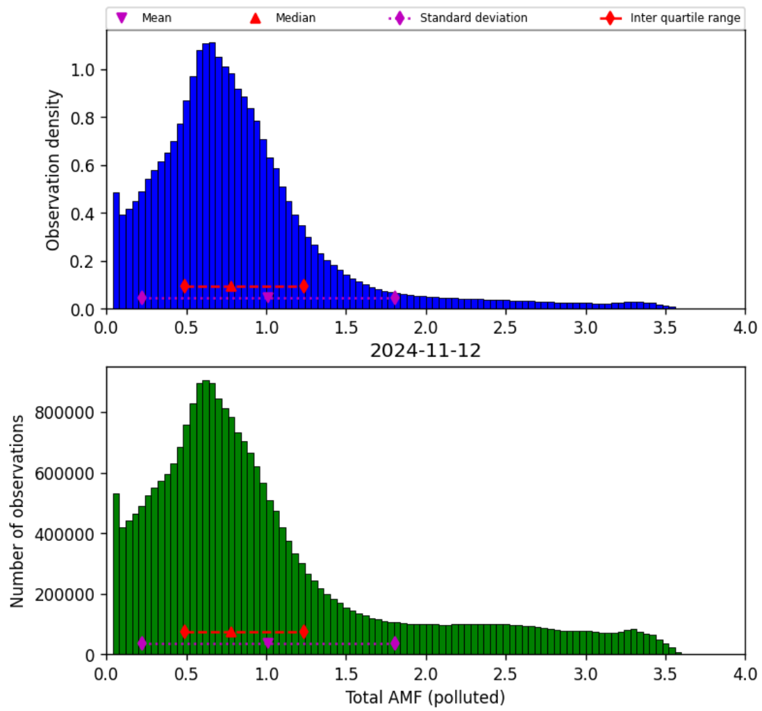
Figure 71: Histogram of “Total AMF (polluted)” for 2024-11-11 to 2024-11-13
