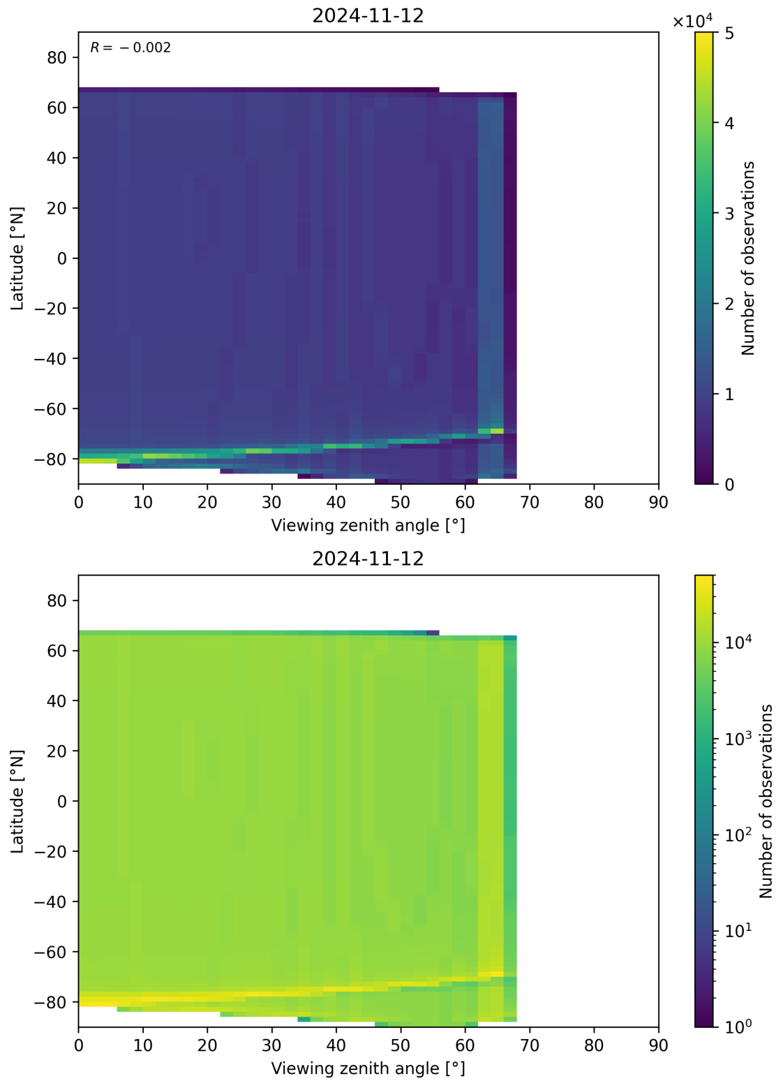
Figure 314: Scatter density plot of “Viewing zenith angle” against “Latitude” for 2024-11-11 to 2024-11-13.
