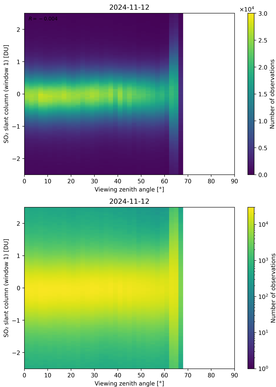
Figure 320: Scatter density plot of “Viewing zenith angle” against “SO 2 slant column (window 1)” for 2024-11-11 to 2024-11-13.
