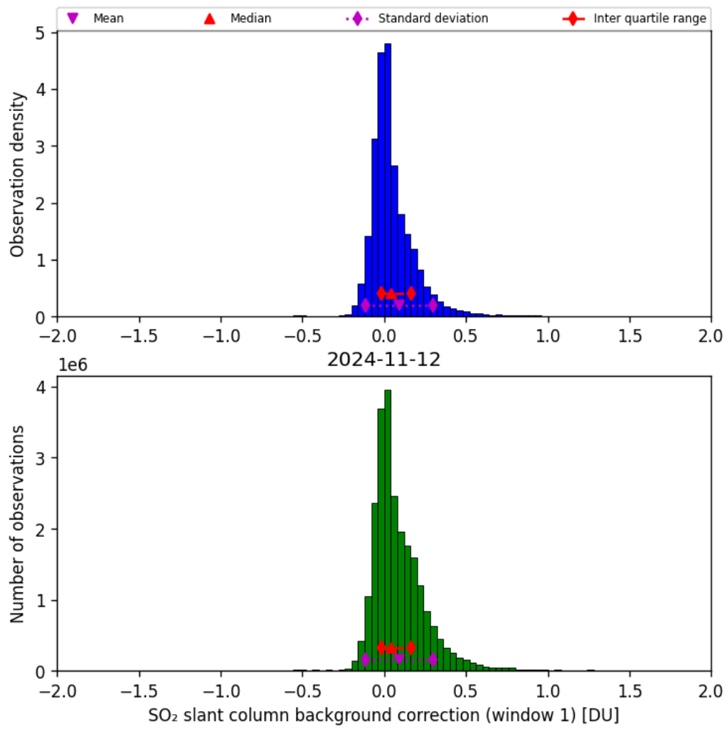
Figure 59: Histogram of “SO 2 slant column background correction (window 1)” for 2024-11-11 to 2024-11-13
