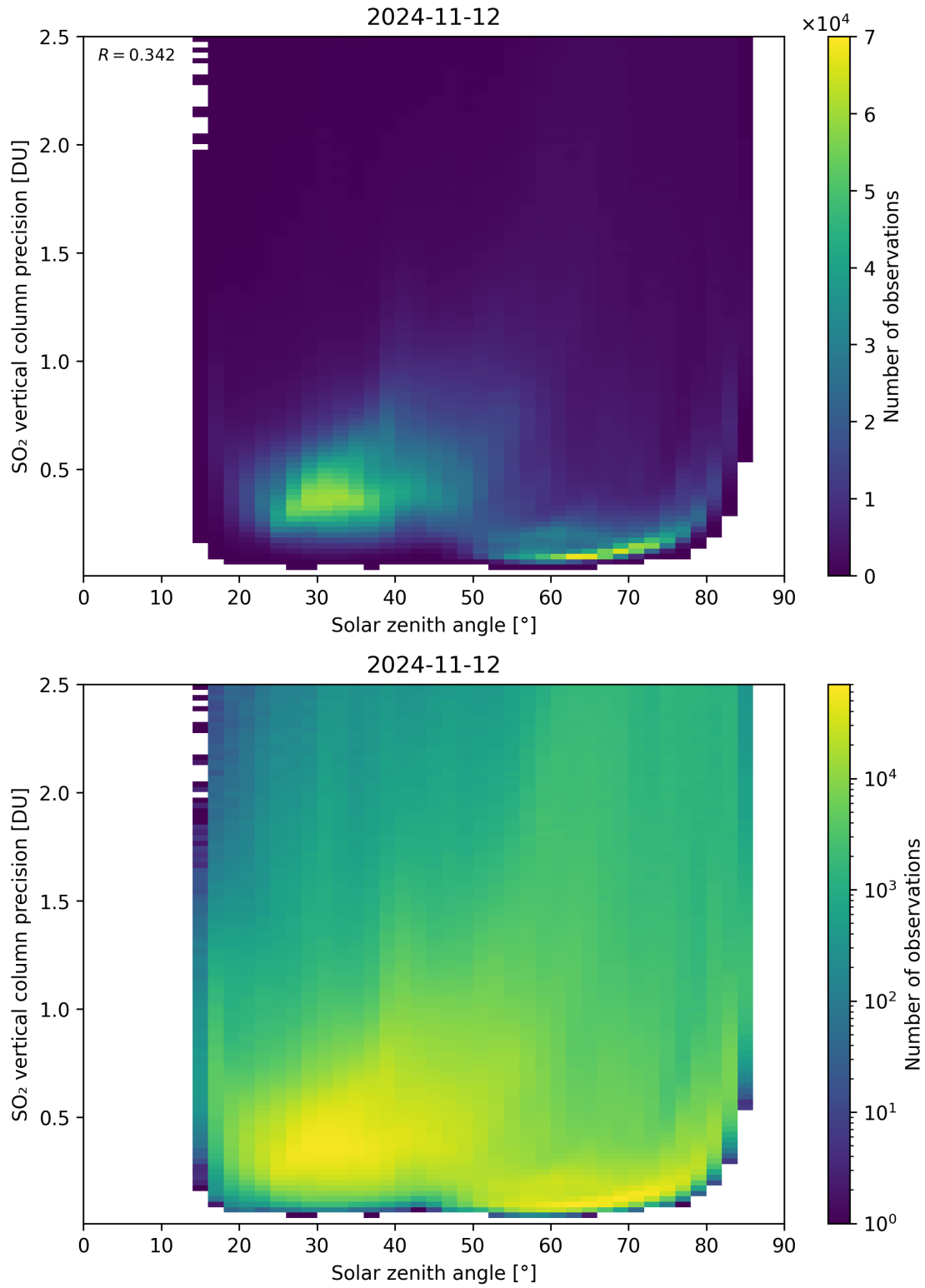
Figure 177: Scatter density plot of “Solar zenith angle” against “SO 2 vertical column precision” for 2024-11-11 to 2024-11-13.
