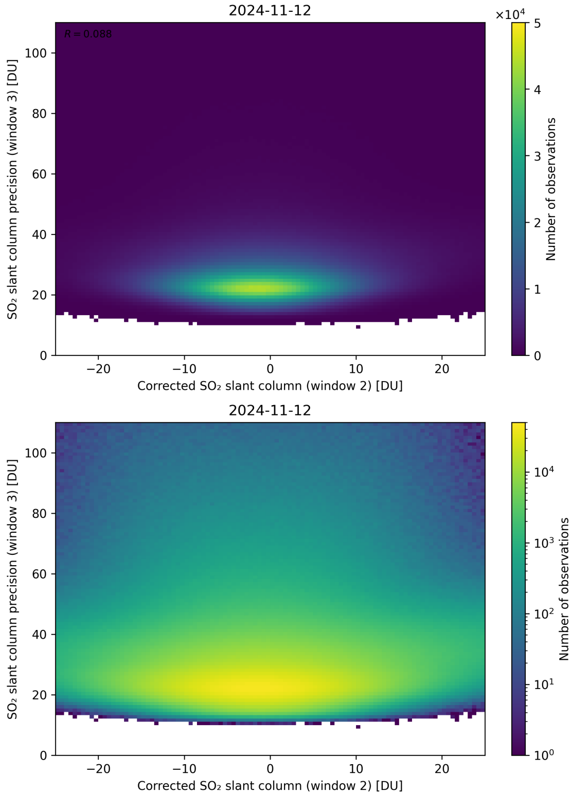
Figure 202: Scatter density plot of “Corrected SO 2 slant column (window 2)” against “SO 2 slant column precision (window 3)” for 2024-11-11 to 2024-11-13.
