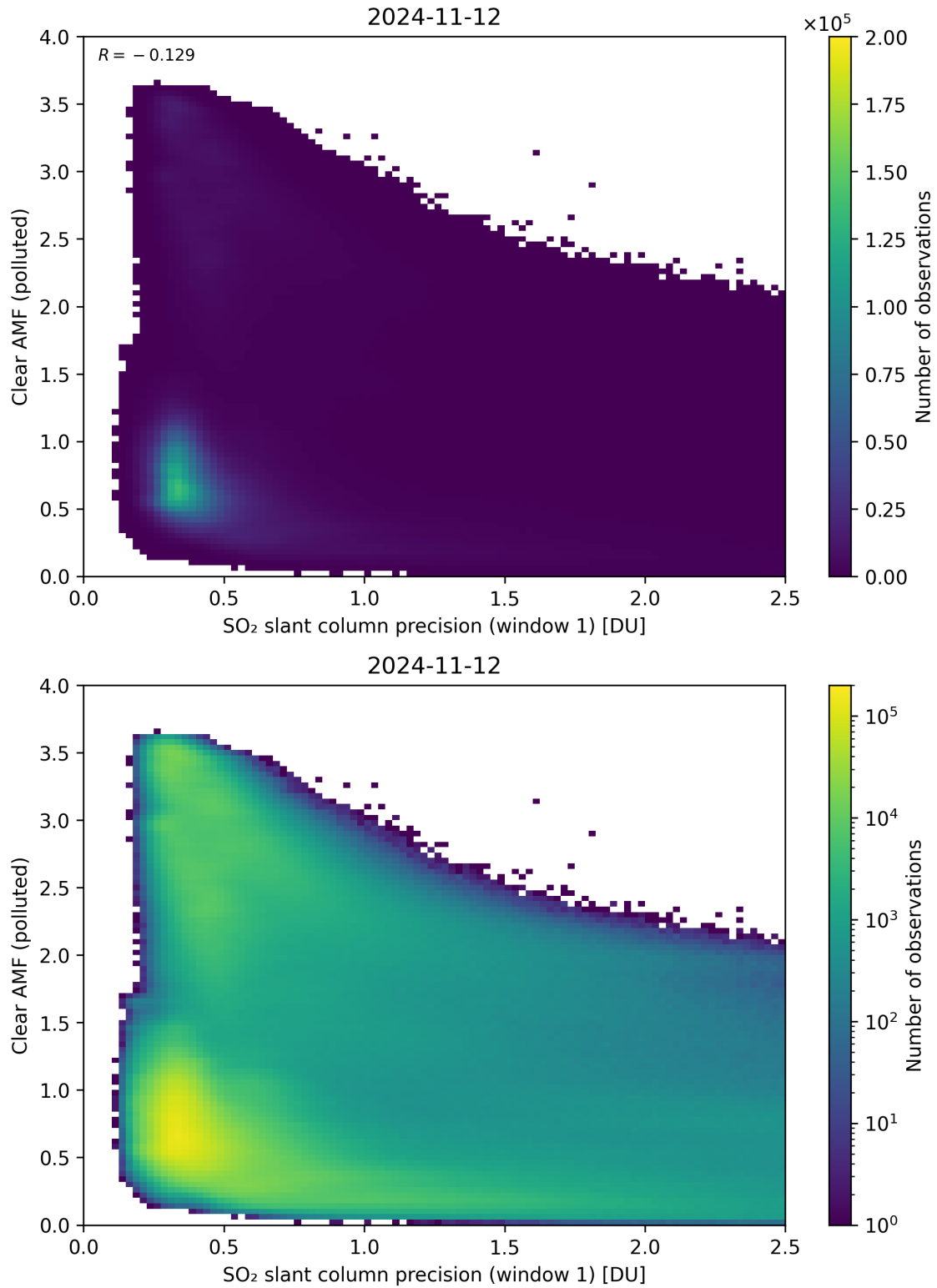
Figure 224: Scatter density plot of “SO 2 slant column precision (window 1)” against “Clear AMF (polluted)” for 2024-11-11 to 2024-11-13.
