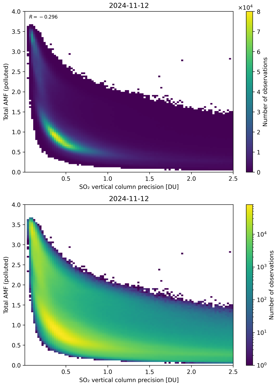
Figure 294: Scatter density plot of “SO 2 vertical column precision” against “Total AMF (polluted)” for 2024-11-11 to 2024-11-13.
