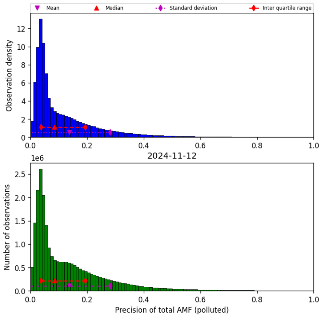
Figure 72: Histogram of “Precision of total AMF (polluted)” for 2024-11-11 to 2024-11-13
