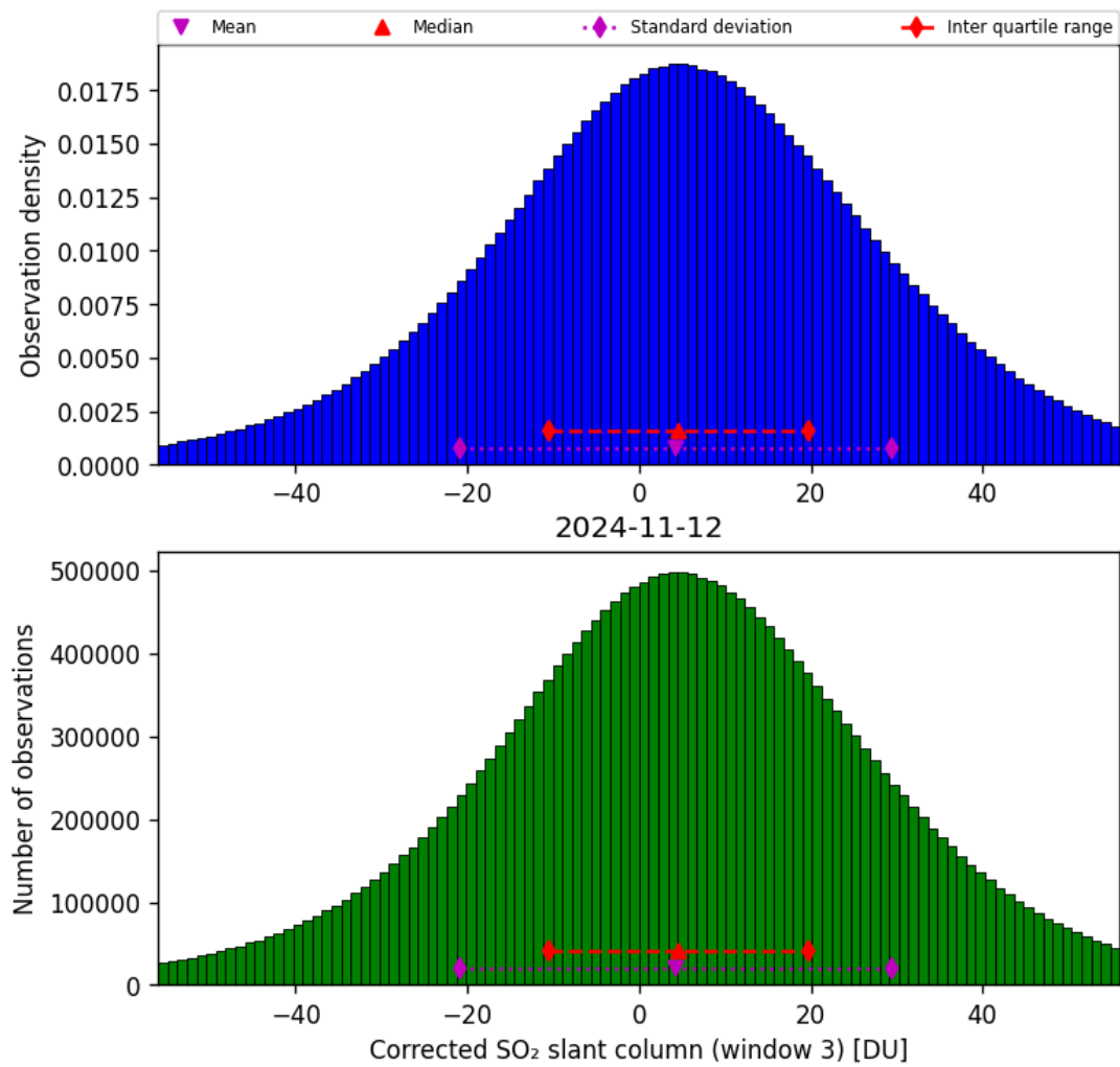
Figure 66: Histogram of “Corrected SO 2 slant column (window 3)” for 2024-11-11 to 2024-11-13
