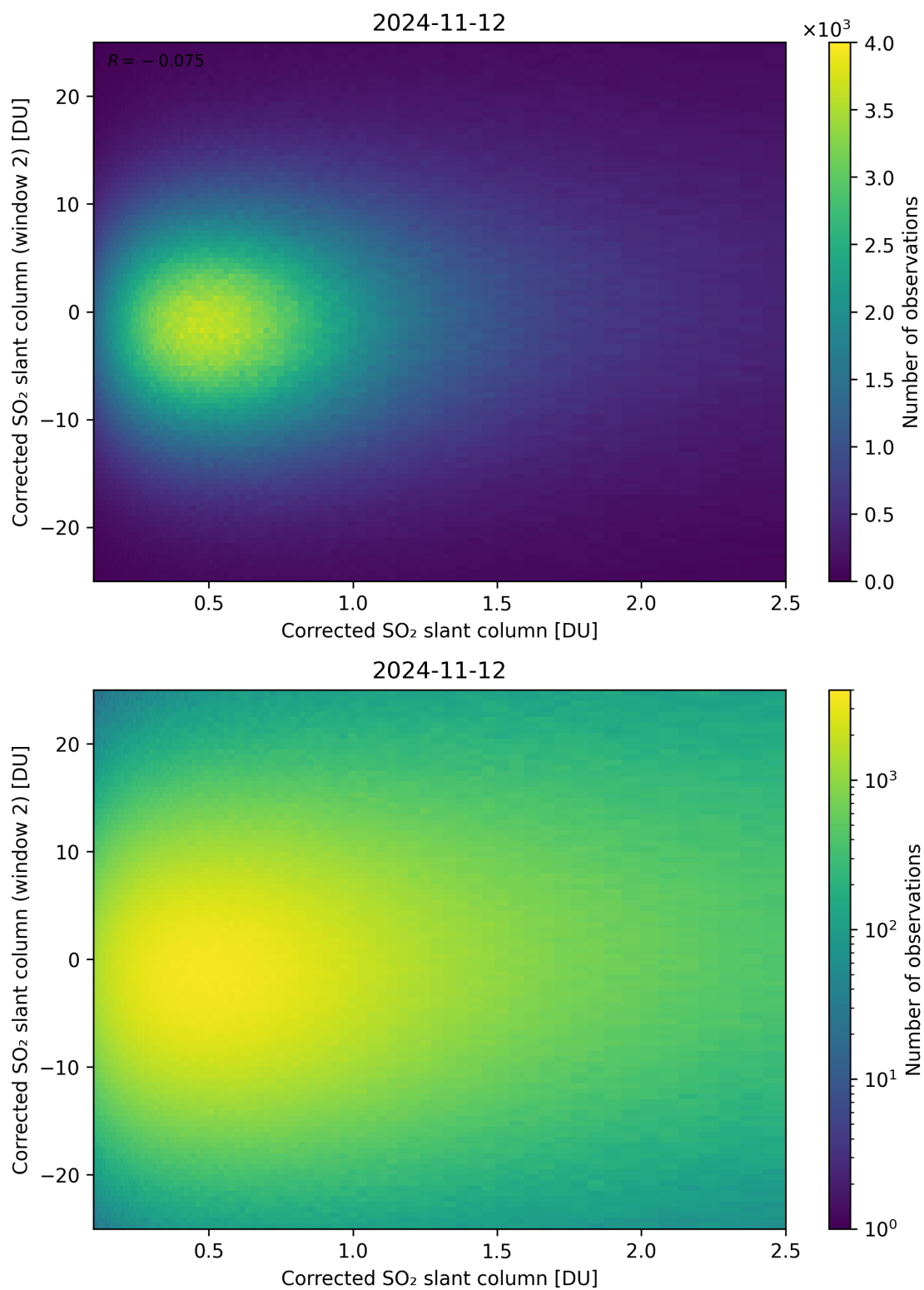
Figure 185: Scatter density plot of “Corrected SO 2 slant column” against “Corrected SO 2 slant column (window 2)” for 2024-11-11 to 2024-11-13.
