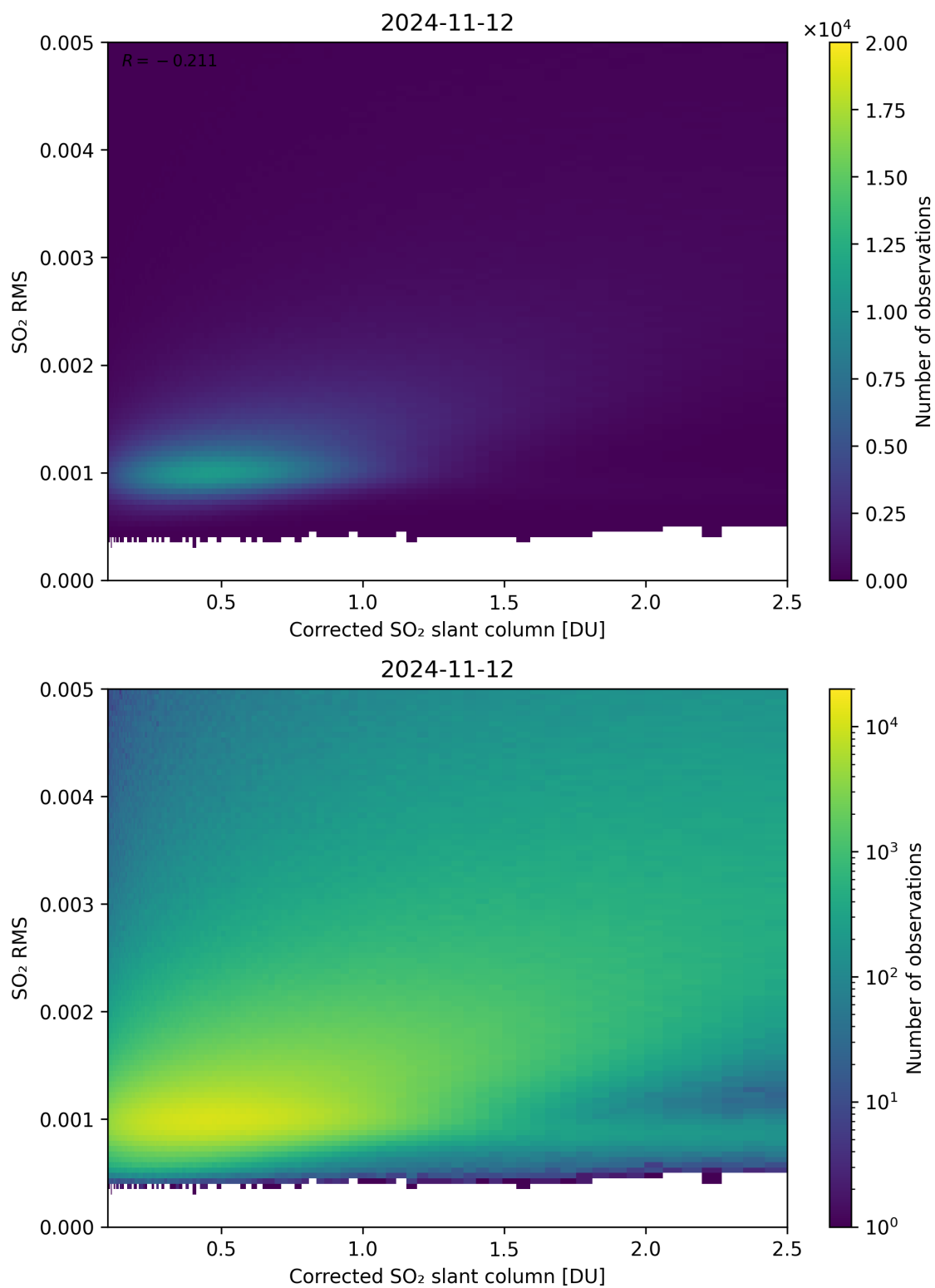
Figure 183: Scatter density plot of “Corrected SO 2 slant column” against “SO 2 RMS” for 2024-11-11 to 2024-11-13.
