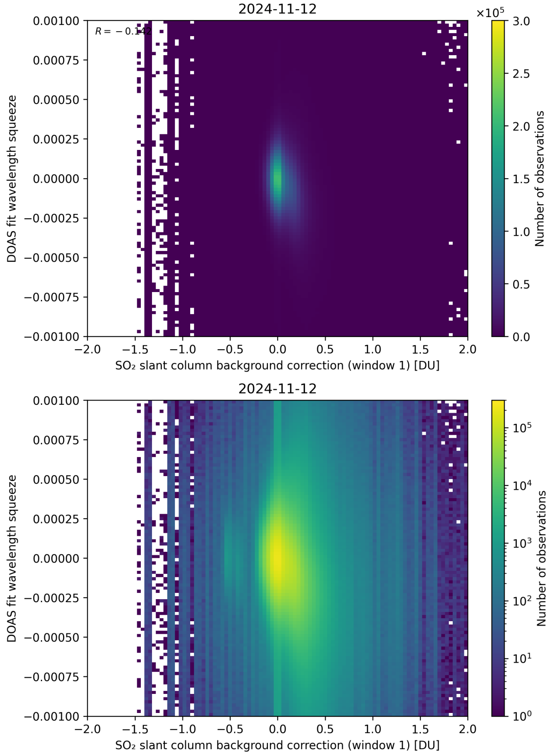
Figure 101: Scatter density plot of “SO 2 slant column background correction (window 1)” against “DOAS fit wavelength squeeze” for 2024-11-11 to 2024-11-13.
