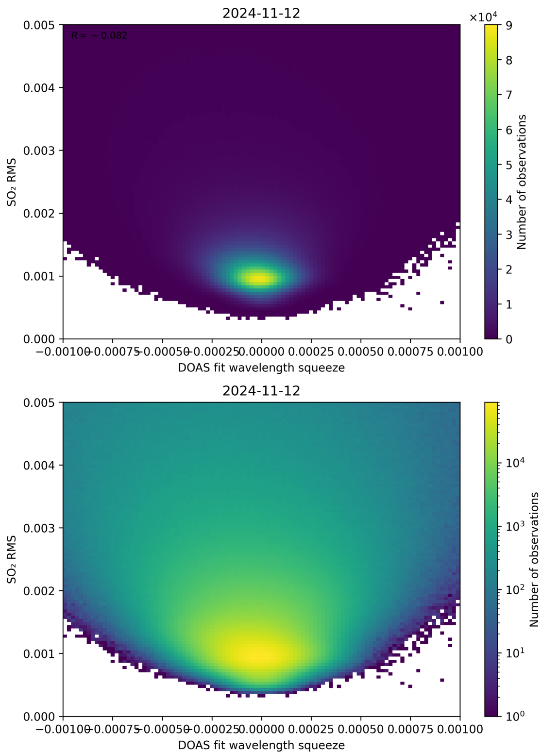
Figure 132: Scatter density plot of “DOAS fit wavelength squeeze” against “SO 2 RMS” for 2024-11-11 to 2024-11-13.
