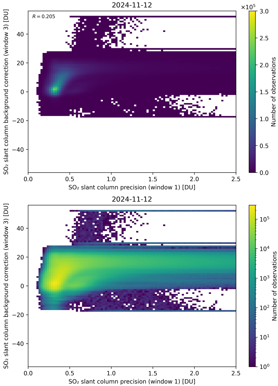
Figure 220: Scatter density plot of “SO 2 slant column precision (window 1)” against “SO 2 slant column background correction (window 3)” for 2024-11-11 to 2024-11-13.
