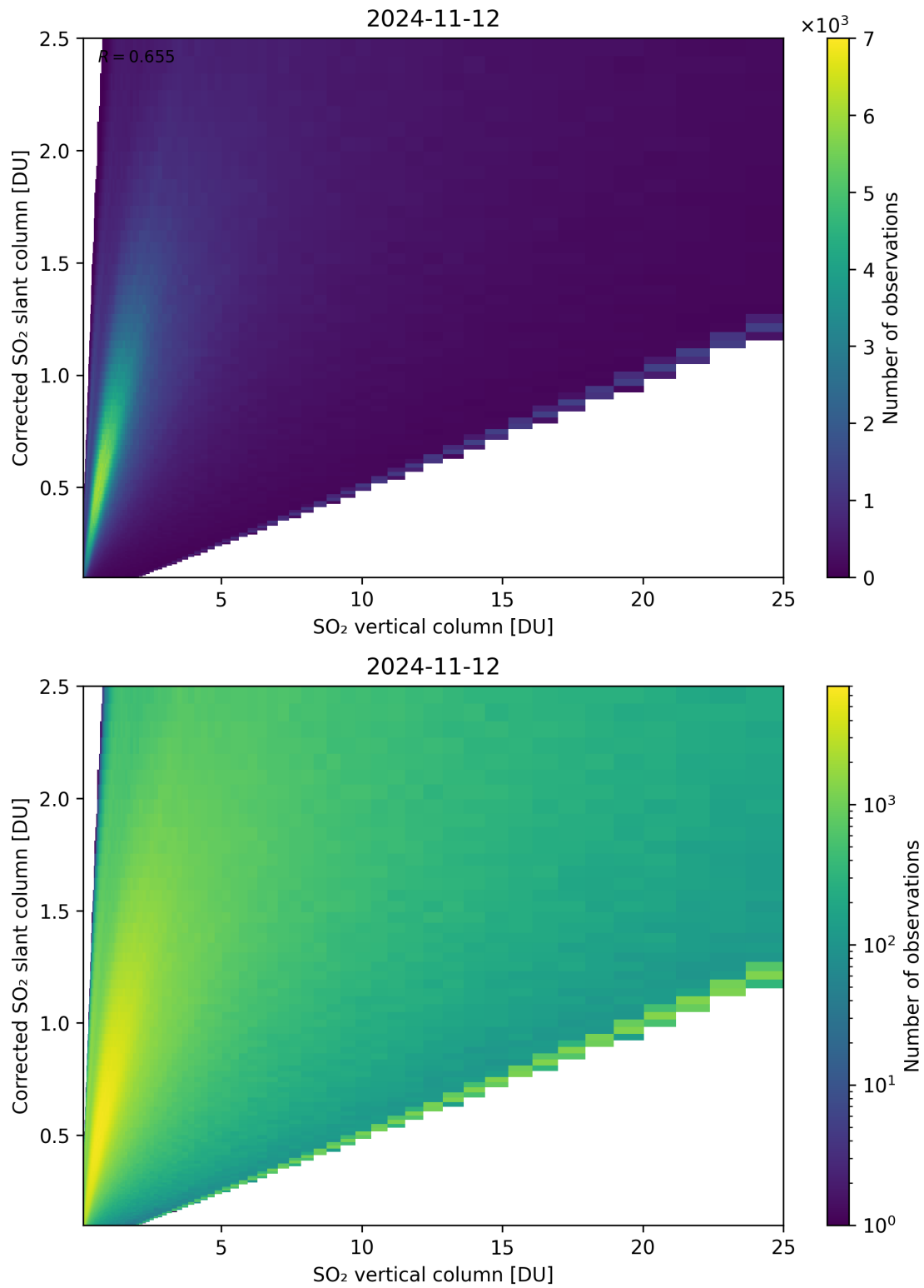
Figure 297: Scatter density plot of “SO 2 vertical column” against “Corrected SO 2 slant column” for 2024-11-11 to 2024-11-13.
