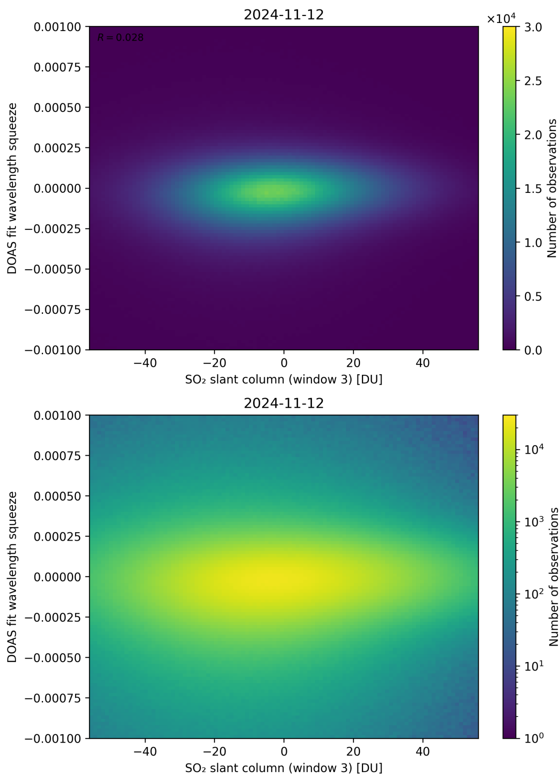
Figure 255: Scatter density plot of “SO 2 slant column (window 3)” against “DOAS fit wavelength squeeze” for 2024-11-11 to 2024-11-13.
