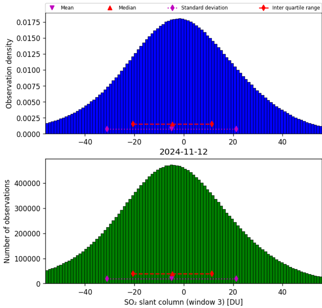
Figure 64: Histogram of “SO 2 slant column (window 3)” for 2024-11-11 to 2024-11-13
