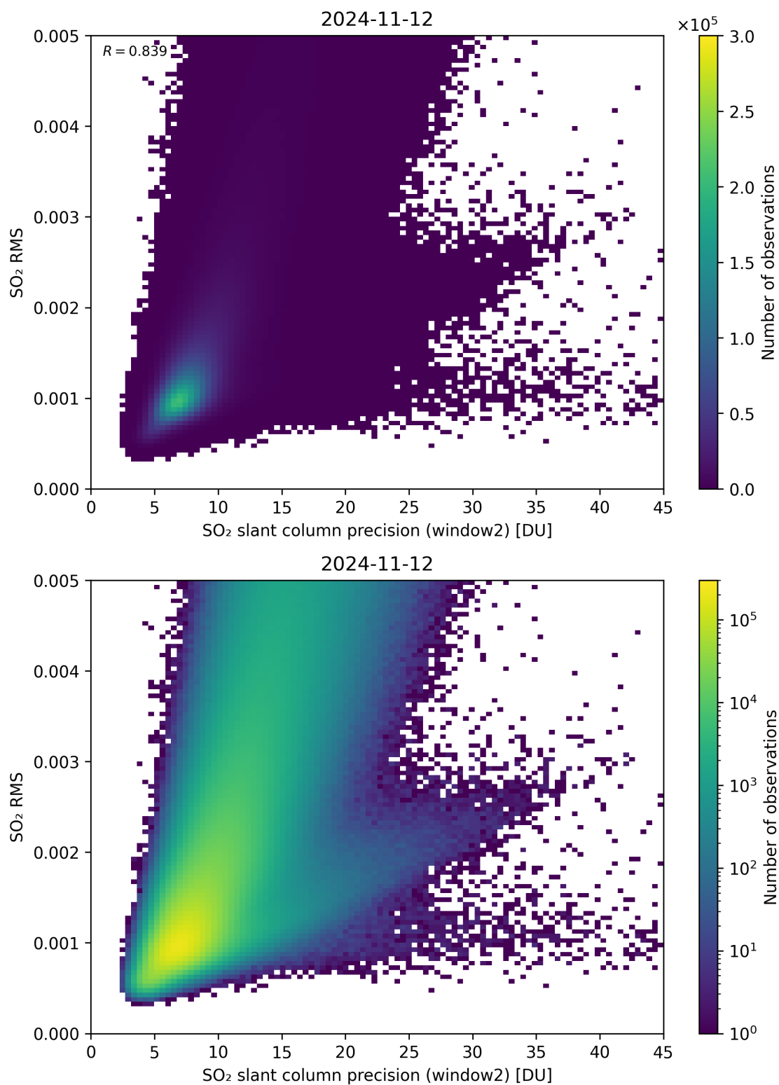
Figure 245: Scatter density plot of “SO 2 slant column precision (window2)” against “SO 2 RMS” for 2024-11-11 to 2024-11-13.
