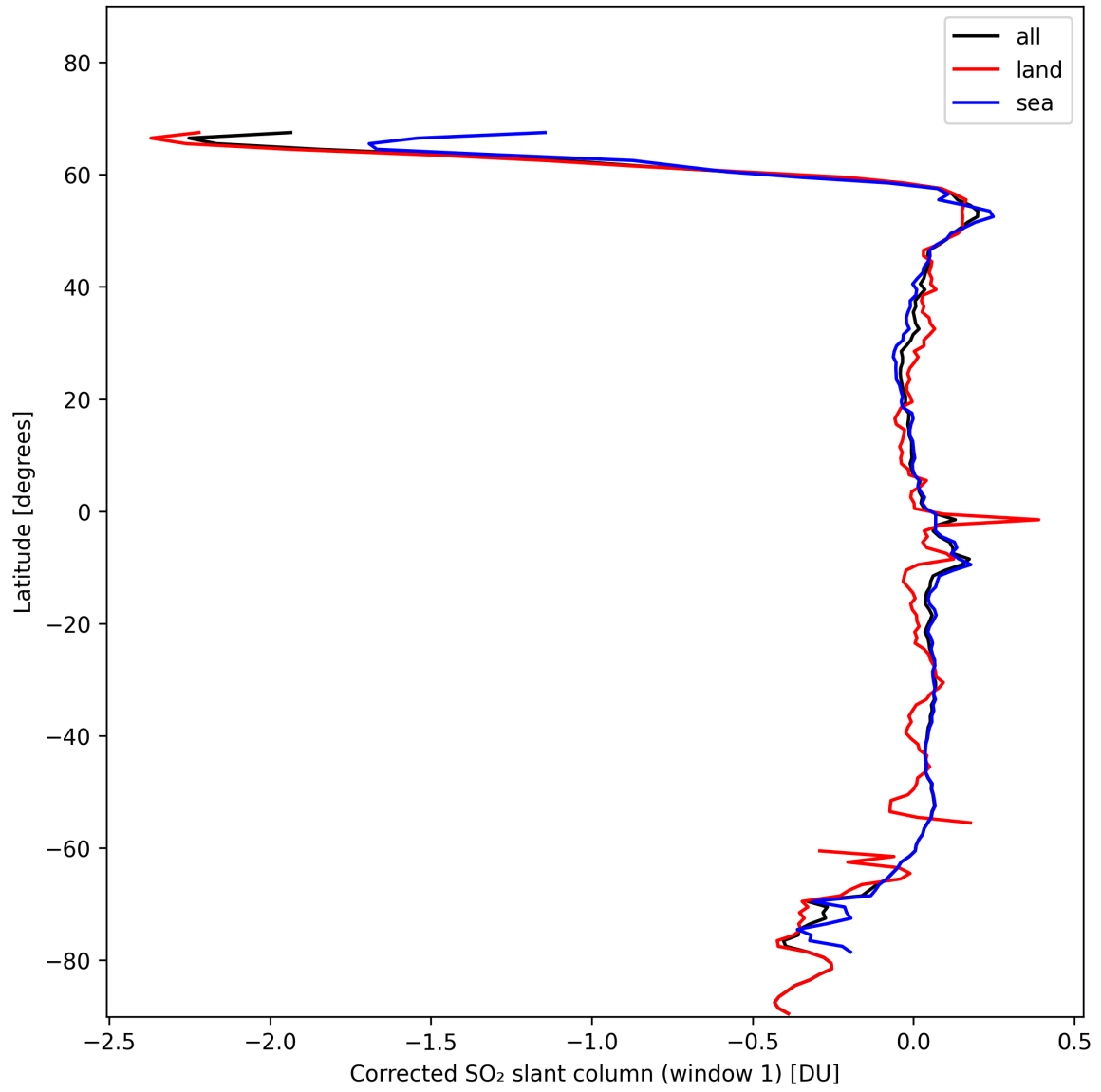
Figure 35: Zonal average of “Corrected SO 2 slant column (window 1)” for 2024-11-11 to 2024-11-13.
