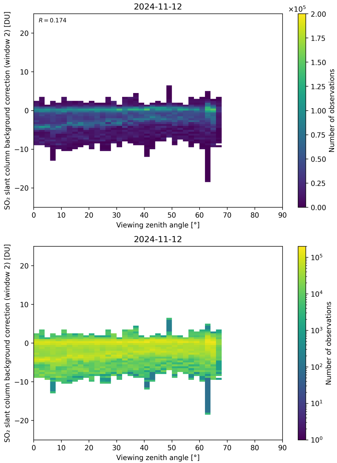
Figure 309: Scatter density plot of “Viewing zenith angle” against “SO 2 slant column background correction (window 2)” for 2024-11-11 to 2024-11-13.
