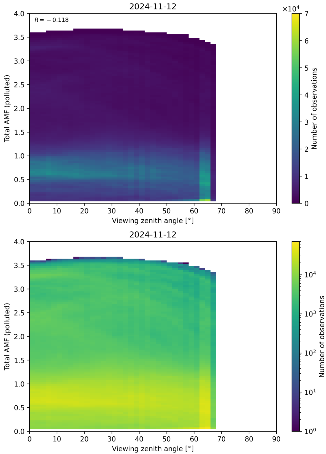
Figure 325: Scatter density plot of “Viewing zenith angle” against “Total AMF (polluted)” for 2024-11-11 to 2024-11-13.
