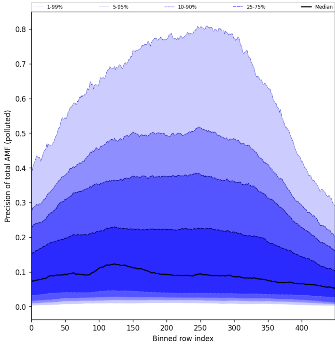
Figure 95: Along track statistics of “Precision of total AMF (polluted)” for 2024-11-11 to 2024-11-13
