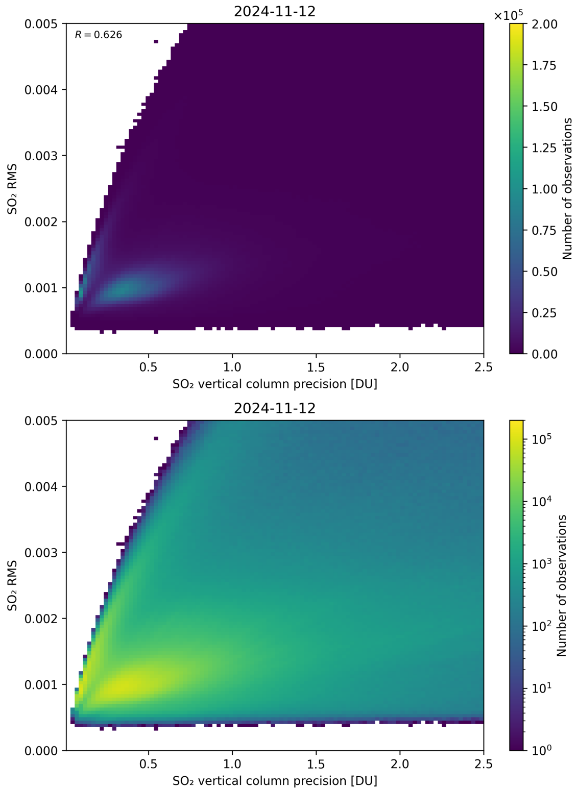
Figure 284: Scatter density plot of “SO 2 vertical column precision” against “SO 2 RMS” for 2024-11-11 to 2024-11-13.
