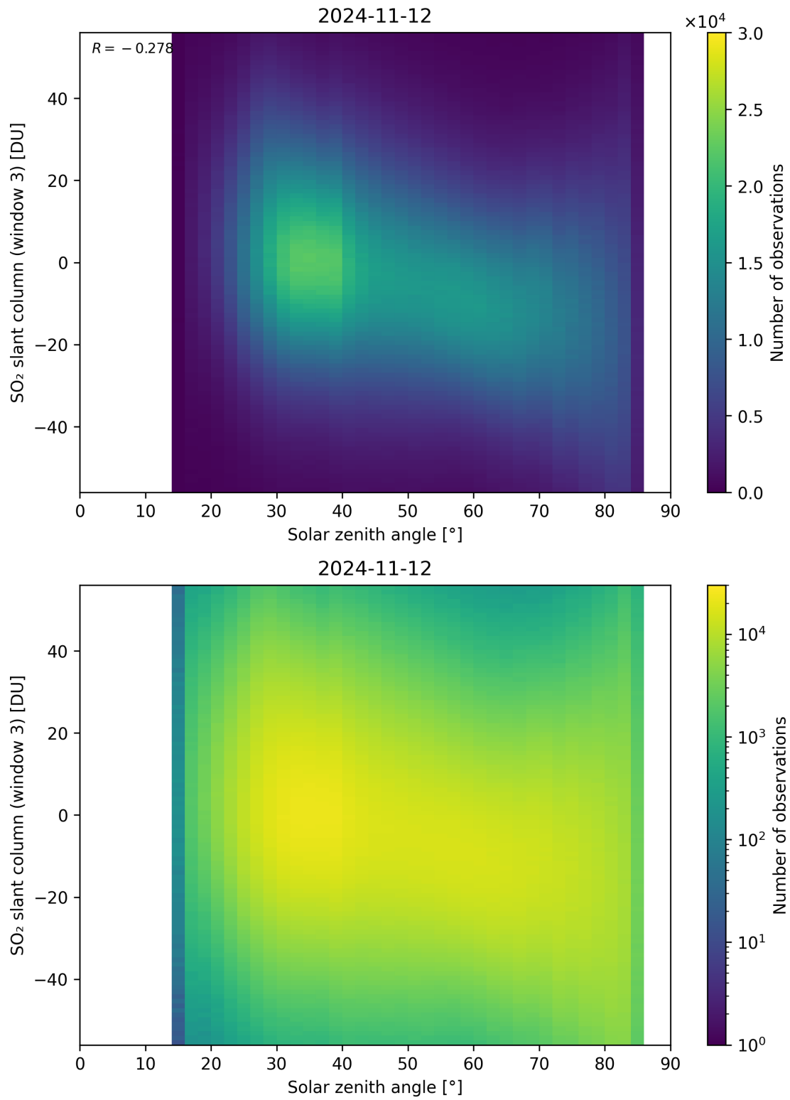
Figure 172: Scatter density plot of “Solar zenith angle” against “SO 2 slant column (window 3)” for 2024-11-11 to 2024-11-13.
