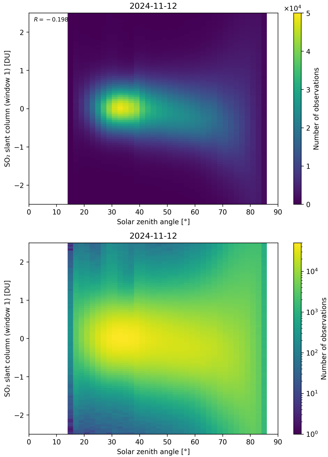
Figure 169: Scatter density plot of “Solar zenith angle” against “SO 2 slant column (window 1)” for 2024-11-11 to 2024-11-13.
