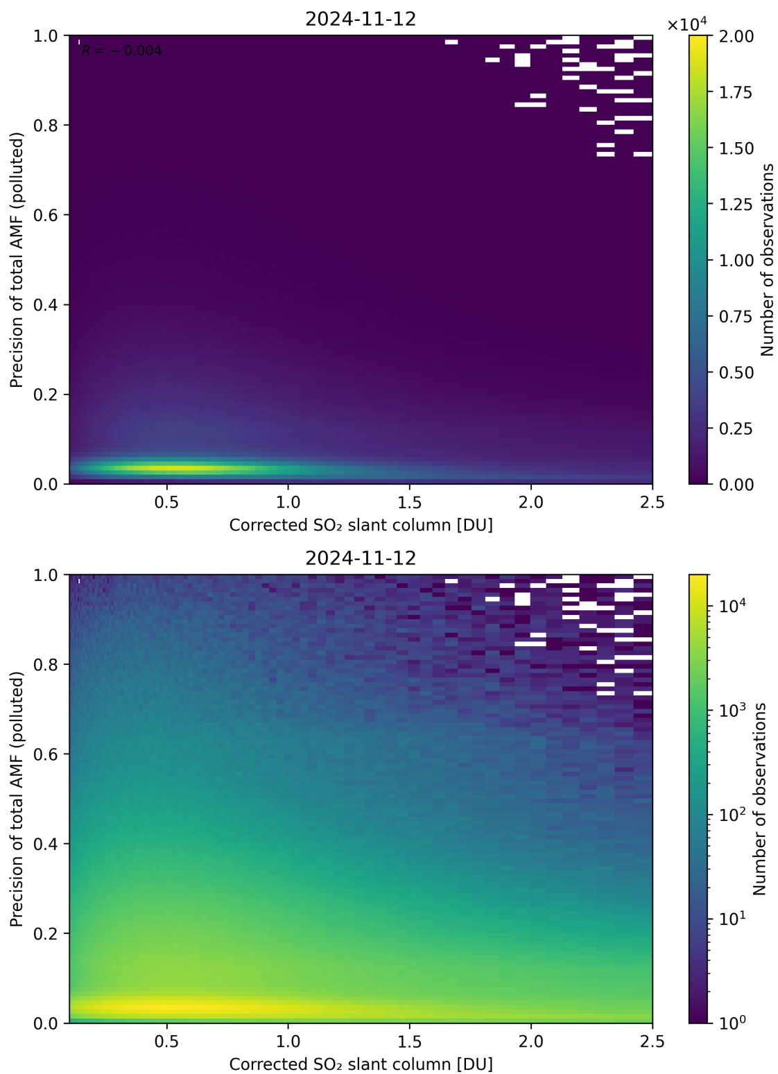
Figure 193: Scatter density plot of “Corrected SO 2 slant column” against “Precision of total AMF (polluted)” for 2024-11-11 to 2024-11-13.
