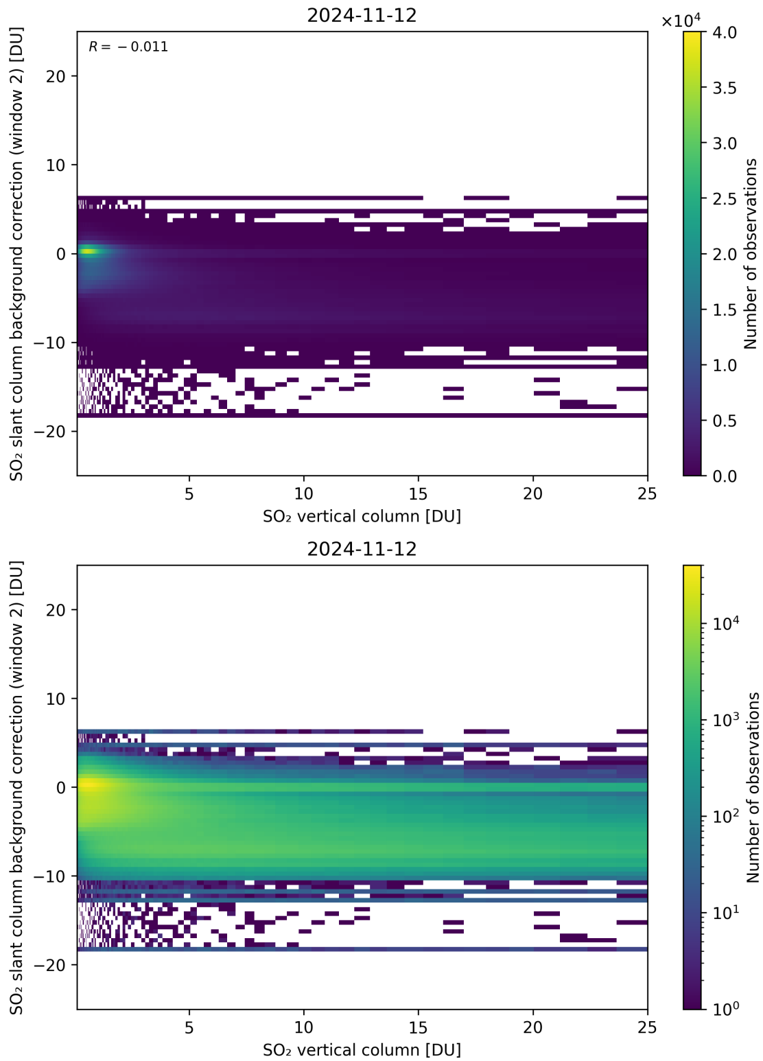
Figure 274: Scatter density plot of “SO 2 vertical column” against “SO 2 slant column background correction (window 2)” for 2024-11-11 to 2024-11-13.
