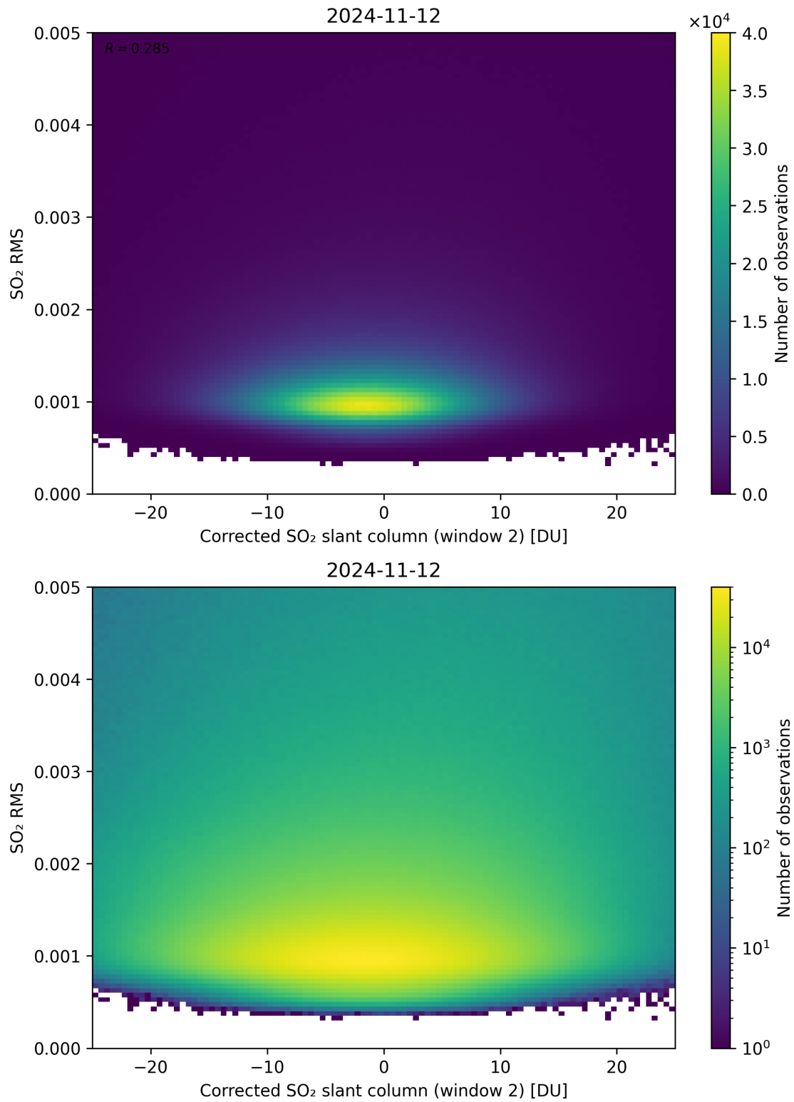
Figure 198: Scatter density plot of “Corrected SO 2 slant column (window 2)” against “SO 2 RMS” for 2024-11-11 to 2024-11-13.
