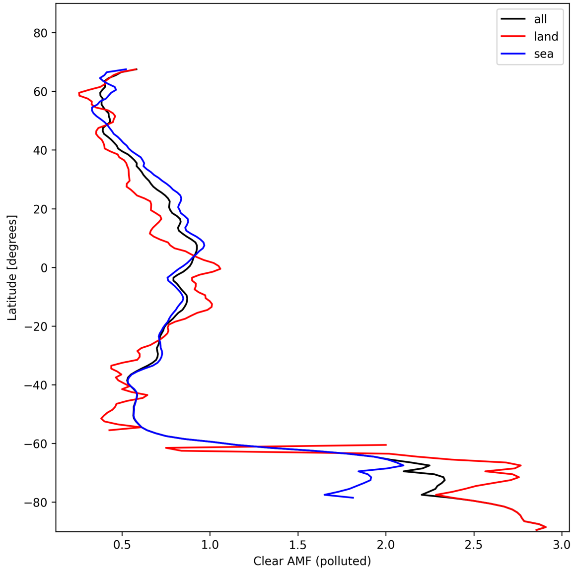
Figure 50: Zonal average of “Clear AMF (polluted)” for 2024-11-11 to 2024-11-13.
