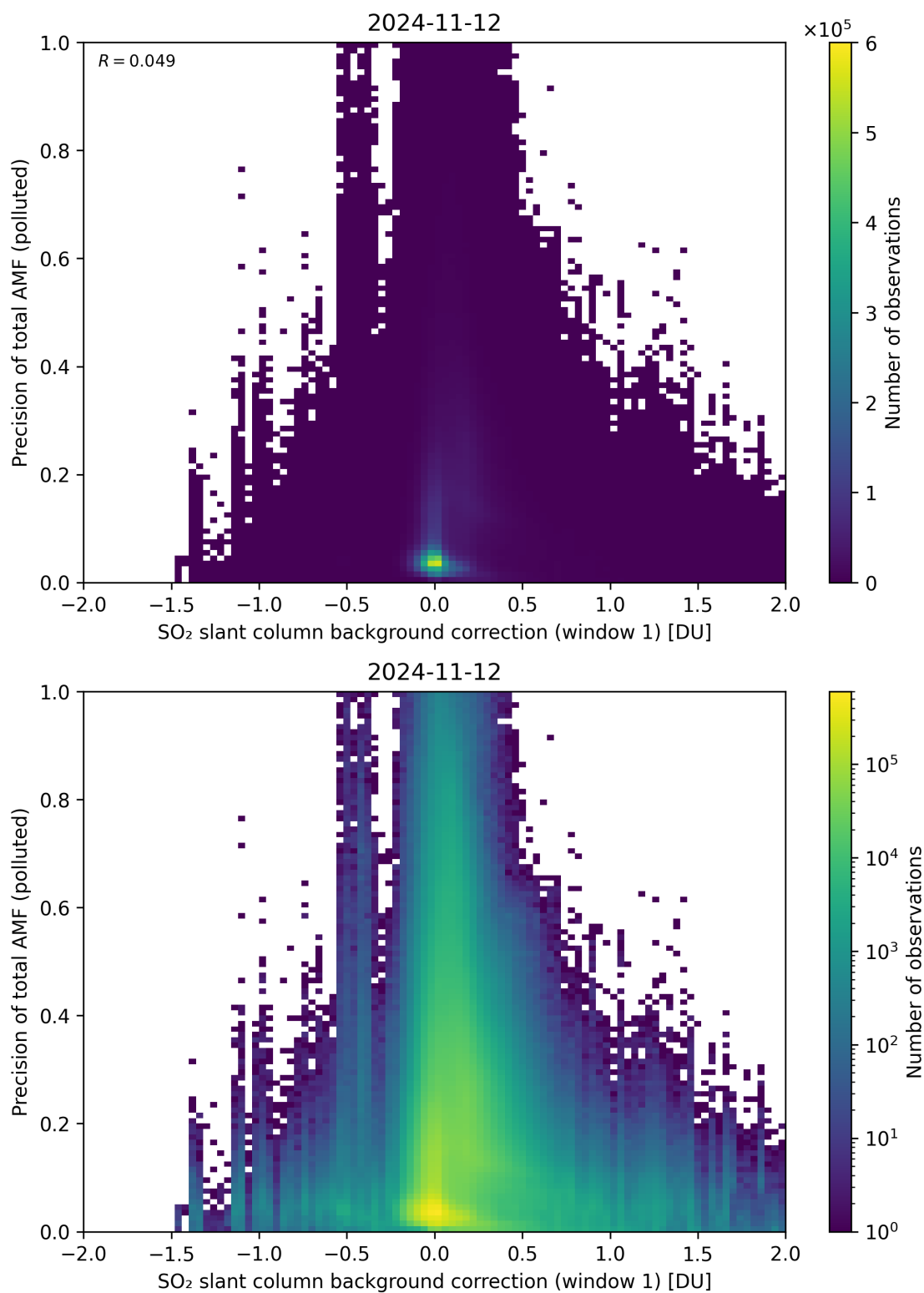
Figure 110: Scatter density plot of “SO 2 slant column background correction (window 1)” against “Precision of total AMF (polluted)” for 2024-11-11 to 2024-11-13.
