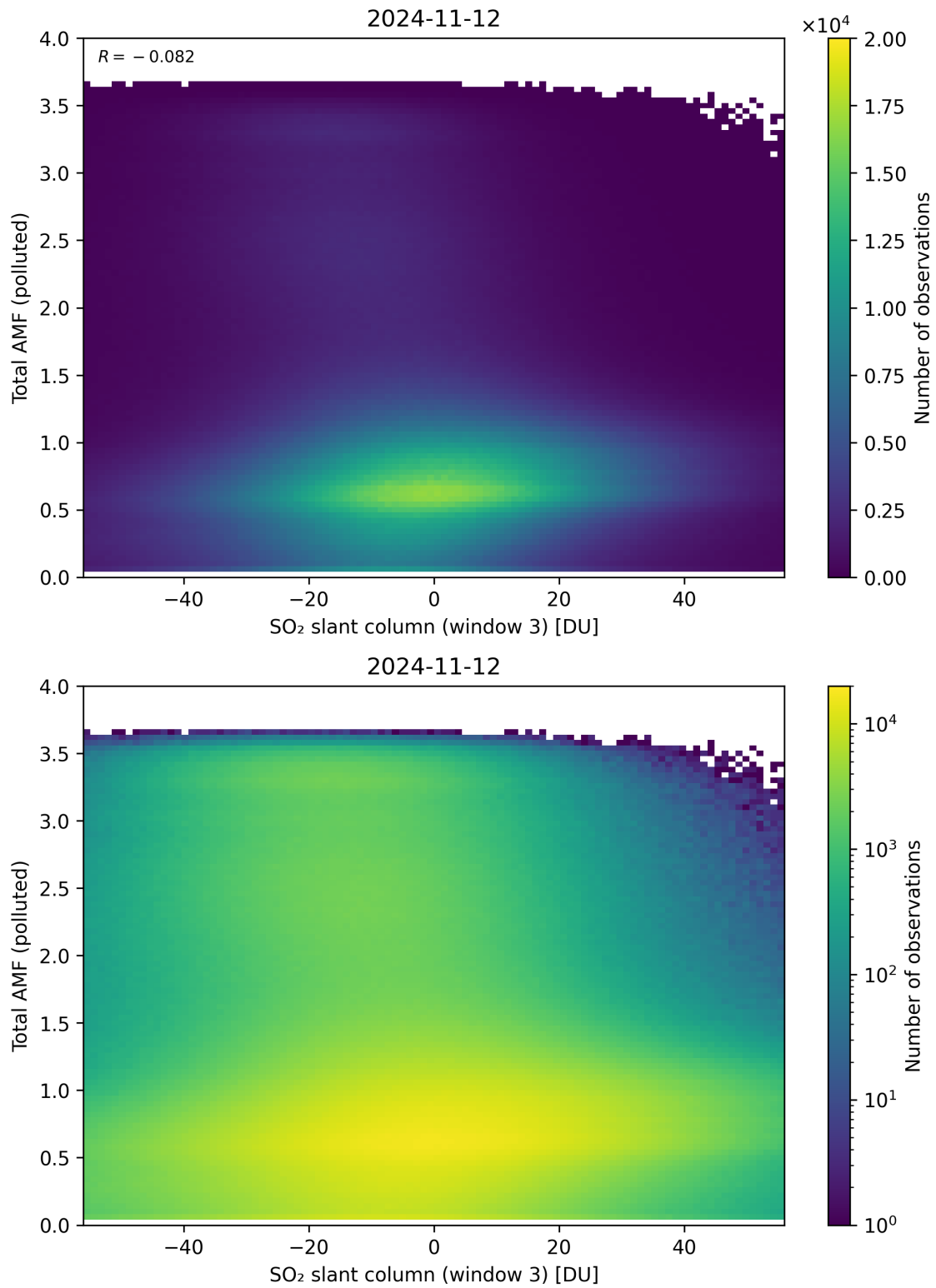
Figure 268: Scatter density plot of “SO 2 slant column (window 3)” against “Total AMF (polluted)” for 2024-11-11 to 2024-11-13.
