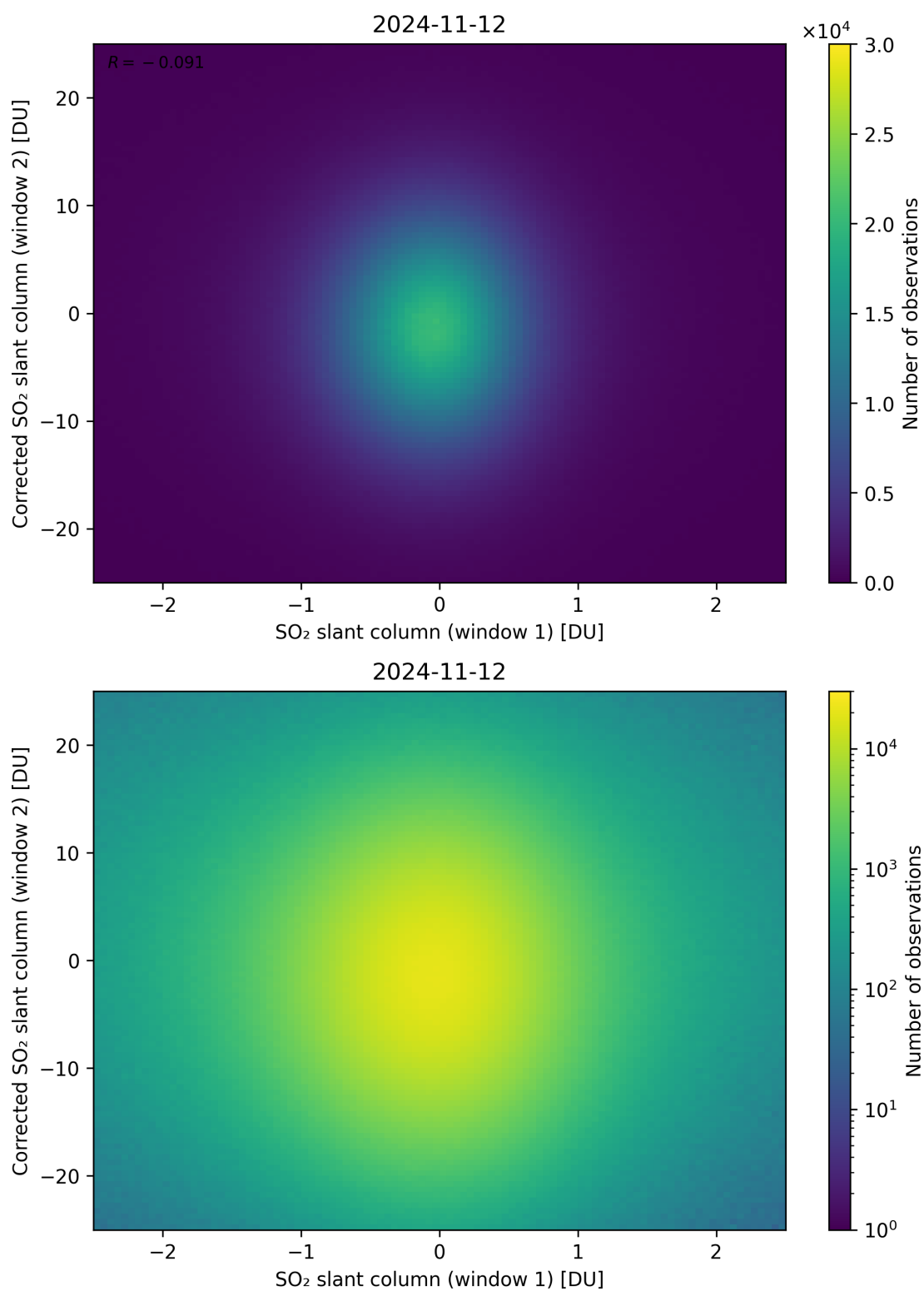
Figure 233: Scatter density plot of “SO 2 slant column (window 1)” against “Corrected SO 2 slant column (window 2)” for 2024-11-11 to 2024-11-13.
