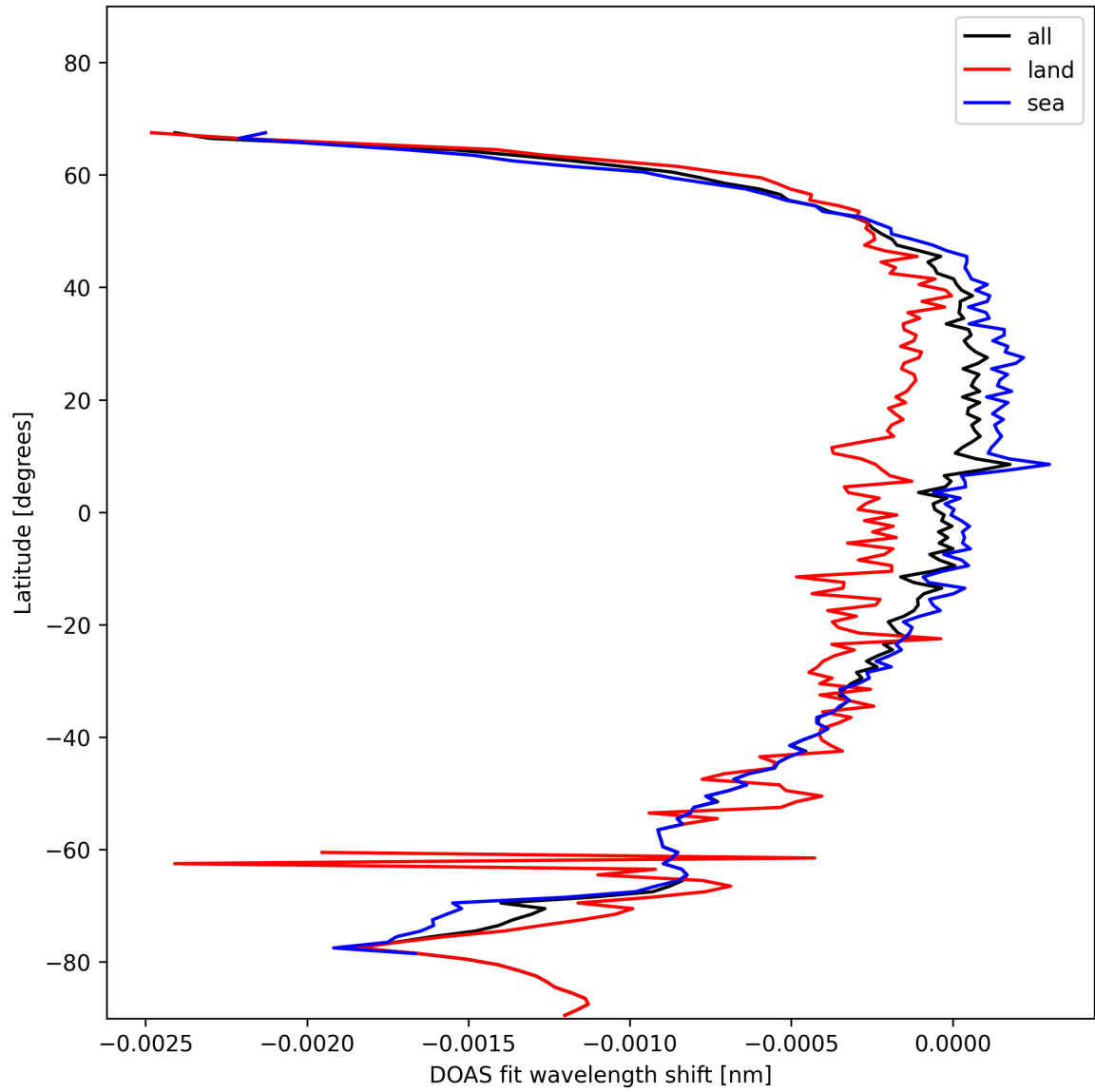
Figure 45: Zonal average of “DOAS fit wavelength shift” for 2024-11-11 to 2024-11-13.
