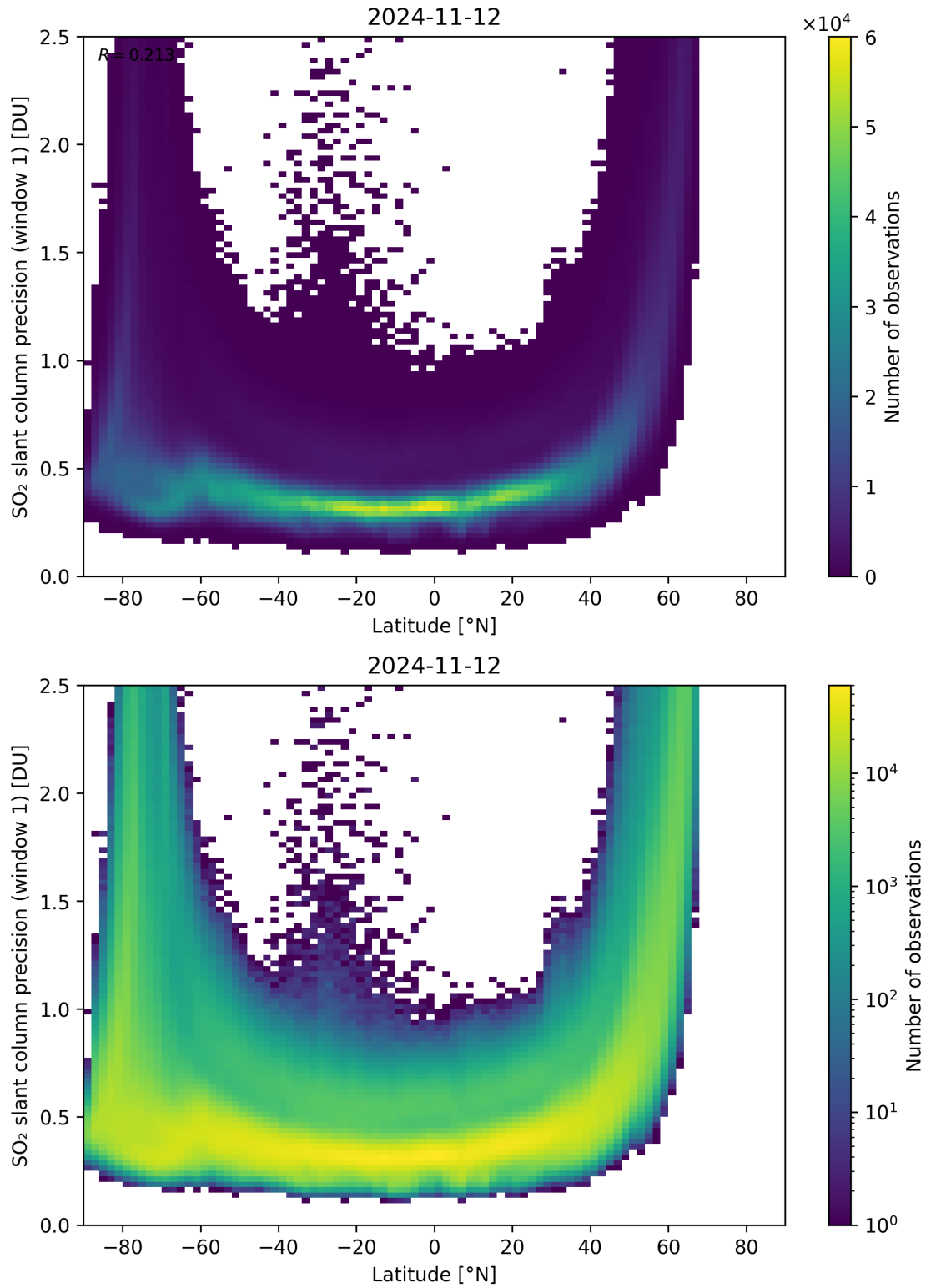
Figure 150: Scatter density plot of “Latitude” against “SO 2 slant column precision (window 1)” for 2024-11-11 to 2024-11-13.
