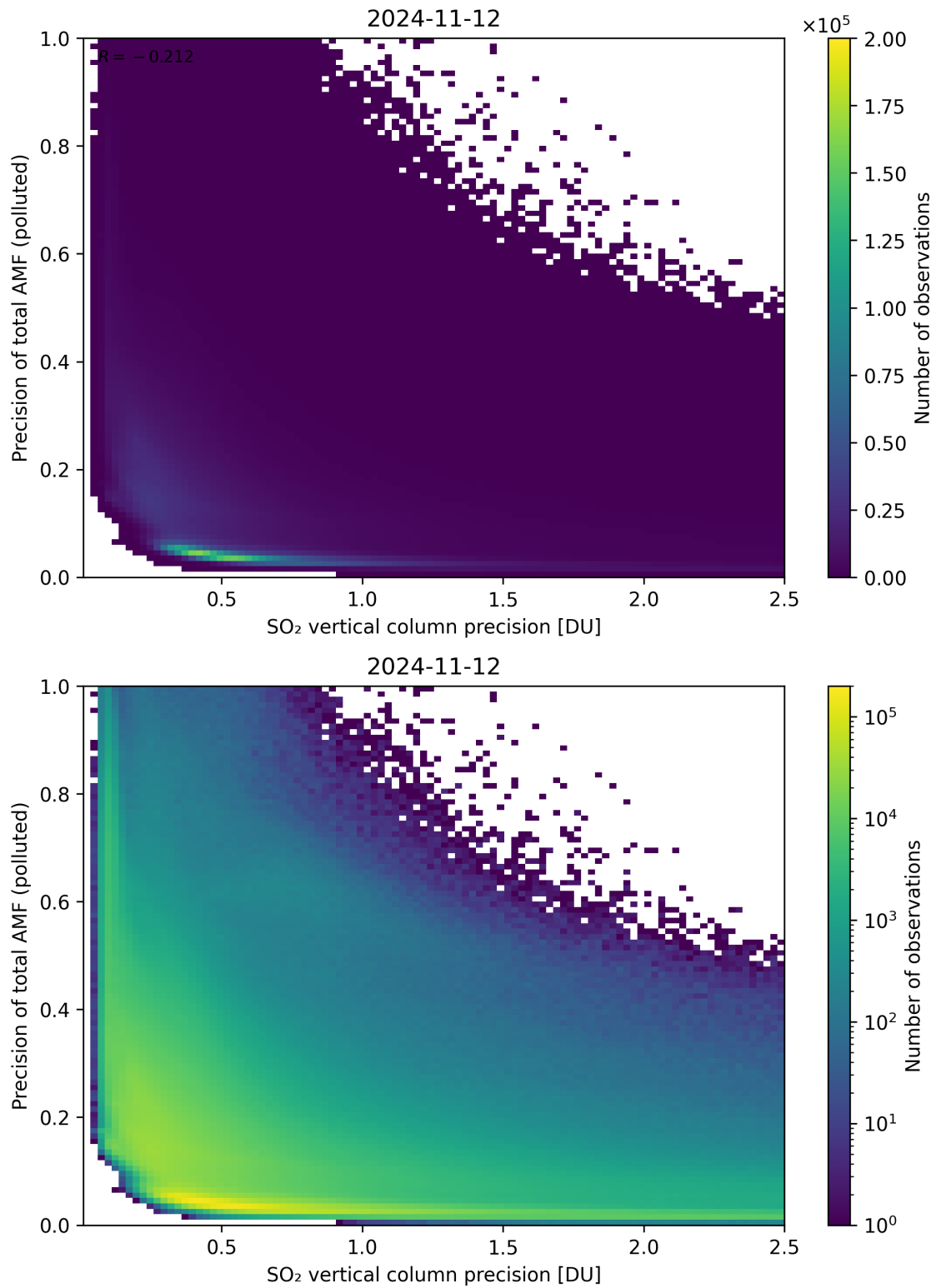
Figure 295: Scatter density plot of “SO 2 vertical column precision” against “Precision of total AMF (polluted)” for 2024-11-11 to 2024-11-13.
