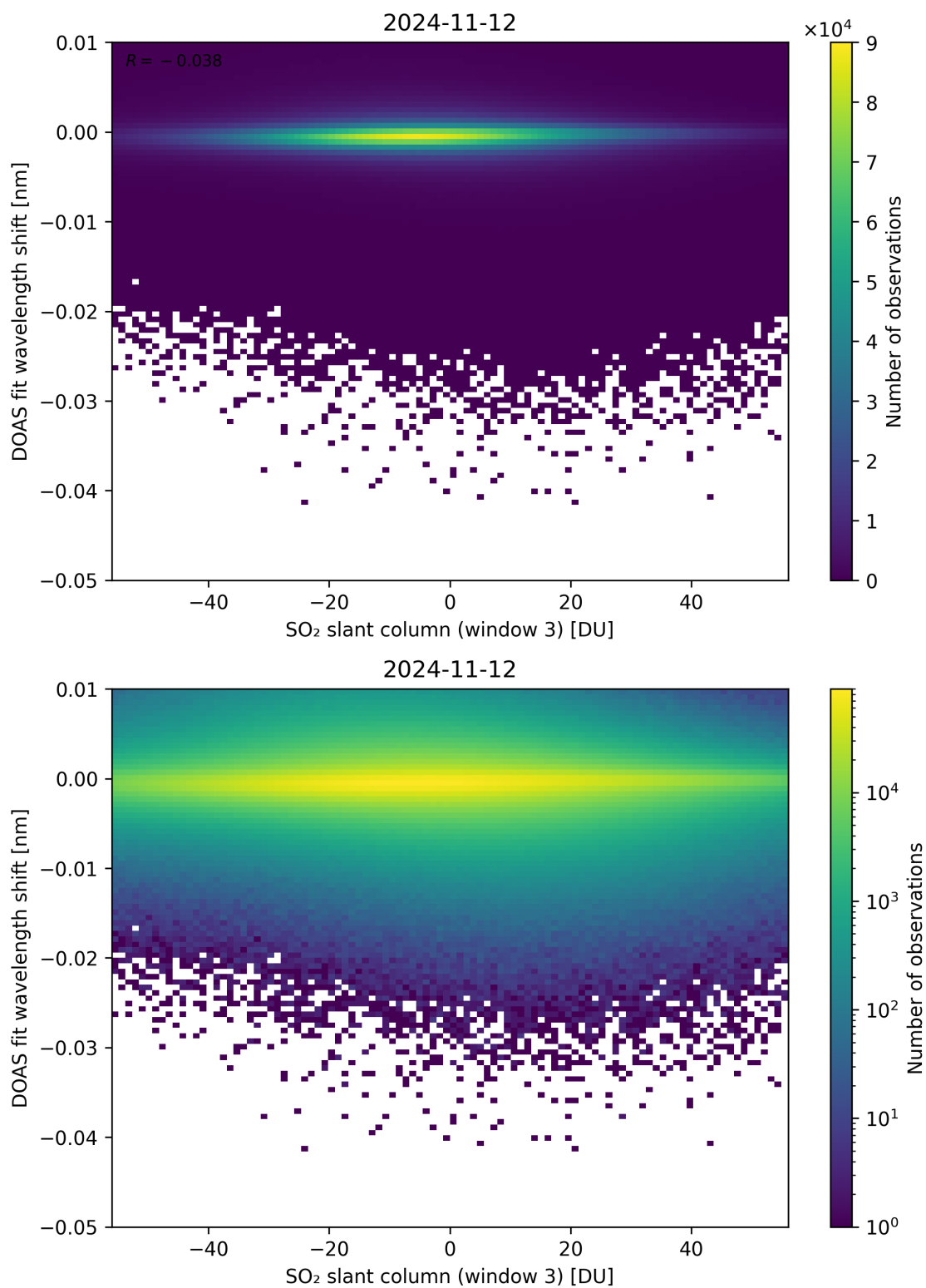
Figure 254: Scatter density plot of “SO 2 slant column (window 3)” against “DOAS fit wavelength shift” for 2024-11-11 to 2024-11-13.
