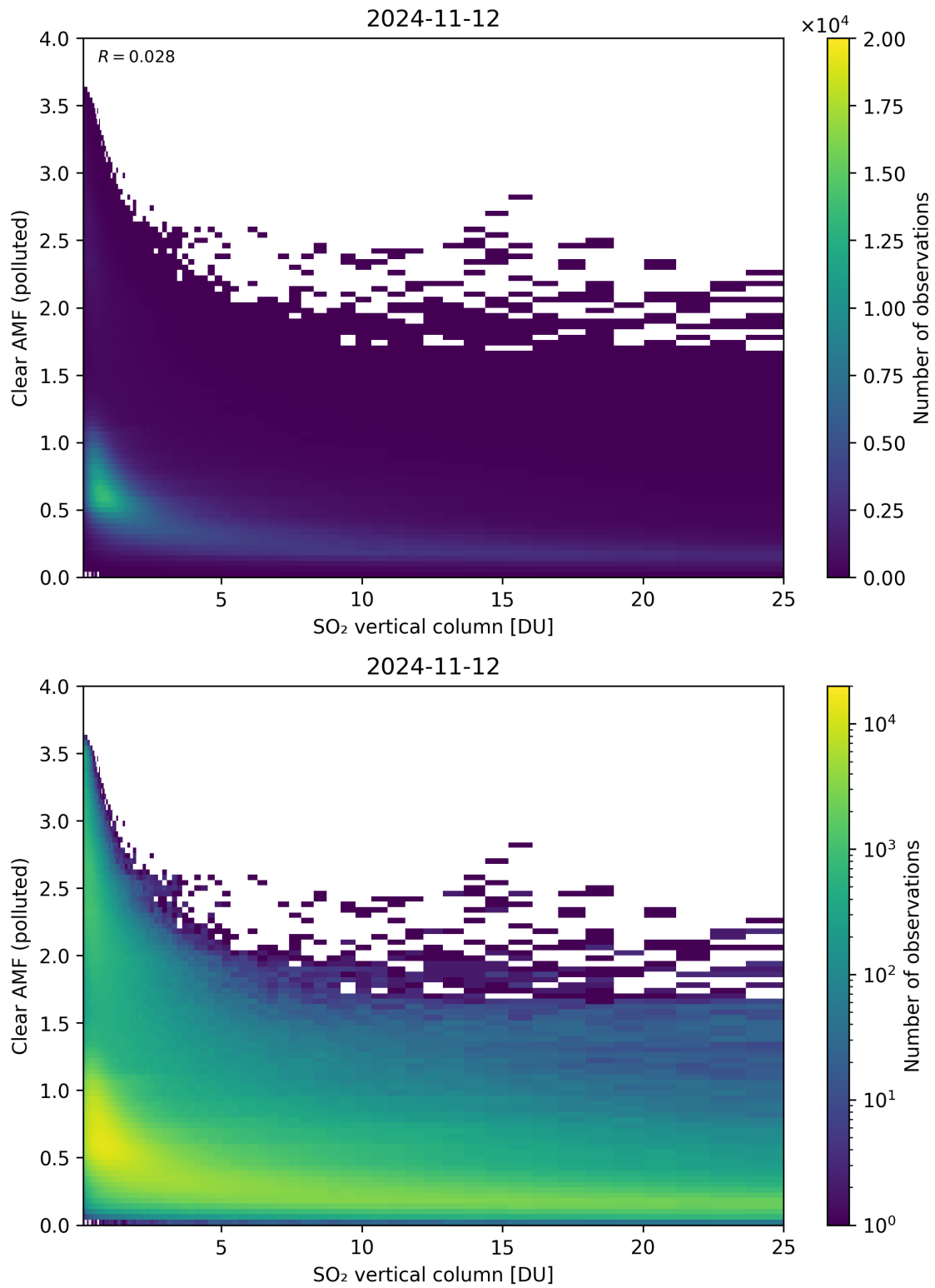
Figure 296: Scatter density plot of “SO 2 vertical column” against “Clear AMF (polluted)” for 2024-11-11 to 2024-11-13.
