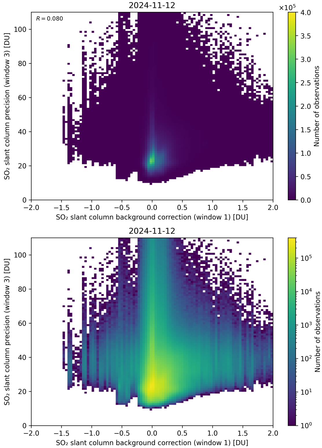
Figure 108: Scatter density plot of “SO 2 slant column background correction (window 1)” against “SO 2 slant column precision (window 3)” for 2024-11-11 to 2024-11-13.
