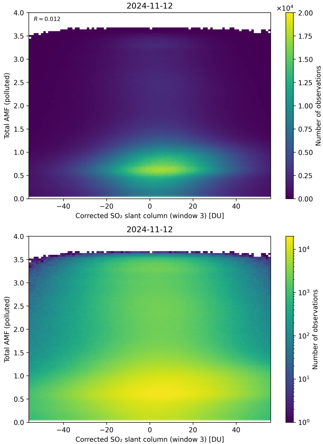
Figure 210: Scatter density plot of “Corrected SO 2 slant column (window 3)” against “Total AMF (polluted)” for 2024-11-11 to 2024-11-13.
