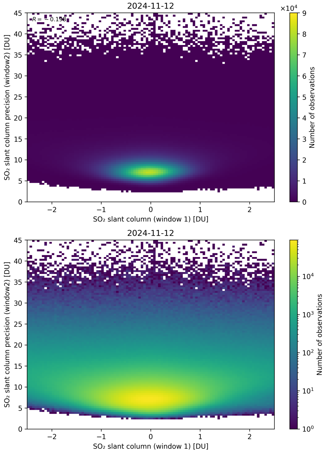
Figure 236: Scatter density plot of “SO 2 slant column (window 1)” against “SO 2 slant column precision (window2)” for 2024-11-11 to 2024-11-13.
