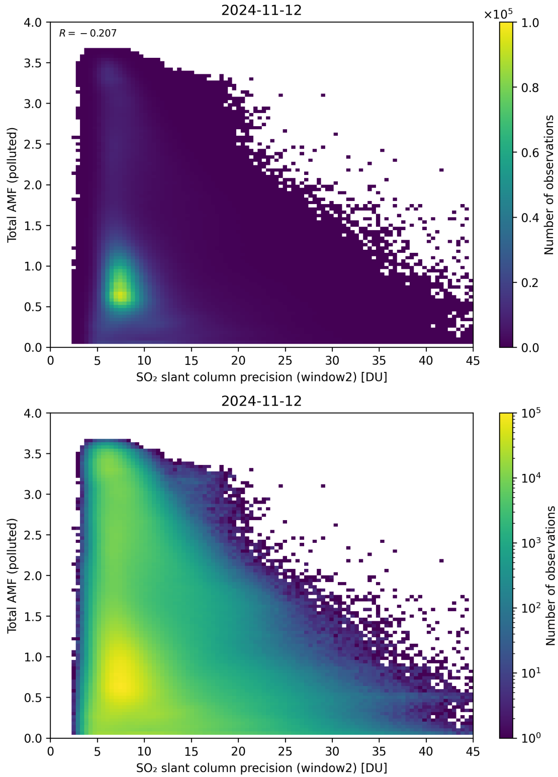
Figure 251: Scatter density plot of “SO 2 slant column precision (window2)” against “Total AMF (polluted)” for 2024-11-11 to 2024-11-13.
