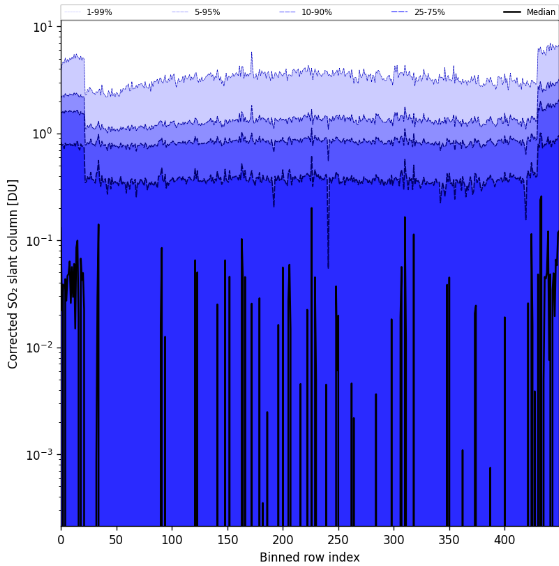
Figure 78: Along track statistics of “Corrected SO 2 slant column” for 2024-11-11 to 2024-11-13
