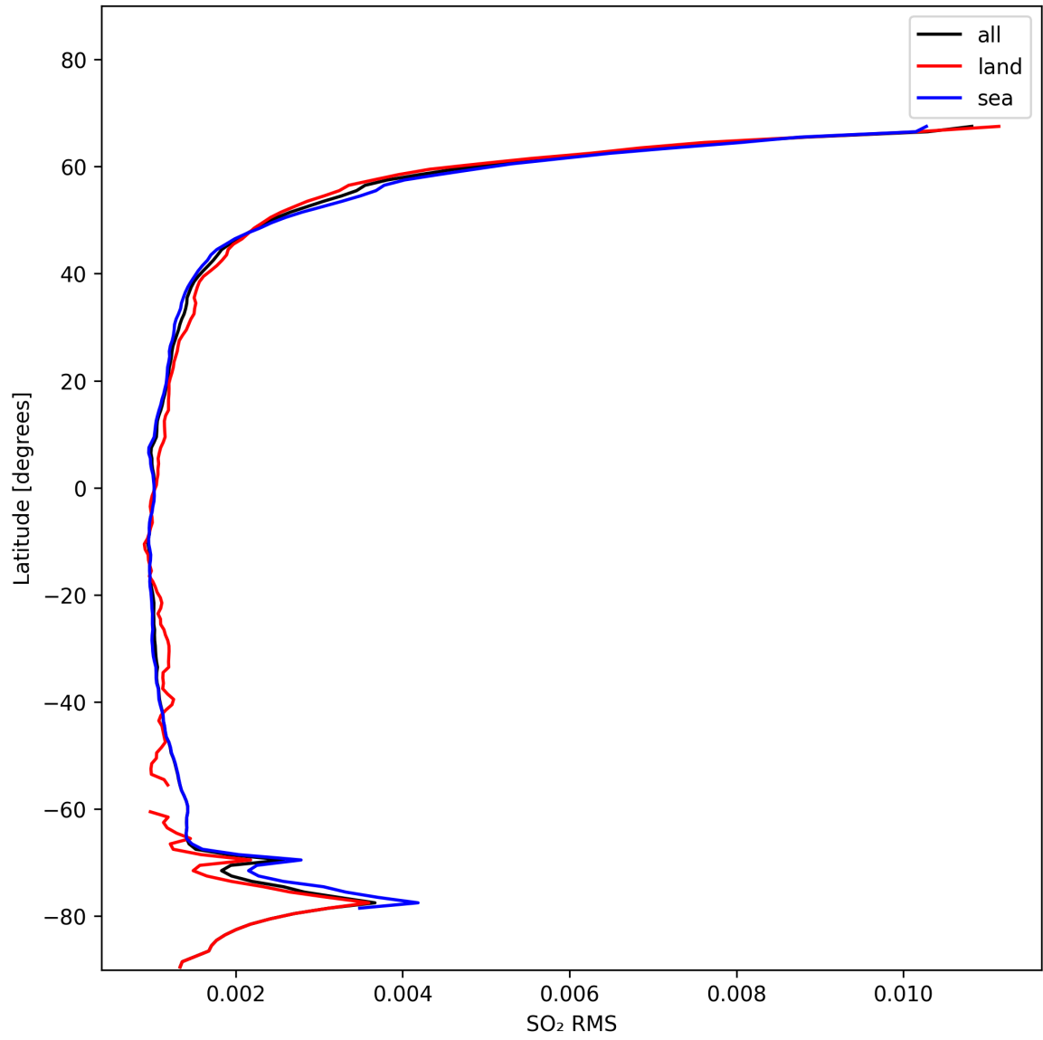
Figure 47: Zonal average of “SO 2 RMS” for 2024-11-11 to 2024-11-13.
