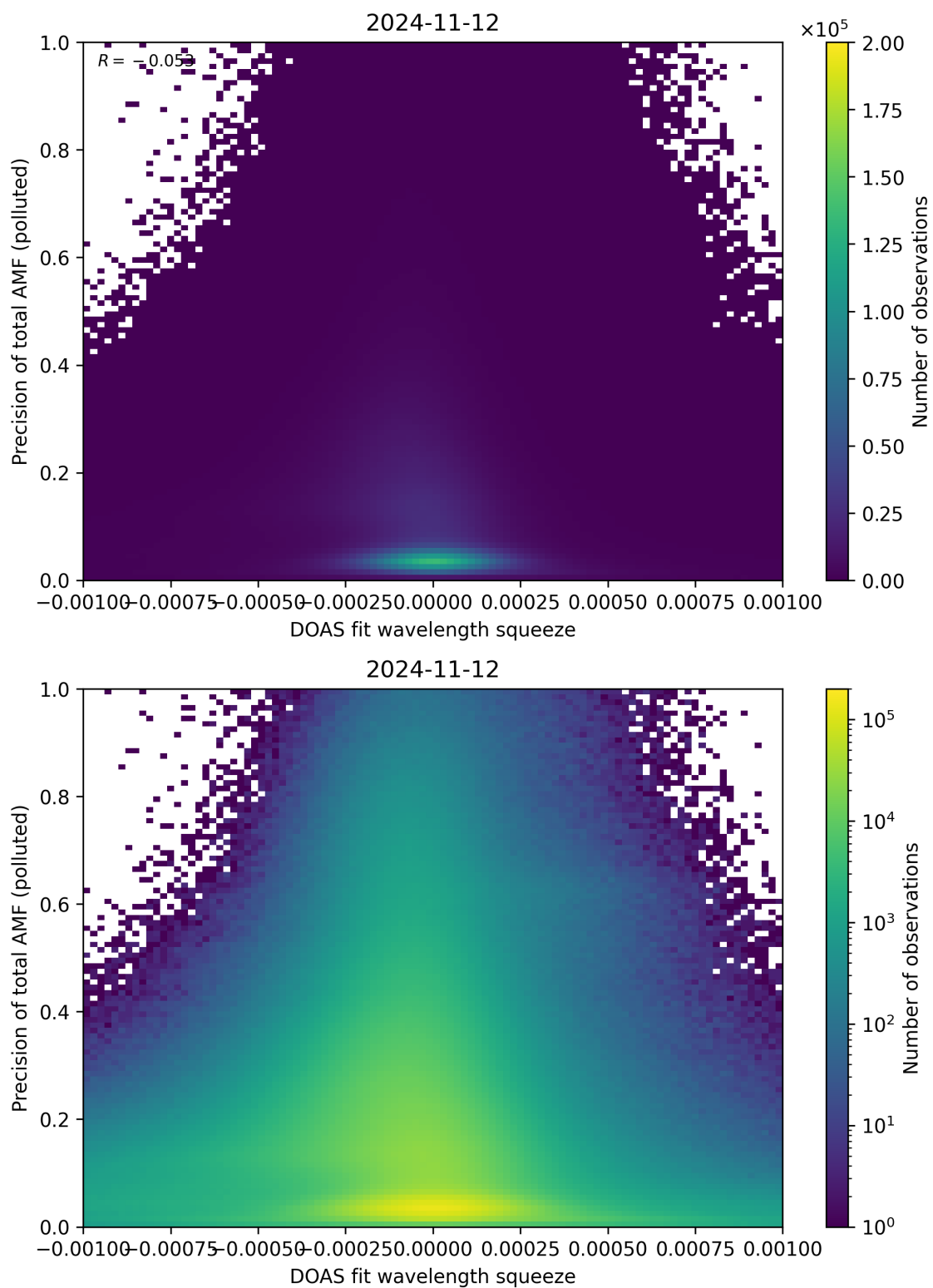
Figure 135: Scatter density plot of “DOAS fit wavelength squeeze” against “Precision of total AMF (polluted)” for 2024-11-11 to 2024-11-13.
