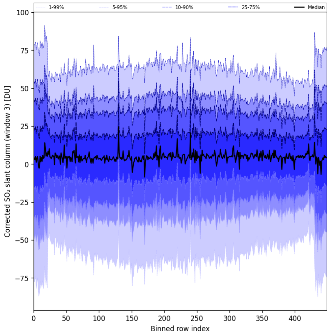
Figure 89: Along track statistics of “Corrected SO 2 slant column (window 3)” for 2024-11-11 to 2024-11-13
