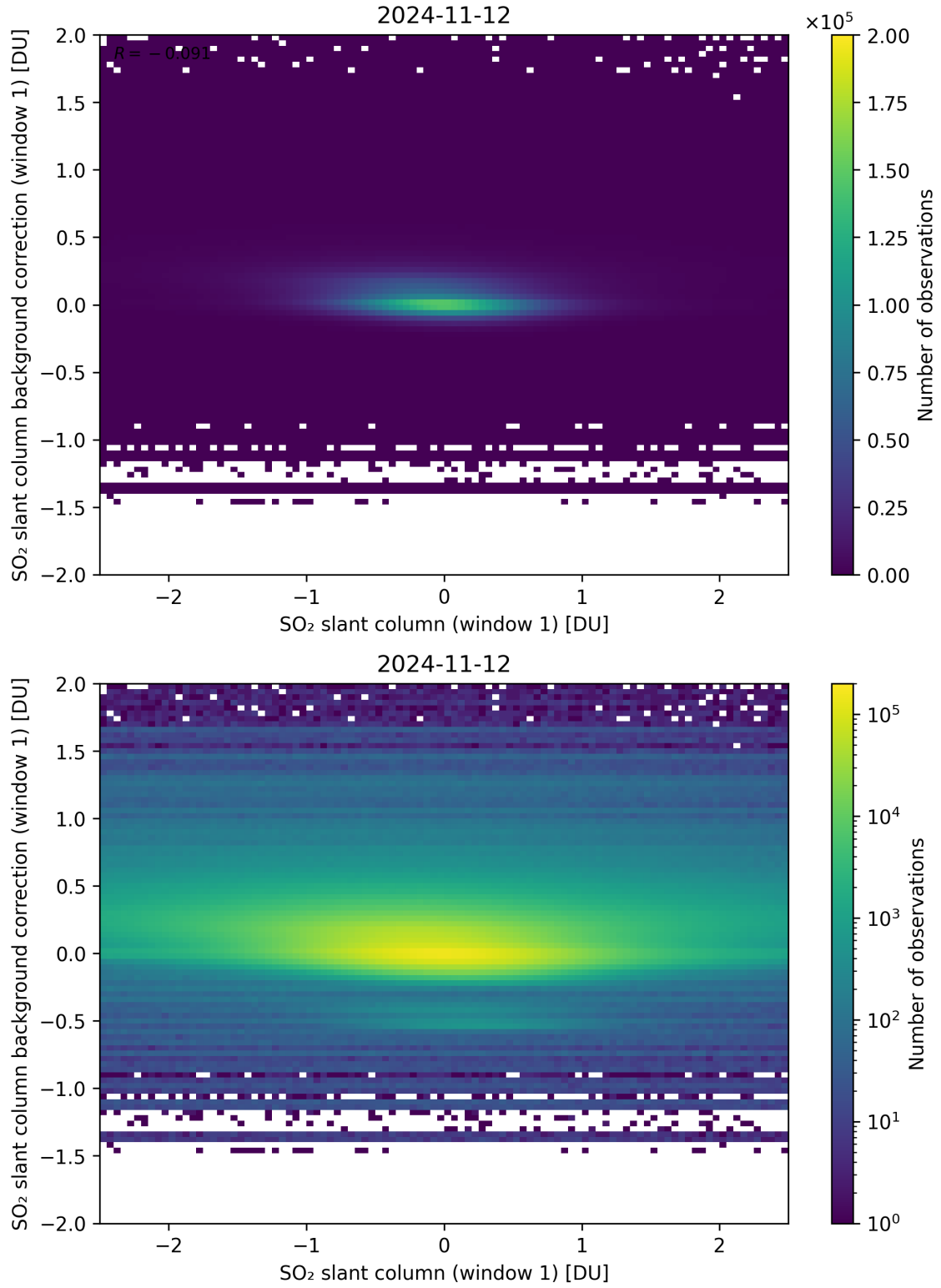
Figure 212: Scatter density plot of “SO 2 slant column (window 1)” against “SO 2 slant column background correction (window 1)” for 2024-11-11 to 2024-11-13.
