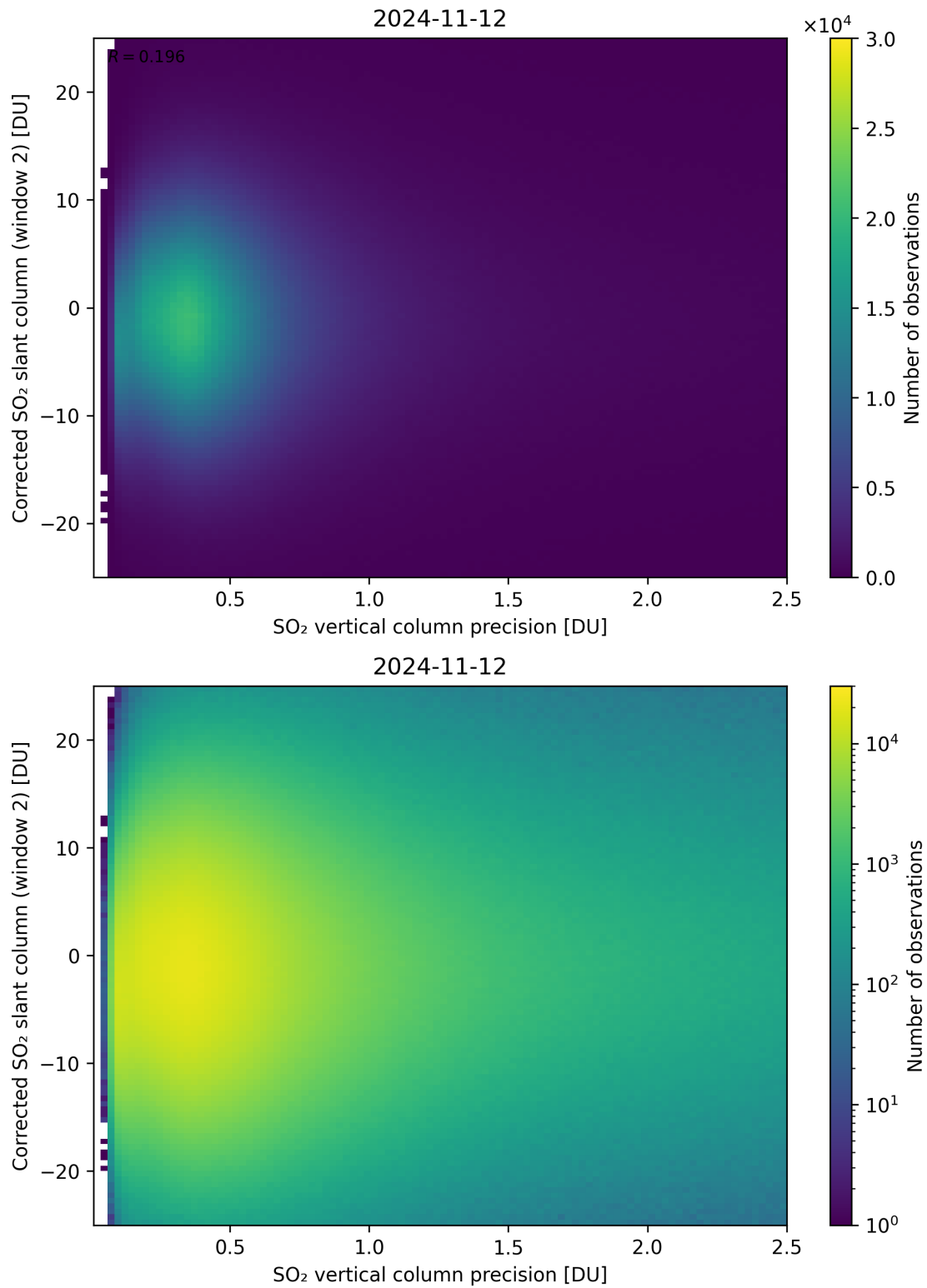
Figure 287: Scatter density plot of “SO 2 vertical column precision” against “Corrected SO 2 slant column (window 2)” for 2024-11-11 to 2024-11-13.
