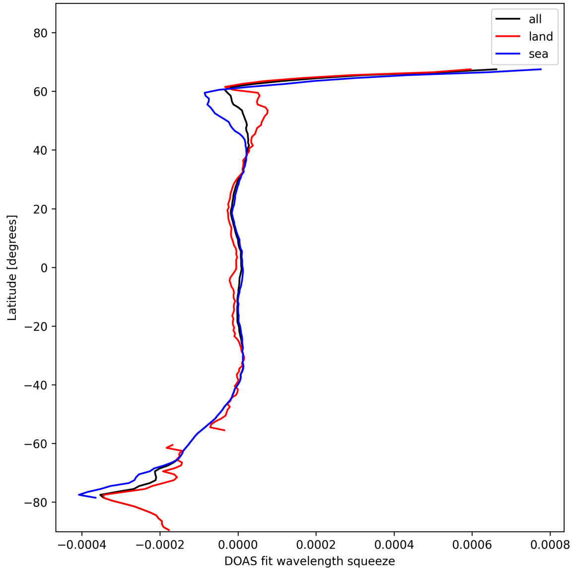
Figure 46: Zonal average of “DOAS fit wavelength squeeze” for 2024-11-11 to 2024-11-13.
