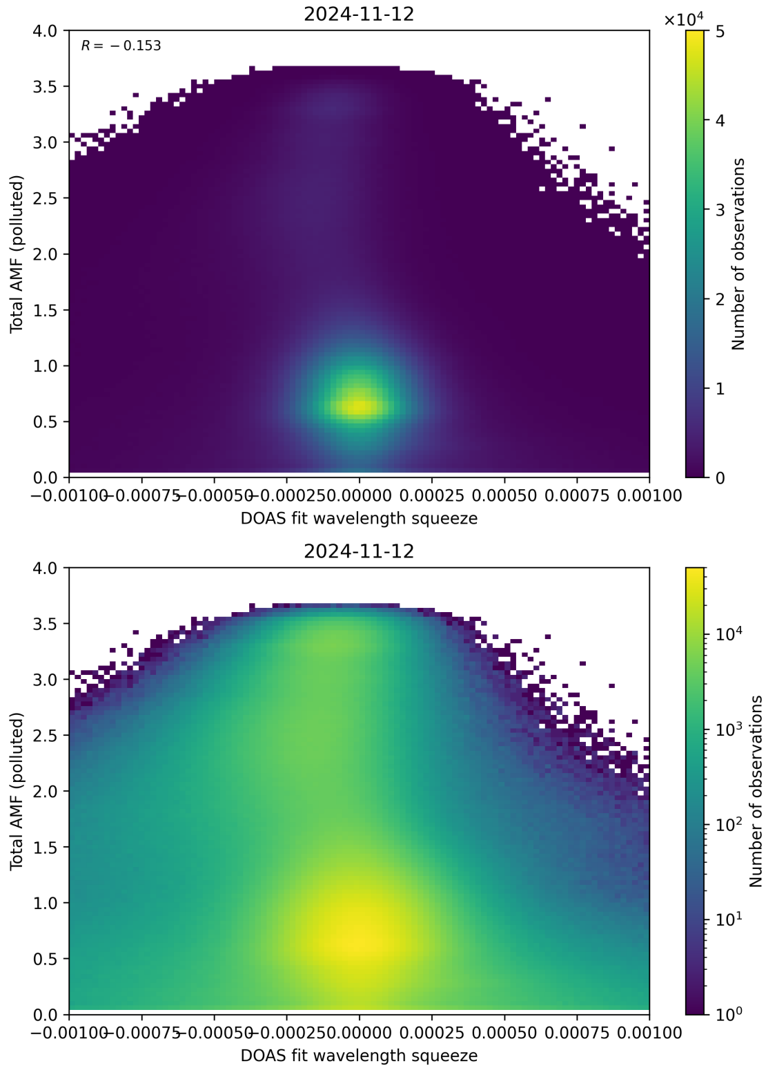
Figure 134: Scatter density plot of “DOAS fit wavelength squeeze” against “Total AMF (polluted)” for 2024-11-11 to 2024-11-13.
