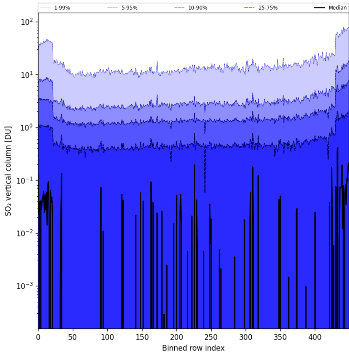
Figure 76: Along track statistics of “SO 2 vertical column” for 2024-11-11 to 2024-11-13
