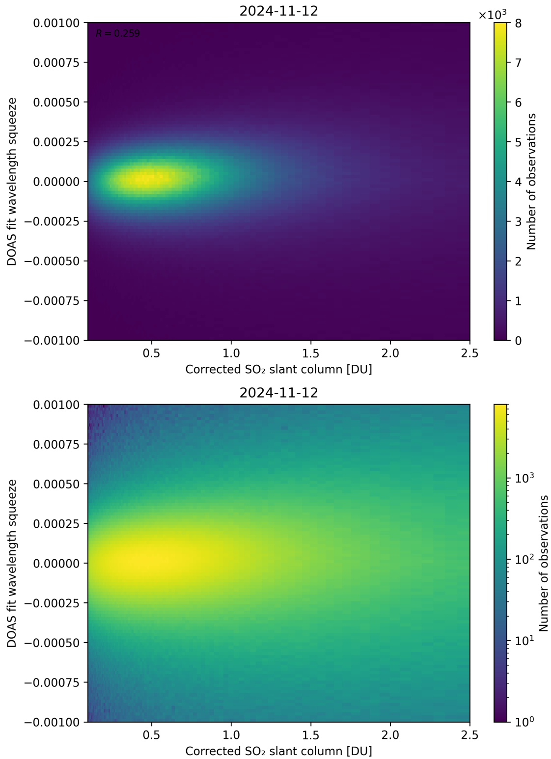
Figure 182: Scatter density plot of “Corrected SO 2 slant column” against “DOAS fit wavelength squeeze” for 2024-11-11 to 2024-11-13.
