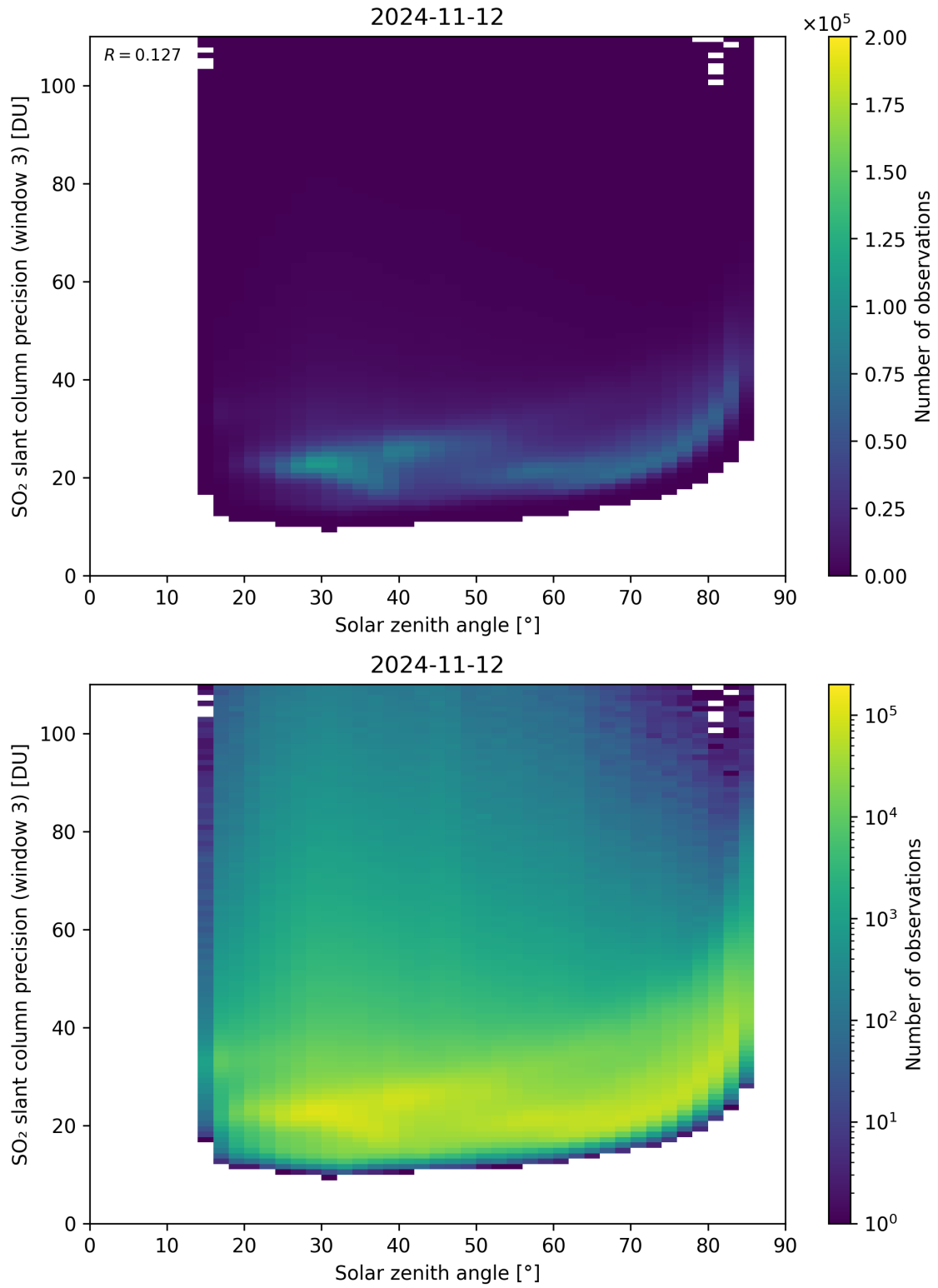
Figure 173: Scatter density plot of “Solar zenith angle” against “SO 2 slant column precision (window 3)” for 2024-11-11 to 2024-11-13.
