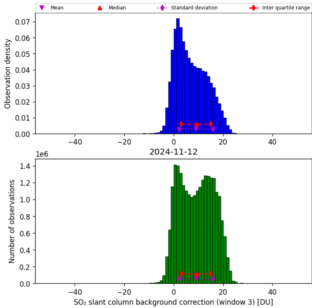
Figure 67: Histogram of “SO 2 slant column background correction (window 3)” for 2024-11-11 to 2024-11-13
