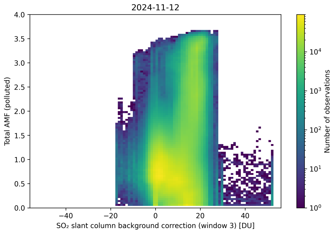
Figure 125: Scatter density plot of “SO 2 slant column background correction (window 3)” against “Total AMF (polluted)” for 2024-11-11 to 2024-11-13.
