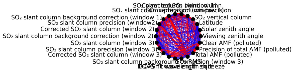
Figure 1: Map of correlation graph for 2024-11-11 to 2024-11-13.
