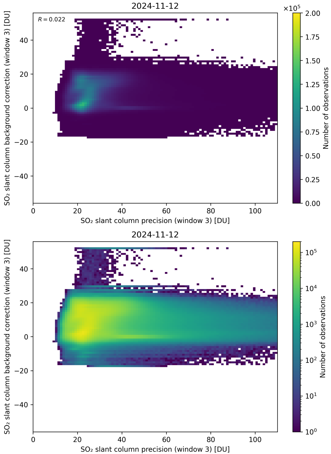
Figure 257: Scatter density plot of “SO 2 slant column precision (window 3)” against “SO 2 slant column background correction (window 3)” for 2024-11-11 to 2024-11-13.
