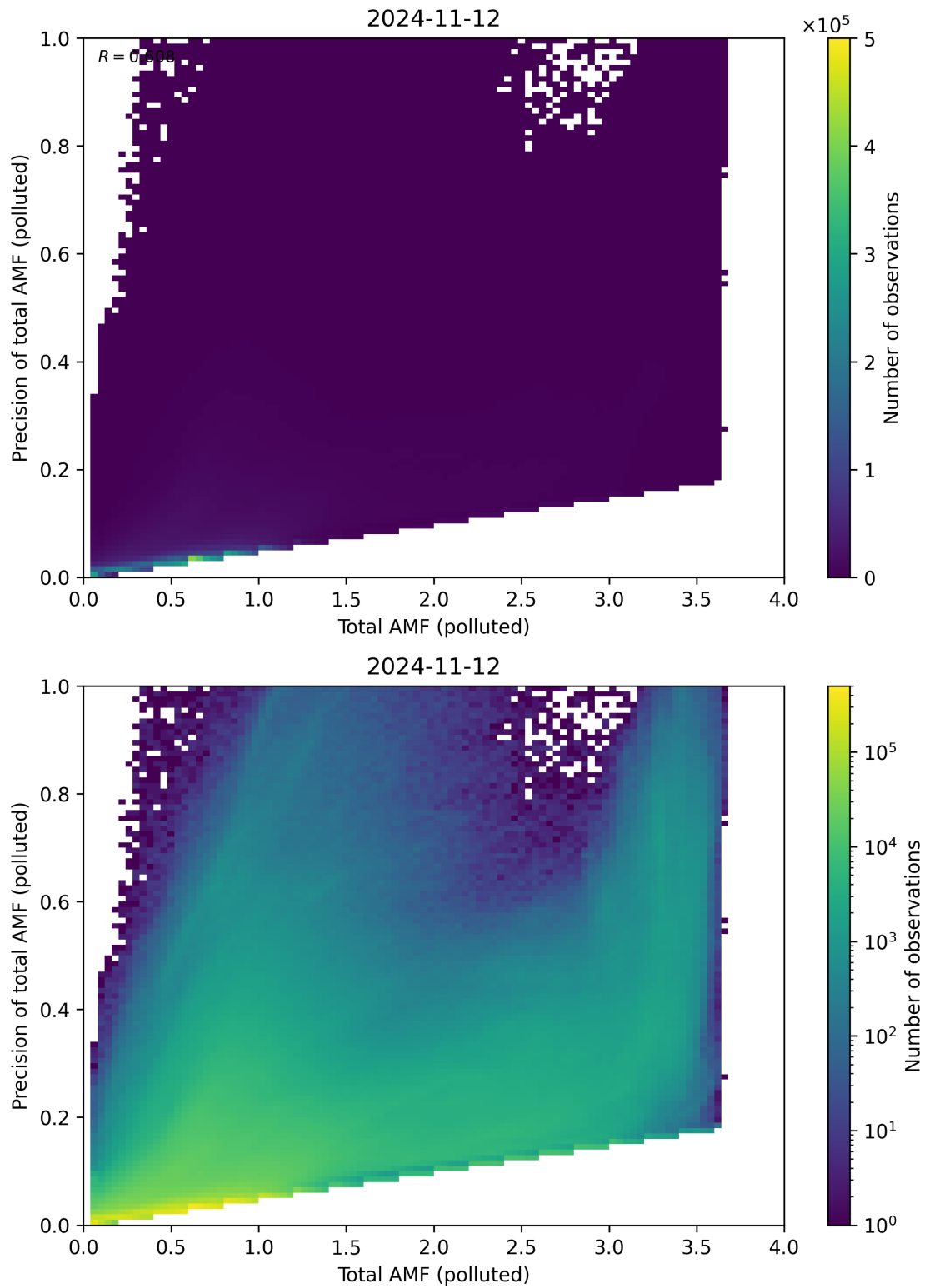
Figure 272: Scatter density plot of “Total AMF (polluted)” against “Precision of total AMF (polluted)” for 2024-11-11 to 2024-11-13.
