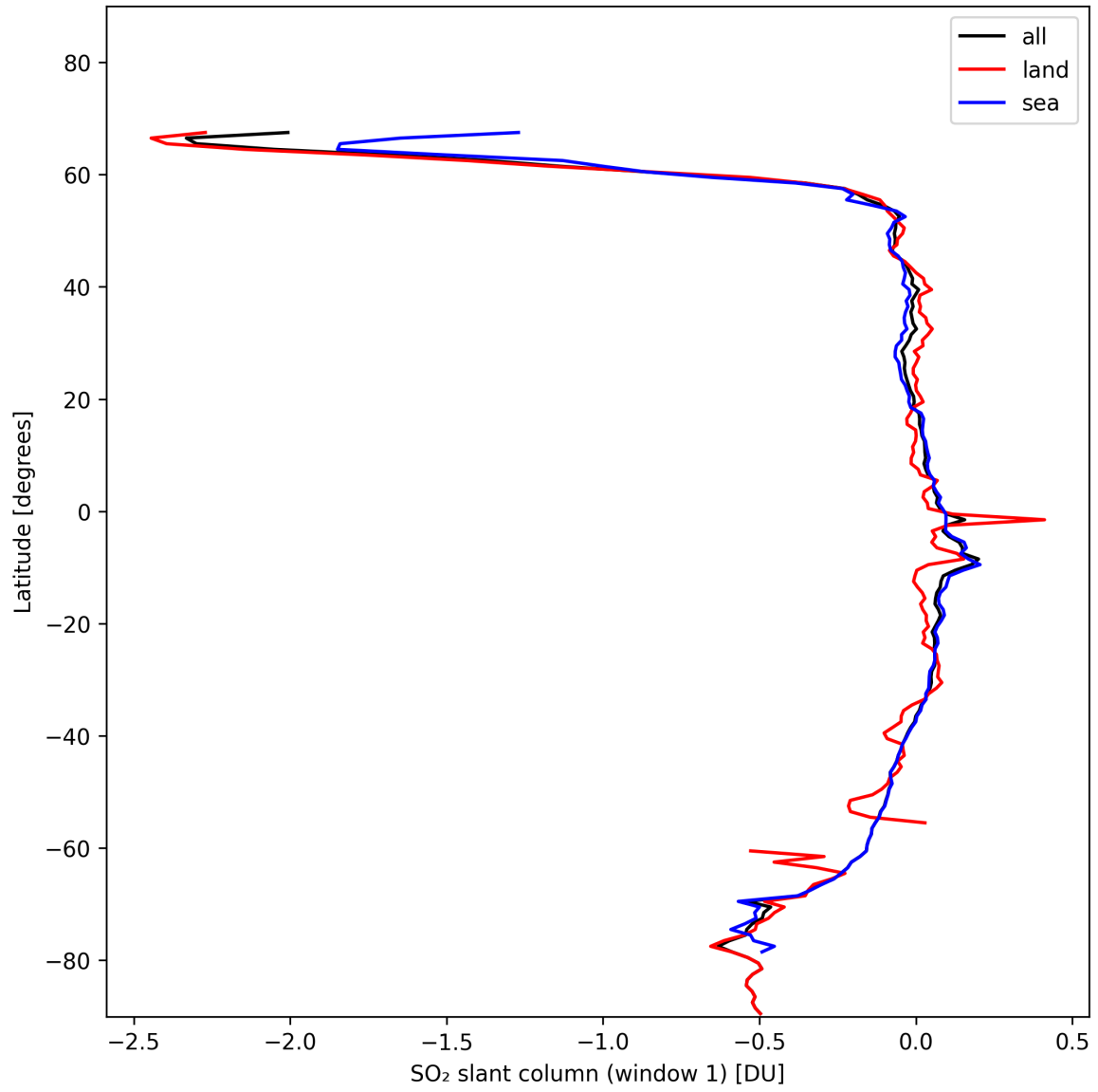
Figure 33: Zonal average of “SO 2 slant column (window 1)” for 2024-11-11 to 2024-11-13.
