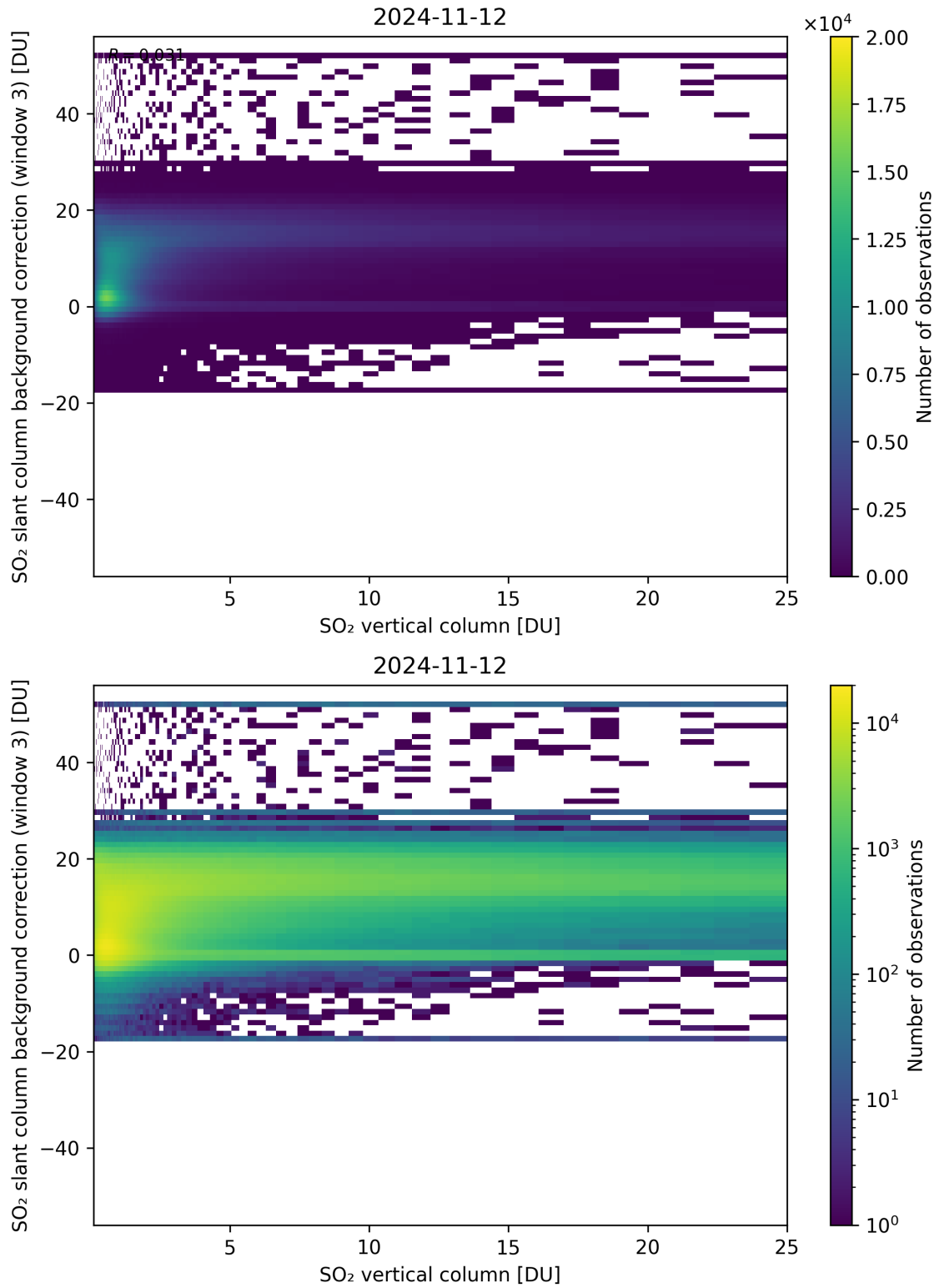
Figure 275: Scatter density plot of “SO 2 vertical column” against “SO 2 slant column background correction (window 3)” for 2024-11-11 to 2024-11-13.
