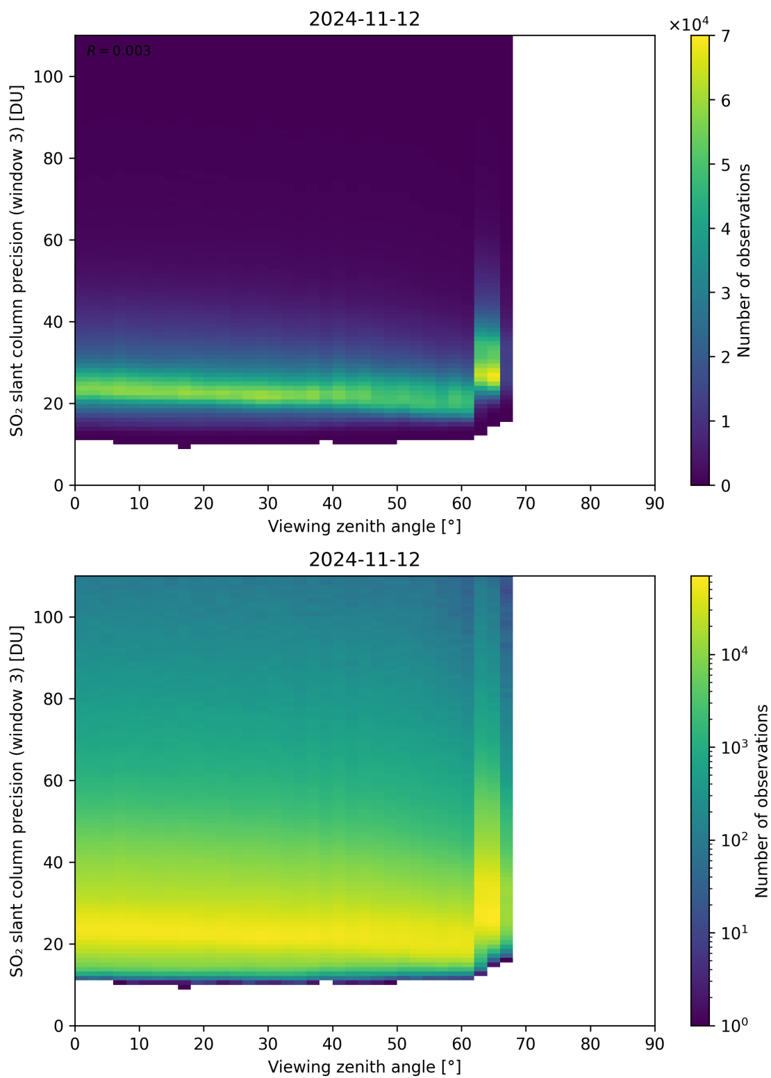
Figure 324: Scatter density plot of “Viewing zenith angle” against “SO 2 slant column precision (window 3)” for 2024-11-11 to 2024-11-13.
