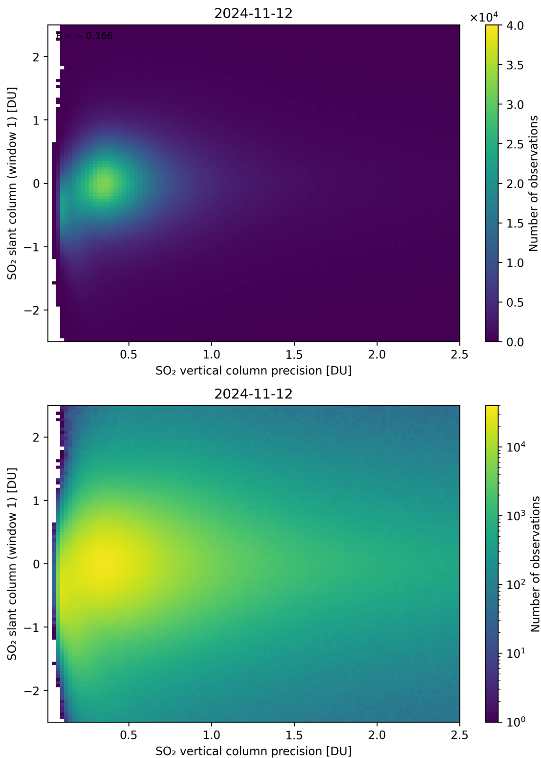
Figure 289: Scatter density plot of “SO 2 vertical column precision” against “SO 2 slant column (window 1)” for 2024-11-11 to 2024-11-13.
