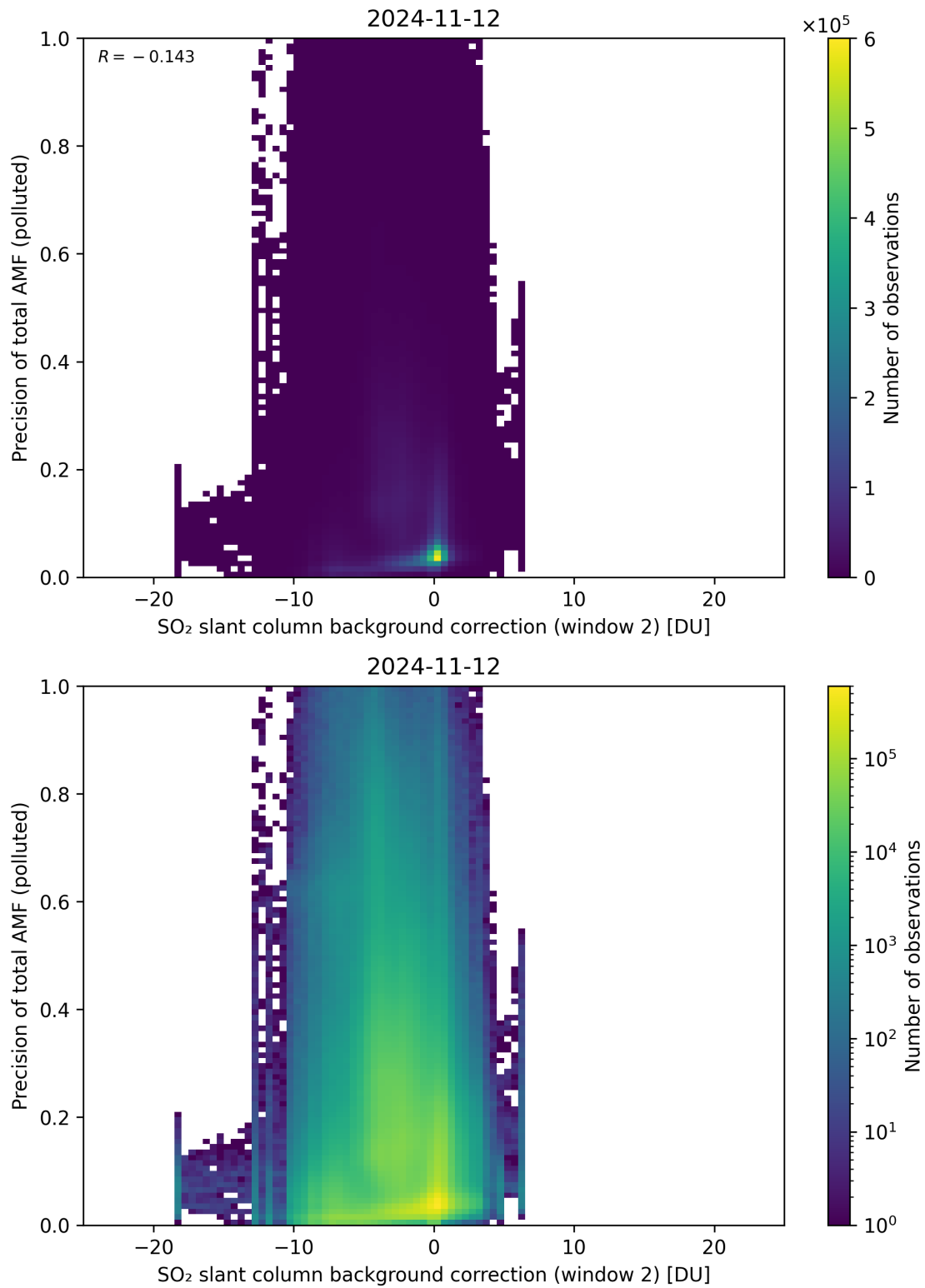
Figure 120: Scatter density plot of “SO 2 slant column background correction (window 2)” against “Precision of total AMF (polluted)” for 2024-11-11 to 2024-11-13.
