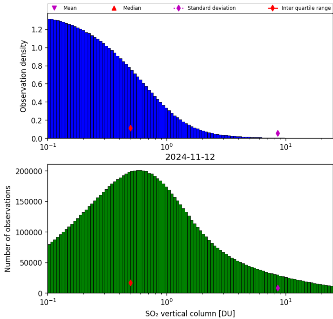
Figure 53: Histogram of “SO 2 vertical column” for 2024-11-11 to 2024-11-13
