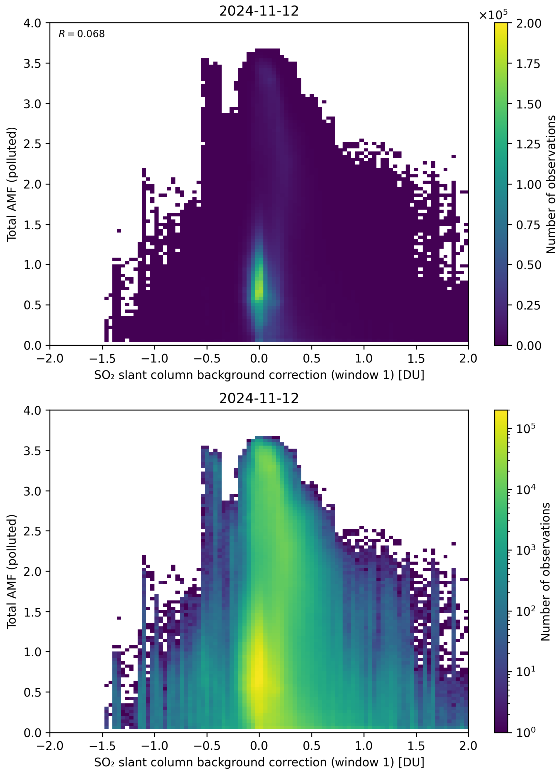
Figure 109: Scatter density plot of “SO 2 slant column background correction (window 1)” against “Total AMF (polluted)” for 2024-11-11 to 2024-11-13.
