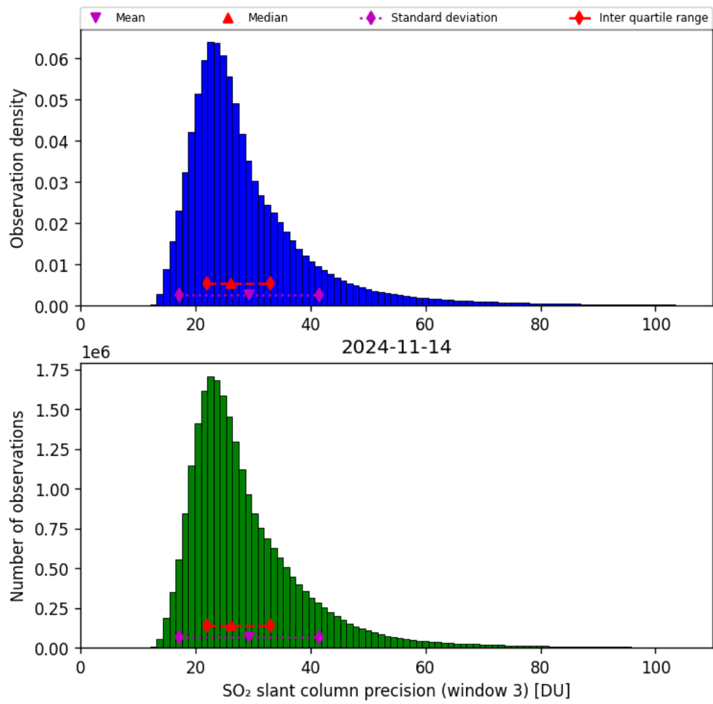
Figure 65: Histogram of “SO 2 slant column precision (window 3)” for 2024-11-14 to 2024-11-15
