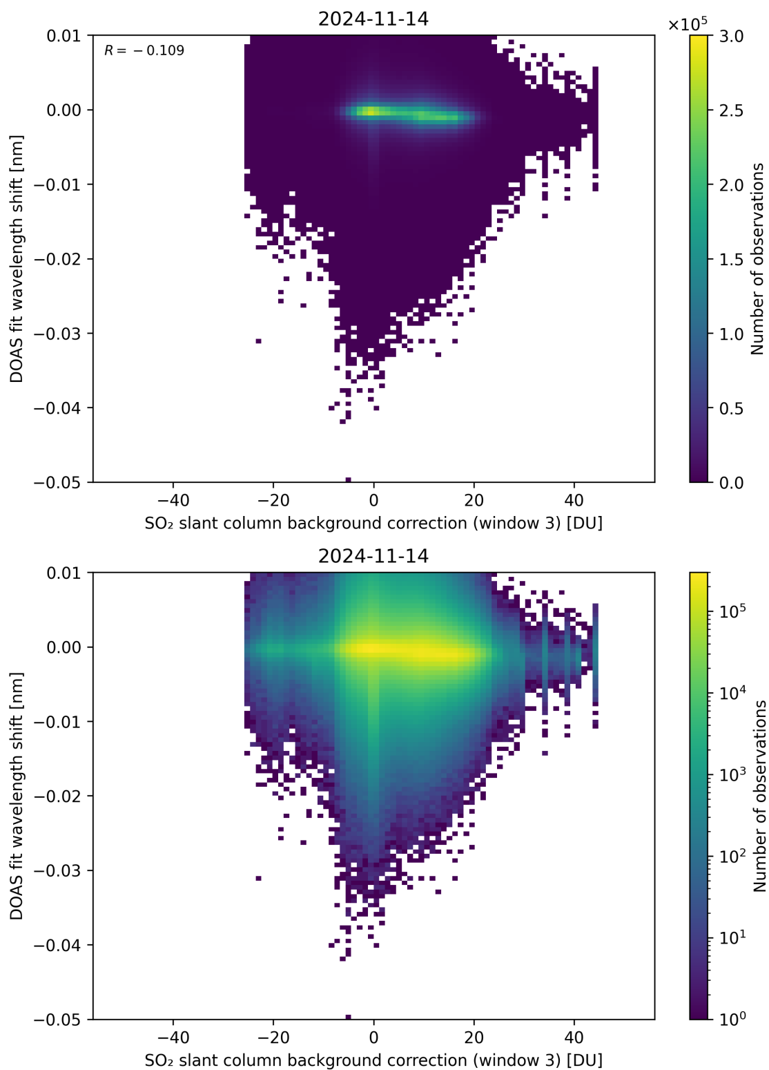
Figure 121: Scatter density plot of “SO 2 slant column background correction (window 3)” against “DOAS fit wavelength shift” for 2024-11-14 to 2024-11-15.
