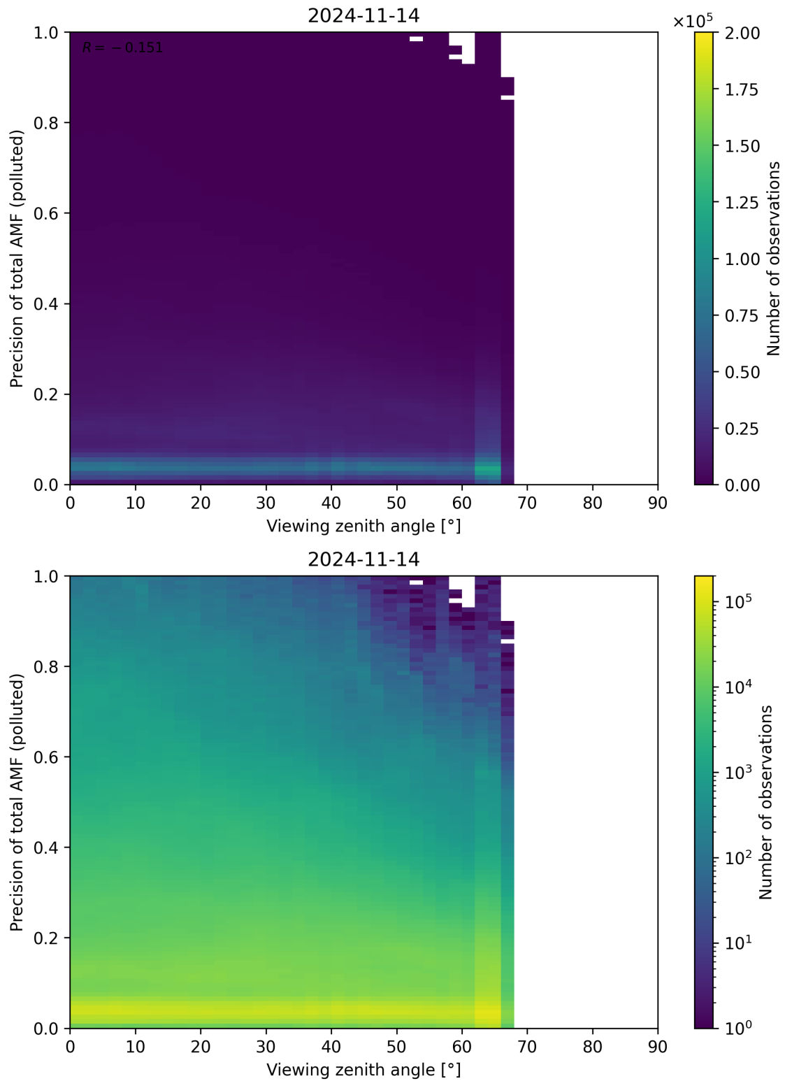
Figure 326: Scatter density plot of “Viewing zenith angle” against “Precision of total AMF (polluted)” for 2024-11-14 to 2024-11-15.
