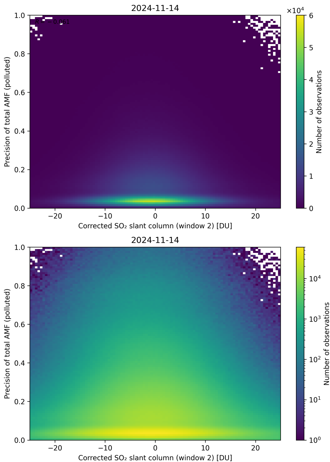
Figure 204: Scatter density plot of “Corrected SO 2 slant column (window 2)” against “Precision of total AMF (polluted)” for 2024-11-14 to 2024-11-15.
