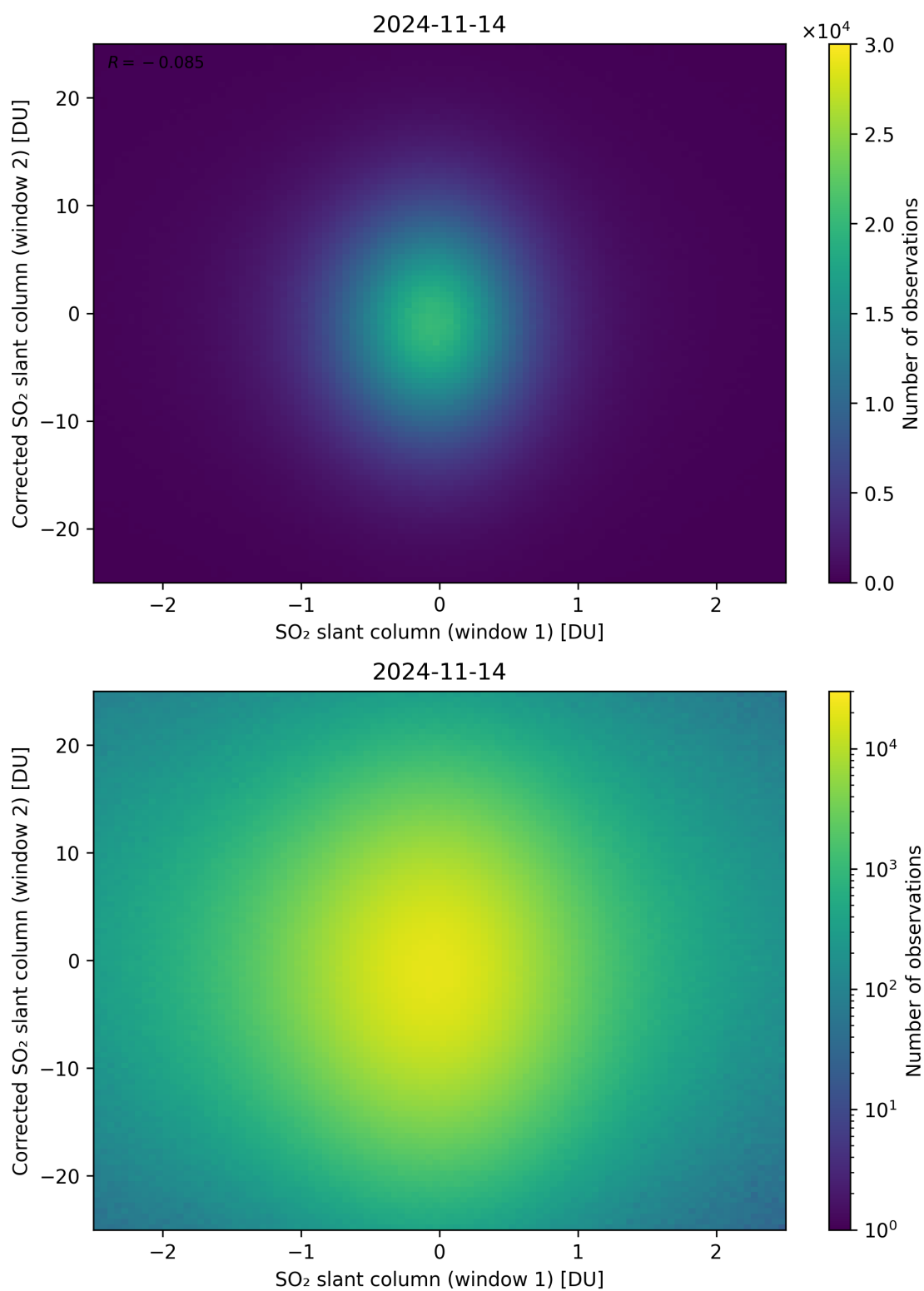
Figure 233: Scatter density plot of “SO 2 slant column (window 1)” against “Corrected SO 2 slant column (window 2)” for 2024-11-14 to 2024-11-15.
