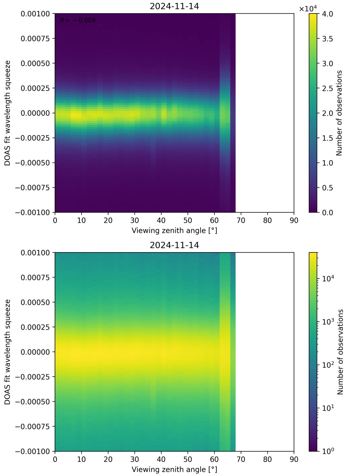
Figure 312: Scatter density plot of “Viewing zenith angle” against “DOAS fit wavelength squeeze” for 2024-11-14 to 2024-11-15.
