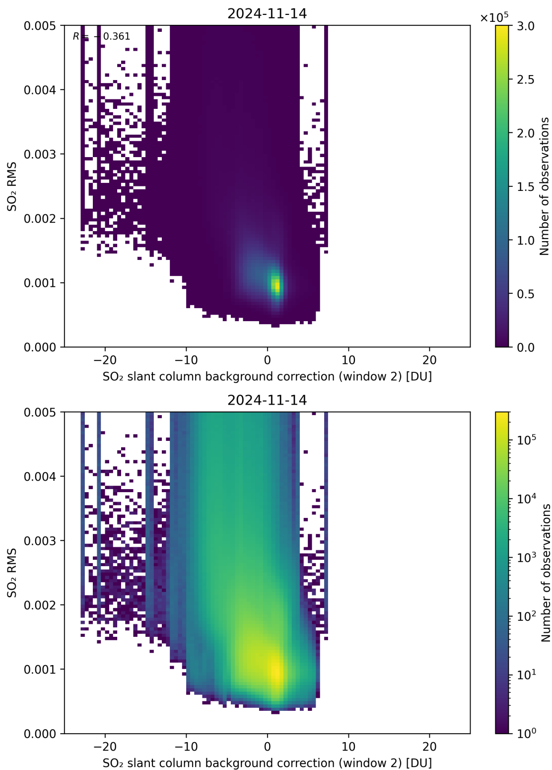
Figure 114: Scatter density plot of “SO 2 slant column background correction (window 2)” against “SO 2 RMS” for 2024-11-14 to 2024-11-15.
