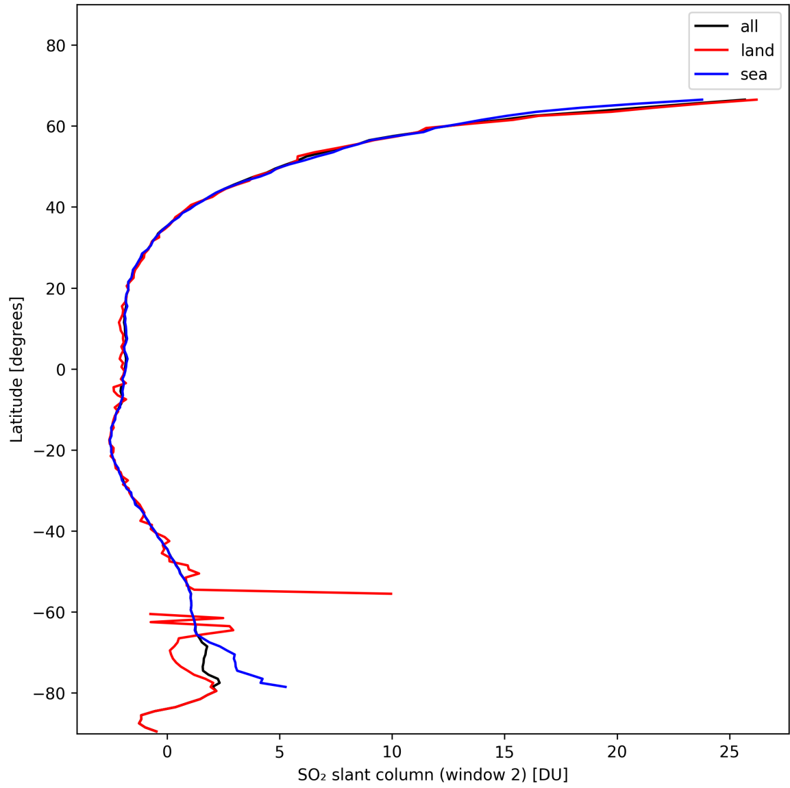
Figure 37: Zonal average of “SO 2 slant column (window 2)” for 2024-11-14 to 2024-11-15.
