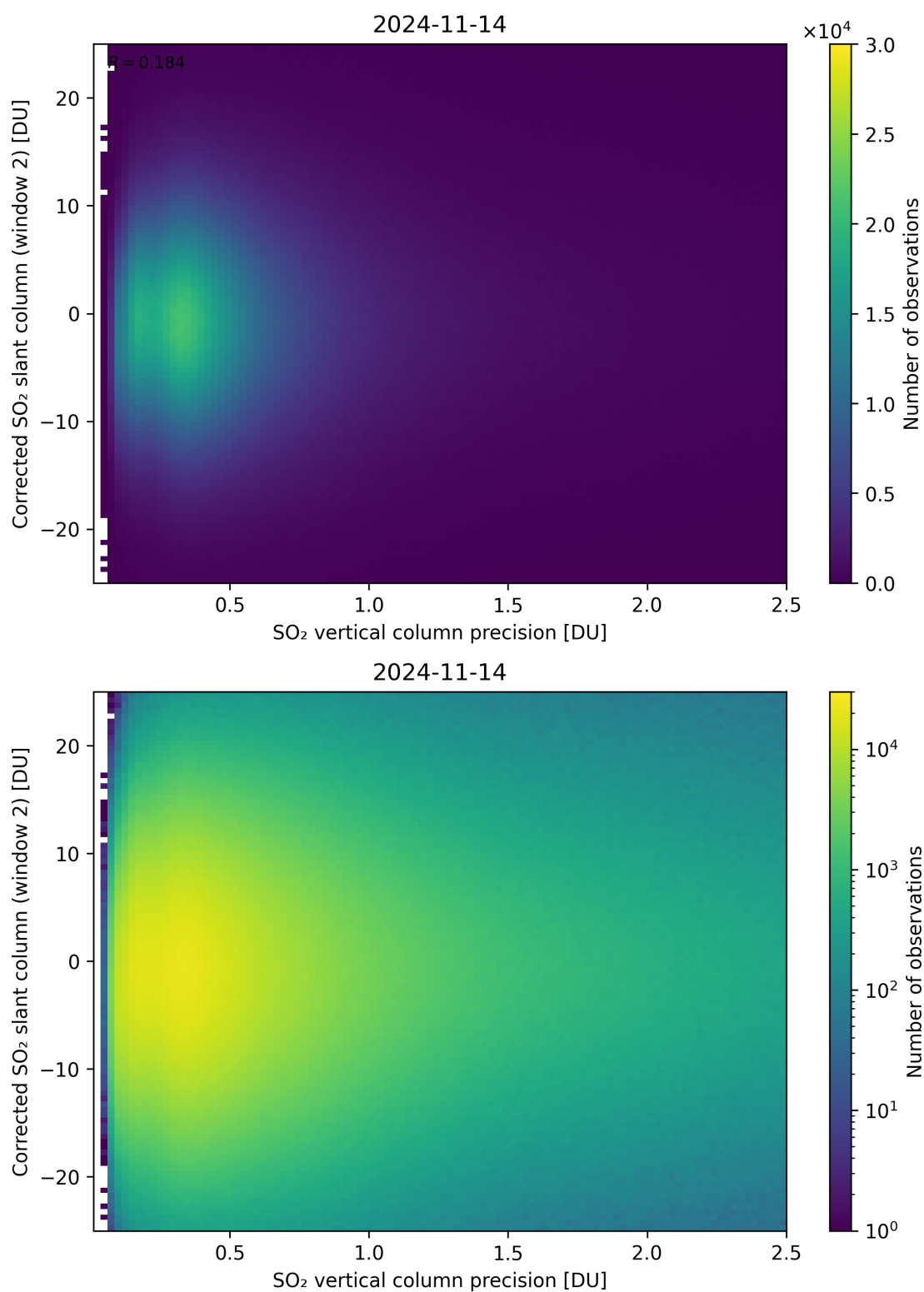
Figure 287: Scatter density plot of “SO 2 vertical column precision” against “Corrected SO 2 slant column (window 2)” for 2024-11-14 to 2024-11-15.
