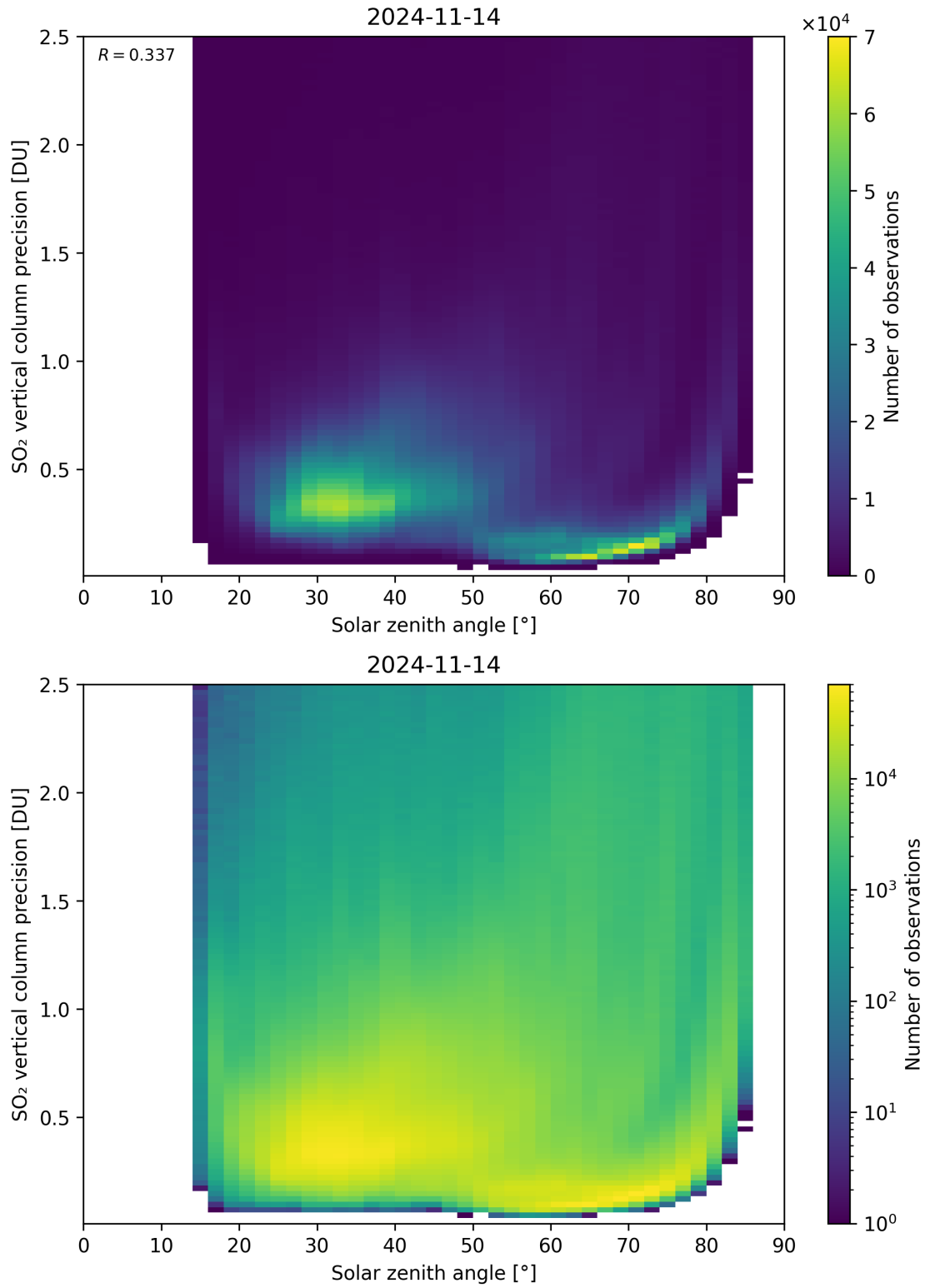
Figure 177: Scatter density plot of “Solar zenith angle” against “SO 2 vertical column precision” for 2024-11-14 to 2024-11-15.
