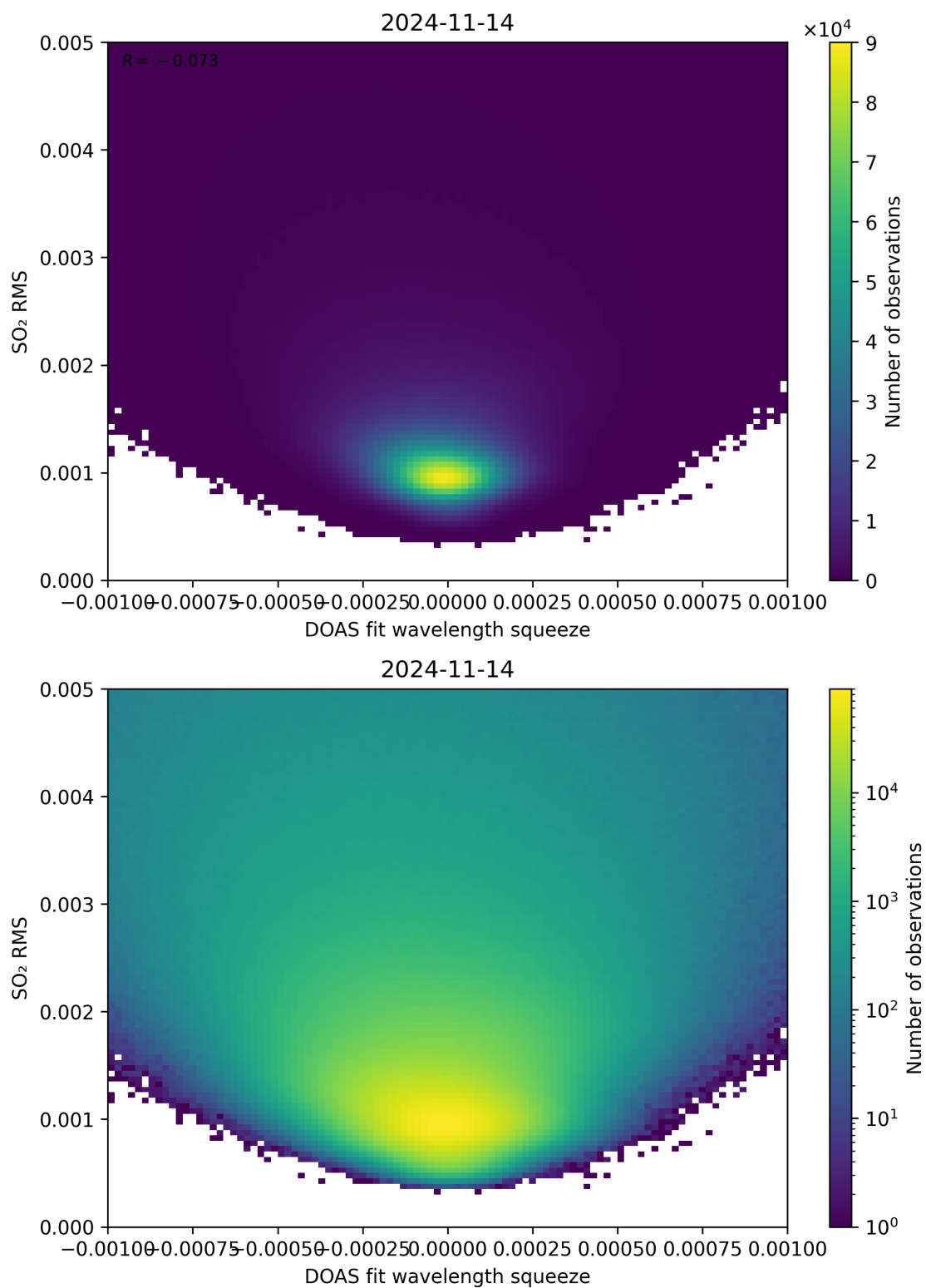
Figure 132: Scatter density plot of “DOAS fit wavelength squeeze” against “SO 2 RMS” for 2024-11-14 to 2024-11-15.
