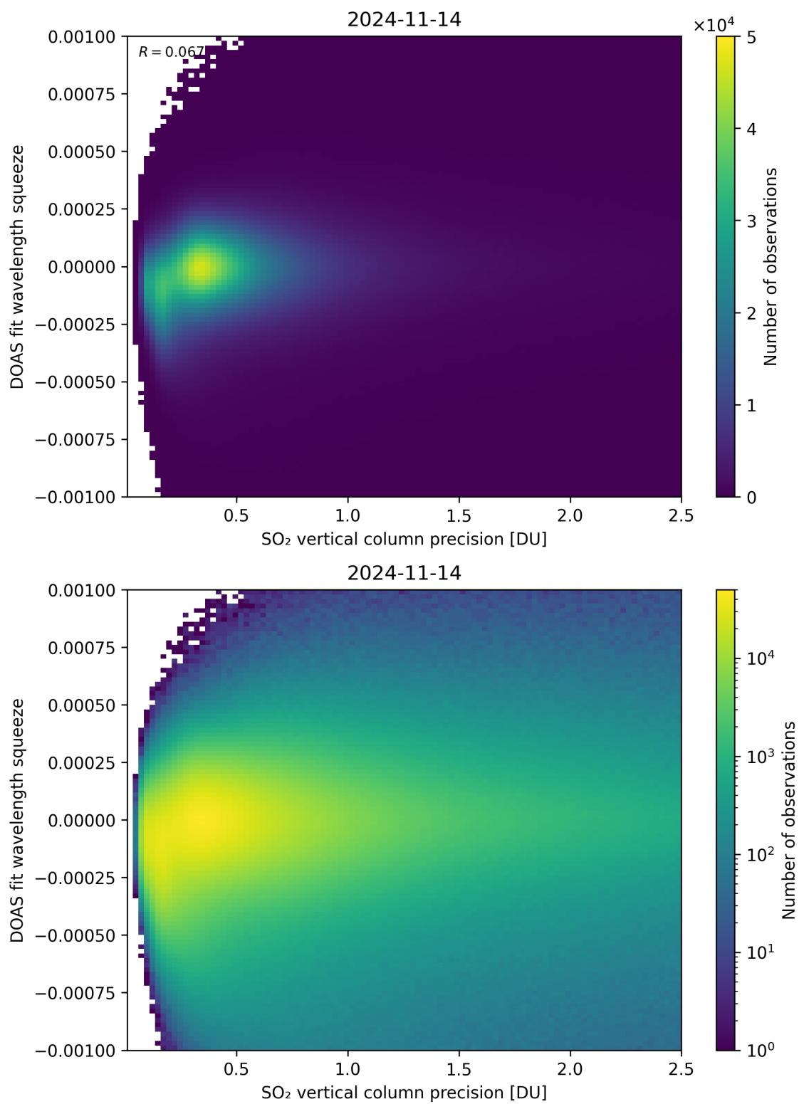
Figure 283: Scatter density plot of “SO 2 vertical column precision” against “DOAS fit wavelength squeeze” for 2024-11-14 to 2024-11-15.
