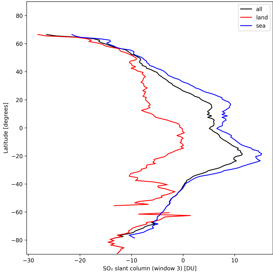
Figure 41: Zonal average of “SO 2 slant column (window 3)” for 2024-11-14 to 2024-11-15.
