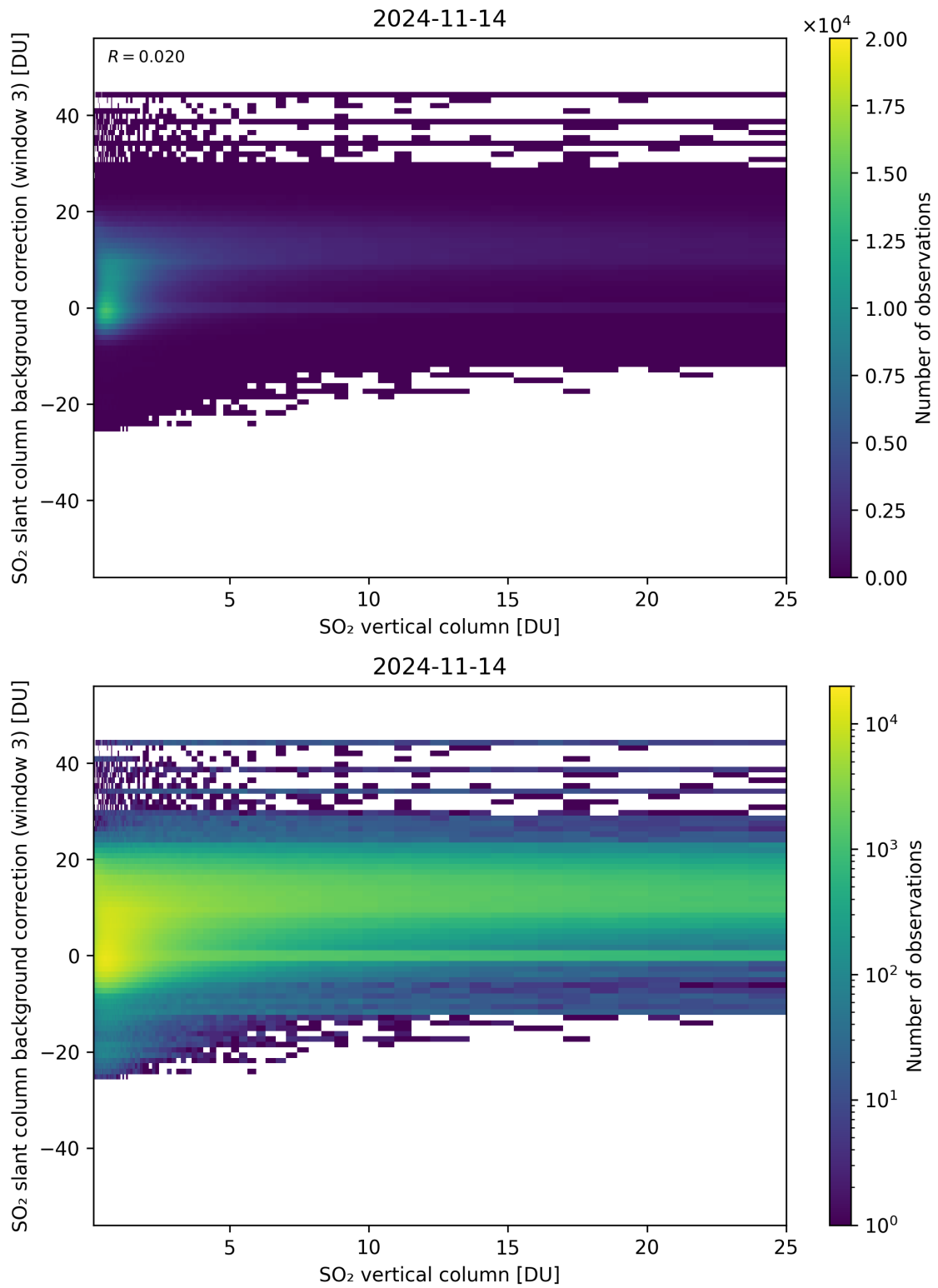
Figure 275: Scatter density plot of “SO 2 vertical column” against “SO 2 slant column background correction (window 3)” for 2024-11-14 to 2024-11-15.
