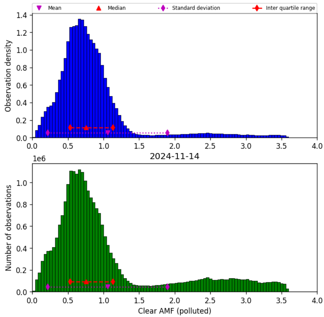
Figure 73: Histogram of “Clear AMF (polluted)” for 2024-11-14 to 2024-11-15
