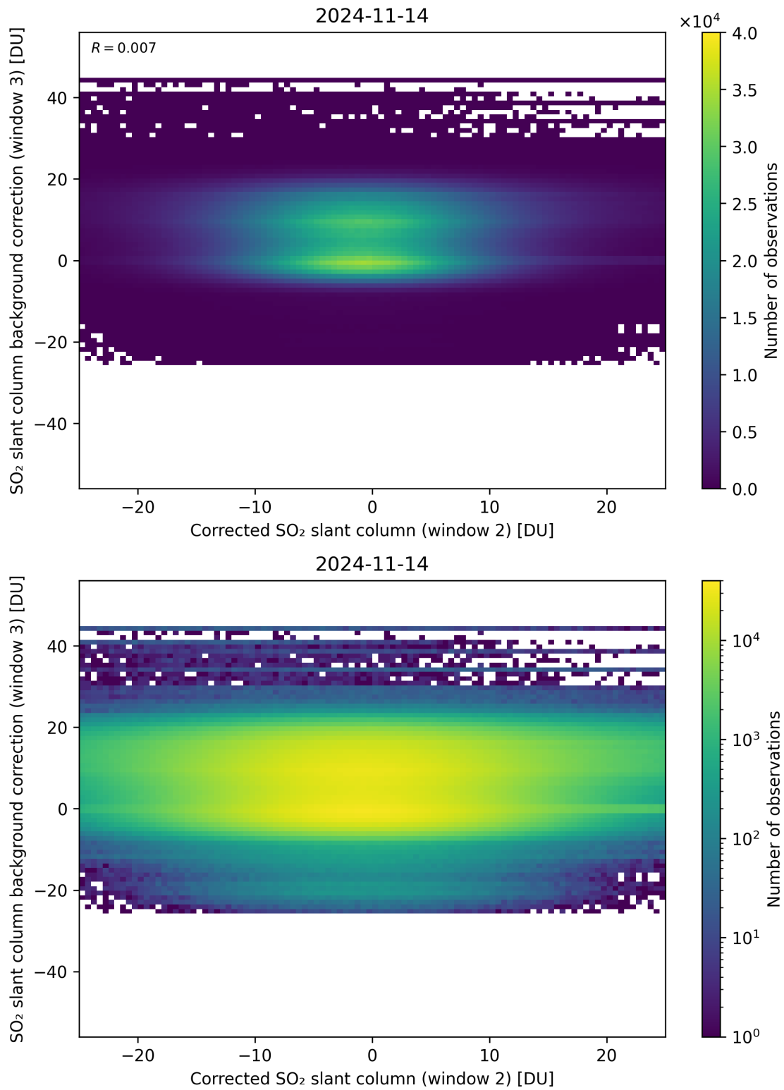
Figure 195: Scatter density plot of “Corrected SO 2 slant column (window 2)” against “SO 2 slant column background correction (window 3)” for 2024-11-14 to 2024-11-15.
