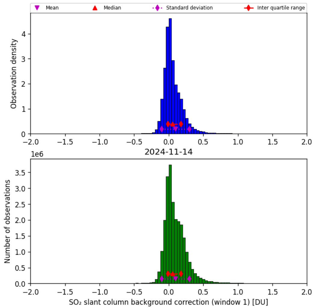
Figure 59: Histogram of “SO 2 slant column background correction (window 1)” for 2024-11-14 to 2024-11-15
