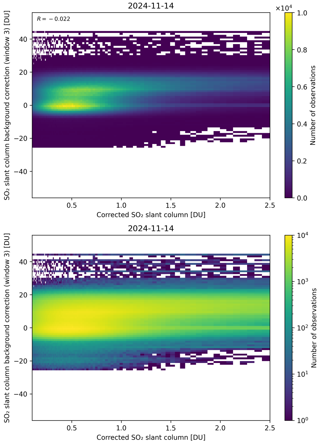
Figure 180: Scatter density plot of “Corrected SO 2 slant column” against “SO 2 slant column background correction (window 3)” for 2024-11-14 to 2024-11-15.
