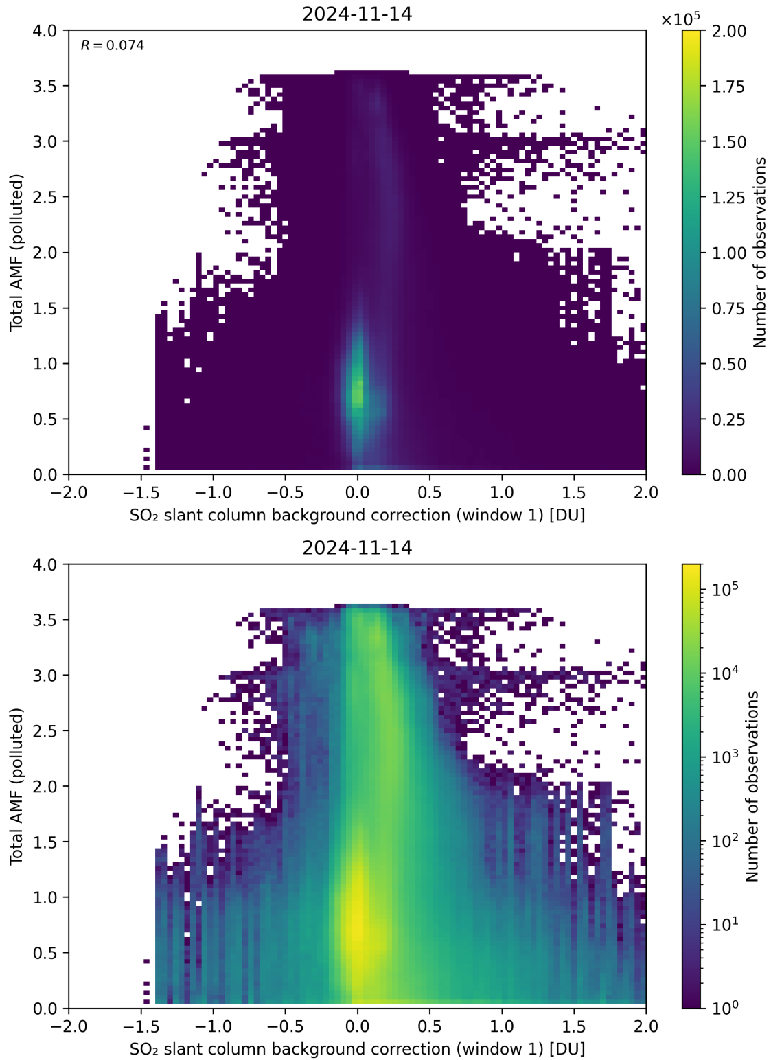
Figure 109: Scatter density plot of “SO 2 slant column background correction (window 1)” against “Total AMF (polluted)” for 2024-11-14 to 2024-11-15.
