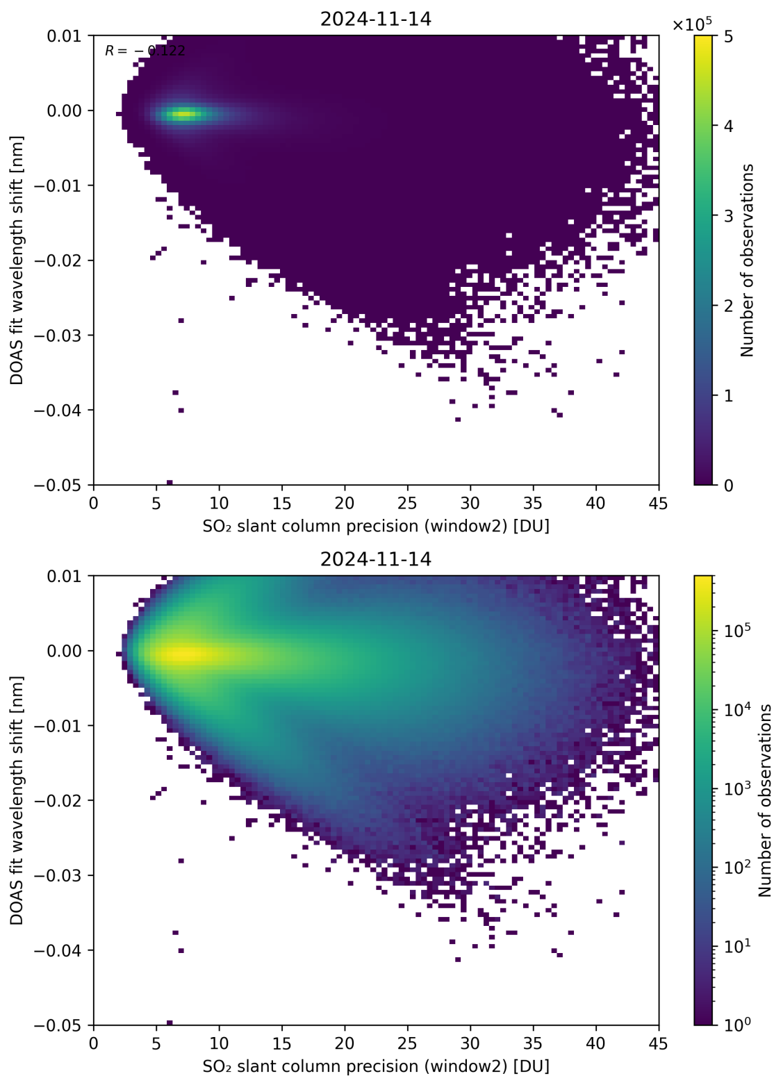
Figure 243: Scatter density plot of “SO 2 slant column precision (window2)” against “DOAS fit wavelength shift” for 2024-11-14 to 2024-11-15.
