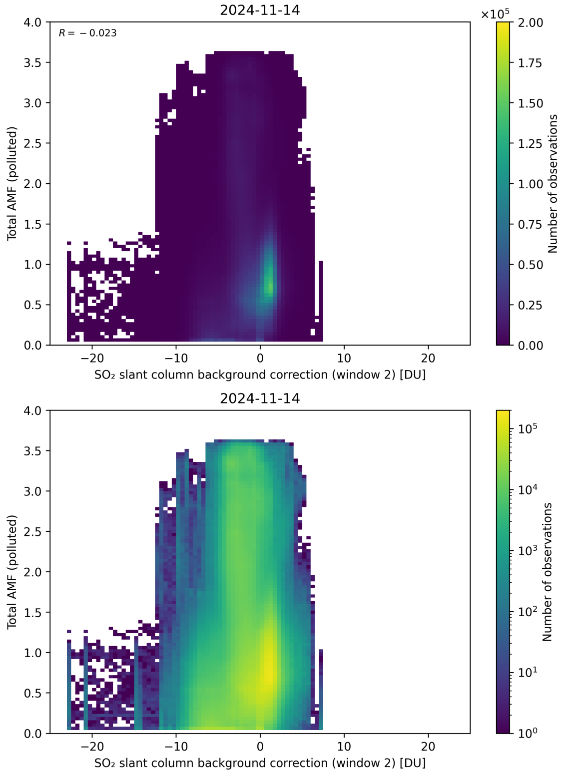
Figure 119: Scatter density plot of “SO 2 slant column background correction (window 2)” against “Total AMF (polluted)” for 2024-11-14 to 2024-11-15.
