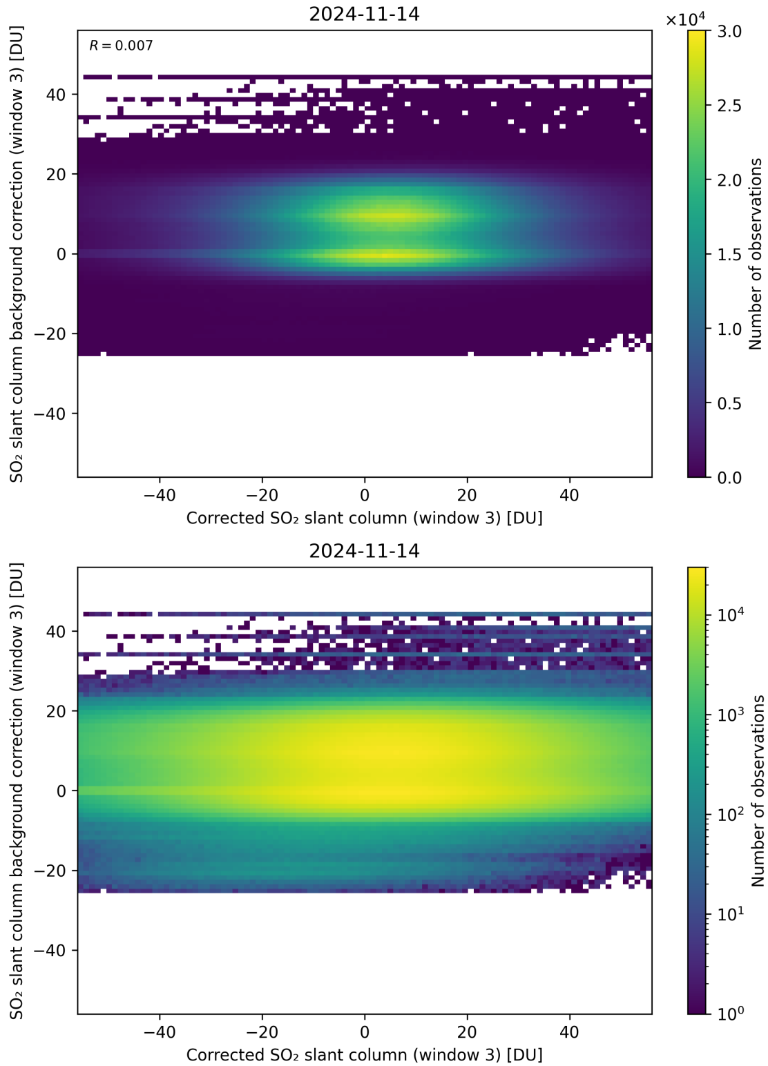
Figure 205: Scatter density plot of “Corrected SO 2 slant column (window 3)” against “SO 2 slant column background correction (window 3)” for 2024-11-14 to 2024-11-15.
