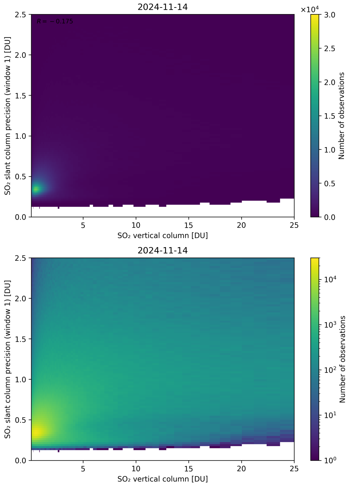
Figure 301: Scatter density plot of “SO 2 vertical column” against “SO 2 slant column precision (window 1)” for 2024-11-14 to 2024-11-15.
