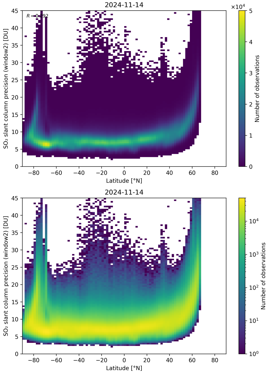
Figure 151: Scatter density plot of “Latitude” against “SO 2 slant column precision (window2)” for 2024-11-14 to 2024-11-15.
