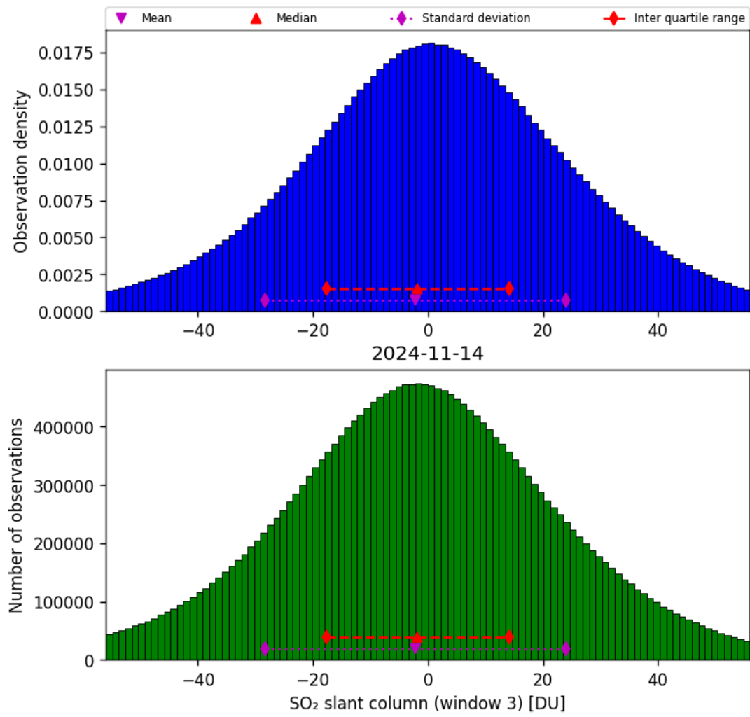
Figure 64: Histogram of “SO 2 slant column (window 3)” for 2024-11-14 to 2024-11-15
