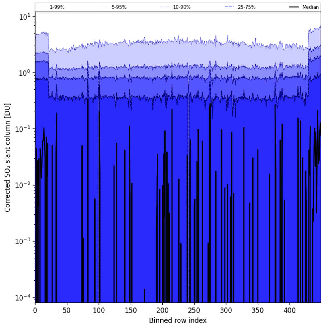
Figure 78: Along track statistics of “Corrected SO 2 slant column” for 2024-11-14 to 2024-11-15
