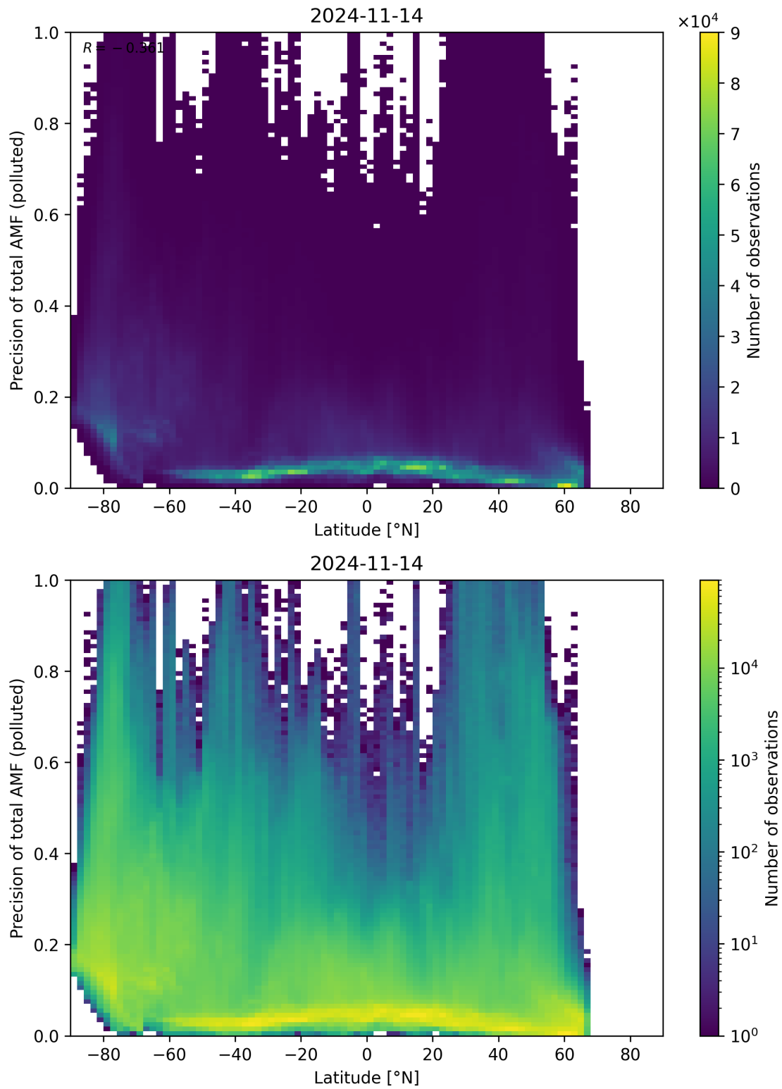
Figure 155: Scatter density plot of “Latitude” against “Precision of total AMF (polluted)” for 2024-11-14 to 2024-11-15.
