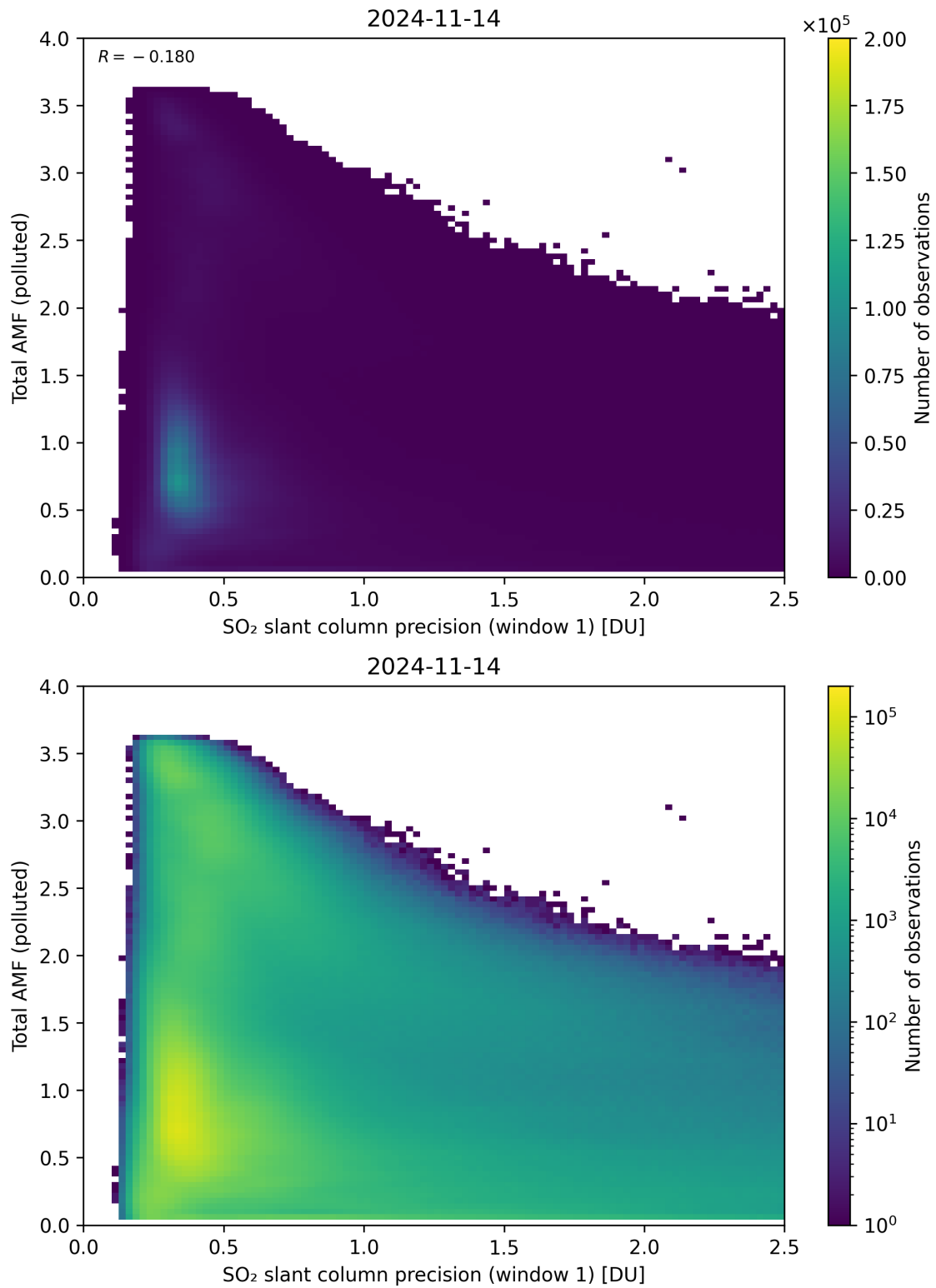
Figure 230: Scatter density plot of “SO 2 slant column precision (window 1)” against “Total AMF (polluted)” for 2024-11-14 to 2024-11-15.
