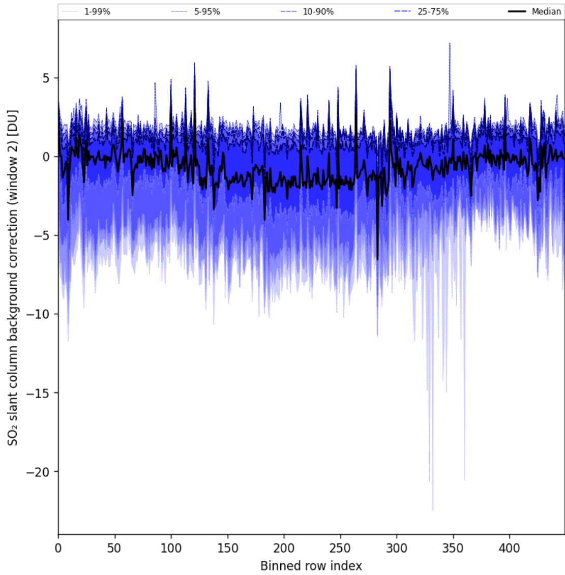
Figure 86: Along track statistics of “SO 2 slant column background correction (window 2)” for 2024-11-14 to 2024-11-15
