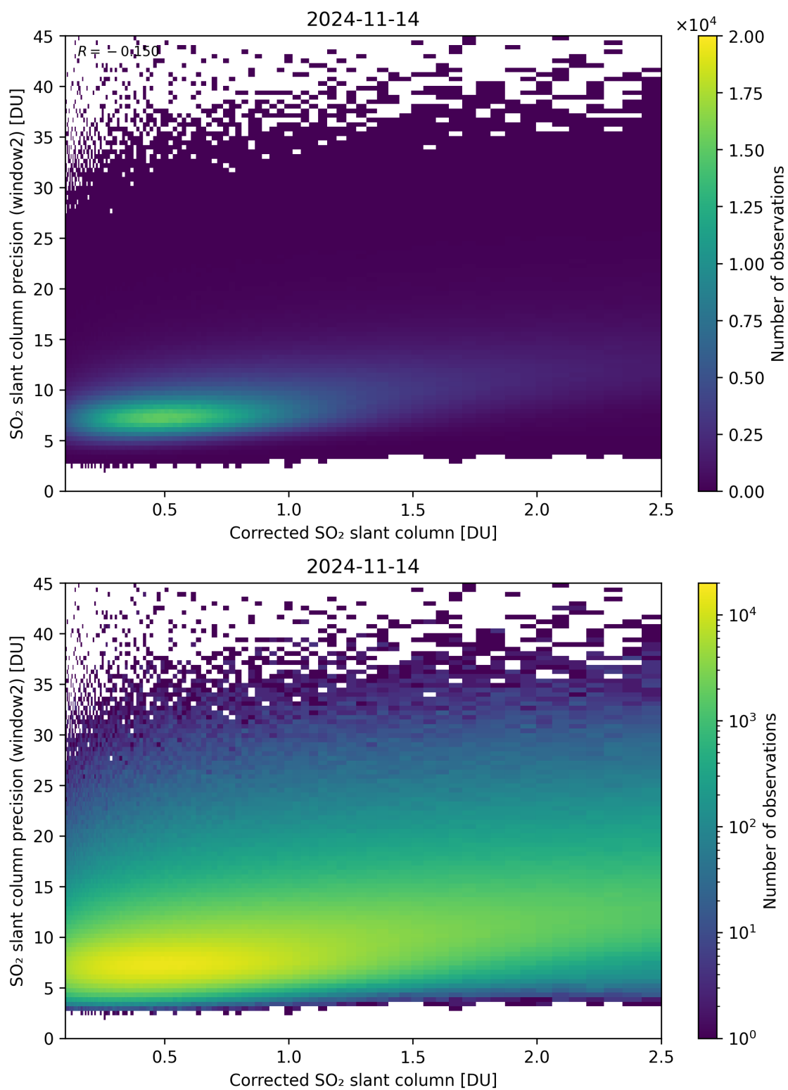
Figure 189: Scatter density plot of “Corrected SO 2 slant column” against “SO 2 slant column precision (window2)” for 2024-11-14 to 2024-11-15.
