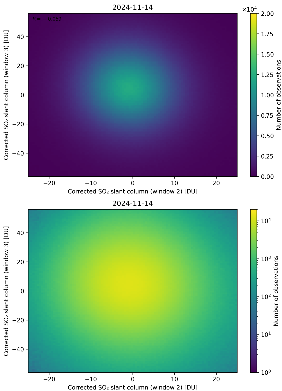
Figure 200: Scatter density plot of “Corrected SO 2 slant column (window 2)” against “Corrected SO 2 slant column (window 3)” for 2024-11-14 to 2024-11-15.
