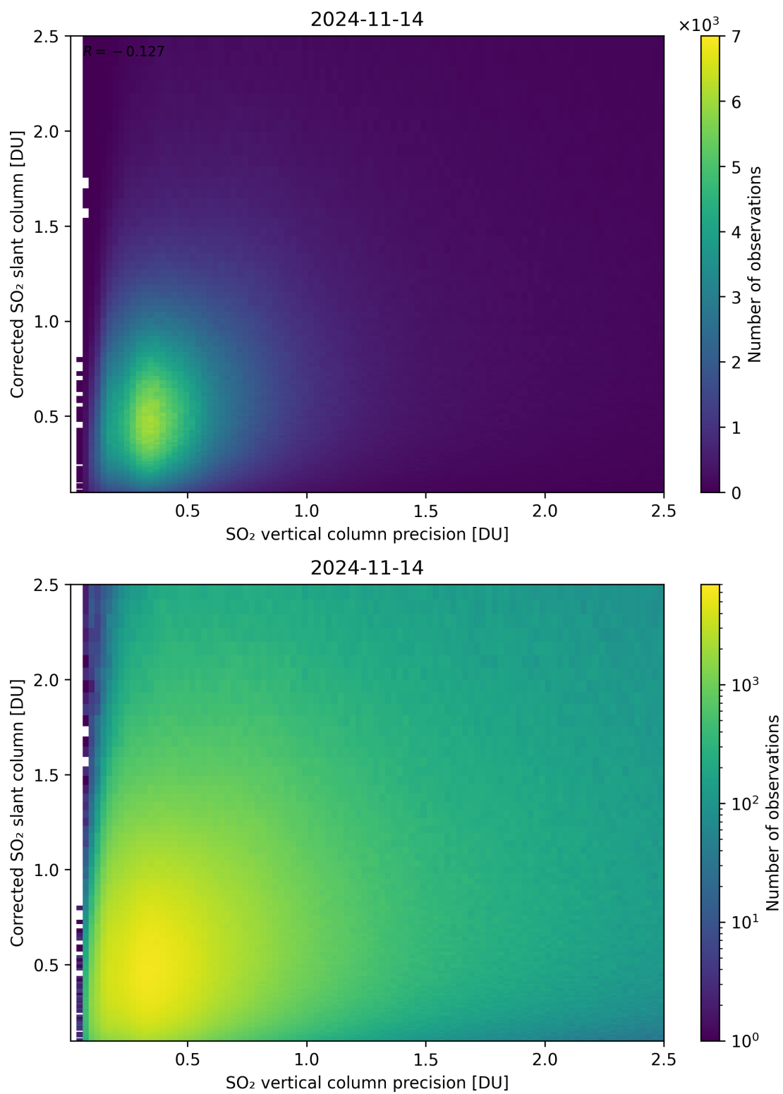
Figure 286: Scatter density plot of “SO 2 vertical column precision” against “Corrected SO 2 slant column” for 2024-11-14 to 2024-11-15.
