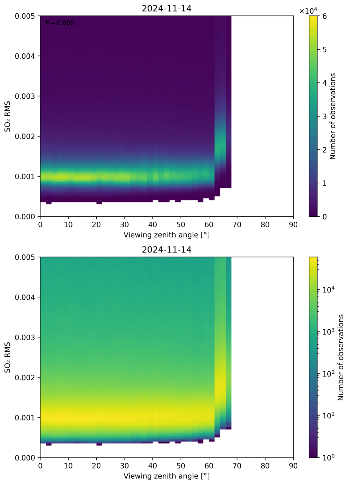
Figure 313: Scatter density plot of “Viewing zenith angle” against “SO 2 RMS” for 2024-11-14 to 2024-11-15.
