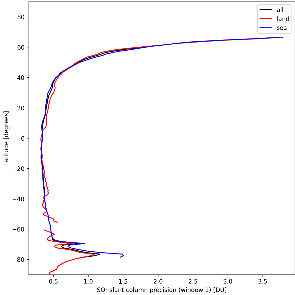
Figure 34: Zonal average of “SO 2 slant column precision (window 1)” for 2024-11-14 to 2024-11-15.
