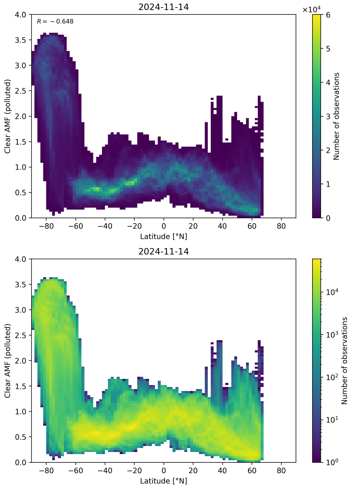
Figure 145: Scatter density plot of “Latitude” against “Clear AMF (polluted)” for 2024-11-14 to 2024-11-15.
