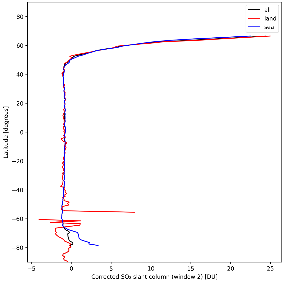
Figure 39: Zonal average of “Corrected SO 2 slant column (window 2)” for 2024-11-14 to 2024-11-15.
