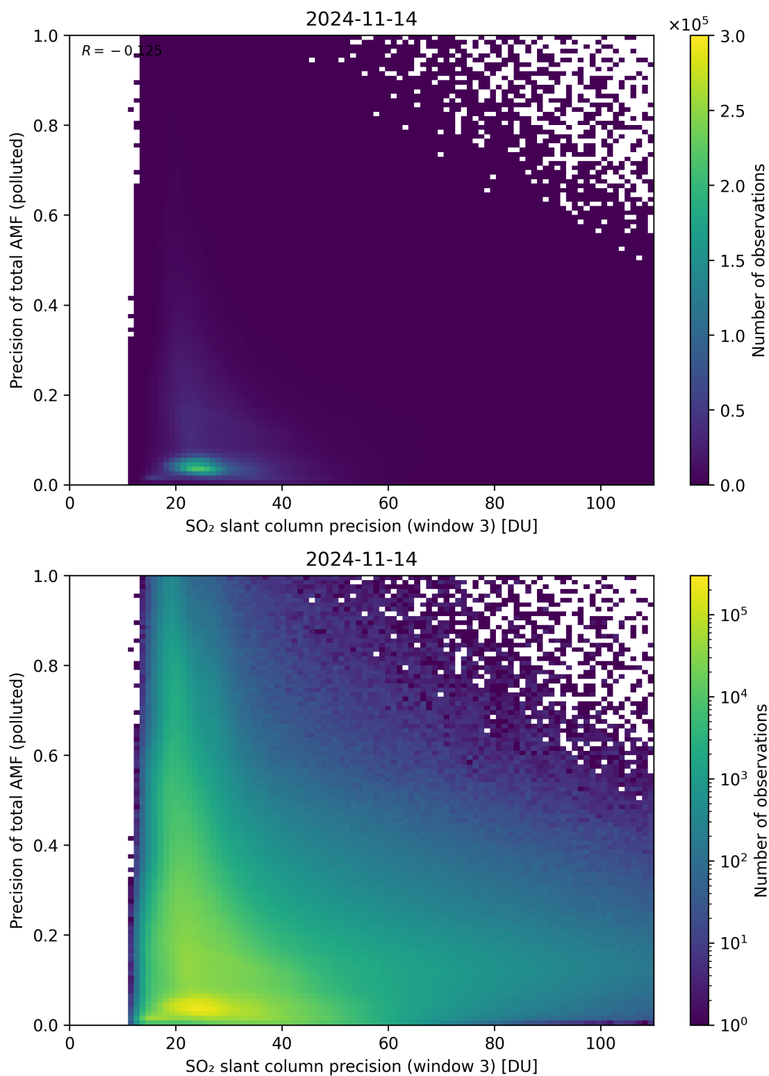
Figure 264: Scatter density plot of “SO 2 slant column precision (window 3)” against “Precision of total AMF (polluted)” for 2024-11-14 to 2024-11-15.
