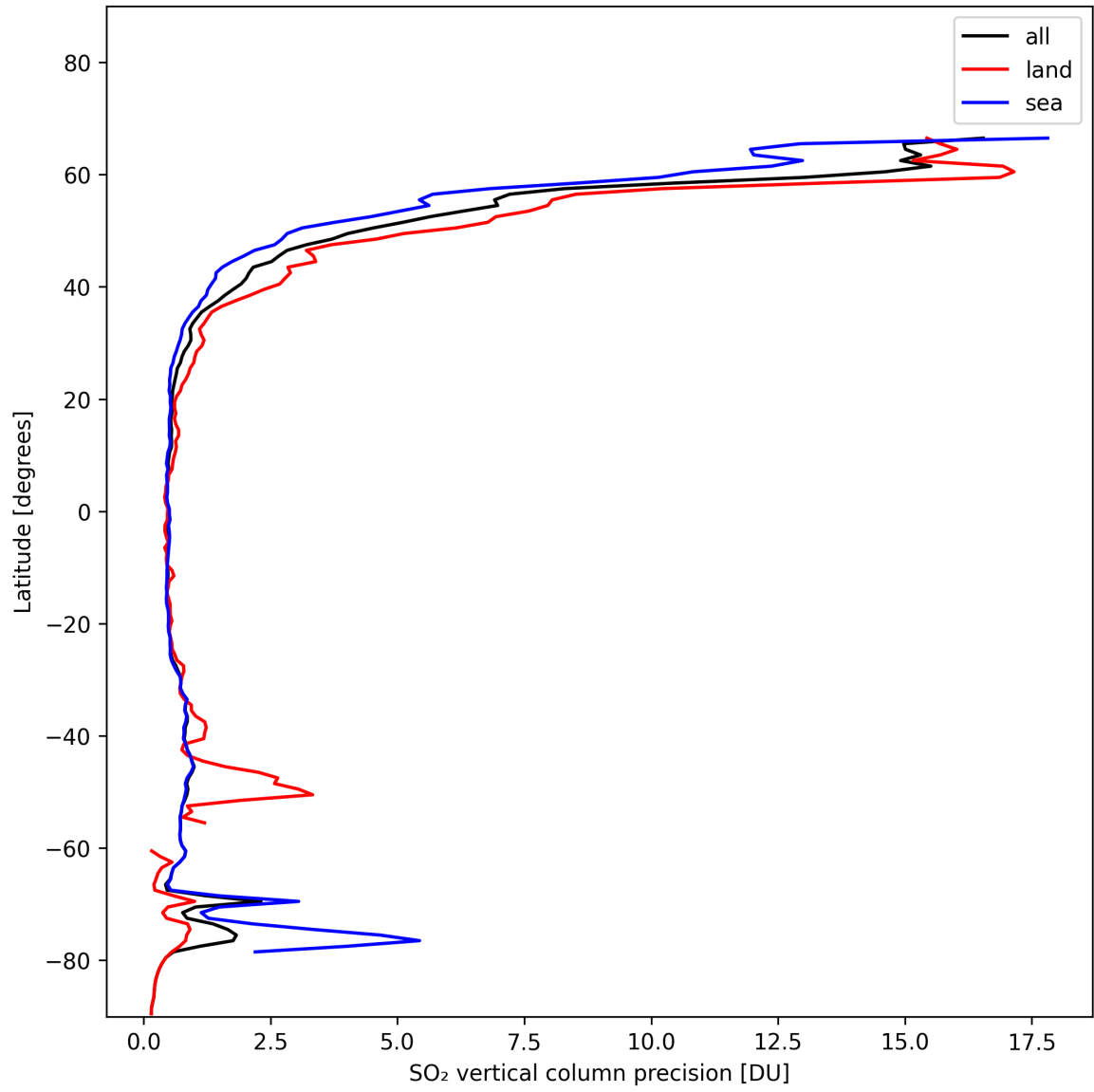
Figure 31: Zonal average of “SO 2 vertical column precision” for 2024-11-14 to 2024-11-15.
