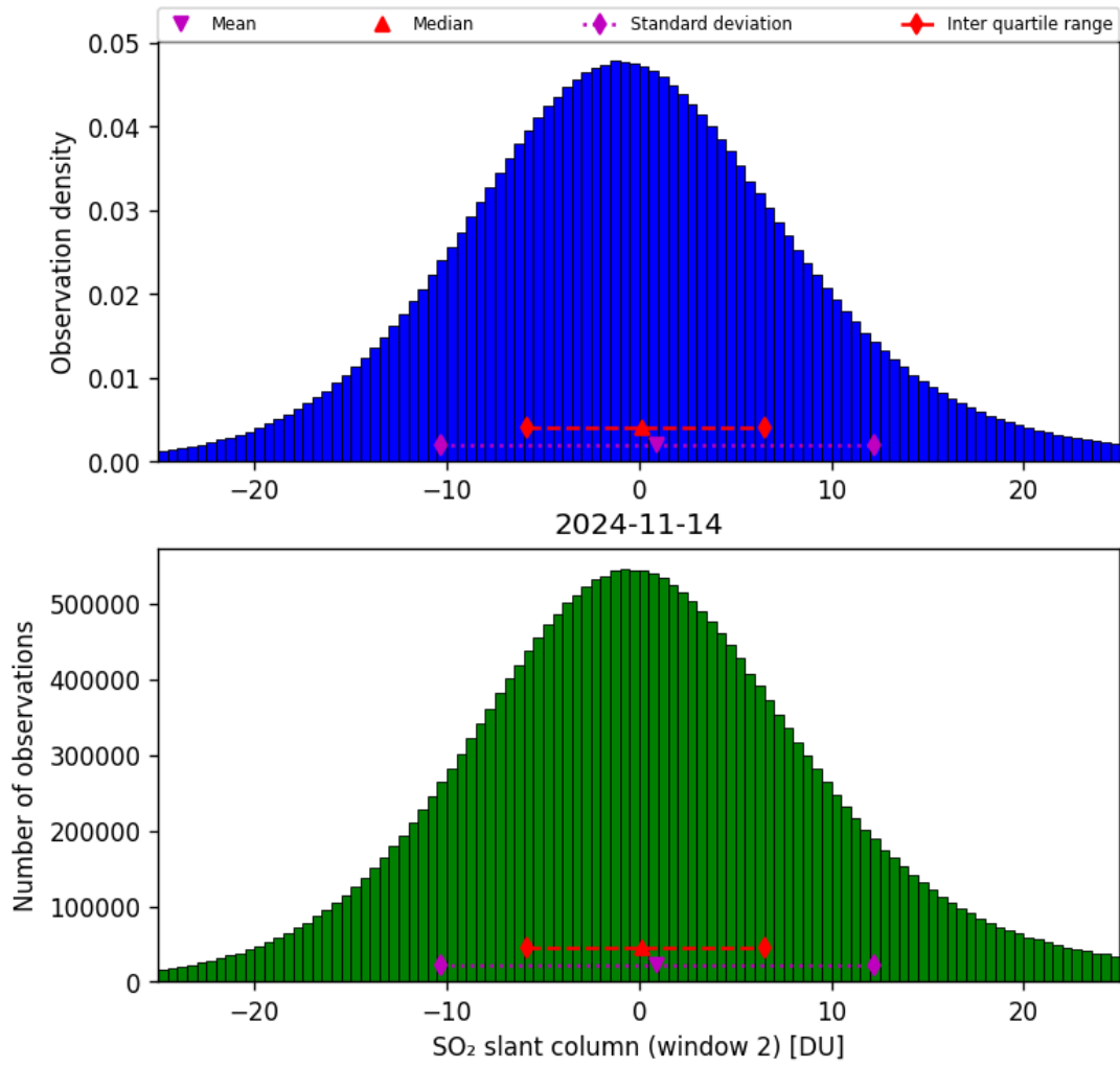
Figure 60: Histogram of “SO 2 slant column (window 2)” for 2024-11-14 to 2024-11-15
