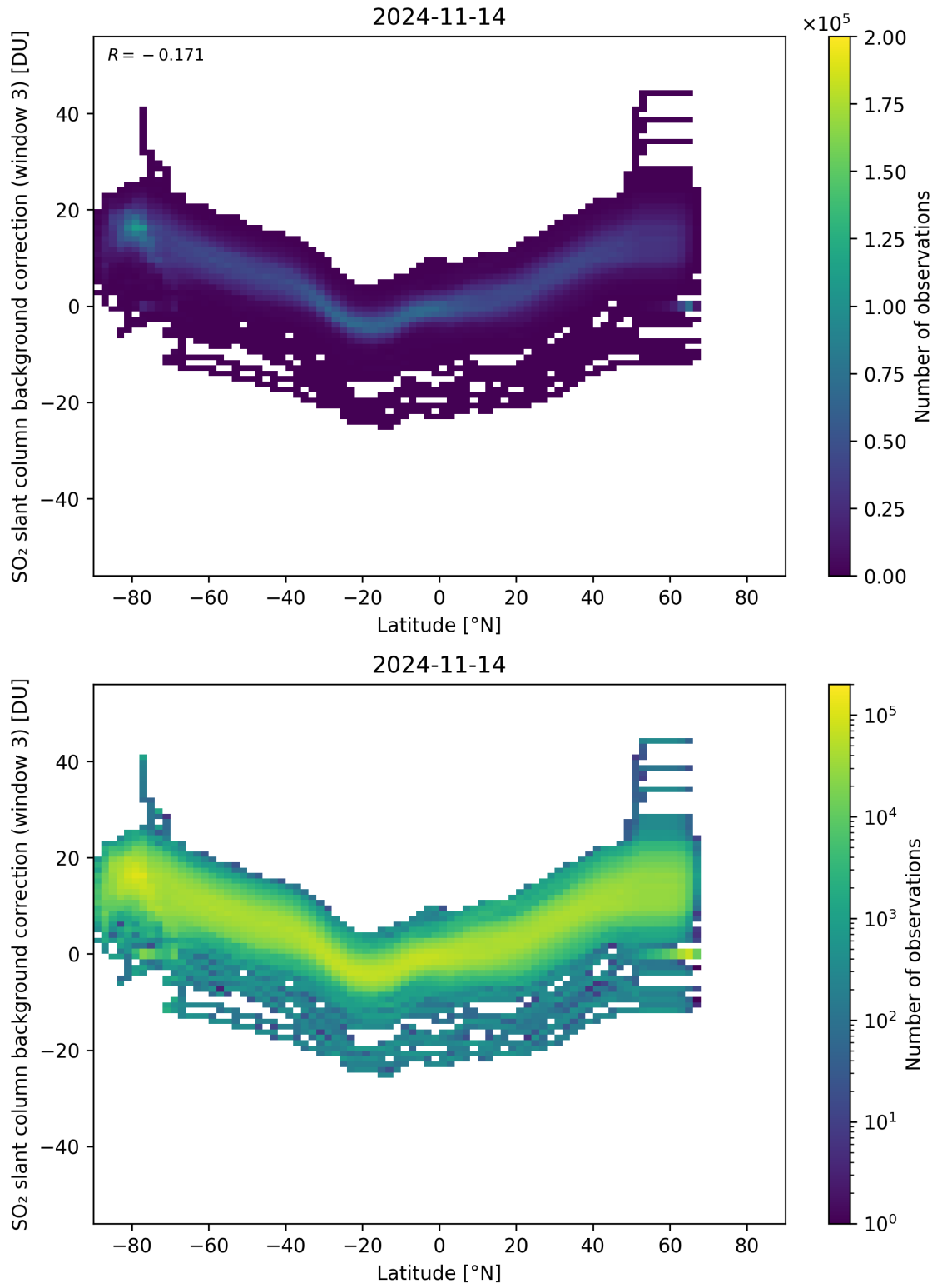
Figure 141: Scatter density plot of “Latitude” against “SO 2 slant column background correction (window 3)” for 2024-11-14 to 2024-11-15.
