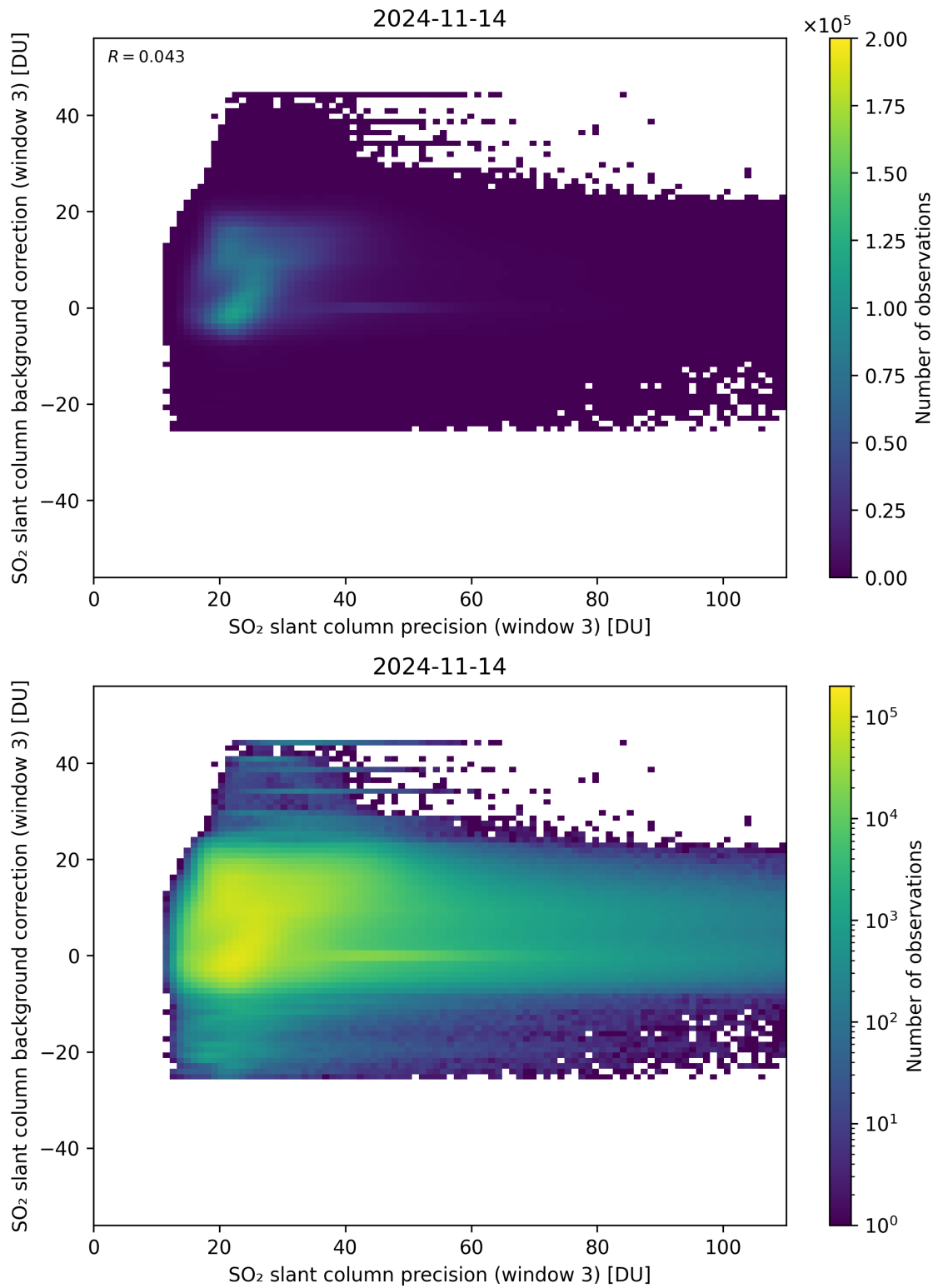
Figure 257: Scatter density plot of “SO 2 slant column precision (window 3)” against “SO 2 slant column background correction (window 3)” for 2024-11-14 to 2024-11-15.
