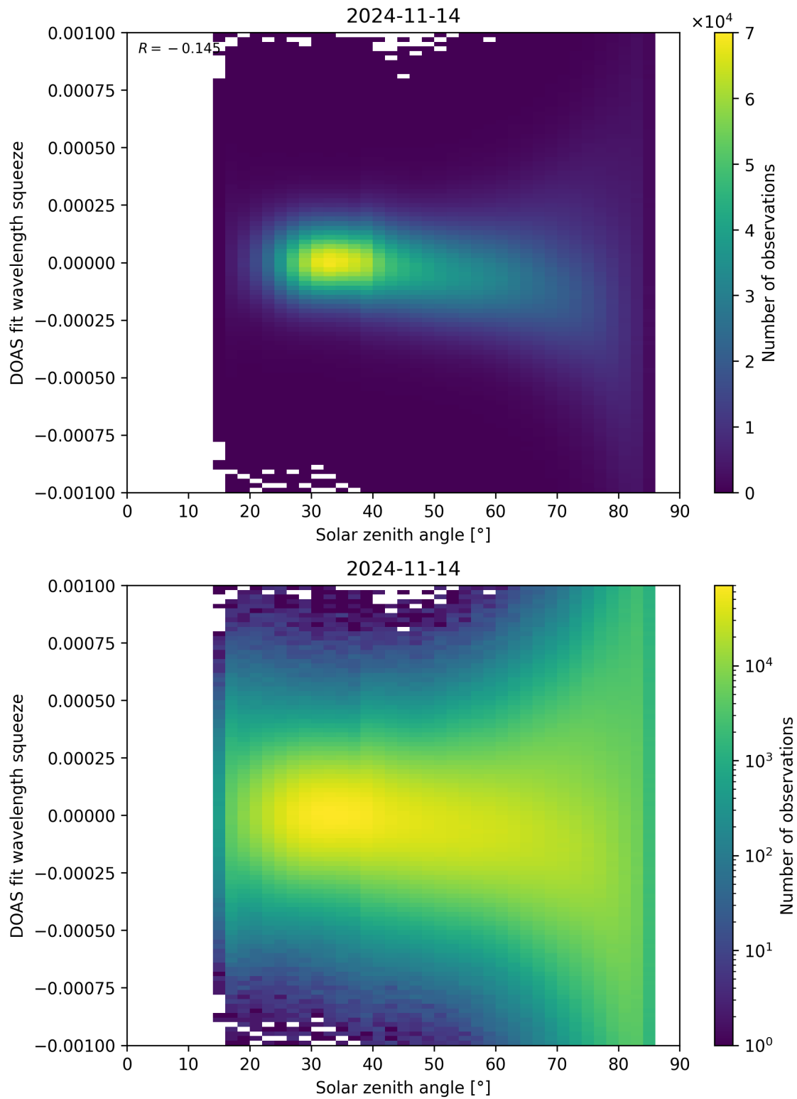
Figure 162: Scatter density plot of “Solar zenith angle” against “DOAS fit wavelength squeeze” for 2024-11-14 to 2024-11-15.
