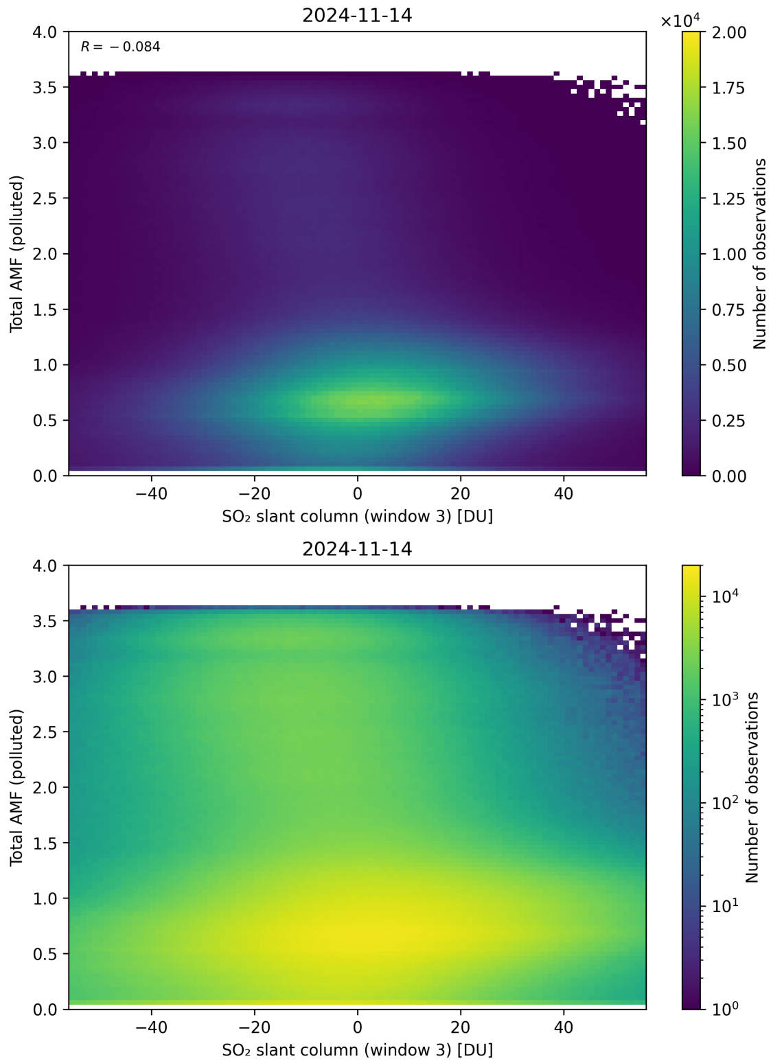
Figure 268: Scatter density plot of “SO 2 slant column (window 3)” against “Total AMF (polluted)” for 2024-11-14 to 2024-11-15.
