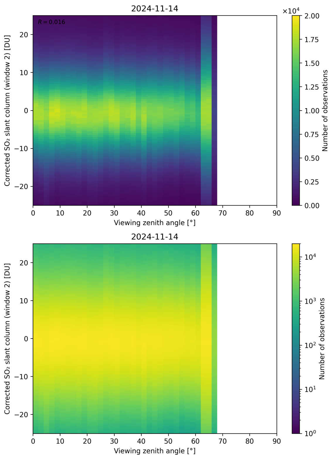
Figure 318: Scatter density plot of “Viewing zenith angle” against “Corrected SO 2 slant column (window 2)” for 2024-11-14 to 2024-11-15.
