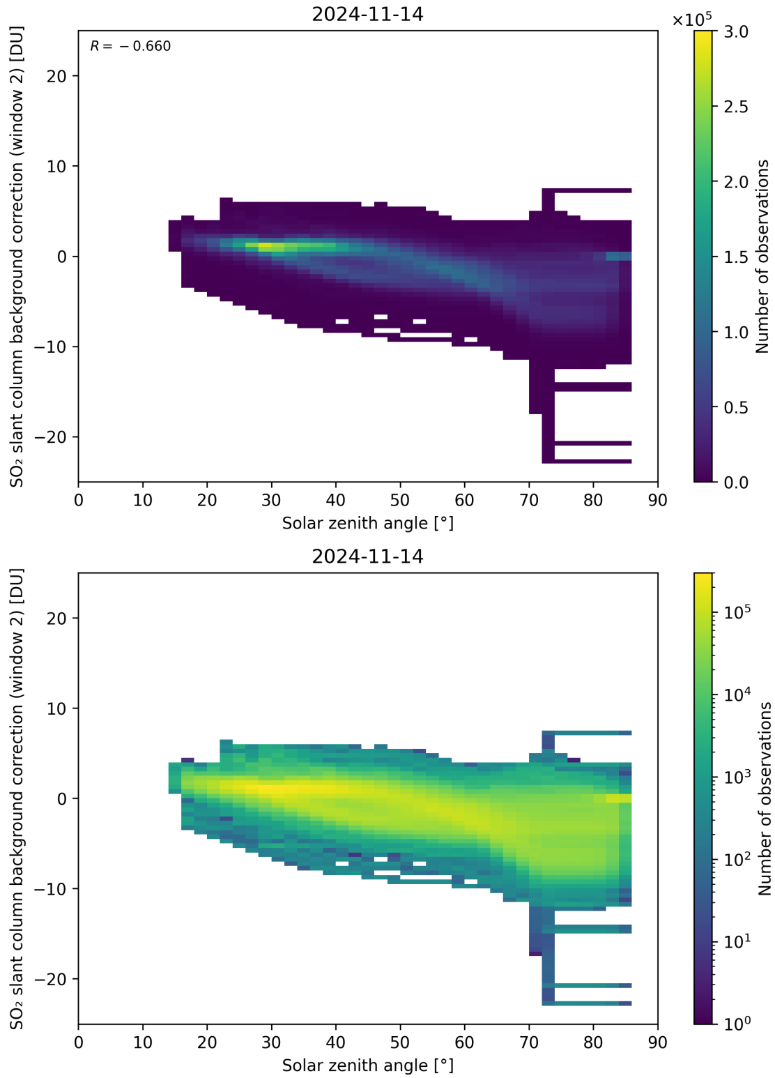
Figure 159: Scatter density plot of “Solar zenith angle” against “SO 2 slant column background correction (window 2)” for 2024-11-14 to 2024-11-15.
