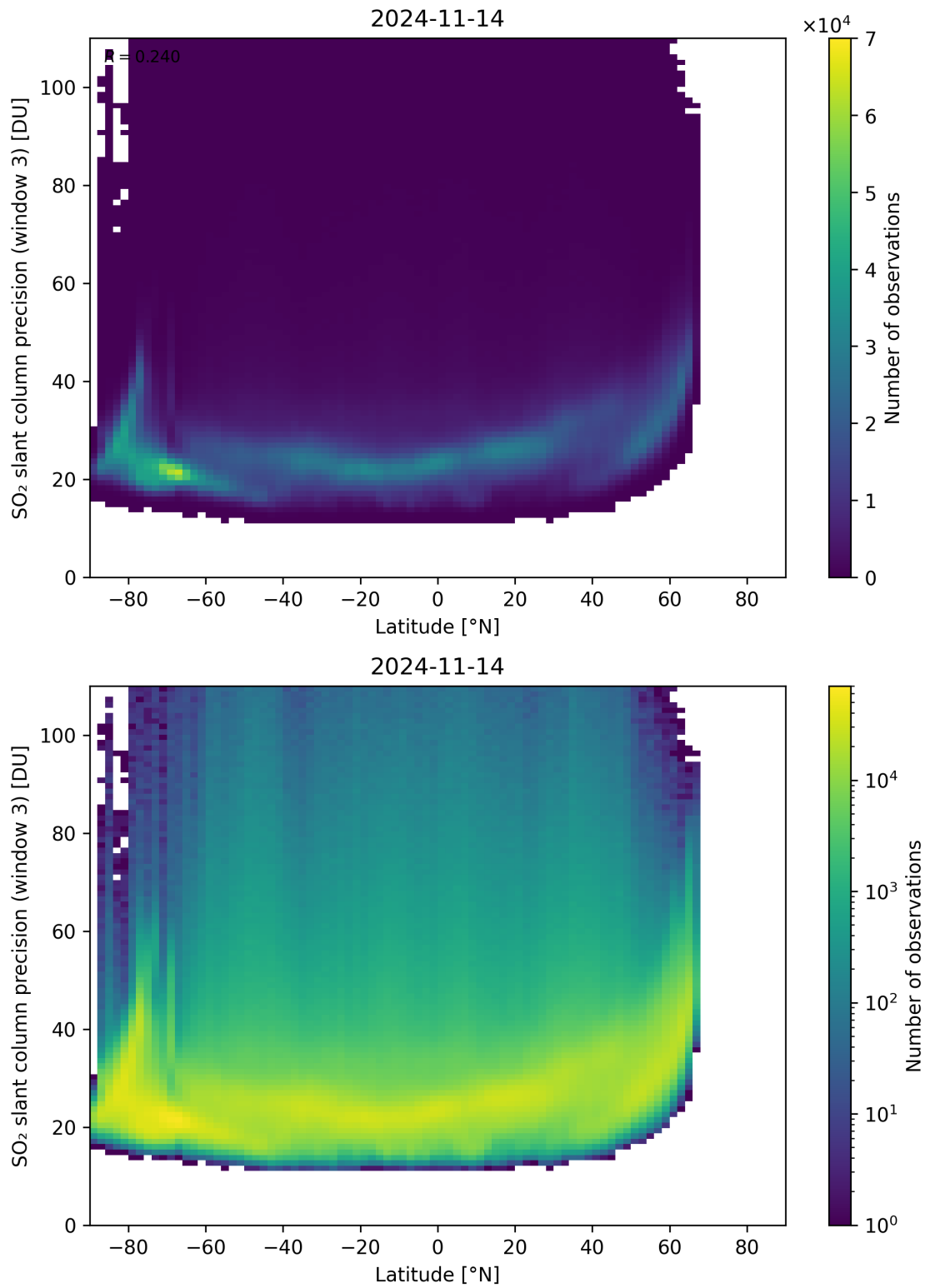
Figure 153: Scatter density plot of “Latitude” against “SO 2 slant column precision (window 3)” for 2024-11-14 to 2024-11-15.
