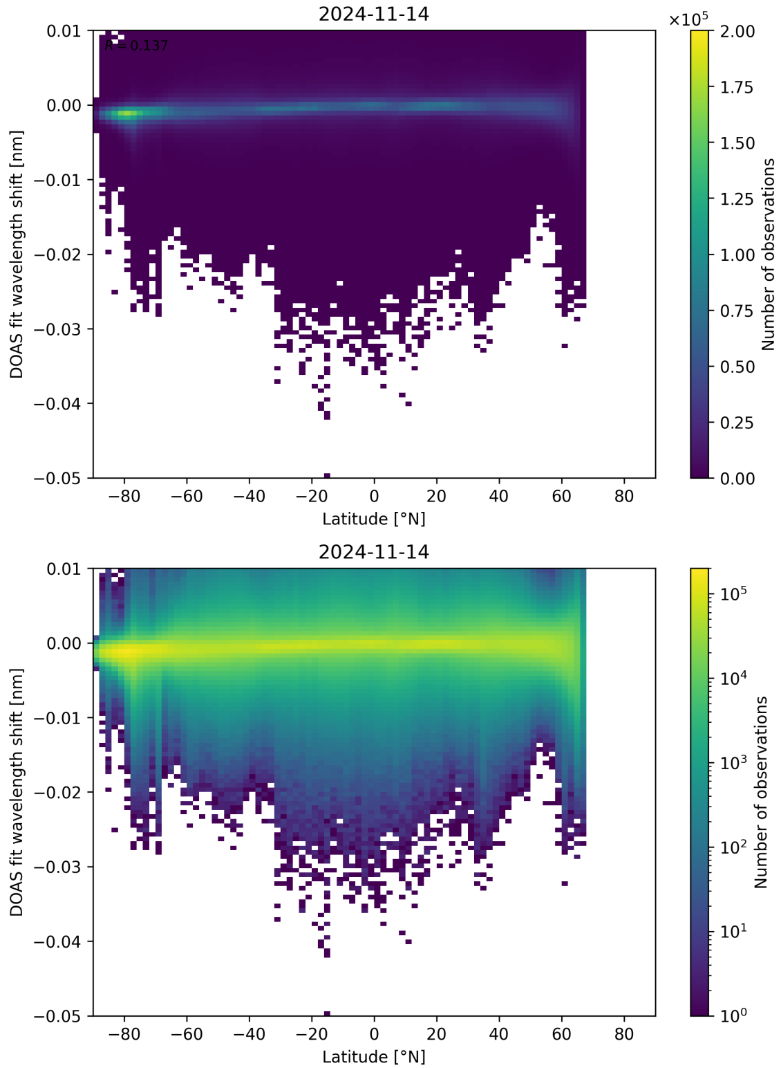
Figure 142: Scatter density plot of “Latitude” against “DOAS fit wavelength shift” for 2024-11-14 to 2024-11-15.
