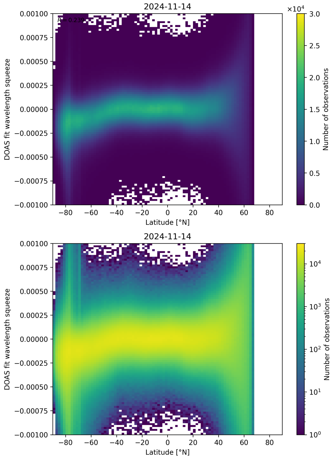
Figure 143: Scatter density plot of “Latitude” against “DOAS fit wavelength squeeze” for 2024-11-14 to 2024-11-15.
