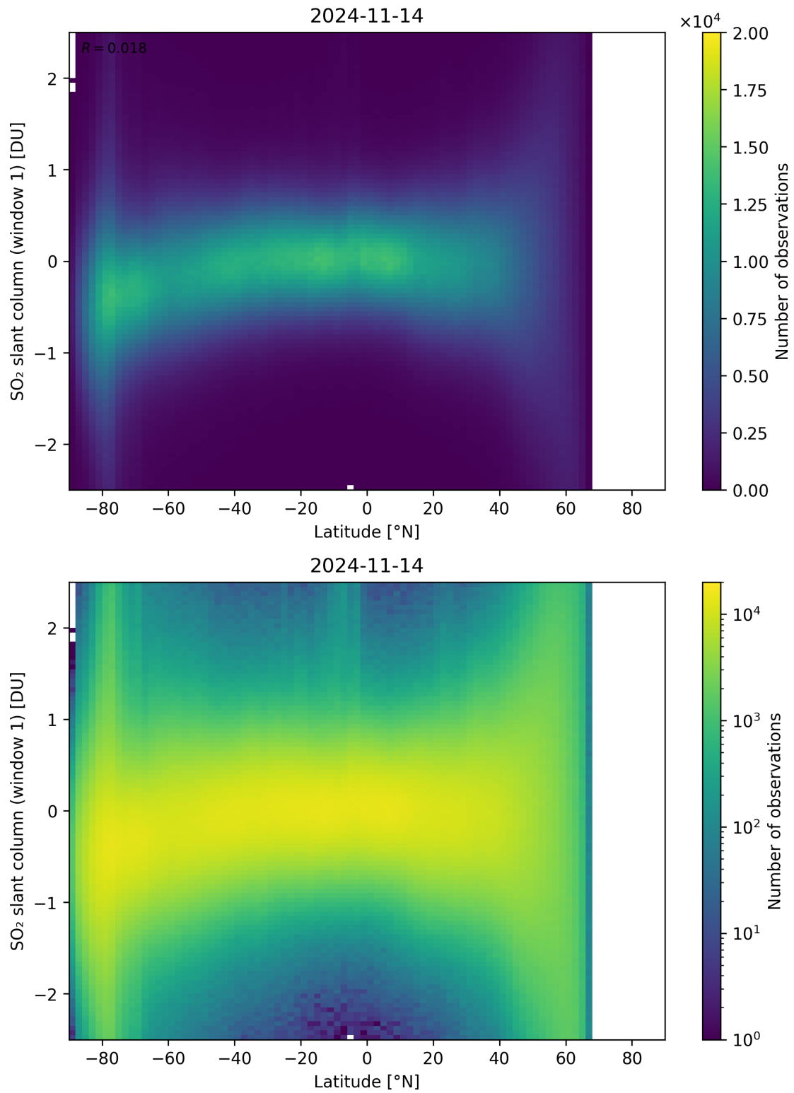
Figure 149: Scatter density plot of “Latitude” against “SO 2 slant column (window 1)” for 2024-11-14 to 2024-11-15.
