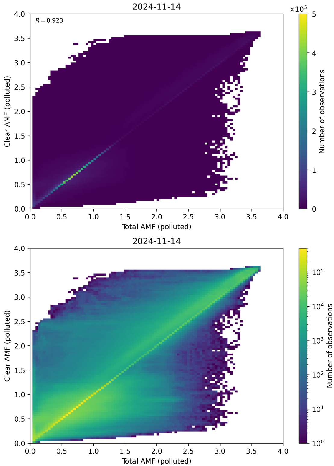
Figure 271: Scatter density plot of “Total AMF (polluted)” against “Clear AMF (polluted)” for 2024-11-14 to 2024-11-15.
