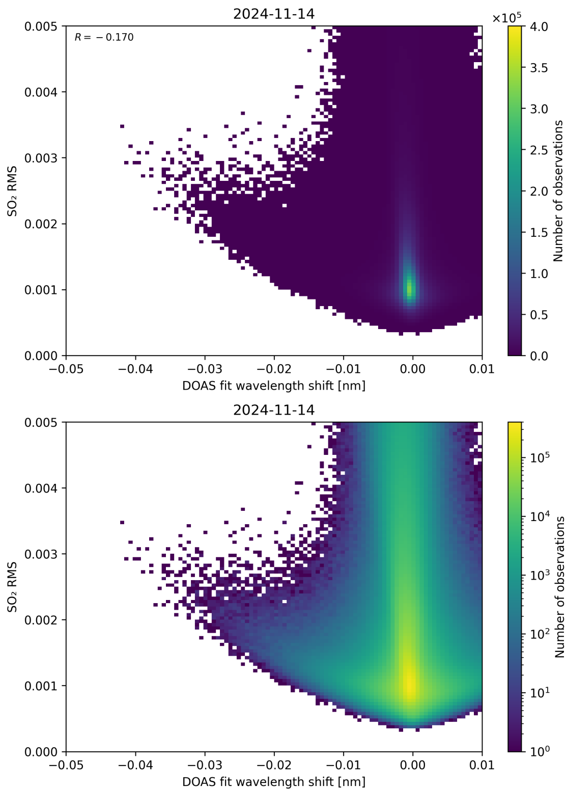
Figure 128: Scatter density plot of “DOAS fit wavelength shift” against “SO 2 RMS” for 2024-11-14 to 2024-11-15.
