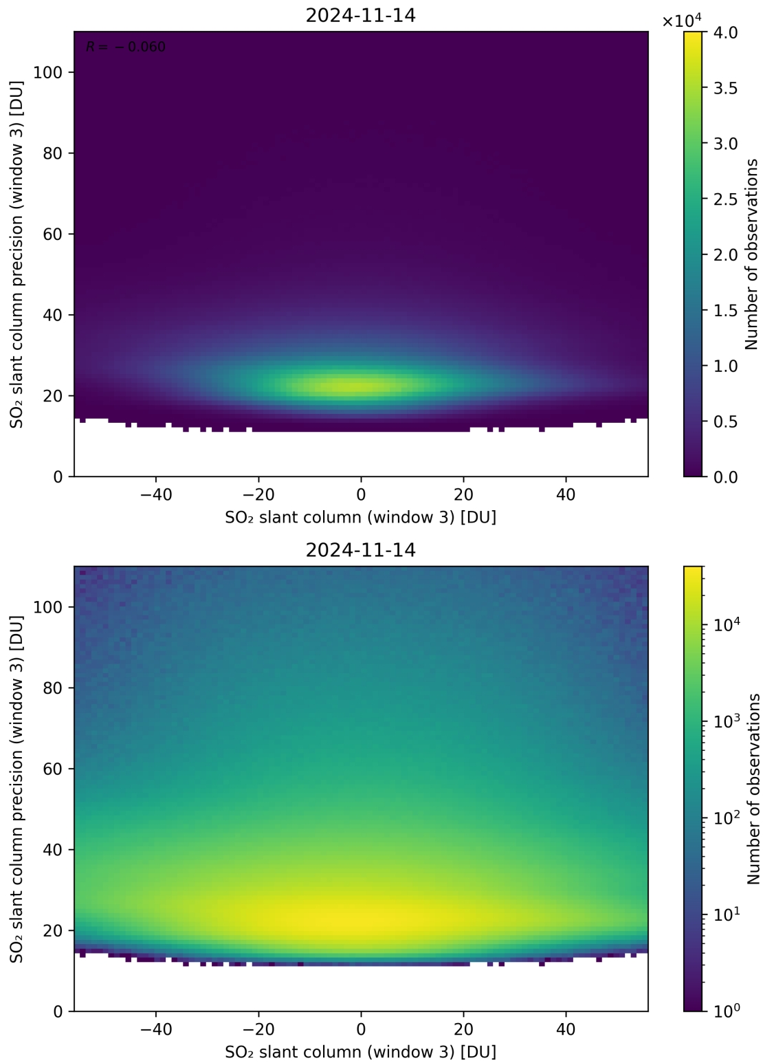
Figure 267: Scatter density plot of “SO 2 slant column (window 3)” against “SO 2 slant column precision (window 3)” for 2024-11-14 to 2024-11-15.
