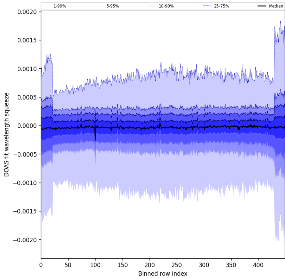
Figure 92: Along track statistics of “DOAS fit wavelength squeeze” for 2024-11-14 to 2024-11-15
