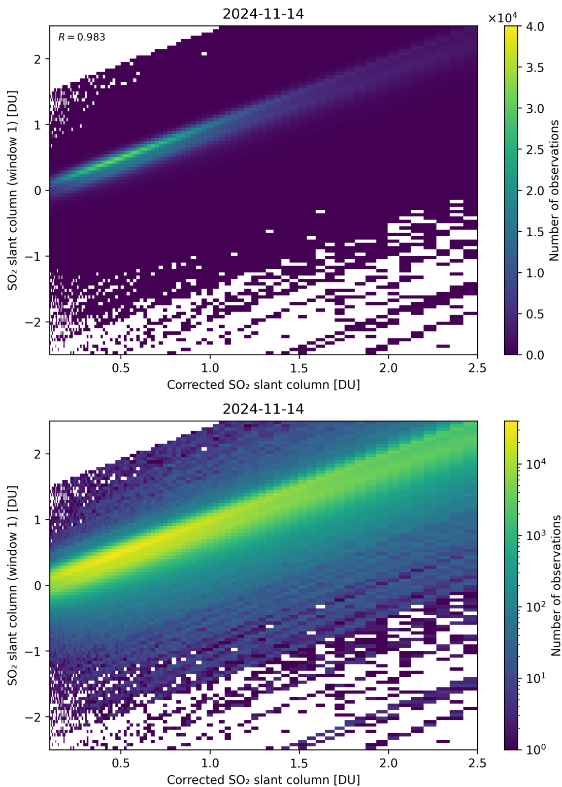
Figure 187: Scatter density plot of “Corrected SO 2 slant column” against “SO 2 slant column (window 1)” for 2024-11-14 to 2024-11-15.
