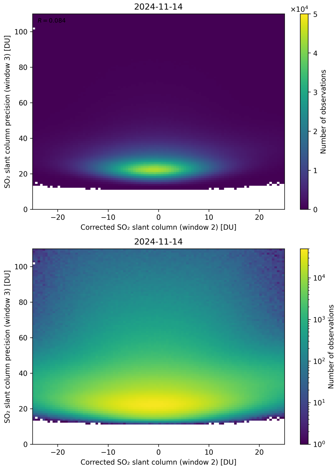
Figure 202: Scatter density plot of “Corrected SO 2 slant column (window 2)” against “SO 2 slant column precision (window 3)” for 2024-11-14 to 2024-11-15.
