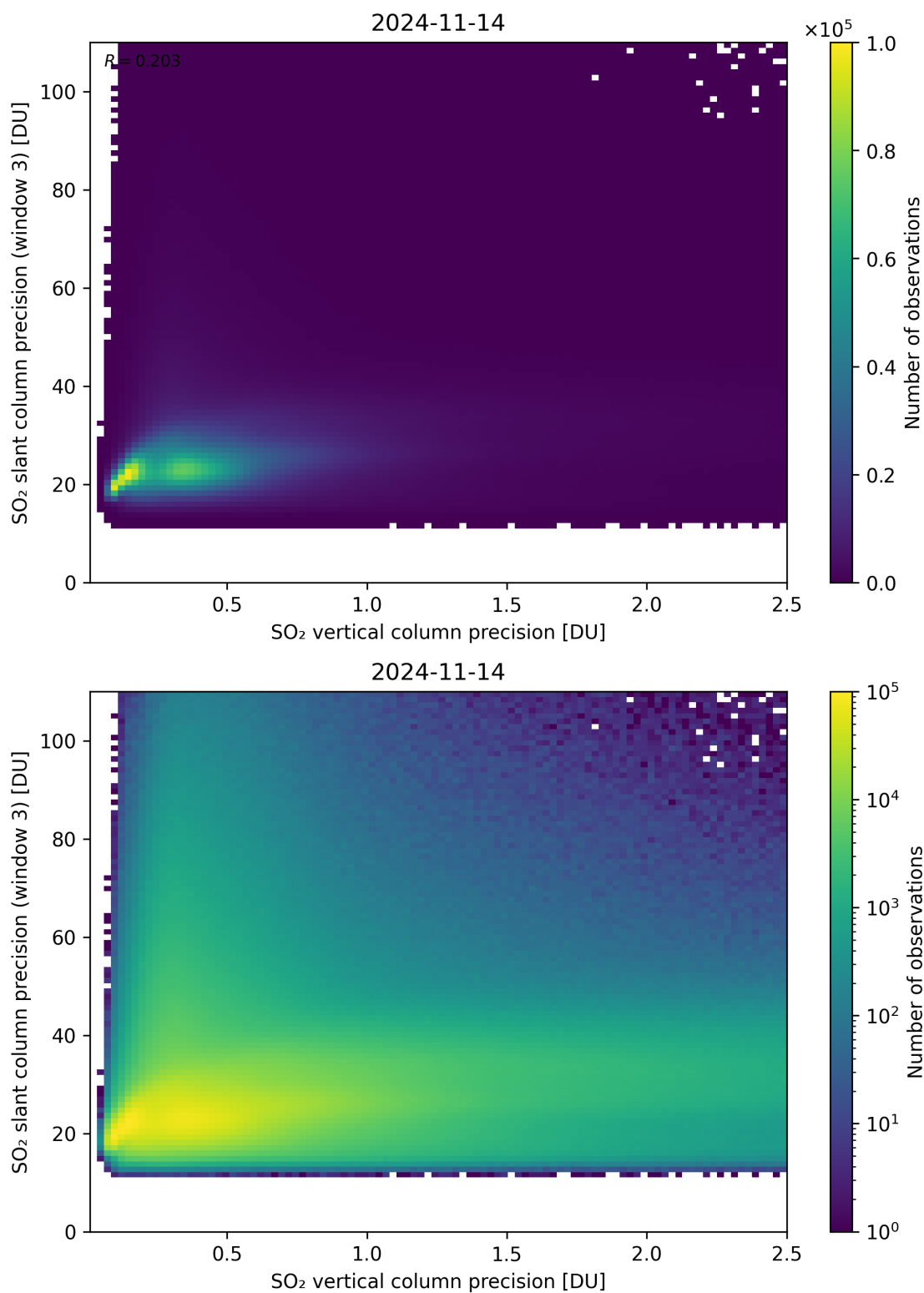
Figure 293: Scatter density plot of “SO 2 vertical column precision” against “SO 2 slant column precision (window 3)” for 2024-11-14 to 2024-11-15.
