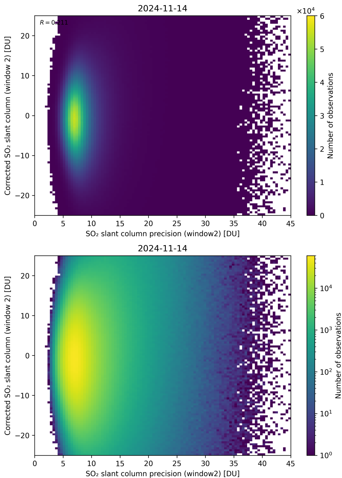
Figure 247: Scatter density plot of “SO 2 slant column precision (window2)” against “Corrected SO 2 slant column (window 2)” for 2024-11-14 to 2024-11-15.
