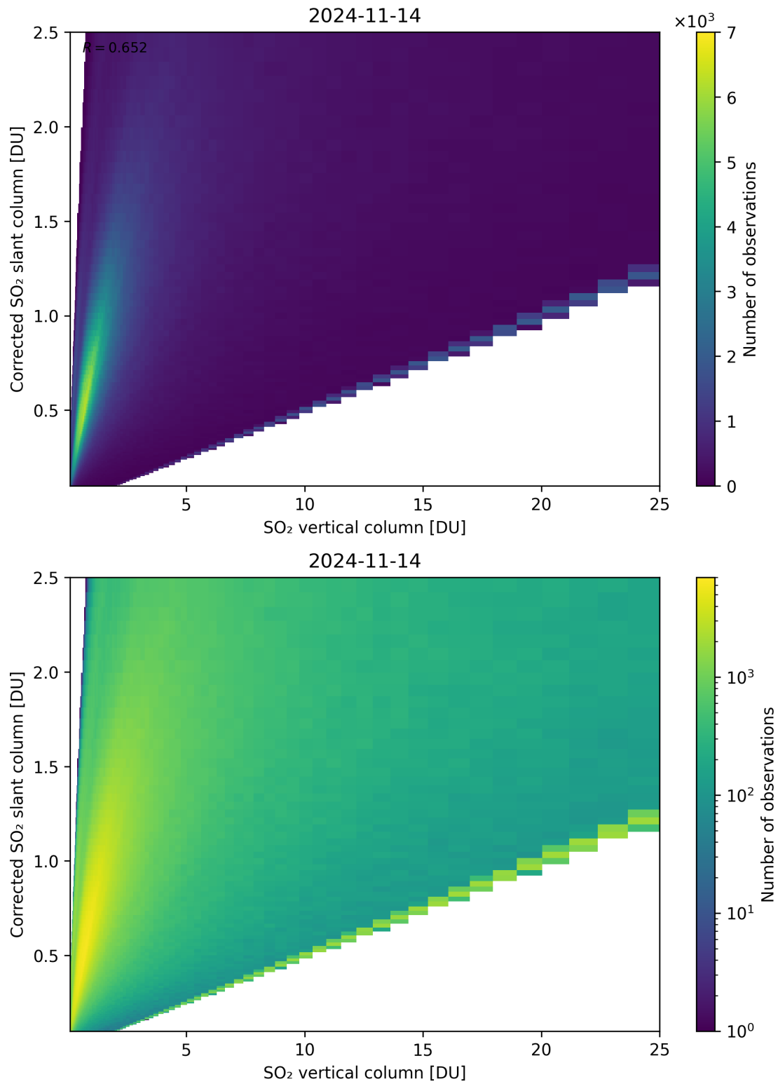
Figure 297: Scatter density plot of “SO 2 vertical column” against “Corrected SO 2 slant column” for 2024-11-14 to 2024-11-15.
