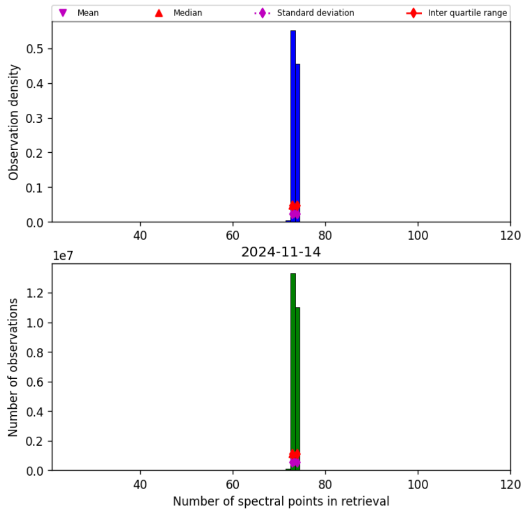
Figure 74: Histogram of “Number of spectral points in retrieval” for 2024-11-14 to 2024-11-15
