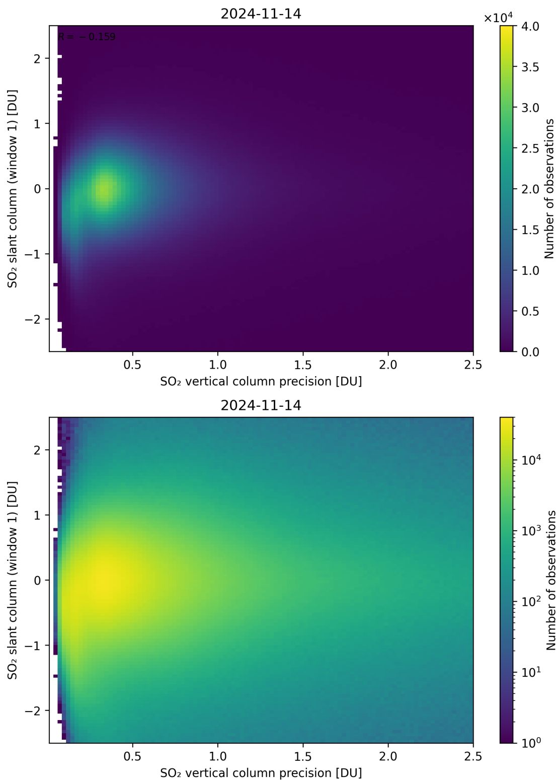
Figure 289: Scatter density plot of “SO 2 vertical column precision” against “SO 2 slant column (window 1)” for 2024-11-14 to 2024-11-15.
