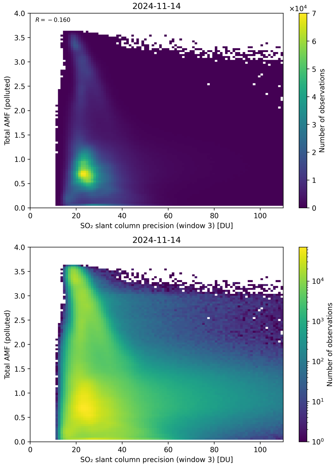
Figure 263: Scatter density plot of “SO 2 slant column precision (window 3)” against “Total AMF (polluted)” for 2024-11-14 to 2024-11-15.
