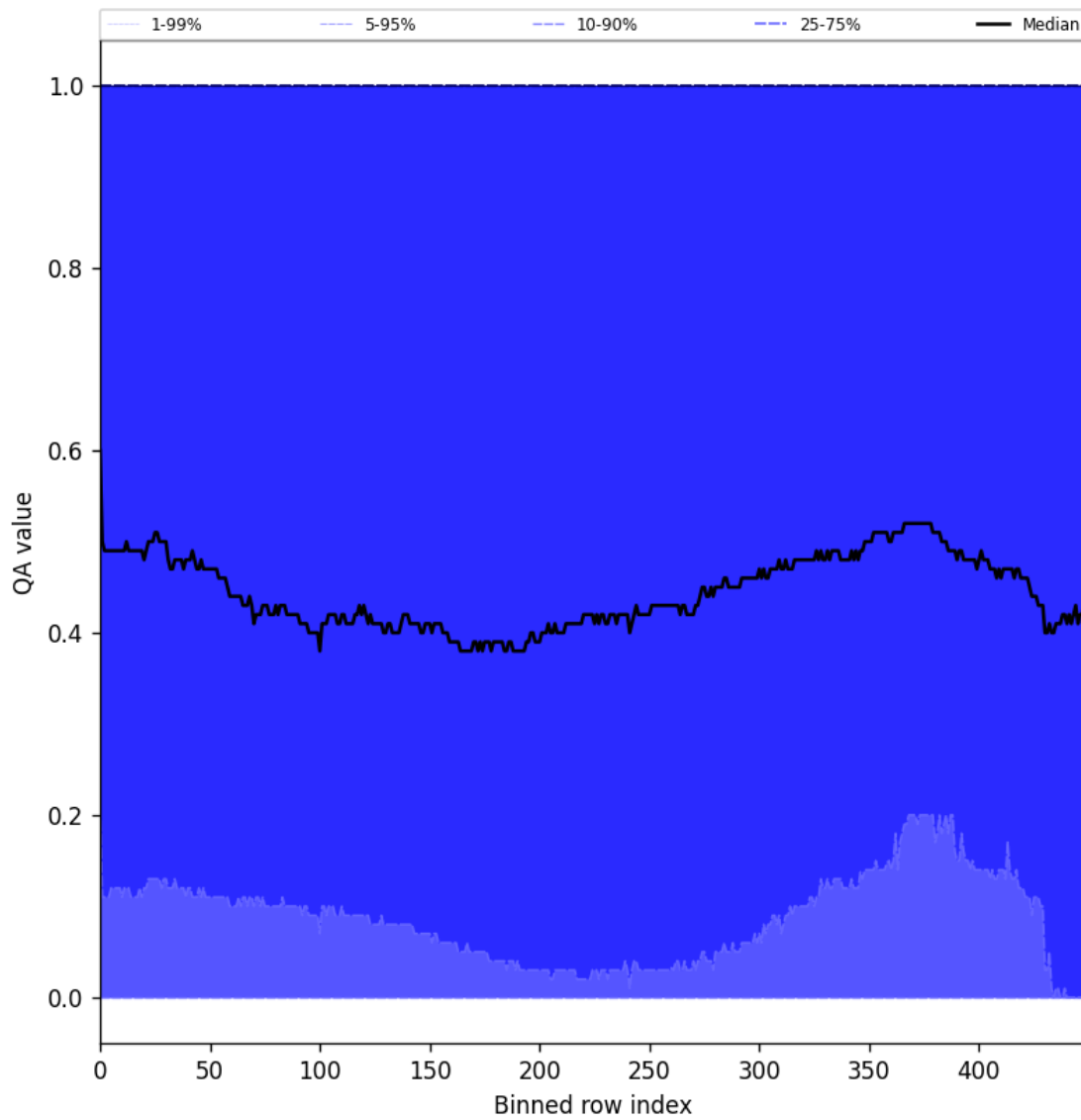
Figure 75: Along track statistics of “QA value” for 2024-11-14 to 2024-11-15
