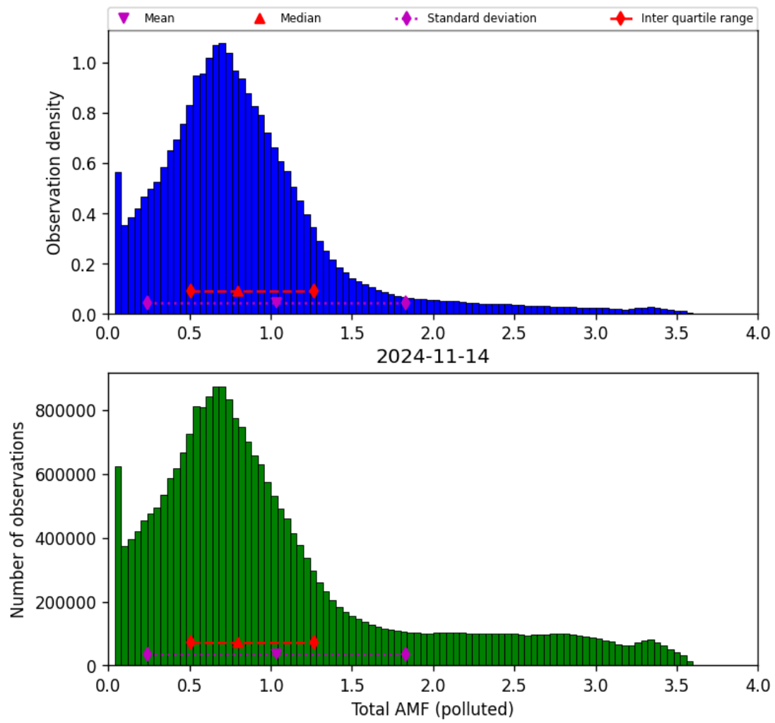
Figure 71: Histogram of “Total AMF (polluted)” for 2024-11-14 to 2024-11-15
