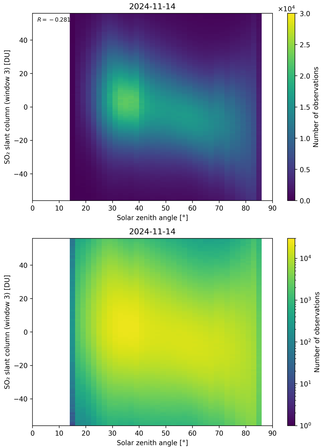
Figure 172: Scatter density plot of “Solar zenith angle” against “SO 2 slant column (window 3)” for 2024-11-14 to 2024-11-15.
