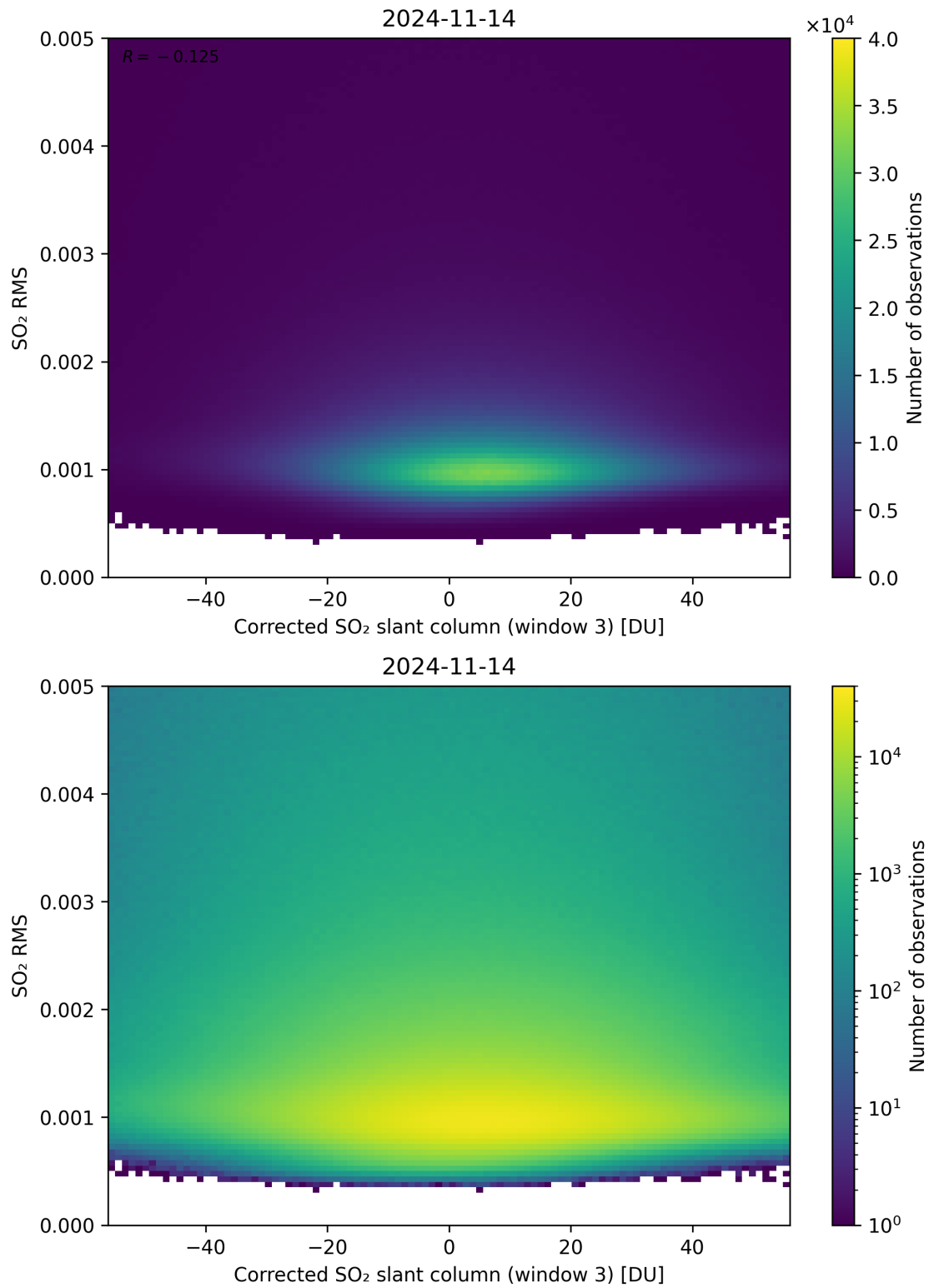
Figure 208: Scatter density plot of “Corrected SO 2 slant column (window 3)” against “SO 2 RMS” for 2024-11-14 to 2024-11-15.
