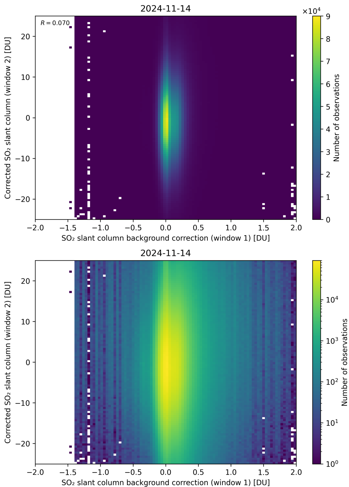
Figure 104: Scatter density plot of “SO 2 slant column background correction (window 1)” against “Corrected SO 2 slant column (window 2)” for 2024-11-14 to 2024-11-15.
