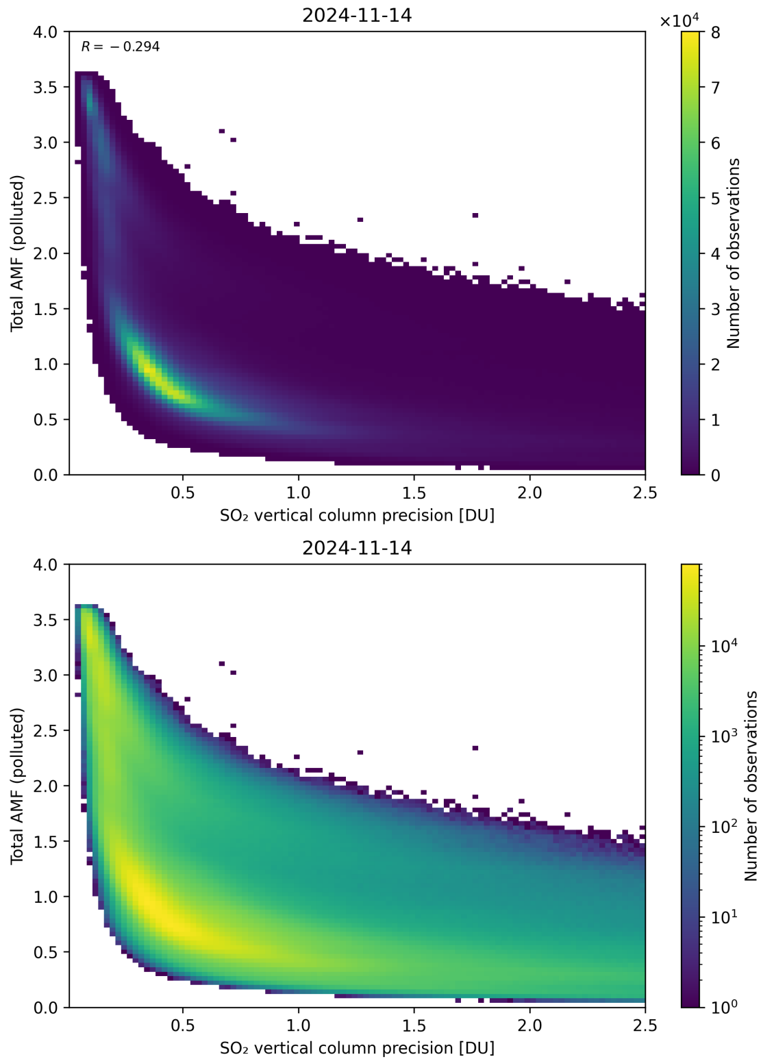
Figure 294: Scatter density plot of “SO 2 vertical column precision” against “Total AMF (polluted)” for 2024-11-14 to 2024-11-15.
