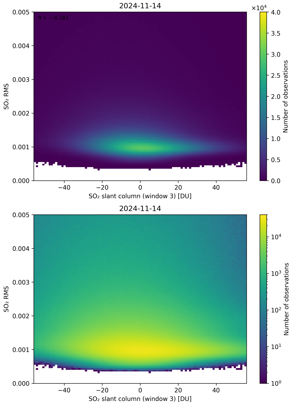
Figure 256: Scatter density plot of “SO 2 slant column (window 3)” against “SO 2 RMS” for 2024-11-14 to 2024-11-15.
