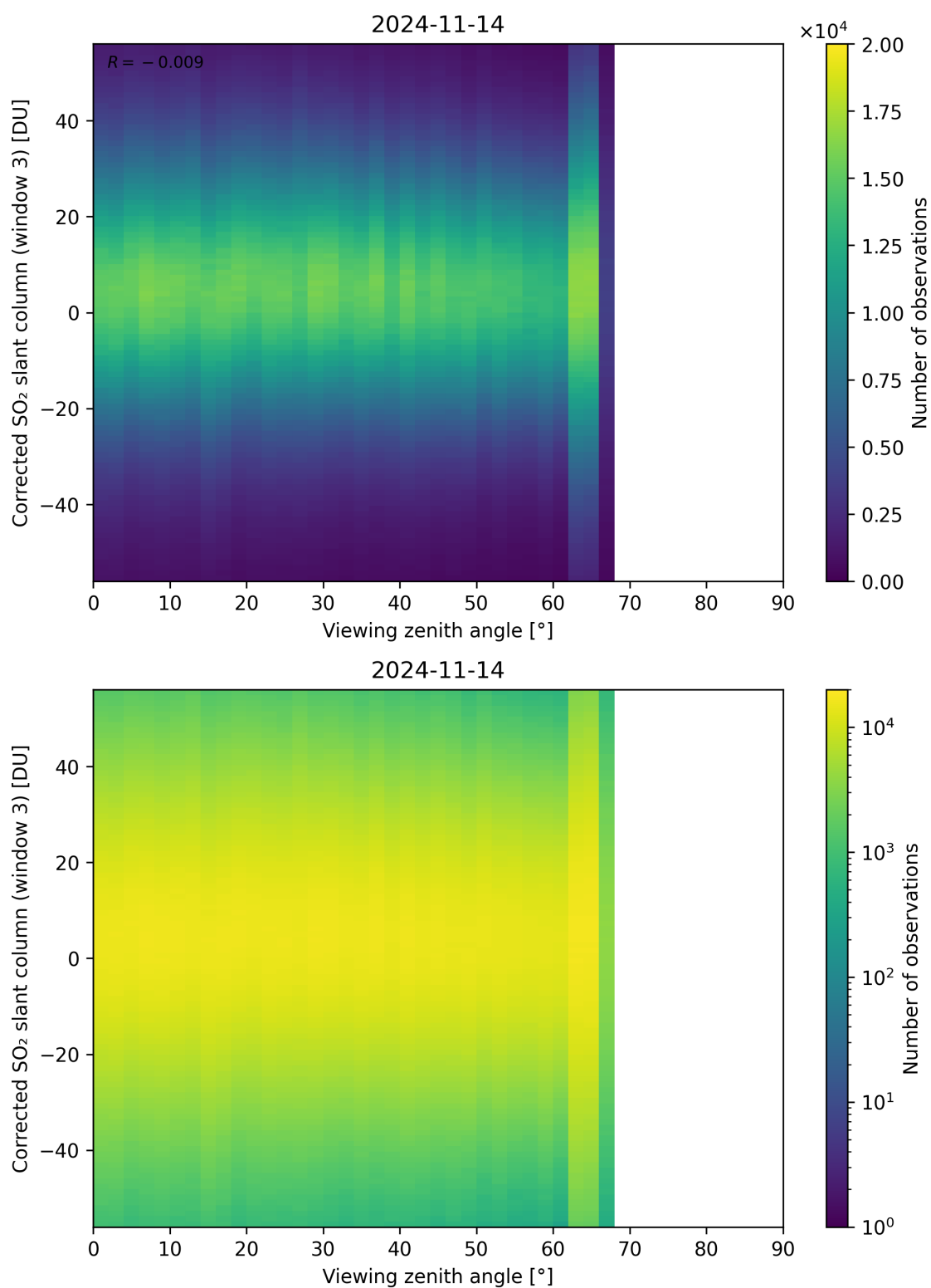
Figure 319: Scatter density plot of “Viewing zenith angle” against “Corrected SO 2 slant column (window 3)” for 2024-11-14 to 2024-11-15.
