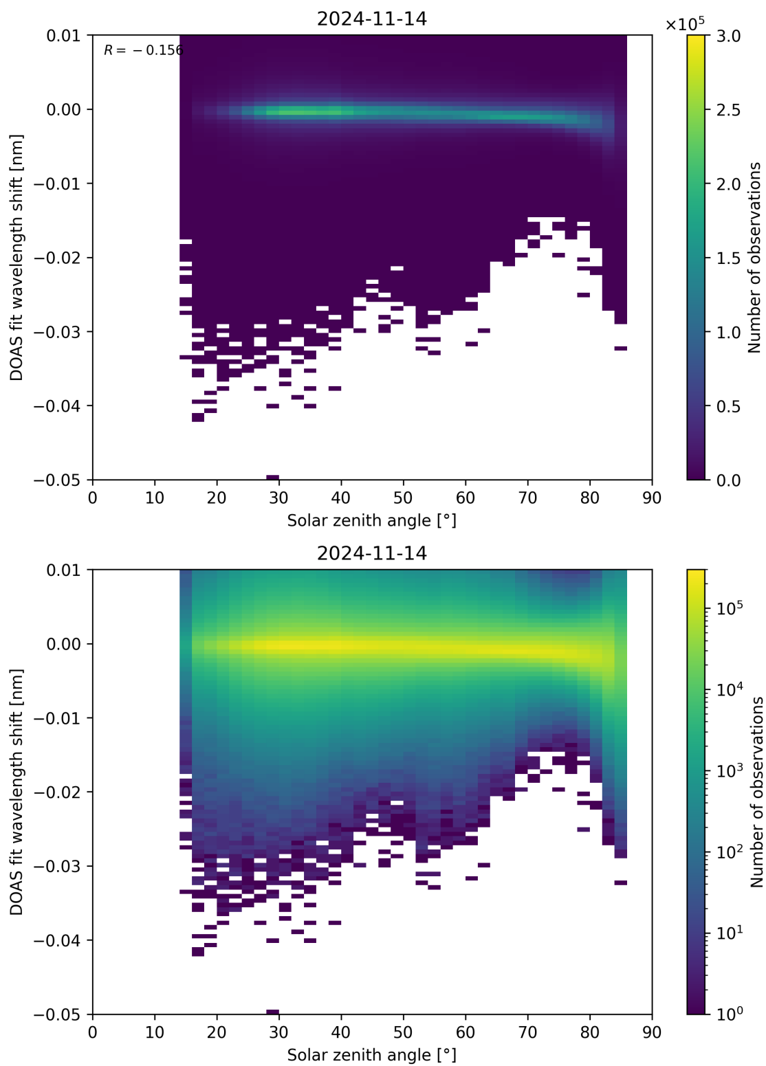
Figure 161: Scatter density plot of “Solar zenith angle” against “DOAS fit wavelength shift” for 2024-11-14 to 2024-11-15.
