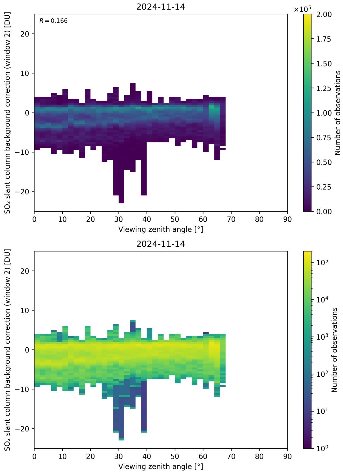
Figure 309: Scatter density plot of “Viewing zenith angle” against “SO 2 slant column background correction (window 2)” for 2024-11-14 to 2024-11-15.
