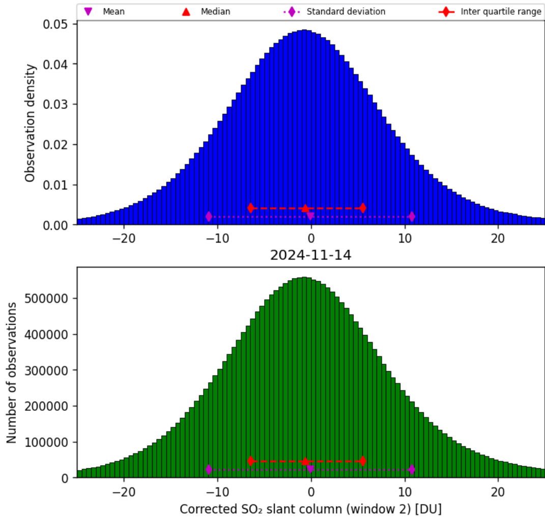
Figure 62: Histogram of “Corrected SO 2 slant column (window 2)” for 2024-11-14 to 2024-11-15
