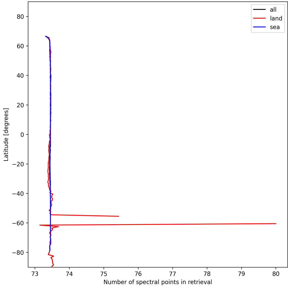
Figure 51: Zonal average of “Number of spectral points in retrieval” for 2024-11-14 to 2024-11-15.
