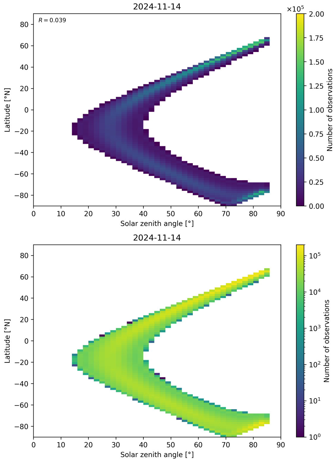
Figure 164: Scatter density plot of “Solar zenith angle” against “Latitude” for 2024-11-14 to 2024-11-15.
