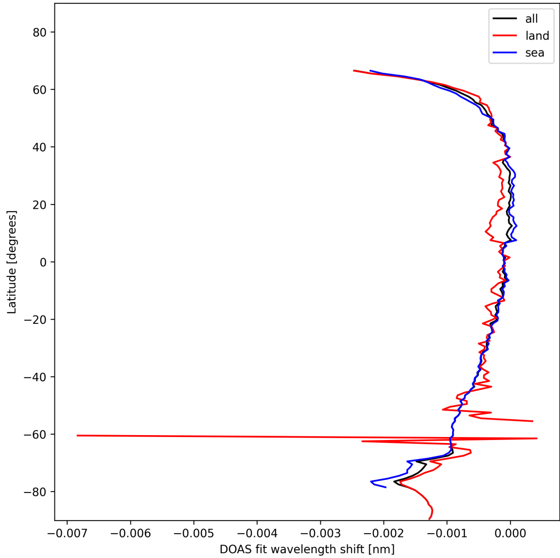
Figure 45: Zonal average of “DOAS fit wavelength shift” for 2024-11-14 to 2024-11-15.
