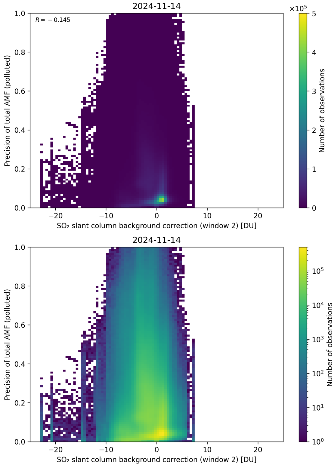
Figure 120: Scatter density plot of “SO 2 slant column background correction (window 2)” against “Precision of total AMF (polluted)” for 2024-11-14 to 2024-11-15.
