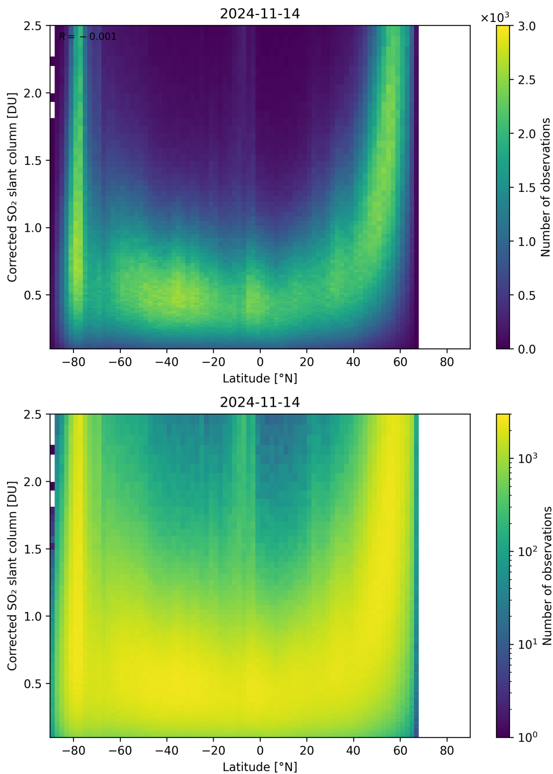
Figure 146: Scatter density plot of “Latitude” against “Corrected SO 2 slant column” for 2024-11-14 to 2024-11-15.
