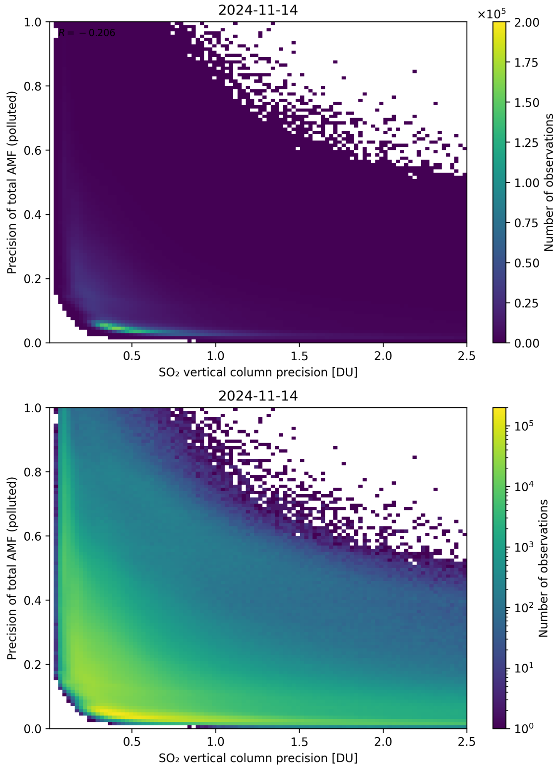
Figure 295: Scatter density plot of “SO 2 vertical column precision” against “Precision of total AMF (polluted)” for 2024-11-14 to 2024-11-15.
