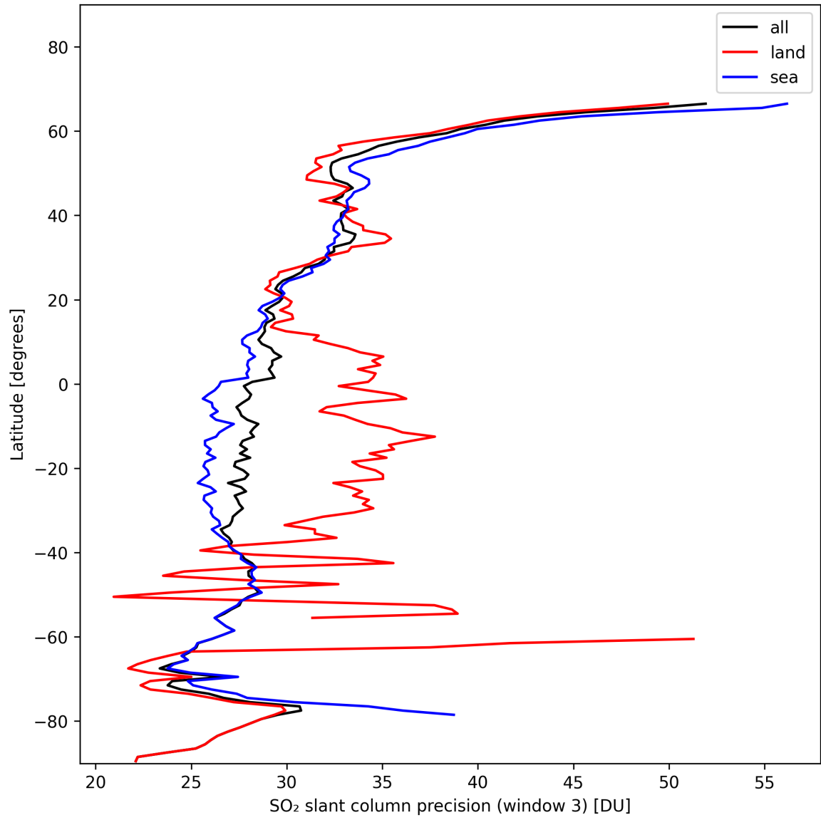
Figure 42: Zonal average of “SO 2 slant column precision (window 3)” for 2024-11-14 to 2024-11-15.
