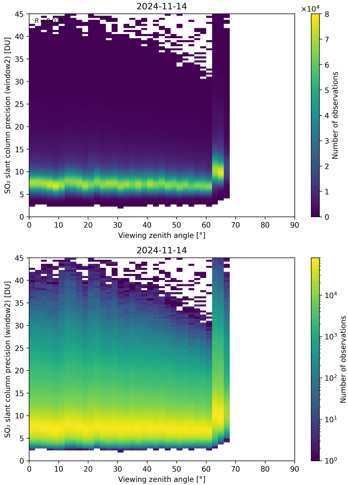
Figure 322: Scatter density plot of “Viewing zenith angle” against “SO 2 slant column precision (window2)” for 2024-11-14 to 2024-11-15.
