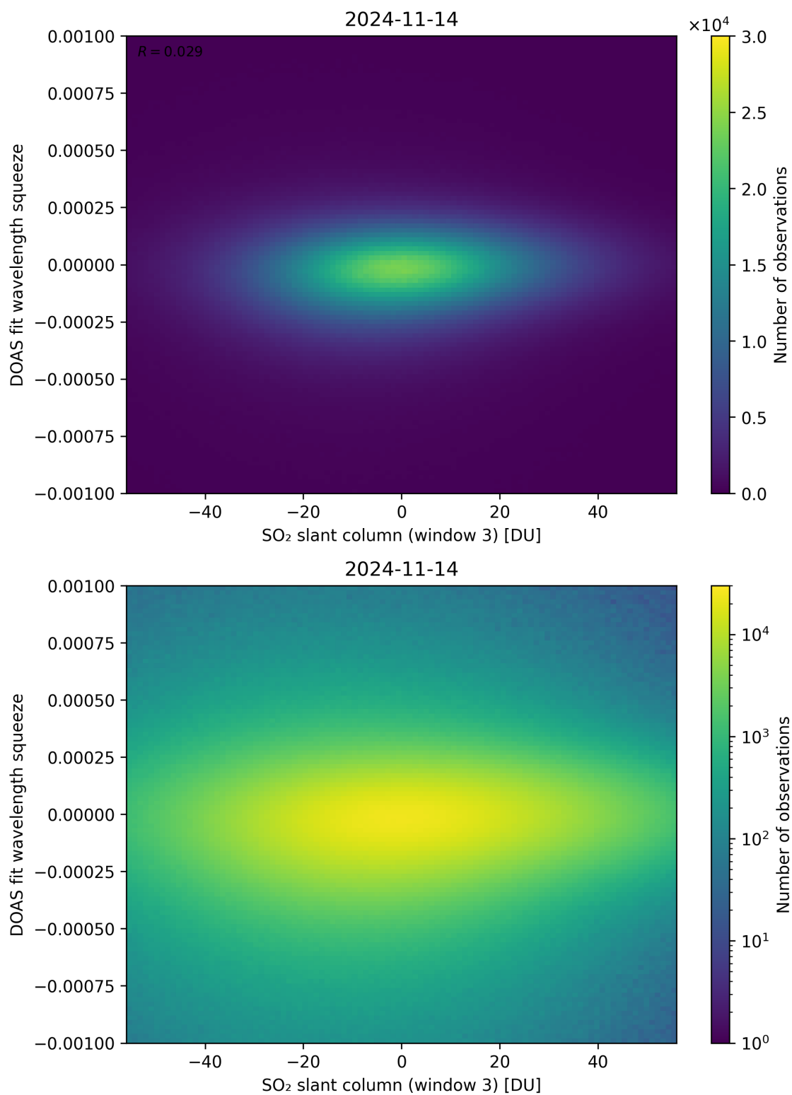
Figure 255: Scatter density plot of “SO 2 slant column (window 3)” against “DOAS fit wavelength squeeze” for 2024-11-14 to 2024-11-15.
