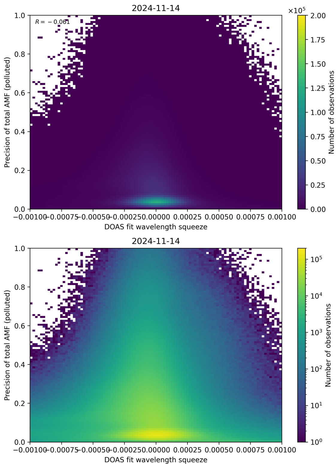
Figure 135: Scatter density plot of “DOAS fit wavelength squeeze” against “Precision of total AMF (polluted)” for 2024-11-14 to 2024-11-15.
