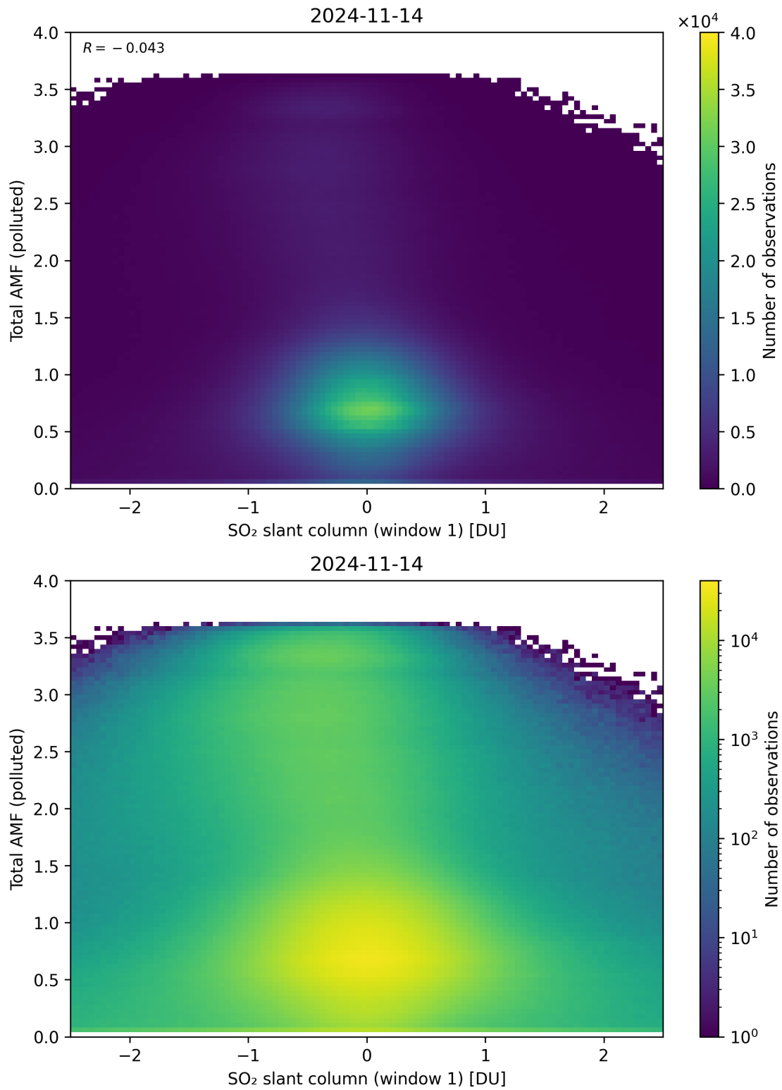
Figure 239: Scatter density plot of “SO 2 slant column (window 1)” against “Total AMF (polluted)” for 2024-11-14 to 2024-11-15.
