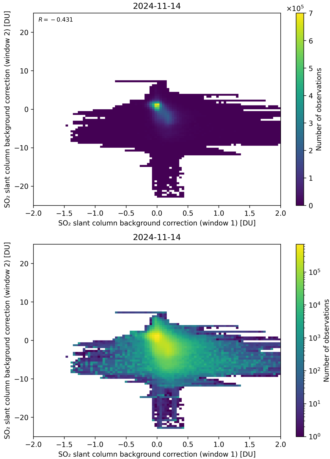
Figure 98: Scatter density plot of “SO 2 slant column background correction (window 1)” against “SO 2 slant column background correction (window 2)” for 2024-11-14 to 2024-11-15.
