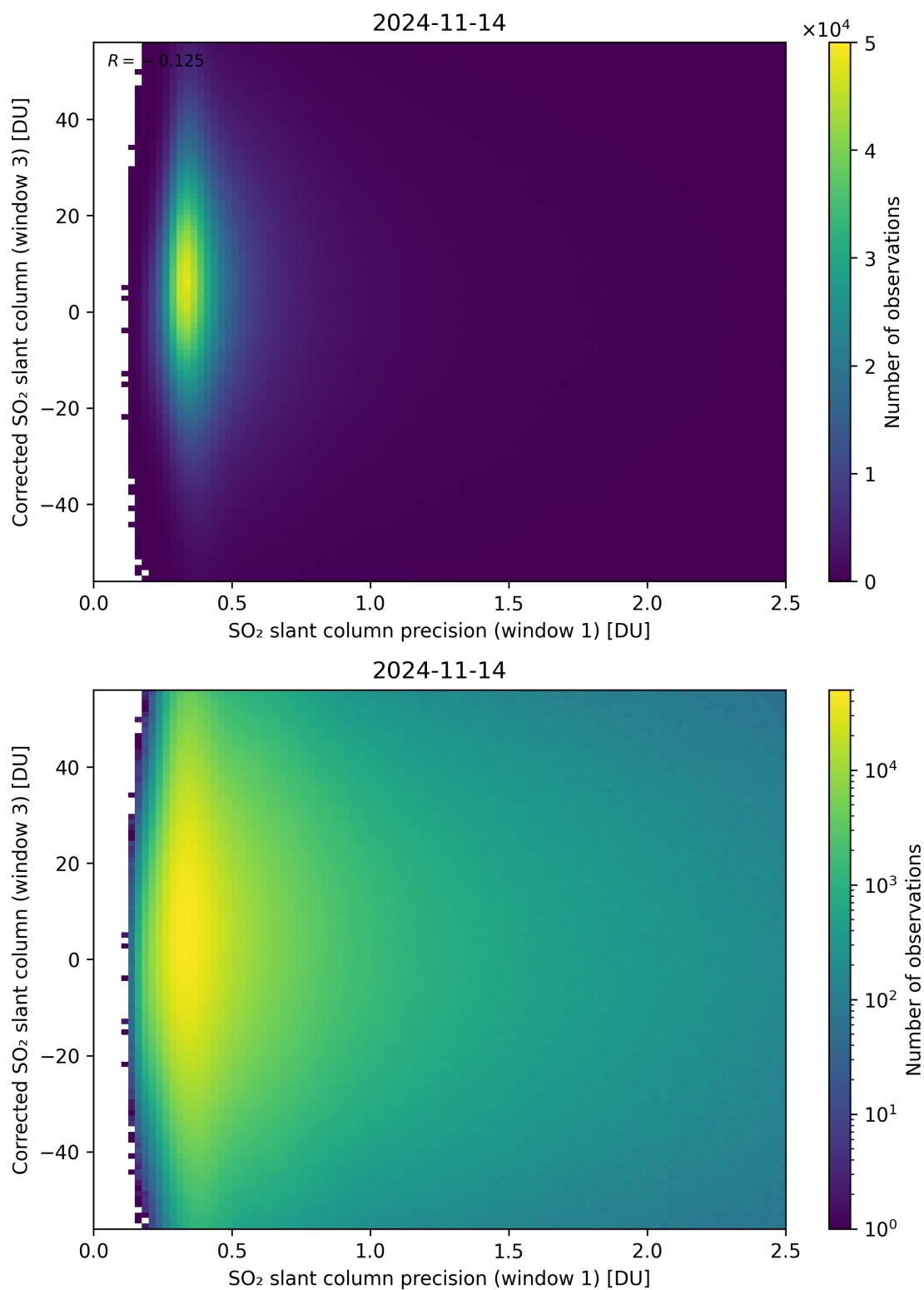
Figure 226: Scatter density plot of “SO 2 slant column precision (window 1)” against “Corrected SO 2 slant column (window 3)” for 2024-11-14 to 2024-11-15.
