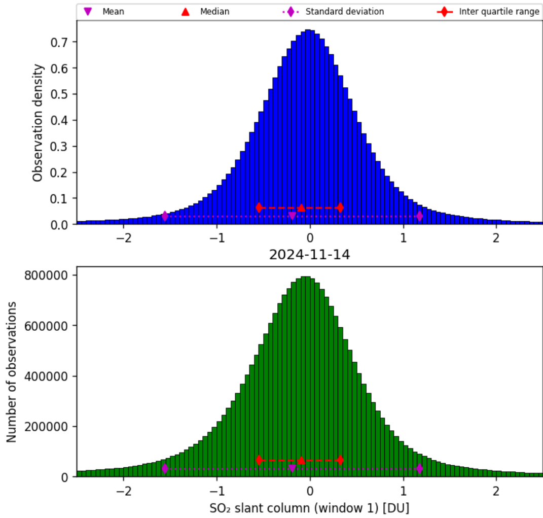
Figure 56: Histogram of “SO 2 slant column (window 1)” for 2024-11-14 to 2024-11-15
