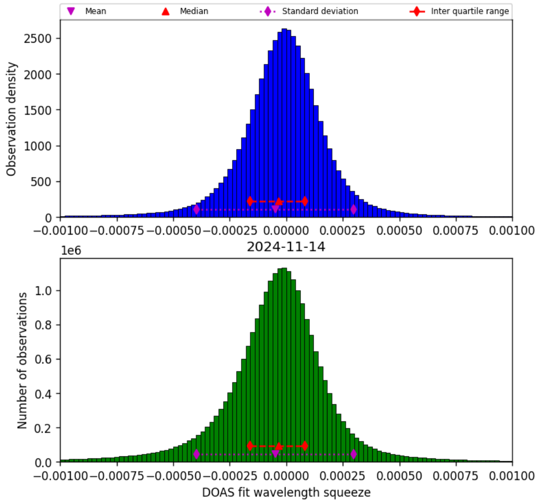
Figure 69: Histogram of “DOAS fit wavelength squeeze” for 2024-11-14 to 2024-11-15
