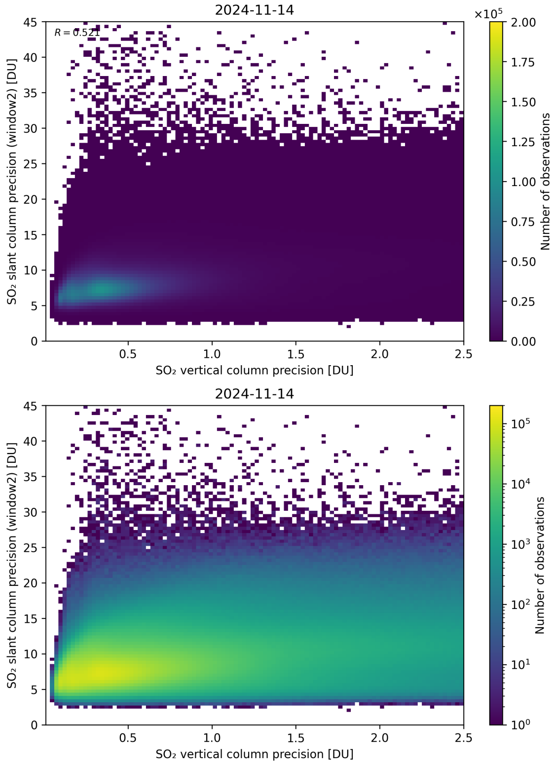
Figure 291: Scatter density plot of “SO 2 vertical column precision” against “SO 2 slant column precision (window2)” for 2024-11-14 to 2024-11-15.
