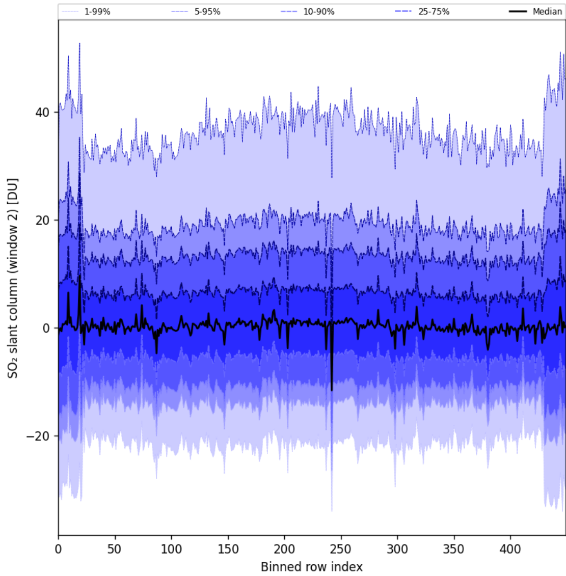
Figure 83: Along track statistics of “SO 2 slant column (window 2)” for 2024-11-14 to 2024-11-15
