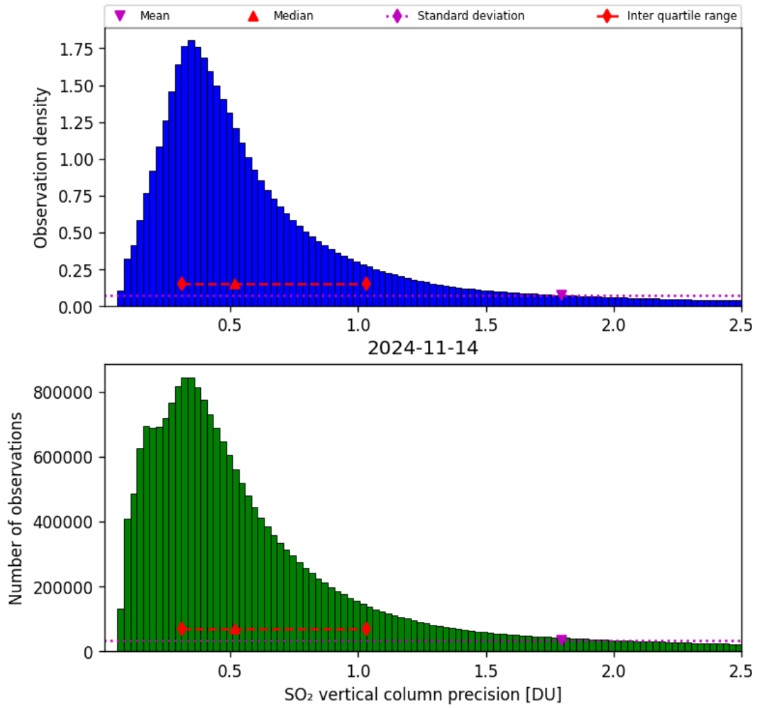
Figure 54: Histogram of “SO 2 vertical column precision” for 2024-11-14 to 2024-11-15
