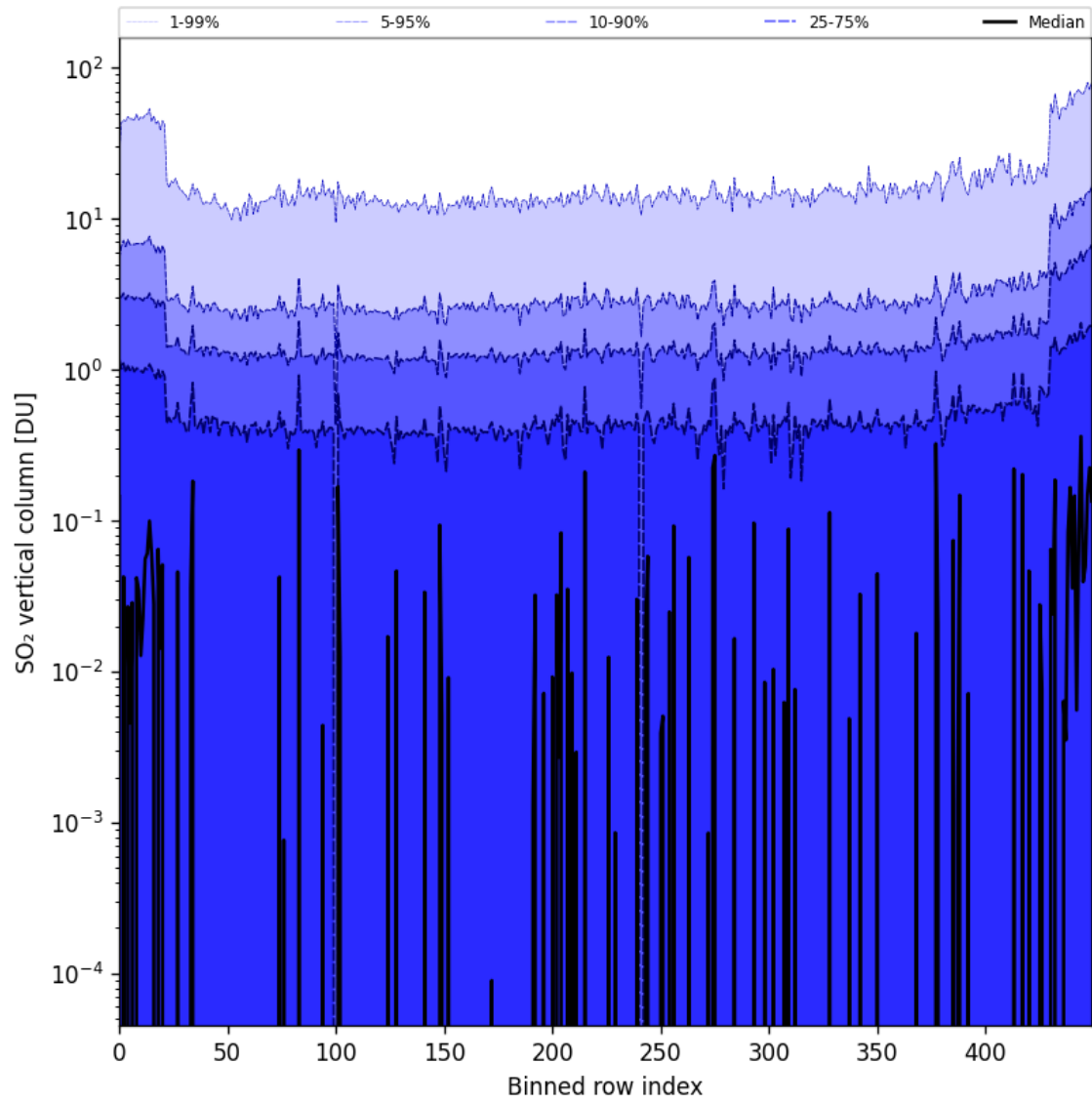
Figure 76: Along track statistics of “SO 2 vertical column” for 2024-11-14 to 2024-11-15
