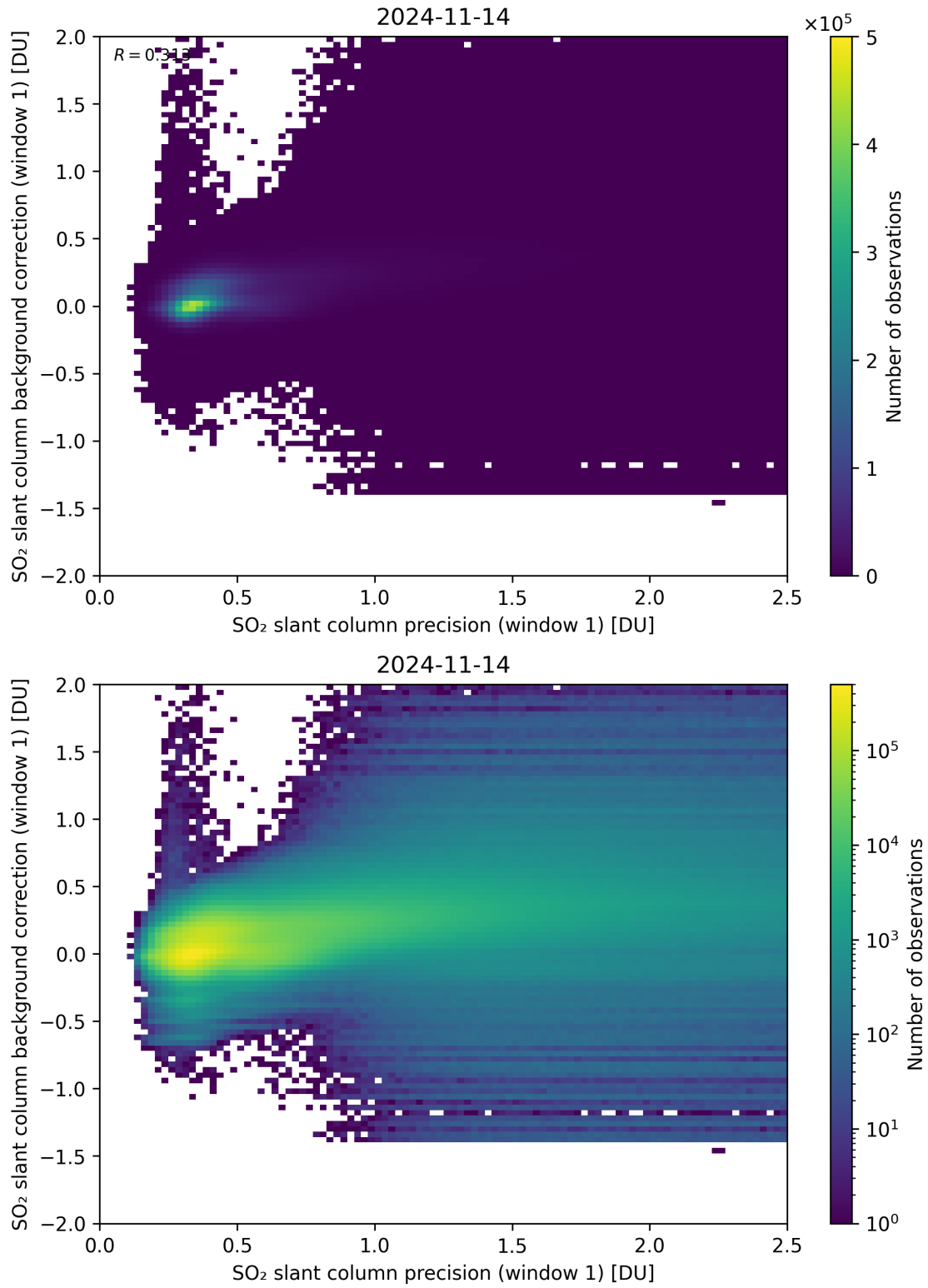
Figure 218: Scatter density plot of “SO 2 slant column precision (window 1)” against “SO 2 slant column background correction (window 1)” for 2024-11-14 to 2024-11-15.
