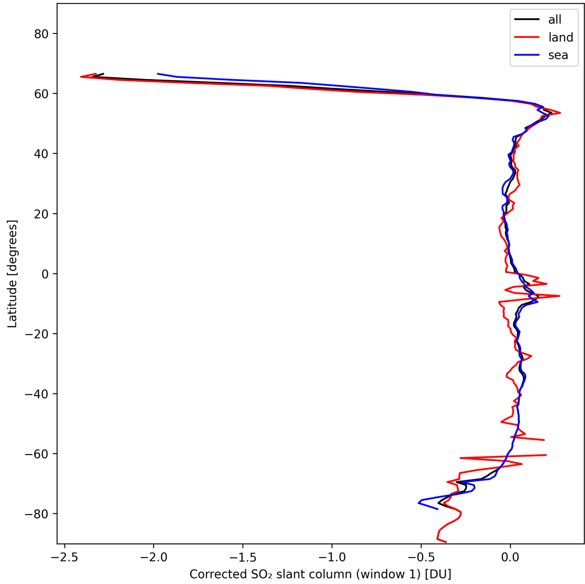
Figure 35: Zonal average of “Corrected SO 2 slant column (window 1)” for 2024-11-14 to 2024-11-15.
