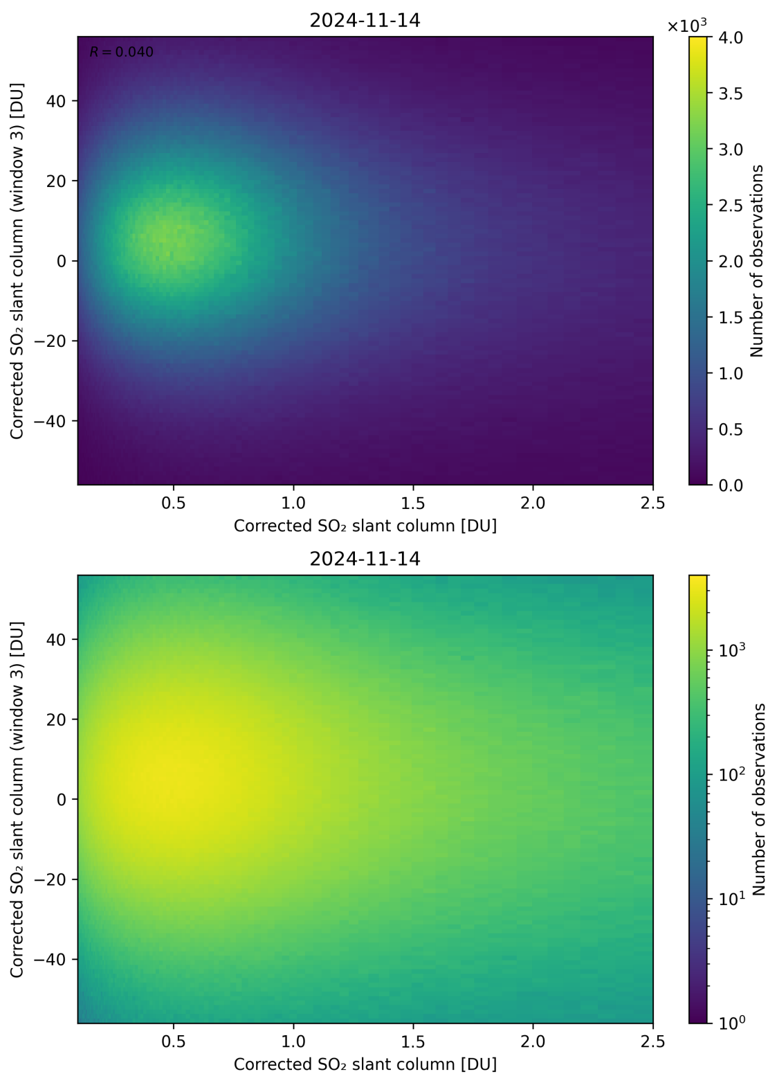
Figure 186: Scatter density plot of “Corrected SO 2 slant column” against “Corrected SO 2 slant column (window 3)” for 2024-11-14 to 2024-11-15.
