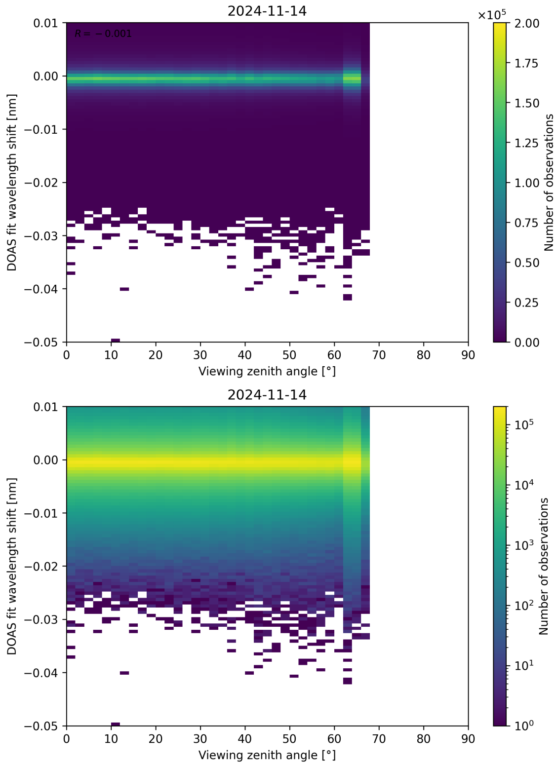
Figure 311: Scatter density plot of “Viewing zenith angle” against “DOAS fit wavelength shift” for 2024-11-14 to 2024-11-15.
