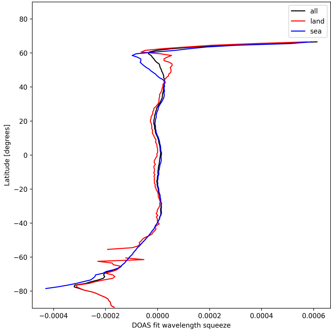
Figure 46: Zonal average of “DOAS fit wavelength squeeze” for 2024-11-14 to 2024-11-15.
