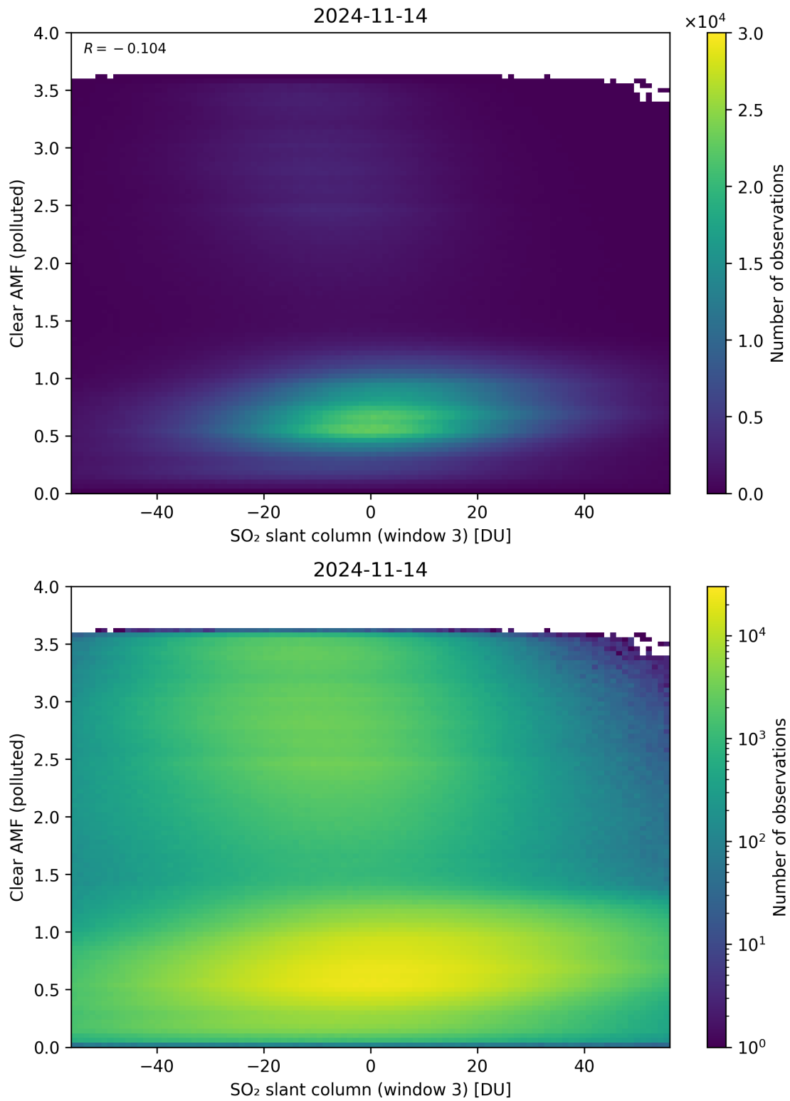
Figure 265: Scatter density plot of “SO 2 slant column (window 3)” against “Clear AMF (polluted)” for 2024-11-14 to 2024-11-15.
