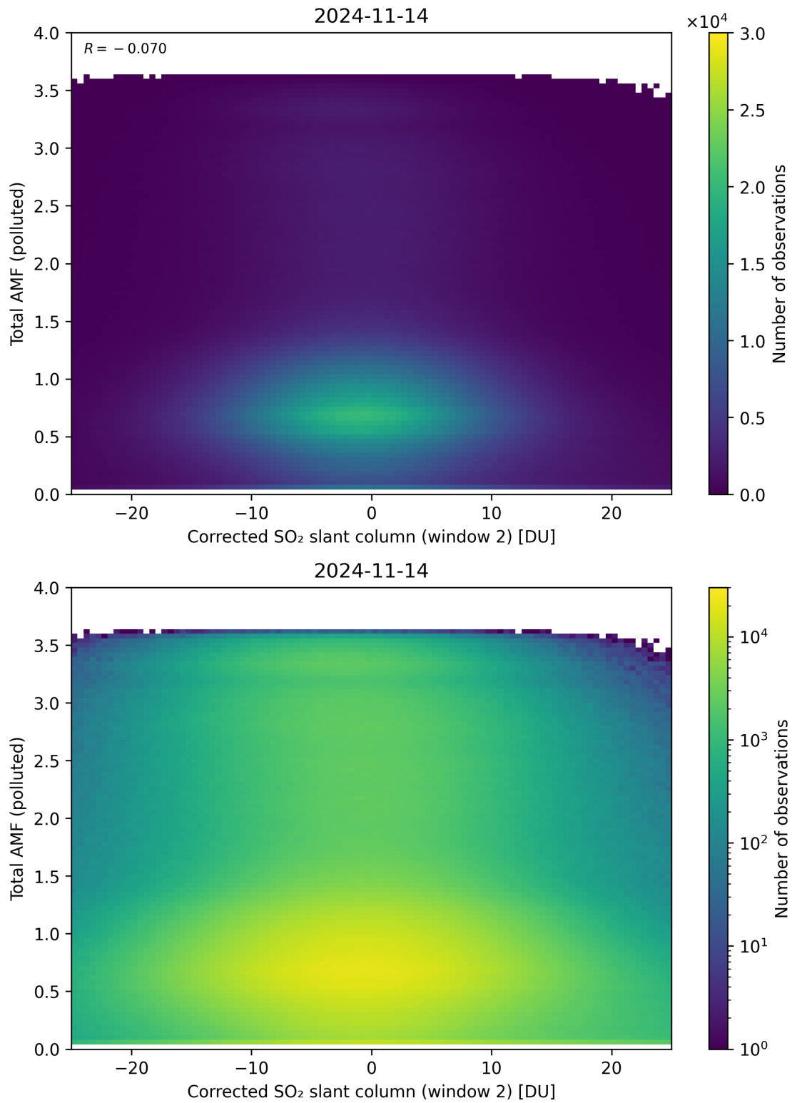
Figure 203: Scatter density plot of “Corrected SO 2 slant column (window 2)” against “Total AMF (polluted)” for 2024-11-14 to 2024-11-15.
