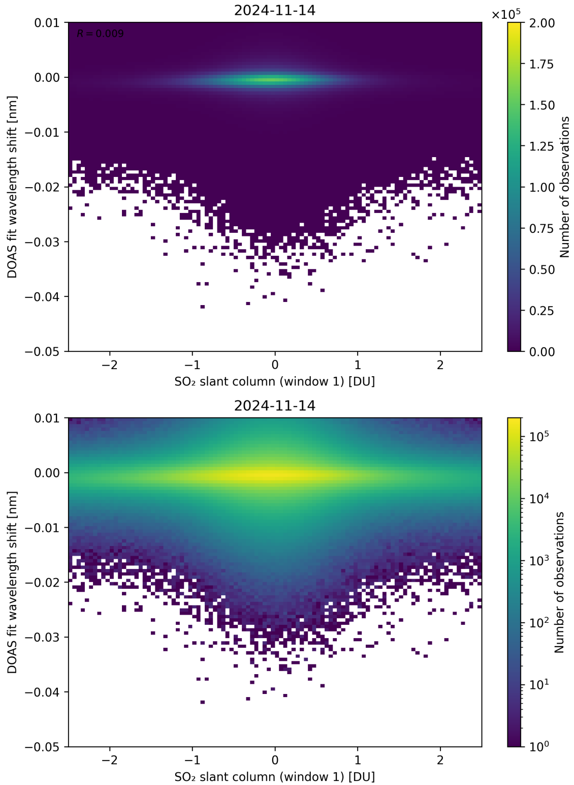
Figure 215: Scatter density plot of “SO 2 slant column (window 1)” against “DOAS fit wavelength shift” for 2024-11-14 to 2024-11-15.
