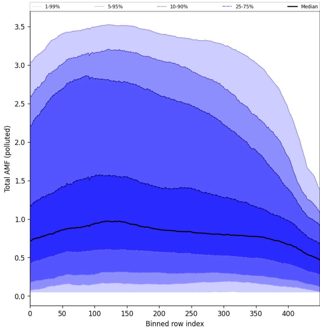
Figure 94: Along track statistics of “Total AMF (polluted)” for 2024-11-14 to 2024-11-15
