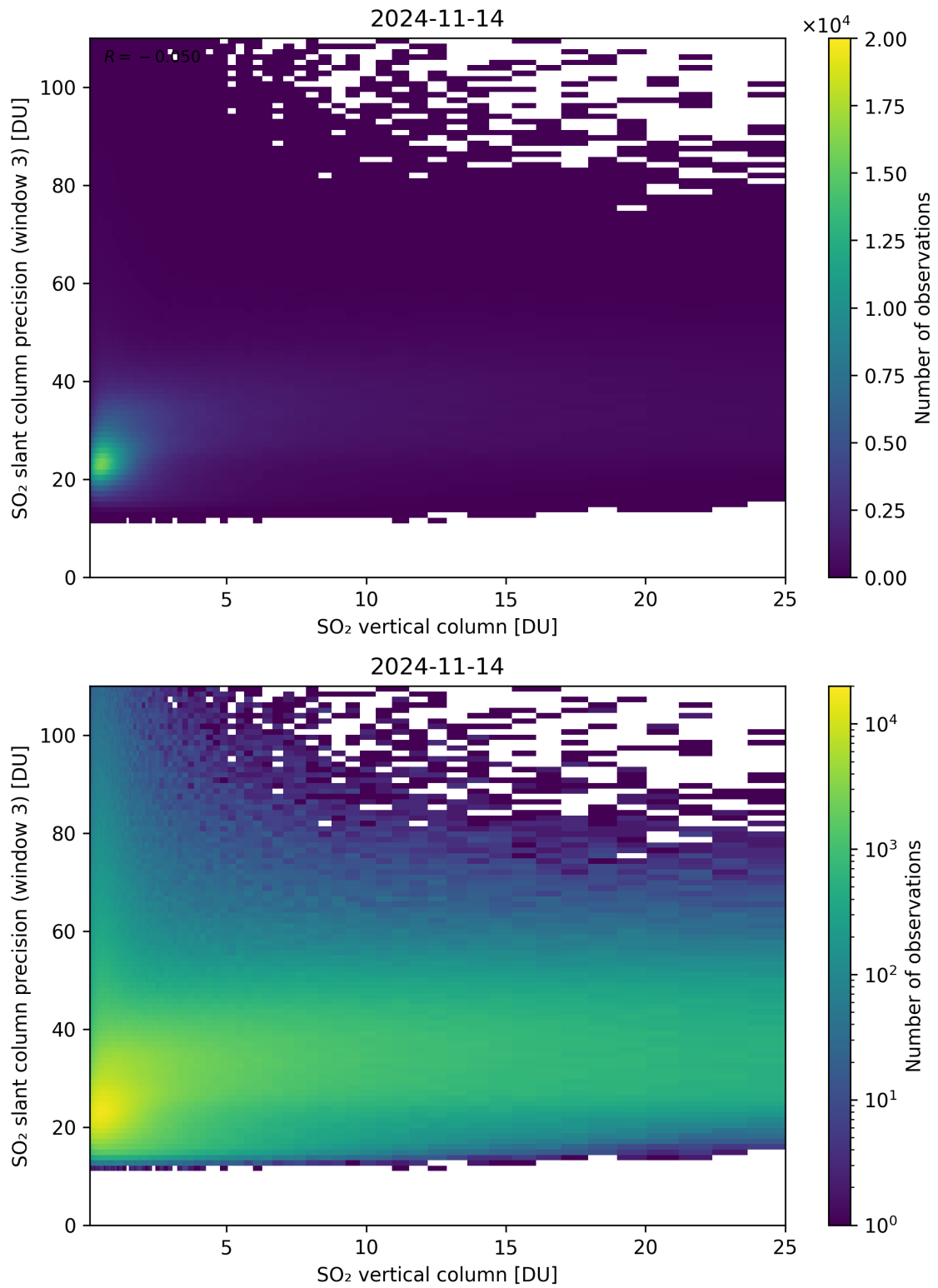
Figure 304: Scatter density plot of “SO 2 vertical column” against “SO 2 slant column precision (window 3)” for 2024-11-14 to 2024-11-15.
