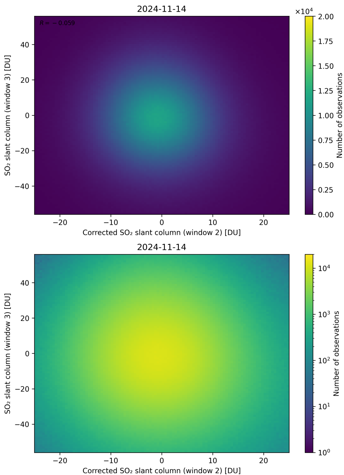
Figure 201: Scatter density plot of “Corrected SO 2 slant column (window 2)” against “SO 2 slant column (window 3)” for 2024-11-14 to 2024-11-15.
