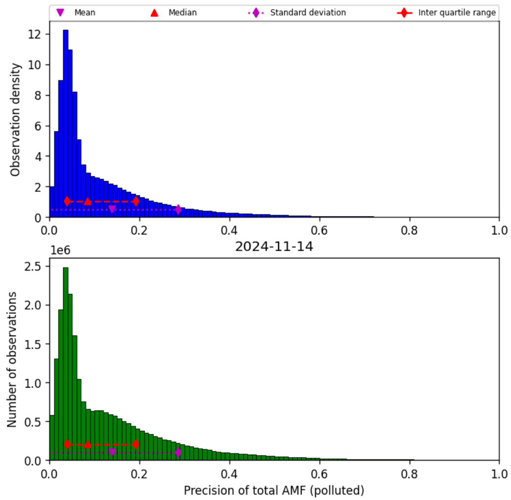
Figure 72: Histogram of “Precision of total AMF (polluted)” for 2024-11-14 to 2024-11-15
