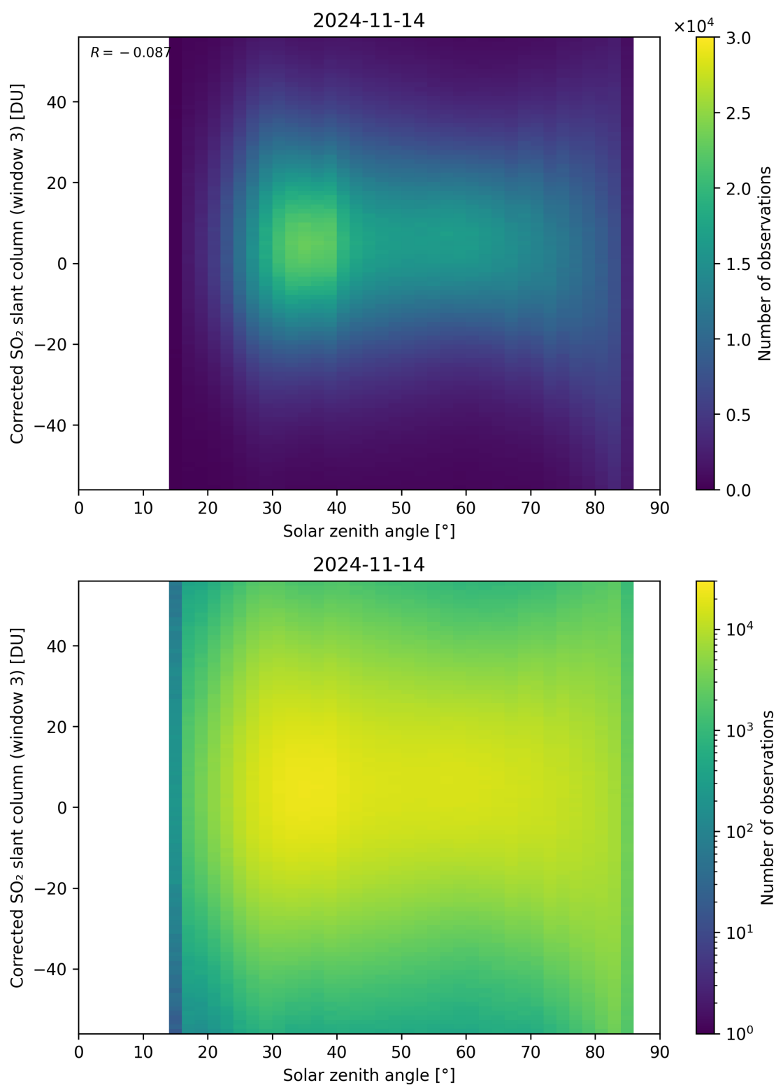
Figure 168: Scatter density plot of “Solar zenith angle” against “Corrected SO 2 slant column (window 3)” for 2024-11-14 to 2024-11-15.
