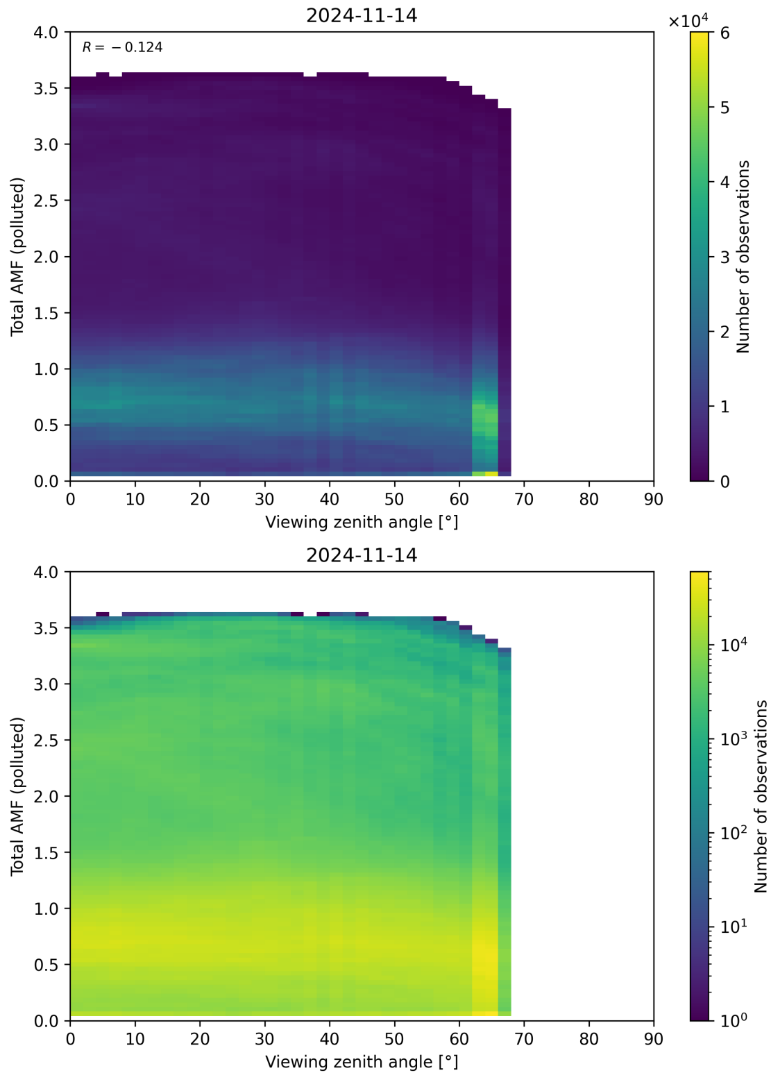
Figure 325: Scatter density plot of “Viewing zenith angle” against “Total AMF (polluted)” for 2024-11-14 to 2024-11-15.
