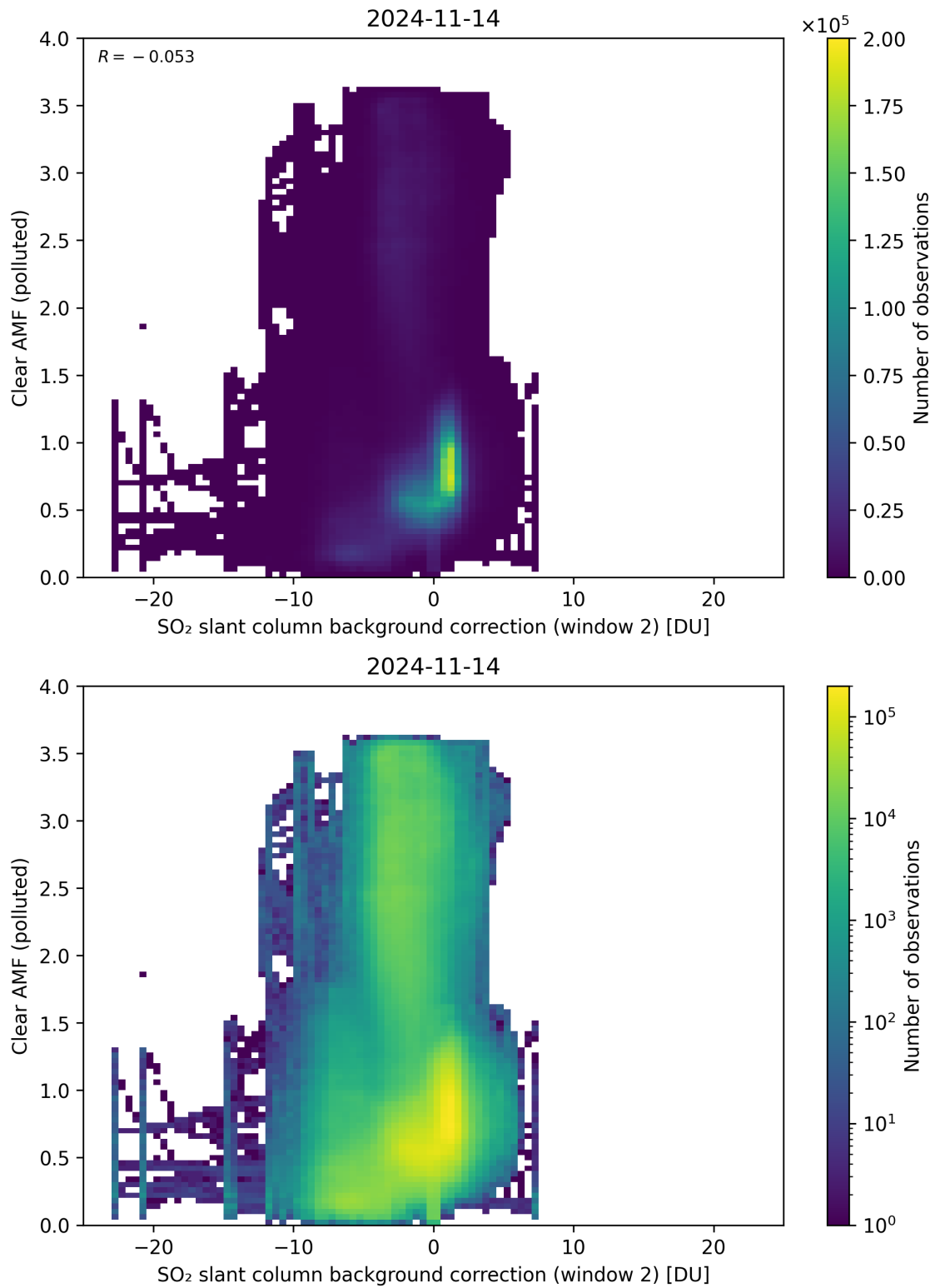
Figure 115: Scatter density plot of “SO 2 slant column background correction (window 2)” against “Clear AMF (polluted)” for 2024-11-14 to 2024-11-15.
