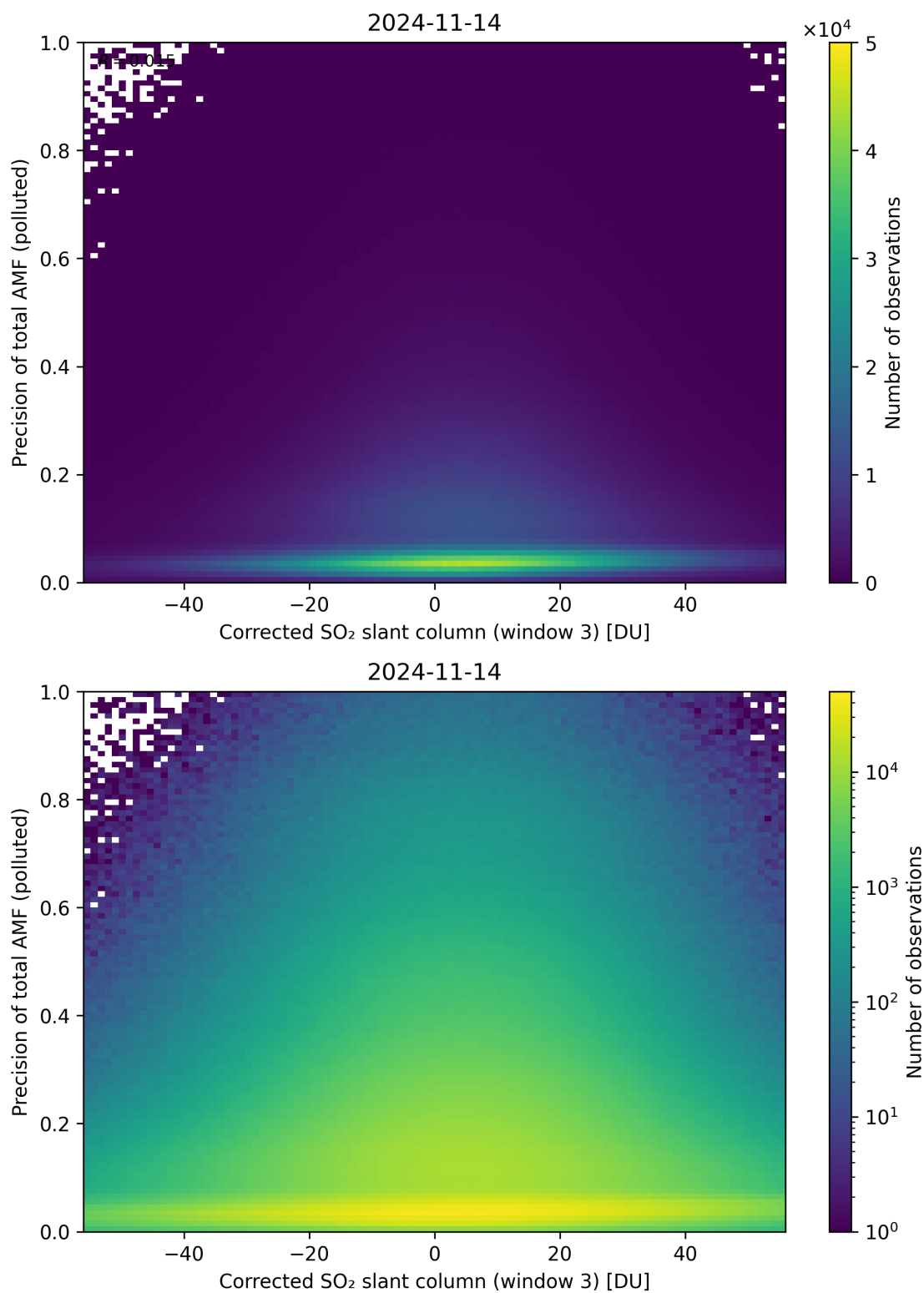
Figure 211: Scatter density plot of “Corrected SO 2 slant column (window 3)” against “Precision of total AMF (polluted)” for 2024-11-14 to 2024-11-15.
