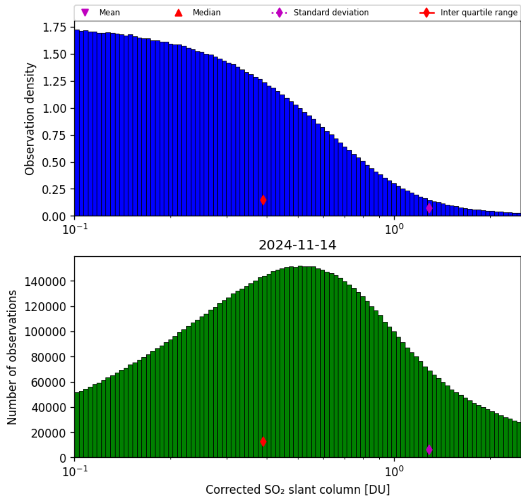
Figure 55: Histogram of “Corrected SO 2 slant column” for 2024-11-14 to 2024-11-15
