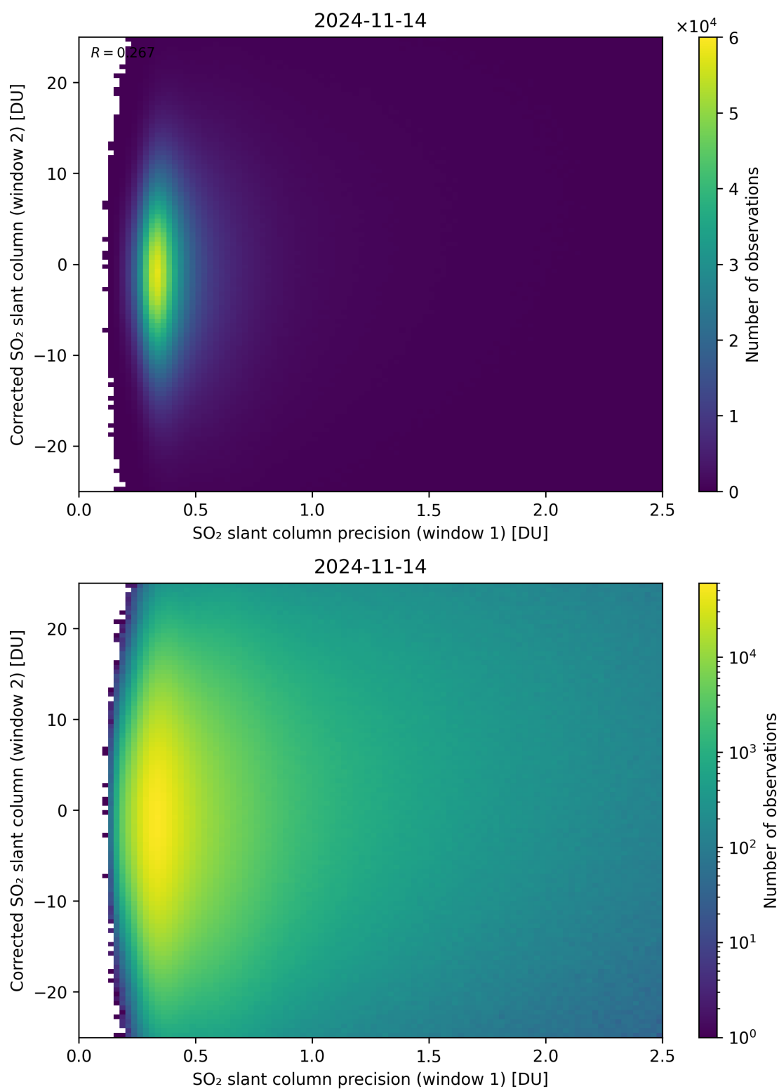
Figure 225: Scatter density plot of “SO 2 slant column precision (window 1)” against “Corrected SO 2 slant column (window 2)” for 2024-11-14 to 2024-11-15.
