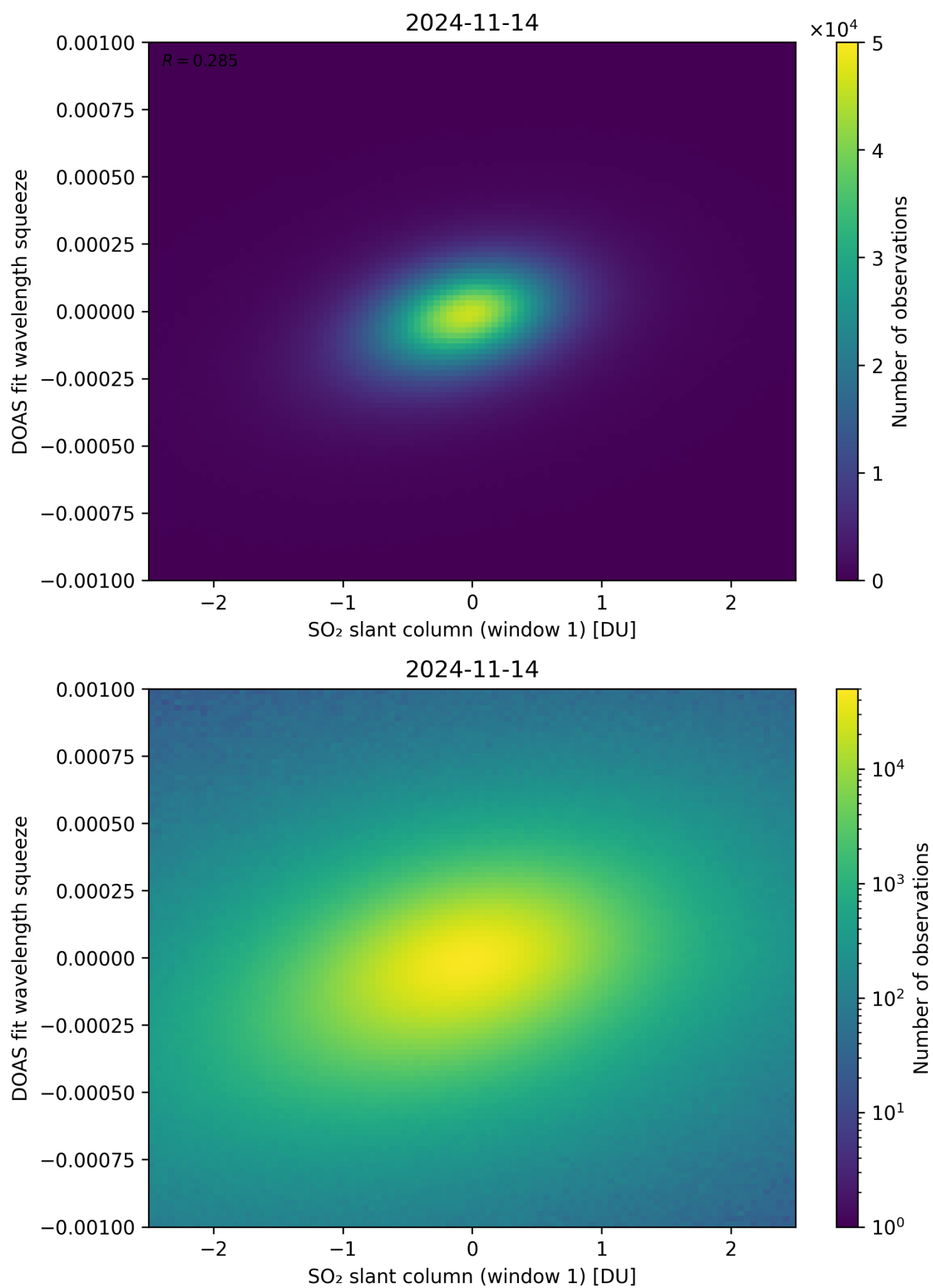
Figure 216: Scatter density plot of “SO 2 slant column (window 1)” against “DOAS fit wavelength squeeze” for 2024-11-14 to 2024-11-15.
