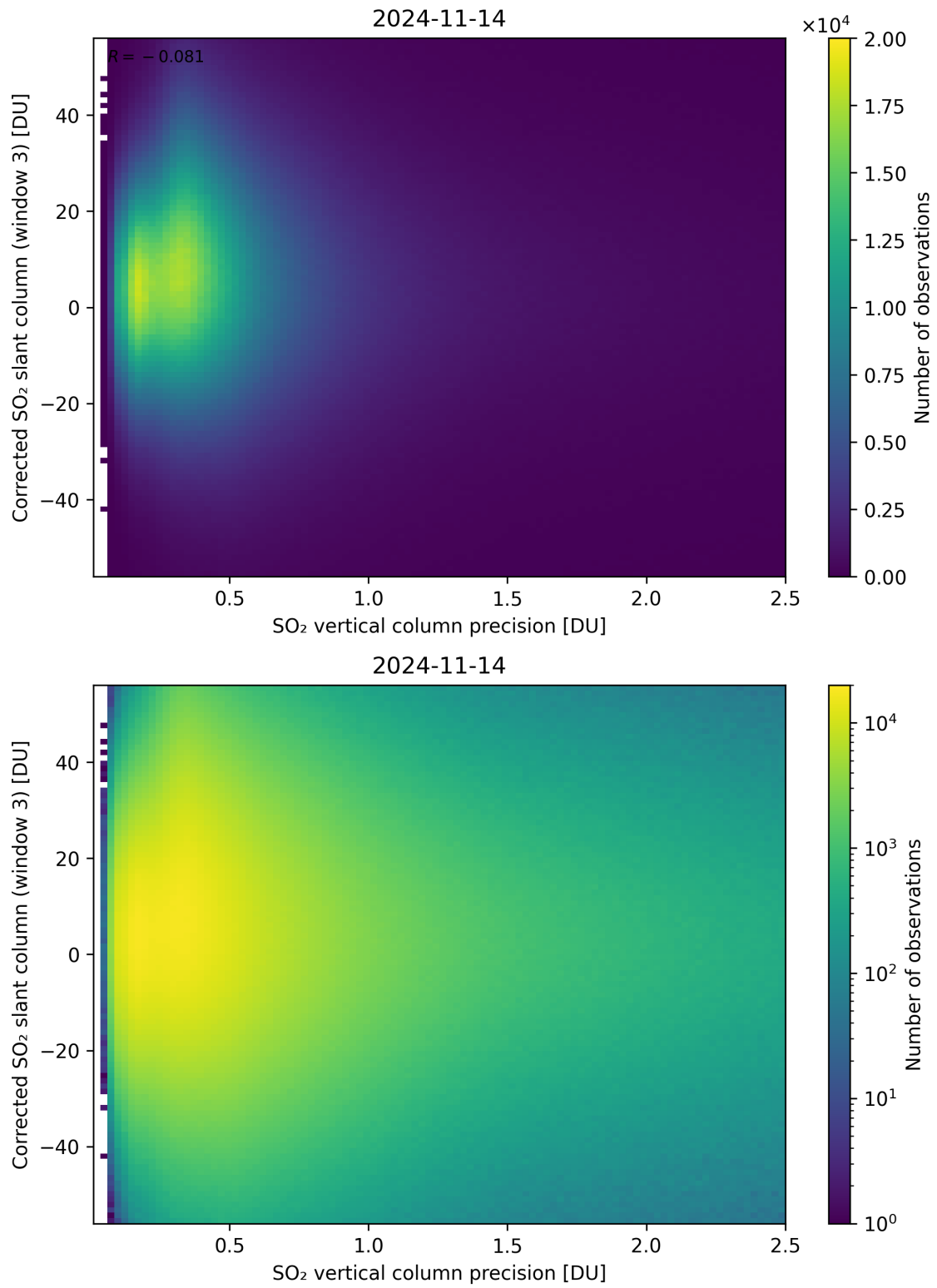
Figure 288: Scatter density plot of “SO 2 vertical column precision” against “Corrected SO 2 slant column (window 3)” for 2024-11-14 to 2024-11-15.
