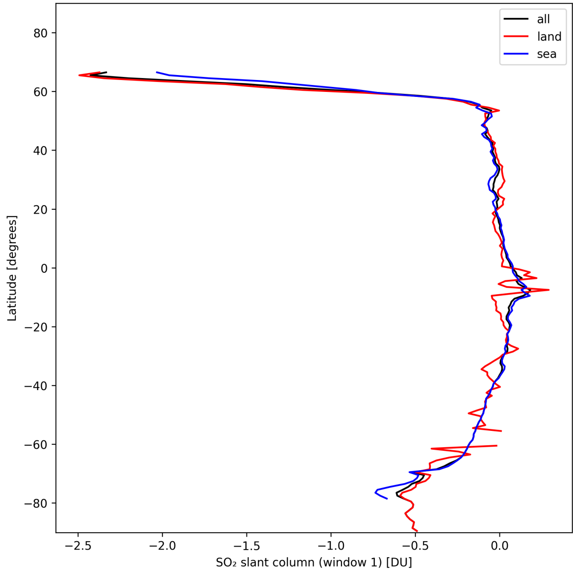
Figure 33: Zonal average of “SO 2 slant column (window 1)” for 2024-11-14 to 2024-11-15.
