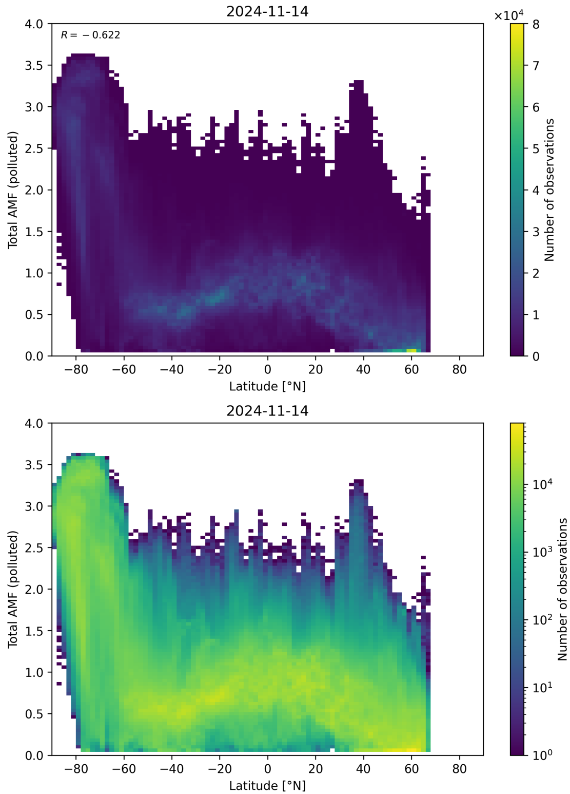
Figure 154: Scatter density plot of “Latitude” against “Total AMF (polluted)” for 2024-11-14 to 2024-11-15.
