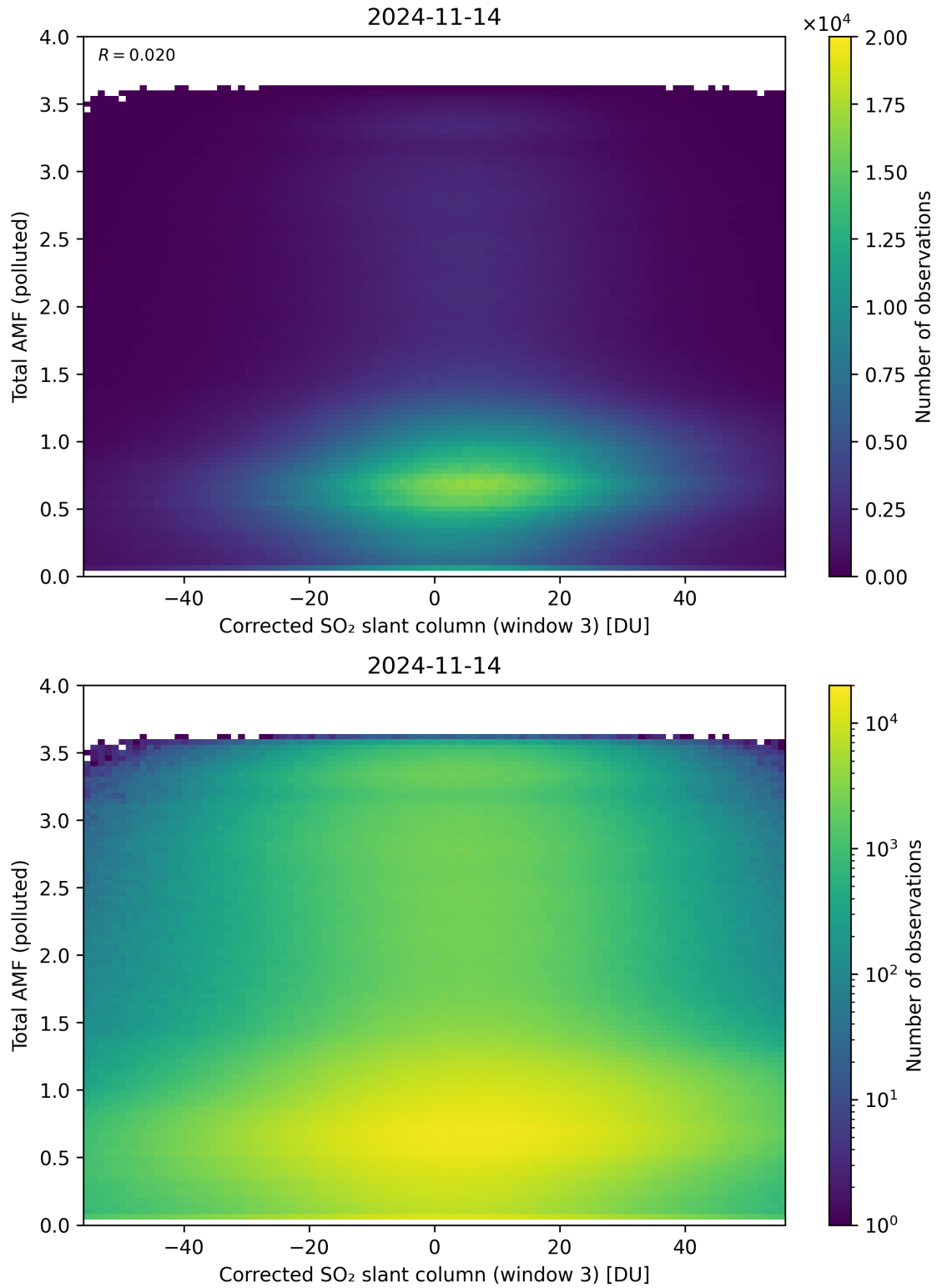
Figure 210: Scatter density plot of “Corrected SO 2 slant column (window 3)” against “Total AMF (polluted)” for 2024-11-14 to 2024-11-15.
