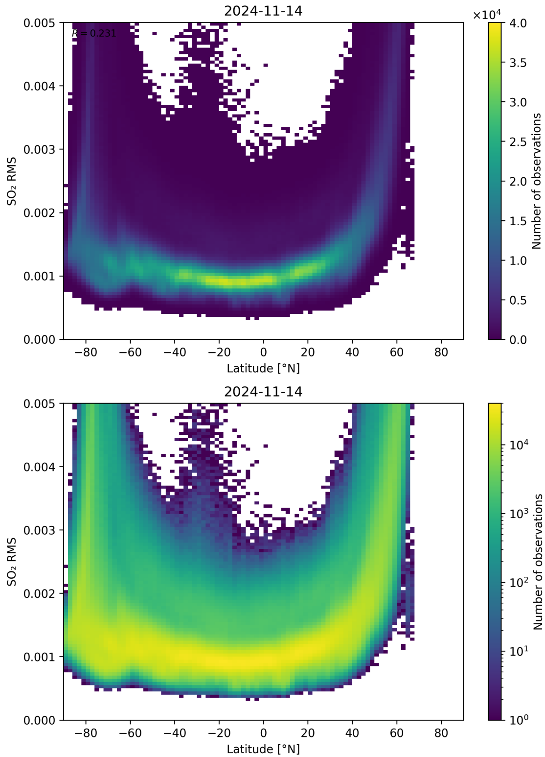
Figure 144: Scatter density plot of “Latitude” against “SO 2 RMS” for 2024-11-14 to 2024-11-15.
