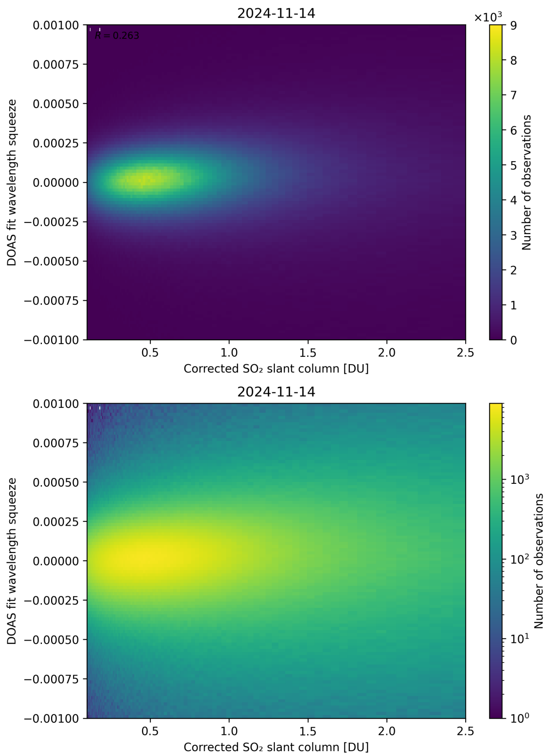
Figure 182: Scatter density plot of “Corrected SO 2 slant column” against “DOAS fit wavelength squeeze” for 2024-11-14 to 2024-11-15.
