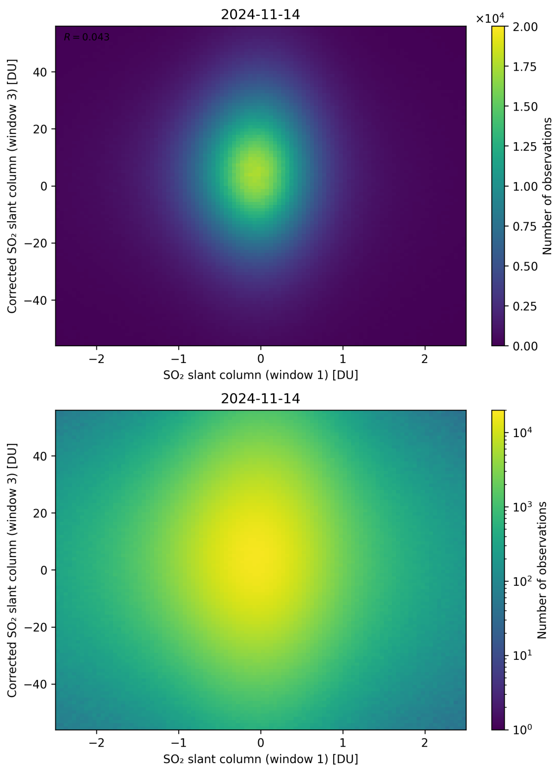
Figure 234: Scatter density plot of “SO 2 slant column (window 1)” against “Corrected SO 2 slant column (window 3)” for 2024-11-14 to 2024-11-15.
