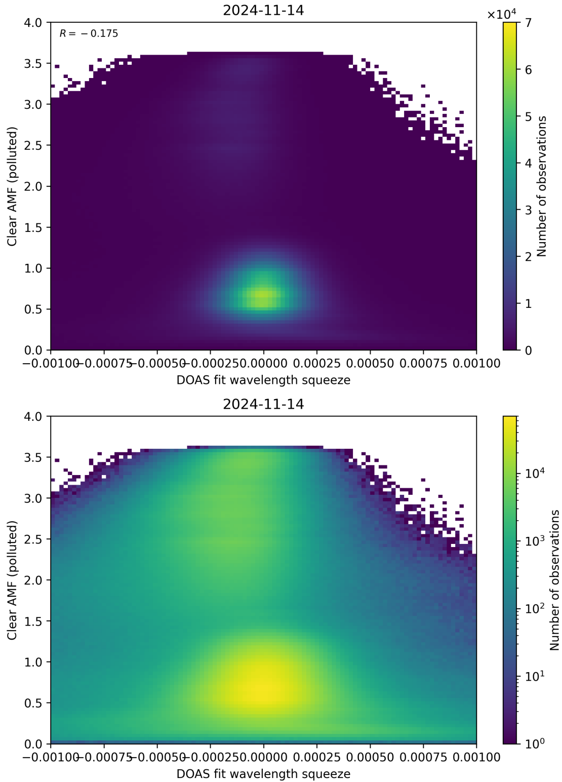
Figure 133: Scatter density plot of “DOAS fit wavelength squeeze” against “Clear AMF (polluted)” for 2024-11-14 to 2024-11-15.
