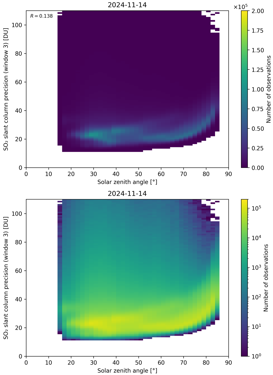
Figure 173: Scatter density plot of “Solar zenith angle” against “SO 2 slant column precision (window 3)” for 2024-11-14 to 2024-11-15.
