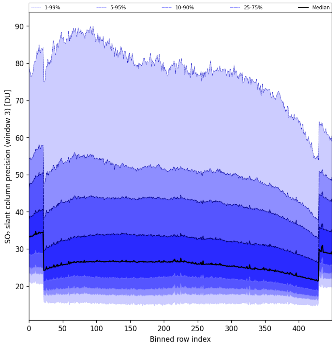
Figure 88: Along track statistics of “SO 2 slant column precision (window 3)” for 2024-11-14 to 2024-11-15
