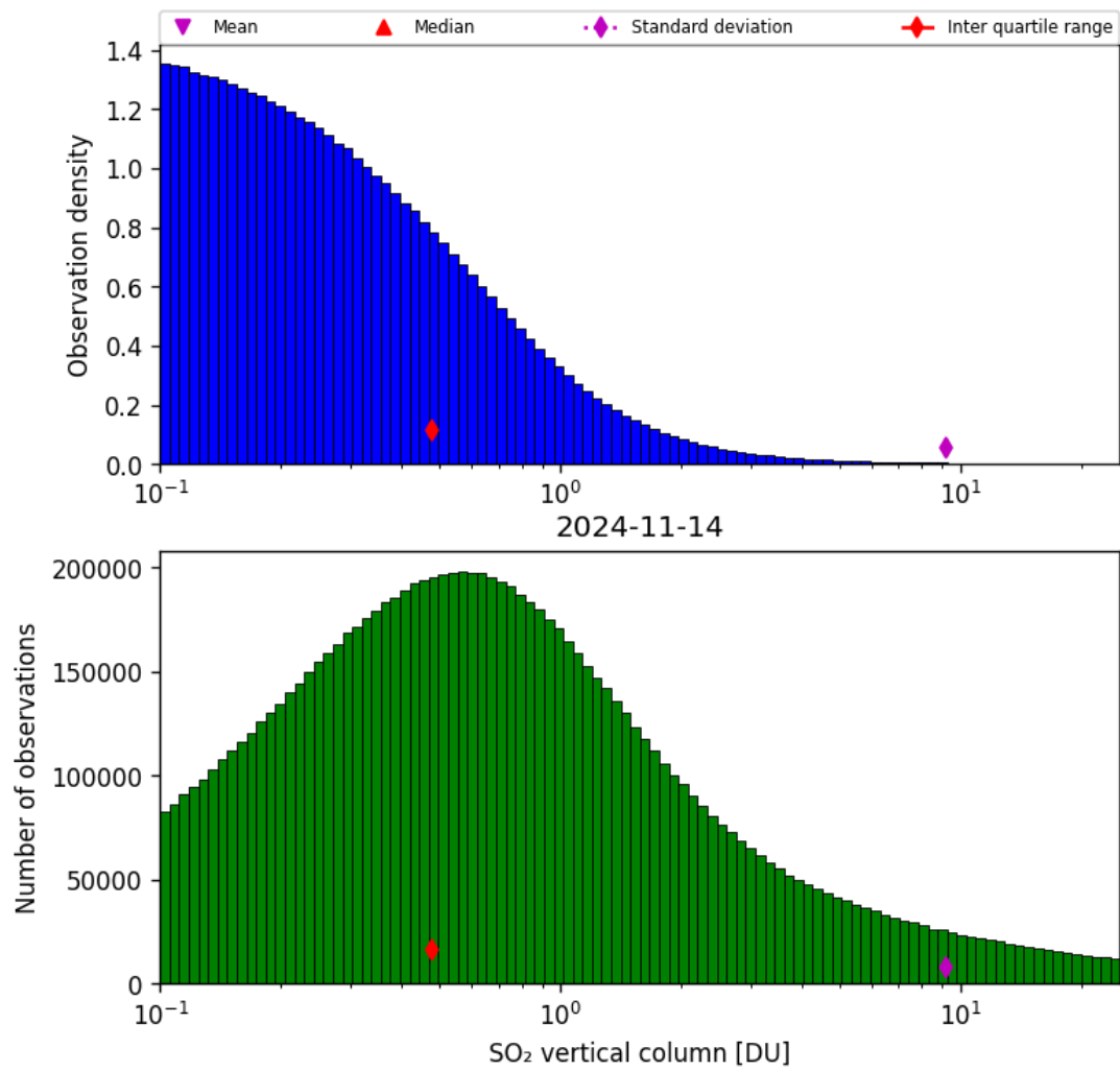
Figure 53: Histogram of “SO 2 vertical column” for 2024-11-14 to 2024-11-15
