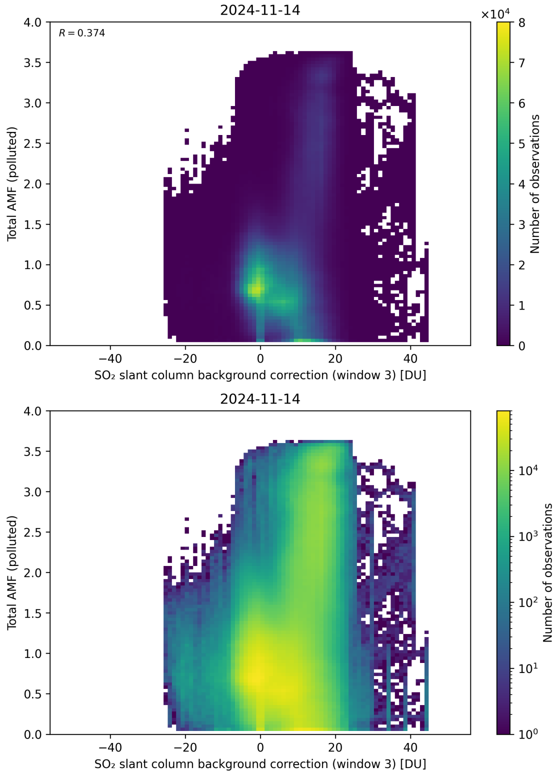
Figure 125: Scatter density plot of “SO 2 slant column background correction (window 3)” against “Total AMF (polluted)” for 2024-11-14 to 2024-11-15.
