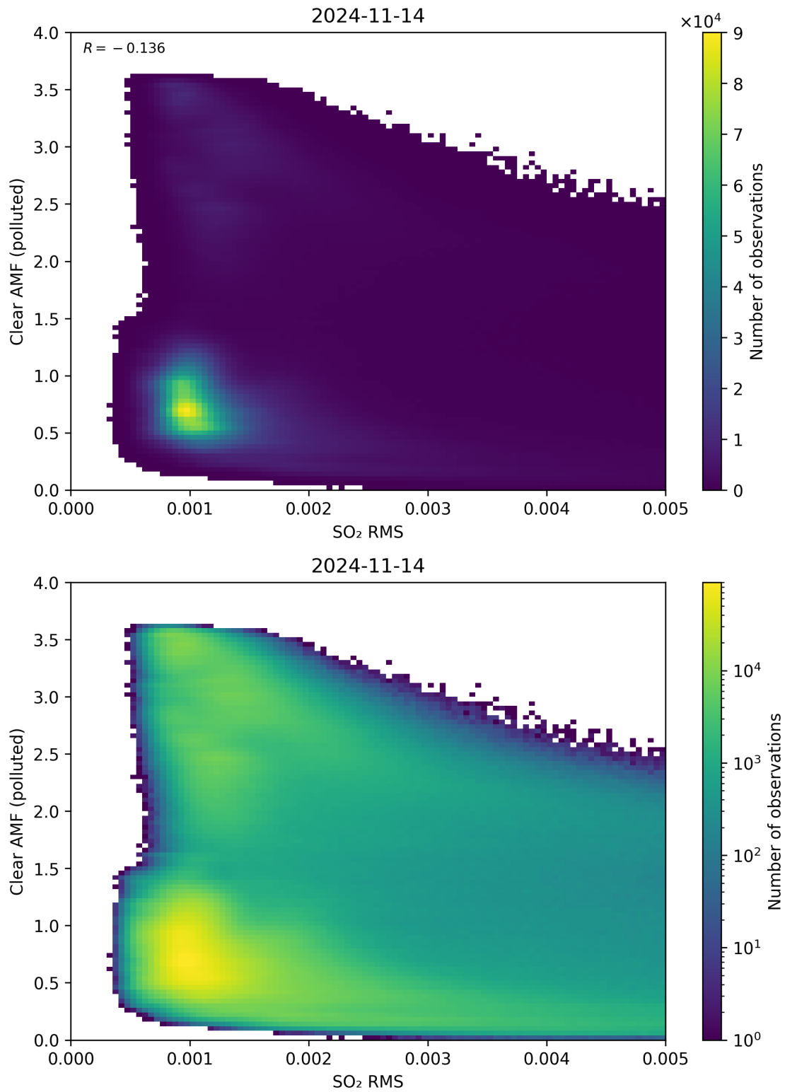
Figure 136: Scatter density plot of “SO 2 RMS” against “Clear AMF (polluted)” for 2024-11-14 to 2024-11-15.
