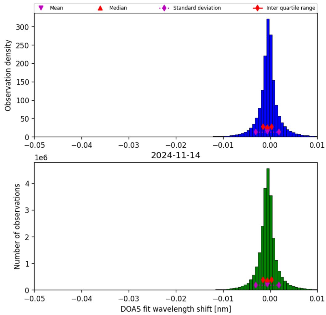
Figure 68: Histogram of “DOAS fit wavelength shift” for 2024-11-14 to 2024-11-15
