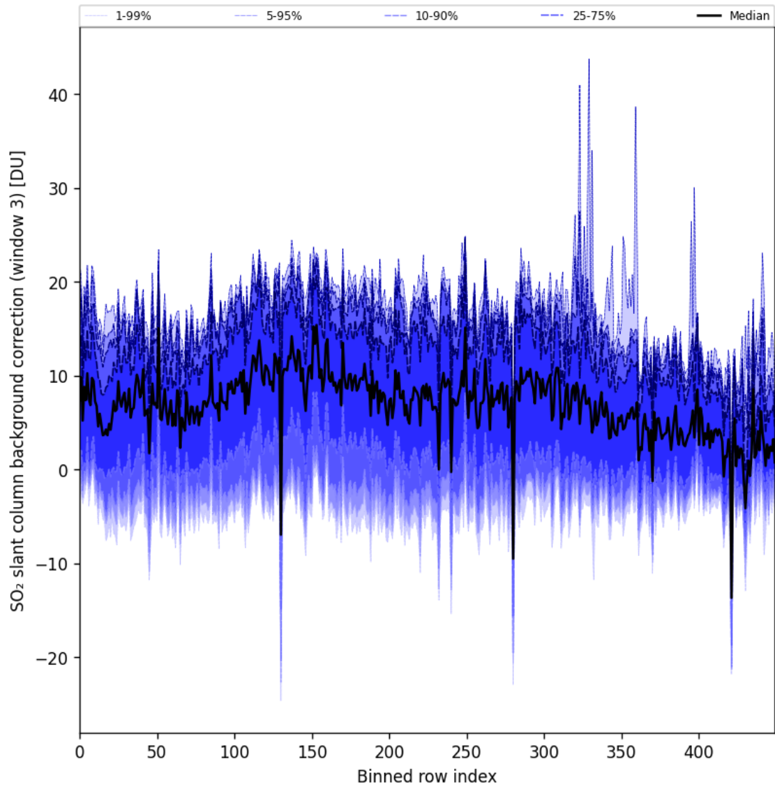
Figure 90: Along track statistics of “SO 2 slant column background correction (window 3)” for 2024-11-14 to 2024-11-15
