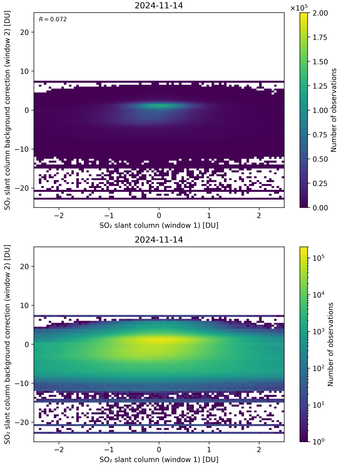
Figure 213: Scatter density plot of “SO 2 slant column (window 1)” against “SO 2 slant column background correction (window 2)” for 2024-11-14 to 2024-11-15.
