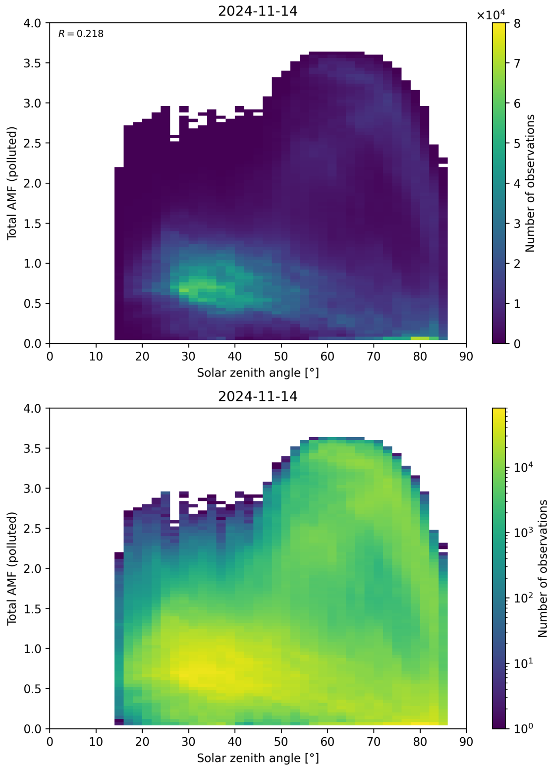
Figure 174: Scatter density plot of “Solar zenith angle” against “Total AMF (polluted)” for 2024-11-14 to 2024-11-15.
