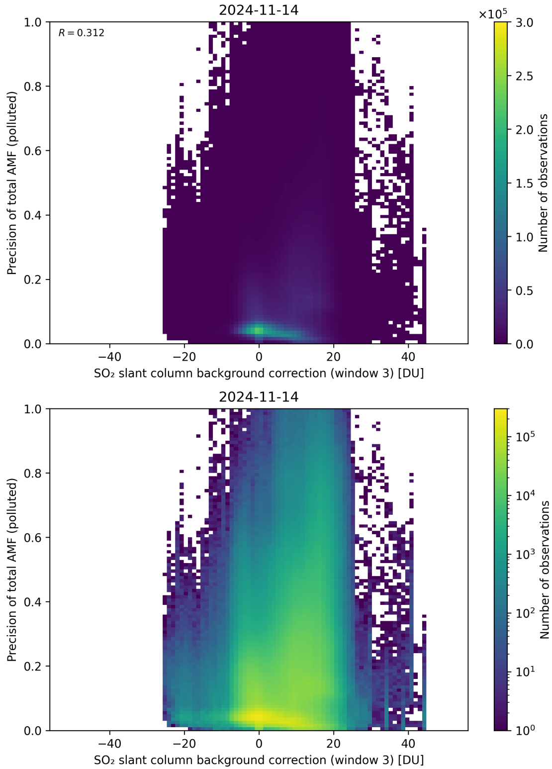
Figure 126: Scatter density plot of “SO 2 slant column background correction (window 3)” against “Precision of total AMF (polluted)” for 2024-11-14 to 2024-11-15.
