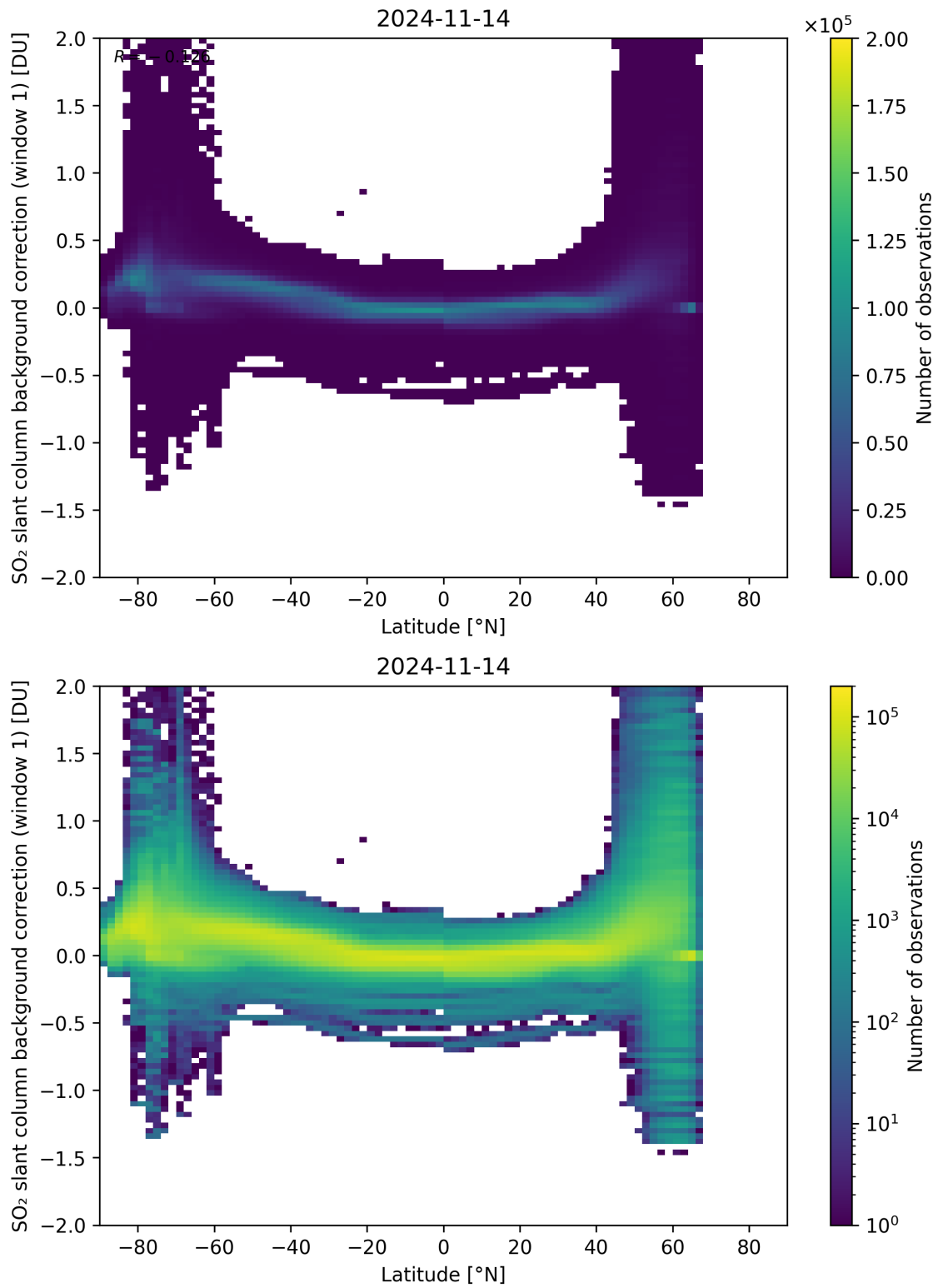
Figure 139: Scatter density plot of “Latitude” against “SO 2 slant column background correction (window 1)” for 2024-11-14 to 2024-11-15.
