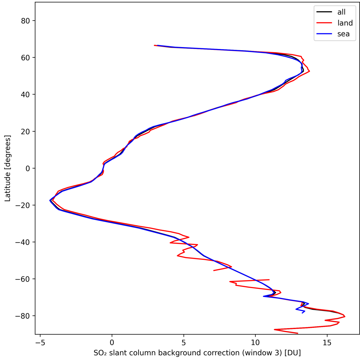
Figure 44: Zonal average of “SO 2 slant column background correction (window 3)” for 2024-11-14 to 2024-11-15.
