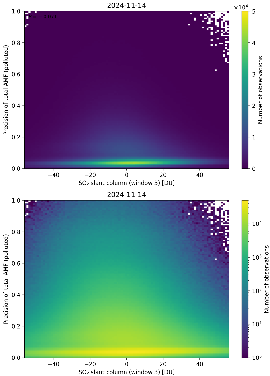
Figure 269: Scatter density plot of “SO 2 slant column (window 3)” against “Precision of total AMF (polluted)” for 2024-11-14 to 2024-11-15.
