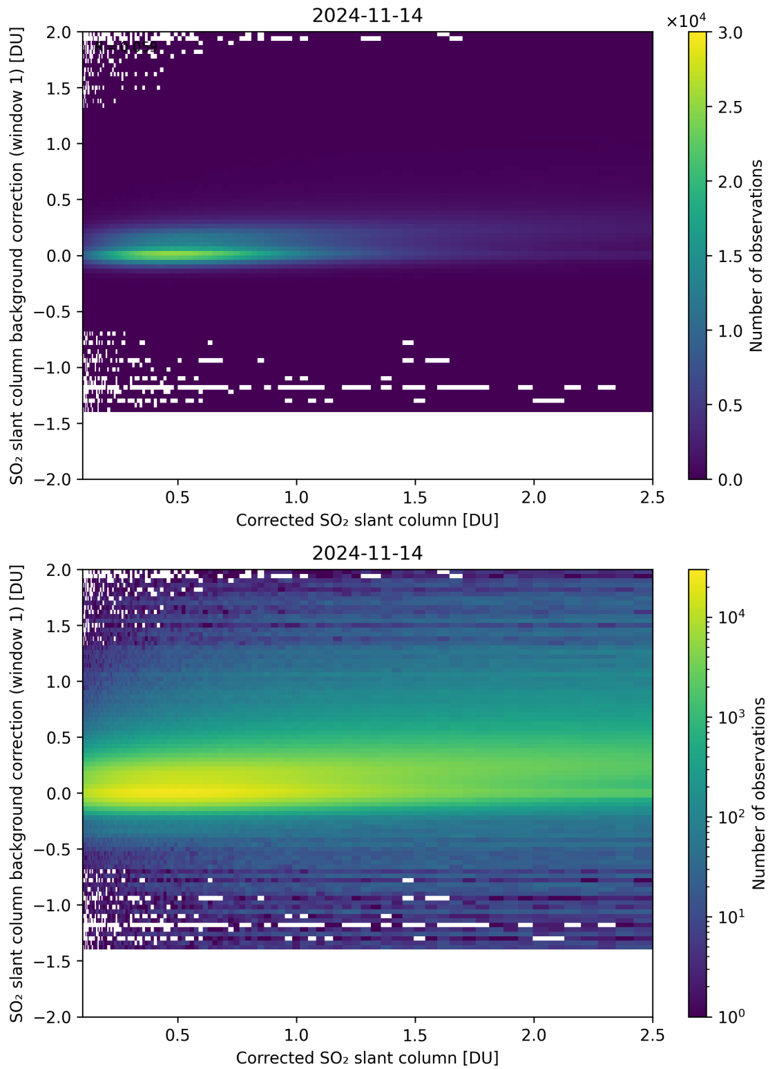
Figure 178: Scatter density plot of “Corrected SO 2 slant column” against “SO 2 slant column background correction (window 1)” for 2024-11-14 to 2024-11-15.
