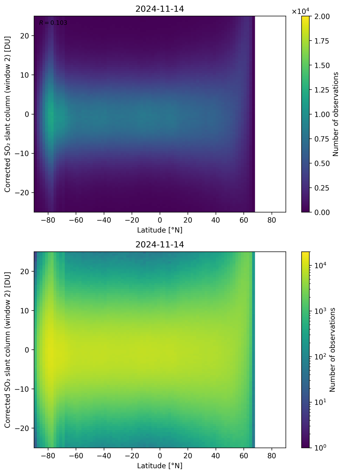
Figure 147: Scatter density plot of “Latitude” against “Corrected SO 2 slant column (window 2)” for 2024-11-14 to 2024-11-15.
