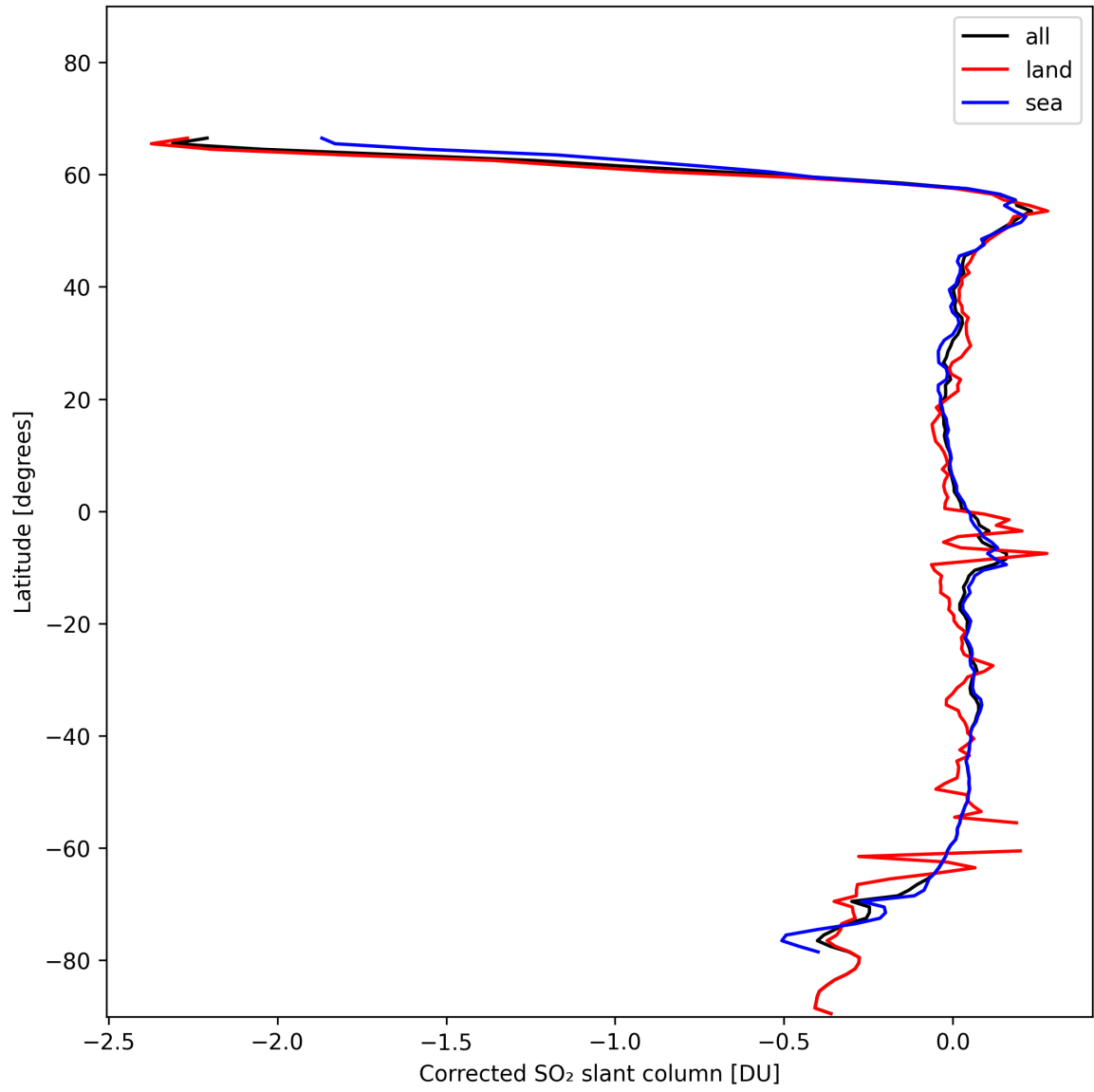
Figure 32: Zonal average of “Corrected SO 2 slant column” for 2024-11-14 to 2024-11-15.
