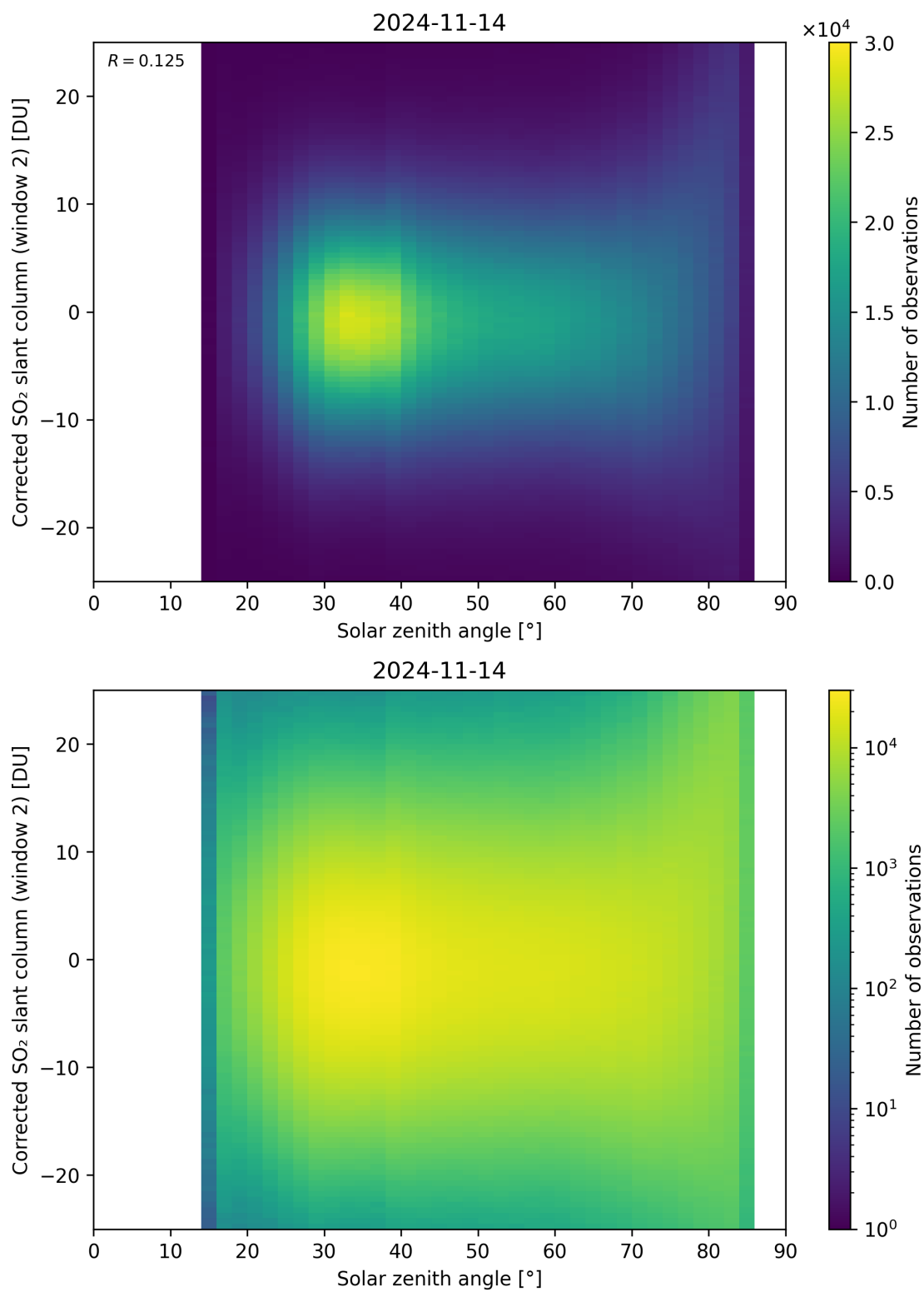
Figure 167: Scatter density plot of “Solar zenith angle” against “Corrected SO 2 slant column (window 2)” for 2024-11-14 to 2024-11-15.
