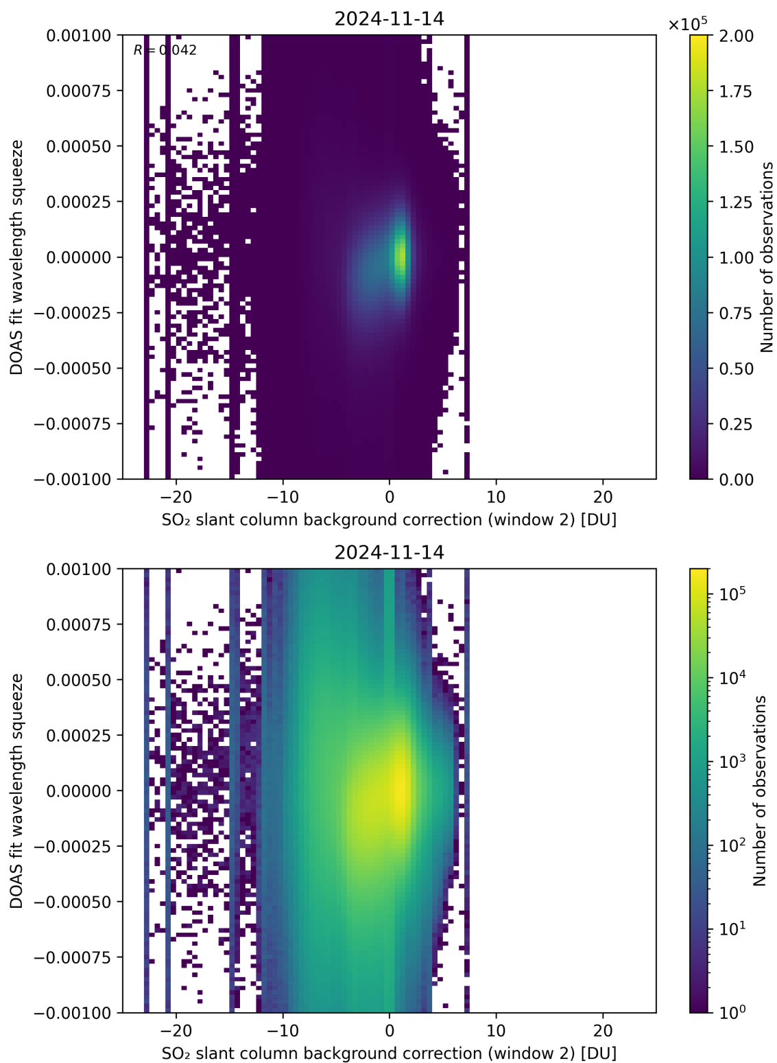
Figure 113: Scatter density plot of “SO 2 slant column background correction (window 2)” against “DOAS fit wavelength squeeze” for 2024-11-14 to 2024-11-15.
