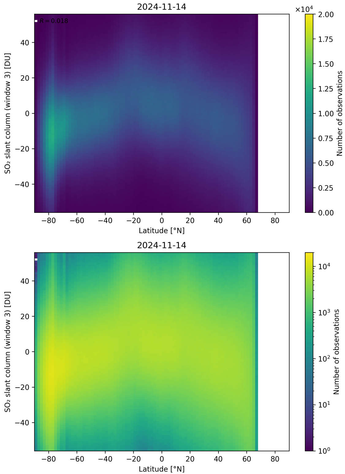
Figure 152: Scatter density plot of “Latitude” against “SO 2 slant column (window 3)” for 2024-11-14 to 2024-11-15.
