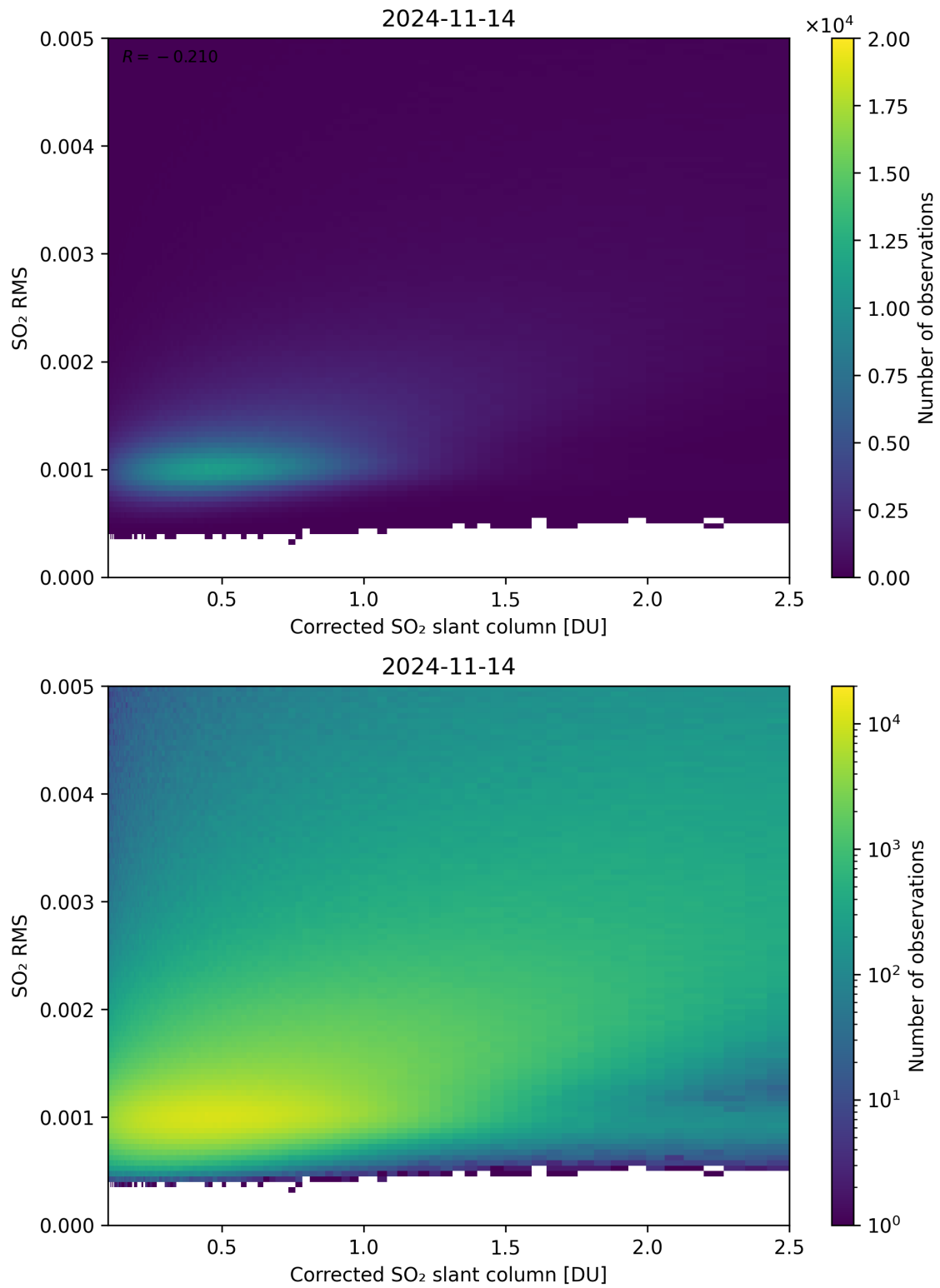
Figure 183: Scatter density plot of “Corrected SO 2 slant column” against “SO 2 RMS” for 2024-11-14 to 2024-11-15.
