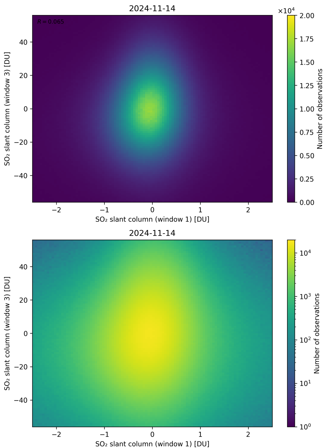
Figure 237: Scatter density plot of “SO 2 slant column (window 1)” against “SO 2 slant column (window 3)” for 2024-11-14 to 2024-11-15.
