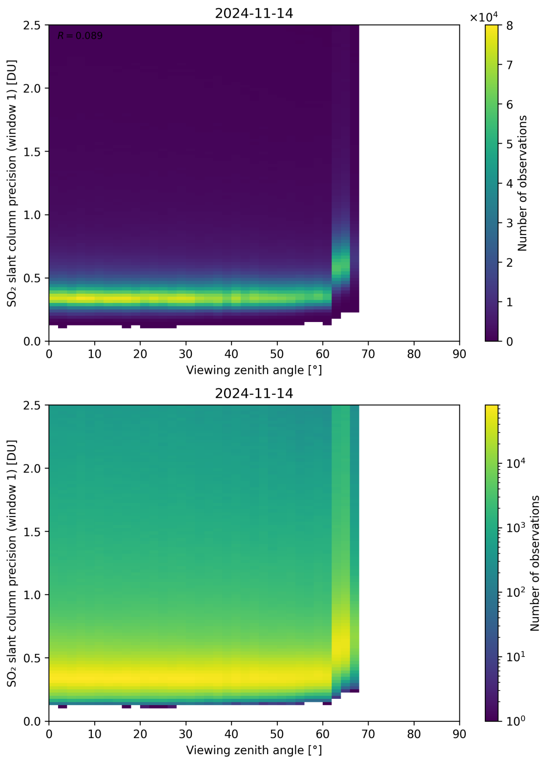
Figure 321: Scatter density plot of “Viewing zenith angle” against “SO 2 slant column precision (window 1)” for 2024-11-14 to 2024-11-15.
