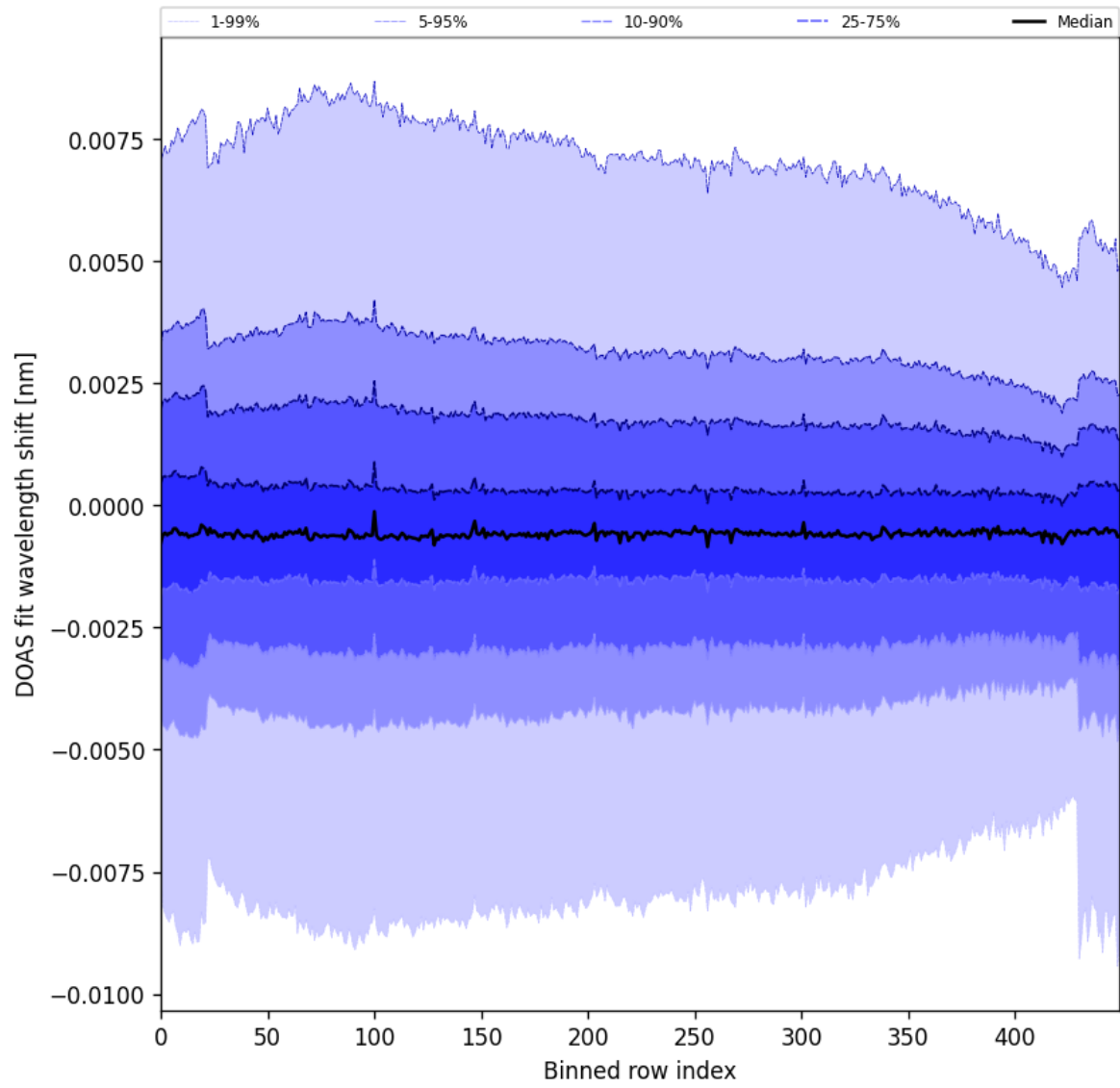
Figure 91: Along track statistics of “DOAS fit wavelength shift” for 2024-11-14 to 2024-11-15
