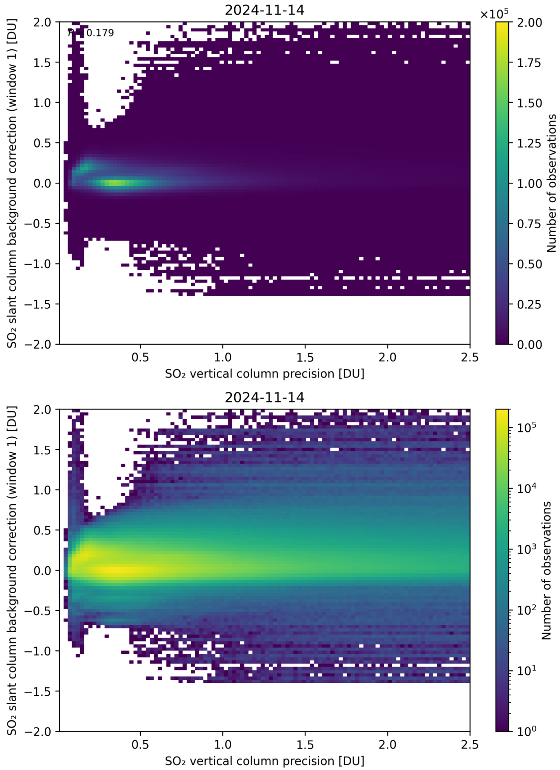
Figure 279: Scatter density plot of “SO 2 vertical column precision” against “SO 2 slant column background correction (window 1)” for 2024-11-14 to 2024-11-15.
