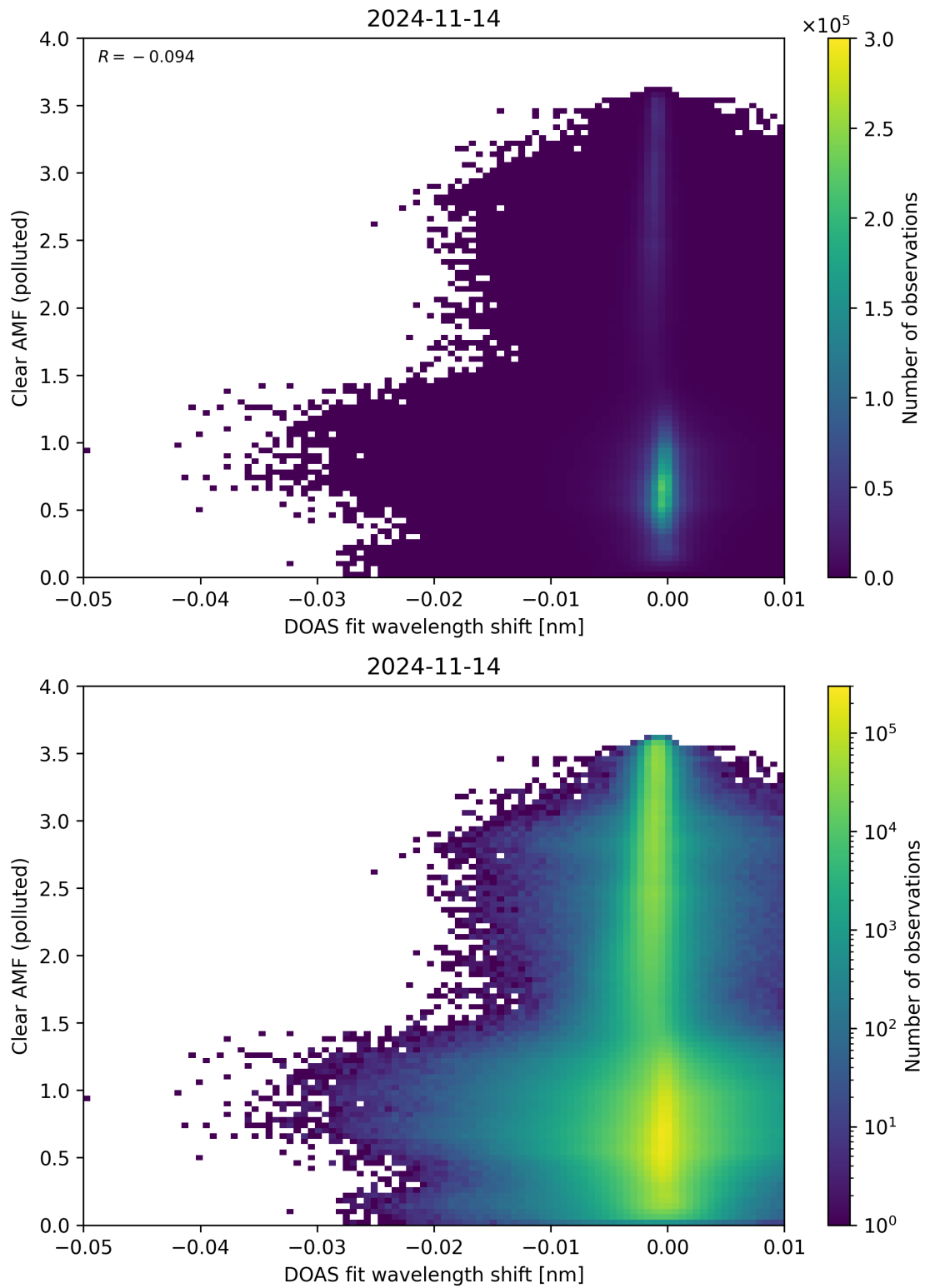
Figure 129: Scatter density plot of “DOAS fit wavelength shift” against “Clear AMF (polluted)” for 2024-11-14 to 2024-11-15.
