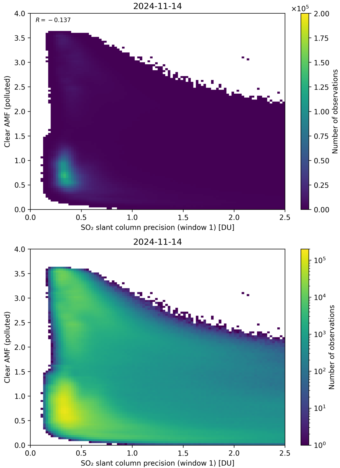
Figure 224: Scatter density plot of “SO 2 slant column precision (window 1)” against “Clear AMF (polluted)” for 2024-11-14 to 2024-11-15.
