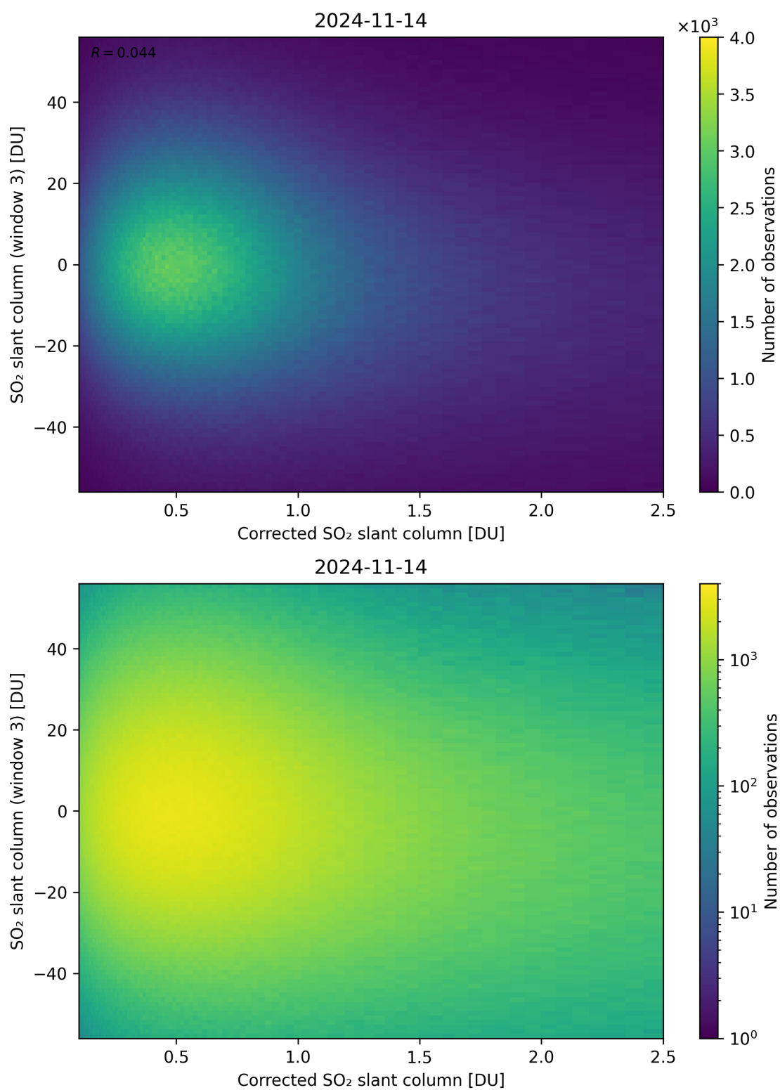
Figure 190: Scatter density plot of “Corrected SO 2 slant column” against “SO 2 slant column (window 3)” for 2024-11-14 to 2024-11-15.
