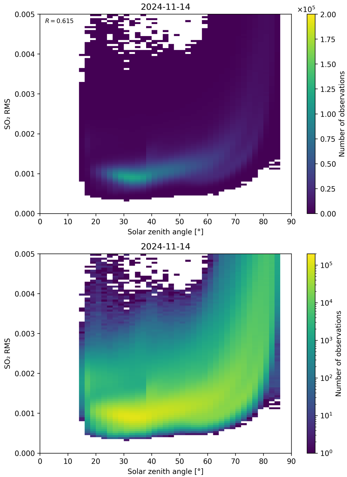
Figure 163: Scatter density plot of “Solar zenith angle” against “SO 2 RMS” for 2024-11-14 to 2024-11-15.
