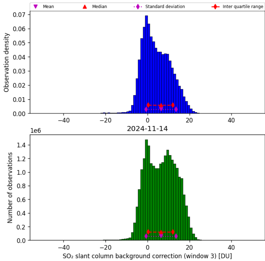
Figure 67: Histogram of “SO 2 slant column background correction (window 3)” for 2024-11-14 to 2024-11-15
