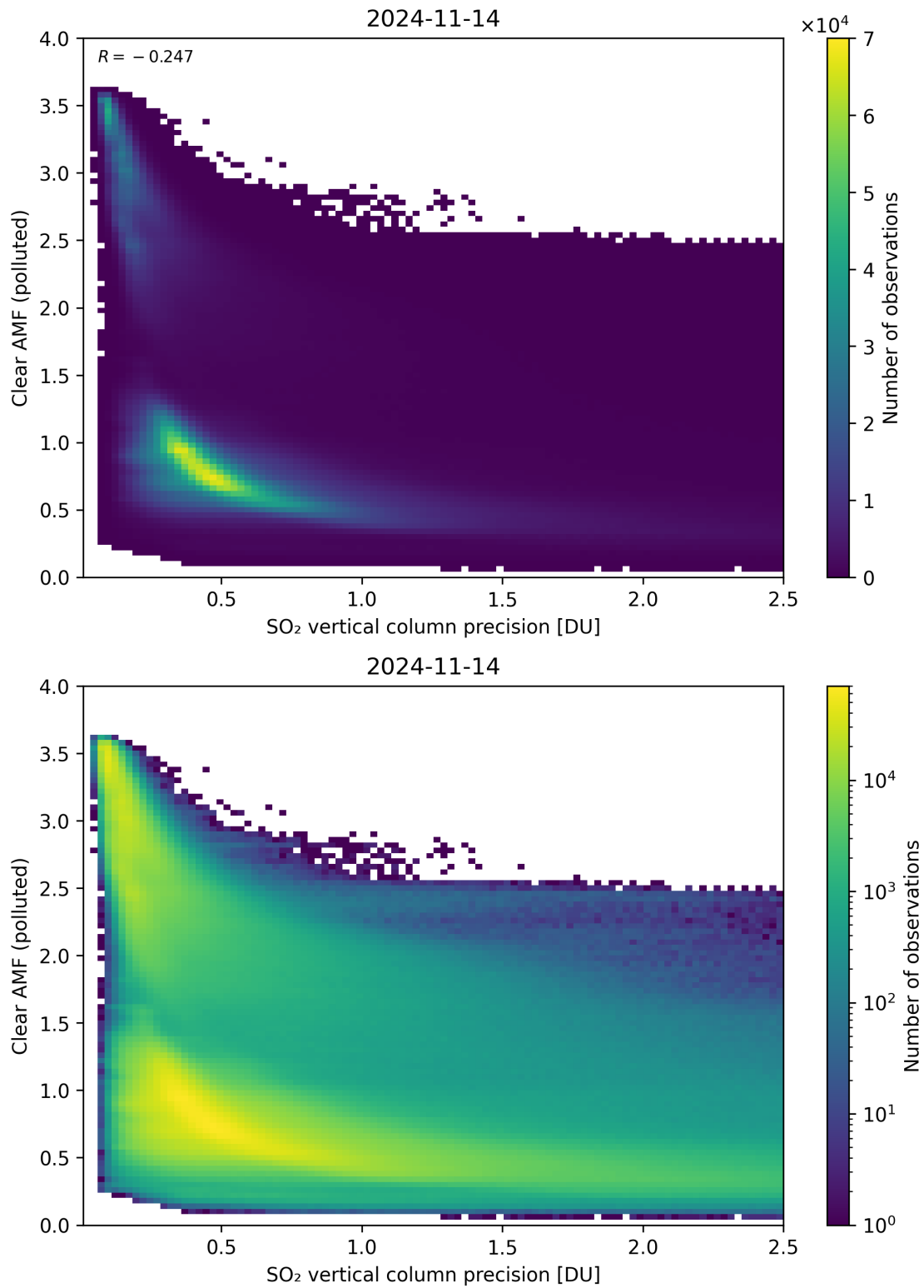
Figure 285: Scatter density plot of “SO 2 vertical column precision” against “Clear AMF (polluted)” for 2024-11-14 to 2024-11-15.
