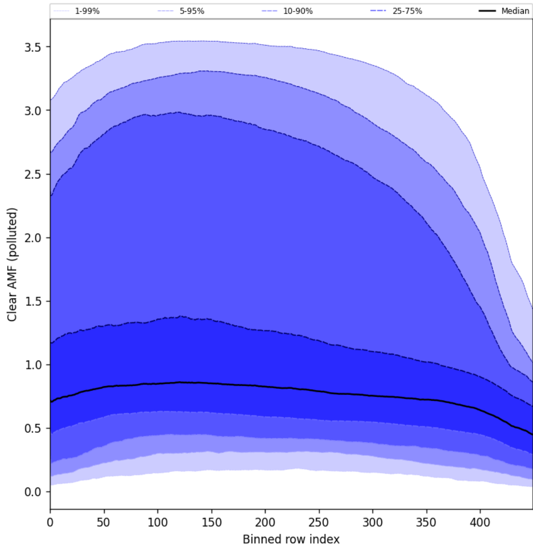
Figure 96: Along track statistics of “Clear AMF (polluted)” for 2024-11-14 to 2024-11-15
