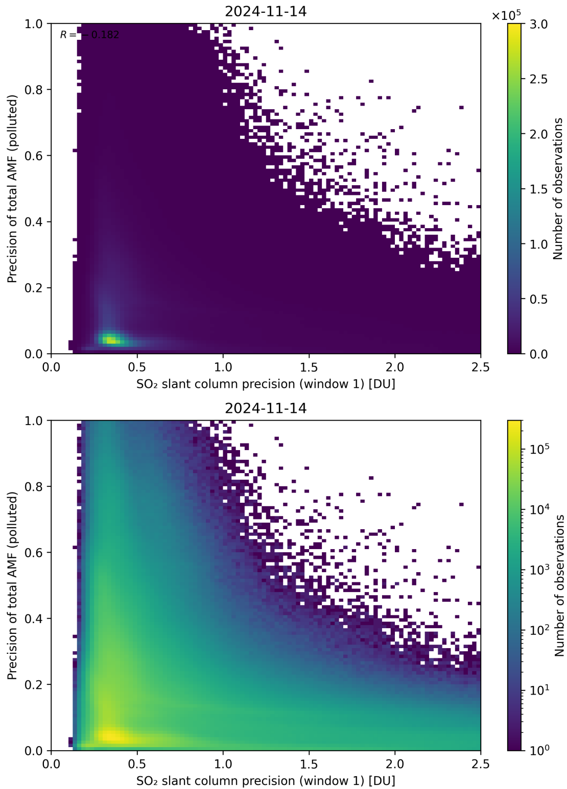
Figure 231: Scatter density plot of “SO 2 slant column precision (window 1)” against “Precision of total AMF (polluted)” for 2024-11-14 to 2024-11-15.
