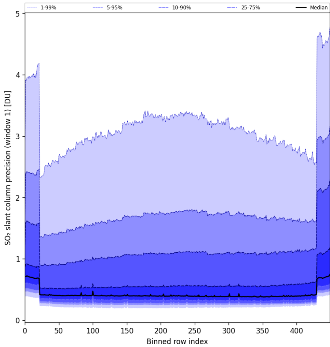
Figure 80: Along track statistics of “SO 2 slant column precision (window 1)” for 2024-11-14 to 2024-11-15
