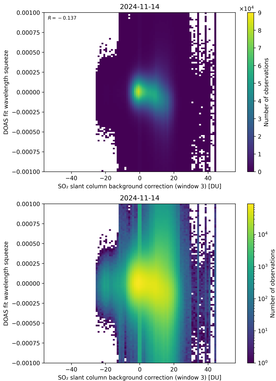
Figure 122: Scatter density plot of “SO 2 slant column background correction (window 3)” against “DOAS fit wavelength squeeze” for 2024-11-14 to 2024-11-15.
