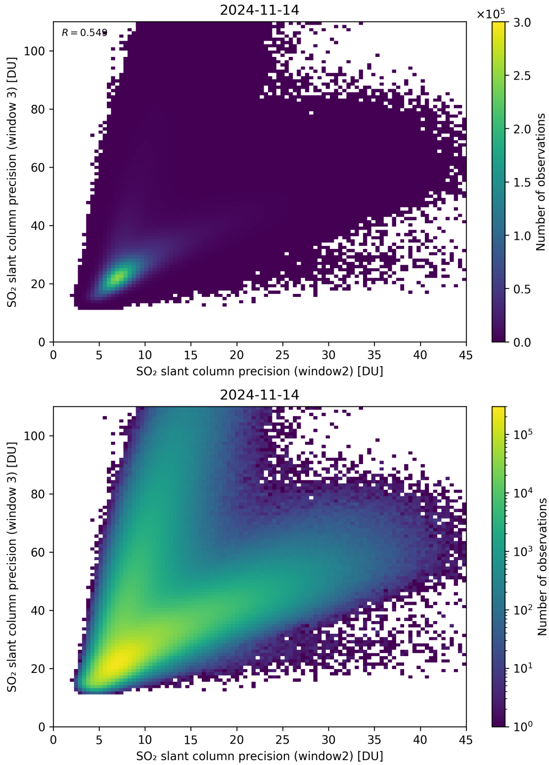
Figure 250: Scatter density plot of “SO 2 slant column precision (window2)” against “SO 2 slant column precision (window 3)” for 2024-11-14 to 2024-11-15.
