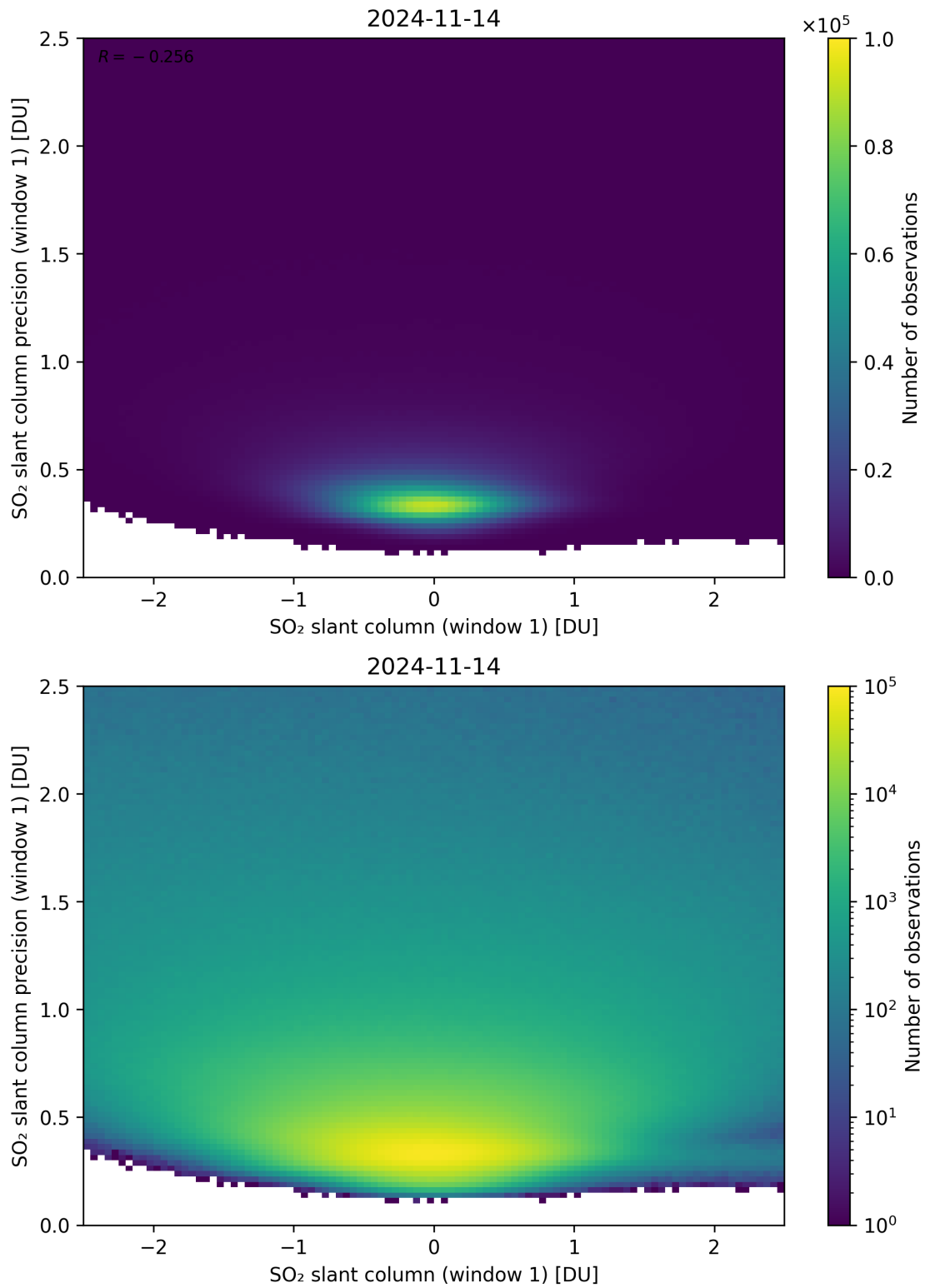
Figure 235: Scatter density plot of “SO 2 slant column (window 1)” against “SO 2 slant column precision (window 1)” for 2024-11-14 to 2024-11-15.
