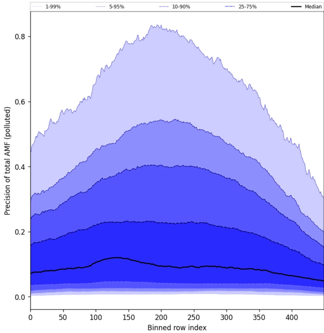
Figure 95: Along track statistics of “Precision of total AMF (polluted)” for 2024-11-14 to 2024-11-15
