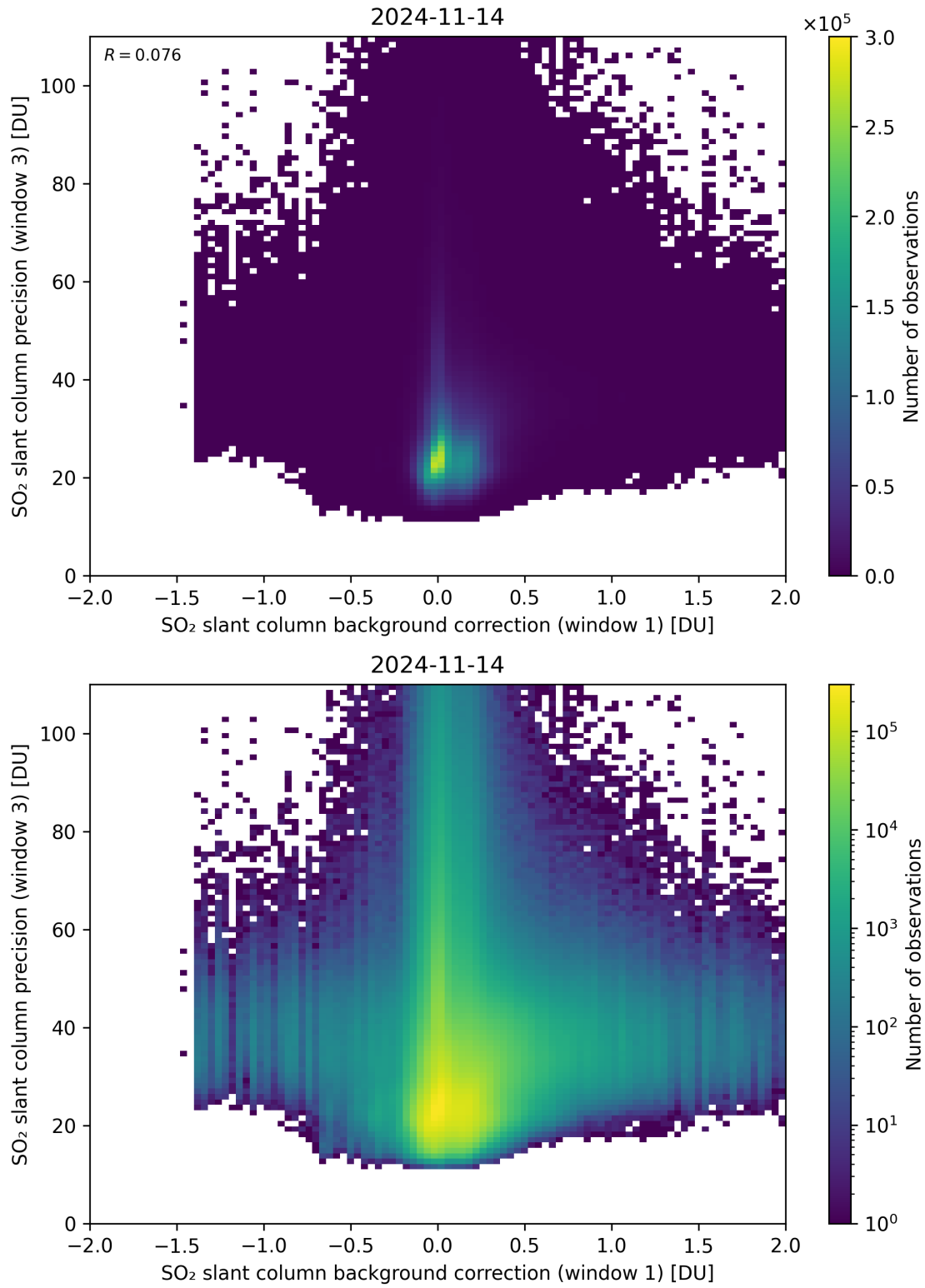
Figure 108: Scatter density plot of “SO 2 slant column background correction (window 1)” against “SO 2 slant column precision (window 3)” for 2024-11-14 to 2024-11-15.
