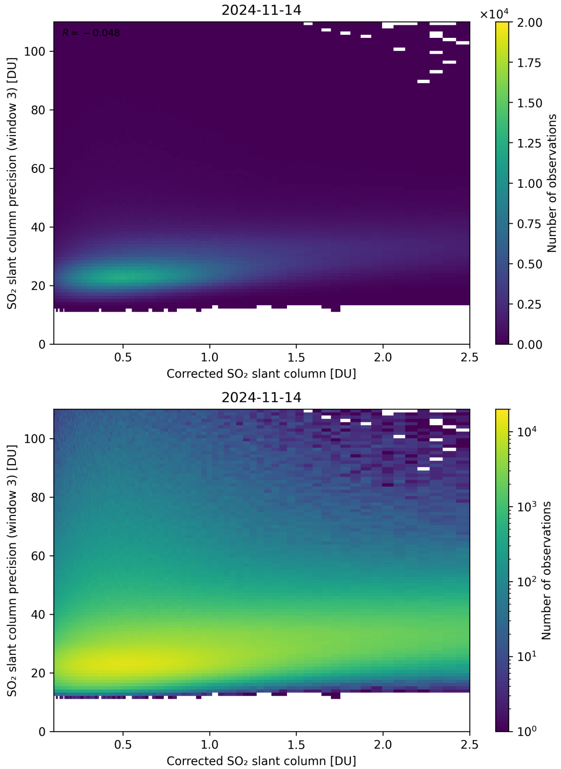
Figure 191: Scatter density plot of “Corrected SO 2 slant column” against “SO 2 slant column precision (window 3)” for 2024-11-14 to 2024-11-15.
