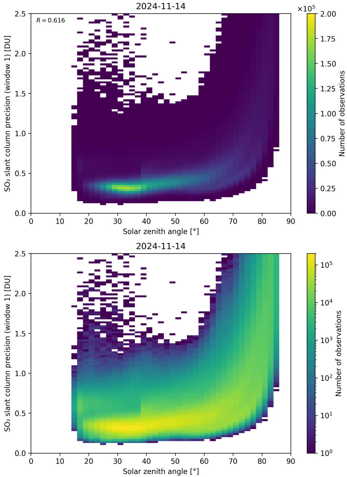
Figure 170: Scatter density plot of “Solar zenith angle” against “SO 2 slant column precision (window 1)” for 2024-11-14 to 2024-11-15.
