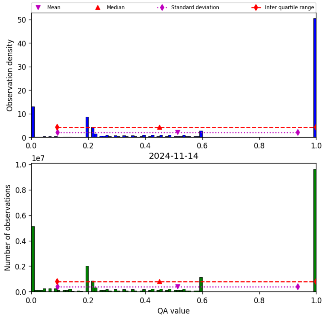
Figure 52: Histogram of “QA value” for 2024-11-14 to 2024-11-15
