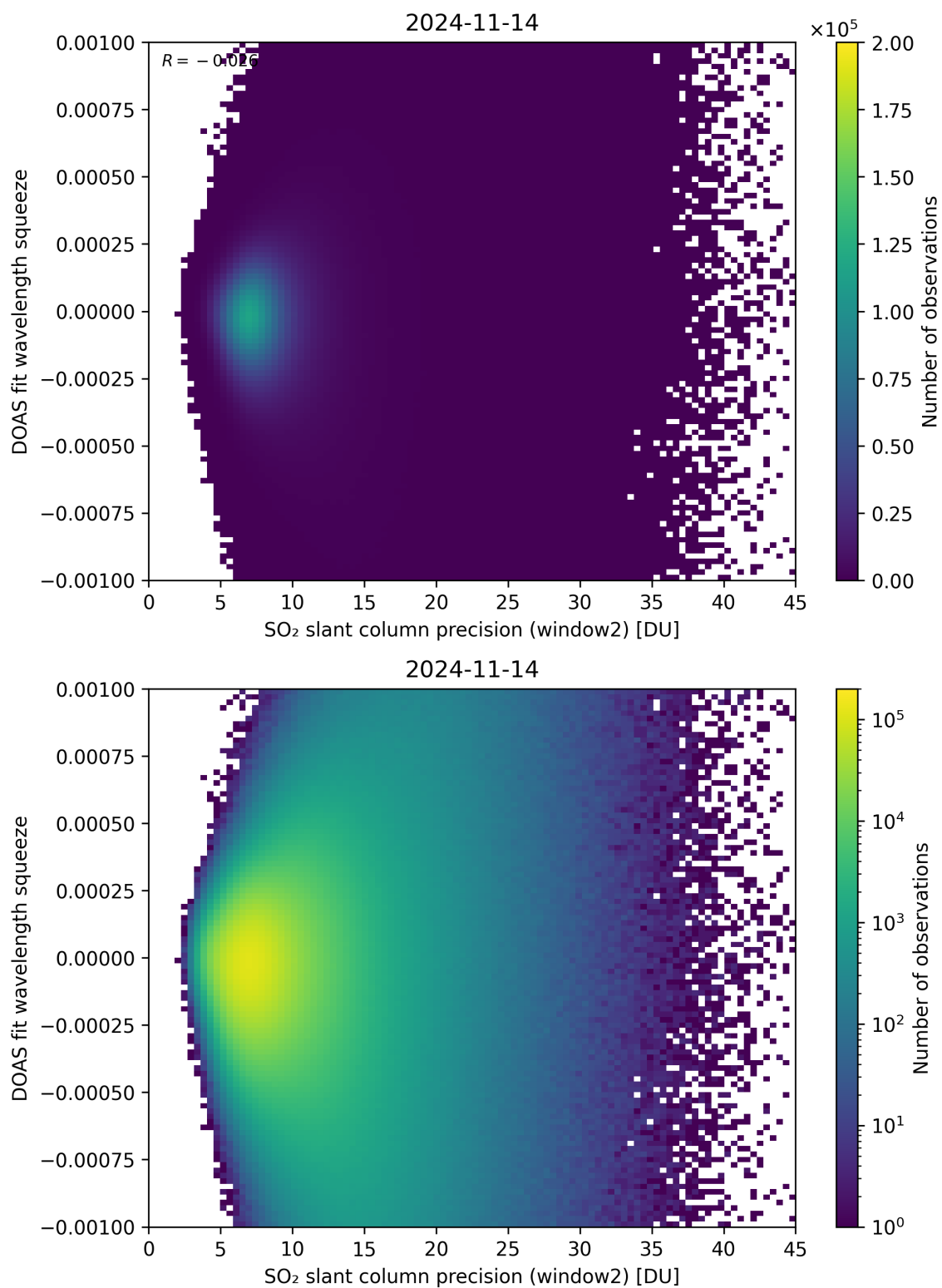
Figure 244: Scatter density plot of “SO 2 slant column precision (window2)” against “DOAS fit wavelength squeeze” for 2024-11-14 to 2024-11-15.
