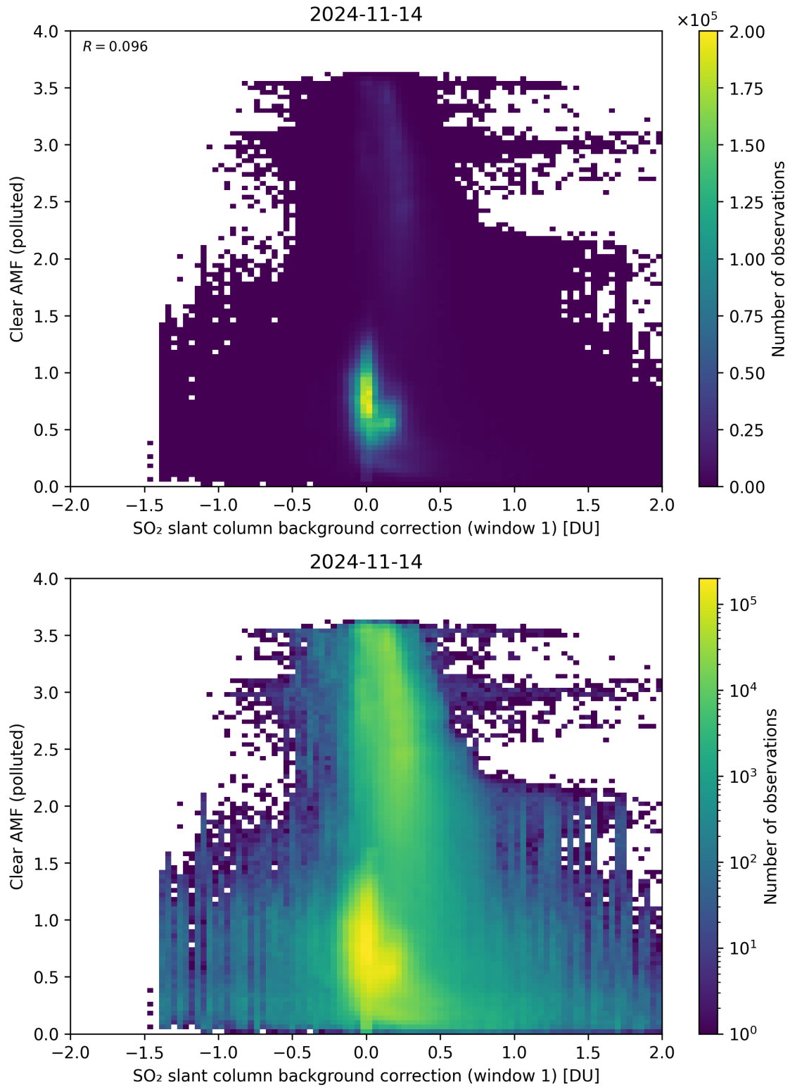
Figure 103: Scatter density plot of “SO 2 slant column background correction (window 1)” against “Clear AMF (polluted)” for 2024-11-14 to 2024-11-15.
