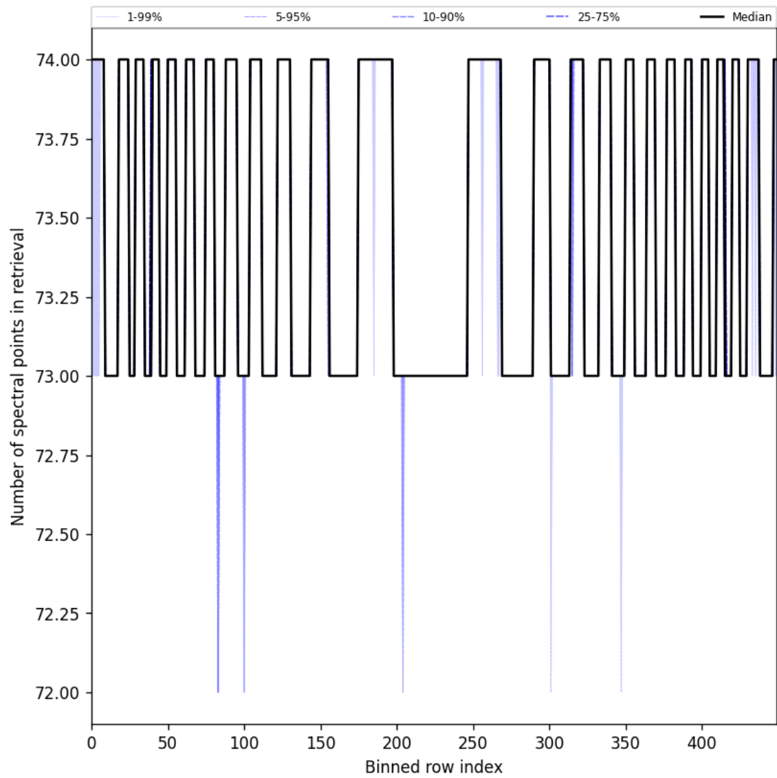
Figure 97: Along track statistics of “Number of spectral points in retrieval” for 2024-11-14 to 2024-11-15
