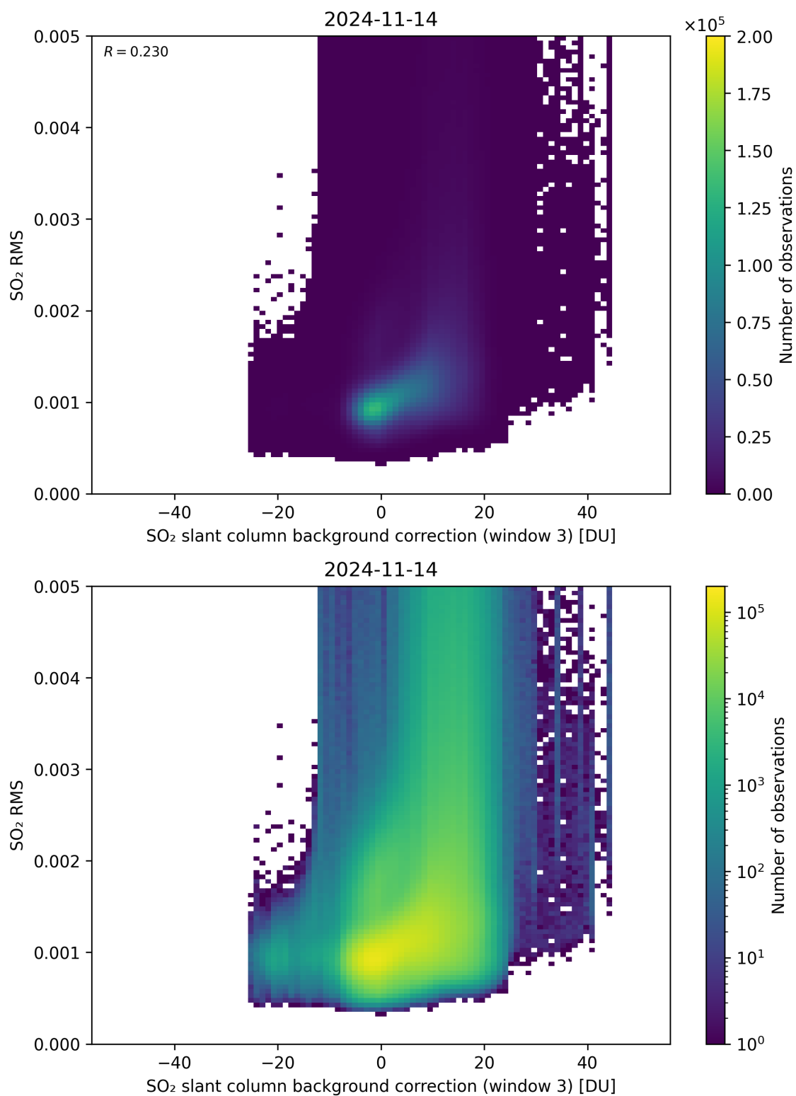
Figure 123: Scatter density plot of “SO 2 slant column background correction (window 3)” against “SO 2 RMS” for 2024-11-14 to 2024-11-15.
