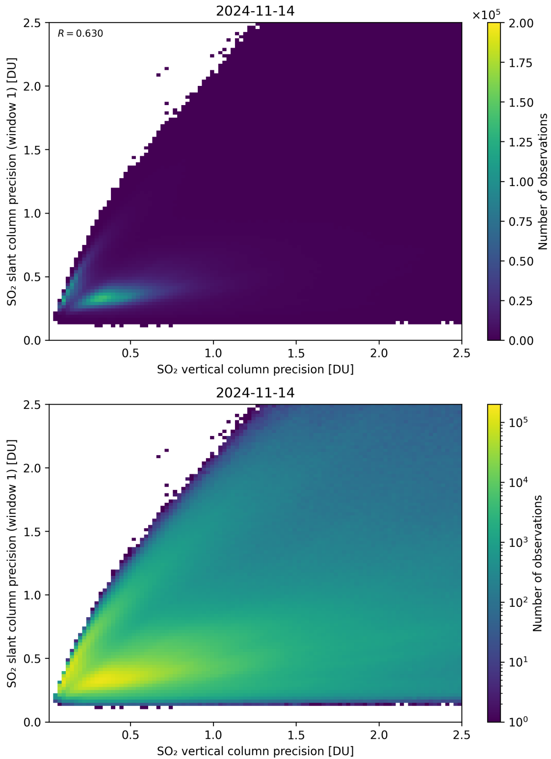
Figure 290: Scatter density plot of “SO 2 vertical column precision” against “SO 2 slant column precision (window 1)” for 2024-11-14 to 2024-11-15.
