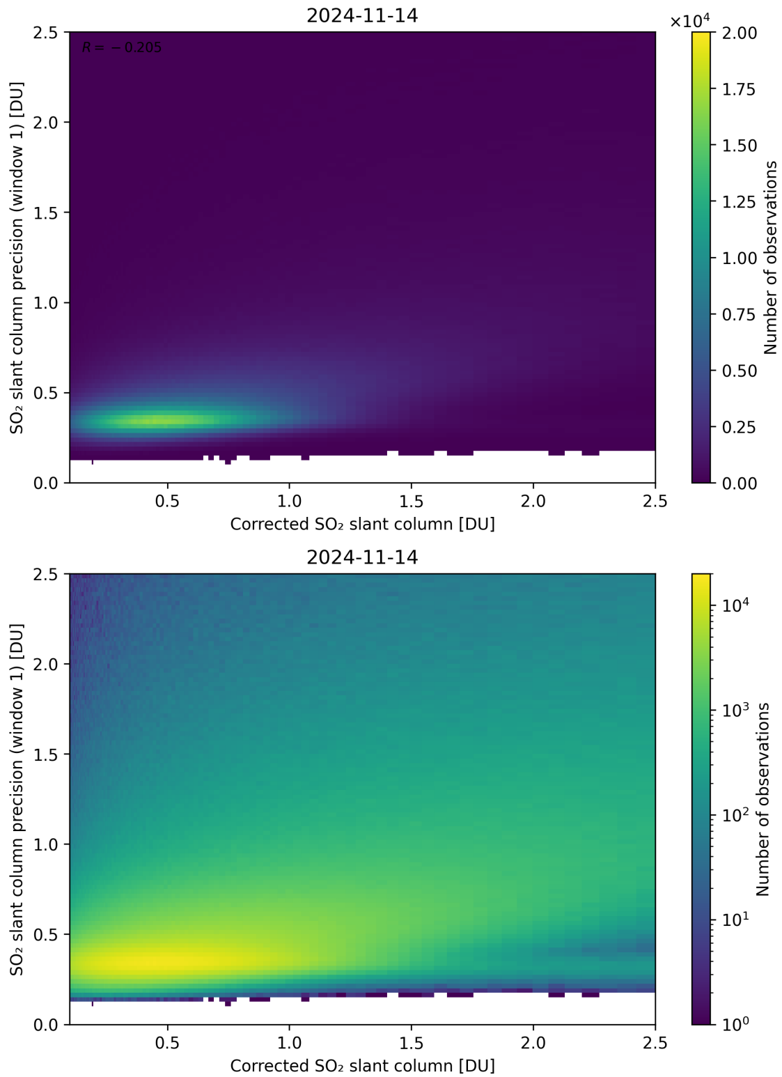
Figure 188: Scatter density plot of “Corrected SO 2 slant column” against “SO 2 slant column precision (window 1)” for 2024-11-14 to 2024-11-15.
