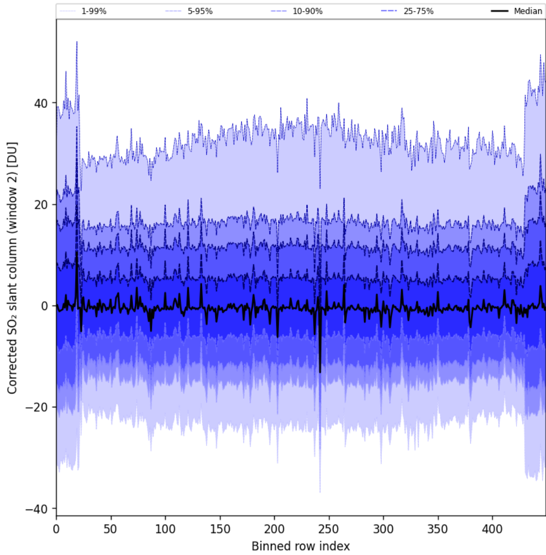
Figure 85: Along track statistics of “Corrected SO 2 slant column (window 2)” for 2024-11-14 to 2024-11-15
