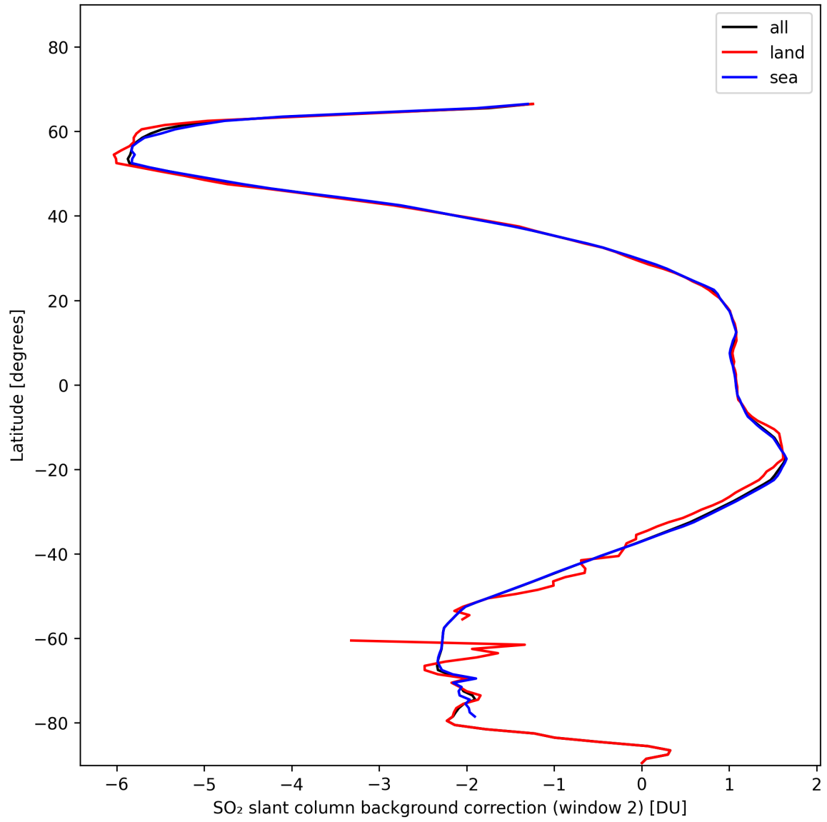
Figure 40: Zonal average of “SO 2 slant column background correction (window 2)” for 2024-11-14 to 2024-11-15.
