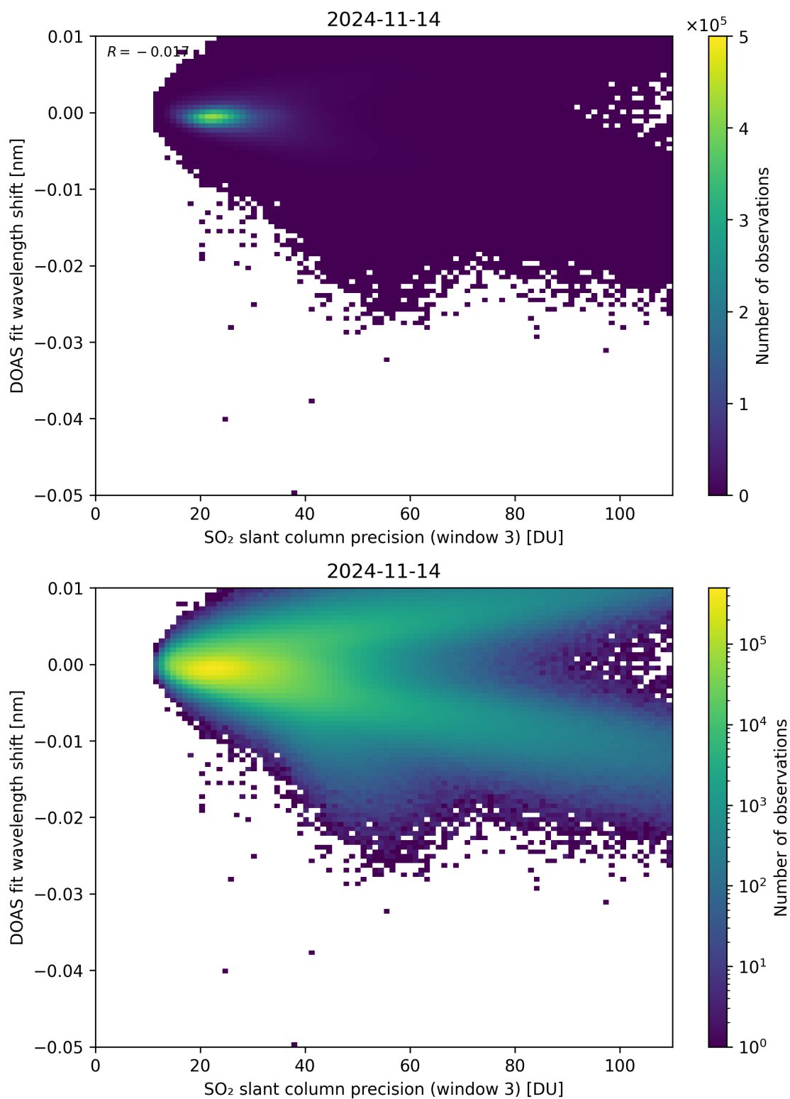
Figure 258: Scatter density plot of “SO 2 slant column precision (window 3)” against “DOAS fit wavelength shift” for 2024-11-14 to 2024-11-15.
