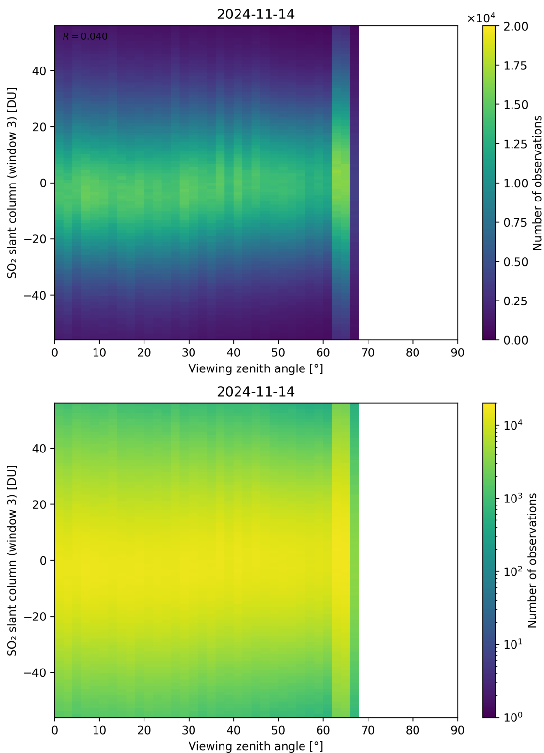
Figure 323: Scatter density plot of “Viewing zenith angle” against “SO 2 slant column (window 3)” for 2024-11-14 to 2024-11-15.
