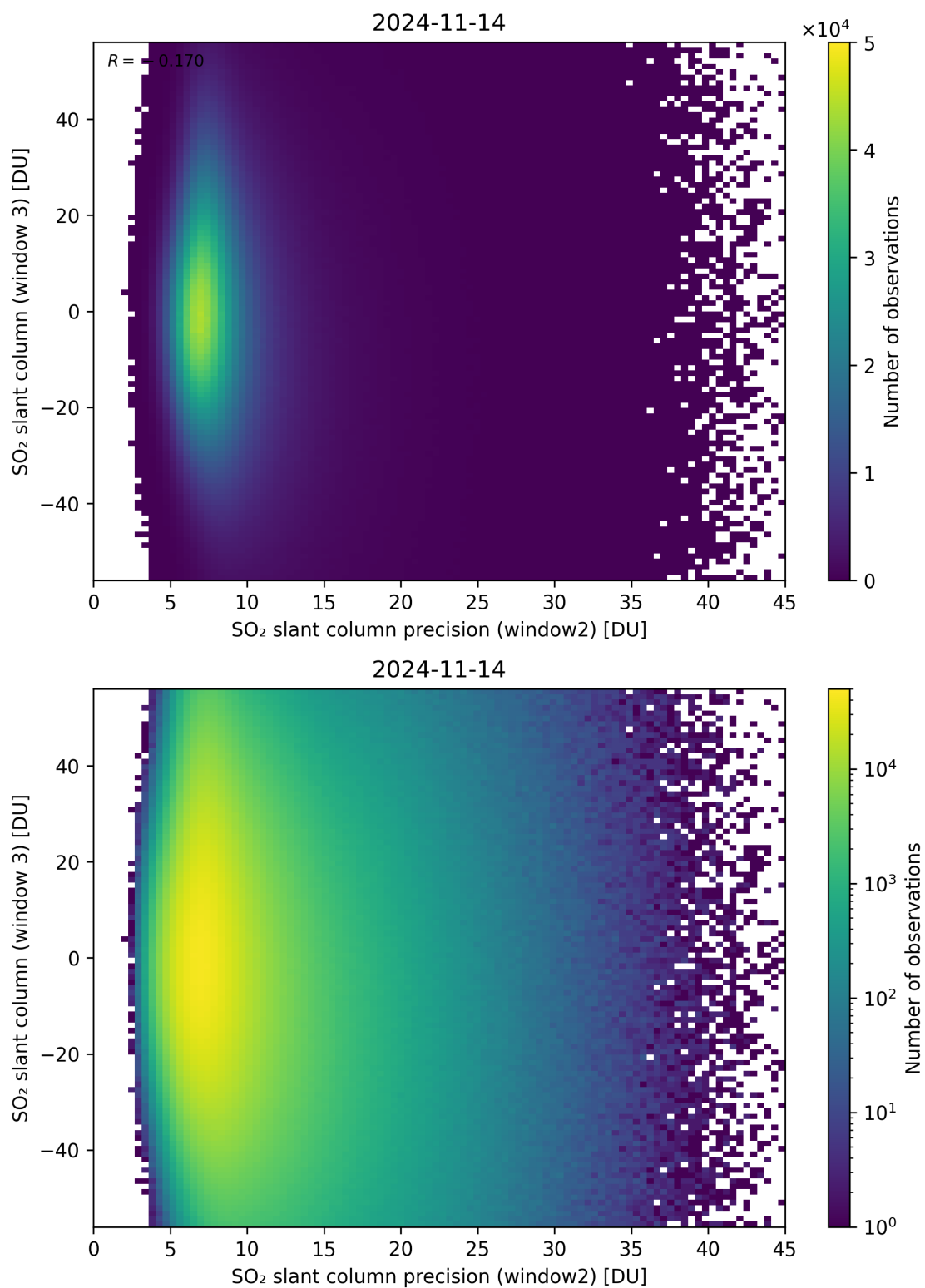
Figure 249: Scatter density plot of “SO 2 slant column precision (window2)” against “SO 2 slant column (window 3)” for 2024-11-14 to 2024-11-15.
