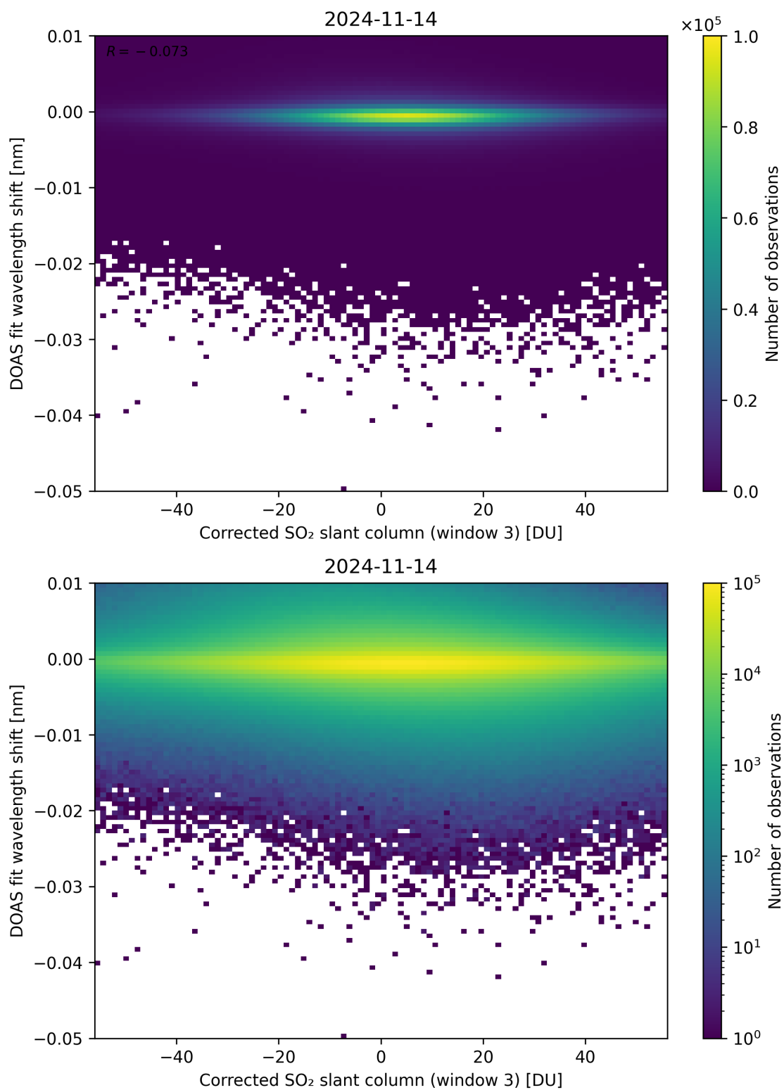
Figure 206: Scatter density plot of “Corrected SO 2 slant column (window 3)” against “DOAS fit wavelength shift” for 2024-11-14 to 2024-11-15.
