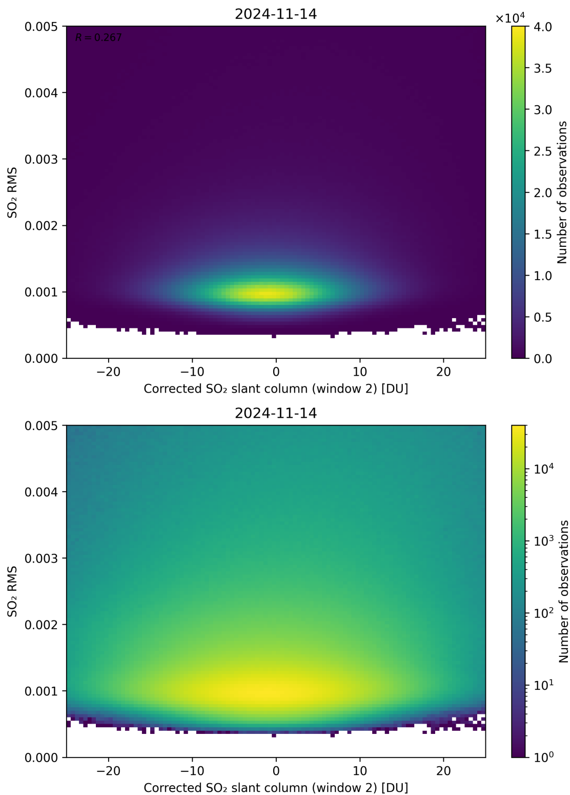
Figure 198: Scatter density plot of “Corrected SO 2 slant column (window 2)” against “SO 2 RMS” for 2024-11-14 to 2024-11-15.
