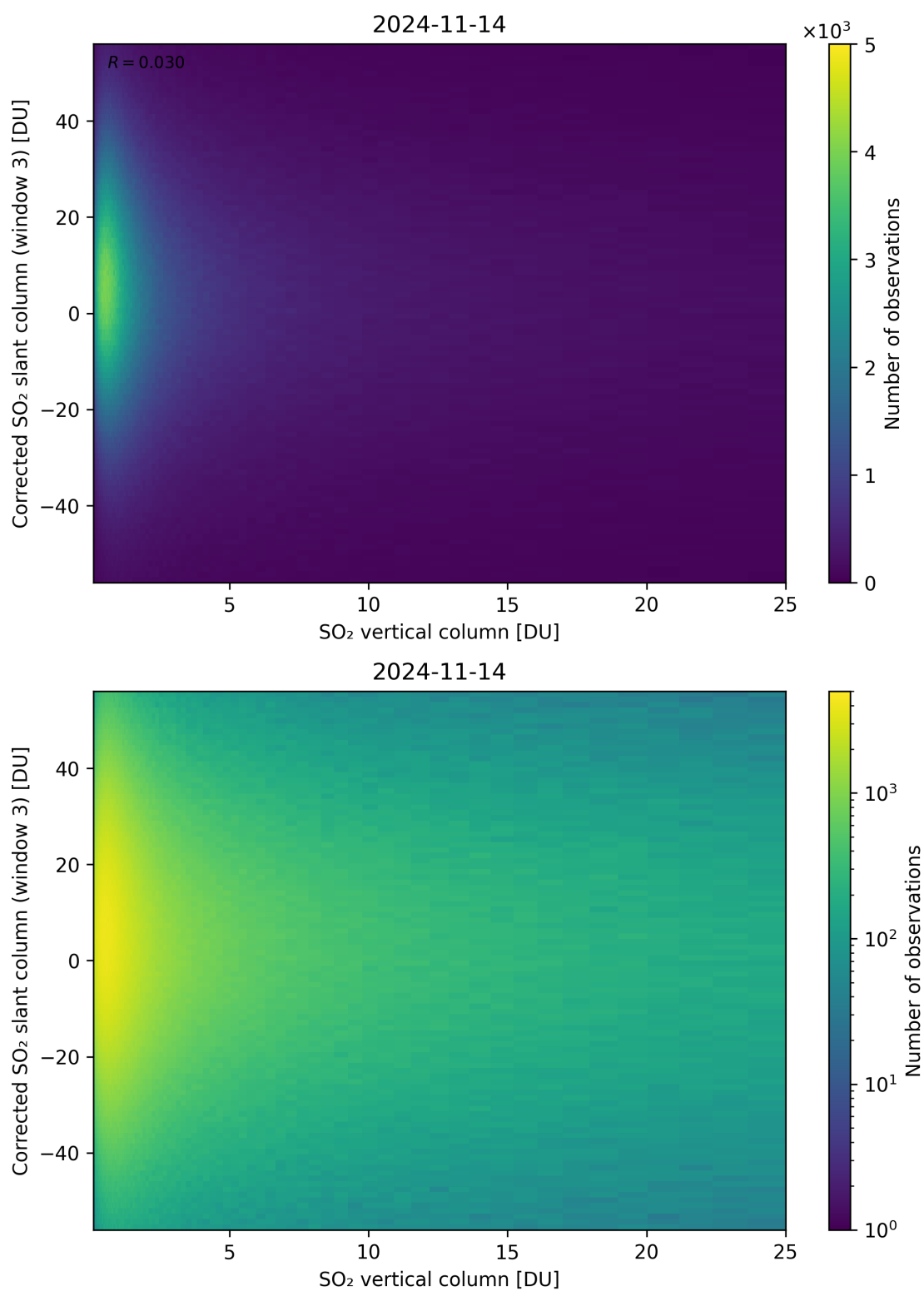
Figure 299: Scatter density plot of “SO 2 vertical column” against “Corrected SO 2 slant column (window 3)” for 2024-11-14 to 2024-11-15.
