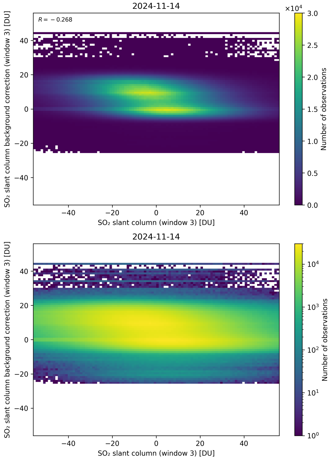
Figure 253: Scatter density plot of “SO 2 slant column (window 3)” against “SO 2 slant column background correction (window 3)” for 2024-11-14 to 2024-11-15.
