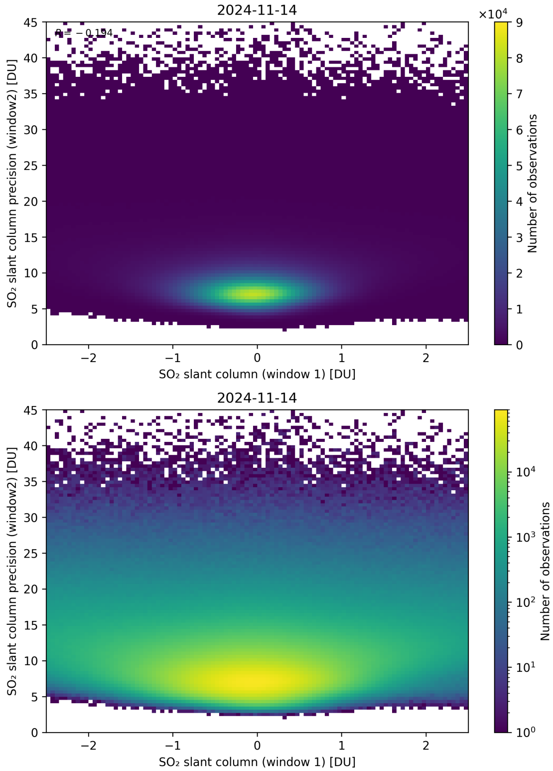
Figure 236: Scatter density plot of “SO 2 slant column (window 1)” against “SO 2 slant column precision (window2)” for 2024-11-14 to 2024-11-15.
