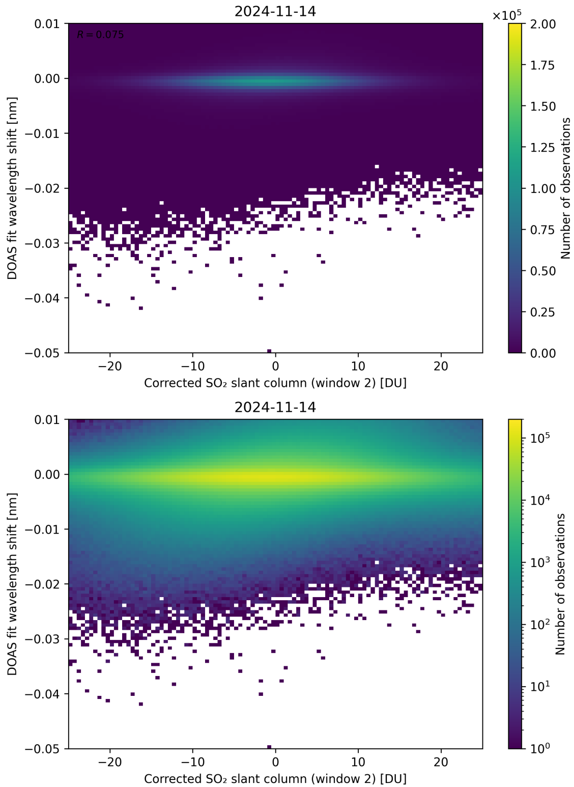
Figure 196: Scatter density plot of “Corrected SO 2 slant column (window 2)” against “DOAS fit wavelength shift” for 2024-11-14 to 2024-11-15.
