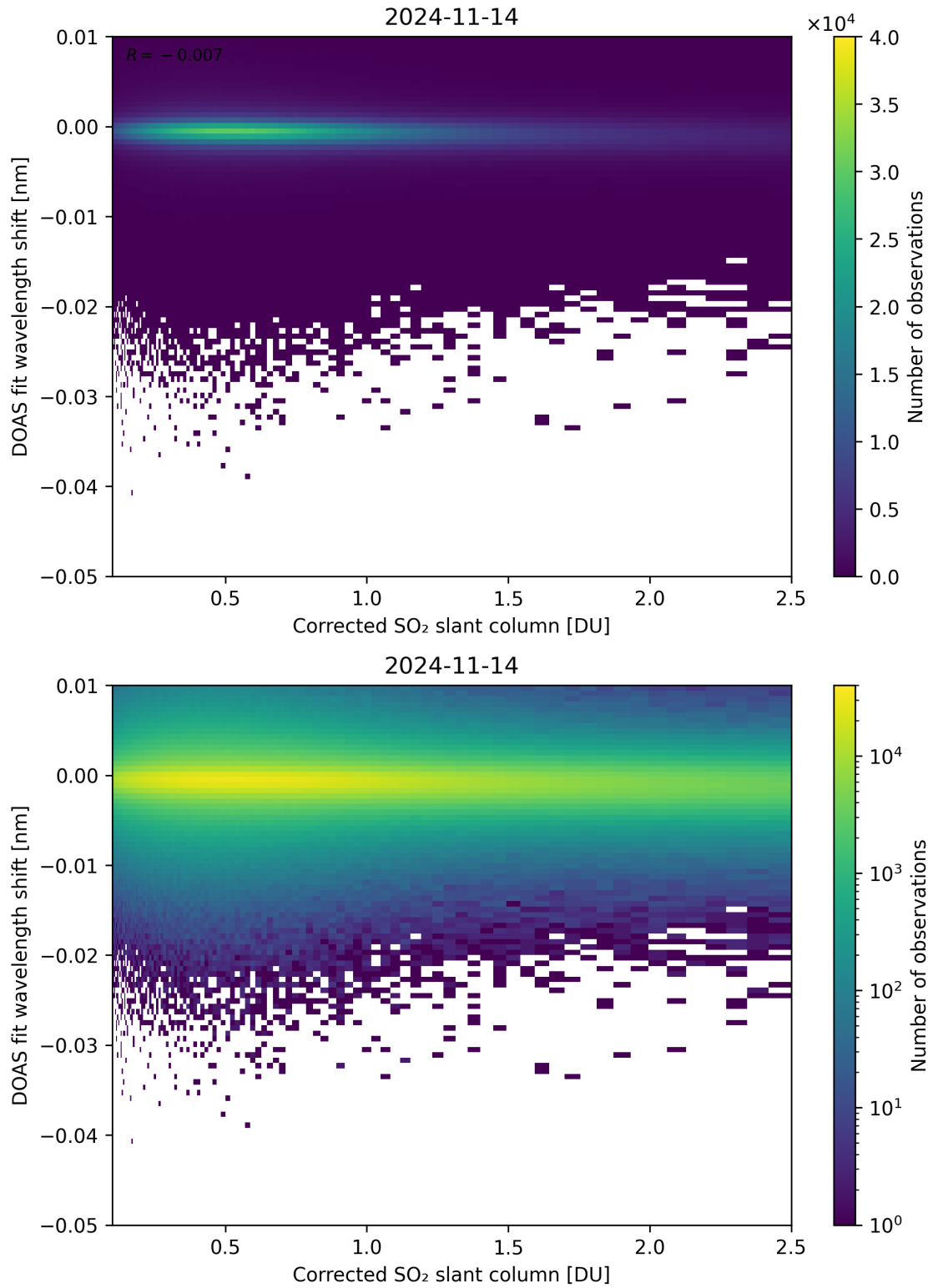
Figure 181: Scatter density plot of “Corrected SO 2 slant column” against “DOAS fit wavelength shift” for 2024-11-14 to 2024-11-15.
