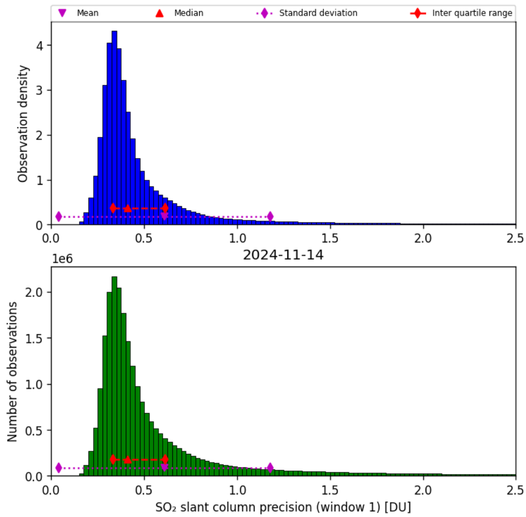
Figure 57: Histogram of “SO 2 slant column precision (window 1)” for 2024-11-14 to 2024-11-15
