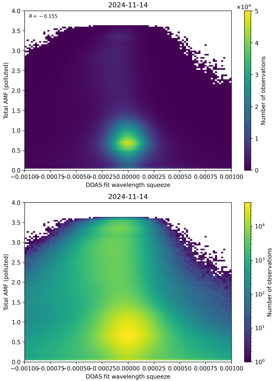
Figure 134: Scatter density plot of “DOAS fit wavelength squeeze” against “Total AMF (polluted)” for 2024-11-14 to 2024-11-15.
