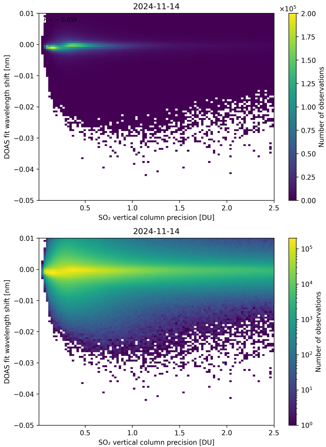
Figure 282: Scatter density plot of “SO 2 vertical column precision” against “DOAS fit wavelength shift” for 2024-11-14 to 2024-11-15.
