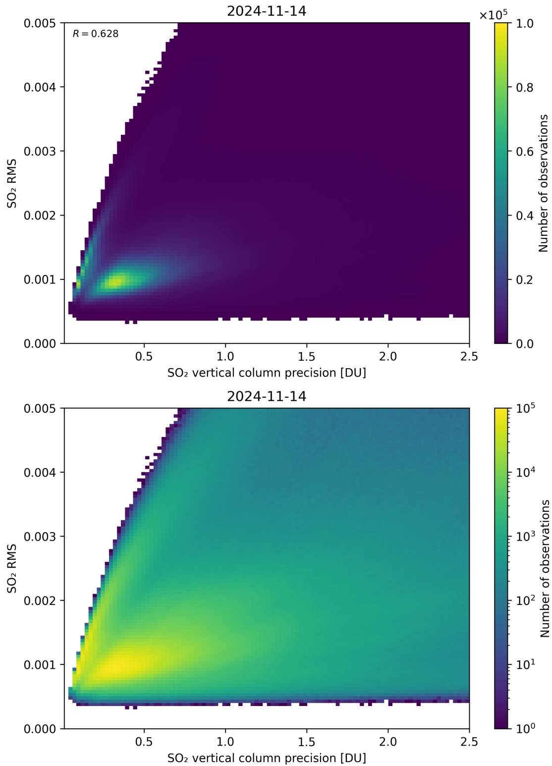
Figure 284: Scatter density plot of “SO 2 vertical column precision” against “SO 2 RMS” for 2024-11-14 to 2024-11-15.
