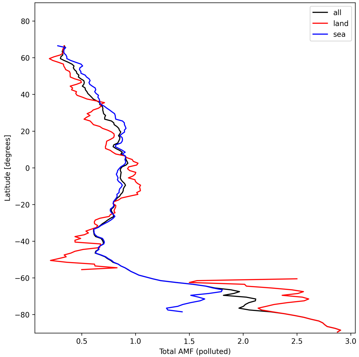
Figure 48: Zonal average of “Total AMF (polluted)” for 2024-11-14 to 2024-11-15.
