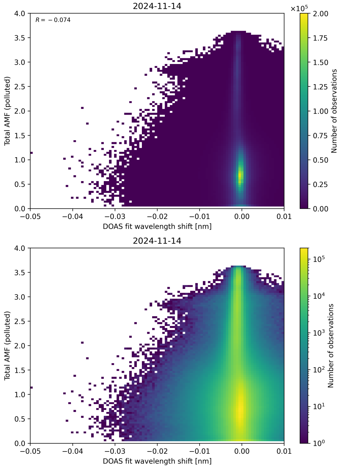
Figure 130: Scatter density plot of “DOAS fit wavelength shift” against “Total AMF (polluted)” for 2024-11-14 to 2024-11-15.
