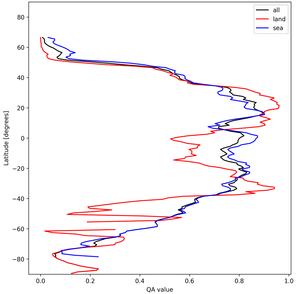
Figure 29: Zonal average of “QA value” for 2024-11-14 to 2024-11-15.
