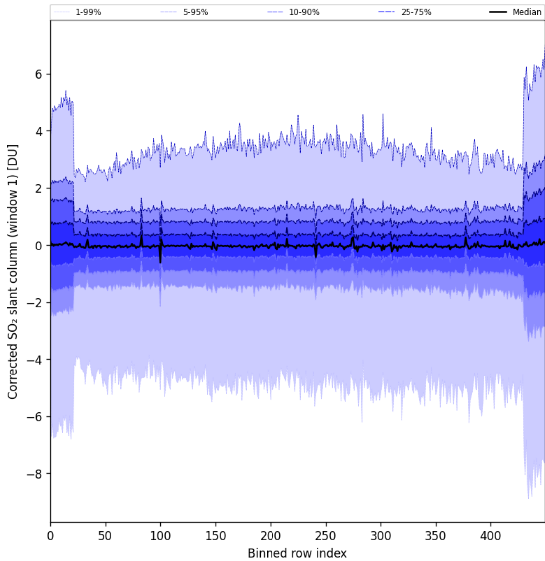
Figure 81: Along track statistics of “Corrected SO 2 slant column (window 1)” for 2024-11-14 to 2024-11-15
