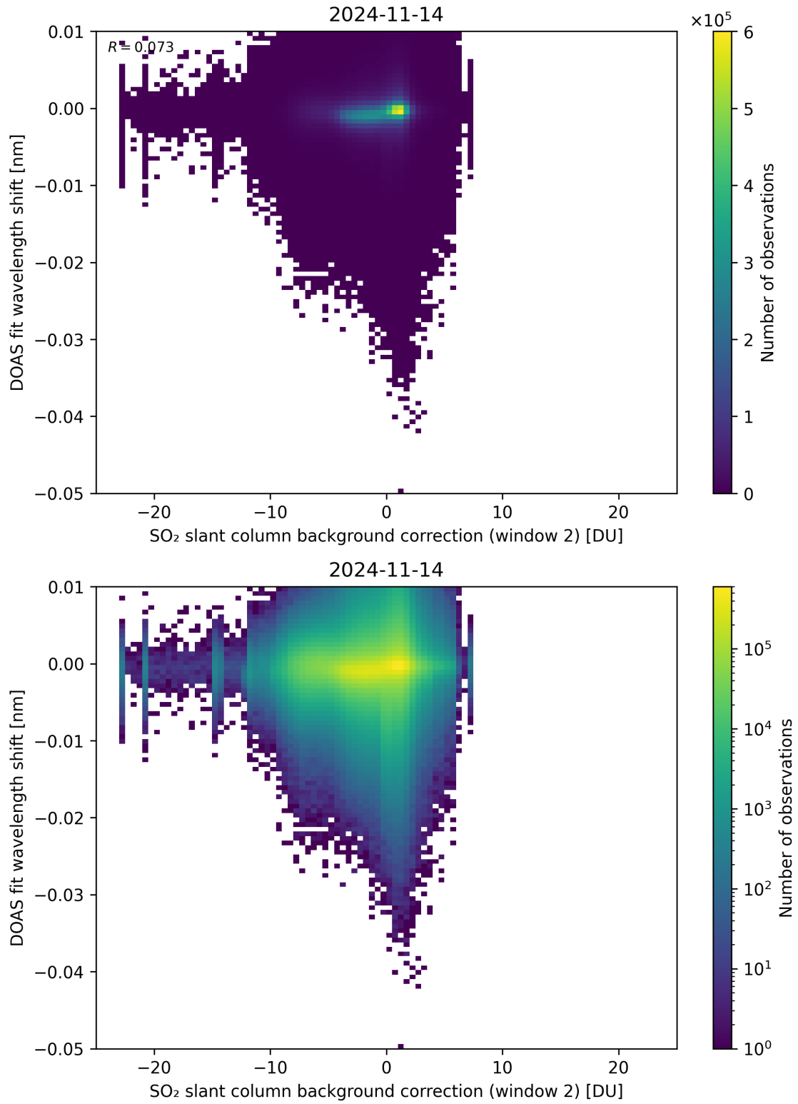
Figure 112: Scatter density plot of “SO 2 slant column background correction (window 2)” against “DOAS fit wavelength shift” for 2024-11-14 to 2024-11-15.
