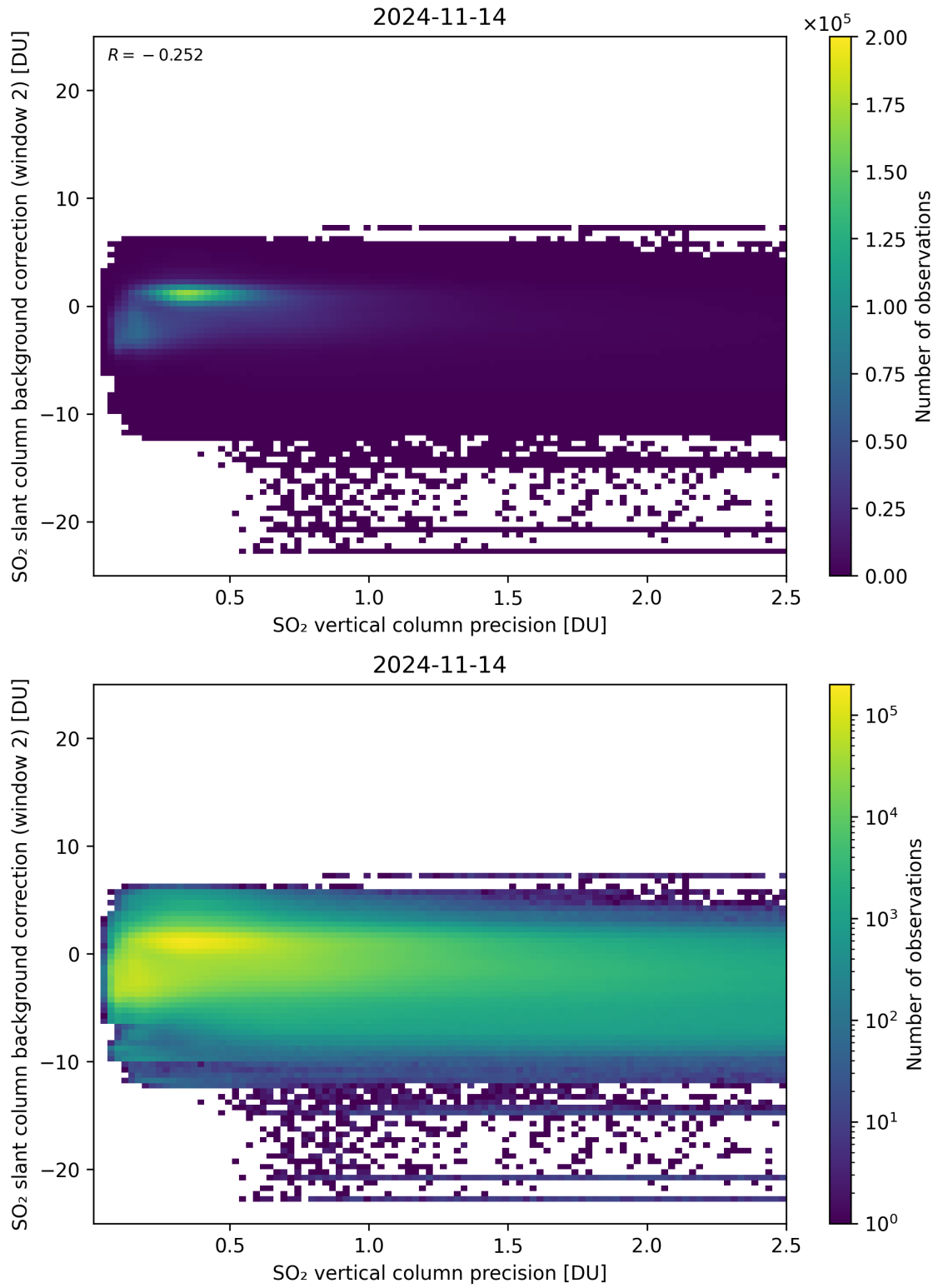
Figure 280: Scatter density plot of “SO 2 vertical column precision” against “SO 2 slant column background correction (window 2)” for 2024-11-14 to 2024-11-15.
