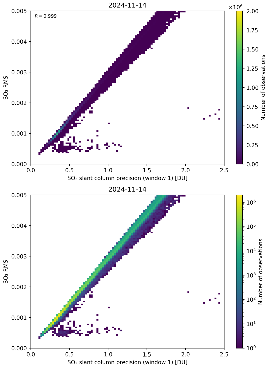
Figure 223: Scatter density plot of “SO 2 slant column precision (window 1)” against “SO 2 RMS” for 2024-11-14 to 2024-11-15.
