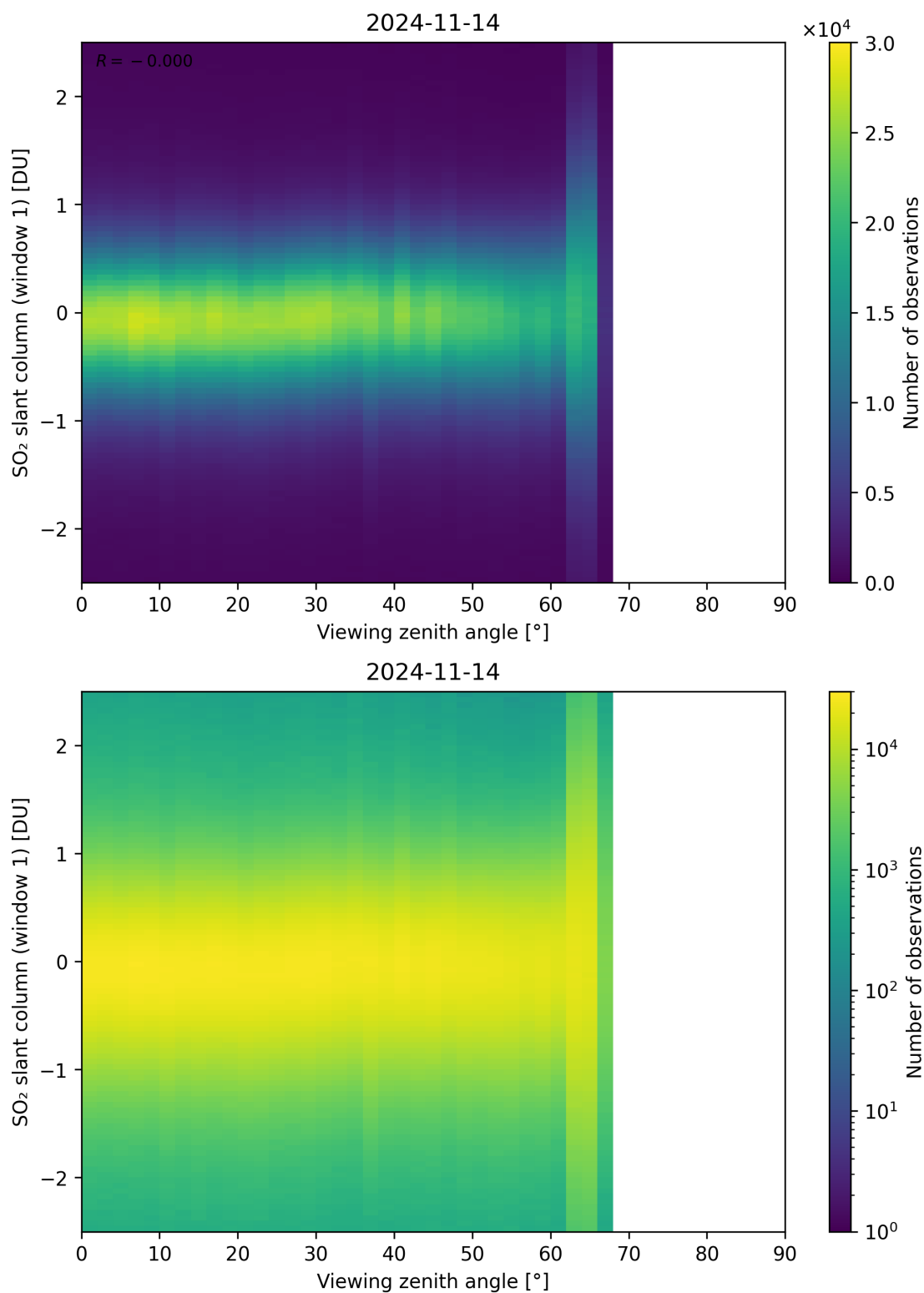
Figure 320: Scatter density plot of “Viewing zenith angle” against “SO 2 slant column (window 1)” for 2024-11-14 to 2024-11-15.
