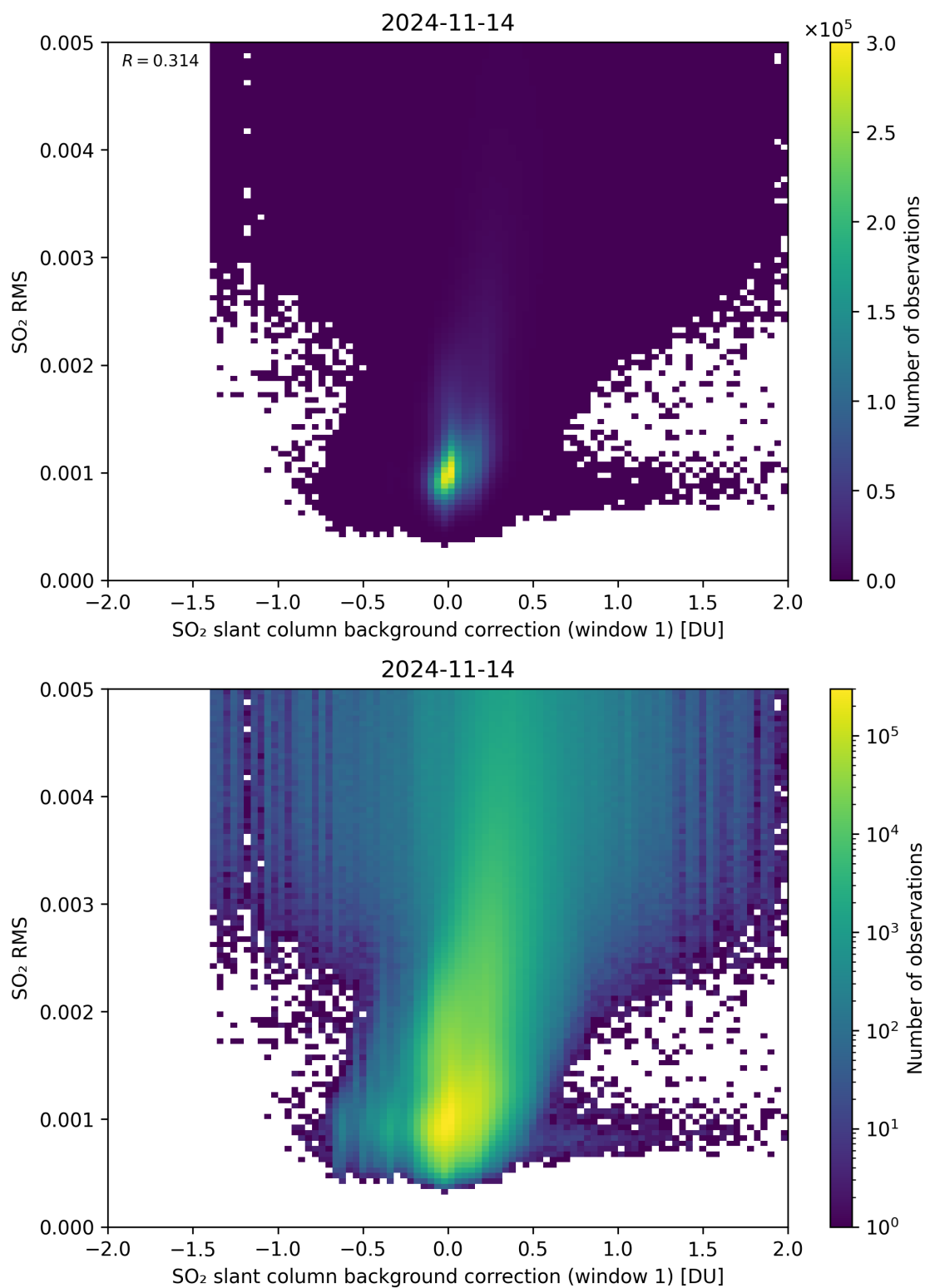
Figure 102: Scatter density plot of “SO 2 slant column background correction (window 1)” against “SO 2 RMS” for 2024-11-14 to 2024-11-15.
