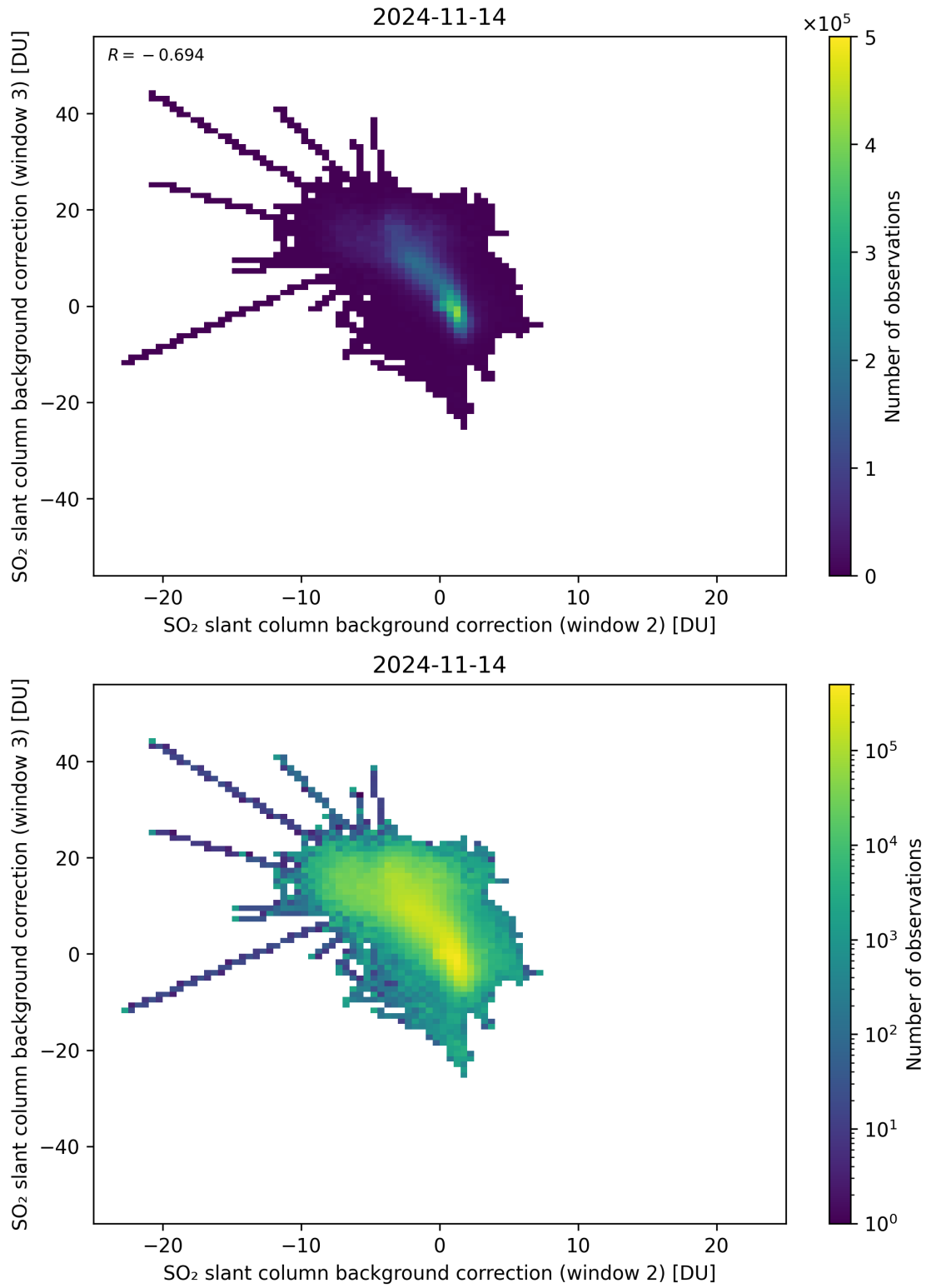
Figure 111: Scatter density plot of “SO 2 slant column background correction (window 2)” against “SO 2 slant column background correction (window 3)” for 2024-11-14 to 2024-11-15.
