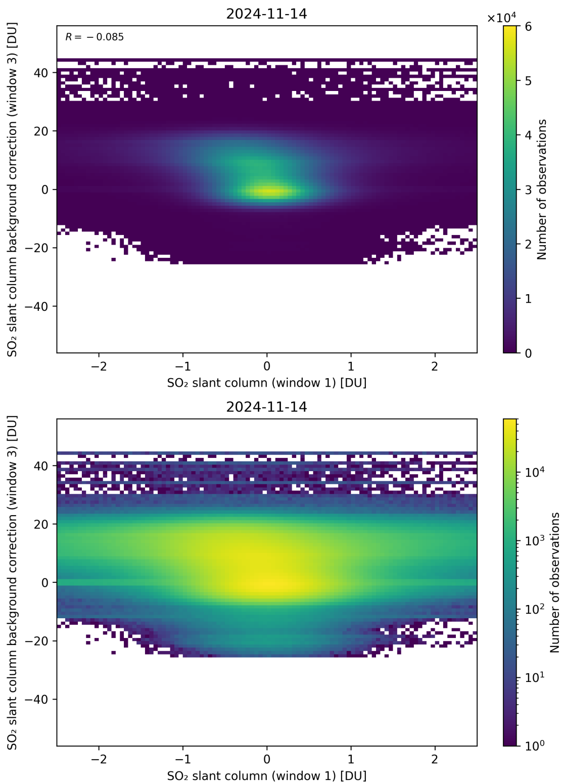
Figure 214: Scatter density plot of “SO 2 slant column (window 1)” against “SO 2 slant column background correction (window 3)” for 2024-11-14 to 2024-11-15.
