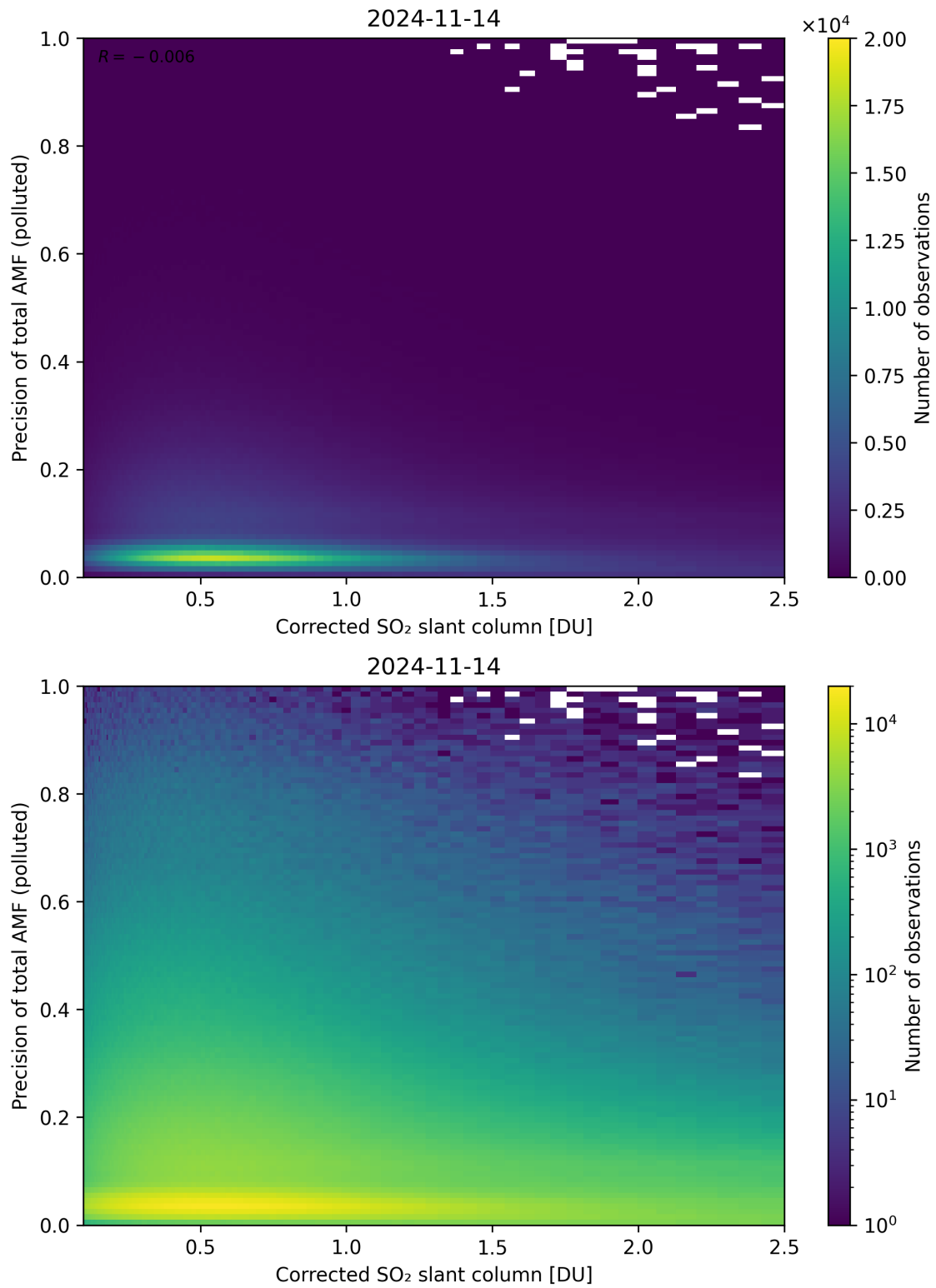
Figure 193: Scatter density plot of “Corrected SO 2 slant column” against “Precision of total AMF (polluted)” for 2024-11-14 to 2024-11-15.
