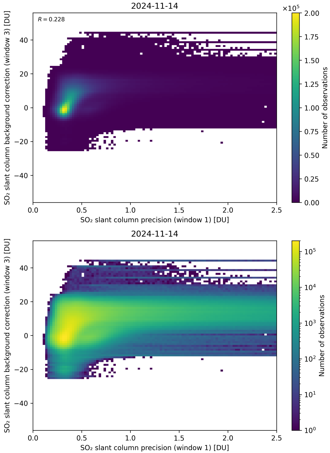
Figure 220: Scatter density plot of “SO 2 slant column precision (window 1)” against “SO 2 slant column background correction (window 3)” for 2024-11-14 to 2024-11-15.
