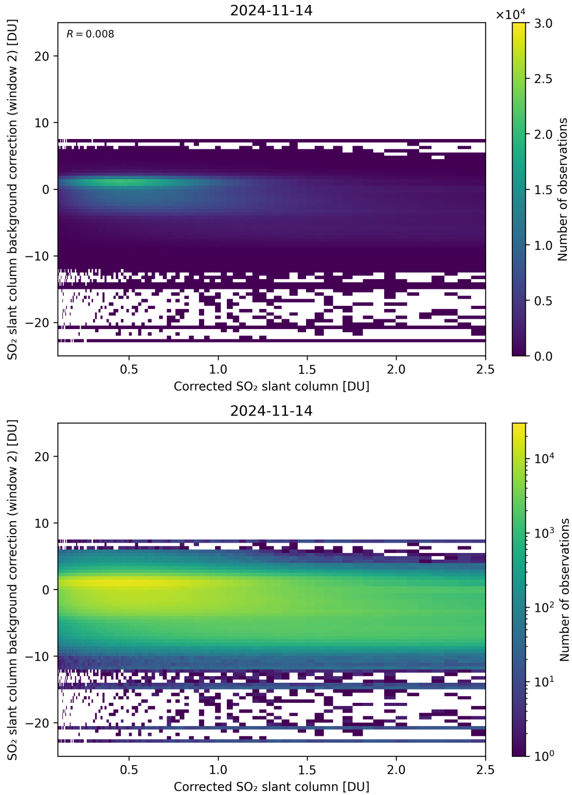
Figure 179: Scatter density plot of “Corrected SO 2 slant column” against “SO 2 slant column background correction (window 2)” for 2024-11-14 to 2024-11-15.
