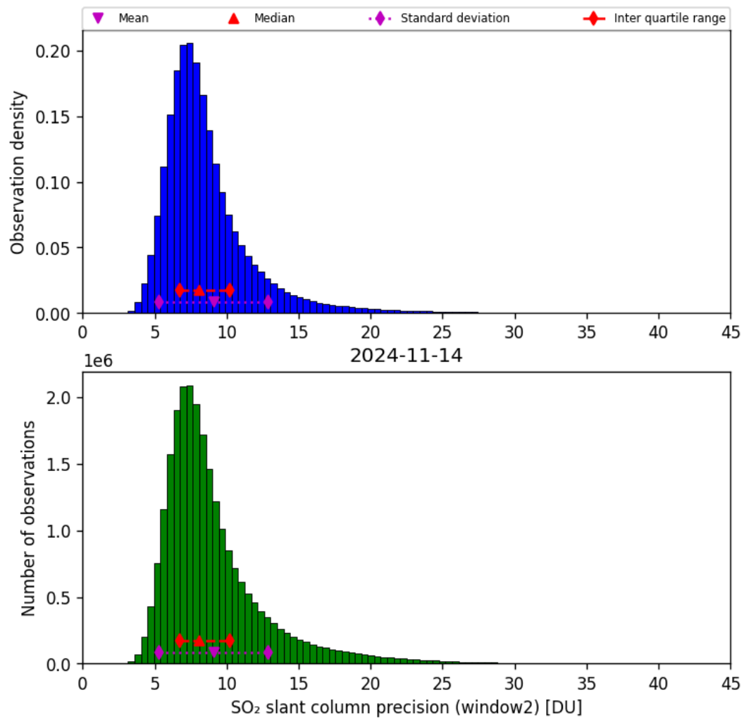
Figure 61: Histogram of “SO 2 slant column precision (window2)” for 2024-11-14 to 2024-11-15
