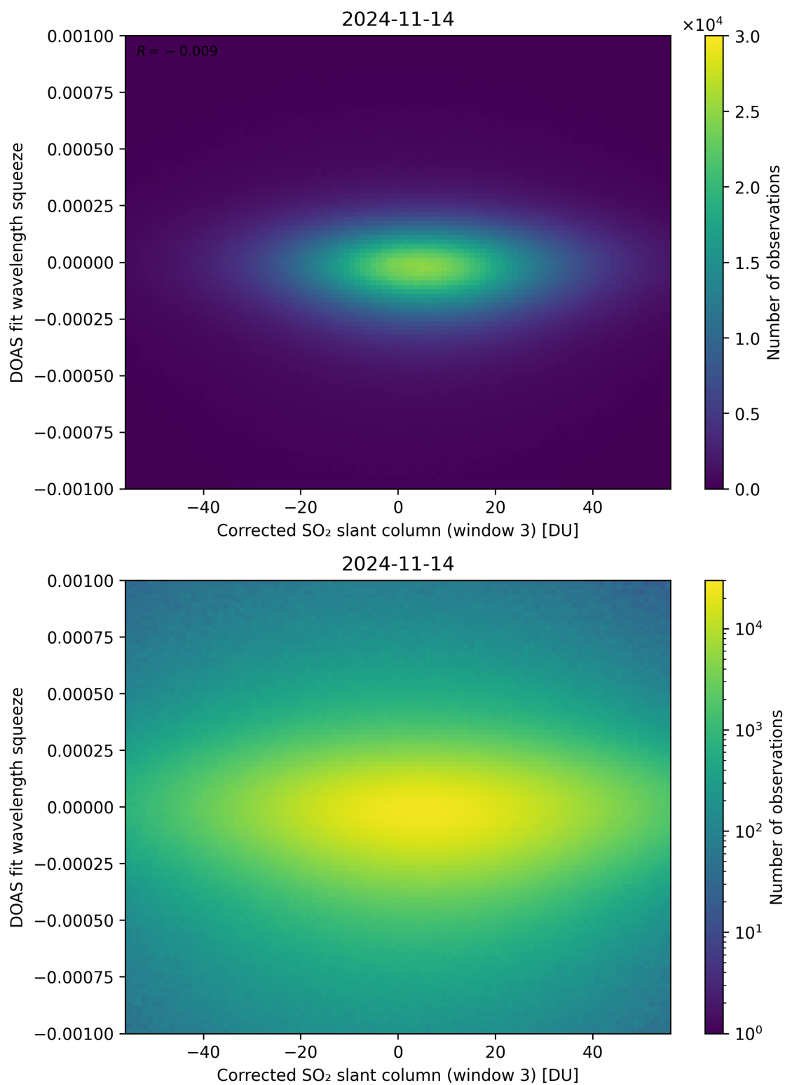
Figure 207: Scatter density plot of “Corrected SO 2 slant column (window 3)” against “DOAS fit wavelength squeeze” for 2024-11-14 to 2024-11-15.
