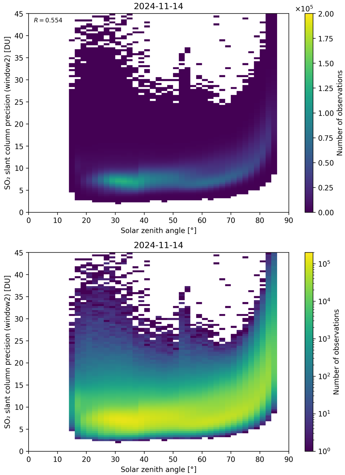
Figure 171: Scatter density plot of “Solar zenith angle” against “SO 2 slant column precision (window2)” for 2024-11-14 to 2024-11-15.
