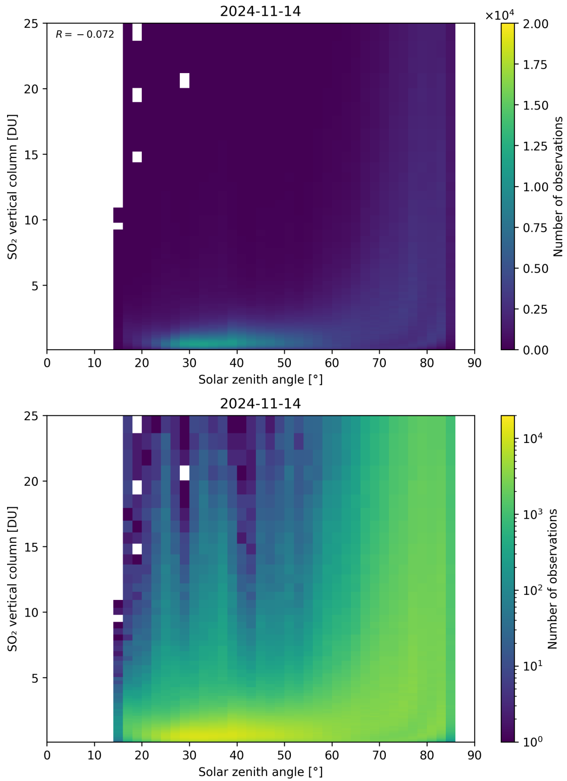
Figure 176: Scatter density plot of “Solar zenith angle” against “SO 2 vertical column” for 2024-11-14 to 2024-11-15.
