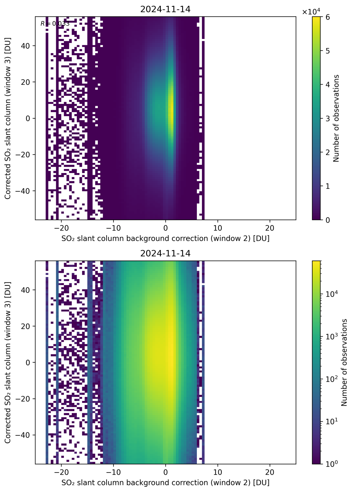
Figure 116: Scatter density plot of “SO 2 slant column background correction (window 2)” against “Corrected SO 2 slant column (window 3)” for 2024-11-14 to 2024-11-15.
