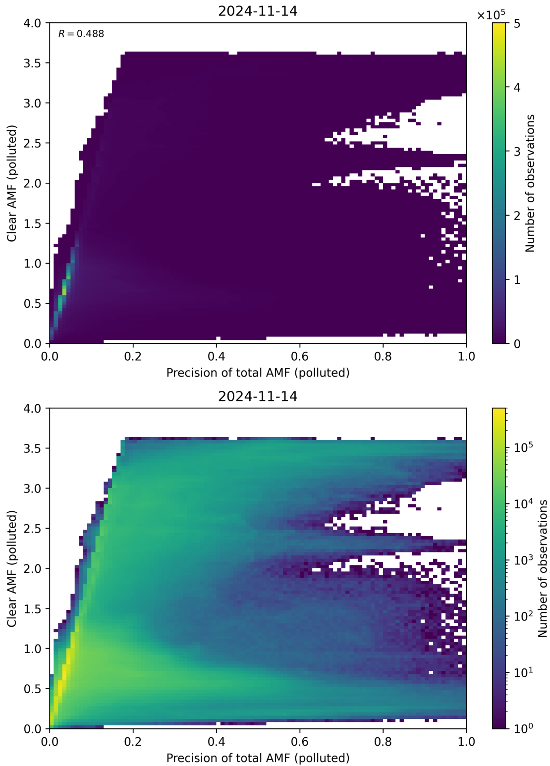
Figure 270: Scatter density plot of “Precision of total AMF (polluted)” against “Clear AMF (polluted)” for 2024-11-14 to 2024-11-15.
