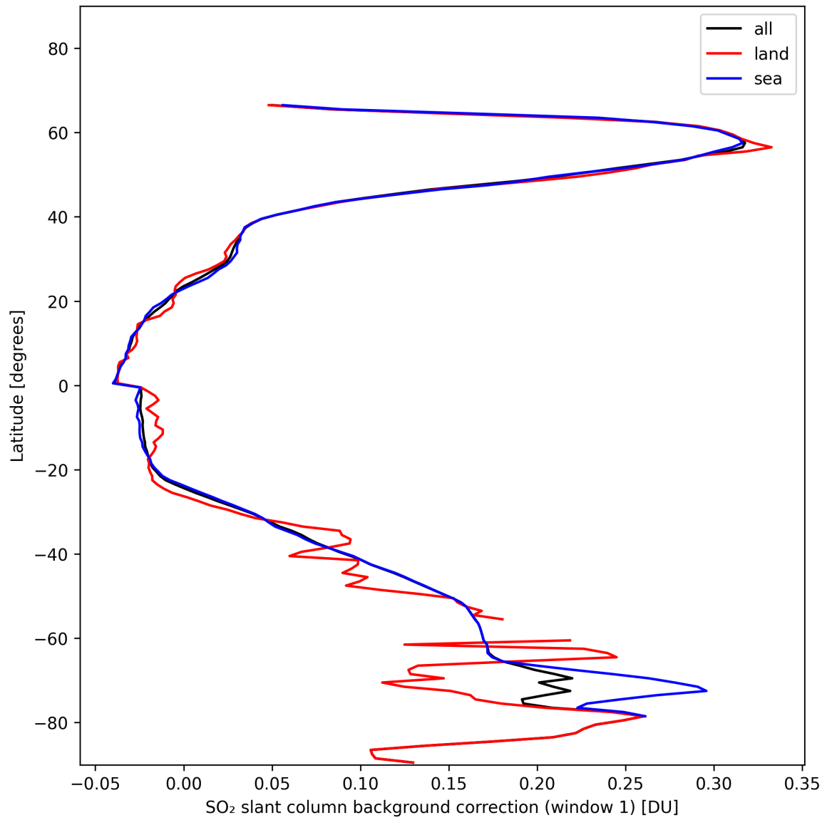
Figure 36: Zonal average of “SO 2 slant column background correction (window 1)” for 2024-11-14 to 2024-11-15.
