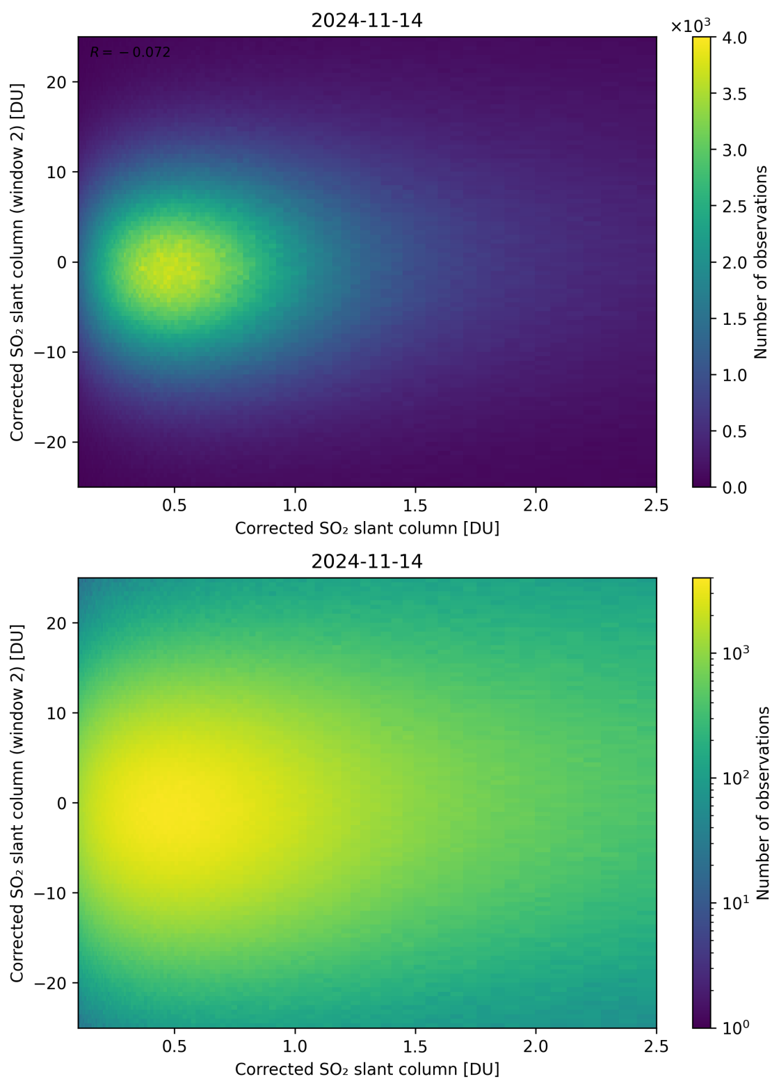
Figure 185: Scatter density plot of “Corrected SO 2 slant column” against “Corrected SO 2 slant column (window 2)” for 2024-11-14 to 2024-11-15.
