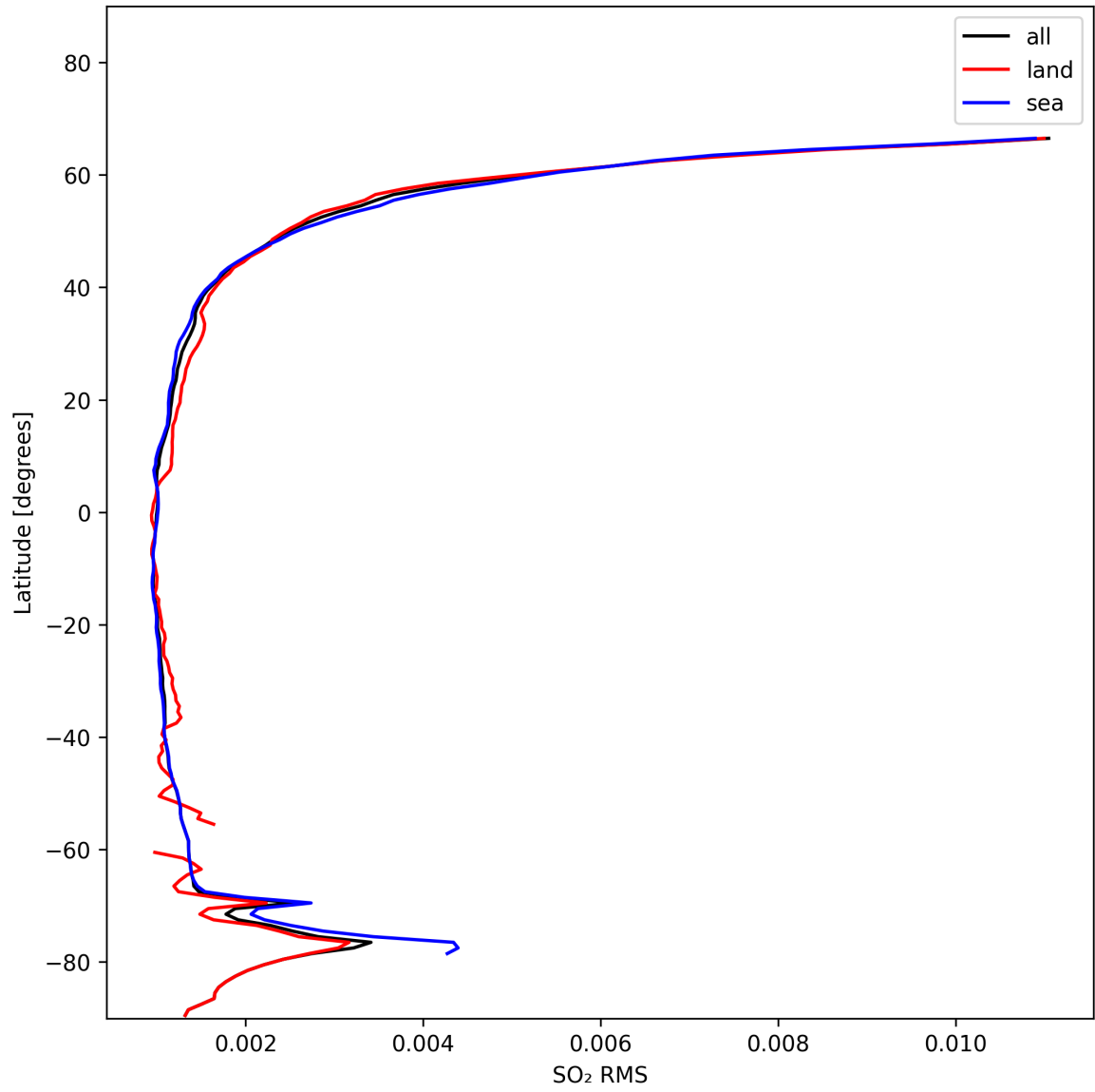
Figure 47: Zonal average of “SO 2 RMS” for 2024-11-14 to 2024-11-15.
