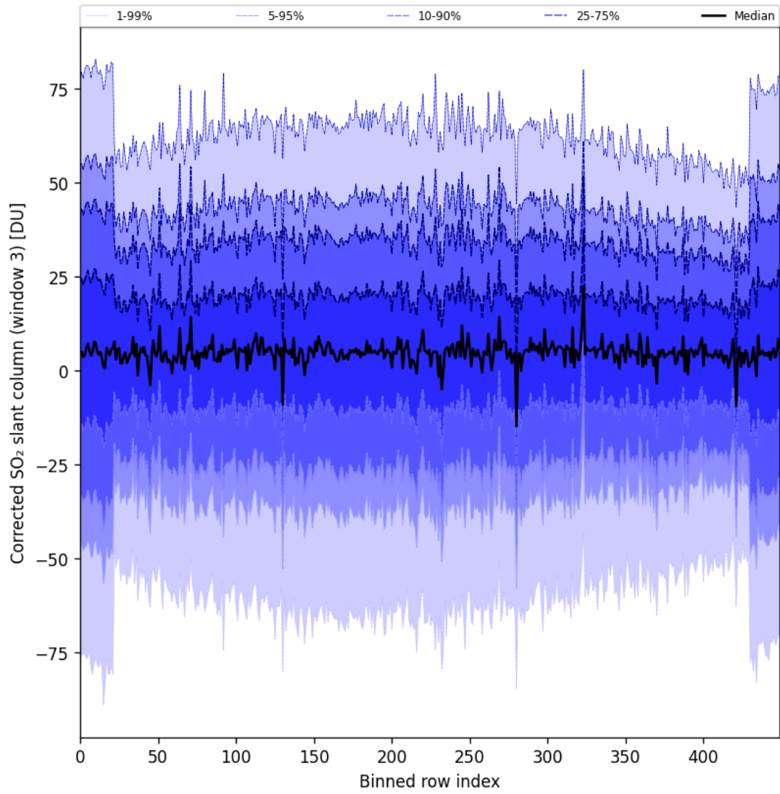
Figure 89: Along track statistics of “Corrected SO 2 slant column (window 3)” for 2024-11-14 to 2024-11-15
