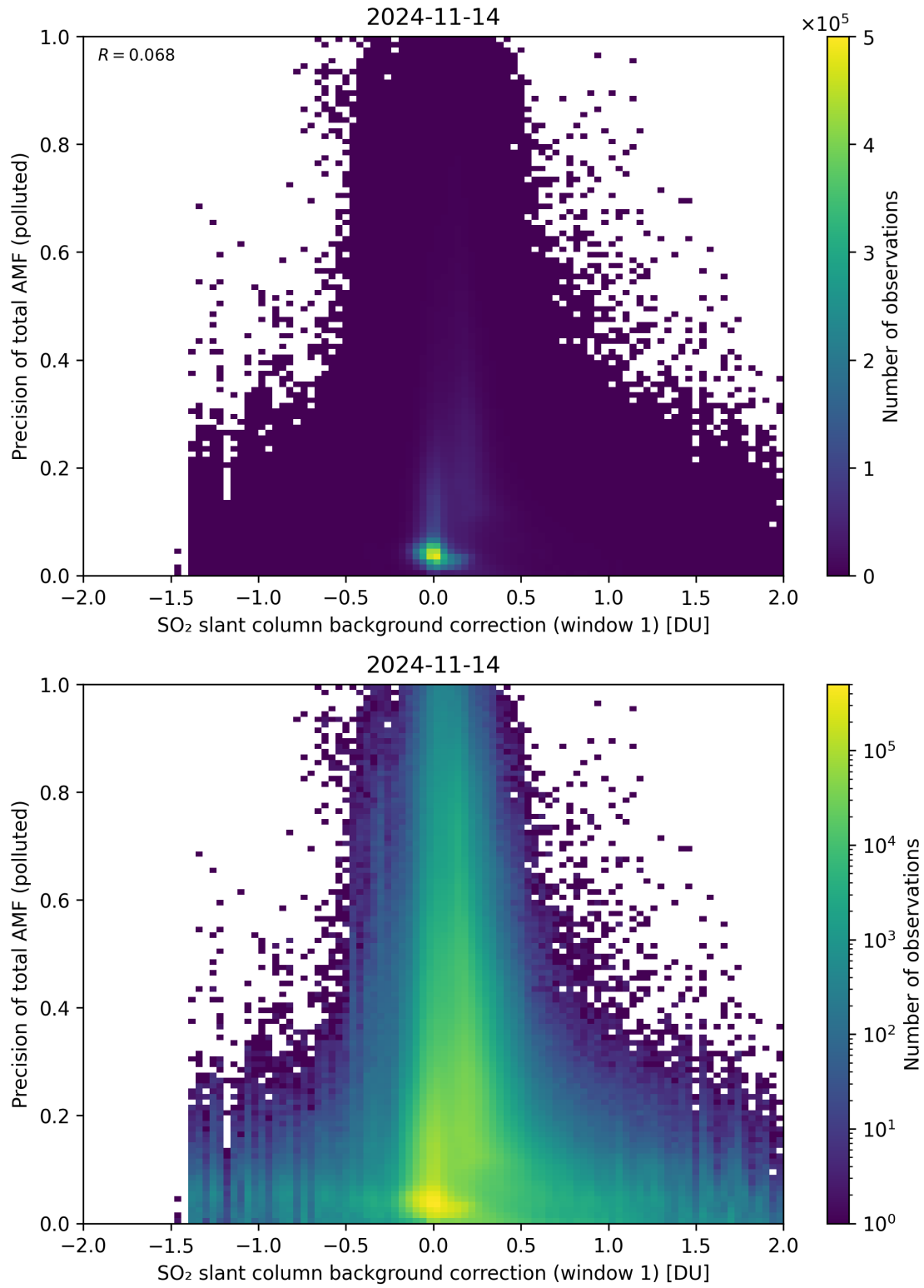
Figure 110: Scatter density plot of “SO 2 slant column background correction (window 1)” against “Precision of total AMF (polluted)” for 2024-11-14 to 2024-11-15.
