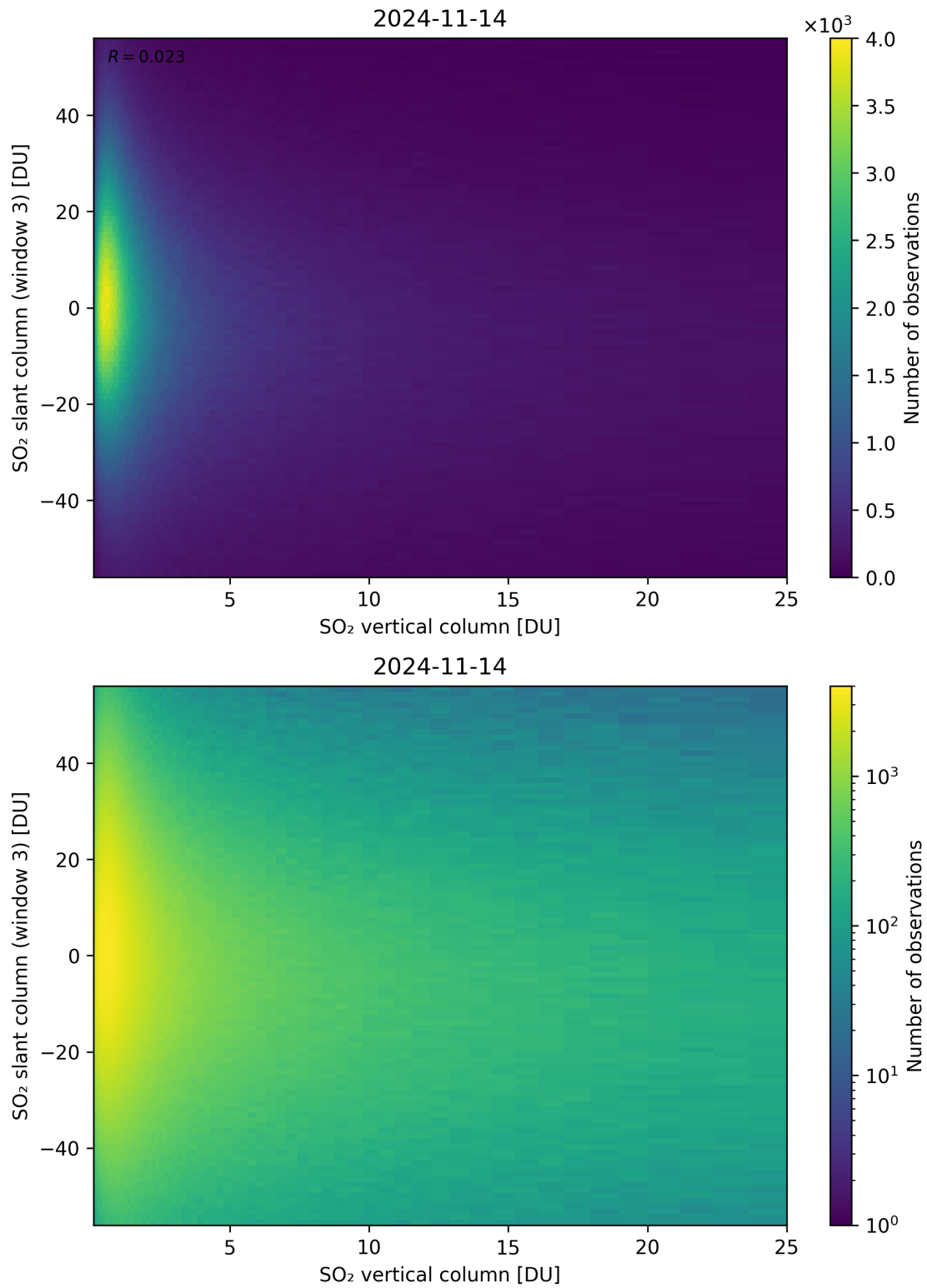
Figure 303: Scatter density plot of “SO 2 vertical column” against “SO 2 slant column (window 3)” for 2024-11-14 to 2024-11-15.
