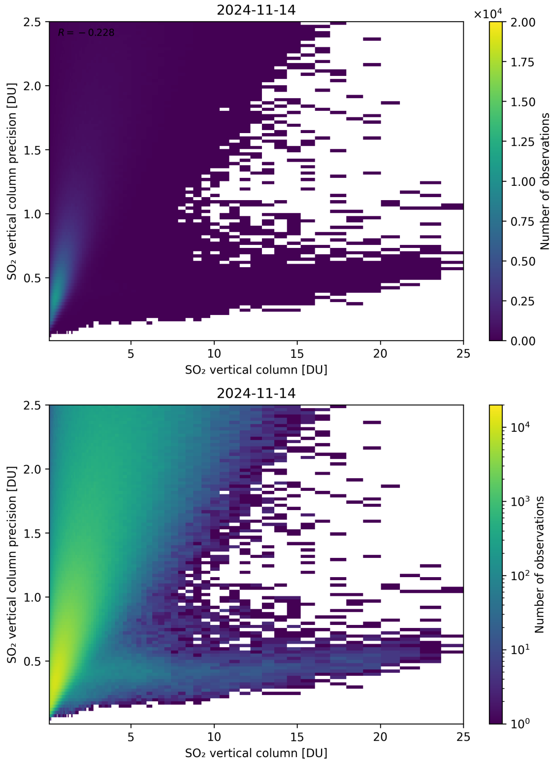
Figure 307: Scatter density plot of “SO 2 vertical column” against “SO 2 vertical column precision” for 2024-11-14 to 2024-11-15.
