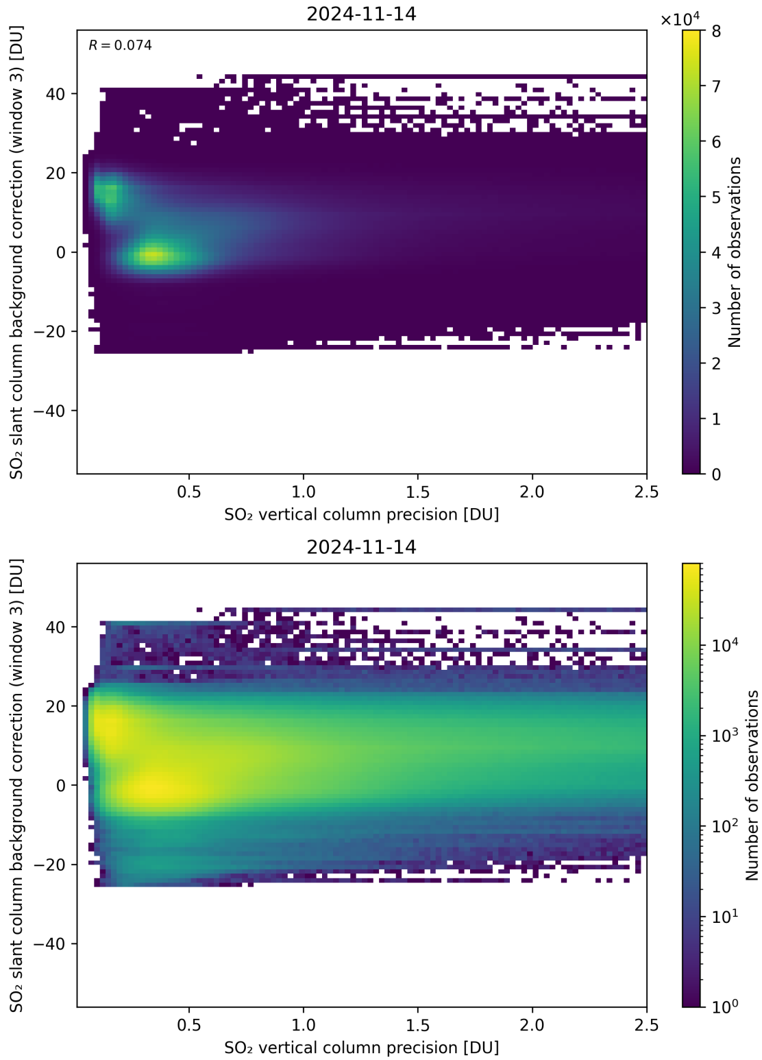
Figure 281: Scatter density plot of “SO 2 vertical column precision” against “SO 2 slant column background correction (window 3)” for 2024-11-14 to 2024-11-15.
