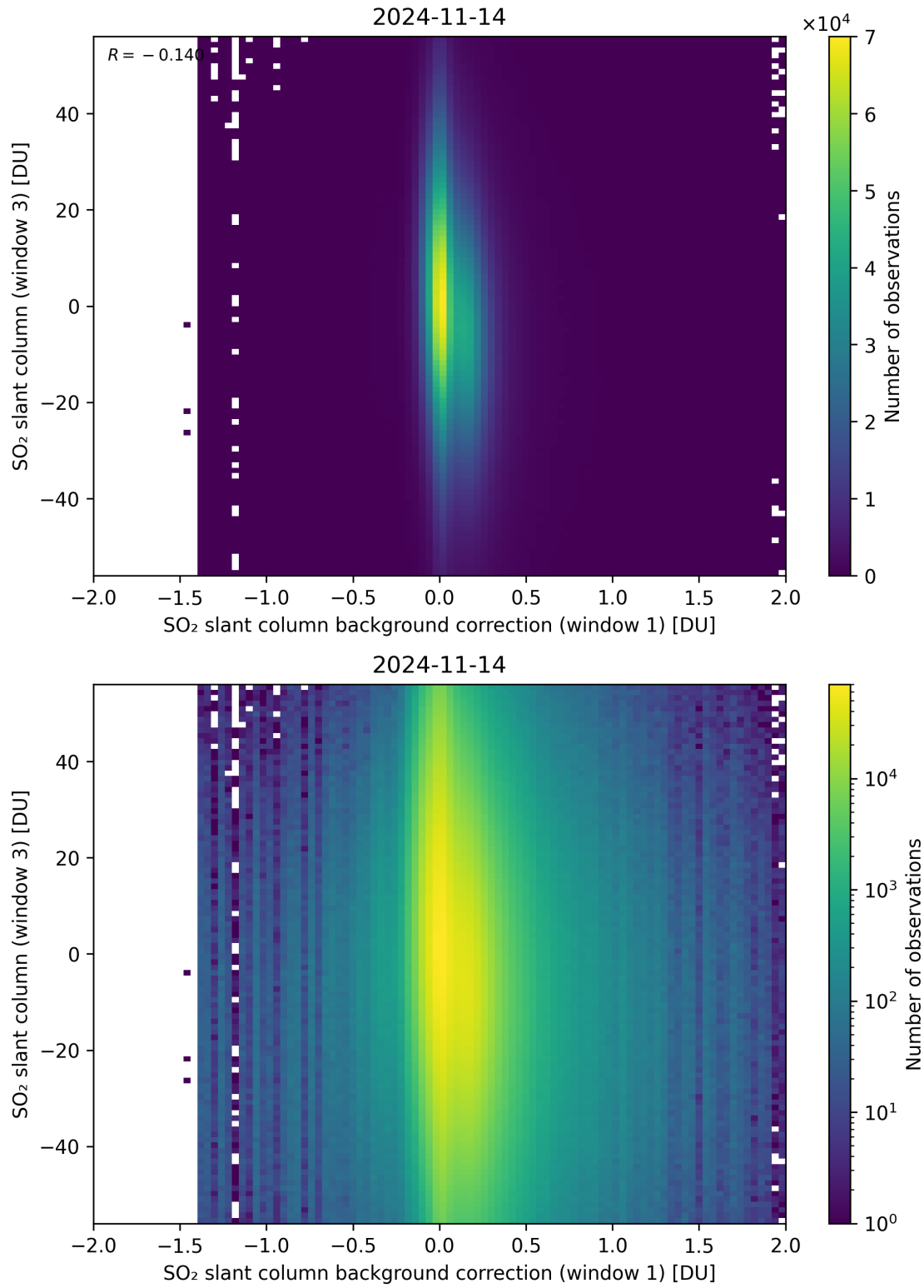
Figure 107: Scatter density plot of “SO 2 slant column background correction (window 1)” against “SO 2 slant column (window 3)” for 2024-11-14 to 2024-11-15.
