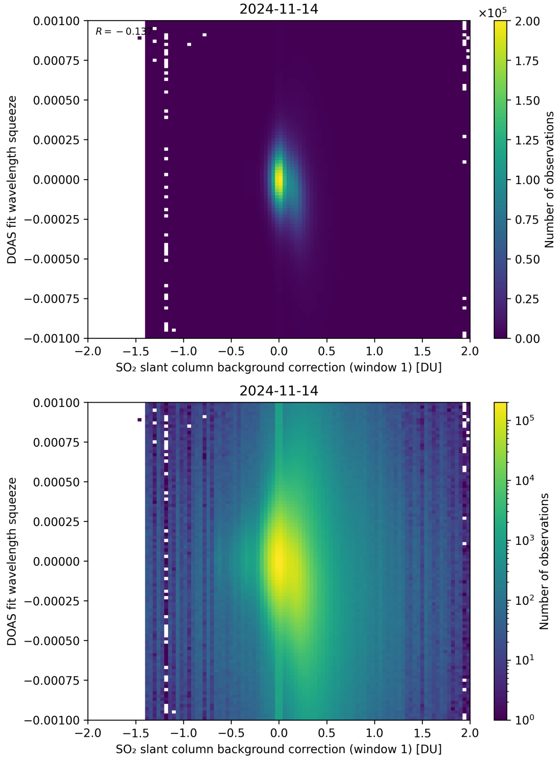
Figure 101: Scatter density plot of “SO 2 slant column background correction (window 1)” against “DOAS fit wavelength squeeze” for 2024-11-14 to 2024-11-15.
