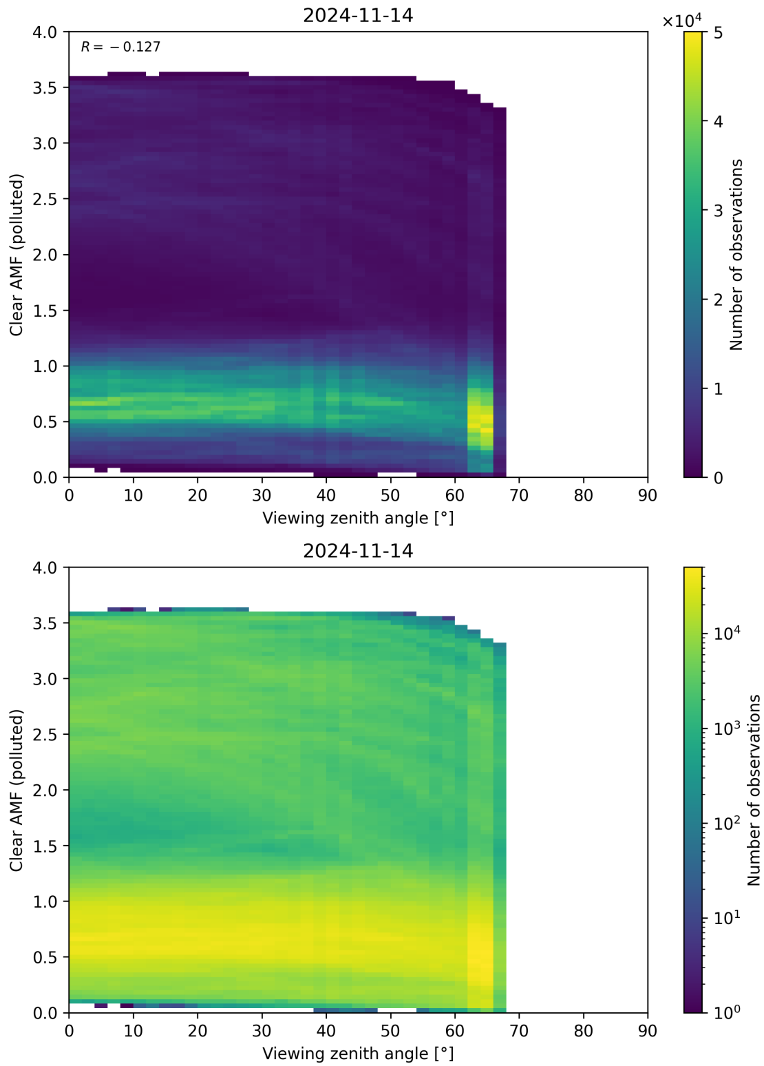
Figure 316: Scatter density plot of “Viewing zenith angle” against “Clear AMF (polluted)” for 2024-11-14 to 2024-11-15.
