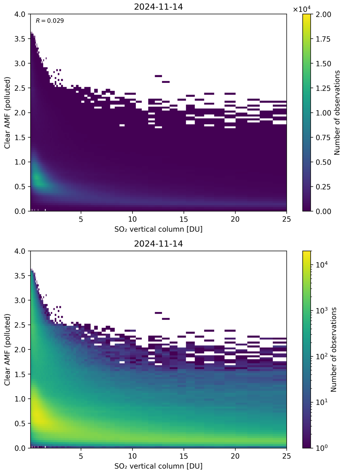
Figure 296: Scatter density plot of “SO 2 vertical column” against “Clear AMF (polluted)” for 2024-11-14 to 2024-11-15.
