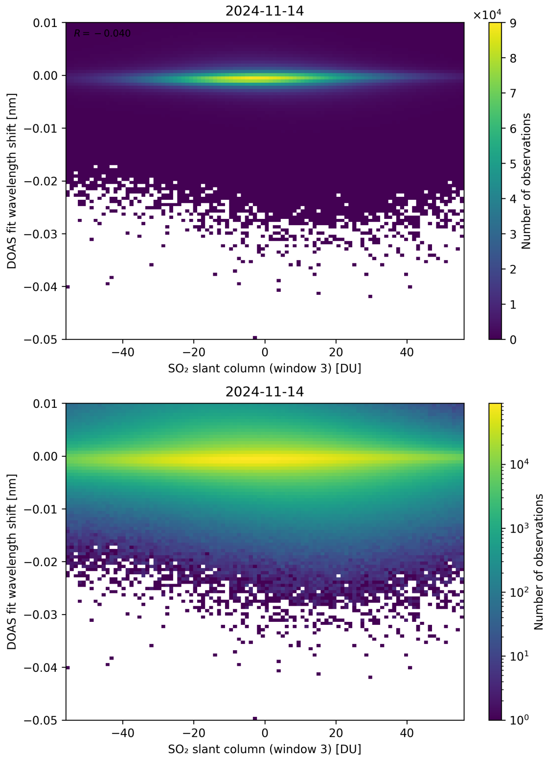
Figure 254: Scatter density plot of “SO 2 slant column (window 3)” against “DOAS fit wavelength shift” for 2024-11-14 to 2024-11-15.
