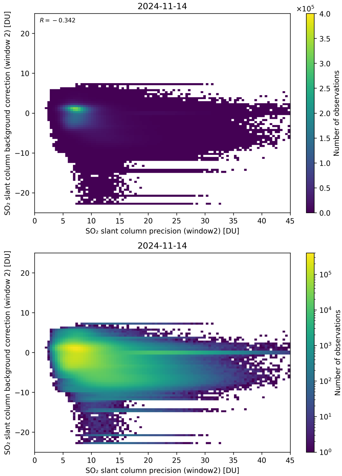
Figure 241: Scatter density plot of “SO 2 slant column precision (window2)” against “SO 2 slant column background correction (window 2)” for 2024-11-14 to 2024-11-15.
