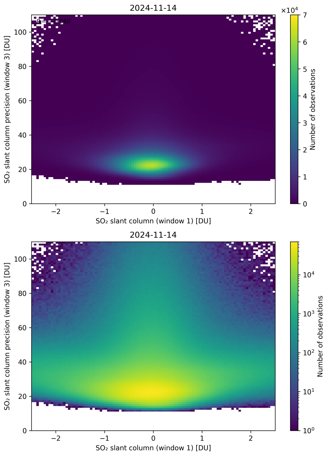
Figure 238: Scatter density plot of “SO 2 slant column (window 1)” against “SO 2 slant column precision (window 3)” for 2024-11-14 to 2024-11-15.
