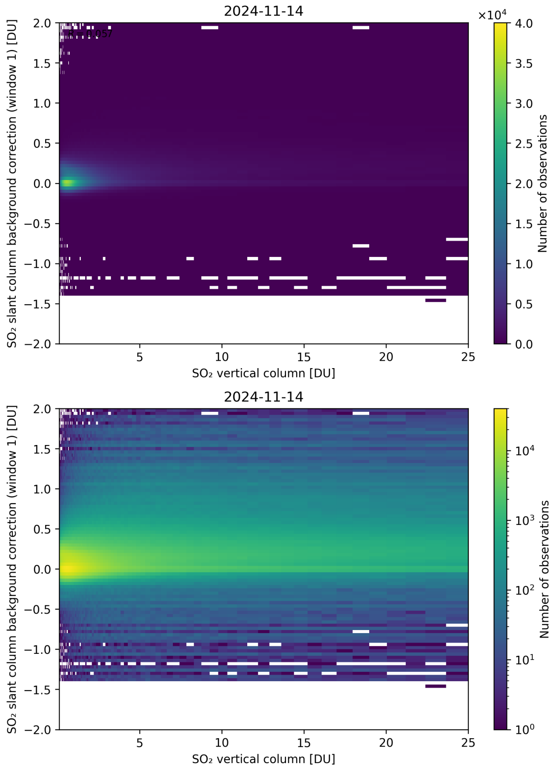
Figure 273: Scatter density plot of “SO 2 vertical column” against “SO 2 slant column background correction (window 1)” for 2024-11-14 to 2024-11-15.
