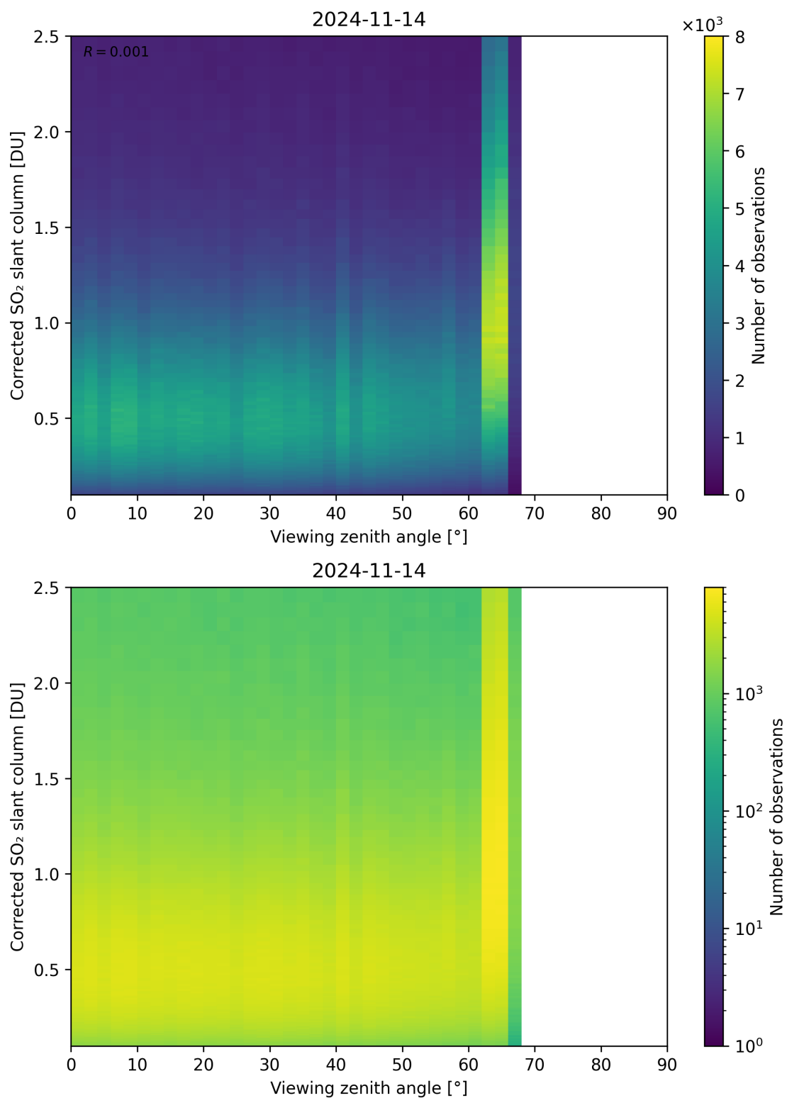
Figure 317: Scatter density plot of “Viewing zenith angle” against “Corrected SO 2 slant column” for 2024-11-14 to 2024-11-15.
