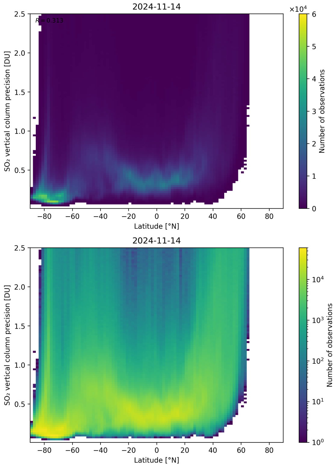
Figure 157: Scatter density plot of “Latitude” against “SO 2 vertical column precision” for 2024-11-14 to 2024-11-15.
