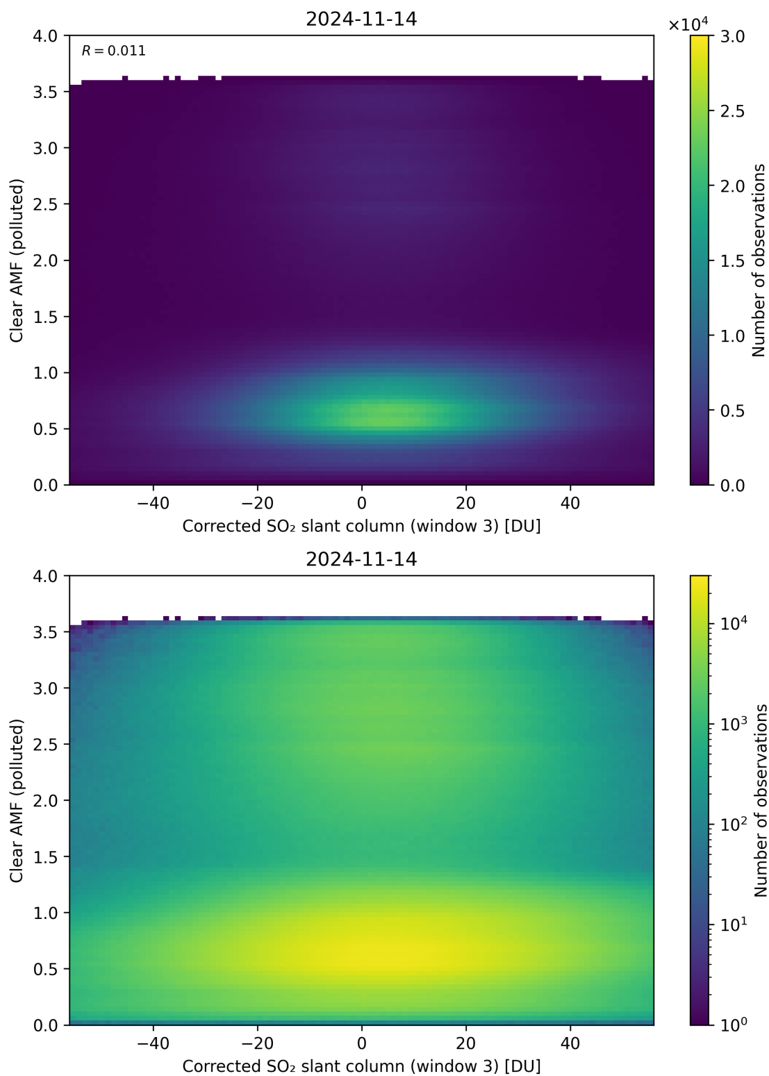
Figure 209: Scatter density plot of “Corrected SO 2 slant column (window 3)” against “Clear AMF (polluted)” for 2024-11-14 to 2024-11-15.
