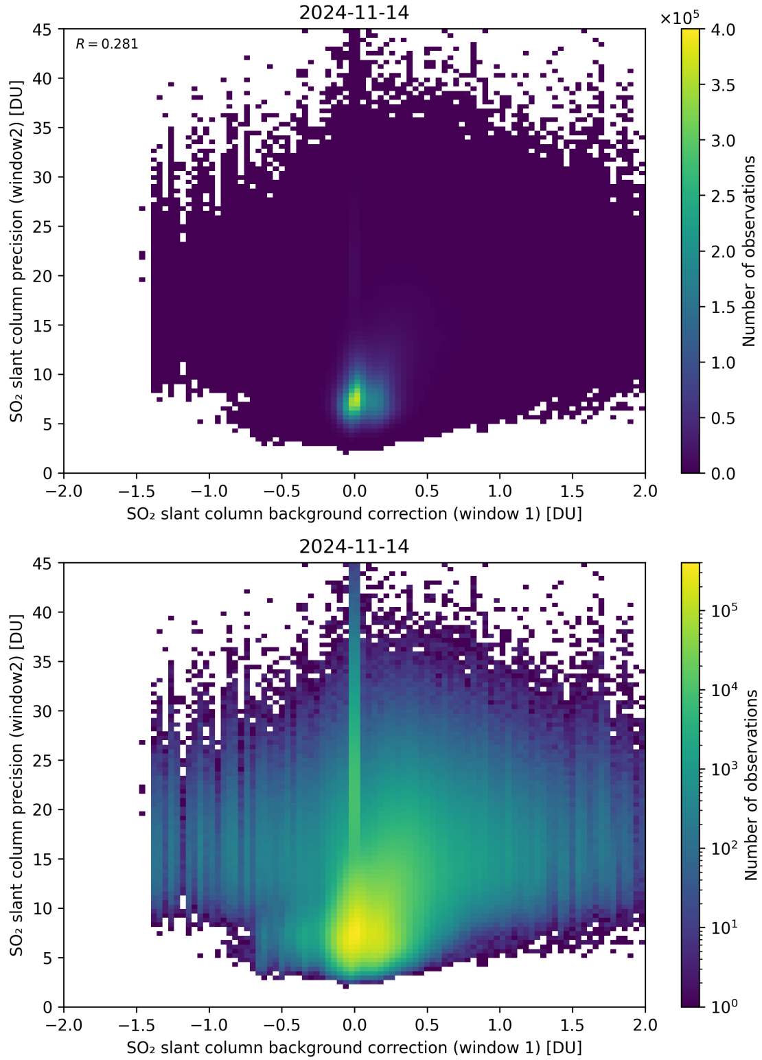
Figure 106: Scatter density plot of “SO 2 slant column background correction (window 1)” against “SO 2 slant column precision (window2)” for 2024-11-14 to 2024-11-15.
