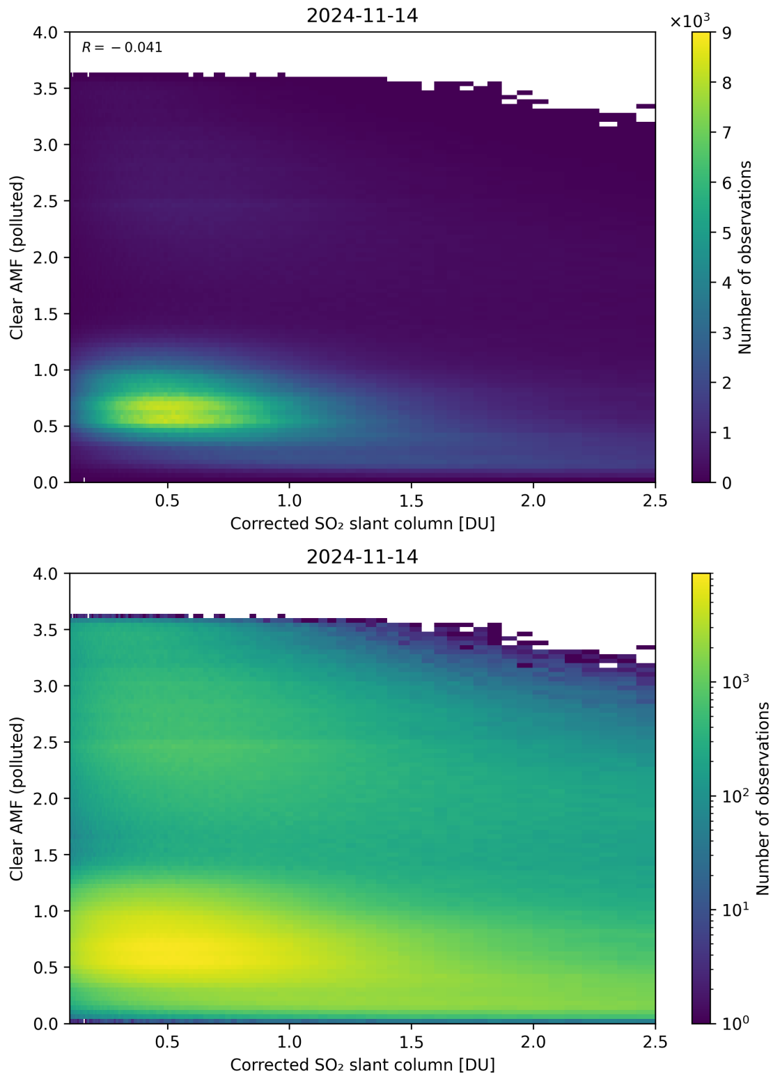
Figure 184: Scatter density plot of “Corrected SO 2 slant column” against “Clear AMF (polluted)” for 2024-11-14 to 2024-11-15.
