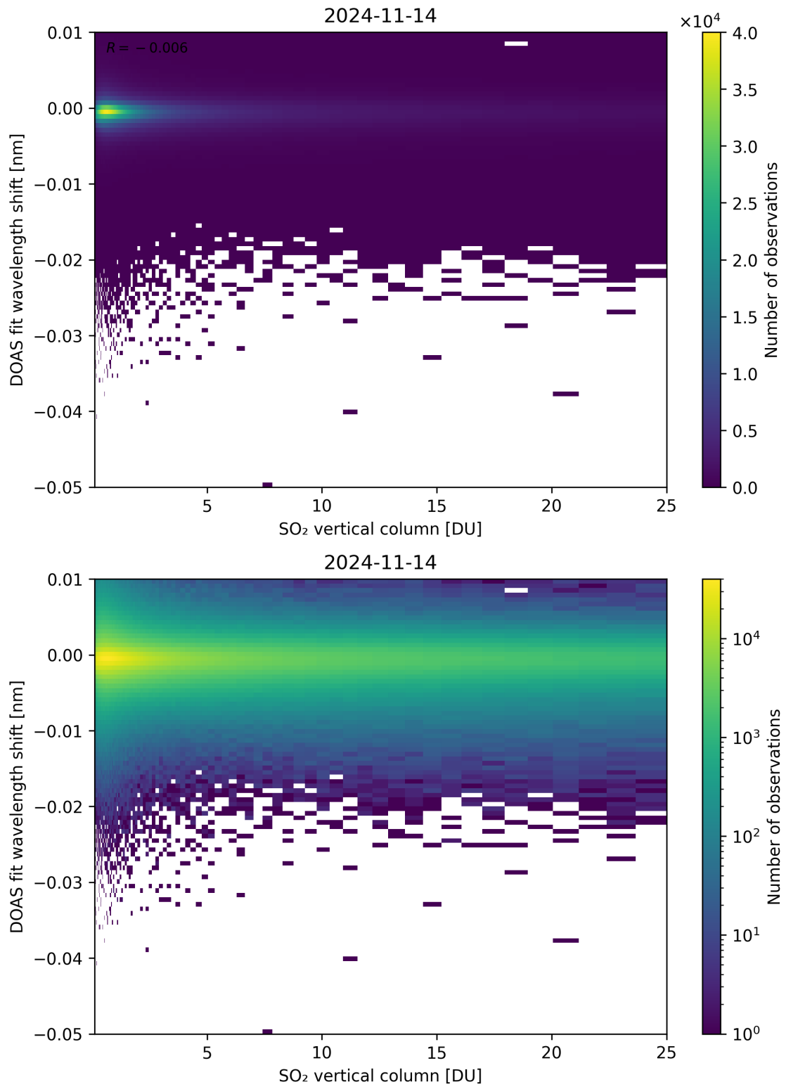
Figure 276: Scatter density plot of “SO 2 vertical column” against “DOAS fit wavelength shift” for 2024-11-14 to 2024-11-15.
