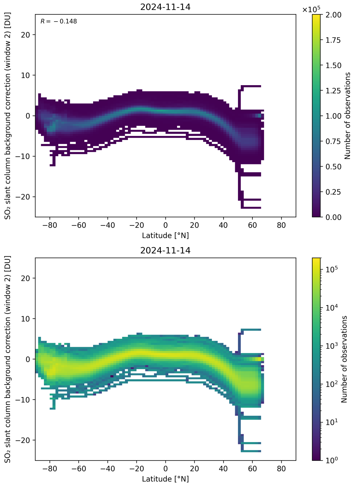
Figure 140: Scatter density plot of “Latitude” against “SO 2 slant column background correction (window 2)” for 2024-11-14 to 2024-11-15.
