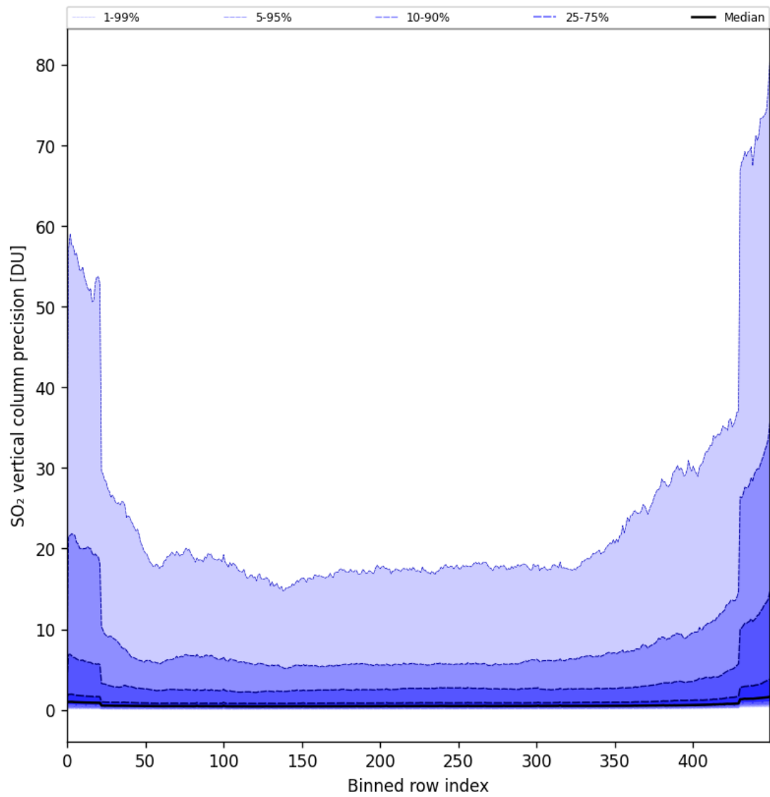
Figure 77: Along track statistics of “SO 2 vertical column precision” for 2024-11-14 to 2024-11-15
