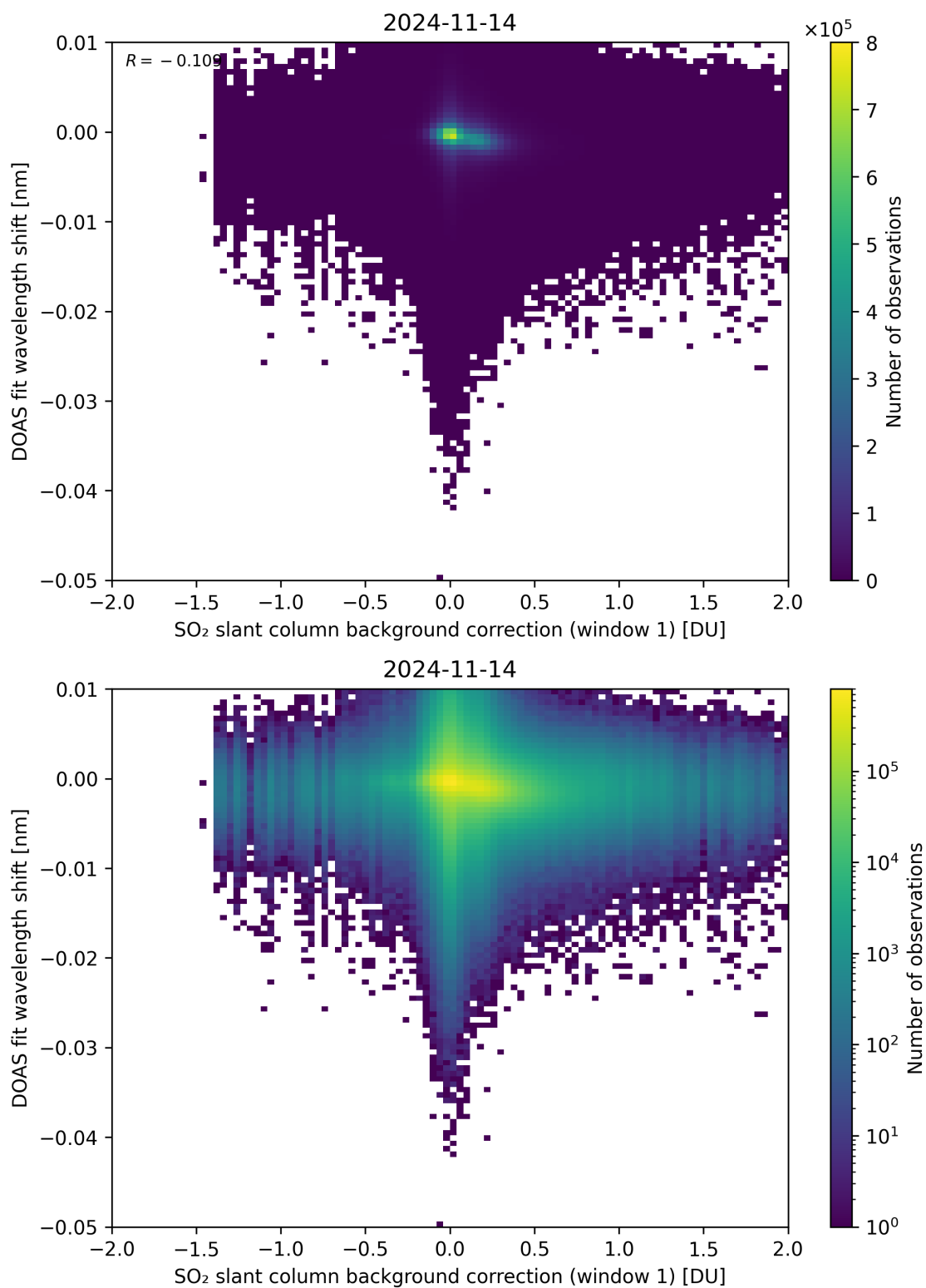
Figure 100: Scatter density plot of “SO 2 slant column background correction (window 1)” against “DOAS fit wavelength shift” for 2024-11-14 to 2024-11-15.
