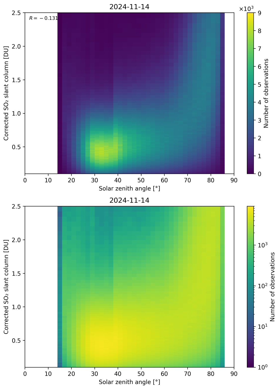
Figure 166: Scatter density plot of “Solar zenith angle” against “Corrected SO 2 slant column” for 2024-11-14 to 2024-11-15.
