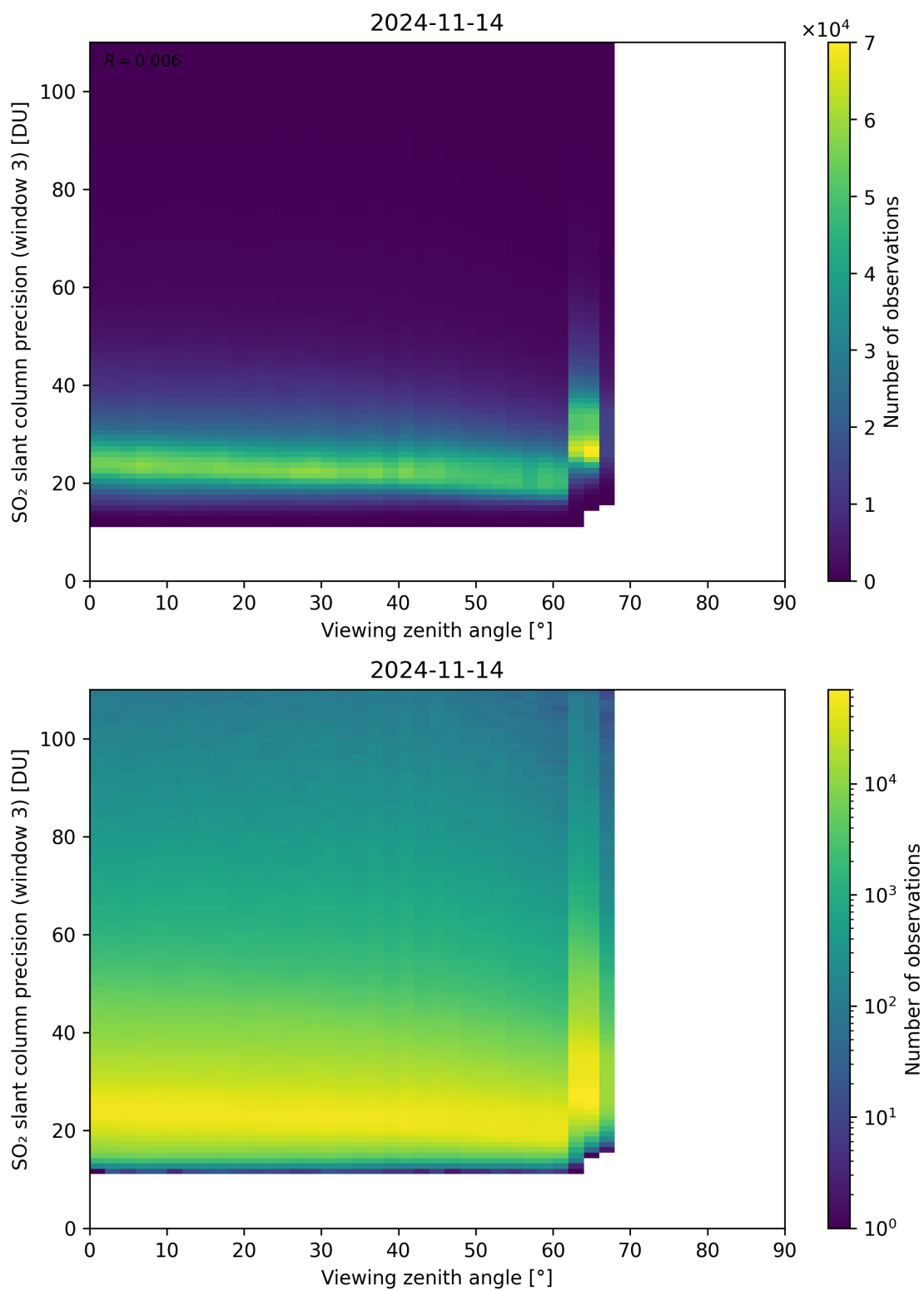
Figure 324: Scatter density plot of “Viewing zenith angle” against “SO 2 slant column precision (window 3)” for 2024-11-14 to 2024-11-15.
