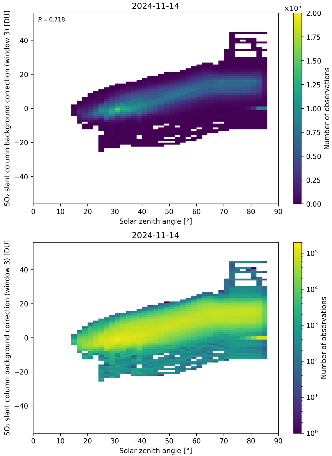
Figure 160: Scatter density plot of “Solar zenith angle” against “SO 2 slant column background correction (window 3)” for 2024-11-14 to 2024-11-15.
