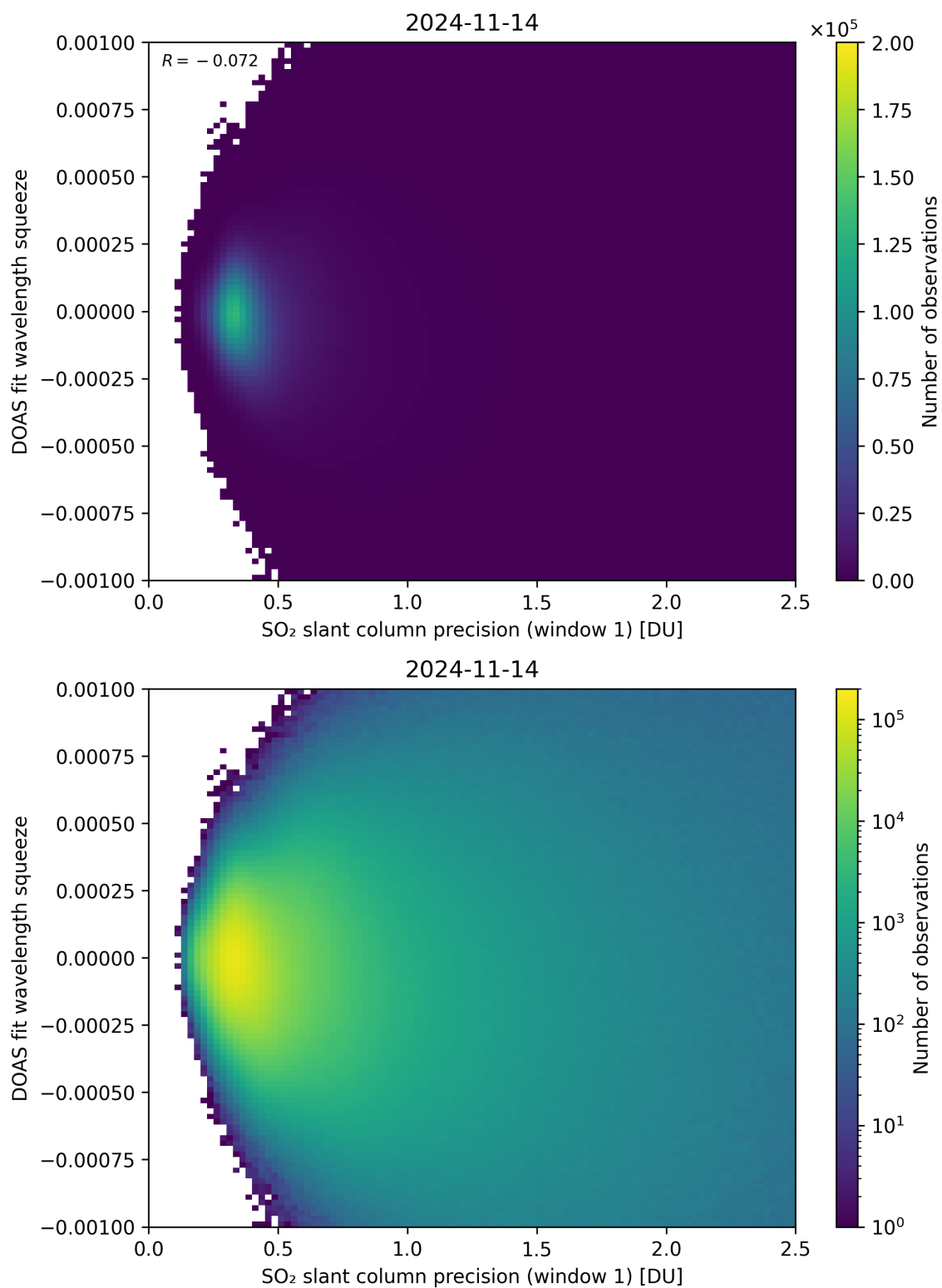
Figure 222: Scatter density plot of “SO 2 slant column precision (window 1)” against “DOAS fit wavelength squeeze” for 2024-11-14 to 2024-11-15.
