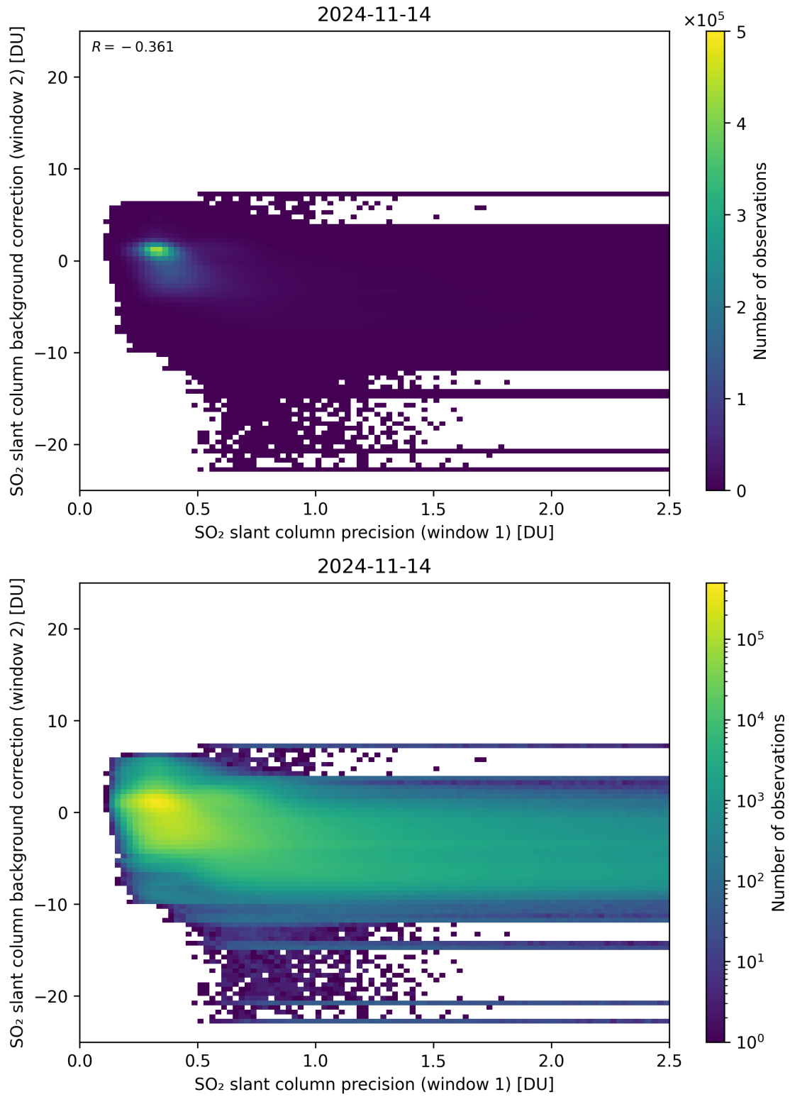
Figure 219: Scatter density plot of “SO 2 slant column precision (window 1)” against “SO 2 slant column background correction (window 2)” for 2024-11-14 to 2024-11-15.
