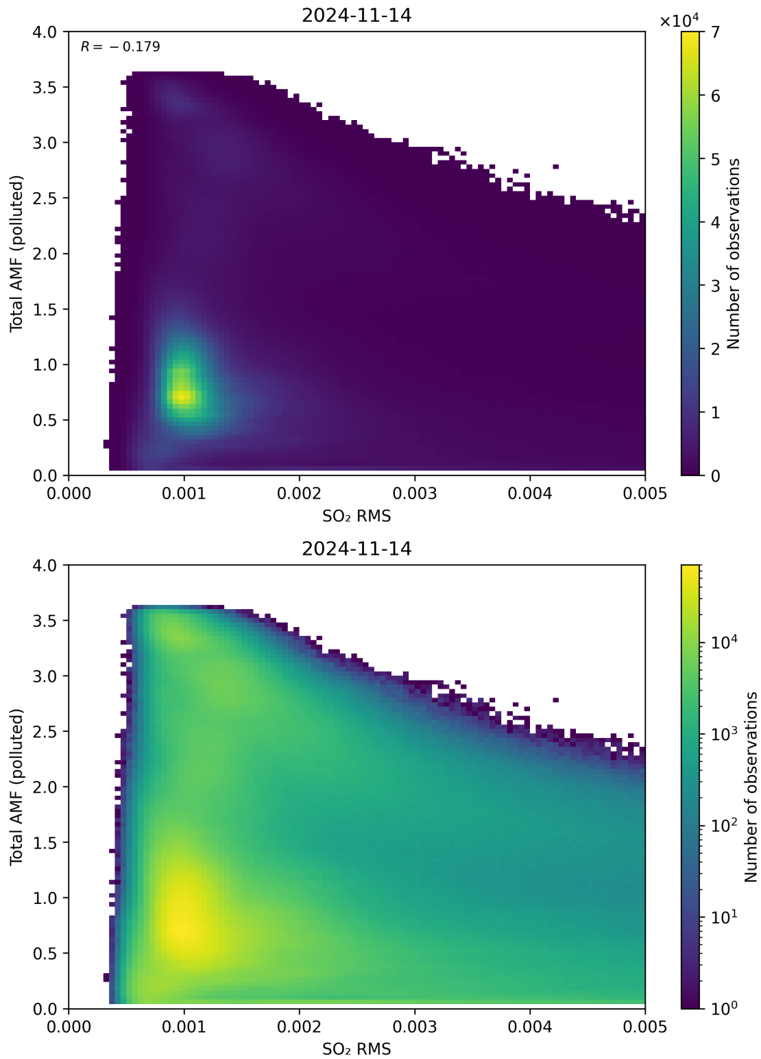
Figure 137: Scatter density plot of “SO 2 RMS” against “Total AMF (polluted)” for 2024-11-14 to 2024-11-15.
