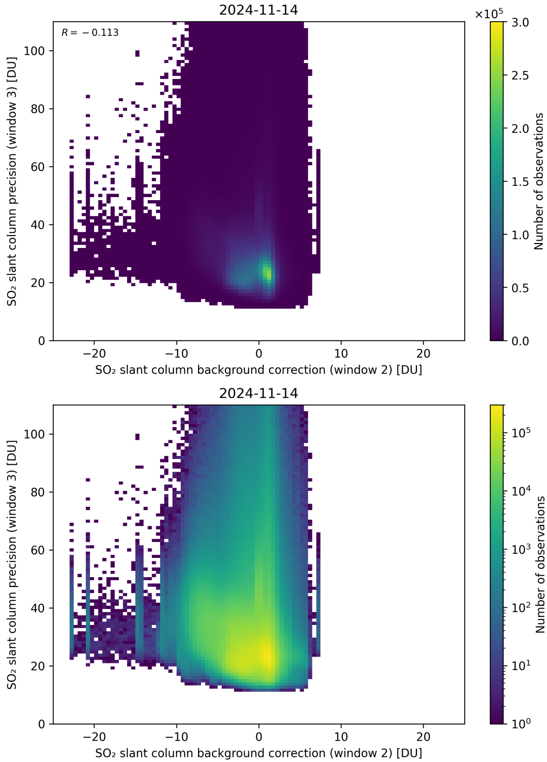
Figure 118: Scatter density plot of “SO 2 slant column background correction (window 2)” against “SO 2 slant column precision (window 3)” for 2024-11-14 to 2024-11-15.
