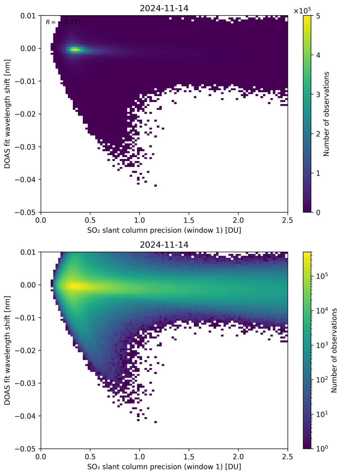
Figure 221: Scatter density plot of “SO 2 slant column precision (window 1)” against “DOAS fit wavelength shift” for 2024-11-14 to 2024-11-15.
