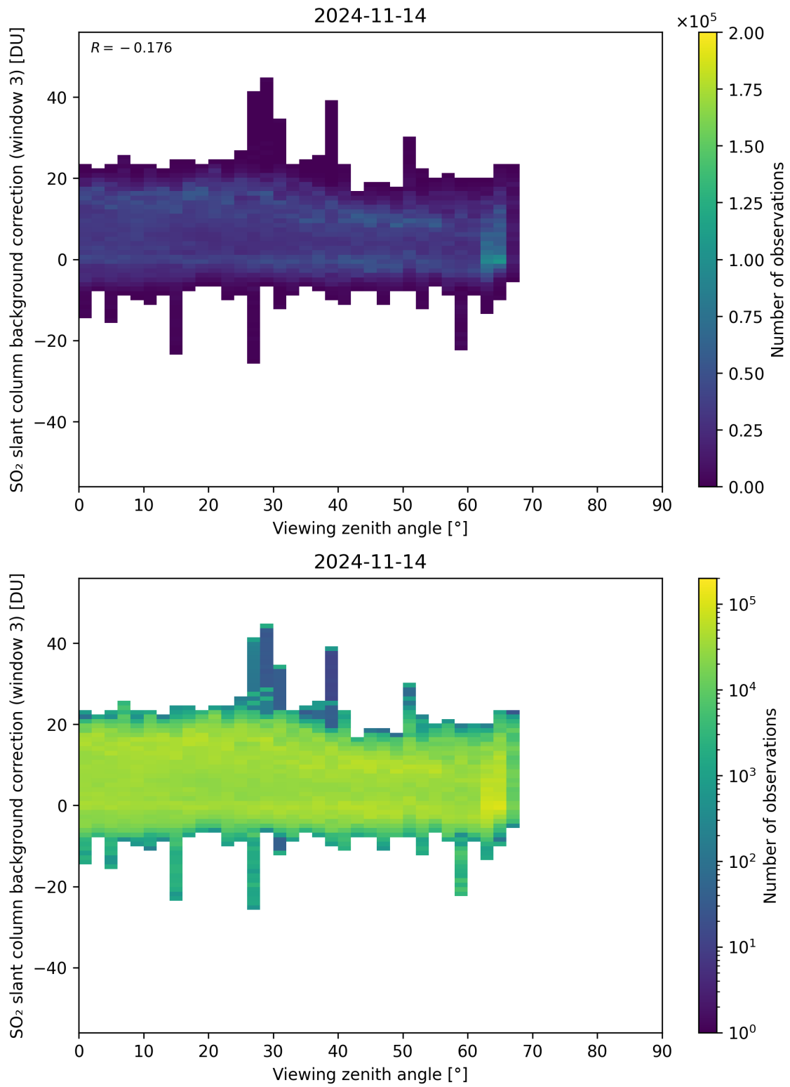
Figure 310: Scatter density plot of “Viewing zenith angle” against “SO 2 slant column background correction (window 3)” for 2024-11-14 to 2024-11-15.
