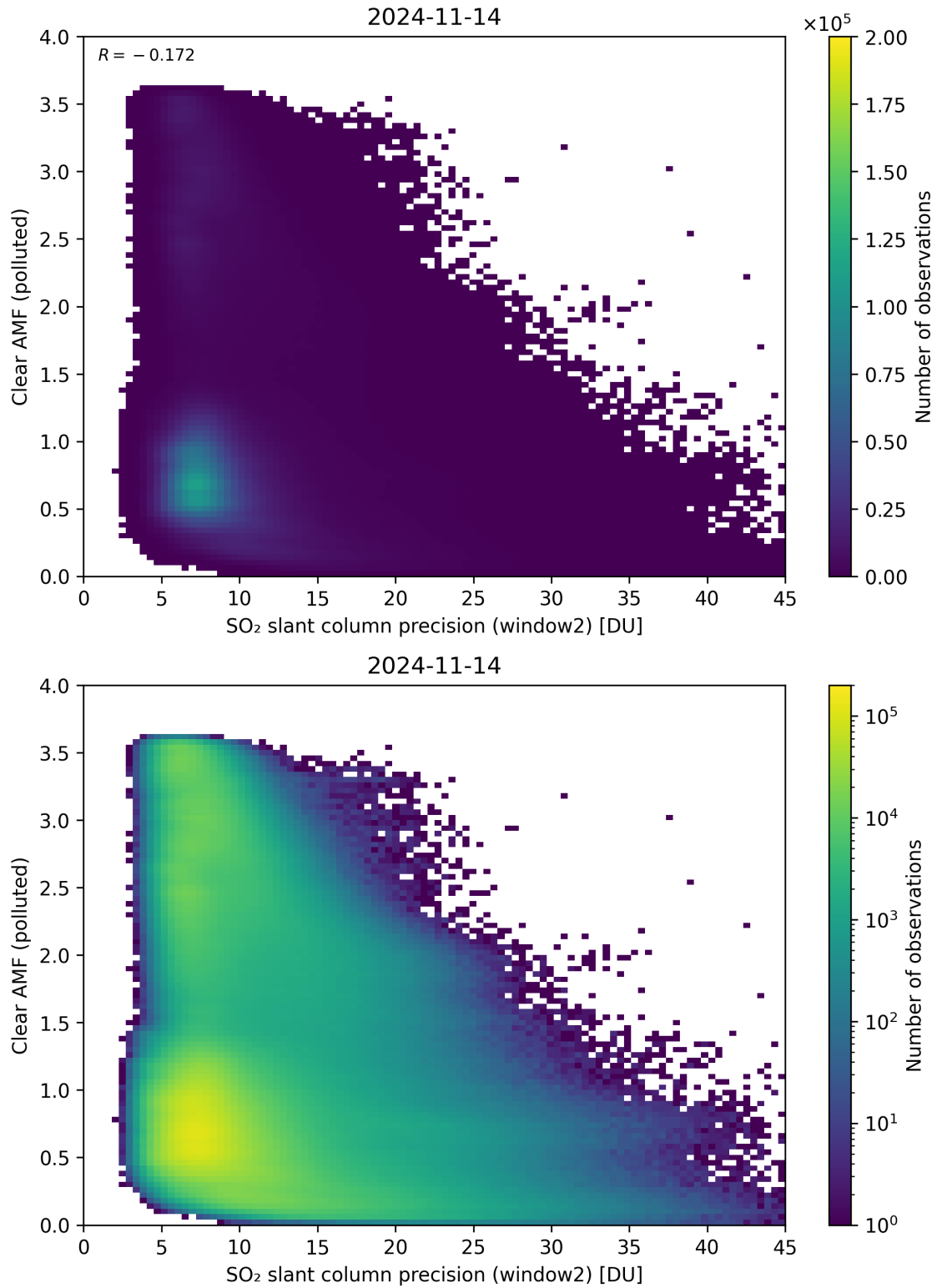
Figure 246: Scatter density plot of “SO 2 slant column precision (window2)” against “Clear AMF (polluted)” for 2024-11-14 to 2024-11-15.
