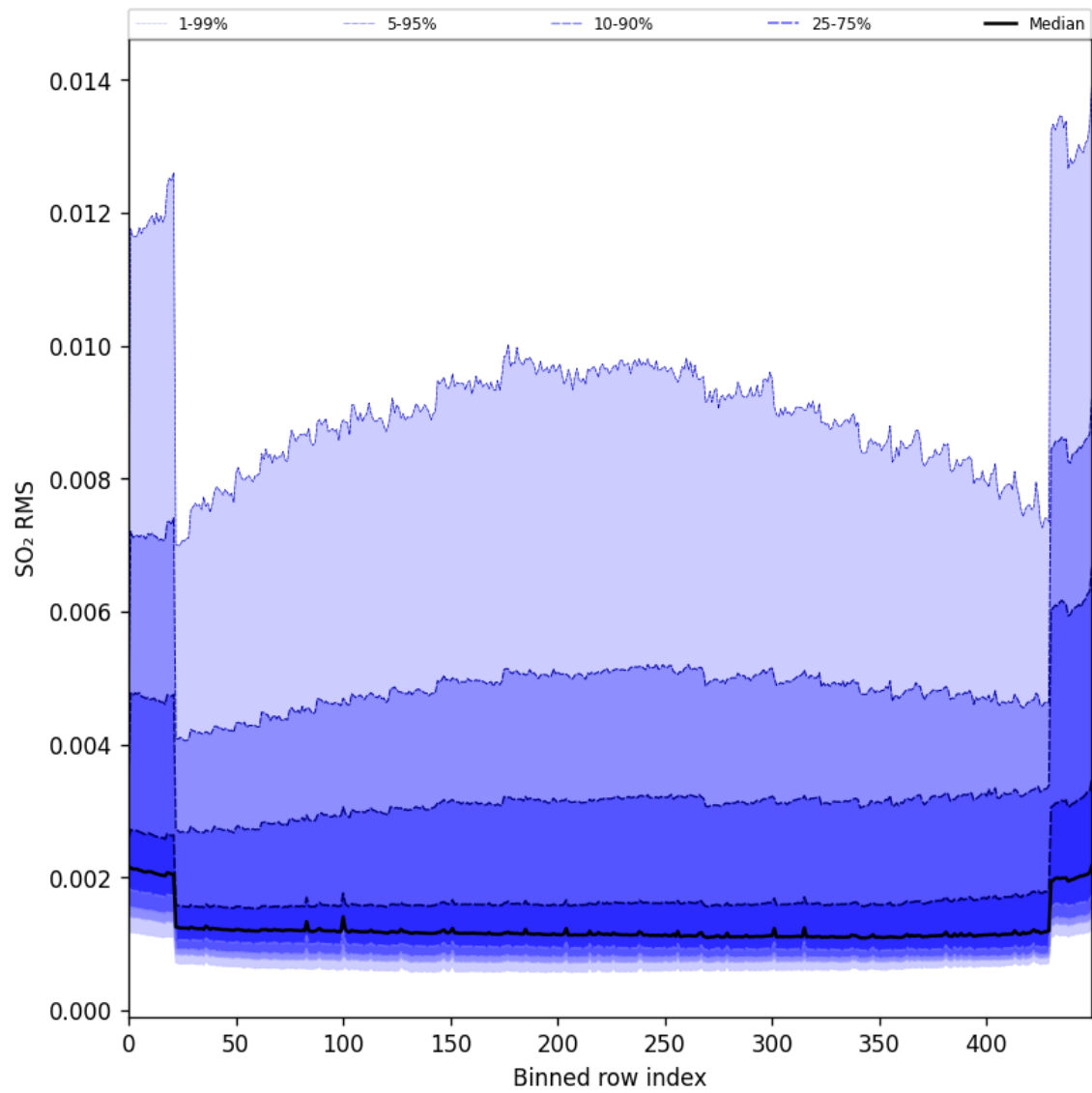
Figure 93: Along track statistics of “SO 2 RMS” for 2024-11-14 to 2024-11-15
