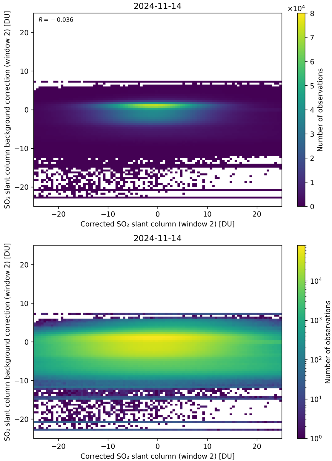
Figure 194: Scatter density plot of “Corrected SO 2 slant column (window 2)” against “SO 2 slant column background correction (window 2)” for 2024-11-14 to 2024-11-15.
