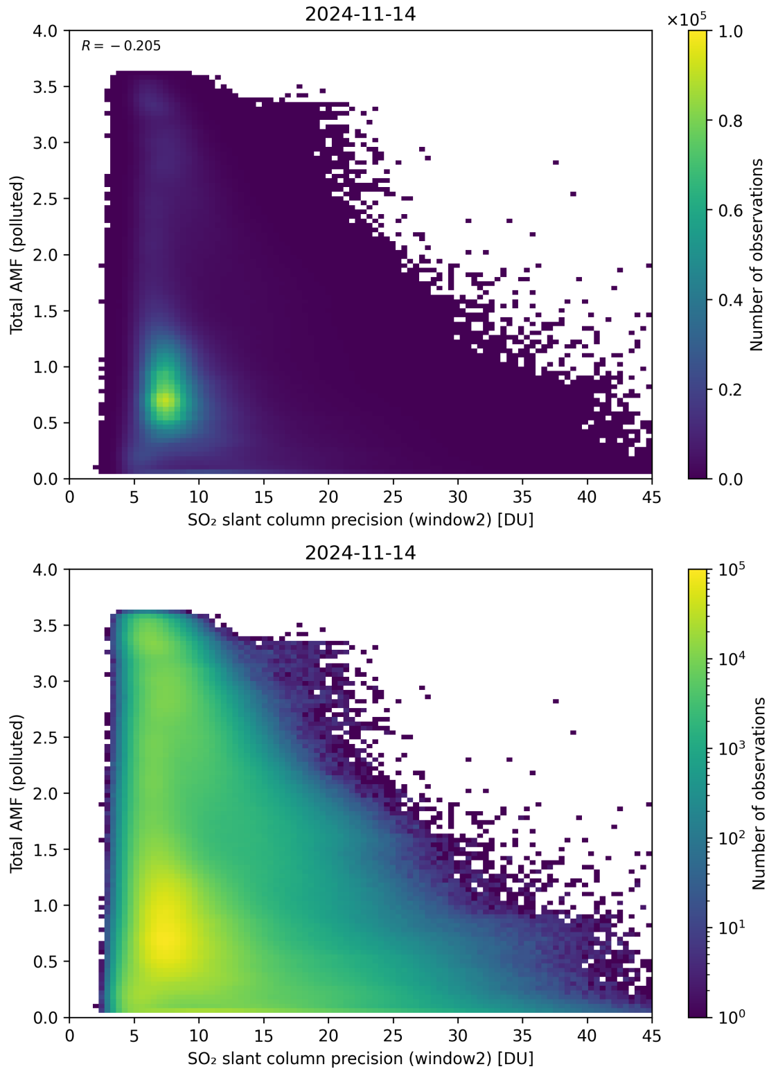
Figure 251: Scatter density plot of “SO 2 slant column precision (window2)” against “Total AMF (polluted)” for 2024-11-14 to 2024-11-15.
