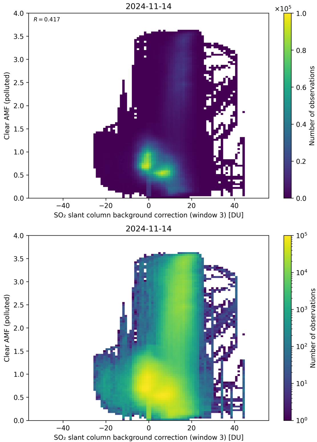
Figure 124: Scatter density plot of “SO 2 slant column background correction (window 3)” against “Clear AMF (polluted)” for 2024-11-14 to 2024-11-15.
