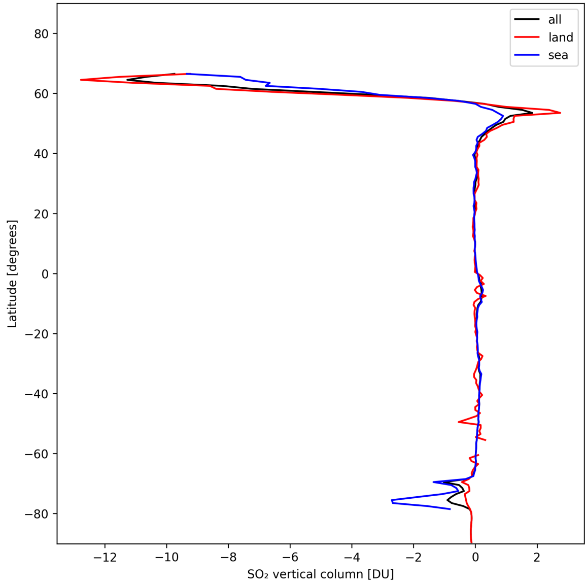
Figure 30: Zonal average of “SO 2 vertical column” for 2024-11-14 to 2024-11-15.
