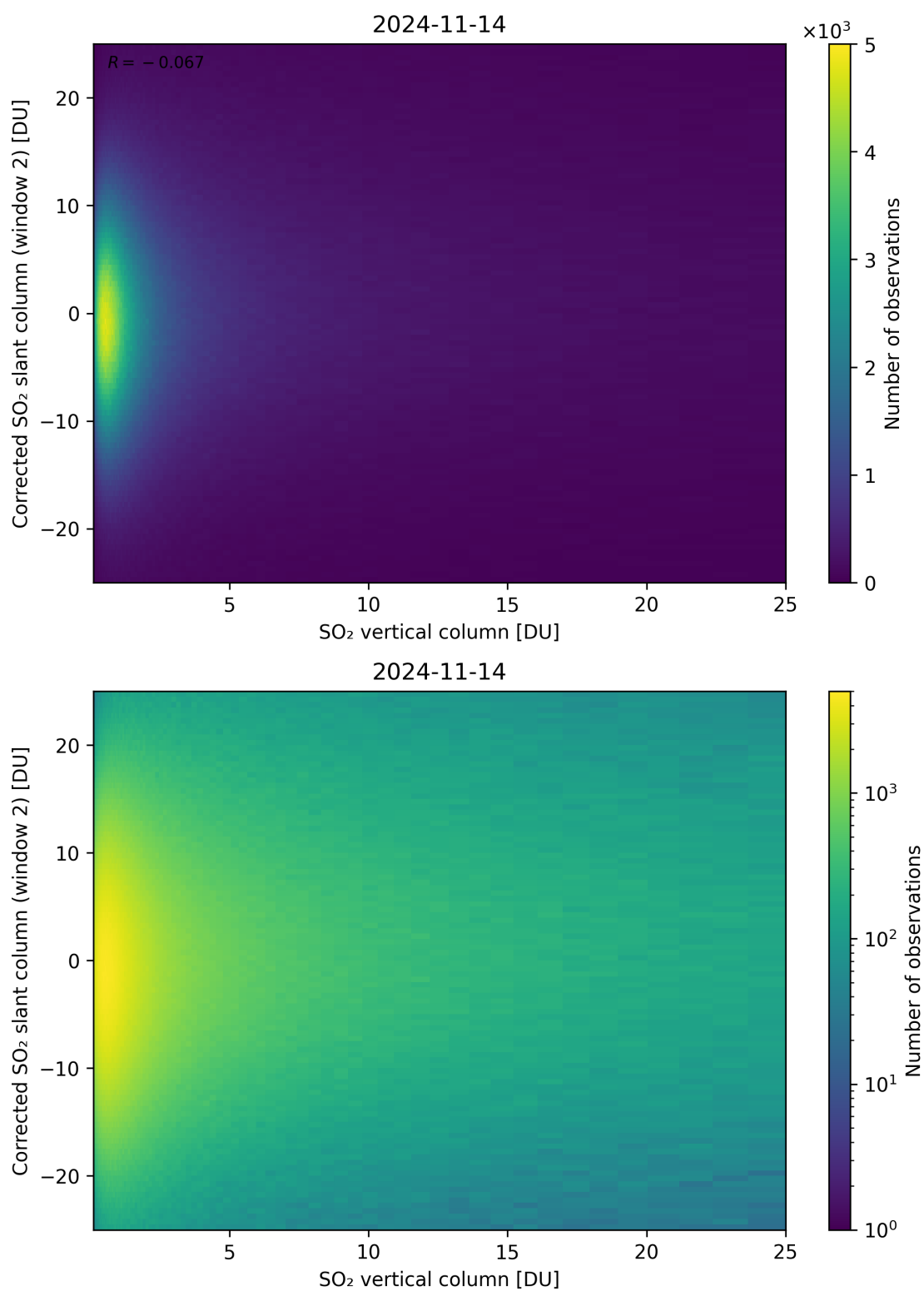
Figure 298: Scatter density plot of “SO 2 vertical column” against “Corrected SO 2 slant column (window 2)” for 2024-11-14 to 2024-11-15.
