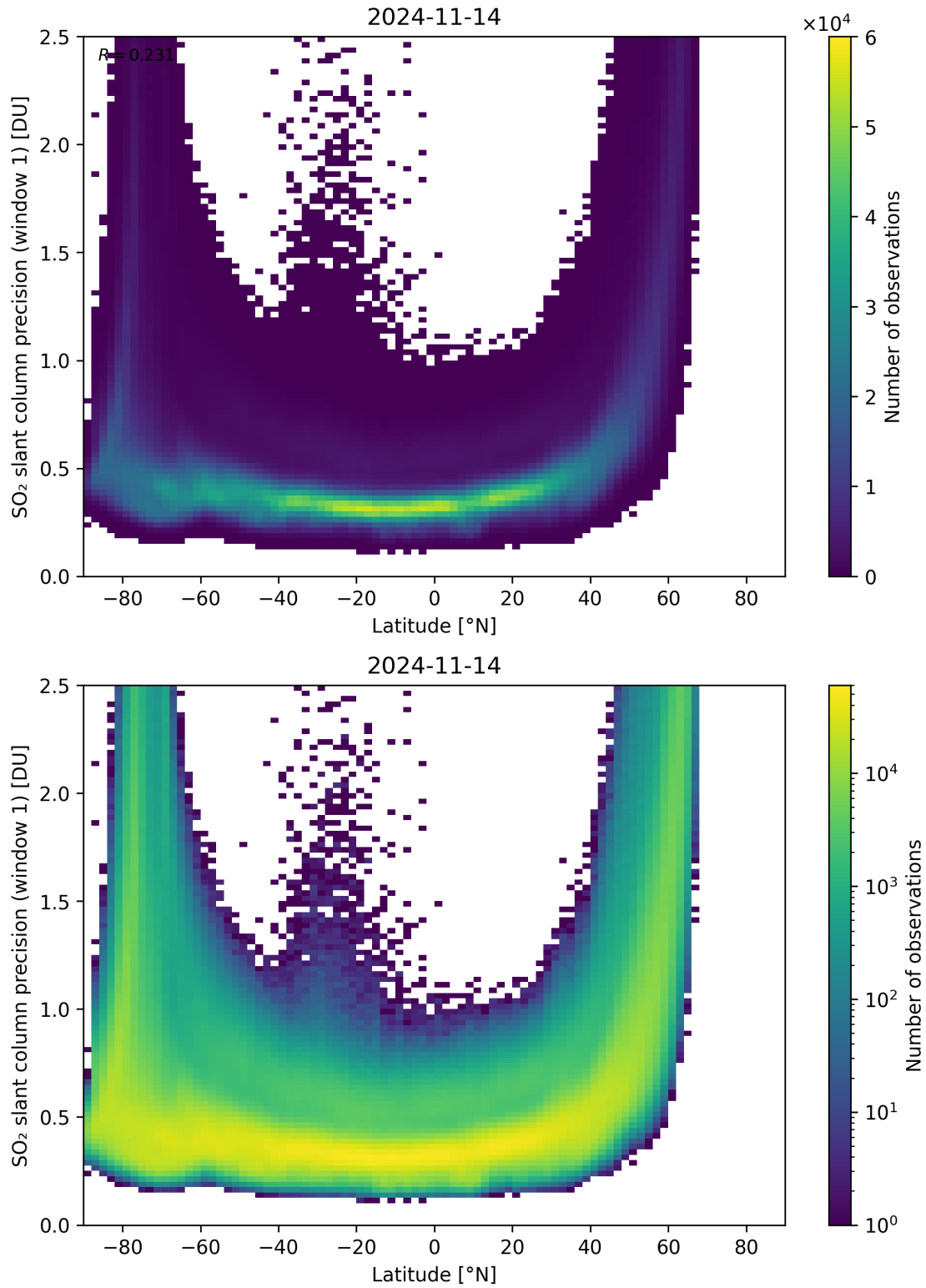
Figure 150: Scatter density plot of “Latitude” against “SO 2 slant column precision (window 1)” for 2024-11-14 to 2024-11-15.
