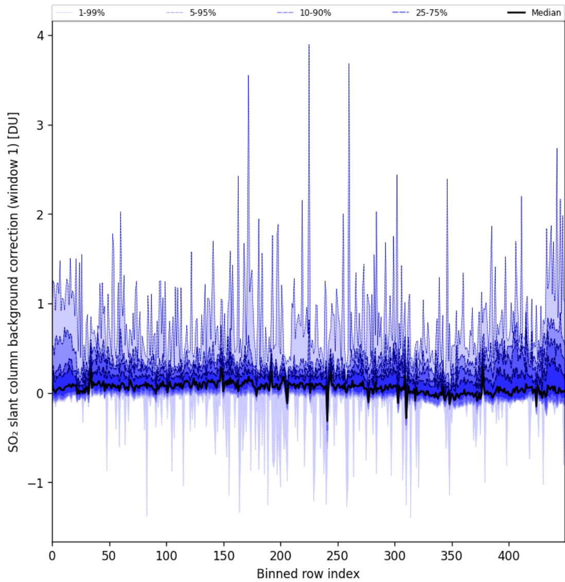
Figure 82: Along track statistics of “SO 2 slant column background correction (window 1)” for 2024-11-14 to 2024-11-15
