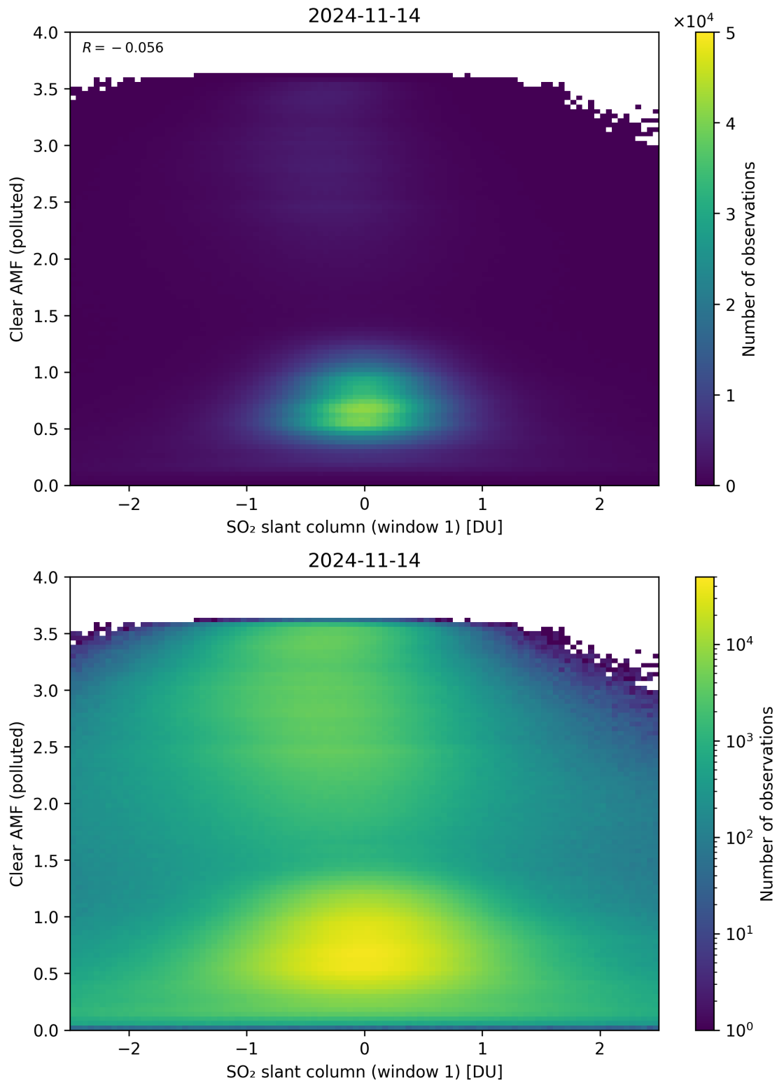
Figure 232: Scatter density plot of “SO 2 slant column (window 1)” against “Clear AMF (polluted)” for 2024-11-14 to 2024-11-15.
