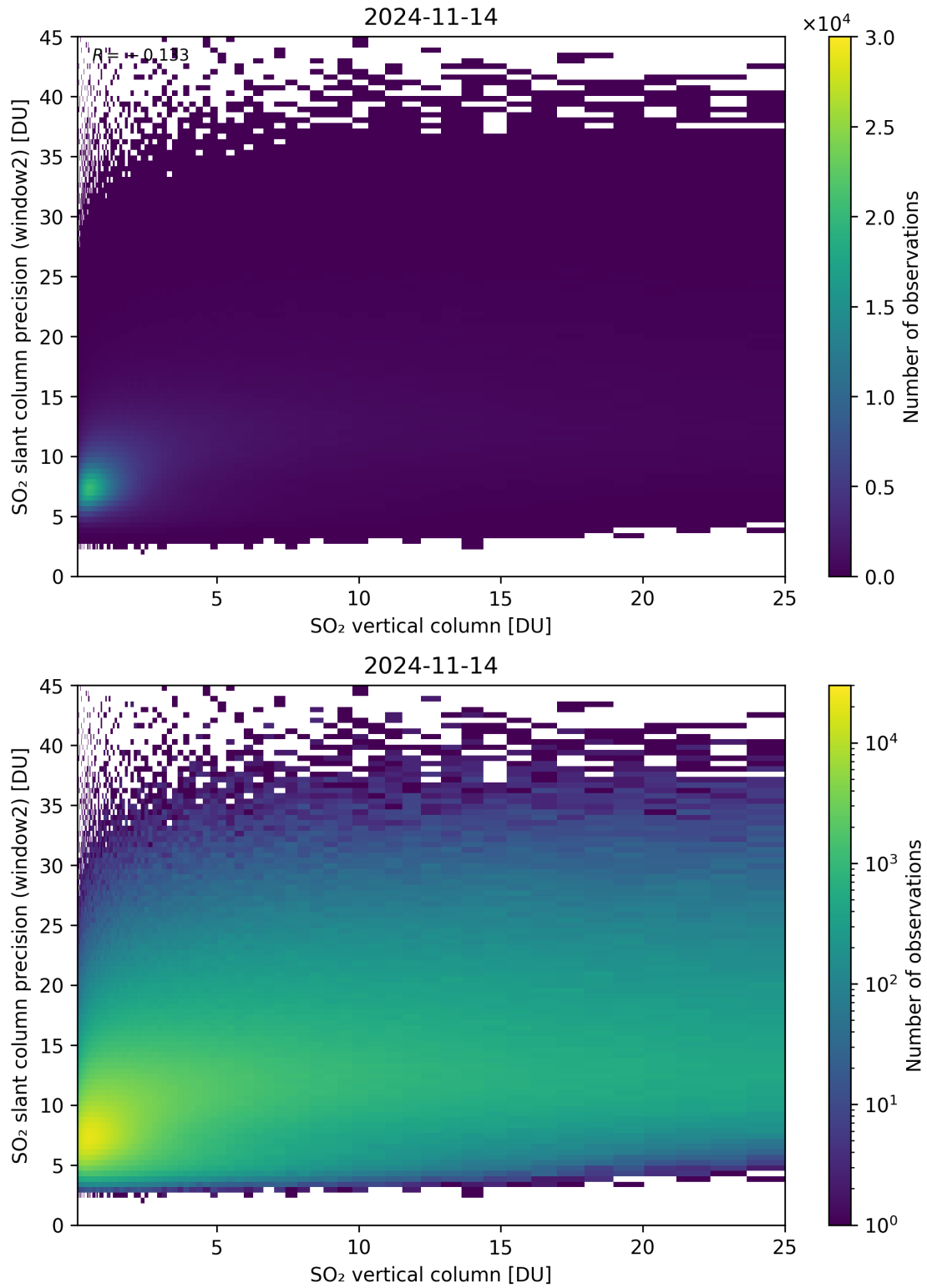
Figure 302: Scatter density plot of “SO 2 vertical column” against “SO 2 slant column precision (window2)” for 2024-11-14 to 2024-11-15.
