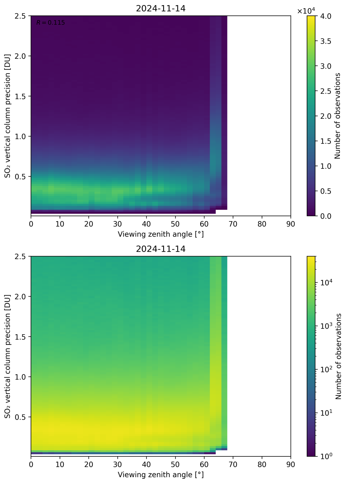
Figure 328: Scatter density plot of “Viewing zenith angle” against “SO 2 vertical column precision” for 2024-11-14 to 2024-11-15.
