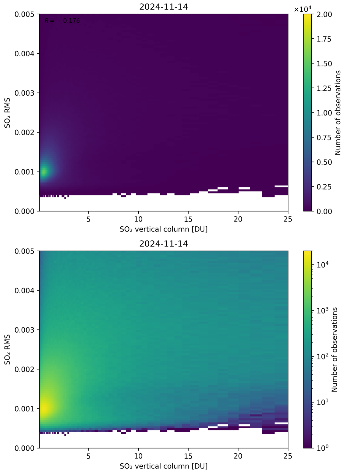
Figure 278: Scatter density plot of “SO 2 vertical column” against “SO 2 RMS” for 2024-11-14 to 2024-11-15.
