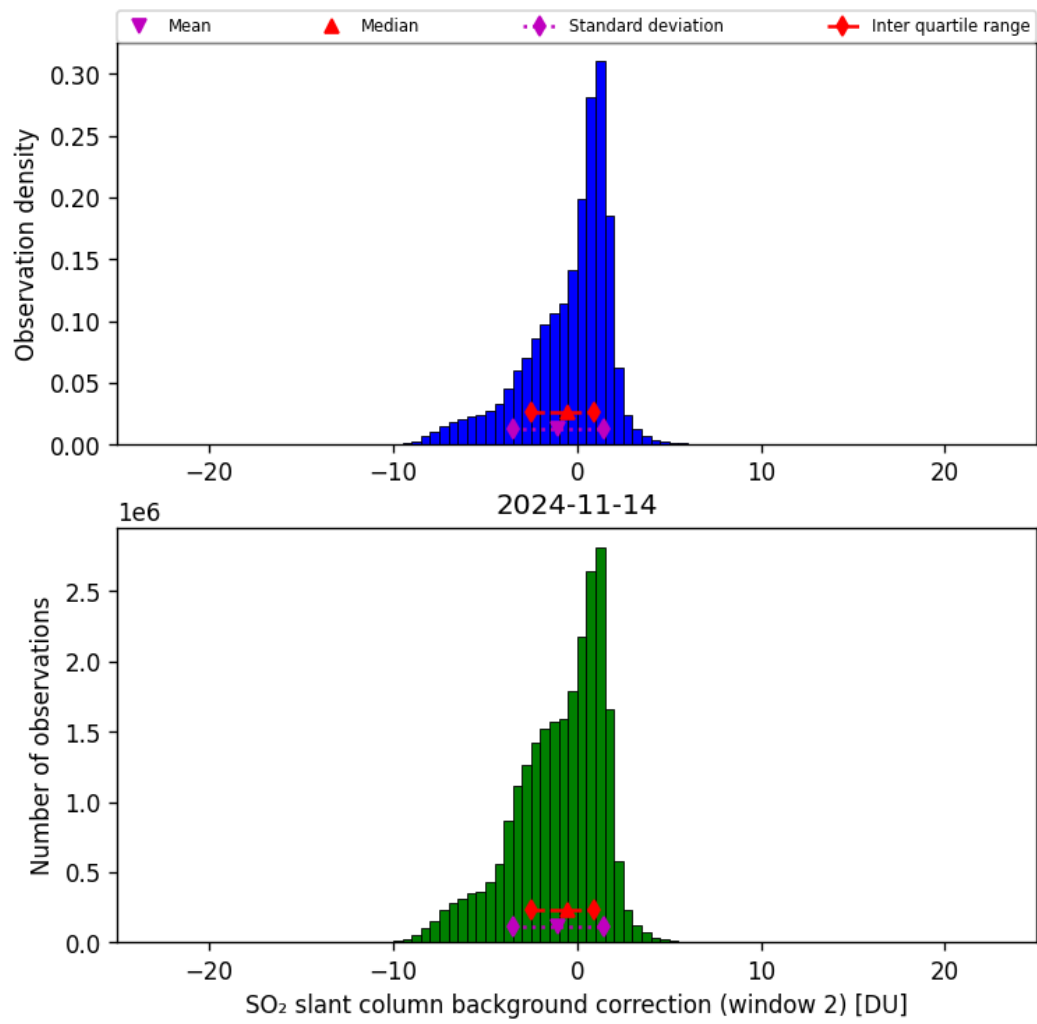
Figure 63: Histogram of “SO 2 slant column background correction (window 2)” for 2024-11-14 to 2024-11-15
