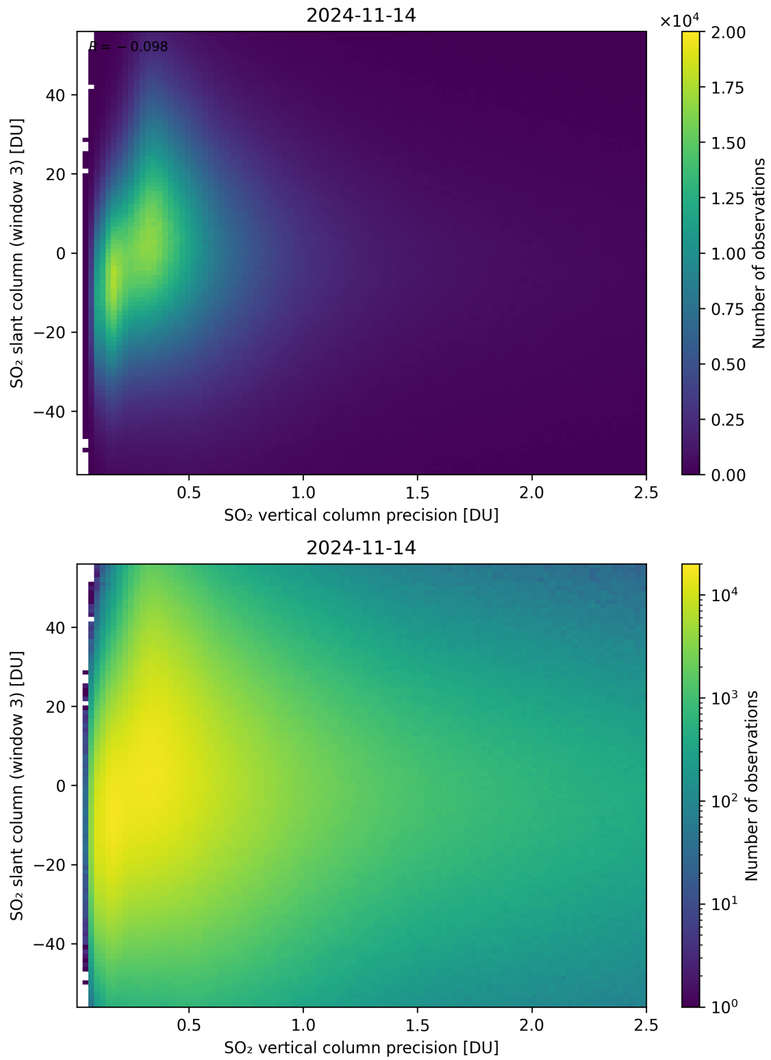
Figure 292: Scatter density plot of “SO 2 vertical column precision” against “SO 2 slant column (window 3)” for 2024-11-14 to 2024-11-15.
