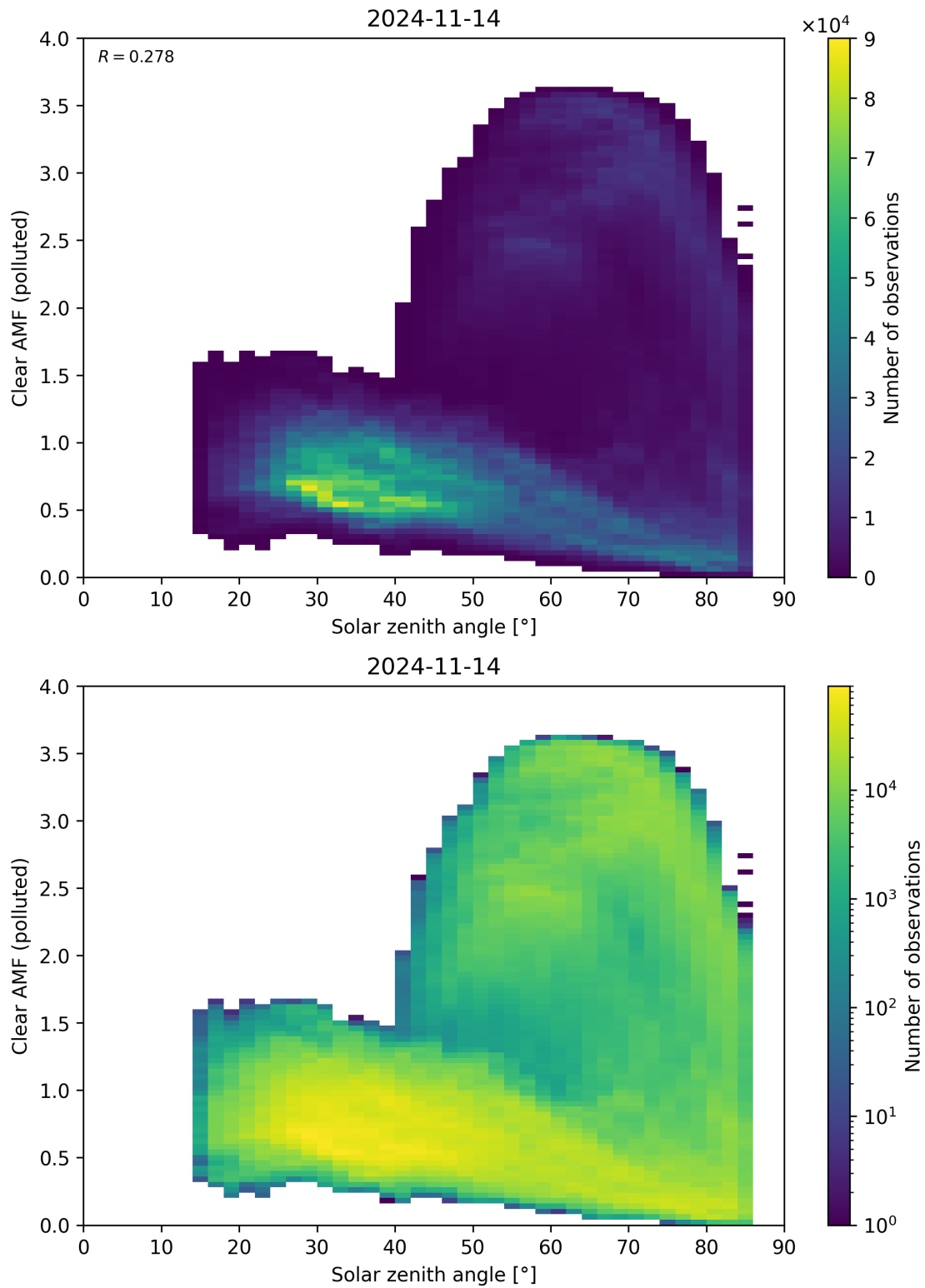
Figure 165: Scatter density plot of “Solar zenith angle” against “Clear AMF (polluted)” for 2024-11-14 to 2024-11-15.
