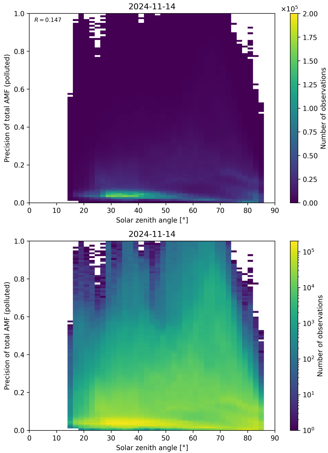
Figure 175: Scatter density plot of “Solar zenith angle” against “Precision of total AMF (polluted)” for 2024-11-14 to 2024-11-15.
