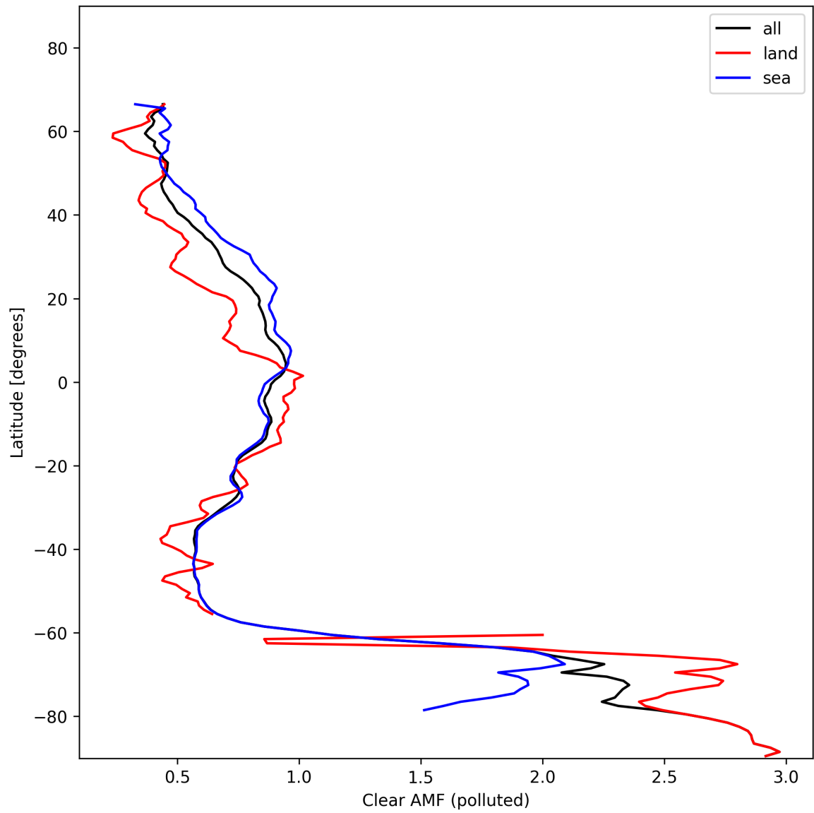
Figure 50: Zonal average of “Clear AMF (polluted)” for 2024-11-14 to 2024-11-15.
