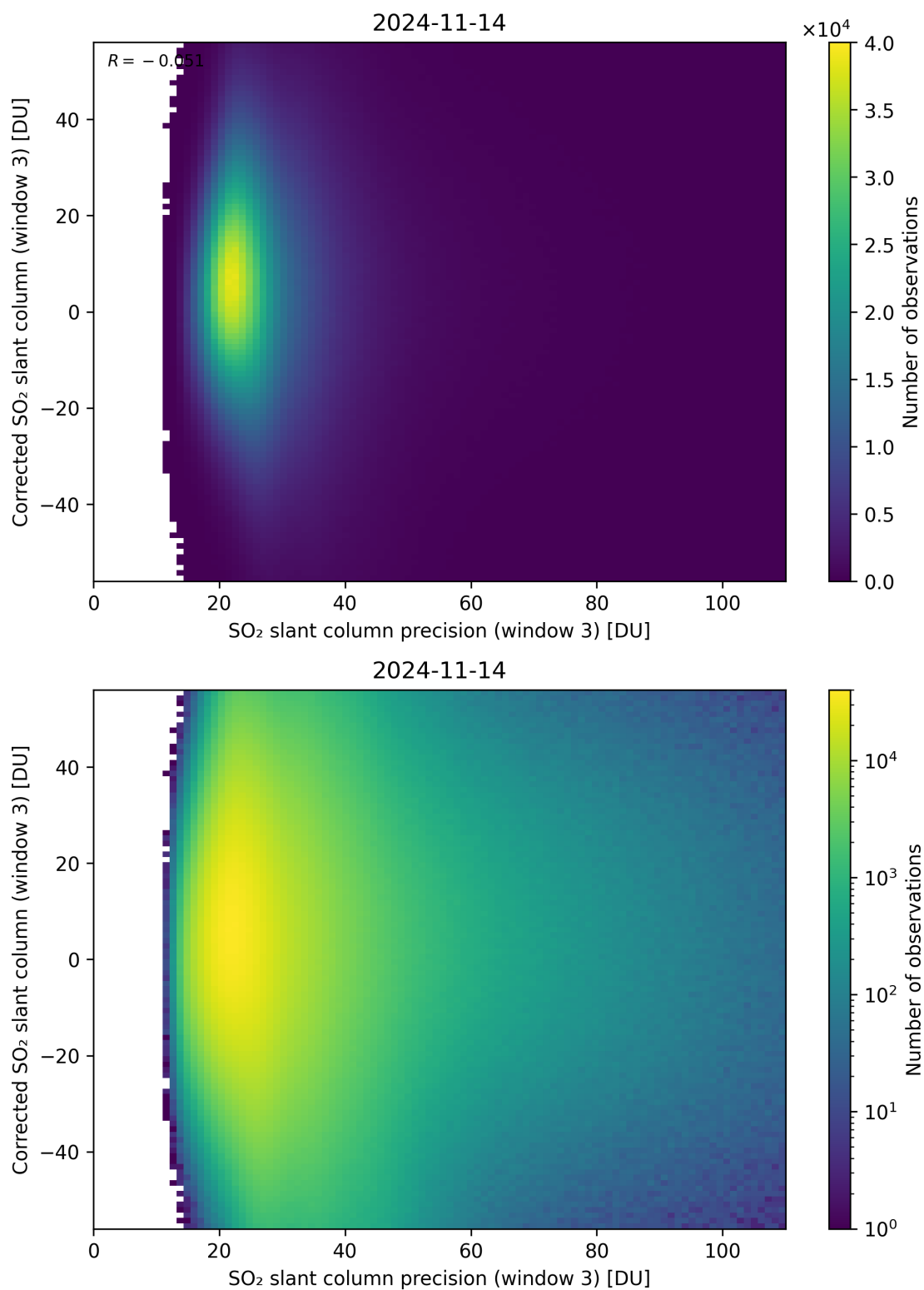
Figure 262: Scatter density plot of “SO 2 slant column precision (window 3)” against “Corrected SO 2 slant column (window 3)” for 2024-11-14 to 2024-11-15.
