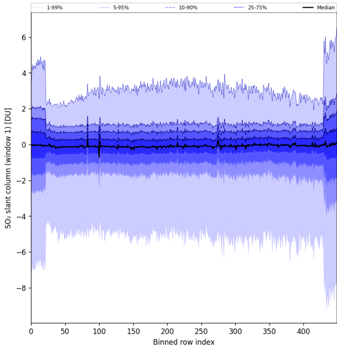
Figure 79: Along track statistics of “SO 2 slant column (window 1)” for 2024-11-14 to 2024-11-15
