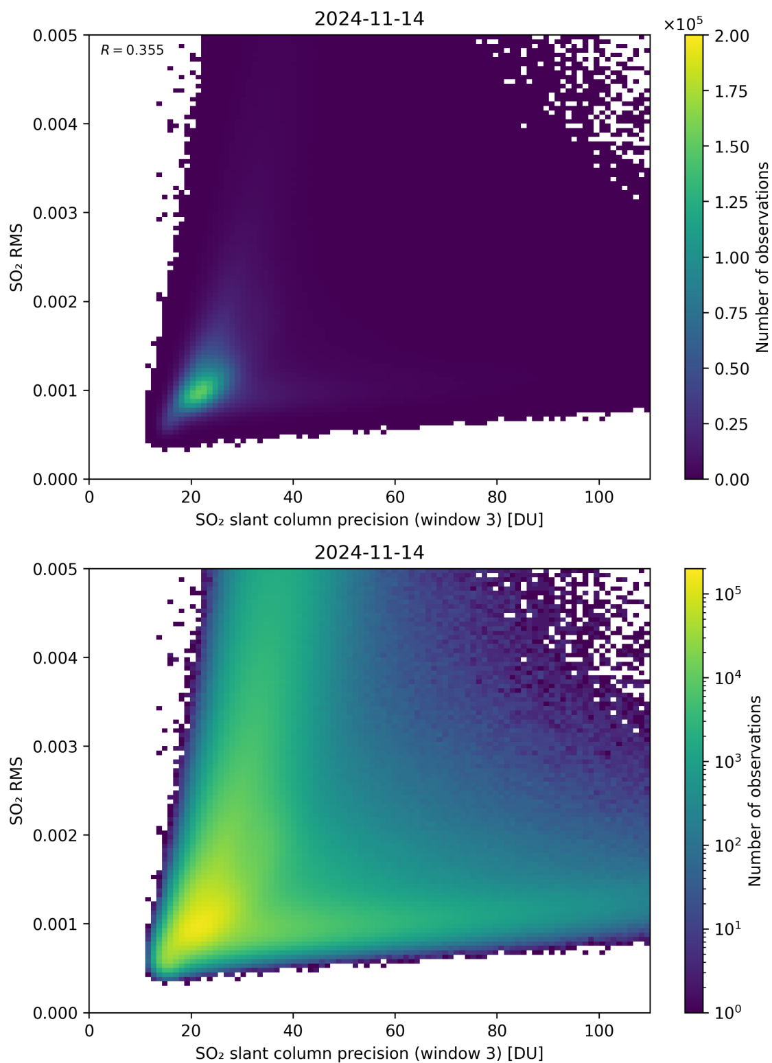
Figure 260: Scatter density plot of “SO 2 slant column precision (window 3)” against “SO 2 RMS” for 2024-11-14 to 2024-11-15.
