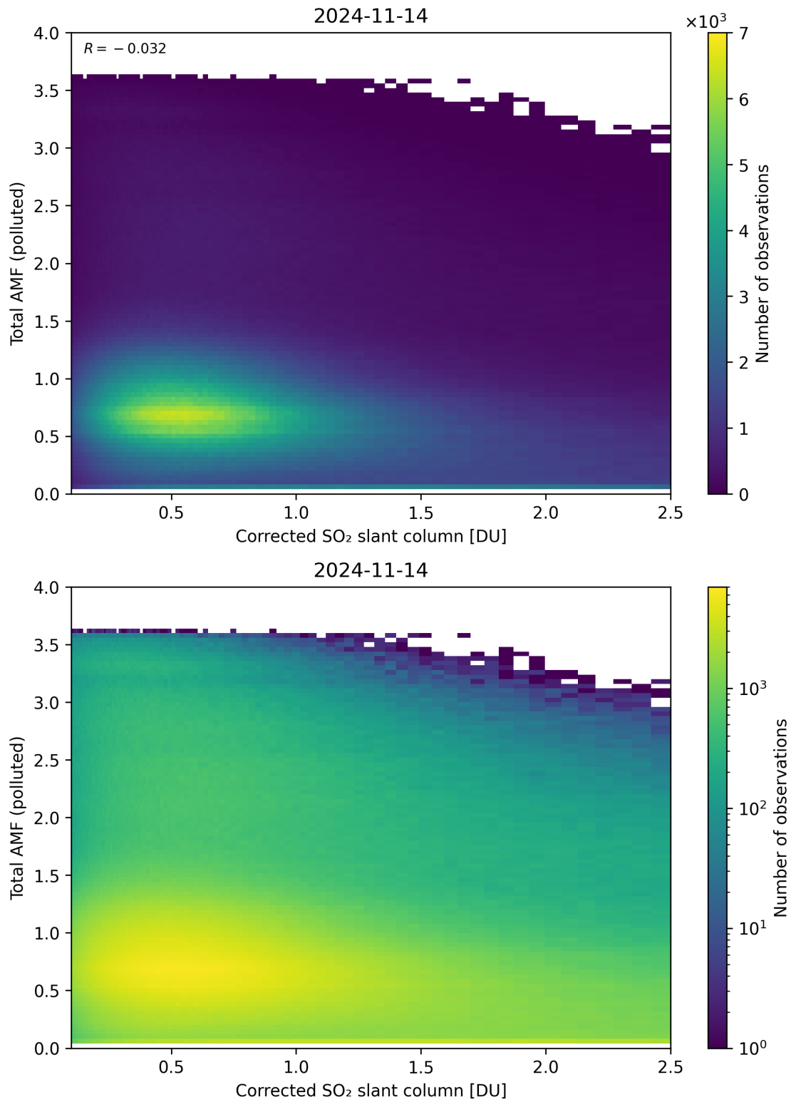
Figure 192: Scatter density plot of “Corrected SO 2 slant column” against “Total AMF (polluted)” for 2024-11-14 to 2024-11-15.
