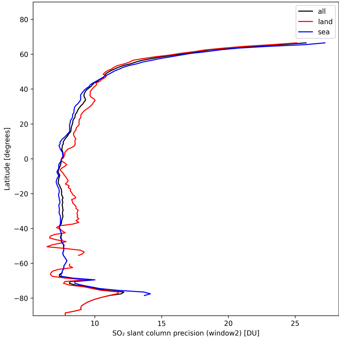
Figure 38: Zonal average of “SO 2 slant column precision (window2)” for 2024-11-14 to 2024-11-15.
