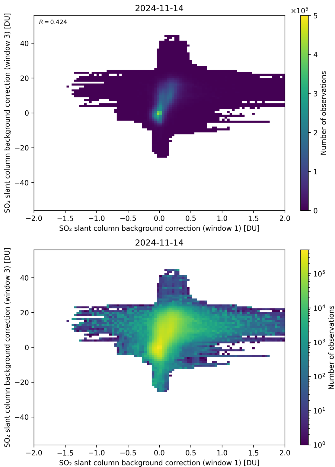
Figure 99: Scatter density plot of “SO 2 slant column background correction (window 1)” against “SO 2 slant column background correction (window 3)” for 2024-11-14 to 2024-11-15.
