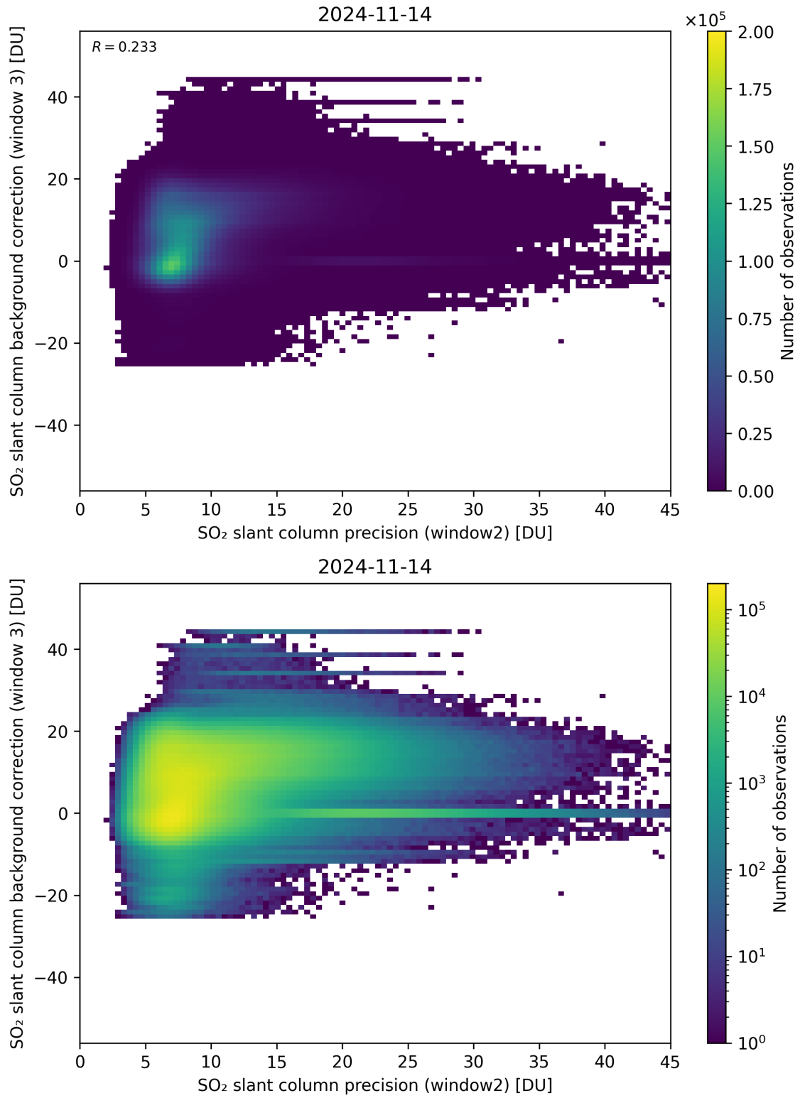
Figure 242: Scatter density plot of “SO 2 slant column precision (window2)” against “SO 2 slant column background correction (window 3)” for 2024-11-14 to 2024-11-15.
