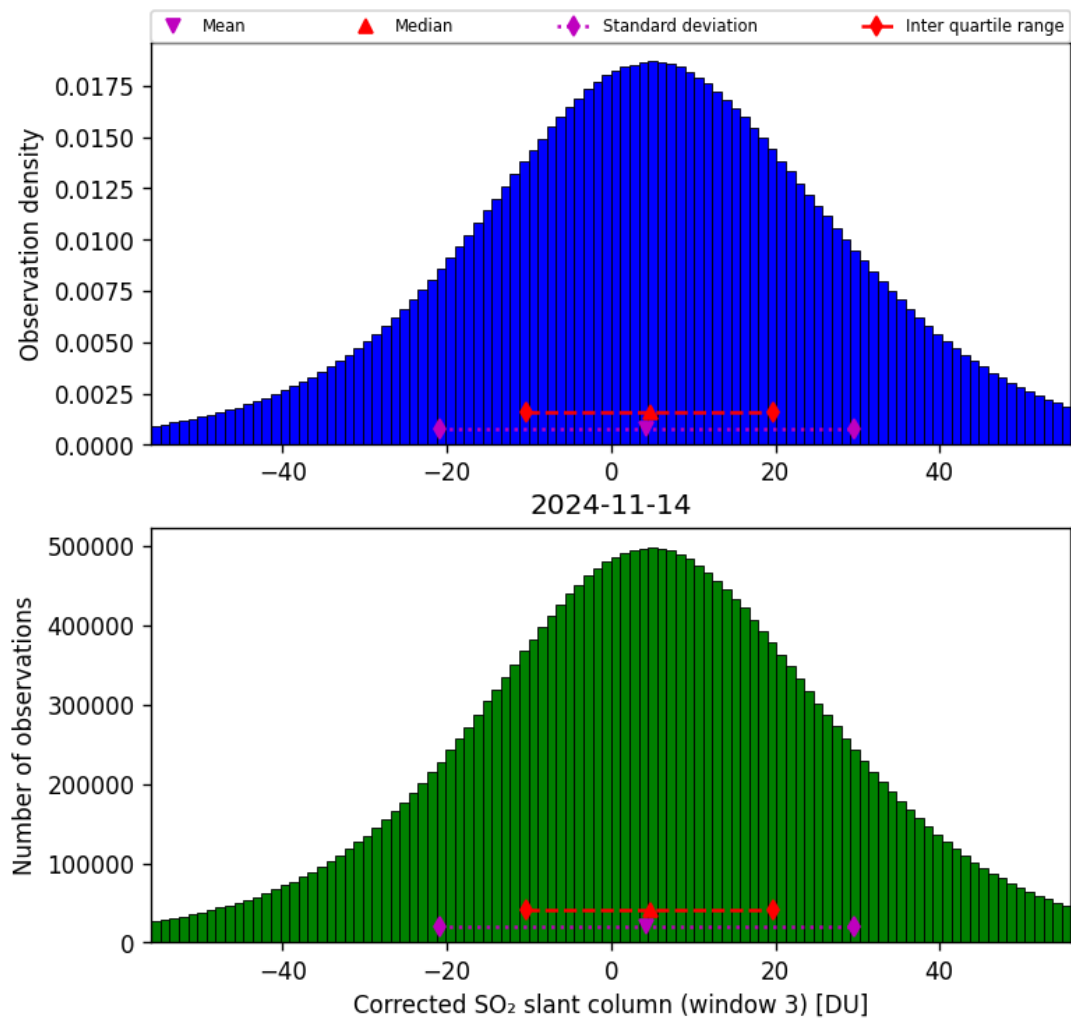
Figure 66: Histogram of “Corrected SO 2 slant column (window 3)” for 2024-11-14 to 2024-11-15
