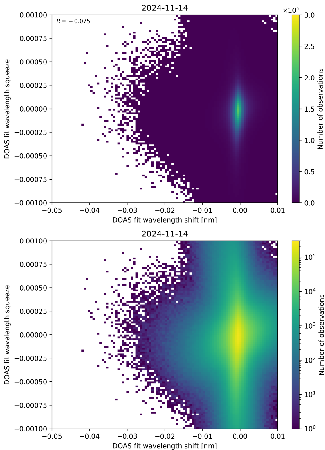
Figure 127: Scatter density plot of “DOAS fit wavelength shift” against “DOAS fit wavelength squeeze” for 2024-11-14 to 2024-11-15.
