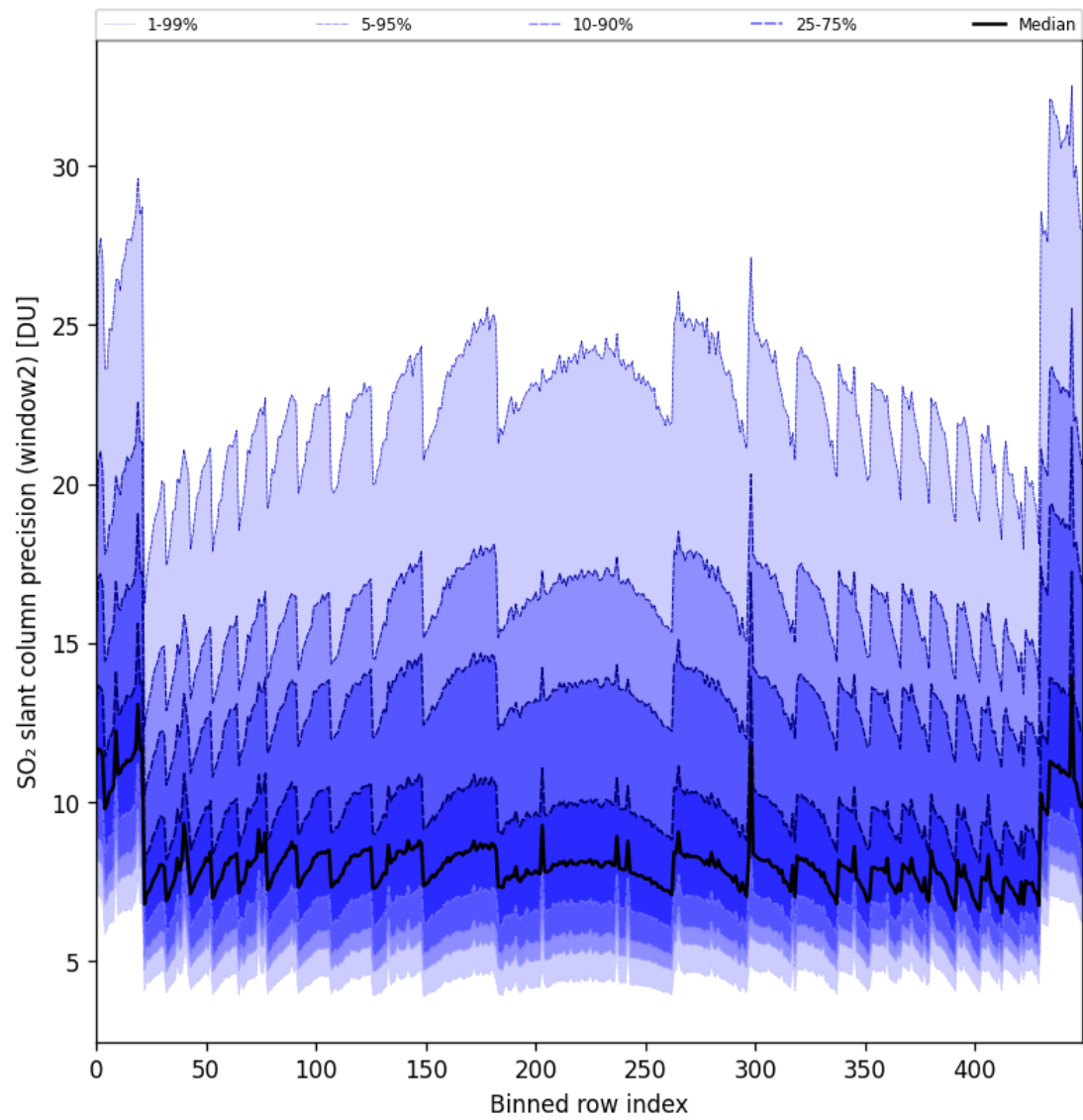
Figure 84: Along track statistics of “SO 2 slant column precision (window2)” for 2024-11-14 to 2024-11-15
