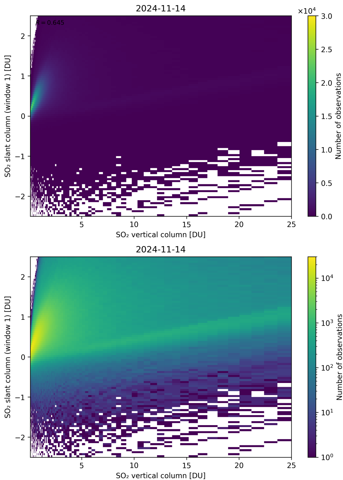
Figure 300: Scatter density plot of “SO 2 vertical column” against “SO 2 slant column (window 1)” for 2024-11-14 to 2024-11-15.
