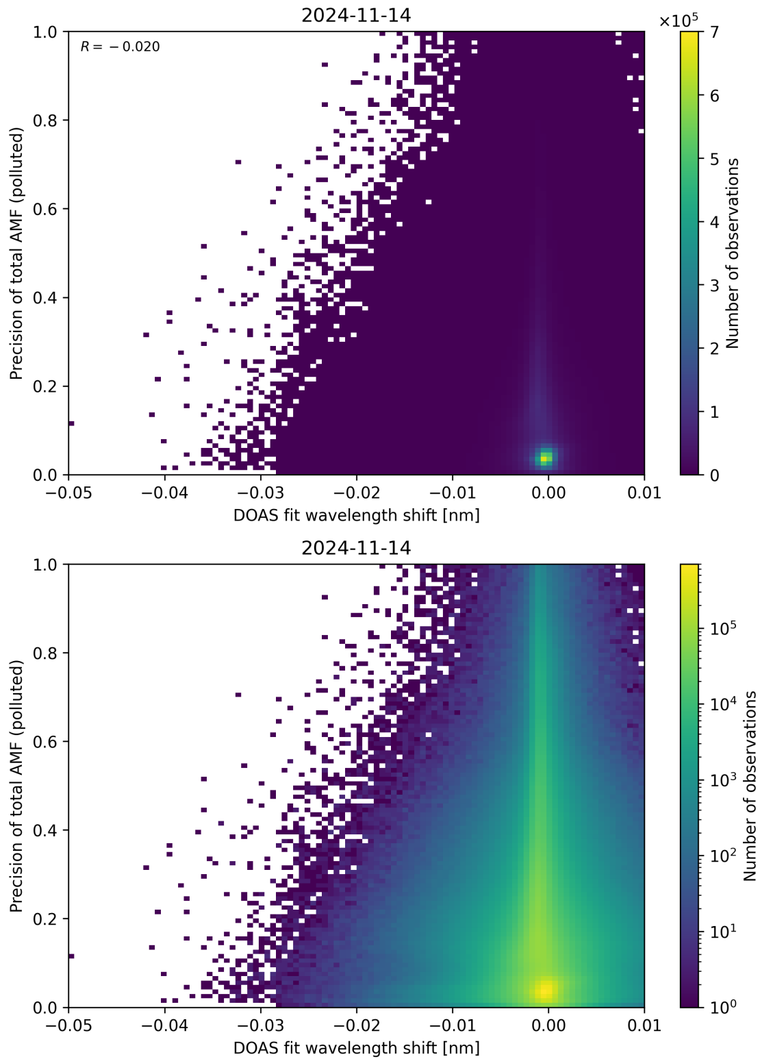
Figure 131: Scatter density plot of “DOAS fit wavelength shift” against “Precision of total AMF (polluted)” for 2024-11-14 to 2024-11-15.
