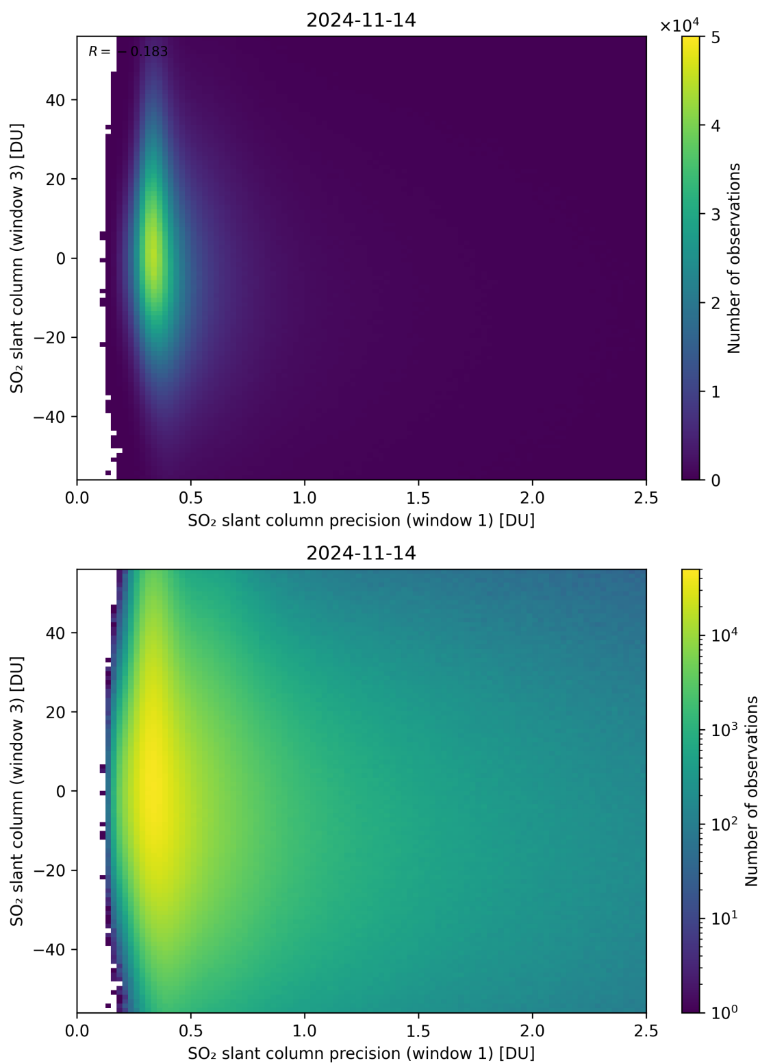
Figure 228: Scatter density plot of “SO 2 slant column precision (window 1)” against “SO 2 slant column (window 3)” for 2024-11-14 to 2024-11-15.
