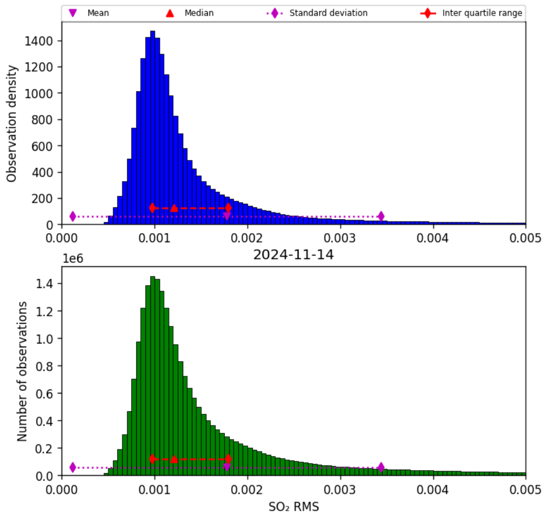
Figure 70: Histogram of “SO 2 RMS” for 2024-11-14 to 2024-11-15
