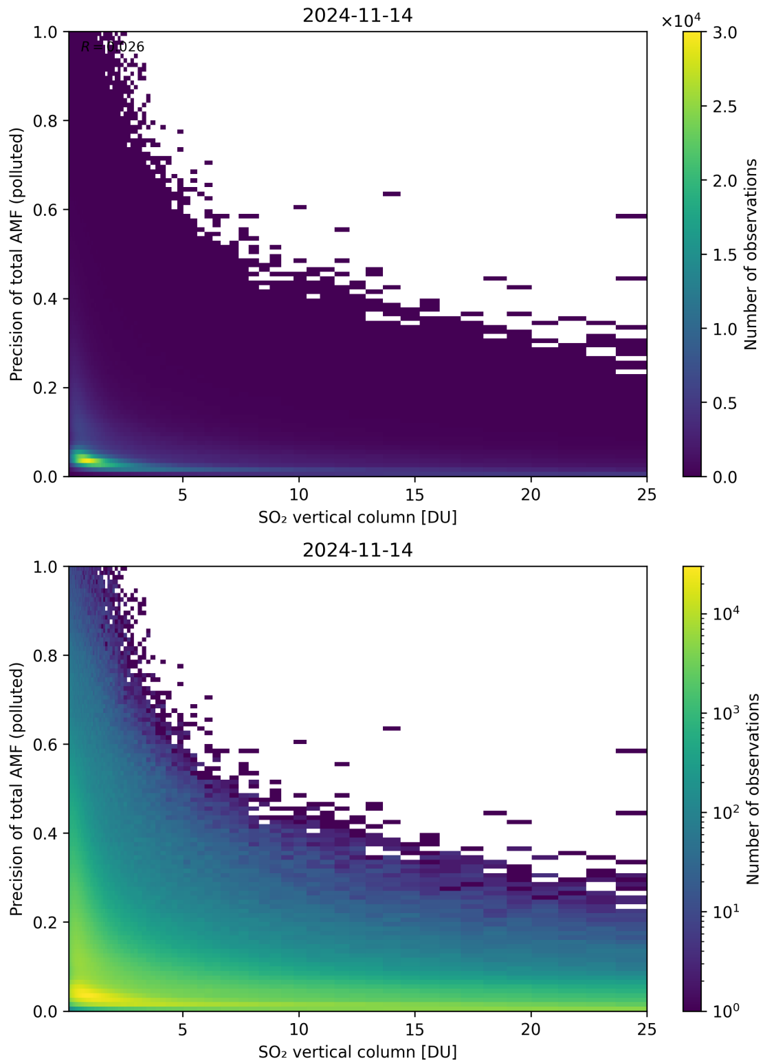
Figure 306: Scatter density plot of “SO 2 vertical column” against “Precision of total AMF (polluted)” for 2024-11-14 to 2024-11-15.
