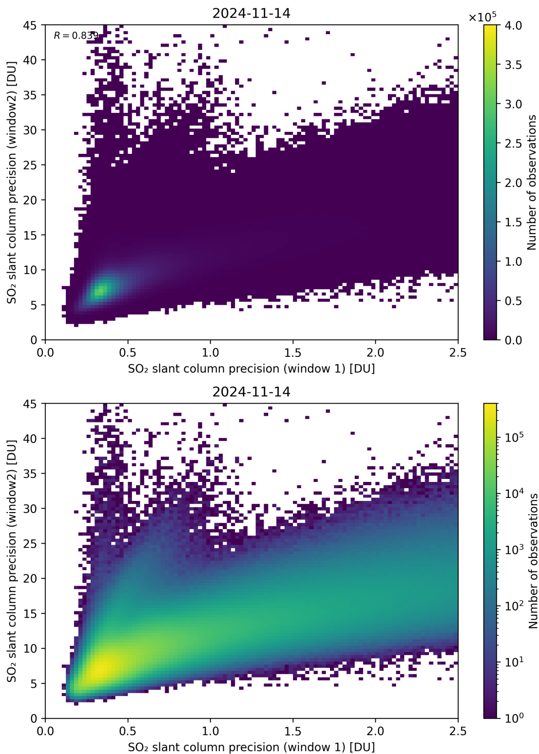
Figure 227: Scatter density plot of “SO 2 slant column precision (window 1)” against “SO 2 slant column precision (window2)” for 2024-11-14 to 2024-11-15.
