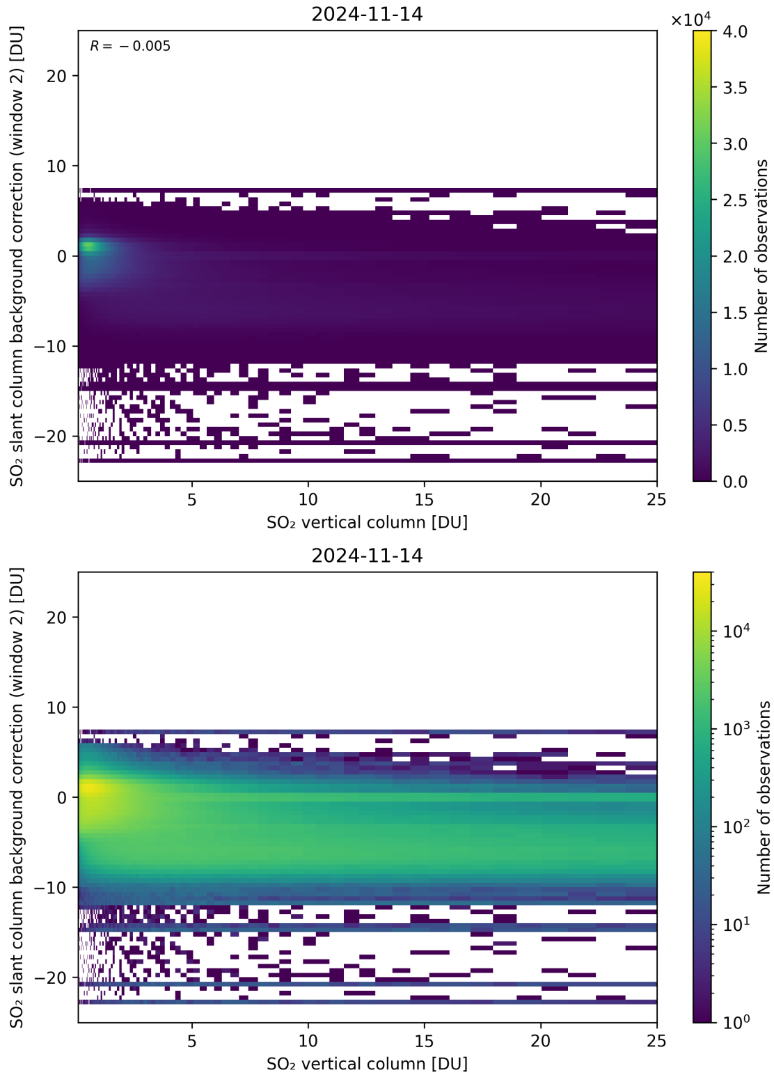
Figure 274: Scatter density plot of “SO 2 vertical column” against “SO 2 slant column background correction (window 2)” for 2024-11-14 to 2024-11-15.
