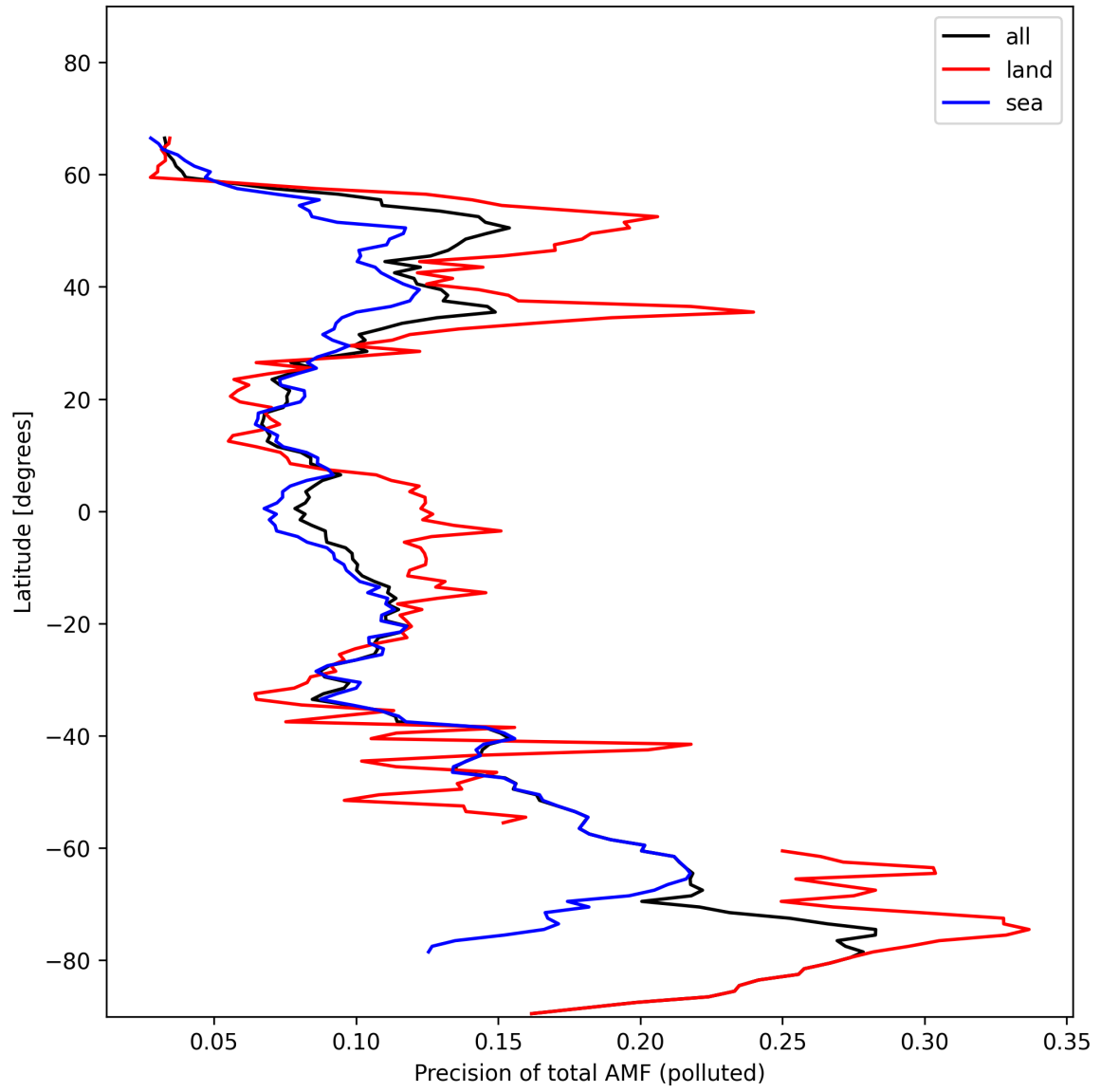
Figure 49: Zonal average of “Precision of total AMF (polluted)” for 2024-11-14 to 2024-11-15.
