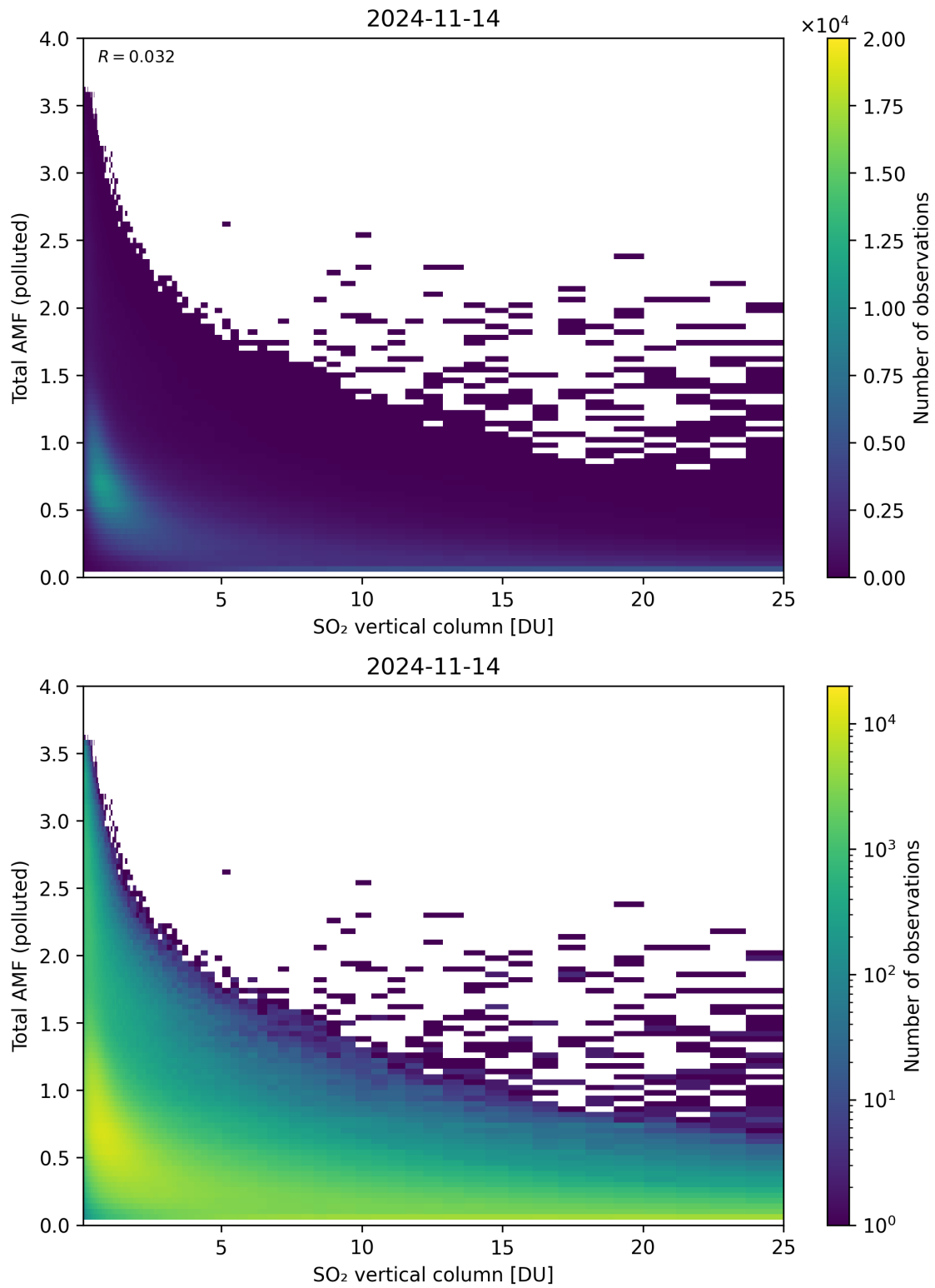
Figure 305: Scatter density plot of “SO 2 vertical column” against “Total AMF (polluted)” for 2024-11-14 to 2024-11-15.
