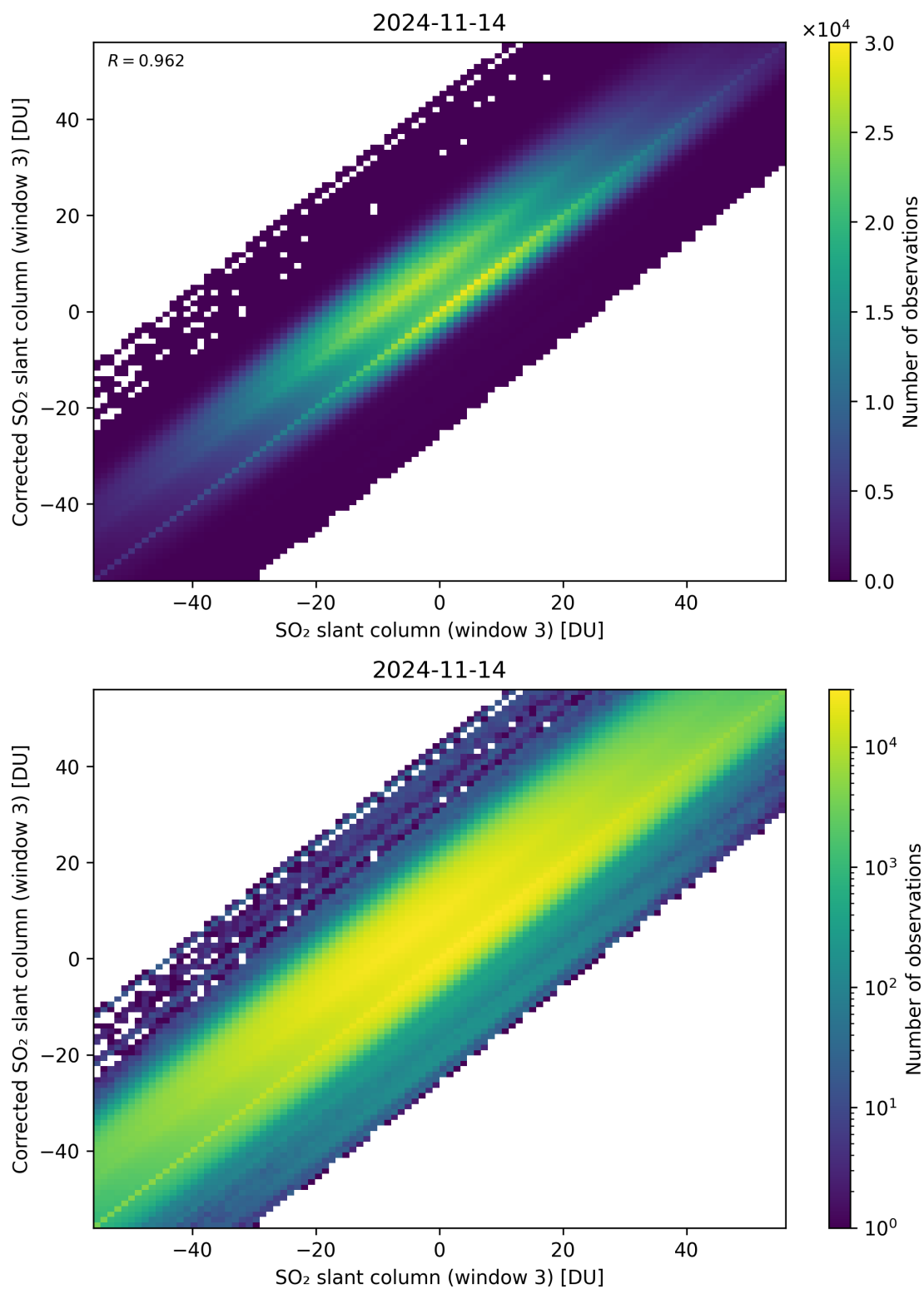
Figure 266: Scatter density plot of “SO 2 slant column (window 3)” against “Corrected SO 2 slant column (window 3)” for 2024-11-14 to 2024-11-15.
