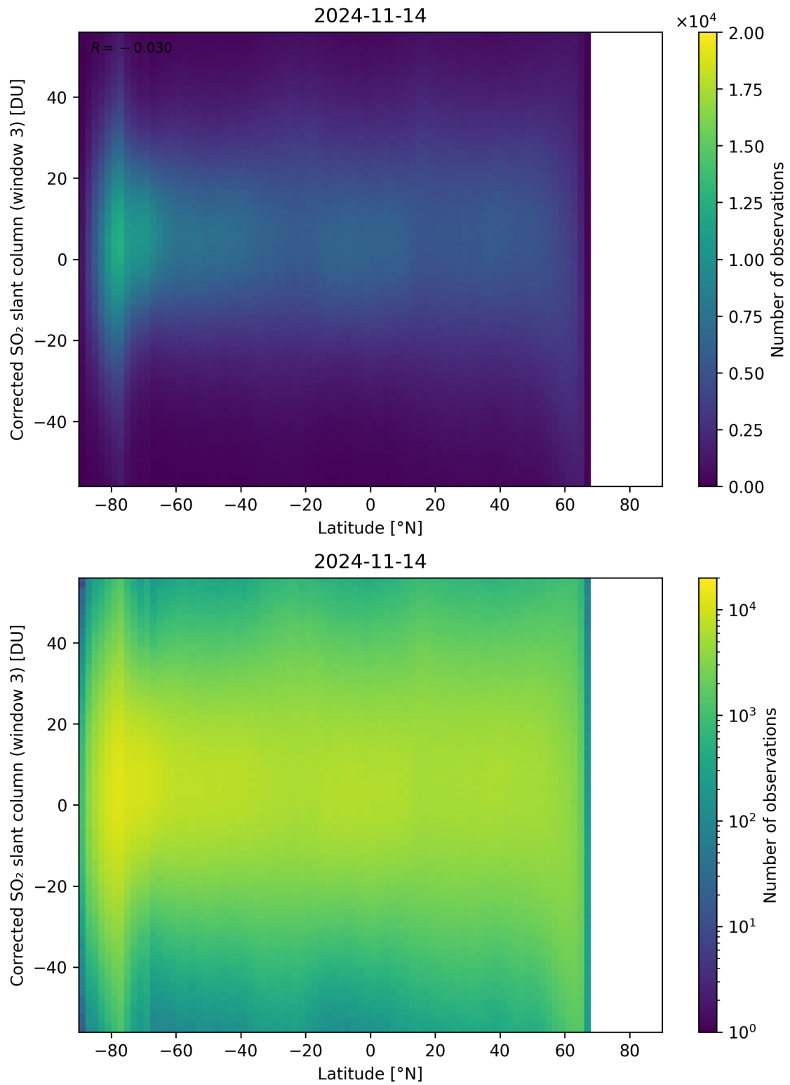
Figure 148: Scatter density plot of “Latitude” against “Corrected SO 2 slant column (window 3)” for 2024-11-14 to 2024-11-15.
