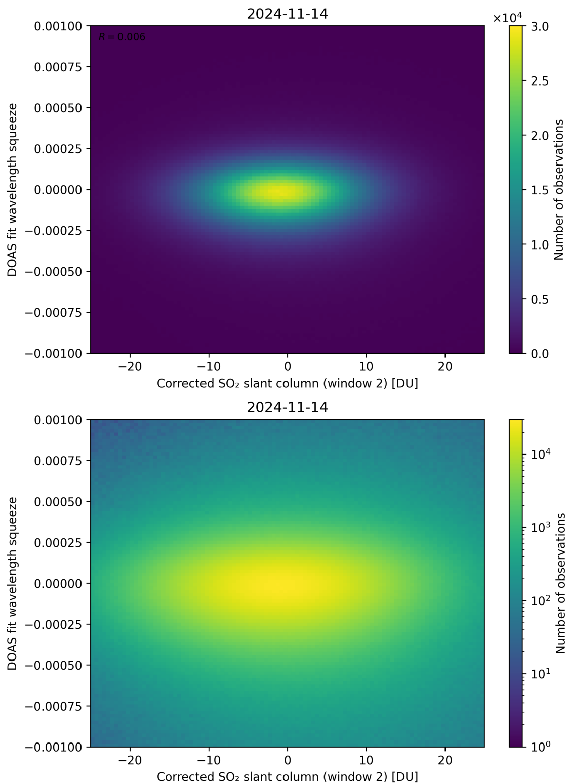
Figure 197: Scatter density plot of “Corrected SO 2 slant column (window 2)” against “DOAS fit wavelength squeeze” for 2024-11-14 to 2024-11-15.
