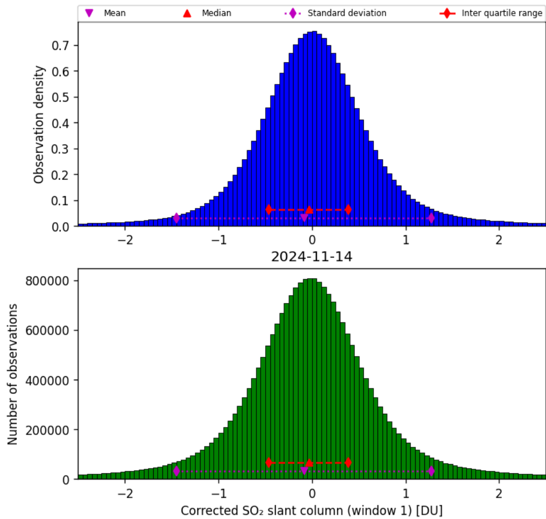
Figure 58: Histogram of “Corrected SO 2 slant column (window 1)” for 2024-11-14 to 2024-11-15
