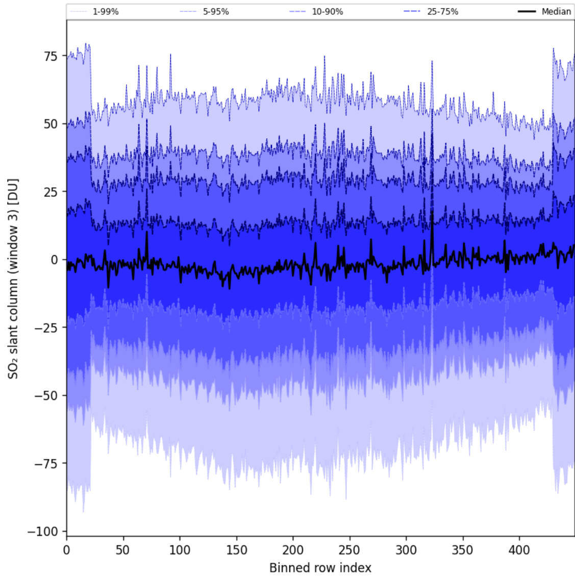
Figure 87: Along track statistics of “SO 2 slant column (window 3)” for 2024-11-14 to 2024-11-15
