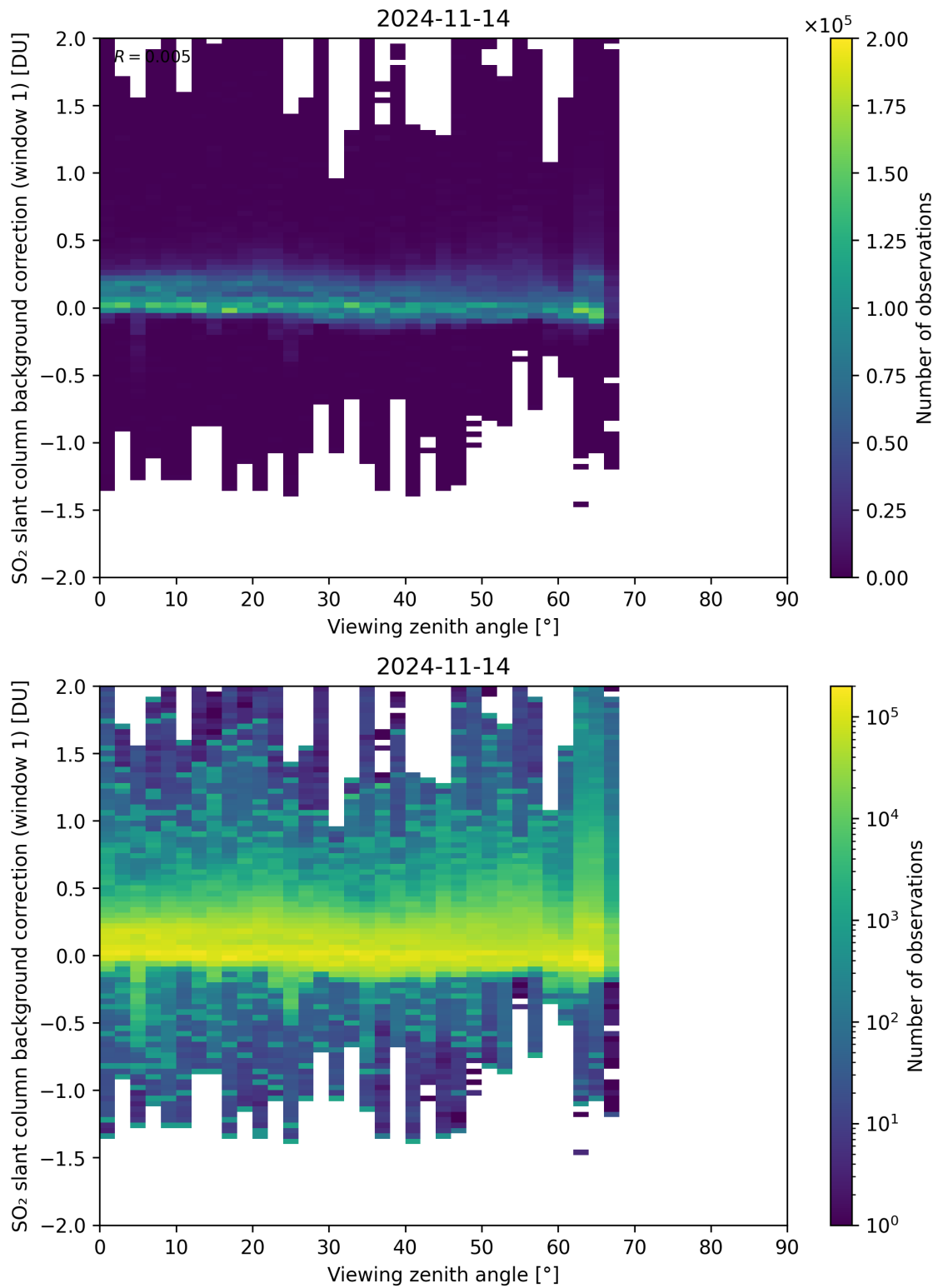
Figure 308: Scatter density plot of “Viewing zenith angle” against “SO 2 slant column background correction (window 1)” for 2024-11-14 to 2024-11-15.
