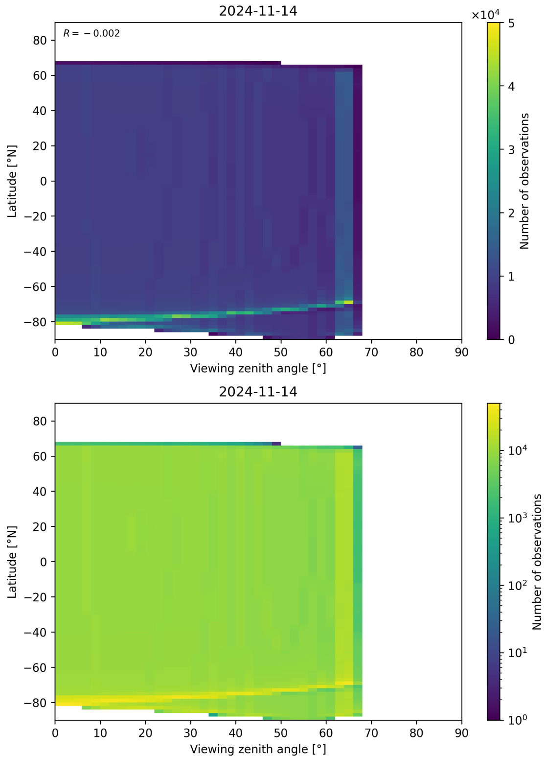
Figure 314: Scatter density plot of “Viewing zenith angle” against “Latitude” for 2024-11-14 to 2024-11-15.
