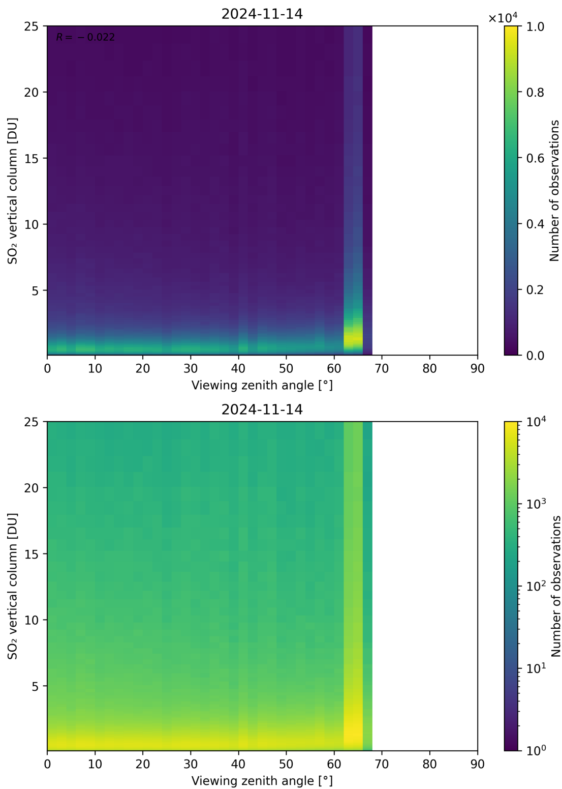
Figure 327: Scatter density plot of “Viewing zenith angle” against “SO 2 vertical column” for 2024-11-14 to 2024-11-15.
