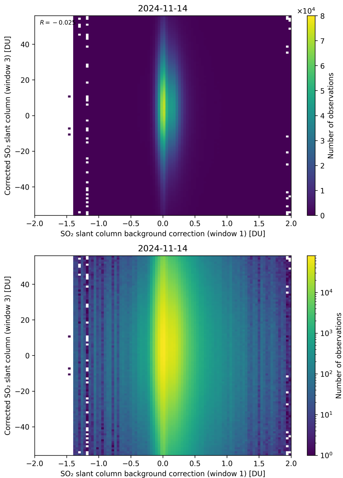
Figure 105: Scatter density plot of “SO 2 slant column background correction (window 1)” against “Corrected SO 2 slant column (window 3)” for 2024-11-14 to 2024-11-15.
