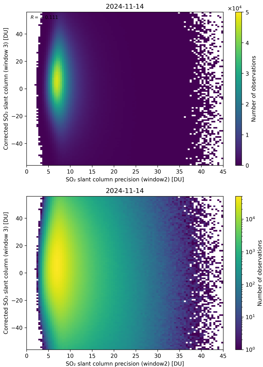
Figure 248: Scatter density plot of “SO 2 slant column precision (window2)” against “Corrected SO 2 slant column (window 3)” for 2024-11-14 to 2024-11-15.
