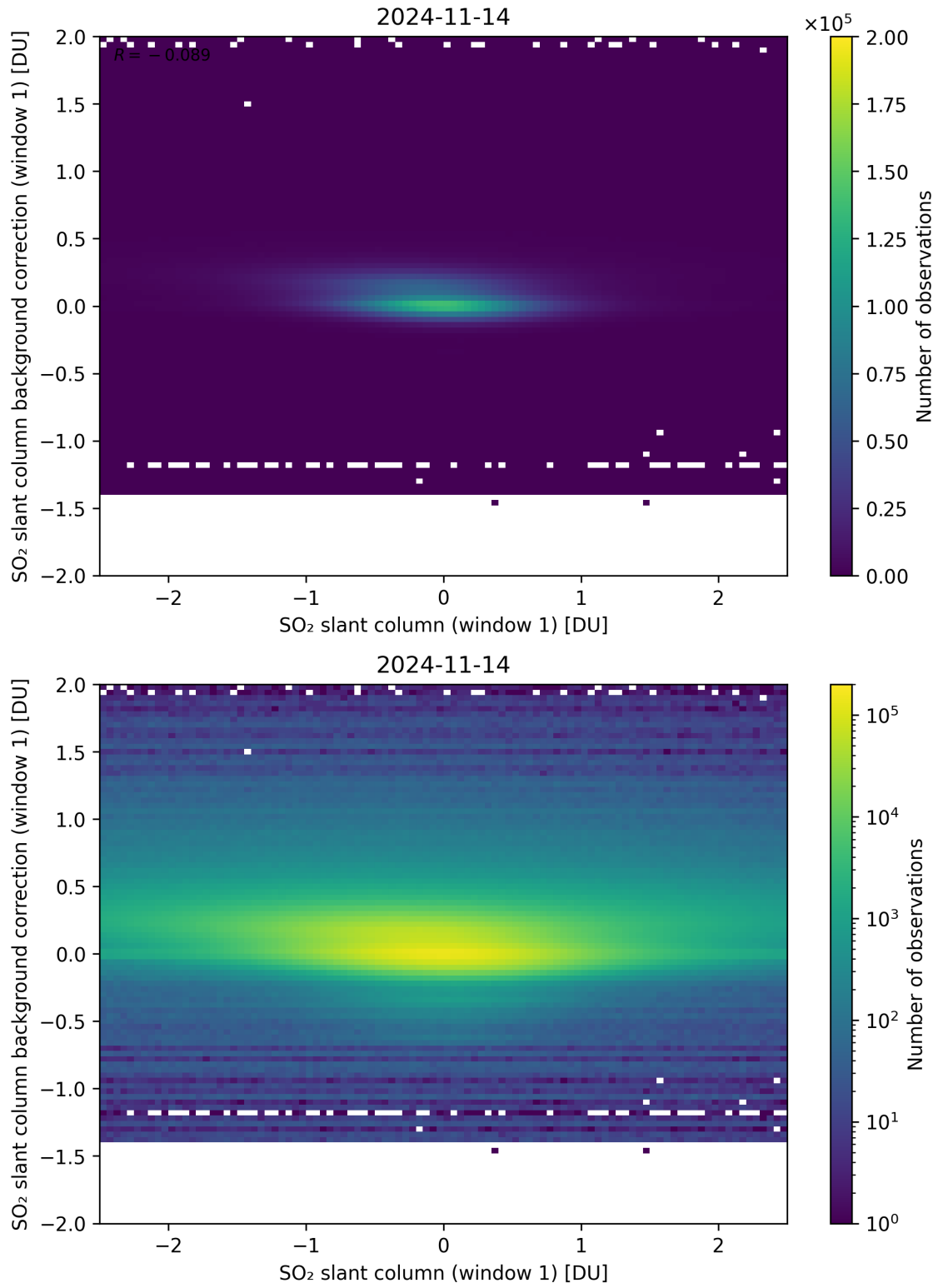
Figure 212: Scatter density plot of “SO 2 slant column (window 1)” against “SO 2 slant column background correction (window 1)” for 2024-11-14 to 2024-11-15.
