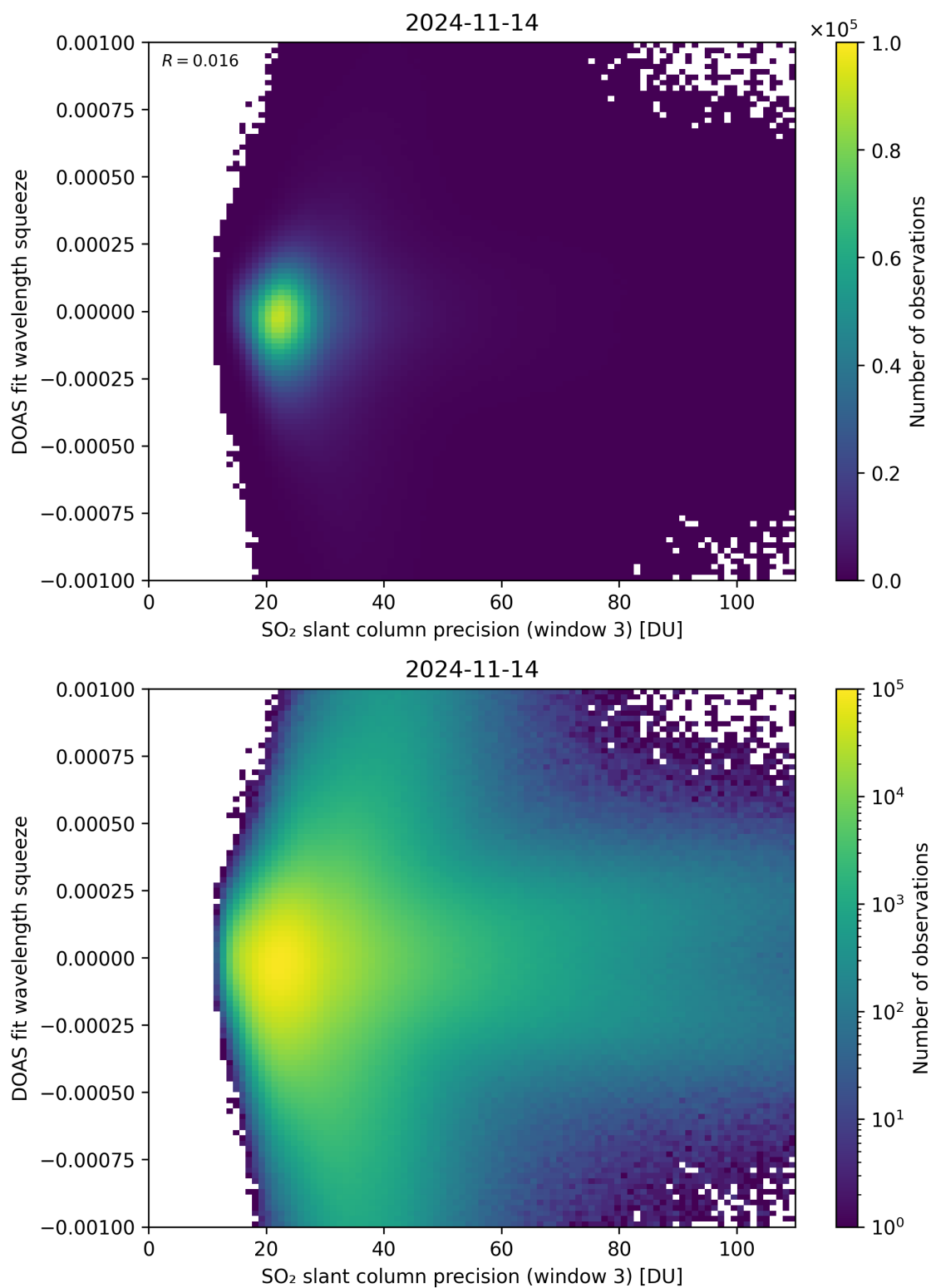
Figure 259: Scatter density plot of “SO 2 slant column precision (window 3)” against “DOAS fit wavelength squeeze” for 2024-11-14 to 2024-11-15.
