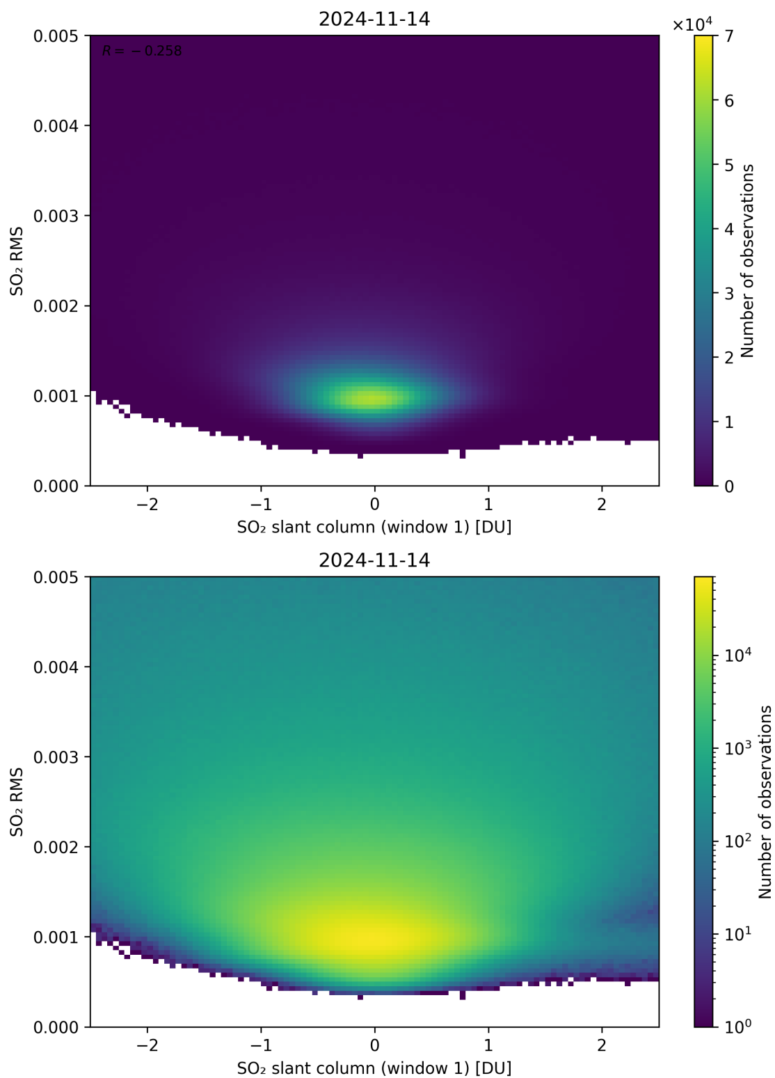
Figure 217: Scatter density plot of “SO 2 slant column (window 1)” against “SO 2 RMS” for 2024-11-14 to 2024-11-15.
