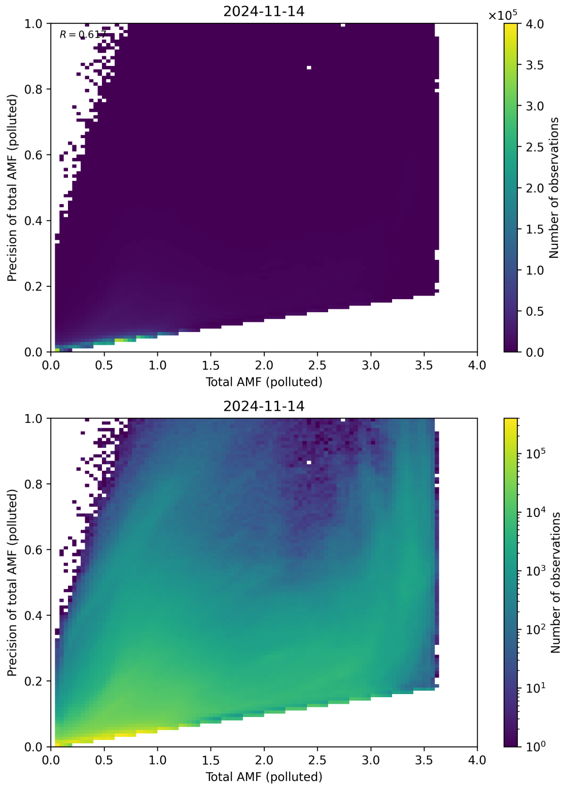
Figure 272: Scatter density plot of “Total AMF (polluted)” against “Precision of total AMF (polluted)” for 2024-11-14 to 2024-11-15.
