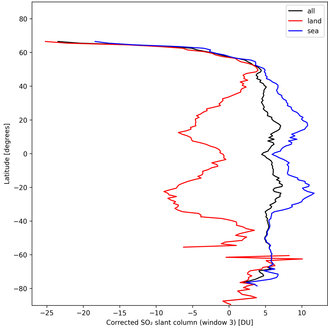
Figure 43: Zonal average of “Corrected SO 2 slant column (window 3)” for 2024-11-14 to 2024-11-15.
