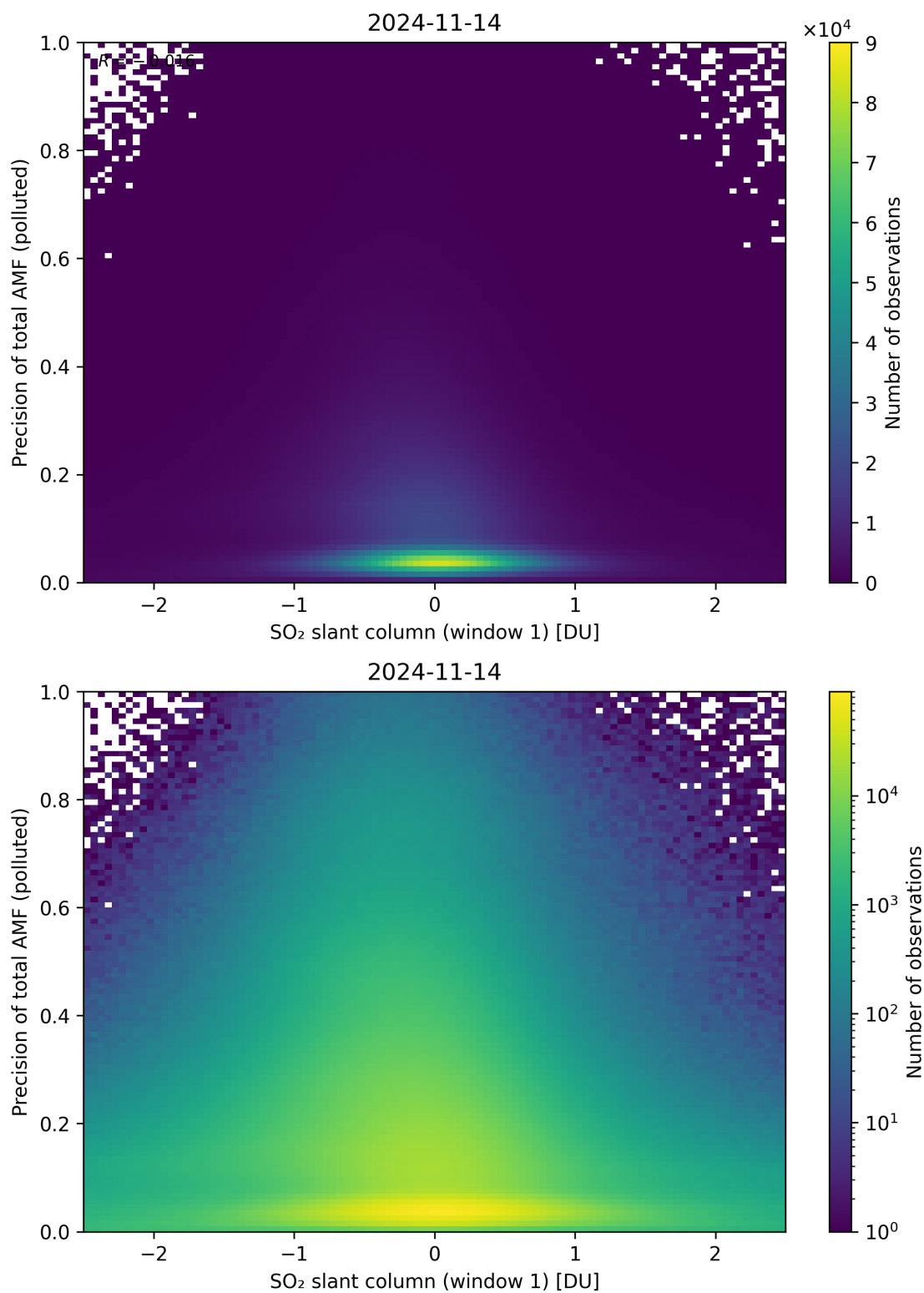
Figure 240: Scatter density plot of “SO 2 slant column (window 1)” against “Precision of total AMF (polluted)” for 2024-11-14 to 2024-11-15.
