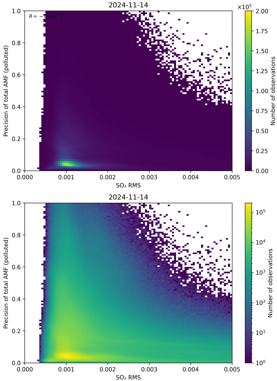
Figure 138: Scatter density plot of “SO 2 RMS” against “Precision of total AMF (polluted)” for 2024-11-14 to 2024-11-15.
