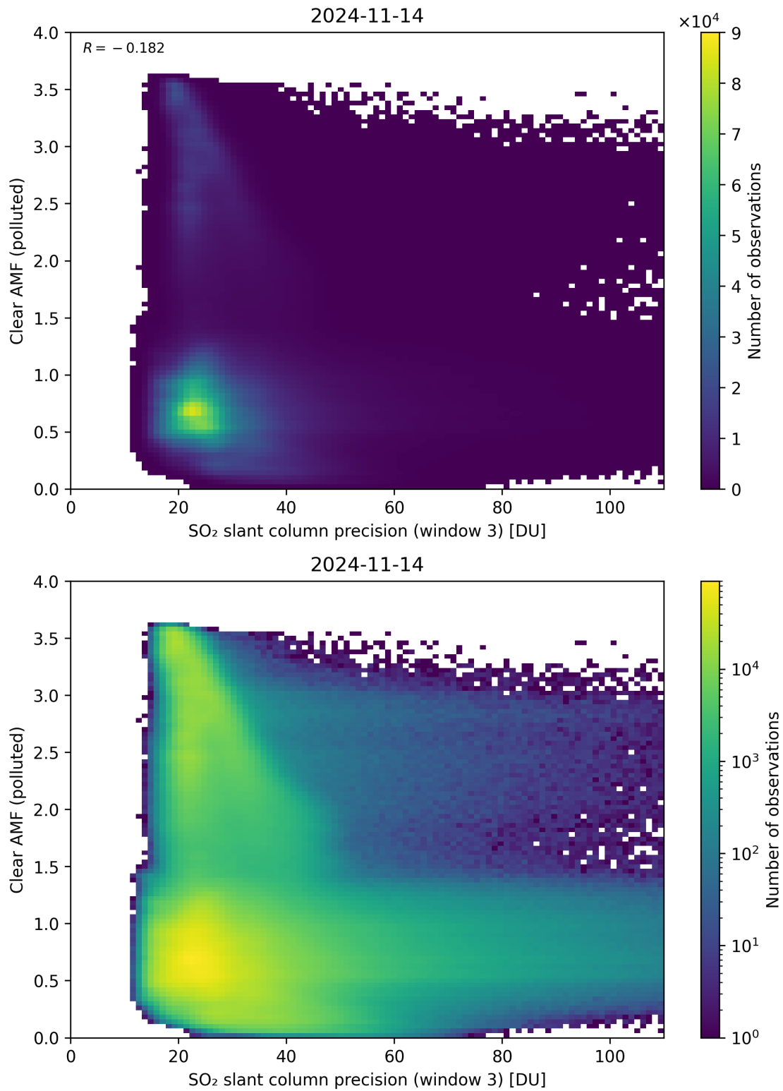
Figure 261: Scatter density plot of “SO 2 slant column precision (window 3)” against “Clear AMF (polluted)” for 2024-11-14 to 2024-11-15.
