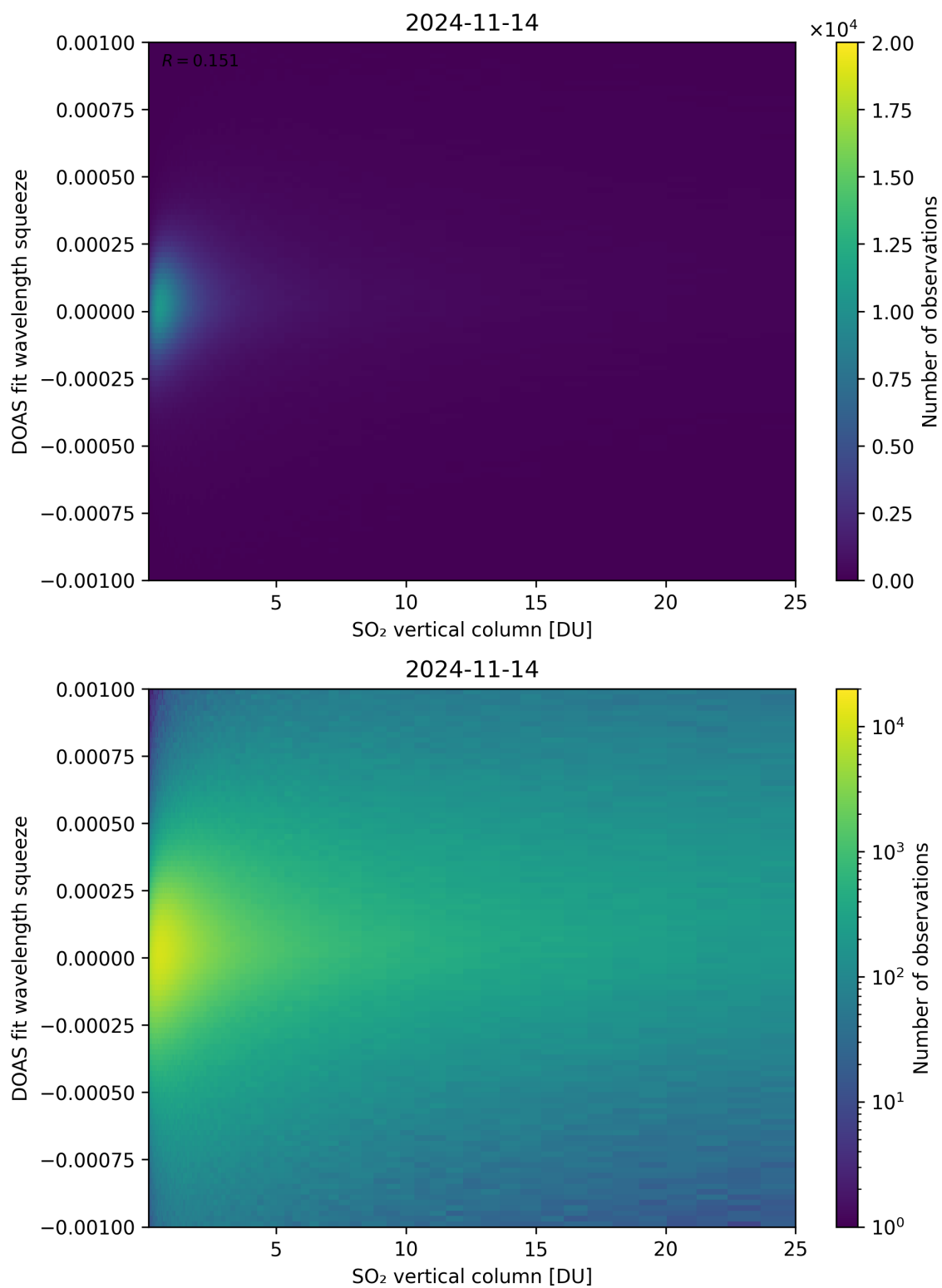
Figure 277: Scatter density plot of “SO 2 vertical column” against “DOAS fit wavelength squeeze” for 2024-11-14 to 2024-11-15.
