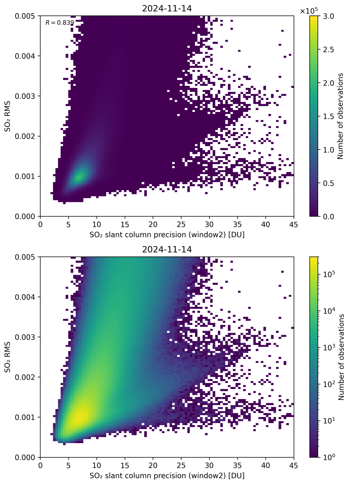
Figure 245: Scatter density plot of “SO 2 slant column precision (window2)” against “SO 2 RMS” for 2024-11-14 to 2024-11-15.
