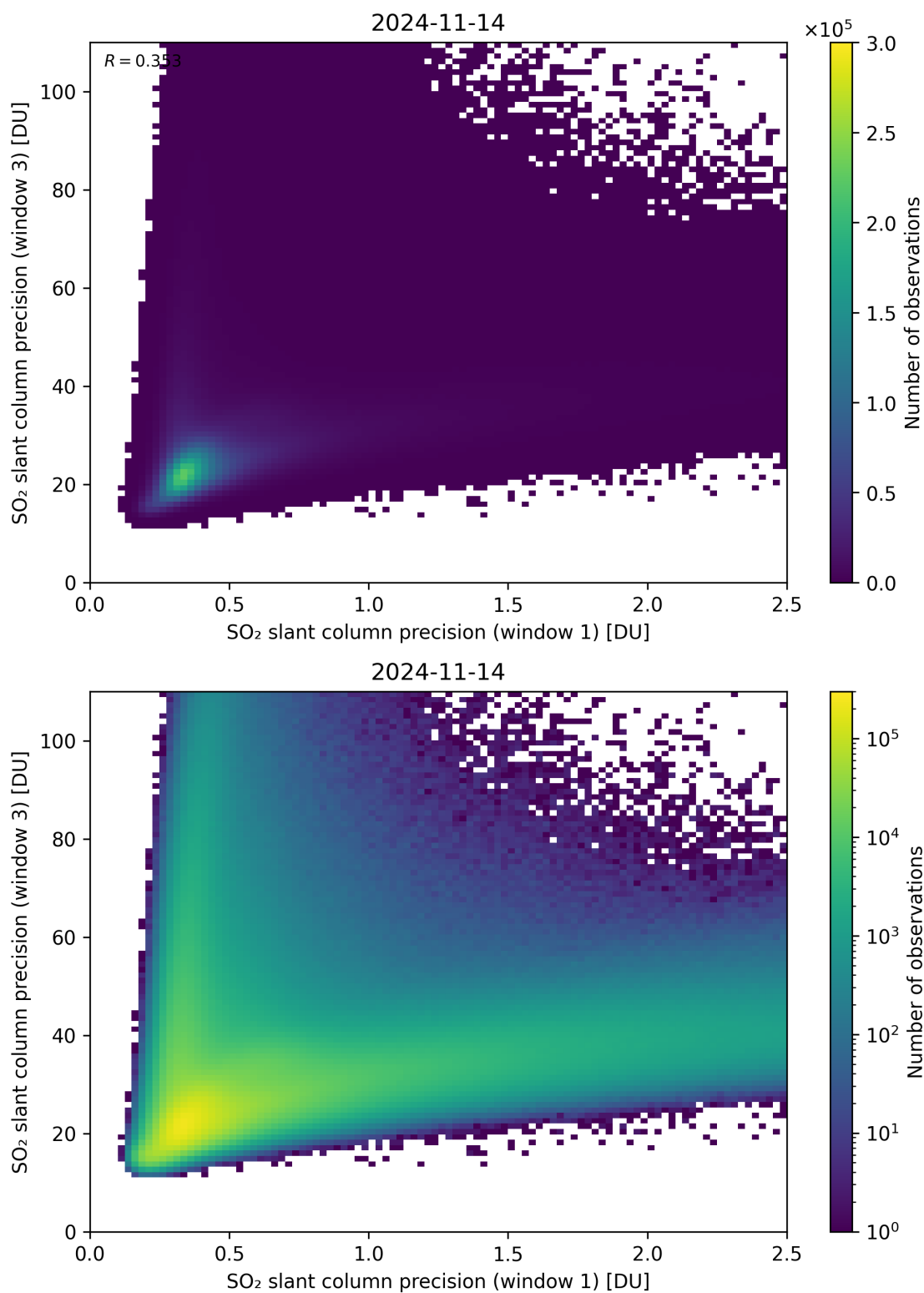
Figure 229: Scatter density plot of “SO 2 slant column precision (window 1)” against “SO 2 slant column precision (window 3)” for 2024-11-14 to 2024-11-15.
