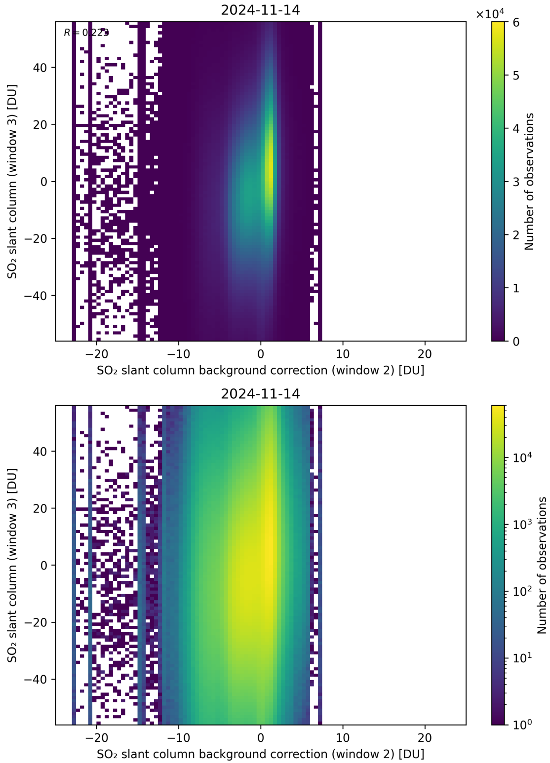
Figure 117: Scatter density plot of “SO 2 slant column background correction (window 2)” against “SO 2 slant column (window 3)” for 2024-11-14 to 2024-11-15.
