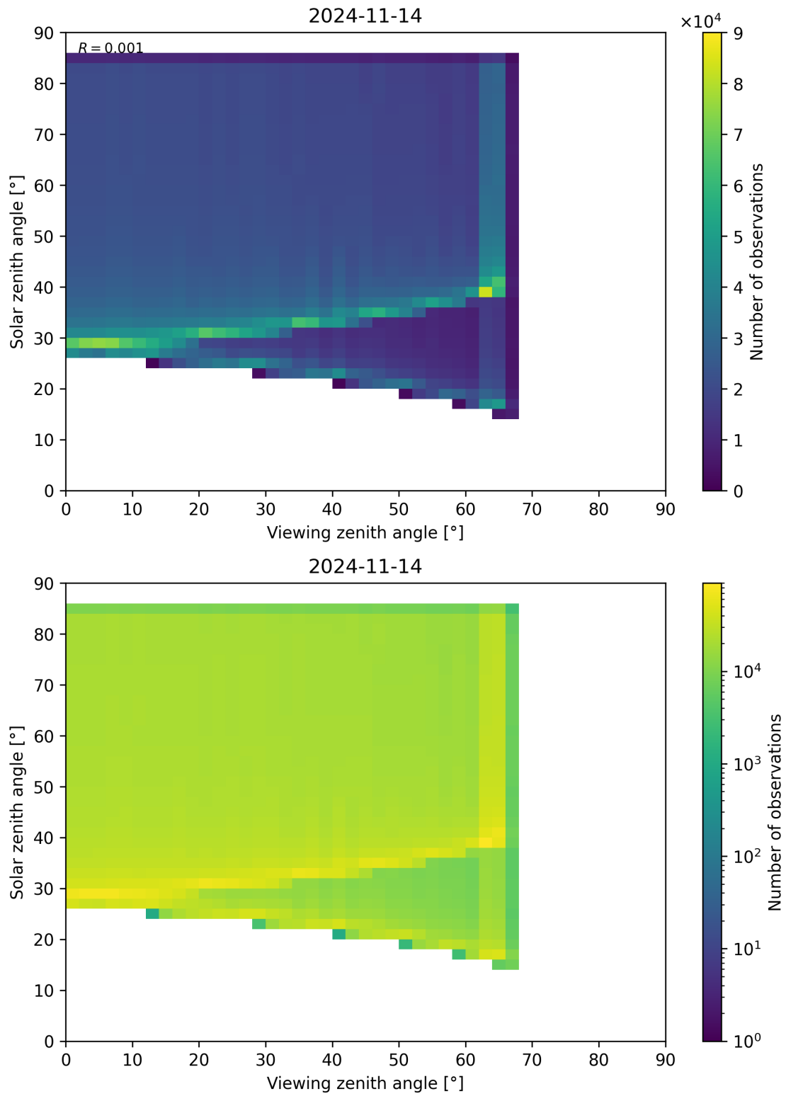
Figure 315: Scatter density plot of “Viewing zenith angle” against “Solar zenith angle” for 2024-11-14 to 2024-11-15.
