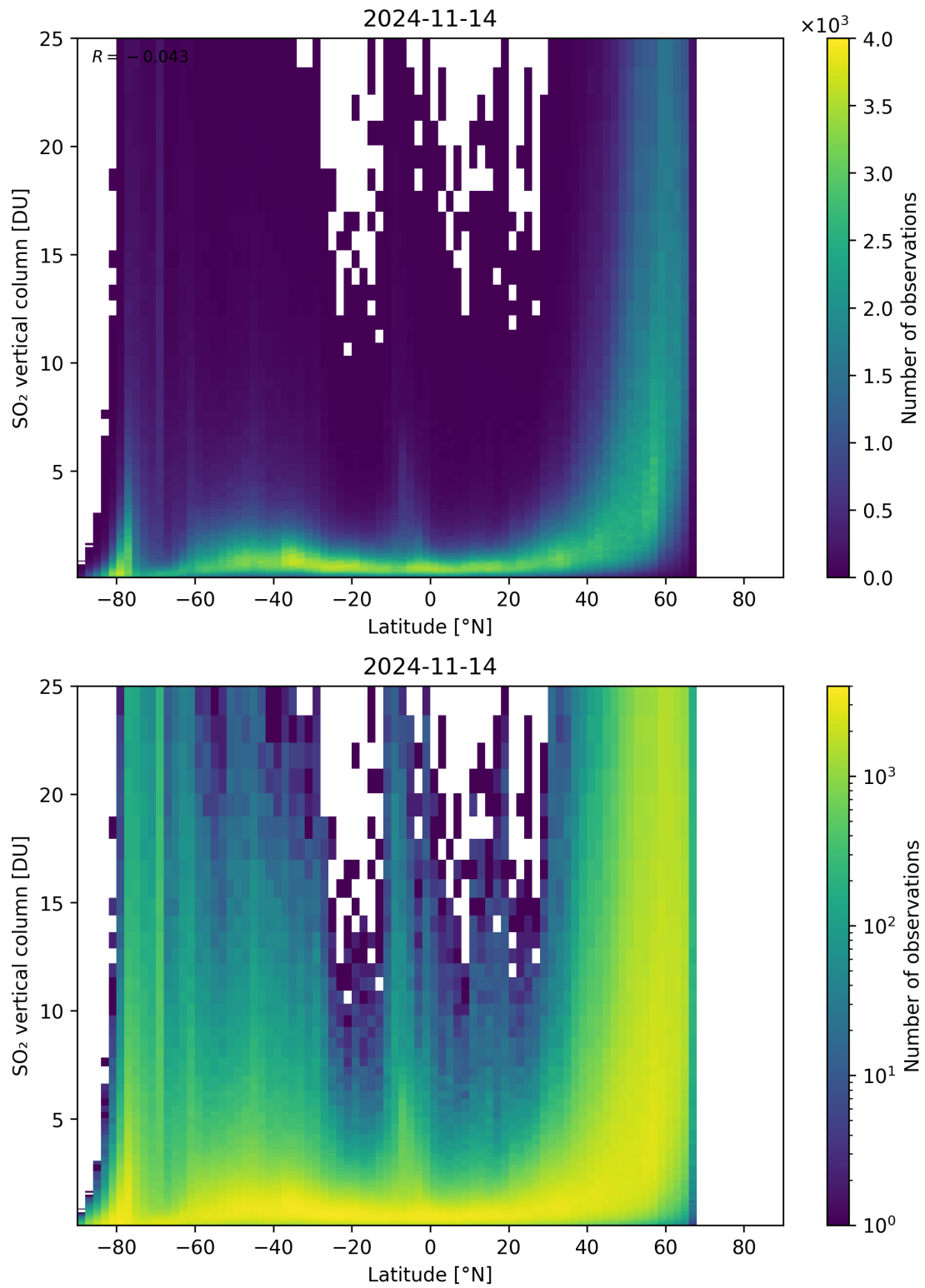
Figure 156: Scatter density plot of “Latitude” against “SO 2 vertical column” for 2024-11-14 to 2024-11-15.
