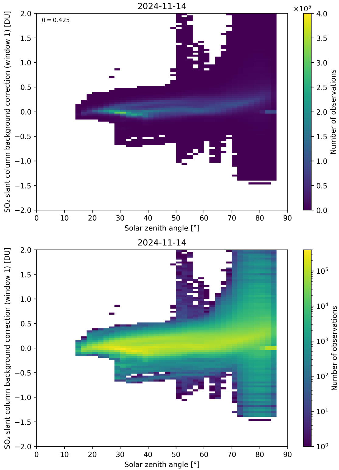
Figure 158: Scatter density plot of “Solar zenith angle” against “SO 2 slant column background correction (window 1)” for 2024-11-14 to 2024-11-15.
