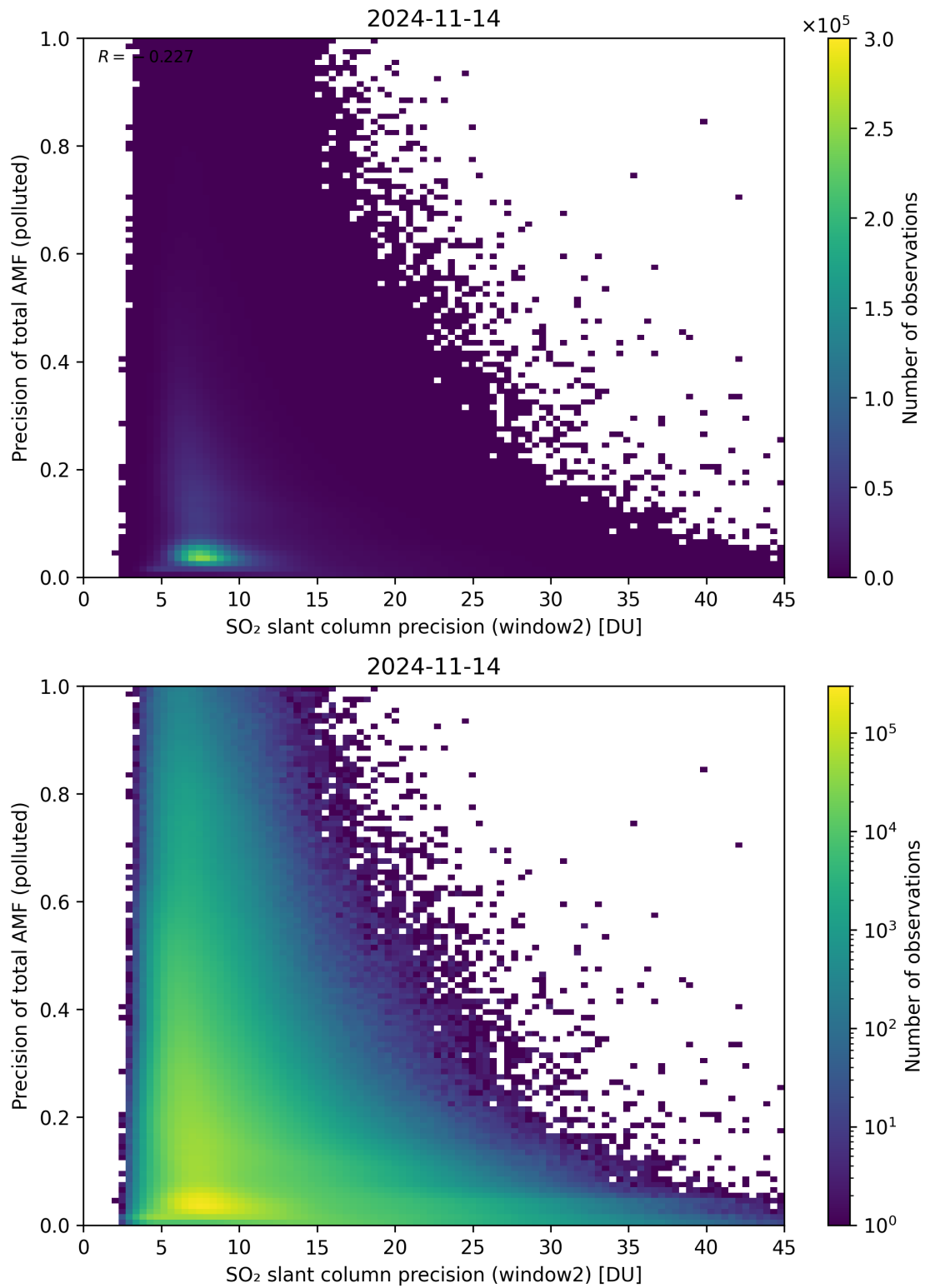
Figure 252: Scatter density plot of “SO 2 slant column precision (window2)” against “Precision of total AMF (polluted)” for 2024-11-14 to 2024-11-15.
