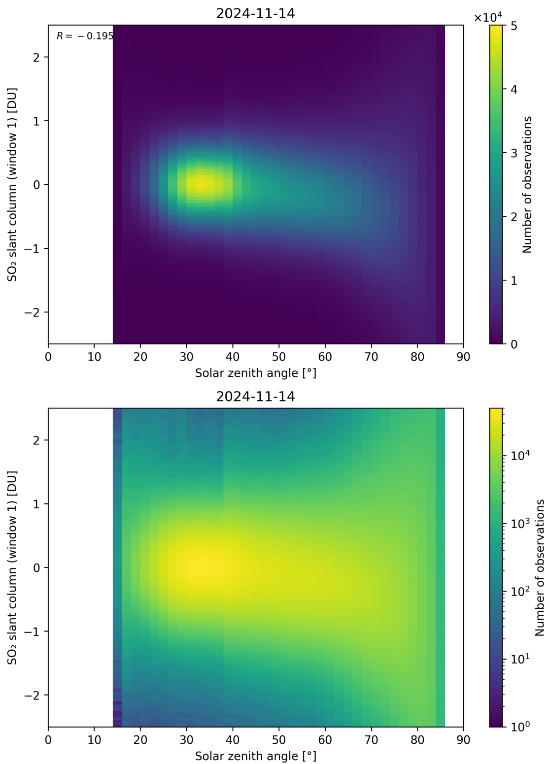
Figure 169: Scatter density plot of “Solar zenith angle” against “SO 2 slant column (window 1)” for 2024-11-14 to 2024-11-15.
