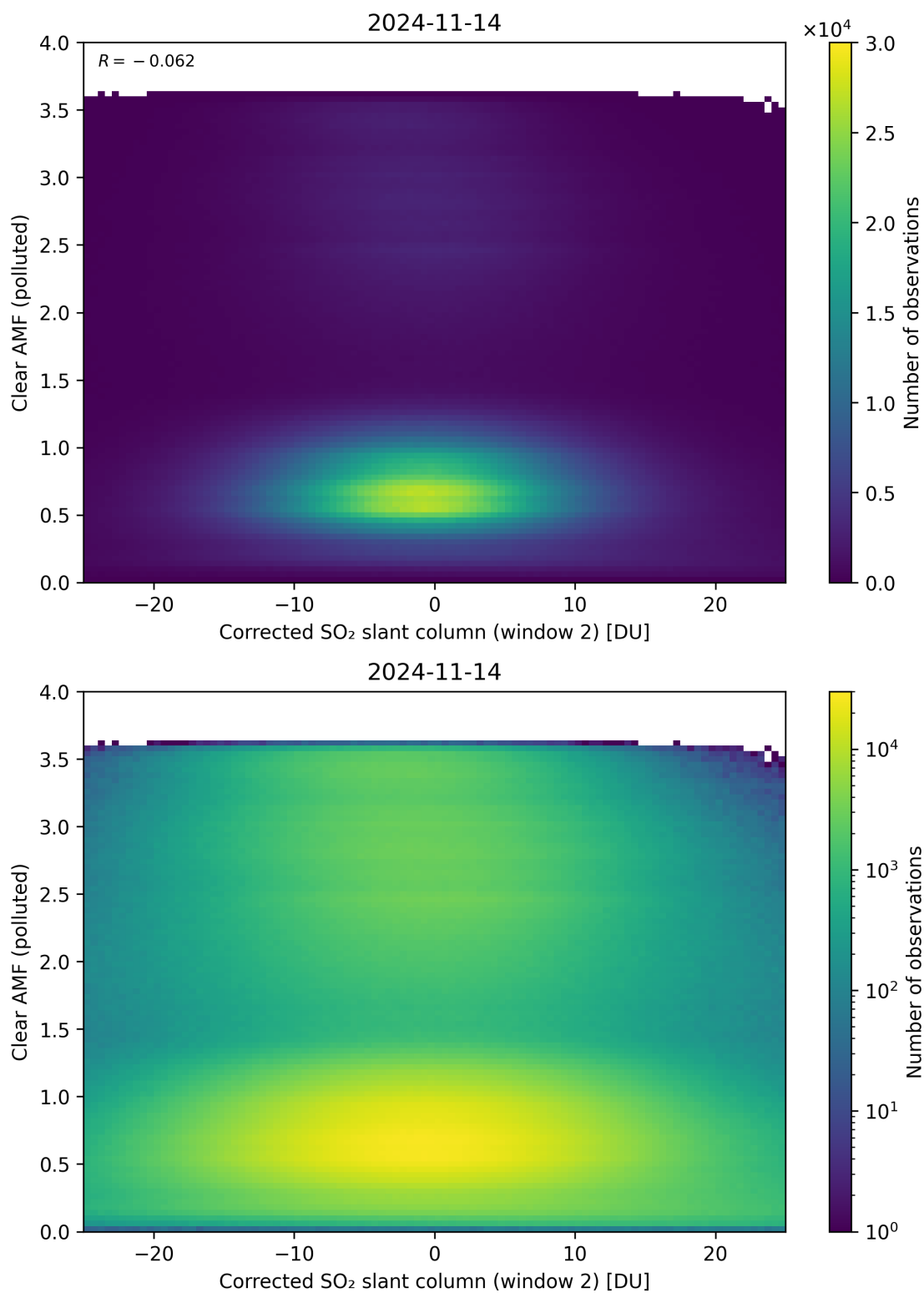
Figure 199: Scatter density plot of “Corrected SO 2 slant column (window 2)” against “Clear AMF (polluted)” for 2024-11-14 to 2024-11-15.
