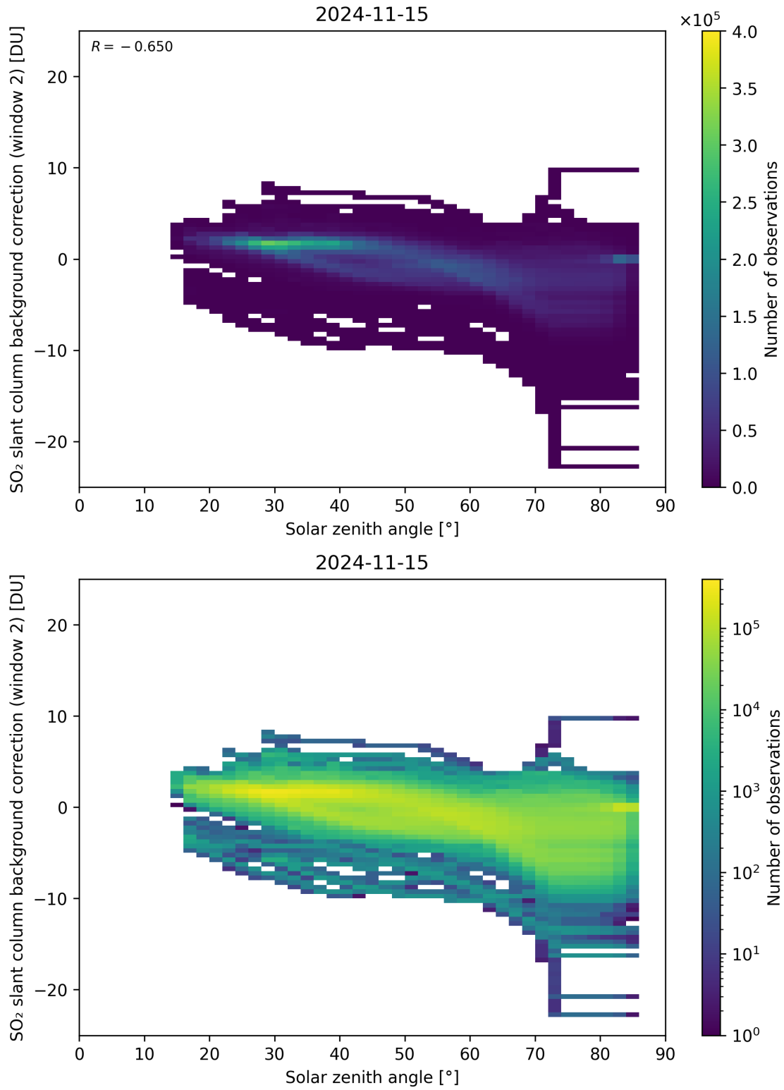
Figure 159: Scatter density plot of “Solar zenith angle” against “SO 2 slant column background correction (window 2)” for 2024-11-14 to 2024-11-16.
