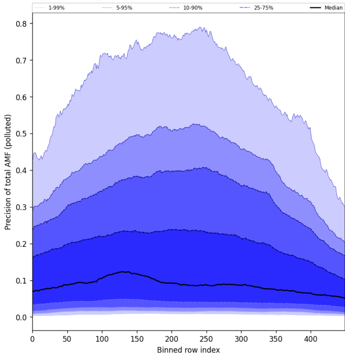
Figure 95: Along track statistics of “Precision of total AMF (polluted)” for 2024-11-14 to 2024-11-16
