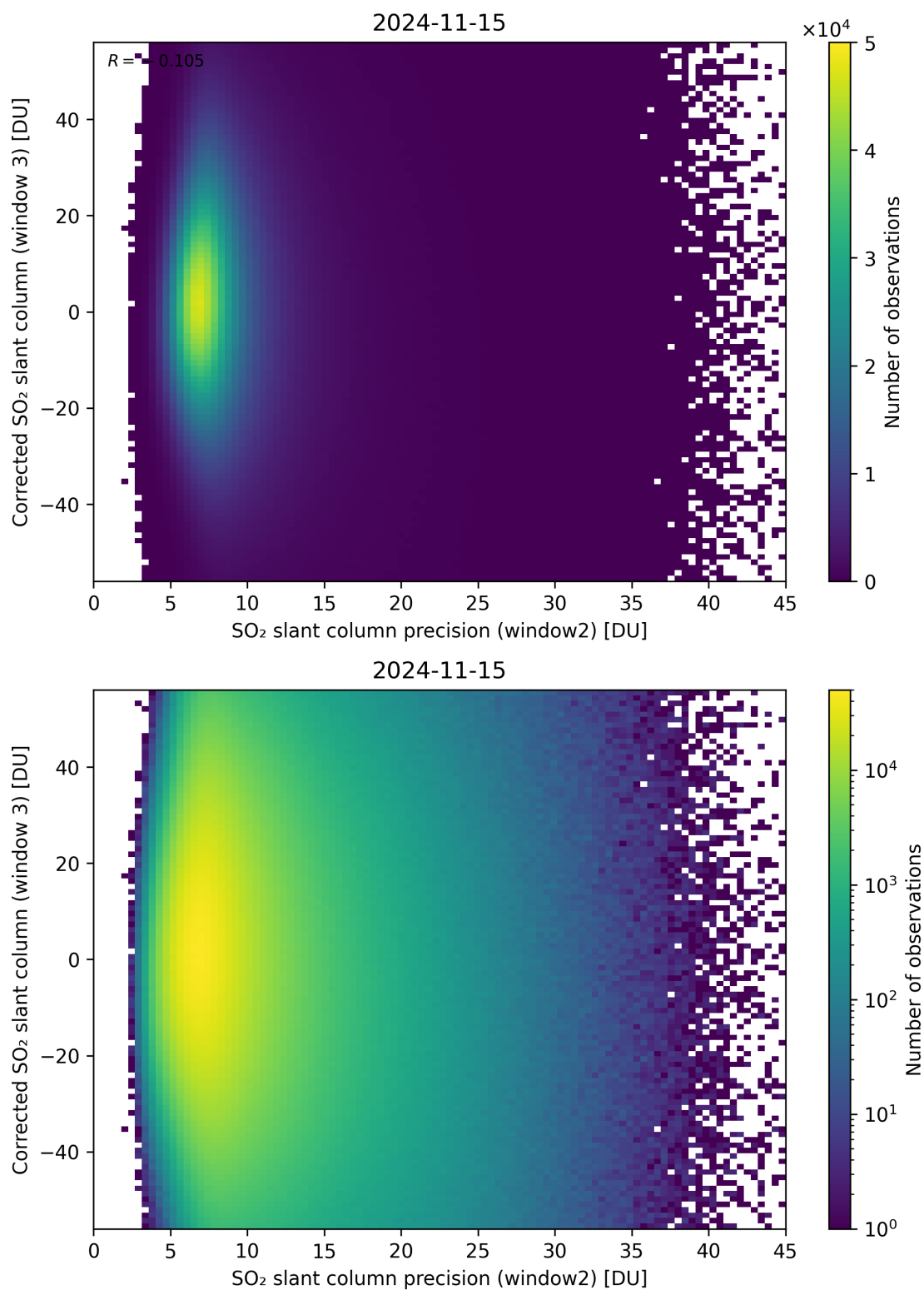
Figure 248: Scatter density plot of “SO 2 slant column precision (window2)” against “Corrected SO 2 slant column (window 3)” for 2024-11-14 to 2024-11-16.
