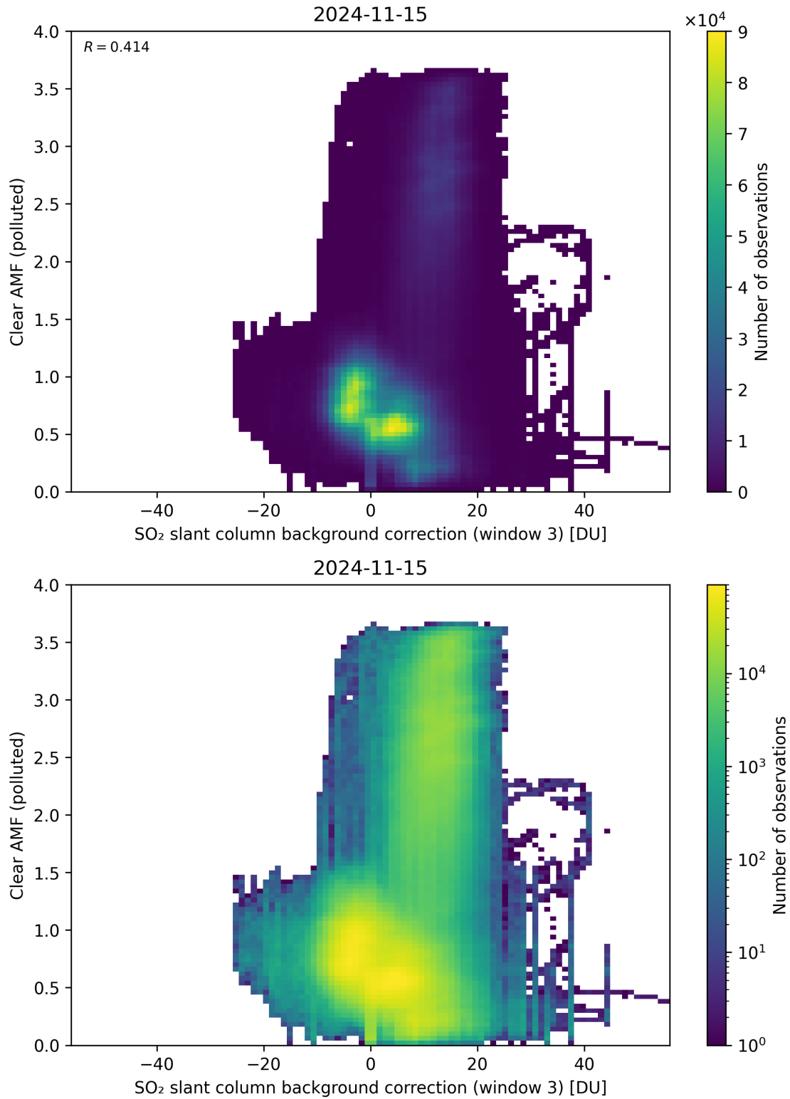
Figure 124: Scatter density plot of “SO 2 slant column background correction (window 3)” against “Clear AMF (polluted)” for 2024-11-14 to 2024-11-16.
