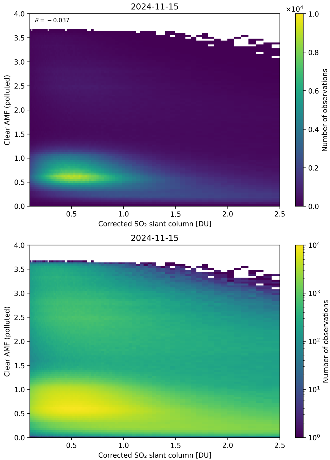
Figure 184: Scatter density plot of “Corrected SO 2 slant column” against “Clear AMF (polluted)” for 2024-11-14 to 2024-11-16.
