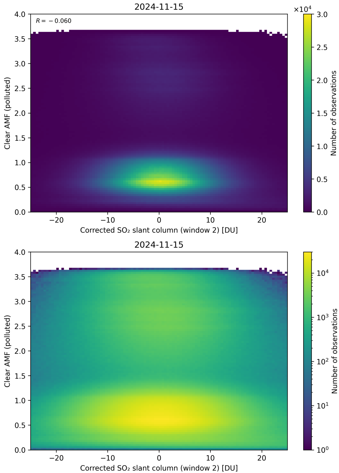
Figure 199: Scatter density plot of “Corrected SO 2 slant column (window 2)” against “Clear AMF (polluted)” for 2024-11-14 to 2024-11-16.
