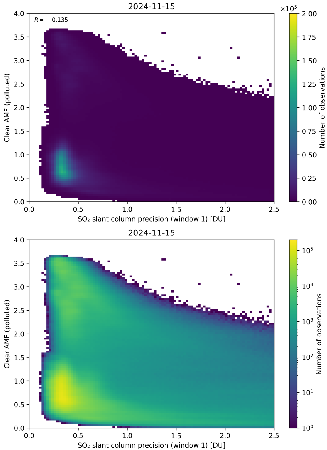
Figure 224: Scatter density plot of “SO 2 slant column precision (window 1)” against “Clear AMF (polluted)” for 2024-11-14 to 2024-11-16.
