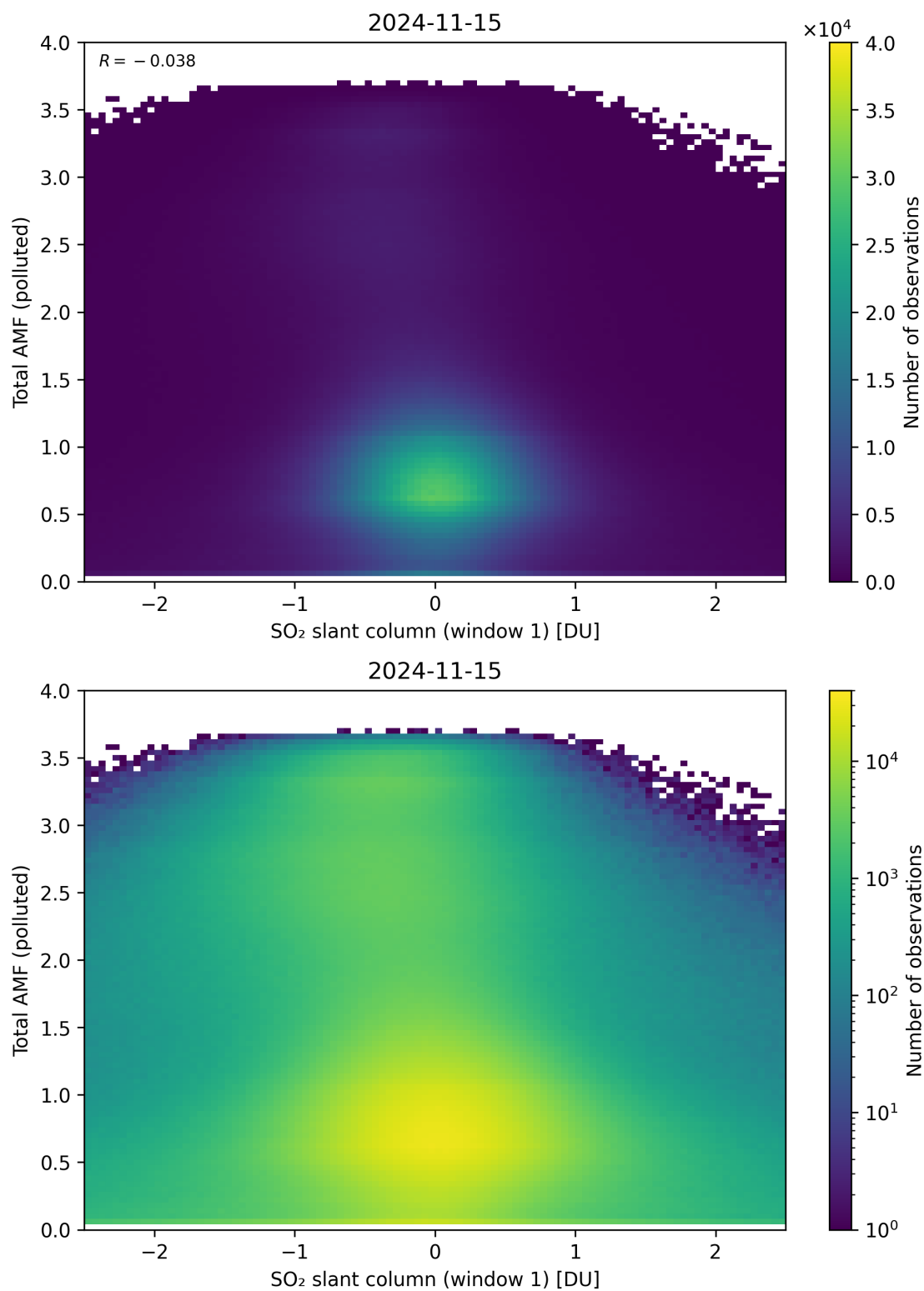
Figure 239: Scatter density plot of “SO 2 slant column (window 1)” against “Total AMF (polluted)” for 2024-11-14 to 2024-11-16.
