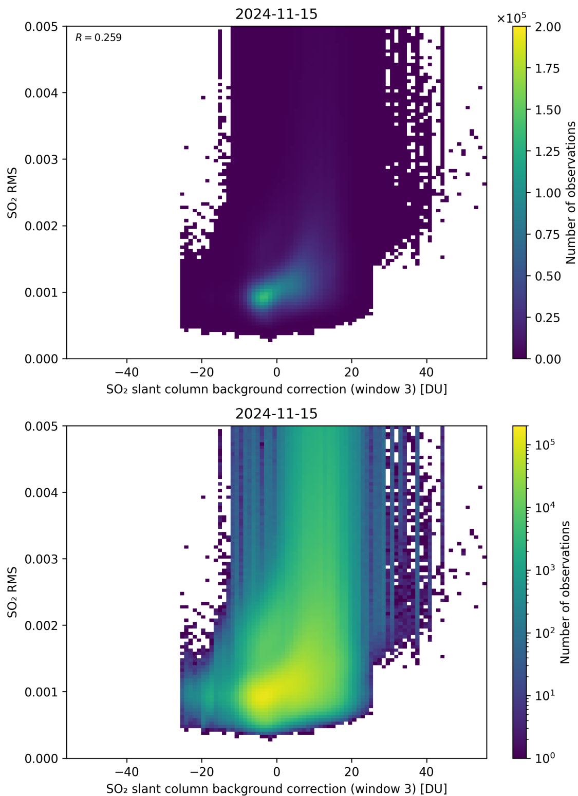
Figure 123: Scatter density plot of “SO 2 slant column background correction (window 3)” against “SO 2 RMS” for 2024-11-14 to 2024-11-16.
