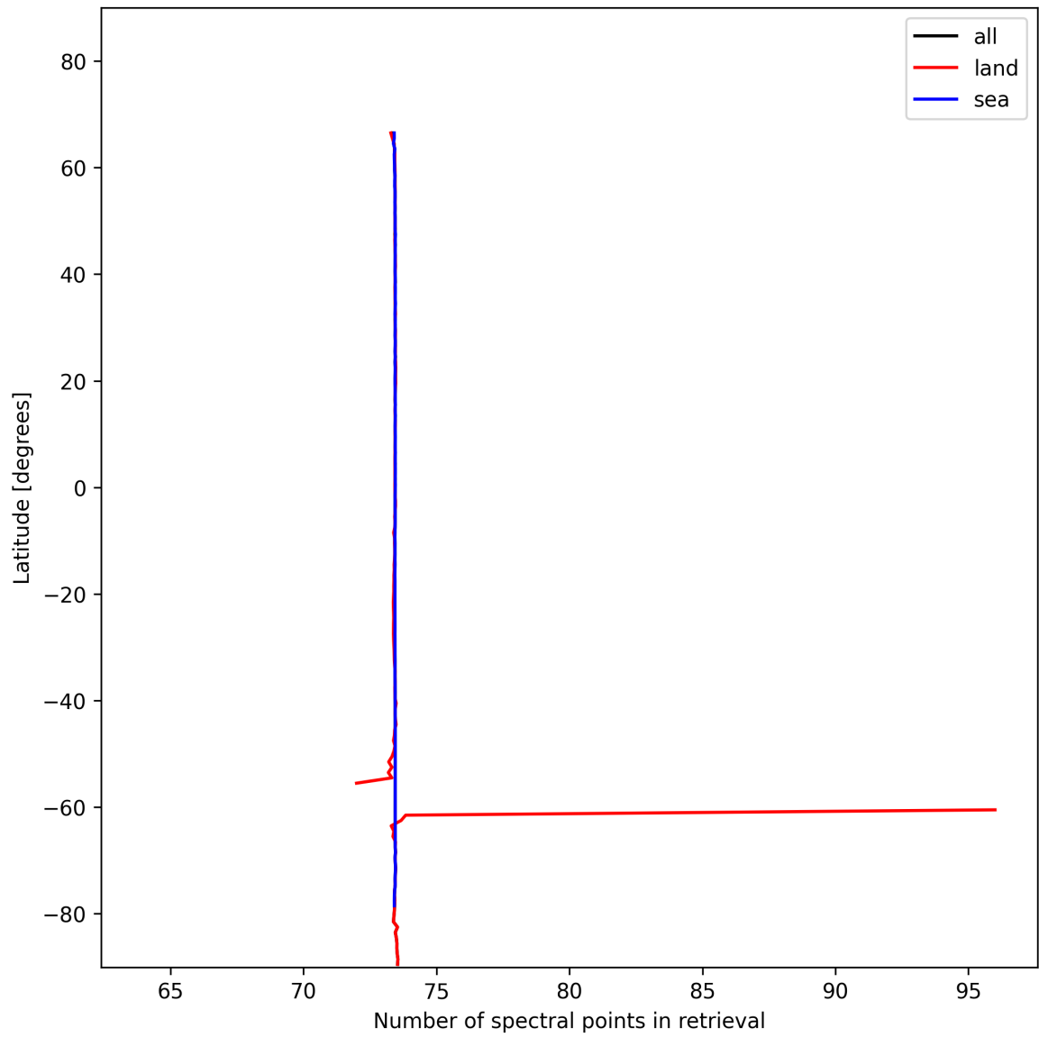
Figure 51: Zonal average of “Number of spectral points in retrieval” for 2024-11-14 to 2024-11-16.
