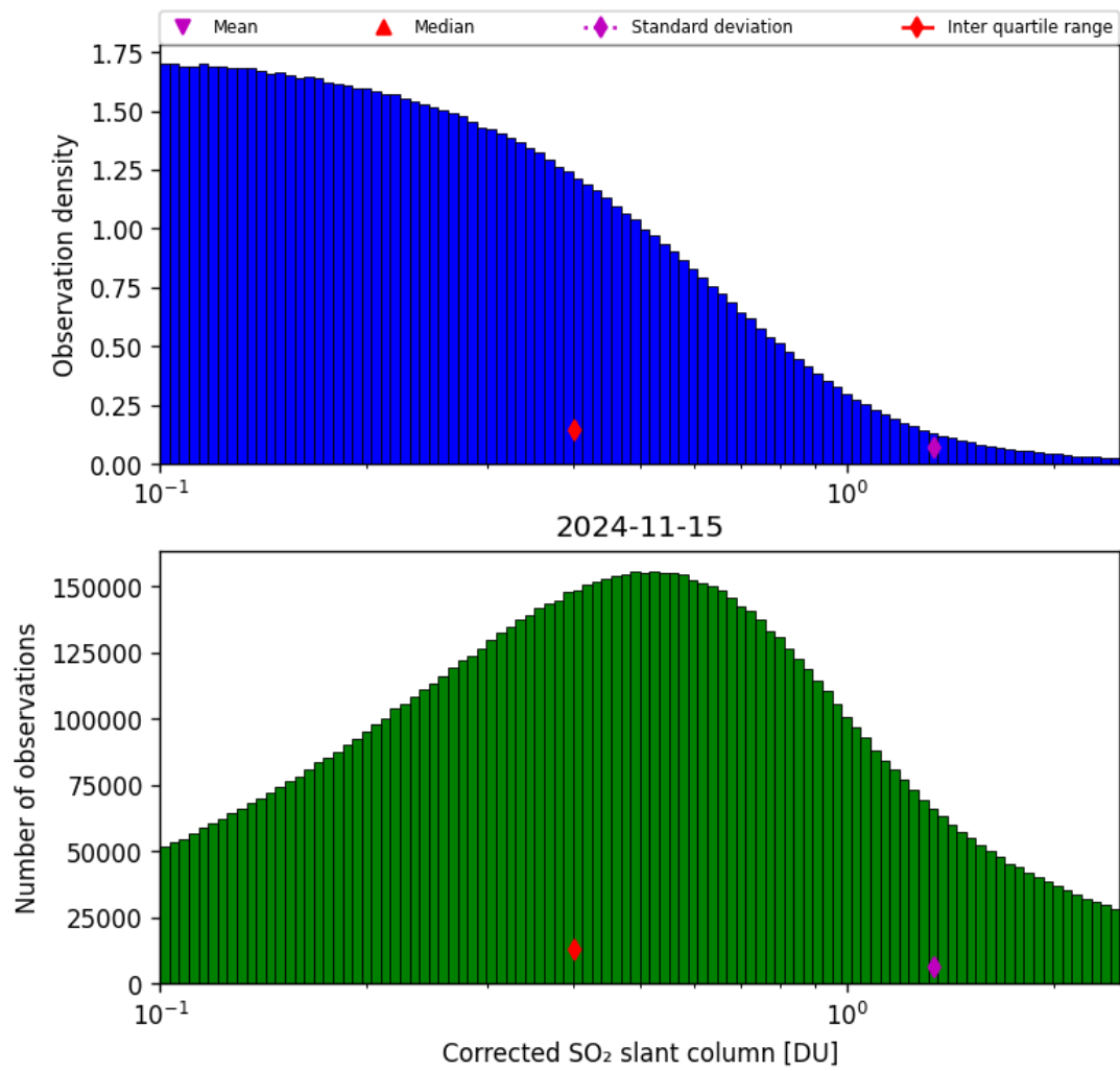
Figure 55: Histogram of “Corrected SO 2 slant column” for 2024-11-14 to 2024-11-16
