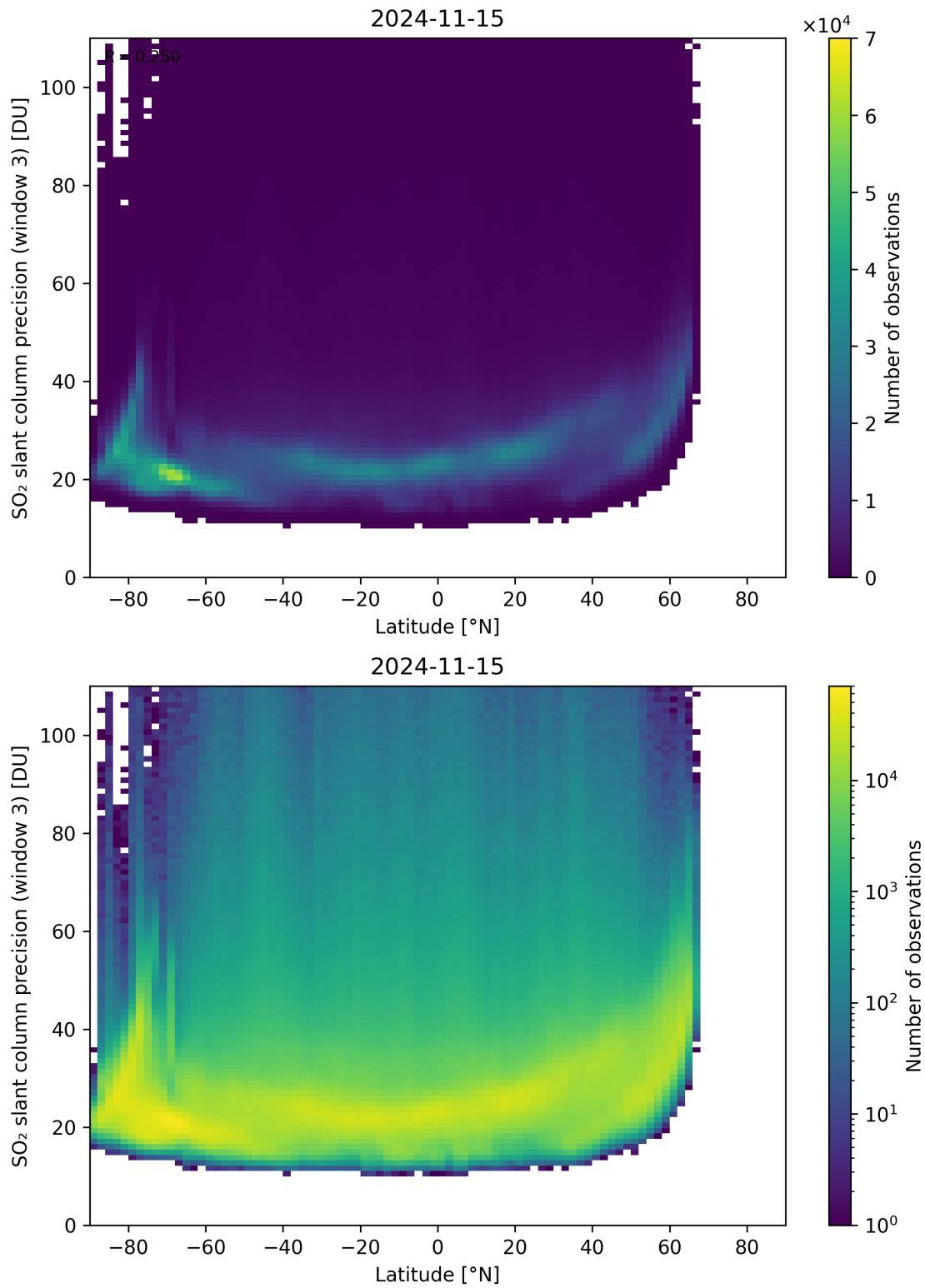
Figure 153: Scatter density plot of “Latitude” against “SO 2 slant column precision (window 3)” for 2024-11-14 to 2024-11-16.
