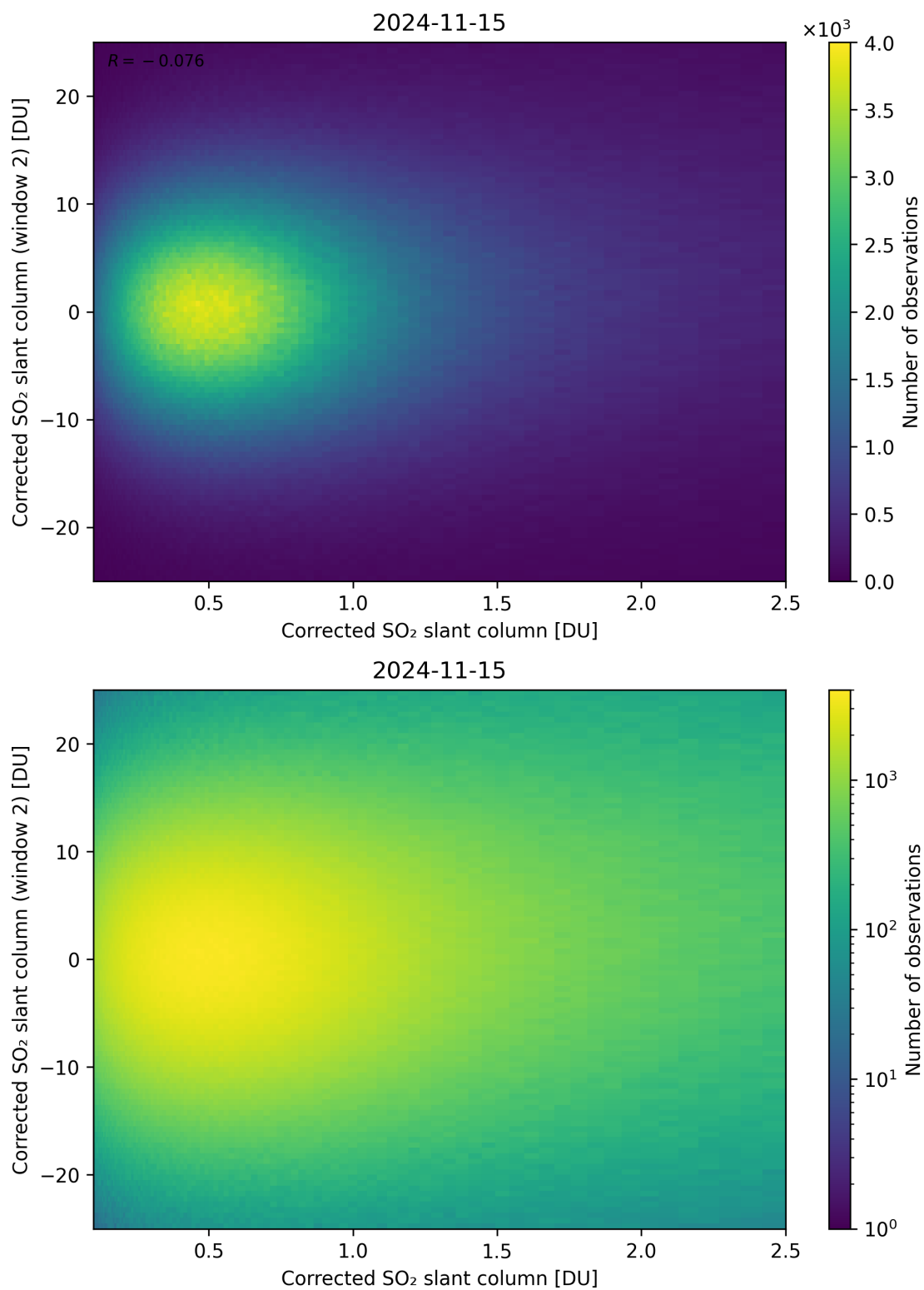
Figure 185: Scatter density plot of “Corrected SO 2 slant column” against “Corrected SO 2 slant column (window 2)” for 2024-11-14 to 2024-11-16.
