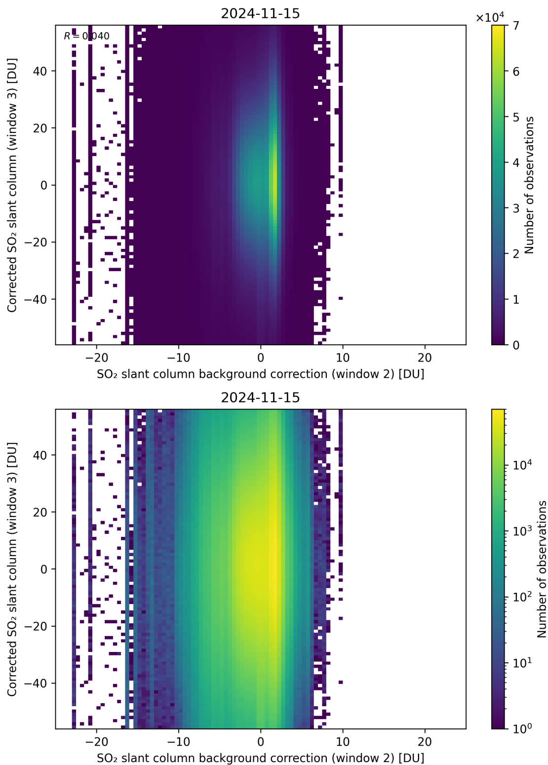
Figure 116: Scatter density plot of “SO 2 slant column background correction (window 2)” against “Corrected SO 2 slant column (window 3)” for 2024-11-14 to 2024-11-16.
