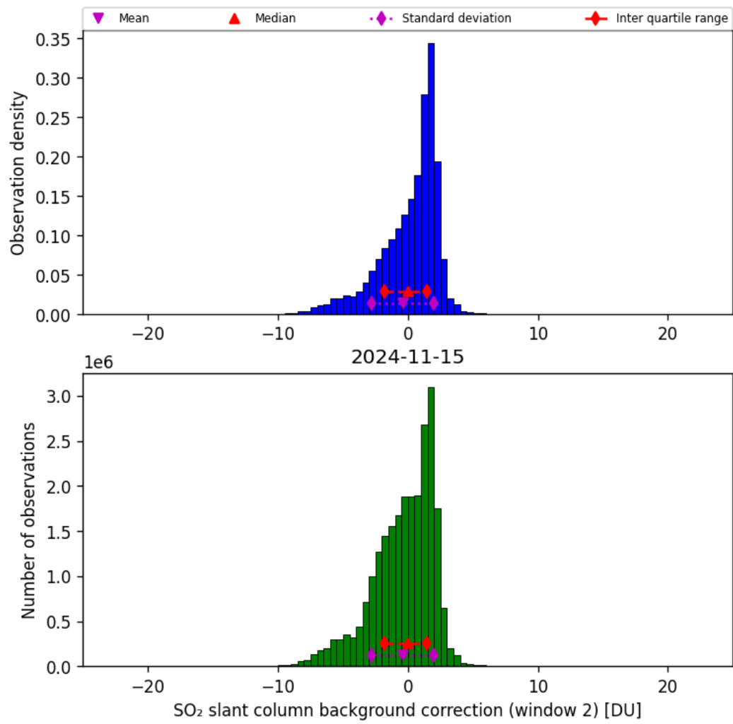
Figure 63: Histogram of “SO 2 slant column background correction (window 2)” for 2024-11-14 to 2024-11-16
