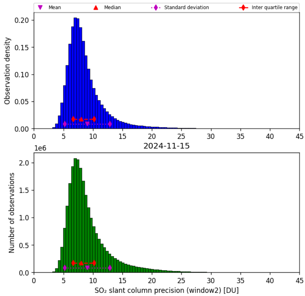
Figure 61: Histogram of “SO 2 slant column precision (window2)” for 2024-11-14 to 2024-11-16
