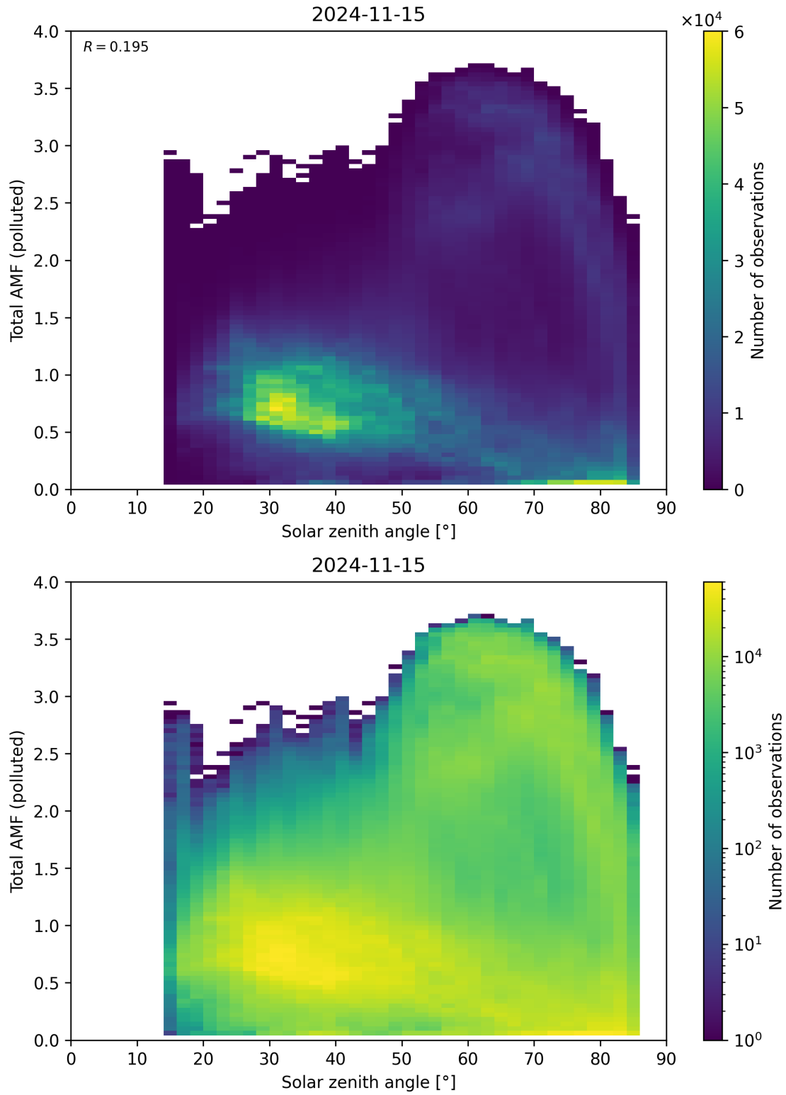
Figure 174: Scatter density plot of “Solar zenith angle” against “Total AMF (polluted)” for 2024-11-14 to 2024-11-16.
