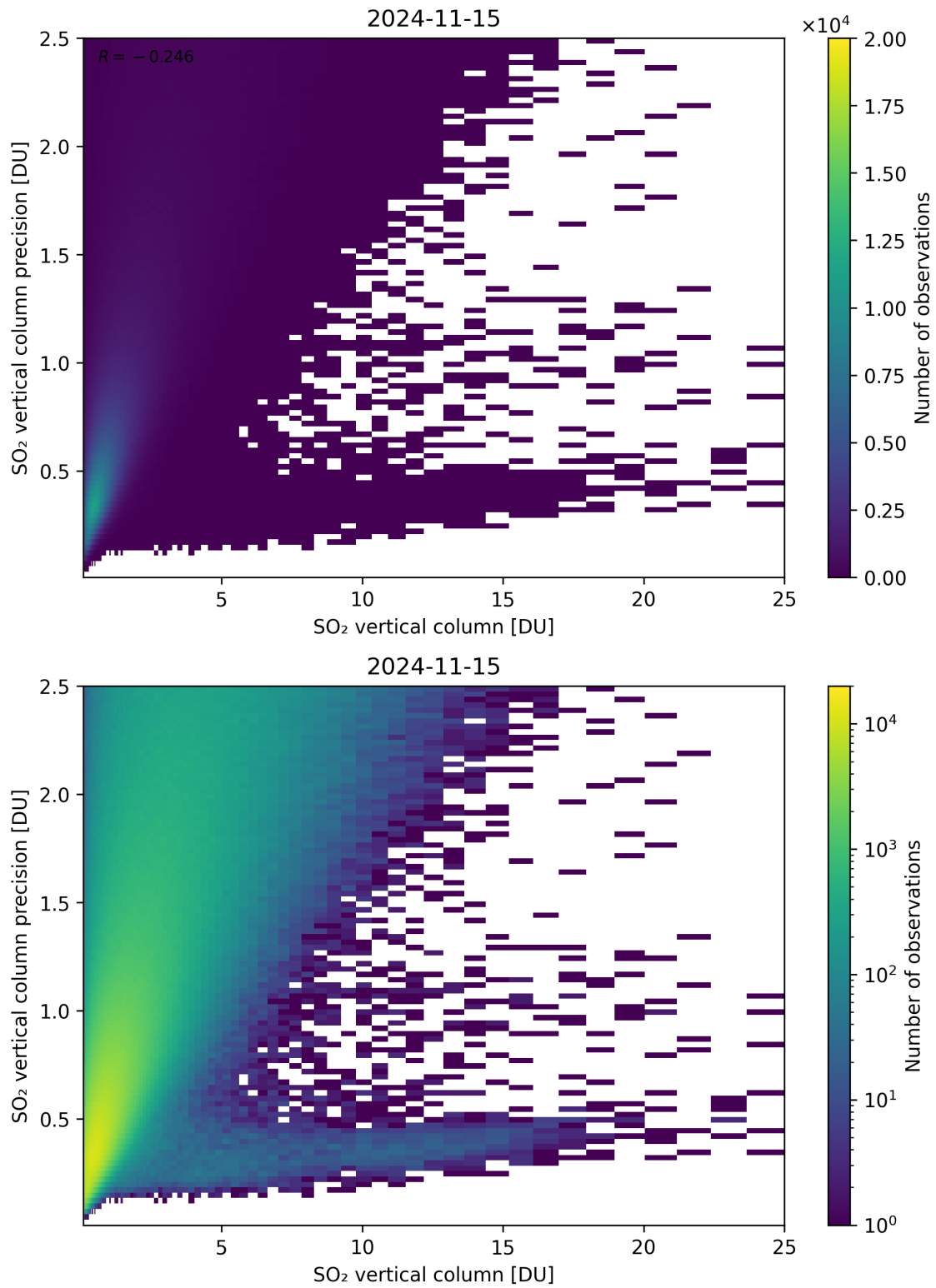
Figure 307: Scatter density plot of “SO 2 vertical column” against “SO 2 vertical column precision” for 2024-11-14 to 2024-11-16.
