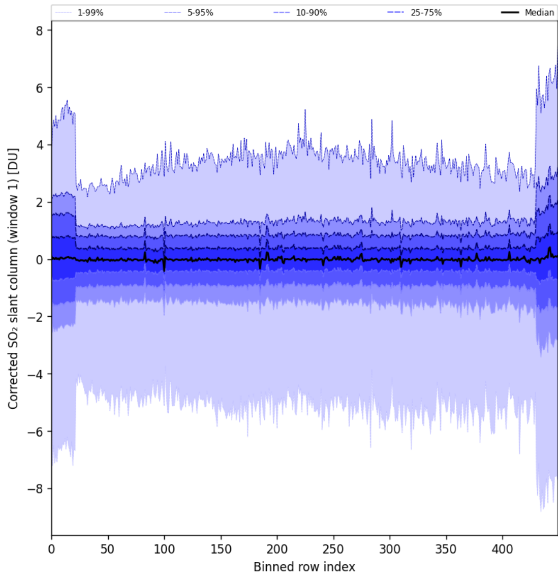
Figure 81: Along track statistics of “Corrected SO 2 slant column (window 1)” for 2024-11-14 to 2024-11-16
