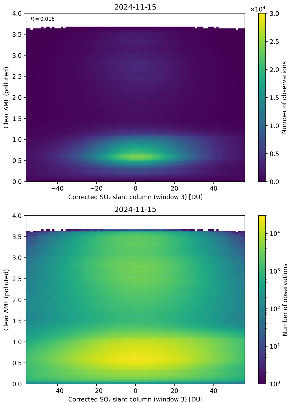
Figure 209: Scatter density plot of “Corrected SO 2 slant column (window 3)” against “Clear AMF (polluted)” for 2024-11-14 to 2024-11-16.
