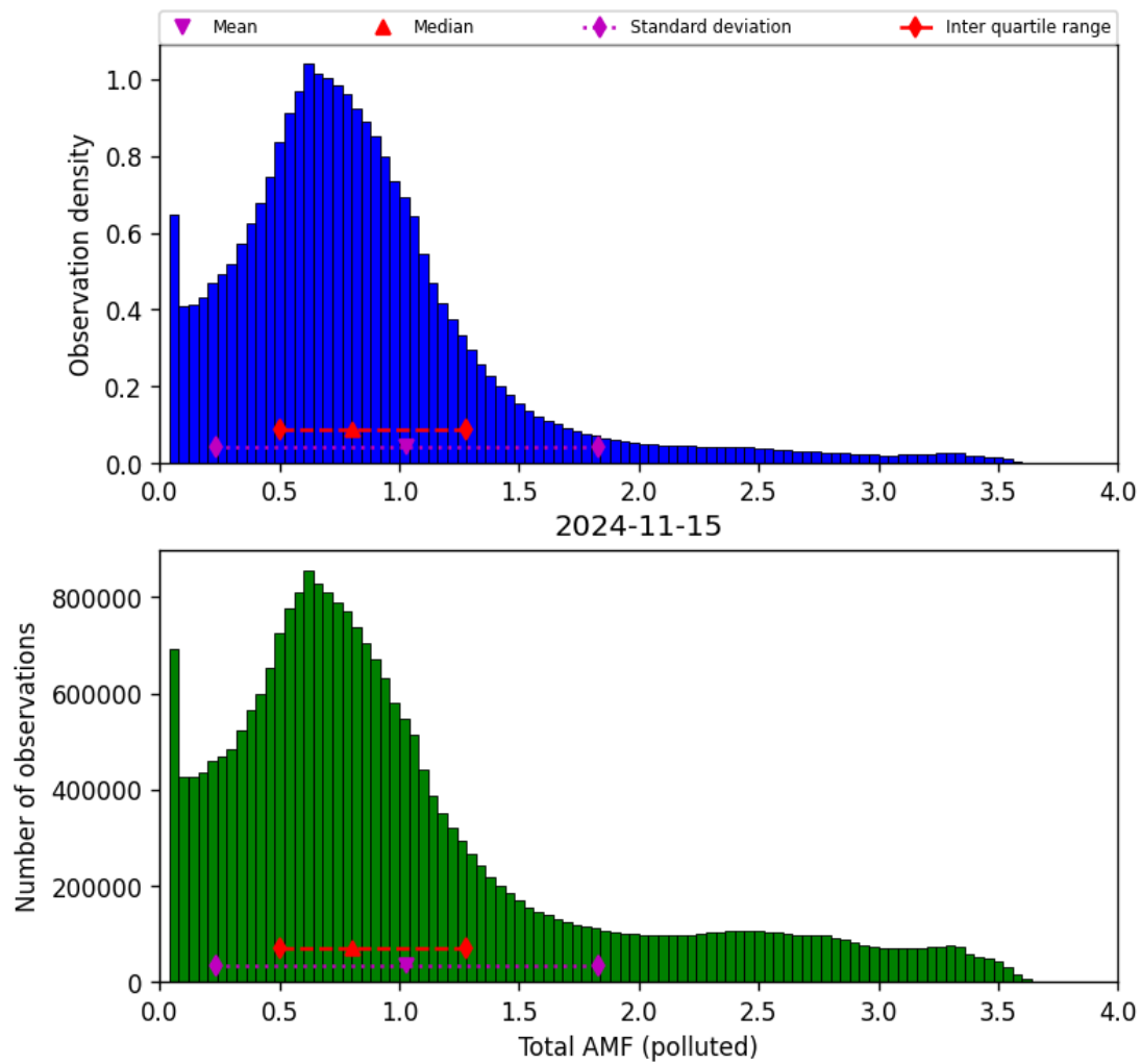
Figure 71: Histogram of “Total AMF (polluted)” for 2024-11-14 to 2024-11-16
