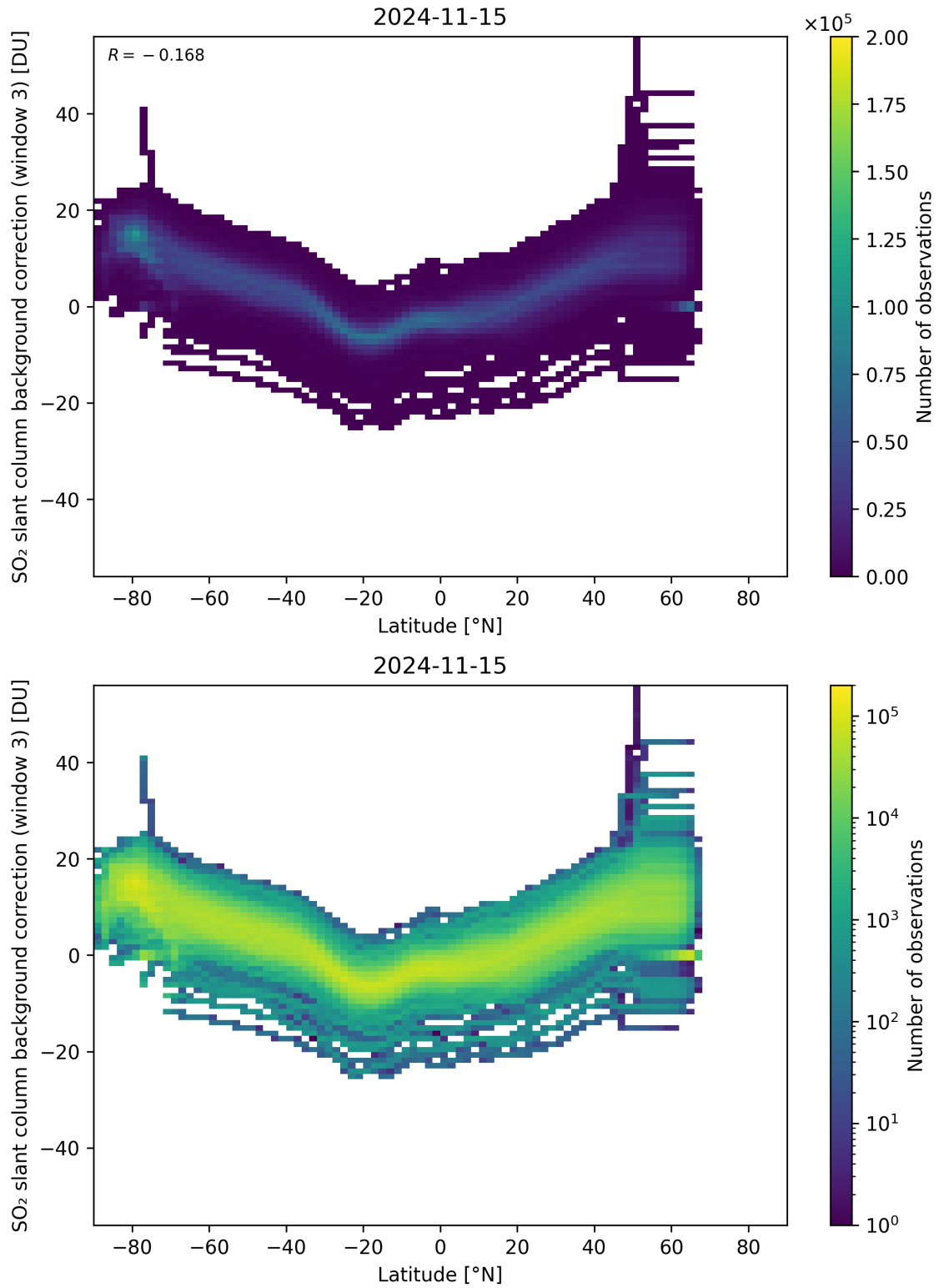
Figure 141: Scatter density plot of “Latitude” against “SO 2 slant column background correction (window 3)” for 2024-11-14 to 2024-11-16.
