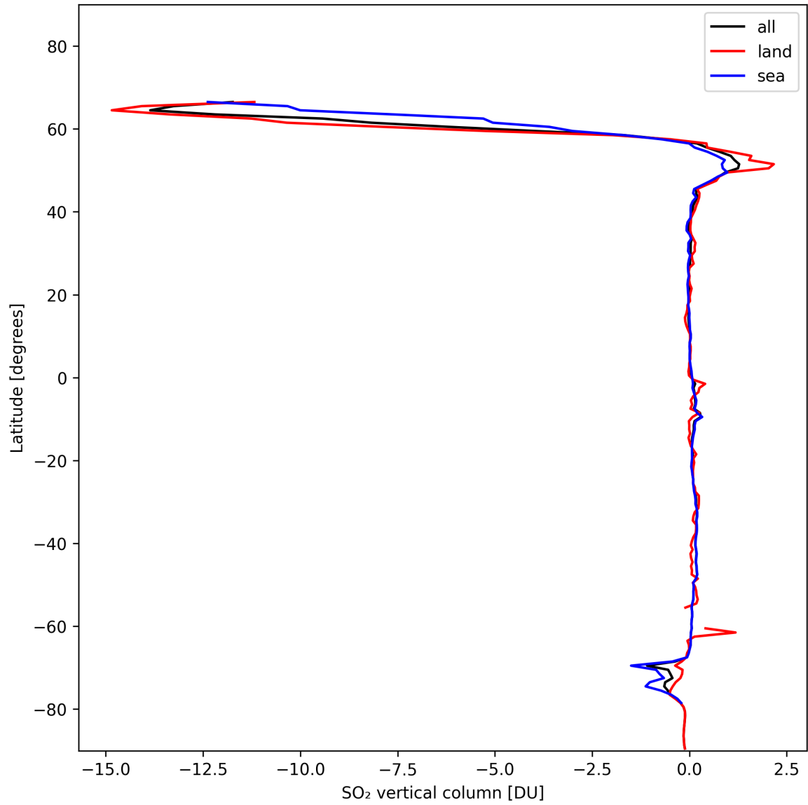
Figure 30: Zonal average of “SO 2 vertical column” for 2024-11-14 to 2024-11-16.
