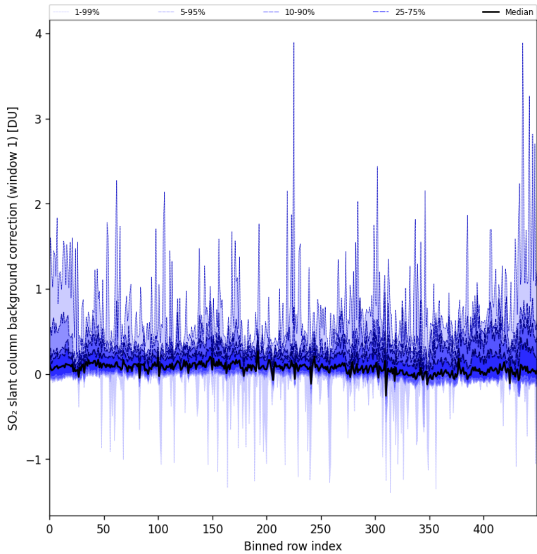
Figure 82: Along track statistics of “SO 2 slant column background correction (window 1)” for 2024-11-14 to 2024-11-16
