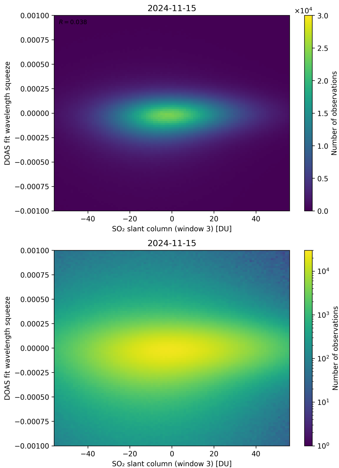
Figure 255: Scatter density plot of “SO 2 slant column (window 3)” against “DOAS fit wavelength squeeze” for 2024-11-14 to 2024-11-16.
