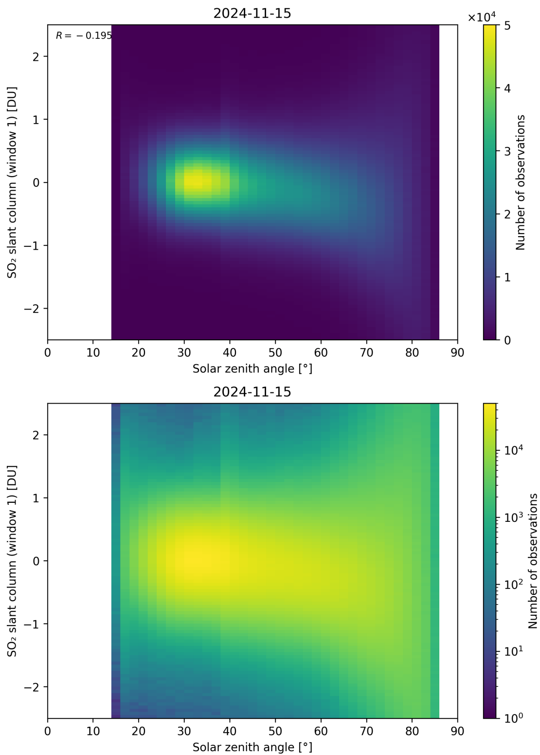
Figure 169: Scatter density plot of “Solar zenith angle” against “SO 2 slant column (window 1)” for 2024-11-14 to 2024-11-16.
