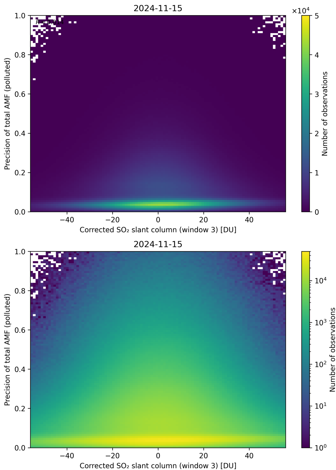
Figure 211: Scatter density plot of “Corrected SO 2 slant column (window 3)” against “Precision of total AMF (polluted)” for 2024-11-14 to 2024-11-16.
