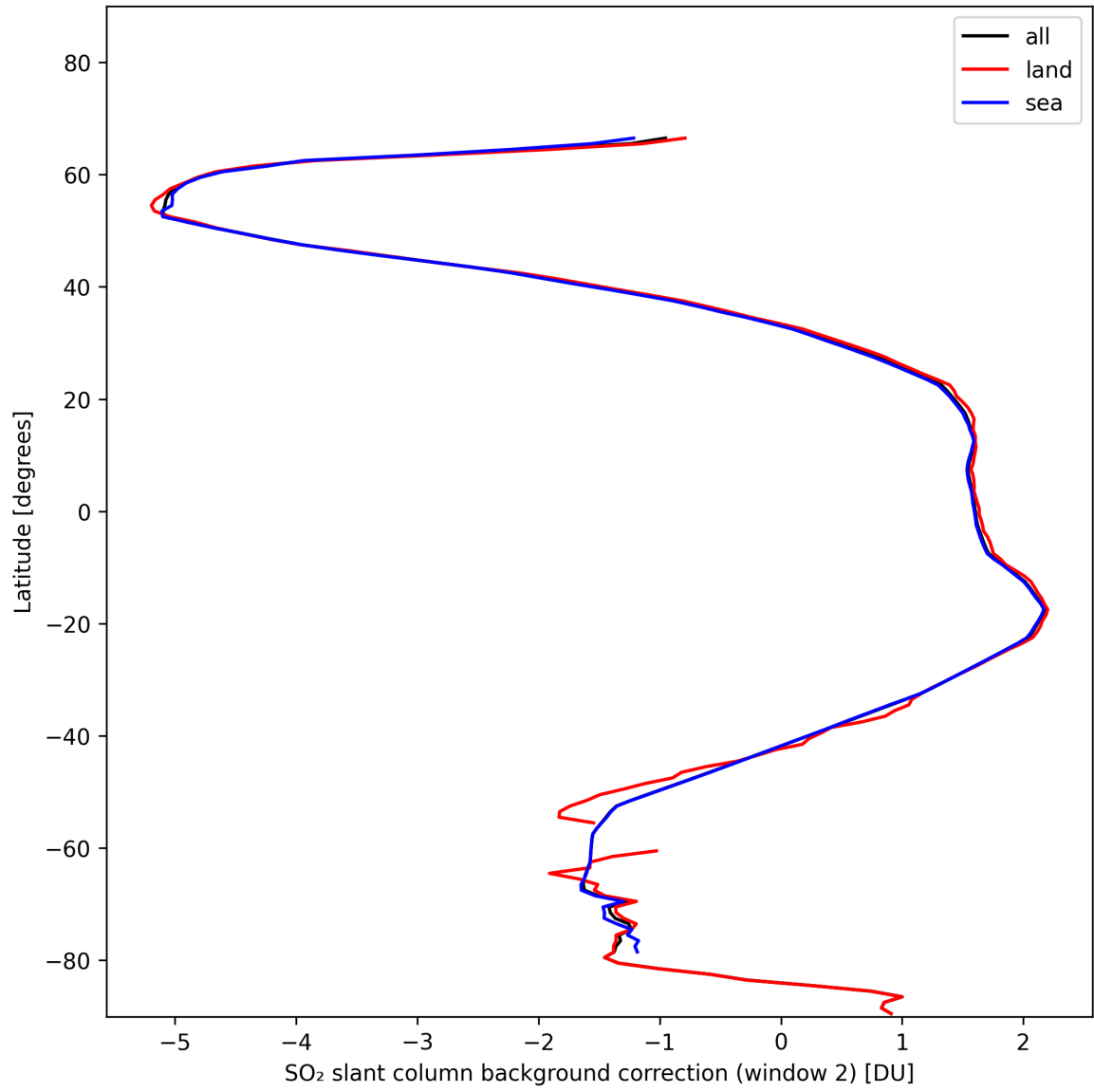
Figure 40: Zonal average of “SO 2 slant column background correction (window 2)” for 2024-11-14 to 2024-11-16.
