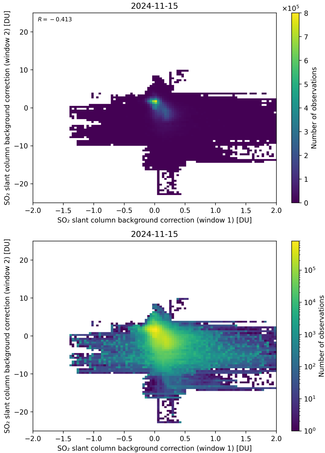
Figure 98: Scatter density plot of “SO 2 slant column background correction (window 1)” against “SO 2 slant column background correction (window 2)” for 2024-11-14 to 2024-11-16.
