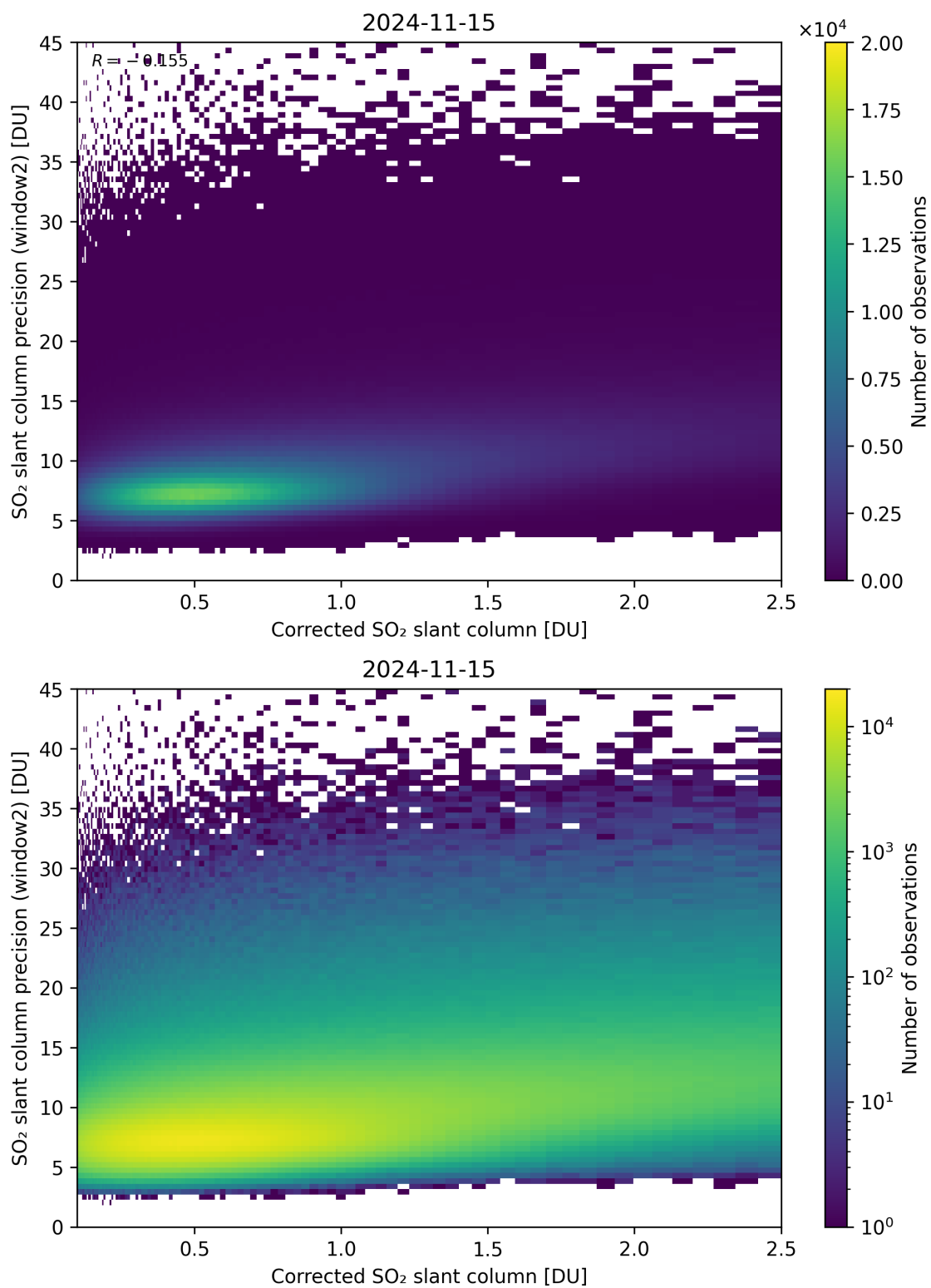
Figure 189: Scatter density plot of “Corrected SO 2 slant column” against “SO 2 slant column precision (window2)” for 2024-11-14 to 2024-11-16.
