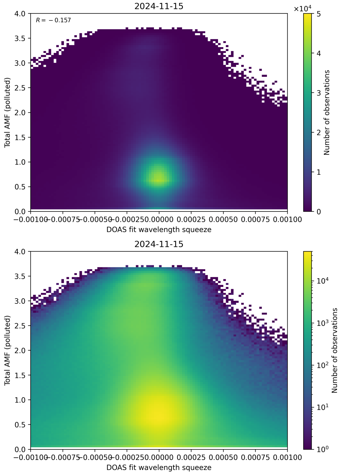
Figure 134: Scatter density plot of “DOAS fit wavelength squeeze” against “Total AMF (polluted)” for 2024-11-14 to 2024-11-16.
