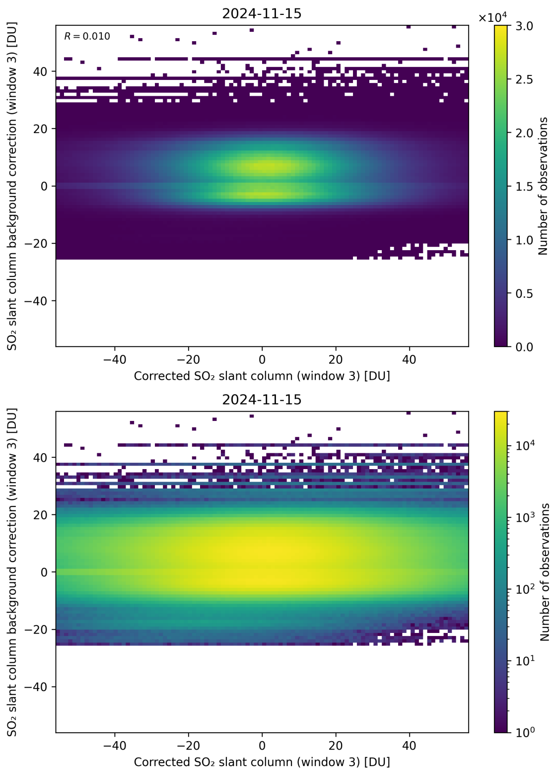
Figure 205: Scatter density plot of “Corrected SO 2 slant column (window 3)” against “SO 2 slant column background correction (window 3)” for 2024-11-14 to 2024-11-16.
