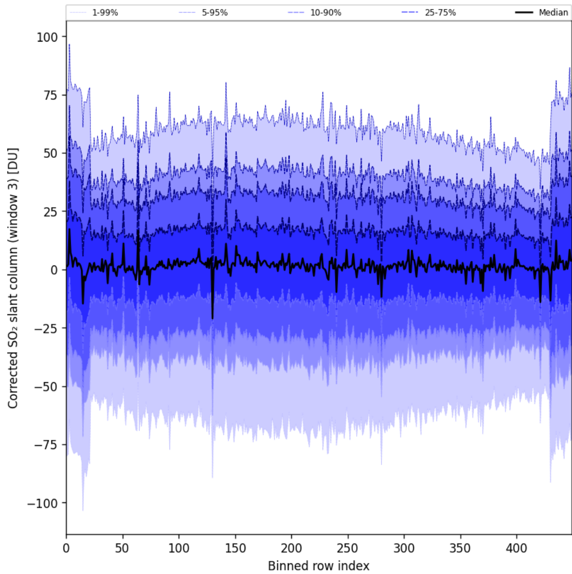
Figure 89: Along track statistics of “Corrected SO 2 slant column (window 3)” for 2024-11-14 to 2024-11-16
