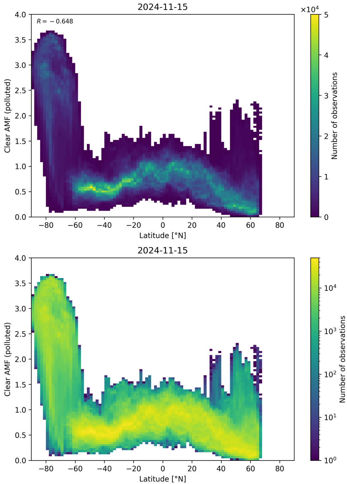
Figure 145: Scatter density plot of “Latitude” against “Clear AMF (polluted)” for 2024-11-14 to 2024-11-16.
