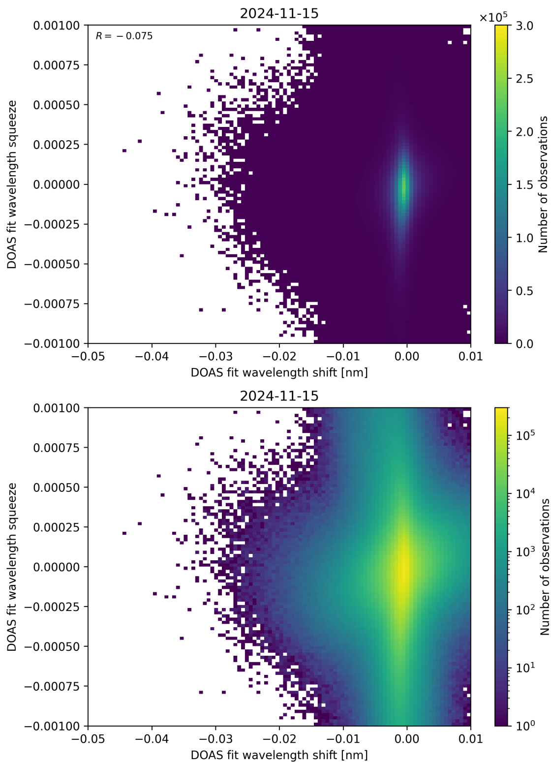
Figure 127: Scatter density plot of “DOAS fit wavelength shift” against “DOAS fit wavelength squeeze” for 2024-11-14 to 2024-11-16.
