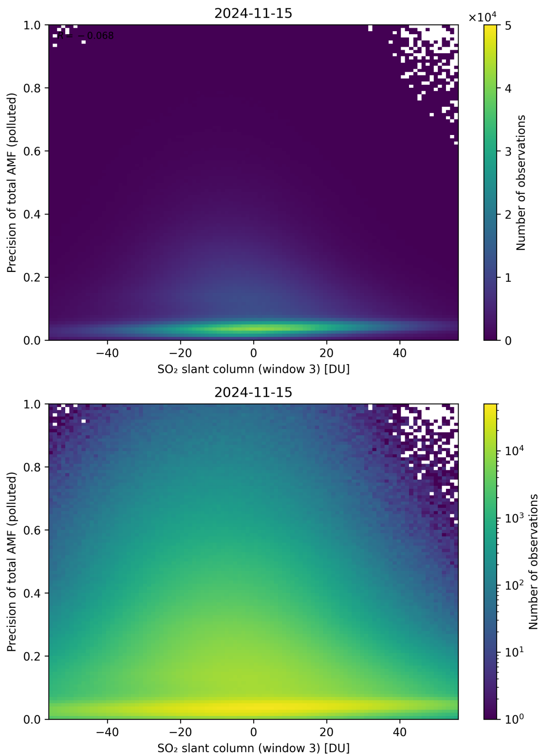
Figure 269: Scatter density plot of “SO 2 slant column (window 3)” against “Precision of total AMF (polluted)” for 2024-11-14 to 2024-11-16.
