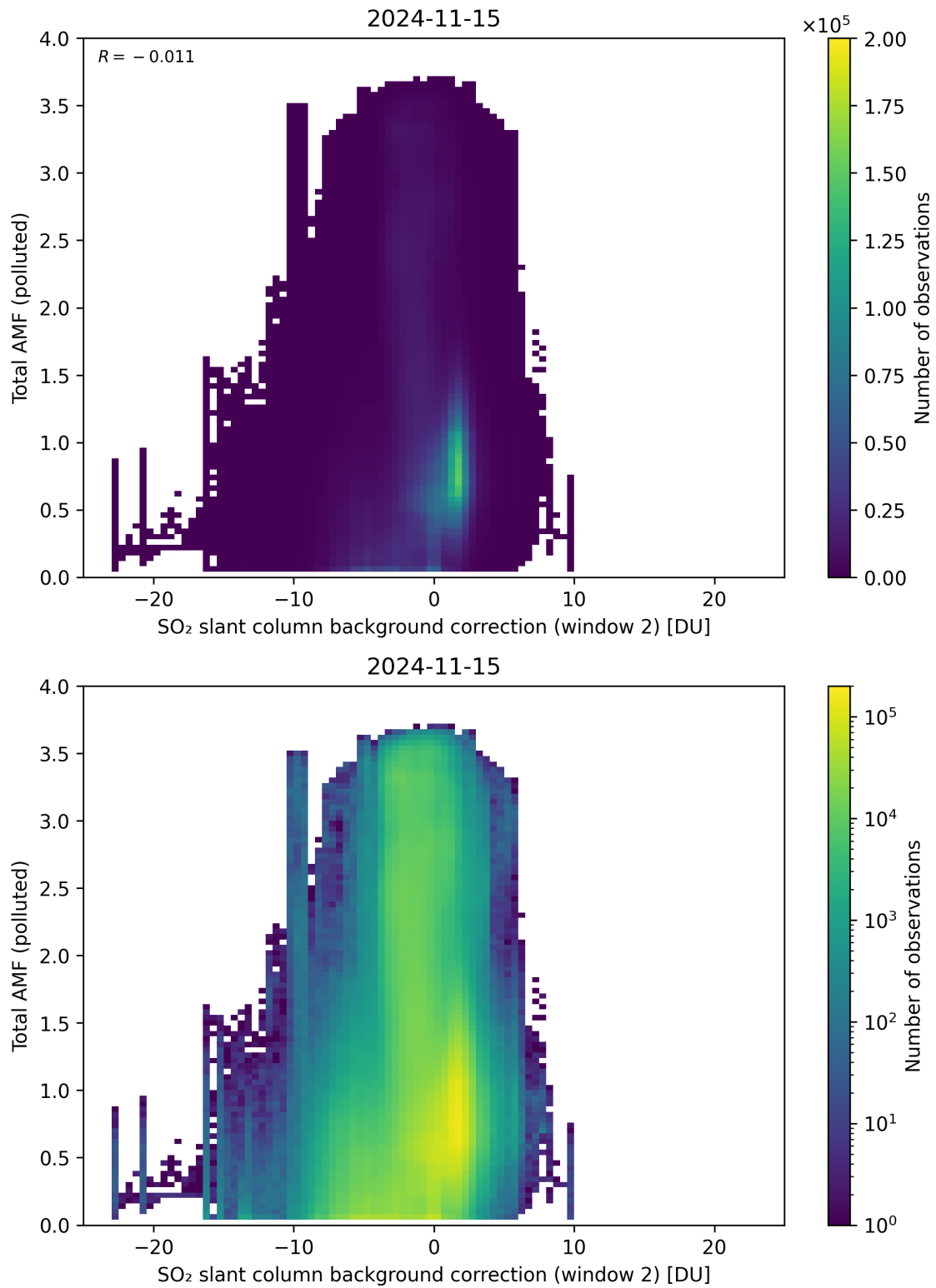
Figure 119: Scatter density plot of “SO 2 slant column background correction (window 2)” against “Total AMF (polluted)” for 2024-11-14 to 2024-11-16.
