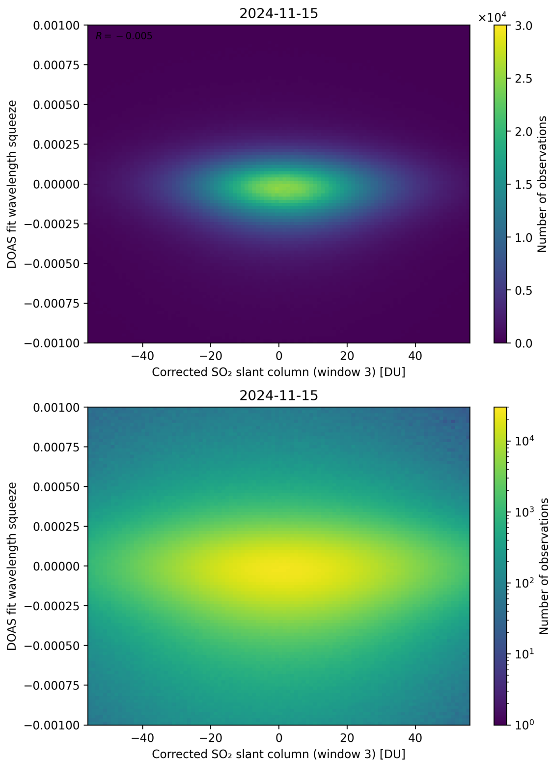
Figure 207: Scatter density plot of “Corrected SO 2 slant column (window 3)” against “DOAS fit wavelength squeeze” for 2024-11-14 to 2024-11-16.
