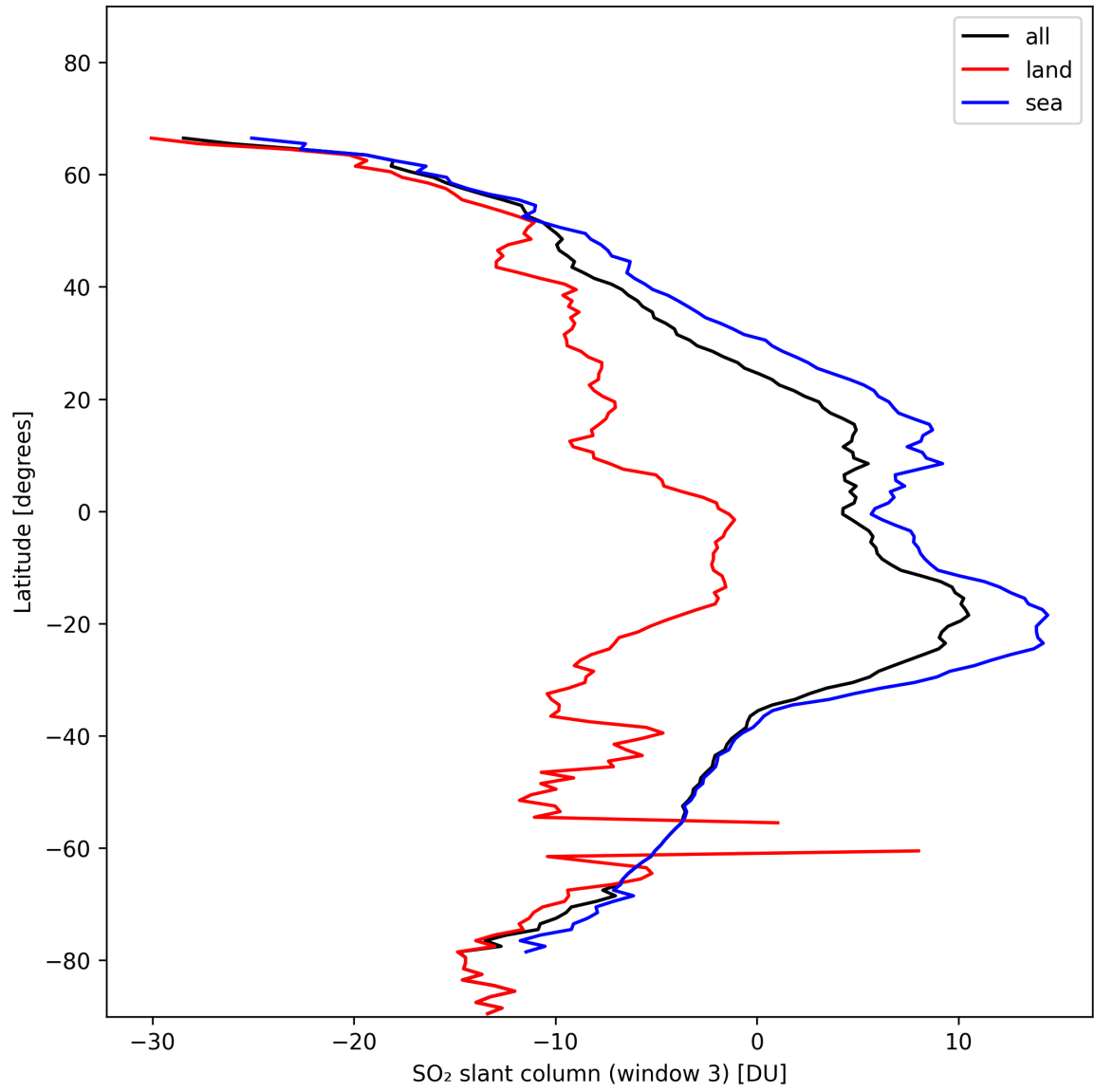
Figure 41: Zonal average of “SO 2 slant column (window 3)” for 2024-11-14 to 2024-11-16.
