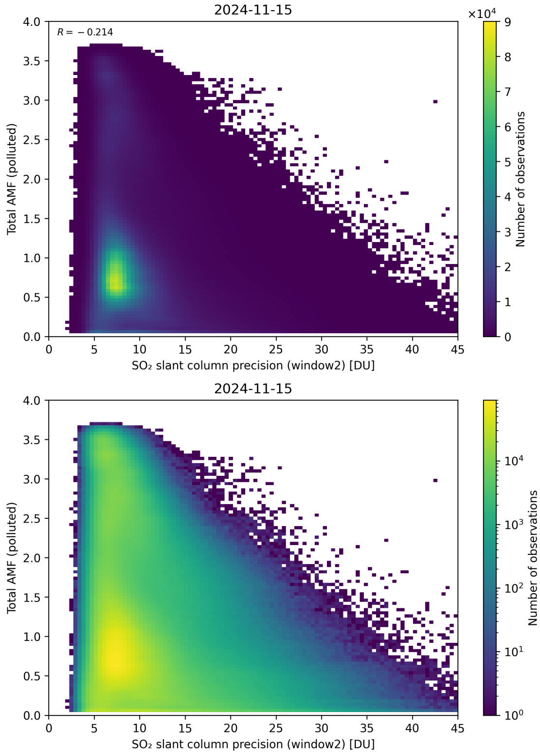
Figure 251: Scatter density plot of “SO 2 slant column precision (window2)” against “Total AMF (polluted)” for 2024-11-14 to 2024-11-16.
