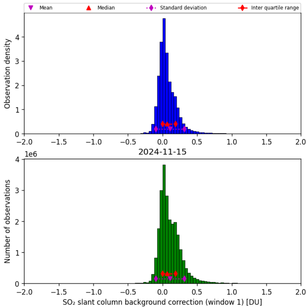
Figure 59: Histogram of “SO 2 slant column background correction (window 1)” for 2024-11-14 to 2024-11-16
