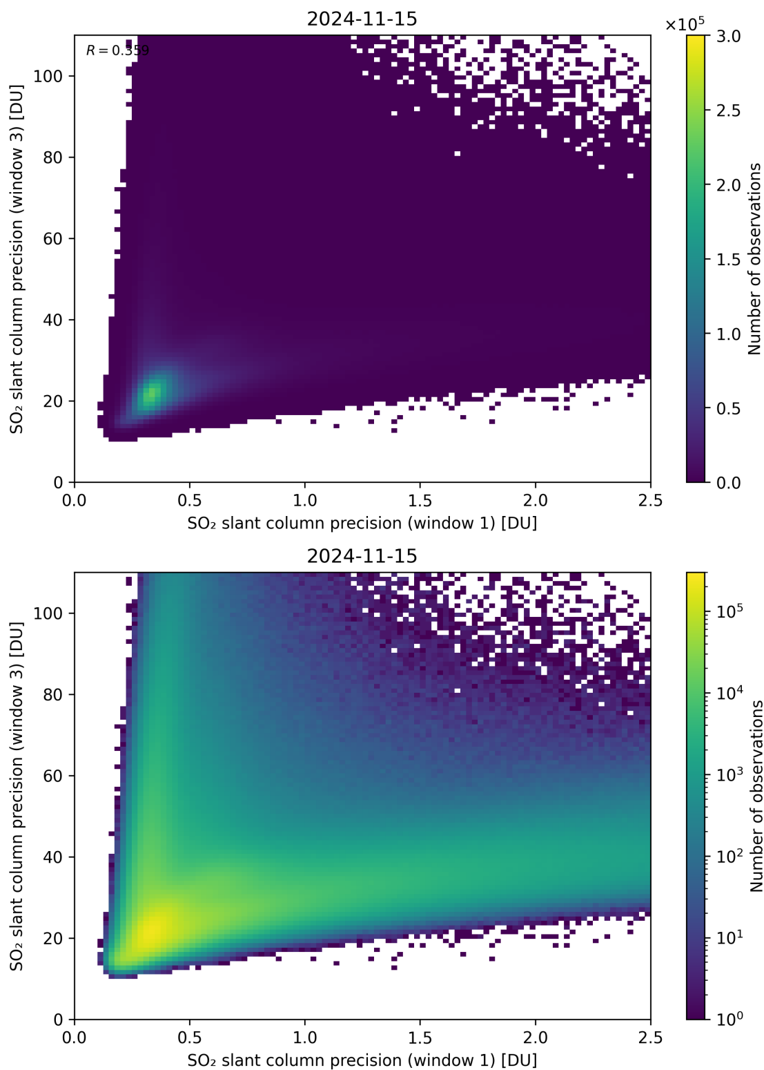
Figure 229: Scatter density plot of “SO 2 slant column precision (window 1)” against “SO 2 slant column precision (window 3)” for 2024-11-14 to 2024-11-16.
