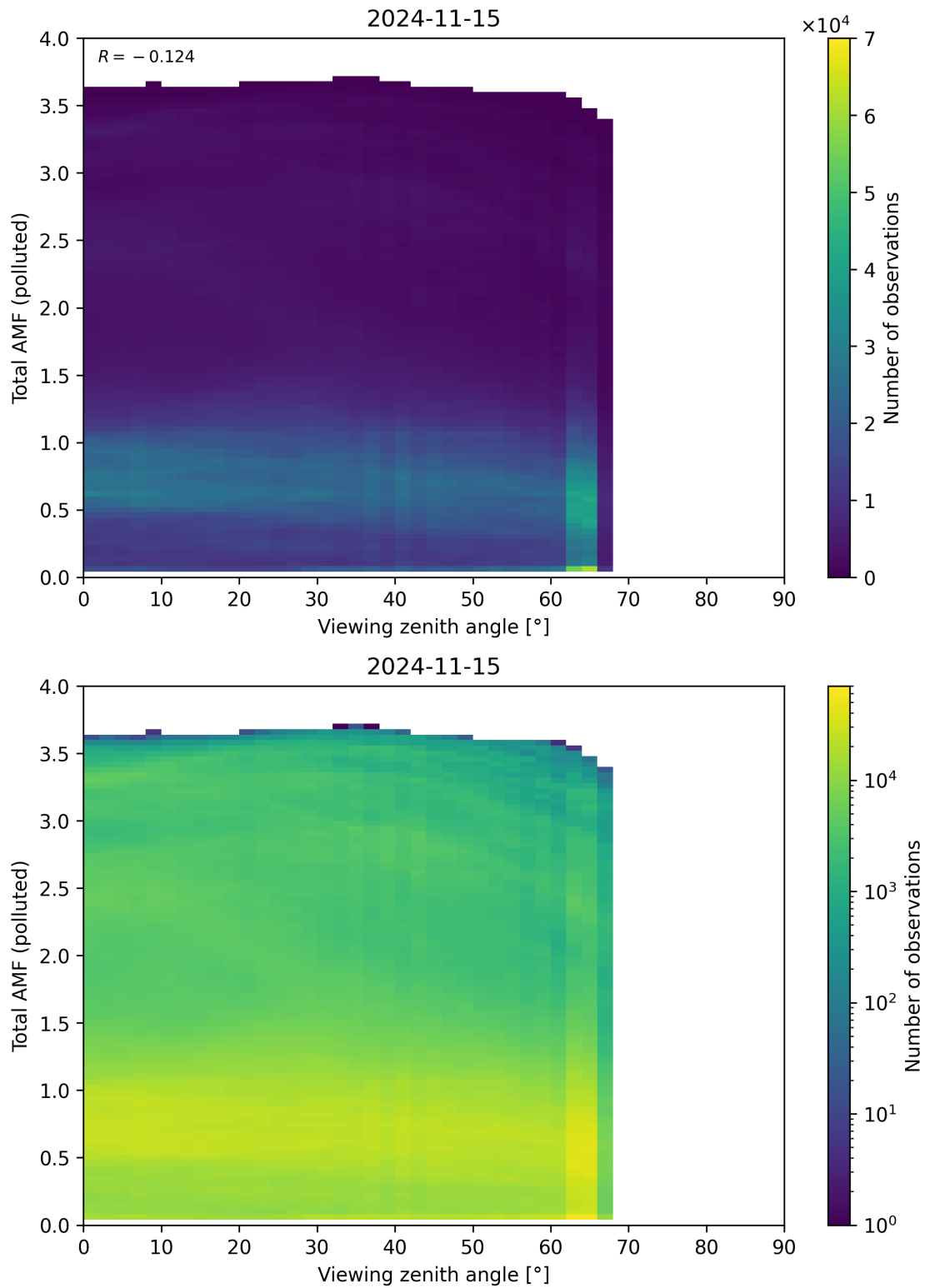
Figure 325: Scatter density plot of “Viewing zenith angle” against “Total AMF (polluted)” for 2024-11-14 to 2024-11-16.
