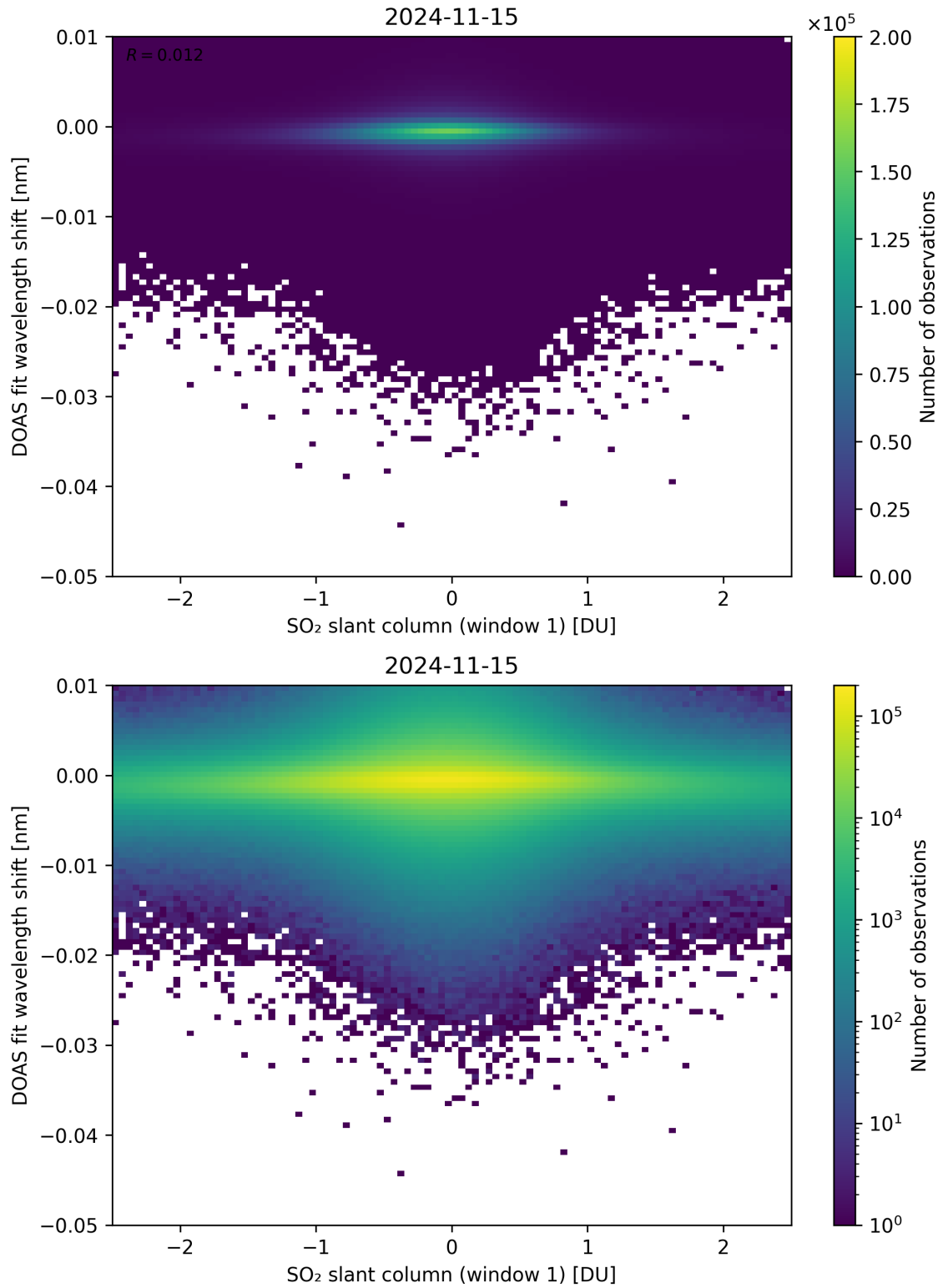
Figure 215: Scatter density plot of “SO 2 slant column (window 1)” against “DOAS fit wavelength shift” for 2024-11-14 to 2024-11-16.
