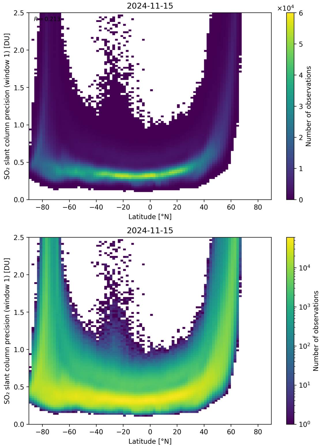
Figure 150: Scatter density plot of “Latitude” against “SO 2 slant column precision (window 1)” for 2024-11-14 to 2024-11-16.
