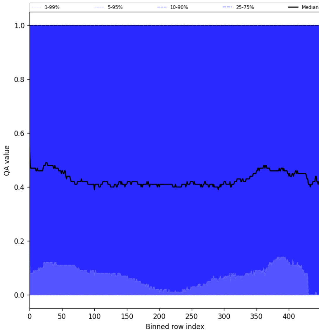
Figure 75: Along track statistics of “QA value” for 2024-11-14 to 2024-11-16
