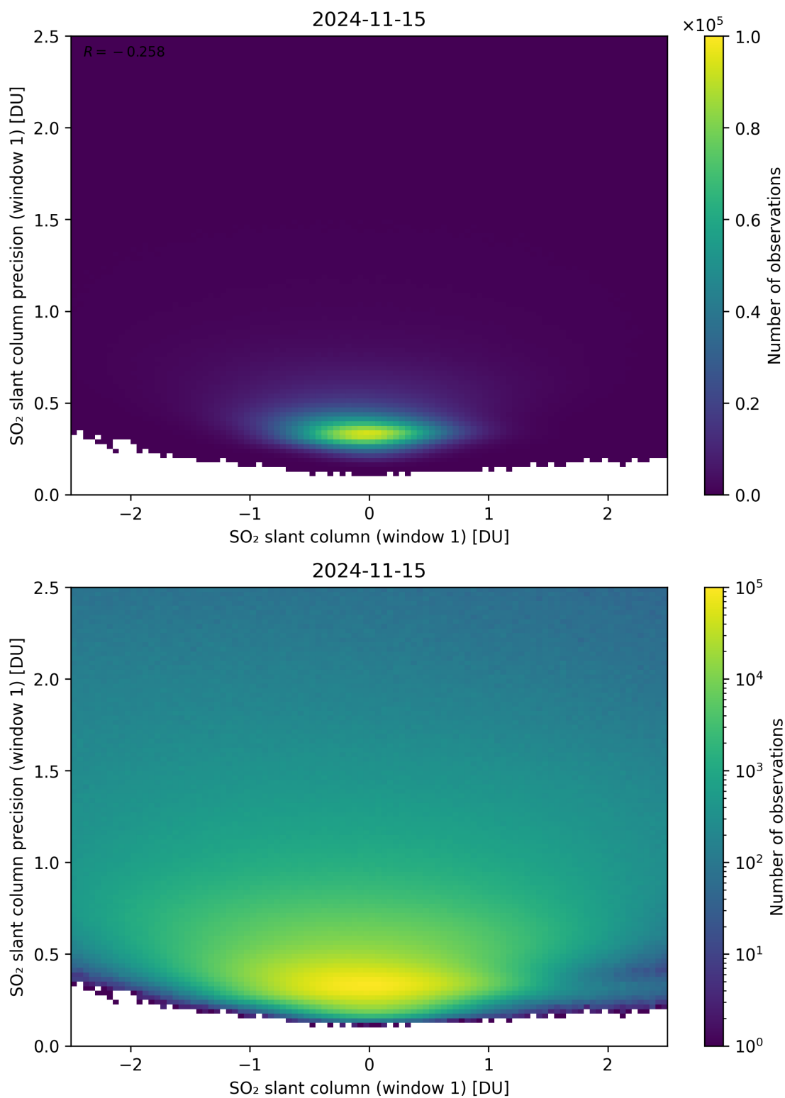
Figure 235: Scatter density plot of “SO 2 slant column (window 1)” against “SO 2 slant column precision (window 1)” for 2024-11-14 to 2024-11-16.
