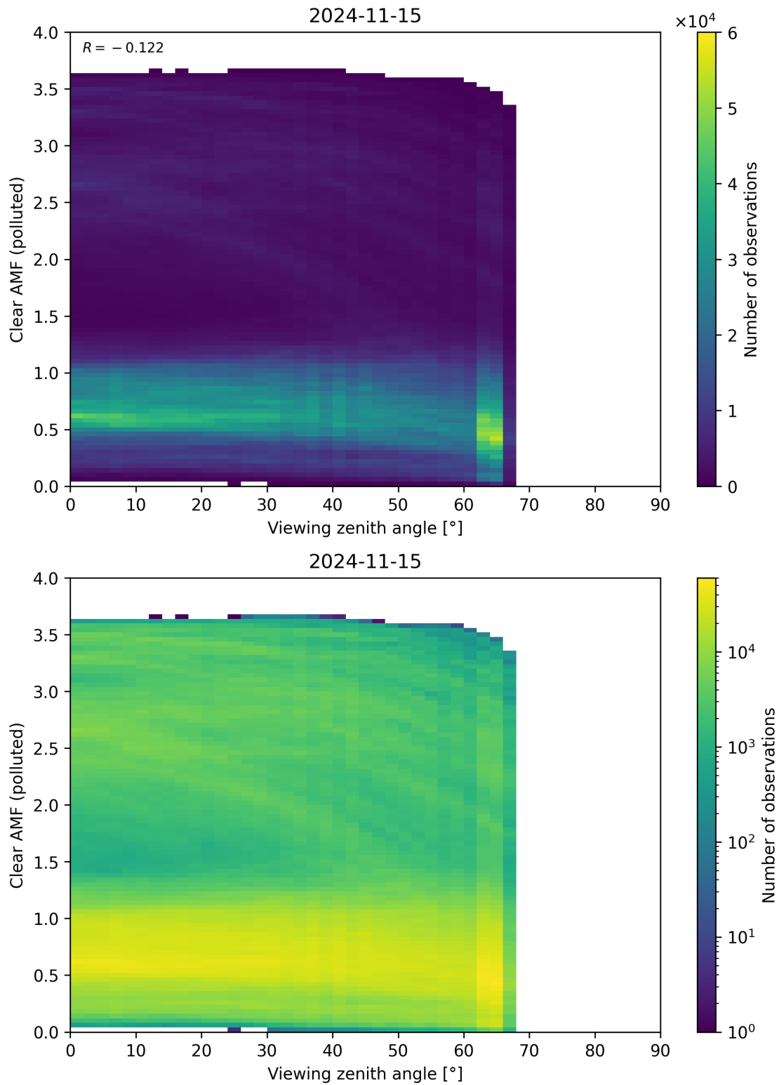
Figure 316: Scatter density plot of “Viewing zenith angle” against “Clear AMF (polluted)” for 2024-11-14 to 2024-11-16.
