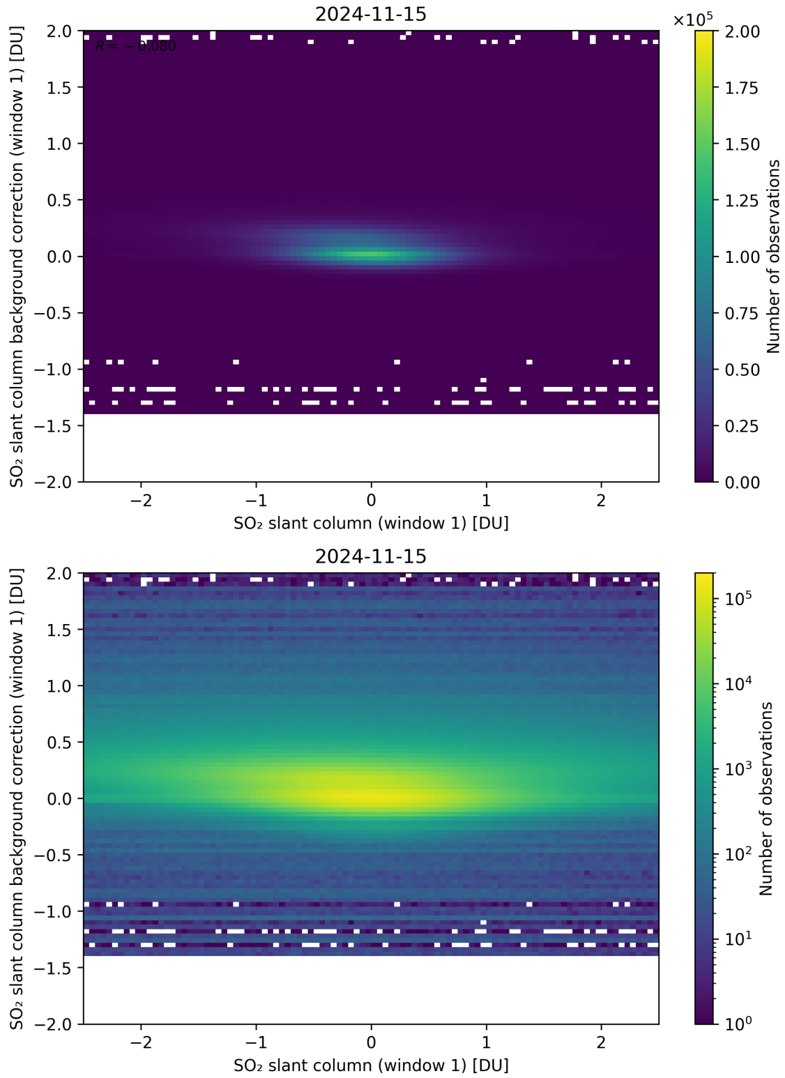
Figure 212: Scatter density plot of “SO 2 slant column (window 1)” against “SO 2 slant column background correction (window 1)” for 2024-11-14 to 2024-11-16.
