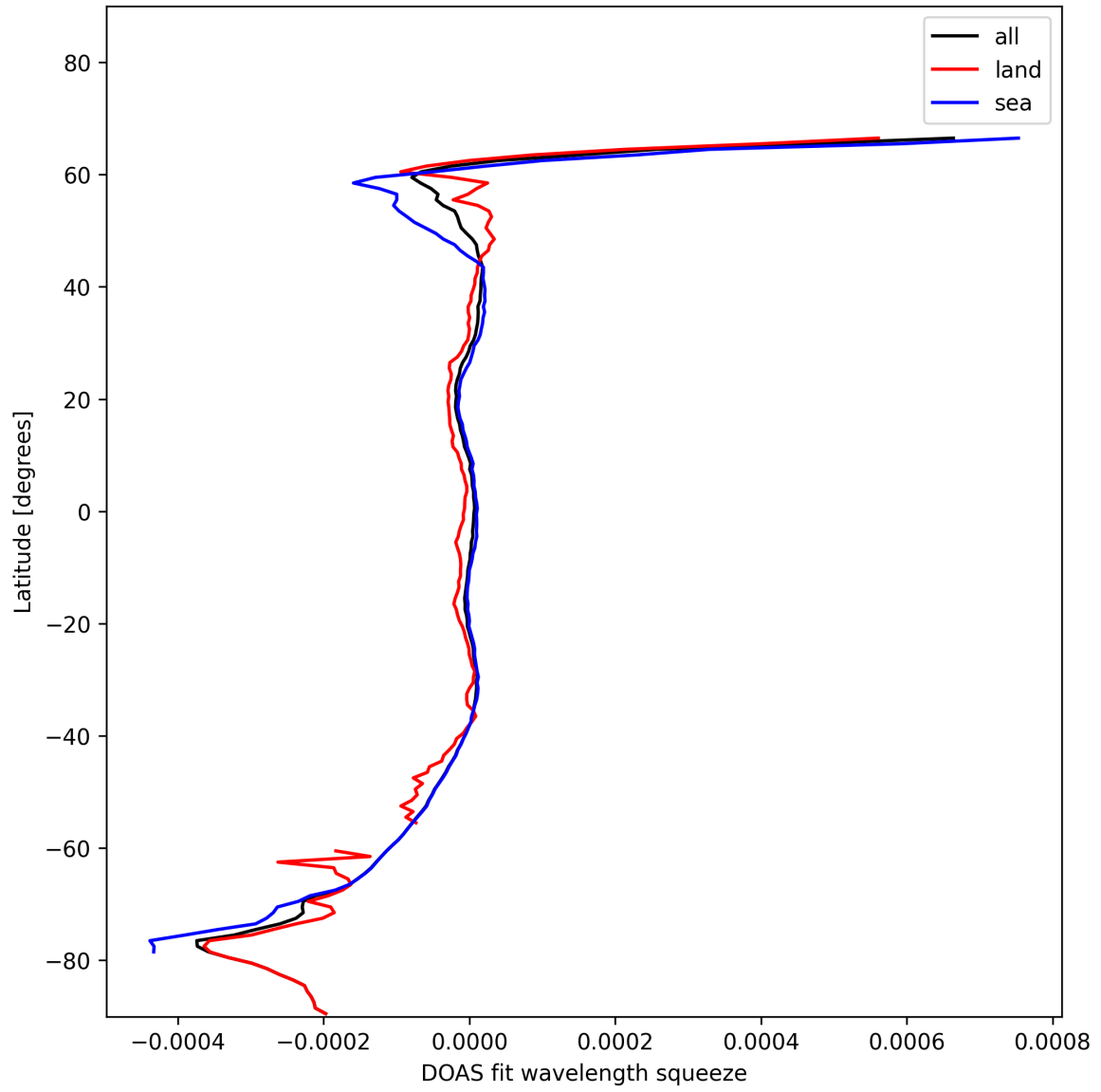
Figure 46: Zonal average of “DOAS fit wavelength squeeze” for 2024-11-14 to 2024-11-16.
