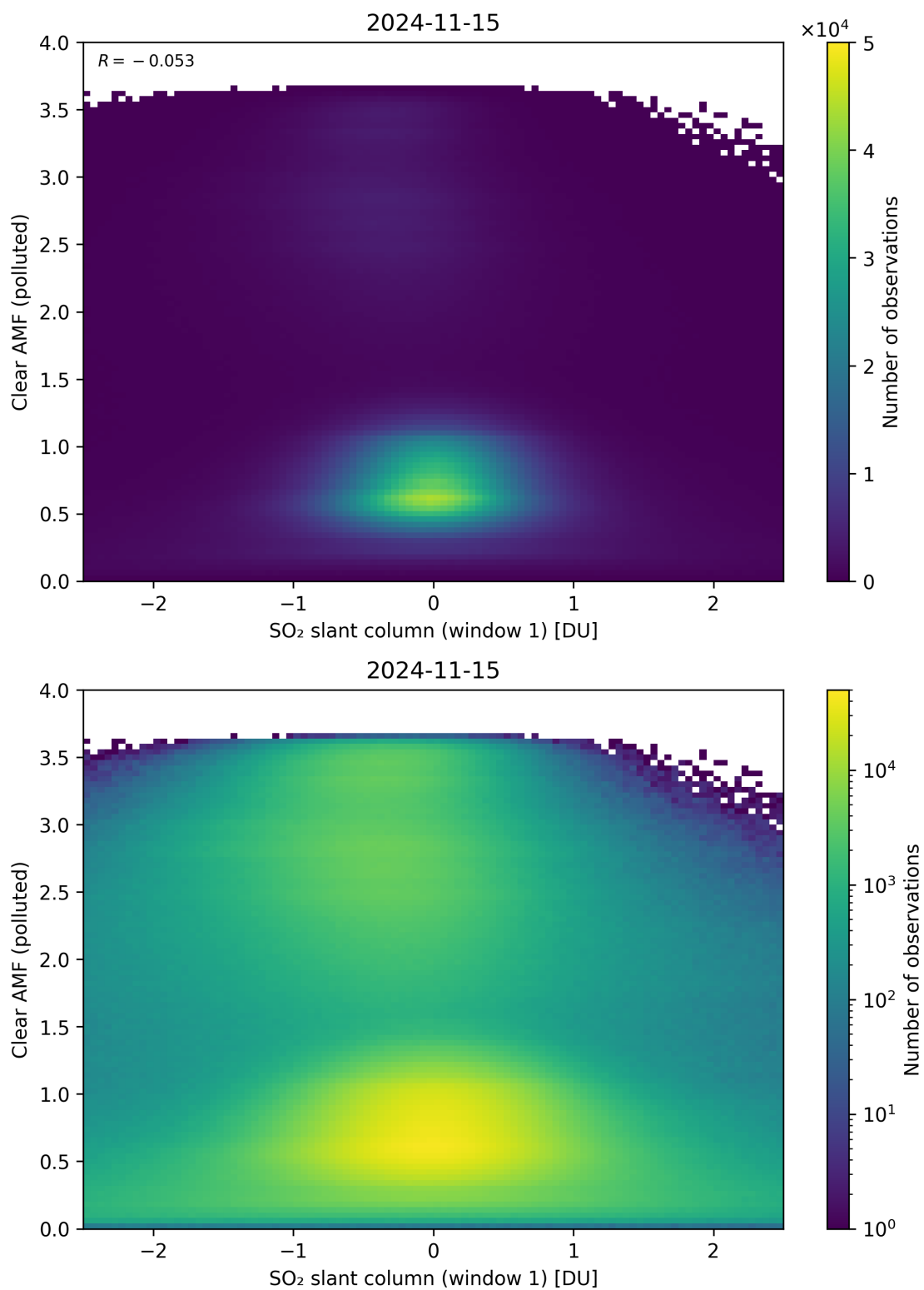
Figure 232: Scatter density plot of “SO 2 slant column (window 1)” against “Clear AMF (polluted)” for 2024-11-14 to 2024-11-16.
