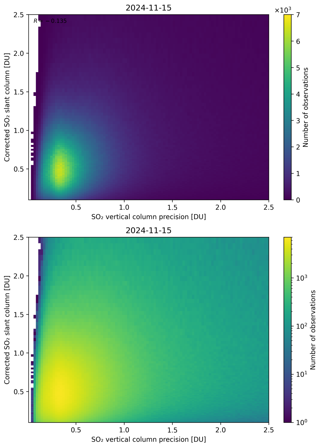
Figure 286: Scatter density plot of “SO 2 vertical column precision” against “Corrected SO 2 slant column” for 2024-11-14 to 2024-11-16.
