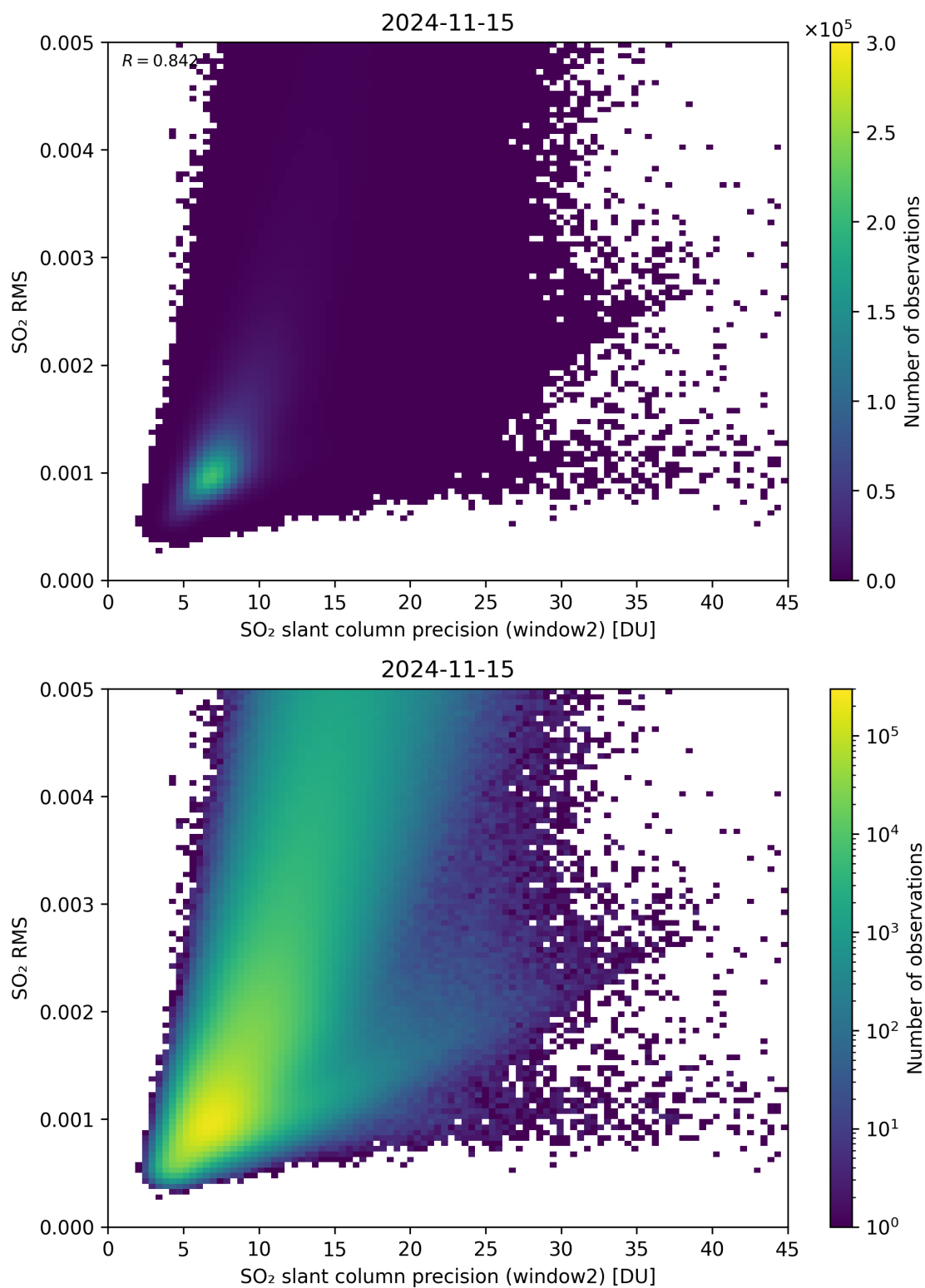
Figure 245: Scatter density plot of “SO 2 slant column precision (window2)” against “SO 2 RMS” for 2024-11-14 to 2024-11-16.
