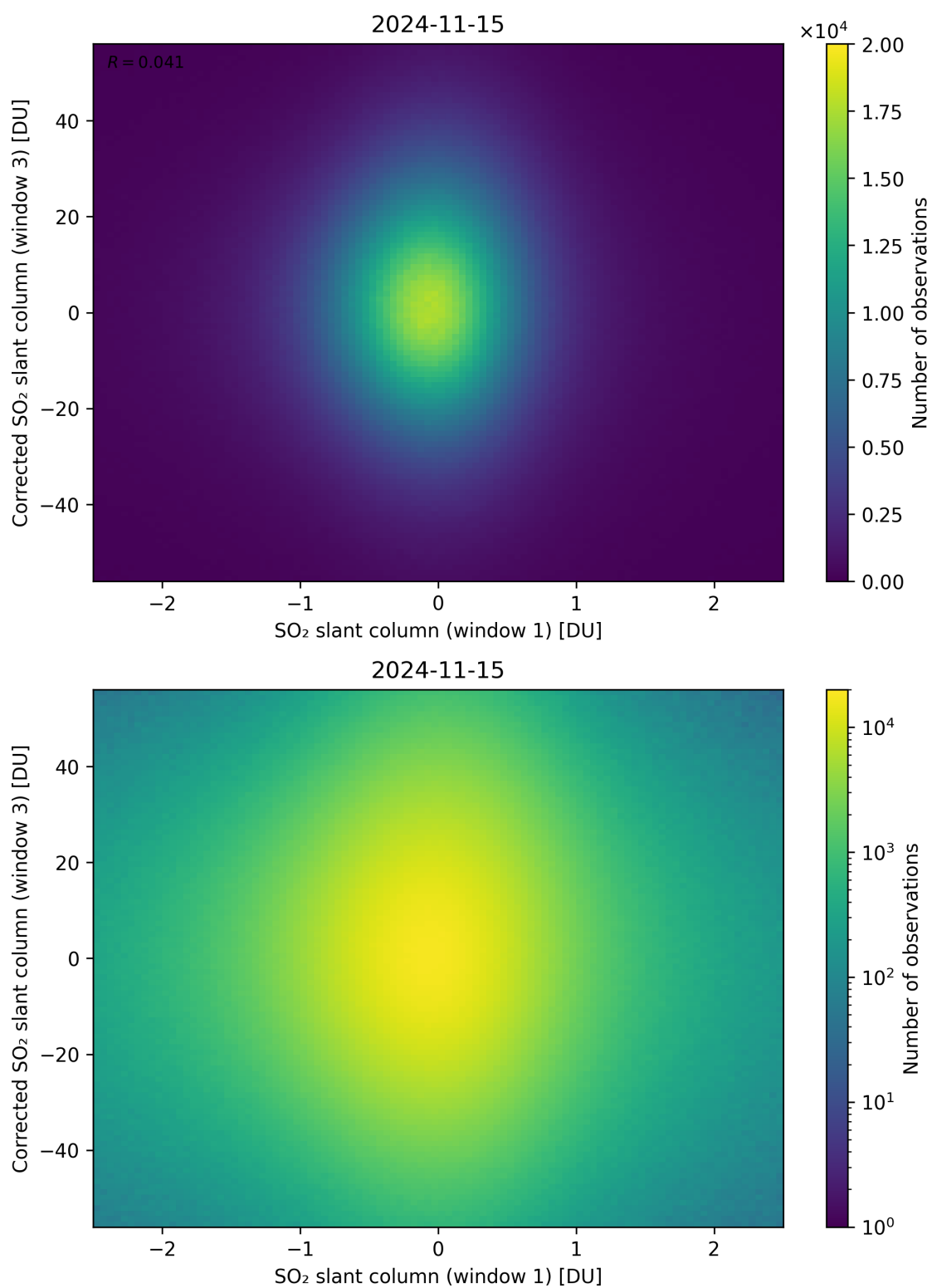
Figure 234: Scatter density plot of “SO 2 slant column (window 1)” against “Corrected SO 2 slant column (window 3)” for 2024-11-14 to 2024-11-16.
