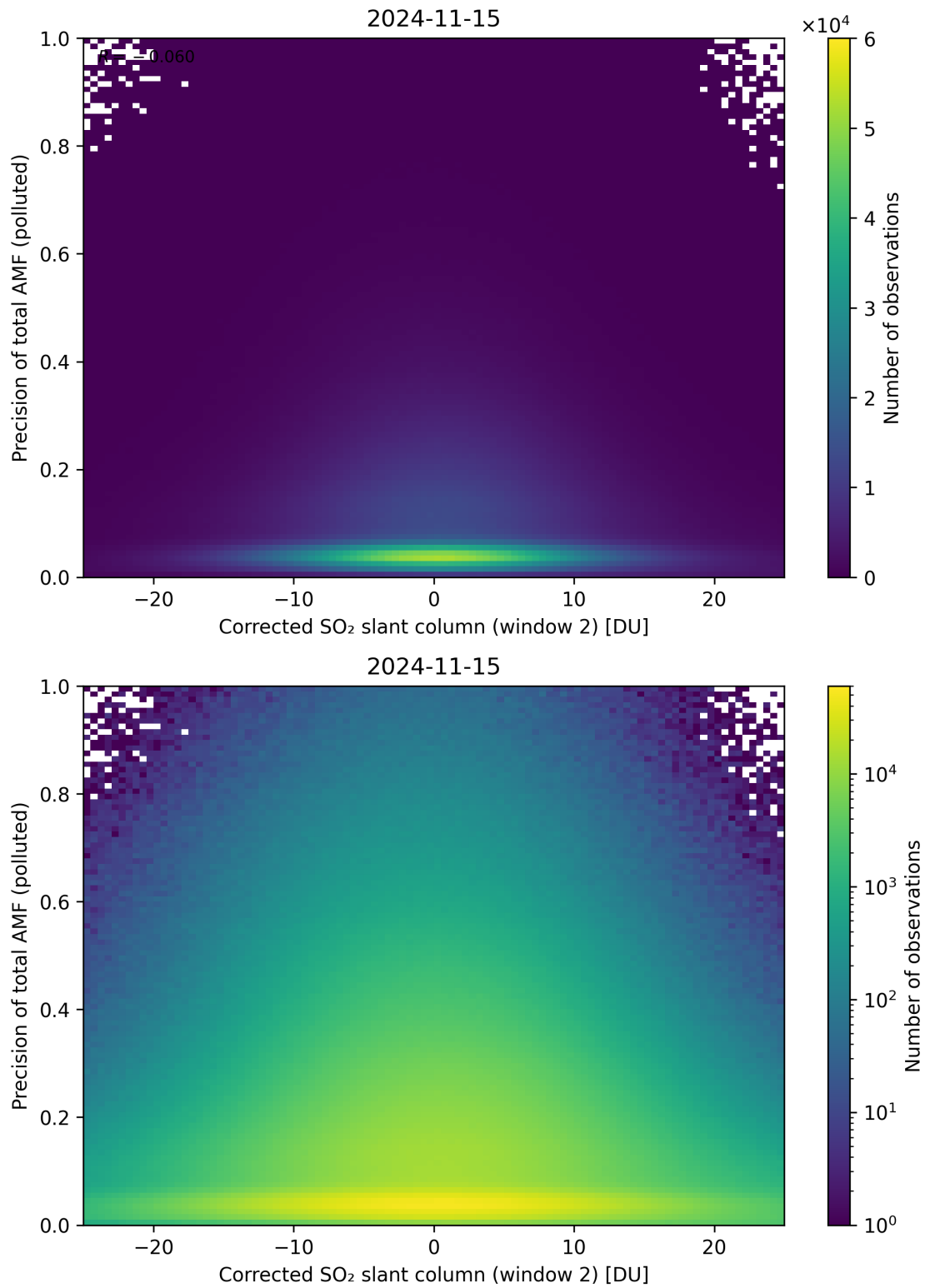
Figure 204: Scatter density plot of “Corrected SO 2 slant column (window 2)” against “Precision of total AMF (polluted)” for 2024-11-14 to 2024-11-16.
