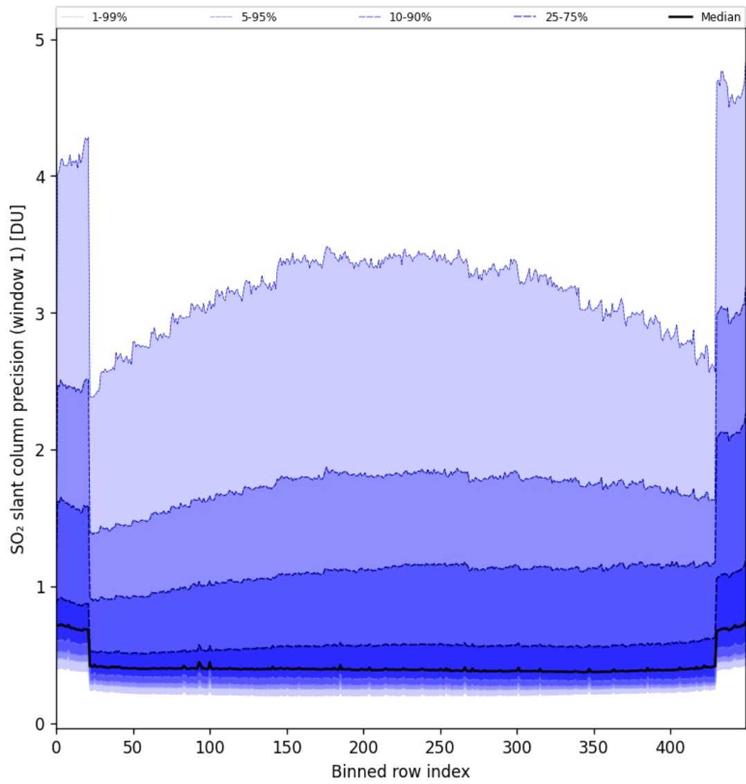
Figure 80: Along track statistics of “SO 2 slant column precision (window 1)” for 2024-11-14 to 2024-11-16
