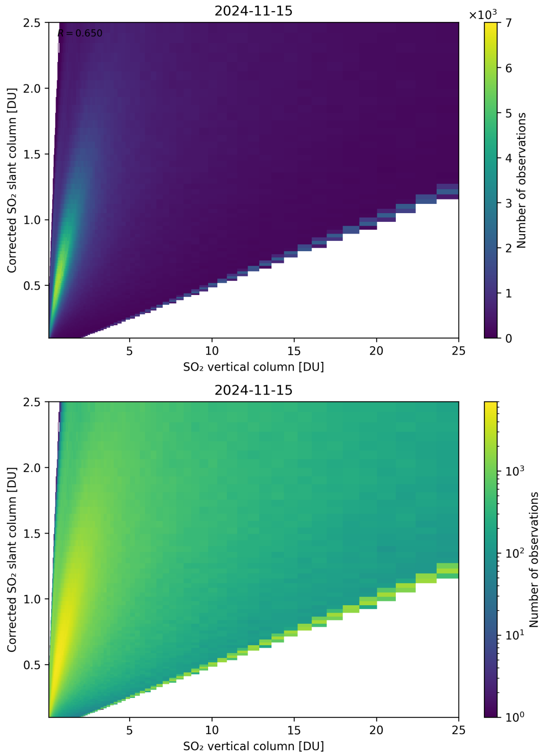
Figure 297: Scatter density plot of “SO 2 vertical column” against “Corrected SO 2 slant column” for 2024-11-14 to 2024-11-16.
