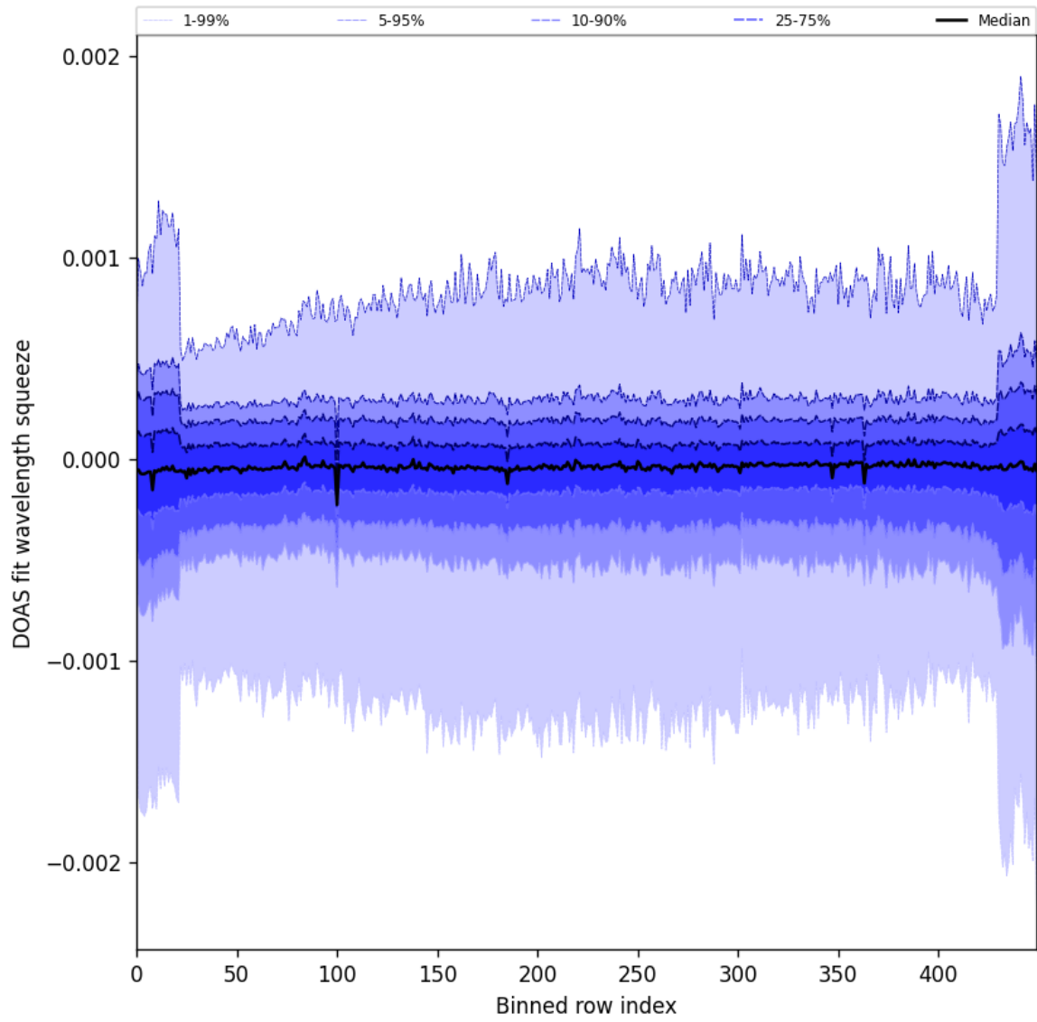
Figure 92: Along track statistics of “DOAS fit wavelength squeeze” for 2024-11-14 to 2024-11-16
