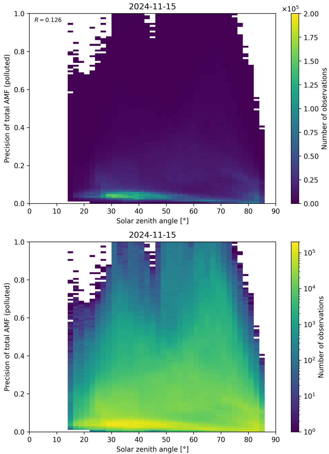
Figure 175: Scatter density plot of “Solar zenith angle” against “Precision of total AMF (polluted)” for 2024-11-14 to 2024-11-16.
