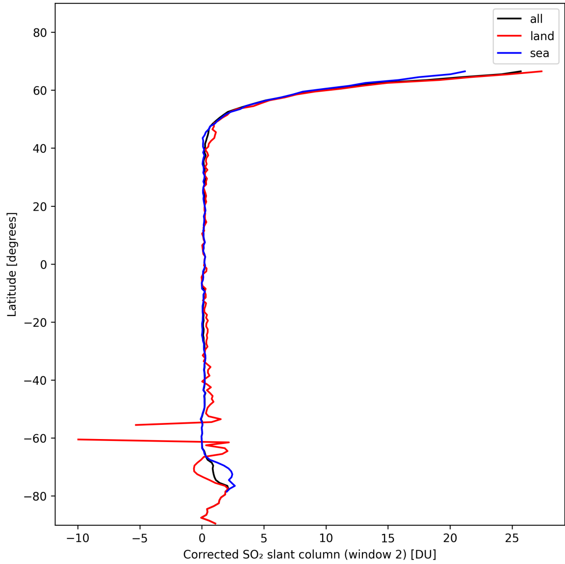
Figure 39: Zonal average of “Corrected SO 2 slant column (window 2)” for 2024-11-14 to 2024-11-16.
