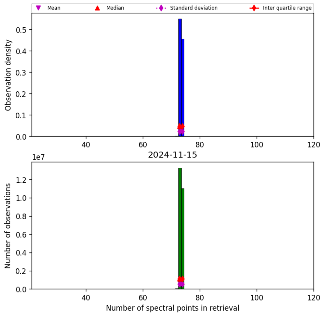
Figure 74: Histogram of “Number of spectral points in retrieval” for 2024-11-14 to 2024-11-16
