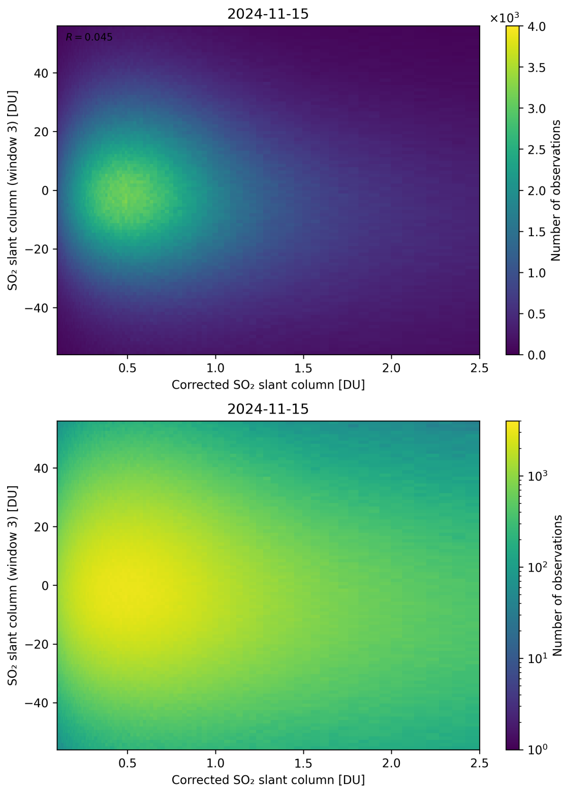
Figure 190: Scatter density plot of “Corrected SO 2 slant column” against “SO 2 slant column (window 3)” for 2024-11-14 to 2024-11-16.
