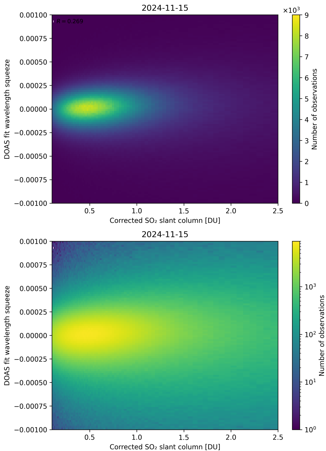
Figure 182: Scatter density plot of “Corrected SO 2 slant column” against “DOAS fit wavelength squeeze” for 2024-11-14 to 2024-11-16.
