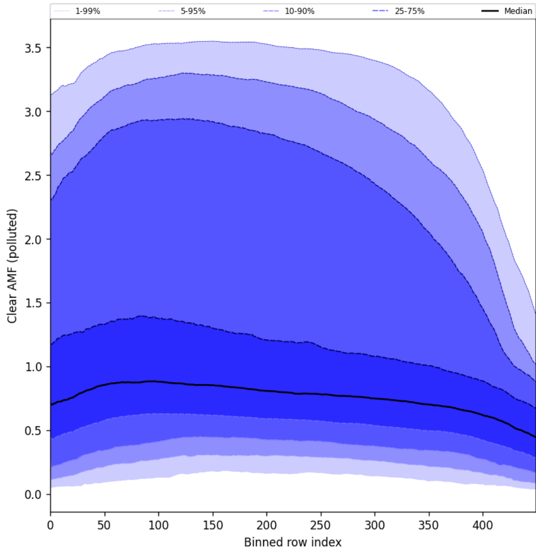
Figure 96: Along track statistics of “Clear AMF (polluted)” for 2024-11-14 to 2024-11-16
