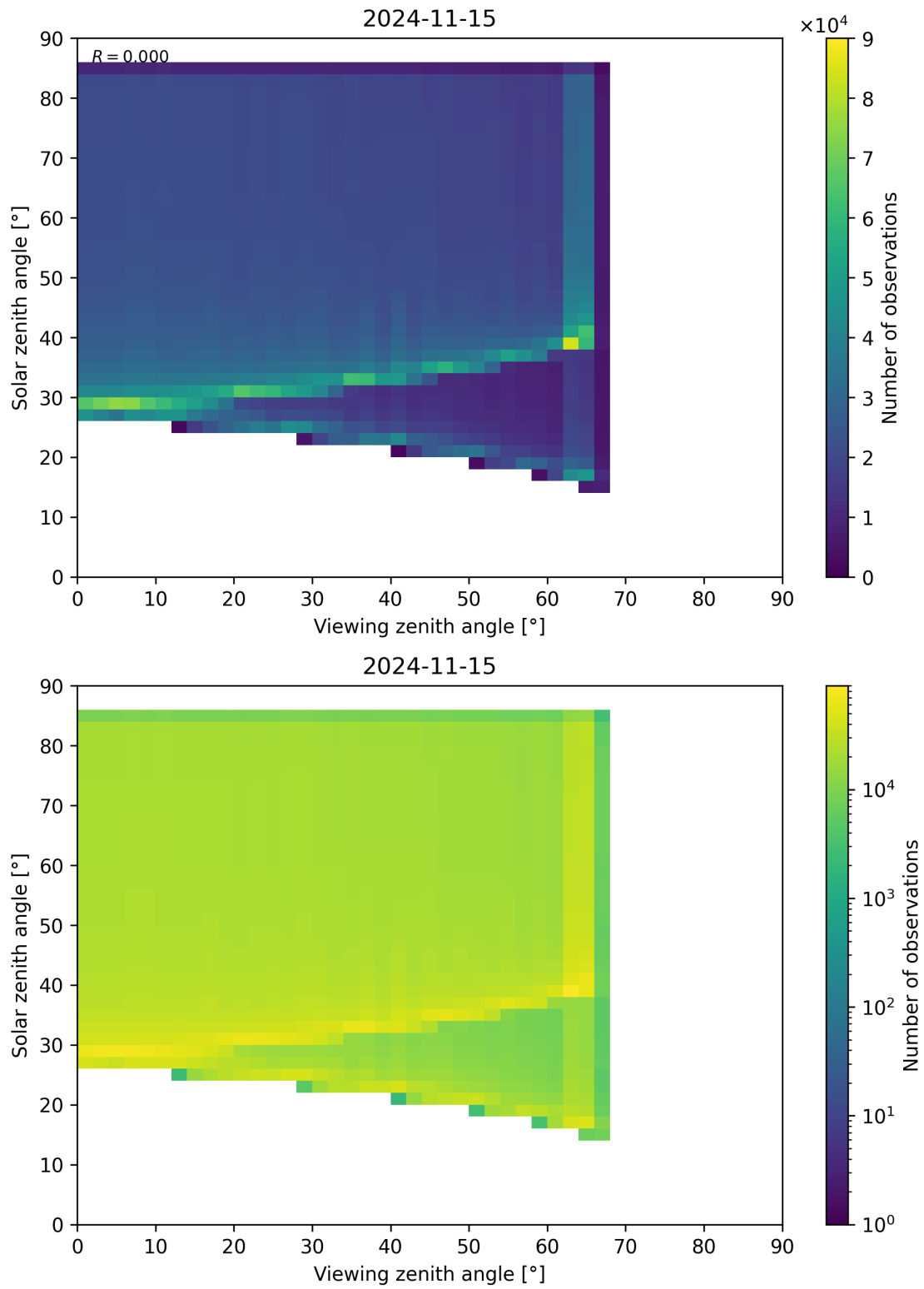
Figure 315: Scatter density plot of “Viewing zenith angle” against “Solar zenith angle” for 2024-11-14 to 2024-11-16.
