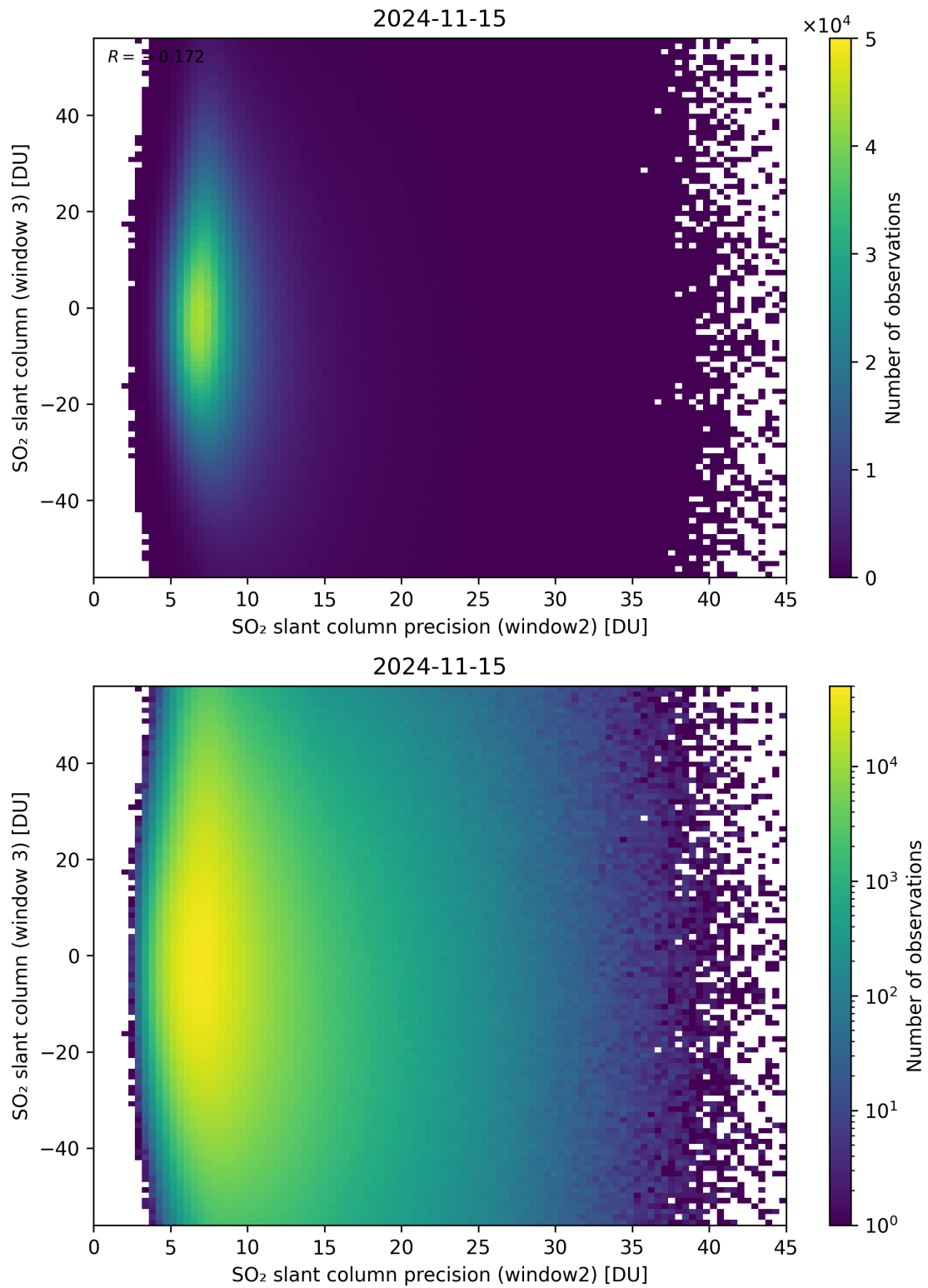
Figure 249: Scatter density plot of “SO 2 slant column precision (window2)” against “SO 2 slant column (window 3)” for 2024-11-14 to 2024-11-16.
