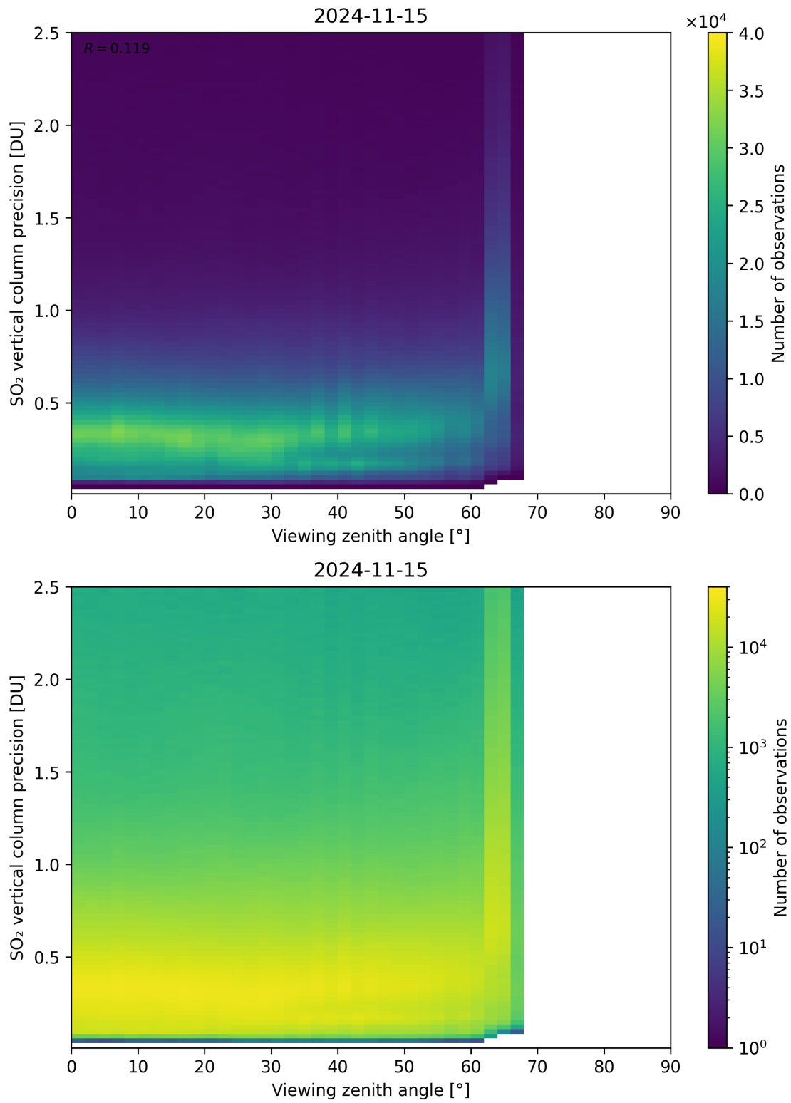
Figure 328: Scatter density plot of “Viewing zenith angle” against “SO 2 vertical column precision” for 2024-11-14 to 2024-11-16.
