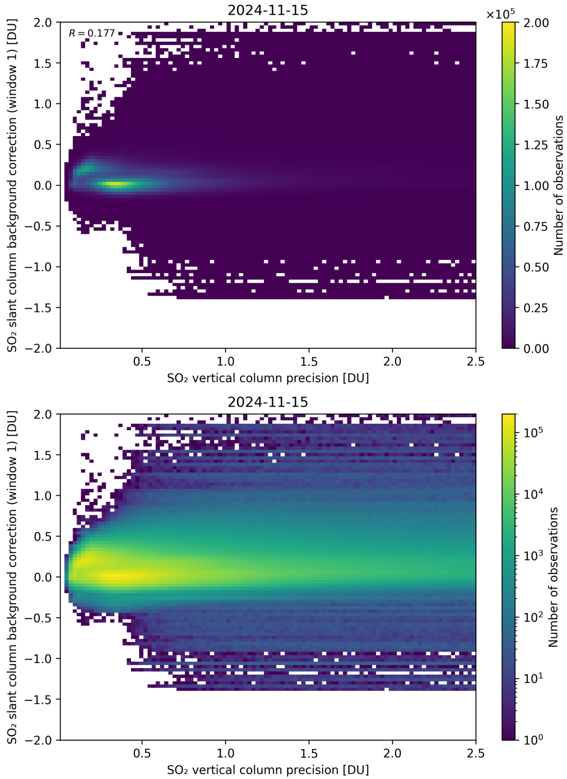
Figure 279: Scatter density plot of “SO 2 vertical column precision” against “SO 2 slant column background correction (window 1)” for 2024-11-14 to 2024-11-16.
