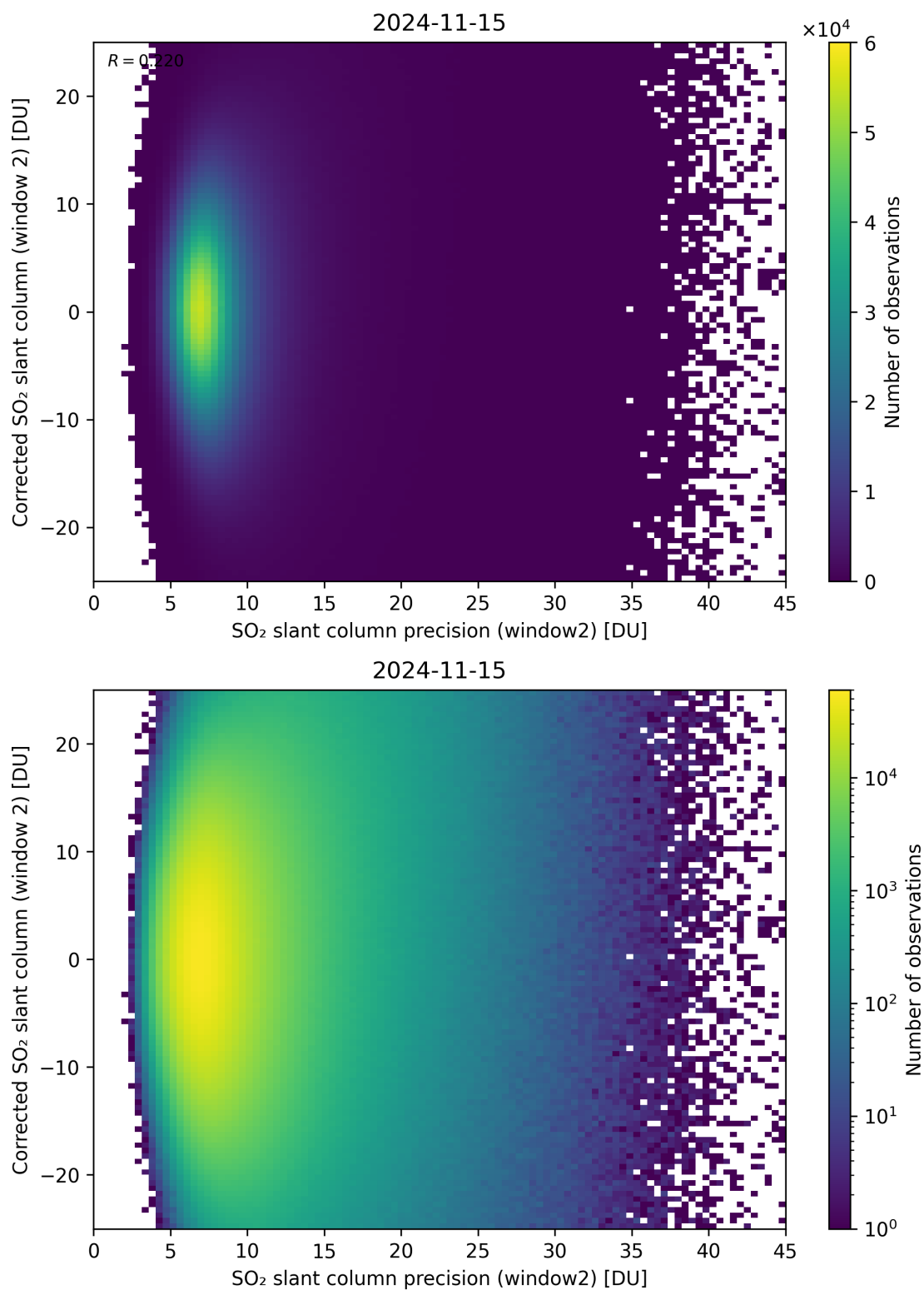
Figure 247: Scatter density plot of “SO 2 slant column precision (window2)” against “Corrected SO 2 slant column (window 2)” for 2024-11-14 to 2024-11-16.
