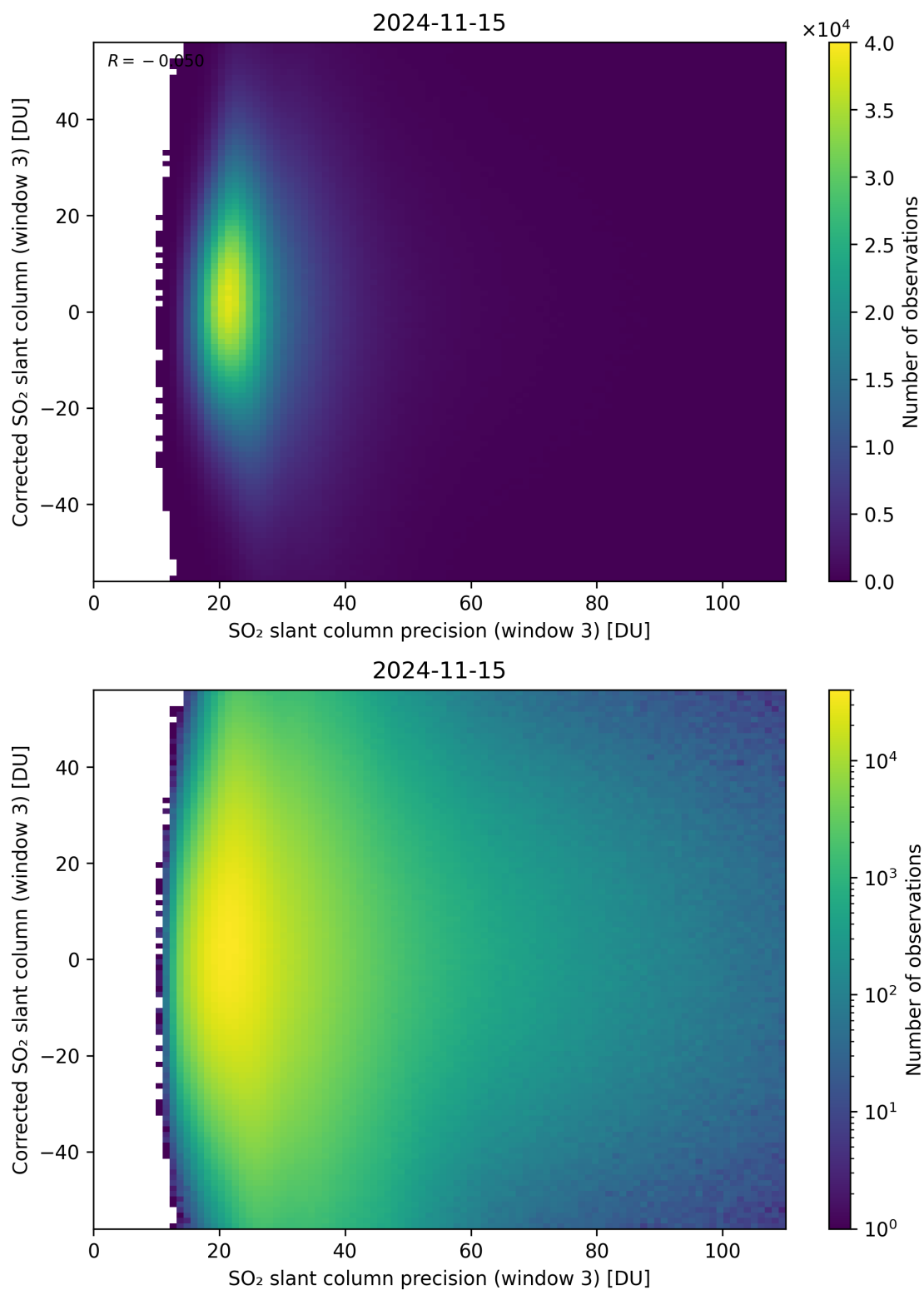
Figure 262: Scatter density plot of “SO 2 slant column precision (window 3)” against “Corrected SO 2 slant column (window 3)” for 2024-11-14 to 2024-11-16.
