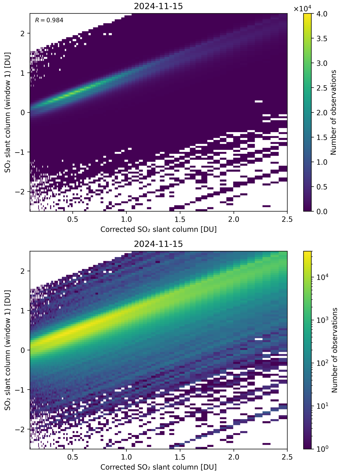
Figure 187: Scatter density plot of “Corrected SO 2 slant column” against “SO 2 slant column (window 1)” for 2024-11-14 to 2024-11-16.
