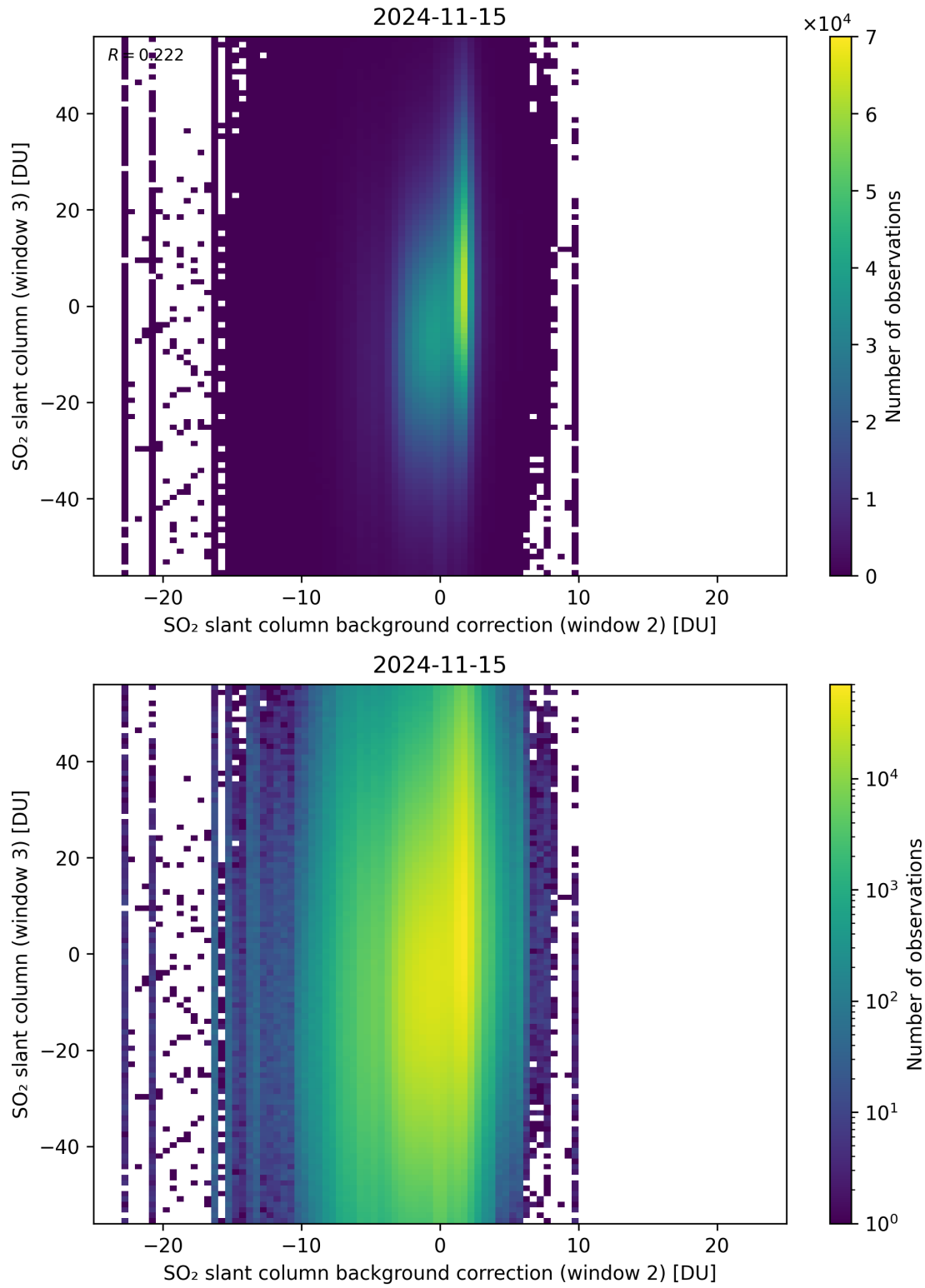
Figure 117: Scatter density plot of “SO 2 slant column background correction (window 2)” against “SO 2 slant column (window 3)” for 2024-11-14 to 2024-11-16.
