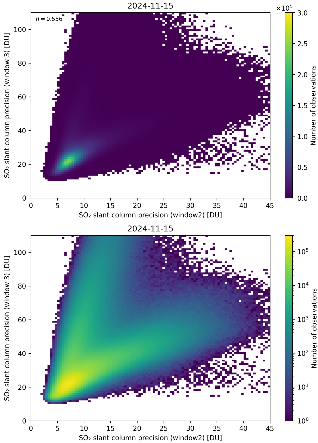
Figure 250: Scatter density plot of “SO 2 slant column precision (window2)” against “SO 2 slant column precision (window 3)” for 2024-11-14 to 2024-11-16.
