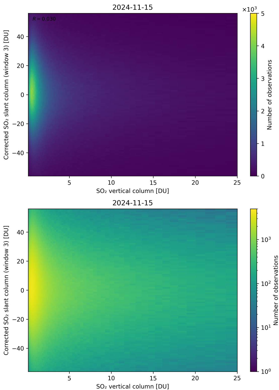
Figure 299: Scatter density plot of “SO 2 vertical column” against “Corrected SO 2 slant column (window 3)” for 2024-11-14 to 2024-11-16.
