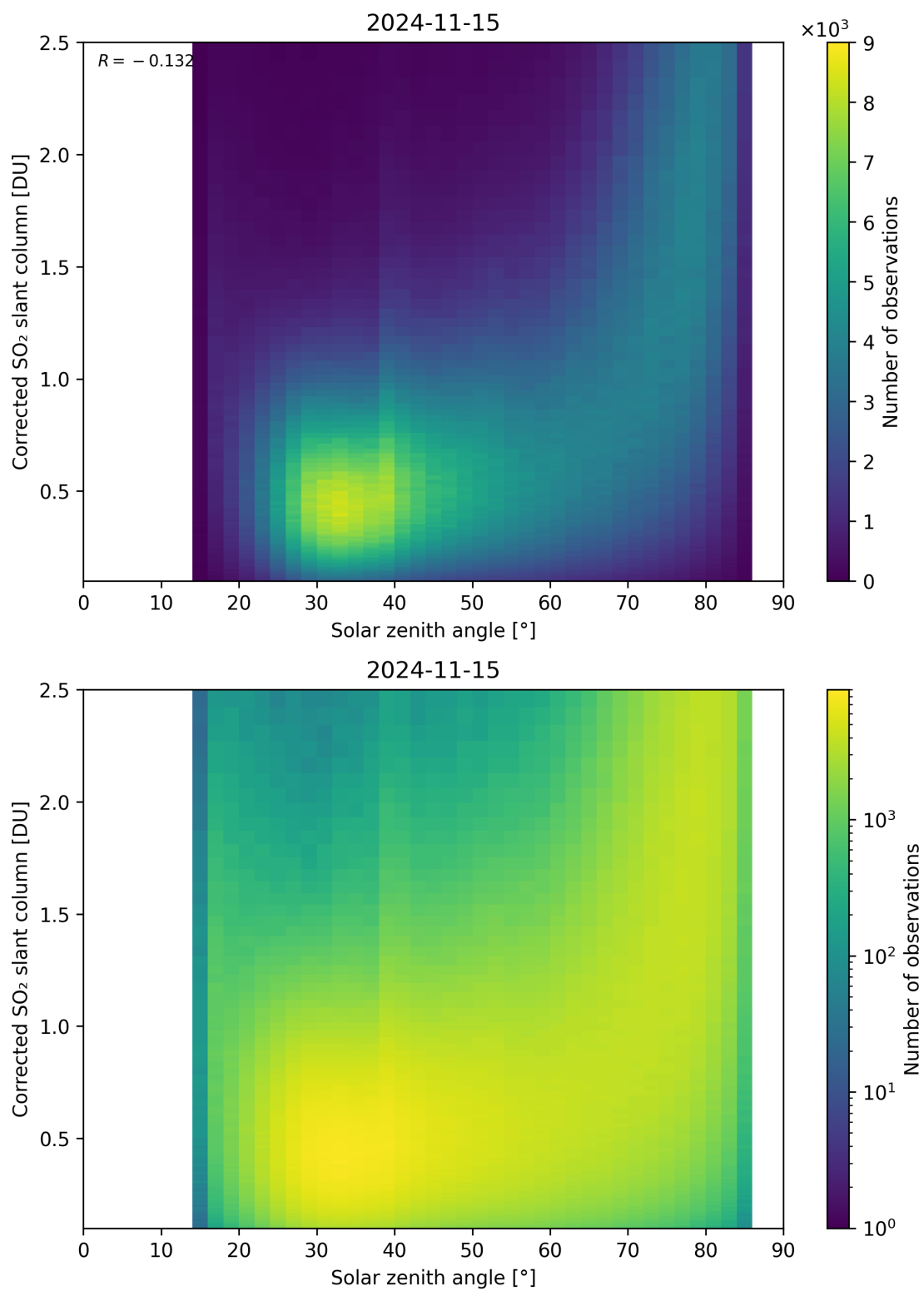
Figure 166: Scatter density plot of “Solar zenith angle” against “Corrected SO 2 slant column” for 2024-11-14 to 2024-11-16.
