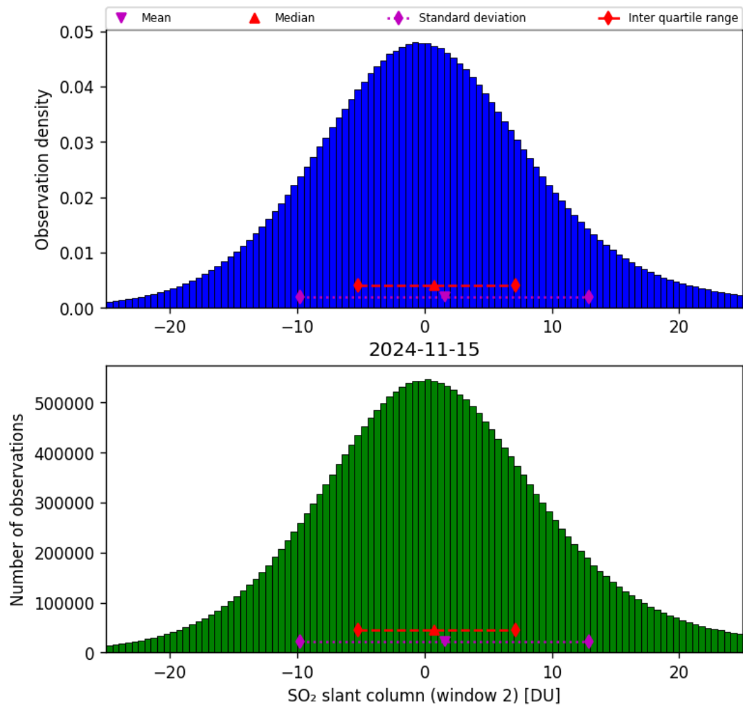
Figure 60: Histogram of “SO 2 slant column (window 2)” for 2024-11-14 to 2024-11-16
