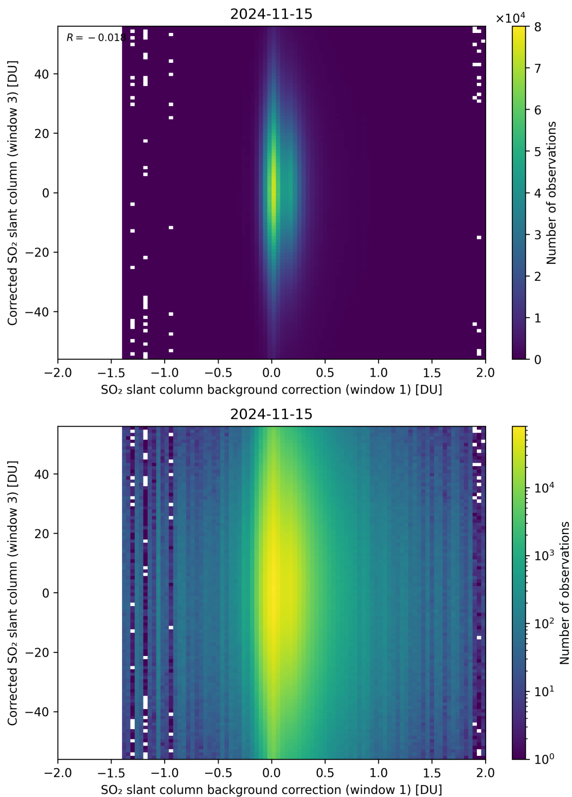
Figure 105: Scatter density plot of “SO 2 slant column background correction (window 1)” against “Corrected SO 2 slant column (window 3)” for 2024-11-14 to 2024-11-16.
