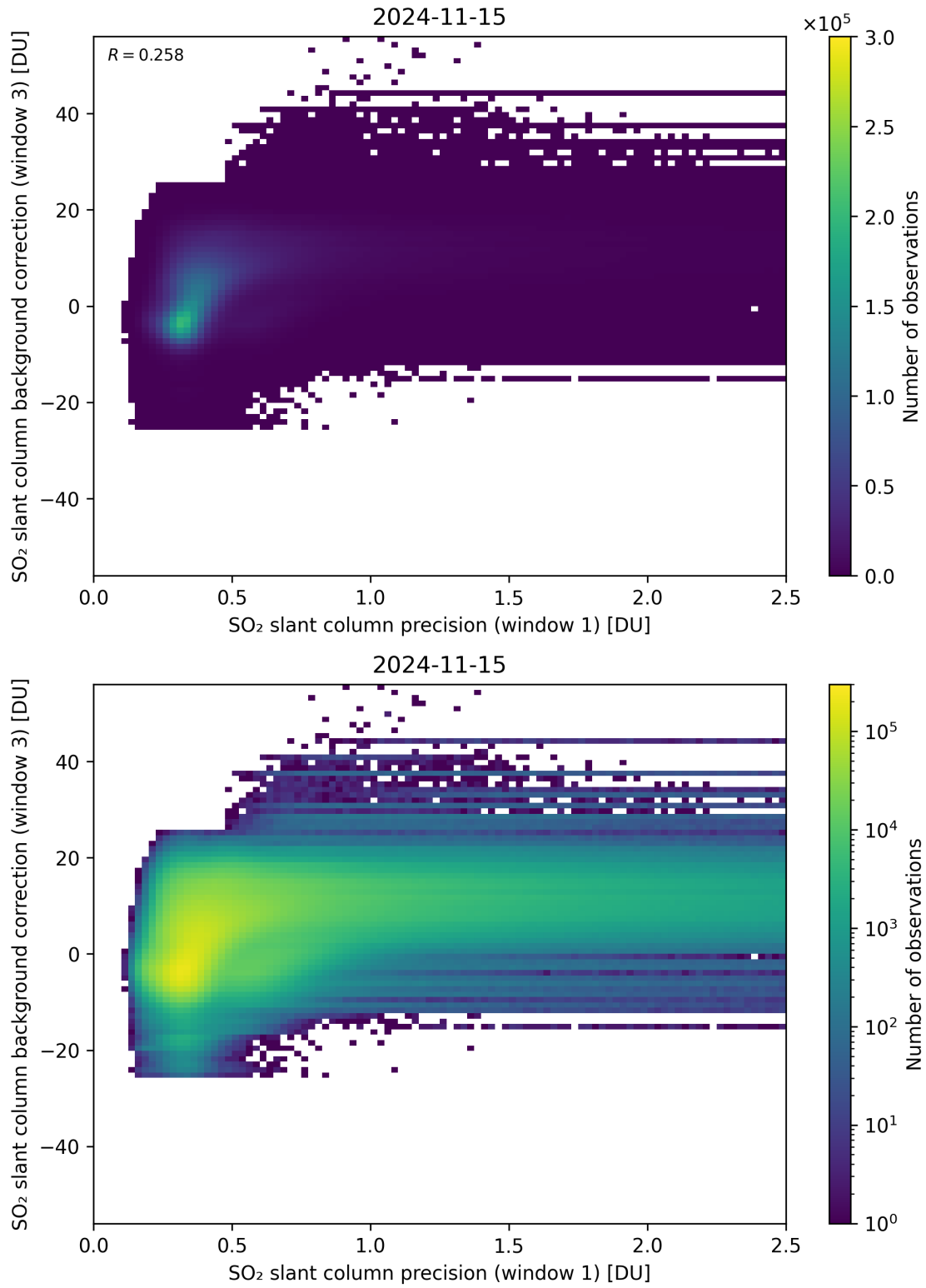
Figure 220: Scatter density plot of “SO 2 slant column precision (window 1)” against “SO 2 slant column background correction (window 3)” for 2024-11-14 to 2024-11-16.
