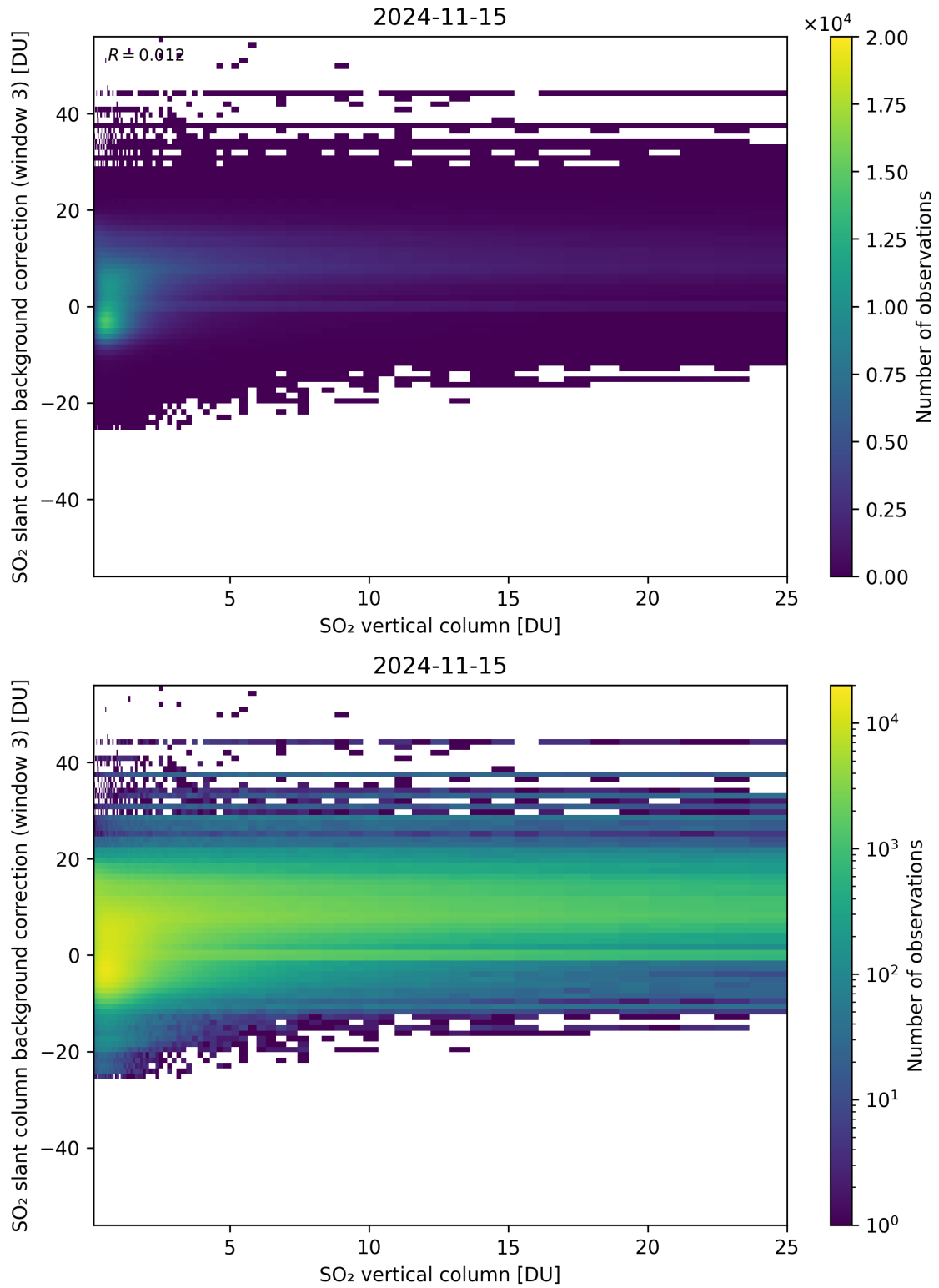
Figure 275: Scatter density plot of “SO 2 vertical column” against “SO 2 slant column background correction (window 3)” for 2024-11-14 to 2024-11-16.
