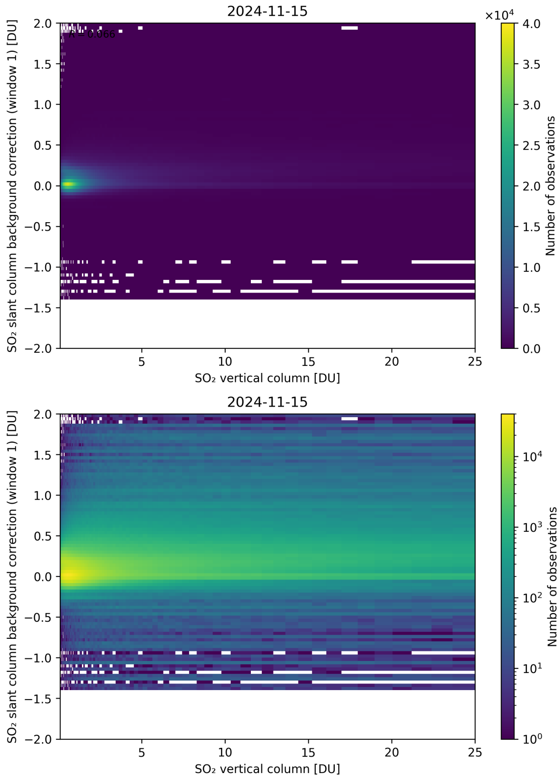
Figure 273: Scatter density plot of “SO 2 vertical column” against “SO 2 slant column background correction (window 1)” for 2024-11-14 to 2024-11-16.
