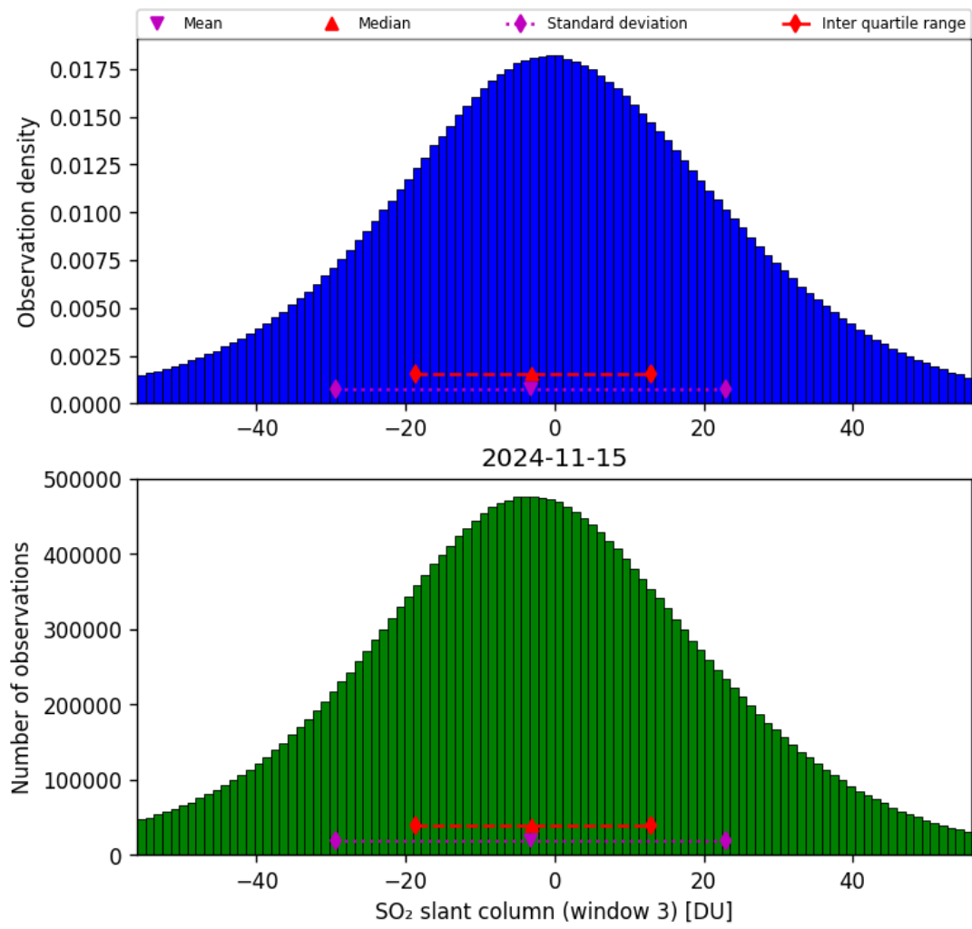
Figure 64: Histogram of “SO 2 slant column (window 3)” for 2024-11-14 to 2024-11-16
