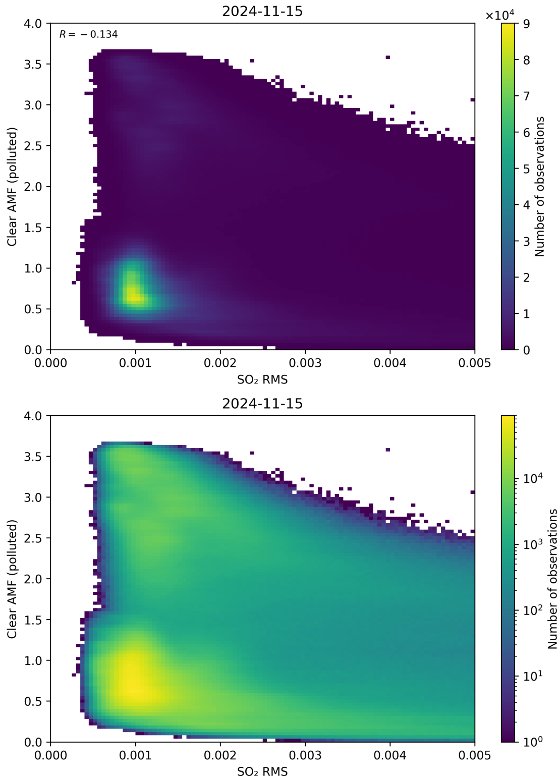
Figure 136: Scatter density plot of “SO 2 RMS” against “Clear AMF (polluted)” for 2024-11-14 to 2024-11-16.
