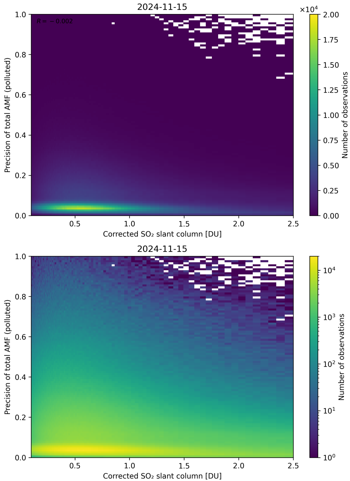
Figure 193: Scatter density plot of “Corrected SO 2 slant column” against “Precision of total AMF (polluted)” for 2024-11-14 to 2024-11-16.
