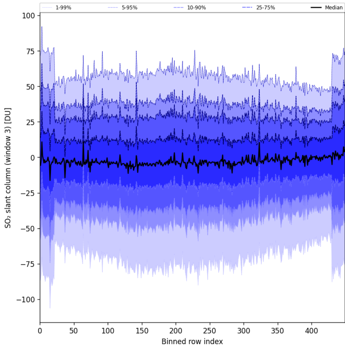
Figure 87: Along track statistics of “SO 2 slant column (window 3)” for 2024-11-14 to 2024-11-16
