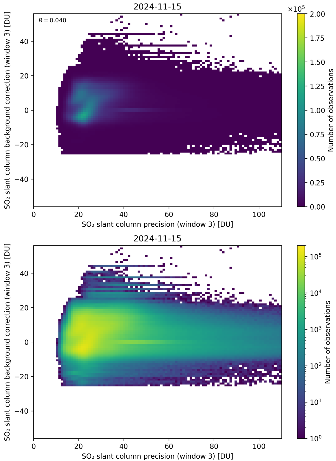
Figure 257: Scatter density plot of “SO 2 slant column precision (window 3)” against “SO 2 slant column background correction (window 3)” for 2024-11-14 to 2024-11-16.
