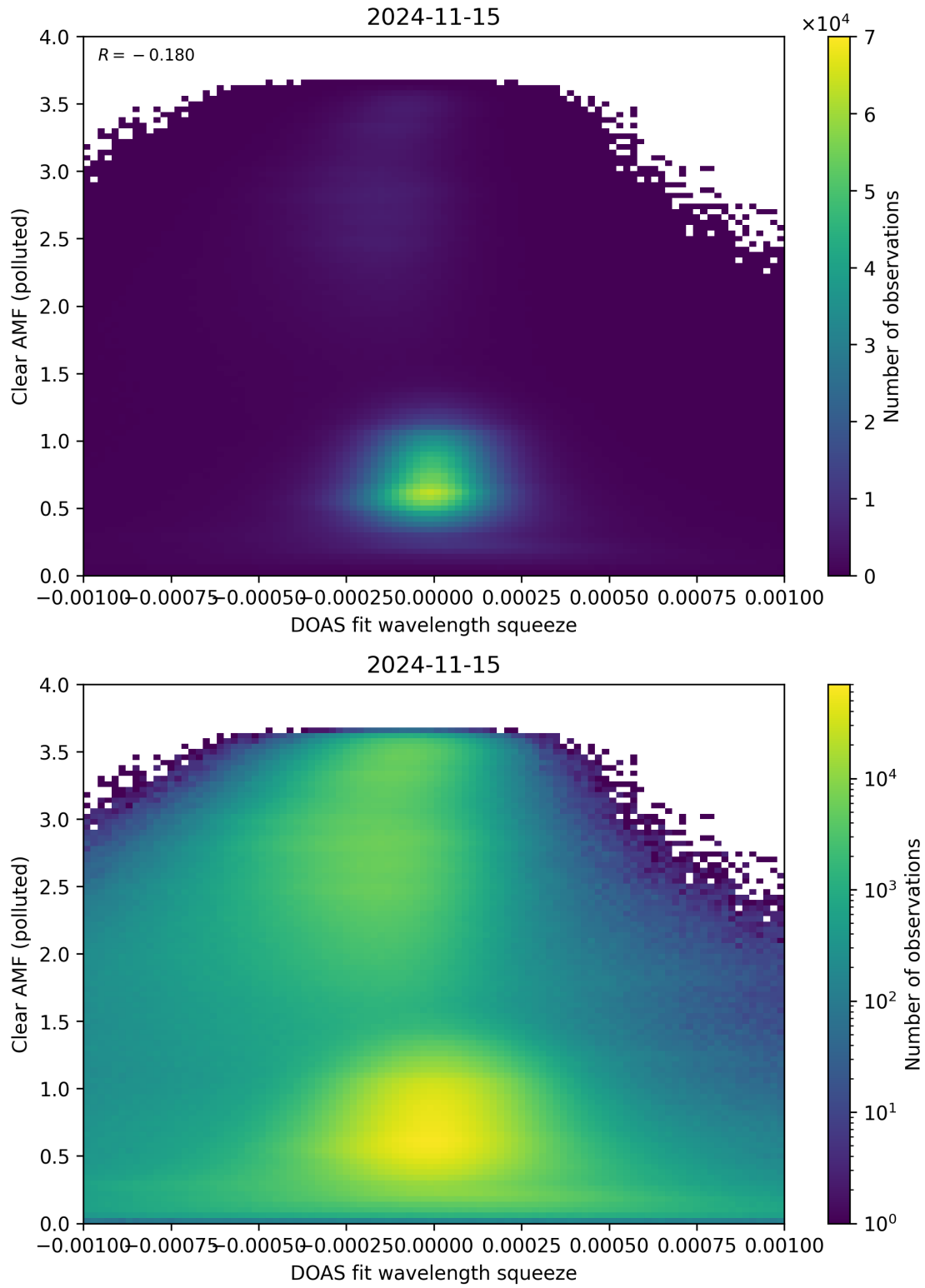
Figure 133: Scatter density plot of “DOAS fit wavelength squeeze” against “Clear AMF (polluted)” for 2024-11-14 to 2024-11-16.
