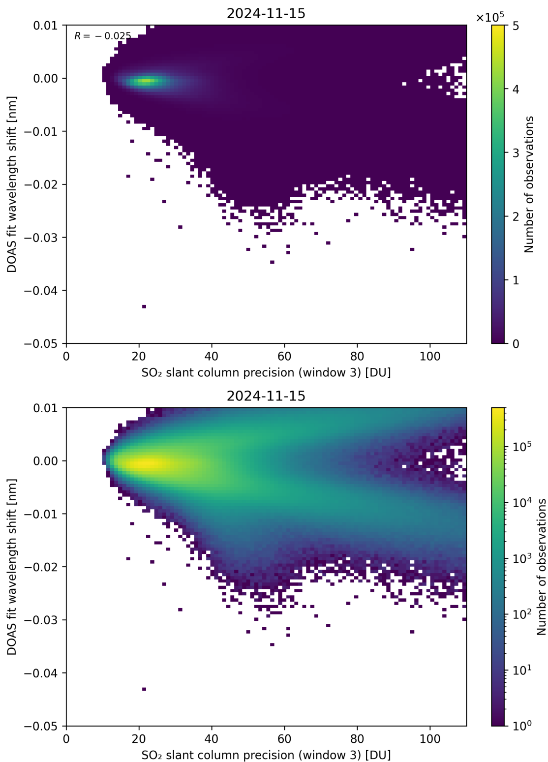
Figure 258: Scatter density plot of “SO 2 slant column precision (window 3)” against “DOAS fit wavelength shift” for 2024-11-14 to 2024-11-16.
