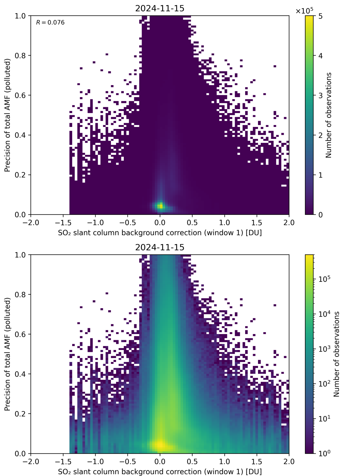
Figure 110: Scatter density plot of “SO 2 slant column background correction (window 1)” against “Precision of total AMF (polluted)” for 2024-11-14 to 2024-11-16.
