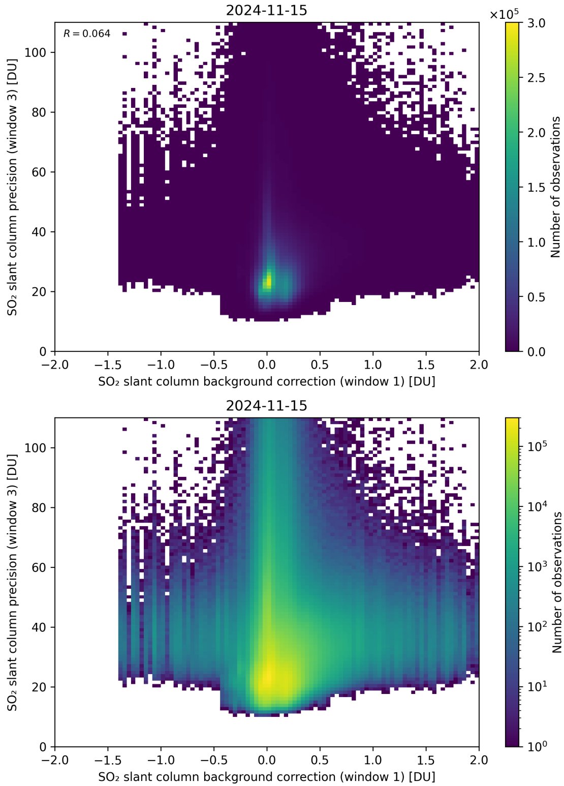
Figure 108: Scatter density plot of “SO 2 slant column background correction (window 1)” against “SO 2 slant column precision (window 3)” for 2024-11-14 to 2024-11-16.
