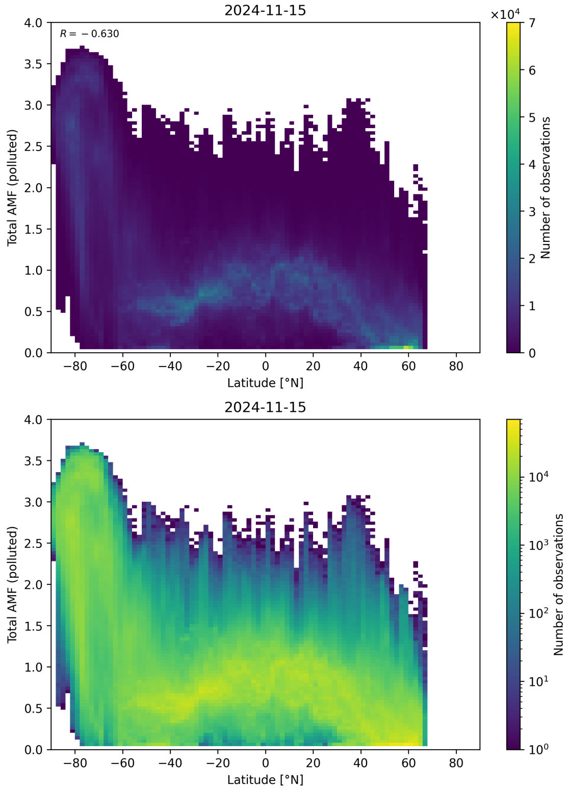
Figure 154: Scatter density plot of “Latitude” against “Total AMF (polluted)” for 2024-11-14 to 2024-11-16.
