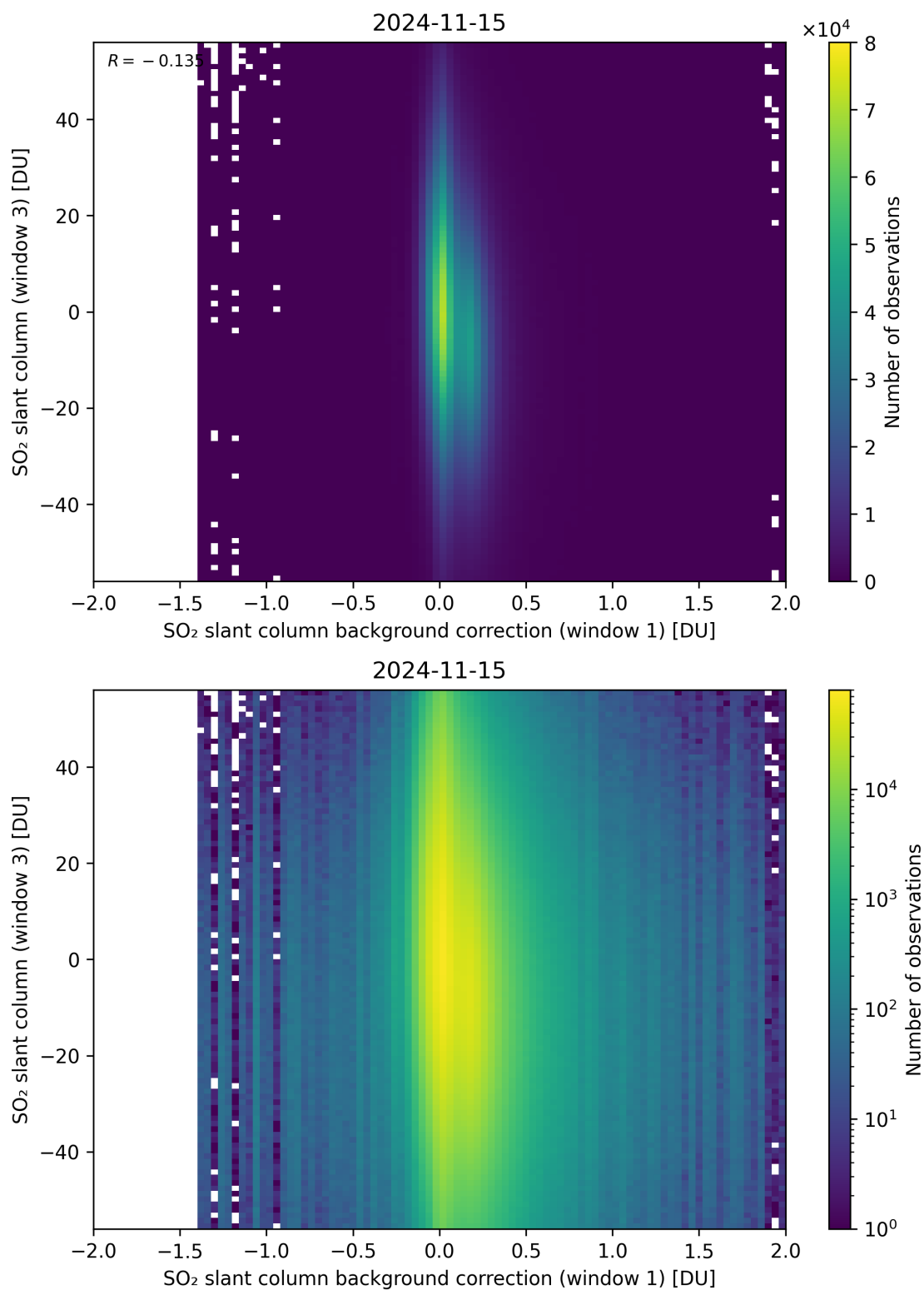
Figure 107: Scatter density plot of “SO 2 slant column background correction (window 1)” against “SO 2 slant column (window 3)” for 2024-11-14 to 2024-11-16.
