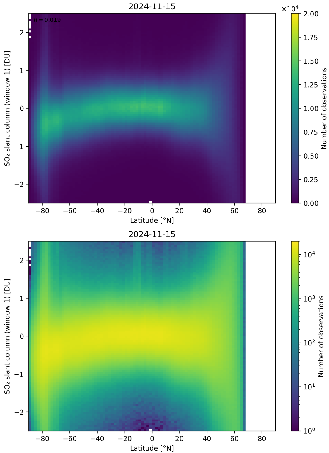
Figure 149: Scatter density plot of “Latitude” against “SO 2 slant column (window 1)” for 2024-11-14 to 2024-11-16.
