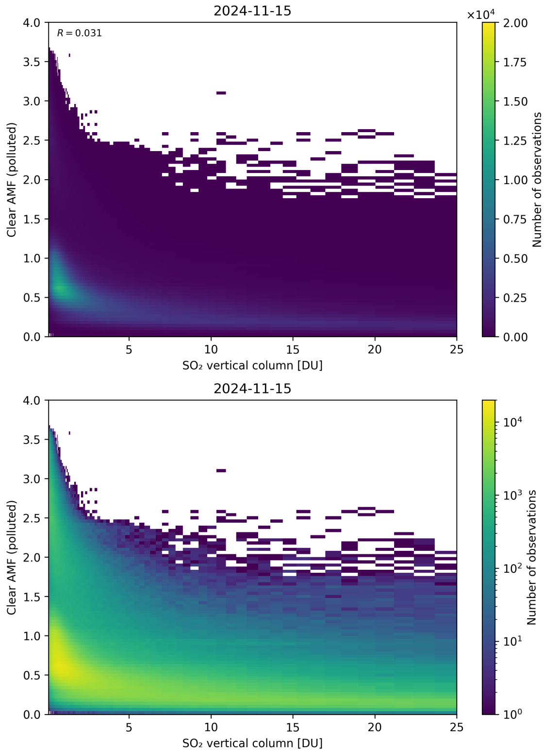
Figure 296: Scatter density plot of “SO 2 vertical column” against “Clear AMF (polluted)” for 2024-11-14 to 2024-11-16.
