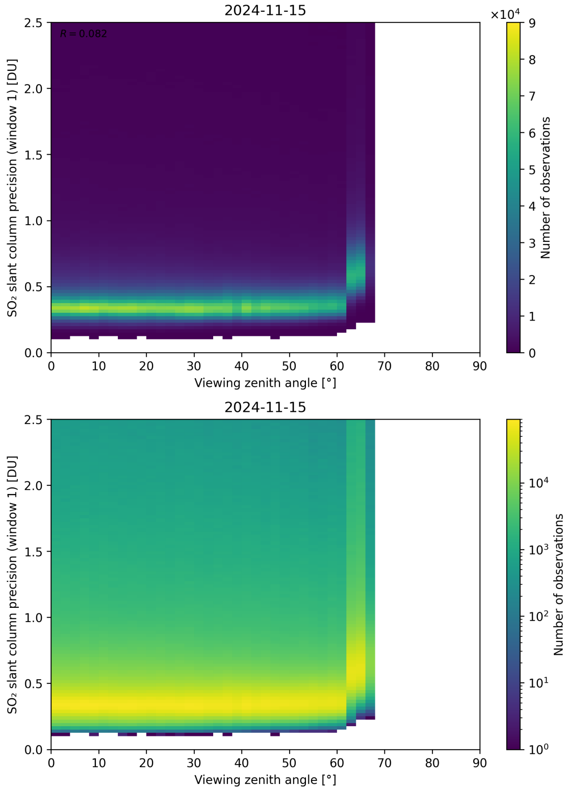
Figure 321: Scatter density plot of “Viewing zenith angle” against “SO 2 slant column precision (window 1)” for 2024-11-14 to 2024-11-16.
