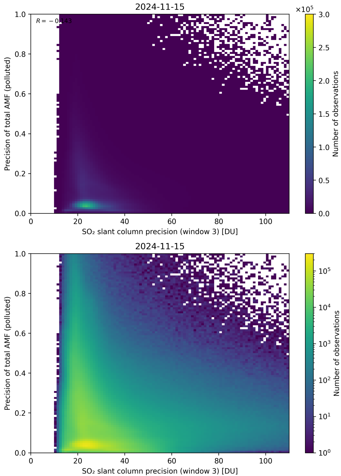
Figure 264: Scatter density plot of “SO 2 slant column precision (window 3)” against “Precision of total AMF (polluted)” for 2024-11-14 to 2024-11-16.
