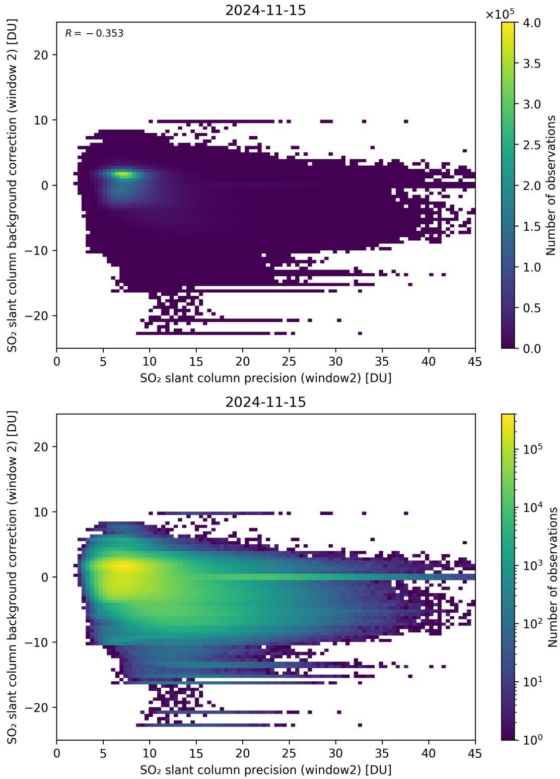
Figure 241: Scatter density plot of “SO 2 slant column precision (window2)” against “SO 2 slant column background correction (window 2)” for 2024-11-14 to 2024-11-16.
