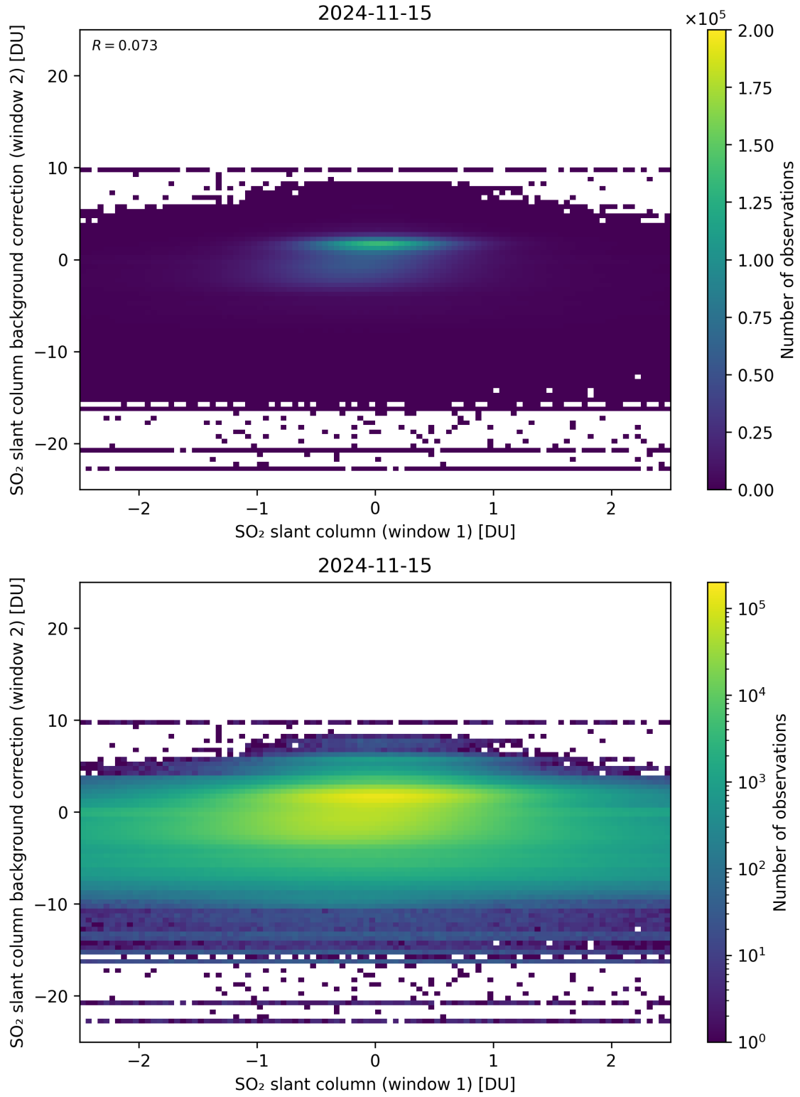
Figure 213: Scatter density plot of “SO 2 slant column (window 1)” against “SO 2 slant column background correction (window 2)” for 2024-11-14 to 2024-11-16.
