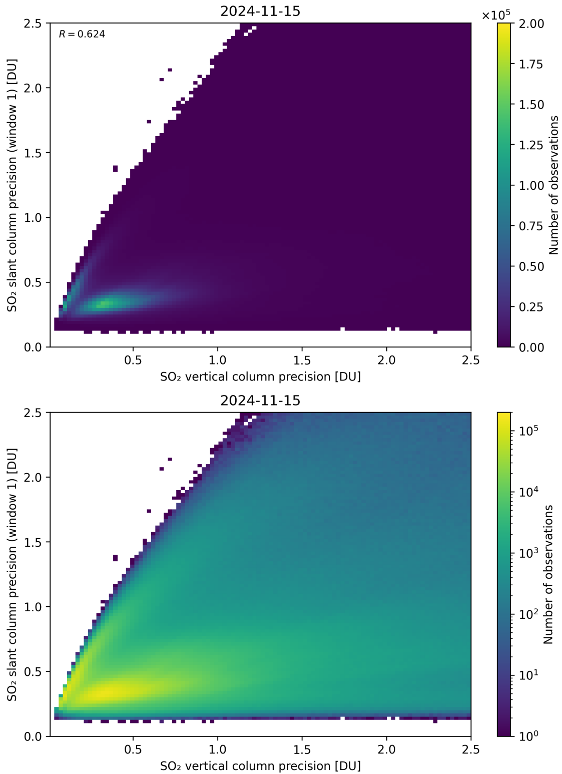
Figure 290: Scatter density plot of “SO 2 vertical column precision” against “SO 2 slant column precision (window 1)” for 2024-11-14 to 2024-11-16.
