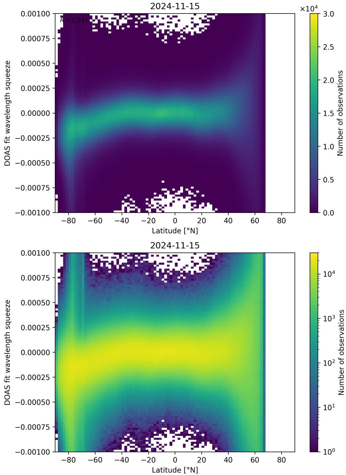
Figure 143: Scatter density plot of “Latitude” against “DOAS fit wavelength squeeze” for 2024-11-14 to 2024-11-16.
