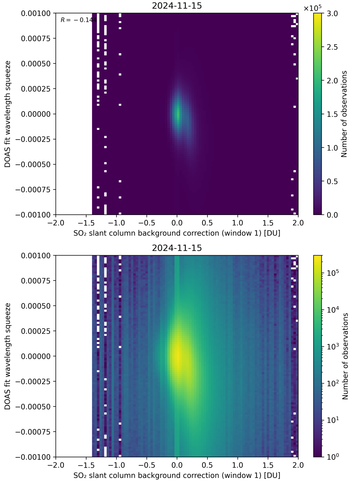
Figure 101: Scatter density plot of “SO 2 slant column background correction (window 1)” against “DOAS fit wavelength squeeze” for 2024-11-14 to 2024-11-16.
