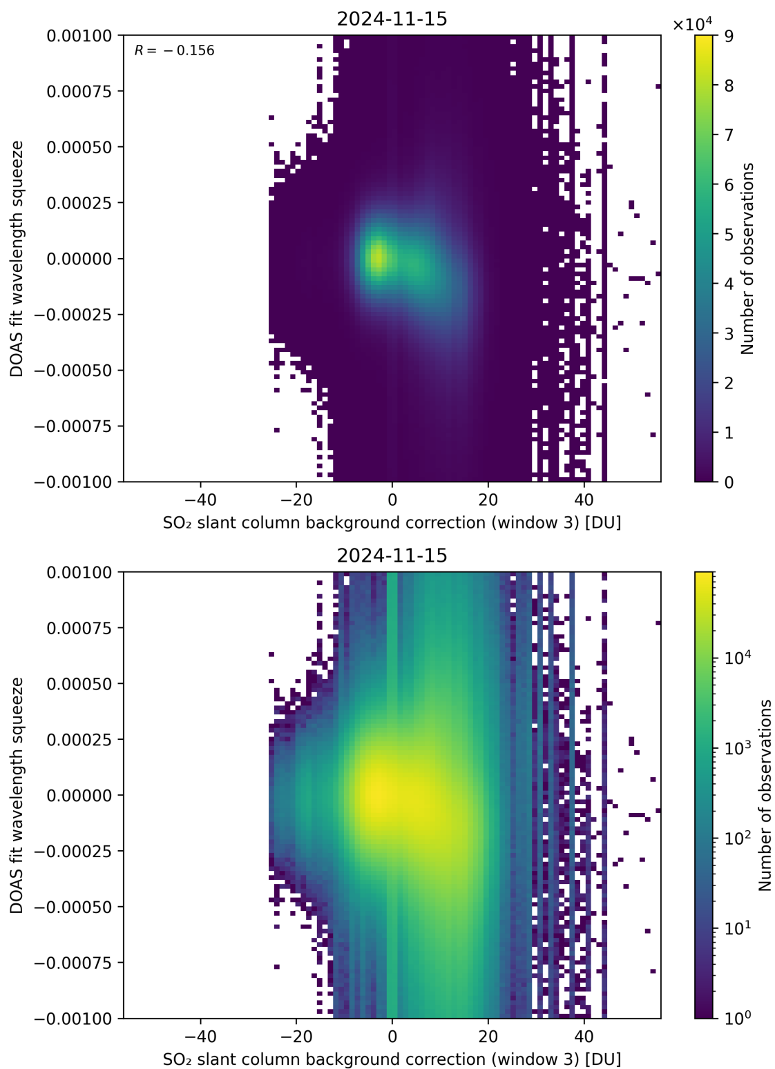
Figure 122: Scatter density plot of “SO 2 slant column background correction (window 3)” against “DOAS fit wavelength squeeze” for 2024-11-14 to 2024-11-16.
