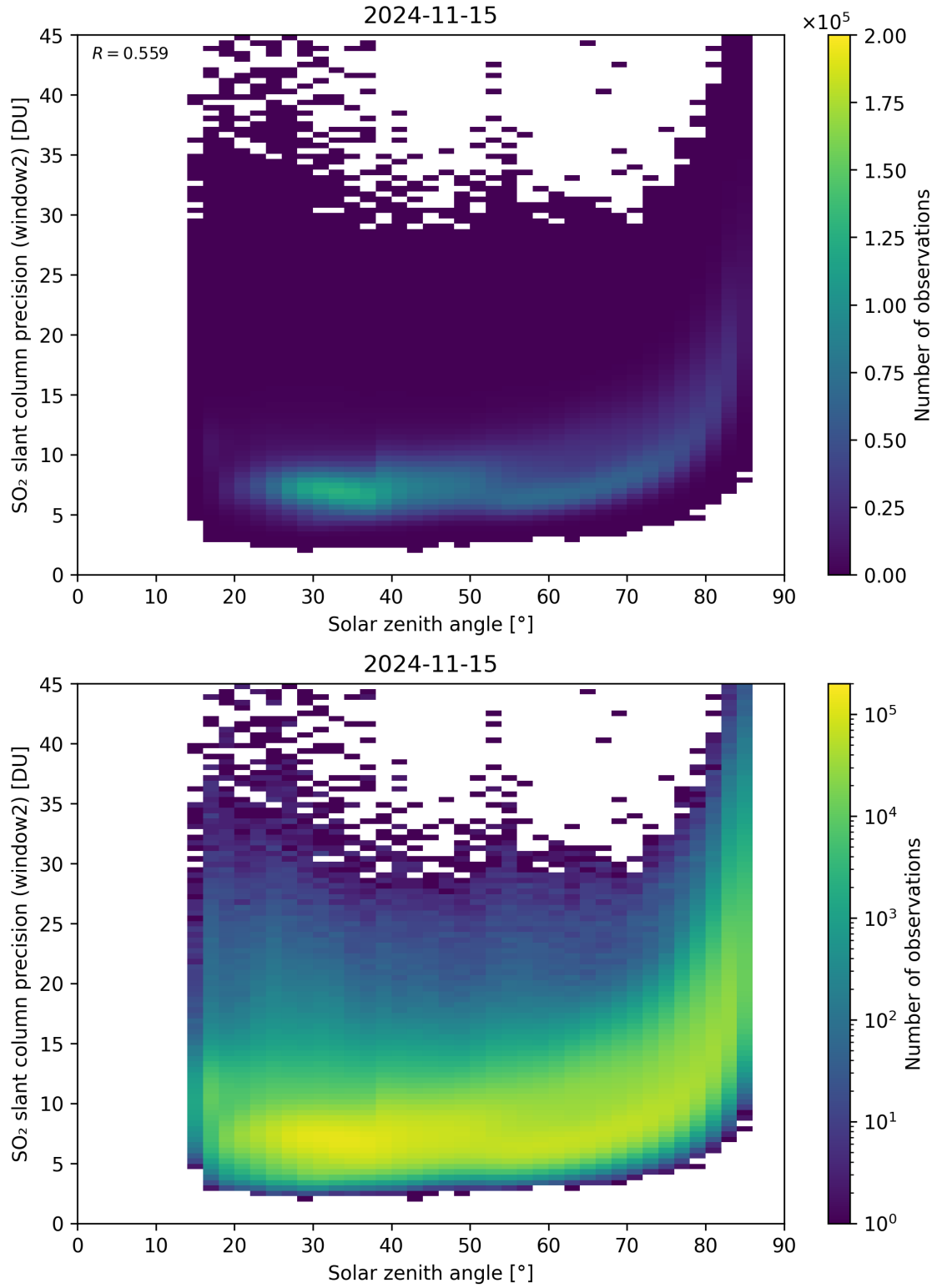
Figure 171: Scatter density plot of “Solar zenith angle” against “SO 2 slant column precision (window2)” for 2024-11-14 to 2024-11-16.
