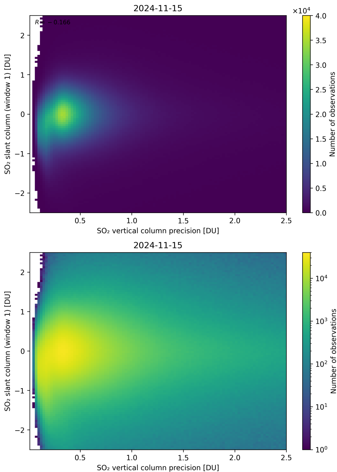
Figure 289: Scatter density plot of “SO 2 vertical column precision” against “SO 2 slant column (window 1)” for 2024-11-14 to 2024-11-16.
