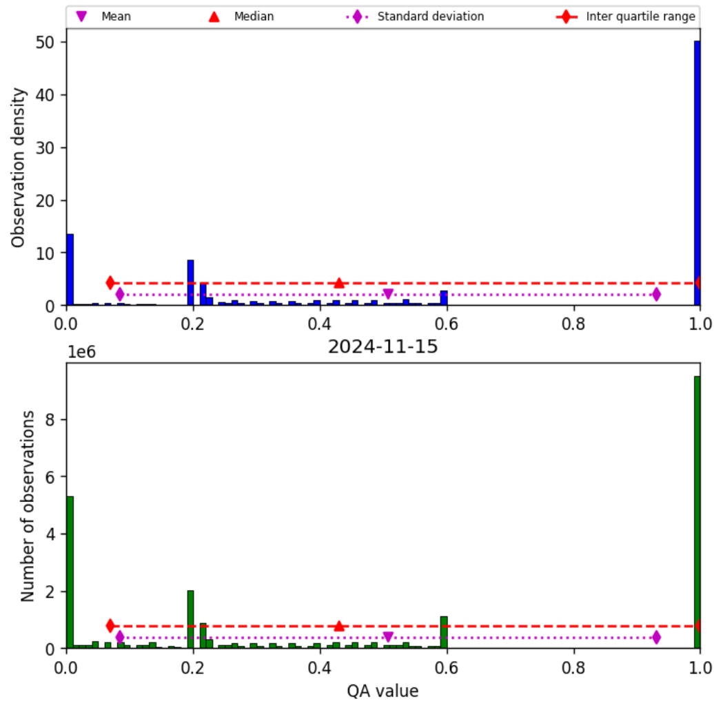
Figure 52: Histogram of “QA value” for 2024-11-14 to 2024-11-16
