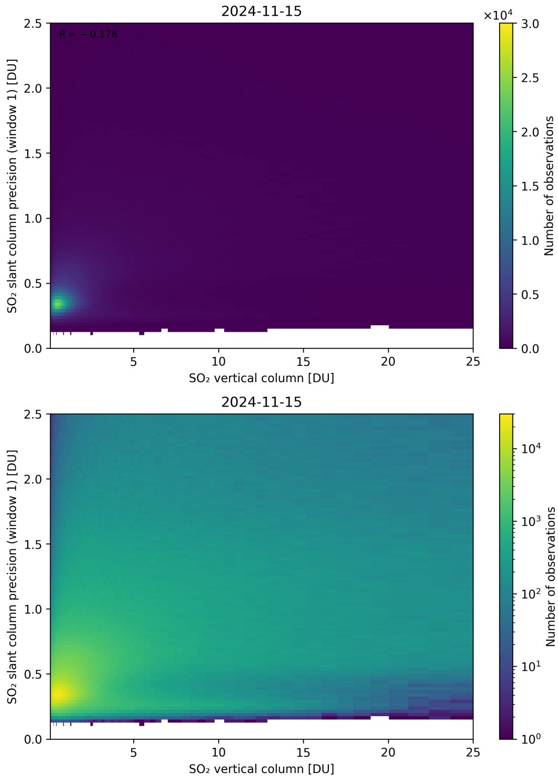
Figure 301: Scatter density plot of “SO 2 vertical column” against “SO 2 slant column precision (window 1)” for 2024-11-14 to 2024-11-16.
