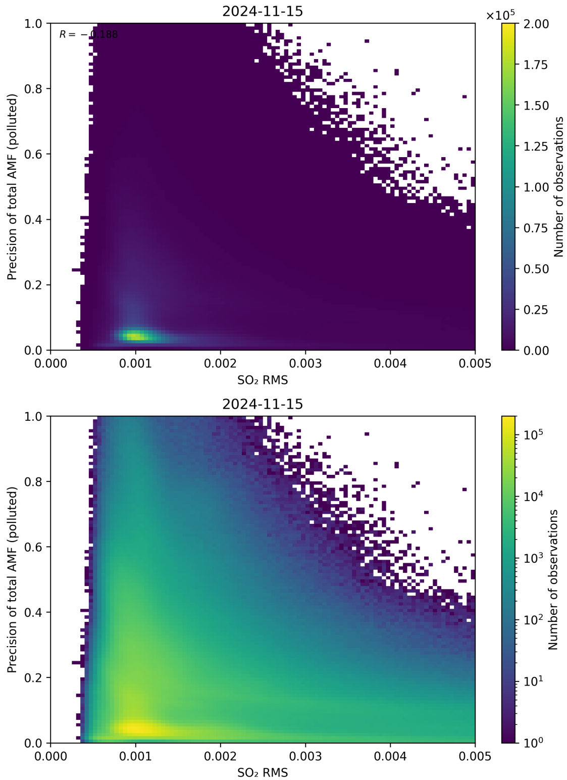
Figure 138: Scatter density plot of “SO 2 RMS” against “Precision of total AMF (polluted)” for 2024-11-14 to 2024-11-16.
