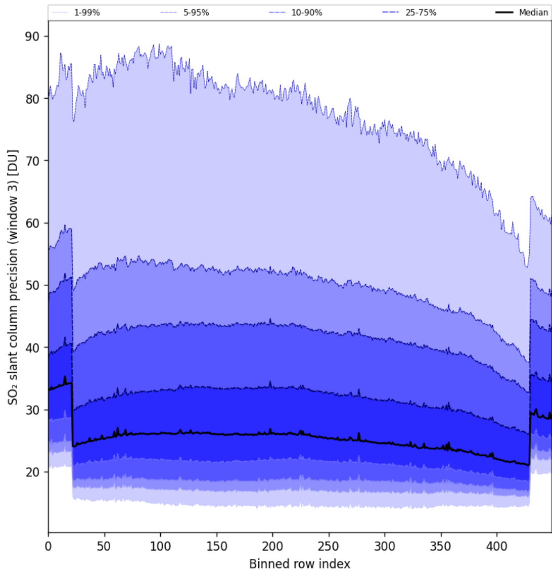
Figure 88: Along track statistics of “SO 2 slant column precision (window 3)” for 2024-11-14 to 2024-11-16
