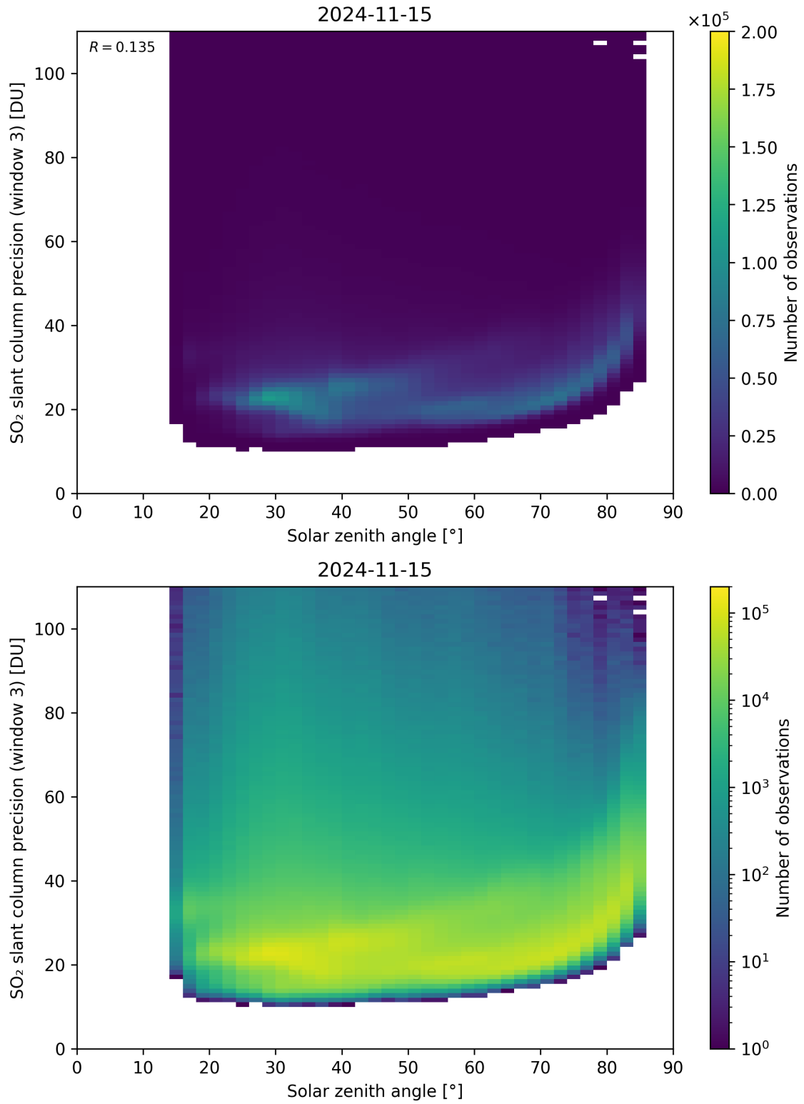
Figure 173: Scatter density plot of “Solar zenith angle” against “SO 2 slant column precision (window 3)” for 2024-11-14 to 2024-11-16.
