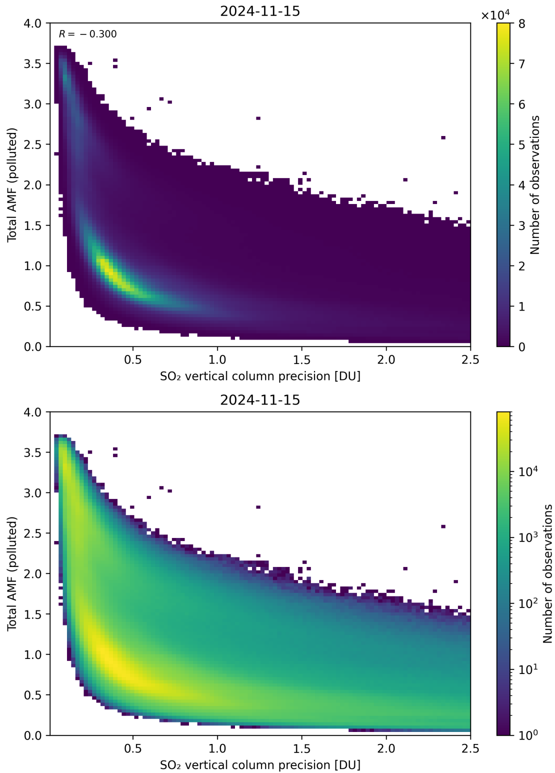
Figure 294: Scatter density plot of “SO 2 vertical column precision” against “Total AMF (polluted)” for 2024-11-14 to 2024-11-16.
