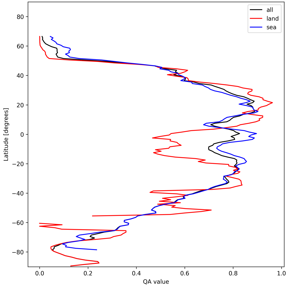
Figure 29: Zonal average of “QA value” for 2024-11-14 to 2024-11-16.
