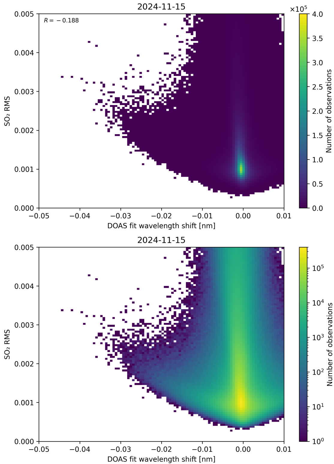
Figure 128: Scatter density plot of “DOAS fit wavelength shift” against “SO 2 RMS” for 2024-11-14 to 2024-11-16.
