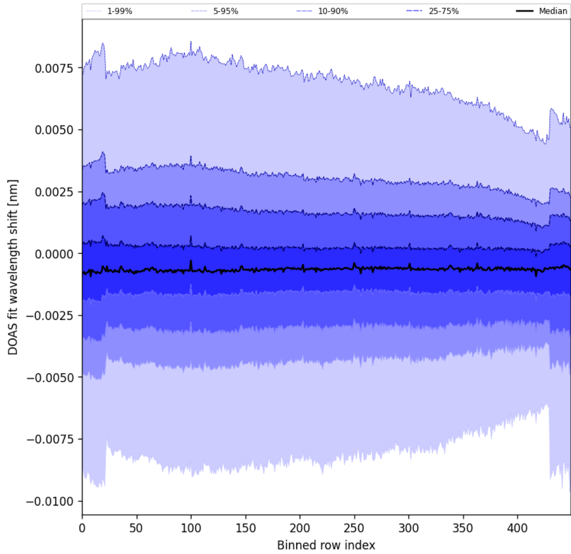
Figure 91: Along track statistics of “DOAS fit wavelength shift” for 2024-11-14 to 2024-11-16
