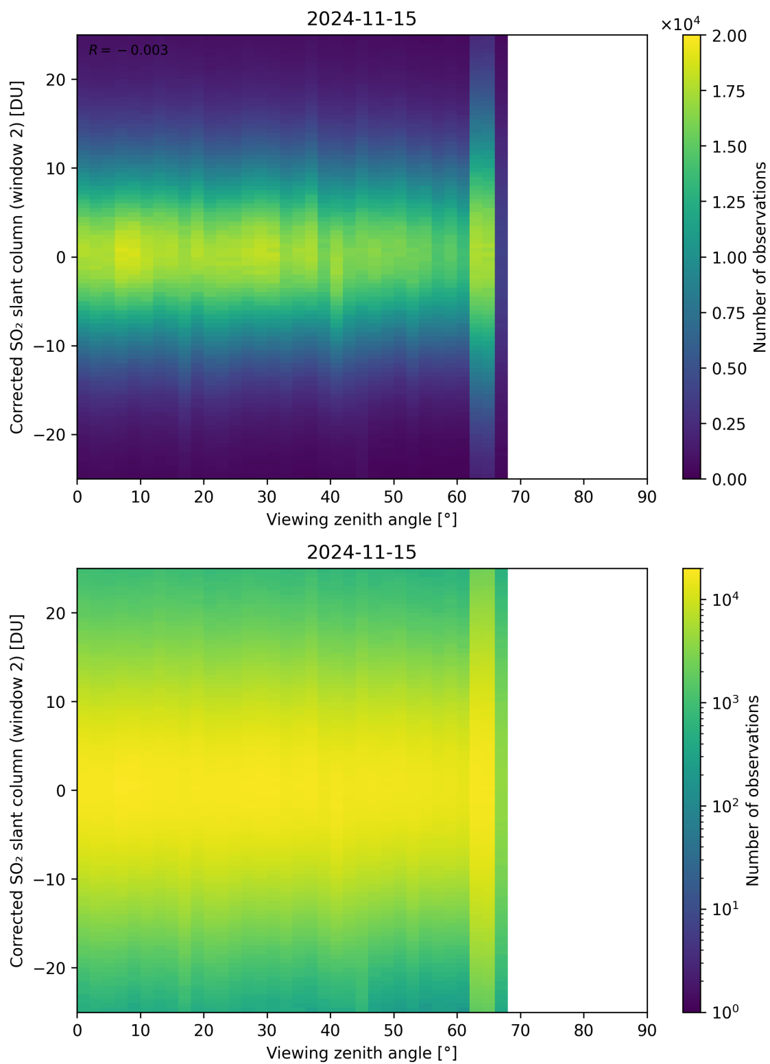
Figure 318: Scatter density plot of “Viewing zenith angle” against “Corrected SO 2 slant column (window 2)” for 2024-11-14 to 2024-11-16.
