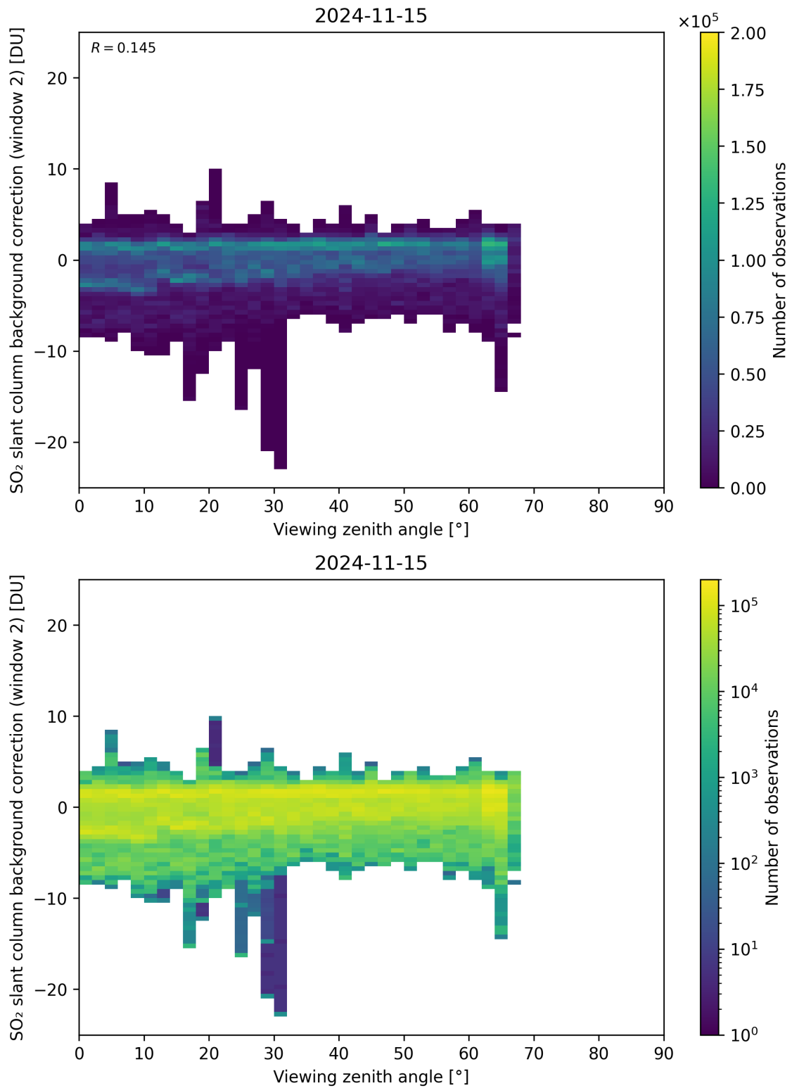
Figure 309: Scatter density plot of “Viewing zenith angle” against “SO 2 slant column background correction (window 2)” for 2024-11-14 to 2024-11-16.
