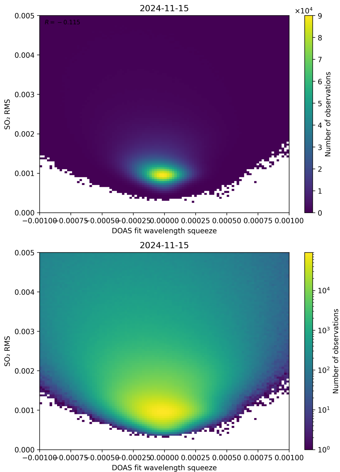
Figure 132: Scatter density plot of “DOAS fit wavelength squeeze” against “SO 2 RMS” for 2024-11-14 to 2024-11-16.
