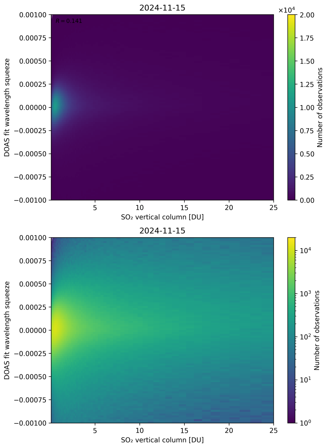
Figure 277: Scatter density plot of “SO 2 vertical column” against “DOAS fit wavelength squeeze” for 2024-11-14 to 2024-11-16.
