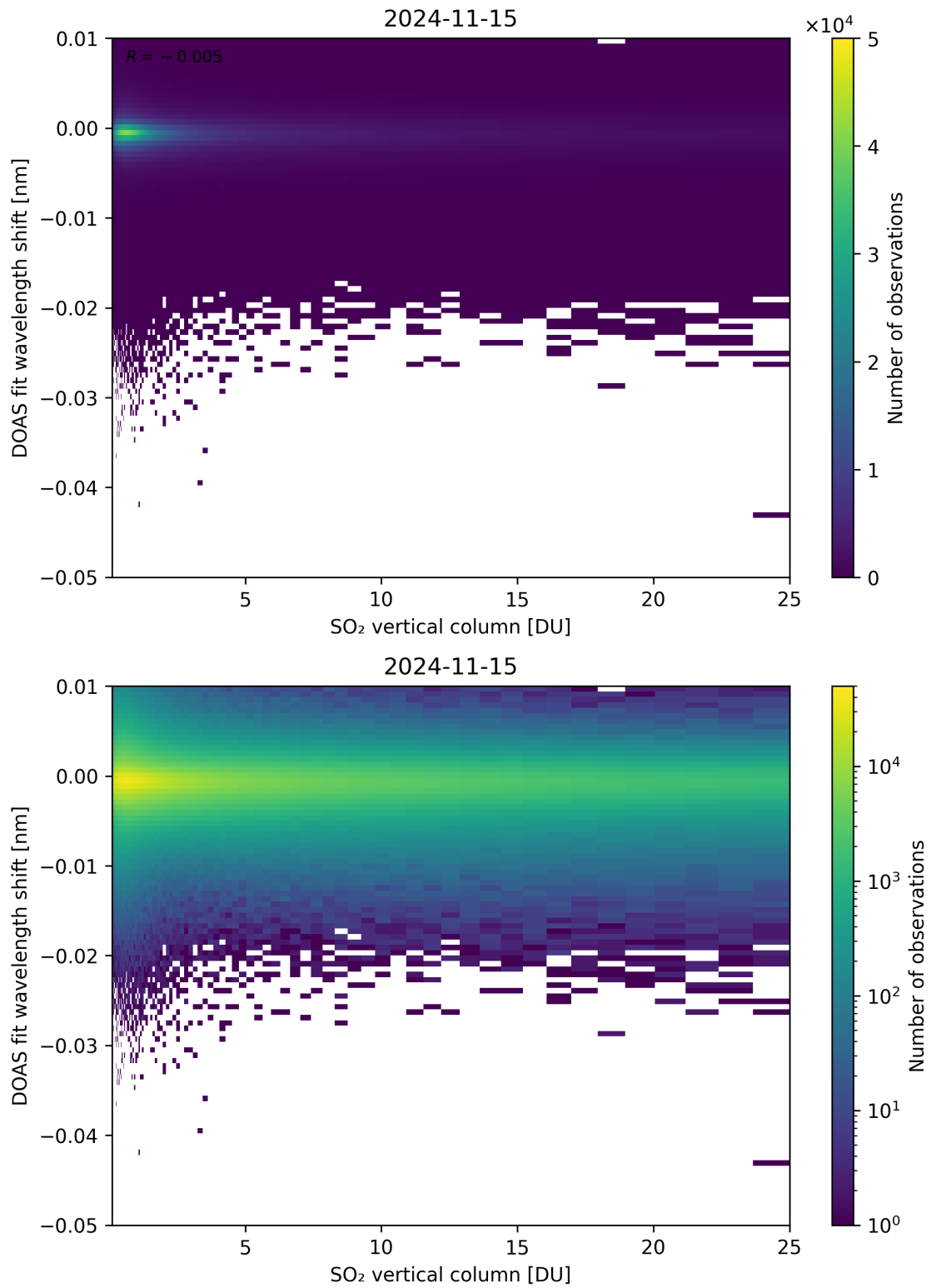
Figure 276: Scatter density plot of “SO 2 vertical column” against “DOAS fit wavelength shift” for 2024-11-14 to 2024-11-16.
