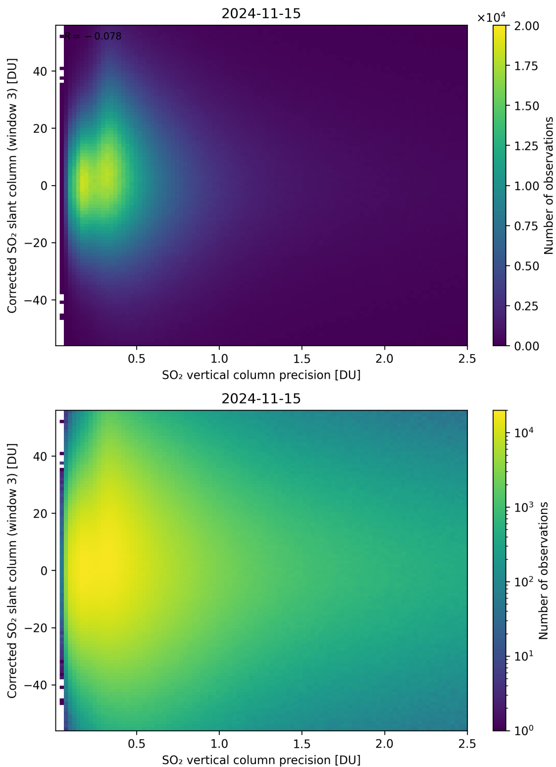
Figure 288: Scatter density plot of “SO 2 vertical column precision” against “Corrected SO 2 slant column (window 3)” for 2024-11-14 to 2024-11-16.
