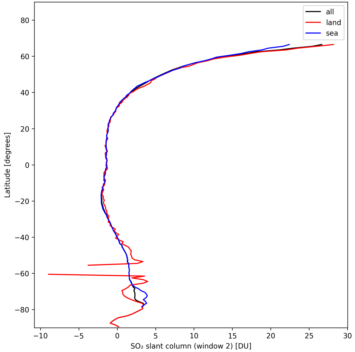
Figure 37: Zonal average of “SO 2 slant column (window 2)” for 2024-11-14 to 2024-11-16.
