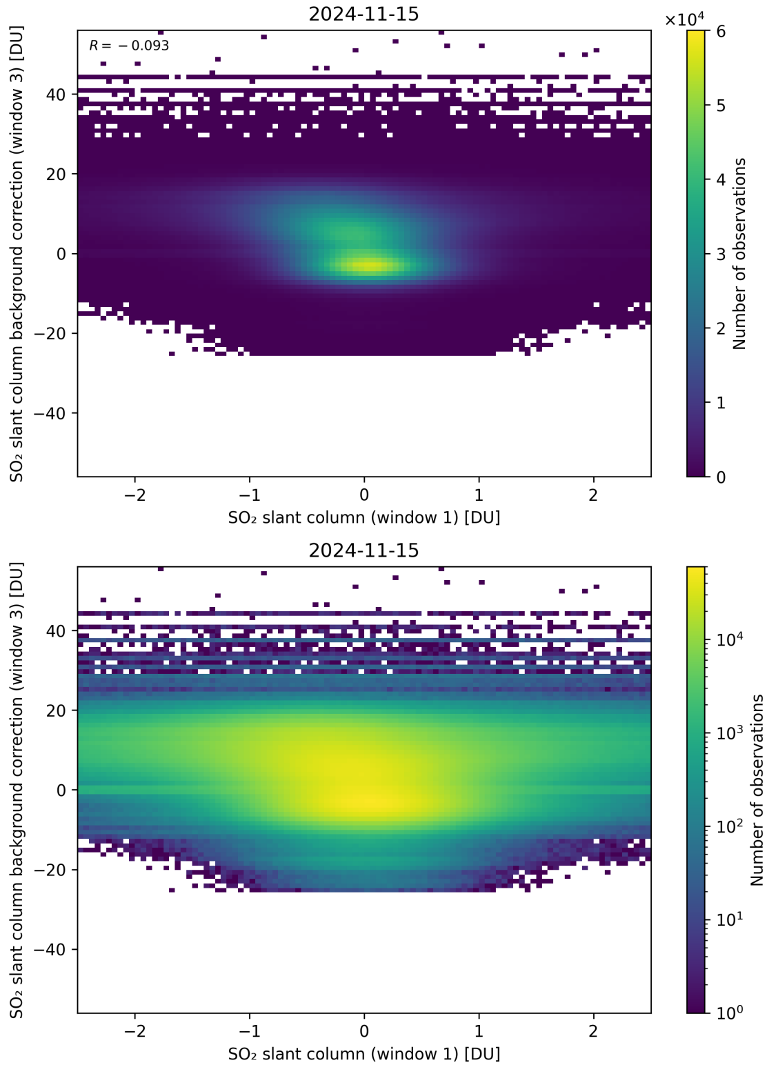
Figure 214: Scatter density plot of “SO 2 slant column (window 1)” against “SO 2 slant column background correction (window 3)” for 2024-11-14 to 2024-11-16.
