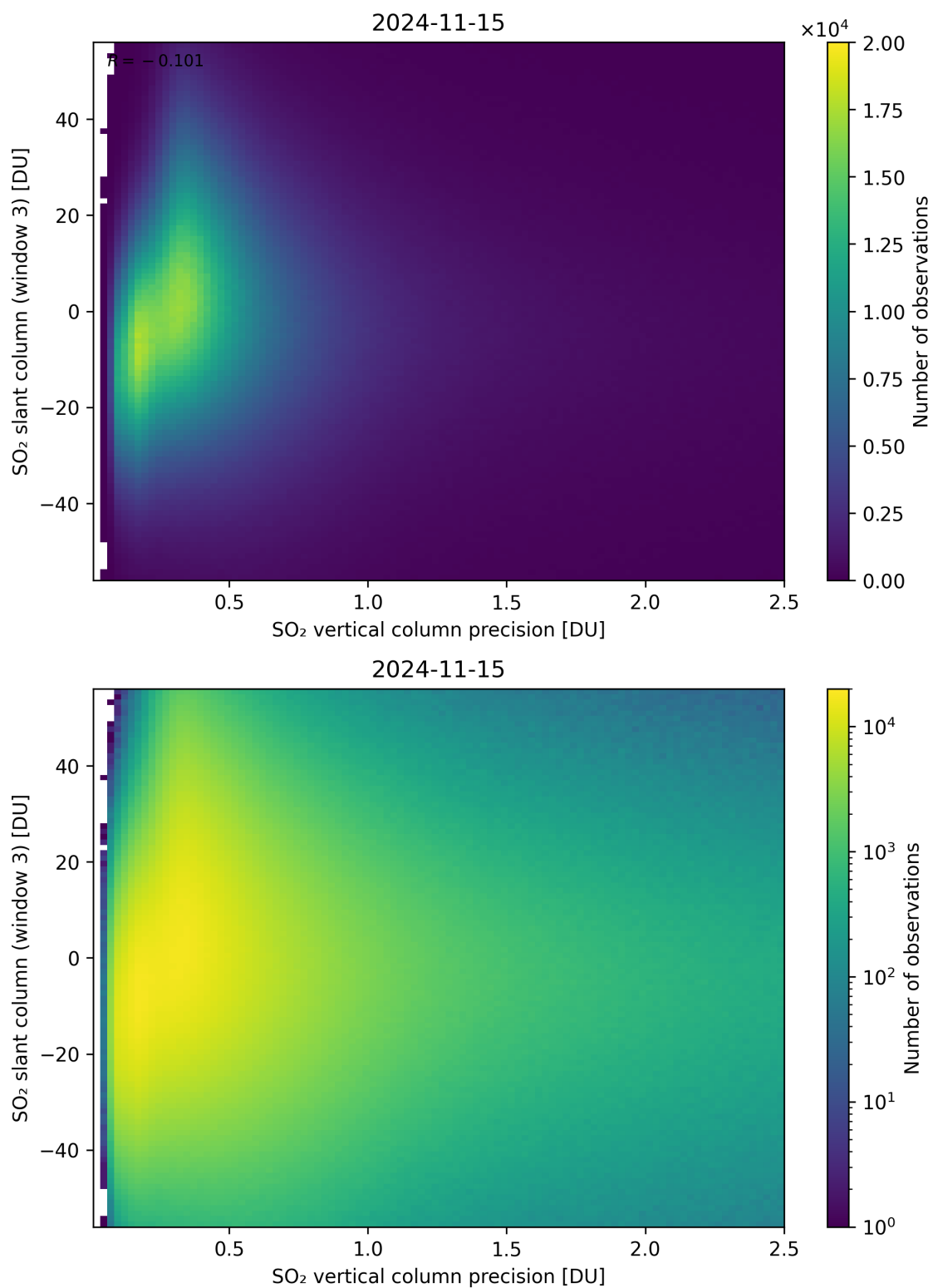
Figure 292: Scatter density plot of “SO 2 vertical column precision” against “SO 2 slant column (window 3)” for 2024-11-14 to 2024-11-16.
