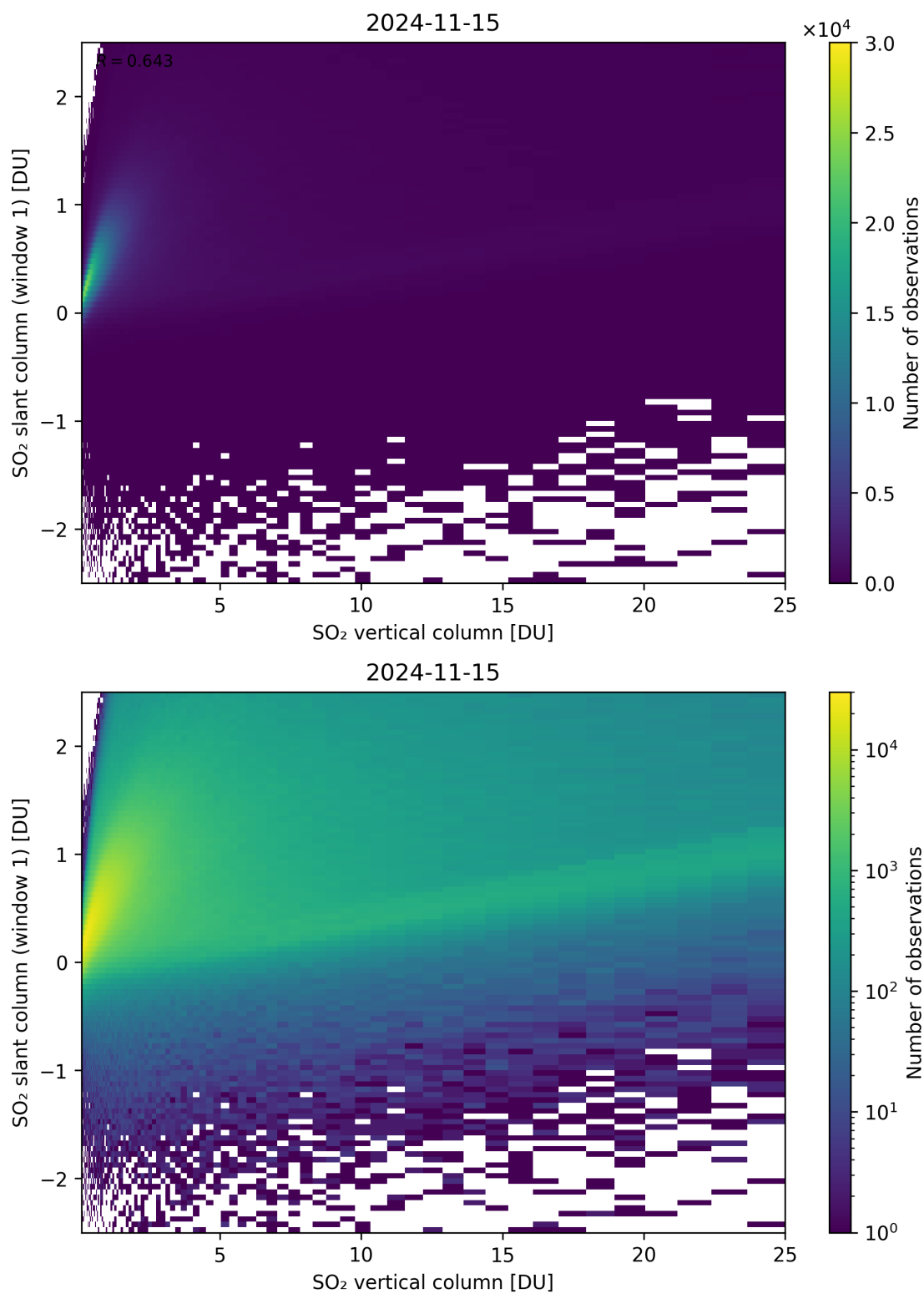
Figure 300: Scatter density plot of “SO 2 vertical column” against “SO 2 slant column (window 1)” for 2024-11-14 to 2024-11-16.
