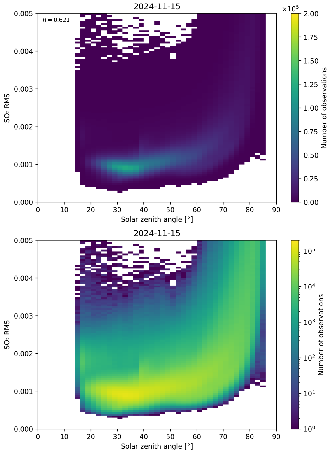
Figure 163: Scatter density plot of “Solar zenith angle” against “SO 2 RMS” for 2024-11-14 to 2024-11-16.
