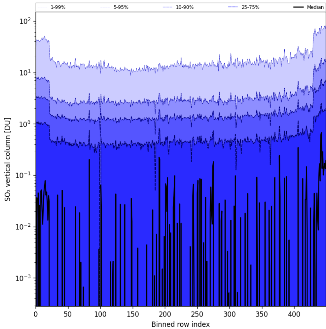
Figure 76: Along track statistics of “SO 2 vertical column” for 2024-11-14 to 2024-11-16
