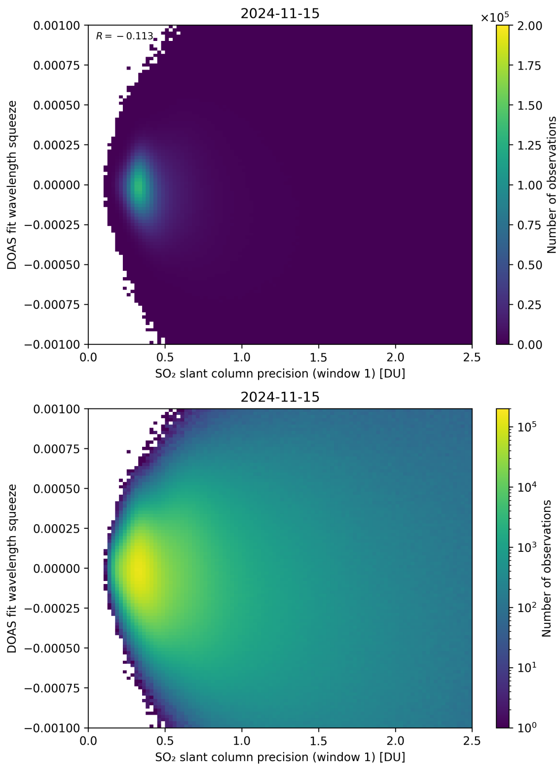
Figure 222: Scatter density plot of “SO 2 slant column precision (window 1)” against “DOAS fit wavelength squeeze” for 2024-11-14 to 2024-11-16.
