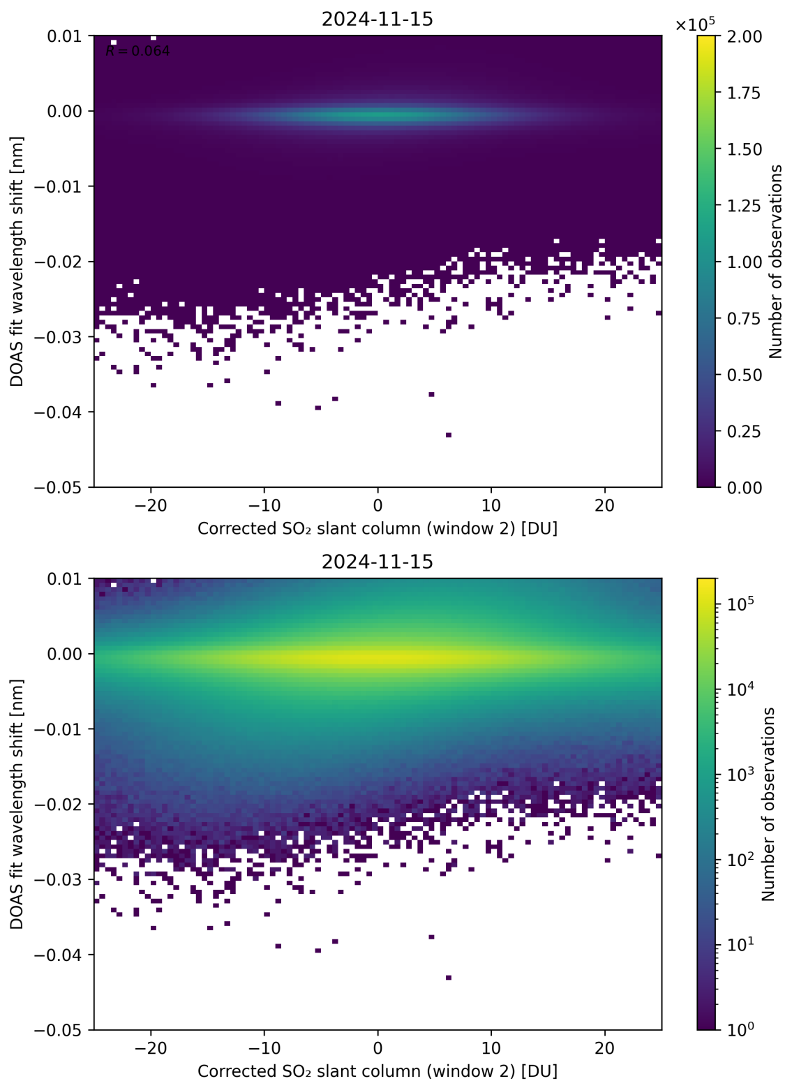
Figure 196: Scatter density plot of “Corrected SO 2 slant column (window 2)” against “DOAS fit wavelength shift” for 2024-11-14 to 2024-11-16.
