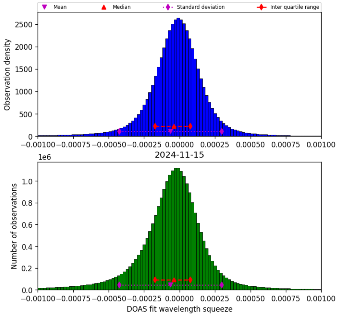
Figure 69: Histogram of “DOAS fit wavelength squeeze” for 2024-11-14 to 2024-11-16
