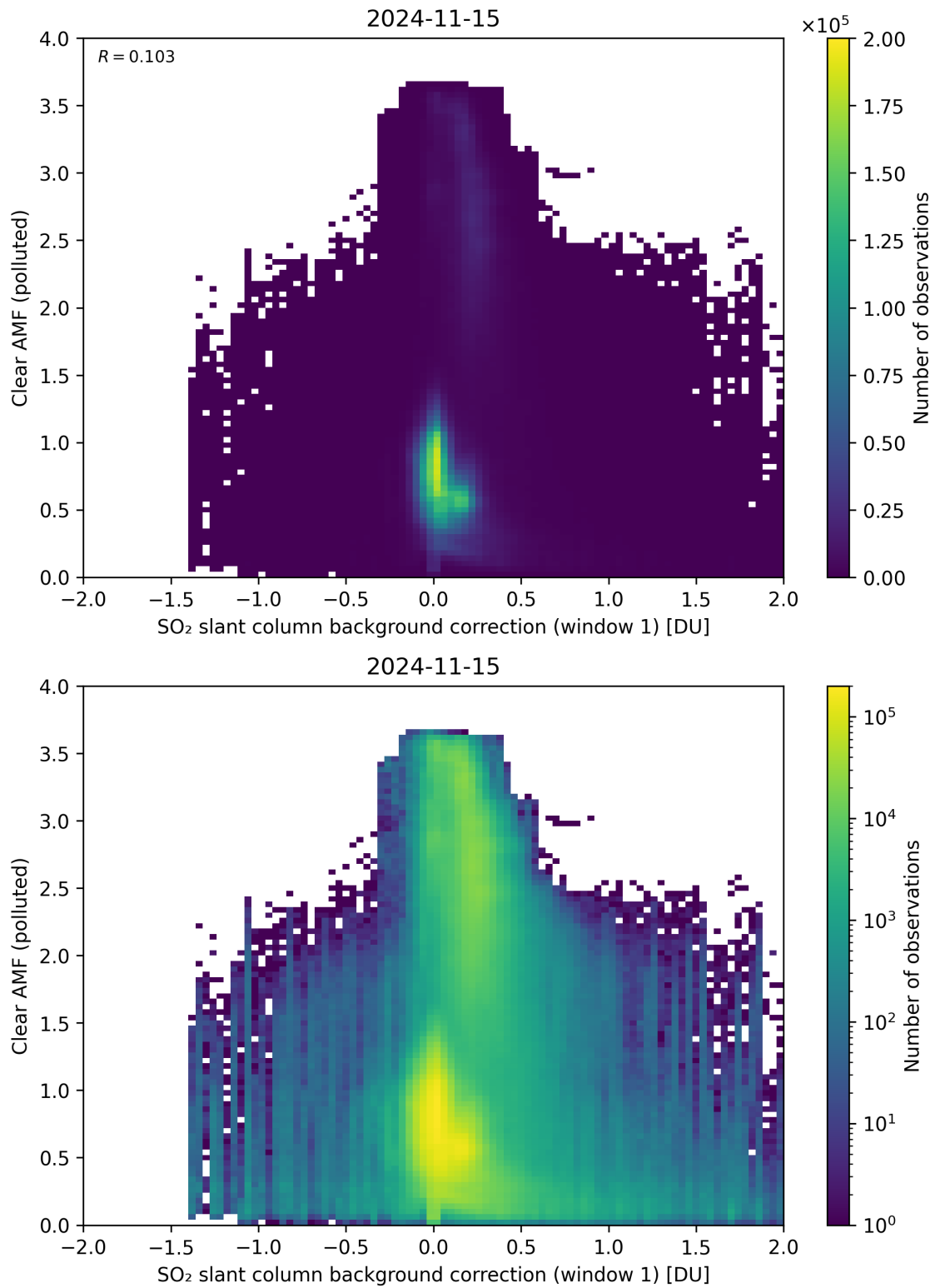
Figure 103: Scatter density plot of “SO 2 slant column background correction (window 1)” against “Clear AMF (polluted)” for 2024-11-14 to 2024-11-16.
