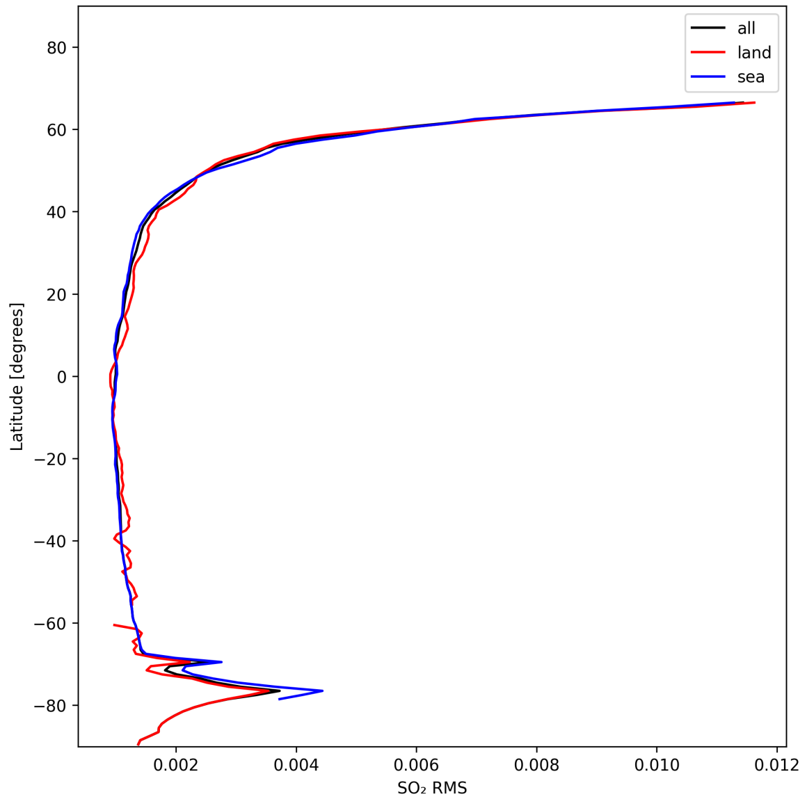
Figure 47: Zonal average of “SO 2 RMS” for 2024-11-14 to 2024-11-16.
