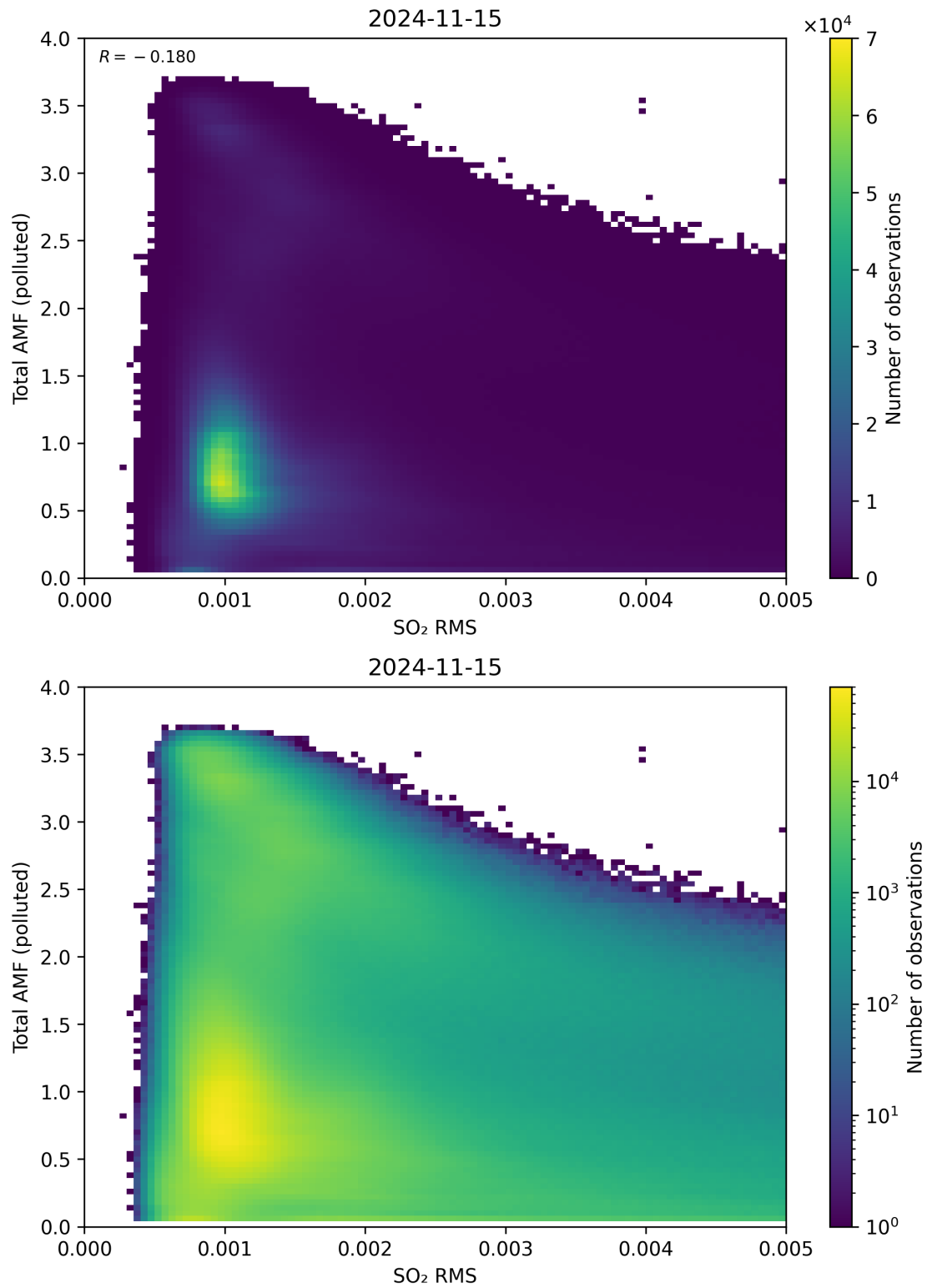
Figure 137: Scatter density plot of “SO 2 RMS” against “Total AMF (polluted)” for 2024-11-14 to 2024-11-16.
