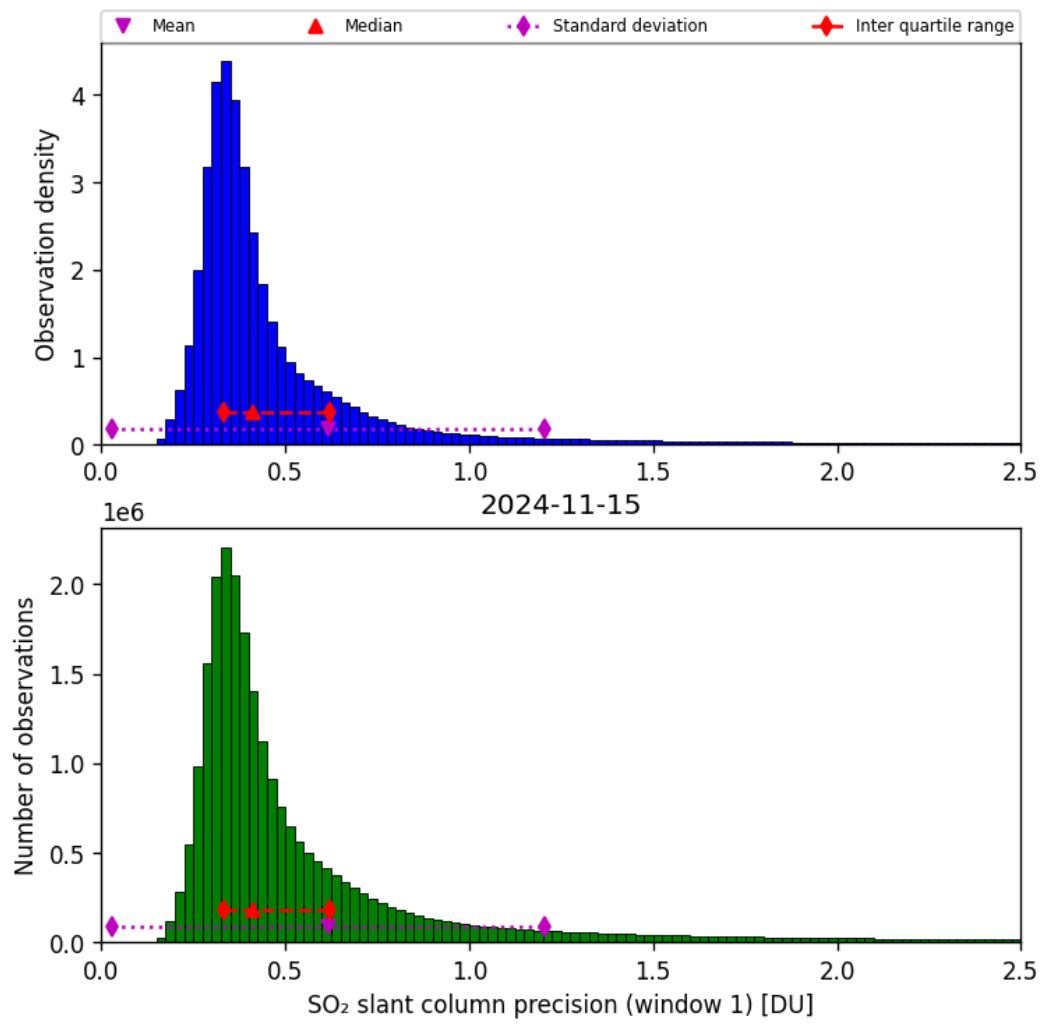
Figure 57: Histogram of “SO 2 slant column precision (window 1)” for 2024-11-14 to 2024-11-16
