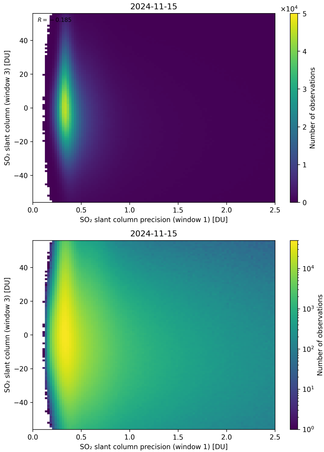
Figure 228: Scatter density plot of “SO 2 slant column precision (window 1)” against “SO 2 slant column (window 3)” for 2024-11-14 to 2024-11-16.
