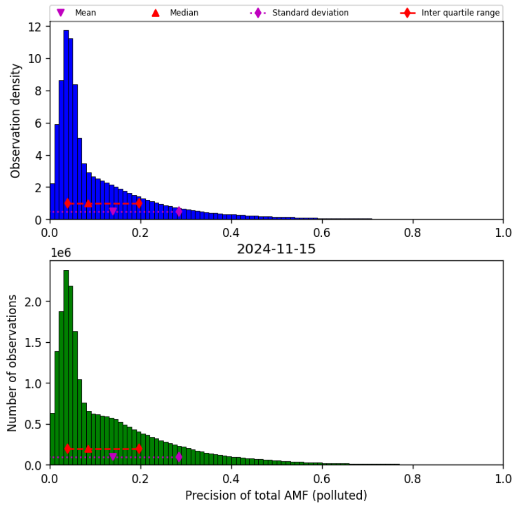
Figure 72: Histogram of “Precision of total AMF (polluted)” for 2024-11-14 to 2024-11-16
