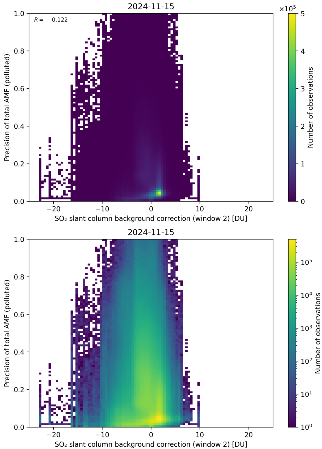
Figure 120: Scatter density plot of “SO 2 slant column background correction (window 2)” against “Precision of total AMF (polluted)” for 2024-11-14 to 2024-11-16.
