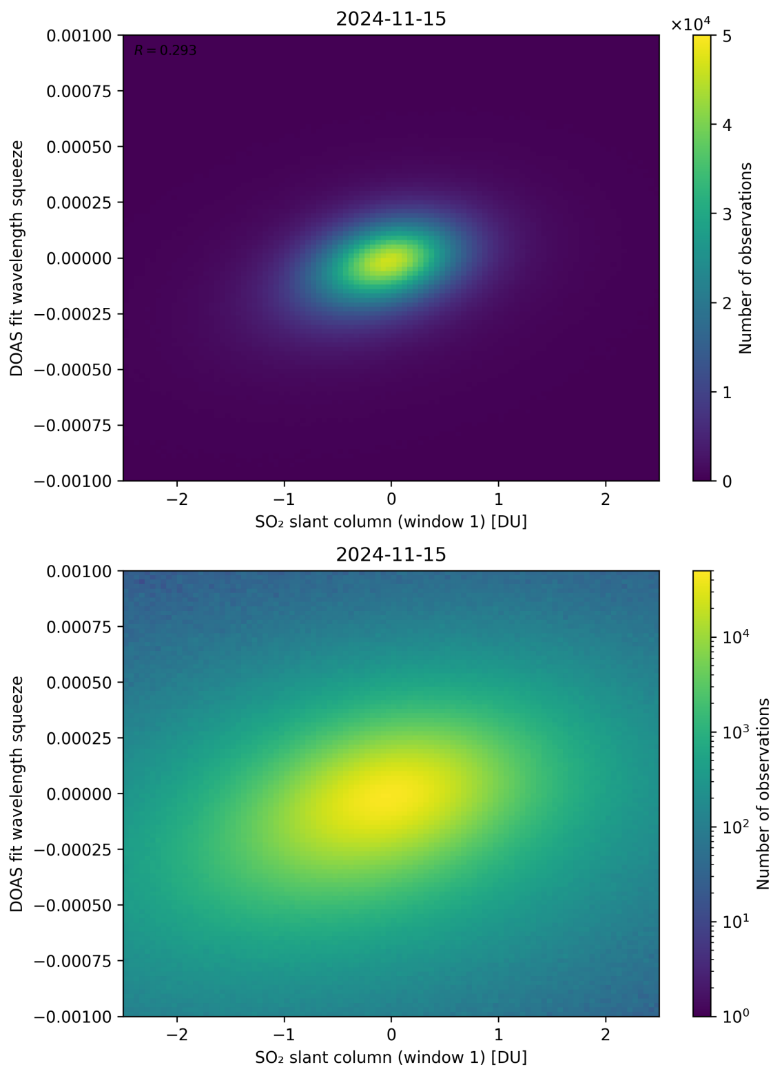
Figure 216: Scatter density plot of “SO 2 slant column (window 1)” against “DOAS fit wavelength squeeze” for 2024-11-14 to 2024-11-16.
