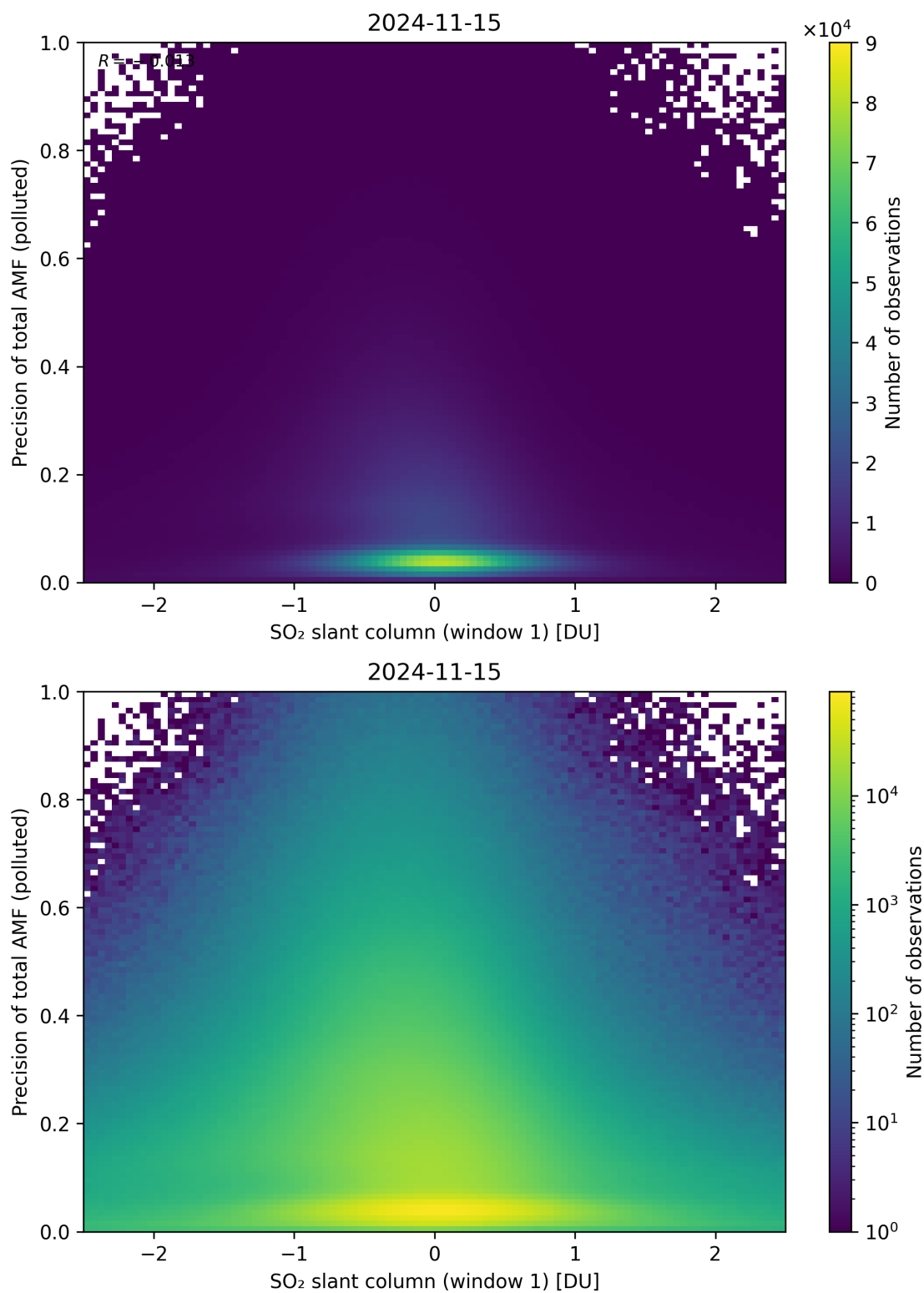
Figure 240: Scatter density plot of “SO 2 slant column (window 1)” against “Precision of total AMF (polluted)” for 2024-11-14 to 2024-11-16.
