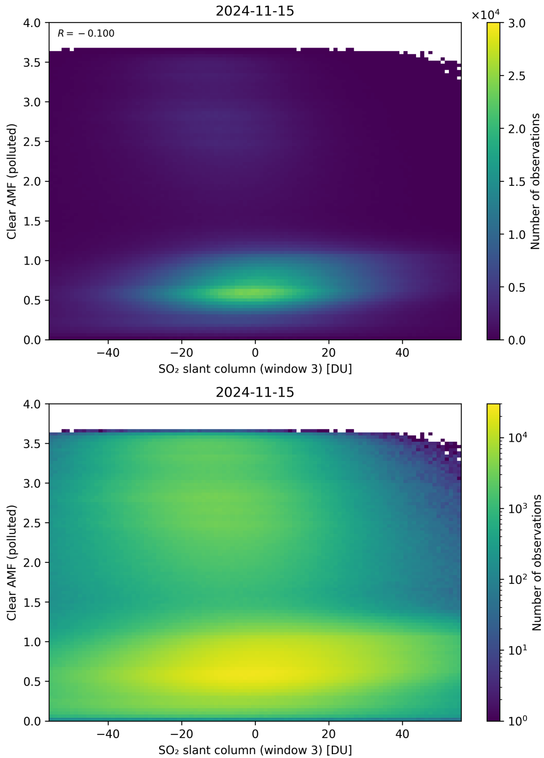
Figure 265: Scatter density plot of “SO 2 slant column (window 3)” against “Clear AMF (polluted)” for 2024-11-14 to 2024-11-16.
