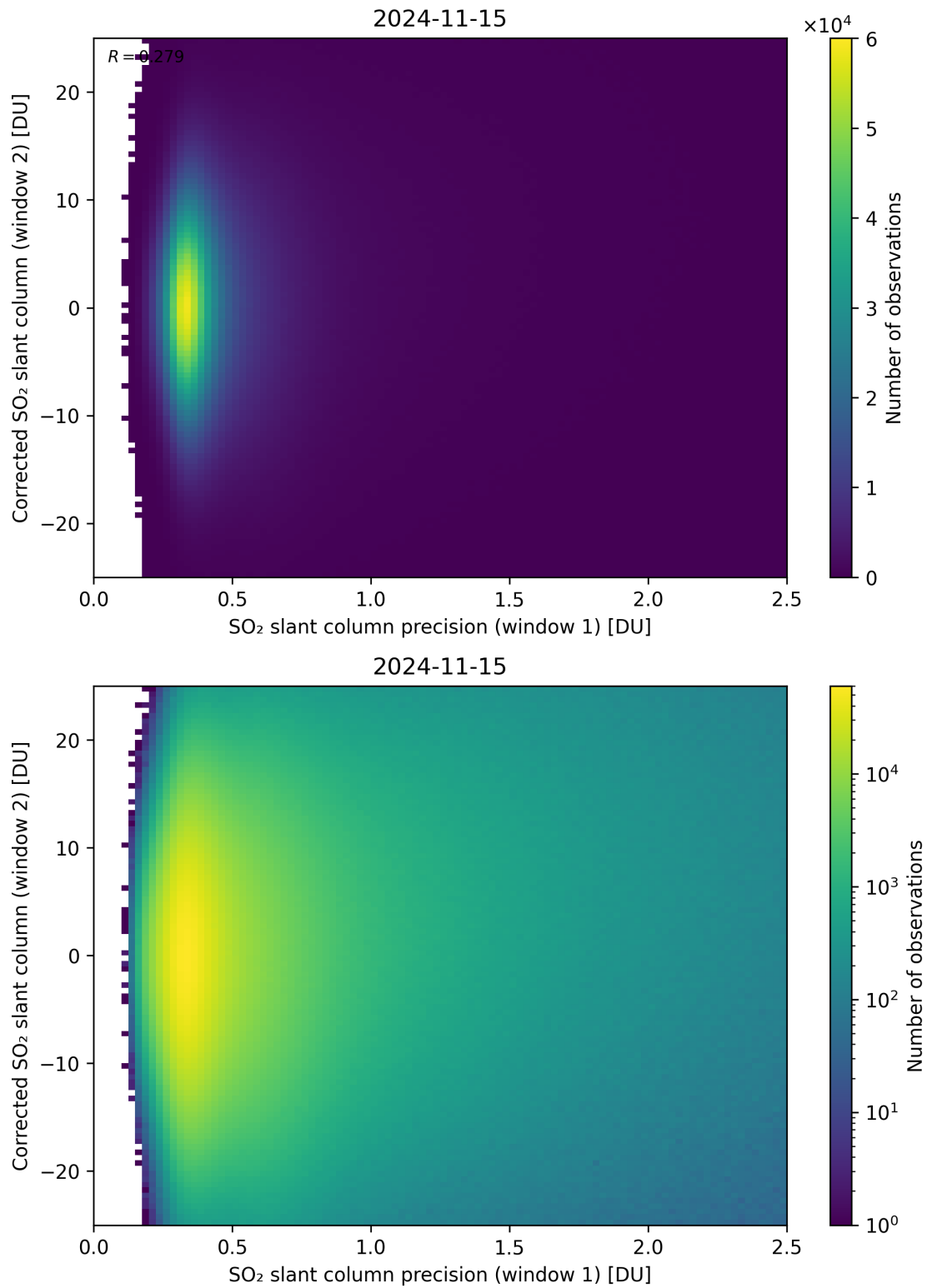
Figure 225: Scatter density plot of “SO 2 slant column precision (window 1)” against “Corrected SO 2 slant column (window 2)” for 2024-11-14 to 2024-11-16.
