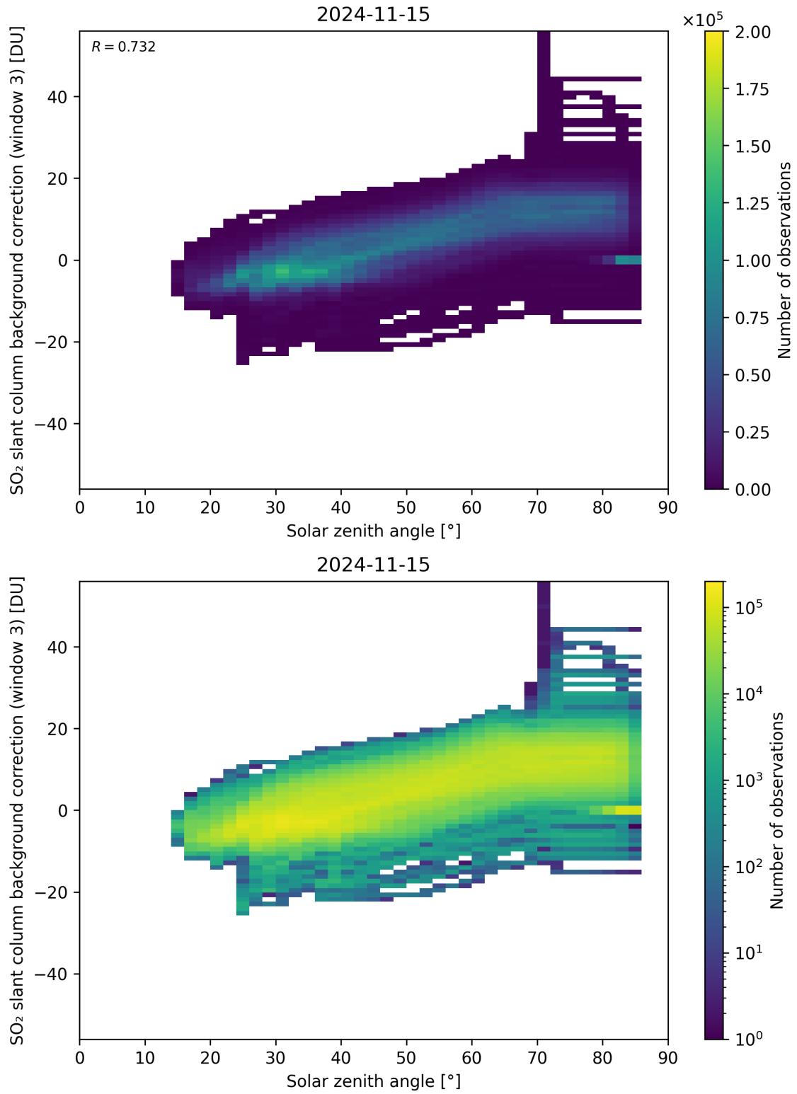
Figure 160: Scatter density plot of “Solar zenith angle” against “SO 2 slant column background correction (window 3)” for 2024-11-14 to 2024-11-16.
