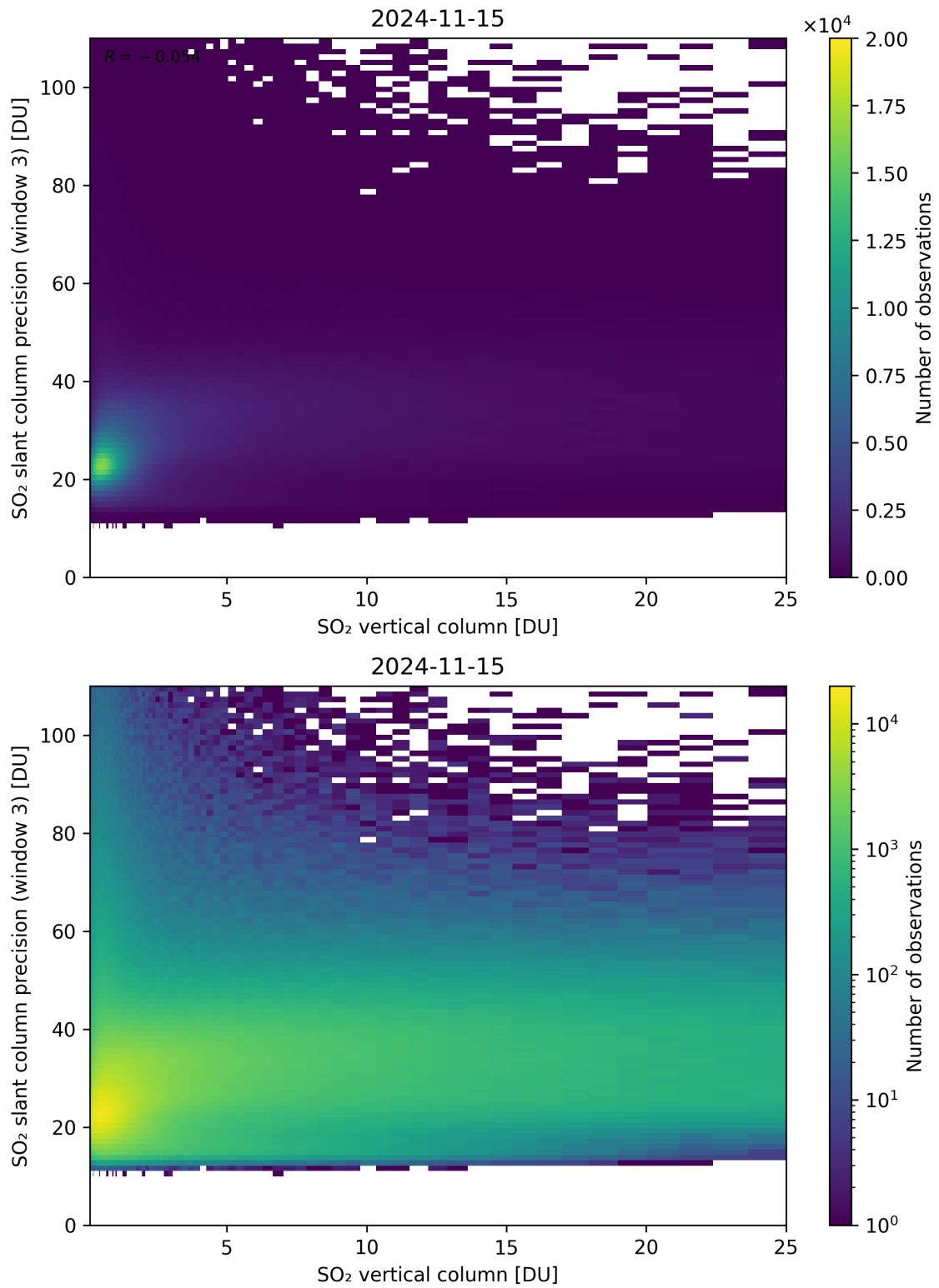
Figure 304: Scatter density plot of “SO 2 vertical column” against “SO 2 slant column precision (window 3)” for 2024-11-14 to 2024-11-16.
