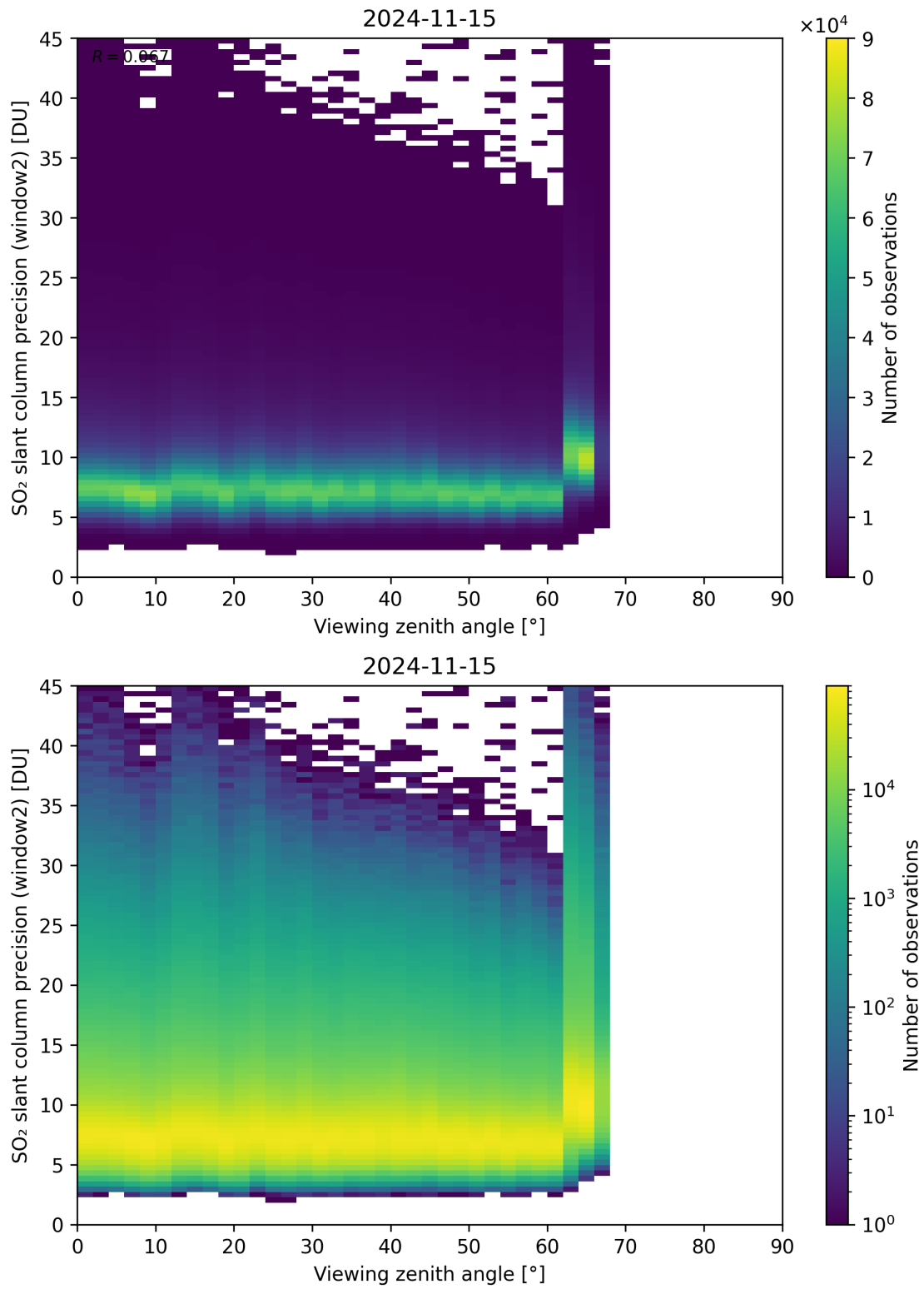
Figure 322: Scatter density plot of “Viewing zenith angle” against “SO 2 slant column precision (window2)” for 2024-11-14 to 2024-11-16.
