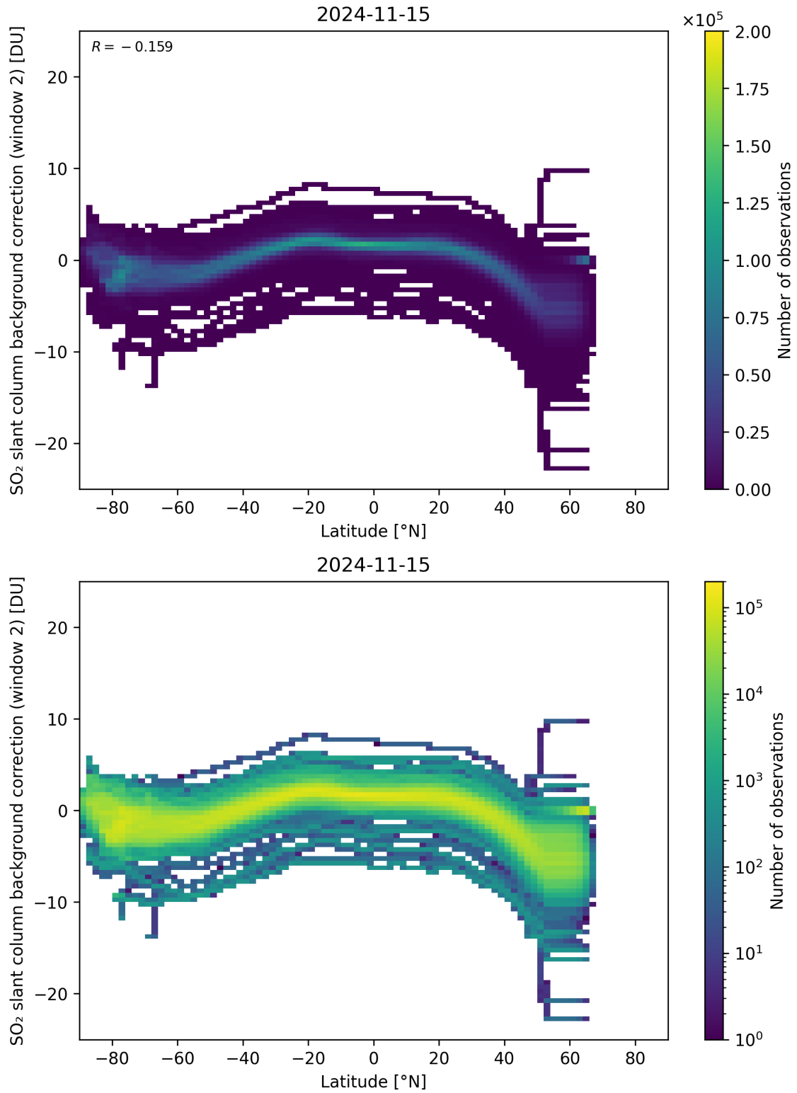
Figure 140: Scatter density plot of “Latitude” against “SO 2 slant column background correction (window 2)” for 2024-11-14 to 2024-11-16.
