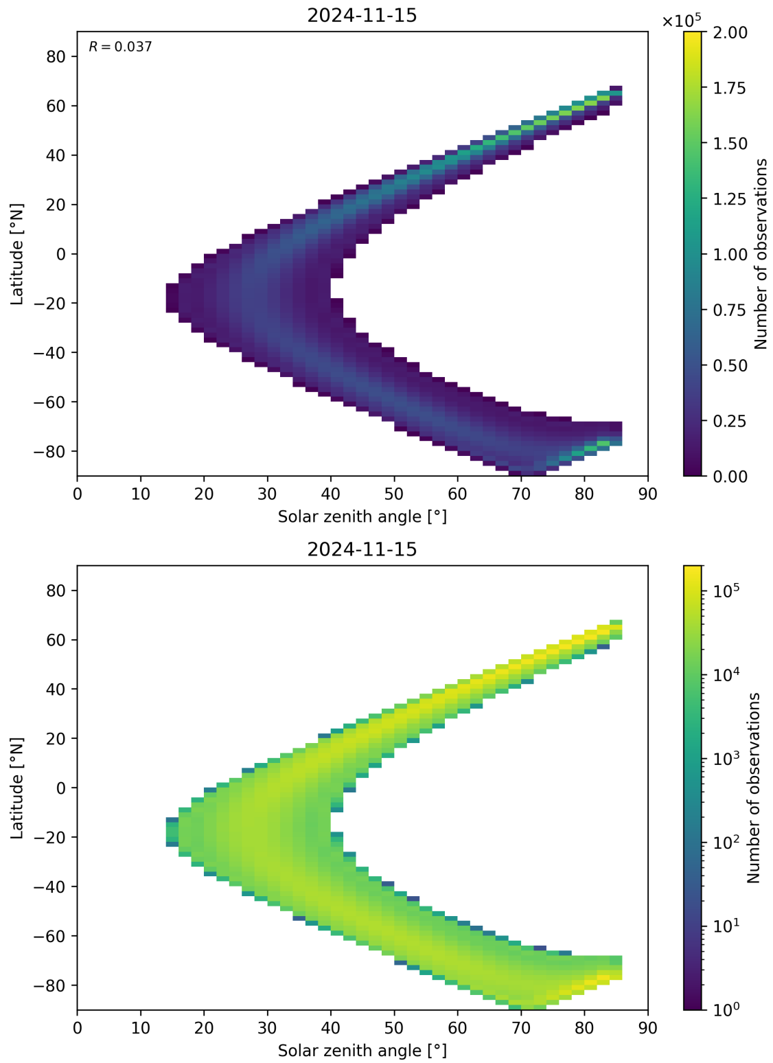
Figure 164: Scatter density plot of “Solar zenith angle” against “Latitude” for 2024-11-14 to 2024-11-16.
