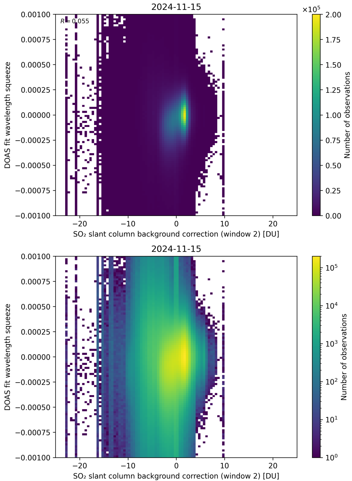
Figure 113: Scatter density plot of “SO 2 slant column background correction (window 2)” against “DOAS fit wavelength squeeze” for 2024-11-14 to 2024-11-16.
