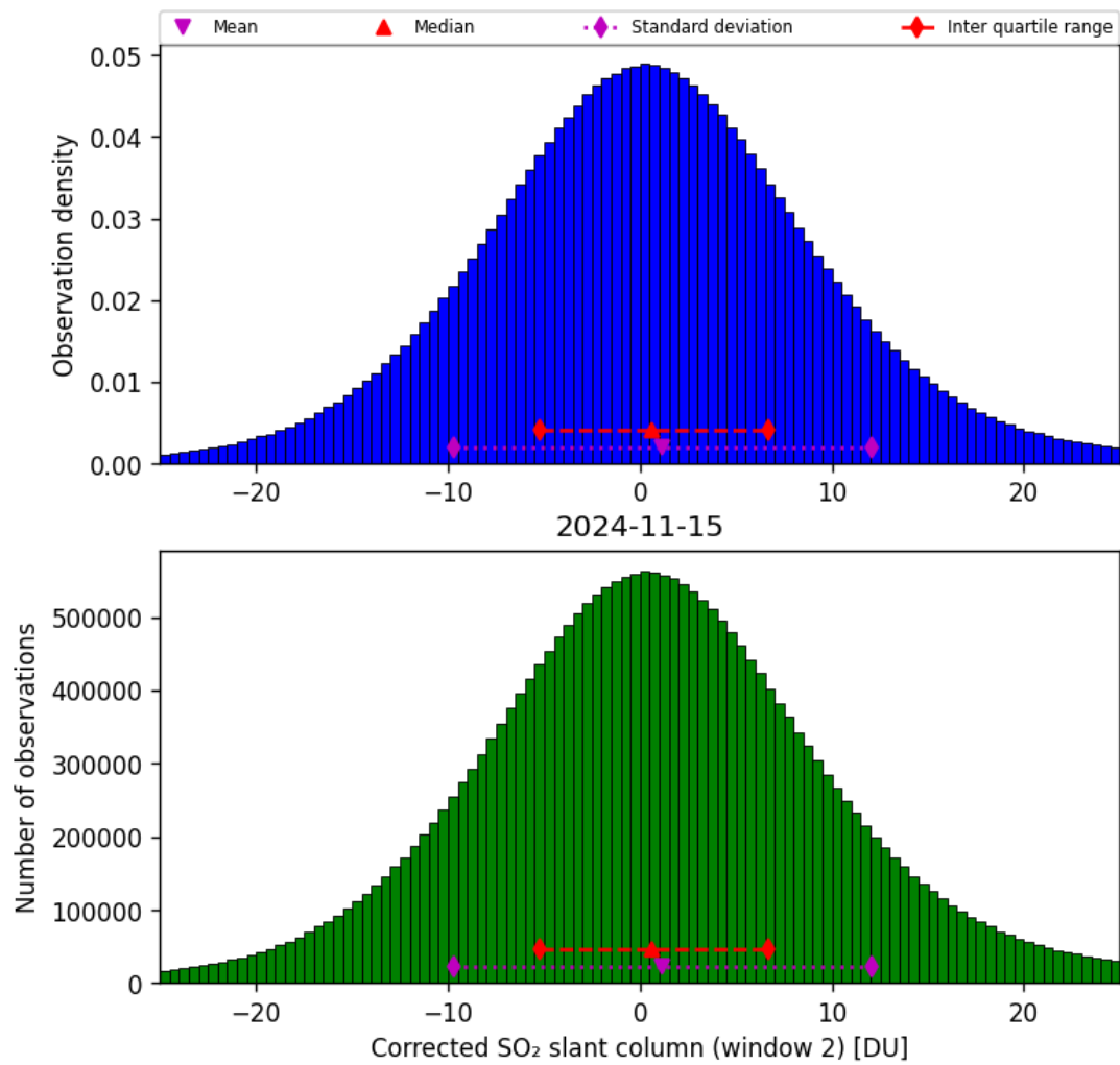
Figure 62: Histogram of “Corrected SO 2 slant column (window 2)” for 2024-11-14 to 2024-11-16
