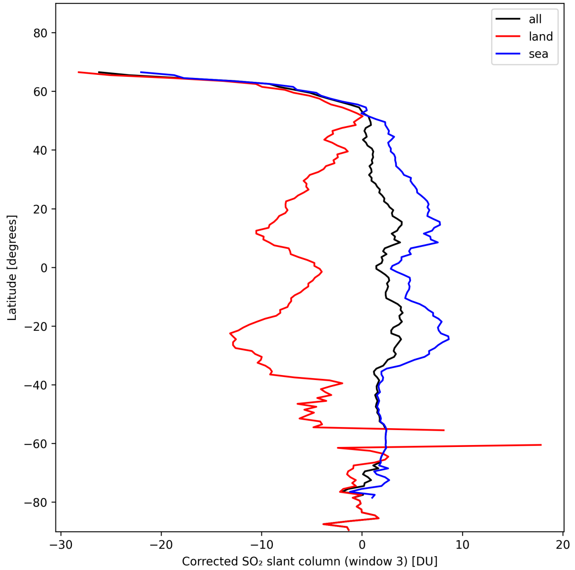
Figure 43: Zonal average of “Corrected SO 2 slant column (window 3)” for 2024-11-14 to 2024-11-16.
