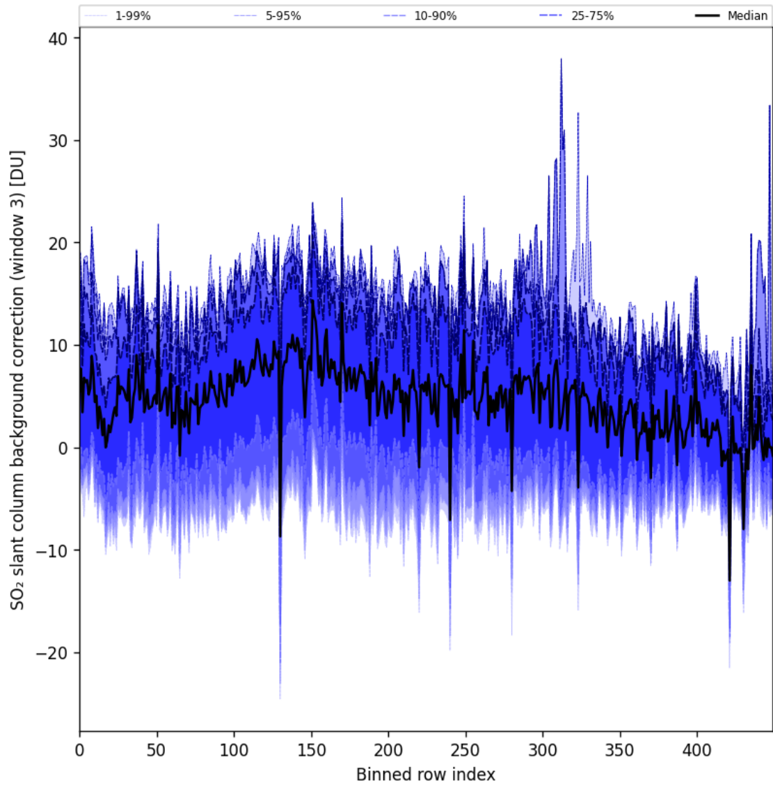
Figure 90: Along track statistics of “SO 2 slant column background correction (window 3)” for 2024-11-14 to 2024-11-16
