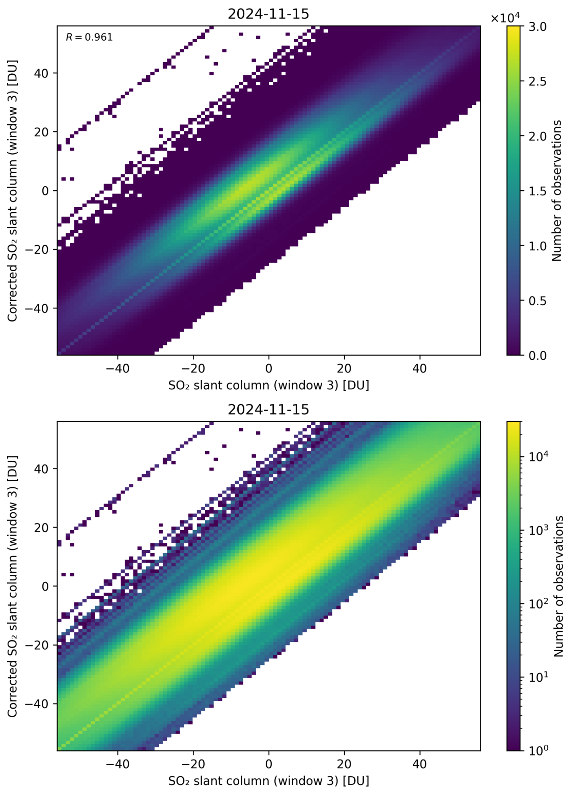
Figure 266: Scatter density plot of “SO 2 slant column (window 3)” against “Corrected SO 2 slant column (window 3)” for 2024-11-14 to 2024-11-16.
