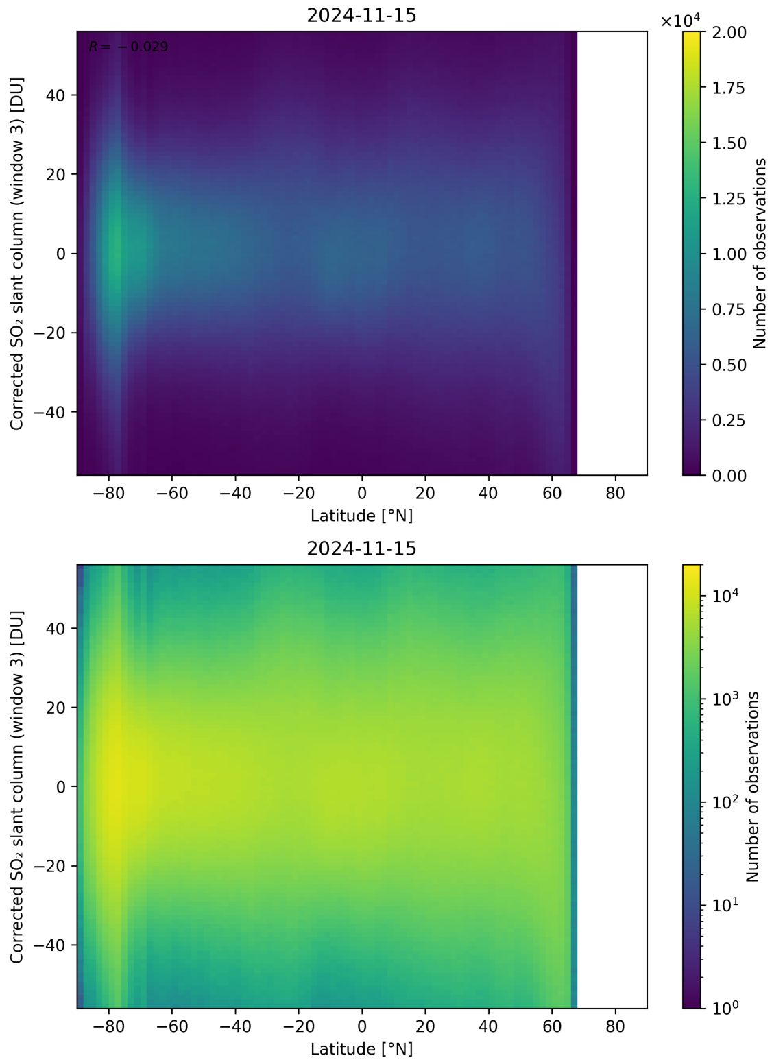
Figure 148: Scatter density plot of “Latitude” against “Corrected SO 2 slant column (window 3)” for 2024-11-14 to 2024-11-16.
