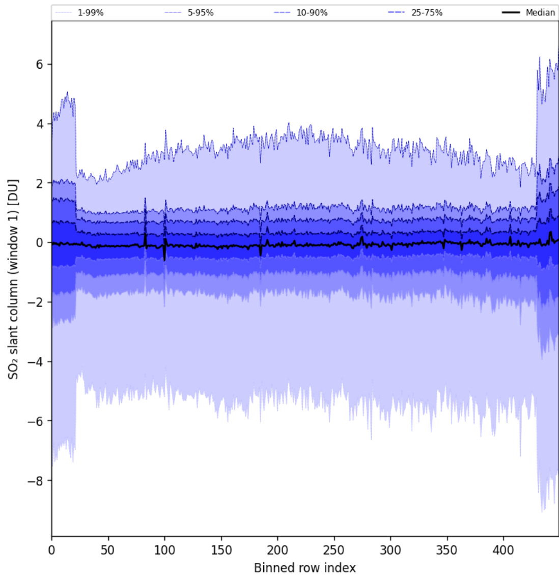
Figure 79: Along track statistics of “SO 2 slant column (window 1)” for 2024-11-14 to 2024-11-16
