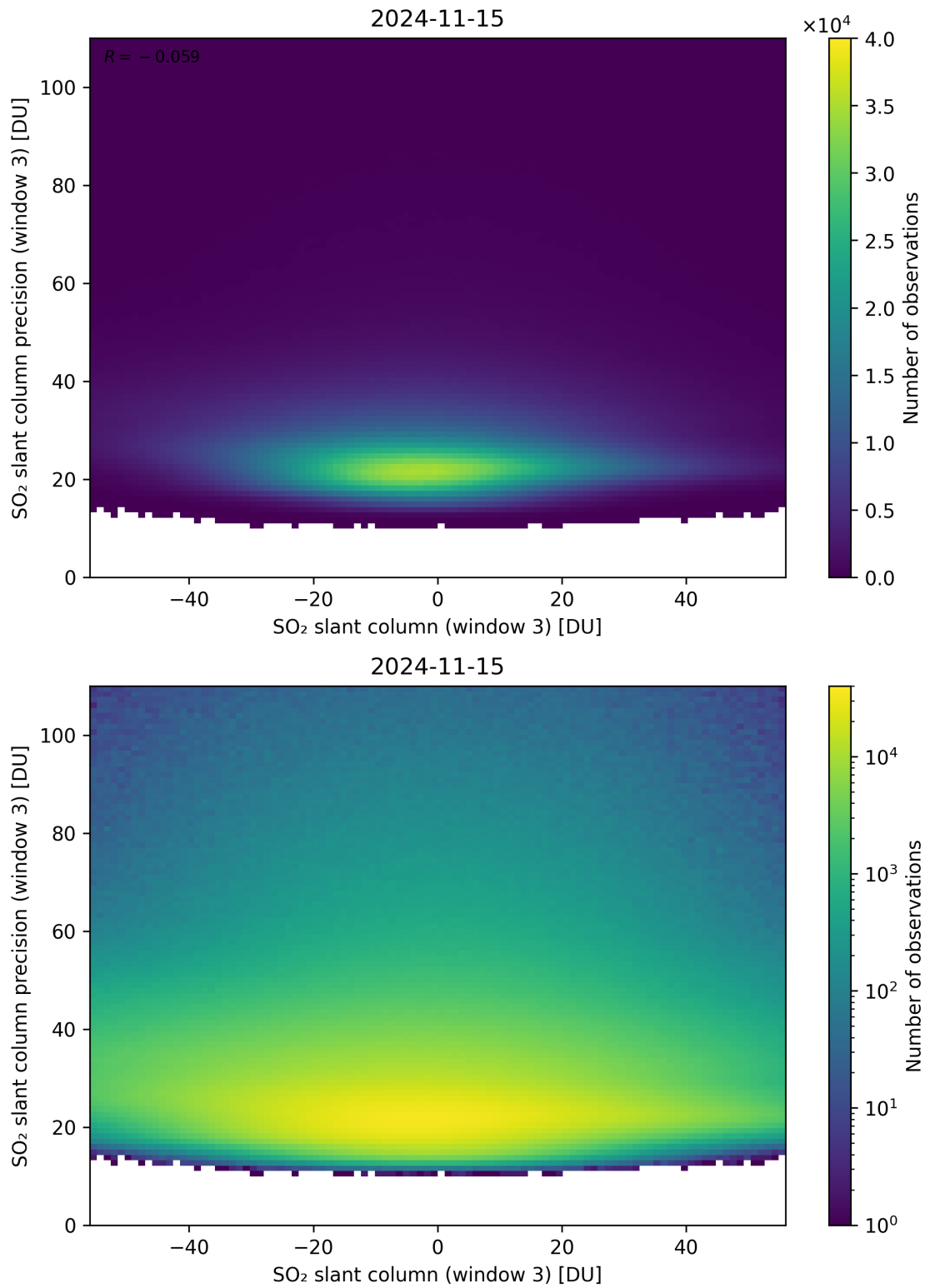
Figure 267: Scatter density plot of “SO 2 slant column (window 3)” against “SO 2 slant column precision (window 3)” for 2024-11-14 to 2024-11-16.
