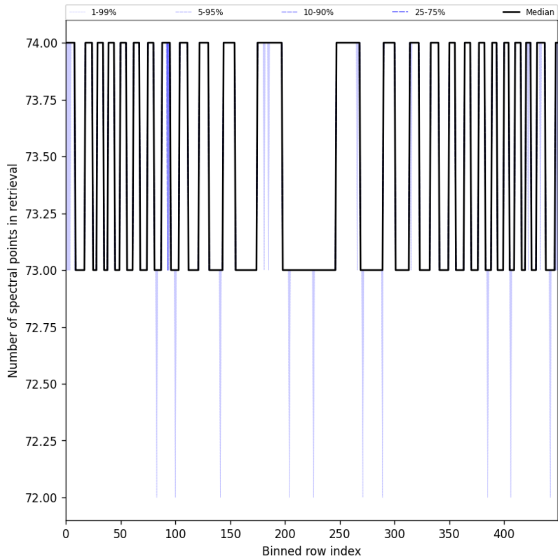
Figure 97: Along track statistics of “Number of spectral points in retrieval” for 2024-11-14 to 2024-11-16
