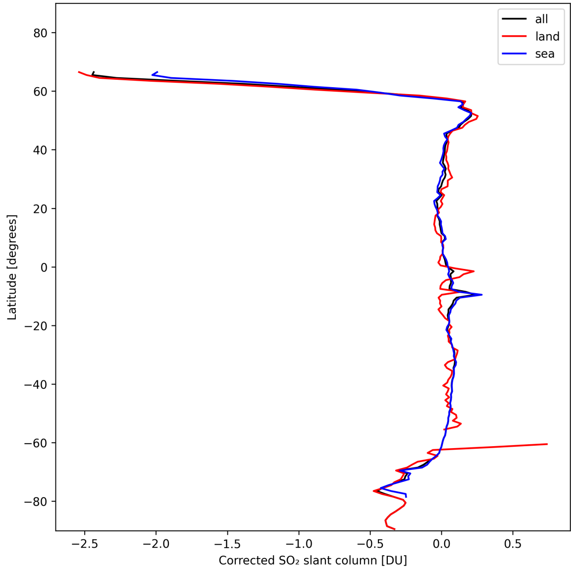
Figure 32: Zonal average of “Corrected SO 2 slant column” for 2024-11-14 to 2024-11-16.
