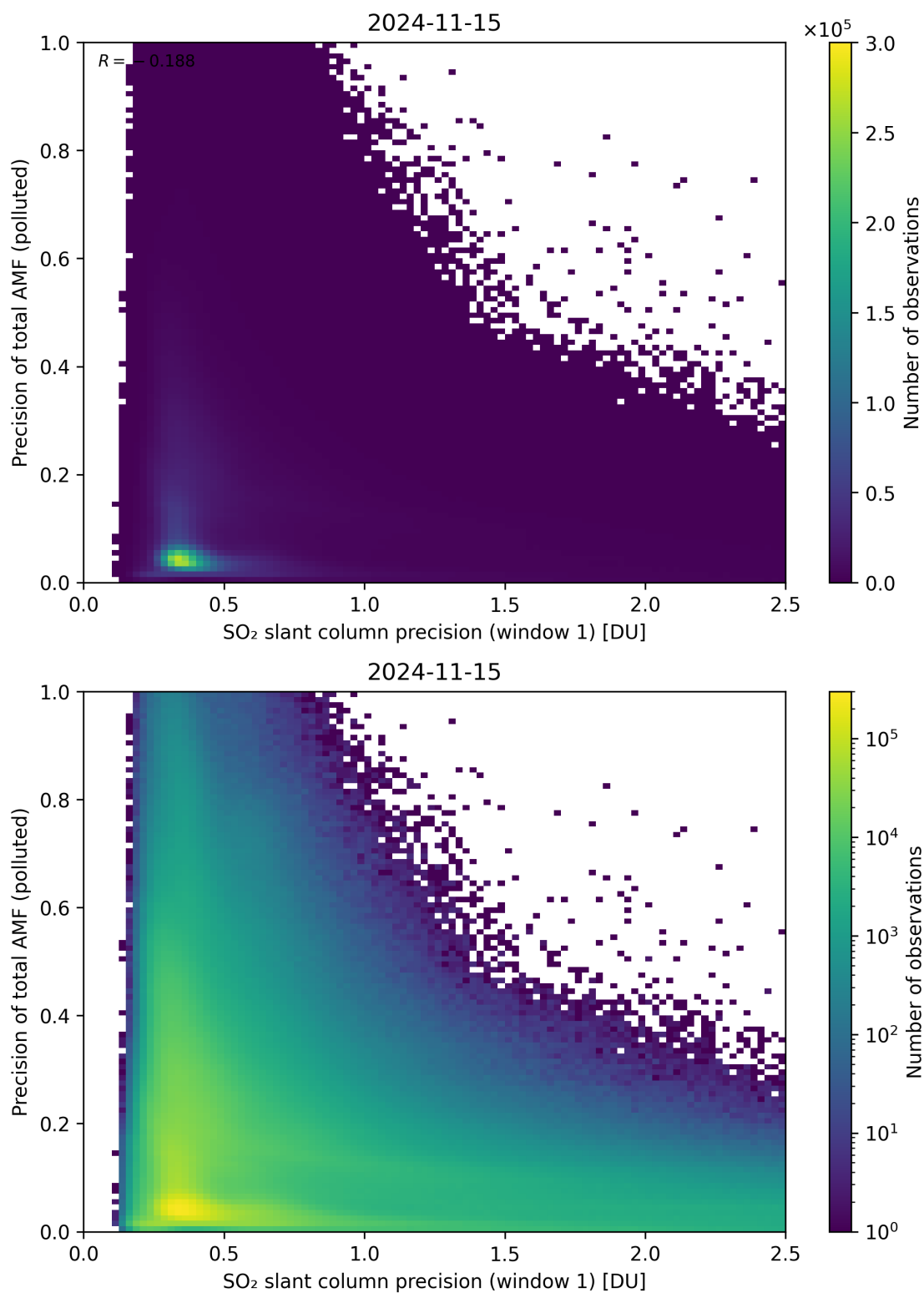
Figure 231: Scatter density plot of “SO 2 slant column precision (window 1)” against “Precision of total AMF (polluted)” for 2024-11-14 to 2024-11-16.
