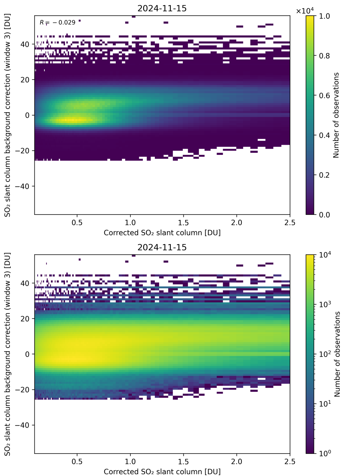
Figure 180: Scatter density plot of “Corrected SO 2 slant column” against “SO 2 slant column background correction (window 3)” for 2024-11-14 to 2024-11-16.
