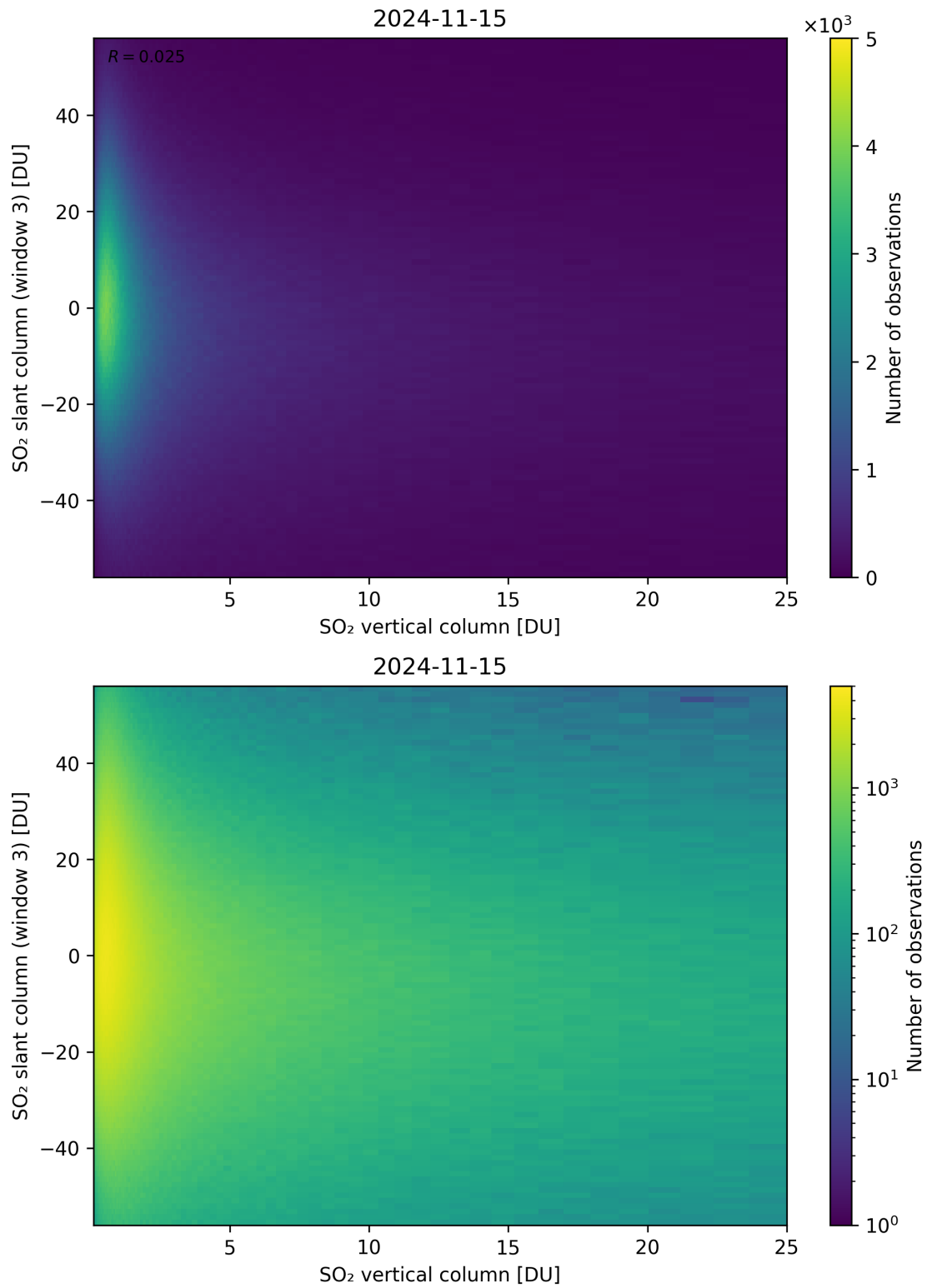
Figure 303: Scatter density plot of “SO 2 vertical column” against “SO 2 slant column (window 3)” for 2024-11-14 to 2024-11-16.
