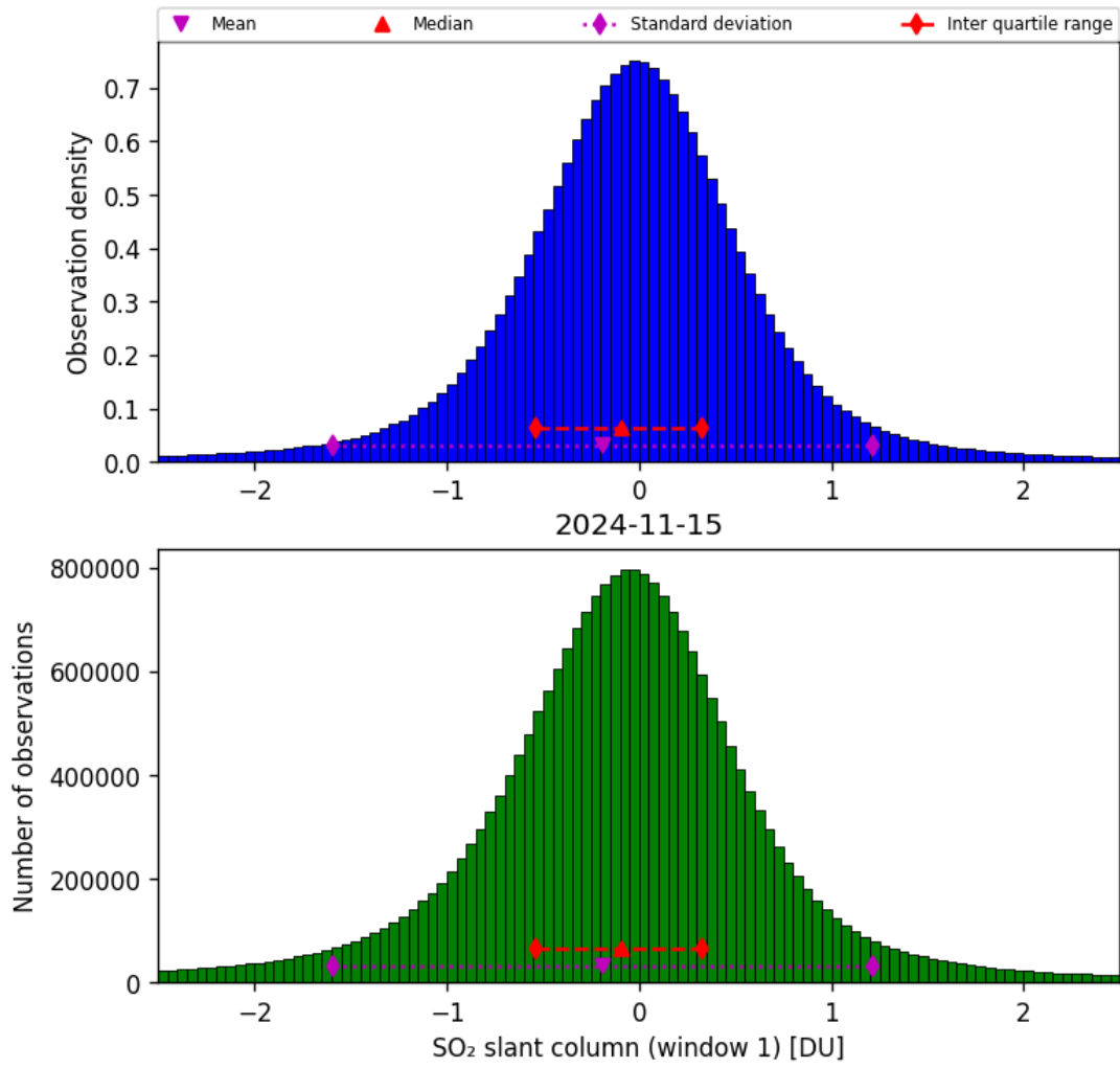
Figure 56: Histogram of “SO 2 slant column (window 1)” for 2024-11-14 to 2024-11-16
