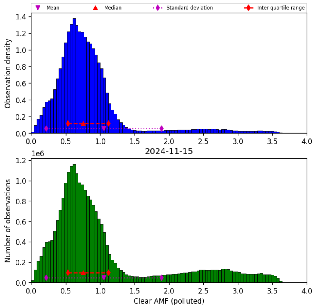
Figure 73: Histogram of “Clear AMF (polluted)” for 2024-11-14 to 2024-11-16
