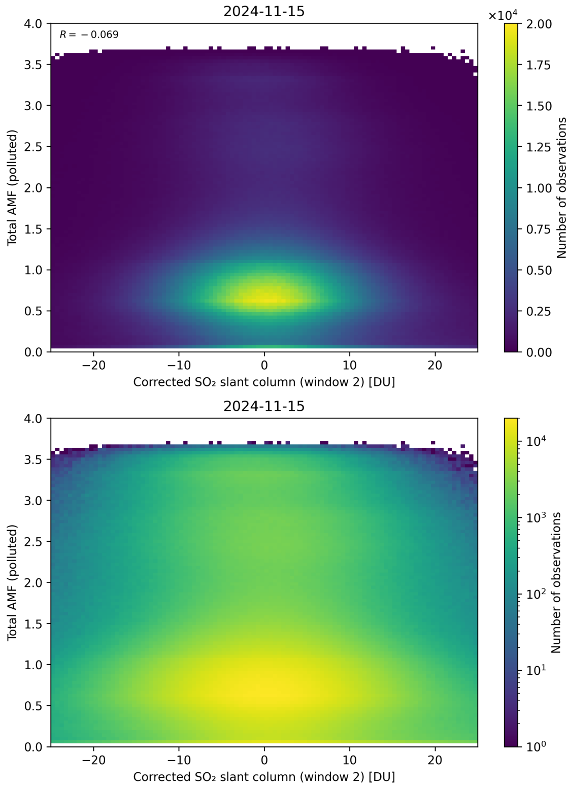
Figure 203: Scatter density plot of “Corrected SO 2 slant column (window 2)” against “Total AMF (polluted)” for 2024-11-14 to 2024-11-16.
