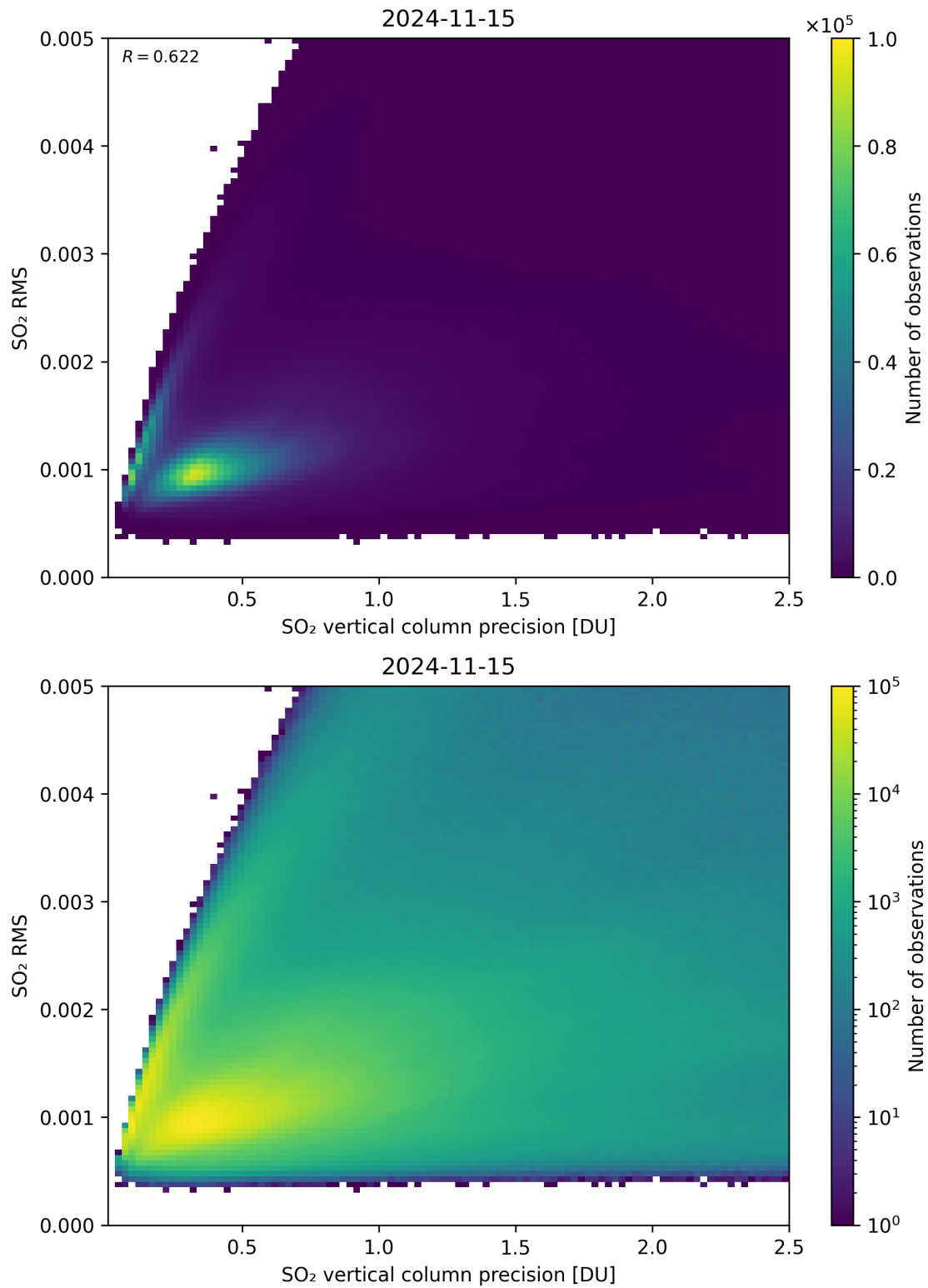
Figure 284: Scatter density plot of “SO 2 vertical column precision” against “SO 2 RMS” for 2024-11-14 to 2024-11-16.
