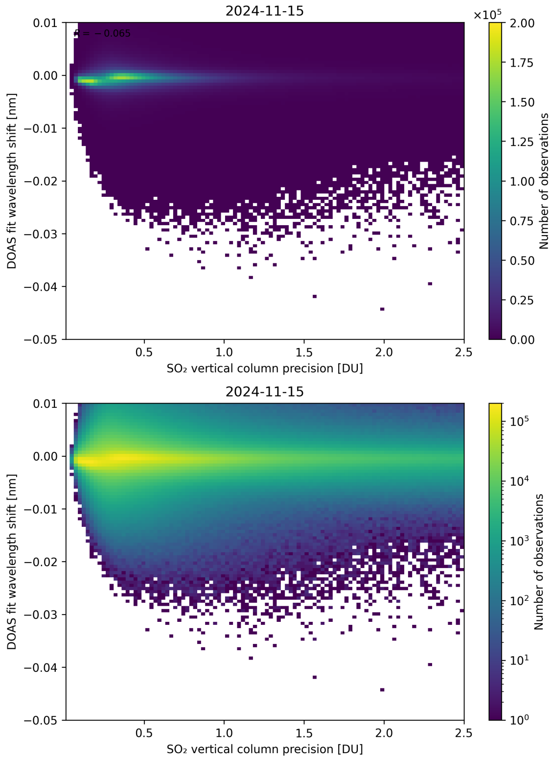
Figure 282: Scatter density plot of “SO 2 vertical column precision” against “DOAS fit wavelength shift” for 2024-11-14 to 2024-11-16.
