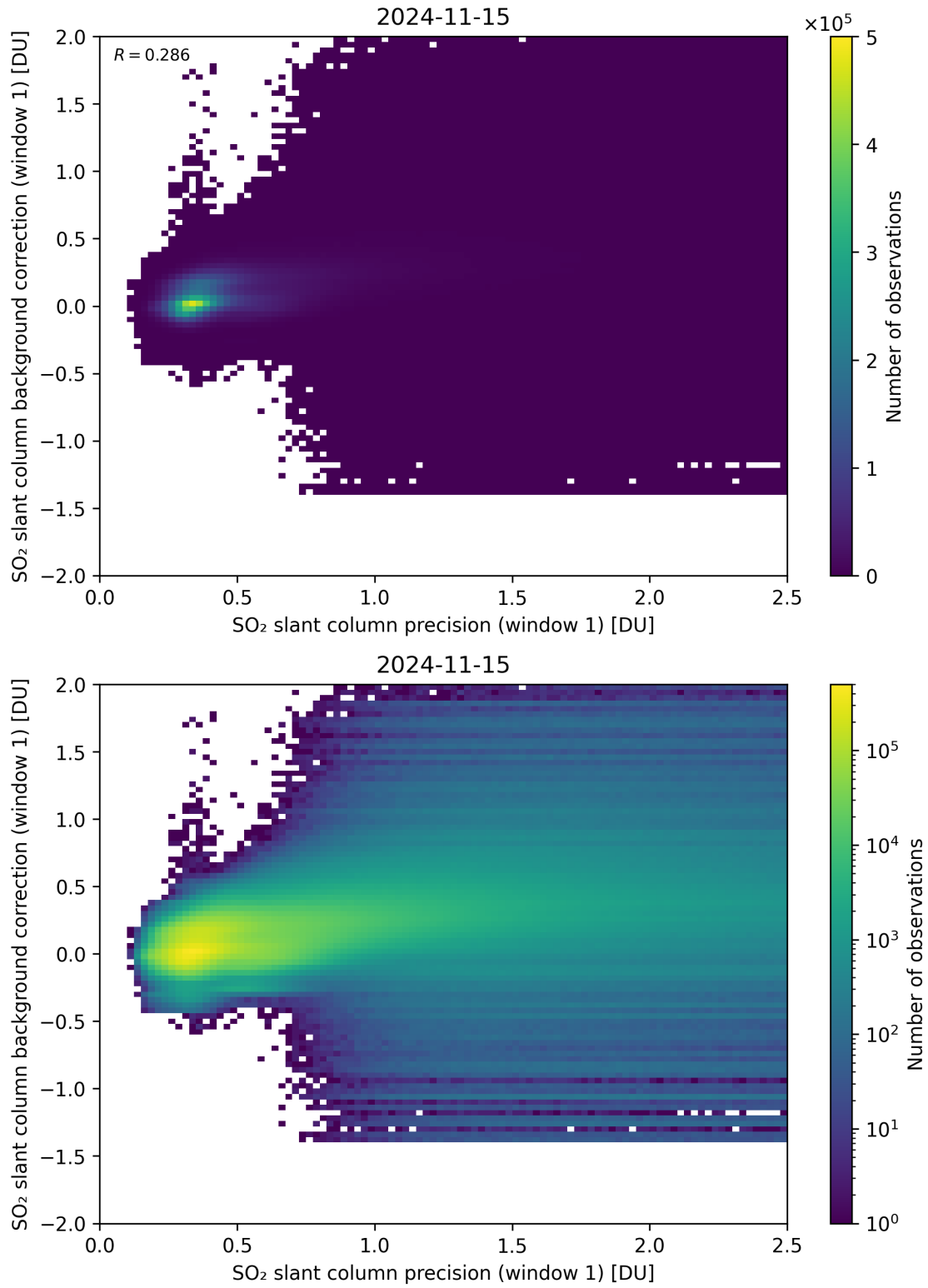
Figure 218: Scatter density plot of “SO 2 slant column precision (window 1)” against “SO 2 slant column background correction (window 1)” for 2024-11-14 to 2024-11-16.
