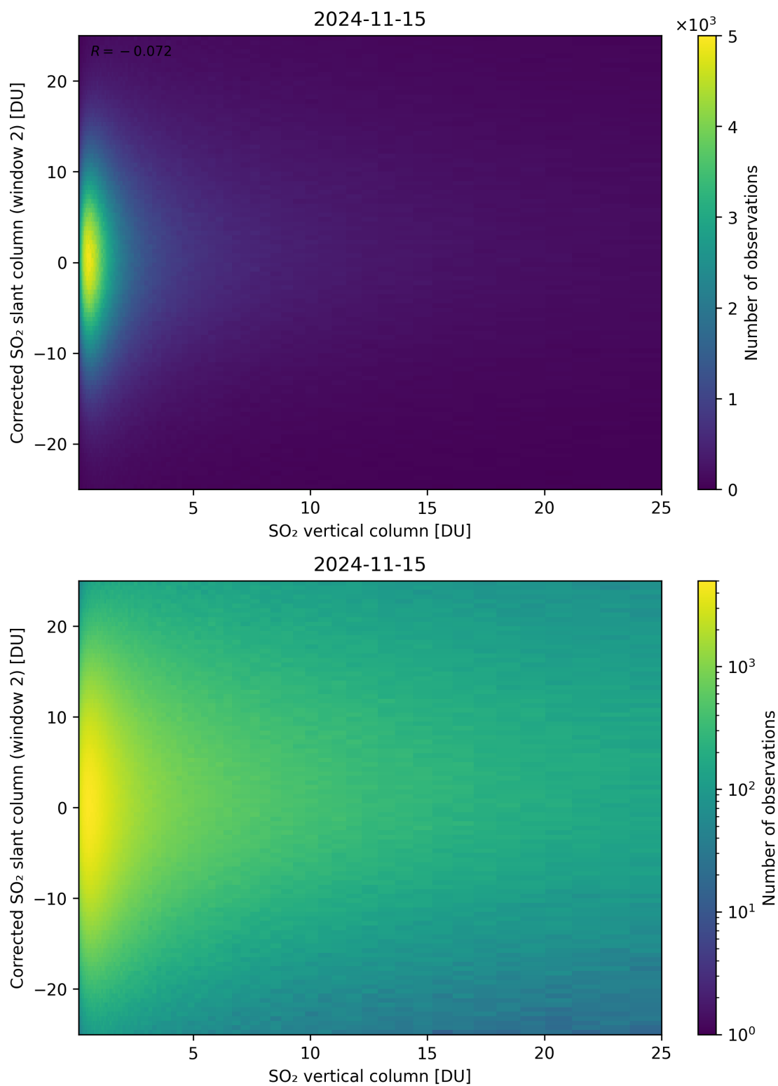
Figure 298: Scatter density plot of “SO 2 vertical column” against “Corrected SO 2 slant column (window 2)” for 2024-11-14 to 2024-11-16.
