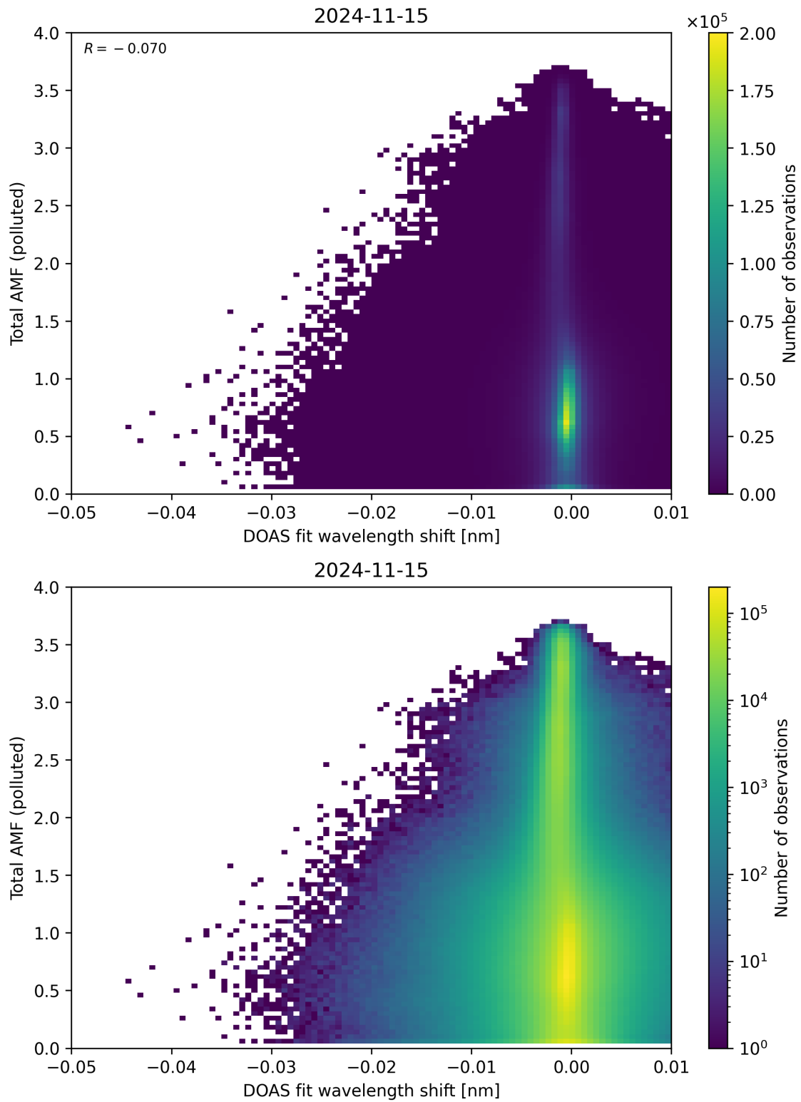
Figure 130: Scatter density plot of “DOAS fit wavelength shift” against “Total AMF (polluted)” for 2024-11-14 to 2024-11-16.
