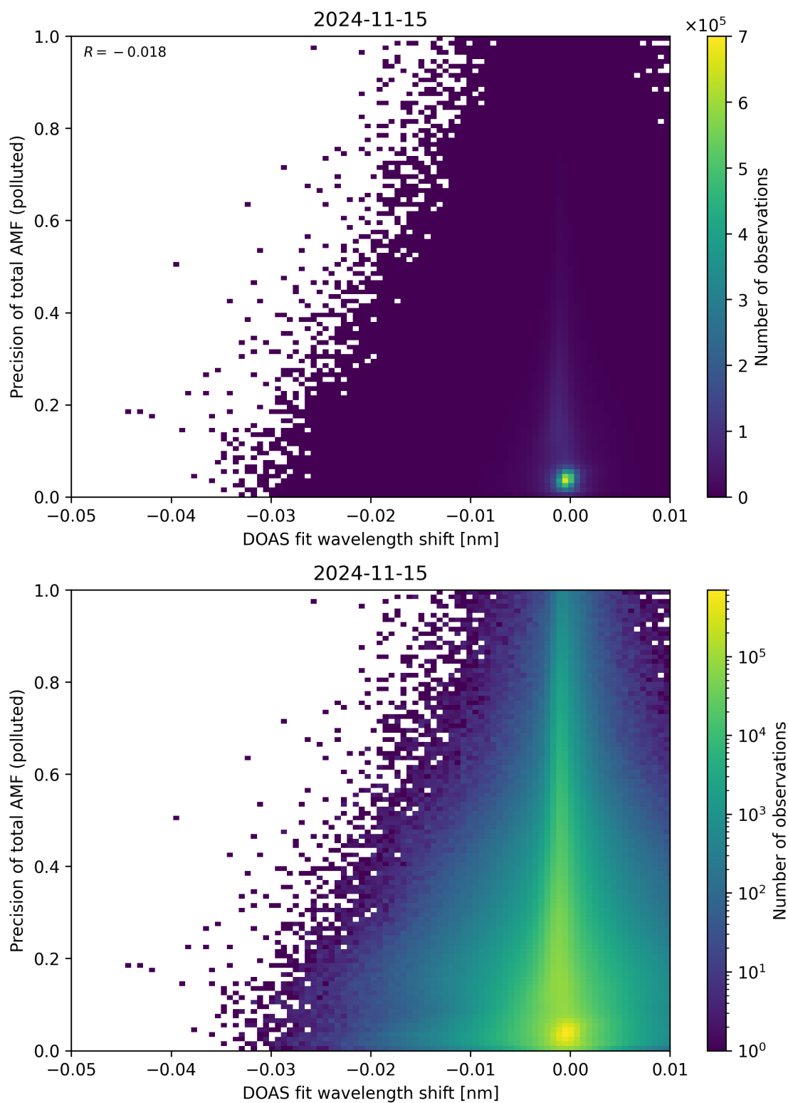
Figure 131: Scatter density plot of “DOAS fit wavelength shift” against “Precision of total AMF (polluted)” for 2024-11-14 to 2024-11-16.
