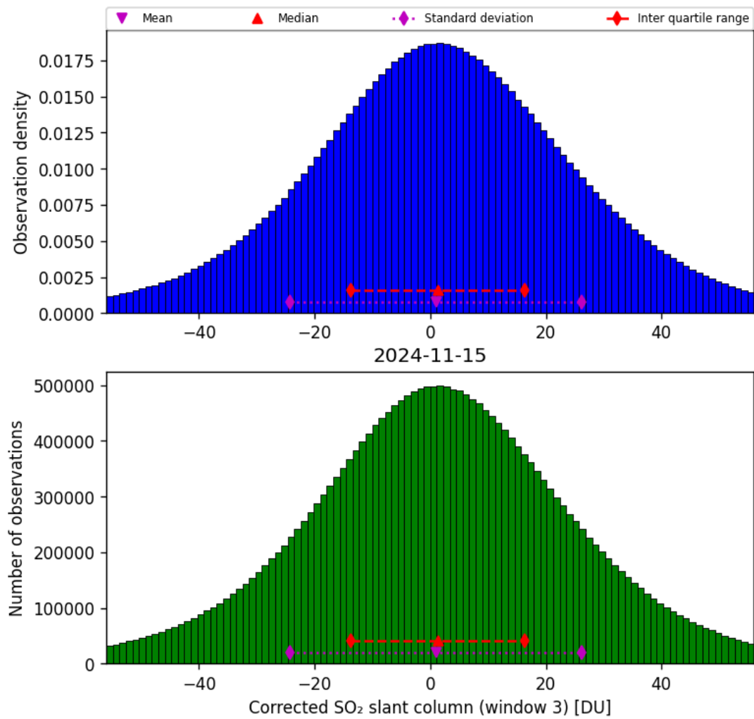
Figure 66: Histogram of “Corrected SO 2 slant column (window 3)” for 2024-11-14 to 2024-11-16
