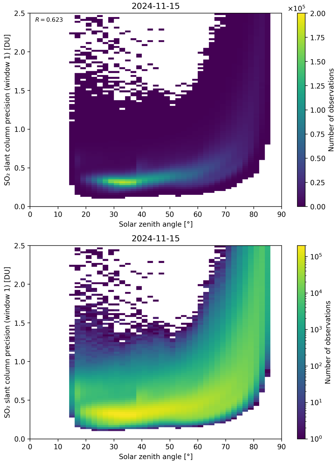
Figure 170: Scatter density plot of “Solar zenith angle” against “SO 2 slant column precision (window 1)” for 2024-11-14 to 2024-11-16.
