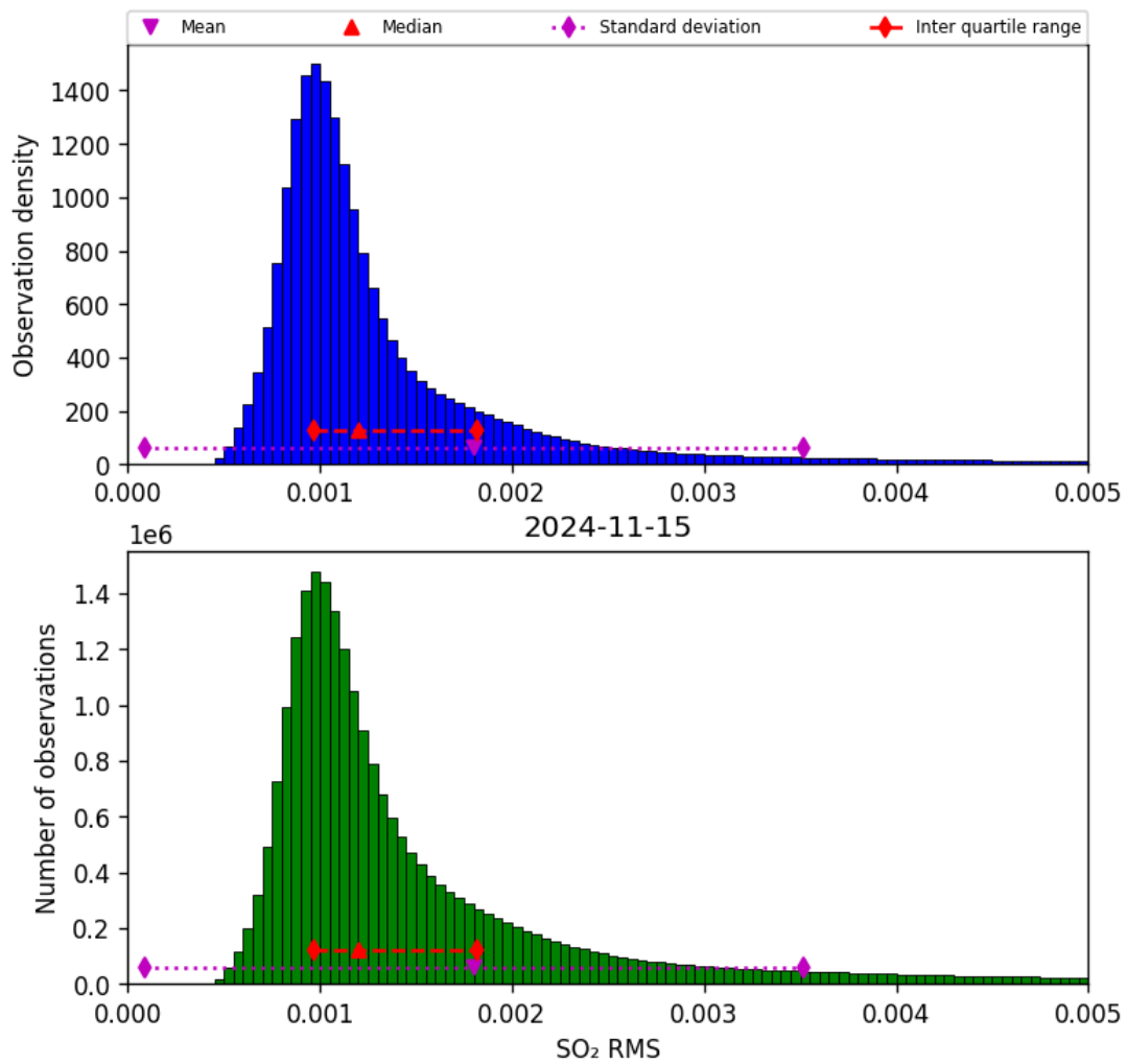
Figure 70: Histogram of “SO 2 RMS” for 2024-11-14 to 2024-11-16
