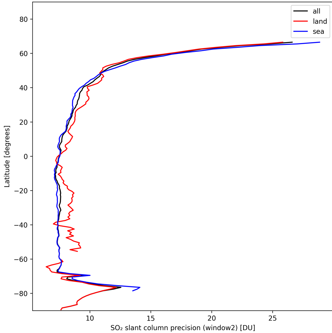
Figure 38: Zonal average of “SO 2 slant column precision (window2)” for 2024-11-14 to 2024-11-16.
