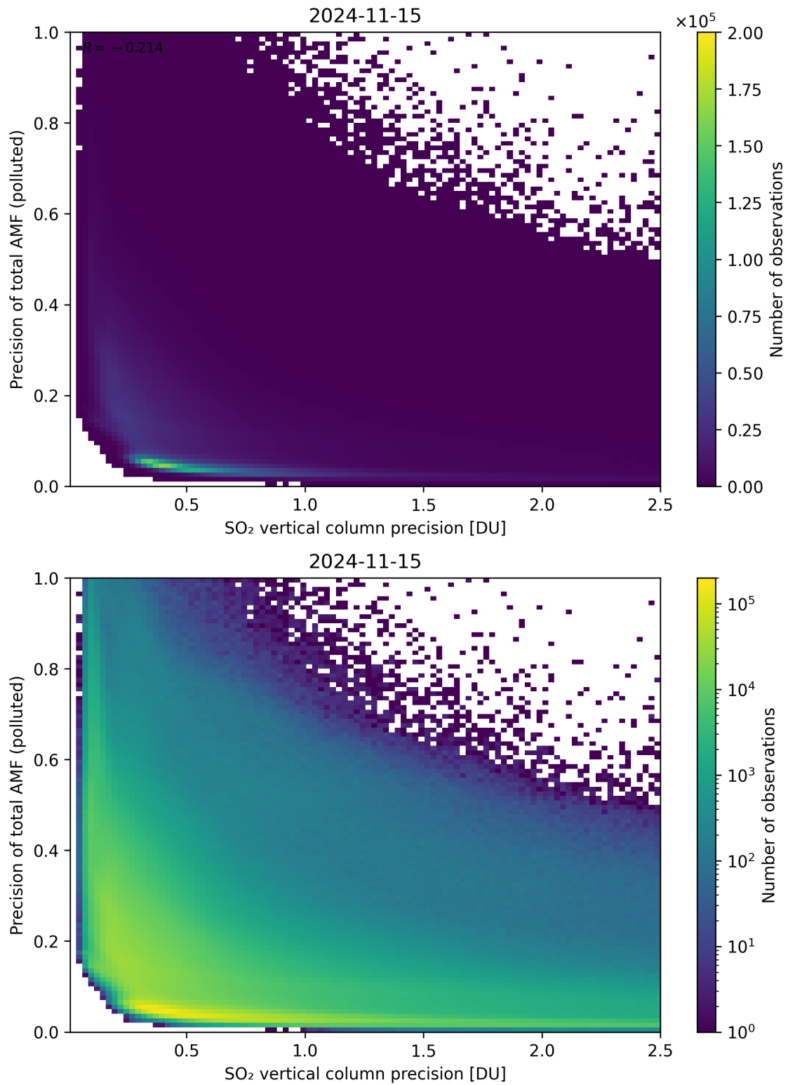
Figure 295: Scatter density plot of “SO 2 vertical column precision” against “Precision of total AMF (polluted)” for 2024-11-14 to 2024-11-16.
