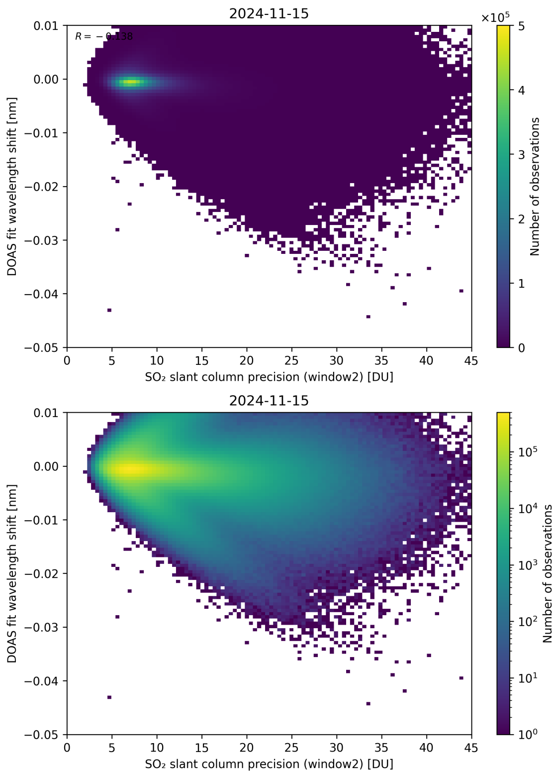
Figure 243: Scatter density plot of “SO 2 slant column precision (window2)” against “DOAS fit wavelength shift” for 2024-11-14 to 2024-11-16.
