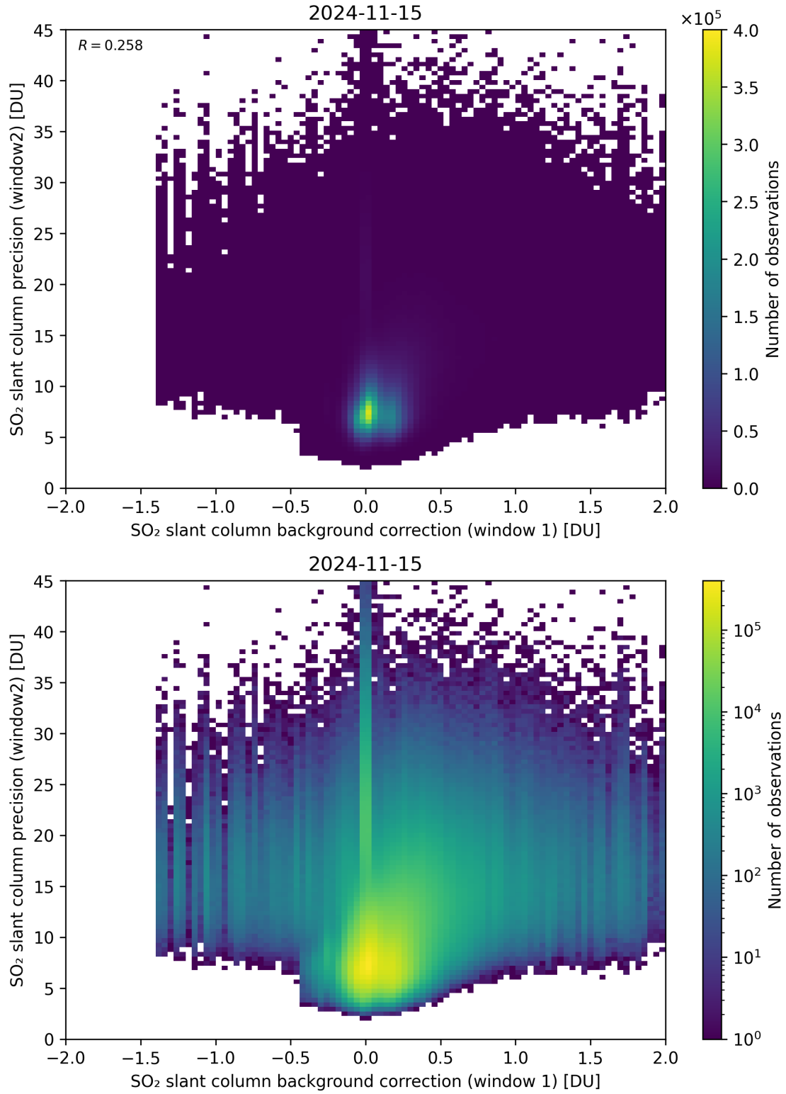
Figure 106: Scatter density plot of “SO 2 slant column background correction (window 1)” against “SO 2 slant column precision (window2)” for 2024-11-14 to 2024-11-16.
