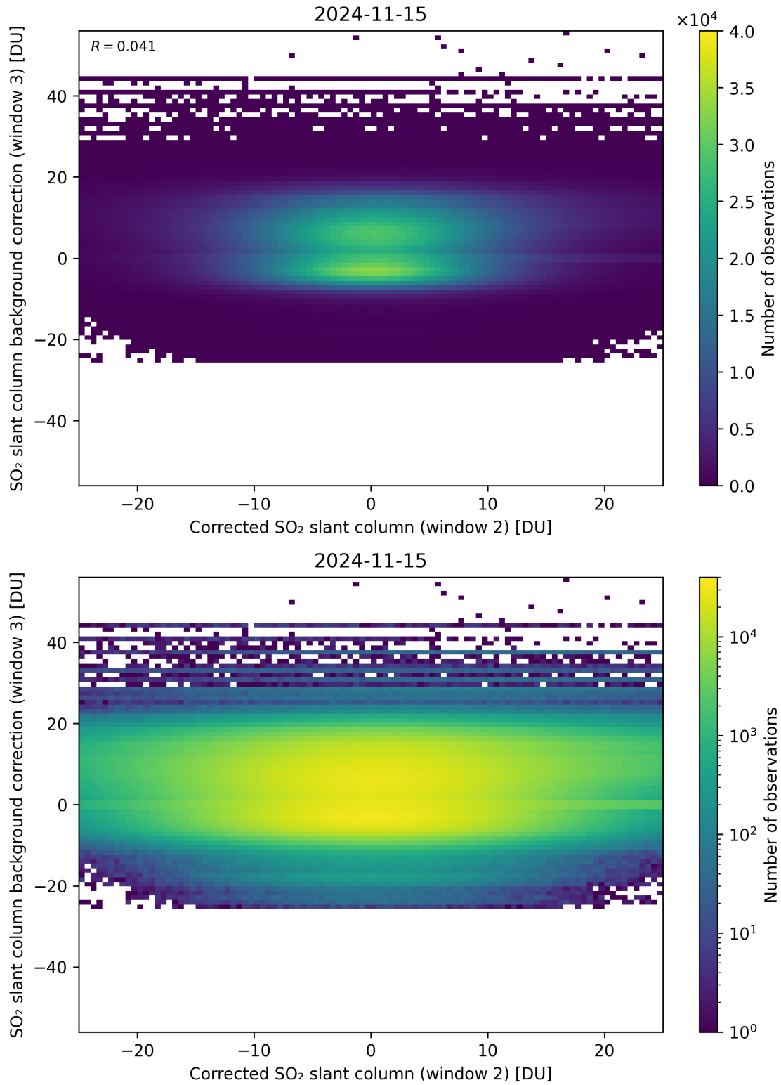
Figure 195: Scatter density plot of “Corrected SO 2 slant column (window 2)” against “SO 2 slant column background correction (window 3)” for 2024-11-14 to 2024-11-16.
