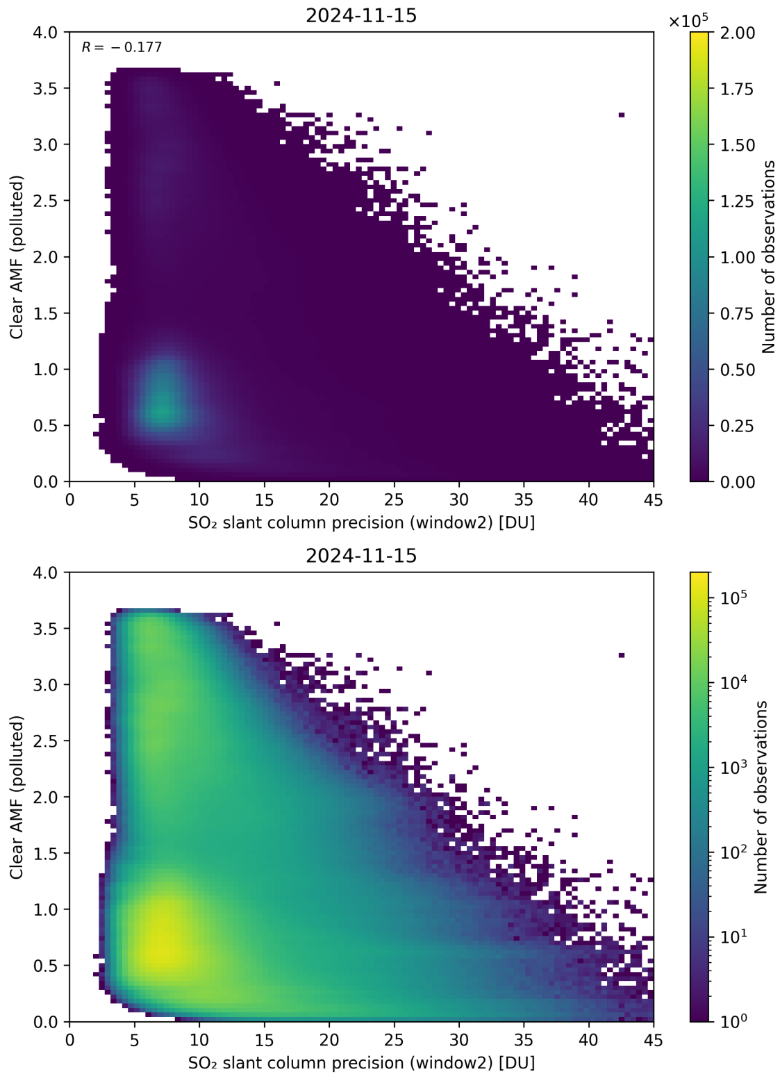
Figure 246: Scatter density plot of “SO 2 slant column precision (window2)” against “Clear AMF (polluted)” for 2024-11-14 to 2024-11-16.
