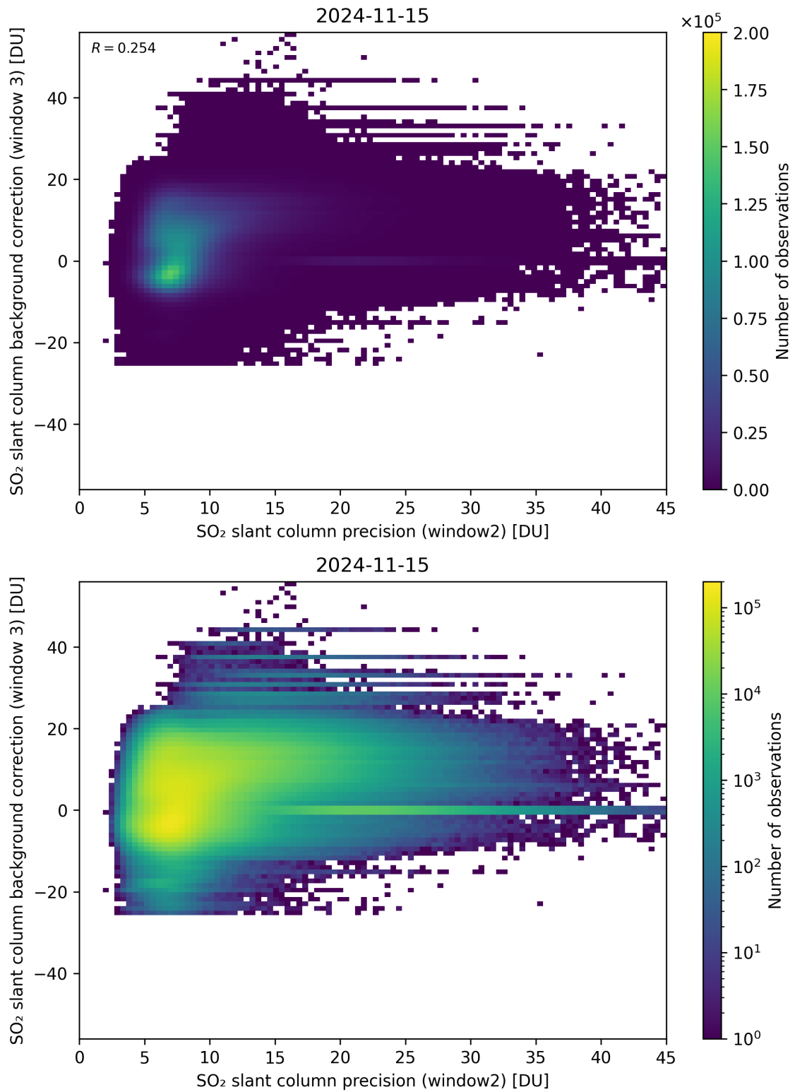
Figure 242: Scatter density plot of “SO 2 slant column precision (window2)” against “SO 2 slant column background correction (window 3)” for 2024-11-14 to 2024-11-16.
