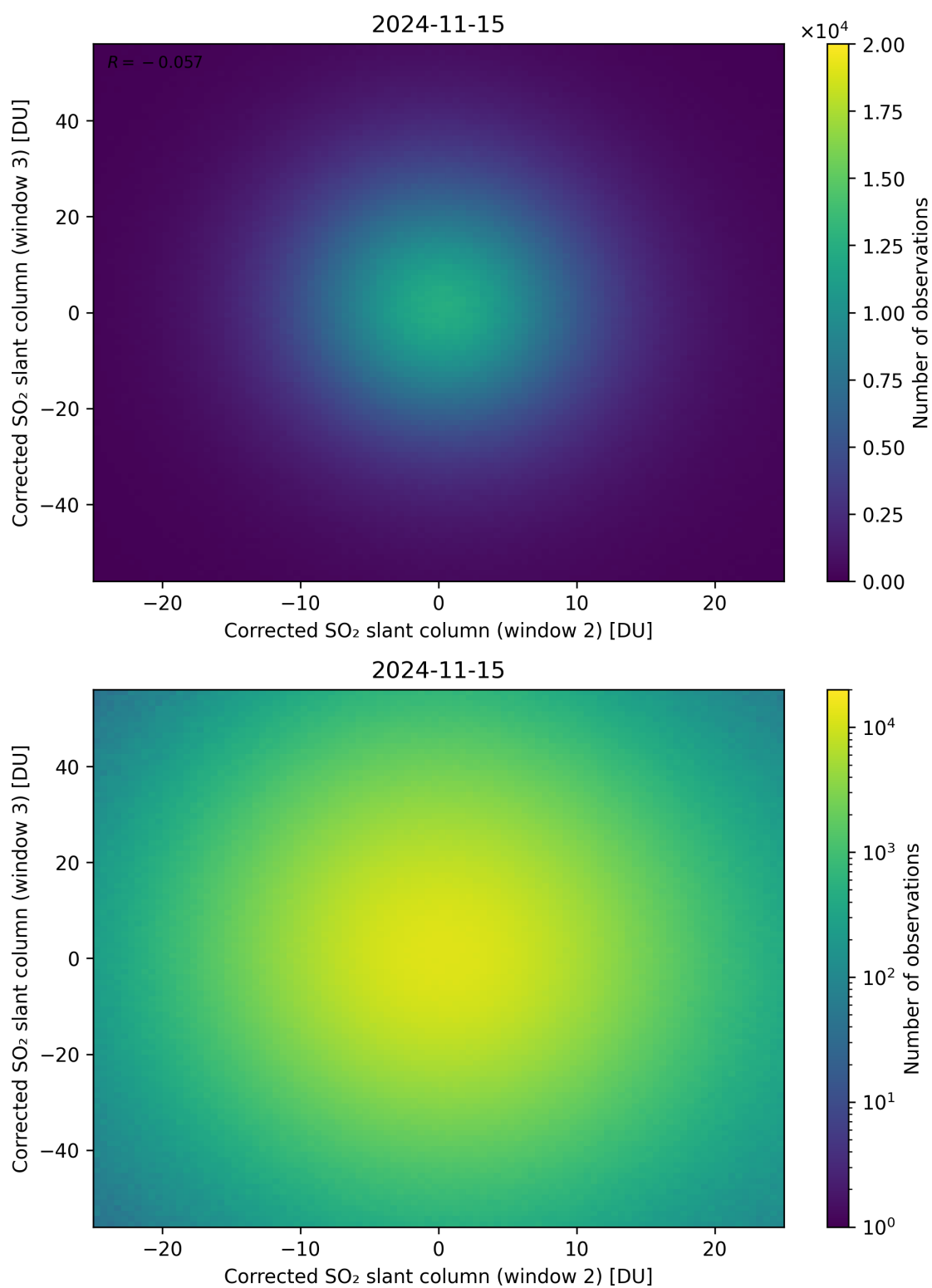
Figure 200: Scatter density plot of “Corrected SO 2 slant column (window 2)” against “Corrected SO 2 slant column (window 3)” for 2024-11-14 to 2024-11-16.
