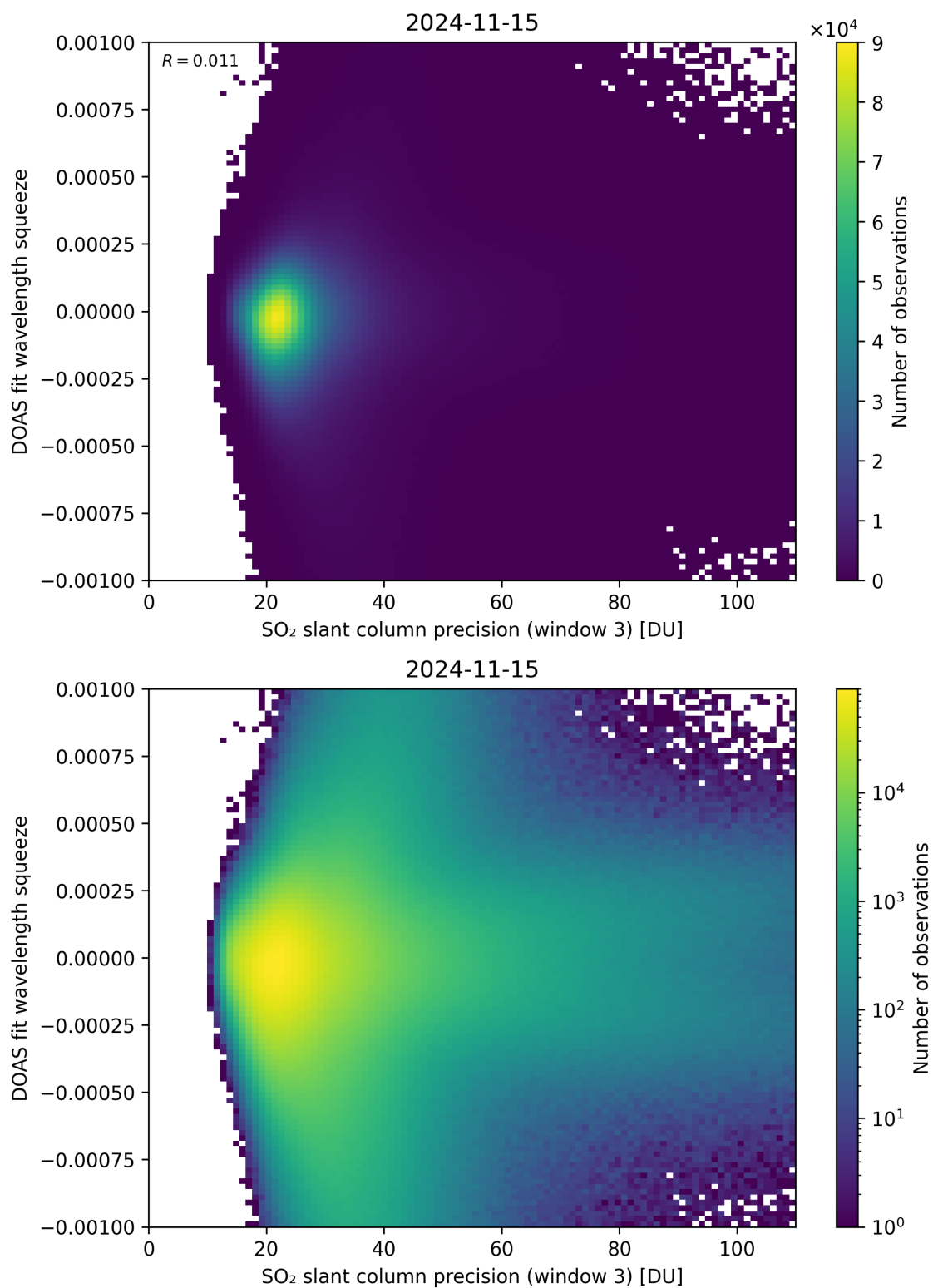
Figure 259: Scatter density plot of “SO 2 slant column precision (window 3)” against “DOAS fit wavelength squeeze” for 2024-11-14 to 2024-11-16.
