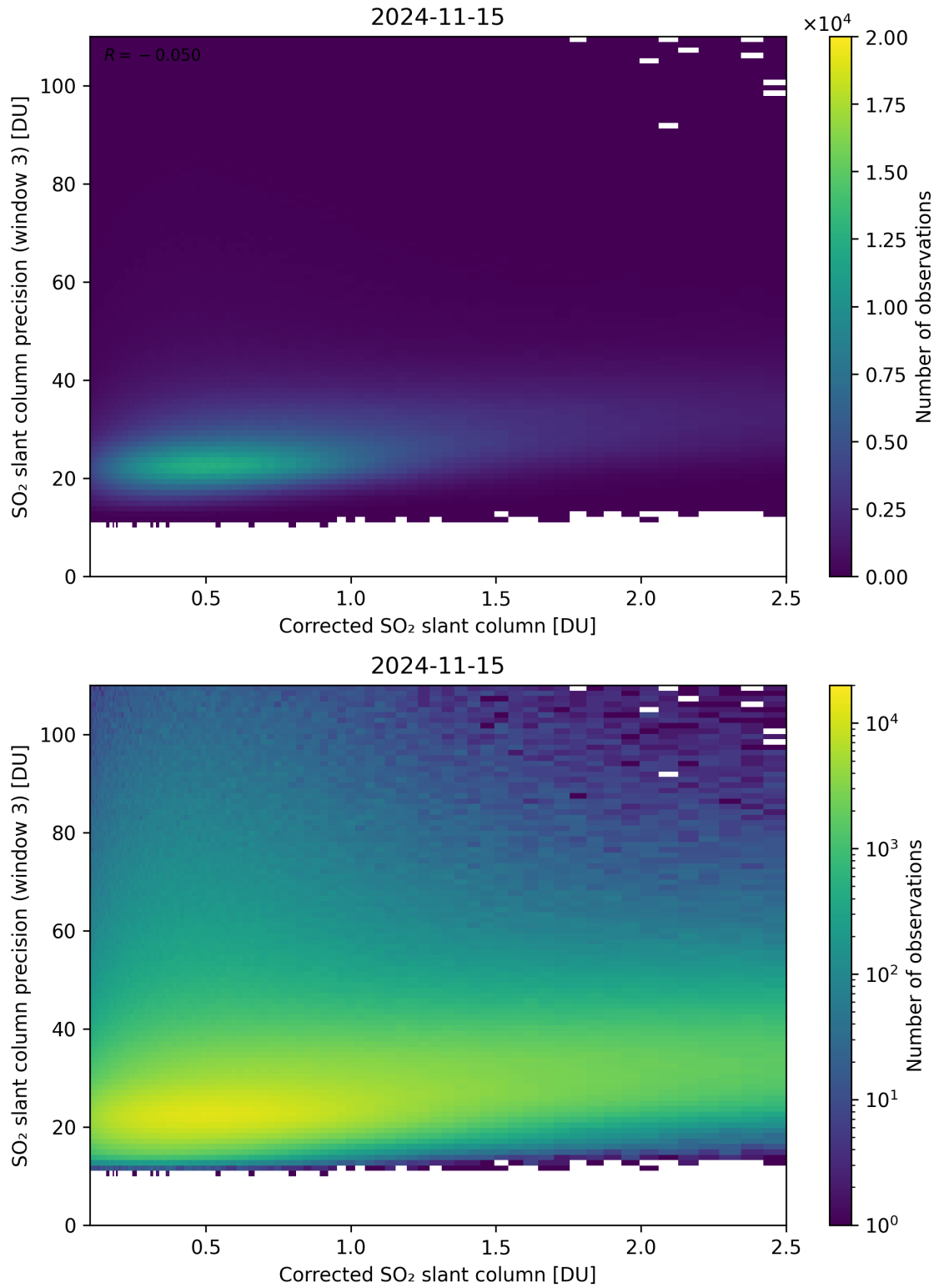
Figure 191: Scatter density plot of “Corrected SO 2 slant column” against “SO 2 slant column precision (window 3)” for 2024-11-14 to 2024-11-16.
