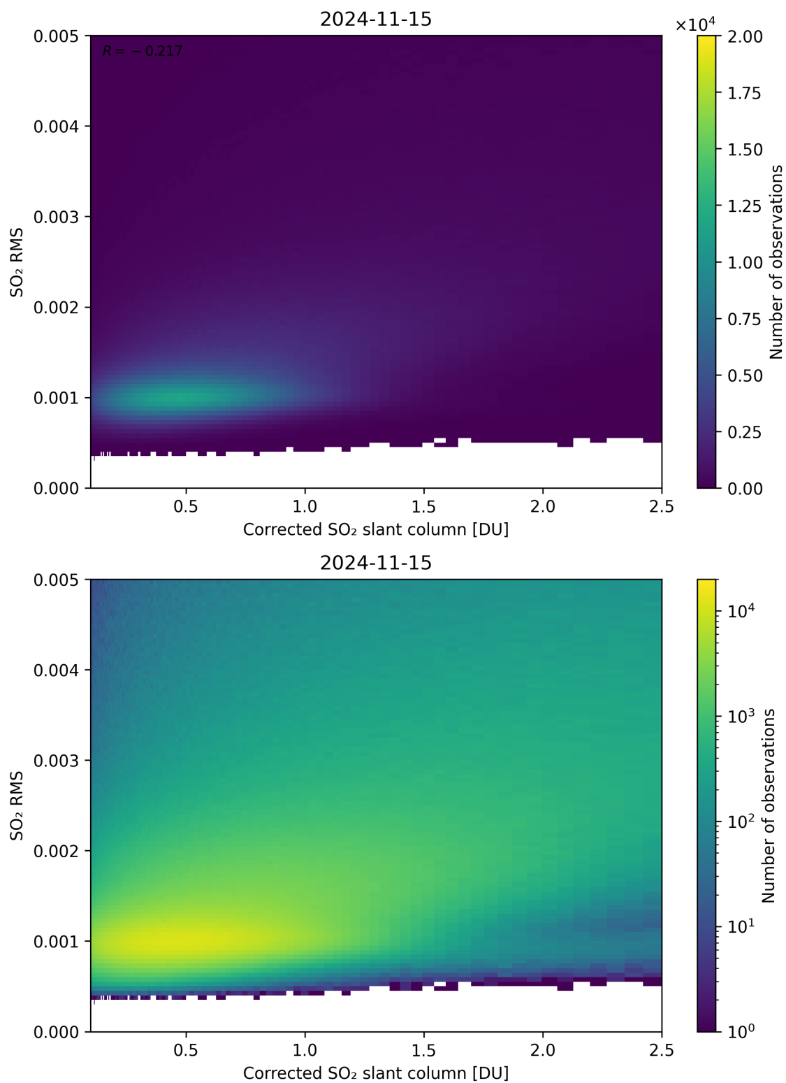
Figure 183: Scatter density plot of “Corrected SO 2 slant column” against “SO 2 RMS” for 2024-11-14 to 2024-11-16.
