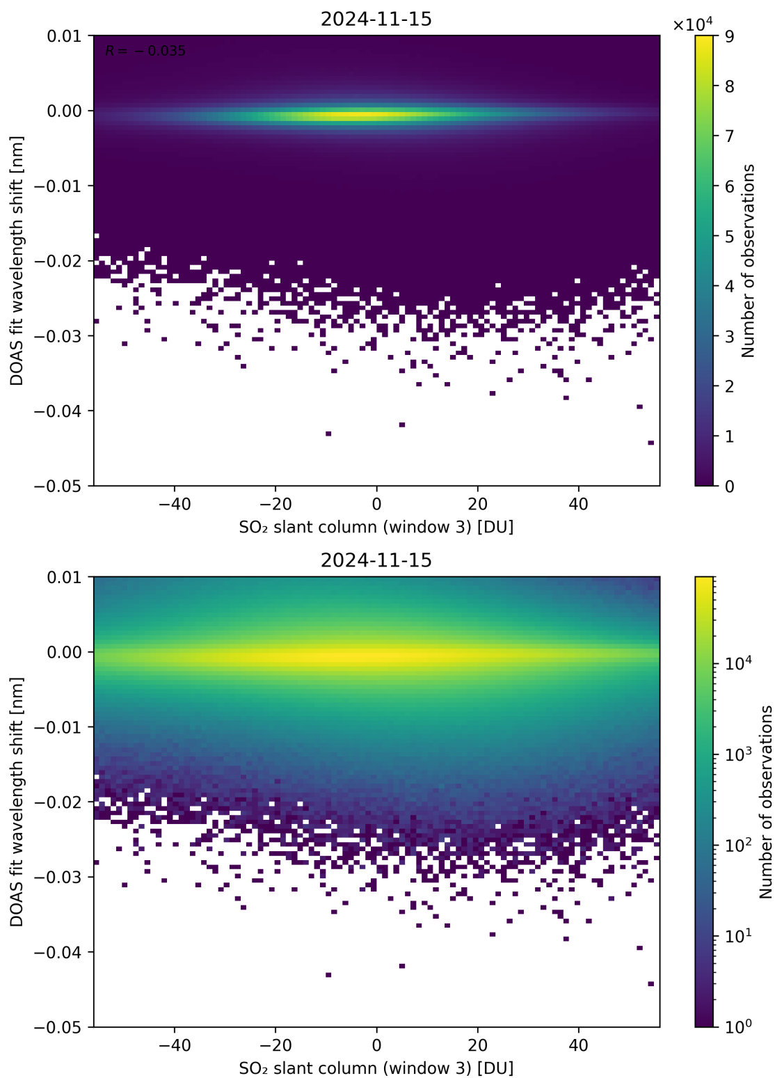
Figure 254: Scatter density plot of “SO 2 slant column (window 3)” against “DOAS fit wavelength shift” for 2024-11-14 to 2024-11-16.
