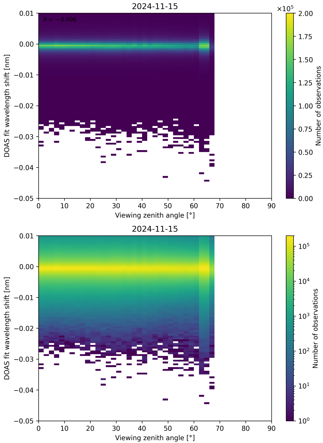
Figure 311: Scatter density plot of “Viewing zenith angle” against “DOAS fit wavelength shift” for 2024-11-14 to 2024-11-16.
