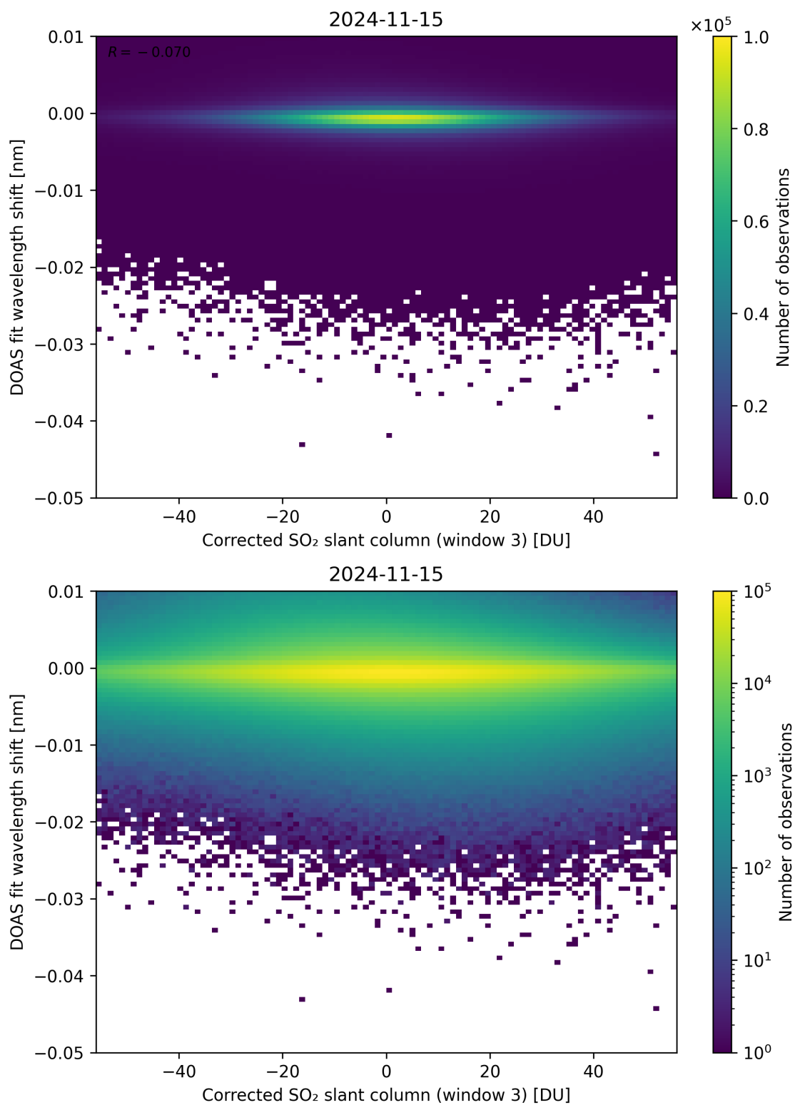
Figure 206: Scatter density plot of “Corrected SO 2 slant column (window 3)” against “DOAS fit wavelength shift” for 2024-11-14 to 2024-11-16.
