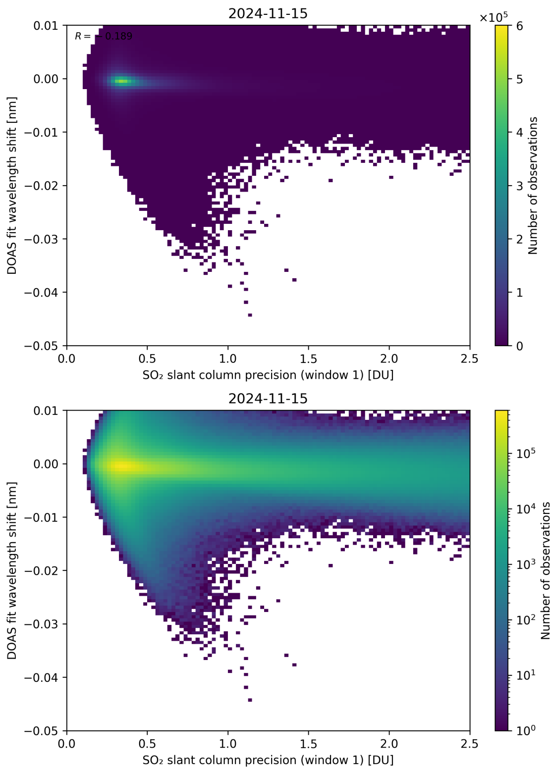
Figure 221: Scatter density plot of “SO 2 slant column precision (window 1)” against “DOAS fit wavelength shift” for 2024-11-14 to 2024-11-16.
