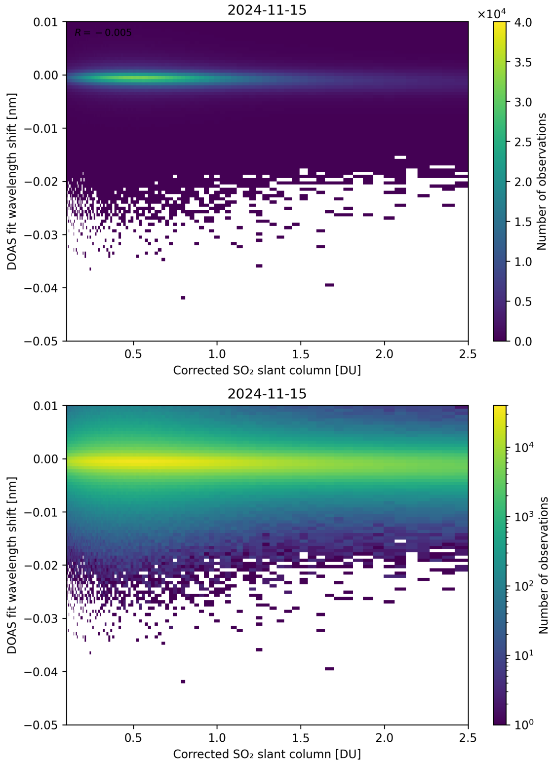
Figure 181: Scatter density plot of “Corrected SO 2 slant column” against “DOAS fit wavelength shift” for 2024-11-14 to 2024-11-16.
