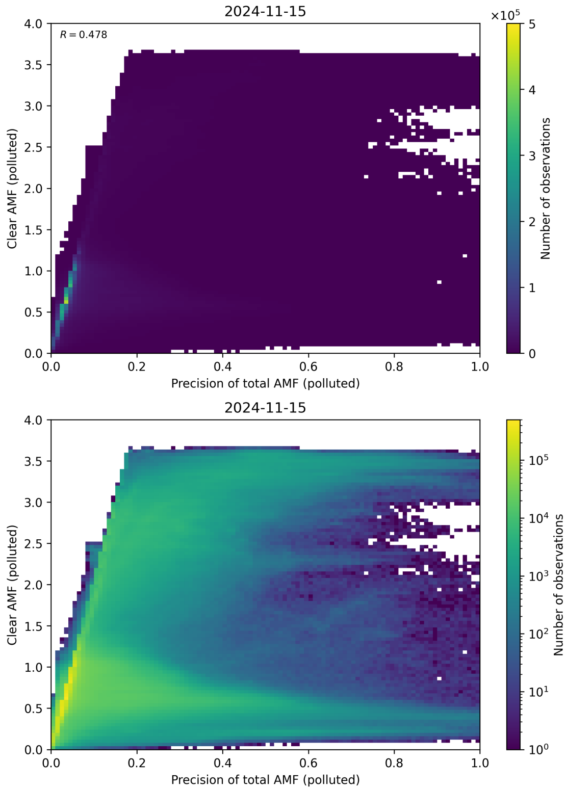
Figure 270: Scatter density plot of “Precision of total AMF (polluted)” against “Clear AMF (polluted)” for 2024-11-14 to 2024-11-16.
