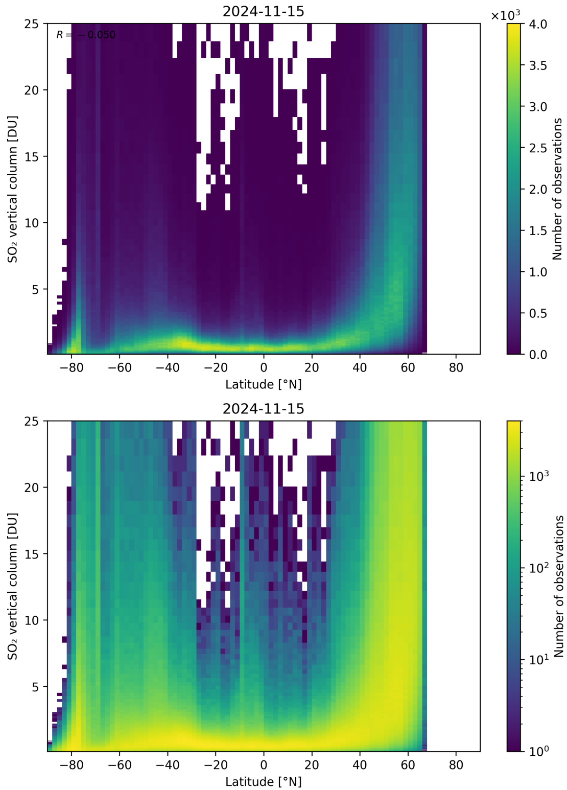
Figure 156: Scatter density plot of “Latitude” against “SO 2 vertical column” for 2024-11-14 to 2024-11-16.
