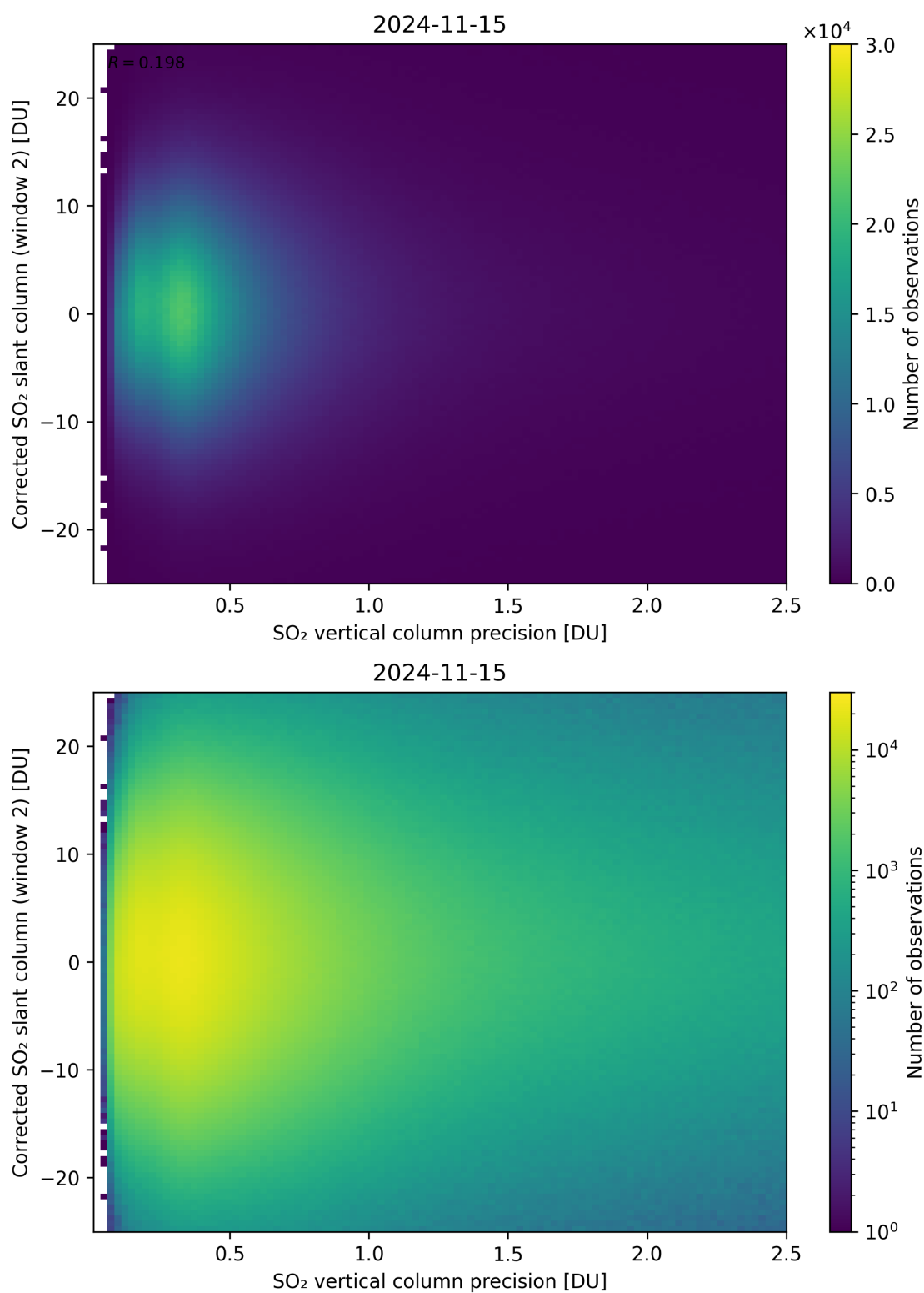
Figure 287: Scatter density plot of “SO 2 vertical column precision” against “Corrected SO 2 slant column (window 2)” for 2024-11-14 to 2024-11-16.
