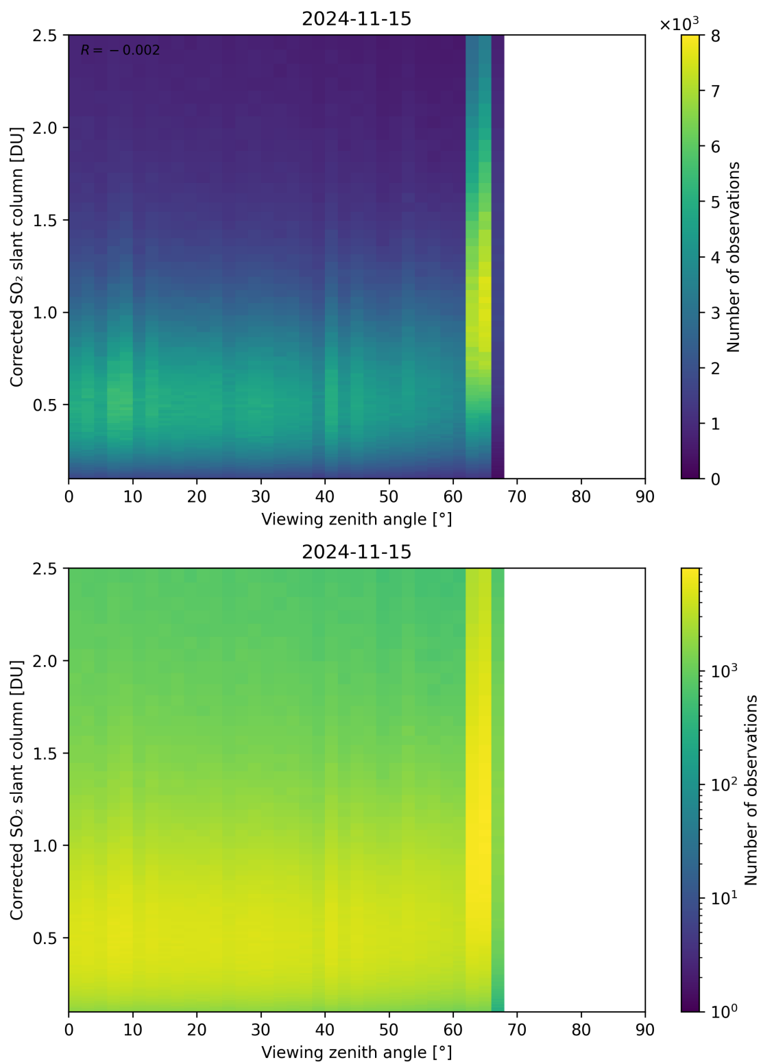
Figure 317: Scatter density plot of “Viewing zenith angle” against “Corrected SO 2 slant column” for 2024-11-14 to 2024-11-16.
