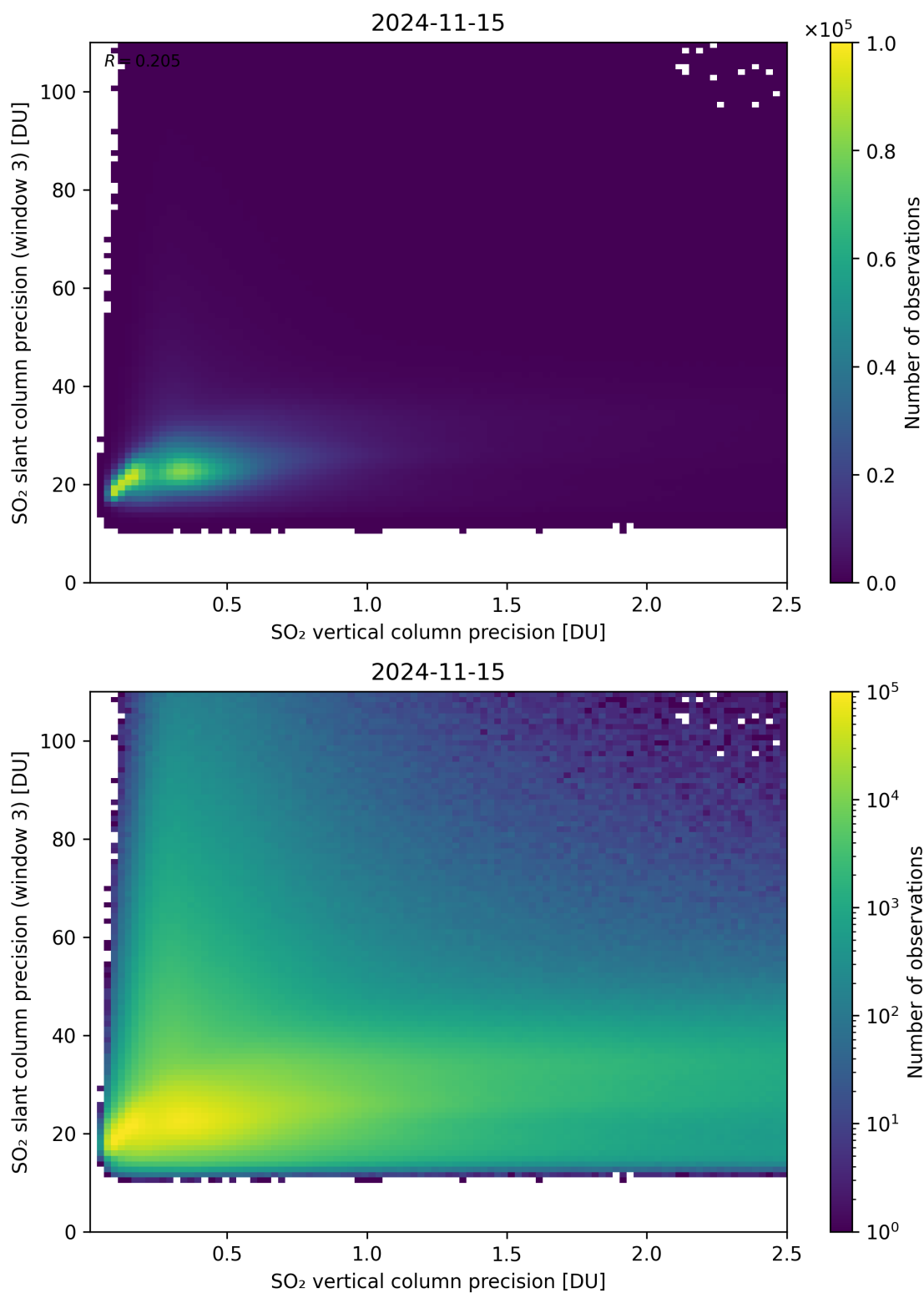
Figure 293: Scatter density plot of “SO 2 vertical column precision” against “SO 2 slant column precision (window 3)” for 2024-11-14 to 2024-11-16.
