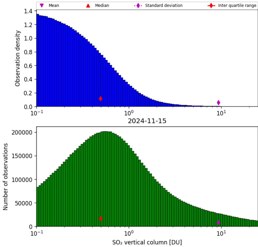
Figure 53: Histogram of “SO 2 vertical column” for 2024-11-14 to 2024-11-16
