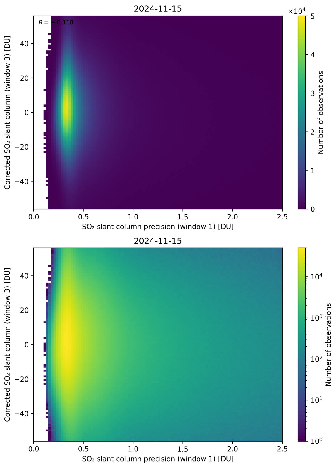
Figure 226: Scatter density plot of “SO 2 slant column precision (window 1)” against “Corrected SO 2 slant column (window 3)” for 2024-11-14 to 2024-11-16.
