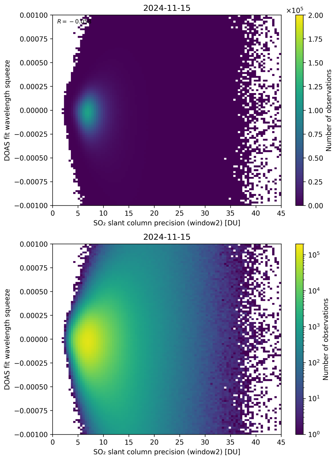
Figure 244: Scatter density plot of “SO 2 slant column precision (window2)” against “DOAS fit wavelength squeeze” for 2024-11-14 to 2024-11-16.
