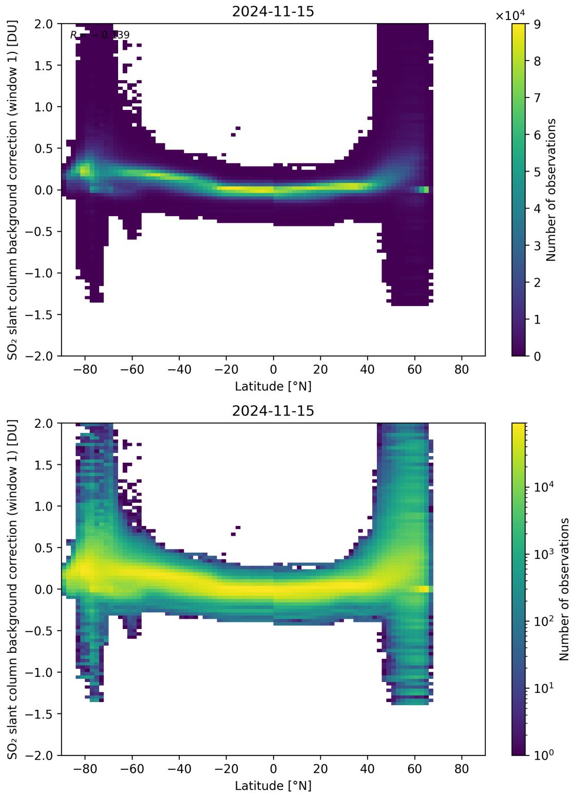
Figure 139: Scatter density plot of “Latitude” against “SO 2 slant column background correction (window 1)” for 2024-11-14 to 2024-11-16.
