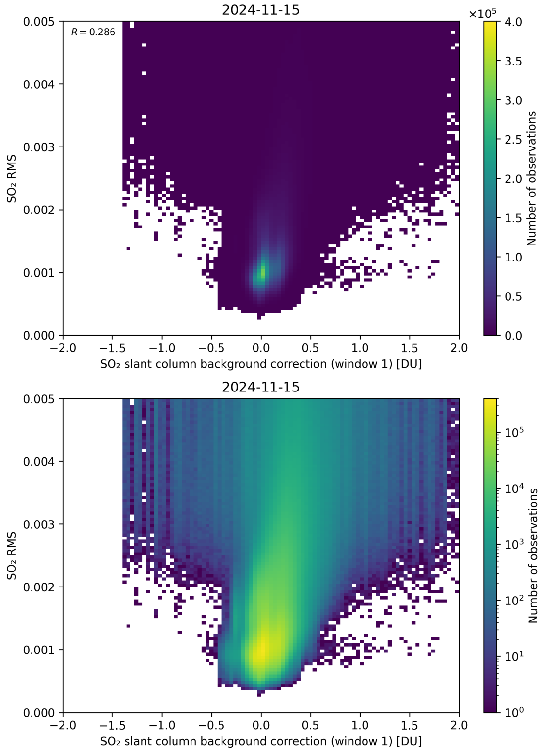
Figure 102: Scatter density plot of “SO 2 slant column background correction (window 1)” against “SO 2 RMS” for 2024-11-14 to 2024-11-16.
