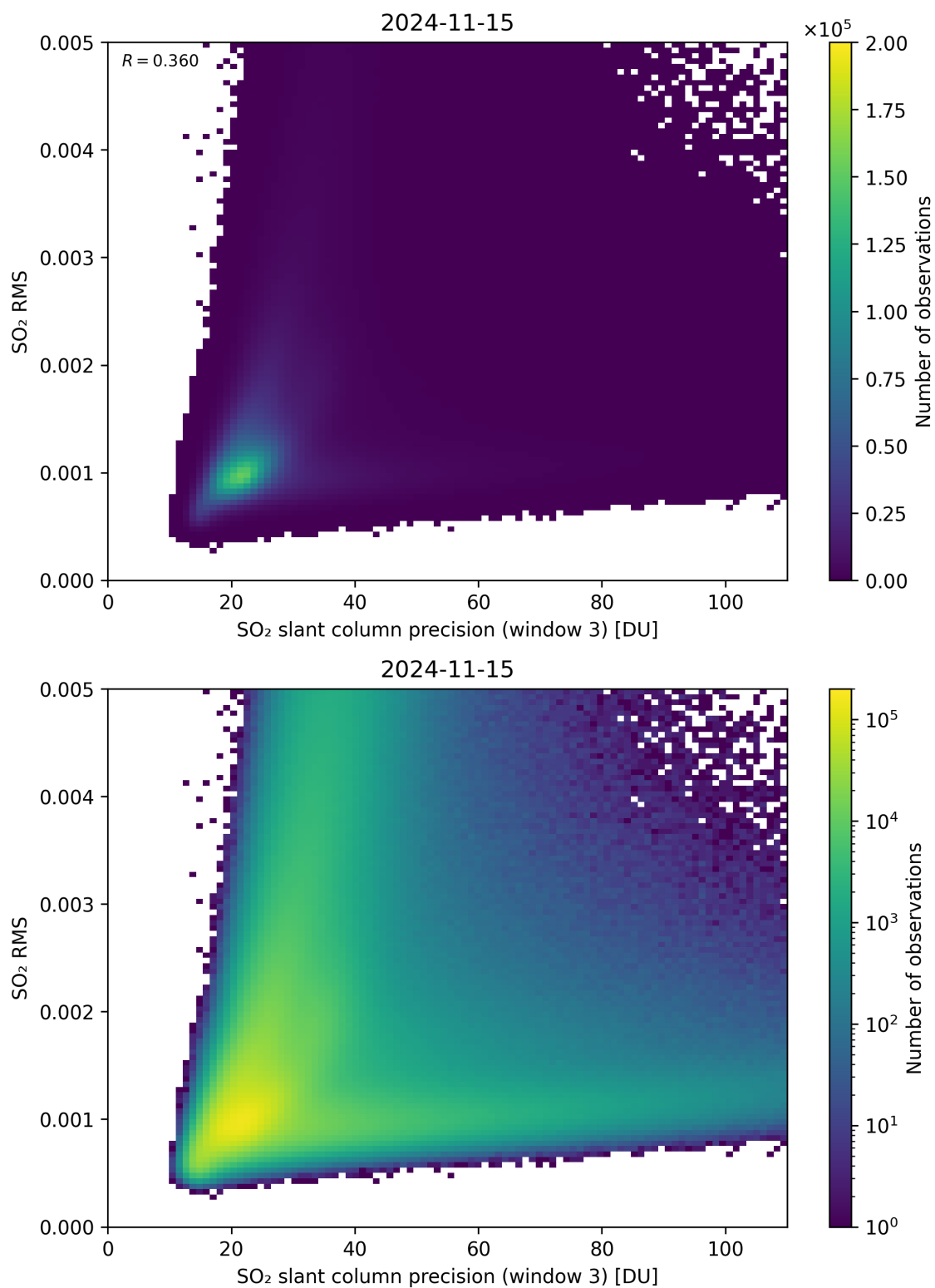
Figure 260: Scatter density plot of “SO 2 slant column precision (window 3)” against “SO 2 RMS” for 2024-11-14 to 2024-11-16.
