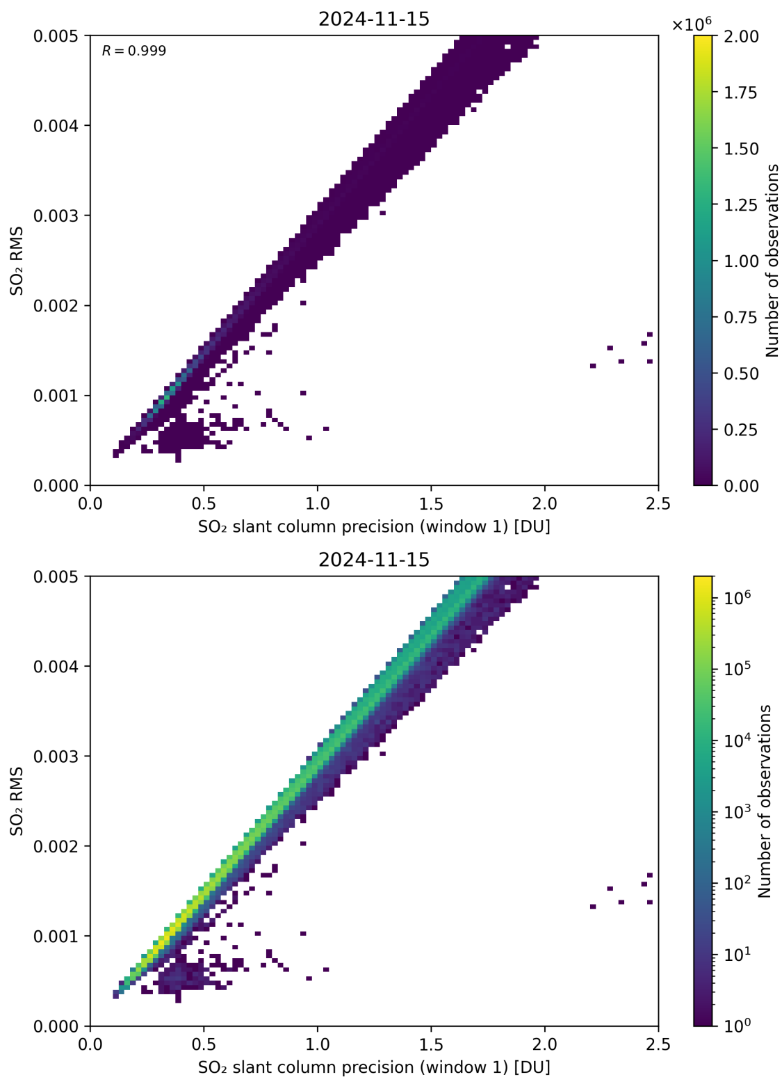
Figure 223: Scatter density plot of “SO 2 slant column precision (window 1)” against “SO 2 RMS” for 2024-11-14 to 2024-11-16.
