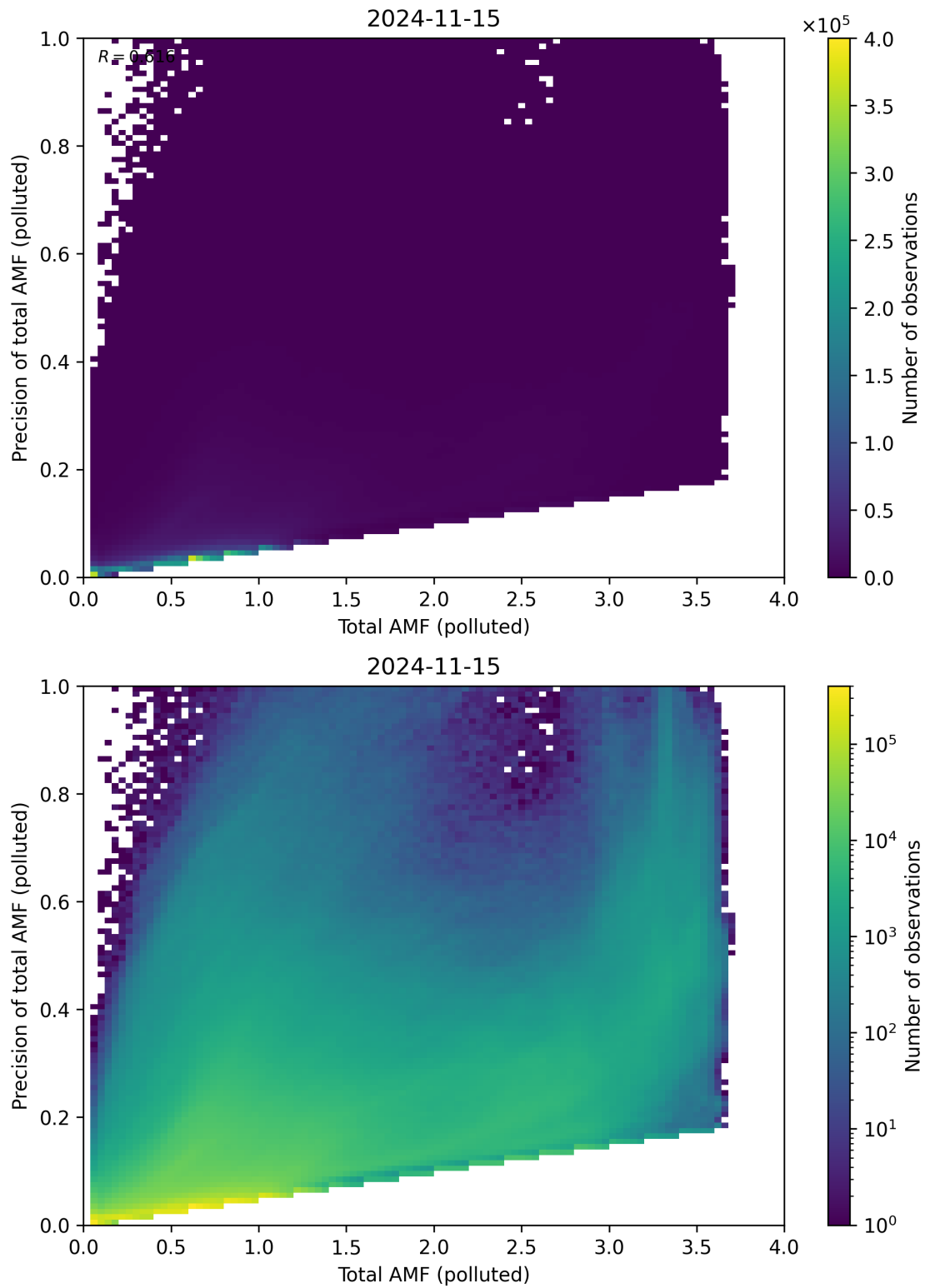
Figure 272: Scatter density plot of “Total AMF (polluted)” against “Precision of total AMF (polluted)” for 2024-11-14 to 2024-11-16.
