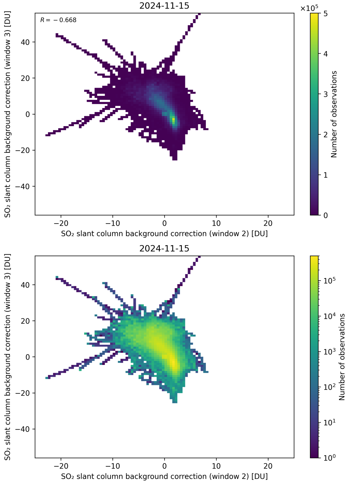
Figure 111: Scatter density plot of “SO 2 slant column background correction (window 2)” against “SO 2 slant column background correction (window 3)” for 2024-11-14 to 2024-11-16.
