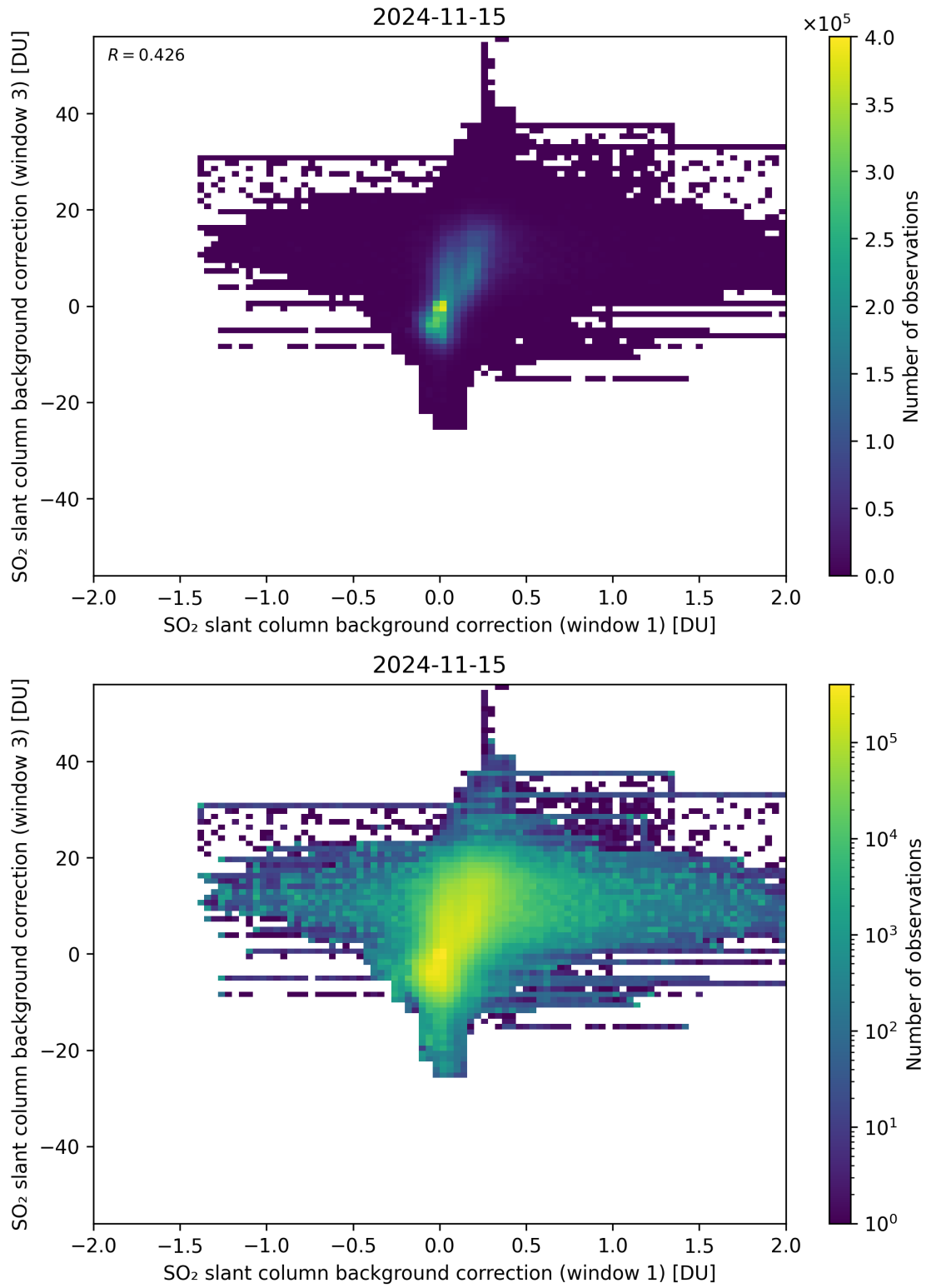
Figure 99: Scatter density plot of “SO 2 slant column background correction (window 1)” against “SO 2 slant column background correction (window 3)” for 2024-11-14 to 2024-11-16.
