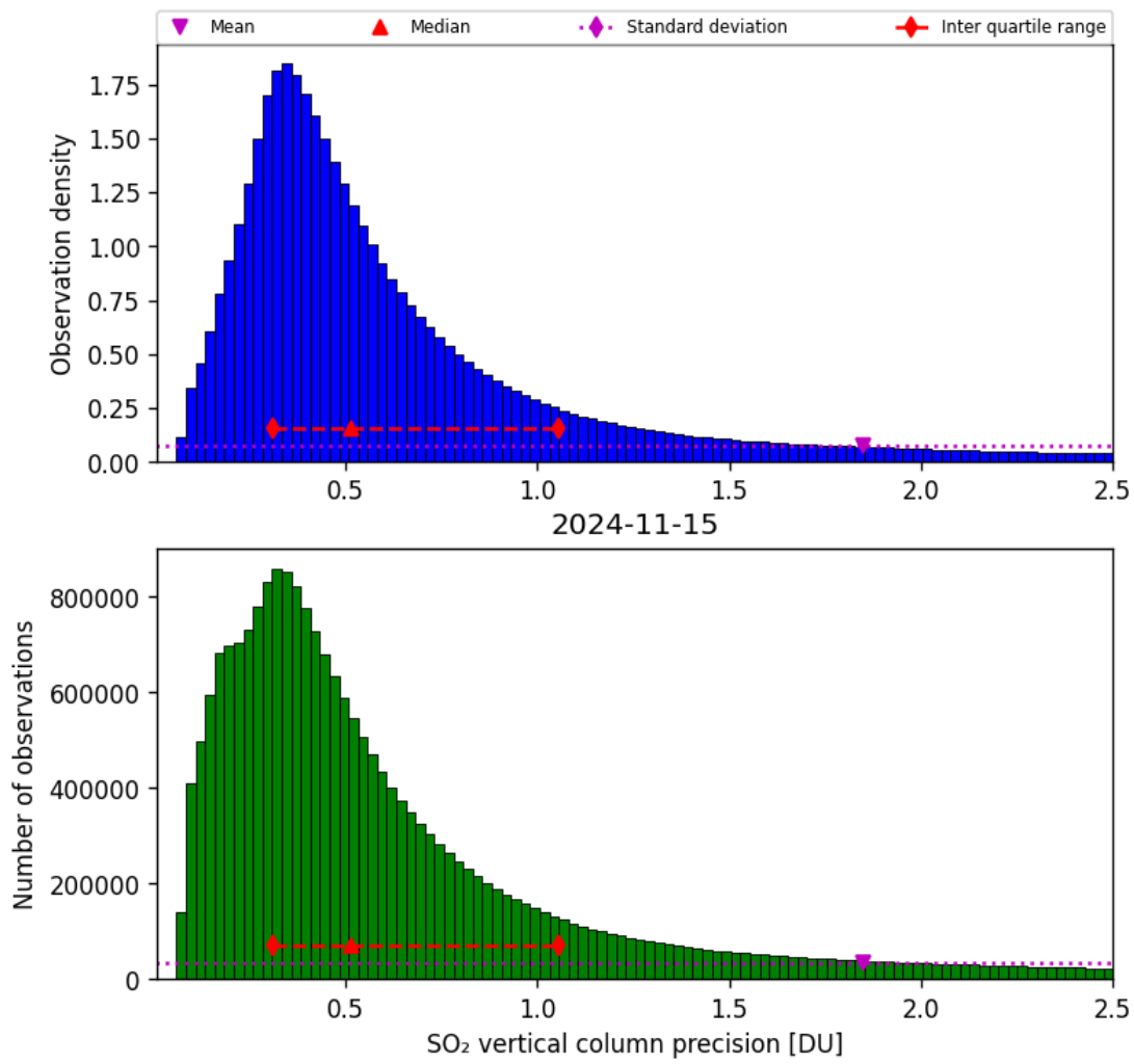
Figure 54: Histogram of “SO 2 vertical column precision” for 2024-11-14 to 2024-11-16
