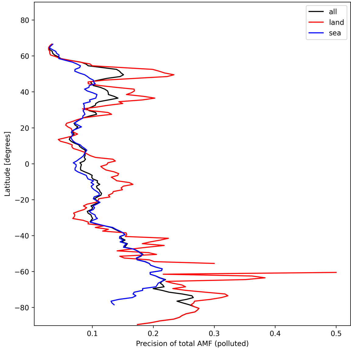
Figure 49: Zonal average of “Precision of total AMF (polluted)” for 2024-11-14 to 2024-11-16.
