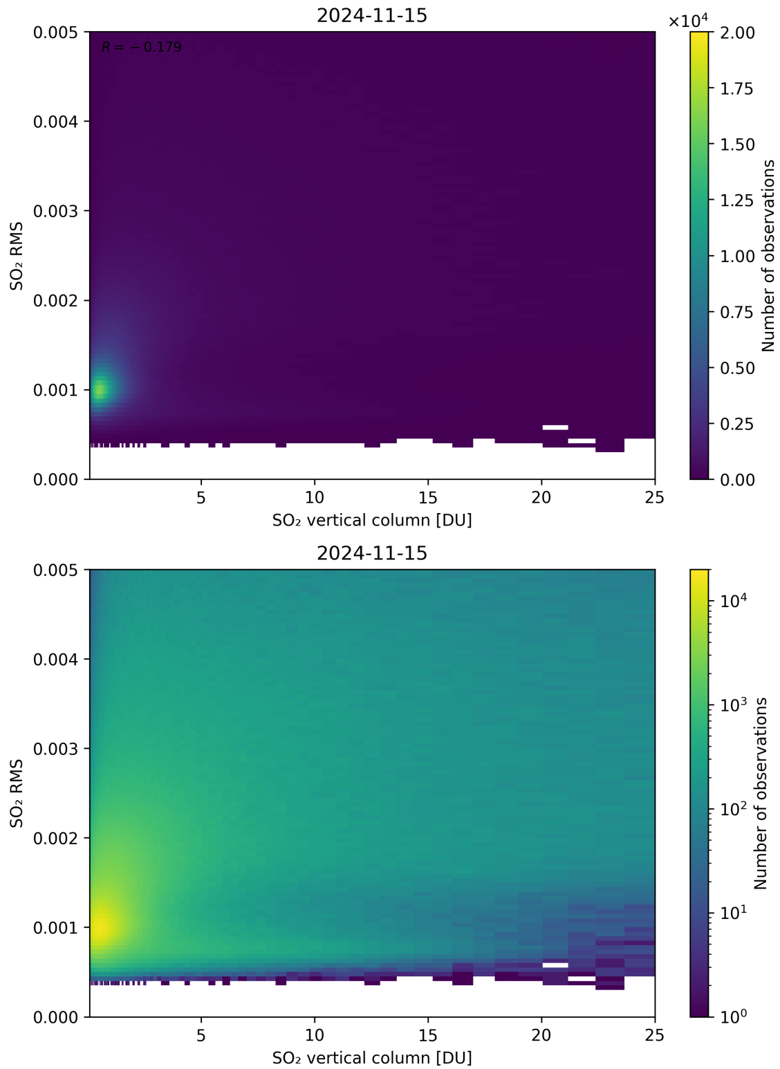
Figure 278: Scatter density plot of “SO 2 vertical column” against “SO 2 RMS” for 2024-11-14 to 2024-11-16.
