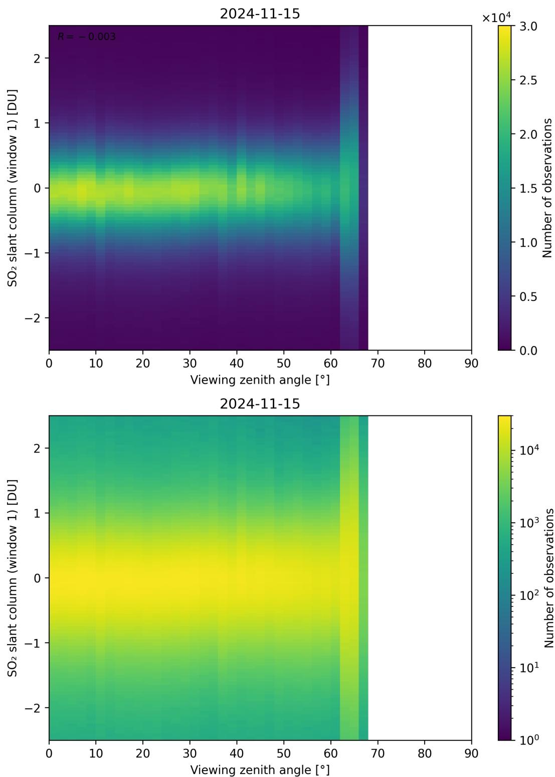
Figure 320: Scatter density plot of “Viewing zenith angle” against “SO 2 slant column (window 1)” for 2024-11-14 to 2024-11-16.
