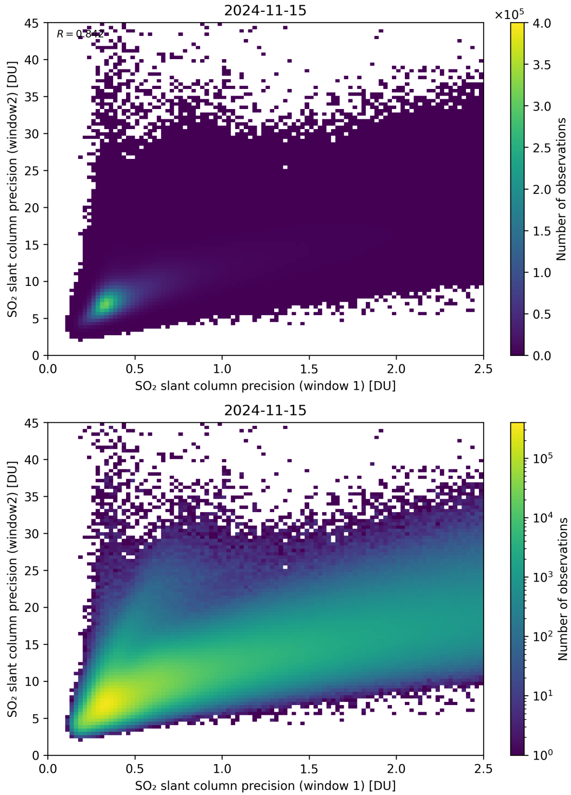
Figure 227: Scatter density plot of “SO 2 slant column precision (window 1)” against “SO 2 slant column precision (window2)” for 2024-11-14 to 2024-11-16.
