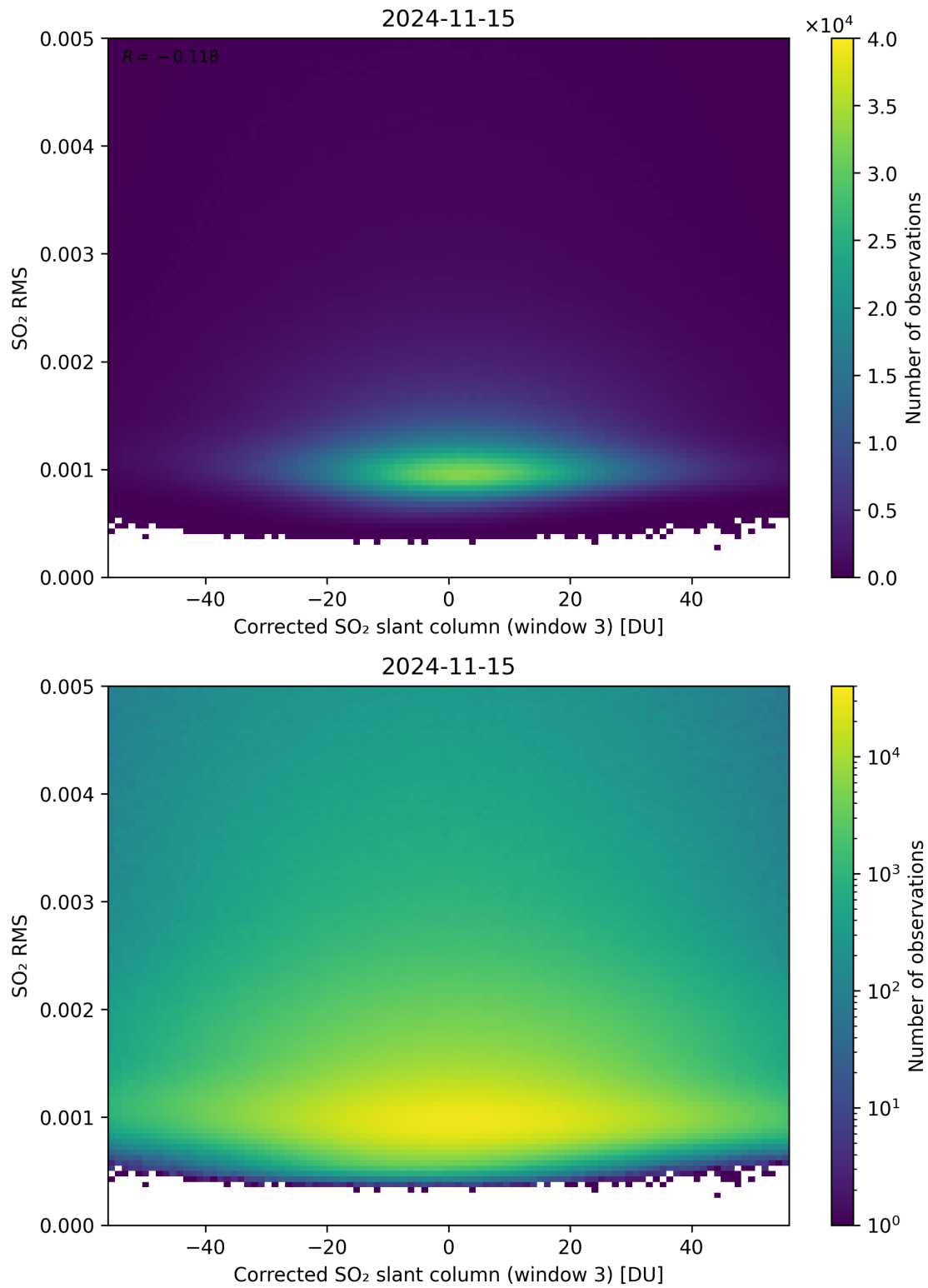
Figure 208: Scatter density plot of “Corrected SO 2 slant column (window 3)” against “SO 2 RMS” for 2024-11-14 to 2024-11-16.
