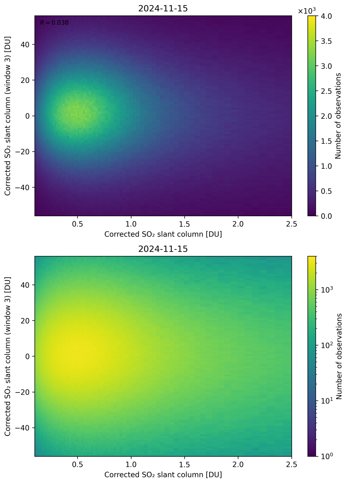
Figure 186: Scatter density plot of “Corrected SO 2 slant column” against “Corrected SO 2 slant column (window 3)” for 2024-11-14 to 2024-11-16.
