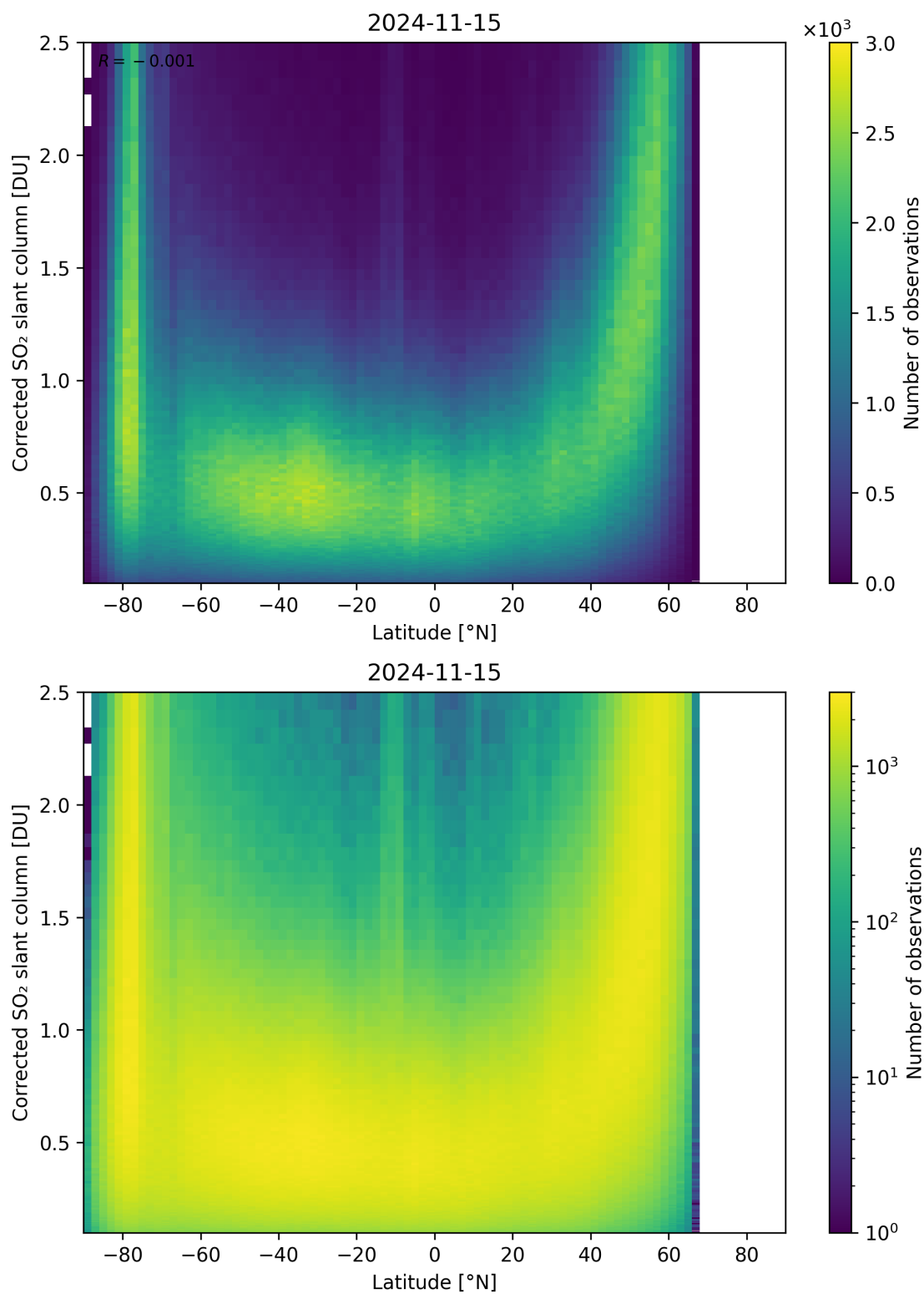
Figure 146: Scatter density plot of “Latitude” against “Corrected SO 2 slant column” for 2024-11-14 to 2024-11-16.
