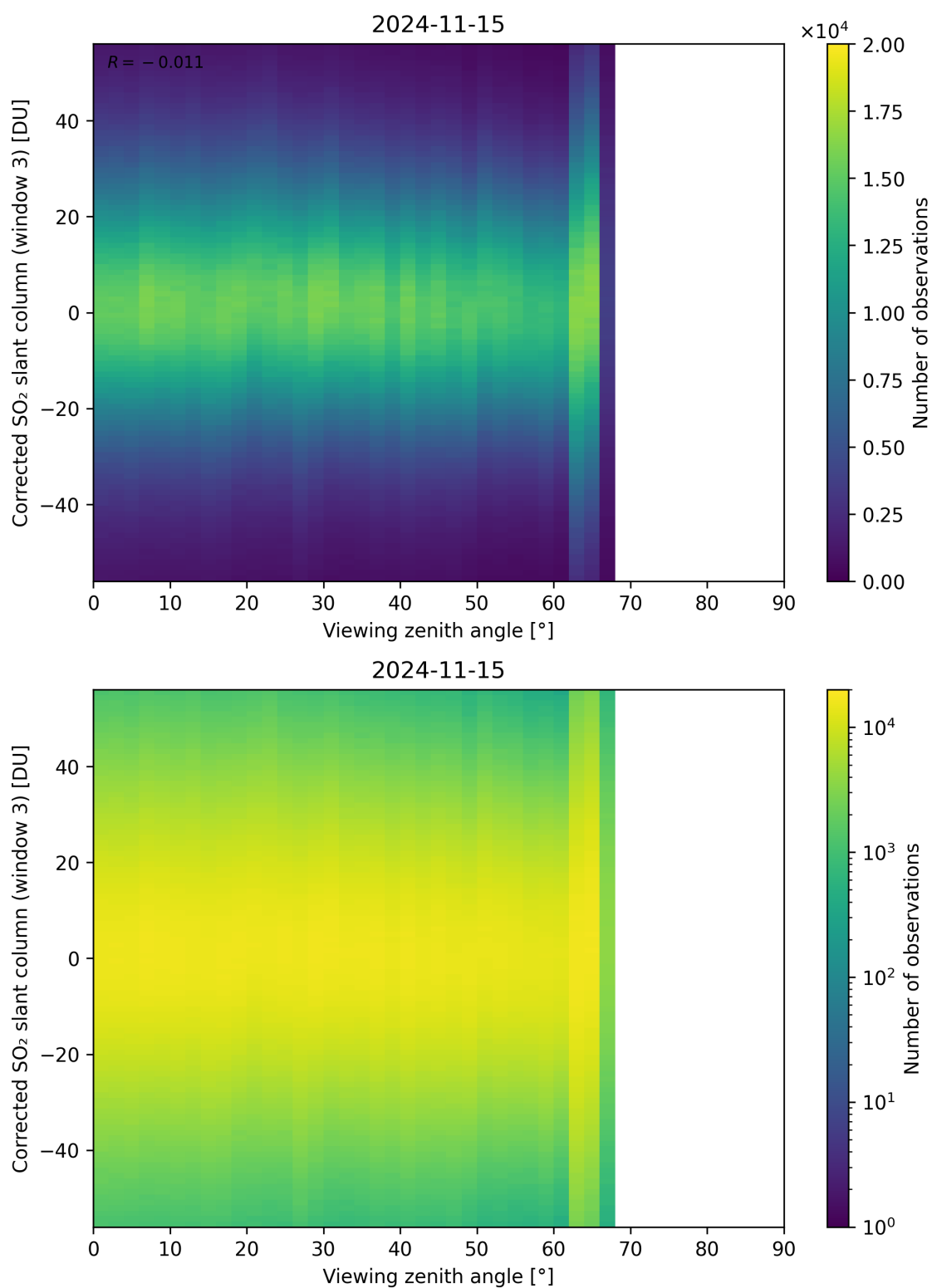
Figure 319: Scatter density plot of “Viewing zenith angle” against “Corrected SO 2 slant column (window 3)” for 2024-11-14 to 2024-11-16.
