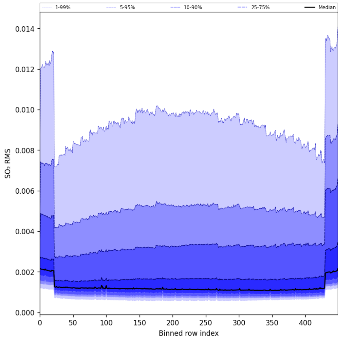
Figure 93: Along track statistics of “SO 2 RMS” for 2024-11-14 to 2024-11-16
