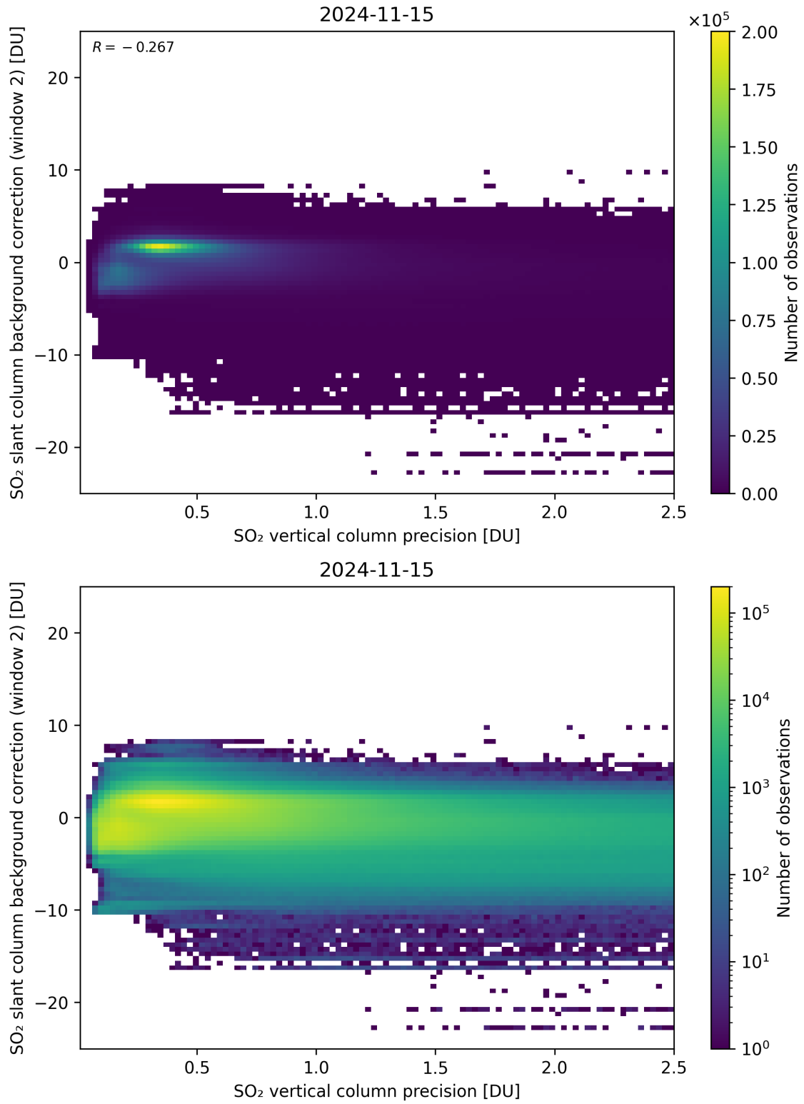
Figure 280: Scatter density plot of “SO 2 vertical column precision” against “SO 2 slant column background correction (window 2)” for 2024-11-14 to 2024-11-16.
