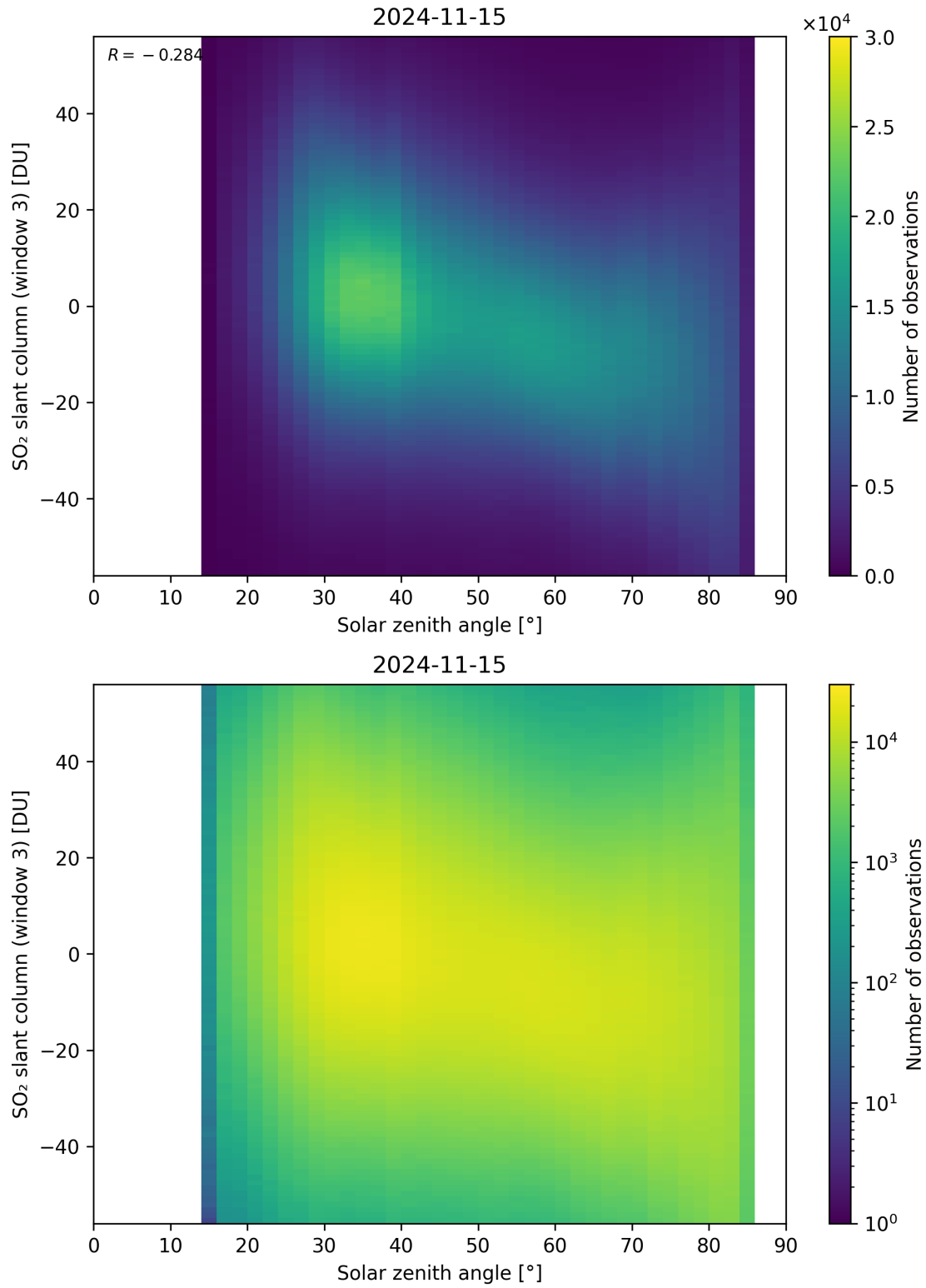
Figure 172: Scatter density plot of “Solar zenith angle” against “SO 2 slant column (window 3)” for 2024-11-14 to 2024-11-16.
