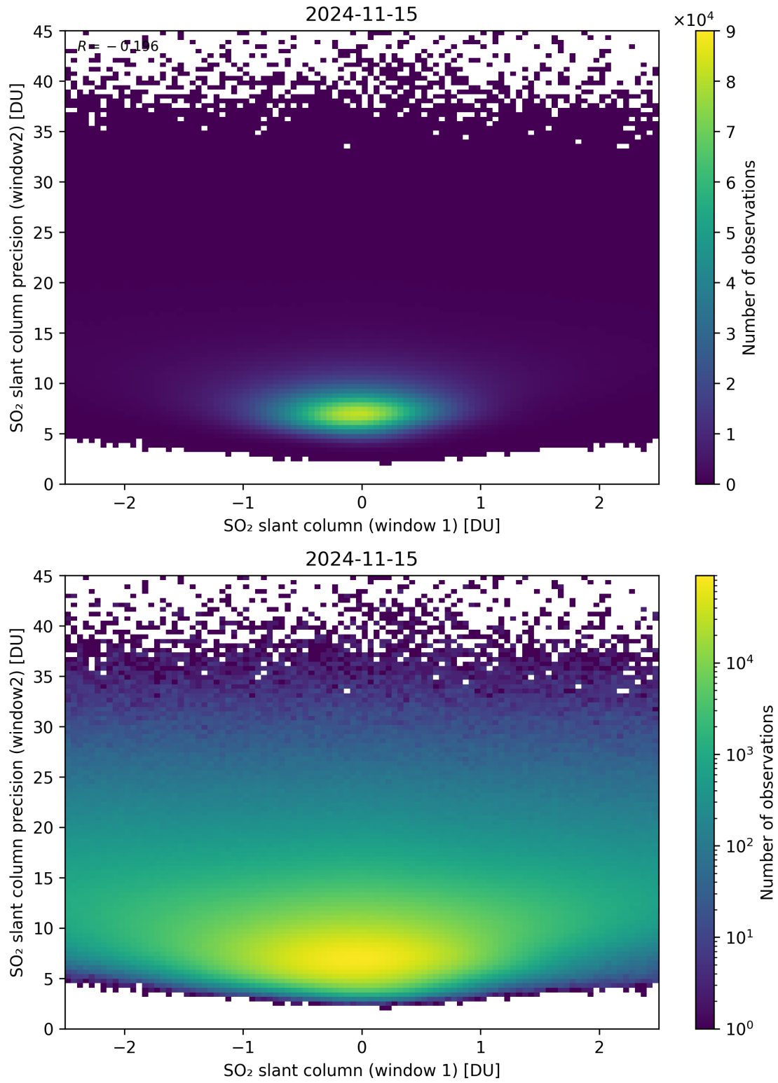
Figure 236: Scatter density plot of “SO 2 slant column (window 1)” against “SO 2 slant column precision (window2)” for 2024-11-14 to 2024-11-16.
