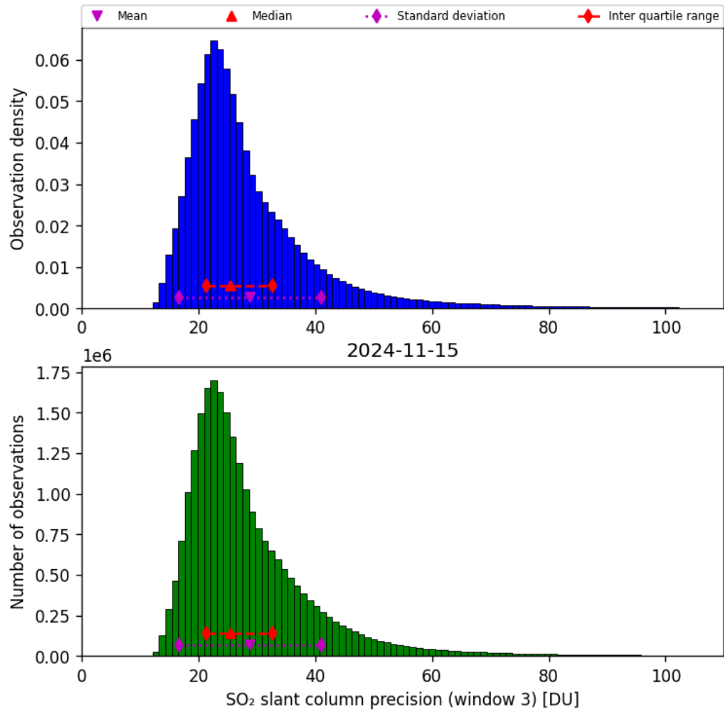
Figure 65: Histogram of “SO 2 slant column precision (window 3)” for 2024-11-14 to 2024-11-16
