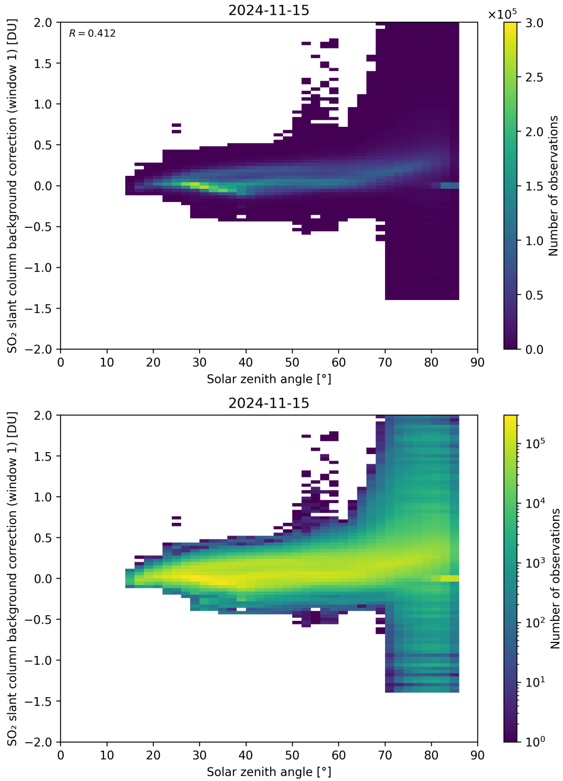
Figure 158: Scatter density plot of “Solar zenith angle” against “SO 2 slant column background correction (window 1)” for 2024-11-14 to 2024-11-16.
