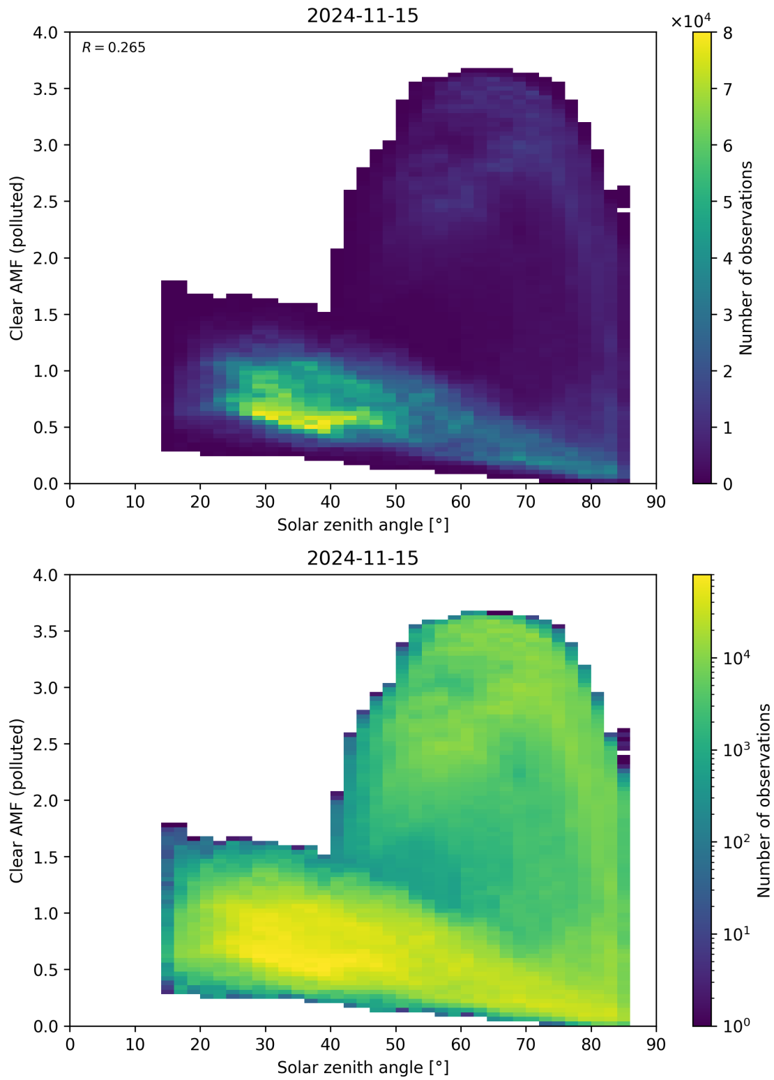
Figure 165: Scatter density plot of “Solar zenith angle” against “Clear AMF (polluted)” for 2024-11-14 to 2024-11-16.
