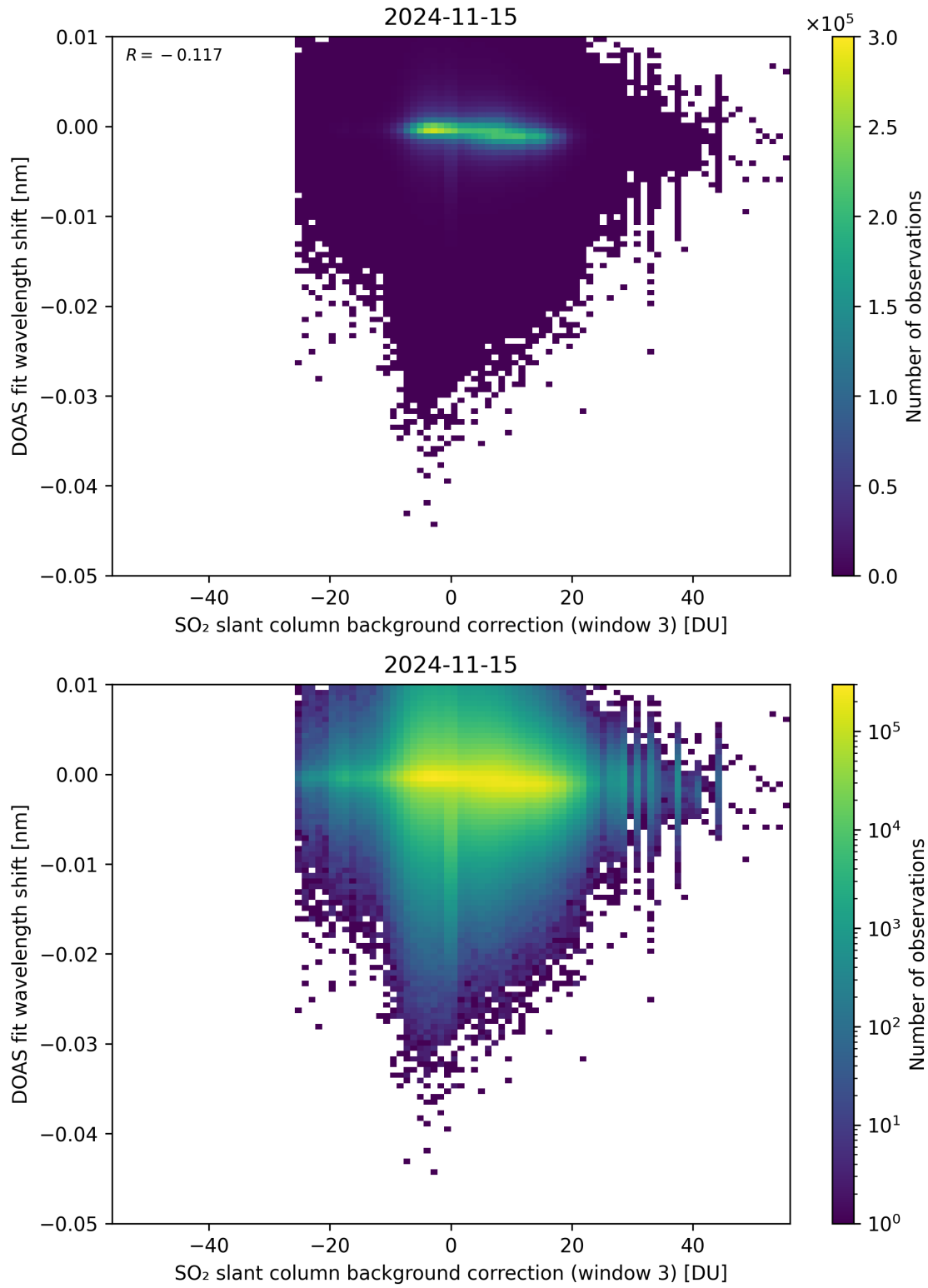
Figure 121: Scatter density plot of “SO 2 slant column background correction (window 3)” against “DOAS fit wavelength shift” for 2024-11-14 to 2024-11-16.
