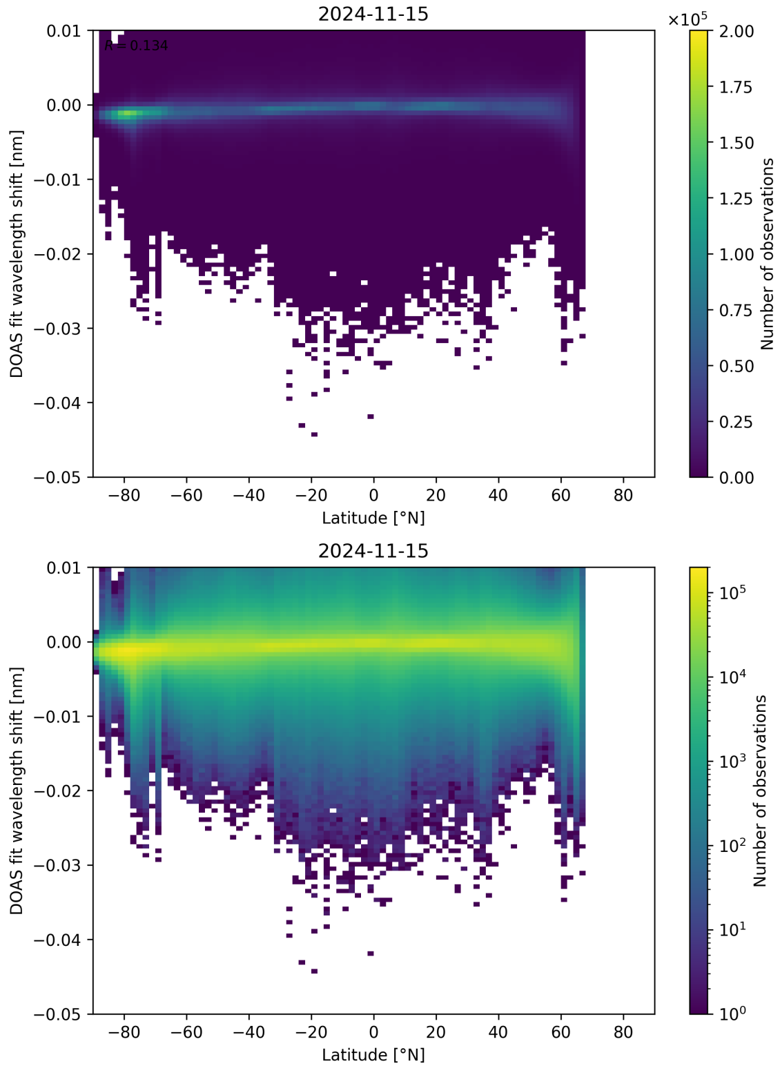
Figure 142: Scatter density plot of “Latitude” against “DOAS fit wavelength shift” for 2024-11-14 to 2024-11-16.
