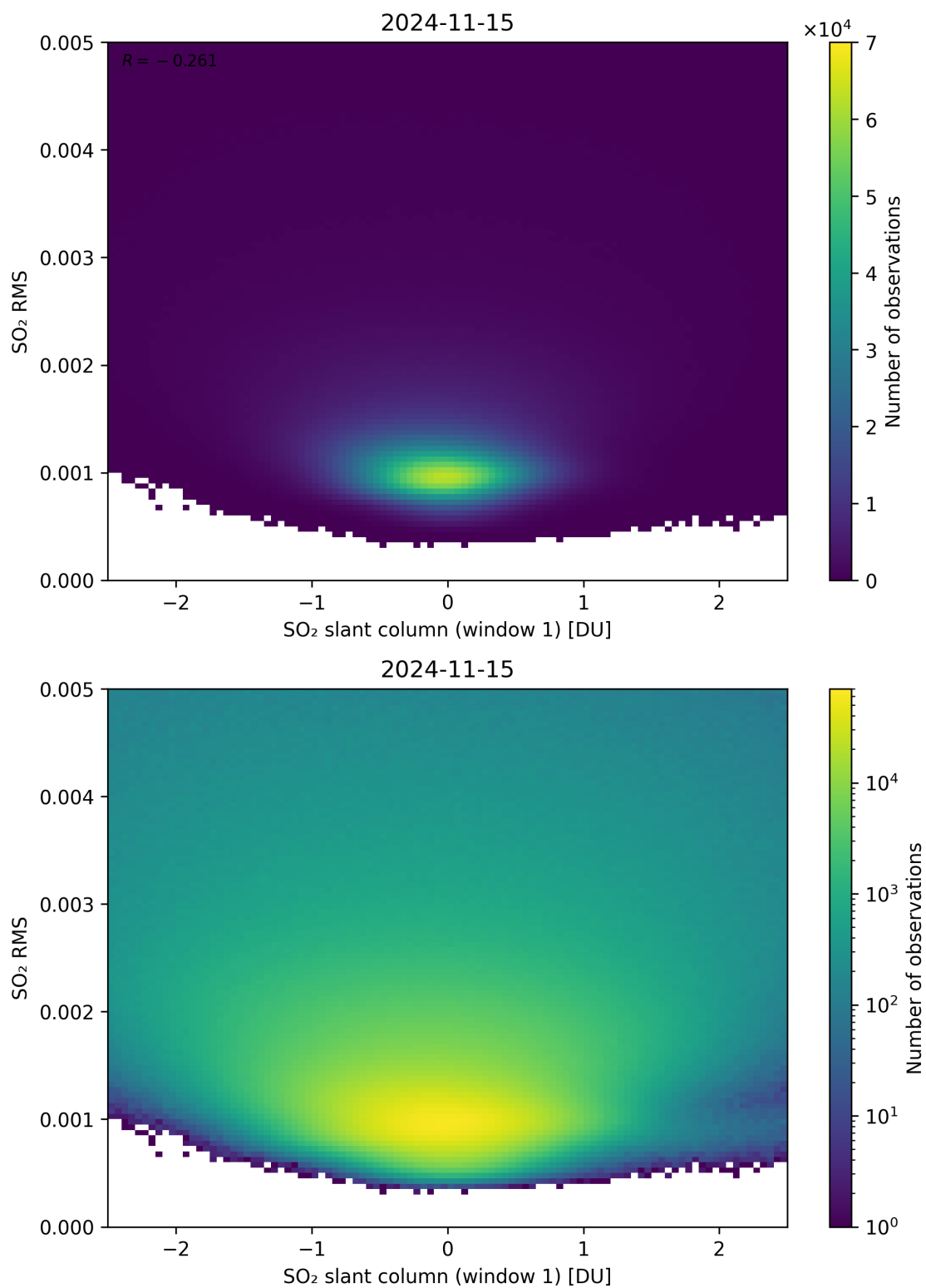
Figure 217: Scatter density plot of “SO 2 slant column (window 1)” against “SO 2 RMS” for 2024-11-14 to 2024-11-16.
