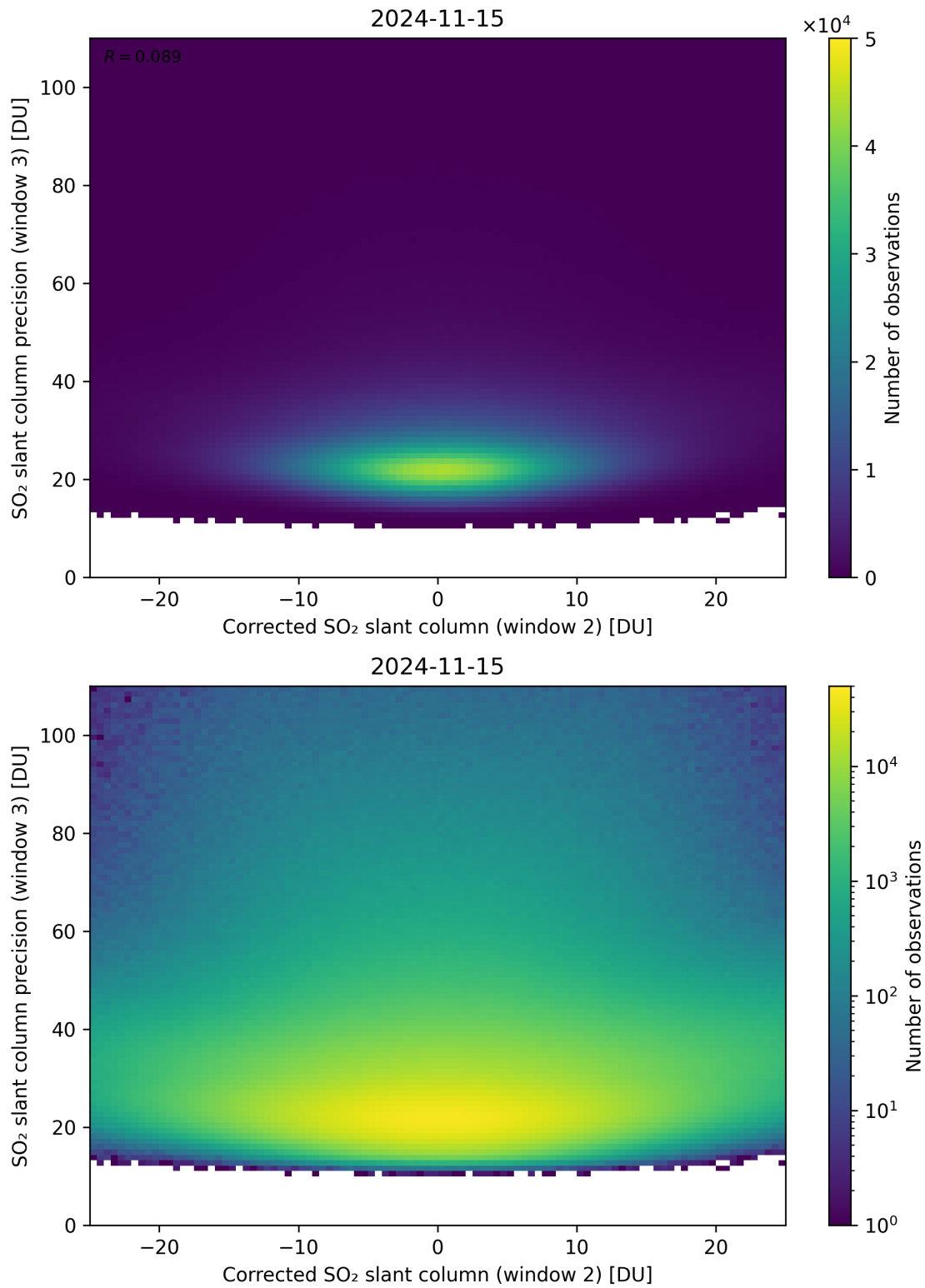
Figure 202: Scatter density plot of “Corrected SO 2 slant column (window 2)” against “SO 2 slant column precision (window 3)” for 2024-11-14 to 2024-11-16.
