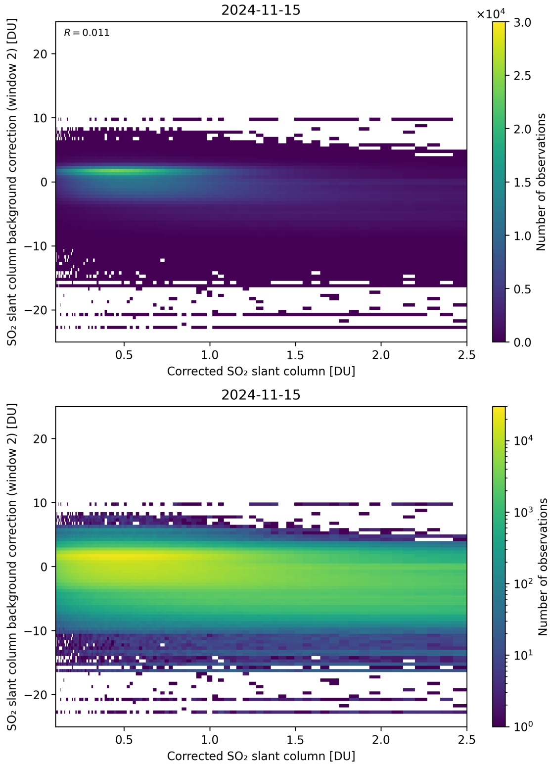
Figure 179: Scatter density plot of “Corrected SO 2 slant column” against “SO 2 slant column background correction (window 2)” for 2024-11-14 to 2024-11-16.
