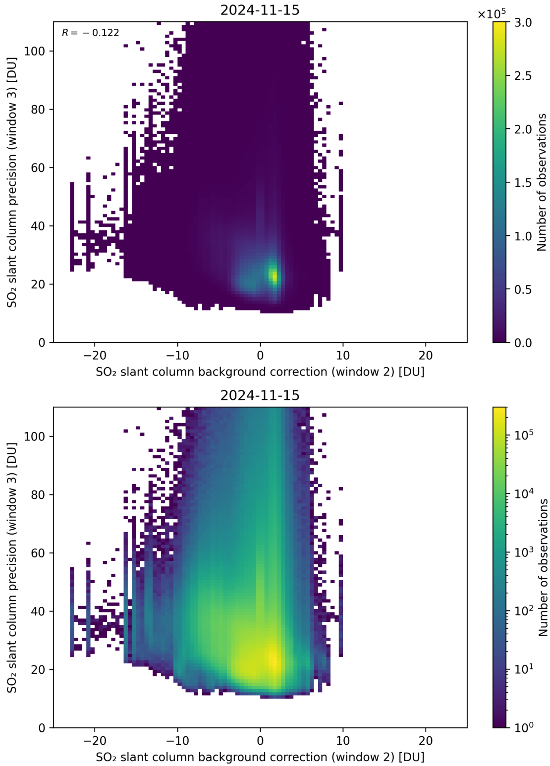
Figure 118: Scatter density plot of “SO 2 slant column background correction (window 2)” against “SO 2 slant column precision (window 3)” for 2024-11-14 to 2024-11-16.
