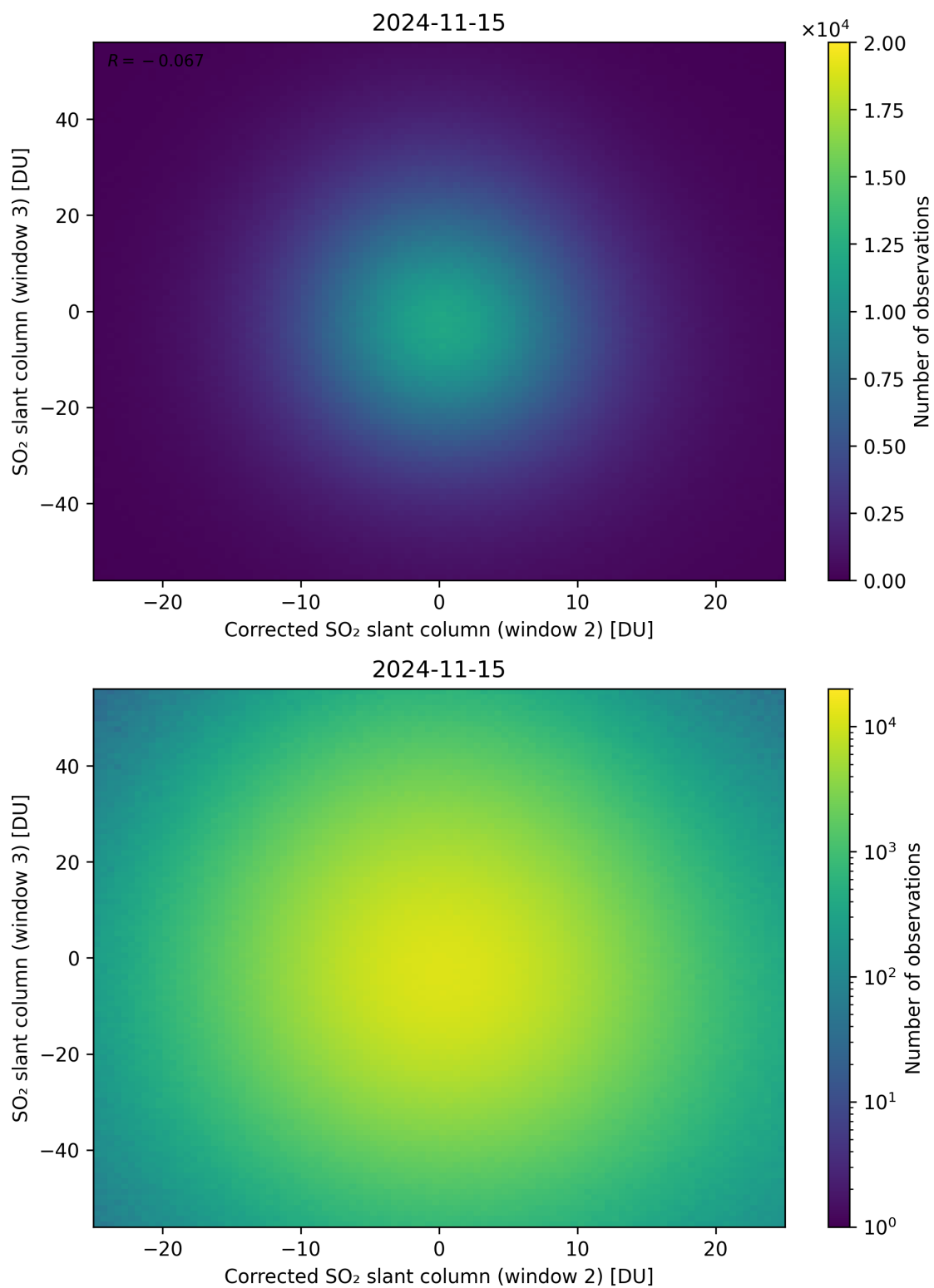
Figure 201: Scatter density plot of “Corrected SO 2 slant column (window 2)” against “SO 2 slant column (window 3)” for 2024-11-14 to 2024-11-16.
