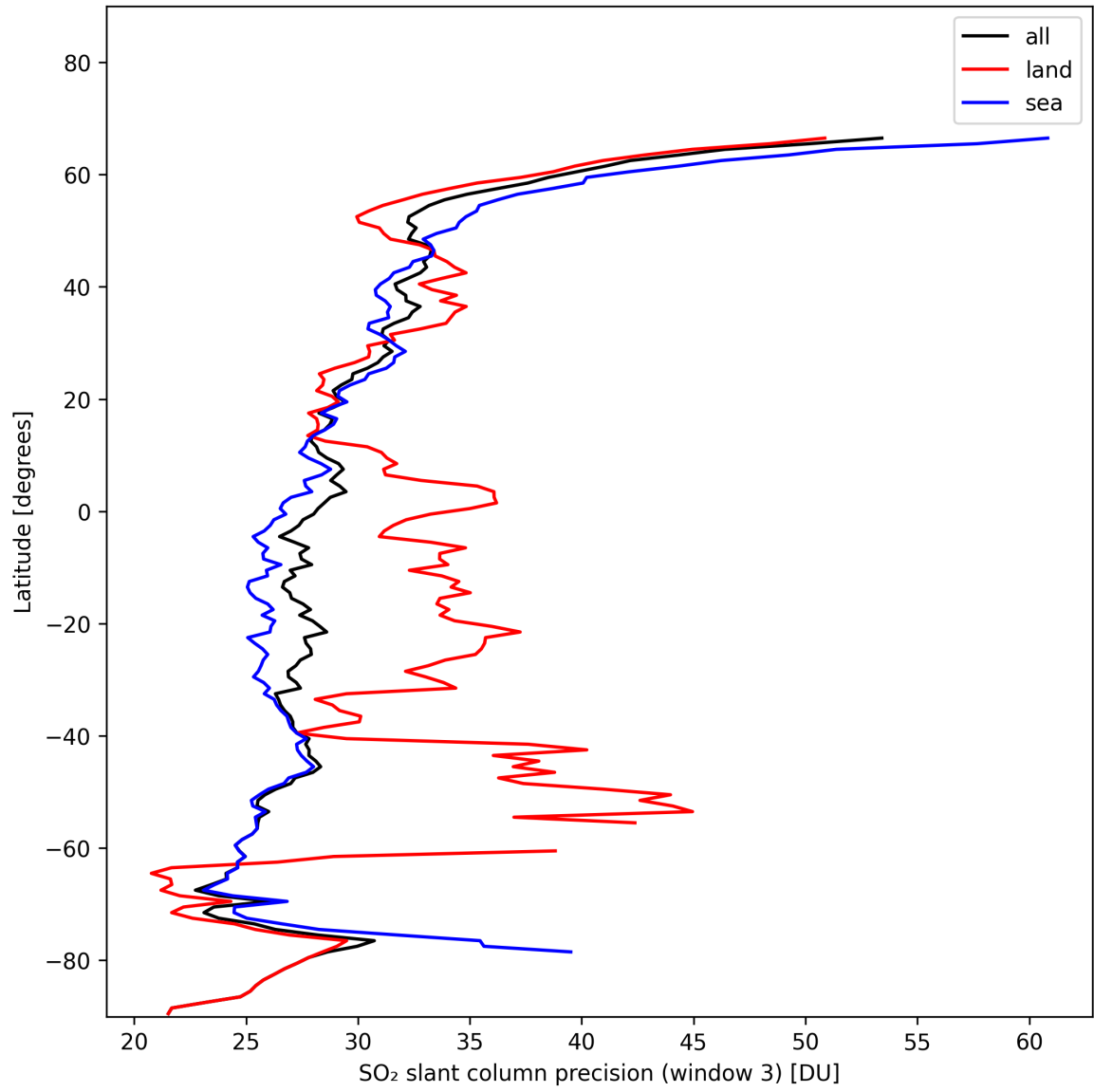
Figure 42: Zonal average of “SO 2 slant column precision (window 3)” for 2024-11-14 to 2024-11-16.
