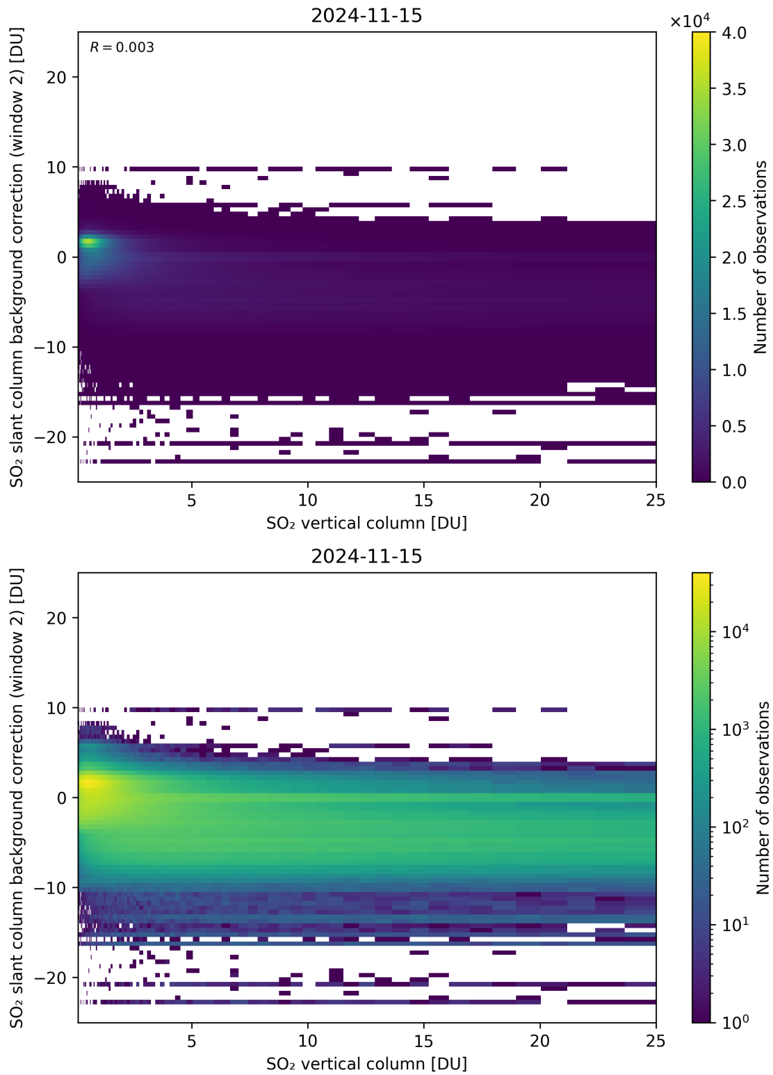
Figure 274: Scatter density plot of “SO 2 vertical column” against “SO 2 slant column background correction (window 2)” for 2024-11-14 to 2024-11-16.
