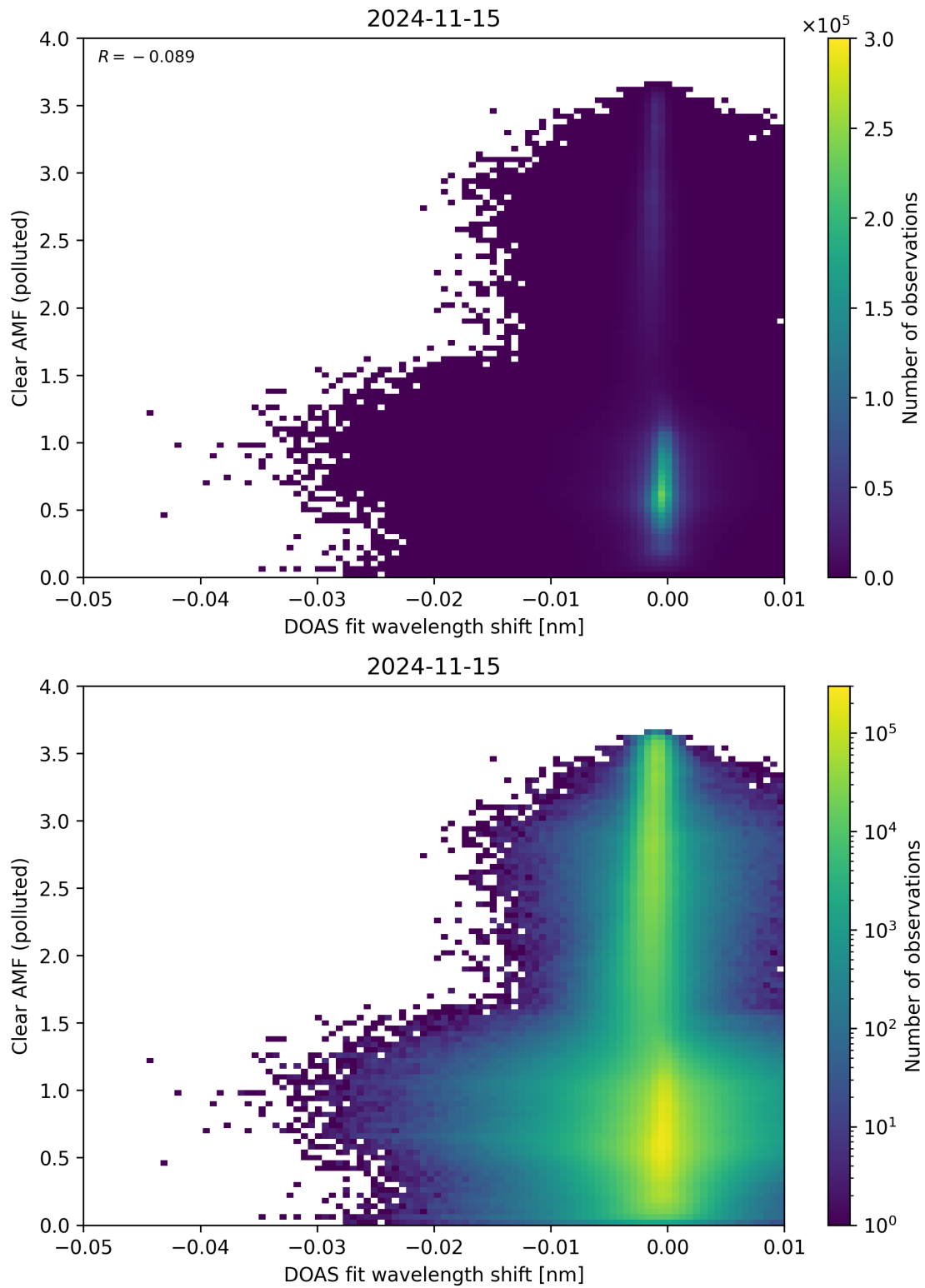
Figure 129: Scatter density plot of “DOAS fit wavelength shift” against “Clear AMF (polluted)” for 2024-11-14 to 2024-11-16.
