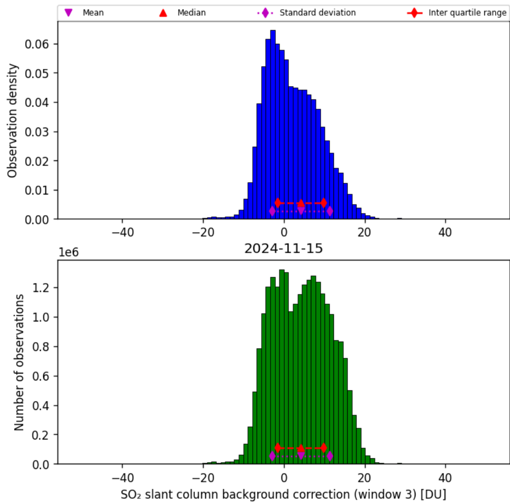
Figure 67: Histogram of “SO 2 slant column background correction (window 3)” for 2024-11-14 to 2024-11-16
