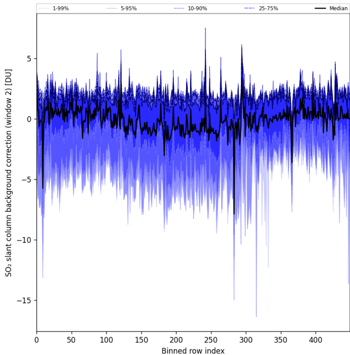
Figure 86: Along track statistics of “SO 2 slant column background correction (window 2)” for 2024-11-14 to 2024-11-16
