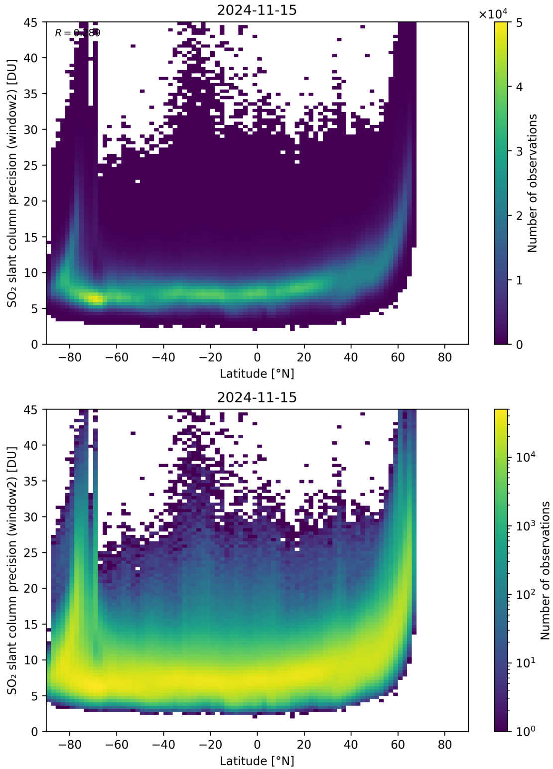
Figure 151: Scatter density plot of “Latitude” against “SO 2 slant column precision (window2)” for 2024-11-14 to 2024-11-16.
