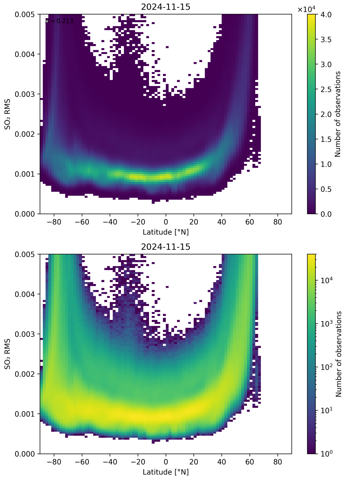
Figure 144: Scatter density plot of “Latitude” against “SO 2 RMS” for 2024-11-14 to 2024-11-16.
