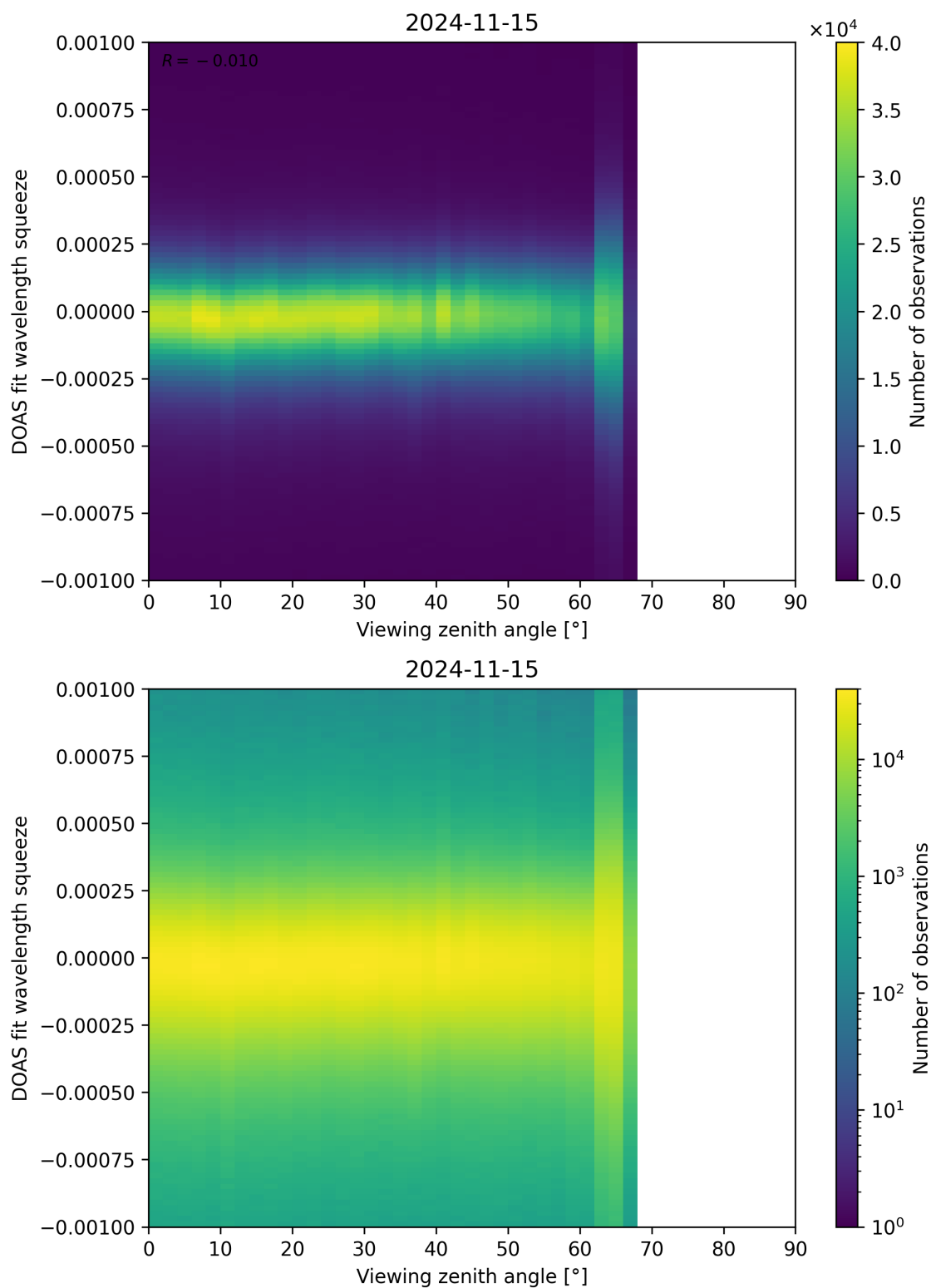
Figure 312: Scatter density plot of “Viewing zenith angle” against “DOAS fit wavelength squeeze” for 2024-11-14 to 2024-11-16.
