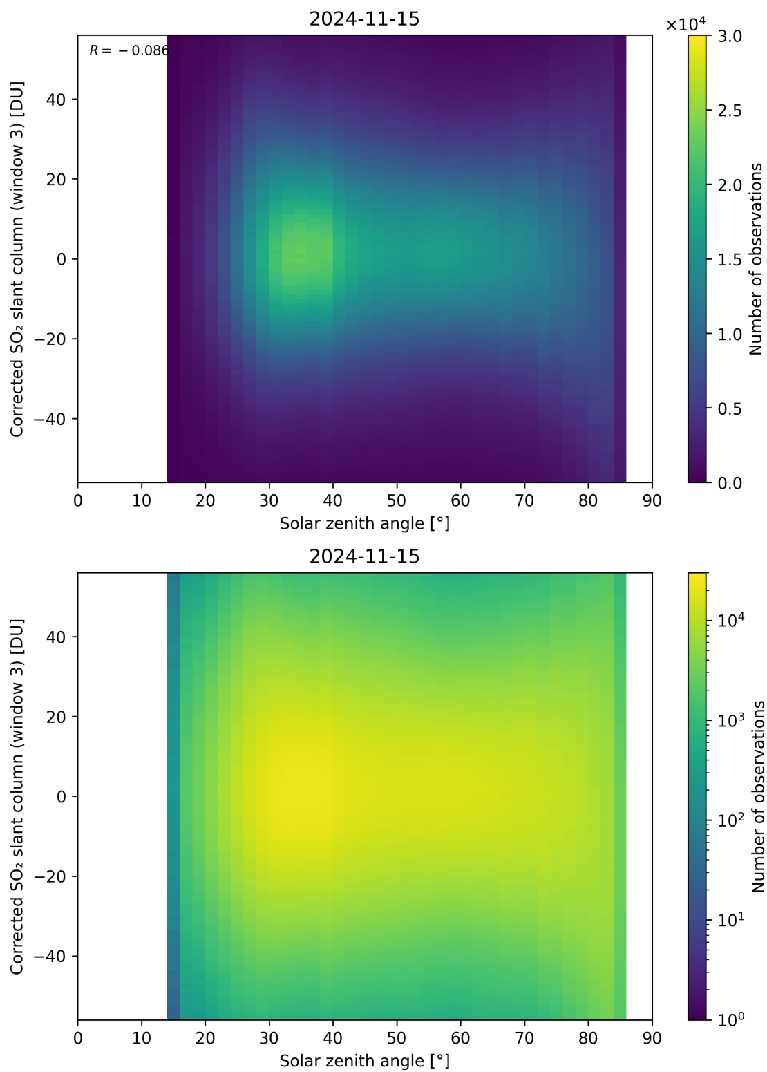
Figure 168: Scatter density plot of “Solar zenith angle” against “Corrected SO 2 slant column (window 3)” for 2024-11-14 to 2024-11-16.
