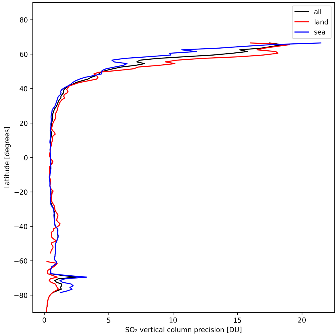
Figure 31: Zonal average of “SO 2 vertical column precision” for 2024-11-14 to 2024-11-16.
