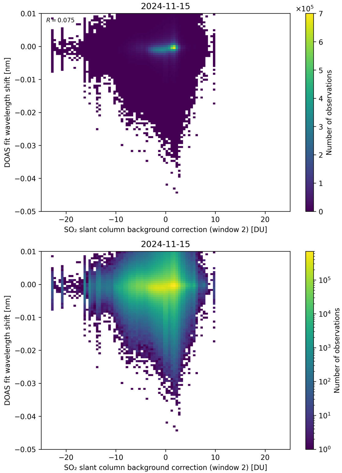
Figure 112: Scatter density plot of “SO 2 slant column background correction (window 2)” against “DOAS fit wavelength shift” for 2024-11-14 to 2024-11-16.
