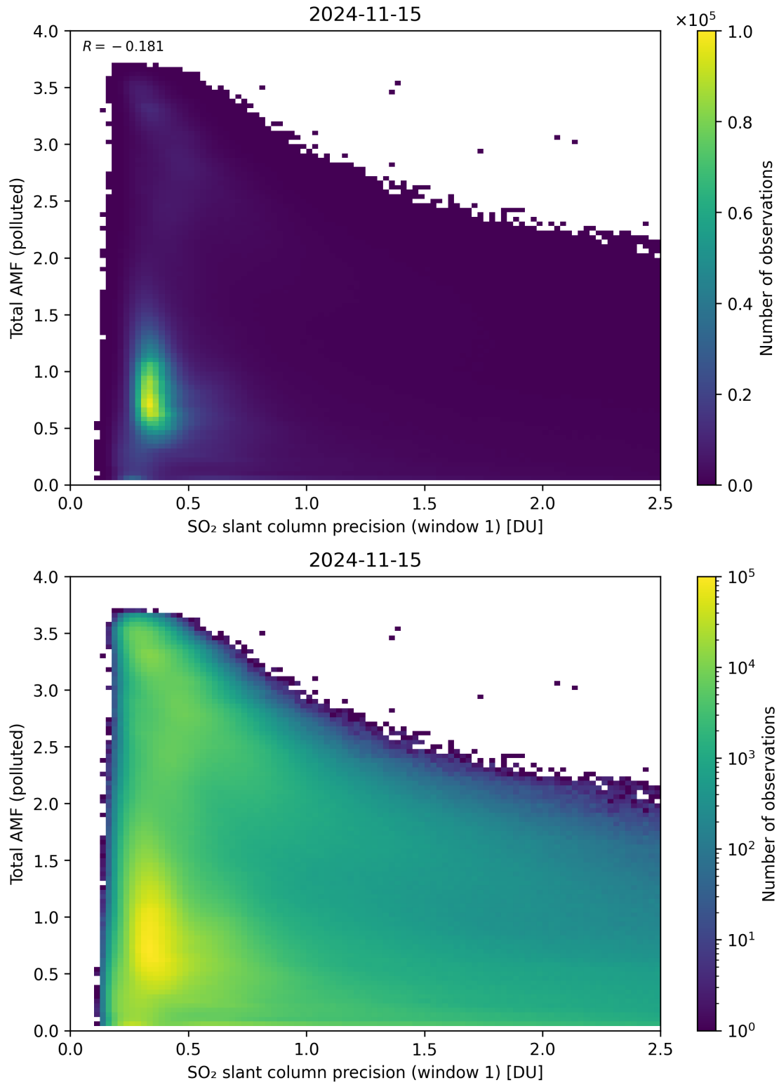
Figure 230: Scatter density plot of “SO 2 slant column precision (window 1)” against “Total AMF (polluted)” for 2024-11-14 to 2024-11-16.
