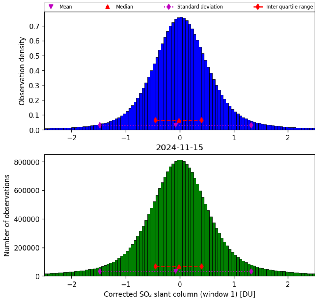
Figure 58: Histogram of “Corrected SO 2 slant column (window 1)” for 2024-11-14 to 2024-11-16
