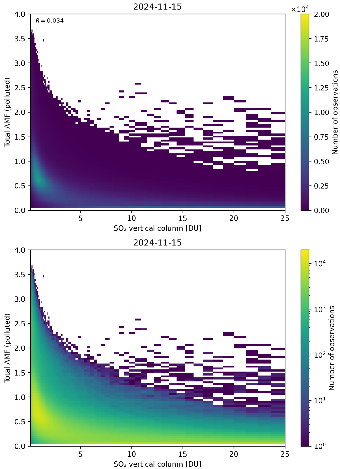
Figure 305: Scatter density plot of “SO 2 vertical column” against “Total AMF (polluted)” for 2024-11-14 to 2024-11-16.
