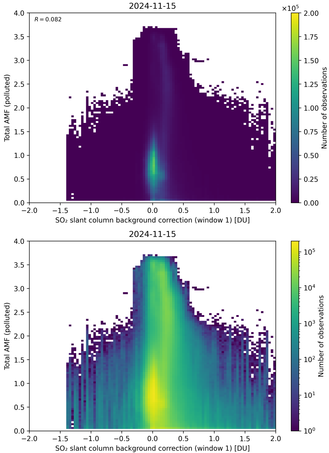
Figure 109: Scatter density plot of “SO 2 slant column background correction (window 1)” against “Total AMF (polluted)” for 2024-11-14 to 2024-11-16.
