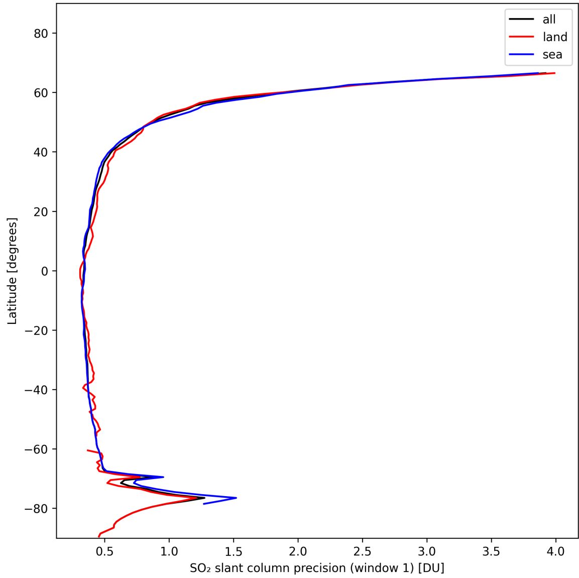
Figure 34: Zonal average of “SO 2 slant column precision (window 1)” for 2024-11-14 to 2024-11-16.
