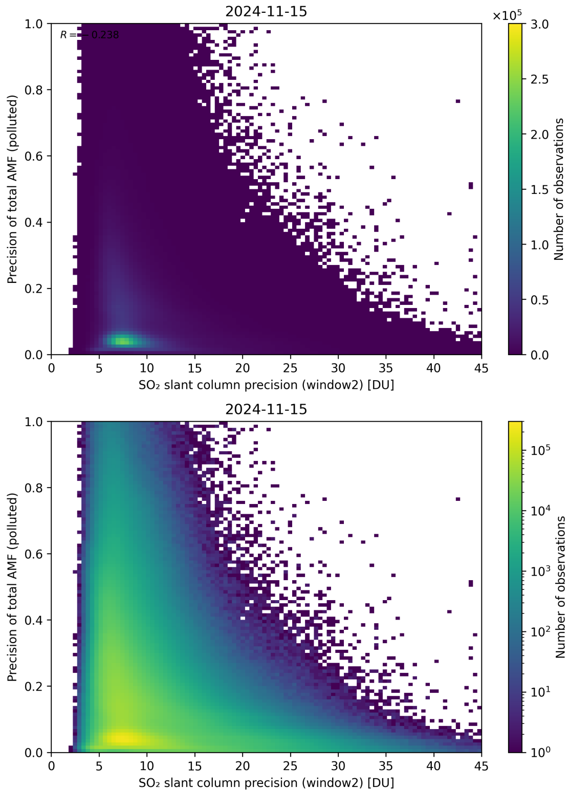
Figure 252: Scatter density plot of “SO 2 slant column precision (window2)” against “Precision of total AMF (polluted)” for 2024-11-14 to 2024-11-16.
