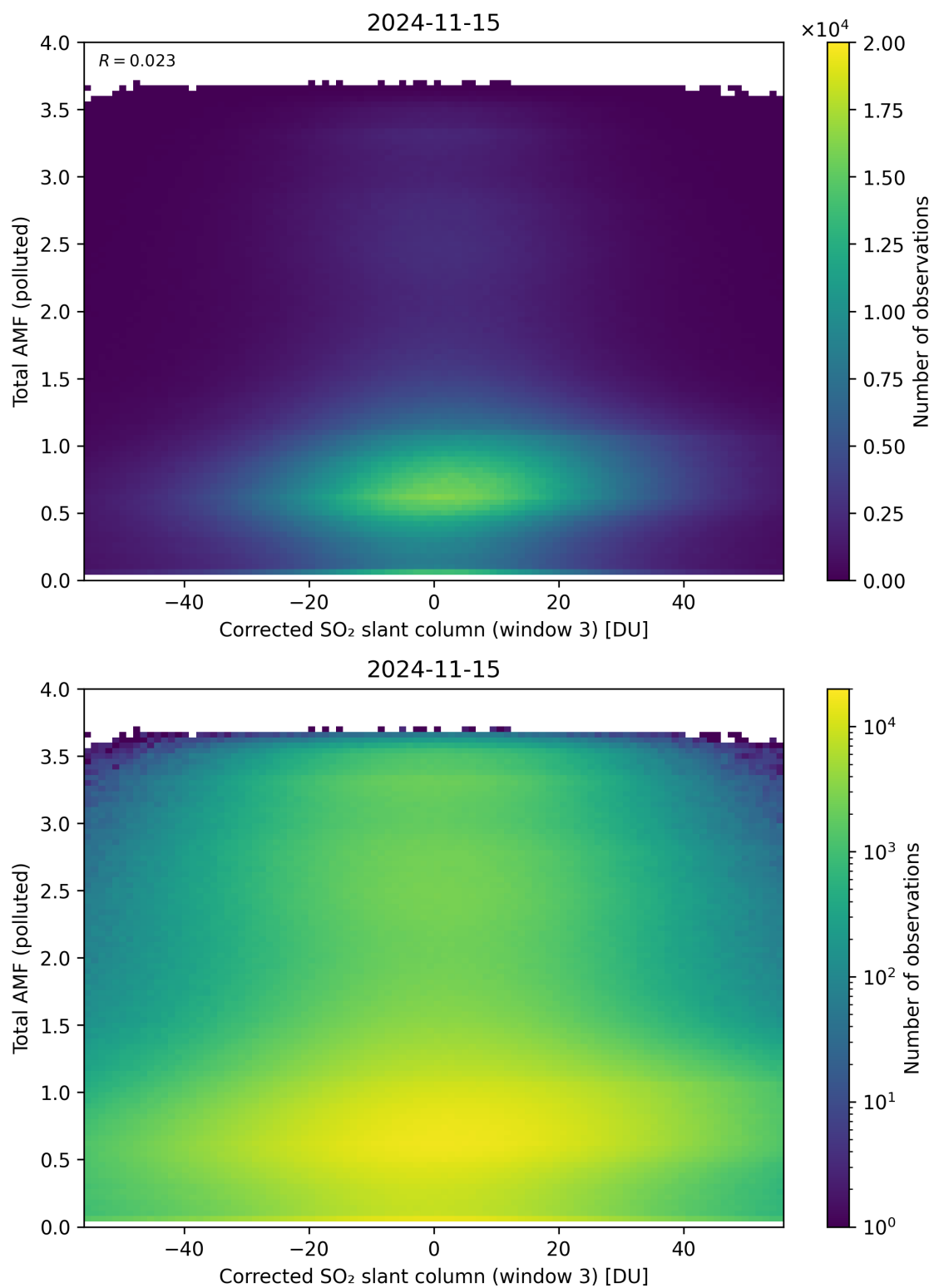
Figure 210: Scatter density plot of “Corrected SO 2 slant column (window 3)” against “Total AMF (polluted)” for 2024-11-14 to 2024-11-16.
