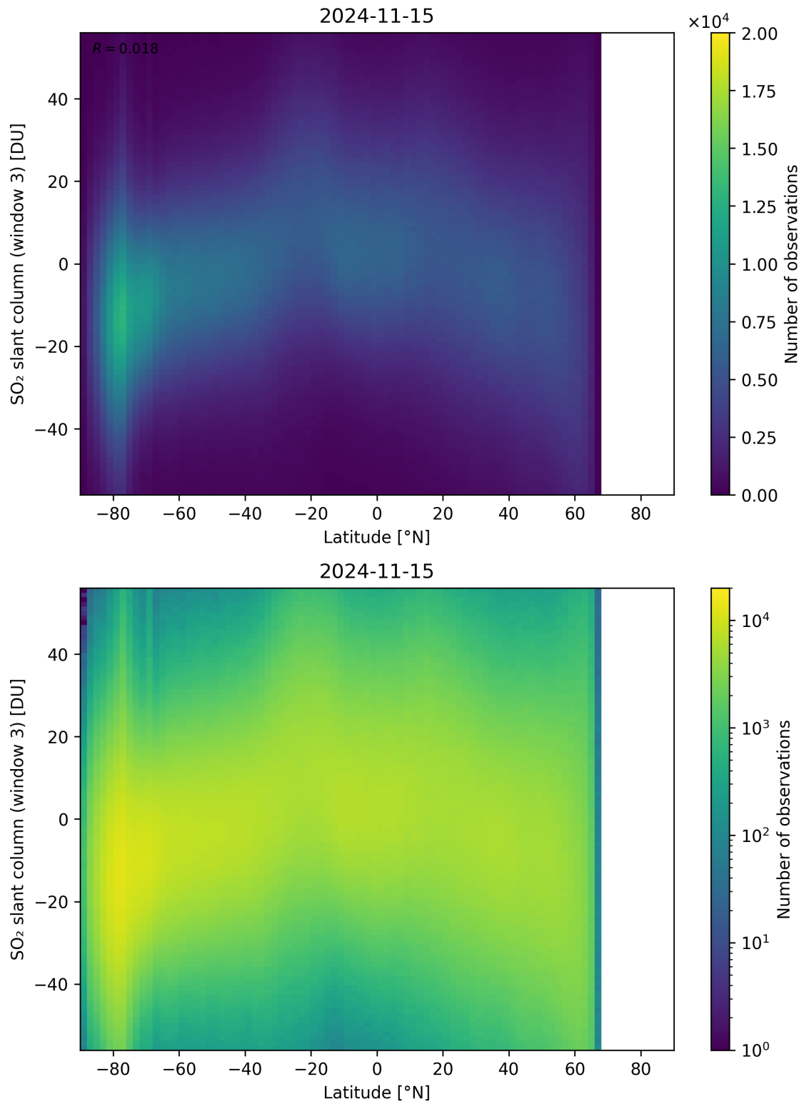
Figure 152: Scatter density plot of “Latitude” against “SO 2 slant column (window 3)” for 2024-11-14 to 2024-11-16.
