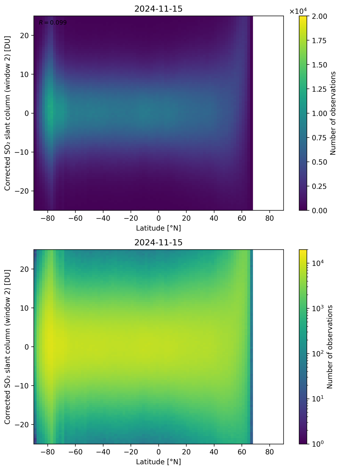
Figure 147: Scatter density plot of “Latitude” against “Corrected SO 2 slant column (window 2)” for 2024-11-14 to 2024-11-16.
