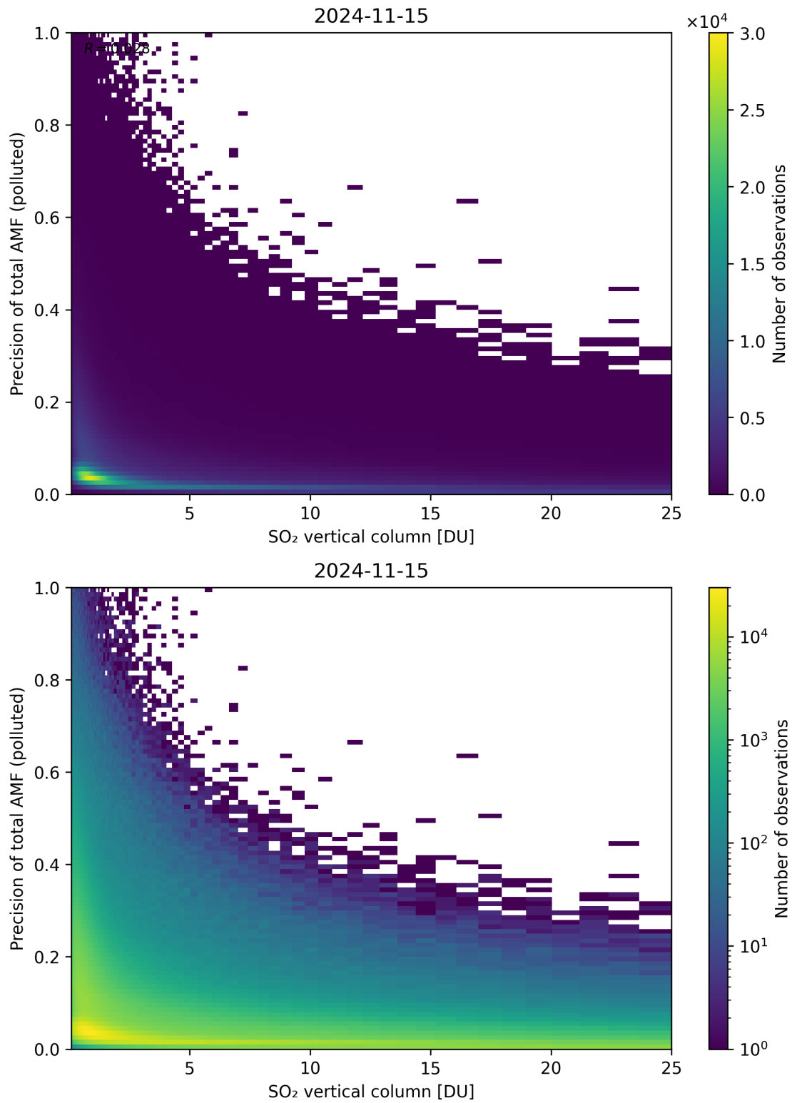
Figure 306: Scatter density plot of “SO 2 vertical column” against “Precision of total AMF (polluted)” for 2024-11-14 to 2024-11-16.
