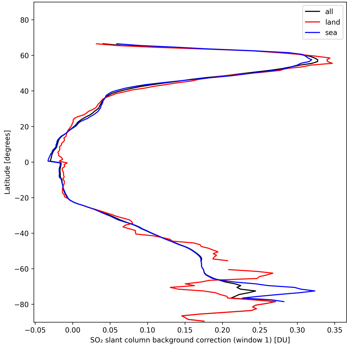
Figure 36: Zonal average of “SO 2 slant column background correction (window 1)” for 2024-11-14 to 2024-11-16.
