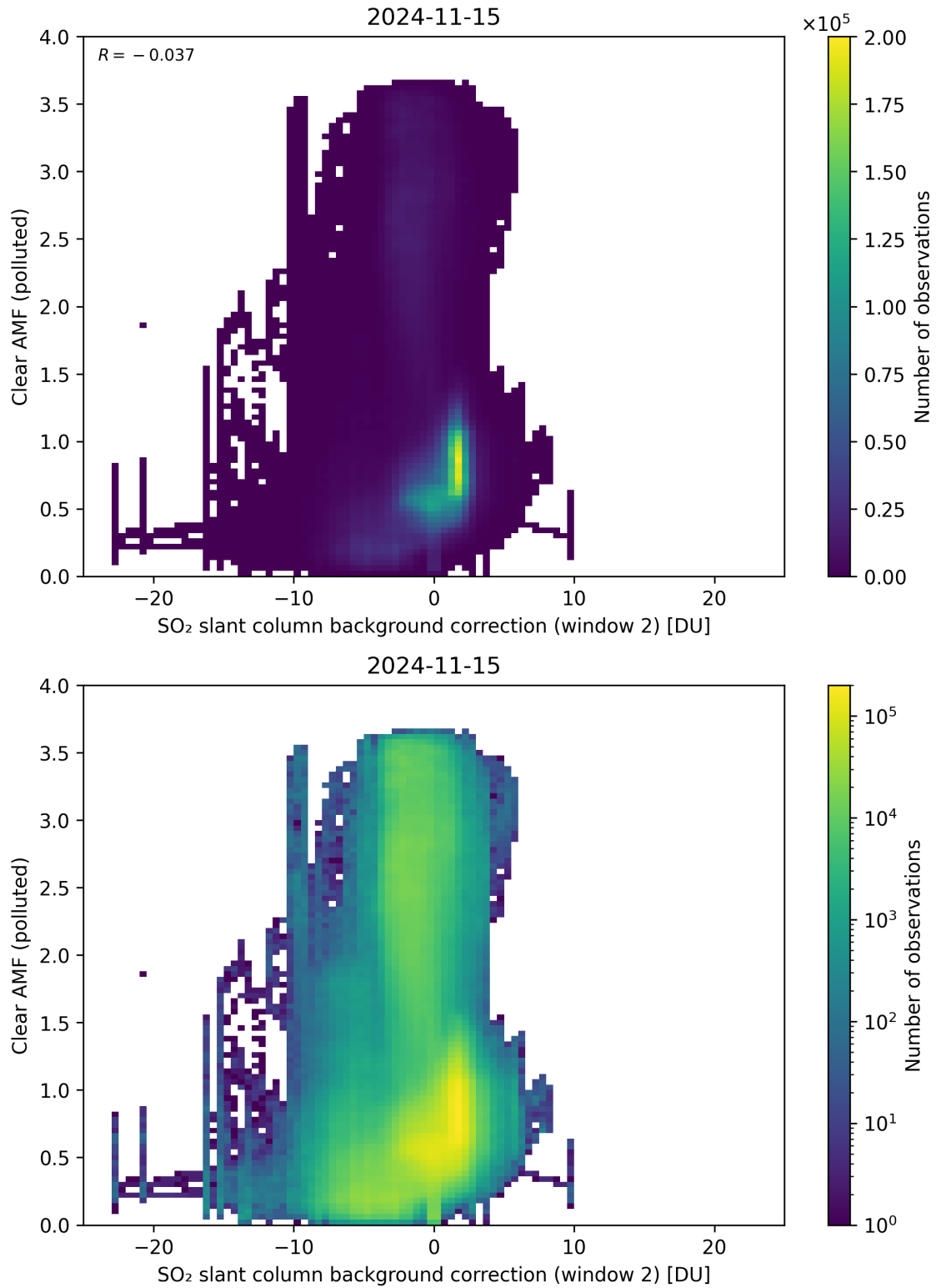
Figure 115: Scatter density plot of “SO 2 slant column background correction (window 2)” against “Clear AMF (polluted)” for 2024-11-14 to 2024-11-16.
