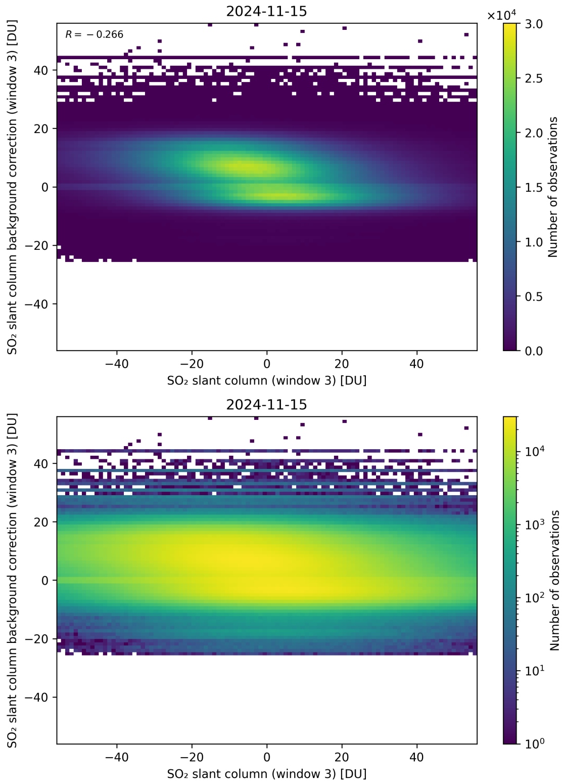
Figure 253: Scatter density plot of “SO 2 slant column (window 3)” against “SO 2 slant column background correction (window 3)” for 2024-11-14 to 2024-11-16.
