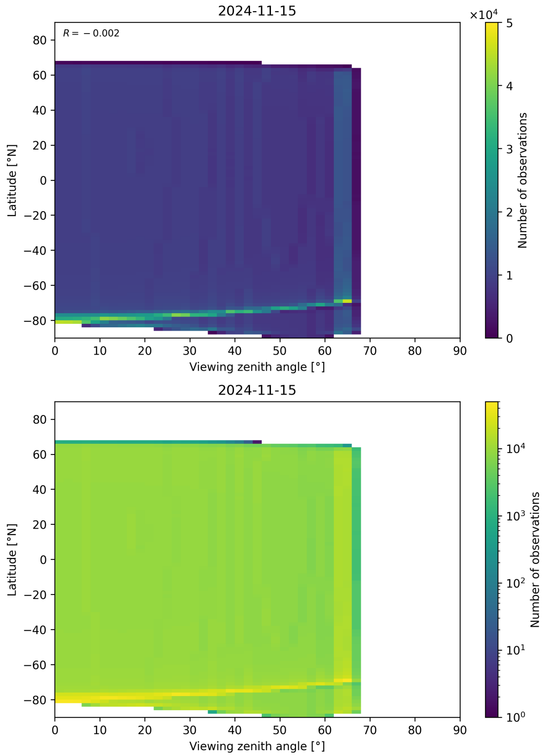
Figure 314: Scatter density plot of “Viewing zenith angle” against “Latitude” for 2024-11-14 to 2024-11-16.
