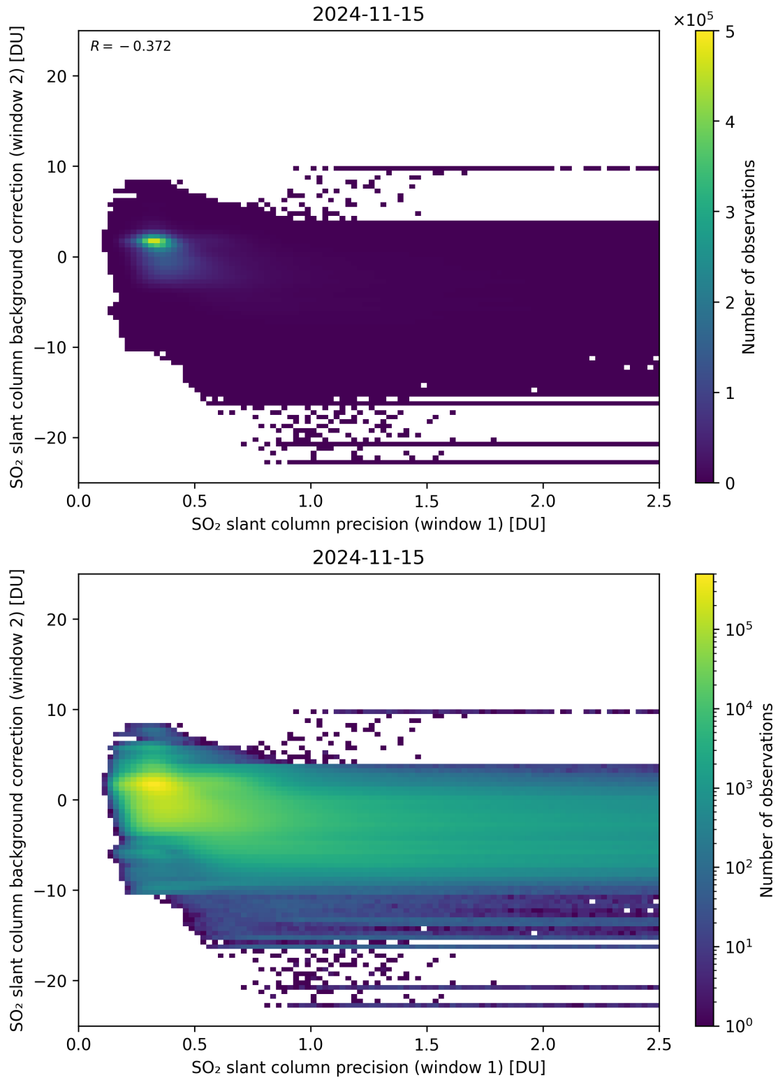
Figure 219: Scatter density plot of “SO 2 slant column precision (window 1)” against “SO 2 slant column background correction (window 2)” for 2024-11-14 to 2024-11-16.
