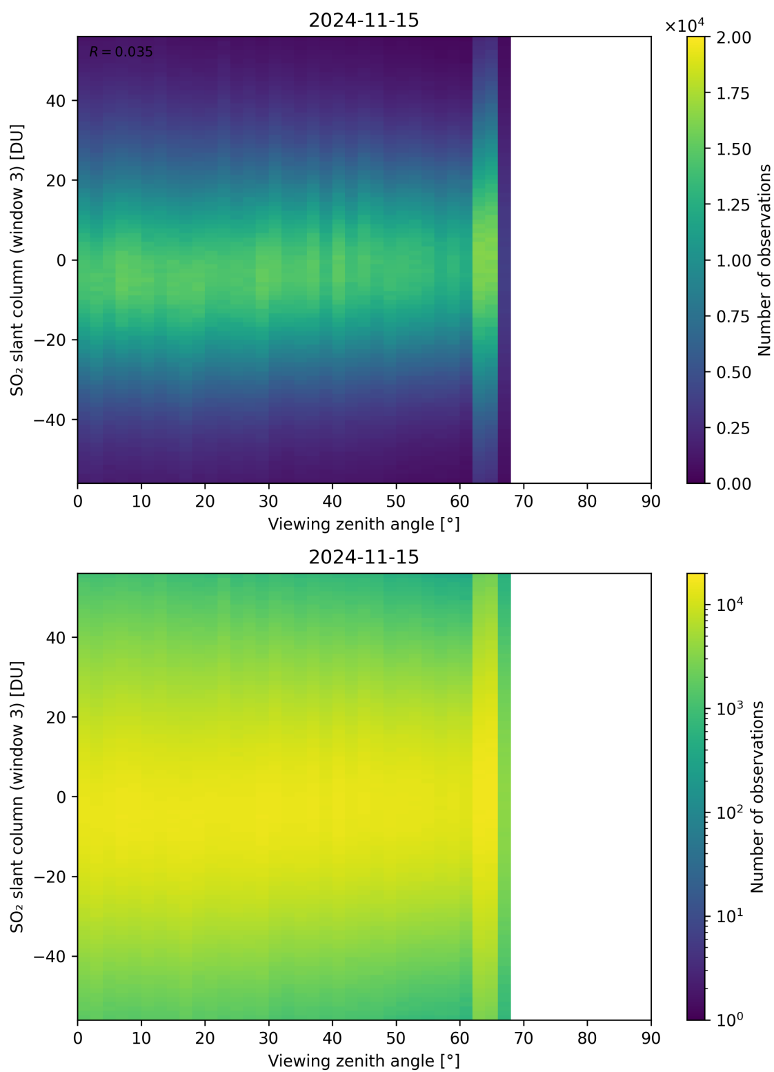
Figure 323: Scatter density plot of “Viewing zenith angle” against “SO 2 slant column (window 3)” for 2024-11-14 to 2024-11-16.
