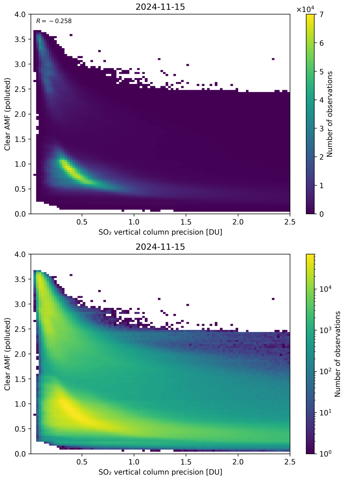
Figure 285: Scatter density plot of “SO 2 vertical column precision” against “Clear AMF (polluted)” for 2024-11-14 to 2024-11-16.
