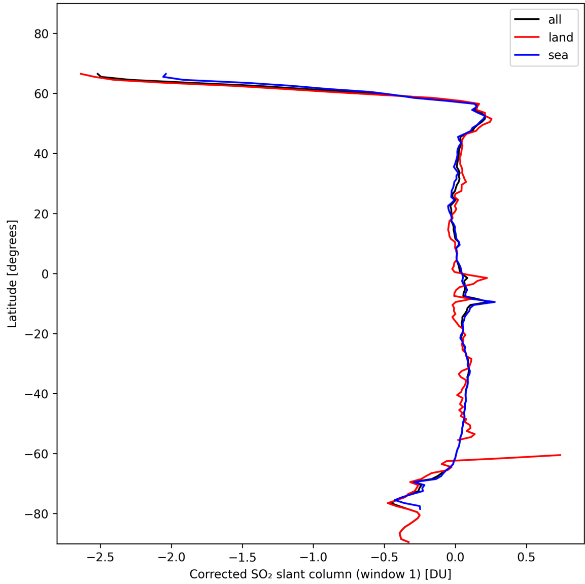
Figure 35: Zonal average of “Corrected SO 2 slant column (window 1)” for 2024-11-14 to 2024-11-16.
