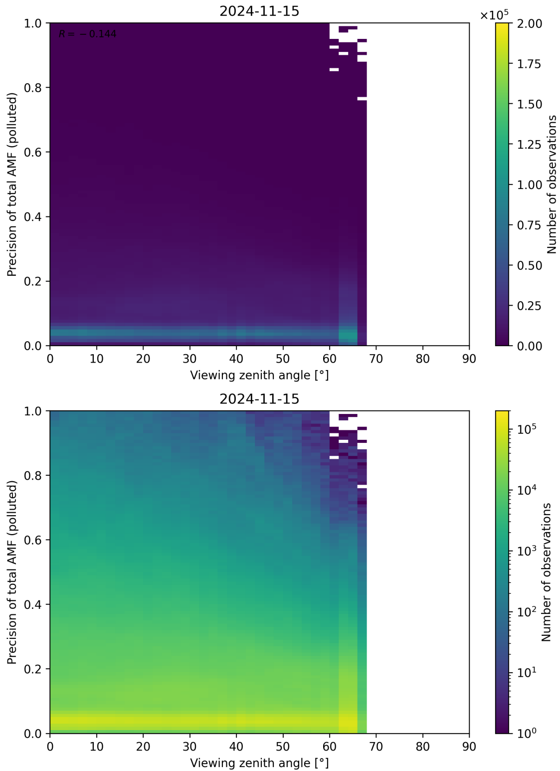
Figure 326: Scatter density plot of “Viewing zenith angle” against “Precision of total AMF (polluted)” for 2024-11-14 to 2024-11-16.
