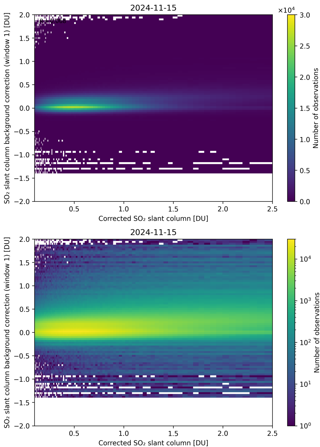
Figure 178: Scatter density plot of “Corrected SO 2 slant column” against “SO 2 slant column background correction (window 1)” for 2024-11-14 to 2024-11-16.
