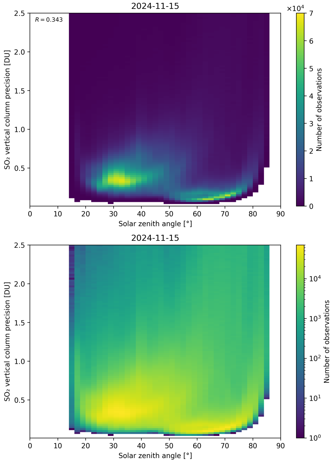
Figure 177: Scatter density plot of “Solar zenith angle” against “SO 2 vertical column precision” for 2024-11-14 to 2024-11-16.
