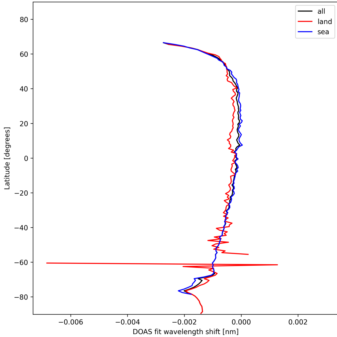
Figure 45: Zonal average of “DOAS fit wavelength shift” for 2024-11-14 to 2024-11-16.
