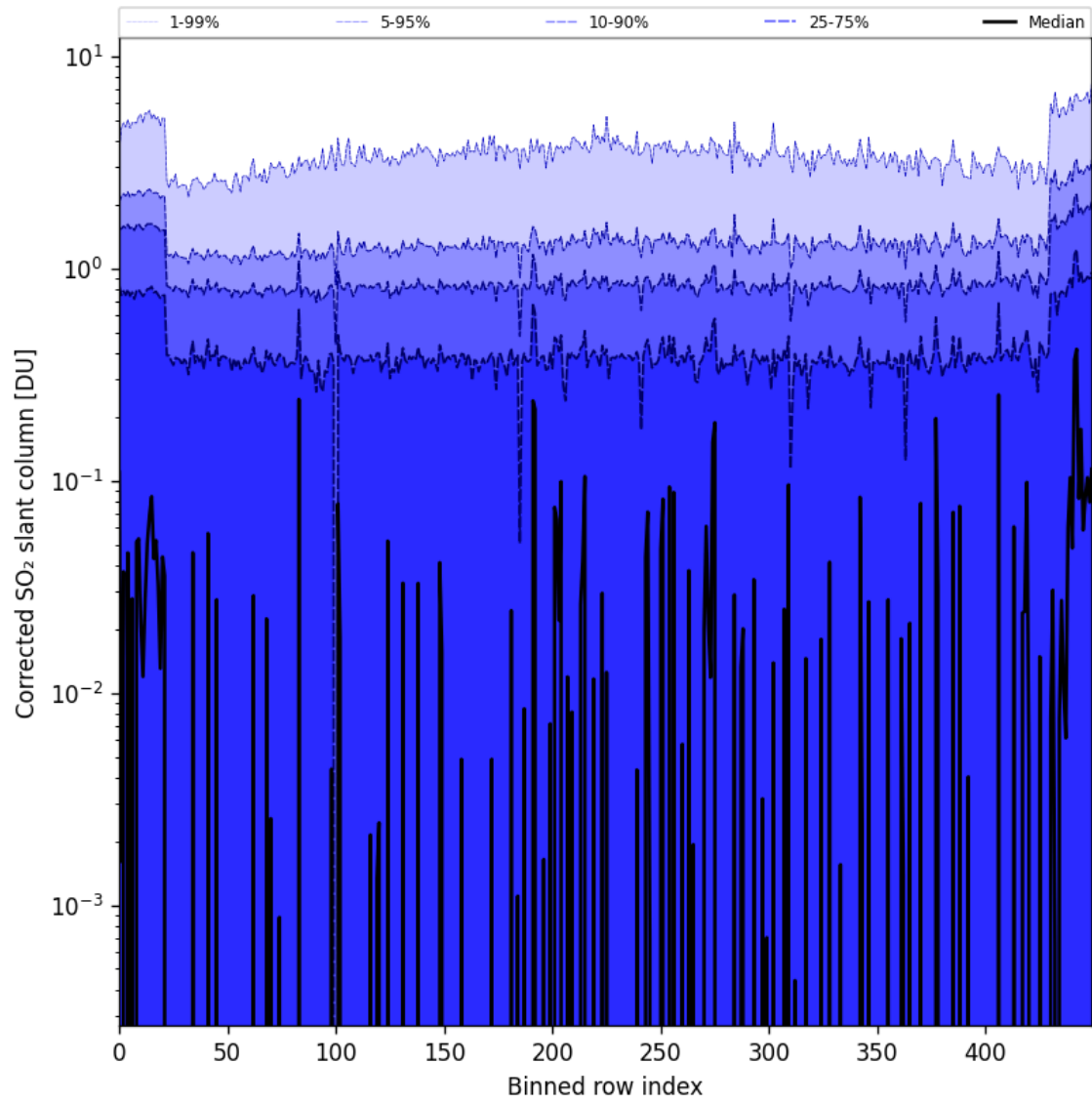
Figure 78: Along track statistics of “Corrected SO 2 slant column” for 2024-11-14 to 2024-11-16
