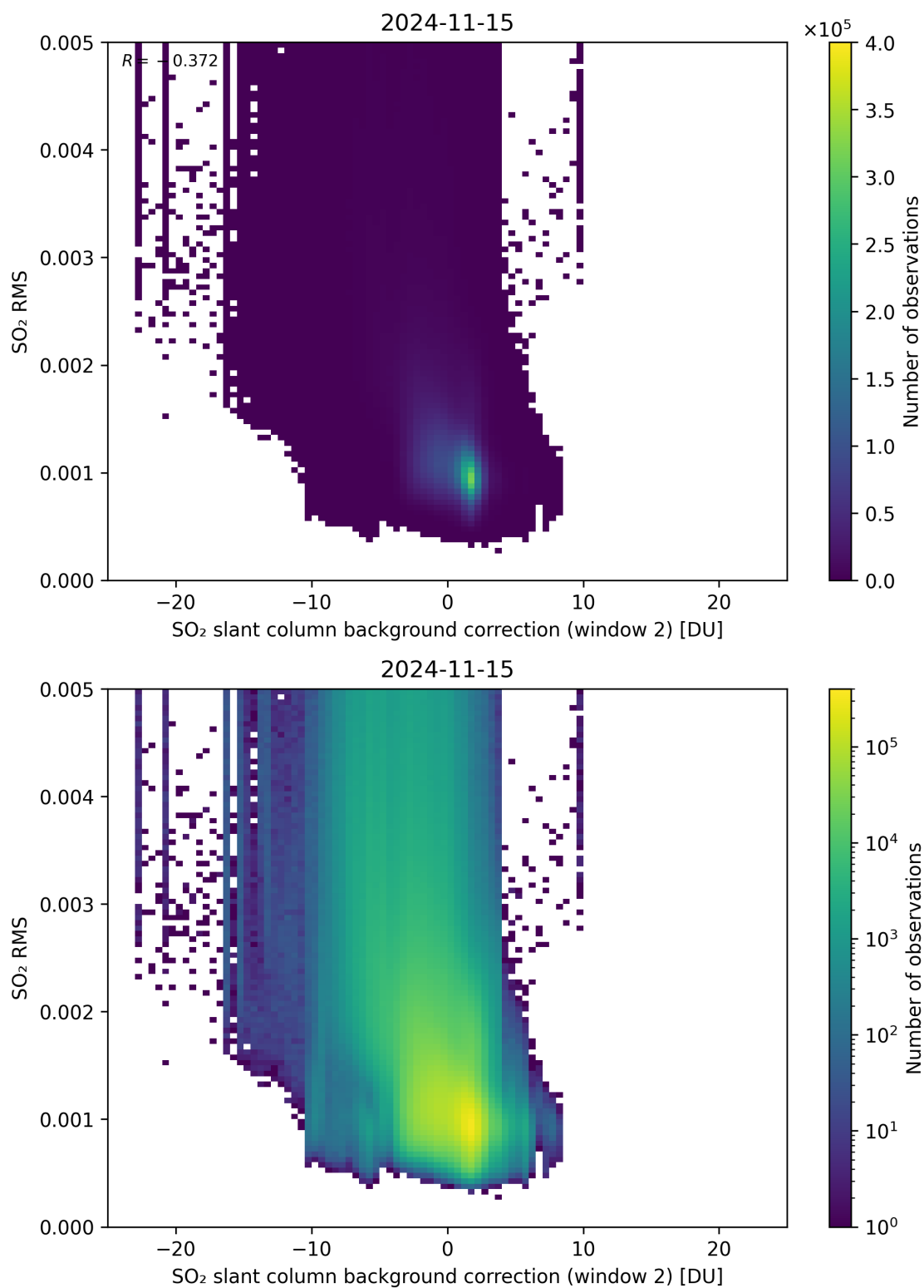
Figure 114: Scatter density plot of “SO 2 slant column background correction (window 2)” against “SO 2 RMS” for 2024-11-14 to 2024-11-16.
