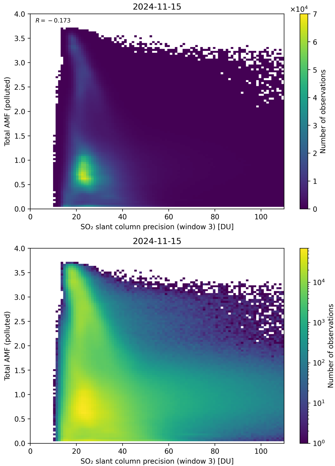
Figure 263: Scatter density plot of “SO 2 slant column precision (window 3)” against “Total AMF (polluted)” for 2024-11-14 to 2024-11-16.
