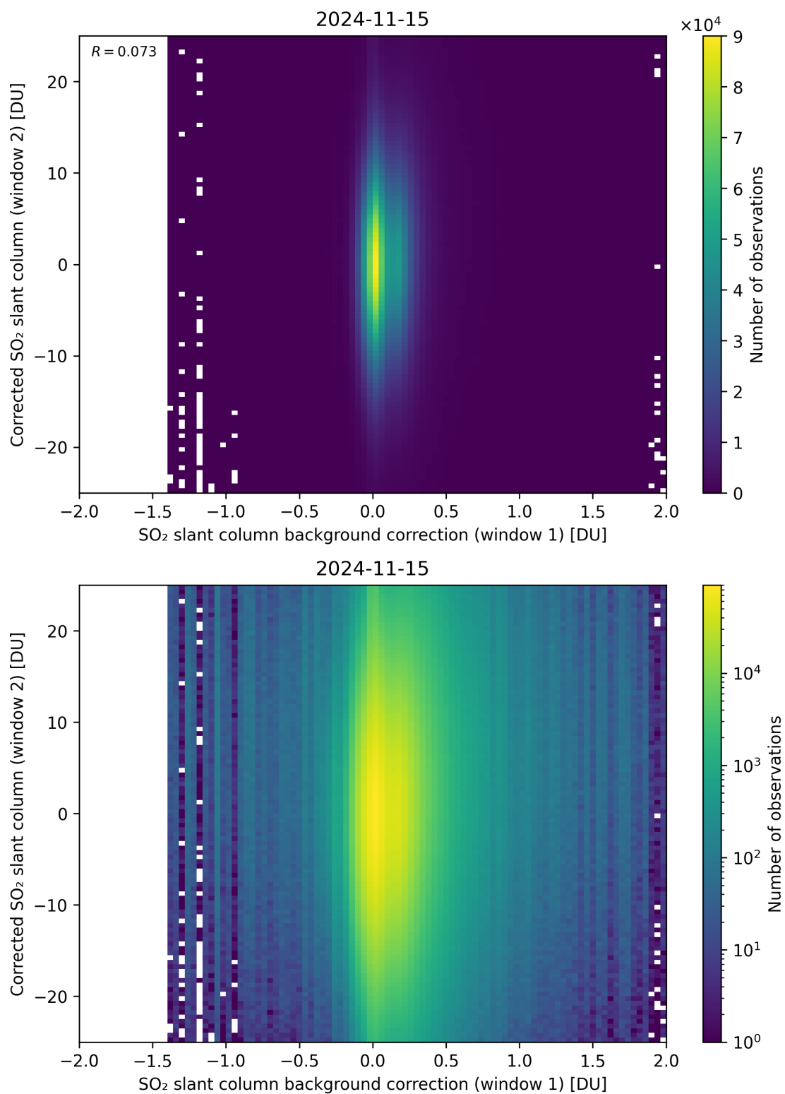
Figure 104: Scatter density plot of “SO 2 slant column background correction (window 1)” against “Corrected SO 2 slant column (window 2)” for 2024-11-14 to 2024-11-16.
