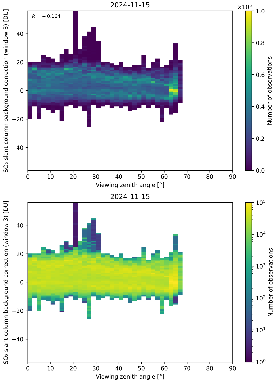
Figure 310: Scatter density plot of “Viewing zenith angle” against “SO 2 slant column background correction (window 3)” for 2024-11-14 to 2024-11-16.
