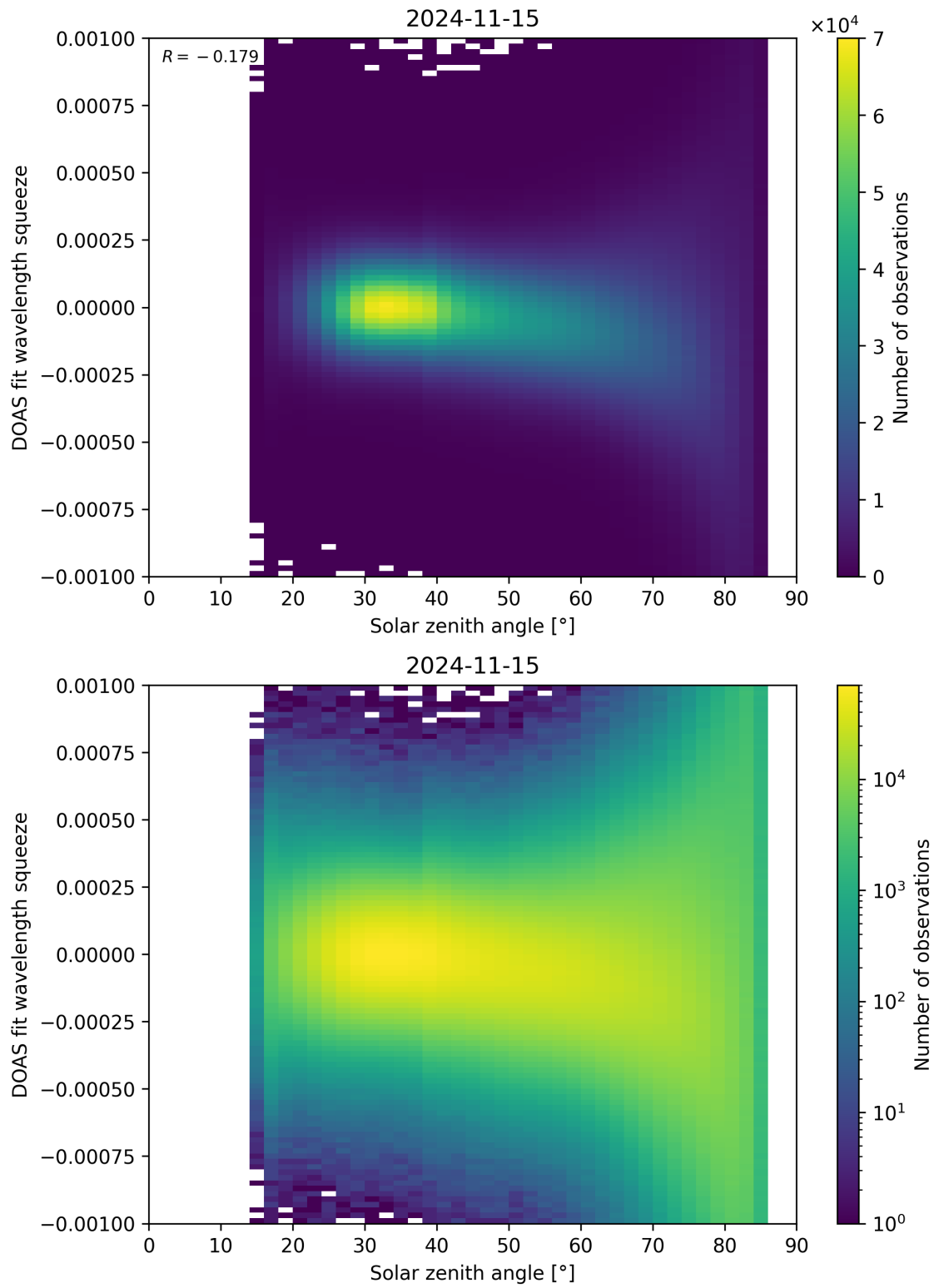
Figure 162: Scatter density plot of “Solar zenith angle” against “DOAS fit wavelength squeeze” for 2024-11-14 to 2024-11-16.
