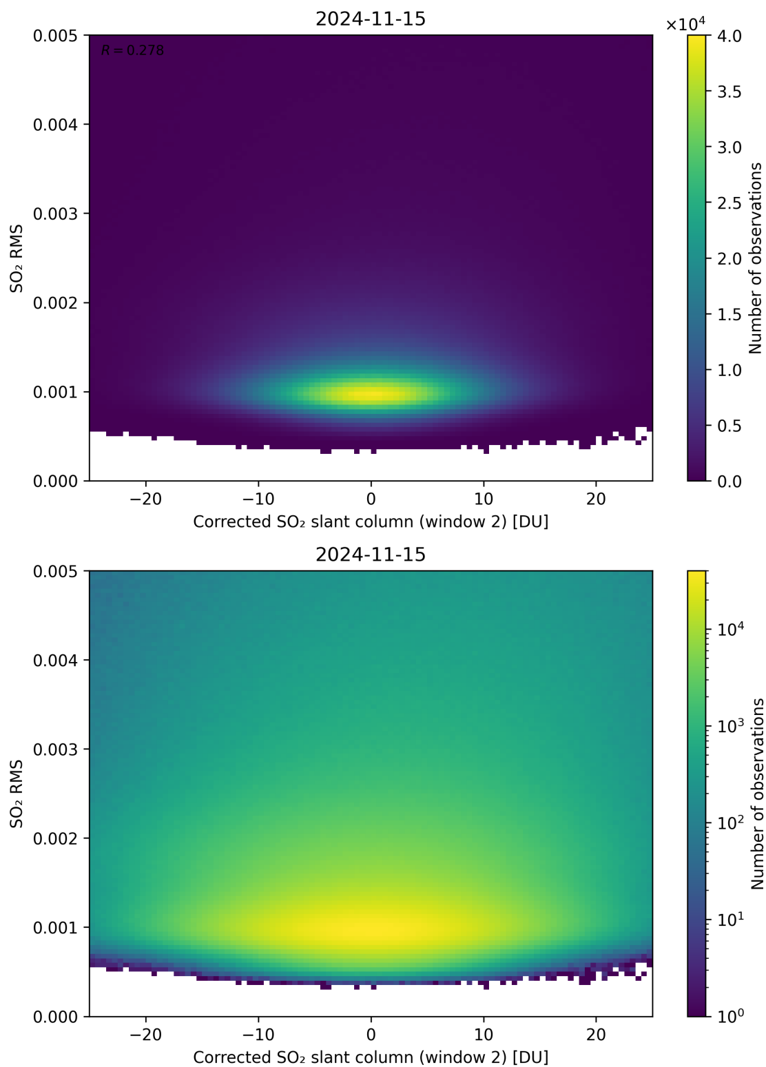
Figure 198: Scatter density plot of “Corrected SO 2 slant column (window 2)” against “SO 2 RMS” for 2024-11-14 to 2024-11-16.
