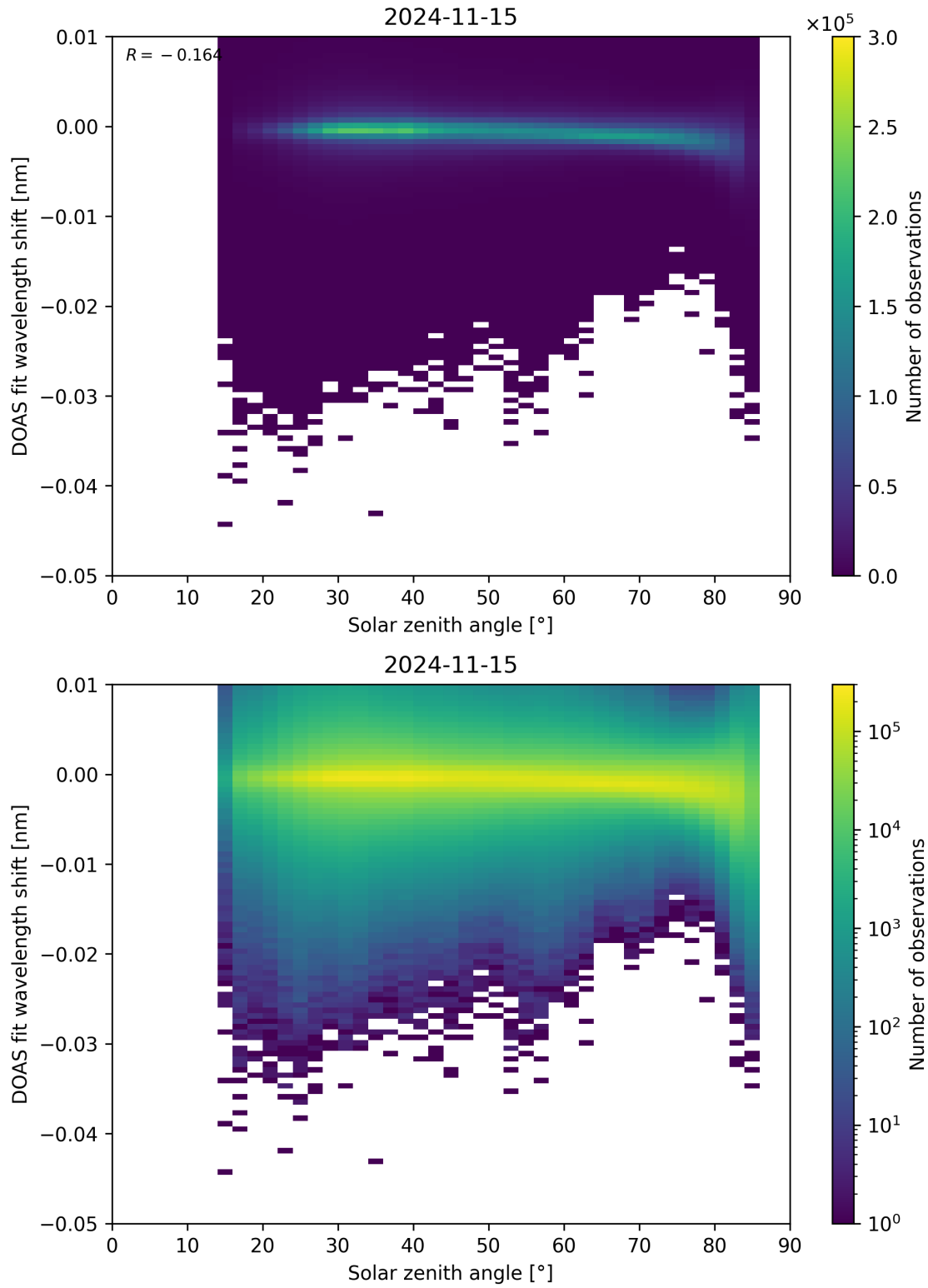
Figure 161: Scatter density plot of “Solar zenith angle” against “DOAS fit wavelength shift” for 2024-11-14 to 2024-11-16.
