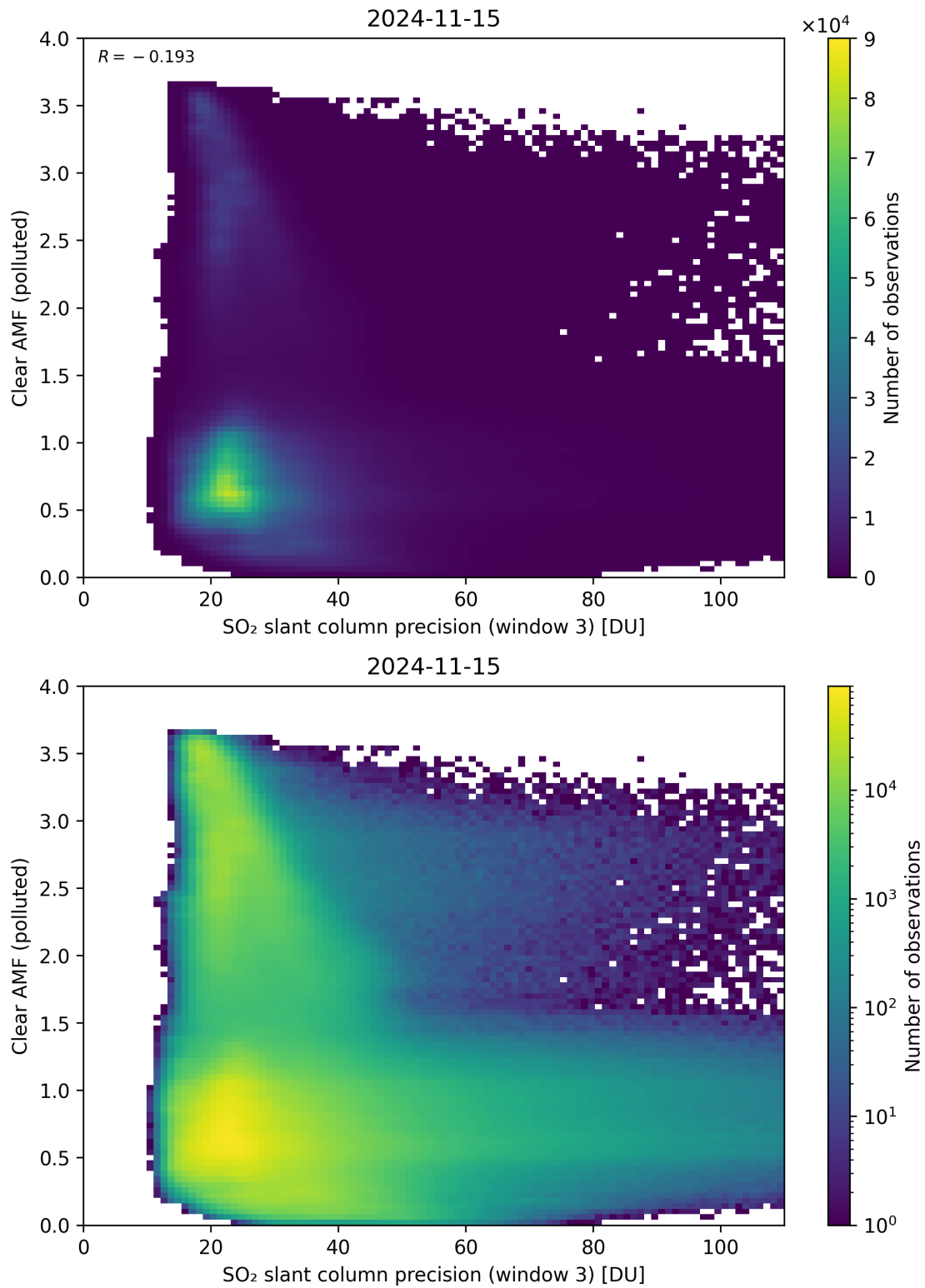
Figure 261: Scatter density plot of “SO 2 slant column precision (window 3)” against “Clear AMF (polluted)” for 2024-11-14 to 2024-11-16.
