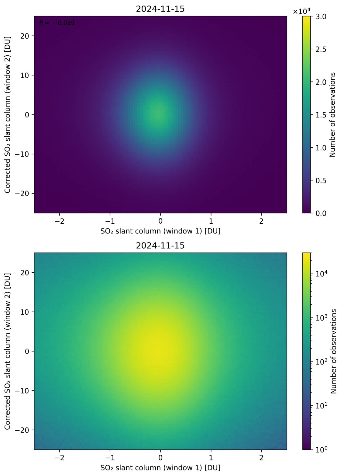
Figure 233: Scatter density plot of “SO 2 slant column (window 1)” against “Corrected SO 2 slant column (window 2)” for 2024-11-14 to 2024-11-16.
