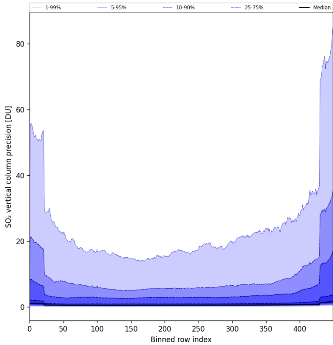
Figure 77: Along track statistics of “SO 2 vertical column precision” for 2024-11-14 to 2024-11-16
