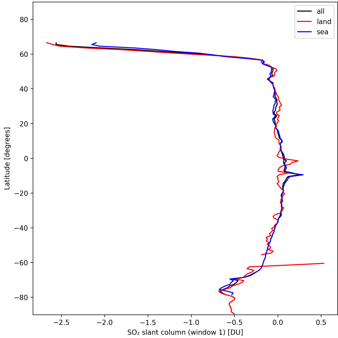
Figure 33: Zonal average of “SO 2 slant column (window 1)” for 2024-11-14 to 2024-11-16.
