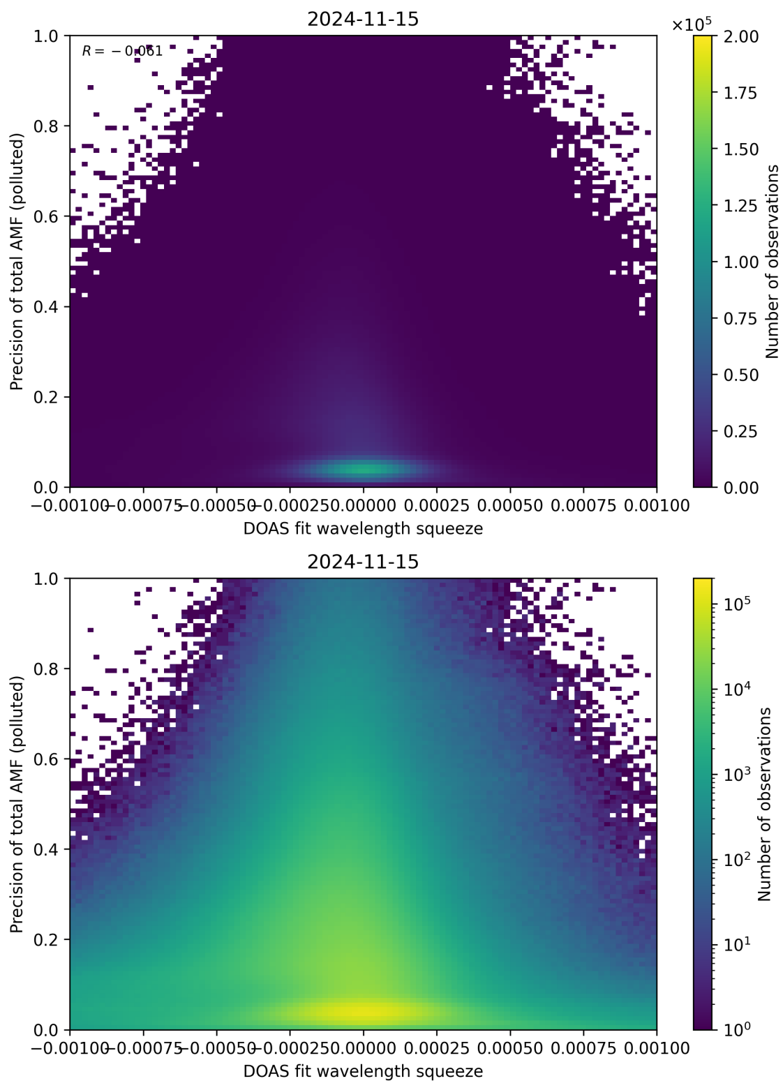
Figure 135: Scatter density plot of “DOAS fit wavelength squeeze” against “Precision of total AMF (polluted)” for 2024-11-14 to 2024-11-16.
