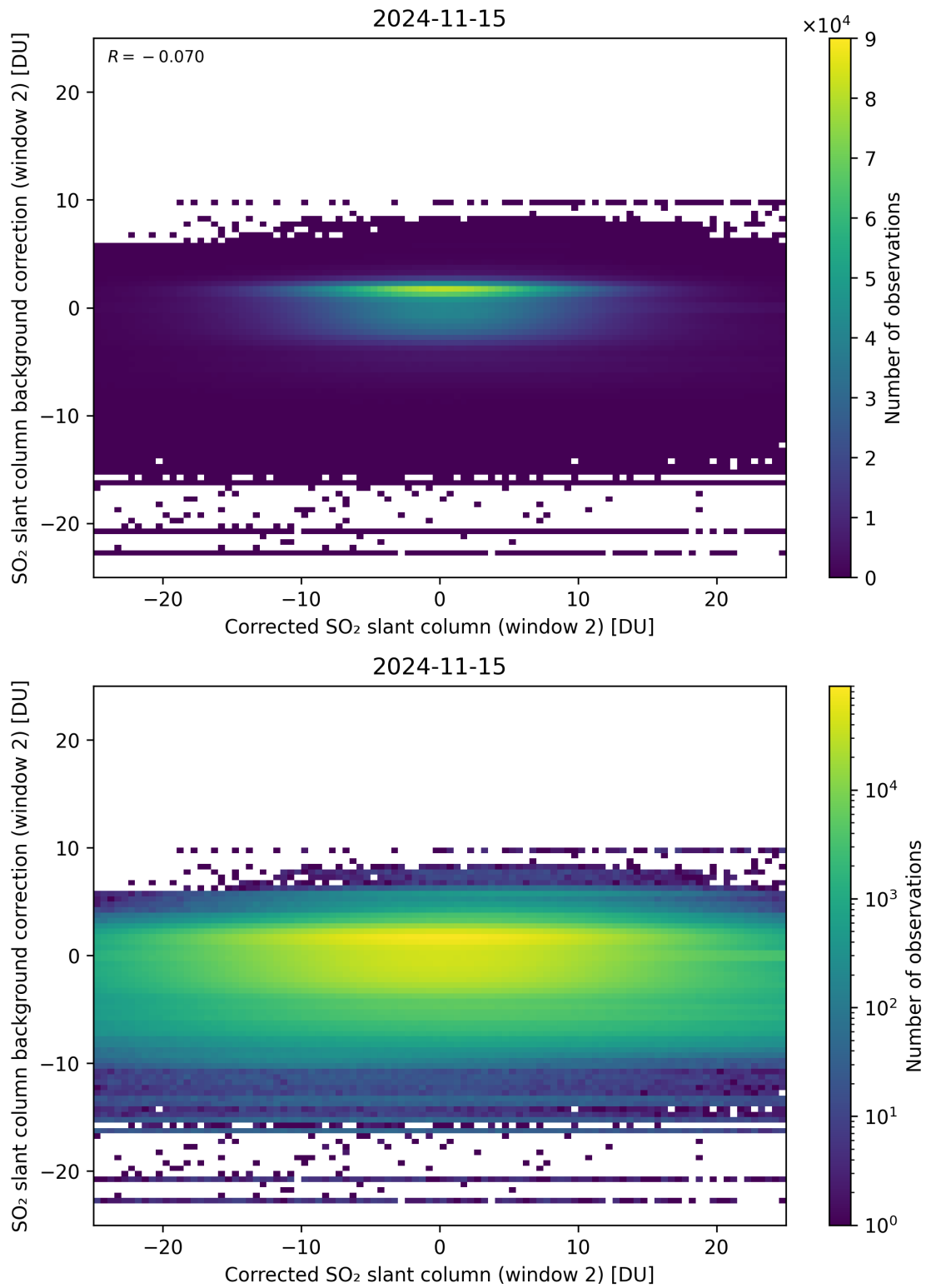
Figure 194: Scatter density plot of “Corrected SO 2 slant column (window 2)” against “SO 2 slant column background correction (window 2)” for 2024-11-14 to 2024-11-16.
