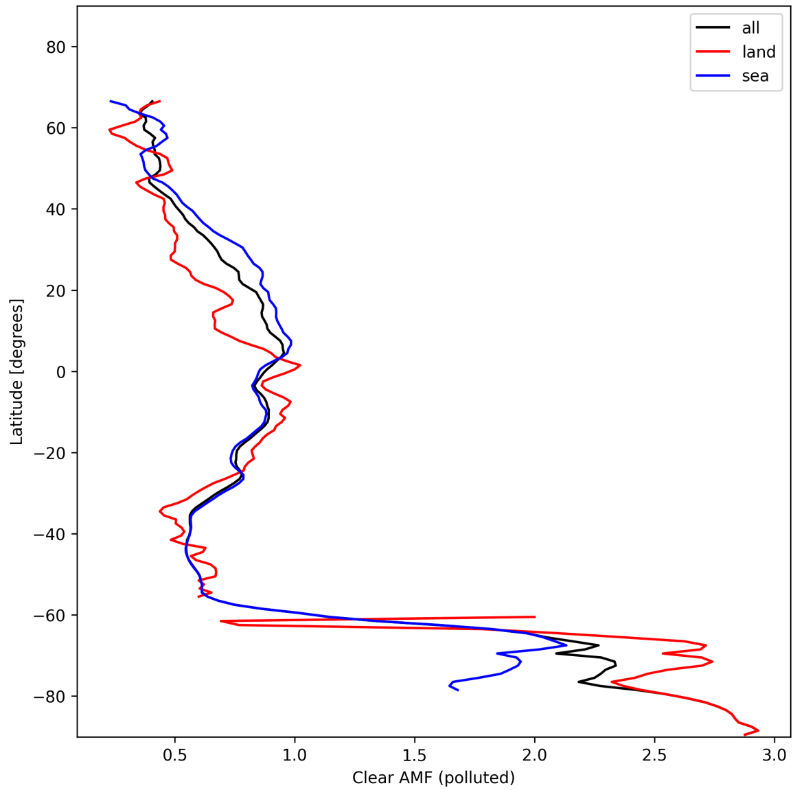
Figure 50: Zonal average of “Clear AMF (polluted)” for 2024-11-14 to 2024-11-16.
