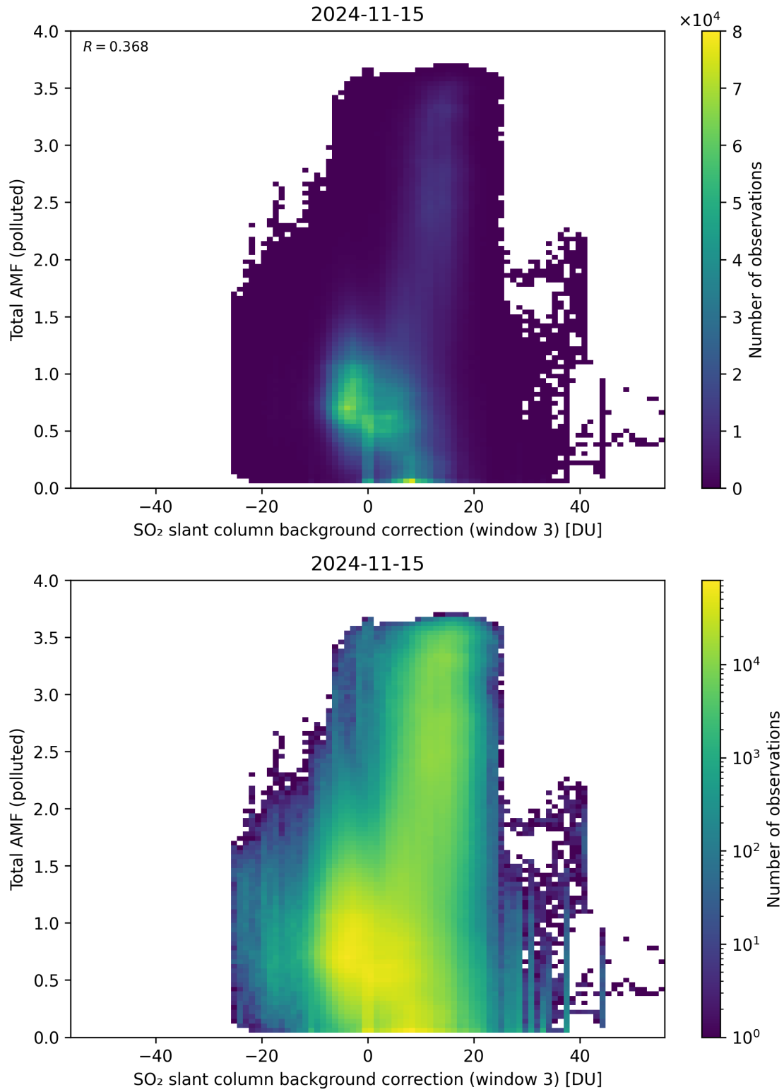
Figure 125: Scatter density plot of “SO 2 slant column background correction (window 3)” against “Total AMF (polluted)” for 2024-11-14 to 2024-11-16.
