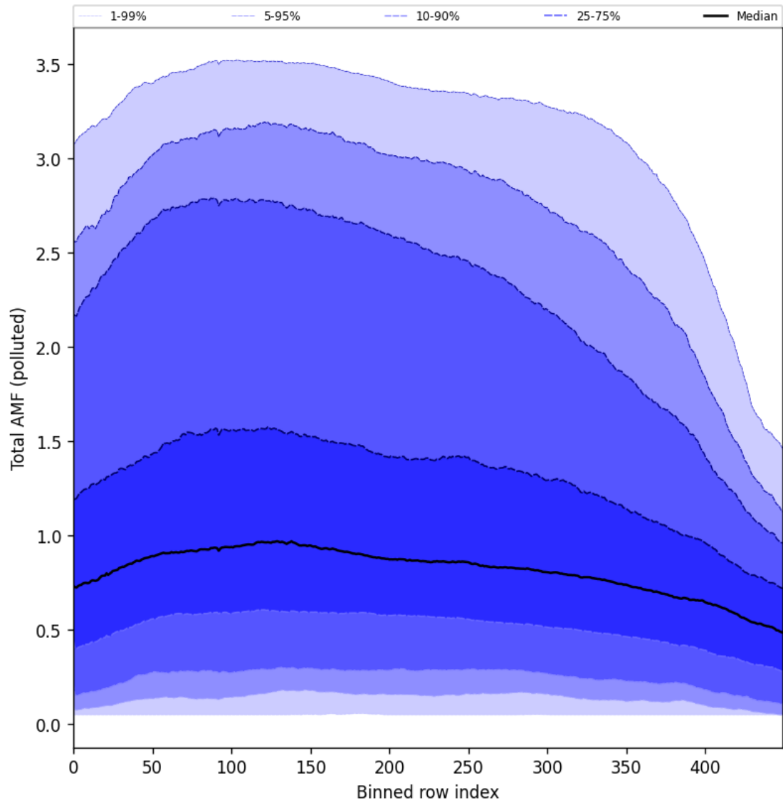
Figure 94: Along track statistics of “Total AMF (polluted)” for 2024-11-14 to 2024-11-16
