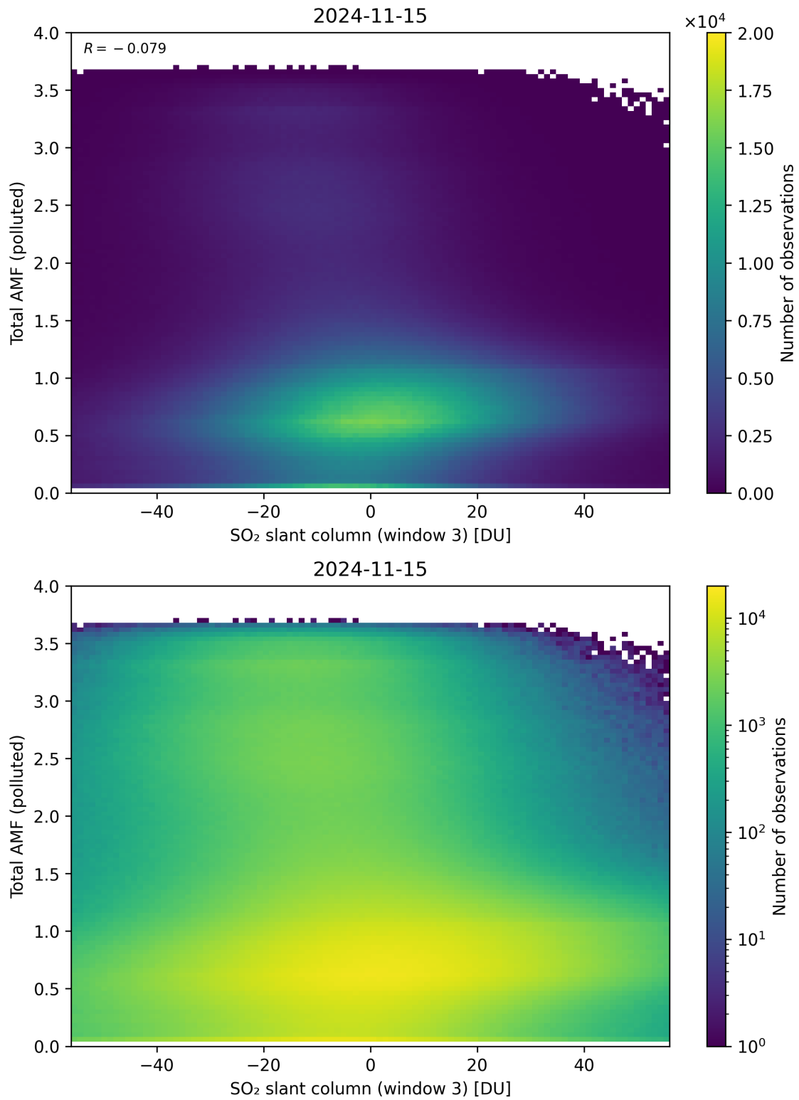
Figure 268: Scatter density plot of “SO 2 slant column (window 3)” against “Total AMF (polluted)” for 2024-11-14 to 2024-11-16.
