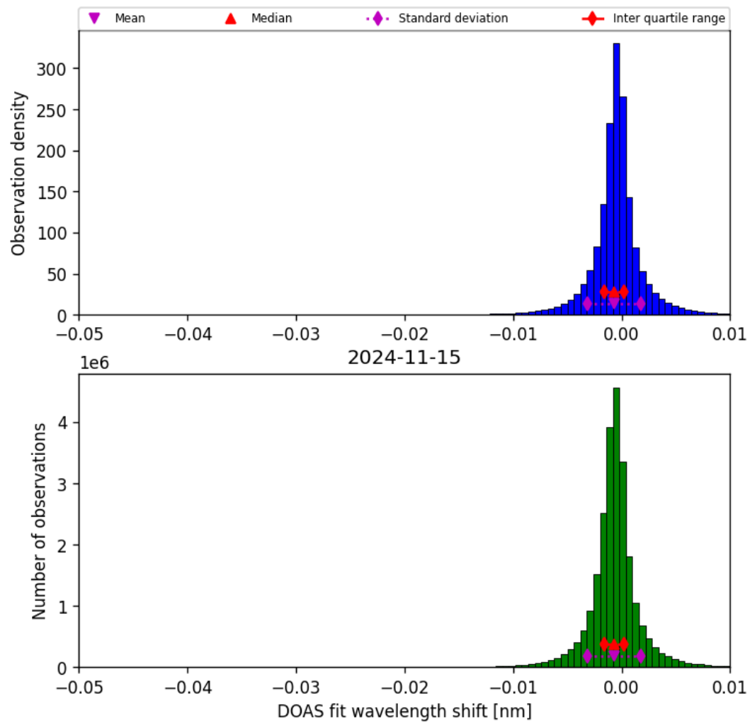
Figure 68: Histogram of “DOAS fit wavelength shift” for 2024-11-14 to 2024-11-16
