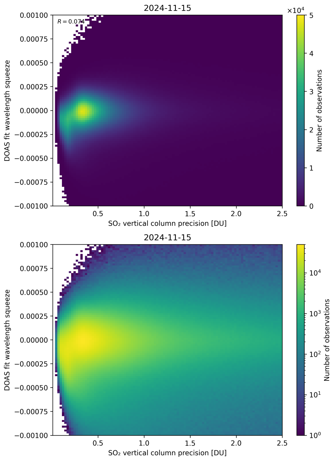
Figure 283: Scatter density plot of “SO 2 vertical column precision” against “DOAS fit wavelength squeeze” for 2024-11-14 to 2024-11-16.
