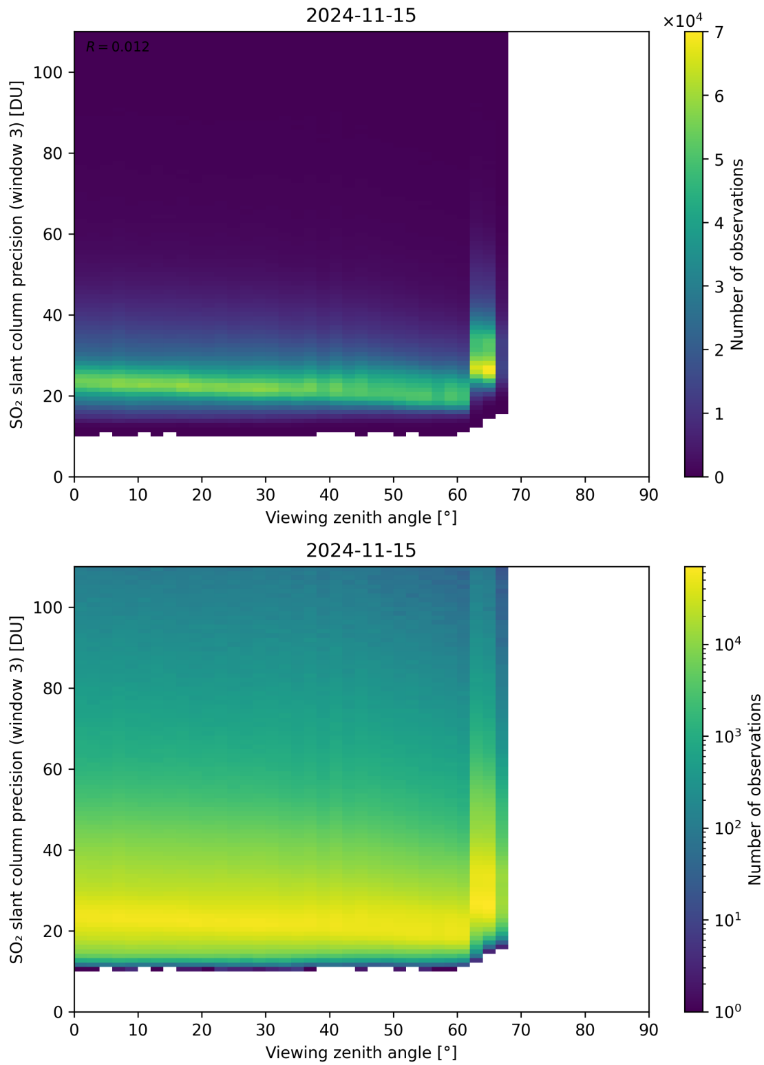
Figure 324: Scatter density plot of “Viewing zenith angle” against “SO 2 slant column precision (window 3)” for 2024-11-14 to 2024-11-16.
