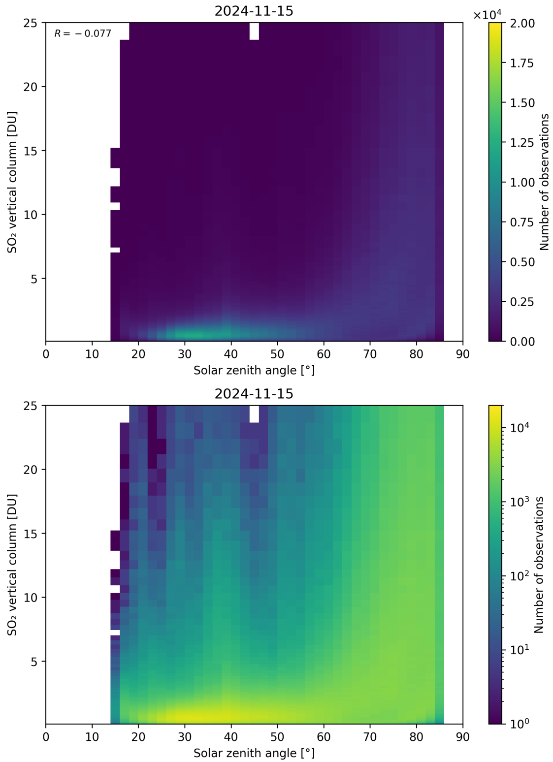
Figure 176: Scatter density plot of “Solar zenith angle” against “SO 2 vertical column” for 2024-11-14 to 2024-11-16.
