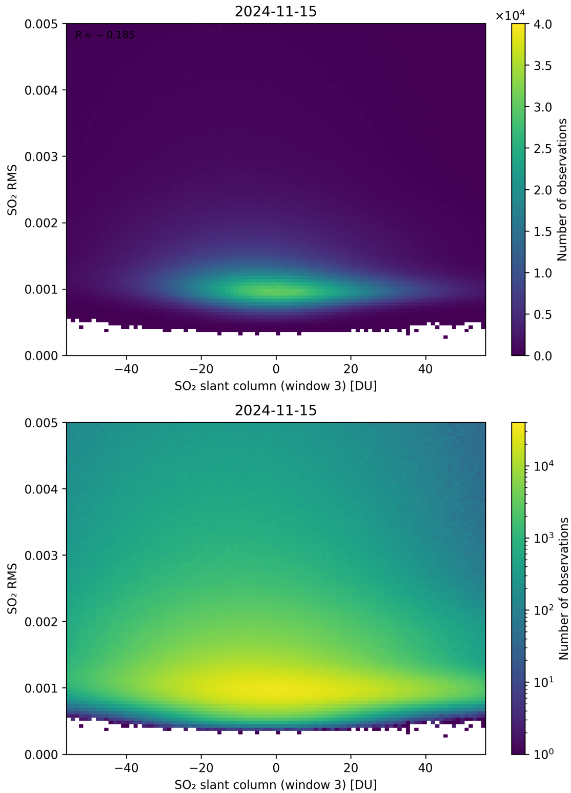
Figure 256: Scatter density plot of “SO 2 slant column (window 3)” against “SO 2 RMS” for 2024-11-14 to 2024-11-16.
