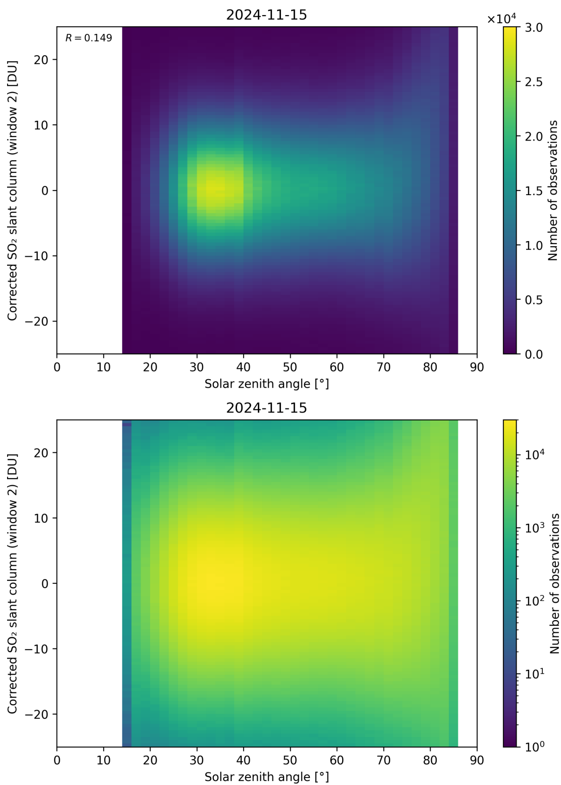
Figure 167: Scatter density plot of “Solar zenith angle” against “Corrected SO 2 slant column (window 2)” for 2024-11-14 to 2024-11-16.
