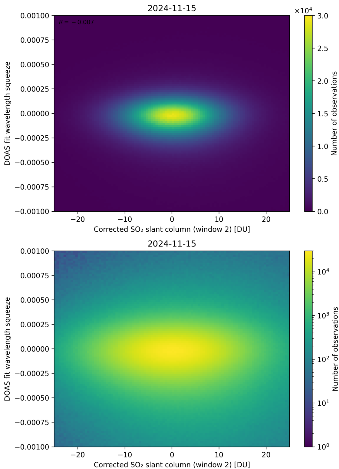
Figure 197: Scatter density plot of “Corrected SO 2 slant column (window 2)” against “DOAS fit wavelength squeeze” for 2024-11-14 to 2024-11-16.
