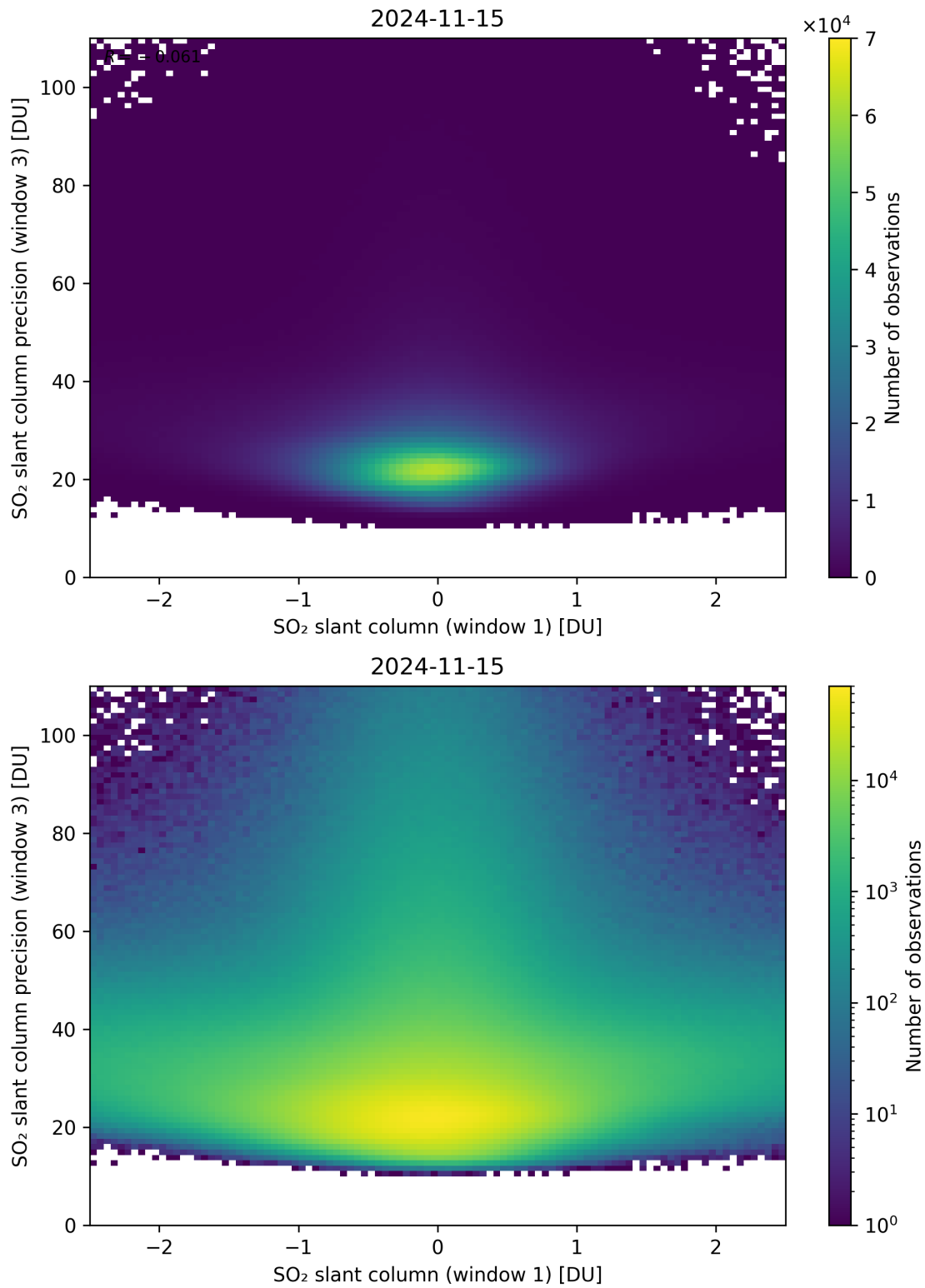
Figure 238: Scatter density plot of “SO 2 slant column (window 1)” against “SO 2 slant column precision (window 3)” for 2024-11-14 to 2024-11-16.
