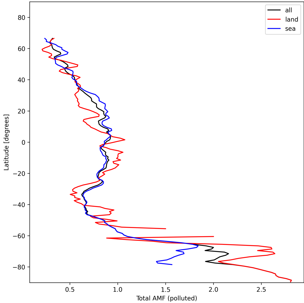
Figure 48: Zonal average of “Total AMF (polluted)” for 2024-11-14 to 2024-11-16.
