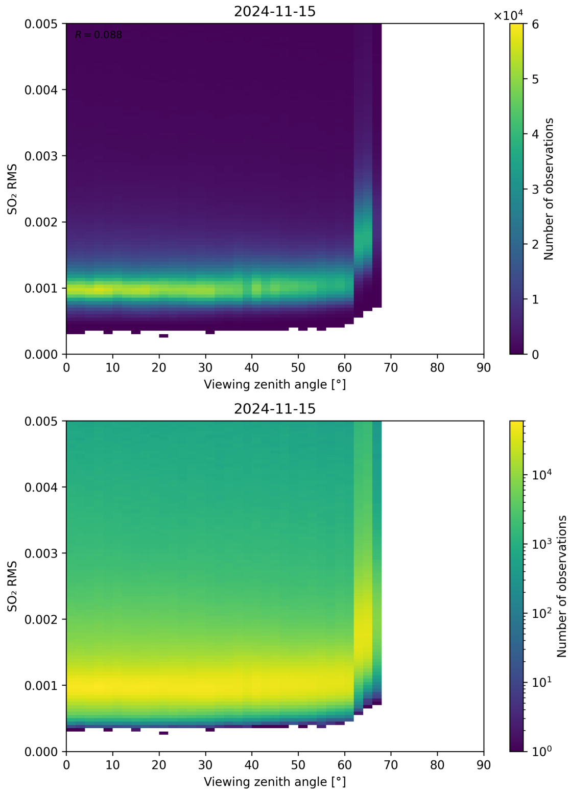
Figure 313: Scatter density plot of “Viewing zenith angle” against “SO 2 RMS” for 2024-11-14 to 2024-11-16.
