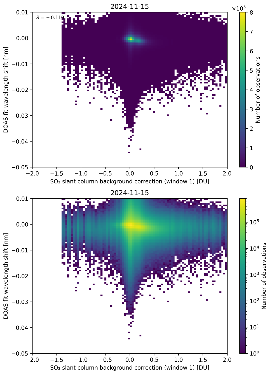
Figure 100: Scatter density plot of “SO 2 slant column background correction (window 1)” against “DOAS fit wavelength shift” for 2024-11-14 to 2024-11-16.
