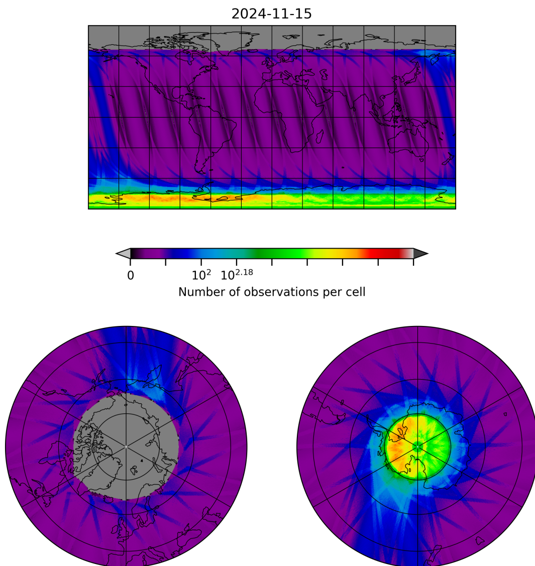
Figure 28: Map of the number of observations for 2024-11-14 to 2024-11-16
