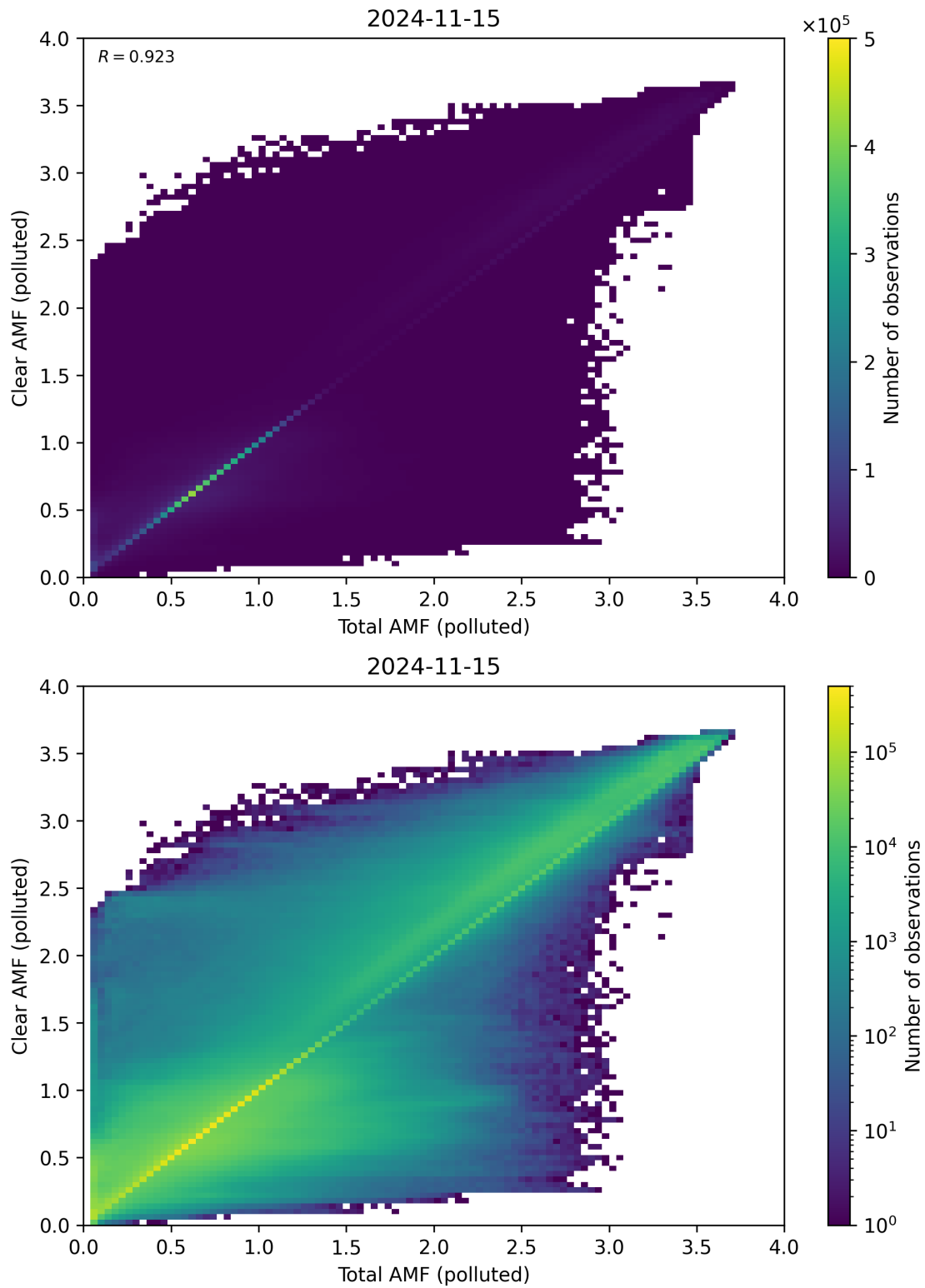
Figure 271: Scatter density plot of “Total AMF (polluted)” against “Clear AMF (polluted)” for 2024-11-14 to 2024-11-16.
