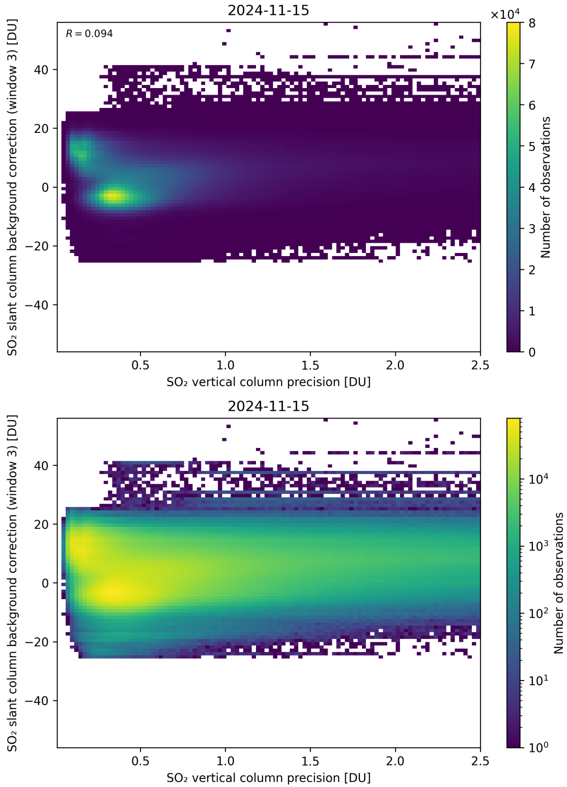
Figure 281: Scatter density plot of “SO 2 vertical column precision” against “SO 2 slant column background correction (window 3)” for 2024-11-14 to 2024-11-16.
