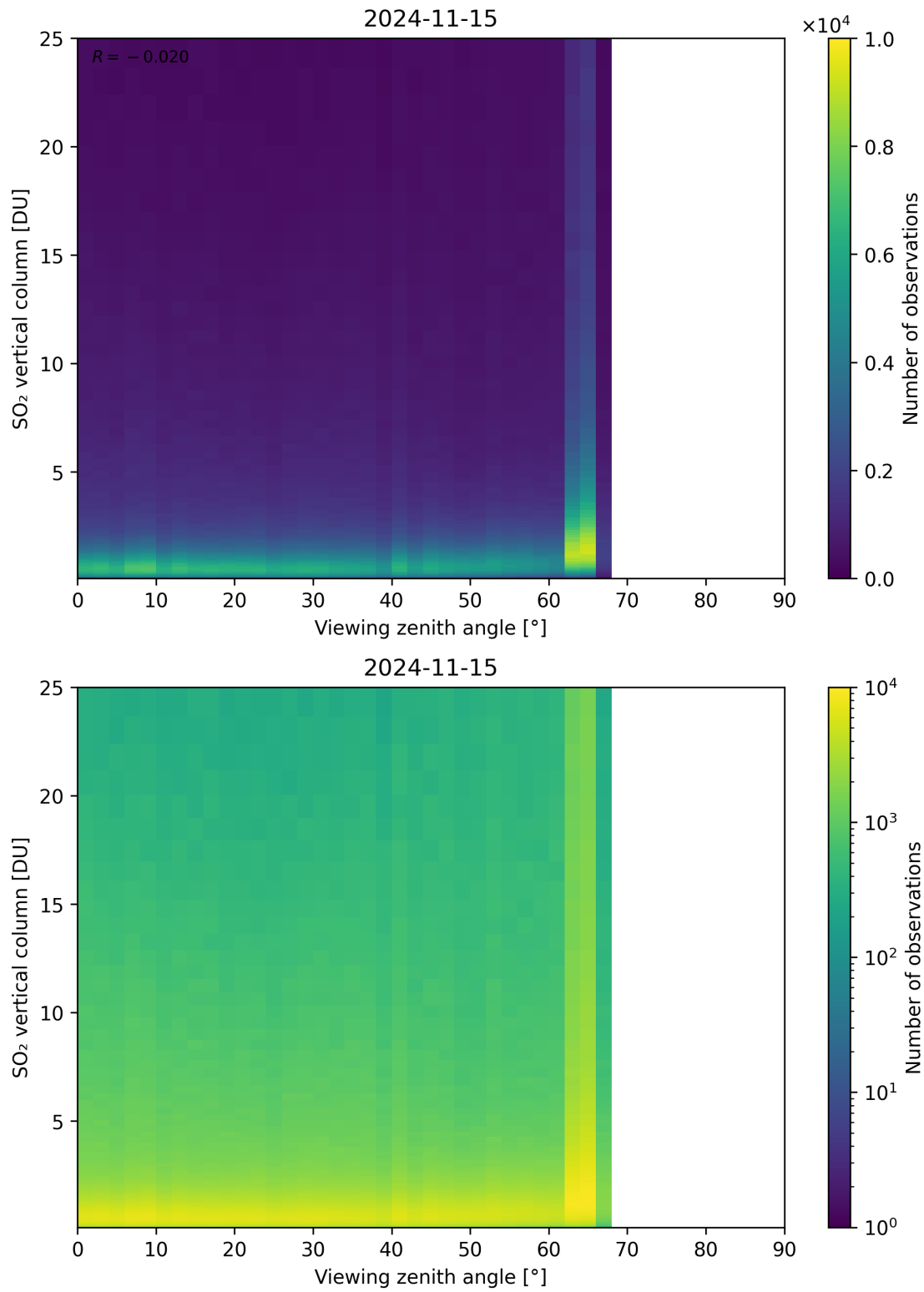
Figure 327: Scatter density plot of “Viewing zenith angle” against “SO 2 vertical column” for 2024-11-14 to 2024-11-16.
