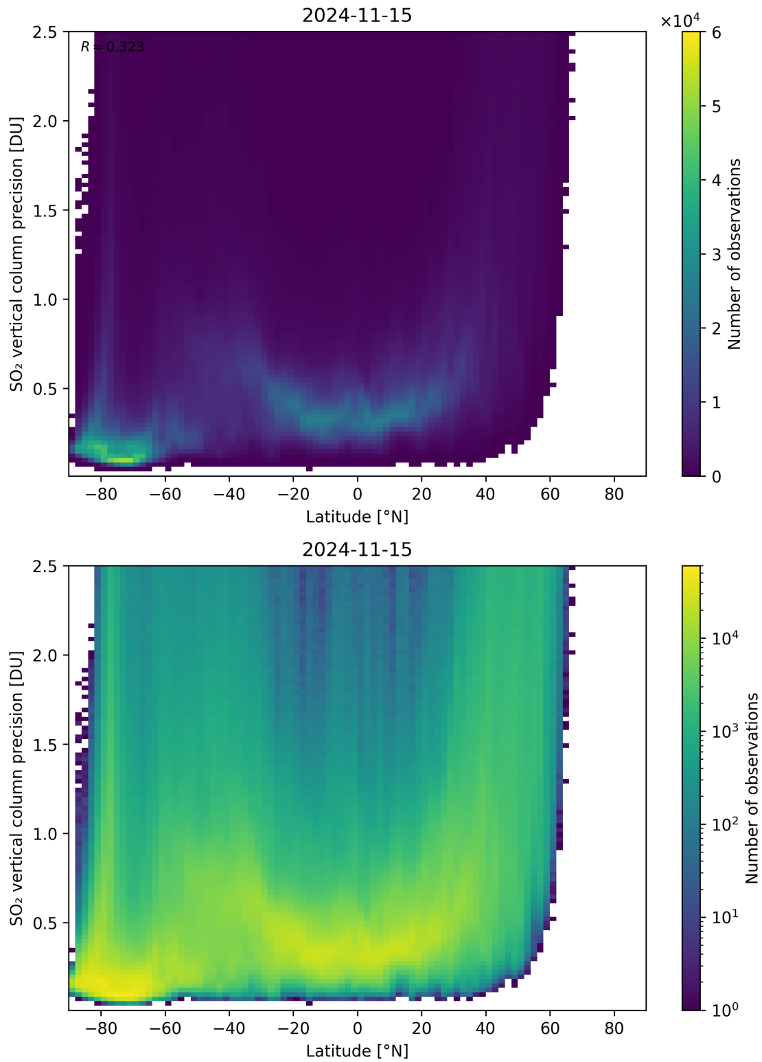
Figure 157: Scatter density plot of “Latitude” against “SO 2 vertical column precision” for 2024-11-14 to 2024-11-16.
