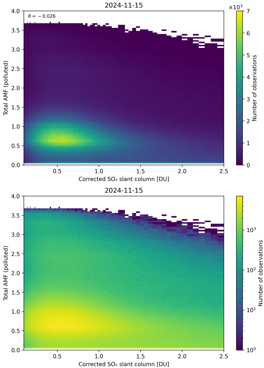
Figure 192: Scatter density plot of “Corrected SO 2 slant column” against “Total AMF (polluted)” for 2024-11-14 to 2024-11-16.
