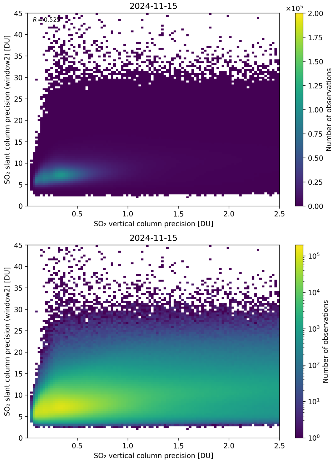
Figure 291: Scatter density plot of “SO 2 vertical column precision” against “SO 2 slant column precision (window2)” for 2024-11-14 to 2024-11-16.
