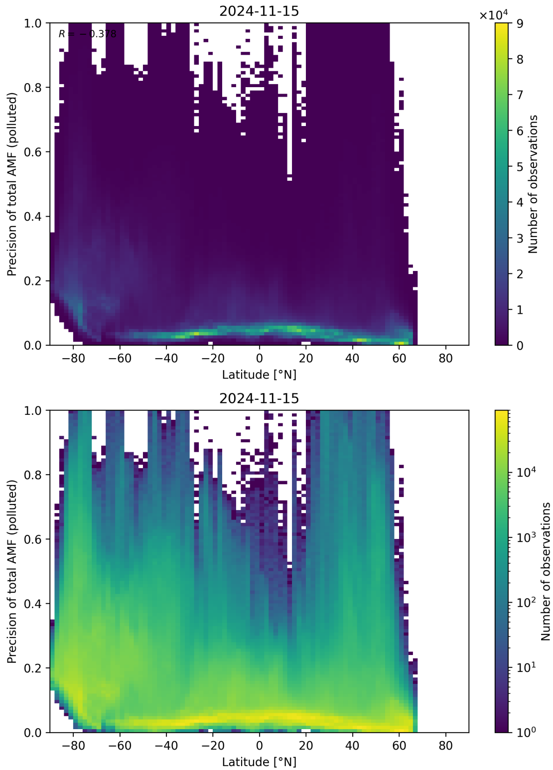
Figure 155: Scatter density plot of “Latitude” against “Precision of total AMF (polluted)” for 2024-11-14 to 2024-11-16.
