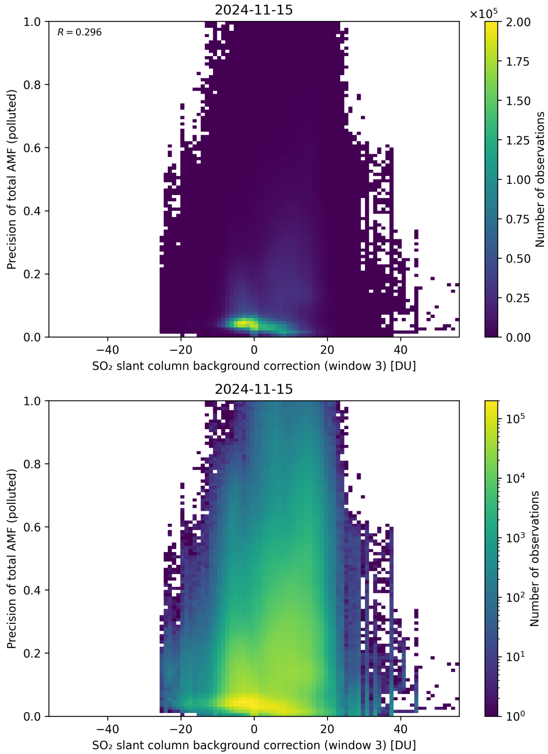
Figure 126: Scatter density plot of “SO 2 slant column background correction (window 3)” against “Precision of total AMF (polluted)” for 2024-11-14 to 2024-11-16.
