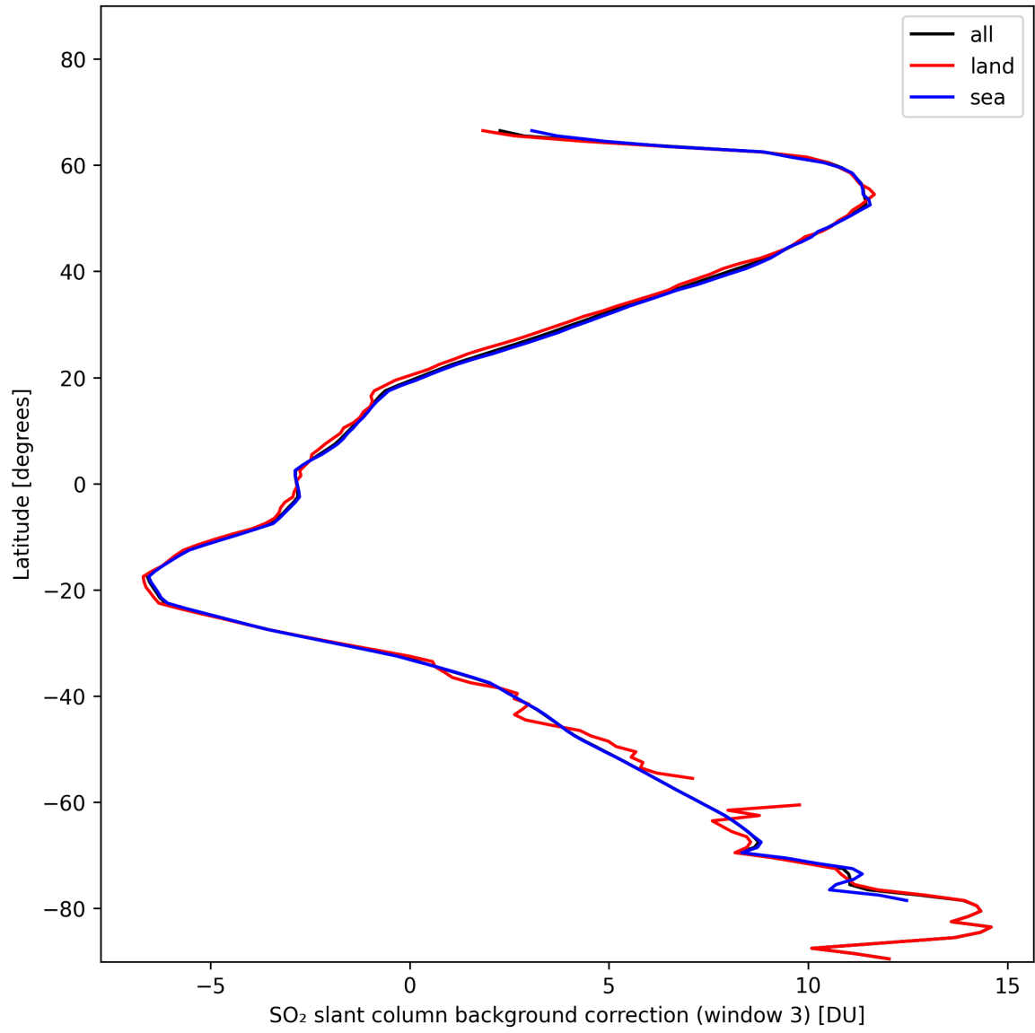
Figure 44: Zonal average of “SO 2 slant column background correction (window 3)” for 2024-11-14 to 2024-11-16.
