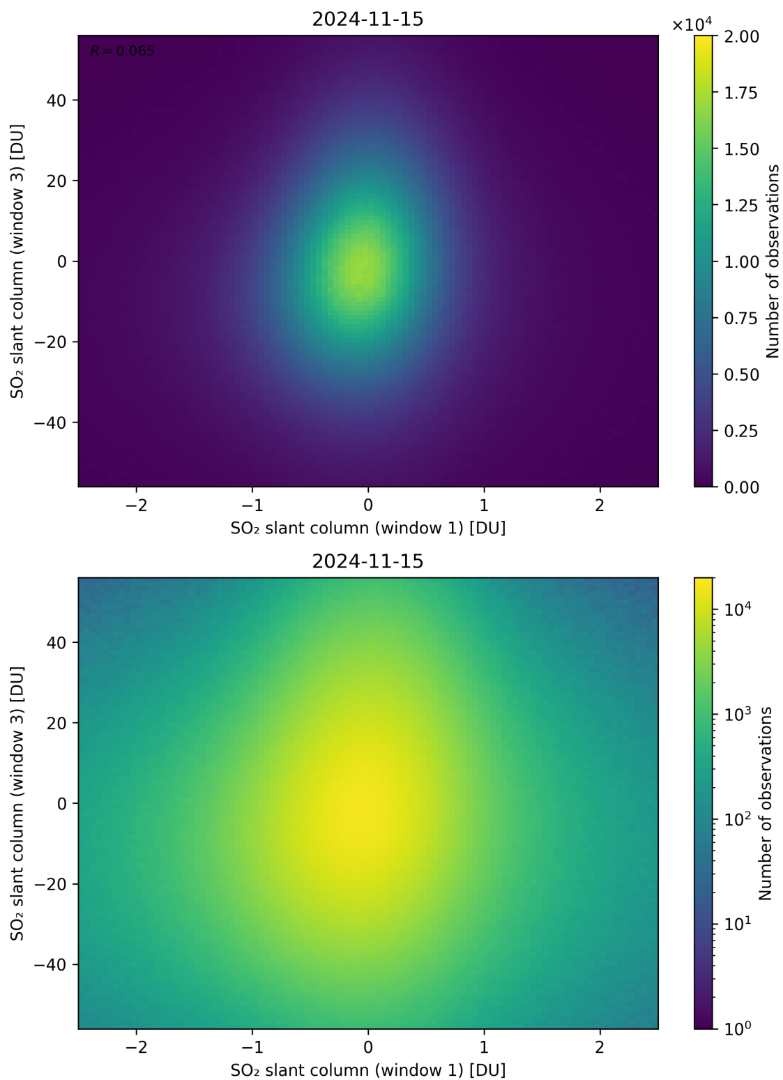
Figure 237: Scatter density plot of “SO 2 slant column (window 1)” against “SO 2 slant column (window 3)” for 2024-11-14 to 2024-11-16.
