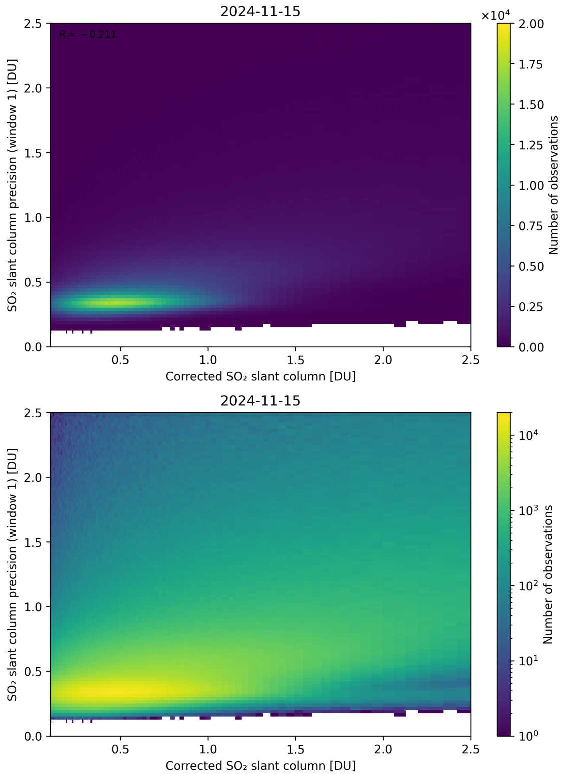
Figure 188: Scatter density plot of “Corrected SO 2 slant column” against “SO 2 slant column precision (window 1)” for 2024-11-14 to 2024-11-16.
