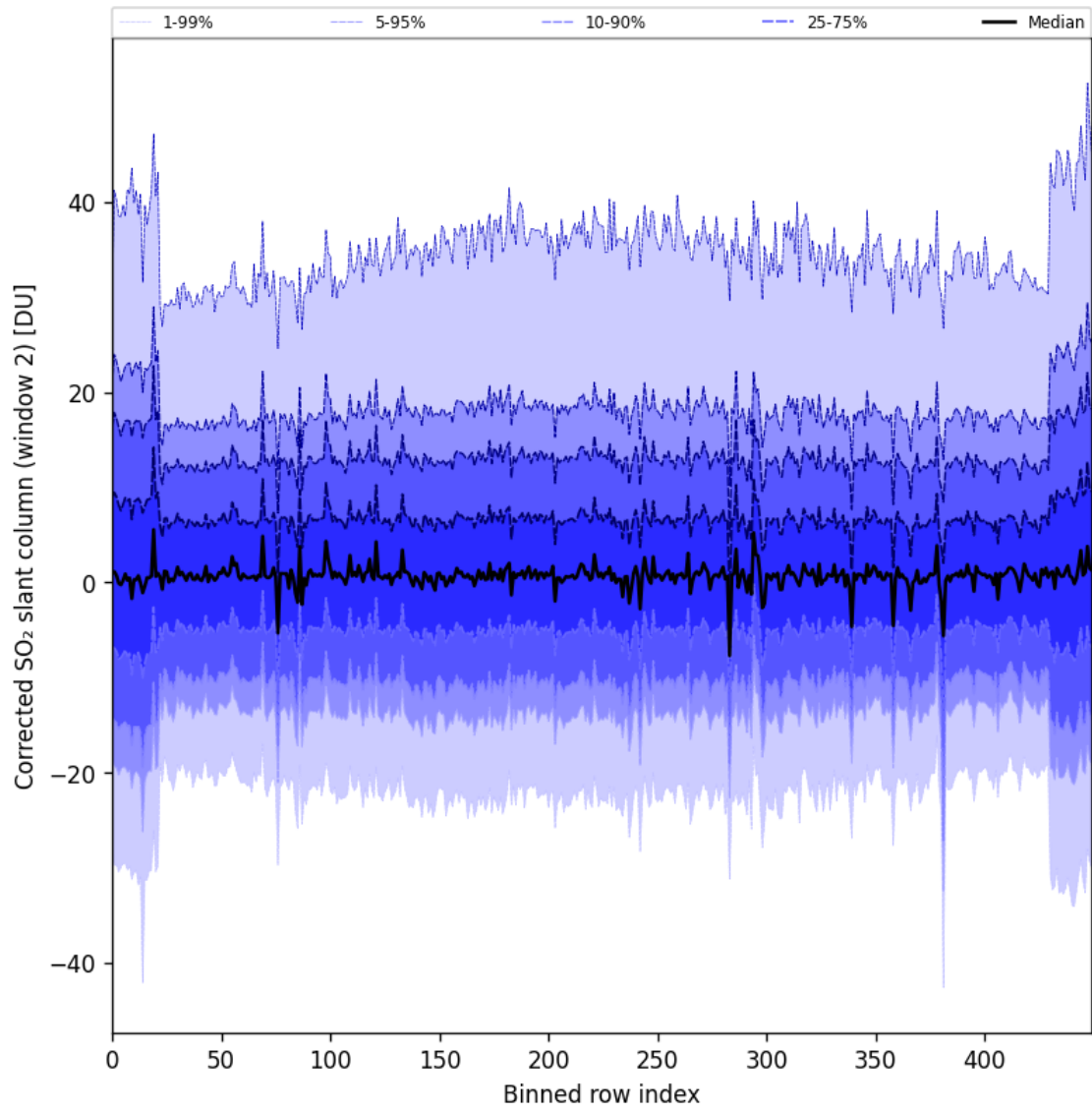
Figure 85: Along track statistics of “Corrected SO 2 slant column (window 2)” for 2024-11-14 to 2024-11-16
