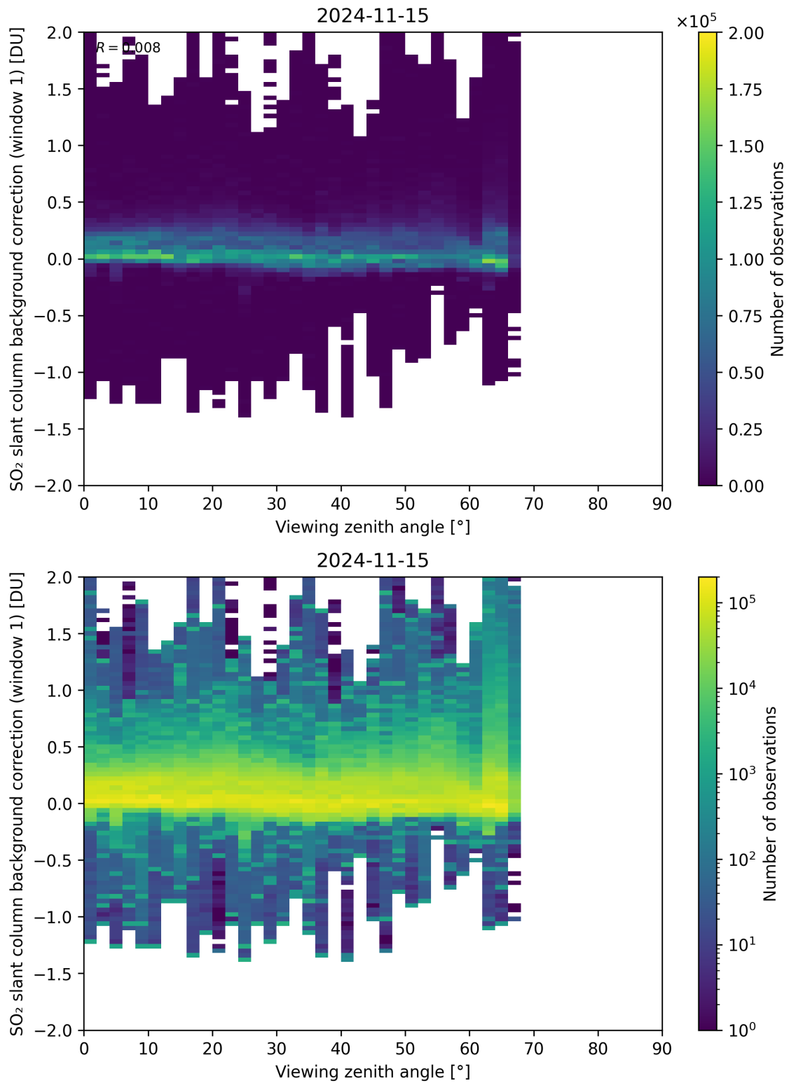
Figure 308: Scatter density plot of “Viewing zenith angle” against “SO 2 slant column background correction (window 1)” for 2024-11-14 to 2024-11-16.
