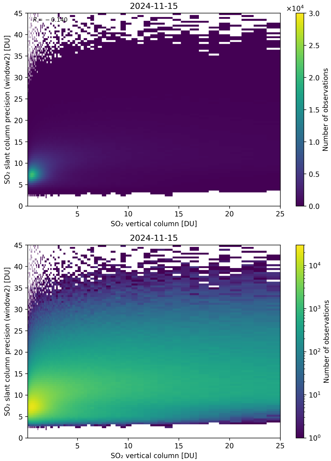
Figure 302: Scatter density plot of “SO 2 vertical column” against “SO 2 slant column precision (window2)” for 2024-11-14 to 2024-11-16.
