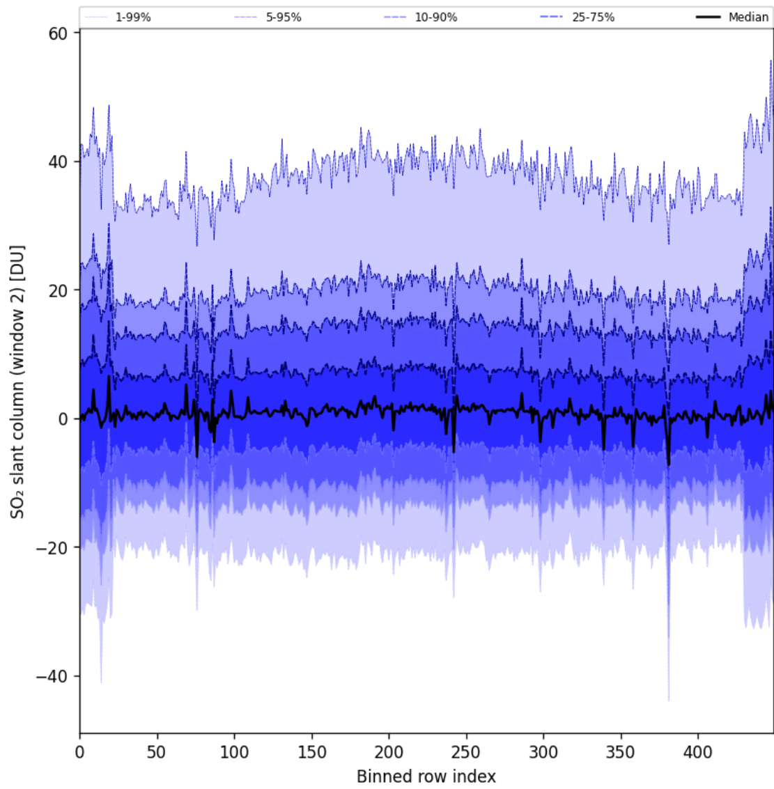
Figure 83: Along track statistics of “SO 2 slant column (window 2)” for 2024-11-14 to 2024-11-16
