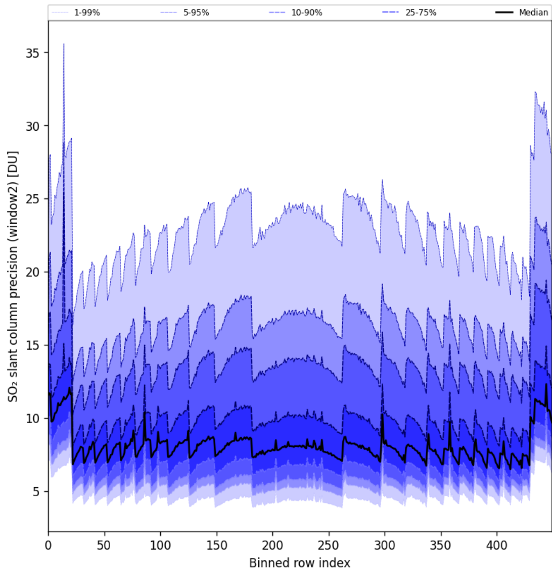
Figure 84: Along track statistics of “SO 2 slant column precision (window2)” for 2024-11-14 to 2024-11-16
