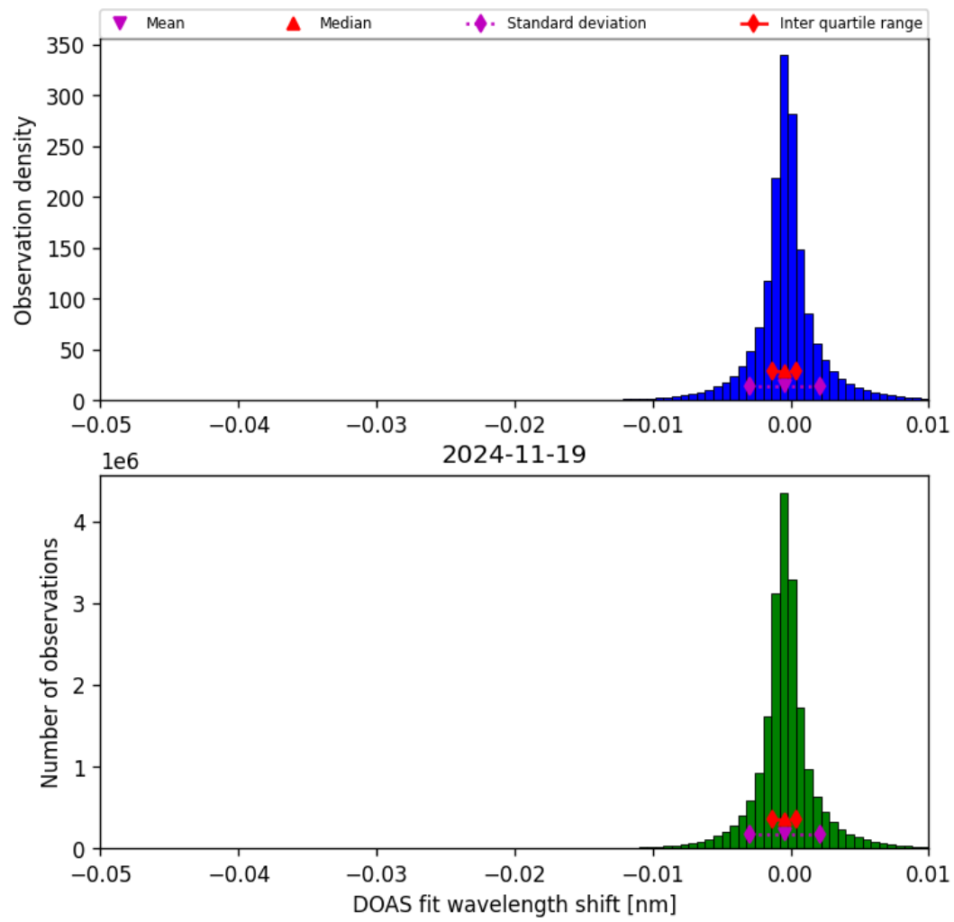
Figure 76: Histogram of “DOAS fit wavelength shift” for 2024-11-18 to 2024-11-20
