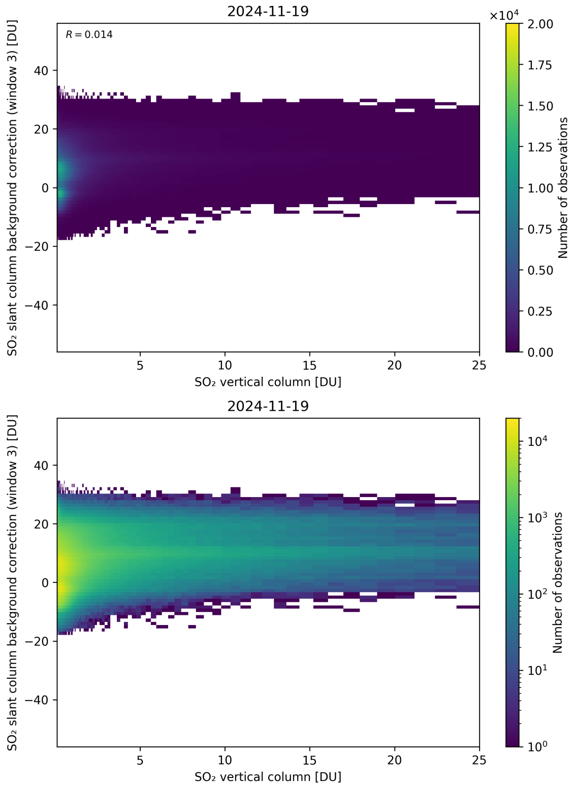
Figure 325: Scatter density plot of “SO 2 vertical column” against “SO 2 slant column background correction (window 3)” for 2024-11-18 to 2024-11-20.
