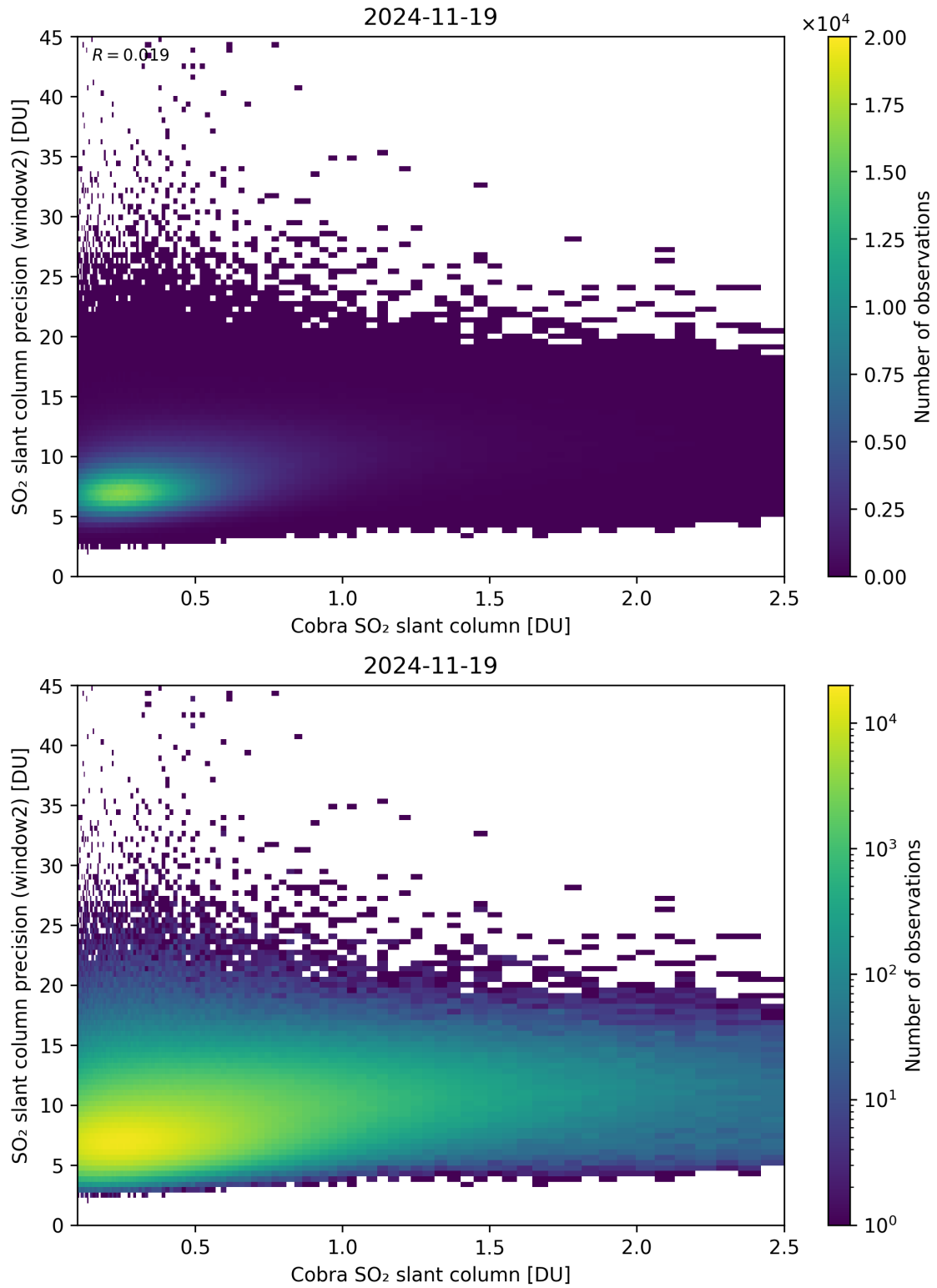
Figure 221: Scatter density plot of “Cobra SO 2 slant column” against “SO 2 slant column precision (window2)” for 2024-11-18 to 2024-11-20.
