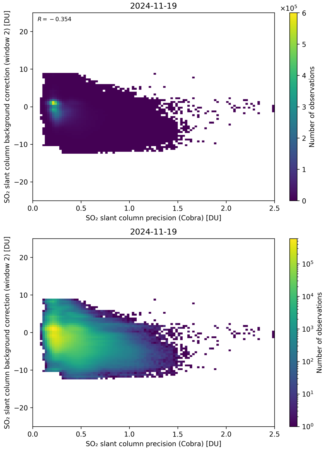
Figure 200: Scatter density plot of “SO 2 slant column precision (Cobra)” against “SO 2 slant column background correction (window 2)” for 2024-11-18 to 2024-11-20.
