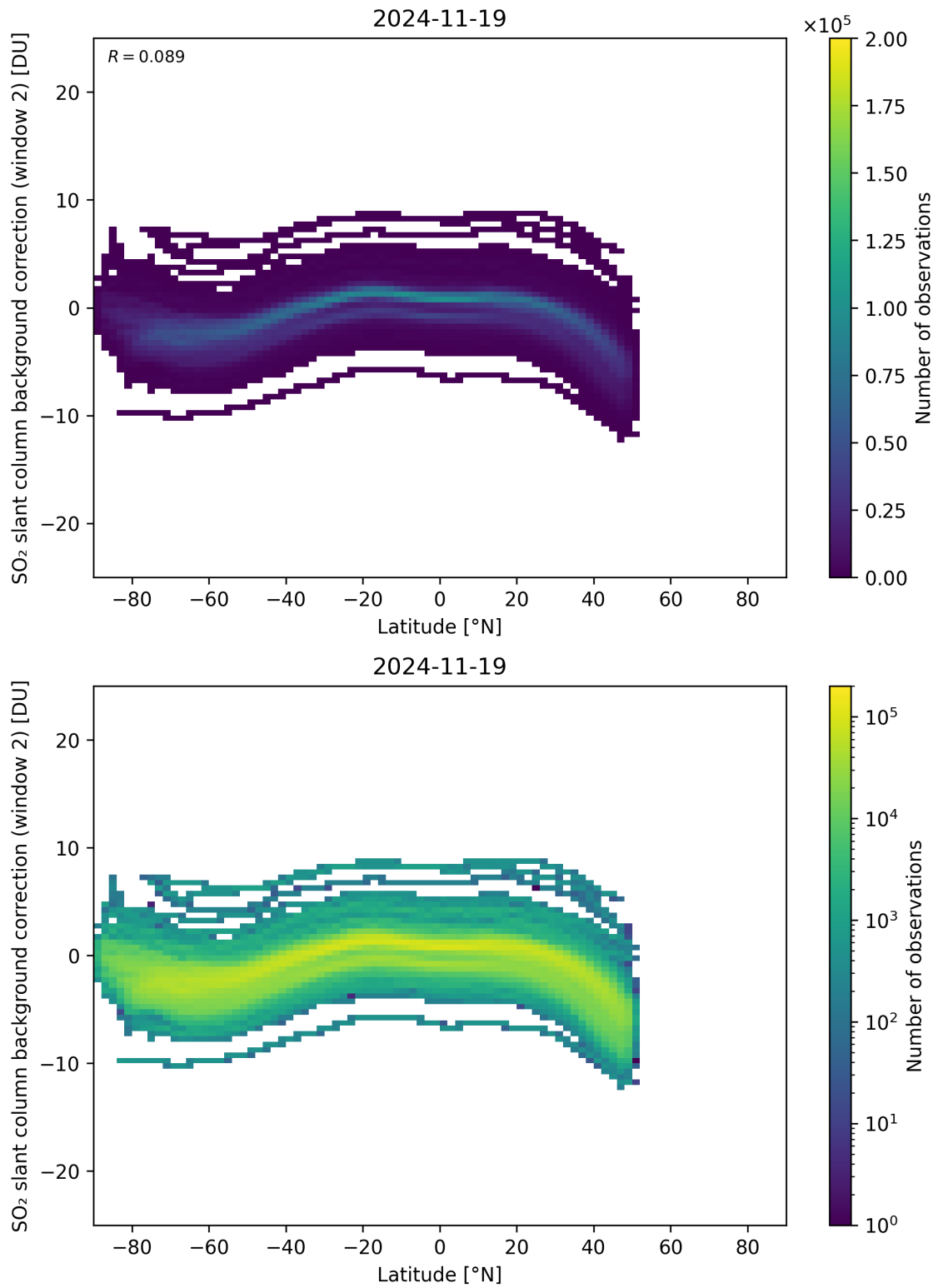
Figure 151: Scatter density plot of “Latitude” against “SO 2 slant column background correction (window 2)” for 2024-11-18 to 2024-11-20.
