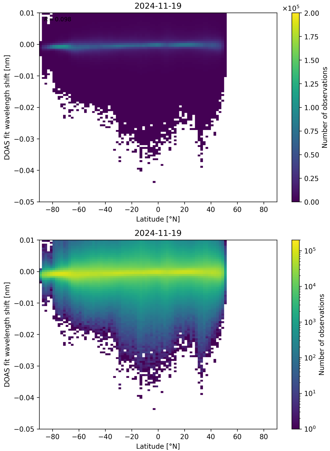
Figure 153: Scatter density plot of “Latitude” against “DOAS fit wavelength shift” for 2024-11-18 to 2024-11-20.
