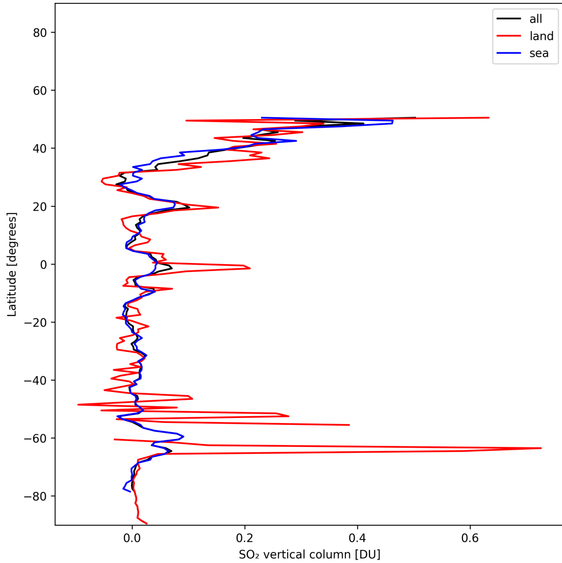
Figure 32: Zonal average of “SO 2 vertical column” for 2024-11-18 to 2024-11-20.
