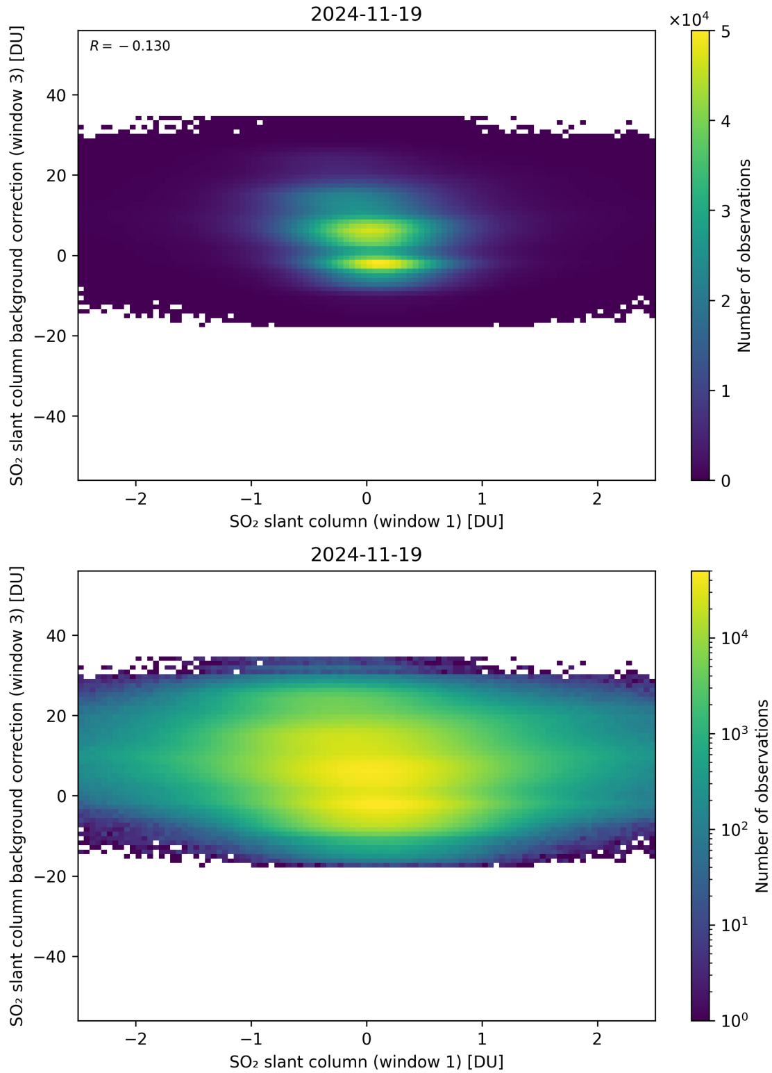
Figure 264: Scatter density plot of “SO 2 slant column (window 1)” against “SO 2 slant column background correction (window 3)” for 2024-11-18 to 2024-11-20.
