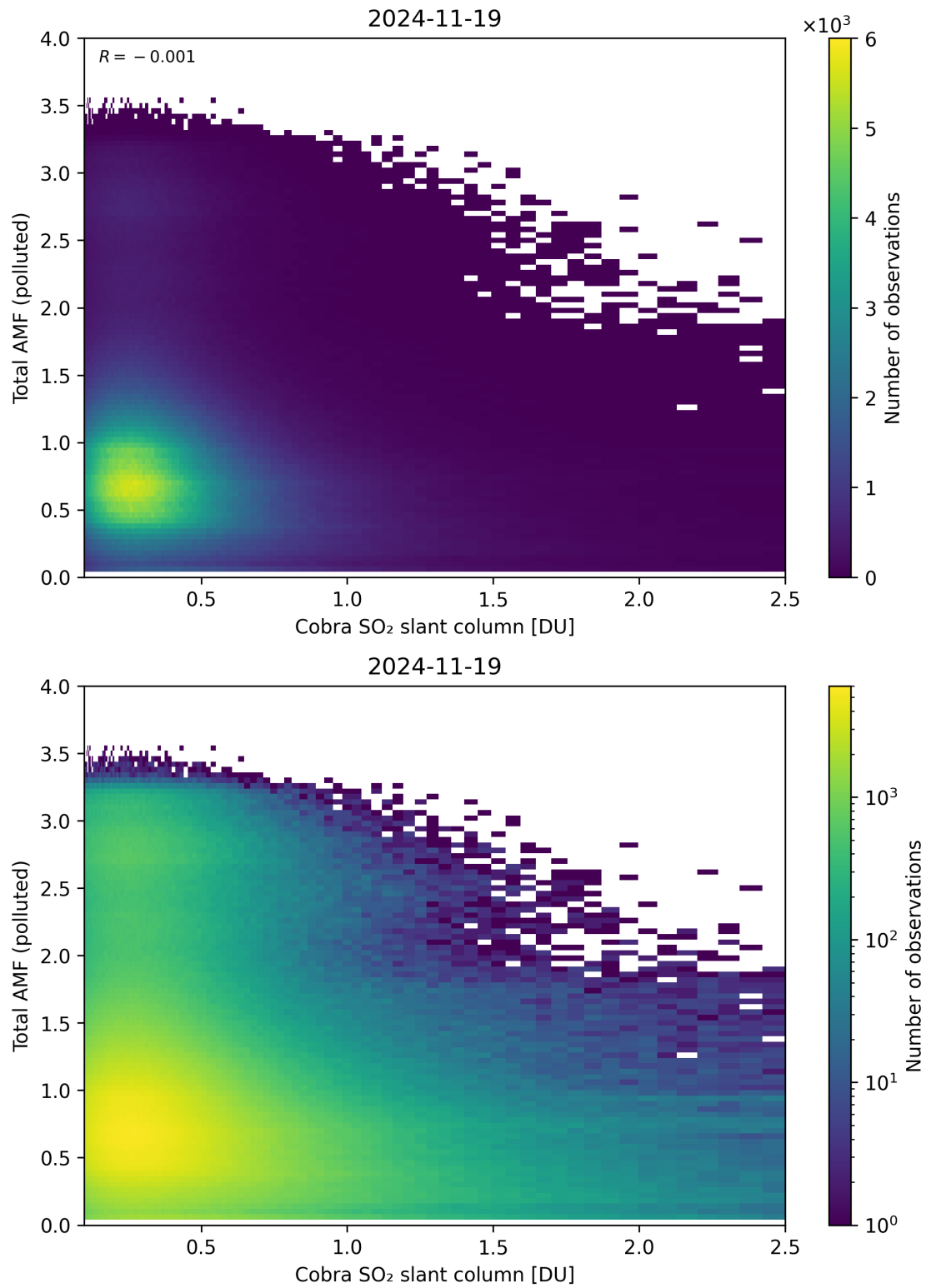
Figure 224: Scatter density plot of “Cobra SO 2 slant column” against “Total AMF (polluted)” for 2024-11-18 to 2024-11-20.
