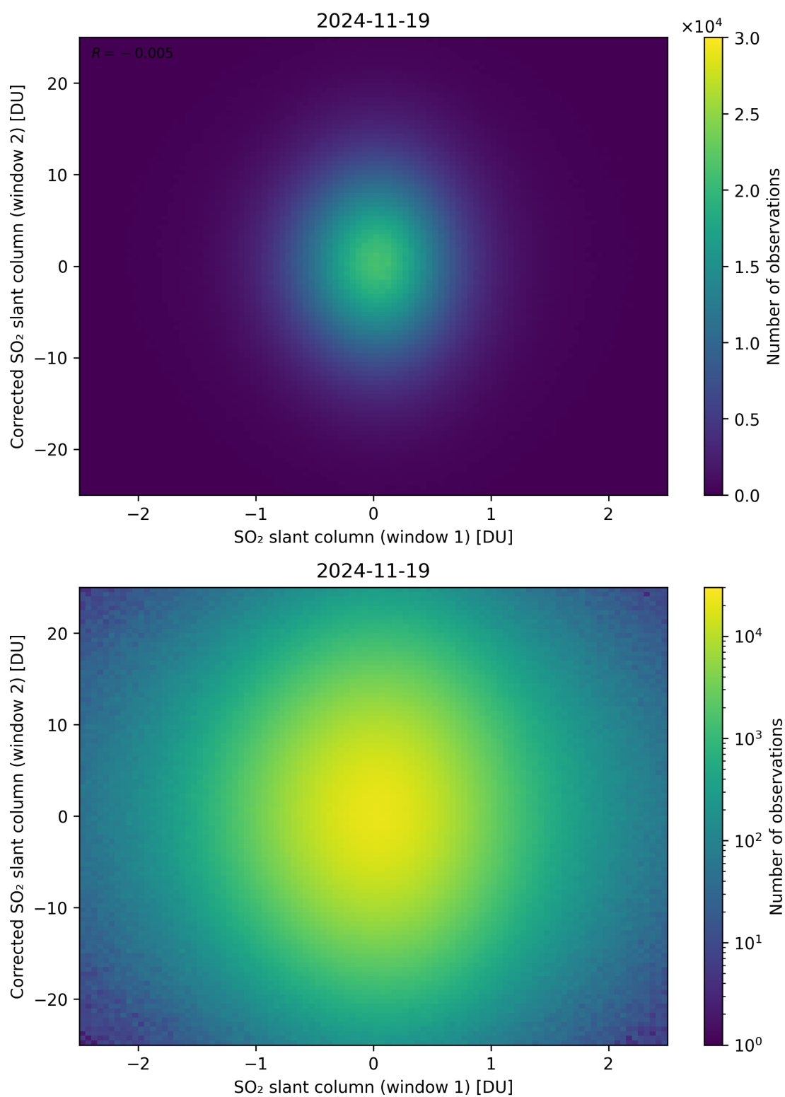
Figure 283: Scatter density plot of “SO 2 slant column (window 1)” against “Corrected SO 2 slant column (window 2)” for 2024-11-18 to 2024-11-20.
