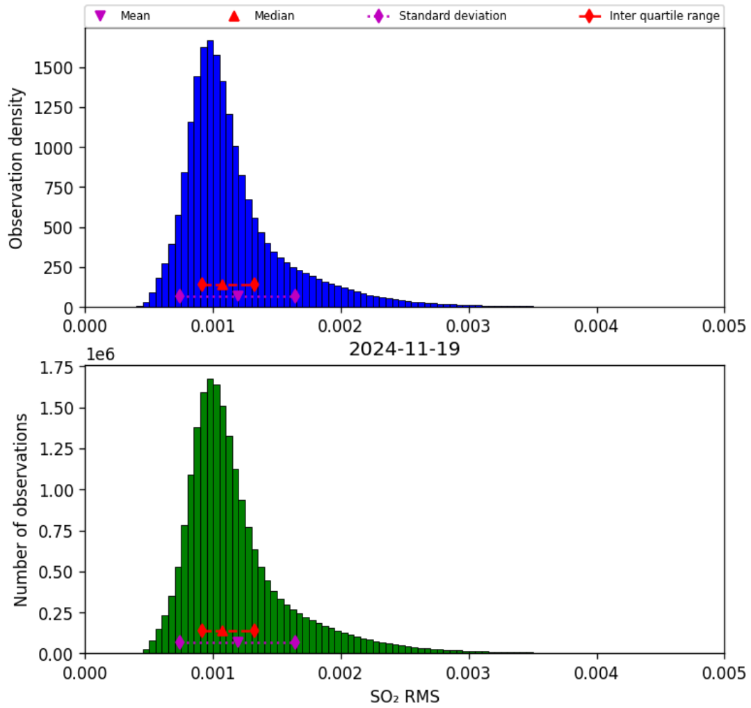
Figure 78: Histogram of “SO 2 RMS” for 2024-11-18 to 2024-11-20
