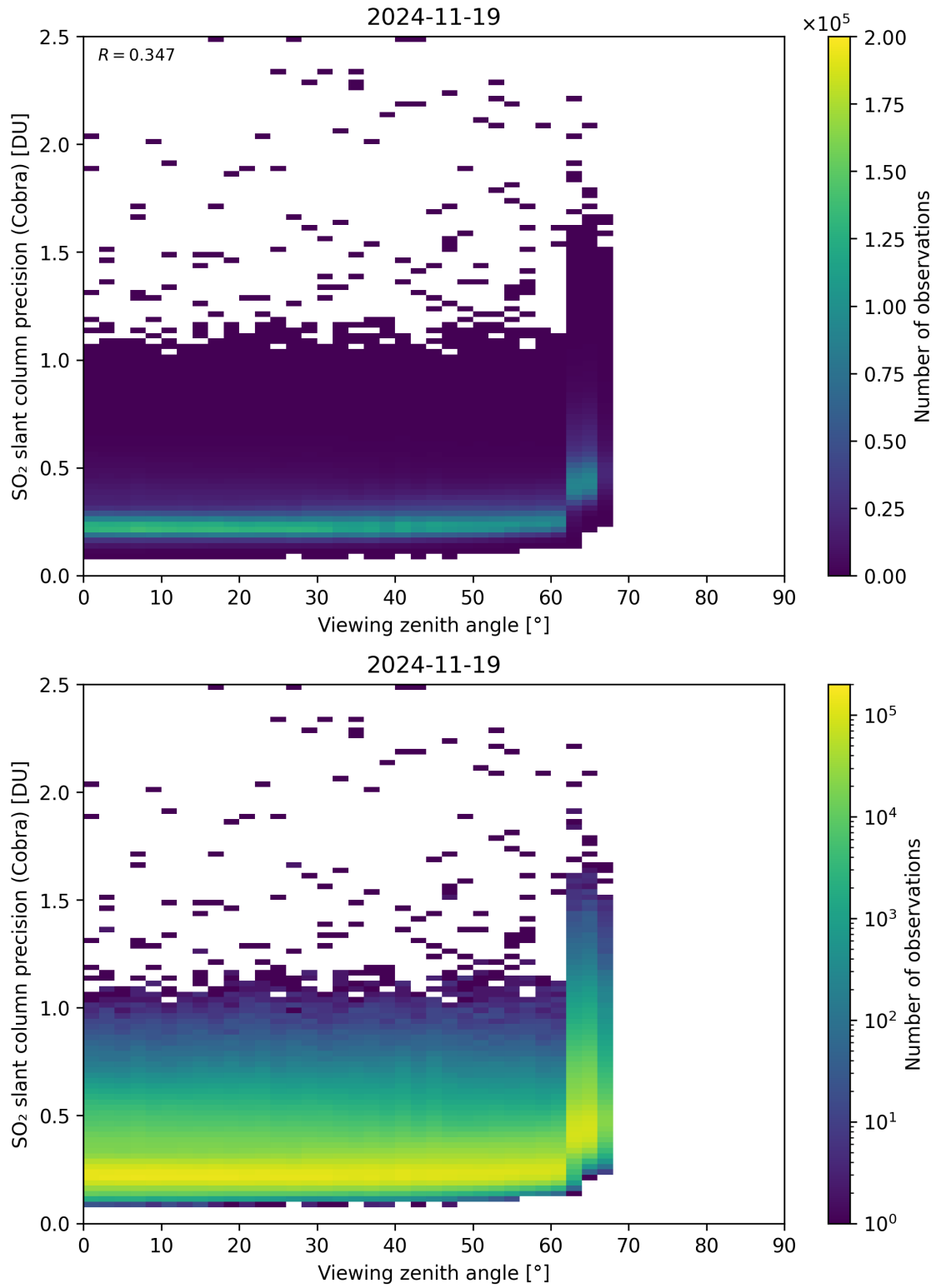
Figure 372: Scatter density plot of “Viewing zenith angle” against “SO 2 slant column precision (Cobra)” for 2024-11-18 to 2024-11-20.
