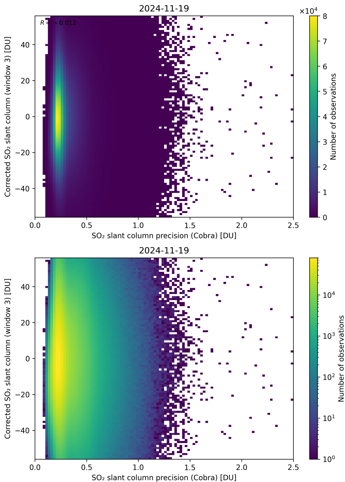
Figure 207: Scatter density plot of “SO 2 slant column precision (Cobra)” against “Corrected SO 2 slant column (window 3)” for 2024-11-18 to 2024-11-20.
