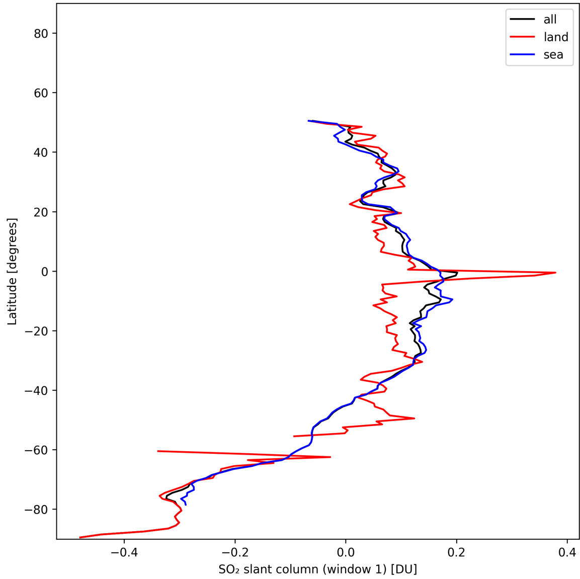
Figure 37: Zonal average of “SO 2 slant column (window 1)” for 2024-11-18 to 2024-11-20.
