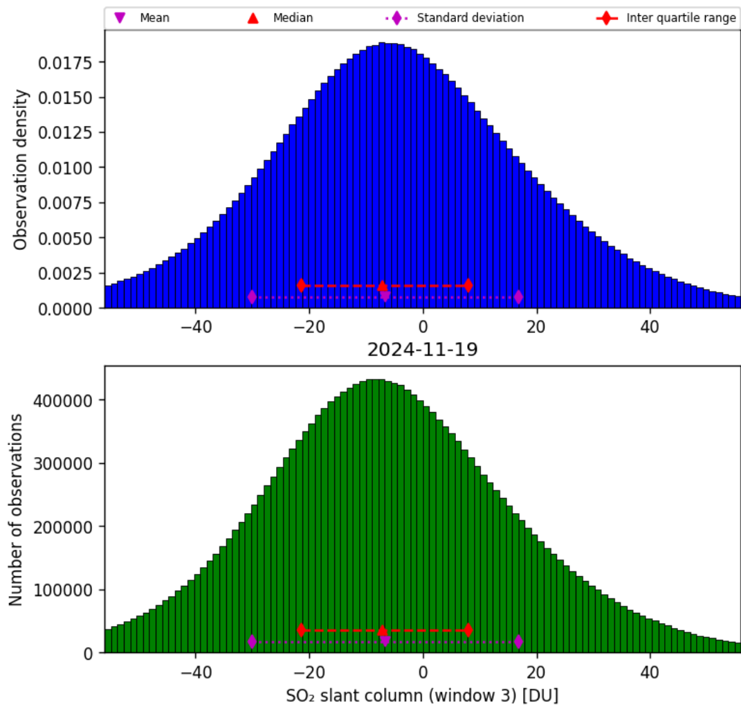
Figure 71: Histogram of “SO 2 slant column (window 3)” for 2024-11-18 to 2024-11-20
