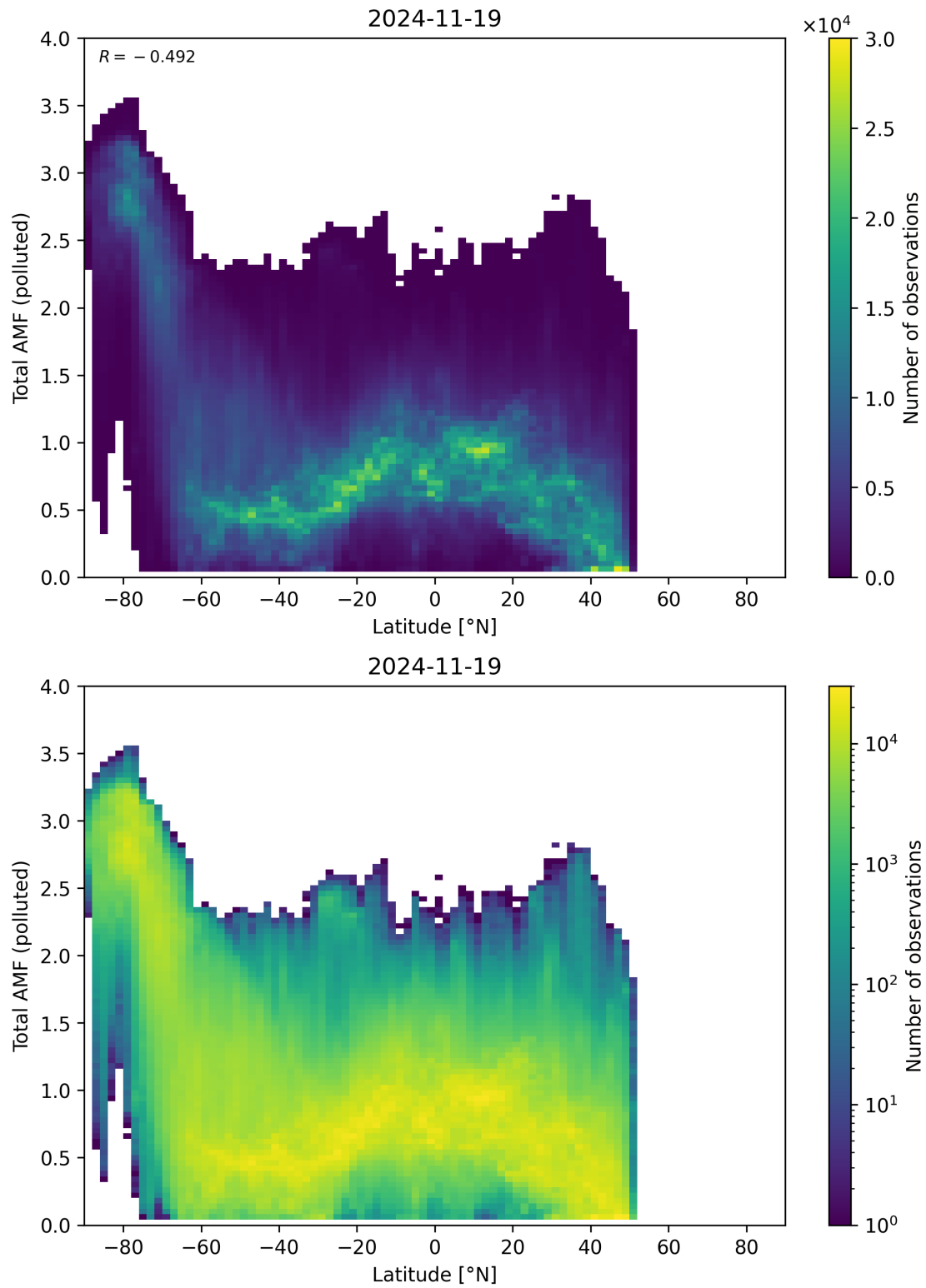
Figure 167: Scatter density plot of “Latitude” against “Total AMF (polluted)” for 2024-11-18 to 2024-11-20.
