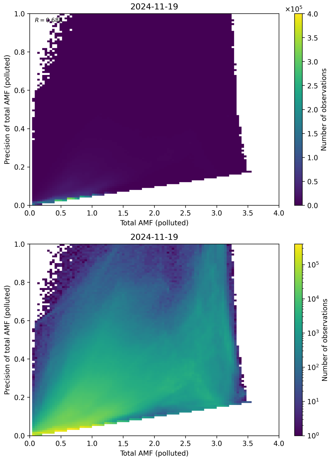
Figure 322: Scatter density plot of “Total AMF (polluted)” against “Precision of total AMF (polluted)” for 2024-11-18 to 2024-11-20.
