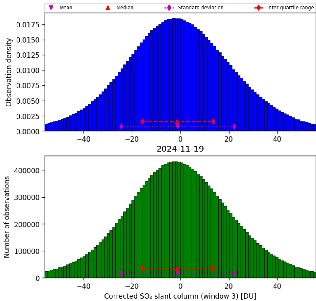
Figure 73: Histogram of “Corrected SO 2 slant column (window 3)” for 2024-11-18 to 2024-11-20
