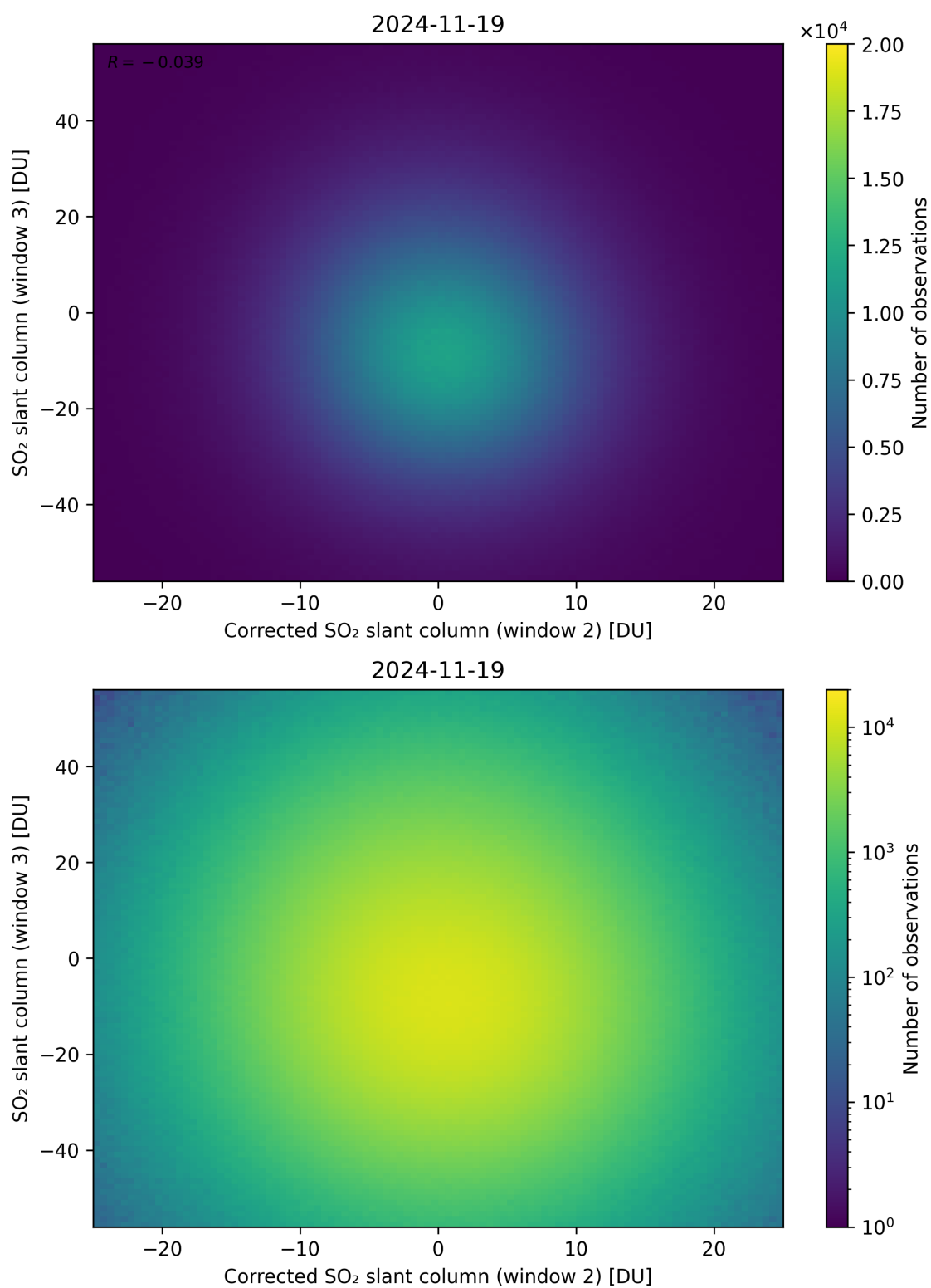
Figure 251: Scatter density plot of “Corrected SO 2 slant column (window 2)” against “SO 2 slant column (window 3)” for 2024-11-18 to 2024-11-20.
