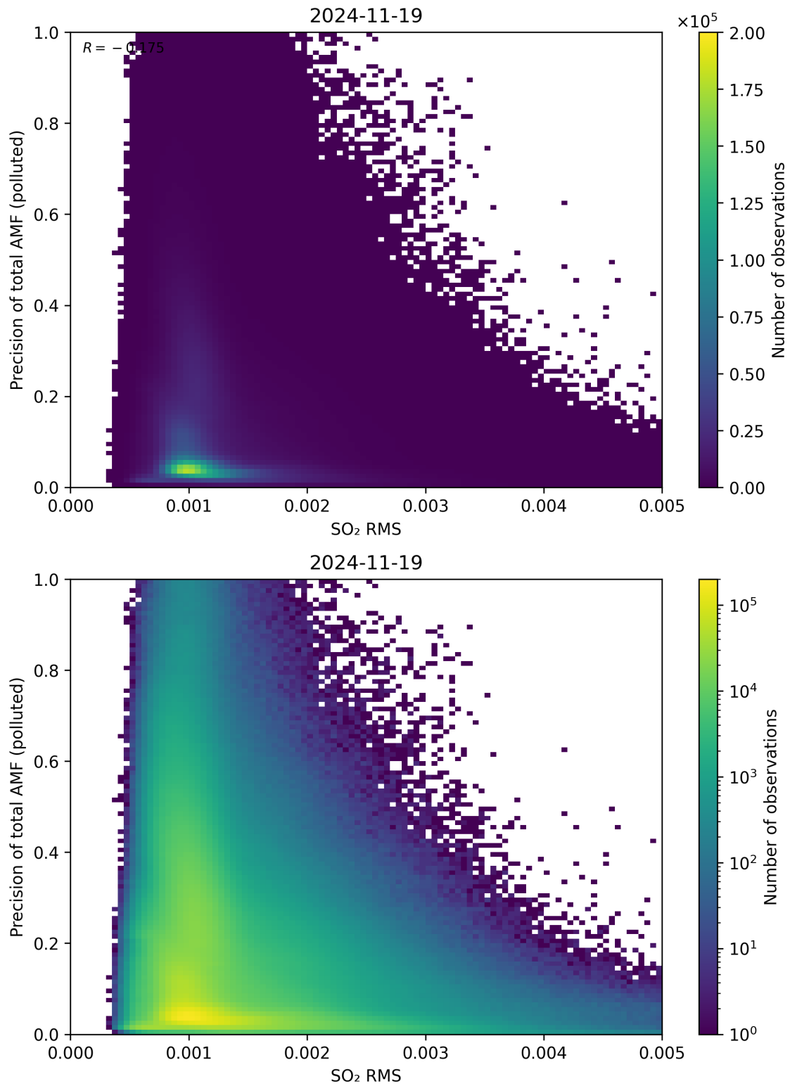
Figure 149: Scatter density plot of “SO 2 RMS” against “Precision of total AMF (polluted)” for 2024-11-18 to 2024-11-20.
