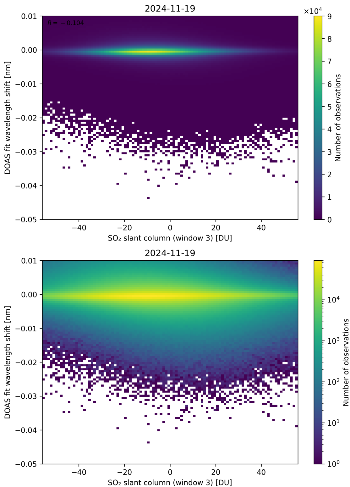
Figure 304: Scatter density plot of “SO 2 slant column (window 3)” against “DOAS fit wavelength shift” for 2024-11-18 to 2024-11-20.
