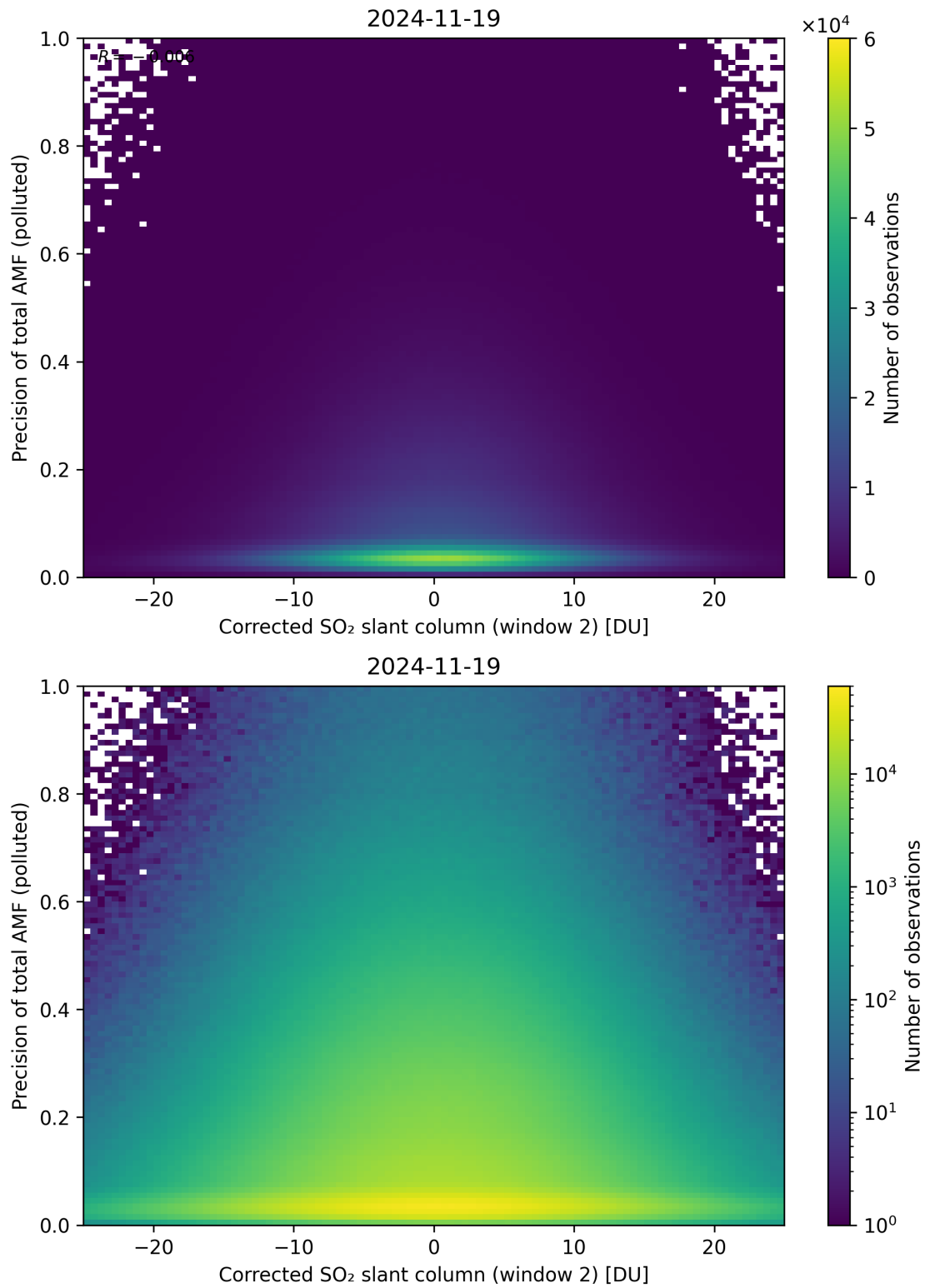
Figure 254: Scatter density plot of “Corrected SO 2 slant column (window 2)” against “Precision of total AMF (polluted)” for 2024-11-18 to 2024-11-20.
