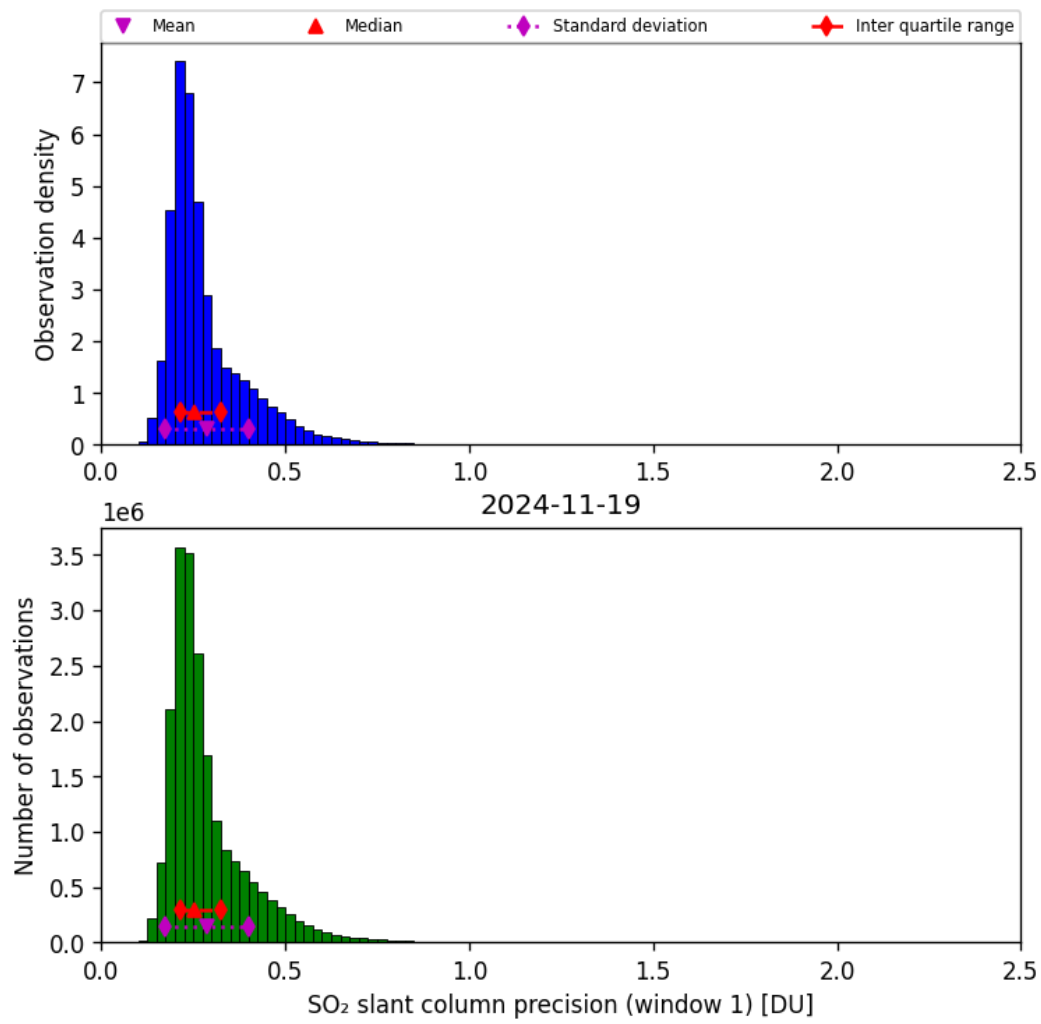
Figure 64: Histogram of “SO 2 slant column precision (window 1)” for 2024-11-18 to 2024-11-20
