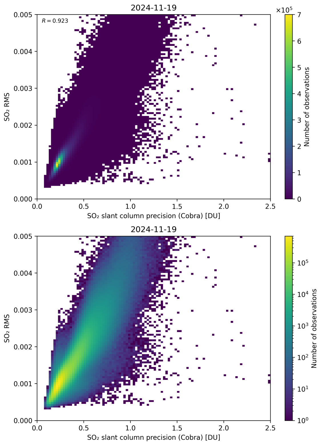
Figure 204: Scatter density plot of “SO 2 slant column precision (Cobra)” against “SO 2 RMS” for 2024-11-18 to 2024-11-20.
