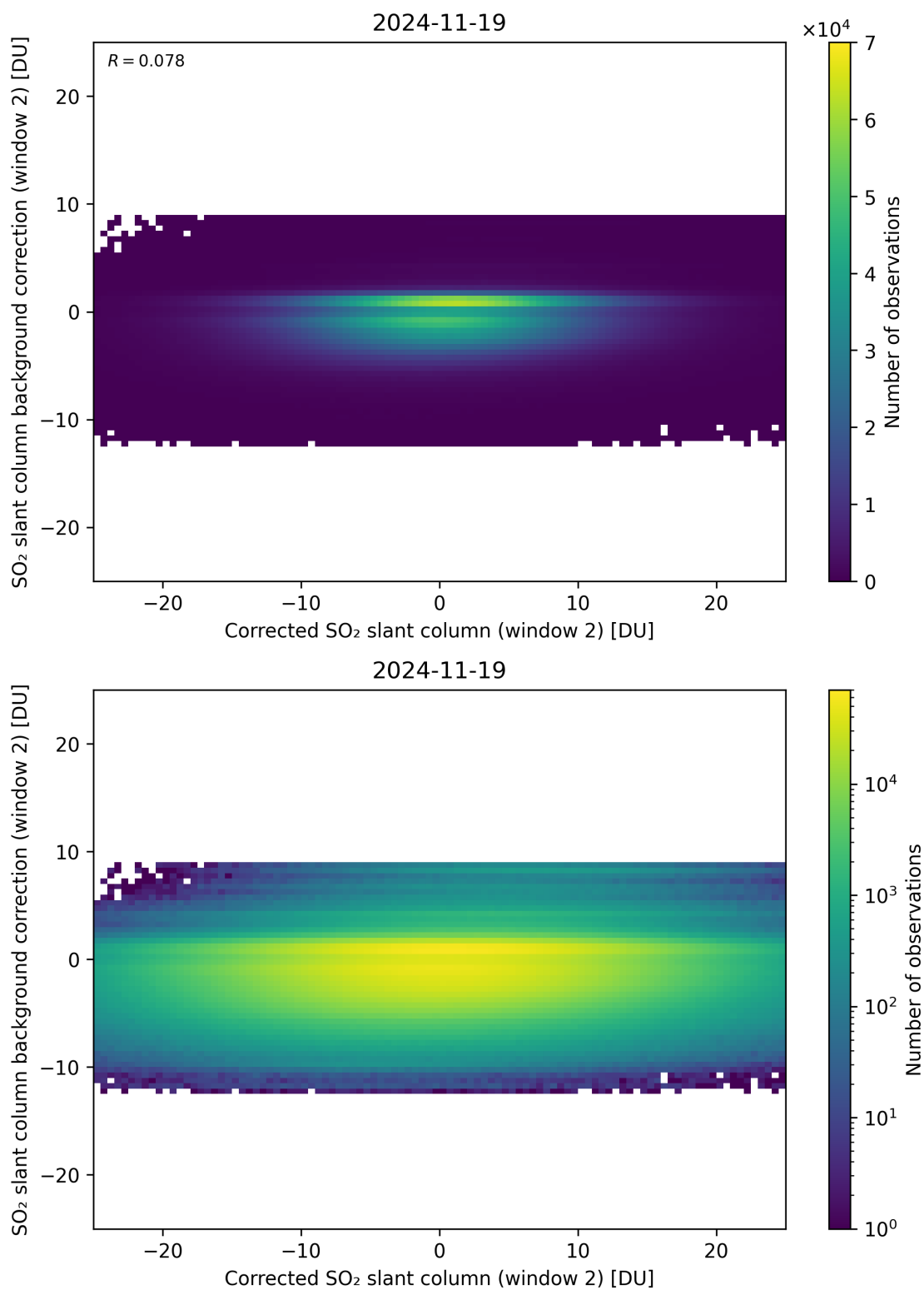
Figure 244: Scatter density plot of “Corrected SO 2 slant column (window 2)” against “SO 2 slant column background correction (window 2)” for 2024-11-18 to 2024-11-20.
