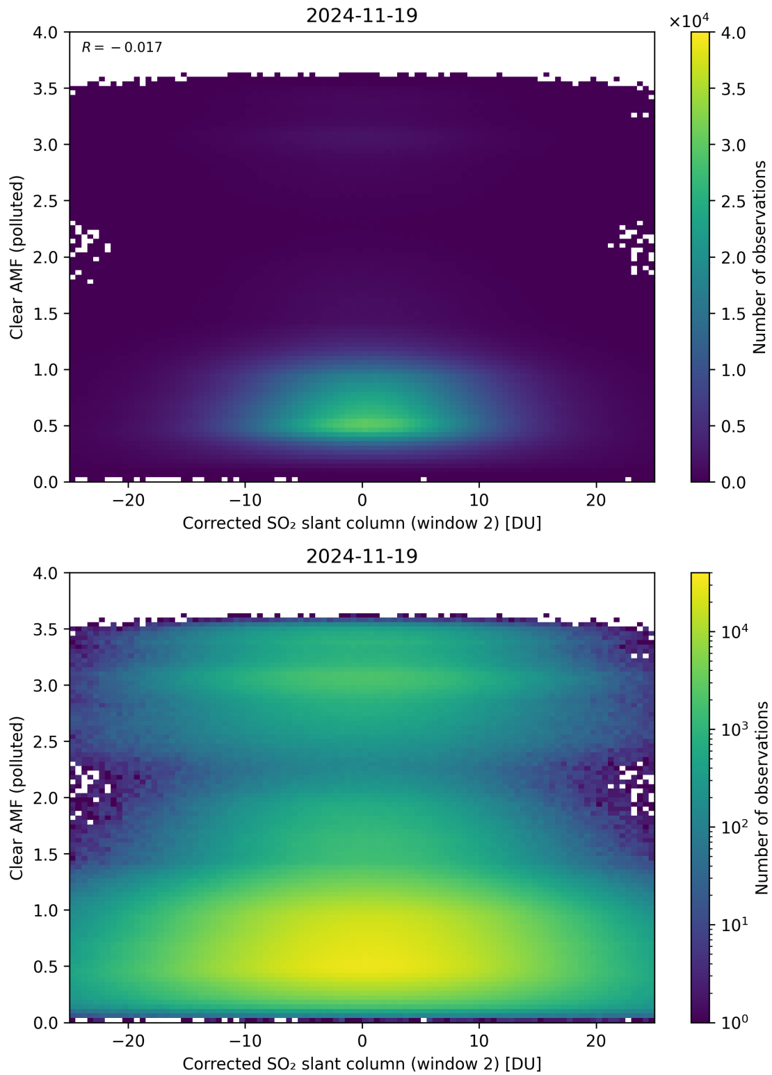
Figure 249: Scatter density plot of “Corrected SO 2 slant column (window 2)” against “Clear AMF (polluted)” for 2024-11-18 to 2024-11-20.
