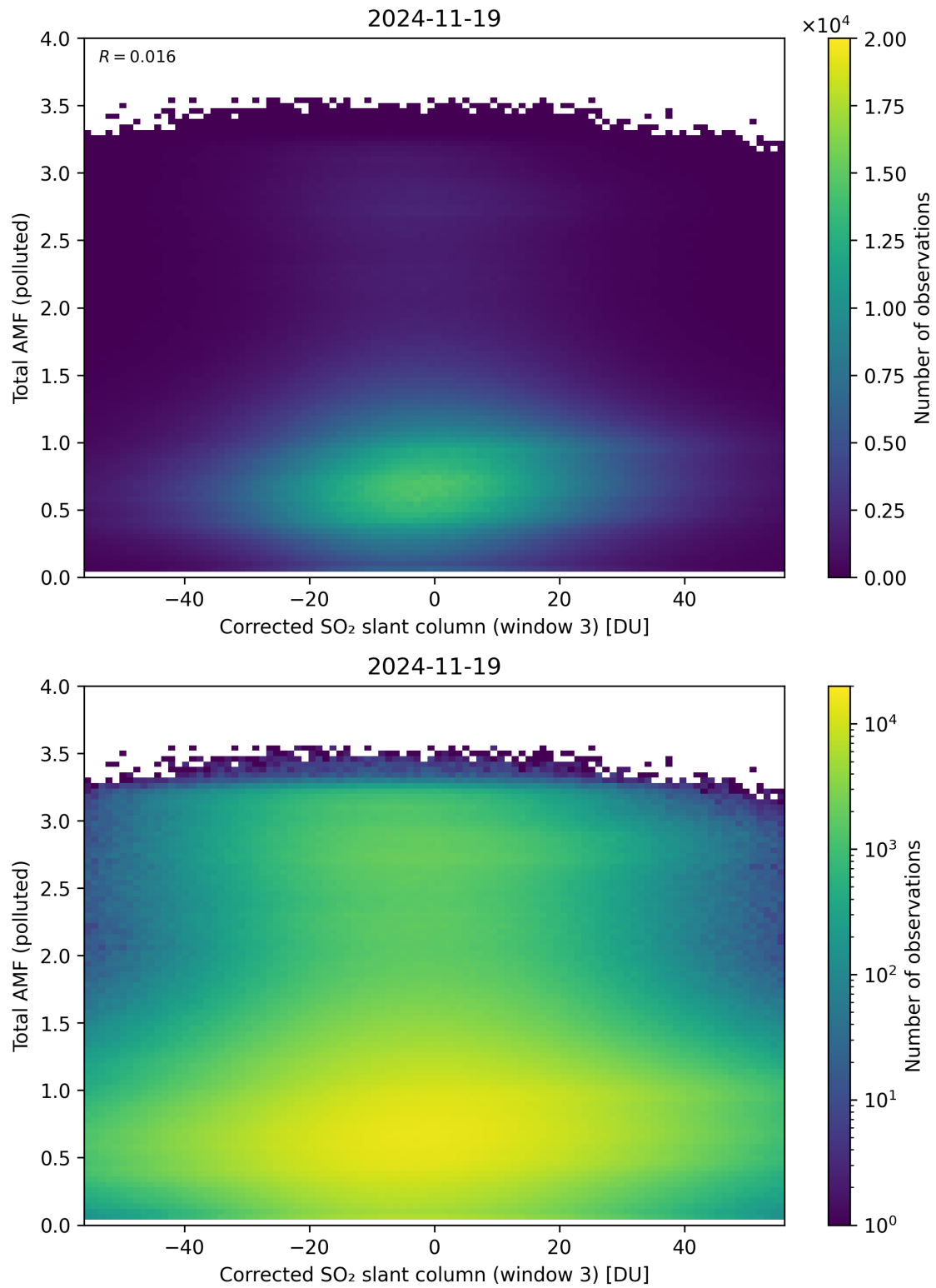
Figure 260: Scatter density plot of “Corrected SO 2 slant column (window 3)” against “Total AMF (polluted)” for 2024-11-18 to 2024-11-20.
