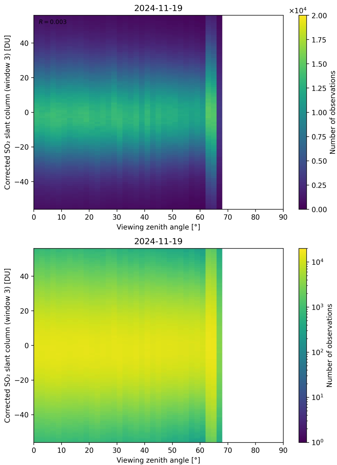
Figure 375: Scatter density plot of “Viewing zenith angle” against “Corrected SO 2 slant column (window 3)” for 2024-11-18 to 2024-11-20.
