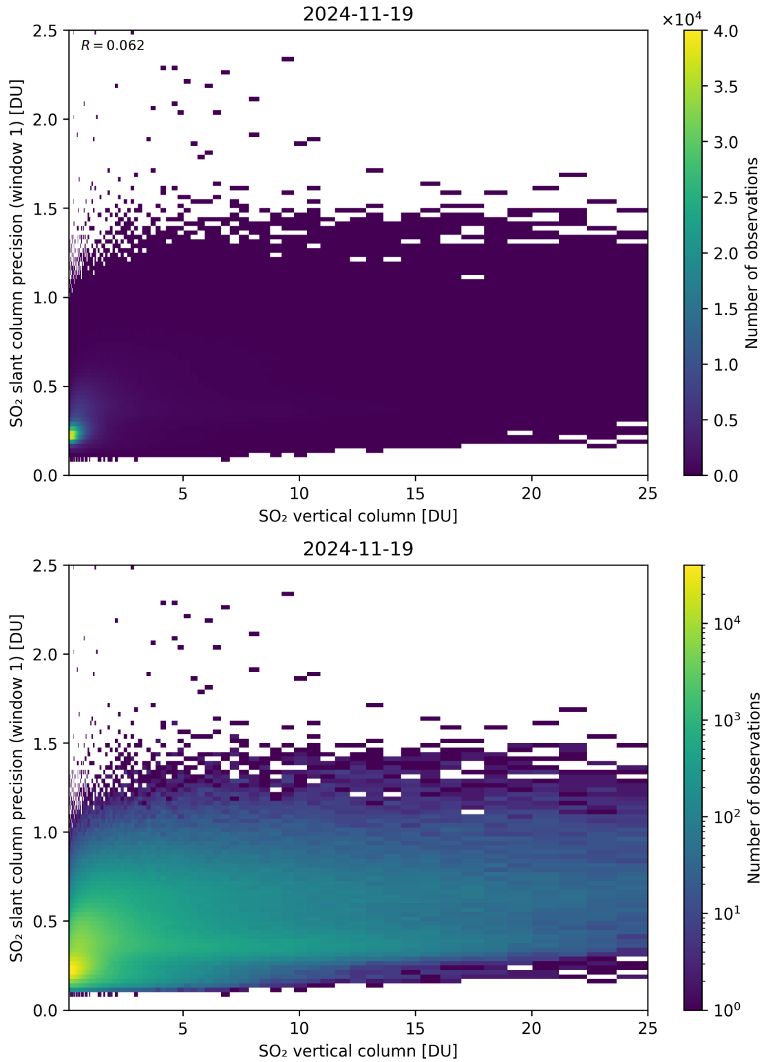
Figure 355: Scatter density plot of “SO 2 vertical column” against “SO 2 slant column precision (window 1)” for 2024-11-18 to 2024-11-20.
