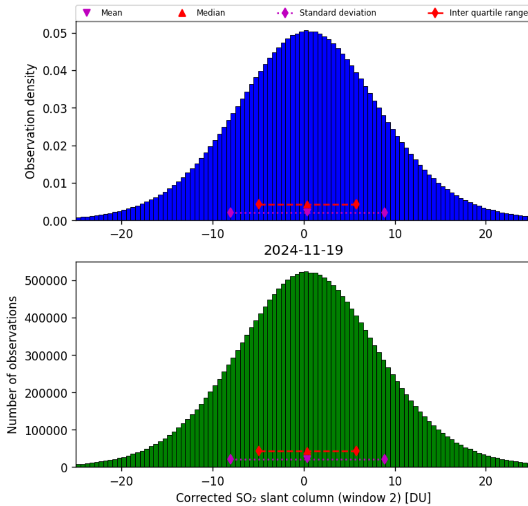
Figure 69: Histogram of “Corrected SO 2 slant column (window 2)” for 2024-11-18 to 2024-11-20
