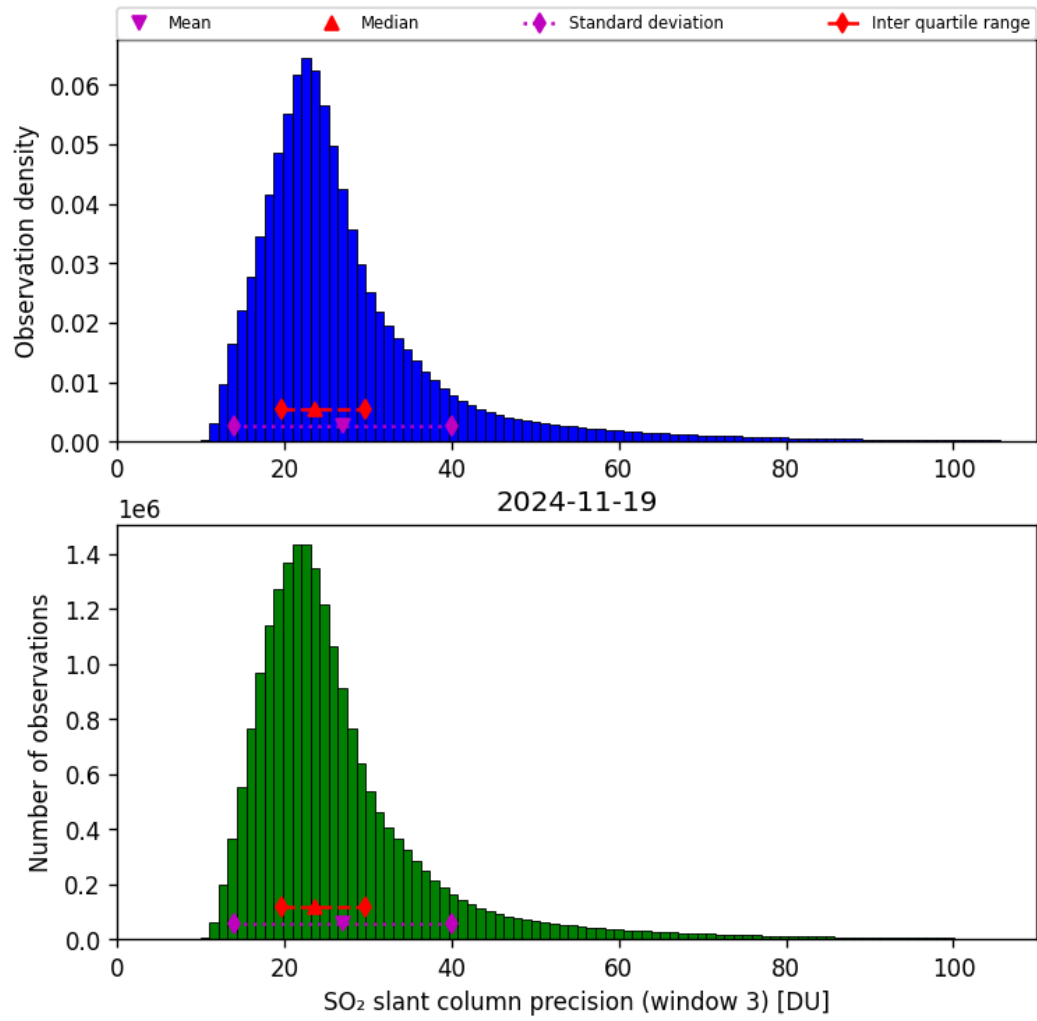
Figure 72: Histogram of “SO 2 slant column precision (window 3)” for 2024-11-18 to 2024-11-20
