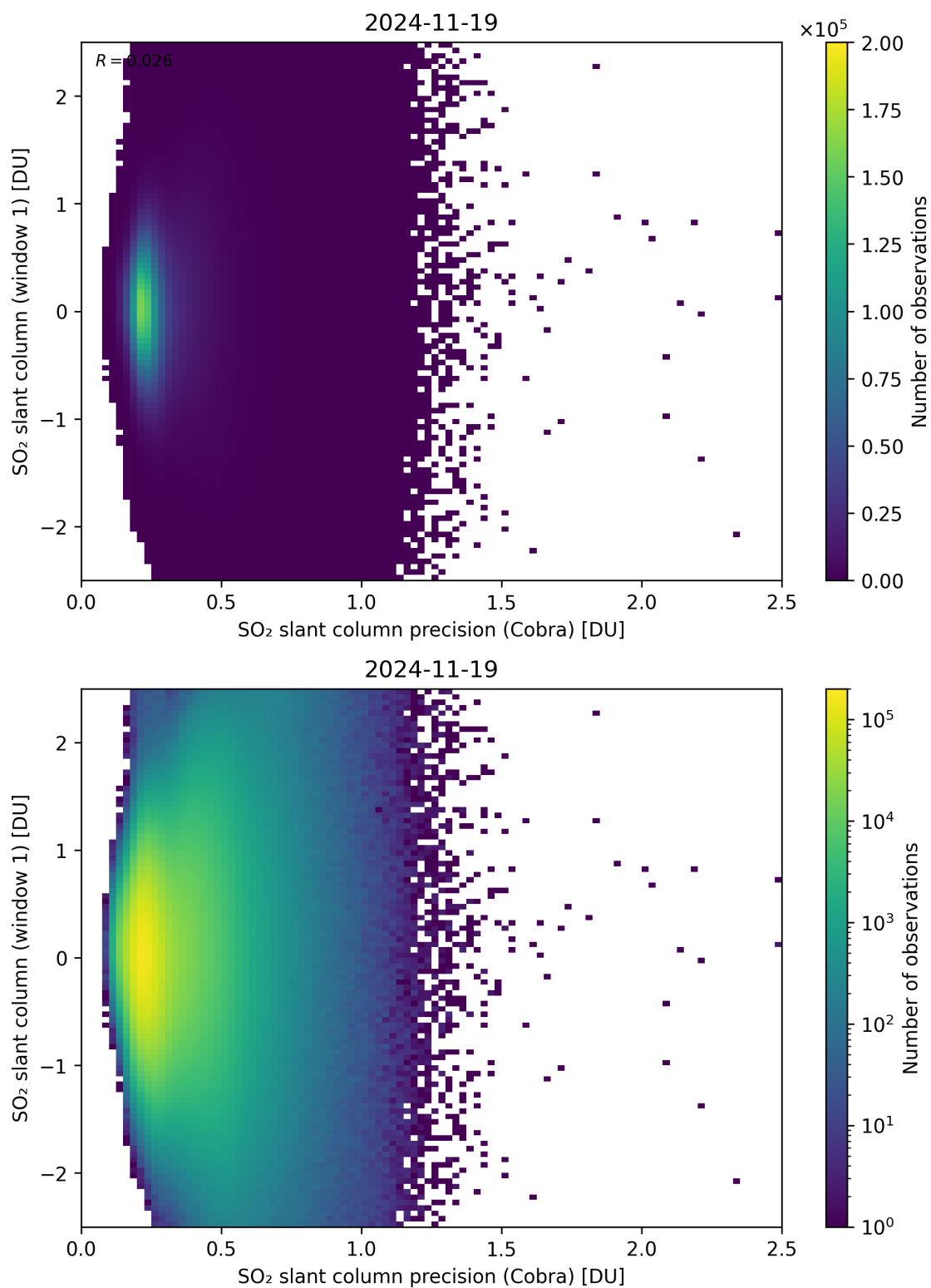
Figure 208: Scatter density plot of “SO 2 slant column precision (Cobra)” against “SO 2 slant column (window 1)” for 2024-11-18 to 2024-11-20.
