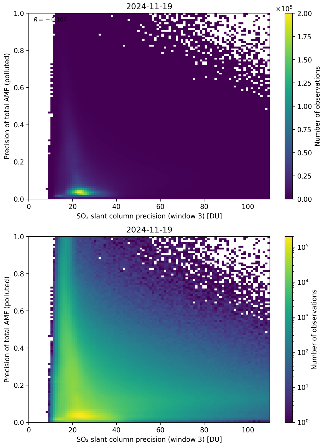
Figure 314: Scatter density plot of “SO 2 slant column precision (window 3)” against “Precision of total AMF (polluted)” for 2024-11-18 to 2024-11-20.
