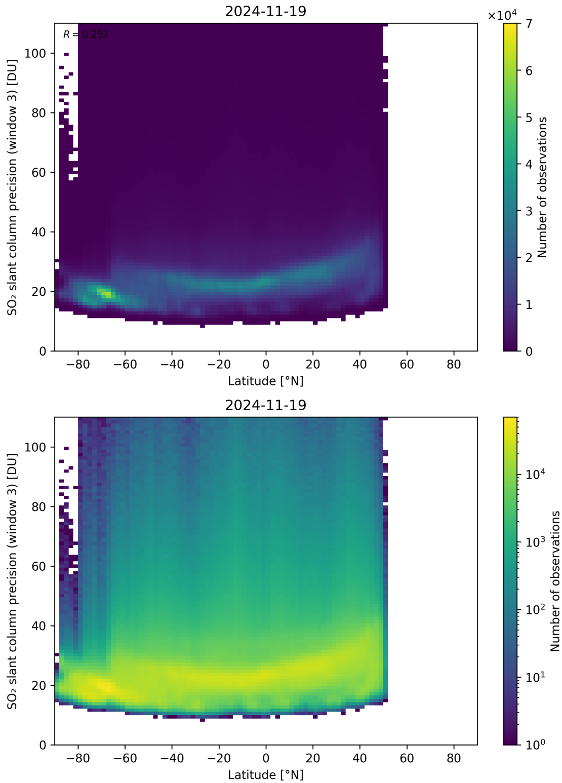
Figure 166: Scatter density plot of “Latitude” against “SO 2 slant column precision (window 3)” for 2024-11-18 to 2024-11-20.
