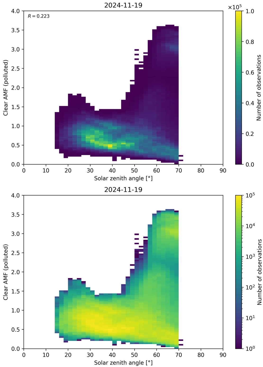
Figure 178: Scatter density plot of “Solar zenith angle” against “Clear AMF (polluted)” for 2024-11-18 to 2024-11-20.
