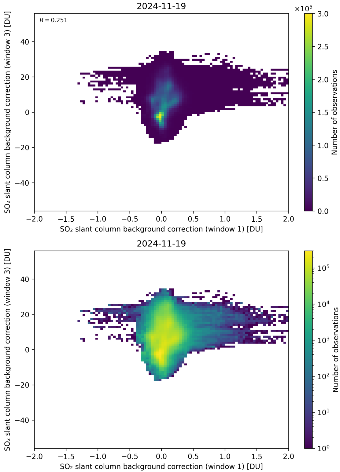
Figure 110: Scatter density plot of “SO 2 slant column background correction (window 1)” against “SO 2 slant column background correction (window 3)” for 2024-11-18 to 2024-11-20.
