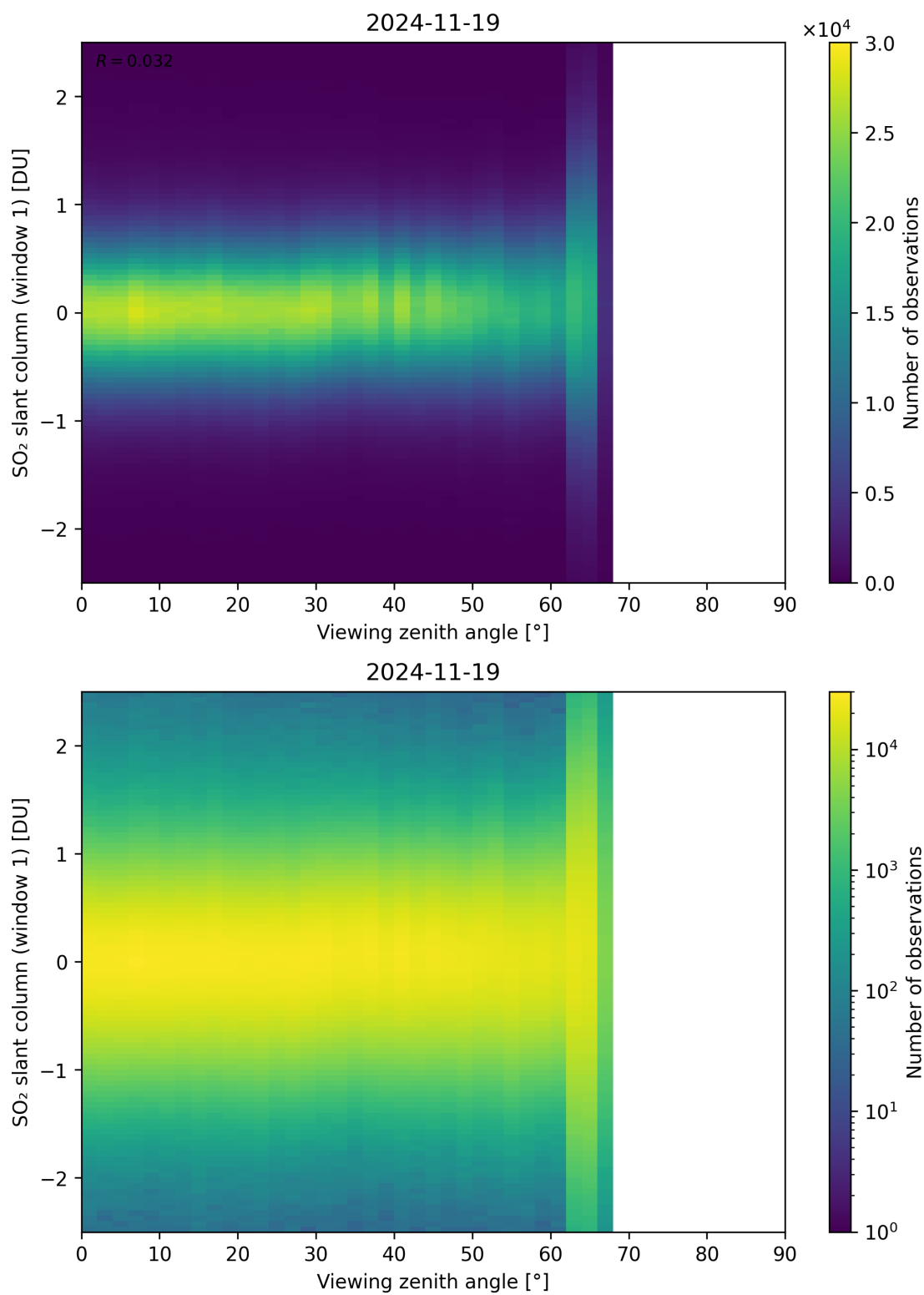
Figure 376: Scatter density plot of “Viewing zenith angle” against “SO 2 slant column (window 1)” for 2024-11-18 to 2024-11-20.
