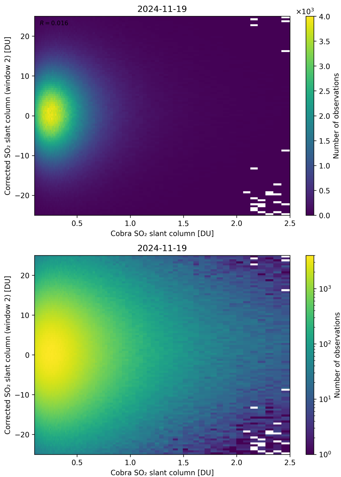
Figure 217: Scatter density plot of “Cobra SO 2 slant column” against “Corrected SO 2 slant column (window 2)” for 2024-11-18 to 2024-11-20.
