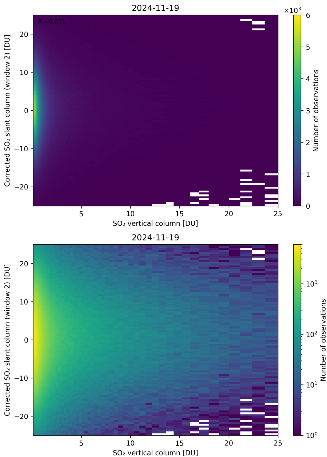
Figure 352: Scatter density plot of “SO 2 vertical column” against “Corrected SO 2 slant column (window 2)” for 2024-11-18 to 2024-11-20.
