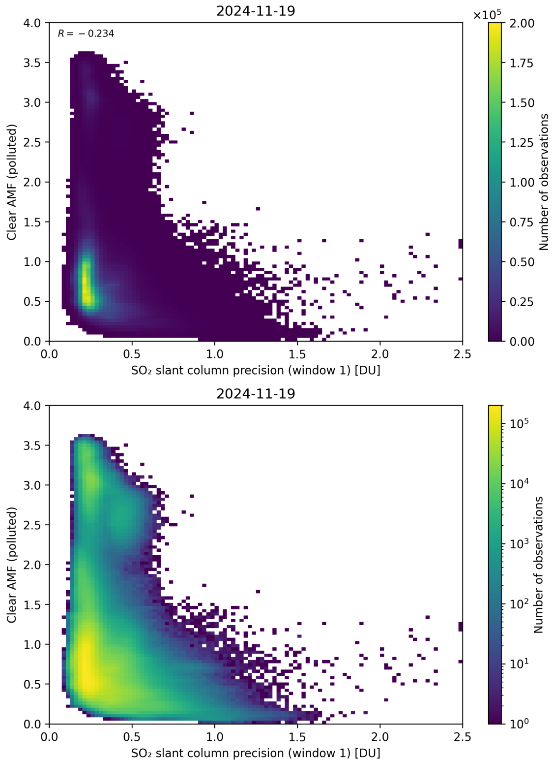
Figure 274: Scatter density plot of “SO 2 slant column precision (window 1)” against “Clear AMF (polluted)” for 2024-11-18 to 2024-11-20.
