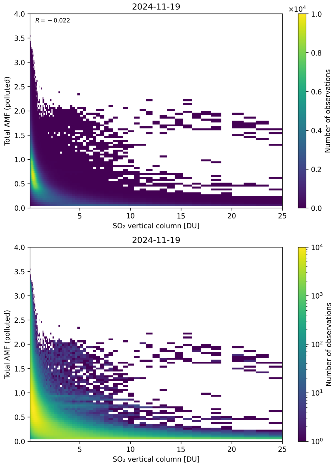
Figure 359: Scatter density plot of “SO 2 vertical column” against “Total AMF (polluted)” for 2024-11-18 to 2024-11-20.
