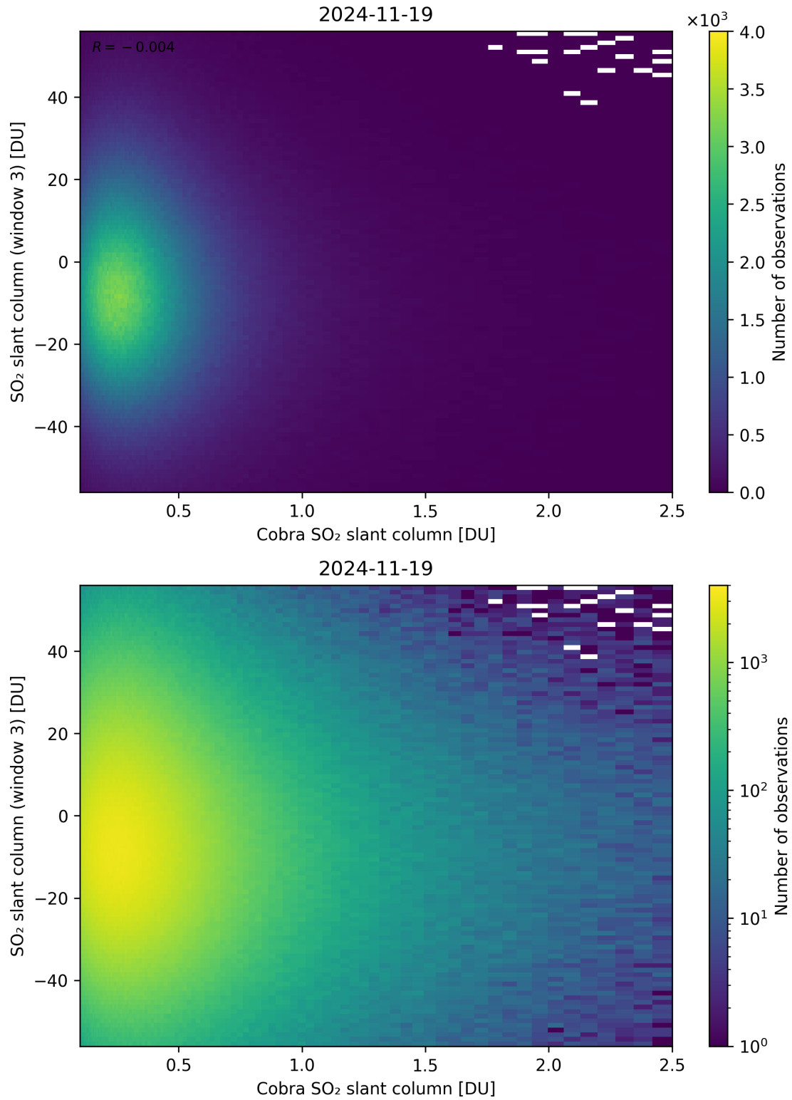
Figure 222: Scatter density plot of “Cobra SO 2 slant column” against “SO 2 slant column (window 3)” for 2024-11-18 to 2024-11-20.
