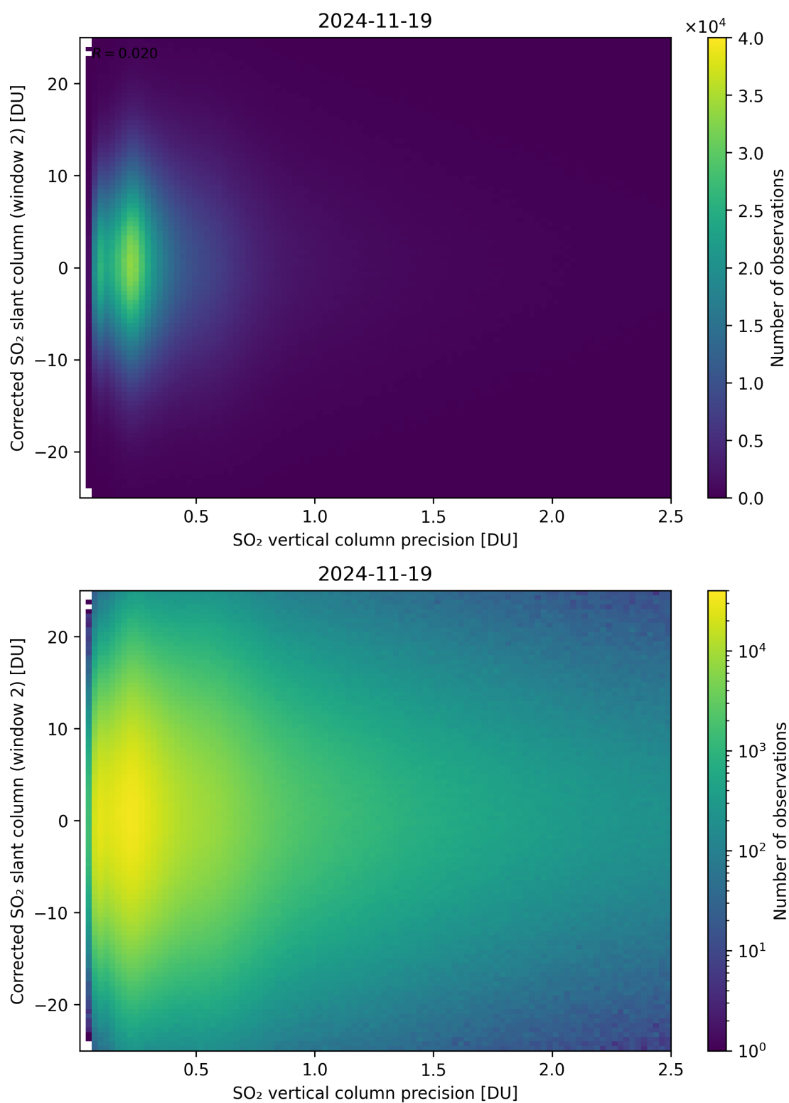
Figure 339: Scatter density plot of “SO 2 vertical column precision” against “Corrected SO 2 slant column (window 2)” for 2024-11-18 to 2024-11-20.
