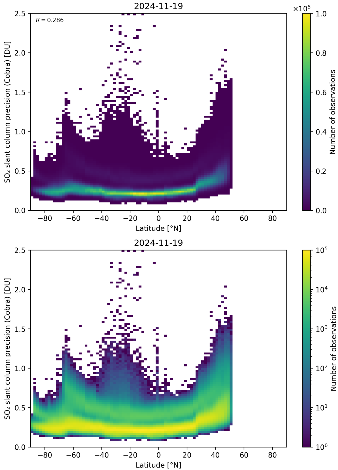
Figure 158: Scatter density plot of “Latitude” against “SO 2 slant column precision (Cobra)” for 2024-11-18 to 2024-11-20.
