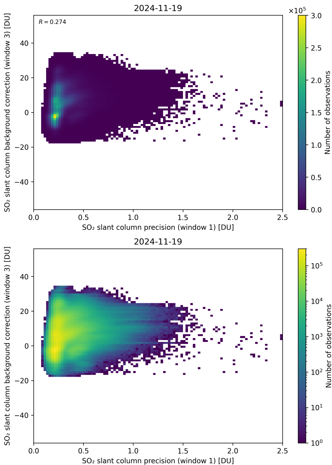
Figure 270: Scatter density plot of “SO 2 slant column precision (window 1)” against “SO 2 slant column background correction (window 3)” for 2024-11-18 to 2024-11-20.
