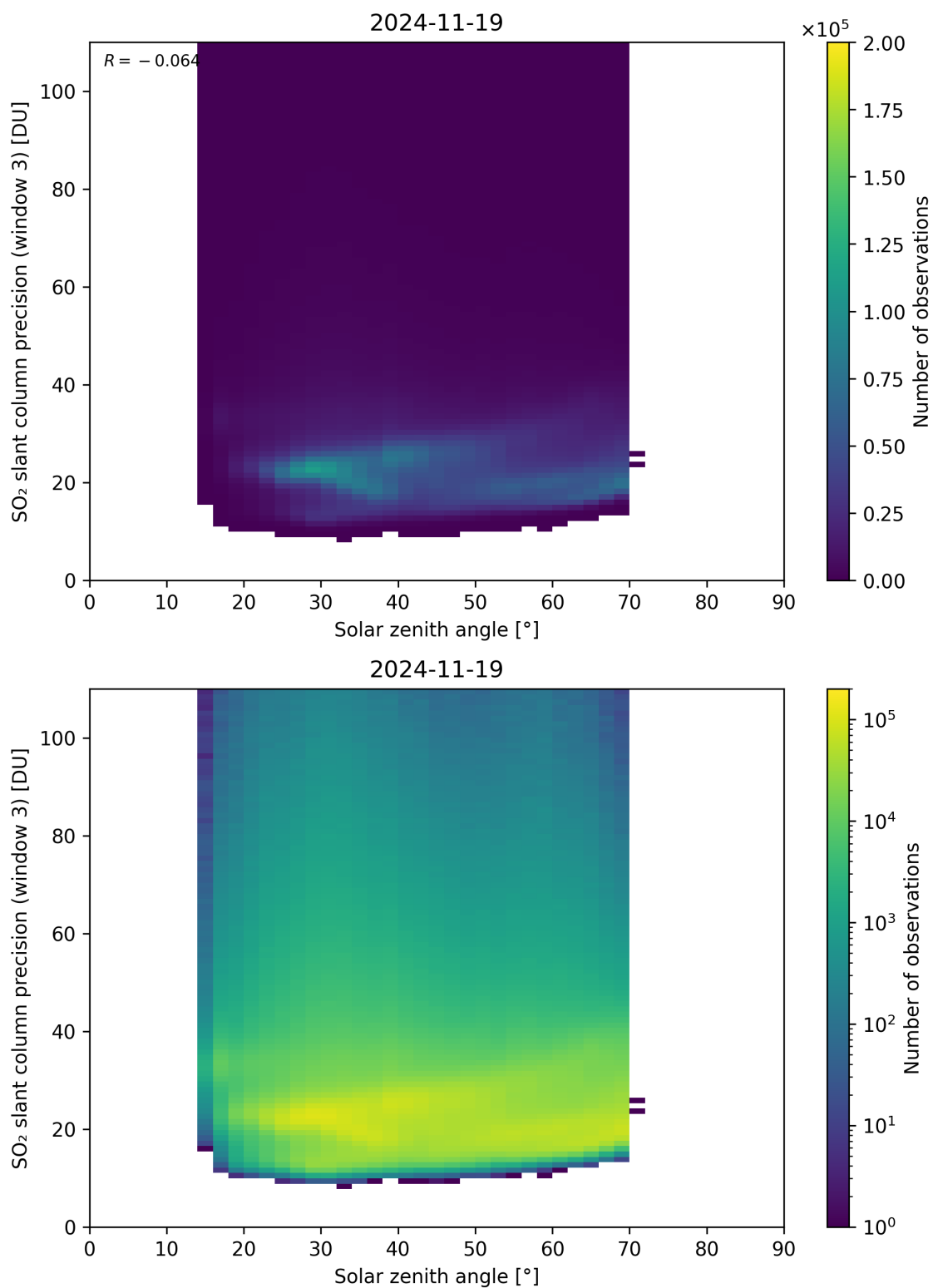
Figure 188: Scatter density plot of “Solar zenith angle” against “SO 2 slant column precision (window 3)” for 2024-11-18 to 2024-11-20.
