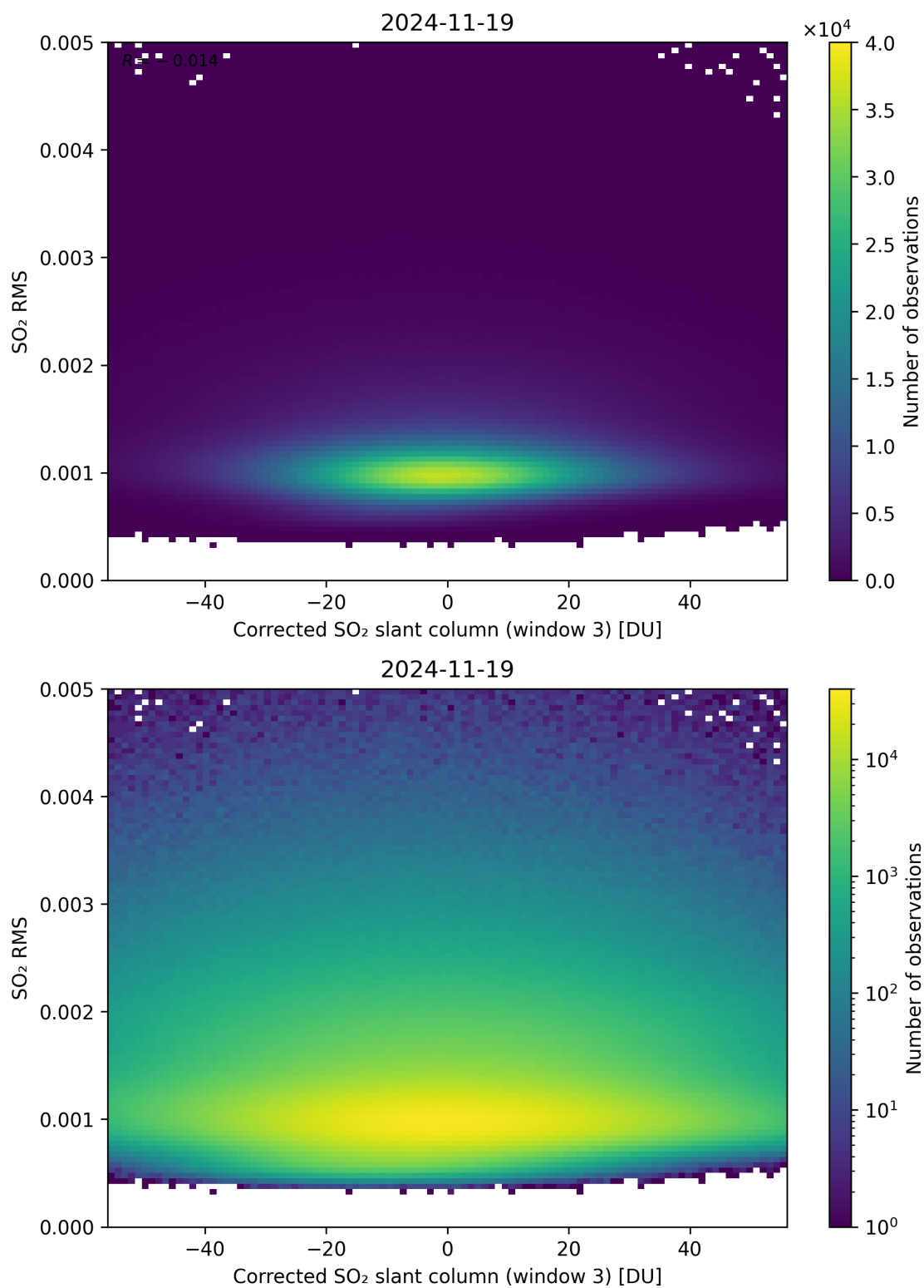
Figure 258: Scatter density plot of “Corrected SO 2 slant column (window 3)” against “SO 2 RMS” for 2024-11-18 to 2024-11-20.
