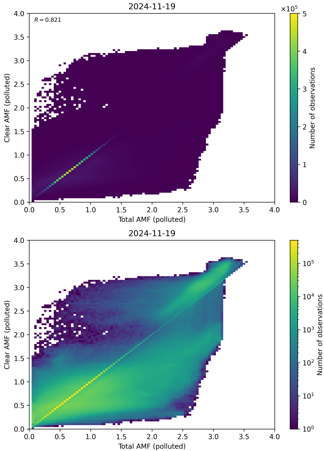
Figure 321: Scatter density plot of “Total AMF (polluted)” against “Clear AMF (polluted)” for 2024-11-18 to 2024-11-20.
