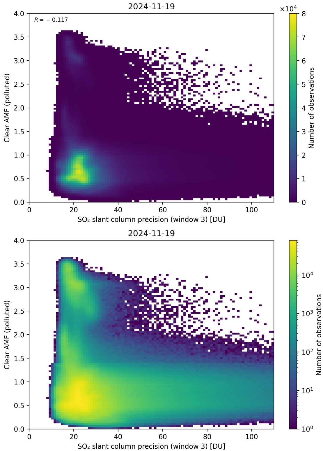
Figure 311: Scatter density plot of “SO 2 slant column precision (window 3)” against “Clear AMF (polluted)” for 2024-11-18 to 2024-11-20.
