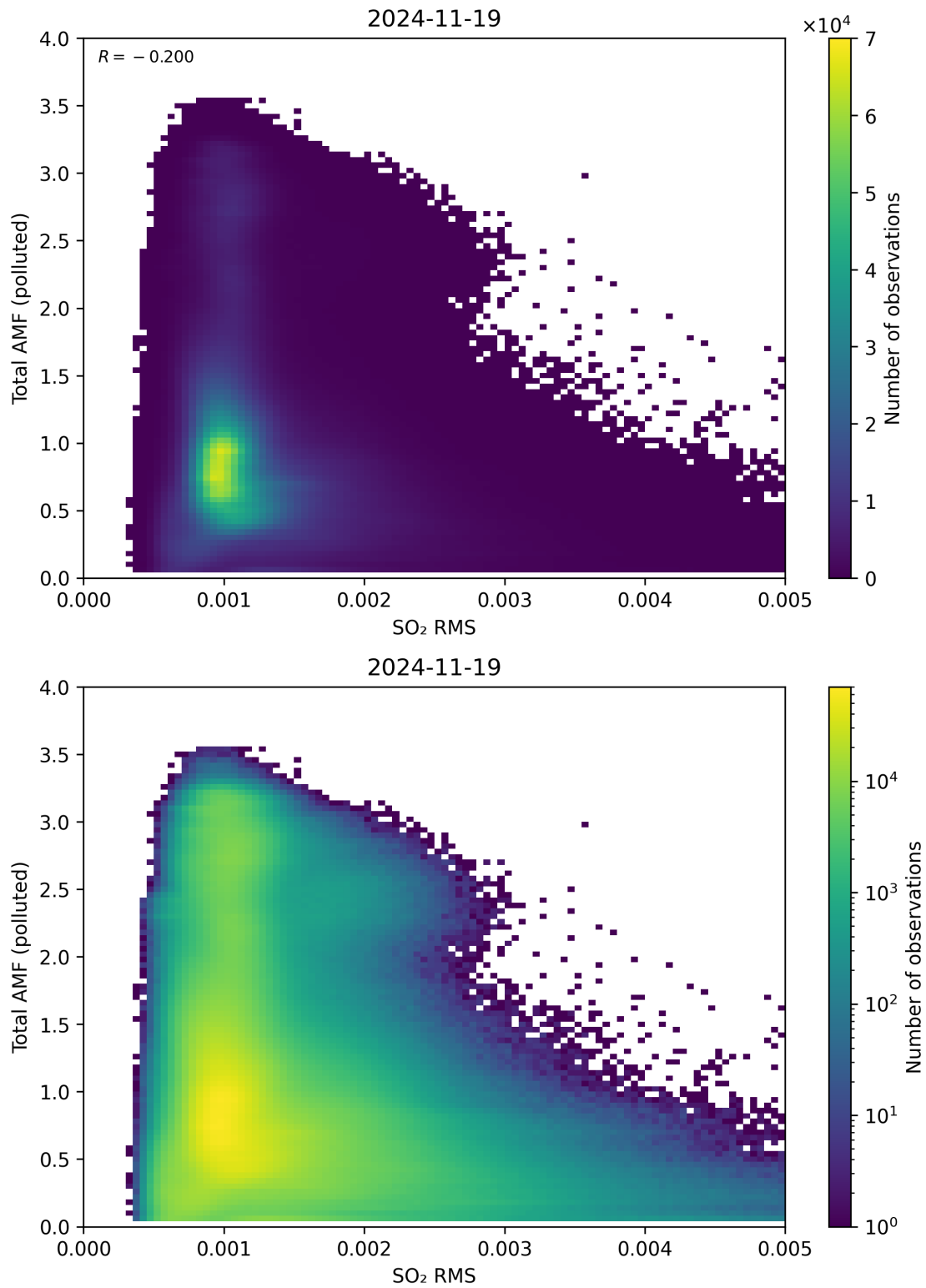
Figure 148: Scatter density plot of “SO 2 RMS” against “Total AMF (polluted)” for 2024-11-18 to 2024-11-20.
