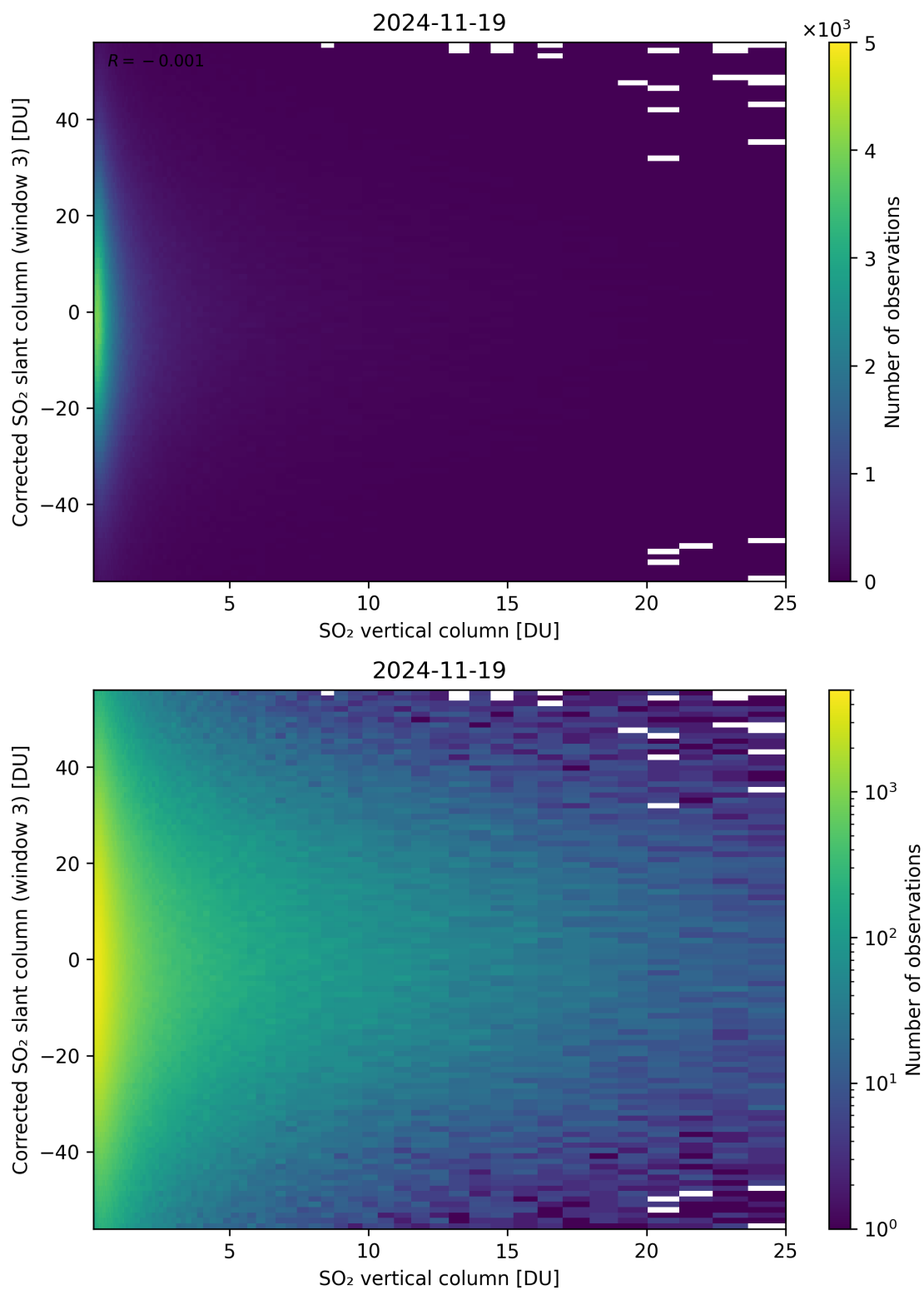
Figure 353: Scatter density plot of “SO 2 vertical column” against “Corrected SO 2 slant column (window 3)” for 2024-11-18 to 2024-11-20.
