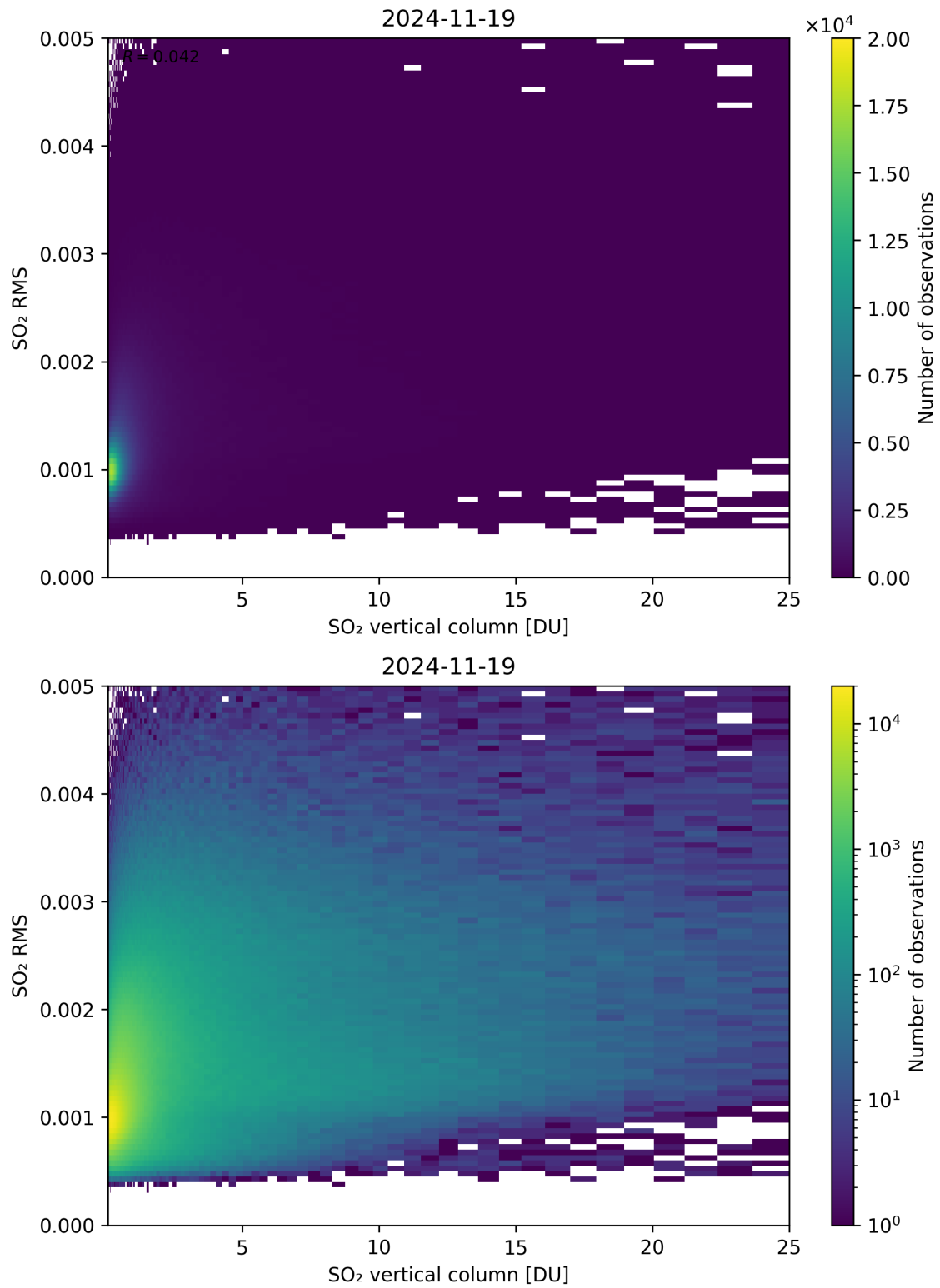
Figure 328: Scatter density plot of “SO 2 vertical column” against “SO 2 RMS” for 2024-11-18 to 2024-11-20.
