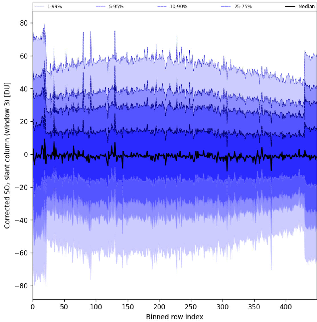
Figure 99: Along track statistics of “Corrected SO 2 slant column (window 3)” for 2024-11-18 to 2024-11-20
