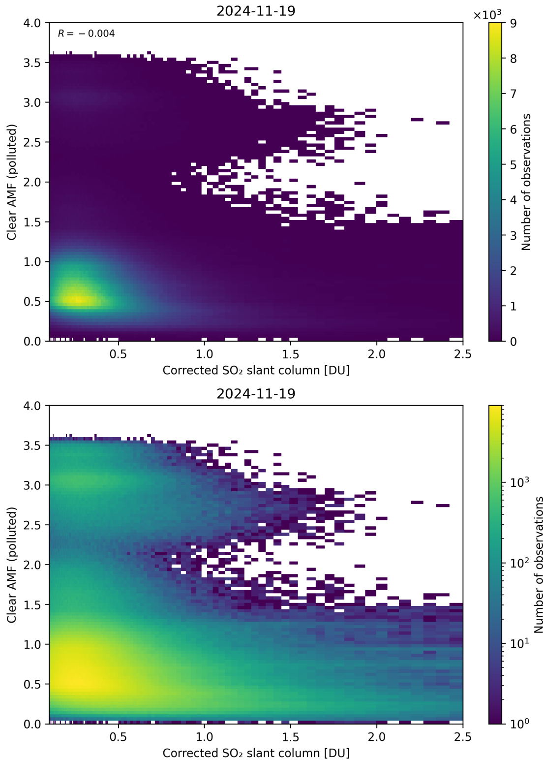
Figure 232: Scatter density plot of “Corrected SO 2 slant column” against “Clear AMF (polluted)” for 2024-11-18 to 2024-11-20.
