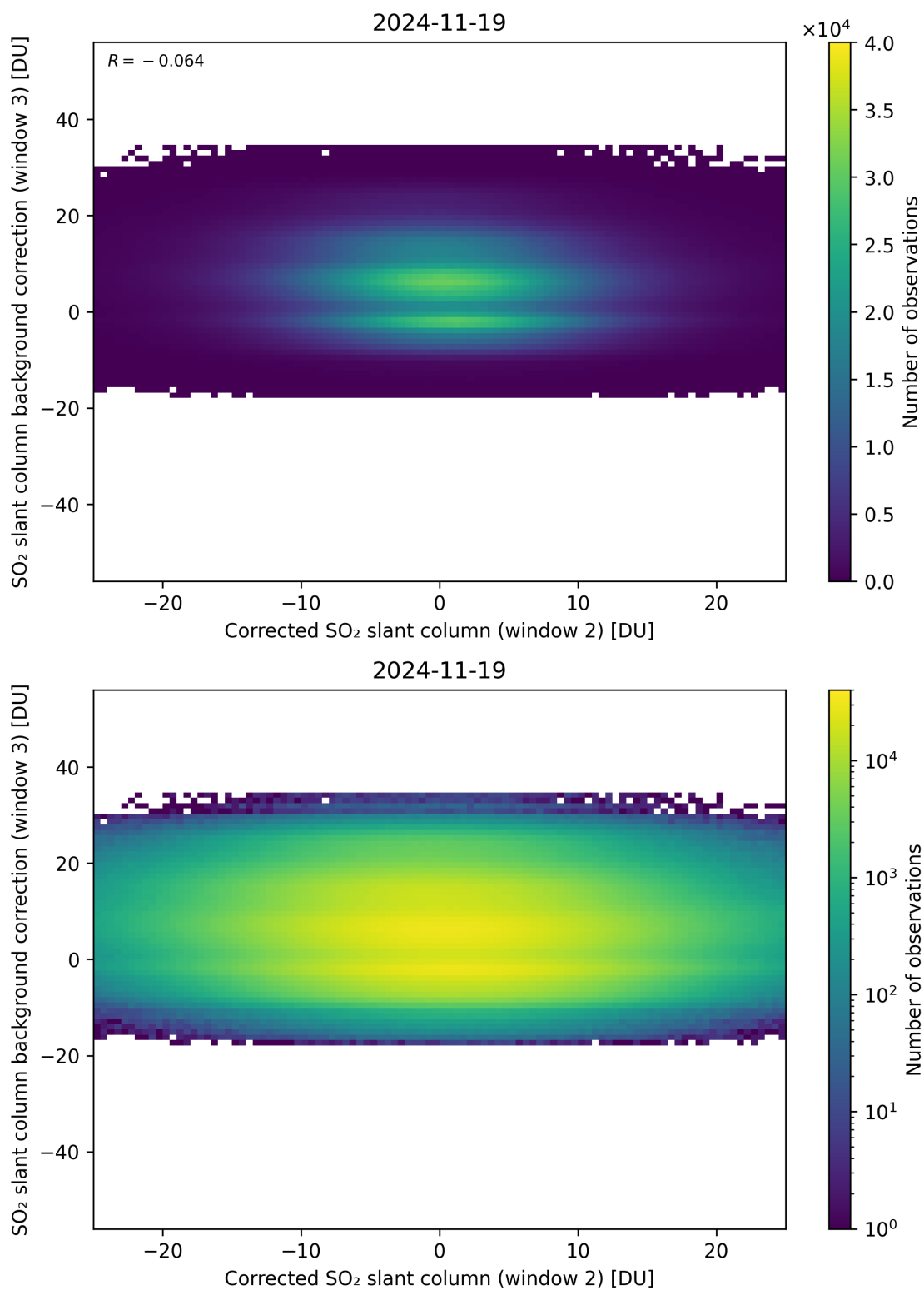
Figure 245: Scatter density plot of “Corrected SO 2 slant column (window 2)” against “SO 2 slant column background correction (window 3)” for 2024-11-18 to 2024-11-20.
