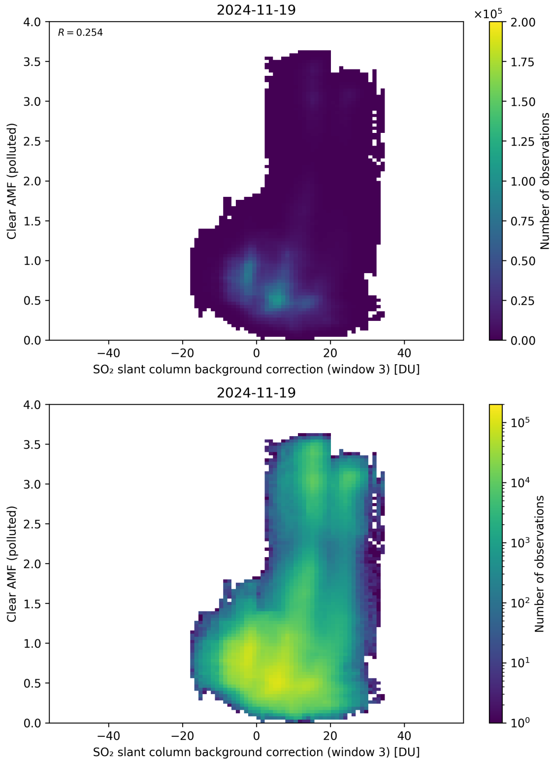
Figure 135: Scatter density plot of “SO 2 slant column background correction (window 3)” against “Clear AMF (polluted)” for 2024-11-18 to 2024-11-20.
