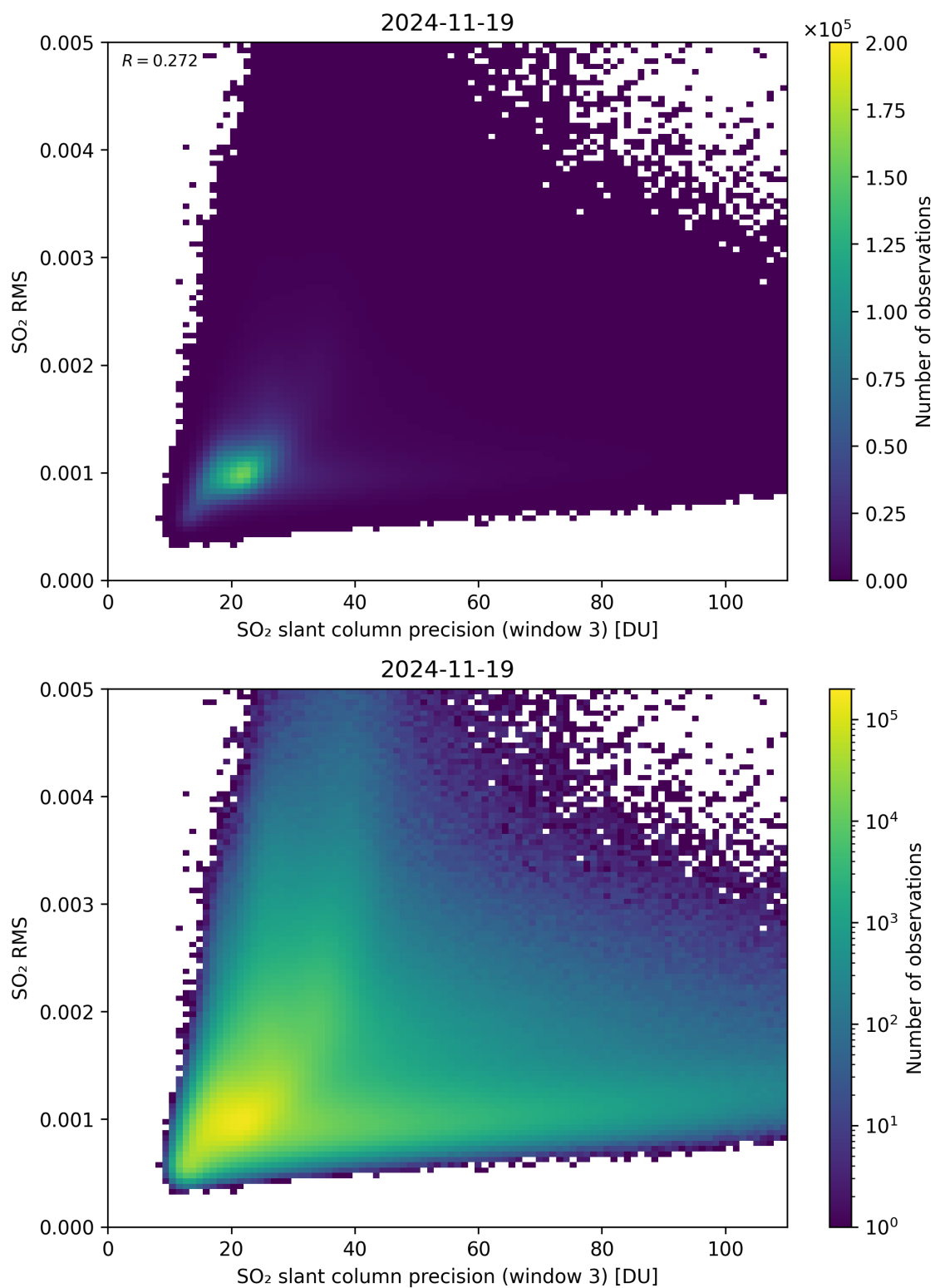
Figure 310: Scatter density plot of “SO 2 slant column precision (window 3)” against “SO 2 RMS” for 2024-11-18 to 2024-11-20.
