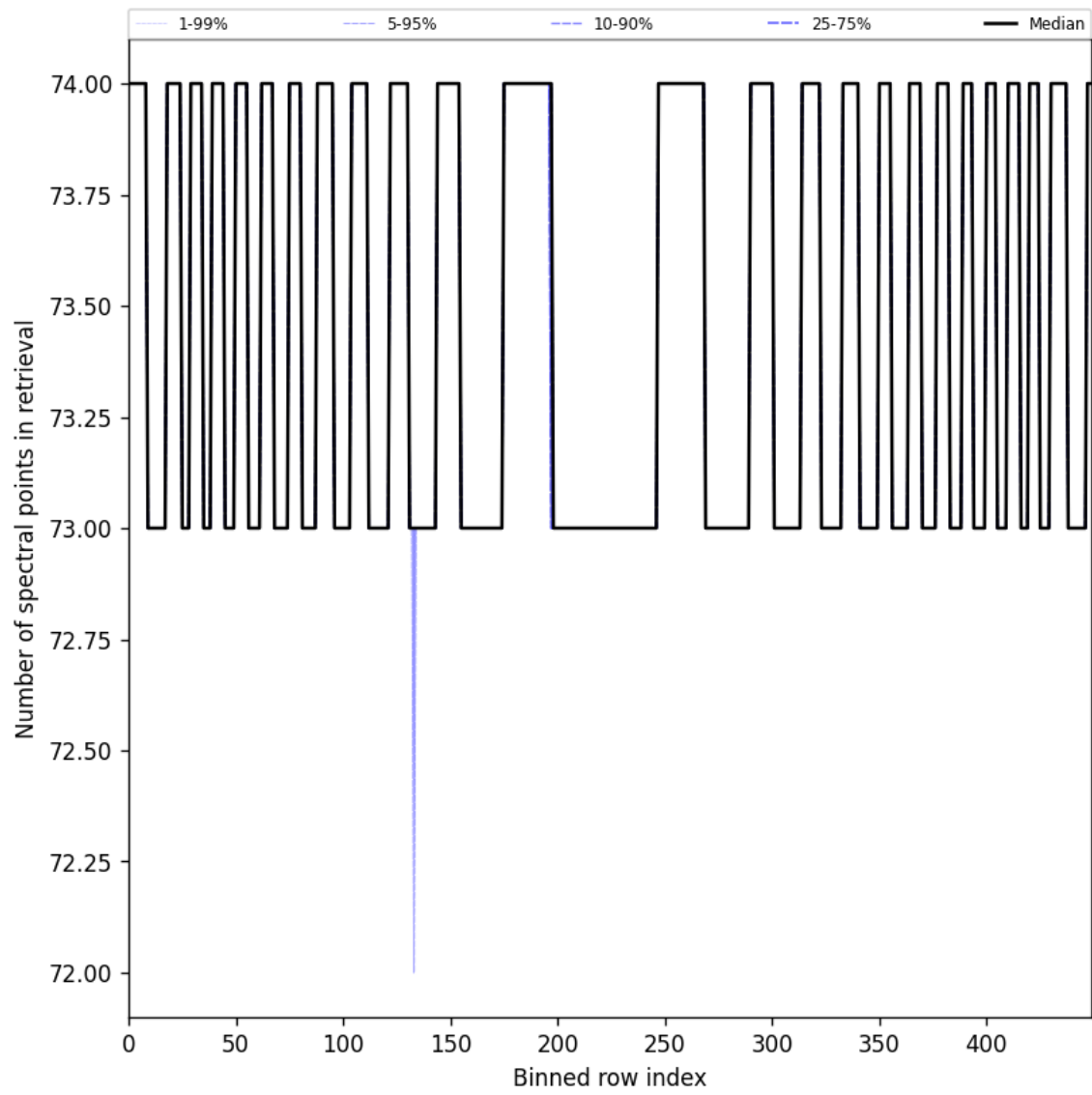
Figure 108: Along track statistics of “Number of spectral points in retrieval” for 2024-11-18 to 2024-11-20
