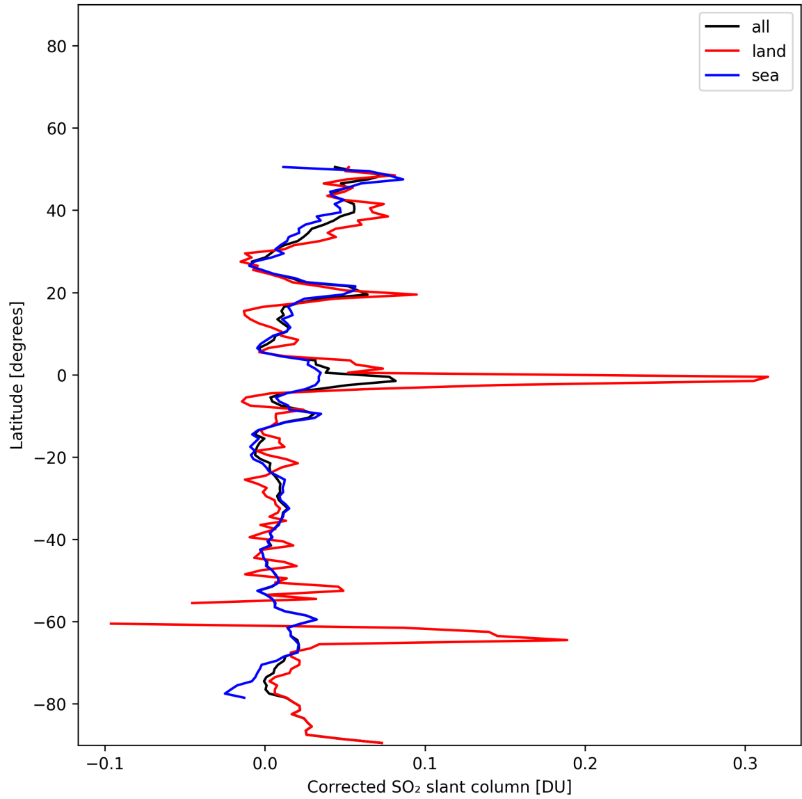
Figure 34: Zonal average of “Corrected SO 2 slant column” for 2024-11-18 to 2024-11-20.
