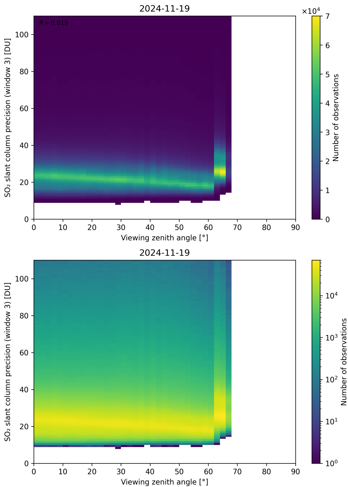
Figure 380: Scatter density plot of “Viewing zenith angle” against “SO 2 slant column precision (window 3)” for 2024-11-18 to 2024-11-20.
