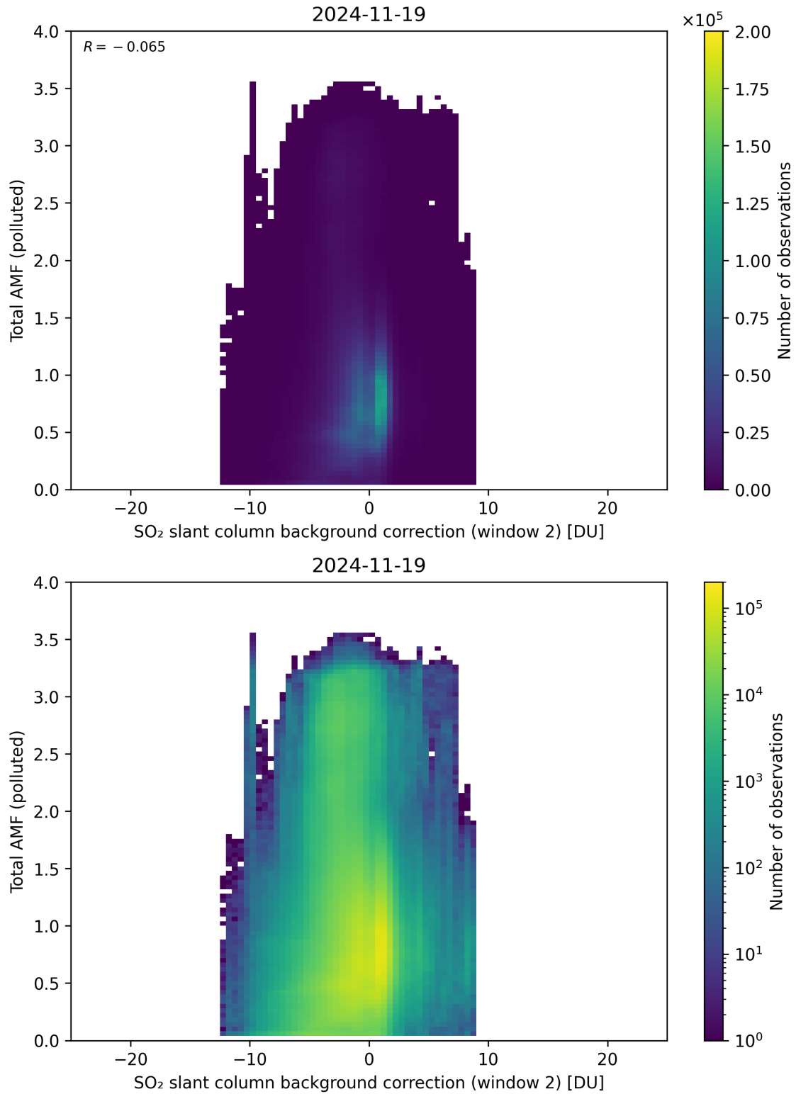
Figure 130: Scatter density plot of “SO 2 slant column background correction (window 2)” against “Total AMF (polluted)” for 2024-11-18 to 2024-11-20.
