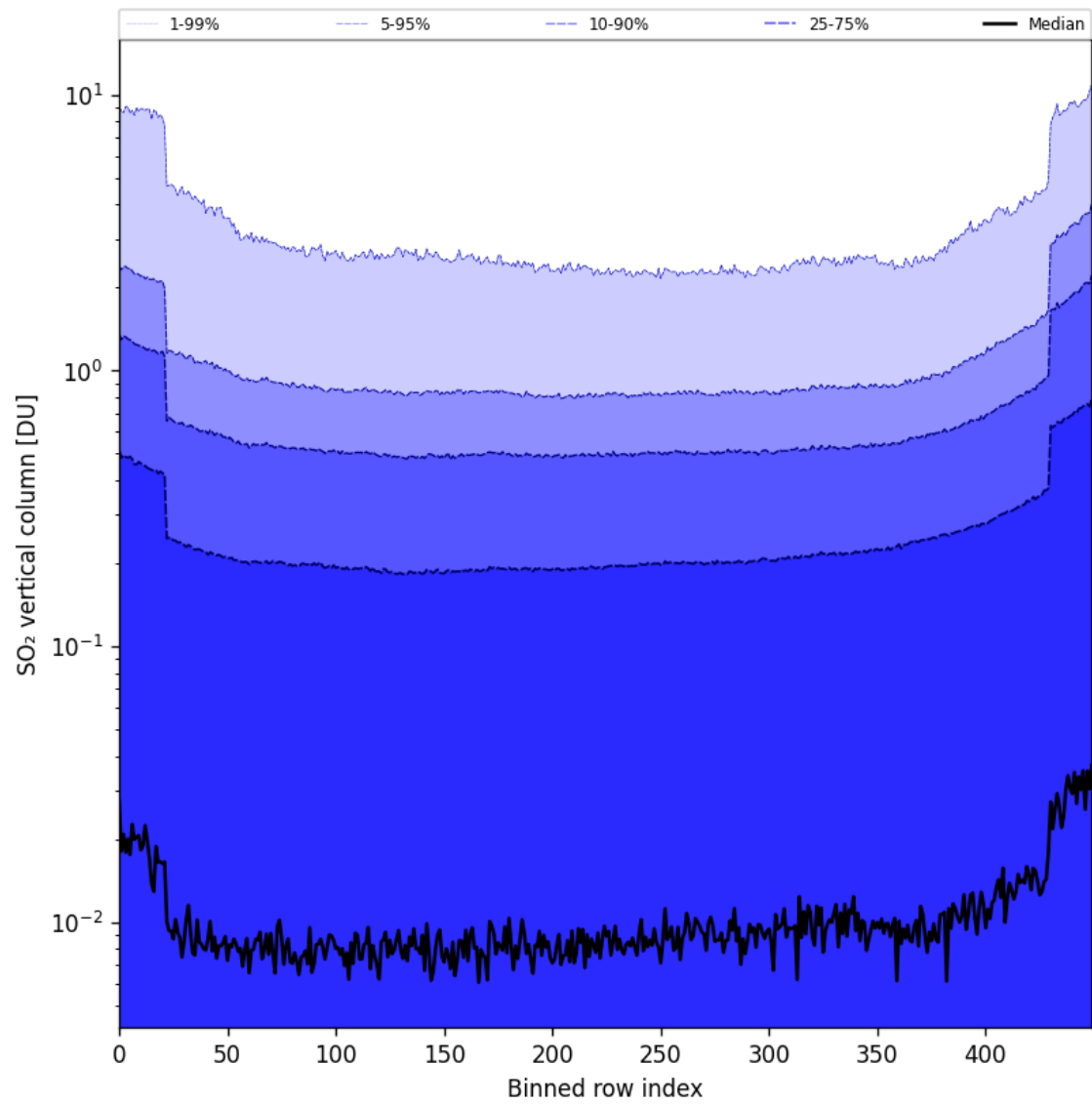
Figure 84: Along track statistics of “SO 2 vertical column” for 2024-11-18 to 2024-11-20
