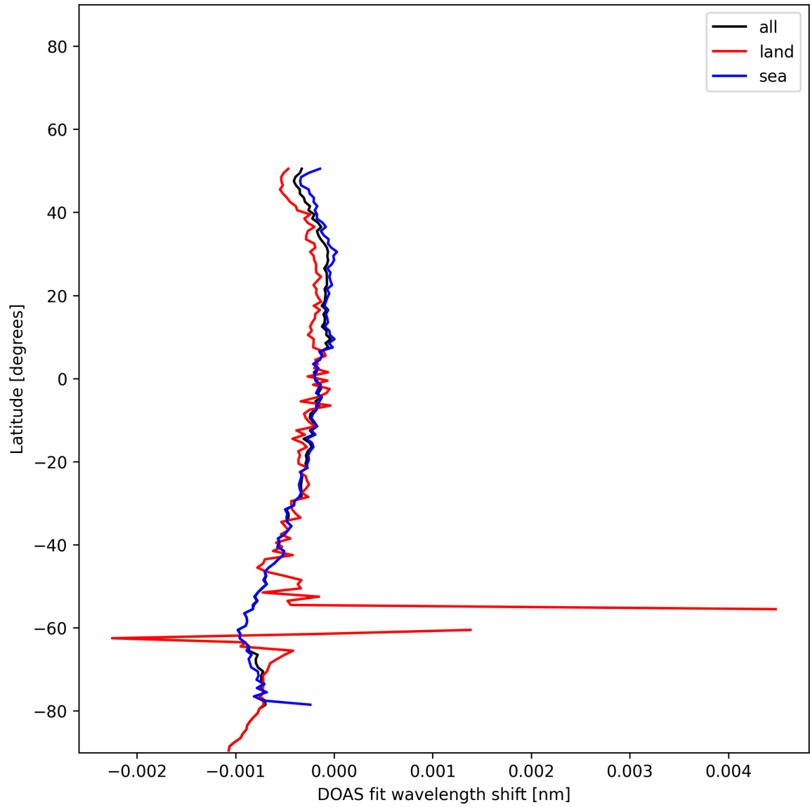
Figure 50: Zonal average of "DOAS fit wavelength shift" for 2024-11-18 to 2024-11-20.
