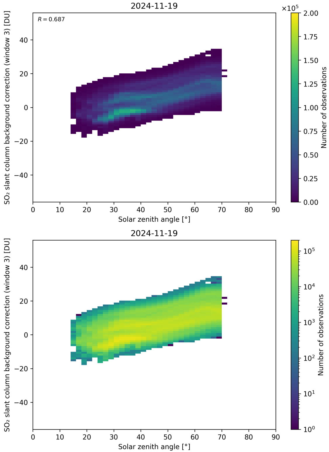
Figure 173: Scatter density plot of “Solar zenith angle” against “SO 2 slant column background correction (window 3)” for 2024-11-18 to 2024-11-20.
