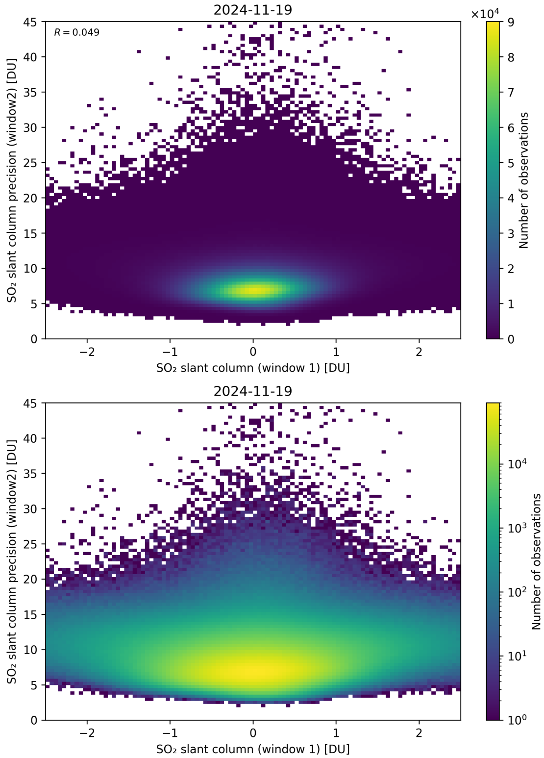
Figure 286: Scatter density plot of “SO 2 slant column (window 1)” against “SO 2 slant column precision (window2)” for 2024-11-18 to 2024-11-20.
