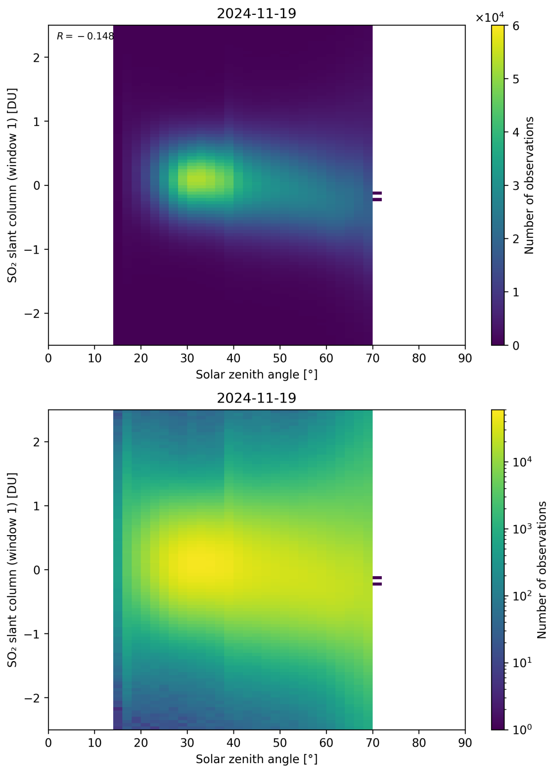
Figure 184: Scatter density plot of “Solar zenith angle” against “SO 2 slant column (window 1)” for 2024-11-18 to 2024-11-20.
