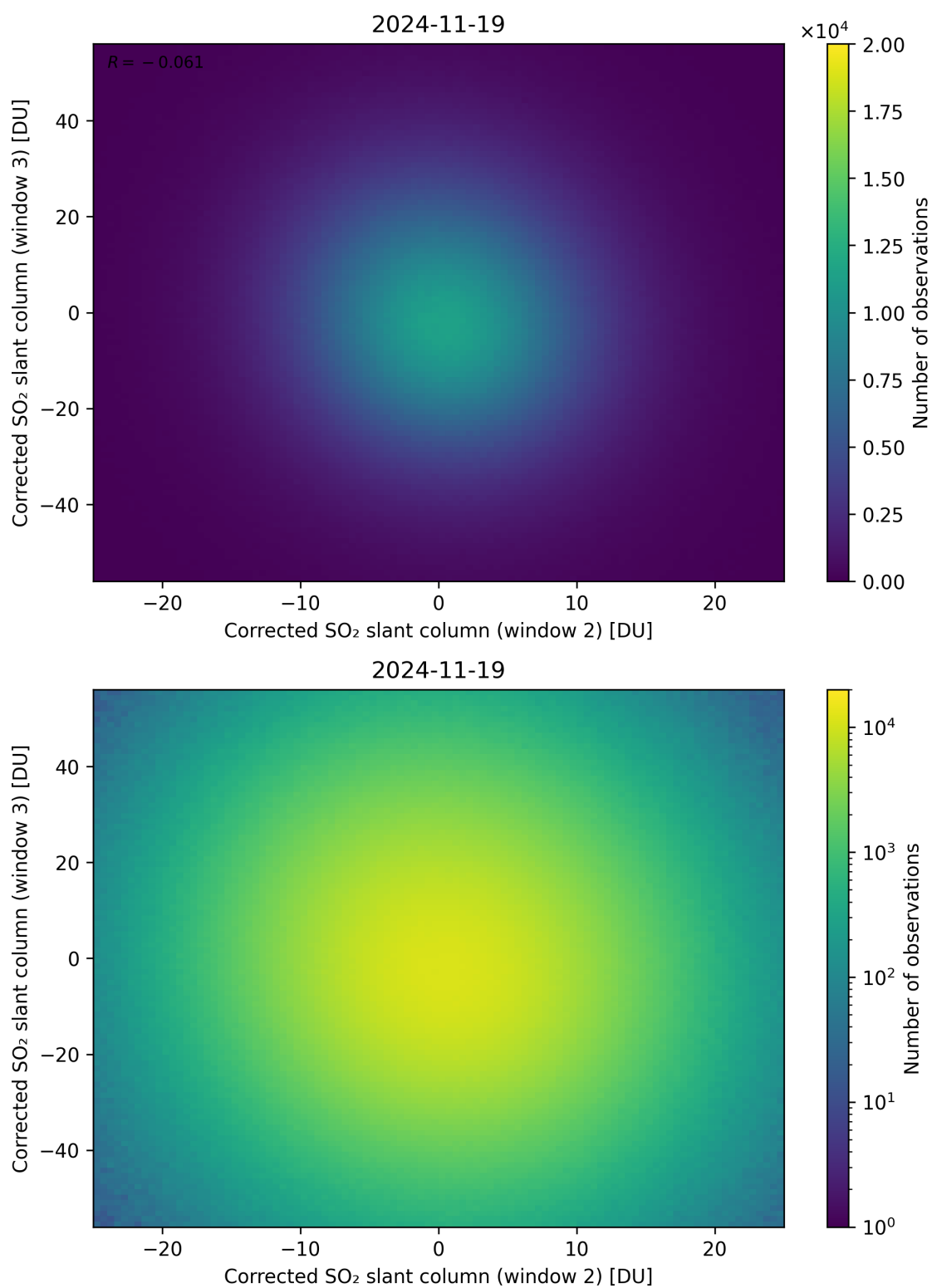
Figure 250: Scatter density plot of “Corrected SO 2 slant column (window 2)” against “Corrected SO 2 slant column (window 3)” for 2024-11-18 to 2024-11-20.
