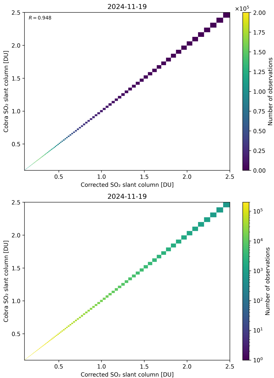
Figure 233: Scatter density plot of “Corrected SO 2 slant column” against “Cobra SO 2 slant column” for 2024-11-18 to 2024-11-20.
