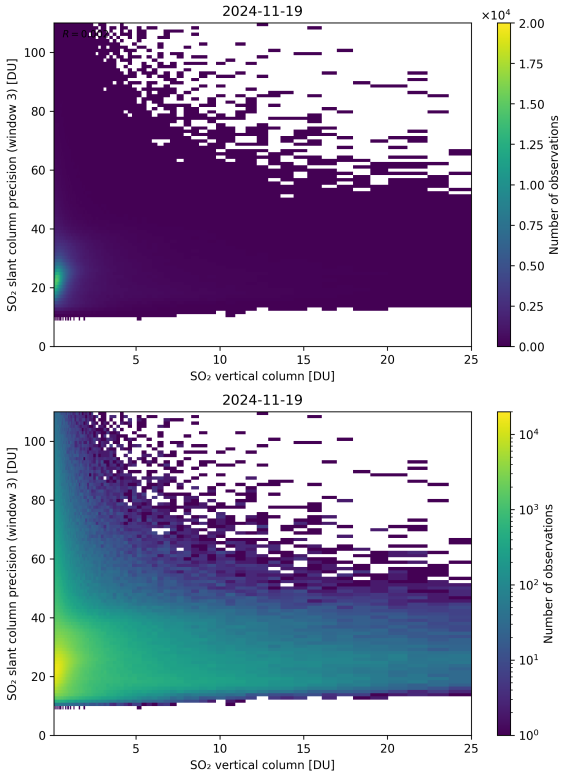
Figure 358: Scatter density plot of “SO 2 vertical column” against “SO 2 slant column precision (window 3)” for 2024-11-18 to 2024-11-20.
