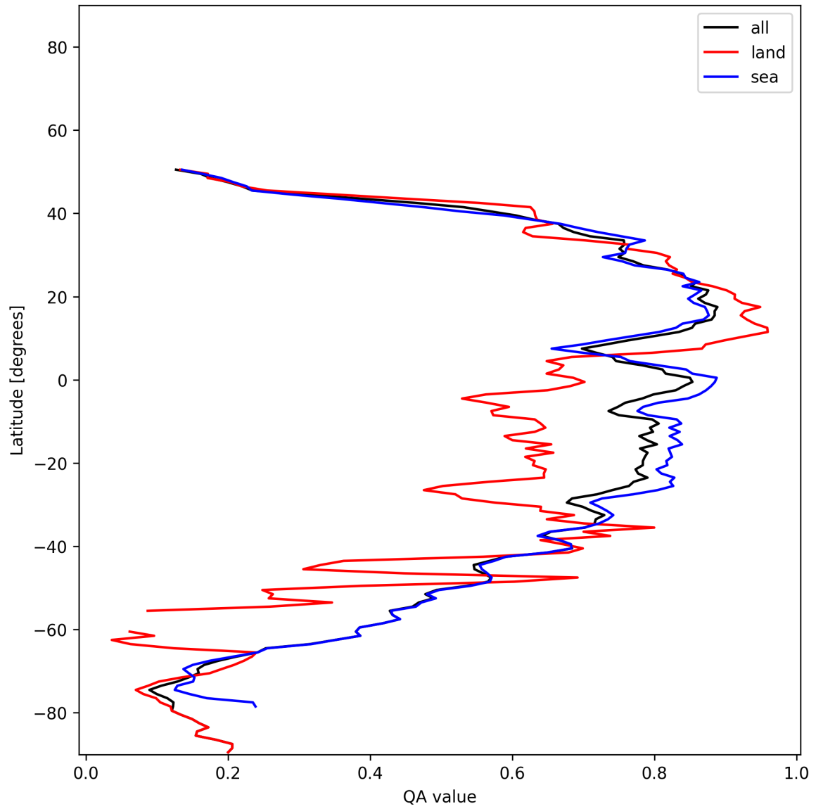
Figure 31: Zonal average of “QA value” for 2024-11-18 to 2024-11-20.
