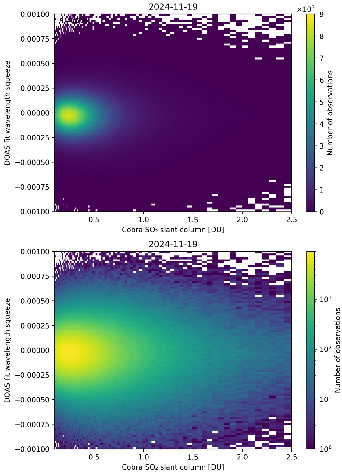
Figure 197: Scatter density plot of “Cobra SO 2 slant column” against “DOAS fit wavelength squeeze” for 2024-11-18 to 2024-11-20.
