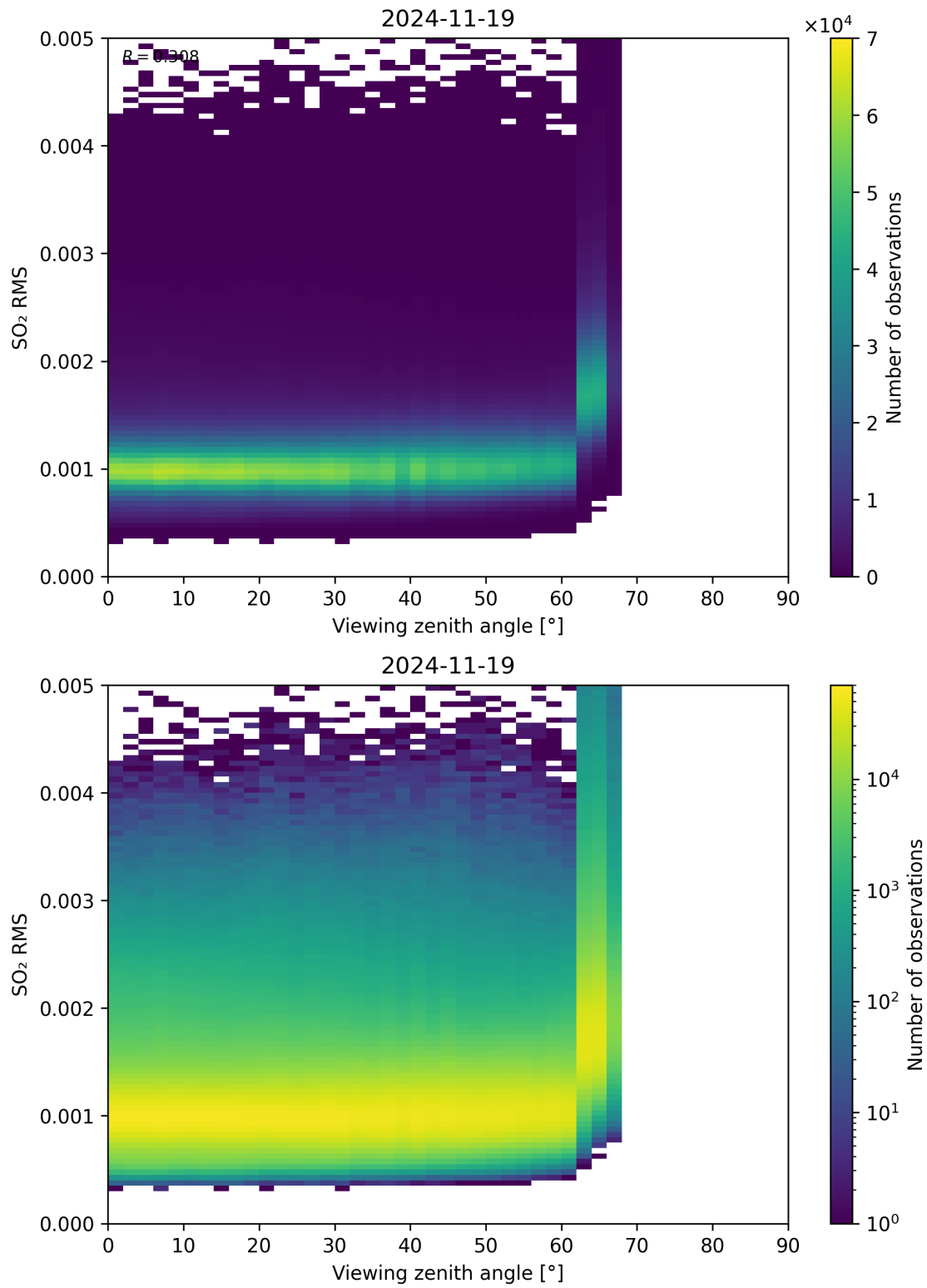
Figure 367: Scatter density plot of “Viewing zenith angle” against “SO 2 RMS” for 2024-11-18 to 2024-11-20.
