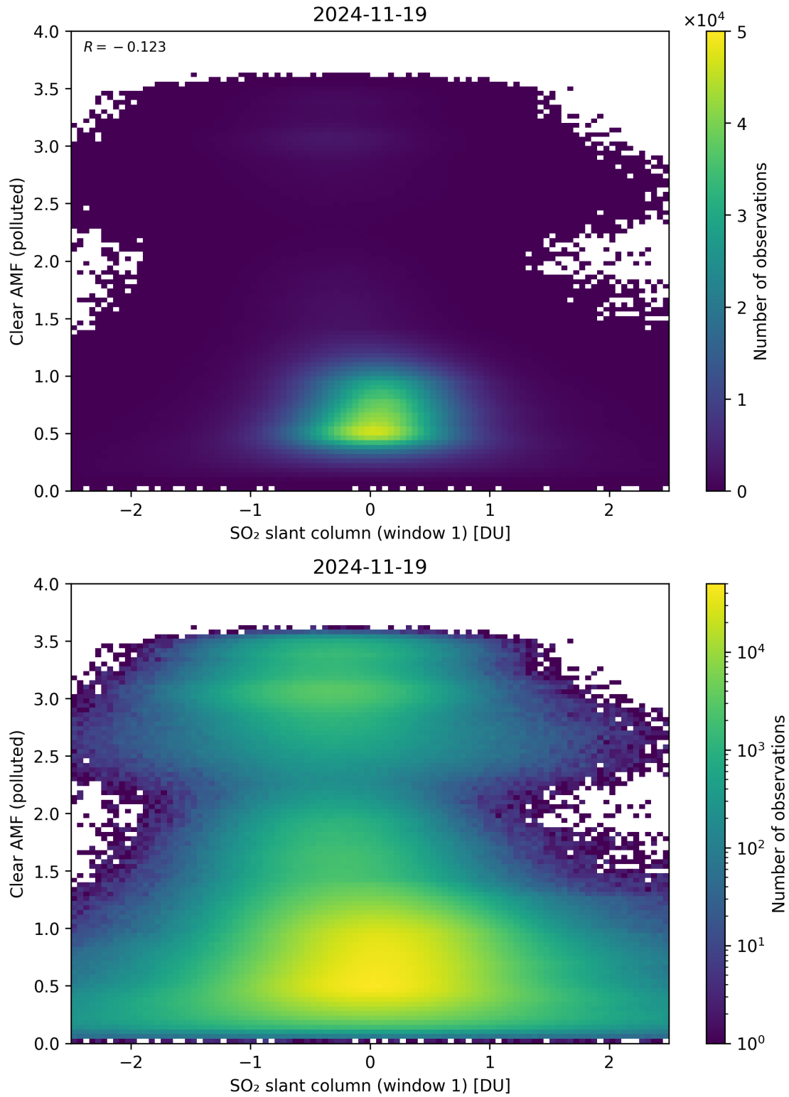
Figure 282: Scatter density plot of “SO 2 slant column (window 1)” against “Clear AMF (polluted)” for 2024-11-18 to 2024-11-20.
