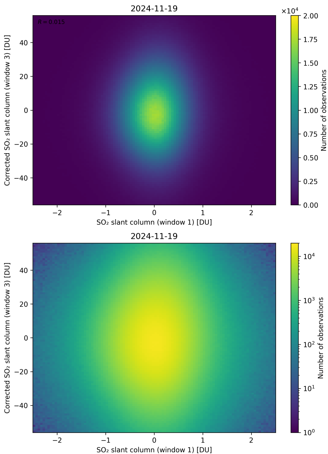
Figure 284: Scatter density plot of “SO 2 slant column (window 1)” against “Corrected SO 2 slant column (window 3)” for 2024-11-18 to 2024-11-20.
