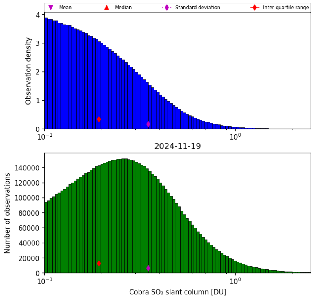
Figure 61: Histogram of “Cobra SO 2 slant column” for 2024-11-18 to 2024-11-20
