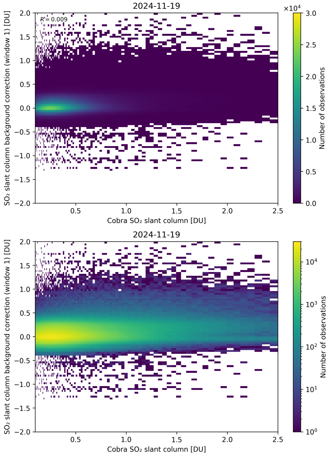
Figure 193: Scatter density plot of “Cobra SO 2 slant column” against “SO 2 slant column background correction (window 1)” for 2024-11-18 to 2024-11-20.
