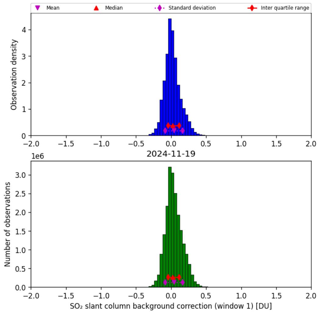
Figure 66: Histogram of “SO 2 slant column background correction (window 1)” for 2024-11-18 to 2024-11-20
