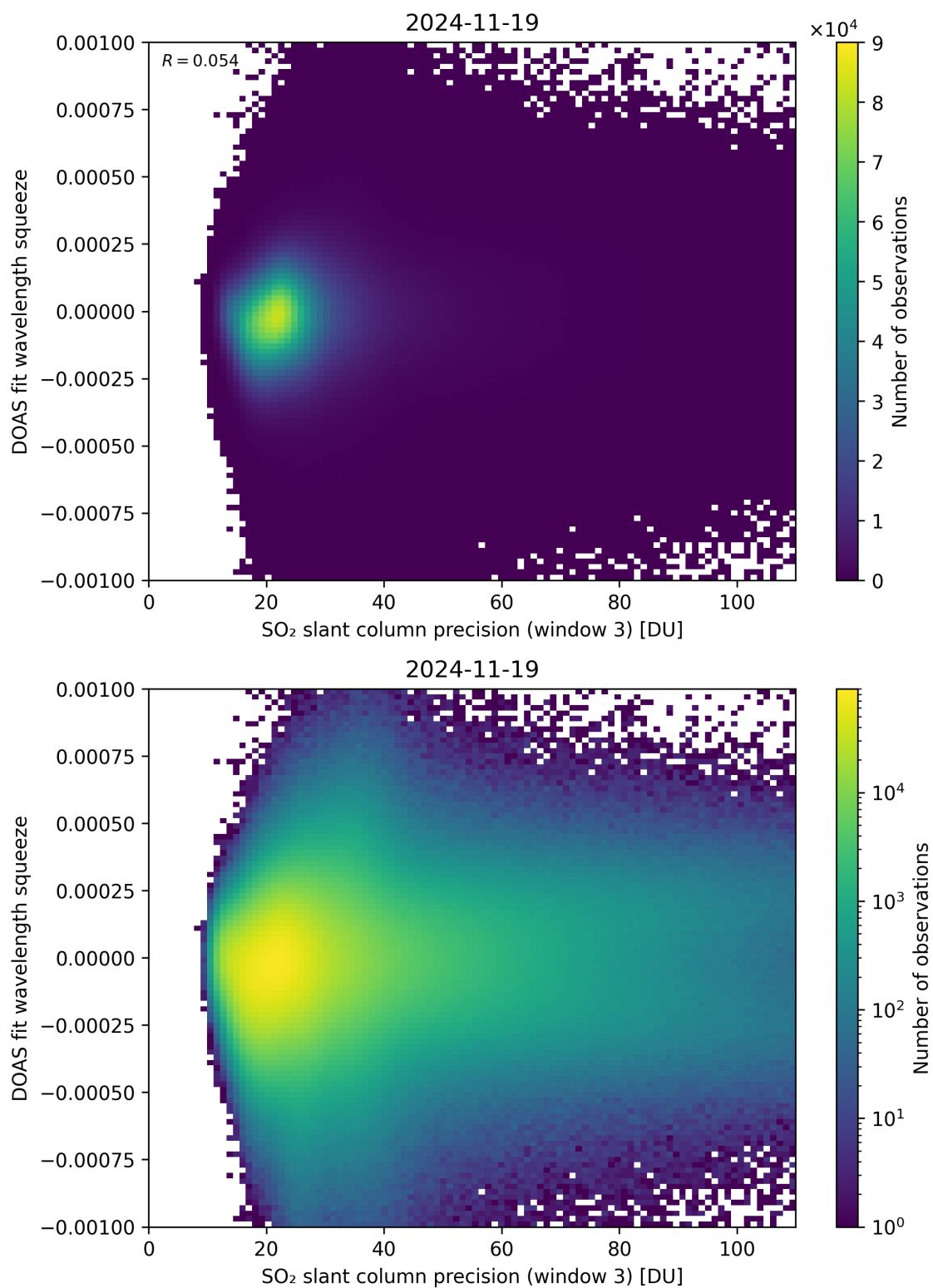
Figure 309: Scatter density plot of “SO 2 slant column precision (window 3)” against “DOAS fit wavelength squeeze” for 2024-11-18 to 2024-11-20.
