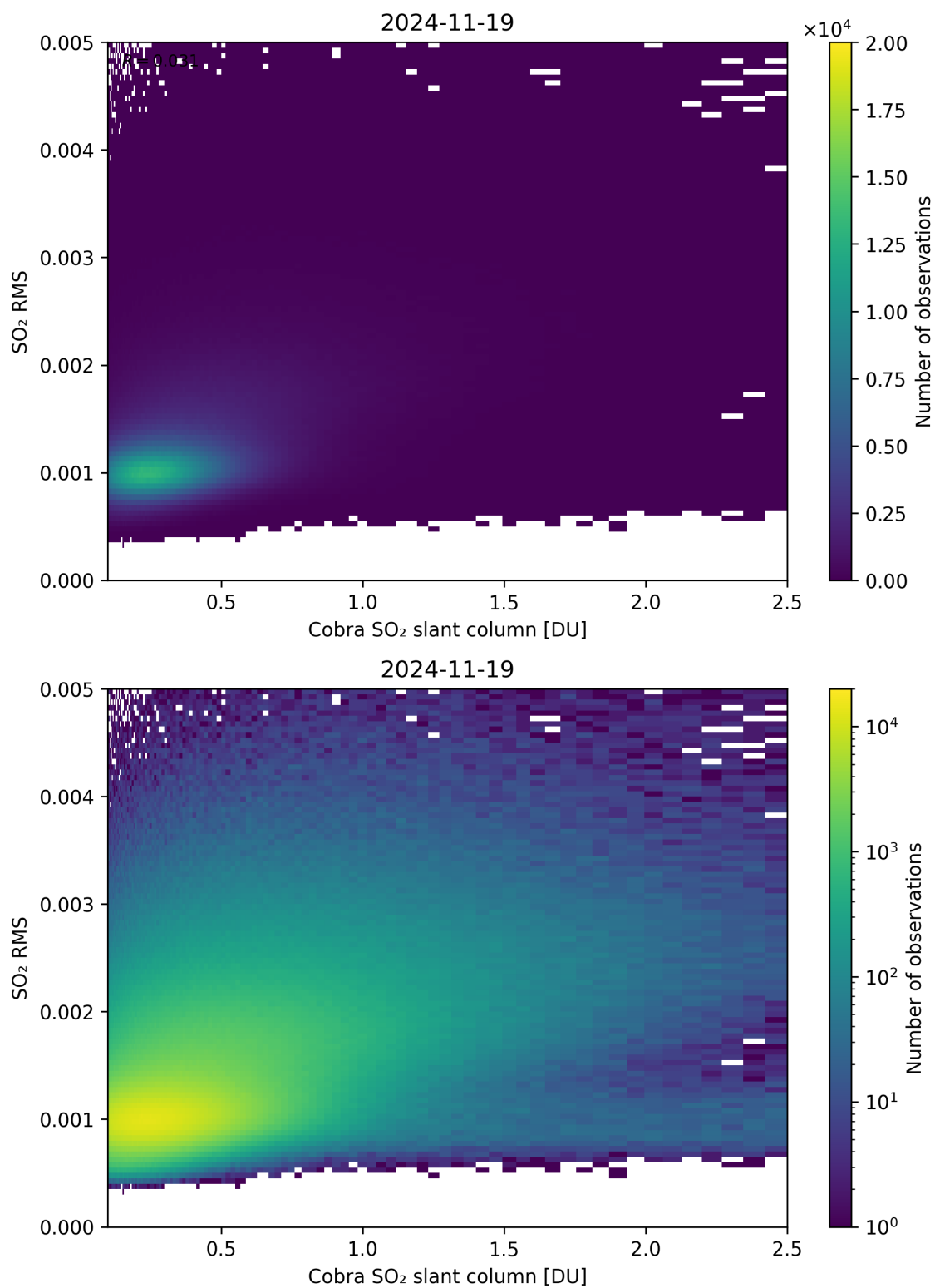
Figure 198: Scatter density plot of “Cobra SO 2 slant column” against “SO 2 RMS” for 2024-11-18 to 2024-11-20.
