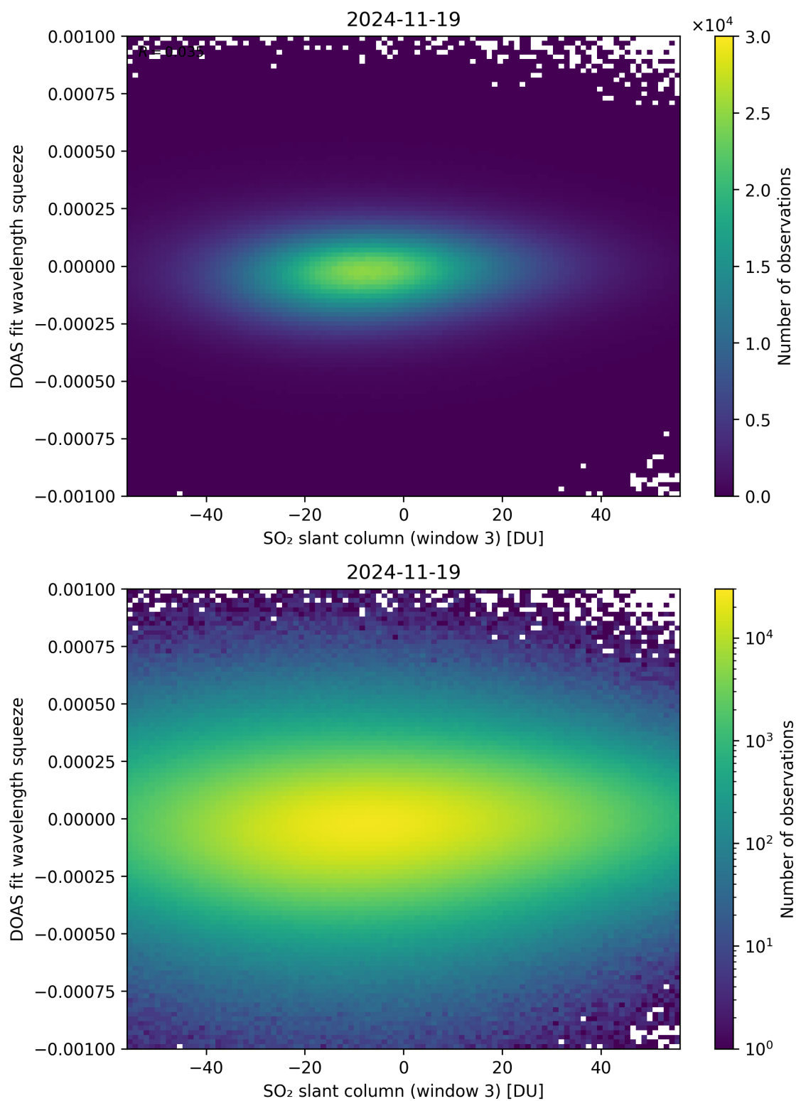
Figure 305: Scatter density plot of “SO 2 slant column (window 3)” against “DOAS fit wavelength squeeze” for 2024-11-18 to 2024-11-20.
