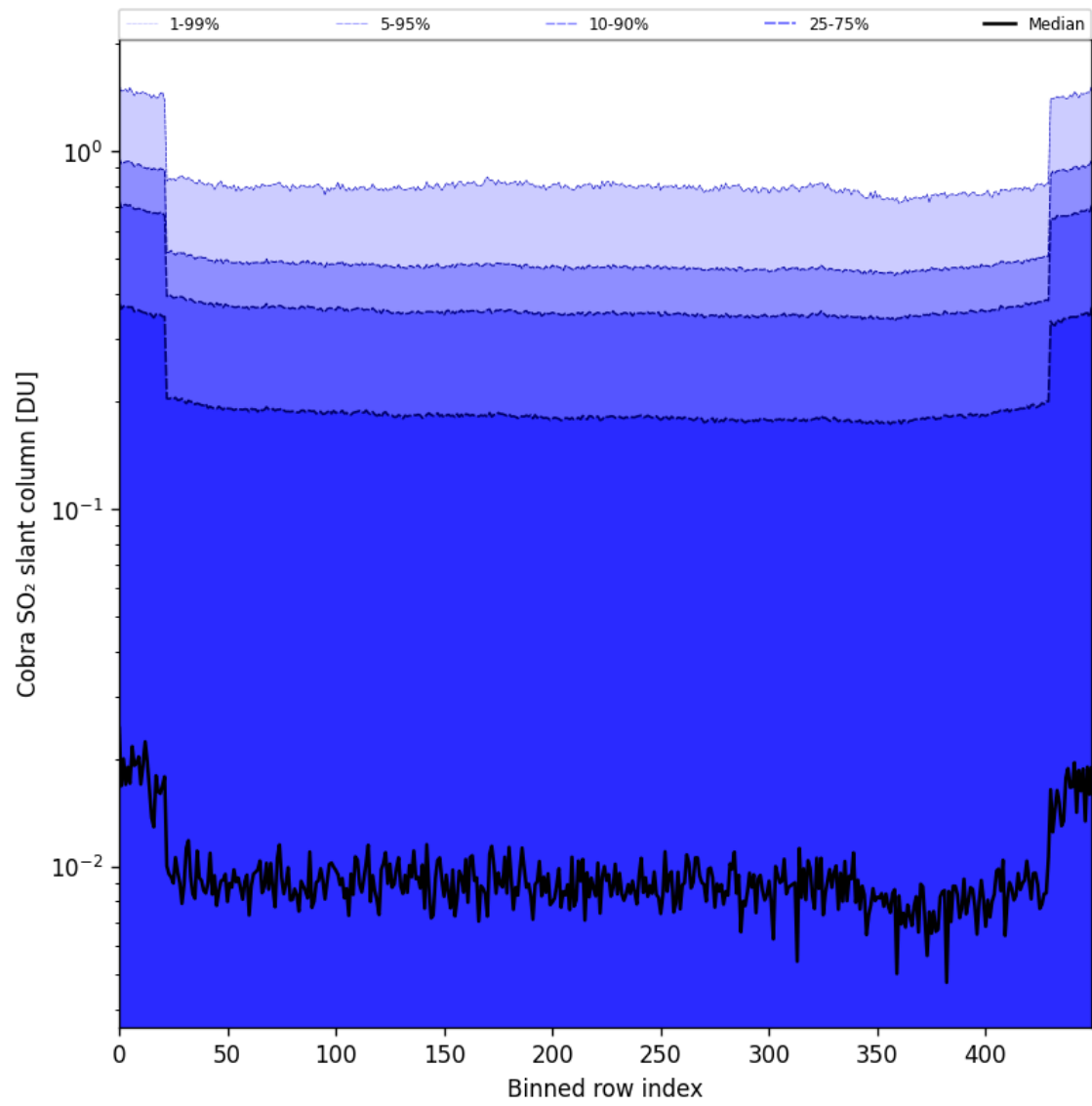
Figure 87: Along track statistics of "Cobra SO 2 slant column" for 2024-11-18 to 2024-11-20
