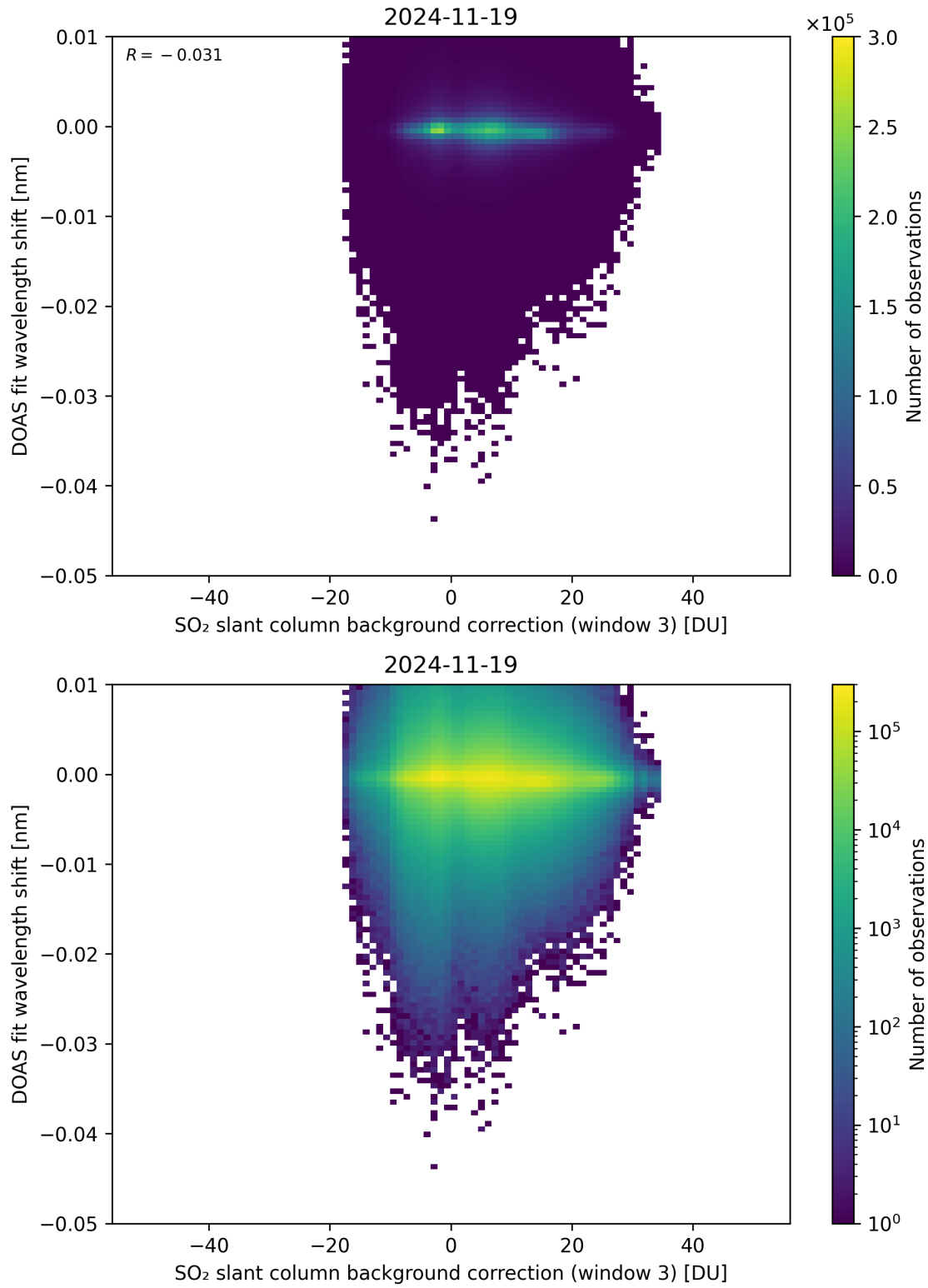
Figure 132: Scatter density plot of “SO 2 slant column background correction (window 3)” against “DOAS fit wavelength shift” for 2024-11-18 to 2024-11-20.
