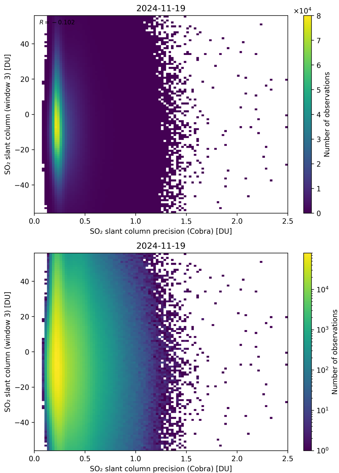
Figure 211: Scatter density plot of “SO 2 slant column precision (Cobra)” against “SO 2 slant column (window 3)” for 2024-11-18 to 2024-11-20.
