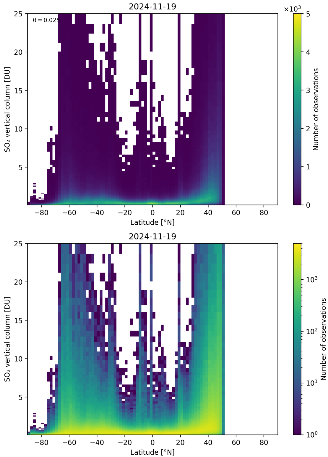
Figure 169: Scatter density plot of “Latitude” against “SO 2 vertical column” for 2024-11-18 to 2024-11-20.
