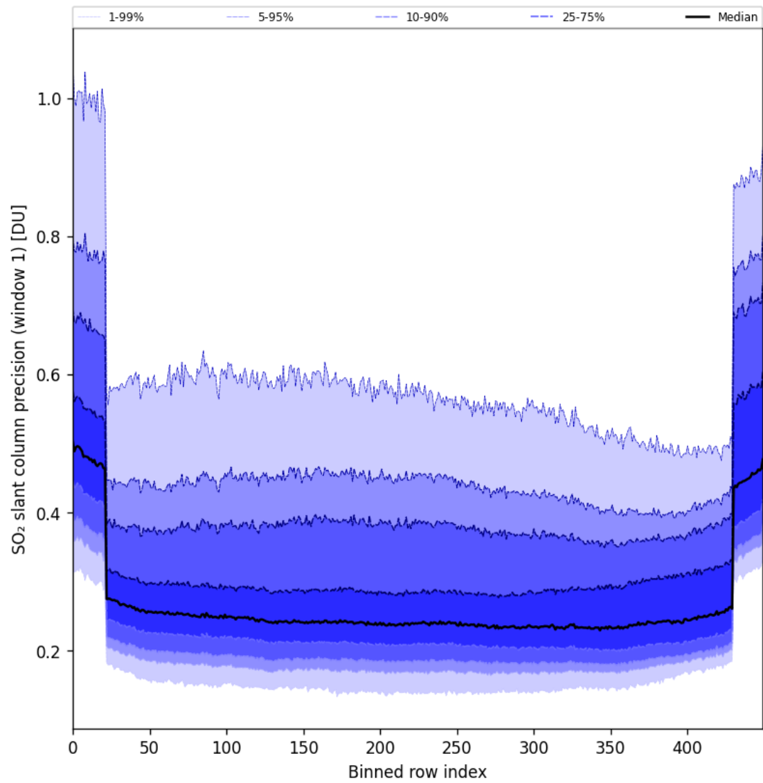
Figure 90: Along track statistics of “SO 2 slant column precision (window 1)” for 2024-11-18 to 2024-11-20
