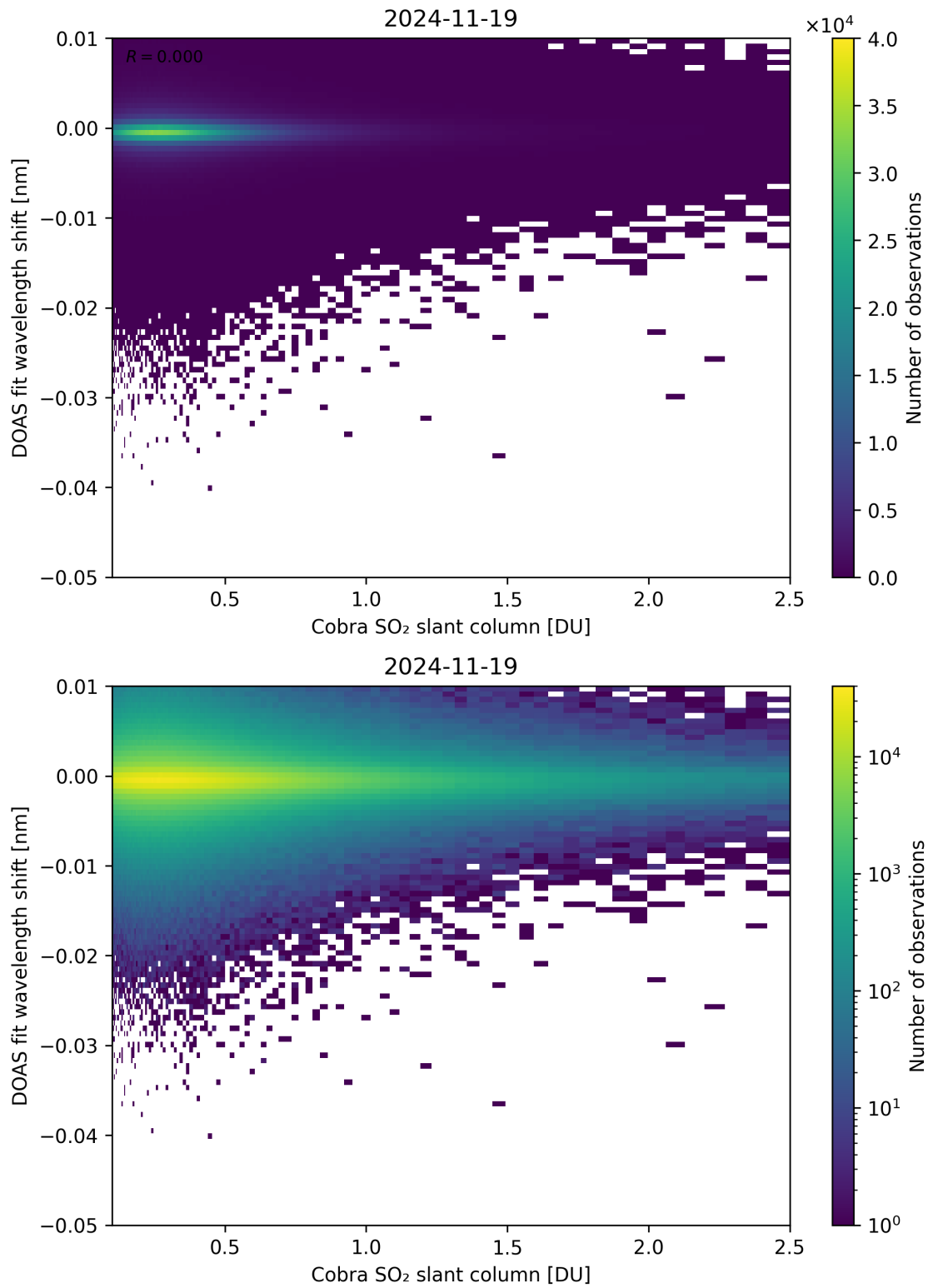
Figure 196: Scatter density plot of “Cobra SO 2 slant column” against “DOAS fit wavelength shift” for 2024-11-18 to 2024-11-20.
