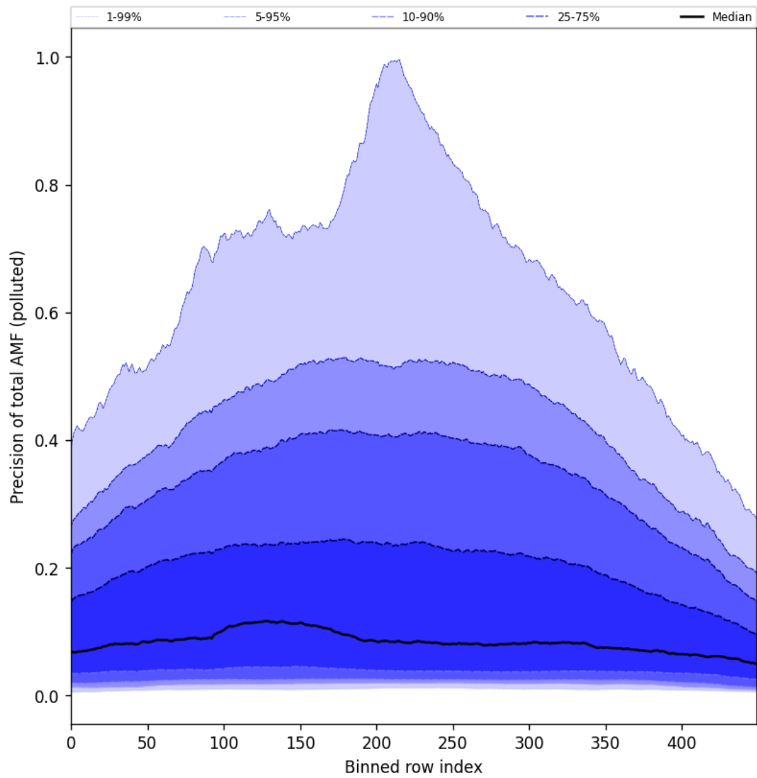
Figure 106: Along track statistics of “Precision of total AMF (polluted)” for 2024-11-18 to 2024-11-20
