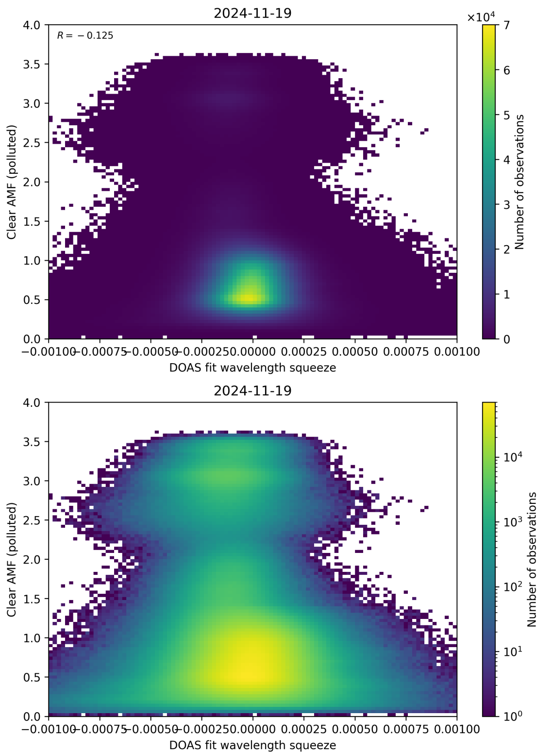
Figure 144: Scatter density plot of “DOAS fit wavelength squeeze” against “Clear AMF (polluted)” for 2024-11-18 to 2024-11-20.
