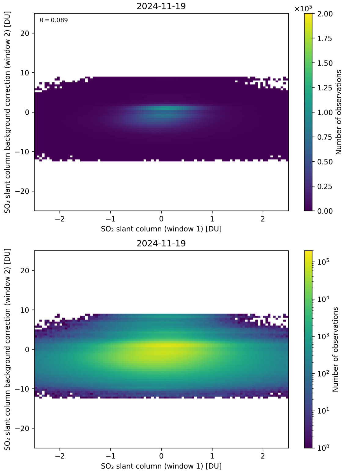
Figure 263: Scatter density plot of “SO 2 slant column (window 1)” against “SO 2 slant column background correction (window 2)” for 2024-11-18 to 2024-11-20.
