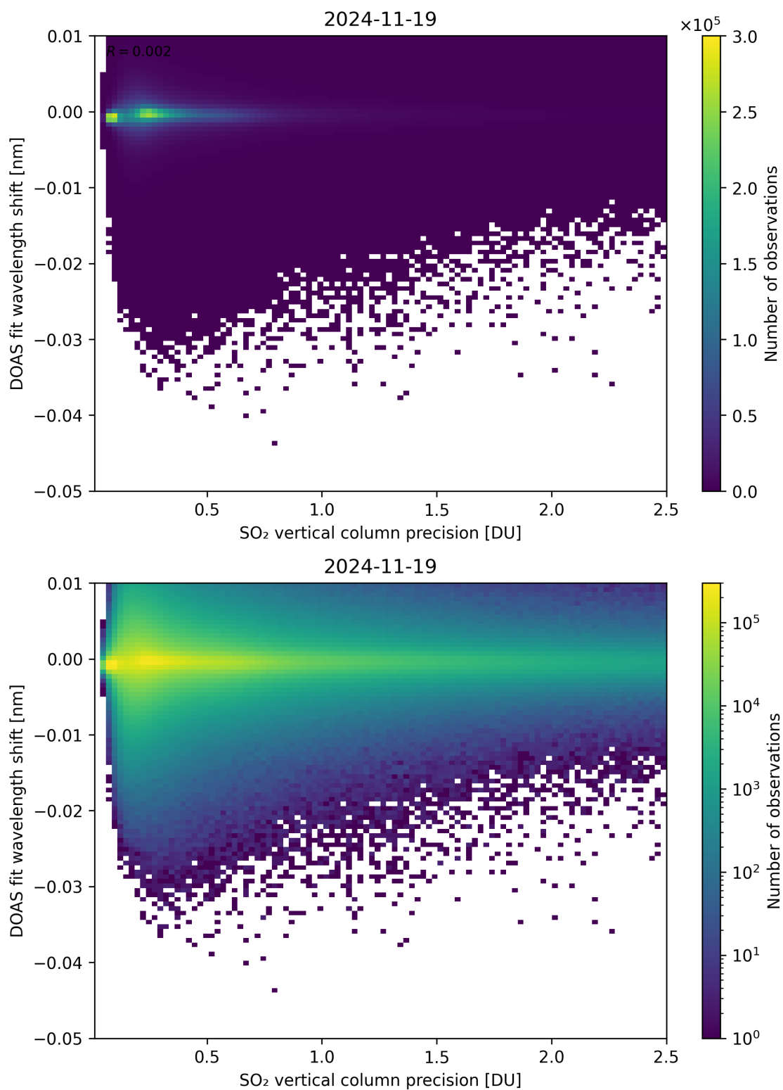
Figure 332: Scatter density plot of “SO 2 vertical column precision” against “DOAS fit wavelength shift” for 2024-11-18 to 2024-11-20.
