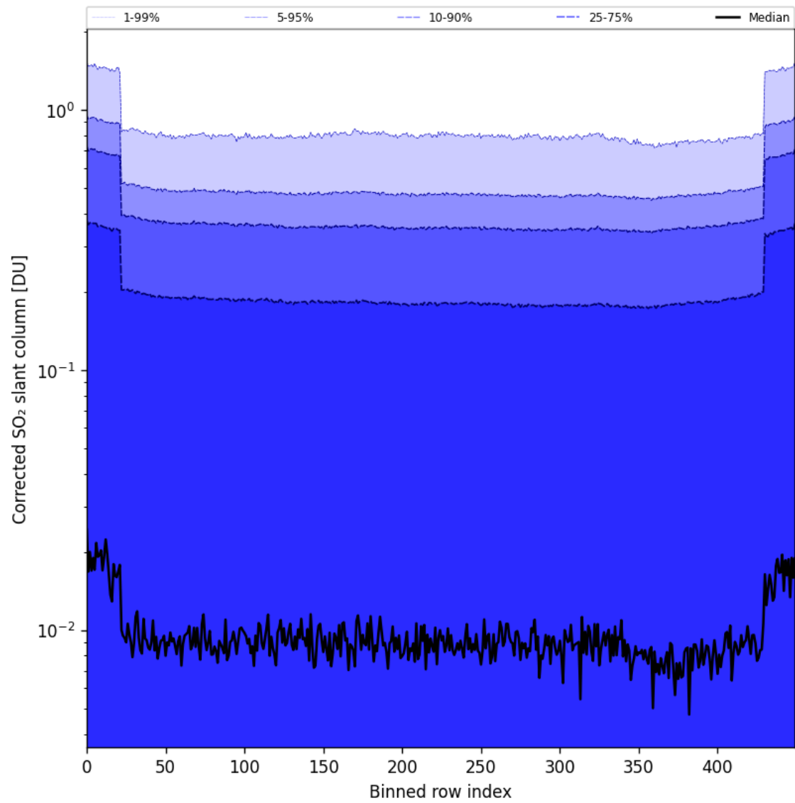
Figure 86: Along track statistics of “Corrected SO 2 slant column” for 2024-11-18 to 2024-11-20
