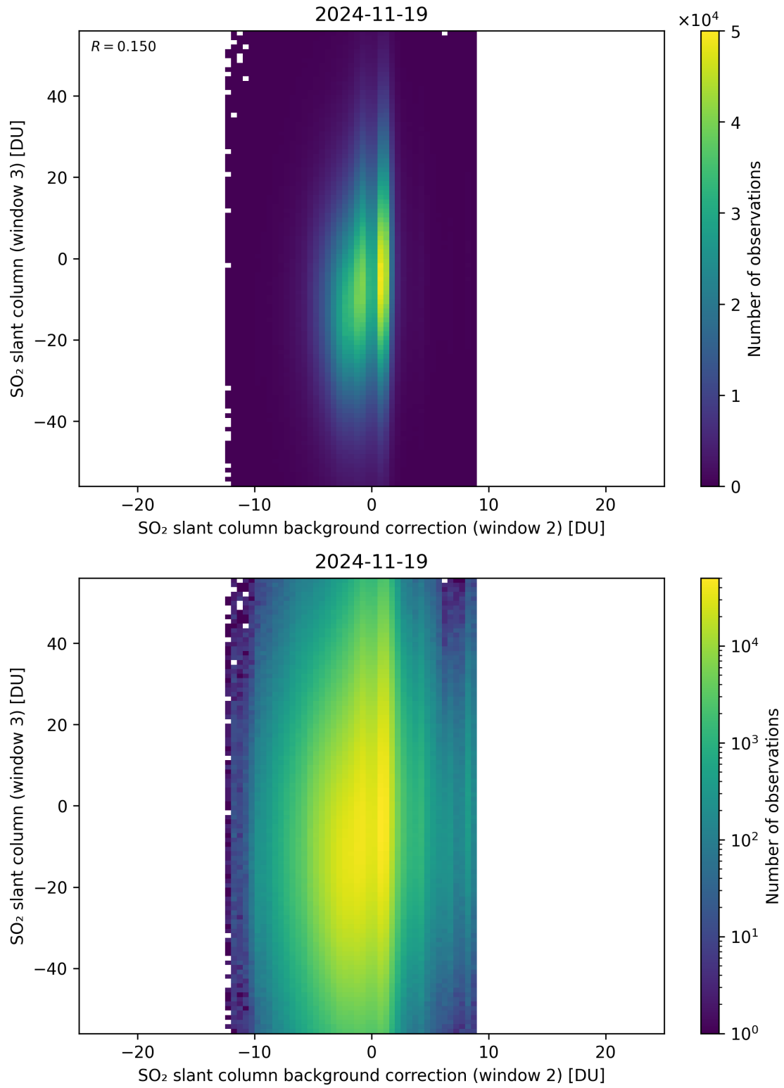
Figure 128: Scatter density plot of “SO 2 slant column background correction (window 2)” against “SO 2 slant column (window 3)” for 2024-11-18 to 2024-11-20.
