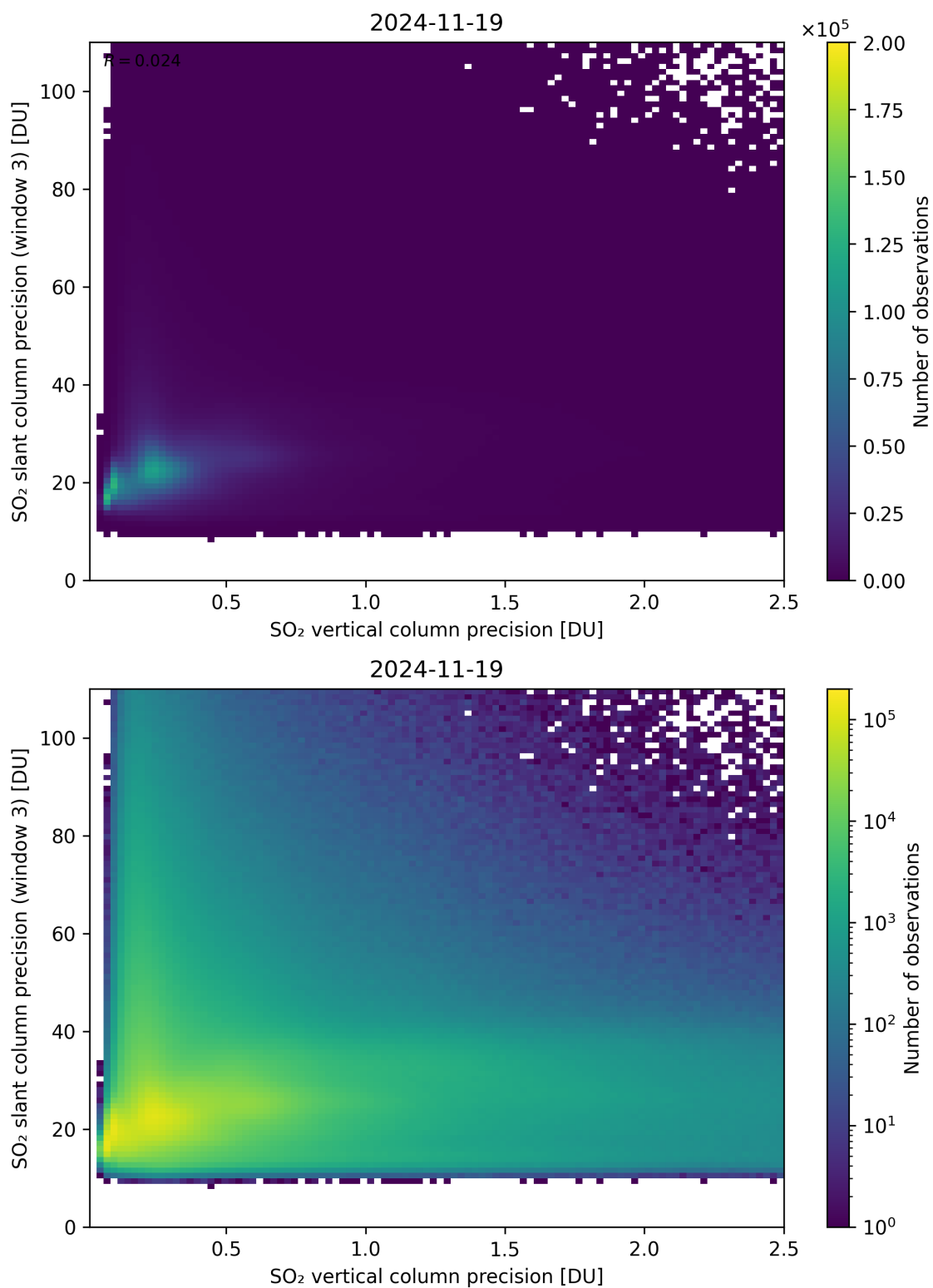
Figure 345: Scatter density plot of “SO 2 vertical column precision” against “SO 2 slant column precision (window 3)” for 2024-11-18 to 2024-11-20.
