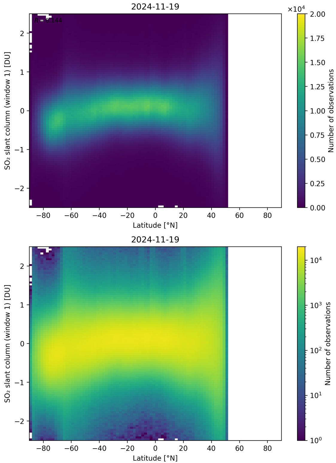
Figure 162: Scatter density plot of “Latitude” against “SO 2 slant column (window 1)” for 2024-11-18 to 2024-11-20.
