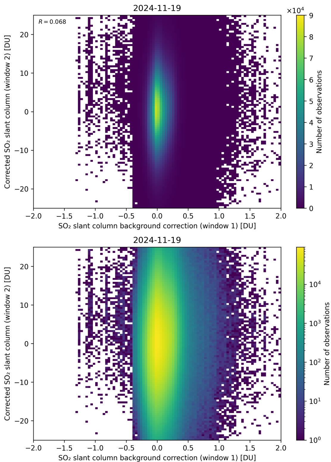
Figure 115: Scatter density plot of “SO 2 slant column background correction (window 1)” against “Corrected SO 2 slant column (window 2)” for 2024-11-18 to 2024-11-20.
