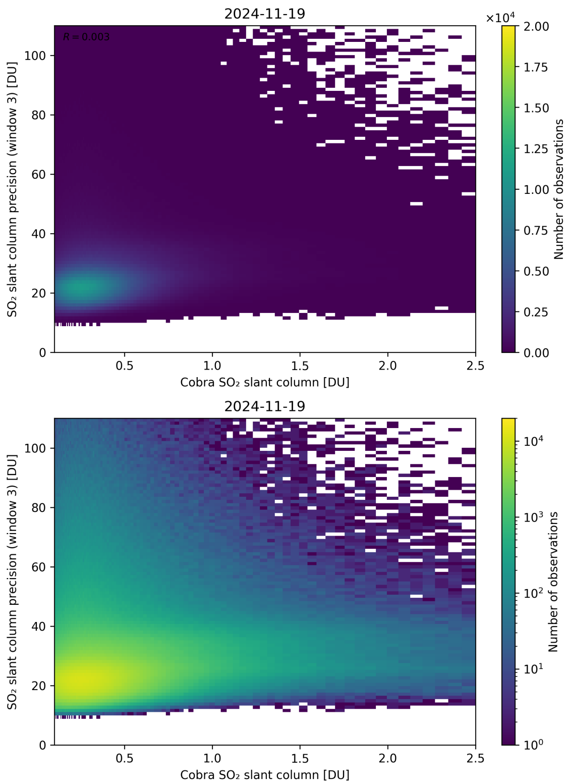
Figure 223: Scatter density plot of “Cobra SO 2 slant column” against “SO 2 slant column precision (window 3)” for 2024-11-18 to 2024-11-20.
