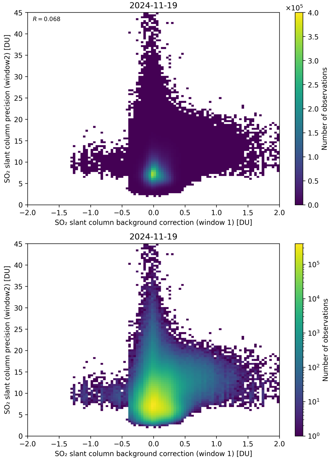
Figure 117: Scatter density plot of “SO 2 slant column background correction (window 1)” against “SO 2 slant column precision (window2)” for 2024-11-18 to 2024-11-20.
