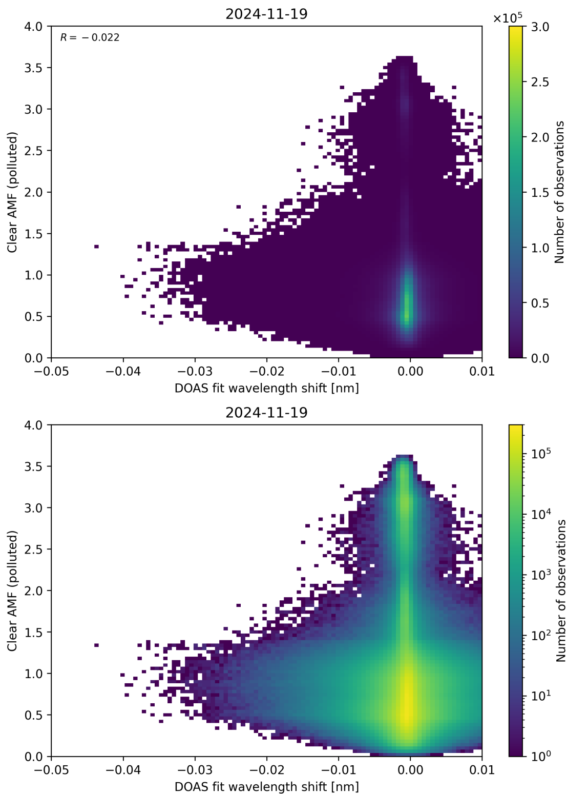
Figure 140: Scatter density plot of “DOAS fit wavelength shift” against “Clear AMF (polluted)” for 2024-11-18 to 2024-11-20.
