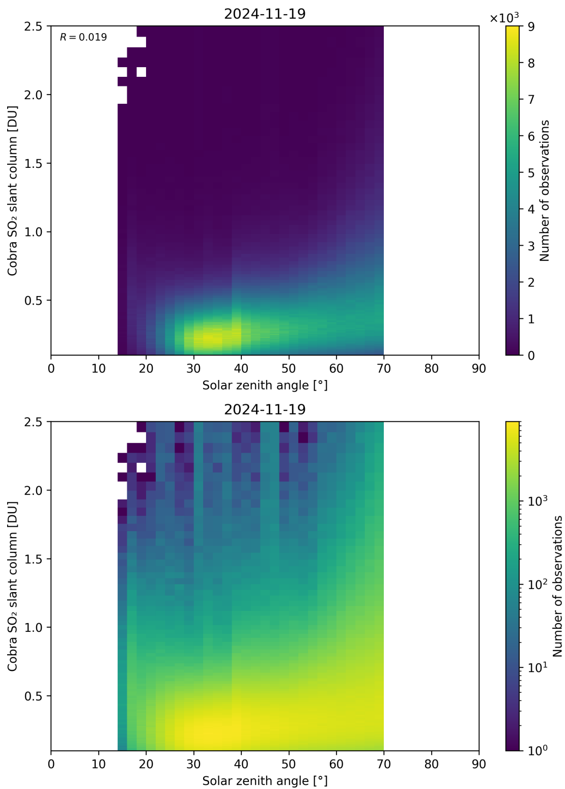
Figure 179: Scatter density plot of “Solar zenith angle” against “Cobra SO 2 slant column” for 2024-11-18 to 2024-11-20.
