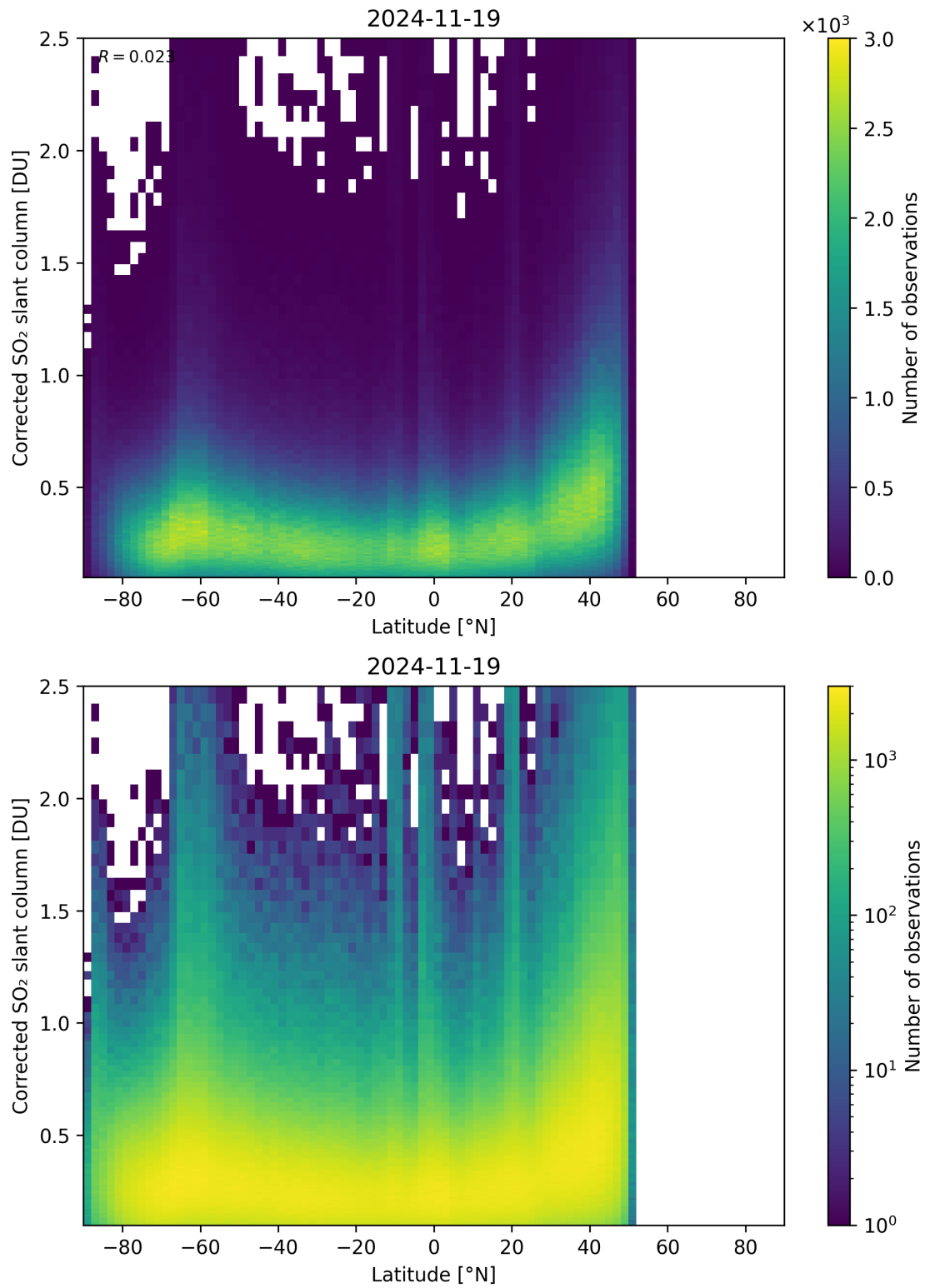
Figure 159: Scatter density plot of “Latitude” against “Corrected SO 2 slant column” for 2024-11-18 to 2024-11-20.
