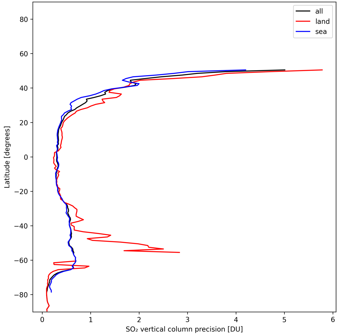
Figure 33: Zonal average of “SO 2 vertical column precision” for 2024-11-18 to 2024-11-20.
