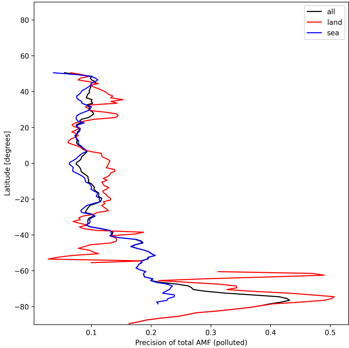
Figure 54: Zonal average of “Precision of total AMF (polluted)” for 2024-11-18 to 2024-11-20.
