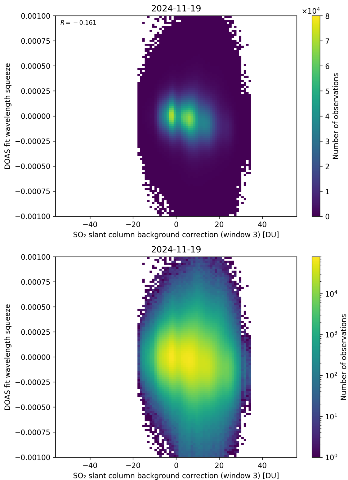
Figure 133: Scatter density plot of “SO 2 slant column background correction (window 3)” against “DOAS fit wavelength squeeze” for 2024-11-18 to 2024-11-20.
