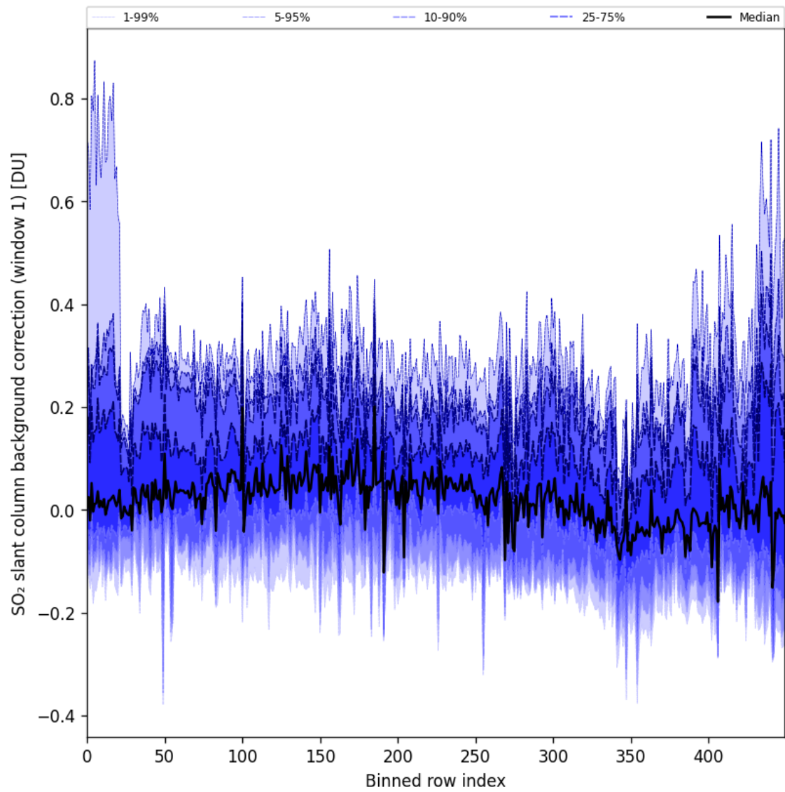
Figure 92: Along track statistics of “SO 2 slant column background correction (window 1)” for 2024-11-18 to 2024-11-20
