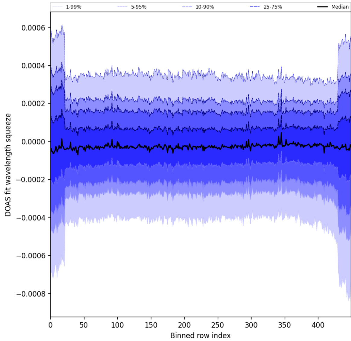
Figure 103: Along track statistics of “DOAS fit wavelength squeeze” for 2024-11-18 to 2024-11-20
