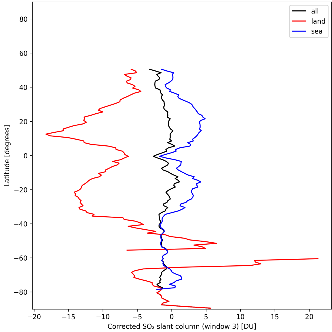
Figure 47: Zonal average of “Corrected SO 2 slant column (window 3)” for 2024-11-18 to 2024-11-20.
