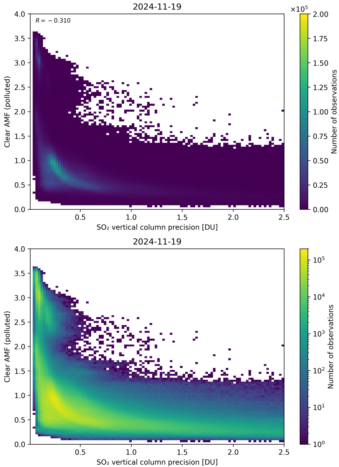
Figure 335: Scatter density plot of “SO 2 vertical column precision” against “Clear AMF (polluted)” for 2024-11-18 to 2024-11-20.
