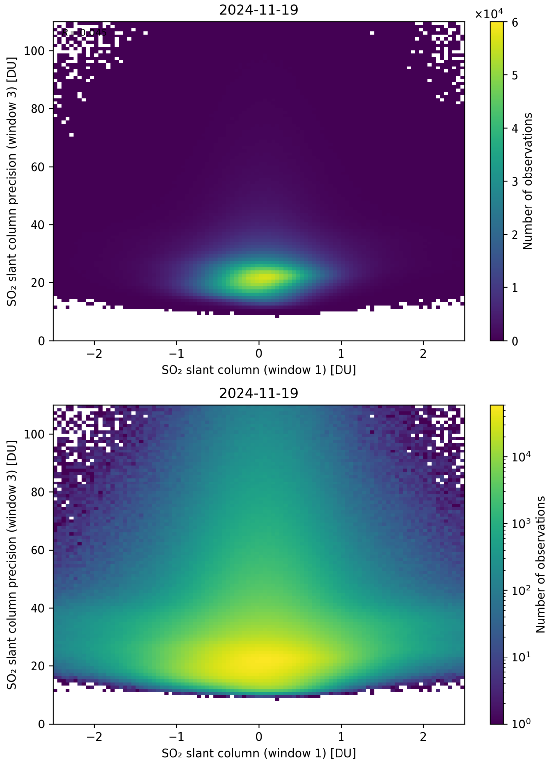
Figure 288: Scatter density plot of “SO 2 slant column (window 1)” against “SO 2 slant column precision (window 3)” for 2024-11-18 to 2024-11-20.
