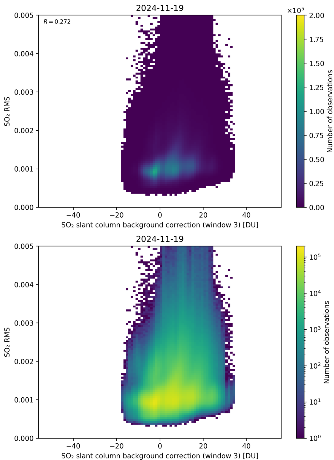
Figure 134: Scatter density plot of “SO 2 slant column background correction (window 3)” against “SO 2 RMS” for 2024-11-18 to 2024-11-20.
