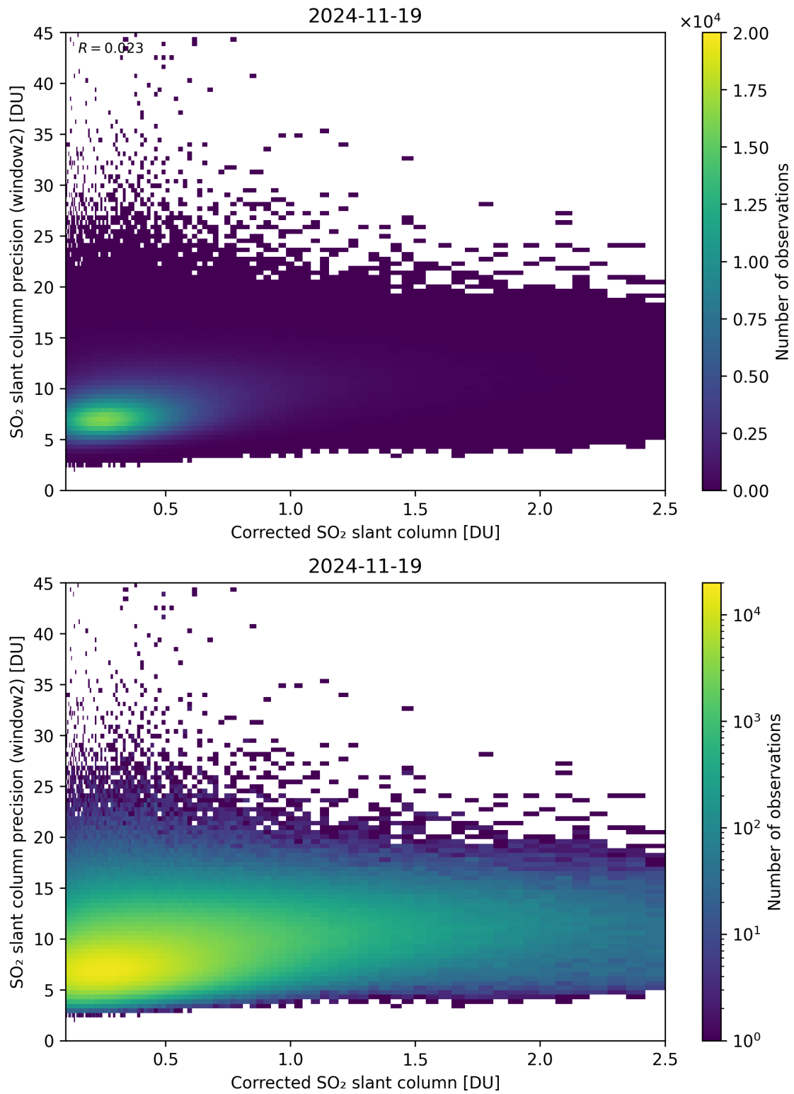
Figure 239: Scatter density plot of “Corrected SO 2 slant column” against “SO 2 slant column precision (window2)” for 2024-11-18 to 2024-11-20.
