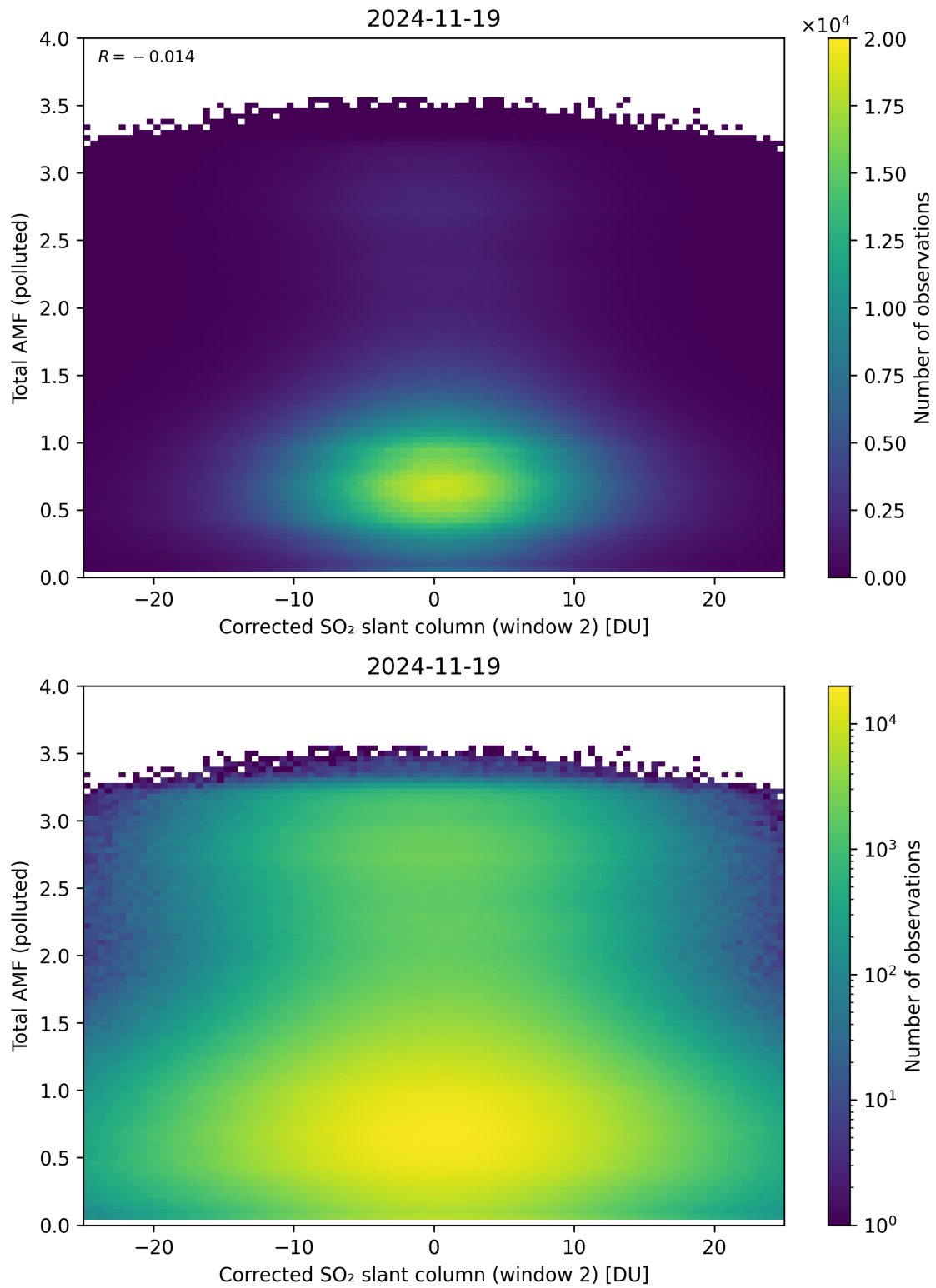
Figure 253: Scatter density plot of “Corrected SO 2 slant column (window 2)” against “Total AMF (polluted)” for 2024-11-18 to 2024-11-20.
