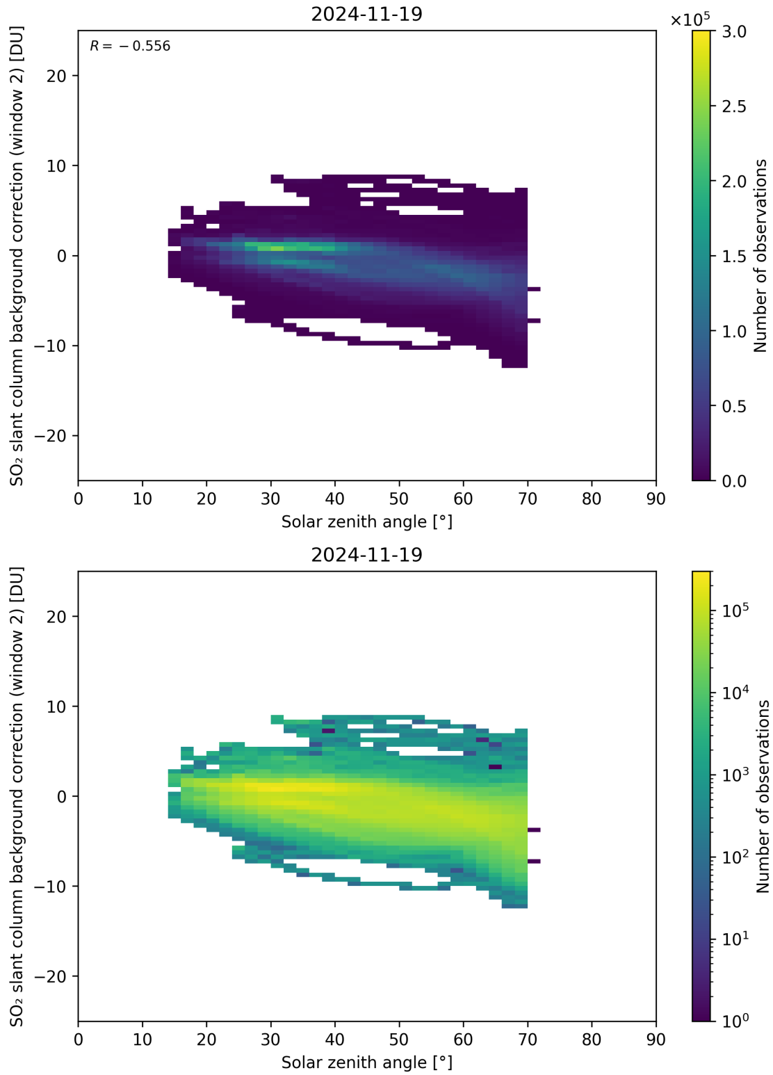
Figure 172: Scatter density plot of “Solar zenith angle” against “SO 2 slant column background correction (window 2)” for 2024-11-18 to 2024-11-20.
