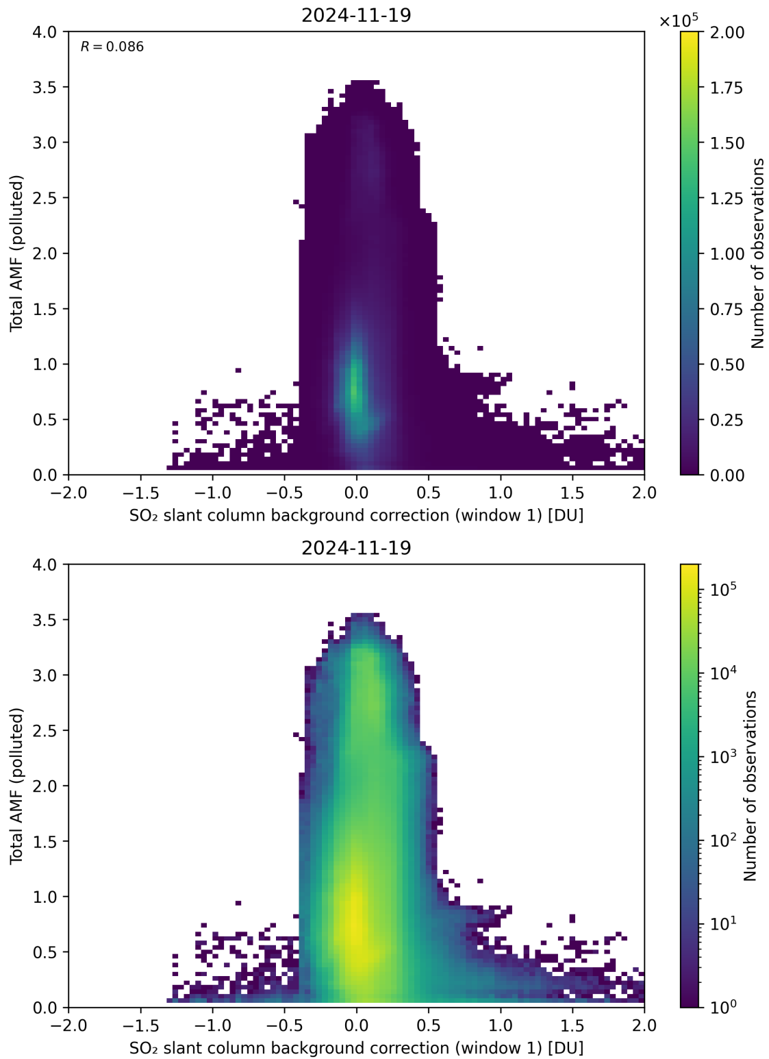
Figure 120: Scatter density plot of “SO 2 slant column background correction (window 1)” against “Total AMF (polluted)” for 2024-11-18 to 2024-11-20.
