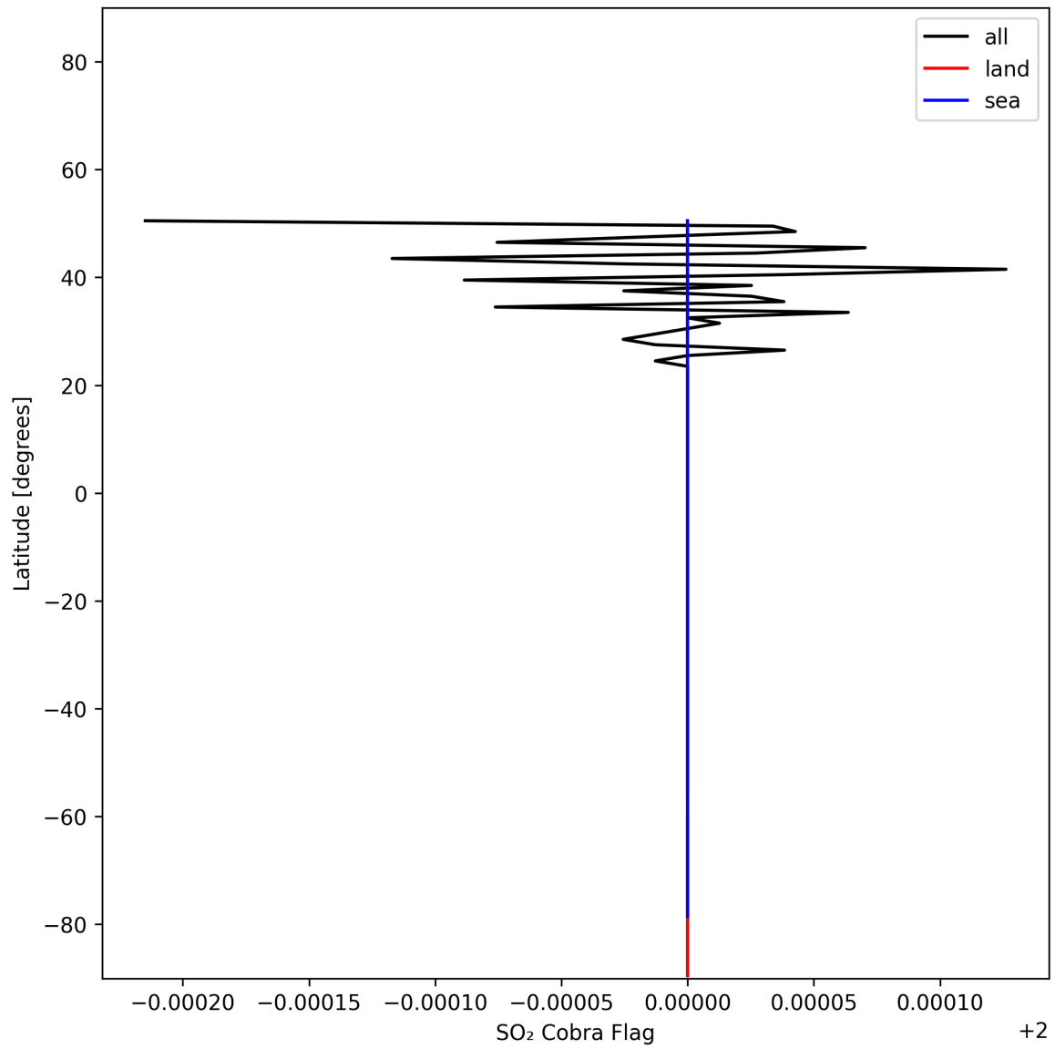
Figure 49: Zonal average of "SO 2 Cobra Flag" for 2024-11-18 to 2024-11-20.
