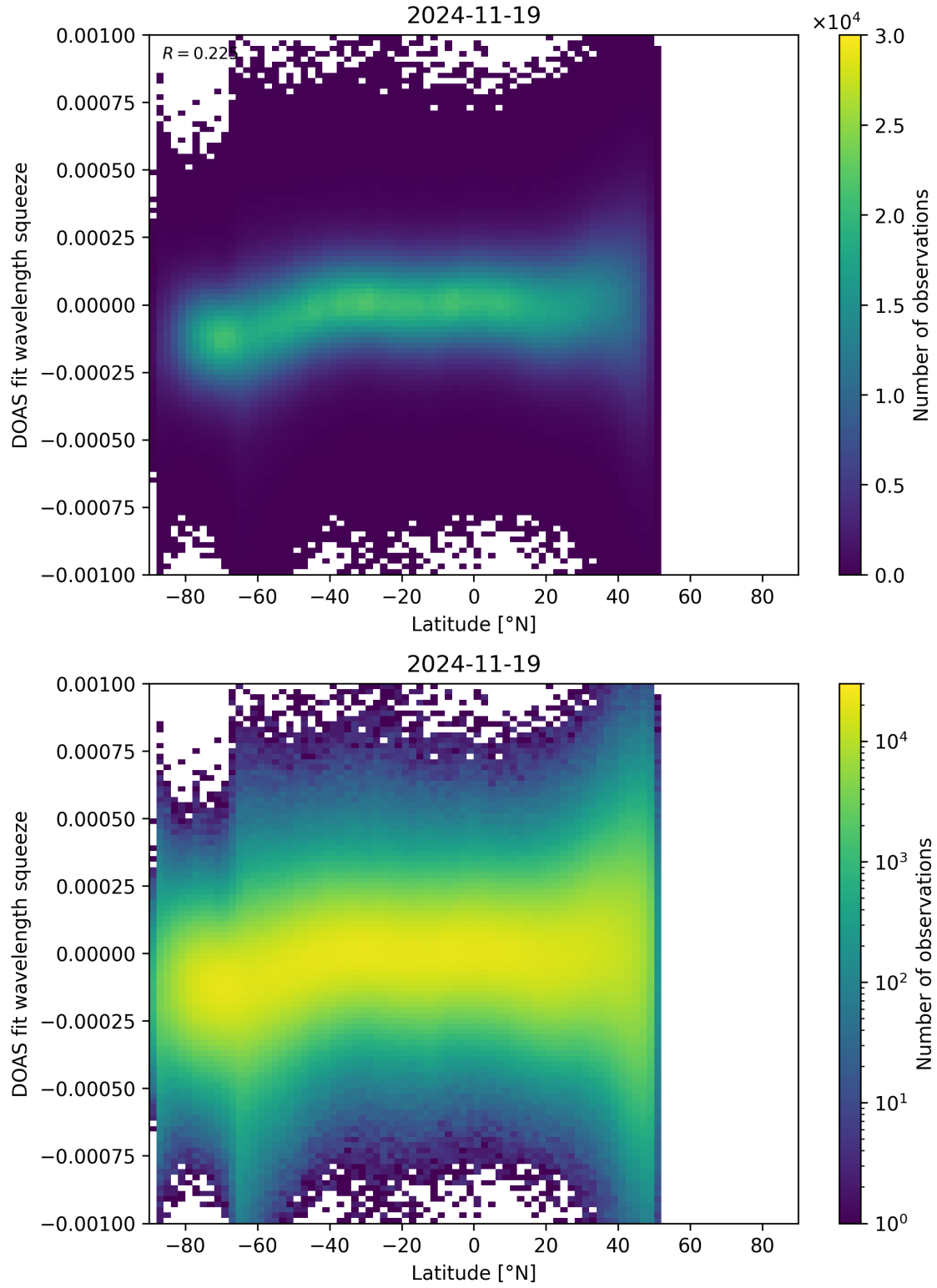
Figure 154: Scatter density plot of “Latitude” against “DOAS fit wavelength squeeze” for 2024-11-18 to 2024-11-20.
