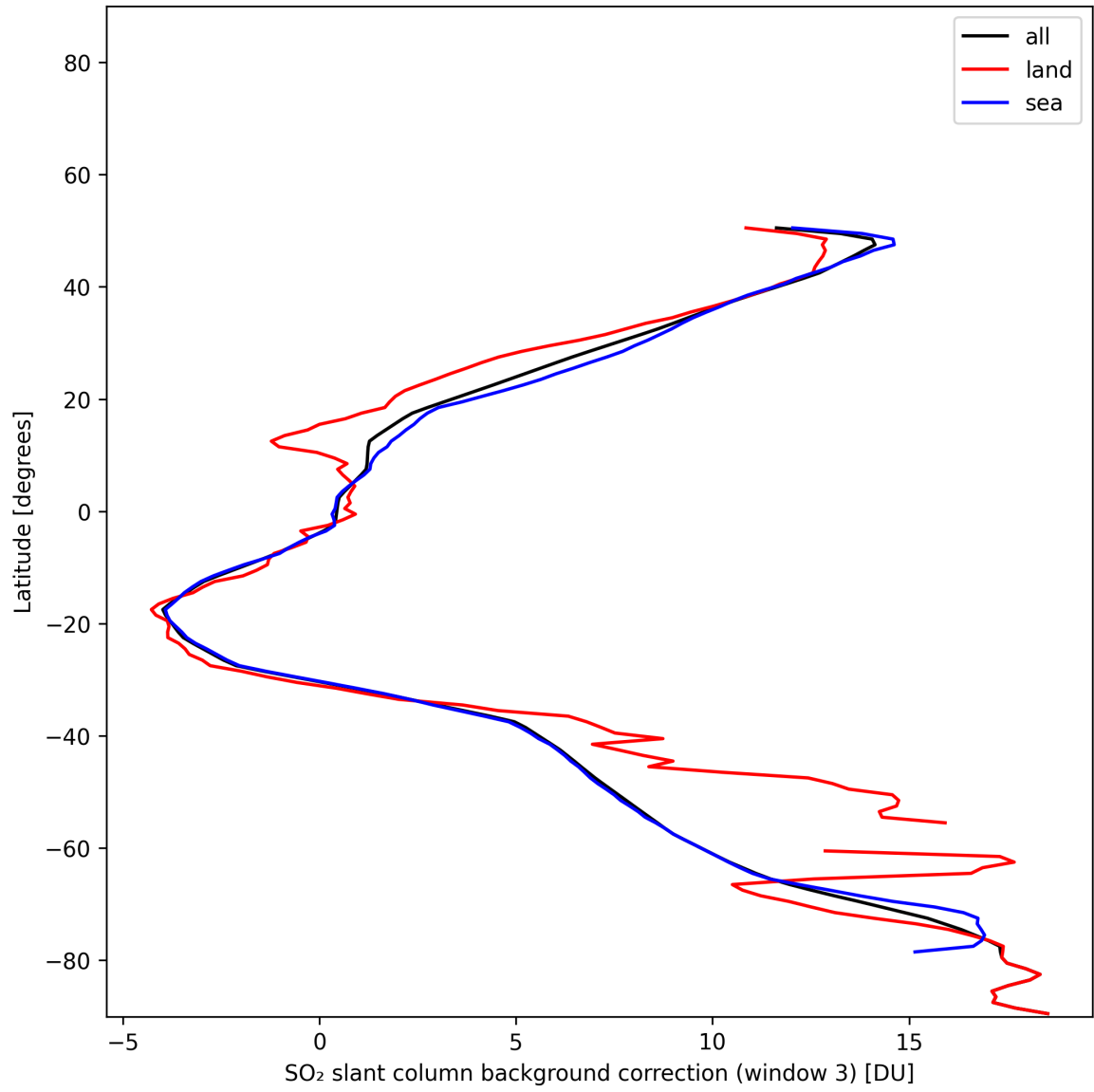
Figure 48: Zonal average of “SO 2 slant column background correction (window 3)” for 2024-11-18 to 2024-11-20.
