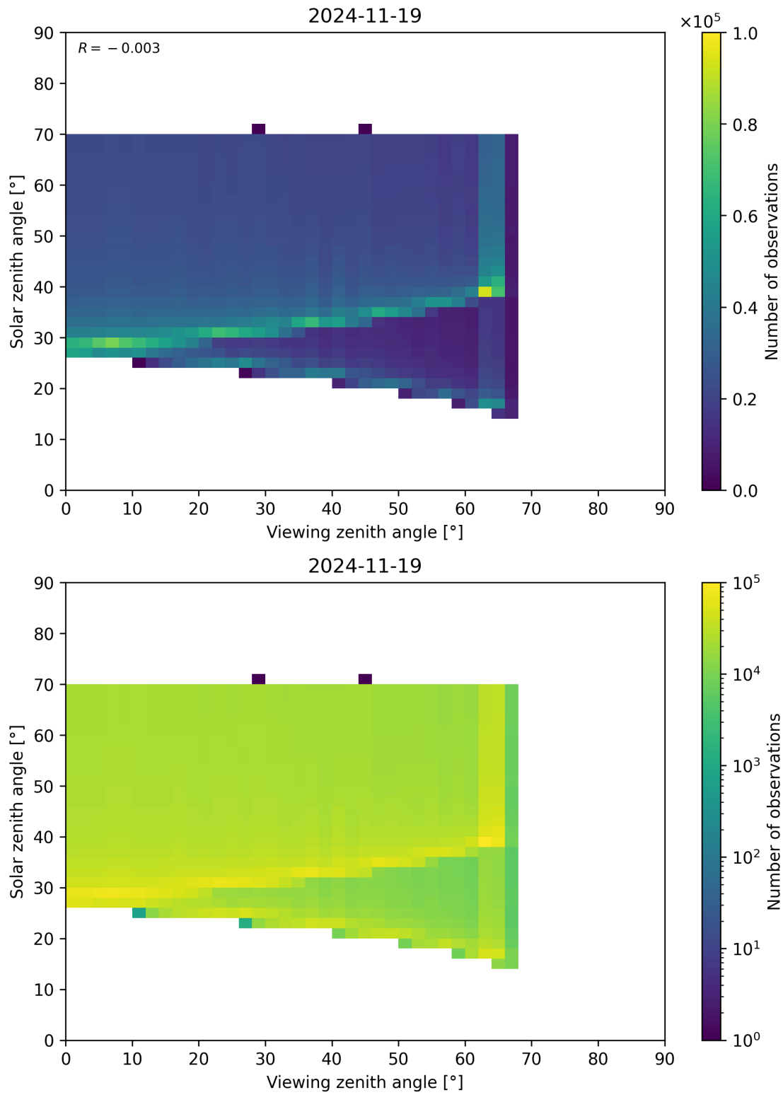
Figure 369: Scatter density plot of “Viewing zenith angle” against “Solar zenith angle” for 2024-11-18 to 2024-11-20.
