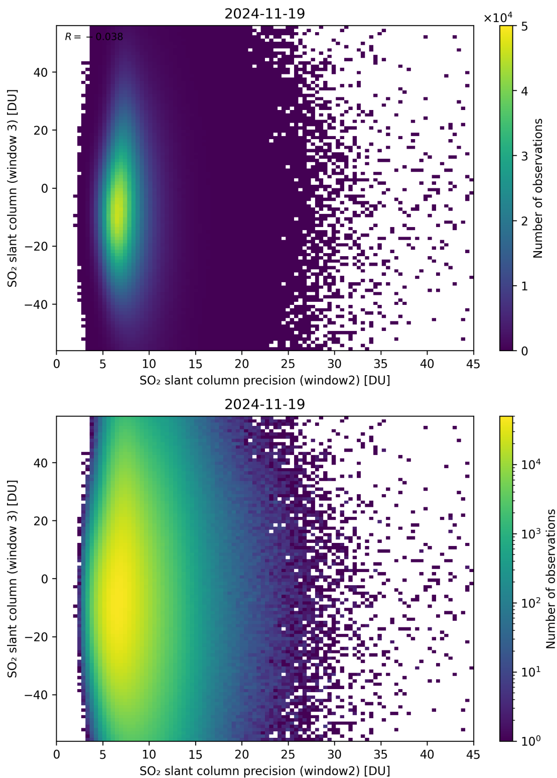
Figure 299: Scatter density plot of “SO 2 slant column precision (window2)” against “SO 2 slant column (window 3)” for 2024-11-18 to 2024-11-20.
