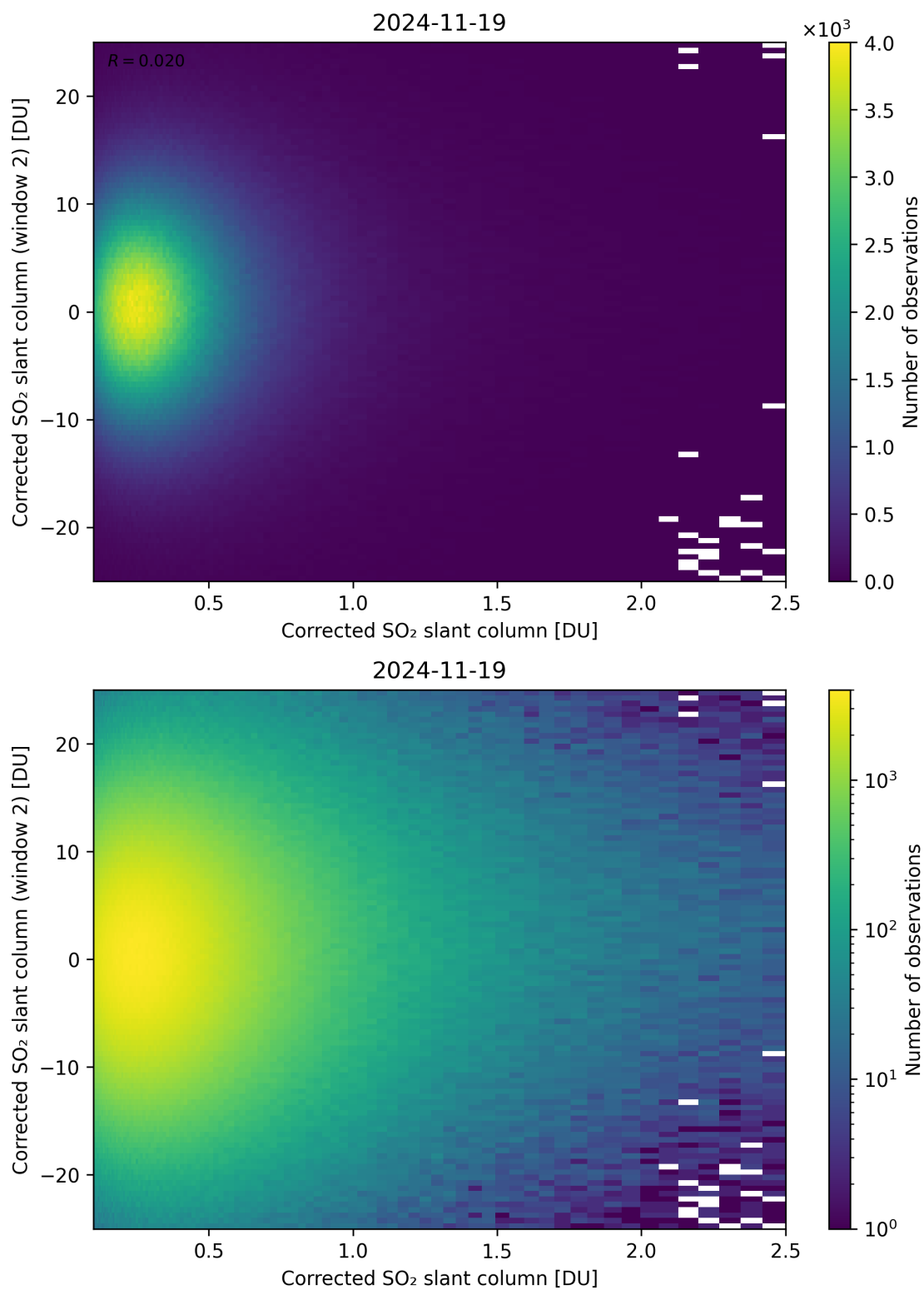
Figure 235: Scatter density plot of “Corrected SO 2 slant column” against “Corrected SO 2 slant column (window 2)” for 2024-11-18 to 2024-11-20.
