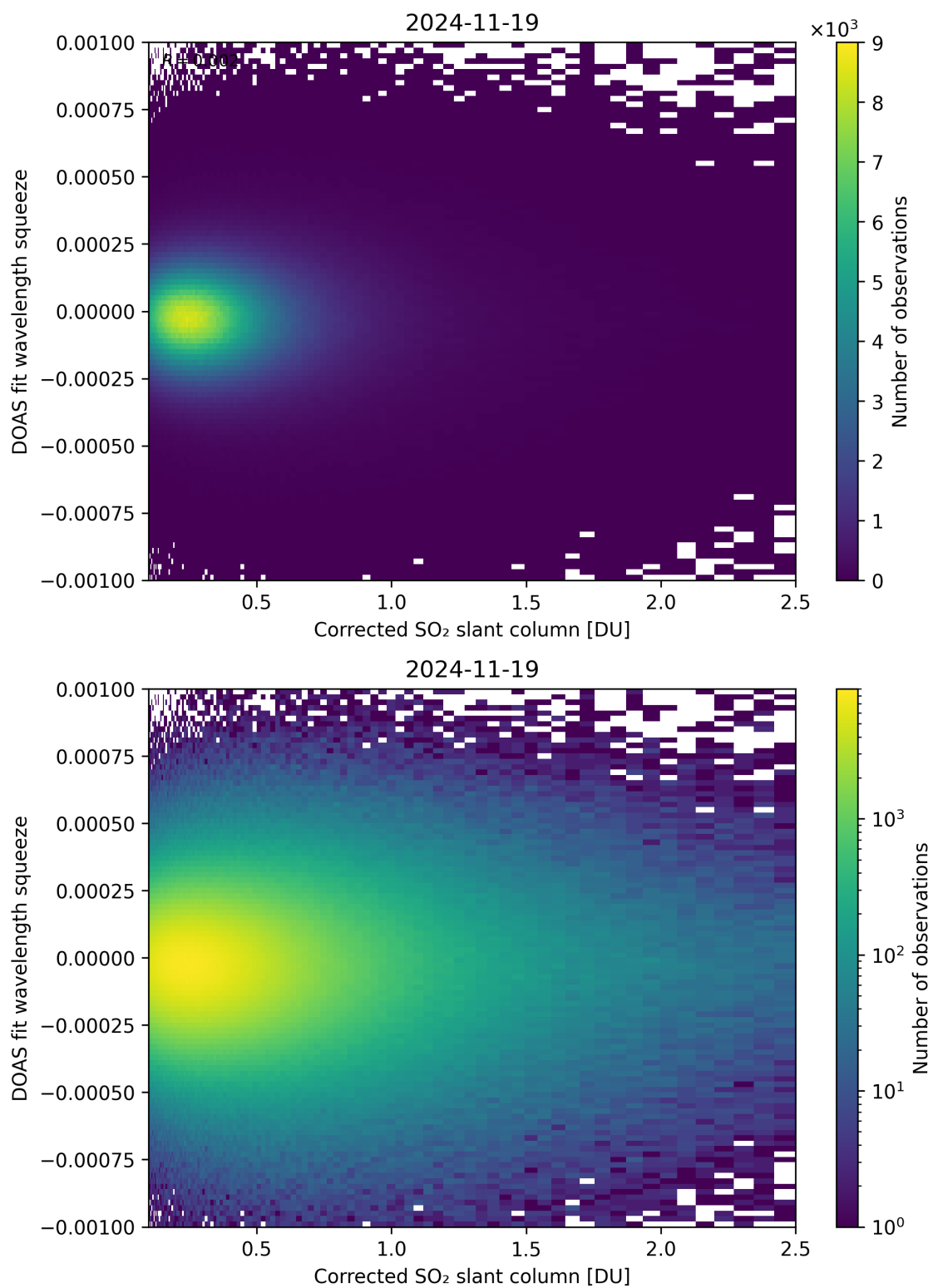
Figure 230: Scatter density plot of "Corrected SO 2 slant column" against "DOAS fit wavelength squeeze" for 2024-11-18 to 2024-11-20.
