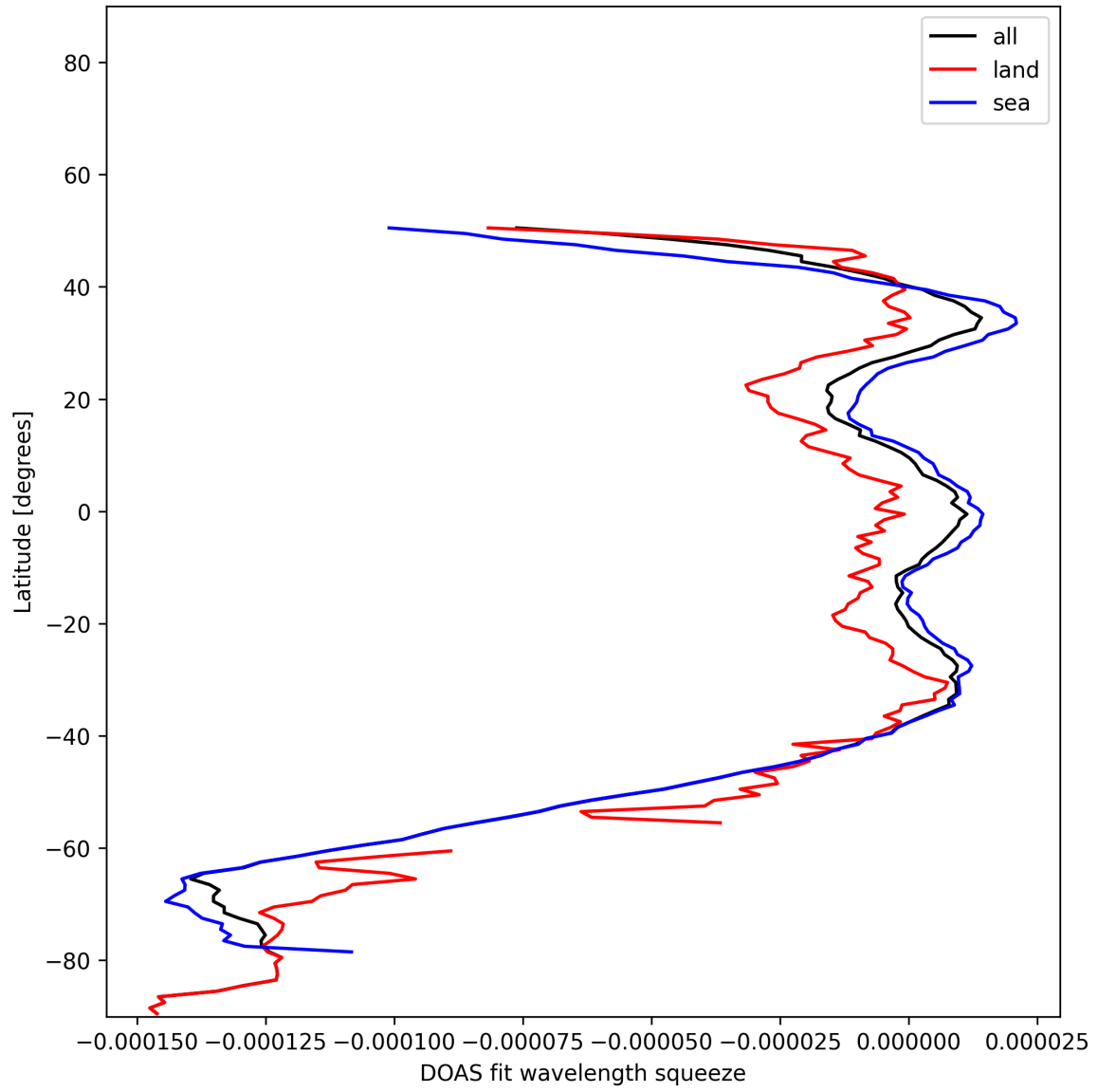
Figure 51: Zonal average of “DOAS fit wavelength squeeze” for 2024-11-18 to 2024-11-20.
