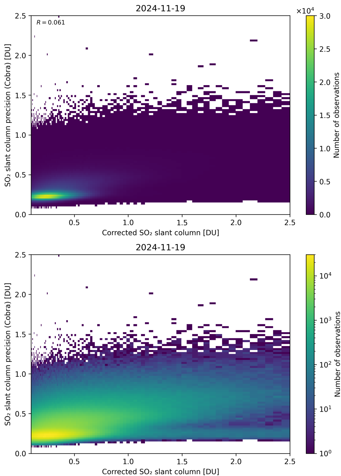
Figure 234: Scatter density plot of “Corrected SO 2 slant column” against “SO 2 slant column precision (Cobra)” for 2024-11-18 to 2024-11-20.
