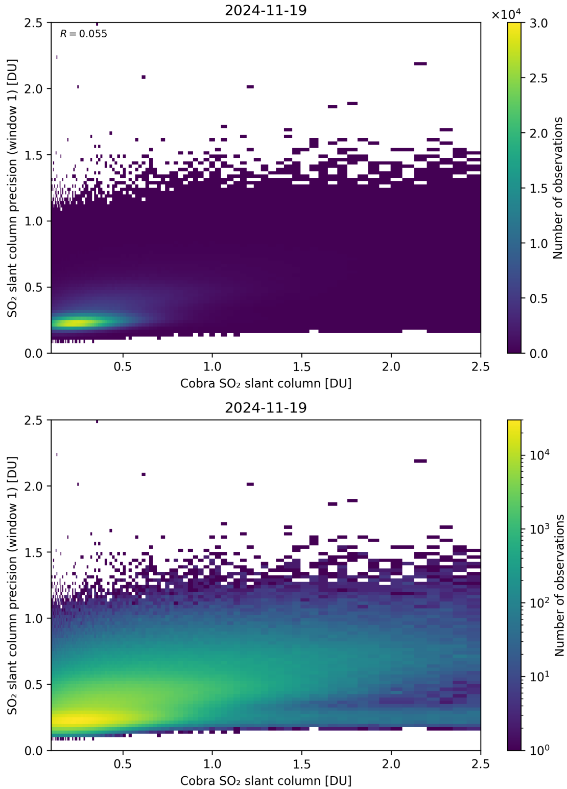
Figure 220: Scatter density plot of “Cobra SO 2 slant column” against “SO 2 slant column precision (window 1)” for 2024-11-18 to 2024-11-20.
