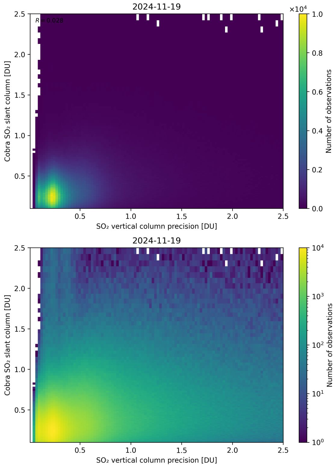
Figure 336: Scatter density plot of “SO 2 vertical column precision” against “Cobra SO 2 slant column” for 2024-11-18 to 2024-11-20.
