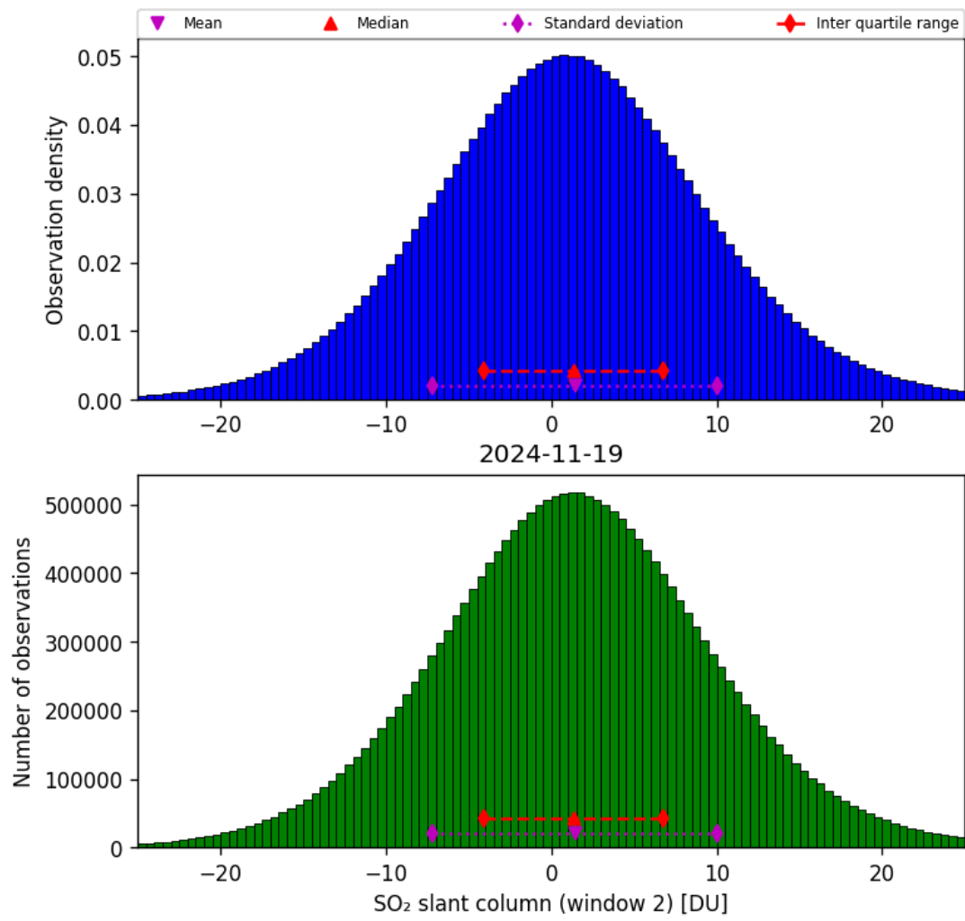
Figure 67: Histogram of “SO 2 slant column (window 2)” for 2024-11-18 to 2024-11-20
