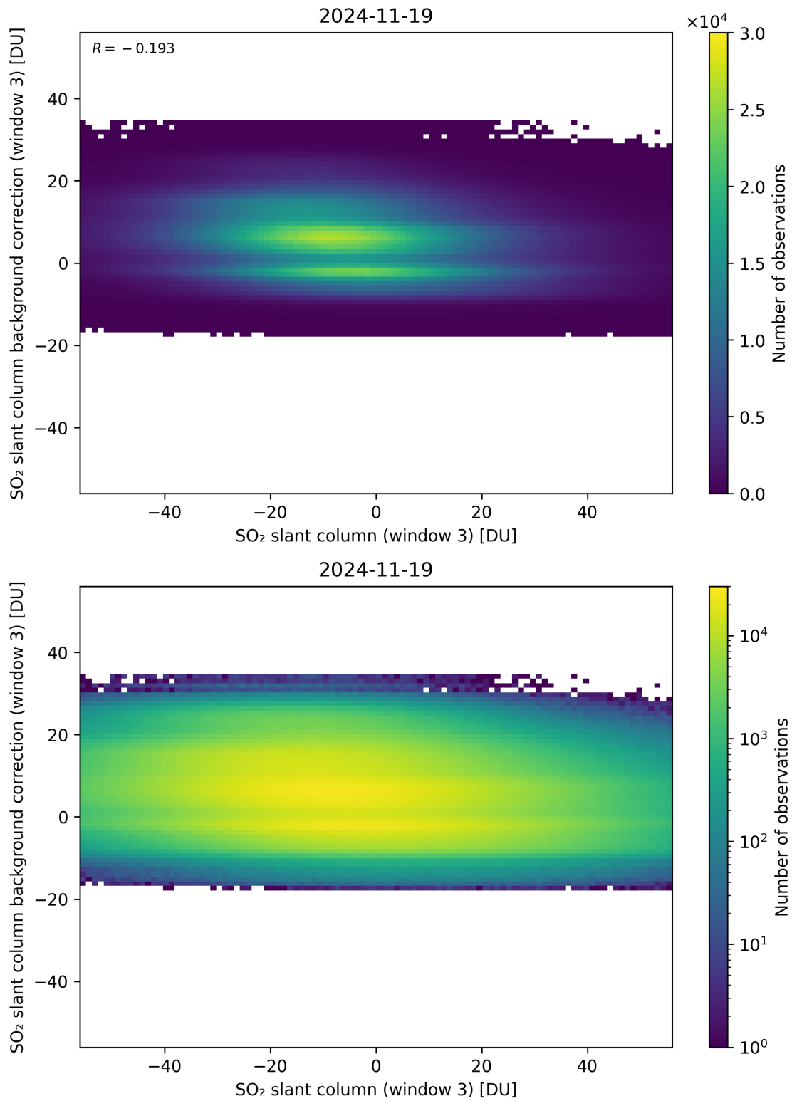
Figure 303: Scatter density plot of “SO 2 slant column (window 3)” against “SO 2 slant column background correction (window 3)” for 2024-11-18 to 2024-11-20.
