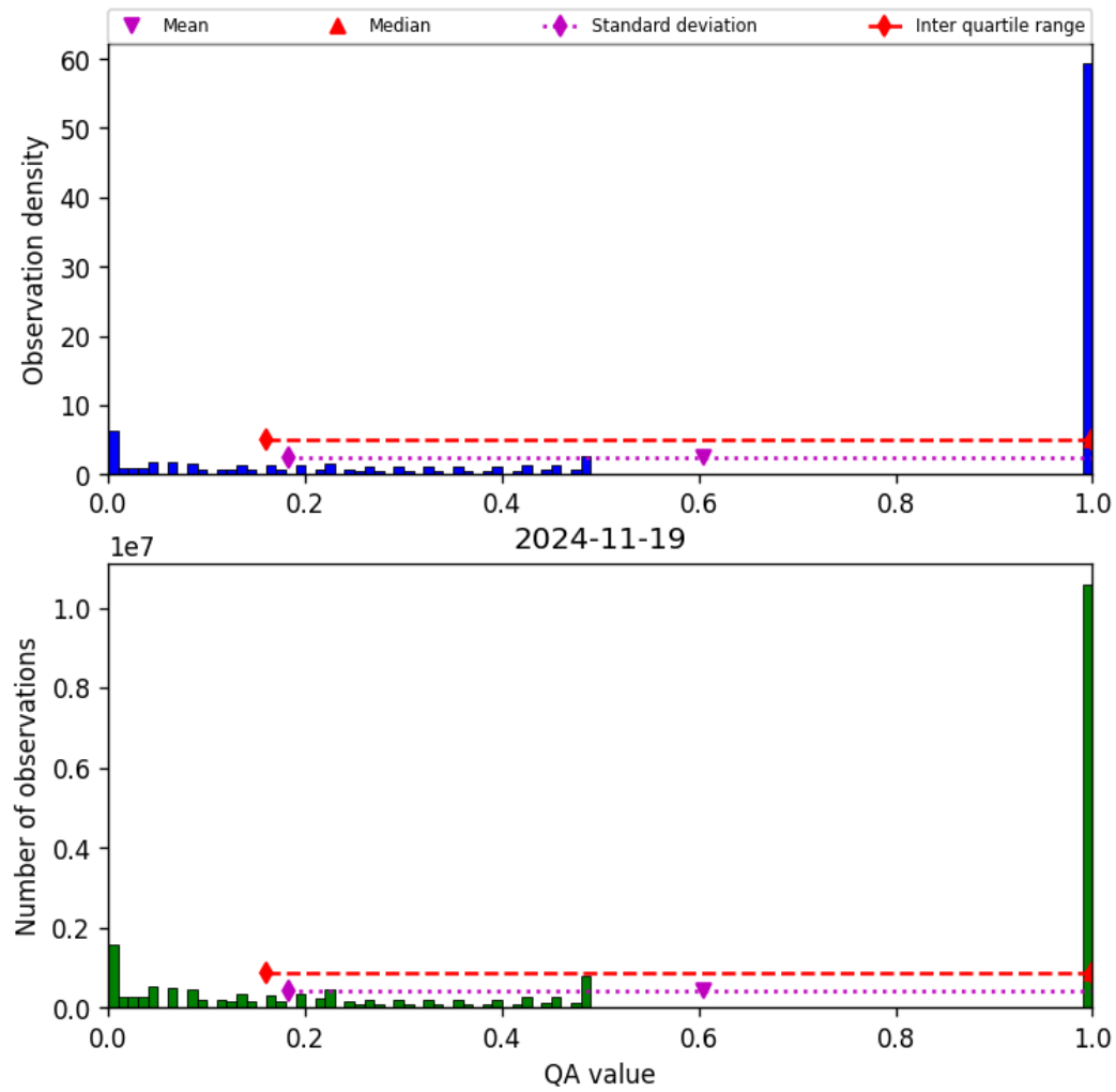
Figure 57: Histogram of “QA value” for 2024-11-18 to 2024-11-20
