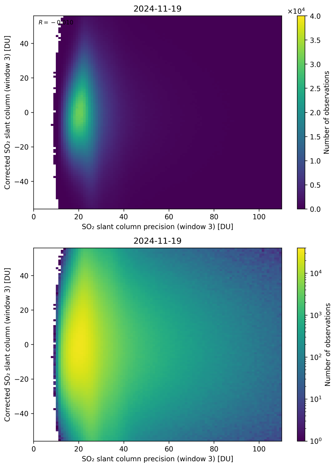
Figure 312: Scatter density plot of “SO 2 slant column precision (window 3)” against “Corrected SO 2 slant column (window 3)” for 2024-11-18 to 2024-11-20.
