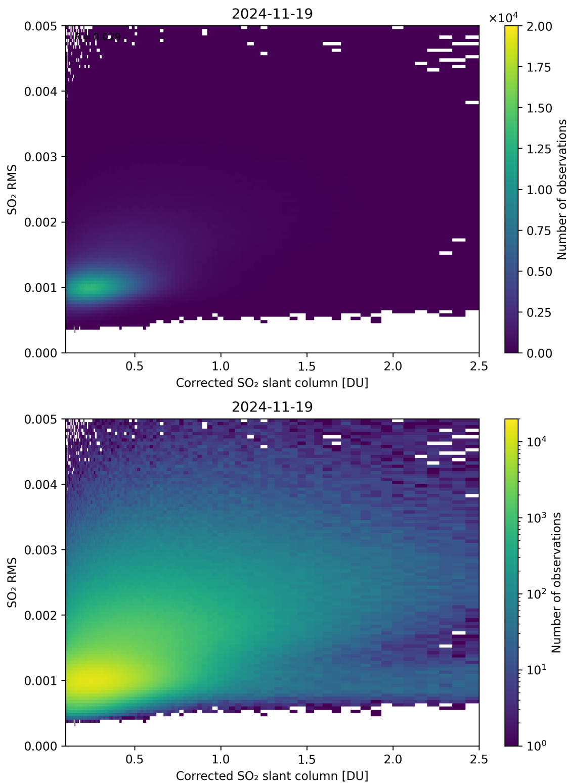
Figure 231: Scatter density plot of “Corrected SO 2 slant column” against “SO 2 RMS” for 2024-11-18 to 2024-11-20.
