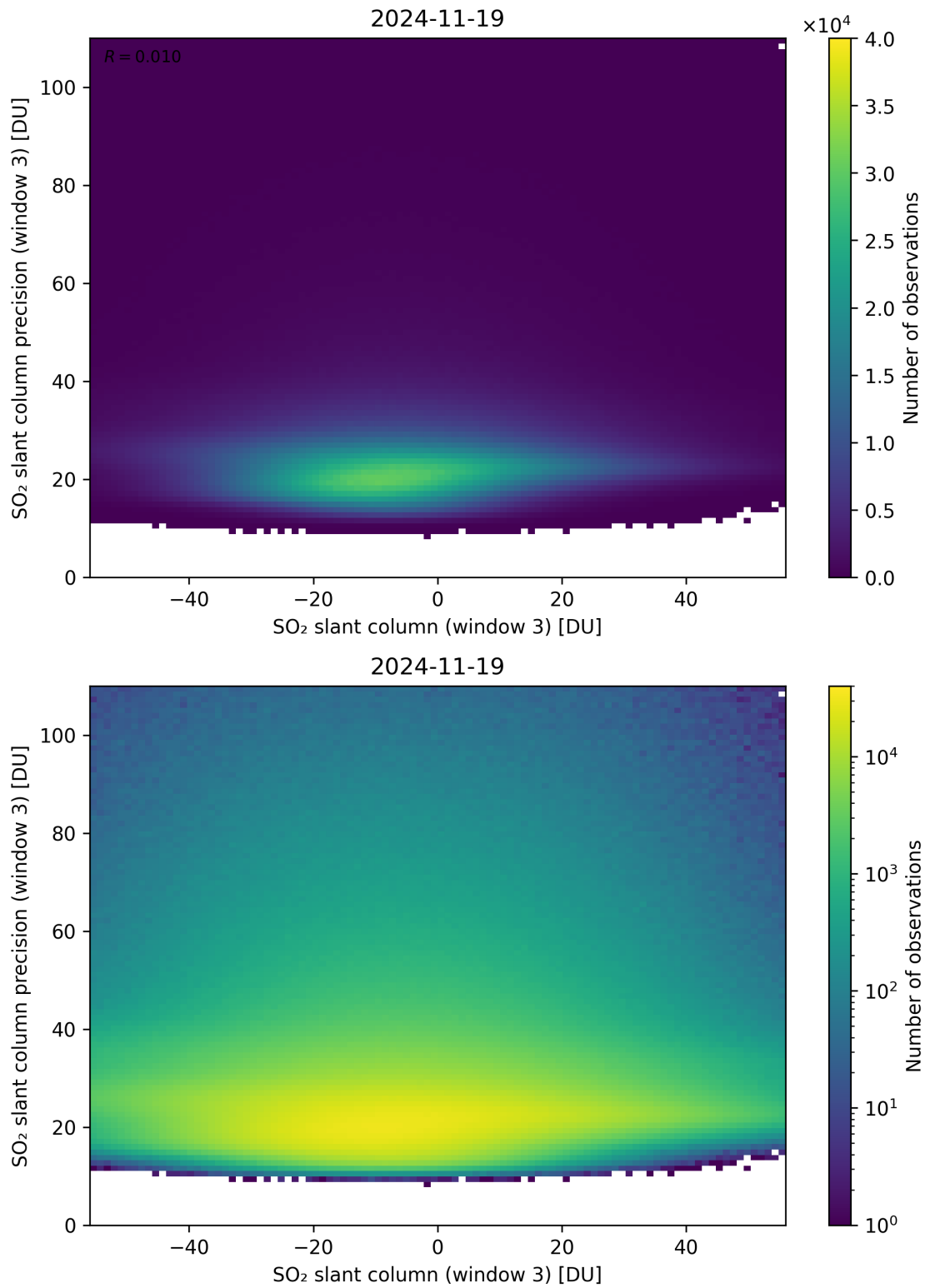
Figure 317: Scatter density plot of “SO 2 slant column (window 3)” against “SO 2 slant column precision (window 3)” for 2024-11-18 to 2024-11-20.
