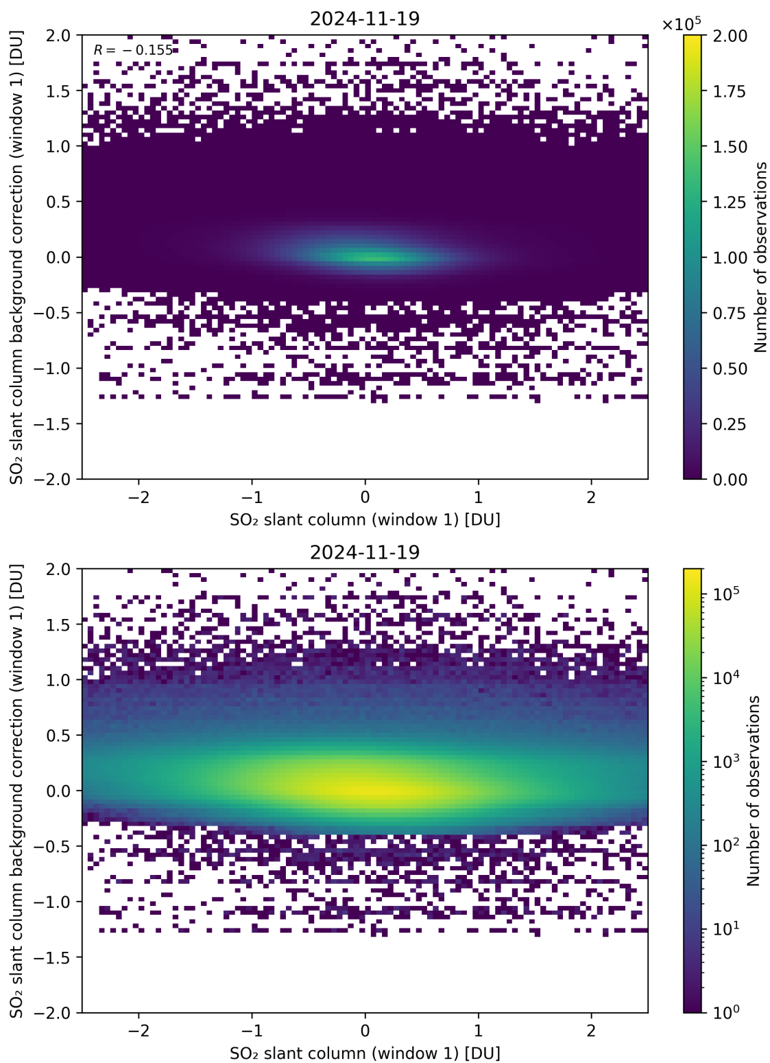
Figure 262: Scatter density plot of “SO 2 slant column (window 1)” against “SO 2 slant column background correction (window 1)” for 2024-11-18 to 2024-11-20.
