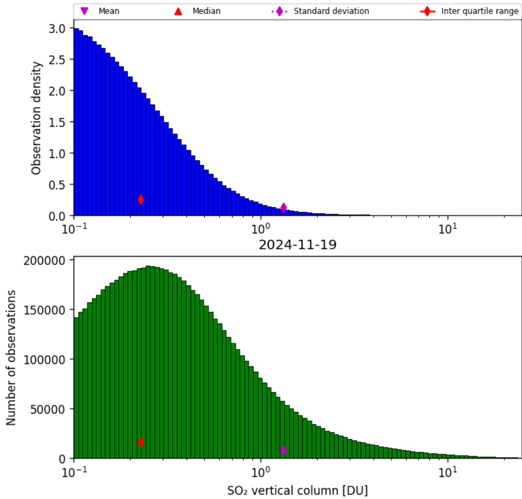
Figure 58: Histogram of “SO 2 vertical column” for 2024-11-18 to 2024-11-20
