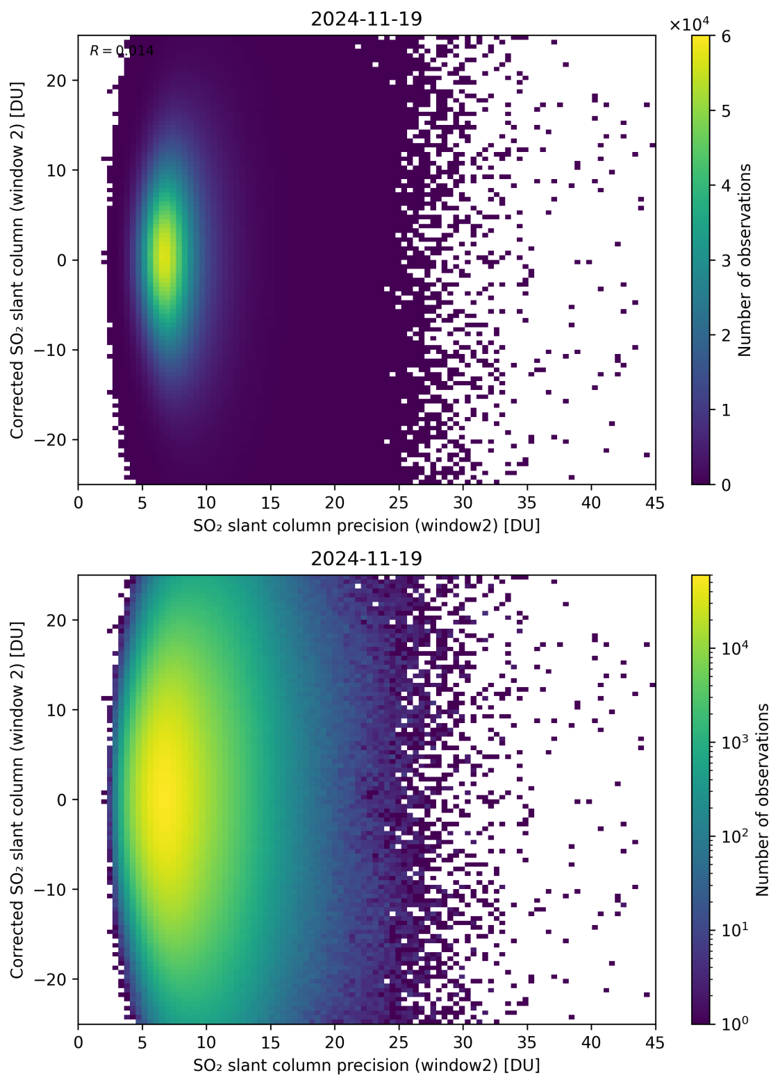
Figure 297: Scatter density plot of “SO 2 slant column precision (window2)” against “Corrected SO 2 slant column (window 2)” for 2024-11-18 to 2024-11-20.
