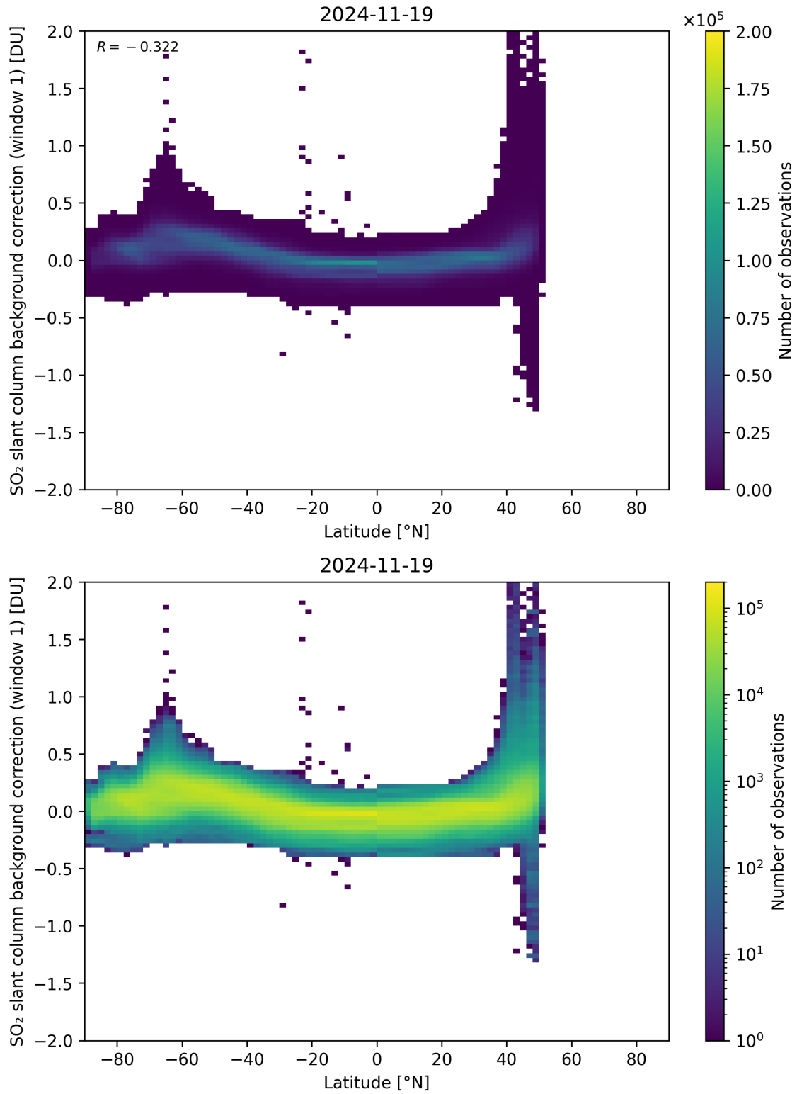
Figure 150: Scatter density plot of “Latitude” against “SO 2 slant column background correction (window 1)” for 2024-11-18 to 2024-11-20.
