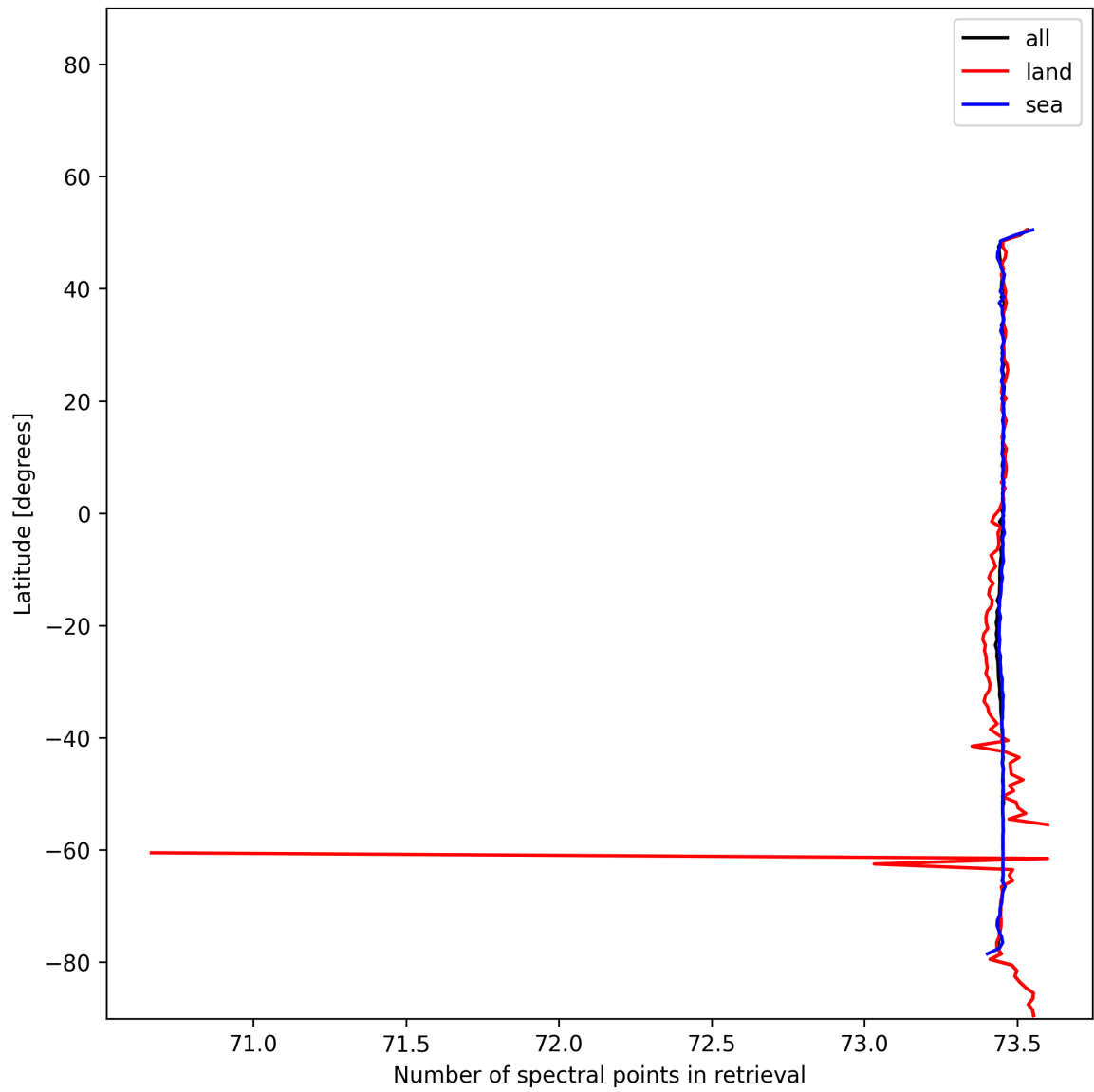
Figure 56: Zonal average of “Number of spectral points in retrieval” for 2024-11-18 to 2024-11-20.
