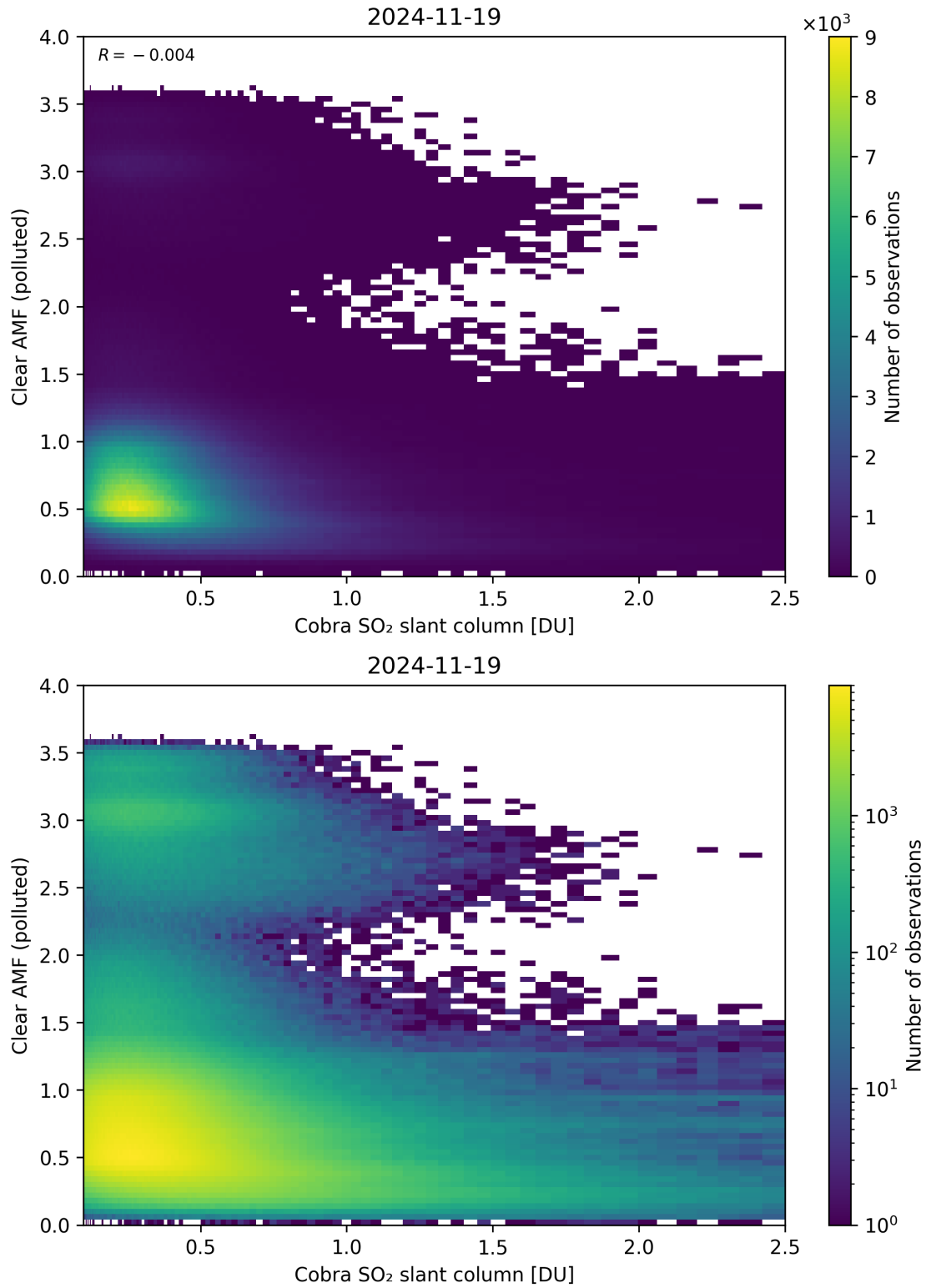
Figure 215: Scatter density plot of “Cobra SO 2 slant column” against “Clear AMF (polluted)” for 2024-11-18 to 2024-11-20.
