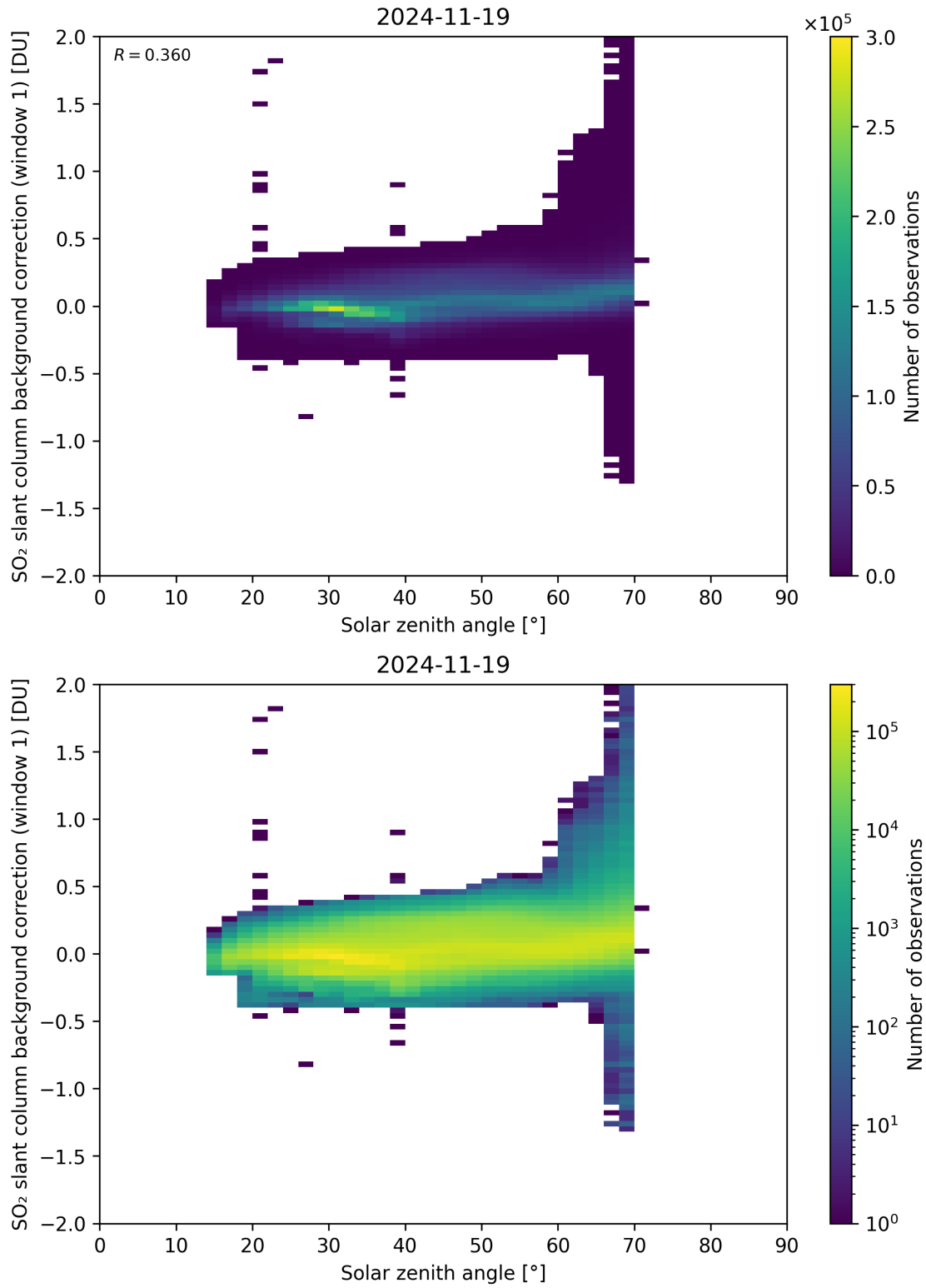
Figure 171: Scatter density plot of “Solar zenith angle” against “SO 2 slant column background correction (window 1)” for 2024-11-18 to 2024-11-20.
