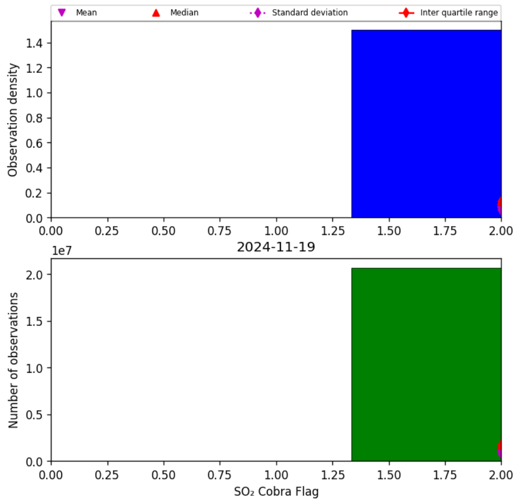
Figure 75: Histogram of “SO 2 Cobra Flag” for 2024-11-18 to 2024-11-20
