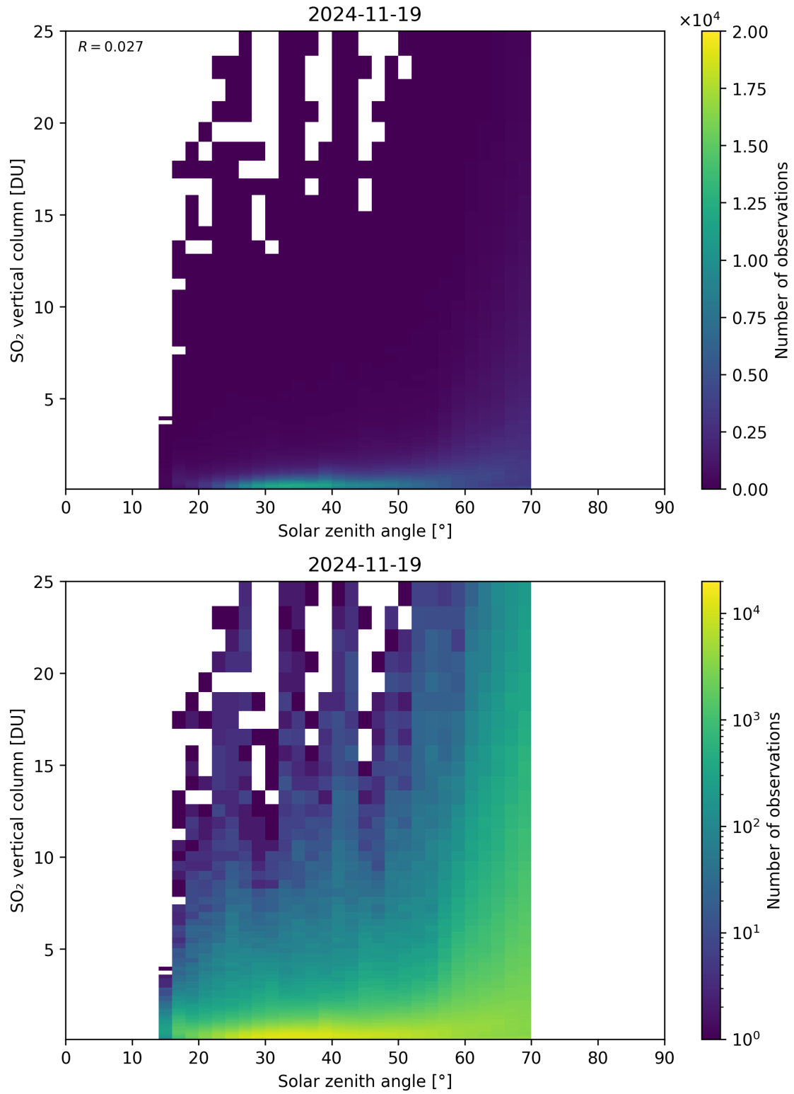
Figure 191: Scatter density plot of “Solar zenith angle” against “SO 2 vertical column” for 2024-11-18 to 2024-11-20.
