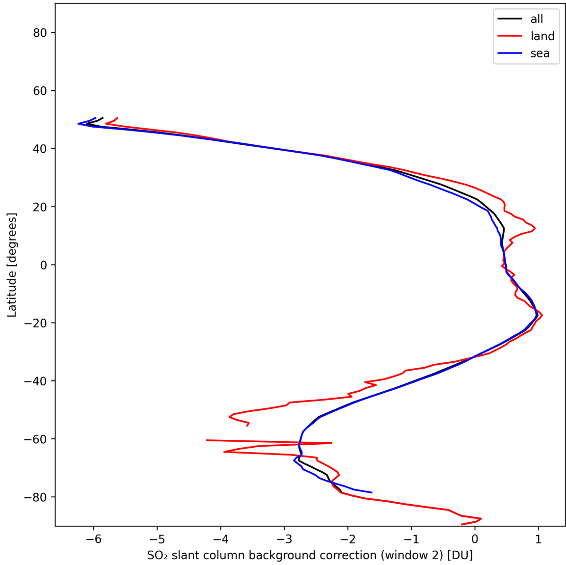
Figure 44: Zonal average of “SO 2 slant column background correction (window 2)” for 2024-11-18 to 2024-11-20.
