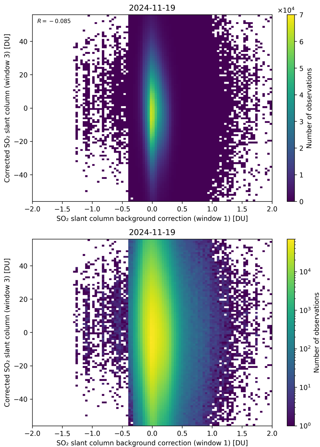
Figure 116: Scatter density plot of “SO 2 slant column background correction (window 1)” against “Corrected SO 2 slant column (window 3)” for 2024-11-18 to 2024-11-20.
