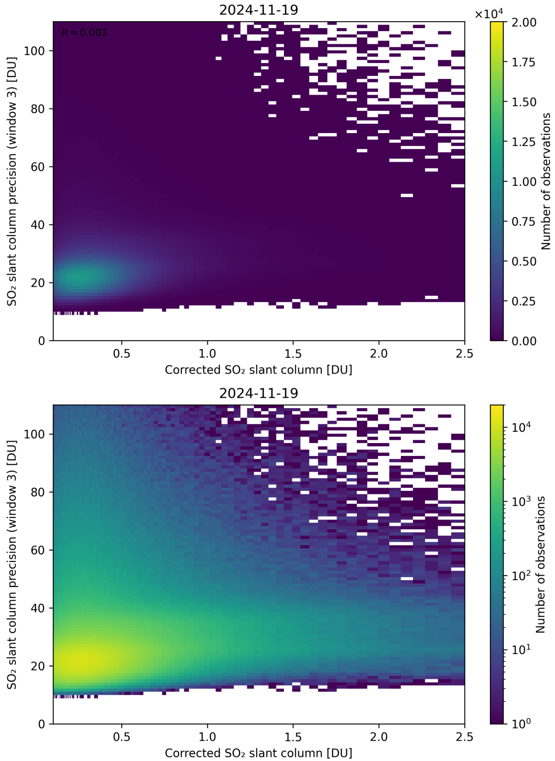
Figure 241: Scatter density plot of “Corrected SO 2 slant column” against “SO 2 slant column precision (window 3)” for 2024-11-18 to 2024-11-20.
