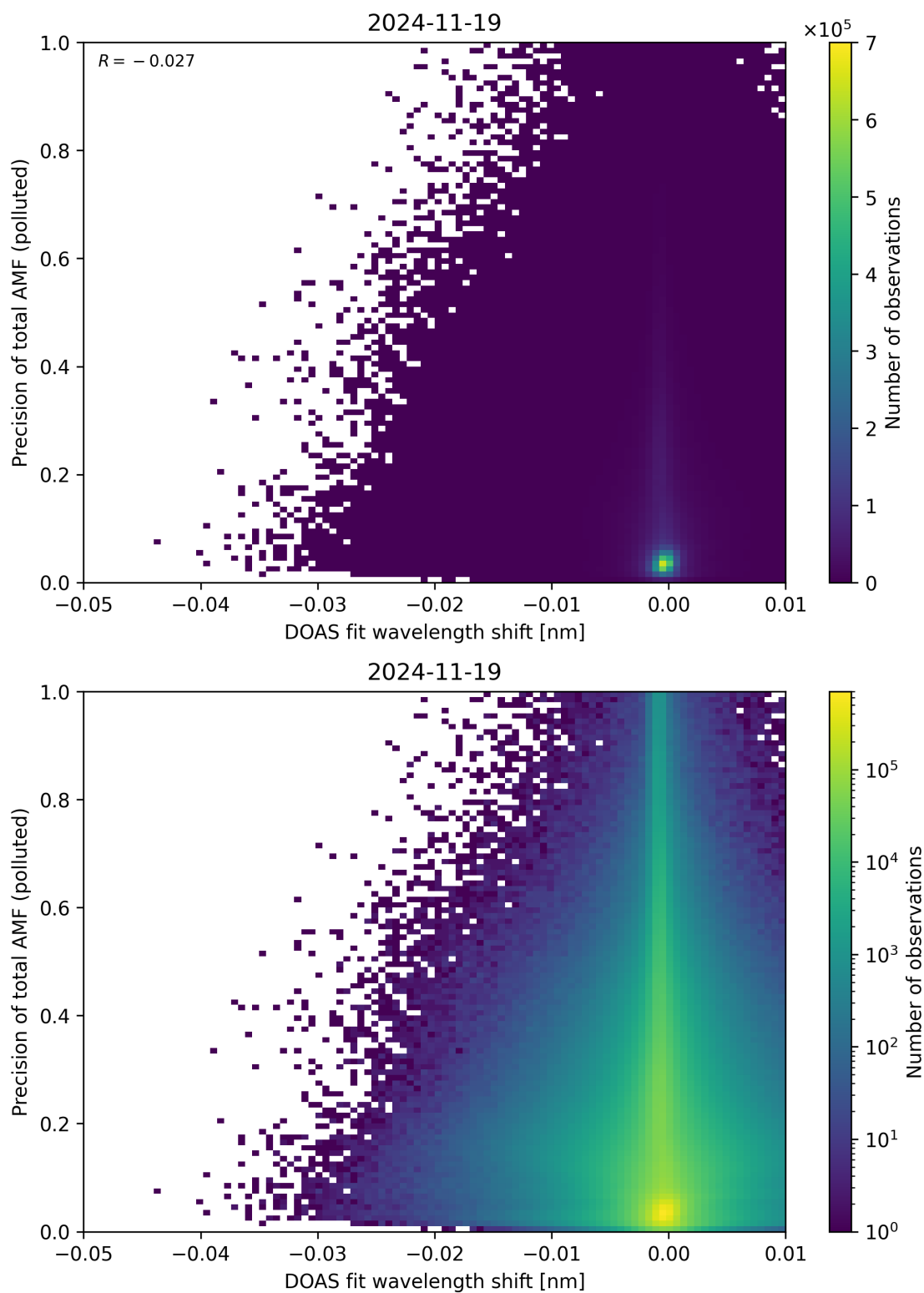
Figure 142: Scatter density plot of “DOAS fit wavelength shift” against “Precision of total AMF (polluted)” for 2024-11-18 to 2024-11-20.
