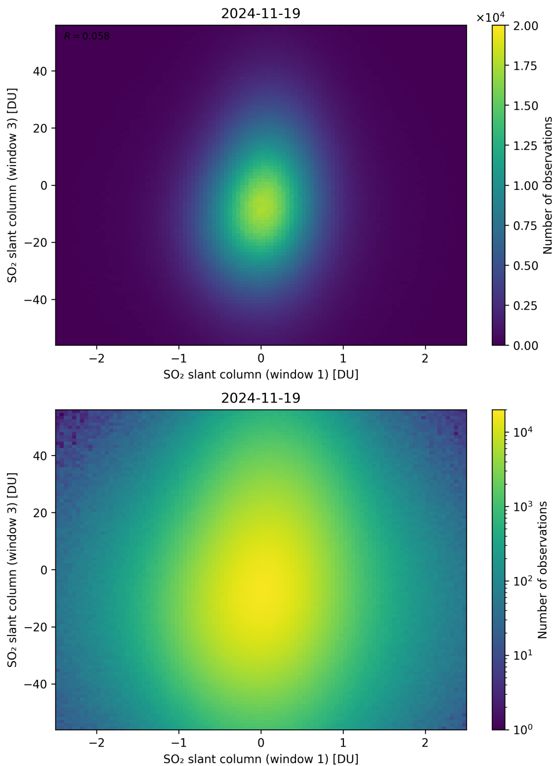
Figure 287: Scatter density plot of “SO 2 slant column (window 1)” against “SO 2 slant column (window 3)” for 2024-11-18 to 2024-11-20.
