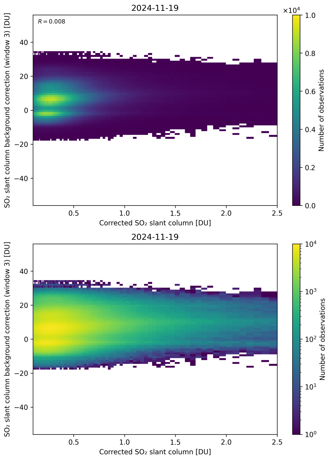
Figure 228: Scatter density plot of “Corrected SO 2 slant column” against “SO 2 slant column background correction (window 3)” for 2024-11-18 to 2024-11-20.
