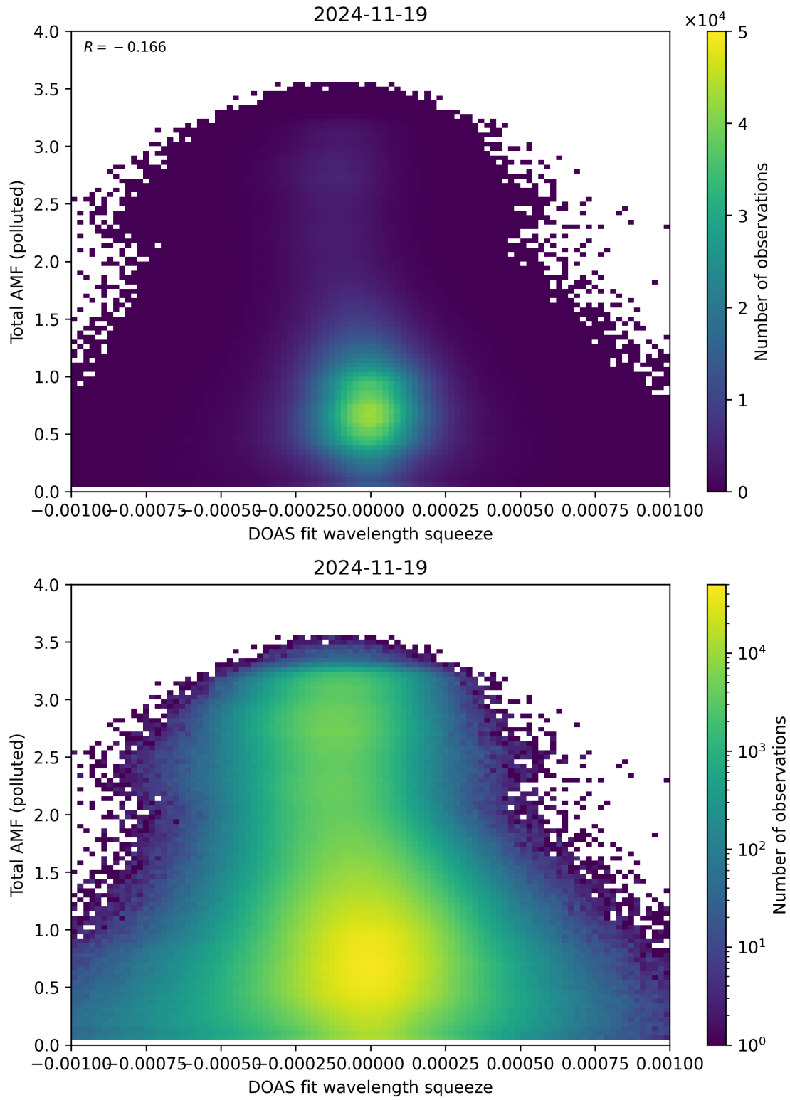
Figure 145: Scatter density plot of “DOAS fit wavelength squeeze” against “Total AMF (polluted)” for 2024-11-18 to 2024-11-20.
