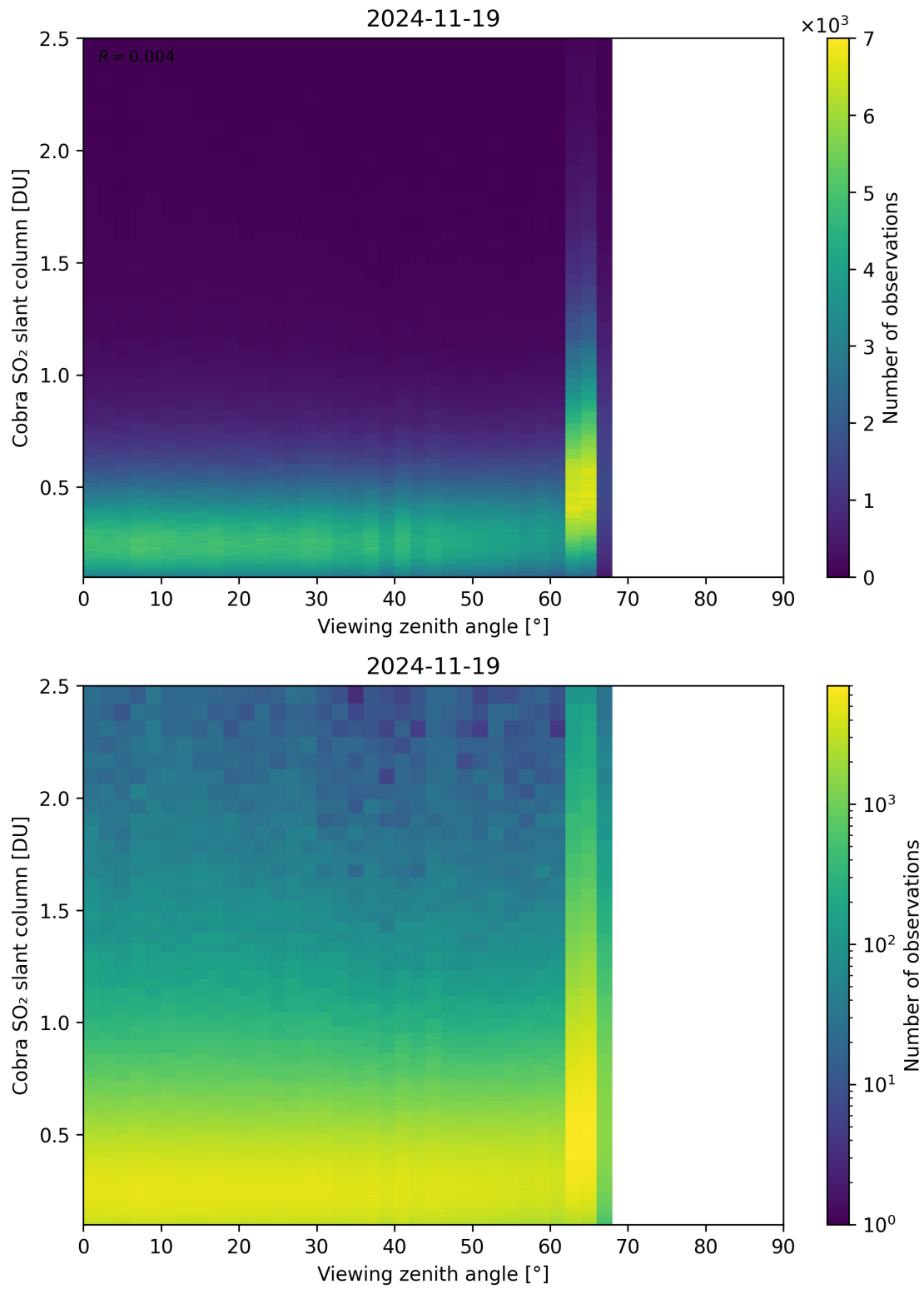
Figure 371: Scatter density plot of “Viewing zenith angle” against “Cobra SO 2 slant column” for 2024-11-18 to 2024-11-20.
