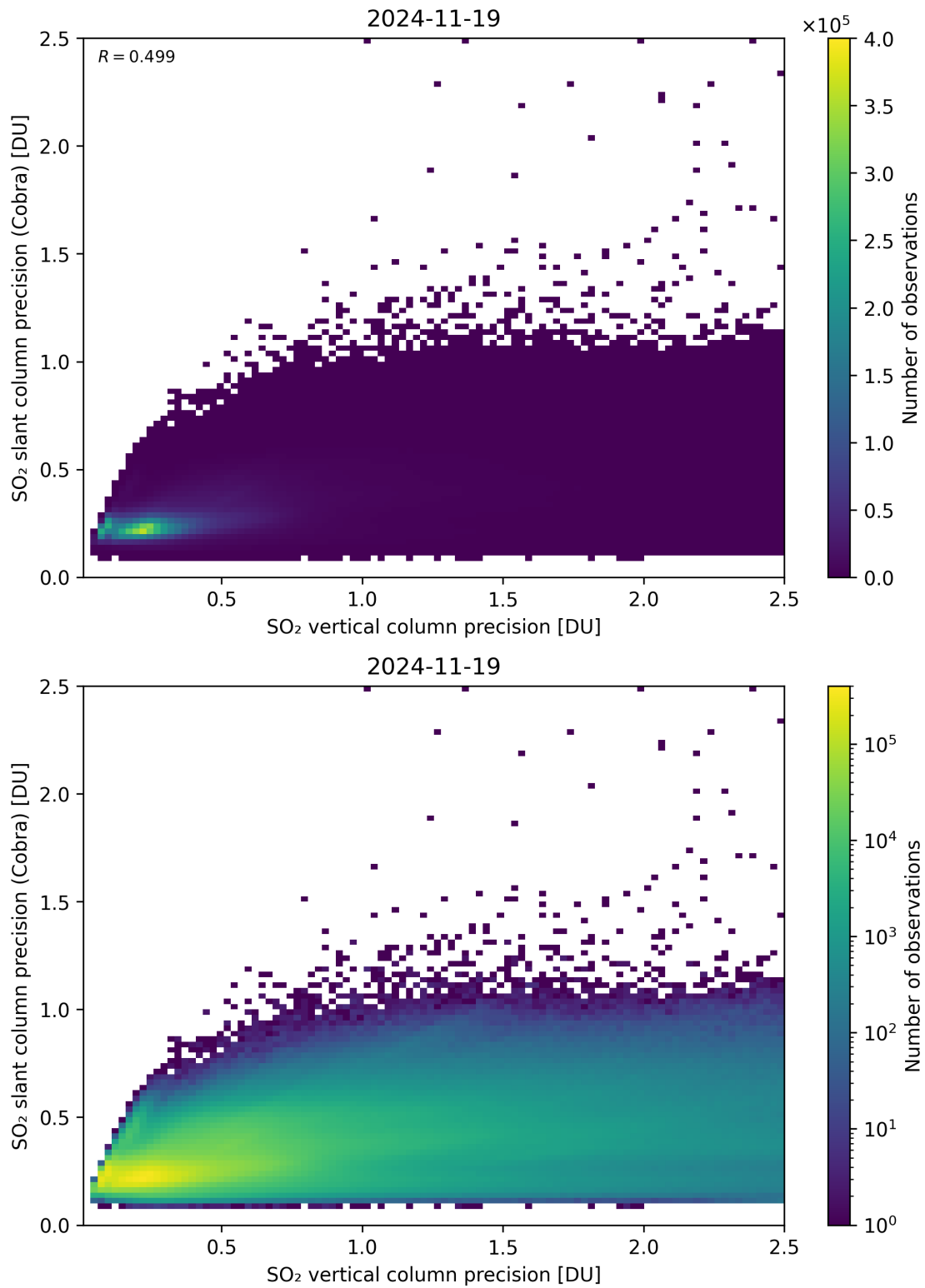
Figure 337: Scatter density plot of “SO 2 vertical column precision” against “SO 2 slant column precision (Cobra)” for 2024-11-18 to 2024-11-20.
