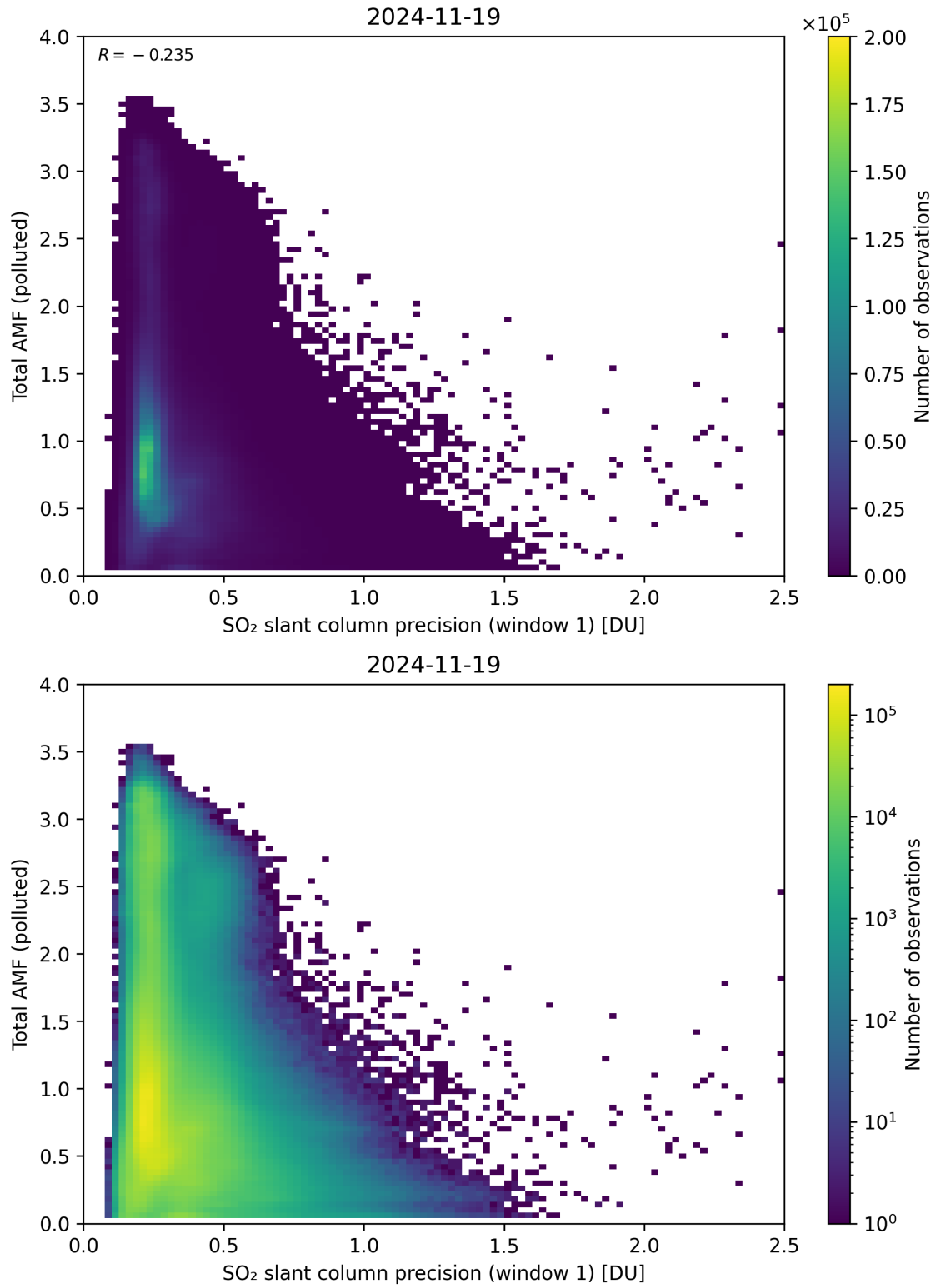
Figure 280: Scatter density plot of “SO 2 slant column precision (window 1)” against “Total AMF (polluted)” for 2024-11-18 to 2024-11-20.
