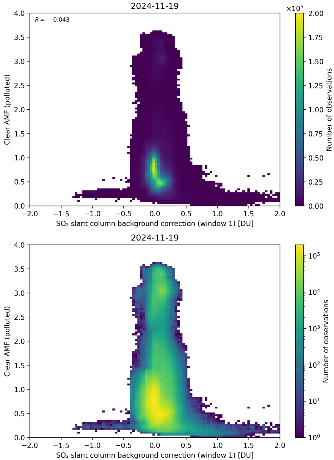
Figure 114: Scatter density plot of “SO 2 slant column background correction (window 1)” against “Clear AMF (polluted)” for 2024-11-18 to 2024-11-20.
