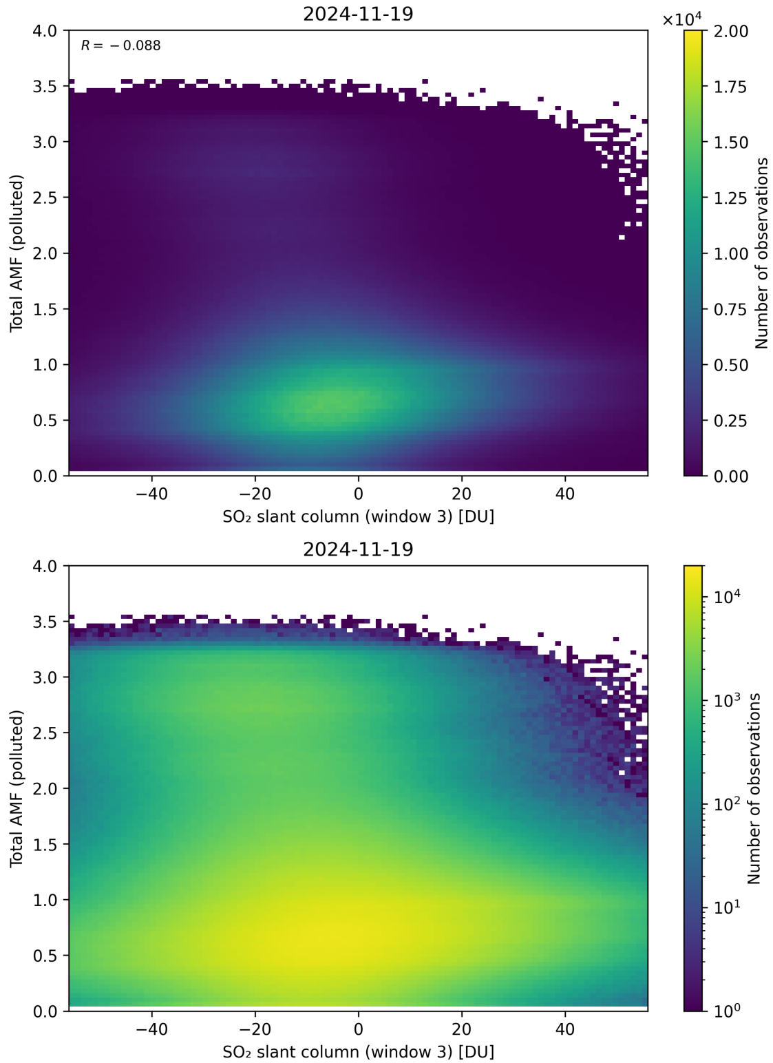
Figure 318: Scatter density plot of “SO 2 slant column (window 3)” against “Total AMF (polluted)” for 2024-11-18 to 2024-11-20.
