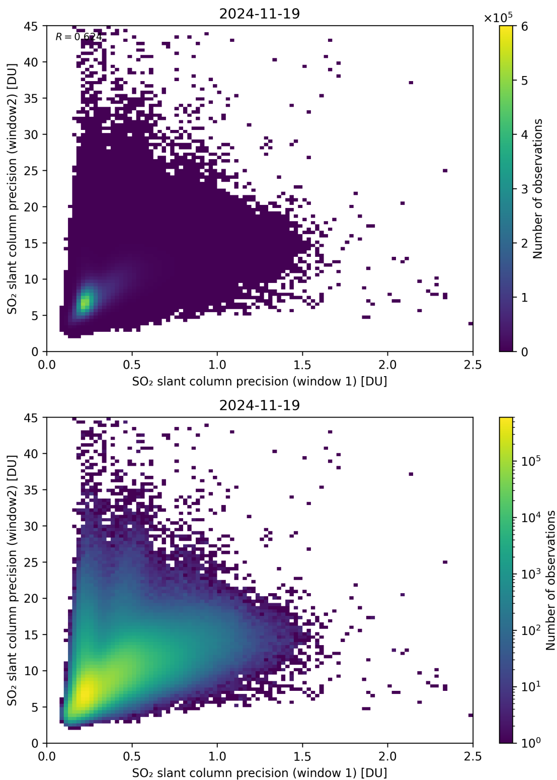
Figure 277: Scatter density plot of “SO 2 slant column precision (window 1)” against “SO 2 slant column precision (window2)” for 2024-11-18 to 2024-11-20.
