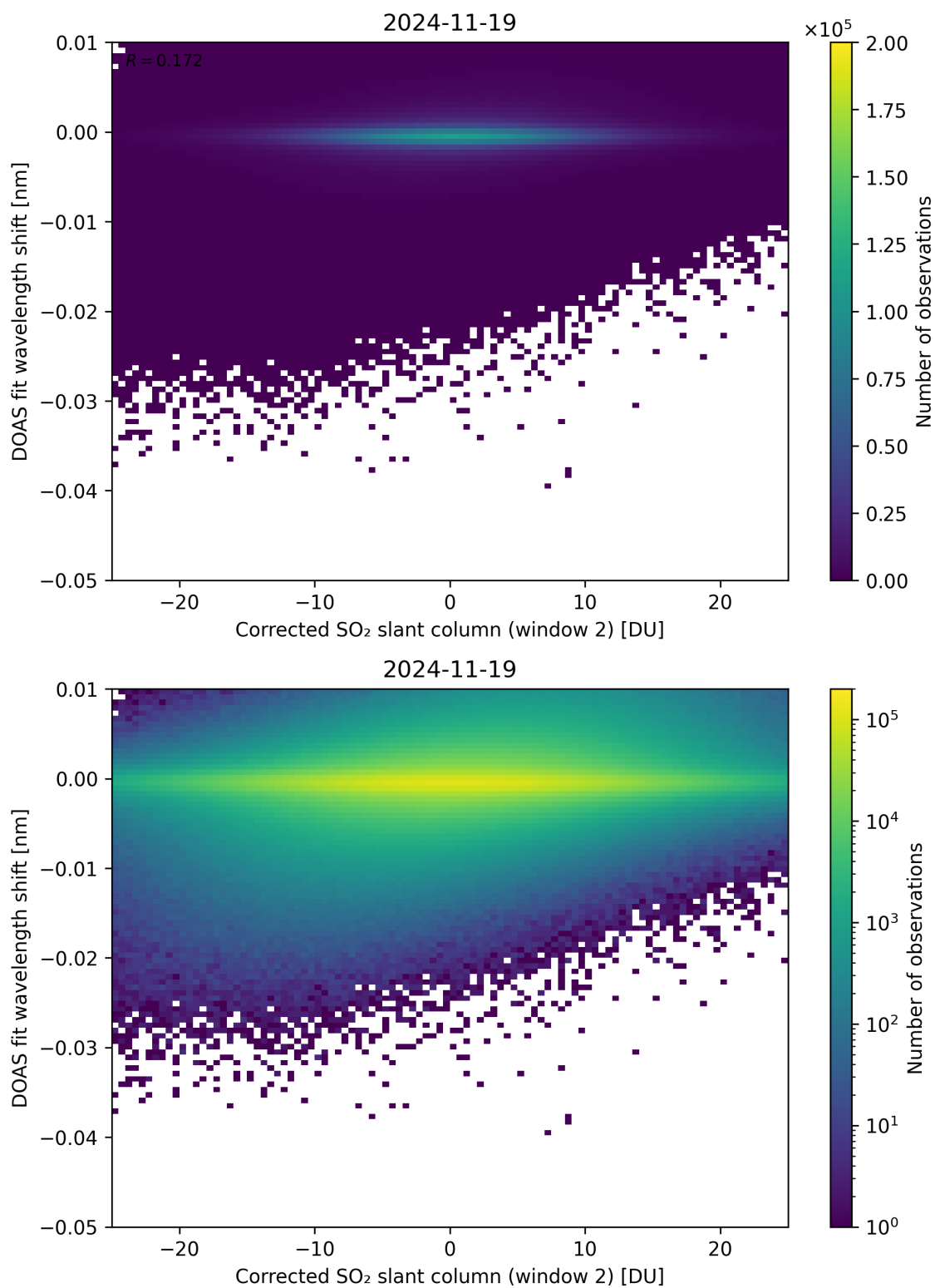
Figure 246: Scatter density plot of “Corrected SO 2 slant column (window 2)” against “DOAS fit wavelength shift” for 2024-11-18 to 2024-11-20.
