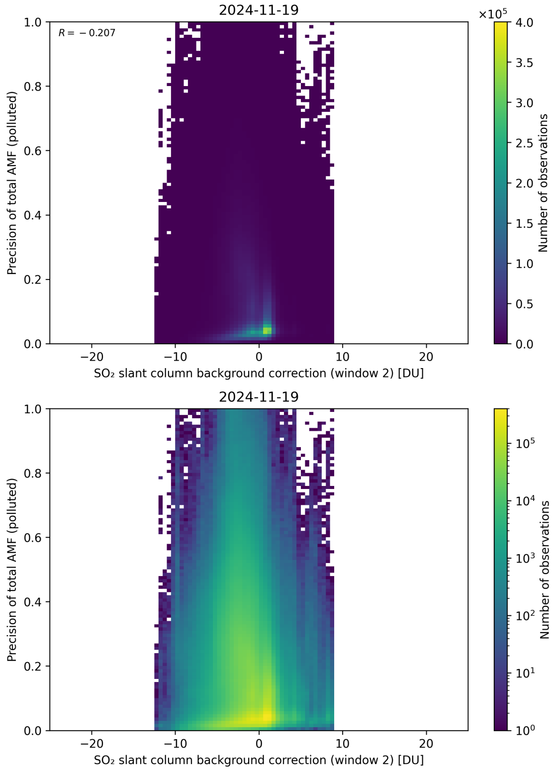
Figure 131: Scatter density plot of “SO 2 slant column background correction (window 2)” against “Precision of total AMF (polluted)” for 2024-11-18 to 2024-11-20.
