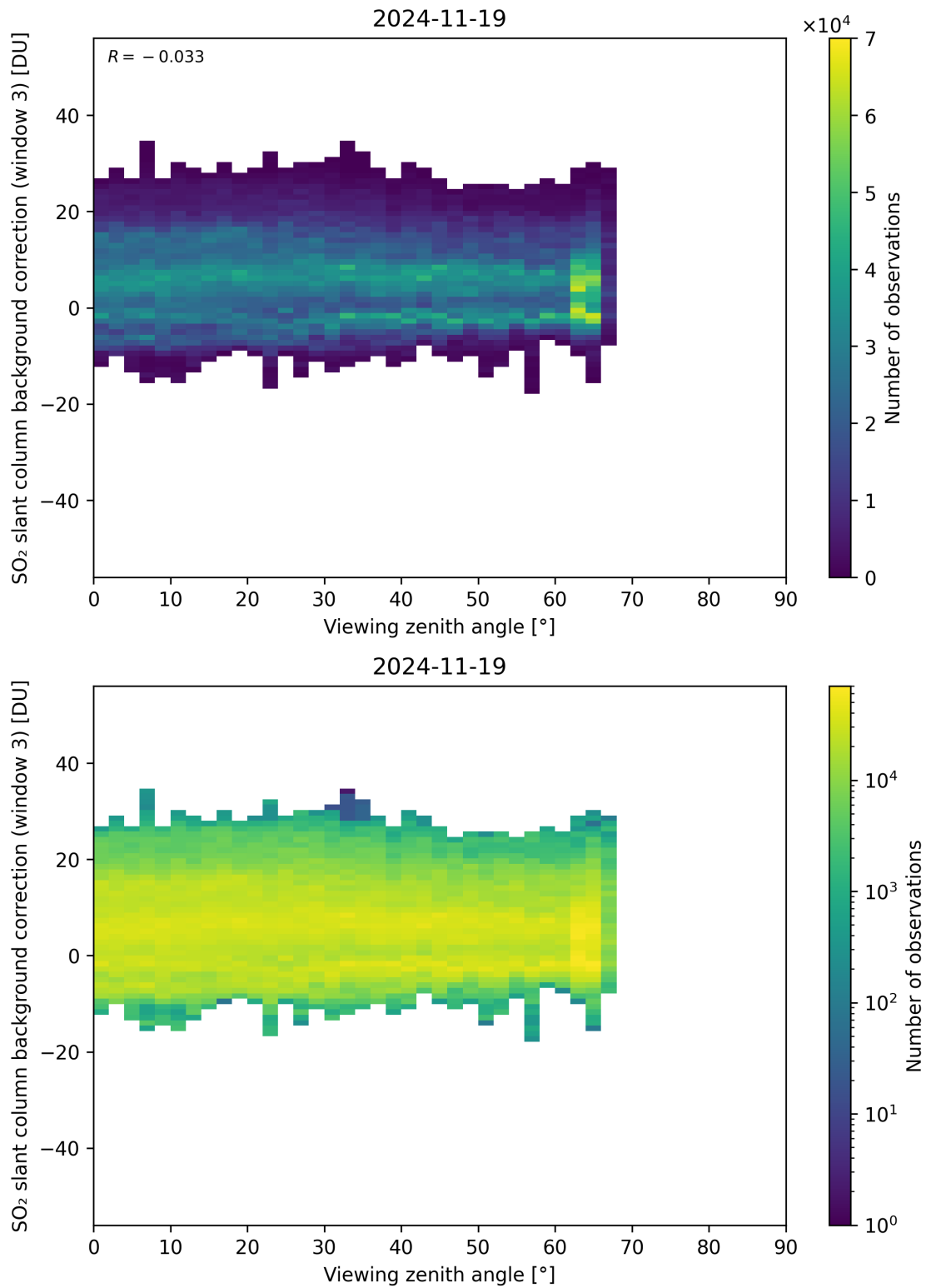
Figure 364: Scatter density plot of “Viewing zenith angle” against “SO 2 slant column background correction (window 3)” for 2024-11-18 to 2024-11-20.
