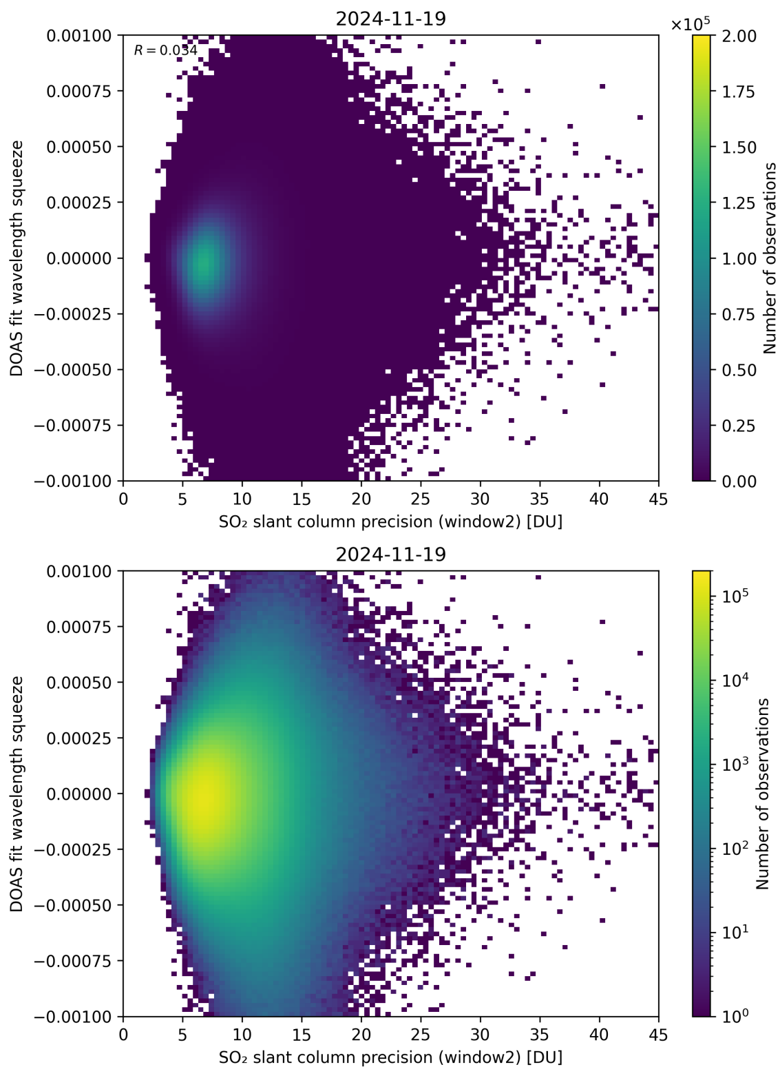
Figure 294: Scatter density plot of “SO 2 slant column precision (window2)” against “DOAS fit wavelength squeeze” for 2024-11-18 to 2024-11-20.
