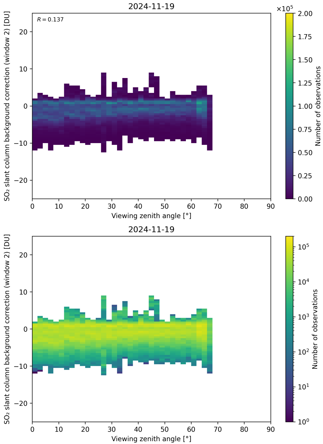
Figure 363: Scatter density plot of “Viewing zenith angle” against “SO 2 slant column background correction (window 2)” for 2024-11-18 to 2024-11-20.
