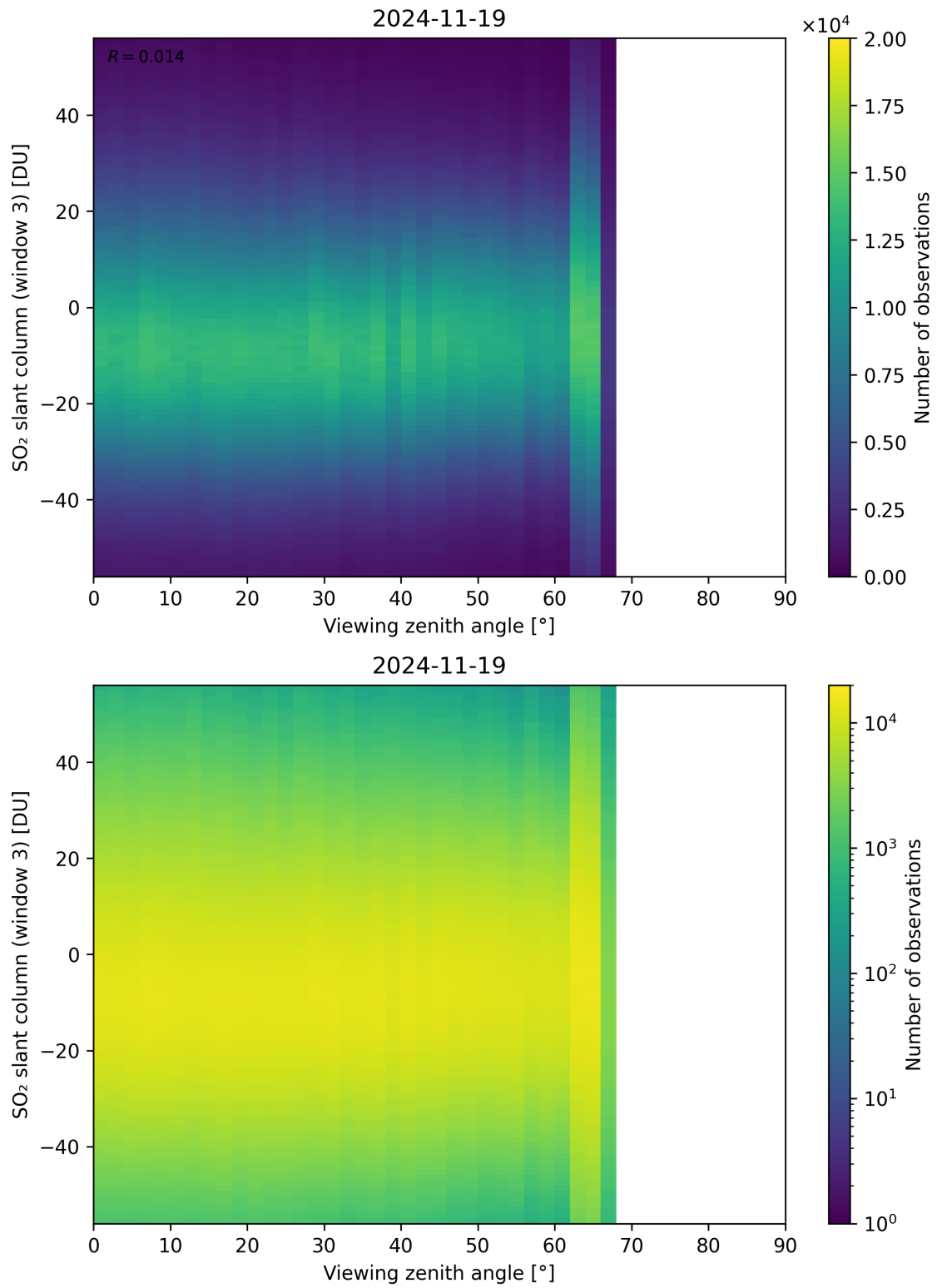
Figure 379: Scatter density plot of “Viewing zenith angle” against “SO 2 slant column (window 3)” for 2024-11-18 to 2024-11-20.
