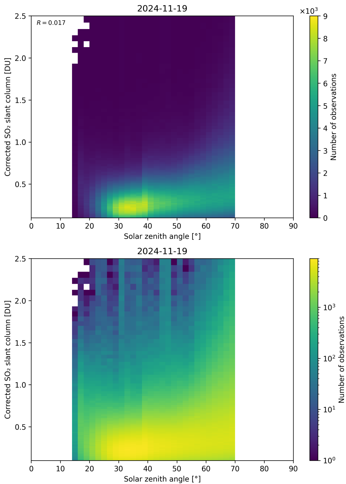
Figure 181: Scatter density plot of “Solar zenith angle” against “Corrected SO 2 slant column” for 2024-11-18 to 2024-11-20.
