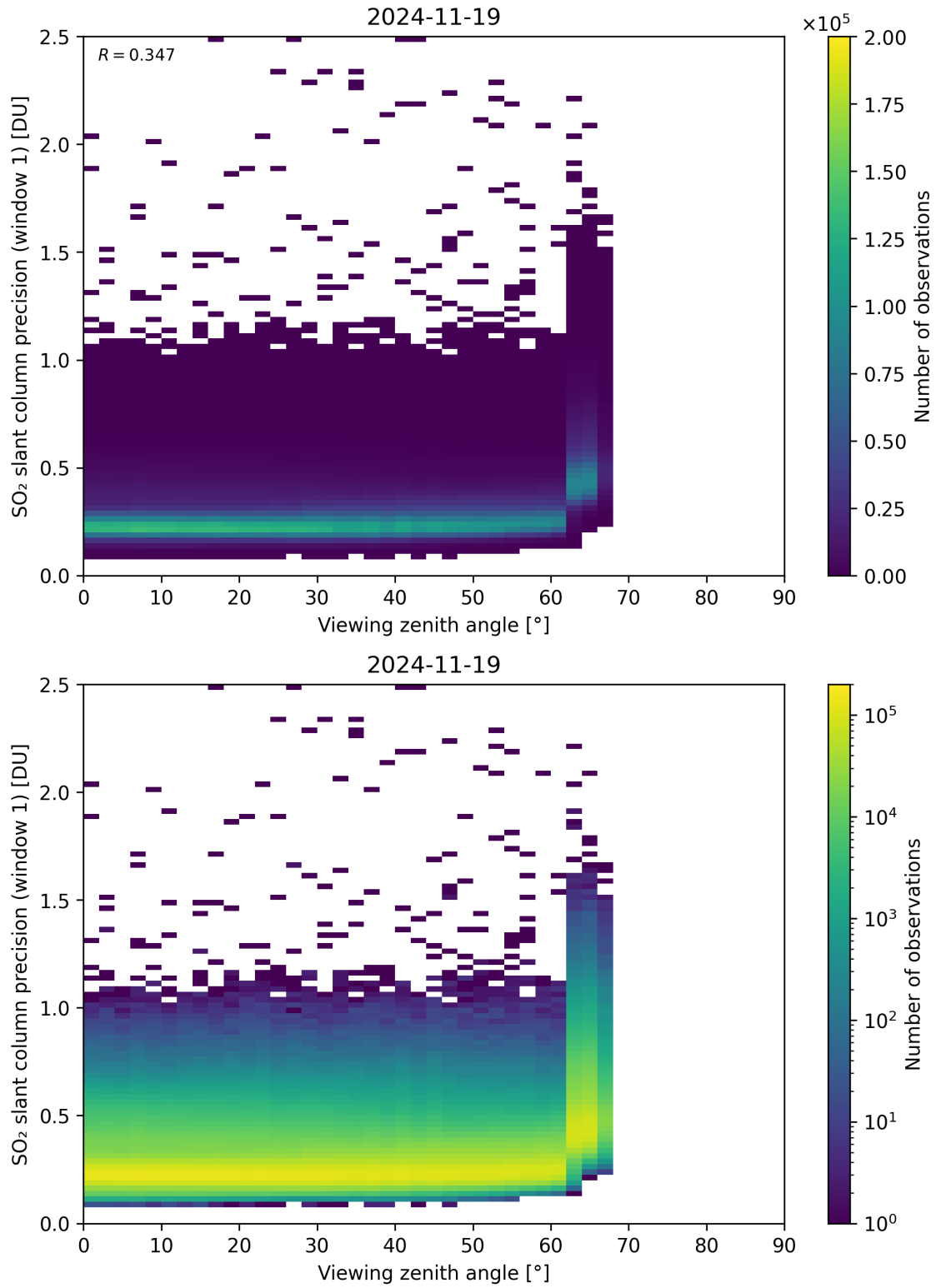
Figure 377: Scatter density plot of “Viewing zenith angle” against “SO 2 slant column precision (window 1)” for 2024-11-18 to 2024-11-20.
