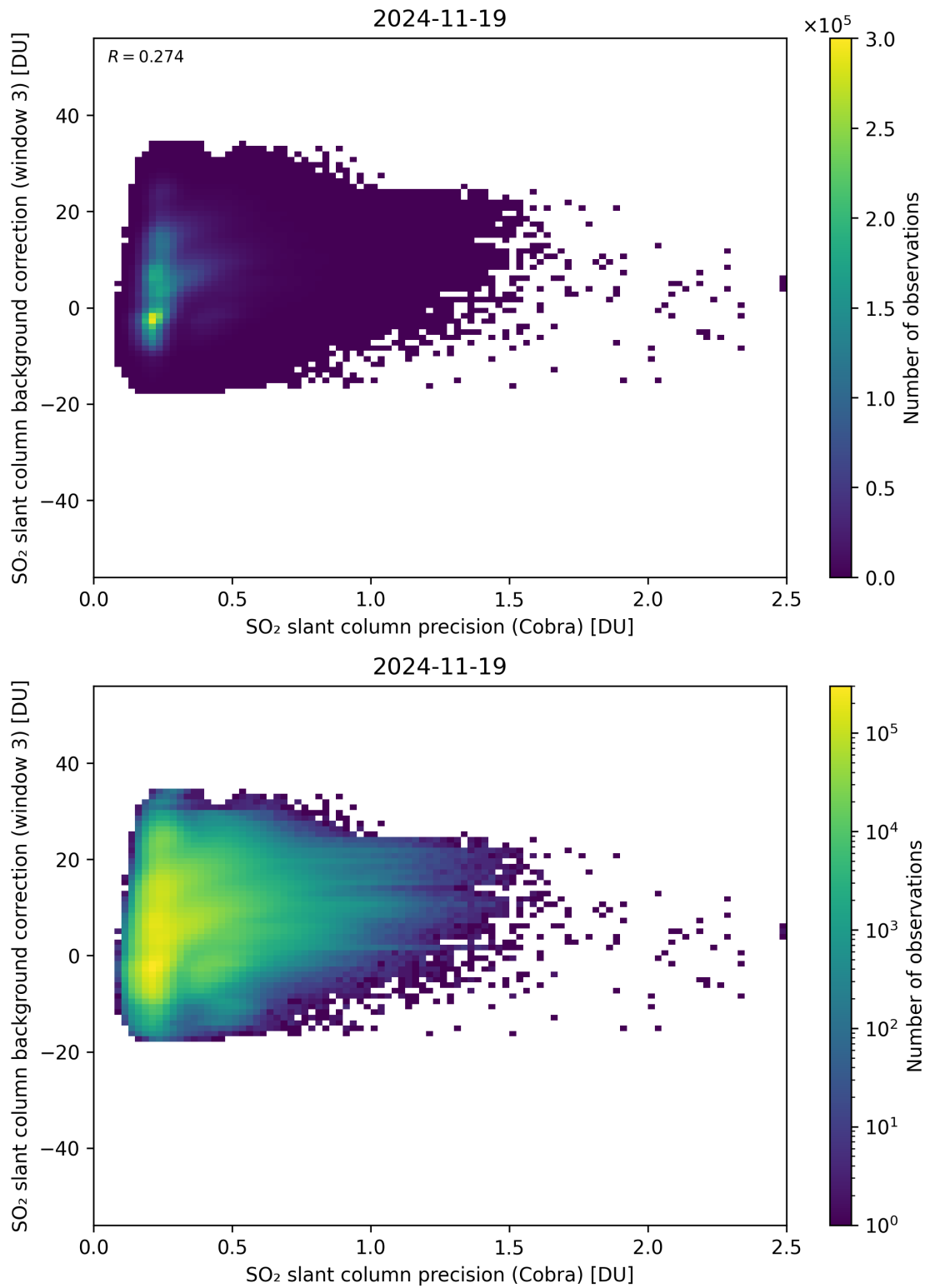
Figure 201: Scatter density plot of “SO 2 slant column precision (Cobra)” against “SO 2 slant column background correction (window 3)” for 2024-11-18 to 2024-11-20.
