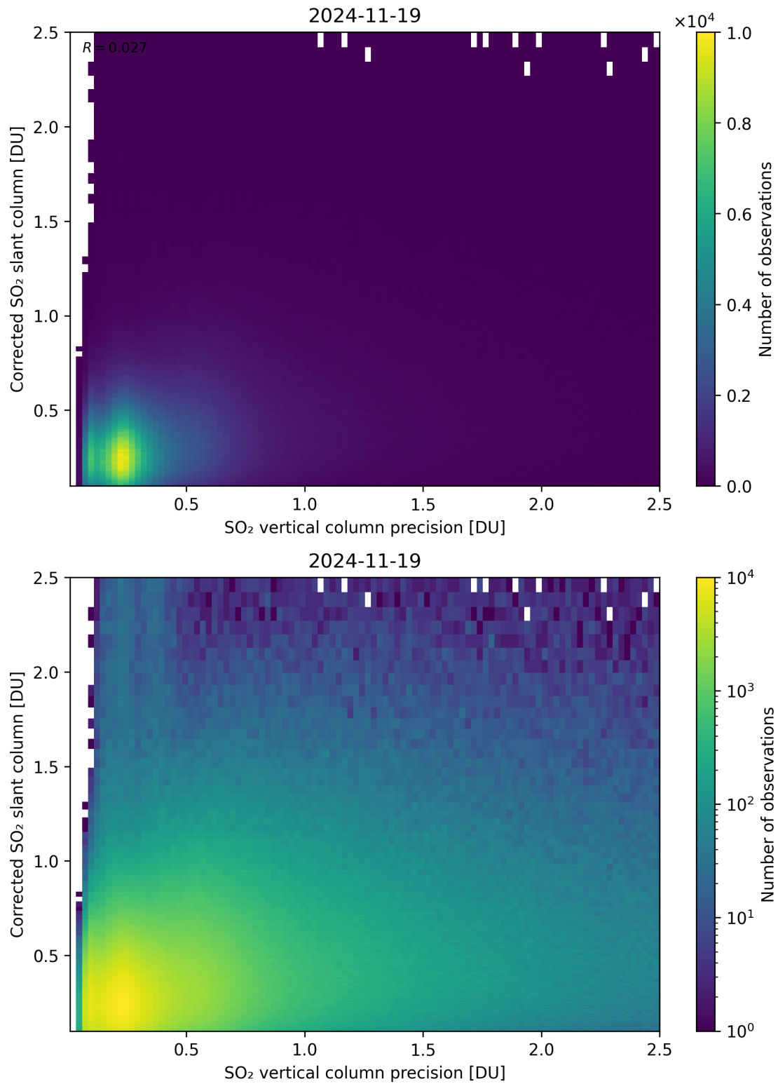
Figure 338: Scatter density plot of “SO 2 vertical column precision” against “Corrected SO 2 slant column” for 2024-11-18 to 2024-11-20.
