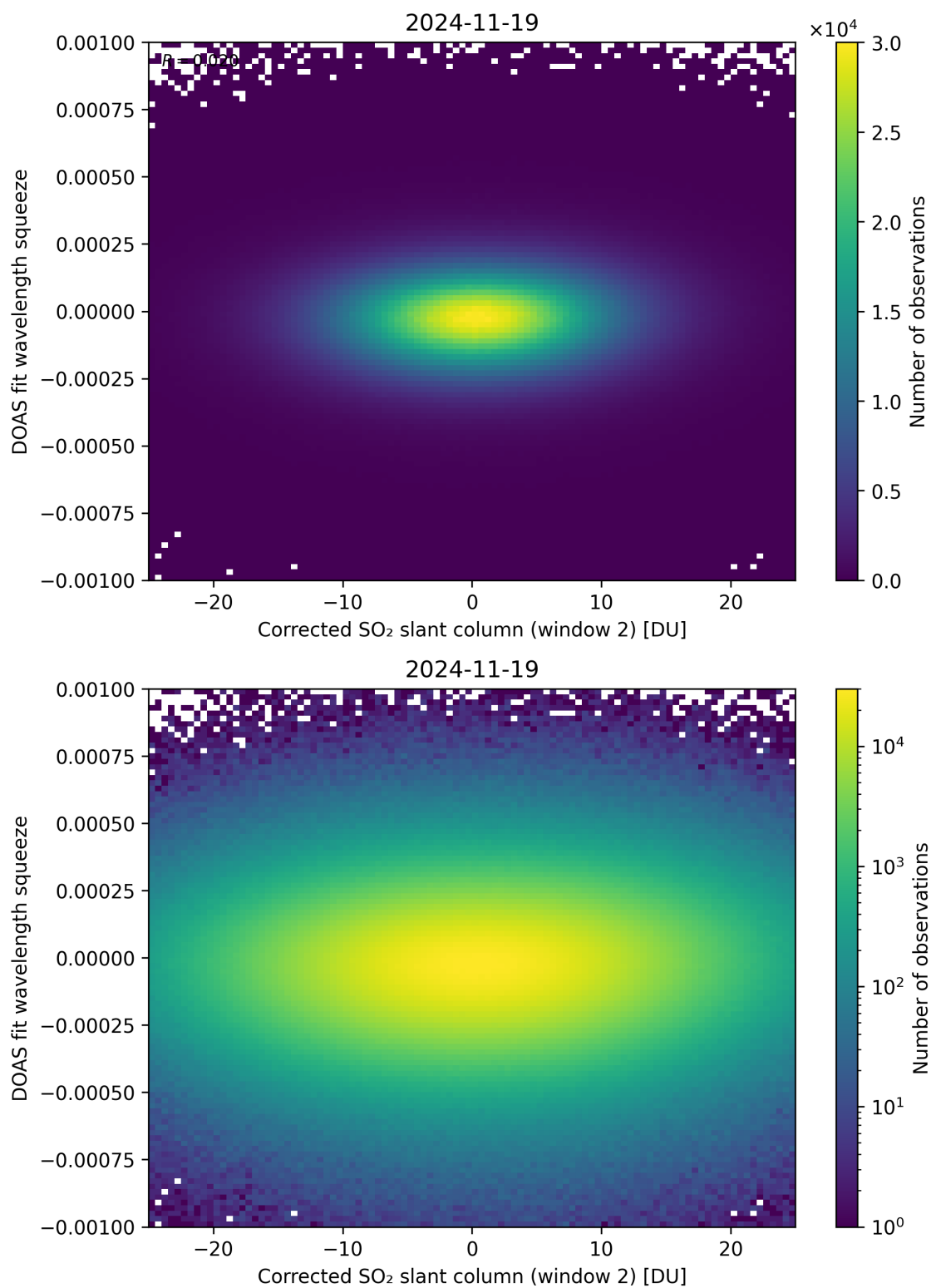
Figure 247: Scatter density plot of “Corrected SO 2 slant column (window 2)” against “DOAS fit wavelength squeeze” for 2024-11-18 to 2024-11-20.
