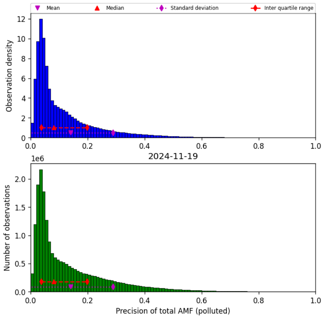
Figure 80: Histogram of “Precision of total AMF (polluted)” for 2024-11-18 to 2024-11-20
