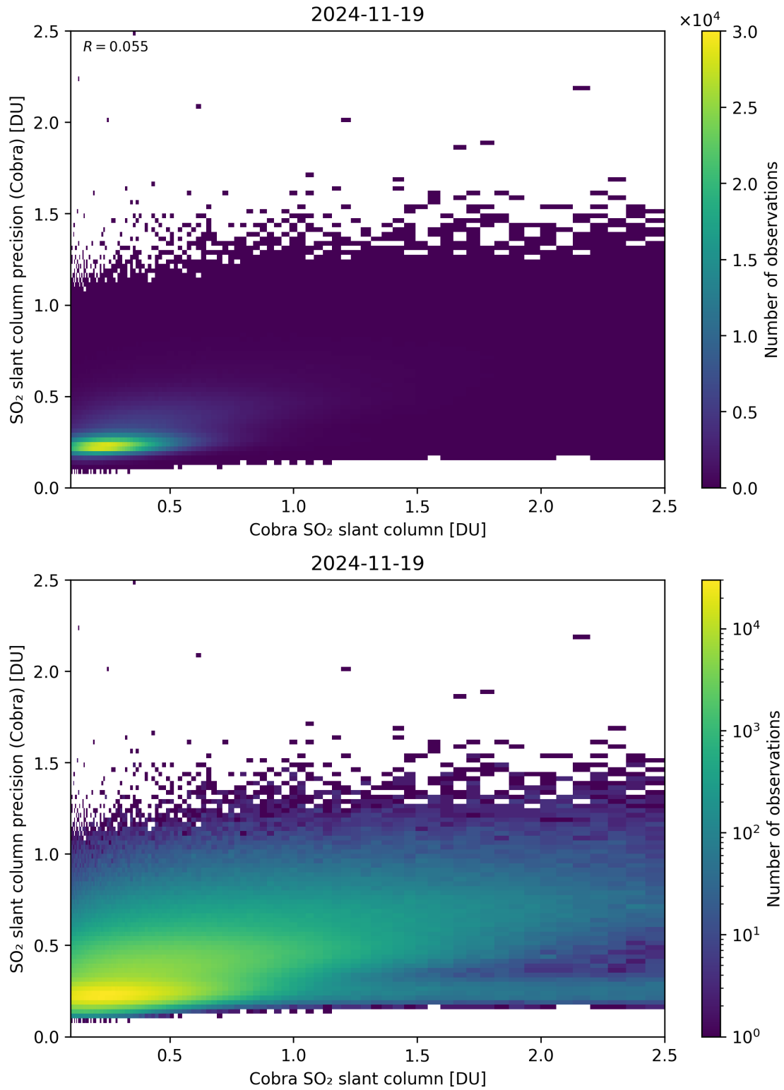
Figure 216: Scatter density plot of “Cobra SO 2 slant column” against “SO 2 slant column precision (Cobra)” for 2024-11-18 to 2024-11-20.
