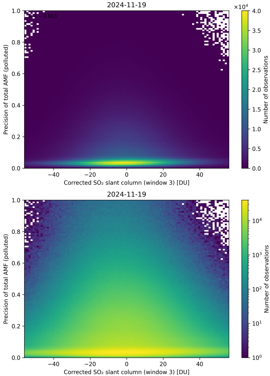
Figure 261: Scatter density plot of “Corrected SO 2 slant column (window 3)” against “Precision of total AMF (polluted)” for 2024-11-18 to 2024-11-20.
