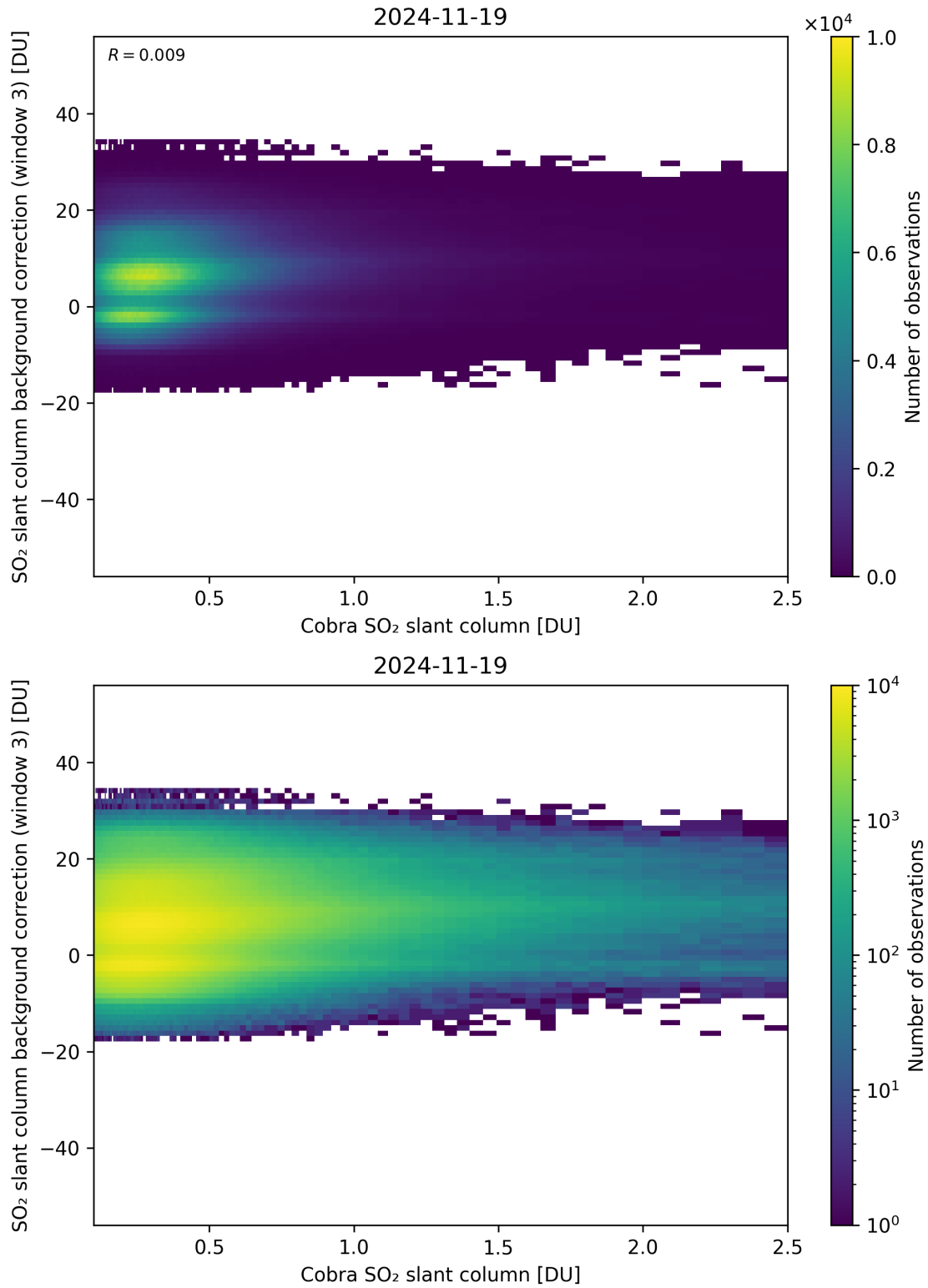
Figure 195: Scatter density plot of “Cobra SO 2 slant column” against “SO 2 slant column background correction (window 3)” for 2024-11-18 to 2024-11-20.
