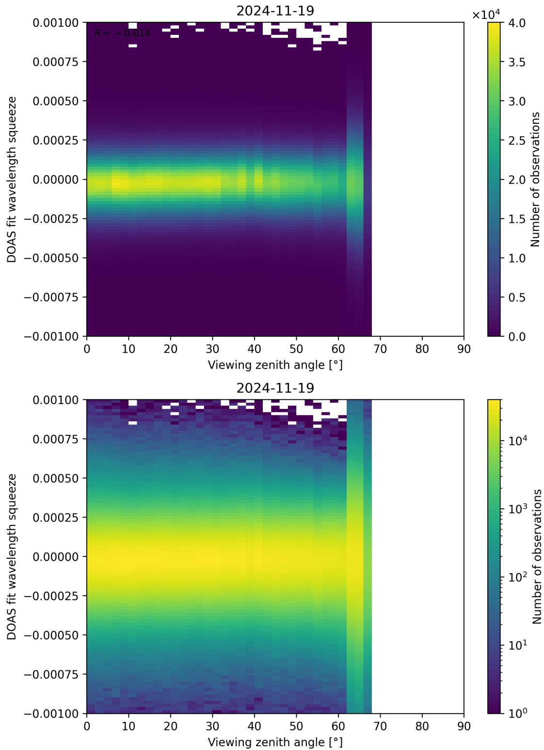
Figure 366: Scatter density plot of “Viewing zenith angle” against “DOAS fit wavelength squeeze” for 2024-11-18 to 2024-11-20.
