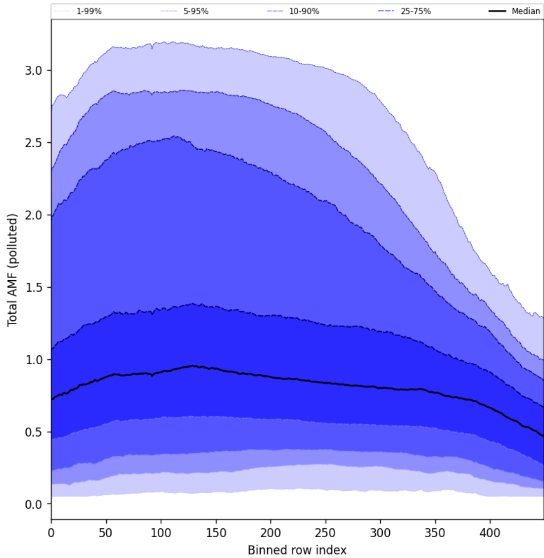
Figure 105: Along track statistics of “Total AMF (polluted)” for 2024-11-18 to 2024-11-20
