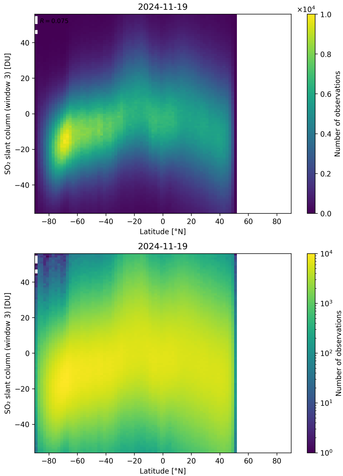
Figure 165: Scatter density plot of “Latitude” against “SO 2 slant column (window 3)” for 2024-11-18 to 2024-11-20.
