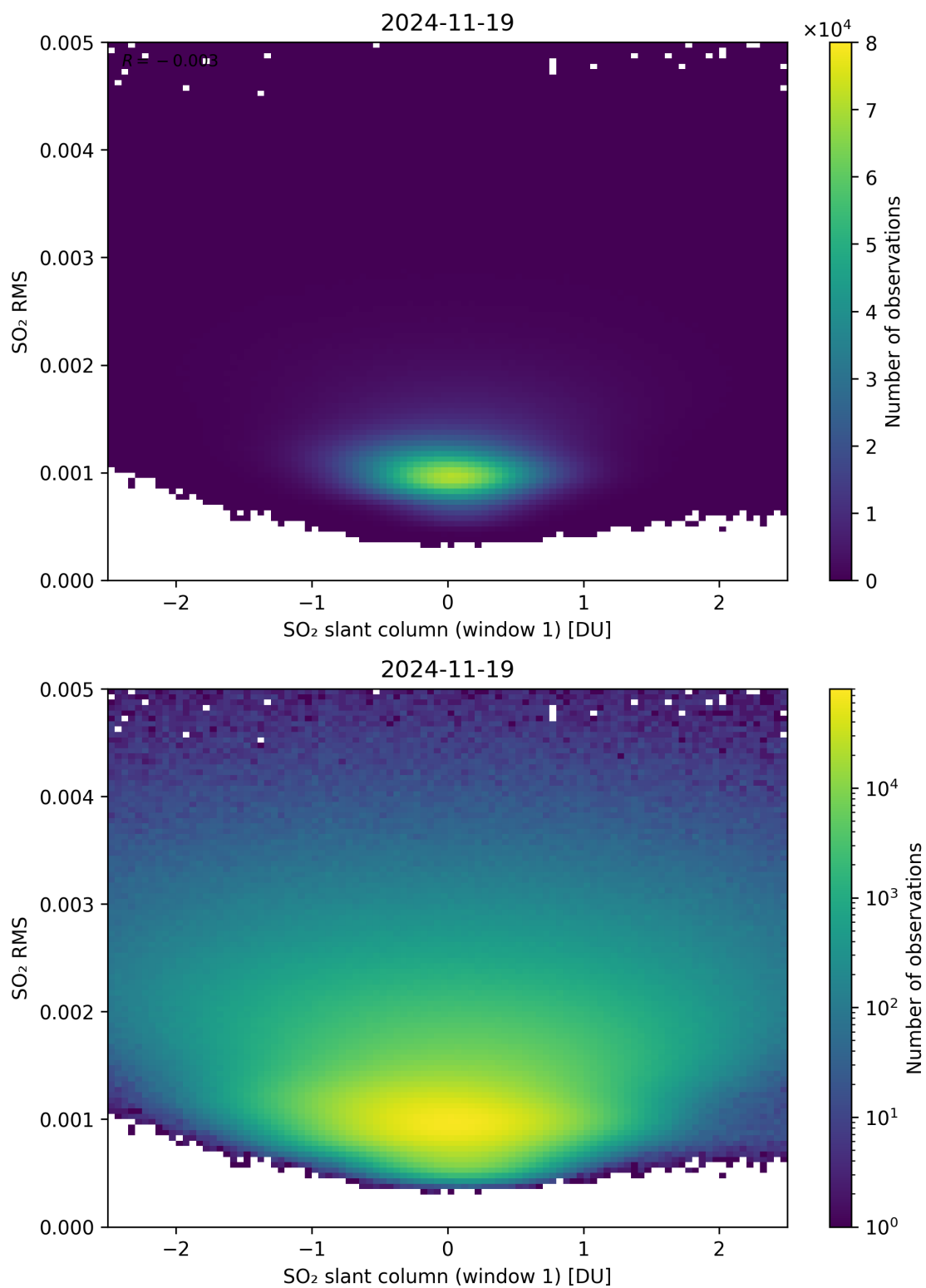
Figure 267: Scatter density plot of “SO 2 slant column (window 1)” against “SO 2 RMS” for 2024-11-18 to 2024-11-20.
