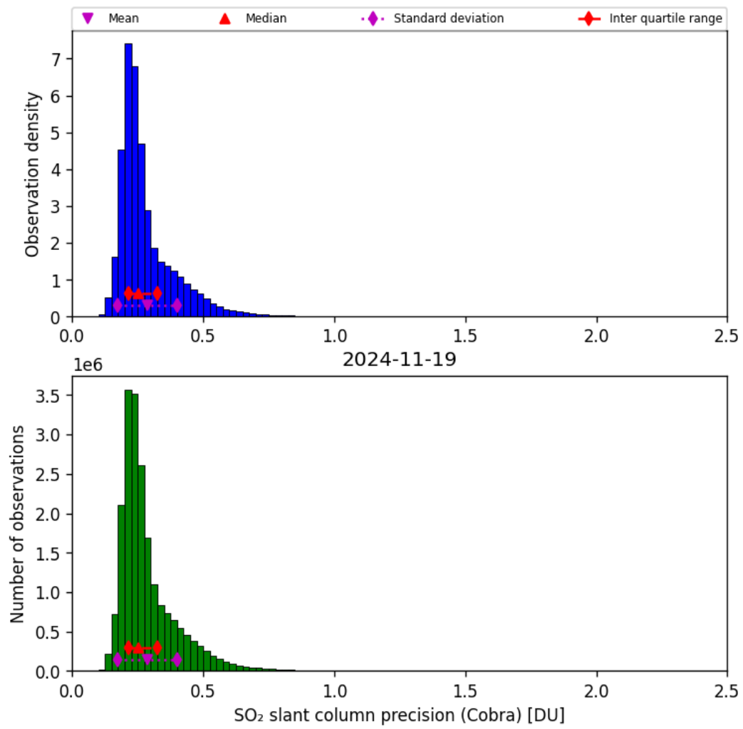
Figure 62: Histogram of “SO 2 slant column precision (Cobra)” for 2024-11-18 to 2024-11-20
