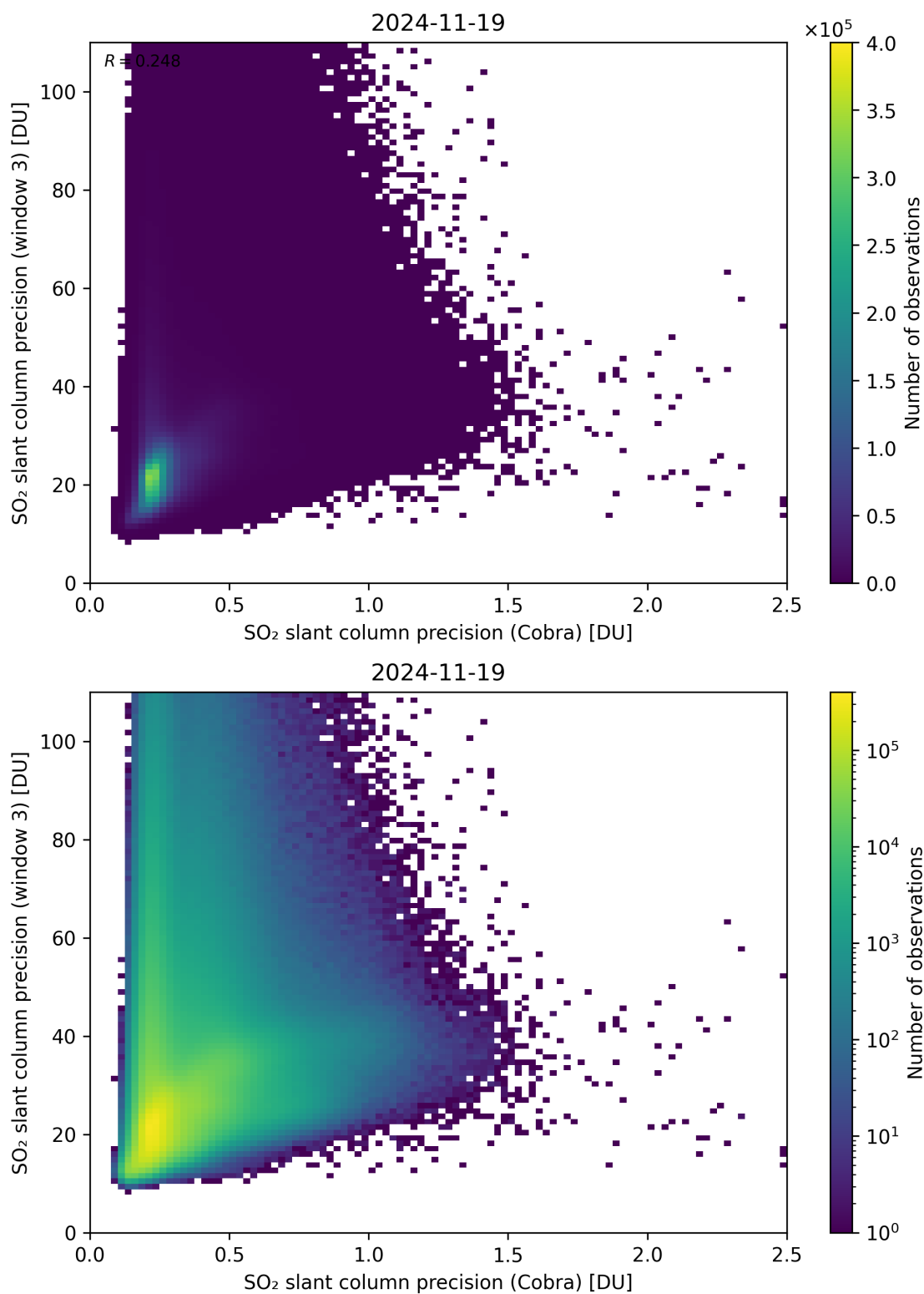
Figure 212: Scatter density plot of “SO 2 slant column precision (Cobra)” against “SO 2 slant column precision (window 3)” for 2024-11-18 to 2024-11-20.
