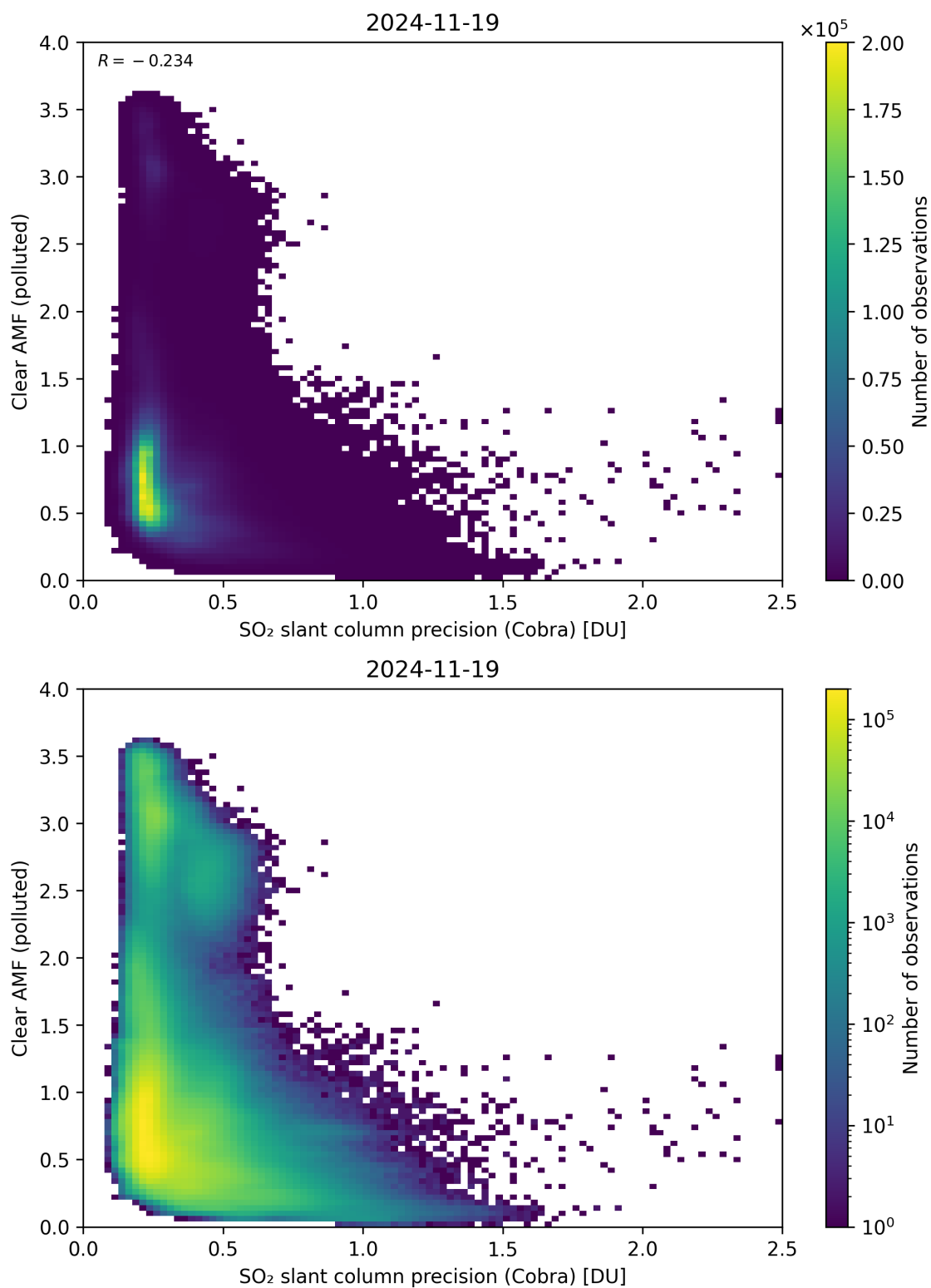
Figure 205: Scatter density plot of “SO 2 slant column precision (Cobra)” against “Clear AMF (polluted)” for 2024-11-18 to 2024-11-20.
