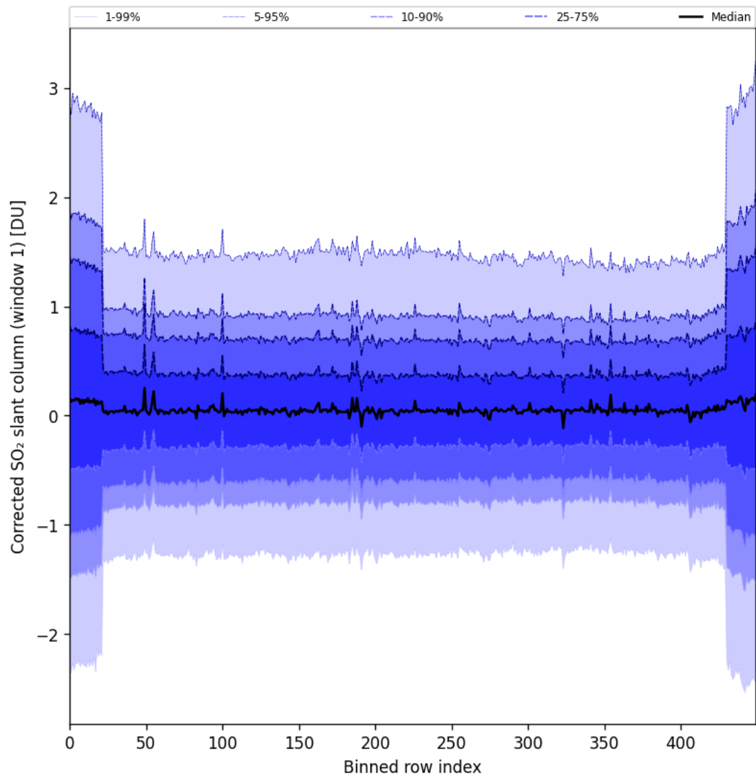
Figure 91: Along track statistics of “Corrected SO 2 slant column (window 1)” for 2024-11-18 to 2024-11-20
