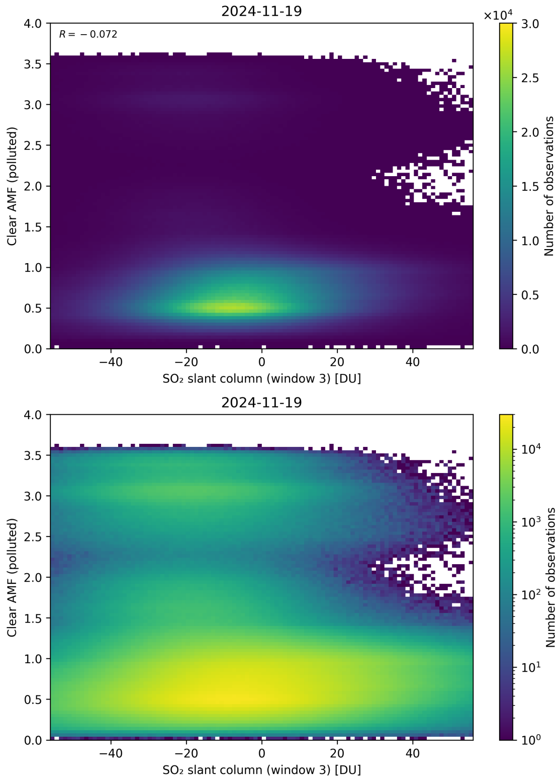
Figure 315: Scatter density plot of “SO 2 slant column (window 3)” against “Clear AMF (polluted)” for 2024-11-18 to 2024-11-20.
