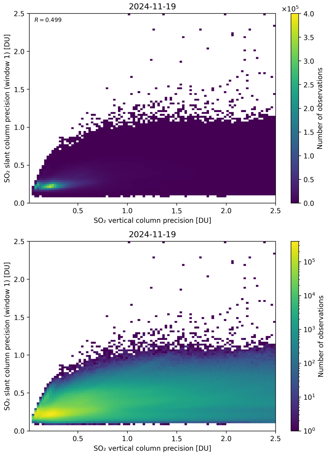
Figure 342: Scatter density plot of “SO 2 vertical column precision” against “SO 2 slant column precision (window 1)” for 2024-11-18 to 2024-11-20.
