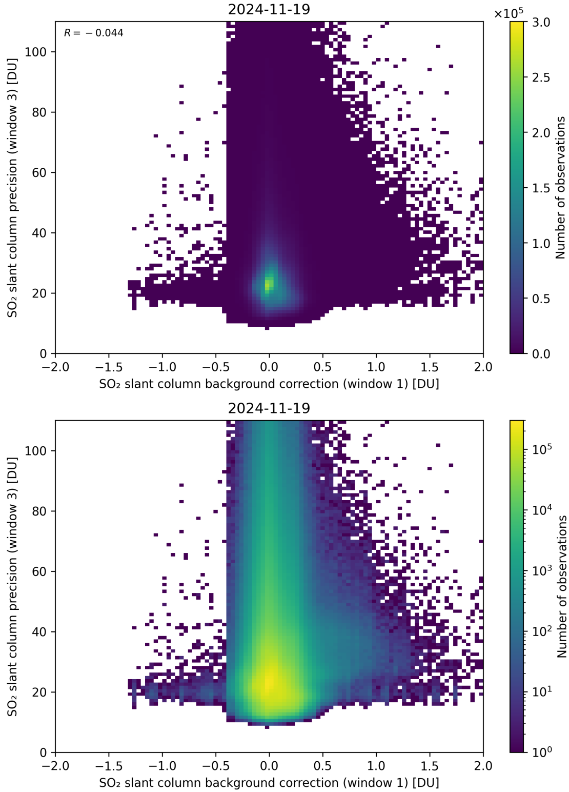
Figure 119: Scatter density plot of “SO 2 slant column background correction (window 1)” against “SO 2 slant column precision (window 3)” for 2024-11-18 to 2024-11-20.
