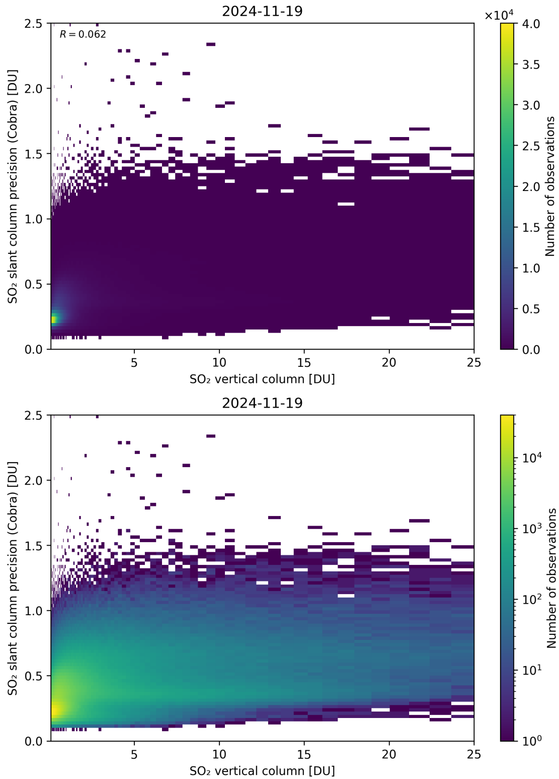
Figure 350: Scatter density plot of “SO 2 vertical column” against “SO 2 slant column precision (Cobra)” for 2024-11-18 to 2024-11-20.
