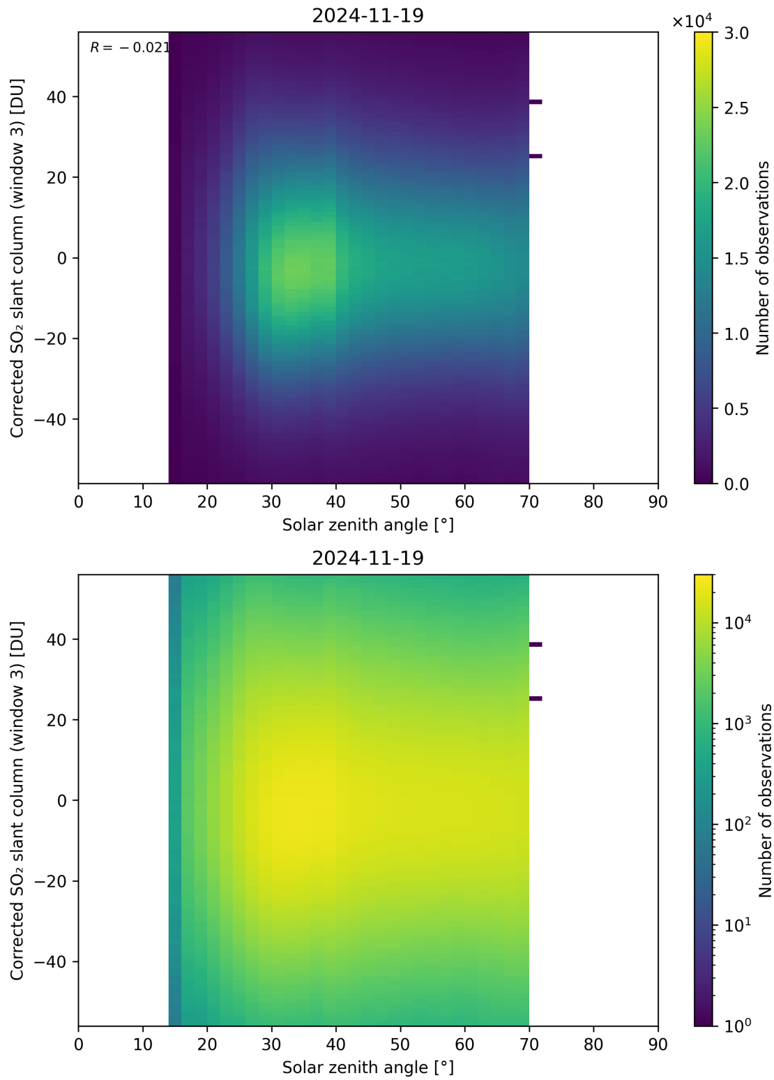
Figure 183: Scatter density plot of “Solar zenith angle” against “Corrected SO 2 slant column (window 3)” for 2024-11-18 to 2024-11-20.
