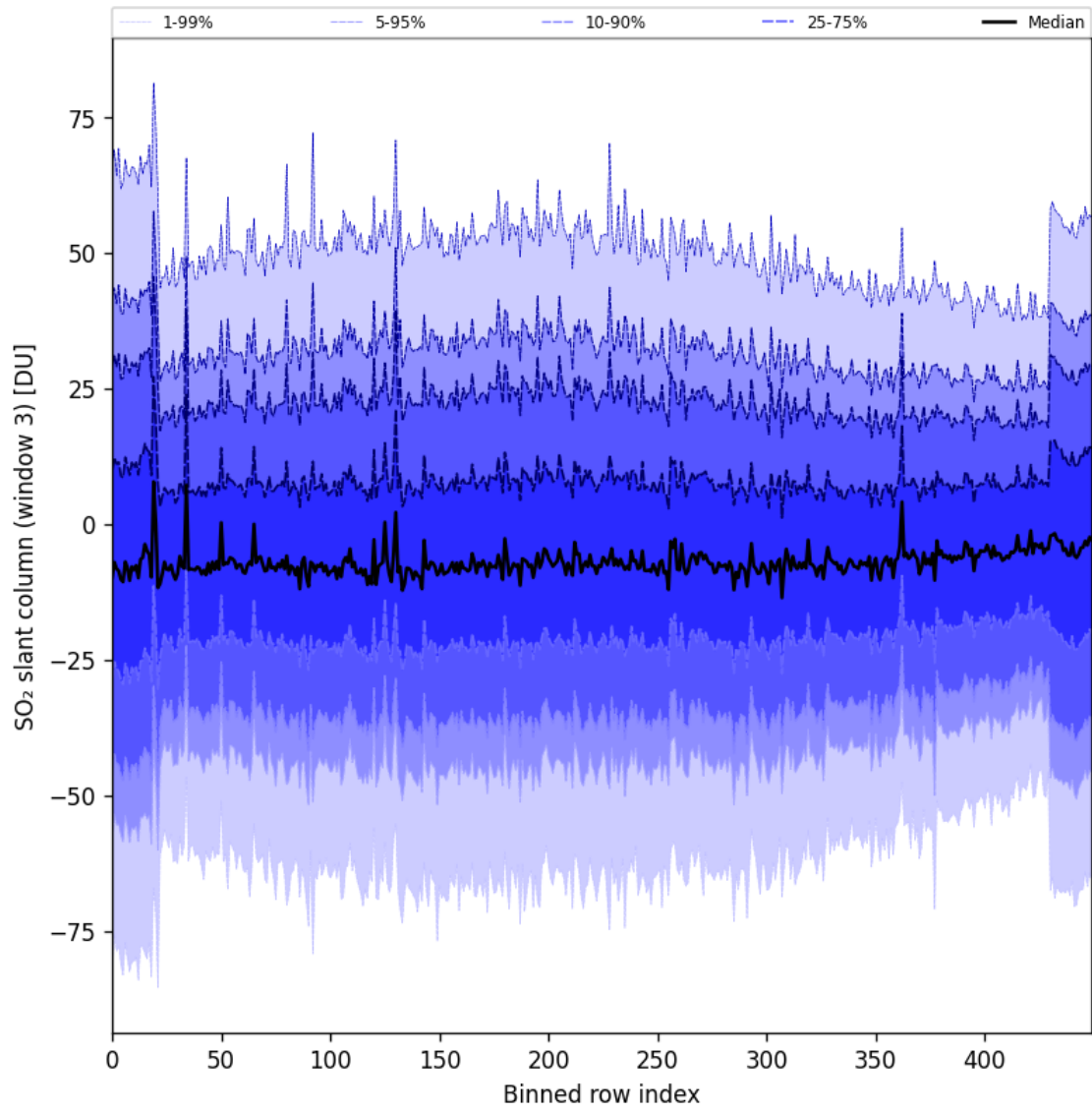
Figure 97: Along track statistics of “SO 2 slant column (window 3)” for 2024-11-18 to 2024-11-20
