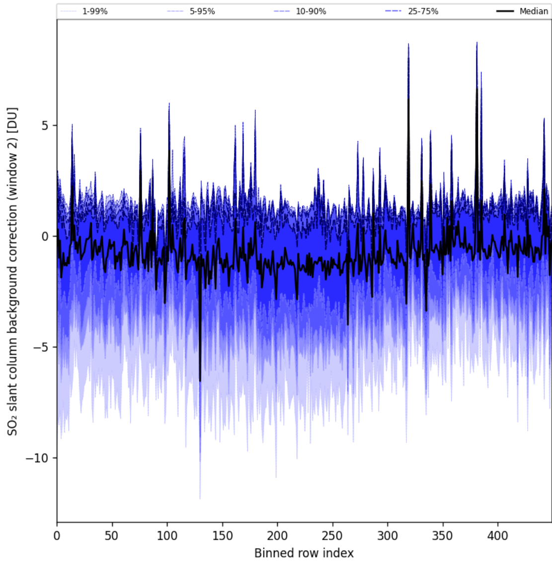
Figure 96: Along track statistics of “SO 2 slant column background correction (window 2)” for 2024-11-18 to 2024-11-20
