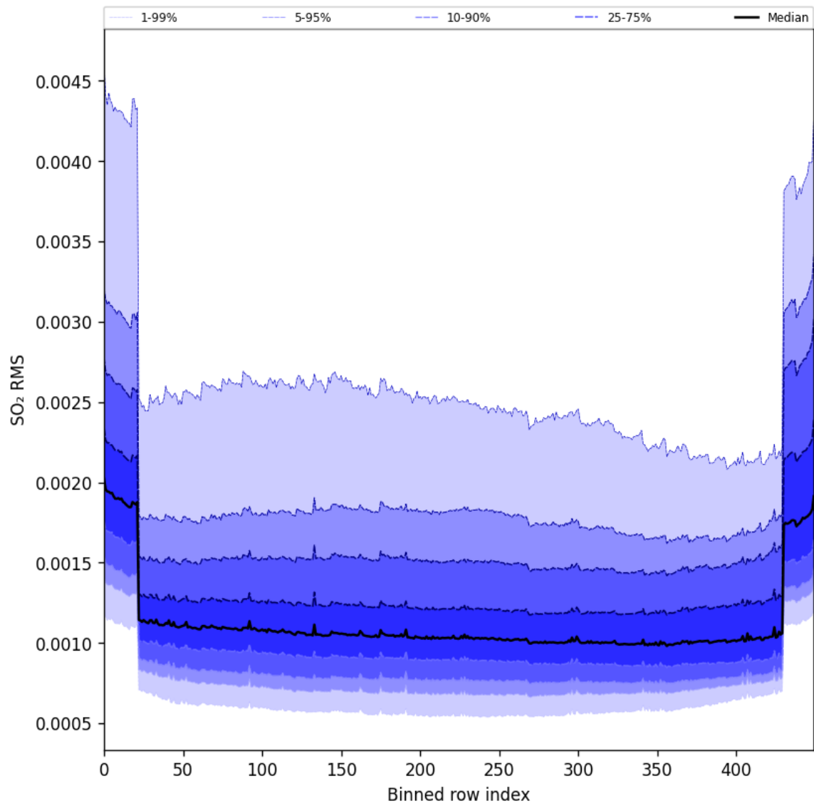
Figure 104: Along track statistics of “SO 2 RMS” for 2024-11-18 to 2024-11-20
