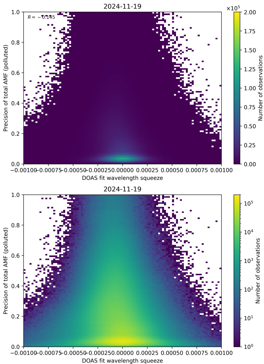
Figure 146: Scatter density plot of “DOAS fit wavelength squeeze” against “Precision of total AMF (polluted)” for 2024-11-18 to 2024-11-20.
