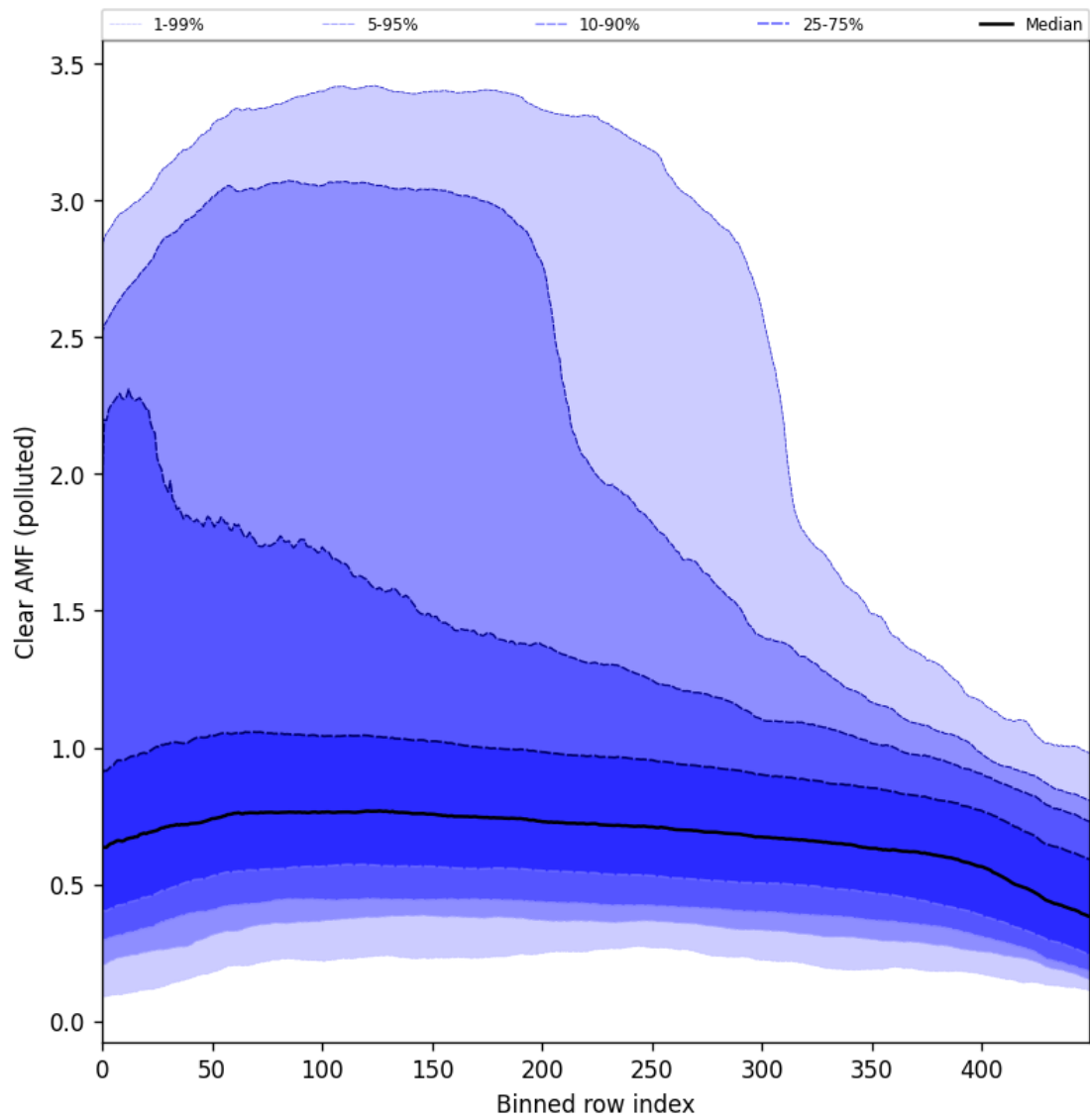
Figure 107: Along track statistics of “Clear AMF (polluted)” for 2024-11-18 to 2024-11-20
