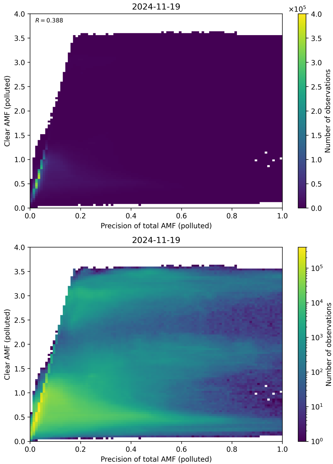
Figure 320: Scatter density plot of “Precision of total AMF (polluted)” against “Clear AMF (polluted)” for 2024-11-18 to 2024-11-20.
