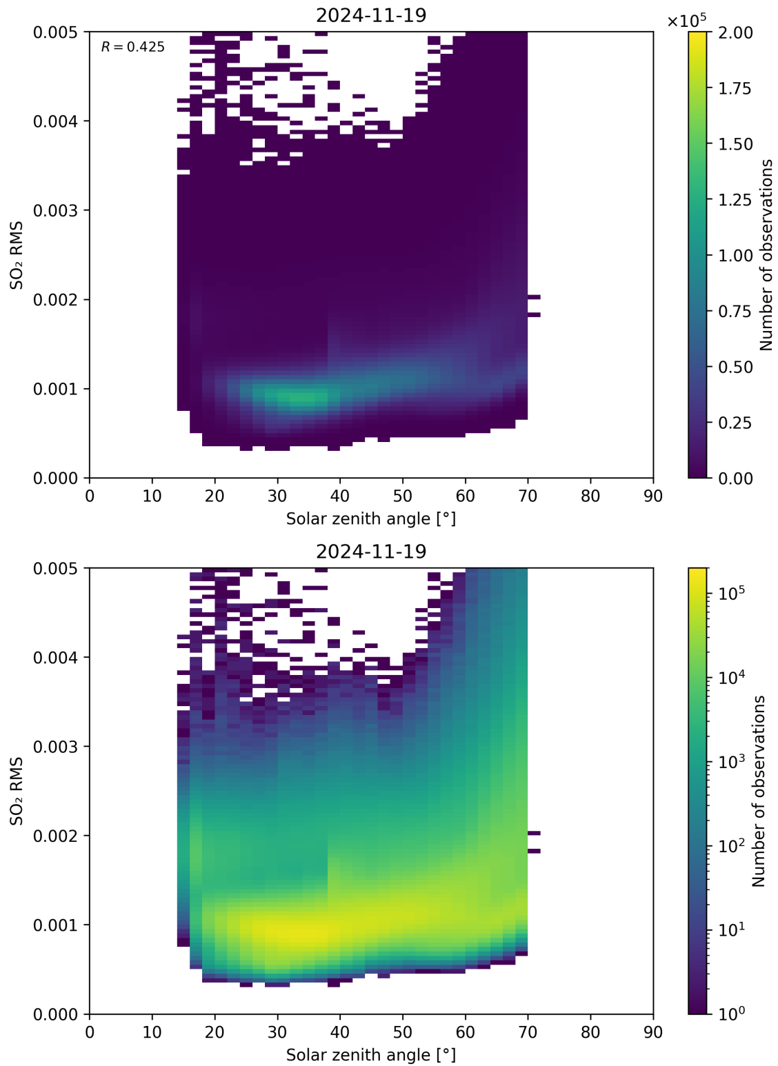
Figure 176: Scatter density plot of “Solar zenith angle” against “SO 2 RMS” for 2024-11-18 to 2024-11-20.
