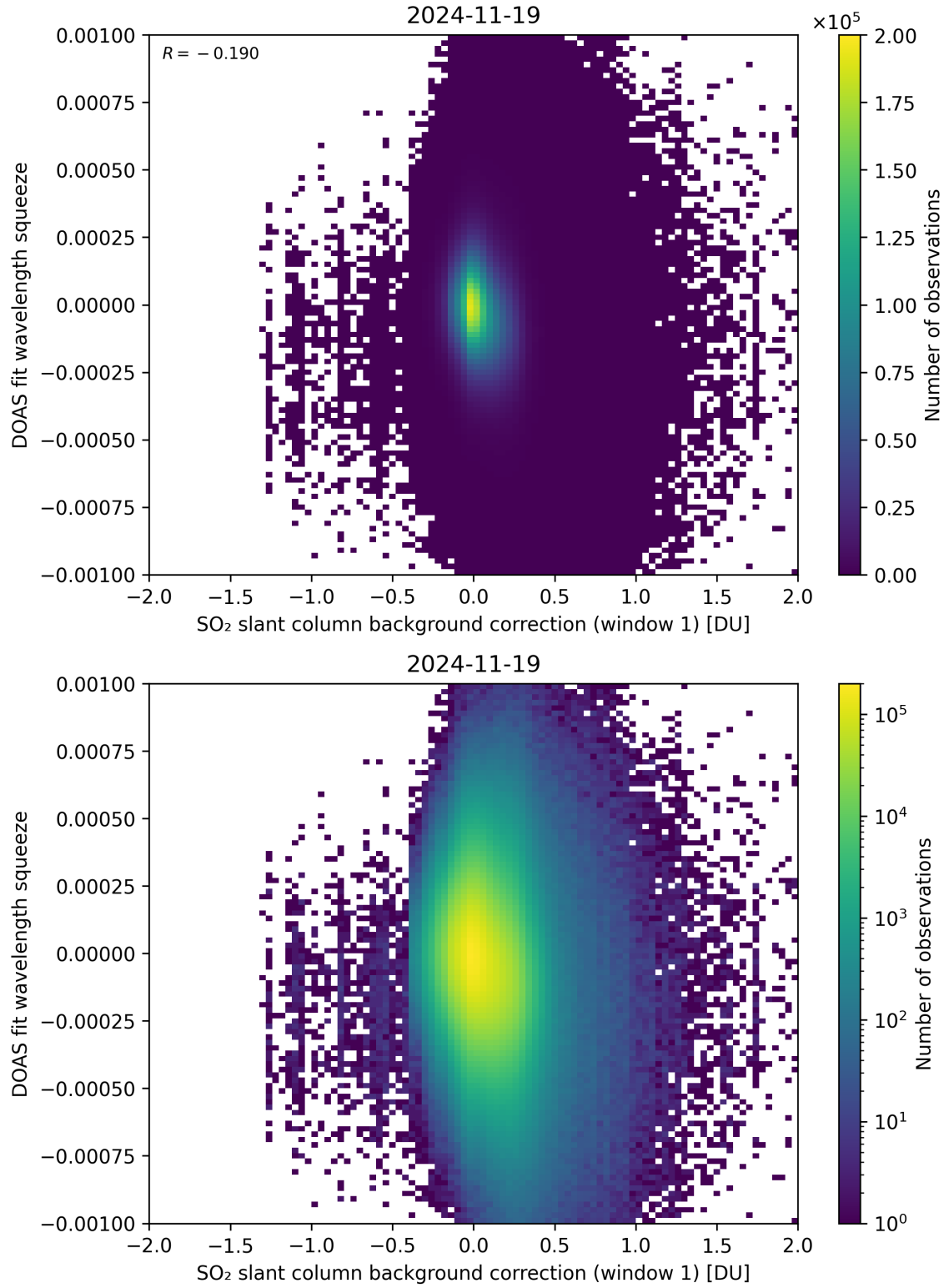
Figure 112: Scatter density plot of “SO 2 slant column background correction (window 1)” against “DOAS fit wavelength squeeze” for 2024-11-18 to 2024-11-20.
