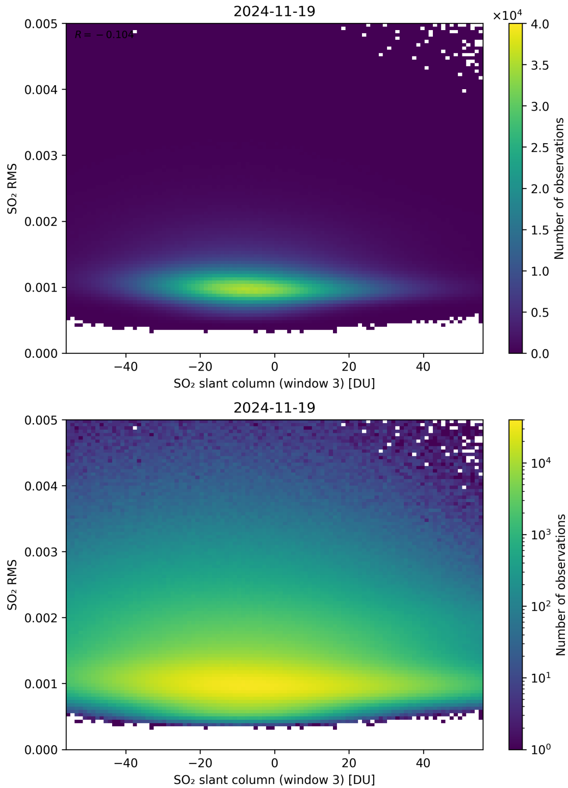
Figure 306: Scatter density plot of “SO 2 slant column (window 3)” against “SO 2 RMS” for 2024-11-18 to 2024-11-20.
