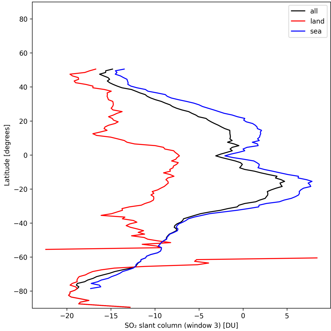
Figure 45: Zonal average of “SO 2 slant column (window 3)” for 2024-11-18 to 2024-11-20.
