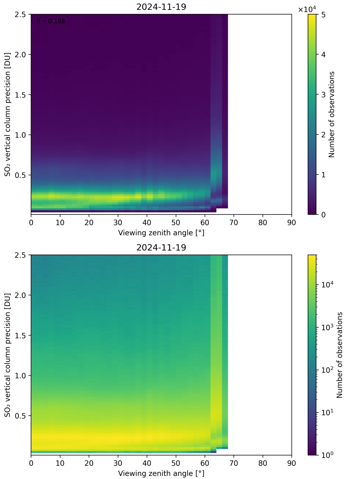
Figure 384: Scatter density plot of “Viewing zenith angle” against “SO 2 vertical column precision” for 2024-11-18 to 2024-11-20.
