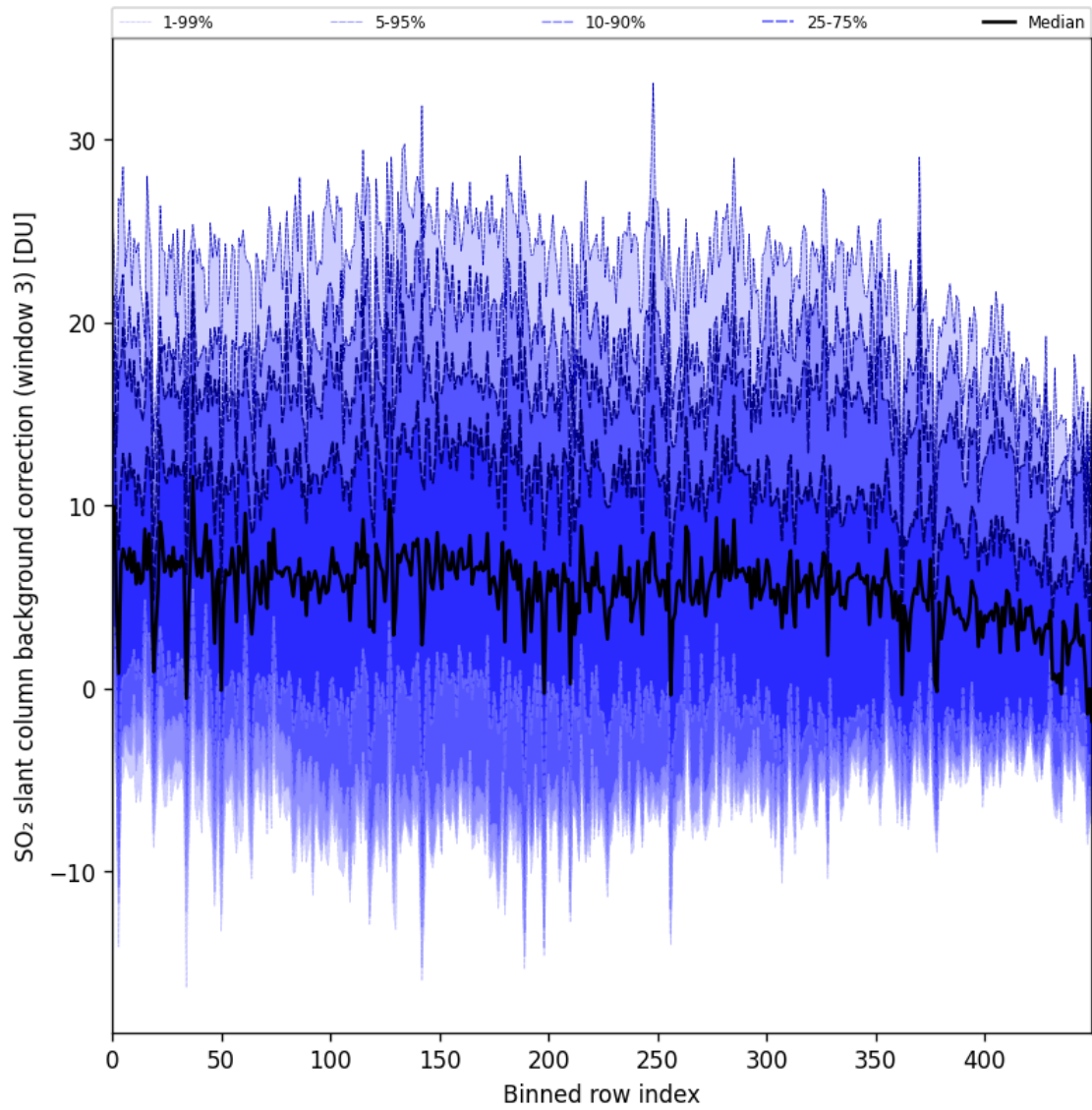
Figure 100: Along track statistics of “SO 2 slant column background correction (window 3)” for 2024-11-18 to 2024-11-20
