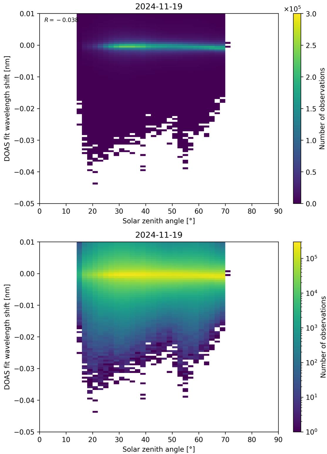
Figure 174: Scatter density plot of “Solar zenith angle” against “DOAS fit wavelength shift” for 2024-11-18 to 2024-11-20.
