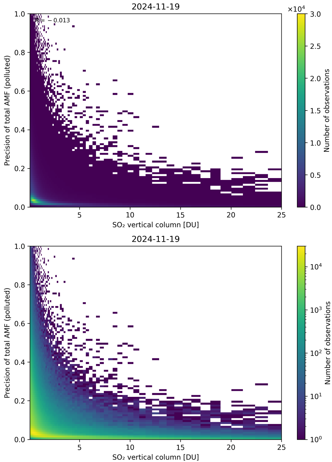
Figure 360: Scatter density plot of “SO 2 vertical column” against “Precision of total AMF (polluted)” for 2024-11-18 to 2024-11-20.
