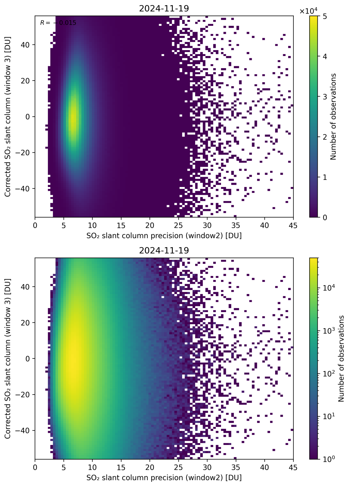
Figure 298: Scatter density plot of “SO 2 slant column precision (window2)” against “Corrected SO 2 slant column (window 3)” for 2024-11-18 to 2024-11-20.
