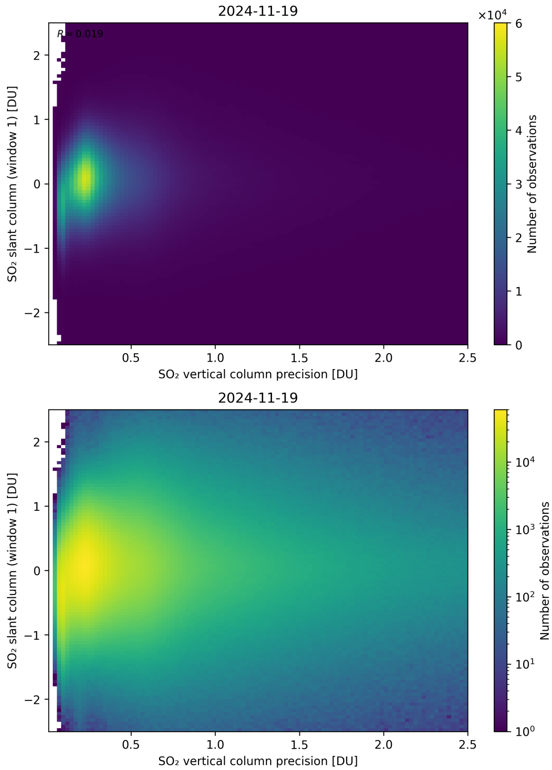
Figure 341: Scatter density plot of “SO 2 vertical column precision” against “SO 2 slant column (window 1)” for 2024-11-18 to 2024-11-20.
