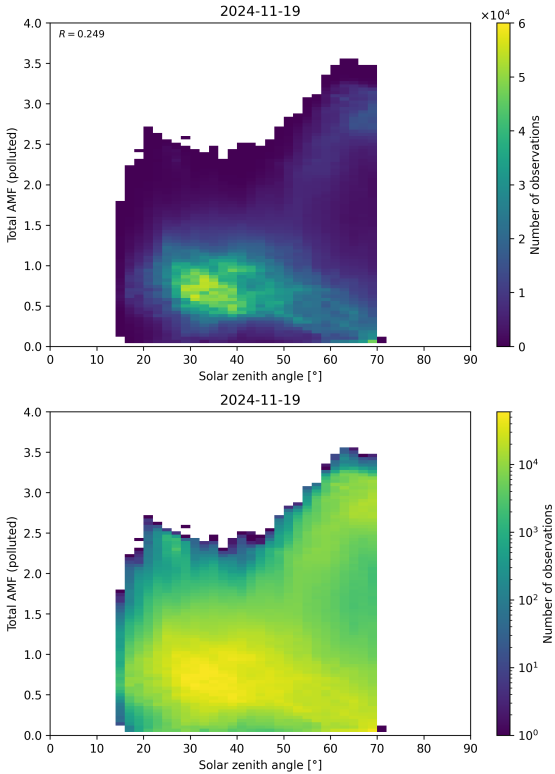
Figure 189: Scatter density plot of “Solar zenith angle” against “Total AMF (polluted)” for 2024-11-18 to 2024-11-20.
