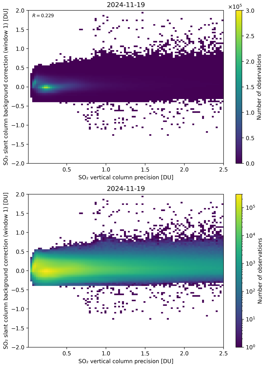
Figure 329: Scatter density plot of “SO 2 vertical column precision” against “SO 2 slant column background correction (window 1)” for 2024-11-18 to 2024-11-20.
