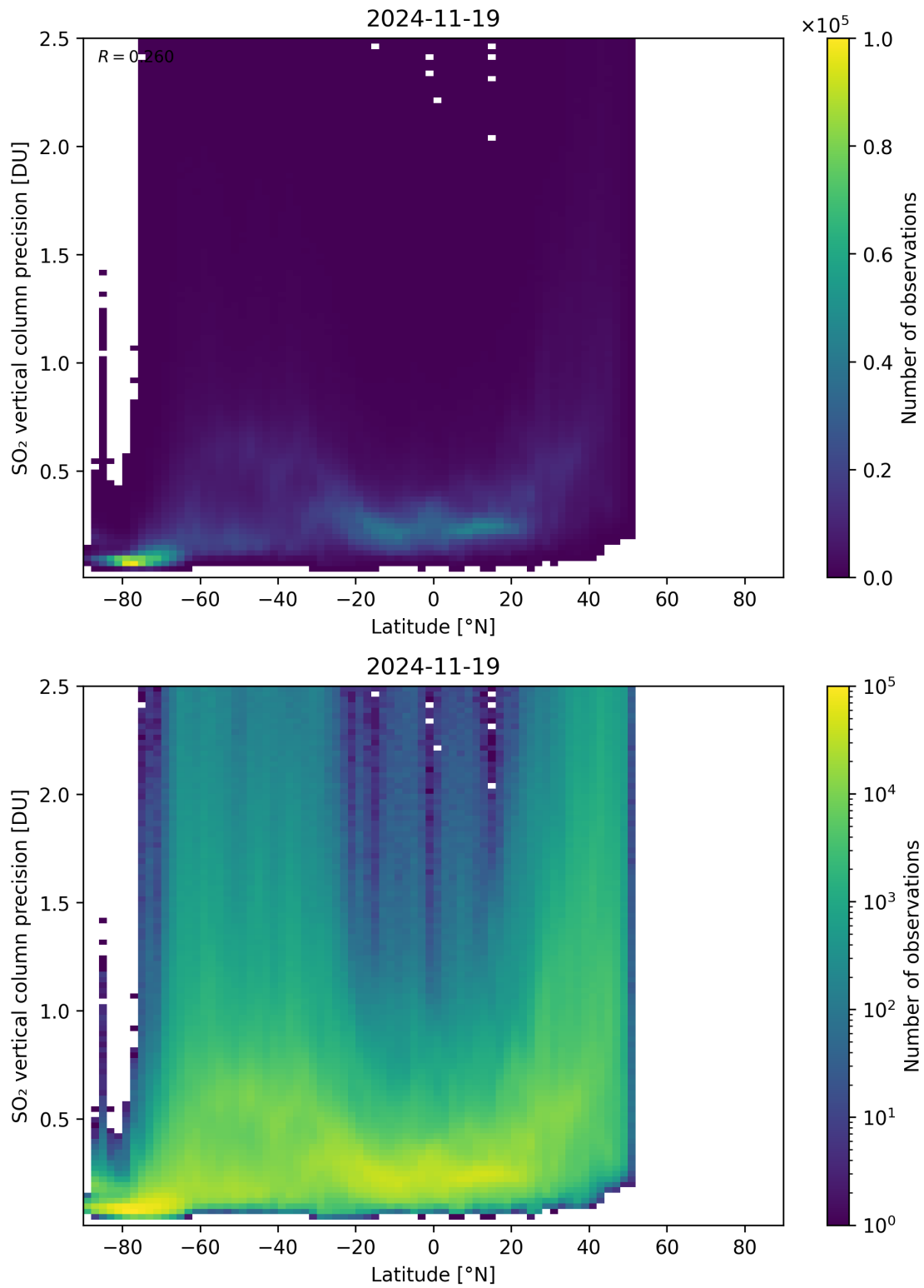
Figure 170: Scatter density plot of “Latitude” against “SO 2 vertical column precision” for 2024-11-18 to 2024-11-20.
