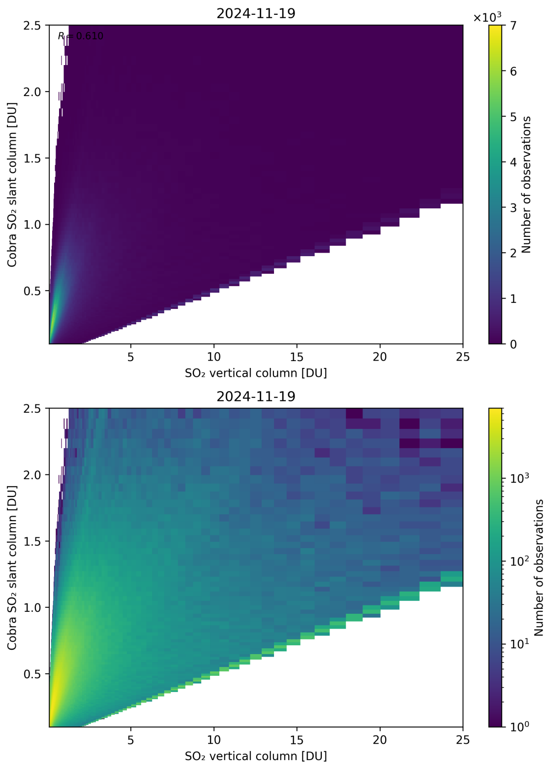
Figure 349: Scatter density plot of “SO 2 vertical column” against “Cobra SO 2 slant column” for 2024-11-18 to 2024-11-20.
