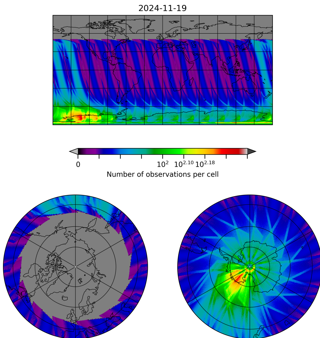
Figure 30: Map of the number of observations for 2024-11-18 to 2024-11-20
