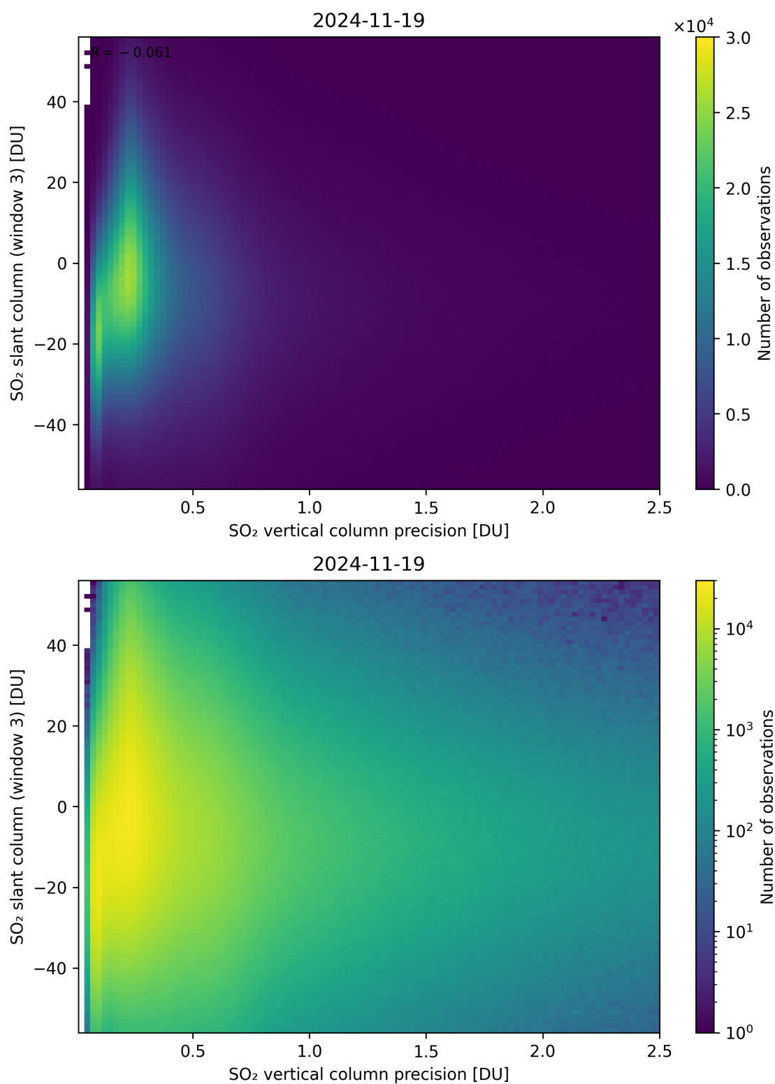
Figure 344: Scatter density plot of “SO 2 vertical column precision” against “SO 2 slant column (window 3)” for 2024-11-18 to 2024-11-20.
