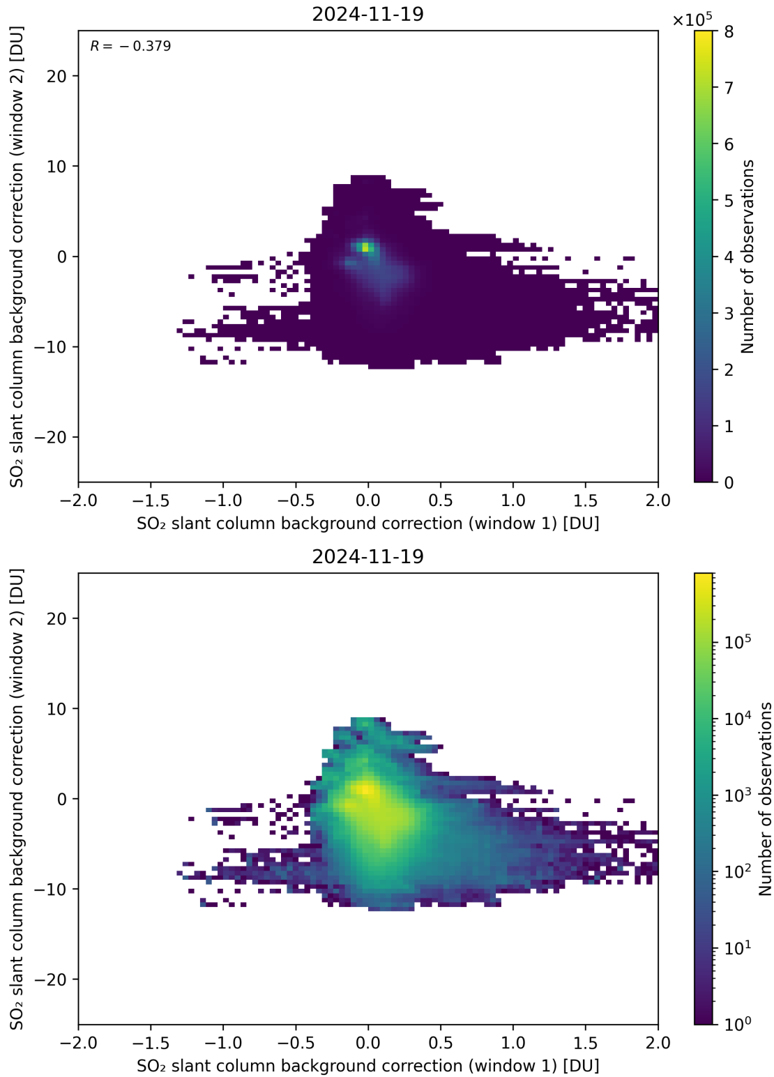
Figure 109: Scatter density plot of “SO 2 slant column background correction (window 1)” against “SO 2 slant column background correction (window 2)” for 2024-11-18 to 2024-11-20.
