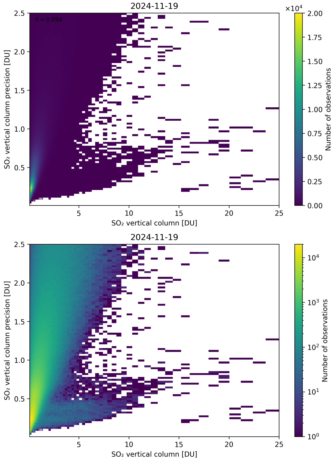
Figure 361: Scatter density plot of “SO 2 vertical column” against “SO 2 vertical column precision” for 2024-11-18 to 2024-11-20.
