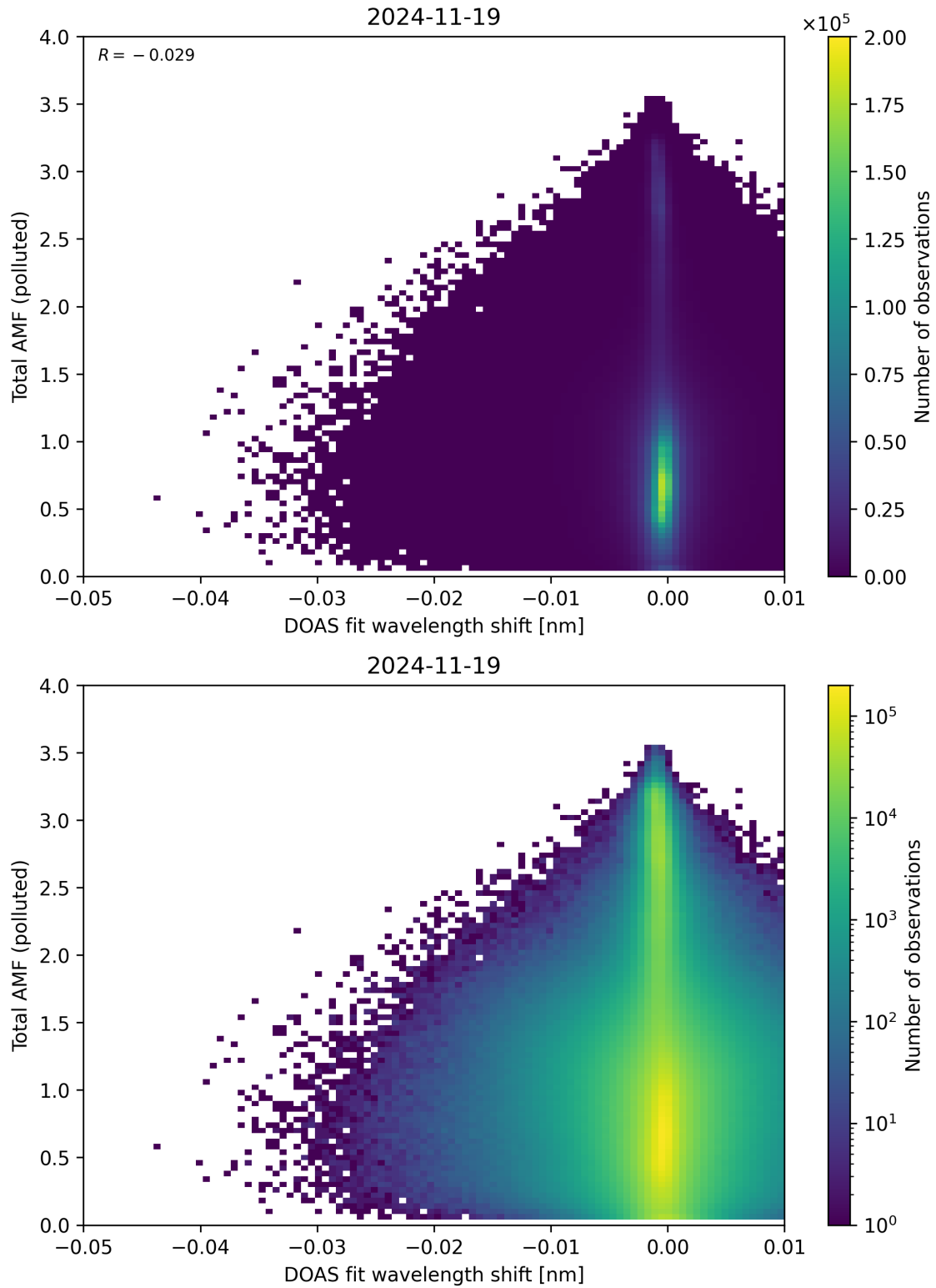
Figure 141: Scatter density plot of “DOAS fit wavelength shift” against “Total AMF (polluted)” for 2024-11-18 to 2024-11-20.
