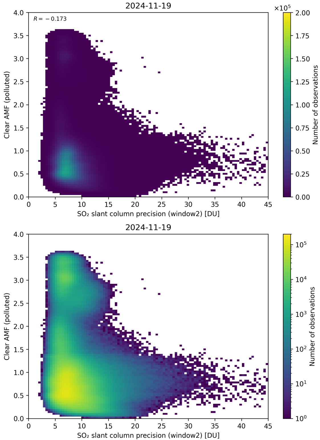
Figure 296: Scatter density plot of “SO 2 slant column precision (window2)” against “Clear AMF (polluted)” for 2024-11-18 to 2024-11-20.
