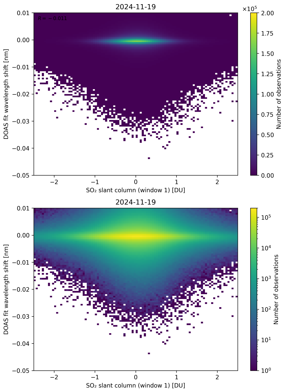
Figure 265: Scatter density plot of “SO 2 slant column (window 1)” against “DOAS fit wavelength shift” for 2024-11-18 to 2024-11-20.
