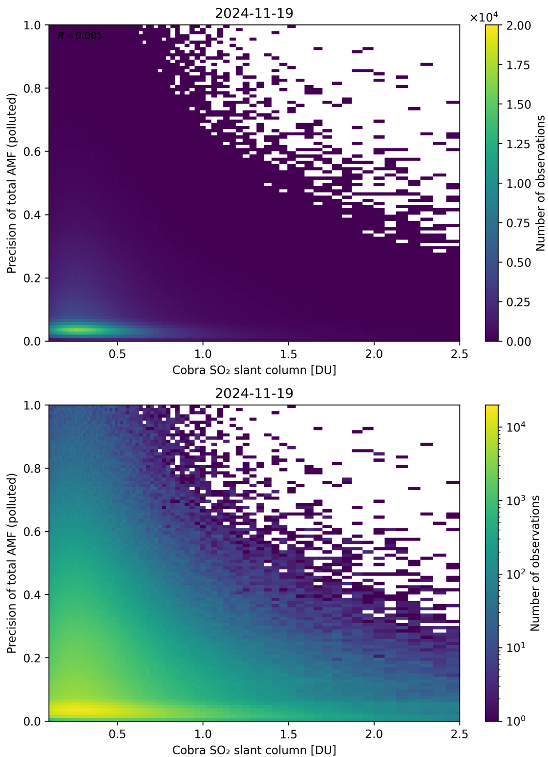
Figure 225: Scatter density plot of “Cobra SO 2 slant column” against “Precision of total AMF (polluted)” for 2024-11-18 to 2024-11-20.
