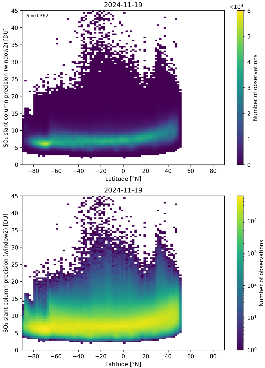
Figure 164: Scatter density plot of “Latitude” against “SO 2 slant column precision (window2)” for 2024-11-18 to 2024-11-20.
