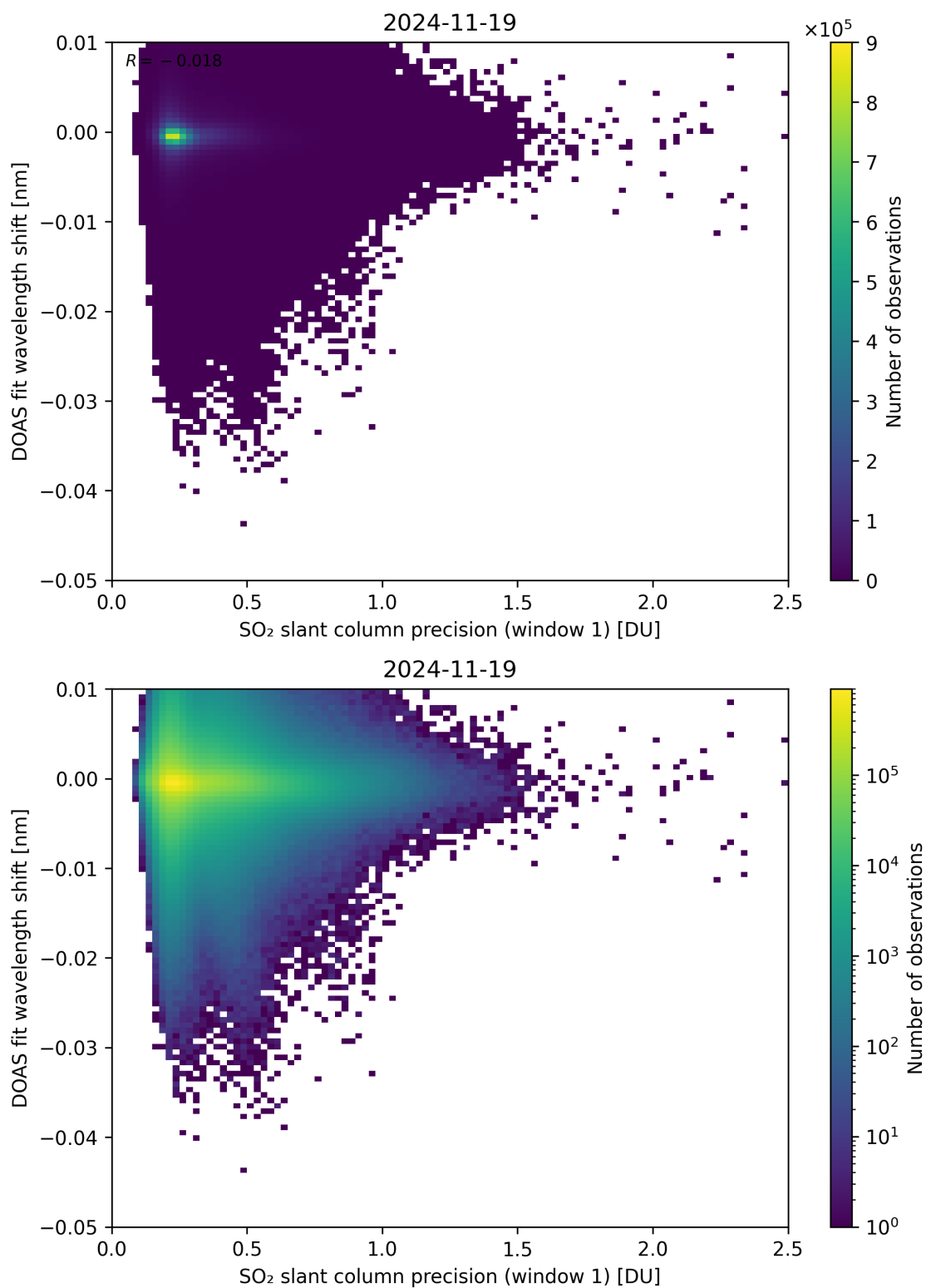
Figure 271: Scatter density plot of “SO 2 slant column precision (window 1)” against “DOAS fit wavelength shift” for 2024-11-18 to 2024-11-20.
