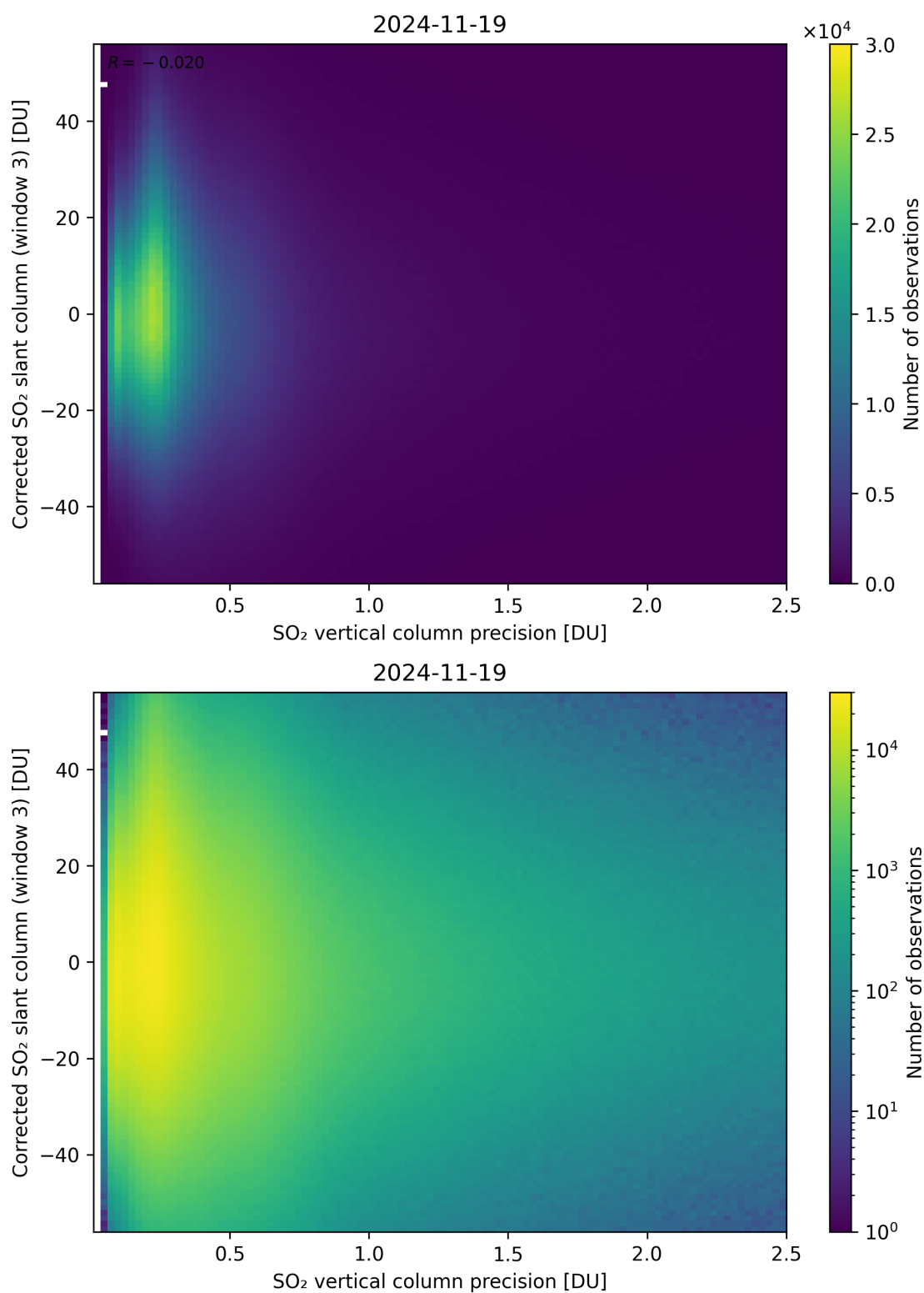
Figure 340: Scatter density plot of “SO 2 vertical column precision” against “Corrected SO 2 slant column (window 3)” for 2024-11-18 to 2024-11-20.
