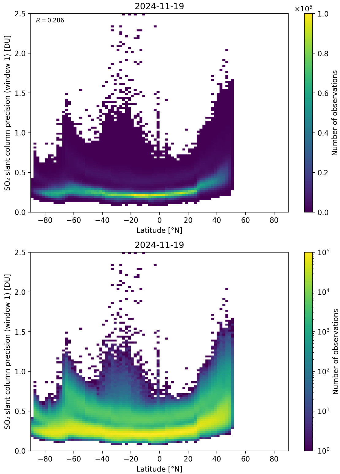
Figure 163: Scatter density plot of “Latitude” against “SO 2 slant column precision (window 1)” for 2024-11-18 to 2024-11-20.
