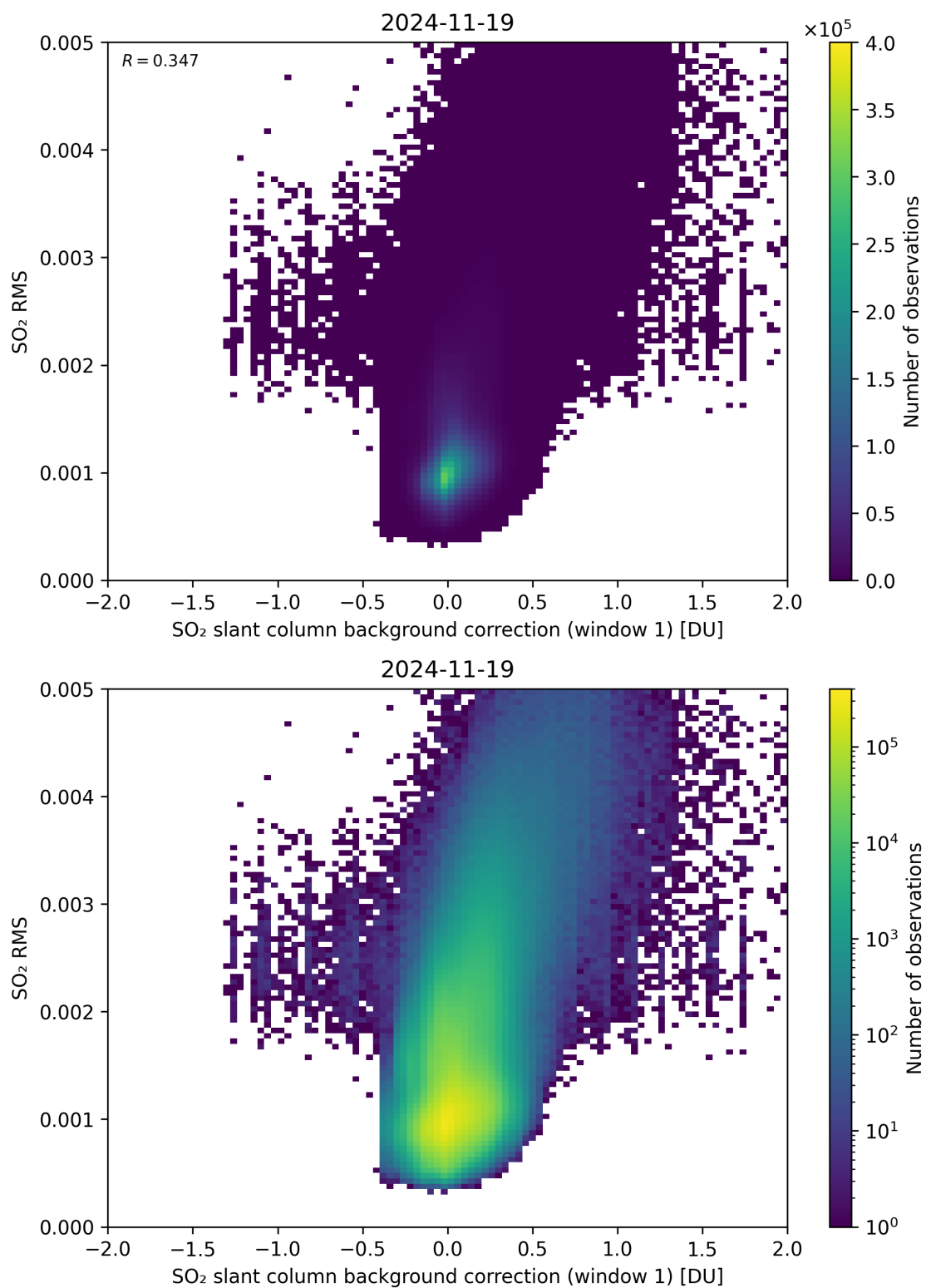
Figure 113: Scatter density plot of “SO 2 slant column background correction (window 1)” against “SO 2 RMS” for 2024-11-18 to 2024-11-20.
