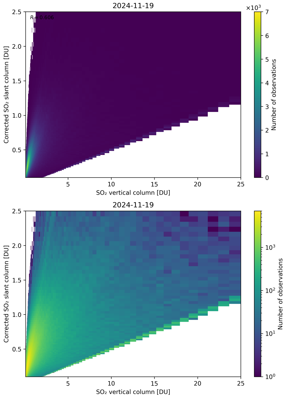
Figure 351: Scatter density plot of “SO 2 vertical column” against “Corrected SO 2 slant column” for 2024-11-18 to 2024-11-20.
