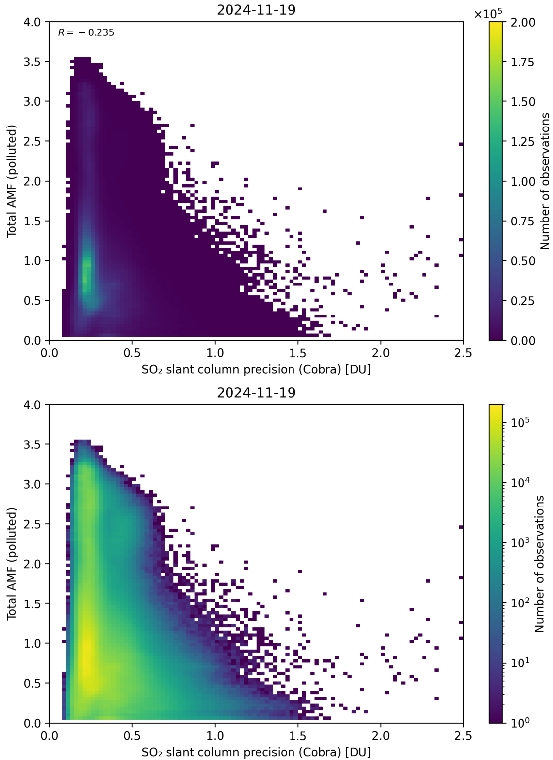
Figure 213: Scatter density plot of “SO 2 slant column precision (Cobra)” against “Total AMF (polluted)” for 2024-11-18 to 2024-11-20.
