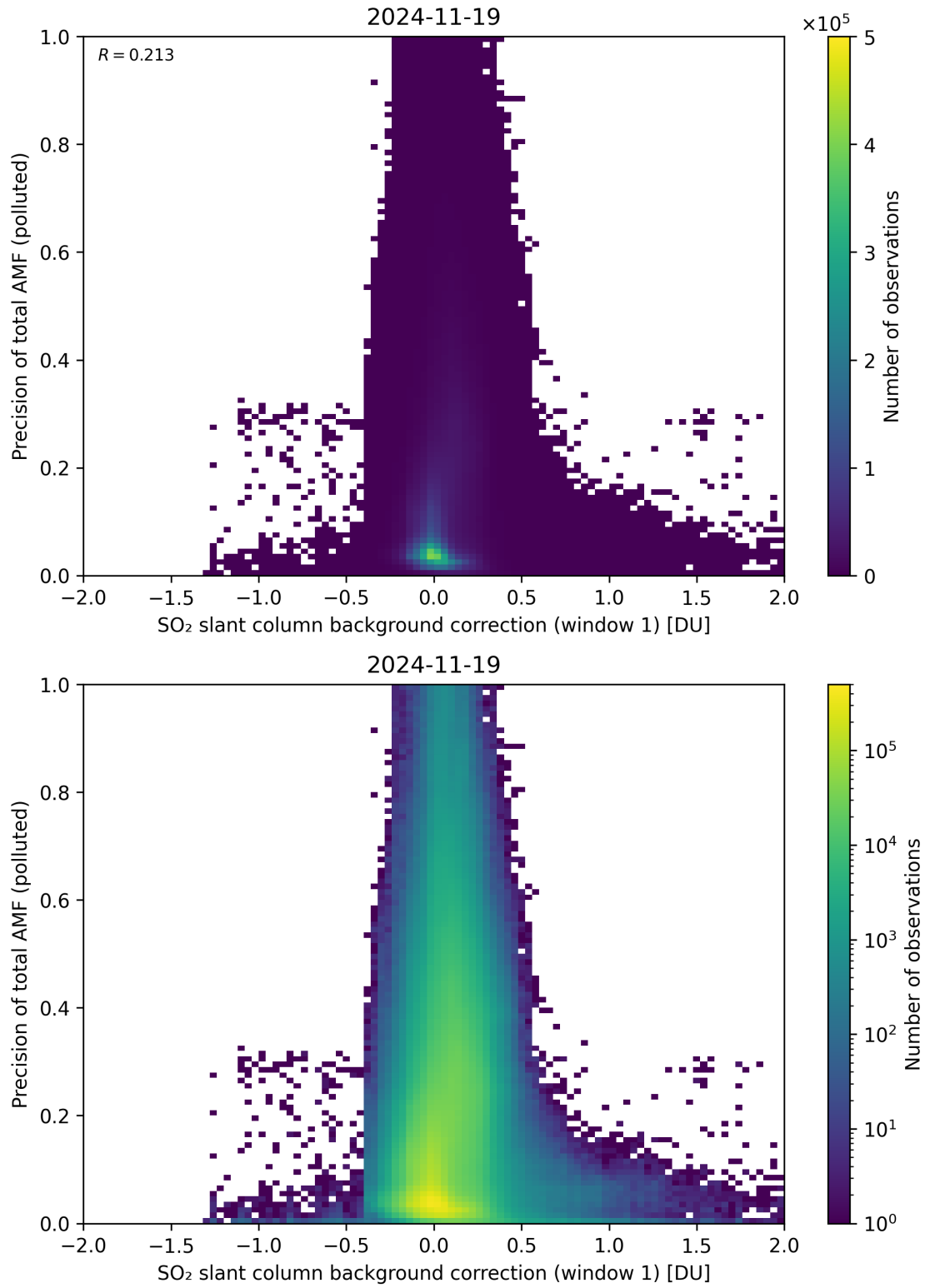
Figure 121: Scatter density plot of “SO 2 slant column background correction (window 1)” against “Precision of total AMF (polluted)” for 2024-11-18 to 2024-11-20.
