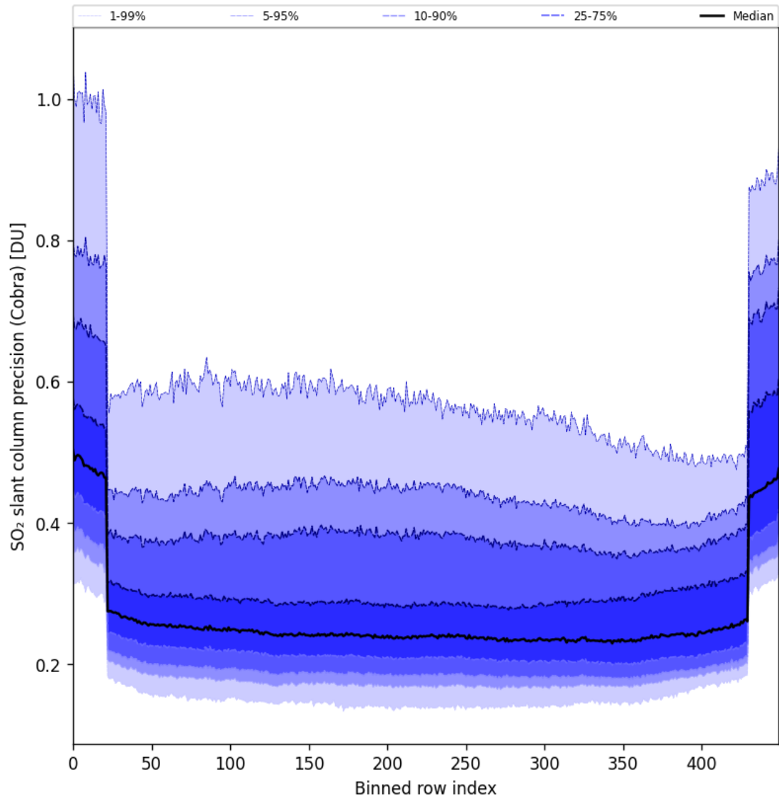
Figure 88: Along track statistics of “SO 2 slant column precision (Cobra)” for 2024-11-18 to 2024-11-20
