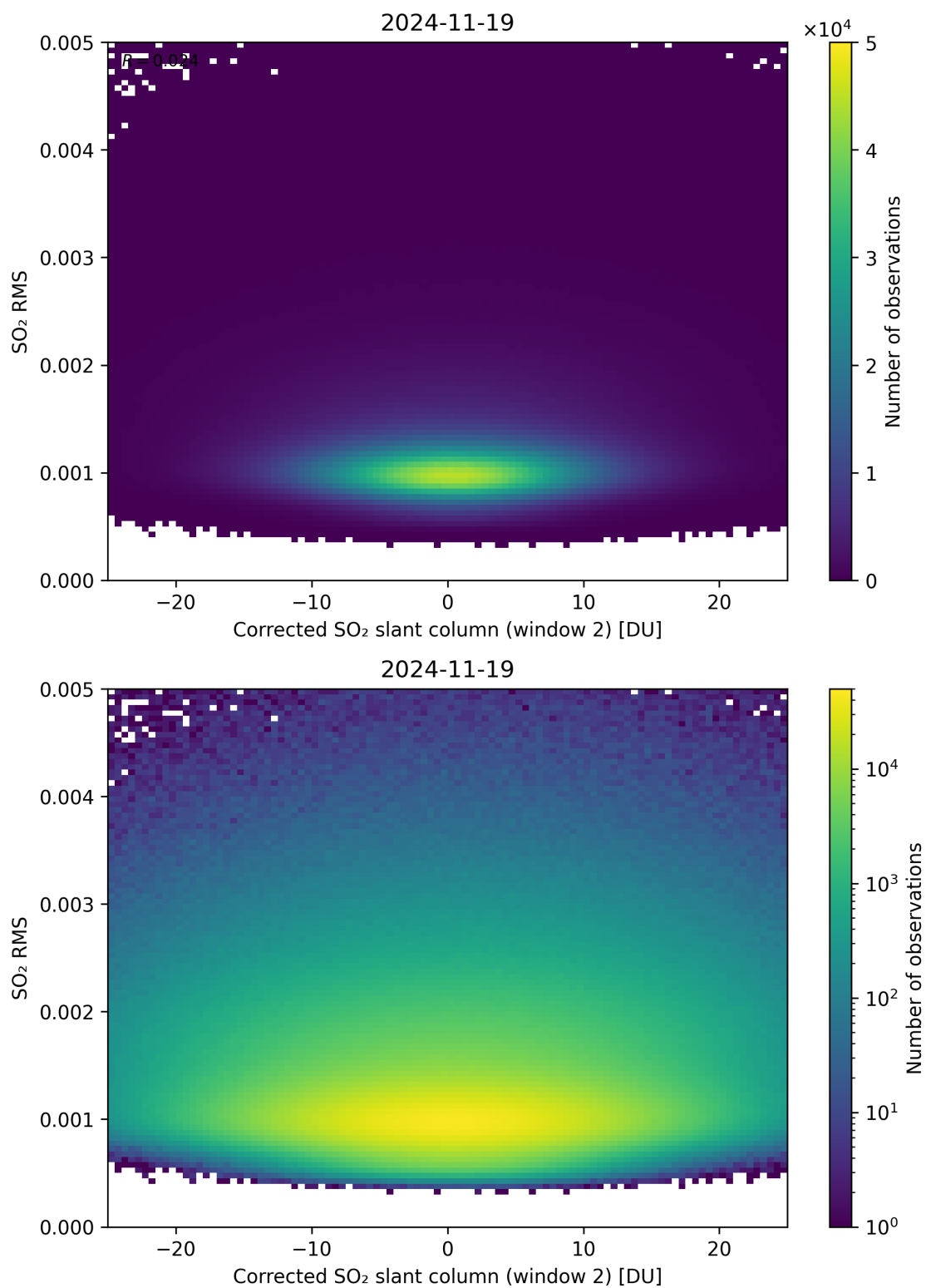
Figure 248: Scatter density plot of “Corrected SO 2 slant column (window 2)” against “SO 2 RMS” for 2024-11-18 to 2024-11-20.
