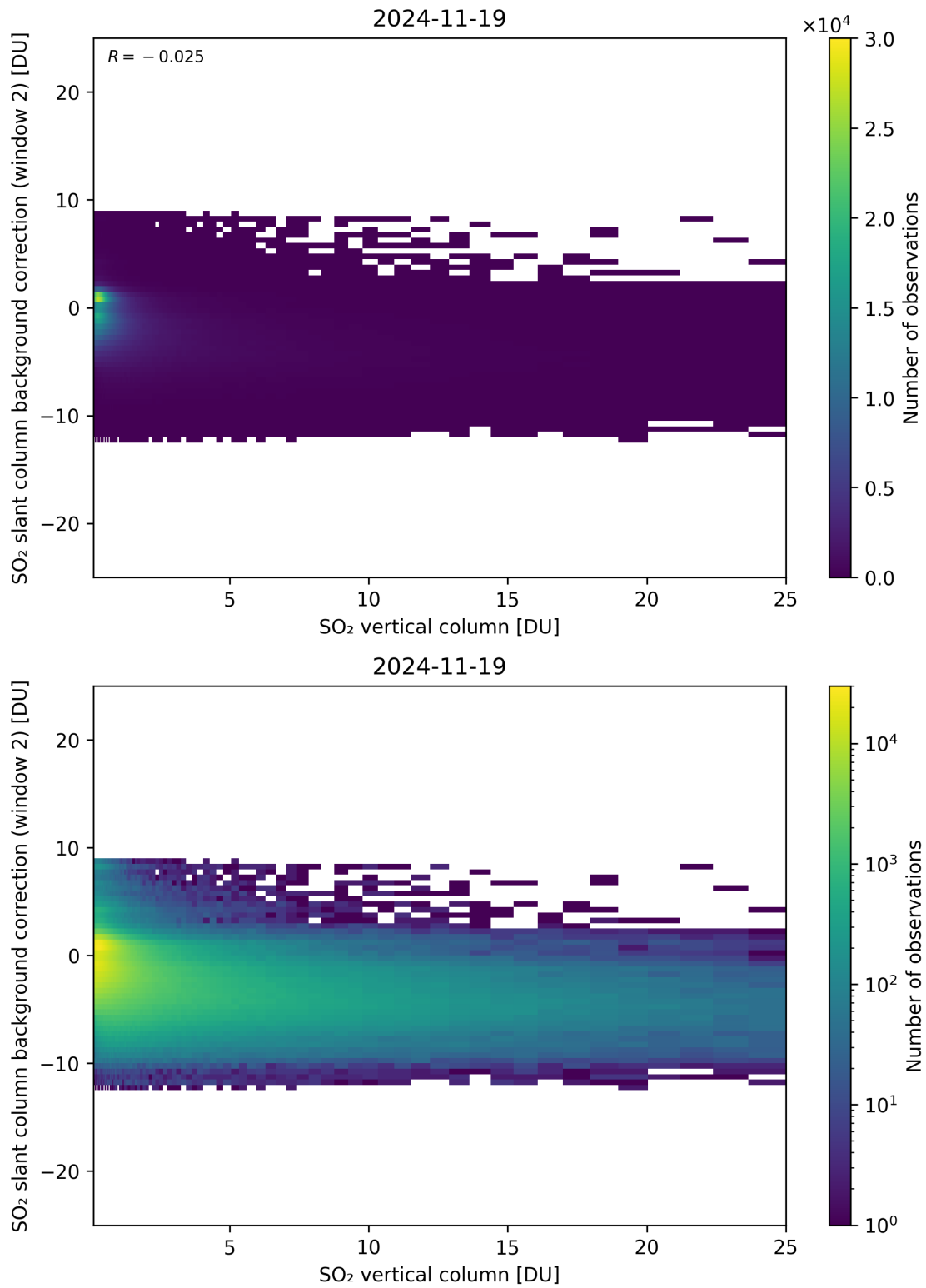
Figure 324: Scatter density plot of “SO 2 vertical column” against “SO 2 slant column background correction (window 2)” for 2024-11-18 to 2024-11-20.
