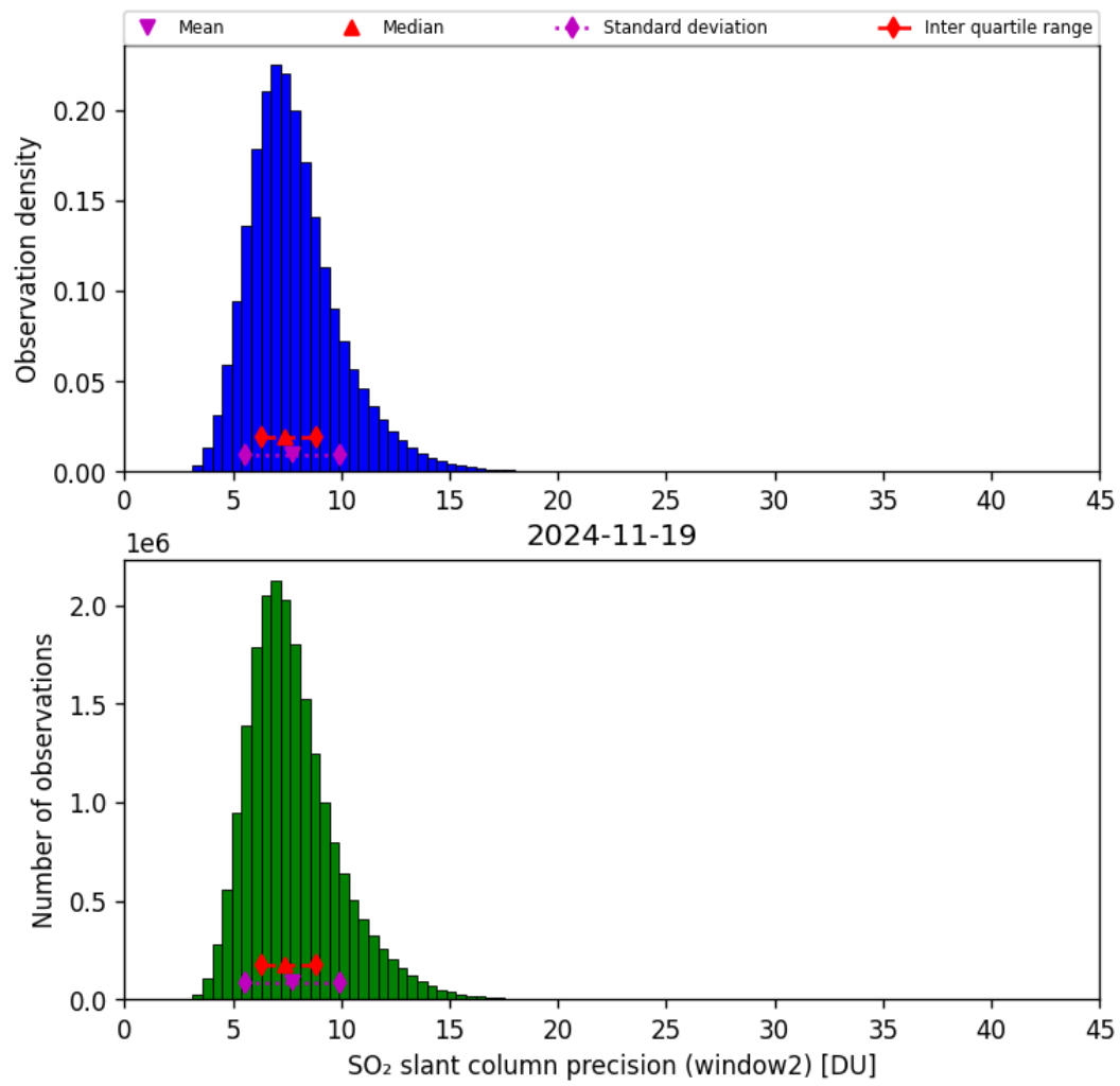
Figure 68: Histogram of “SO 2 slant column precision (window2)” for 2024-11-18 to 2024-11-20
