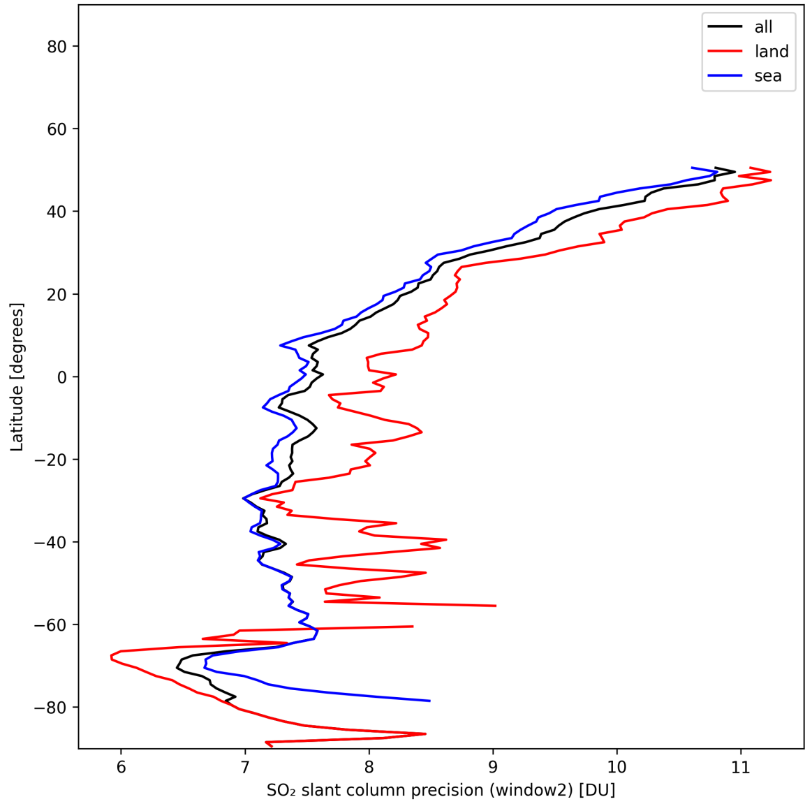
Figure 42: Zonal average of “SO 2 slant column precision (window2)” for 2024-11-18 to 2024-11-20.
