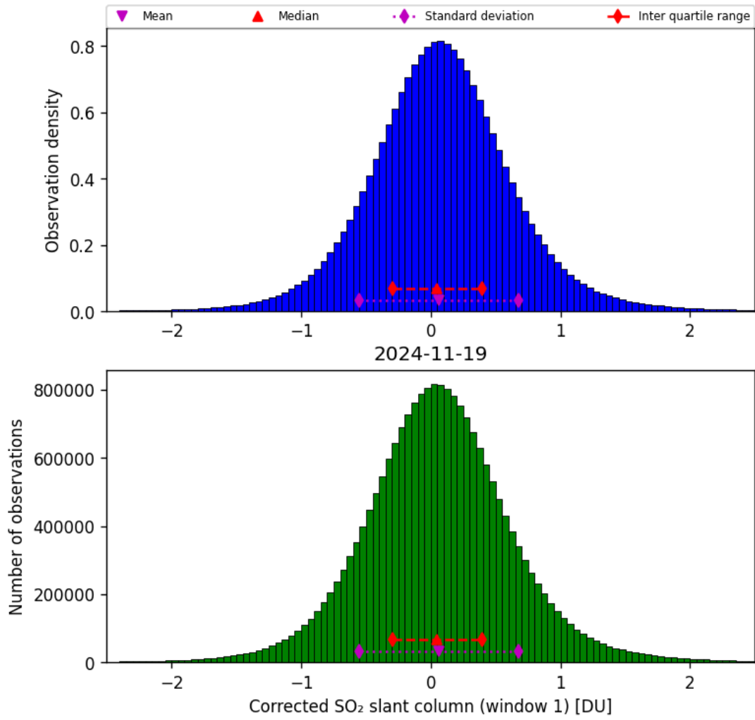
Figure 65: Histogram of “Corrected SO 2 slant column (window 1)” for 2024-11-18 to 2024-11-20
