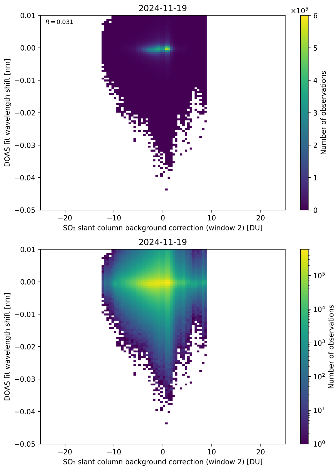
Figure 123: Scatter density plot of “SO 2 slant column background correction (window 2)” against “DOAS fit wavelength shift” for 2024-11-18 to 2024-11-20.
