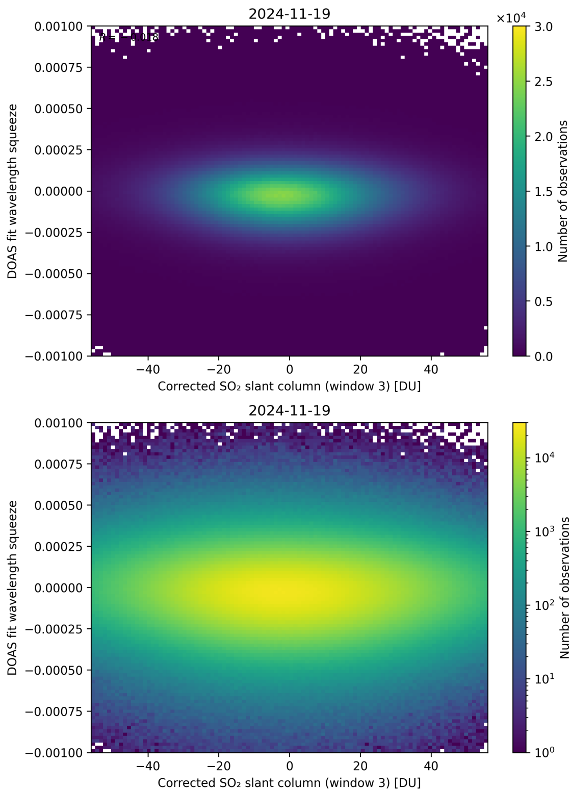
Figure 257: Scatter density plot of “Corrected SO 2 slant column (window 3)” against “DOAS fit wavelength squeeze” for 2024-11-18 to 2024-11-20.
