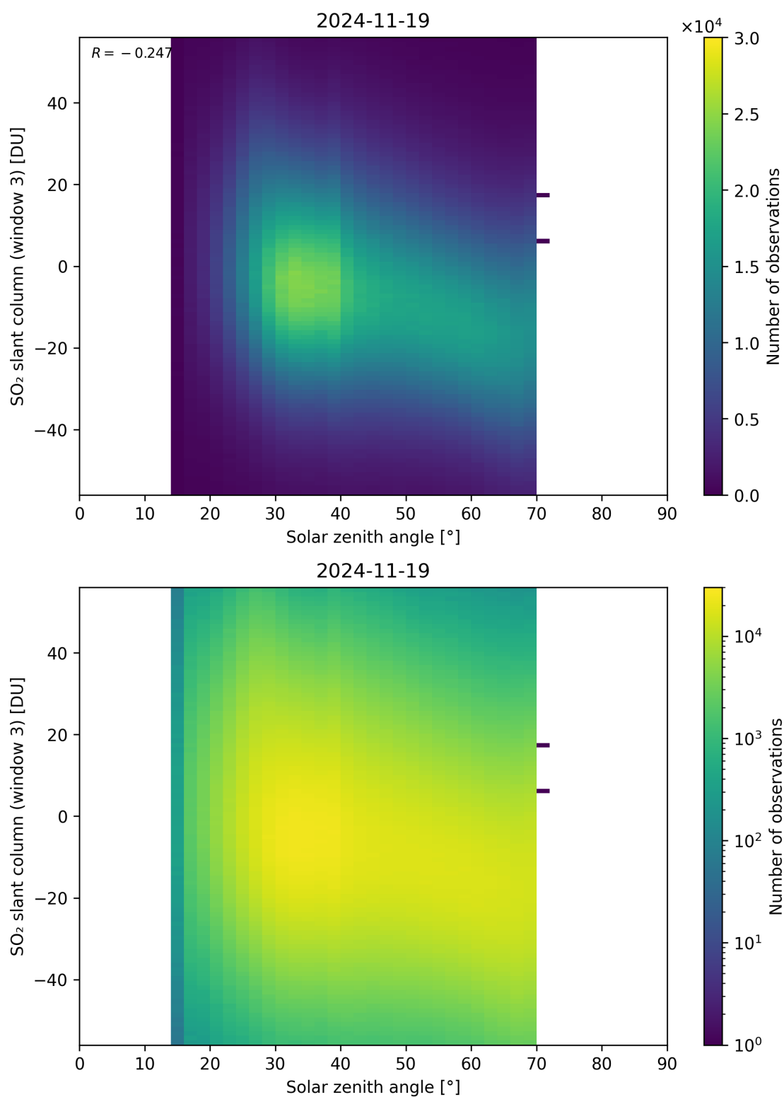
Figure 187: Scatter density plot of “Solar zenith angle” against “SO 2 slant column (window 3)” for 2024-11-18 to 2024-11-20.
