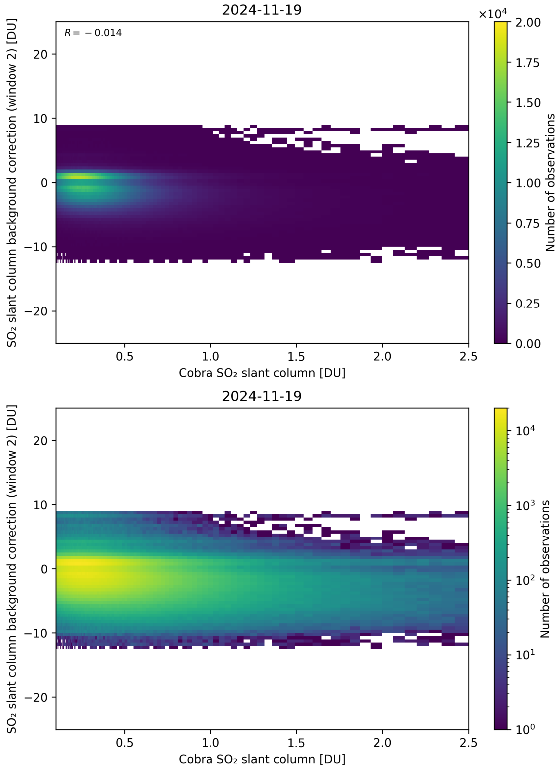
Figure 194: Scatter density plot of “Cobra SO 2 slant column” against “SO 2 slant column background correction (window 2)” for 2024-11-18 to 2024-11-20.
