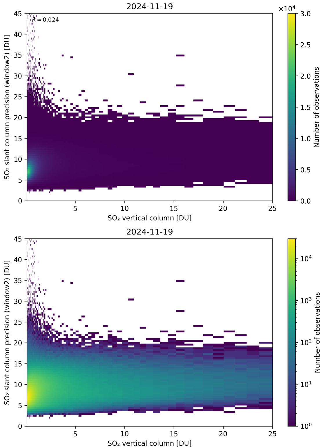
Figure 356: Scatter density plot of “SO 2 vertical column” against “SO 2 slant column precision (window2)” for 2024-11-18 to 2024-11-20.
