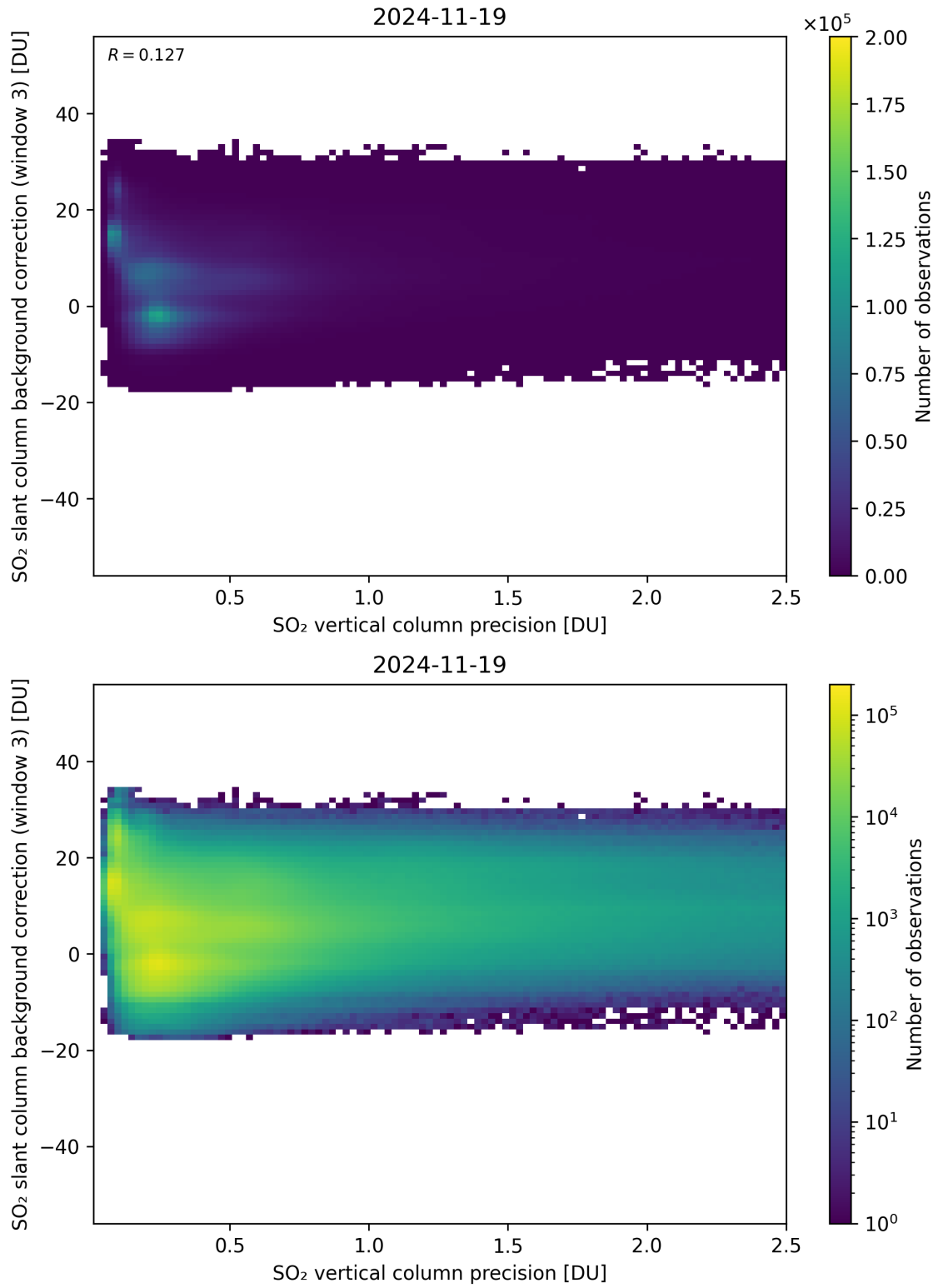
Figure 331: Scatter density plot of “SO 2 vertical column precision” against “SO 2 slant column background correction (window 3)” for 2024-11-18 to 2024-11-20.
