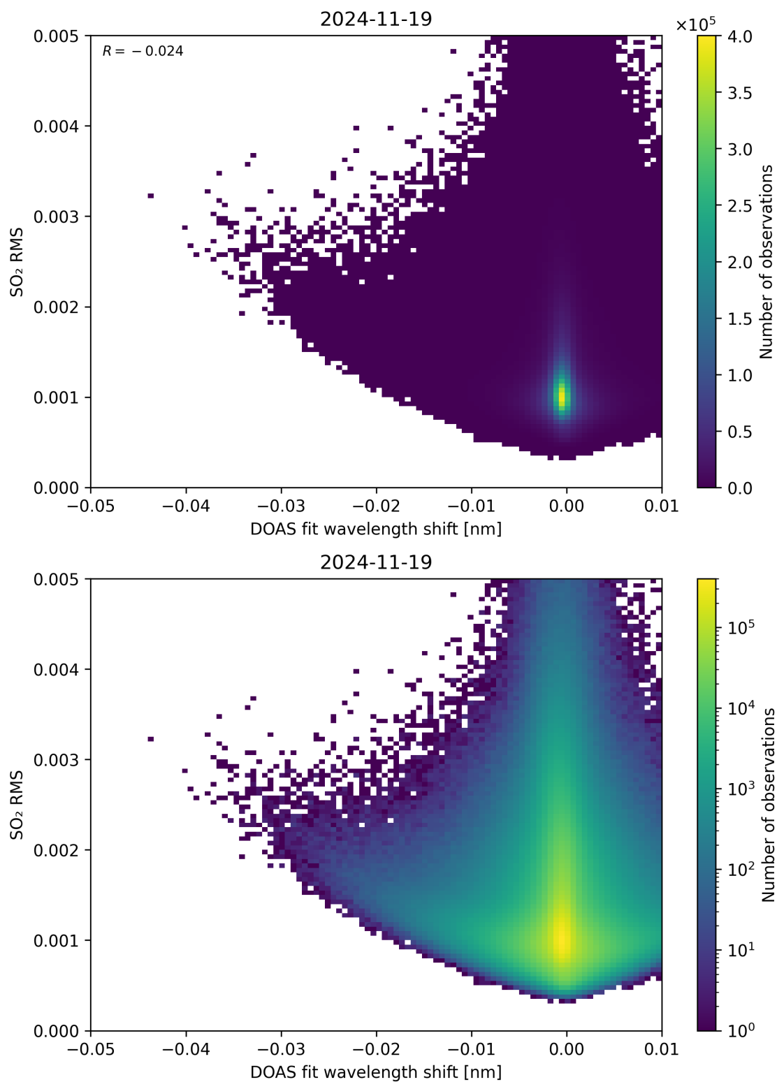
Figure 139: Scatter density plot of “DOAS fit wavelength shift” against “SO 2 RMS” for 2024-11-18 to 2024-11-20.
