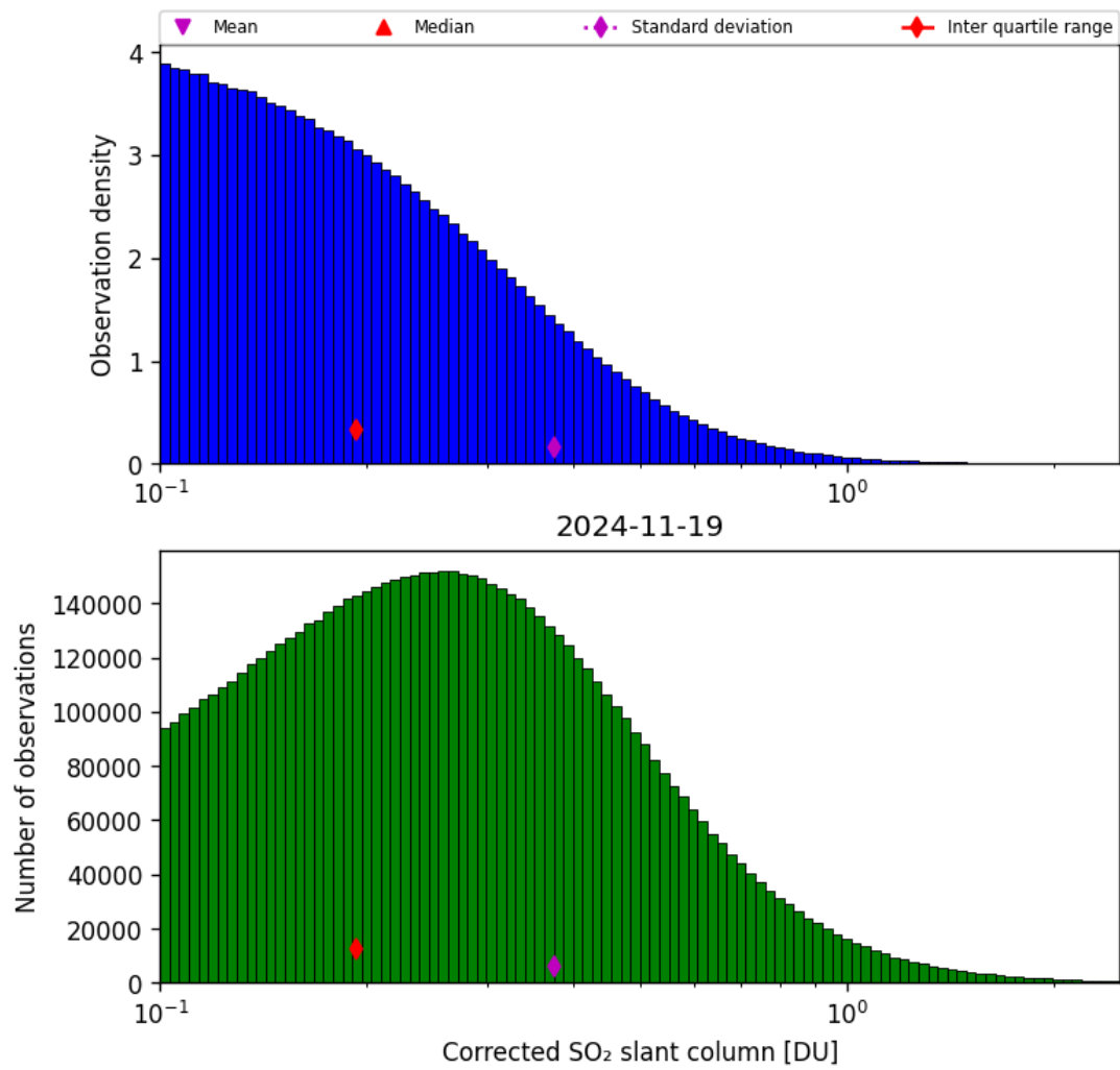
Figure 60: Histogram of “Corrected SO 2 slant column” for 2024-11-18 to 2024-11-20
