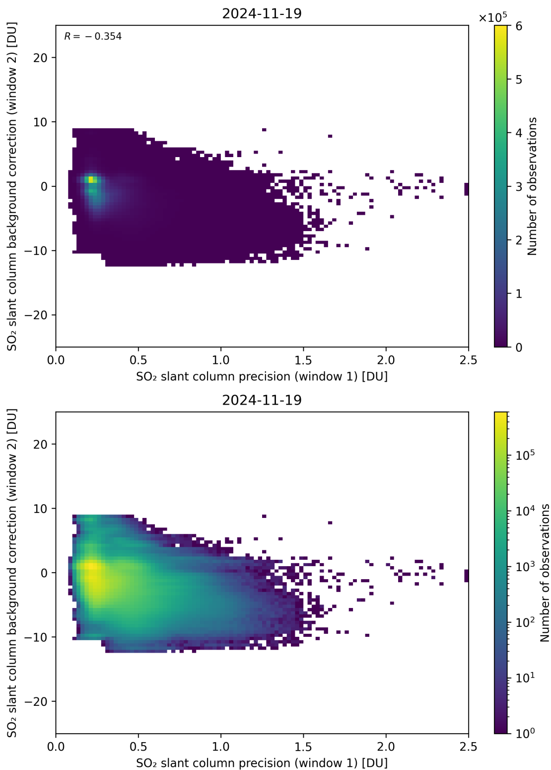
Figure 269: Scatter density plot of “SO 2 slant column precision (window 1)” against “SO 2 slant column background correction (window 2)” for 2024-11-18 to 2024-11-20.
