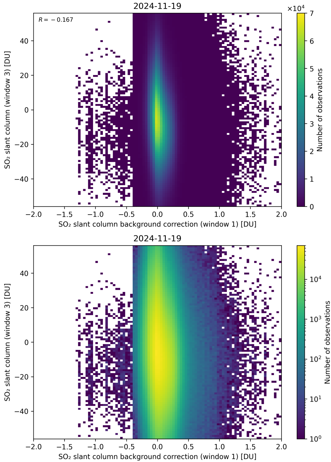
Figure 118: Scatter density plot of “SO 2 slant column background correction (window 1)” against “SO 2 slant column (window 3)” for 2024-11-18 to 2024-11-20.
