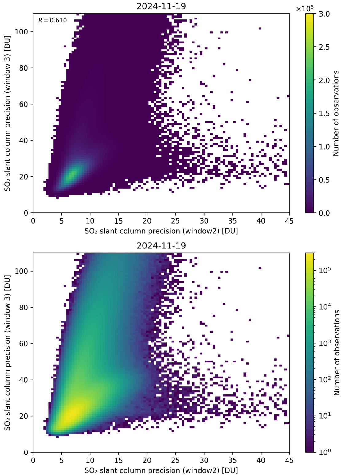
Figure 300: Scatter density plot of “SO 2 slant column precision (window2)” against “SO 2 slant column precision (window 3)” for 2024-11-18 to 2024-11-20.
