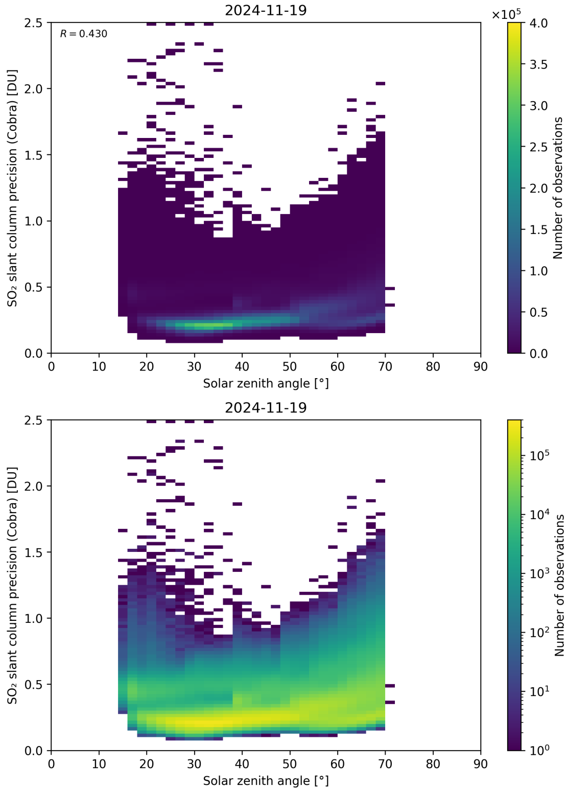
Figure 180: Scatter density plot of “Solar zenith angle” against “SO 2 slant column precision (Cobra)” for 2024-11-18 to 2024-11-20.
