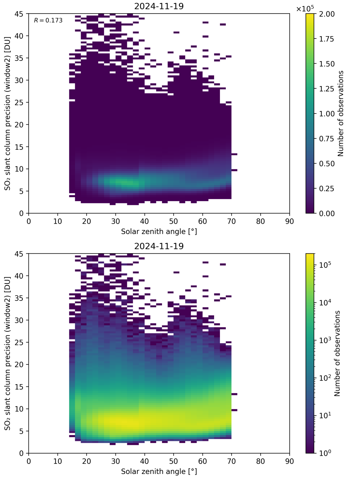
Figure 186: Scatter density plot of “Solar zenith angle” against “SO 2 slant column precision (window2)” for 2024-11-18 to 2024-11-20.
