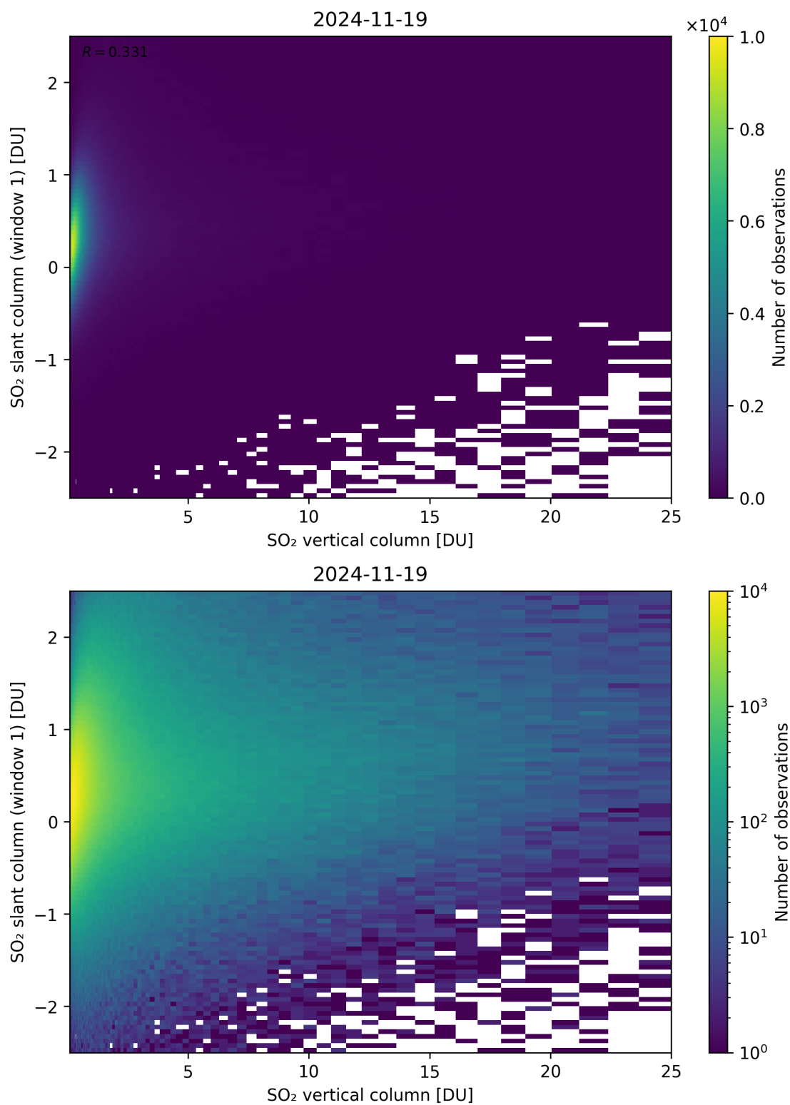
Figure 354: Scatter density plot of “SO 2 vertical column” against “SO 2 slant column (window 1)” for 2024-11-18 to 2024-11-20.
