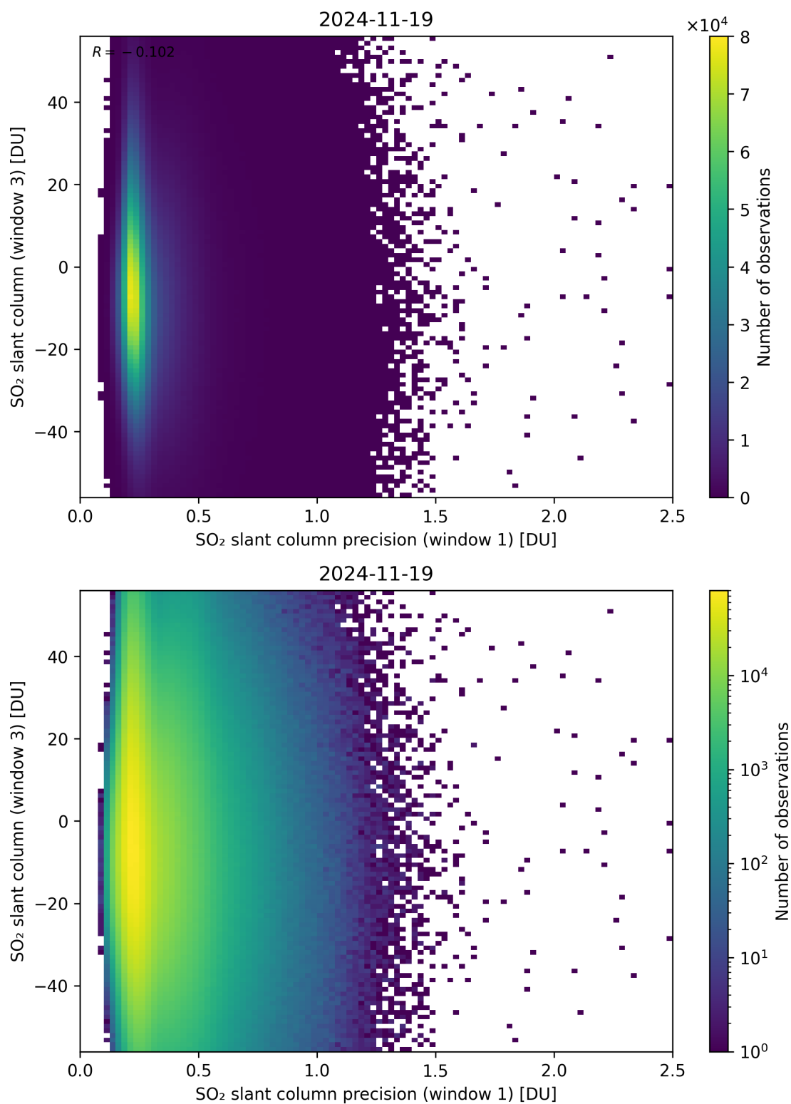
Figure 278: Scatter density plot of “SO 2 slant column precision (window 1)” against “SO 2 slant column (window 3)” for 2024-11-18 to 2024-11-20.
