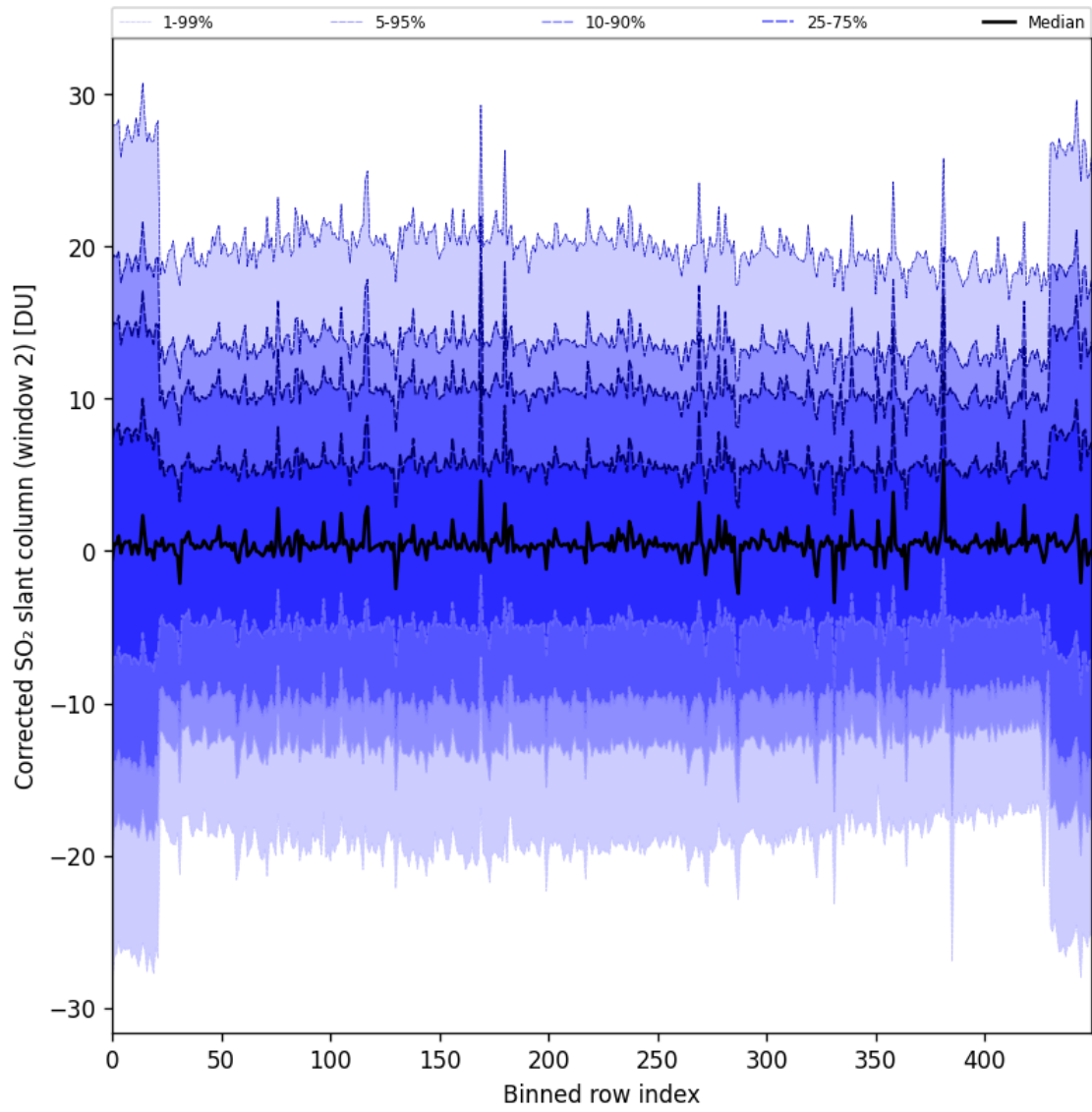
Figure 95: Along track statistics of “Corrected SO 2 slant column (window 2)” for 2024-11-18 to 2024-11-20
