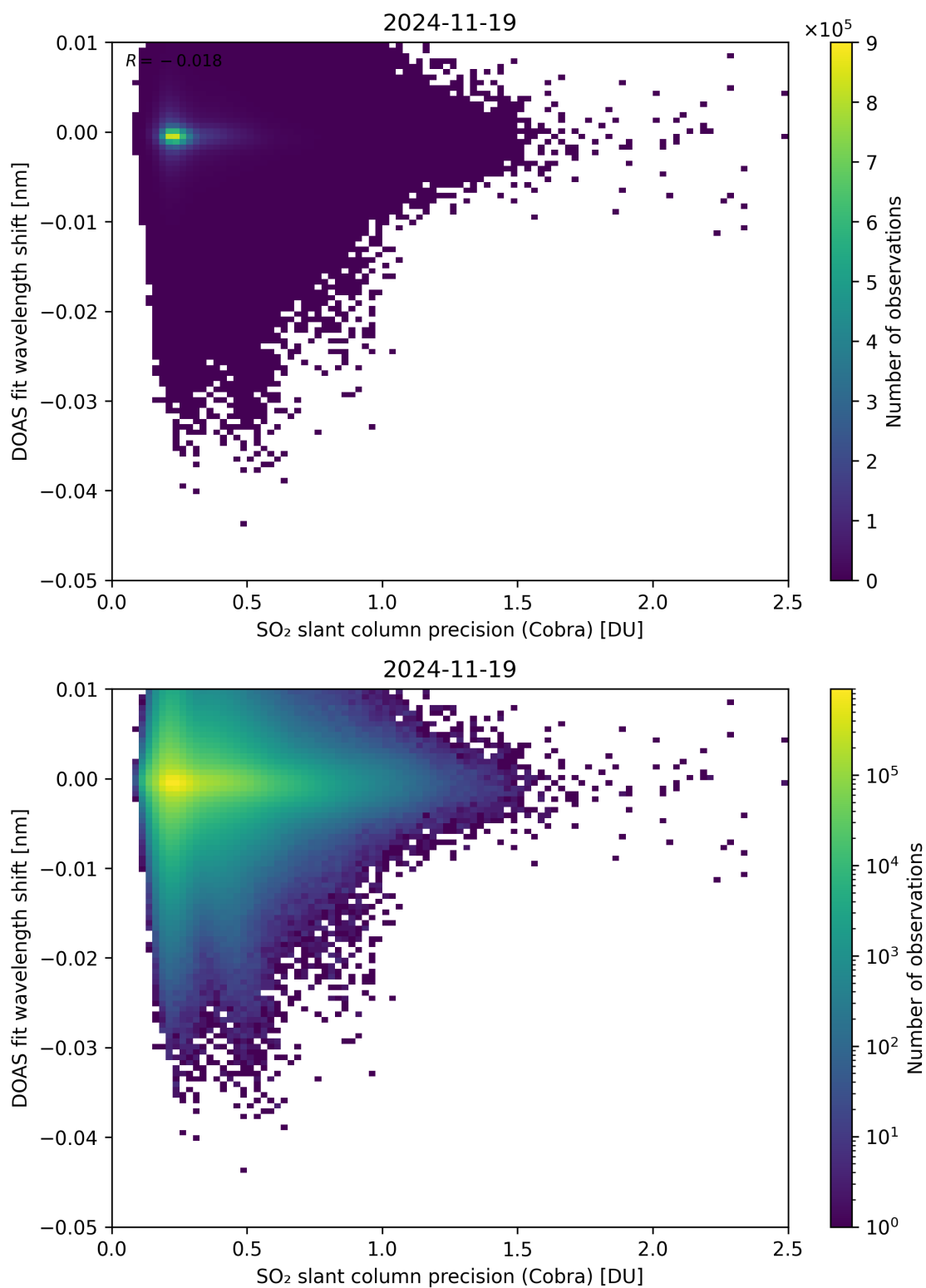
Figure 202: Scatter density plot of “SO 2 slant column precision (Cobra)” against “DOAS fit wavelength shift” for 2024-11-18 to 2024-11-20.
