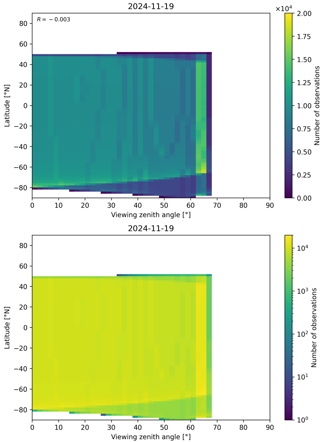
Figure 368: Scatter density plot of “Viewing zenith angle” against “Latitude” for 2024-11-18 to 2024-11-20.
