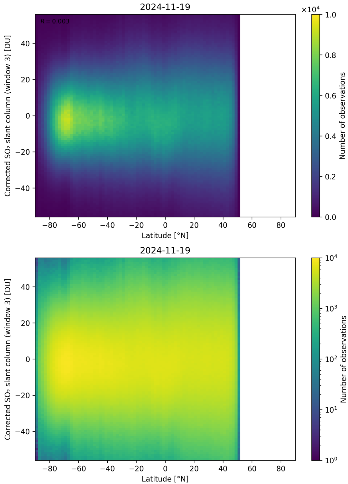
Figure 161: Scatter density plot of “Latitude” against “Corrected SO 2 slant column (window 3)” for 2024-11-18 to 2024-11-20.
