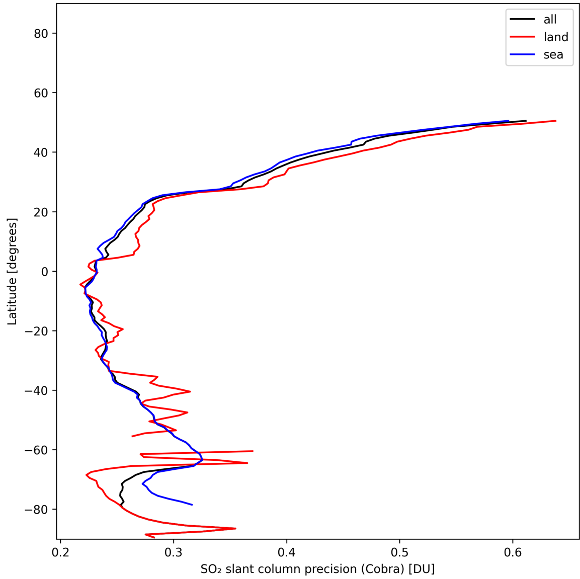
Figure 36: Zonal average of "SO 2 slant column precision (Cobra)" for 2024-11-18 to 2024-11-20.
