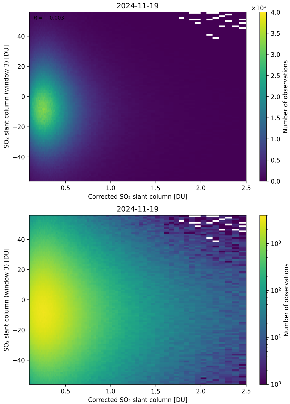
Figure 240: Scatter density plot of “Corrected SO 2 slant column” against “SO 2 slant column (window 3)” for 2024-11-18 to 2024-11-20.
