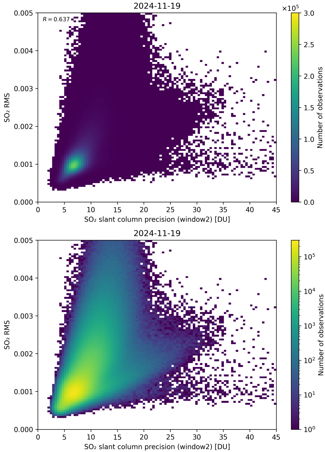
Figure 295: Scatter density plot of “SO 2 slant column precision (window2)” against “SO 2 RMS” for 2024-11-18 to 2024-11-20.
