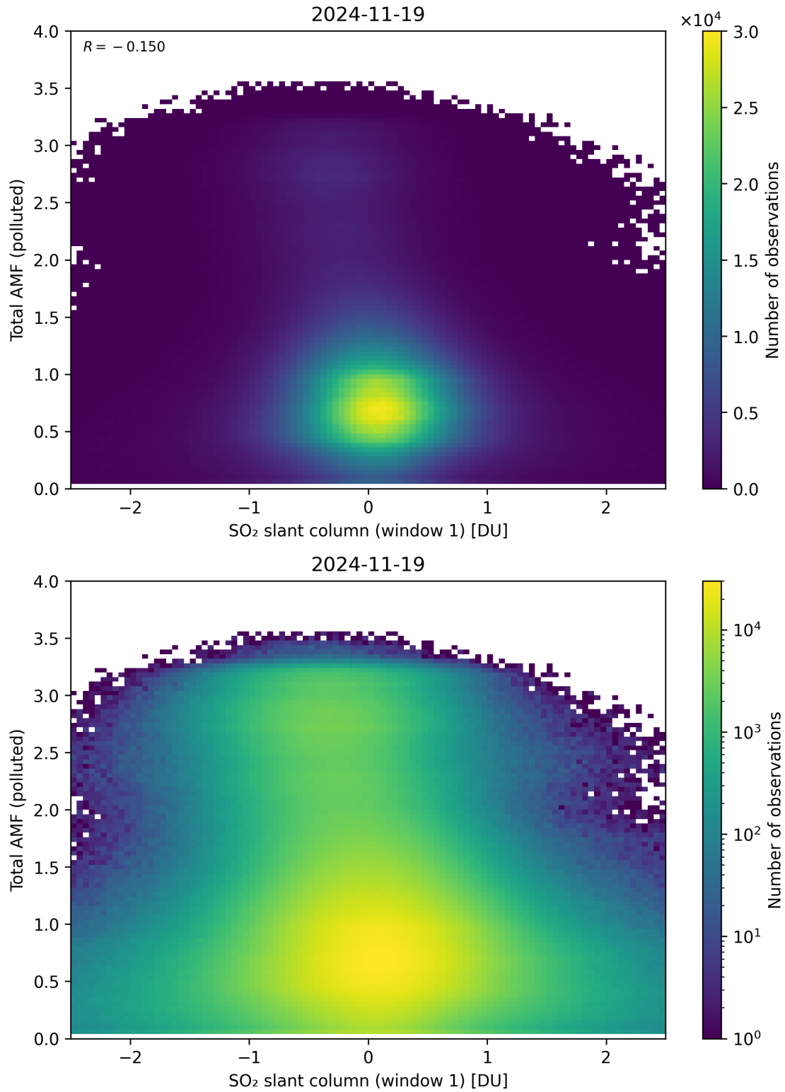
Figure 289: Scatter density plot of “SO 2 slant column (window 1)” against “Total AMF (polluted)” for 2024-11-18 to 2024-11-20.
