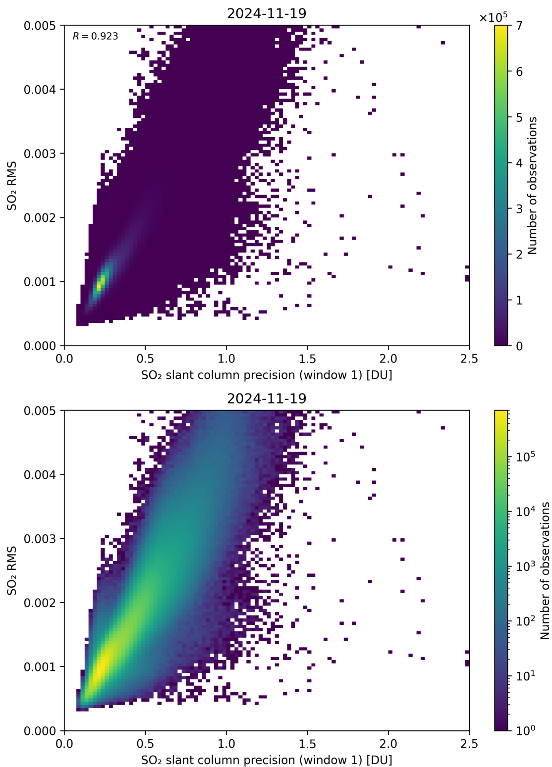
Figure 273: Scatter density plot of “SO 2 slant column precision (window 1)” against “SO 2 RMS” for 2024-11-18 to 2024-11-20.
