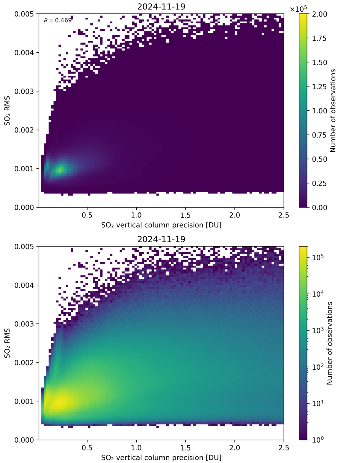
Figure 334: Scatter density plot of “SO 2 vertical column precision” against “SO 2 RMS” for 2024-11-18 to 2024-11-20.
