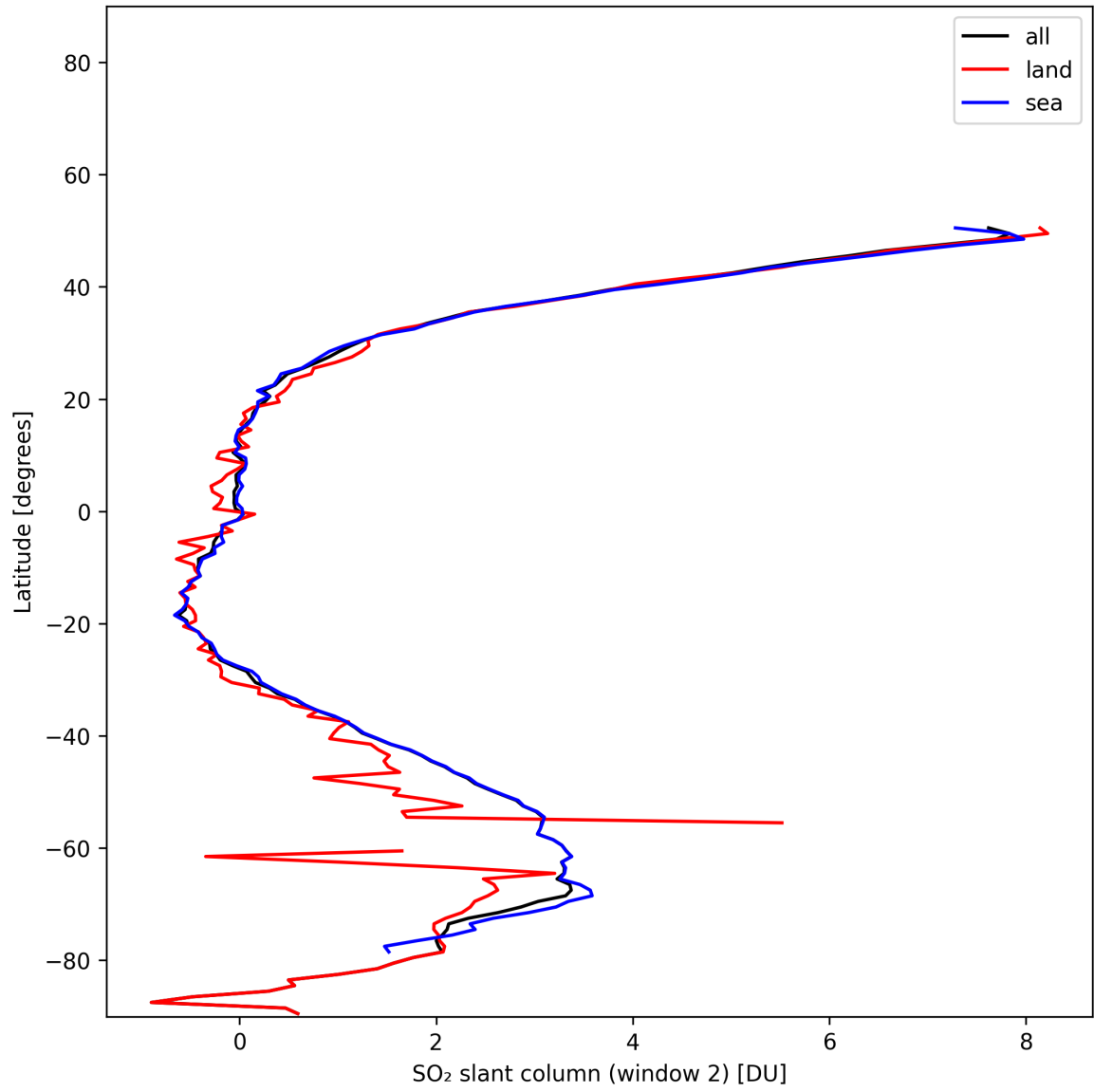
Figure 41: Zonal average of “SO 2 slant column (window 2)” for 2024-11-18 to 2024-11-20.
