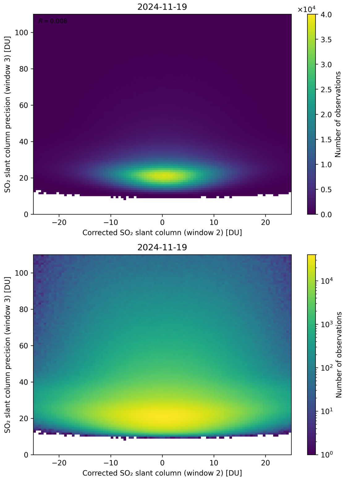
Figure 252: Scatter density plot of “Corrected SO 2 slant column (window 2)” against “SO 2 slant column precision (window 3)” for 2024-11-18 to 2024-11-20.
