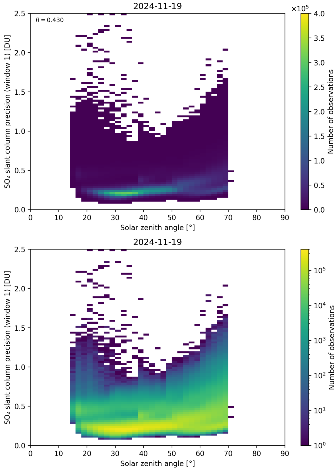
Figure 185: Scatter density plot of “Solar zenith angle” against “SO 2 slant column precision (window 1)” for 2024-11-18 to 2024-11-20.
