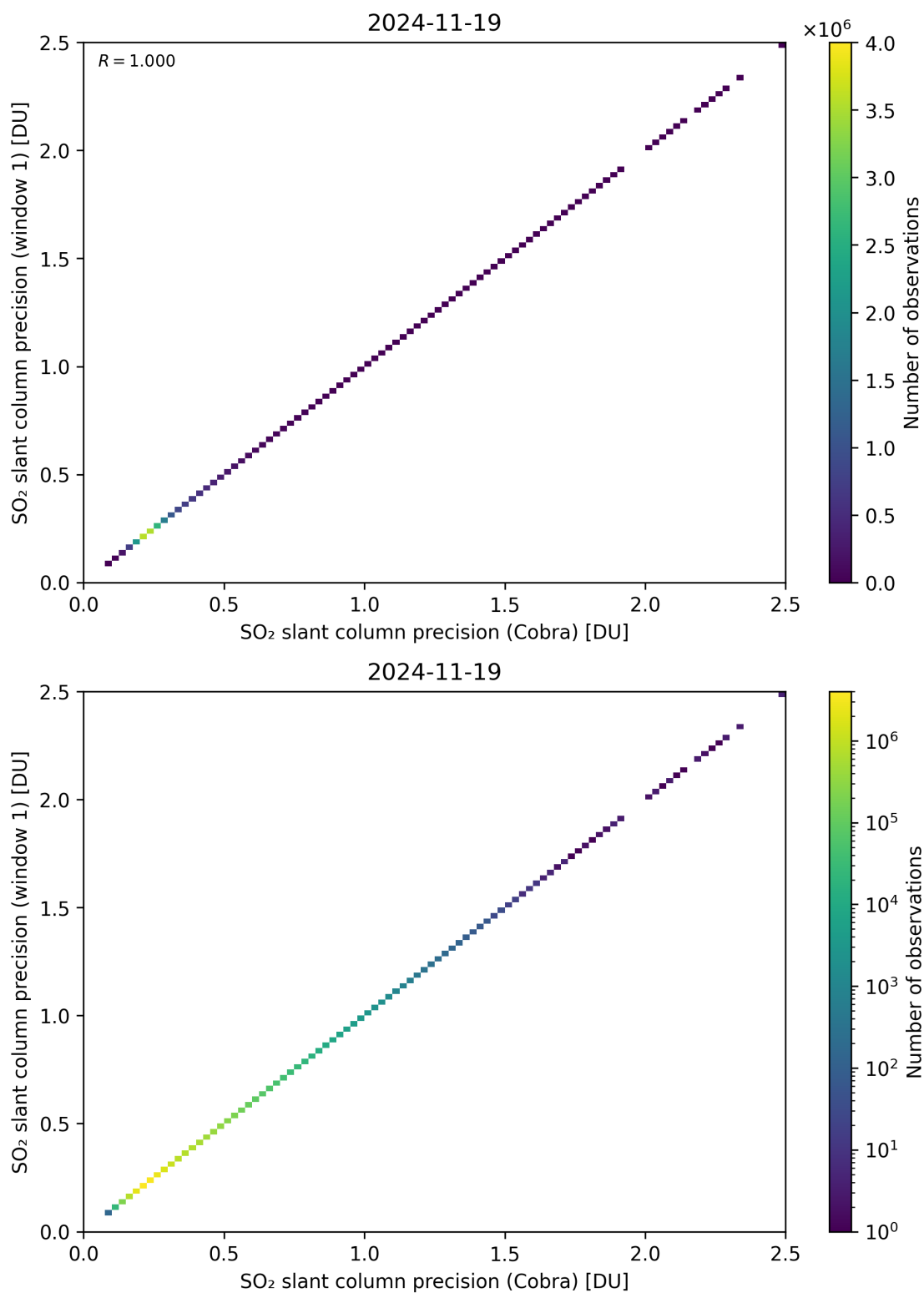
Figure 209: Scatter density plot of “SO 2 slant column precision (Cobra)” against “SO 2 slant column precision (window 1)” for 2024-11-18 to 2024-11-20.
