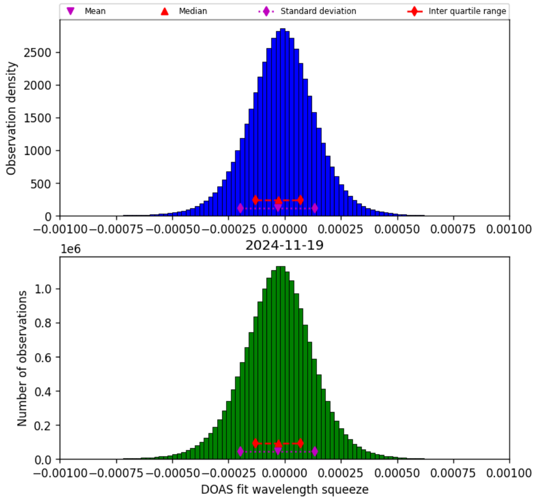
Figure 77: Histogram of “DOAS fit wavelength squeeze” for 2024-11-18 to 2024-11-20
