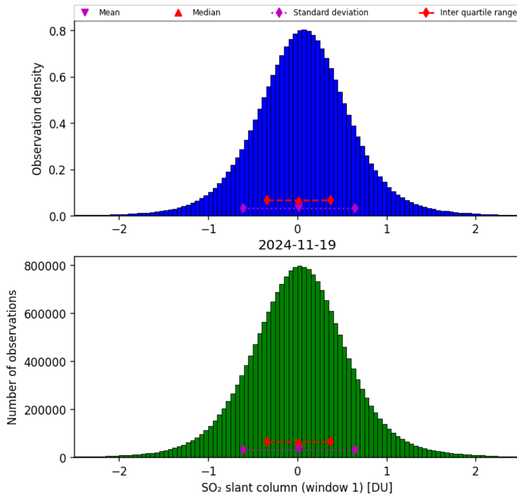
Figure 63: Histogram of “SO 2 slant column (window 1)” for 2024-11-18 to 2024-11-20
