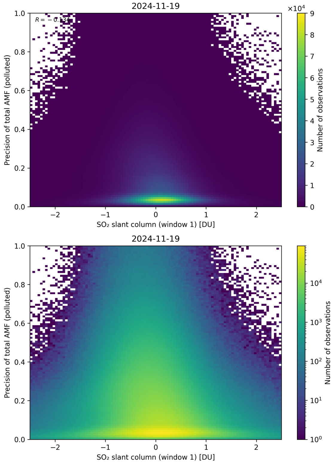
Figure 290: Scatter density plot of “SO 2 slant column (window 1)” against “Precision of total AMF (polluted)” for 2024-11-18 to 2024-11-20.
