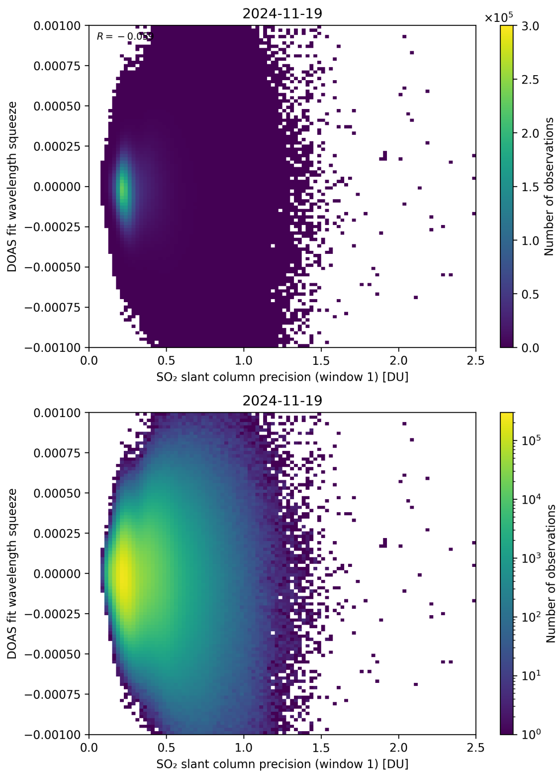
Figure 272: Scatter density plot of “SO 2 slant column precision (window 1)” against “DOAS fit wavelength squeeze” for 2024-11-18 to 2024-11-20.
