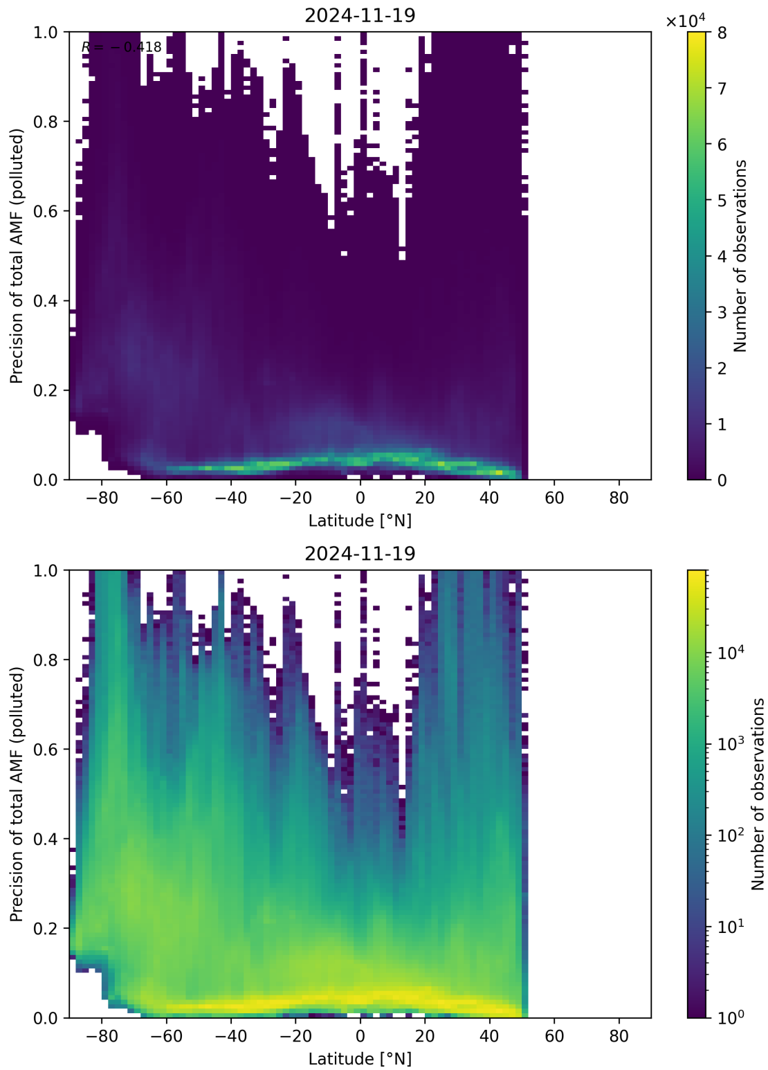
Figure 168: Scatter density plot of “Latitude” against “Precision of total AMF (polluted)” for 2024-11-18 to 2024-11-20.
