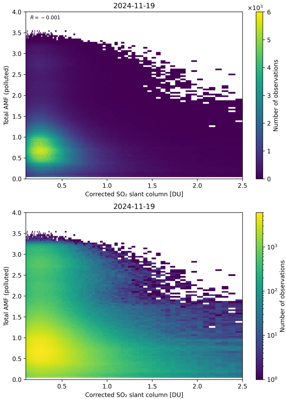
Figure 242: Scatter density plot of “Corrected SO 2 slant column” against “Total AMF (polluted)” for 2024-11-18 to 2024-11-20.
