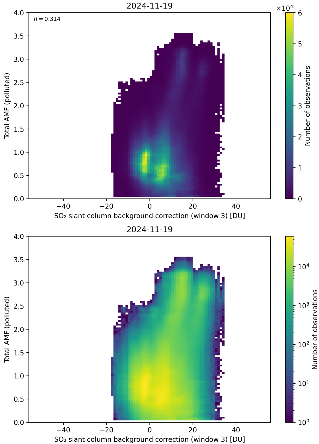
Figure 136: Scatter density plot of “SO 2 slant column background correction (window 3)” against “Total AMF (polluted)” for 2024-11-18 to 2024-11-20.
