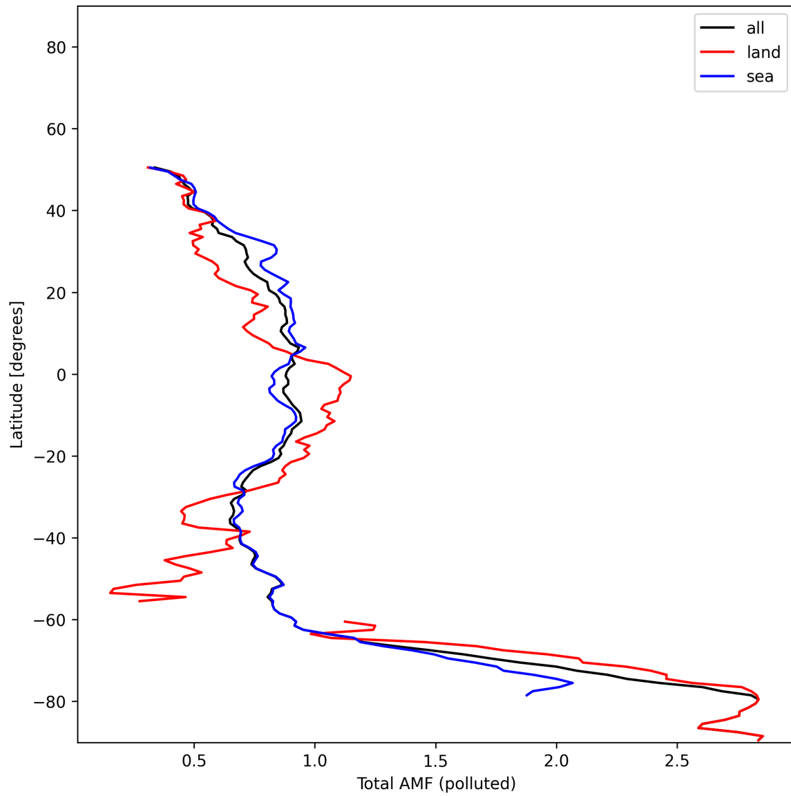
Figure 53: Zonal average of “Total AMF (polluted)” for 2024-11-18 to 2024-11-20.
