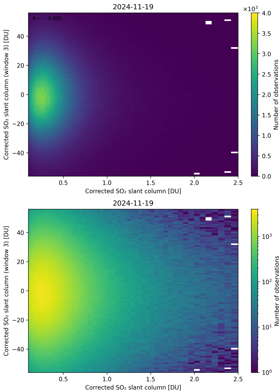
Figure 236: Scatter density plot of “Corrected SO 2 slant column” against “Corrected SO 2 slant column (window 3)” for 2024-11-18 to 2024-11-20.
