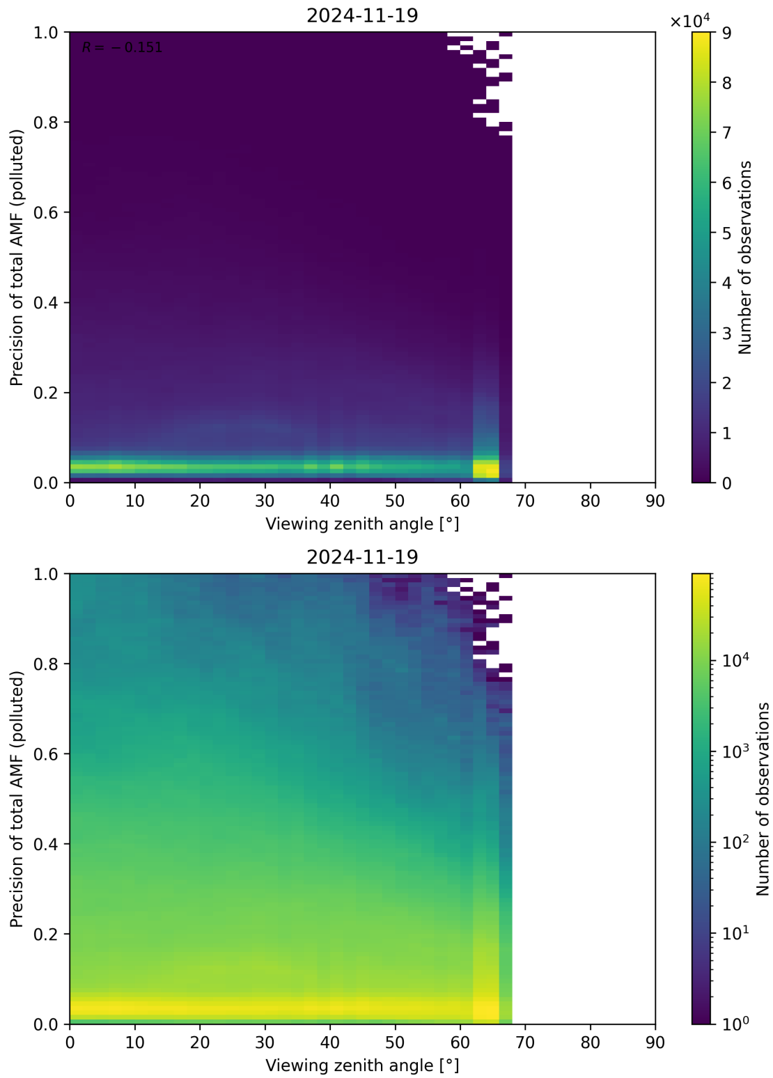
Figure 382: Scatter density plot of “Viewing zenith angle” against “Precision of total AMF (polluted)” for 2024-11-18 to 2024-11-20.
