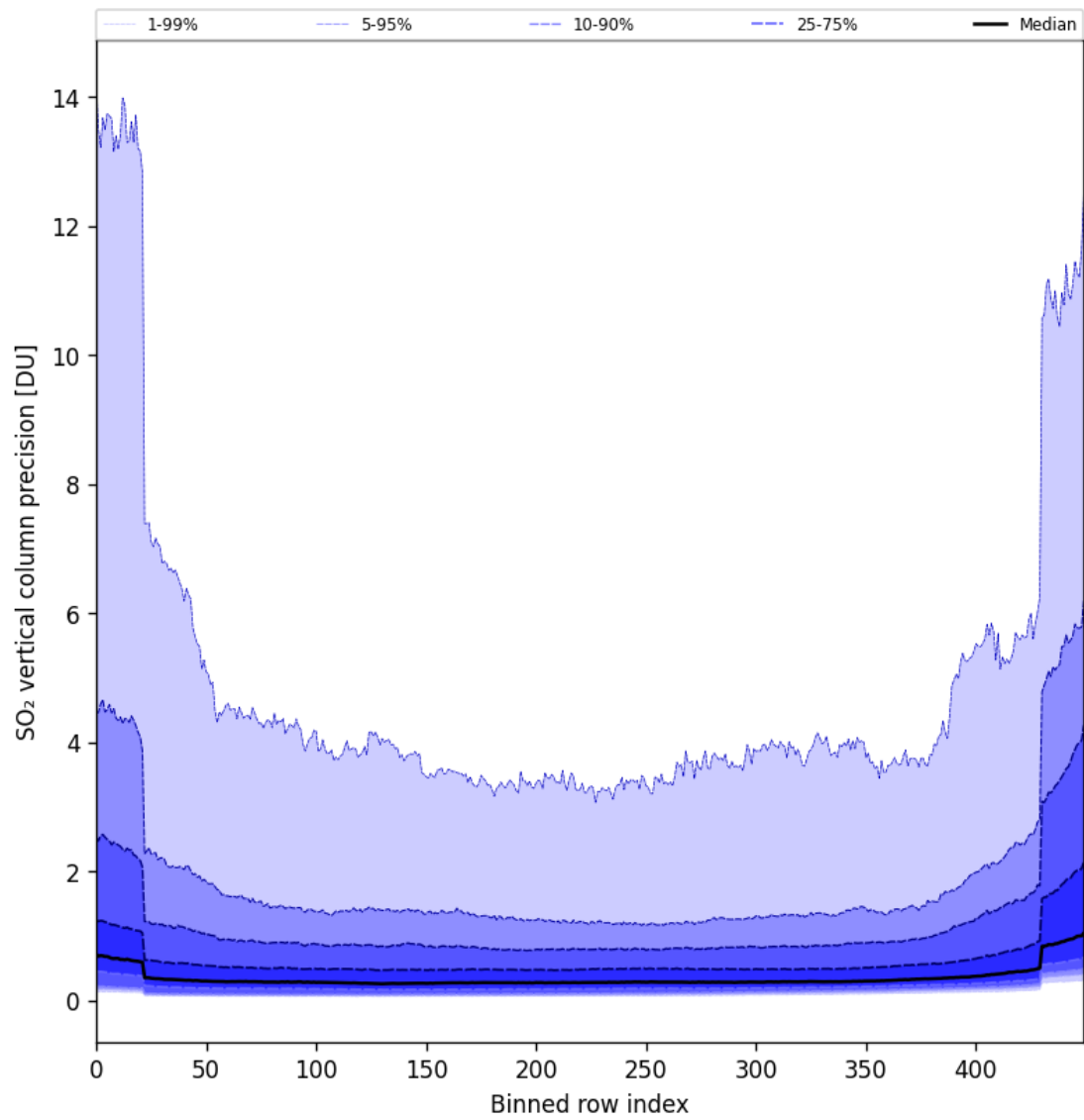
Figure 85: Along track statistics of “SO 2 vertical column precision” for 2024-11-18 to 2024-11-20
