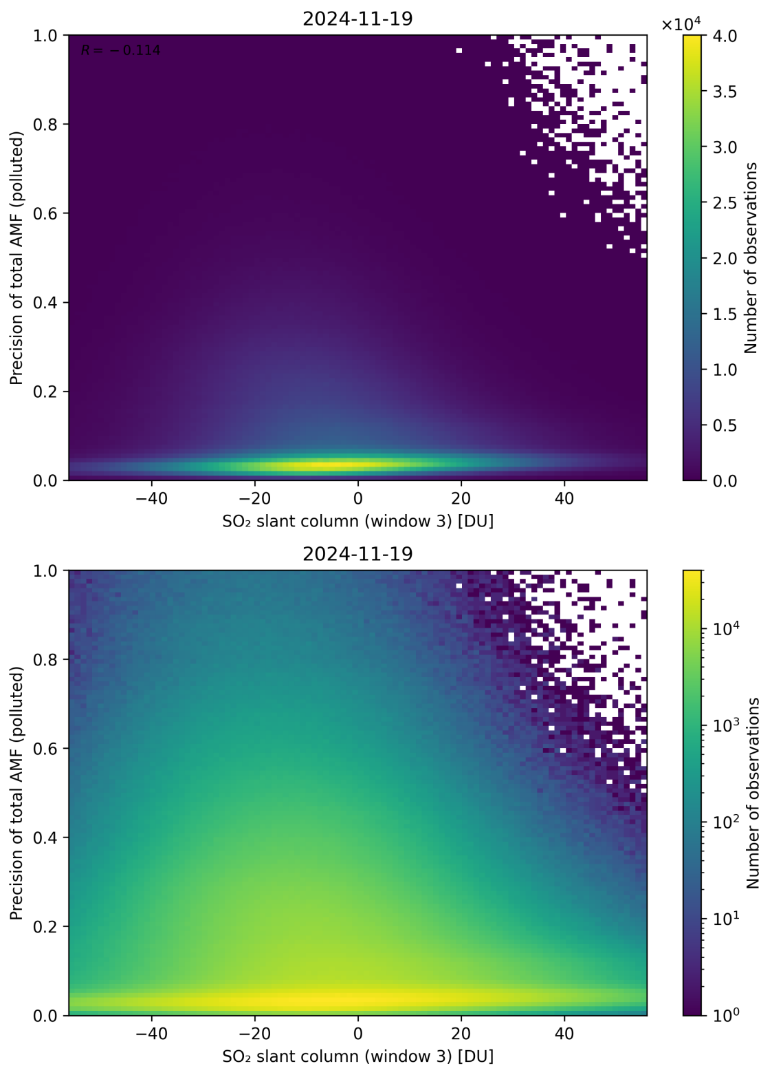
Figure 319: Scatter density plot of “SO 2 slant column (window 3)” against “Precision of total AMF (polluted)” for 2024-11-18 to 2024-11-20.
