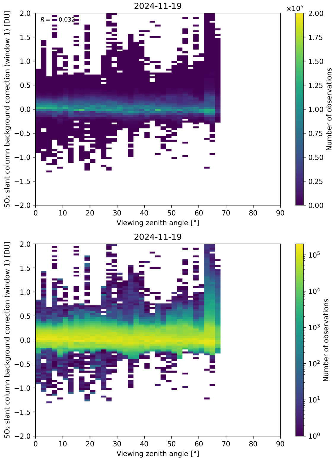
Figure 362: Scatter density plot of “Viewing zenith angle” against “SO 2 slant column background correction (window 1)” for 2024-11-18 to 2024-11-20.
