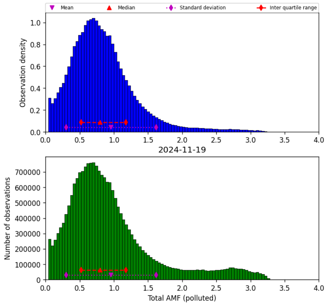
Figure 79: Histogram of “Total AMF (polluted)” for 2024-11-18 to 2024-11-20
