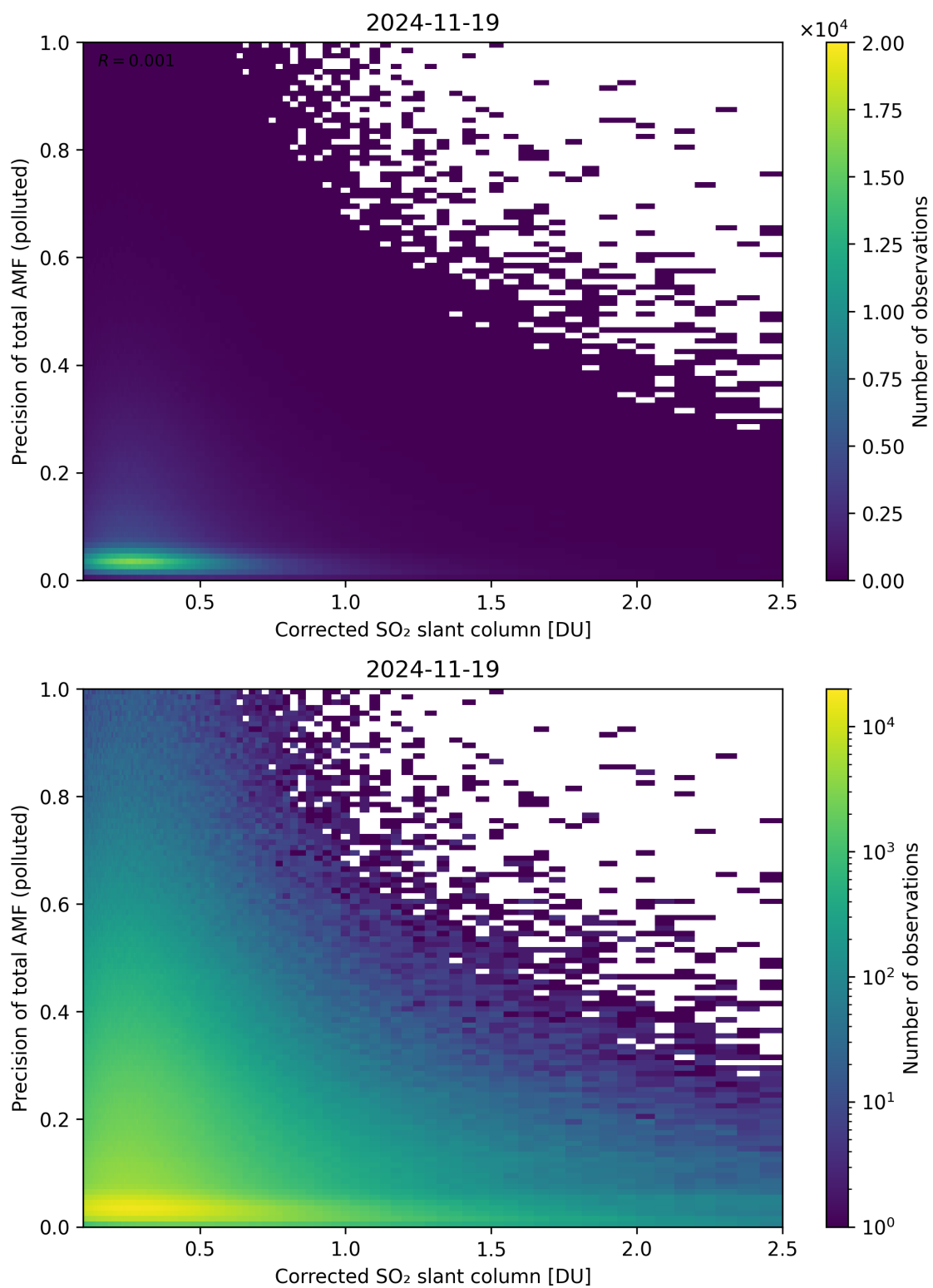
Figure 243: Scatter density plot of “Corrected SO 2 slant column” against “Precision of total AMF (polluted)” for 2024-11-18 to 2024-11-20.
