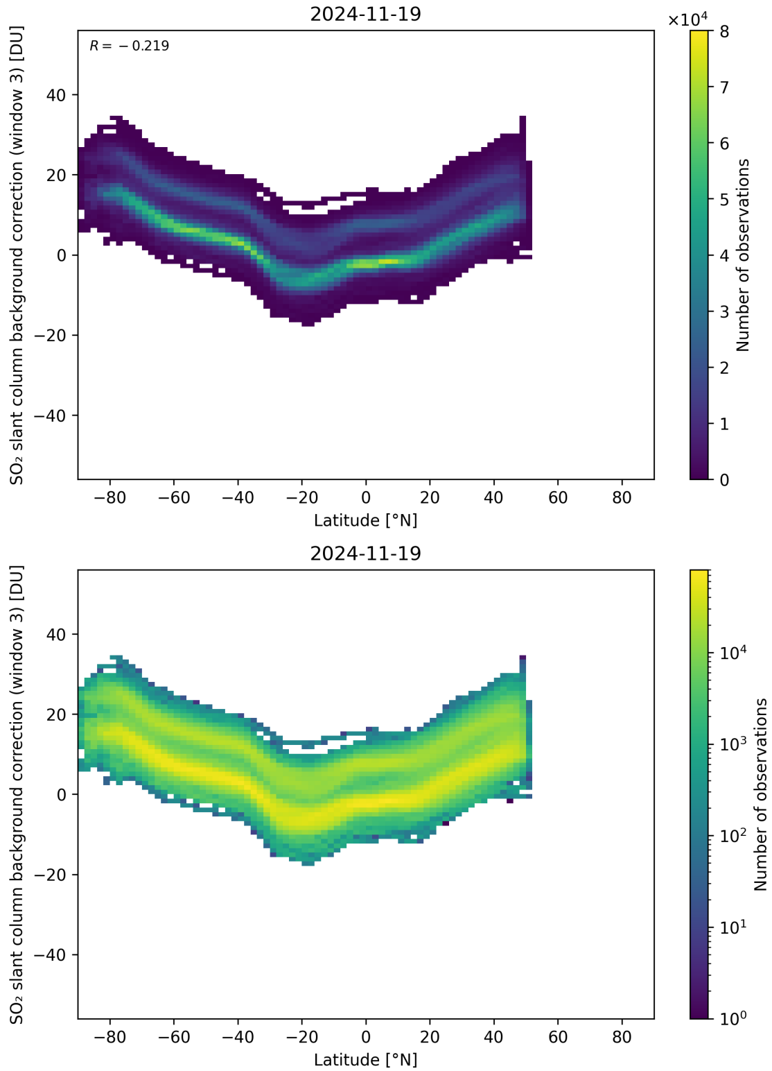
Figure 152: Scatter density plot of “Latitude” against “SO 2 slant column background correction (window 3)” for 2024-11-18 to 2024-11-20.
