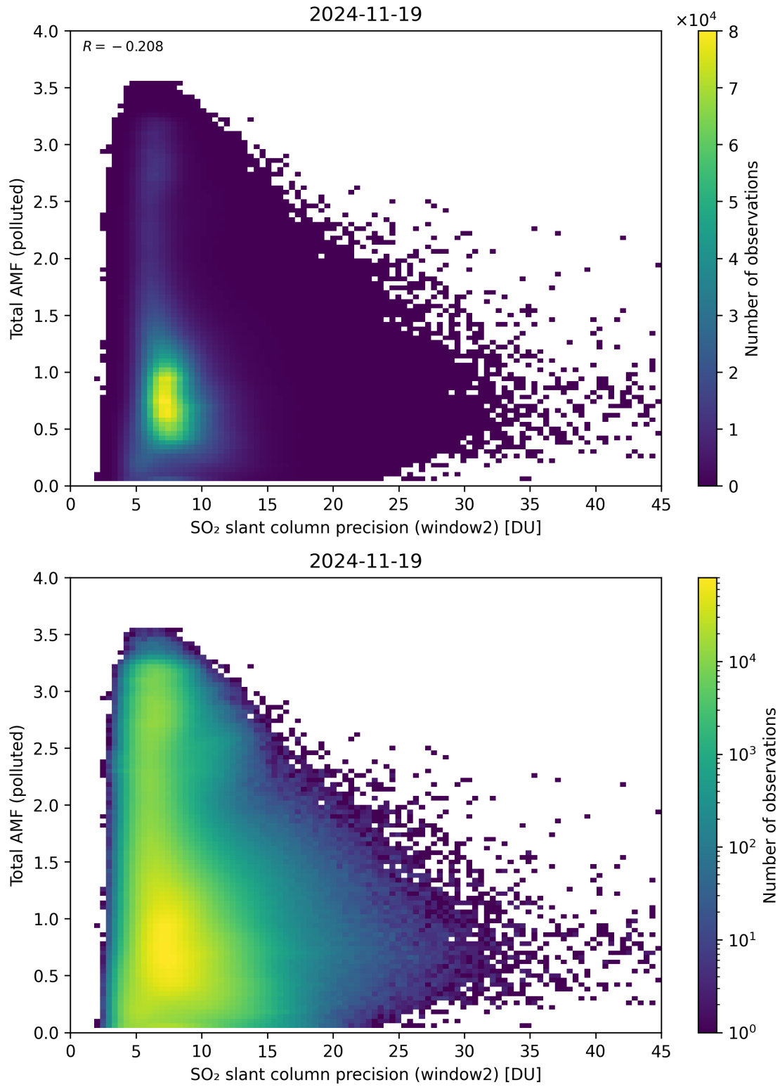
Figure 301: Scatter density plot of “SO 2 slant column precision (window2)” against “Total AMF (polluted)” for 2024-11-18 to 2024-11-20.
