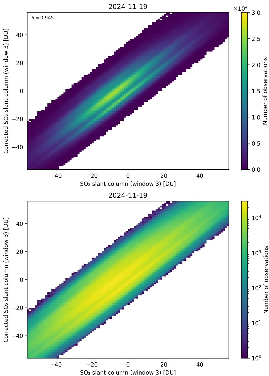
Figure 316: Scatter density plot of “SO 2 slant column (window 3)” against “Corrected SO 2 slant column (window 3)” for 2024-11-18 to 2024-11-20.
