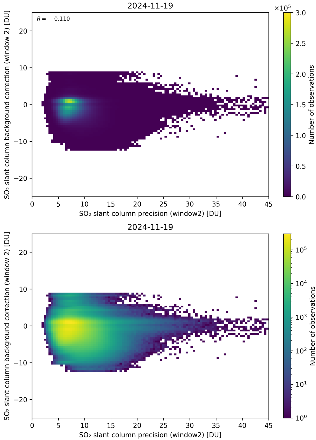
Figure 291: Scatter density plot of “SO 2 slant column precision (window2)” against “SO 2 slant column background correction (window 2)” for 2024-11-18 to 2024-11-20.
