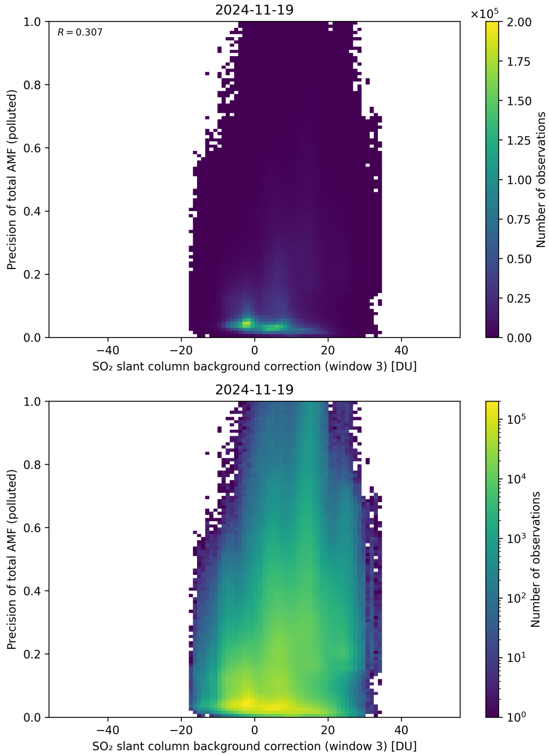
Figure 137: Scatter density plot of “SO 2 slant column background correction (window 3)” against “Precision of total AMF (polluted)” for 2024-11-18 to 2024-11-20.
