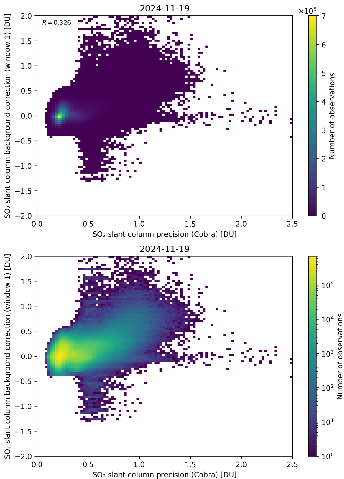
Figure 199: Scatter density plot of “SO 2 slant column precision (Cobra)” against “SO 2 slant column background correction (window 1)” for 2024-11-18 to 2024-11-20.
