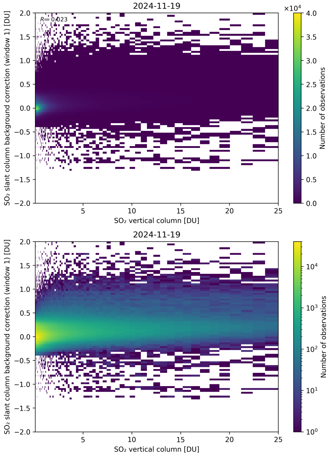
Figure 323: Scatter density plot of “SO 2 vertical column” against “SO 2 slant column background correction (window 1)” for 2024-11-18 to 2024-11-20.
