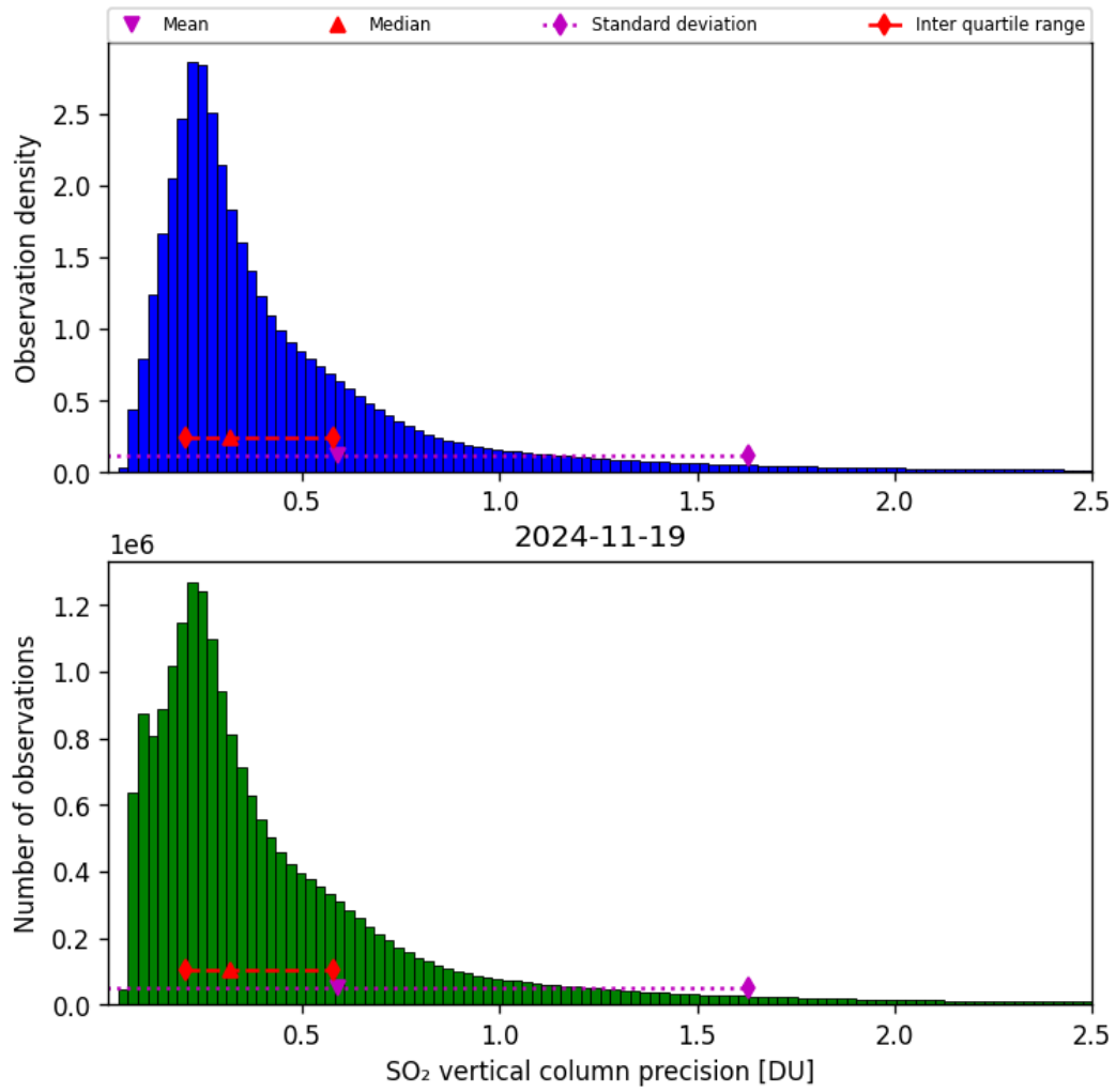
Figure 59: Histogram of “SO 2 vertical column precision” for 2024-11-18 to 2024-11-20
