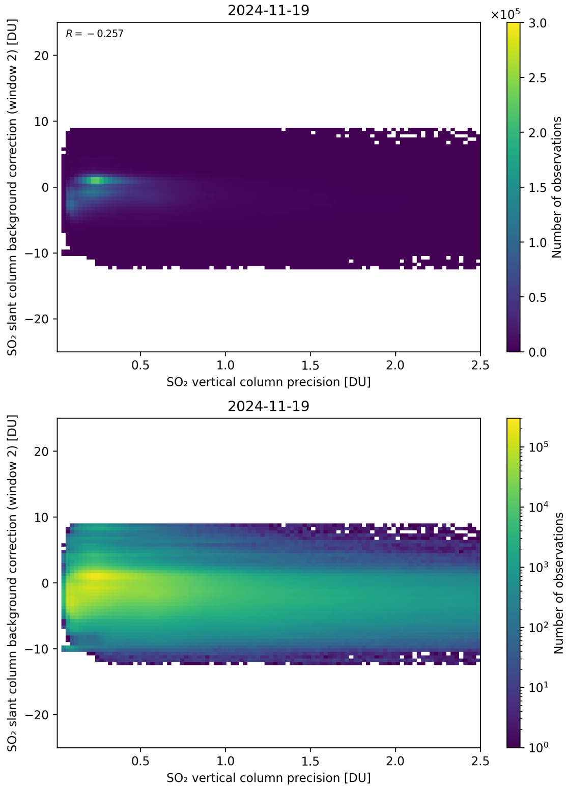
Figure 330: Scatter density plot of “SO 2 vertical column precision” against “SO 2 slant column background correction (window 2)” for 2024-11-18 to 2024-11-20.
