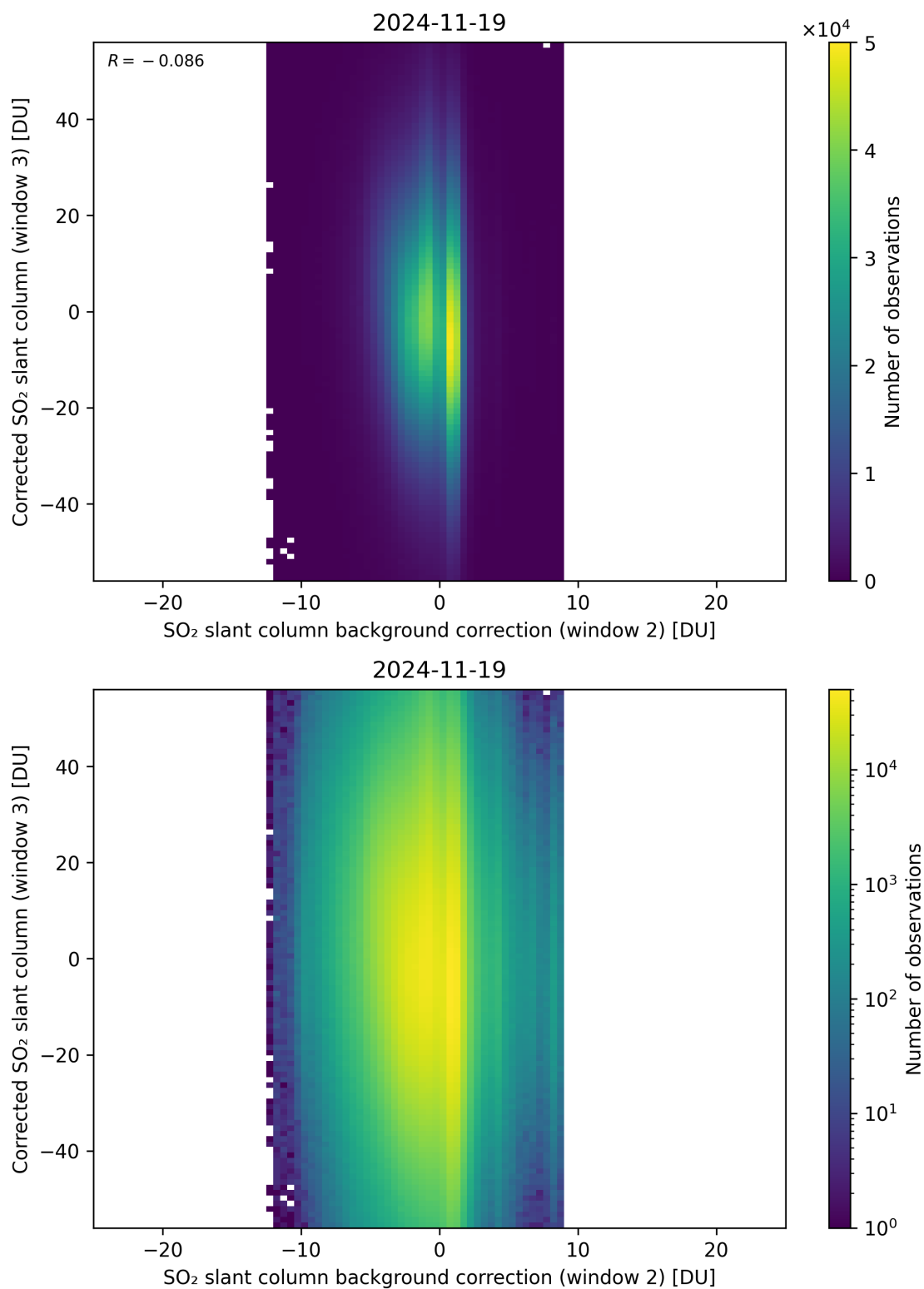
Figure 127: Scatter density plot of “SO 2 slant column background correction (window 2)” against “Corrected SO 2 slant column (window 3)” for 2024-11-18 to 2024-11-20.
