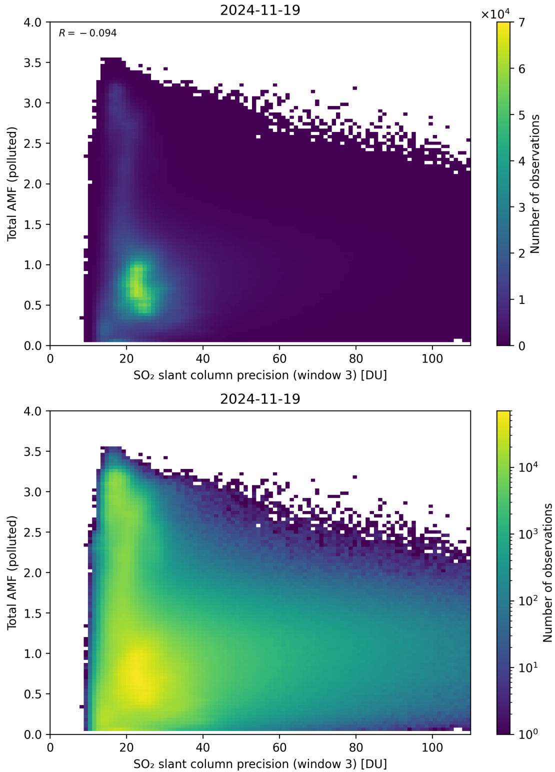
Figure 313: Scatter density plot of “SO 2 slant column precision (window 3)” against “Total AMF (polluted)” for 2024-11-18 to 2024-11-20.
