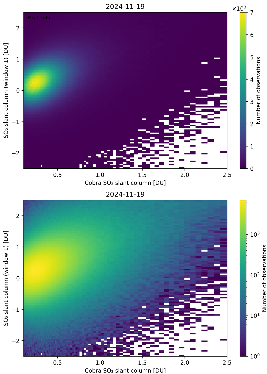
Figure 219: Scatter density plot of “Cobra SO 2 slant column” against “SO 2 slant column (window 1)” for 2024-11-18 to 2024-11-20.
