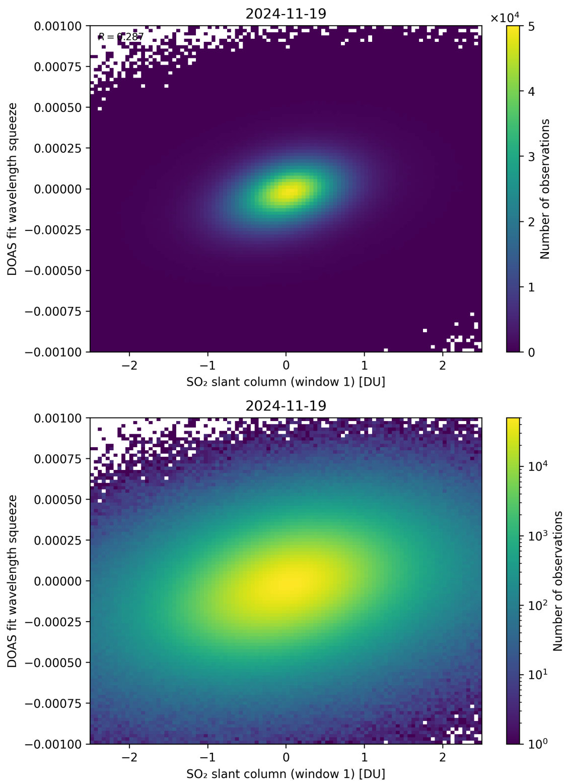
Figure 266: Scatter density plot of “SO 2 slant column (window 1)” against “DOAS fit wavelength squeeze” for 2024-11-18 to 2024-11-20.
