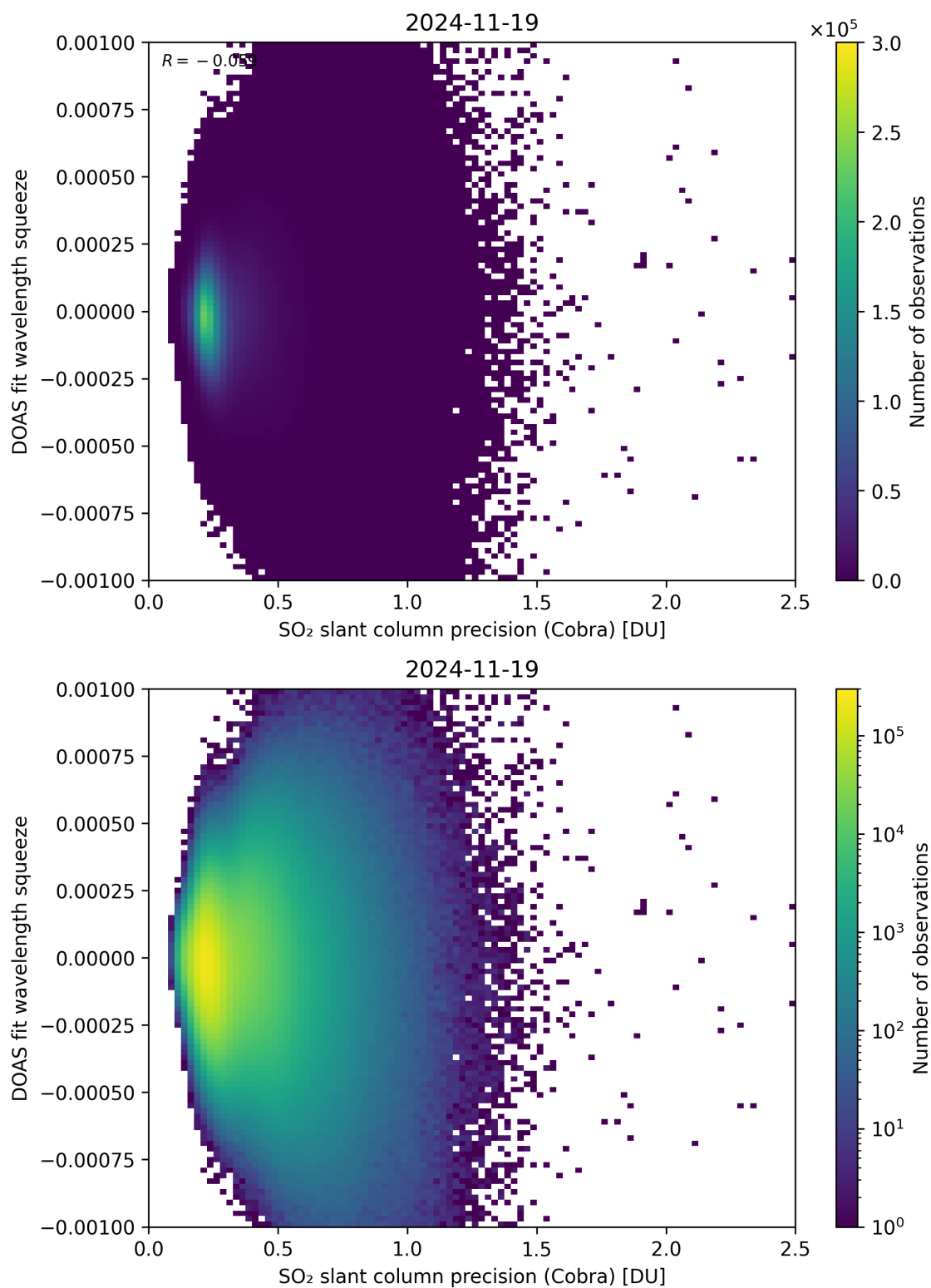
Figure 203: Scatter density plot of “SO 2 slant column precision (Cobra)” against “DOAS fit wavelength squeeze” for 2024-11-18 to 2024-11-20.
