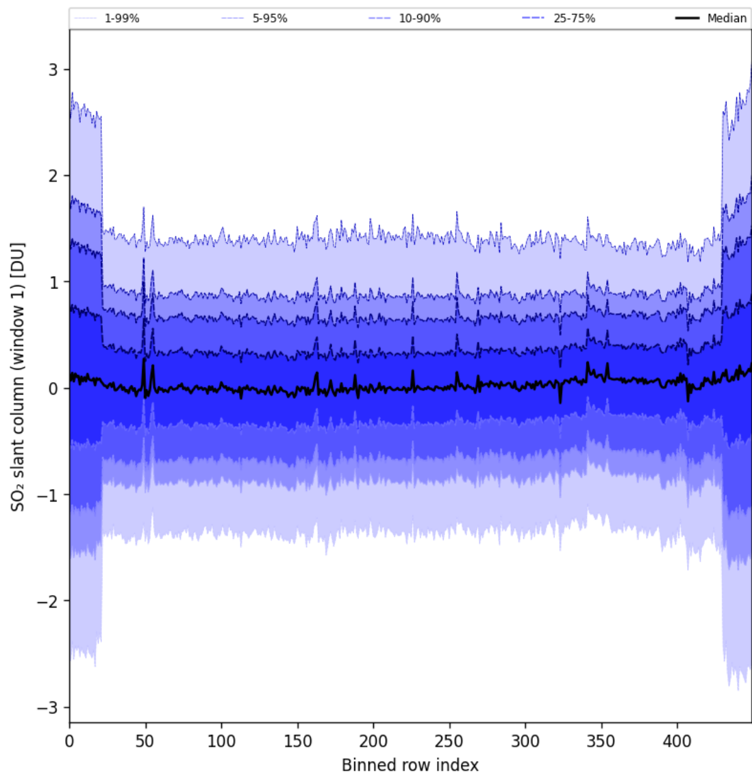
Figure 89: Along track statistics of “SO 2 slant column (window 1)” for 2024-11-18 to 2024-11-20
