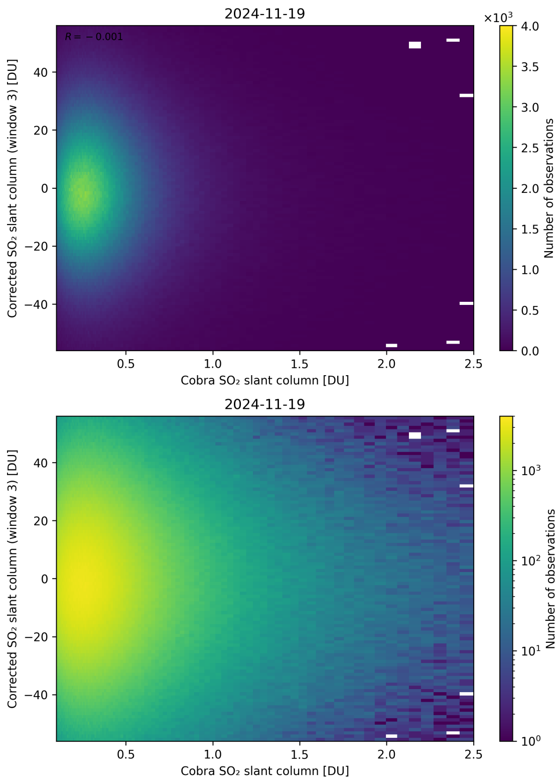
Figure 218: Scatter density plot of “Cobra SO 2 slant column” against “Corrected SO 2 slant column (window 3)” for 2024-11-18 to 2024-11-20.
