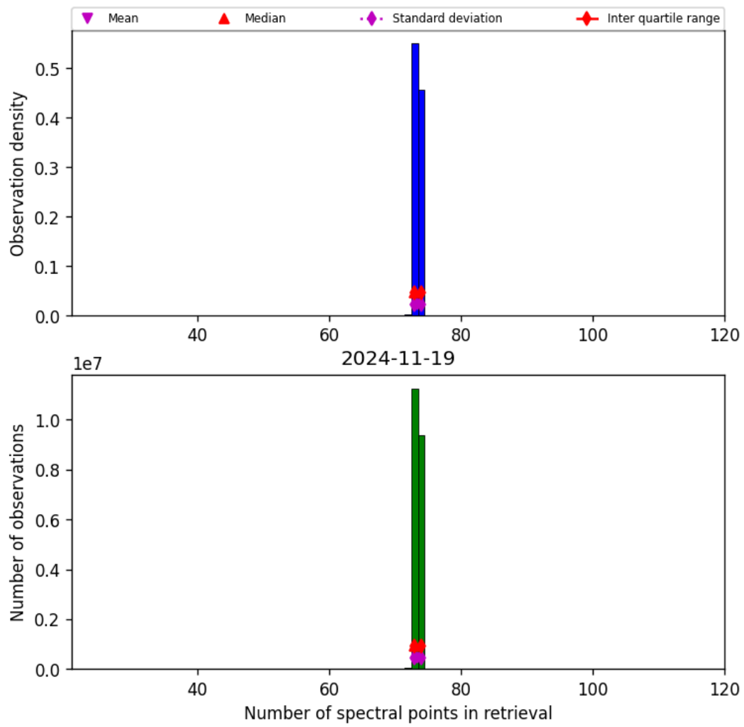
Figure 82: Histogram of “Number of spectral points in retrieval” for 2024-11-18 to 2024-11-20
