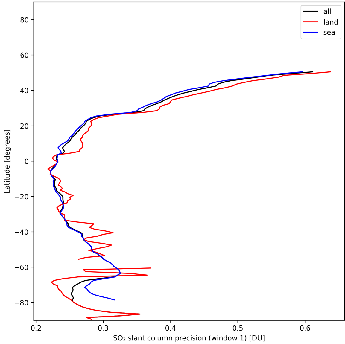
Figure 38: Zonal average of “SO 2 slant column precision (window 1)” for 2024-11-18 to 2024-11-20.
