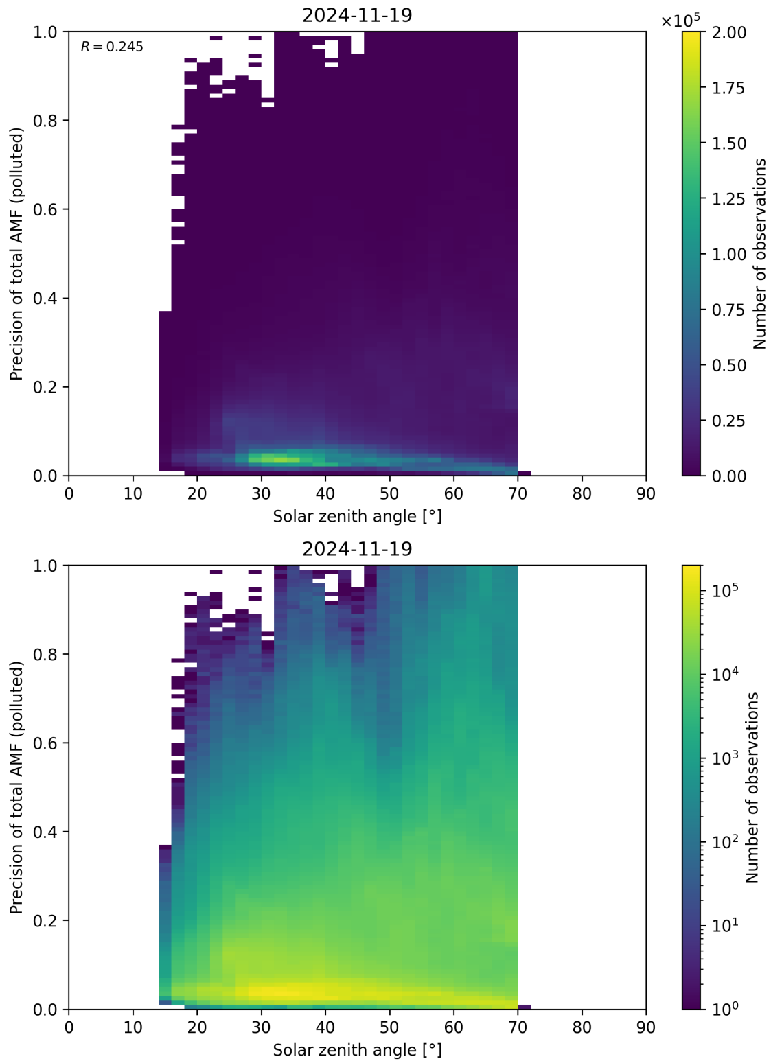
Figure 190: Scatter density plot of “Solar zenith angle” against “Precision of total AMF (polluted)” for 2024-11-18 to 2024-11-20.
