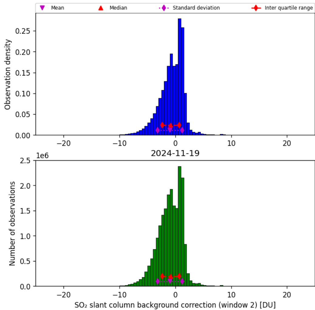
Figure 70: Histogram of “SO 2 slant column background correction (window 2)” for 2024-11-18 to 2024-11-20
