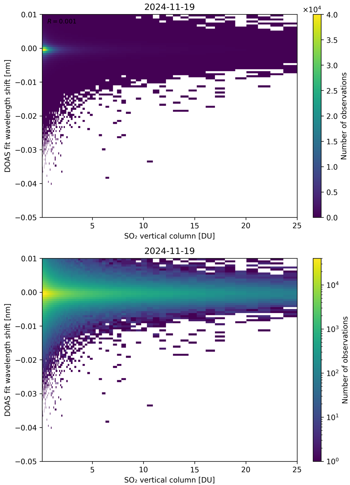
Figure 326: Scatter density plot of “SO 2 vertical column” against “DOAS fit wavelength shift” for 2024-11-18 to 2024-11-20.
