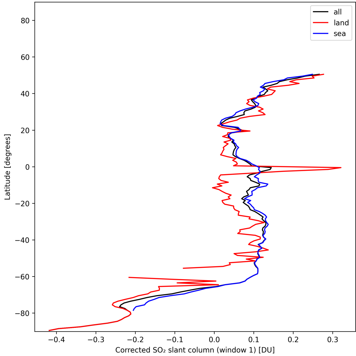
Figure 39: Zonal average of “Corrected SO 2 slant column (window 1)” for 2024-11-18 to 2024-11-20.
