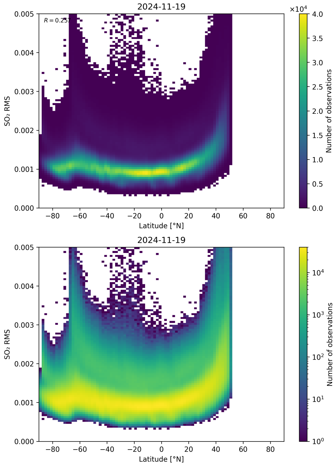
Figure 155: Scatter density plot of “Latitude” against “SO 2 RMS” for 2024-11-18 to 2024-11-20.
