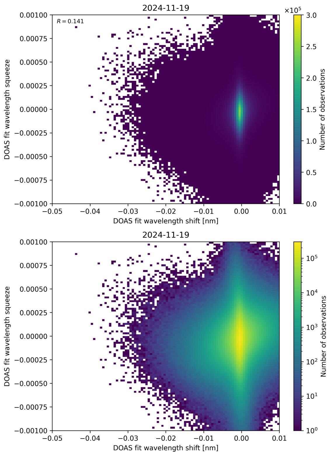
Figure 138: Scatter density plot of “DOAS fit wavelength shift” against “DOAS fit wavelength squeeze” for 2024-11-18 to 2024-11-20.
