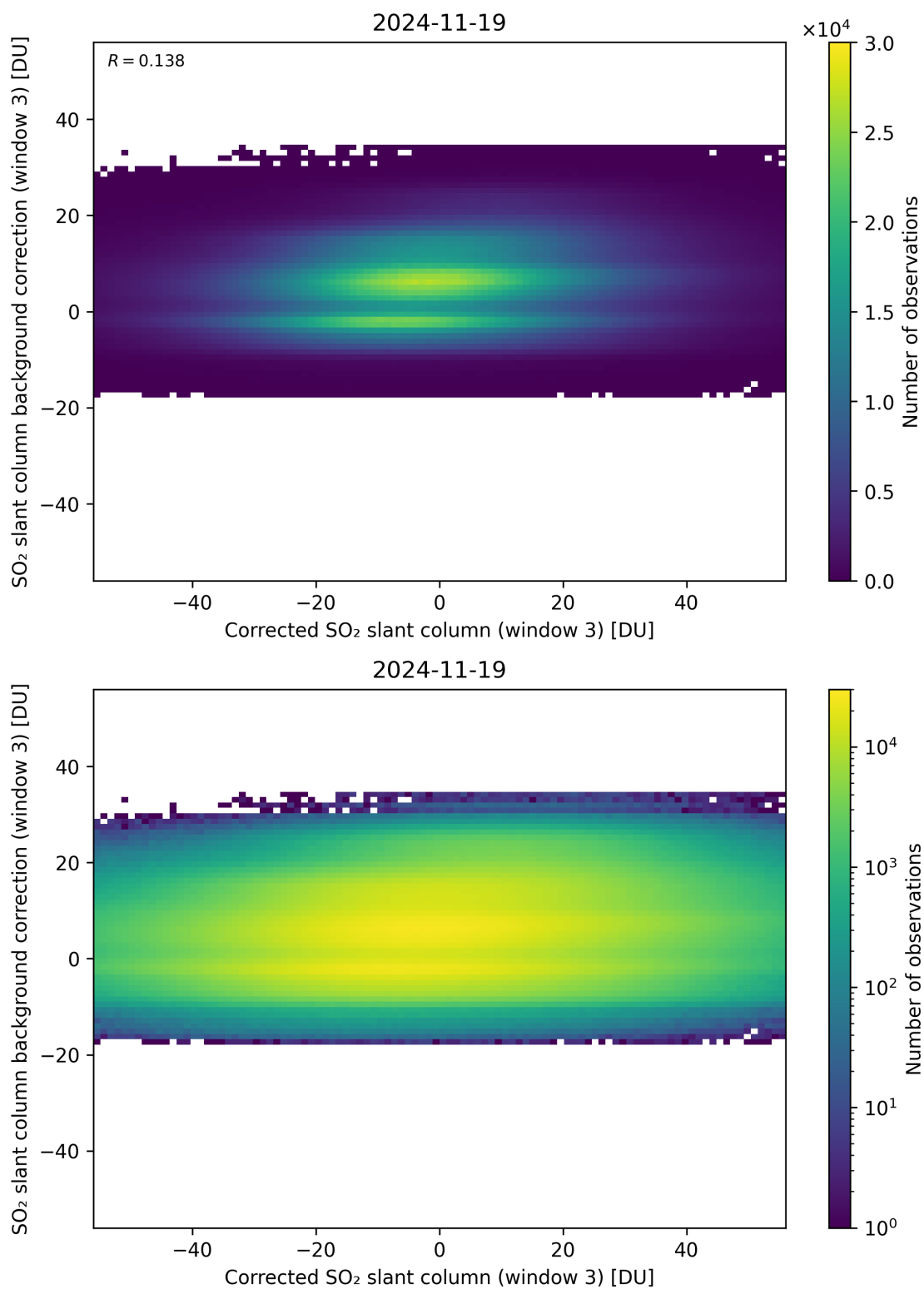
Figure 255: Scatter density plot of “Corrected SO 2 slant column (window 3)” against “SO 2 slant column background correction (window 3)” for 2024-11-18 to 2024-11-20.
