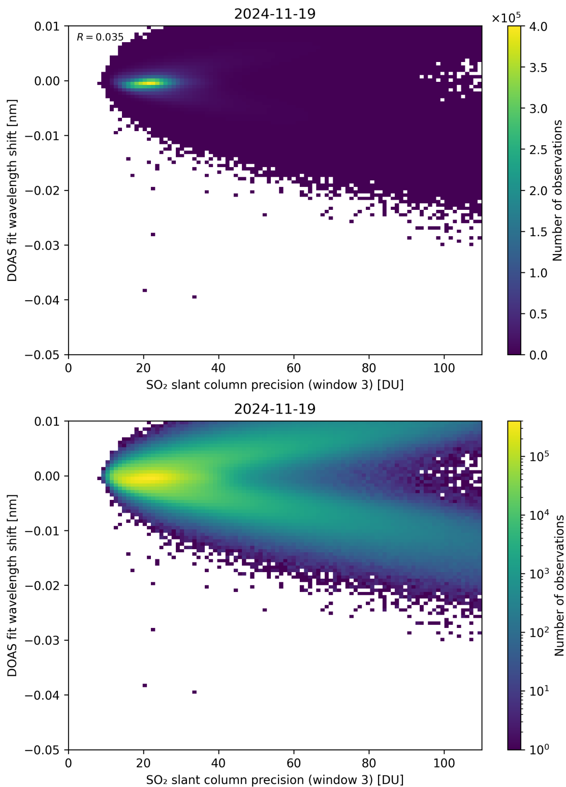
Figure 308: Scatter density plot of “SO 2 slant column precision (window 3)” against “DOAS fit wavelength shift” for 2024-11-18 to 2024-11-20.
