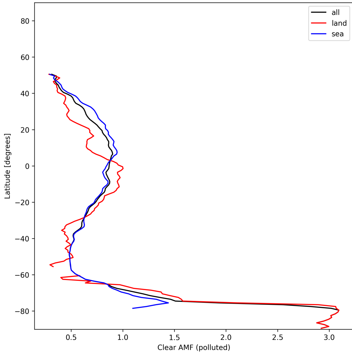
Figure 55: Zonal average of “Clear AMF (polluted)” for 2024-11-18 to 2024-11-20.
