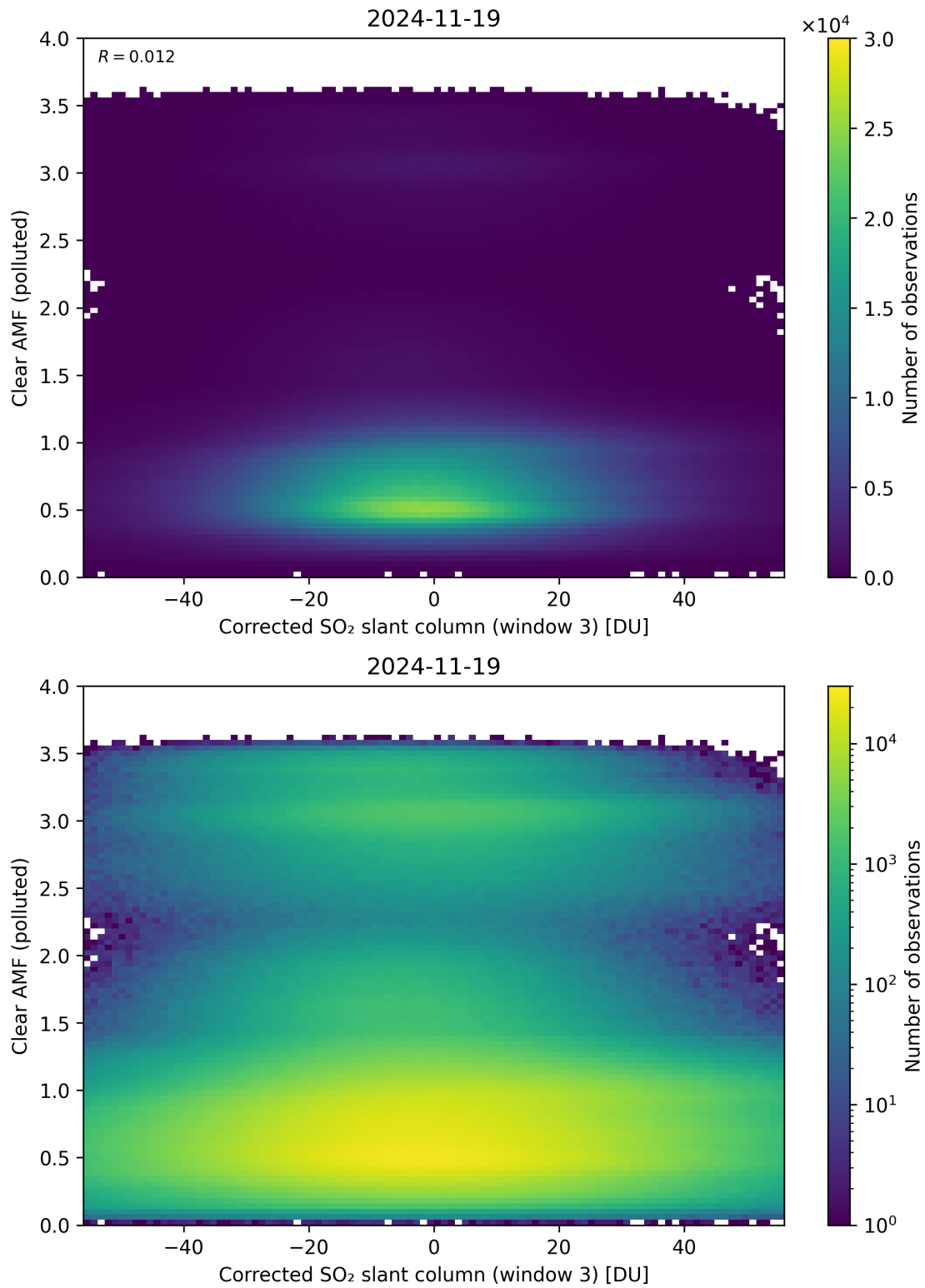
Figure 259: Scatter density plot of “Corrected SO 2 slant column (window 3)” against “Clear AMF (polluted)” for 2024-11-18 to 2024-11-20.
