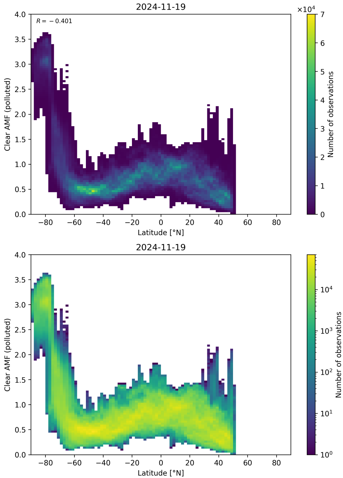
Figure 156: Scatter density plot of “Latitude” against “Clear AMF (polluted)” for 2024-11-18 to 2024-11-20.
