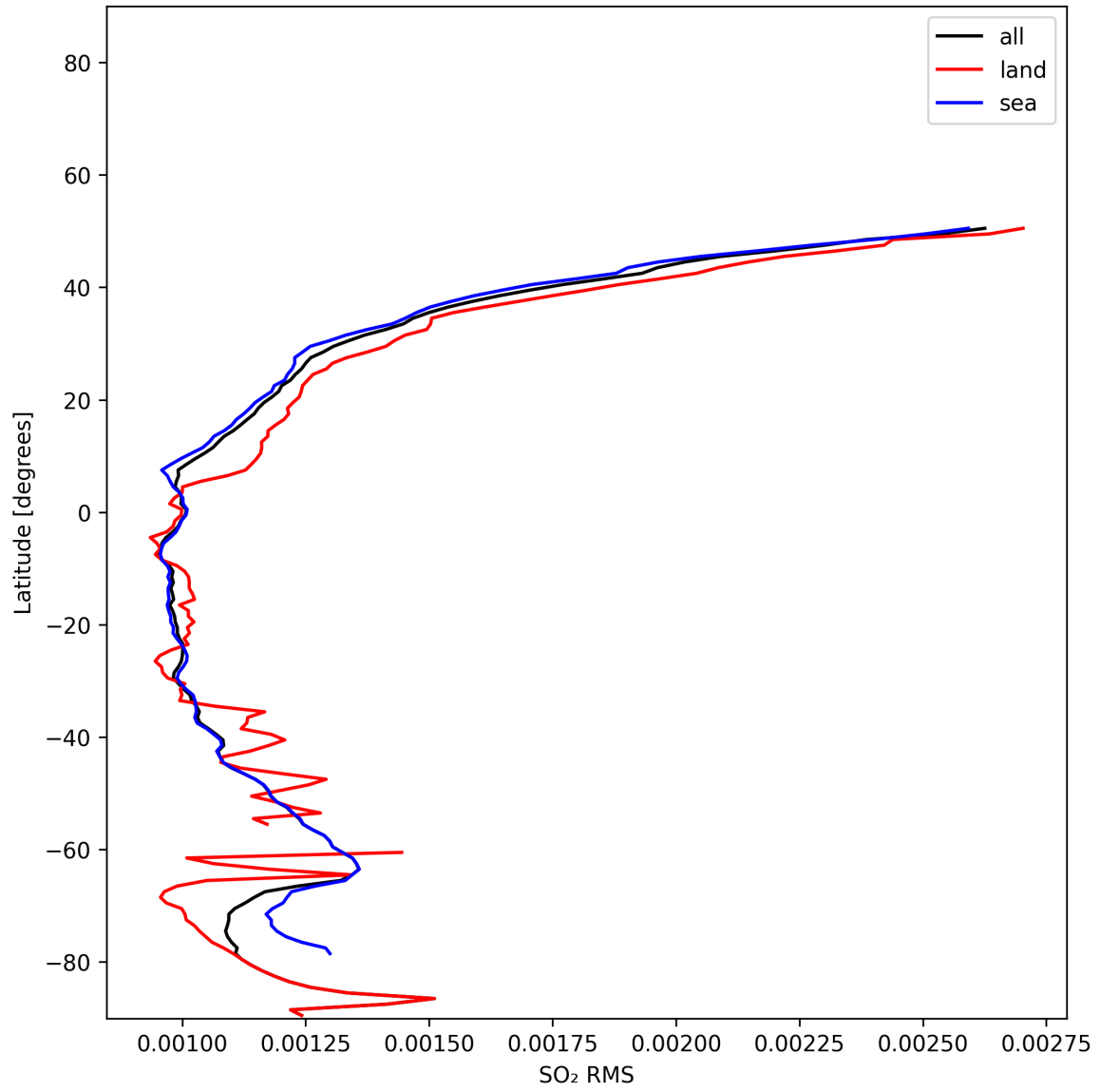
Figure 52: Zonal average of “SO 2 RMS” for 2024-11-18 to 2024-11-20.
