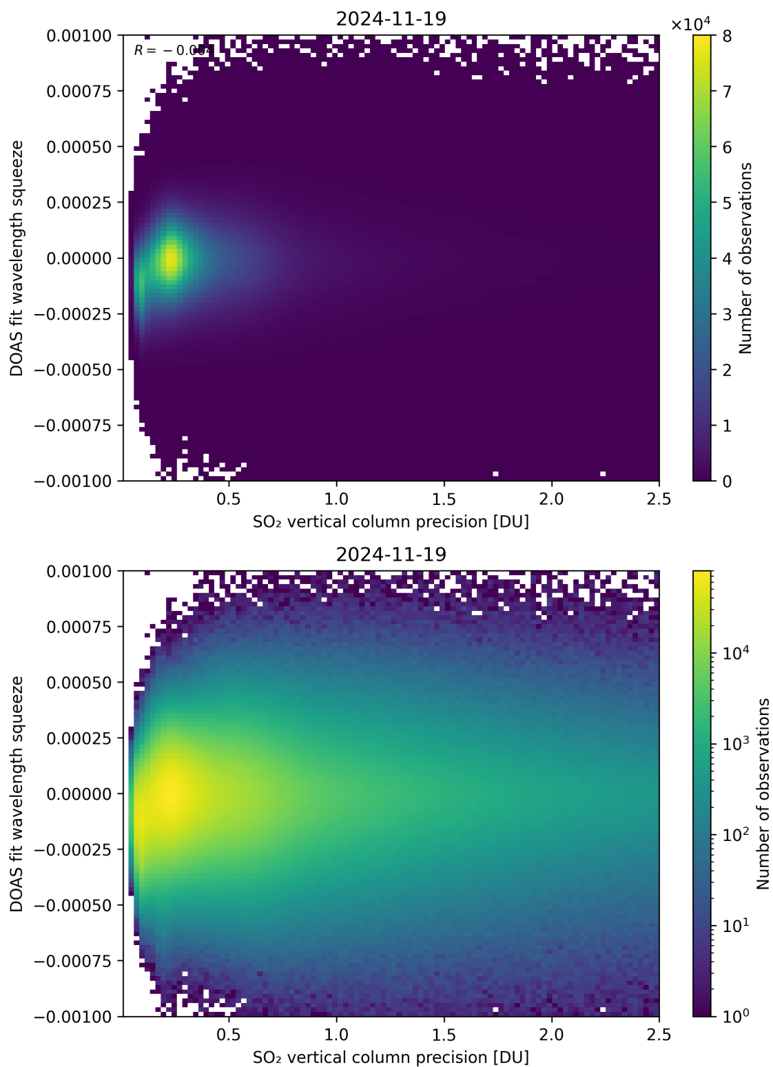
Figure 333: Scatter density plot of “SO 2 vertical column precision” against “DOAS fit wavelength squeeze” for 2024-11-18 to 2024-11-20.
