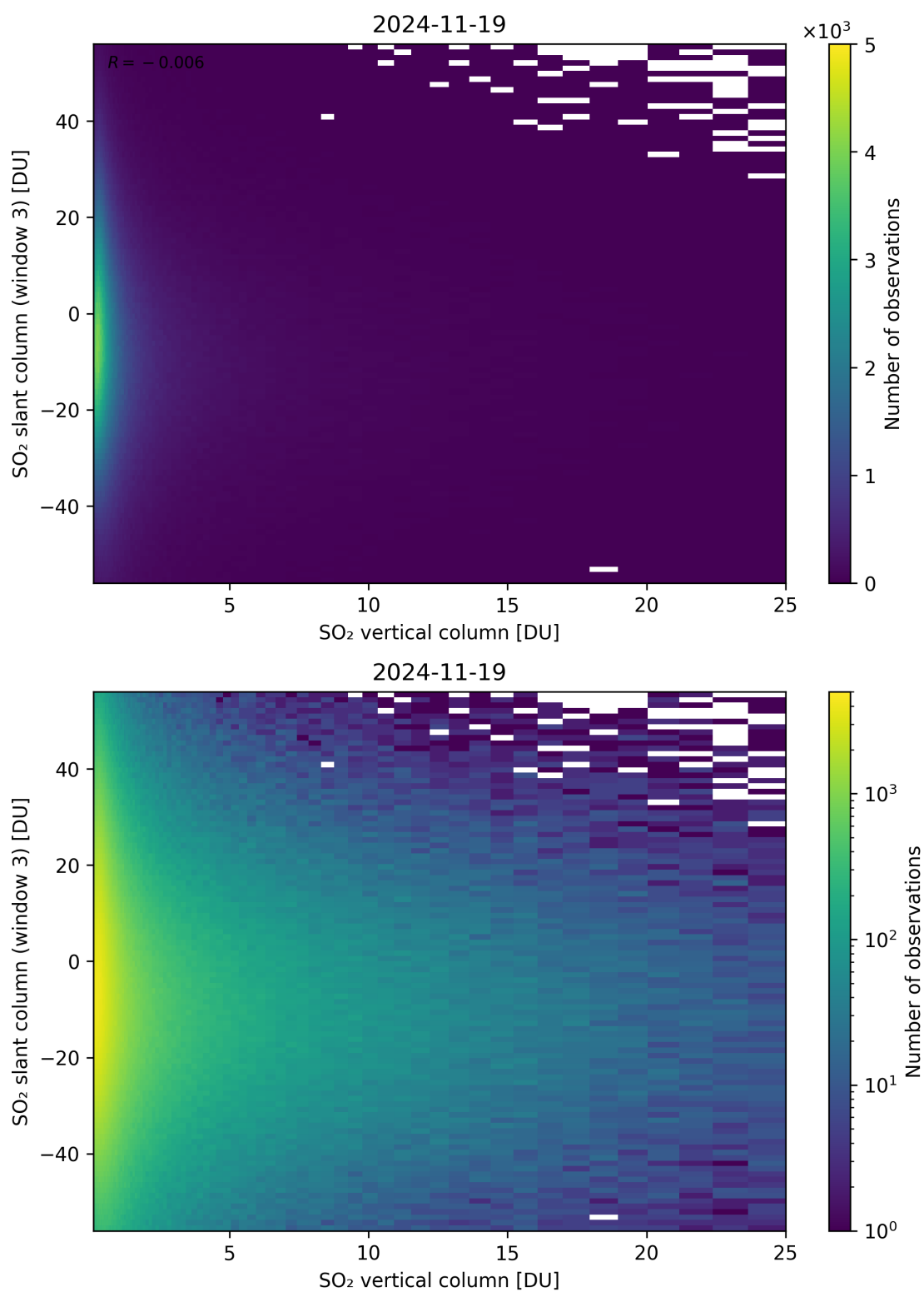
Figure 357: Scatter density plot of “SO 2 vertical column” against “SO 2 slant column (window 3)” for 2024-11-18 to 2024-11-20.
