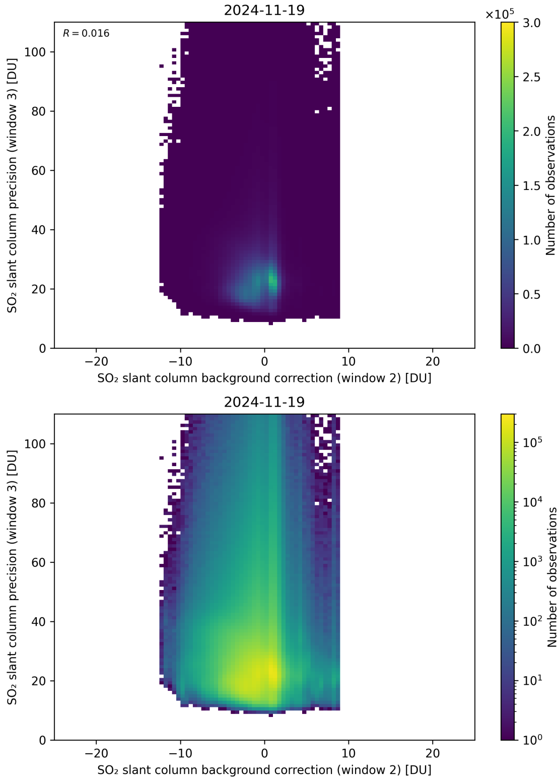
Figure 129: Scatter density plot of “SO 2 slant column background correction (window 2)” against “SO 2 slant column precision (window 3)” for 2024-11-18 to 2024-11-20.
