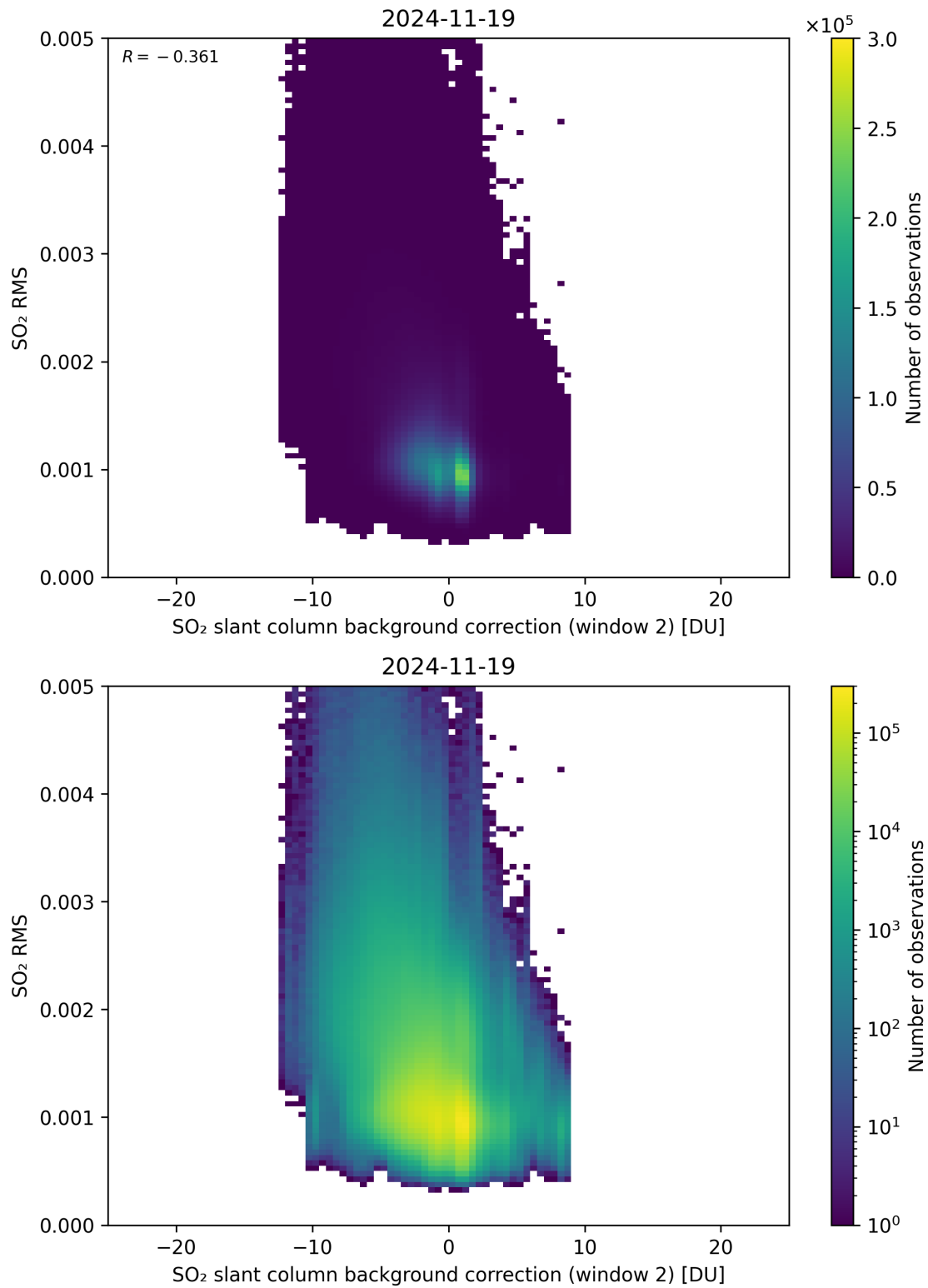
Figure 125: Scatter density plot of “SO 2 slant column background correction (window 2)” against “SO 2 RMS” for 2024-11-18 to 2024-11-20.
