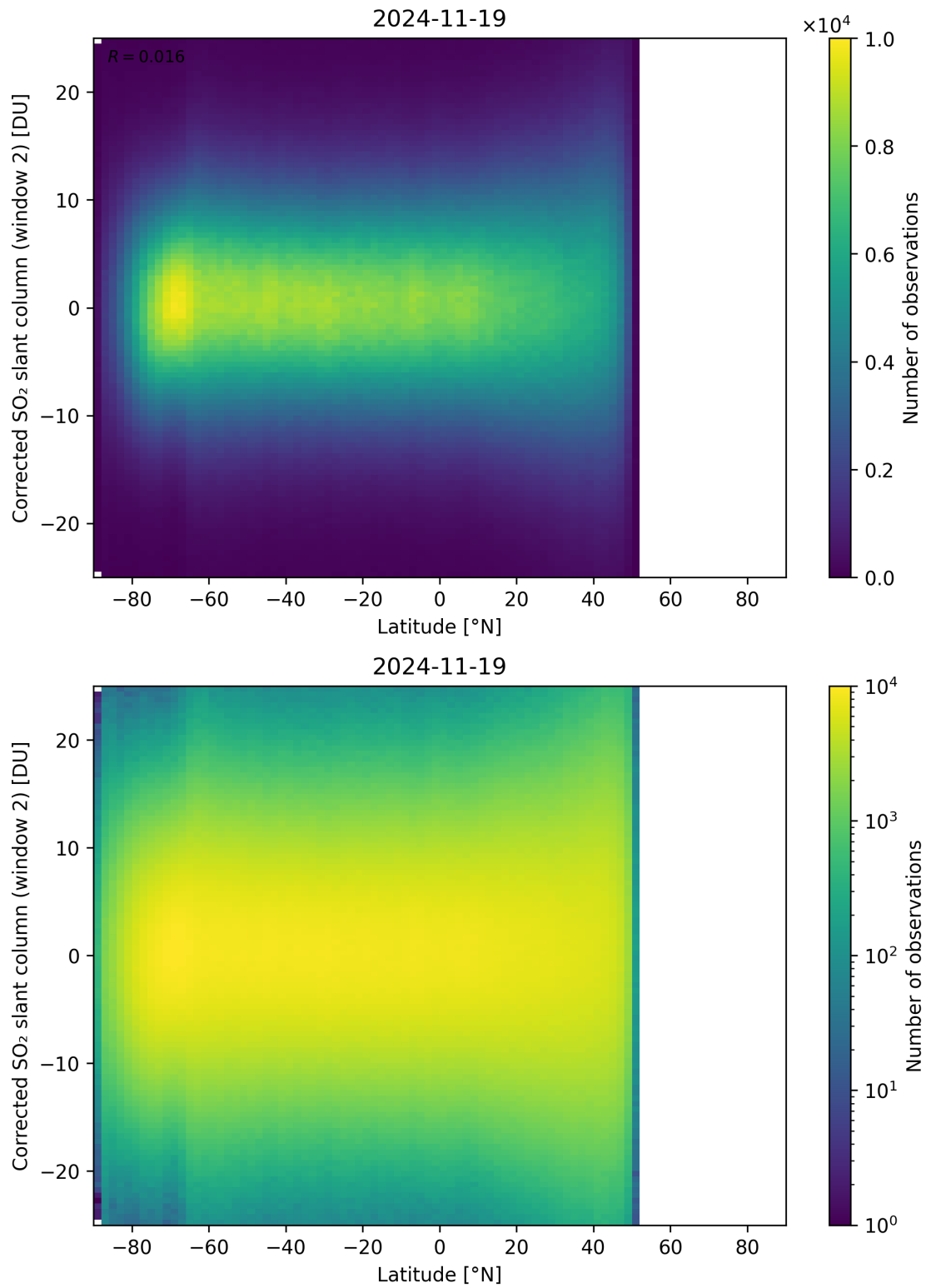
Figure 160: Scatter density plot of “Latitude” against “Corrected SO 2 slant column (window 2)” for 2024-11-18 to 2024-11-20.
