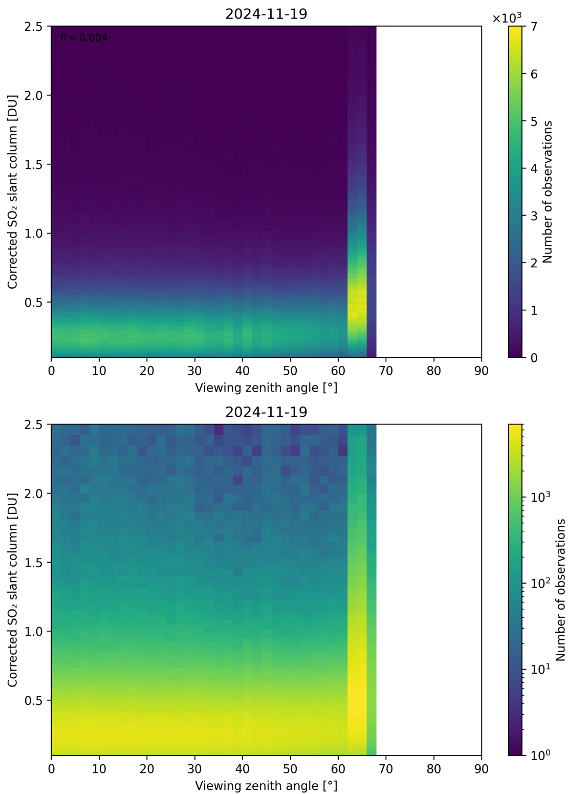
Figure 373: Scatter density plot of “Viewing zenith angle” against “Corrected SO 2 slant column” for 2024-11-18 to 2024-11-20.
