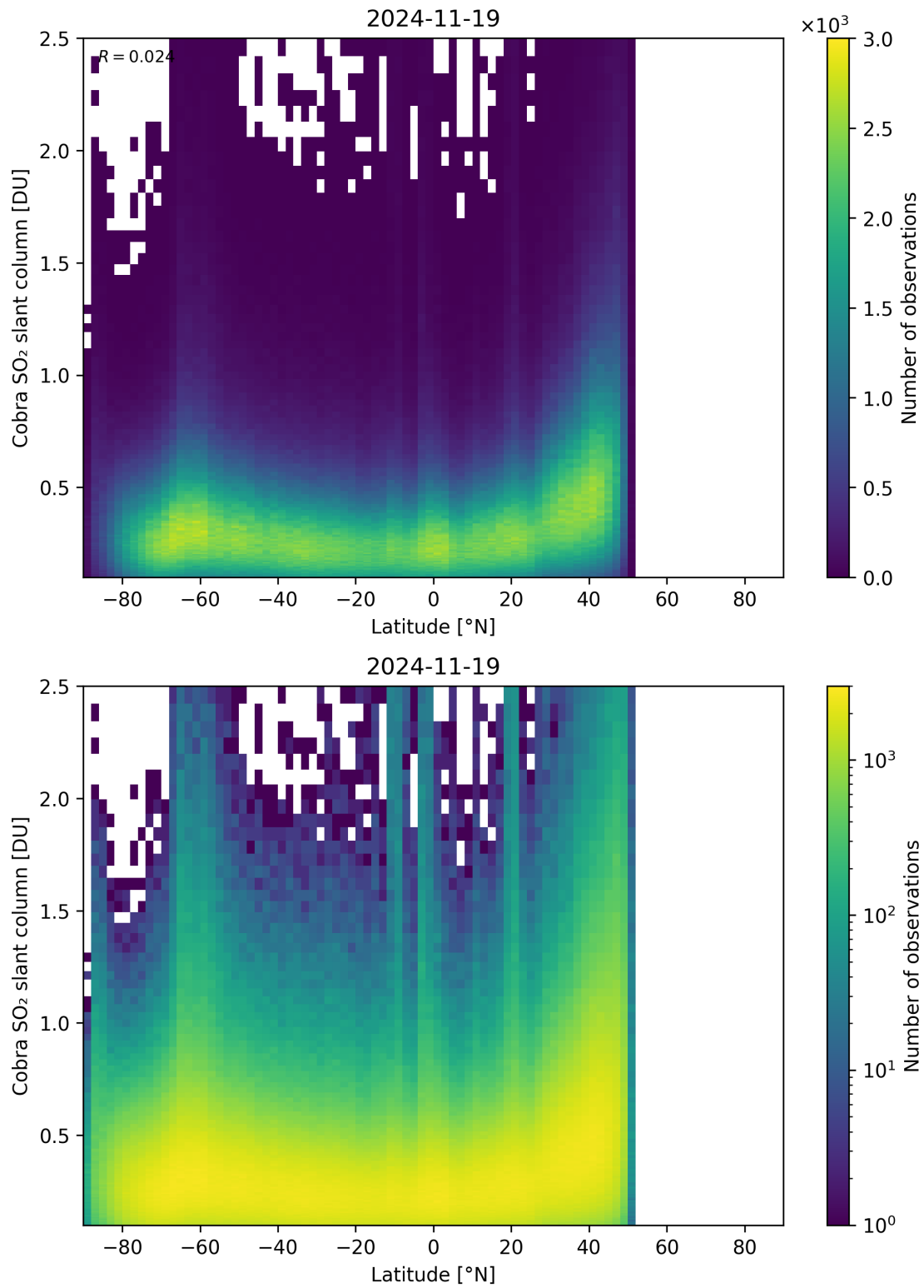
Figure 157: Scatter density plot of “Latitude” against “Cobra SO 2 slant column” for 2024-11-18 to 2024-11-20.
