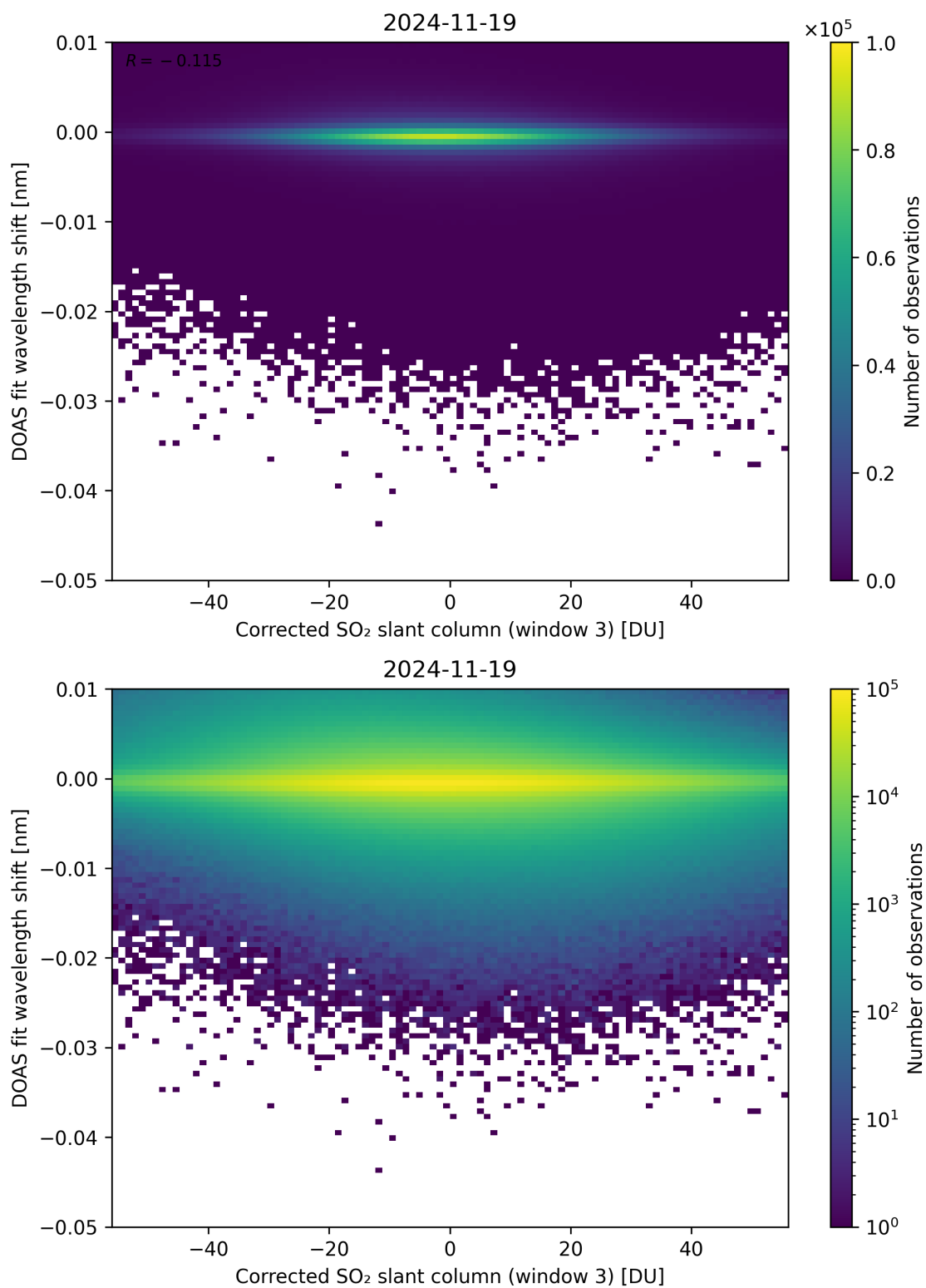
Figure 256: Scatter density plot of “Corrected SO 2 slant column (window 3)” against “DOAS fit wavelength shift” for 2024-11-18 to 2024-11-20.
