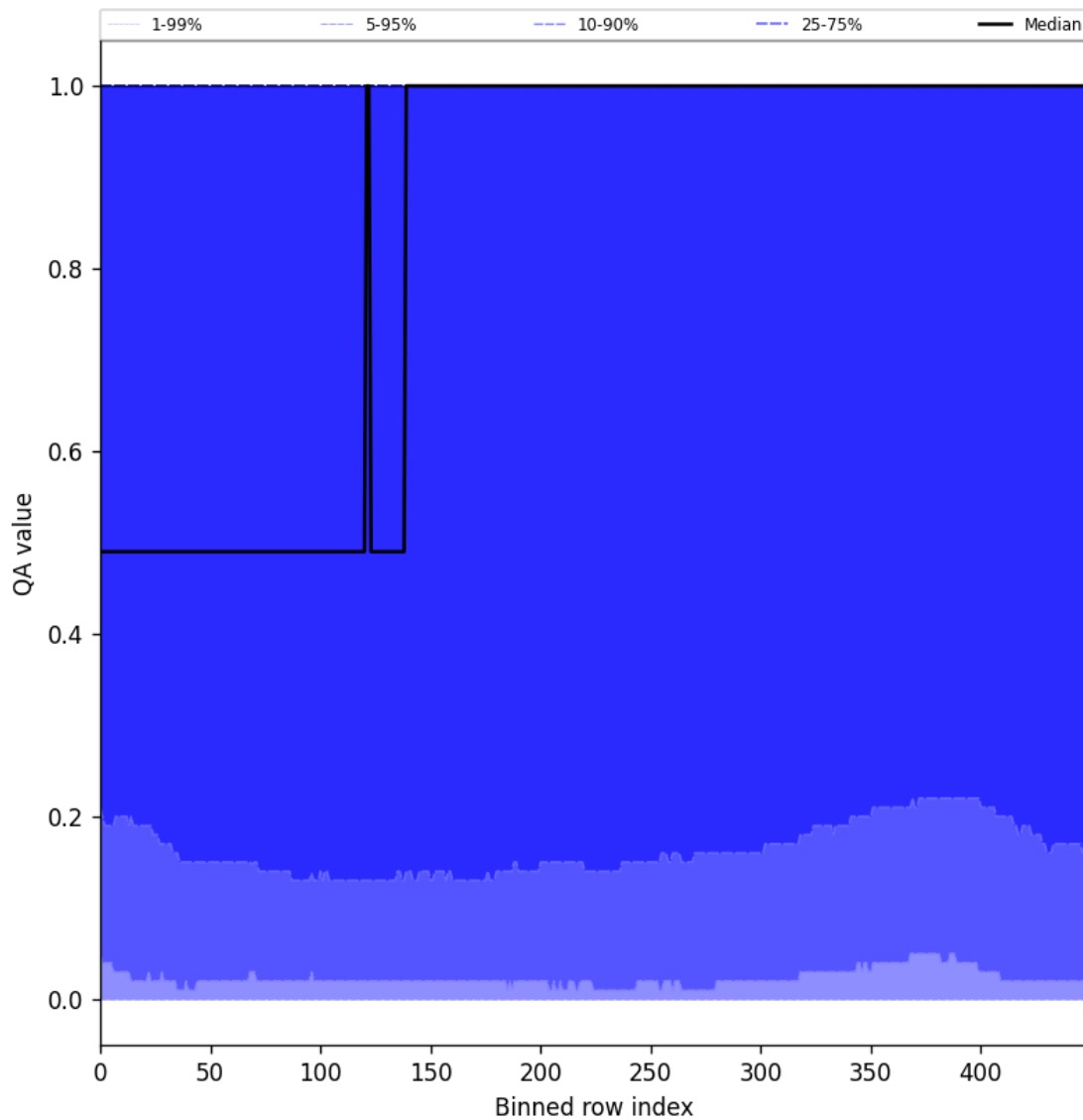
Figure 83: Along track statistics of “QA value” for 2024-11-18 to 2024-11-20
