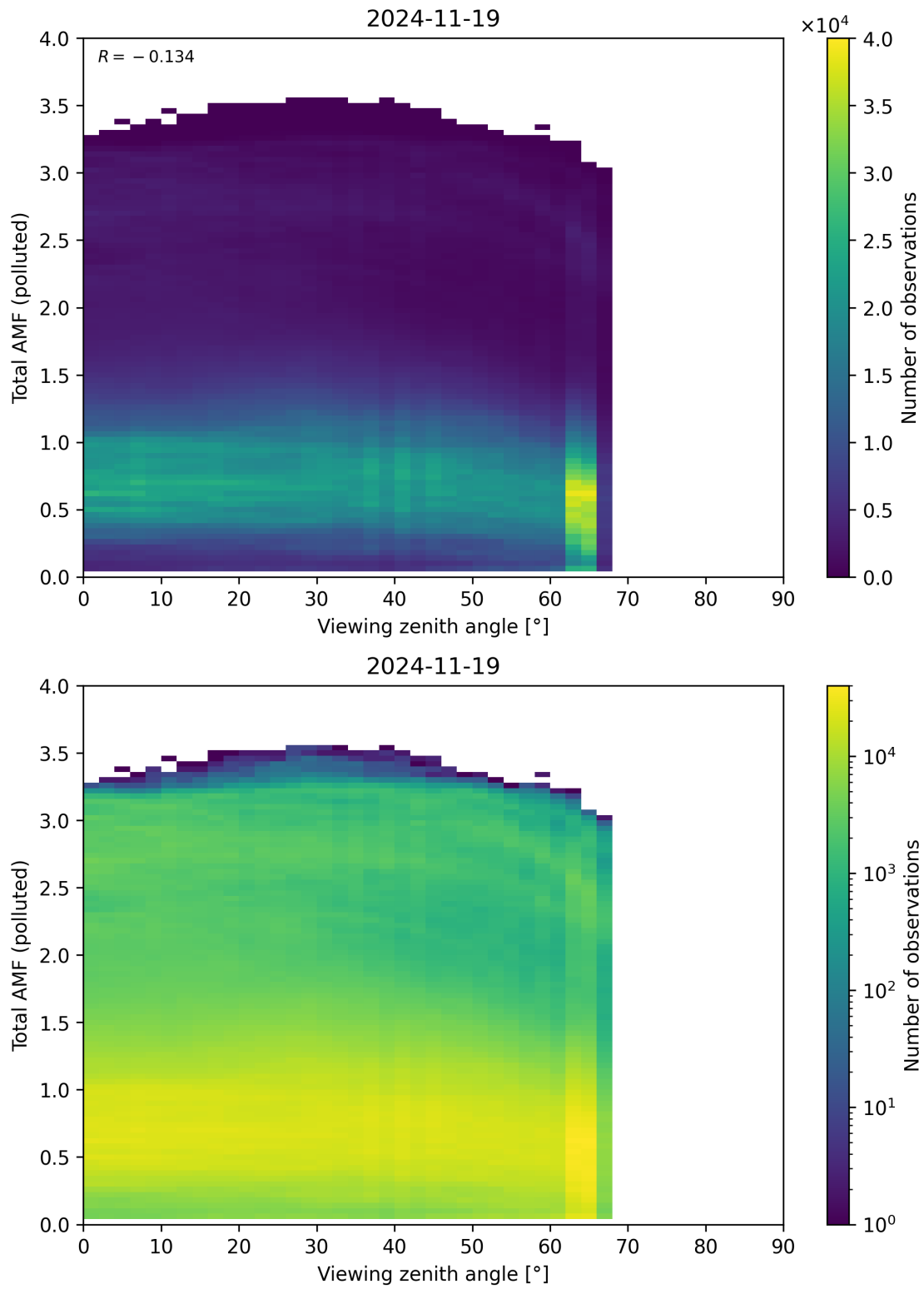
Figure 381: Scatter density plot of “Viewing zenith angle” against “Total AMF (polluted)” for 2024-11-18 to 2024-11-20.
