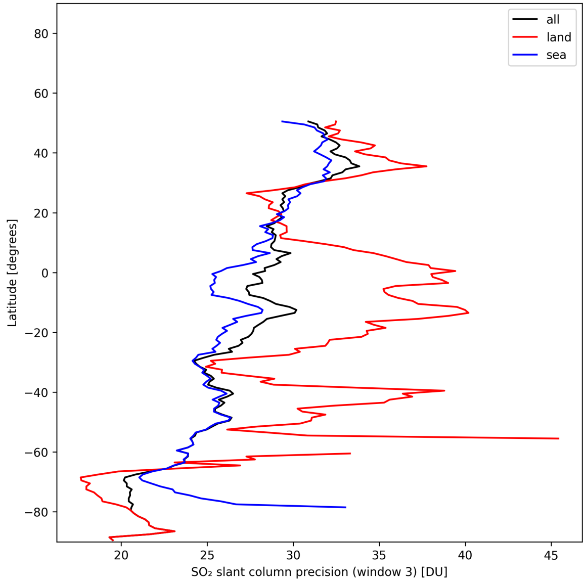
Figure 46: Zonal average of “SO 2 slant column precision (window 3)” for 2024-11-18 to 2024-11-20.
