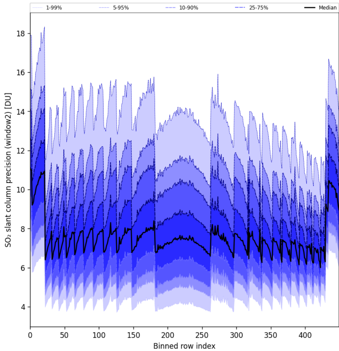
Figure 94: Along track statistics of “SO 2 slant column precision (window2)” for 2024-11-18 to 2024-11-20
