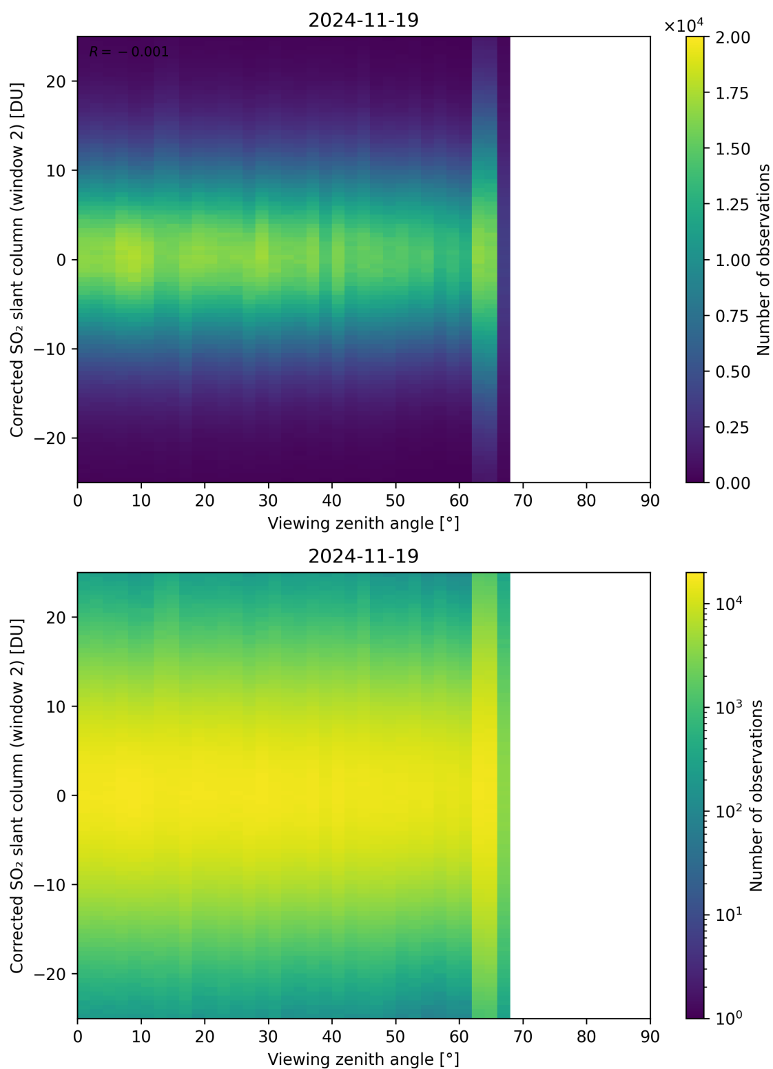
Figure 374: Scatter density plot of “Viewing zenith angle” against “Corrected SO 2 slant column (window 2)” for 2024-11-18 to 2024-11-20.
