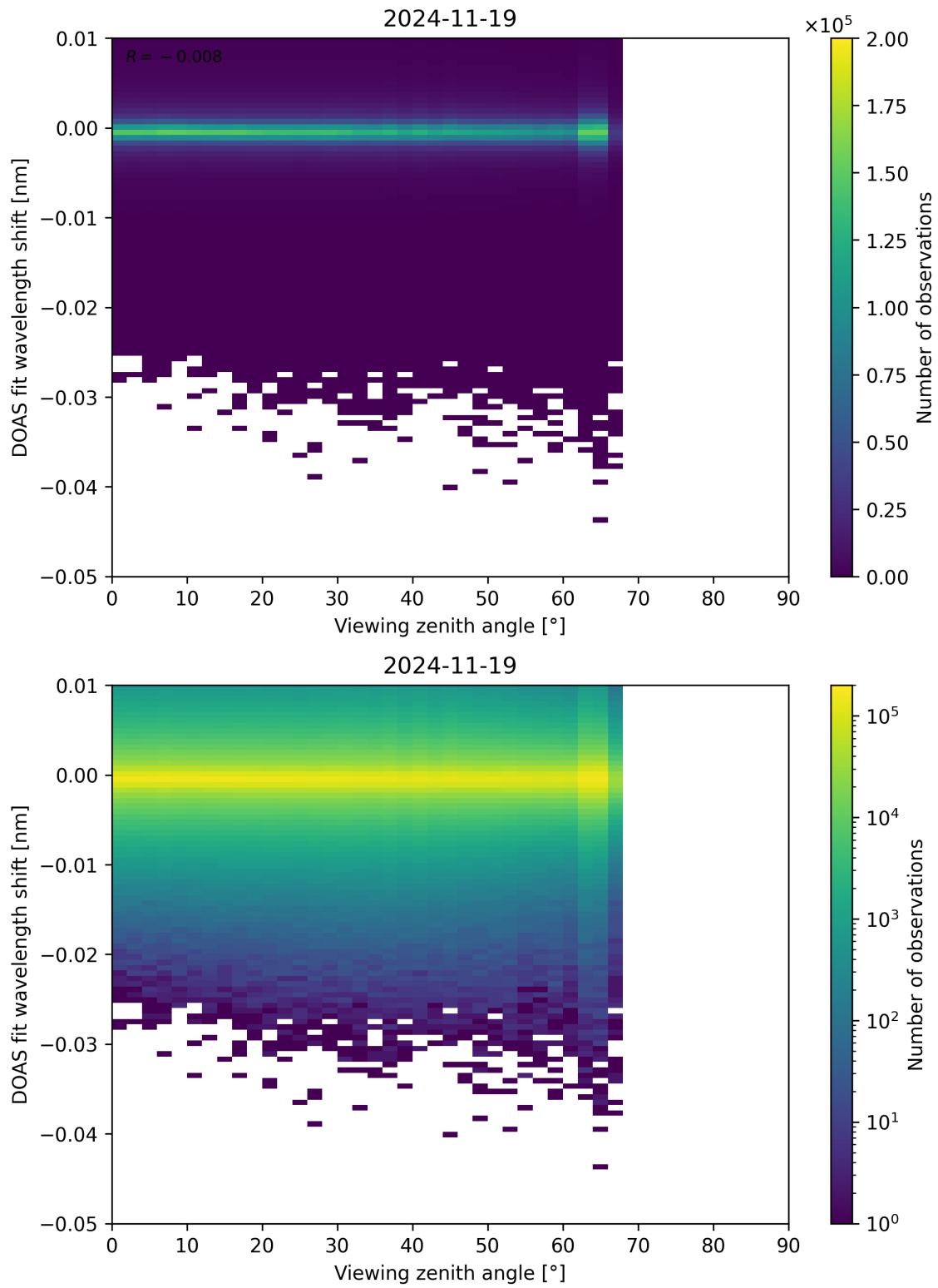
Figure 365: Scatter density plot of “Viewing zenith angle” against “DOAS fit wavelength shift” for 2024-11-18 to 2024-11-20.
