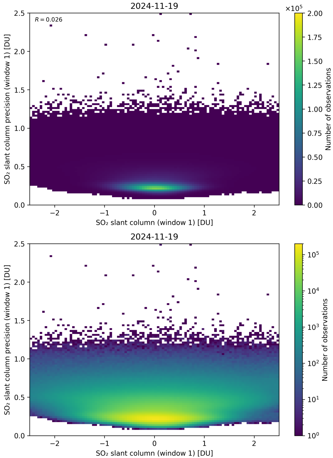
Figure 285: Scatter density plot of “SO 2 slant column (window 1)” against “SO 2 slant column precision (window 1)” for 2024-11-18 to 2024-11-20.
