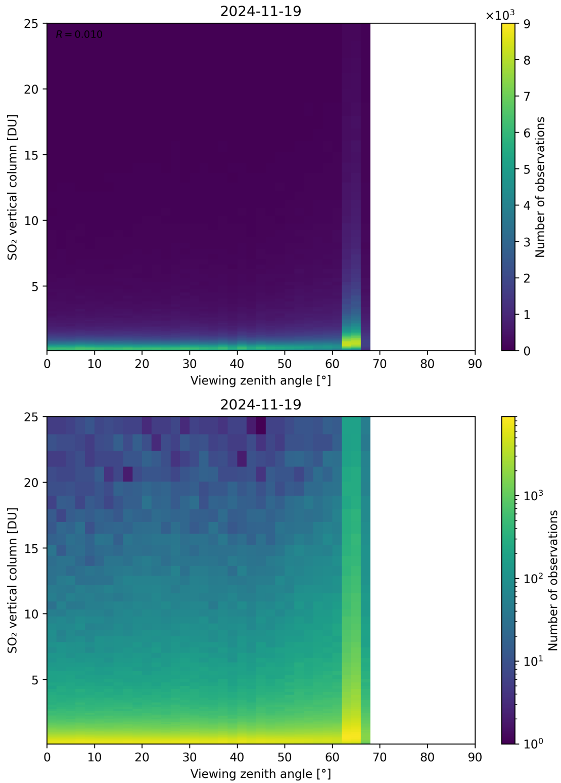
Figure 383: Scatter density plot of “Viewing zenith angle” against “SO 2 vertical column” for 2024-11-18 to 2024-11-20.
