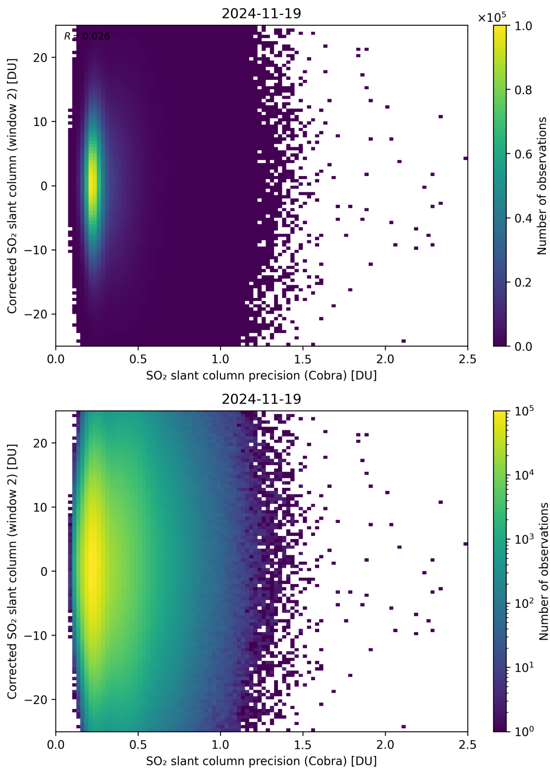
Figure 206: Scatter density plot of “SO 2 slant column precision (Cobra)” against “Corrected SO 2 slant column (window 2)” for 2024-11-18 to 2024-11-20.
