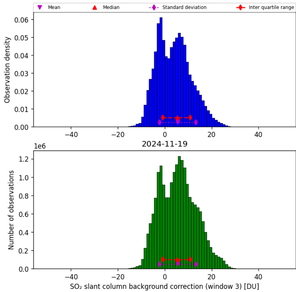
Figure 74: Histogram of "SO 2 slant column background correction (window 3)" for 2024-11-18 to 2024-11-20
