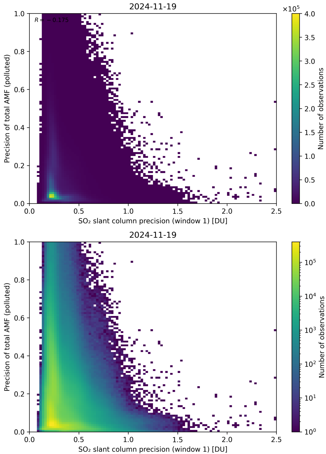
Figure 281: Scatter density plot of “SO 2 slant column precision (window 1)” against “Precision of total AMF (polluted)” for 2024-11-18 to 2024-11-20.
