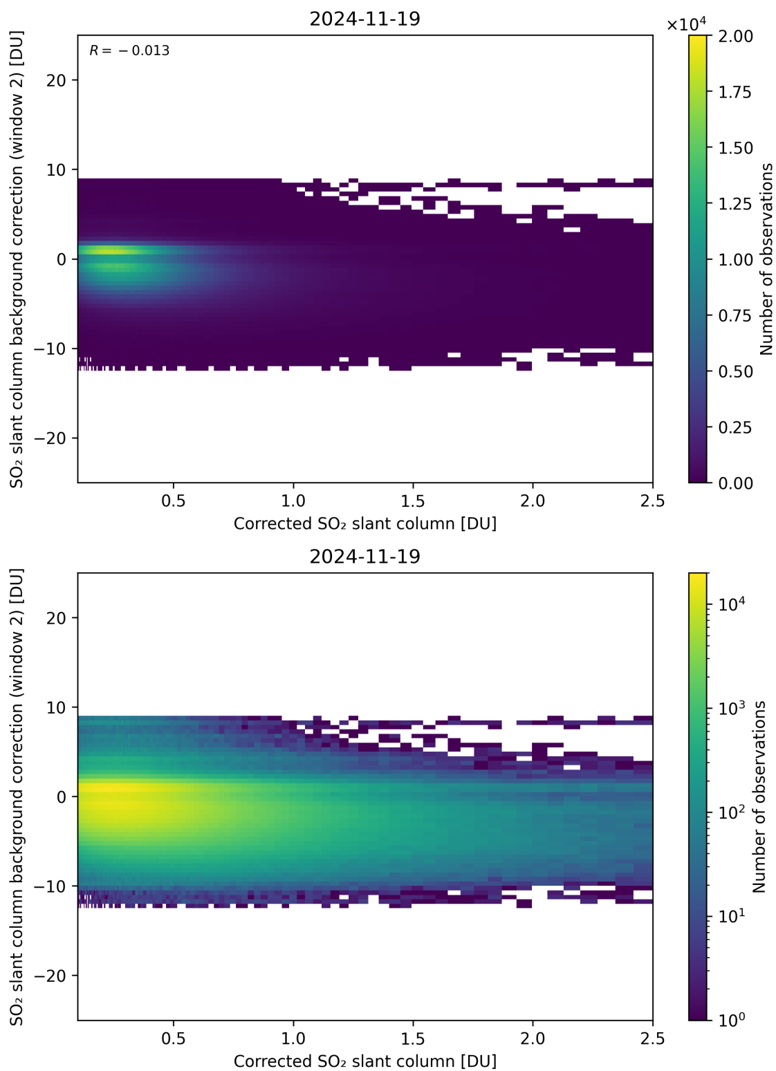
Figure 227: Scatter density plot of “Corrected SO 2 slant column” against “SO 2 slant column background correction (window 2)” for 2024-11-18 to 2024-11-20.
