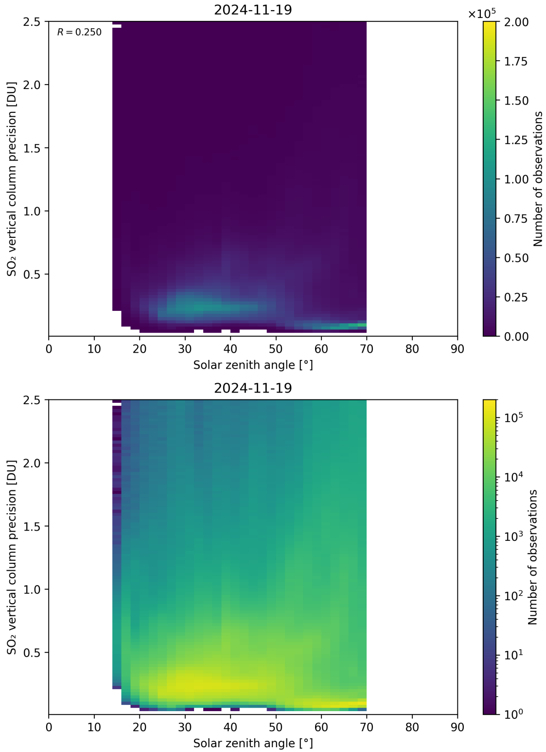
Figure 192: Scatter density plot of “Solar zenith angle” against “SO 2 vertical column precision” for 2024-11-18 to 2024-11-20.
