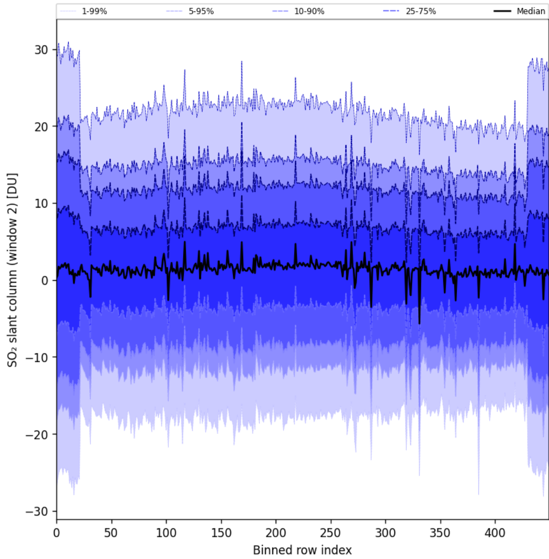
Figure 93: Along track statistics of “SO 2 slant column (window 2)” for 2024-11-18 to 2024-11-20
