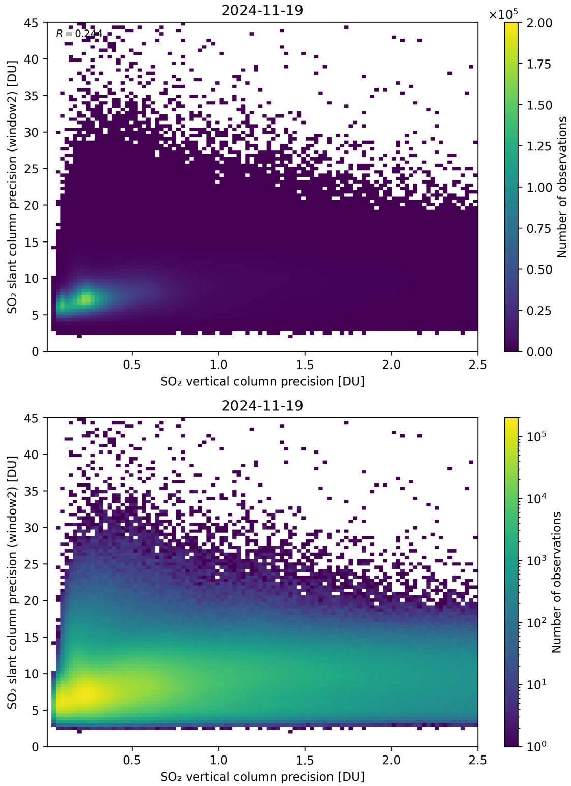
Figure 343: Scatter density plot of “SO 2 vertical column precision” against “SO 2 slant column precision (window2)” for 2024-11-18 to 2024-11-20.
