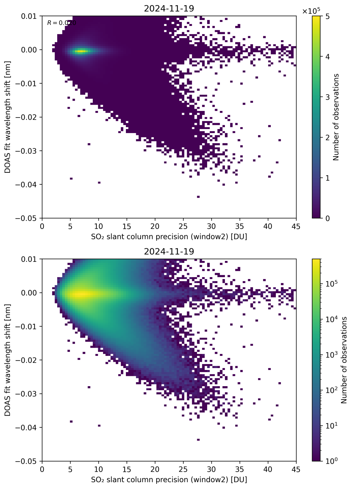
Figure 293: Scatter density plot of “SO 2 slant column precision (window2)” against “DOAS fit wavelength shift” for 2024-11-18 to 2024-11-20.
