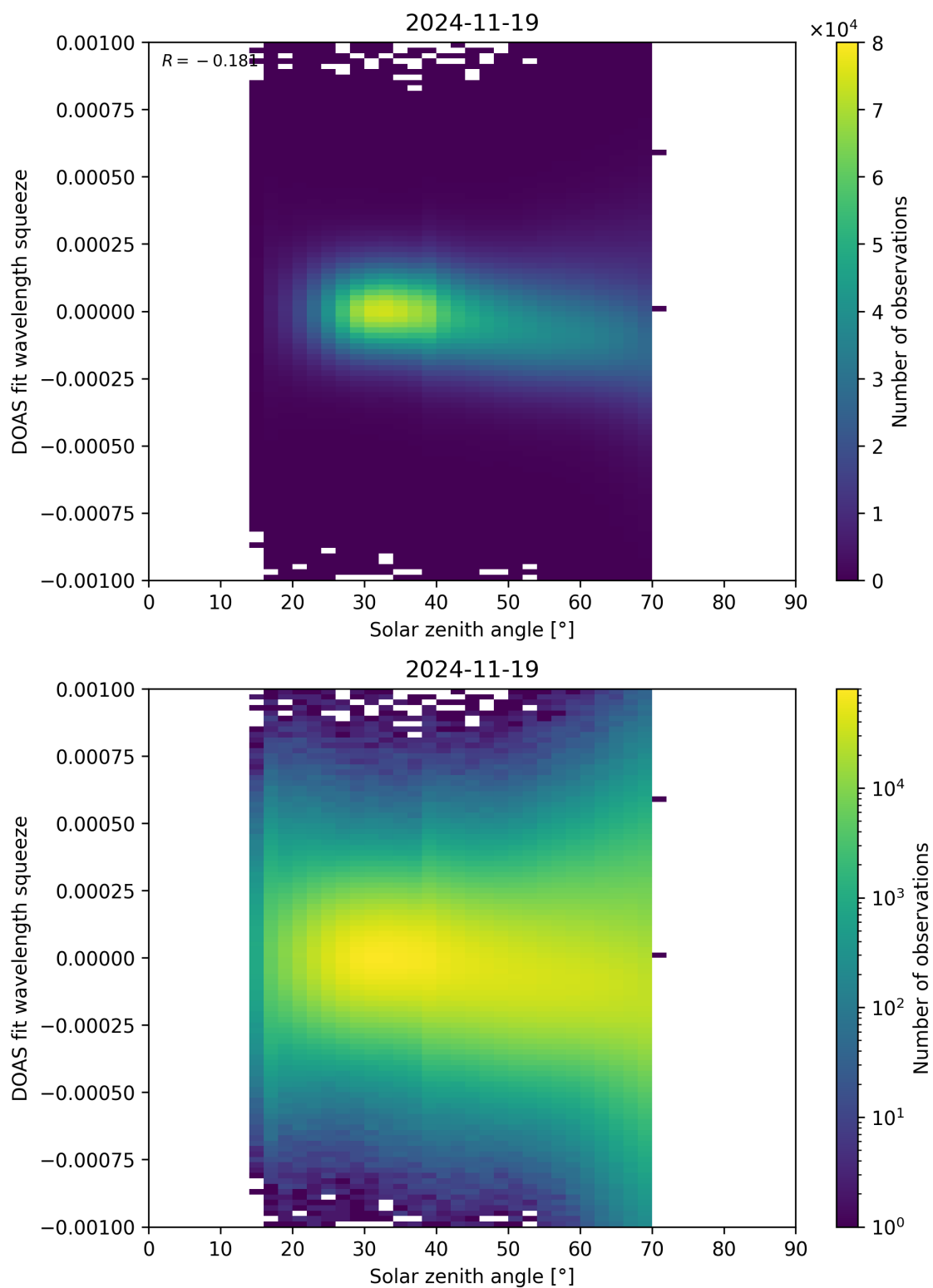
Figure 175: Scatter density plot of “Solar zenith angle” against “DOAS fit wavelength squeeze” for 2024-11-18 to 2024-11-20.
