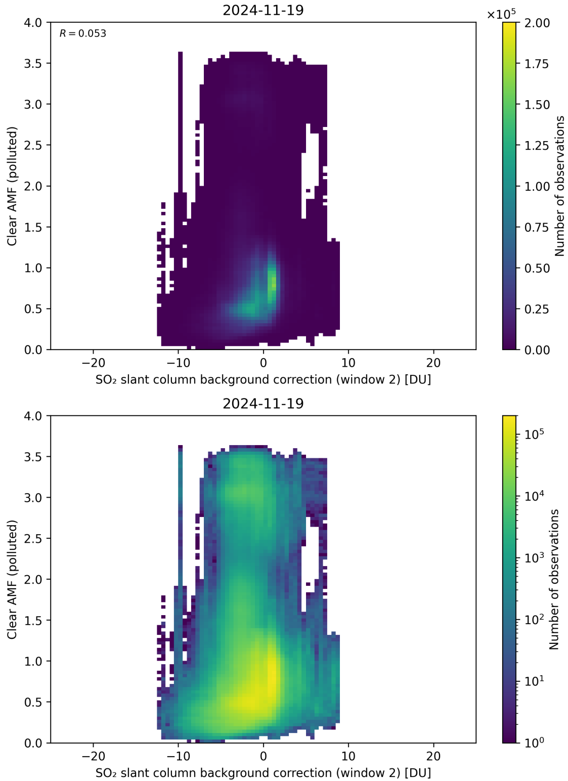
Figure 126: Scatter density plot of “SO 2 slant column background correction (window 2)” against “Clear AMF (polluted)” for 2024-11-18 to 2024-11-20.
