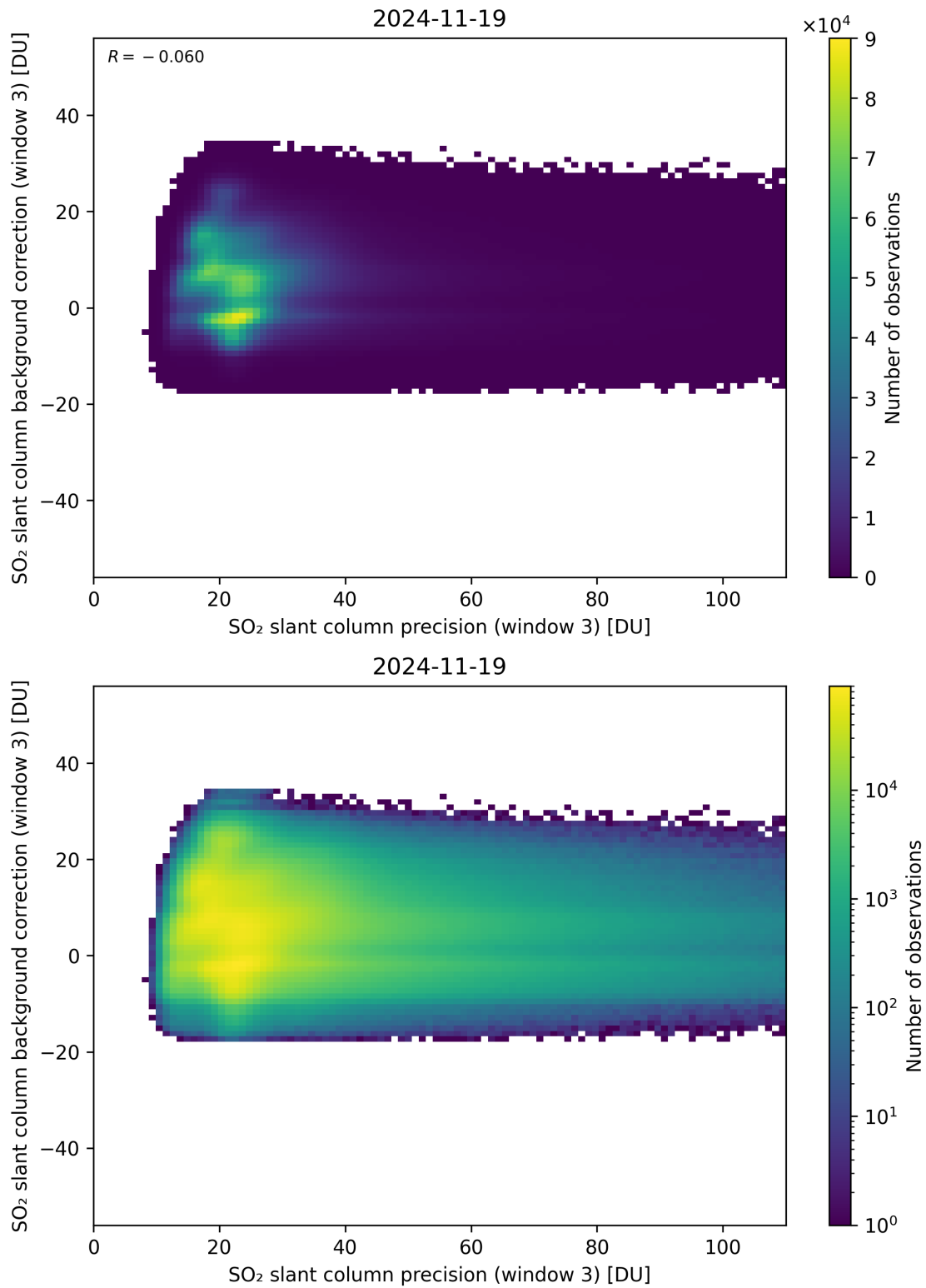
Figure 307: Scatter density plot of “SO 2 slant column precision (window 3)” against “SO 2 slant column background correction (window 3)” for 2024-11-18 to 2024-11-20.
