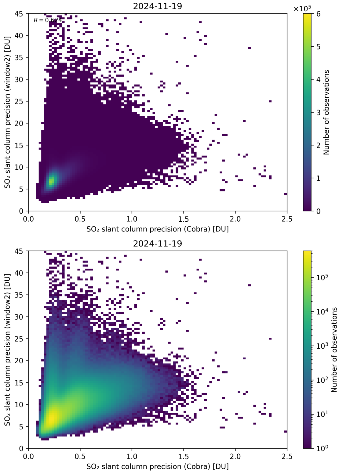
Figure 210: Scatter density plot of “SO 2 slant column precision (Cobra)” against “SO 2 slant column precision (window2)” for 2024-11-18 to 2024-11-20.
