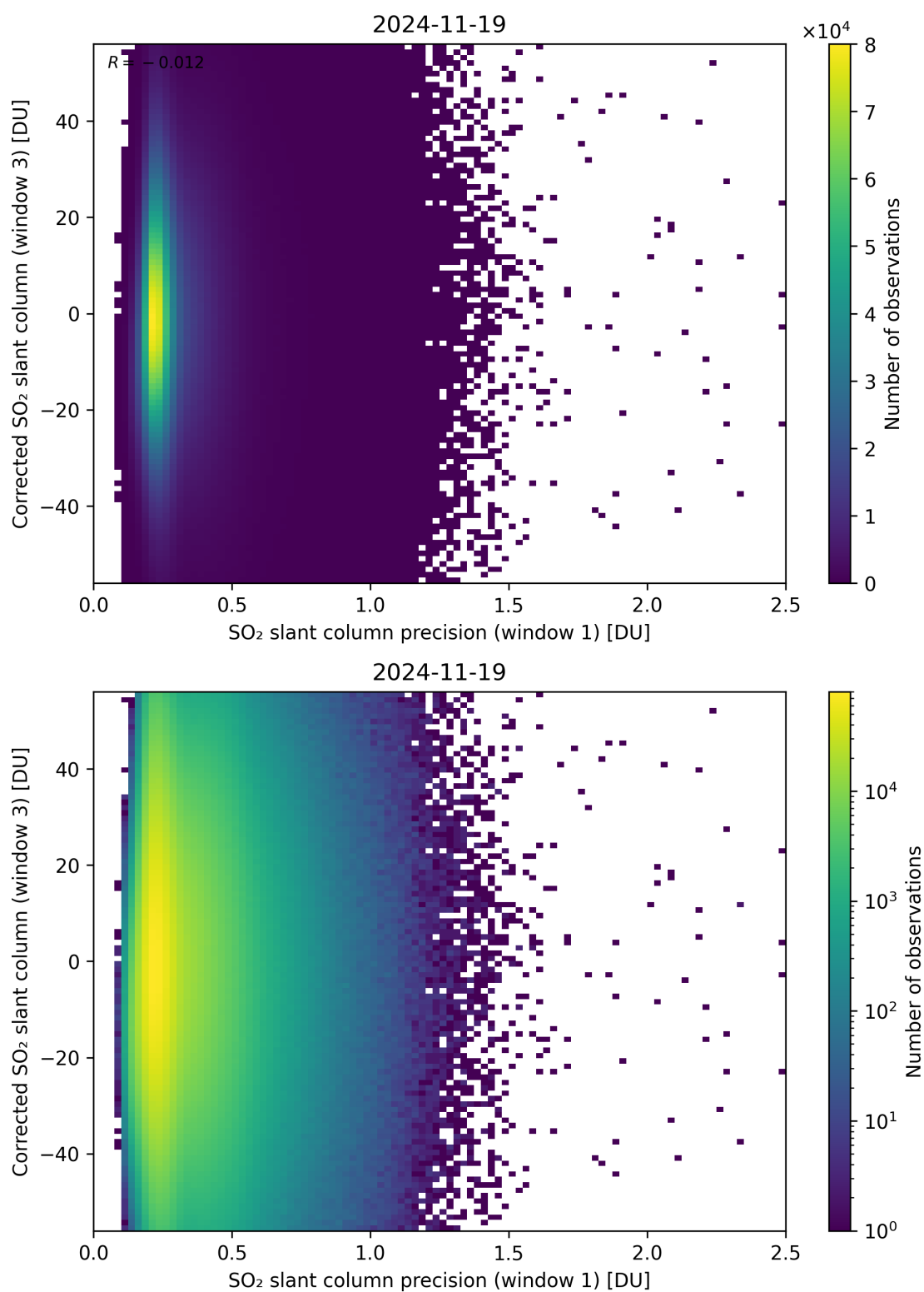
Figure 276: Scatter density plot of “SO 2 slant column precision (window 1)” against “Corrected SO 2 slant column (window 3)” for 2024-11-18 to 2024-11-20.
