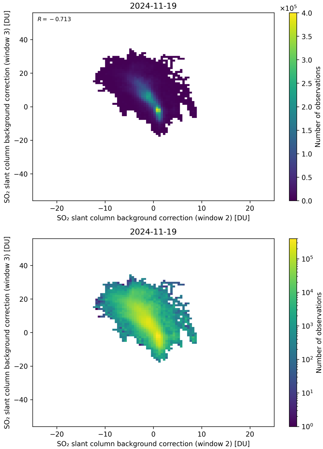
Figure 122: Scatter density plot of “SO 2 slant column background correction (window 2)” against “SO 2 slant column background correction (window 3)” for 2024-11-18 to 2024-11-20.
