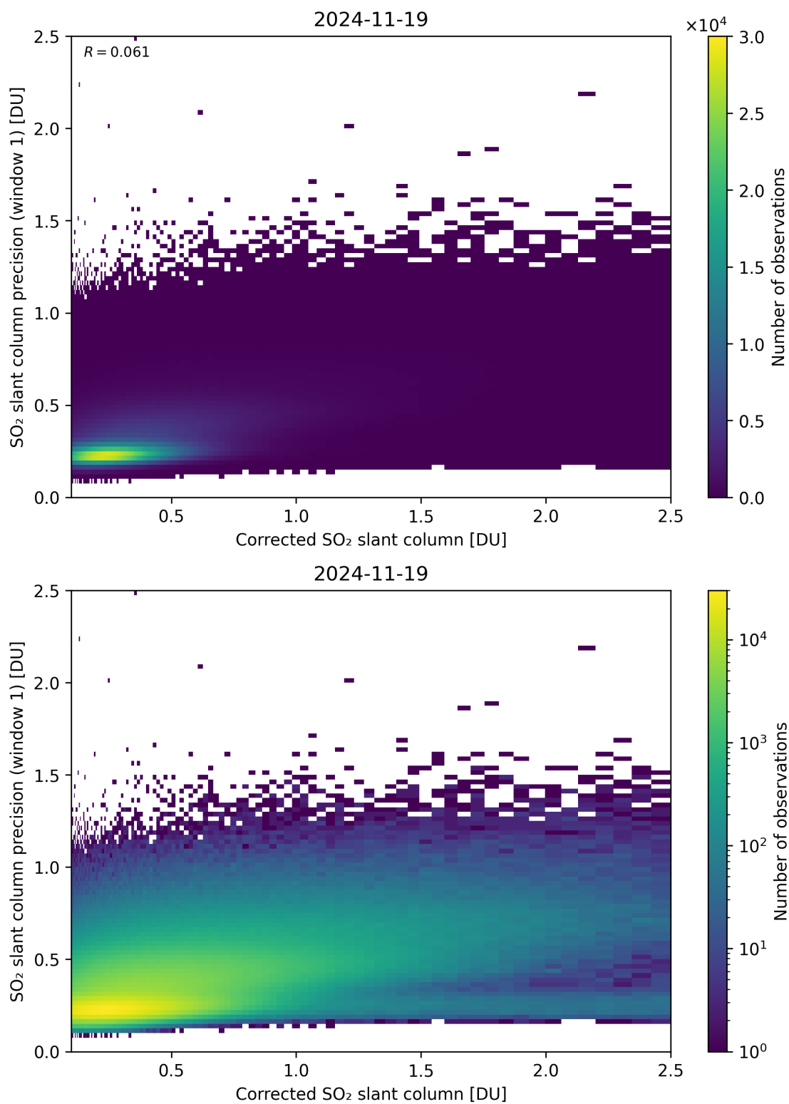
Figure 238: Scatter density plot of “Corrected SO 2 slant column” against “SO 2 slant column precision (window 1)” for 2024-11-18 to 2024-11-20.
