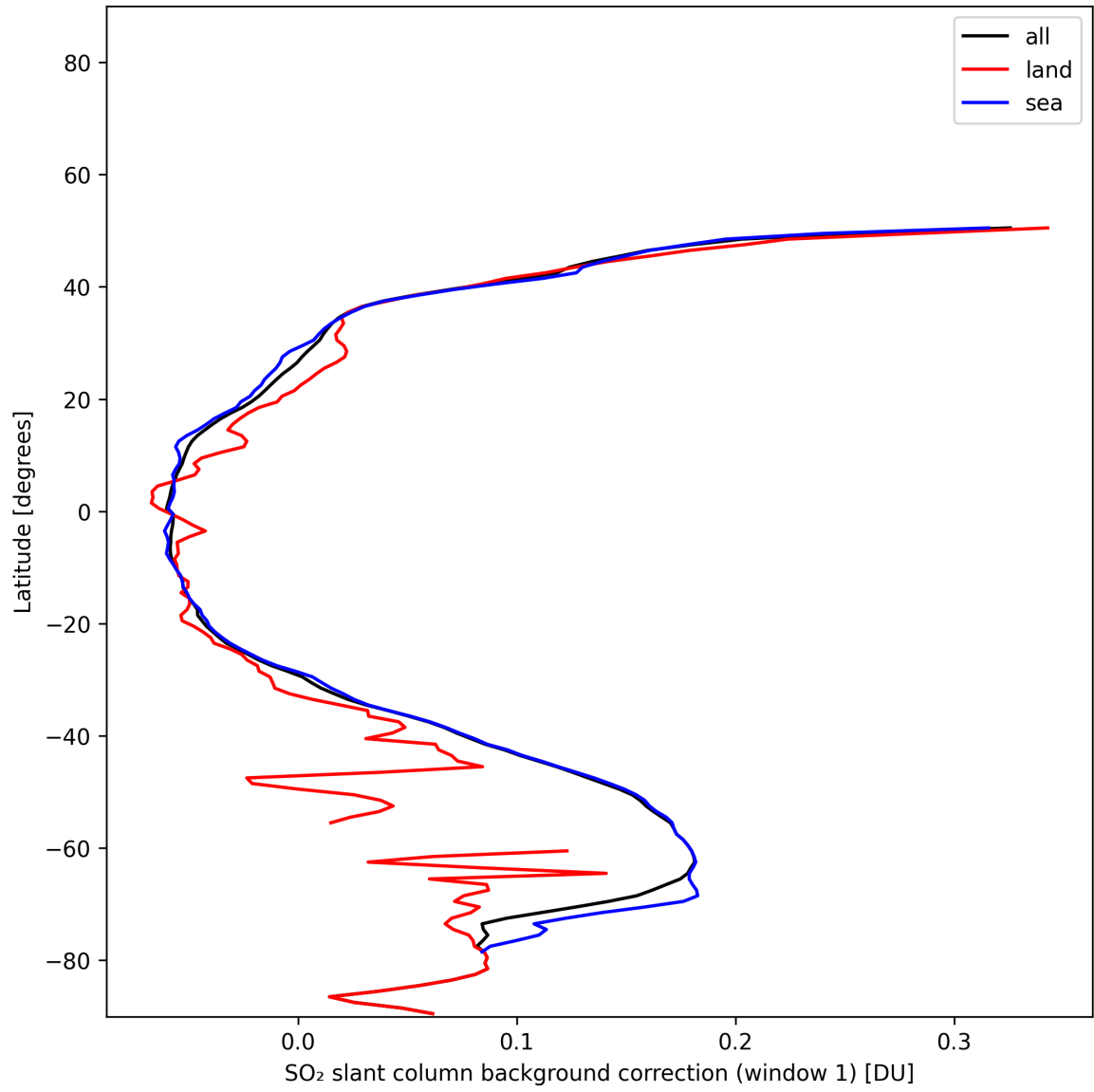
Figure 40: Zonal average of “SO 2 slant column background correction (window 1)” for 2024-11-18 to 2024-11-20.
