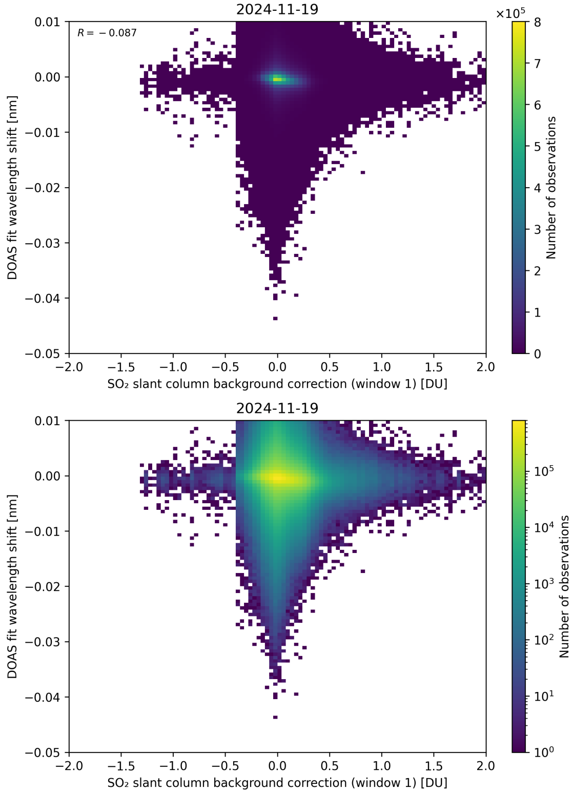
Figure 111: Scatter density plot of “SO 2 slant column background correction (window 1)” against “DOAS fit wavelength shift” for 2024-11-18 to 2024-11-20.
