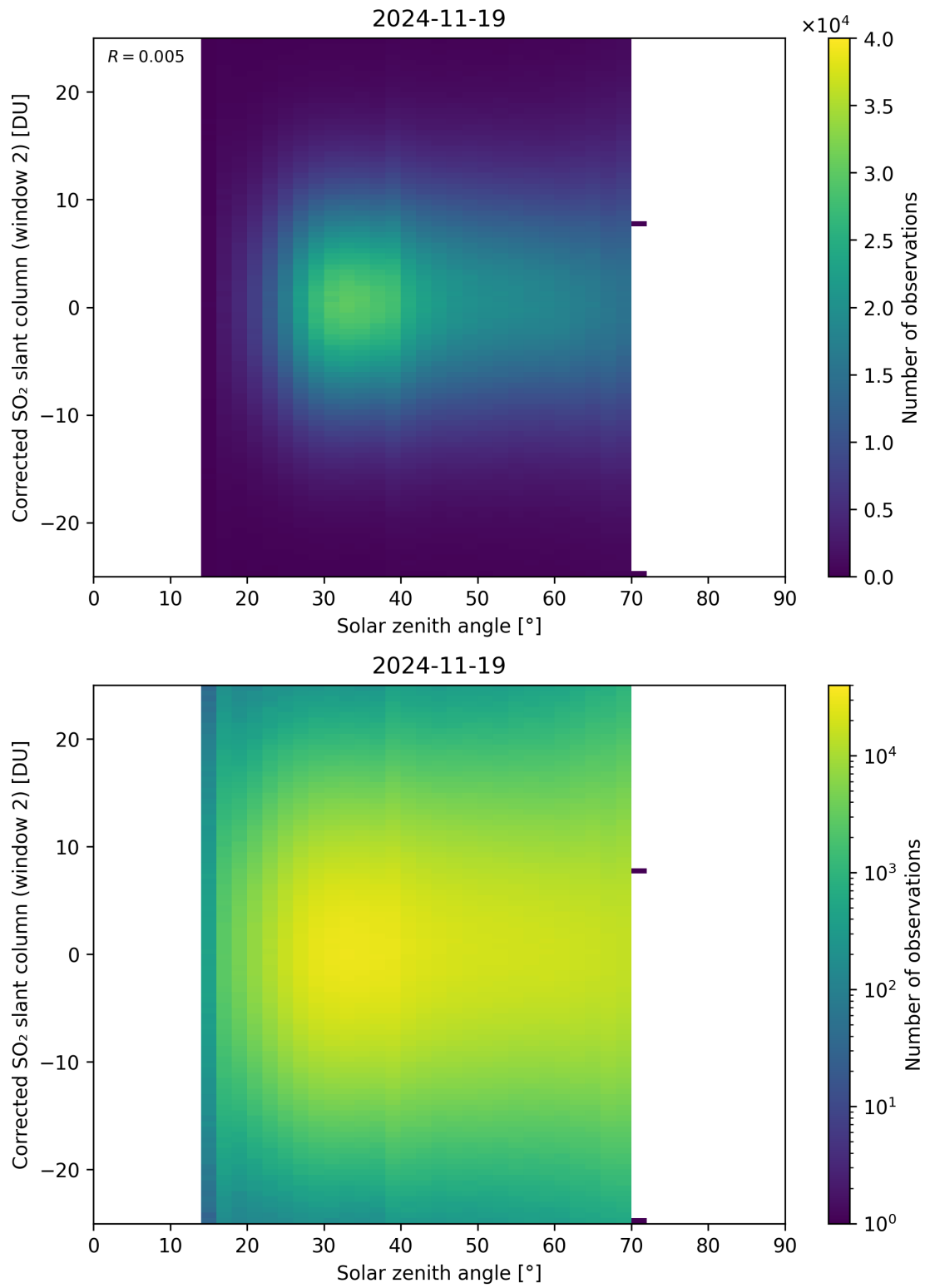
Figure 182: Scatter density plot of “Solar zenith angle” against “Corrected SO 2 slant column (window 2)” for 2024-11-18 to 2024-11-20.
