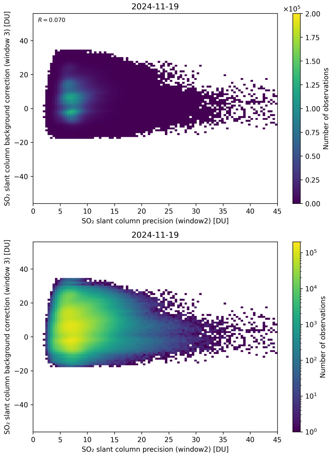
Figure 292: Scatter density plot of “SO 2 slant column precision (window2)” against “SO 2 slant column background correction (window 3)” for 2024-11-18 to 2024-11-20.
