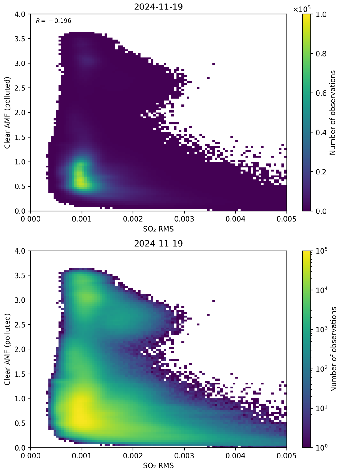
Figure 147: Scatter density plot of “SO 2 RMS” against “Clear AMF (polluted)” for 2024-11-18 to 2024-11-20.
