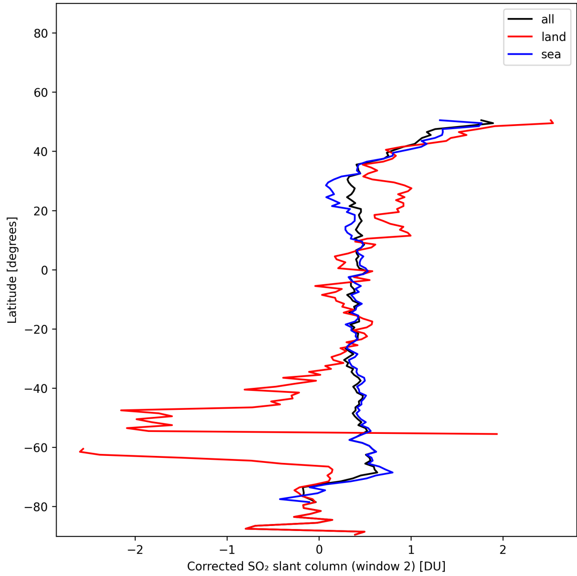
Figure 43: Zonal average of “Corrected SO 2 slant column (window 2)” for 2024-11-18 to 2024-11-20.
