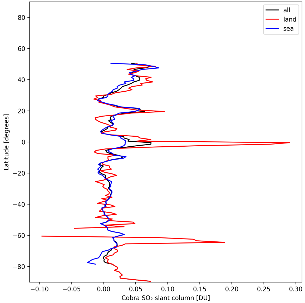
Figure 35: Zonal average of “Cobra SO 2 slant column” for 2024-11-18 to 2024-11-20.
