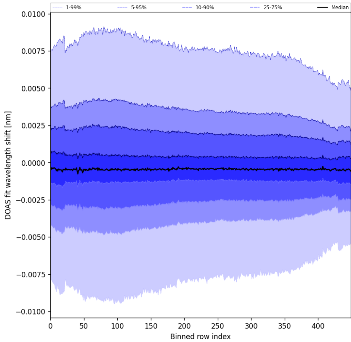
Figure 102: Along track statistics of “DOAS fit wavelength shift” for 2024-11-18 to 2024-11-20
