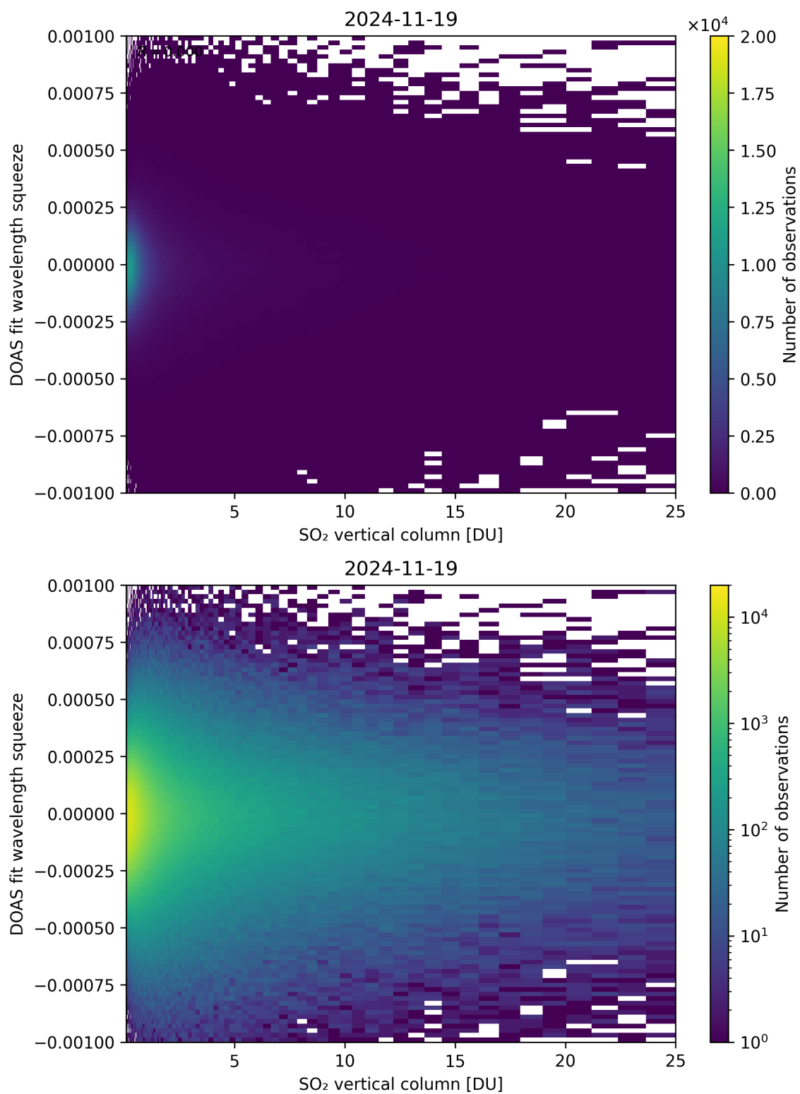
Figure 327: Scatter density plot of “SO 2 vertical column” against “DOAS fit wavelength squeeze” for 2024-11-18 to 2024-11-20.
