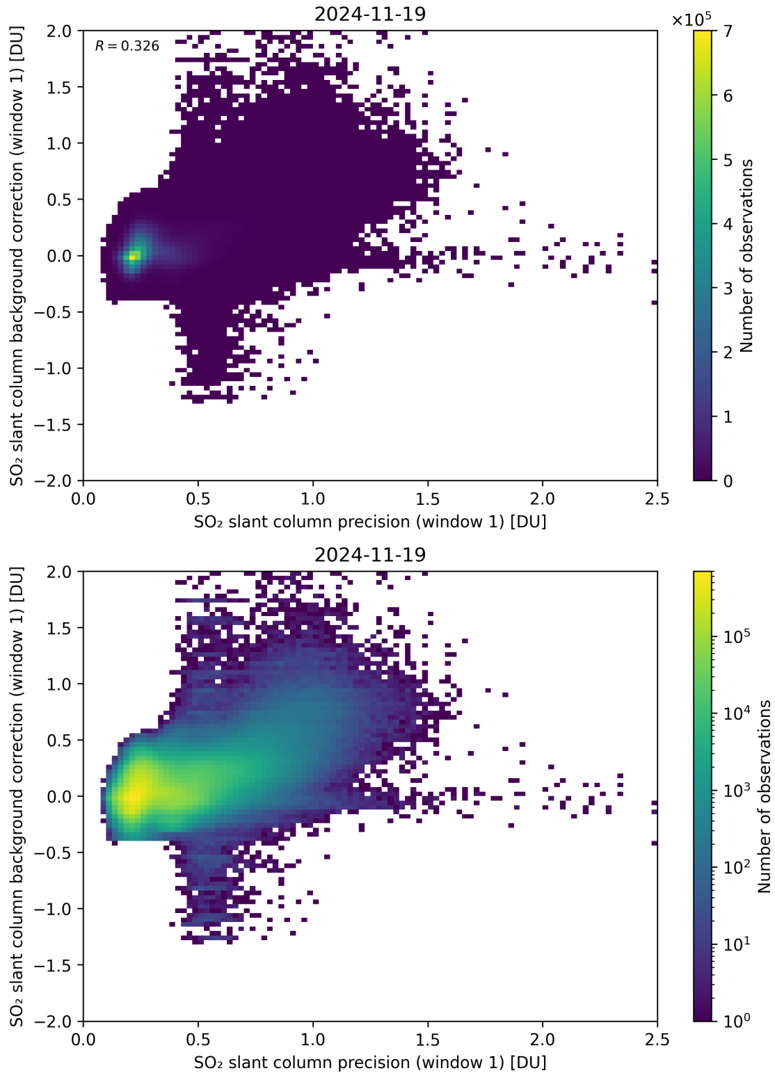
Figure 268: Scatter density plot of “SO 2 slant column precision (window 1)” against “SO 2 slant column background correction (window 1)” for 2024-11-18 to 2024-11-20.
