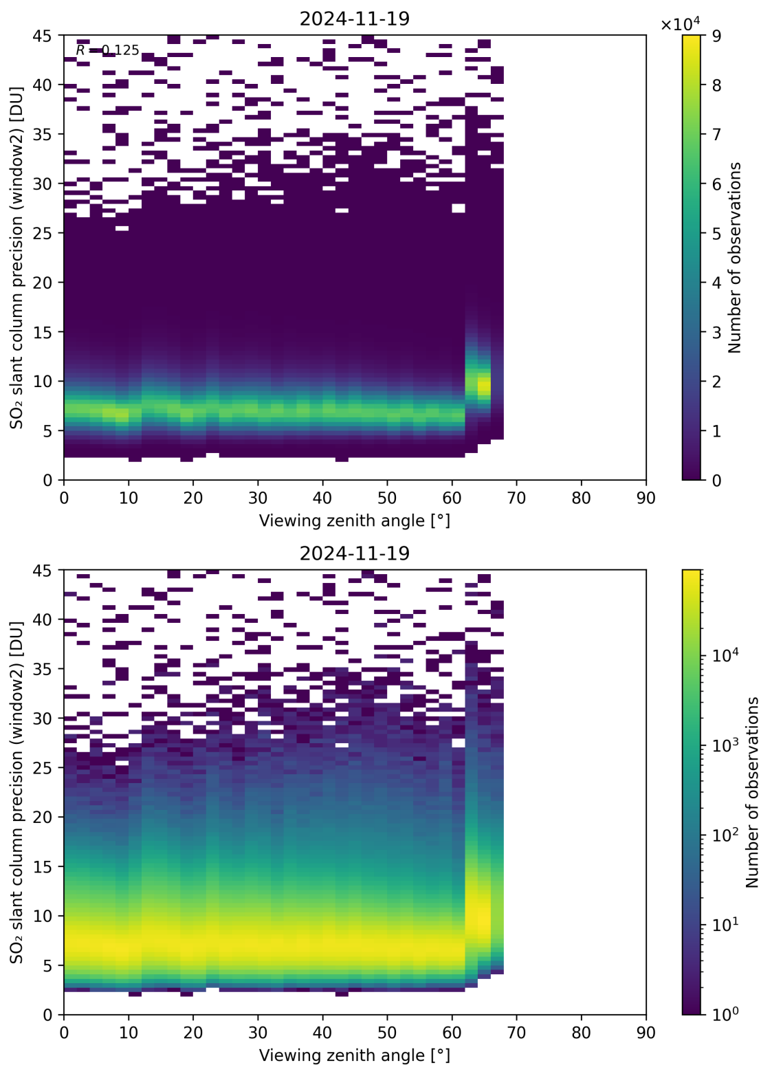
Figure 378: Scatter density plot of “Viewing zenith angle” against “SO 2 slant column precision (window2)” for 2024-11-18 to 2024-11-20.
