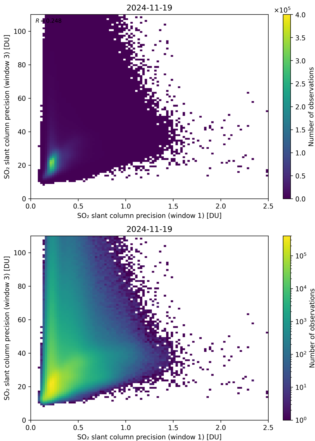
Figure 279: Scatter density plot of “SO 2 slant column precision (window 1)” against “SO 2 slant column precision (window 3)” for 2024-11-18 to 2024-11-20.
