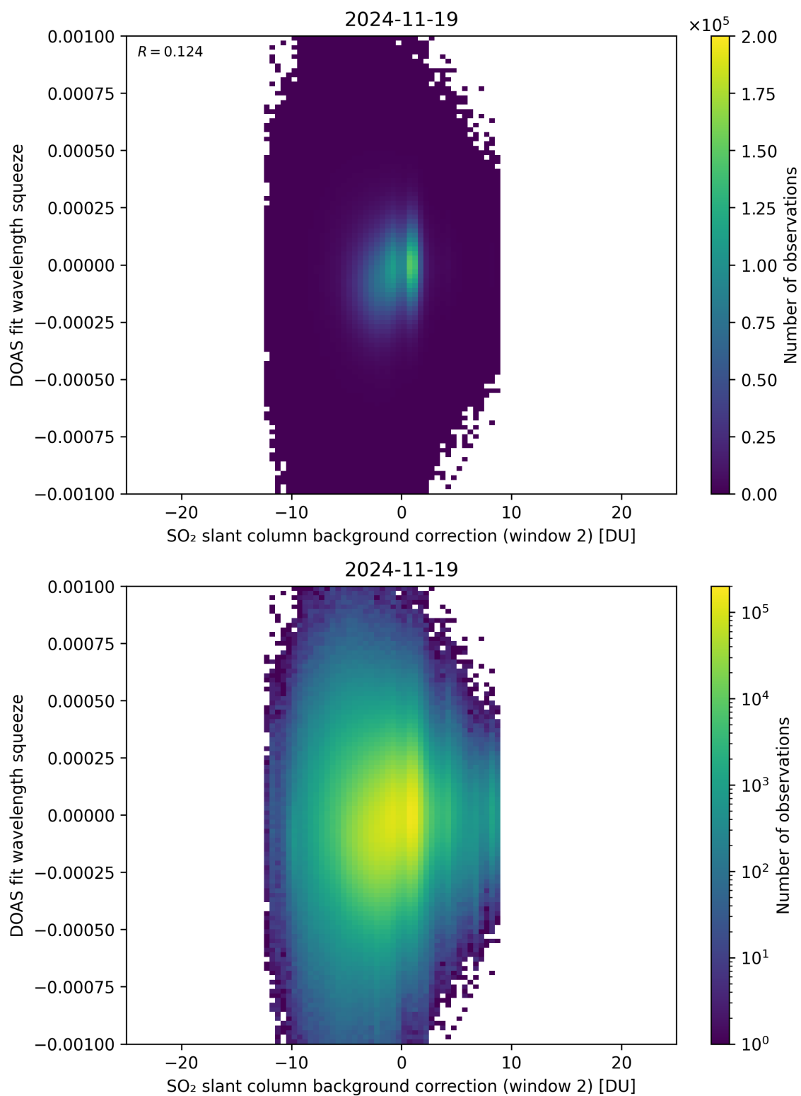
Figure 124: Scatter density plot of “SO 2 slant column background correction (window 2)” against “DOAS fit wavelength squeeze” for 2024-11-18 to 2024-11-20.
