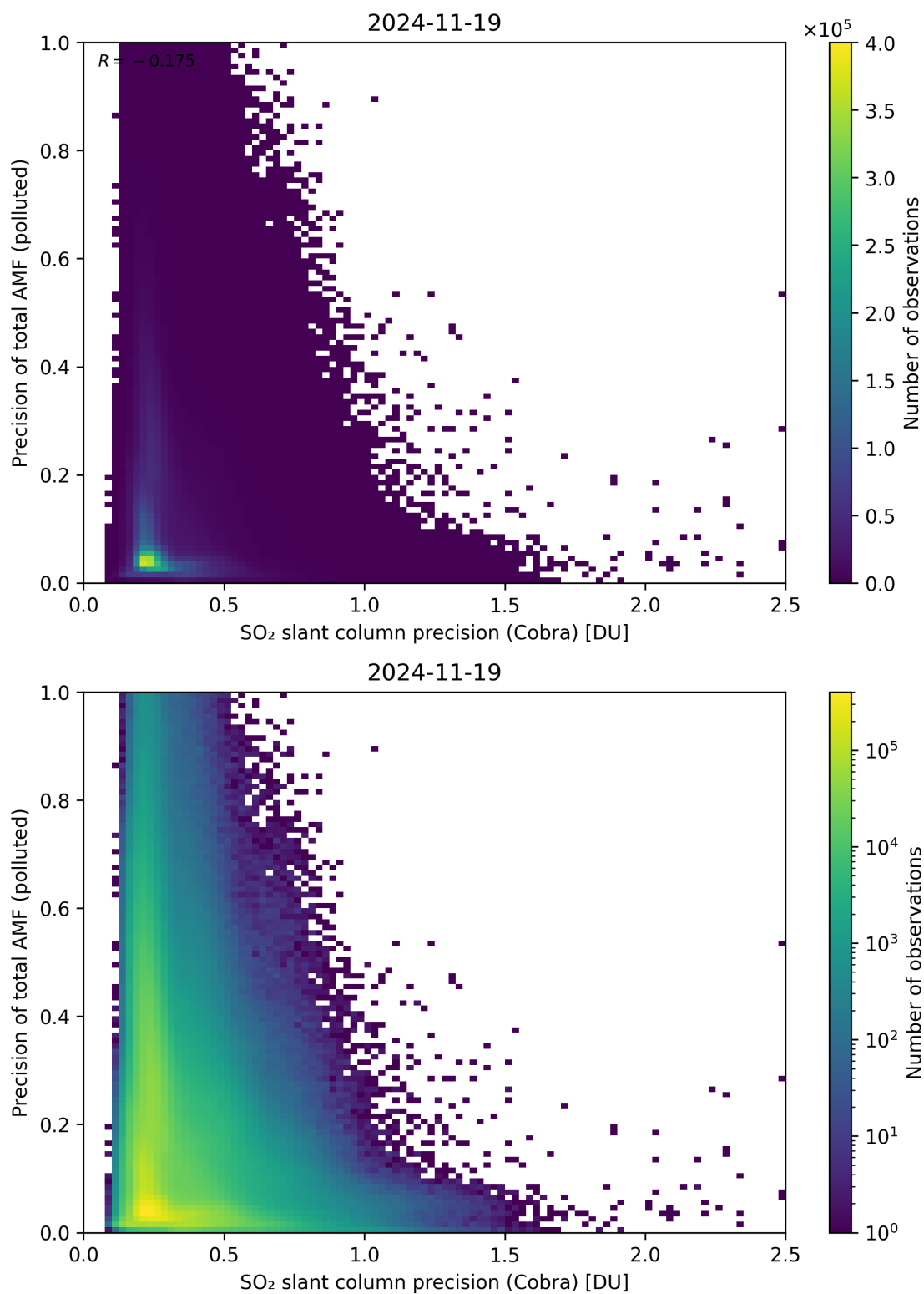
Figure 214: Scatter density plot of “SO 2 slant column precision (Cobra)” against “Precision of total AMF (polluted)” for 2024-11-18 to 2024-11-20.
