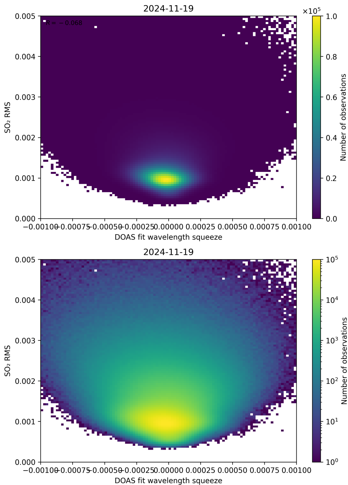
Figure 143: Scatter density plot of “DOAS fit wavelength squeeze” against “SO 2 RMS” for 2024-11-18 to 2024-11-20.
