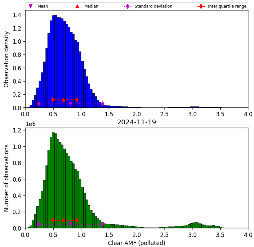
Figure 81: Histogram of “Clear AMF (polluted)” for 2024-11-18 to 2024-11-20
