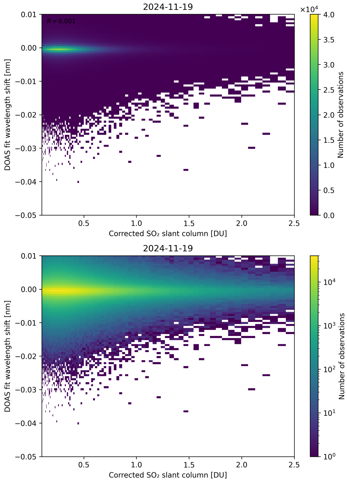
Figure 229: Scatter density plot of “Corrected SO 2 slant column” against “DOAS fit wavelength shift” for 2024-11-18 to 2024-11-20.
