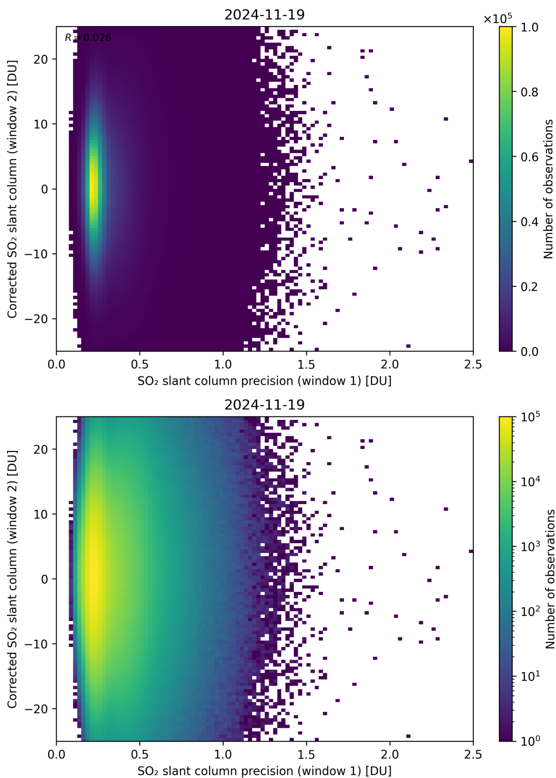
Figure 275: Scatter density plot of “SO 2 slant column precision (window 1)” against “Corrected SO 2 slant column (window 2)” for 2024-11-18 to 2024-11-20.
