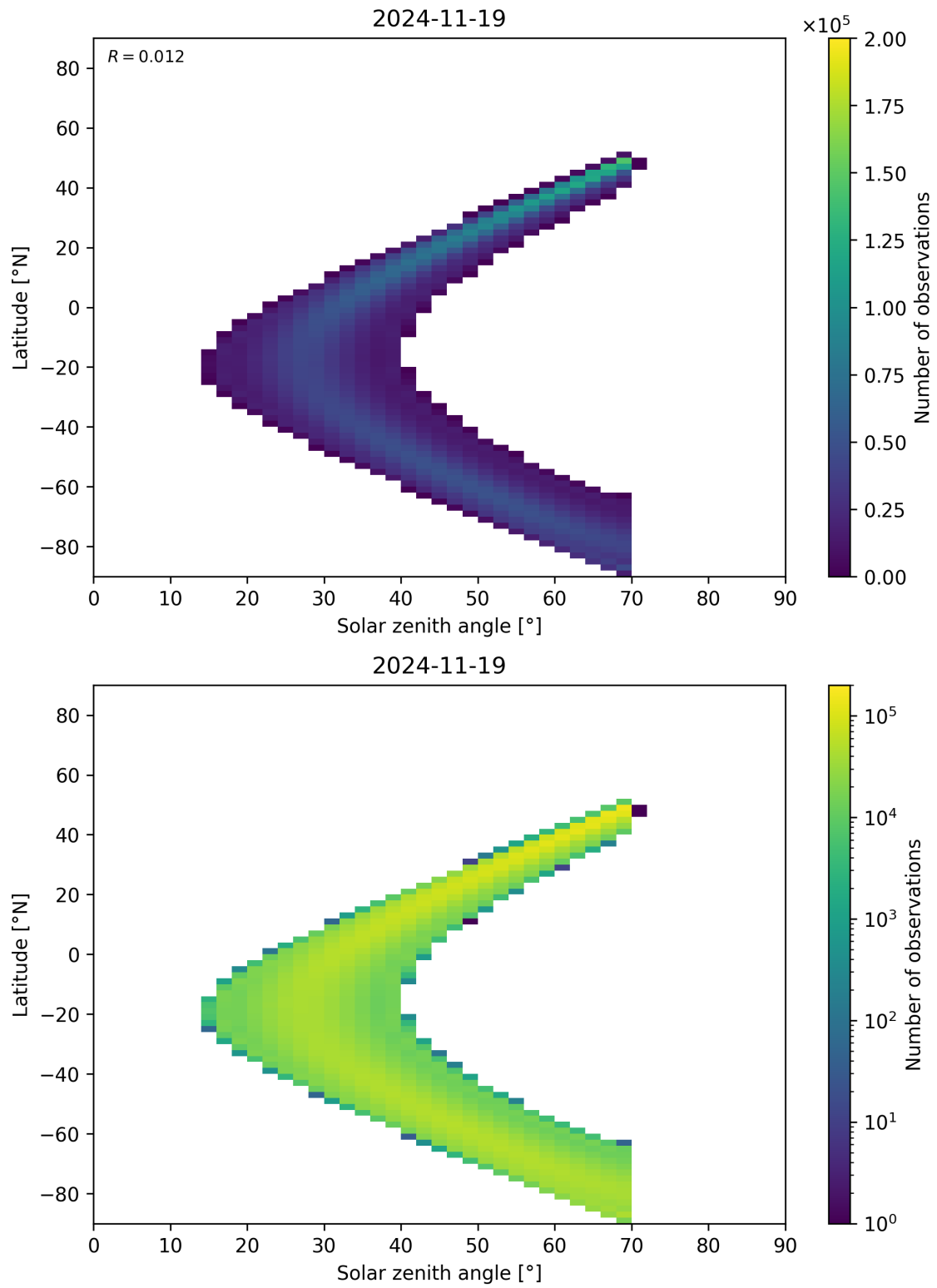
Figure 177: Scatter density plot of “Solar zenith angle” against “Latitude” for 2024-11-18 to 2024-11-20.
