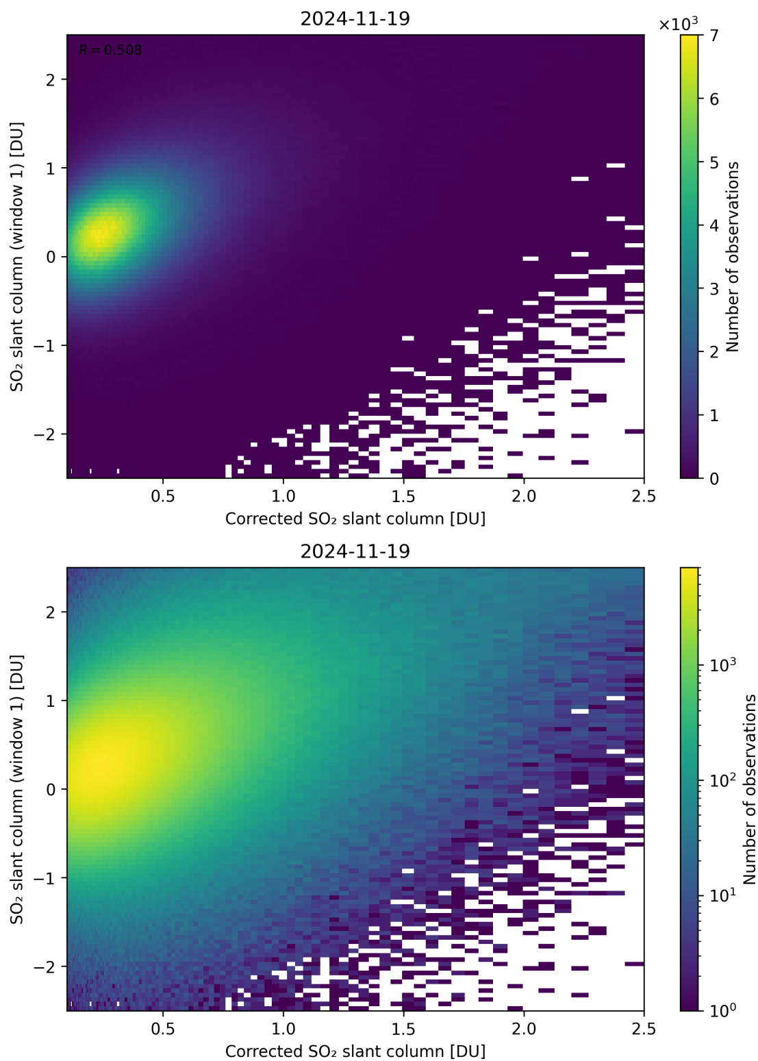
Figure 237: Scatter density plot of “Corrected SO 2 slant column” against “SO 2 slant column (window 1)” for 2024-11-18 to 2024-11-20.
