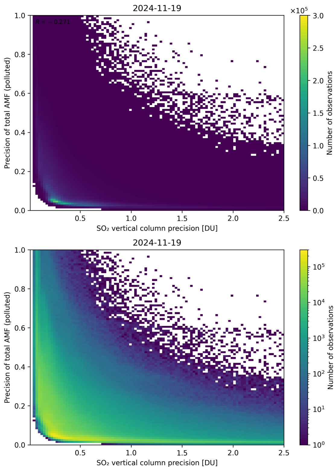
Figure 347: Scatter density plot of “SO 2 vertical column precision” against “Precision of total AMF (polluted)” for 2024-11-18 to 2024-11-20.
