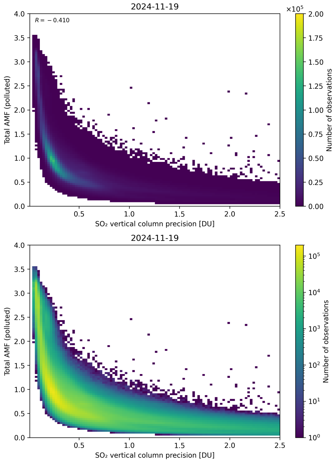
Figure 346: Scatter density plot of “SO 2 vertical column precision” against “Total AMF (polluted)” for 2024-11-18 to 2024-11-20.
