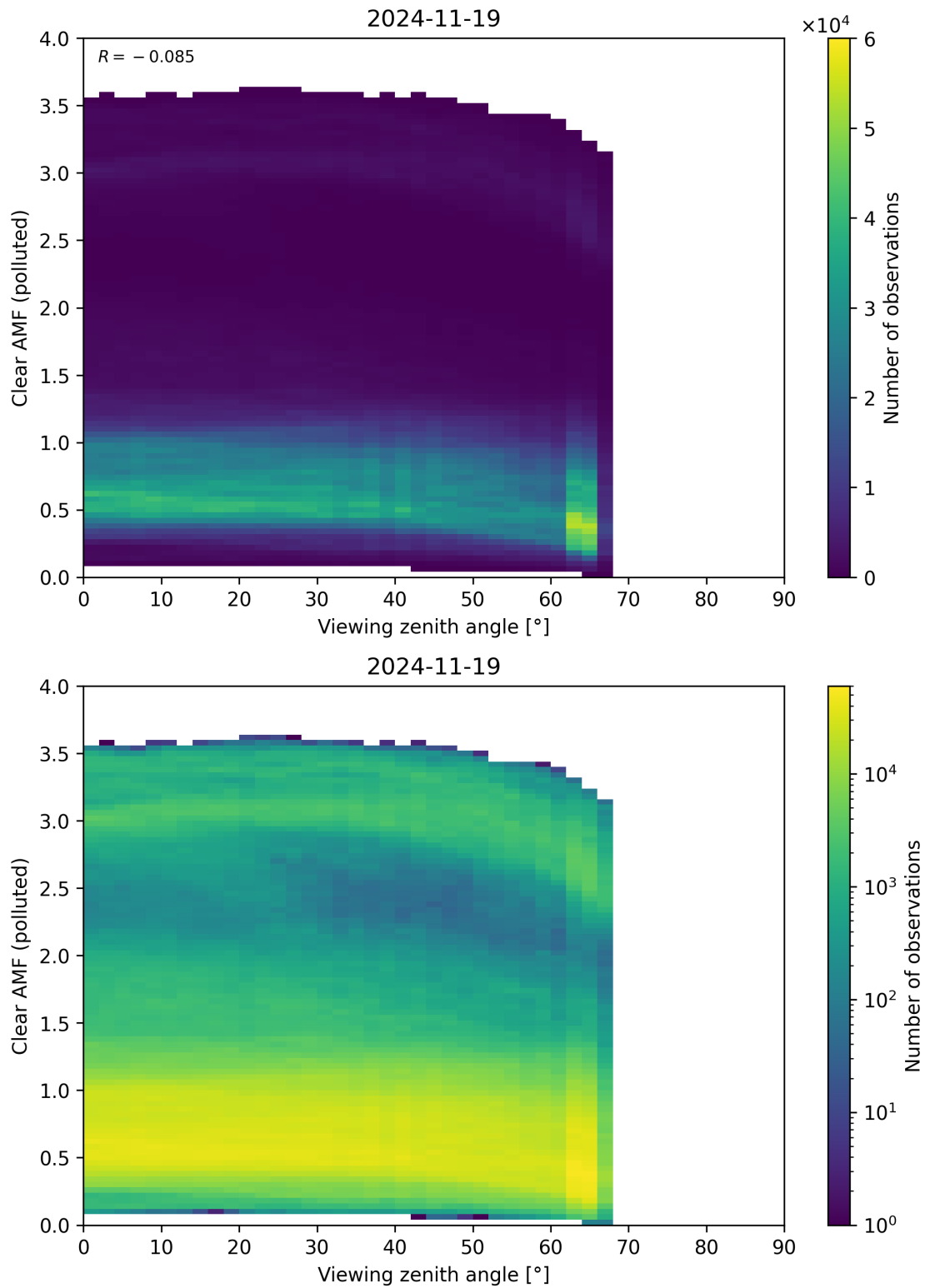
Figure 370: Scatter density plot of “Viewing zenith angle” against “Clear AMF (polluted)” for 2024-11-18 to 2024-11-20.
