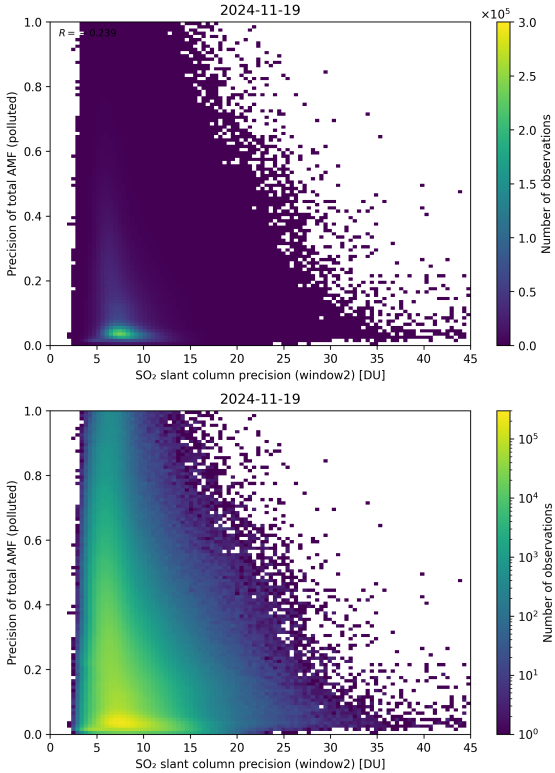
Figure 302: Scatter density plot of “SO 2 slant column precision (window2)” against “Precision of total AMF (polluted)” for 2024-11-18 to 2024-11-20.
