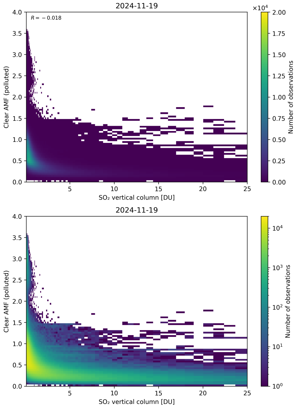
Figure 348: Scatter density plot of “SO 2 vertical column” against “Clear AMF (polluted)” for 2024-11-18 to 2024-11-20.
