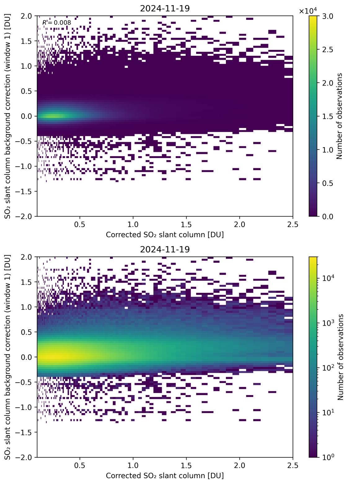
Figure 226: Scatter density plot of “Corrected SO 2 slant column” against “SO 2 slant column background correction (window 1)” for 2024-11-18 to 2024-11-20.
