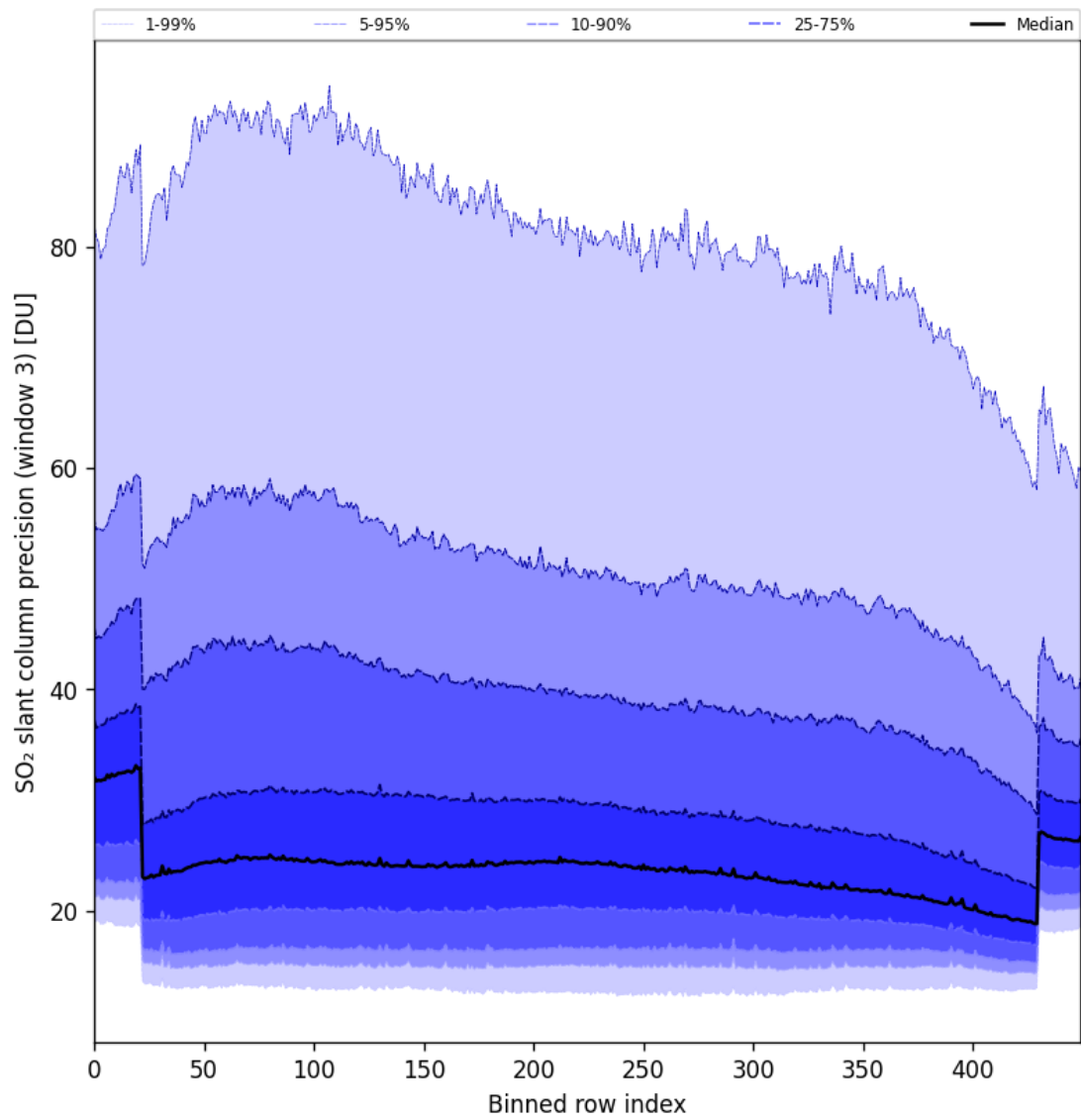
Figure 98: Along track statistics of “SO 2 slant column precision (window 3)” for 2024-11-18 to 2024-11-20
