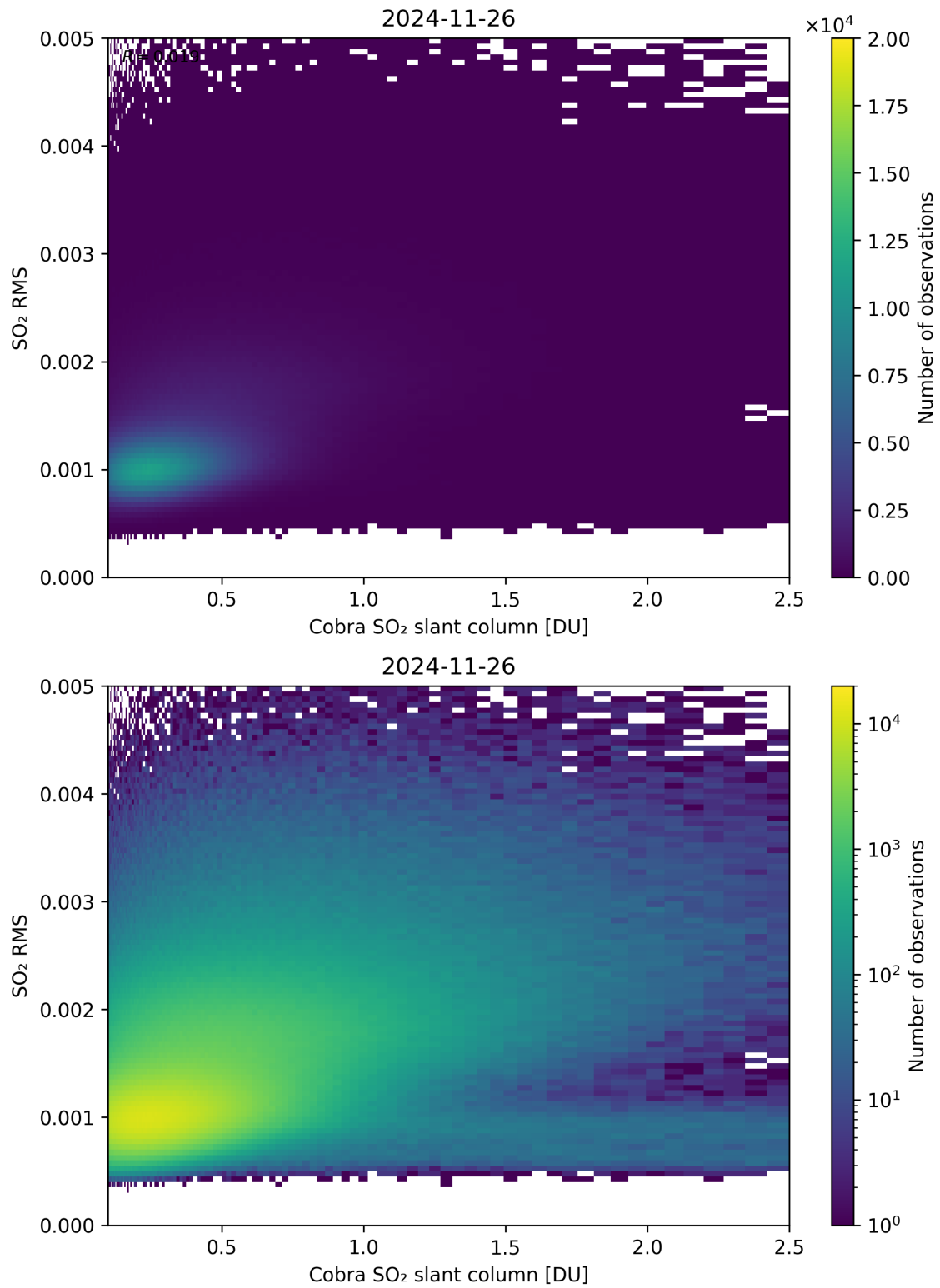
Figure 198: Scatter density plot of “Cobra SO 2 slant column” against “SO 2 RMS” for 2024-11-25 to 2024-11-27.
