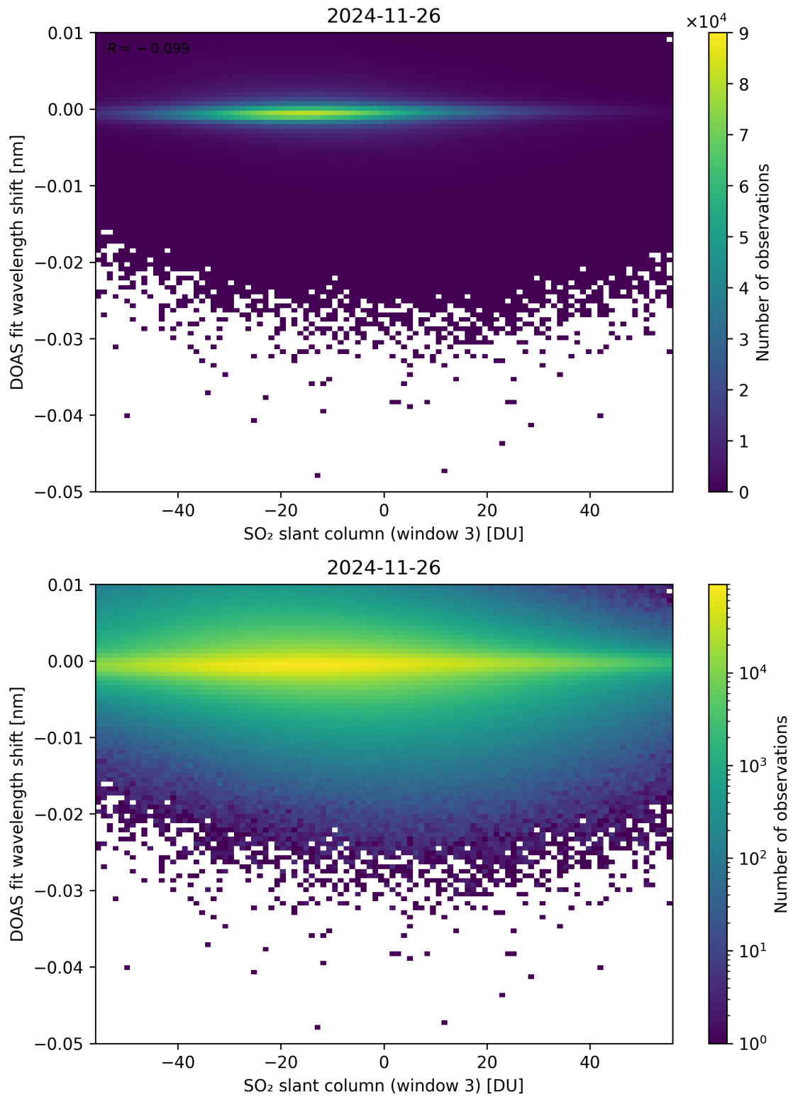
Figure 304: Scatter density plot of “SO 2 slant column (window 3)” against “DOAS fit wavelength shift” for 2024-11-25 to 2024-11-27.
