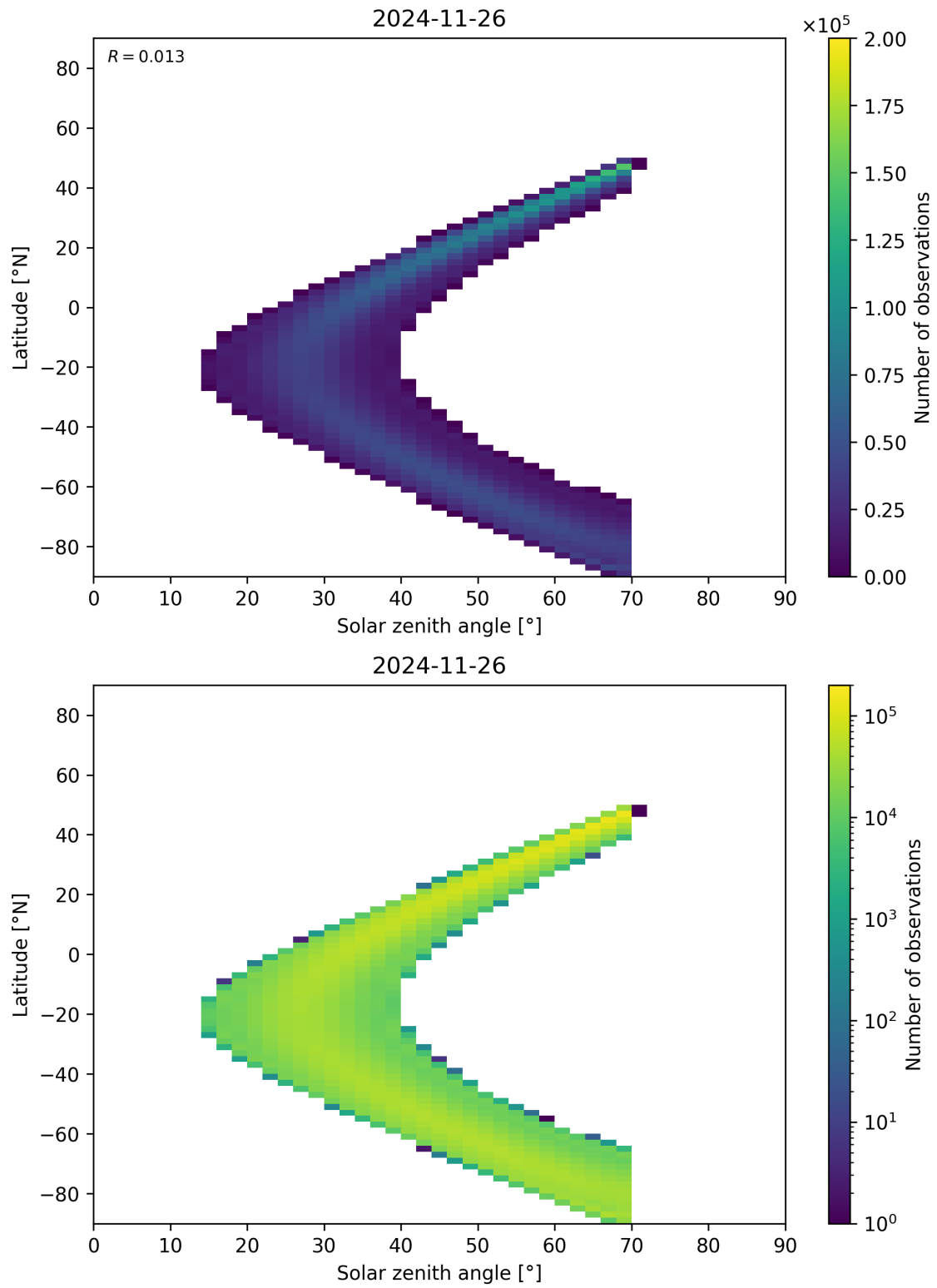
Figure 177: Scatter density plot of “Solar zenith angle” against “Latitude” for 2024-11-25 to 2024-11-27.
