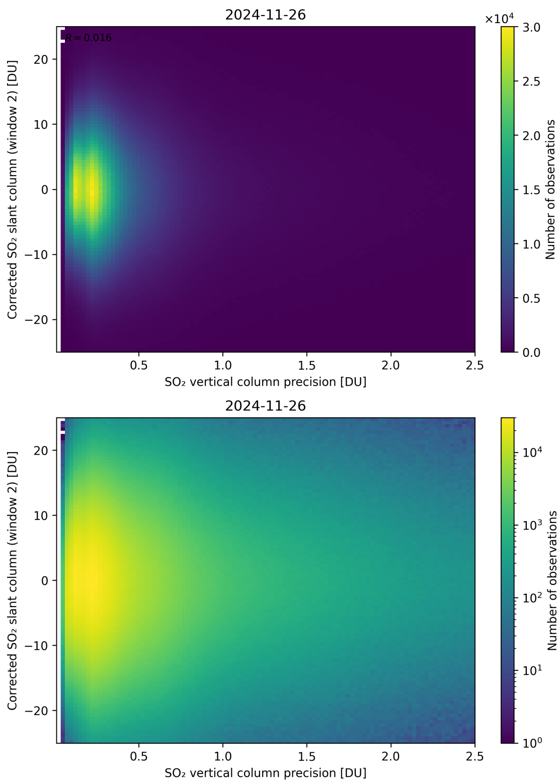
Figure 339: Scatter density plot of “SO 2 vertical column precision” against “Corrected SO 2 slant column (window 2)” for 2024-11-25 to 2024-11-27.
