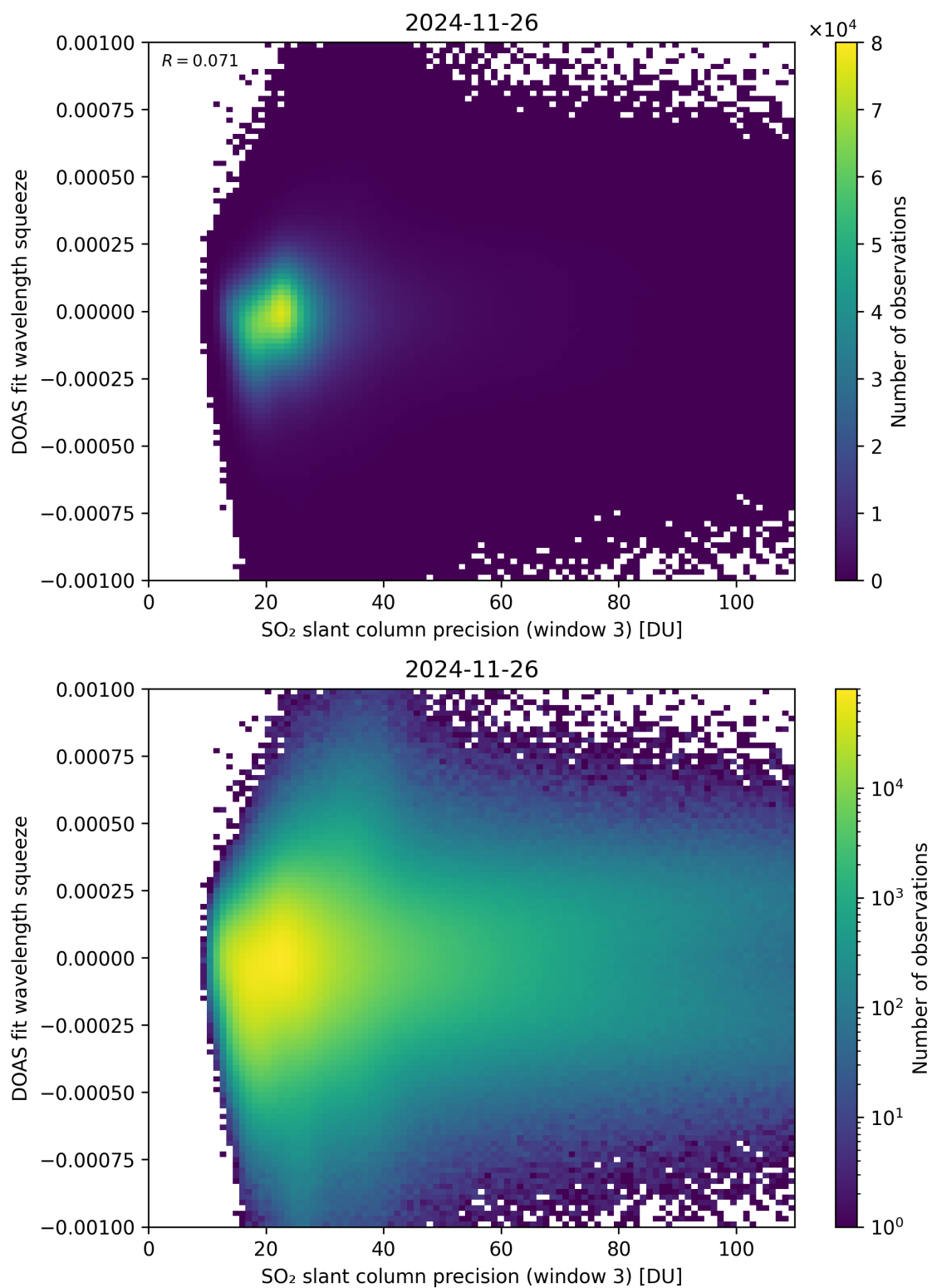
Figure 309: Scatter density plot of “SO 2 slant column precision (window 3)” against “DOAS fit wavelength squeeze” for 2024-11-25 to 2024-11-27.
