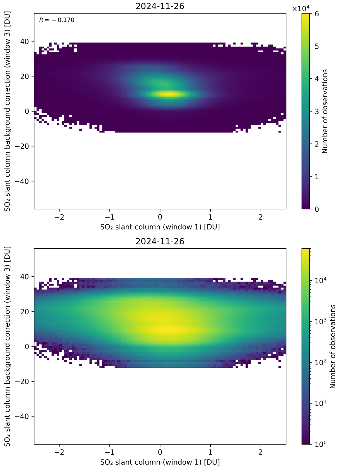
Figure 264: Scatter density plot of “SO 2 slant column (window 1)” against “SO 2 slant column background correction (window 3)” for 2024-11-25 to 2024-11-27.
