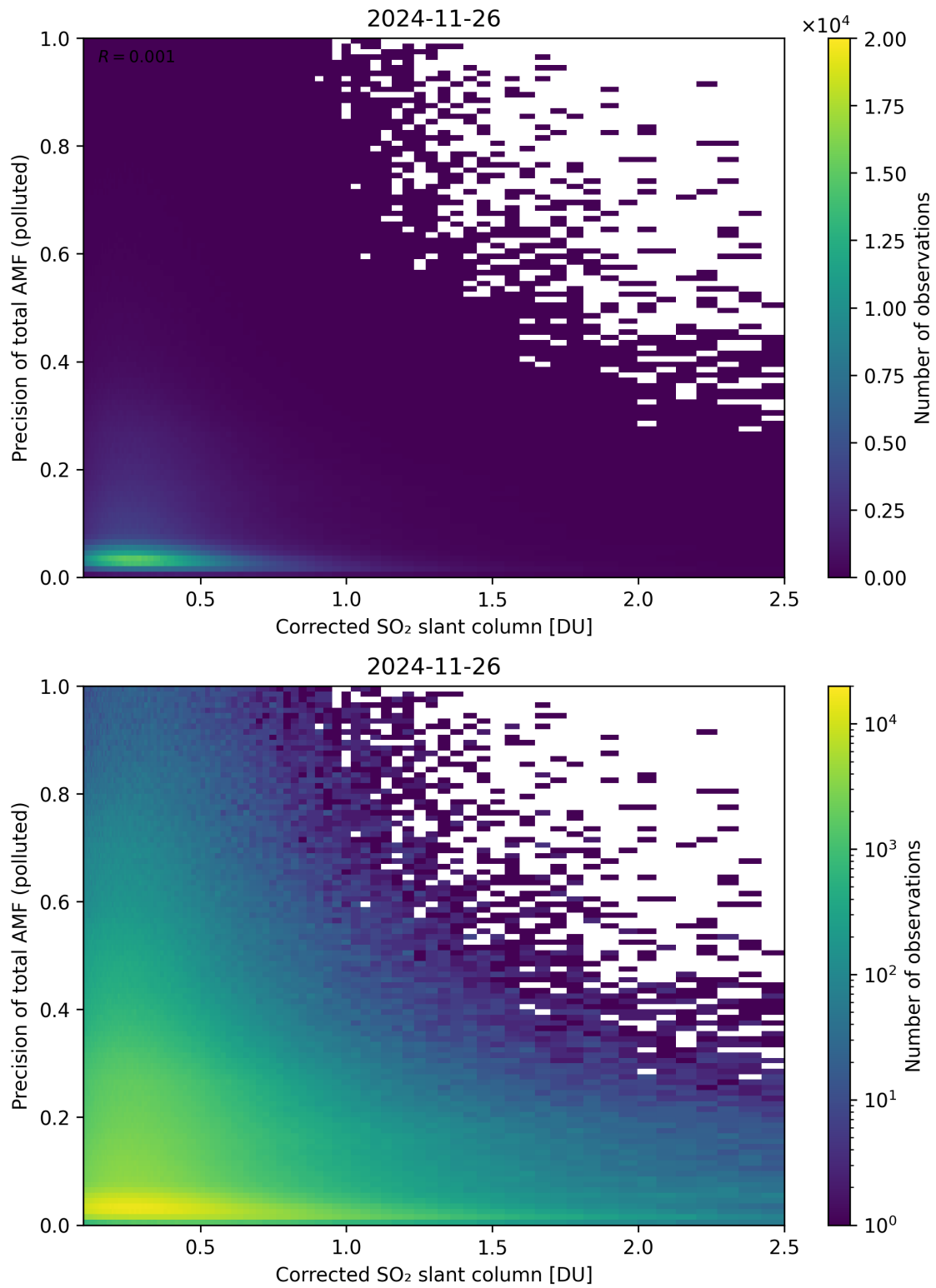
Figure 243: Scatter density plot of “Corrected SO 2 slant column” against “Precision of total AMF (polluted)” for 2024-11-25 to 2024-11-27.
