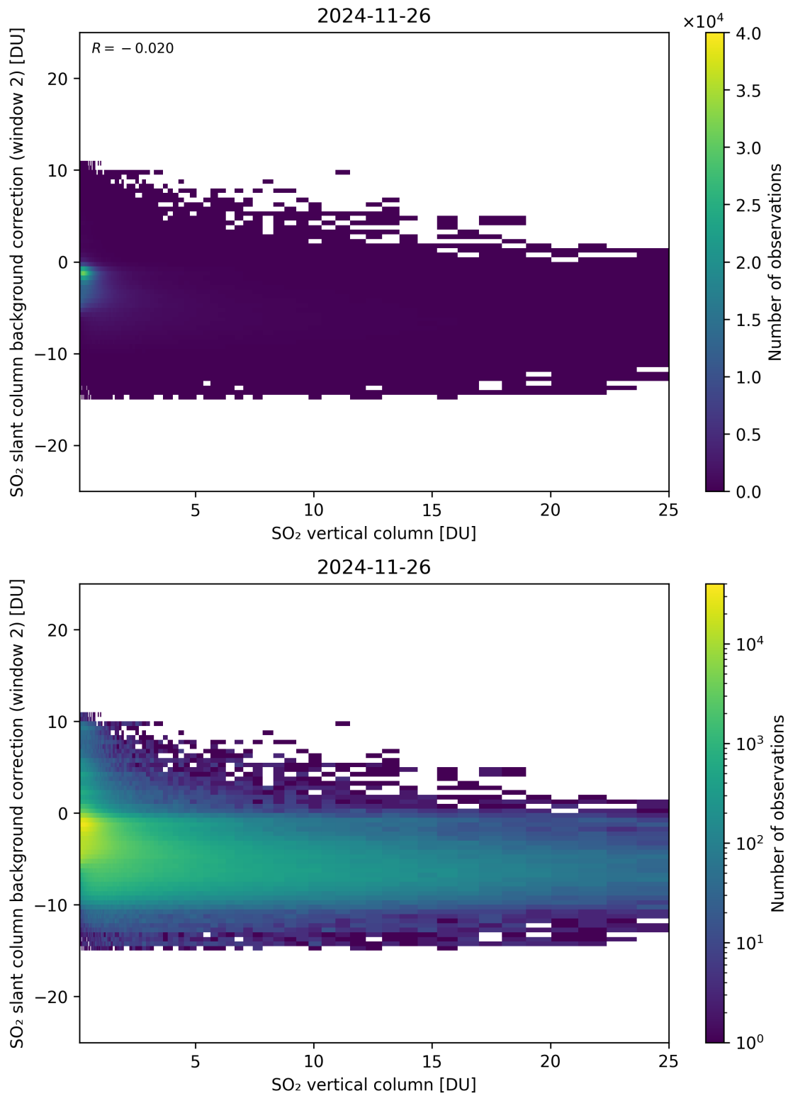
Figure 324: Scatter density plot of “SO 2 vertical column” against “SO 2 slant column background correction (window 2)” for 2024-11-25 to 2024-11-27.
