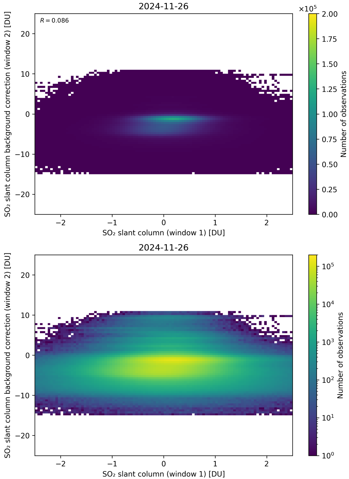
Figure 263: Scatter density plot of “SO 2 slant column (window 1)” against “SO 2 slant column background correction (window 2)” for 2024-11-25 to 2024-11-27.
