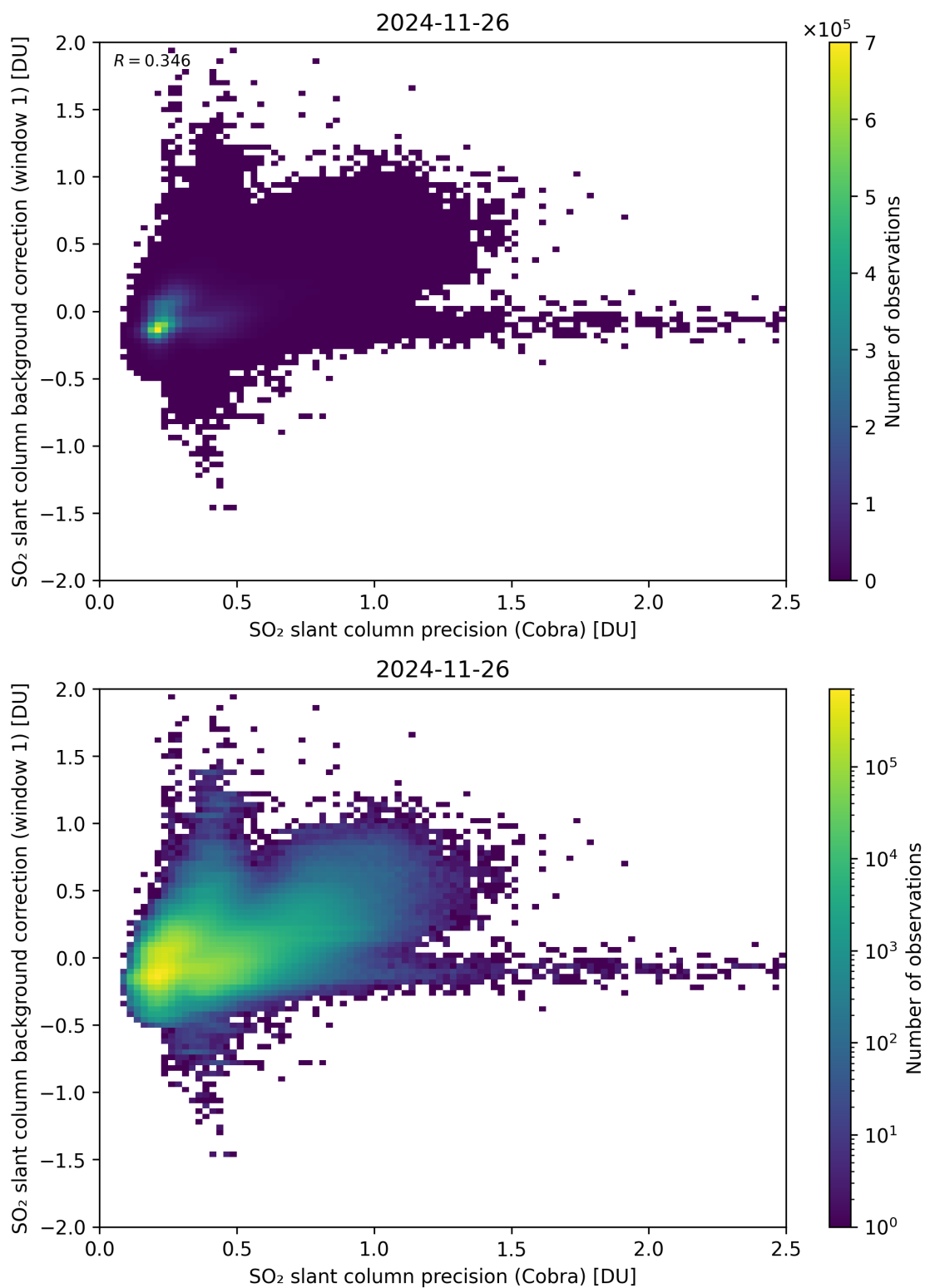
Figure 199: Scatter density plot of “SO 2 slant column precision (Cobra)” against “SO 2 slant column background correction (window 1)” for 2024-11-25 to 2024-11-27.
