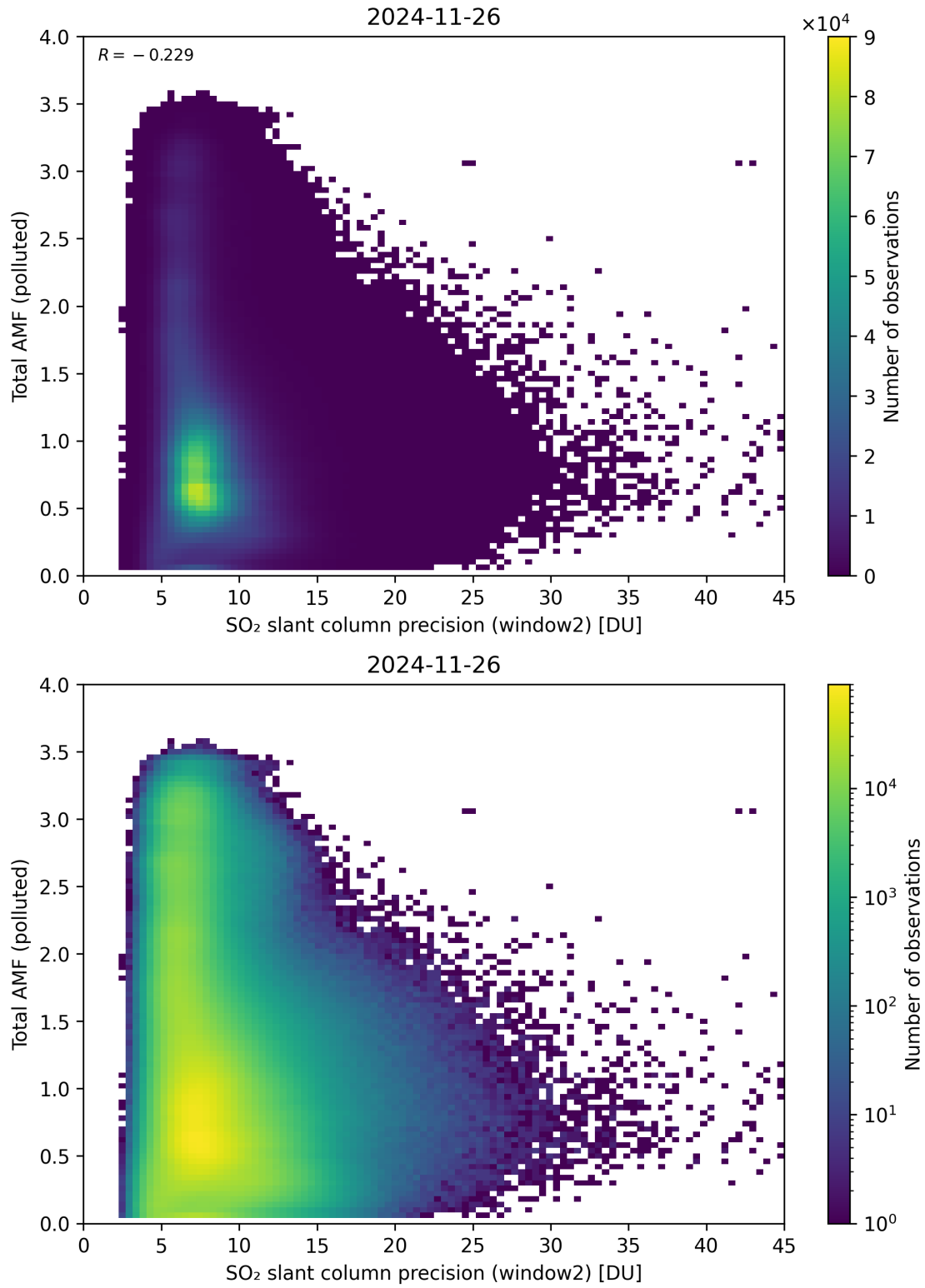
Figure 301: Scatter density plot of “SO 2 slant column precision (window2)” against “Total AMF (polluted)” for 2024-11-25 to 2024-11-27.
