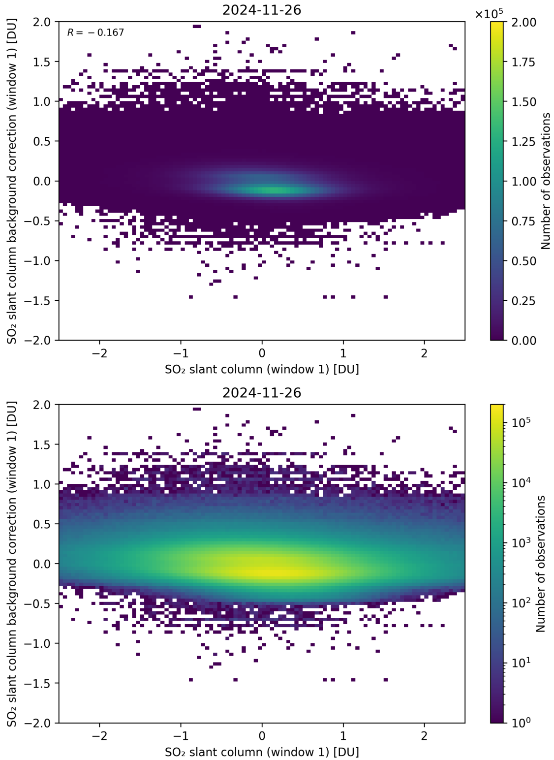
Figure 262: Scatter density plot of “SO 2 slant column (window 1)” against “SO 2 slant column background correction (window 1)” for 2024-11-25 to 2024-11-27.
