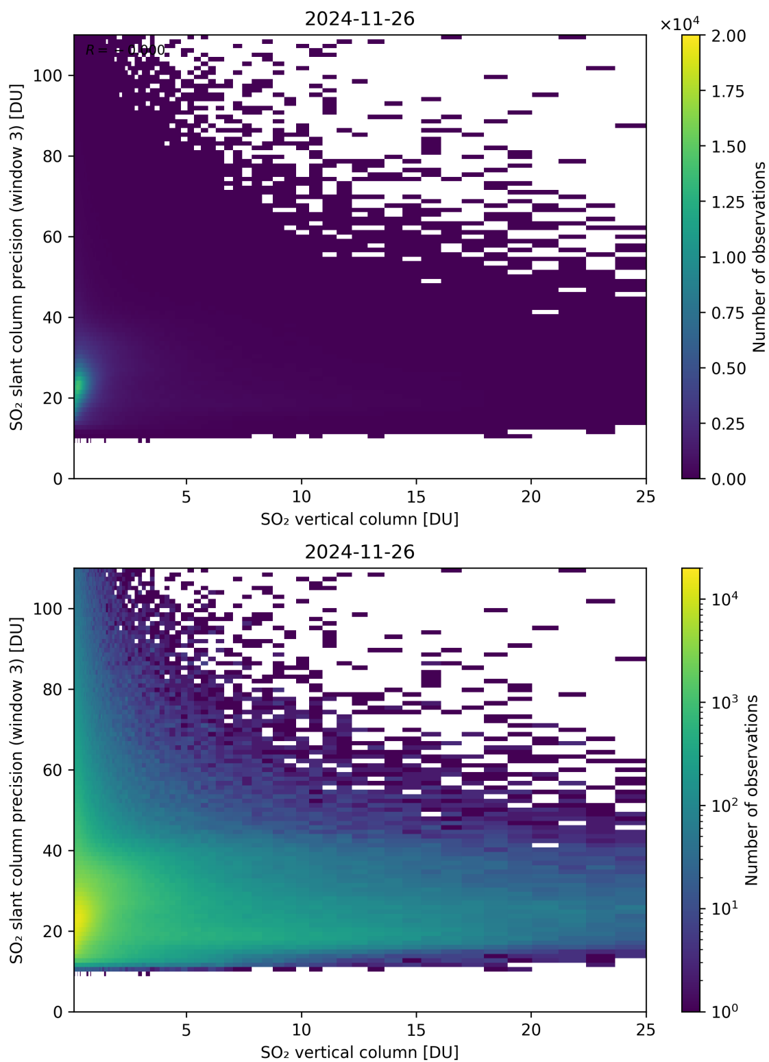
Figure 358: Scatter density plot of “SO 2 vertical column” against “SO 2 slant column precision (window 3)” for 2024-11-25 to 2024-11-27.
