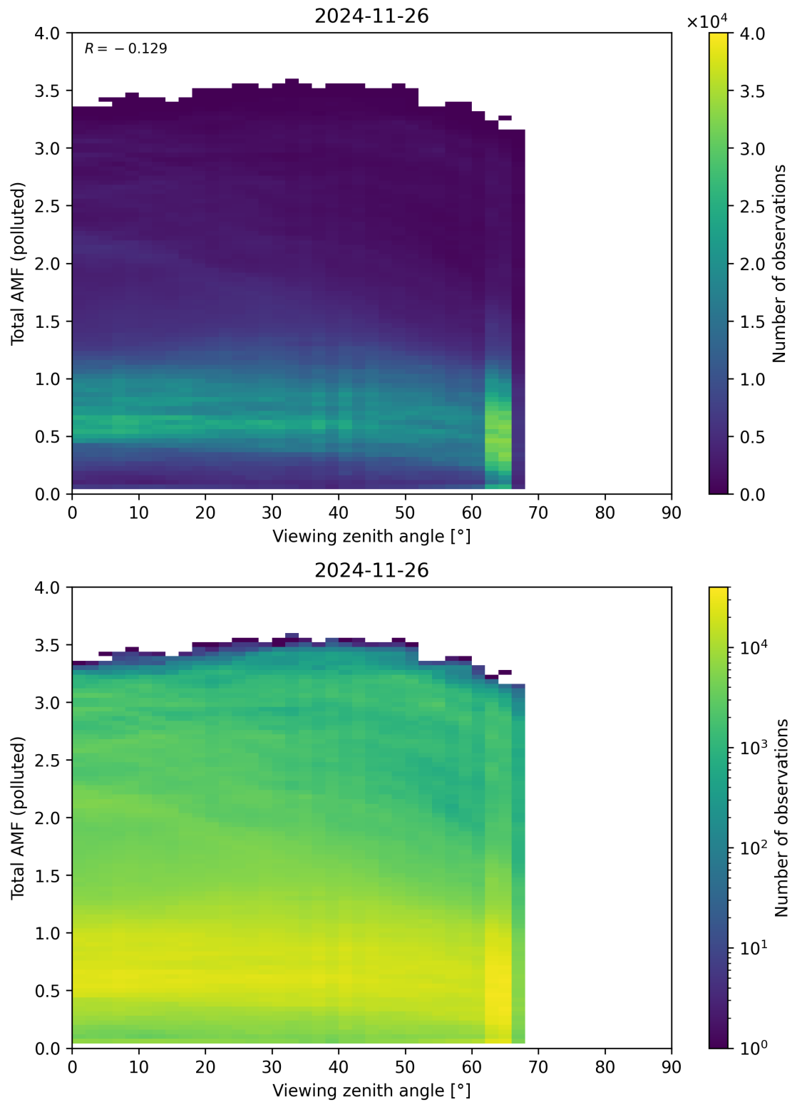
Figure 381: Scatter density plot of “Viewing zenith angle” against “Total AMF (polluted)” for 2024-11-25 to 2024-11-27.
