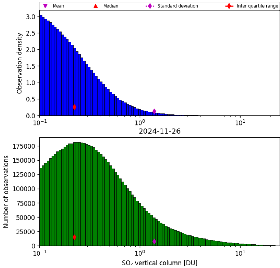
Figure 58: Histogram of “SO 2 vertical column” for 2024-11-25 to 2024-11-27
