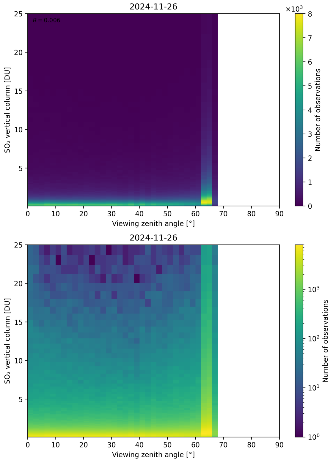
Figure 383: Scatter density plot of “Viewing zenith angle” against “SO 2 vertical column” for 2024-11-25 to 2024-11-27.
