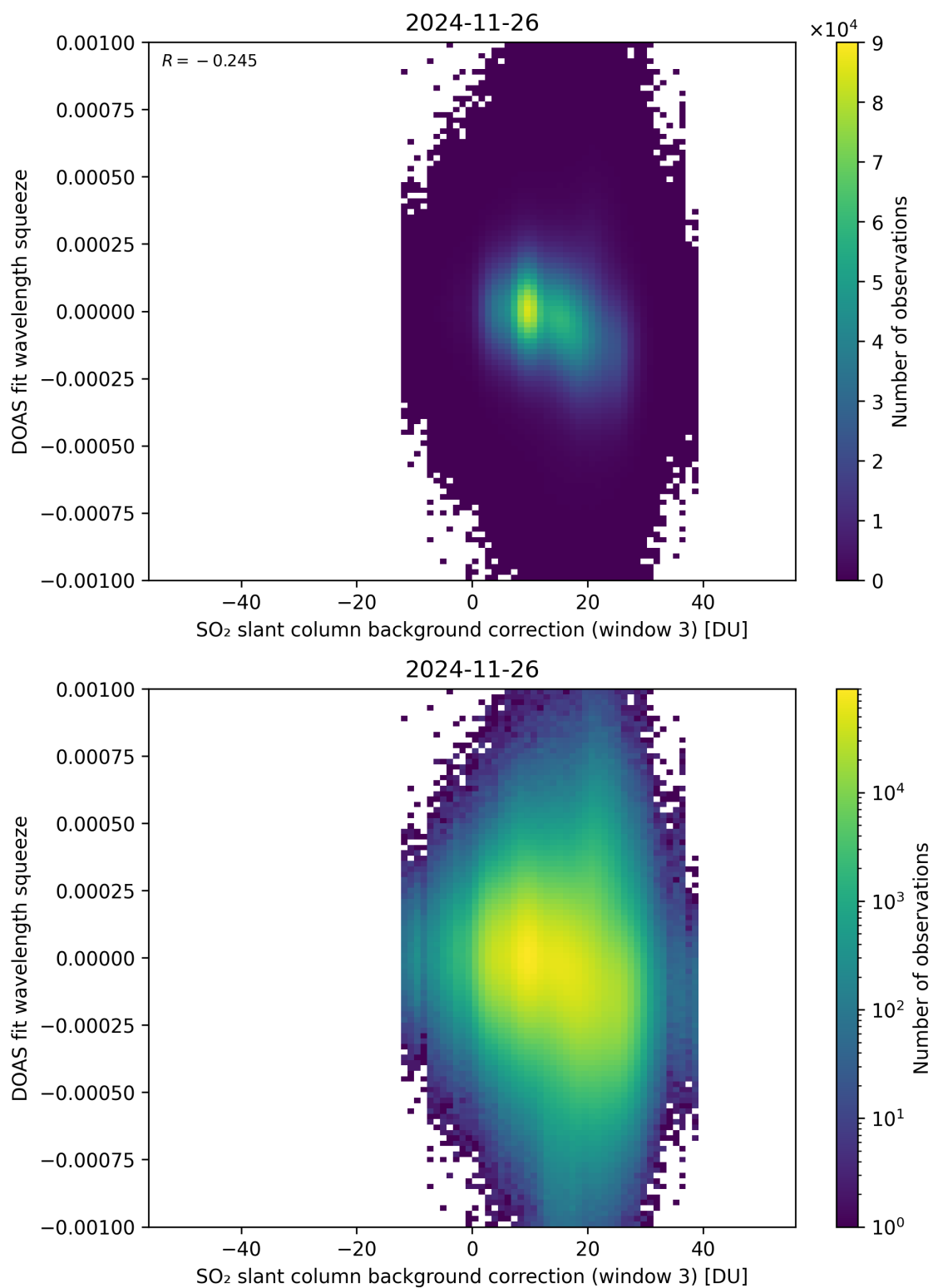
Figure 133: Scatter density plot of “SO 2 slant column background correction (window 3)” against “DOAS fit wavelength squeeze” for 2024-11-25 to 2024-11-27.
