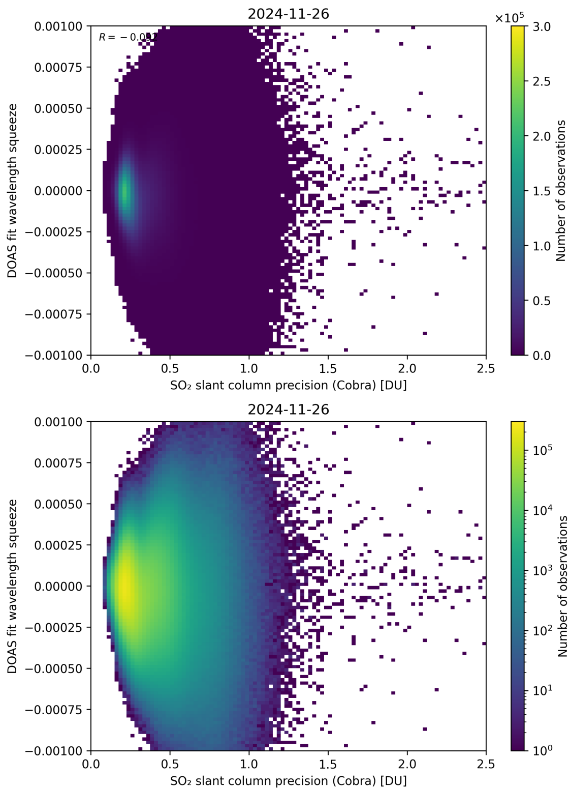
Figure 203: Scatter density plot of “SO 2 slant column precision (Cobra)” against “DOAS fit wavelength squeeze” for 2024-11-25 to 2024-11-27.
