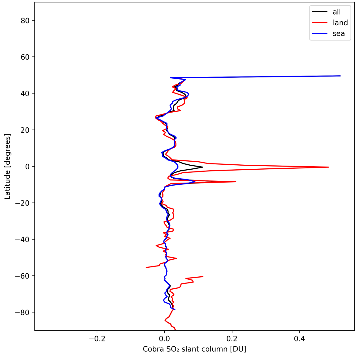
Figure 35: Zonal average of “Cobra SO 2 slant column” for 2024-11-25 to 2024-11-27.
