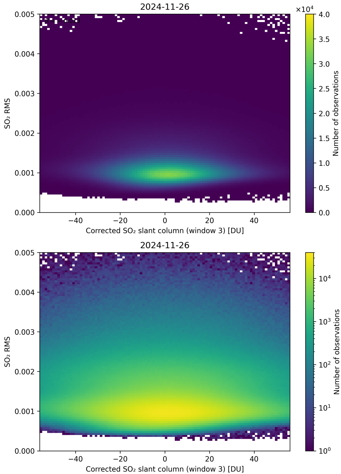
Figure 258: Scatter density plot of “Corrected SO 2 slant column (window 3)” against “SO 2 RMS” for 2024-11-25 to 2024-11-27.
