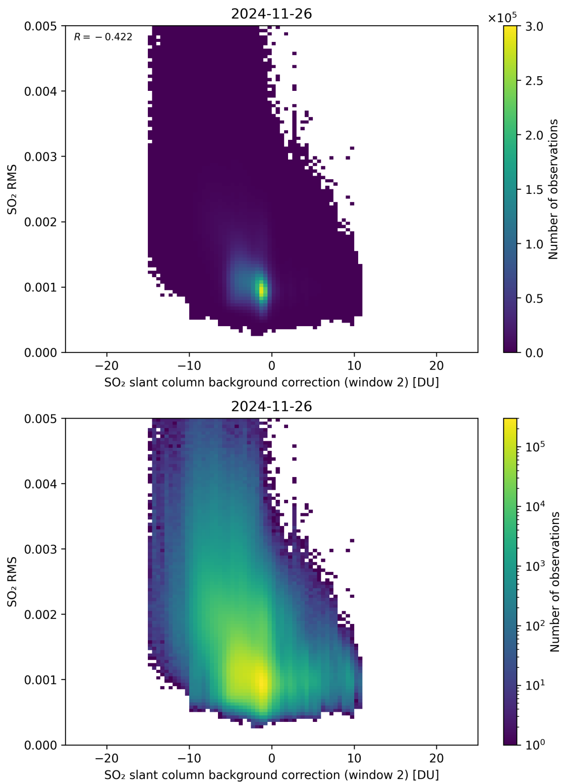
Figure 125: Scatter density plot of “SO 2 slant column background correction (window 2)” against “SO 2 RMS” for 2024-11-25 to 2024-11-27.
