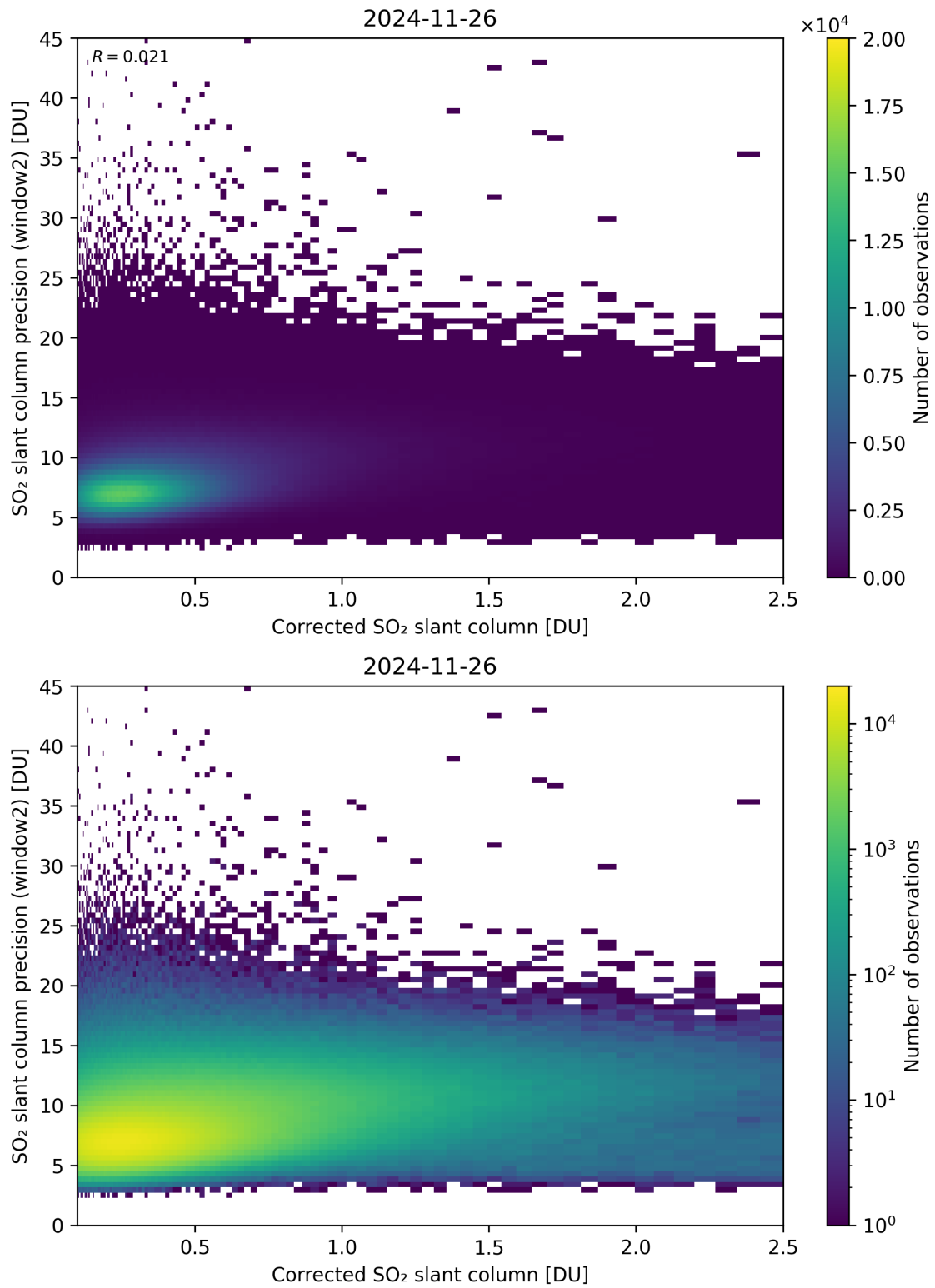
Figure 239: Scatter density plot of “Corrected SO 2 slant column” against “SO 2 slant column precision (window2)” for 2024-11-25 to 2024-11-27.
