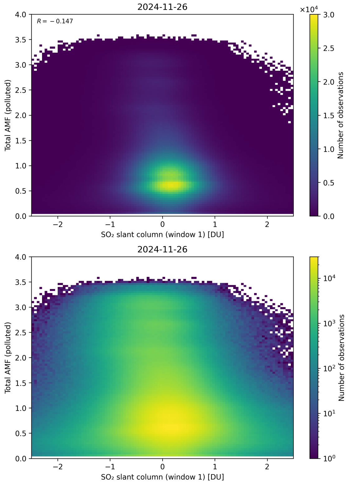
Figure 289: Scatter density plot of “SO 2 slant column (window 1)” against “Total AMF (polluted)” for 2024-11-25 to 2024-11-27.
