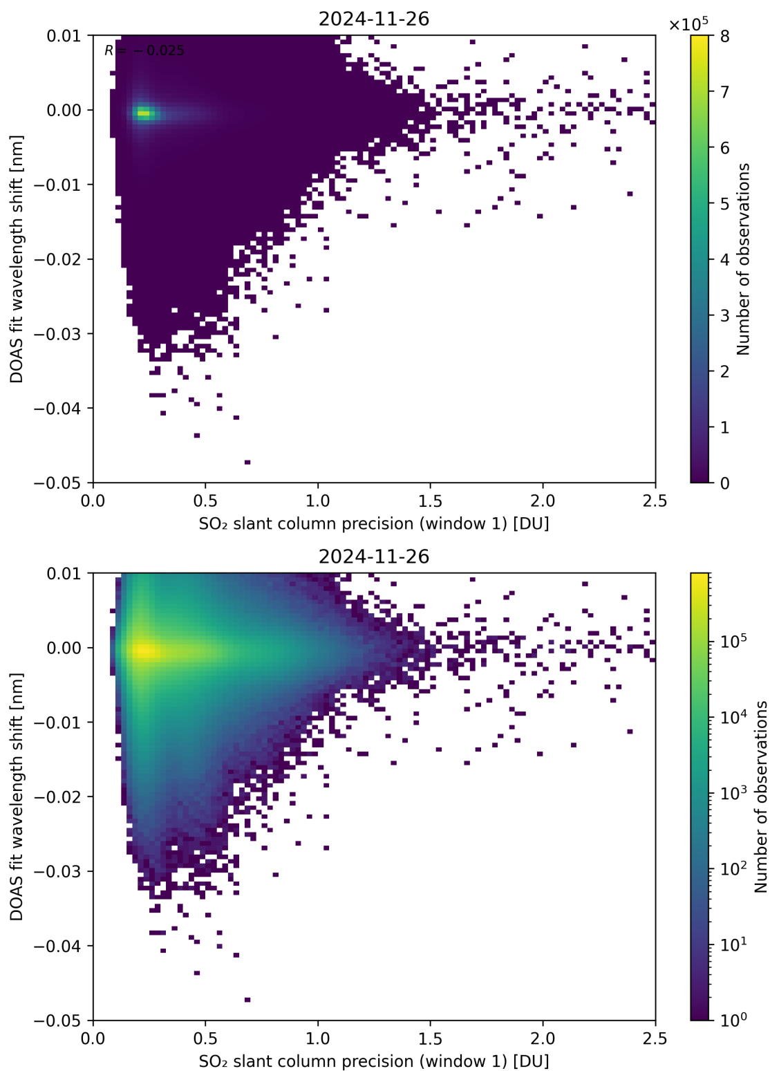
Figure 271: Scatter density plot of “SO 2 slant column precision (window 1)” against “DOAS fit wavelength shift” for 2024-11-25 to 2024-11-27.
