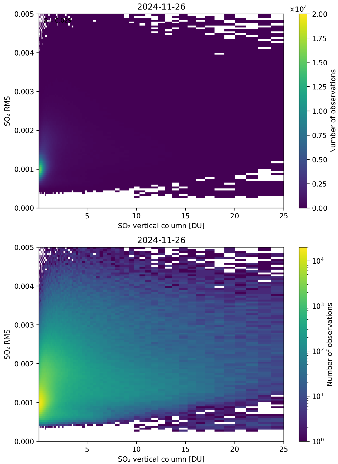
Figure 328: Scatter density plot of “SO 2 vertical column” against “SO 2 RMS” for 2024-11-25 to 2024-11-27.
