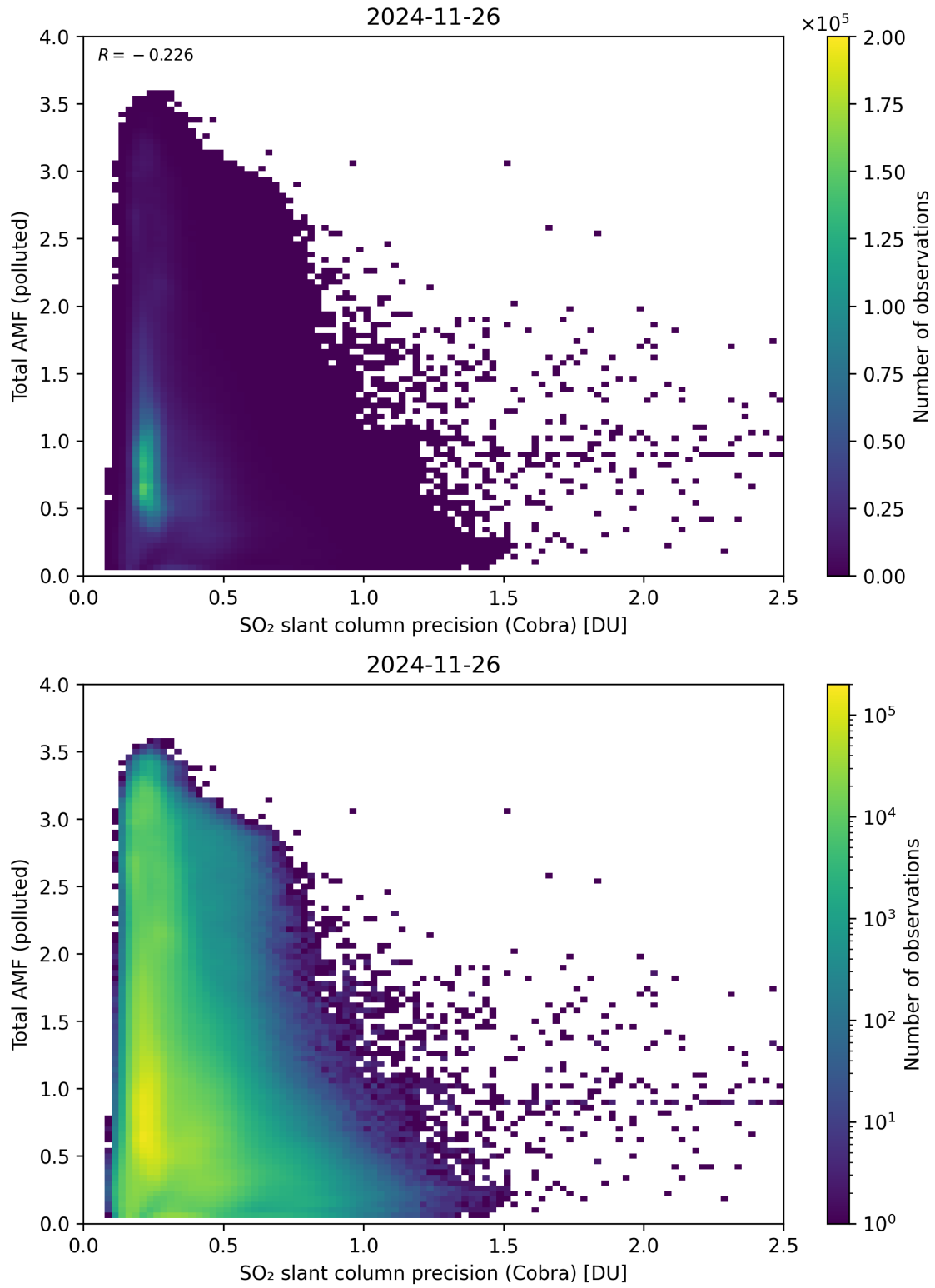
Figure 213: Scatter density plot of “SO 2 slant column precision (Cobra)” against “Total AMF (polluted)” for 2024-11-25 to 2024-11-27.
