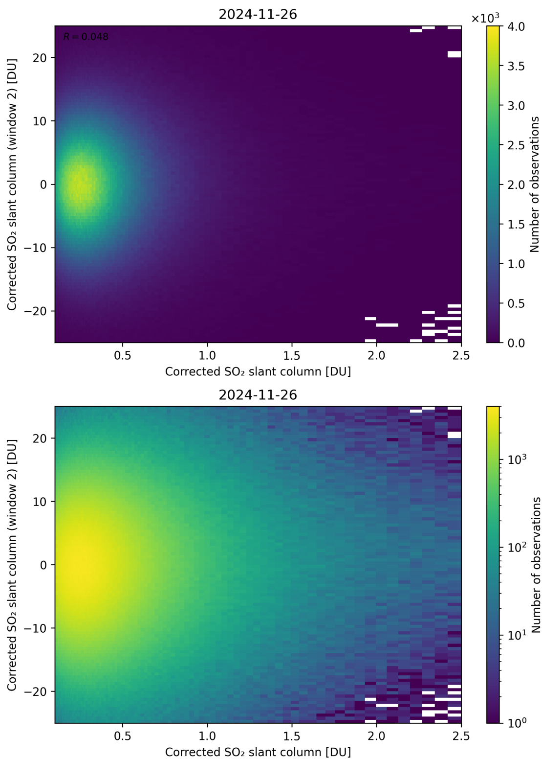
Figure 235: Scatter density plot of “Corrected SO 2 slant column” against “Corrected SO 2 slant column (window 2)” for 2024-11-25 to 2024-11-27.
