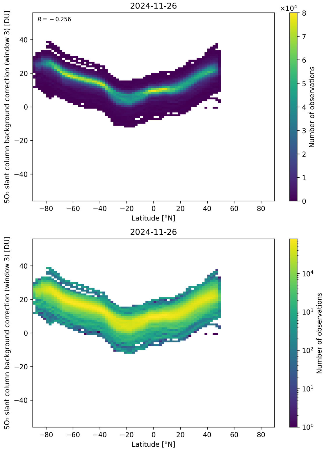
Figure 152: Scatter density plot of “Latitude” against “SO 2 slant column background correction (window 3)” for 2024-11-25 to 2024-11-27.
