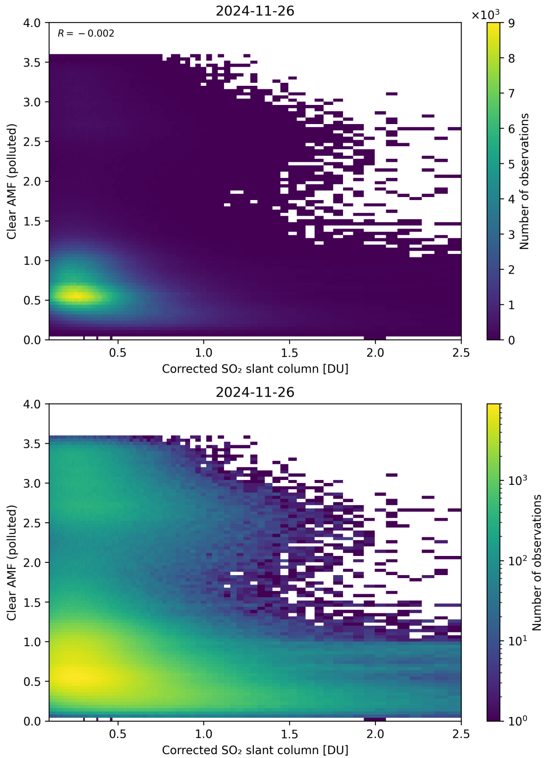
Figure 232: Scatter density plot of “Corrected SO 2 slant column” against “Clear AMF (polluted)” for 2024-11-25 to 2024-11-27.
