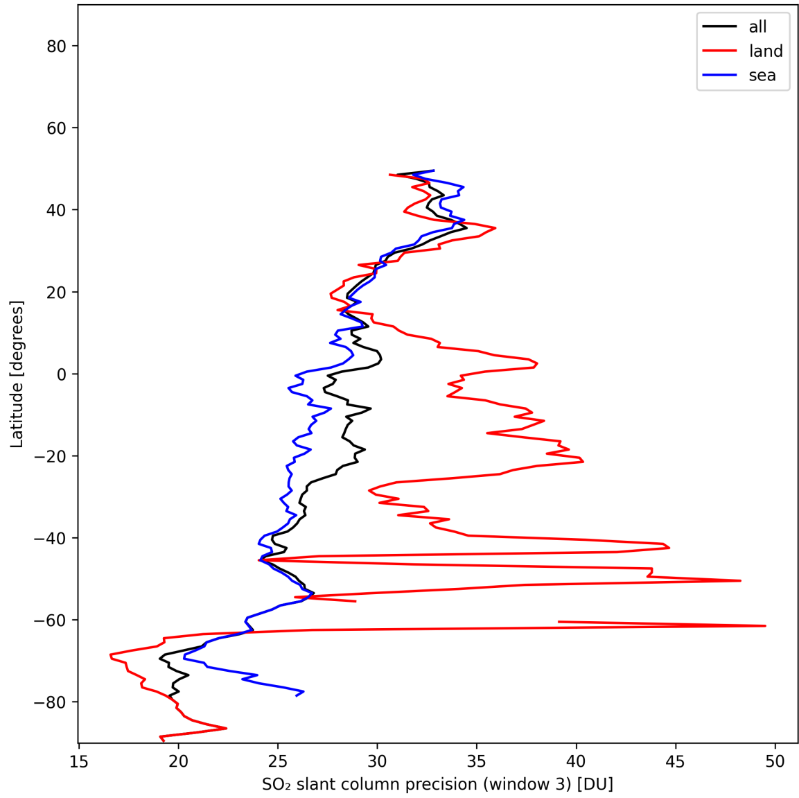
Figure 46: Zonal average of “SO 2 slant column precision (window 3)” for 2024-11-25 to 2024-11-27.
