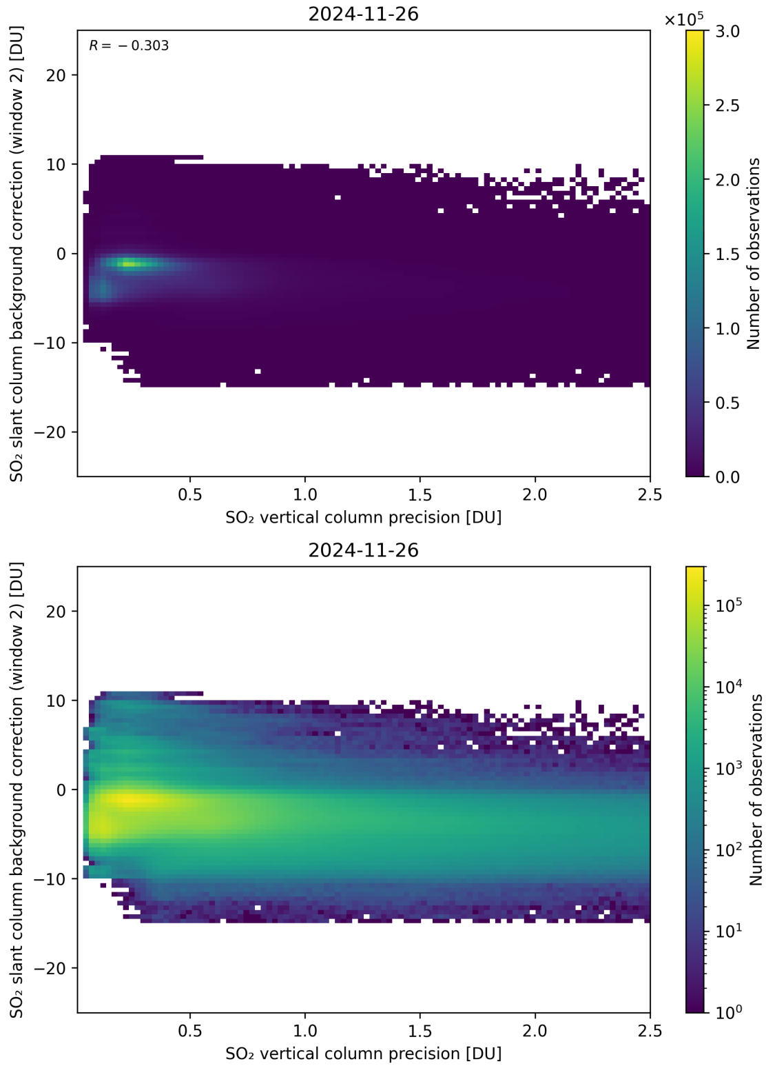
Figure 330: Scatter density plot of “SO 2 vertical column precision” against “SO 2 slant column background correction (window 2)” for 2024-11-25 to 2024-11-27.
