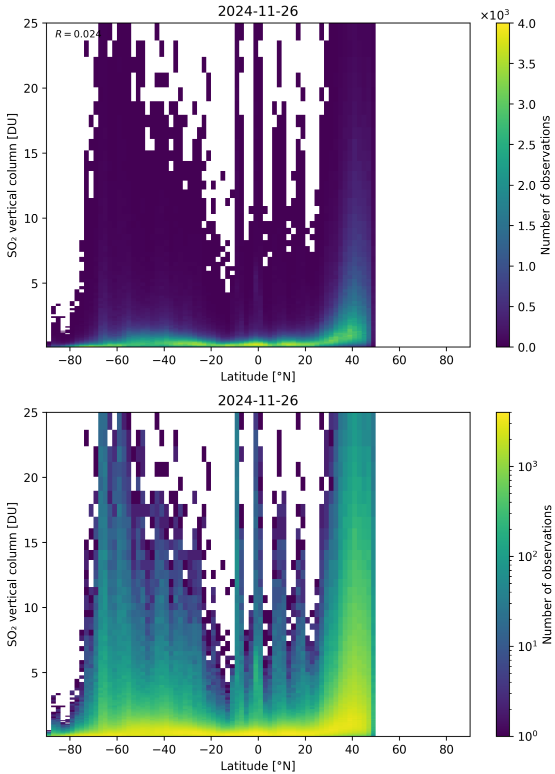
Figure 169: Scatter density plot of “Latitude” against “SO 2 vertical column” for 2024-11-25 to 2024-11-27.
