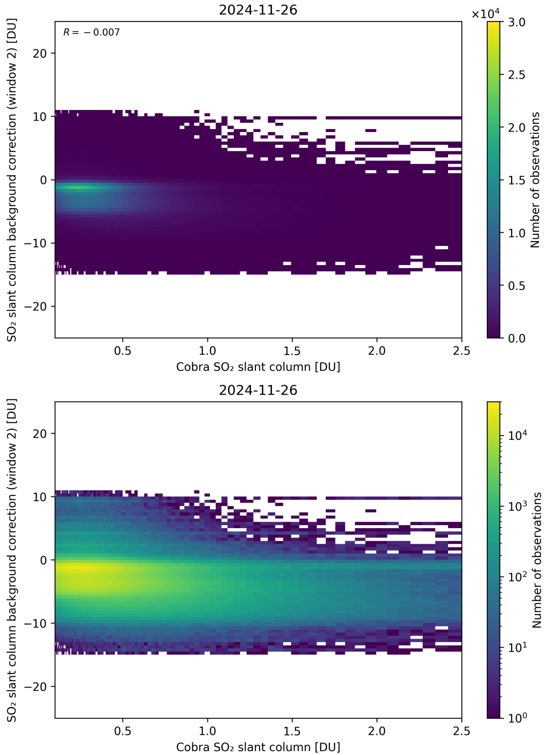
Figure 194: Scatter density plot of “Cobra SO 2 slant column” against “SO 2 slant column background correction (window 2)” for 2024-11-25 to 2024-11-27.
