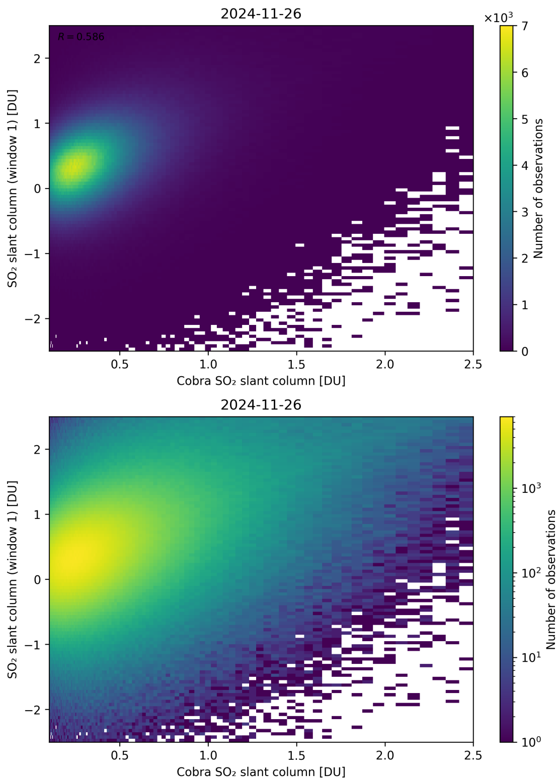
Figure 219: Scatter density plot of “Cobra SO 2 slant column” against “SO 2 slant column (window 1)” for 2024-11-25 to 2024-11-27.
