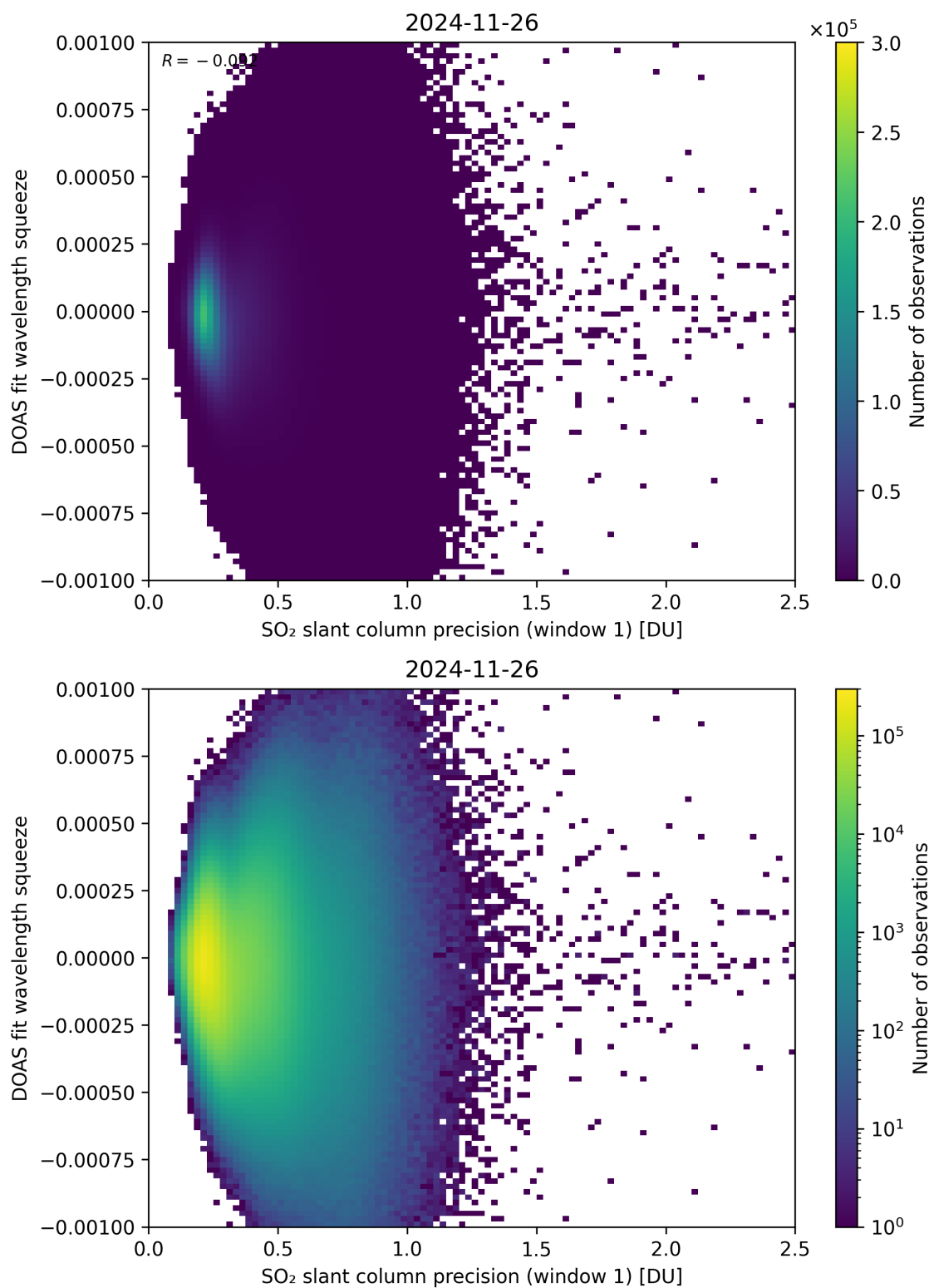
Figure 272: Scatter density plot of “SO 2 slant column precision (window 1)” against “DOAS fit wavelength squeeze” for 2024-11-25 to 2024-11-27.
