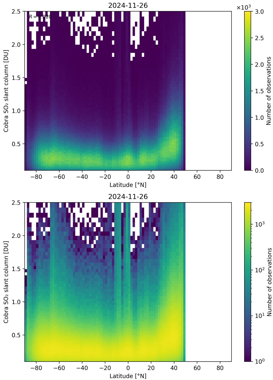
Figure 157: Scatter density plot of “Latitude” against “Cobra SO 2 slant column” for 2024-11-25 to 2024-11-27.
