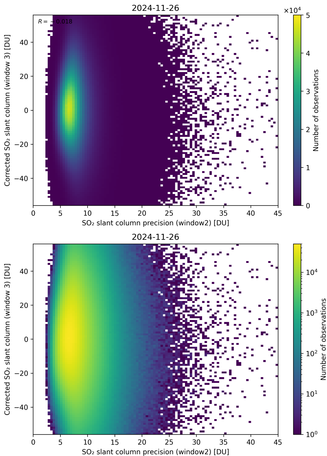
Figure 298: Scatter density plot of “SO 2 slant column precision (window2)” against “Corrected SO 2 slant column (window 3)” for 2024-11-25 to 2024-11-27.
