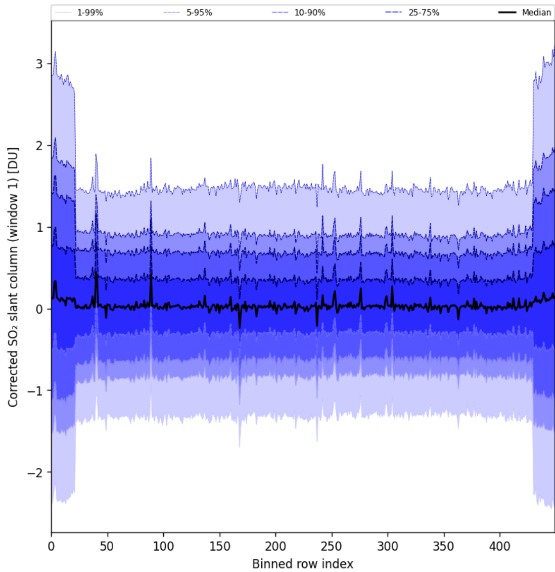
Figure 91: Along track statistics of “Corrected SO 2 slant column (window 1)” for 2024-11-25 to 2024-11-27
