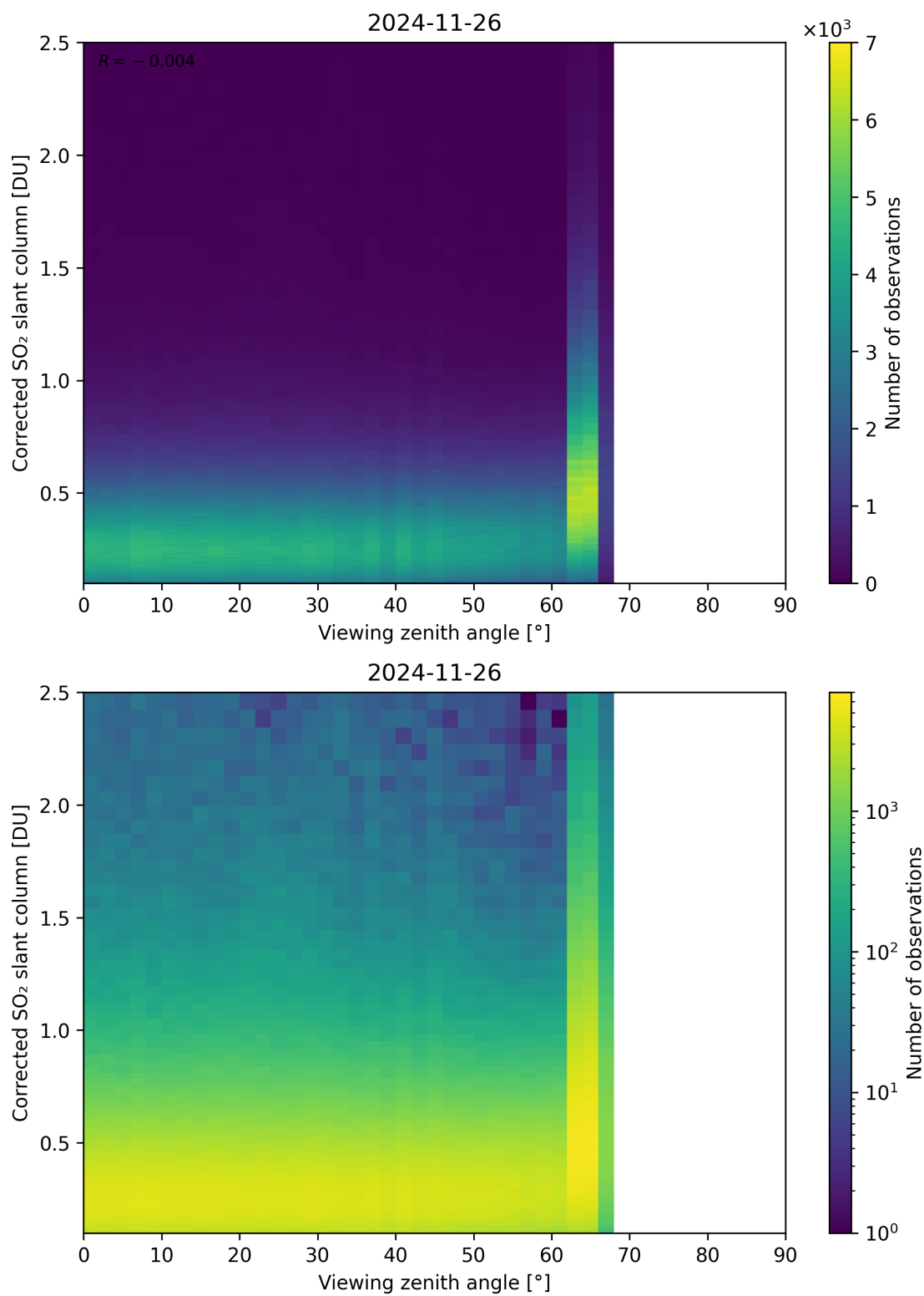
Figure 373: Scatter density plot of “Viewing zenith angle” against “Corrected SO 2 slant column” for 2024-11-25 to 2024-11-27.
