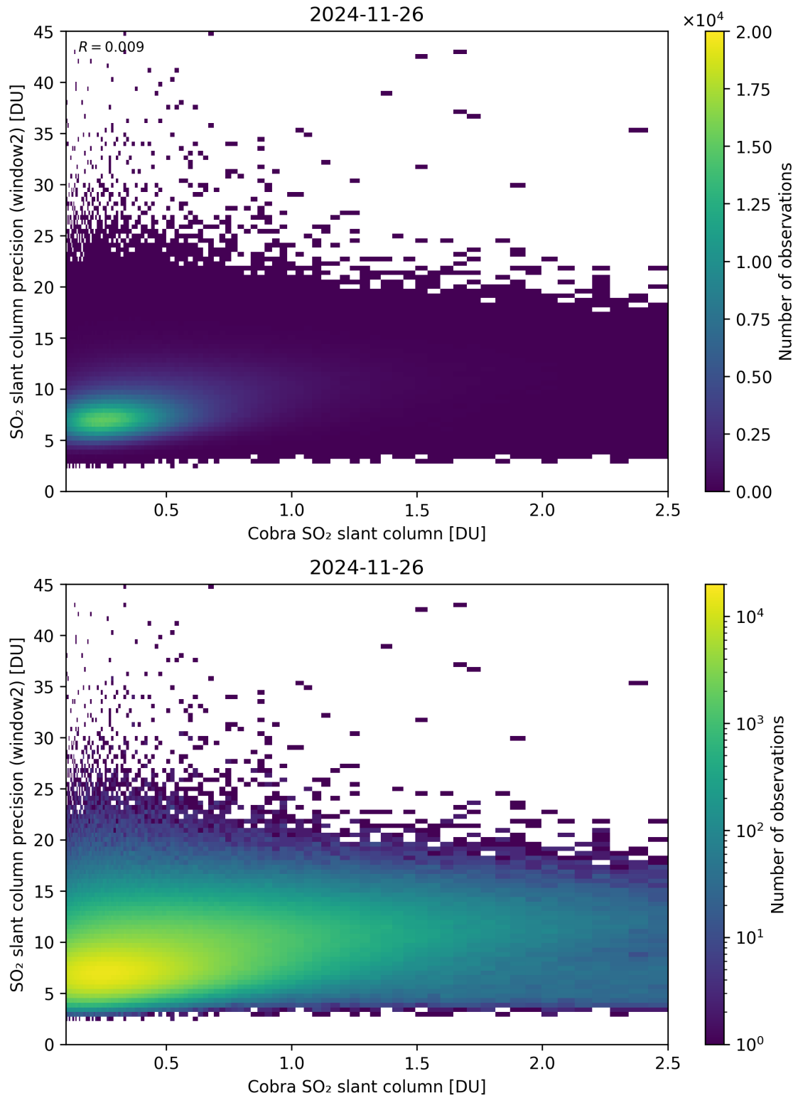
Figure 221: Scatter density plot of “Cobra SO 2 slant column” against “SO 2 slant column precision (window2)” for 2024-11-25 to 2024-11-27.
