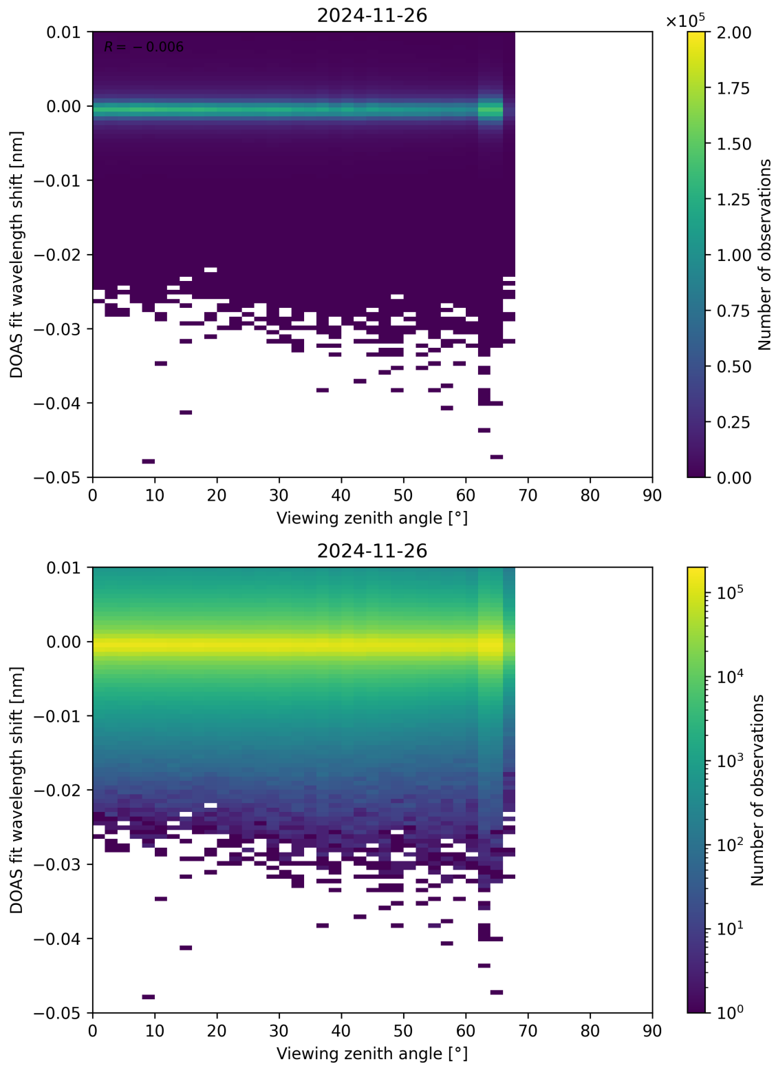
Figure 365: Scatter density plot of “Viewing zenith angle” against “DOAS fit wavelength shift” for 2024-11-25 to 2024-11-27.
