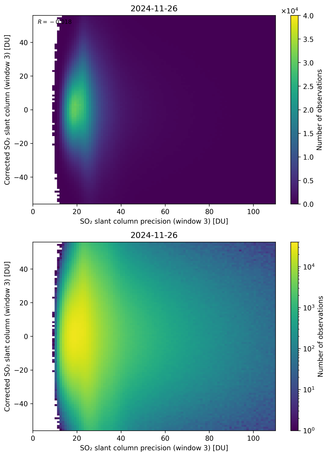
Figure 312: Scatter density plot of “SO 2 slant column precision (window 3)” against “Corrected SO 2 slant column (window 3)” for 2024-11-25 to 2024-11-27.
