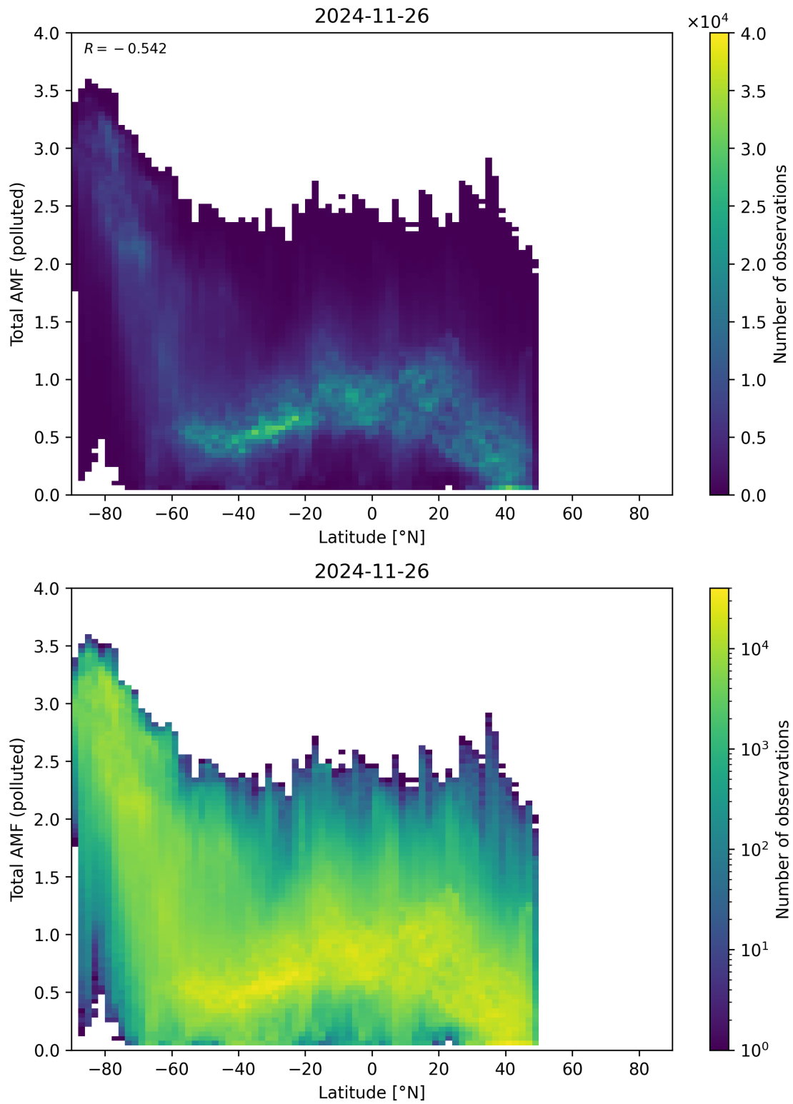
Figure 167: Scatter density plot of “Latitude” against “Total AMF (polluted)” for 2024-11-25 to 2024-11-27.
