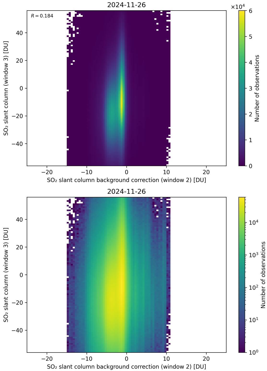
Figure 128: Scatter density plot of “SO 2 slant column background correction (window 2)” against “SO 2 slant column (window 3)” for 2024-11-25 to 2024-11-27.
