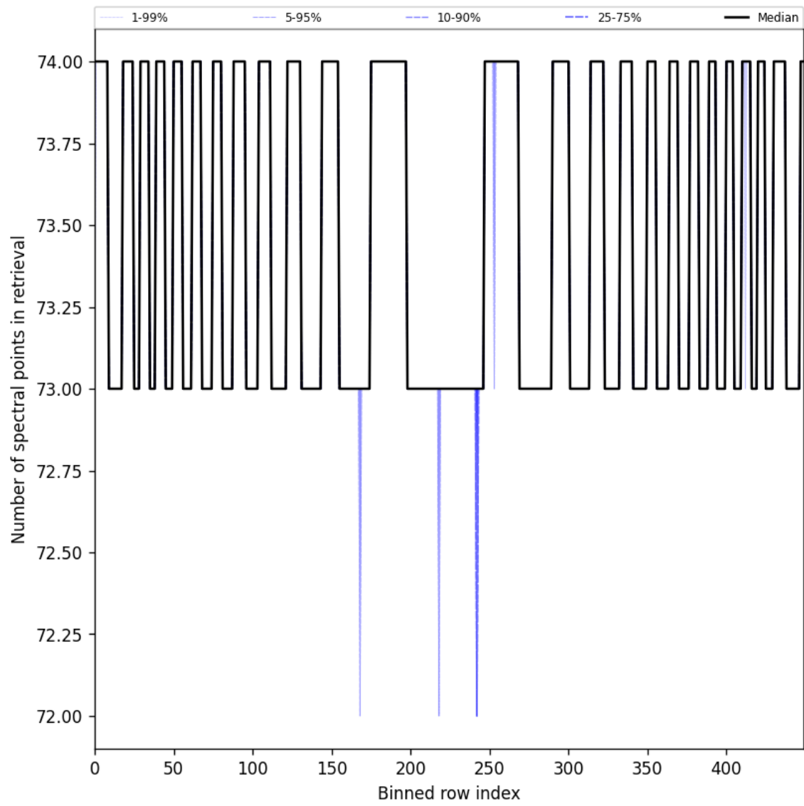
Figure 108: Along track statistics of “Number of spectral points in retrieval” for 2024-11-25 to 2024-11-27
