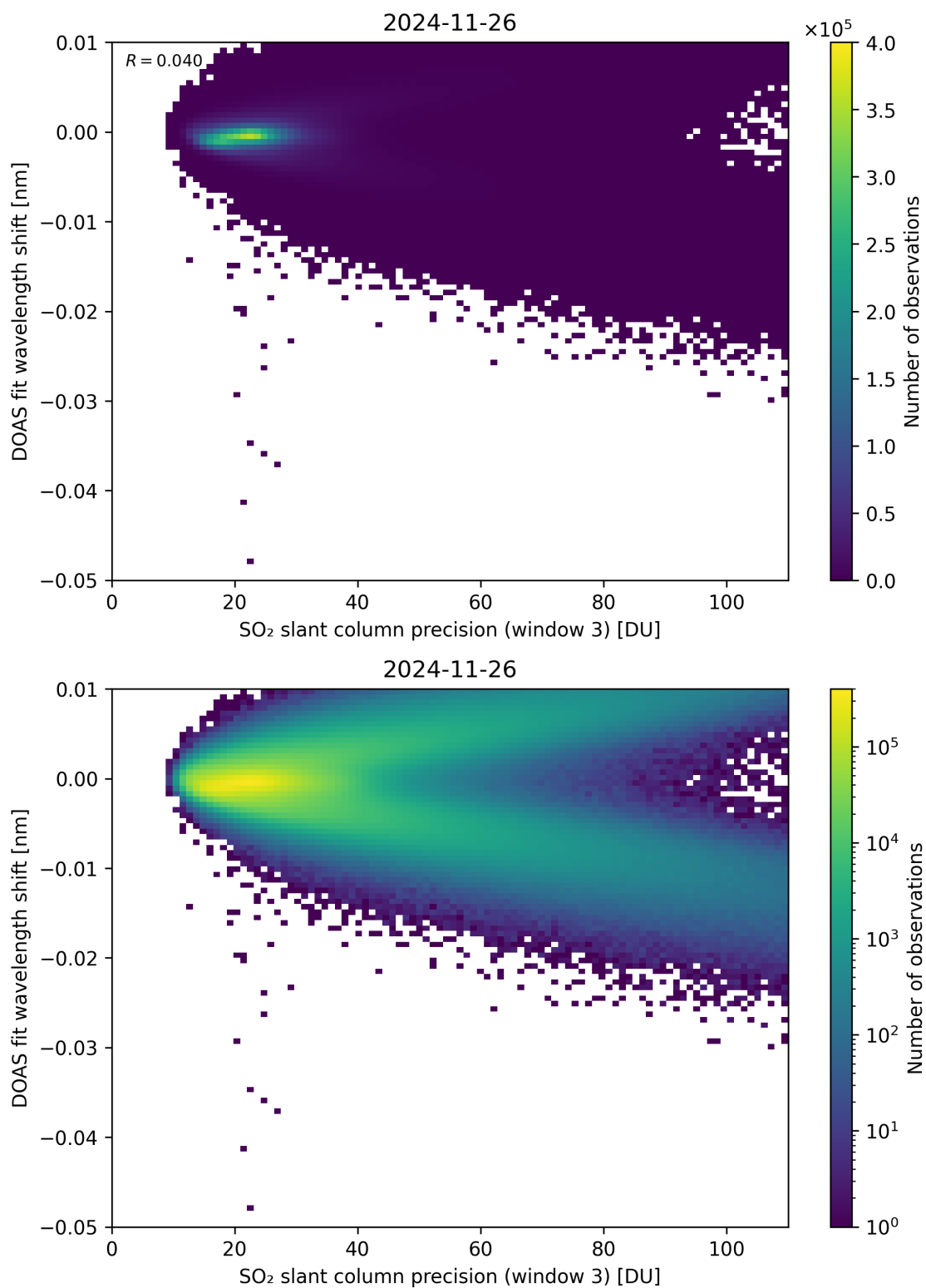
Figure 308: Scatter density plot of “SO 2 slant column precision (window 3)” against “DOAS fit wavelength shift” for 2024-11-25 to 2024-11-27.
