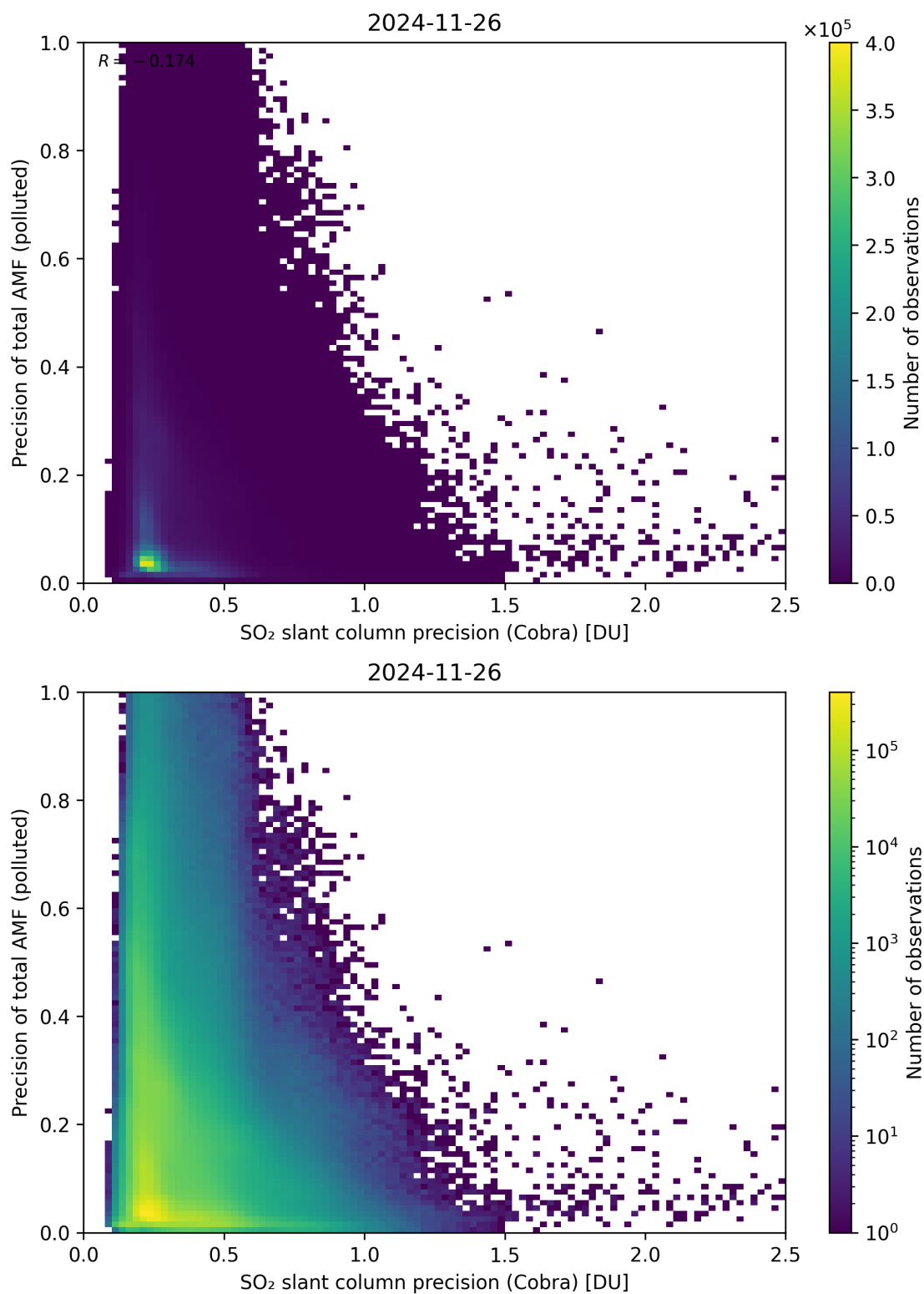
Figure 214: Scatter density plot of “SO 2 slant column precision (Cobra)” against “Precision of total AMF (polluted)” for 2024-11-25 to 2024-11-27.
