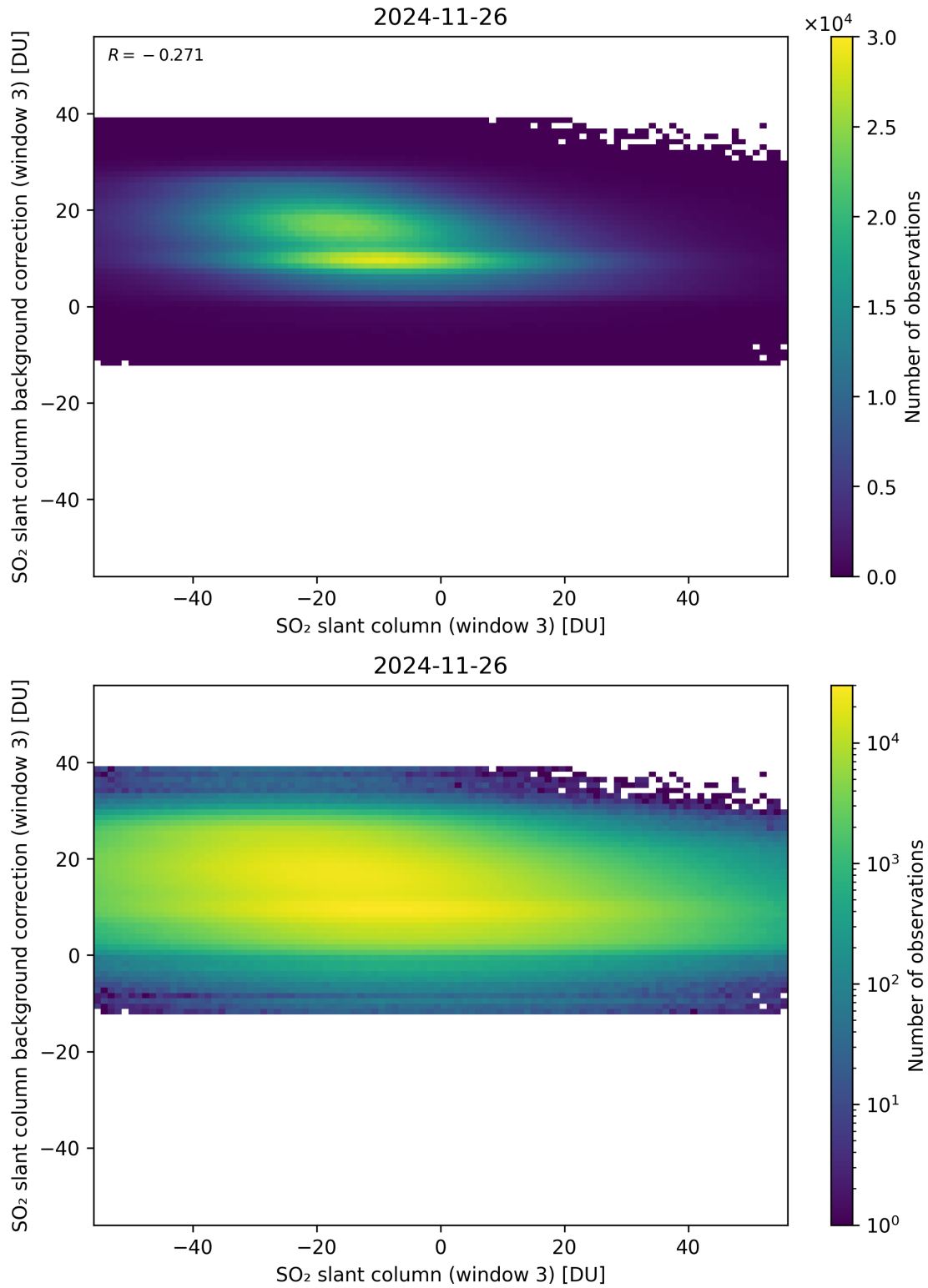
Figure 303: Scatter density plot of “SO 2 slant column (window 3)” against “SO 2 slant column background correction (window 3)” for 2024-11-25 to 2024-11-27.
