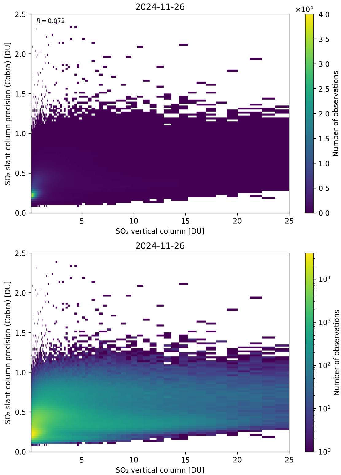
Figure 350: Scatter density plot of “SO 2 vertical column” against “SO 2 slant column precision (Cobra)” for 2024-11-25 to 2024-11-27.
