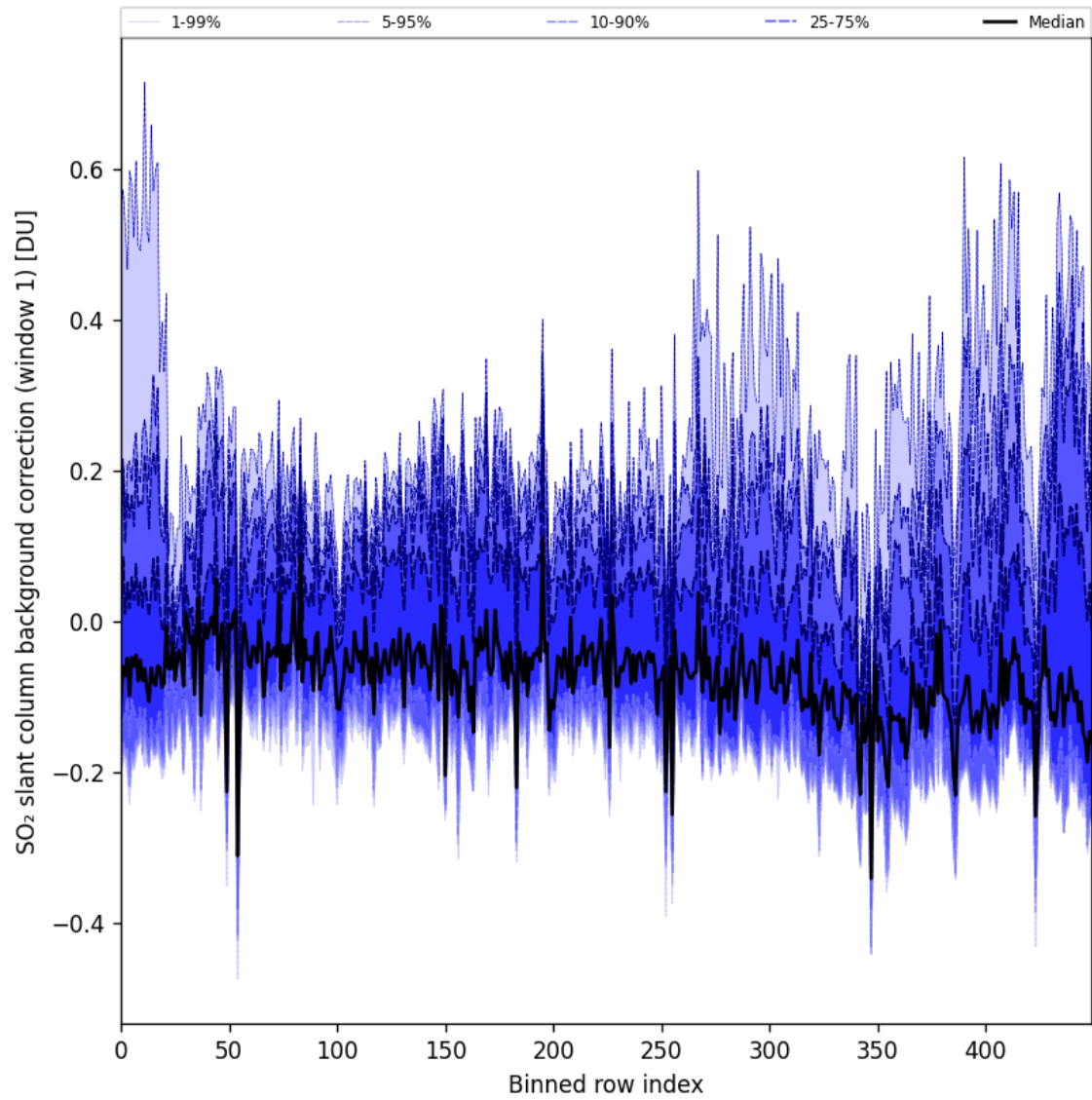
Figure 92: Along track statistics of “SO 2 slant column background correction (window 1)” for 2024-11-25 to 2024-11-27
