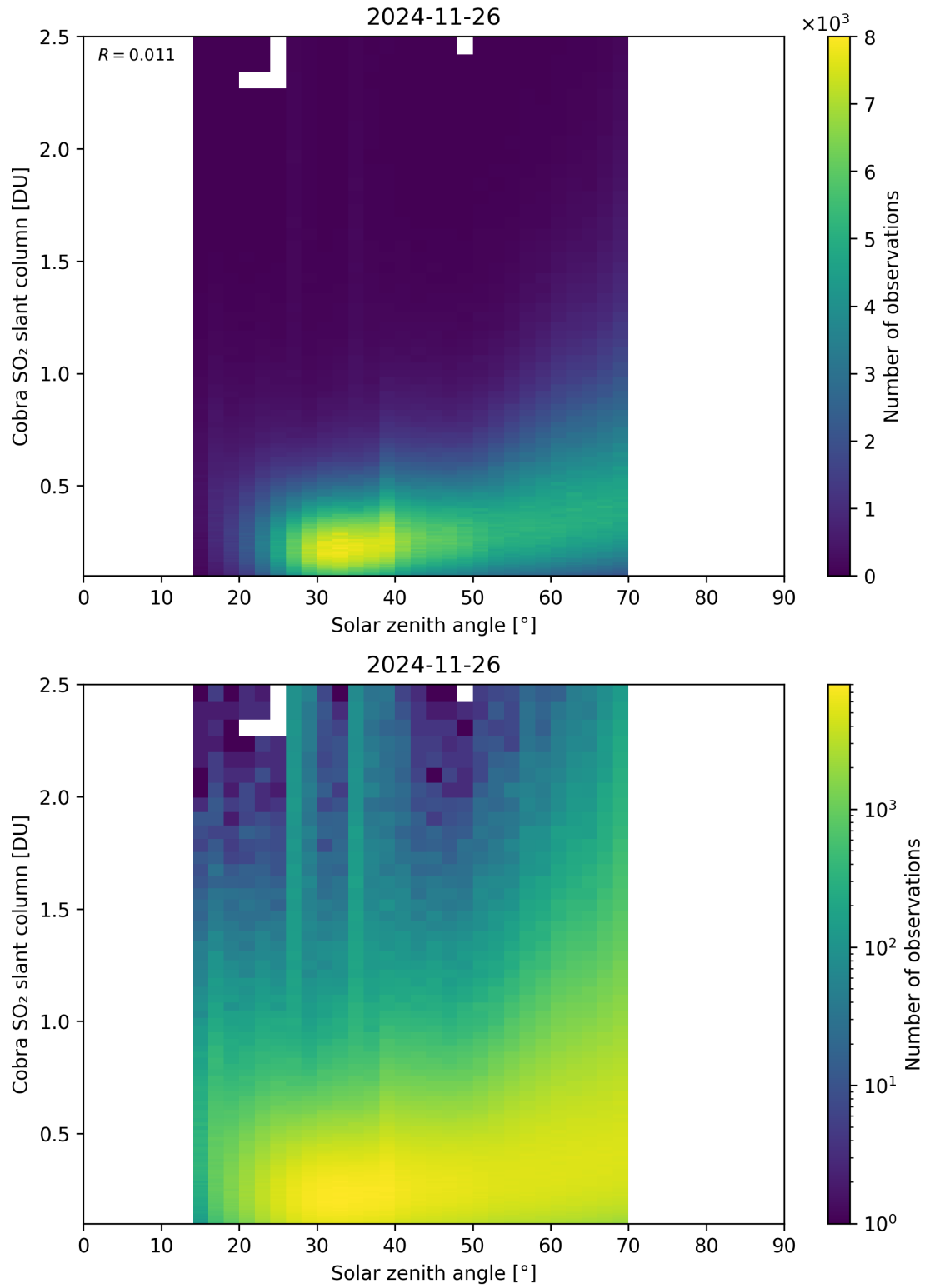
Figure 179: Scatter density plot of “Solar zenith angle” against “Cobra SO 2 slant column” for 2024-11-25 to 2024-11-27.
