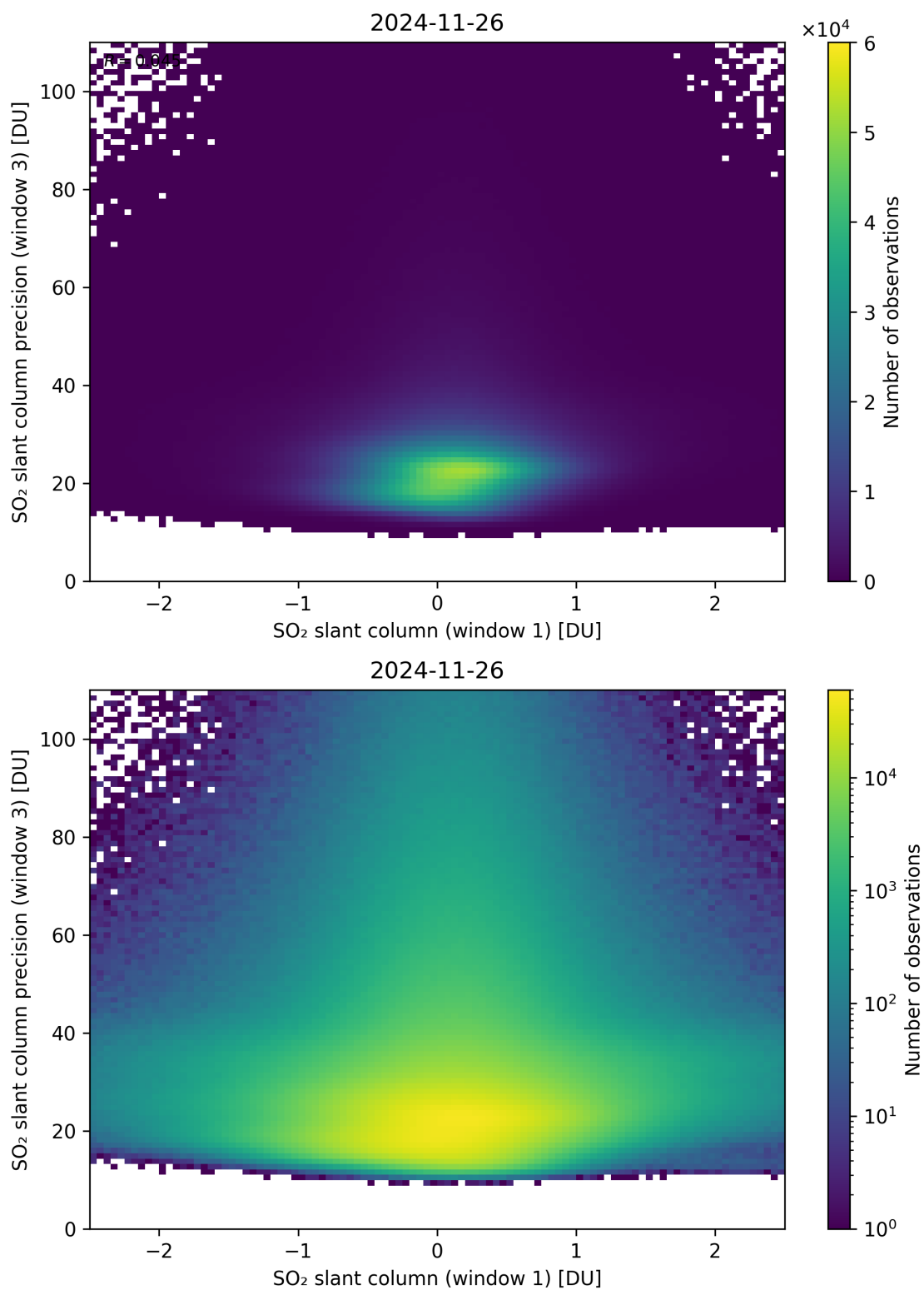
Figure 288: Scatter density plot of “SO 2 slant column (window 1)” against “SO 2 slant column precision (window 3)” for 2024-11-25 to 2024-11-27.
