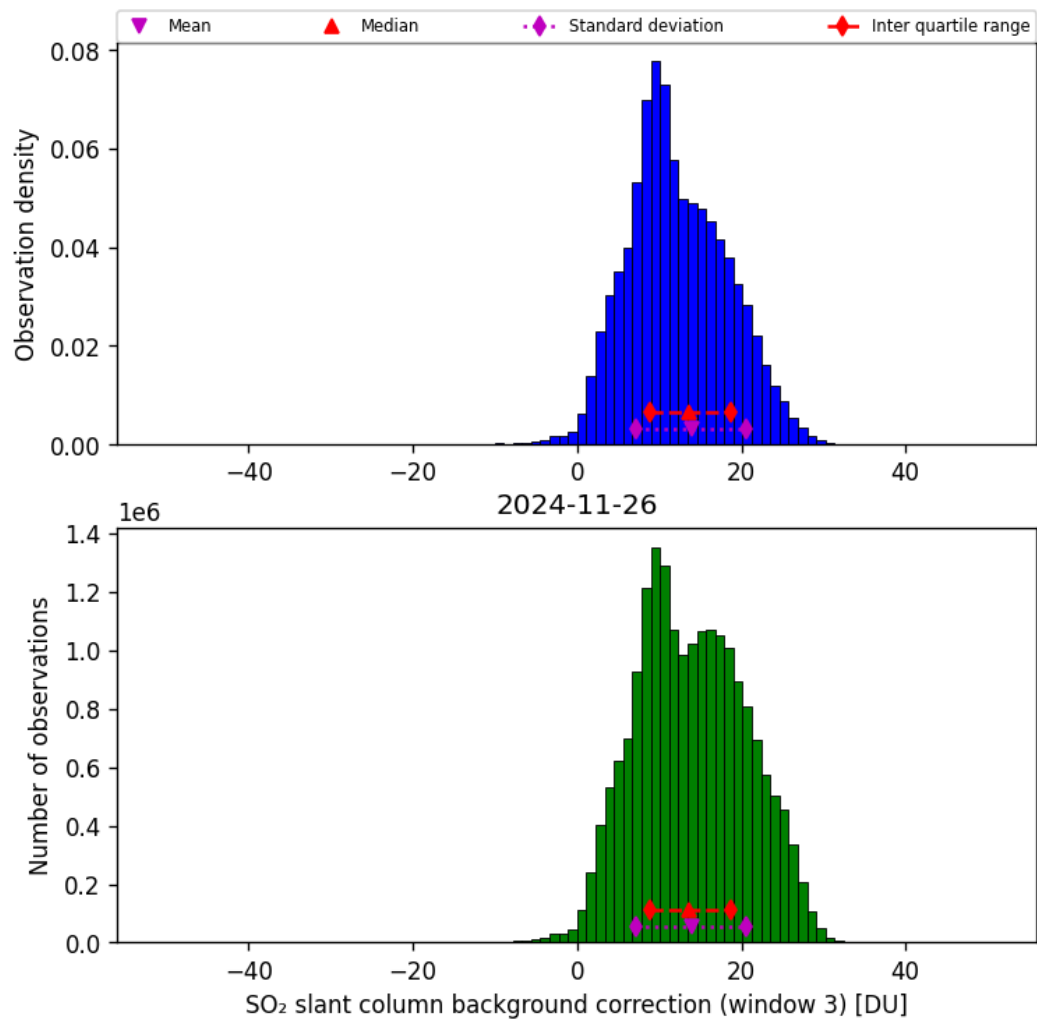
Figure 74: Histogram of “SO 2 slant column background correction (window 3)” for 2024-11-25 to 2024-11-27
