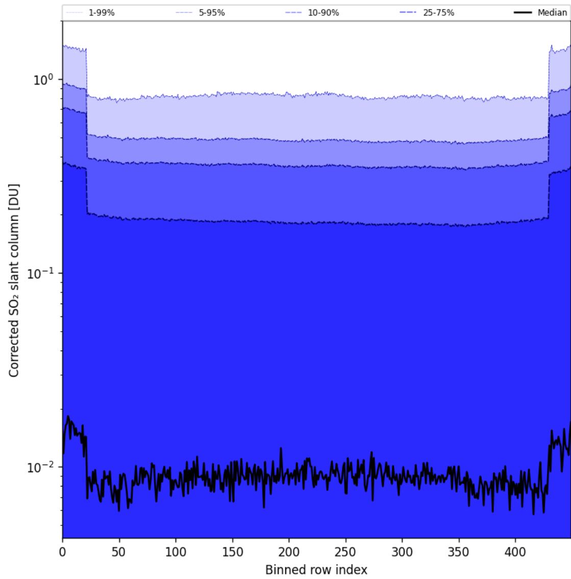
Figure 86: Along track statistics of “Corrected SO 2 slant column” for 2024-11-25 to 2024-11-27
