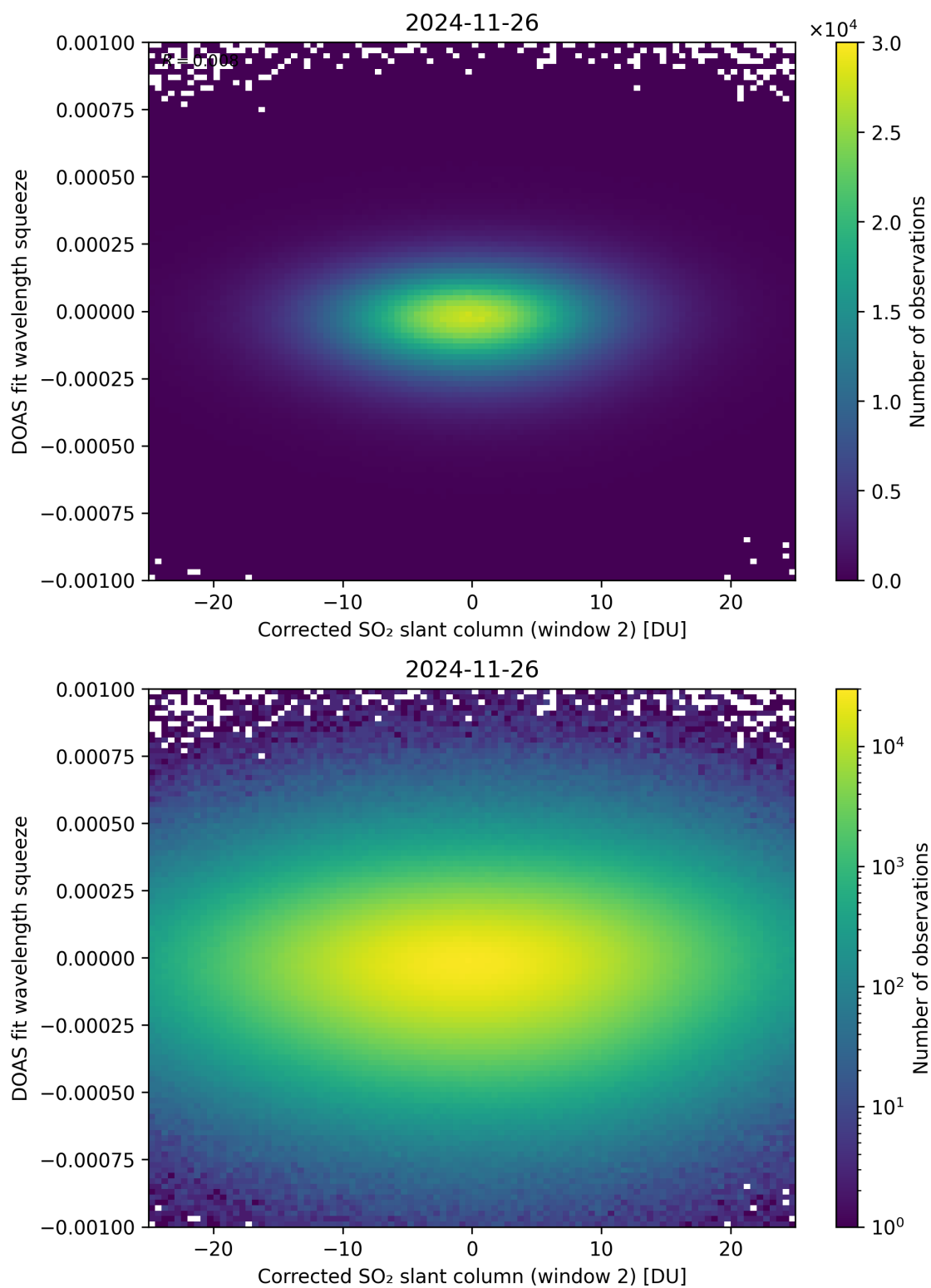
Figure 247: Scatter density plot of “Corrected SO 2 slant column (window 2)” against “DOAS fit wavelength squeeze” for 2024-11-25 to 2024-11-27.
