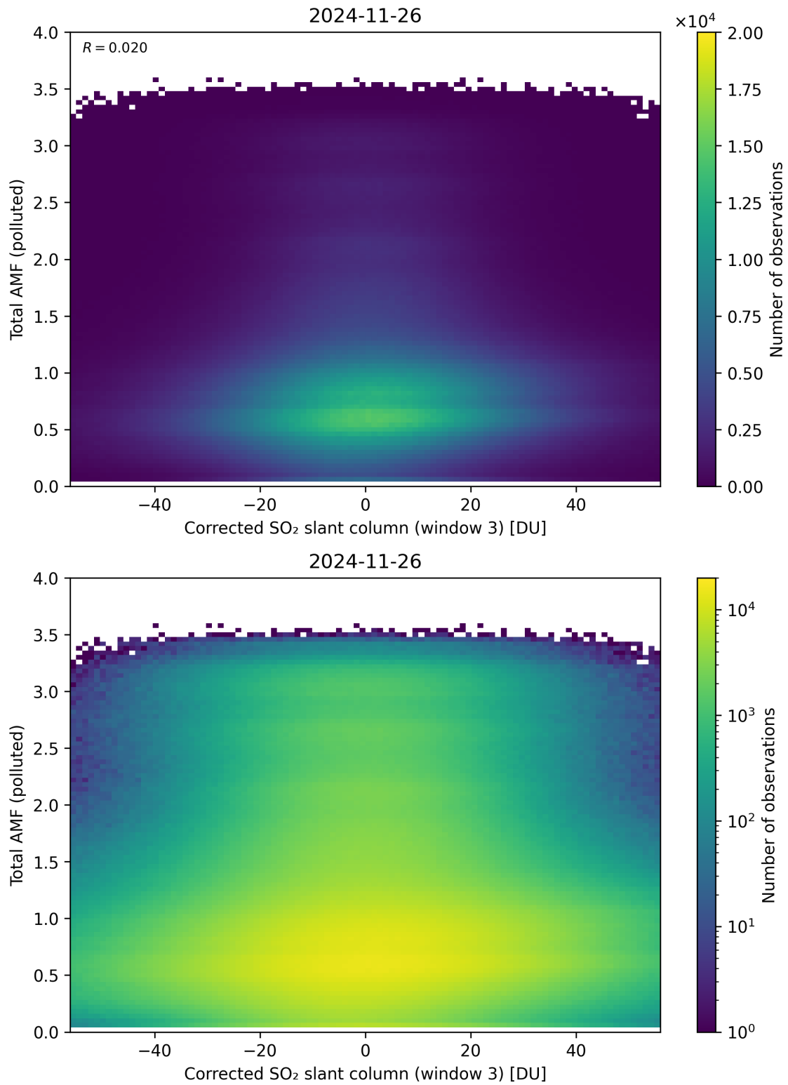
Figure 260: Scatter density plot of “Corrected SO 2 slant column (window 3)” against “Total AMF (polluted)” for 2024-11-25 to 2024-11-27.
