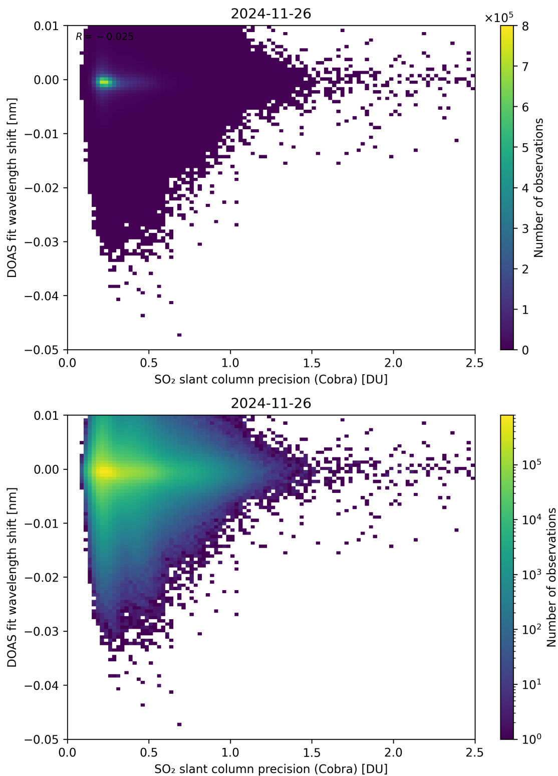
Figure 202: Scatter density plot of “SO 2 slant column precision (Cobra)” against “DOAS fit wavelength shift” for 2024-11-25 to 2024-11-27.
