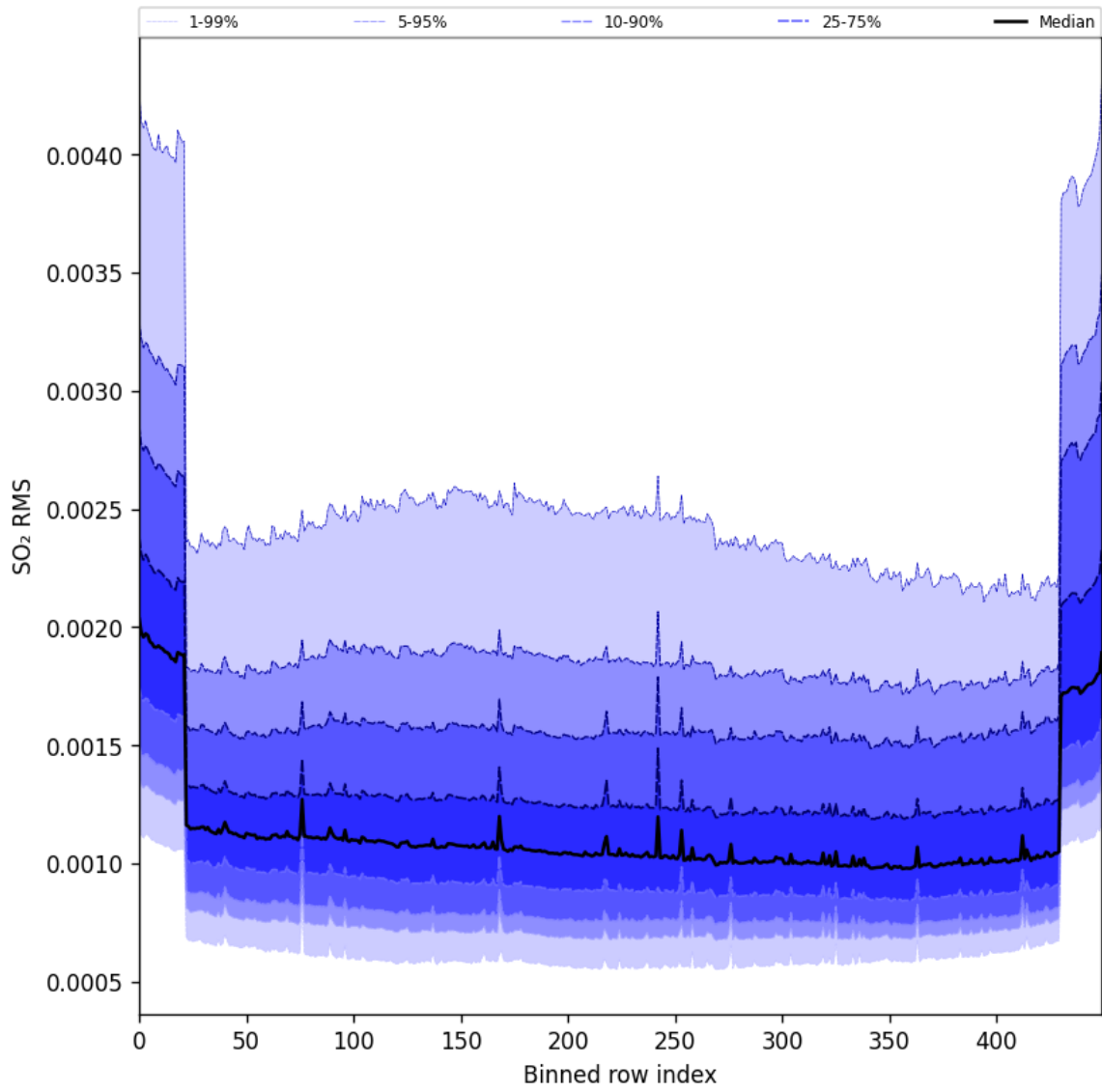
Figure 104: Along track statistics of “SO 2 RMS” for 2024-11-25 to 2024-11-27
