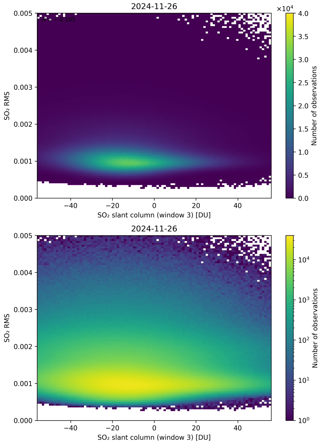
Figure 306: Scatter density plot of “SO 2 slant column (window 3)” against “SO 2 RMS” for 2024-11-25 to 2024-11-27.
