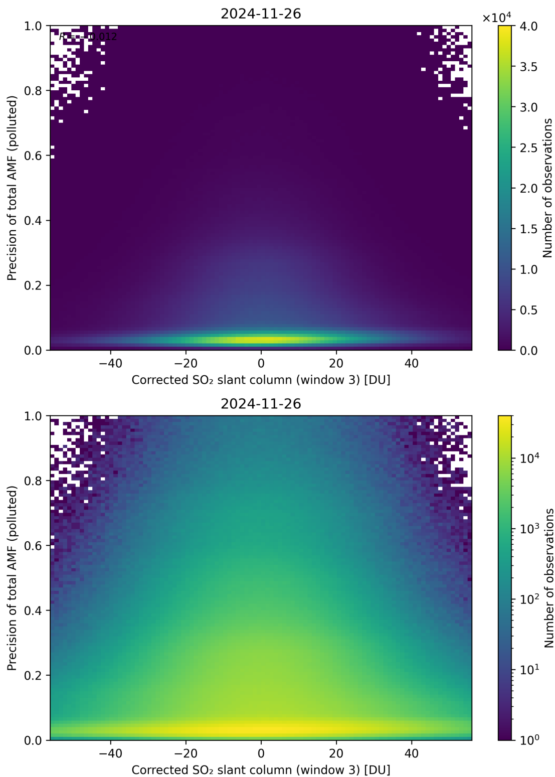
Figure 261: Scatter density plot of “Corrected SO 2 slant column (window 3)” against “Precision of total AMF (polluted)” for 2024-11-25 to 2024-11-27.
