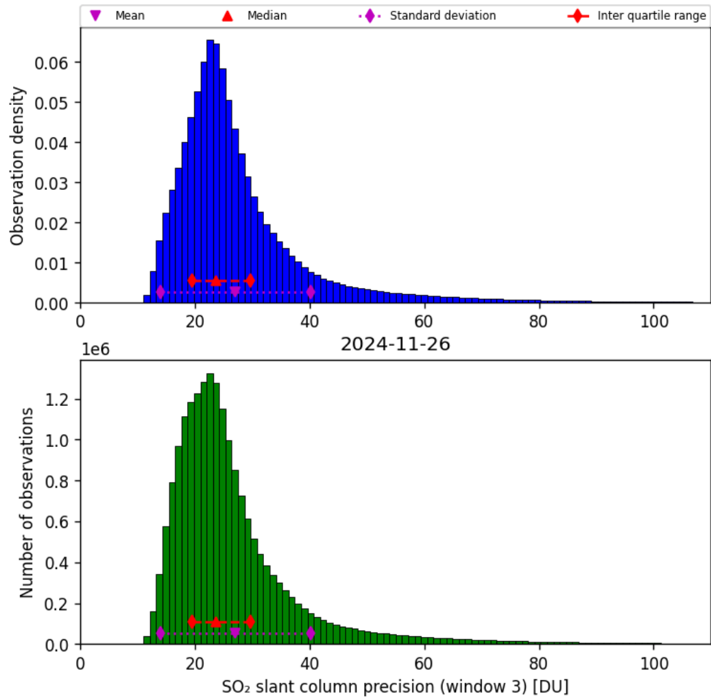
Figure 72: Histogram of “SO 2 slant column precision (window 3)” for 2024-11-25 to 2024-11-27
