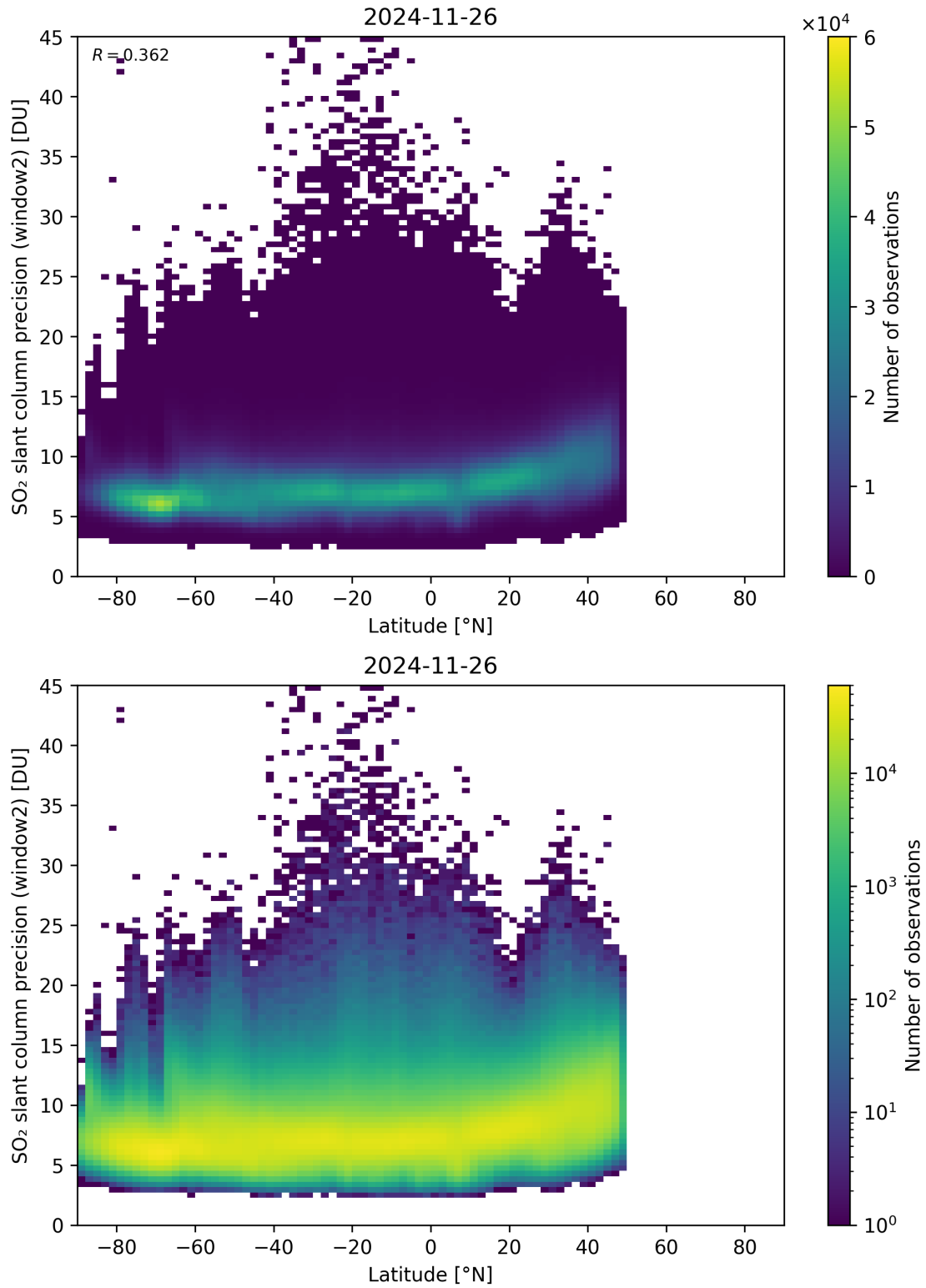
Figure 164: Scatter density plot of “Latitude” against “SO 2 slant column precision (window2)” for 2024-11-25 to 2024-11-27.
