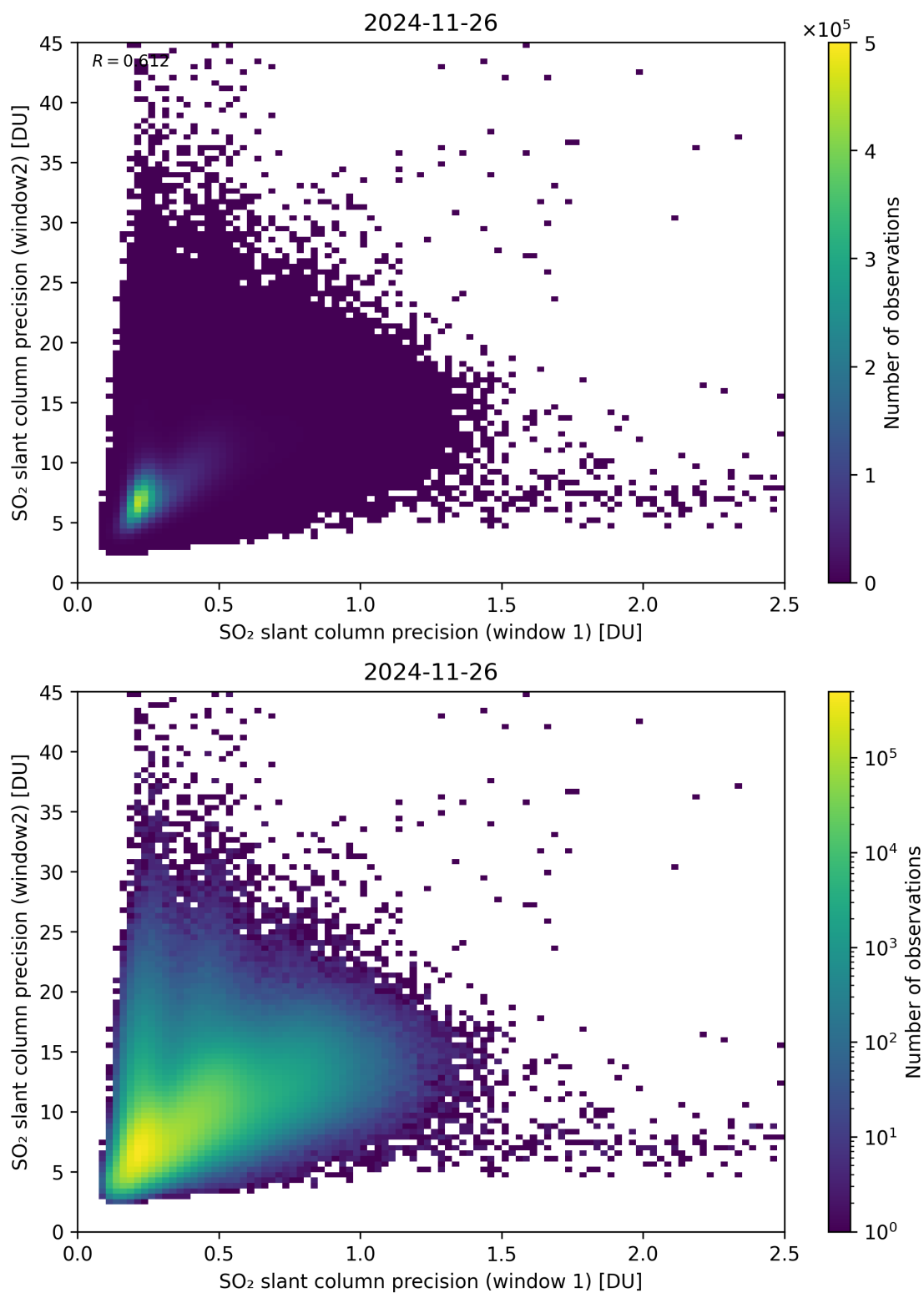
Figure 277: Scatter density plot of “SO 2 slant column precision (window 1)” against “SO 2 slant column precision (window2)” for 2024-11-25 to 2024-11-27.
