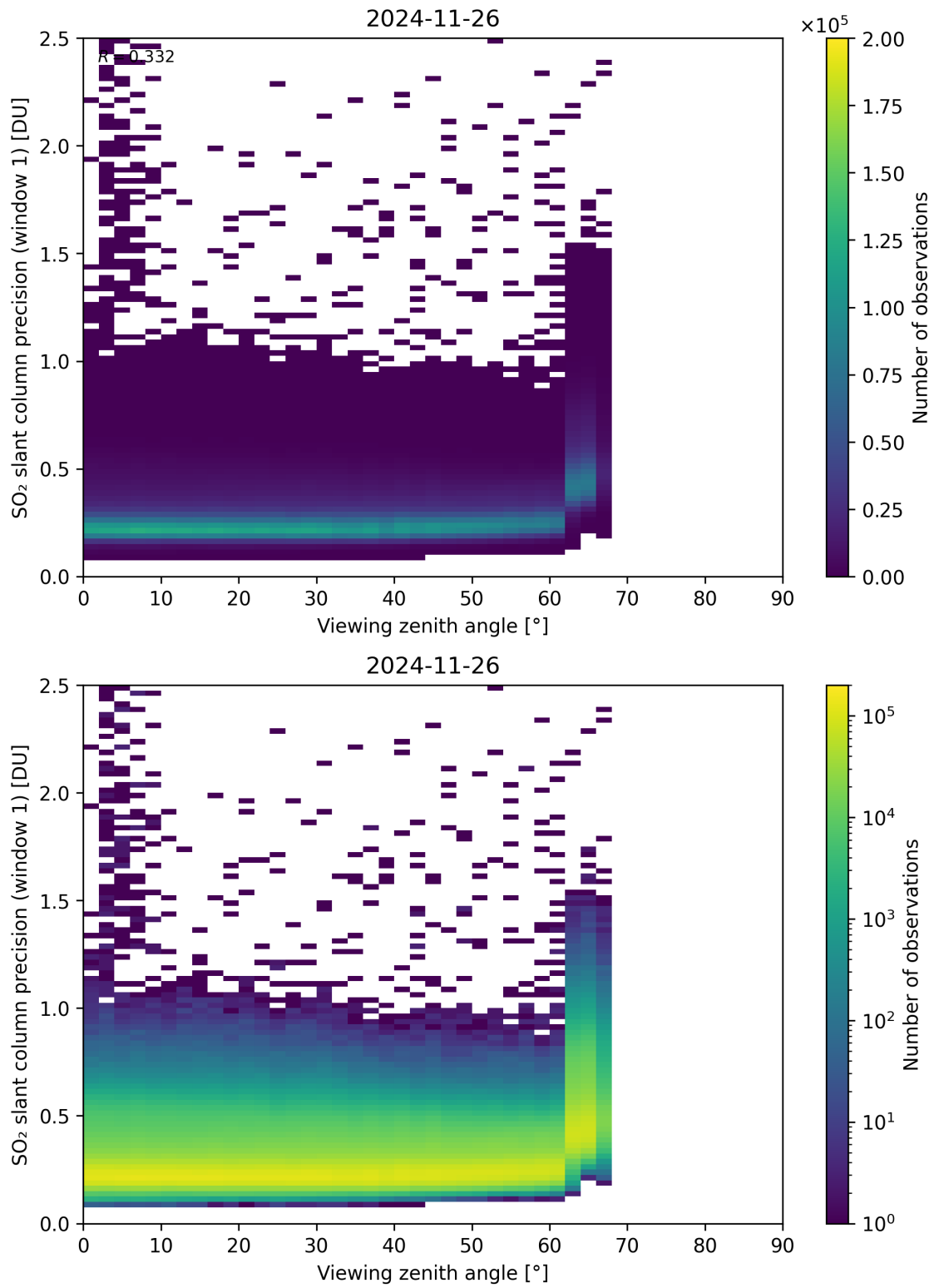
Figure 377: Scatter density plot of “Viewing zenith angle” against “SO 2 slant column precision (window 1)” for 2024-11-25 to 2024-11-27.
