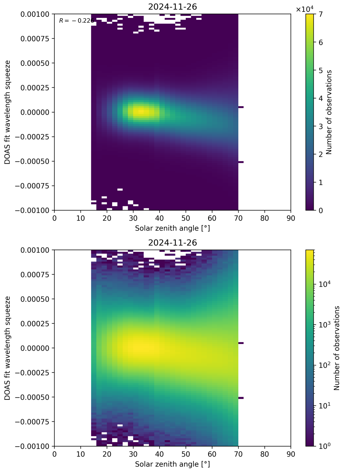
Figure 175: Scatter density plot of “Solar zenith angle” against “DOAS fit wavelength squeeze” for 2024-11-25 to 2024-11-27.
