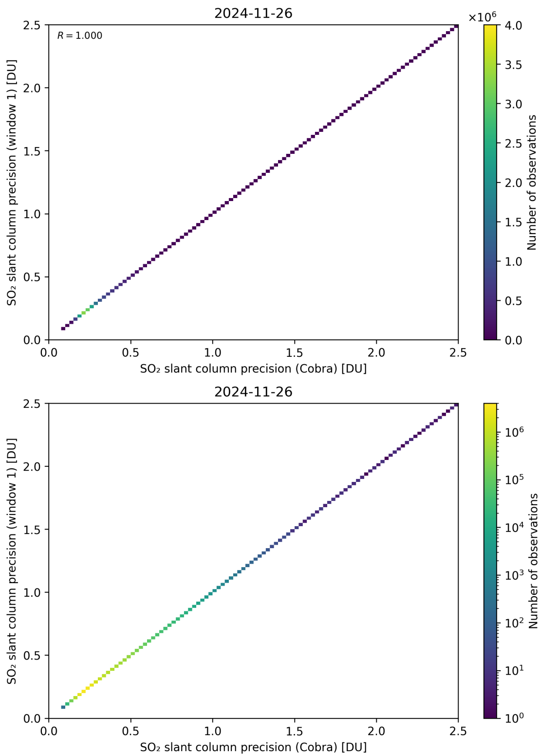
Figure 209: Scatter density plot of “SO 2 slant column precision (Cobra)” against “SO 2 slant column precision (window 1)” for 2024-11-25 to 2024-11-27.
