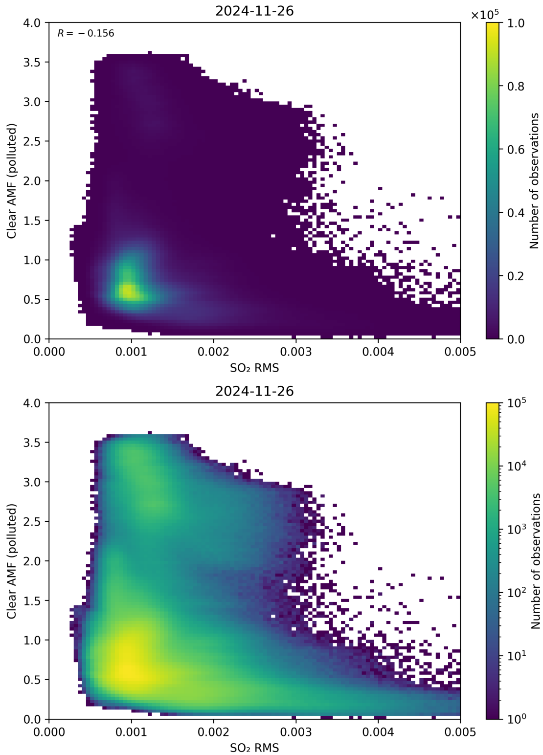
Figure 147: Scatter density plot of “SO 2 RMS” against “Clear AMF (polluted)” for 2024-11-25 to 2024-11-27.
