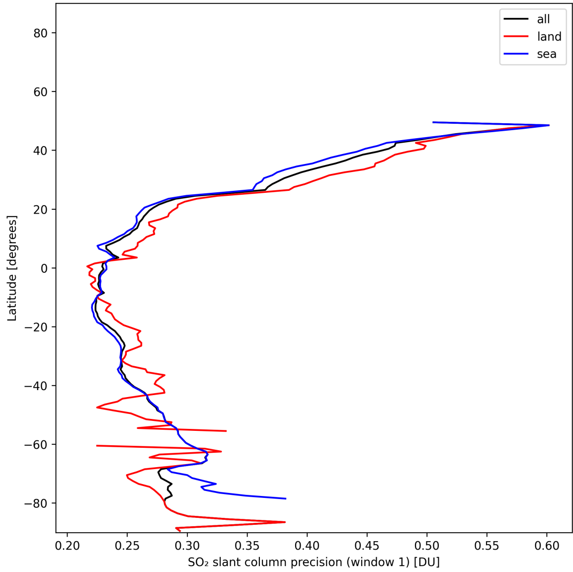
Figure 38: Zonal average of "SO 2 slant column precision (window 1)" for 2024-11-25 to 2024-11-27.
