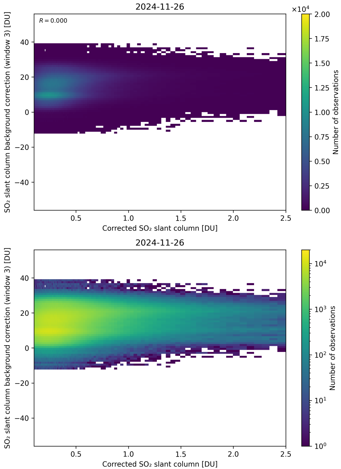
Figure 228: Scatter density plot of “Corrected SO 2 slant column” against “SO 2 slant column background correction (window 3)” for 2024-11-25 to 2024-11-27.
