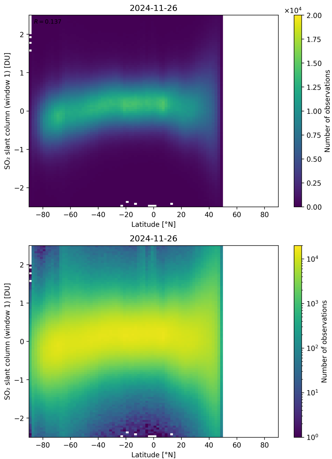
Figure 162: Scatter density plot of “Latitude” against “SO 2 slant column (window 1)” for 2024-11-25 to 2024-11-27.
