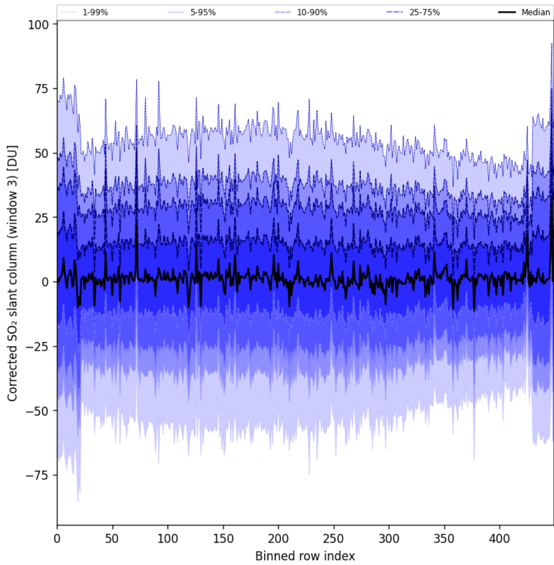
Figure 99: Along track statistics of “Corrected SO 2 slant column (window 3)” for 2024-11-25 to 2024-11-27
