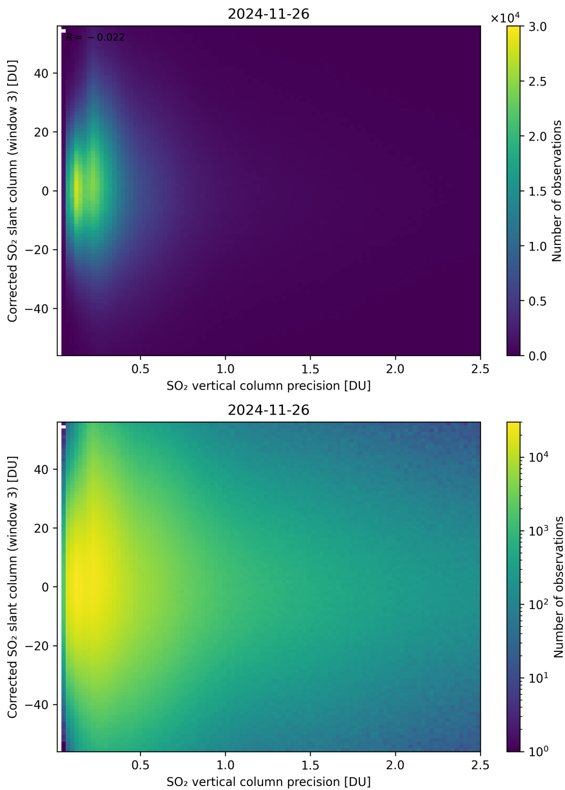
Figure 340: Scatter density plot of “SO 2 vertical column precision” against “Corrected SO 2 slant column (window 3)” for 2024-11-25 to 2024-11-27.
