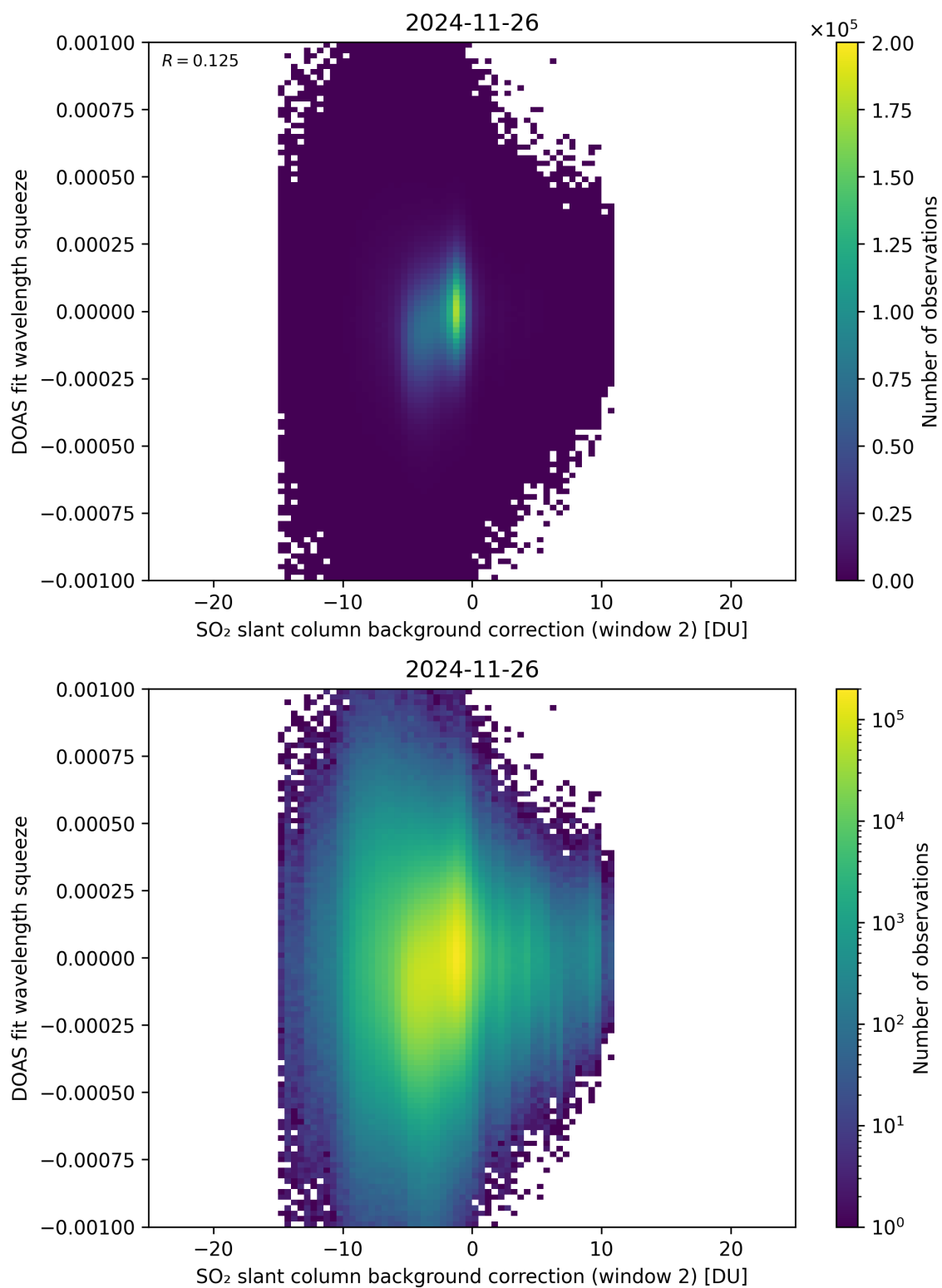
Figure 124: Scatter density plot of “SO 2 slant column background correction (window 2)” against “DOAS fit wavelength squeeze” for 2024-11-25 to 2024-11-27.
