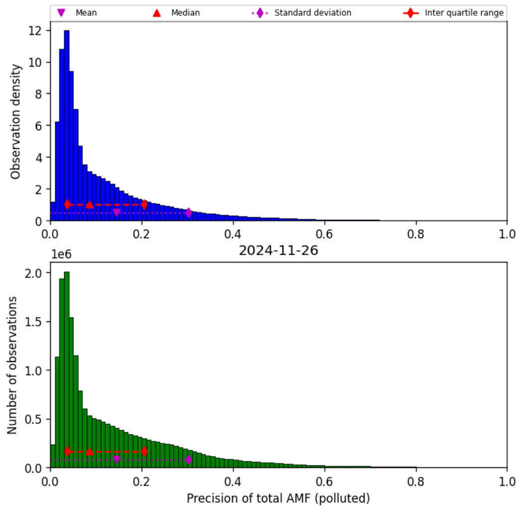
Figure 80: Histogram of “Precision of total AMF (polluted)” for 2024-11-25 to 2024-11-27
