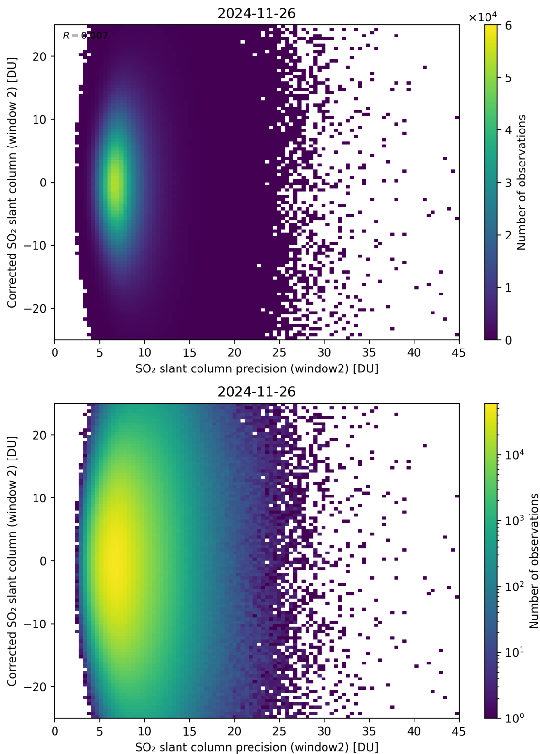
Figure 297: Scatter density plot of “SO 2 slant column precision (window2)” against “Corrected SO 2 slant column (window 2)” for 2024-11-25 to 2024-11-27.
