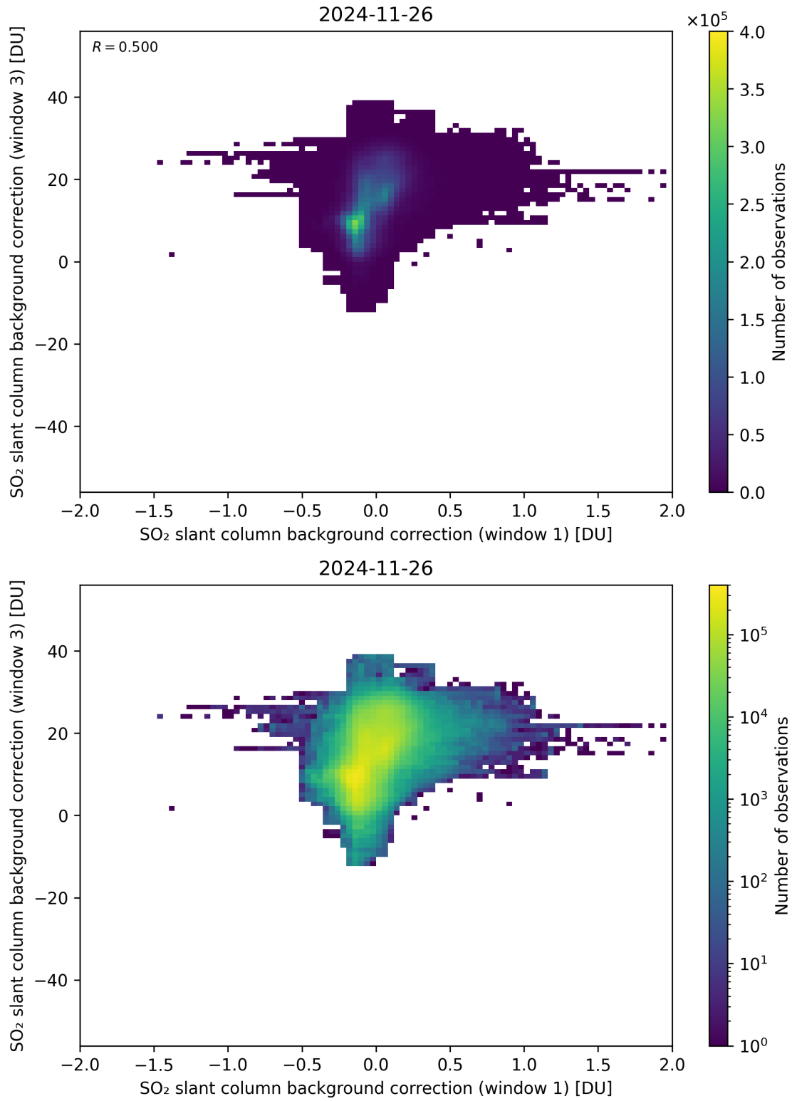
Figure 110: Scatter density plot of “SO 2 slant column background correction (window 1)” against “SO 2 slant column background correction (window 3)” for 2024-11-25 to 2024-11-27.
