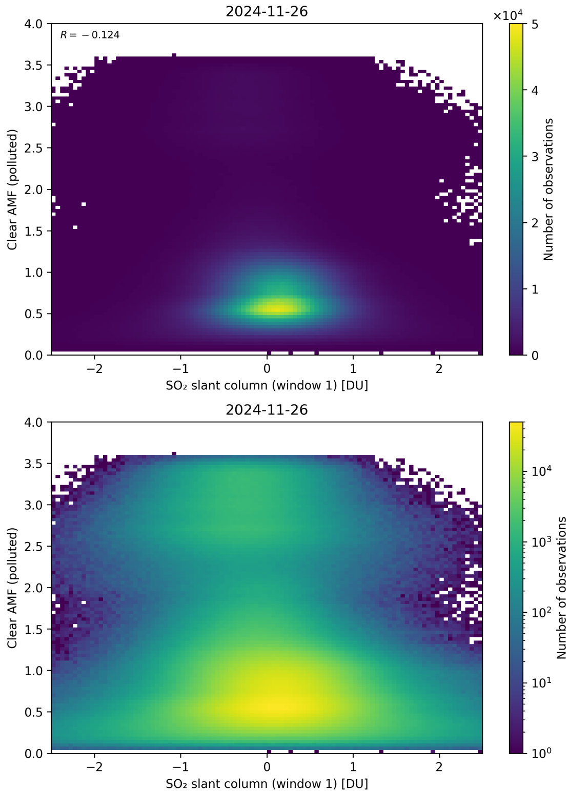
Figure 282: Scatter density plot of “SO 2 slant column (window 1)” against “Clear AMF (polluted)” for 2024-11-25 to 2024-11-27.
