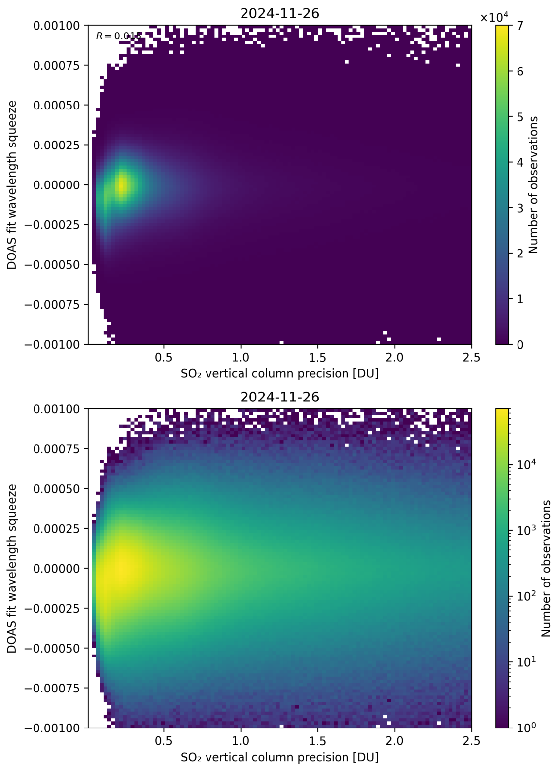
Figure 333: Scatter density plot of “SO 2 vertical column precision” against “DOAS fit wavelength squeeze” for 2024-11-25 to 2024-11-27.
