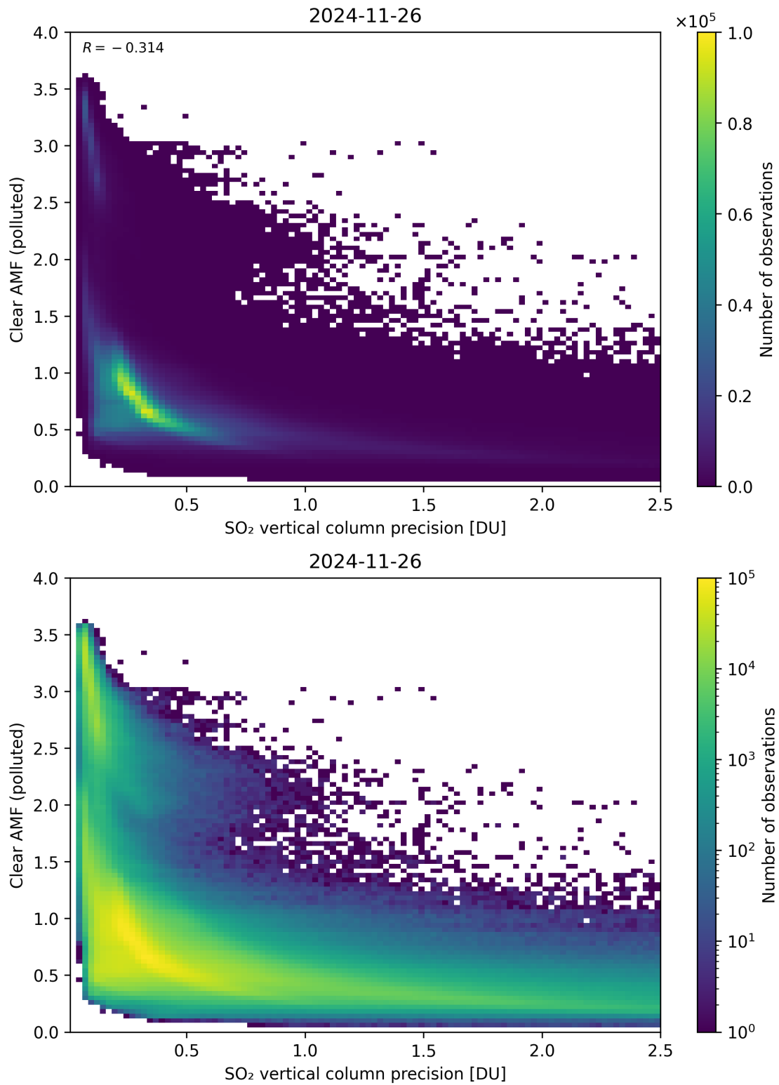
Figure 335: Scatter density plot of “SO 2 vertical column precision” against “Clear AMF (polluted)” for 2024-11-25 to 2024-11-27.
