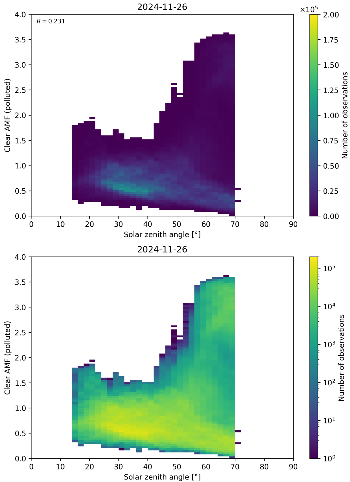
Figure 178: Scatter density plot of “Solar zenith angle” against “Clear AMF (polluted)” for 2024-11-25 to 2024-11-27.
