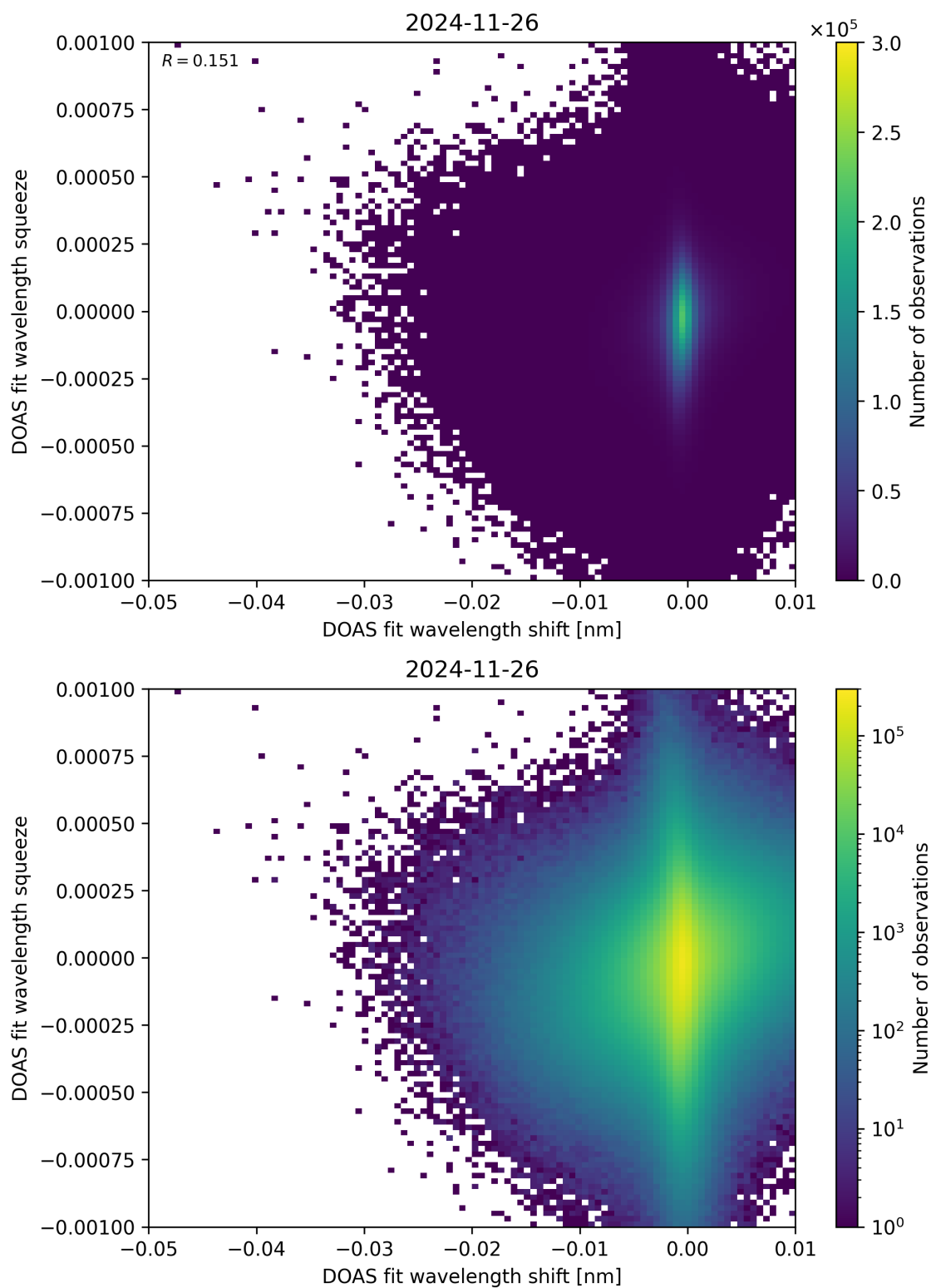
Figure 138: Scatter density plot of “DOAS fit wavelength shift” against “DOAS fit wavelength squeeze” for 2024-11-25 to 2024-11-27.
