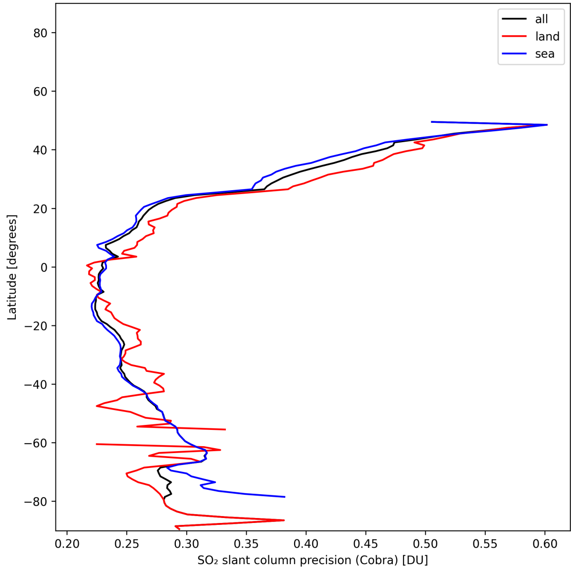
Figure 36: Zonal average of “SO 2 slant column precision (Cobra)” for 2024-11-25 to 2024-11-27.
