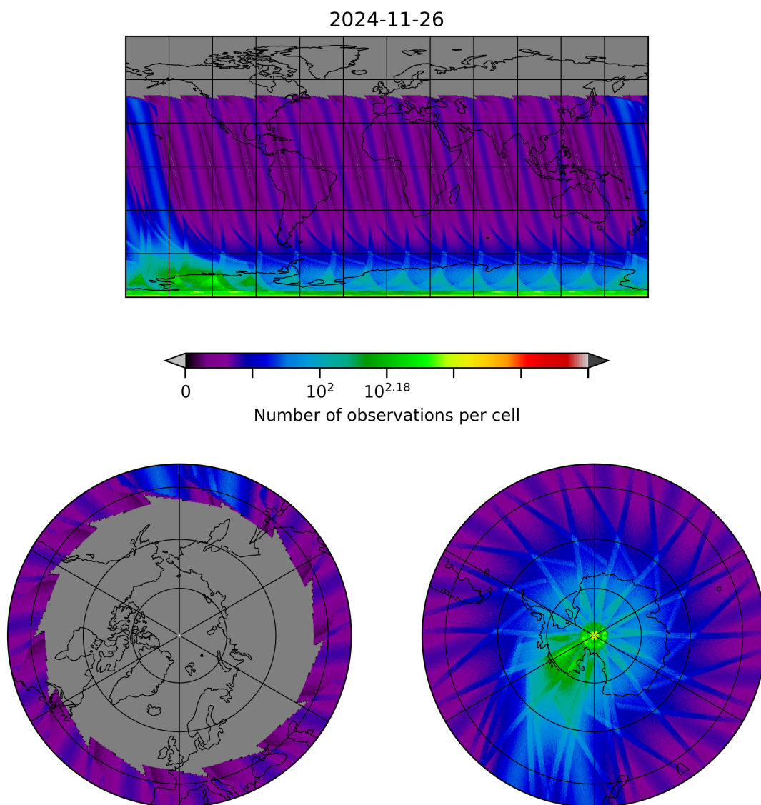
Figure 30: Map of the number of observations for 2024-11-25 to 2024-11-27
