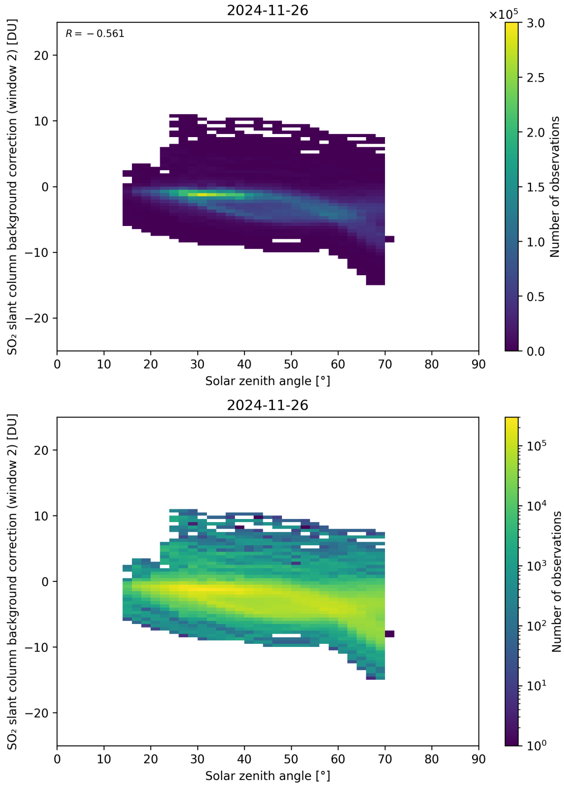
Figure 172: Scatter density plot of “Solar zenith angle” against “SO 2 slant column background correction (window 2)” for 2024-11-25 to 2024-11-27.
