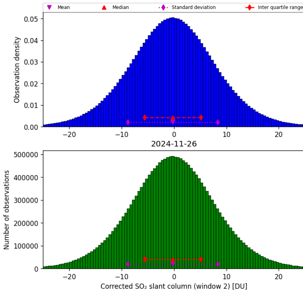
Figure 69: Histogram of “Corrected SO 2 slant column (window 2)” for 2024-11-25 to 2024-11-27
