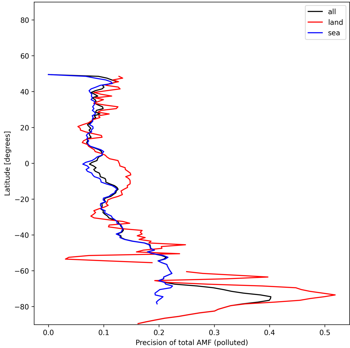
Figure 54: Zonal average of “Precision of total AMF (polluted)” for 2024-11-25 to 2024-11-27.
