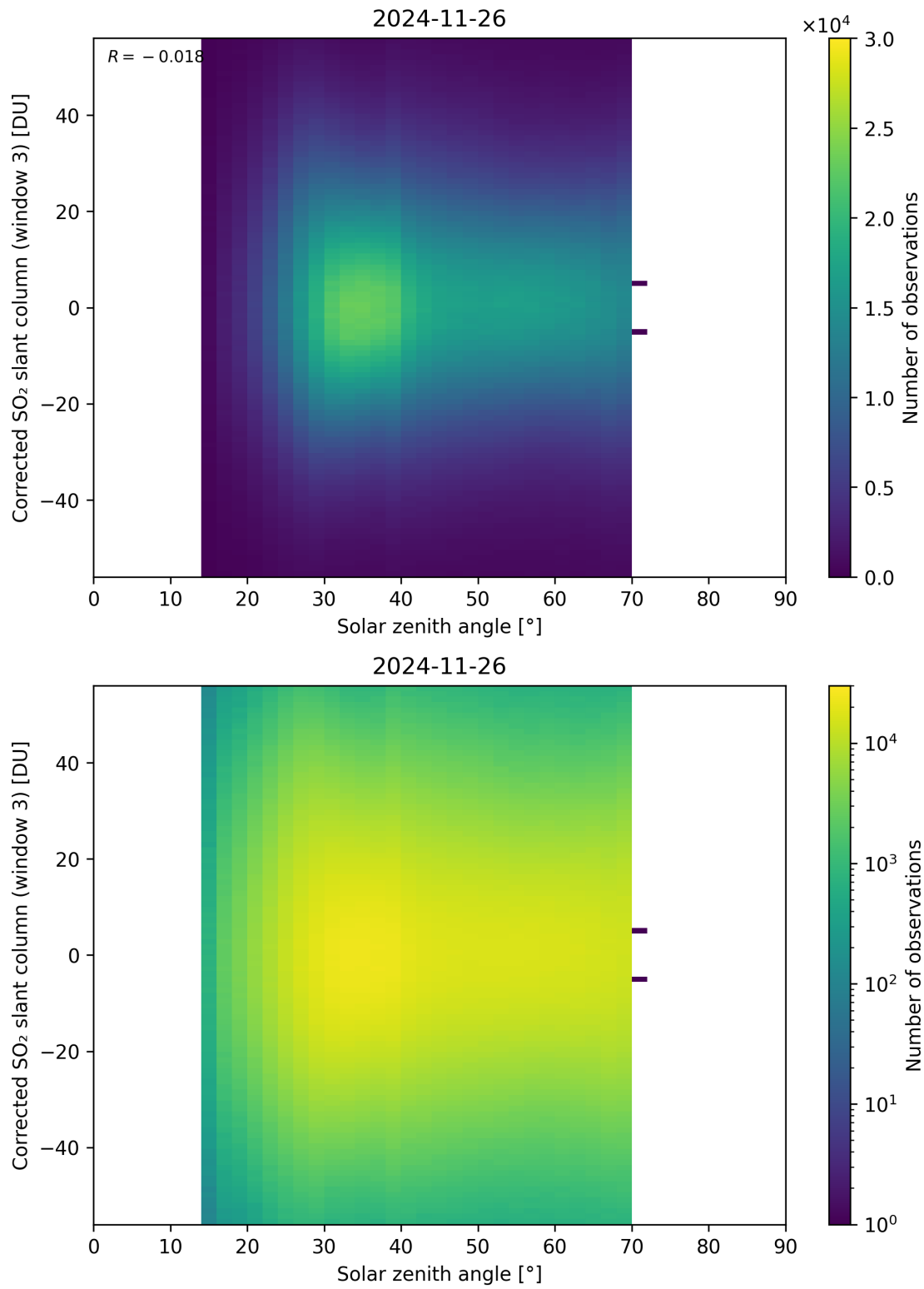
Figure 183: Scatter density plot of “Solar zenith angle” against “Corrected SO 2 slant column (window 3)” for 2024-11-25 to 2024-11-27.
