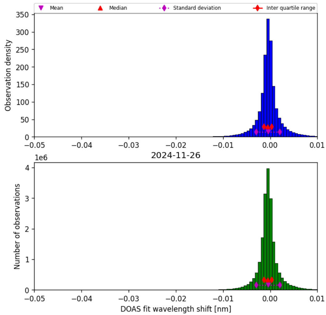
Figure 76: Histogram of “DOAS fit wavelength shift” for 2024-11-25 to 2024-11-27
