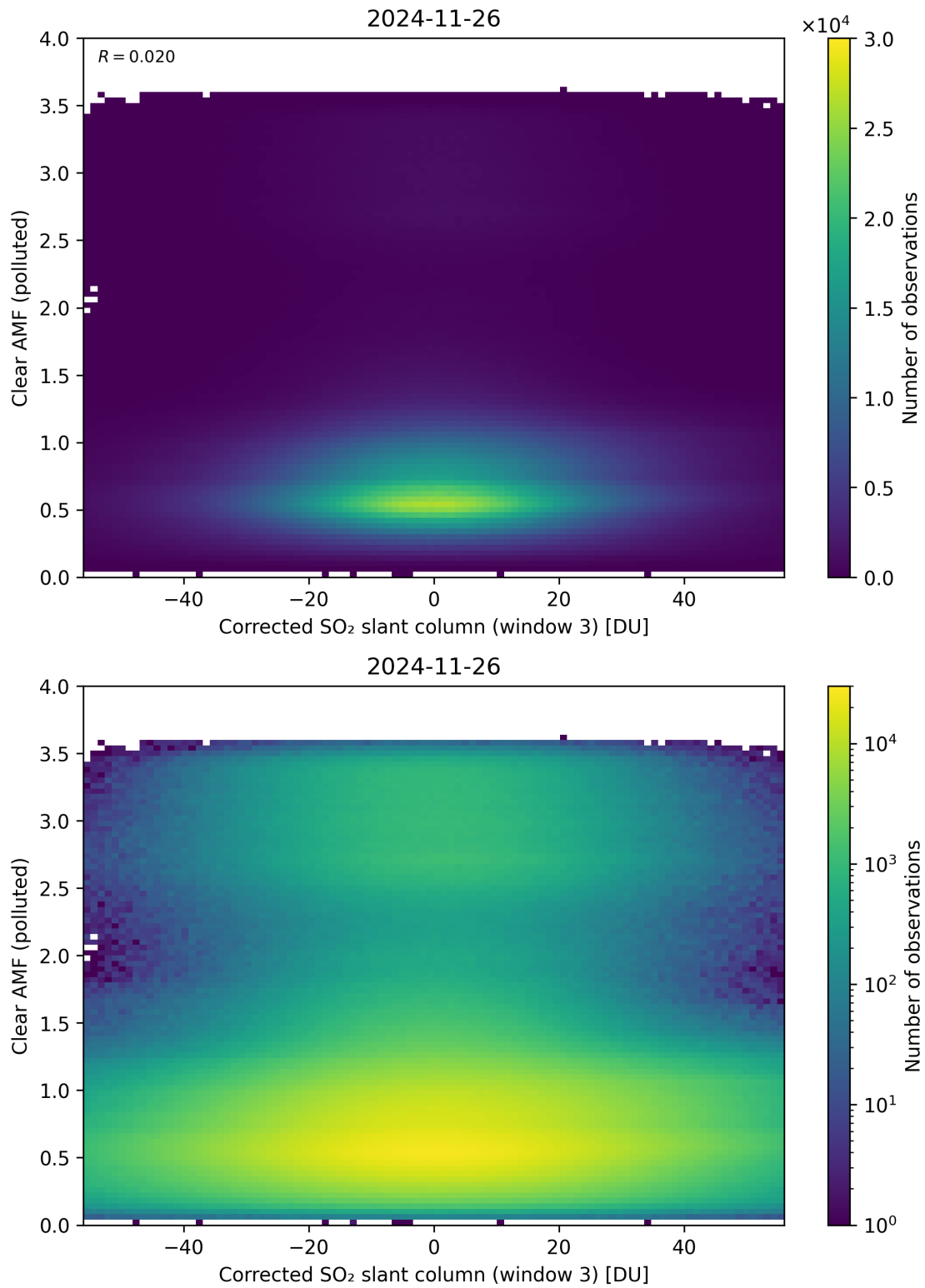
Figure 259: Scatter density plot of “Corrected SO 2 slant column (window 3)” against “Clear AMF (polluted)” for 2024-11-25 to 2024-11-27.
