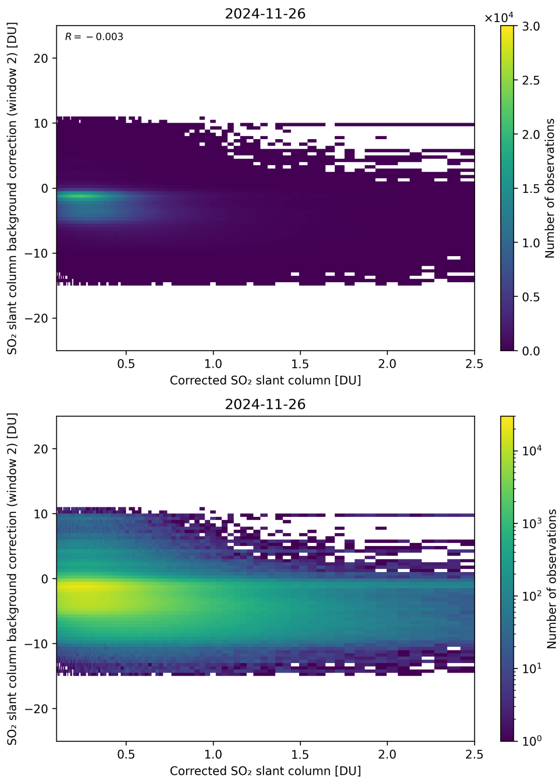
Figure 227: Scatter density plot of “Corrected SO 2 slant column” against “SO 2 slant column background correction (window 2)” for 2024-11-25 to 2024-11-27.
