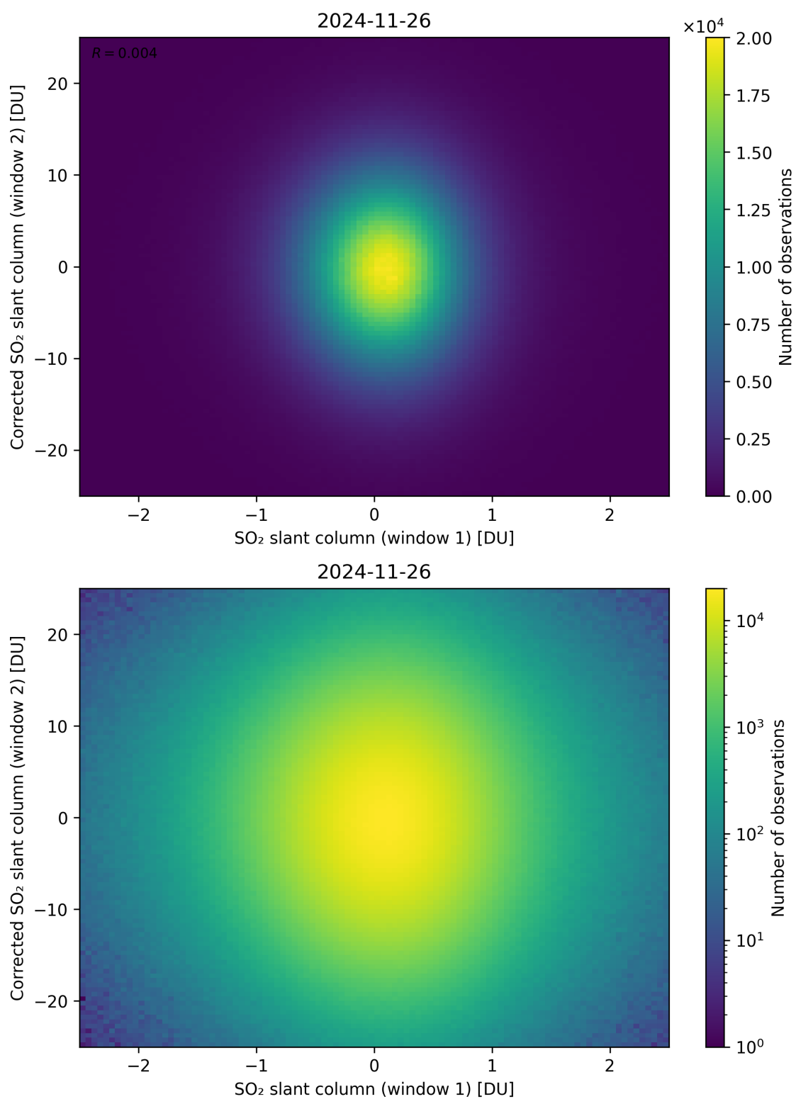
Figure 283: Scatter density plot of “SO 2 slant column (window 1)” against “Corrected SO 2 slant column (window 2)” for 2024-11-25 to 2024-11-27.
