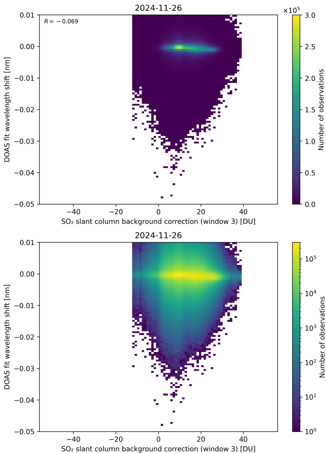
Figure 132: Scatter density plot of “SO 2 slant column background correction (window 3)” against “DOAS fit wavelength shift” for 2024-11-25 to 2024-11-27.
