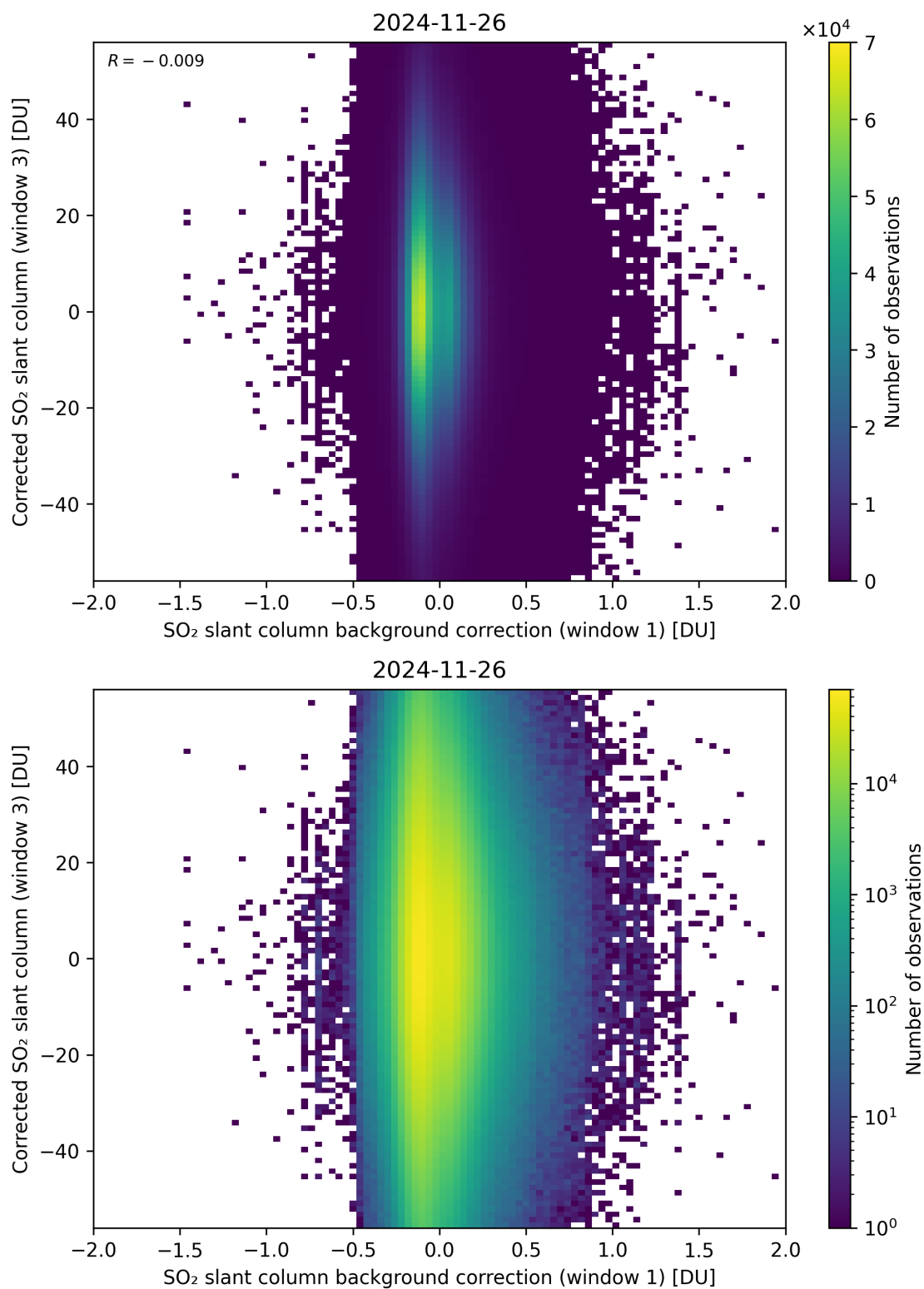
Figure 116: Scatter density plot of “SO 2 slant column background correction (window 1)” against “Corrected SO 2 slant column (window 3)” for 2024-11-25 to 2024-11-27.
