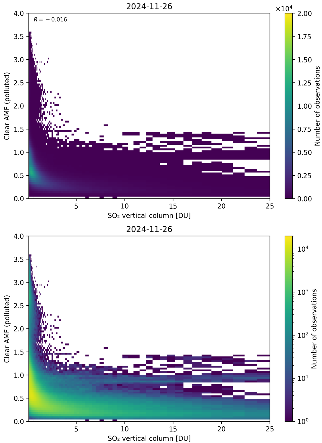
Figure 348: Scatter density plot of “SO 2 vertical column” against “Clear AMF (polluted)” for 2024-11-25 to 2024-11-27.
