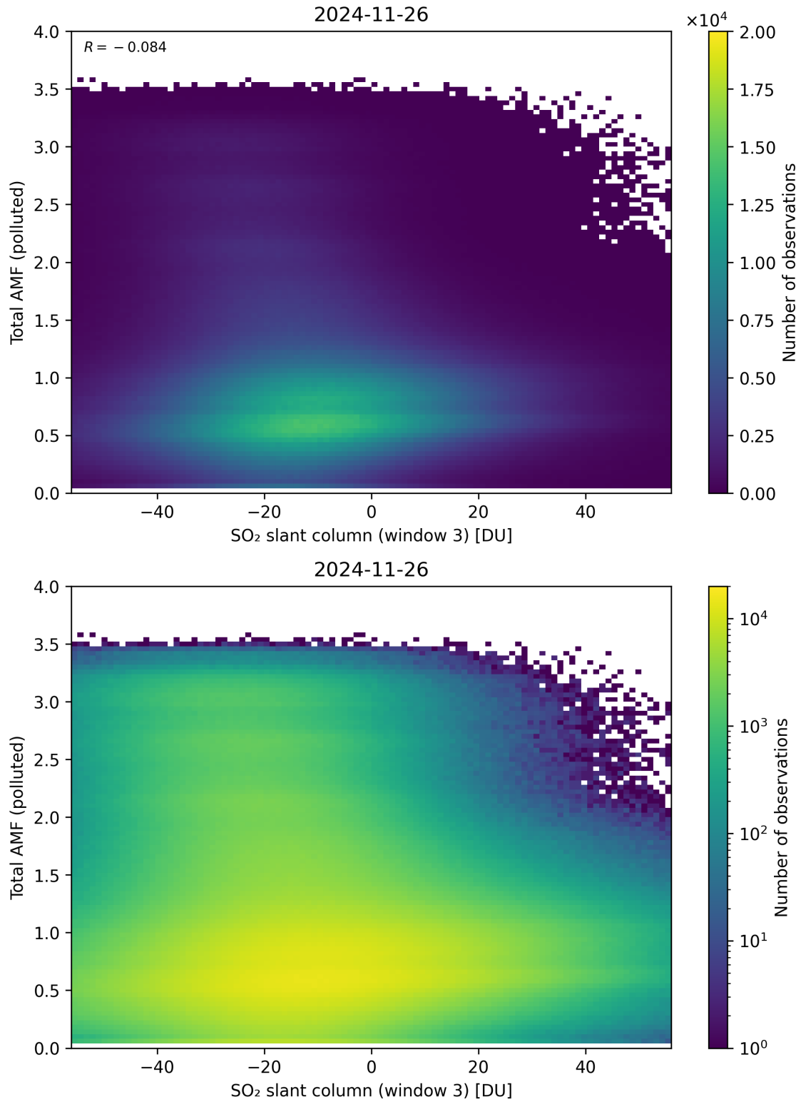
Figure 318: Scatter density plot of “SO 2 slant column (window 3)” against “Total AMF (polluted)” for 2024-11-25 to 2024-11-27.
