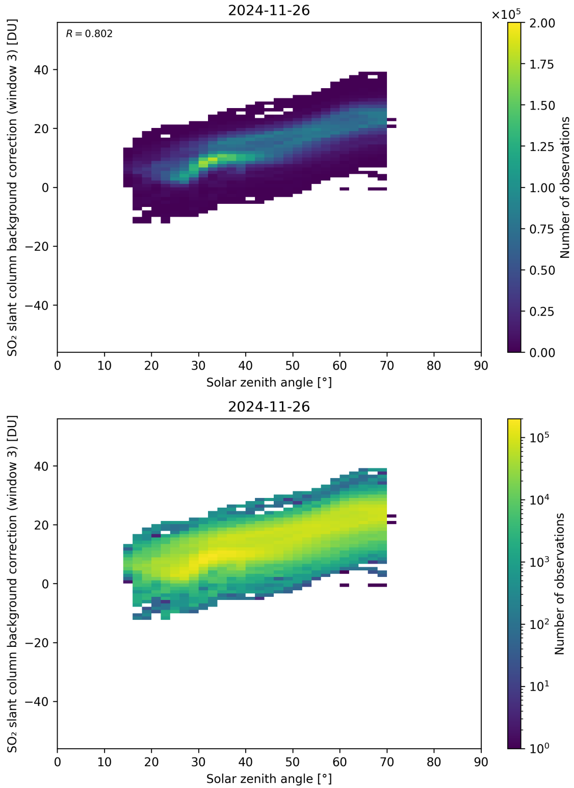
Figure 173: Scatter density plot of “Solar zenith angle” against “SO 2 slant column background correction (window 3)” for 2024-11-25 to 2024-11-27.
