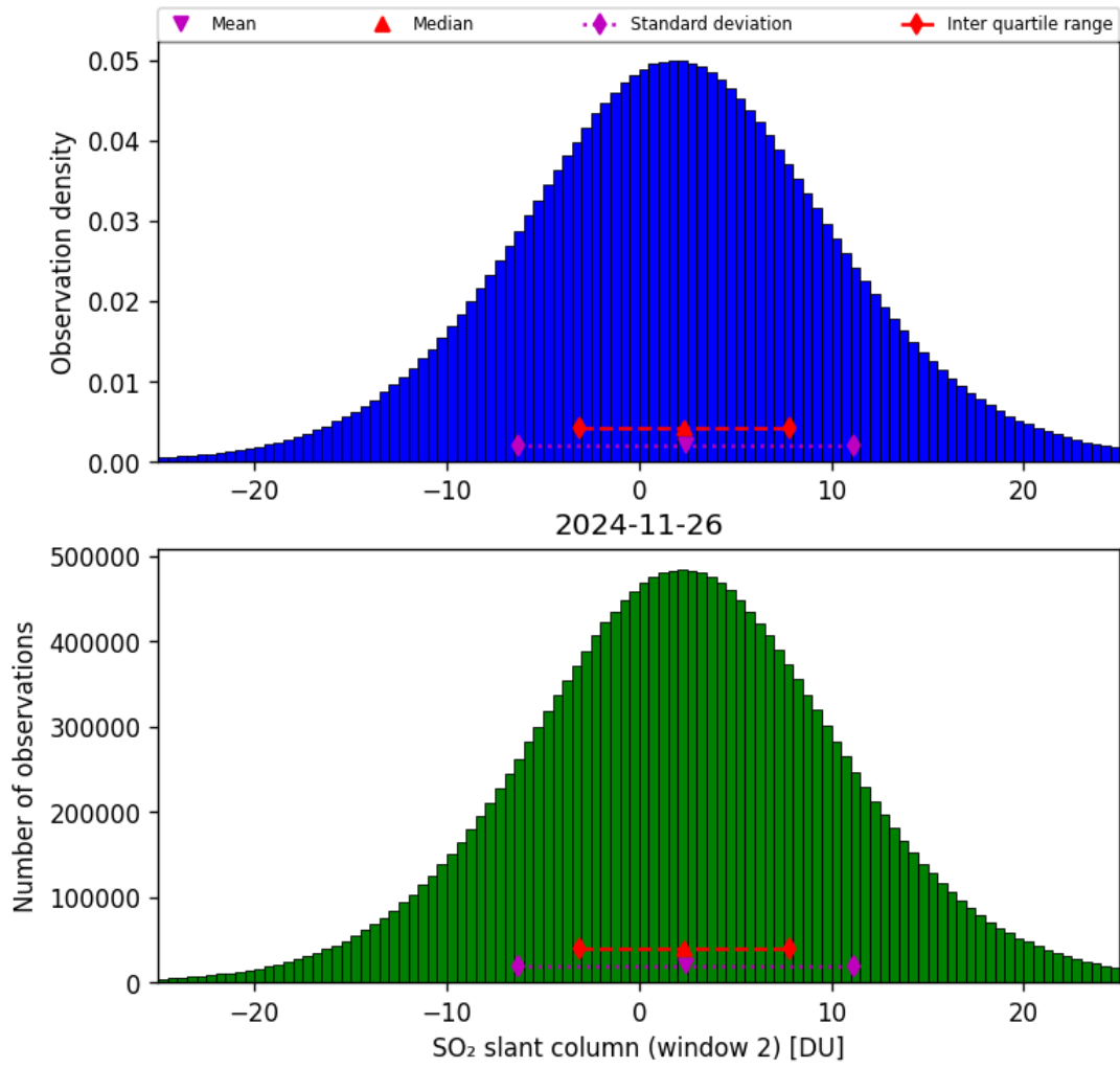
Figure 67: Histogram of “SO 2 slant column (window 2)” for 2024-11-25 to 2024-11-27
