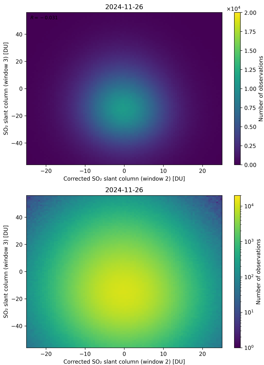
Figure 251: Scatter density plot of “Corrected SO 2 slant column (window 2)” against “SO 2 slant column (window 3)” for 2024-11-25 to 2024-11-27.
