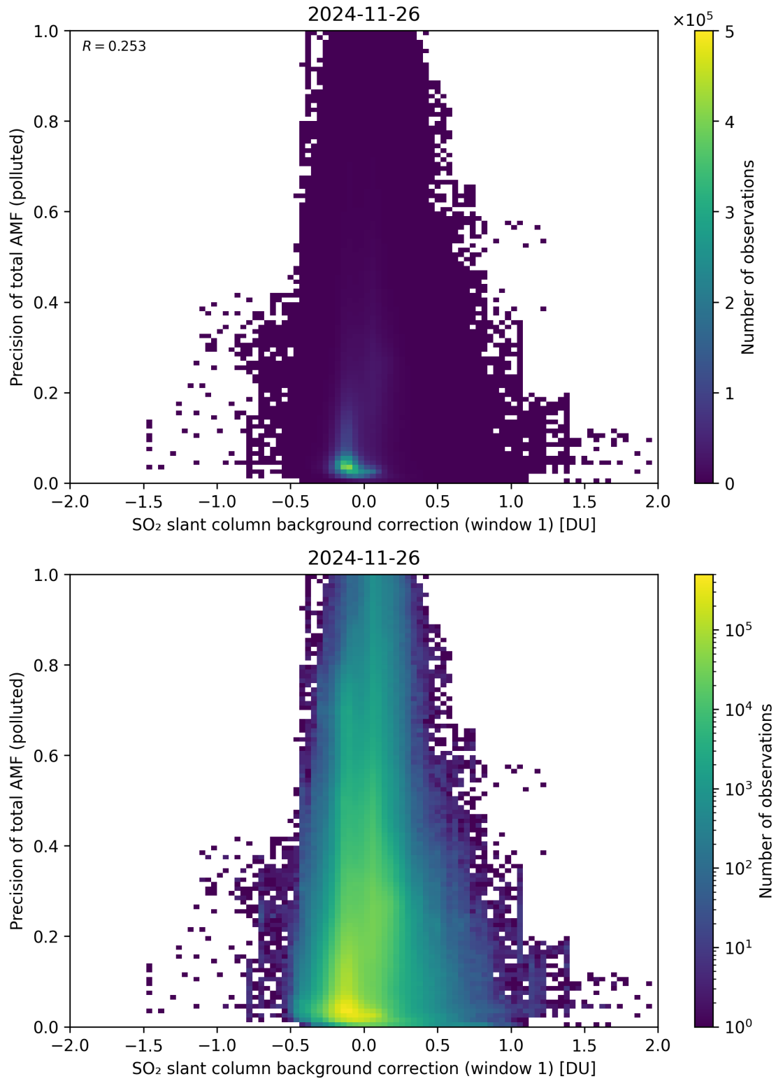
Figure 121: Scatter density plot of “SO 2 slant column background correction (window 1)” against “Precision of total AMF (polluted)” for 2024-11-25 to 2024-11-27.
