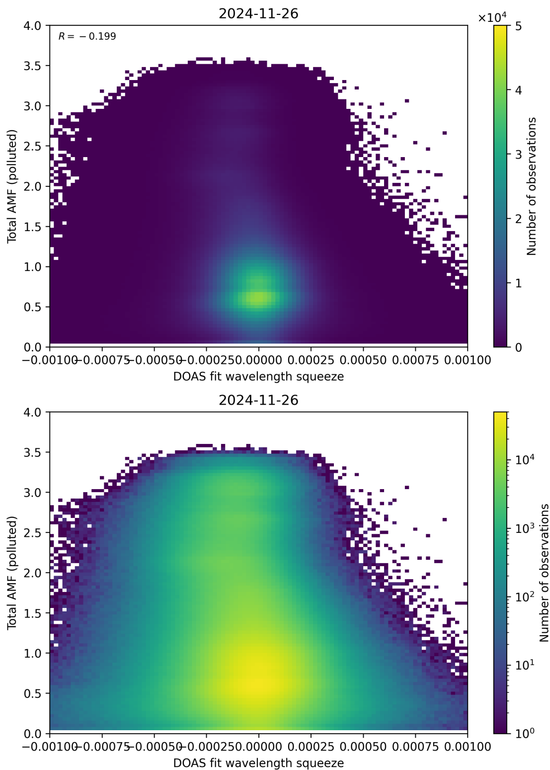
Figure 145: Scatter density plot of “DOAS fit wavelength squeeze” against “Total AMF (polluted)” for 2024-11-25 to 2024-11-27.
