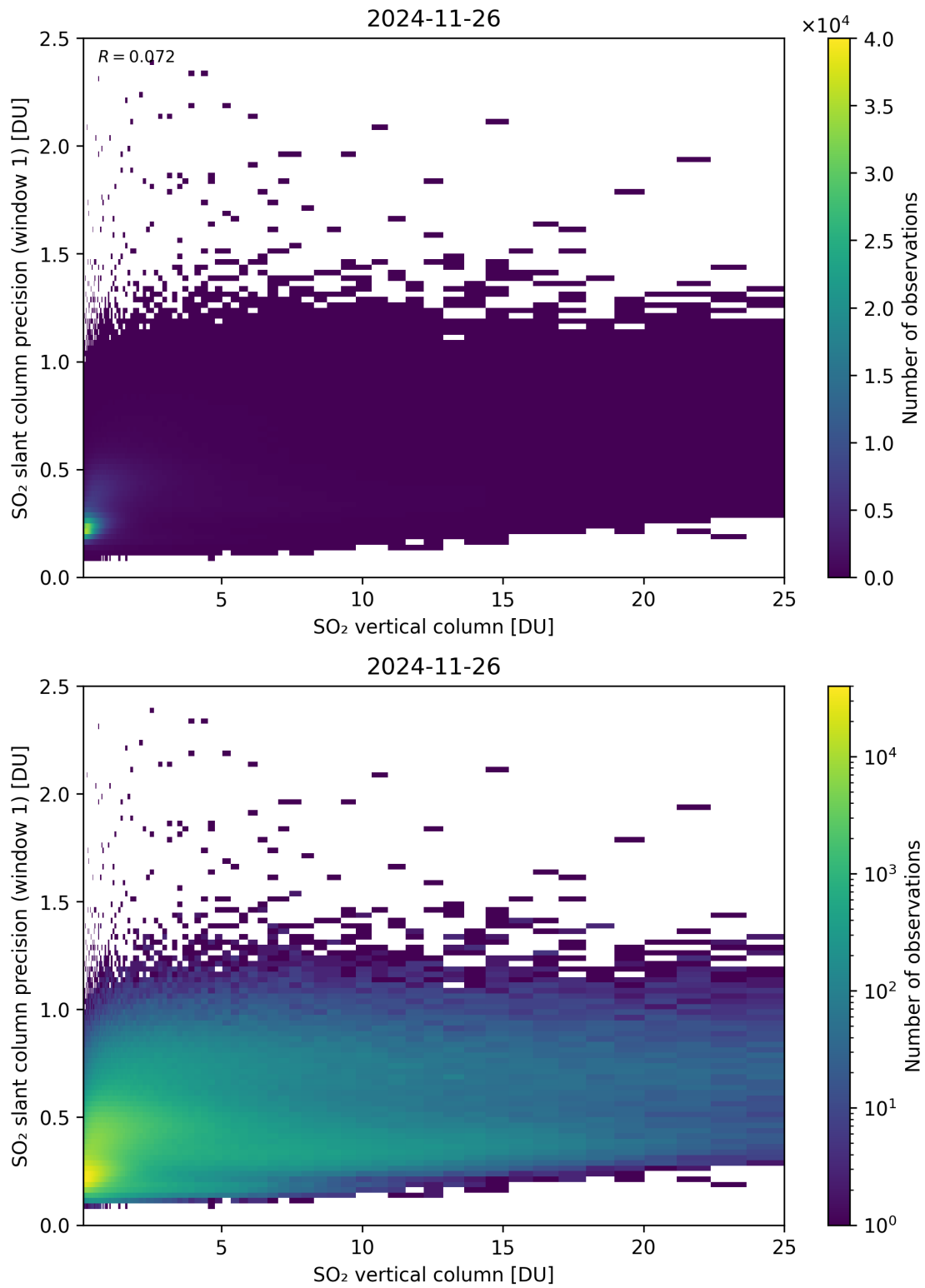
Figure 355: Scatter density plot of “SO 2 vertical column” against “SO 2 slant column precision (window 1)” for 2024-11-25 to 2024-11-27.
