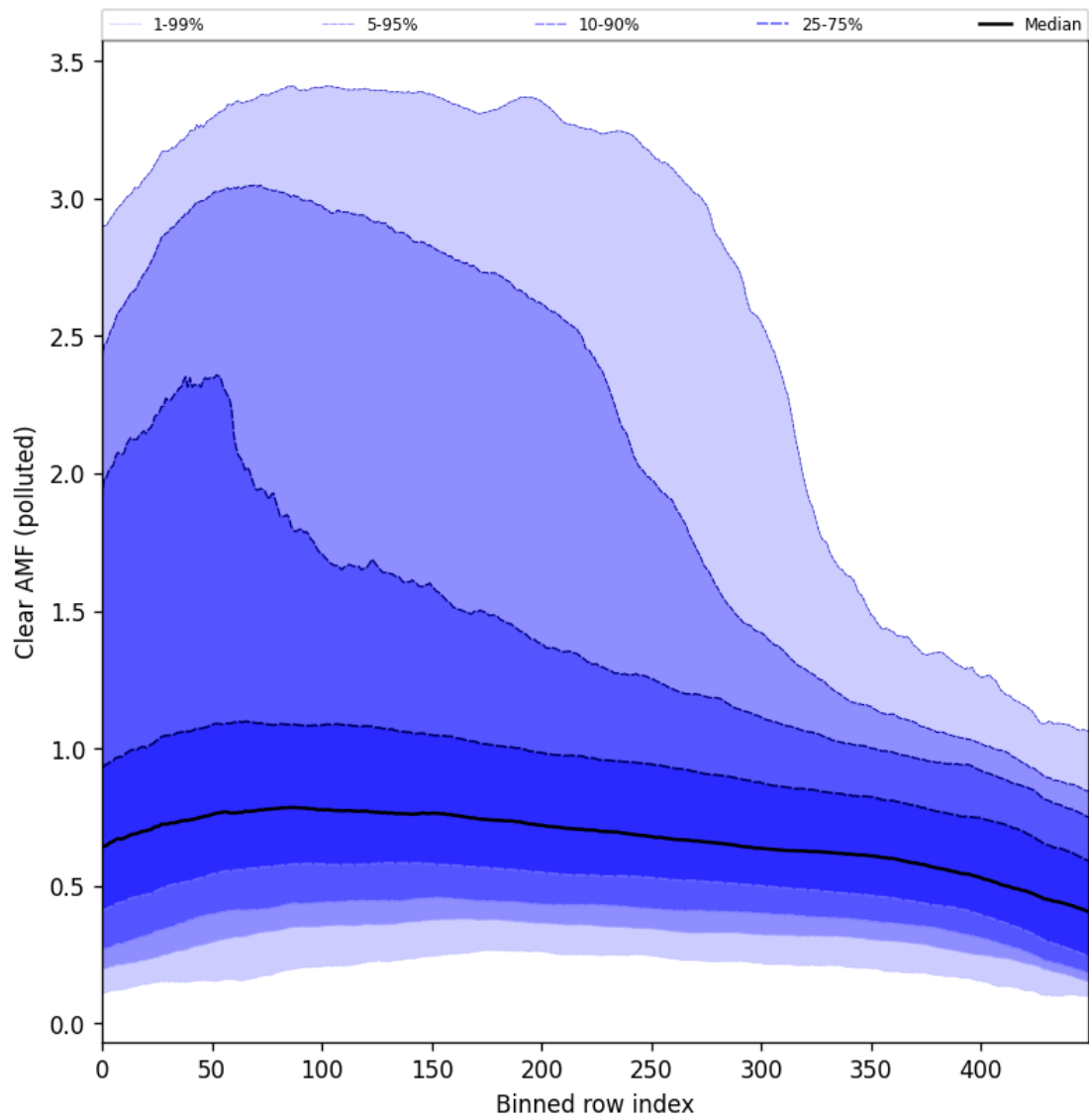
Figure 107: Along track statistics of “Clear AMF (polluted)” for 2024-11-25 to 2024-11-27
