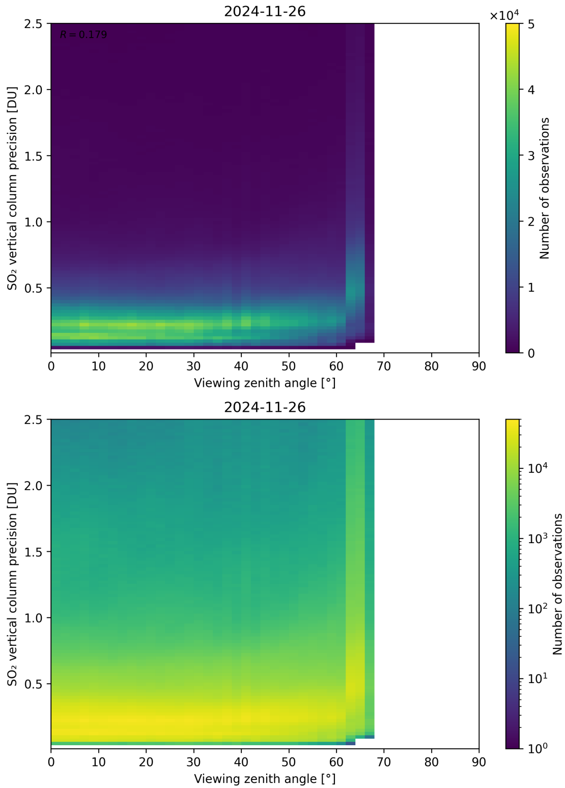
Figure 384: Scatter density plot of “Viewing zenith angle” against “SO 2 vertical column precision” for 2024-11-25 to 2024-11-27.
