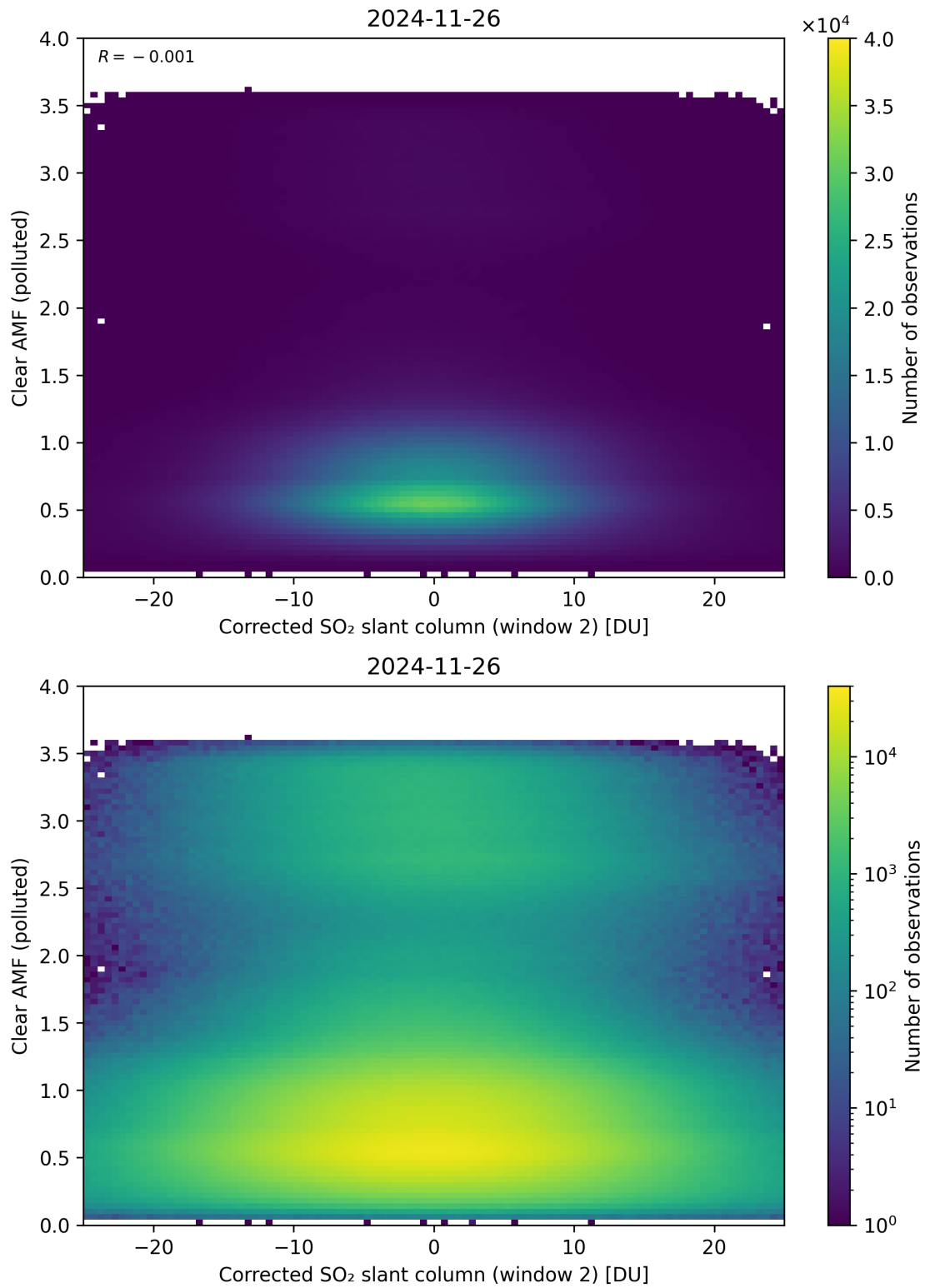
Figure 249: Scatter density plot of “Corrected SO 2 slant column (window 2)” against “Clear AMF (polluted)” for 2024-11-25 to 2024-11-27.
