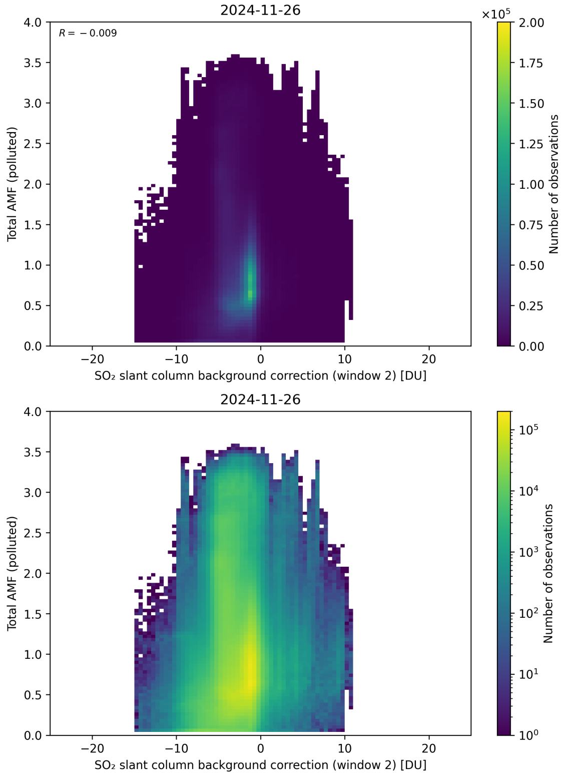
Figure 130: Scatter density plot of “SO 2 slant column background correction (window 2)” against “Total AMF (polluted)” for 2024-11-25 to 2024-11-27.
