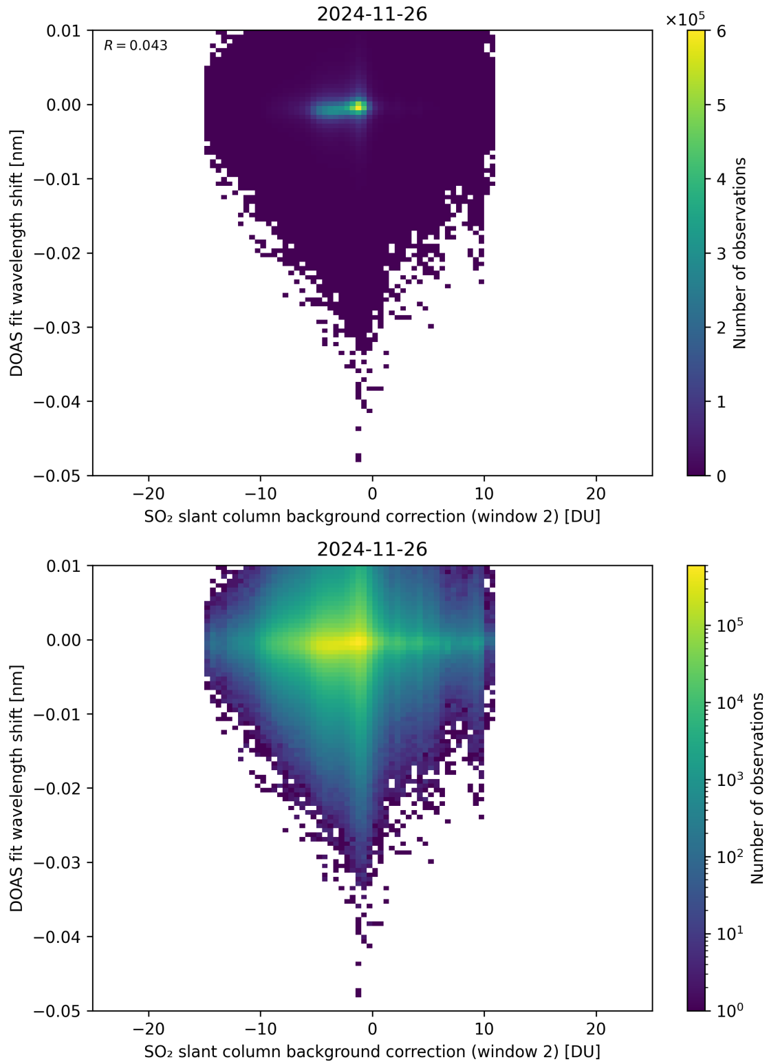
Figure 123: Scatter density plot of “SO 2 slant column background correction (window 2)” against “DOAS fit wavelength shift” for 2024-11-25 to 2024-11-27.
