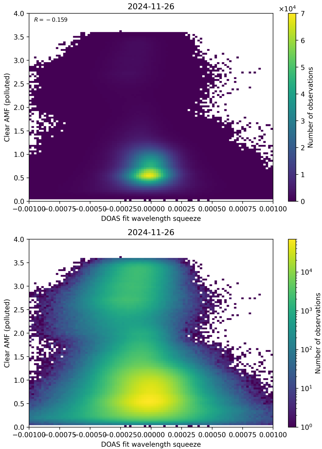
Figure 144: Scatter density plot of “DOAS fit wavelength squeeze” against “Clear AMF (polluted)” for 2024-11-25 to 2024-11-27.
