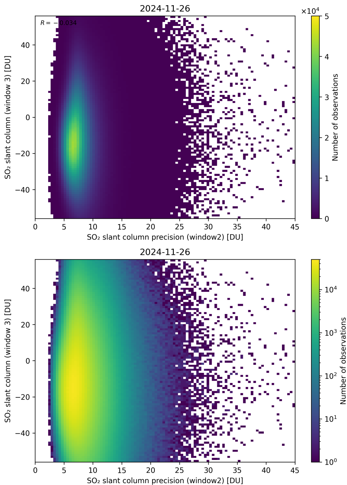
Figure 299: Scatter density plot of “SO 2 slant column precision (window2)” against “SO 2 slant column (window 3)” for 2024-11-25 to 2024-11-27.
