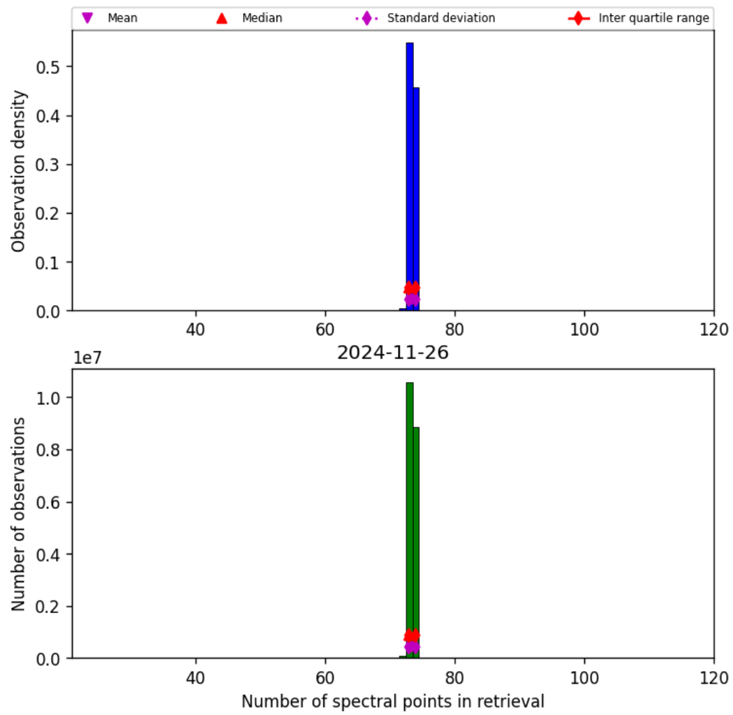
Figure 82: Histogram of “Number of spectral points in retrieval” for 2024-11-25 to 2024-11-27
