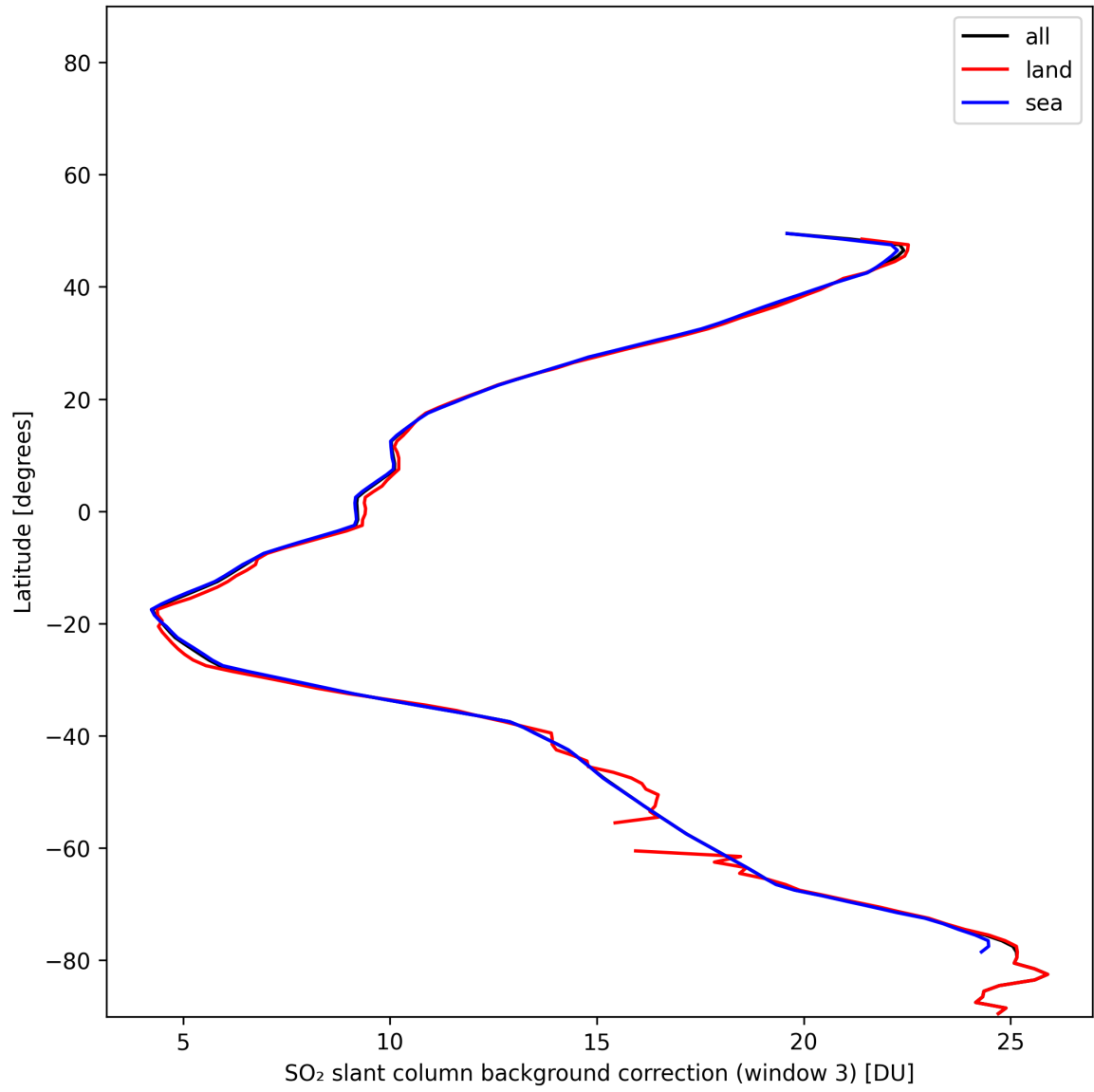
Figure 48: Zonal average of “SO 2 slant column background correction (window 3)” for 2024-11-25 to 2024-11-27.
