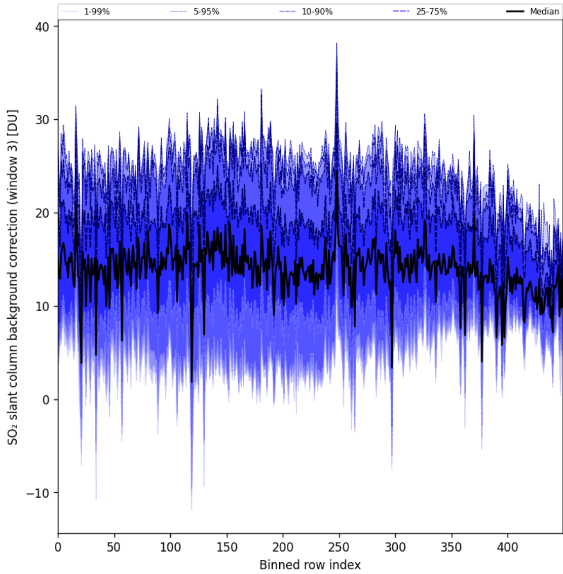
Figure 100: Along track statistics of “SO 2 slant column background correction (window 3)” for 2024-11-25 to 2024-11-27
