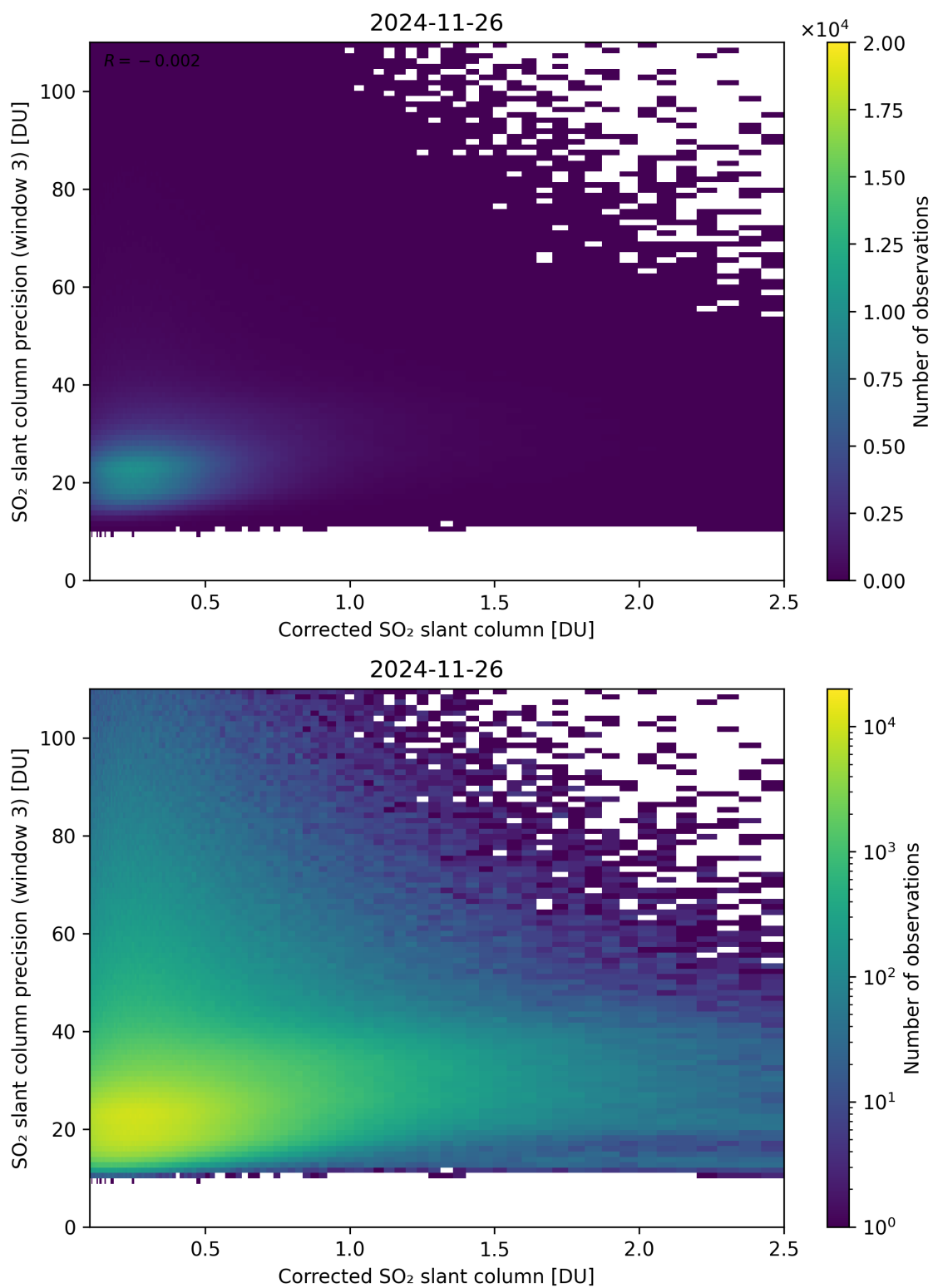
Figure 241: Scatter density plot of “Corrected SO 2 slant column” against “SO 2 slant column precision (window 3)” for 2024-11-25 to 2024-11-27.
