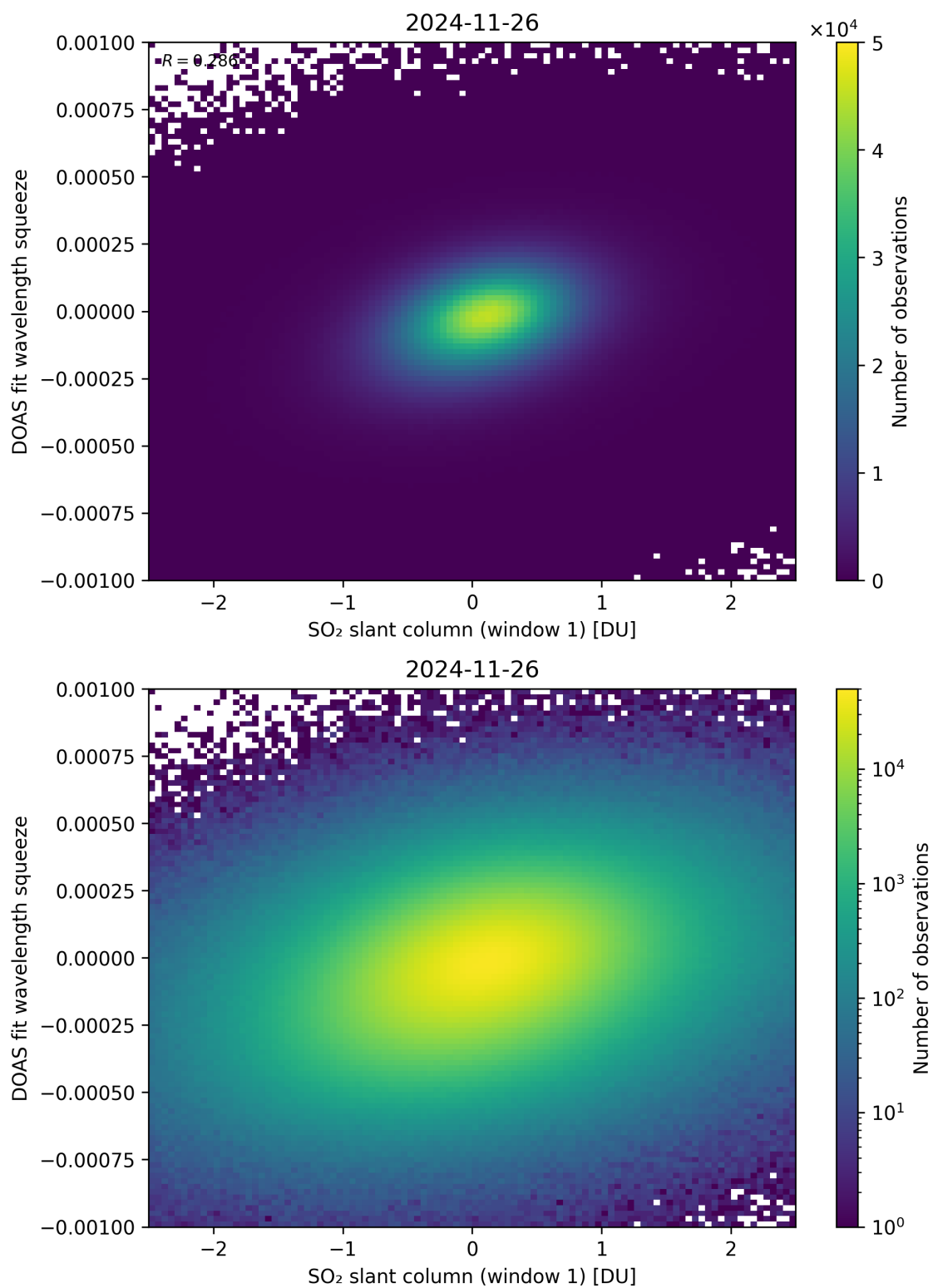
Figure 266: Scatter density plot of “SO 2 slant column (window 1)” against “DOAS fit wavelength squeeze” for 2024-11-25 to 2024-11-27.
