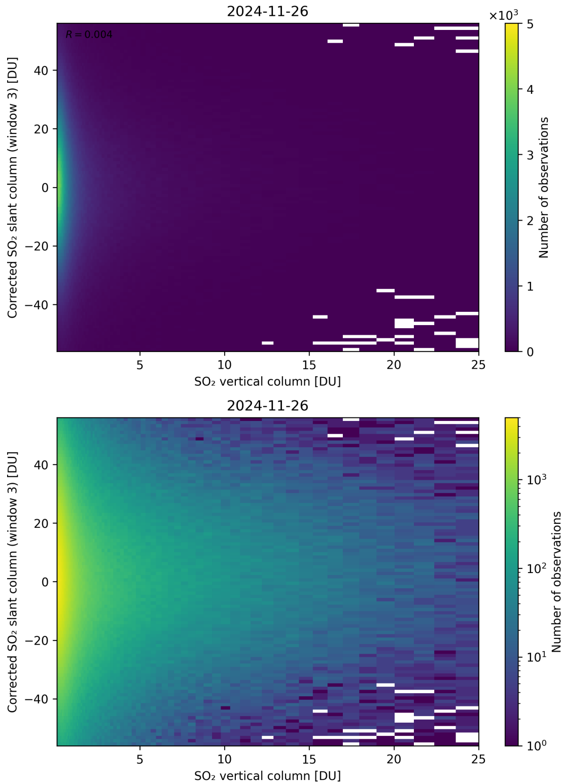
Figure 353: Scatter density plot of “SO 2 vertical column” against “Corrected SO 2 slant column (window 3)” for 2024-11-25 to 2024-11-27.
