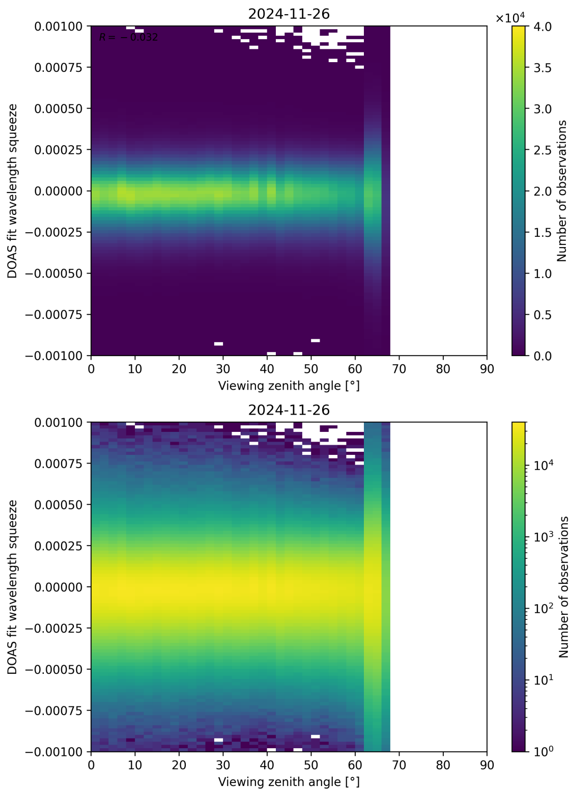
Figure 366: Scatter density plot of “Viewing zenith angle” against “DOAS fit wavelength squeeze” for 2024-11-25 to 2024-11-27.
