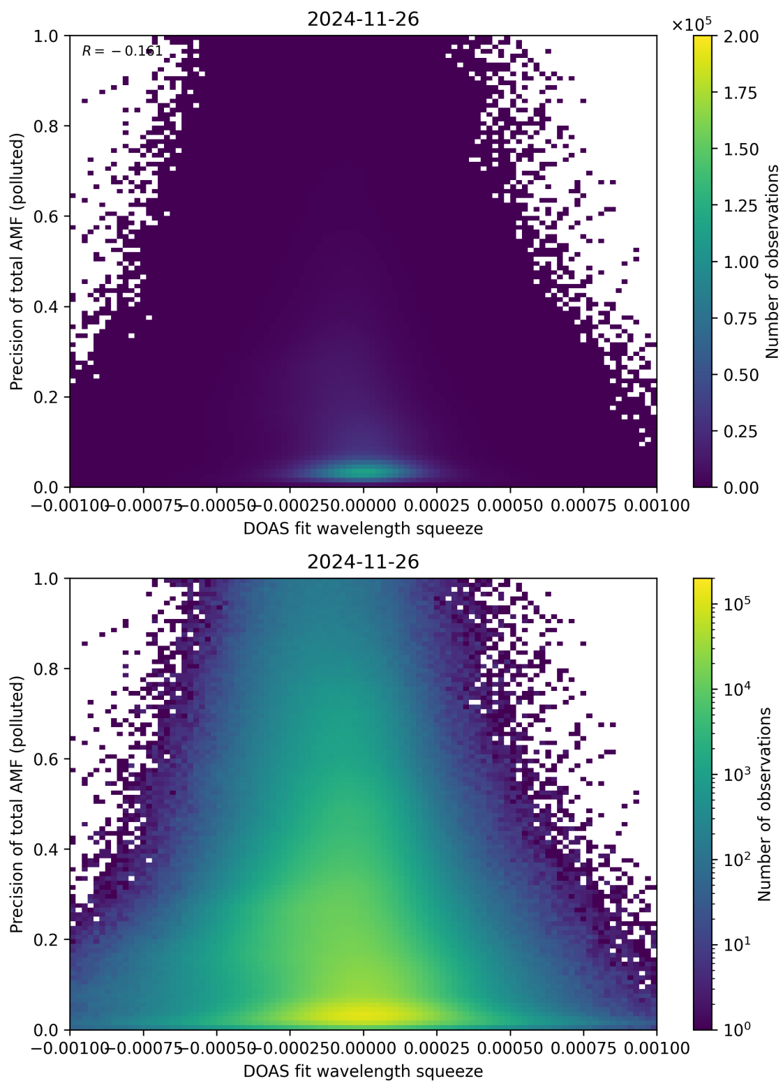
Figure 146: Scatter density plot of “DOAS fit wavelength squeeze” against “Precision of total AMF (polluted)” for 2024-11-25 to 2024-11-27.
