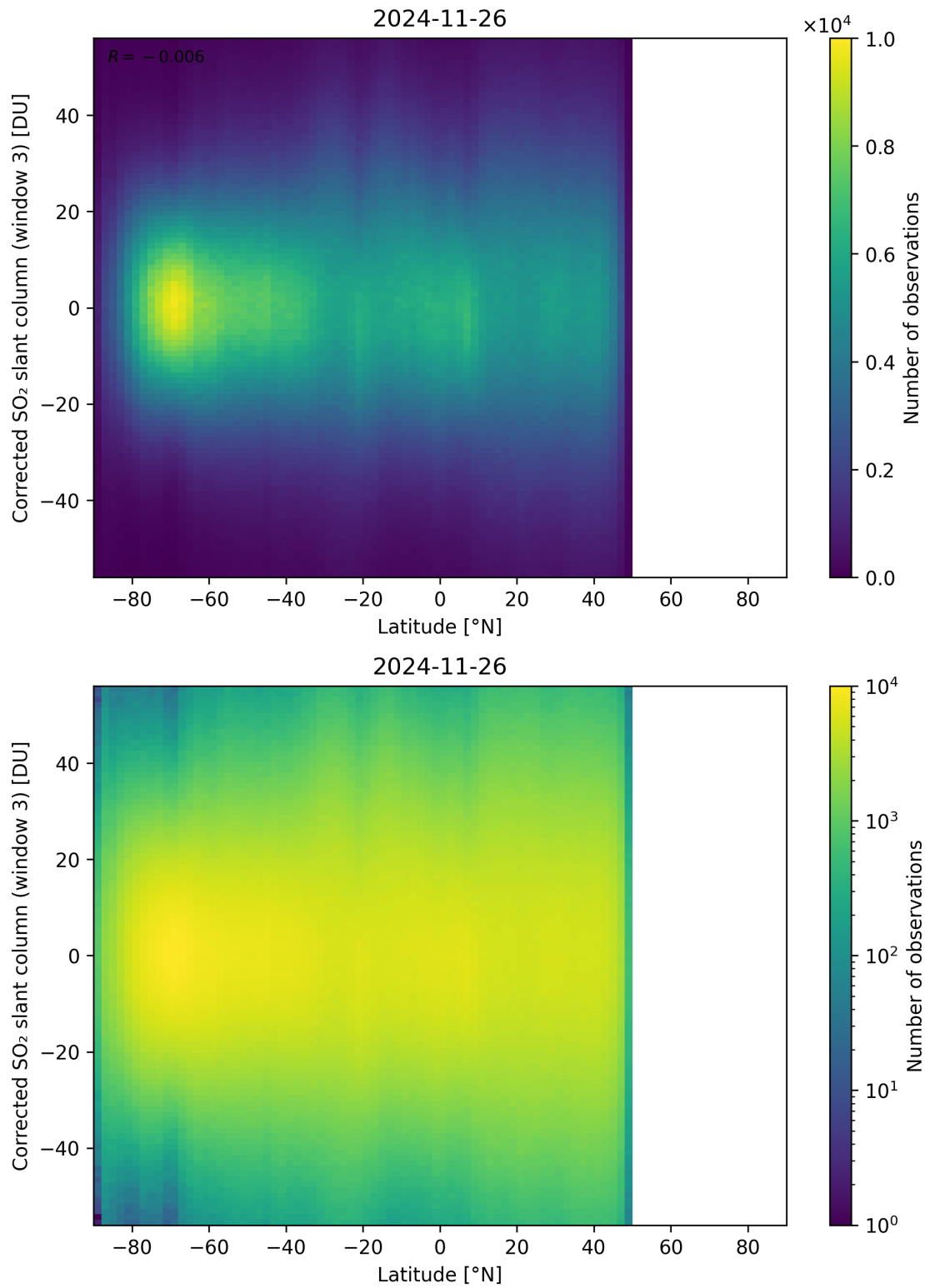
Figure 161: Scatter density plot of “Latitude” against “Corrected SO 2 slant column (window 3)” for 2024-11-25 to 2024-11-27.
