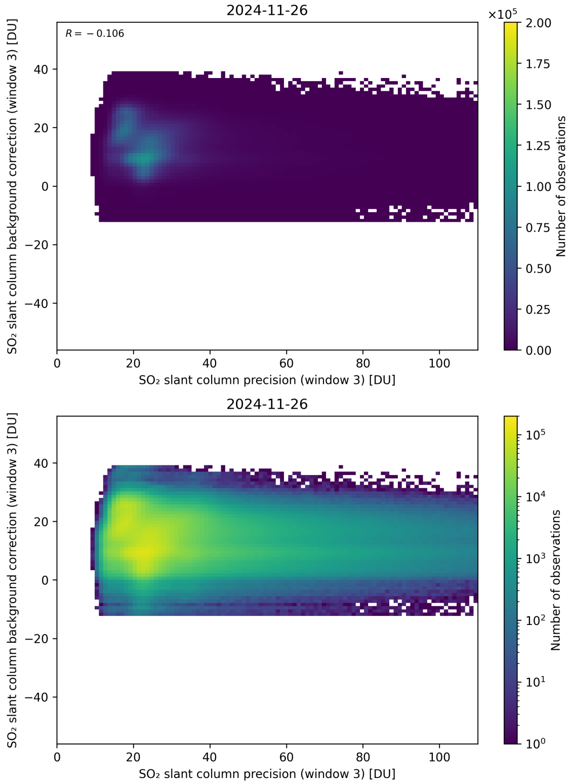
Figure 307: Scatter density plot of “SO 2 slant column precision (window 3)” against “SO 2 slant column background correction (window 3)” for 2024-11-25 to 2024-11-27.
