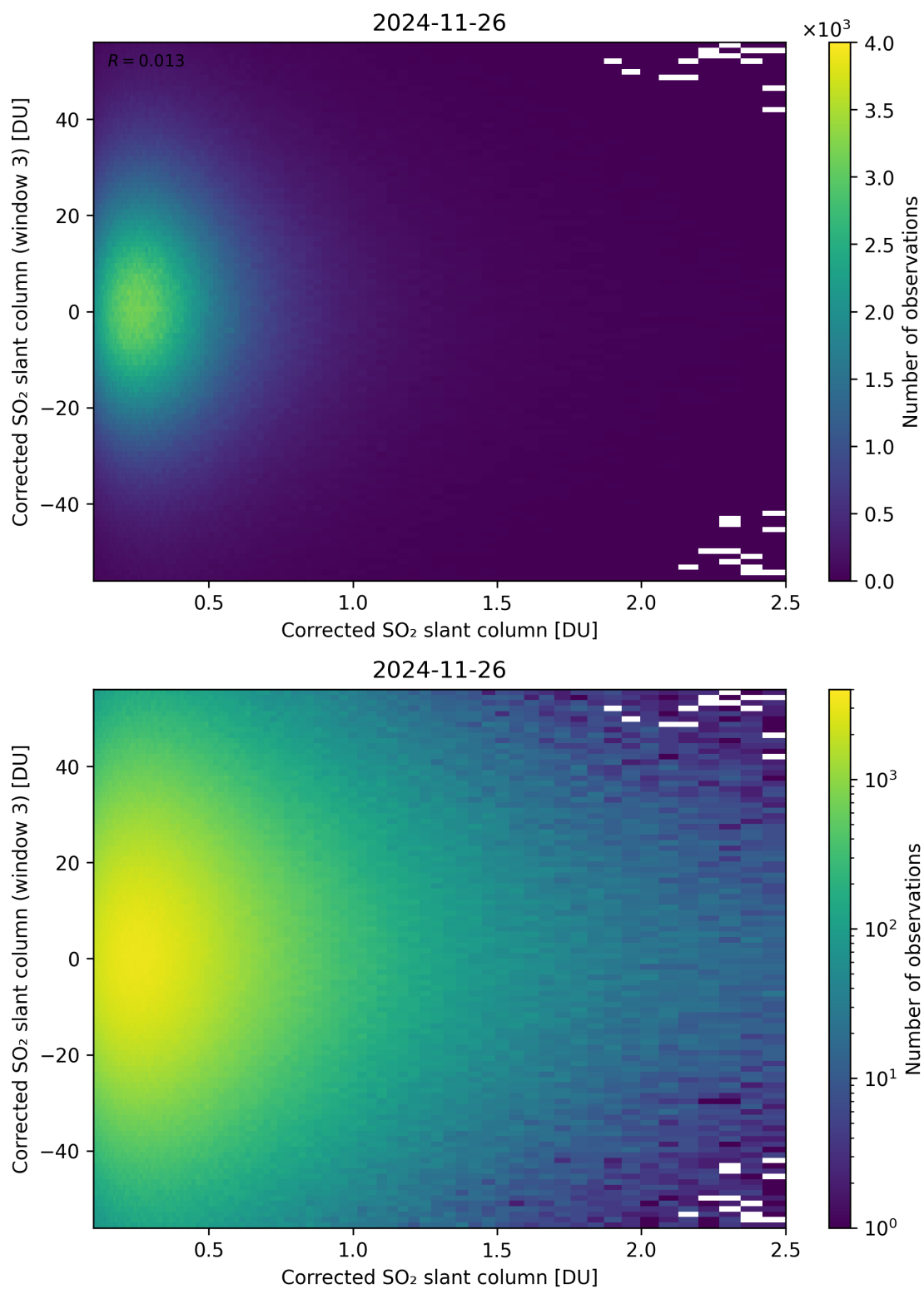
Figure 236: Scatter density plot of “Corrected SO 2 slant column” against “Corrected SO 2 slant column (window 3)” for 2024-11-25 to 2024-11-27.
