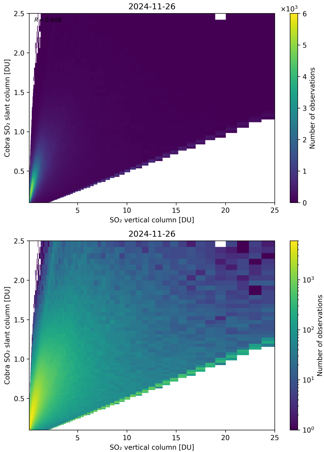
Figure 349: Scatter density plot of “SO 2 vertical column” against “Cobra SO 2 slant column” for 2024-11-25 to 2024-11-27.
