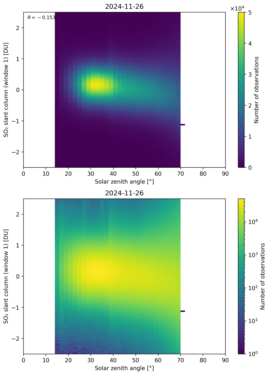
Figure 184: Scatter density plot of “Solar zenith angle” against “SO 2 slant column (window 1)” for 2024-11-25 to 2024-11-27.
