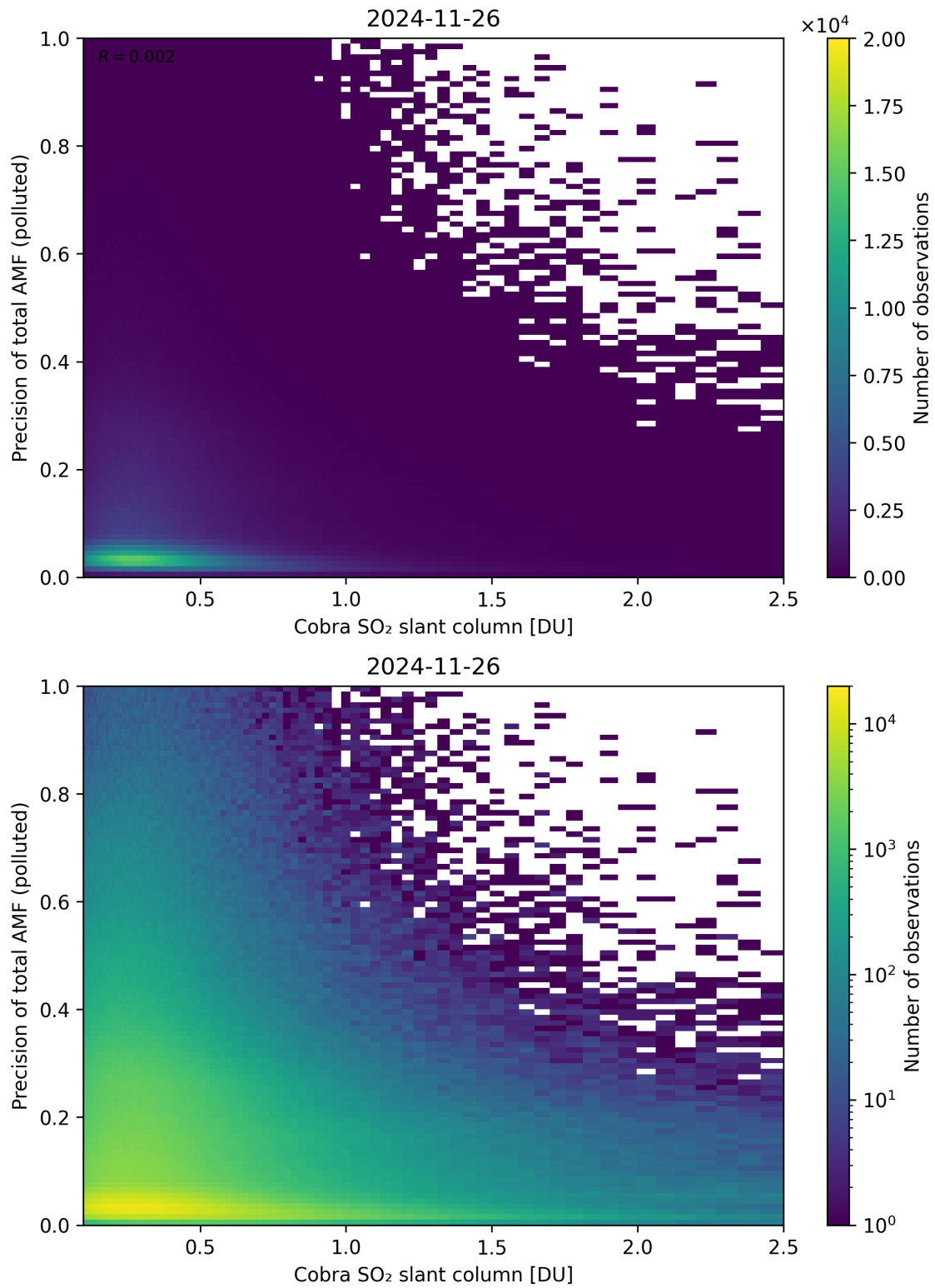
Figure 225: Scatter density plot of “Cobra SO 2 slant column” against “Precision of total AMF (polluted)” for 2024-11-25 to 2024-11-27.
