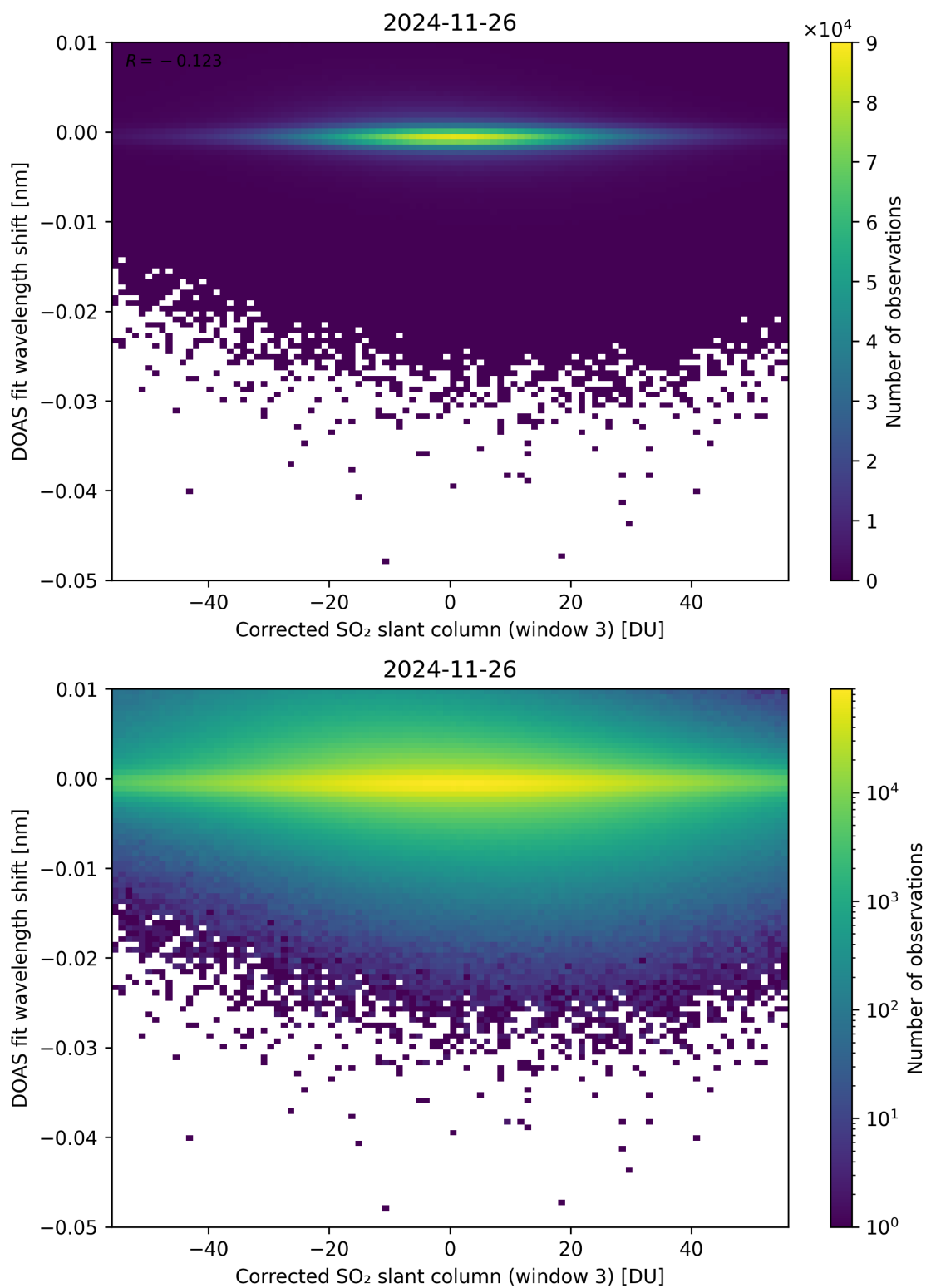
Figure 256: Scatter density plot of “Corrected SO 2 slant column (window 3)” against “DOAS fit wavelength shift” for 2024-11-25 to 2024-11-27.
