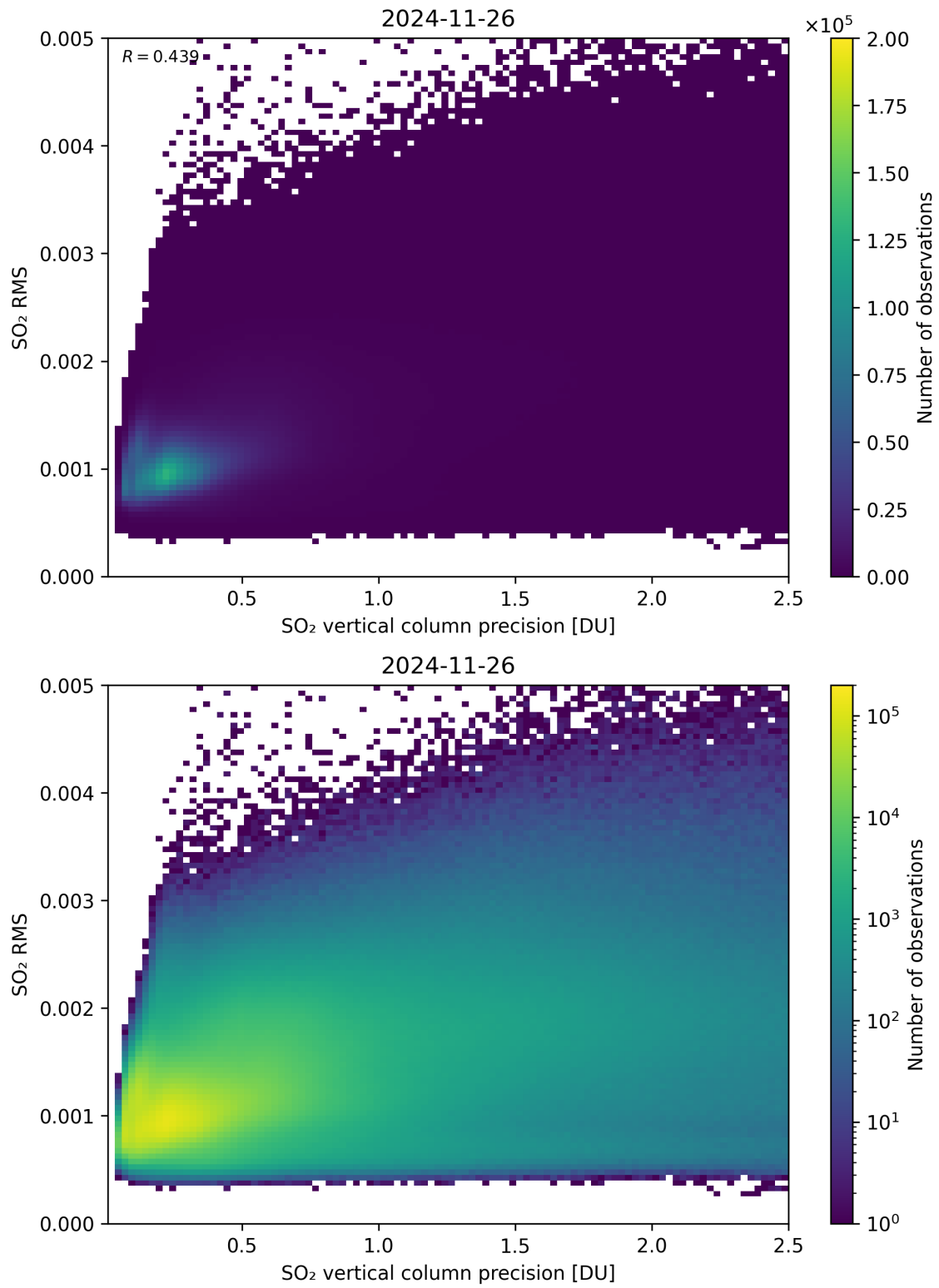
Figure 334: Scatter density plot of “SO 2 vertical column precision” against “SO 2 RMS” for 2024-11-25 to 2024-11-27.
