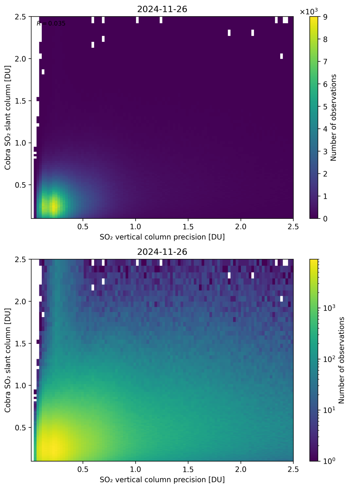
Figure 336: Scatter density plot of “SO 2 vertical column precision” against “Cobra SO 2 slant column” for 2024-11-25 to 2024-11-27.
