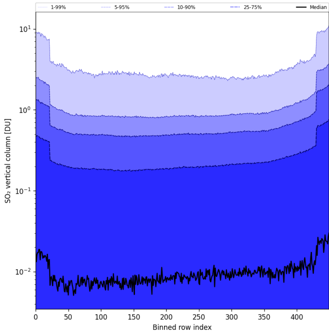
Figure 84: Along track statistics of “SO 2 vertical column” for 2024-11-25 to 2024-11-27
