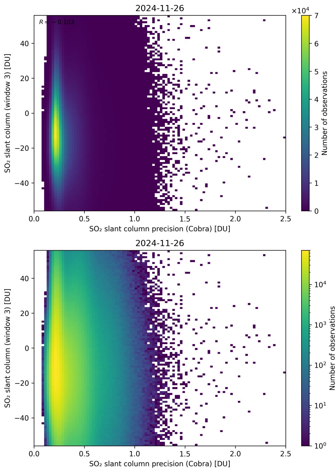
Figure 211: Scatter density plot of “SO 2 slant column precision (Cobra)” against “SO 2 slant column (window 3)” for 2024-11-25 to 2024-11-27.
