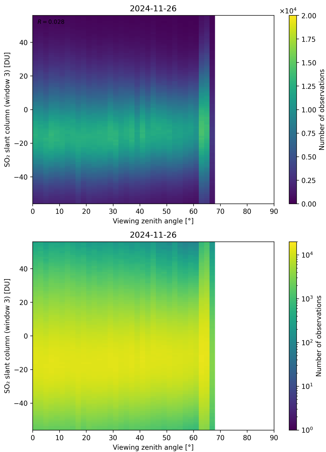
Figure 379: Scatter density plot of “Viewing zenith angle” against “SO 2 slant column (window 3)” for 2024-11-25 to 2024-11-27.
