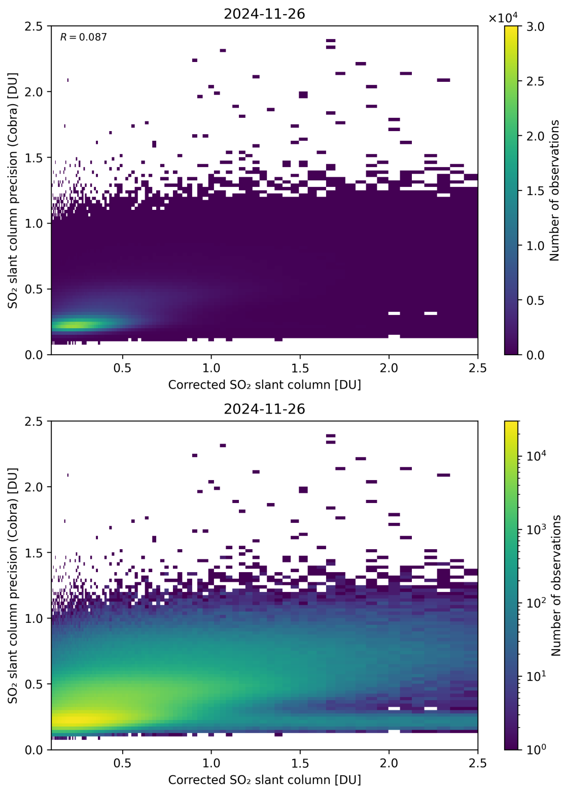
Figure 234: Scatter density plot of “Corrected SO 2 slant column” against “SO 2 slant column precision (Cobra)” for 2024-11-25 to 2024-11-27.
