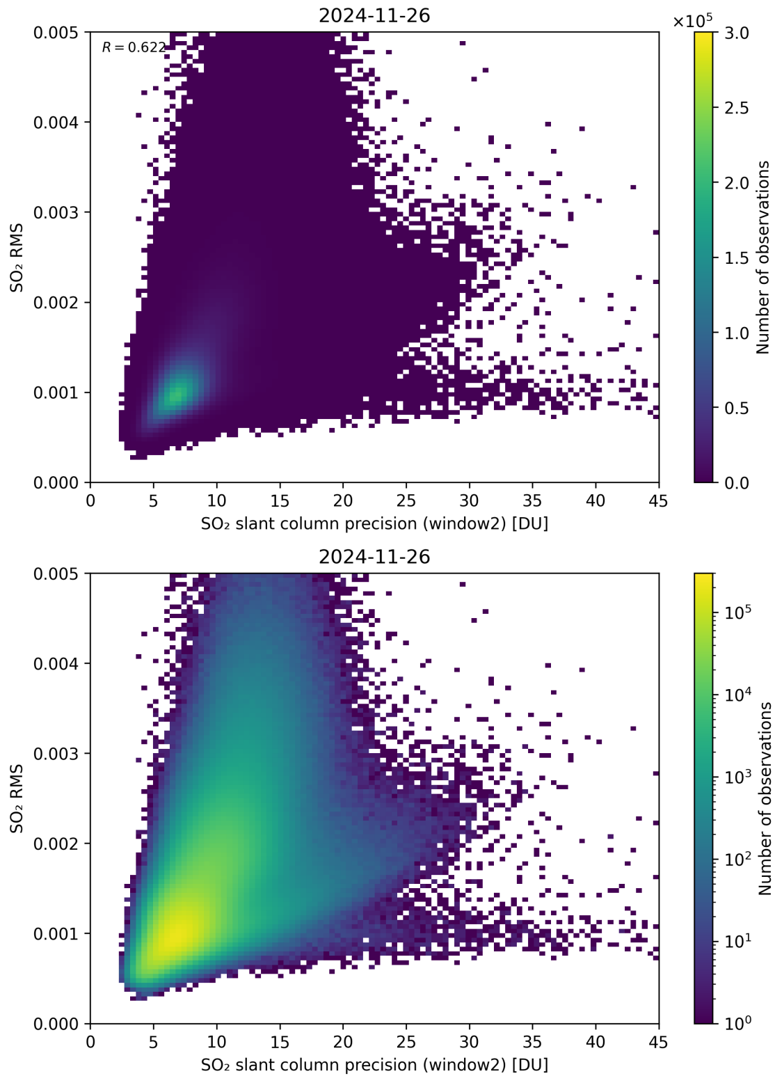
Figure 295: Scatter density plot of “SO 2 slant column precision (window2)” against “SO 2 RMS” for 2024-11-25 to 2024-11-27.
