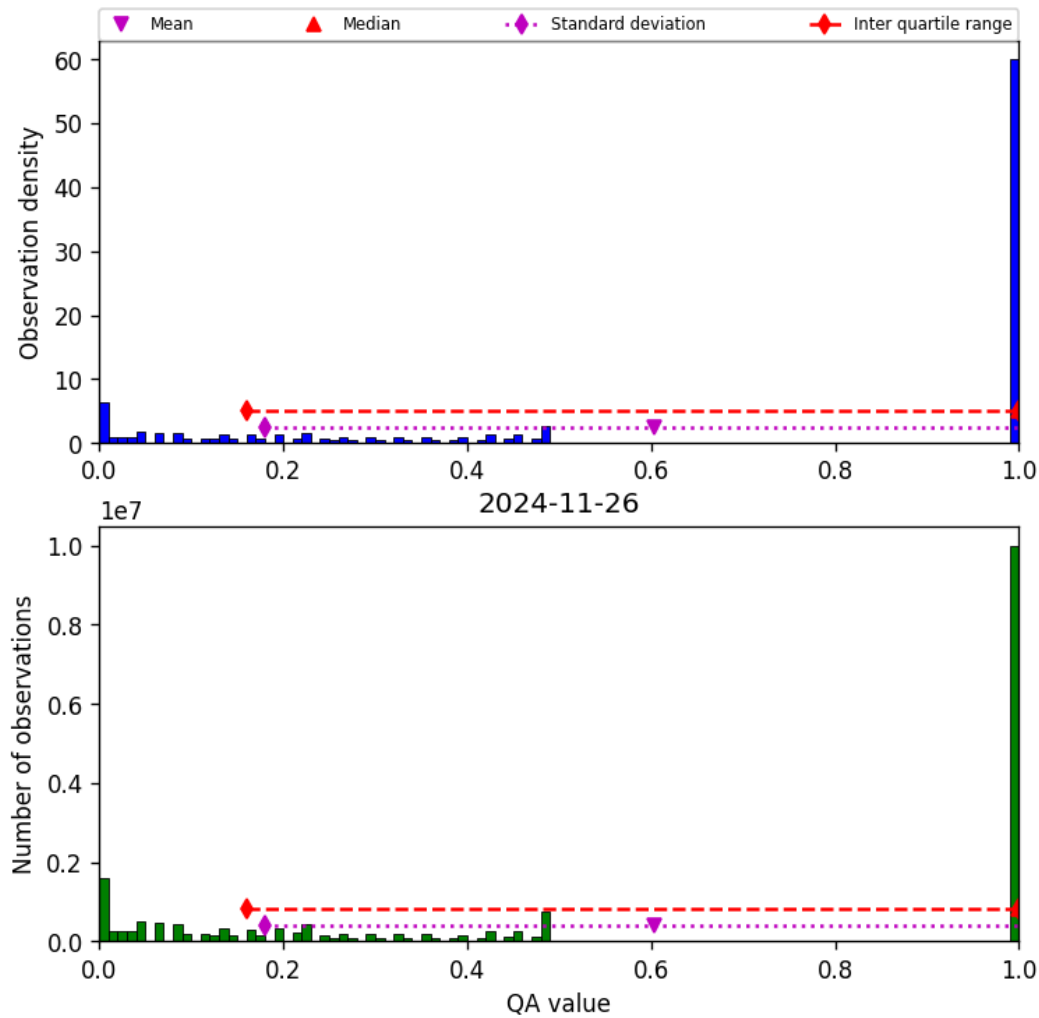
Figure 57: Histogram of “QA value” for 2024-11-25 to 2024-11-27
