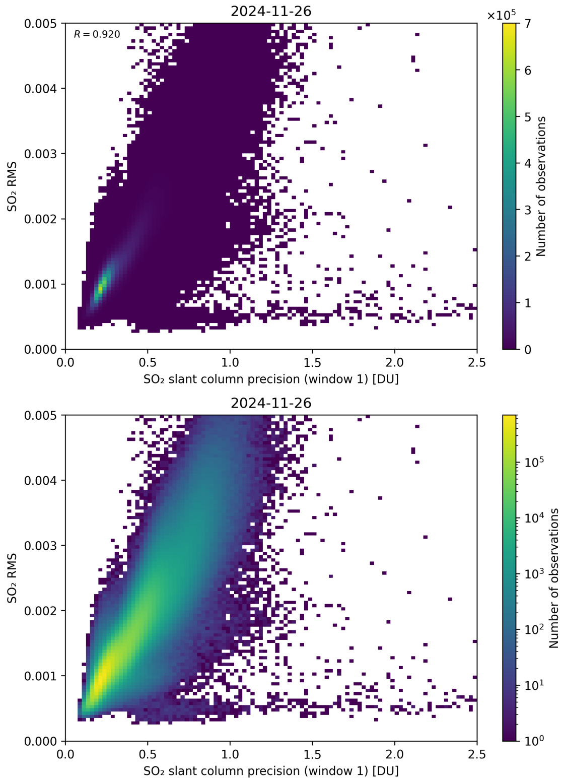
Figure 273: Scatter density plot of “SO 2 slant column precision (window 1)” against “SO 2 RMS” for 2024-11-25 to 2024-11-27.
