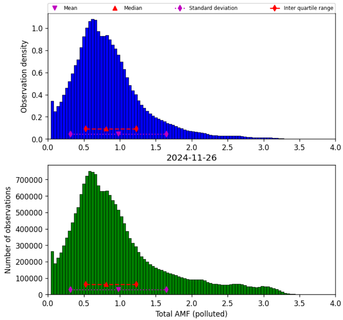
Figure 79: Histogram of “Total AMF (polluted)” for 2024-11-25 to 2024-11-27
