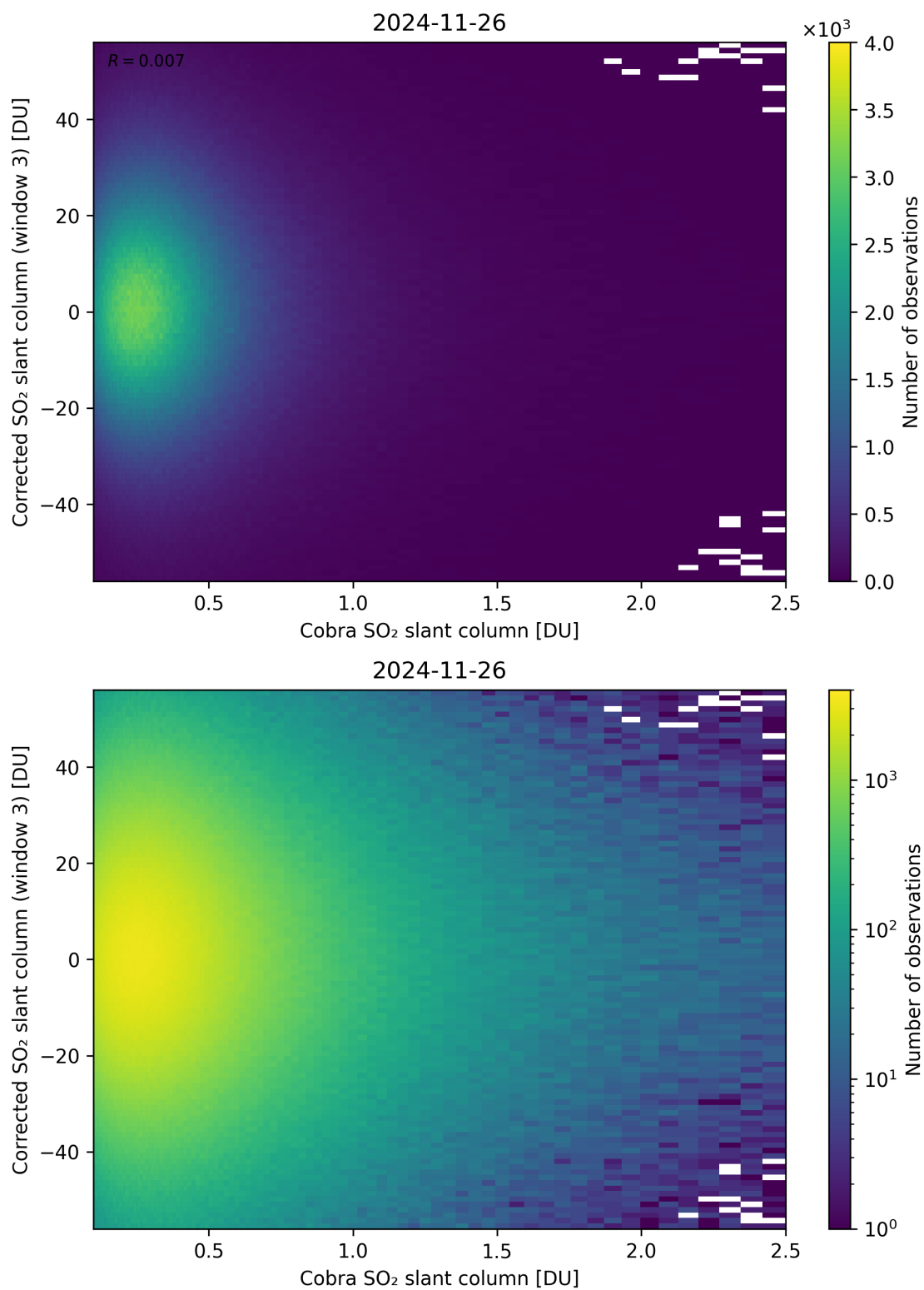
Figure 218: Scatter density plot of “Cobra SO 2 slant column” against “Corrected SO 2 slant column (window 3)” for 2024-11-25 to 2024-11-27.
