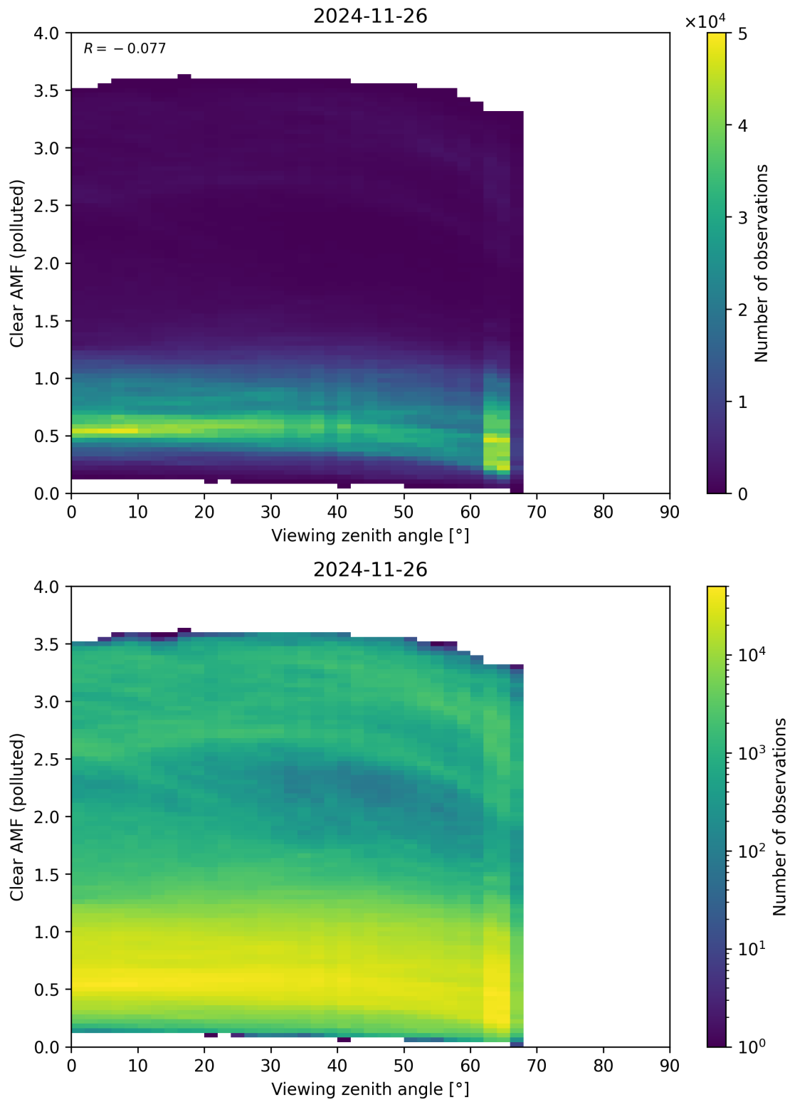
Figure 370: Scatter density plot of “Viewing zenith angle” against “Clear AMF (polluted)” for 2024-11-25 to 2024-11-27.
