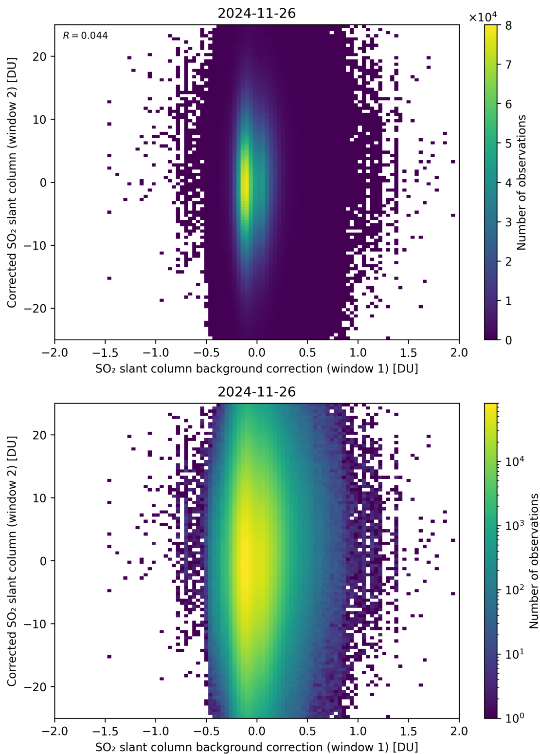
Figure 115: Scatter density plot of “SO 2 slant column background correction (window 1)” against “Corrected SO 2 slant column (window 2)” for 2024-11-25 to 2024-11-27.
