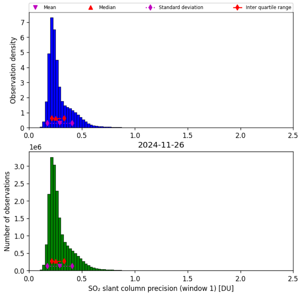
Figure 64: Histogram of “SO 2 slant column precision (window 1)” for 2024-11-25 to 2024-11-27
