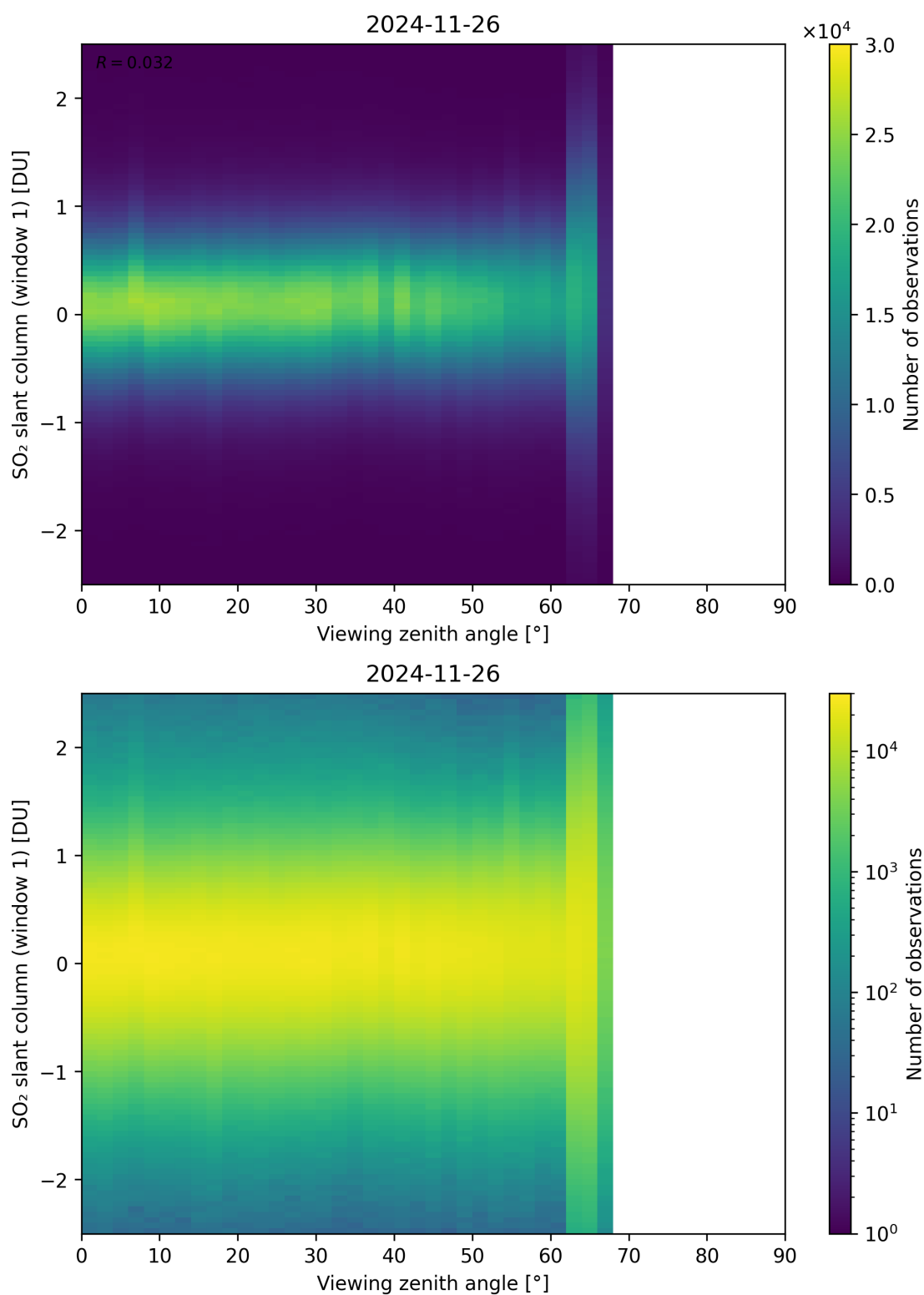
Figure 376: Scatter density plot of “Viewing zenith angle” against “SO 2 slant column (window 1)” for 2024-11-25 to 2024-11-27.
