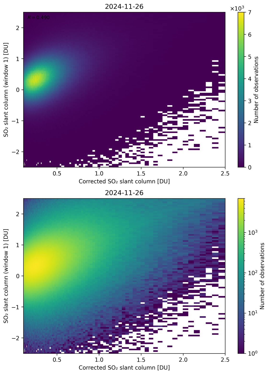
Figure 237: Scatter density plot of “Corrected SO 2 slant column” against “SO 2 slant column (window 1)” for 2024-11-25 to 2024-11-27.
