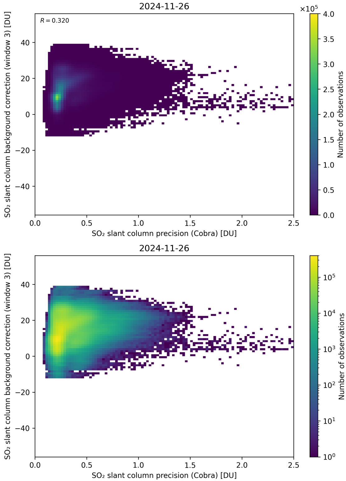
Figure 201: Scatter density plot of “SO 2 slant column precision (Cobra)” against “SO 2 slant column background correction (window 3)” for 2024-11-25 to 2024-11-27.
