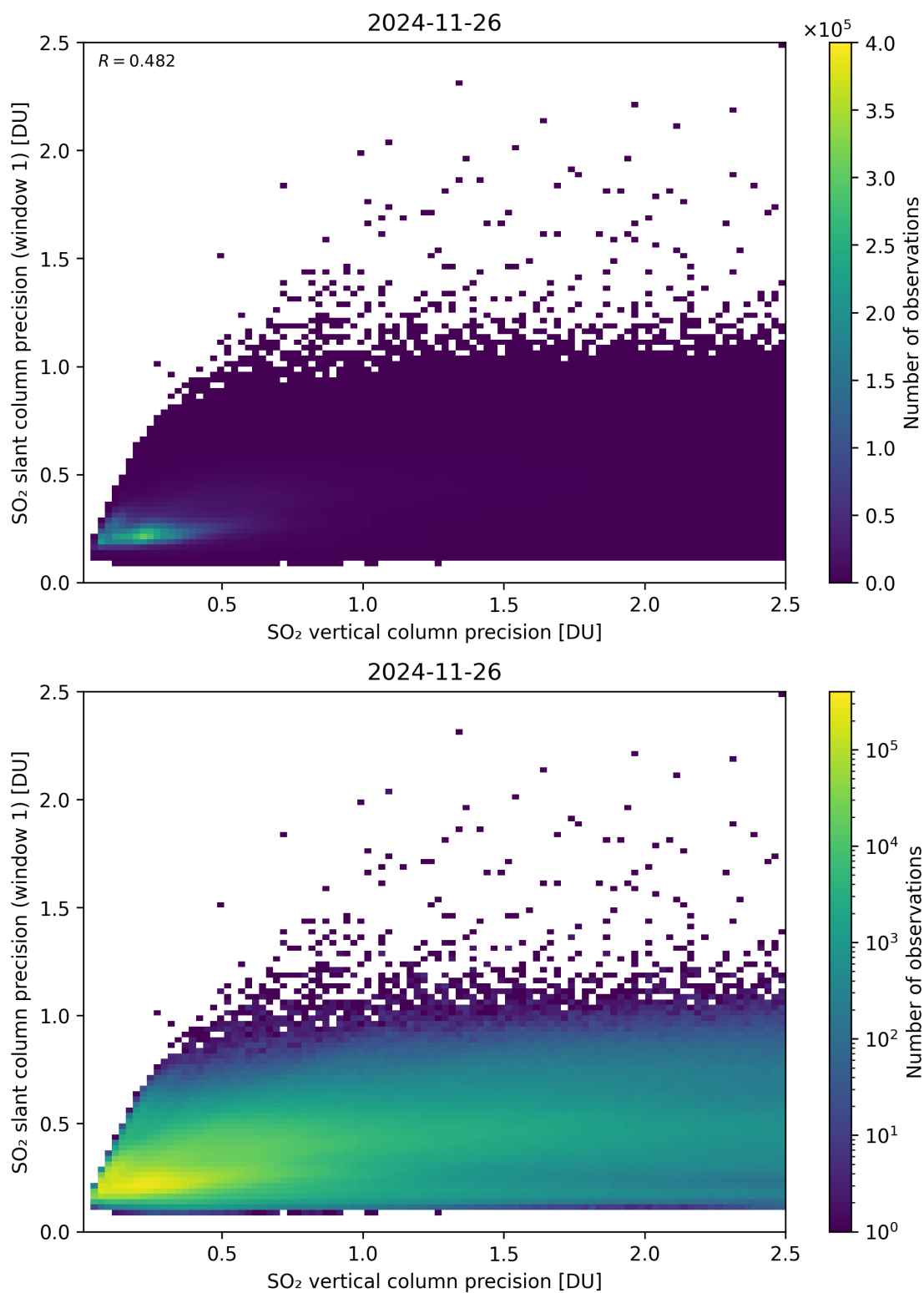
Figure 342: Scatter density plot of “SO 2 vertical column precision” against “SO 2 slant column precision (window 1)” for 2024-11-25 to 2024-11-27.
