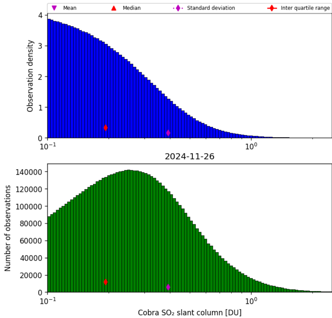
Figure 61: Histogram of “Cobra SO 2 slant column” for 2024-11-25 to 2024-11-27
