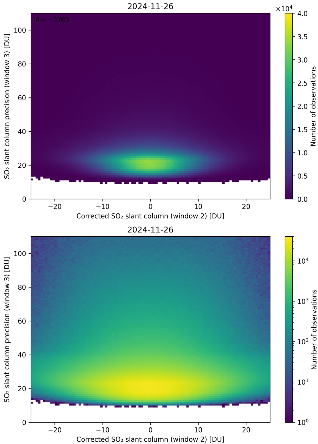
Figure 252: Scatter density plot of “Corrected SO 2 slant column (window 2)” against “SO 2 slant column precision (window 3)” for 2024-11-25 to 2024-11-27.
