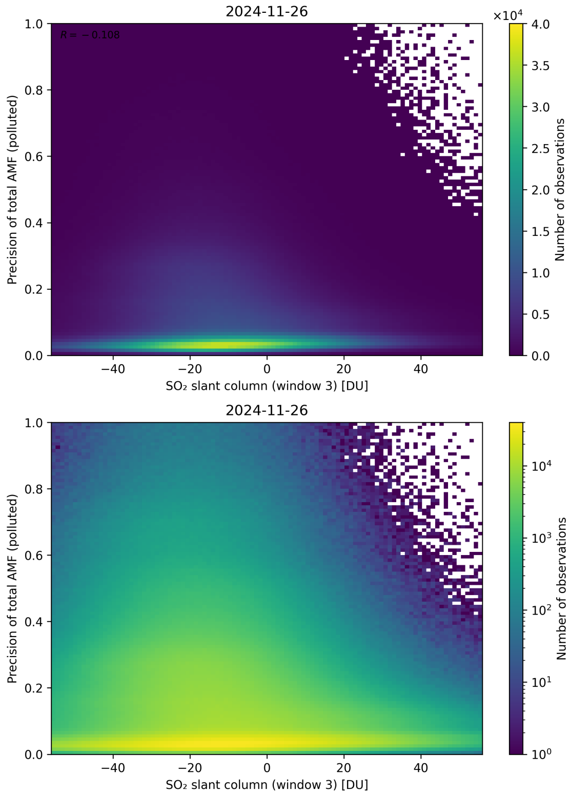
Figure 319: Scatter density plot of “SO 2 slant column (window 3)” against “Precision of total AMF (polluted)” for 2024-11-25 to 2024-11-27.
