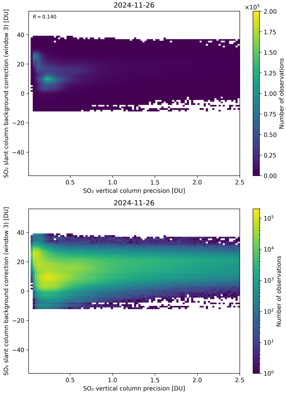
Figure 331: Scatter density plot of “SO 2 vertical column precision” against “SO 2 slant column background correction (window 3)” for 2024-11-25 to 2024-11-27.
