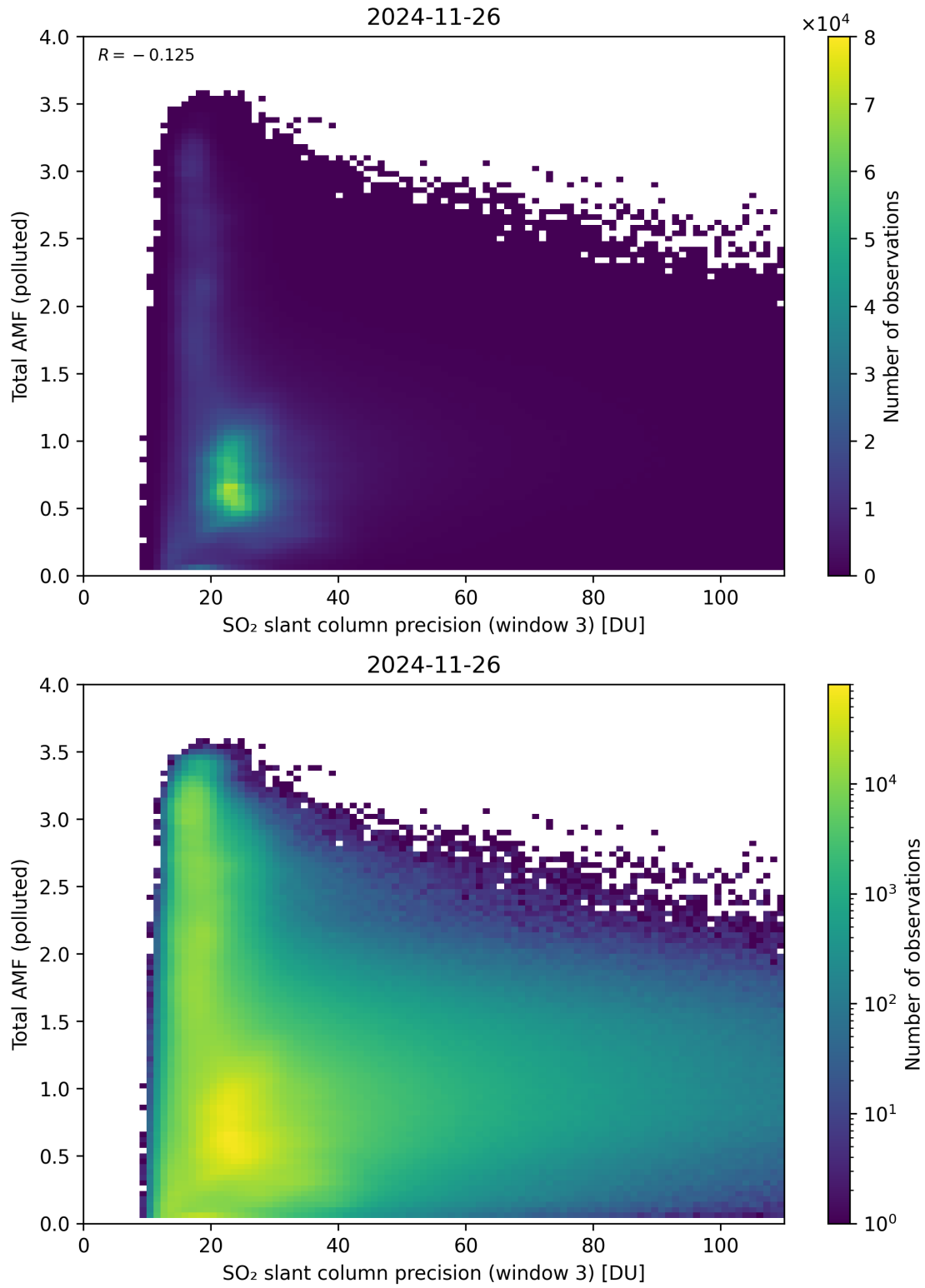
Figure 313: Scatter density plot of “SO 2 slant column precision (window 3)” against “Total AMF (polluted)” for 2024-11-25 to 2024-11-27.
