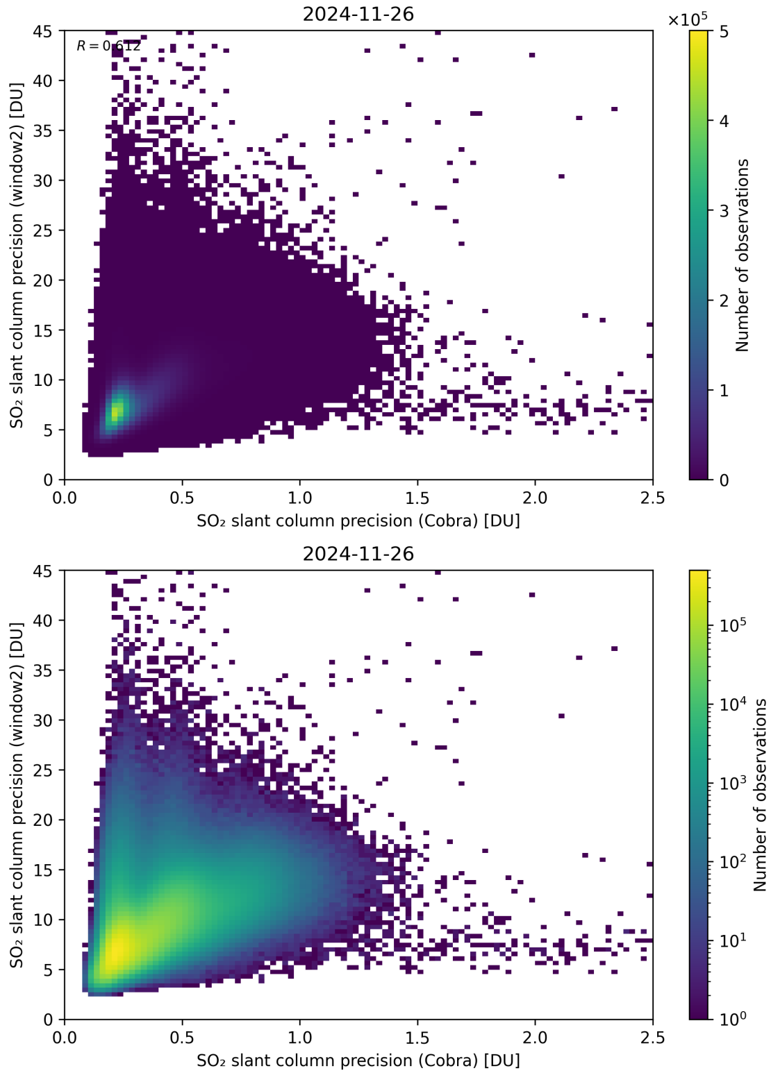
Figure 210: Scatter density plot of “SO 2 slant column precision (Cobra)” against “SO 2 slant column precision (window2)” for 2024-11-25 to 2024-11-27.
