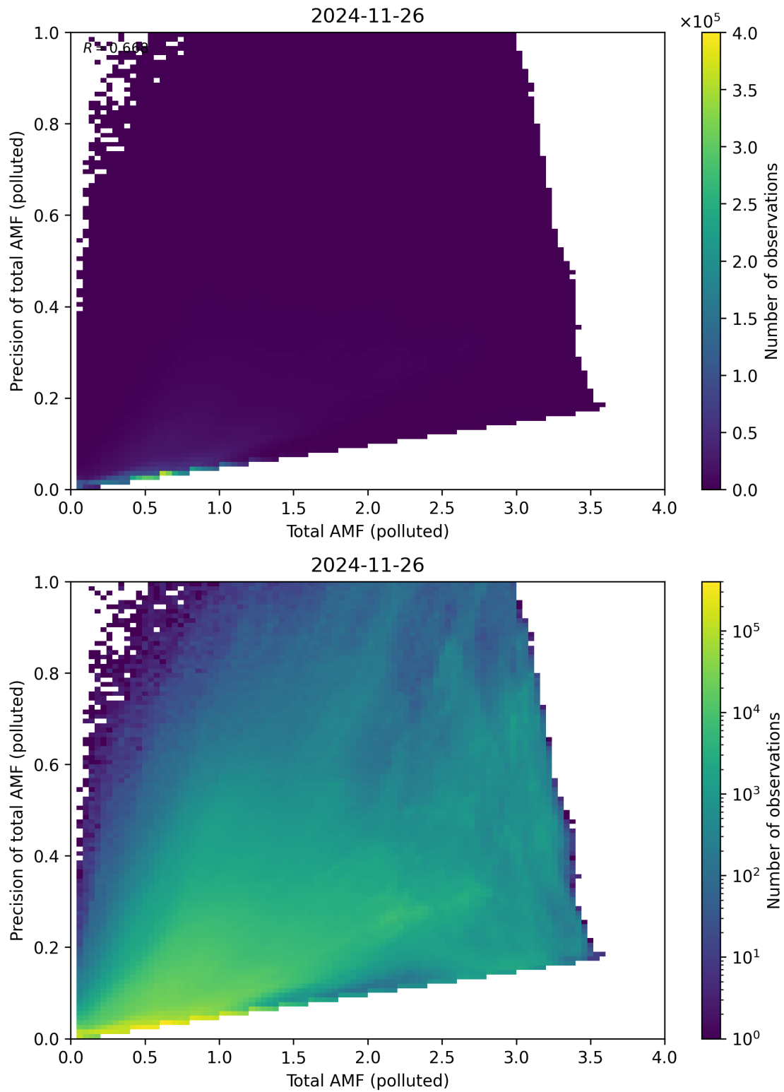
Figure 322: Scatter density plot of “Total AMF (polluted)” against “Precision of total AMF (polluted)” for 2024-11-25 to 2024-11-27.
