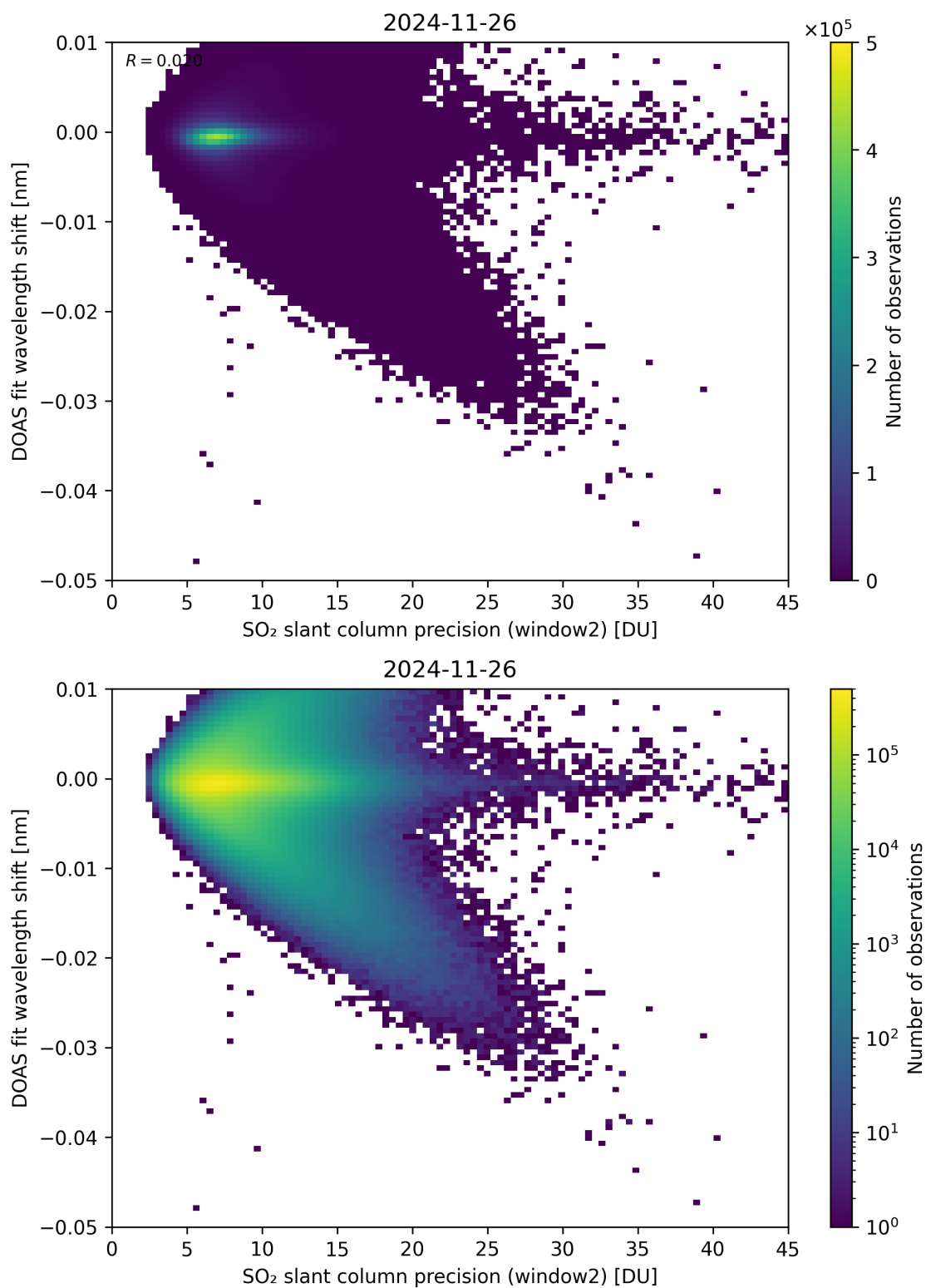
Figure 293: Scatter density plot of “SO 2 slant column precision (window2)” against “DOAS fit wavelength shift” for 2024-11-25 to 2024-11-27.
