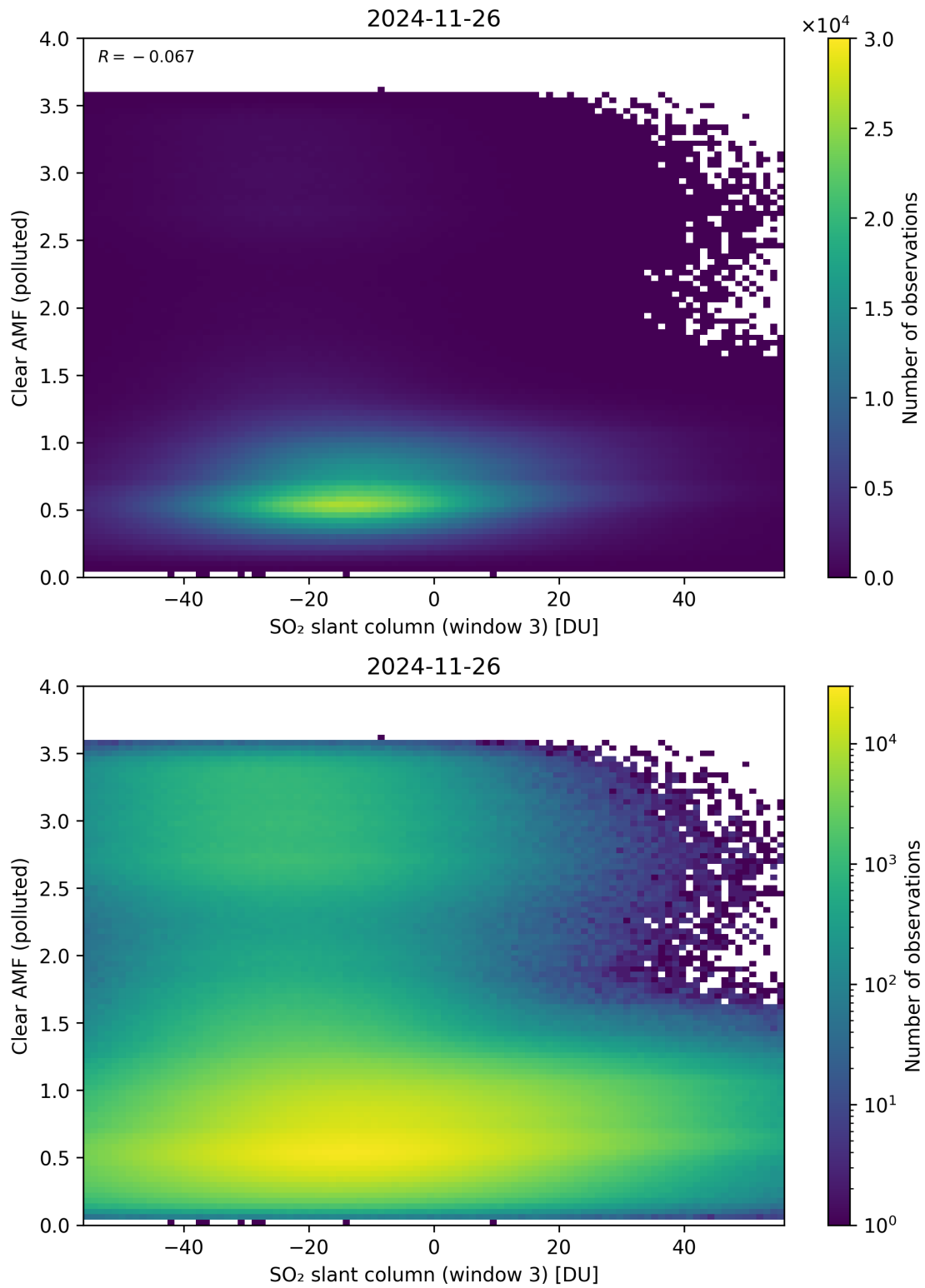
Figure 315: Scatter density plot of “SO 2 slant column (window 3)” against “Clear AMF (polluted)” for 2024-11-25 to 2024-11-27.
