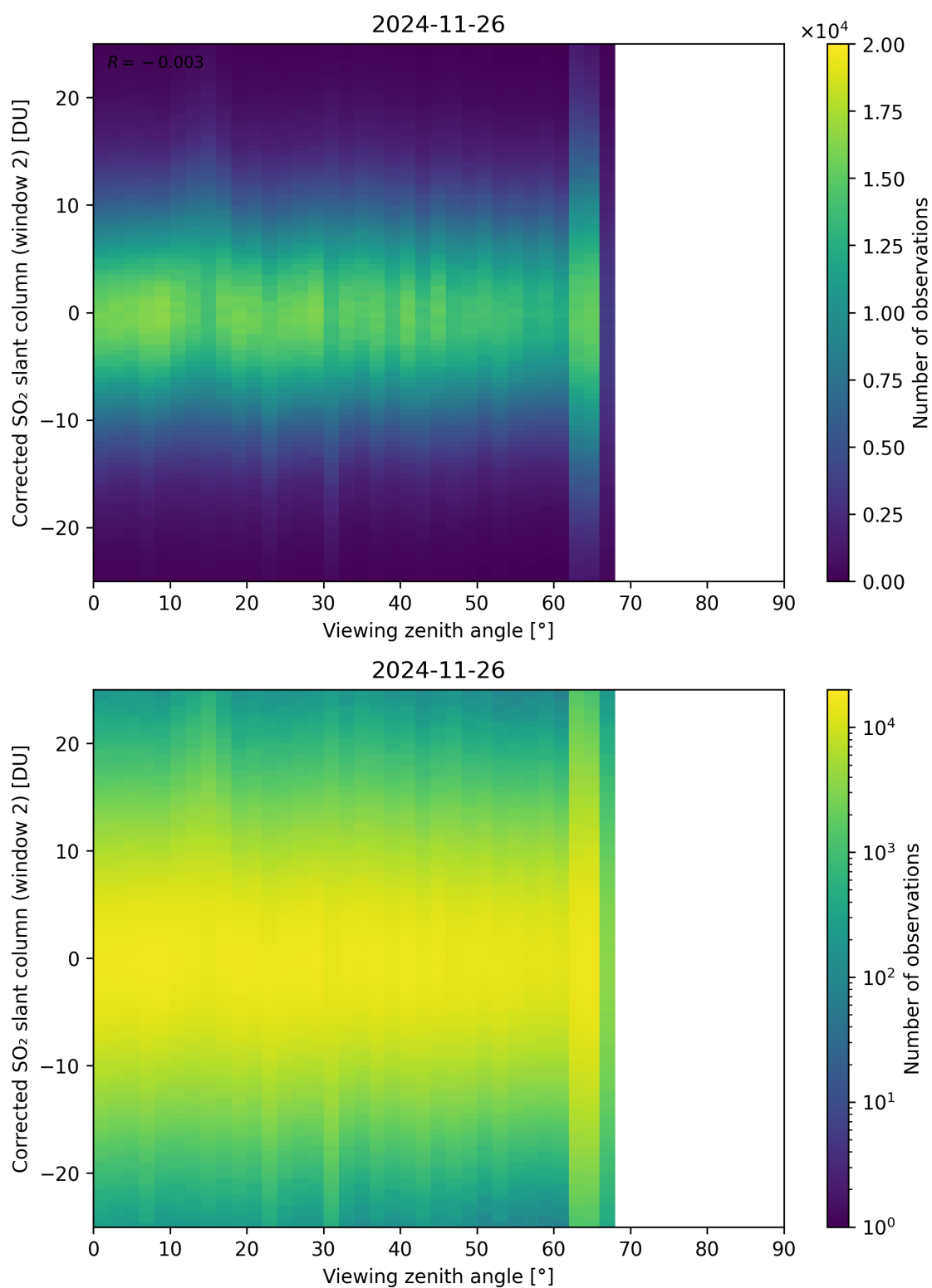
Figure 374: Scatter density plot of “Viewing zenith angle” against “Corrected SO 2 slant column (window 2)” for 2024-11-25 to 2024-11-27.
