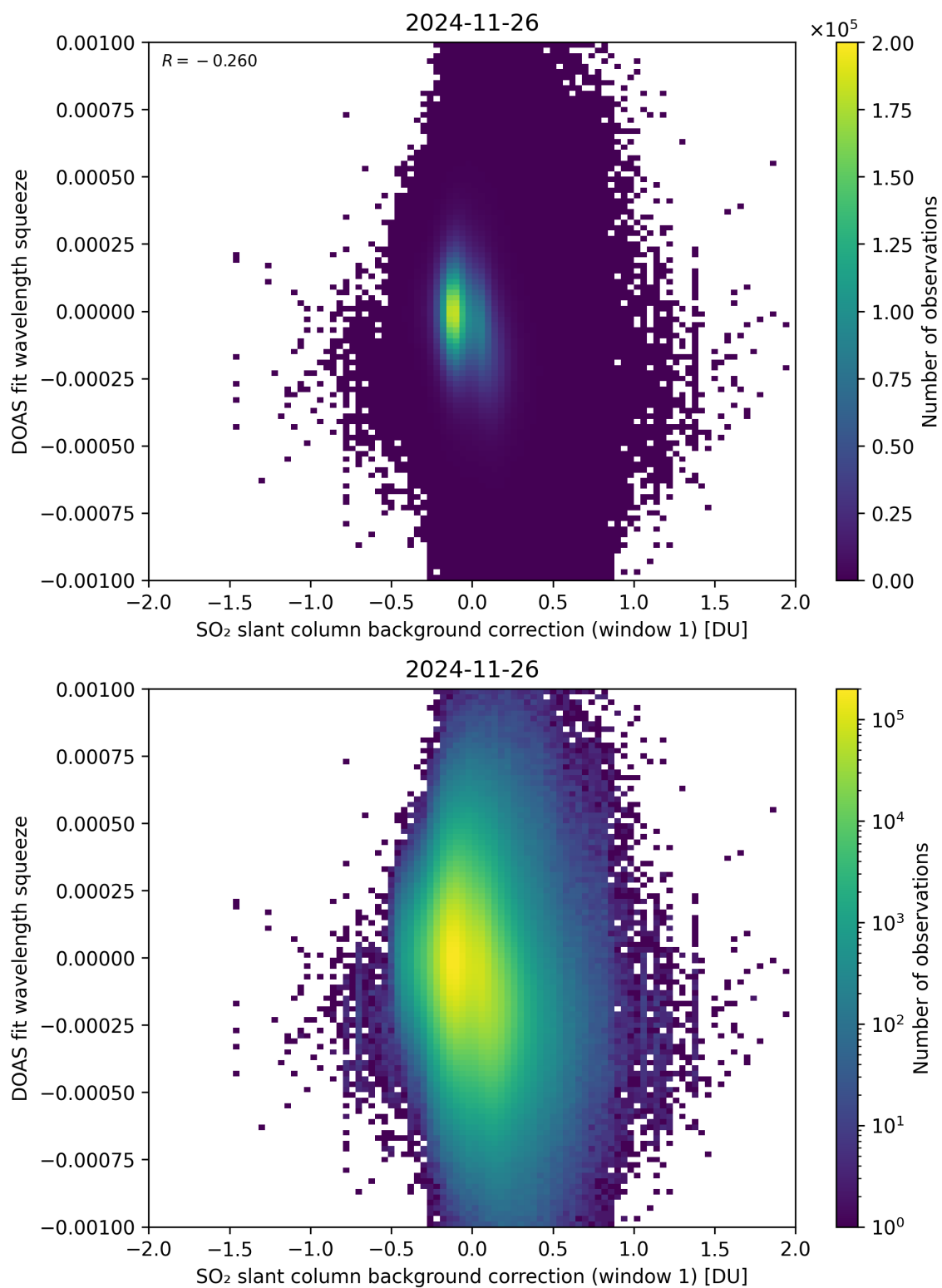
Figure 112: Scatter density plot of “SO 2 slant column background correction (window 1)” against “DOAS fit wavelength squeeze” for 2024-11-25 to 2024-11-27.
