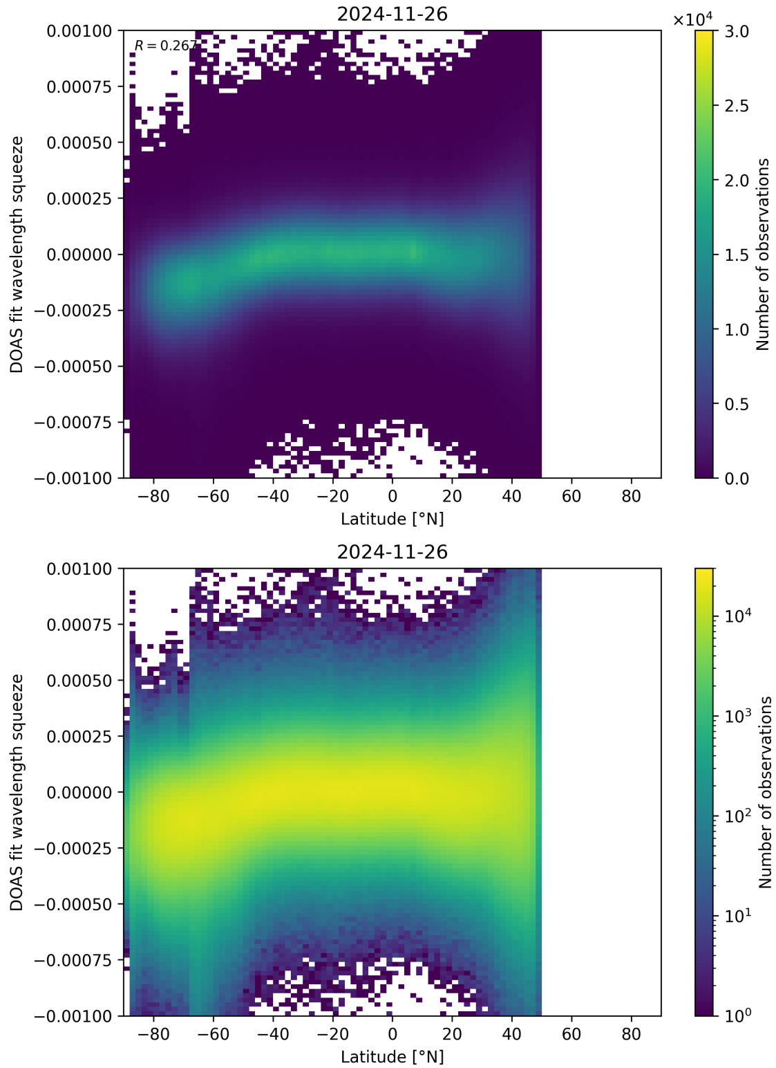
Figure 154: Scatter density plot of “Latitude” against “DOAS fit wavelength squeeze” for 2024-11-25 to 2024-11-27.
