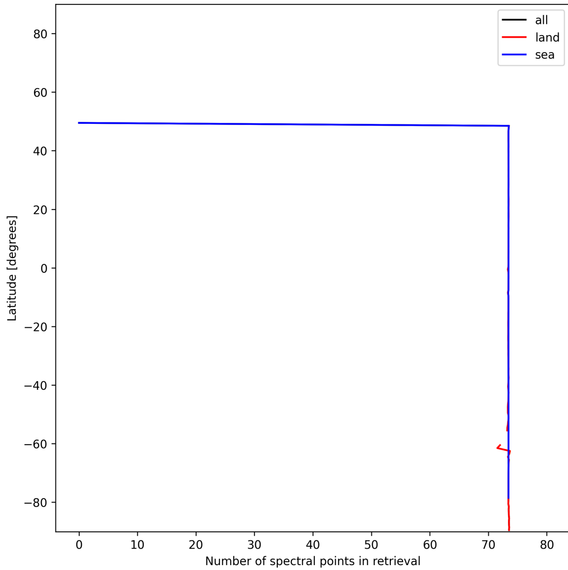
Figure 56: Zonal average of “Number of spectral points in retrieval” for 2024-11-25 to 2024-11-27.
