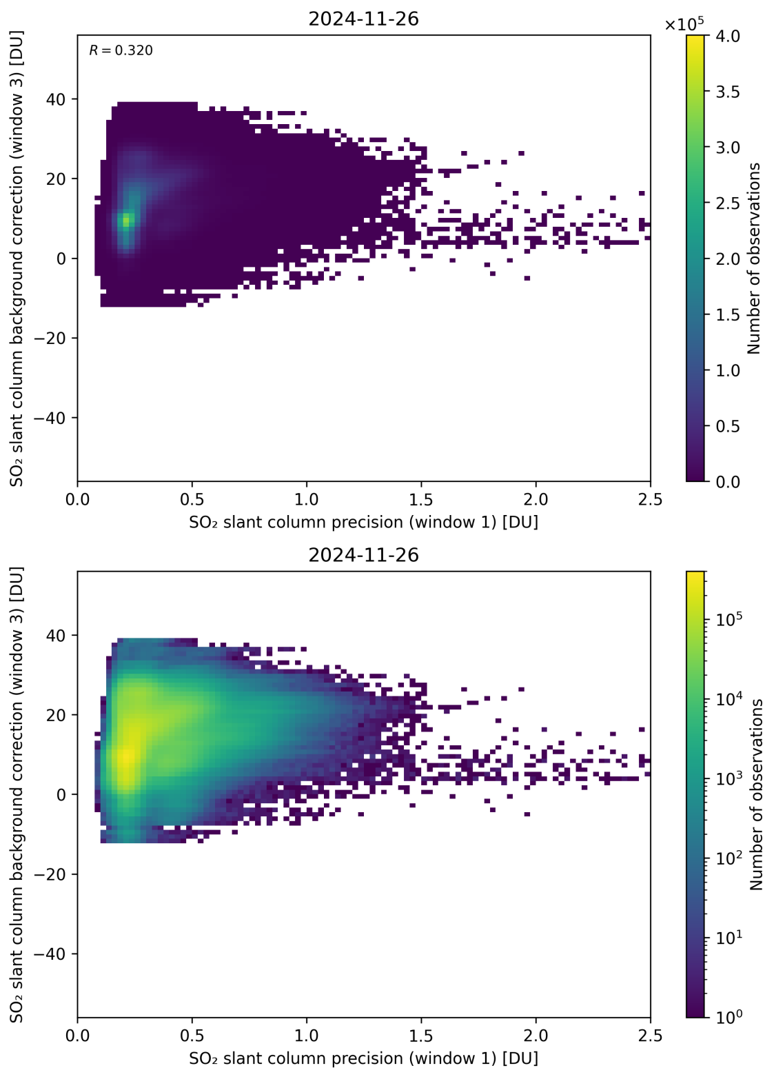
Figure 270: Scatter density plot of “SO 2 slant column precision (window 1)” against “SO 2 slant column background correction (window 3)” for 2024-11-25 to 2024-11-27.
