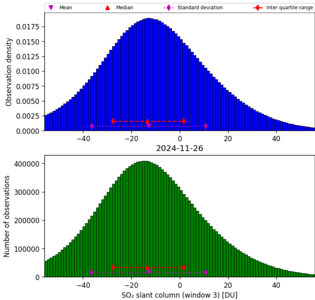
Figure 71: Histogram of “SO 2 slant column (window 3)” for 2024-11-25 to 2024-11-27
