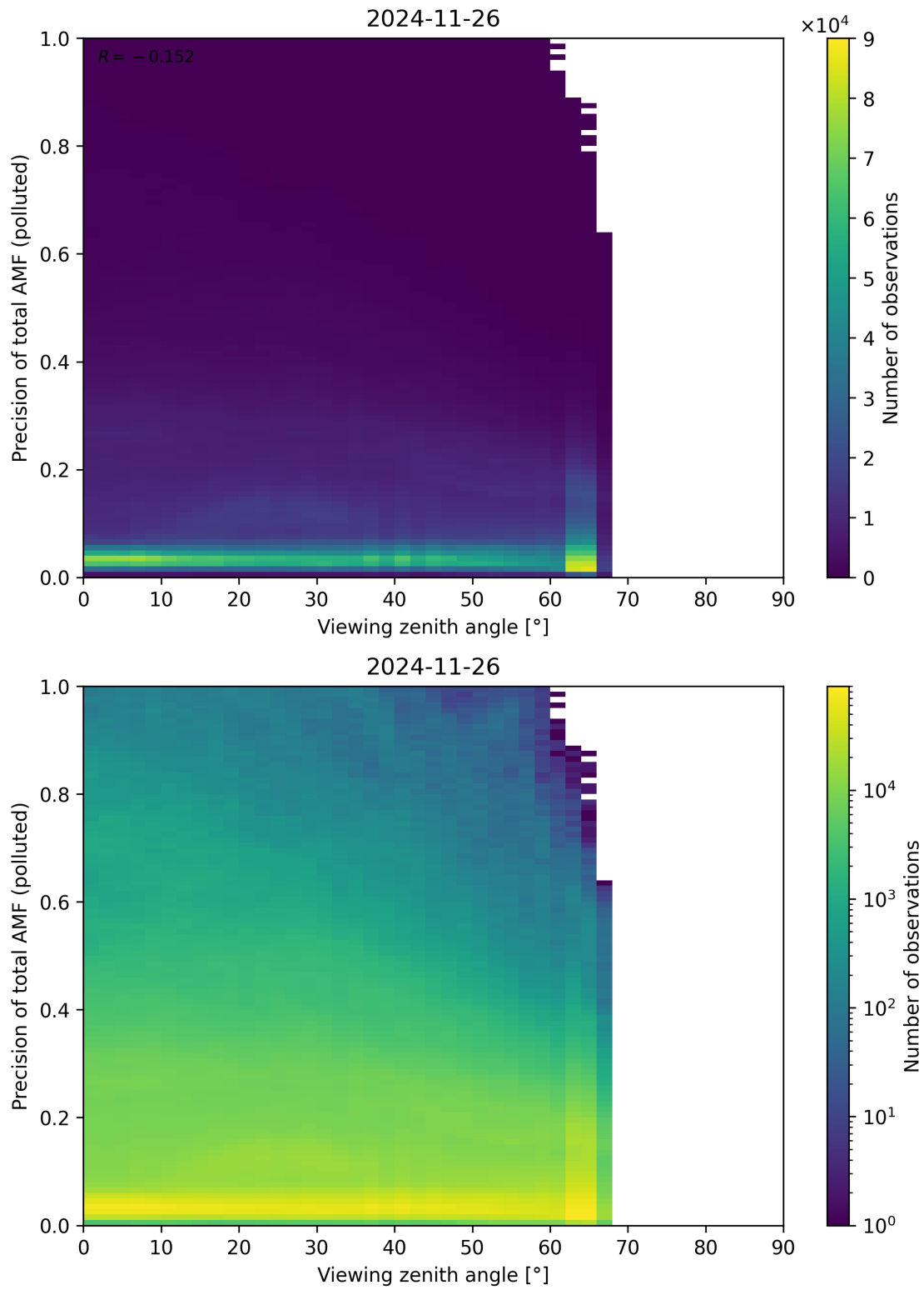
Figure 382: Scatter density plot of “Viewing zenith angle” against “Precision of total AMF (polluted)” for 2024-11-25 to 2024-11-27.
