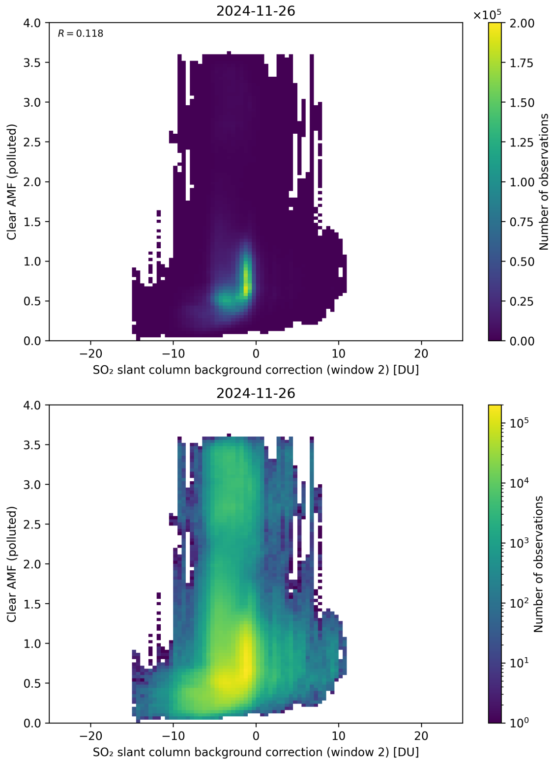
Figure 126: Scatter density plot of “SO 2 slant column background correction (window 2)” against “Clear AMF (polluted)” for 2024-11-25 to 2024-11-27.
