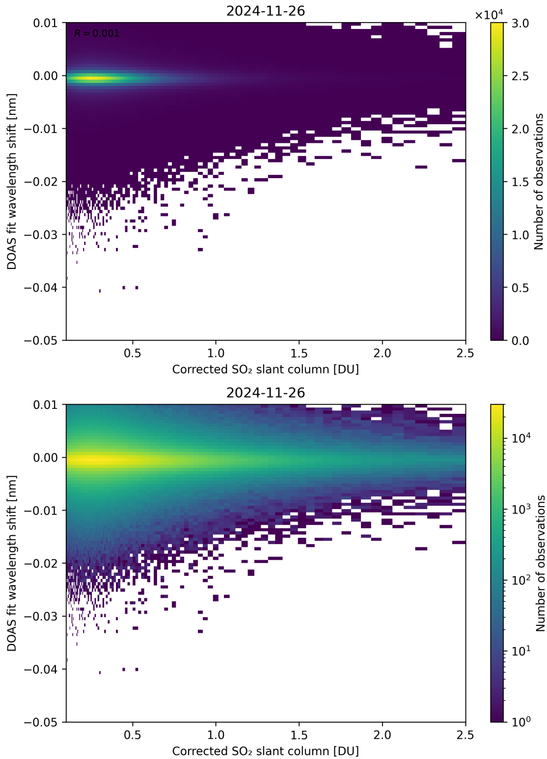
Figure 229: Scatter density plot of “Corrected SO 2 slant column” against “DOAS fit wavelength shift” for 2024-11-25 to 2024-11-27.
