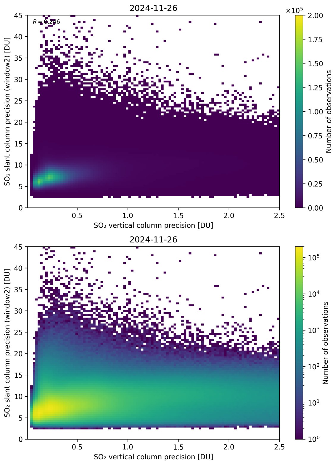
Figure 343: Scatter density plot of “SO 2 vertical column precision” against “SO 2 slant column precision (window2)” for 2024-11-25 to 2024-11-27.
