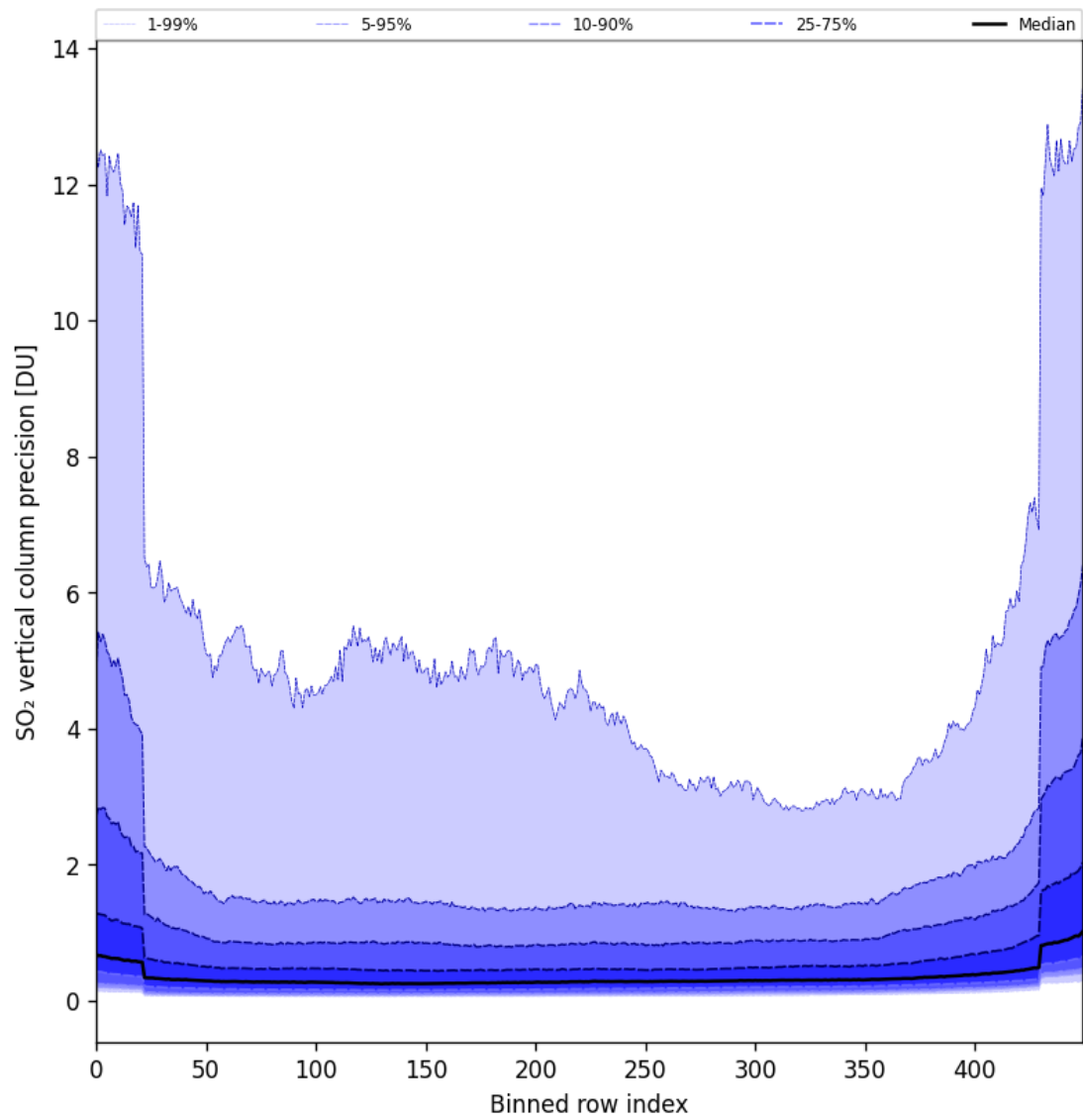
Figure 85: Along track statistics of “SO 2 vertical column precision” for 2024-11-25 to 2024-11-27
