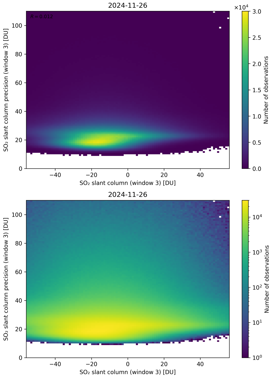
Figure 317: Scatter density plot of “SO 2 slant column (window 3)” against “SO 2 slant column precision (window 3)” for 2024-11-25 to 2024-11-27.
