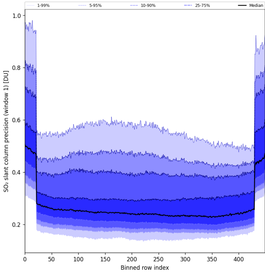
Figure 90: Along track statistics of “SO 2 slant column precision (window 1)” for 2024-11-25 to 2024-11-27
