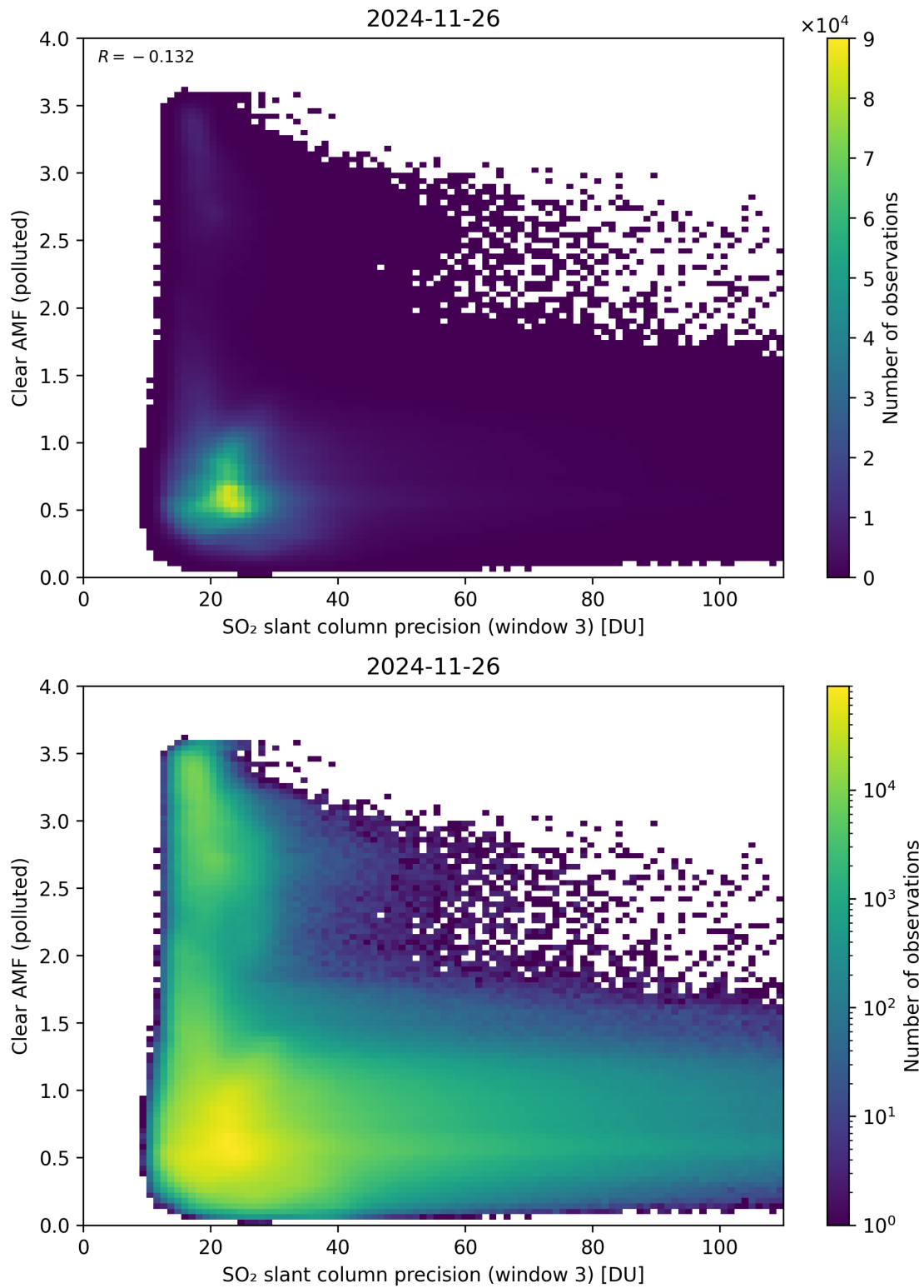
Figure 311: Scatter density plot of “SO 2 slant column precision (window 3)” against “Clear AMF (polluted)” for 2024-11-25 to 2024-11-27.
