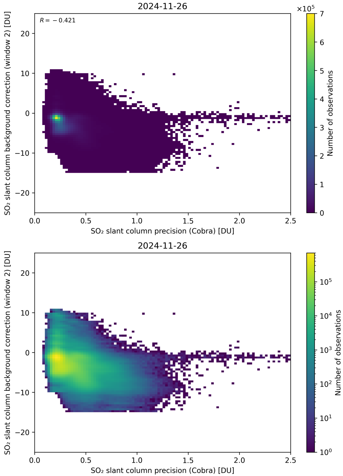
Figure 200: Scatter density plot of “SO 2 slant column precision (Cobra)” against “SO 2 slant column background correction (window 2)” for 2024-11-25 to 2024-11-27.
