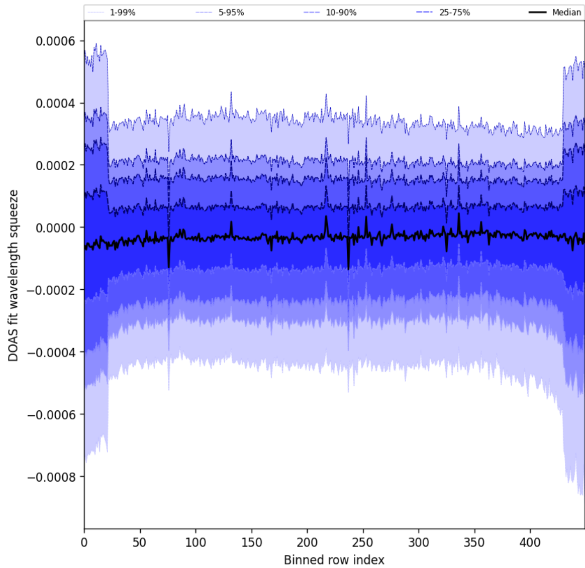
Figure 103: Along track statistics of “DOAS fit wavelength squeeze” for 2024-11-25 to 2024-11-27
