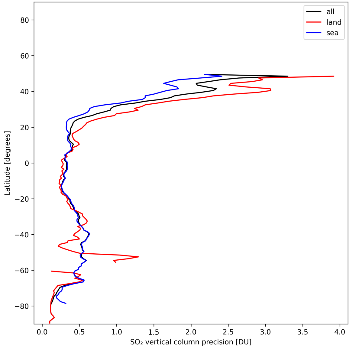
Figure 33: Zonal average of “SO 2 vertical column precision” for 2024-11-25 to 2024-11-27.
