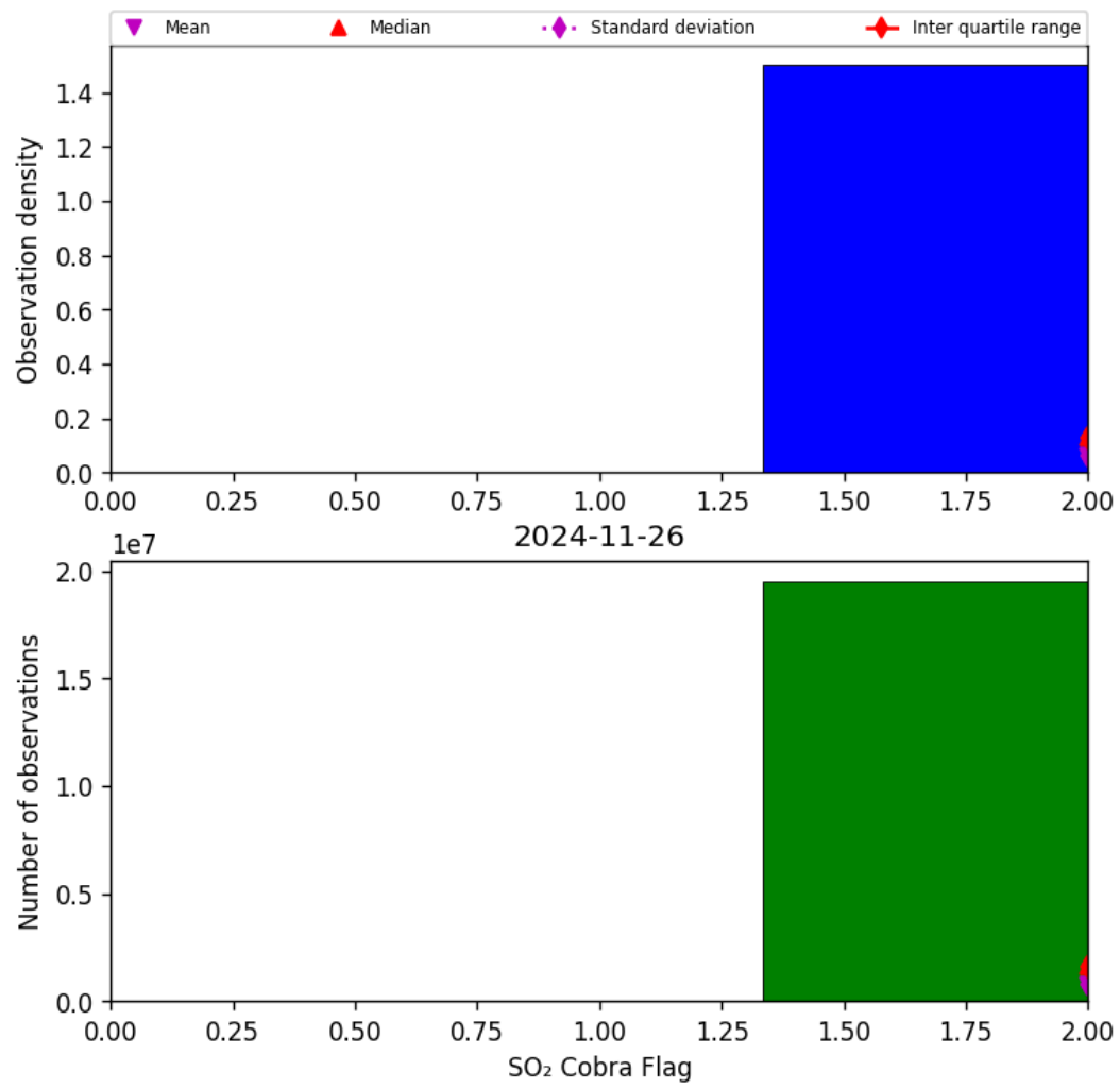
Figure 75: Histogram of “SO 2 Cobra Flag” for 2024-11-25 to 2024-11-27
