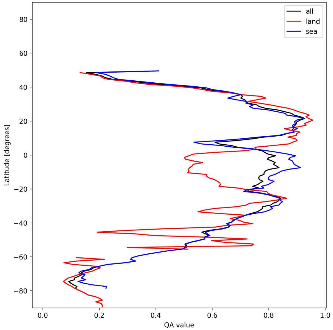
Figure 31: Zonal average of “QA value” for 2024-11-25 to 2024-11-27.
