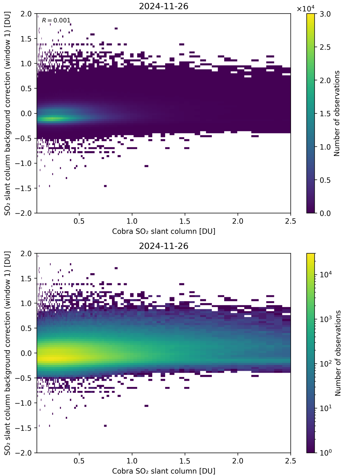
Figure 193: Scatter density plot of “Cobra SO 2 slant column” against “SO 2 slant column background correction (window 1)” for 2024-11-25 to 2024-11-27.
