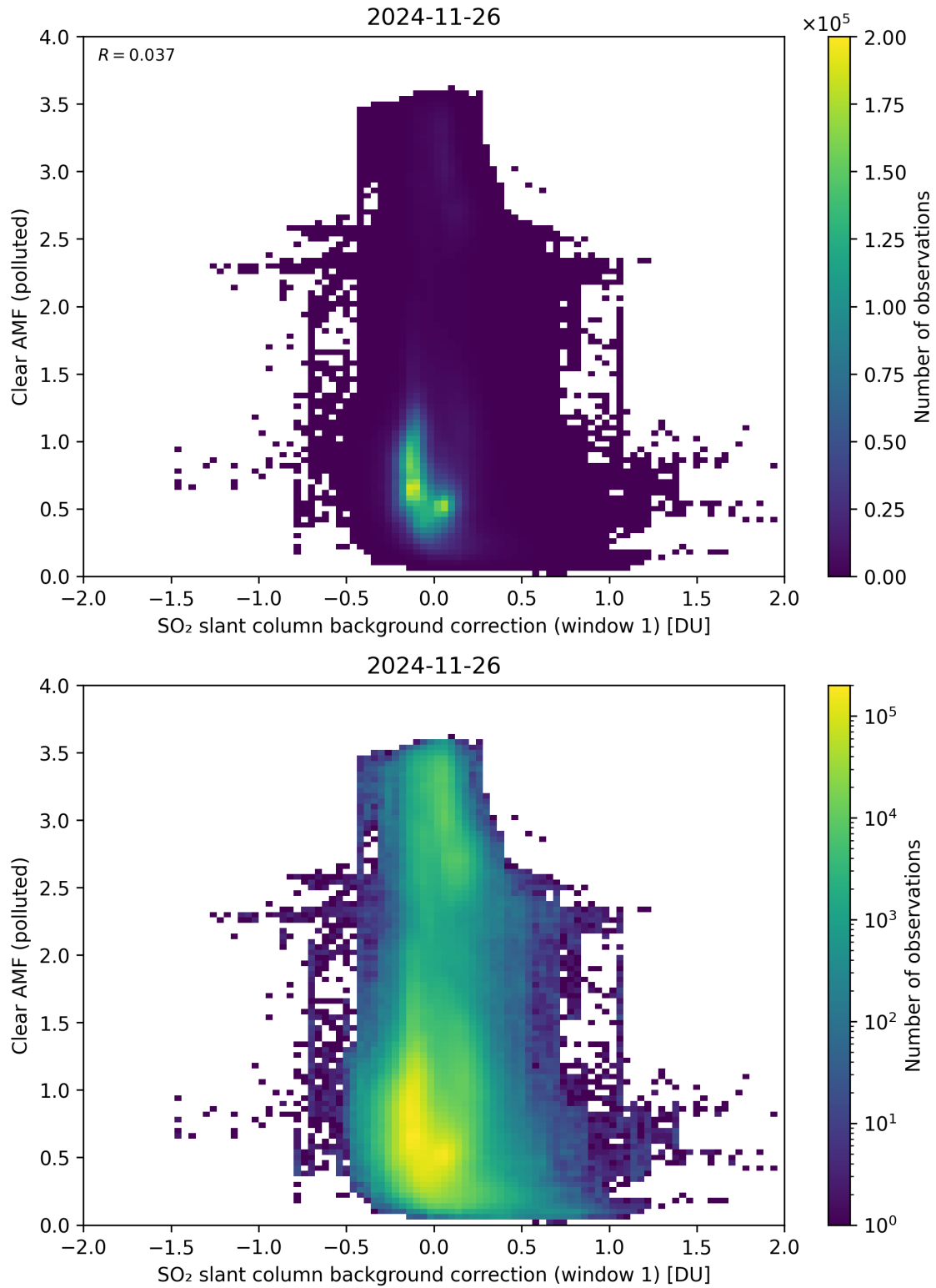
Figure 114: Scatter density plot of “SO 2 slant column background correction (window 1)” against “Clear AMF (polluted)” for 2024-11-25 to 2024-11-27.
