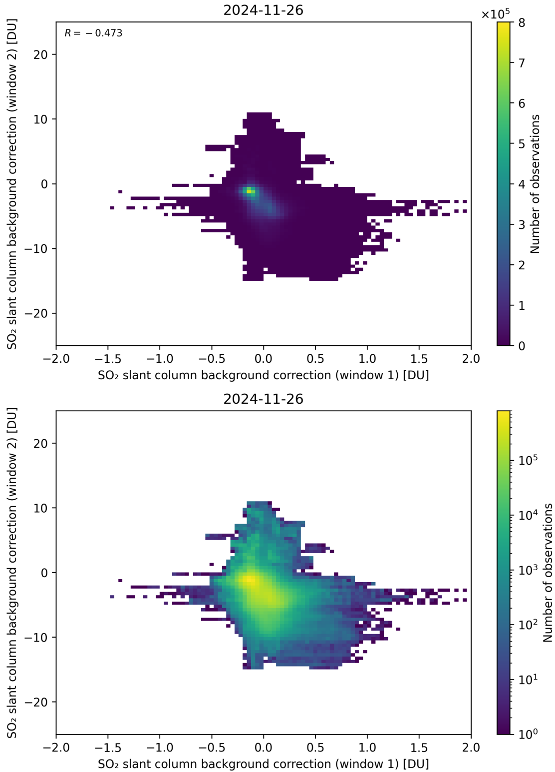
Figure 109: Scatter density plot of “SO 2 slant column background correction (window 1)” against “SO 2 slant column background correction (window 2)” for 2024-11-25 to 2024-11-27.
