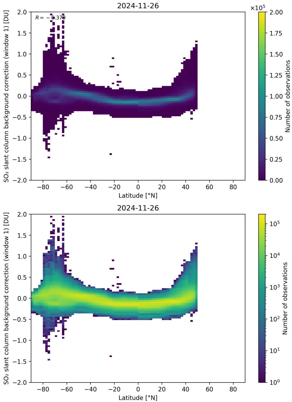
Figure 150: Scatter density plot of “Latitude” against “SO 2 slant column background correction (window 1)” for 2024-11-25 to 2024-11-27.
