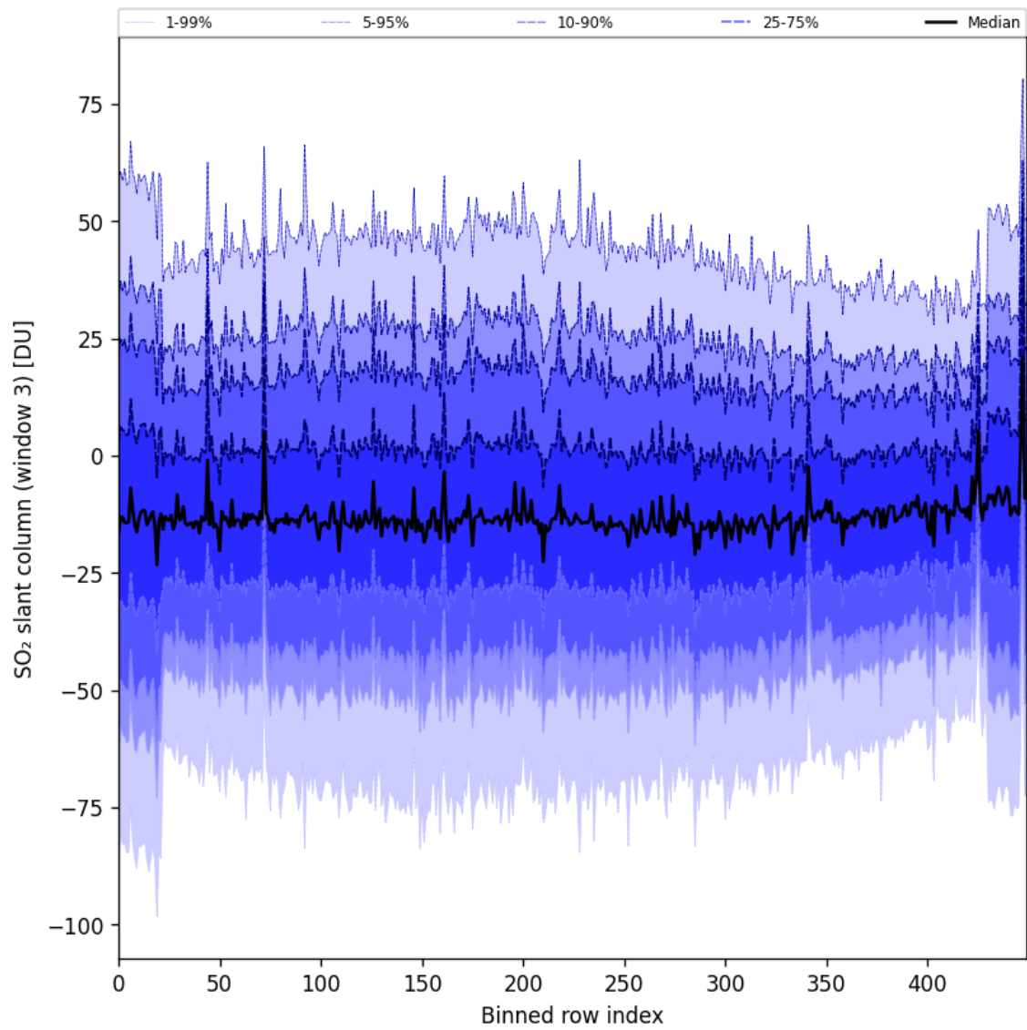
Figure 97: Along track statistics of “SO 2 slant column (window 3)” for 2024-11-25 to 2024-11-27
