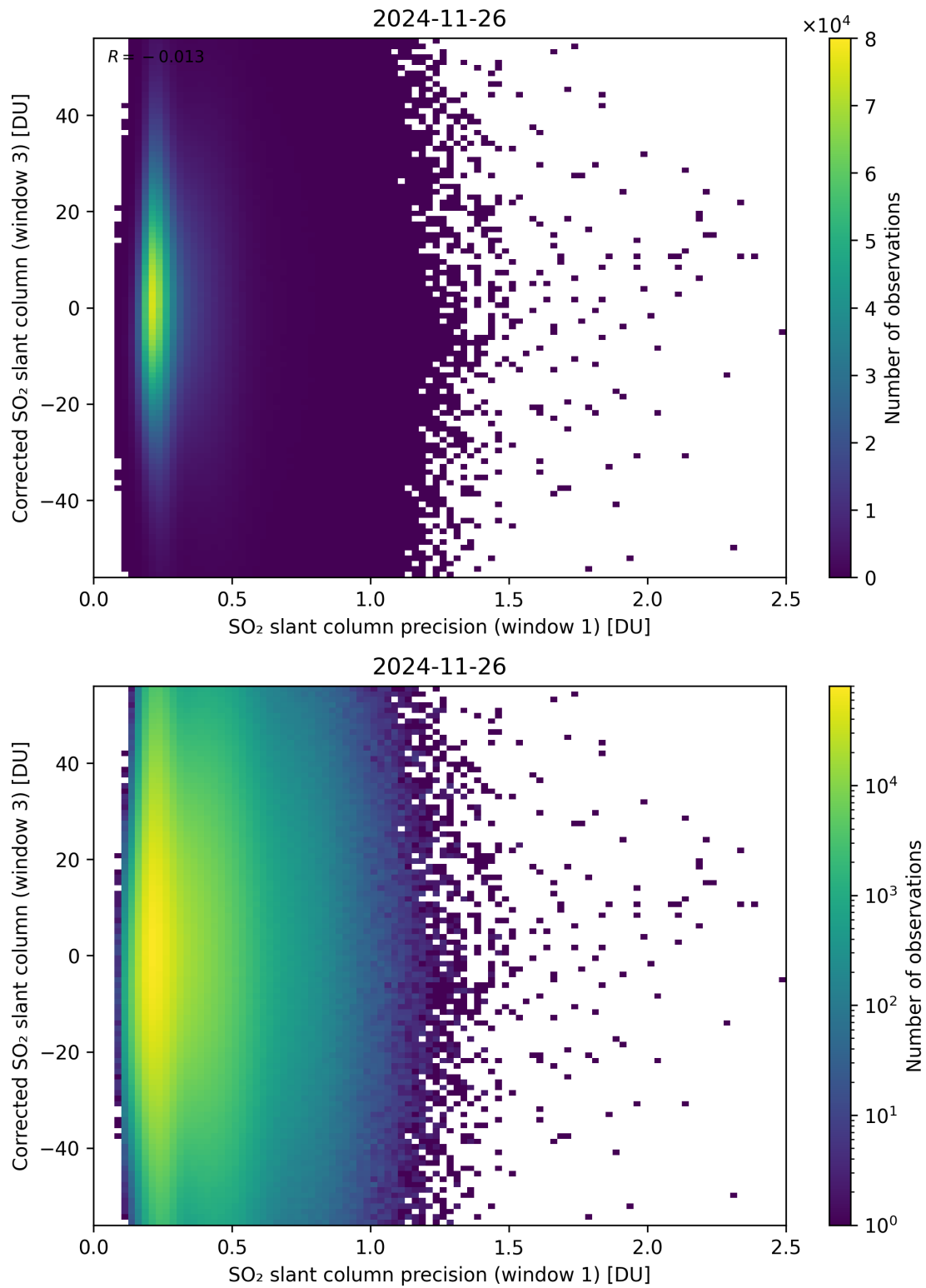
Figure 276: Scatter density plot of “SO 2 slant column precision (window 1)” against “Corrected SO 2 slant column (window 3)” for 2024-11-25 to 2024-11-27.
