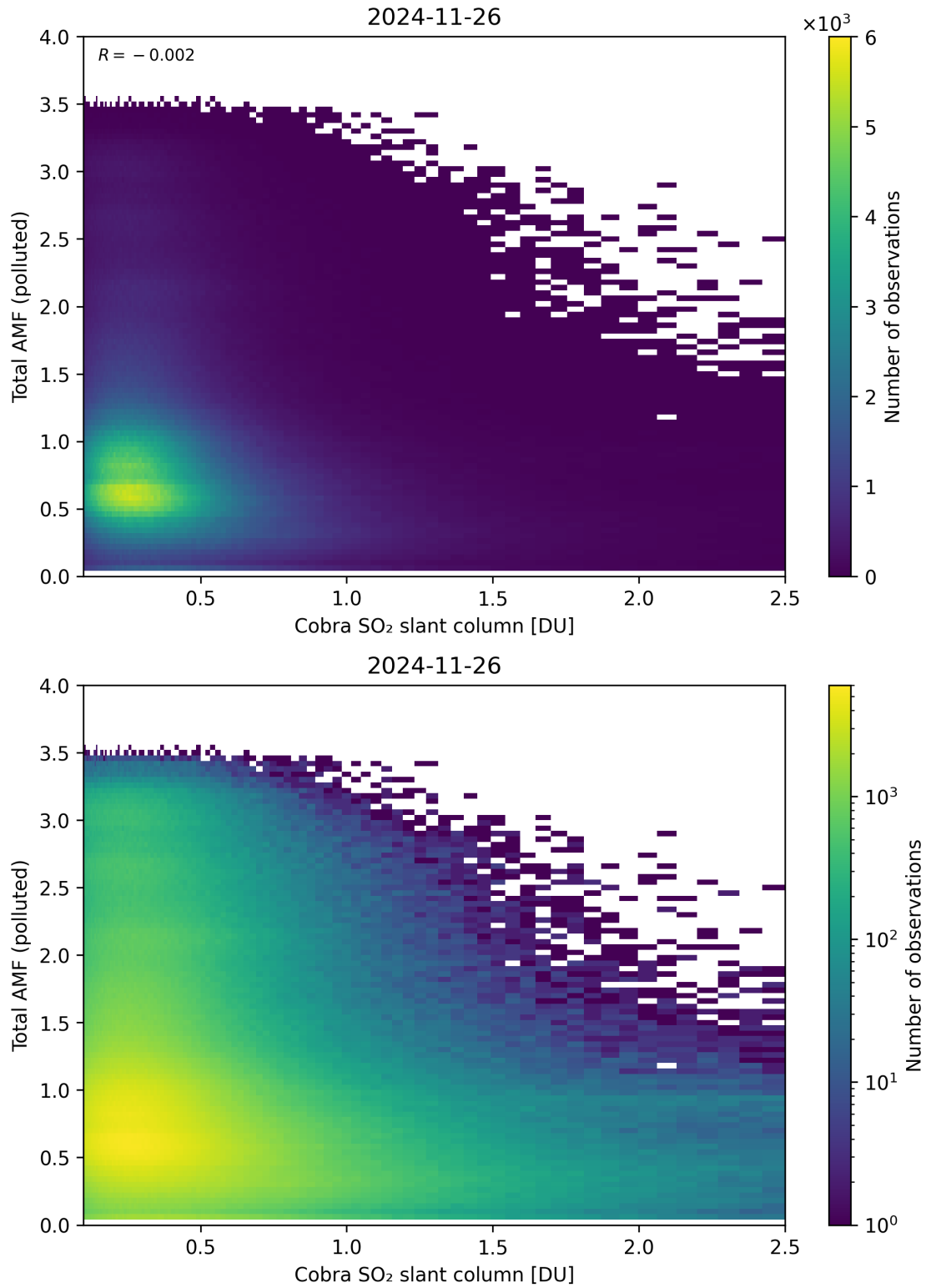
Figure 224: Scatter density plot of “Cobra SO 2 slant column” against “Total AMF (polluted)” for 2024-11-25 to 2024-11-27.
