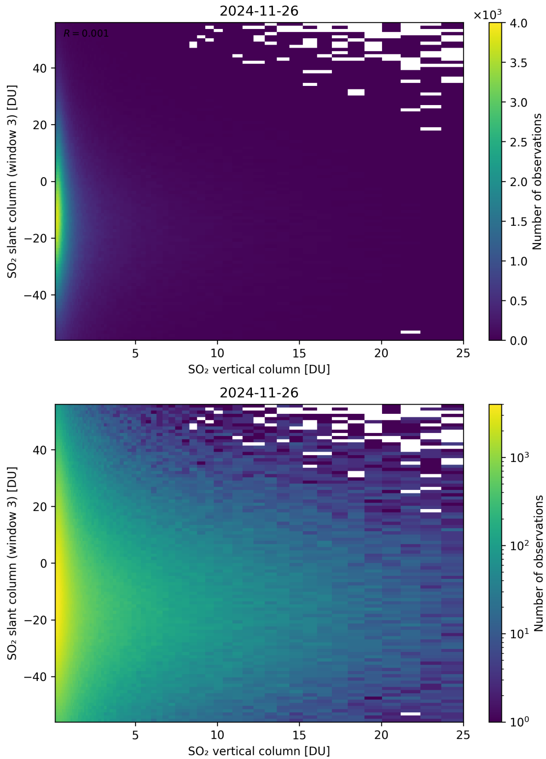
Figure 357: Scatter density plot of “SO 2 vertical column” against “SO 2 slant column (window 3)” for 2024-11-25 to 2024-11-27.
