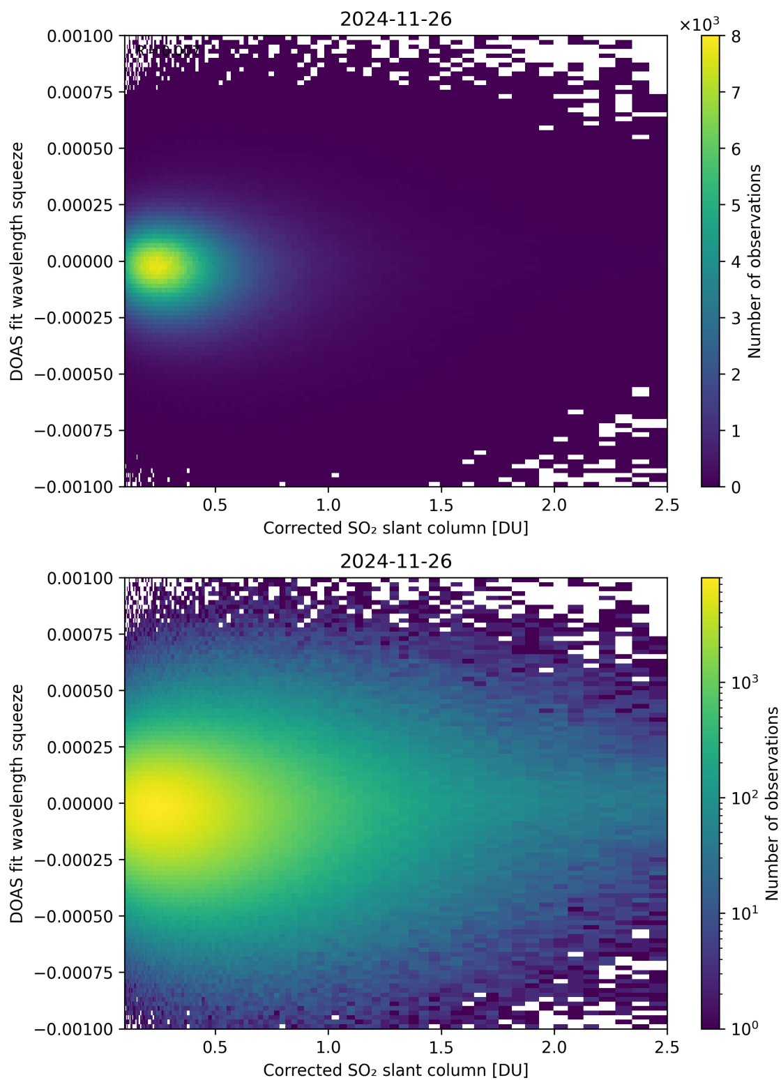
Figure 230: Scatter density plot of “Corrected SO 2 slant column” against “DOAS fit wavelength squeeze” for 2024-11-25 to 2024-11-27.
