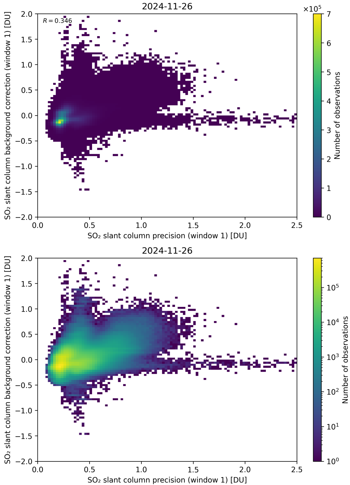
Figure 268: Scatter density plot of “SO 2 slant column precision (window 1)” against “SO 2 slant column background correction (window 1)” for 2024-11-25 to 2024-11-27.
