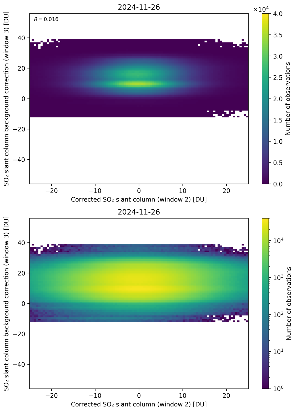
Figure 245: Scatter density plot of “Corrected SO 2 slant column (window 2)” against “SO 2 slant column background correction (window 3)” for 2024-11-25 to 2024-11-27.
