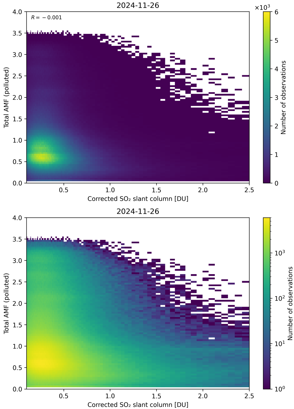
Figure 242: Scatter density plot of “Corrected SO 2 slant column” against “Total AMF (polluted)” for 2024-11-25 to 2024-11-27.
