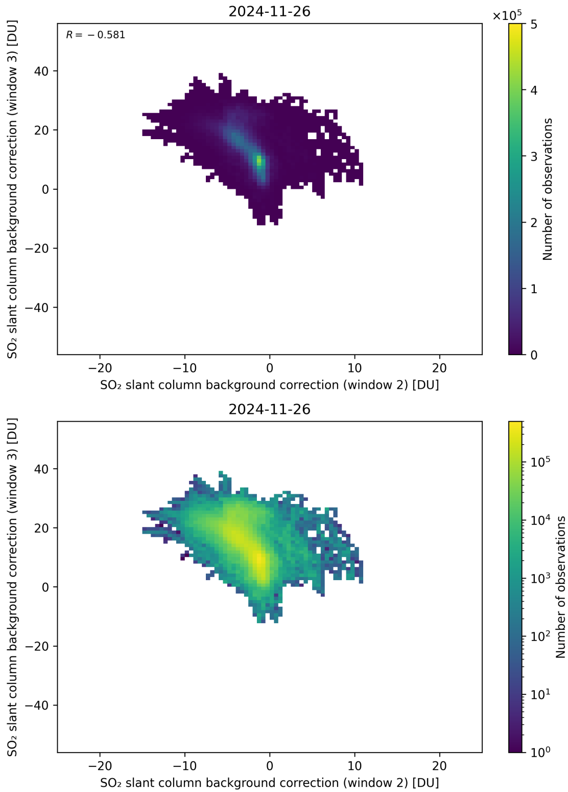
Figure 122: Scatter density plot of “SO 2 slant column background correction (window 2)” against “SO 2 slant column background correction (window 3)” for 2024-11-25 to 2024-11-27.
