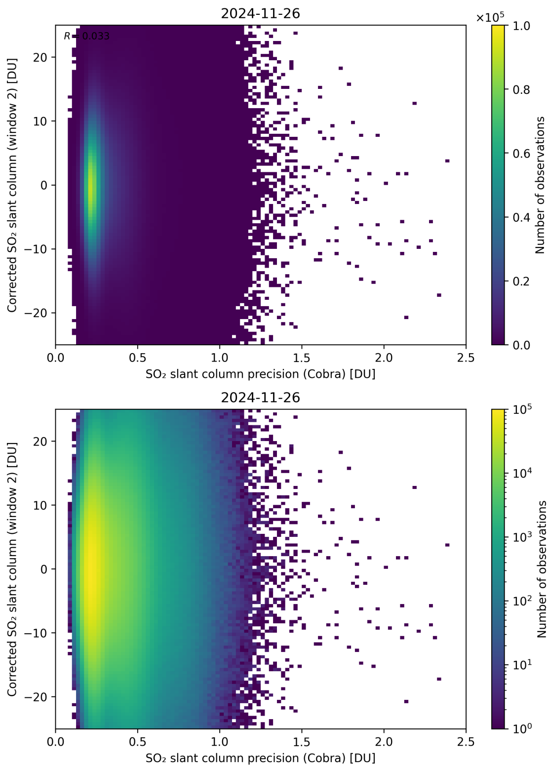
Figure 206: Scatter density plot of “SO 2 slant column precision (Cobra)” against “Corrected SO 2 slant column (window 2)” for 2024-11-25 to 2024-11-27.
