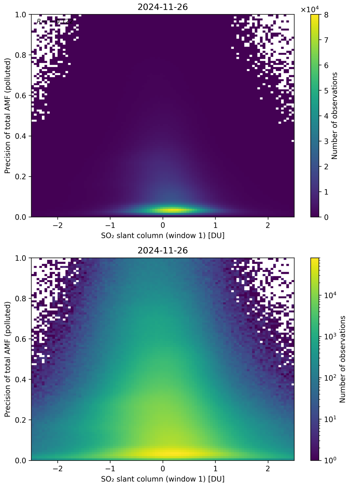
Figure 290: Scatter density plot of “SO 2 slant column (window 1)” against “Precision of total AMF (polluted)” for 2024-11-25 to 2024-11-27.
