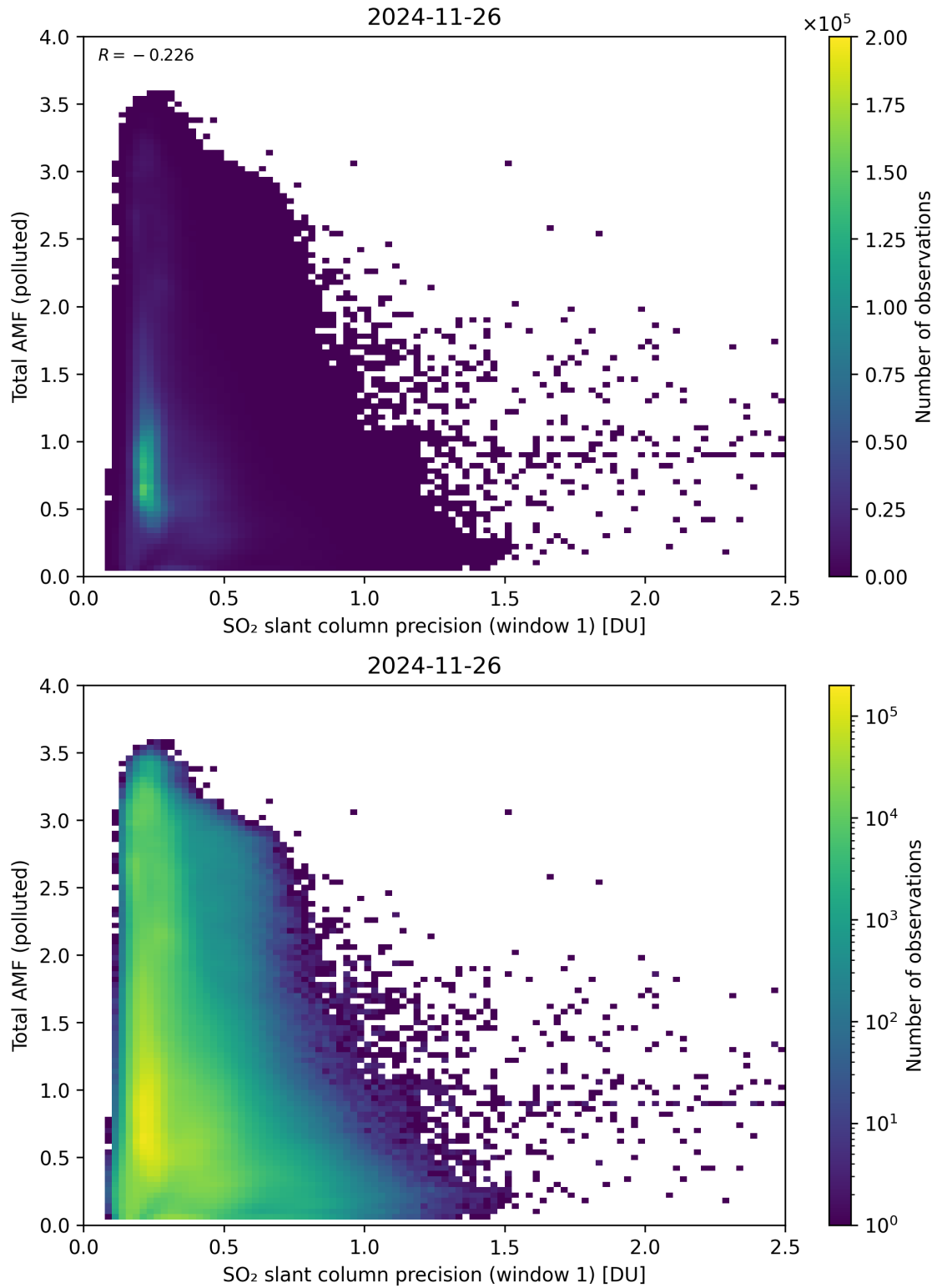
Figure 280: Scatter density plot of “SO 2 slant column precision (window 1)” against “Total AMF (polluted)” for 2024-11-25 to 2024-11-27.
