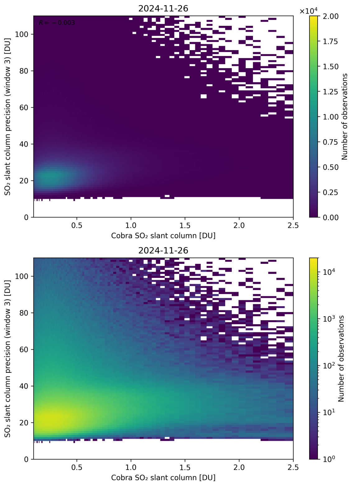
Figure 223: Scatter density plot of “Cobra SO 2 slant column” against “SO 2 slant column precision (window 3)” for 2024-11-25 to 2024-11-27.
