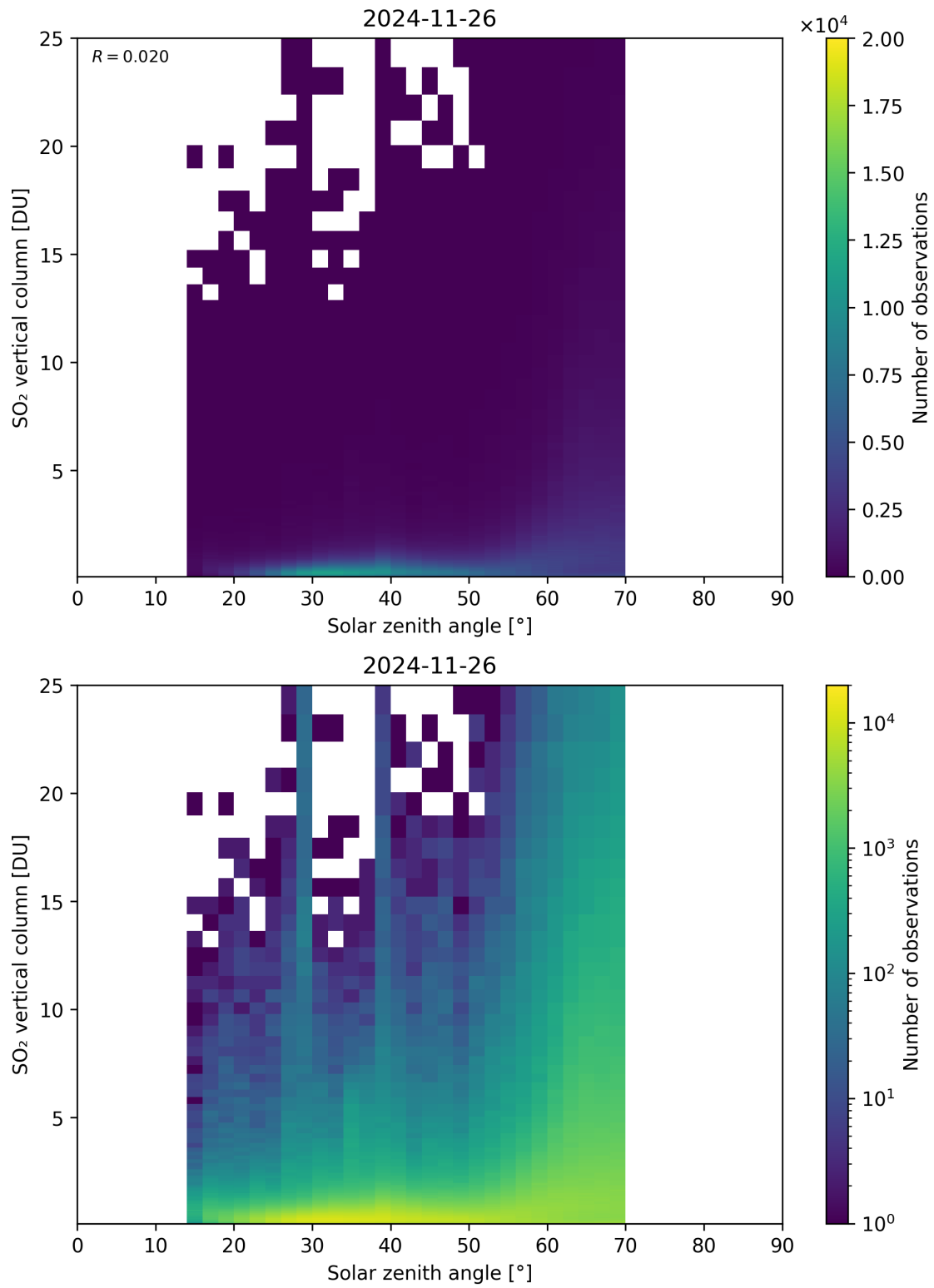
Figure 191: Scatter density plot of “Solar zenith angle” against “SO 2 vertical column” for 2024-11-25 to 2024-11-27.
