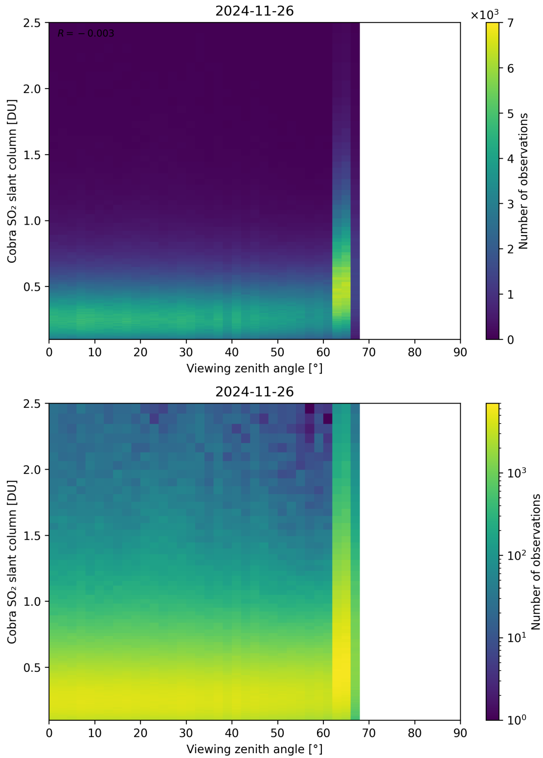
Figure 371: Scatter density plot of “Viewing zenith angle” against “Cobra SO 2 slant column” for 2024-11-25 to 2024-11-27.
