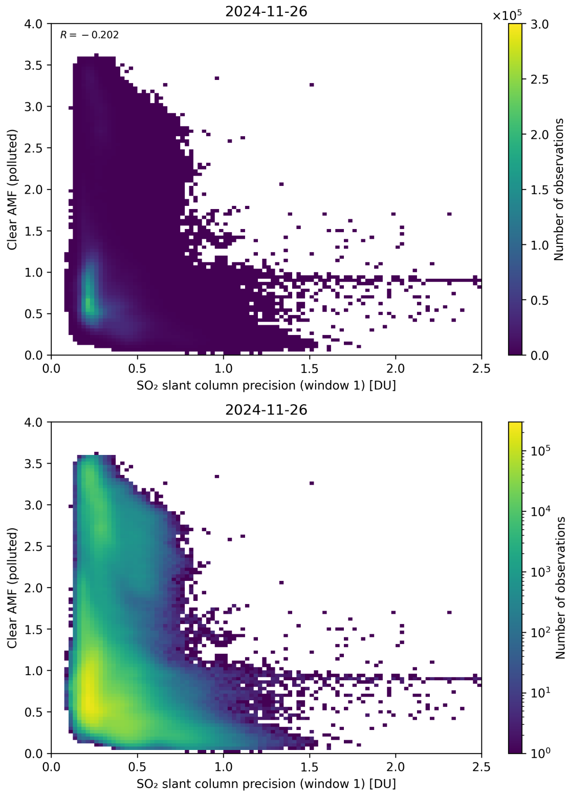
Figure 274: Scatter density plot of “SO 2 slant column precision (window 1)” against “Clear AMF (polluted)” for 2024-11-25 to 2024-11-27.
