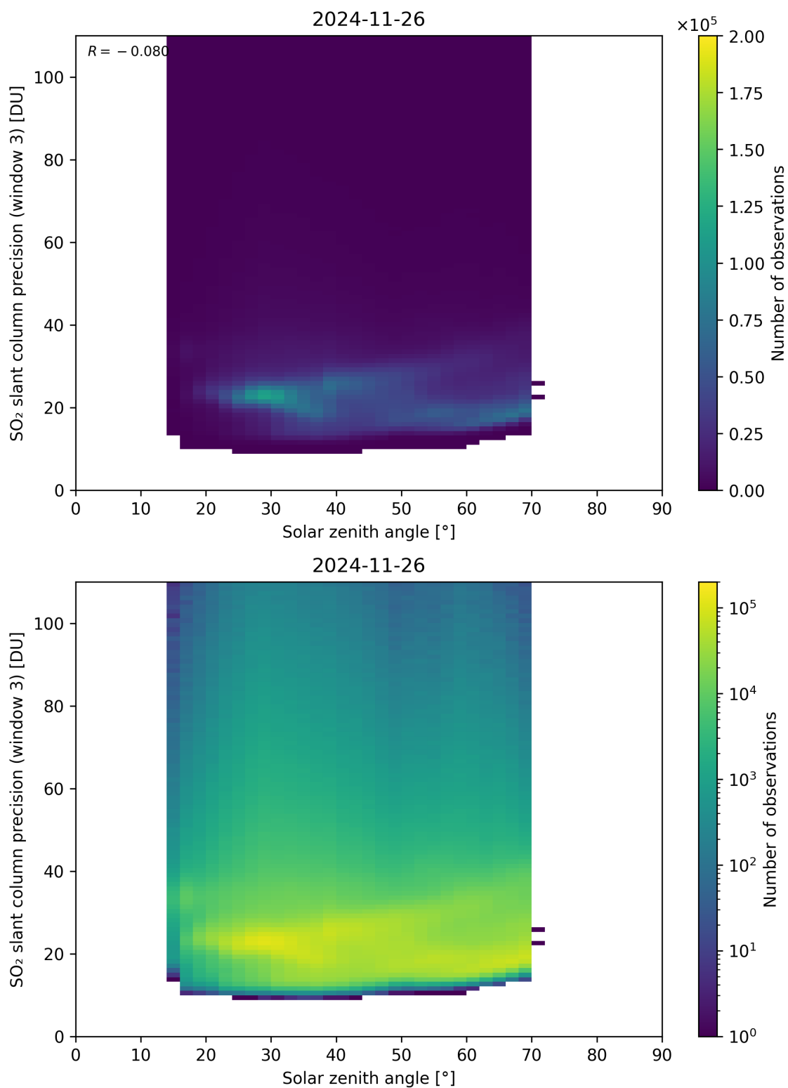
Figure 188: Scatter density plot of “Solar zenith angle” against “SO 2 slant column precision (window 3)” for 2024-11-25 to 2024-11-27.
