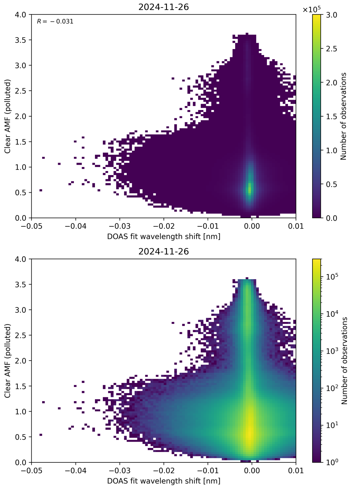
Figure 140: Scatter density plot of “DOAS fit wavelength shift” against “Clear AMF (polluted)” for 2024-11-25 to 2024-11-27.
