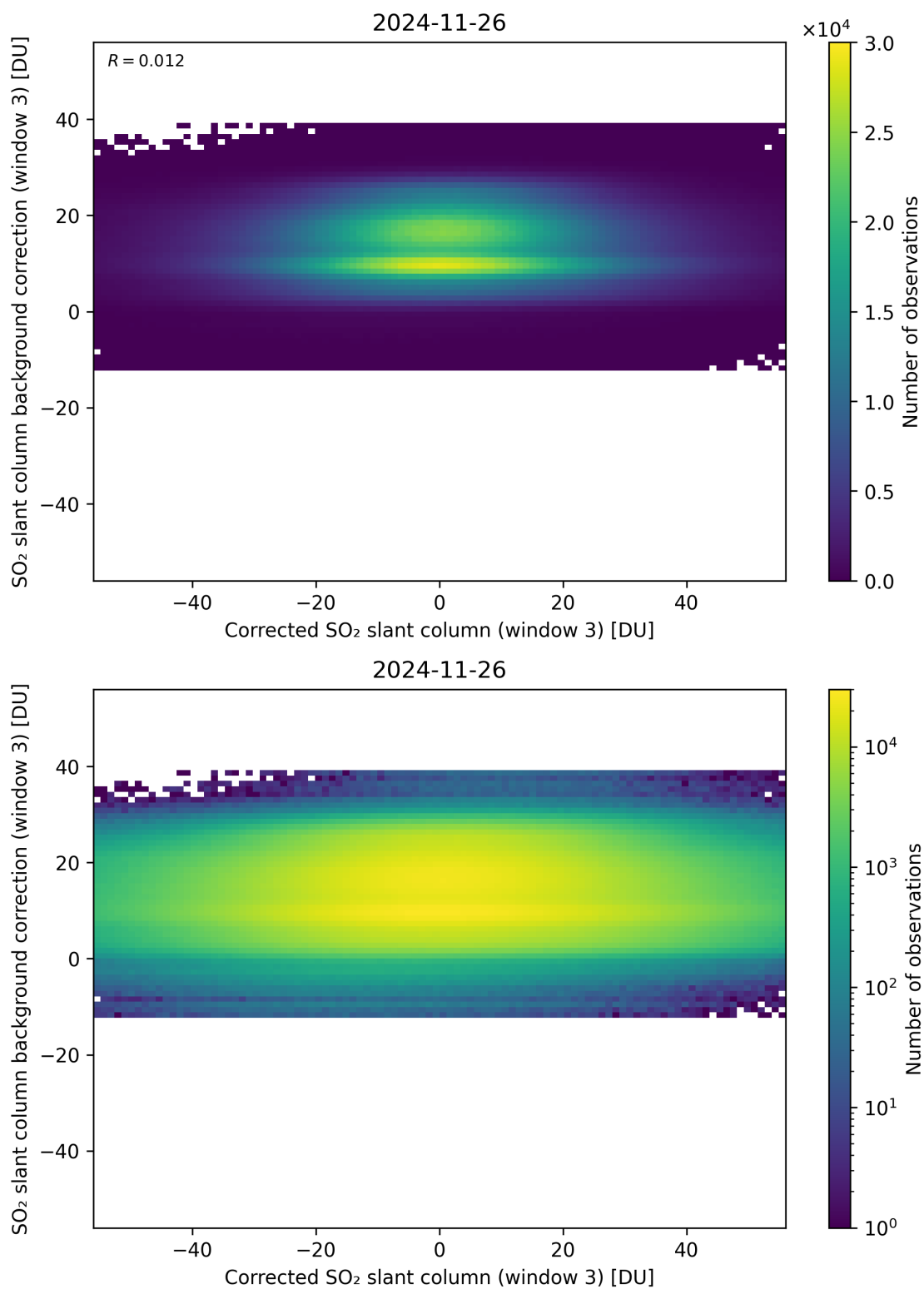
Figure 255: Scatter density plot of “Corrected SO 2 slant column (window 3)” against “SO 2 slant column background correction (window 3)” for 2024-11-25 to 2024-11-27.
