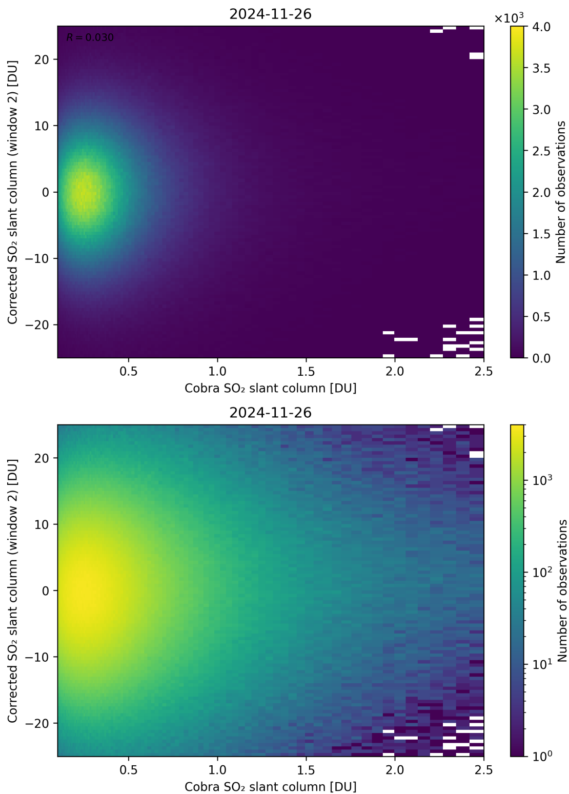
Figure 217: Scatter density plot of “Cobra SO 2 slant column” against “Corrected SO 2 slant column (window 2)” for 2024-11-25 to 2024-11-27.
