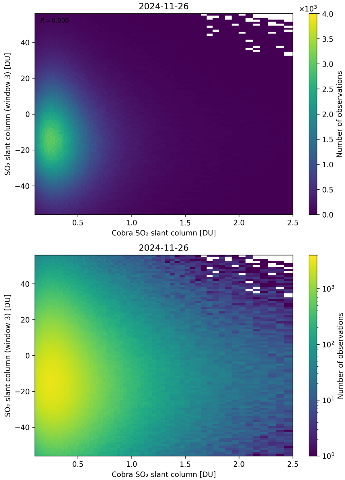
Figure 222: Scatter density plot of “Cobra SO 2 slant column” against “SO 2 slant column (window 3)” for 2024-11-25 to 2024-11-27.
