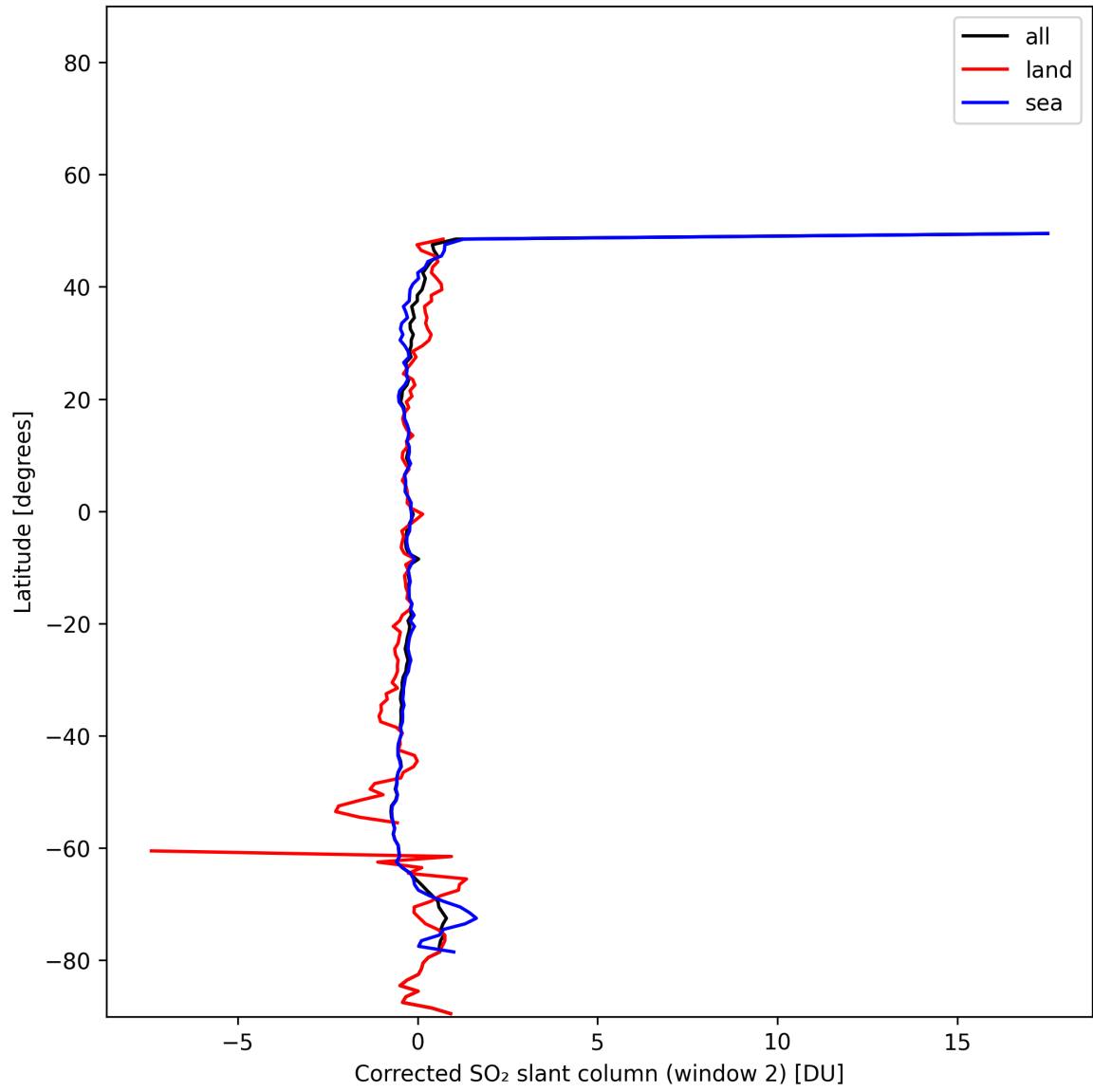
Figure 43: Zonal average of “Corrected SO 2 slant column (window 2)” for 2024-11-25 to 2024-11-27.
