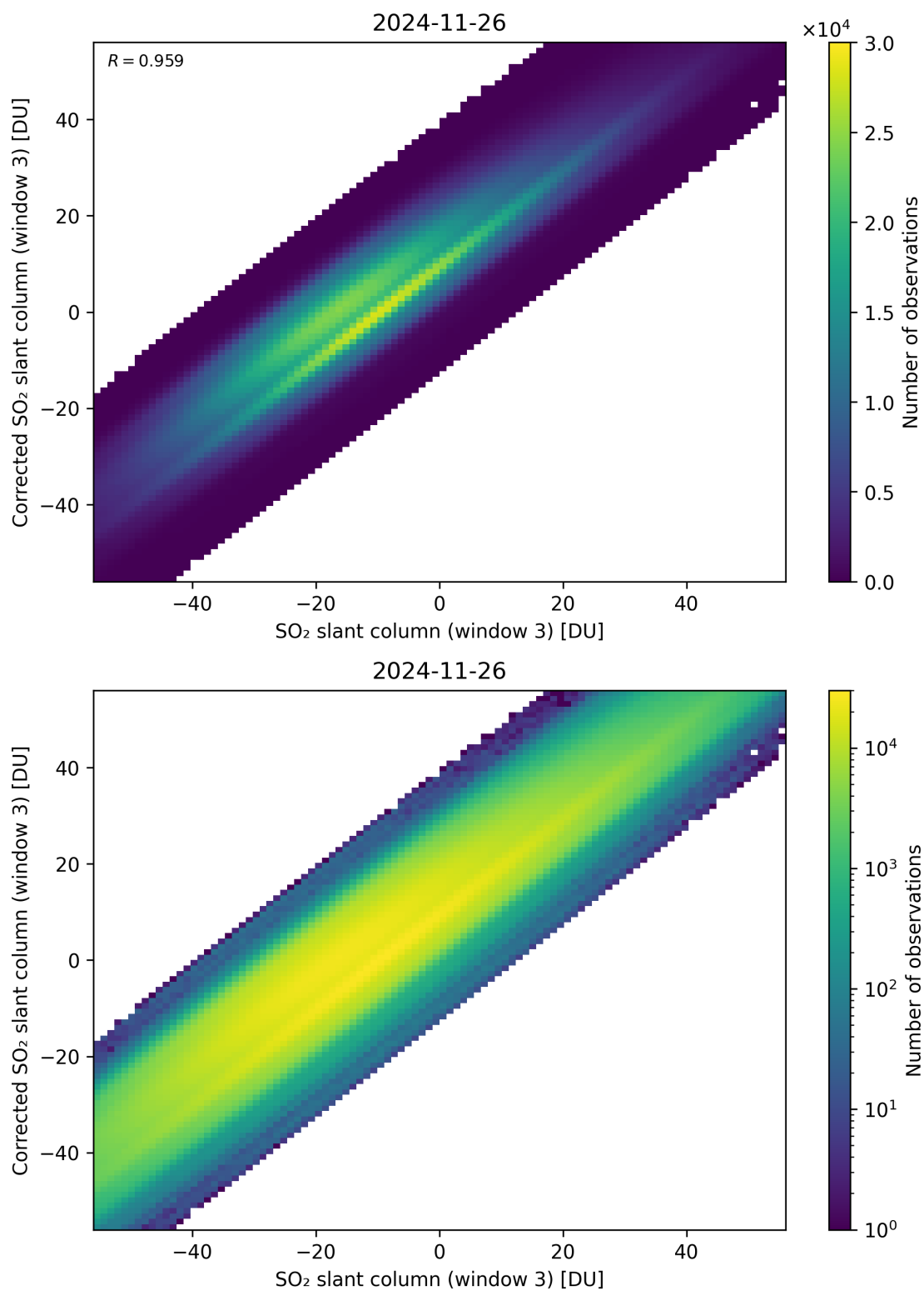
Figure 316: Scatter density plot of “SO 2 slant column (window 3)” against “Corrected SO 2 slant column (window 3)” for 2024-11-25 to 2024-11-27.
