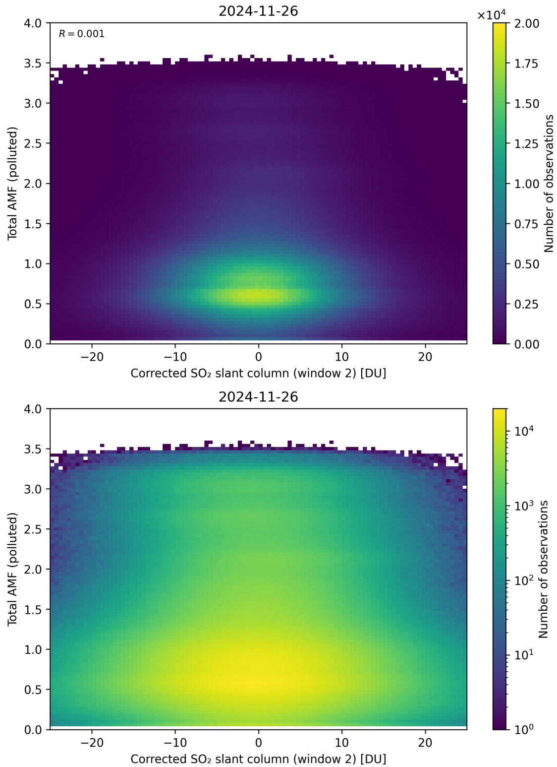
Figure 253: Scatter density plot of “Corrected SO 2 slant column (window 2)” against “Total AMF (polluted)” for 2024-11-25 to 2024-11-27.
