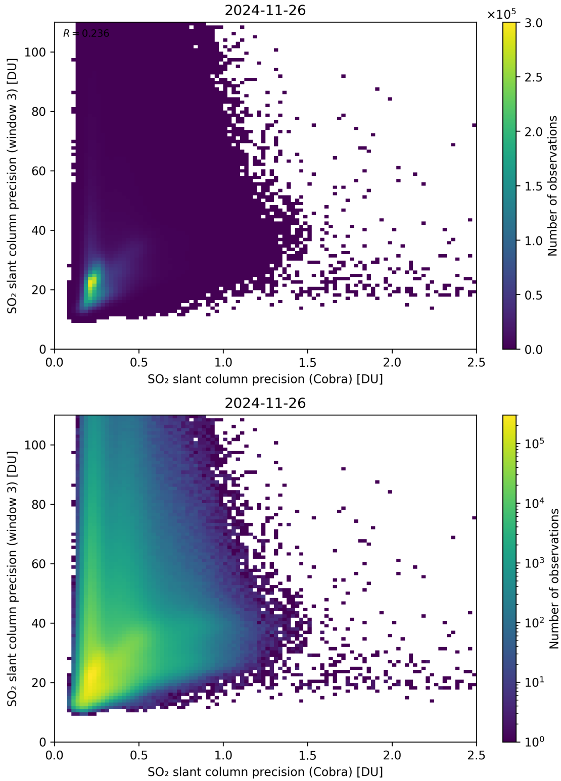
Figure 212: Scatter density plot of “SO 2 slant column precision (Cobra)” against “SO 2 slant column precision (window 3)” for 2024-11-25 to 2024-11-27.
