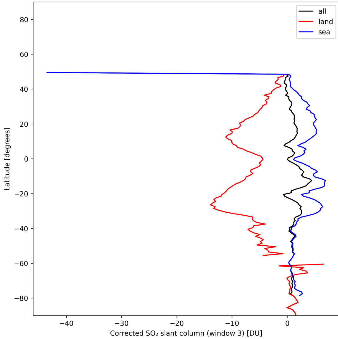
Figure 47: Zonal average of “Corrected SO 2 slant column (window 3)” for 2024-11-25 to 2024-11-27.
