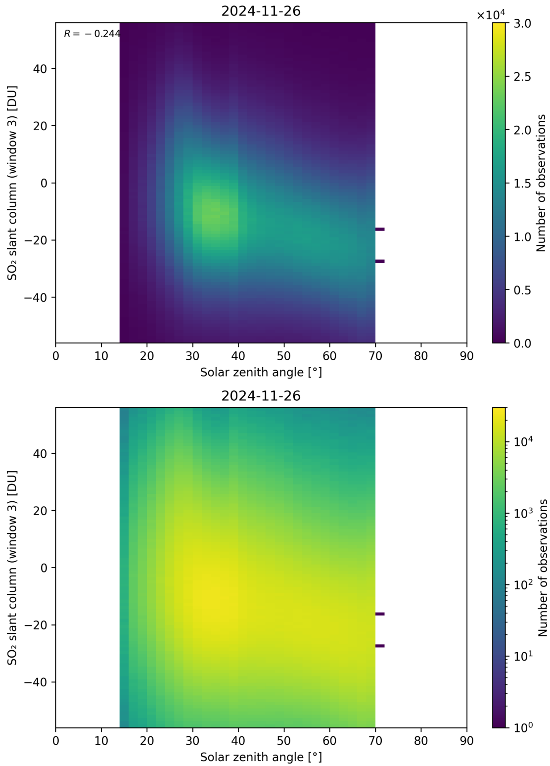
Figure 187: Scatter density plot of “Solar zenith angle” against “SO 2 slant column (window 3)” for 2024-11-25 to 2024-11-27.
