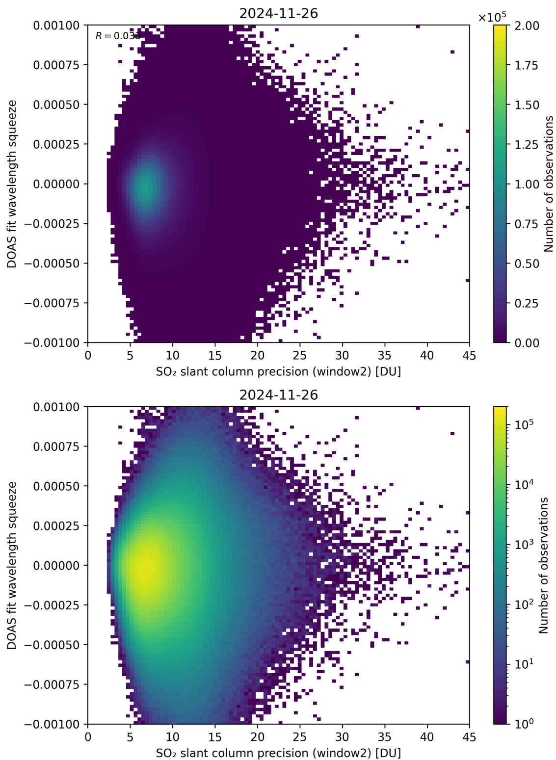
Figure 294: Scatter density plot of “SO 2 slant column precision (window2)” against “DOAS fit wavelength squeeze” for 2024-11-25 to 2024-11-27.
