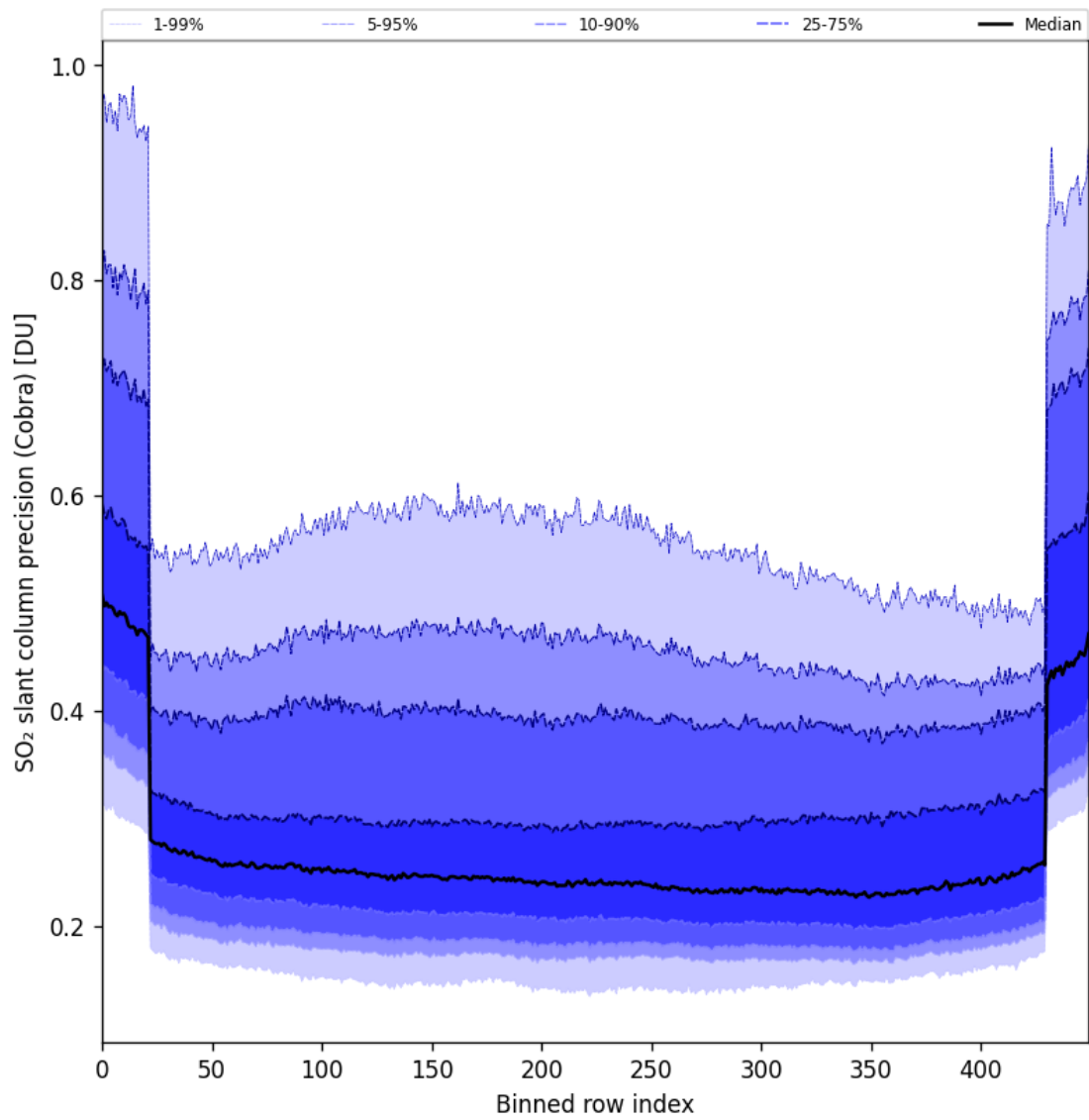
Figure 88: Along track statistics of “SO 2 slant column precision (Cobra)” for 2024-11-25 to 2024-11-27
