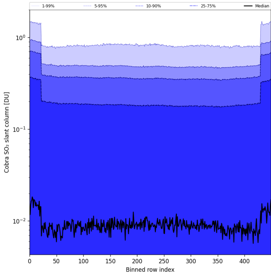
Figure 87: Along track statistics of "Cobra SO 2 slant column" for 2024-11-25 to 2024-11-27
