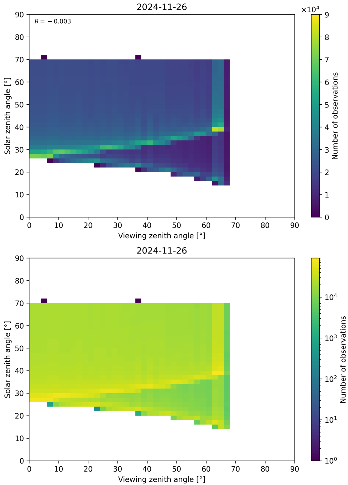
Figure 369: Scatter density plot of “Viewing zenith angle” against “Solar zenith angle” for 2024-11-25 to 2024-11-27.
