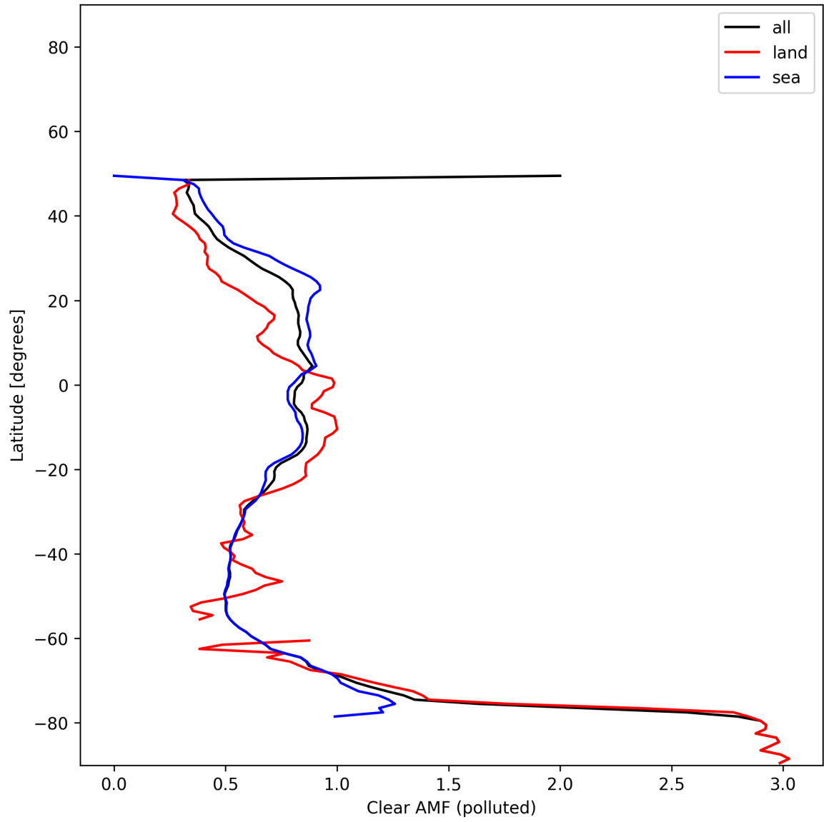
Figure 55: Zonal average of “Clear AMF (polluted)” for 2024-11-25 to 2024-11-27.
