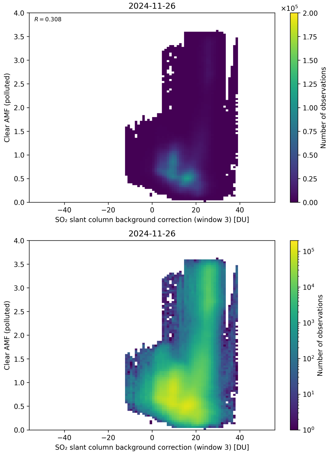
Figure 135: Scatter density plot of “SO 2 slant column background correction (window 3)” against “Clear AMF (polluted)” for 2024-11-25 to 2024-11-27.
