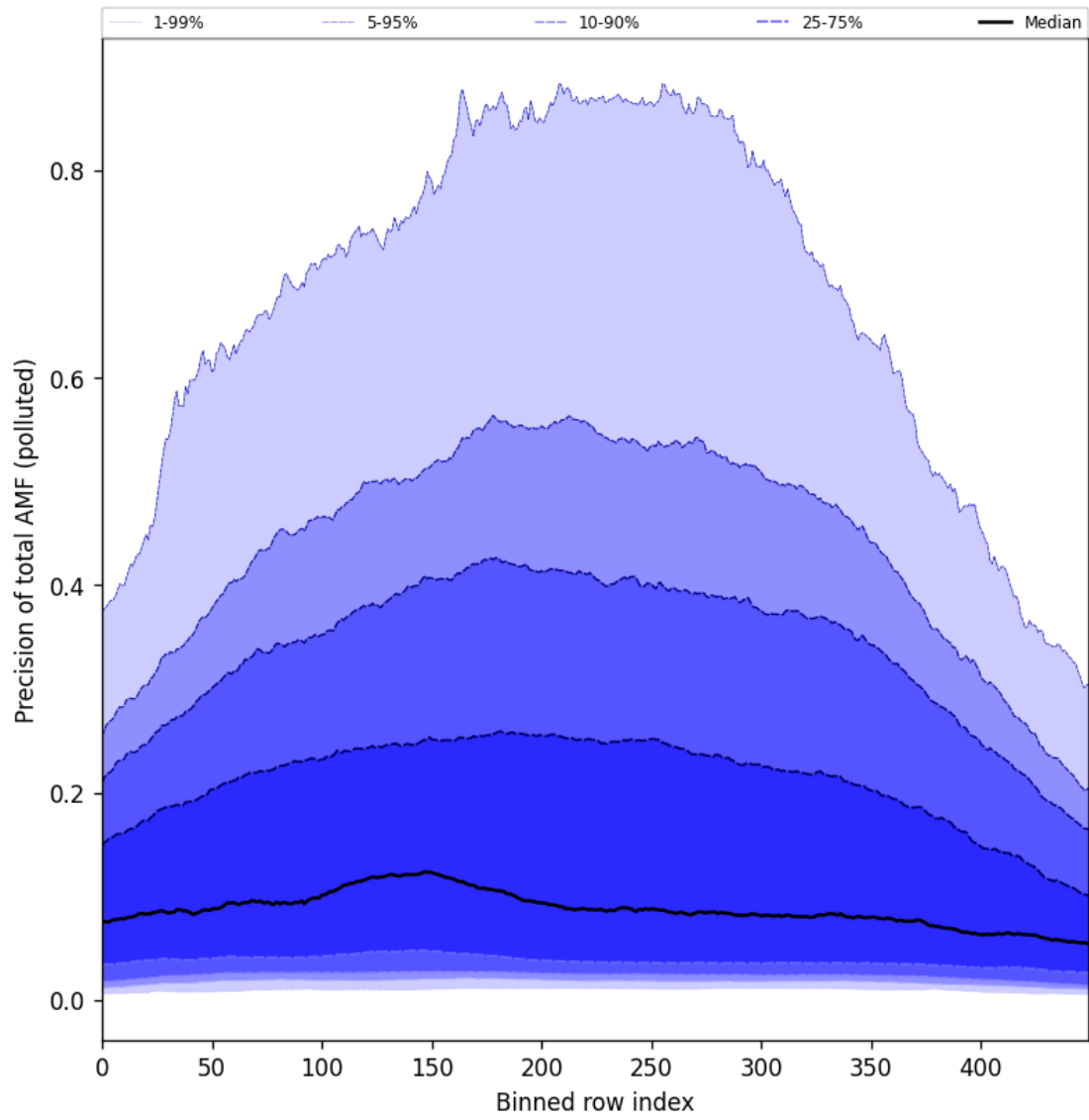
Figure 106: Along track statistics of “Precision of total AMF (polluted)” for 2024-11-25 to 2024-11-27
