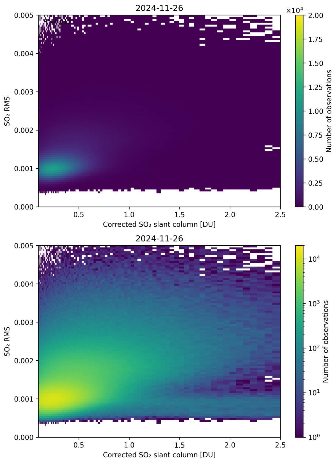
Figure 231: Scatter density plot of “Corrected SO 2 slant column” against “SO 2 RMS” for 2024-11-25 to 2024-11-27.
