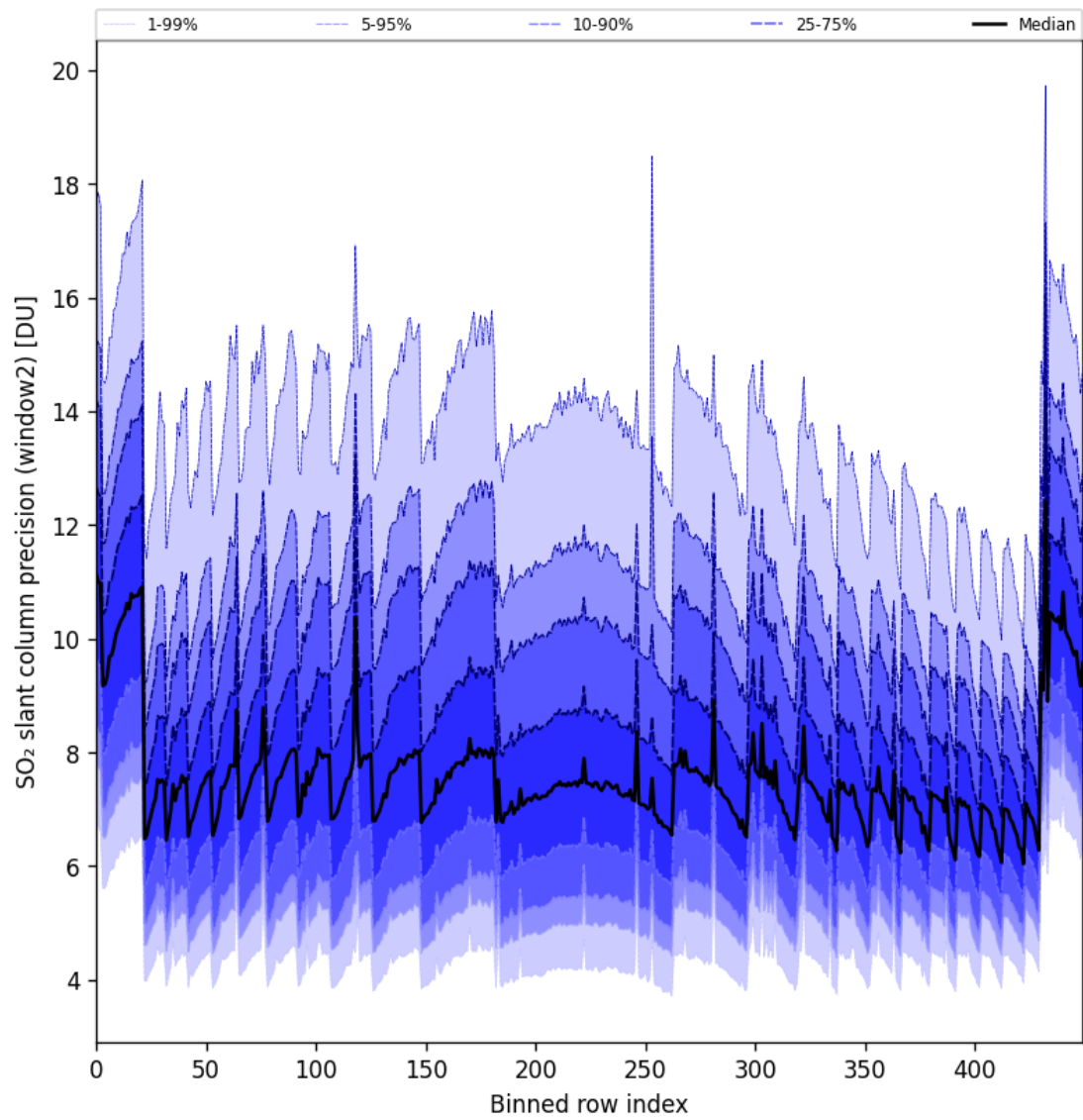
Figure 94: Along track statistics of “SO 2 slant column precision (window2)” for 2024-11-25 to 2024-11-27
