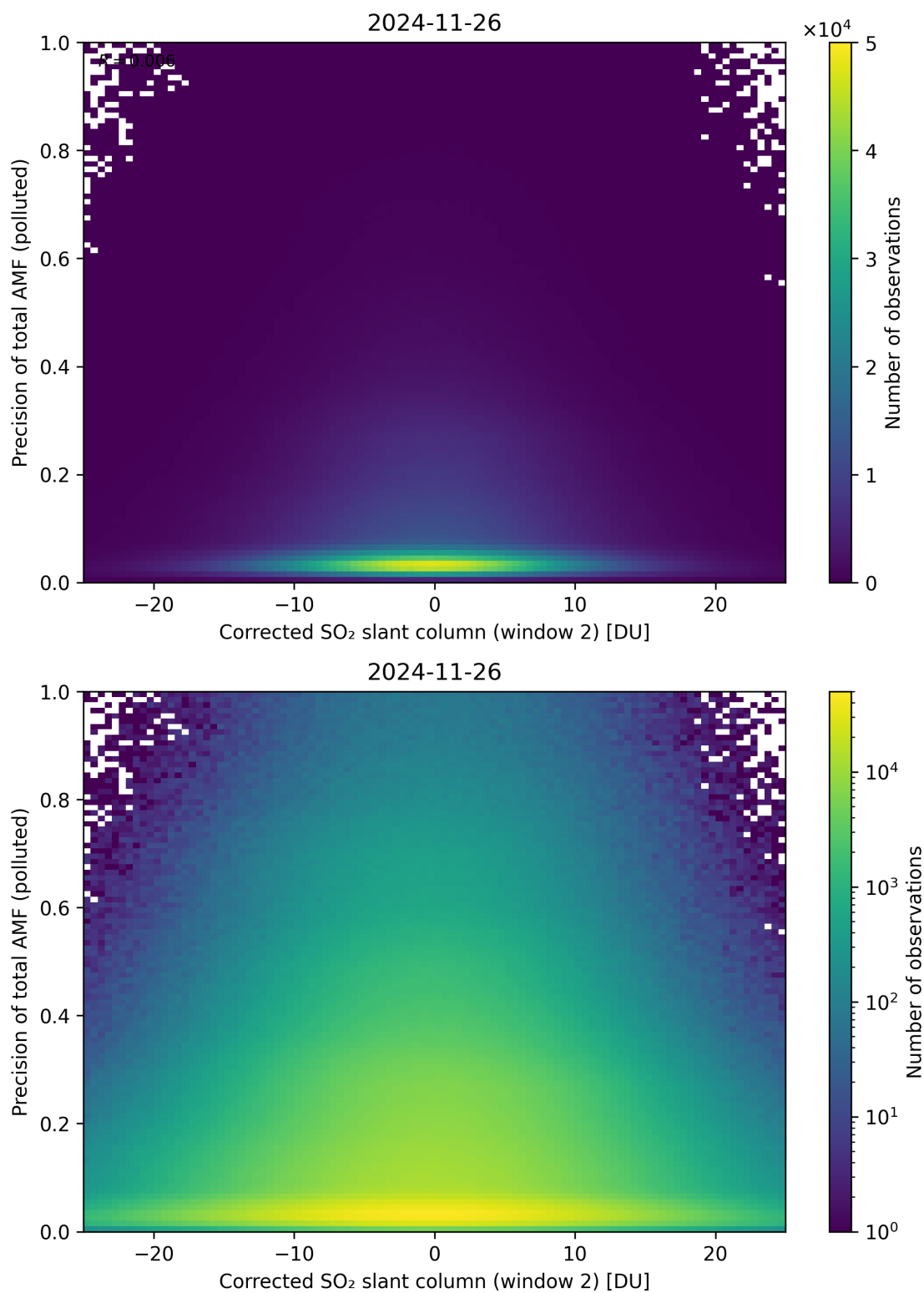
Figure 254: Scatter density plot of “Corrected SO 2 slant column (window 2)” against “Precision of total AMF (polluted)” for 2024-11-25 to 2024-11-27.
