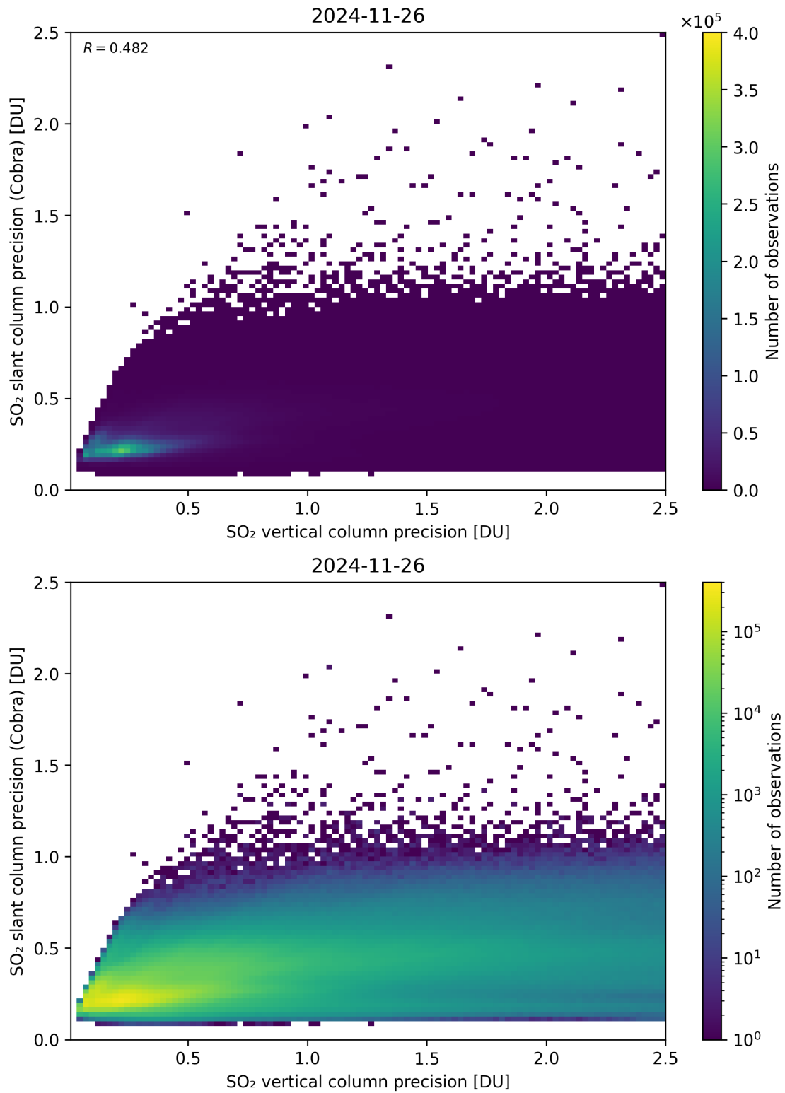
Figure 337: Scatter density plot of “SO 2 vertical column precision” against “SO 2 slant column precision (Cobra)” for 2024-11-25 to 2024-11-27.
