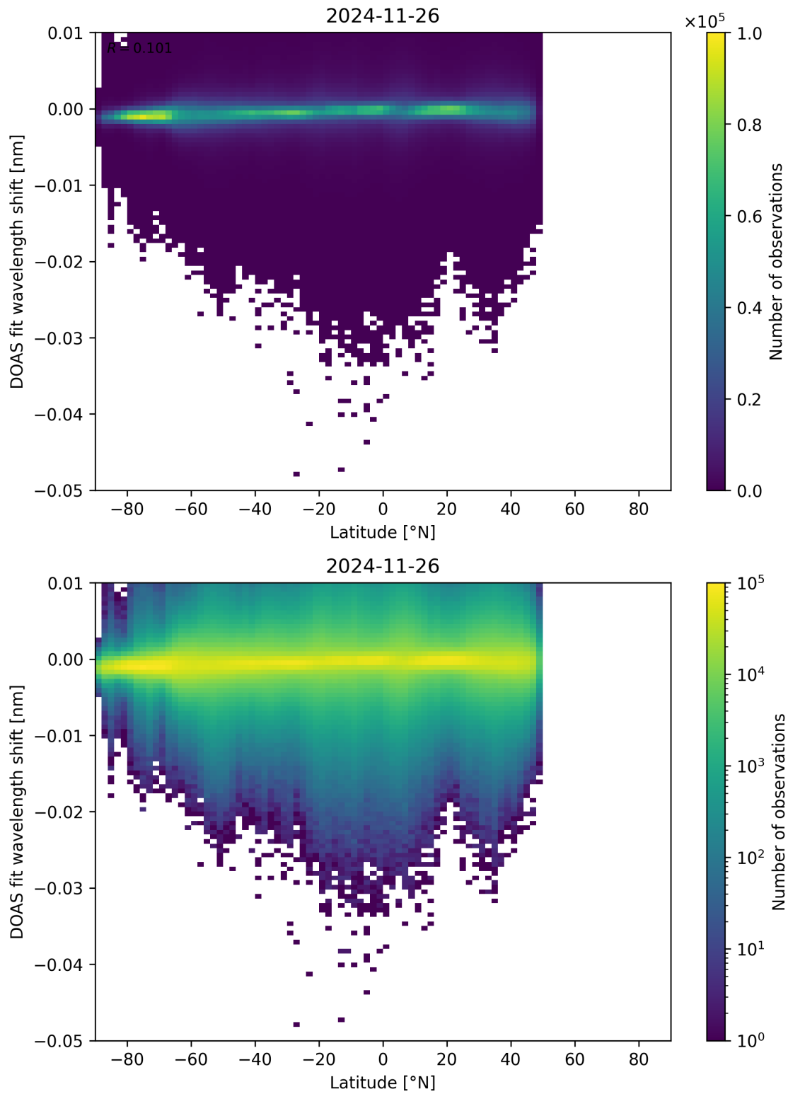
Figure 153: Scatter density plot of “Latitude” against “DOAS fit wavelength shift” for 2024-11-25 to 2024-11-27.
