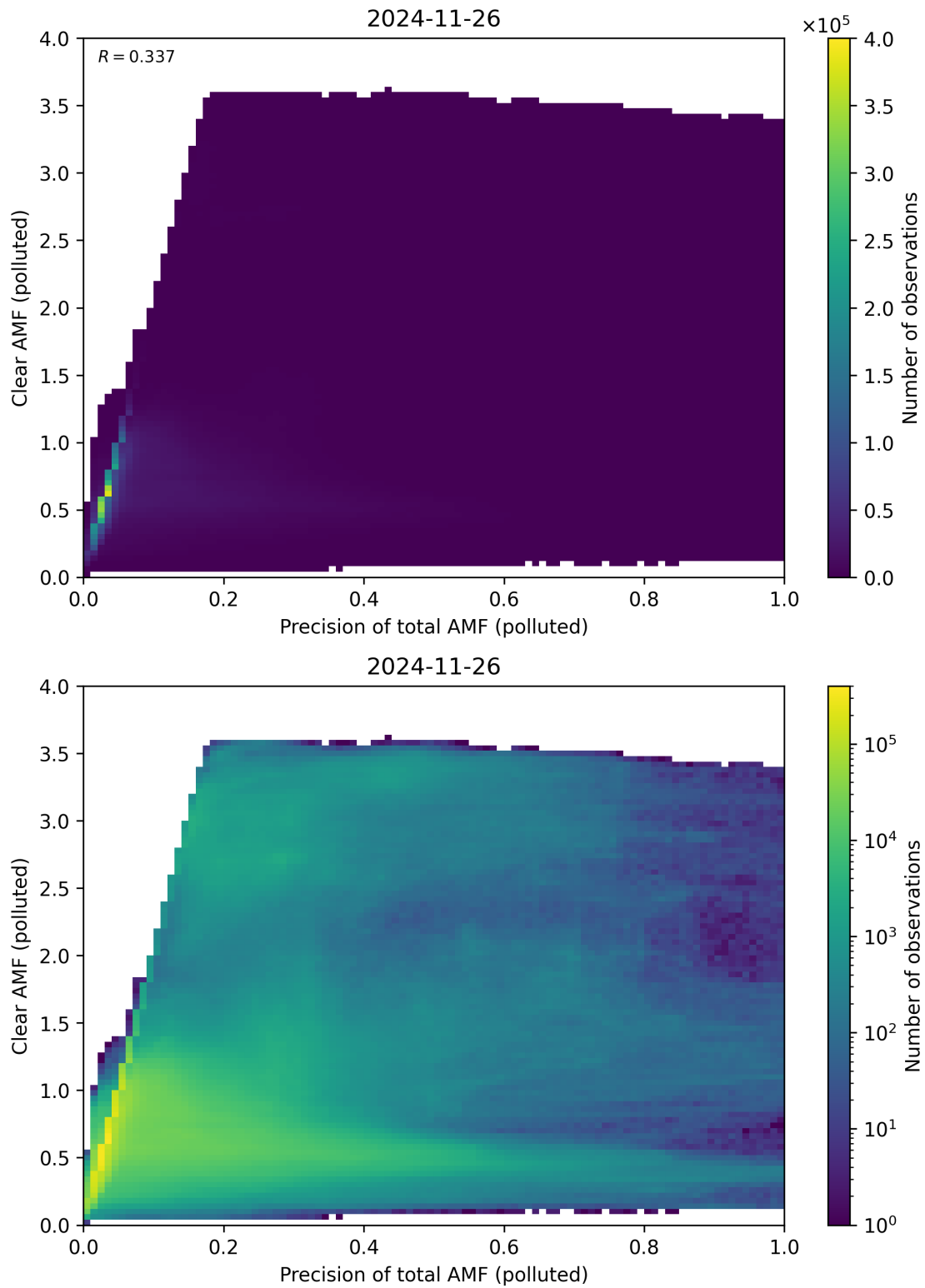
Figure 320: Scatter density plot of “Precision of total AMF (polluted)” against “Clear AMF (polluted)” for 2024-11-25 to 2024-11-27.
