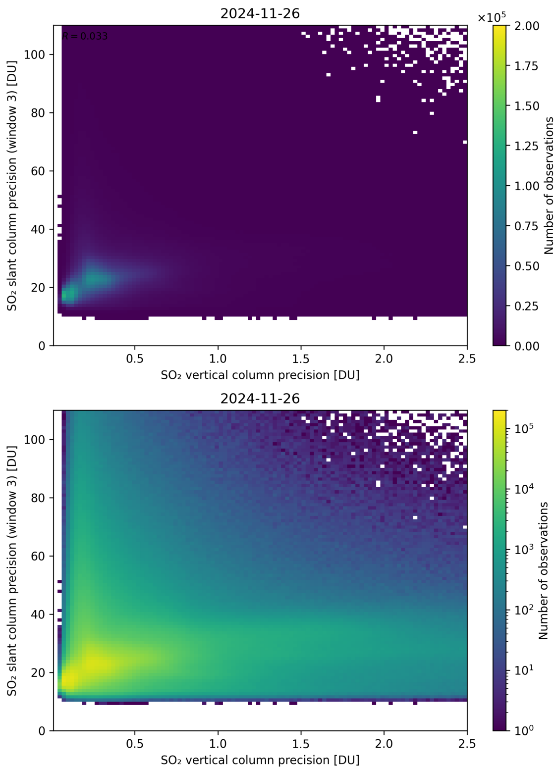
Figure 345: Scatter density plot of “SO 2 vertical column precision” against “SO 2 slant column precision (window 3)” for 2024-11-25 to 2024-11-27.
