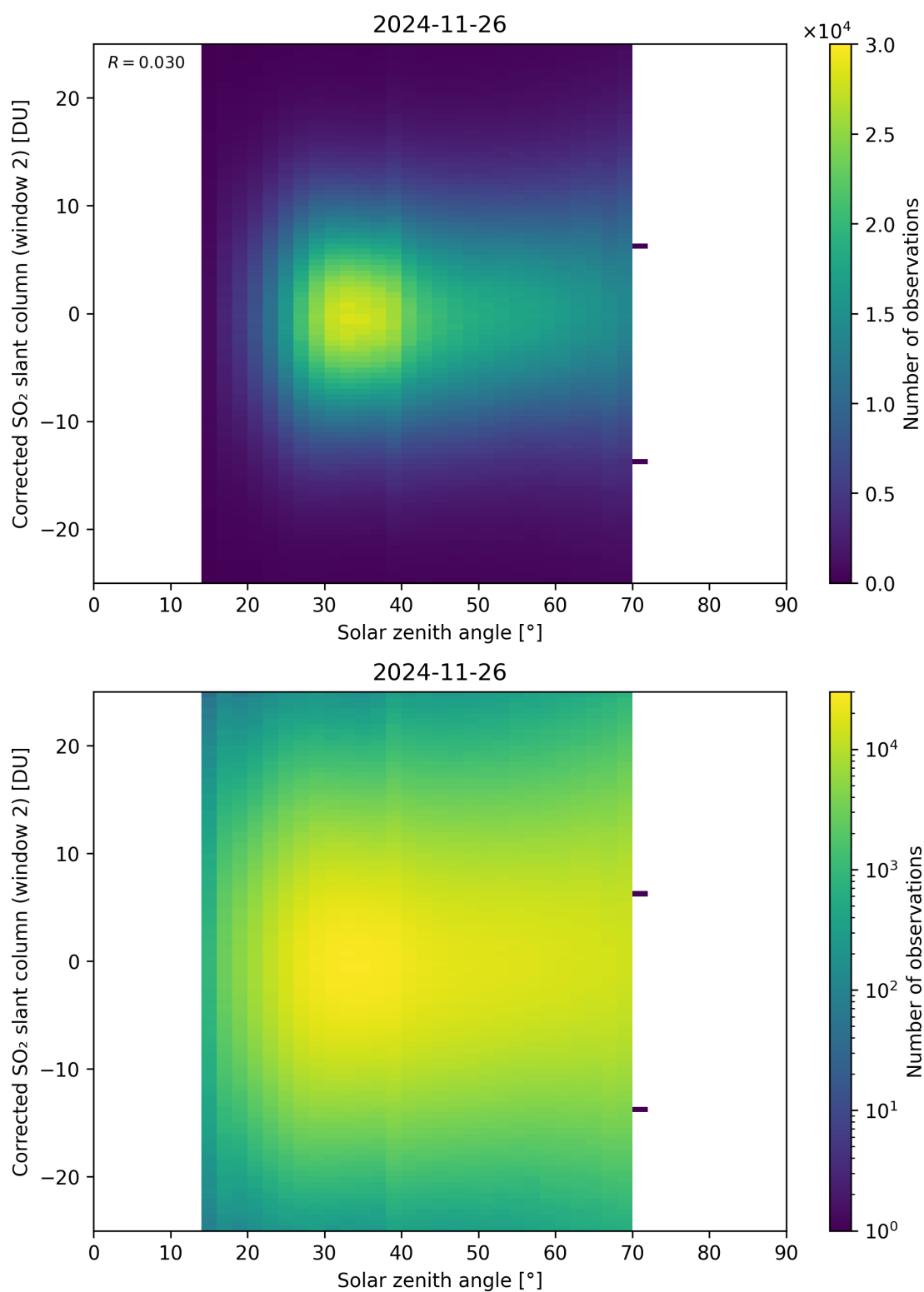
Figure 182: Scatter density plot of “Solar zenith angle” against “Corrected SO 2 slant column (window 2)” for 2024-11-25 to 2024-11-27.
