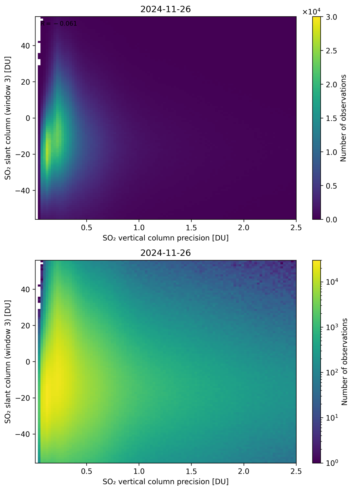
Figure 344: Scatter density plot of “SO 2 vertical column precision” against “SO 2 slant column (window 3)” for 2024-11-25 to 2024-11-27.
