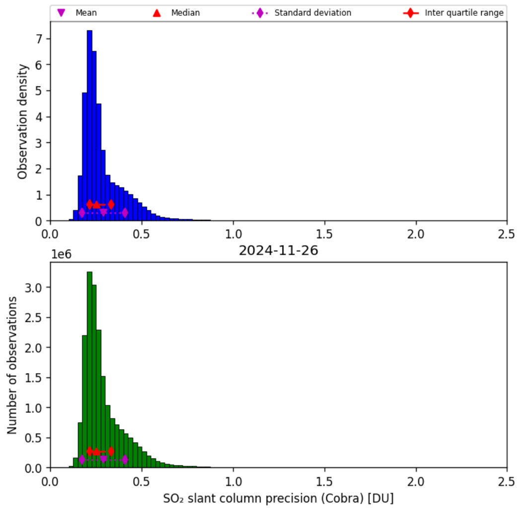
Figure 62: Histogram of “SO 2 slant column precision (Cobra)” for 2024-11-25 to 2024-11-27
