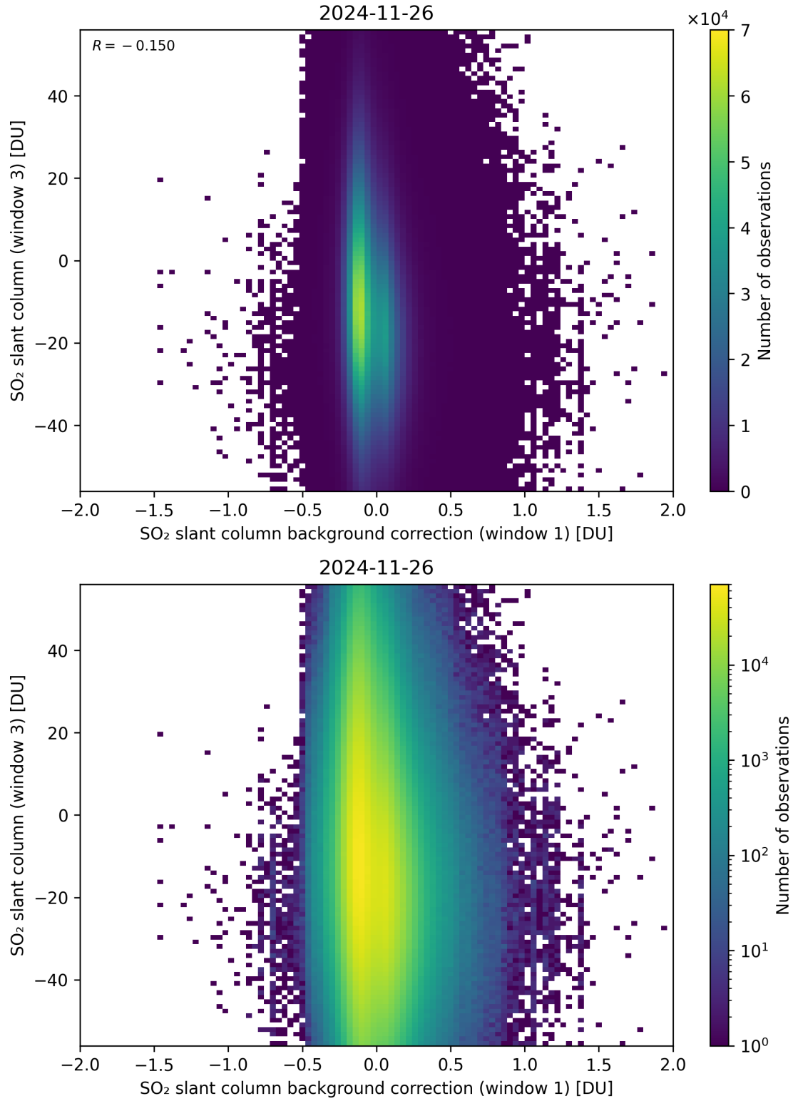
Figure 118: Scatter density plot of “SO 2 slant column background correction (window 1)” against “SO 2 slant column (window 3)” for 2024-11-25 to 2024-11-27.
