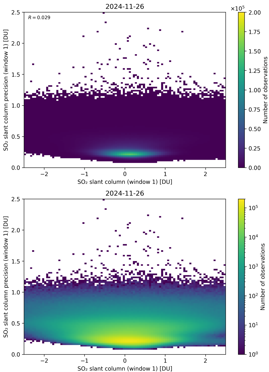
Figure 285: Scatter density plot of “SO 2 slant column (window 1)” against “SO 2 slant column precision (window 1)” for 2024-11-25 to 2024-11-27.
