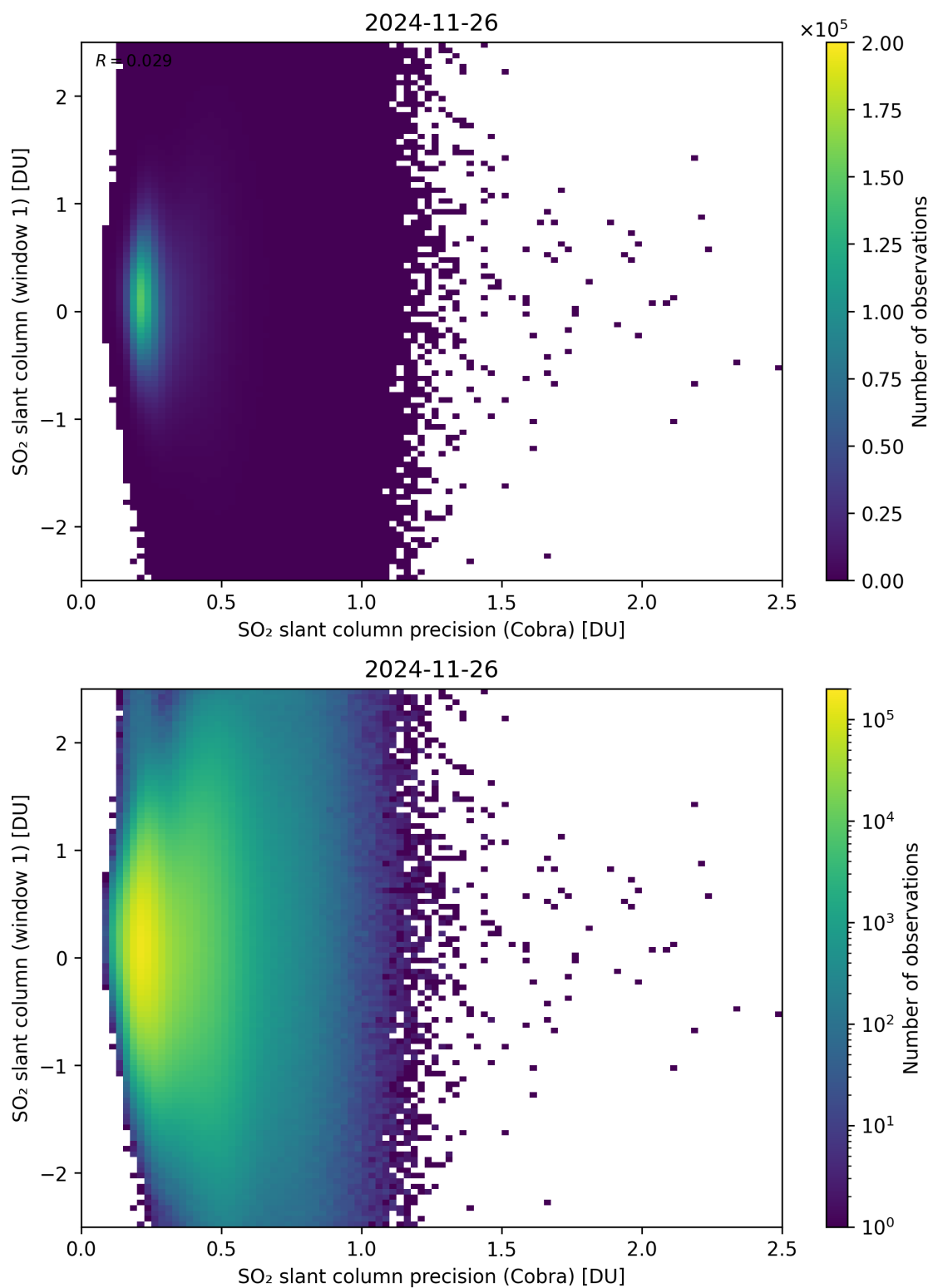
Figure 208: Scatter density plot of “SO 2 slant column precision (Cobra)” against “SO 2 slant column (window 1)” for 2024-11-25 to 2024-11-27.
