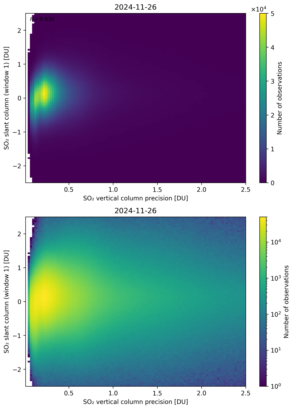
Figure 341: Scatter density plot of “SO 2 vertical column precision” against “SO 2 slant column (window 1)” for 2024-11-25 to 2024-11-27.
