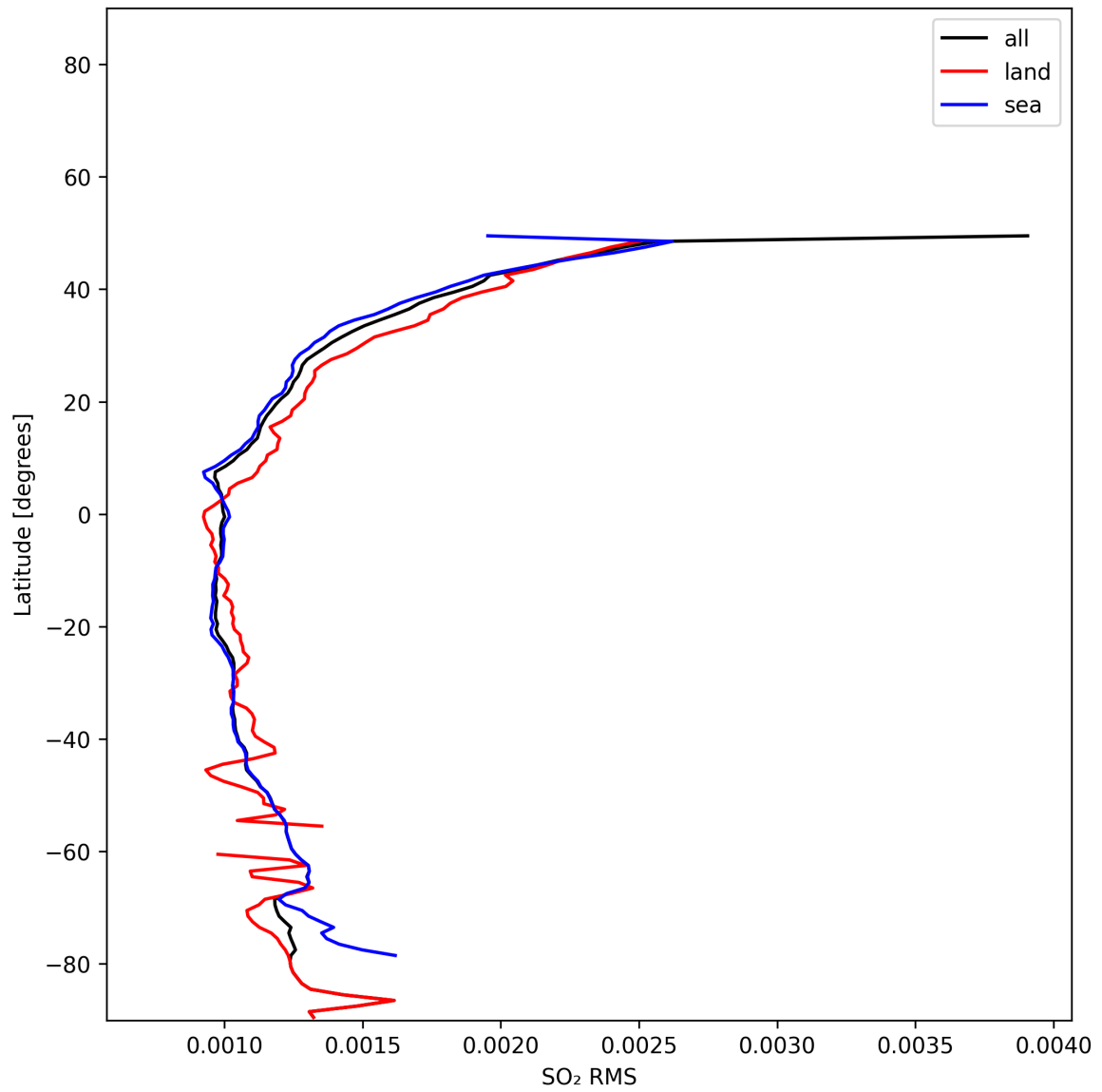
Figure 52: Zonal average of “SO 2 RMS” for 2024-11-25 to 2024-11-27.
