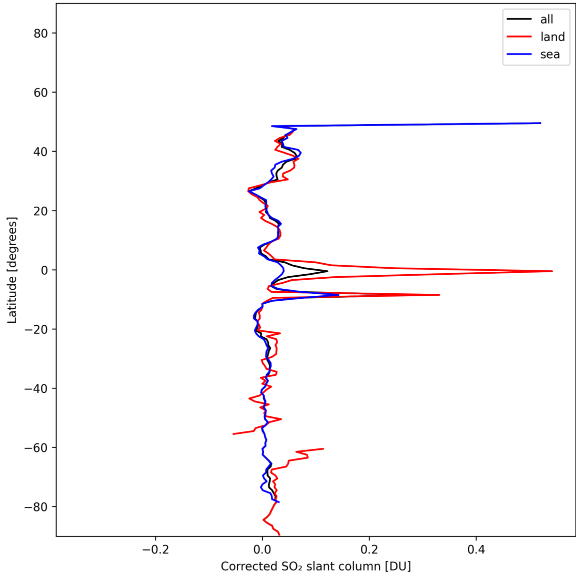
Figure 34: Zonal average of “Corrected SO 2 slant column” for 2024-11-25 to 2024-11-27.
