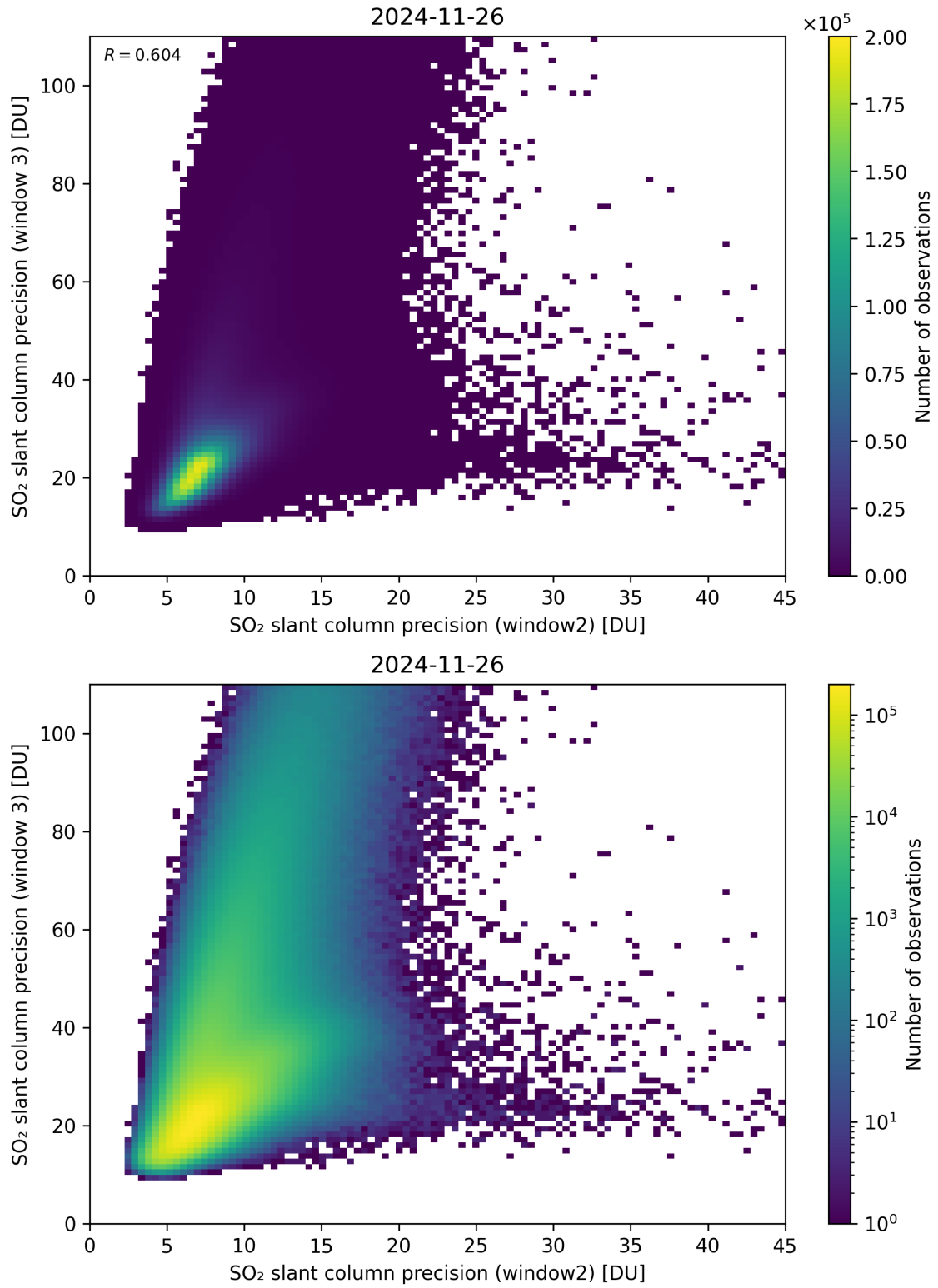
Figure 300: Scatter density plot of “SO 2 slant column precision (window2)” against “SO 2 slant column precision (window 3)” for 2024-11-25 to 2024-11-27.
