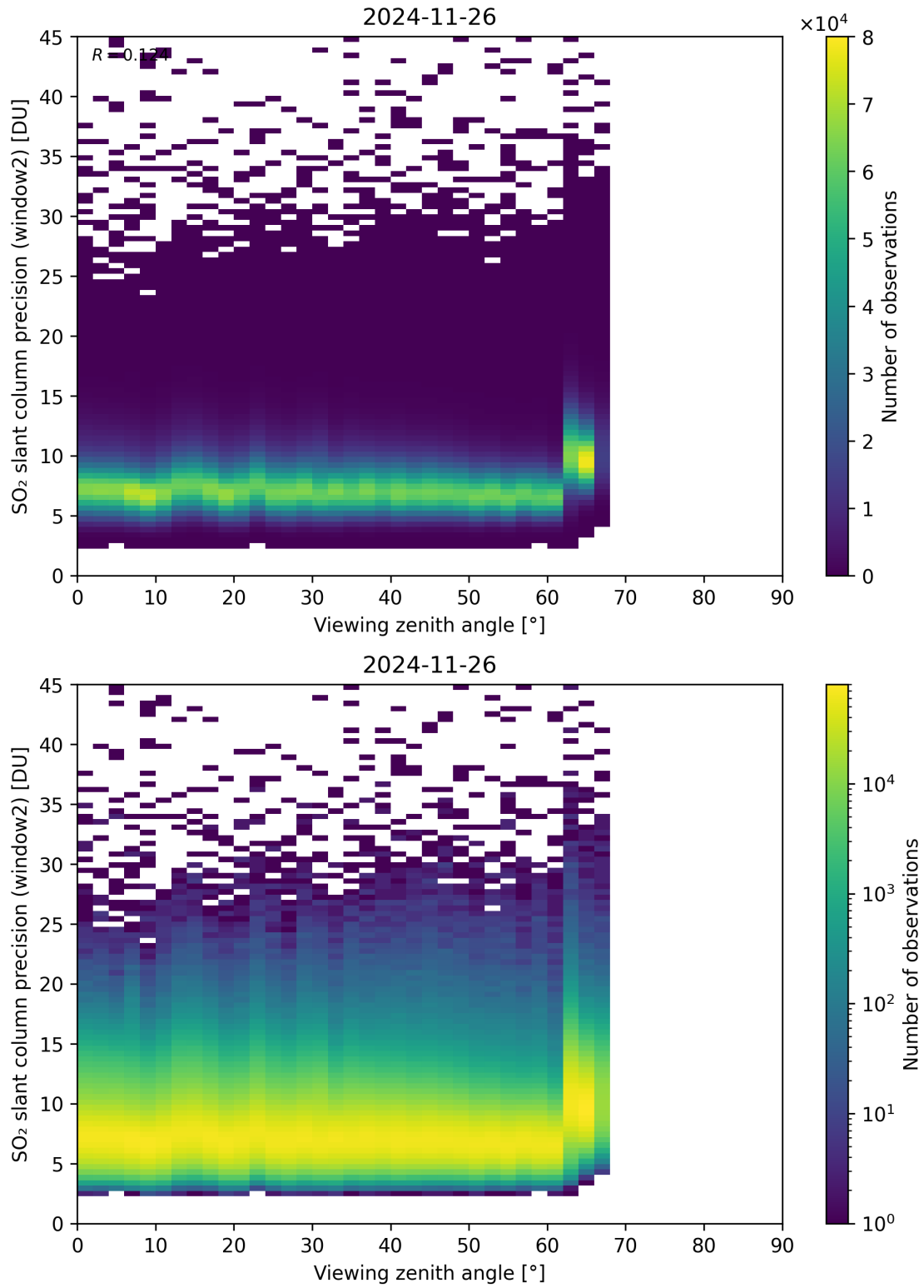
Figure 378: Scatter density plot of “Viewing zenith angle” against “SO 2 slant column precision (window2)” for 2024-11-25 to 2024-11-27.
