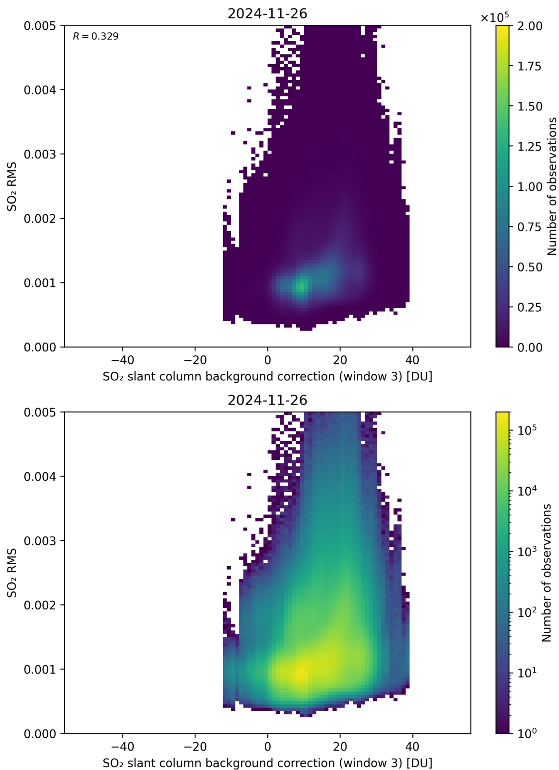
Figure 134: Scatter density plot of “SO 2 slant column background correction (window 3)” against “SO 2 RMS” for 2024-11-25 to 2024-11-27.
