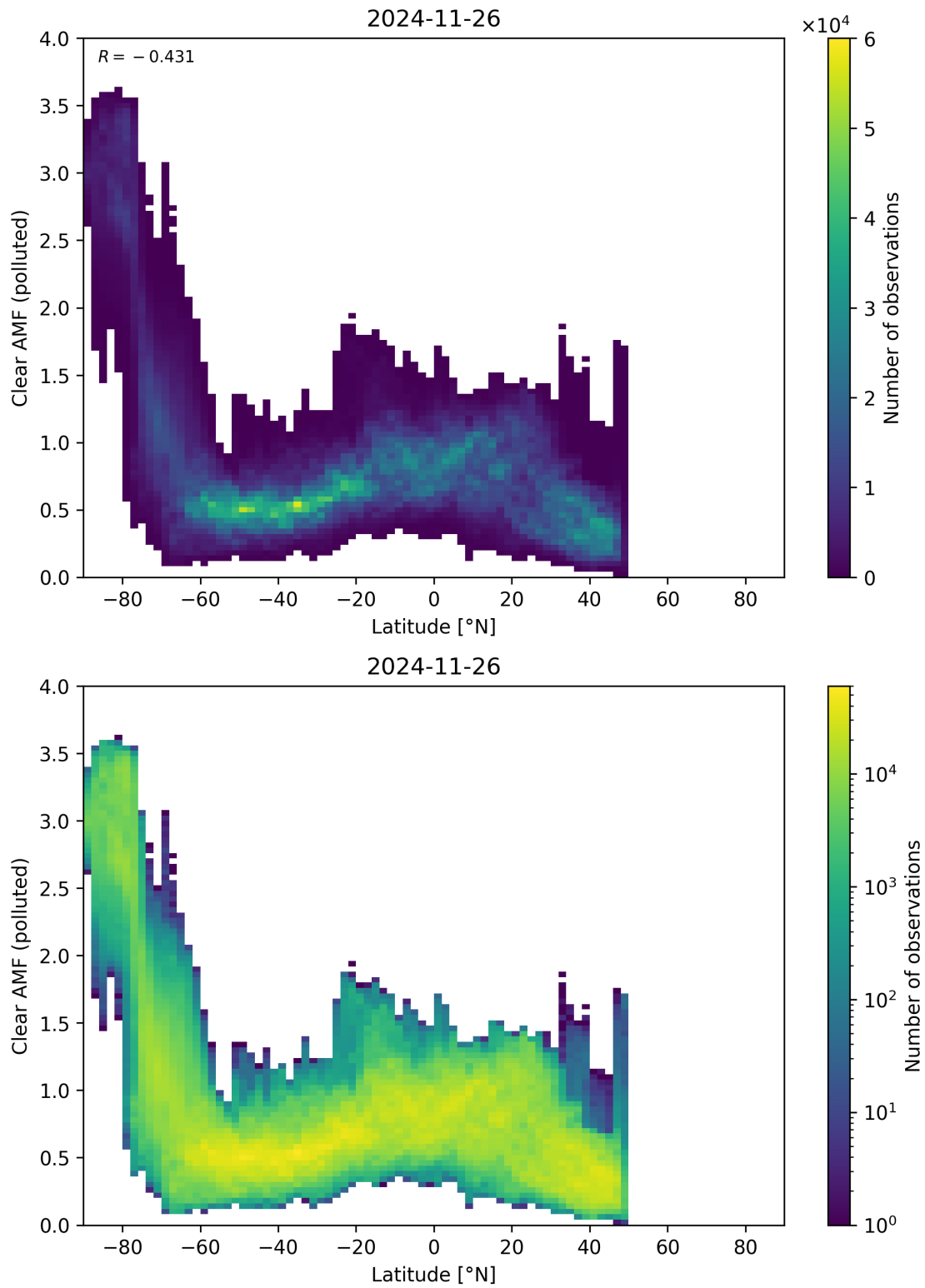
Figure 156: Scatter density plot of “Latitude” against “Clear AMF (polluted)” for 2024-11-25 to 2024-11-27.
