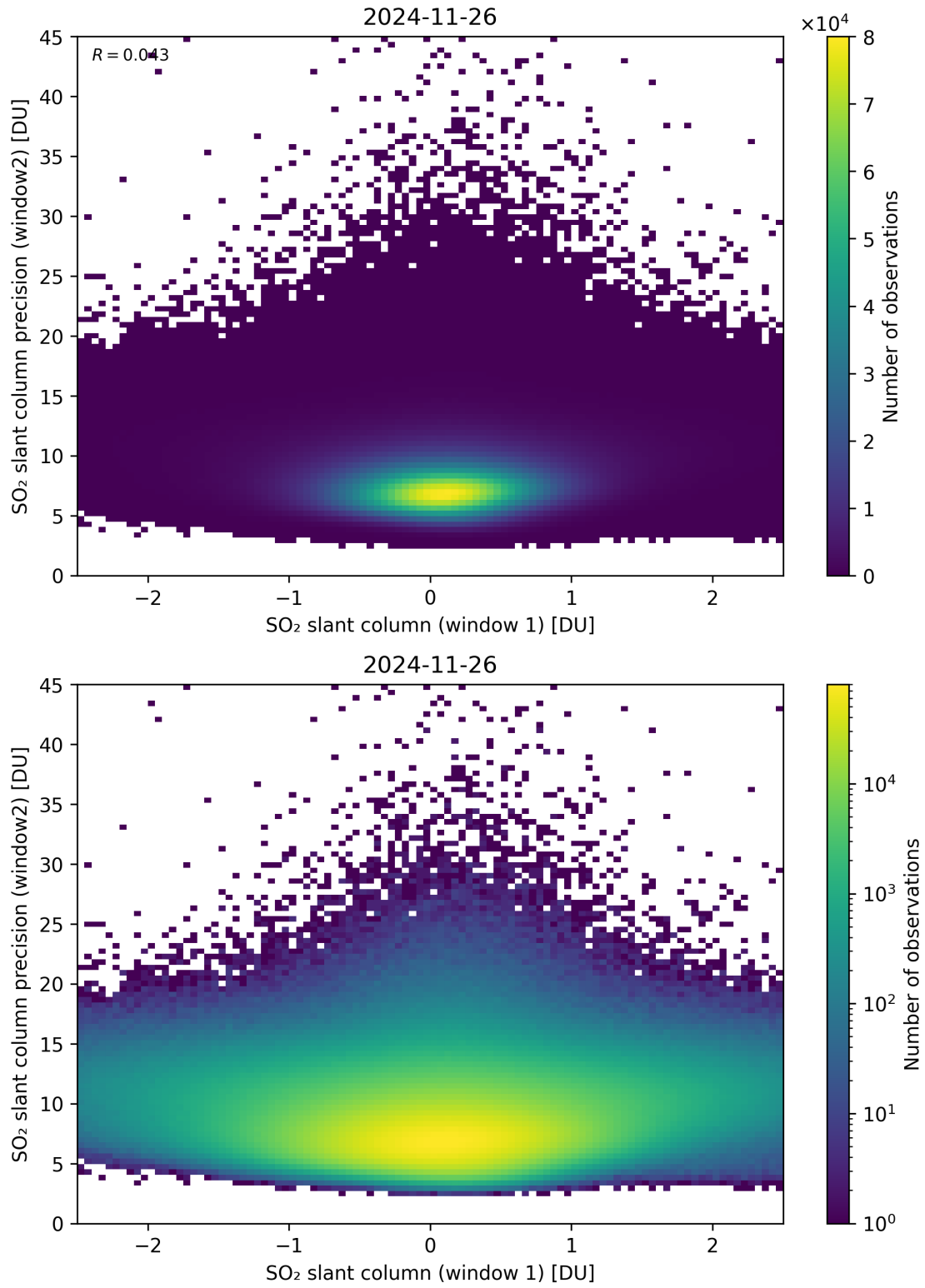
Figure 286: Scatter density plot of “SO 2 slant column (window 1)” against “SO 2 slant column precision (window2)” for 2024-11-25 to 2024-11-27.
