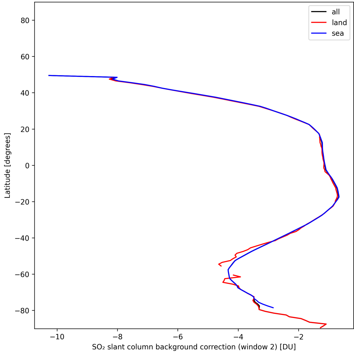
Figure 44: Zonal average of “SO 2 slant column background correction (window 2)” for 2024-11-25 to 2024-11-27.
