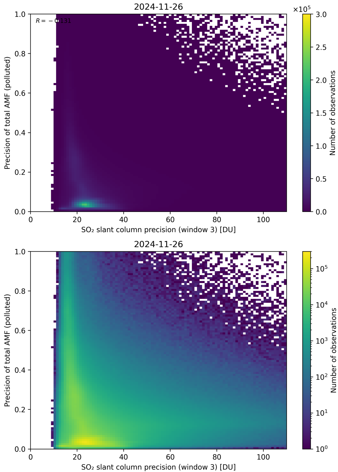
Figure 314: Scatter density plot of “SO 2 slant column precision (window 3)” against “Precision of total AMF (polluted)” for 2024-11-25 to 2024-11-27.
