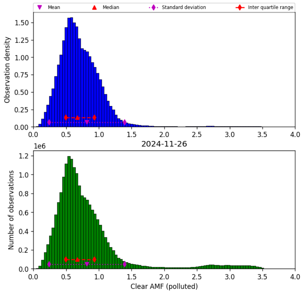
Figure 81: Histogram of “Clear AMF (polluted)” for 2024-11-25 to 2024-11-27
