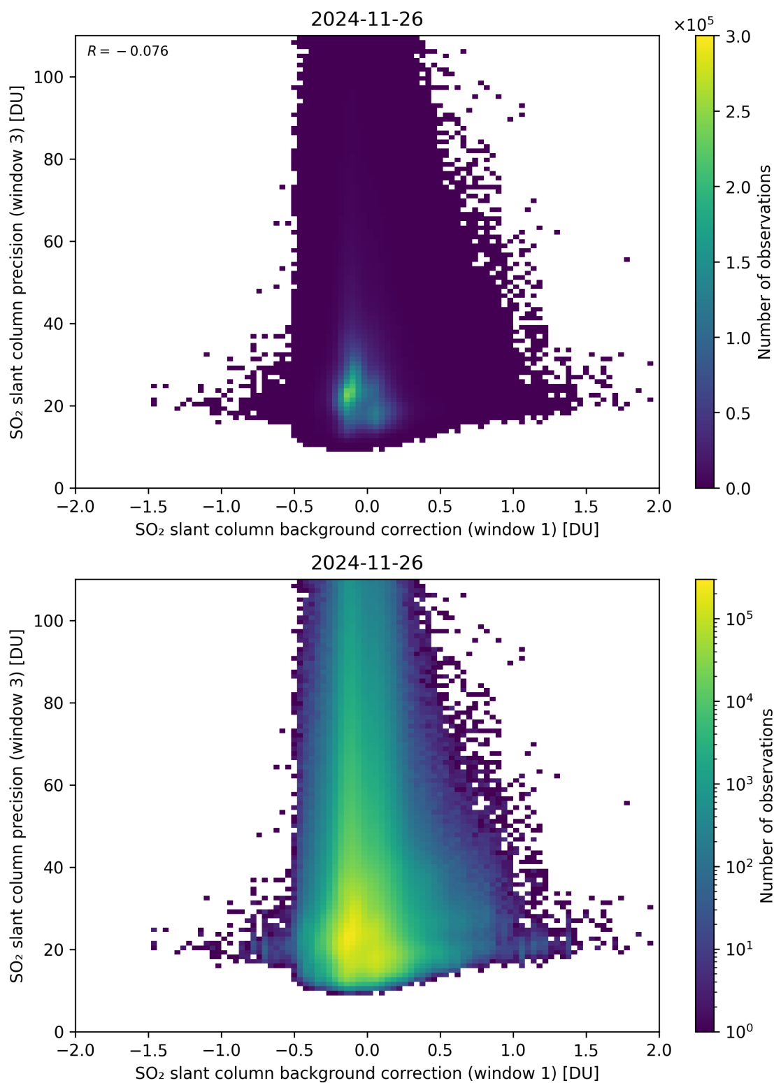
Figure 119: Scatter density plot of “SO 2 slant column background correction (window 1)” against “SO 2 slant column precision (window 3)” for 2024-11-25 to 2024-11-27.
