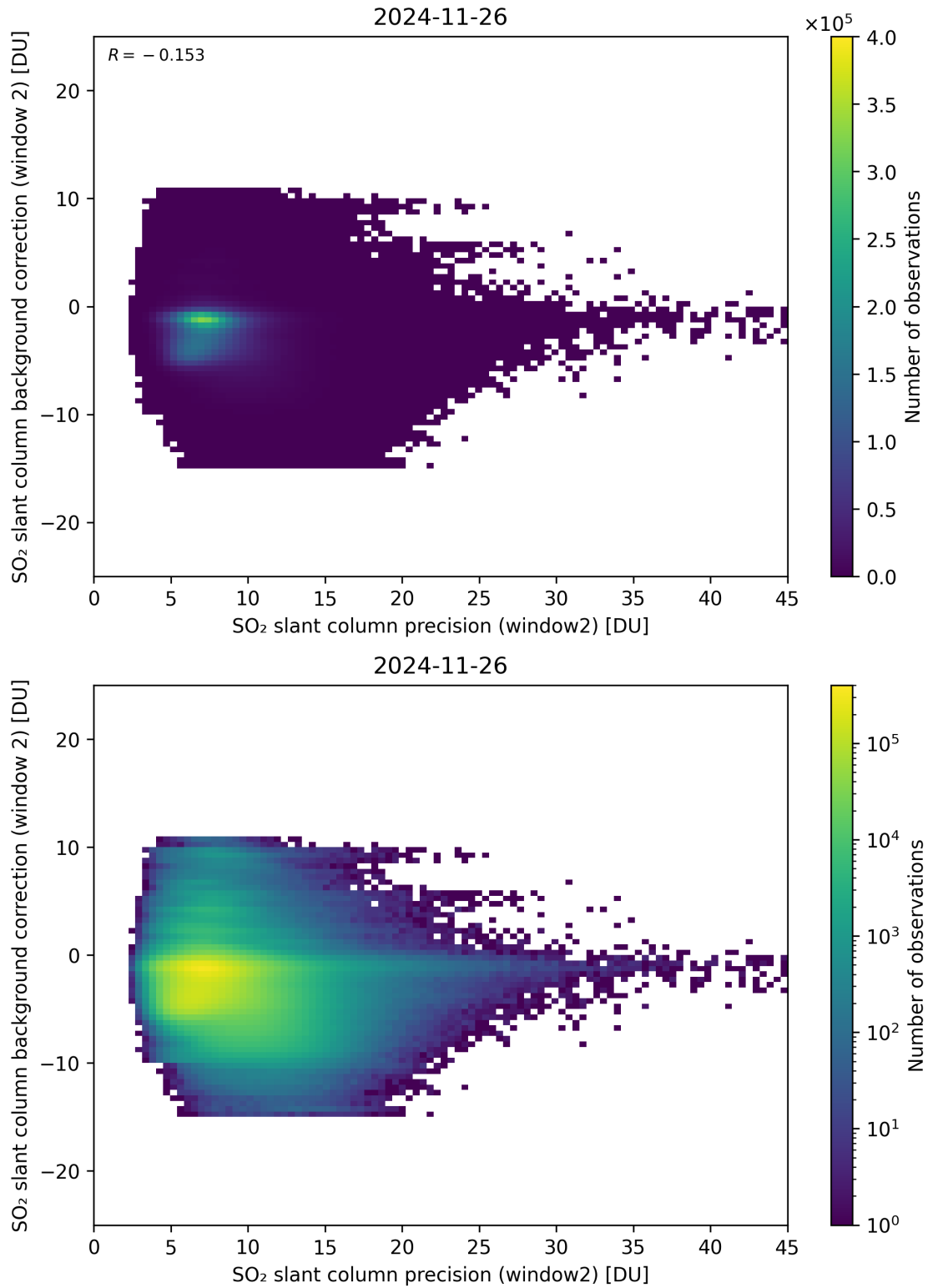
Figure 291: Scatter density plot of “SO 2 slant column precision (window2)” against “SO 2 slant column background correction (window 2)” for 2024-11-25 to 2024-11-27.
