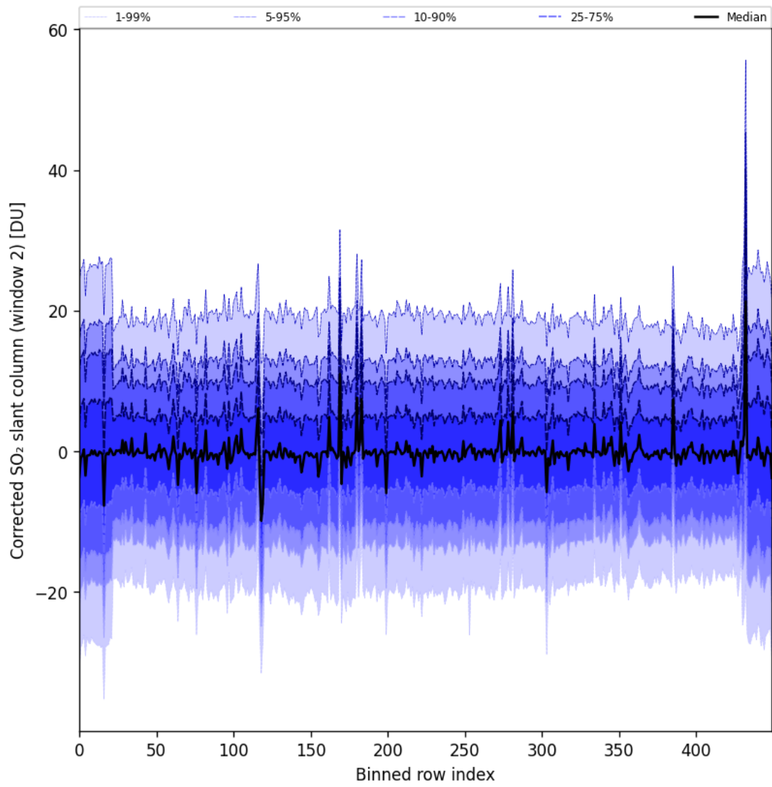
Figure 95: Along track statistics of “Corrected SO 2 slant column (window 2)” for 2024-11-25 to 2024-11-27
