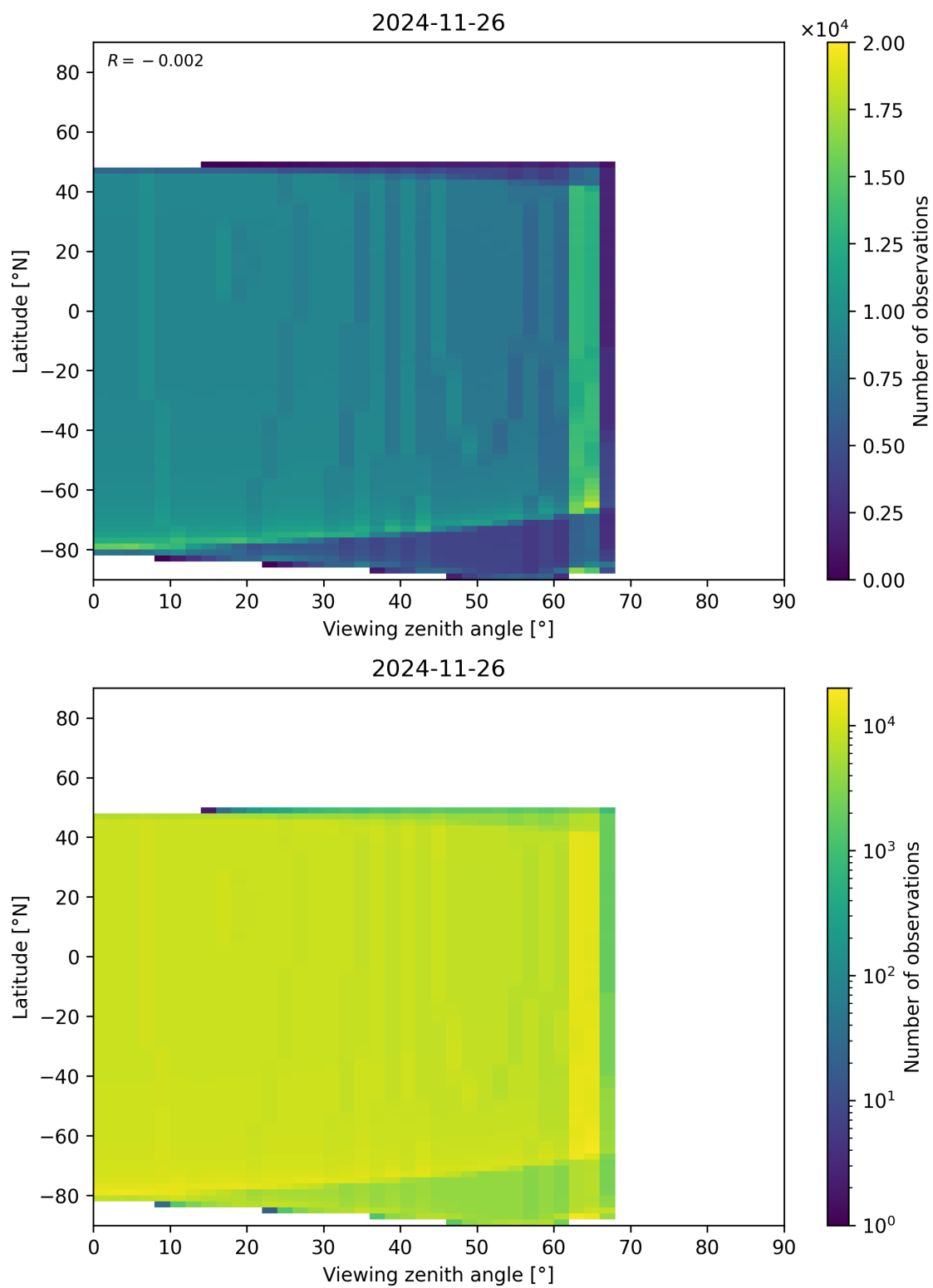
Figure 368: Scatter density plot of “Viewing zenith angle” against “Latitude” for 2024-11-25 to 2024-11-27.
