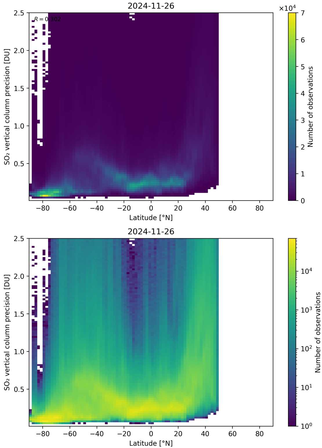
Figure 170: Scatter density plot of “Latitude” against “SO 2 vertical column precision” for 2024-11-25 to 2024-11-27.
