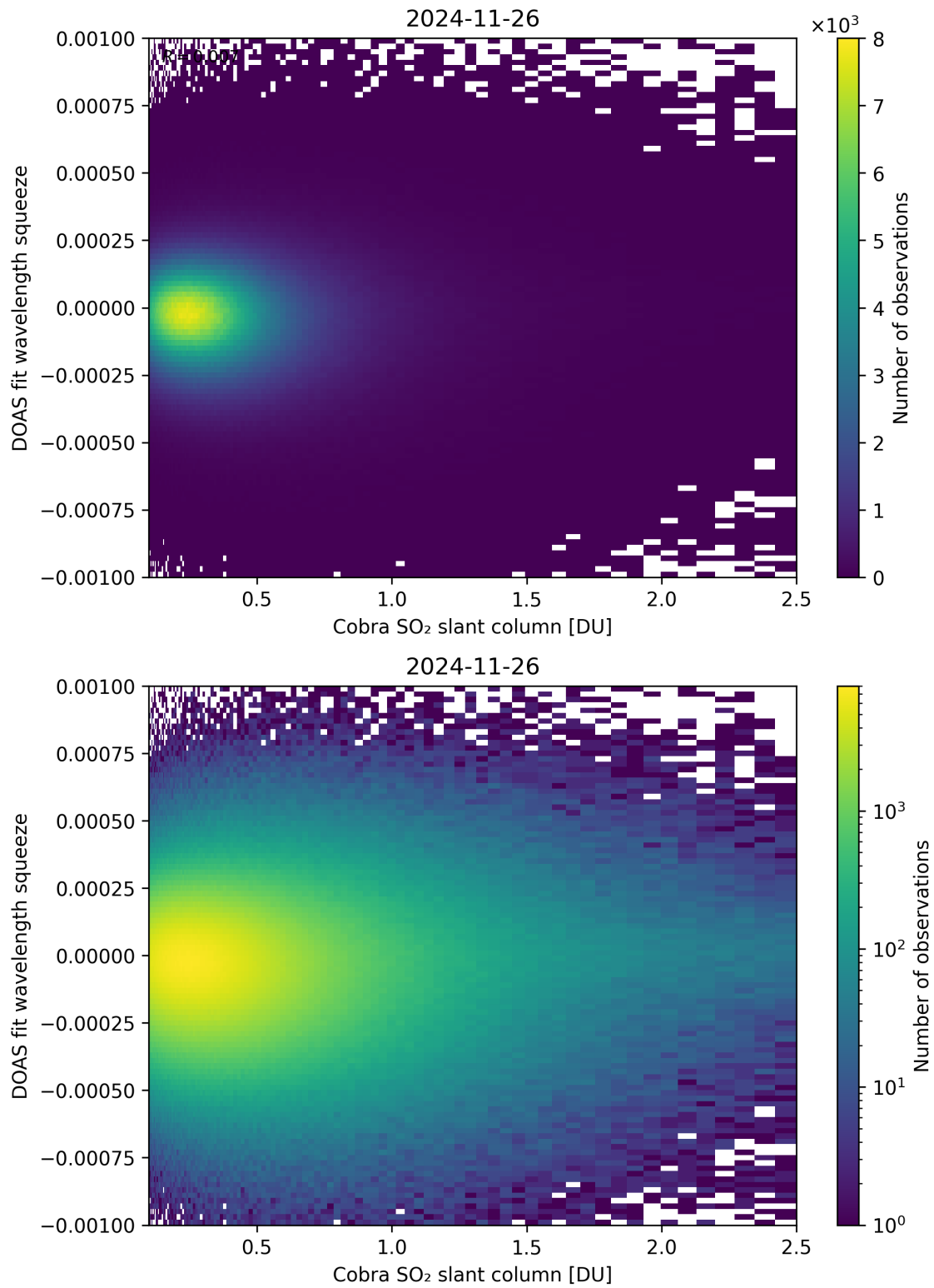
Figure 197: Scatter density plot of “Cobra SO 2 slant column” against “DOAS fit wavelength squeeze” for 2024-11-25 to 2024-11-27.
