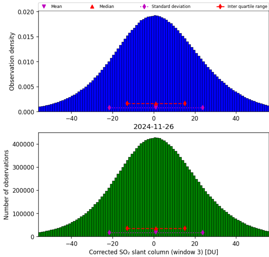
Figure 73: Histogram of “Corrected SO 2 slant column (window 3)” for 2024-11-25 to 2024-11-27
