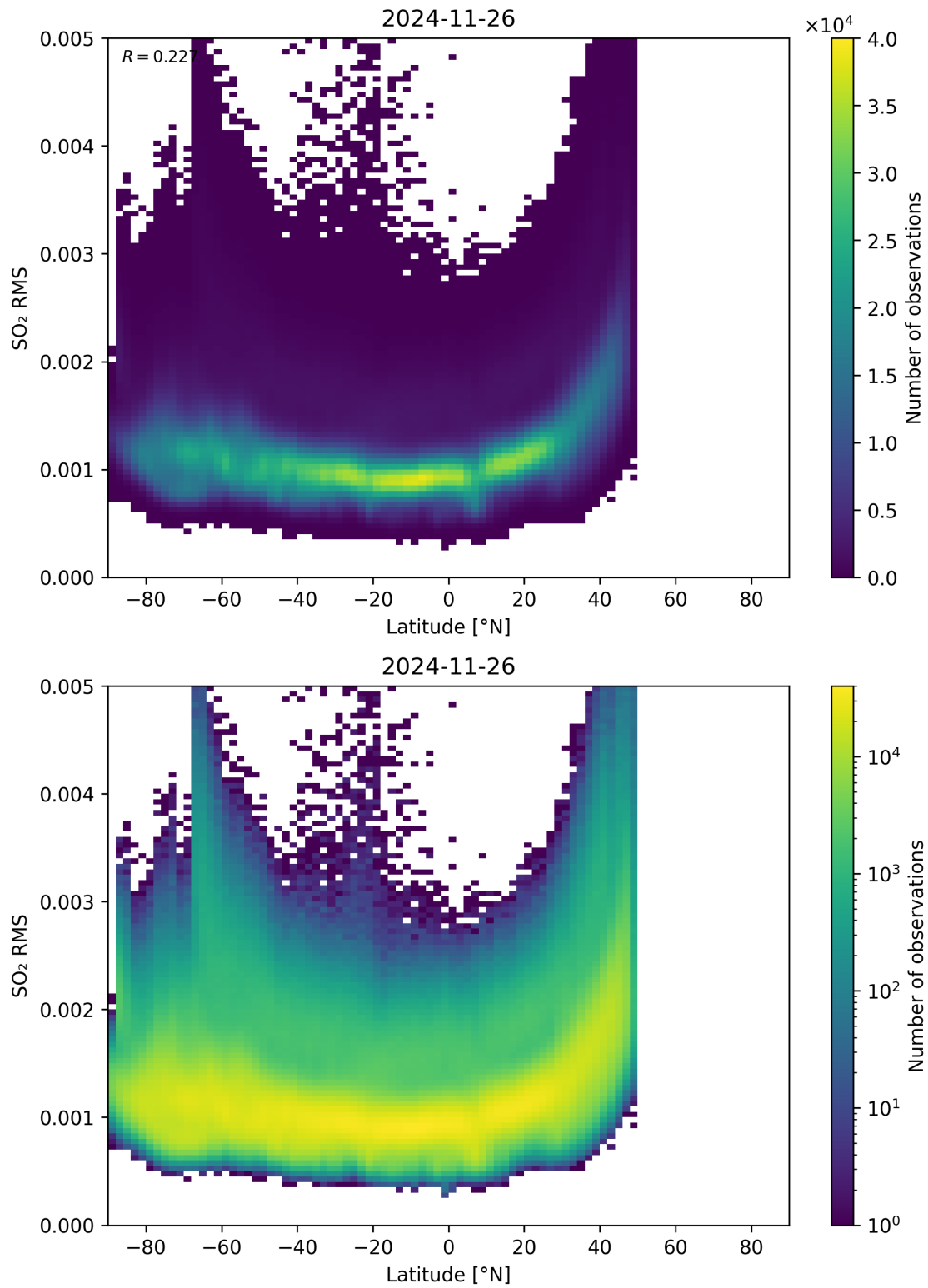
Figure 155: Scatter density plot of “Latitude” against “SO 2 RMS” for 2024-11-25 to 2024-11-27.
