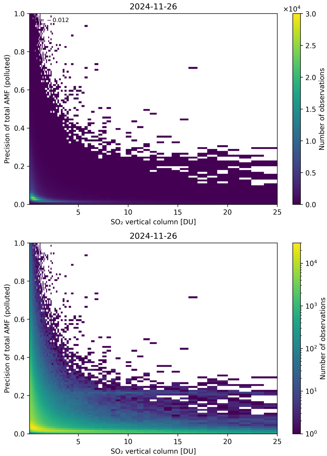
Figure 360: Scatter density plot of “SO 2 vertical column” against “Precision of total AMF (polluted)” for 2024-11-25 to 2024-11-27.
