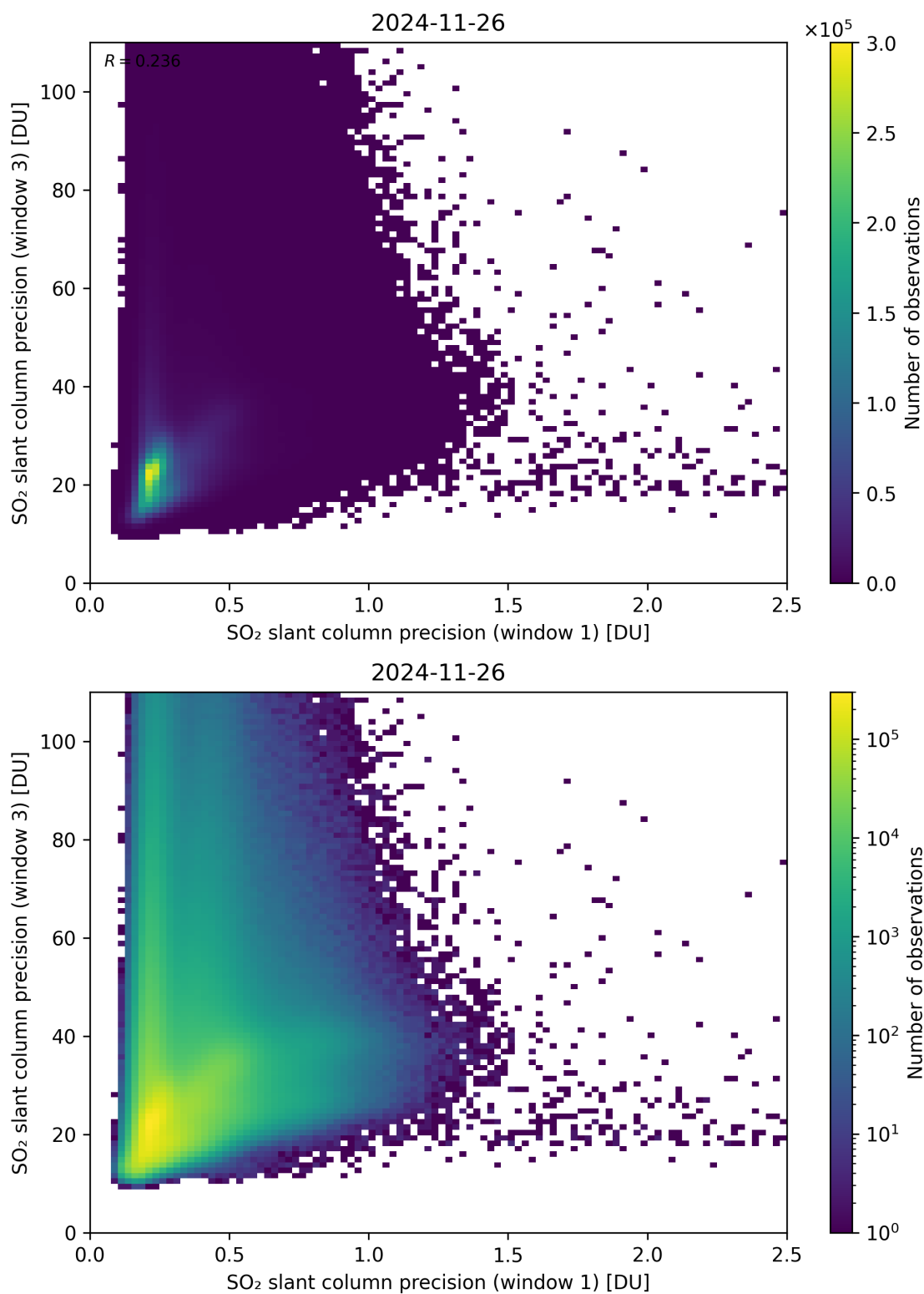
Figure 279: Scatter density plot of “SO 2 slant column precision (window 1)” against “SO 2 slant column precision (window 3)” for 2024-11-25 to 2024-11-27.
