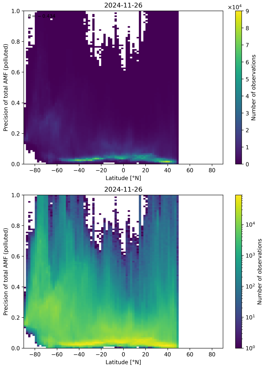
Figure 168: Scatter density plot of “Latitude” against “Precision of total AMF (polluted)” for 2024-11-25 to 2024-11-27.
