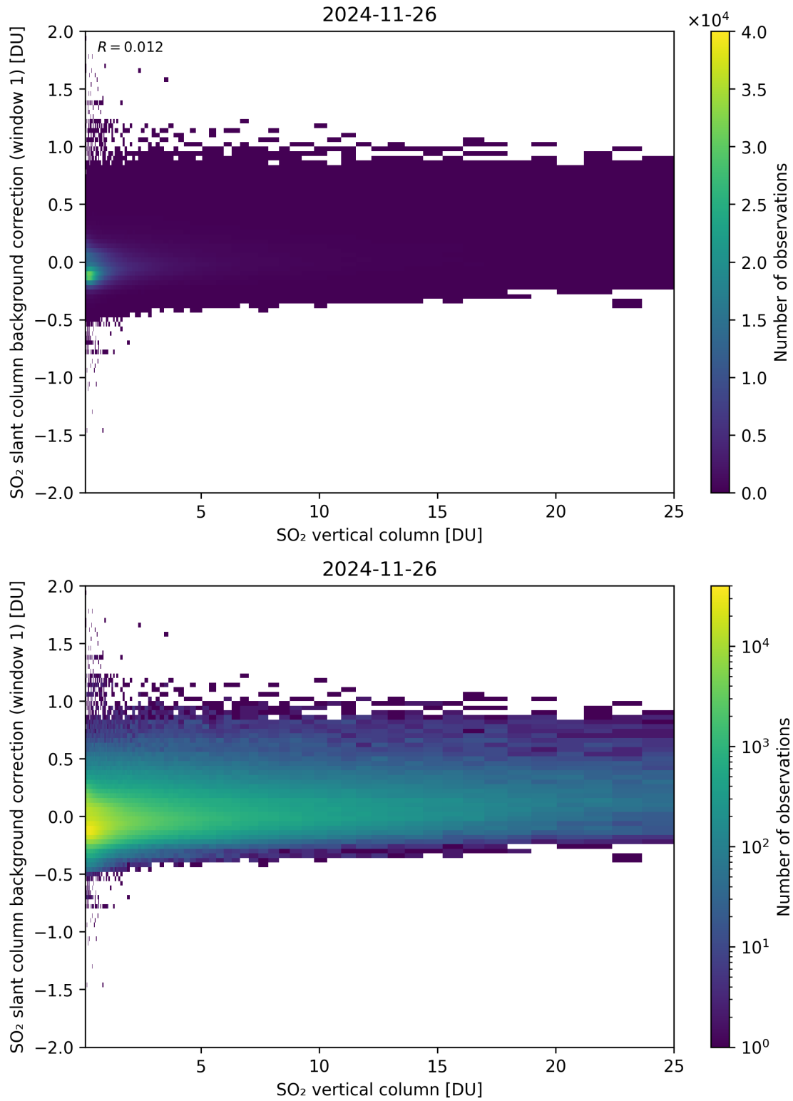
Figure 323: Scatter density plot of “SO 2 vertical column” against “SO 2 slant column background correction (window 1)” for 2024-11-25 to 2024-11-27.
