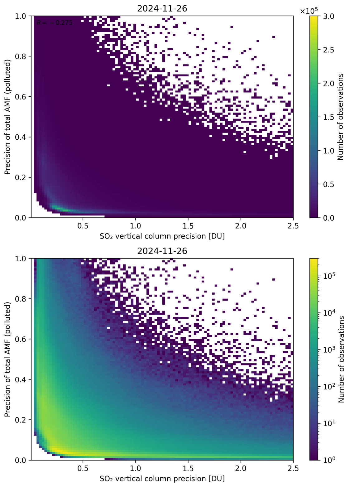
Figure 347: Scatter density plot of “SO 2 vertical column precision” against “Precision of total AMF (polluted)” for 2024-11-25 to 2024-11-27.
