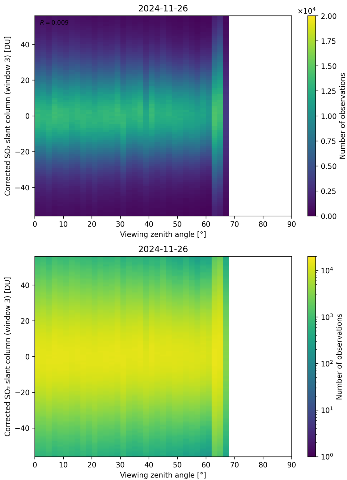
Figure 375: Scatter density plot of “Viewing zenith angle” against “Corrected SO 2 slant column (window 3)” for 2024-11-25 to 2024-11-27.
