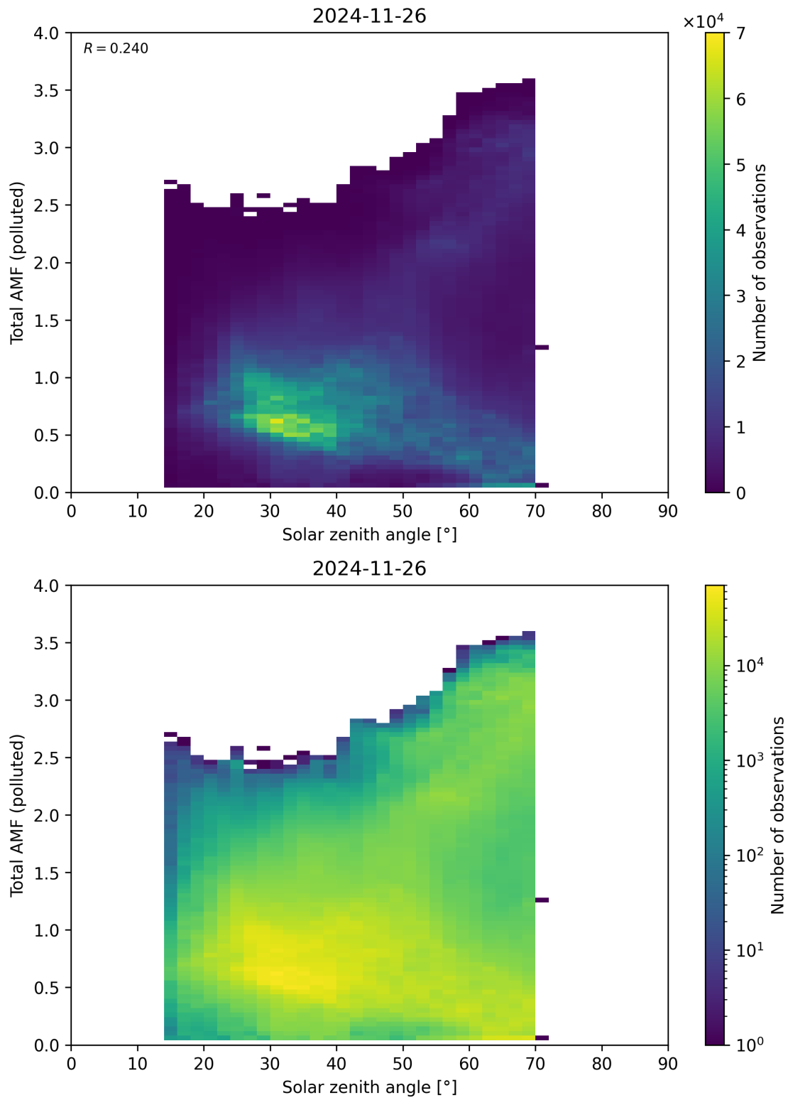
Figure 189: Scatter density plot of “Solar zenith angle” against “Total AMF (polluted)” for 2024-11-25 to 2024-11-27.
