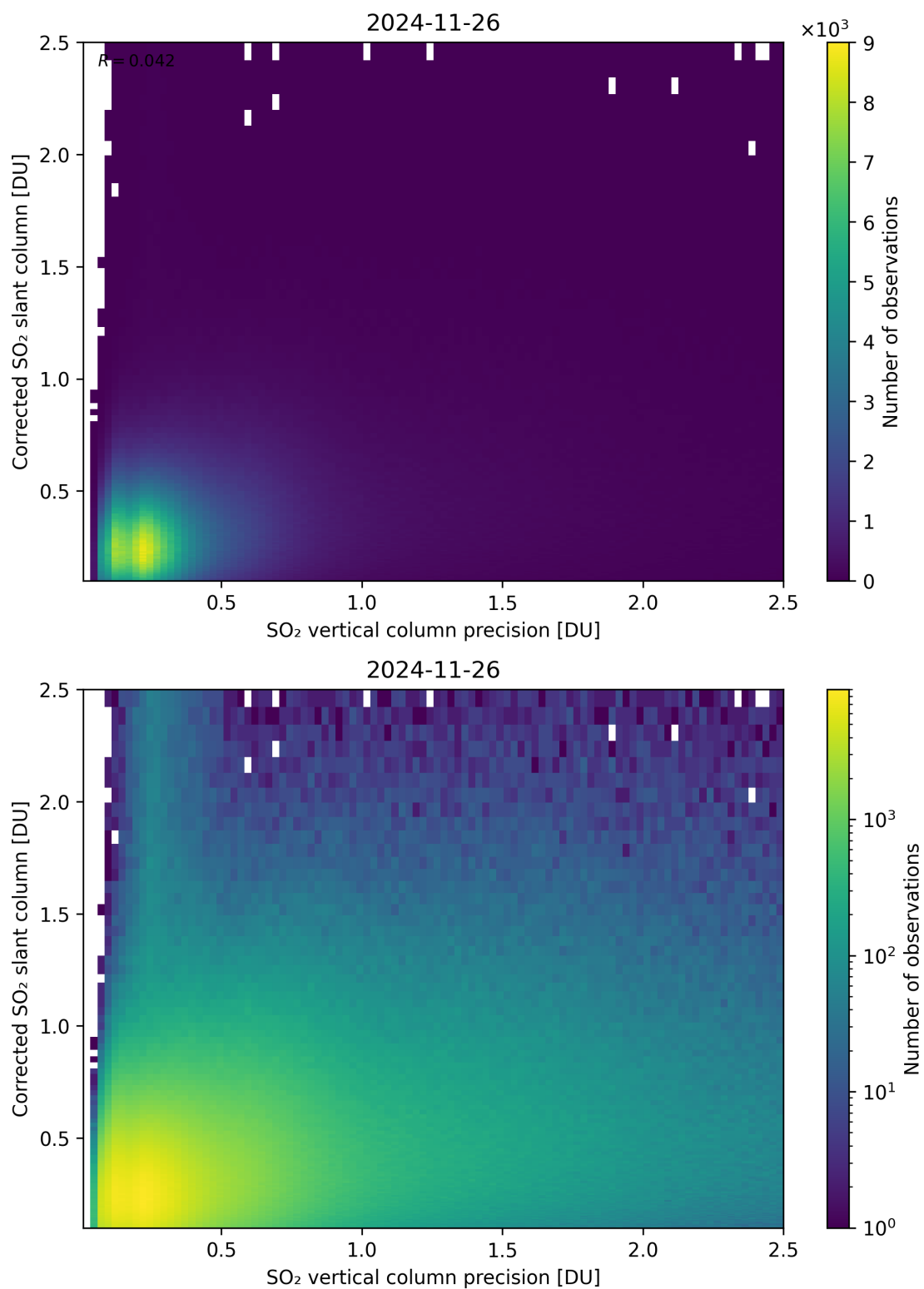
Figure 338: Scatter density plot of “SO 2 vertical column precision” against “Corrected SO 2 slant column” for 2024-11-25 to 2024-11-27.
