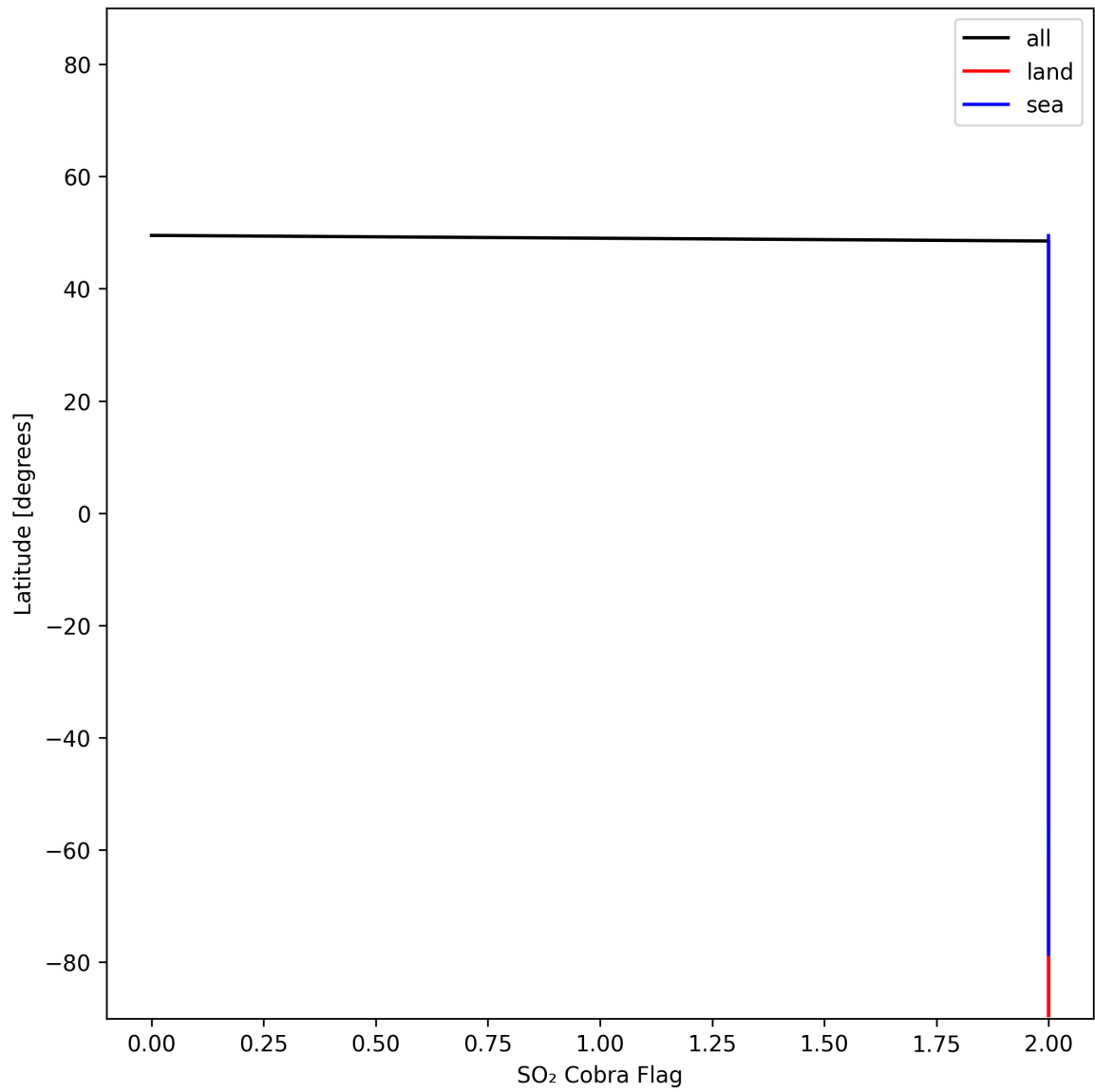
Figure 49: Zonal average of “SO 2 Cobra Flag” for 2024-11-25 to 2024-11-27.
