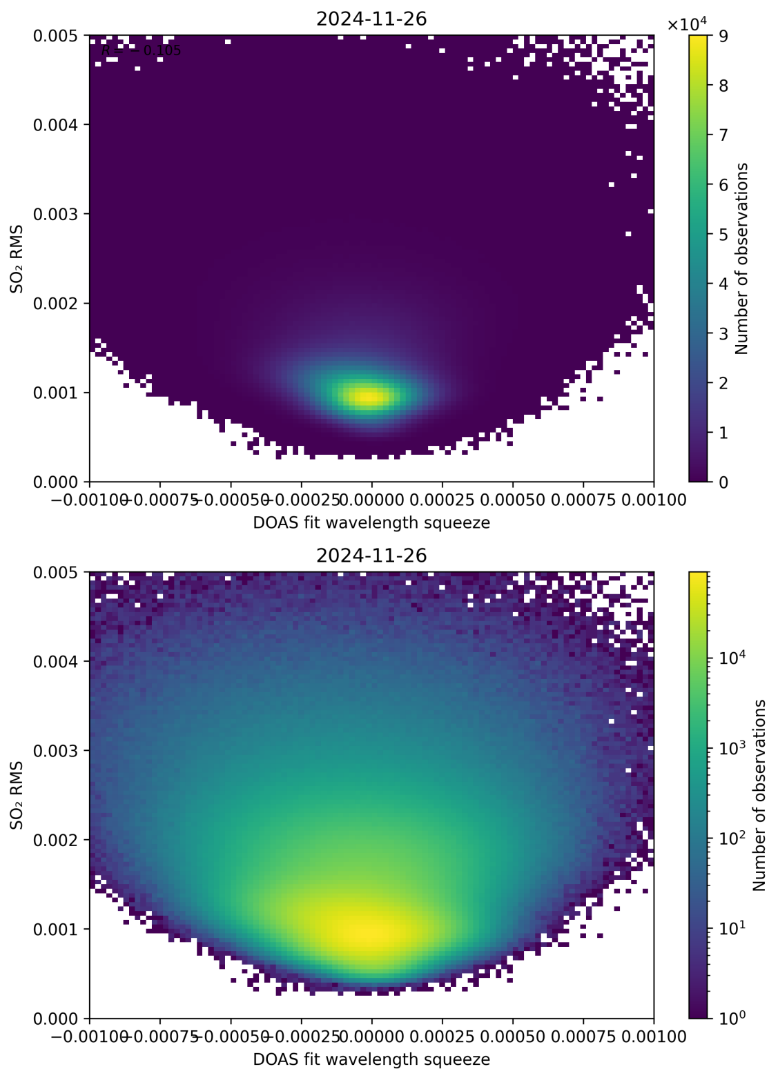
Figure 143: Scatter density plot of “DOAS fit wavelength squeeze” against “SO 2 RMS” for 2024-11-25 to 2024-11-27.
