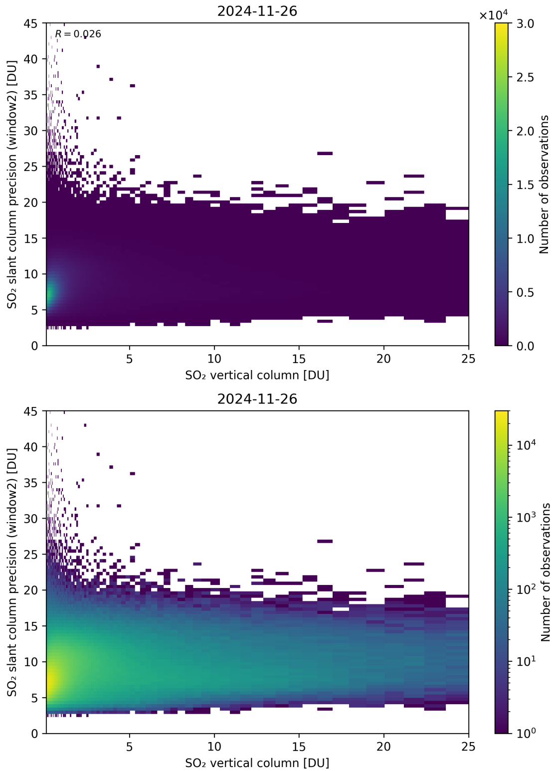
Figure 356: Scatter density plot of “SO 2 vertical column” against “SO 2 slant column precision (window2)” for 2024-11-25 to 2024-11-27.
