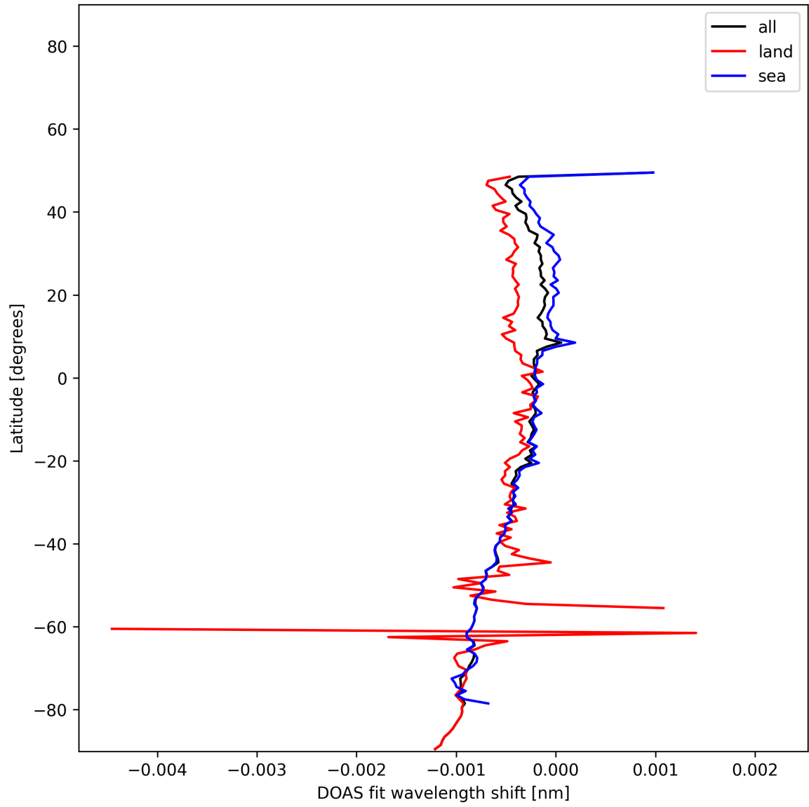
Figure 50: Zonal average of “DOAS fit wavelength shift” for 2024-11-25 to 2024-11-27.
