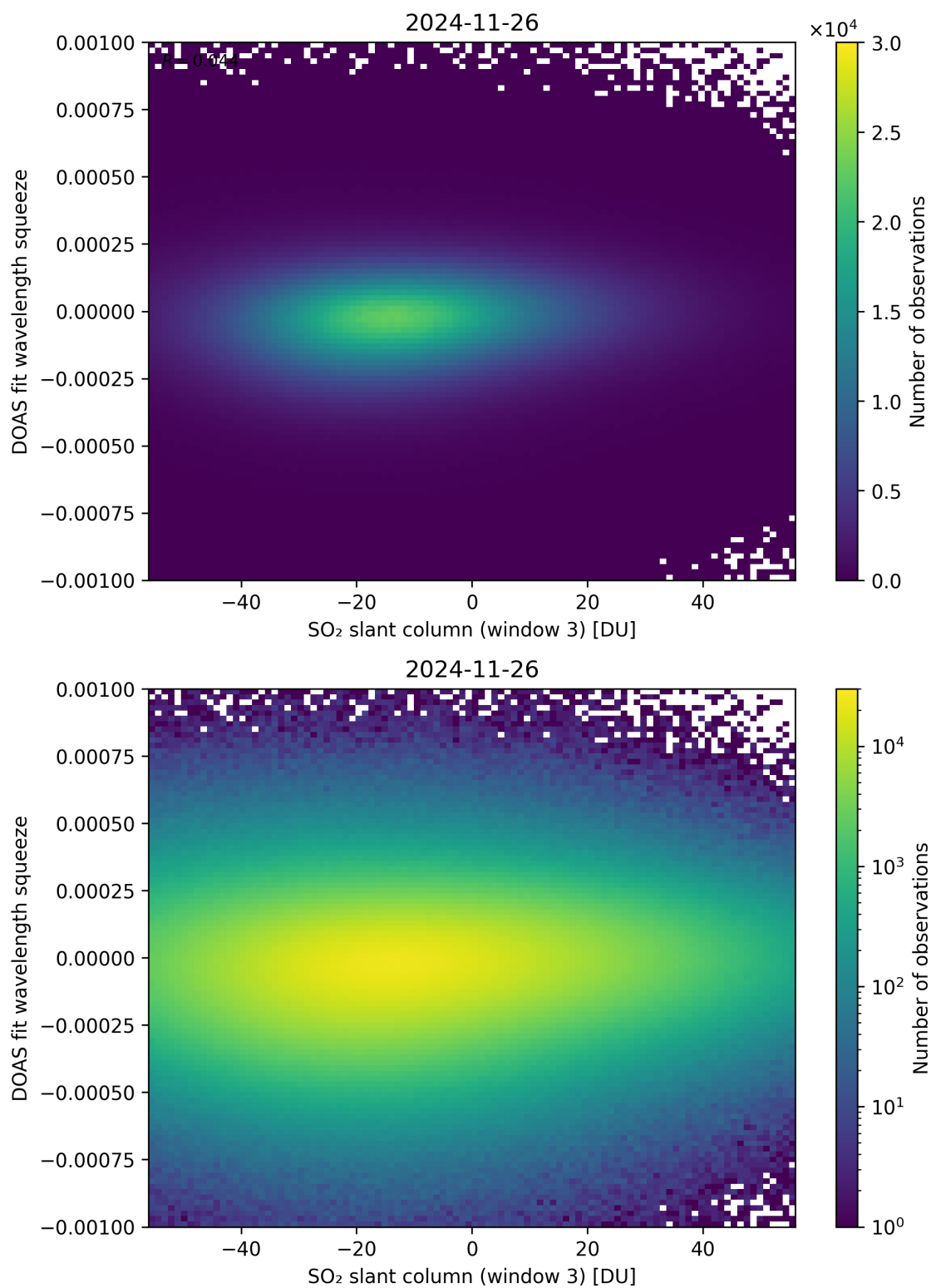
Figure 305: Scatter density plot of “SO 2 slant column (window 3)” against “DOAS fit wavelength squeeze” for 2024-11-25 to 2024-11-27.
