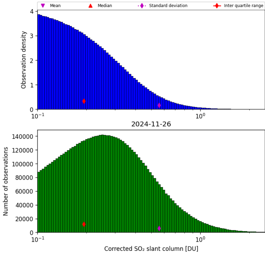
Figure 60: Histogram of “Corrected SO 2 slant column” for 2024-11-25 to 2024-11-27
