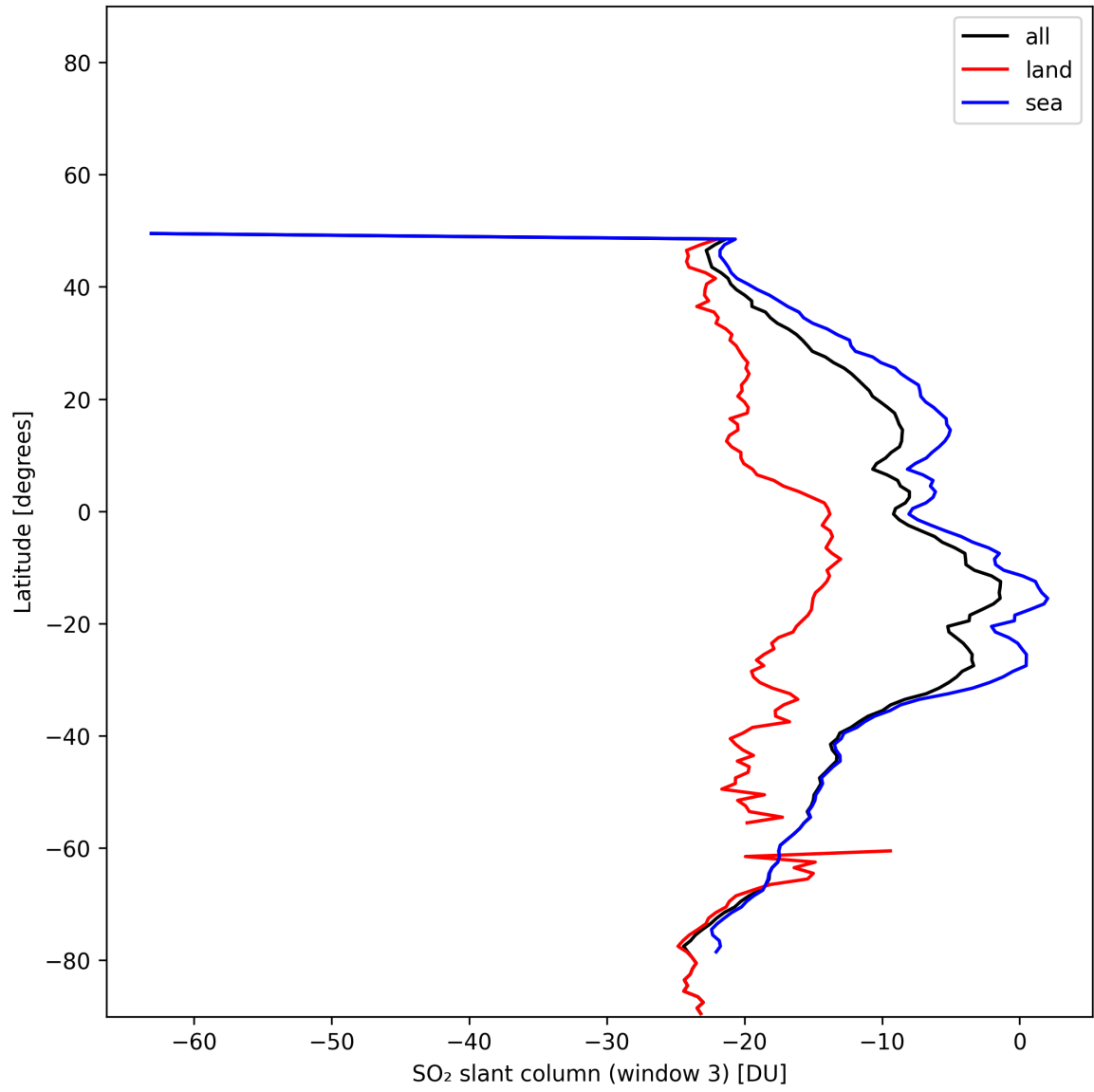
Figure 45: Zonal average of “SO 2 slant column (window 3)” for 2024-11-25 to 2024-11-27.
