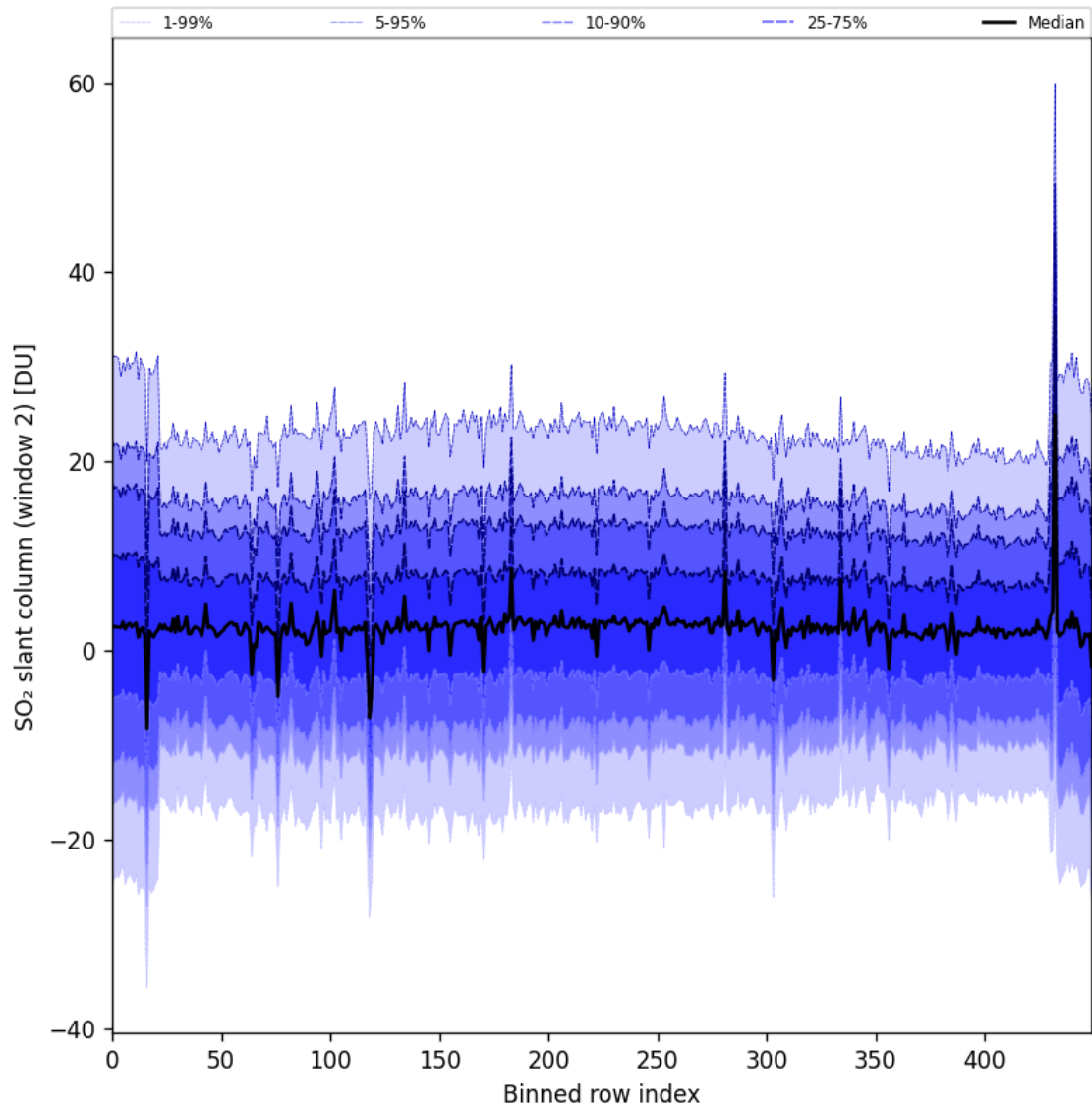
Figure 93: Along track statistics of “SO 2 slant column (window 2)” for 2024-11-25 to 2024-11-27
