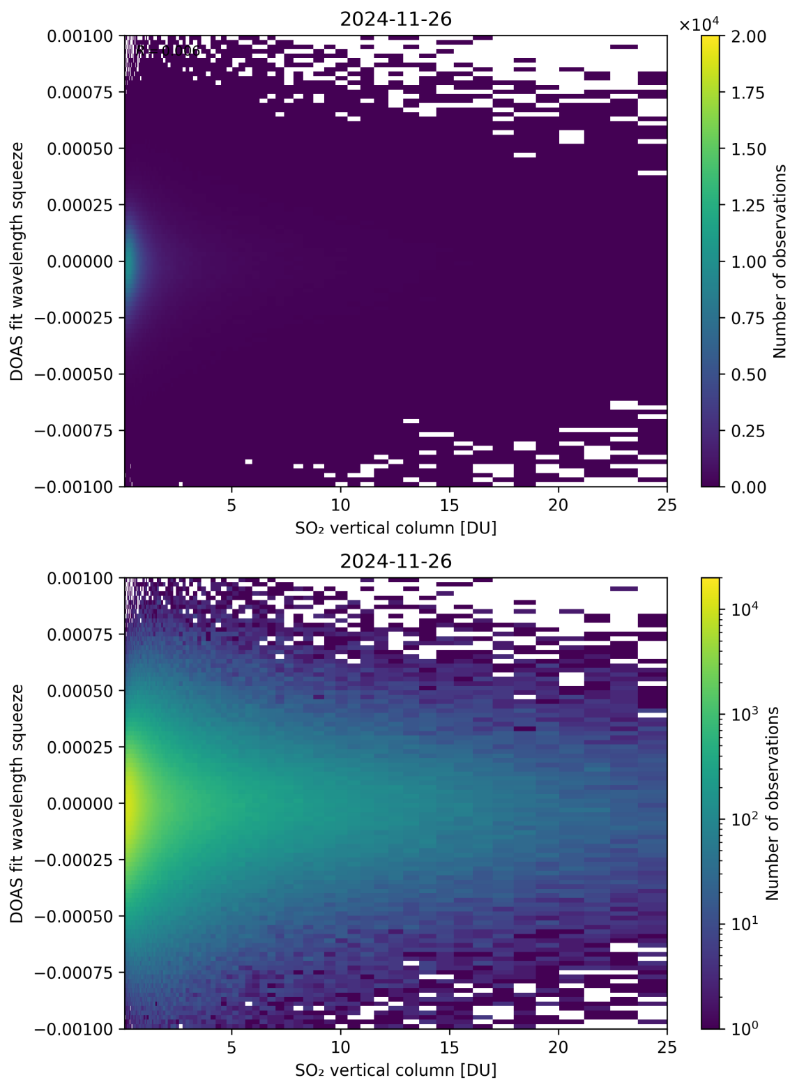
Figure 327: Scatter density plot of “SO 2 vertical column” against “DOAS fit wavelength squeeze” for 2024-11-25 to 2024-11-27.
