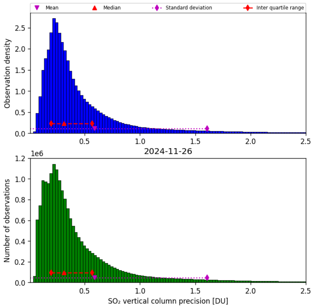
Figure 59: Histogram of “SO 2 vertical column precision” for 2024-11-25 to 2024-11-27
