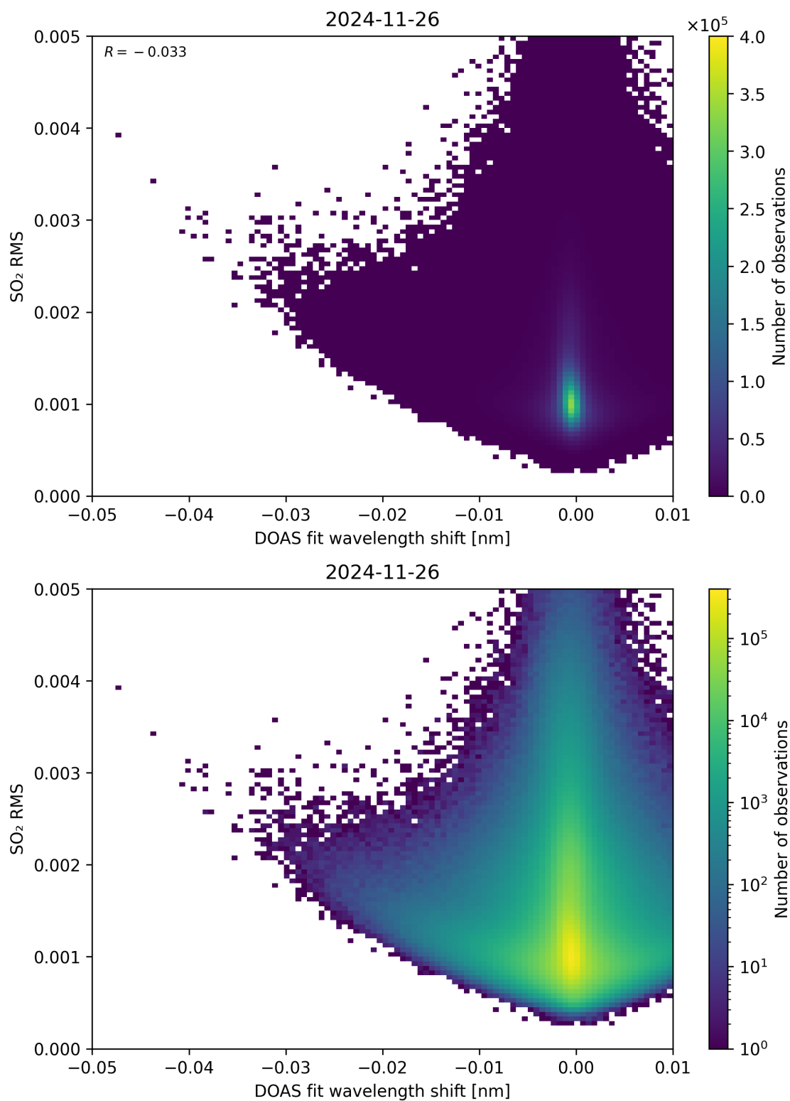
Figure 139: Scatter density plot of “DOAS fit wavelength shift” against “SO 2 RMS” for 2024-11-25 to 2024-11-27.
