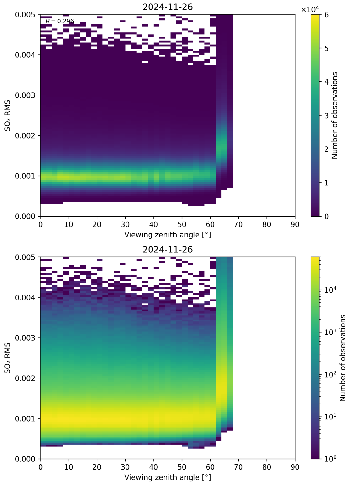
Figure 367: Scatter density plot of “Viewing zenith angle” against “SO 2 RMS” for 2024-11-25 to 2024-11-27.
