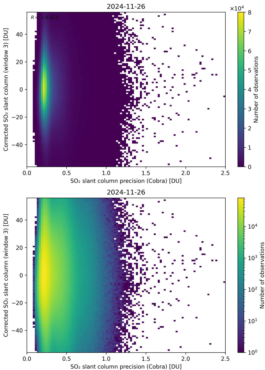
Figure 207: Scatter density plot of “SO 2 slant column precision (Cobra)” against “Corrected SO 2 slant column (window 3)” for 2024-11-25 to 2024-11-27.
