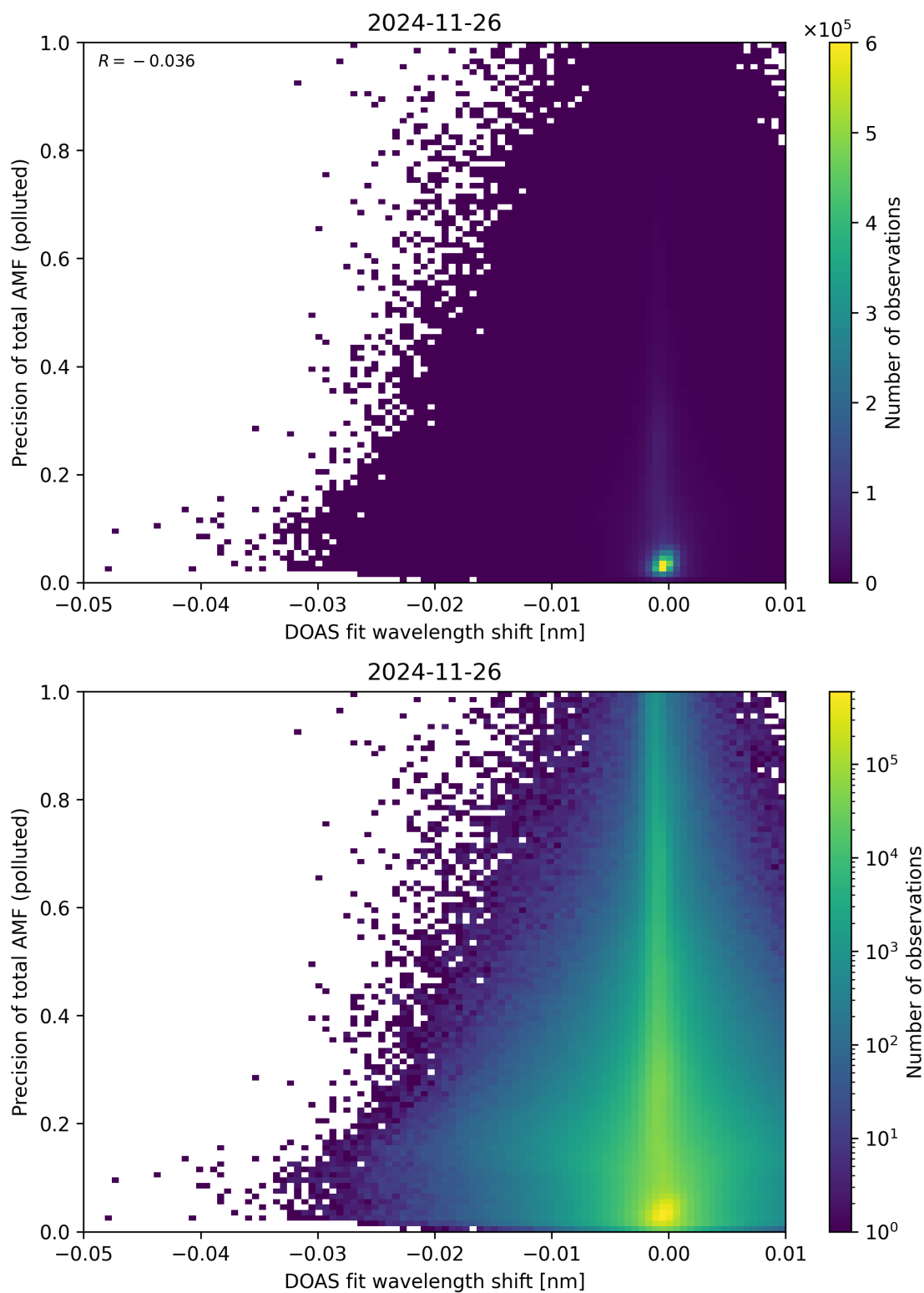
Figure 142: Scatter density plot of “DOAS fit wavelength shift” against “Precision of total AMF (polluted)” for 2024-11-25 to 2024-11-27.
