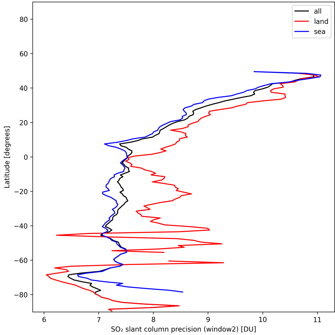
Figure 42: Zonal average of “SO 2 slant column precision (window2)” for 2024-11-25 to 2024-11-27.
