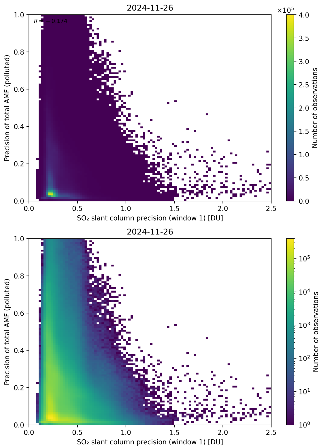
Figure 281: Scatter density plot of “SO 2 slant column precision (window 1)” against “Precision of total AMF (polluted)” for 2024-11-25 to 2024-11-27.
