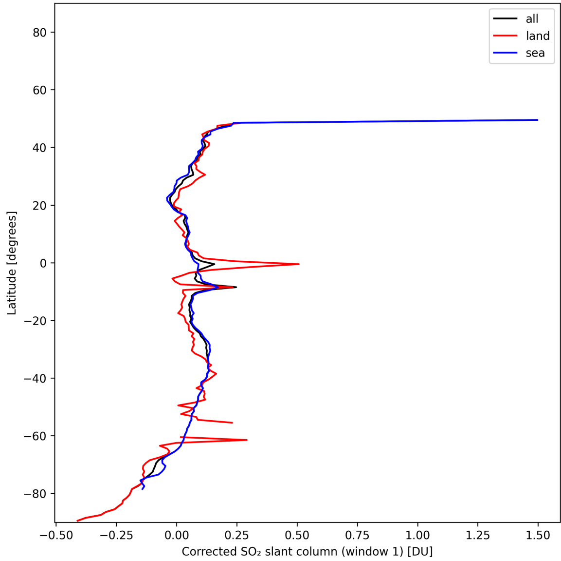
Figure 39: Zonal average of “Corrected SO 2 slant column (window 1)” for 2024-11-25 to 2024-11-27.
