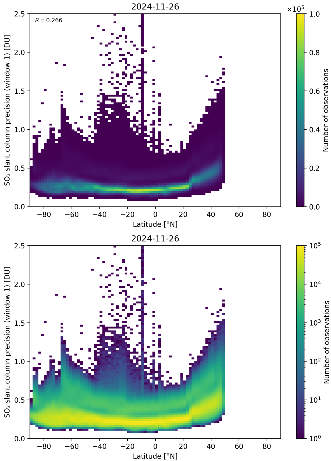
Figure 163: Scatter density plot of “Latitude” against “SO 2 slant column precision (window 1)” for 2024-11-25 to 2024-11-27.
