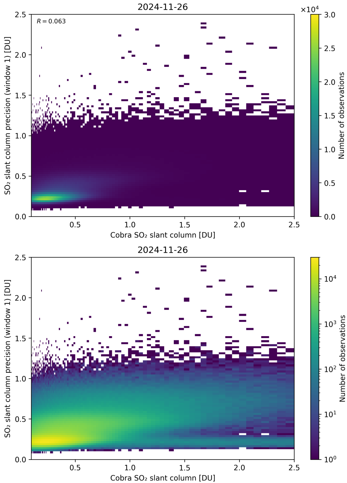
Figure 220: Scatter density plot of “Cobra SO 2 slant column” against “SO 2 slant column precision (window 1)” for 2024-11-25 to 2024-11-27.
