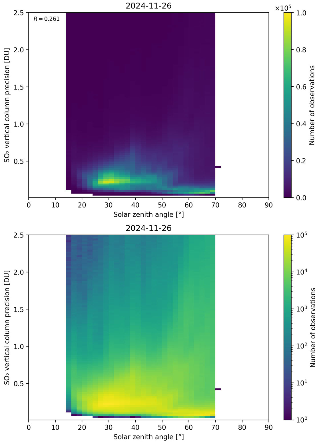
Figure 192: Scatter density plot of “Solar zenith angle” against “SO 2 vertical column precision” for 2024-11-25 to 2024-11-27.
