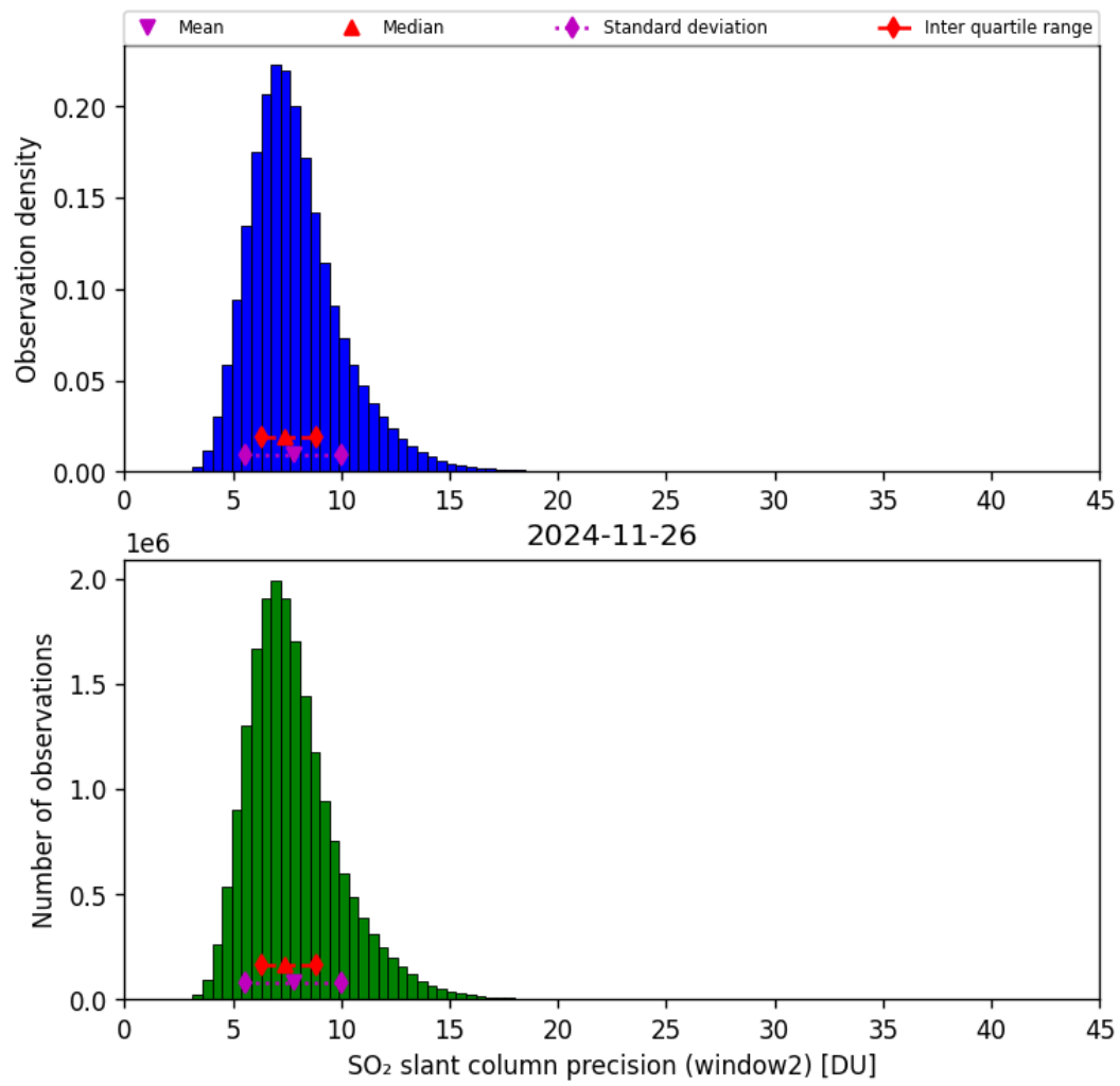
Figure 68: Histogram of “SO 2 slant column precision (window2)” for 2024-11-25 to 2024-11-27
