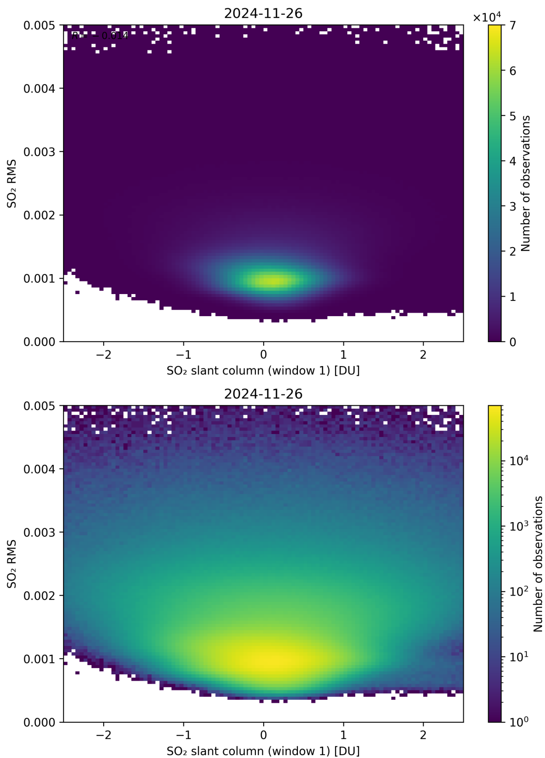
Figure 267: Scatter density plot of “SO 2 slant column (window 1)” against “SO 2 RMS” for 2024-11-25 to 2024-11-27.
