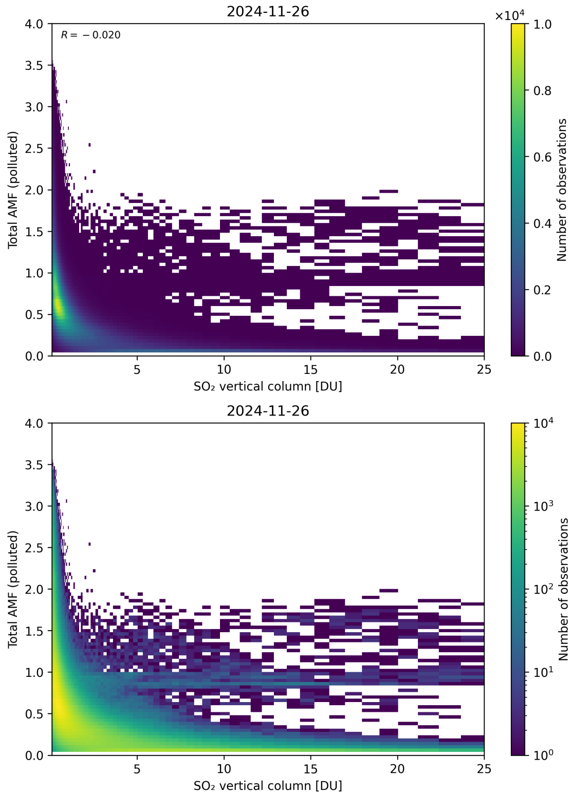
Figure 359: Scatter density plot of “SO 2 vertical column” against “Total AMF (polluted)” for 2024-11-25 to 2024-11-27.
