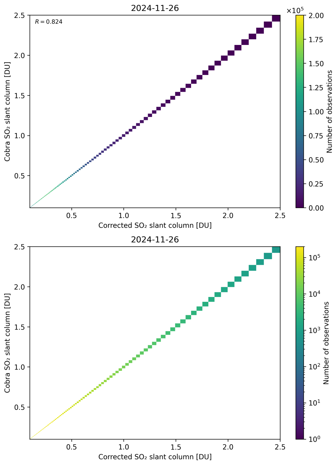
Figure 233: Scatter density plot of “Corrected SO 2 slant column” against “Cobra SO 2 slant column” for 2024-11-25 to 2024-11-27.
