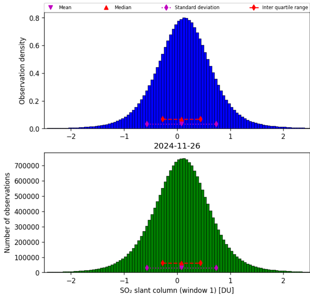
Figure 63: Histogram of “SO 2 slant column (window 1)” for 2024-11-25 to 2024-11-27
