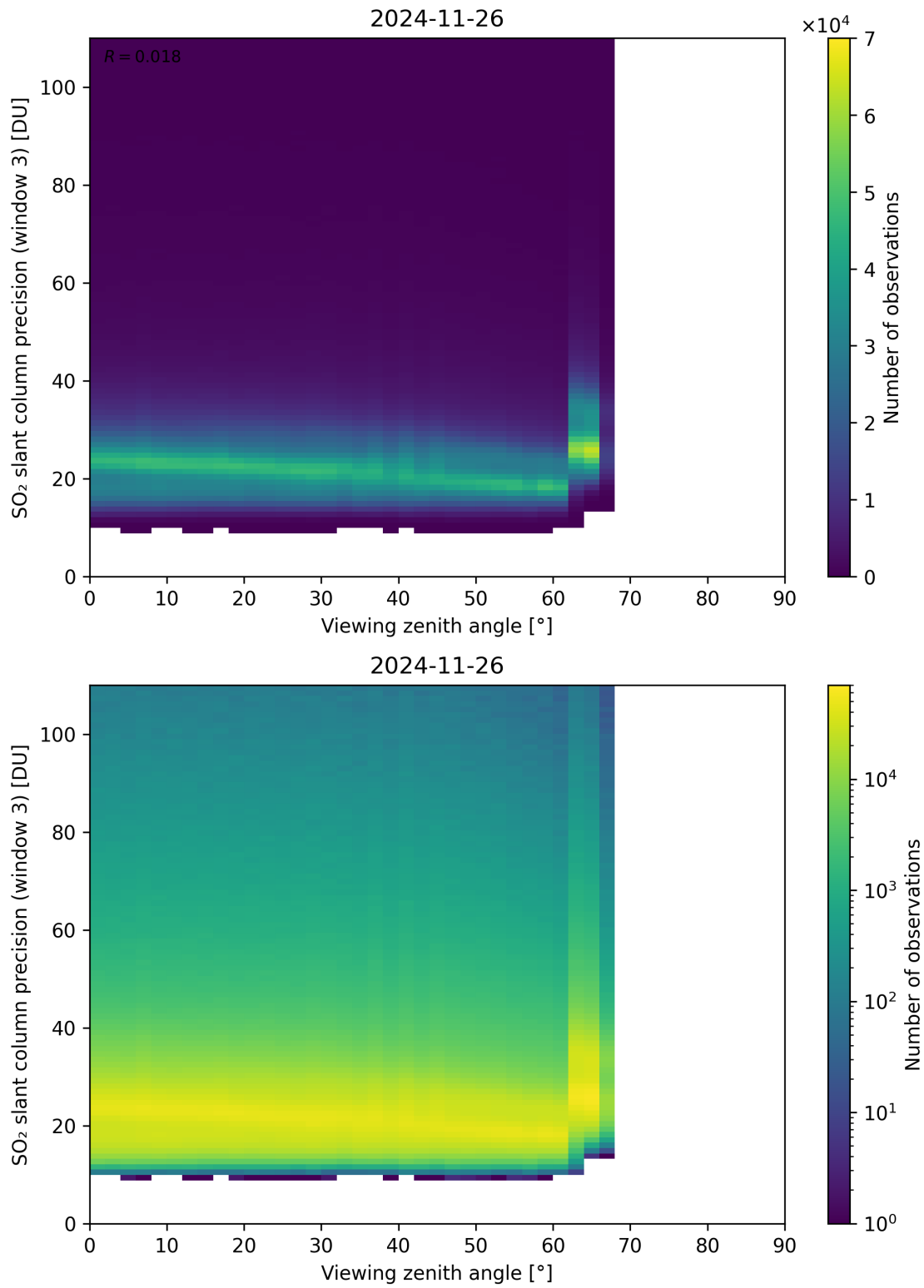
Figure 380: Scatter density plot of “Viewing zenith angle” against “SO 2 slant column precision (window 3)” for 2024-11-25 to 2024-11-27.
