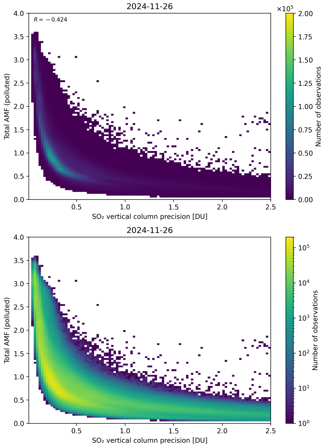
Figure 346: Scatter density plot of “SO 2 vertical column precision” against “Total AMF (polluted)” for 2024-11-25 to 2024-11-27.
