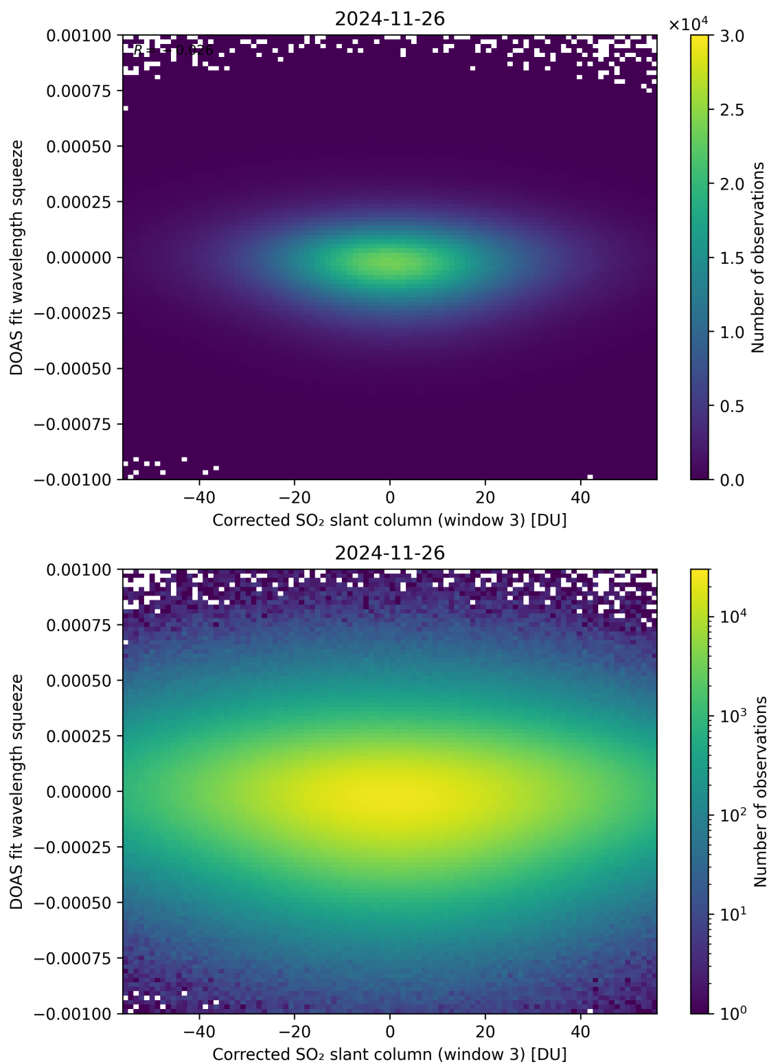
Figure 257: Scatter density plot of “Corrected SO 2 slant column (window 3)” against “DOAS fit wavelength squeeze” for 2024-11-25 to 2024-11-27.
