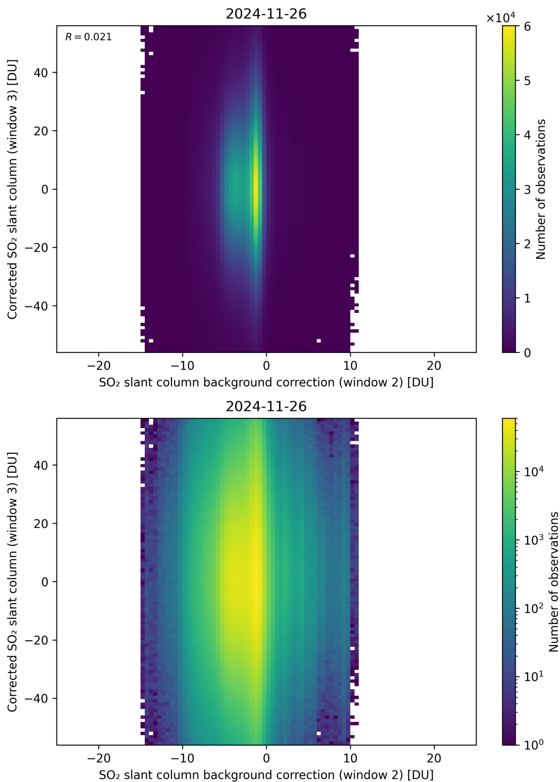
Figure 127: Scatter density plot of “SO 2 slant column background correction (window 2)” against “Corrected SO 2 slant column (window 3)” for 2024-11-25 to 2024-11-27.
