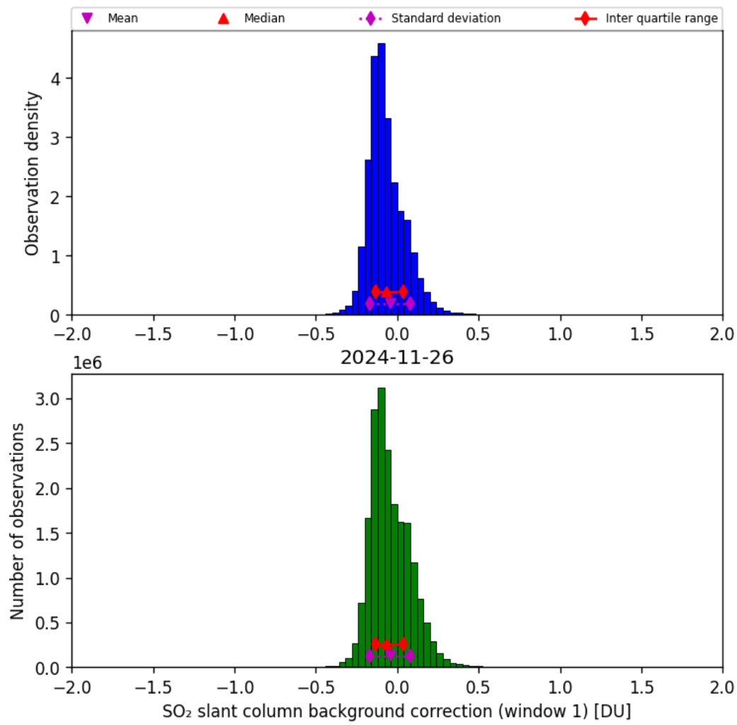
Figure 66: Histogram of “SO 2 slant column background correction (window 1)” for 2024-11-25 to 2024-11-27
