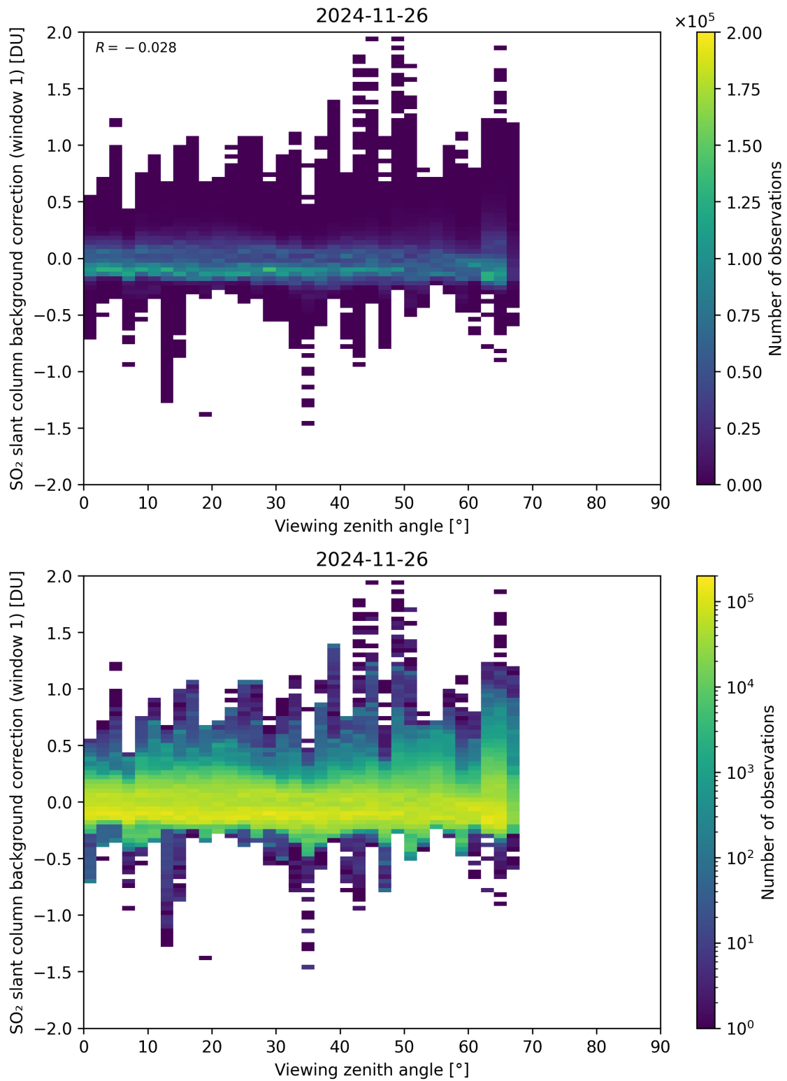
Figure 362: Scatter density plot of “Viewing zenith angle” against “SO 2 slant column background correction (window 1)” for 2024-11-25 to 2024-11-27.
