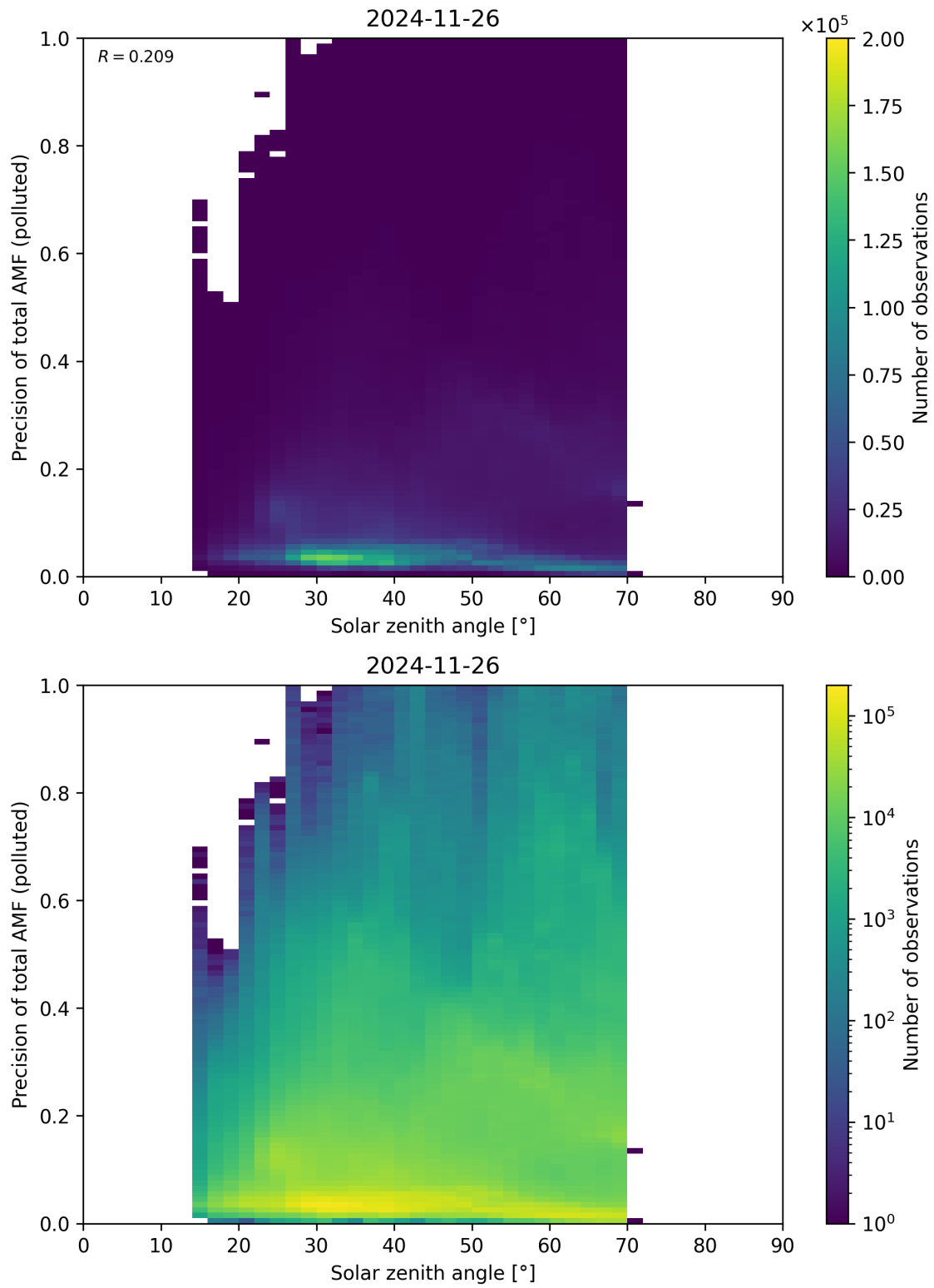
Figure 190: Scatter density plot of “Solar zenith angle” against “Precision of total AMF (polluted)” for 2024-11-25 to 2024-11-27.
