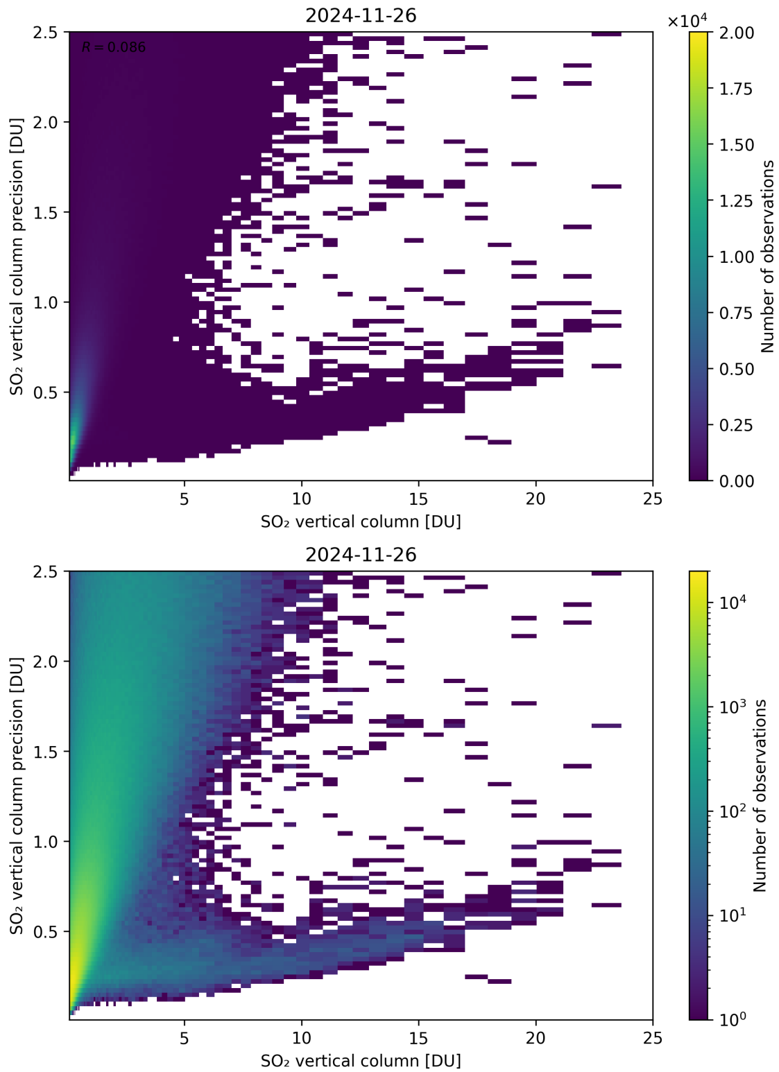
Figure 361: Scatter density plot of “SO 2 vertical column” against “SO 2 vertical column precision” for 2024-11-25 to 2024-11-27.
