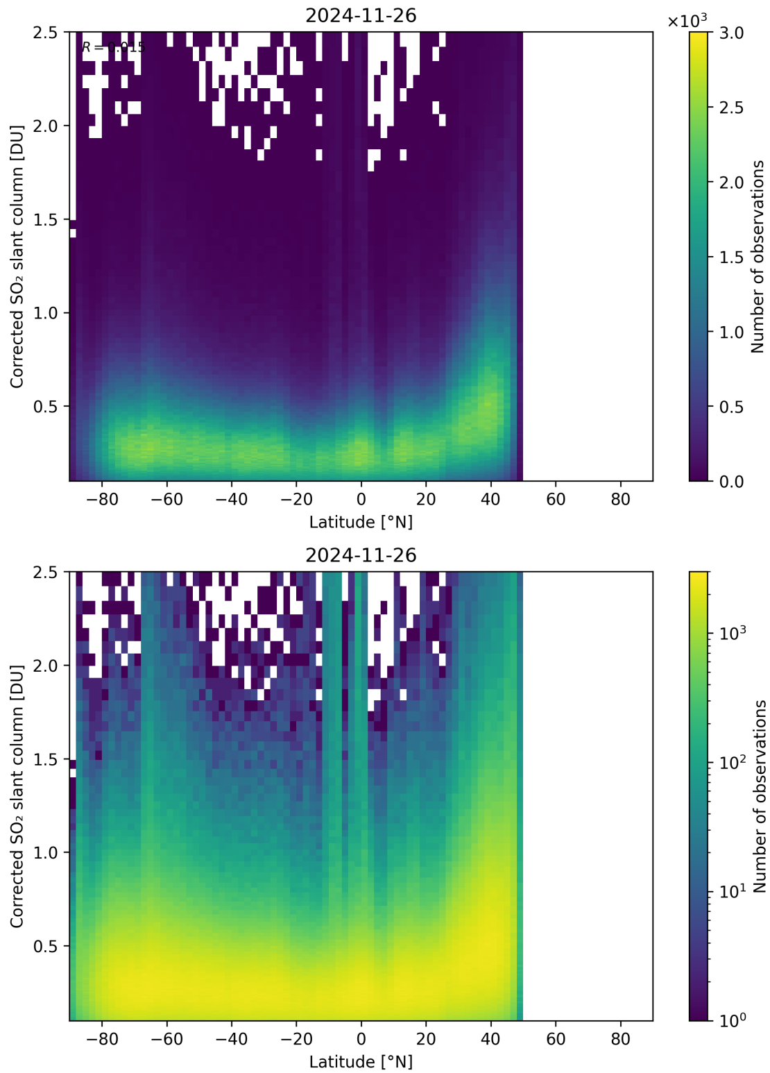
Figure 159: Scatter density plot of “Latitude” against “Corrected SO 2 slant column” for 2024-11-25 to 2024-11-27.
