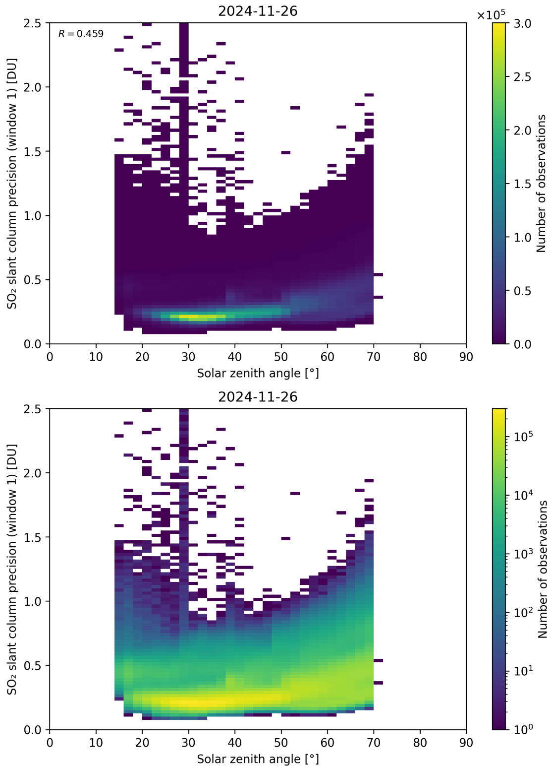
Figure 185: Scatter density plot of “Solar zenith angle” against “SO 2 slant column precision (window 1)” for 2024-11-25 to 2024-11-27.
