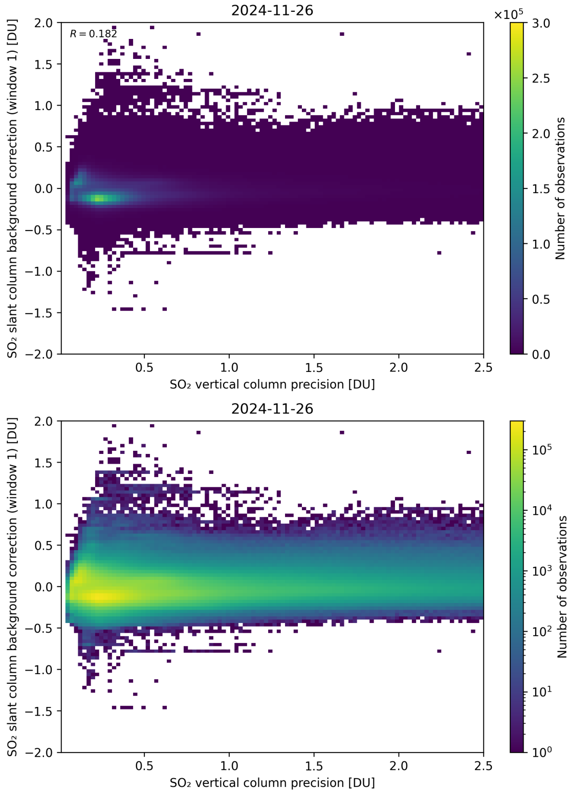
Figure 329: Scatter density plot of “SO 2 vertical column precision” against “SO 2 slant column background correction (window 1)” for 2024-11-25 to 2024-11-27.
