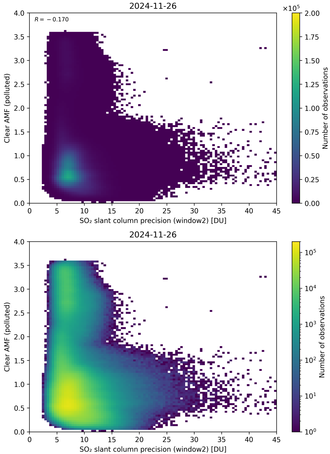
Figure 296: Scatter density plot of “SO 2 slant column precision (window2)” against “Clear AMF (polluted)” for 2024-11-25 to 2024-11-27.
