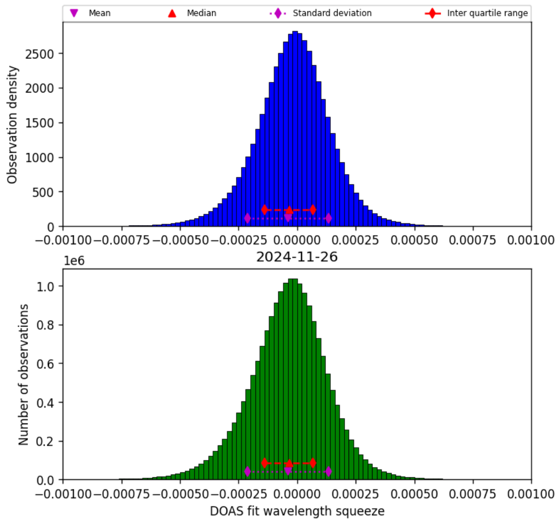
Figure 77: Histogram of “DOAS fit wavelength squeeze” for 2024-11-25 to 2024-11-27
