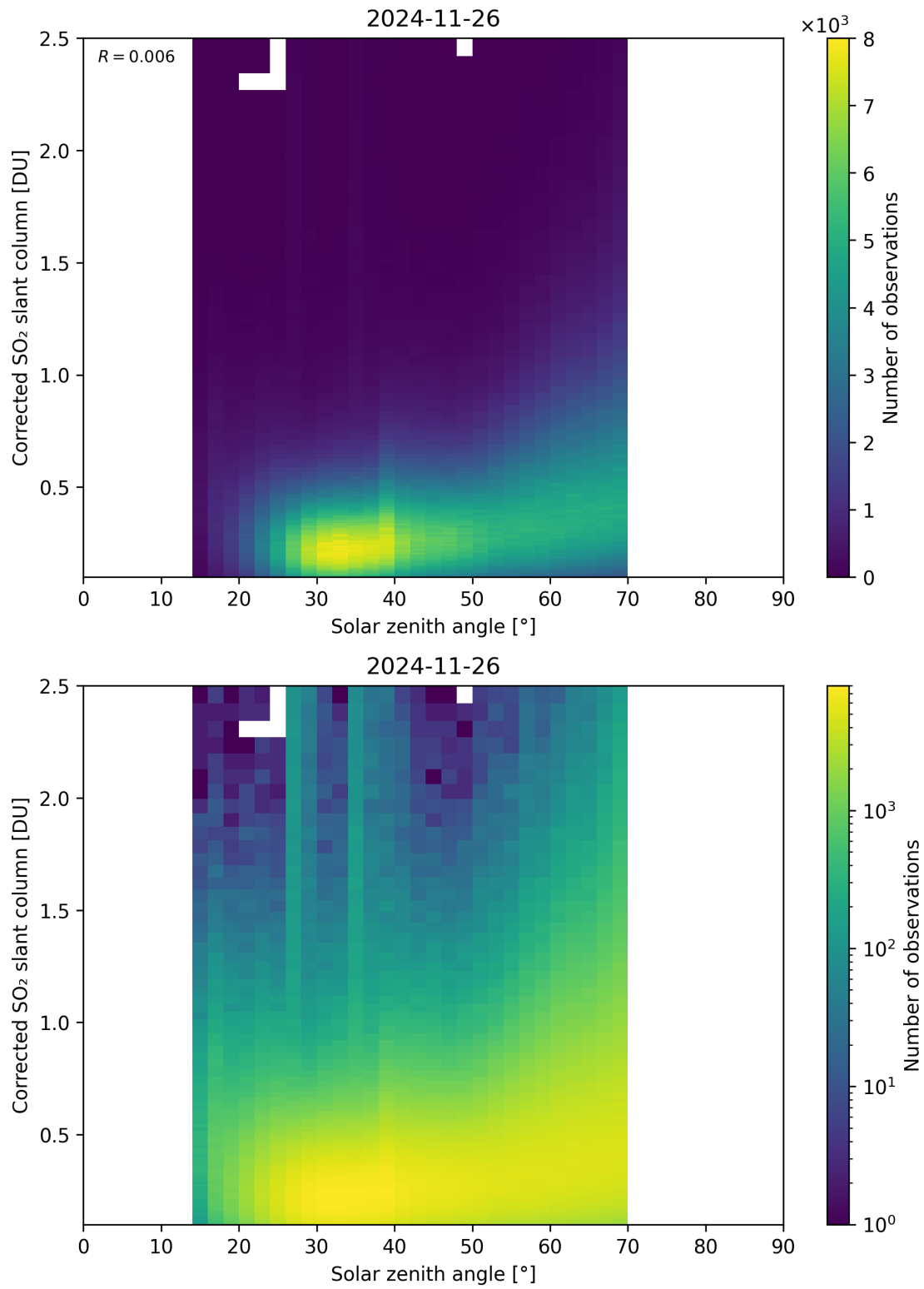
Figure 181: Scatter density plot of “Solar zenith angle” against “Corrected SO 2 slant column” for 2024-11-25 to 2024-11-27.
