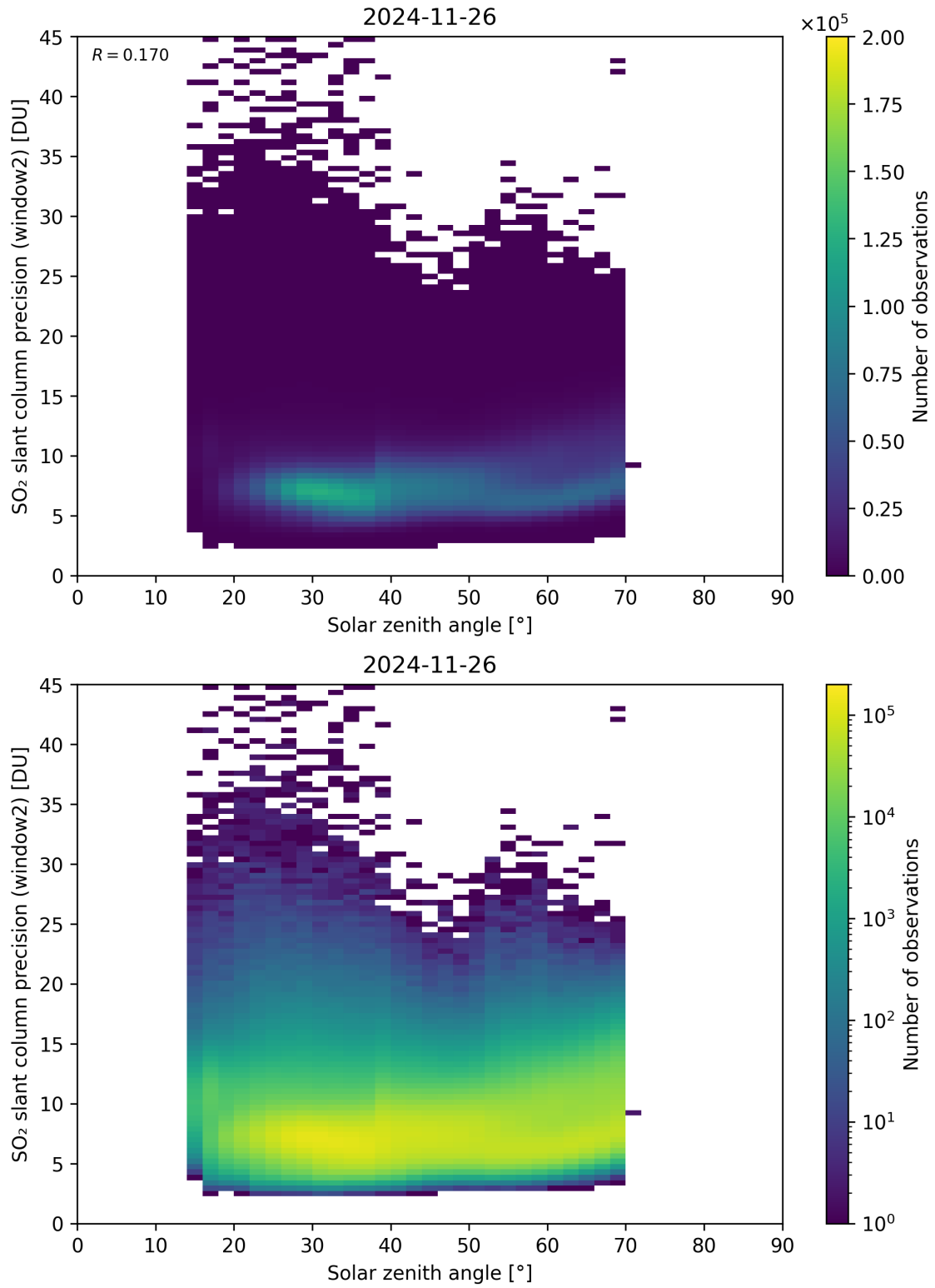
Figure 186: Scatter density plot of “Solar zenith angle” against “SO 2 slant column precision (window2)” for 2024-11-25 to 2024-11-27.
