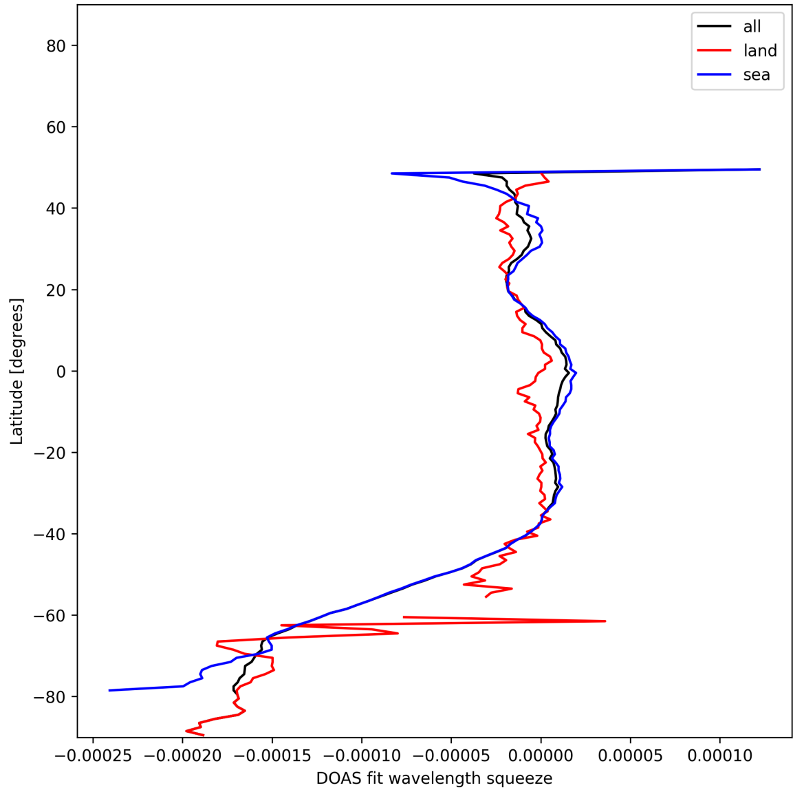
Figure 51: Zonal average of “DOAS fit wavelength squeeze” for 2024-11-25 to 2024-11-27.
