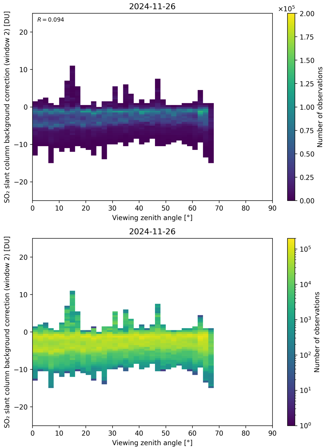
Figure 363: Scatter density plot of “Viewing zenith angle” against “SO 2 slant column background correction (window 2)” for 2024-11-25 to 2024-11-27.
