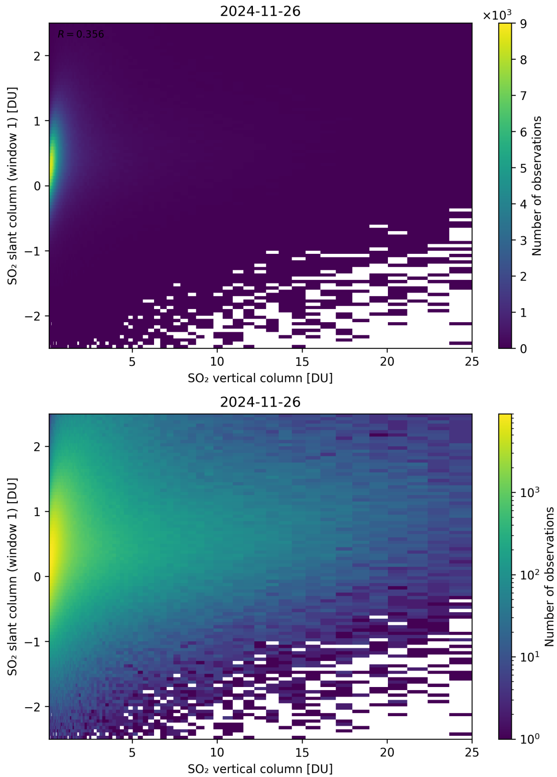
Figure 354: Scatter density plot of “SO 2 vertical column” against “SO 2 slant column (window 1)” for 2024-11-25 to 2024-11-27.
