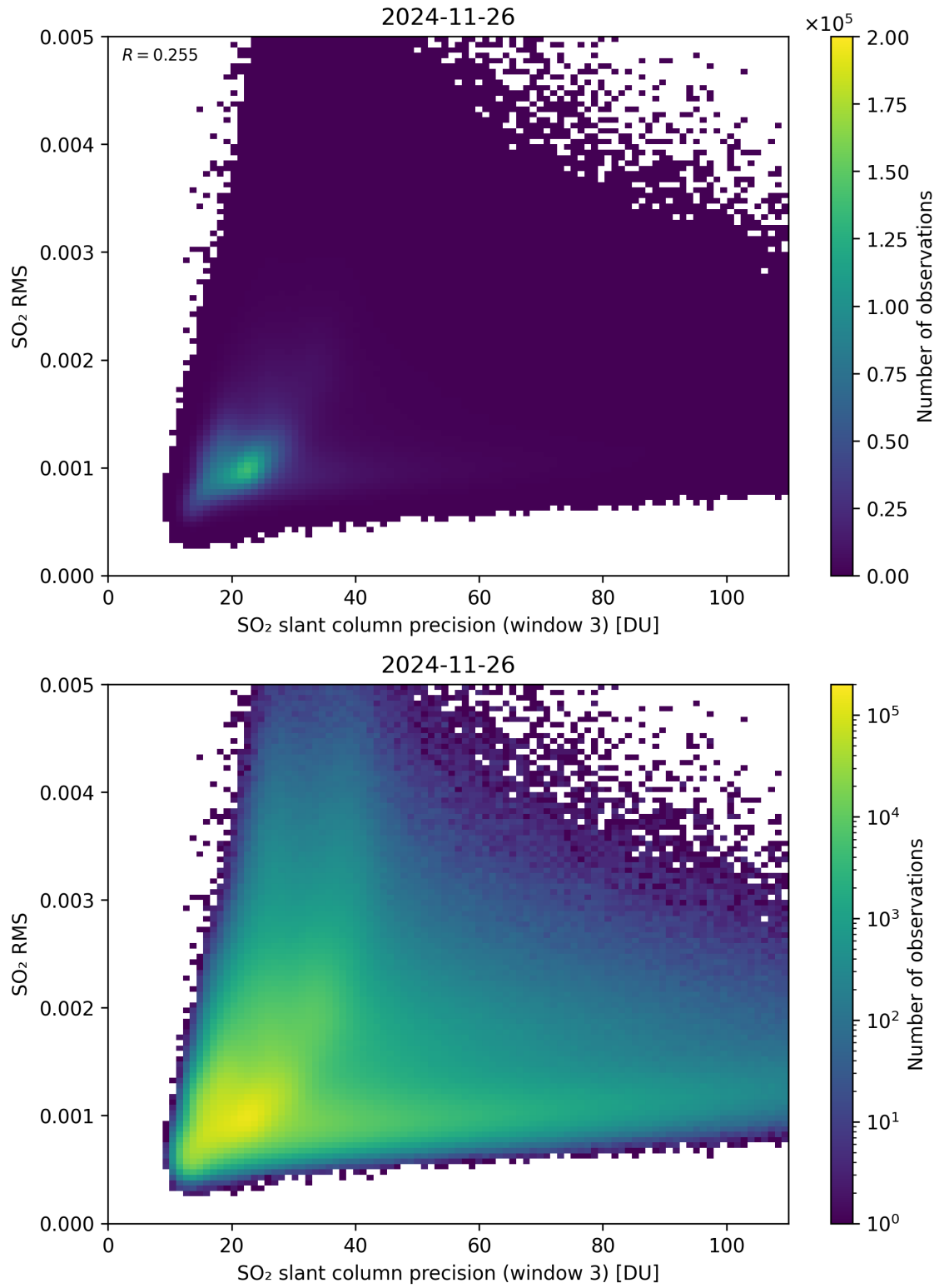
Figure 310: Scatter density plot of “SO 2 slant column precision (window 3)” against “SO 2 RMS” for 2024-11-25 to 2024-11-27.
