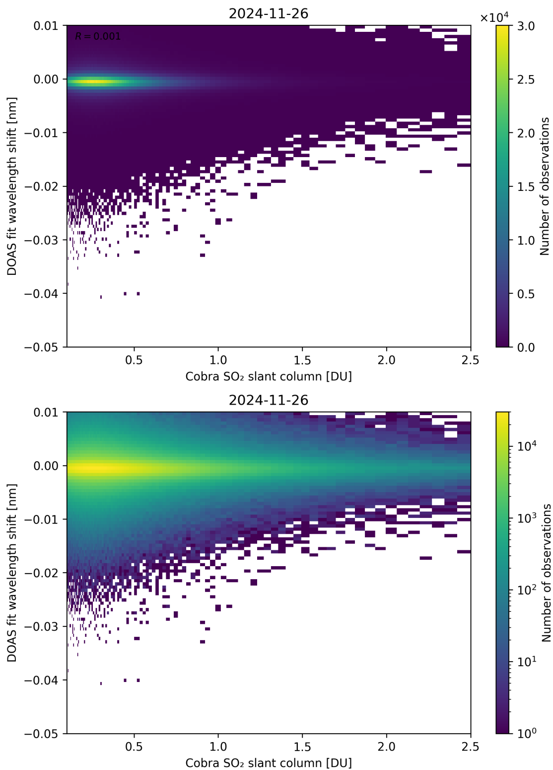
Figure 196: Scatter density plot of “Cobra SO 2 slant column” against “DOAS fit wavelength shift” for 2024-11-25 to 2024-11-27.
