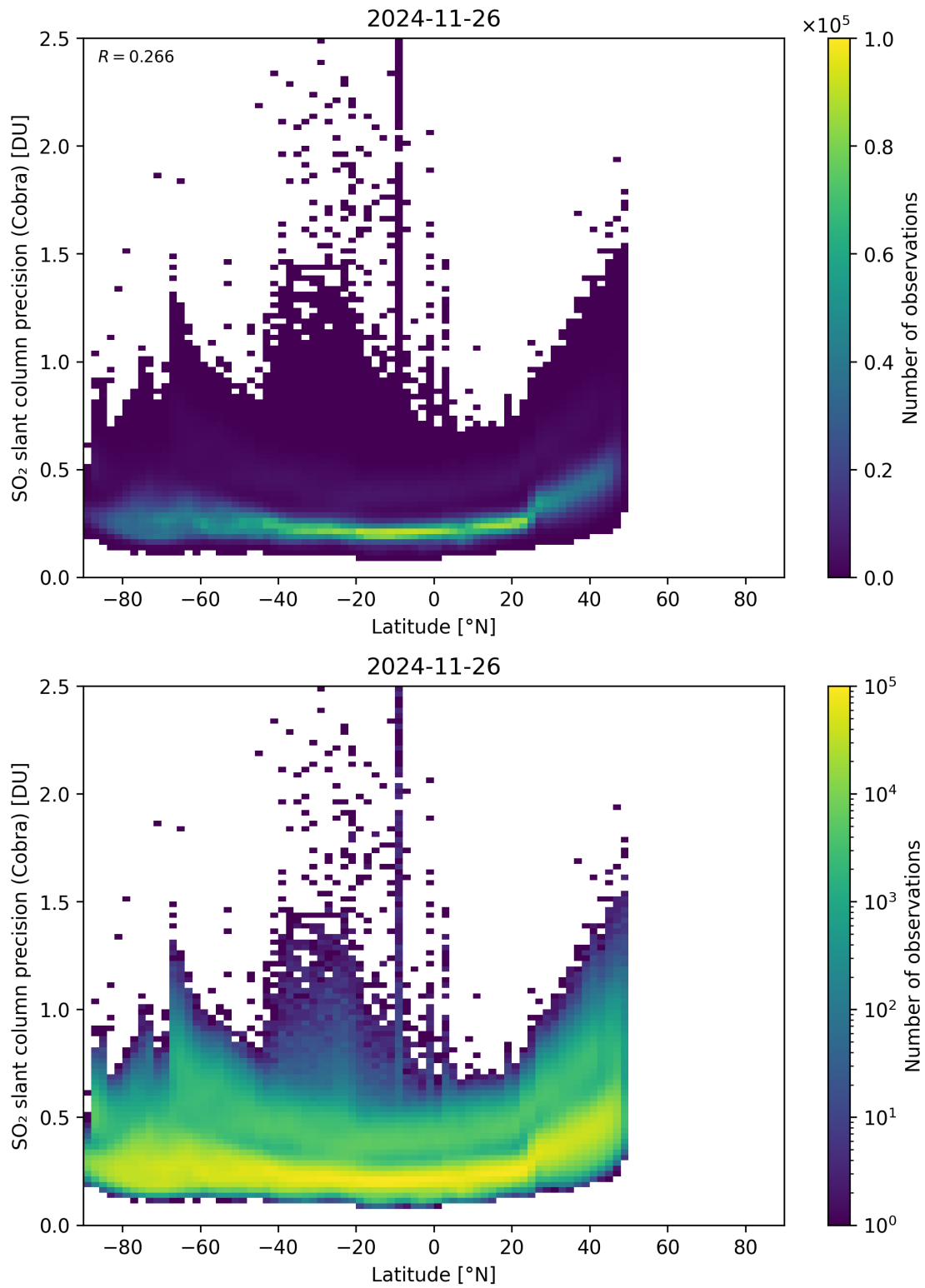
Figure 158: Scatter density plot of “Latitude” against “SO 2 slant column precision (Cobra)” for 2024-11-25 to 2024-11-27.
