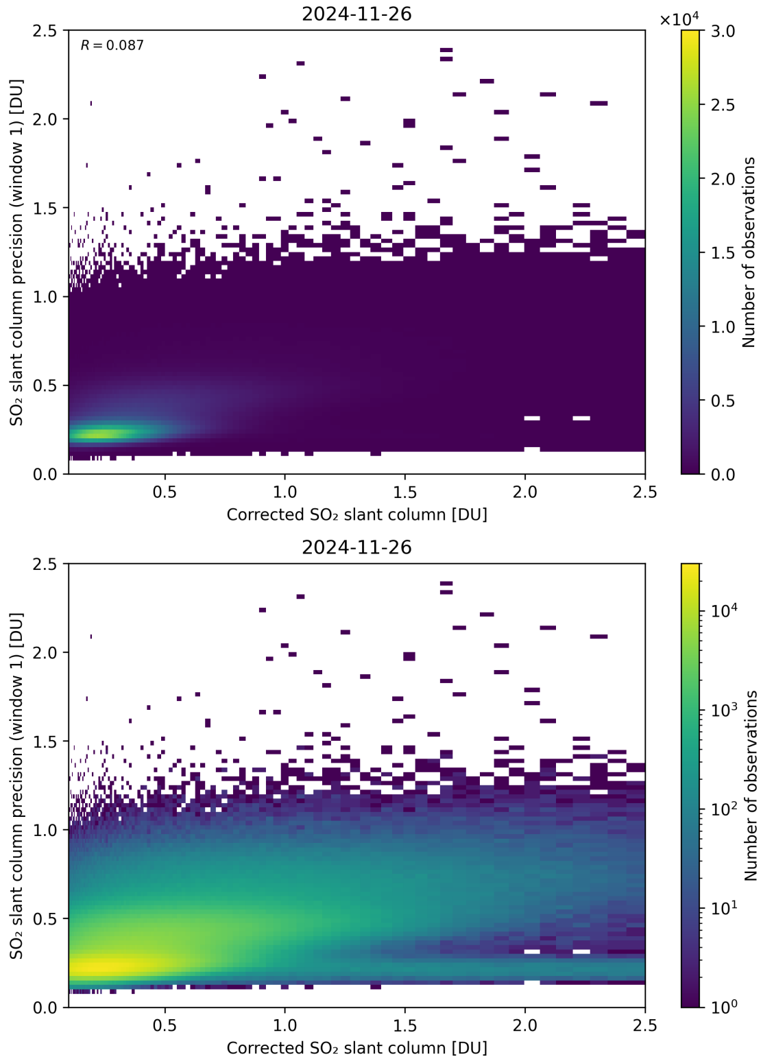
Figure 238: Scatter density plot of “Corrected SO 2 slant column” against “SO 2 slant column precision (window 1)” for 2024-11-25 to 2024-11-27.
