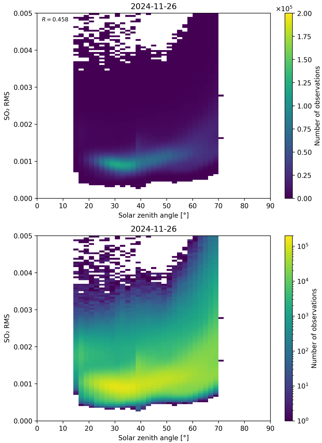
Figure 176: Scatter density plot of “Solar zenith angle” against “SO 2 RMS” for 2024-11-25 to 2024-11-27.
