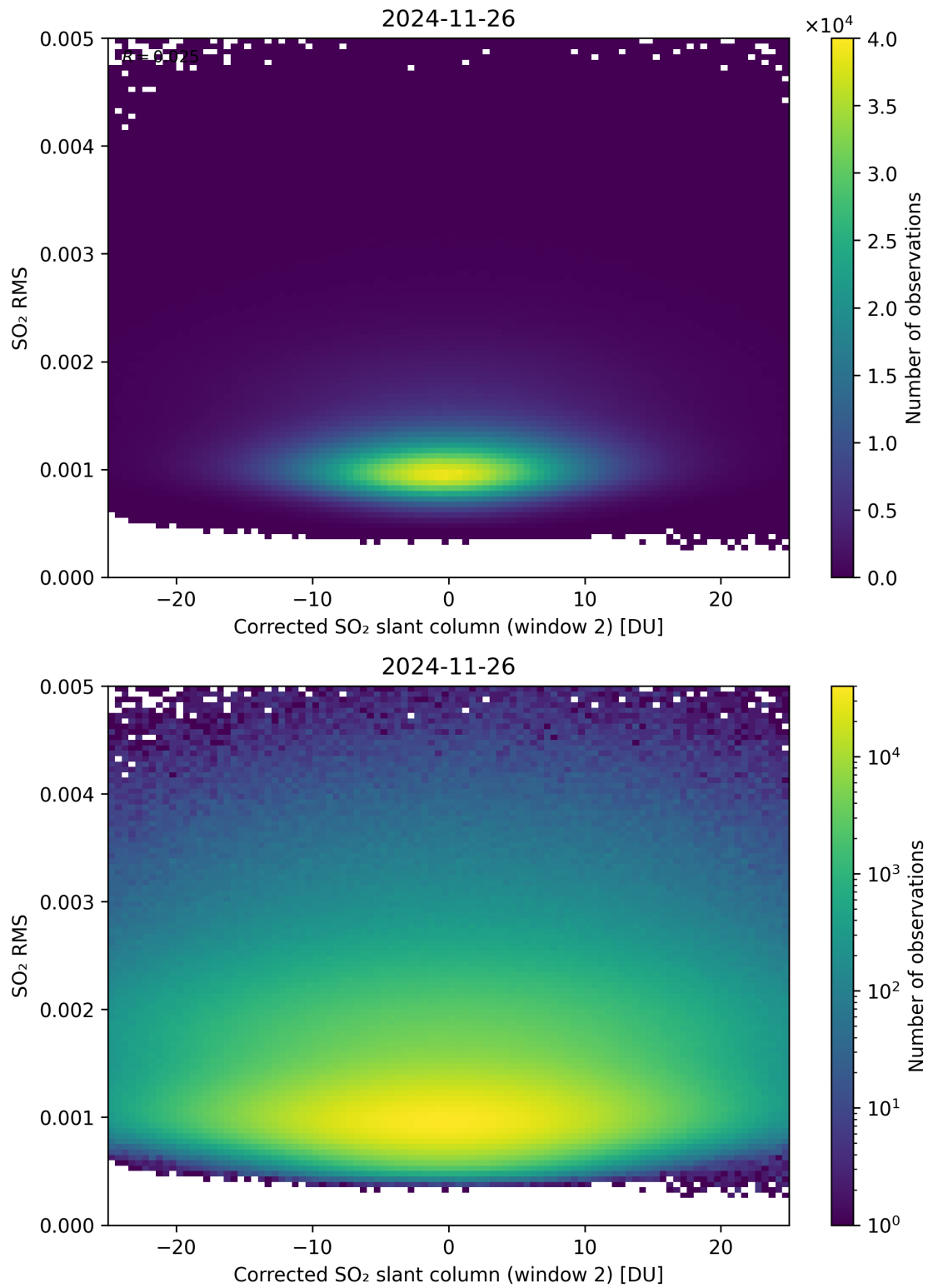
Figure 248: Scatter density plot of “Corrected SO 2 slant column (window 2)” against “SO 2 RMS” for 2024-11-25 to 2024-11-27.
