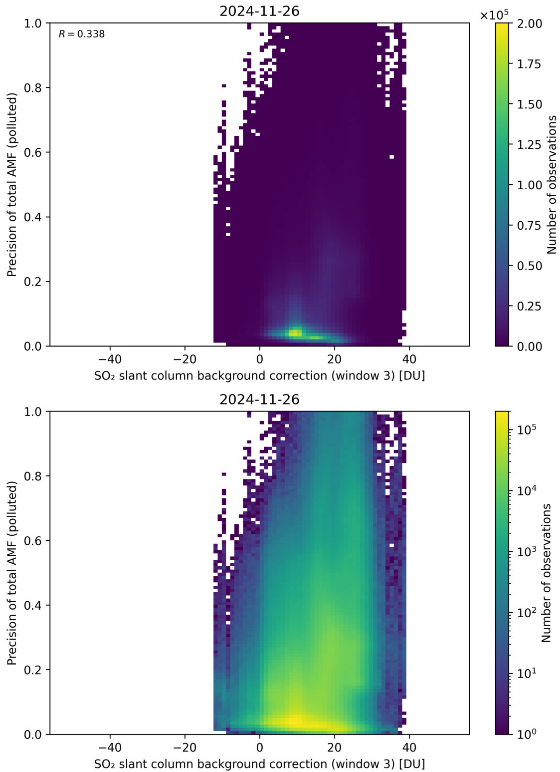
Figure 137: Scatter density plot of “SO 2 slant column background correction (window 3)” against “Precision of total AMF (polluted)” for 2024-11-25 to 2024-11-27.
