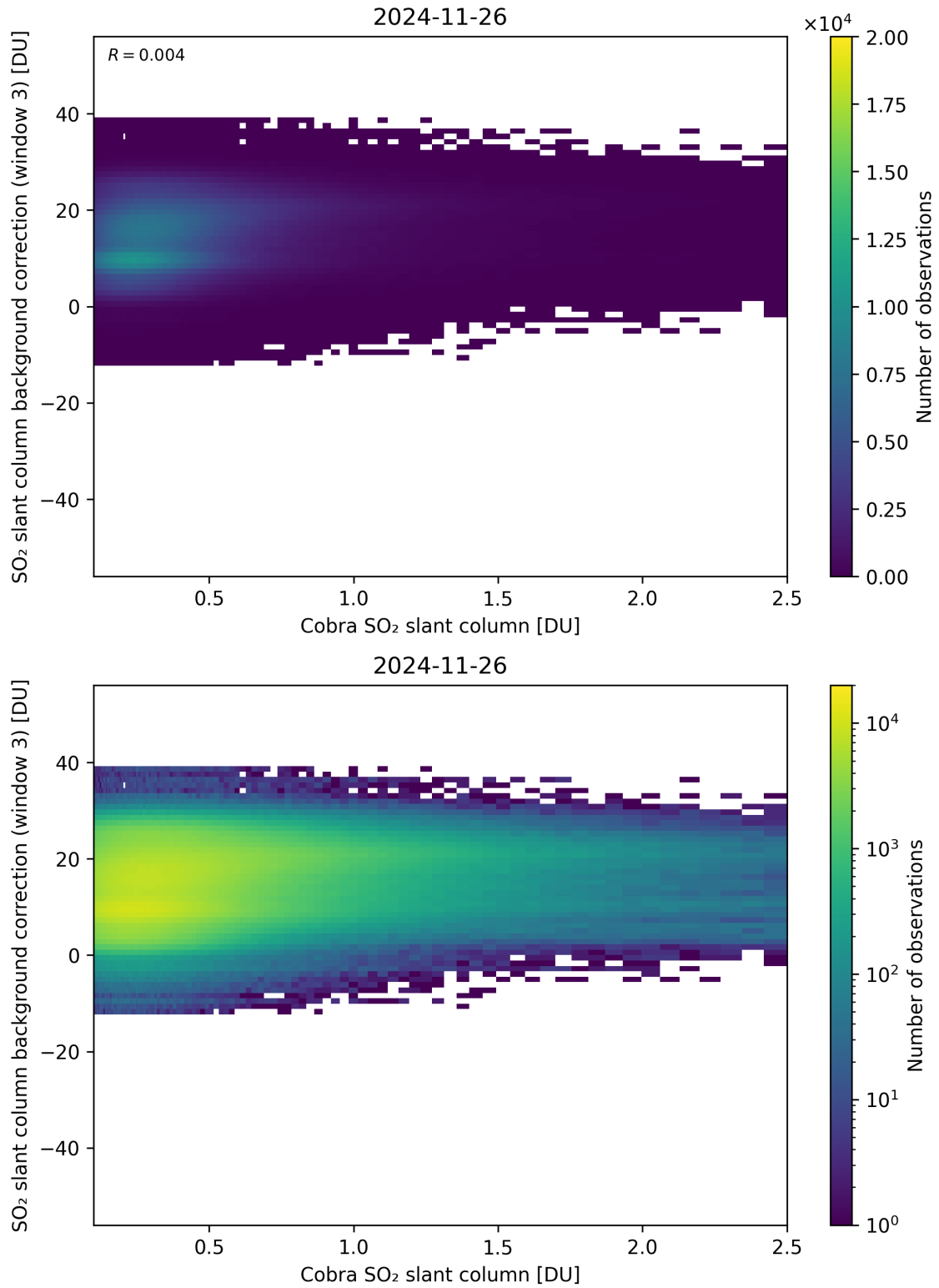
Figure 195: Scatter density plot of “Cobra SO 2 slant column” against “SO 2 slant column background correction (window 3)” for 2024-11-25 to 2024-11-27.
