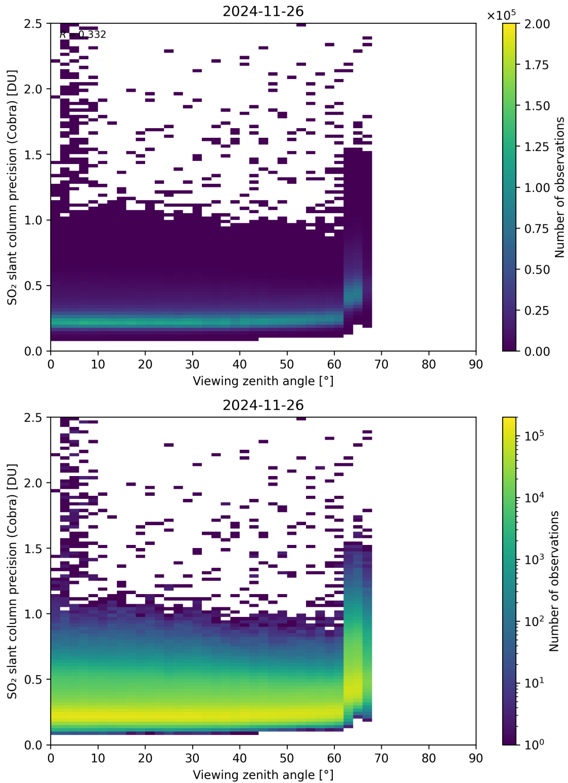
Figure 372: Scatter density plot of “Viewing zenith angle” against “SO 2 slant column precision (Cobra)” for 2024-11-25 to 2024-11-27.
