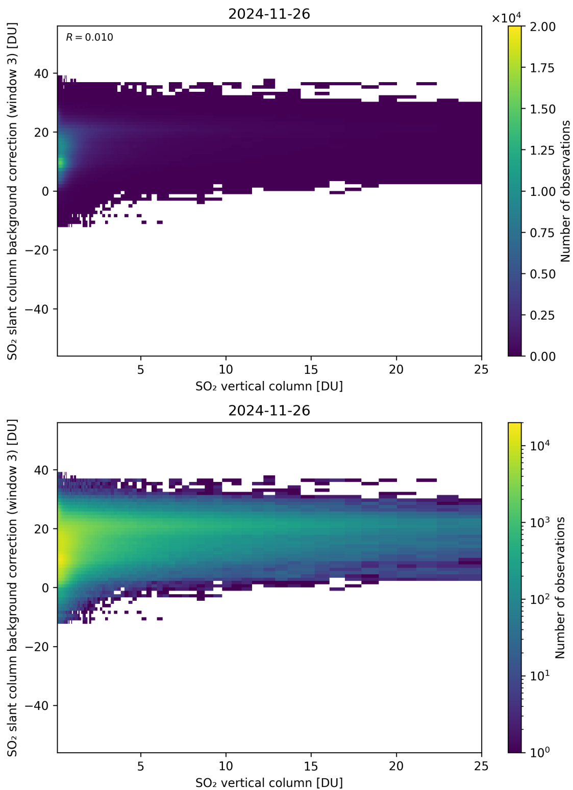
Figure 325: Scatter density plot of “SO 2 vertical column” against “SO 2 slant column background correction (window 3)” for 2024-11-25 to 2024-11-27.
