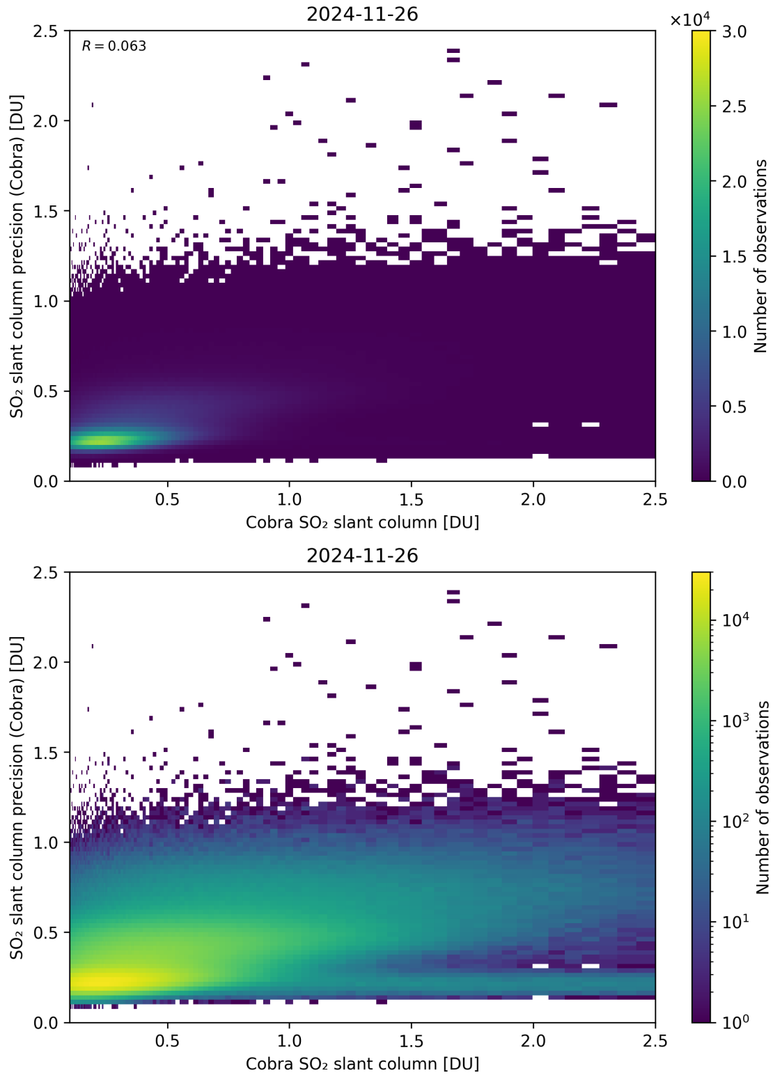
Figure 216: Scatter density plot of “Cobra SO 2 slant column” against “SO 2 slant column precision (Cobra)” for 2024-11-25 to 2024-11-27.
