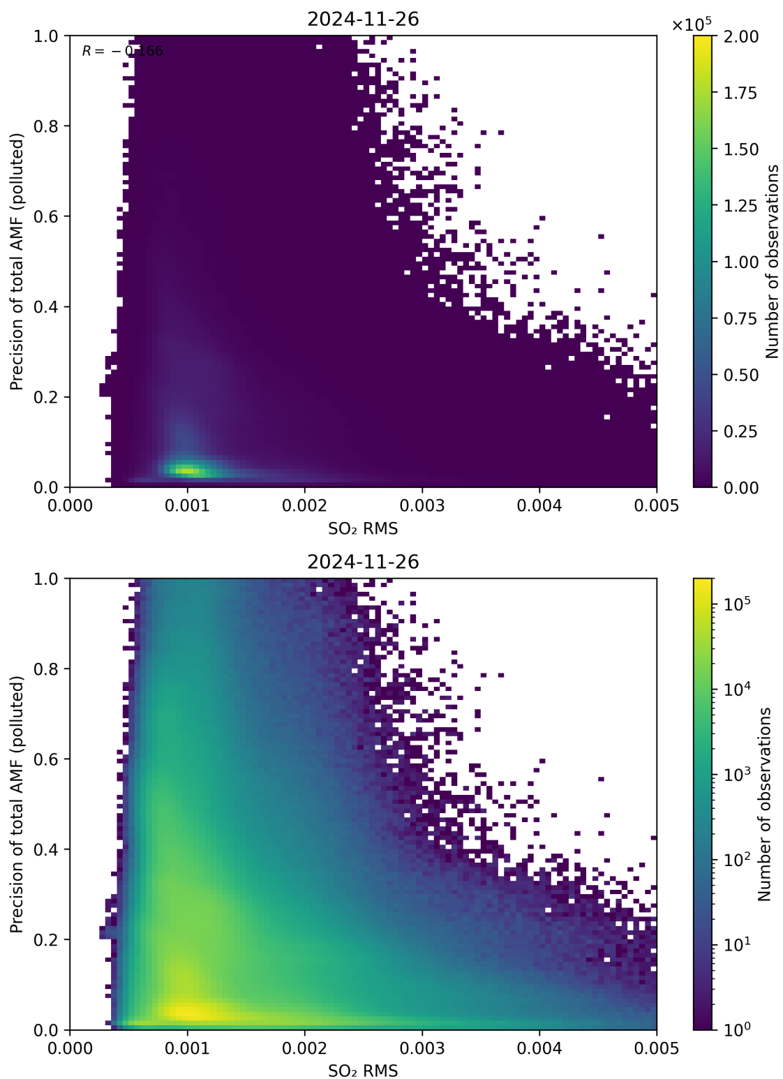
Figure 149: Scatter density plot of “SO 2 RMS” against “Precision of total AMF (polluted)” for 2024-11-25 to 2024-11-27.
