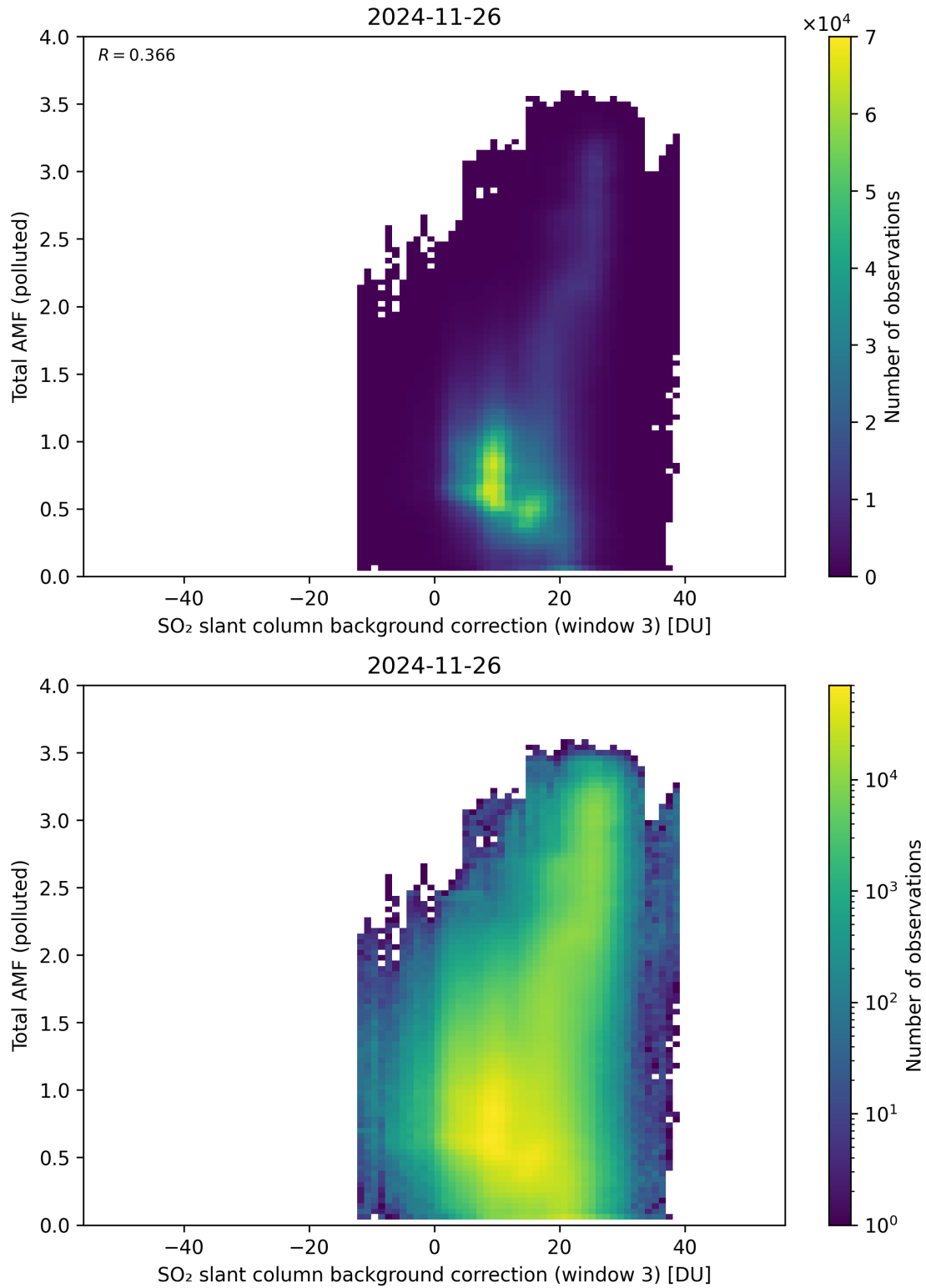
Figure 136: Scatter density plot of “SO 2 slant column background correction (window 3)” against “Total AMF (polluted)” for 2024-11-25 to 2024-11-27.
