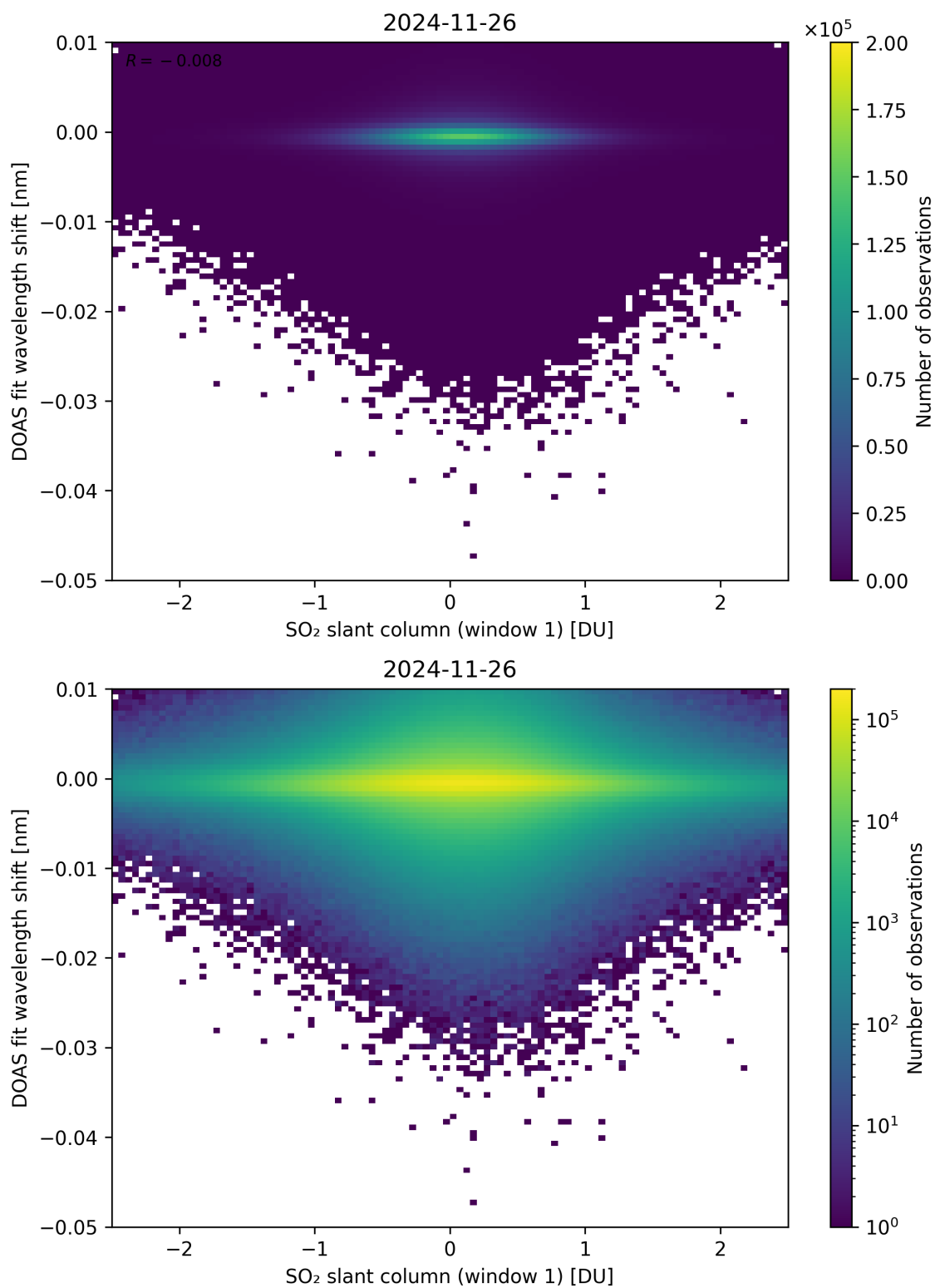
Figure 265: Scatter density plot of “SO 2 slant column (window 1)” against “DOAS fit wavelength shift” for 2024-11-25 to 2024-11-27.
