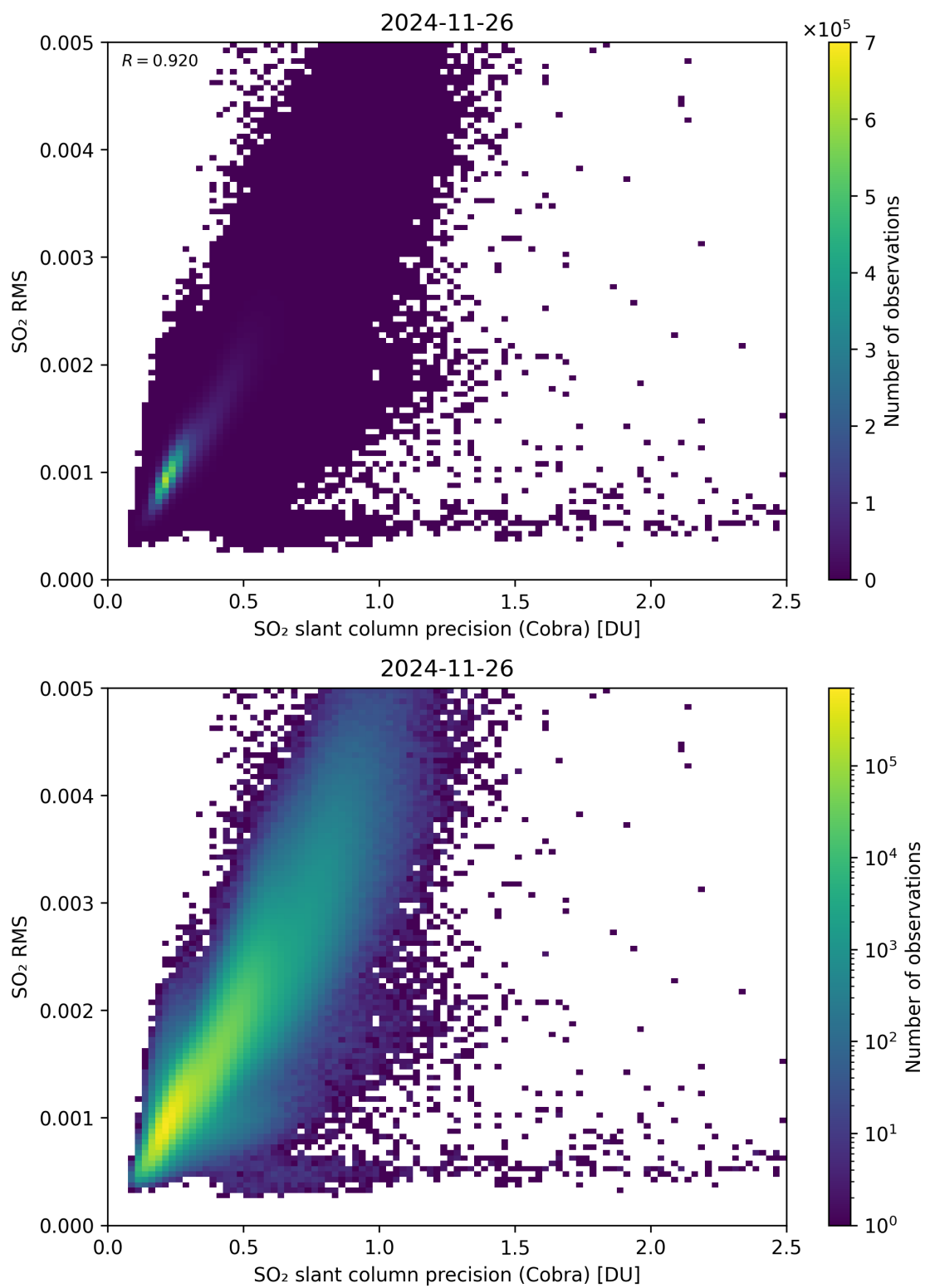
Figure 204: Scatter density plot of “SO 2 slant column precision (Cobra)” against “SO 2 RMS” for 2024-11-25 to 2024-11-27.
