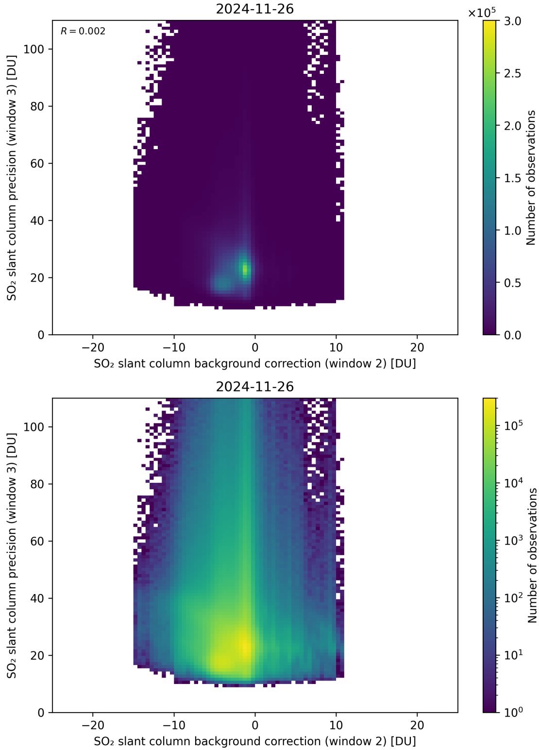
Figure 129: Scatter density plot of “SO 2 slant column background correction (window 2)” against “SO 2 slant column precision (window 3)” for 2024-11-25 to 2024-11-27.
