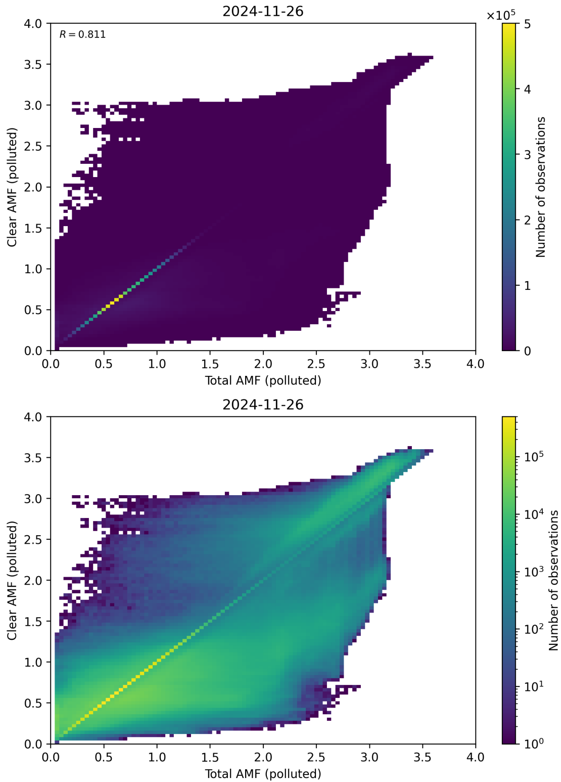
Figure 321: Scatter density plot of “Total AMF (polluted)” against “Clear AMF (polluted)” for 2024-11-25 to 2024-11-27.
