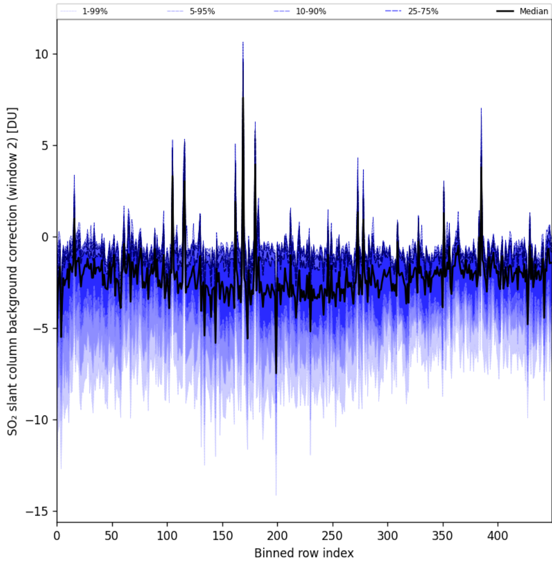
Figure 96: Along track statistics of “SO 2 slant column background correction (window 2)” for 2024-11-25 to 2024-11-27
