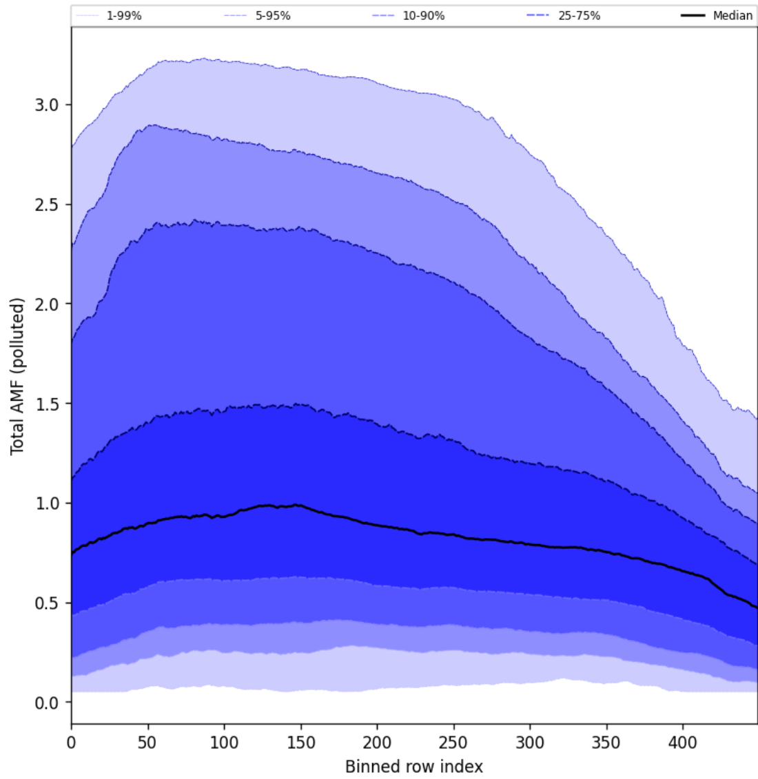
Figure 105: Along track statistics of “Total AMF (polluted)” for 2024-11-25 to 2024-11-27
