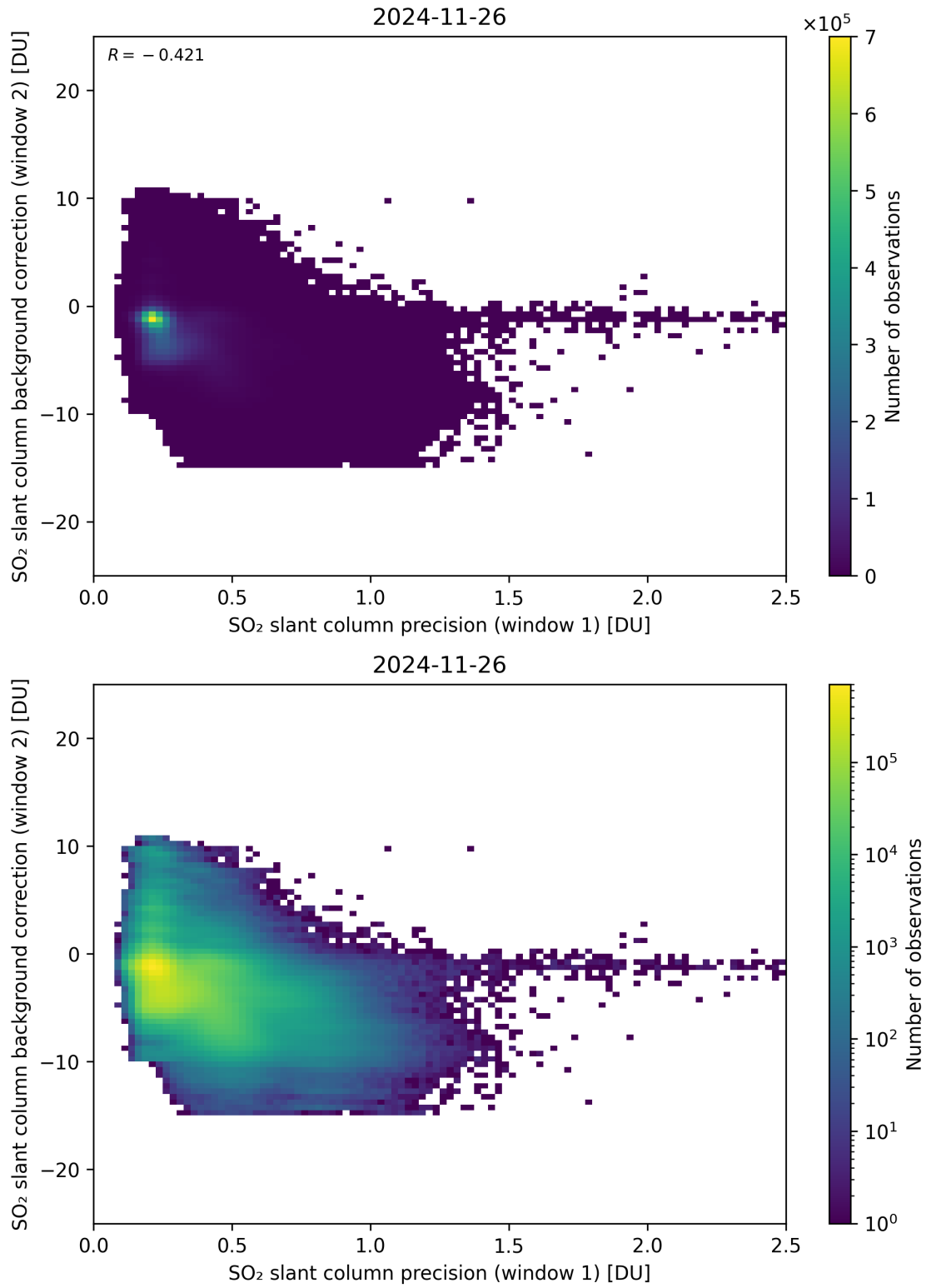
Figure 269: Scatter density plot of “SO 2 slant column precision (window 1)” against “SO 2 slant column background correction (window 2)” for 2024-11-25 to 2024-11-27.
