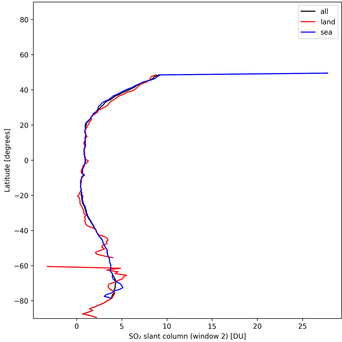
Figure 41: Zonal average of “SO 2 slant column (window 2)” for 2024-11-25 to 2024-11-27.
