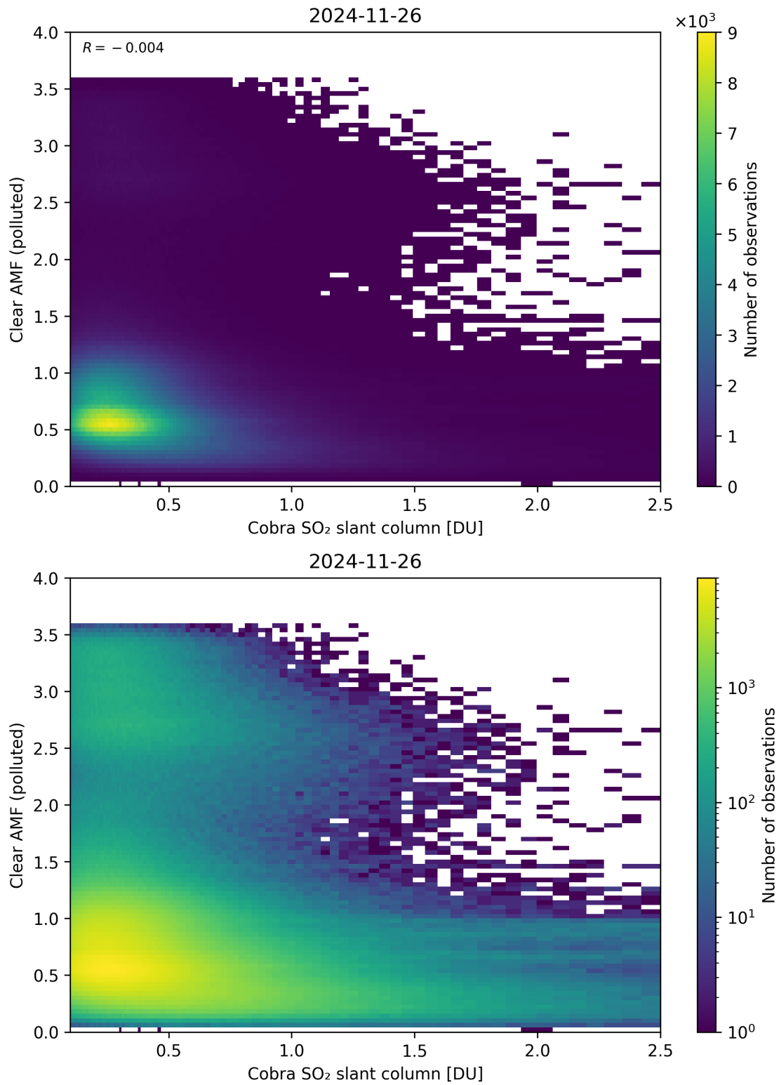
Figure 215: Scatter density plot of “Cobra SO 2 slant column” against “Clear AMF (polluted)” for 2024-11-25 to 2024-11-27.
