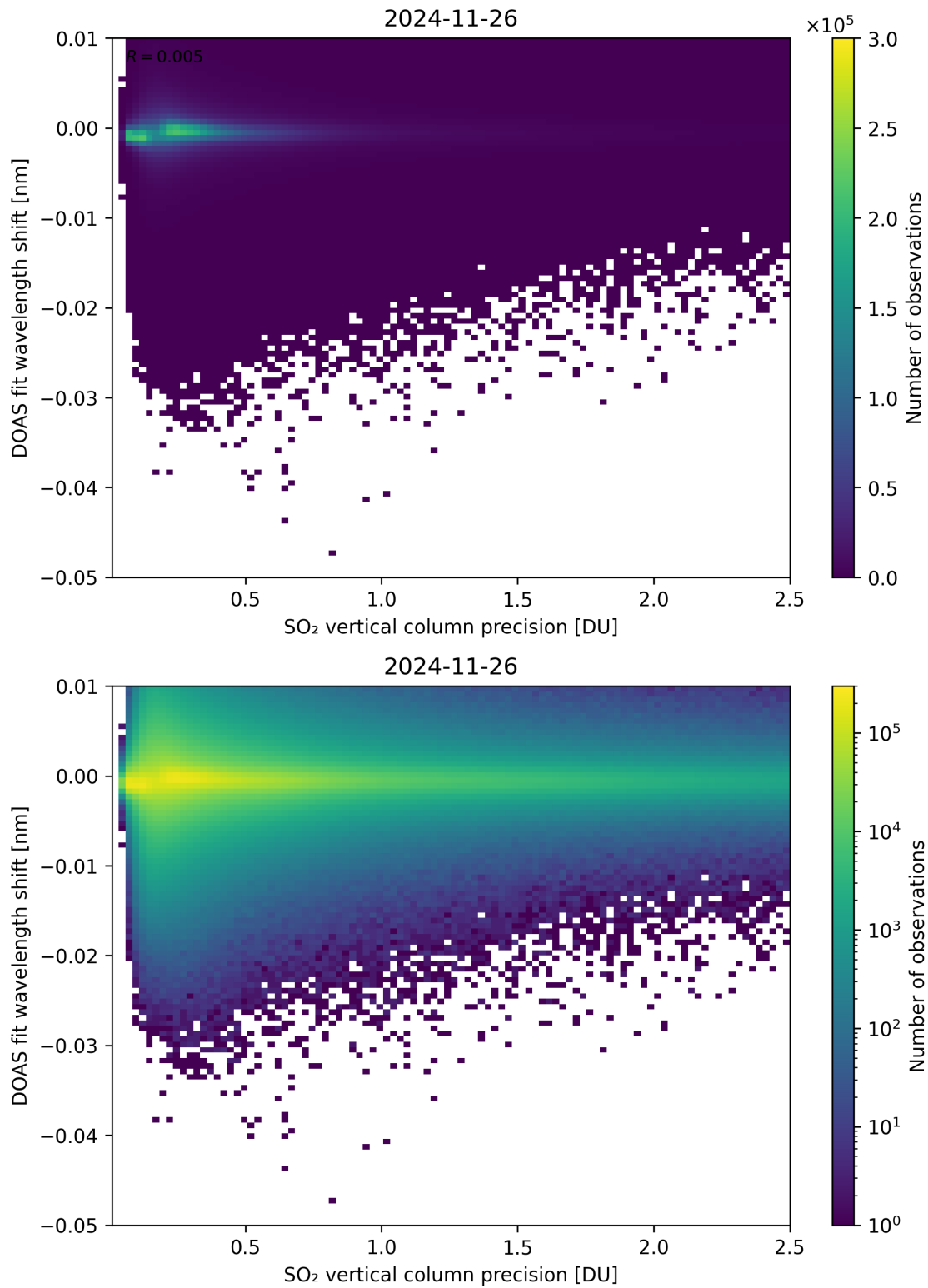
Figure 332: Scatter density plot of “SO 2 vertical column precision” against “DOAS fit wavelength shift” for 2024-11-25 to 2024-11-27.
