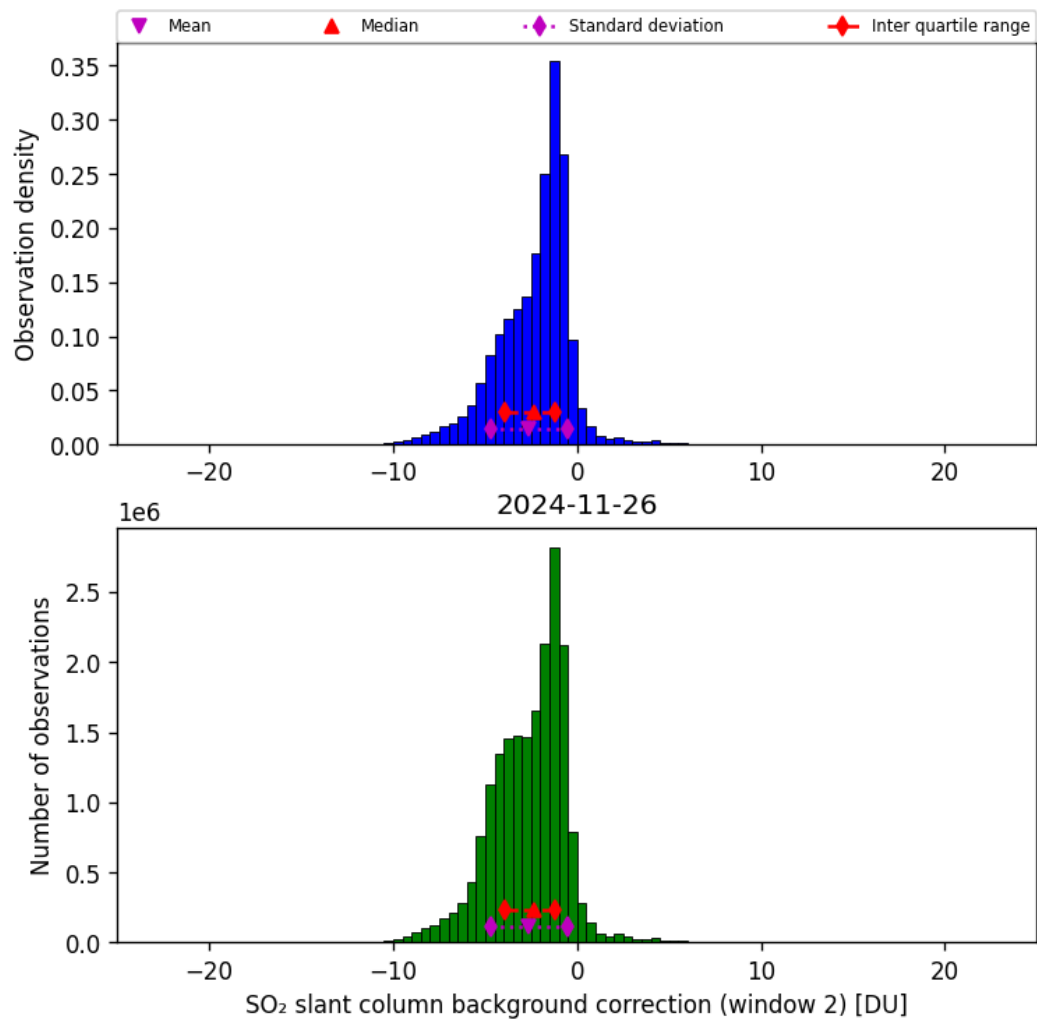
Figure 70: Histogram of “SO 2 slant column background correction (window 2)” for 2024-11-25 to 2024-11-27
