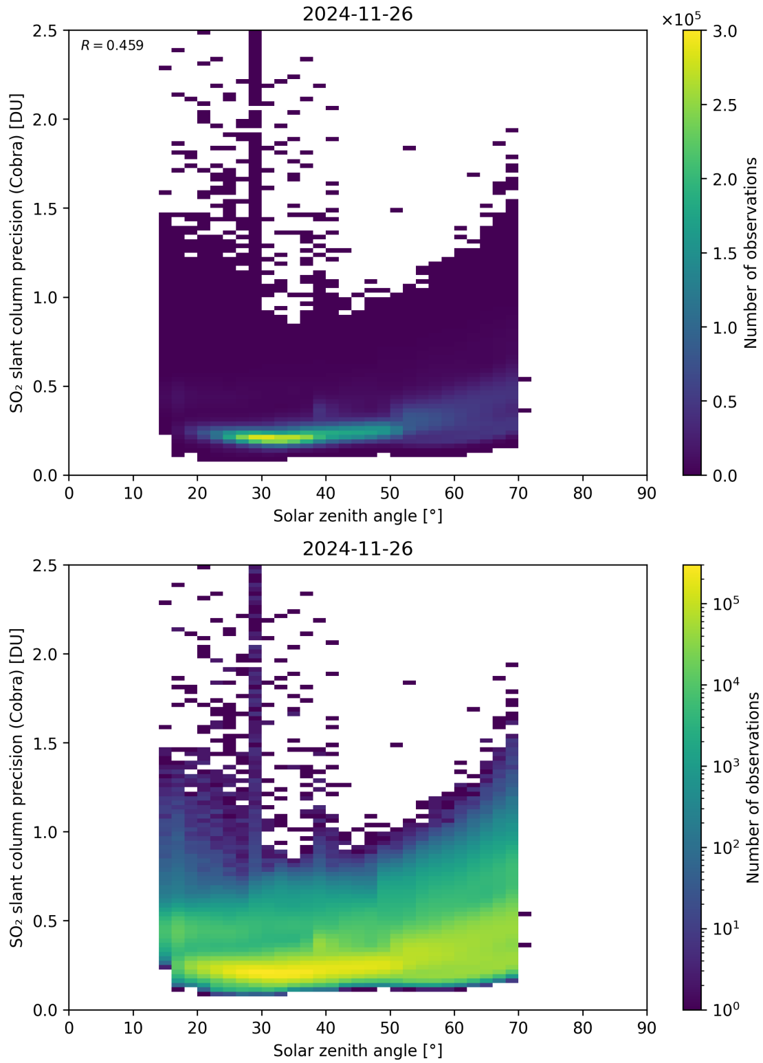
Figure 180: Scatter density plot of “Solar zenith angle” against “SO 2 slant column precision (Cobra)” for 2024-11-25 to 2024-11-27.
