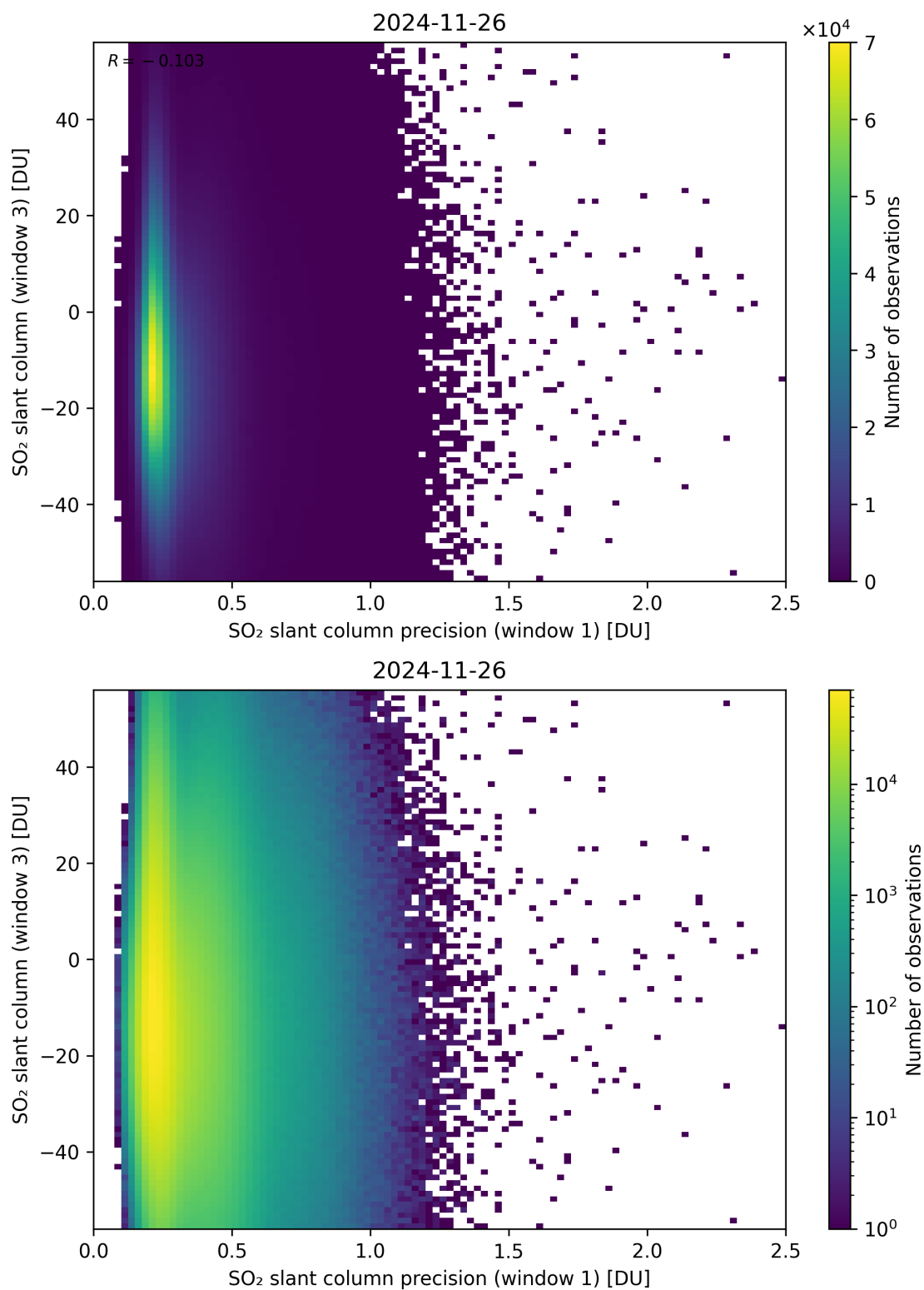
Figure 278: Scatter density plot of “SO 2 slant column precision (window 1)” against “SO 2 slant column (window 3)” for 2024-11-25 to 2024-11-27.
