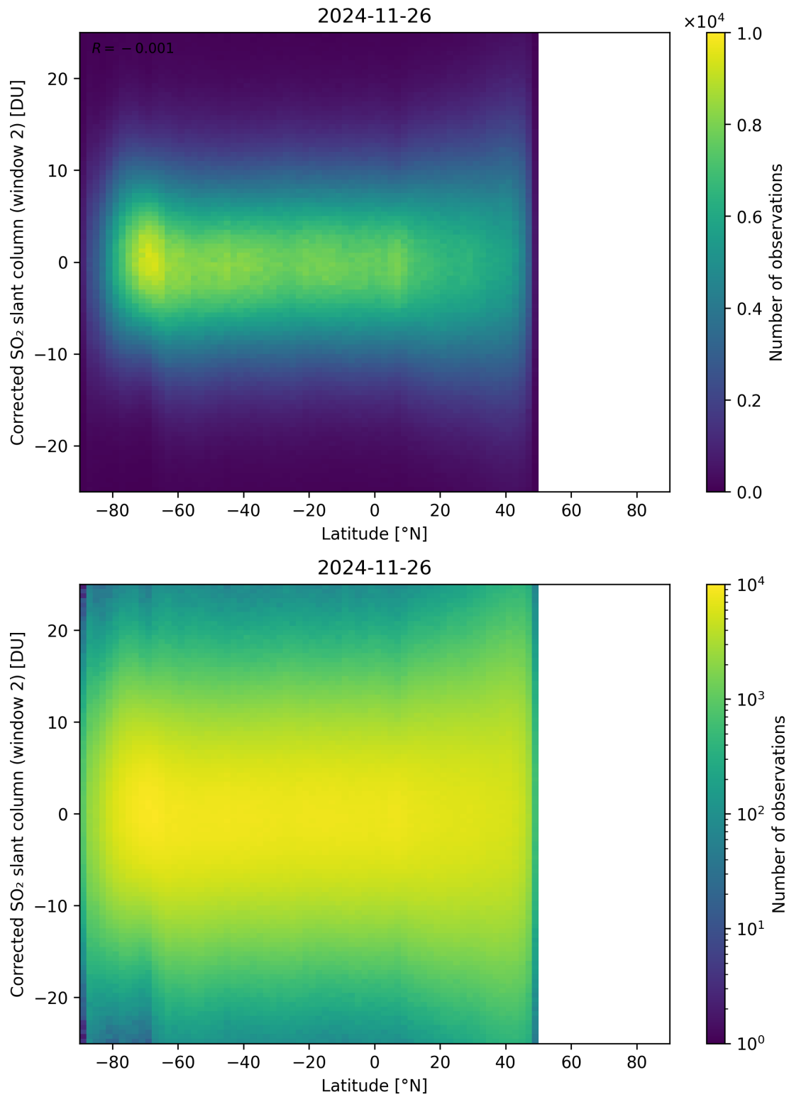
Figure 160: Scatter density plot of “Latitude” against “Corrected SO 2 slant column (window 2)” for 2024-11-25 to 2024-11-27.
