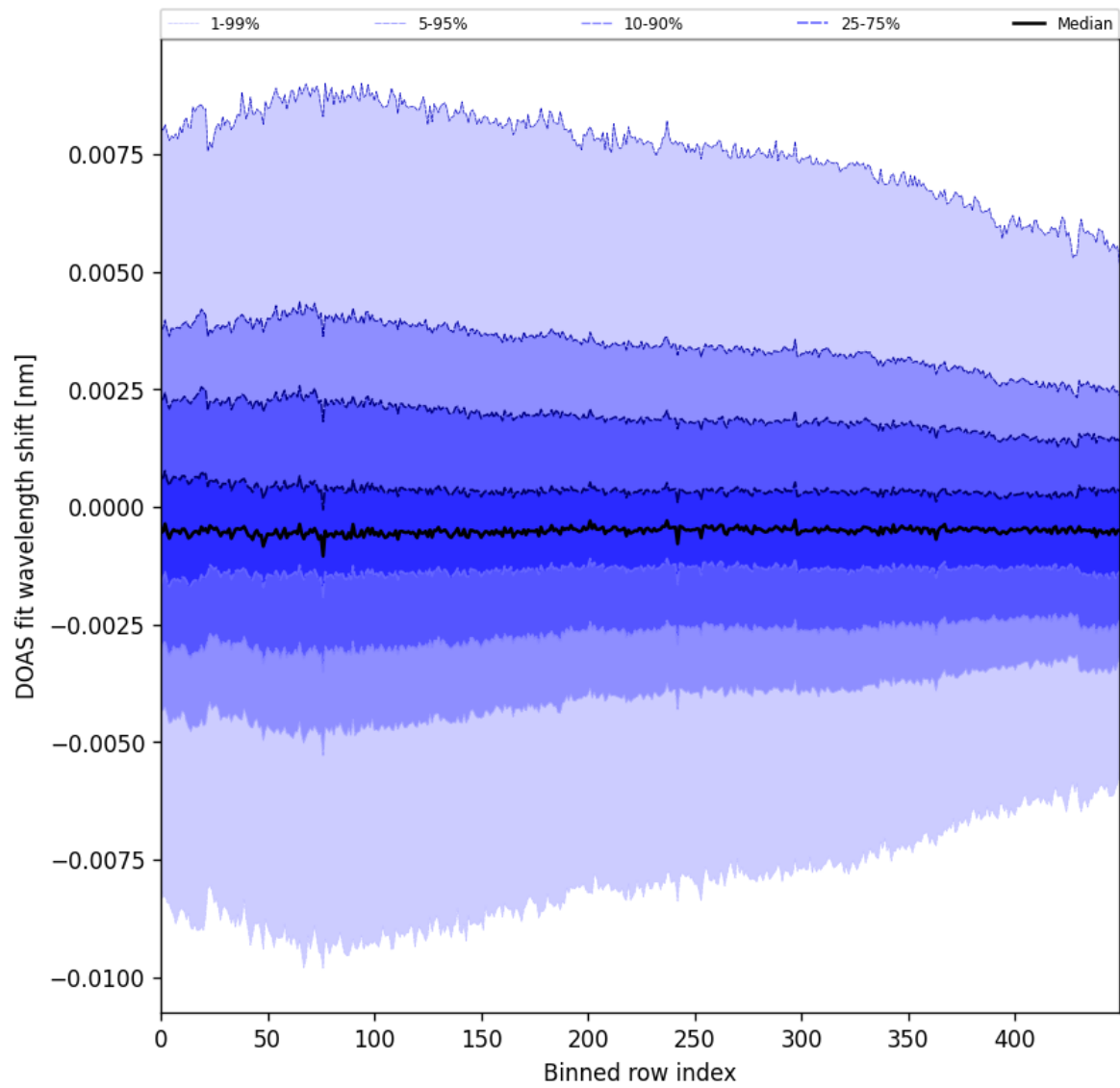
Figure 102: Along track statistics of “DOAS fit wavelength shift” for 2024-11-25 to 2024-11-27
