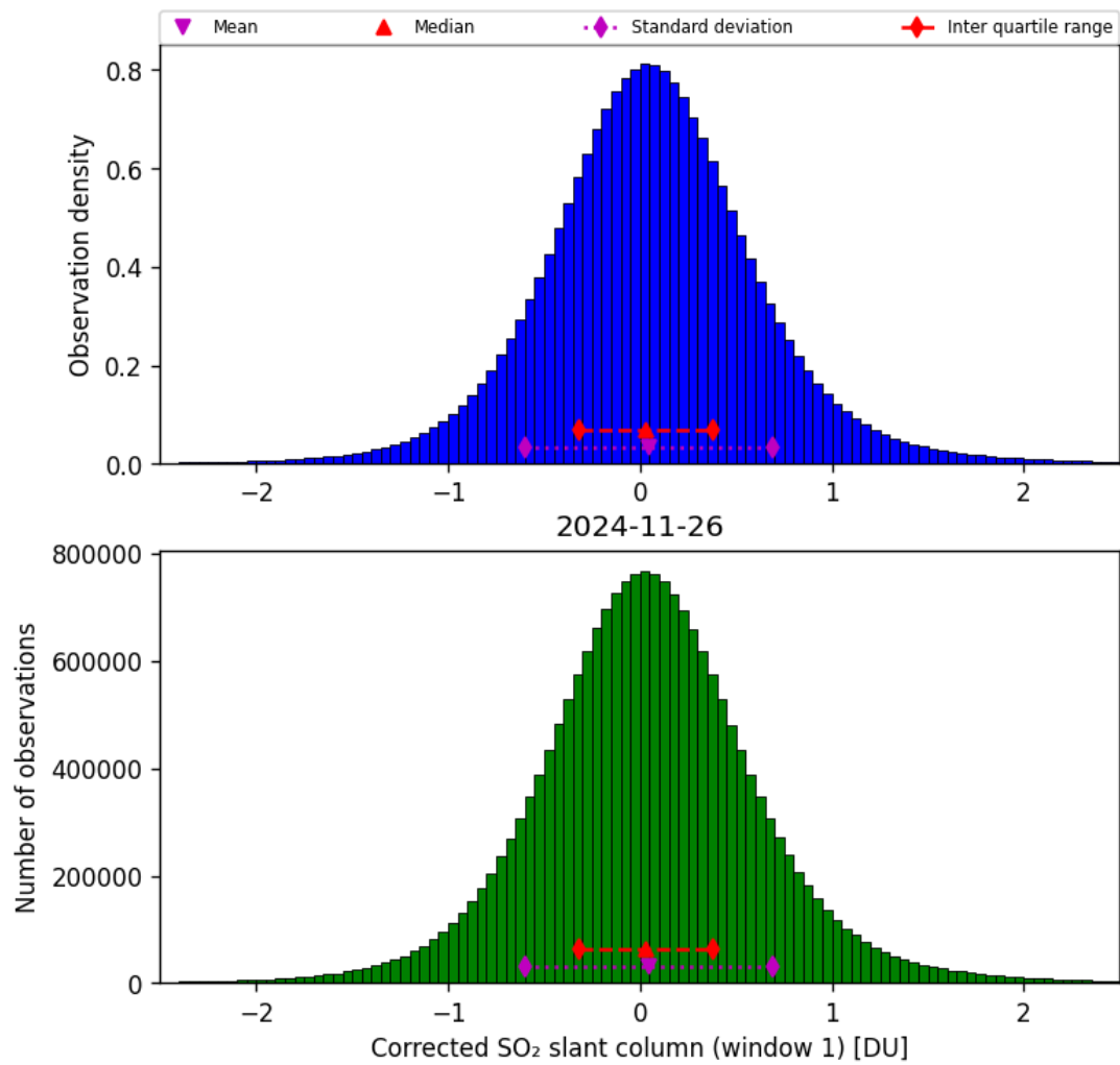
Figure 65: Histogram of “Corrected SO 2 slant column (window 1)” for 2024-11-25 to 2024-11-27
