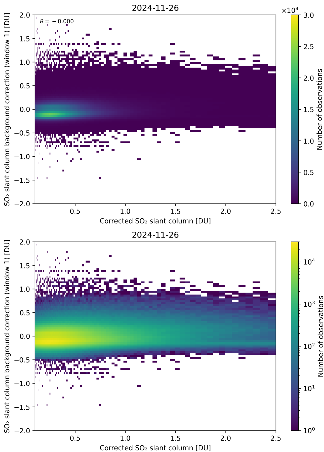
Figure 226: Scatter density plot of “Corrected SO 2 slant column” against “SO 2 slant column background correction (window 1)” for 2024-11-25 to 2024-11-27.
