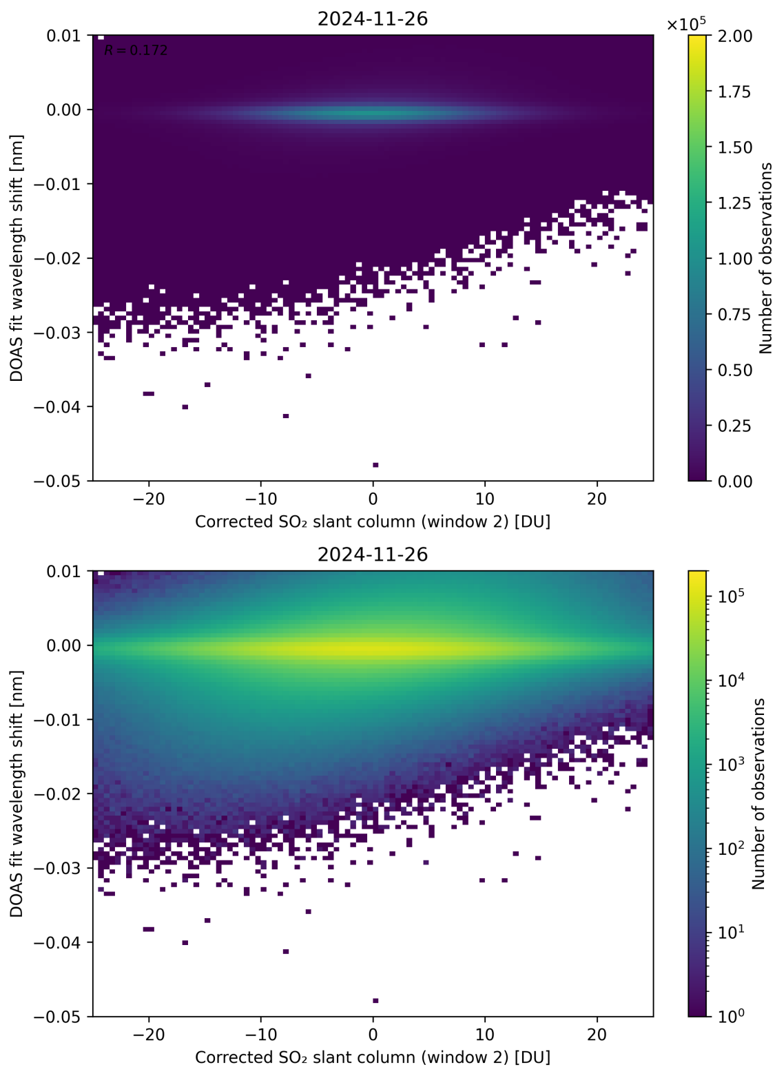
Figure 246: Scatter density plot of “Corrected SO 2 slant column (window 2)” against “DOAS fit wavelength shift” for 2024-11-25 to 2024-11-27.
