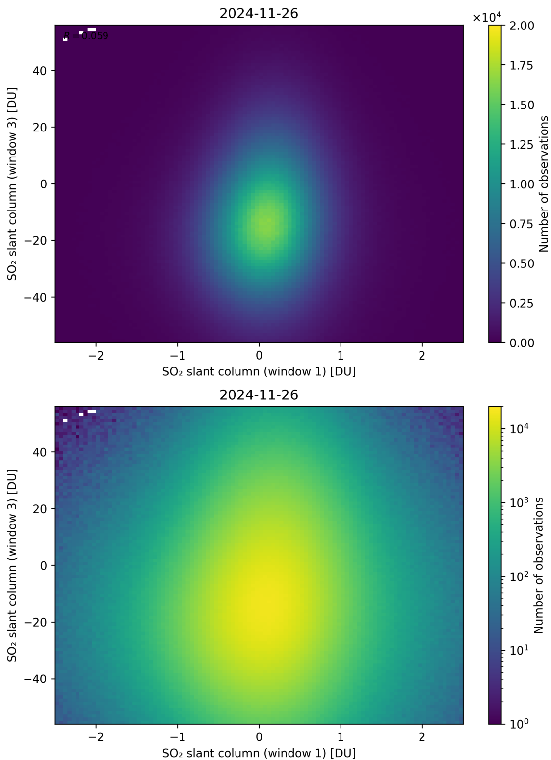
Figure 287: Scatter density plot of “SO 2 slant column (window 1)” against “SO 2 slant column (window 3)” for 2024-11-25 to 2024-11-27.
