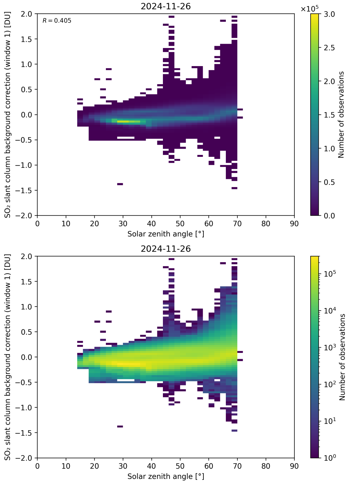
Figure 171: Scatter density plot of “Solar zenith angle” against “SO 2 slant column background correction (window 1)” for 2024-11-25 to 2024-11-27.
