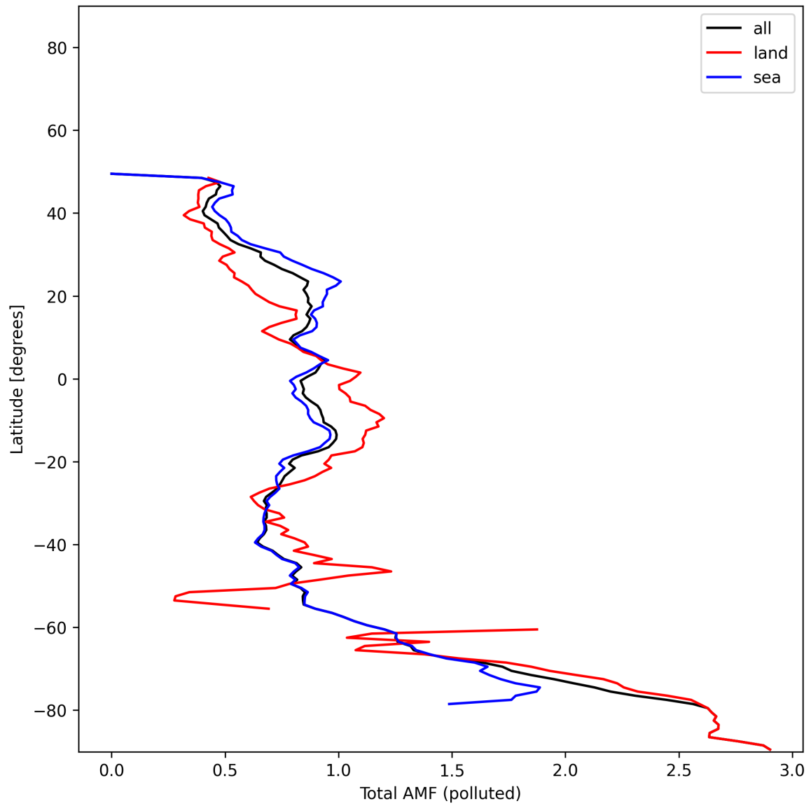
Figure 53: Zonal average of “Total AMF (polluted)” for 2024-11-25 to 2024-11-27.
