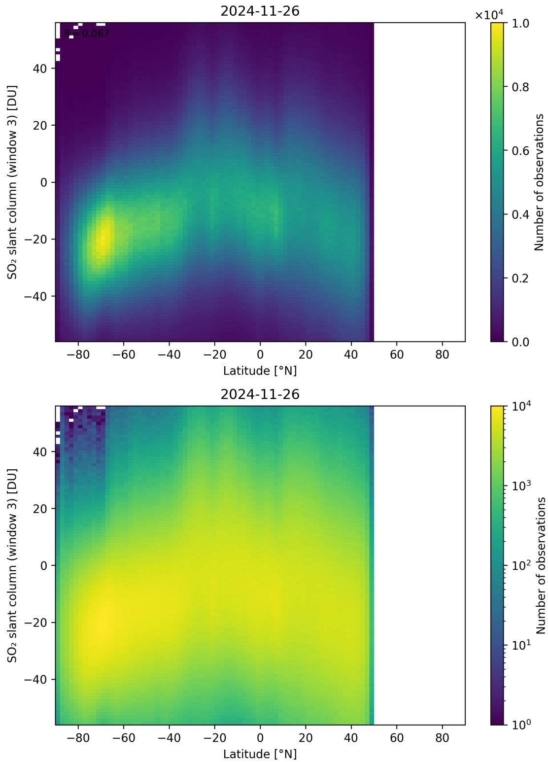
Figure 165: Scatter density plot of “Latitude” against “SO 2 slant column (window 3)” for 2024-11-25 to 2024-11-27.
