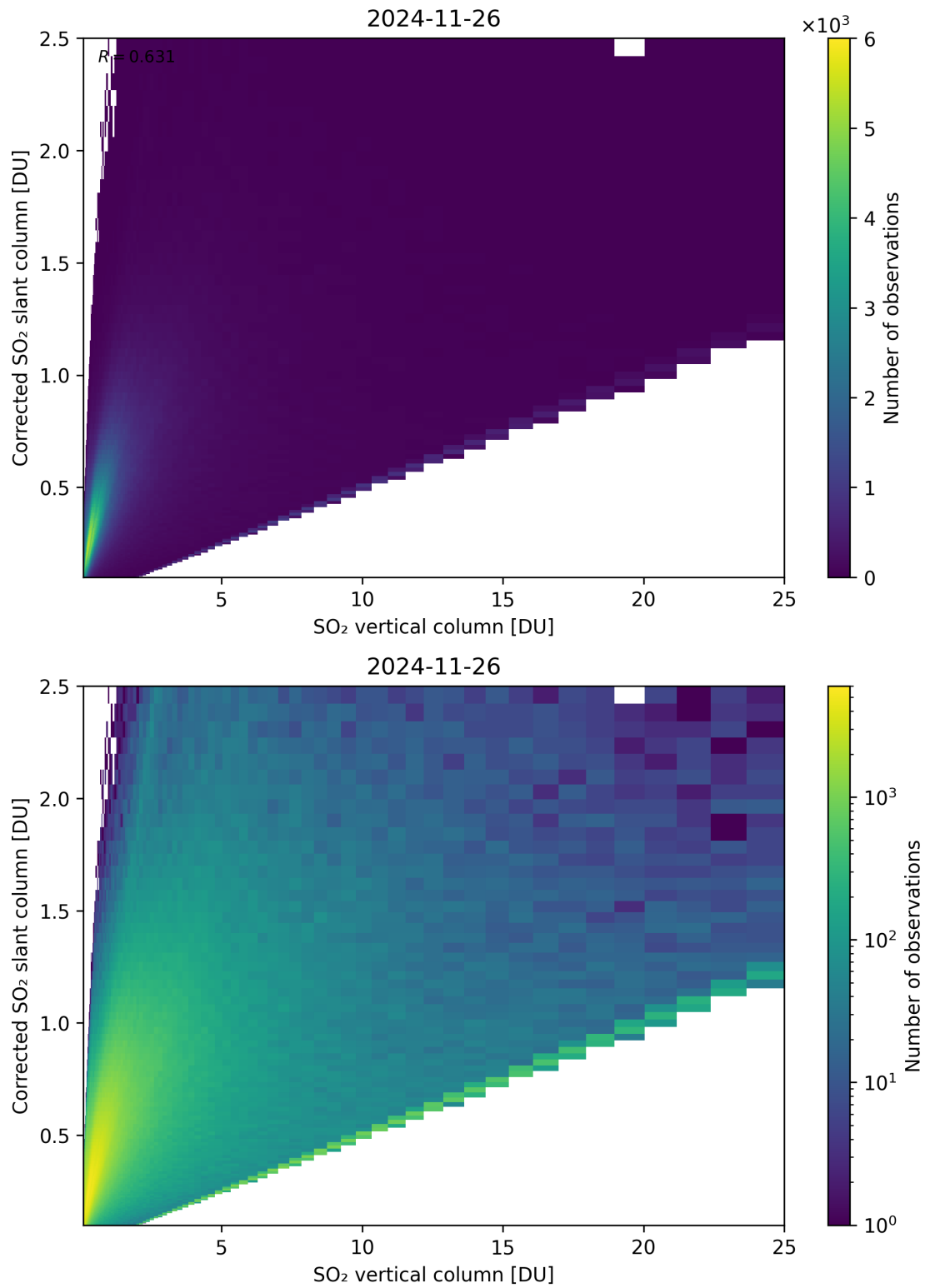
Figure 351: Scatter density plot of “SO 2 vertical column” against “Corrected SO 2 slant column” for 2024-11-25 to 2024-11-27.
