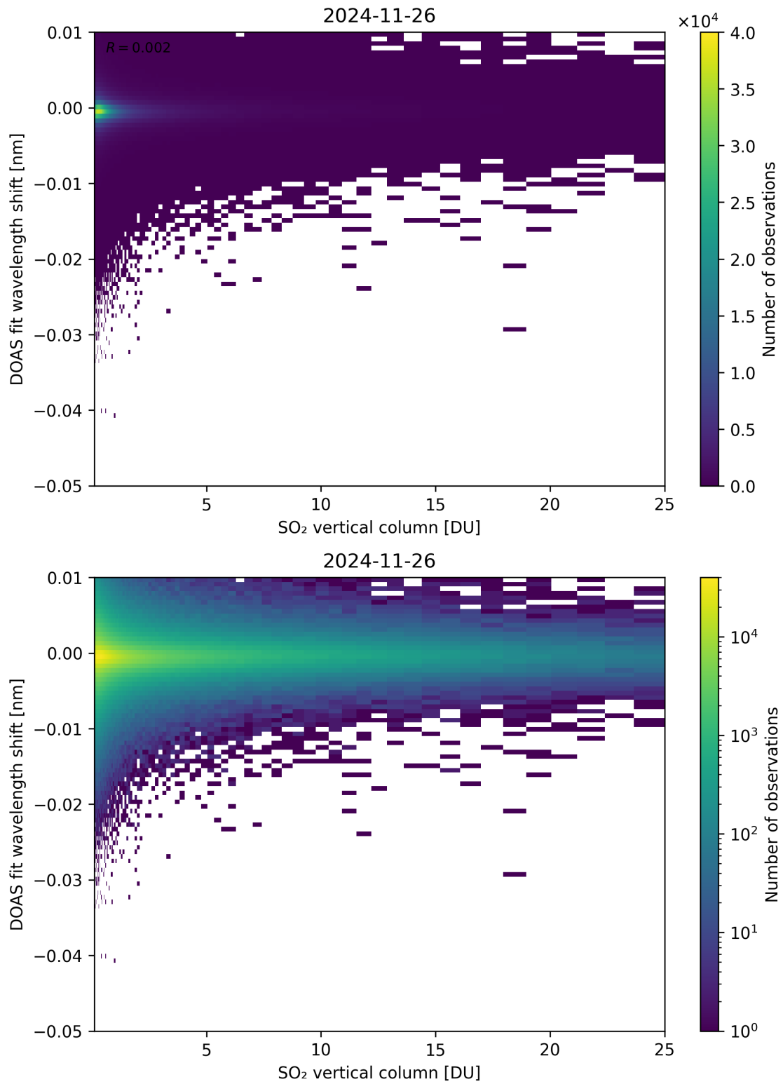
Figure 326: Scatter density plot of “SO 2 vertical column” against “DOAS fit wavelength shift” for 2024-11-25 to 2024-11-27.
