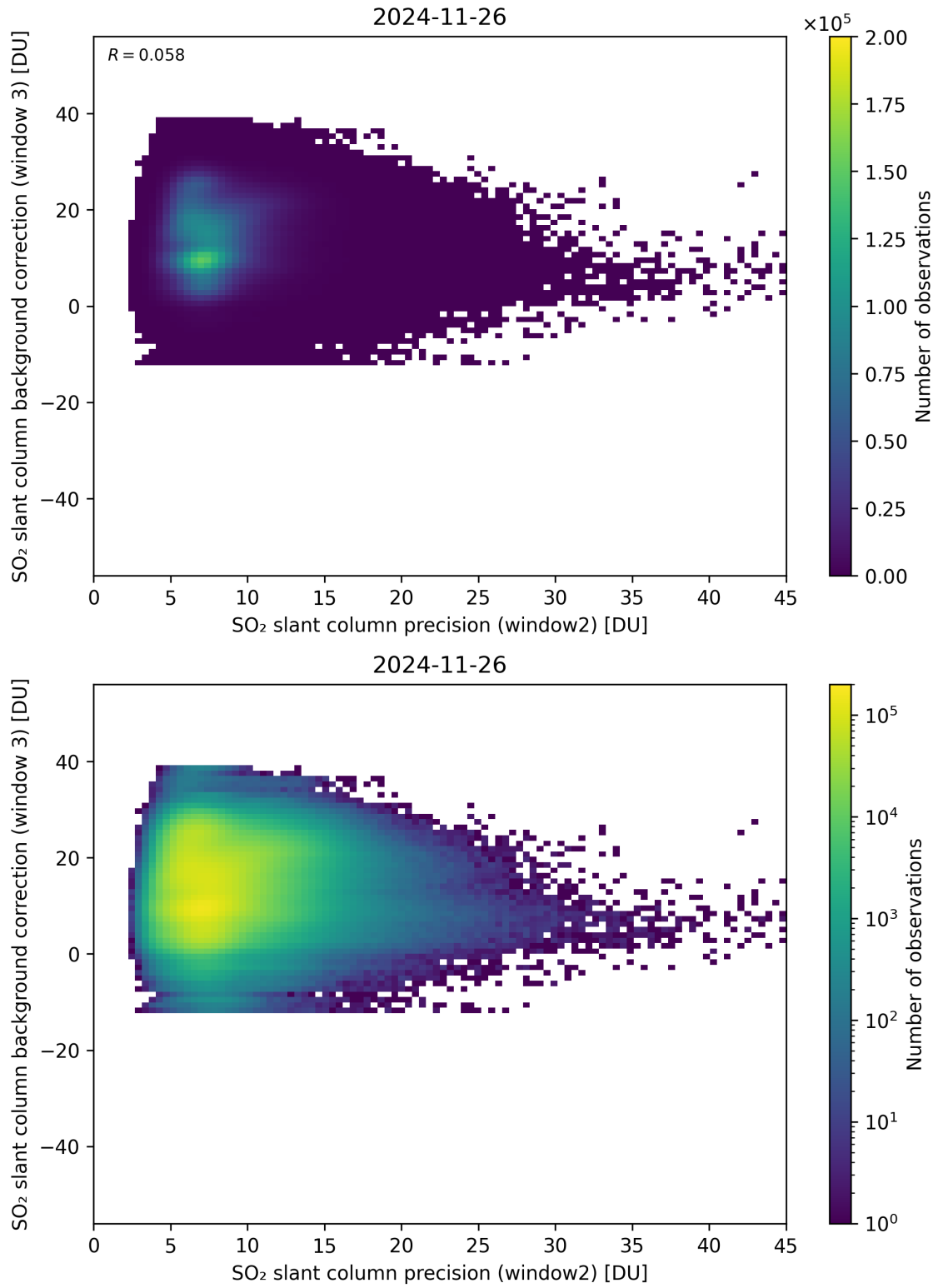
Figure 292: Scatter density plot of “SO 2 slant column precision (window2)” against “SO 2 slant column background correction (window 3)” for 2024-11-25 to 2024-11-27.
