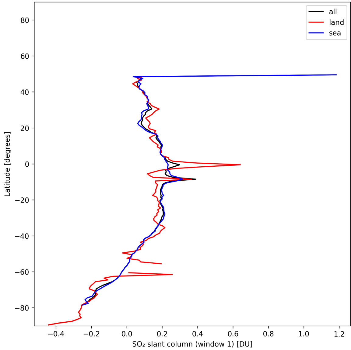
Figure 37: Zonal average of “SO 2 slant column (window 1)” for 2024-11-25 to 2024-11-27.
