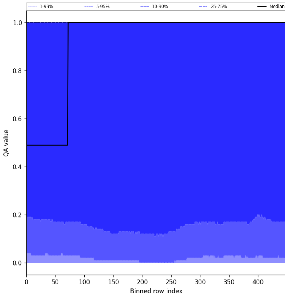
Figure 83: Along track statistics of “QA value” for 2024-11-25 to 2024-11-27
