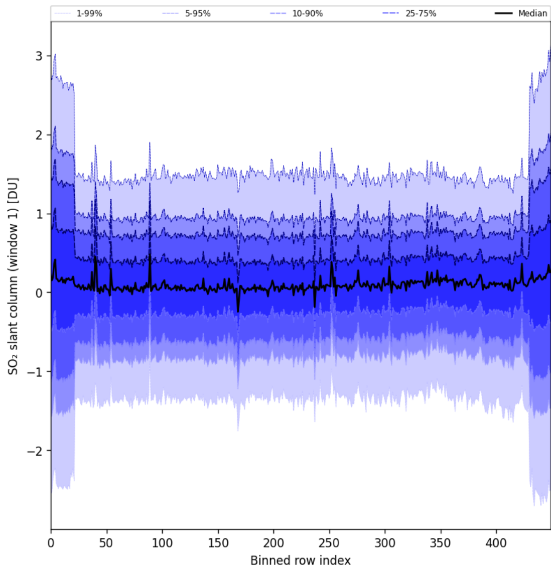
Figure 89: Along track statistics of “SO 2 slant column (window 1)” for 2024-11-25 to 2024-11-27
