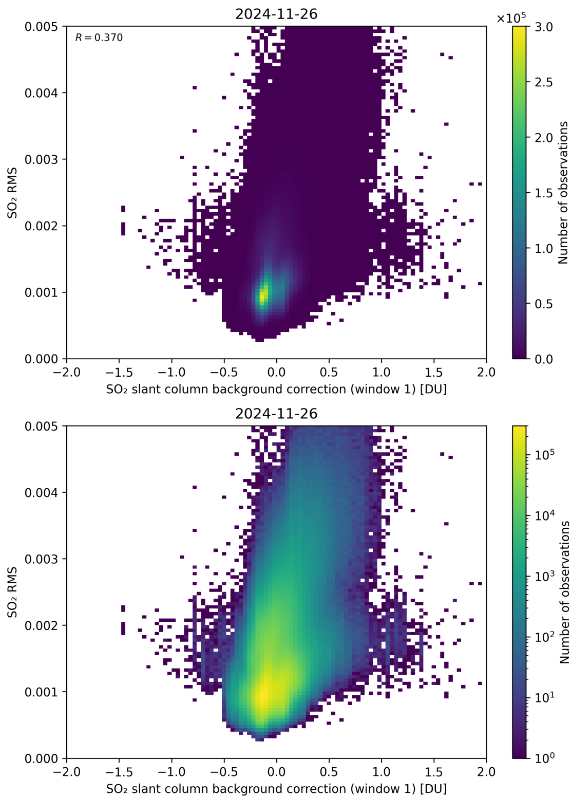
Figure 113: Scatter density plot of “SO 2 slant column background correction (window 1)” against “SO 2 RMS” for 2024-11-25 to 2024-11-27.
