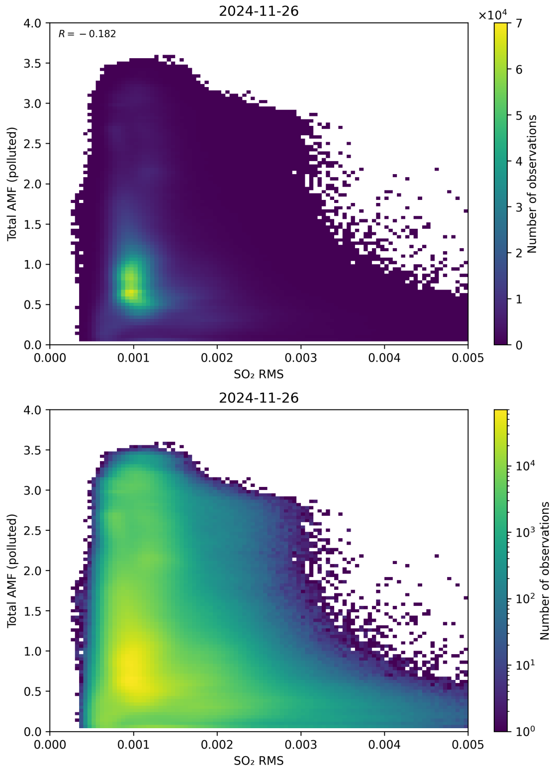
Figure 148: Scatter density plot of “SO 2 RMS” against “Total AMF (polluted)” for 2024-11-25 to 2024-11-27.
