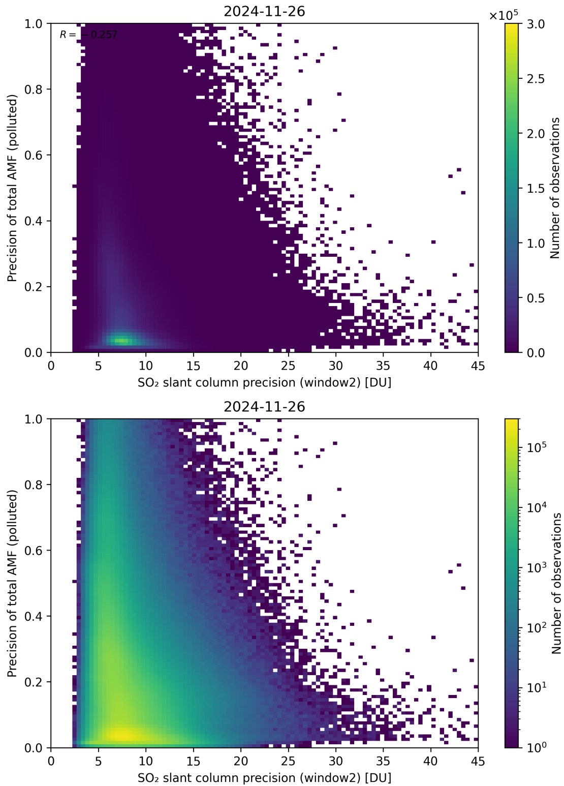
Figure 302: Scatter density plot of “SO 2 slant column precision (window2)” against “Precision of total AMF (polluted)” for 2024-11-25 to 2024-11-27.
