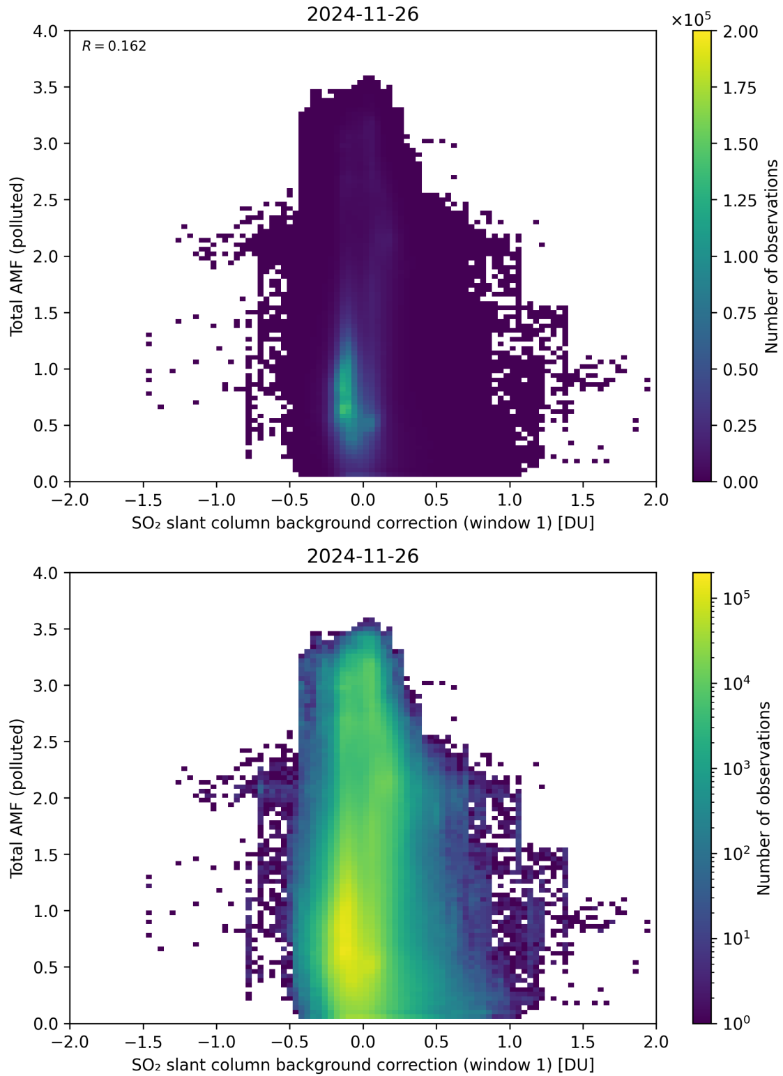
Figure 120: Scatter density plot of “SO 2 slant column background correction (window 1)” against “Total AMF (polluted)” for 2024-11-25 to 2024-11-27.
