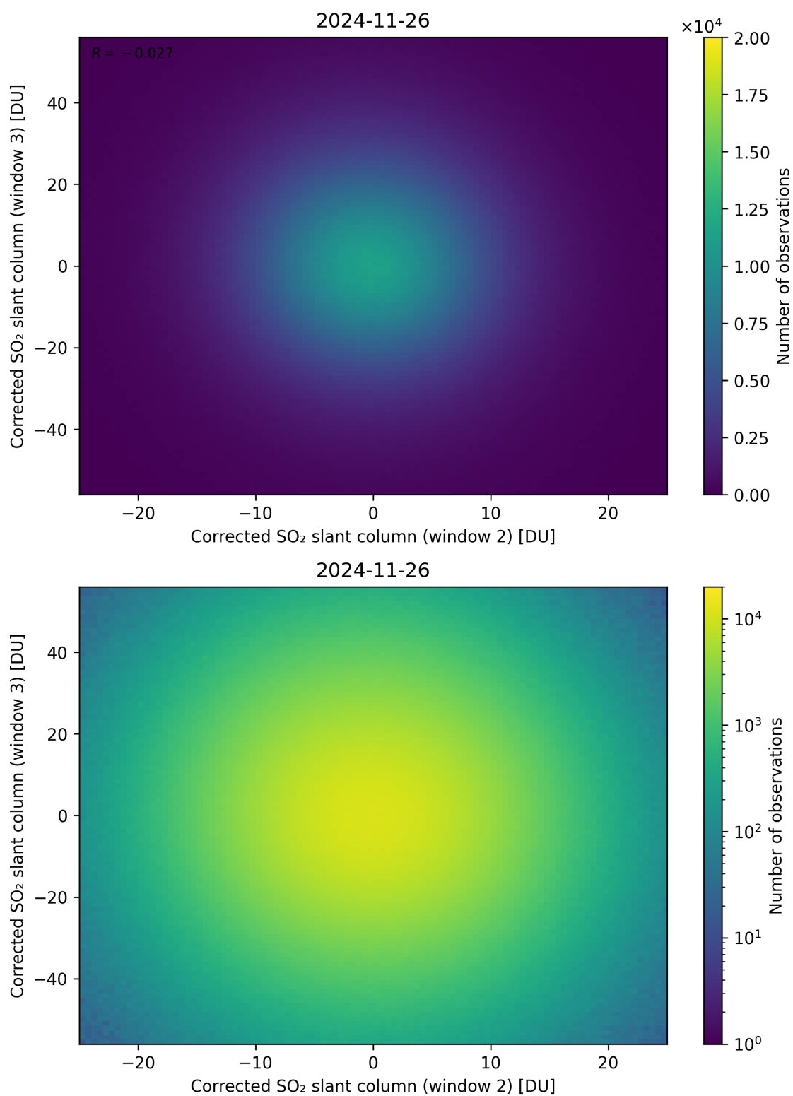
Figure 250: Scatter density plot of “Corrected SO 2 slant column (window 2)” against “Corrected SO 2 slant column (window 3)” for 2024-11-25 to 2024-11-27.
