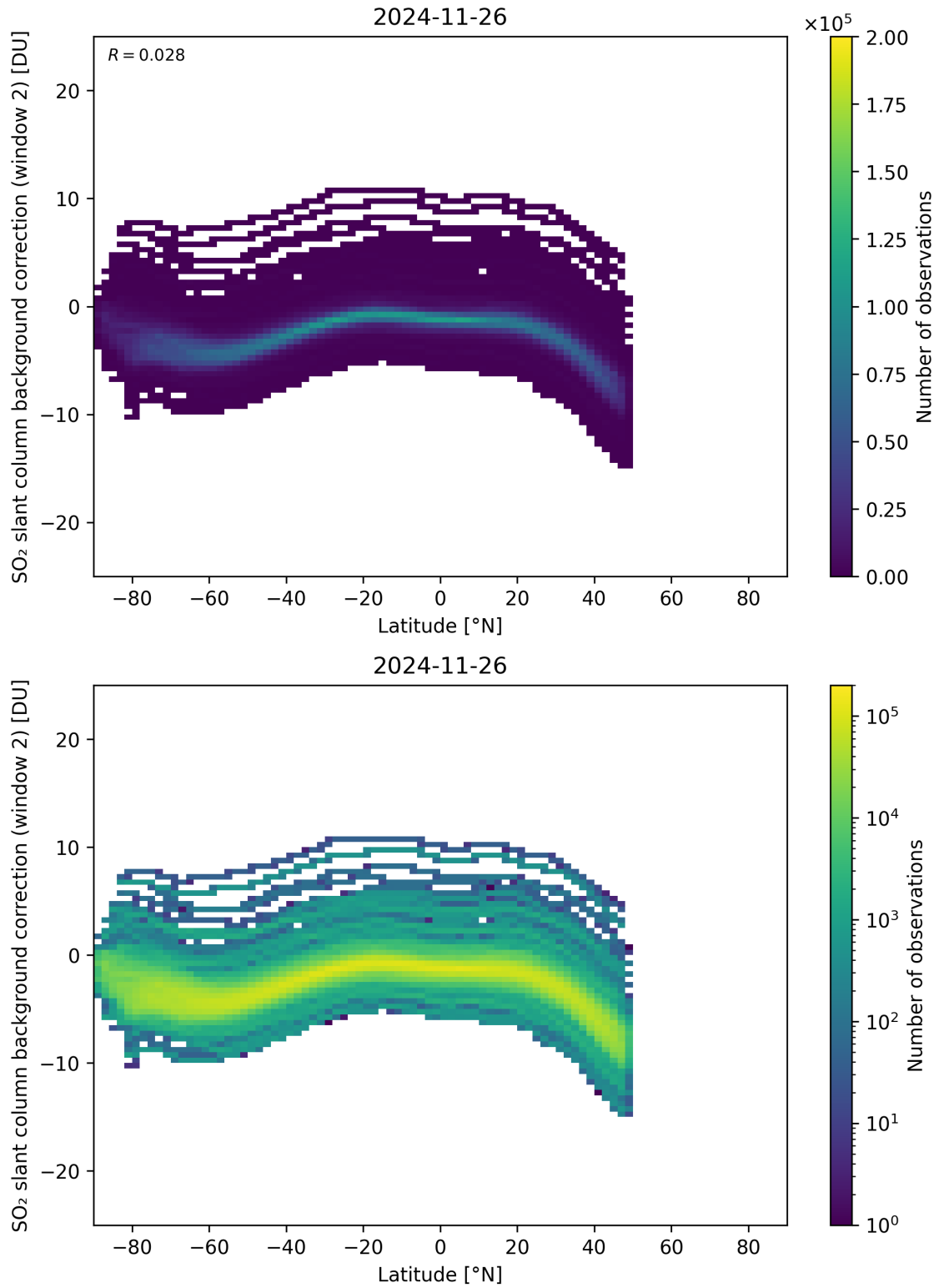
Figure 151: Scatter density plot of “Latitude” against “SO 2 slant column background correction (window 2)” for 2024-11-25 to 2024-11-27.
