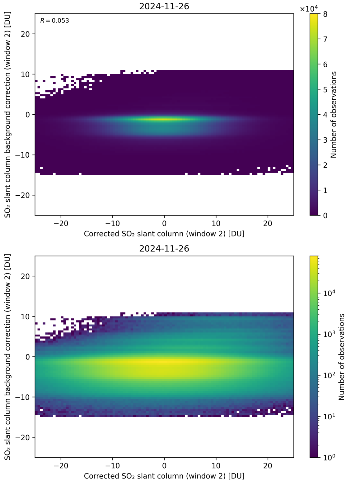
Figure 244: Scatter density plot of “Corrected SO 2 slant column (window 2)” against “SO 2 slant column background correction (window 2)” for 2024-11-25 to 2024-11-27.
