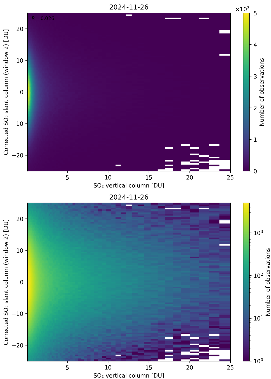
Figure 352: Scatter density plot of “SO 2 vertical column” against “Corrected SO 2 slant column (window 2)” for 2024-11-25 to 2024-11-27.
