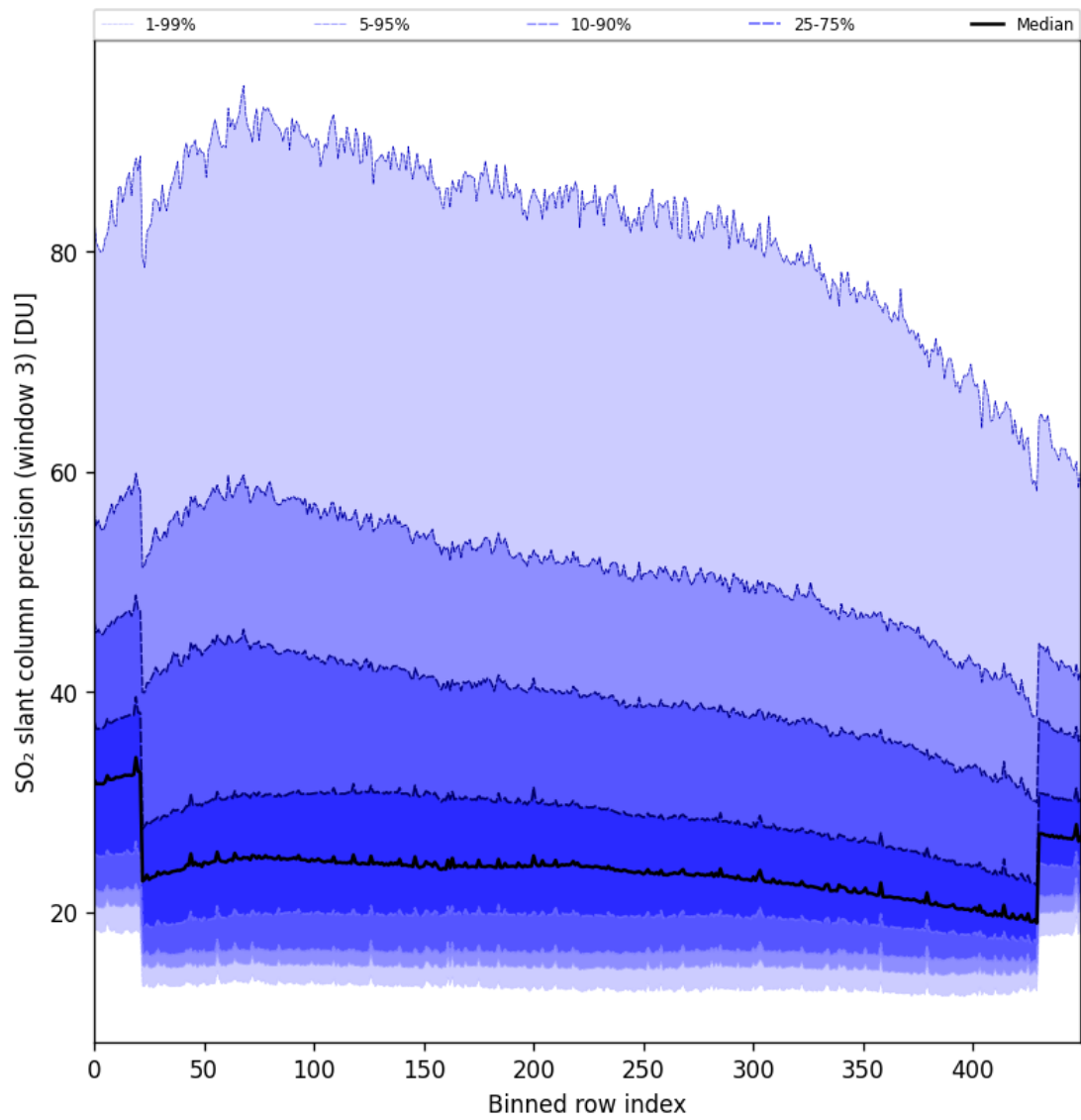
Figure 98: Along track statistics of “SO 2 slant column precision (window 3)” for 2024-11-25 to 2024-11-27
