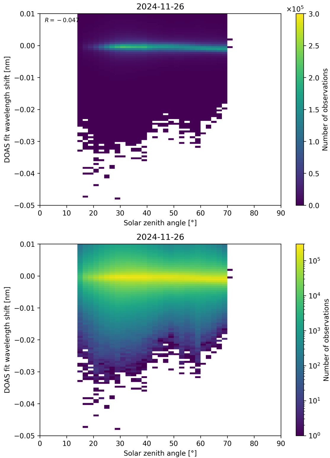
Figure 174: Scatter density plot of “Solar zenith angle” against “DOAS fit wavelength shift” for 2024-11-25 to 2024-11-27.
