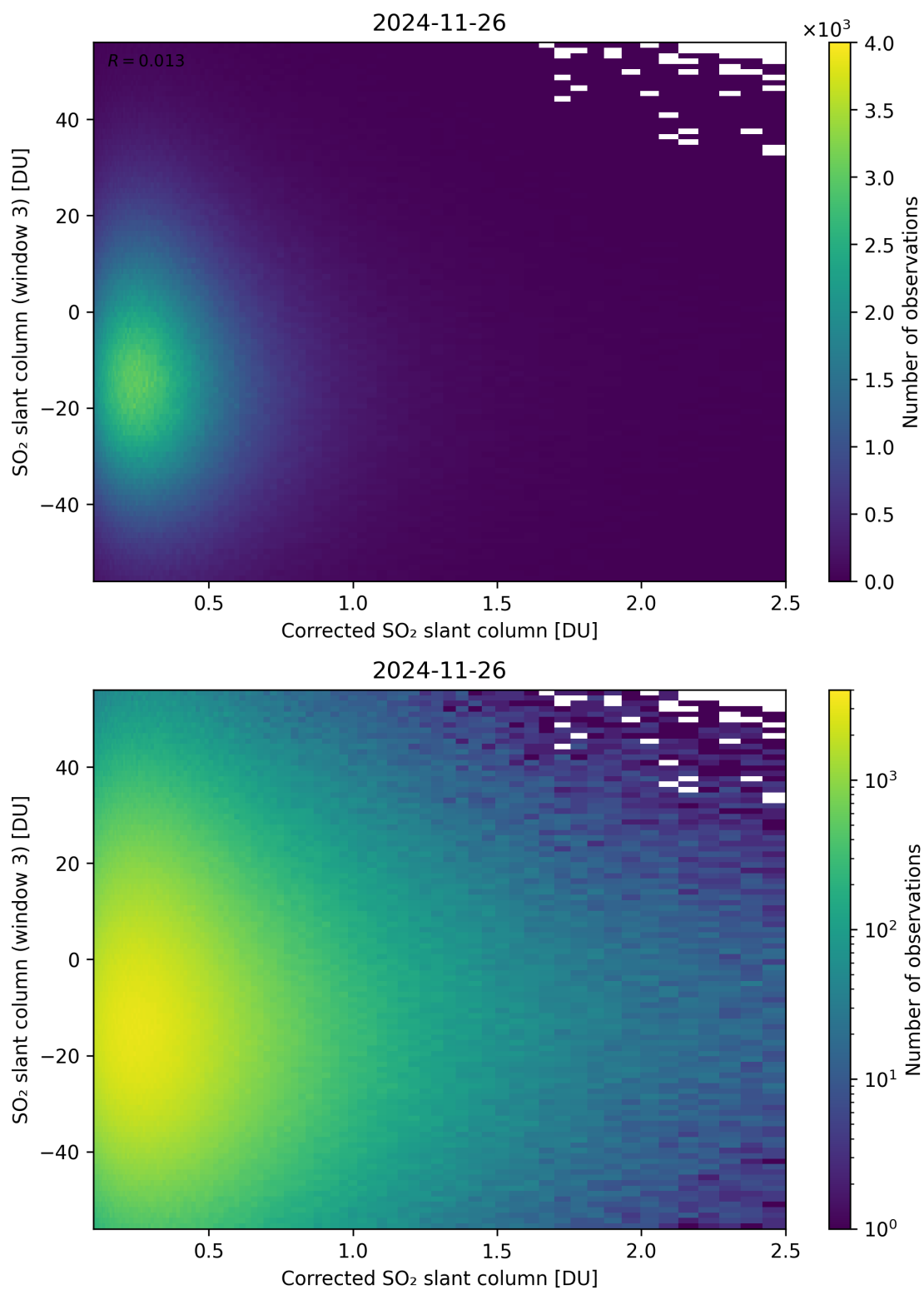
Figure 240: Scatter density plot of “Corrected SO 2 slant column” against “SO 2 slant column (window 3)” for 2024-11-25 to 2024-11-27.
