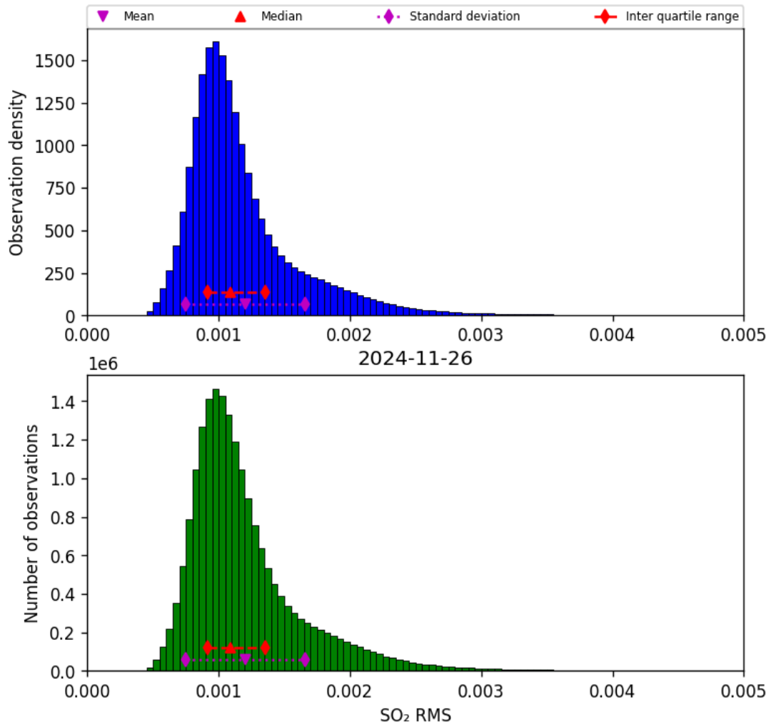
Figure 78: Histogram of “SO 2 RMS” for 2024-11-25 to 2024-11-27
