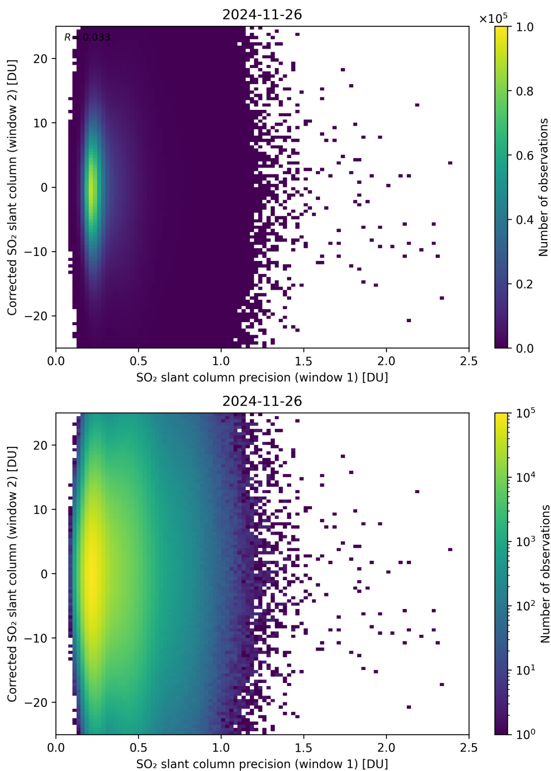
Figure 275: Scatter density plot of “SO 2 slant column precision (window 1)” against “Corrected SO 2 slant column (window 2)” for 2024-11-25 to 2024-11-27.
