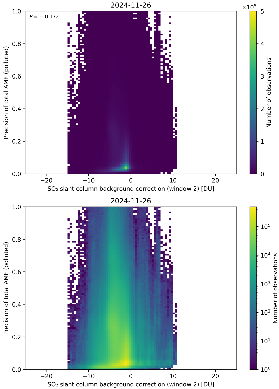
Figure 131: Scatter density plot of “SO 2 slant column background correction (window 2)” against “Precision of total AMF (polluted)” for 2024-11-25 to 2024-11-27.
