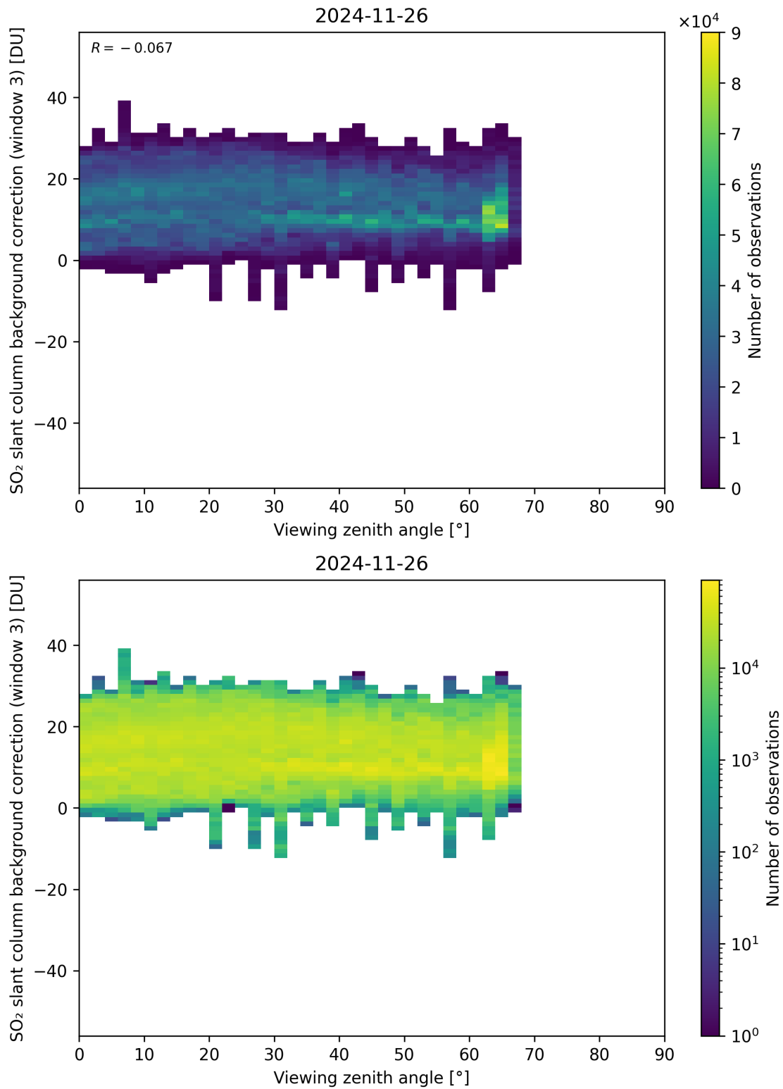
Figure 364: Scatter density plot of “Viewing zenith angle” against “SO 2 slant column background correction (window 3)” for 2024-11-25 to 2024-11-27.
