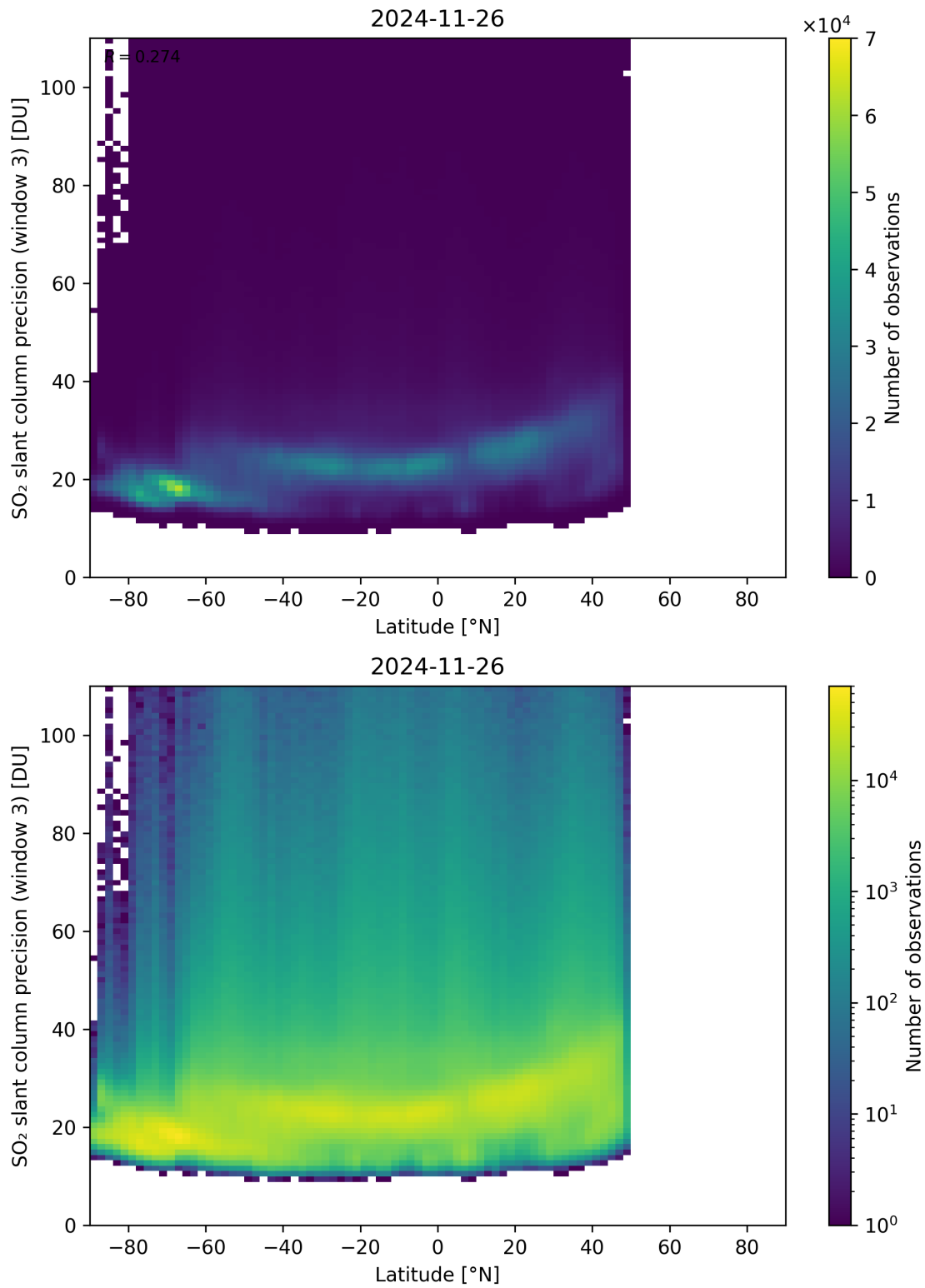
Figure 166: Scatter density plot of “Latitude” against “SO 2 slant column precision (window 3)” for 2024-11-25 to 2024-11-27.
