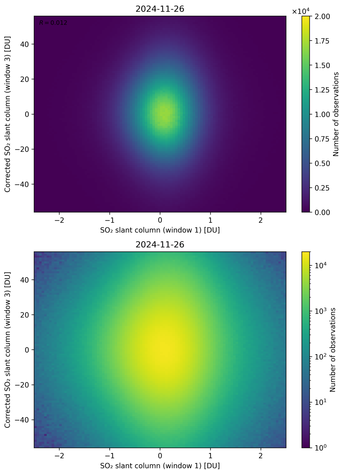
Figure 284: Scatter density plot of “SO 2 slant column (window 1)” against “Corrected SO 2 slant column (window 3)” for 2024-11-25 to 2024-11-27.
