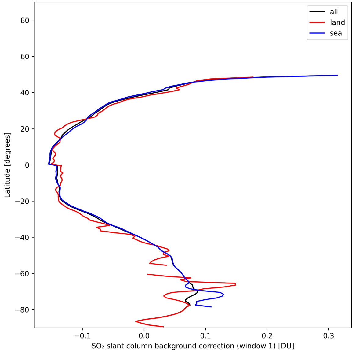
Figure 40: Zonal average of “SO 2 slant column background correction (window 1)” for 2024-11-25 to 2024-11-27.
