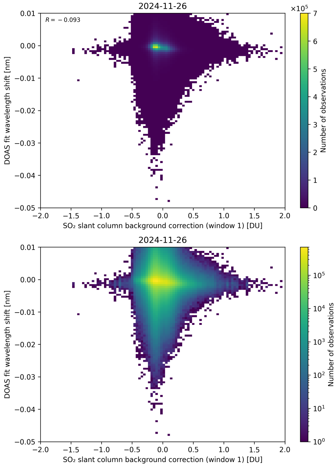
Figure 111: Scatter density plot of “SO 2 slant column background correction (window 1)” against “DOAS fit wavelength shift” for 2024-11-25 to 2024-11-27.
