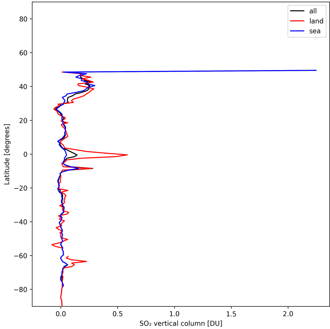
Figure 32: Zonal average of “SO 2 vertical column” for 2024-11-25 to 2024-11-27.
