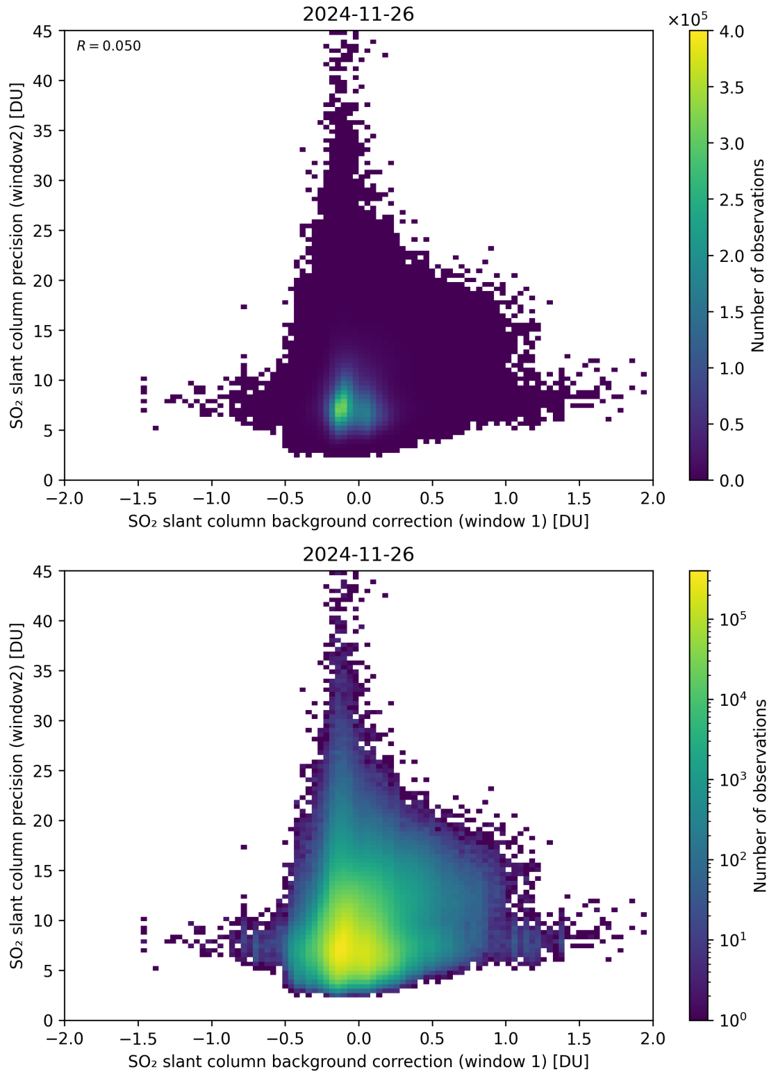
Figure 117: Scatter density plot of “SO 2 slant column background correction (window 1)” against “SO 2 slant column precision (window2)” for 2024-11-25 to 2024-11-27.
