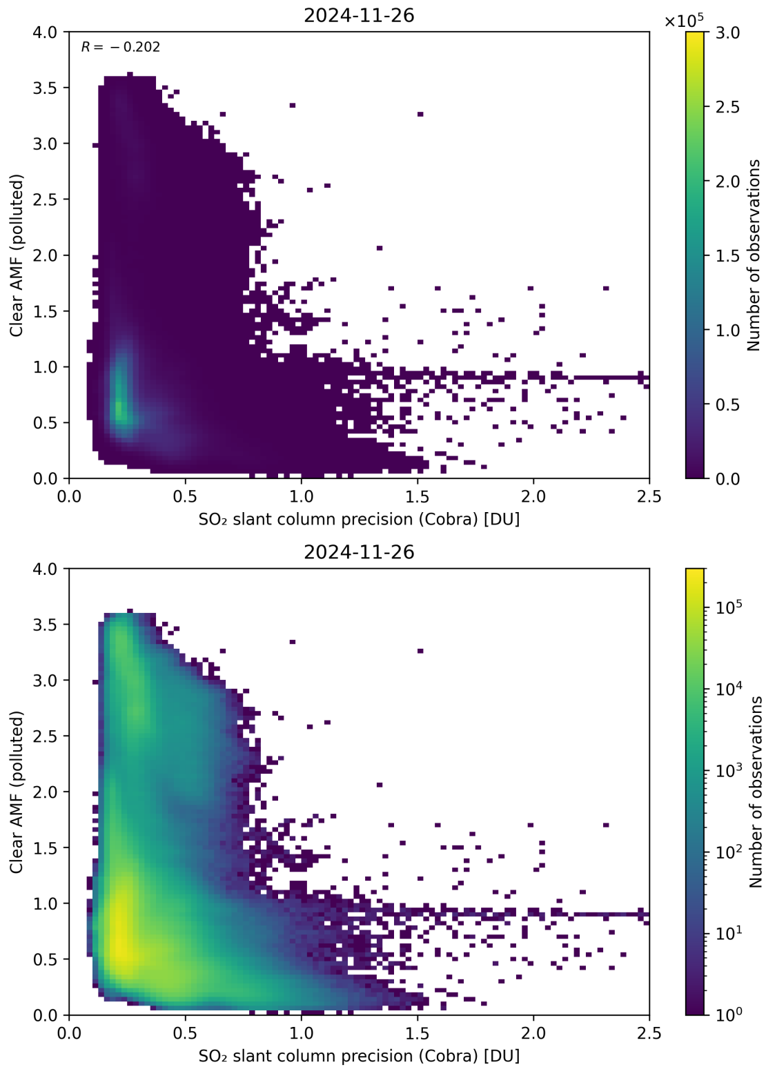
Figure 205: Scatter density plot of “SO 2 slant column precision (Cobra)” against “Clear AMF (polluted)” for 2024-11-25 to 2024-11-27.
