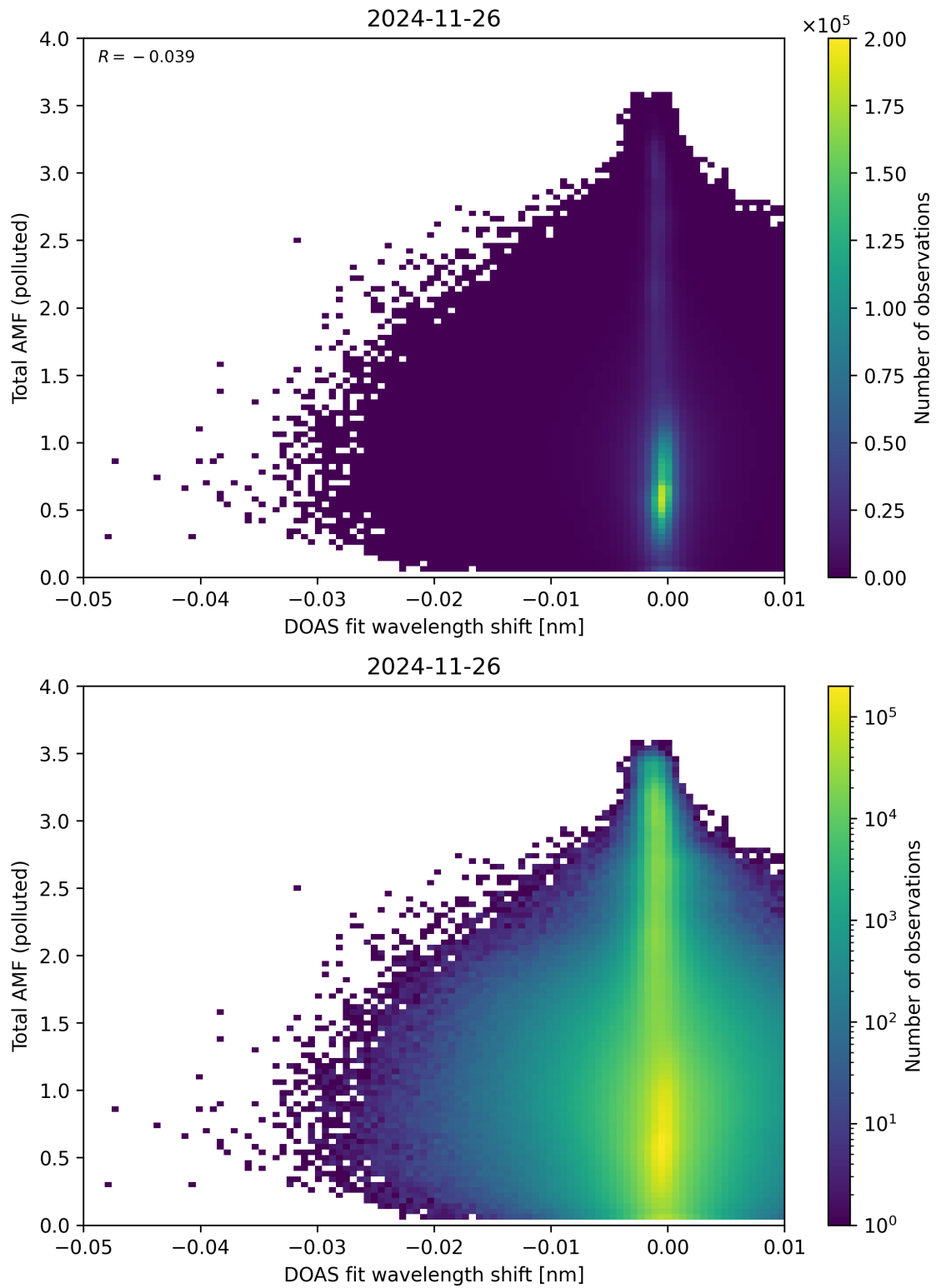
Figure 141: Scatter density plot of “DOAS fit wavelength shift” against “Total AMF (polluted)” for 2024-11-25 to 2024-11-27.
