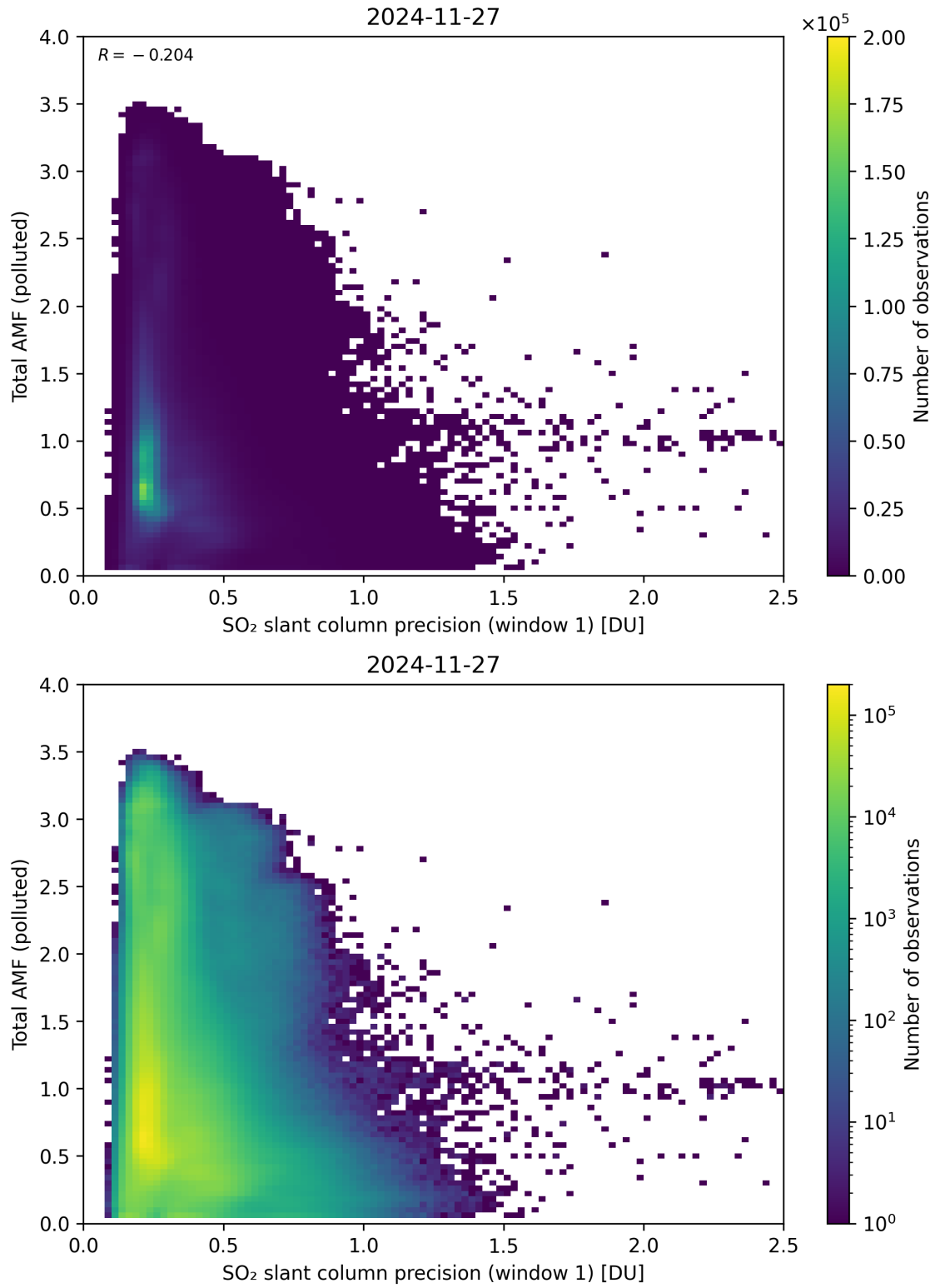
Figure 280: Scatter density plot of “SO 2 slant column precision (window 1)” against “Total AMF (polluted)” for 2024-11-26 to 2024-11-28.
