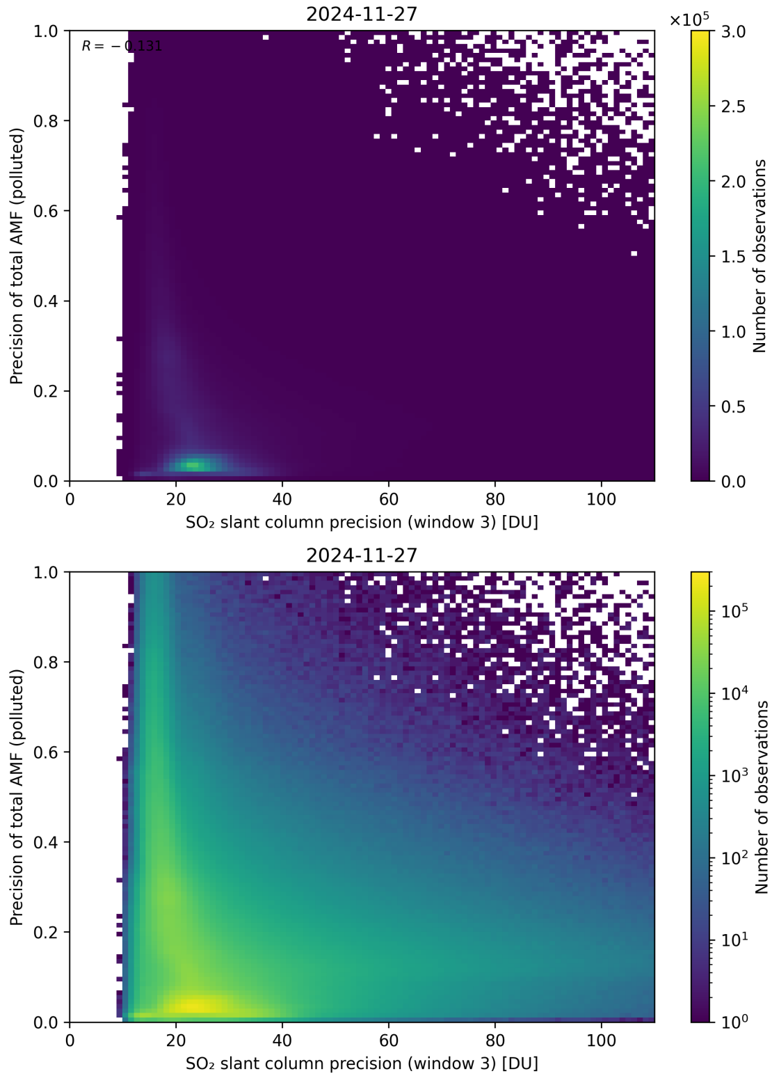
Figure 314: Scatter density plot of “SO 2 slant column precision (window 3)” against “Precision of total AMF (polluted)” for 2024-11-26 to 2024-11-28.
