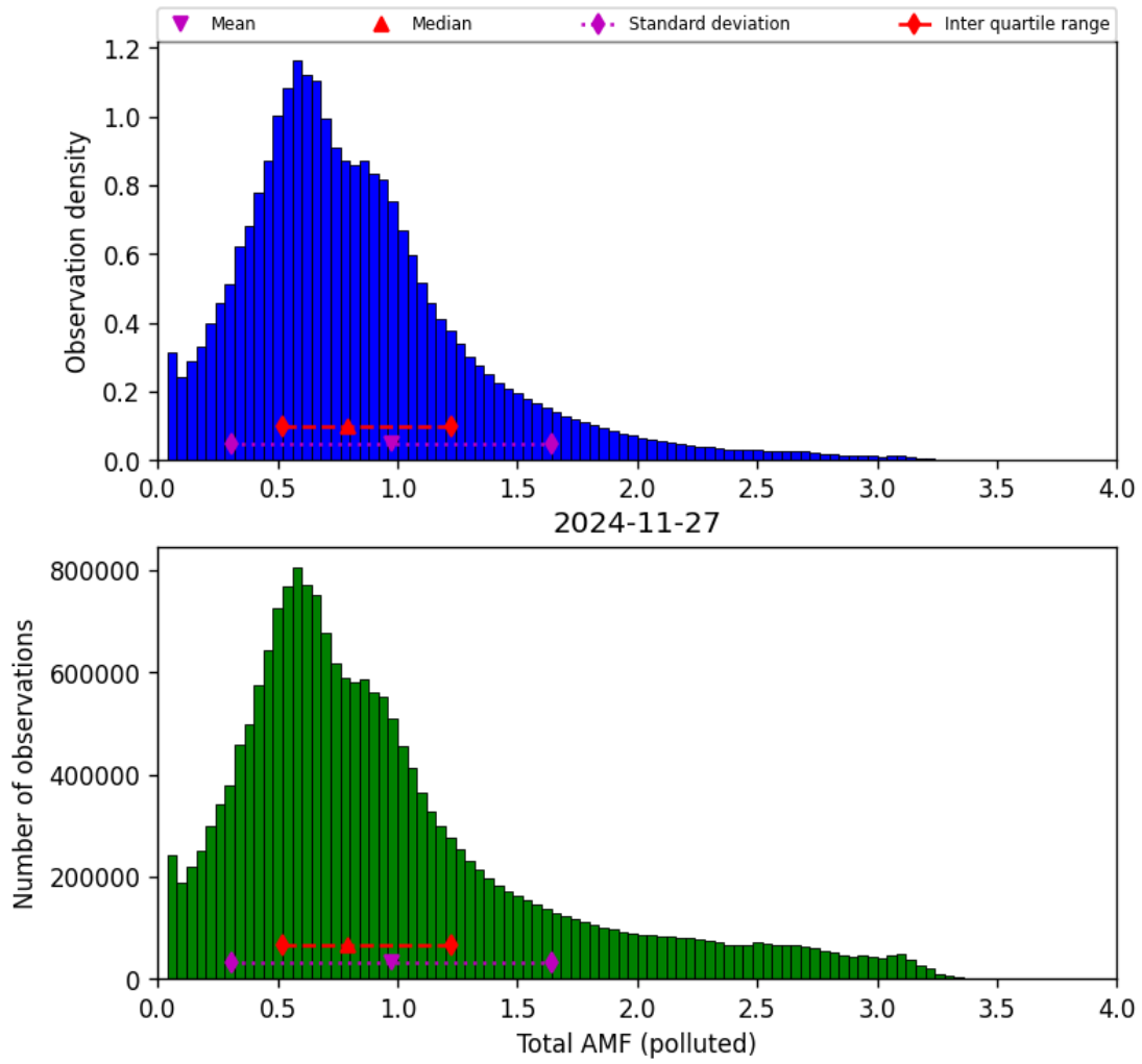
Figure 79: Histogram of “Total AMF (polluted)” for 2024-11-26 to 2024-11-28
