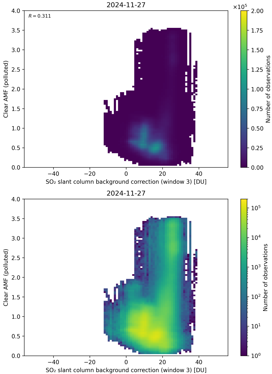
Figure 135: Scatter density plot of “SO 2 slant column background correction (window 3)” against “Clear AMF (polluted)” for 2024-11-26 to 2024-11-28.
