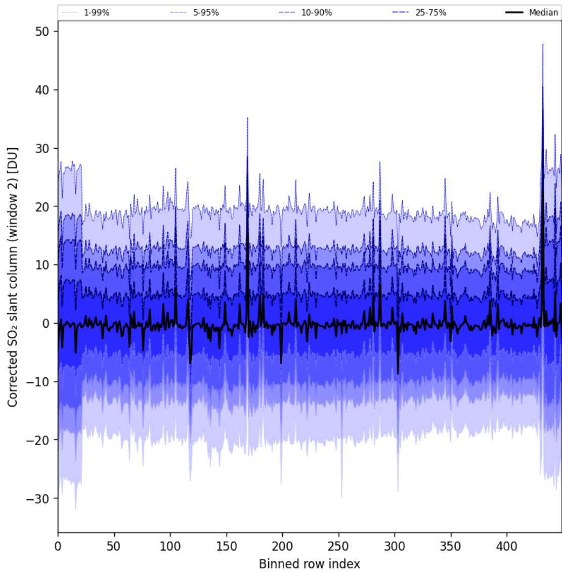
Figure 95: Along track statistics of “Corrected SO 2 slant column (window 2)” for 2024-11-26 to 2024-11-28
