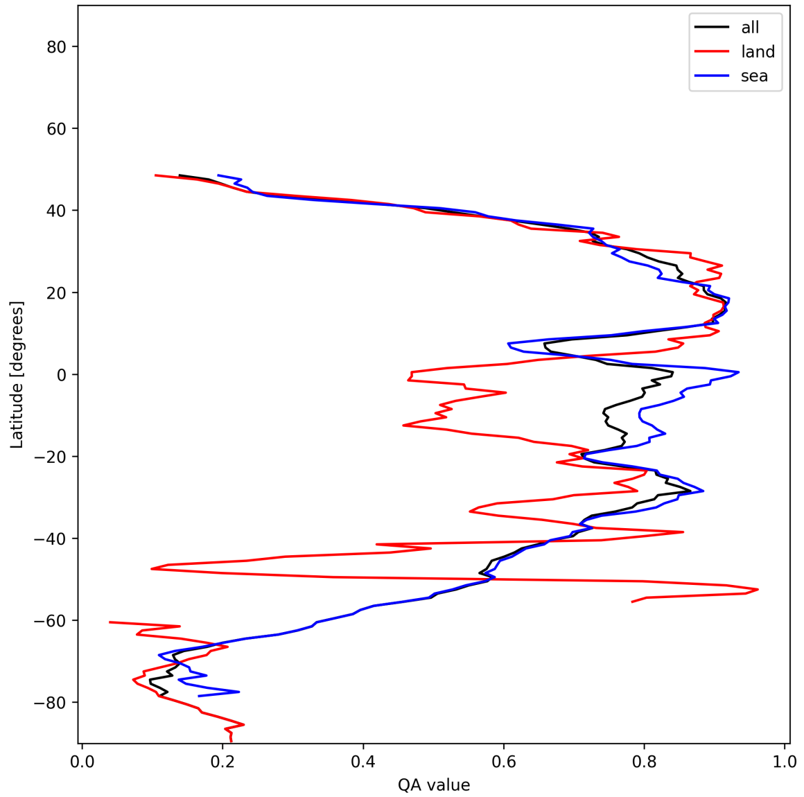
Figure 31: Zonal average of “QA value” for 2024-11-26 to 2024-11-28.
