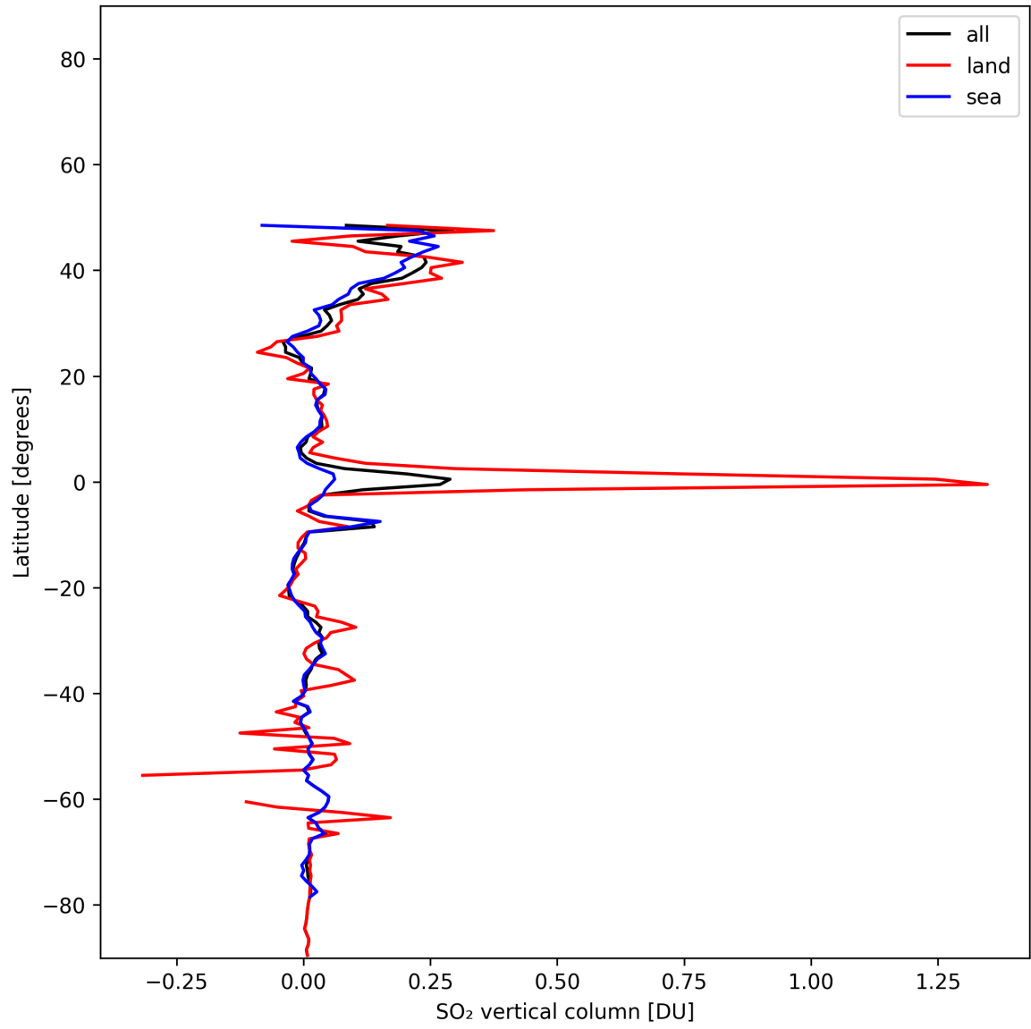
Figure 32: Zonal average of “SO 2 vertical column” for 2024-11-26 to 2024-11-28.
