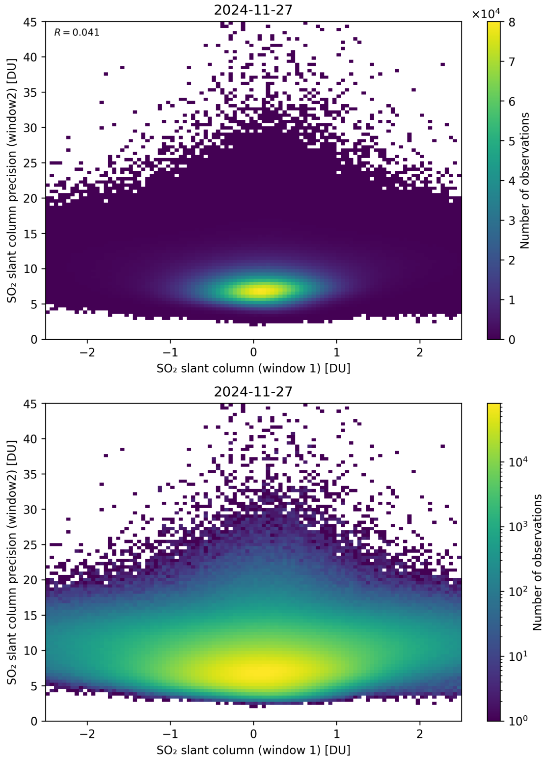
Figure 286: Scatter density plot of “SO 2 slant column (window 1)” against “SO 2 slant column precision (window2)” for 2024-11-26 to 2024-11-28.
