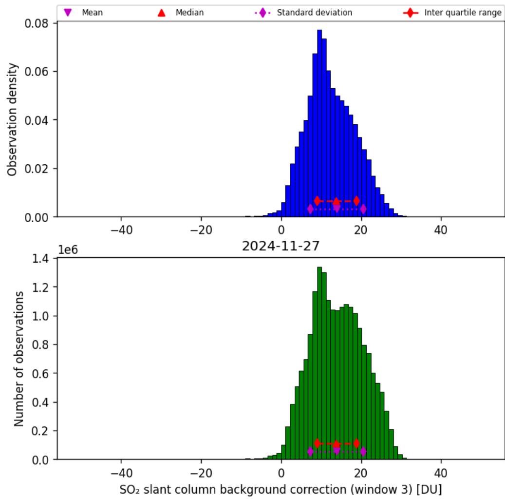
Figure 74: Histogram of “SO 2 slant column background correction (window 3)” for 2024-11-26 to 2024-11-28
