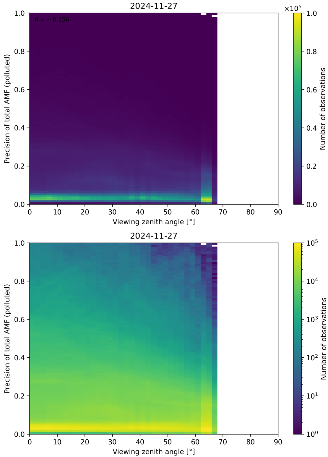
Figure 382: Scatter density plot of “Viewing zenith angle” against “Precision of total AMF (polluted)” for 2024-11-26 to 2024-11-28.
