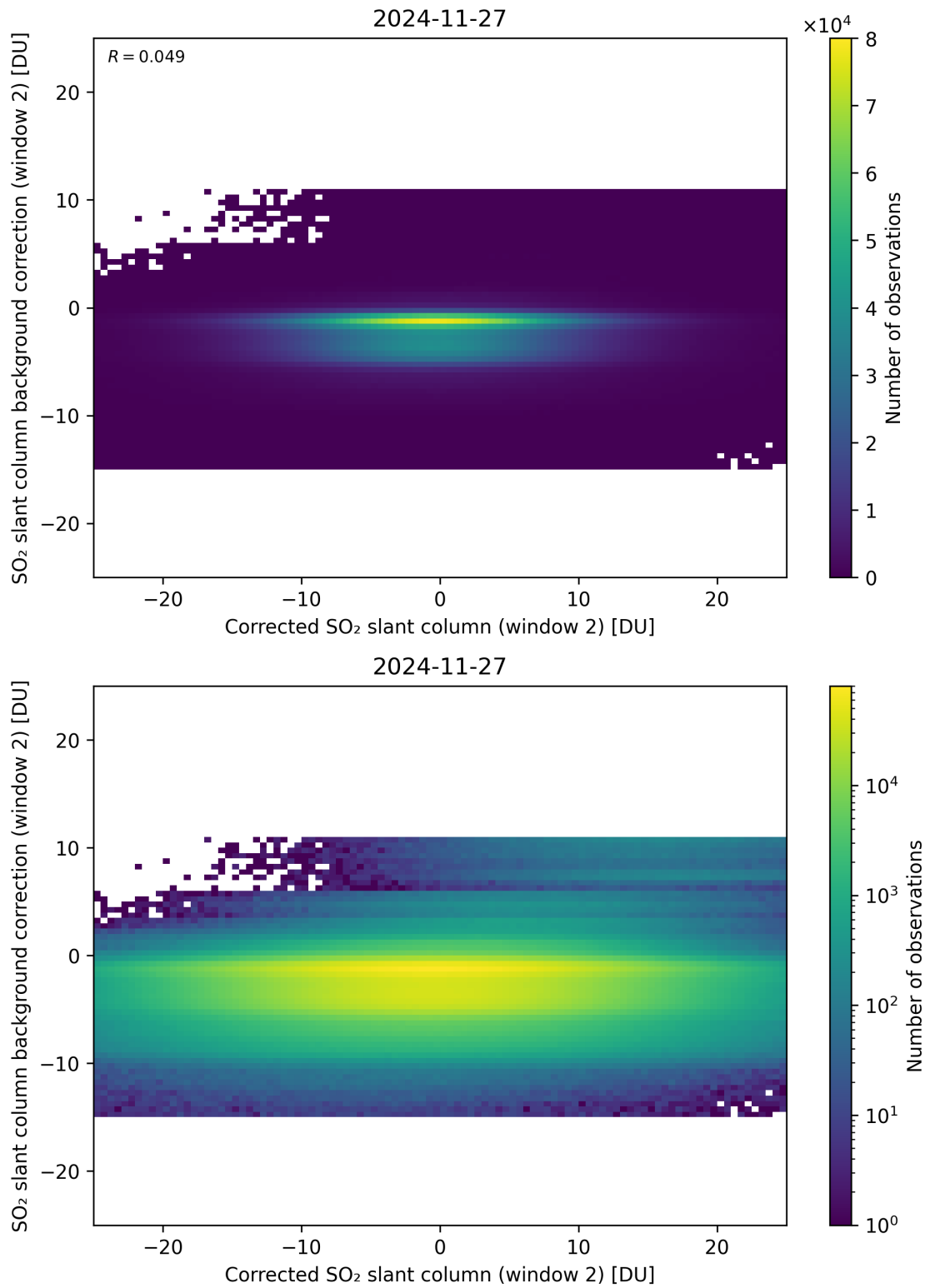
Figure 244: Scatter density plot of “Corrected SO 2 slant column (window 2)” against “SO 2 slant column background correction (window 2)” for 2024-11-26 to 2024-11-28.
