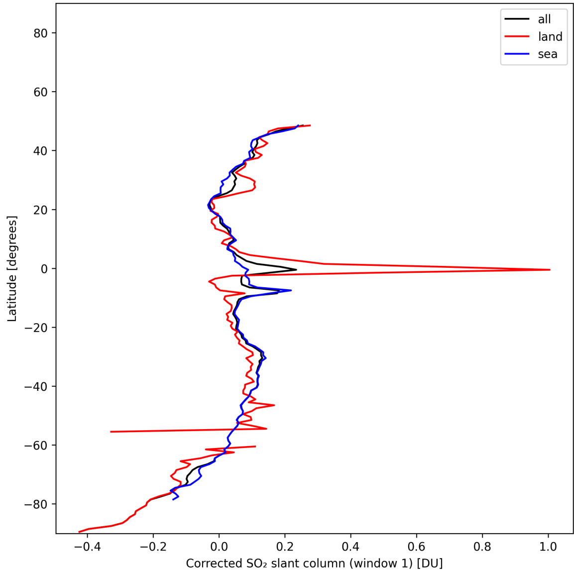
Figure 39: Zonal average of “Corrected SO 2 slant column (window 1)” for 2024-11-26 to 2024-11-28.
