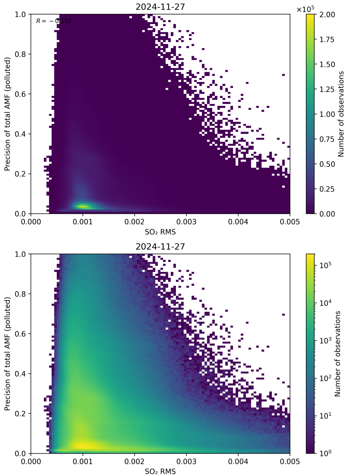
Figure 149: Scatter density plot of “SO 2 RMS” against “Precision of total AMF (polluted)” for 2024-11-26 to 2024-11-28.
