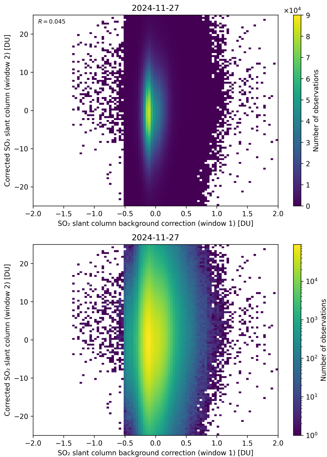
Figure 115: Scatter density plot of “SO 2 slant column background correction (window 1)” against “Corrected SO 2 slant column (window 2)” for 2024-11-26 to 2024-11-28.
