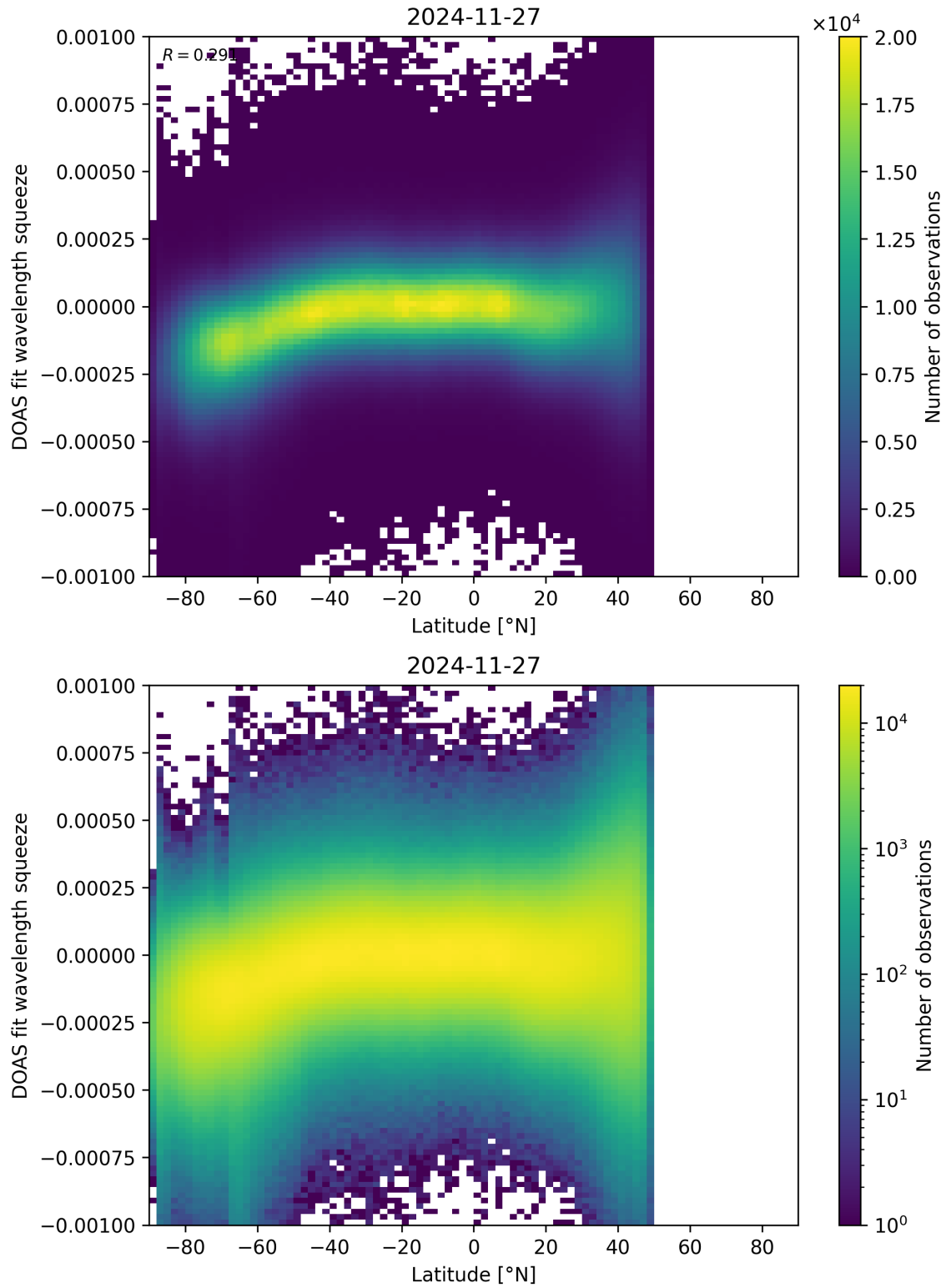
Figure 154: Scatter density plot of “Latitude” against “DOAS fit wavelength squeeze” for 2024-11-26 to 2024-11-28.
