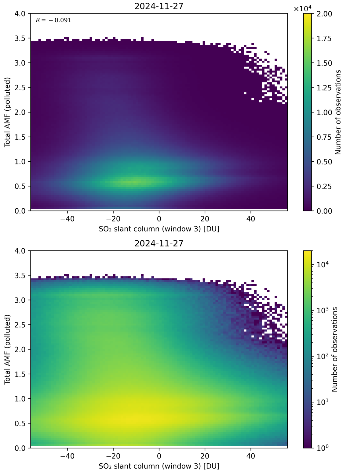
Figure 318: Scatter density plot of “SO 2 slant column (window 3)” against “Total AMF (polluted)” for 2024-11-26 to 2024-11-28.
