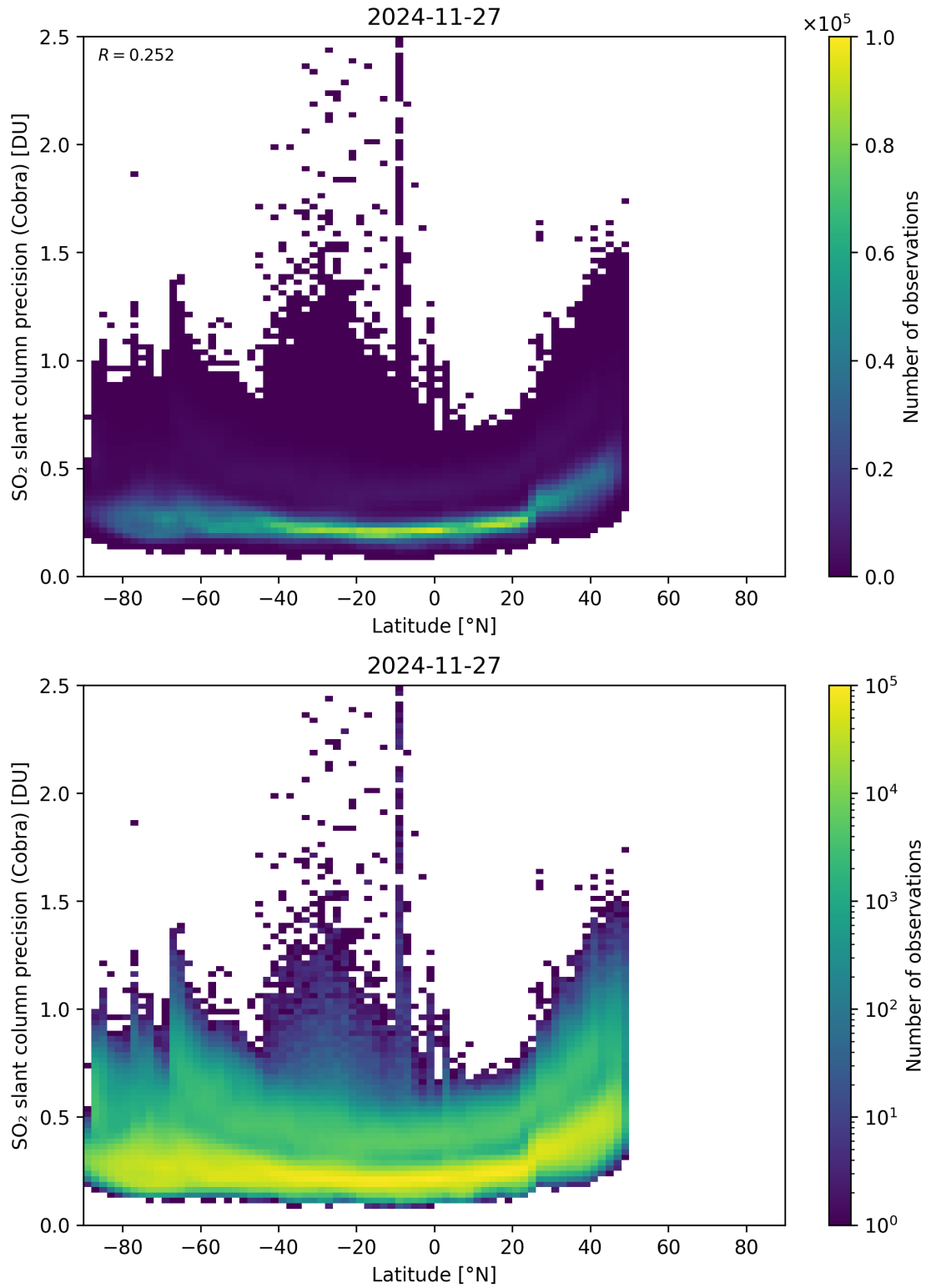
Figure 158: Scatter density plot of “Latitude” against “SO 2 slant column precision (Cobra)” for 2024-11-26 to 2024-11-28.
