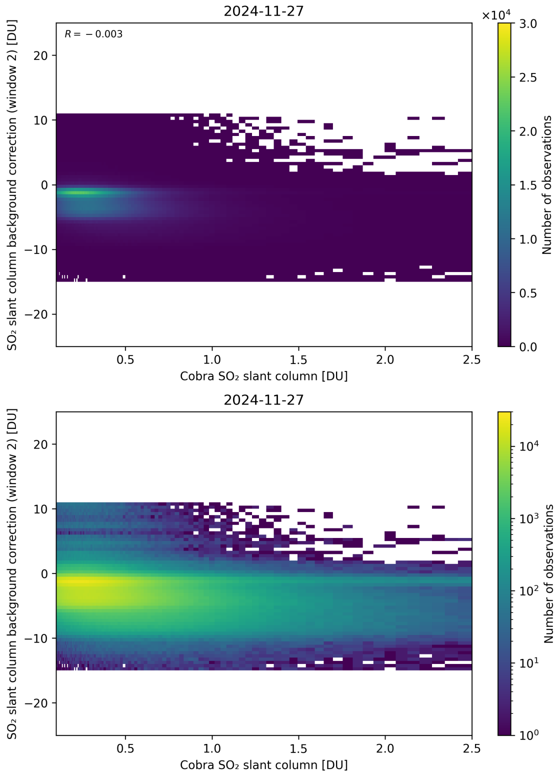
Figure 194: Scatter density plot of “Cobra SO 2 slant column” against “SO 2 slant column background correction (window 2)” for 2024-11-26 to 2024-11-28.
