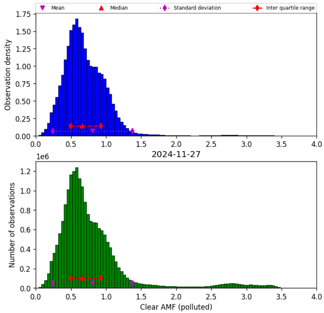
Figure 81: Histogram of “Clear AMF (polluted)” for 2024-11-26 to 2024-11-28
