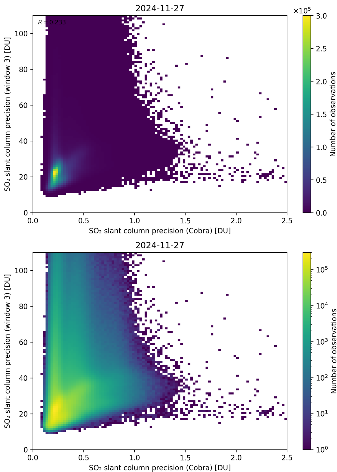
Figure 212: Scatter density plot of “SO 2 slant column precision (Cobra)” against “SO 2 slant column precision (window 3)” for 2024-11-26 to 2024-11-28.
