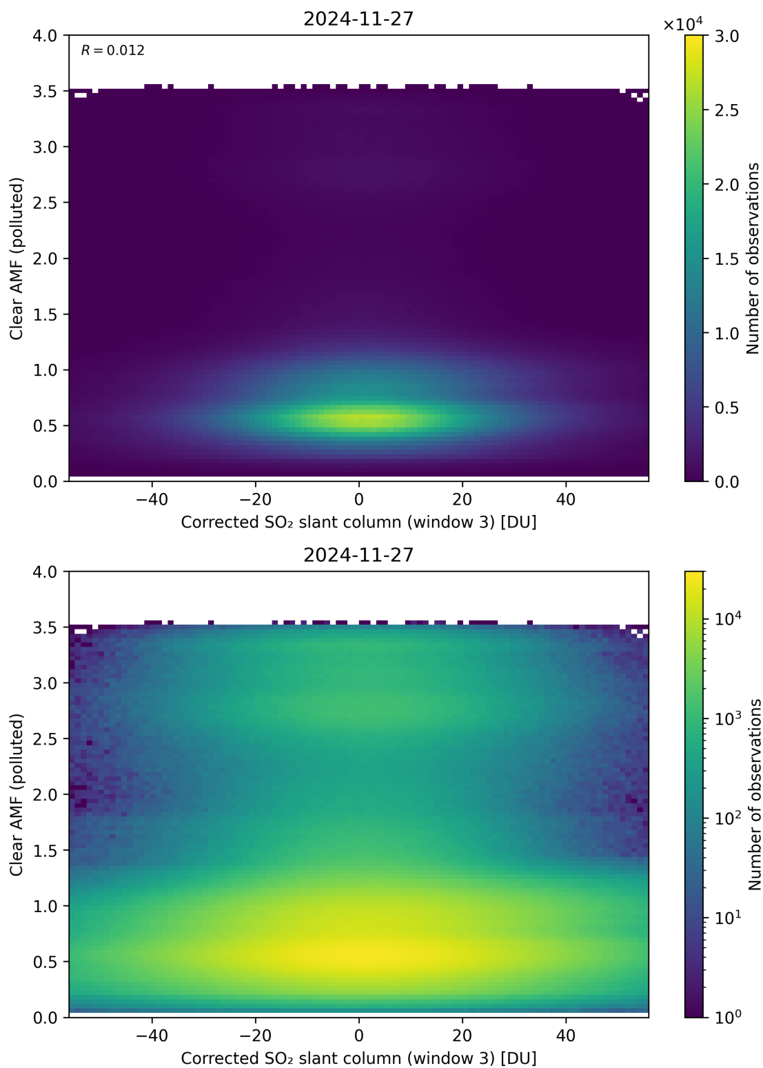
Figure 259: Scatter density plot of “Corrected SO 2 slant column (window 3)” against “Clear AMF (polluted)” for 2024-11-26 to 2024-11-28.
