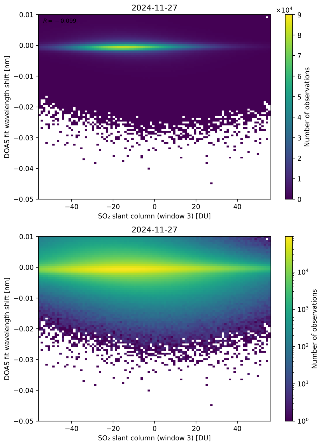
Figure 304: Scatter density plot of “SO 2 slant column (window 3)” against “DOAS fit wavelength shift” for 2024-11-26 to 2024-11-28.
