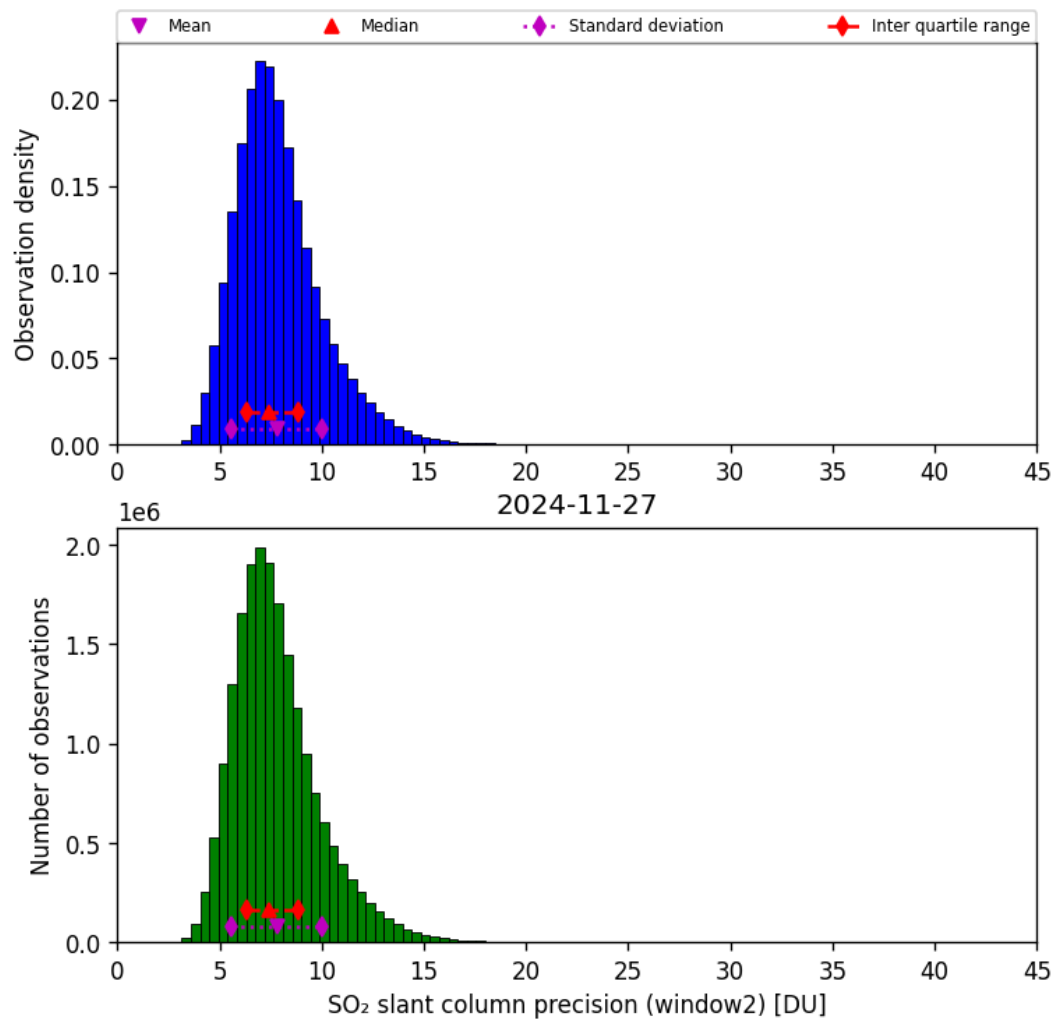
Figure 68: Histogram of “SO 2 slant column precision (window2)” for 2024-11-26 to 2024-11-28
