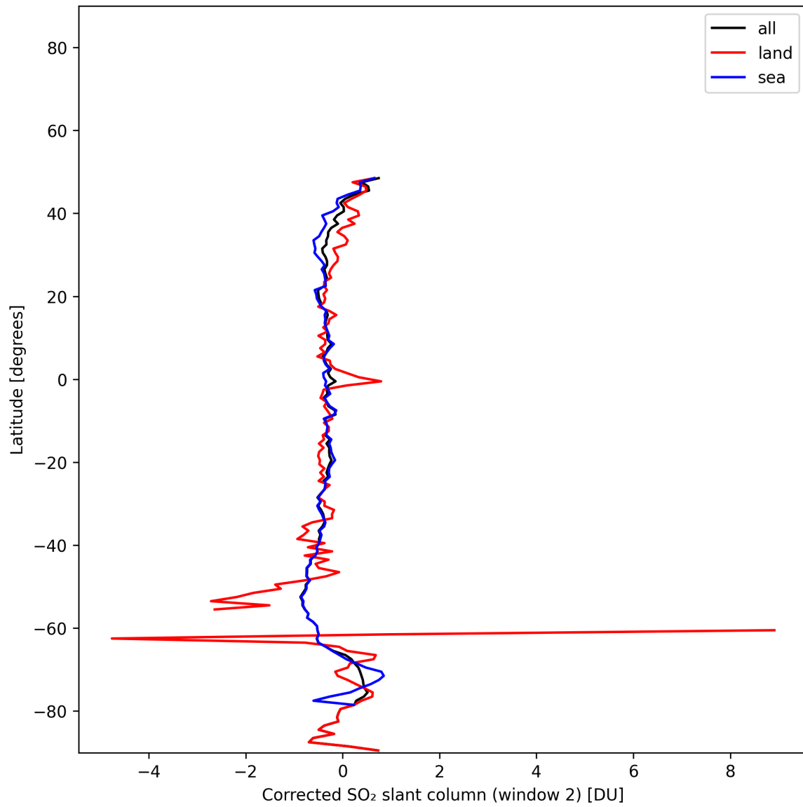
Figure 43: Zonal average of “Corrected SO 2 slant column (window 2)” for 2024-11-26 to 2024-11-28.
