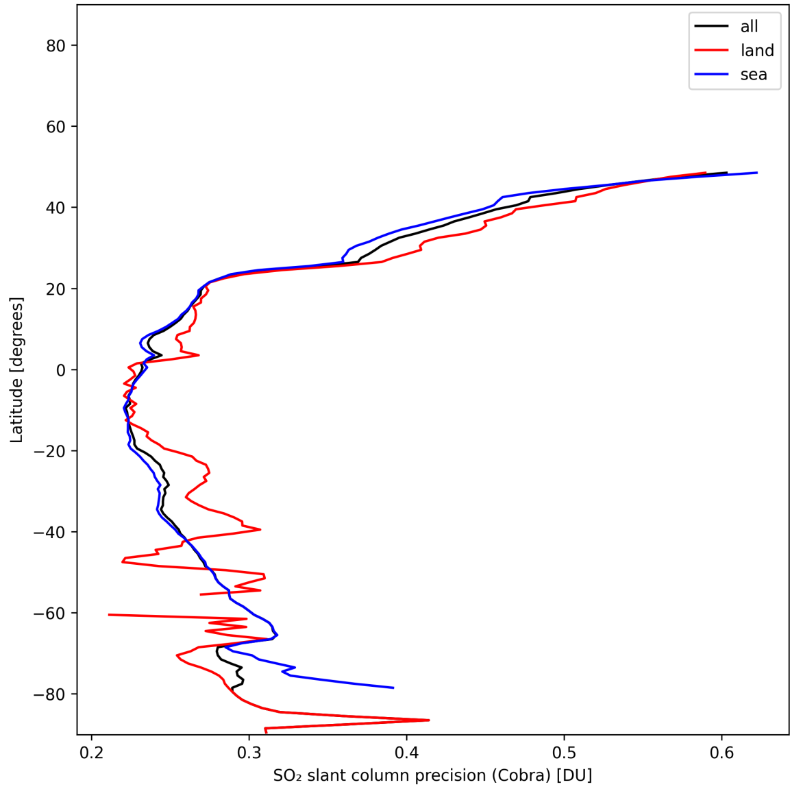
Figure 36: Zonal average of “SO 2 slant column precision (Cobra)” for 2024-11-26 to 2024-11-28.
