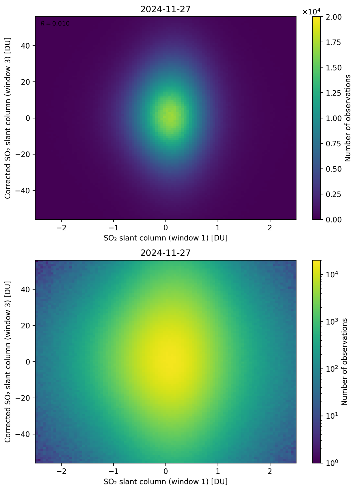
Figure 284: Scatter density plot of “SO 2 slant column (window 1)” against “Corrected SO 2 slant column (window 3)” for 2024-11-26 to 2024-11-28.
