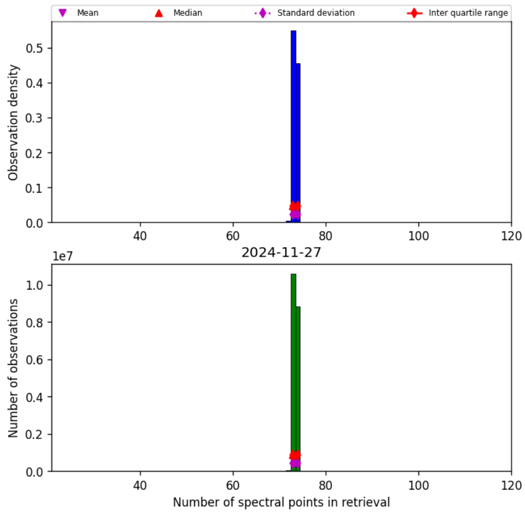
Figure 82: Histogram of “Number of spectral points in retrieval” for 2024-11-26 to 2024-11-28
