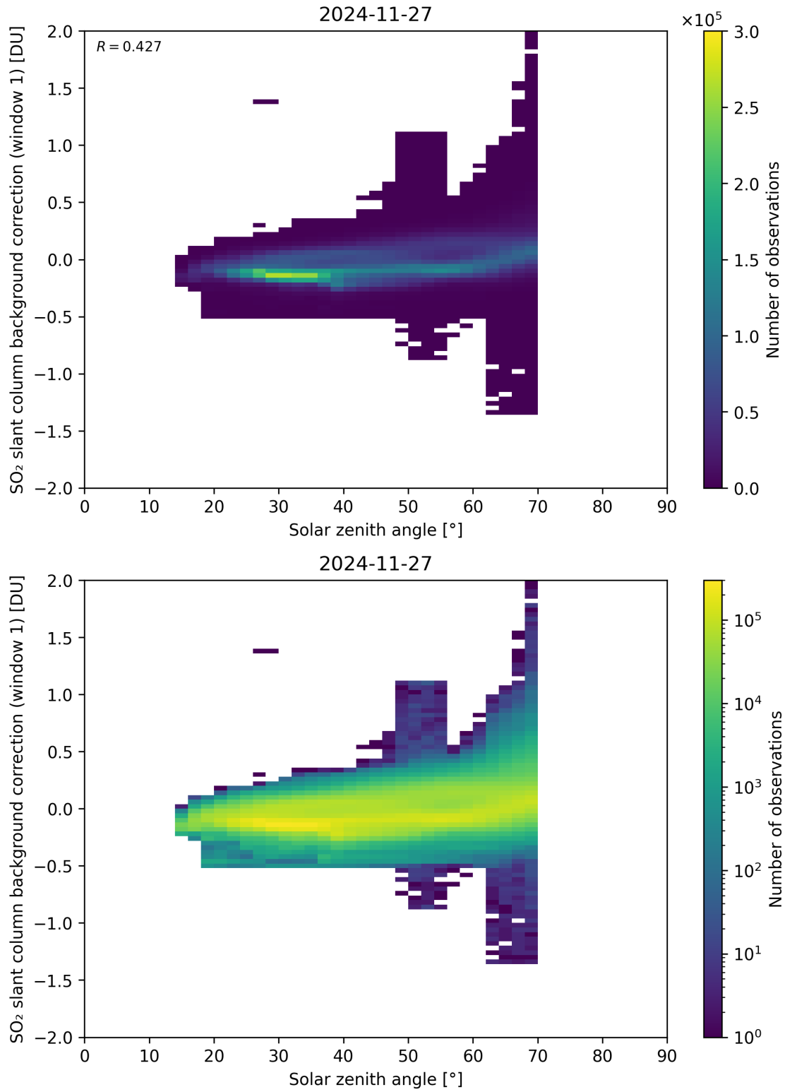
Figure 171: Scatter density plot of “Solar zenith angle” against “SO 2 slant column background correction (window 1)” for 2024-11-26 to 2024-11-28.
