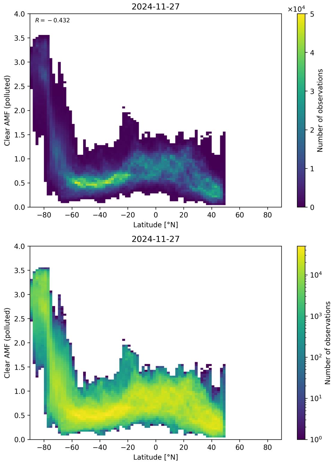
Figure 156: Scatter density plot of “Latitude” against “Clear AMF (polluted)” for 2024-11-26 to 2024-11-28.
