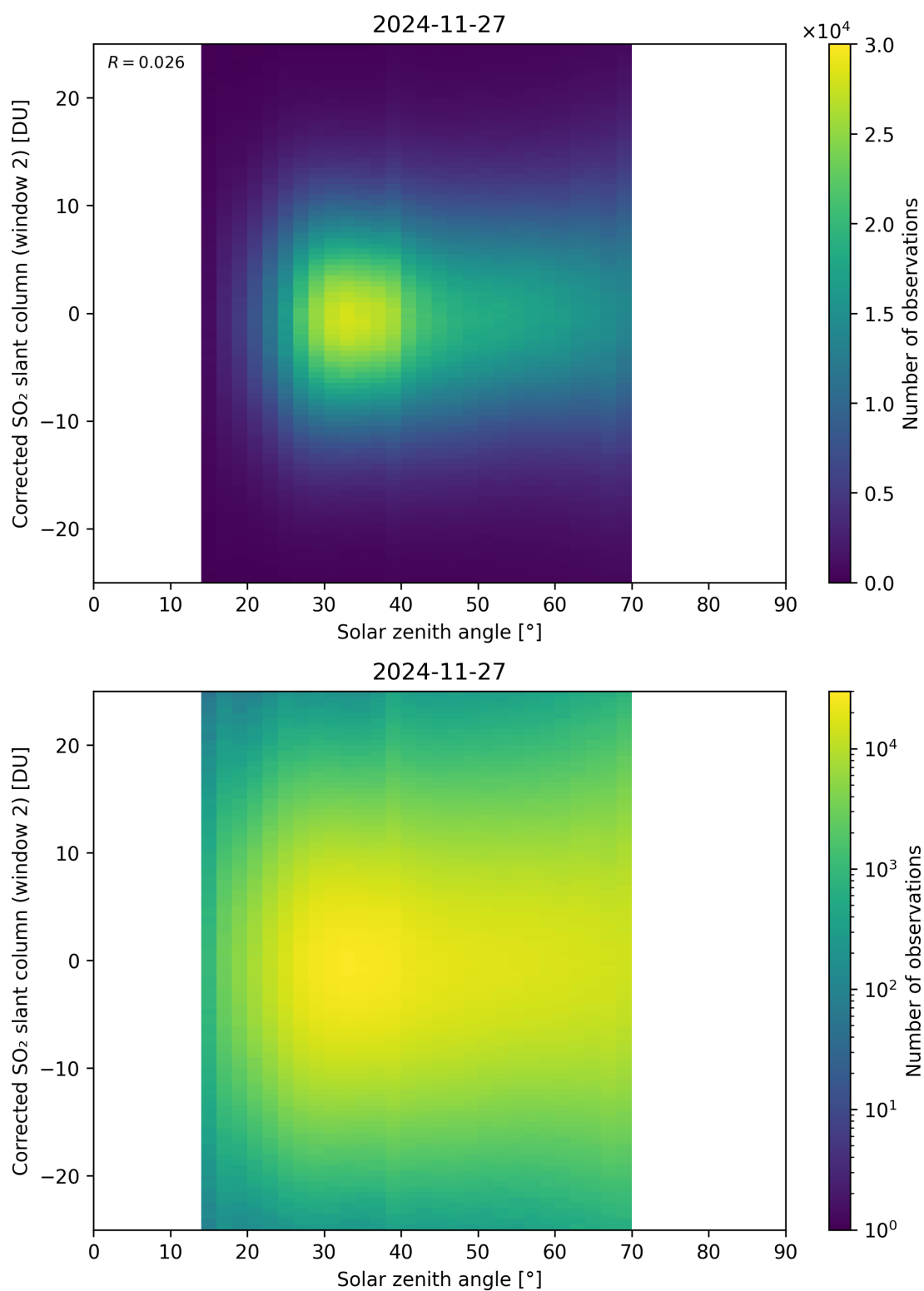
Figure 182: Scatter density plot of “Solar zenith angle” against “Corrected SO 2 slant column (window 2)” for 2024-11-26 to 2024-11-28.
