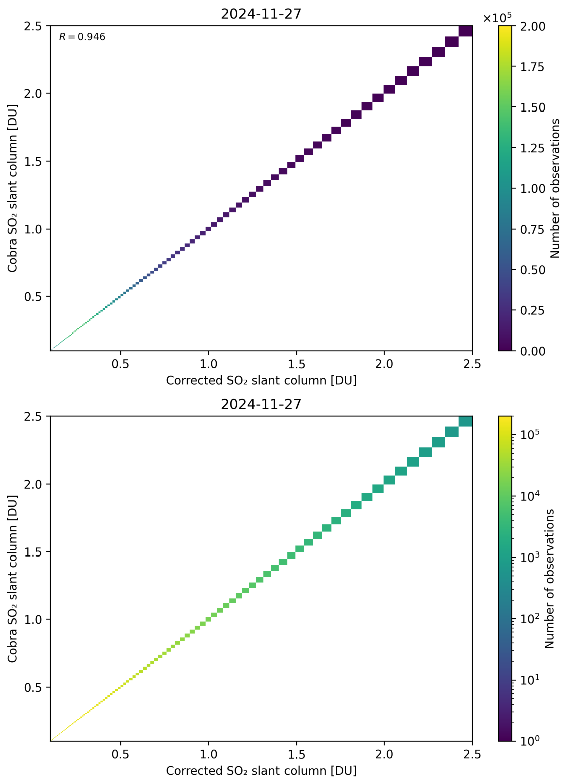
Figure 233: Scatter density plot of “Corrected SO 2 slant column” against “Cobra SO 2 slant column” for 2024-11-26 to 2024-11-28.
