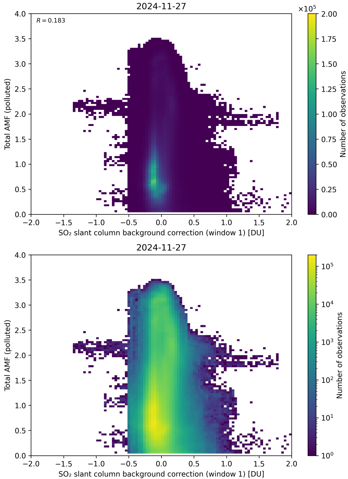
Figure 120: Scatter density plot of “SO 2 slant column background correction (window 1)” against “Total AMF (polluted)” for 2024-11-26 to 2024-11-28.
