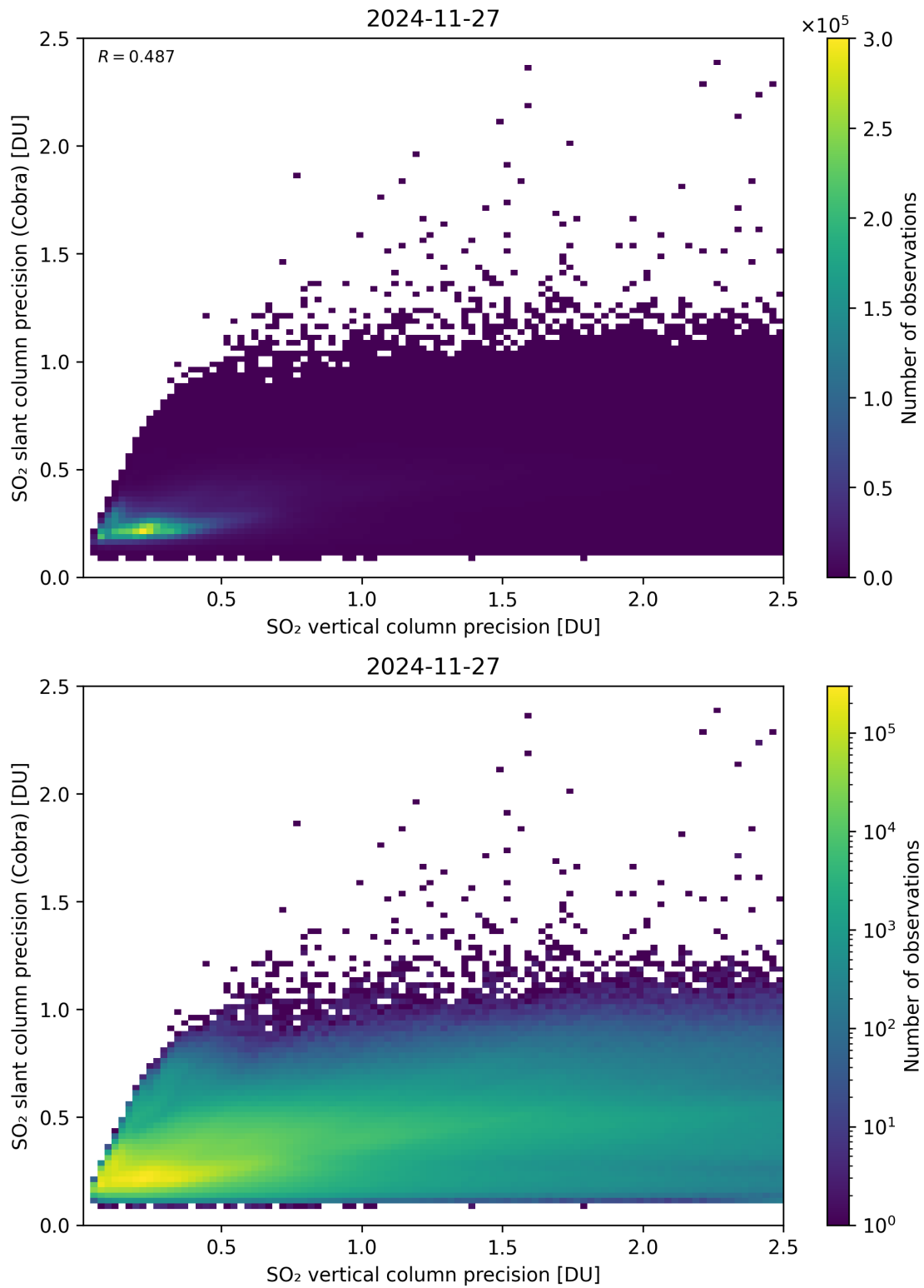
Figure 337: Scatter density plot of “SO 2 vertical column precision” against “SO 2 slant column precision (Cobra)” for 2024-11-26 to 2024-11-28.
