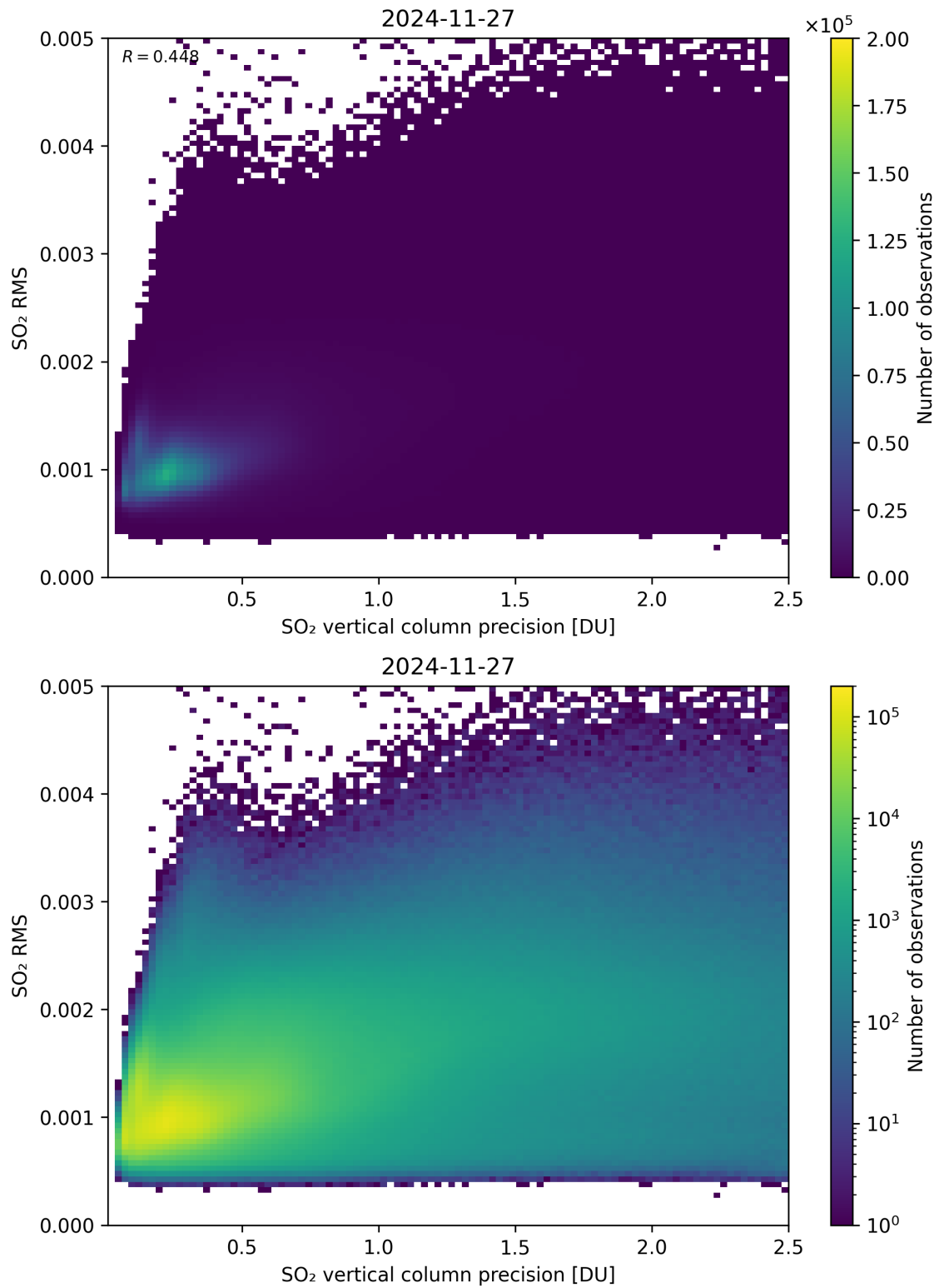
Figure 334: Scatter density plot of “SO 2 vertical column precision” against “SO 2 RMS” for 2024-11-26 to 2024-11-28.
