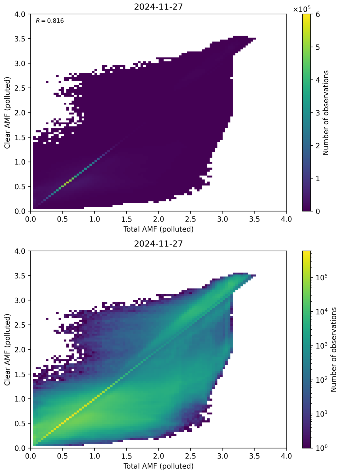
Figure 321: Scatter density plot of “Total AMF (polluted)” against “Clear AMF (polluted)” for 2024-11-26 to 2024-11-28.
