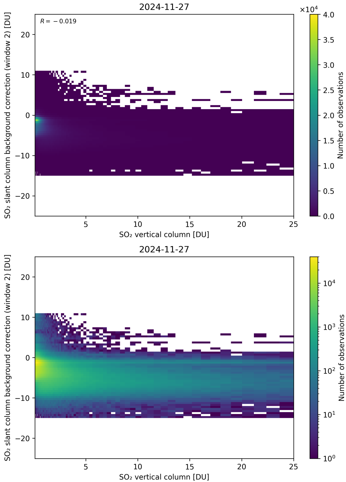
Figure 324: Scatter density plot of “SO 2 vertical column” against “SO 2 slant column background correction (window 2)” for 2024-11-26 to 2024-11-28.
