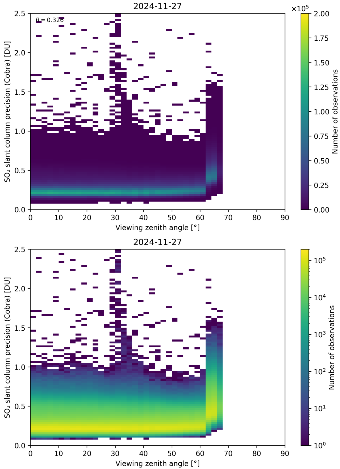
Figure 372: Scatter density plot of “Viewing zenith angle” against “SO 2 slant column precision (Cobra)” for 2024-11-26 to 2024-11-28.
