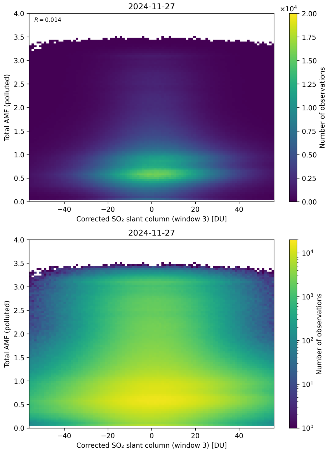
Figure 260: Scatter density plot of “Corrected SO 2 slant column (window 3)” against “Total AMF (polluted)” for 2024-11-26 to 2024-11-28.
