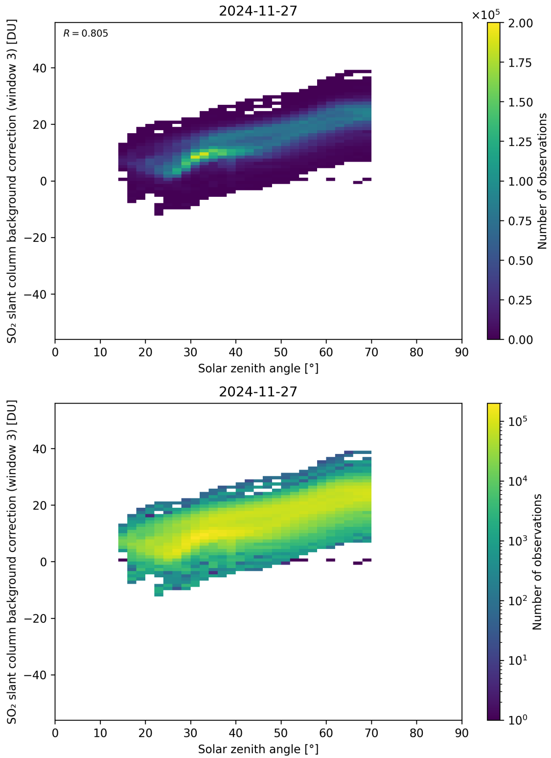
Figure 173: Scatter density plot of “Solar zenith angle” against “SO 2 slant column background correction (window 3)” for 2024-11-26 to 2024-11-28.
