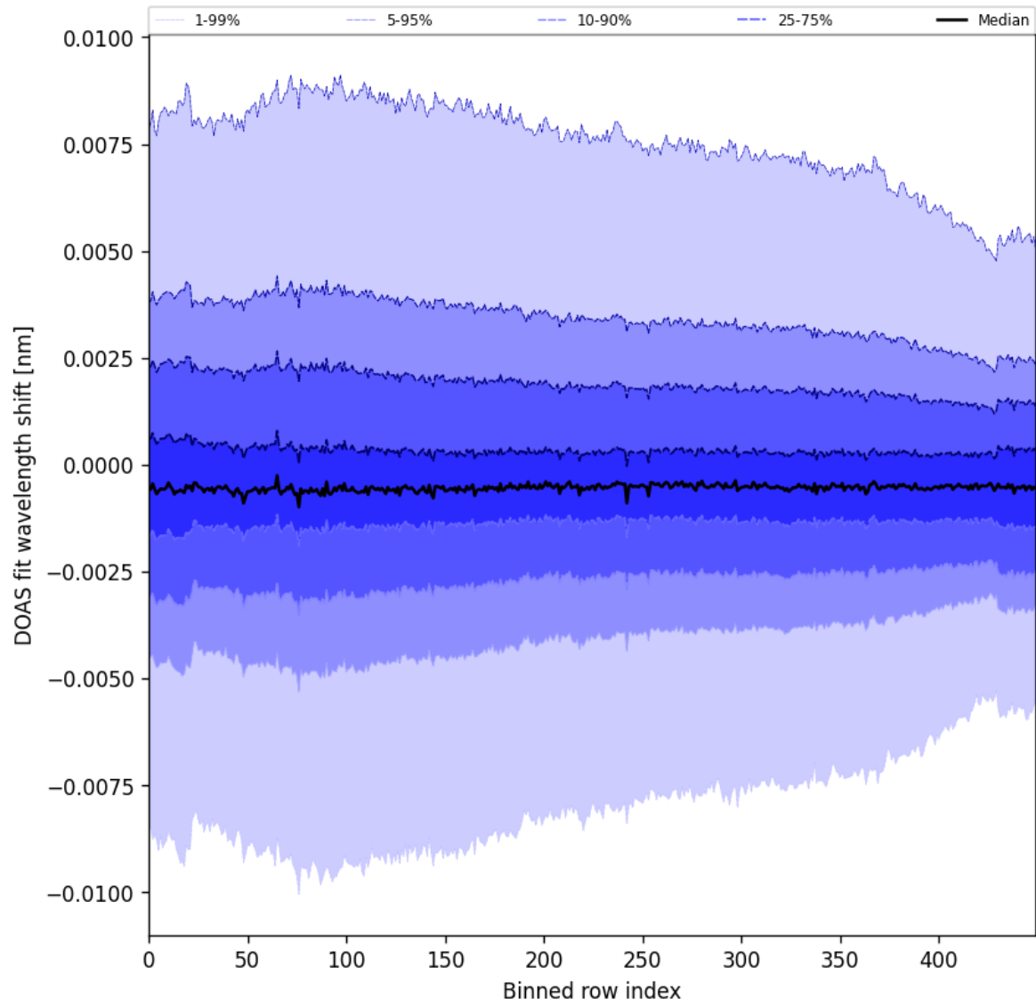
Figure 102: Along track statistics of “DOAS fit wavelength shift” for 2024-11-26 to 2024-11-28
