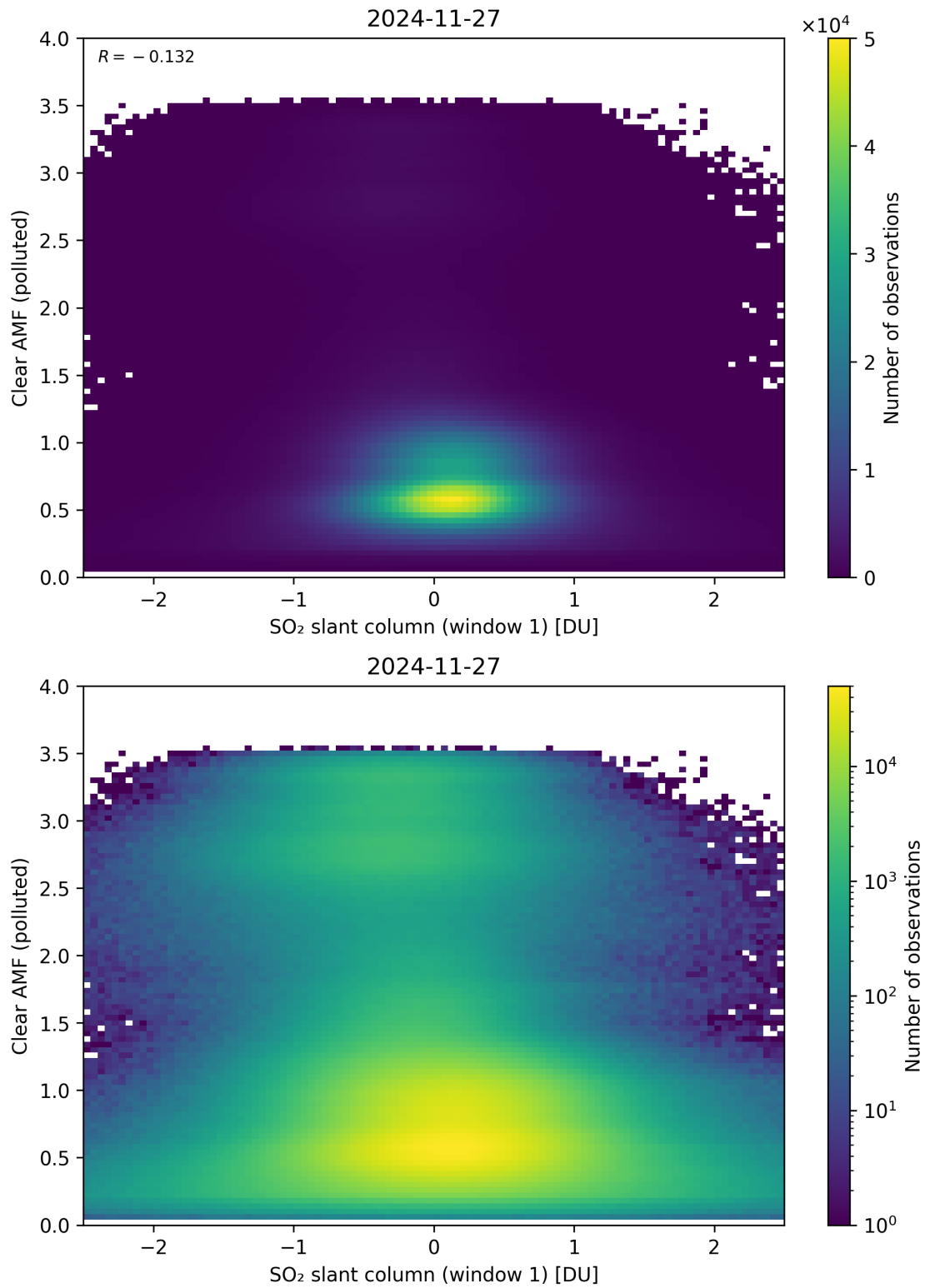
Figure 282: Scatter density plot of “SO 2 slant column (window 1)” against “Clear AMF (polluted)” for 2024-11-26 to 2024-11-28.
