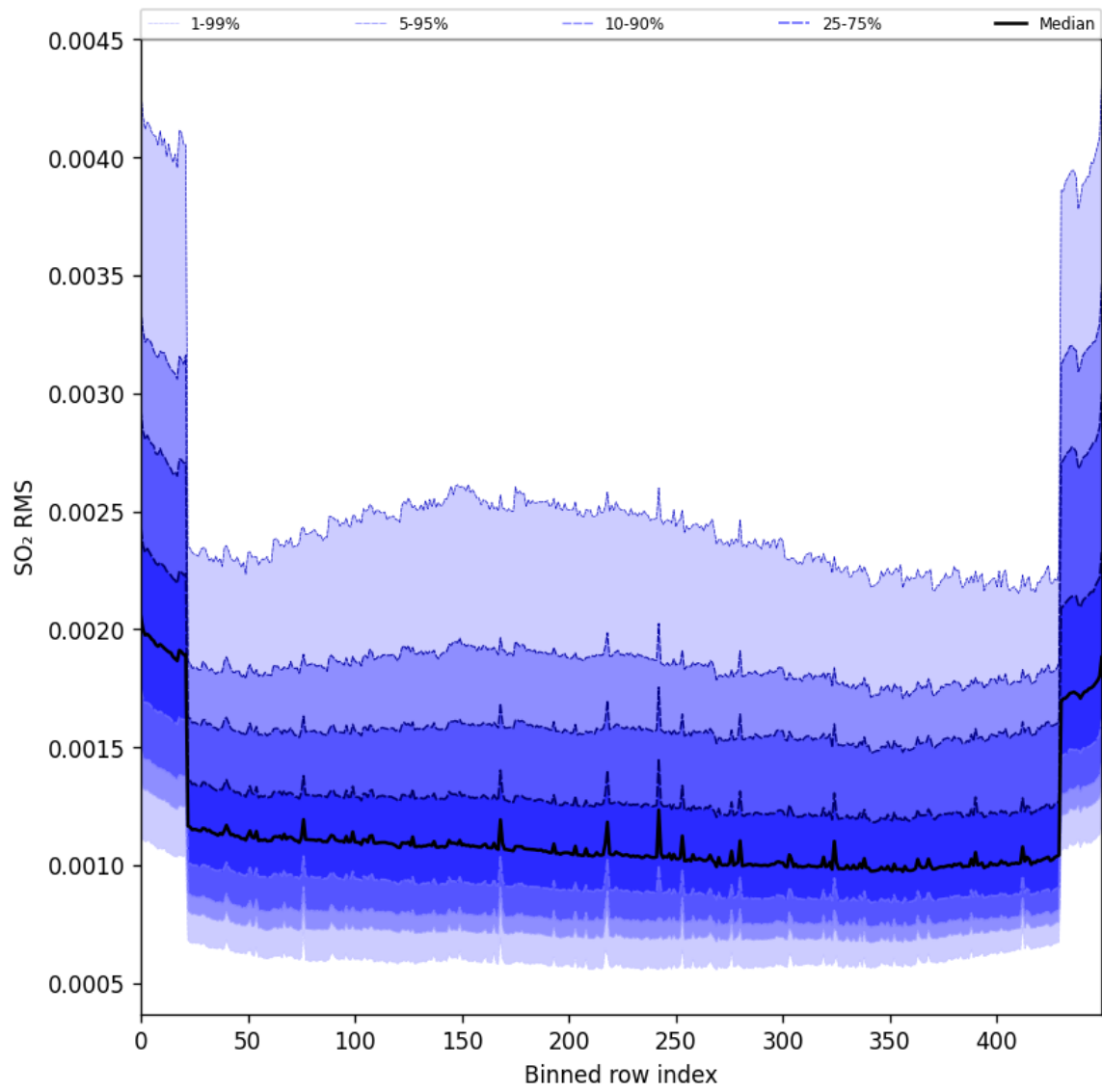
Figure 104: Along track statistics of “SO 2 RMS” for 2024-11-26 to 2024-11-28
