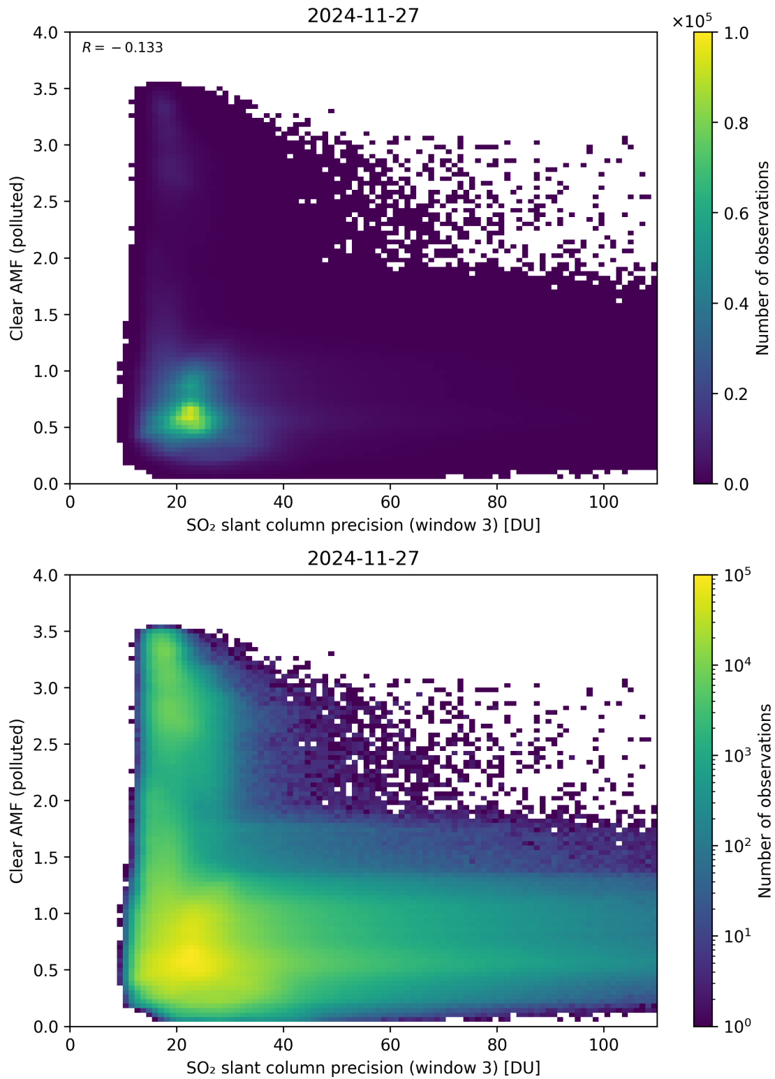
Figure 311: Scatter density plot of “SO 2 slant column precision (window 3)” against “Clear AMF (polluted)” for 2024-11-26 to 2024-11-28.
