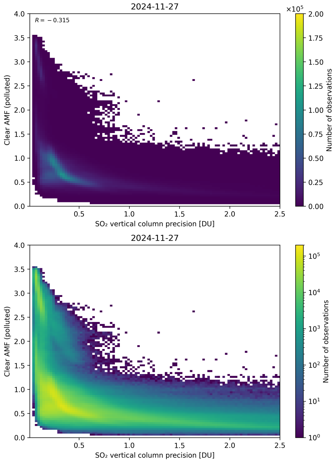
Figure 335: Scatter density plot of “SO 2 vertical column precision” against “Clear AMF (polluted)” for 2024-11-26 to 2024-11-28.
