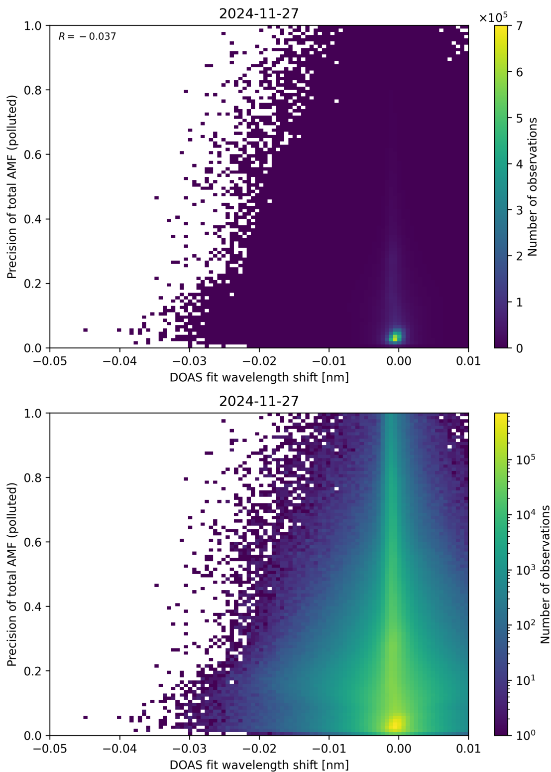
Figure 142: Scatter density plot of “DOAS fit wavelength shift” against “Precision of total AMF (polluted)” for 2024-11-26 to 2024-11-28.
