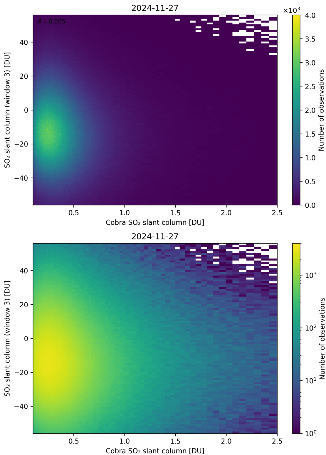
Figure 222: Scatter density plot of “Cobra SO 2 slant column” against “SO 2 slant column (window 3)” for 2024-11-26 to 2024-11-28.
