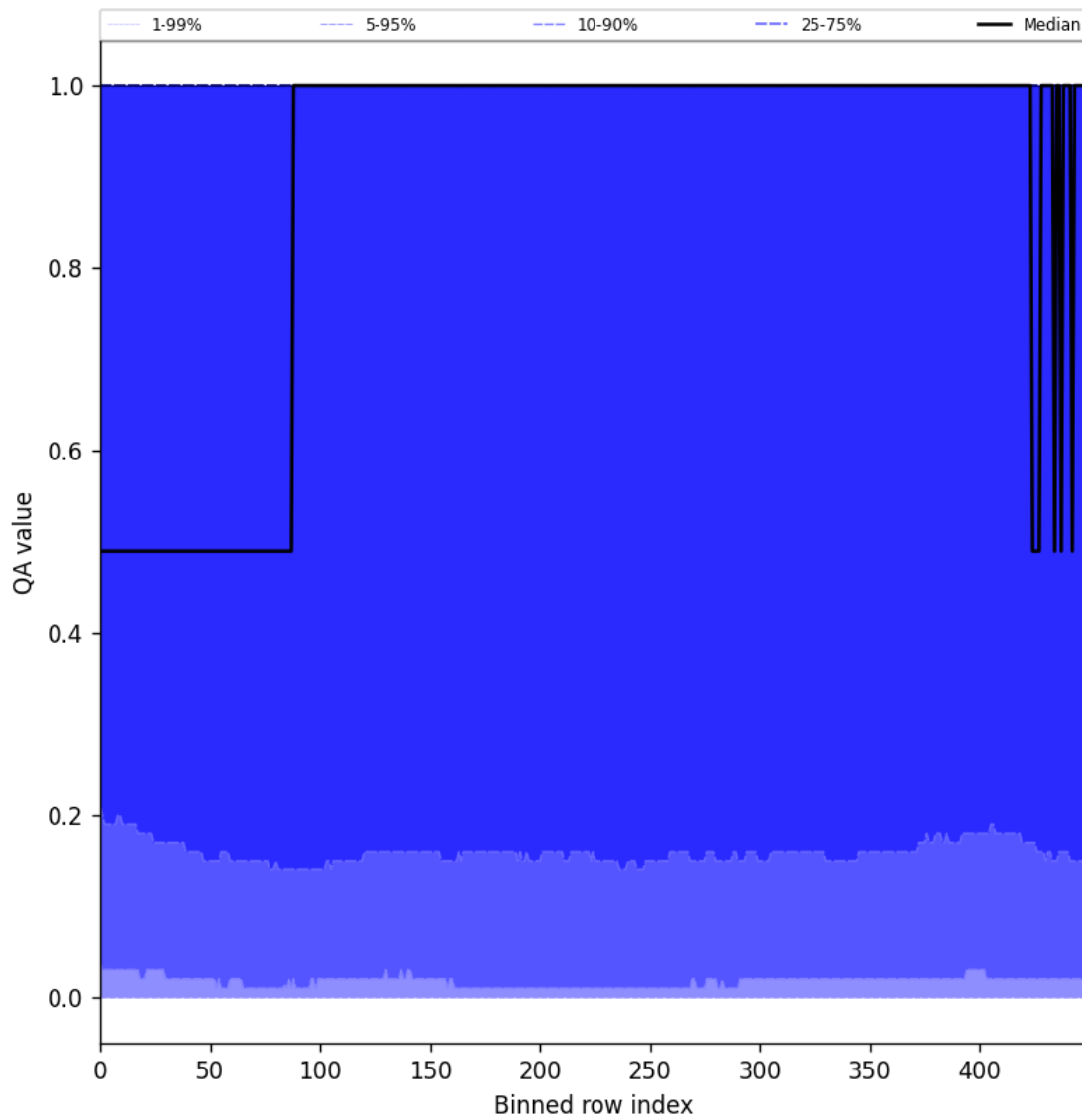
Figure 83: Along track statistics of “QA value” for 2024-11-26 to 2024-11-28
