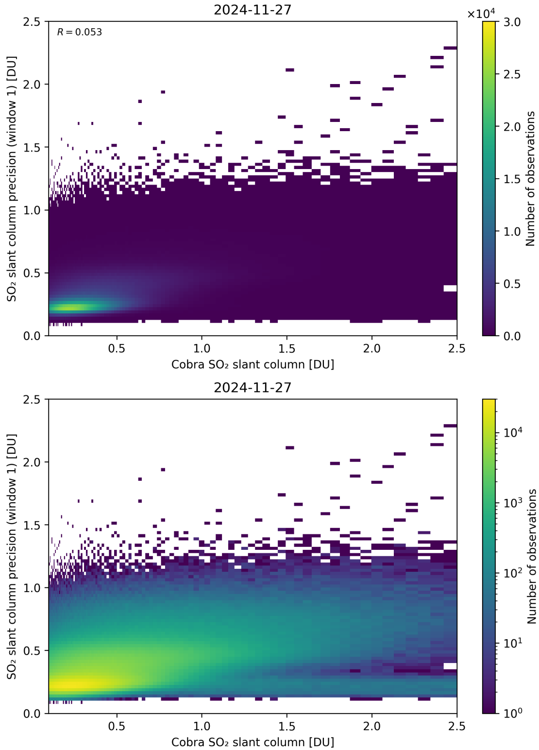
Figure 220: Scatter density plot of “Cobra SO 2 slant column” against “SO 2 slant column precision (window 1)” for 2024-11-26 to 2024-11-28.
