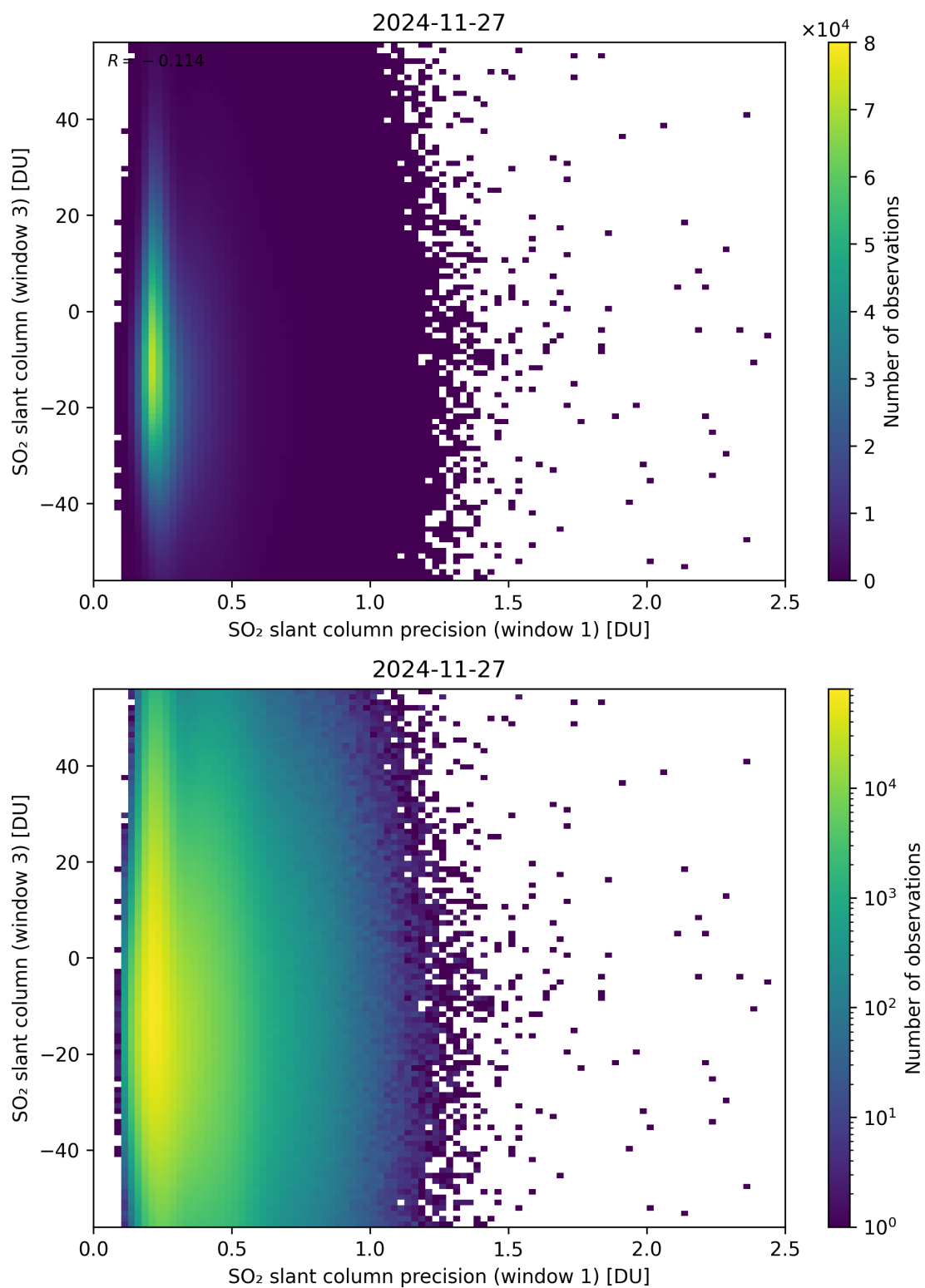
Figure 278: Scatter density plot of “SO 2 slant column precision (window 1)” against “SO 2 slant column (window 3)” for 2024-11-26 to 2024-11-28.
