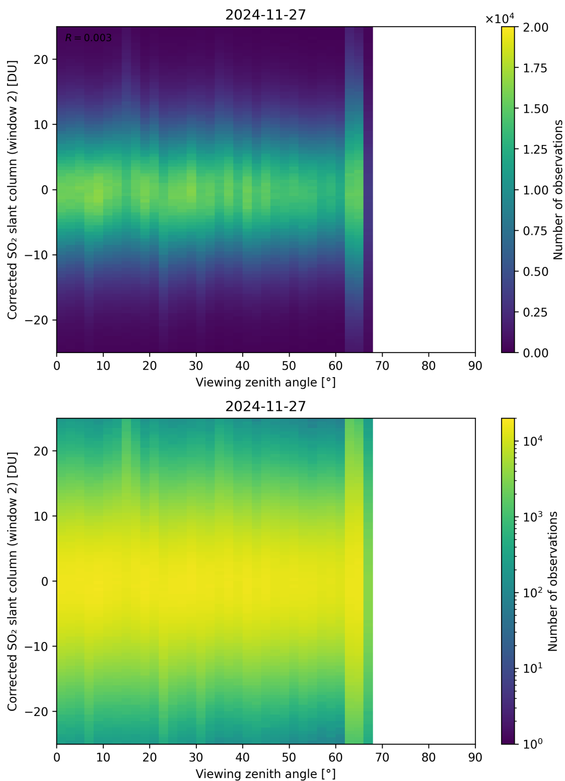
Figure 374: Scatter density plot of “Viewing zenith angle” against “Corrected SO 2 slant column (window 2)” for 2024-11-26 to 2024-11-28.
