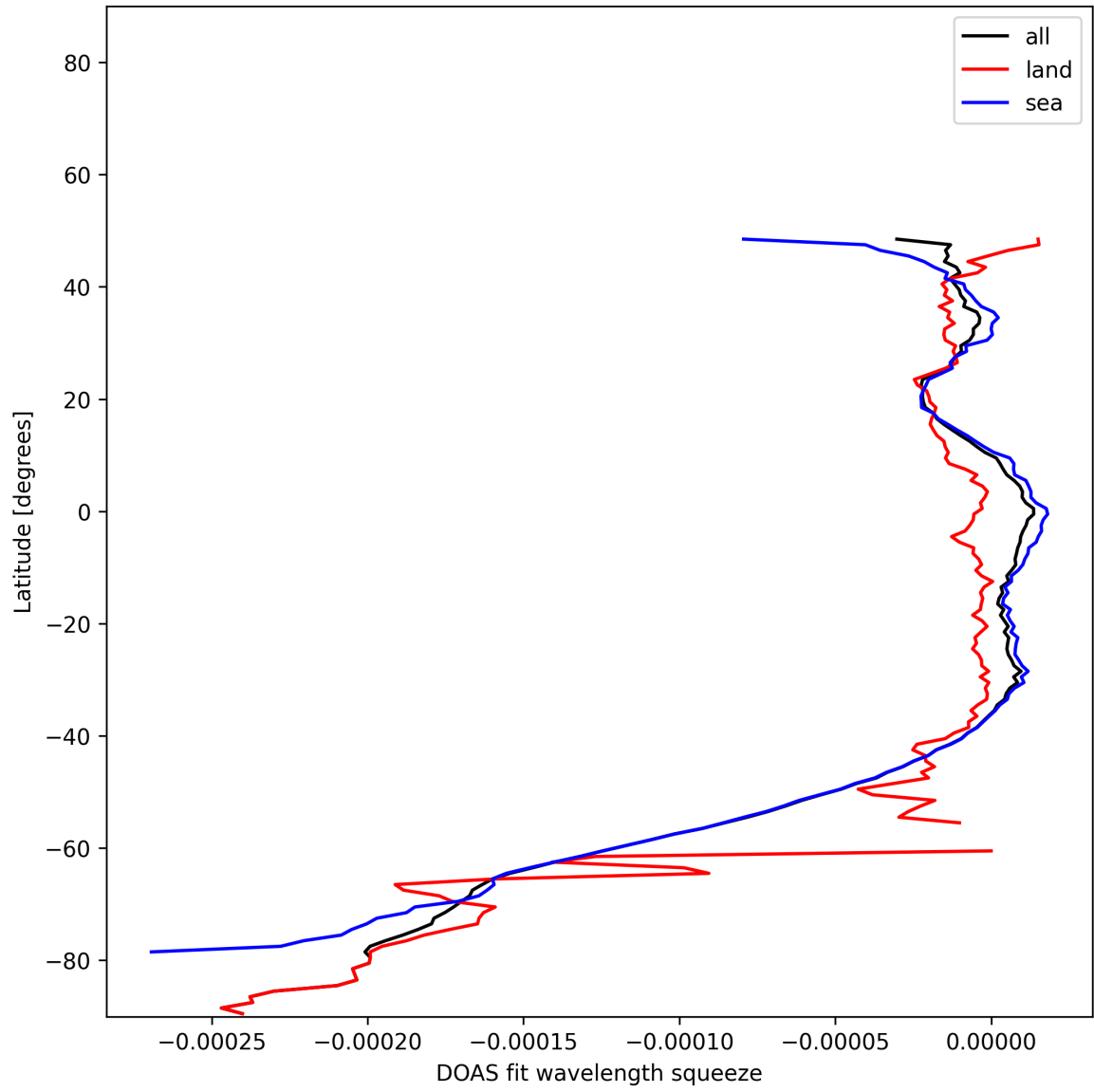
Figure 51: Zonal average of “DOAS fit wavelength squeeze” for 2024-11-26 to 2024-11-28.
