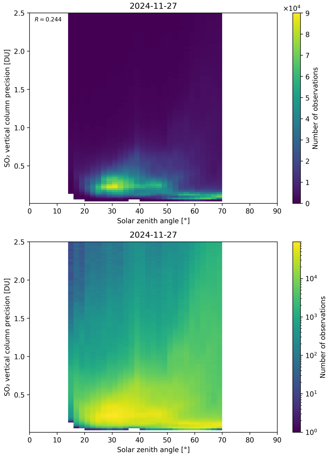
Figure 192: Scatter density plot of “Solar zenith angle” against “SO 2 vertical column precision” for 2024-11-26 to 2024-11-28.
