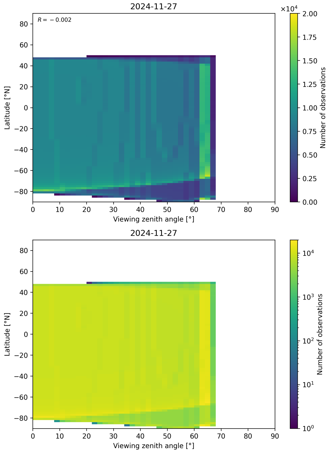
Figure 368: Scatter density plot of “Viewing zenith angle” against “Latitude” for 2024-11-26 to 2024-11-28.
