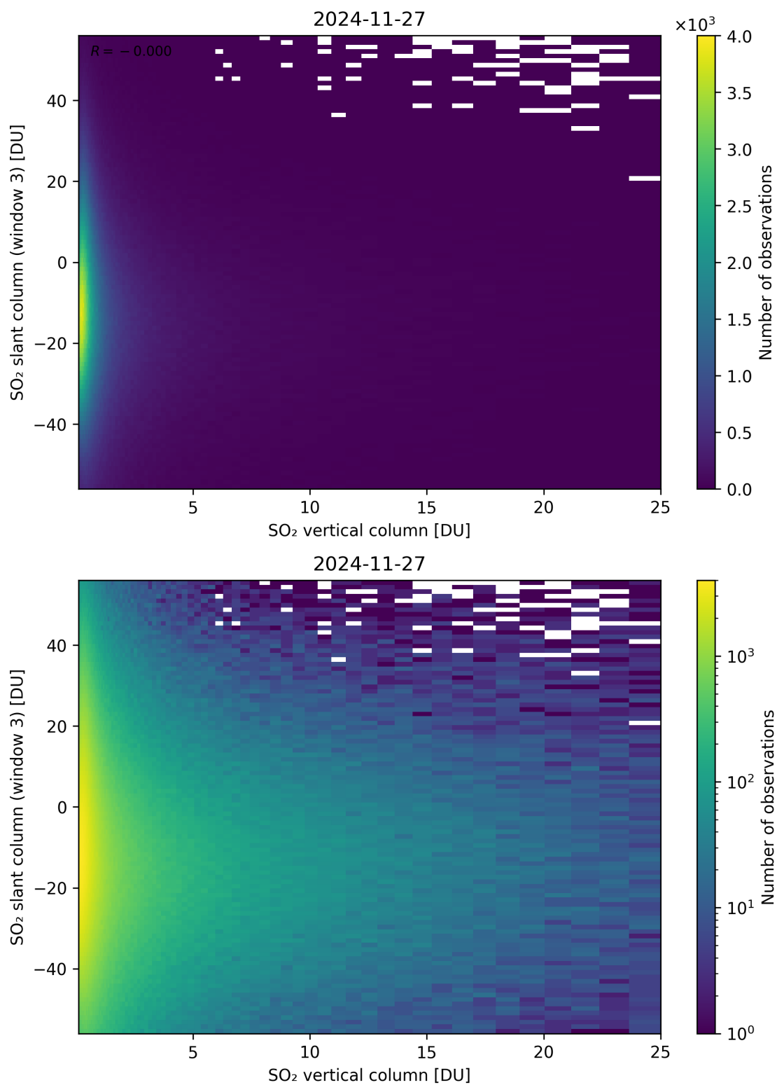
Figure 357: Scatter density plot of “SO 2 vertical column” against “SO 2 slant column (window 3)” for 2024-11-26 to 2024-11-28.
