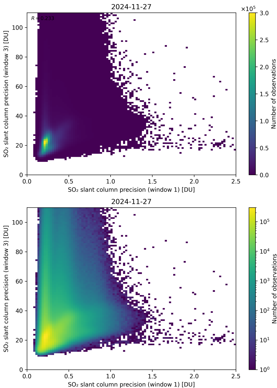
Figure 279: Scatter density plot of “SO 2 slant column precision (window 1)” against “SO 2 slant column precision (window 3)” for 2024-11-26 to 2024-11-28.
