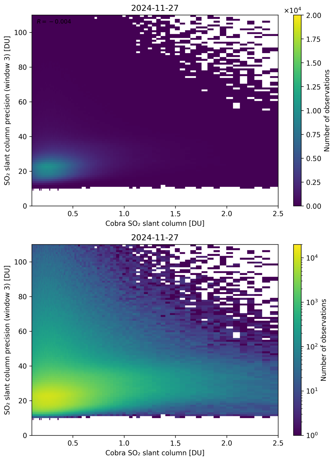
Figure 223: Scatter density plot of “Cobra SO 2 slant column” against “SO 2 slant column precision (window 3)” for 2024-11-26 to 2024-11-28.
