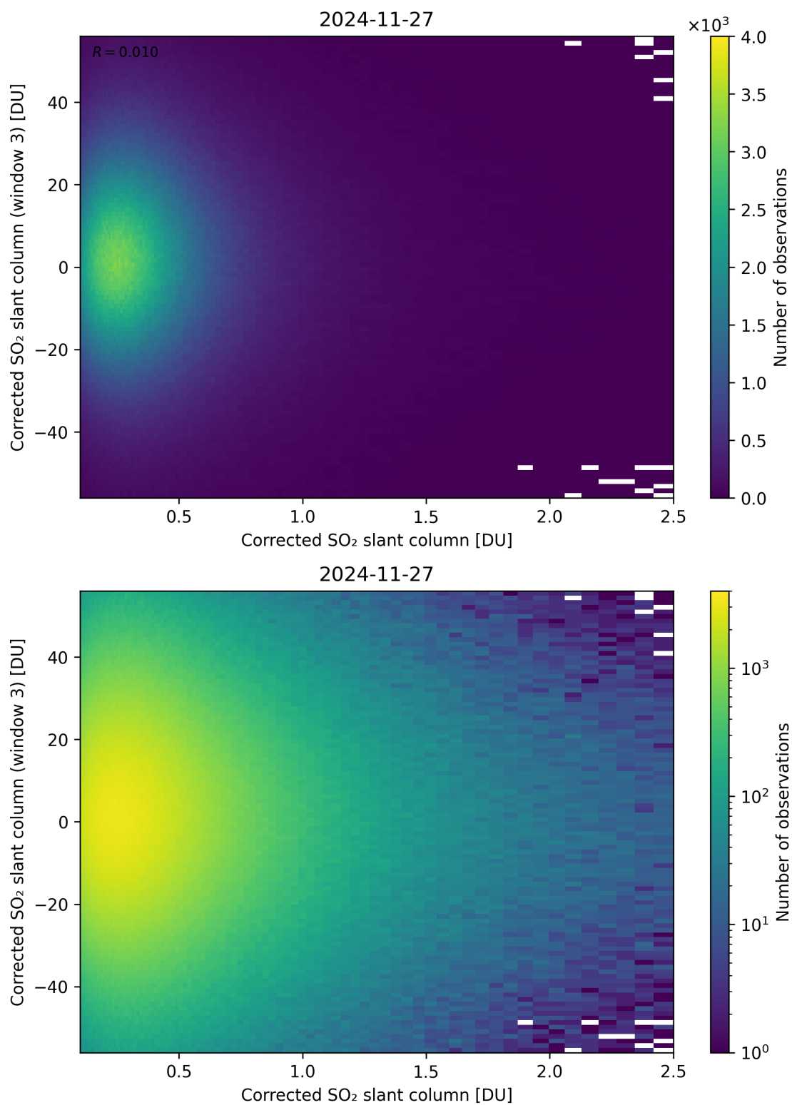
Figure 236: Scatter density plot of “Corrected SO 2 slant column” against “Corrected SO 2 slant column (window 3)” for 2024-11-26 to 2024-11-28.
