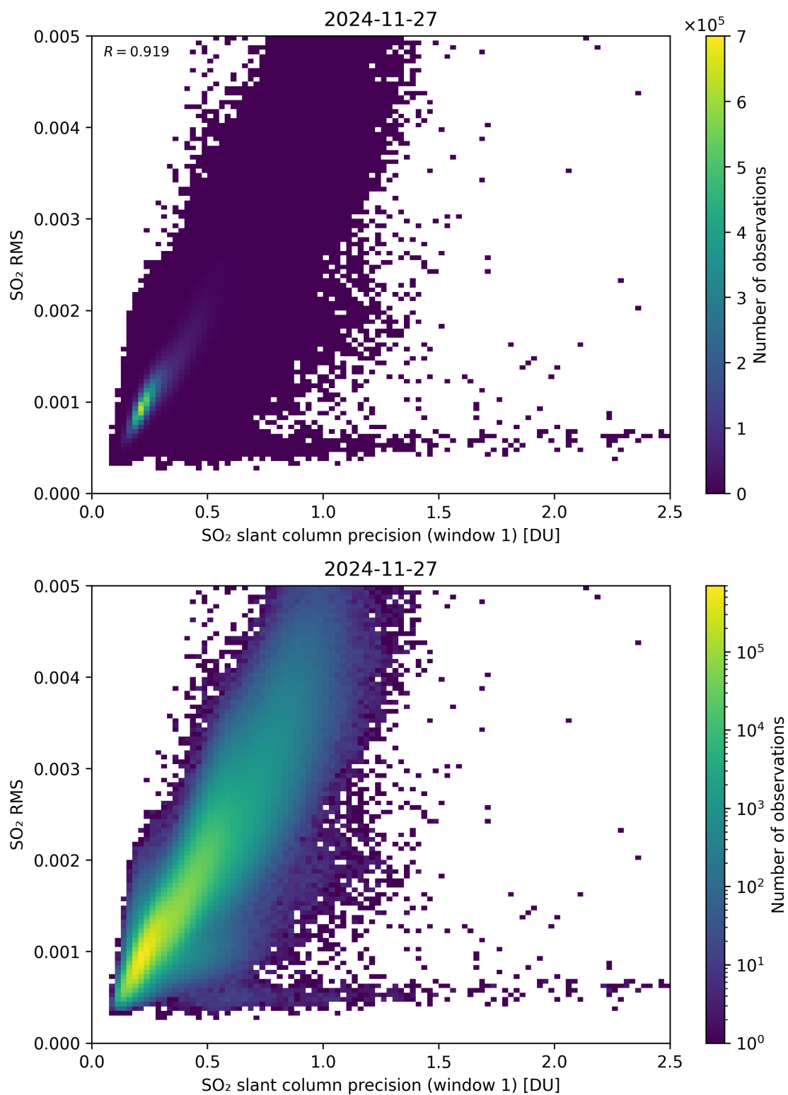
Figure 273: Scatter density plot of “SO 2 slant column precision (window 1)” against “SO 2 RMS” for 2024-11-26 to 2024-11-28.
