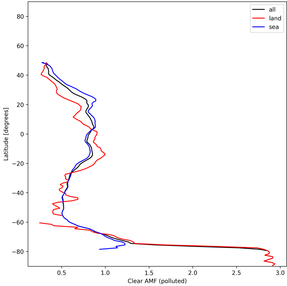
Figure 55: Zonal average of “Clear AMF (polluted)” for 2024-11-26 to 2024-11-28.
