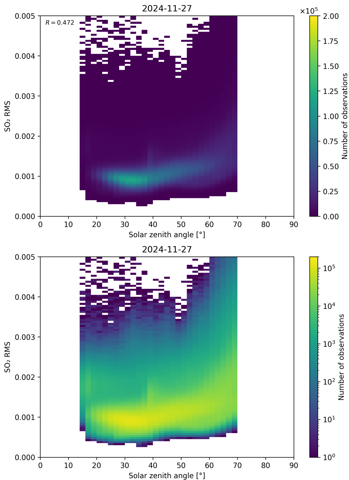
Figure 176: Scatter density plot of “Solar zenith angle” against “SO 2 RMS” for 2024-11-26 to 2024-11-28.
