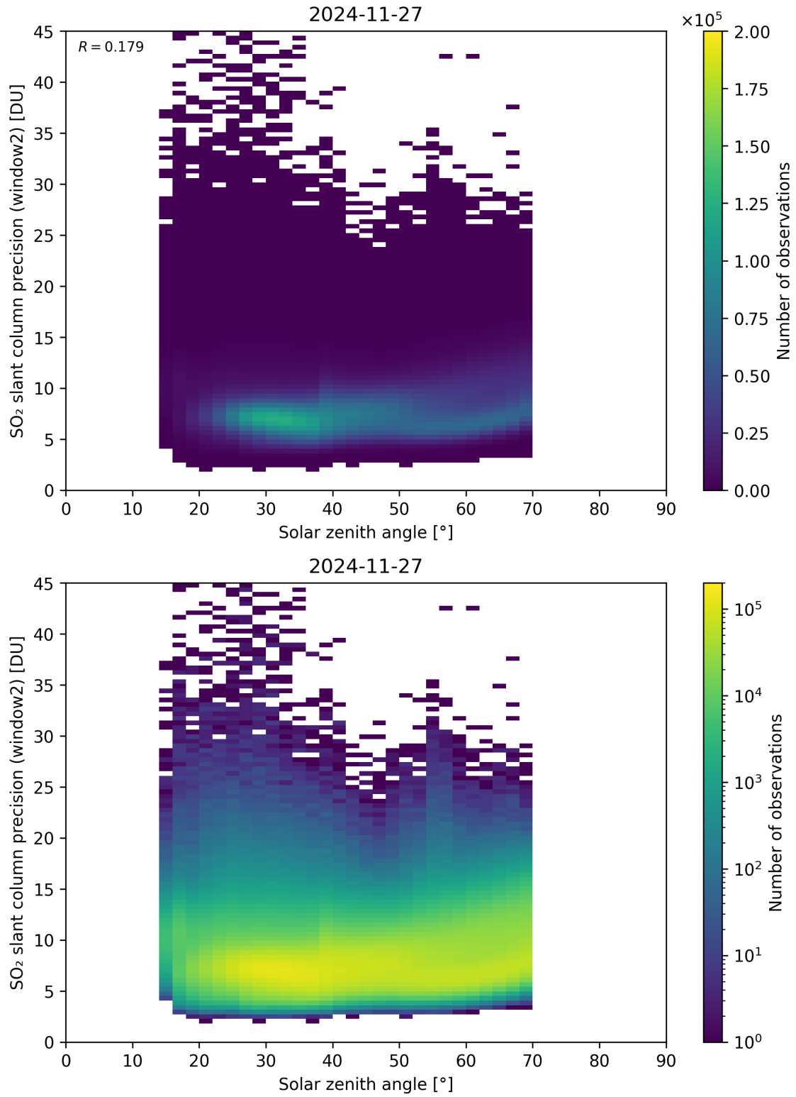
Figure 186: Scatter density plot of “Solar zenith angle” against “SO 2 slant column precision (window2)” for 2024-11-26 to 2024-11-28.
