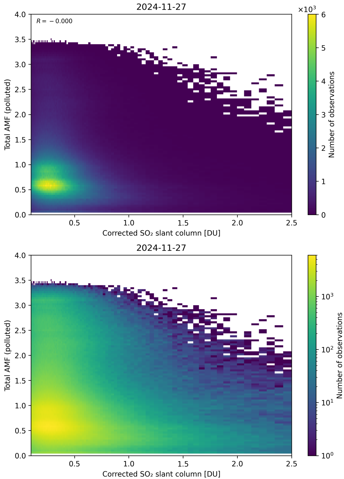
Figure 242: Scatter density plot of “Corrected SO 2 slant column” against “Total AMF (polluted)” for 2024-11-26 to 2024-11-28.
