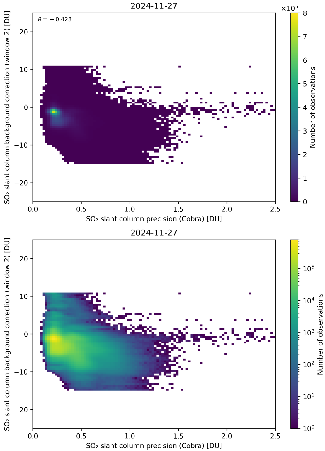
Figure 200: Scatter density plot of “SO 2 slant column precision (Cobra)” against “SO 2 slant column background correction (window 2)” for 2024-11-26 to 2024-11-28.
