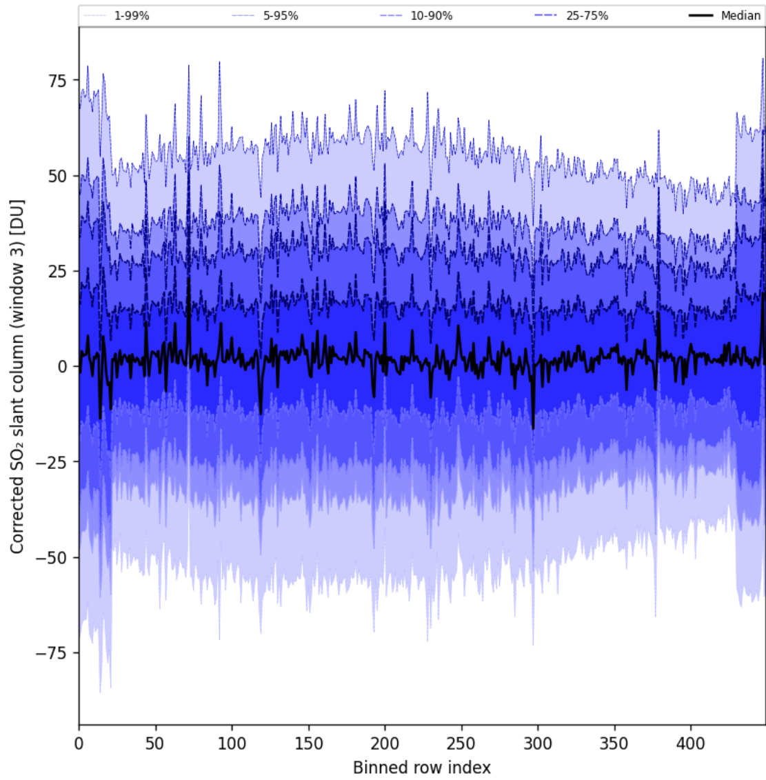
Figure 99: Along track statistics of “Corrected SO 2 slant column (window 3)” for 2024-11-26 to 2024-11-28
