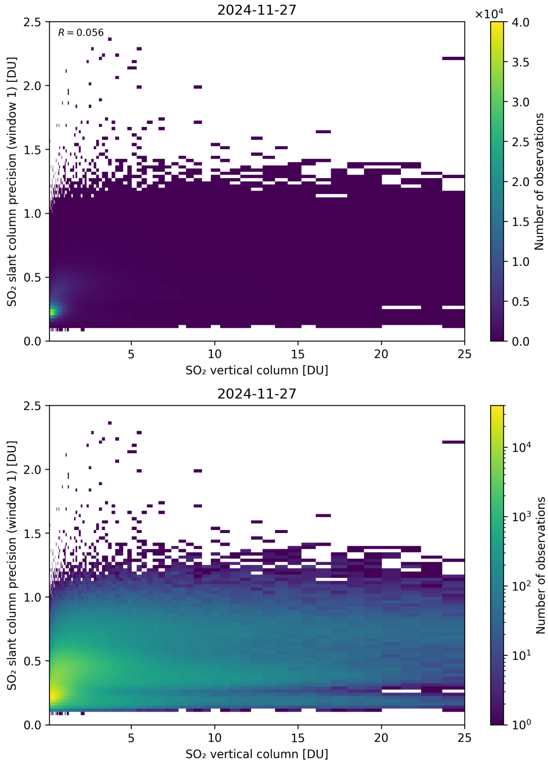
Figure 355: Scatter density plot of “SO 2 vertical column” against “SO 2 slant column precision (window 1)” for 2024-11-26 to 2024-11-28.
