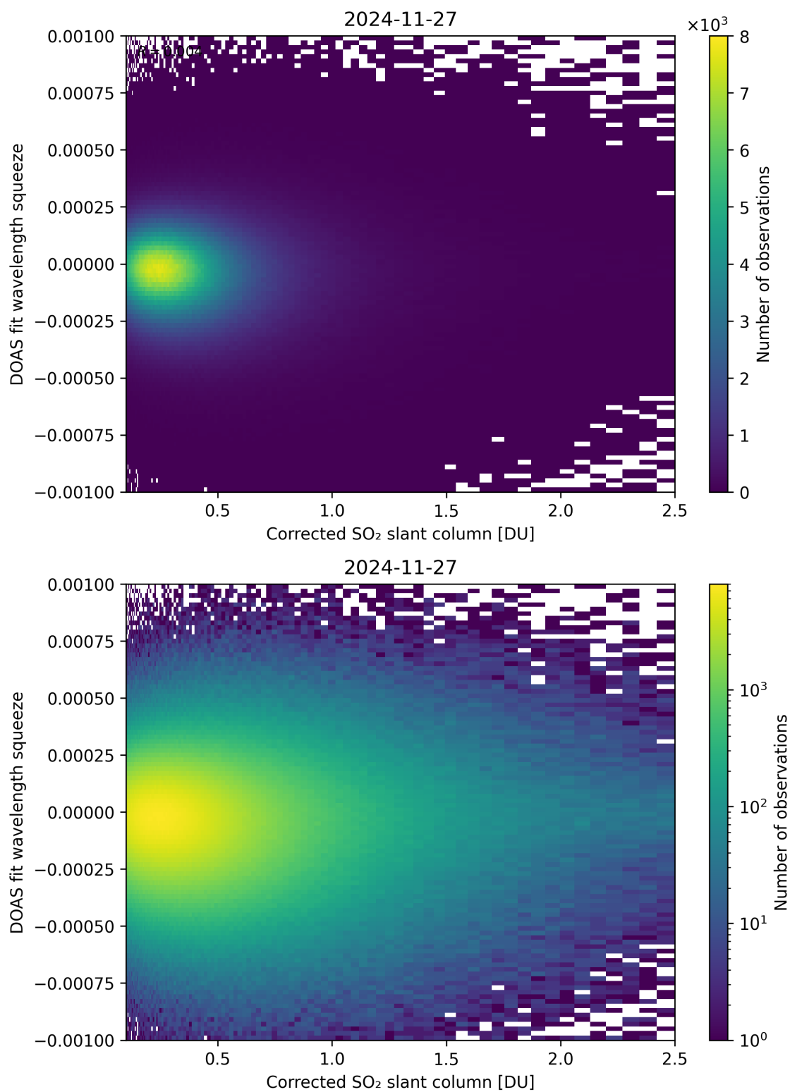
Figure 230: Scatter density plot of “Corrected SO 2 slant column” against “DOAS fit wavelength squeeze” for 2024-11-26 to 2024-11-28.
