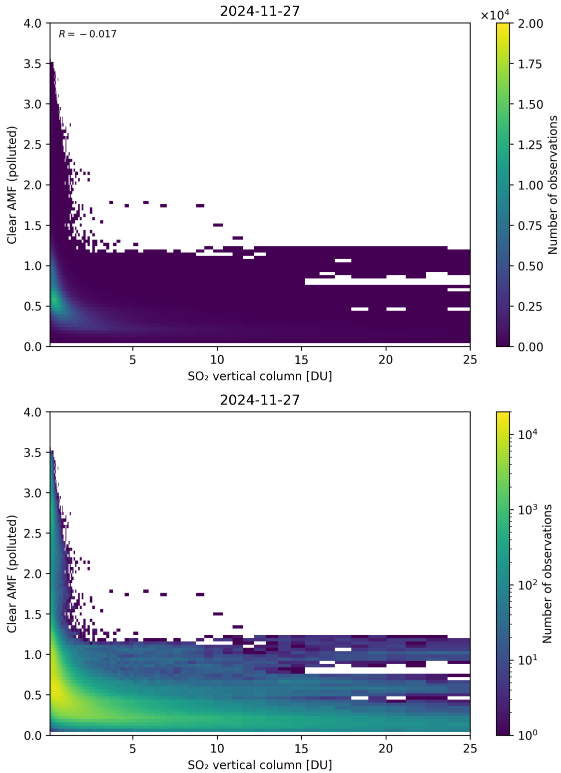
Figure 348: Scatter density plot of “SO 2 vertical column” against “Clear AMF (polluted)” for 2024-11-26 to 2024-11-28.
