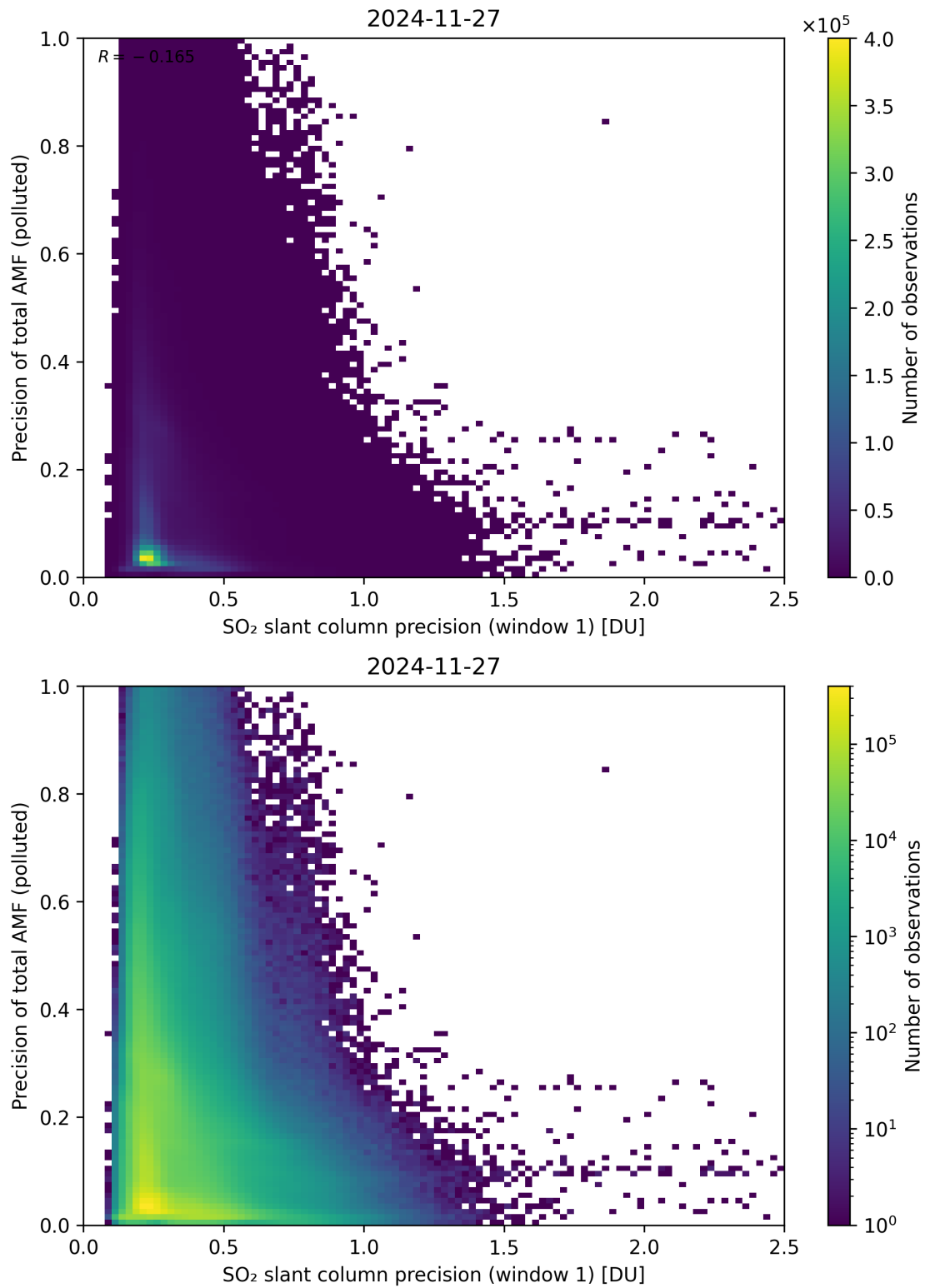
Figure 281: Scatter density plot of “SO 2 slant column precision (window 1)” against “Precision of total AMF (polluted)” for 2024-11-26 to 2024-11-28.
