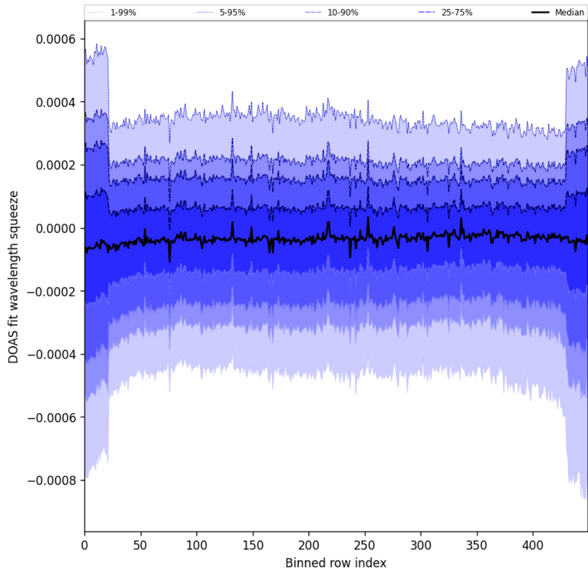
Figure 103: Along track statistics of “DOAS fit wavelength squeeze” for 2024-11-26 to 2024-11-28
