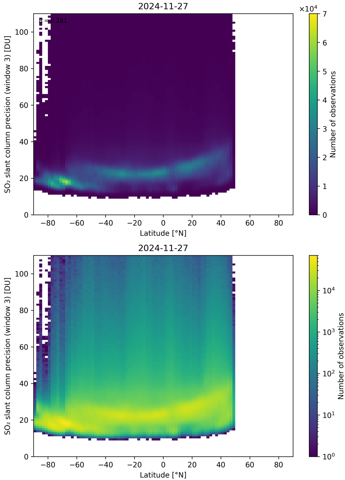
Figure 166: Scatter density plot of “Latitude” against “SO 2 slant column precision (window 3)” for 2024-11-26 to 2024-11-28.
