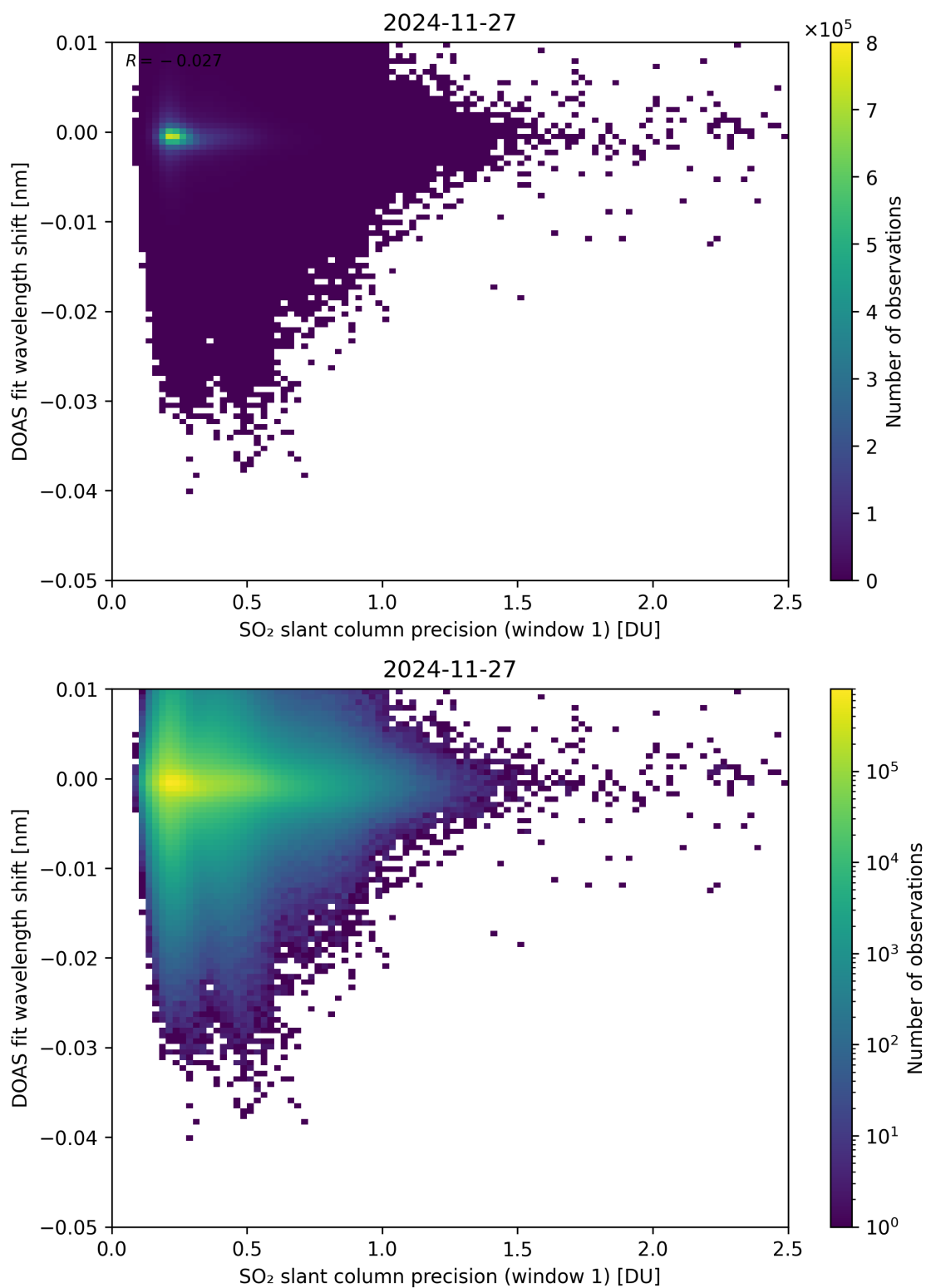
Figure 271: Scatter density plot of “SO 2 slant column precision (window 1)” against “DOAS fit wavelength shift” for 2024-11-26 to 2024-11-28.
