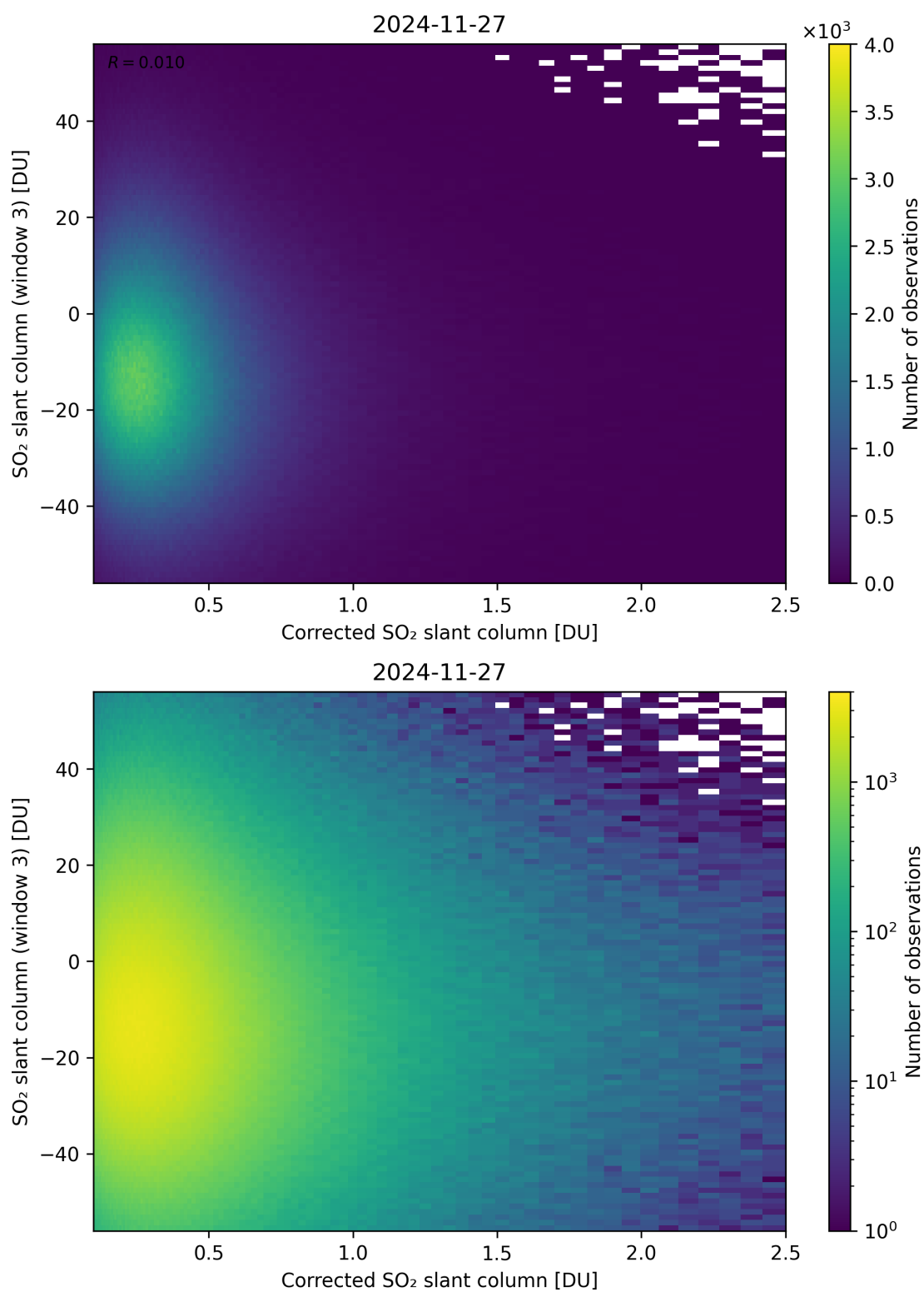
Figure 240: Scatter density plot of “Corrected SO 2 slant column” against “SO 2 slant column (window 3)” for 2024-11-26 to 2024-11-28.
