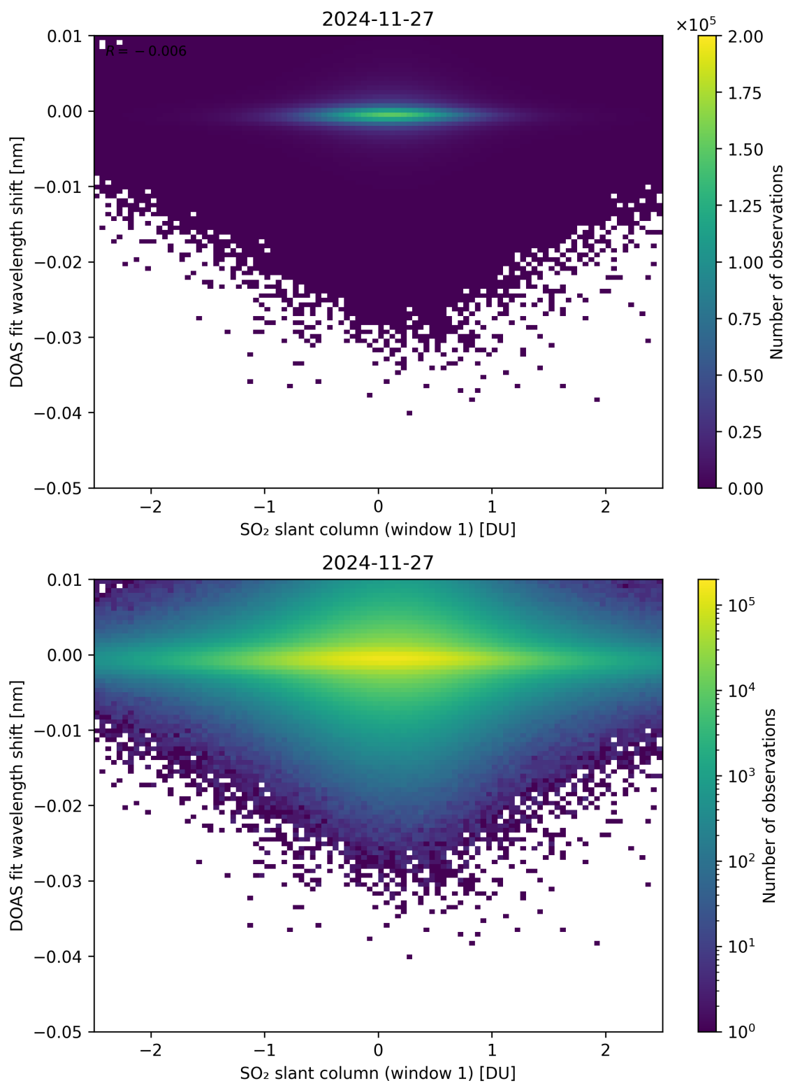
Figure 265: Scatter density plot of “SO 2 slant column (window 1)” against “DOAS fit wavelength shift” for 2024-11-26 to 2024-11-28.
