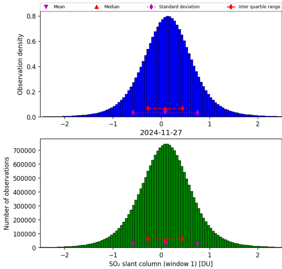
Figure 63: Histogram of “SO 2 slant column (window 1)” for 2024-11-26 to 2024-11-28
