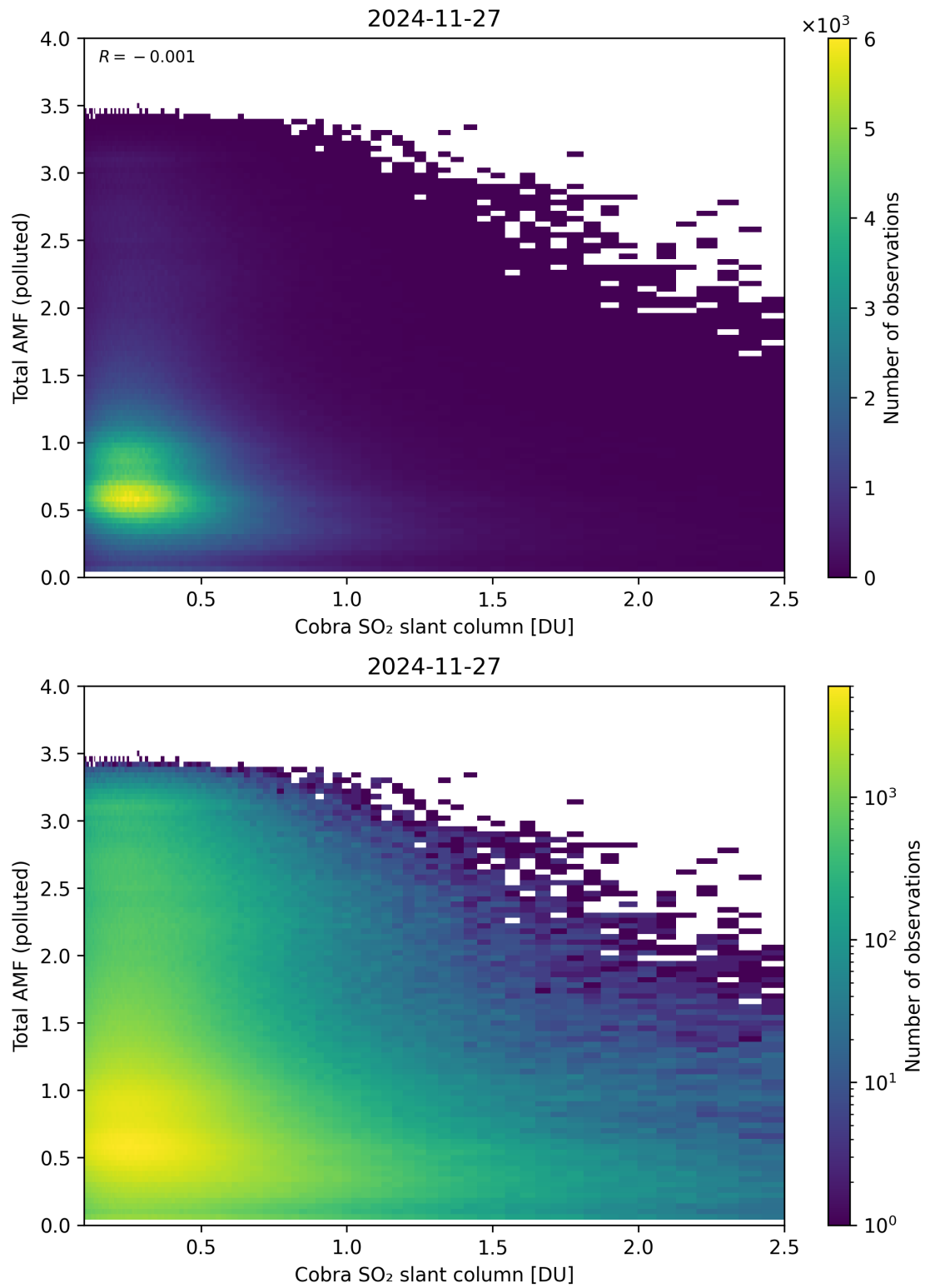
Figure 224: Scatter density plot of “Cobra SO 2 slant column” against “Total AMF (polluted)” for 2024-11-26 to 2024-11-28.
