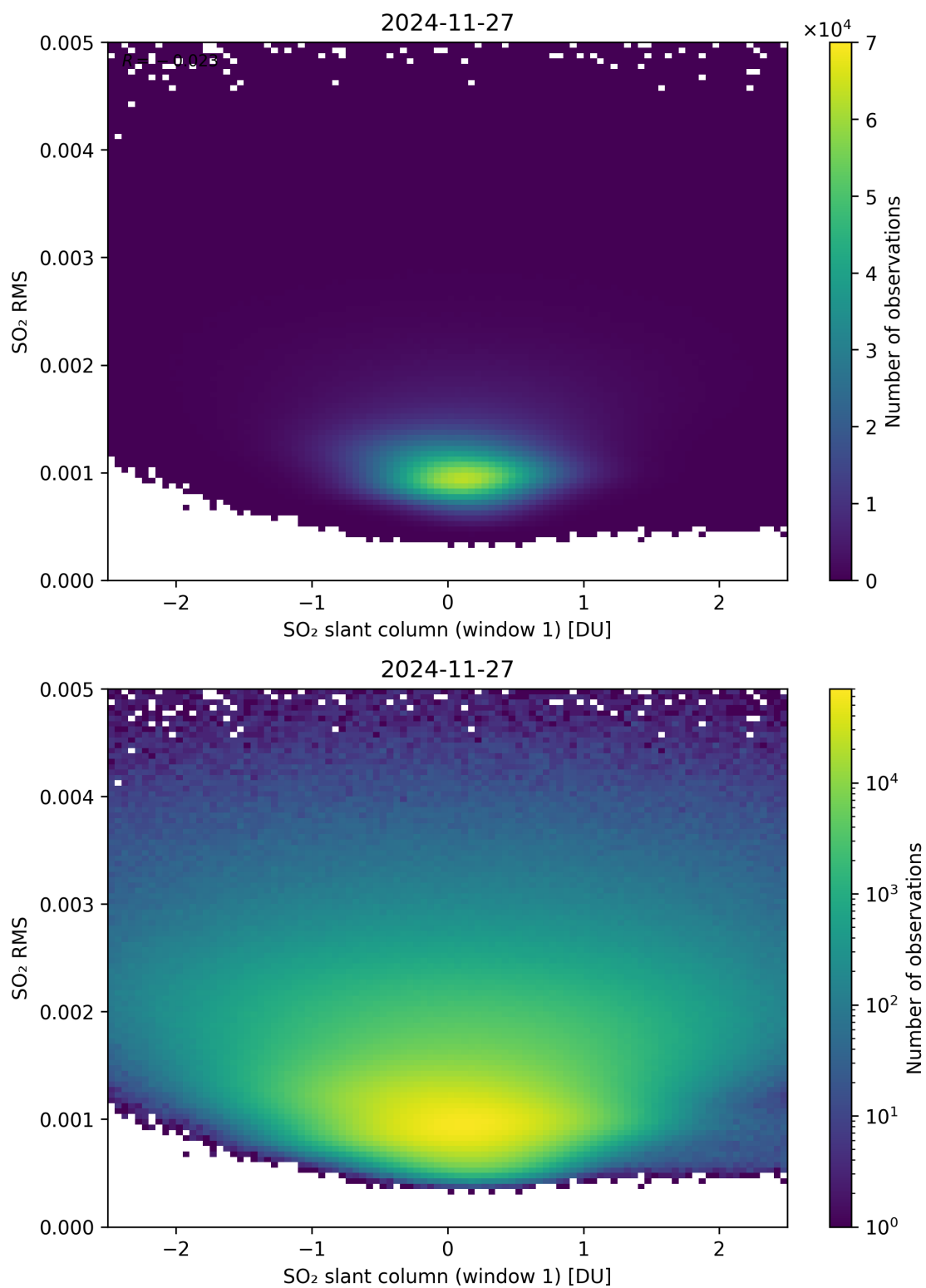
Figure 267: Scatter density plot of “SO 2 slant column (window 1)” against “SO 2 RMS” for 2024-11-26 to 2024-11-28.
