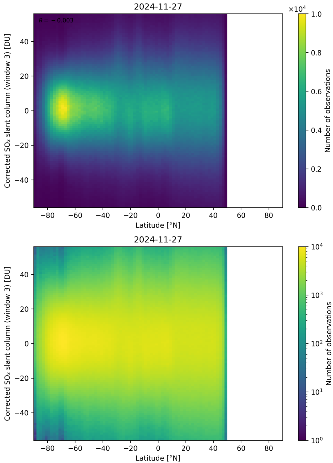
Figure 161: Scatter density plot of “Latitude” against “Corrected SO 2 slant column (window 3)” for 2024-11-26 to 2024-11-28.
