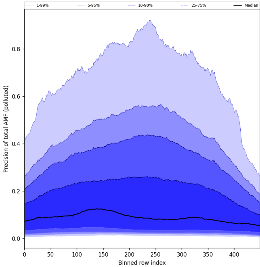
Figure 106: Along track statistics of “Precision of total AMF (polluted)” for 2024-11-26 to 2024-11-28
