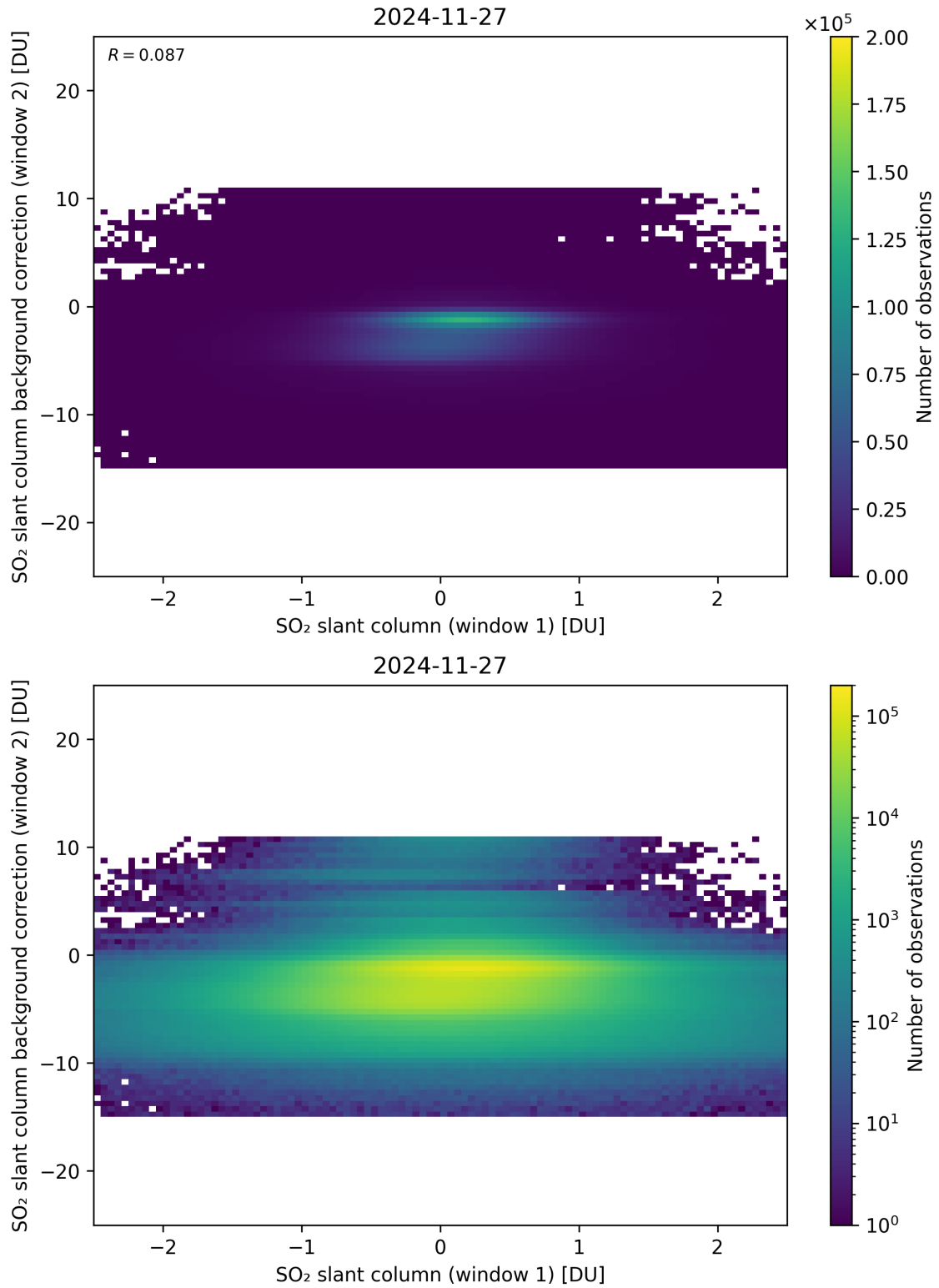
Figure 263: Scatter density plot of “SO 2 slant column (window 1)” against “SO 2 slant column background correction (window 2)” for 2024-11-26 to 2024-11-28.
