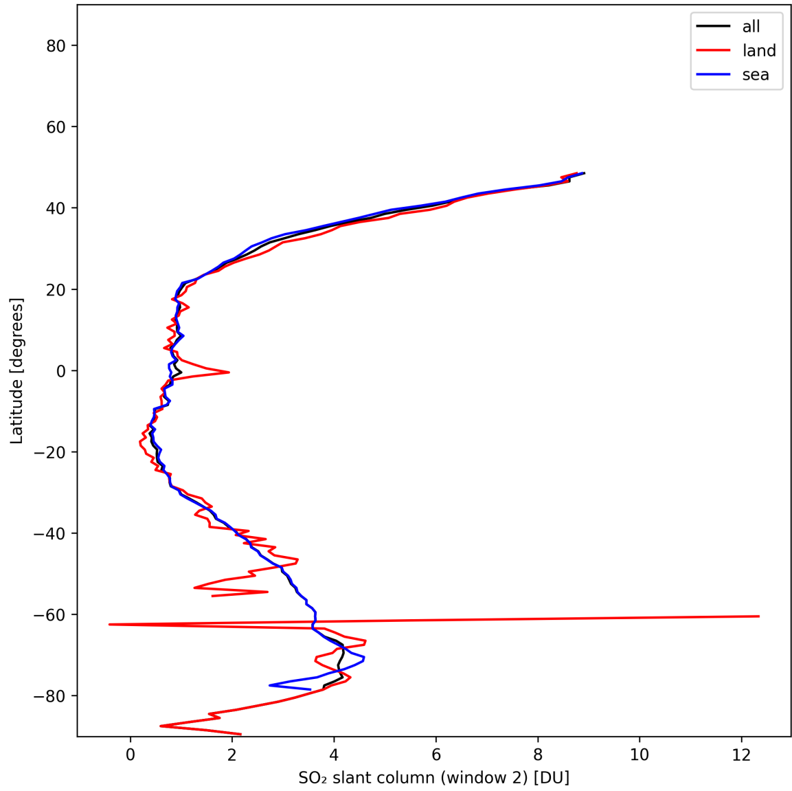
Figure 41: Zonal average of “SO 2 slant column (window 2)” for 2024-11-26 to 2024-11-28.
