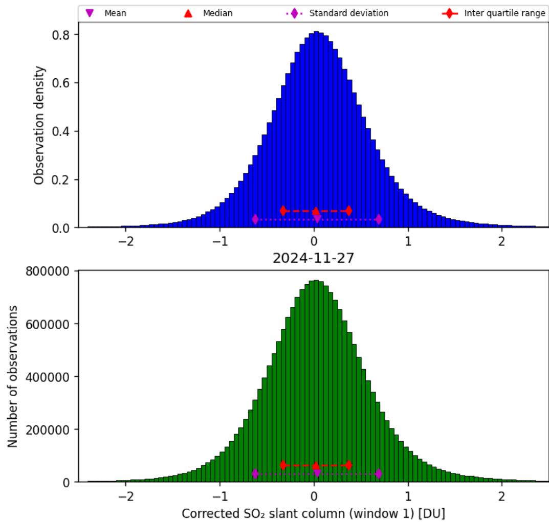
Figure 65: Histogram of “Corrected SO 2 slant column (window 1)” for 2024-11-26 to 2024-11-28
