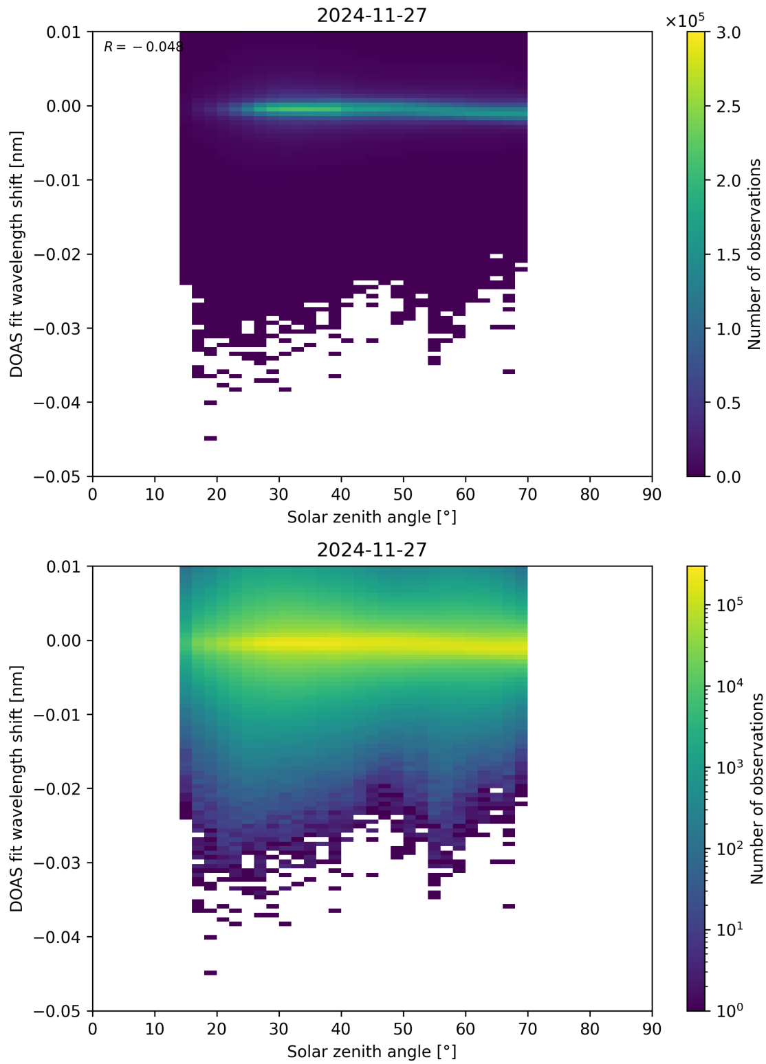
Figure 174: Scatter density plot of “Solar zenith angle” against “DOAS fit wavelength shift” for 2024-11-26 to 2024-11-28.
