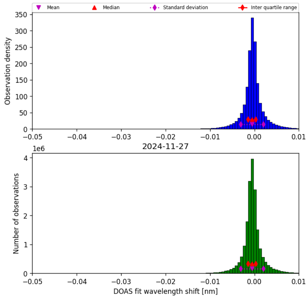
Figure 76: Histogram of “DOAS fit wavelength shift” for 2024-11-26 to 2024-11-28
