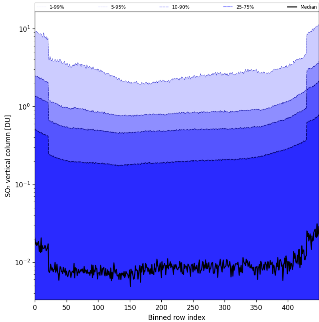
Figure 84: Along track statistics of “SO 2 vertical column” for 2024-11-26 to 2024-11-28
