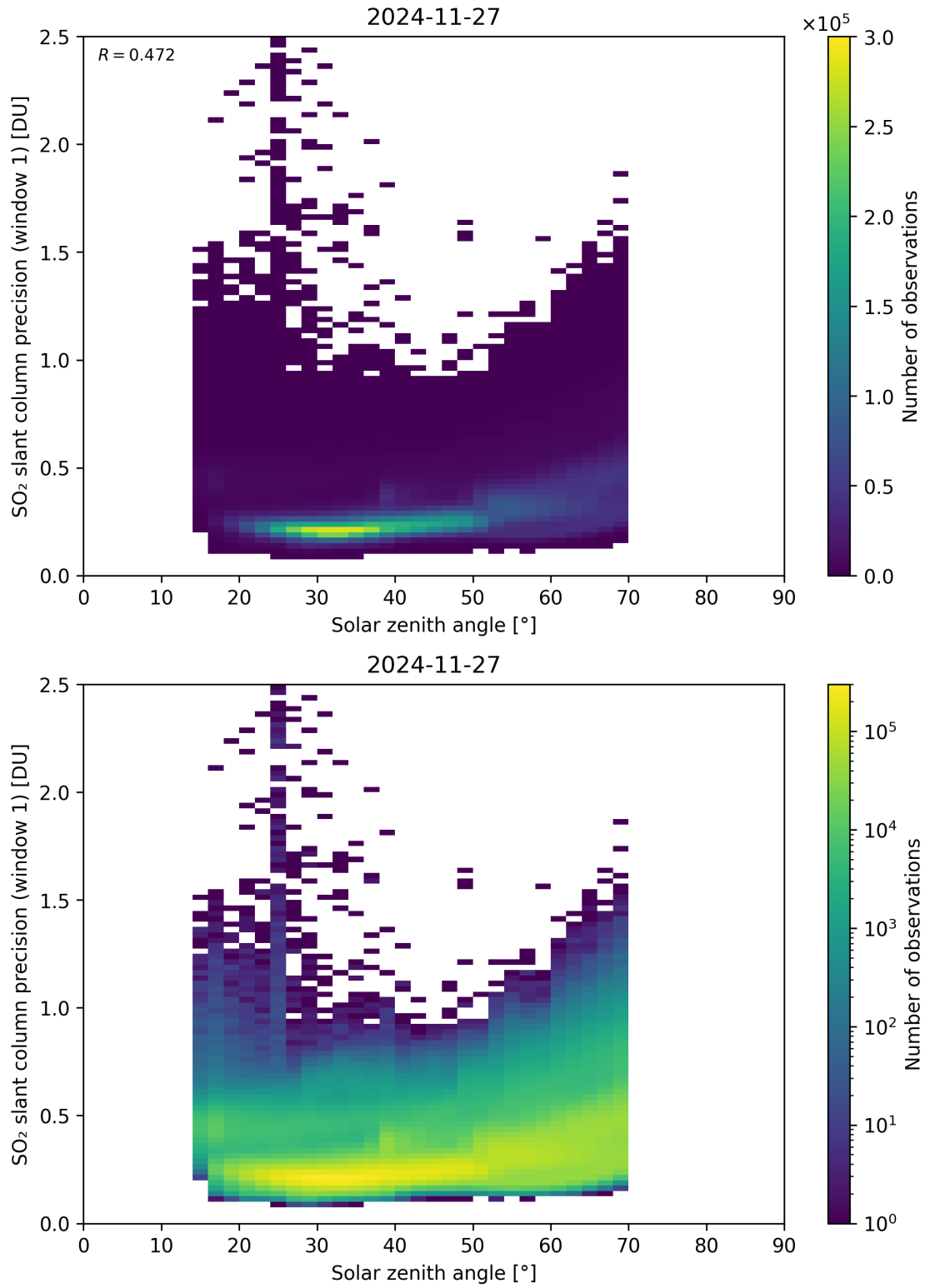
Figure 185: Scatter density plot of “Solar zenith angle” against “SO 2 slant column precision (window 1)” for 2024-11-26 to 2024-11-28.
