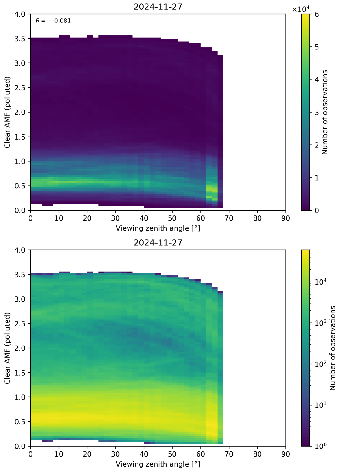
Figure 370: Scatter density plot of “Viewing zenith angle” against “Clear AMF (polluted)” for 2024-11-26 to 2024-11-28.
