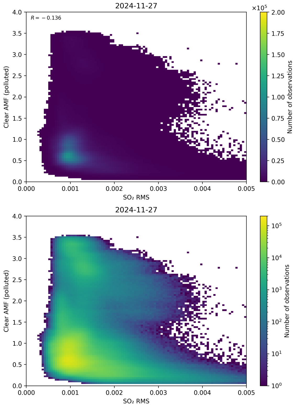
Figure 147: Scatter density plot of “SO 2 RMS” against “Clear AMF (polluted)” for 2024-11-26 to 2024-11-28.
