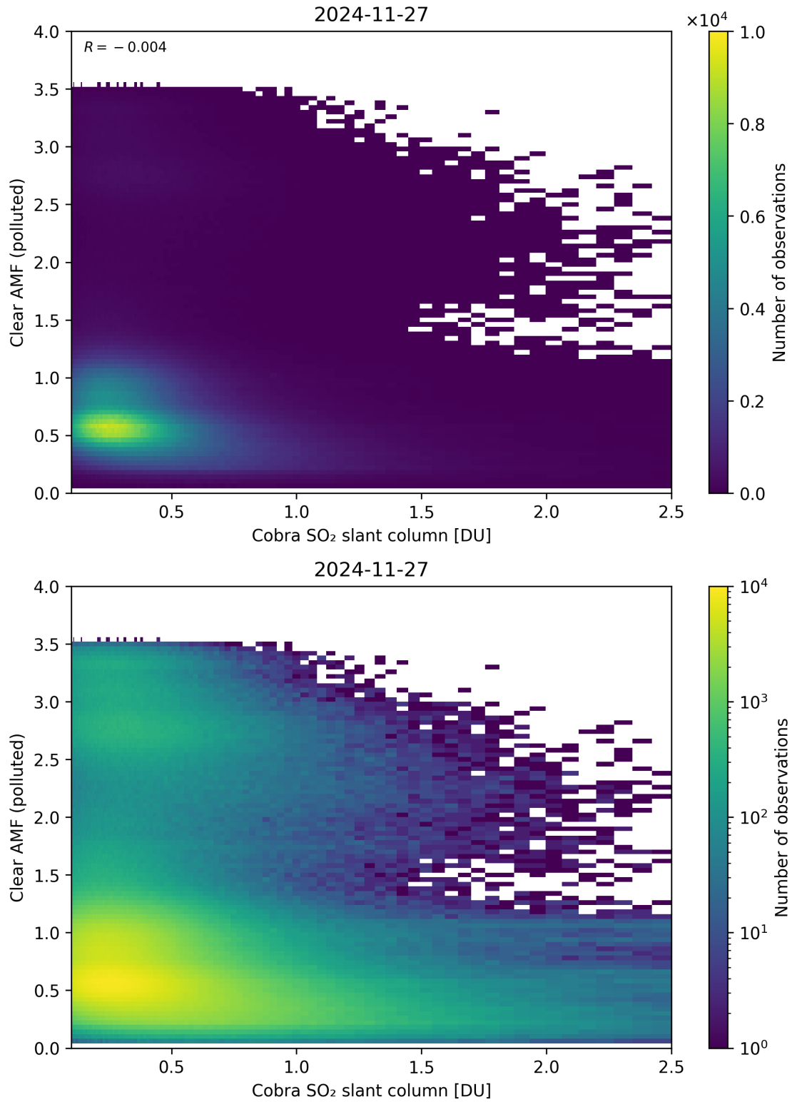
Figure 215: Scatter density plot of “Cobra SO 2 slant column” against “Clear AMF (polluted)” for 2024-11-26 to 2024-11-28.
