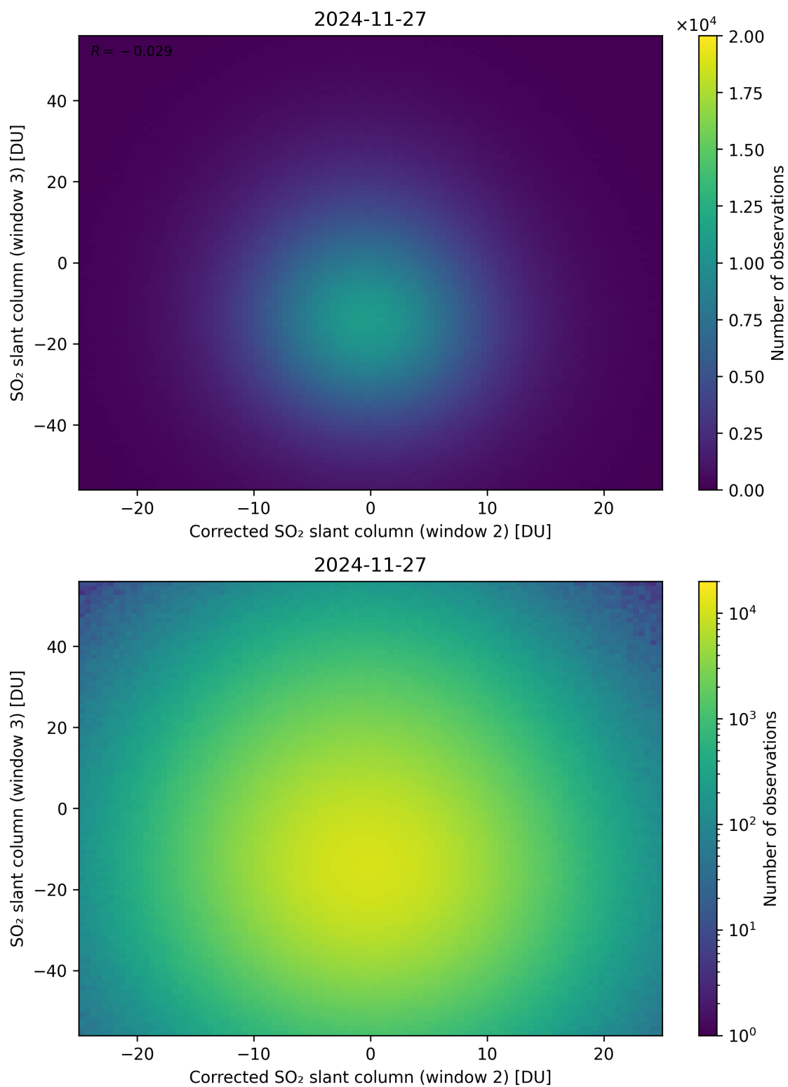
Figure 251: Scatter density plot of “Corrected SO 2 slant column (window 2)” against “SO 2 slant column (window 3)” for 2024-11-26 to 2024-11-28.
