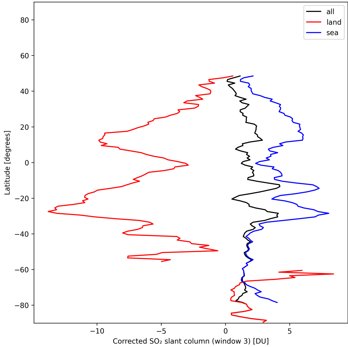
Figure 47: Zonal average of “Corrected SO 2 slant column (window 3)” for 2024-11-26 to 2024-11-28.
