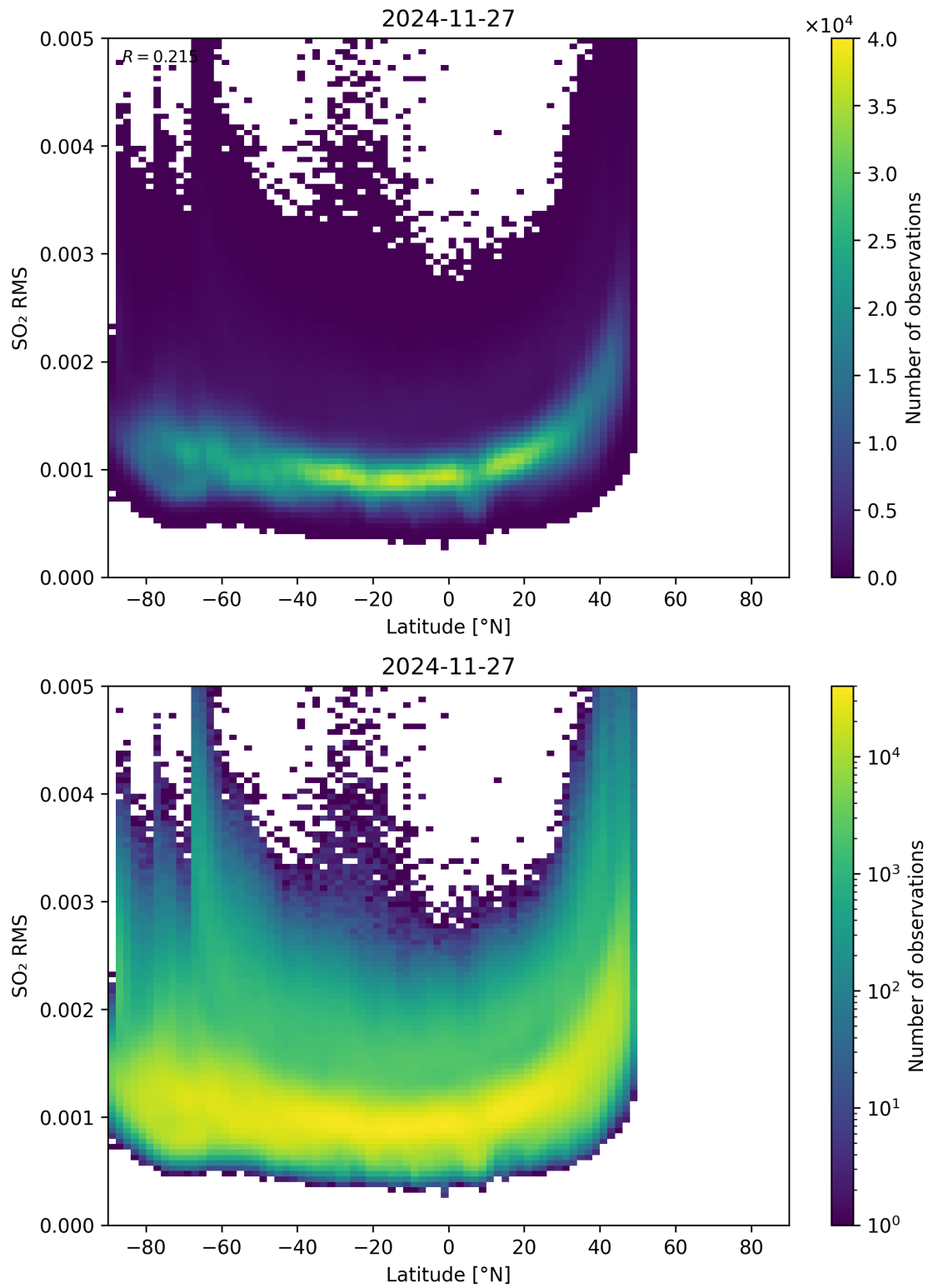
Figure 155: Scatter density plot of “Latitude” against “SO 2 RMS” for 2024-11-26 to 2024-11-28.
