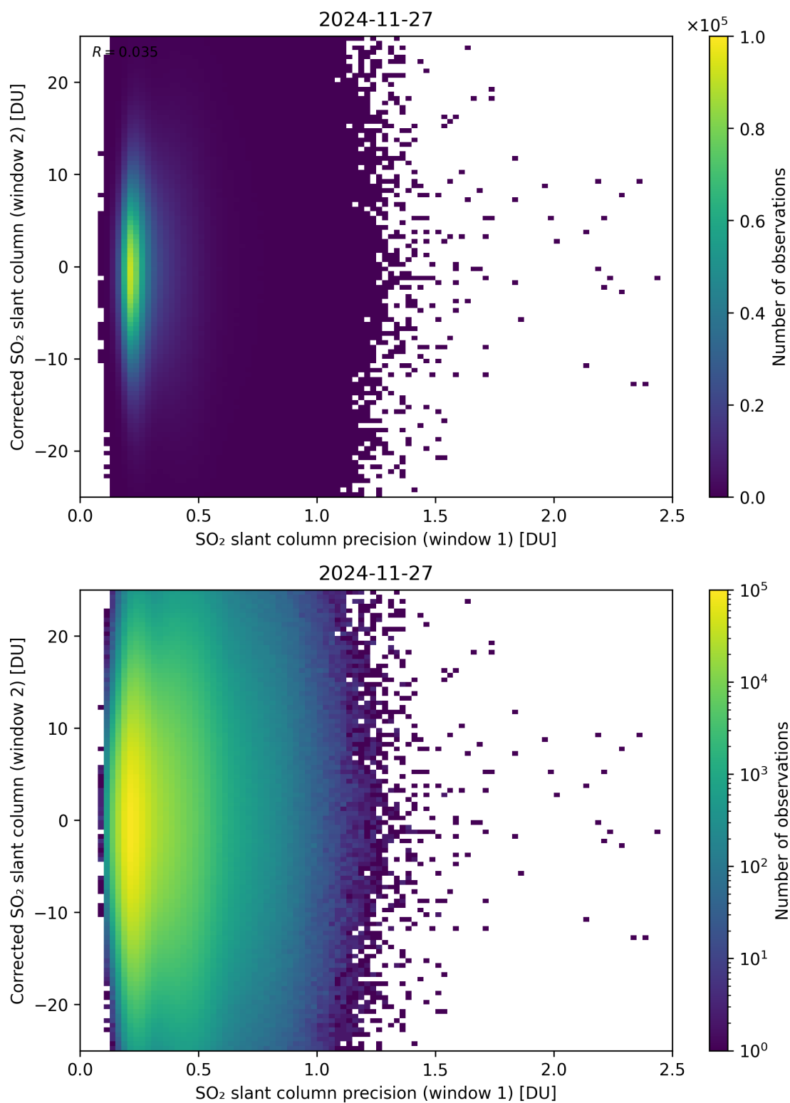
Figure 275: Scatter density plot of “SO 2 slant column precision (window 1)” against “Corrected SO 2 slant column (window 2)” for 2024-11-26 to 2024-11-28.
