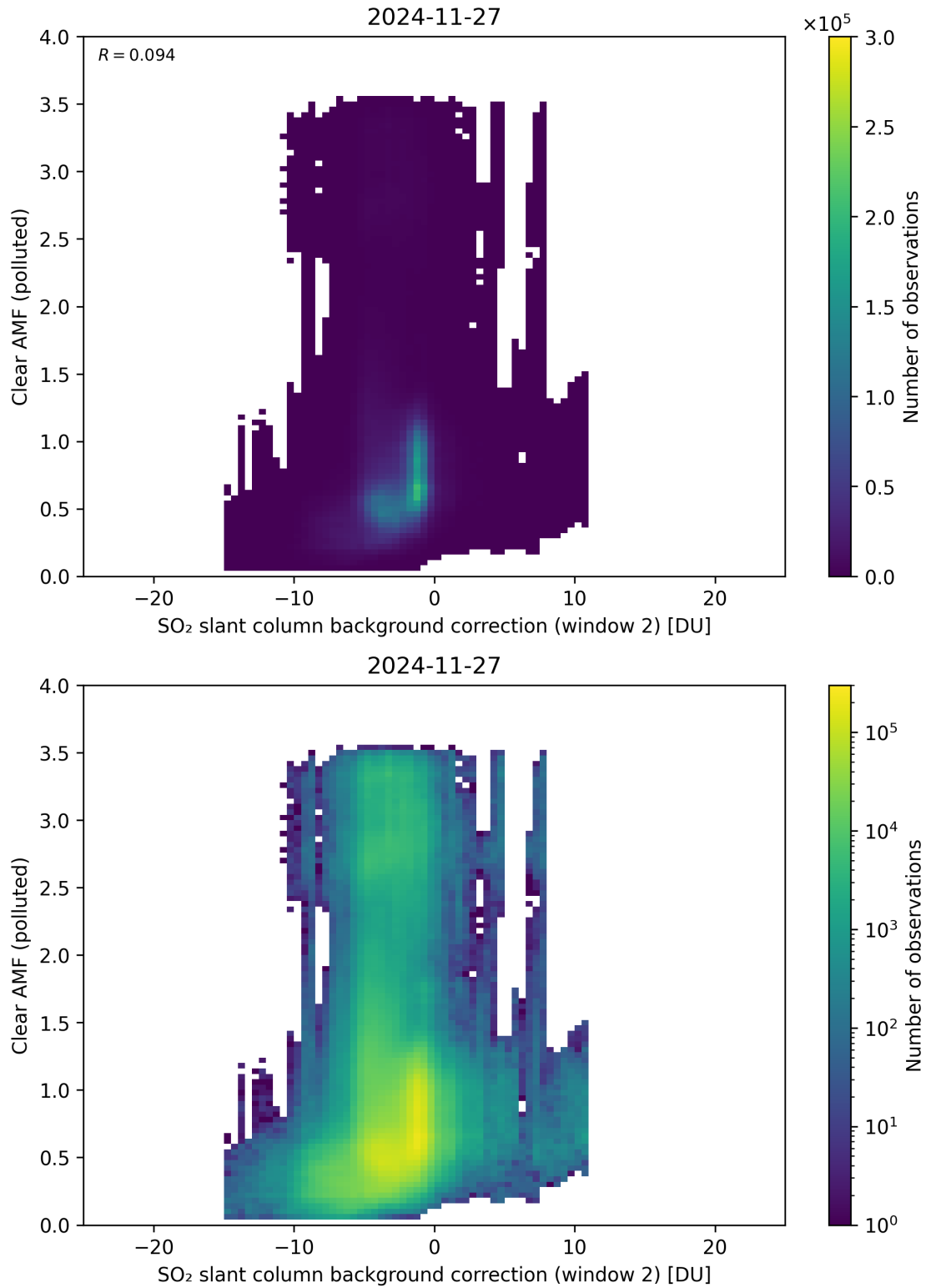
Figure 126: Scatter density plot of “SO 2 slant column background correction (window 2)” against “Clear AMF (polluted)” for 2024-11-26 to 2024-11-28.
