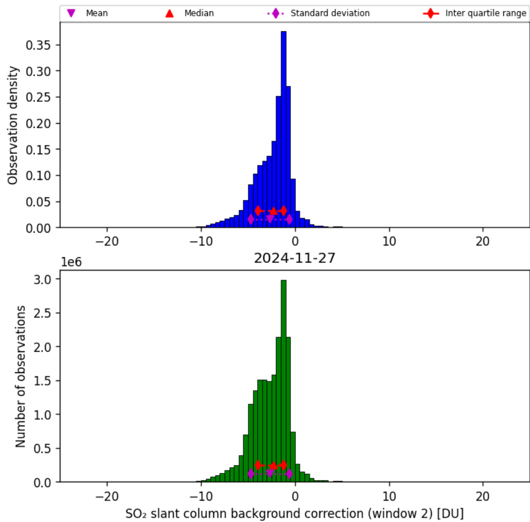
Figure 70: Histogram of “SO 2 slant column background correction (window 2)” for 2024-11-26 to 2024-11-28
