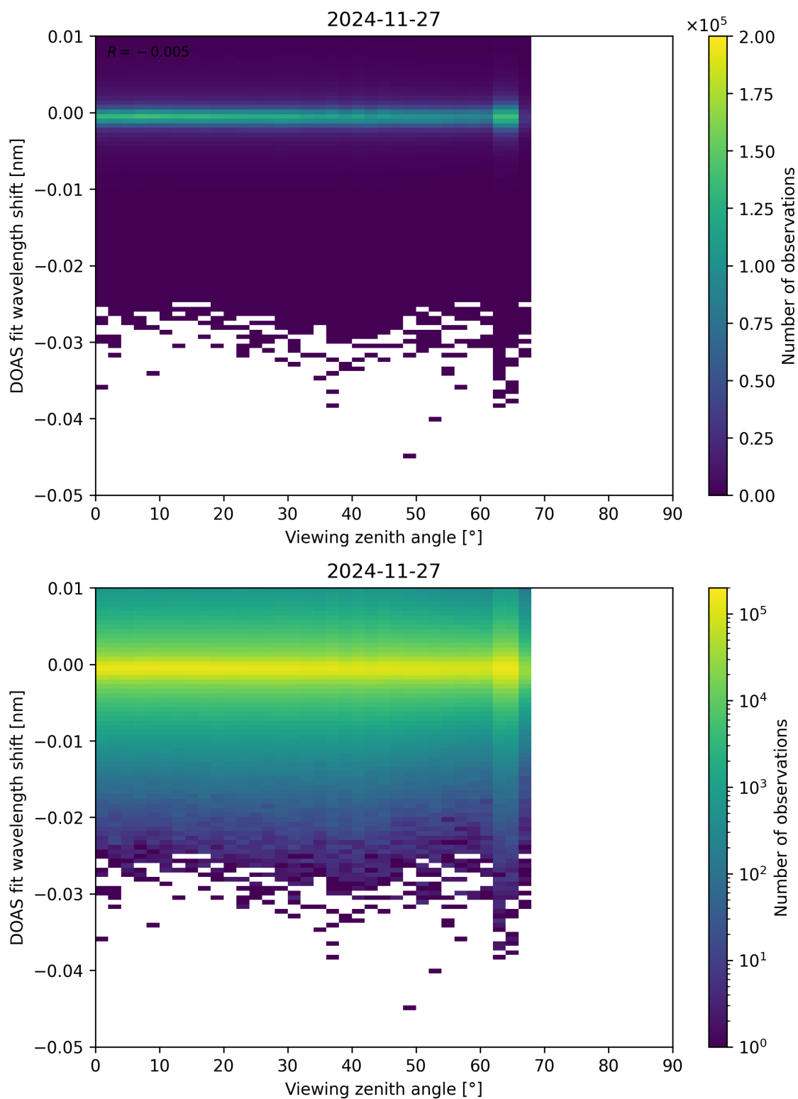
Figure 365: Scatter density plot of “Viewing zenith angle” against “DOAS fit wavelength shift” for 2024-11-26 to 2024-11-28.
