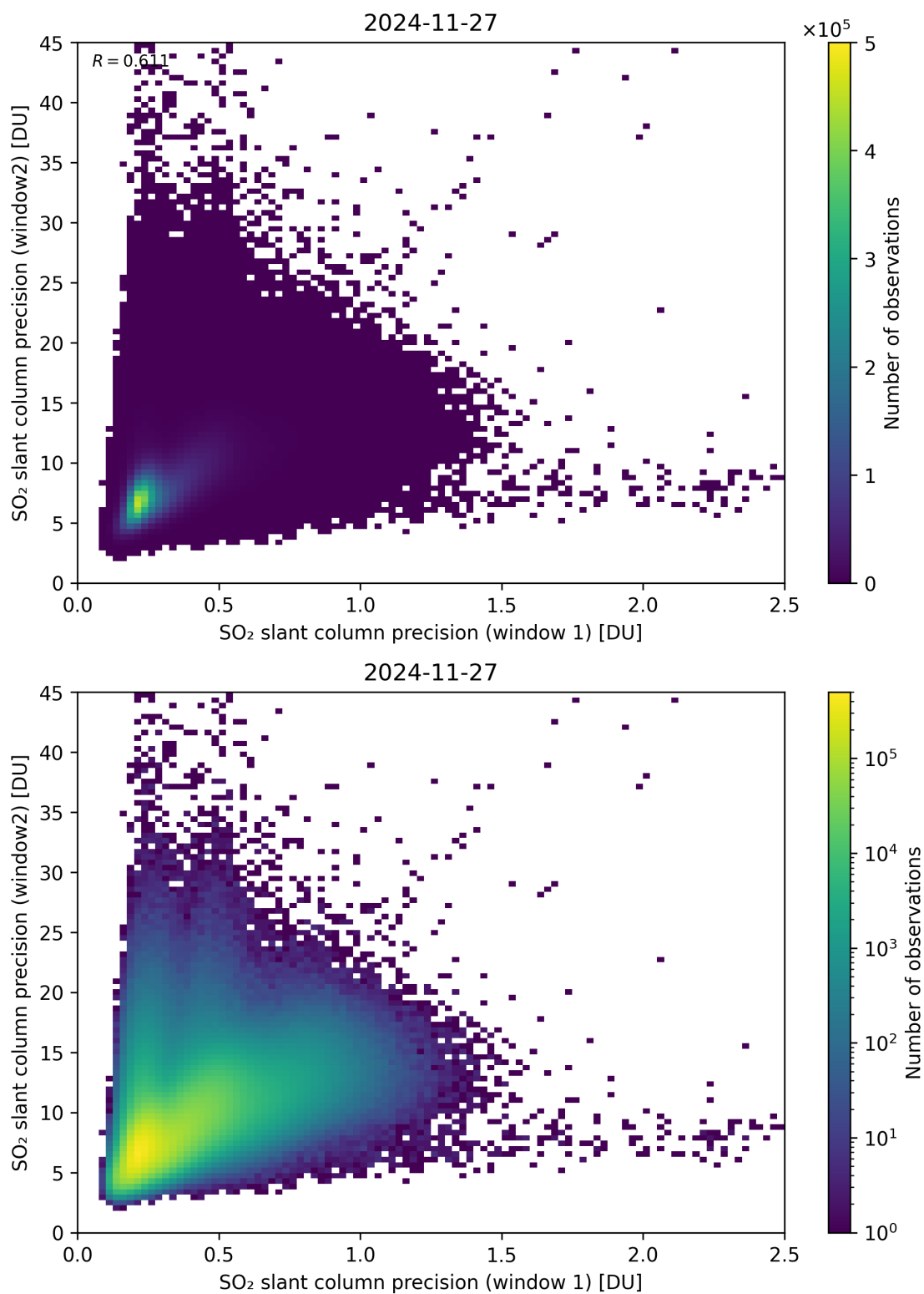
Figure 277: Scatter density plot of “SO 2 slant column precision (window 1)” against “SO 2 slant column precision (window2)” for 2024-11-26 to 2024-11-28.
