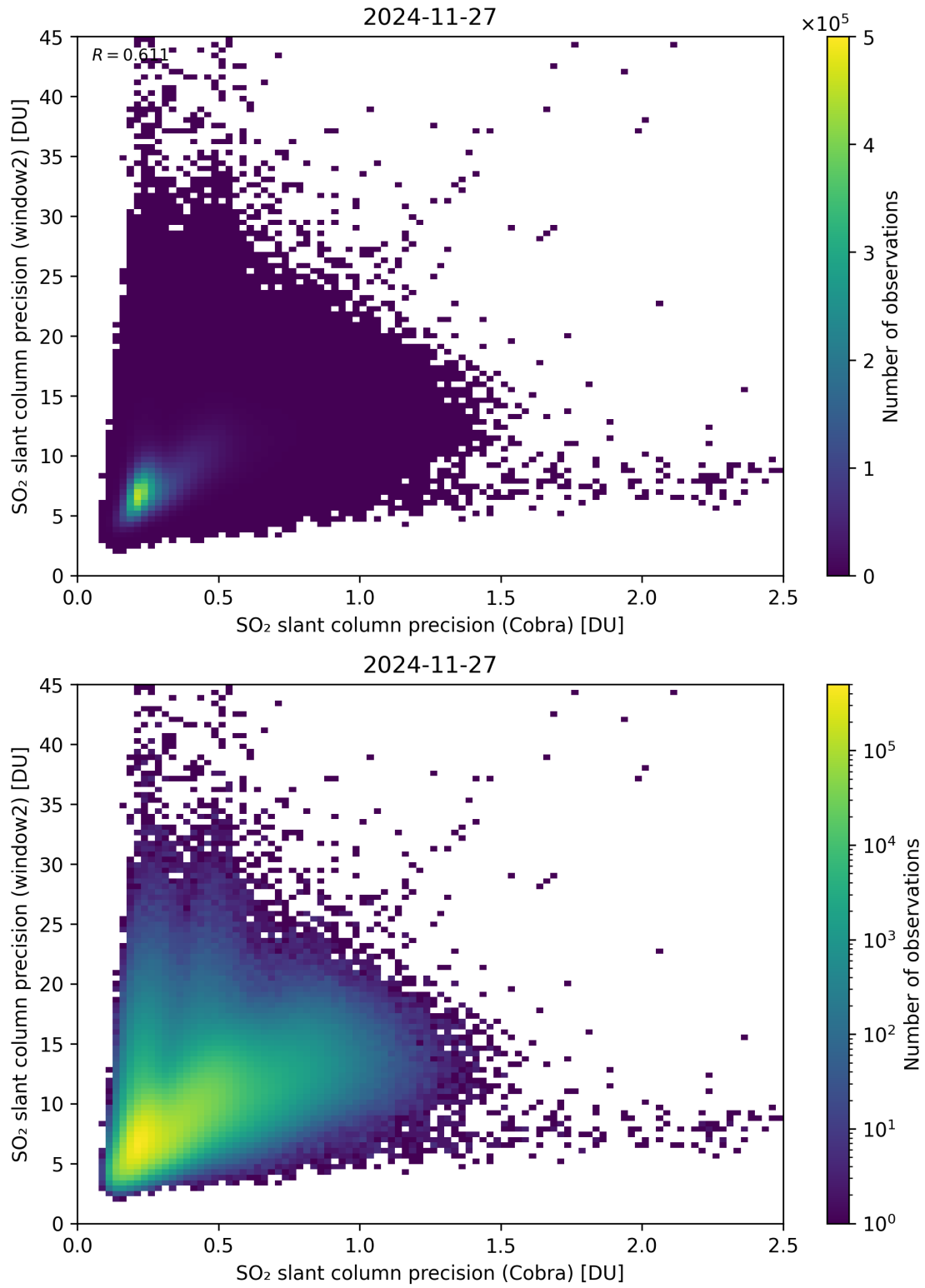
Figure 210: Scatter density plot of “SO 2 slant column precision (Cobra)” against “SO 2 slant column precision (window2)” for 2024-11-26 to 2024-11-28.
