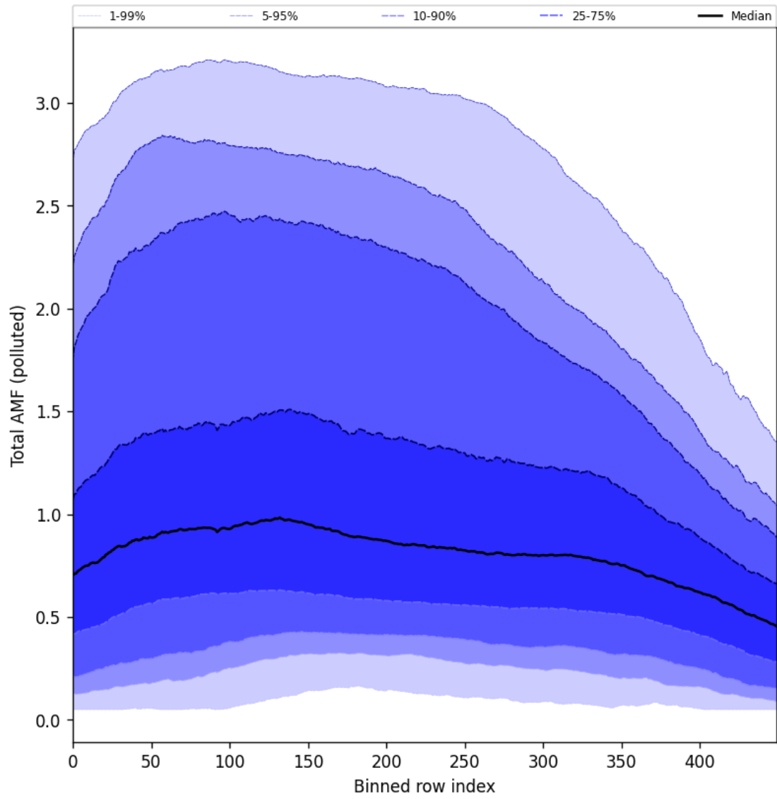
Figure 105: Along track statistics of “Total AMF (polluted)” for 2024-11-26 to 2024-11-28
