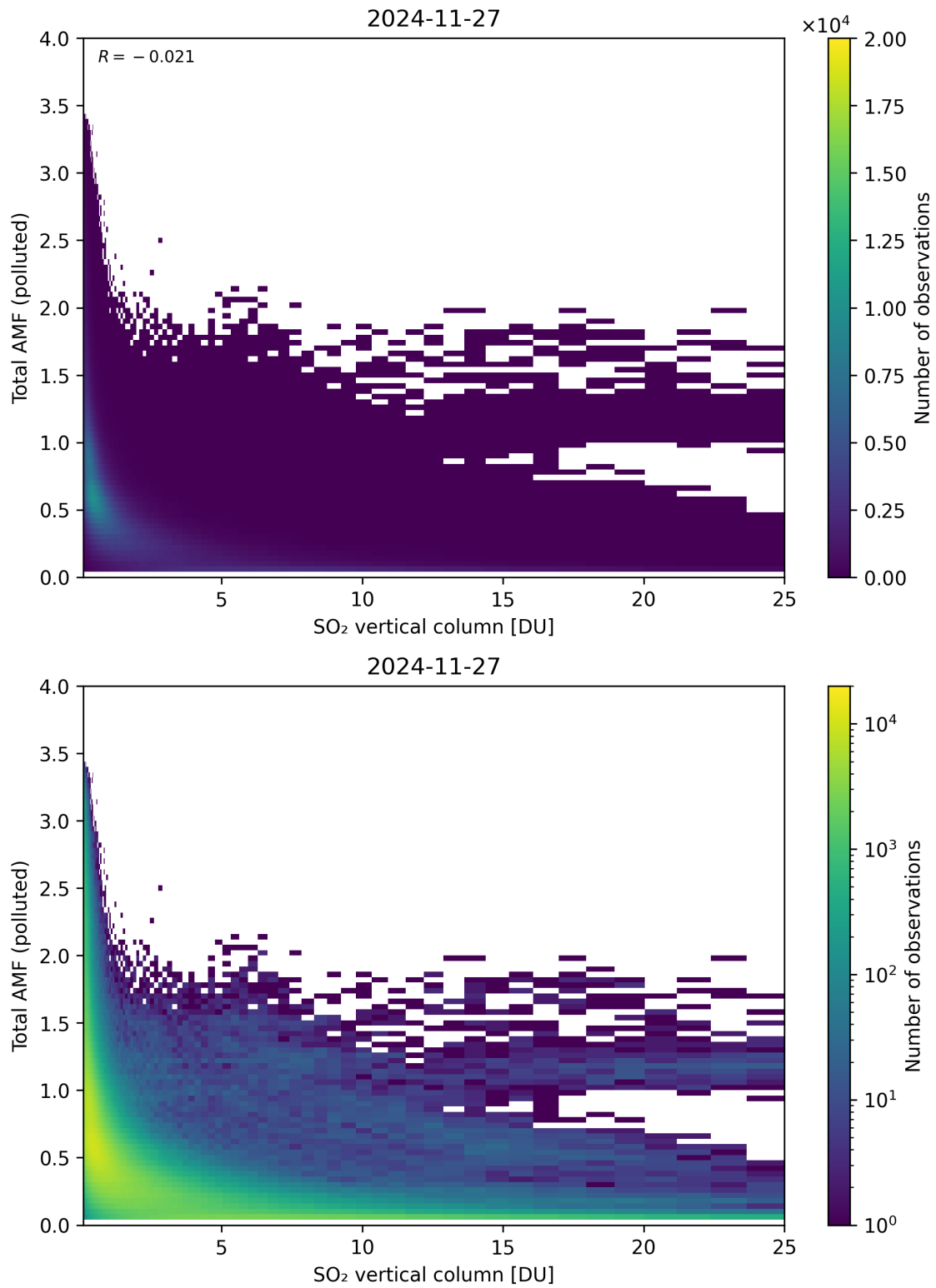
Figure 359: Scatter density plot of “SO 2 vertical column” against “Total AMF (polluted)” for 2024-11-26 to 2024-11-28.
