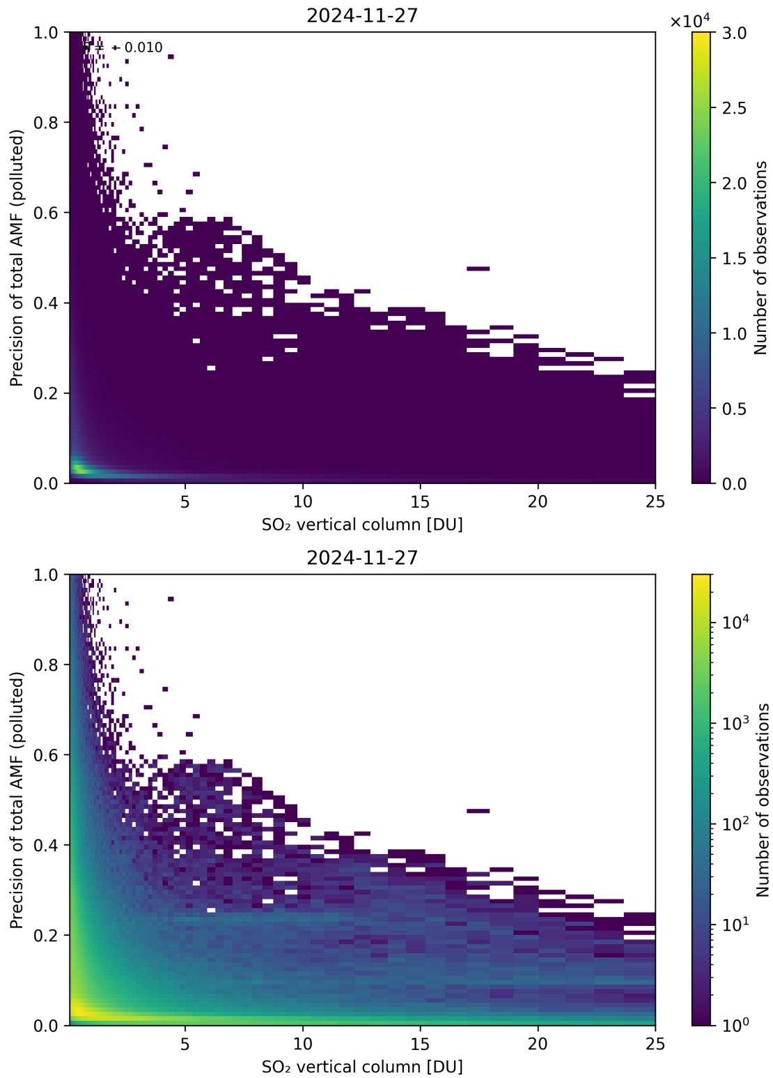
Figure 360: Scatter density plot of “SO 2 vertical column” against “Precision of total AMF (polluted)” for 2024-11-26 to 2024-11-28.
