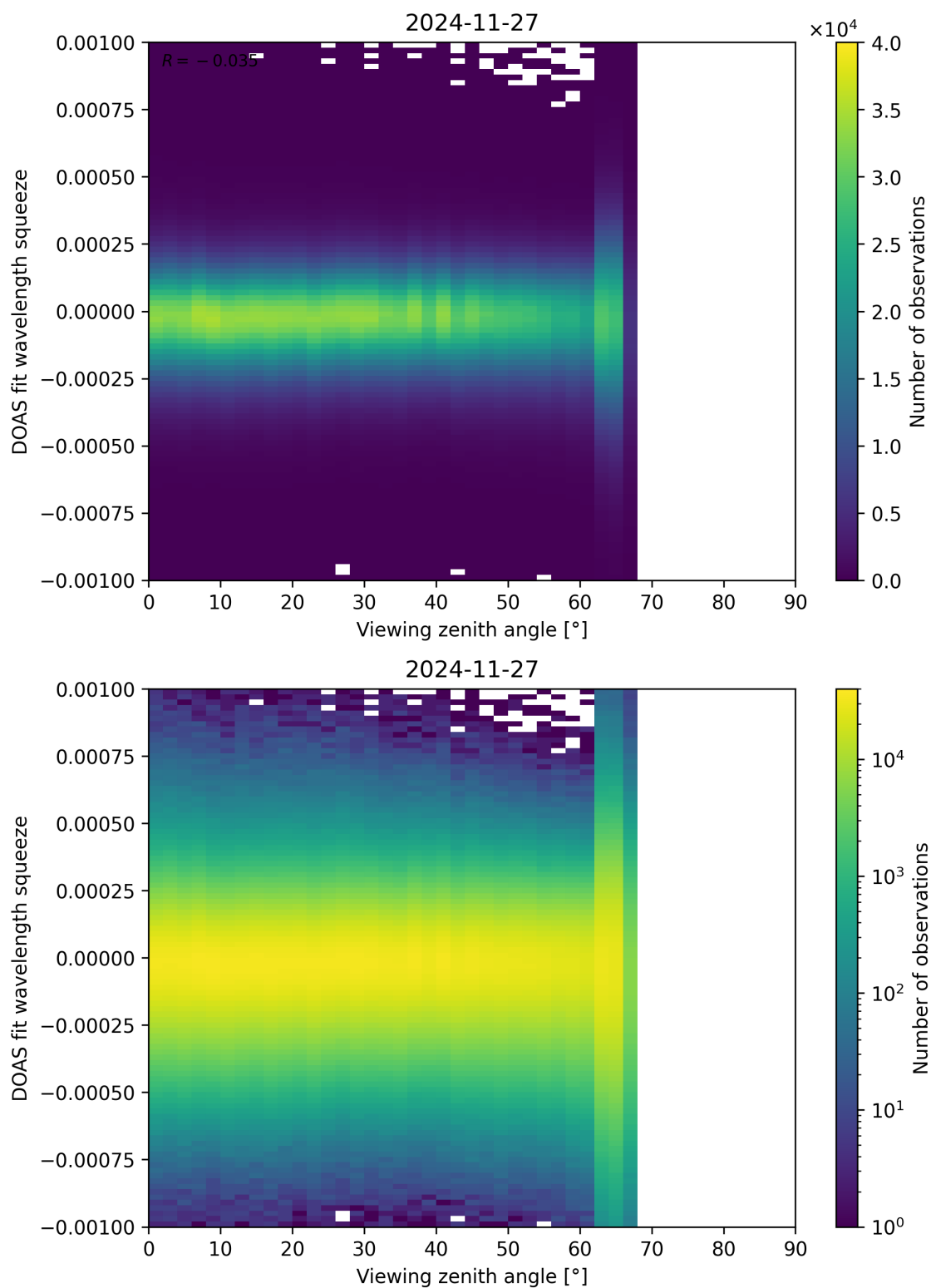
Figure 366: Scatter density plot of “Viewing zenith angle” against “DOAS fit wavelength squeeze” for 2024-11-26 to 2024-11-28.
