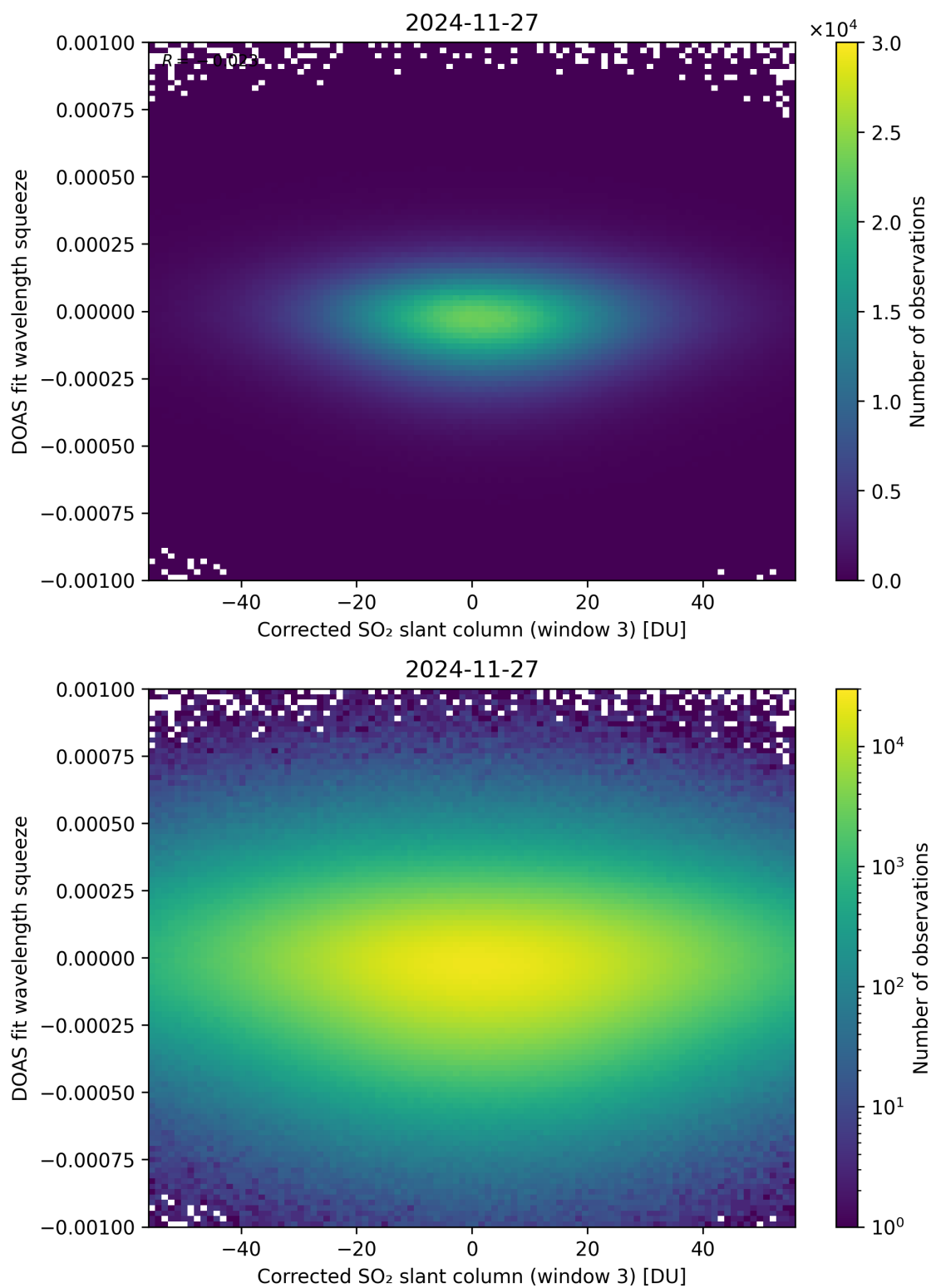
Figure 257: Scatter density plot of “Corrected SO 2 slant column (window 3)” against “DOAS fit wavelength squeeze” for 2024-11-26 to 2024-11-28.
