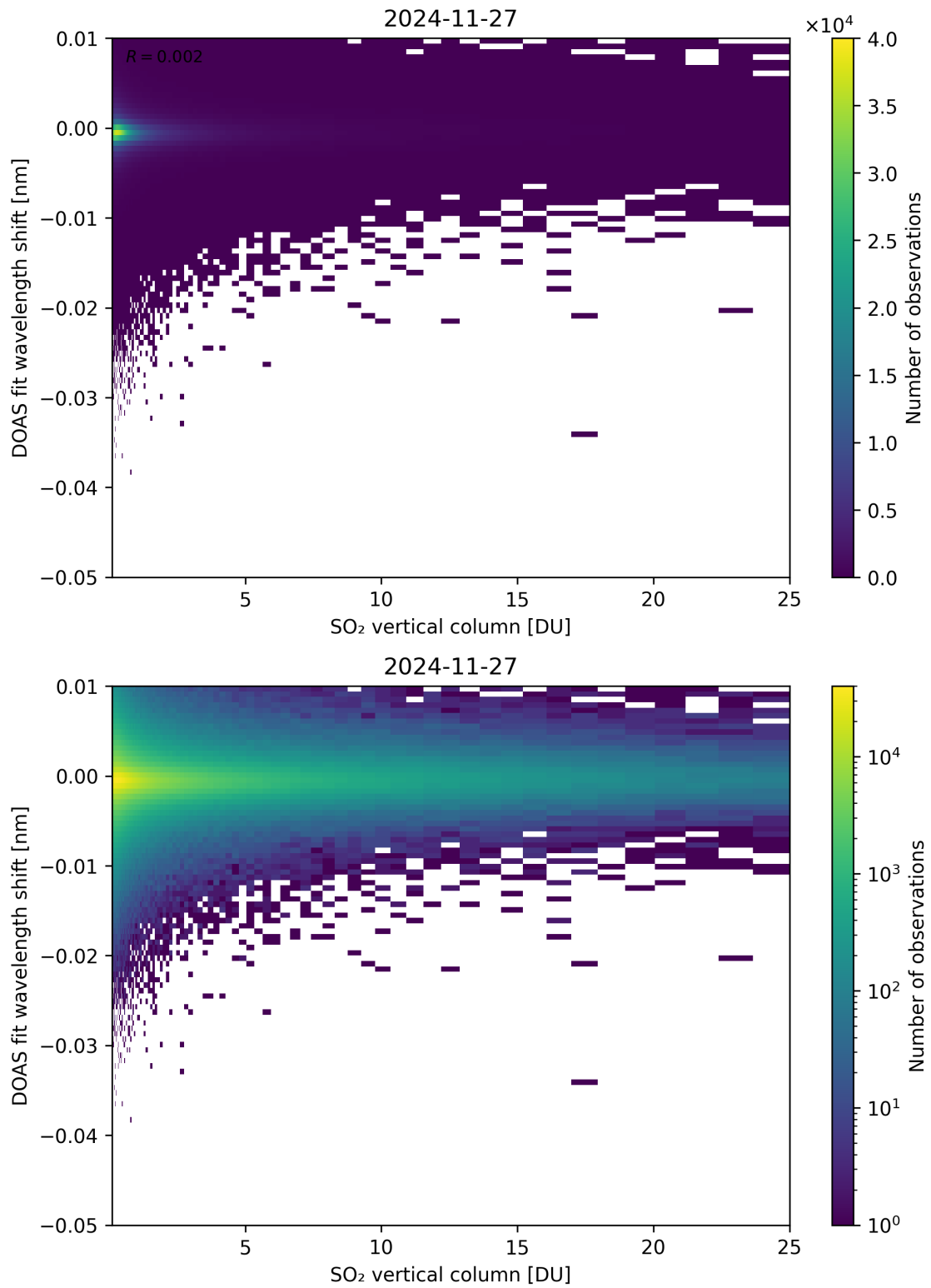
Figure 326: Scatter density plot of “SO 2 vertical column” against “DOAS fit wavelength shift” for 2024-11-26 to 2024-11-28.
