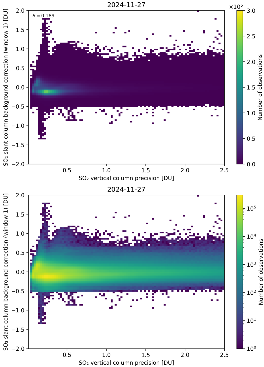
Figure 329: Scatter density plot of “SO 2 vertical column precision” against “SO 2 slant column background correction (window 1)” for 2024-11-26 to 2024-11-28.
