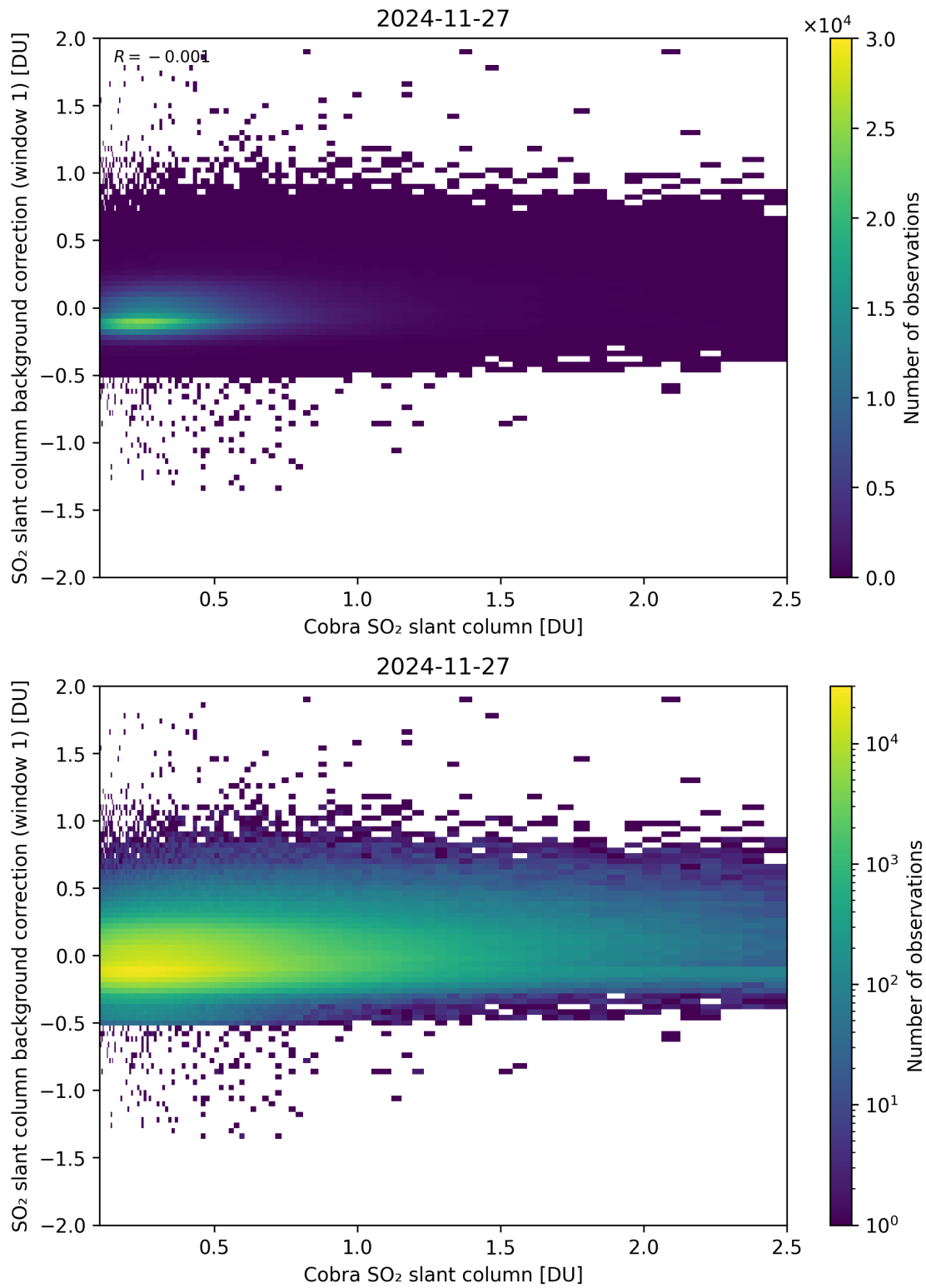
Figure 193: Scatter density plot of “Cobra SO 2 slant column” against “SO 2 slant column background correction (window 1)” for 2024-11-26 to 2024-11-28.
