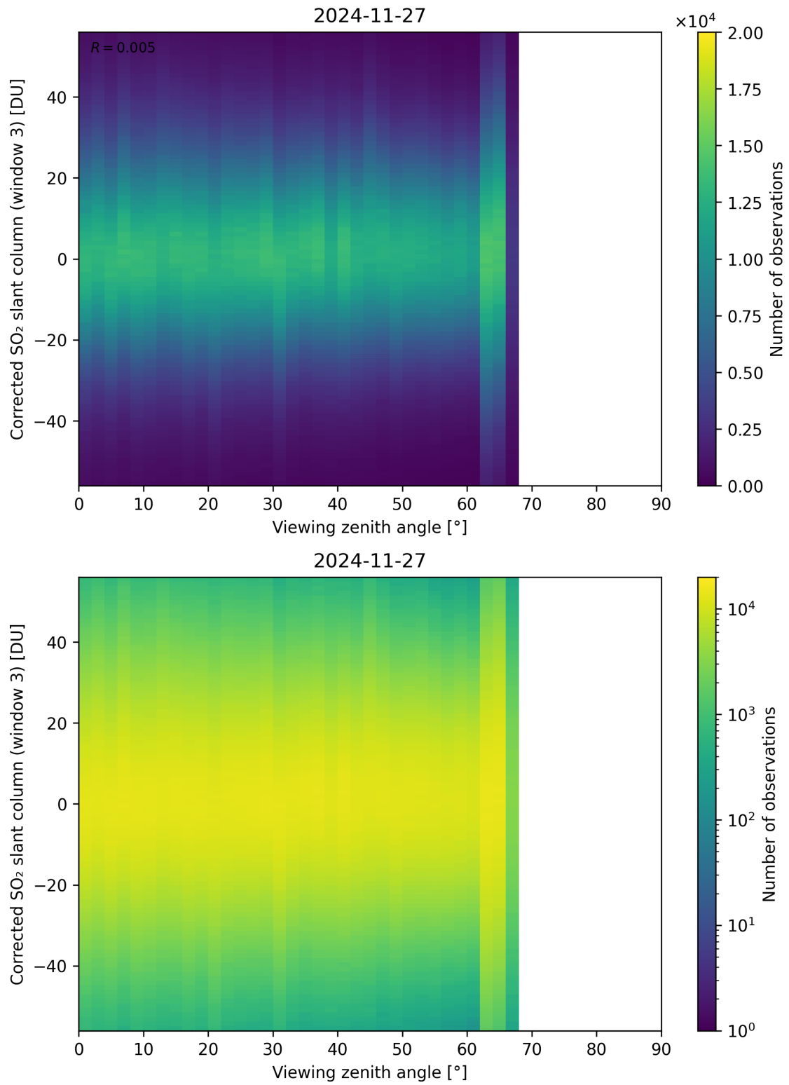
Figure 375: Scatter density plot of “Viewing zenith angle” against “Corrected SO 2 slant column (window 3)” for 2024-11-26 to 2024-11-28.
