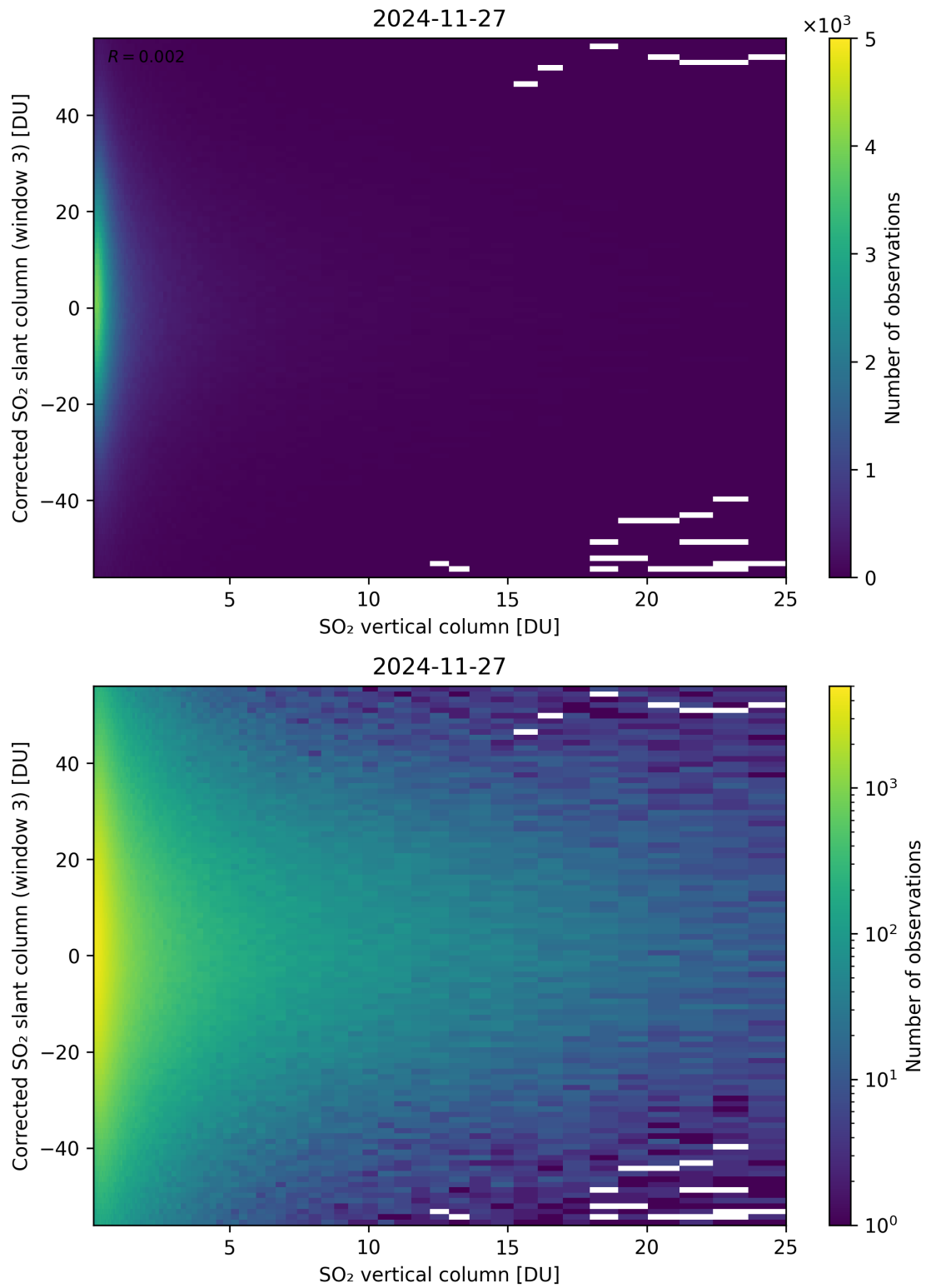
Figure 353: Scatter density plot of “SO 2 vertical column” against “Corrected SO 2 slant column (window 3)” for 2024-11-26 to 2024-11-28.
