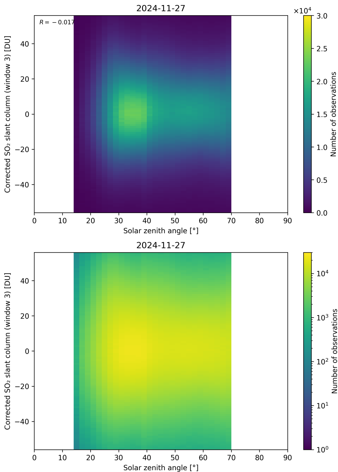
Figure 183: Scatter density plot of “Solar zenith angle” against “Corrected SO 2 slant column (window 3)” for 2024-11-26 to 2024-11-28.
