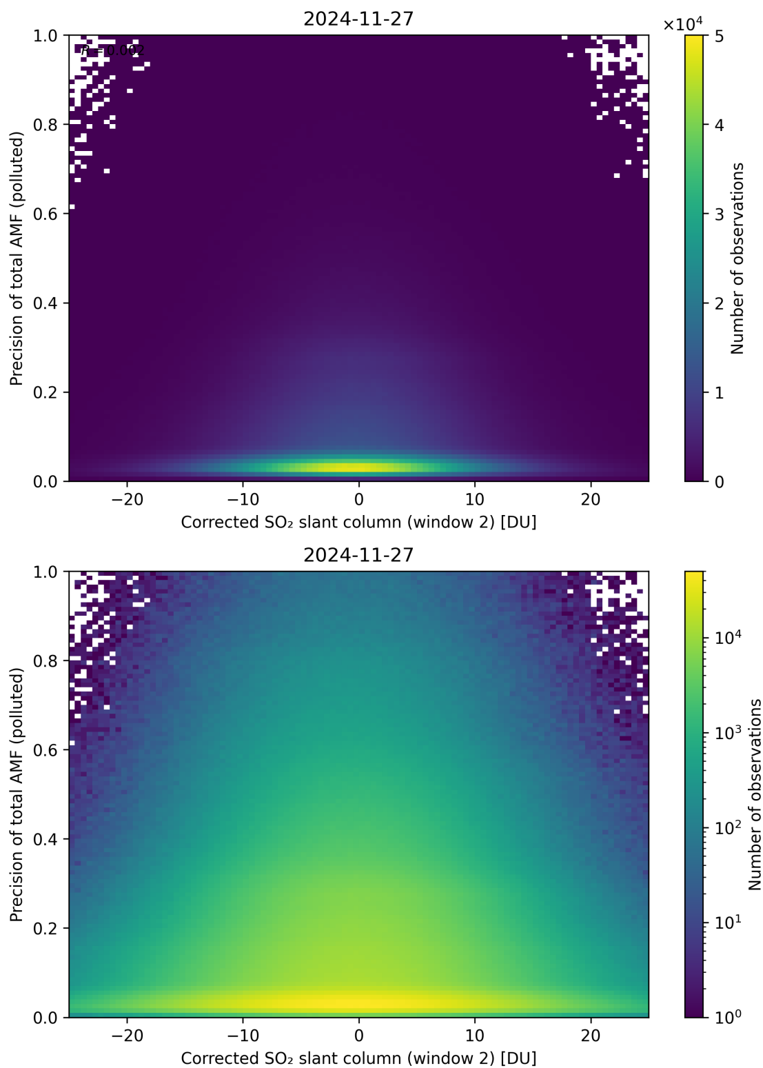
Figure 254: Scatter density plot of “Corrected SO 2 slant column (window 2)” against “Precision of total AMF (polluted)” for 2024-11-26 to 2024-11-28.
