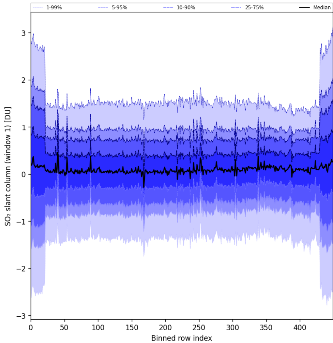
Figure 89: Along track statistics of “SO 2 slant column (window 1)” for 2024-11-26 to 2024-11-28
