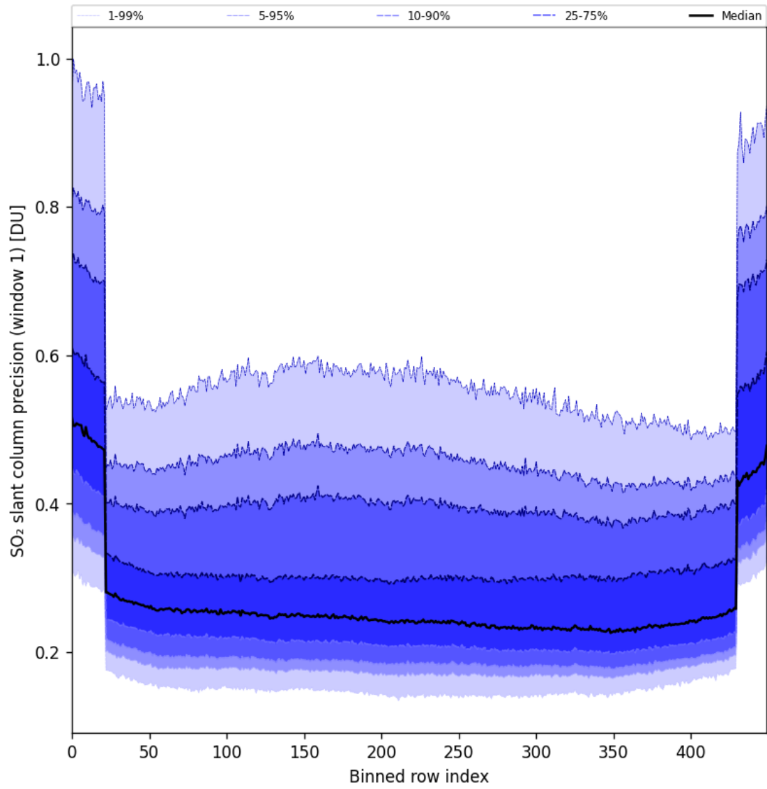
Figure 90: Along track statistics of “SO 2 slant column precision (window 1)” for 2024-11-26 to 2024-11-28
