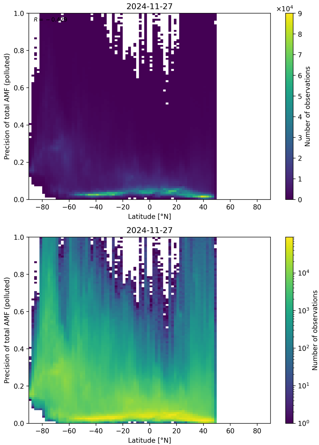
Figure 168: Scatter density plot of “Latitude” against “Precision of total AMF (polluted)” for 2024-11-26 to 2024-11-28.
