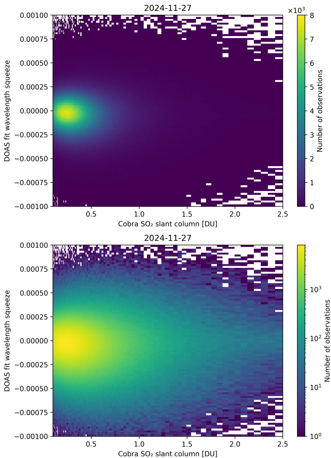
Figure 197: Scatter density plot of “Cobra SO 2 slant column” against “DOAS fit wavelength squeeze” for 2024-11-26 to 2024-11-28.
