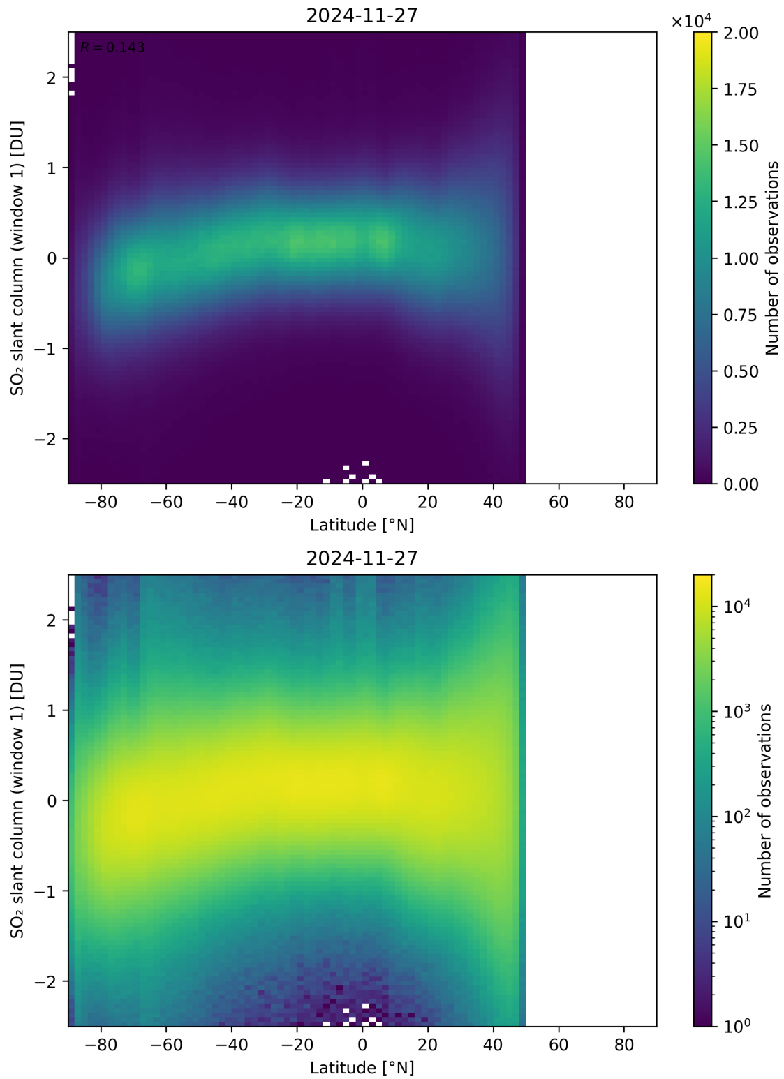
Figure 162: Scatter density plot of “Latitude” against “SO 2 slant column (window 1)” for 2024-11-26 to 2024-11-28.
