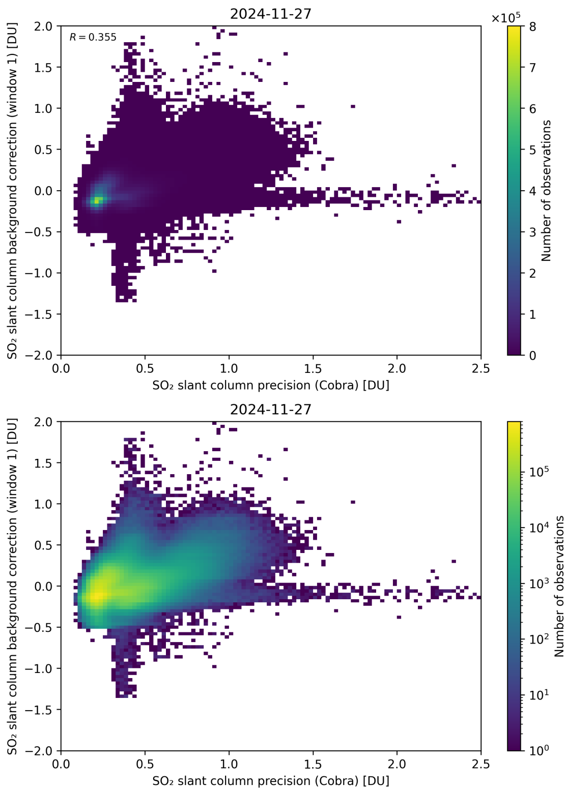
Figure 199: Scatter density plot of “SO 2 slant column precision (Cobra)” against “SO 2 slant column background correction (window 1)” for 2024-11-26 to 2024-11-28.
