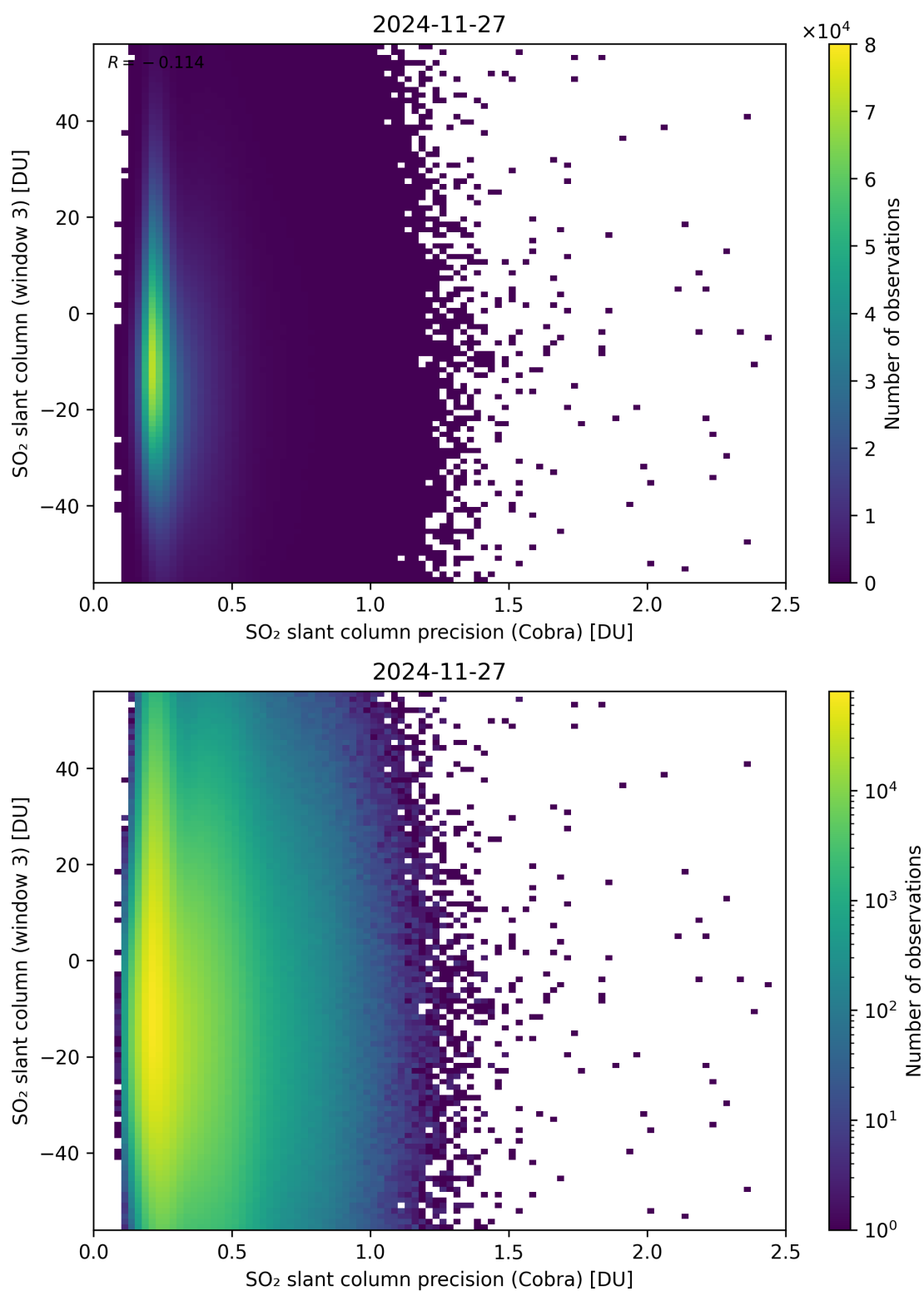
Figure 211: Scatter density plot of “SO 2 slant column precision (Cobra)” against “SO 2 slant column (window 3)” for 2024-11-26 to 2024-11-28.
