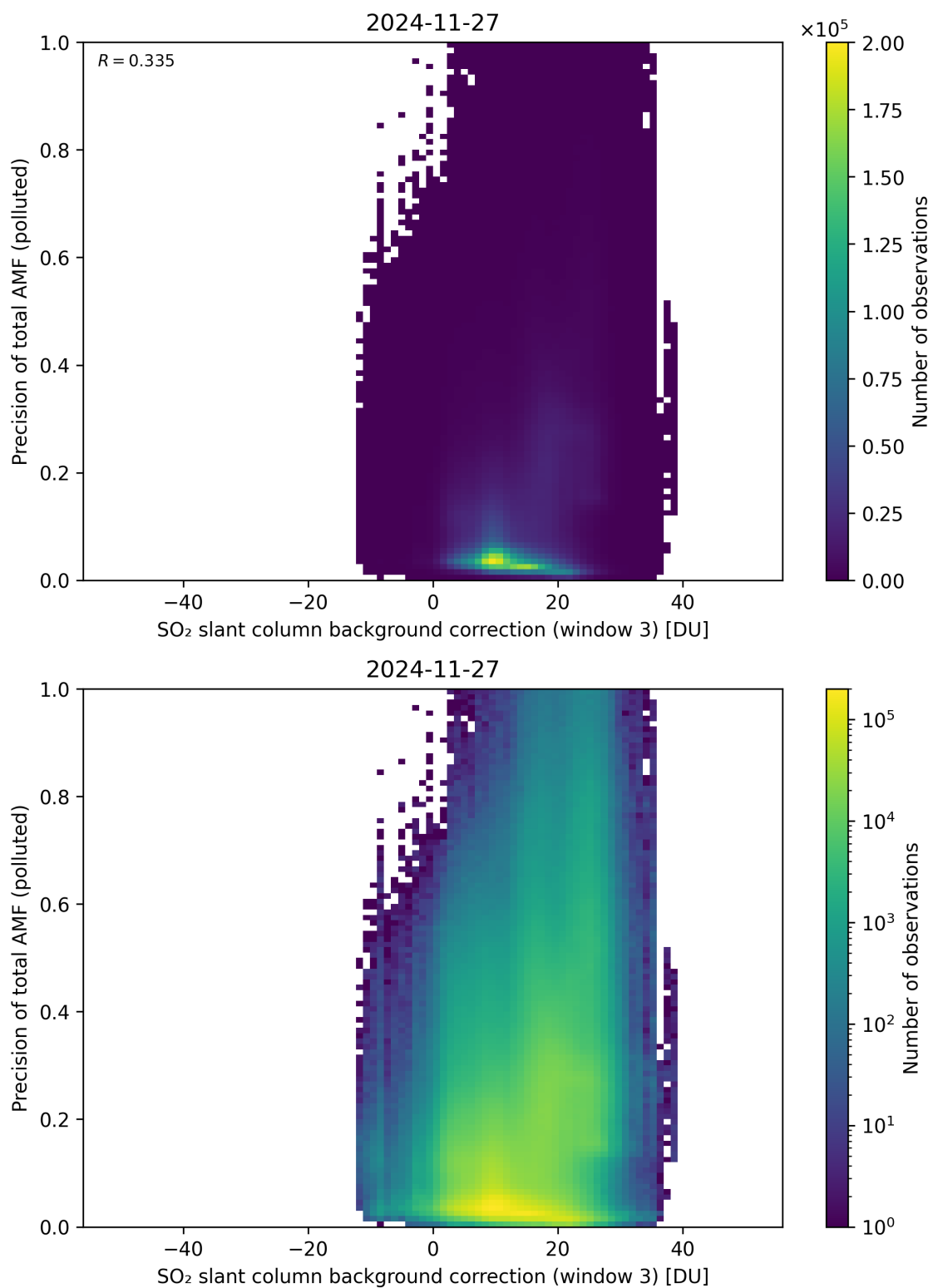
Figure 137: Scatter density plot of “SO 2 slant column background correction (window 3)” against “Precision of total AMF (polluted)” for 2024-11-26 to 2024-11-28.
