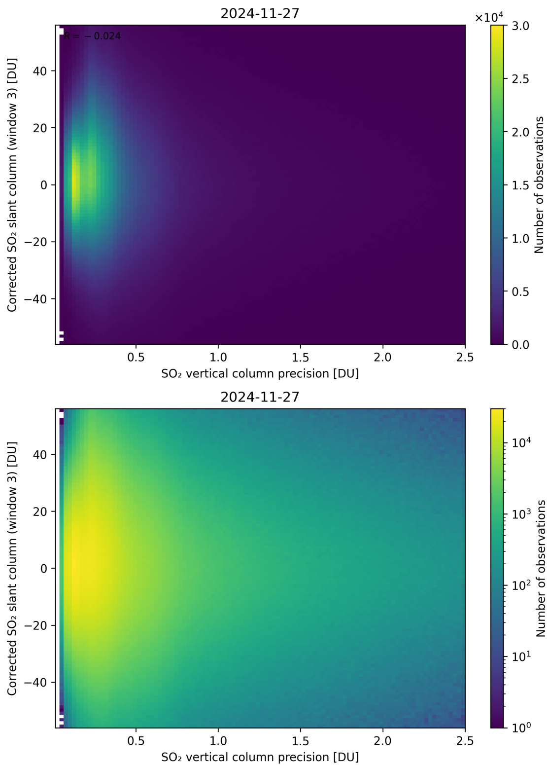
Figure 340: Scatter density plot of “SO 2 vertical column precision” against “Corrected SO 2 slant column (window 3)” for 2024-11-26 to 2024-11-28.
