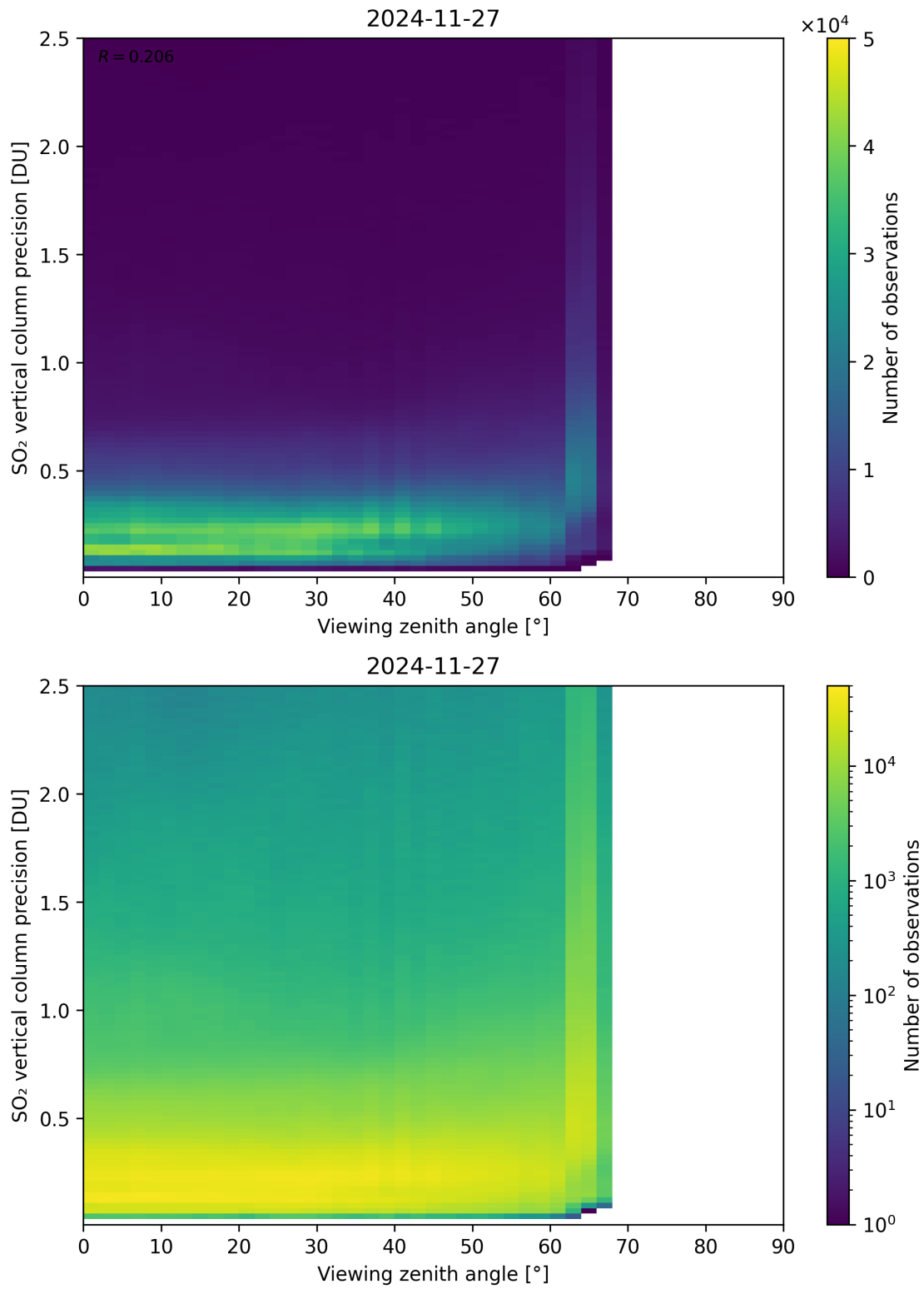
Figure 384: Scatter density plot of “Viewing zenith angle” against “SO 2 vertical column precision” for 2024-11-26 to 2024-11-28.
