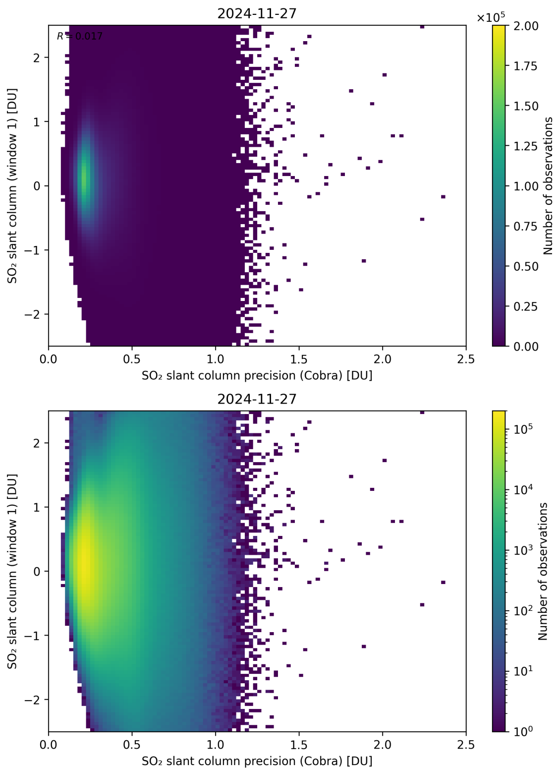
Figure 208: Scatter density plot of “SO 2 slant column precision (Cobra)” against “SO 2 slant column (window 1)” for 2024-11-26 to 2024-11-28.
