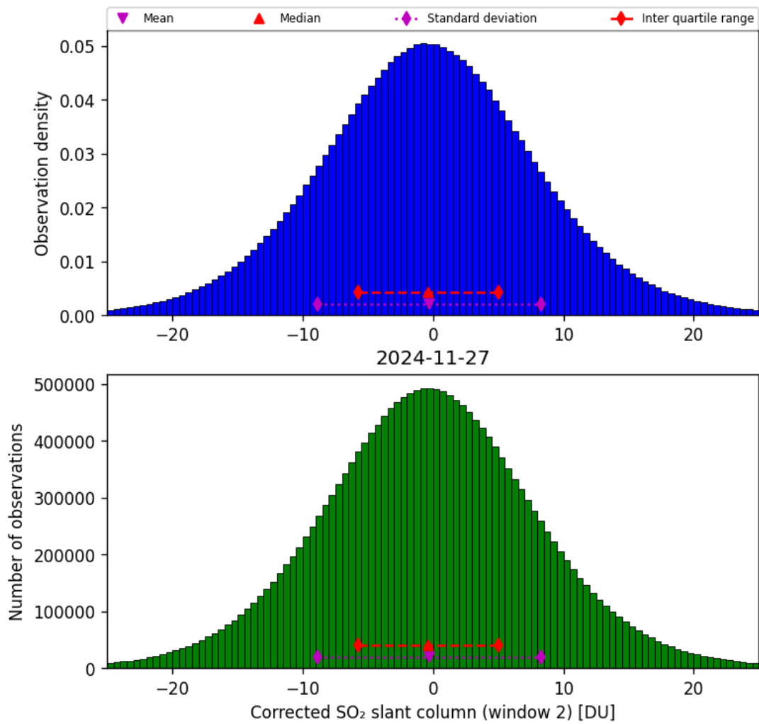
Figure 69: Histogram of “Corrected SO 2 slant column (window 2)” for 2024-11-26 to 2024-11-28
