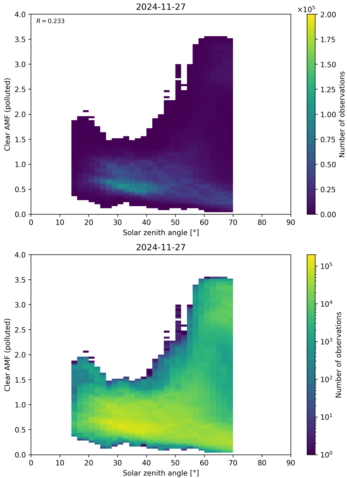
Figure 178: Scatter density plot of “Solar zenith angle” against “Clear AMF (polluted)” for 2024-11-26 to 2024-11-28.
