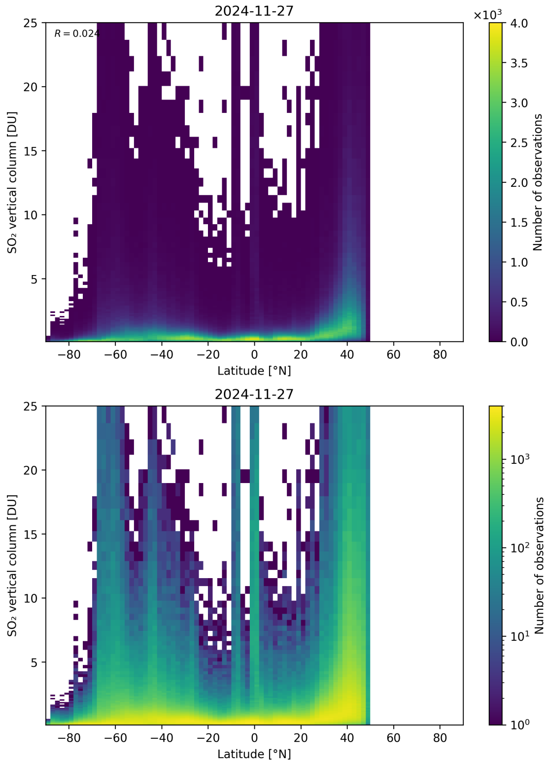
Figure 169: Scatter density plot of “Latitude” against “SO 2 vertical column” for 2024-11-26 to 2024-11-28.
