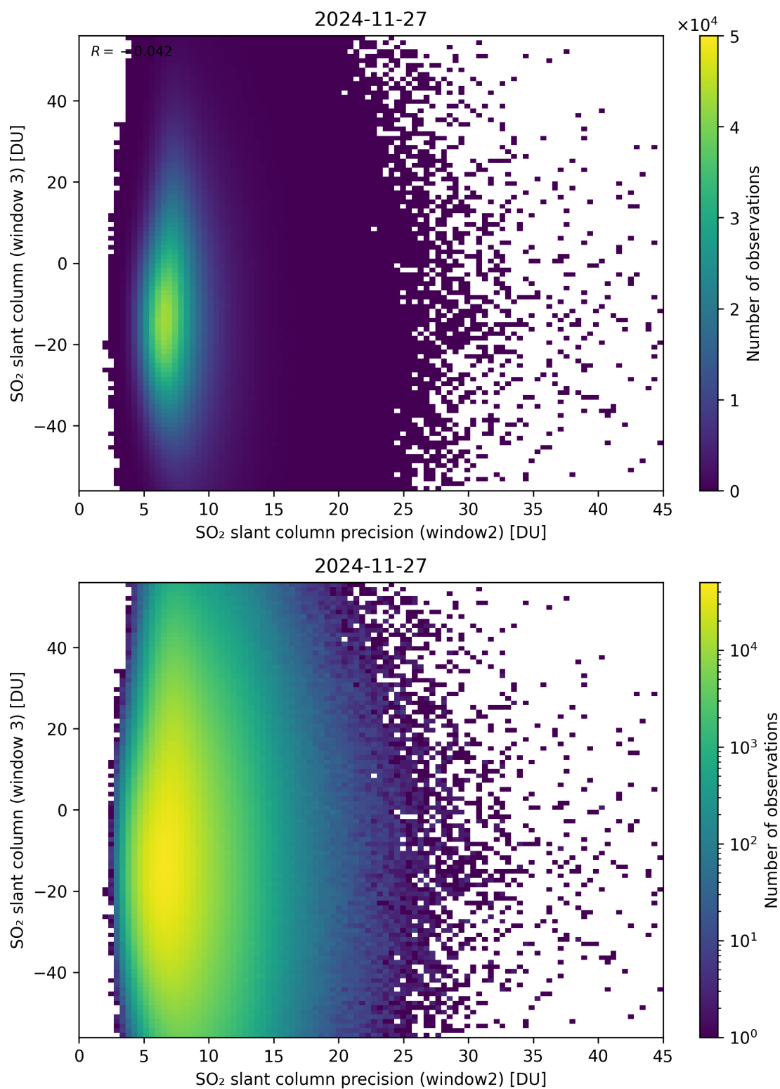
Figure 299: Scatter density plot of “SO 2 slant column precision (window2)” against “SO 2 slant column (window 3)” for 2024-11-26 to 2024-11-28.
