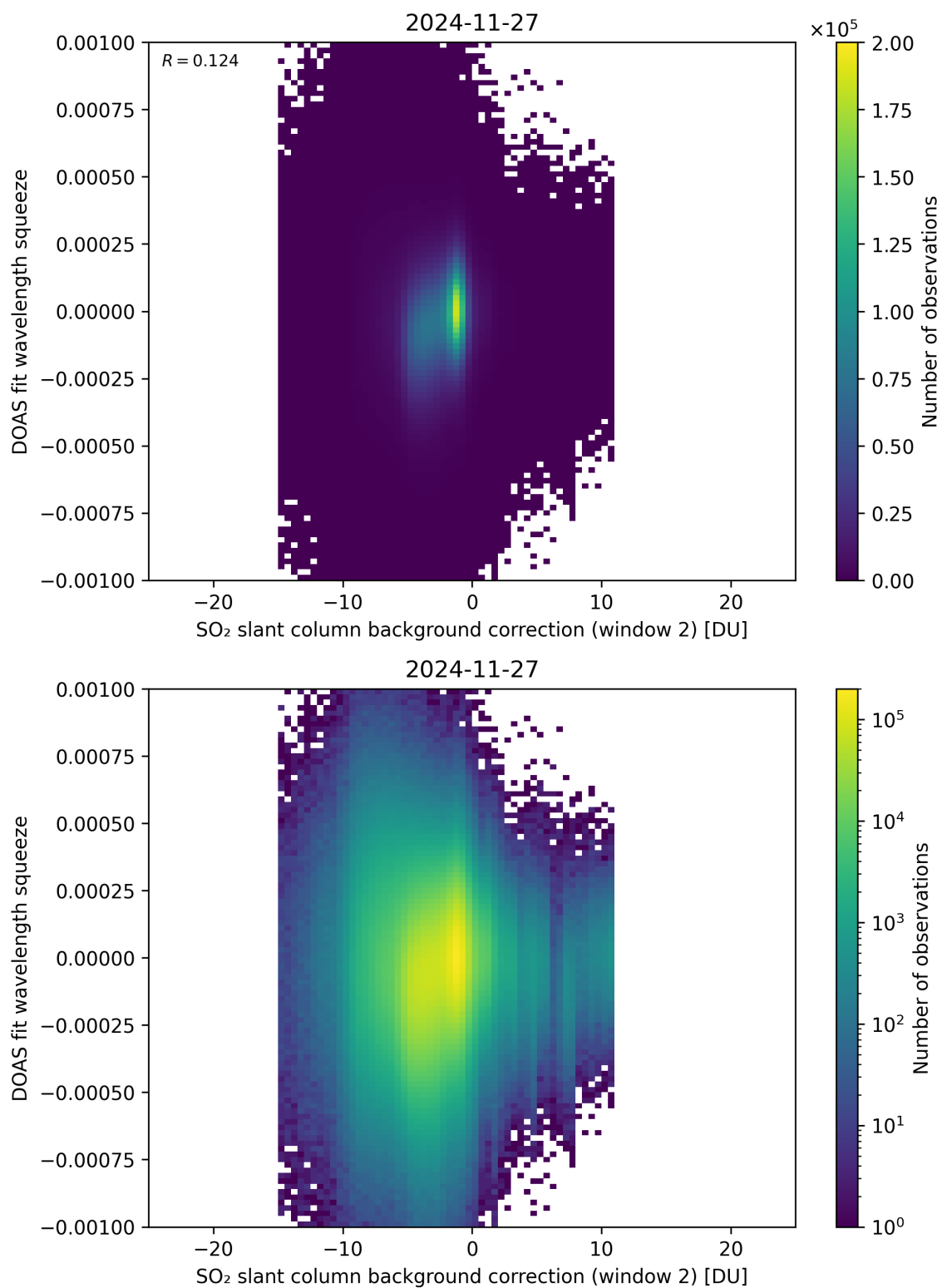
Figure 124: Scatter density plot of “SO 2 slant column background correction (window 2)” against “DOAS fit wavelength squeeze” for 2024-11-26 to 2024-11-28.
