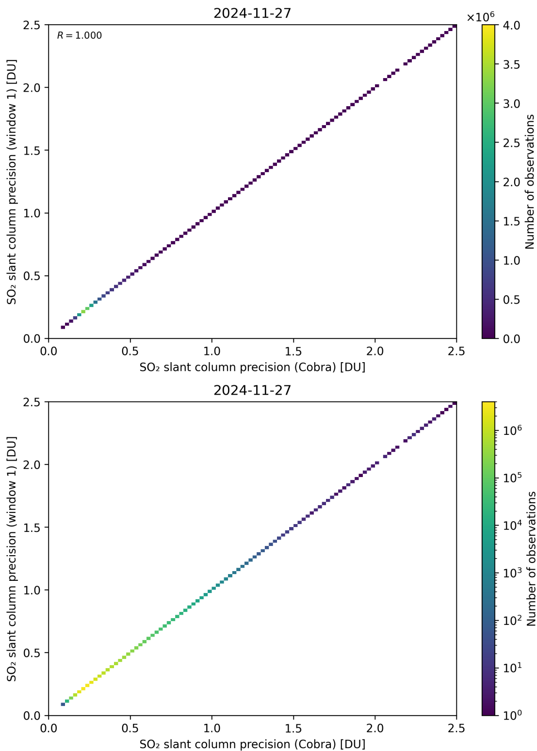
Figure 209: Scatter density plot of “SO 2 slant column precision (Cobra)” against “SO 2 slant column precision (window 1)” for 2024-11-26 to 2024-11-28.
