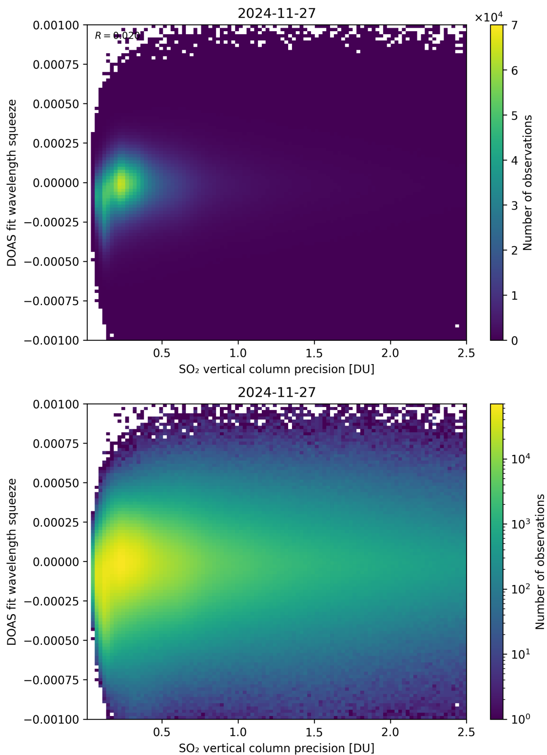
Figure 333: Scatter density plot of “SO 2 vertical column precision” against “DOAS fit wavelength squeeze” for 2024-11-26 to 2024-11-28.
