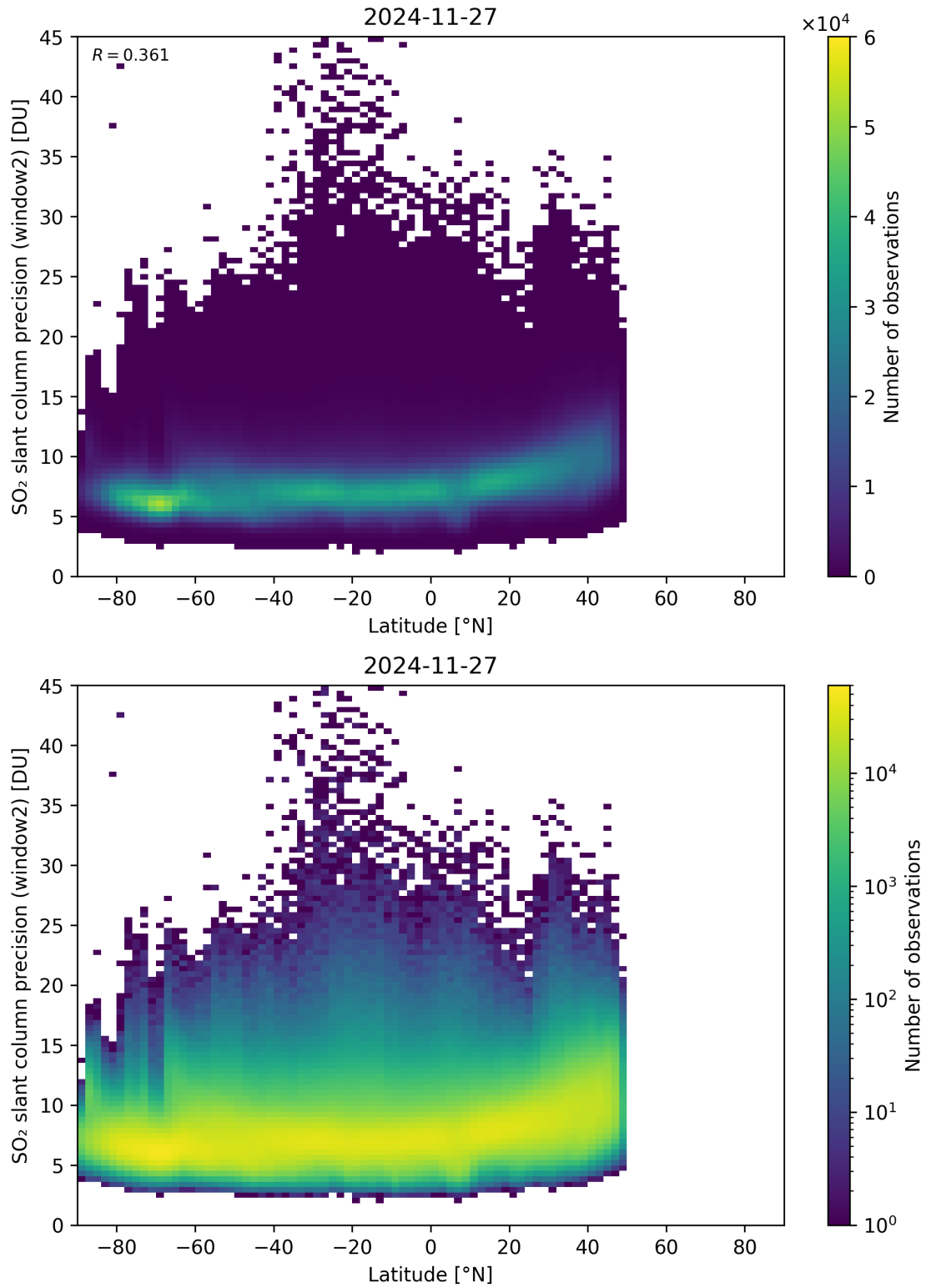
Figure 164: Scatter density plot of “Latitude” against “SO 2 slant column precision (window2)” for 2024-11-26 to 2024-11-28.
