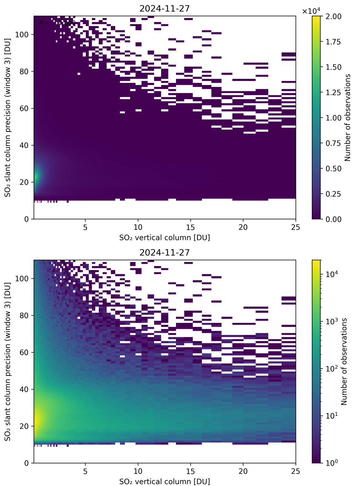
Figure 358: Scatter density plot of “SO 2 vertical column” against “SO 2 slant column precision (window 3)” for 2024-11-26 to 2024-11-28.
