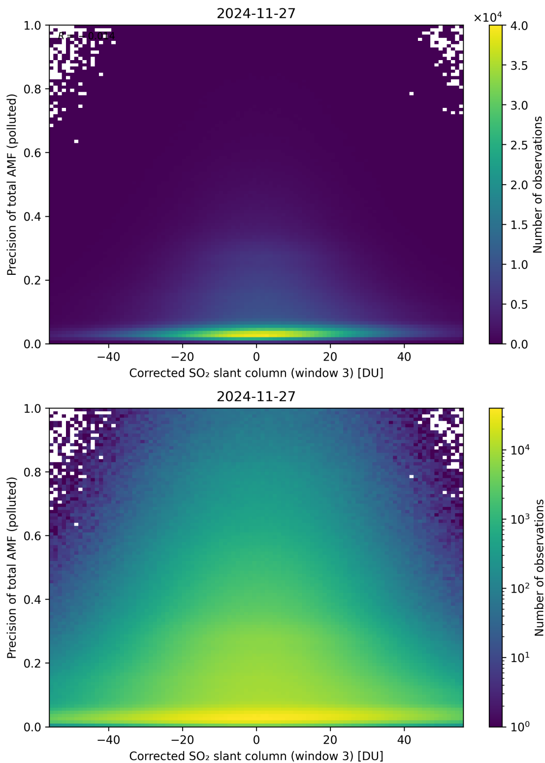
Figure 261: Scatter density plot of “Corrected SO 2 slant column (window 3)” against “Precision of total AMF (polluted)” for 2024-11-26 to 2024-11-28.
