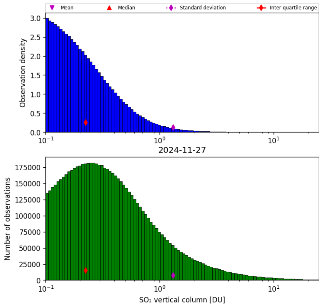
Figure 58: Histogram of “SO 2 vertical column” for 2024-11-26 to 2024-11-28
