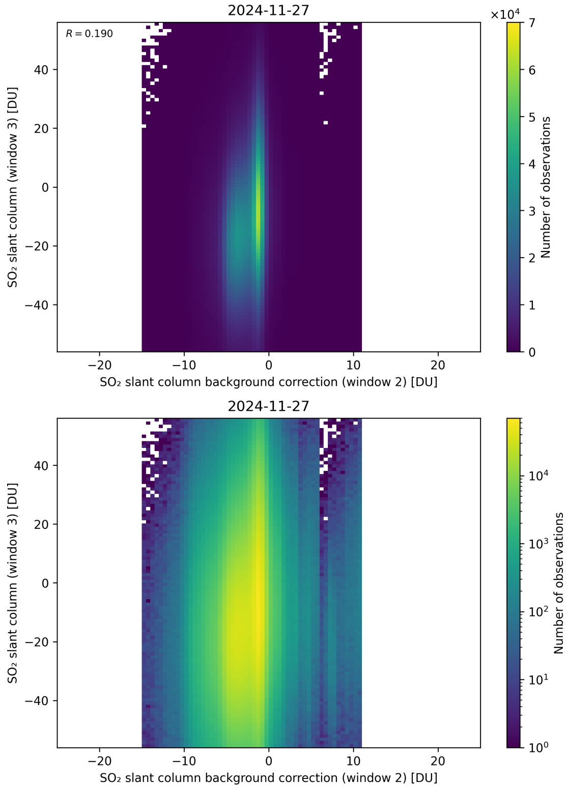
Figure 128: Scatter density plot of “SO 2 slant column background correction (window 2)” against “SO 2 slant column (window 3)” for 2024-11-26 to 2024-11-28.
