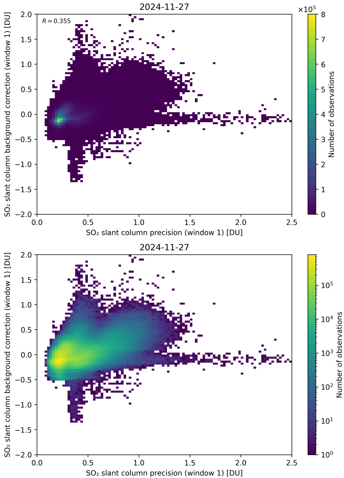
Figure 268: Scatter density plot of “SO 2 slant column precision (window 1)” against “SO 2 slant column background correction (window 1)” for 2024-11-26 to 2024-11-28.
