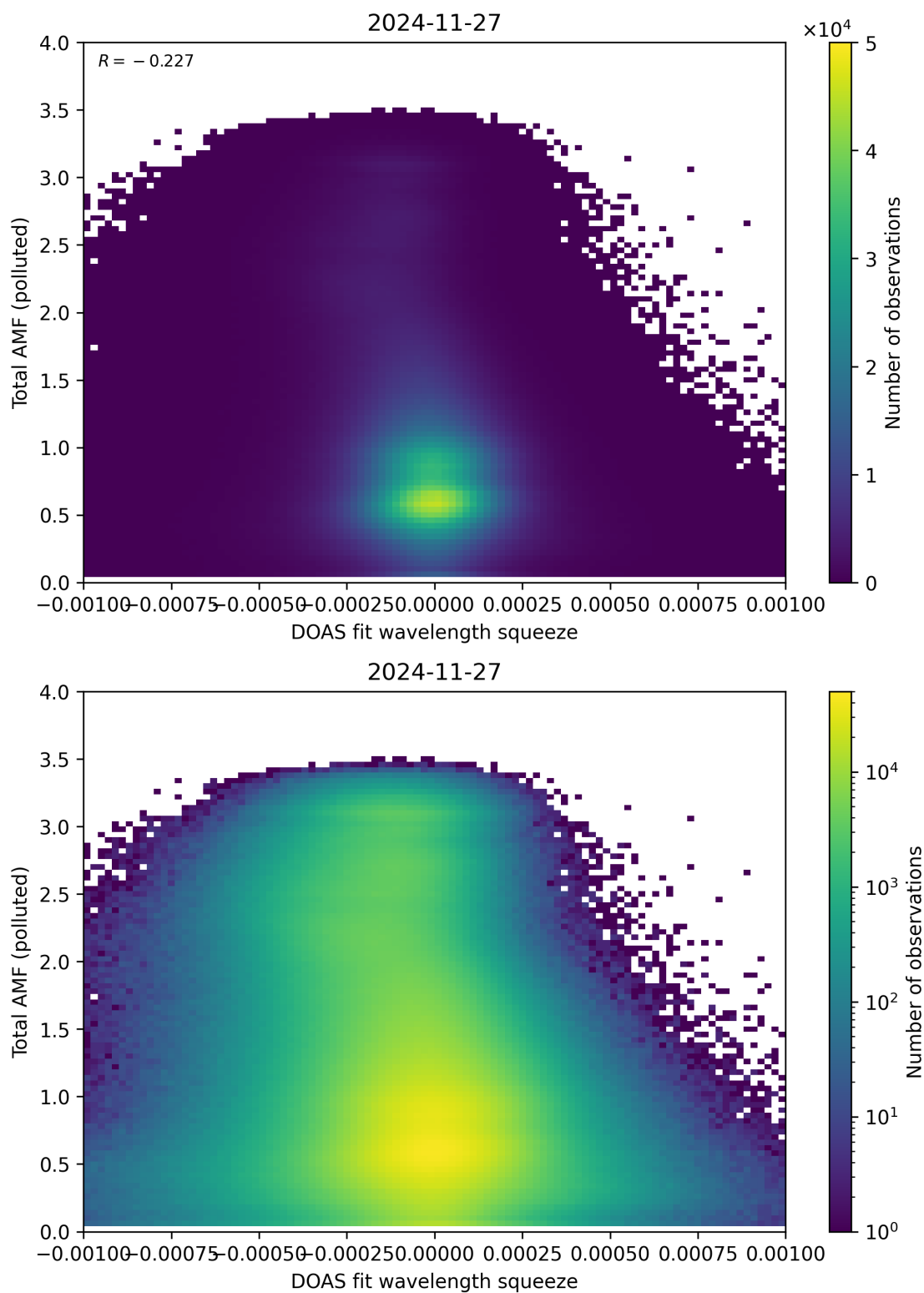
Figure 145: Scatter density plot of “DOAS fit wavelength squeeze” against “Total AMF (polluted)” for 2024-11-26 to 2024-11-28.
