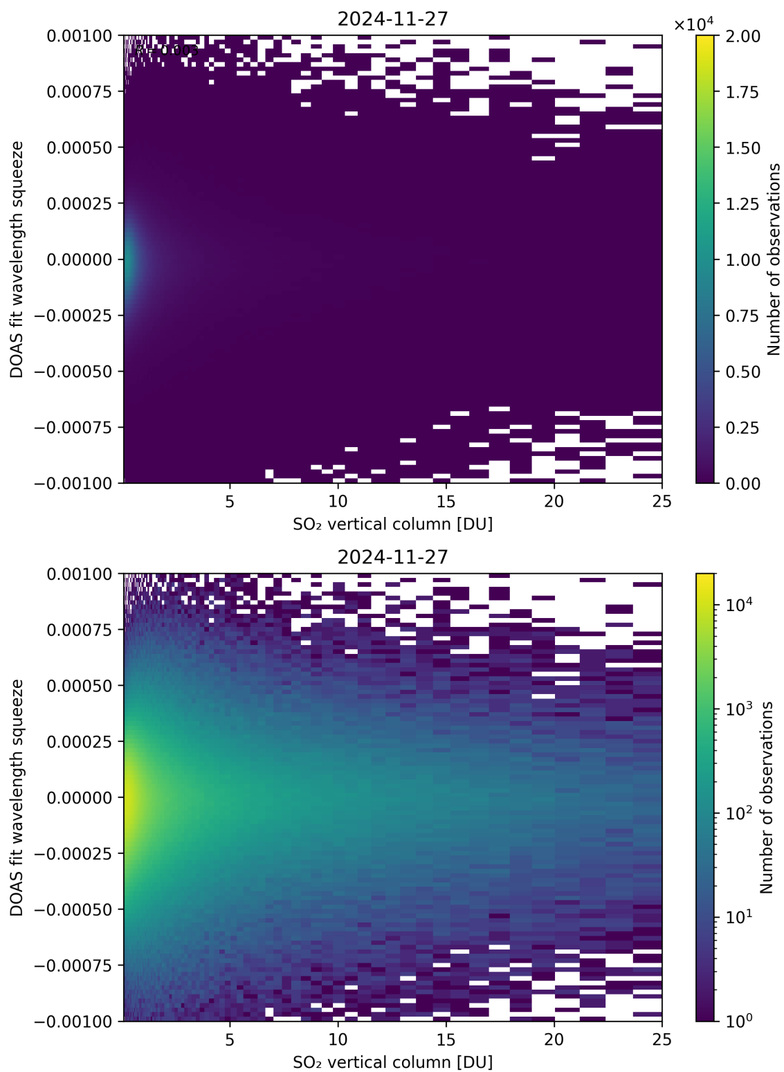
Figure 327: Scatter density plot of “SO 2 vertical column” against “DOAS fit wavelength squeeze” for 2024-11-26 to 2024-11-28.
