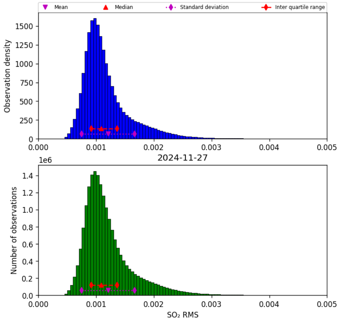
Figure 78: Histogram of “SO 2 RMS” for 2024-11-26 to 2024-11-28
