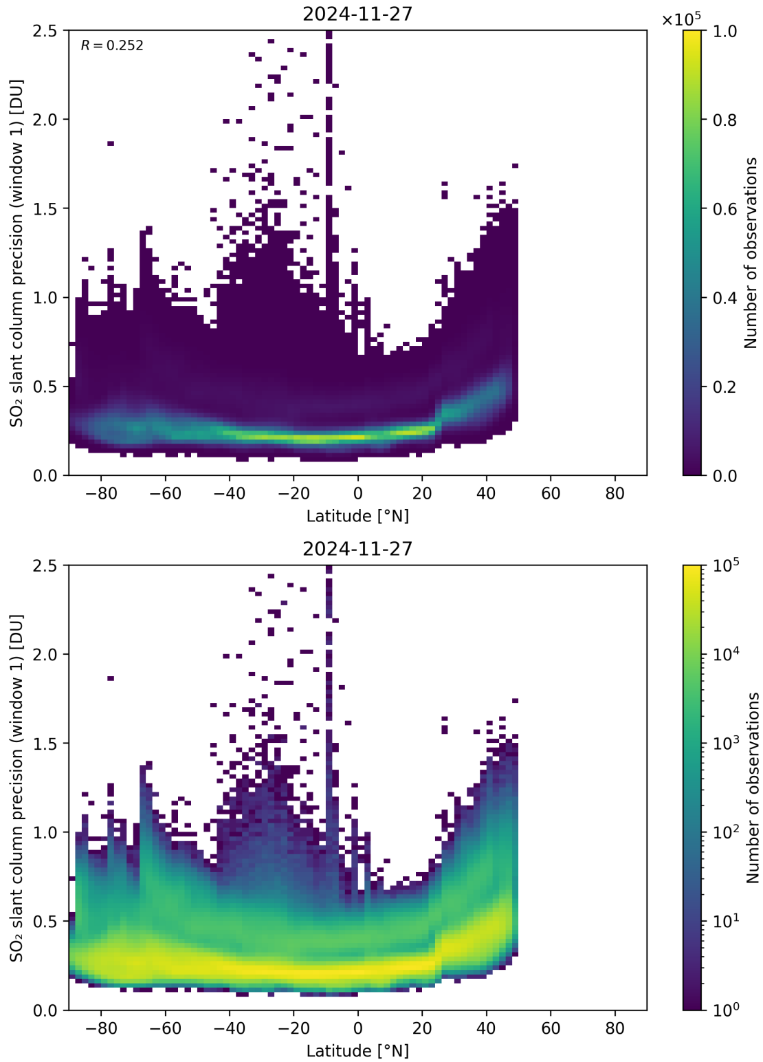
Figure 163: Scatter density plot of “Latitude” against “SO 2 slant column precision (window 1)” for 2024-11-26 to 2024-11-28.
