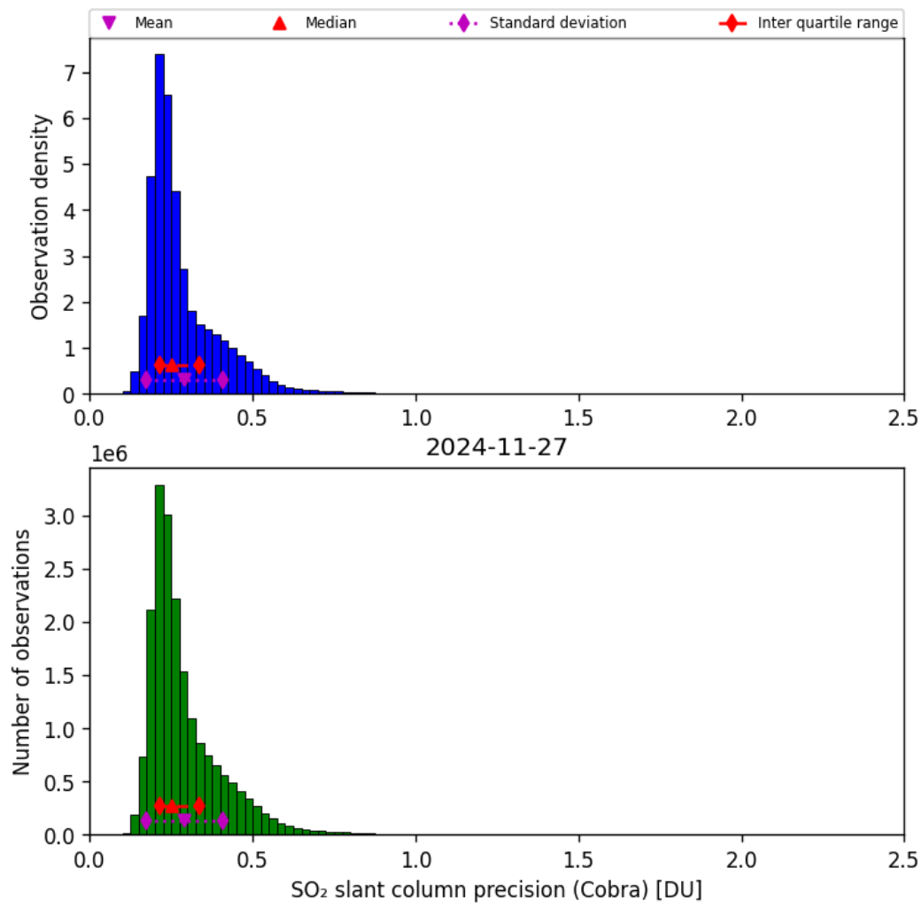
Figure 62: Histogram of “SO 2 slant column precision (Cobra)” for 2024-11-26 to 2024-11-28
