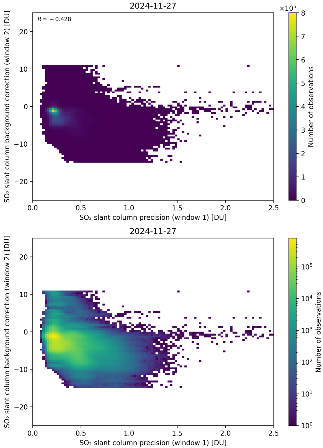
Figure 269: Scatter density plot of “SO 2 slant column precision (window 1)” against “SO 2 slant column background correction (window 2)” for 2024-11-26 to 2024-11-28.
