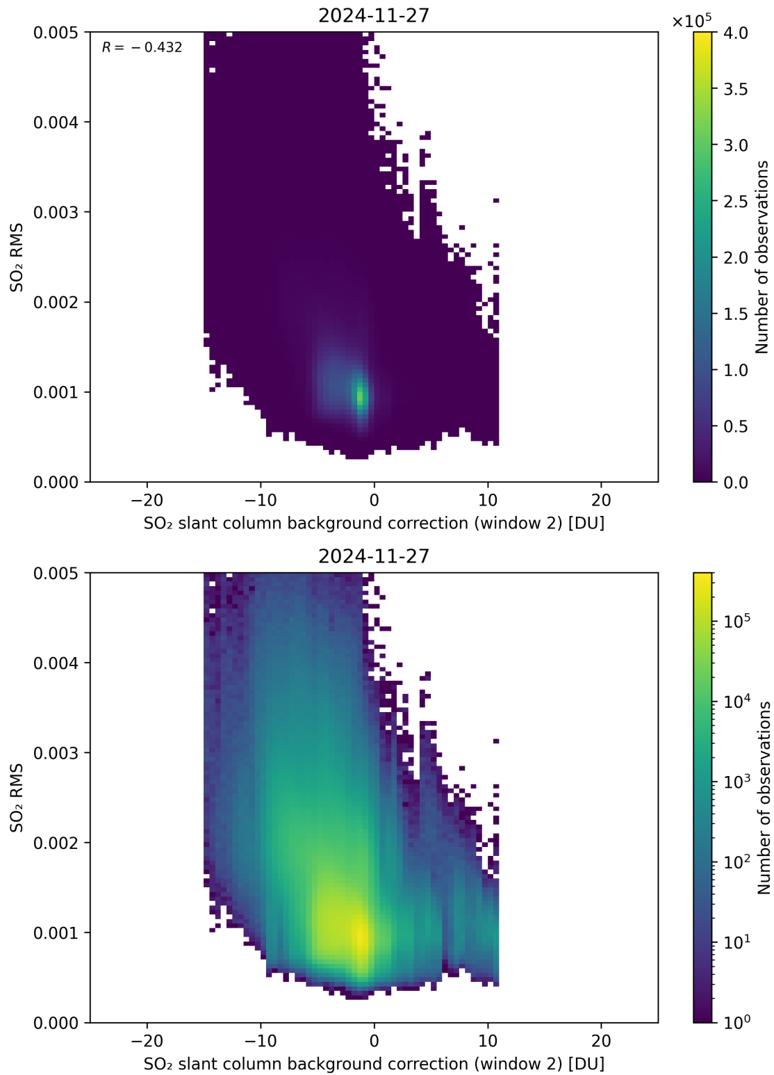
Figure 125: Scatter density plot of “SO 2 slant column background correction (window 2)” against “SO 2 RMS” for 2024-11-26 to 2024-11-28.
