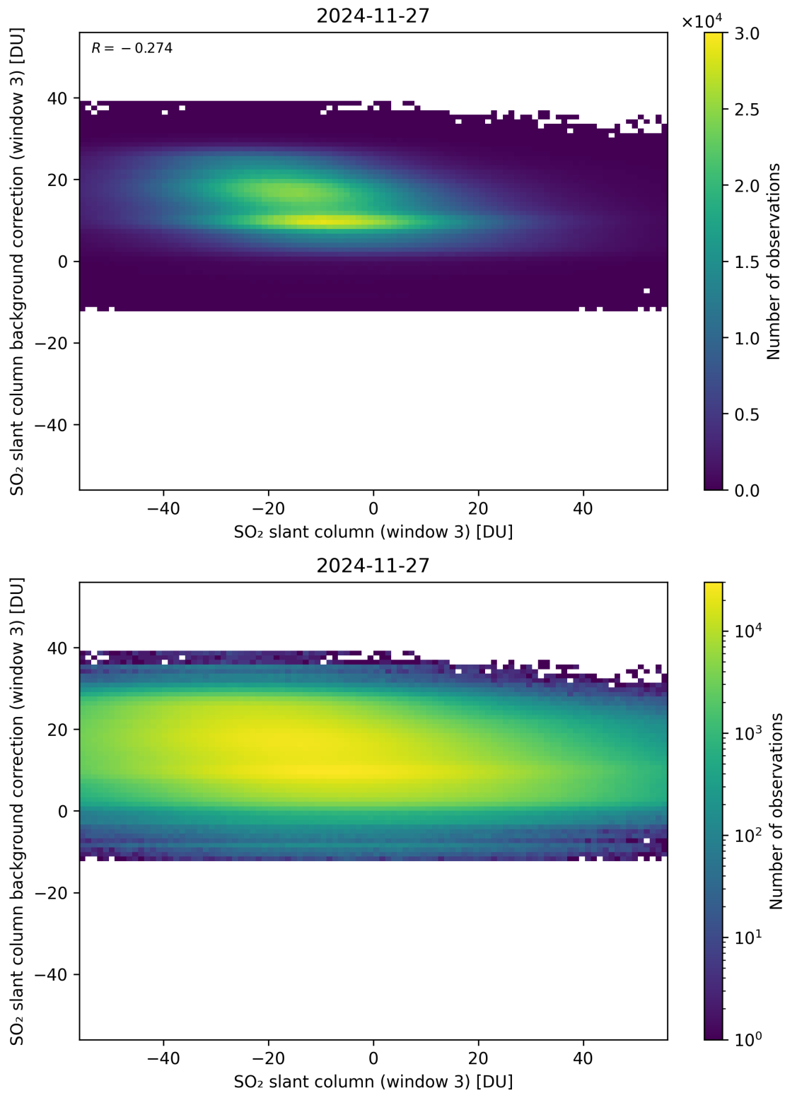
Figure 303: Scatter density plot of “SO 2 slant column (window 3)” against “SO 2 slant column background correction (window 3)” for 2024-11-26 to 2024-11-28.
