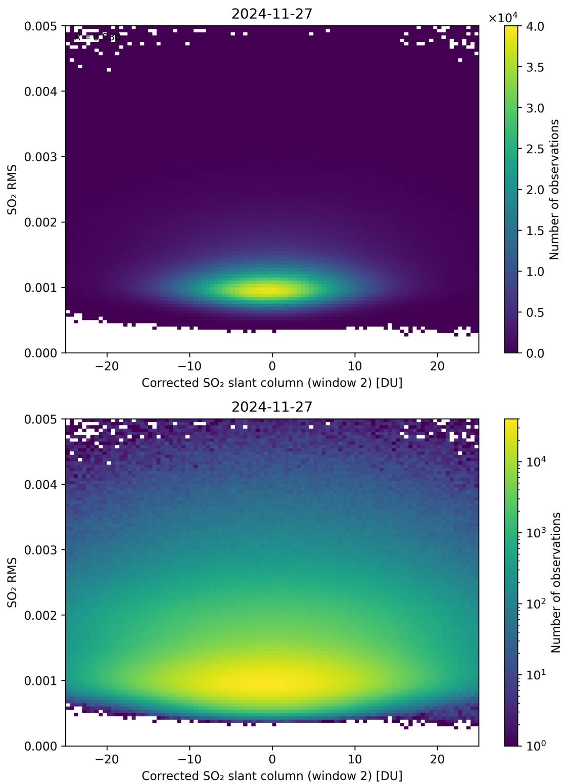
Figure 248: Scatter density plot of “Corrected SO 2 slant column (window 2)” against “SO 2 RMS” for 2024-11-26 to 2024-11-28.
