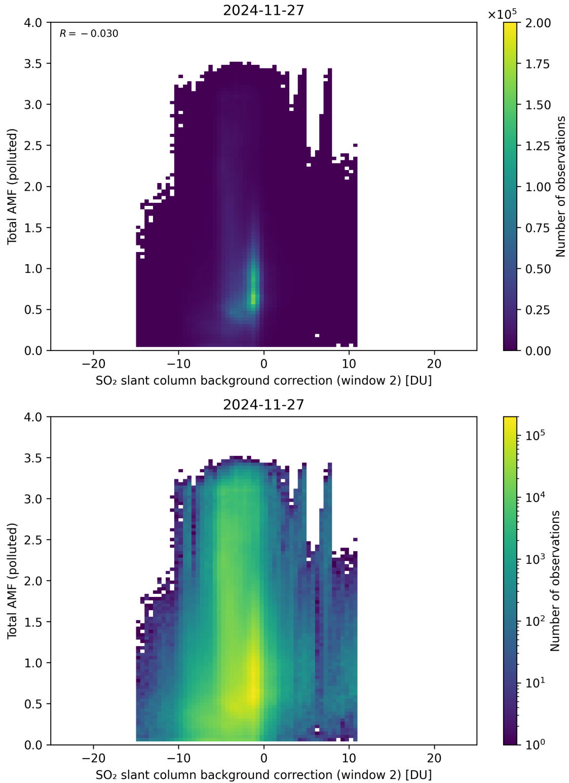
Figure 130: Scatter density plot of “SO 2 slant column background correction (window 2)” against “Total AMF (polluted)” for 2024-11-26 to 2024-11-28.
