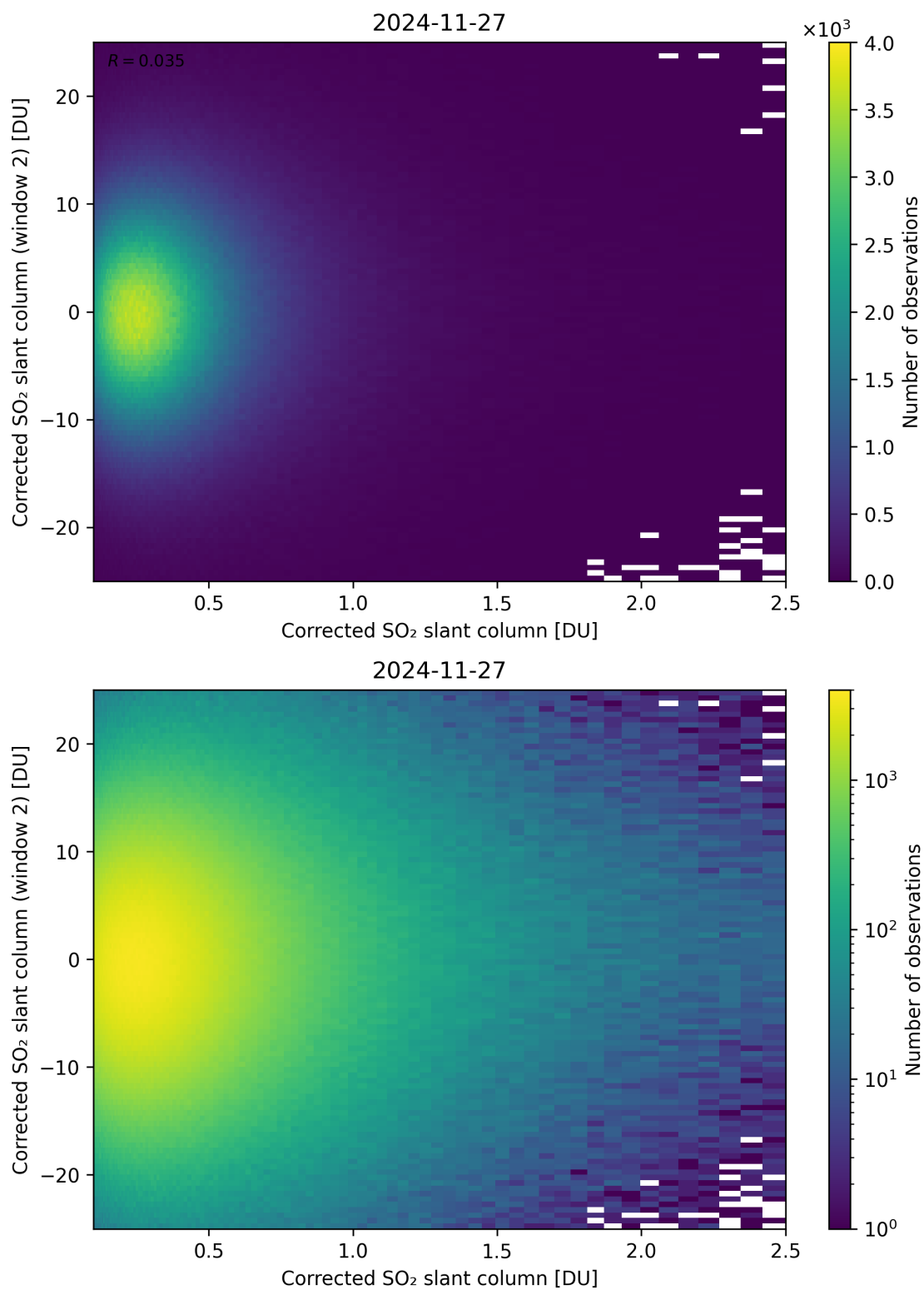
Figure 235: Scatter density plot of “Corrected SO 2 slant column” against “Corrected SO 2 slant column (window 2)” for 2024-11-26 to 2024-11-28.
