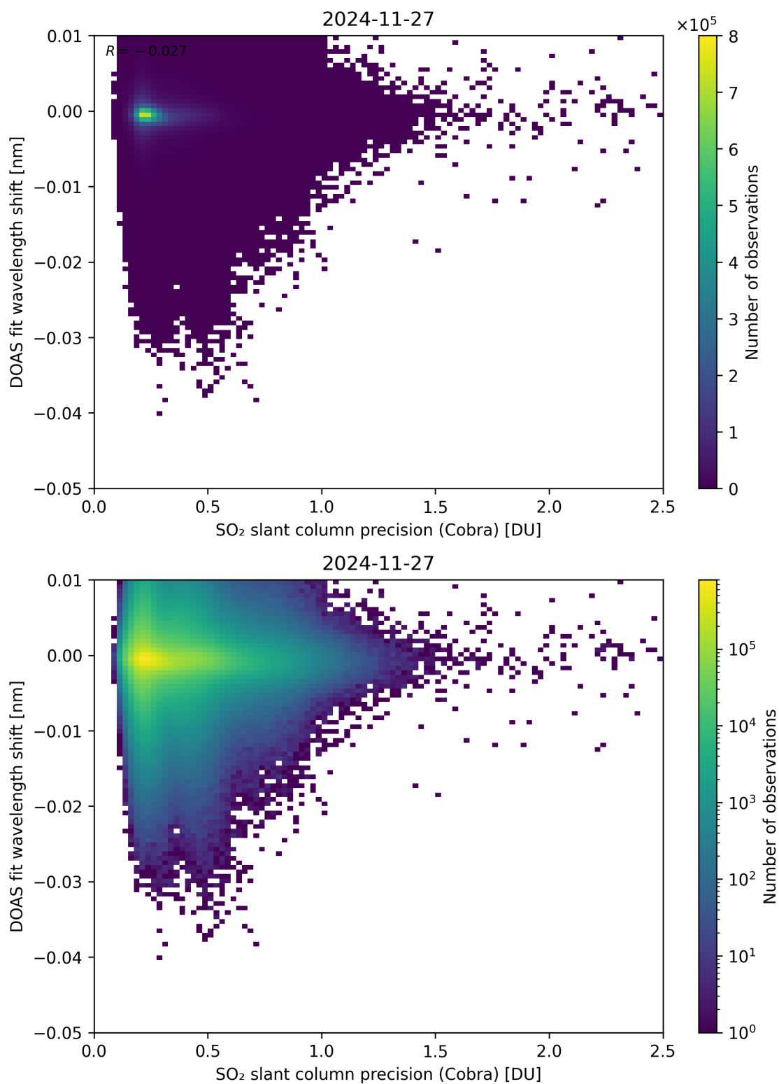
Figure 202: Scatter density plot of “SO 2 slant column precision (Cobra)” against “DOAS fit wavelength shift” for 2024-11-26 to 2024-11-28.
