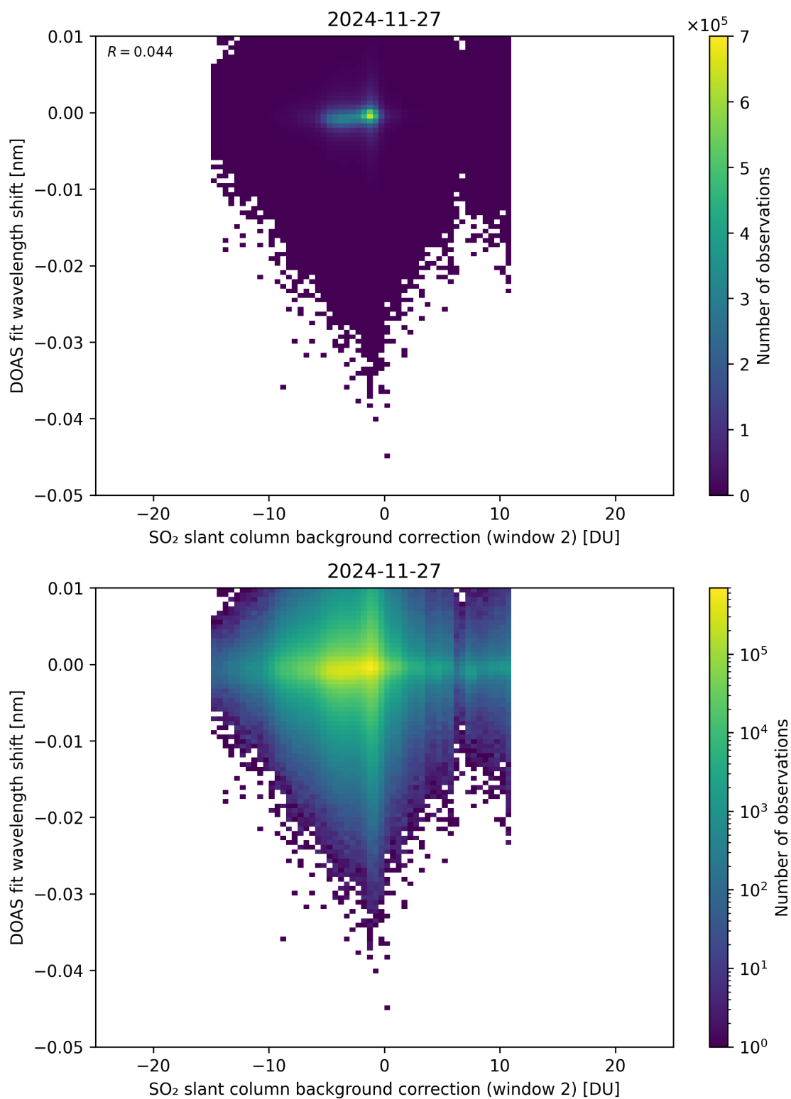
Figure 123: Scatter density plot of “SO 2 slant column background correction (window 2)” against “DOAS fit wavelength shift” for 2024-11-26 to 2024-11-28.
