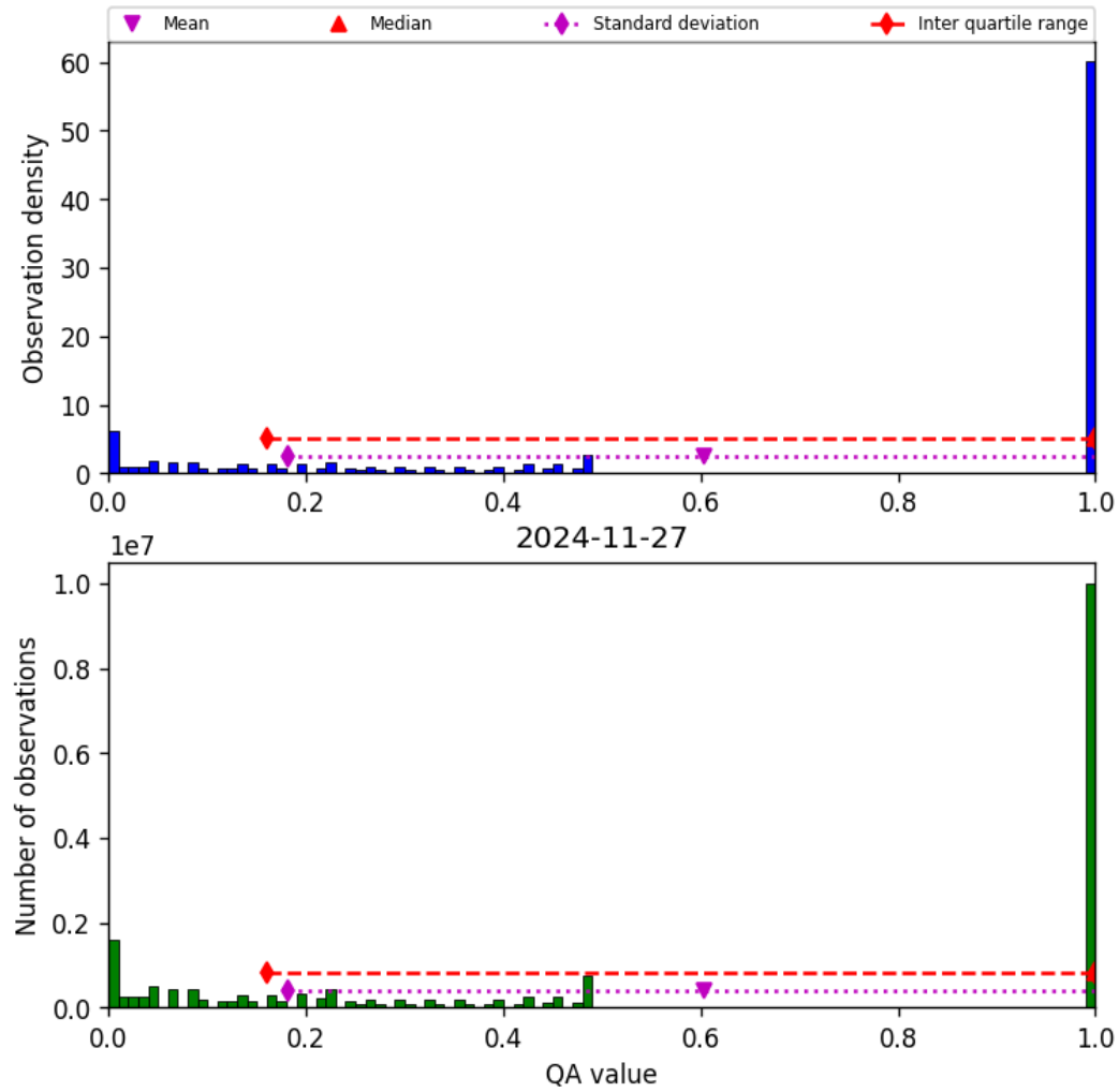
Figure 57: Histogram of “QA value” for 2024-11-26 to 2024-11-28
