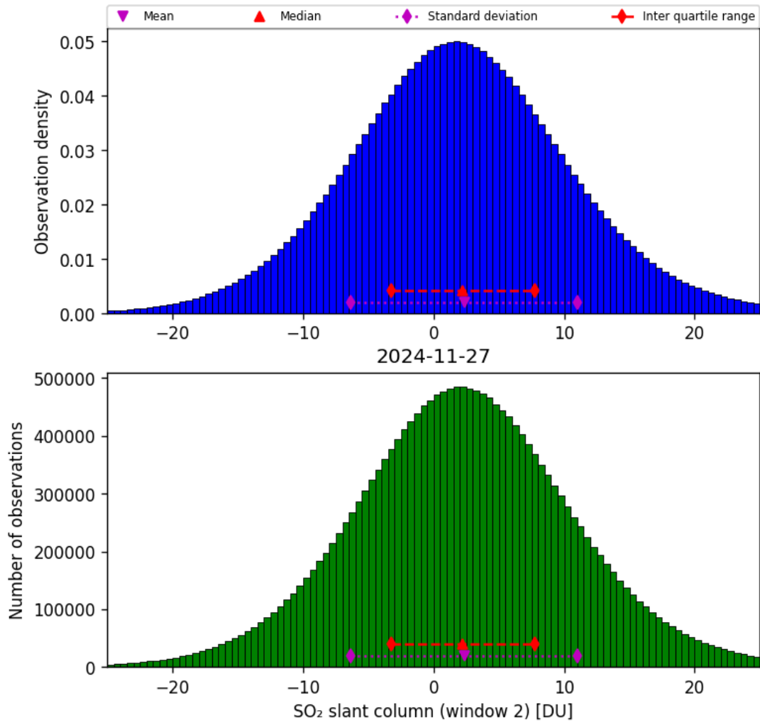
Figure 67: Histogram of “SO 2 slant column (window 2)” for 2024-11-26 to 2024-11-28
