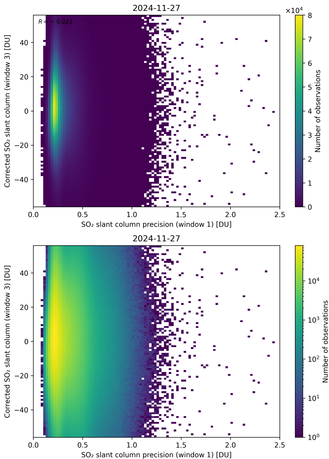
Figure 276: Scatter density plot of “SO 2 slant column precision (window 1)” against “Corrected SO 2 slant column (window 3)” for 2024-11-26 to 2024-11-28.
