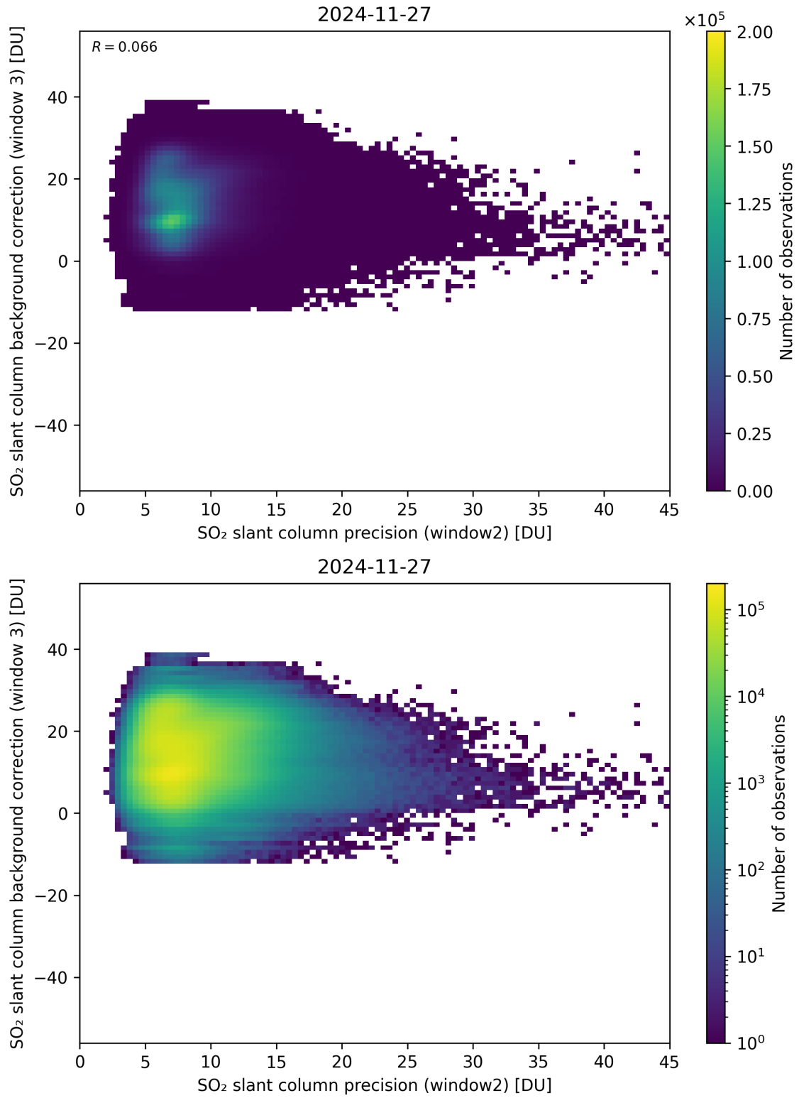
Figure 292: Scatter density plot of “SO 2 slant column precision (window2)” against “SO 2 slant column background correction (window 3)” for 2024-11-26 to 2024-11-28.
