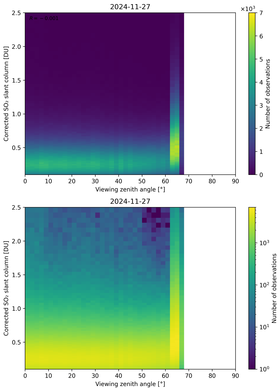
Figure 373: Scatter density plot of “Viewing zenith angle” against “Corrected SO 2 slant column” for 2024-11-26 to 2024-11-28.
