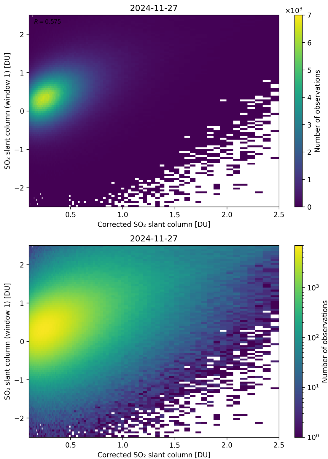
Figure 237: Scatter density plot of “Corrected SO 2 slant column” against “SO 2 slant column (window 1)” for 2024-11-26 to 2024-11-28.
