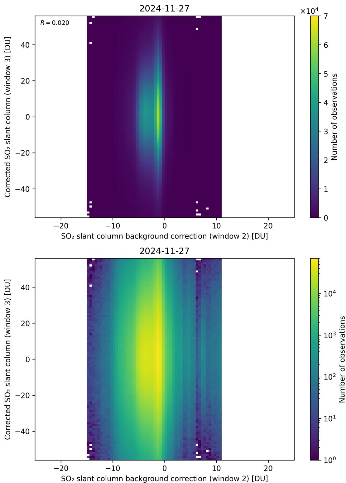
Figure 127: Scatter density plot of “SO 2 slant column background correction (window 2)” against “Corrected SO 2 slant column (window 3)” for 2024-11-26 to 2024-11-28.
