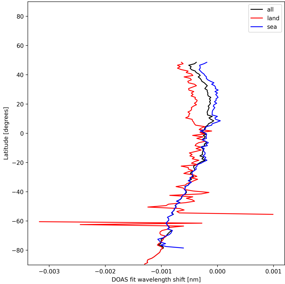
Figure 50: Zonal average of “DOAS fit wavelength shift” for 2024-11-26 to 2024-11-28.
