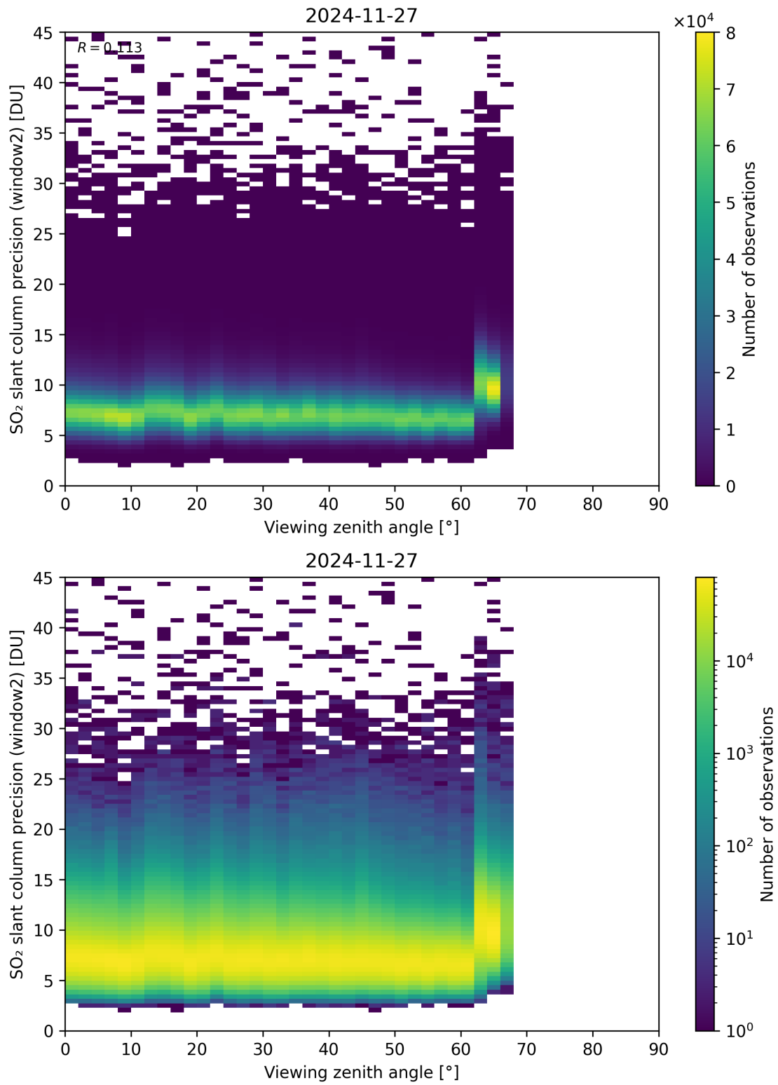
Figure 378: Scatter density plot of “Viewing zenith angle” against “SO 2 slant column precision (window2)” for 2024-11-26 to 2024-11-28.
