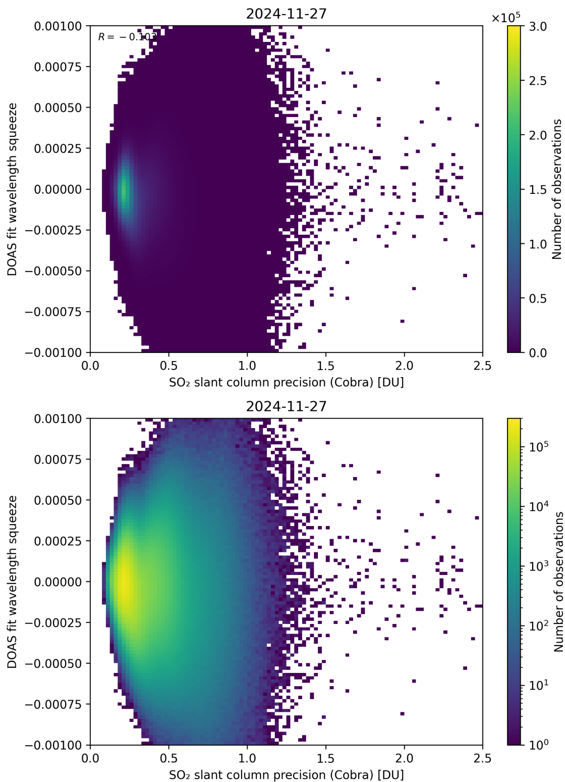
Figure 203: Scatter density plot of “SO 2 slant column precision (Cobra)” against “DOAS fit wavelength squeeze” for 2024-11-26 to 2024-11-28.
