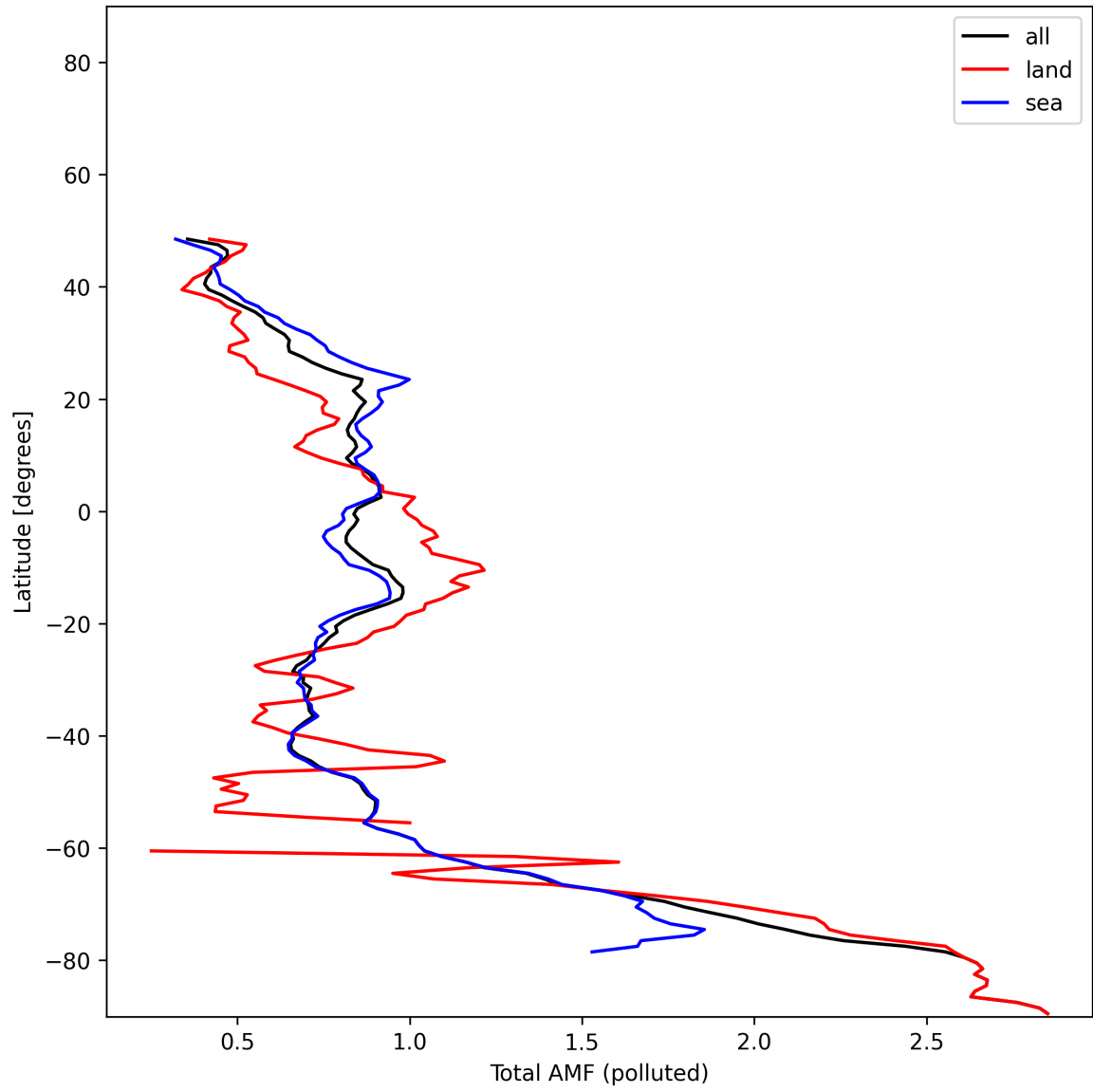
Figure 53: Zonal average of “Total AMF (polluted)” for 2024-11-26 to 2024-11-28.
