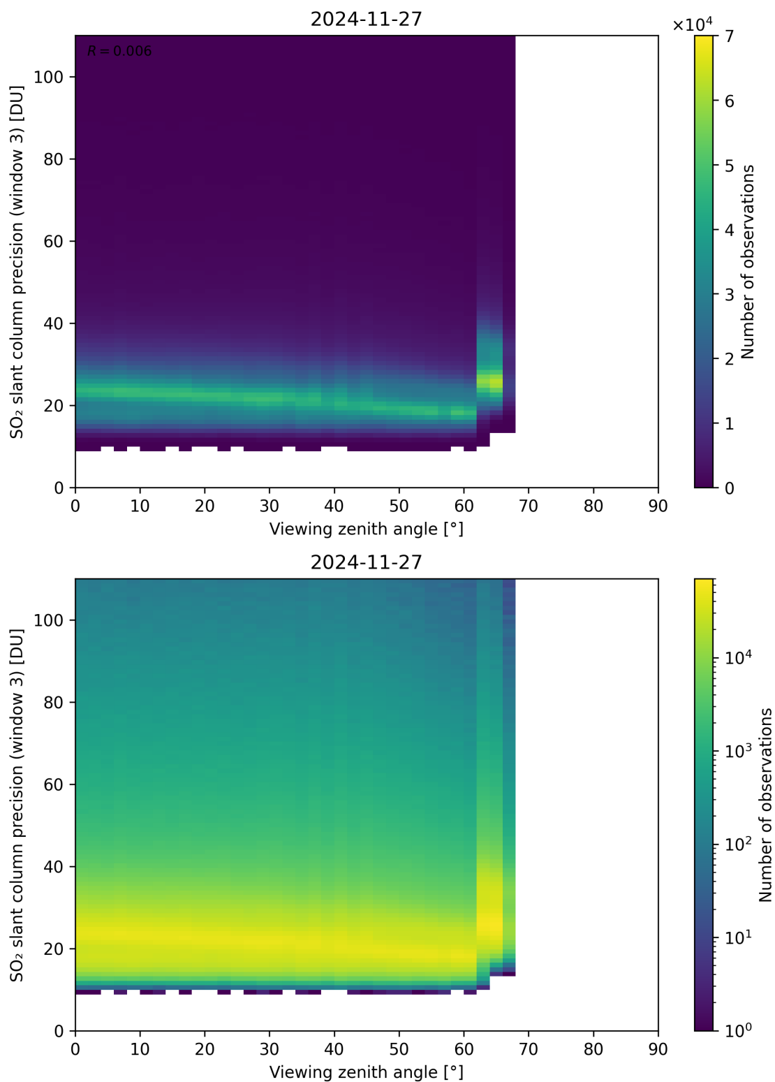
Figure 380: Scatter density plot of “Viewing zenith angle” against “SO 2 slant column precision (window 3)” for 2024-11-26 to 2024-11-28.
