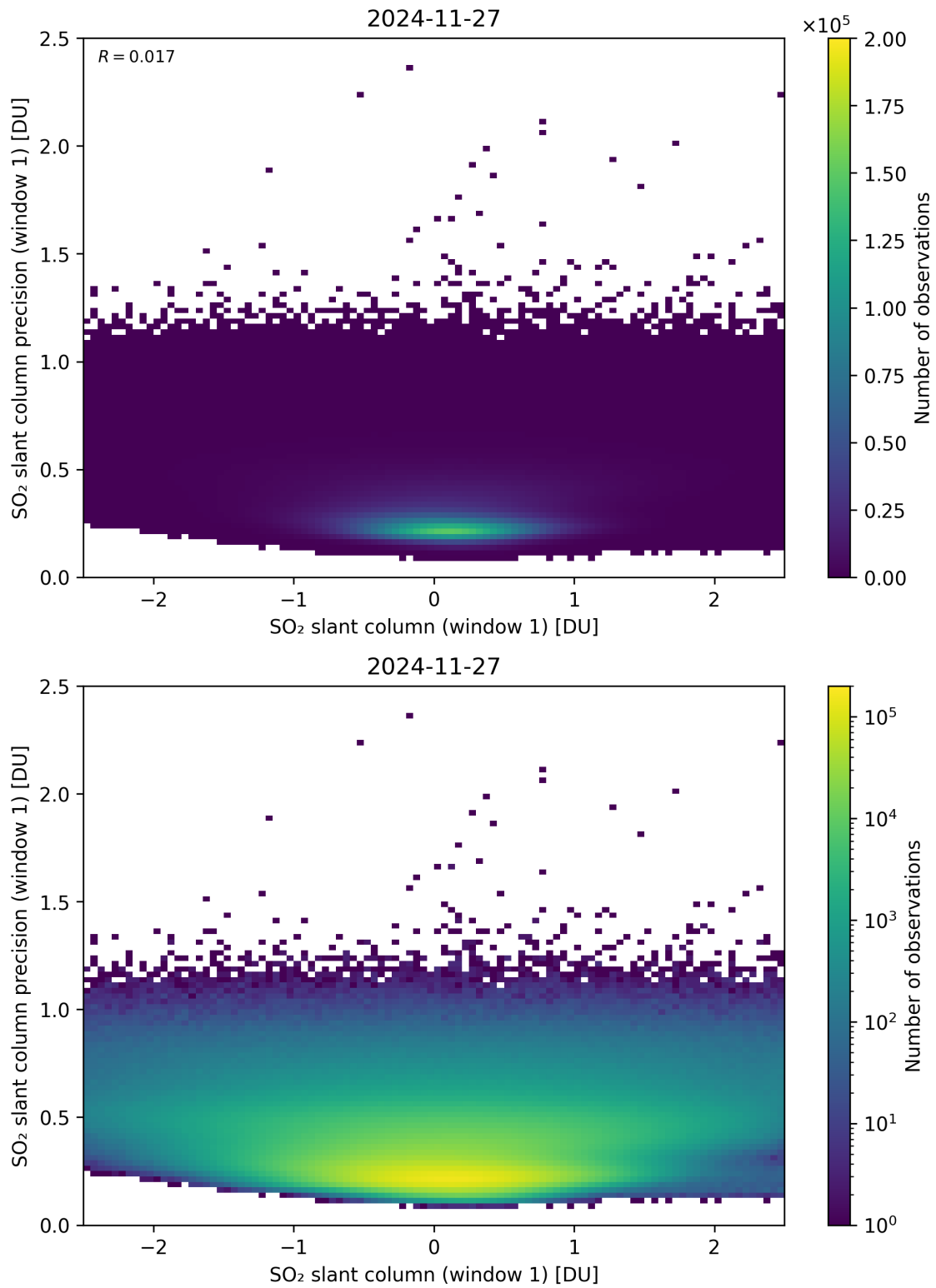
Figure 285: Scatter density plot of “SO 2 slant column (window 1)” against “SO 2 slant column precision (window 1)” for 2024-11-26 to 2024-11-28.
