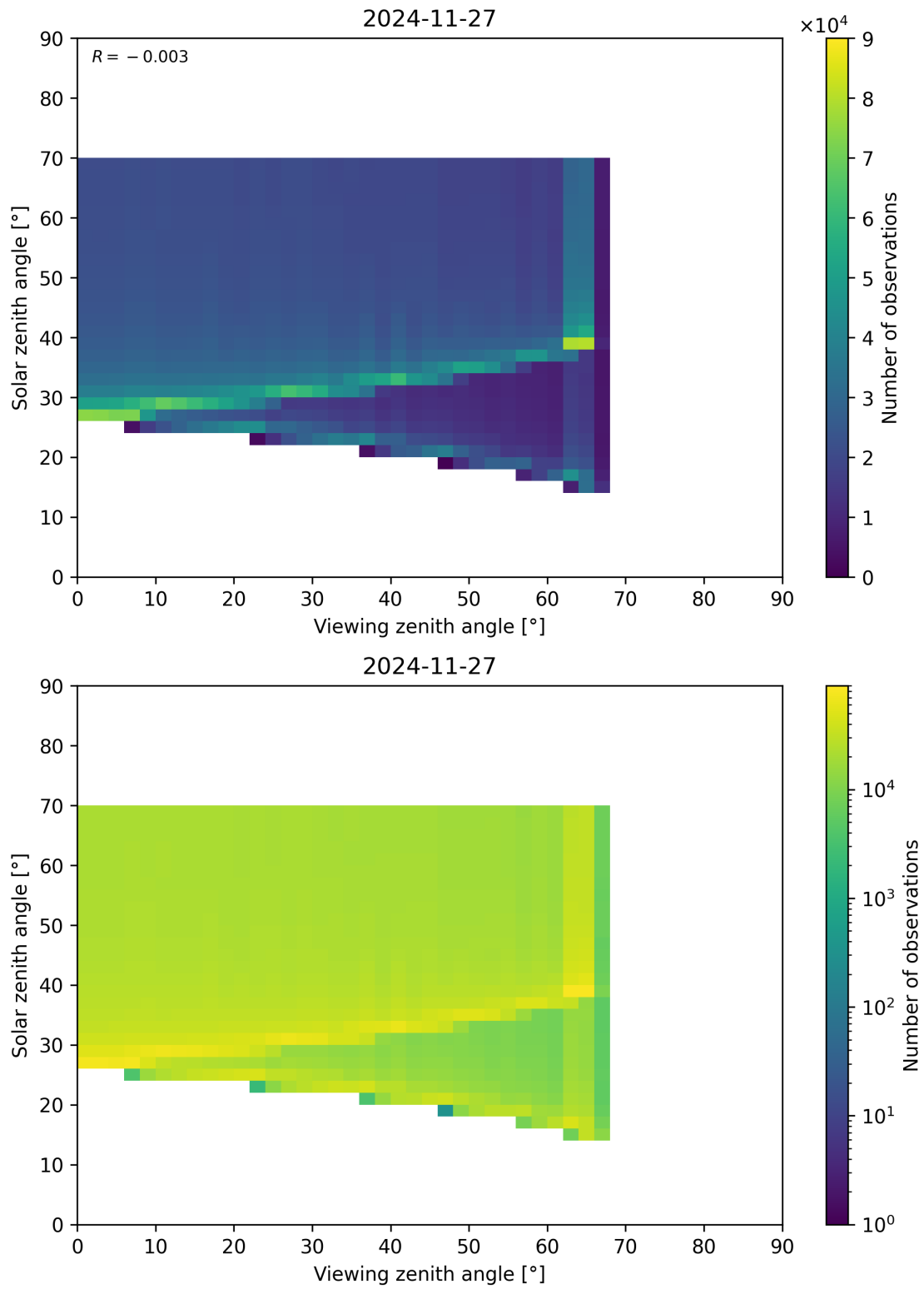
Figure 369: Scatter density plot of “Viewing zenith angle” against “Solar zenith angle” for 2024-11-26 to 2024-11-28.
