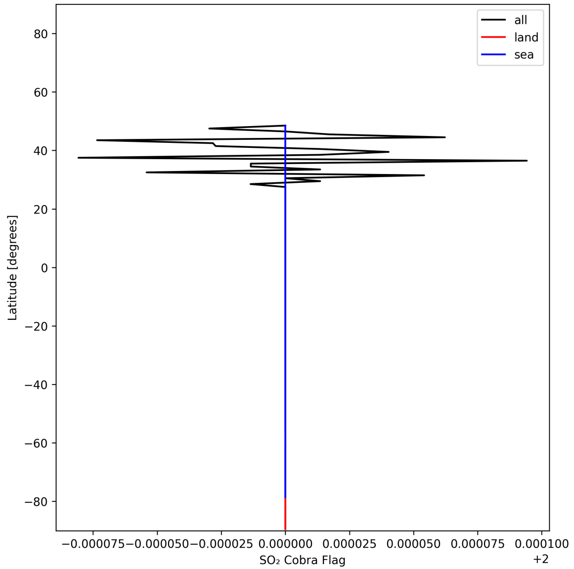
Figure 49: Zonal average of “SO 2 Cobra Flag” for 2024-11-26 to 2024-11-28.
