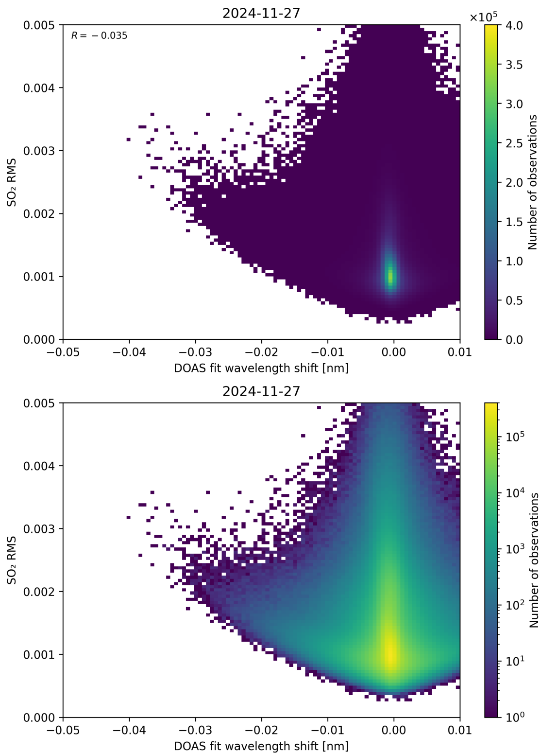
Figure 139: Scatter density plot of “DOAS fit wavelength shift” against “SO 2 RMS” for 2024-11-26 to 2024-11-28.
