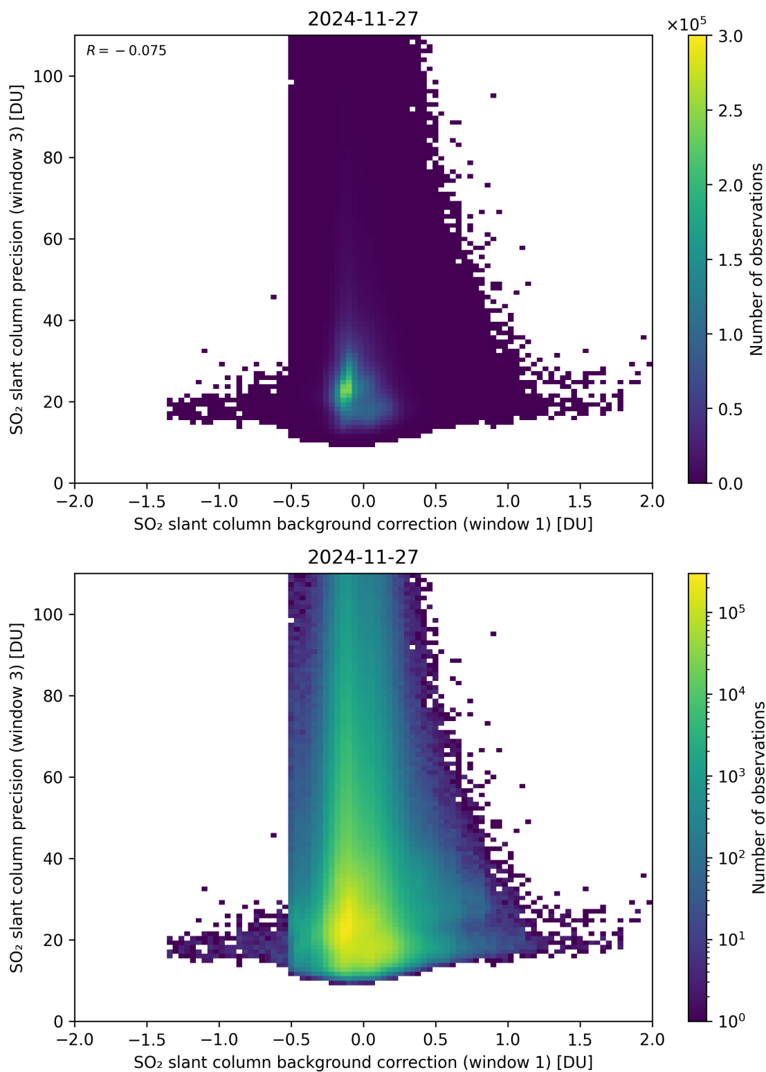
Figure 119: Scatter density plot of “SO 2 slant column background correction (window 1)” against “SO 2 slant column precision (window 3)” for 2024-11-26 to 2024-11-28.
