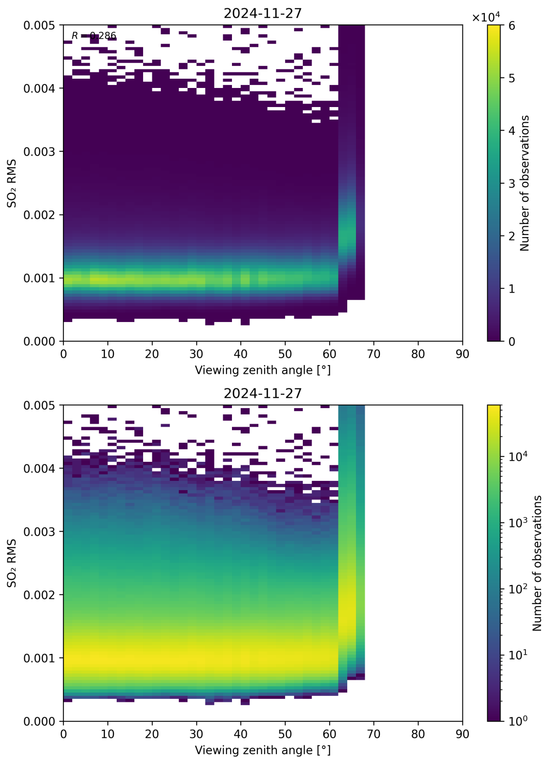
Figure 367: Scatter density plot of “Viewing zenith angle” against “SO 2 RMS” for 2024-11-26 to 2024-11-28.
