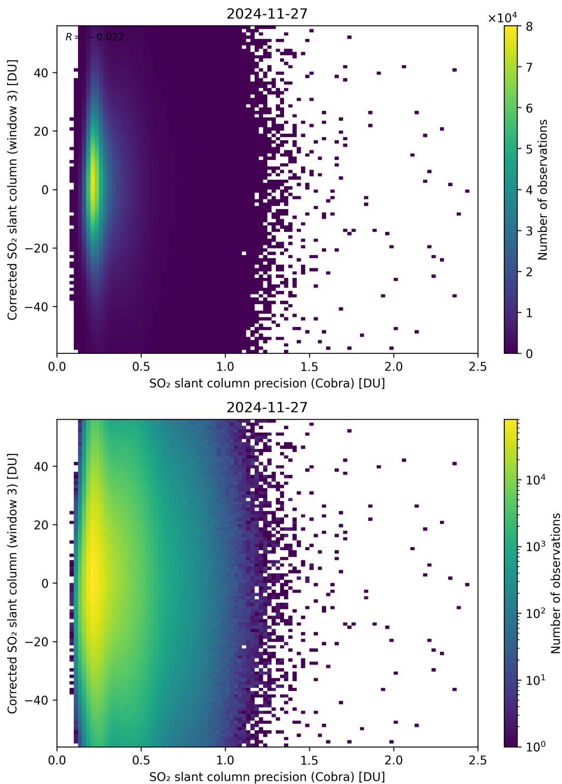
Figure 207: Scatter density plot of “SO 2 slant column precision (Cobra)” against “Corrected SO 2 slant column (window 3)” for 2024-11-26 to 2024-11-28.
