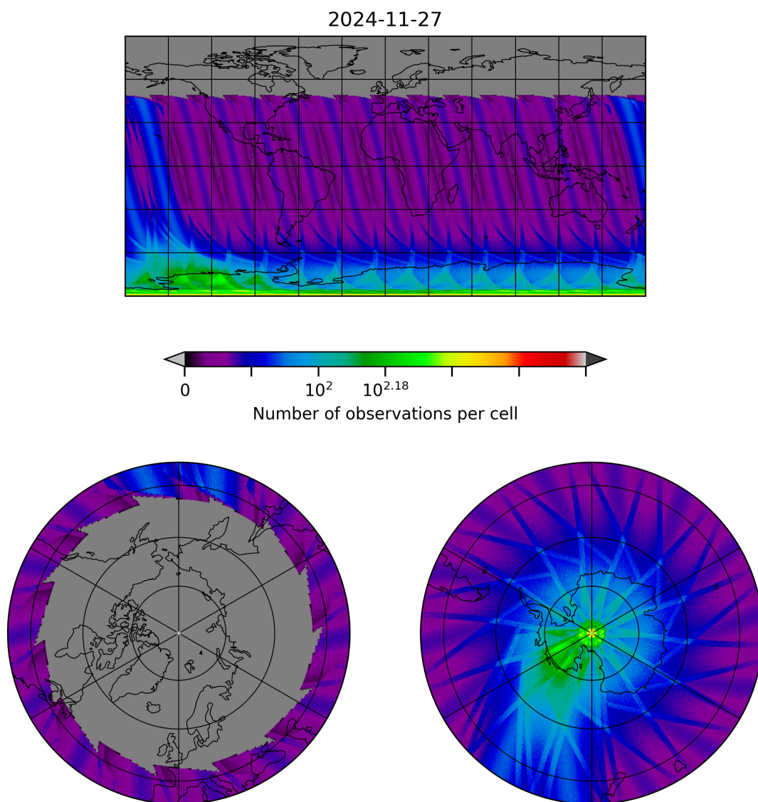
Figure 30: Map of the number of observations for 2024-11-26 to 2024-11-28
