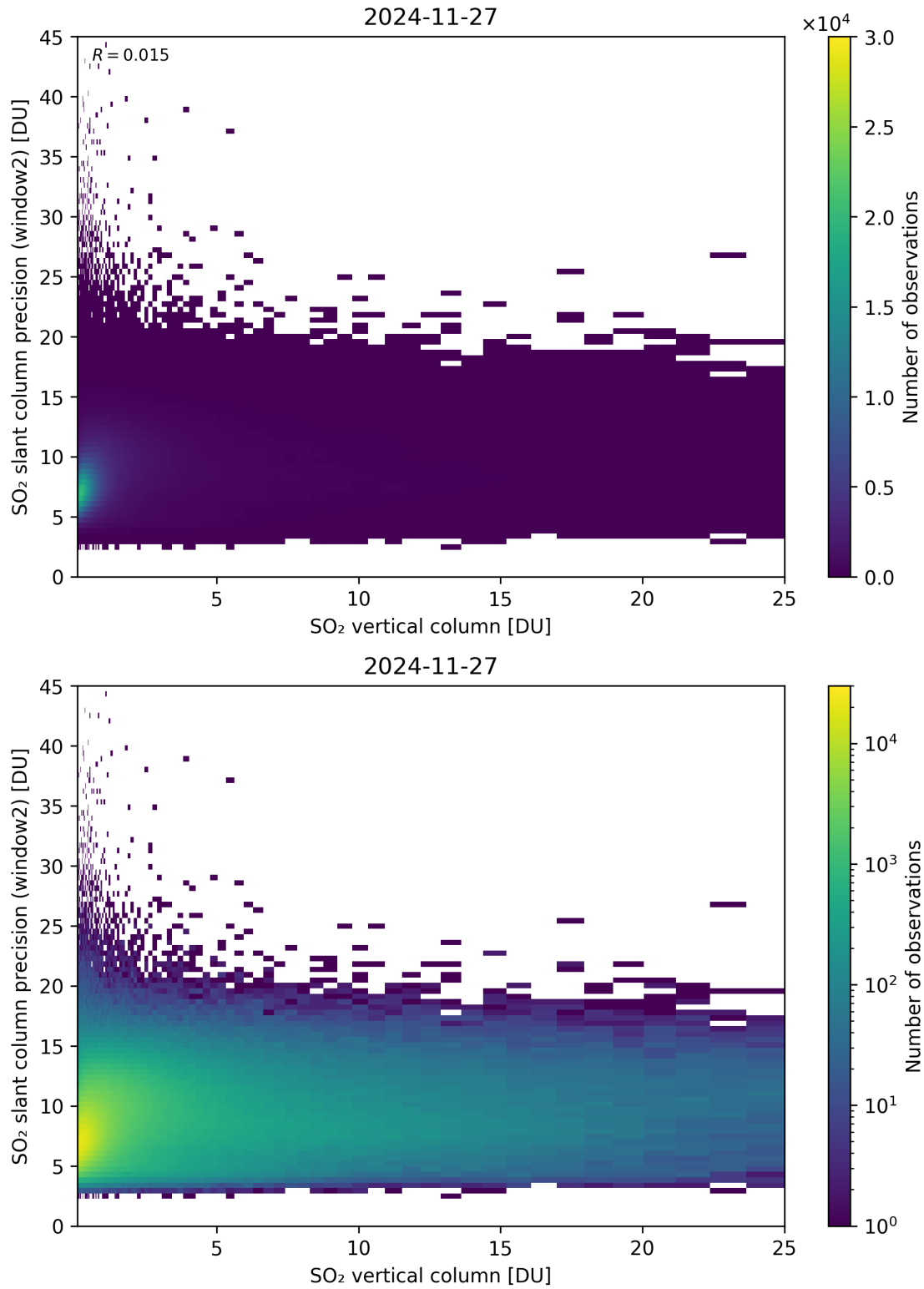
Figure 356: Scatter density plot of “SO 2 vertical column” against “SO 2 slant column precision (window2)” for 2024-11-26 to 2024-11-28.
