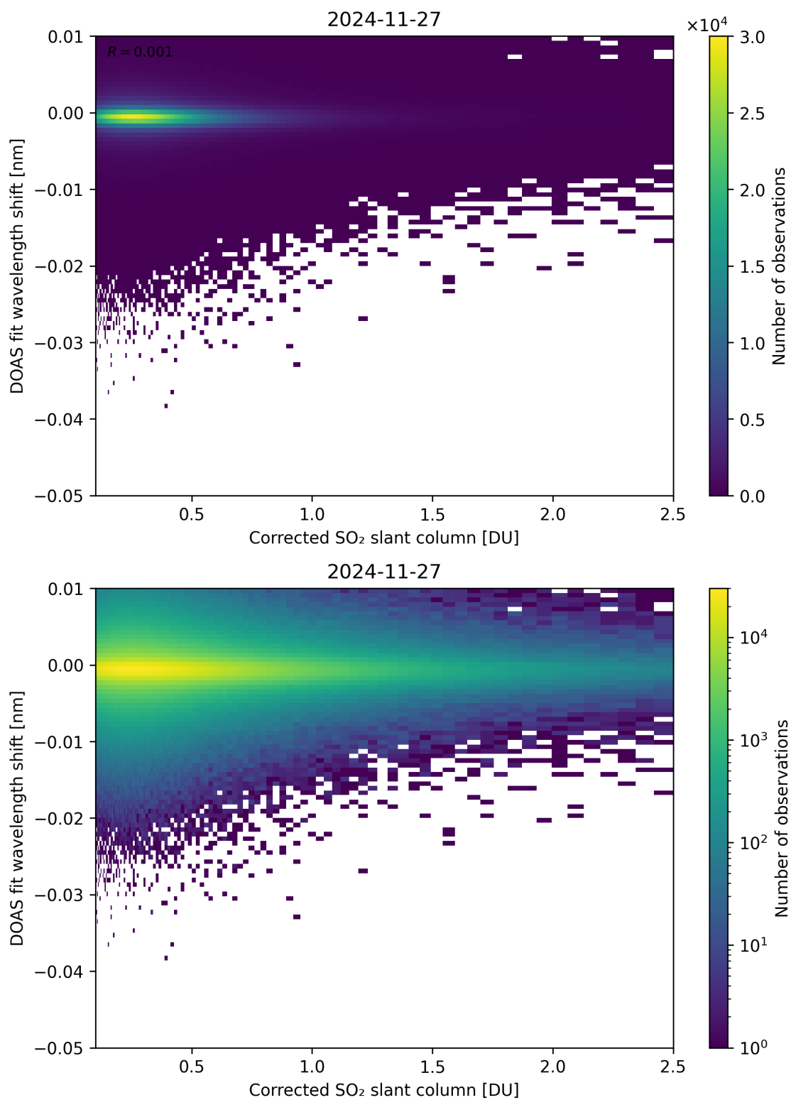
Figure 229: Scatter density plot of “Corrected SO 2 slant column” against “DOAS fit wavelength shift” for 2024-11-26 to 2024-11-28.
