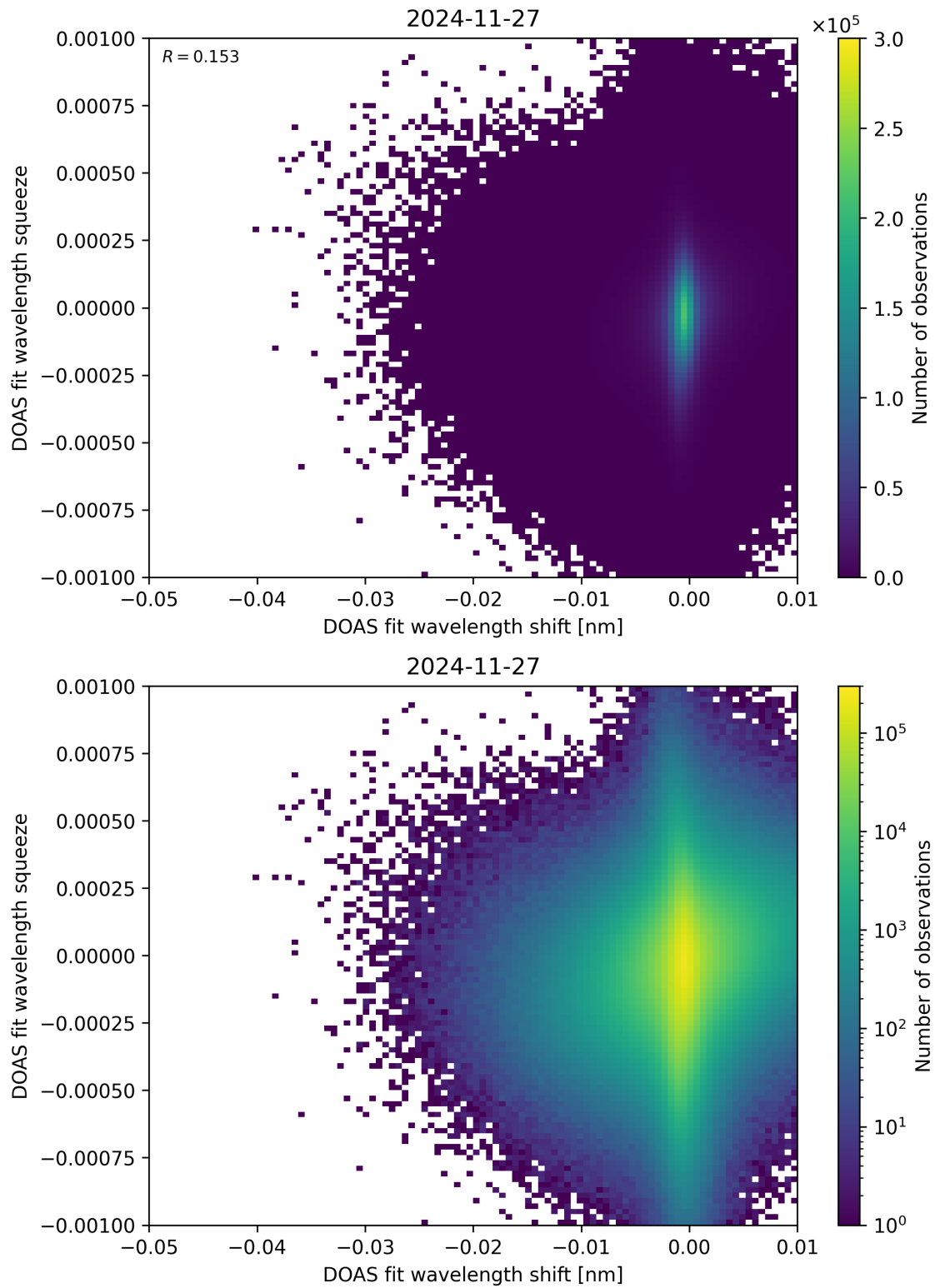
Figure 138: Scatter density plot of “DOAS fit wavelength shift” against “DOAS fit wavelength squeeze” for 2024-11-26 to 2024-11-28.
