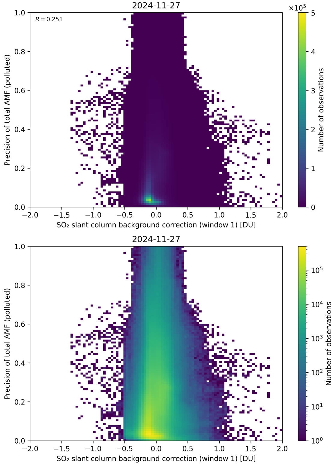
Figure 121: Scatter density plot of “SO 2 slant column background correction (window 1)” against “Precision of total AMF (polluted)” for 2024-11-26 to 2024-11-28.
