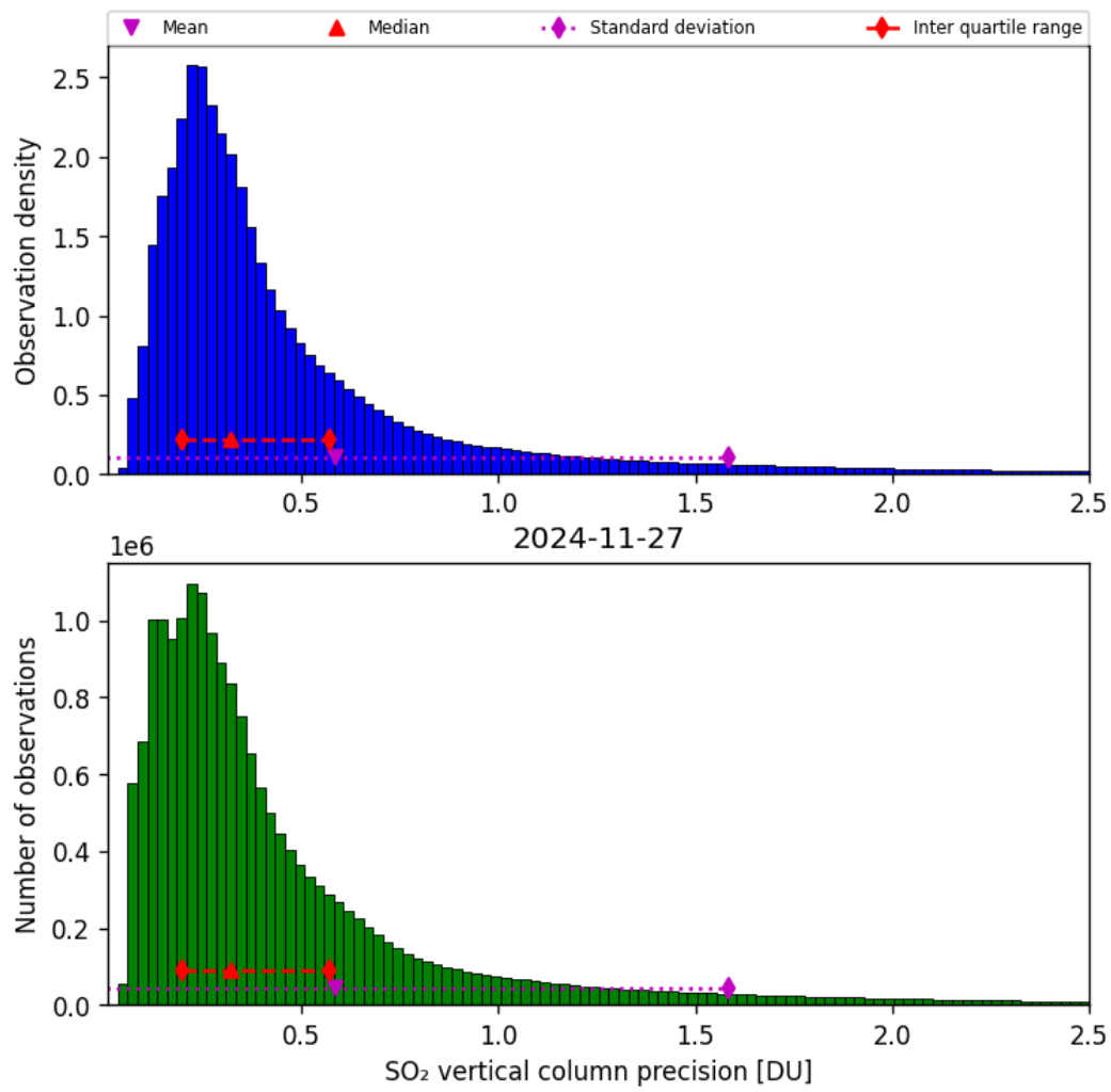
Figure 59: Histogram of “SO 2 vertical column precision” for 2024-11-26 to 2024-11-28
