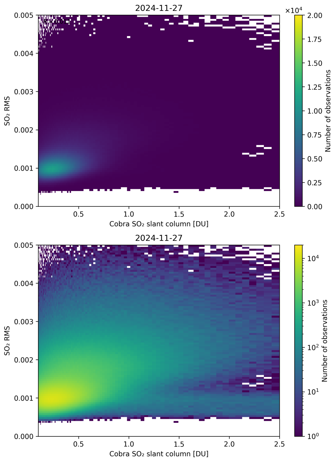
Figure 198: Scatter density plot of “Cobra SO 2 slant column” against “SO 2 RMS” for 2024-11-26 to 2024-11-28.
