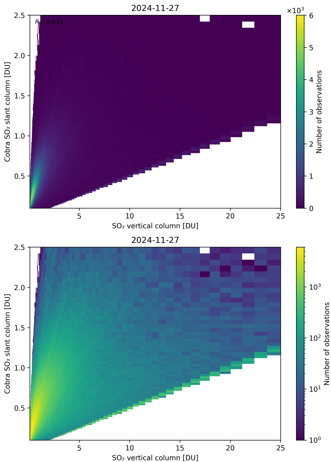
Figure 349: Scatter density plot of “SO 2 vertical column” against “Cobra SO 2 slant column” for 2024-11-26 to 2024-11-28.
