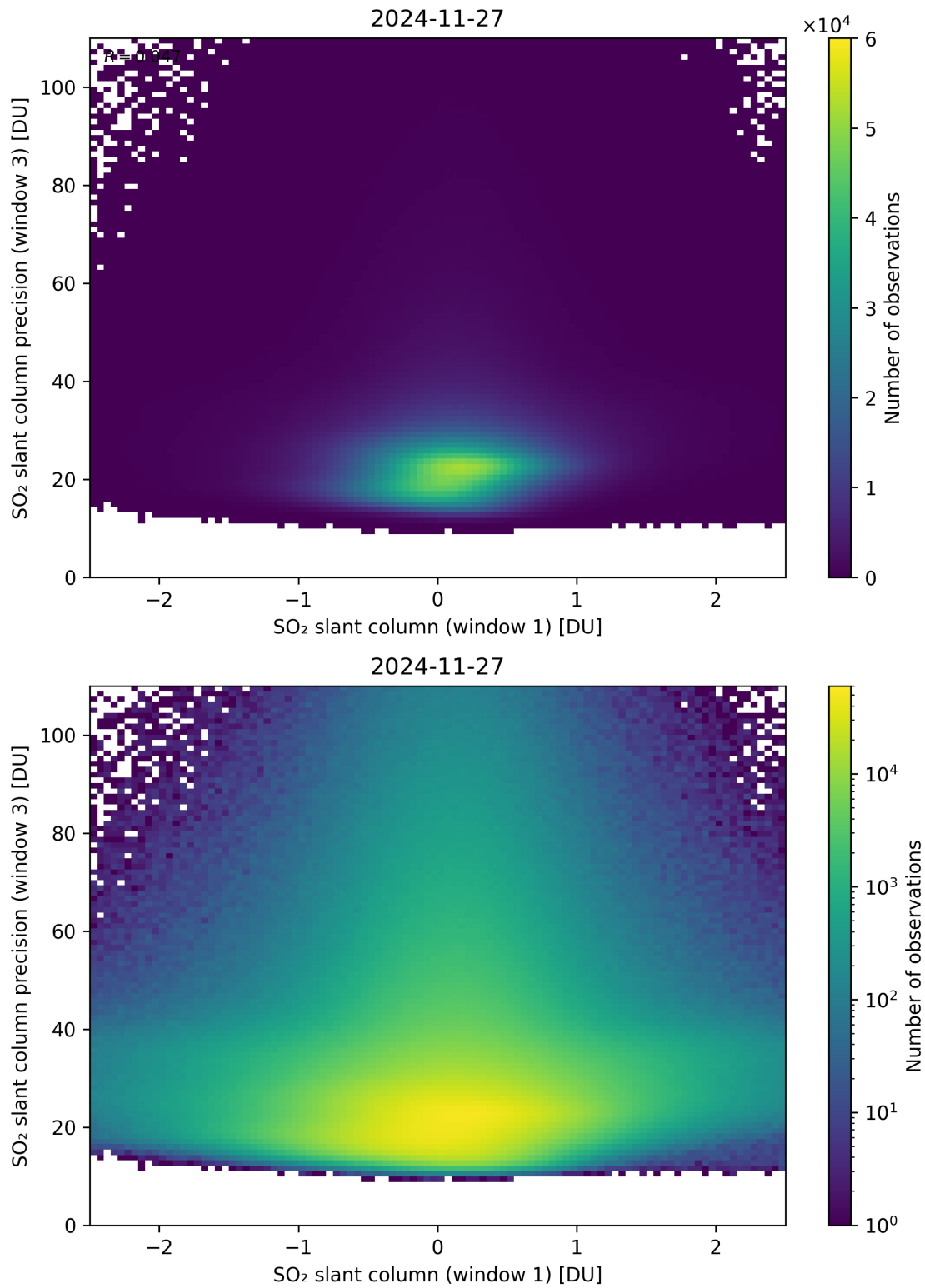
Figure 288: Scatter density plot of “SO 2 slant column (window 1)” against “SO 2 slant column precision (window 3)” for 2024-11-26 to 2024-11-28.
