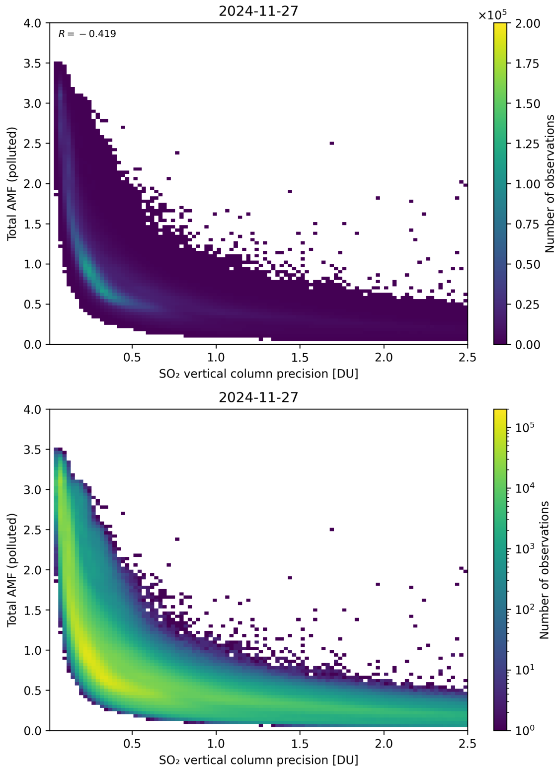
Figure 346: Scatter density plot of “SO 2 vertical column precision” against “Total AMF (polluted)” for 2024-11-26 to 2024-11-28.
