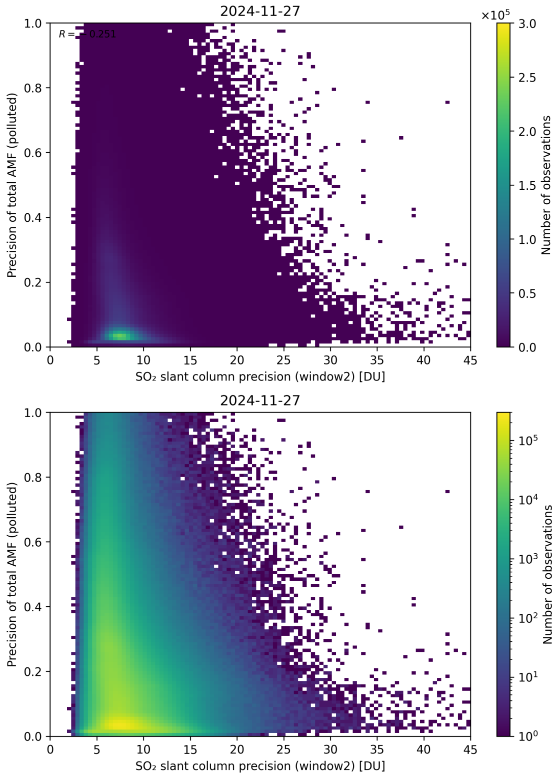
Figure 302: Scatter density plot of “SO 2 slant column precision (window2)” against “Precision of total AMF (polluted)” for 2024-11-26 to 2024-11-28.
