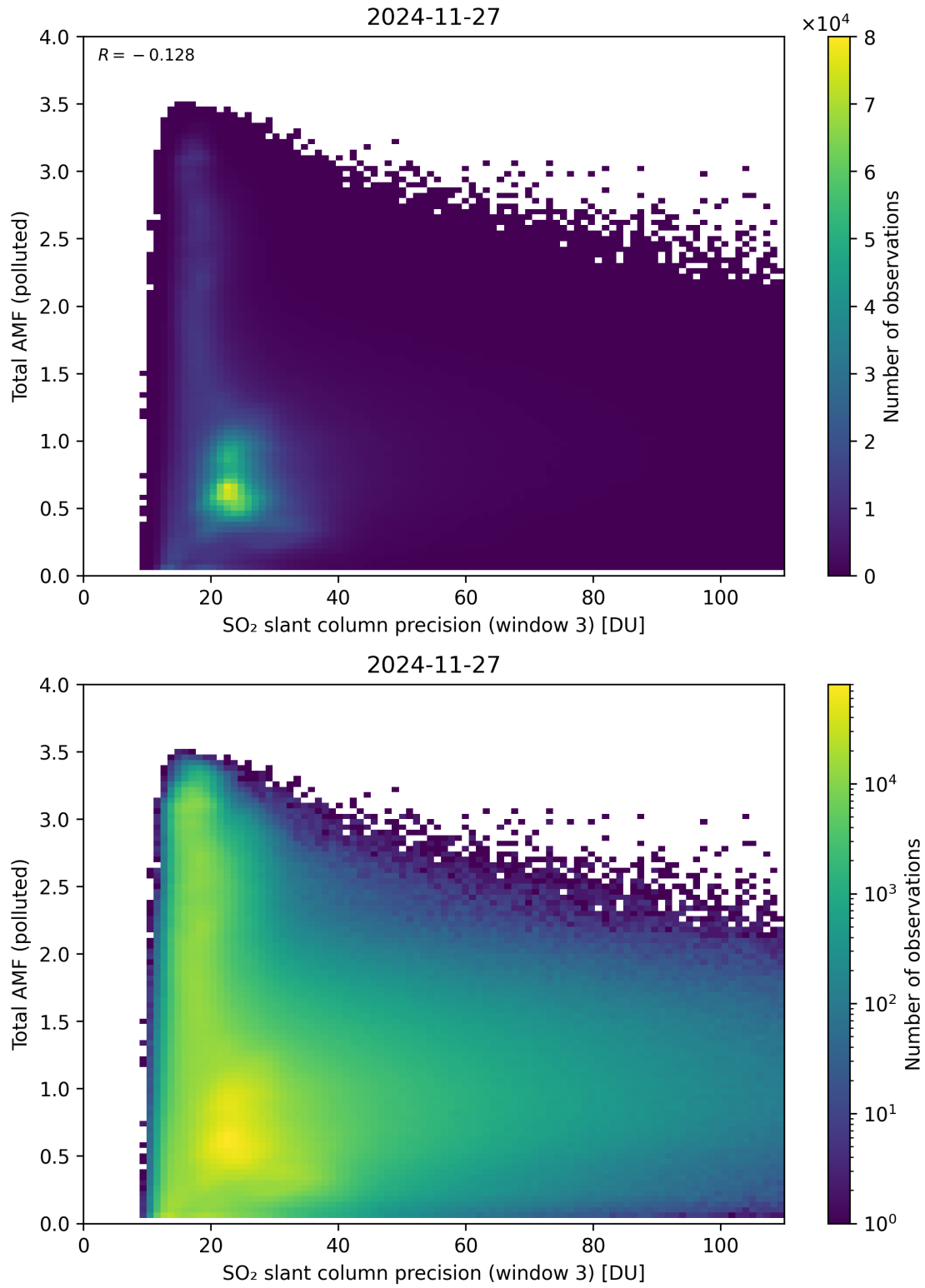
Figure 313: Scatter density plot of “SO 2 slant column precision (window 3)” against “Total AMF (polluted)” for 2024-11-26 to 2024-11-28.
