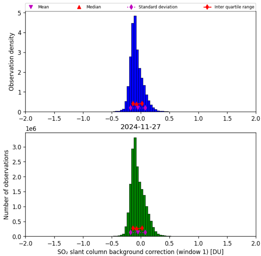
Figure 66: Histogram of “SO 2 slant column background correction (window 1)” for 2024-11-26 to 2024-11-28
