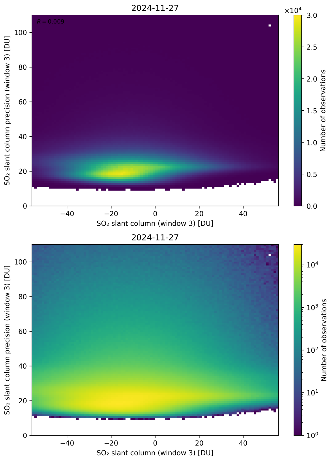
Figure 317: Scatter density plot of “SO 2 slant column (window 3)” against “SO 2 slant column precision (window 3)” for 2024-11-26 to 2024-11-28.
