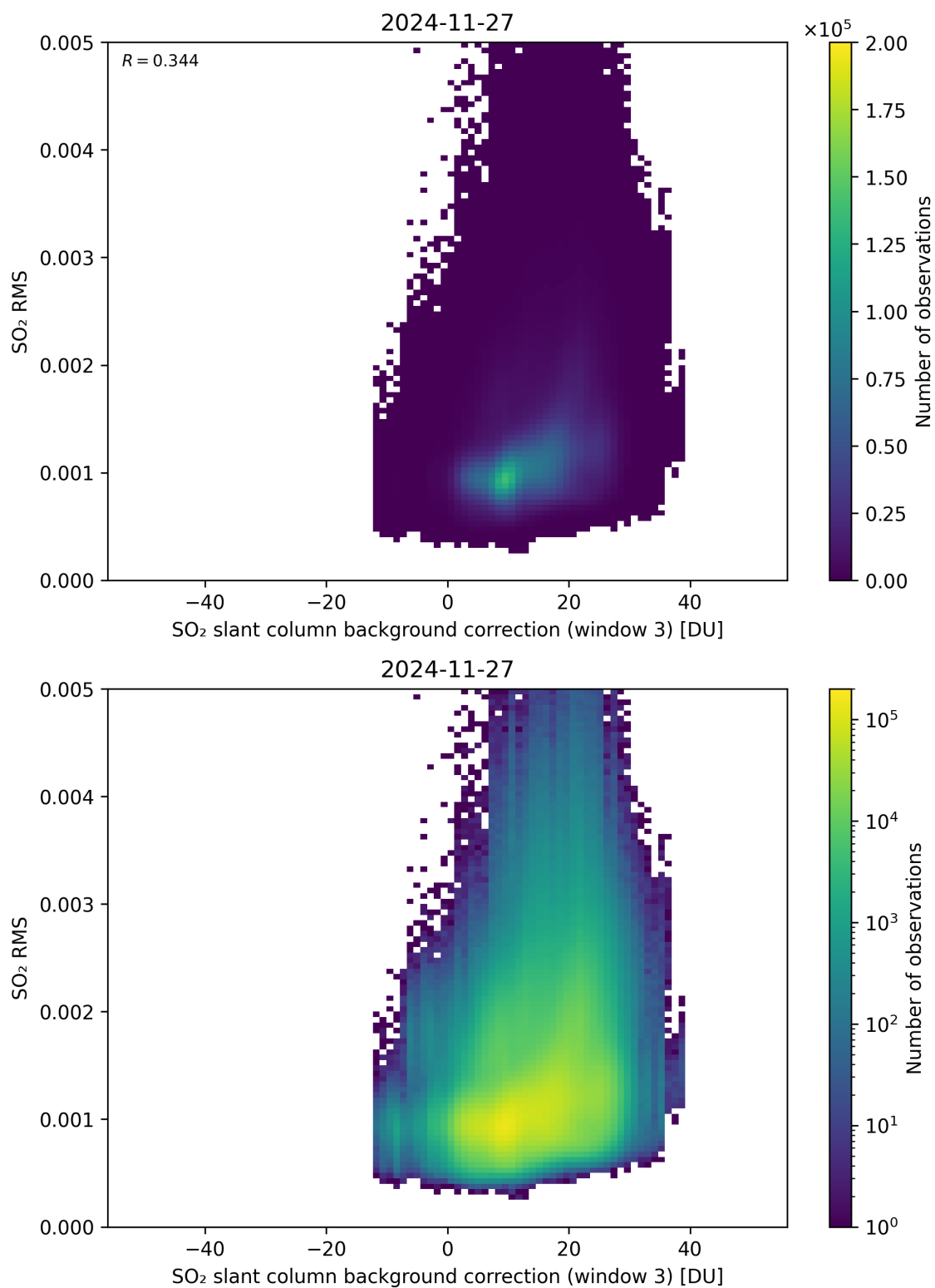
Figure 134: Scatter density plot of “SO 2 slant column background correction (window 3)” against “SO 2 RMS” for 2024-11-26 to 2024-11-28.
