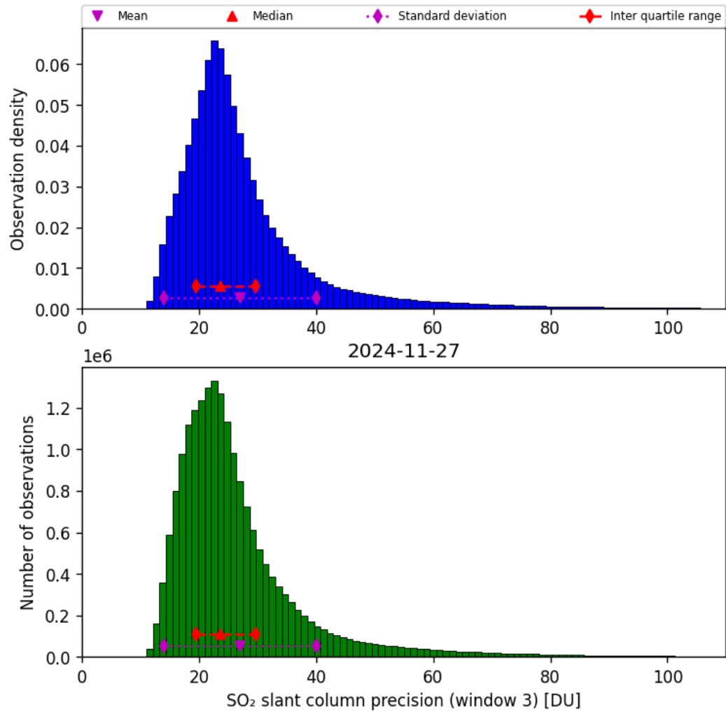
Figure 72: Histogram of “SO 2 slant column precision (window 3)” for 2024-11-26 to 2024-11-28
