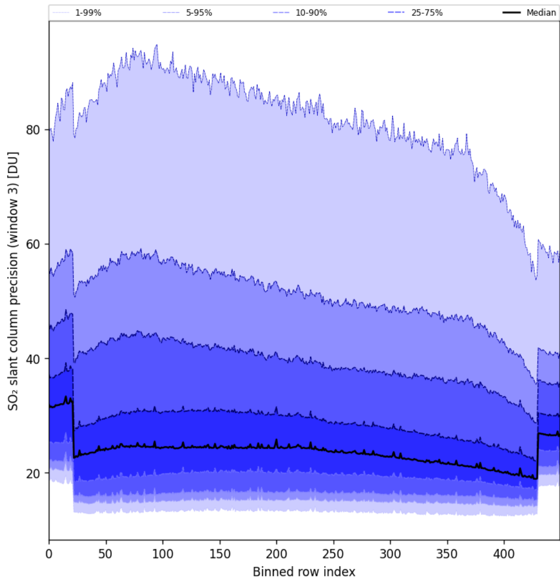
Figure 98: Along track statistics of “SO 2 slant column precision (window 3)” for 2024-11-26 to 2024-11-28
