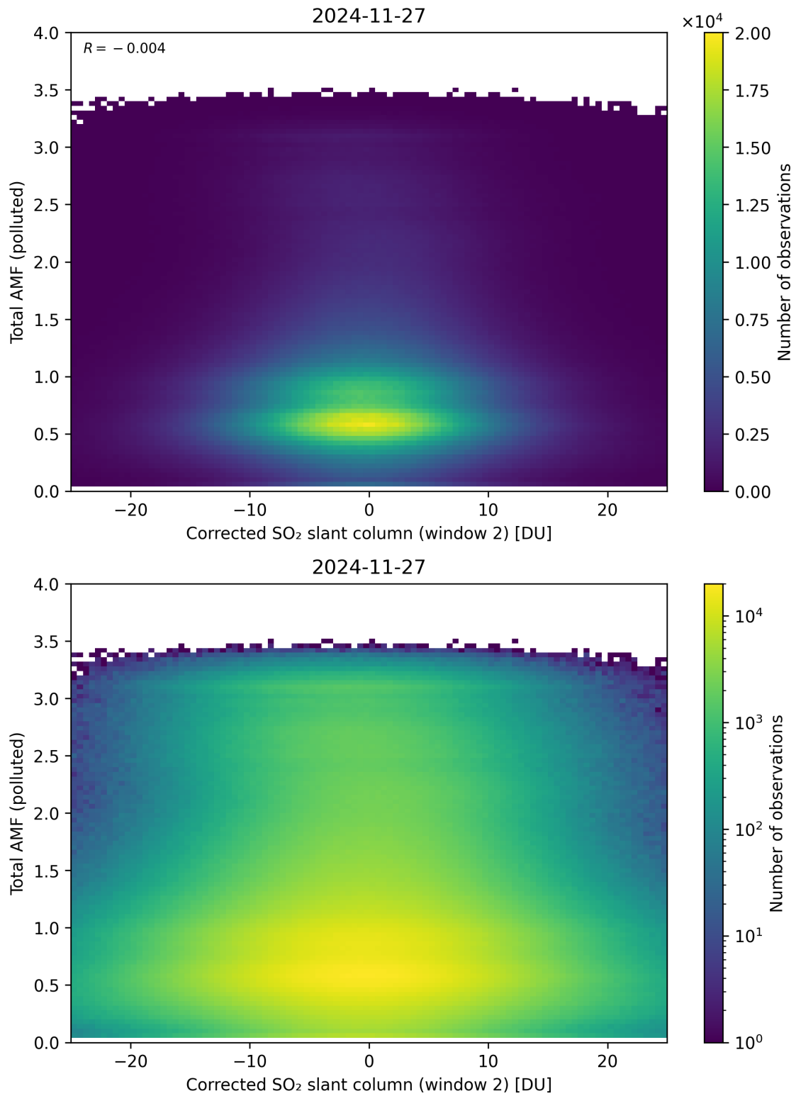
Figure 253: Scatter density plot of “Corrected SO 2 slant column (window 2)” against “Total AMF (polluted)” for 2024-11-26 to 2024-11-28.
