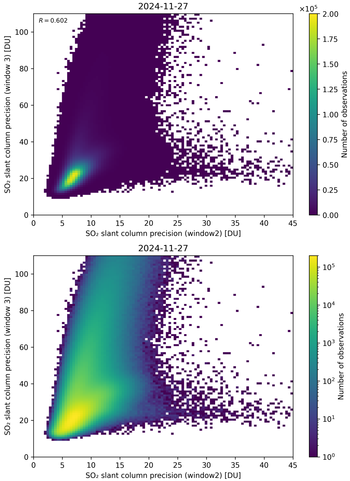
Figure 300: Scatter density plot of “SO 2 slant column precision (window2)” against “SO 2 slant column precision (window 3)” for 2024-11-26 to 2024-11-28.
