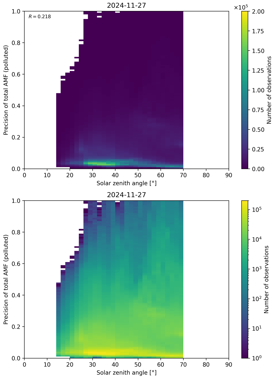
Figure 190: Scatter density plot of “Solar zenith angle” against “Precision of total AMF (polluted)” for 2024-11-26 to 2024-11-28.
