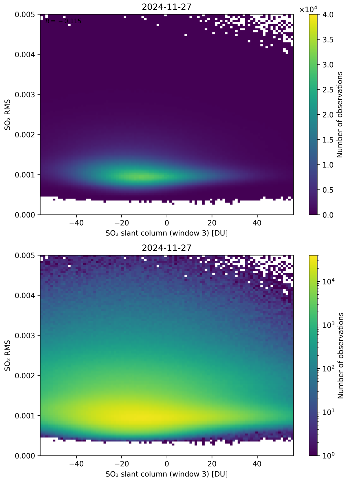
Figure 306: Scatter density plot of “SO 2 slant column (window 3)” against “SO 2 RMS” for 2024-11-26 to 2024-11-28.
