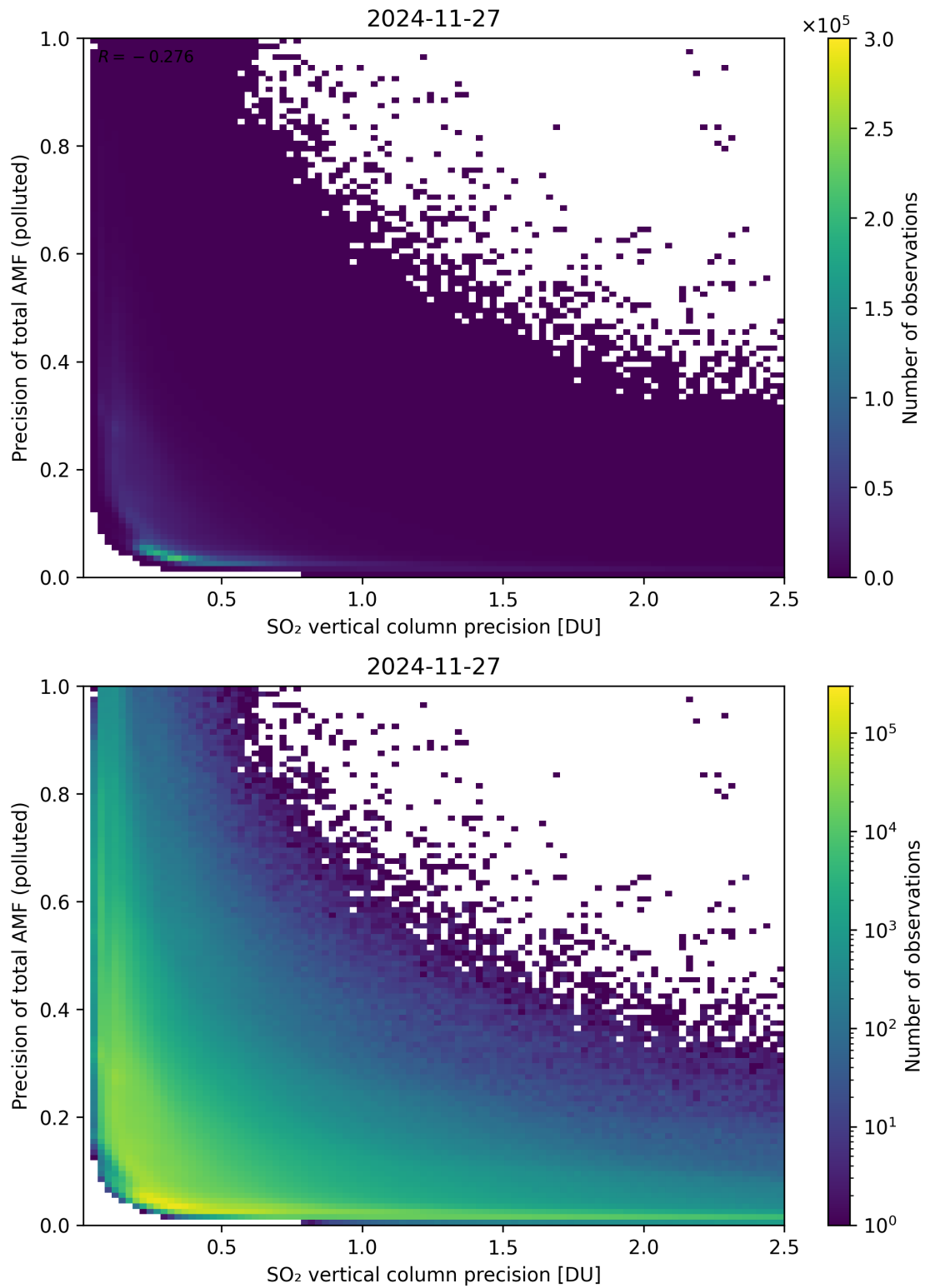
Figure 347: Scatter density plot of “SO 2 vertical column precision” against “Precision of total AMF (polluted)” for 2024-11-26 to 2024-11-28.
