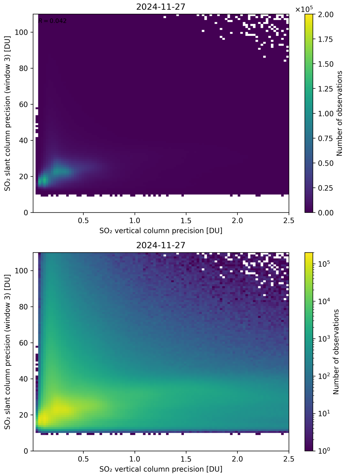
Figure 345: Scatter density plot of “SO 2 vertical column precision” against “SO 2 slant column precision (window 3)” for 2024-11-26 to 2024-11-28.
