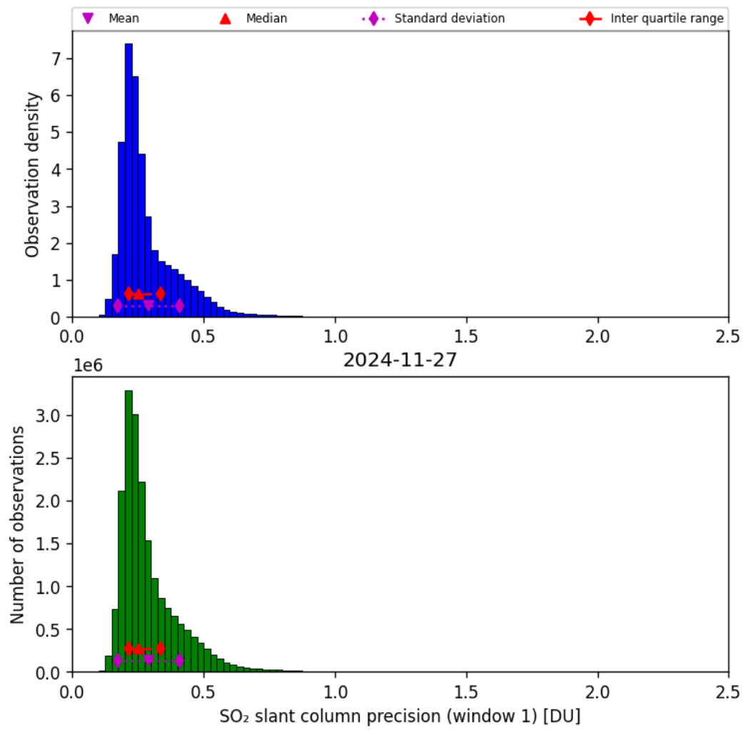
Figure 64: Histogram of “SO 2 slant column precision (window 1)” for 2024-11-26 to 2024-11-28
