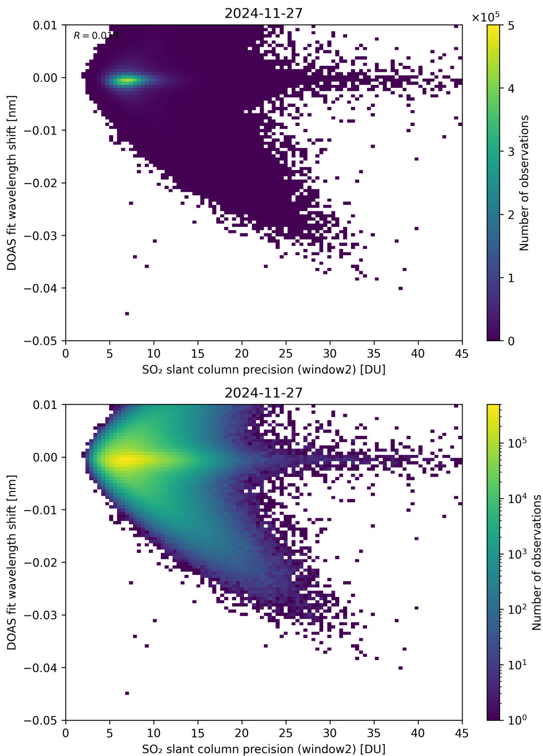
Figure 293: Scatter density plot of “SO 2 slant column precision (window2)” against “DOAS fit wavelength shift” for 2024-11-26 to 2024-11-28.
