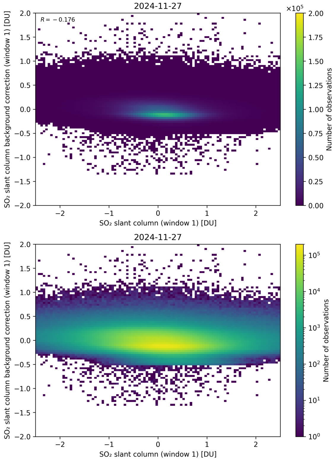
Figure 262: Scatter density plot of “SO 2 slant column (window 1)” against “SO 2 slant column background correction (window 1)” for 2024-11-26 to 2024-11-28.
