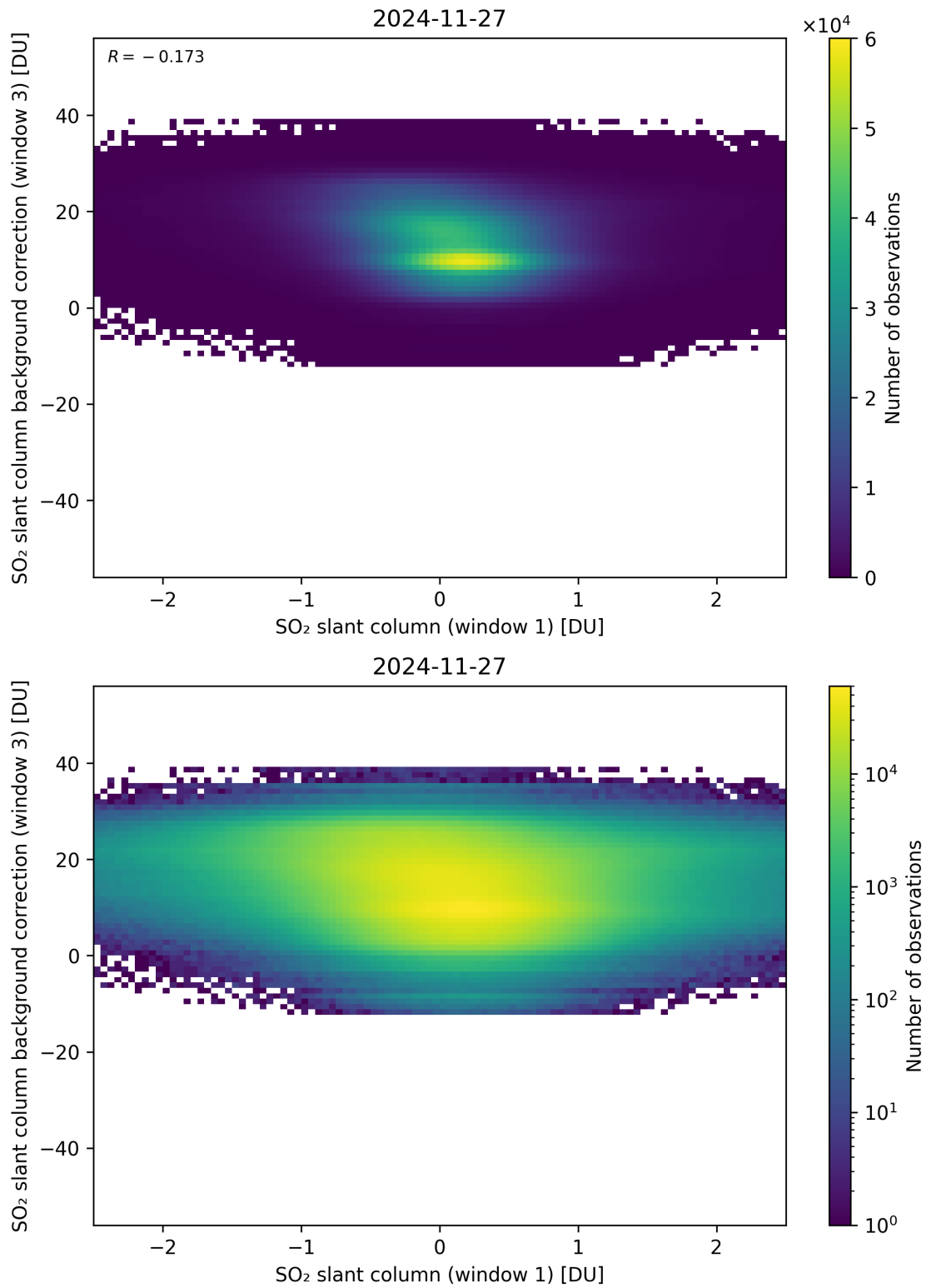
Figure 264: Scatter density plot of “SO 2 slant column (window 1)” against “SO 2 slant column background correction (window 3)” for 2024-11-26 to 2024-11-28.
