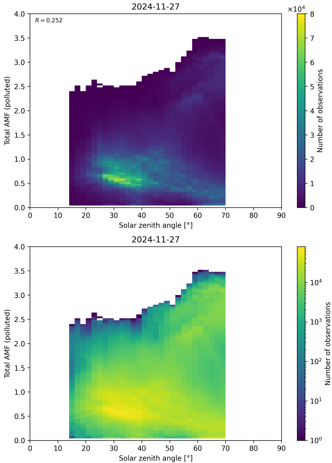
Figure 189: Scatter density plot of “Solar zenith angle” against “Total AMF (polluted)” for 2024-11-26 to 2024-11-28.
