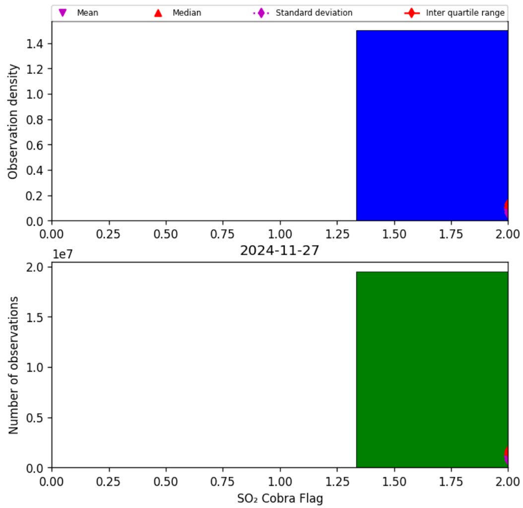
Figure 75: Histogram of “SO 2 Cobra Flag” for 2024-11-26 to 2024-11-28
