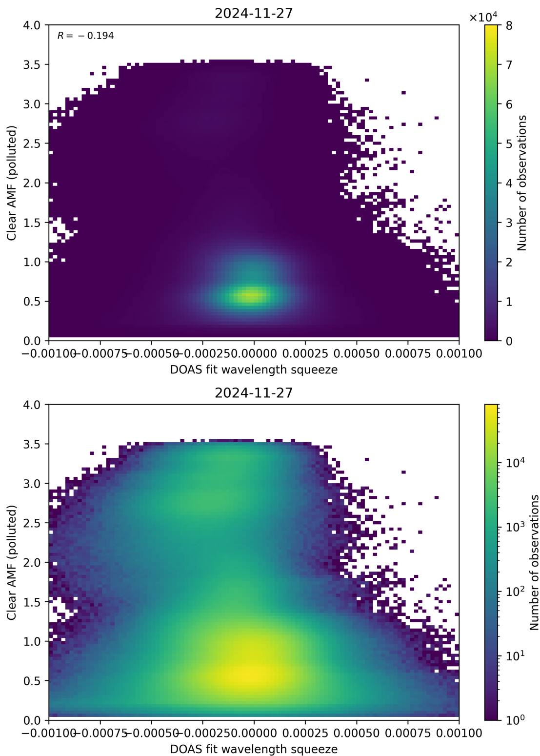
Figure 144: Scatter density plot of “DOAS fit wavelength squeeze” against “Clear AMF (polluted)” for 2024-11-26 to 2024-11-28.
