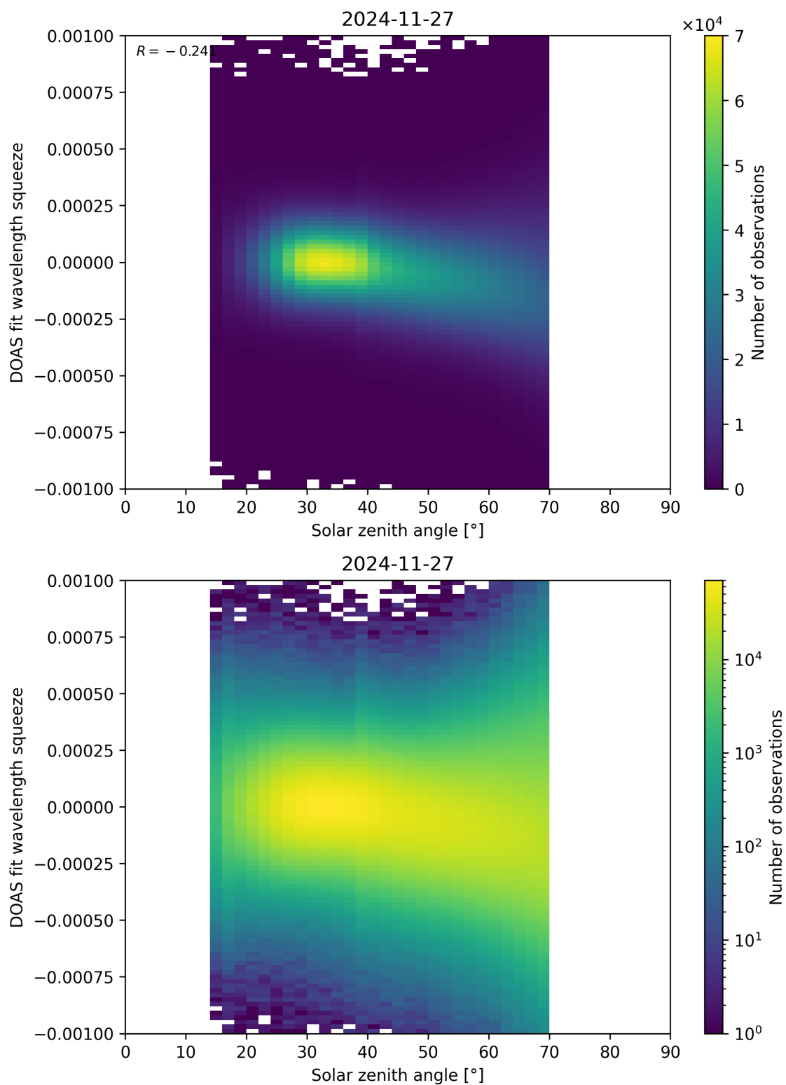
Figure 175: Scatter density plot of “Solar zenith angle” against “DOAS fit wavelength squeeze” for 2024-11-26 to 2024-11-28.
