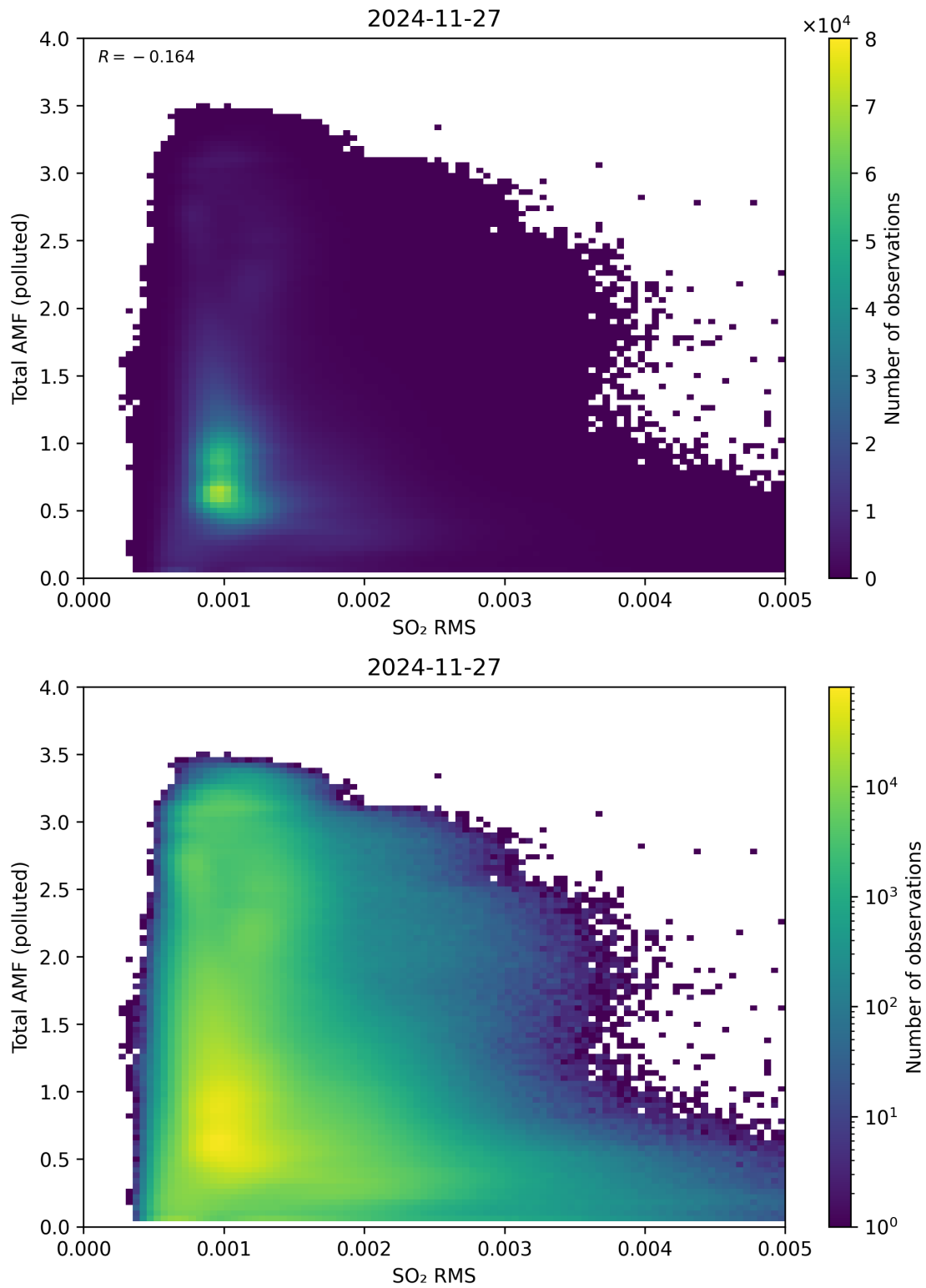
Figure 148: Scatter density plot of “SO 2 RMS” against “Total AMF (polluted)” for 2024-11-26 to 2024-11-28.
