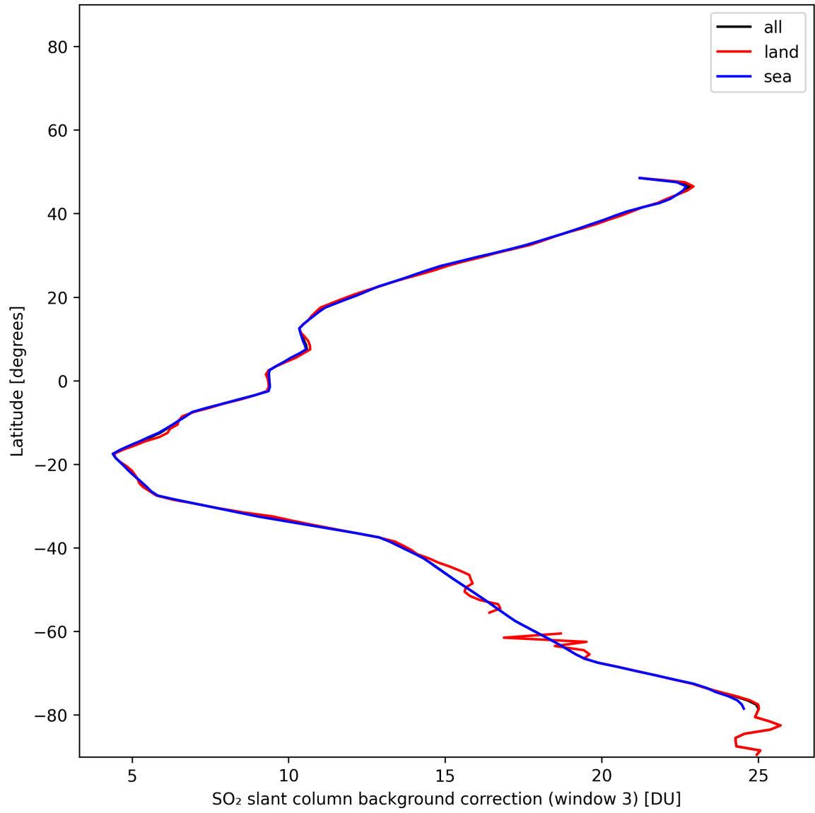
Figure 48: Zonal average of “SO 2 slant column background correction (window 3)” for 2024-11-26 to 2024-11-28.
