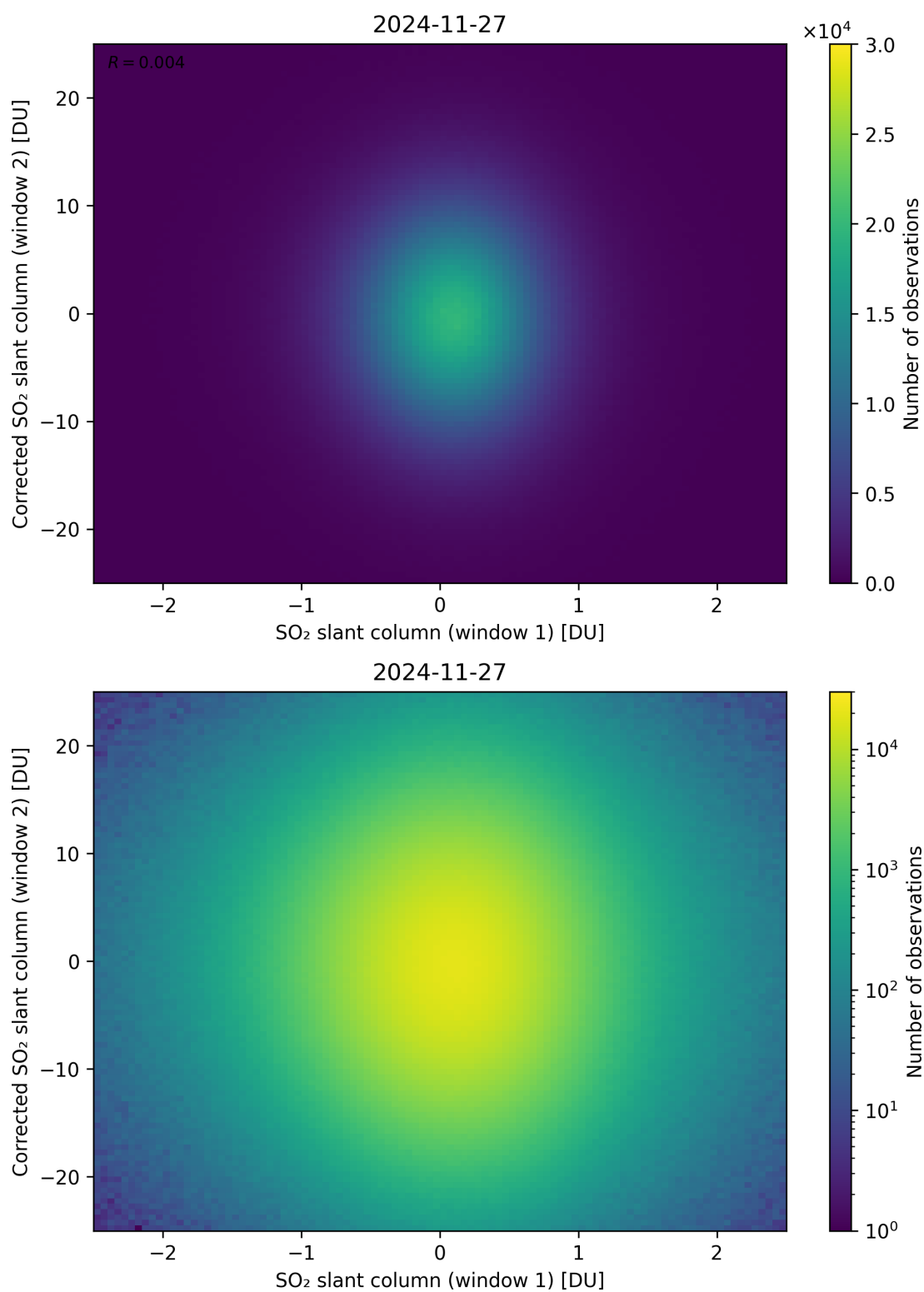
Figure 283: Scatter density plot of “SO 2 slant column (window 1)” against “Corrected SO 2 slant column (window 2)” for 2024-11-26 to 2024-11-28.
