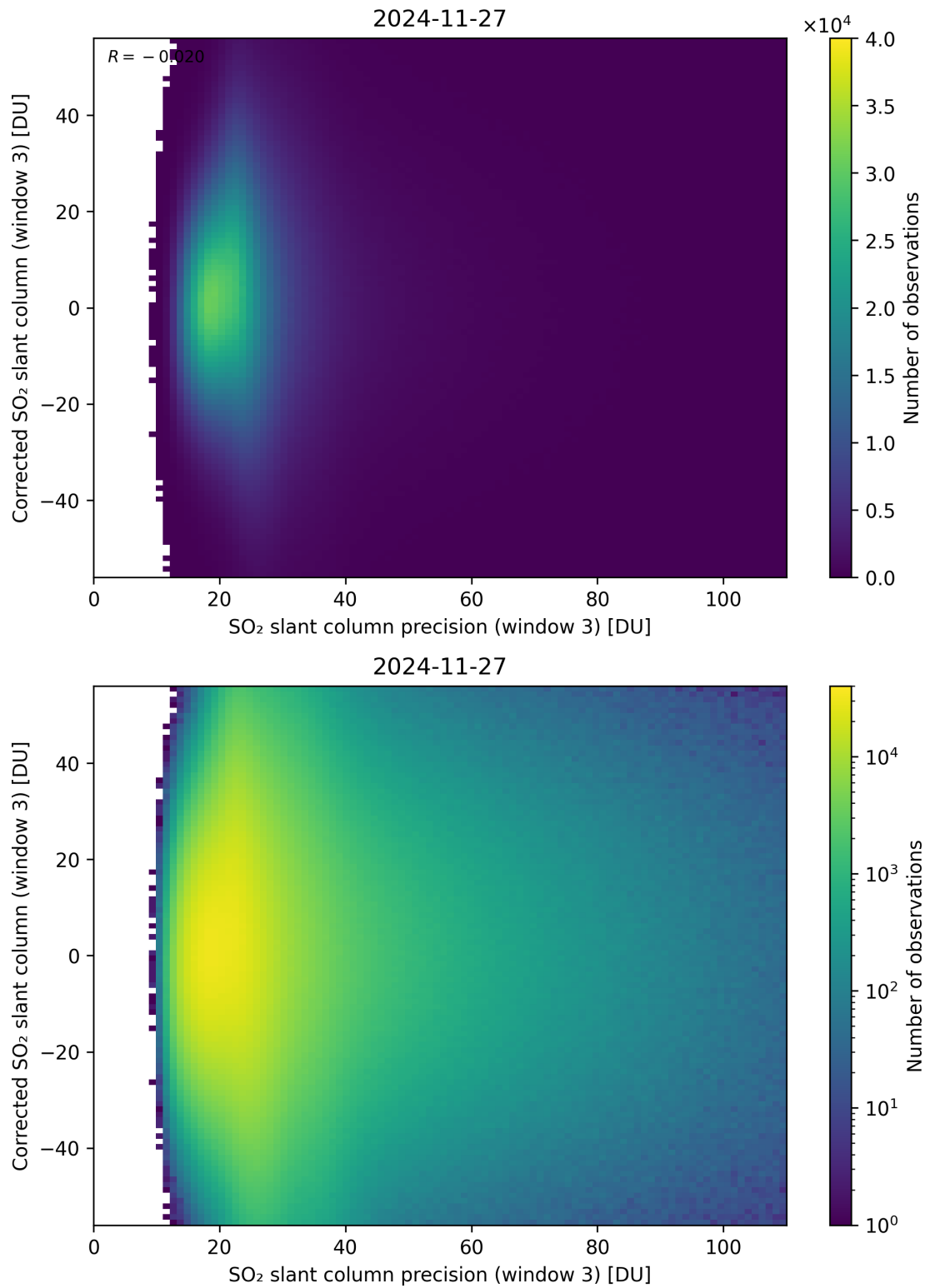
Figure 312: Scatter density plot of “SO 2 slant column precision (window 3)” against “Corrected SO 2 slant column (window 3)” for 2024-11-26 to 2024-11-28.
