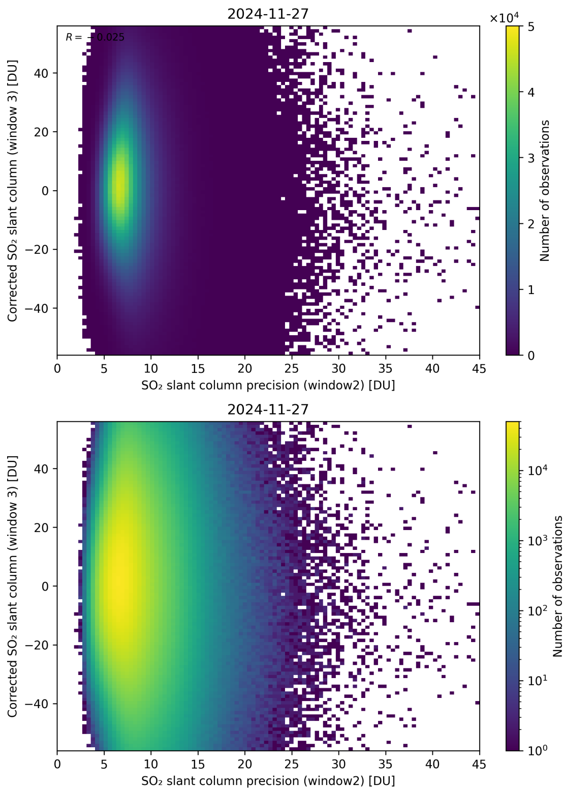
Figure 298: Scatter density plot of “SO 2 slant column precision (window2)” against “Corrected SO 2 slant column (window 3)” for 2024-11-26 to 2024-11-28.
