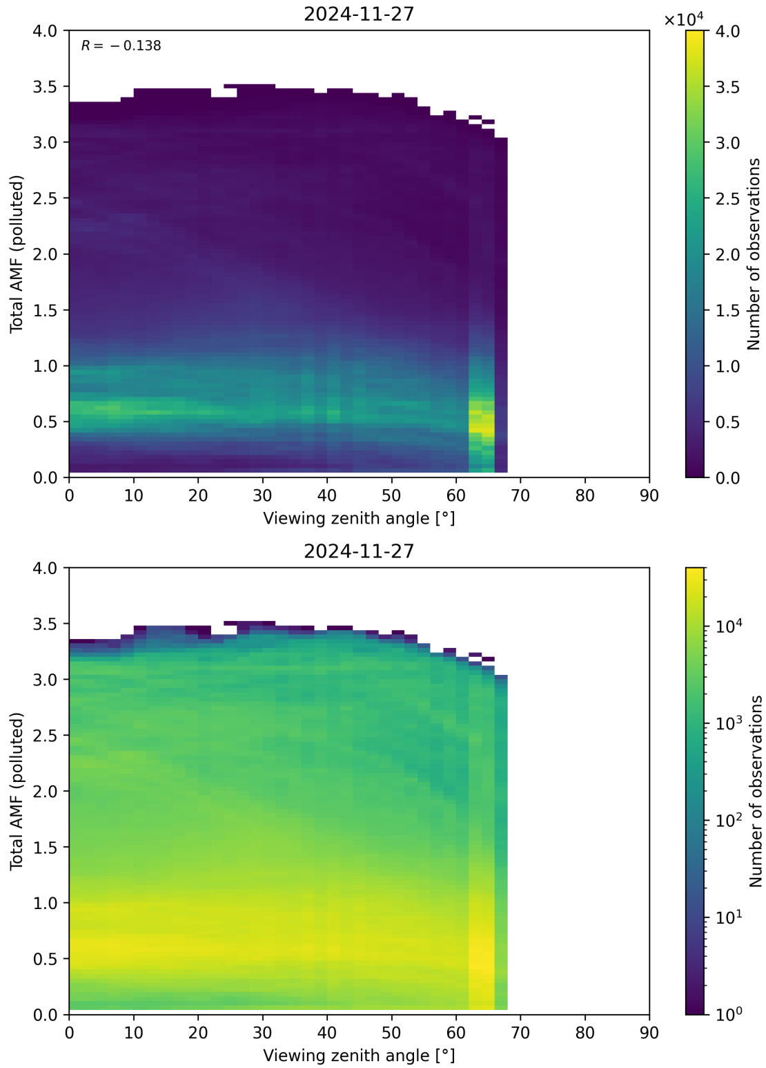
Figure 381: Scatter density plot of “Viewing zenith angle” against “Total AMF (polluted)” for 2024-11-26 to 2024-11-28.
