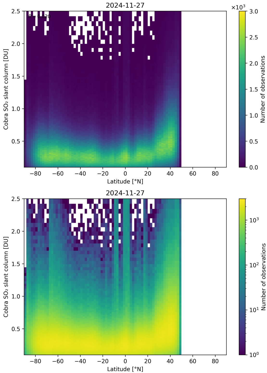
Figure 157: Scatter density plot of “Latitude” against “Cobra SO 2 slant column” for 2024-11-26 to 2024-11-28.
