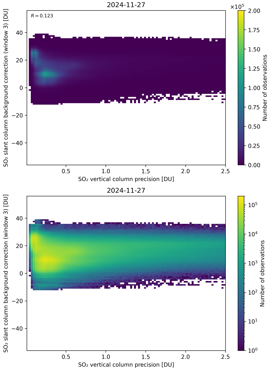
Figure 331: Scatter density plot of “SO 2 vertical column precision” against “SO 2 slant column background correction (window 3)” for 2024-11-26 to 2024-11-28.
