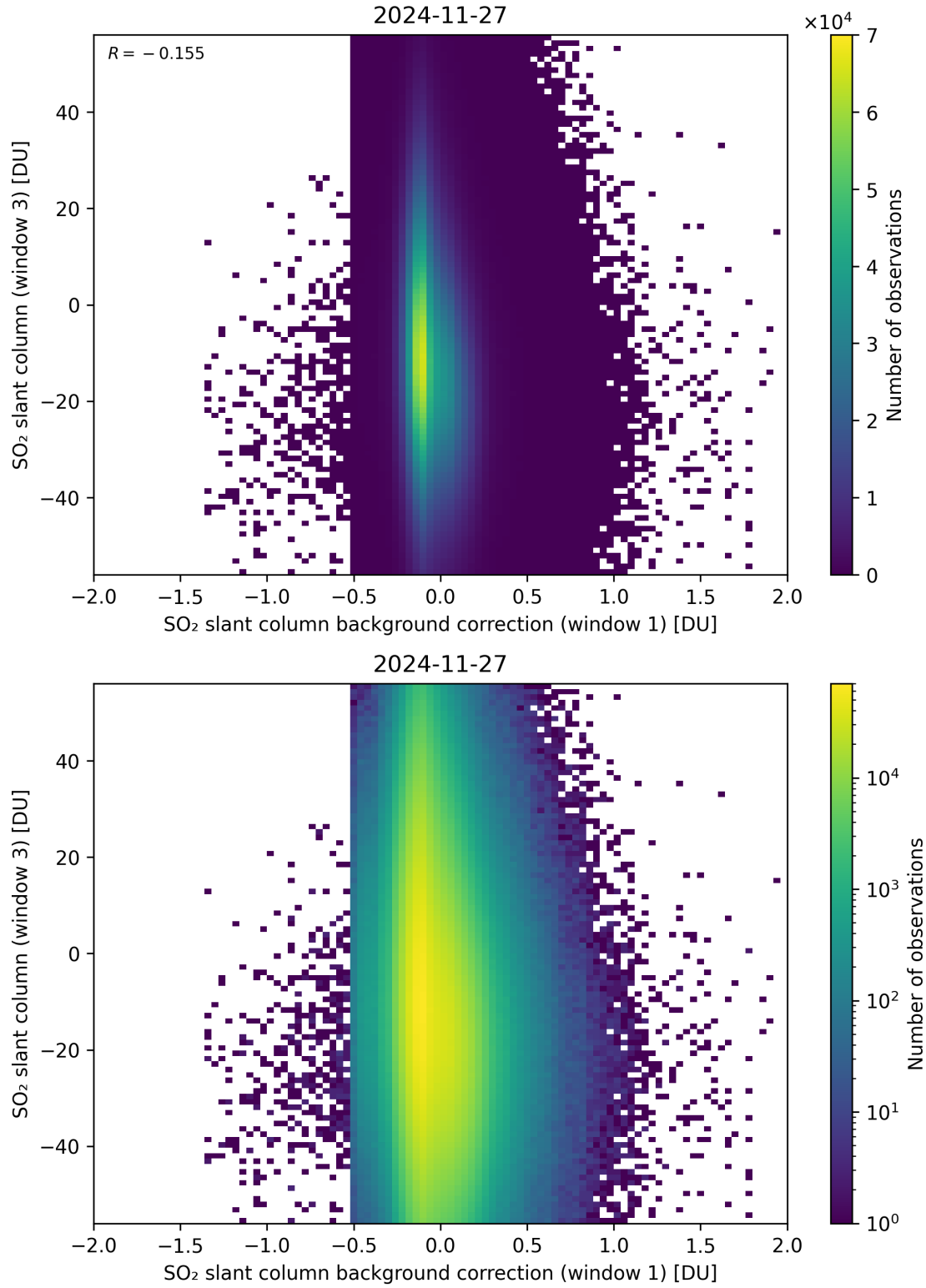
Figure 118: Scatter density plot of “SO 2 slant column background correction (window 1)” against “SO 2 slant column (window 3)” for 2024-11-26 to 2024-11-28.
