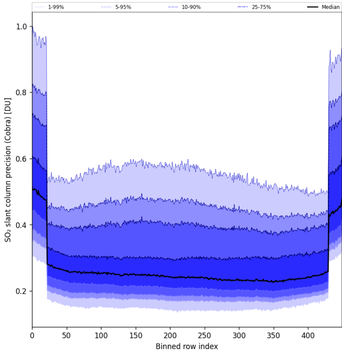
Figure 88: Along track statistics of “SO 2 slant column precision (Cobra)” for 2024-11-26 to 2024-11-28
