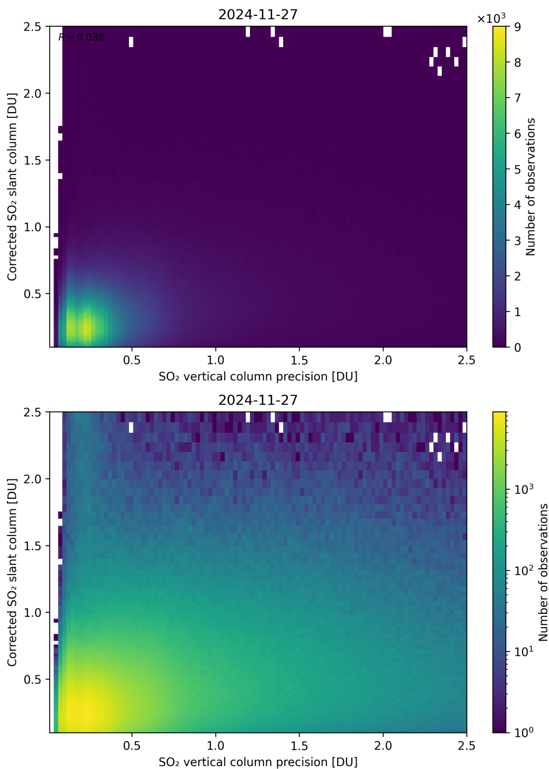
Figure 338: Scatter density plot of “SO 2 vertical column precision” against “Corrected SO 2 slant column” for 2024-11-26 to 2024-11-28.
