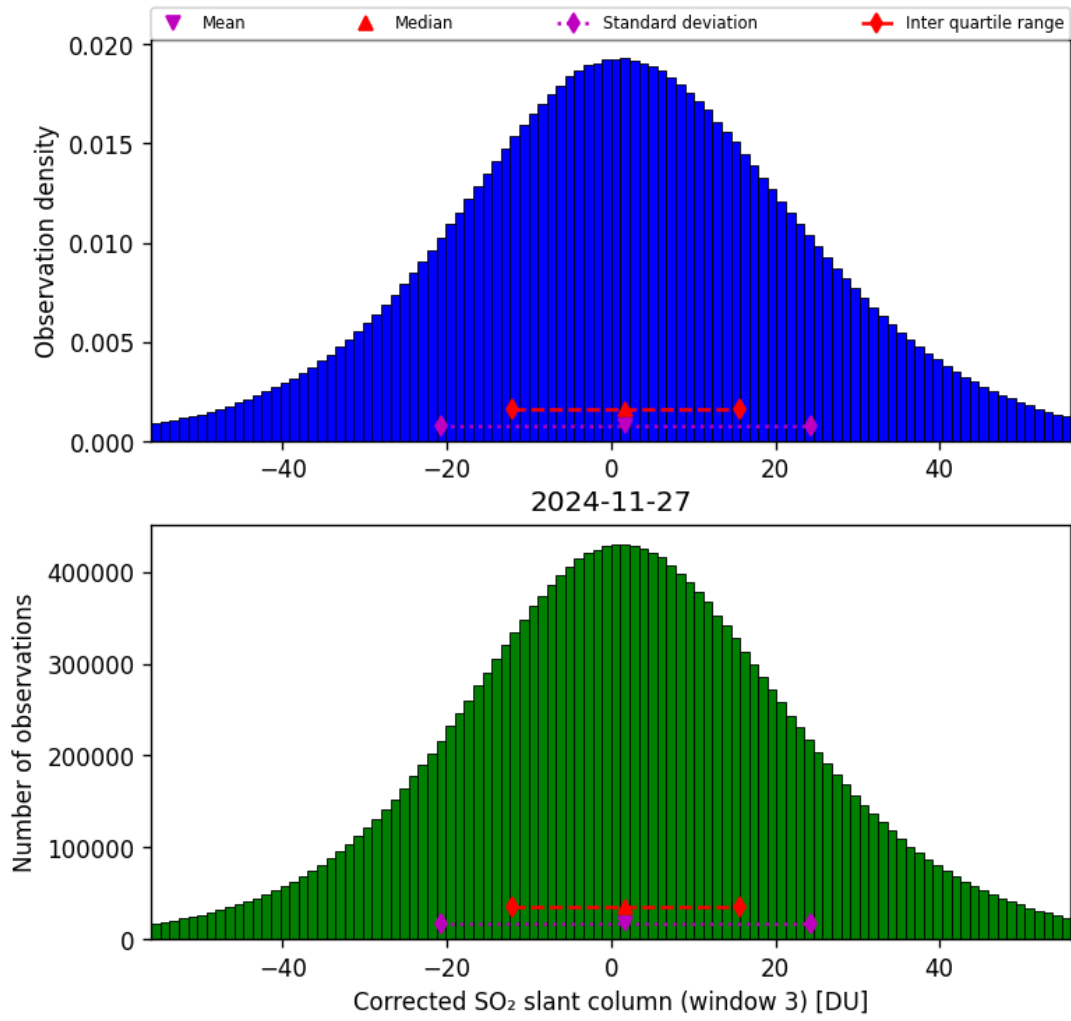
Figure 73: Histogram of “Corrected SO 2 slant column (window 3)” for 2024-11-26 to 2024-11-28
