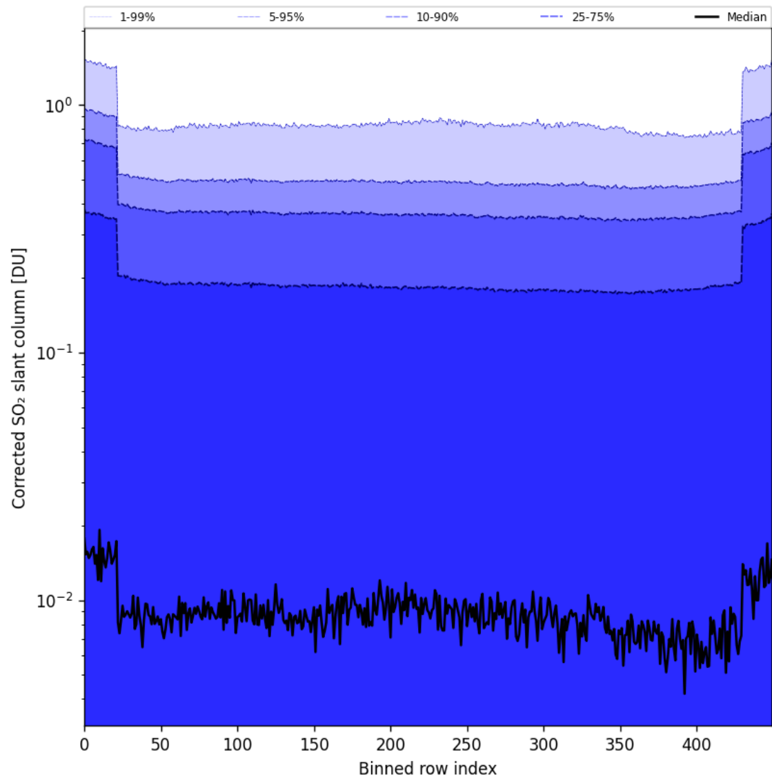
Figure 86: Along track statistics of “Corrected SO 2 slant column” for 2024-11-26 to 2024-11-28
