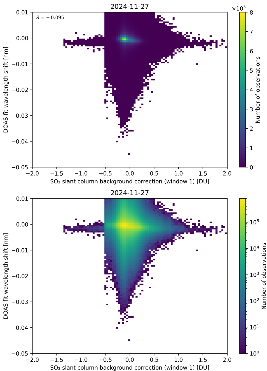
Figure 111: Scatter density plot of “SO 2 slant column background correction (window 1)” against “DOAS fit wavelength shift” for 2024-11-26 to 2024-11-28.
