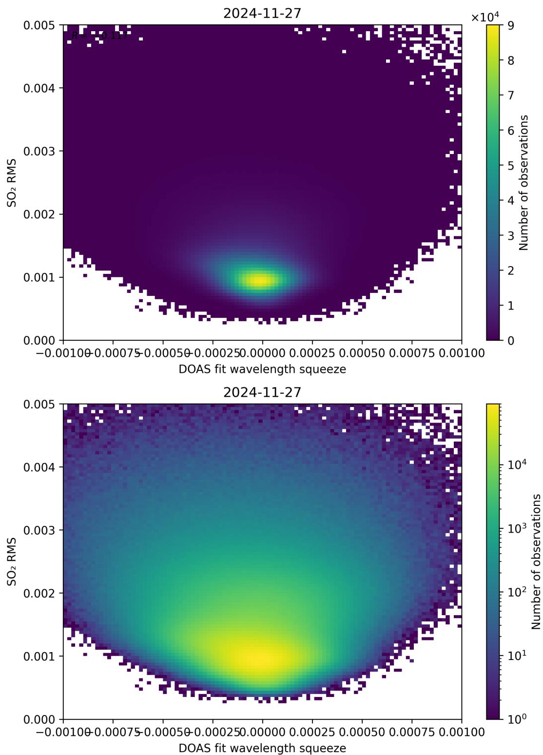
Figure 143: Scatter density plot of “DOAS fit wavelength squeeze” against “SO 2 RMS” for 2024-11-26 to 2024-11-28.
