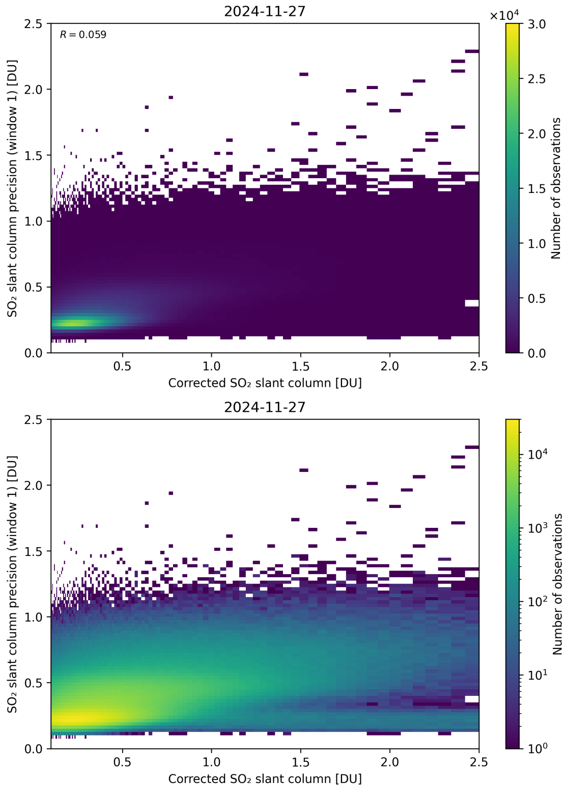
Figure 238: Scatter density plot of “Corrected SO 2 slant column” against “SO 2 slant column precision (window 1)” for 2024-11-26 to 2024-11-28.
