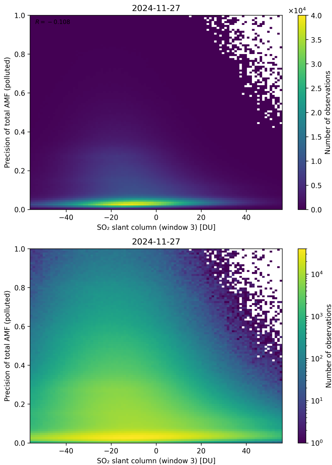
Figure 319: Scatter density plot of “SO 2 slant column (window 3)” against “Precision of total AMF (polluted)” for 2024-11-26 to 2024-11-28.
