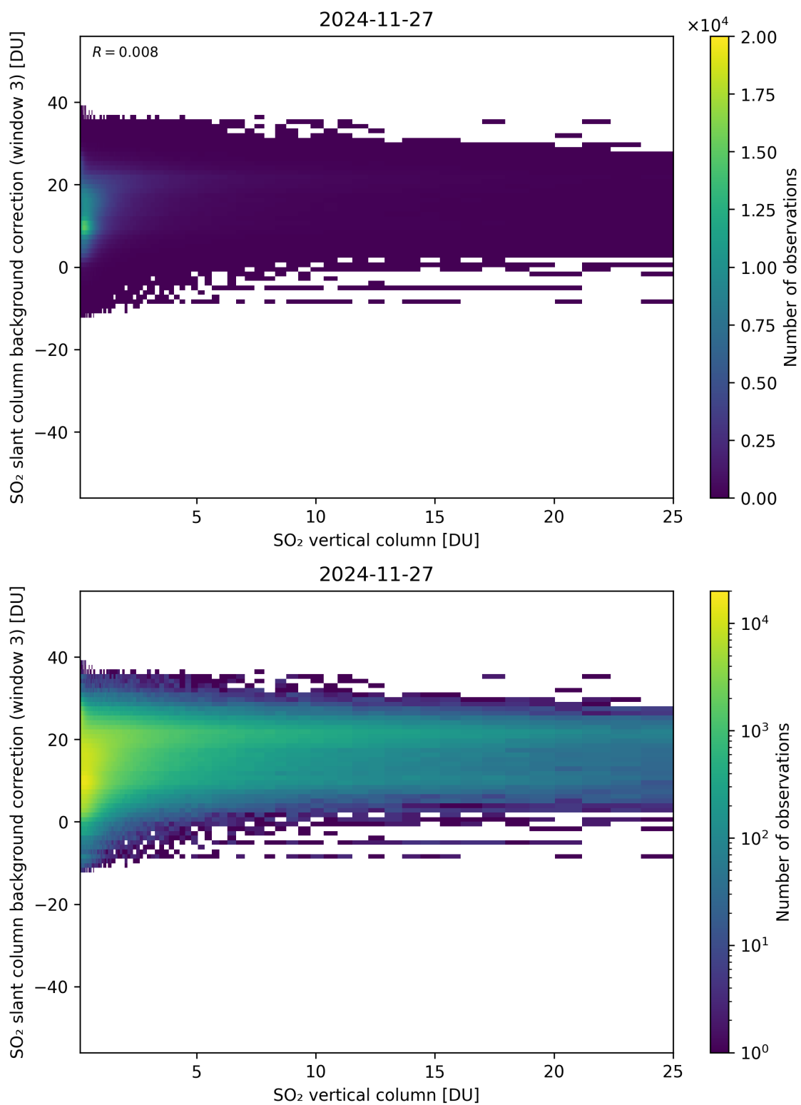
Figure 325: Scatter density plot of “SO 2 vertical column” against “SO 2 slant column background correction (window 3)” for 2024-11-26 to 2024-11-28.
