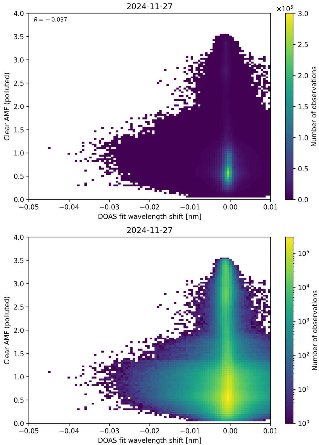
Figure 140: Scatter density plot of “DOAS fit wavelength shift” against “Clear AMF (polluted)” for 2024-11-26 to 2024-11-28.
