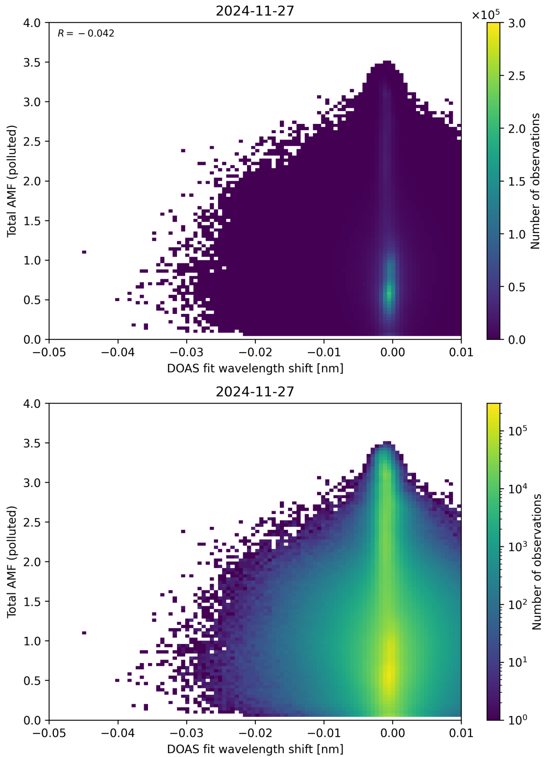
Figure 141: Scatter density plot of “DOAS fit wavelength shift” against “Total AMF (polluted)” for 2024-11-26 to 2024-11-28.
