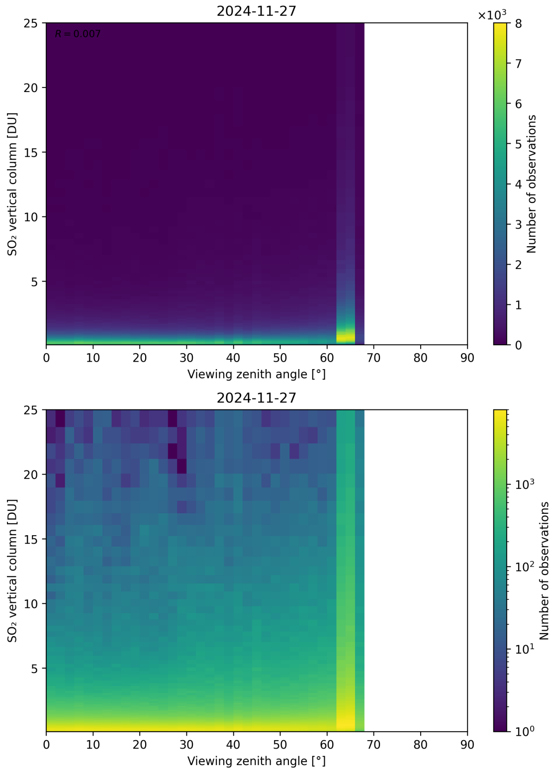
Figure 383: Scatter density plot of “Viewing zenith angle” against “SO 2 vertical column” for 2024-11-26 to 2024-11-28.
