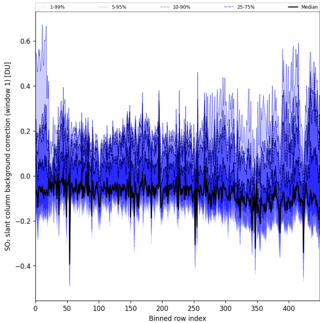
Figure 92: Along track statistics of “SO 2 slant column background correction (window 1)” for 2024-11-26 to 2024-11-28
