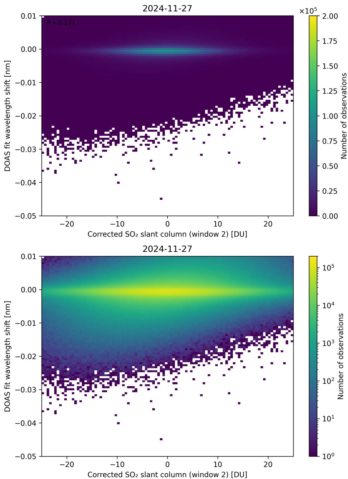
Figure 246: Scatter density plot of “Corrected SO 2 slant column (window 2)” against “DOAS fit wavelength shift” for 2024-11-26 to 2024-11-28.
