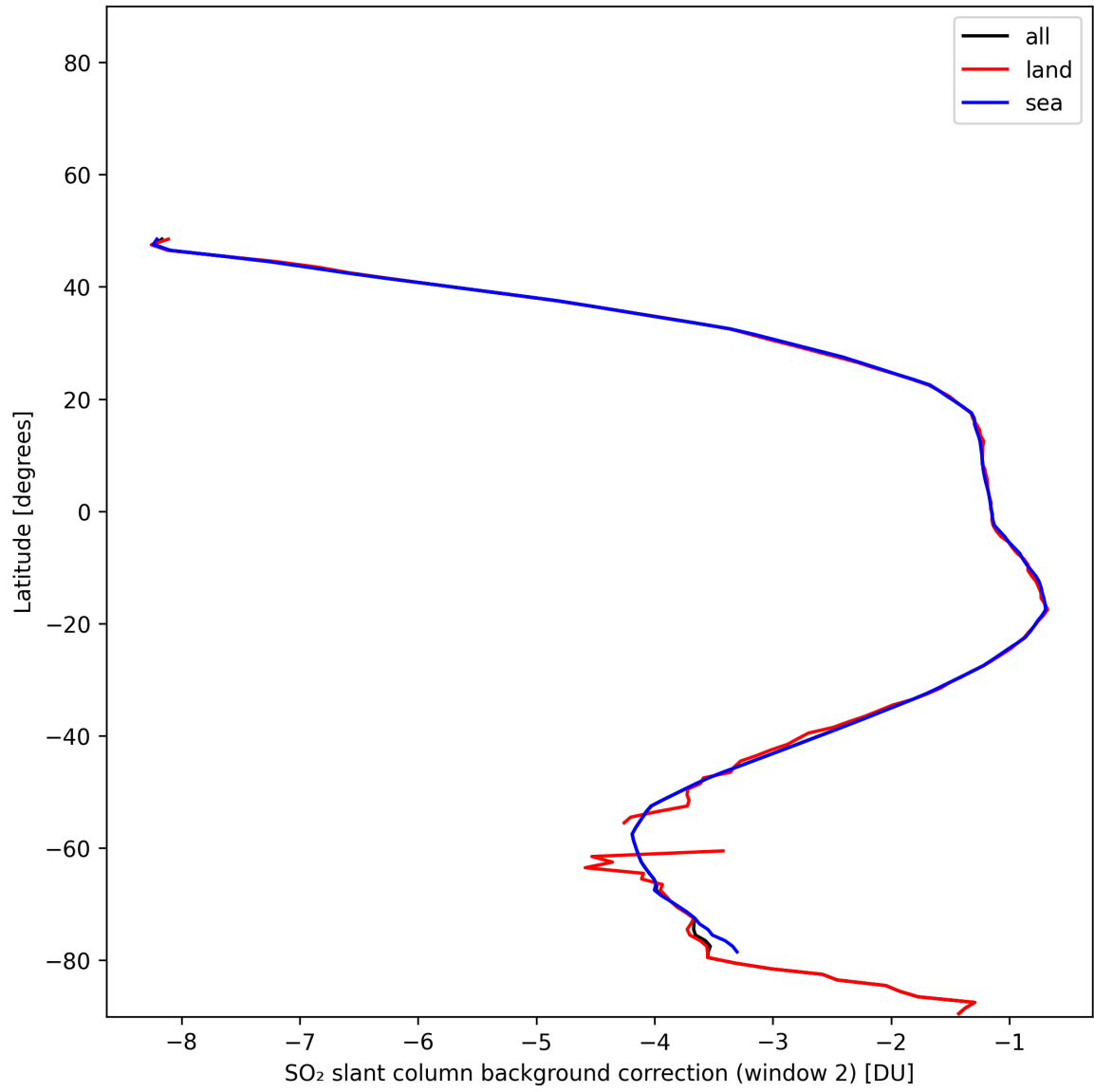
Figure 44: Zonal average of “SO 2 slant column background correction (window 2)” for 2024-11-26 to 2024-11-28.
