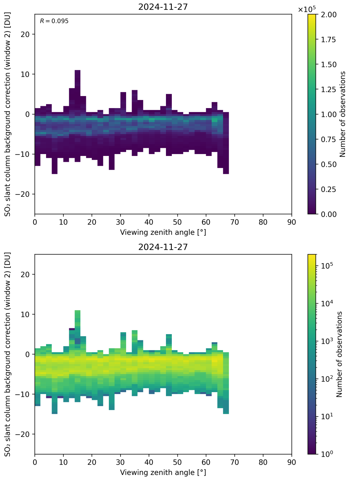
Figure 363: Scatter density plot of “Viewing zenith angle” against “SO 2 slant column background correction (window 2)” for 2024-11-26 to 2024-11-28.
