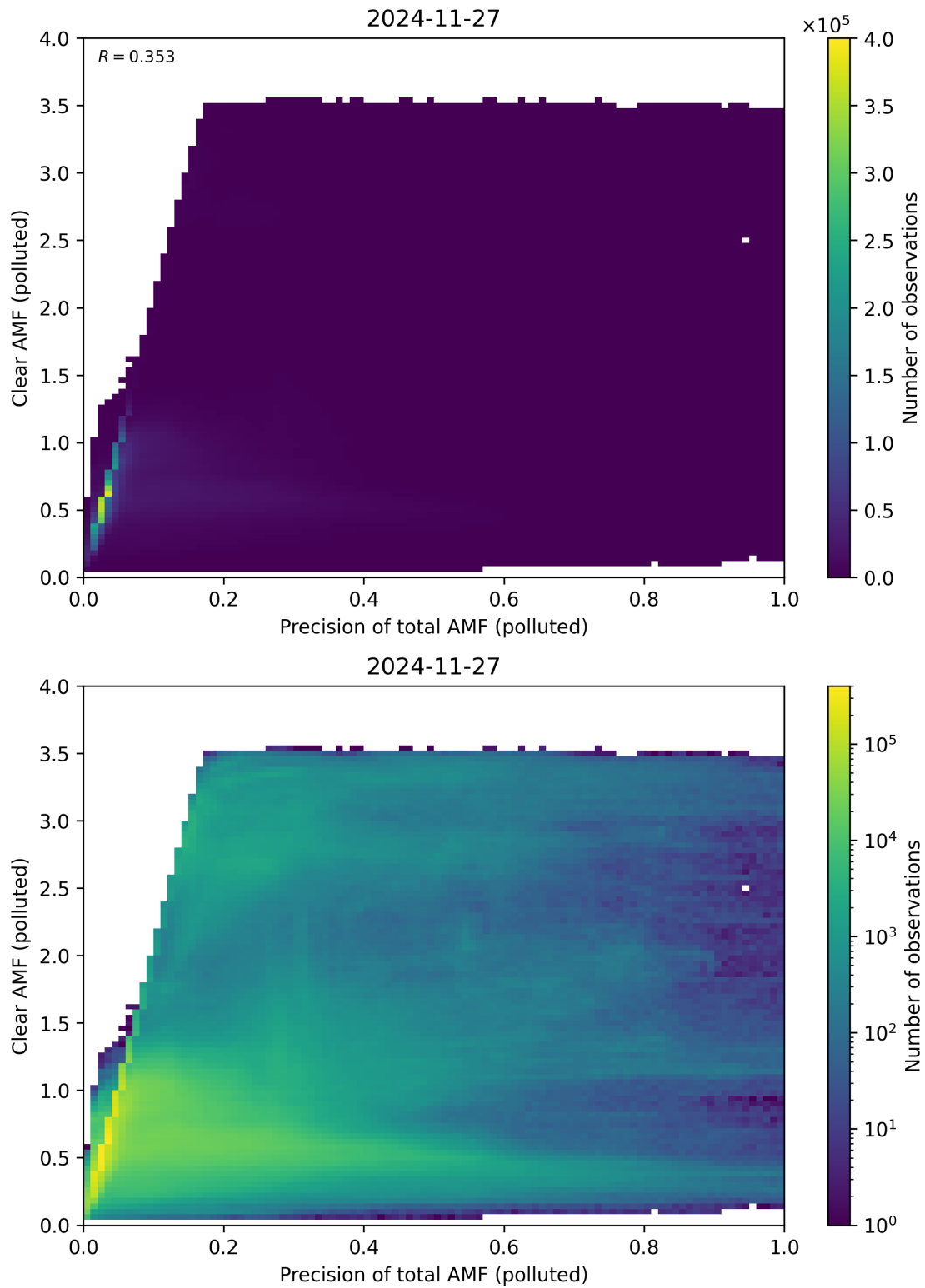
Figure 320: Scatter density plot of “Precision of total AMF (polluted)” against “Clear AMF (polluted)” for 2024-11-26 to 2024-11-28.
