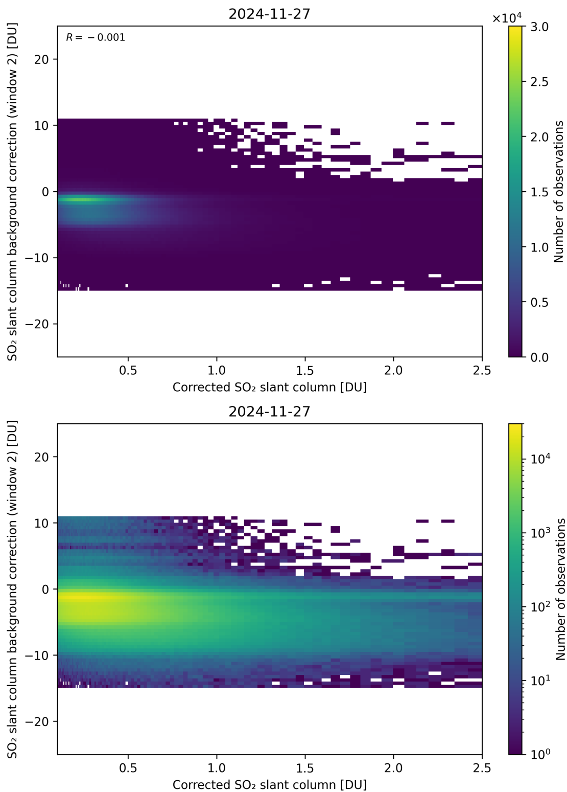
Figure 227: Scatter density plot of “Corrected SO 2 slant column” against “SO 2 slant column background correction (window 2)” for 2024-11-26 to 2024-11-28.
