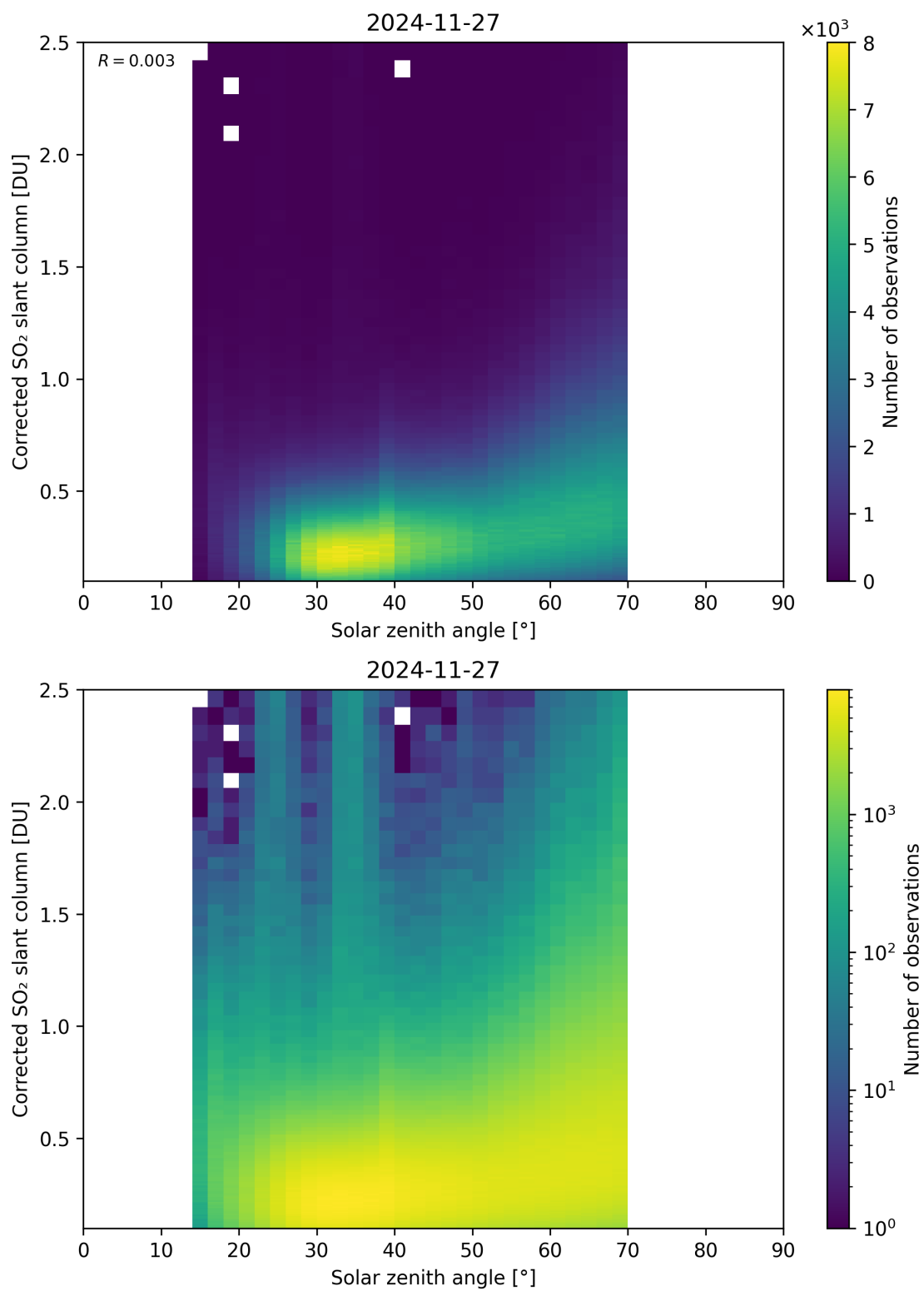
Figure 181: Scatter density plot of “Solar zenith angle” against “Corrected SO 2 slant column” for 2024-11-26 to 2024-11-28.
