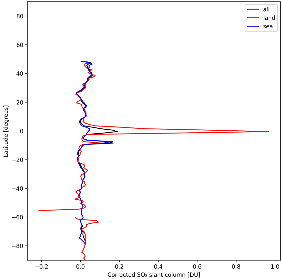
Figure 34: Zonal average of “Corrected SO 2 slant column” for 2024-11-26 to 2024-11-28.
