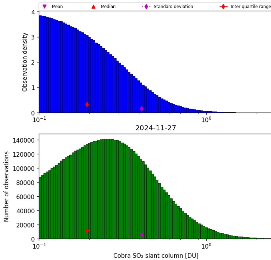
Figure 61: Histogram of “Cobra SO 2 slant column” for 2024-11-26 to 2024-11-28
