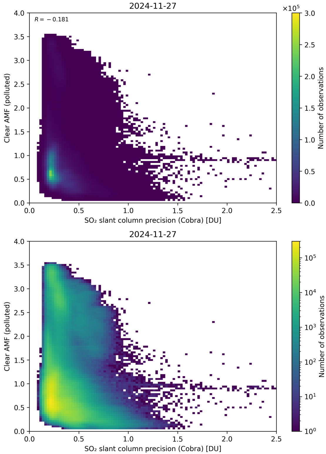
Figure 205: Scatter density plot of “SO 2 slant column precision (Cobra)” against “Clear AMF (polluted)” for 2024-11-26 to 2024-11-28.
