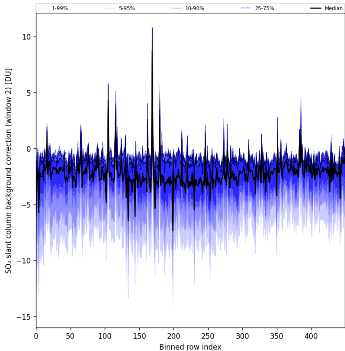
Figure 96: Along track statistics of “SO 2 slant column background correction (window 2)” for 2024-11-26 to 2024-11-28
