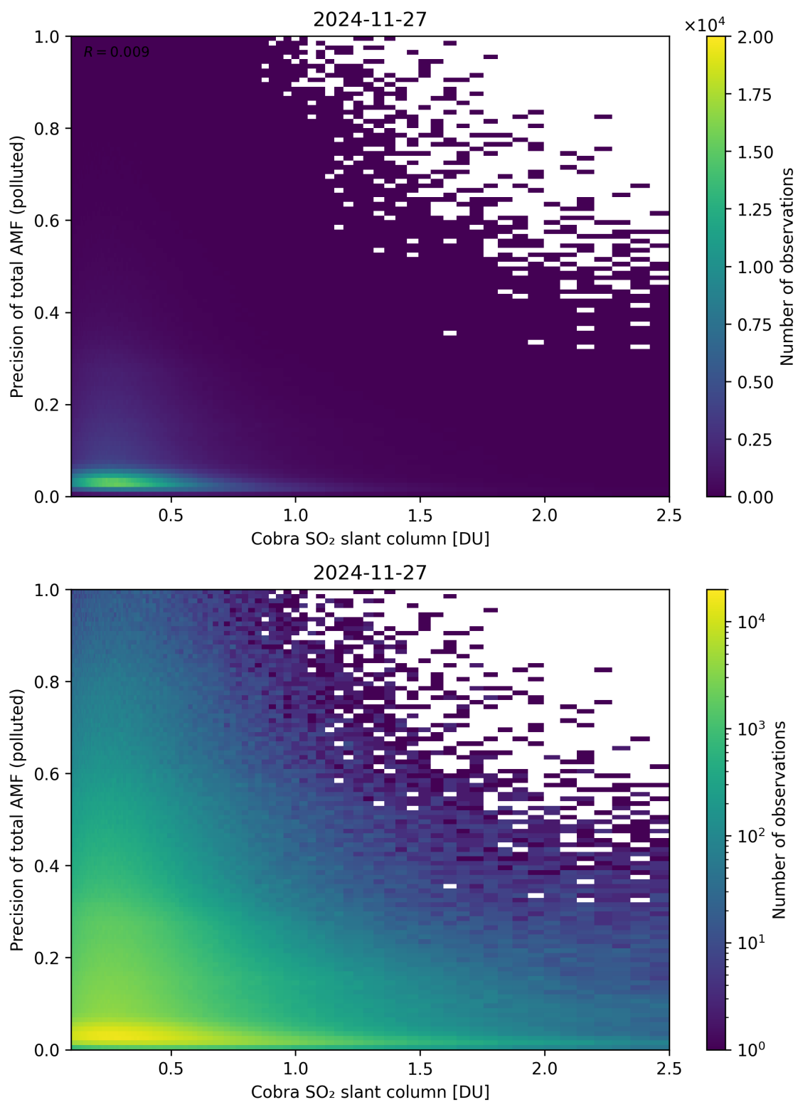
Figure 225: Scatter density plot of “Cobra SO 2 slant column” against “Precision of total AMF (polluted)” for 2024-11-26 to 2024-11-28.
