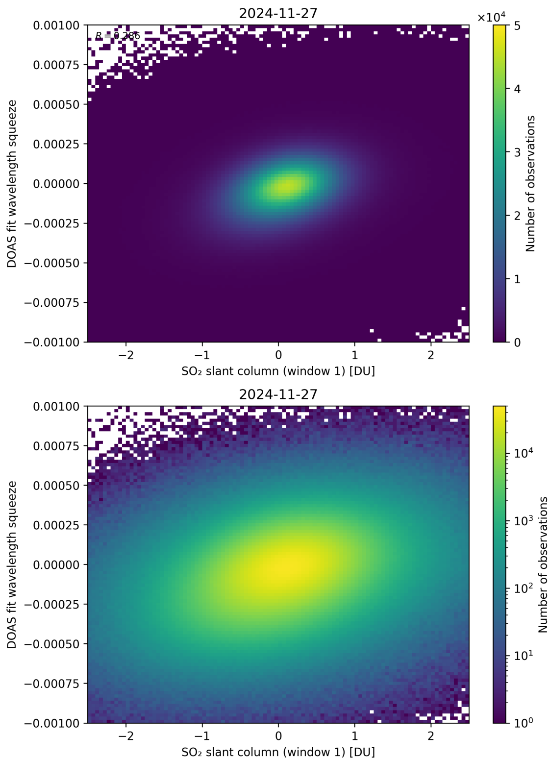
Figure 266: Scatter density plot of “SO 2 slant column (window 1)” against “DOAS fit wavelength squeeze” for 2024-11-26 to 2024-11-28.
