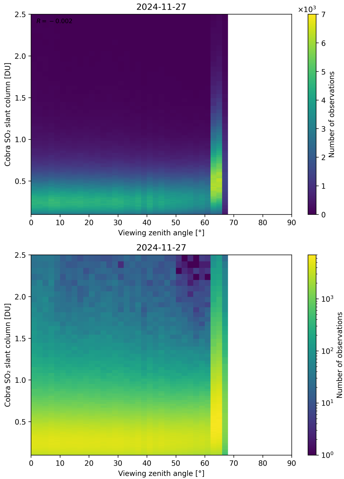
Figure 371: Scatter density plot of “Viewing zenith angle” against “Cobra SO 2 slant column” for 2024-11-26 to 2024-11-28.
