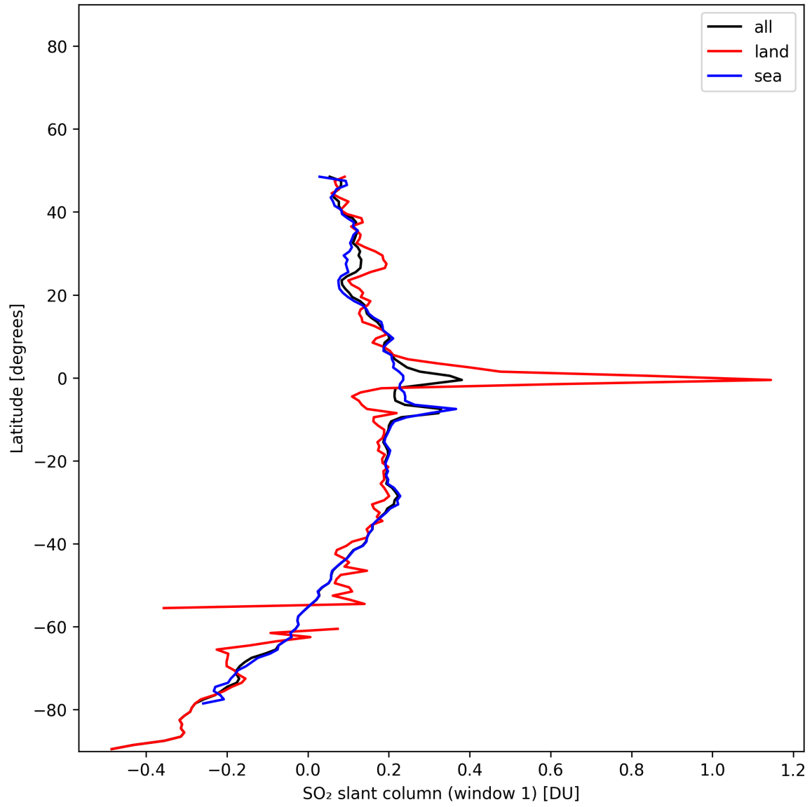
Figure 37: Zonal average of “SO 2 slant column (window 1)” for 2024-11-26 to 2024-11-28.
