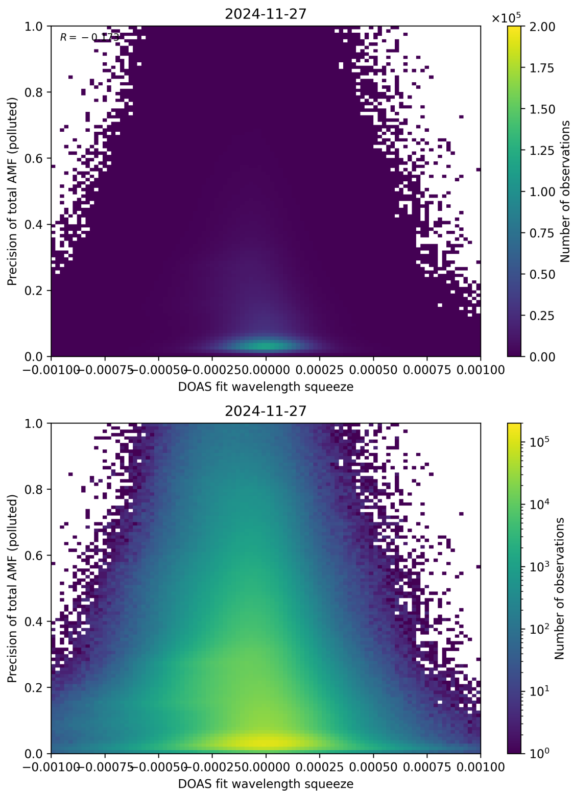
Figure 146: Scatter density plot of “DOAS fit wavelength squeeze” against “Precision of total AMF (polluted)” for 2024-11-26 to 2024-11-28.
