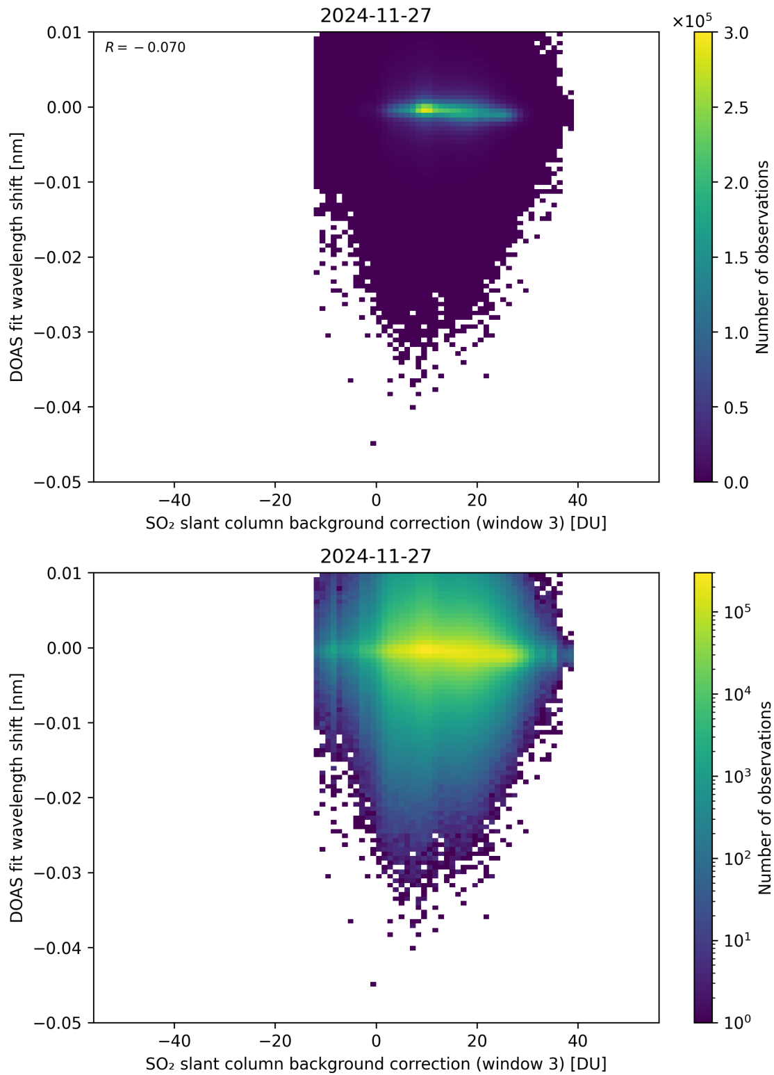
Figure 132: Scatter density plot of “SO 2 slant column background correction (window 3)” against “DOAS fit wavelength shift” for 2024-11-26 to 2024-11-28.
