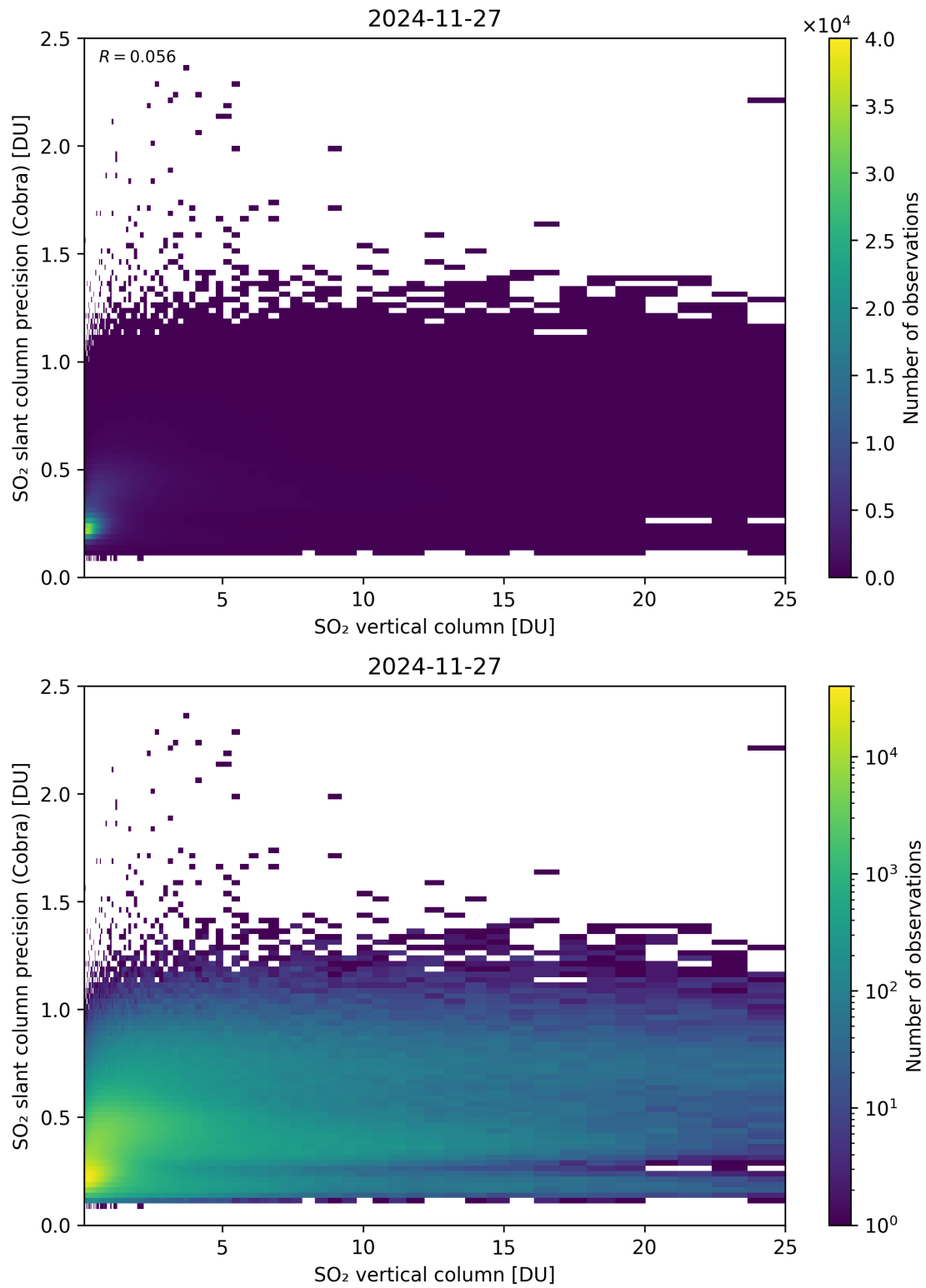
Figure 350: Scatter density plot of “SO 2 vertical column” against “SO 2 slant column precision (Cobra)” for 2024-11-26 to 2024-11-28.
