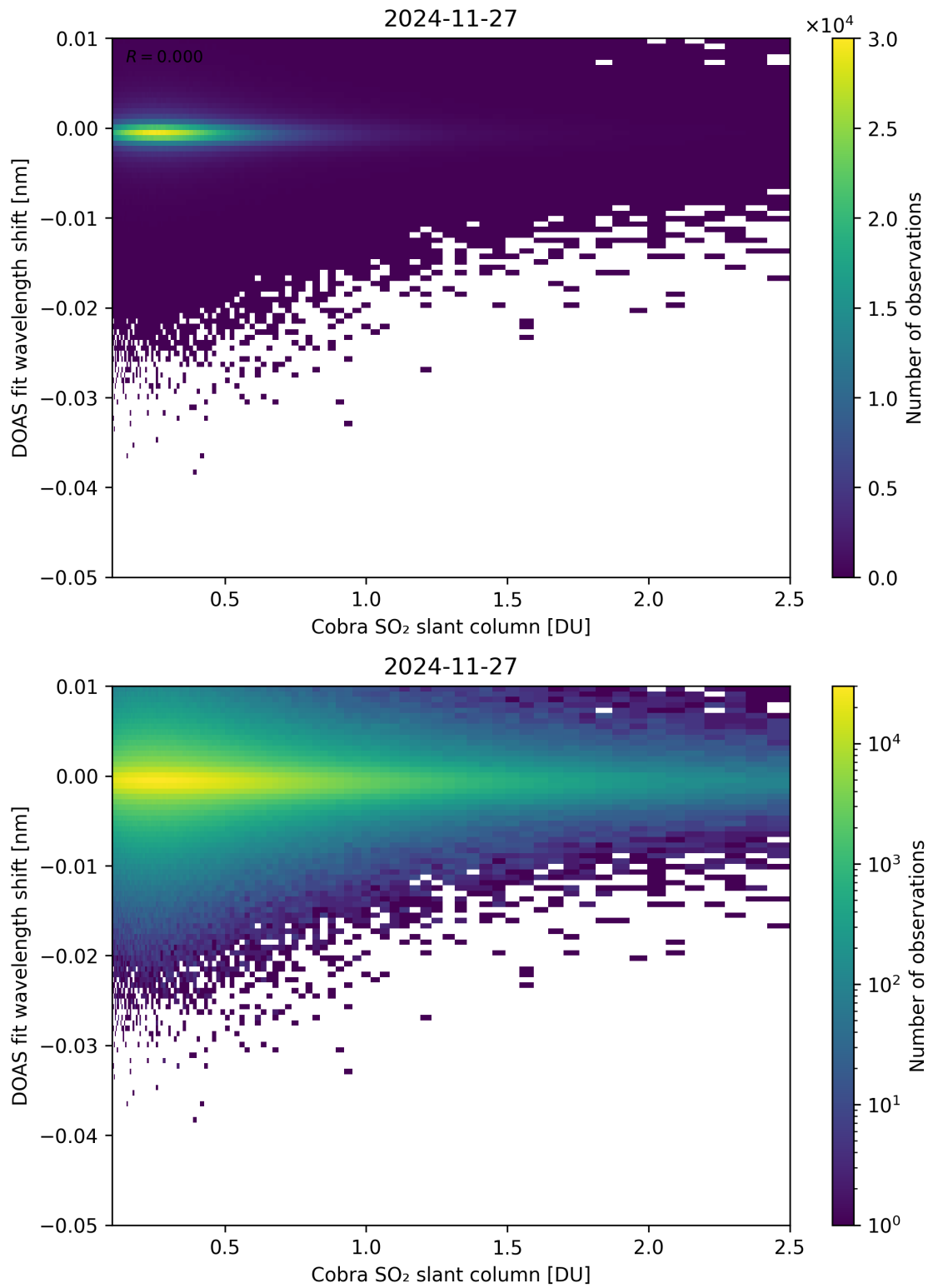
Figure 196: Scatter density plot of “Cobra SO 2 slant column” against “DOAS fit wavelength shift” for 2024-11-26 to 2024-11-28.
