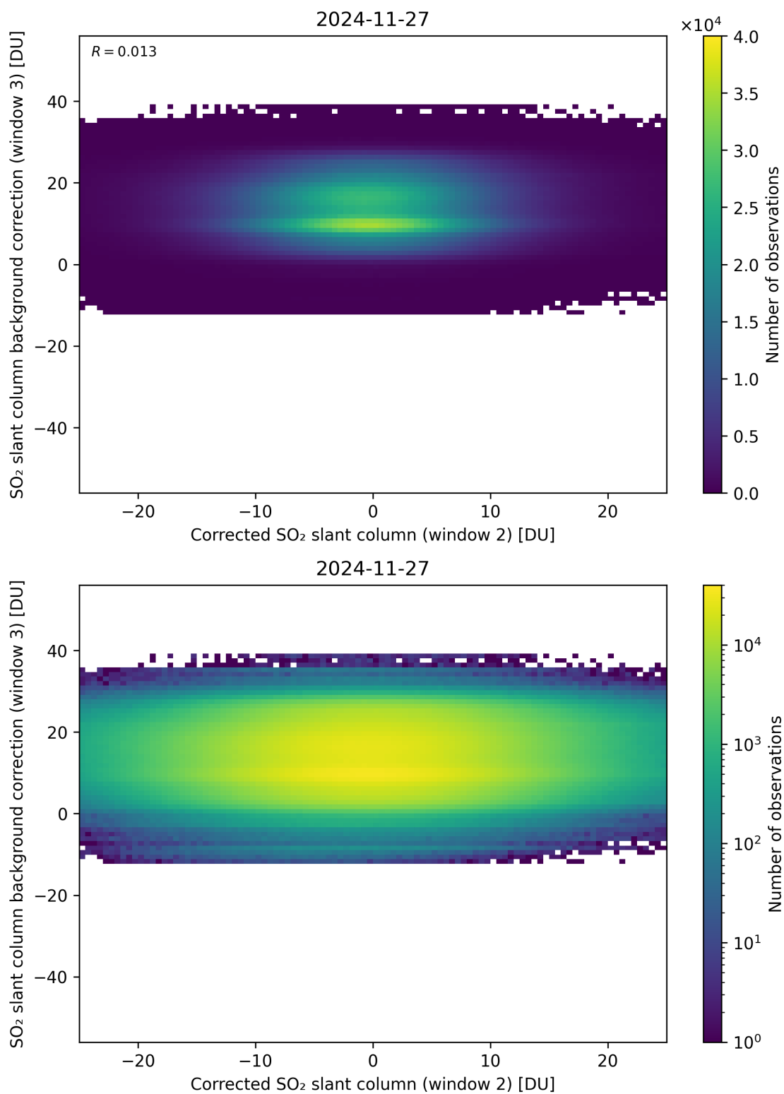
Figure 245: Scatter density plot of “Corrected SO 2 slant column (window 2)” against “SO 2 slant column background correction (window 3)” for 2024-11-26 to 2024-11-28.
