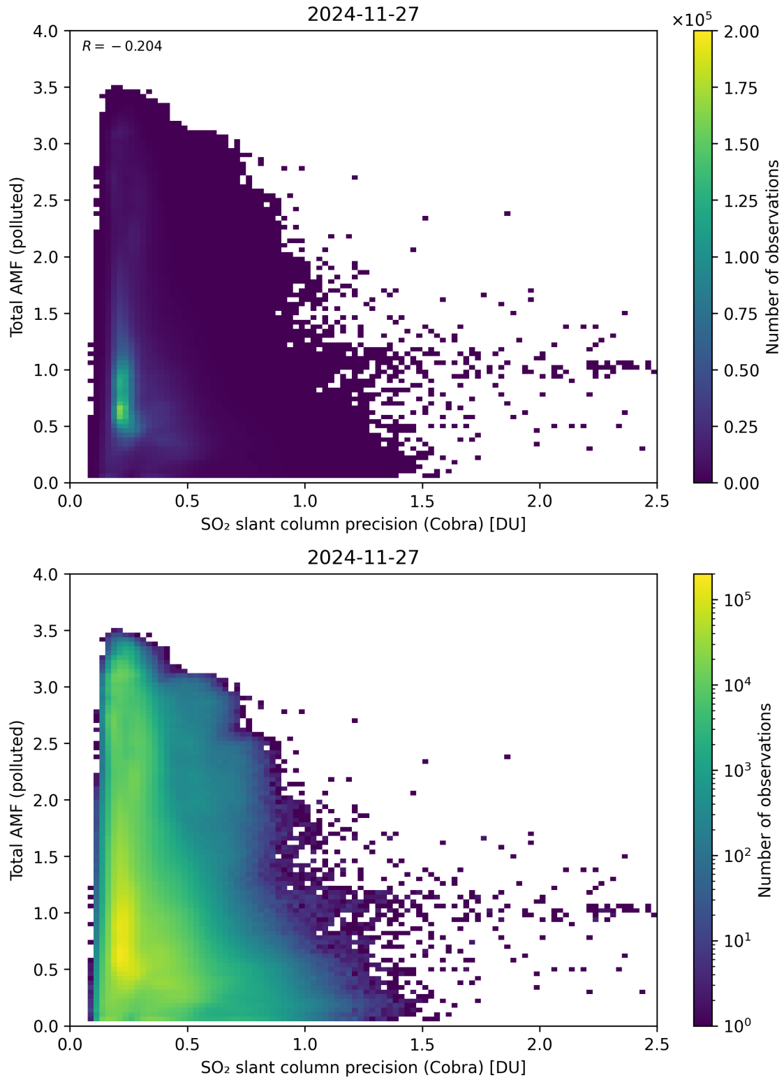
Figure 213: Scatter density plot of “SO 2 slant column precision (Cobra)” against “Total AMF (polluted)” for 2024-11-26 to 2024-11-28.
