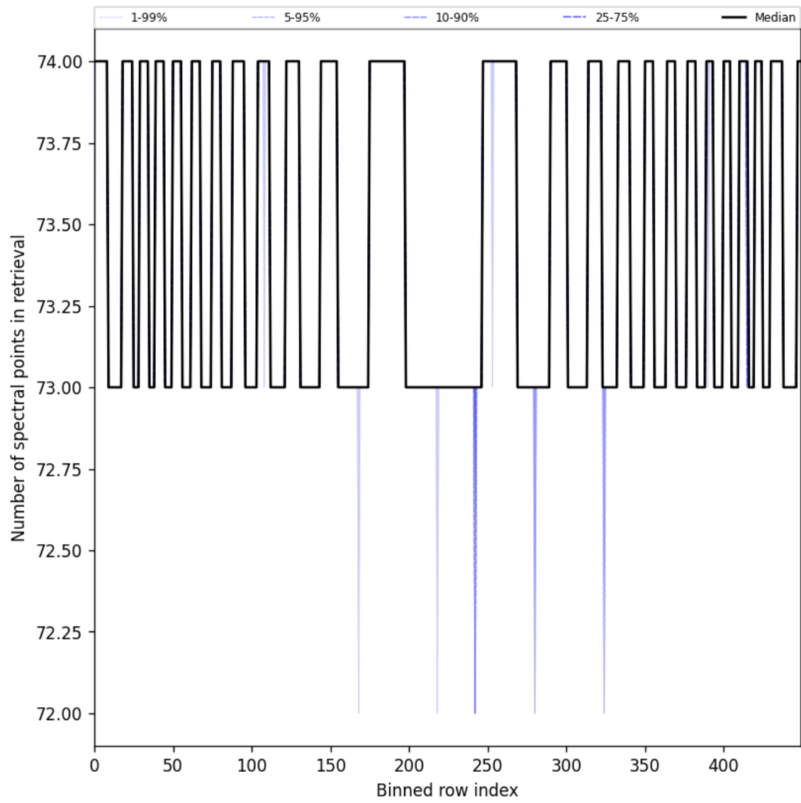
Figure 108: Along track statistics of “Number of spectral points in retrieval” for 2024-11-26 to 2024-11-28
