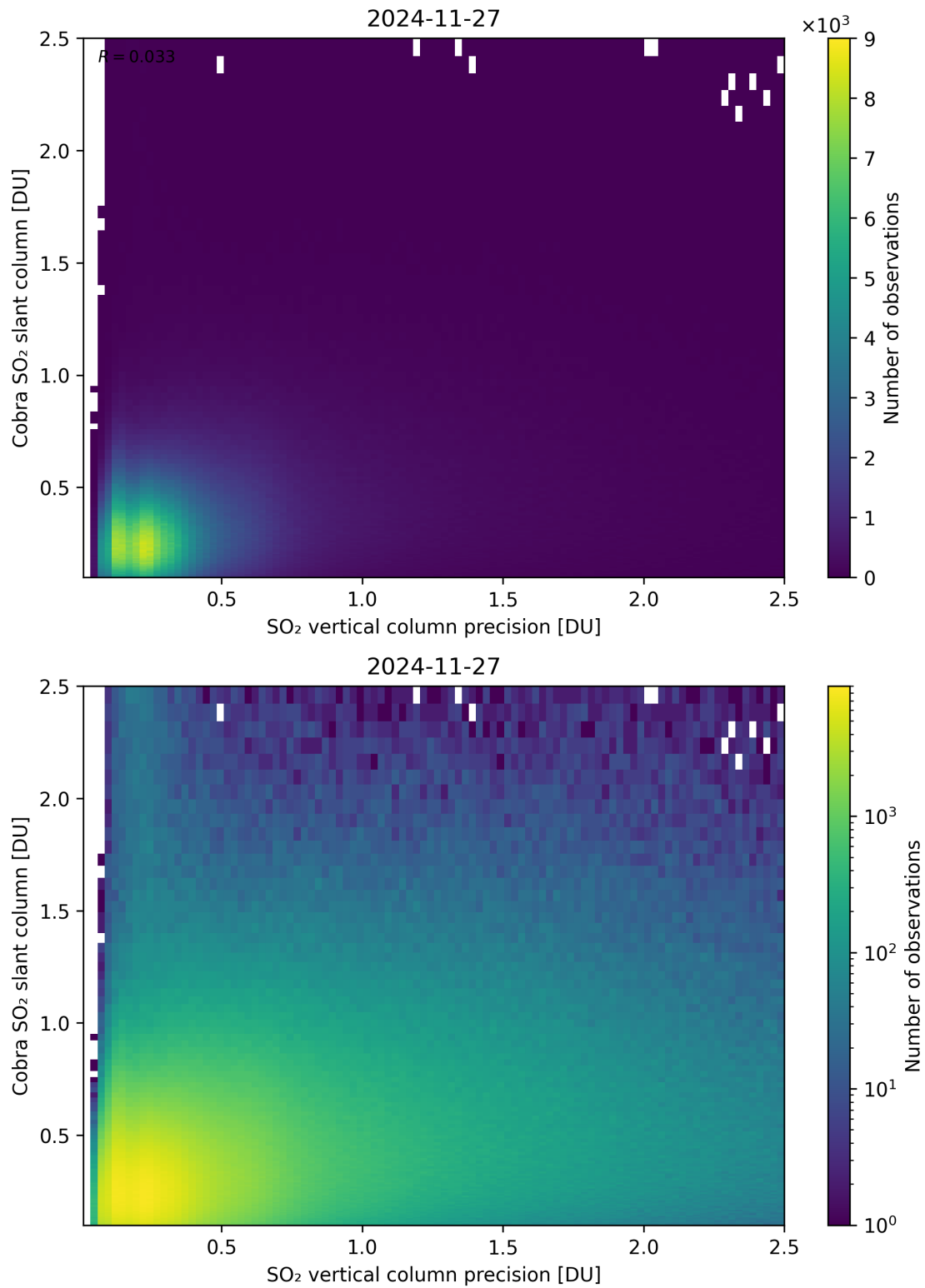
Figure 336: Scatter density plot of “SO 2 vertical column precision” against “Cobra SO 2 slant column” for 2024-11-26 to 2024-11-28.
