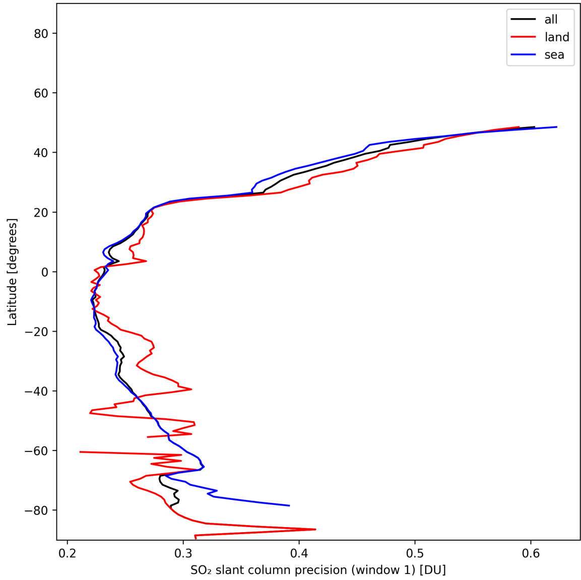
Figure 38: Zonal average of “SO 2 slant column precision (window 1)” for 2024-11-26 to 2024-11-28.
