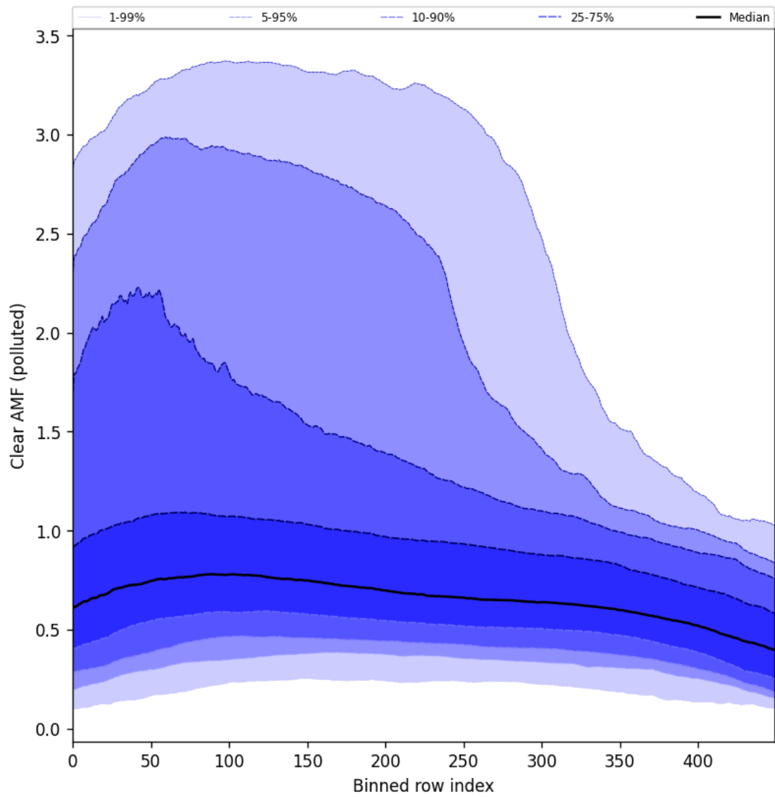
Figure 107: Along track statistics of “Clear AMF (polluted)” for 2024-11-26 to 2024-11-28
