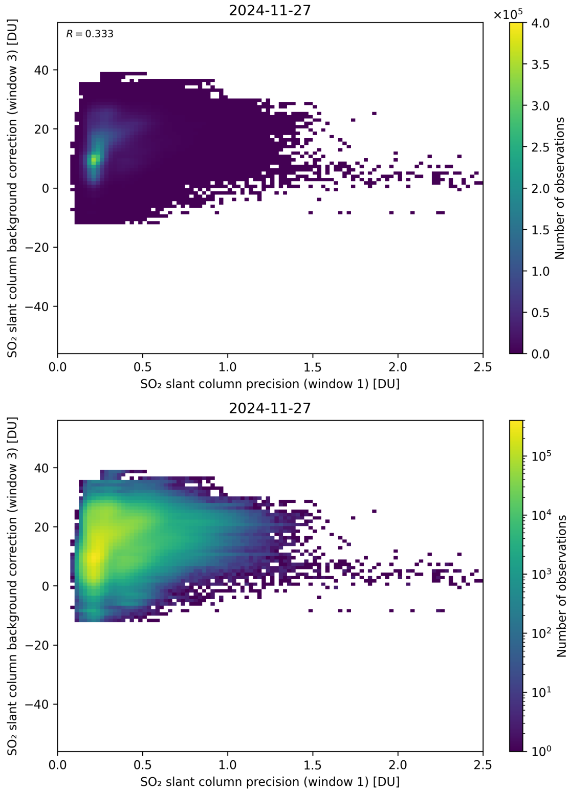
Figure 270: Scatter density plot of “SO 2 slant column precision (window 1)” against “SO 2 slant column background correction (window 3)” for 2024-11-26 to 2024-11-28.
