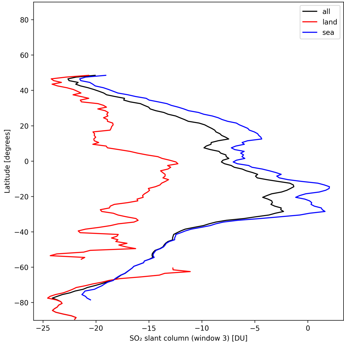
Figure 45: Zonal average of “SO 2 slant column (window 3)” for 2024-11-26 to 2024-11-28.
