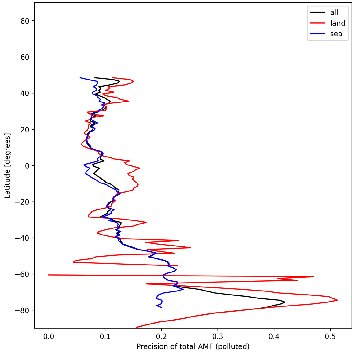
Figure 54: Zonal average of “Precision of total AMF (polluted)” for 2024-11-26 to 2024-11-28.
