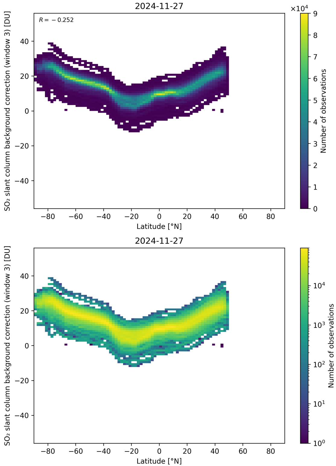
Figure 152: Scatter density plot of “Latitude” against “SO 2 slant column background correction (window 3)” for 2024-11-26 to 2024-11-28.
