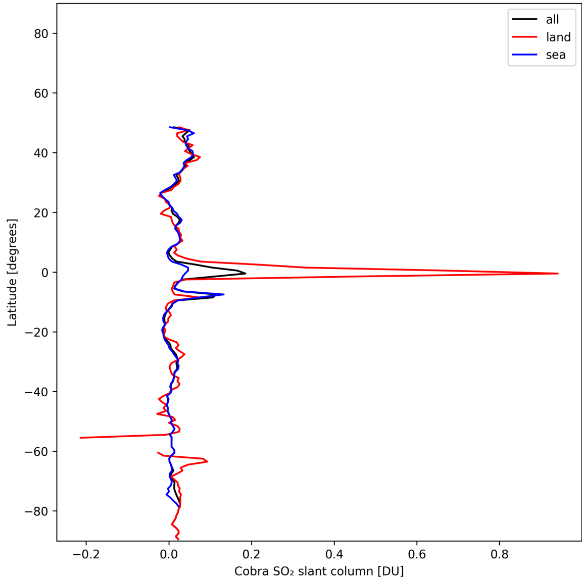
Figure 35: Zonal average of “Cobra SO 2 slant column” for 2024-11-26 to 2024-11-28.
