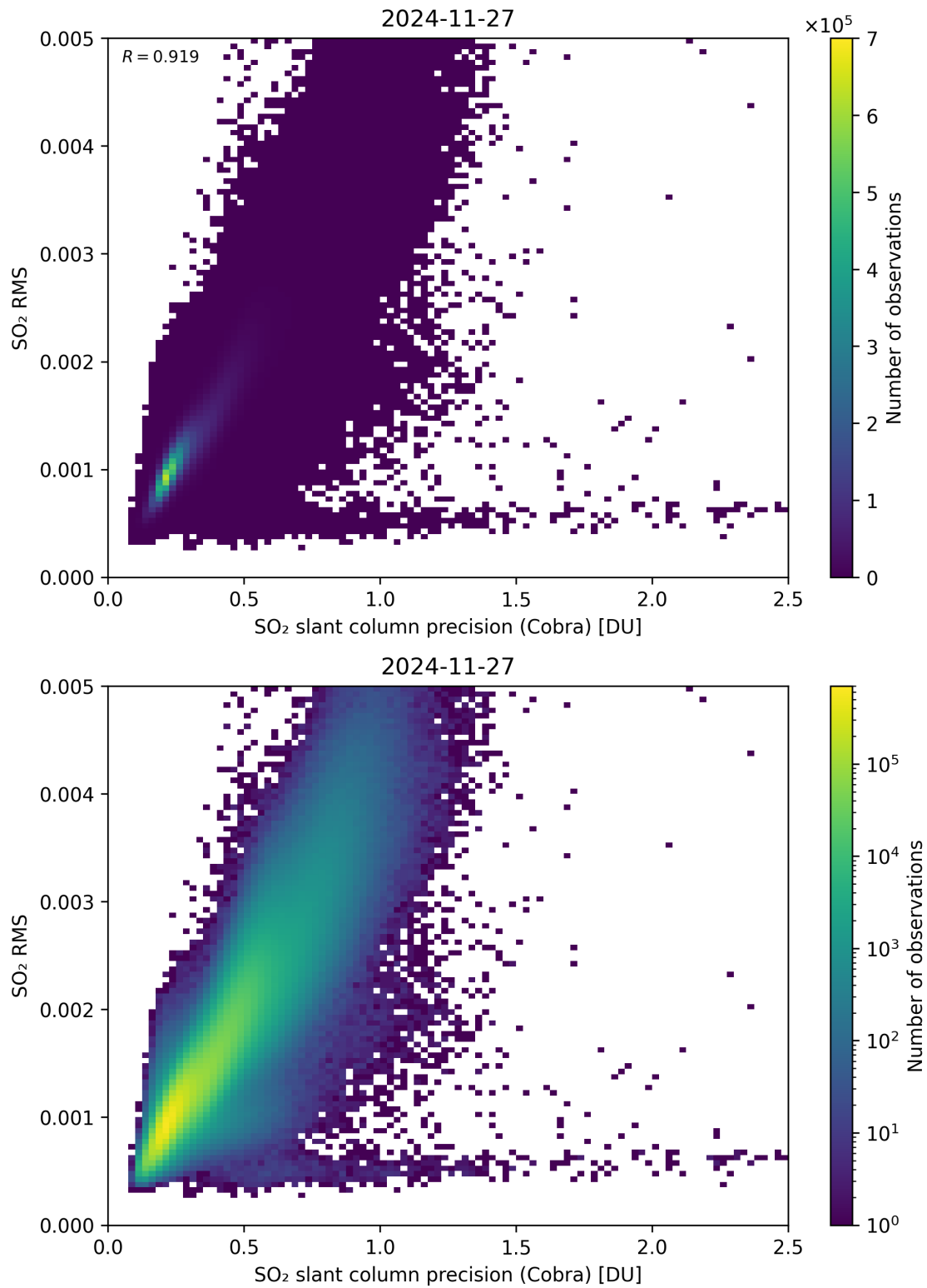
Figure 204: Scatter density plot of “SO 2 slant column precision (Cobra)” against “SO 2 RMS” for 2024-11-26 to 2024-11-28.
