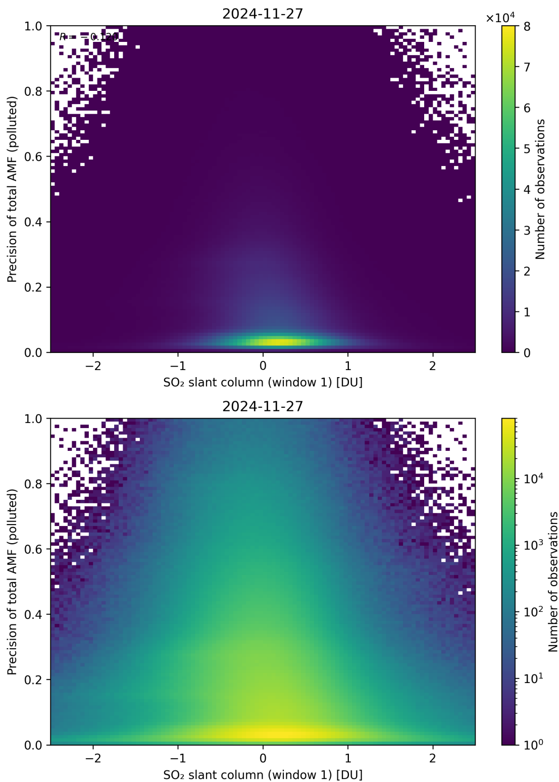
Figure 290: Scatter density plot of “SO 2 slant column (window 1)” against “Precision of total AMF (polluted)” for 2024-11-26 to 2024-11-28.
