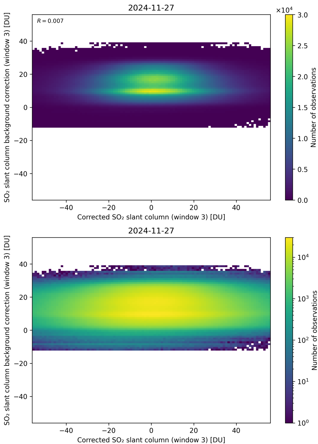
Figure 255: Scatter density plot of “Corrected SO 2 slant column (window 3)” against “SO 2 slant column background correction (window 3)” for 2024-11-26 to 2024-11-28.
