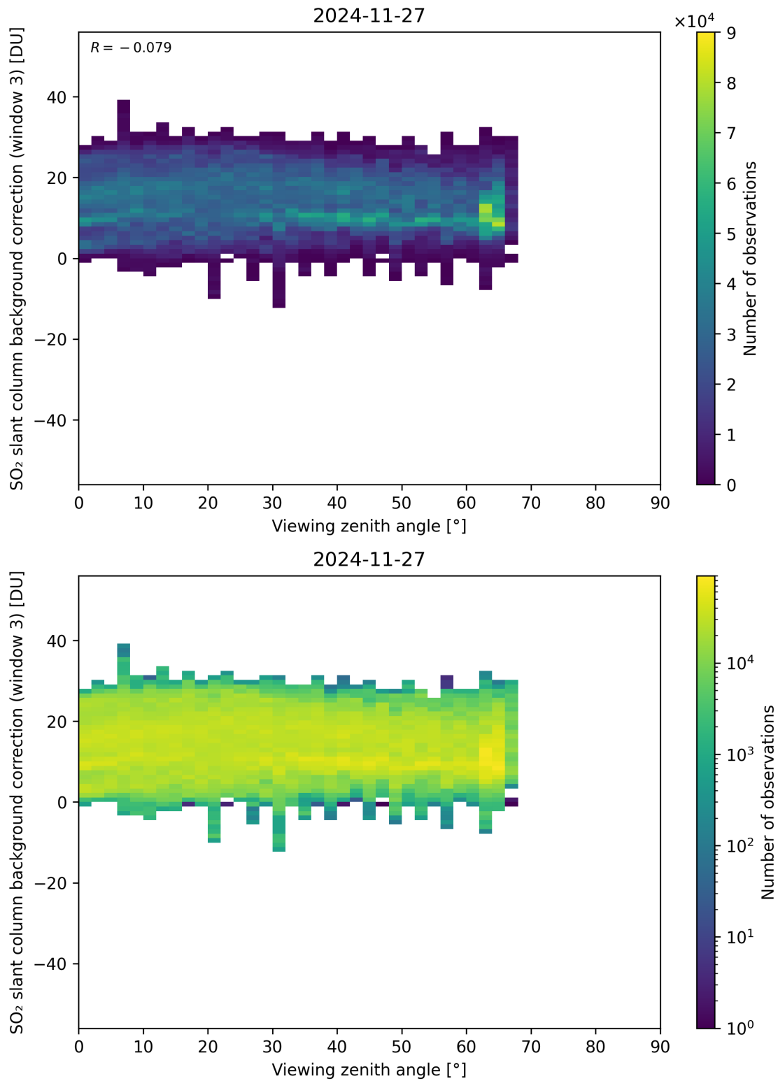
Figure 364: Scatter density plot of “Viewing zenith angle” against “SO 2 slant column background correction (window 3)” for 2024-11-26 to 2024-11-28.
