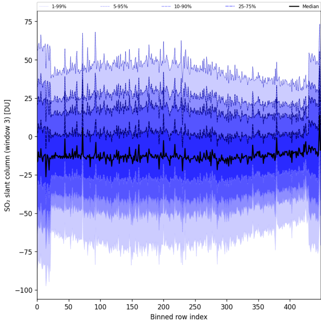
Figure 97: Along track statistics of “SO 2 slant column (window 3)” for 2024-11-26 to 2024-11-28
