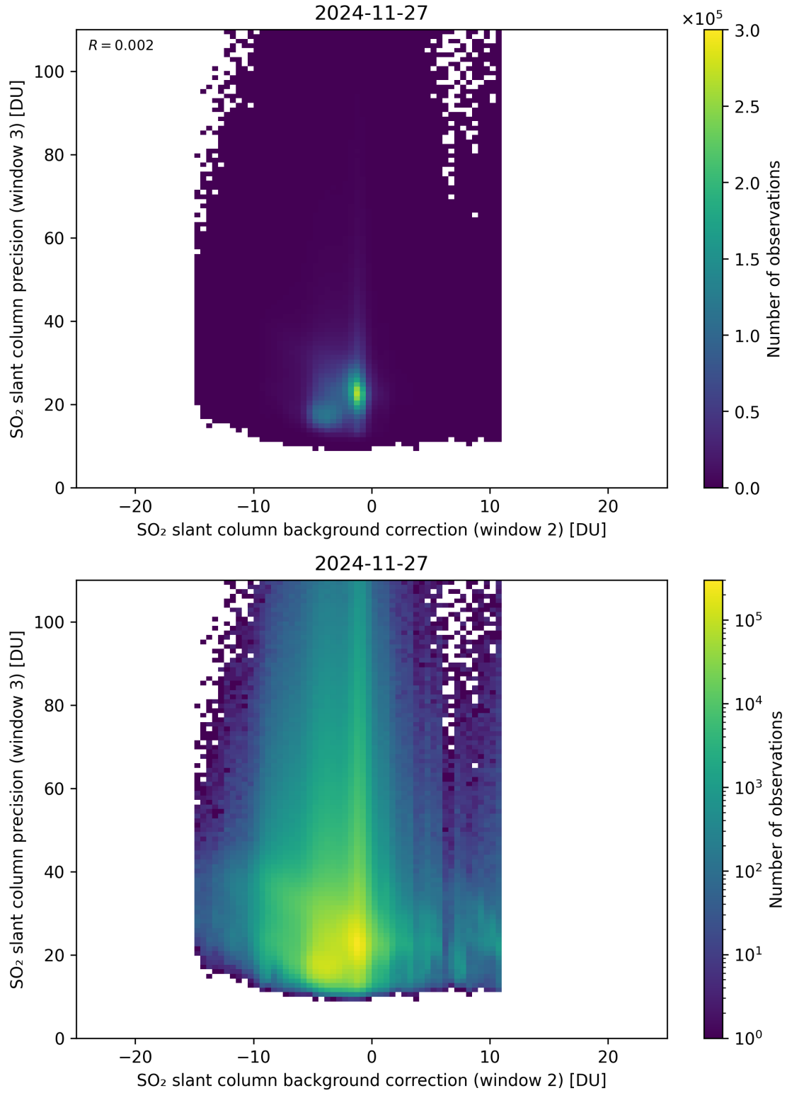
Figure 129: Scatter density plot of “SO 2 slant column background correction (window 2)” against “SO 2 slant column precision (window 3)” for 2024-11-26 to 2024-11-28.
