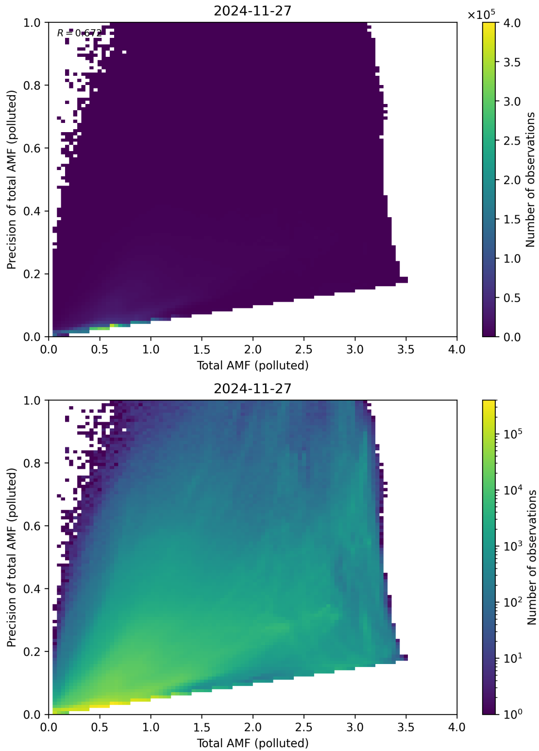
Figure 322: Scatter density plot of “Total AMF (polluted)” against “Precision of total AMF (polluted)” for 2024-11-26 to 2024-11-28.
