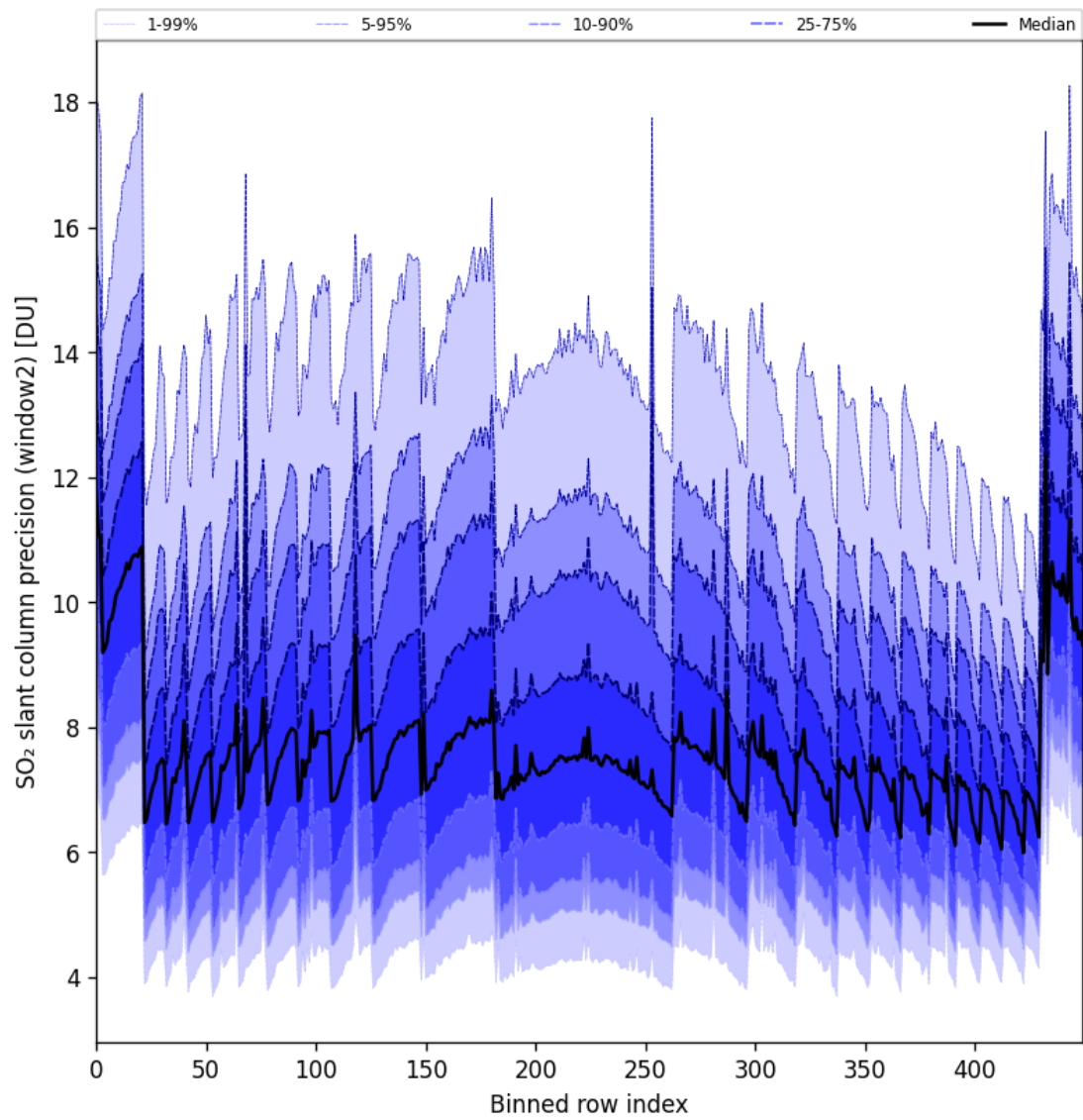
Figure 94: Along track statistics of “SO 2 slant column precision (window2)” for 2024-11-26 to 2024-11-28
