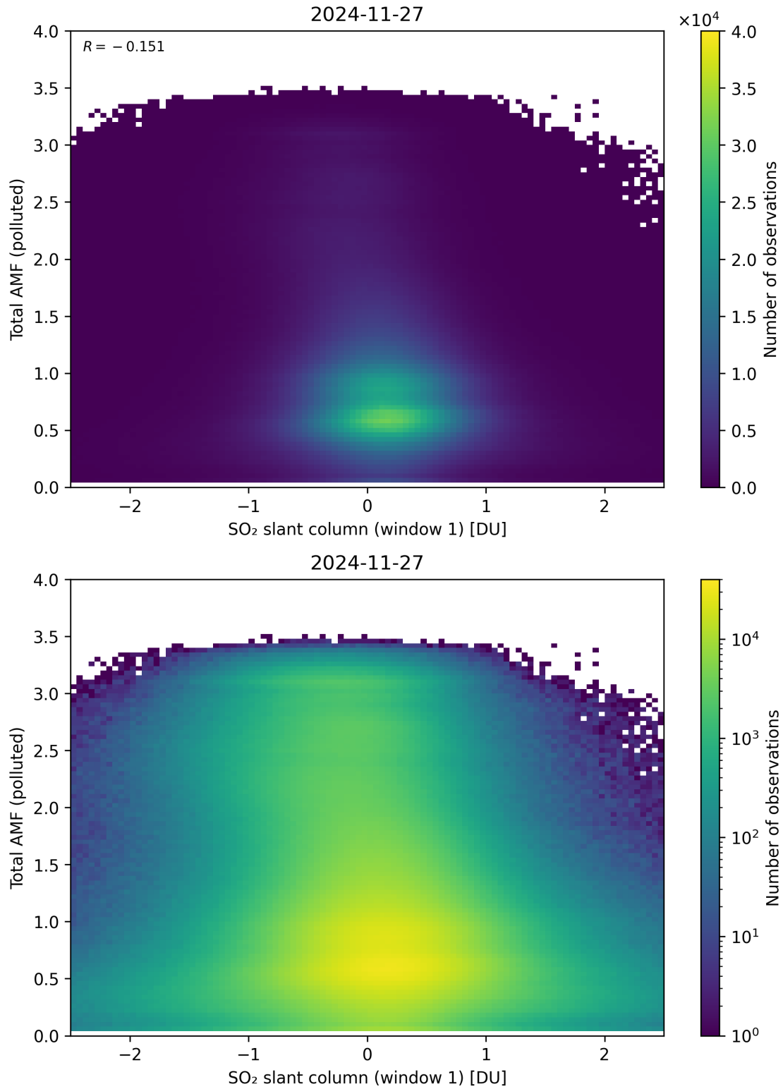
Figure 289: Scatter density plot of “SO 2 slant column (window 1)” against “Total AMF (polluted)” for 2024-11-26 to 2024-11-28.
