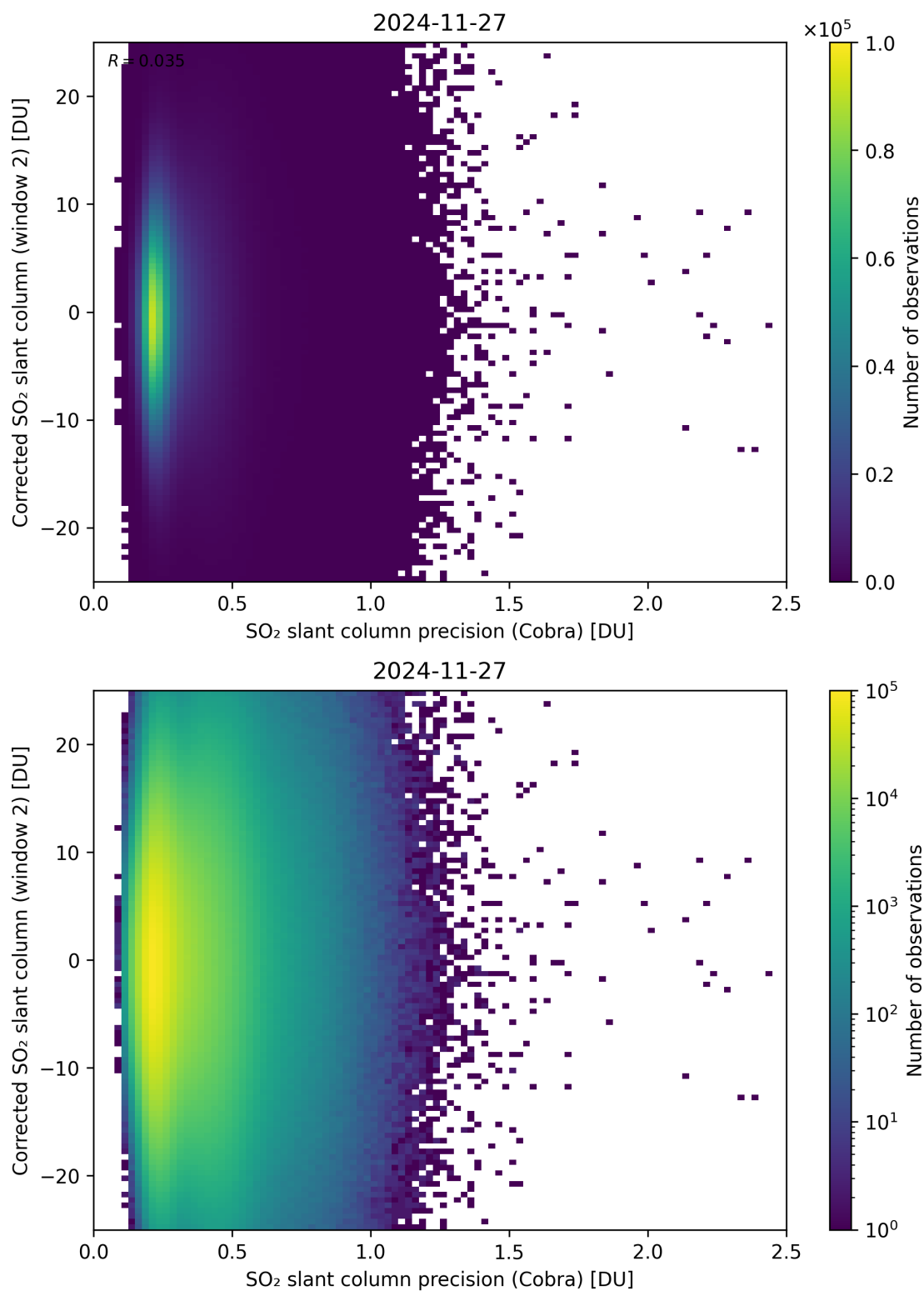
Figure 206: Scatter density plot of “SO 2 slant column precision (Cobra)” against “Corrected SO 2 slant column (window 2)” for 2024-11-26 to 2024-11-28.
