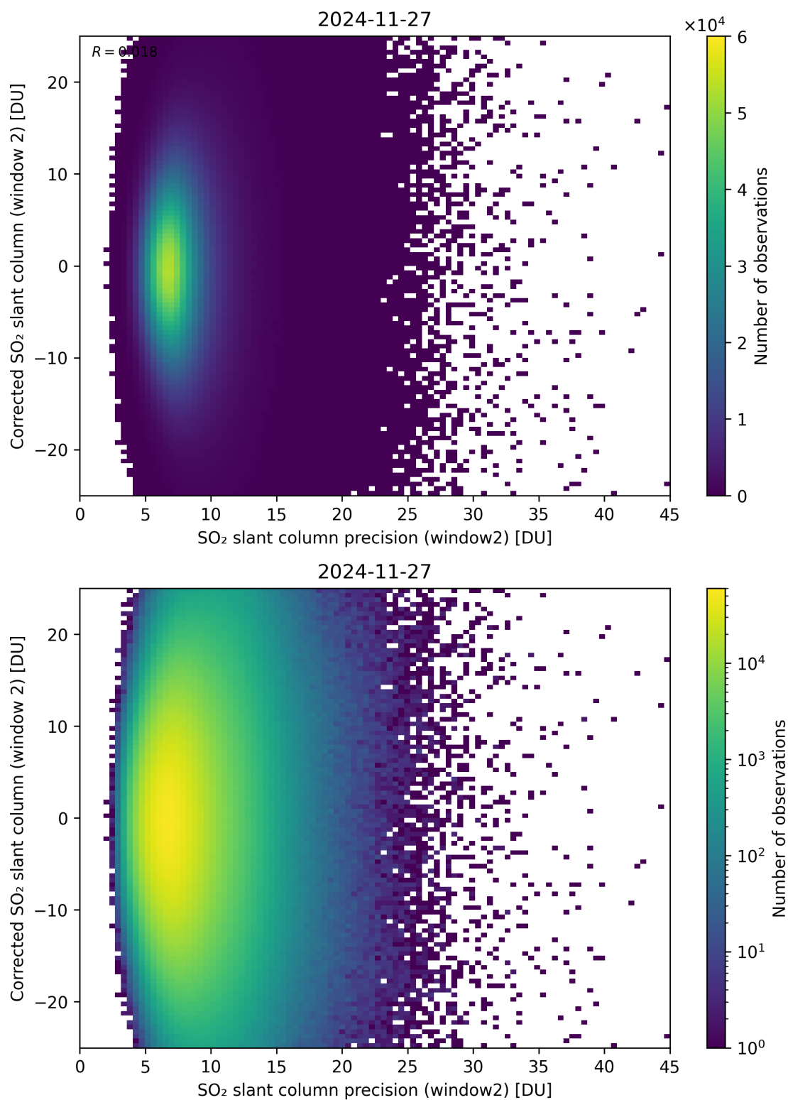
Figure 297: Scatter density plot of “SO 2 slant column precision (window2)” against “Corrected SO 2 slant column (window 2)” for 2024-11-26 to 2024-11-28.
