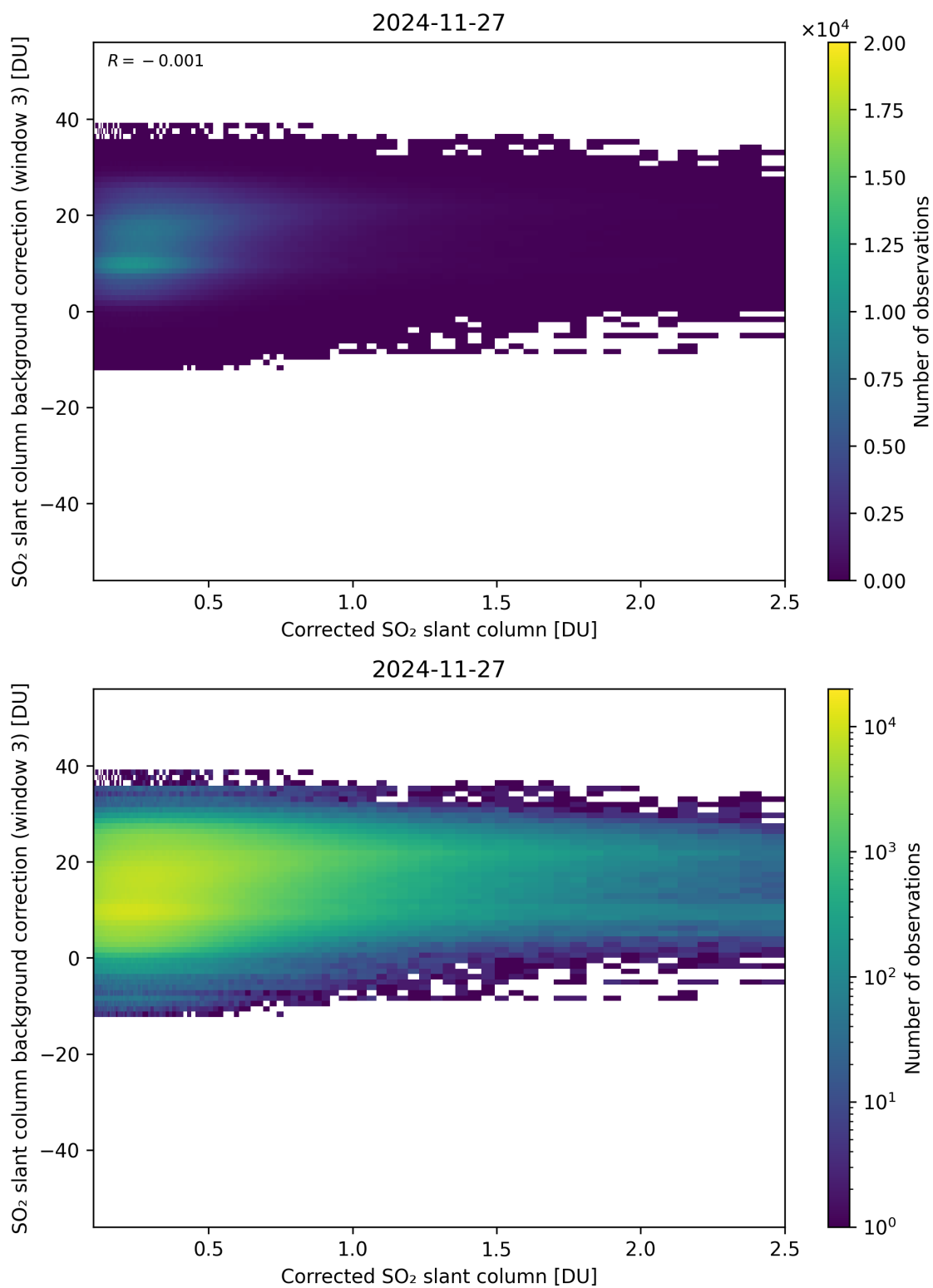
Figure 228: Scatter density plot of “Corrected SO 2 slant column” against “SO 2 slant column background correction (window 3)” for 2024-11-26 to 2024-11-28.
