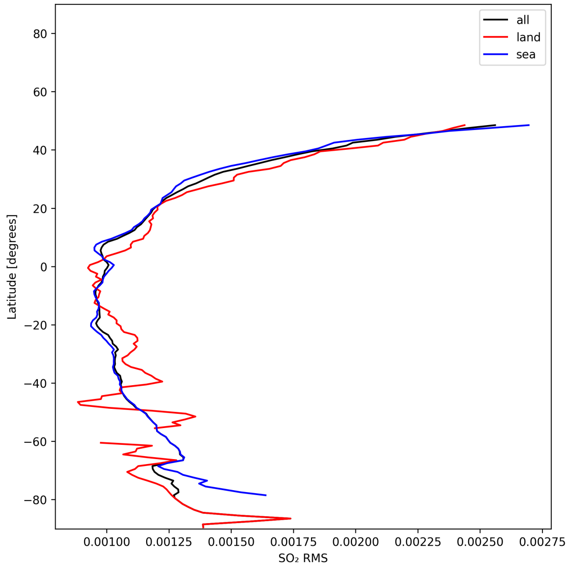
Figure 52: Zonal average of “SO 2 RMS” for 2024-11-26 to 2024-11-28.
