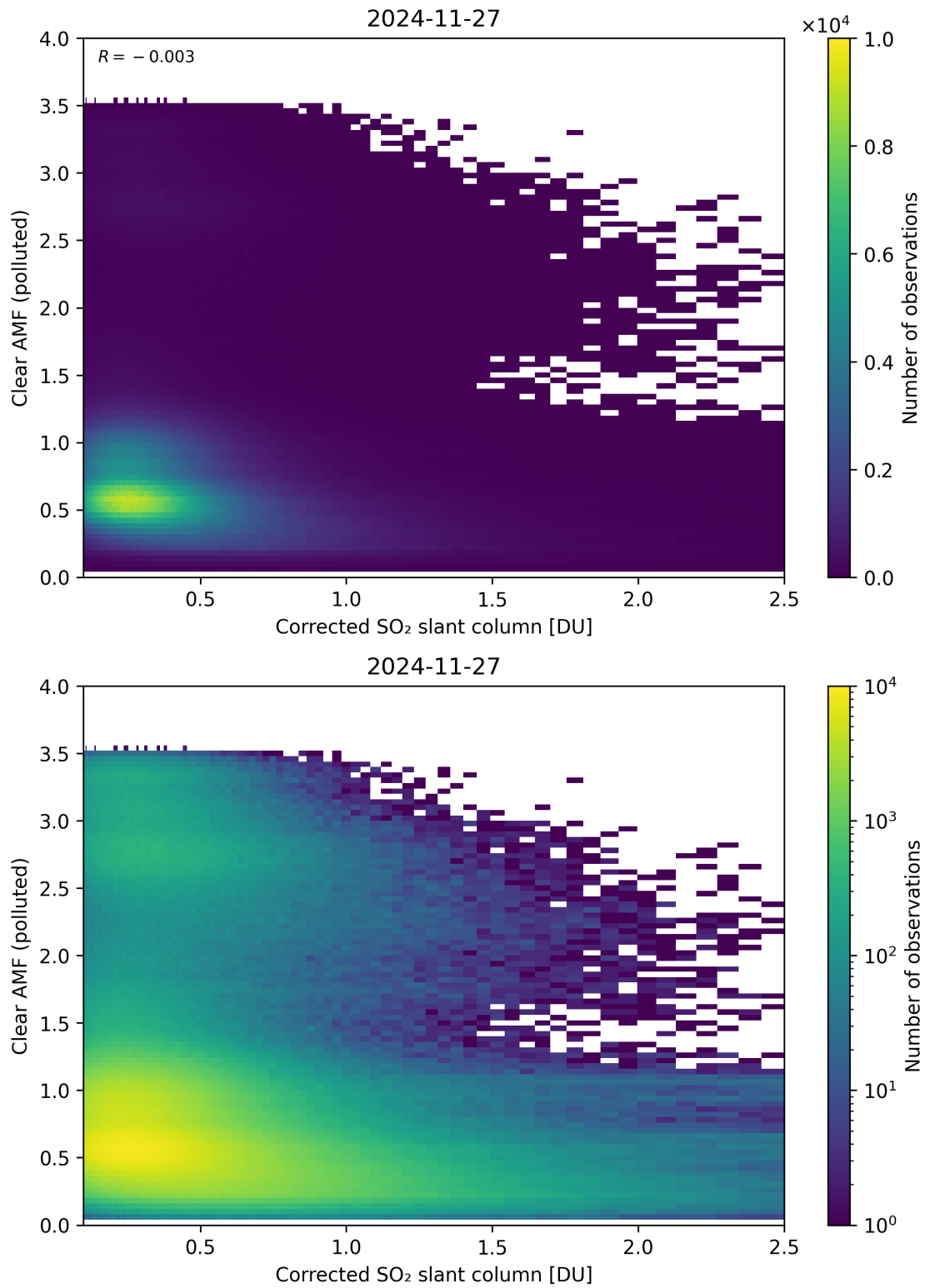
Figure 232: Scatter density plot of “Corrected SO 2 slant column” against “Clear AMF (polluted)” for 2024-11-26 to 2024-11-28.
