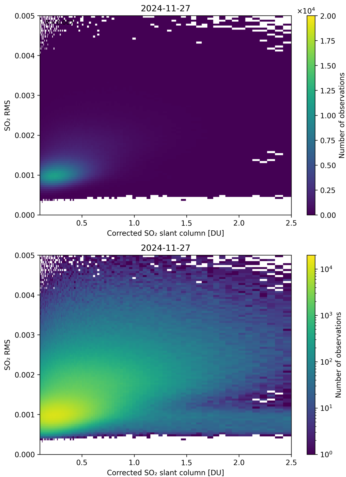
Figure 231: Scatter density plot of “Corrected SO 2 slant column” against “SO 2 RMS” for 2024-11-26 to 2024-11-28.
