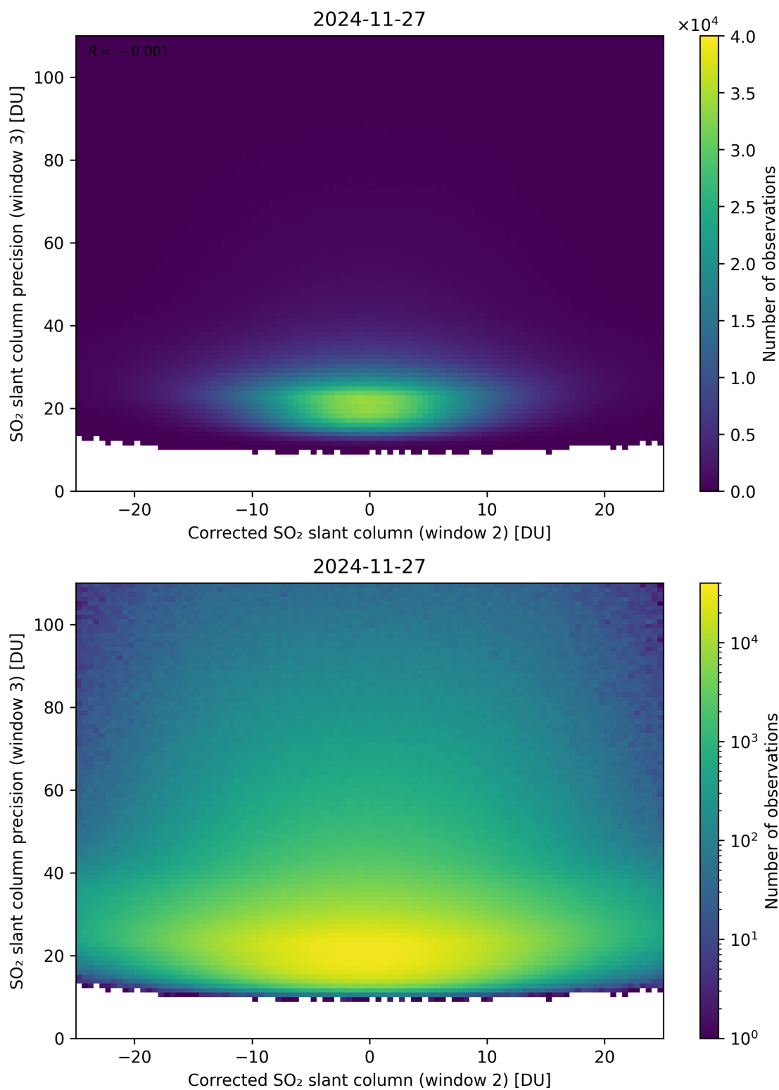
Figure 252: Scatter density plot of “Corrected SO 2 slant column (window 2)” against “SO 2 slant column precision (window 3)” for 2024-11-26 to 2024-11-28.
