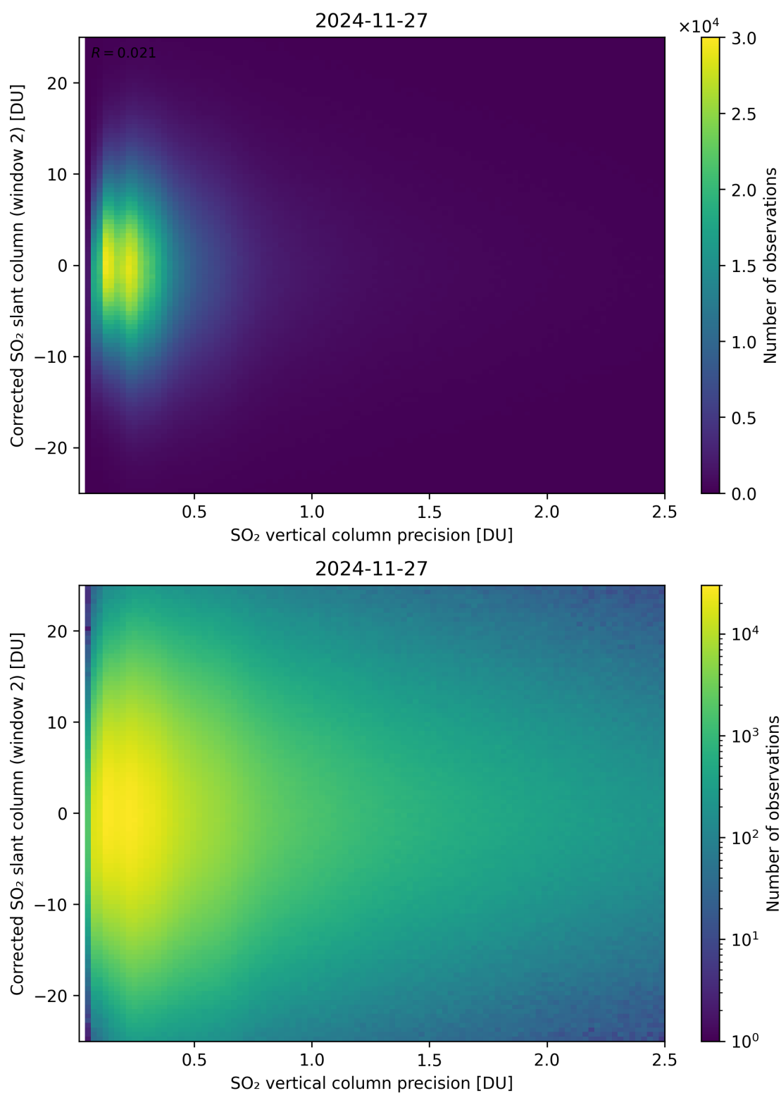
Figure 339: Scatter density plot of “SO 2 vertical column precision” against “Corrected SO 2 slant column (window 2)” for 2024-11-26 to 2024-11-28.
