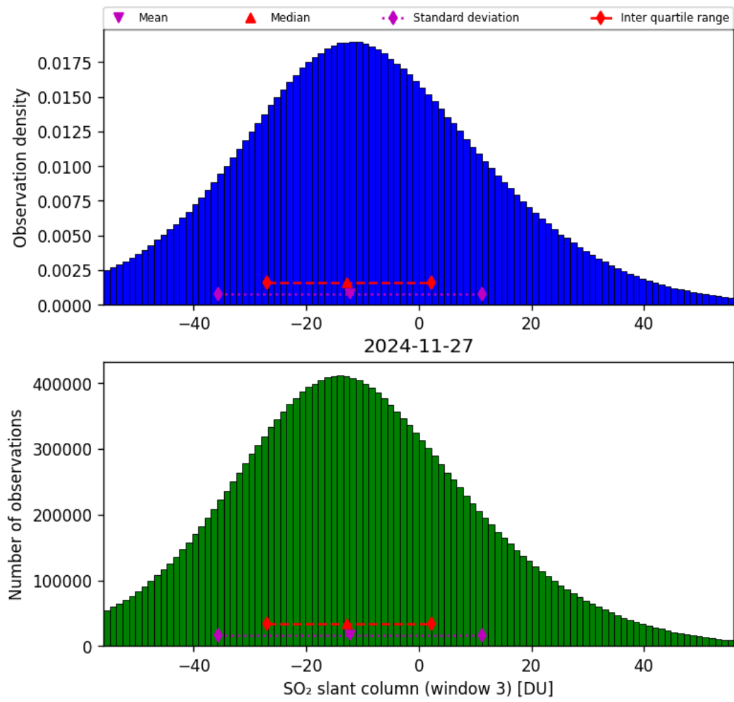
Figure 71: Histogram of “SO 2 slant column (window 3)” for 2024-11-26 to 2024-11-28
