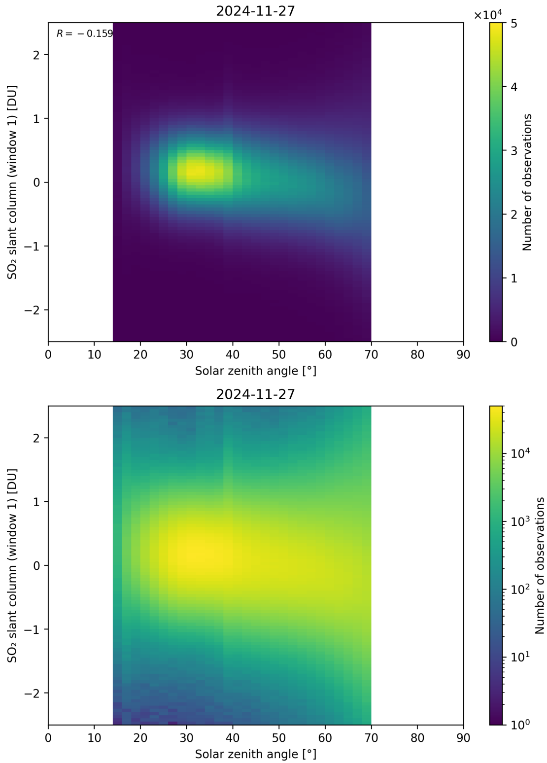
Figure 184: Scatter density plot of “Solar zenith angle” against “SO 2 slant column (window 1)” for 2024-11-26 to 2024-11-28.
