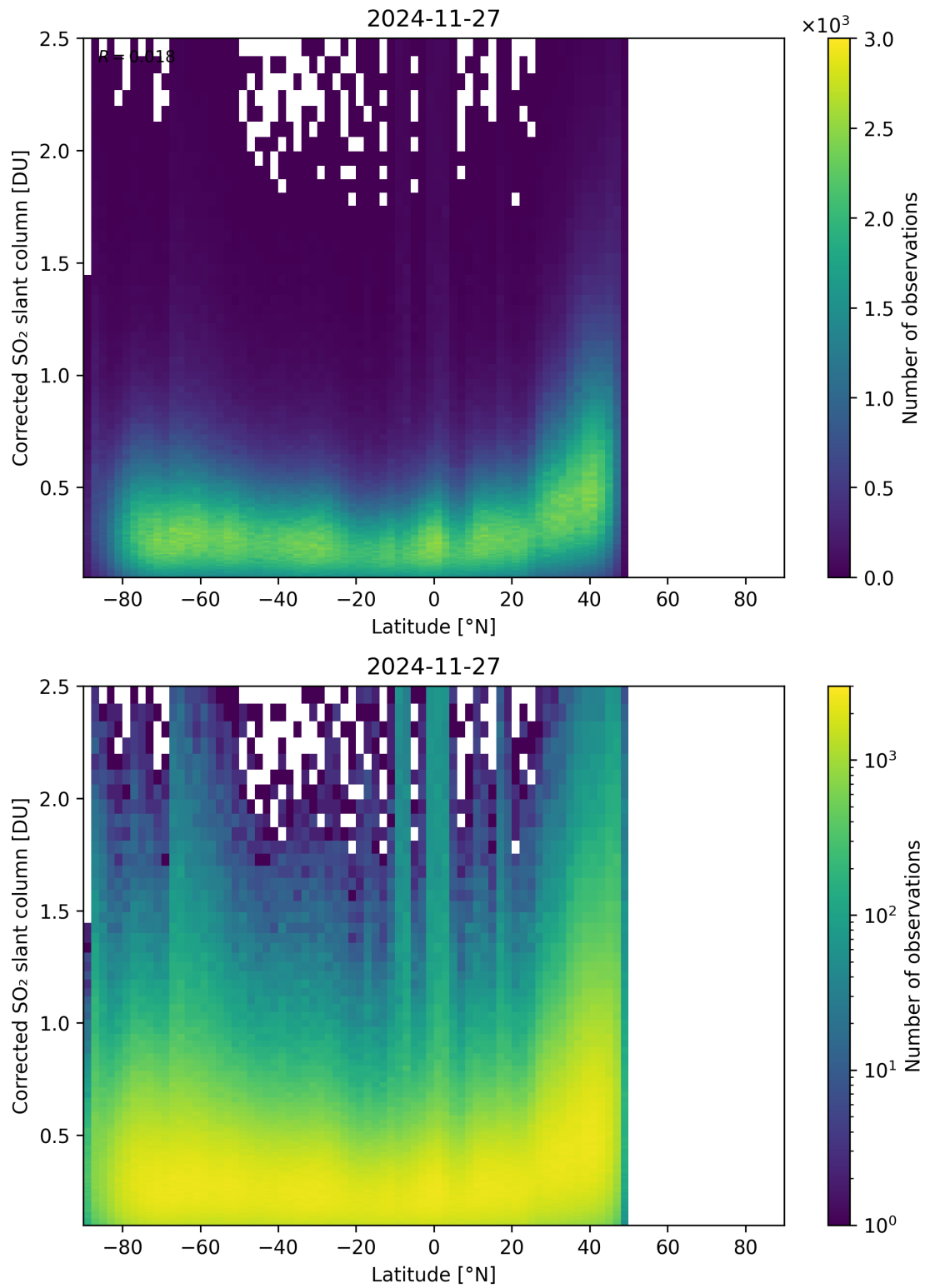
Figure 159: Scatter density plot of “Latitude” against “Corrected SO 2 slant column” for 2024-11-26 to 2024-11-28.
