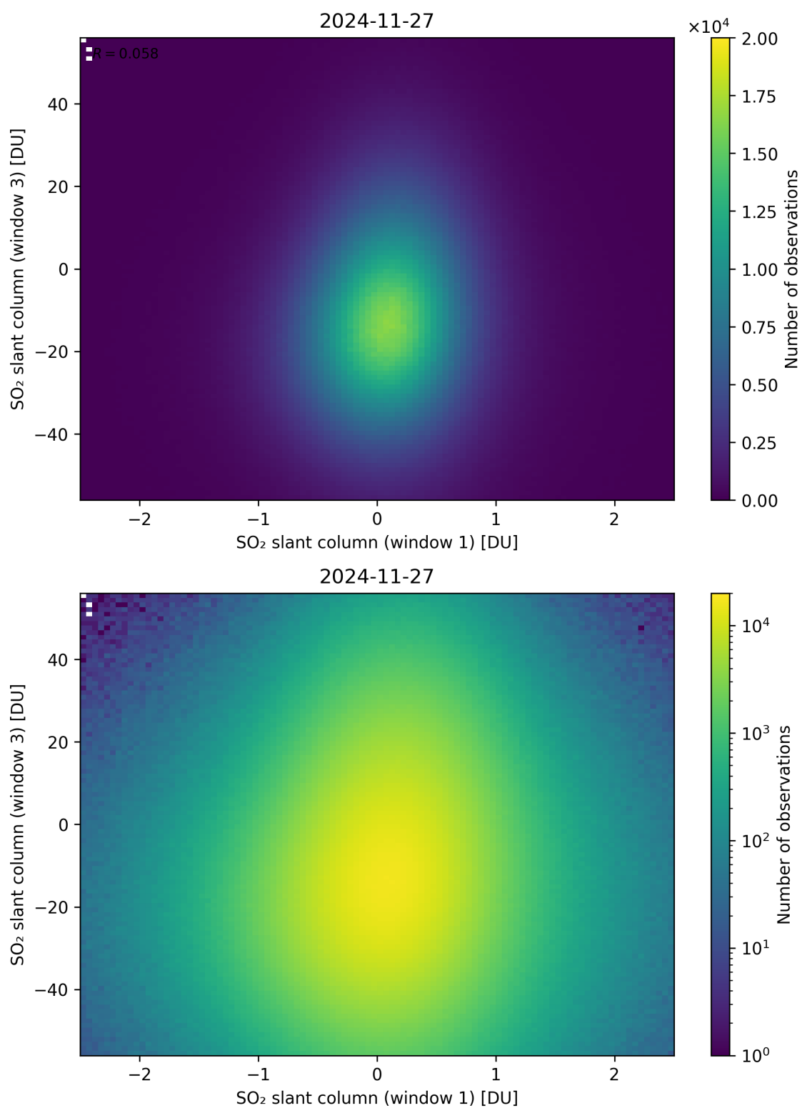
Figure 287: Scatter density plot of “SO 2 slant column (window 1)” against “SO 2 slant column (window 3)” for 2024-11-26 to 2024-11-28.
