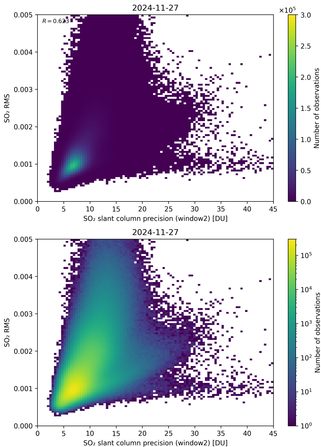
Figure 295: Scatter density plot of “SO 2 slant column precision (window2)” against “SO 2 RMS” for 2024-11-26 to 2024-11-28.
