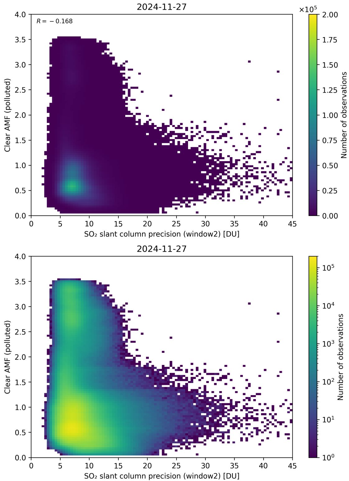
Figure 296: Scatter density plot of “SO 2 slant column precision (window2)” against “Clear AMF (polluted)” for 2024-11-26 to 2024-11-28.
