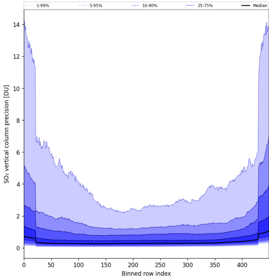
Figure 85: Along track statistics of “SO 2 vertical column precision” for 2024-11-26 to 2024-11-28
