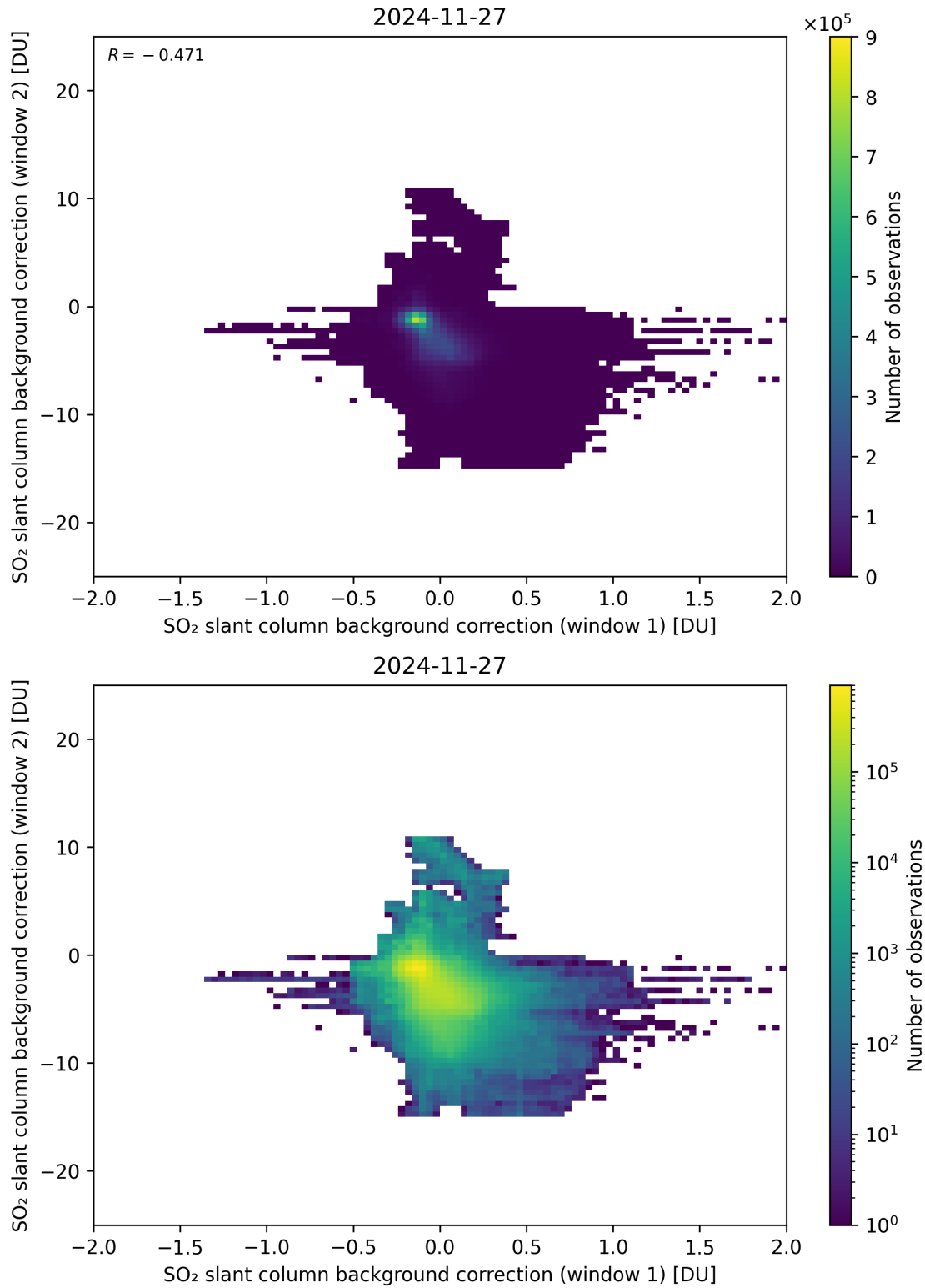
Figure 109: Scatter density plot of “SO 2 slant column background correction (window 1)” against “SO 2 slant column background correction (window 2)” for 2024-11-26 to 2024-11-28.
