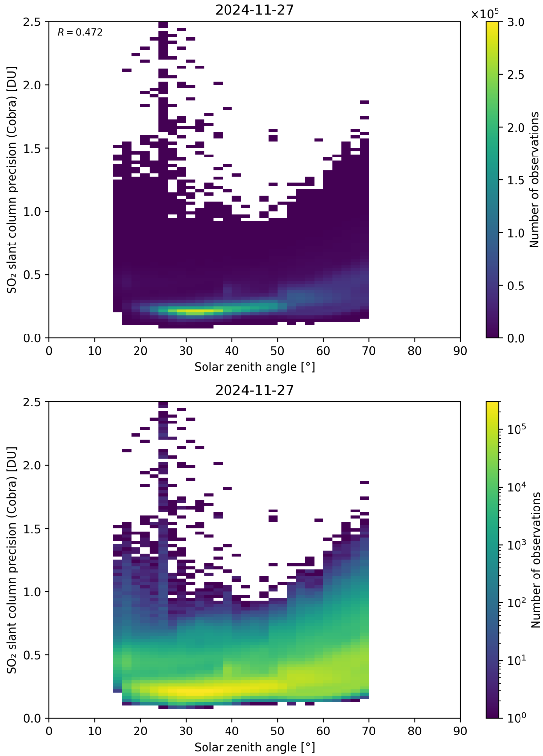
Figure 180: Scatter density plot of “Solar zenith angle” against “SO 2 slant column precision (Cobra)” for 2024-11-26 to 2024-11-28.
