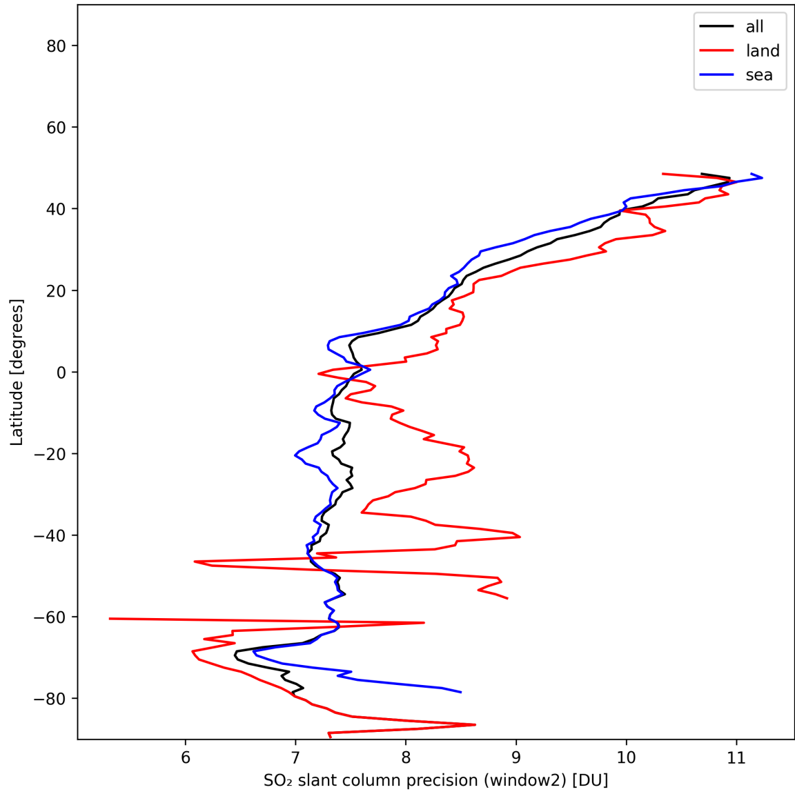
Figure 42: Zonal average of “SO 2 slant column precision (window2)” for 2024-11-26 to 2024-11-28.
