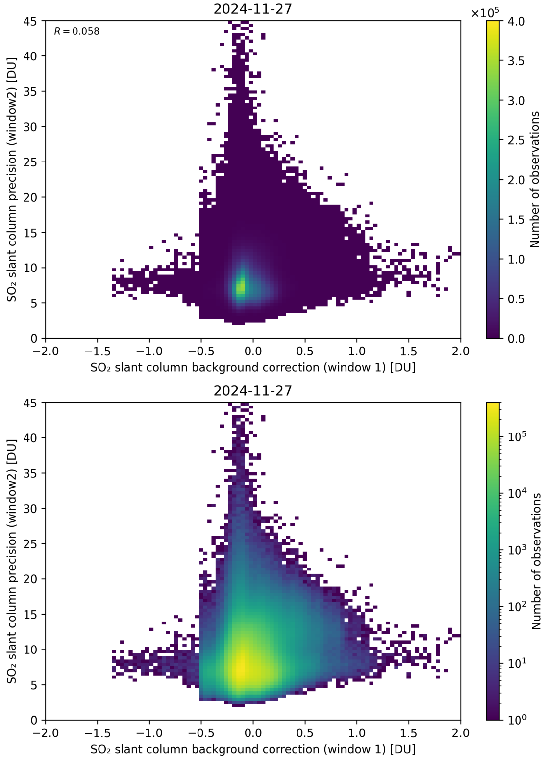
Figure 117: Scatter density plot of “SO 2 slant column background correction (window 1)” against “SO 2 slant column precision (window2)” for 2024-11-26 to 2024-11-28.
