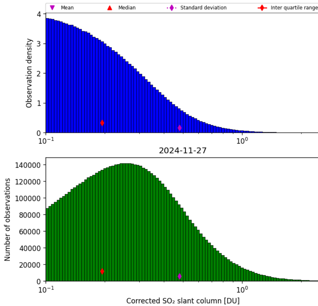
Figure 60: Histogram of “Corrected SO 2 slant column” for 2024-11-26 to 2024-11-28
