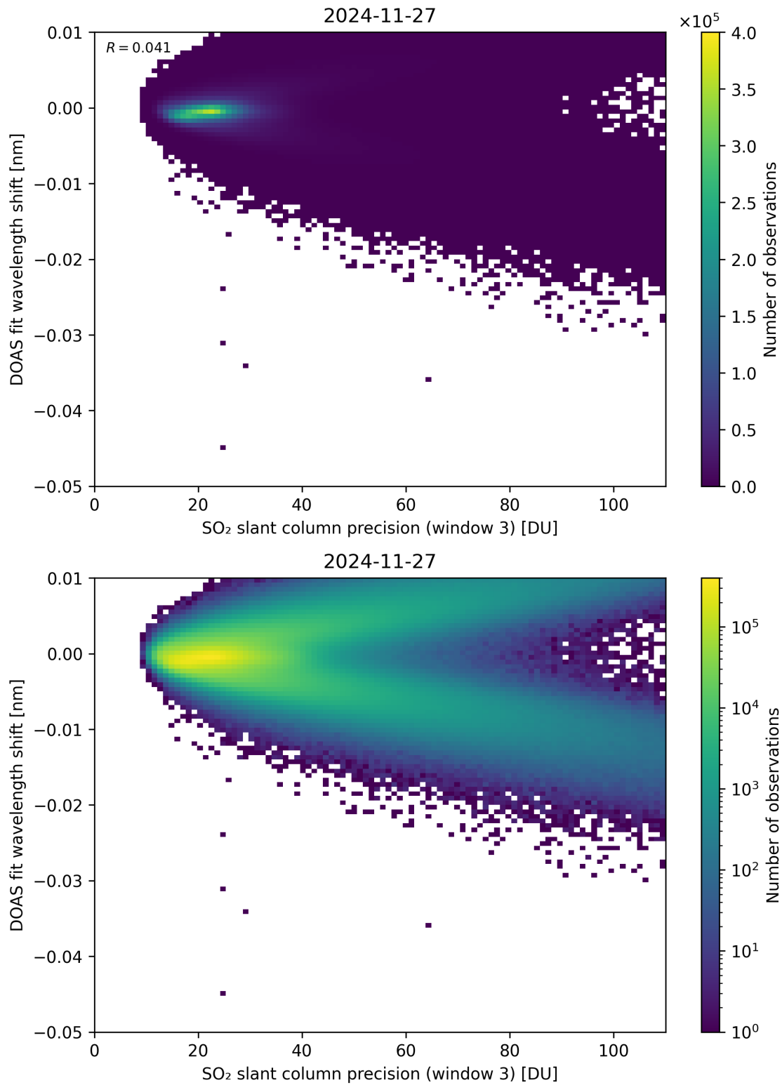
Figure 308: Scatter density plot of “SO 2 slant column precision (window 3)” against “DOAS fit wavelength shift” for 2024-11-26 to 2024-11-28.
