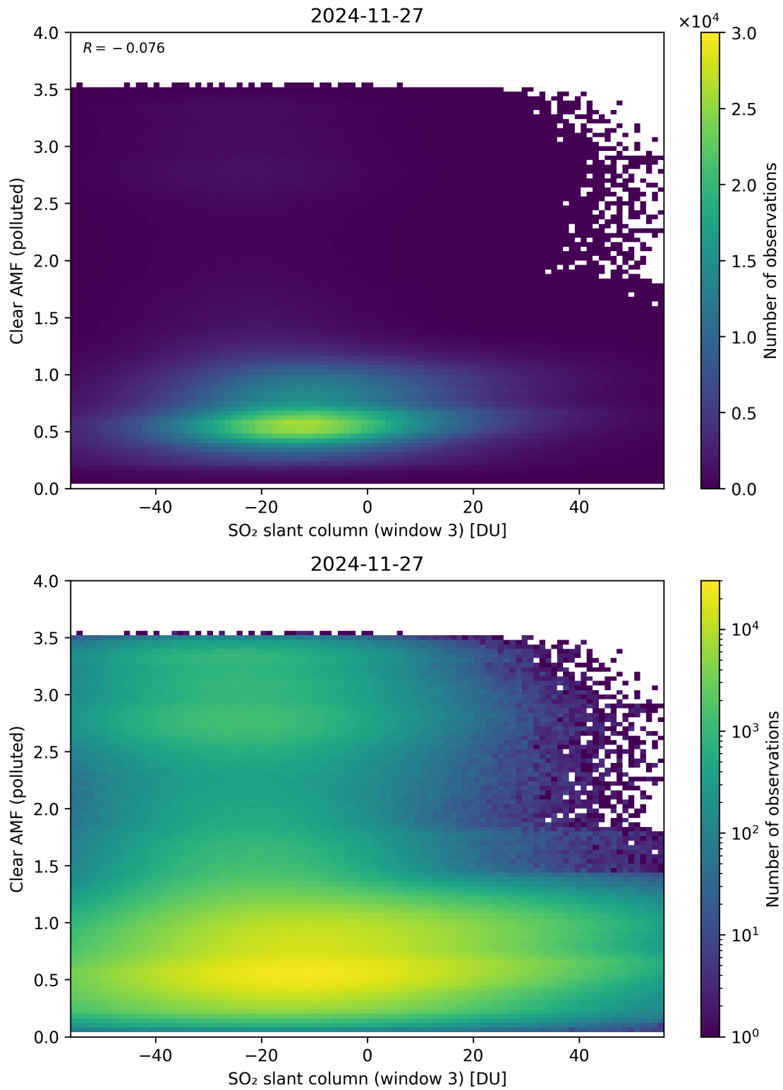
Figure 315: Scatter density plot of “SO 2 slant column (window 3)” against “Clear AMF (polluted)” for 2024-11-26 to 2024-11-28.
