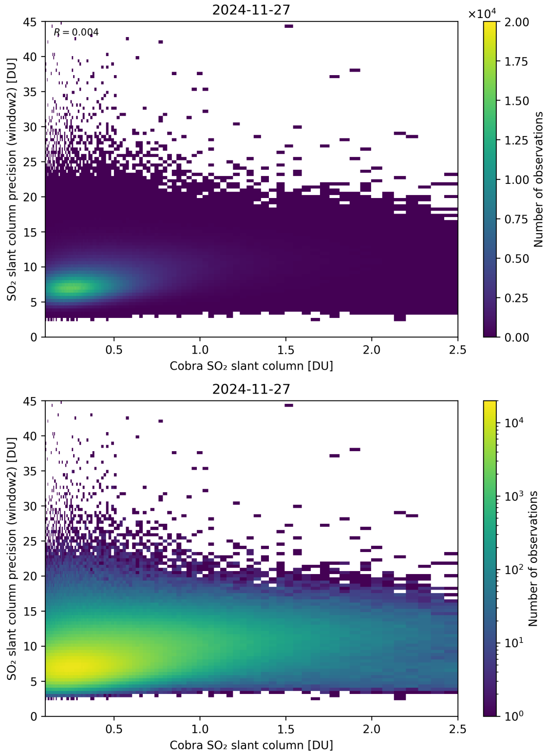
Figure 221: Scatter density plot of “Cobra SO 2 slant column” against “SO 2 slant column precision (window2)” for 2024-11-26 to 2024-11-28.
