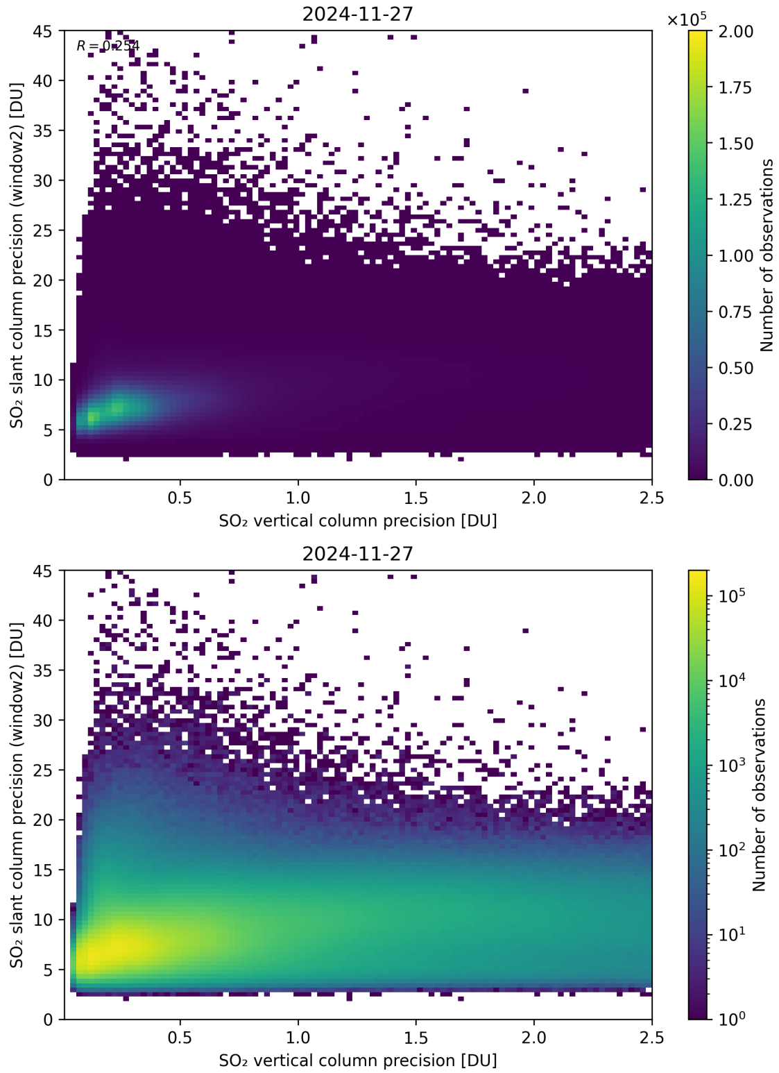
Figure 343: Scatter density plot of “SO 2 vertical column precision” against “SO 2 slant column precision (window2)” for 2024-11-26 to 2024-11-28.
