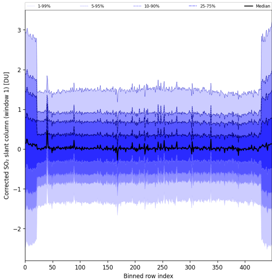
Figure 91: Along track statistics of “Corrected SO 2 slant column (window 1)” for 2024-11-26 to 2024-11-28
