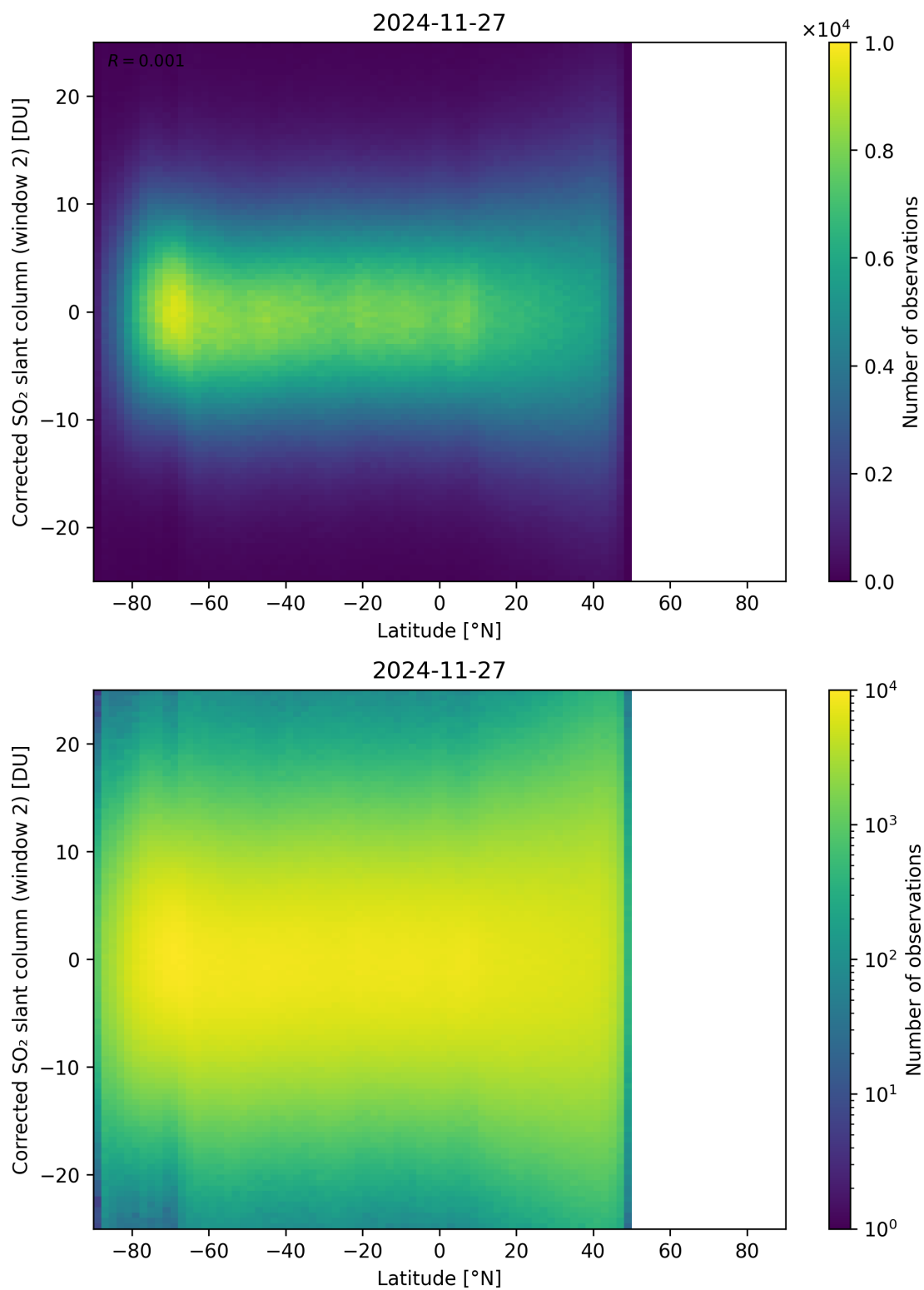
Figure 160: Scatter density plot of “Latitude” against “Corrected SO 2 slant column (window 2)” for 2024-11-26 to 2024-11-28.
