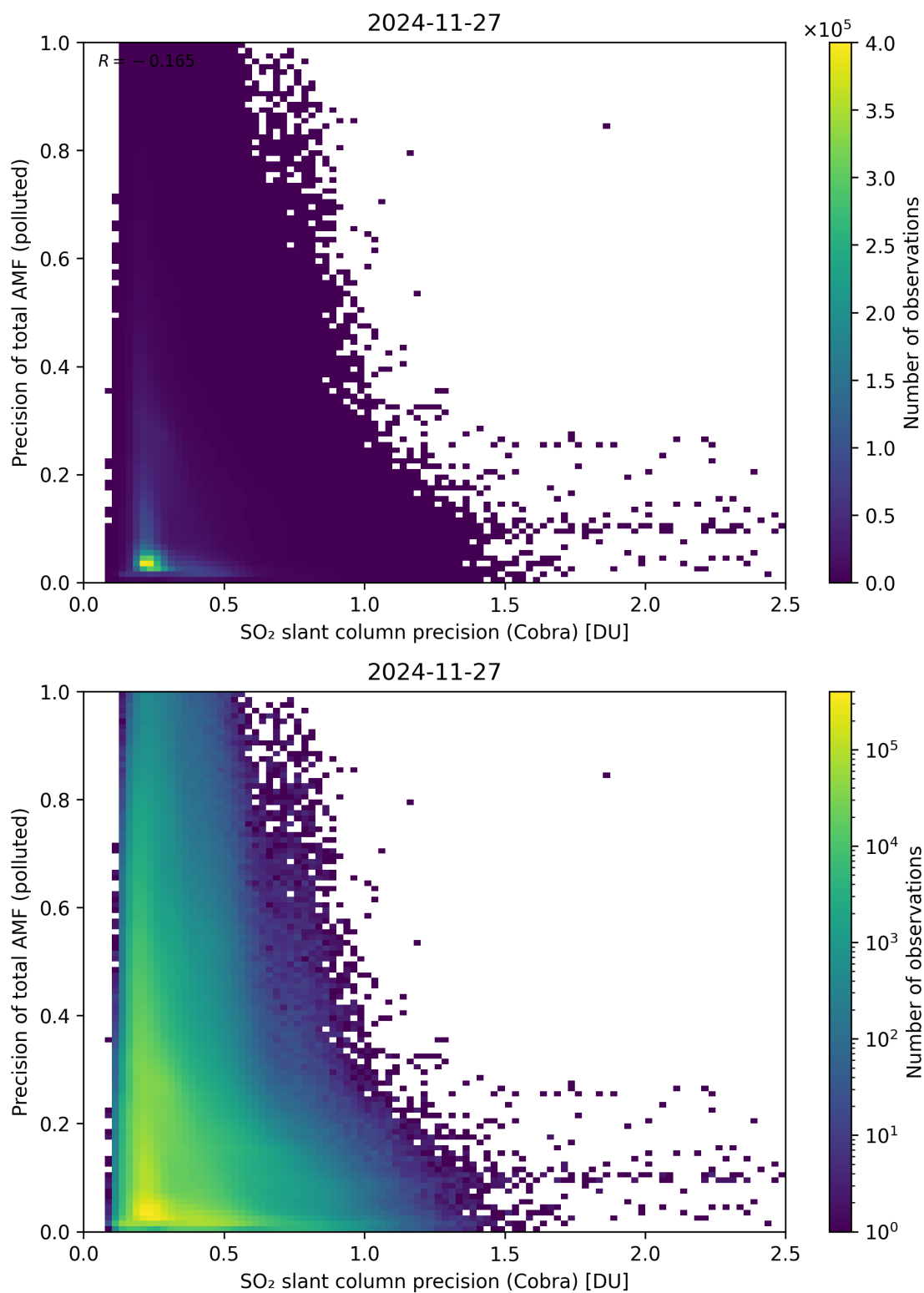
Figure 214: Scatter density plot of “SO 2 slant column precision (Cobra)” against “Precision of total AMF (polluted)” for 2024-11-26 to 2024-11-28.
