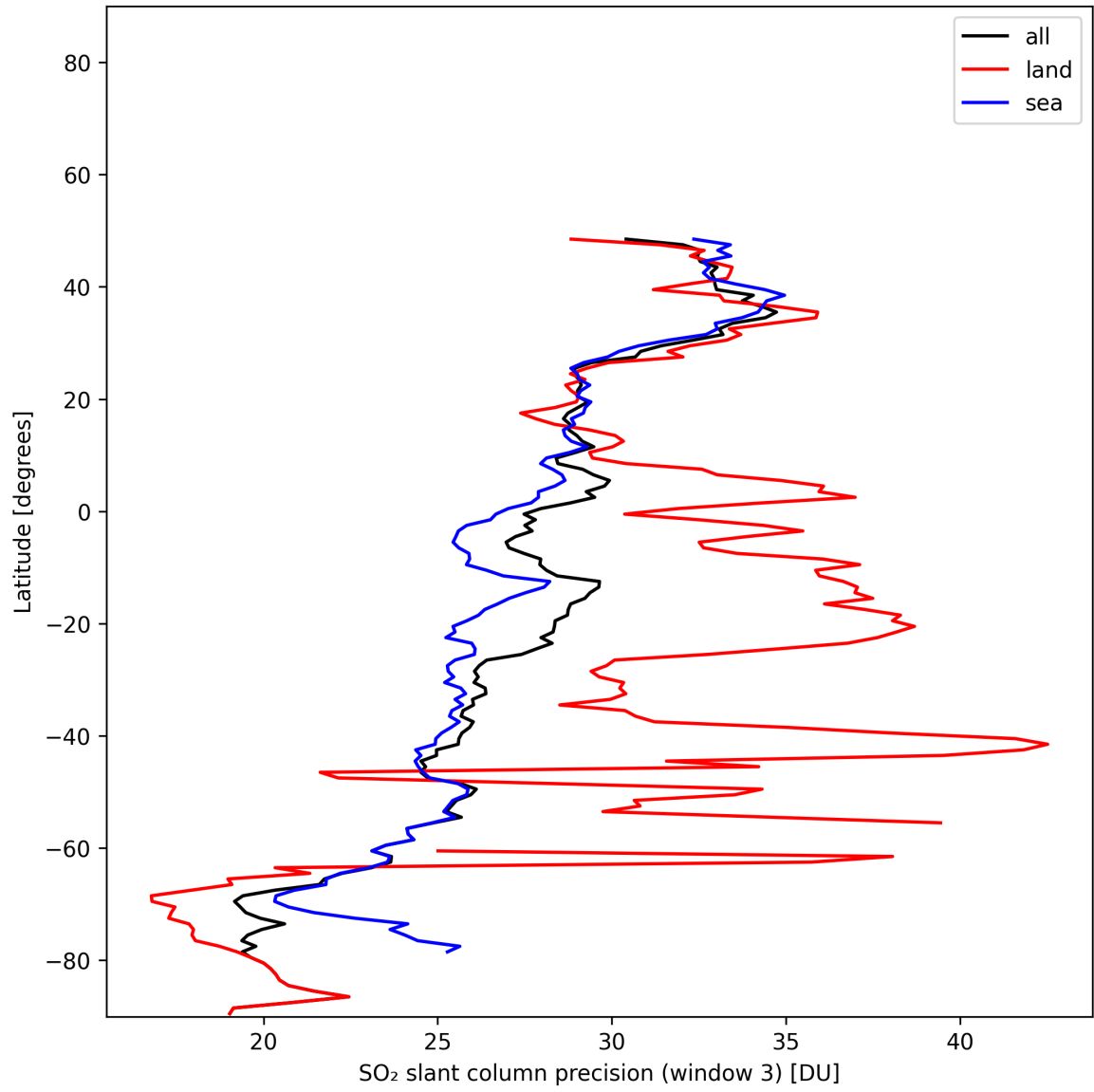
Figure 46: Zonal average of “SO 2 slant column precision (window 3)” for 2024-11-26 to 2024-11-28.
