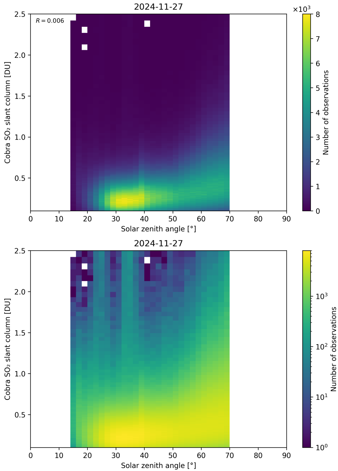
Figure 179: Scatter density plot of “Solar zenith angle” against “Cobra SO 2 slant column” for 2024-11-26 to 2024-11-28.
