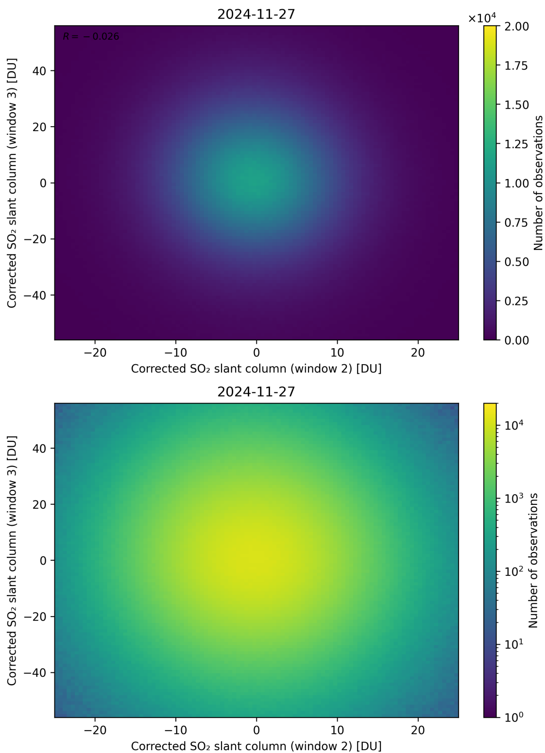
Figure 250: Scatter density plot of “Corrected SO 2 slant column (window 2)” against “Corrected SO 2 slant column (window 3)” for 2024-11-26 to 2024-11-28.
