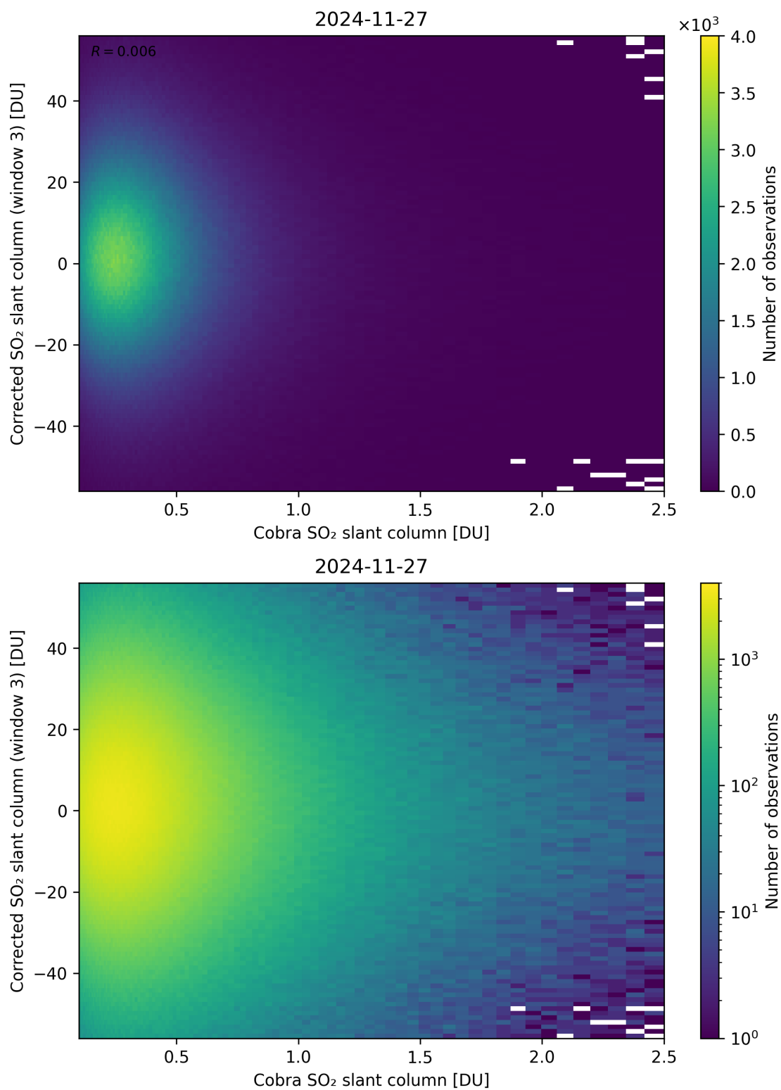
Figure 218: Scatter density plot of “Cobra SO 2 slant column” against “Corrected SO 2 slant column (window 3)” for 2024-11-26 to 2024-11-28.
