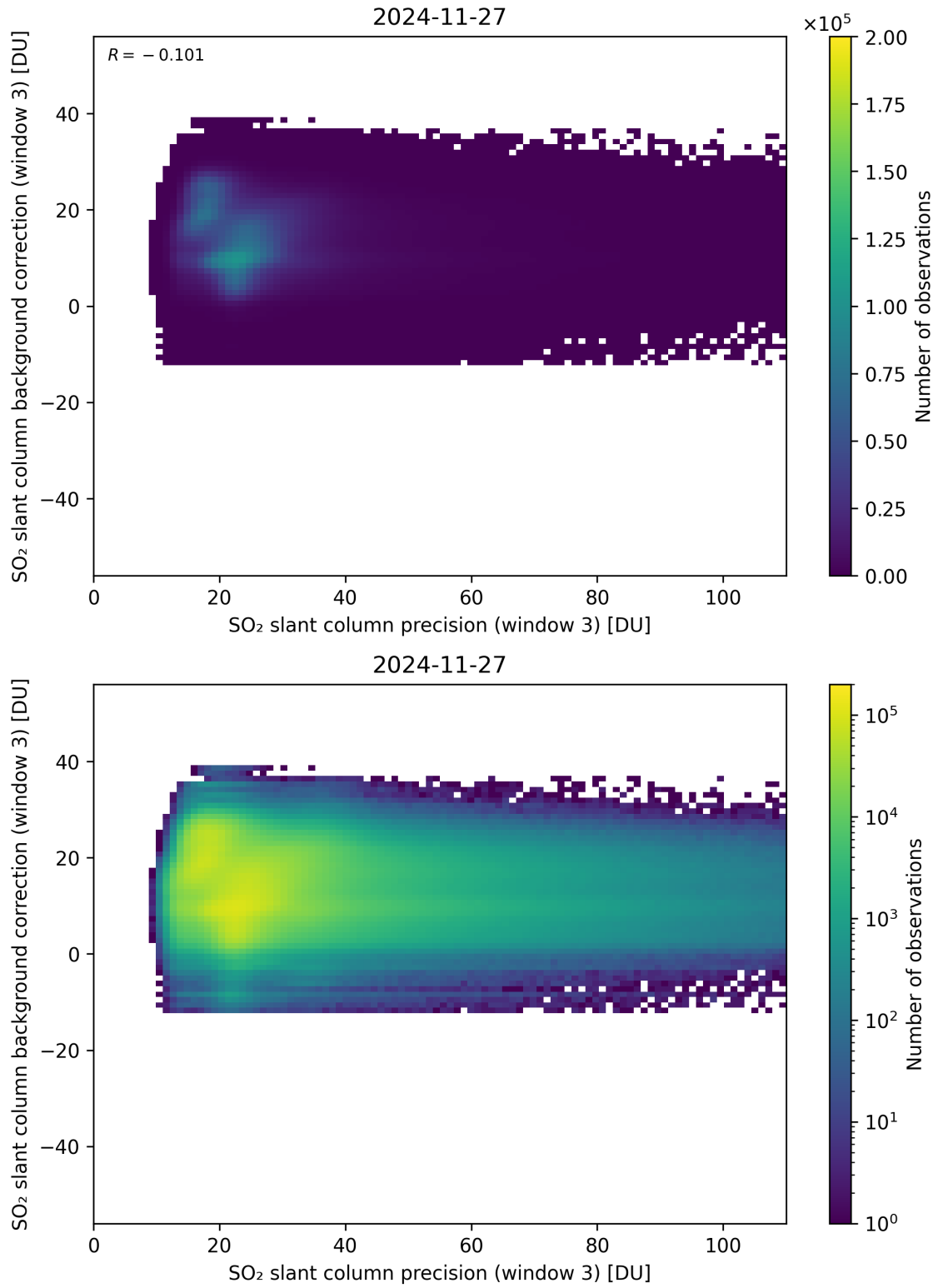
Figure 307: Scatter density plot of “SO 2 slant column precision (window 3)” against “SO 2 slant column background correction (window 3)” for 2024-11-26 to 2024-11-28.
