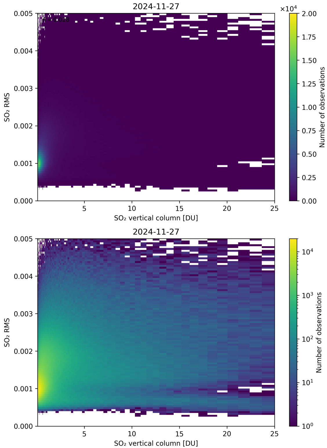
Figure 328: Scatter density plot of “SO 2 vertical column” against “SO 2 RMS” for 2024-11-26 to 2024-11-28.
