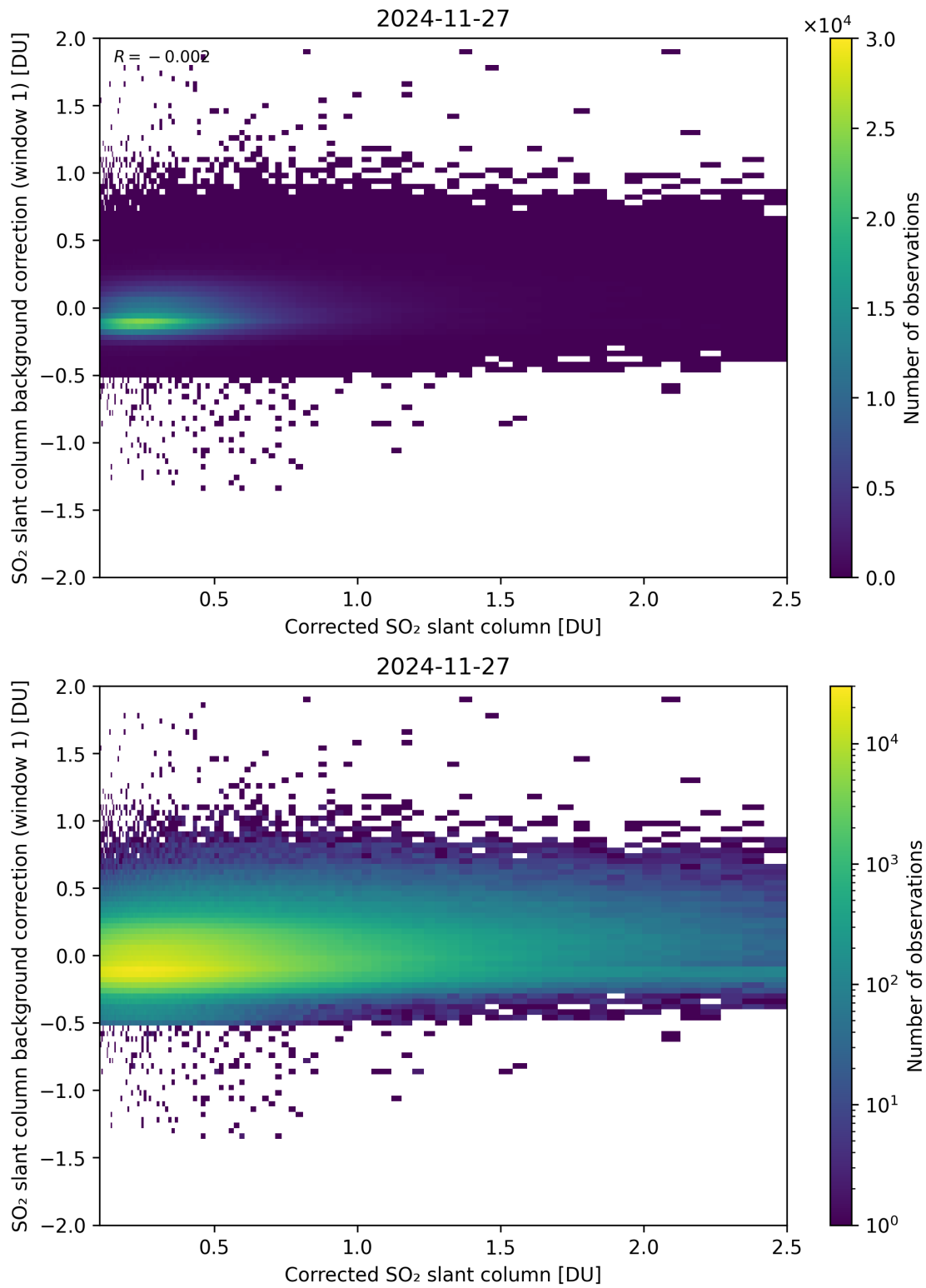
Figure 226: Scatter density plot of “Corrected SO 2 slant column” against “SO 2 slant column background correction (window 1)” for 2024-11-26 to 2024-11-28.
