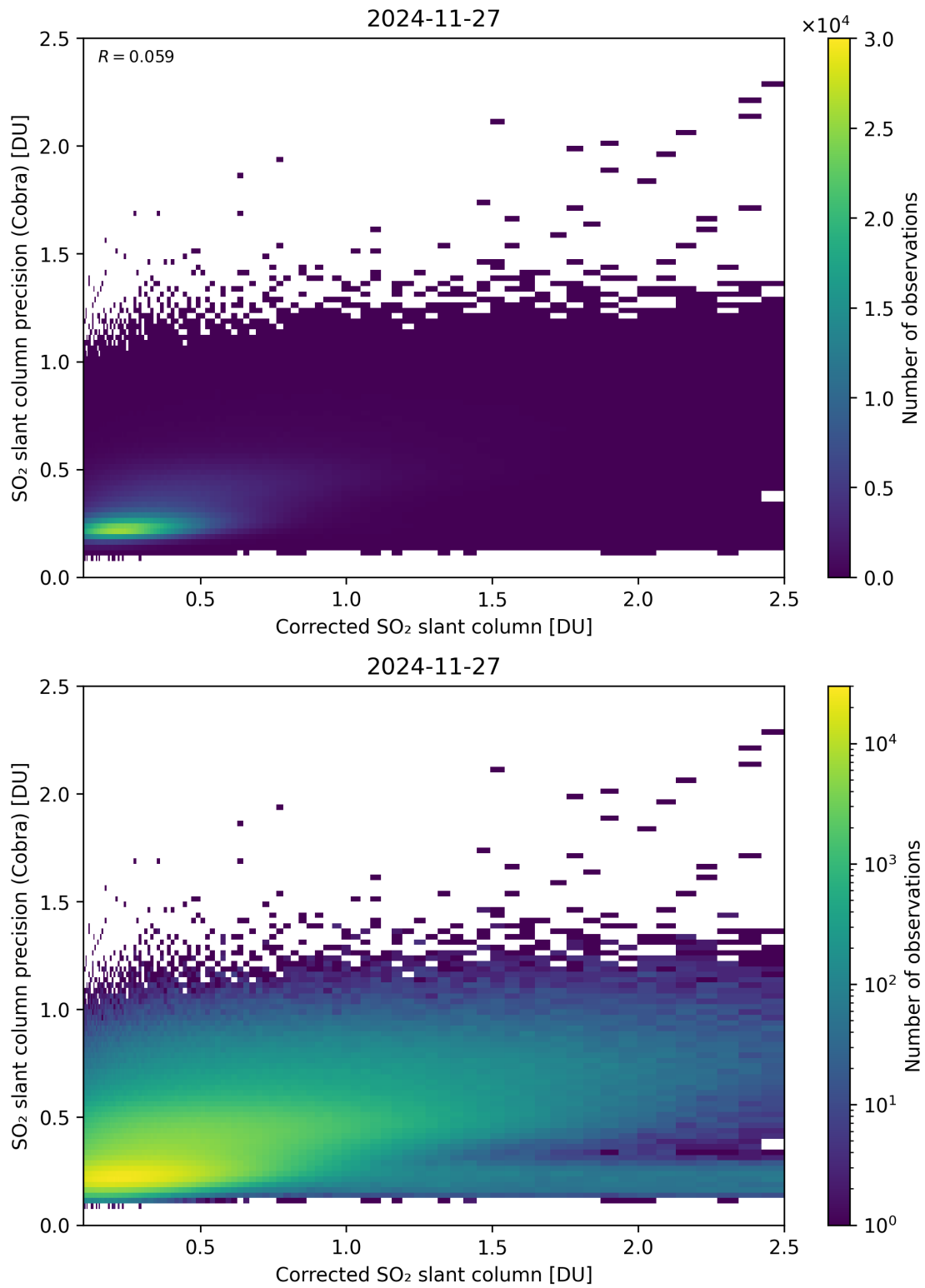
Figure 234: Scatter density plot of “Corrected SO 2 slant column” against “SO 2 slant column precision (Cobra)” for 2024-11-26 to 2024-11-28.
