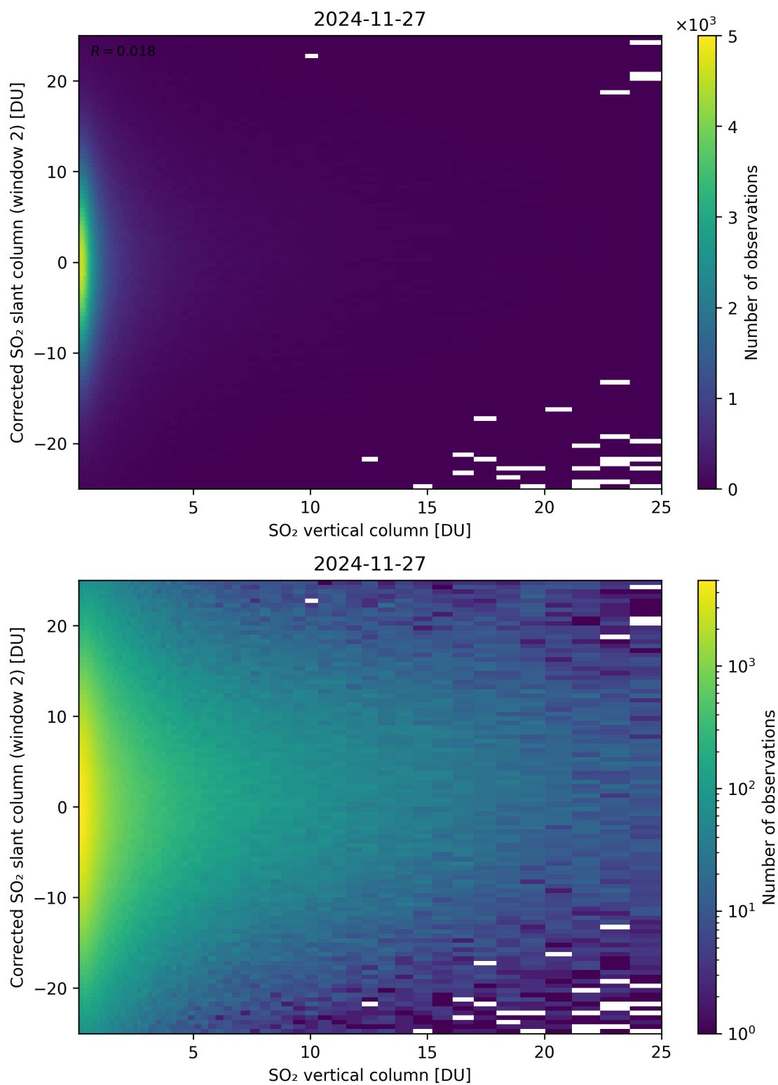
Figure 352: Scatter density plot of “SO 2 vertical column” against “Corrected SO 2 slant column (window 2)” for 2024-11-26 to 2024-11-28.
