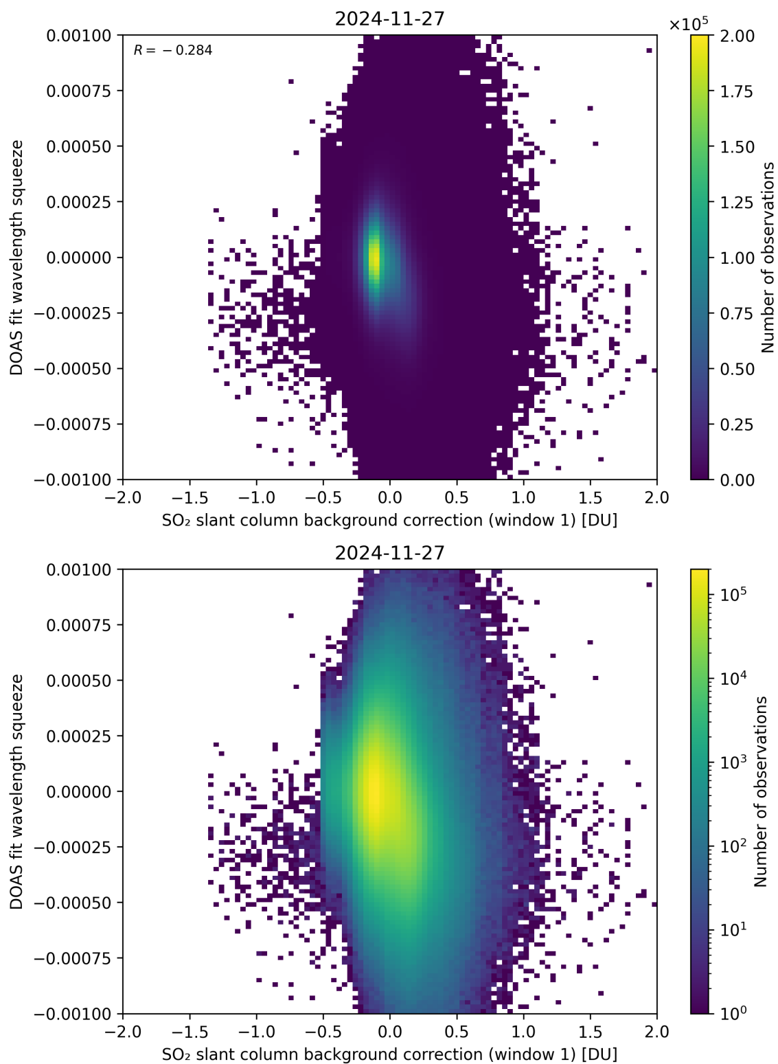
Figure 112: Scatter density plot of “SO 2 slant column background correction (window 1)” against “DOAS fit wavelength squeeze” for 2024-11-26 to 2024-11-28.
