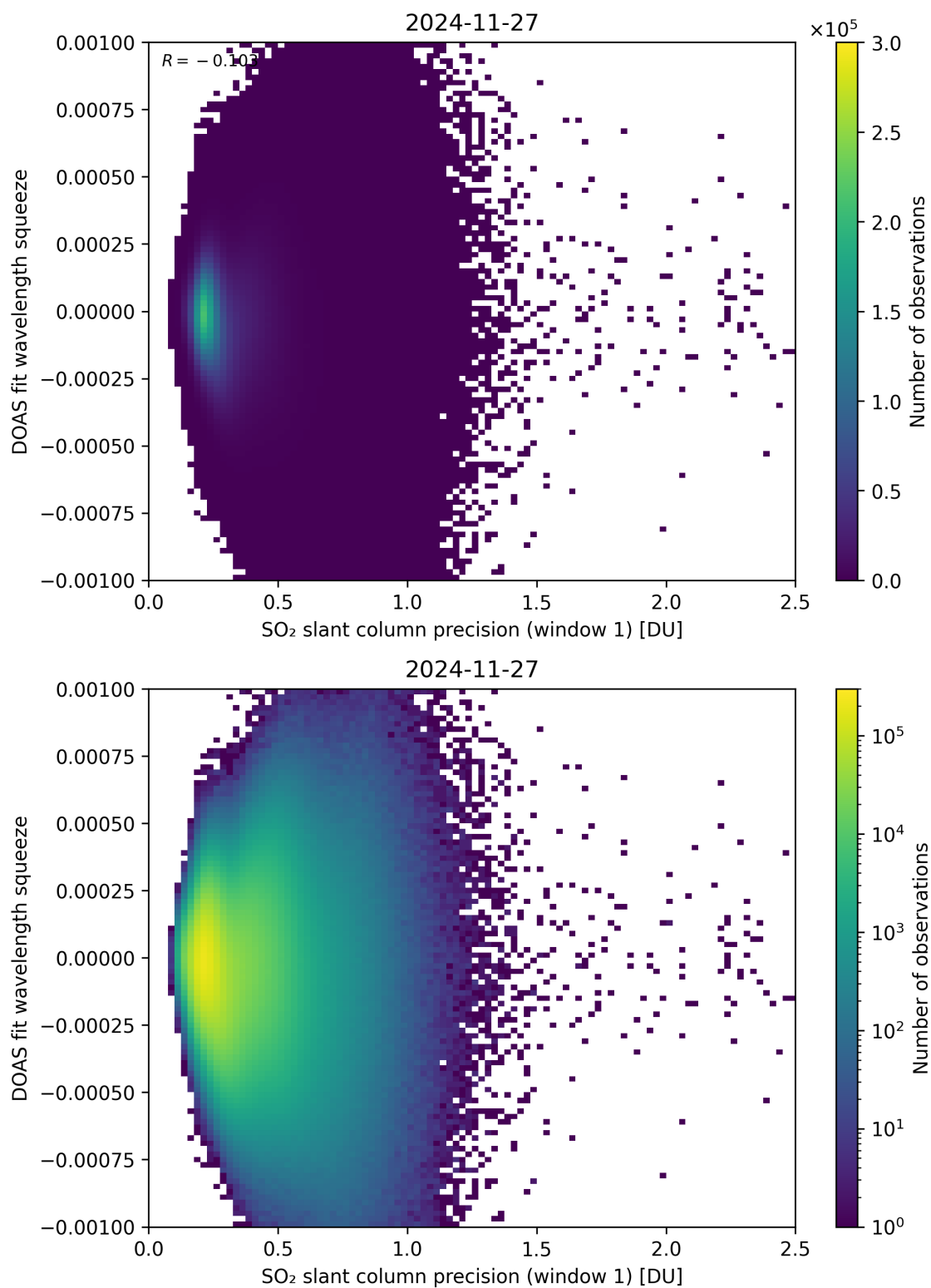
Figure 272: Scatter density plot of “SO 2 slant column precision (window 1)” against “DOAS fit wavelength squeeze” for 2024-11-26 to 2024-11-28.
