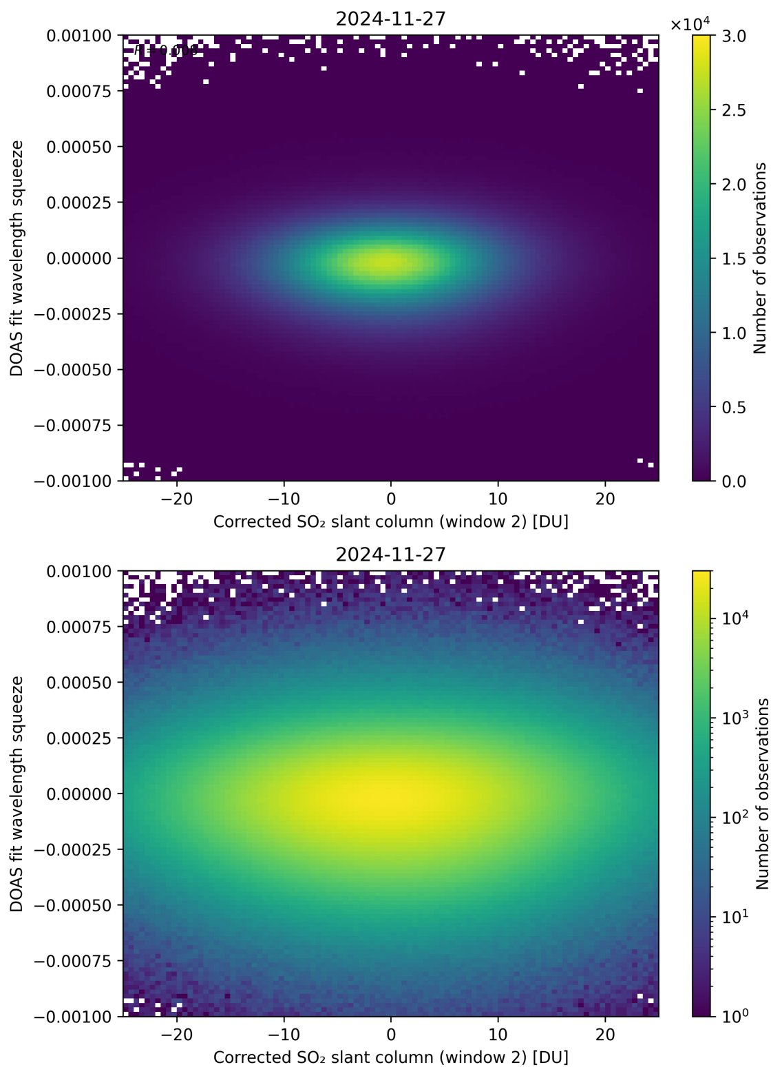
Figure 247: Scatter density plot of “Corrected SO 2 slant column (window 2)” against “DOAS fit wavelength squeeze” for 2024-11-26 to 2024-11-28.
