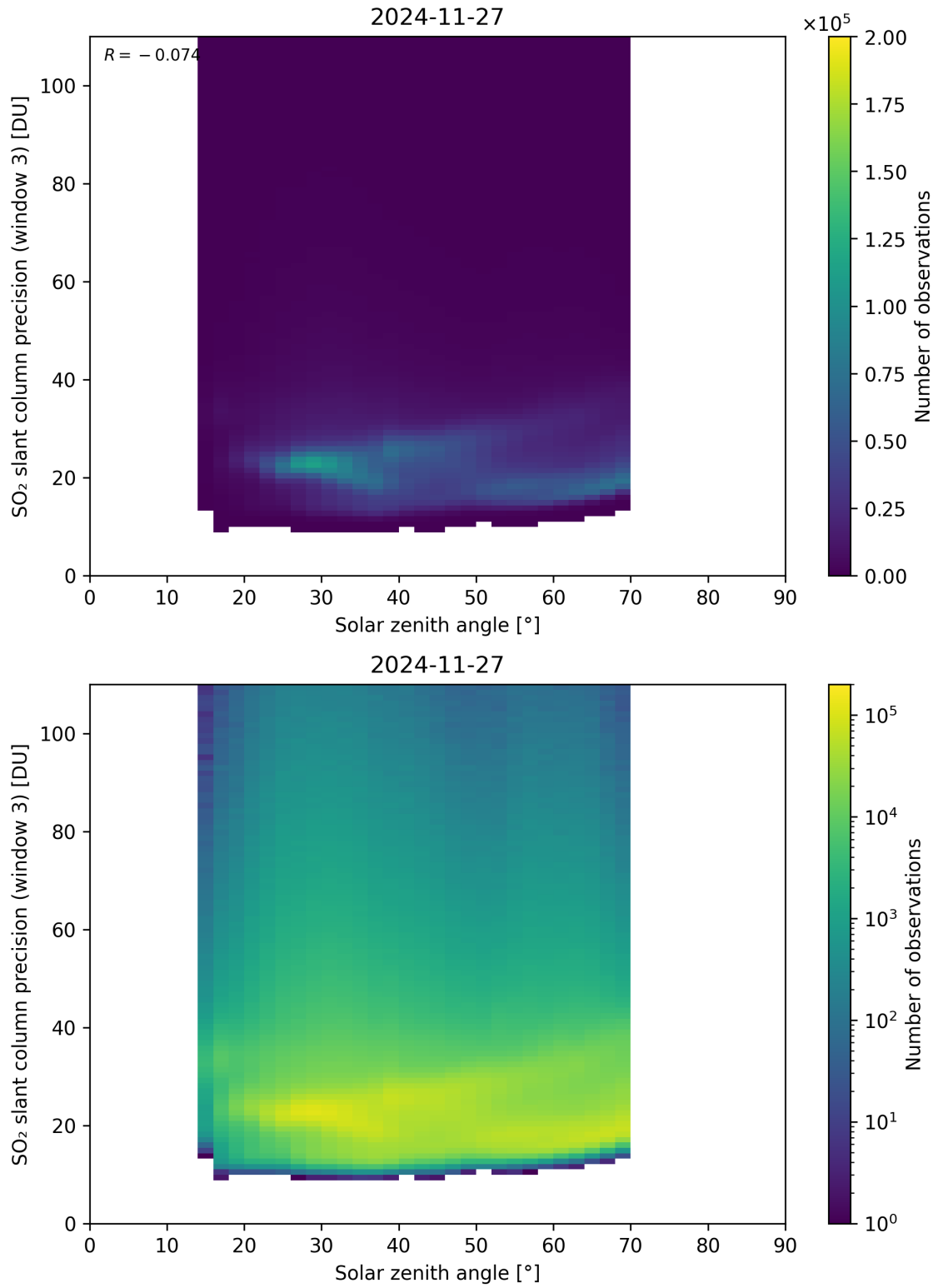
Figure 188: Scatter density plot of “Solar zenith angle” against “SO 2 slant column precision (window 3)” for 2024-11-26 to 2024-11-28.
