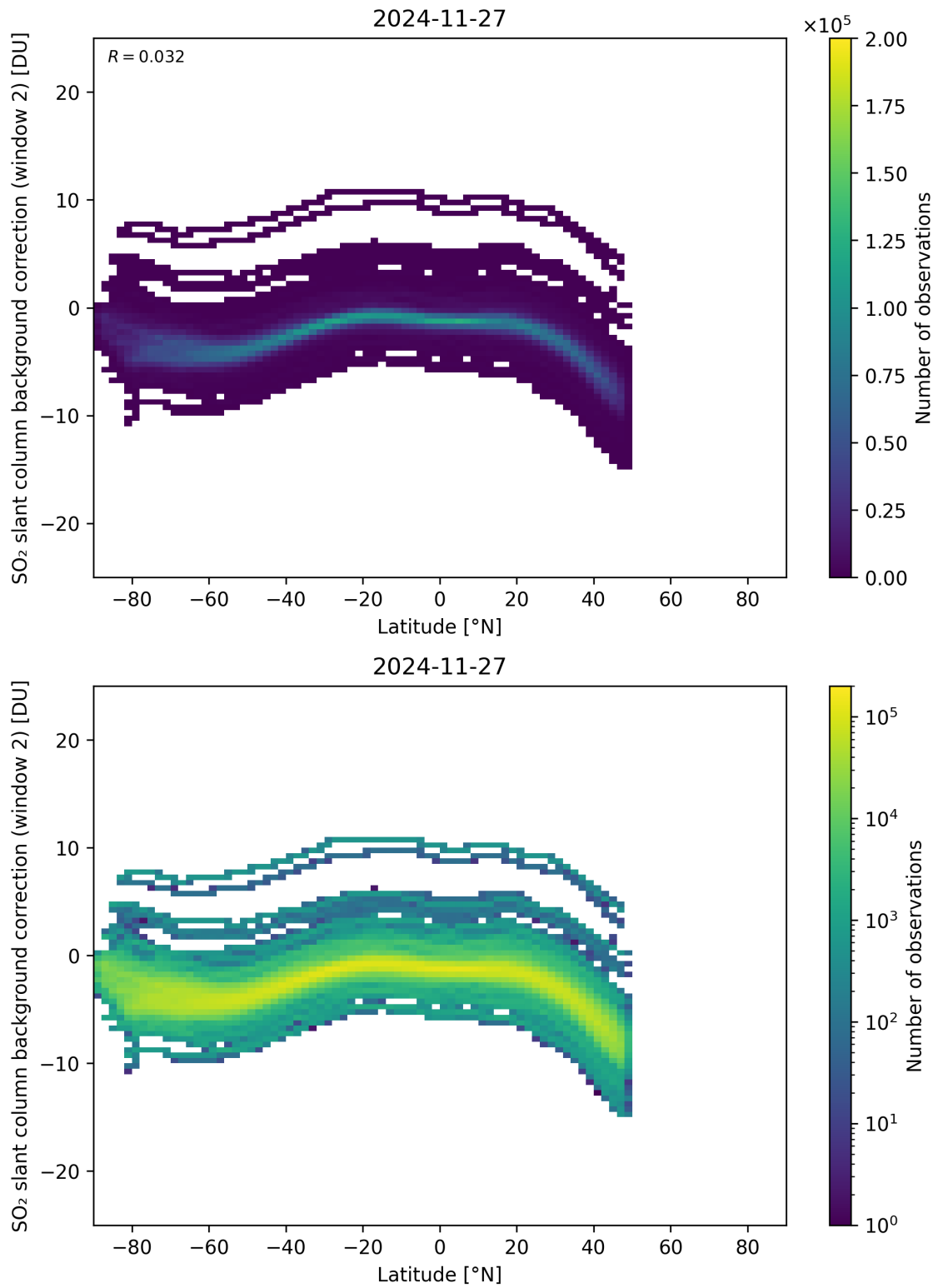
Figure 151: Scatter density plot of “Latitude” against “SO 2 slant column background correction (window 2)” for 2024-11-26 to 2024-11-28.
