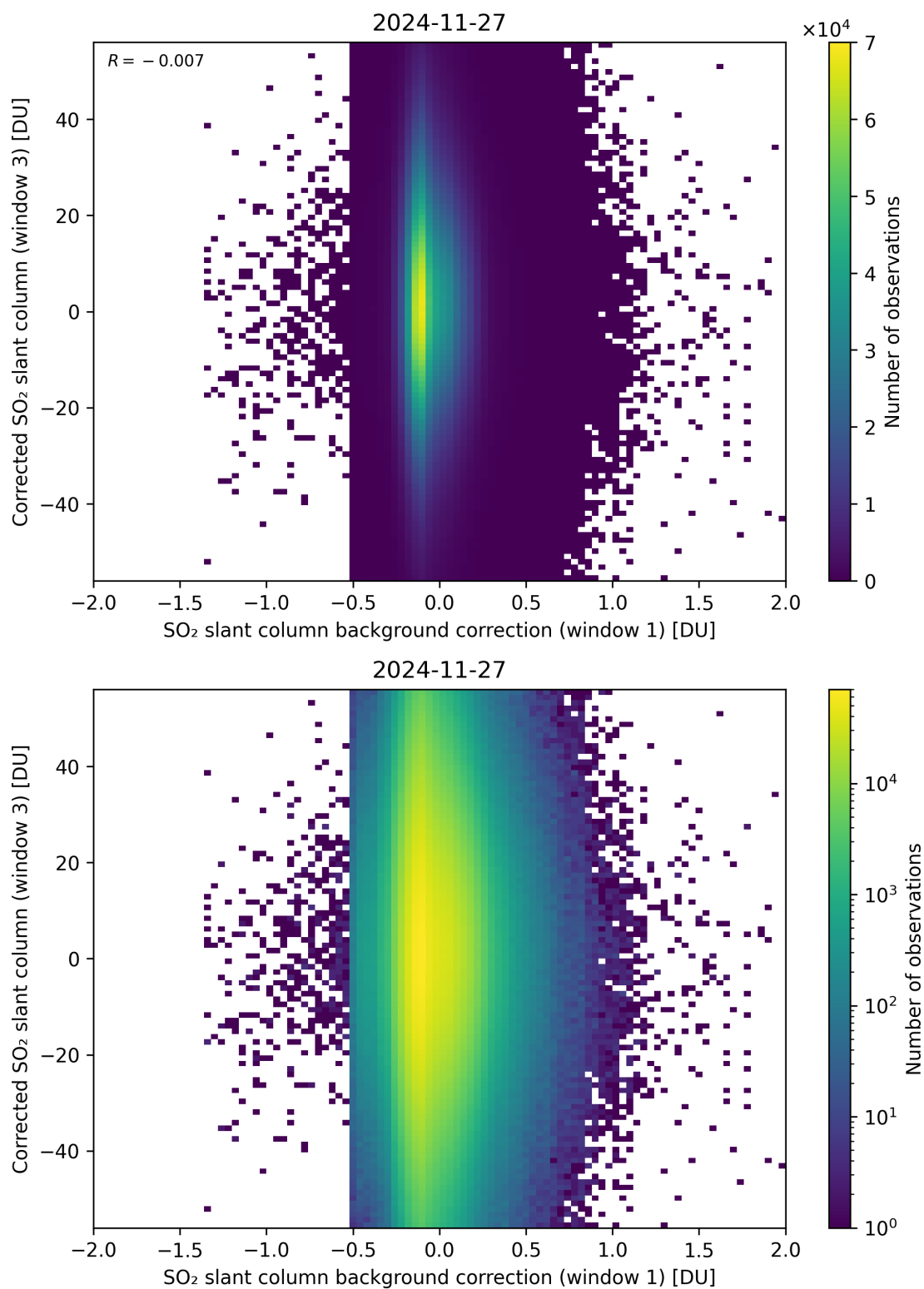
Figure 116: Scatter density plot of “SO 2 slant column background correction (window 1)” against “Corrected SO 2 slant column (window 3)” for 2024-11-26 to 2024-11-28.
