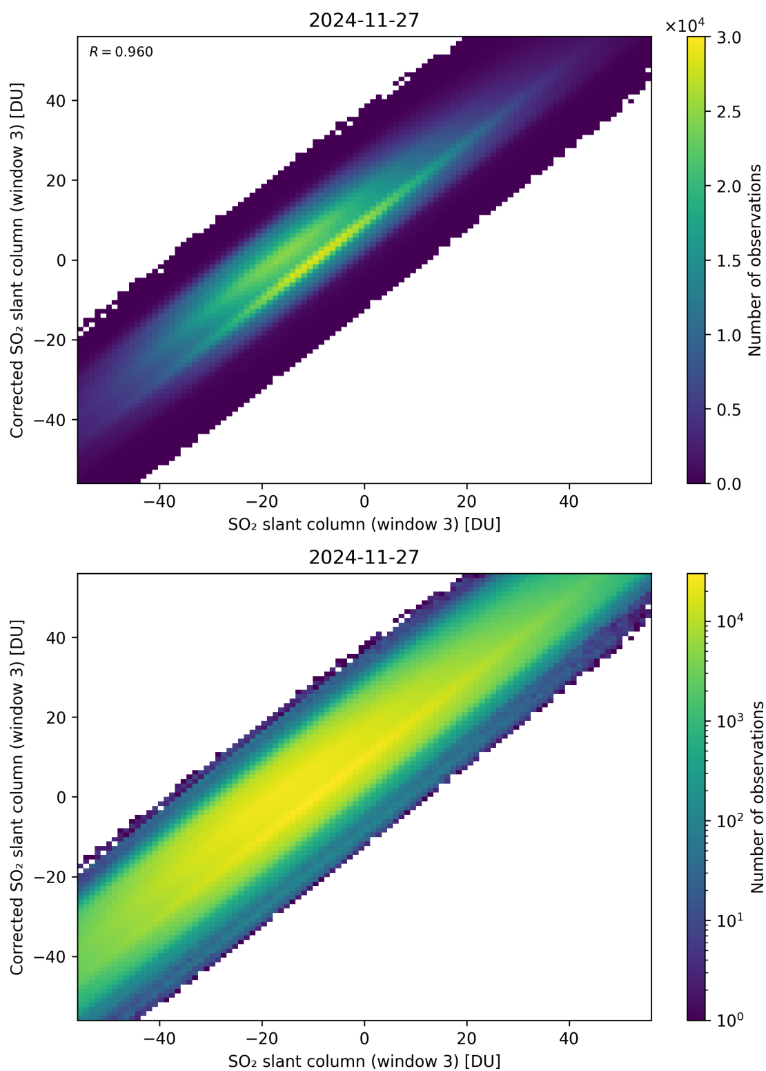
Figure 316: Scatter density plot of “SO 2 slant column (window 3)” against “Corrected SO 2 slant column (window 3)” for 2024-11-26 to 2024-11-28.
