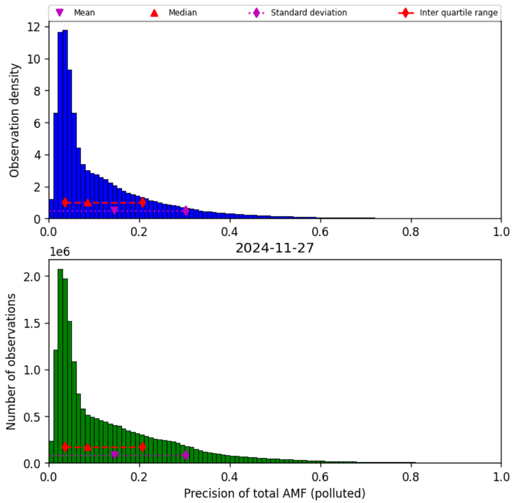
Figure 80: Histogram of “Precision of total AMF (polluted)” for 2024-11-26 to 2024-11-28
