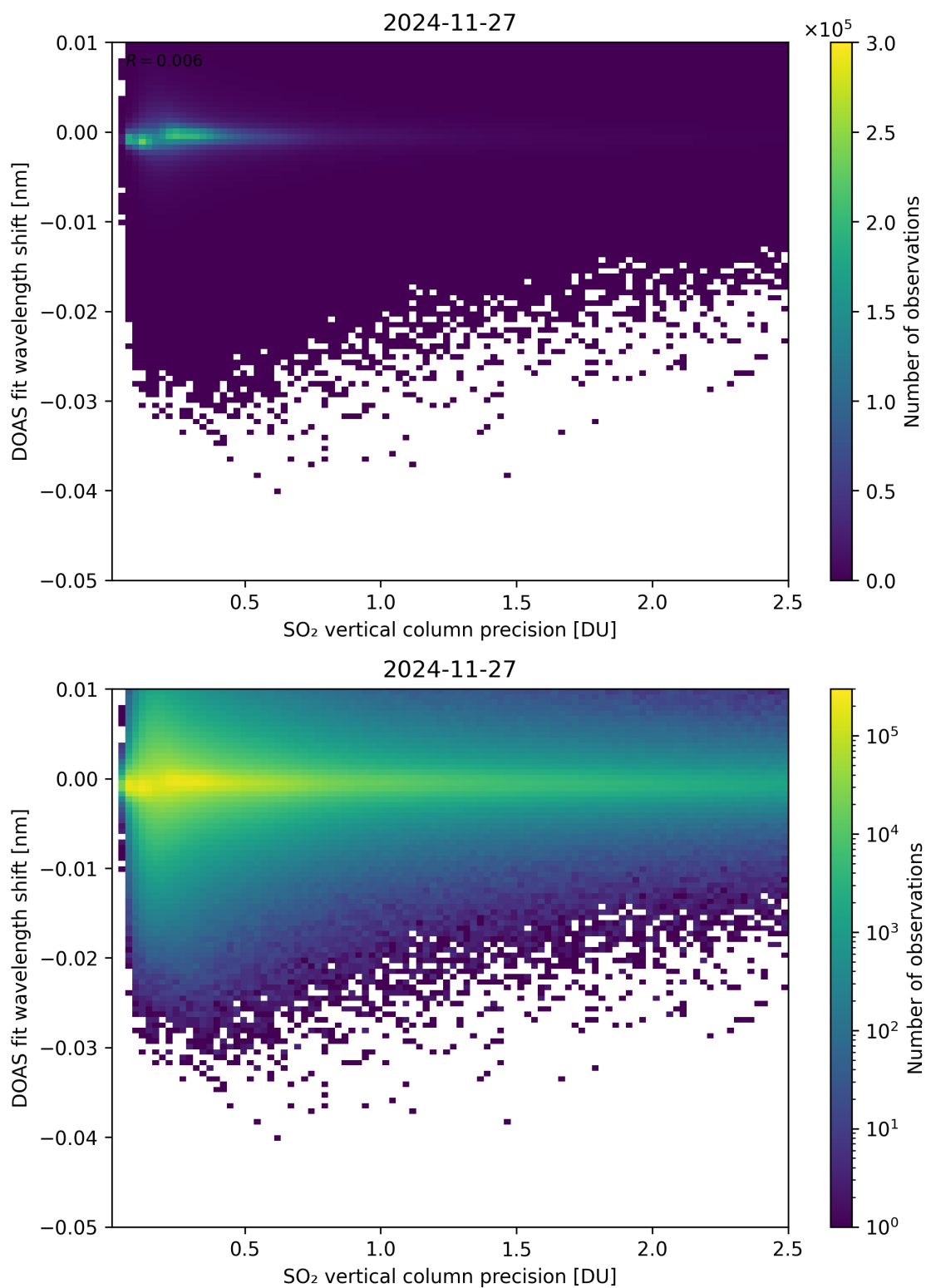
Figure 332: Scatter density plot of “SO 2 vertical column precision” against “DOAS fit wavelength shift” for 2024-11-26 to 2024-11-28.
