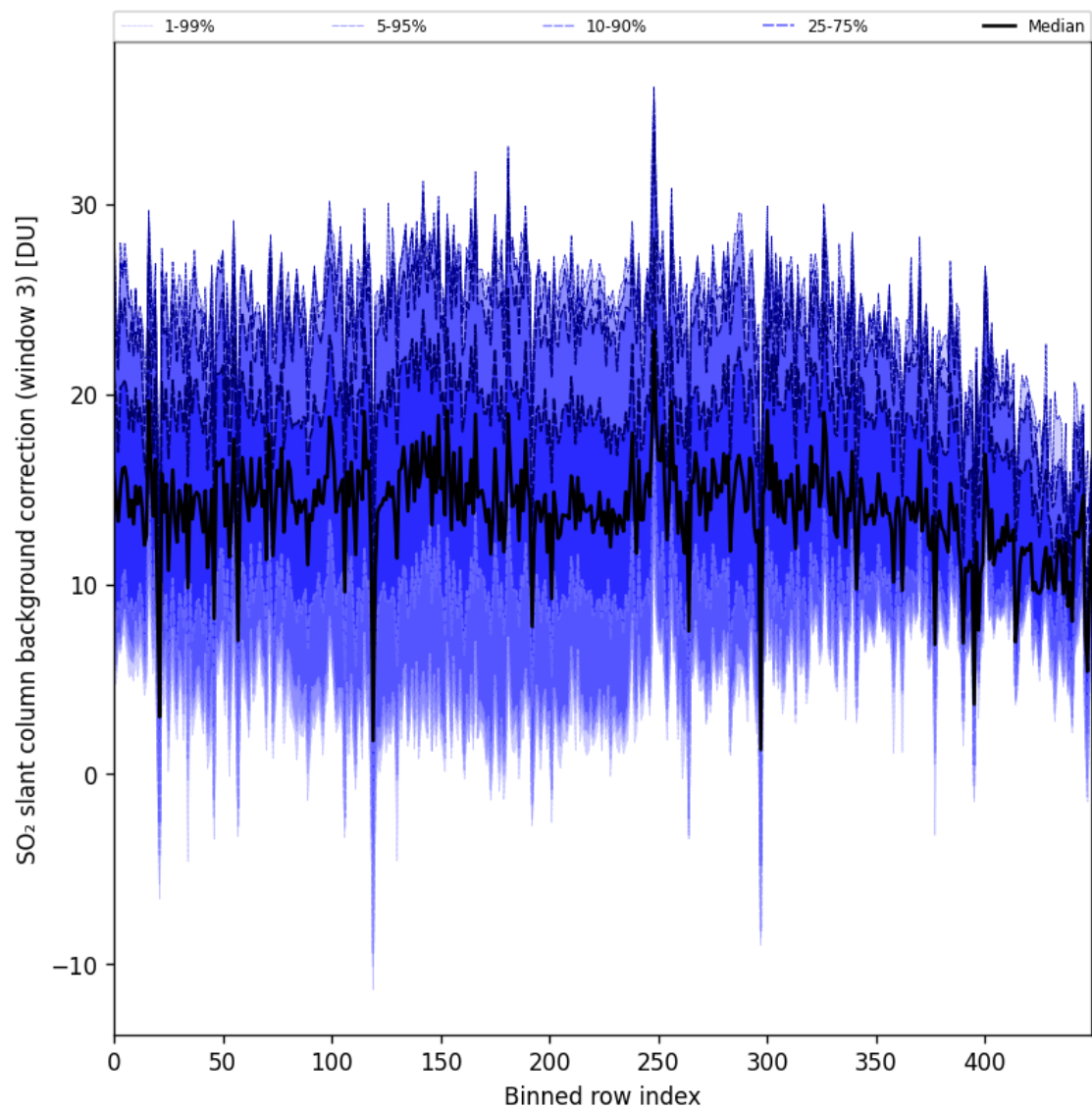
Figure 100: Along track statistics of “SO 2 slant column background correction (window 3)” for 2024-11-26 to 2024-11-28
