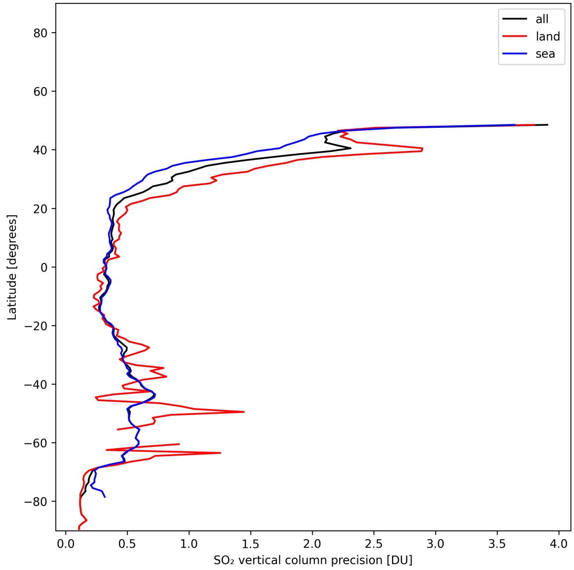
Figure 33: Zonal average of “SO 2 vertical column precision” for 2024-11-26 to 2024-11-28.
