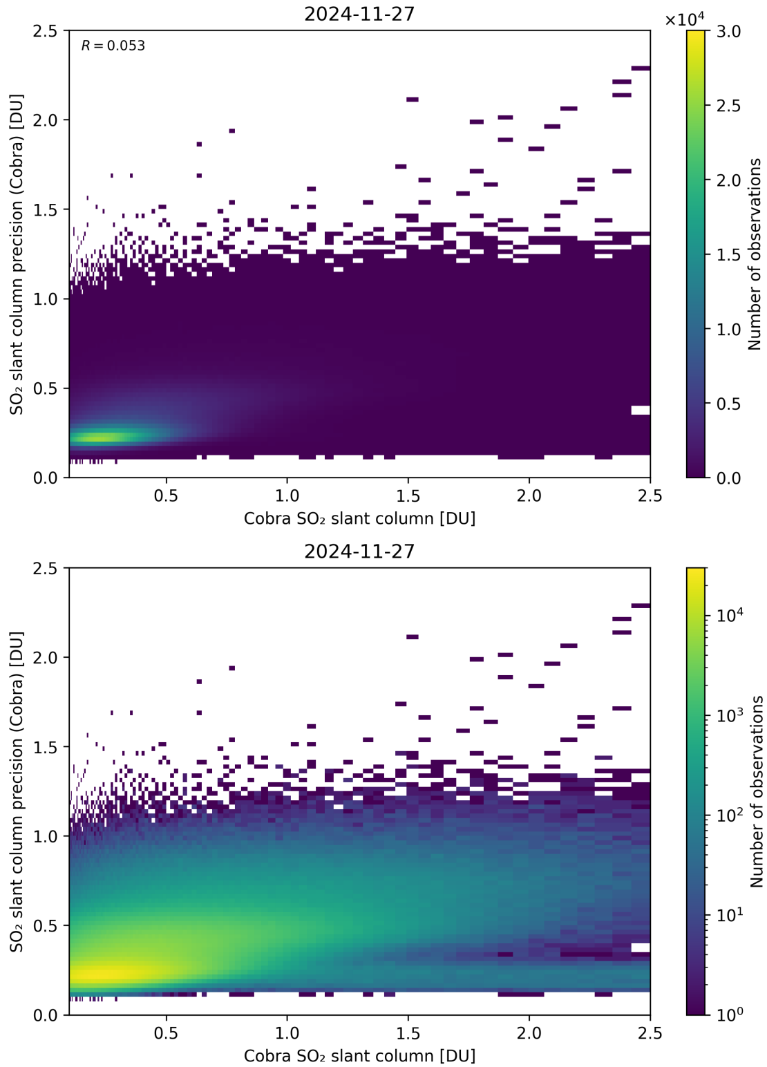
Figure 216: Scatter density plot of “Cobra SO 2 slant column” against “SO 2 slant column precision (Cobra)” for 2024-11-26 to 2024-11-28.
