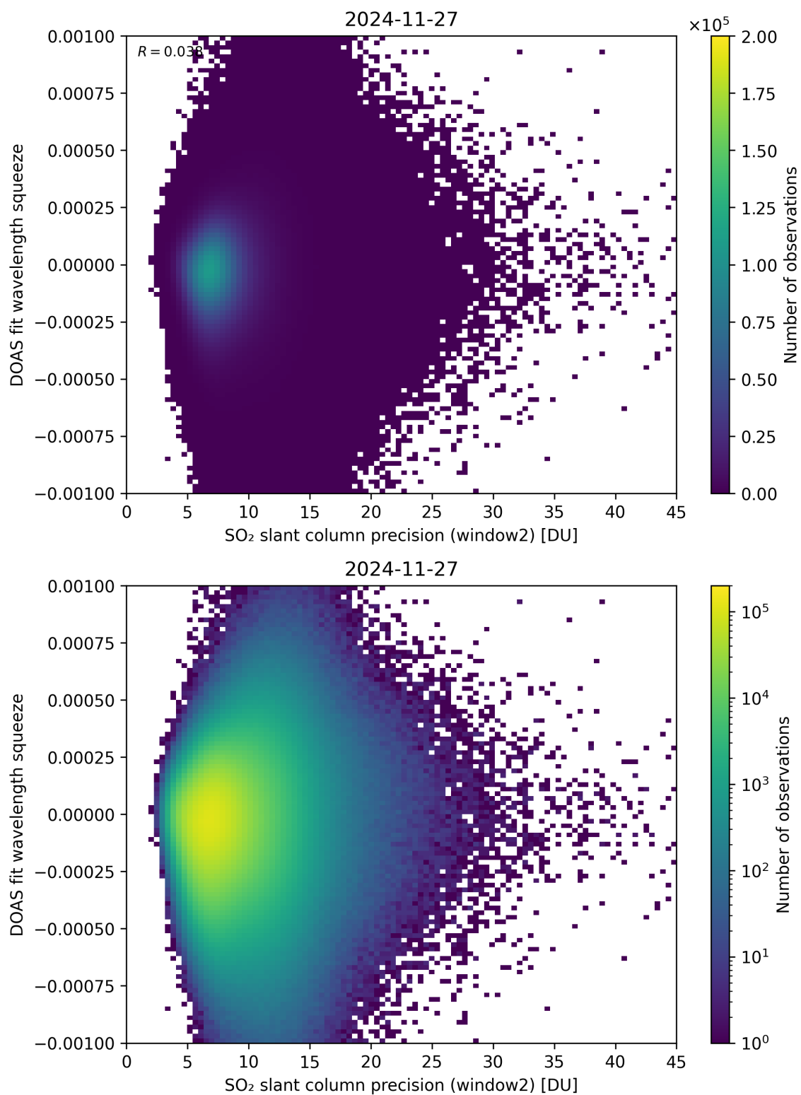
Figure 294: Scatter density plot of “SO 2 slant column precision (window2)” against “DOAS fit wavelength squeeze” for 2024-11-26 to 2024-11-28.
