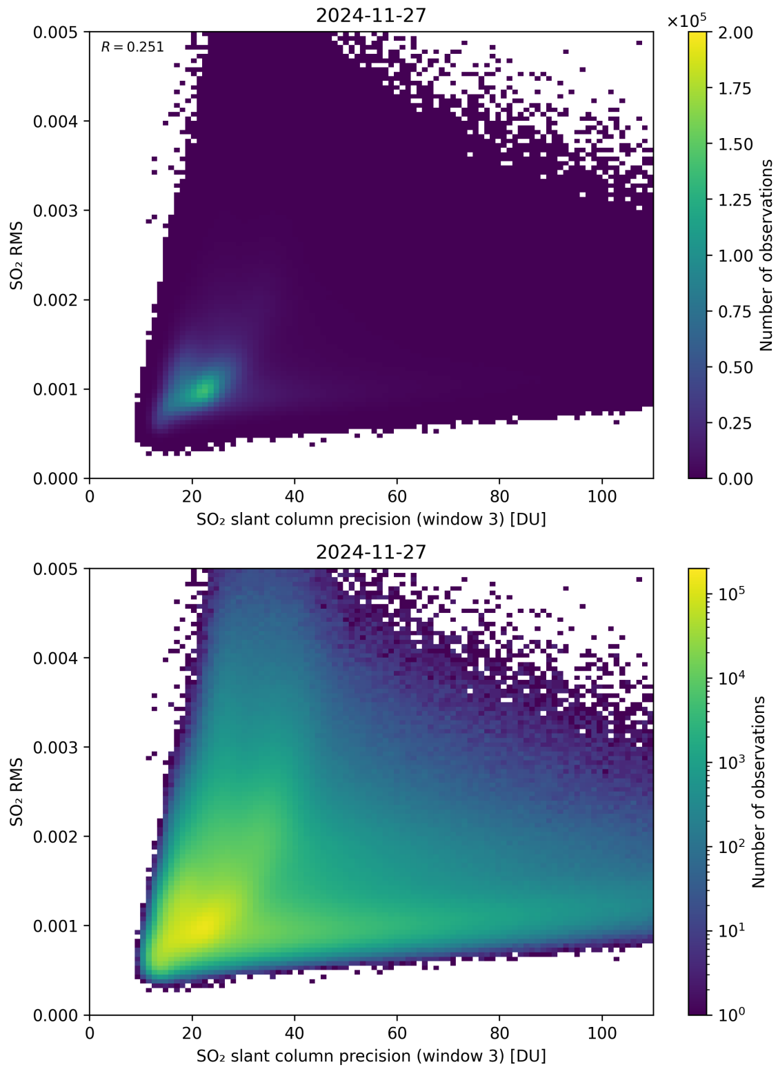
Figure 310: Scatter density plot of “SO 2 slant column precision (window 3)” against “SO 2 RMS” for 2024-11-26 to 2024-11-28.
