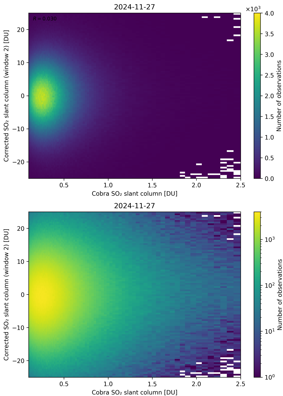
Figure 217: Scatter density plot of “Cobra SO 2 slant column” against “Corrected SO 2 slant column (window 2)” for 2024-11-26 to 2024-11-28.
