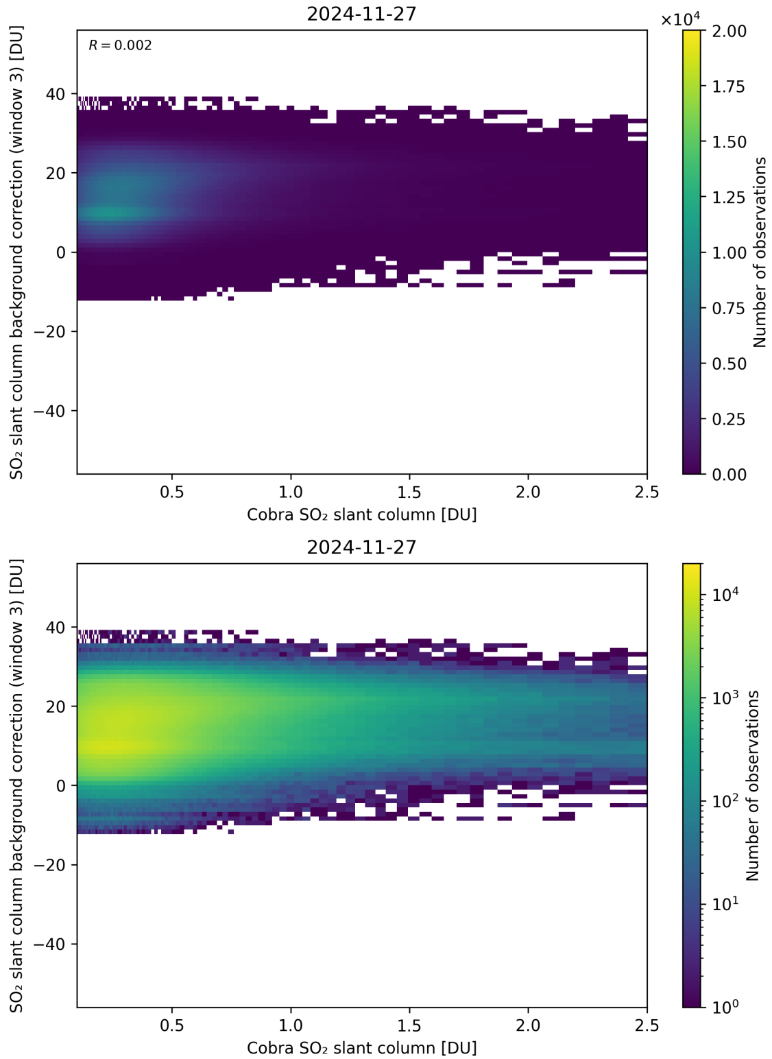
Figure 195: Scatter density plot of “Cobra SO 2 slant column” against “SO 2 slant column background correction (window 3)” for 2024-11-26 to 2024-11-28.
