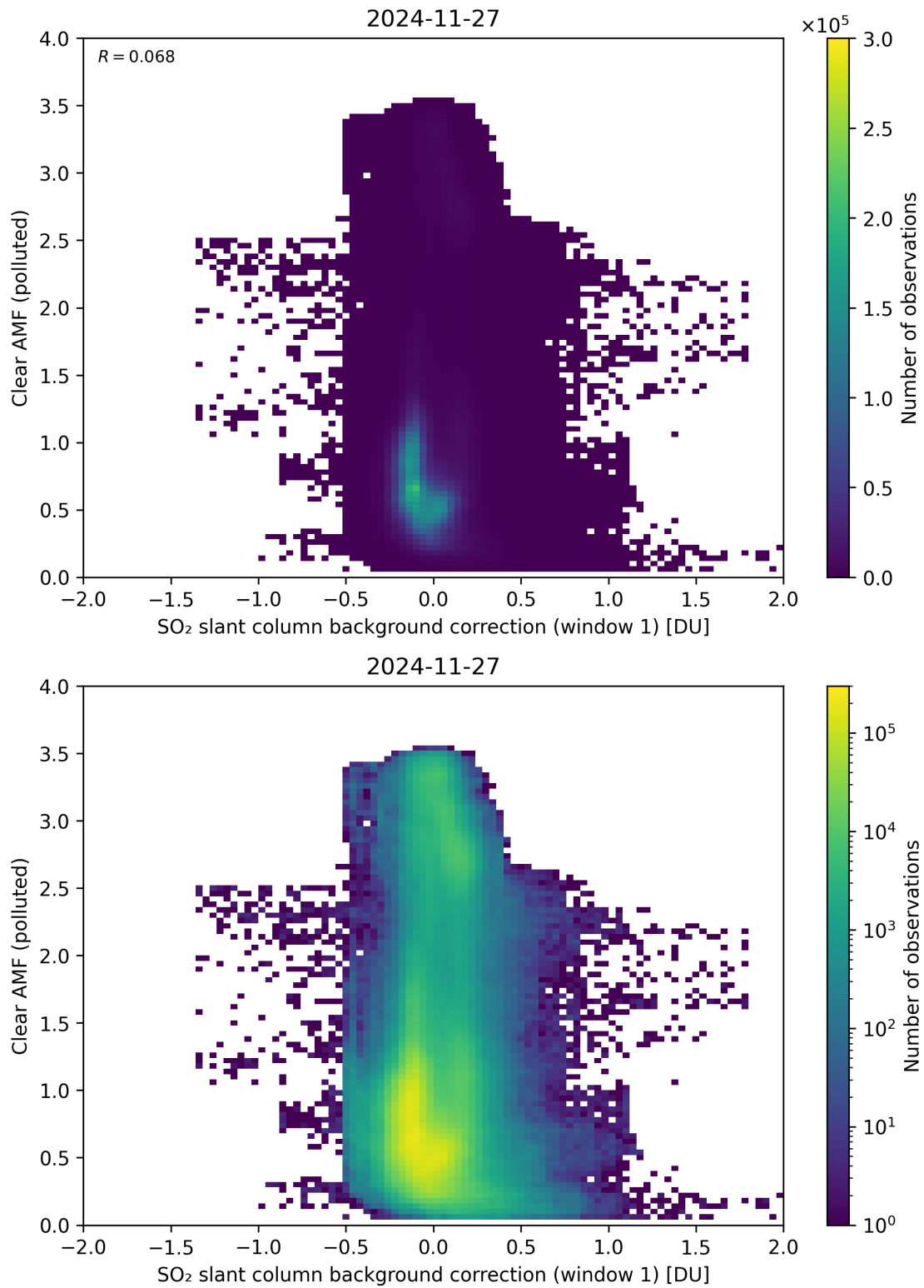
Figure 114: Scatter density plot of “SO 2 slant column background correction (window 1)” against “Clear AMF (polluted)” for 2024-11-26 to 2024-11-28.
