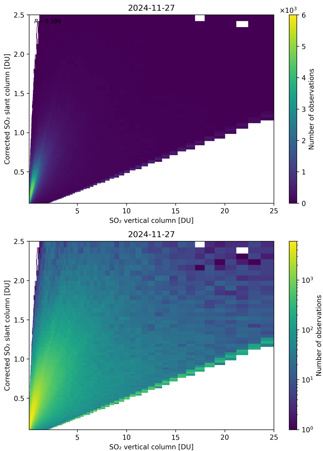
Figure 351: Scatter density plot of “SO 2 vertical column” against “Corrected SO 2 slant column” for 2024-11-26 to 2024-11-28.
