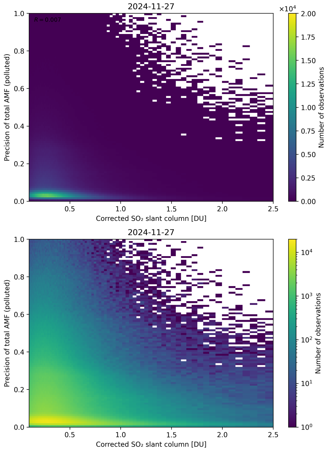
Figure 243: Scatter density plot of “Corrected SO 2 slant column” against “Precision of total AMF (polluted)” for 2024-11-26 to 2024-11-28.
