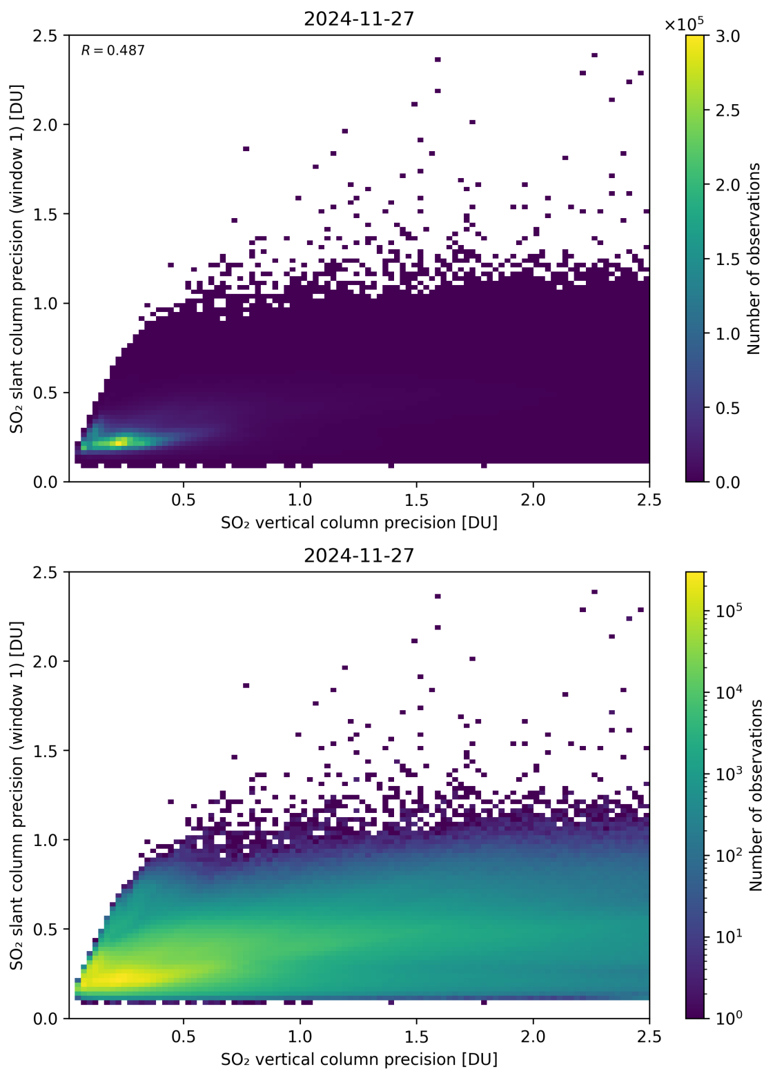
Figure 342: Scatter density plot of “SO 2 vertical column precision” against “SO 2 slant column precision (window 1)” for 2024-11-26 to 2024-11-28.
