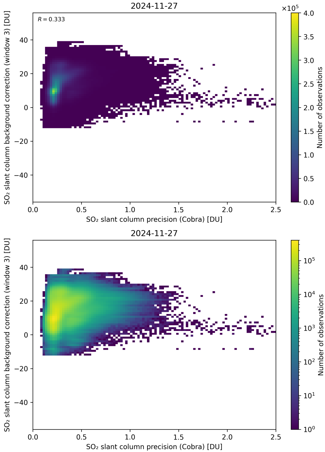
Figure 201: Scatter density plot of “SO 2 slant column precision (Cobra)” against “SO 2 slant column background correction (window 3)” for 2024-11-26 to 2024-11-28.
