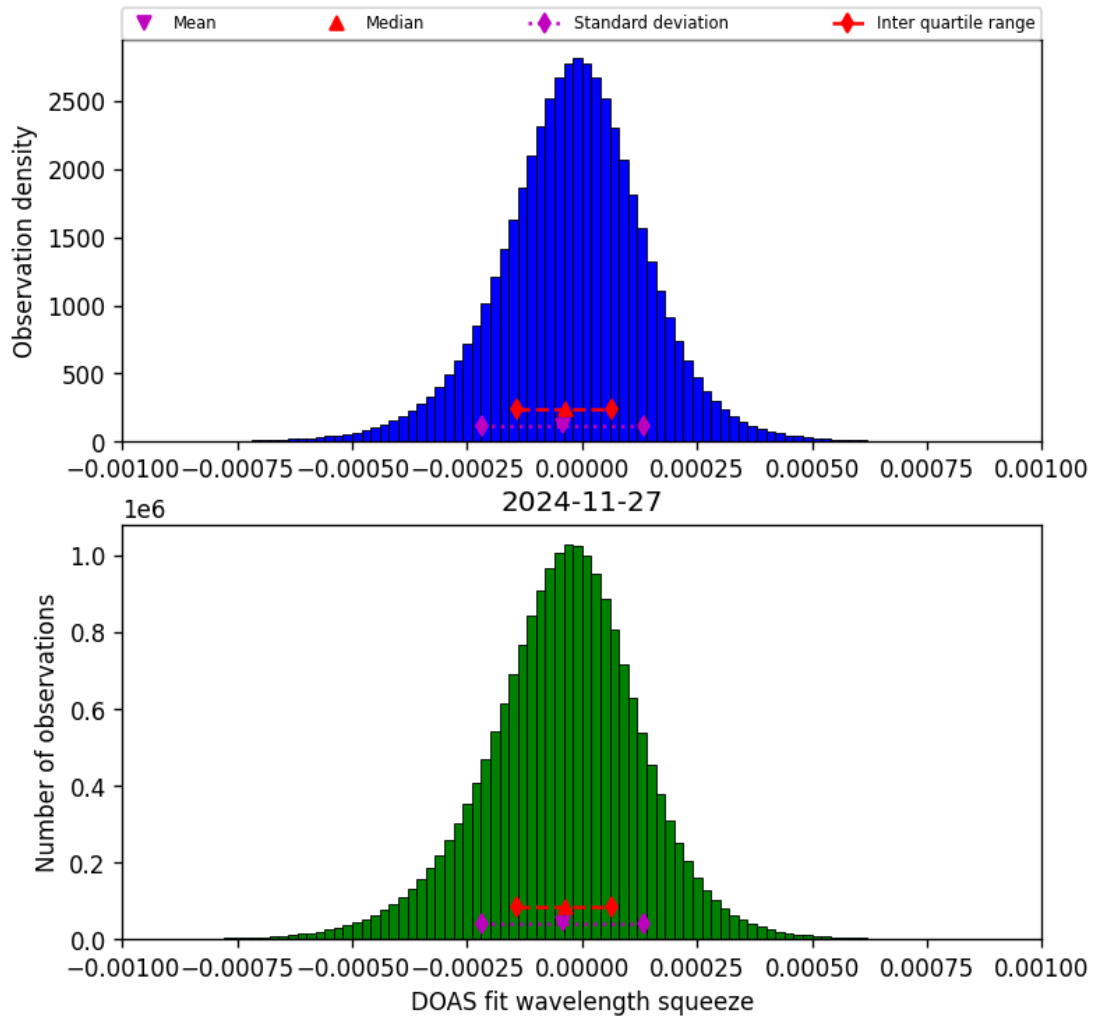
Figure 77: Histogram of “DOAS fit wavelength squeeze” for 2024-11-26 to 2024-11-28
