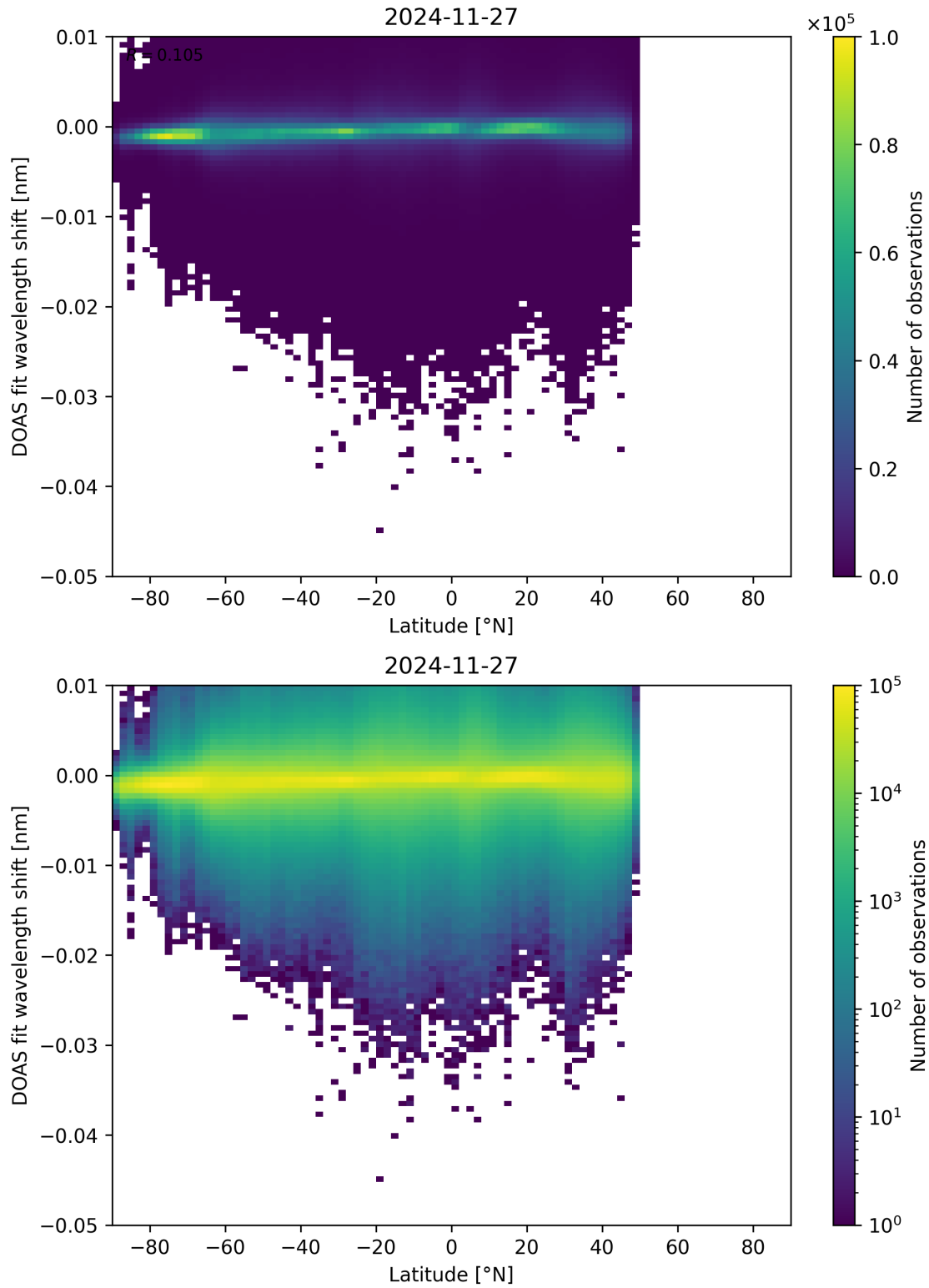
Figure 153: Scatter density plot of “Latitude” against “DOAS fit wavelength shift” for 2024-11-26 to 2024-11-28.
