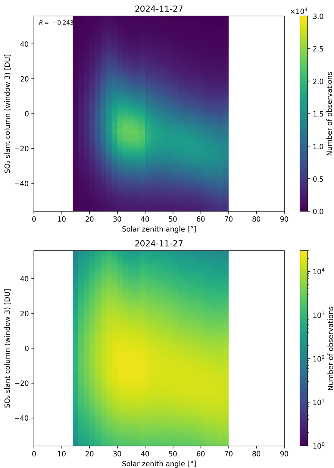
Figure 187: Scatter density plot of “Solar zenith angle” against “SO 2 slant column (window 3)” for 2024-11-26 to 2024-11-28.
