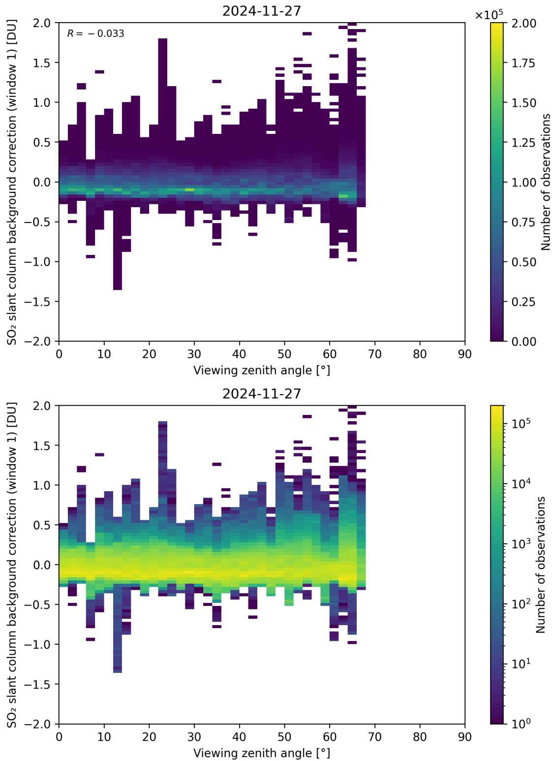
Figure 362: Scatter density plot of “Viewing zenith angle” against “SO 2 slant column background correction (window 1)” for 2024-11-26 to 2024-11-28.
