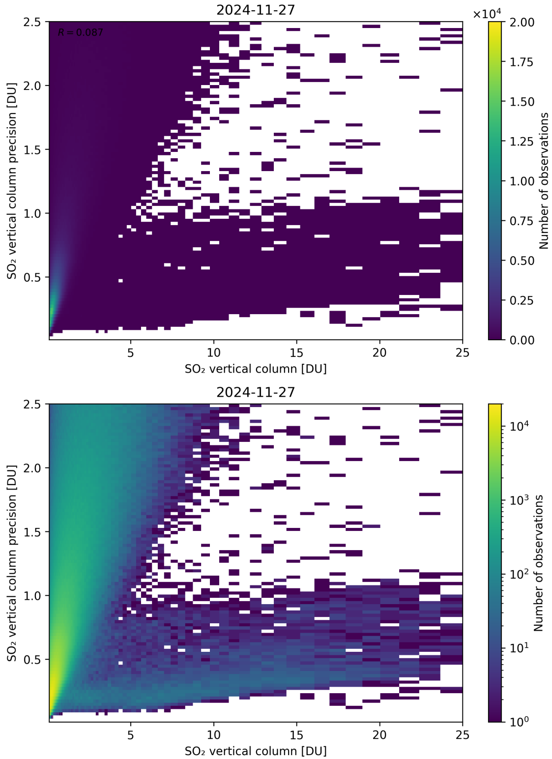
Figure 361: Scatter density plot of “SO 2 vertical column” against “SO 2 vertical column precision” for 2024-11-26 to 2024-11-28.
