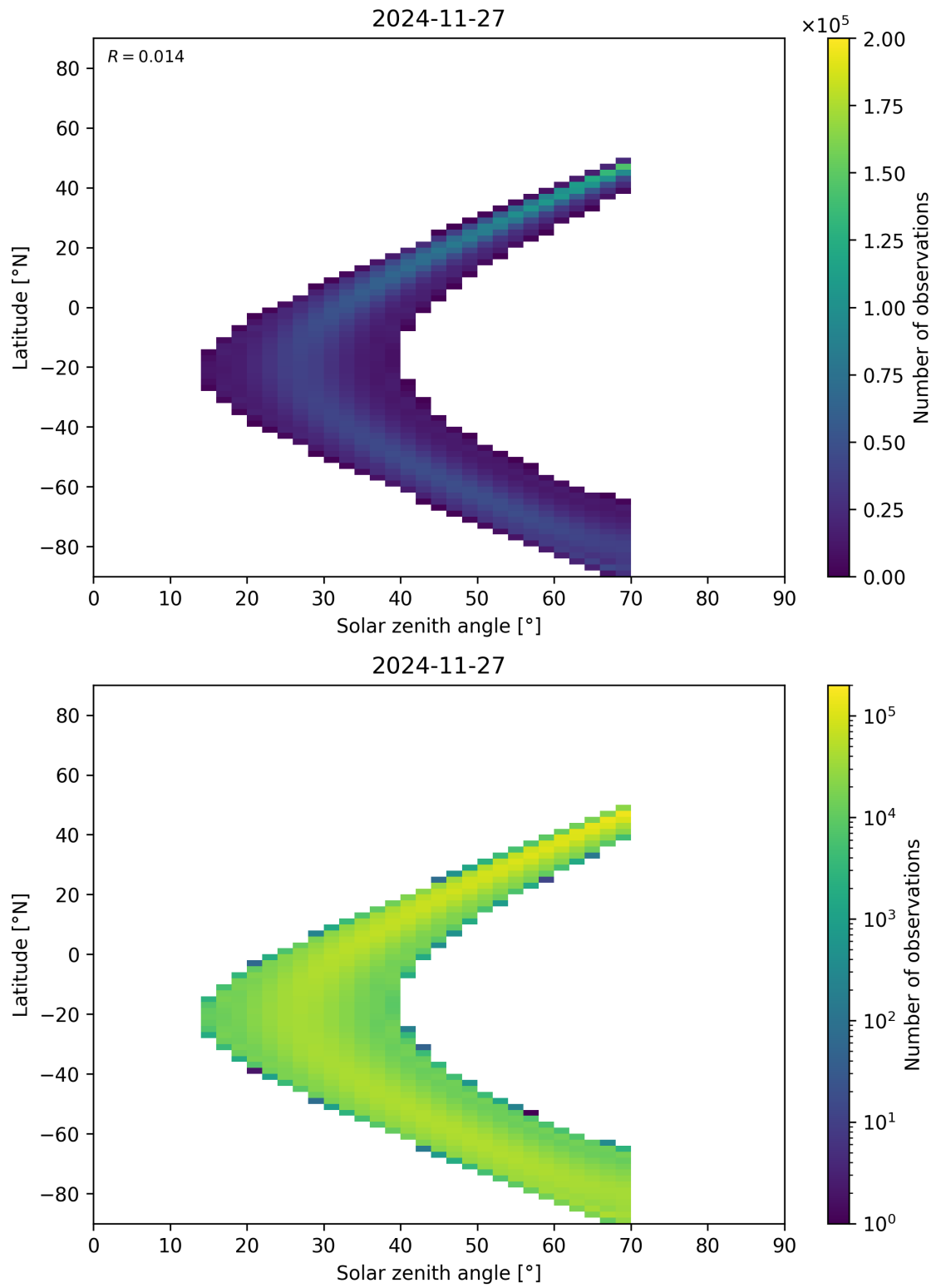
Figure 177: Scatter density plot of “Solar zenith angle” against “Latitude” for 2024-11-26 to 2024-11-28.
