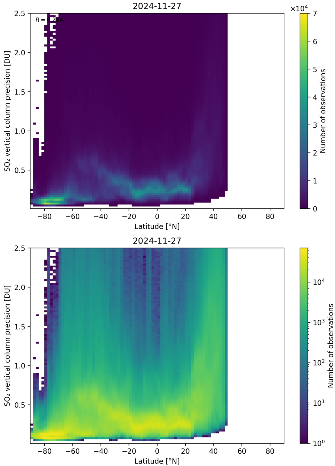
Figure 170: Scatter density plot of “Latitude” against “SO 2 vertical column precision” for 2024-11-26 to 2024-11-28.
