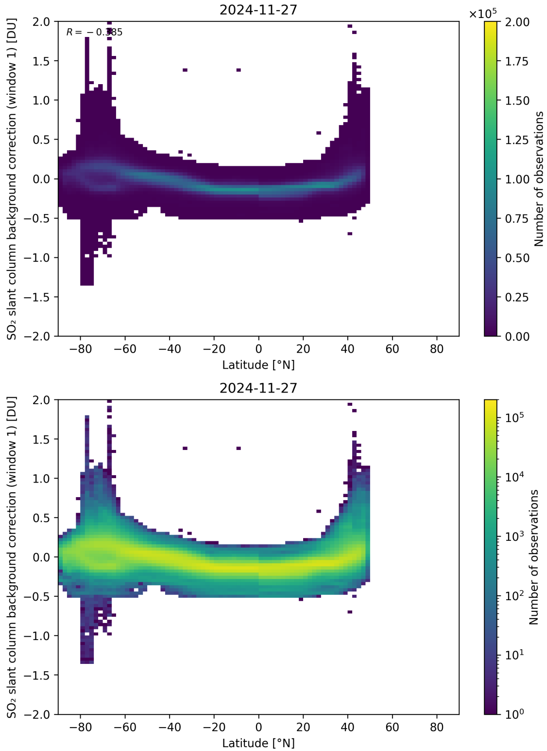
Figure 150: Scatter density plot of “Latitude” against “SO 2 slant column background correction (window 1)” for 2024-11-26 to 2024-11-28.
