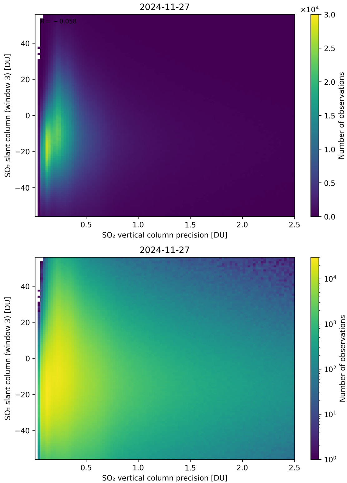
Figure 344: Scatter density plot of “SO 2 vertical column precision” against “SO 2 slant column (window 3)” for 2024-11-26 to 2024-11-28.
