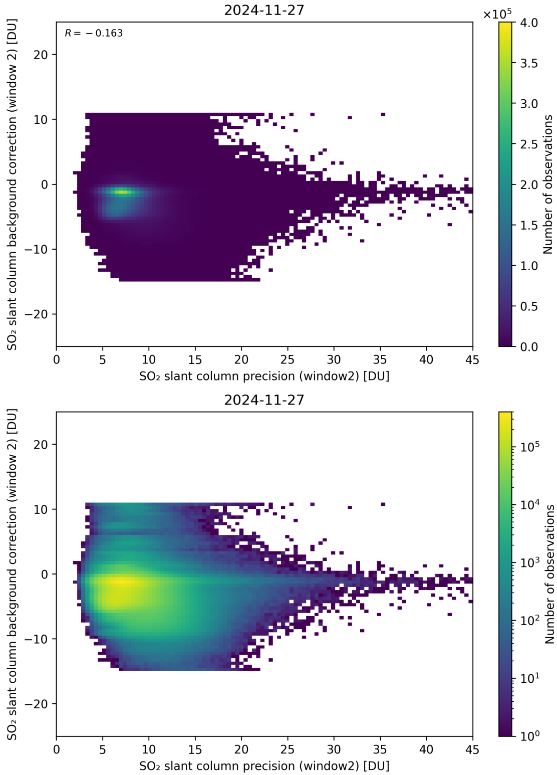
Figure 291: Scatter density plot of “SO 2 slant column precision (window2)” against “SO 2 slant column background correction (window 2)” for 2024-11-26 to 2024-11-28.
