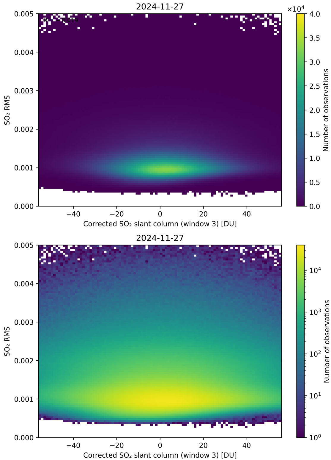
Figure 258: Scatter density plot of “Corrected SO 2 slant column (window 3)” against “SO 2 RMS” for 2024-11-26 to 2024-11-28.
