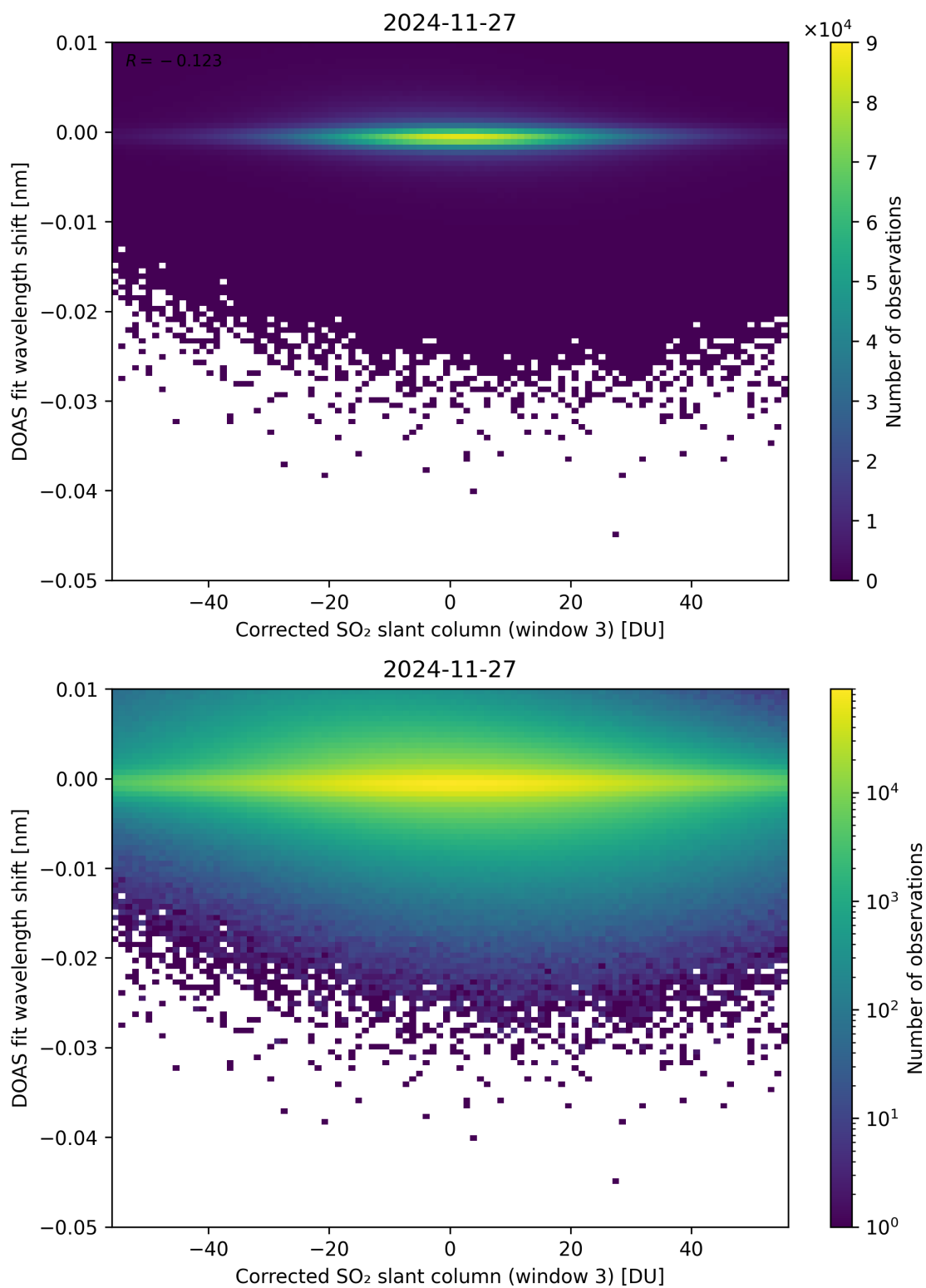
Figure 256: Scatter density plot of “Corrected SO 2 slant column (window 3)” against “DOAS fit wavelength shift” for 2024-11-26 to 2024-11-28.
