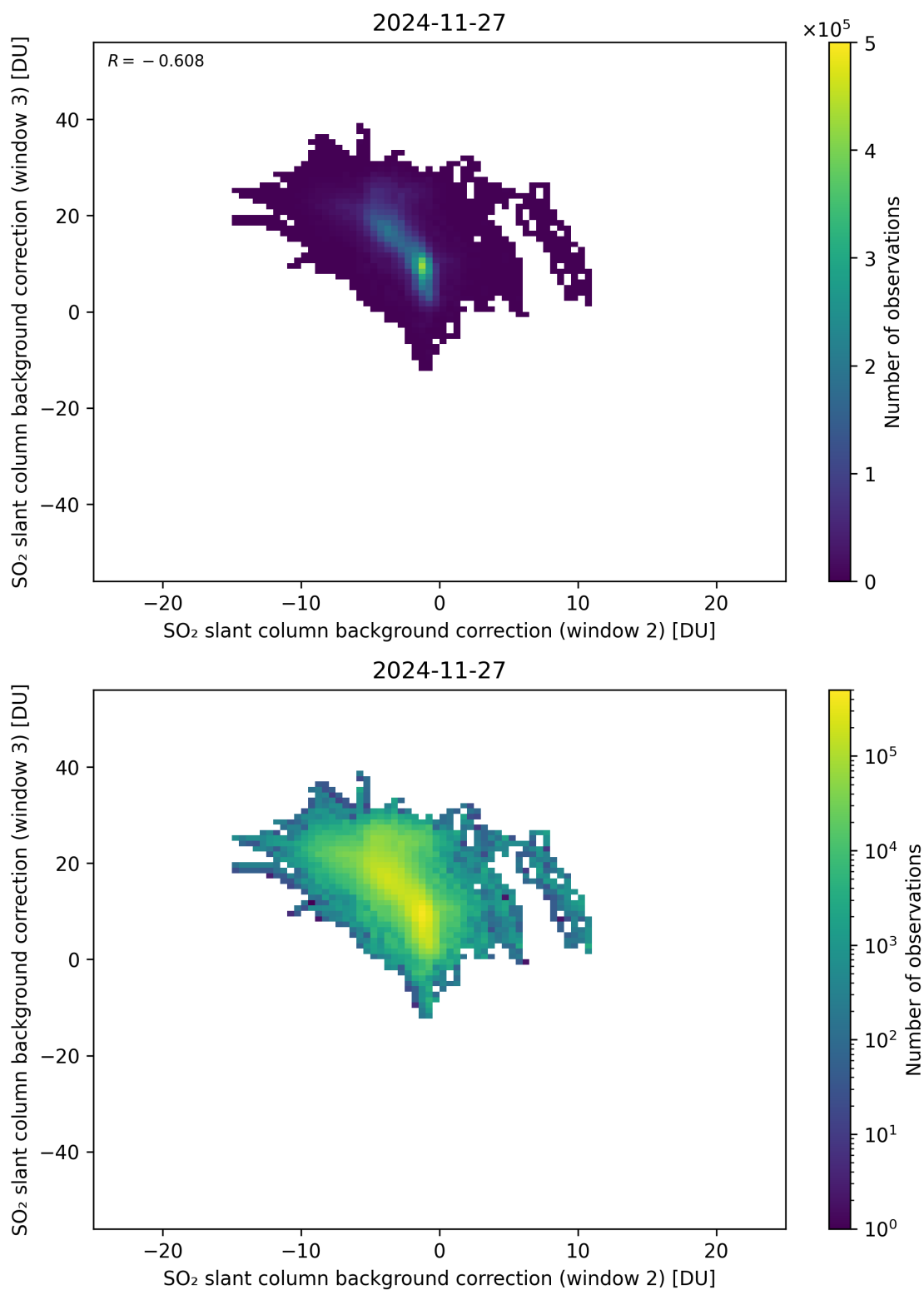
Figure 122: Scatter density plot of “SO 2 slant column background correction (window 2)” against “SO 2 slant column background correction (window 3)” for 2024-11-26 to 2024-11-28.
