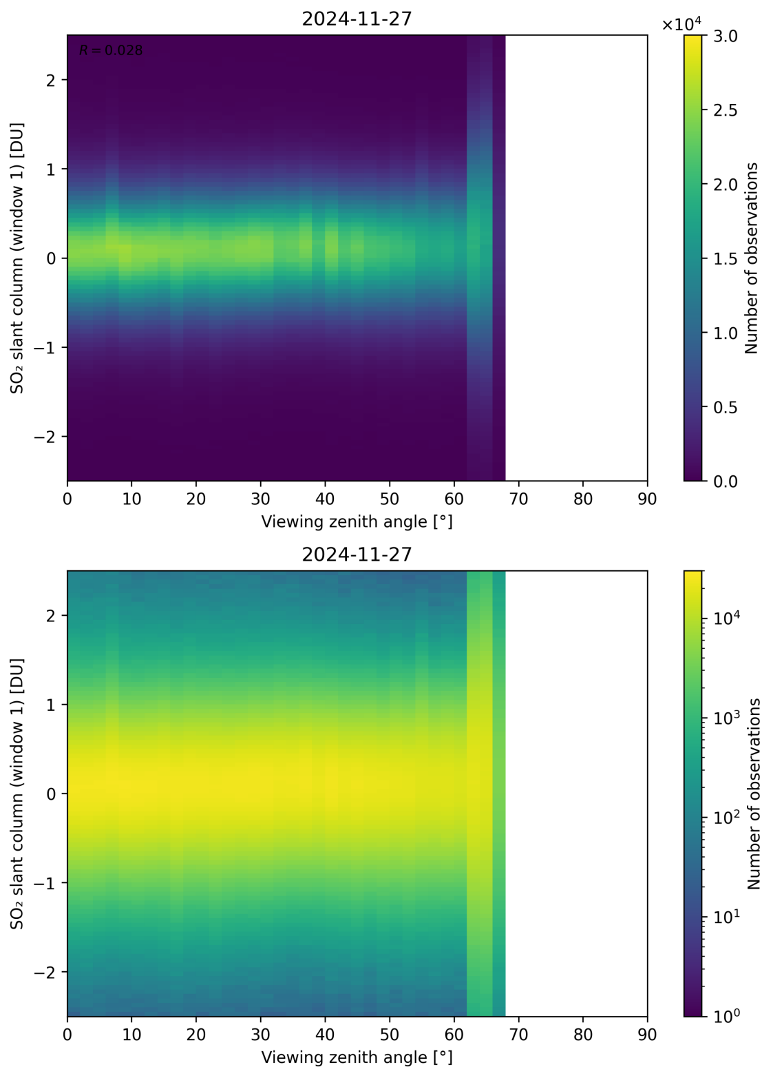
Figure 376: Scatter density plot of “Viewing zenith angle” against “SO 2 slant column (window 1)” for 2024-11-26 to 2024-11-28.
