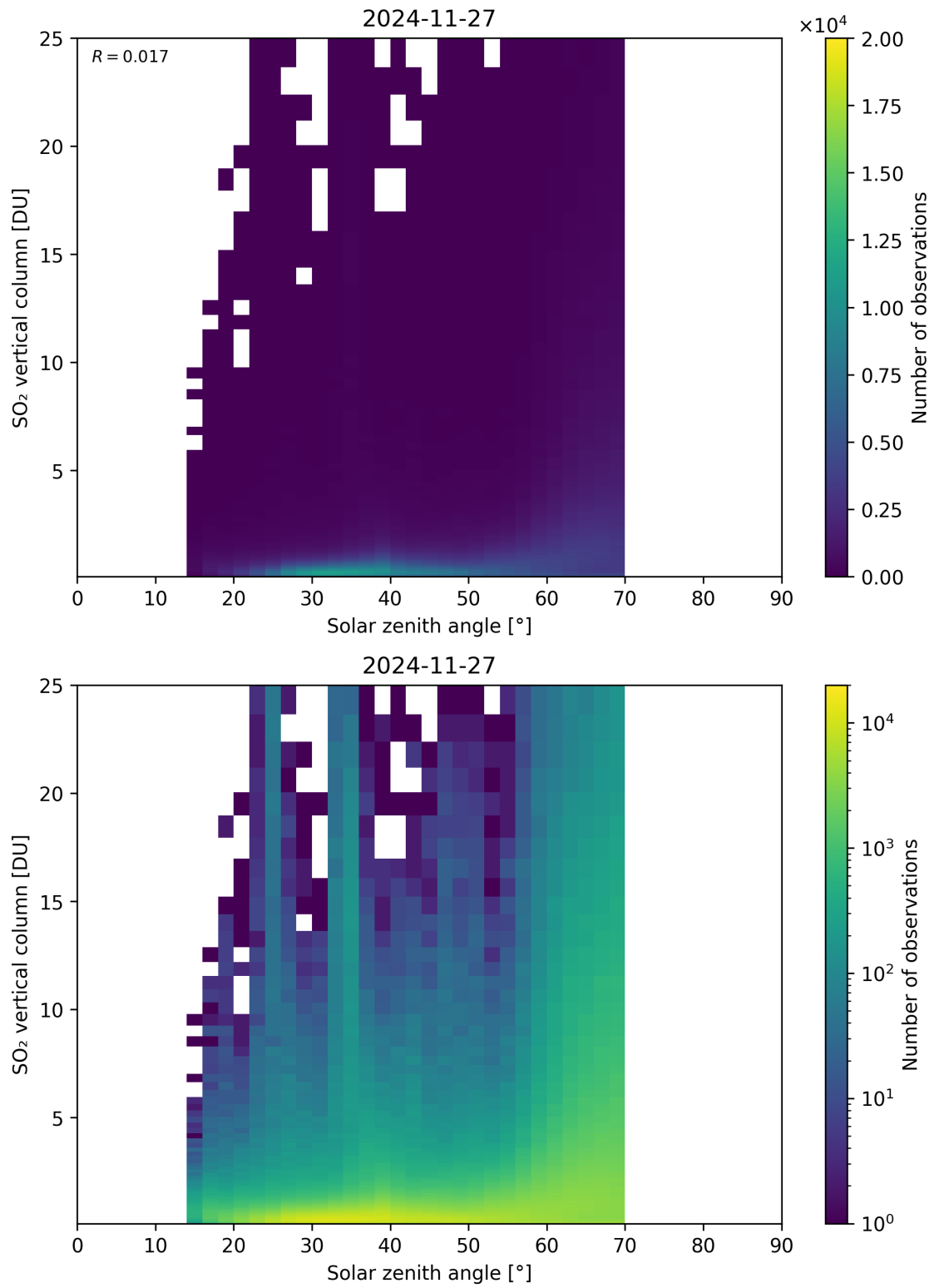
Figure 191: Scatter density plot of “Solar zenith angle” against “SO 2 vertical column” for 2024-11-26 to 2024-11-28.
