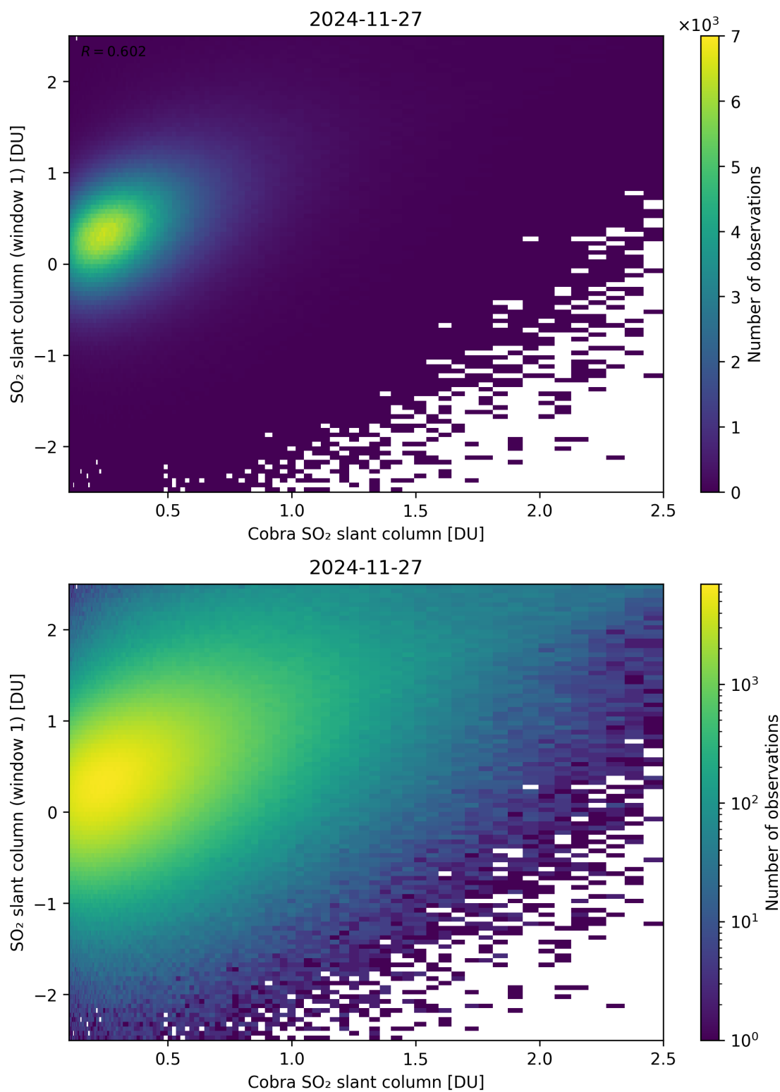
Figure 219: Scatter density plot of “Cobra SO 2 slant column” against “SO 2 slant column (window 1)” for 2024-11-26 to 2024-11-28.
