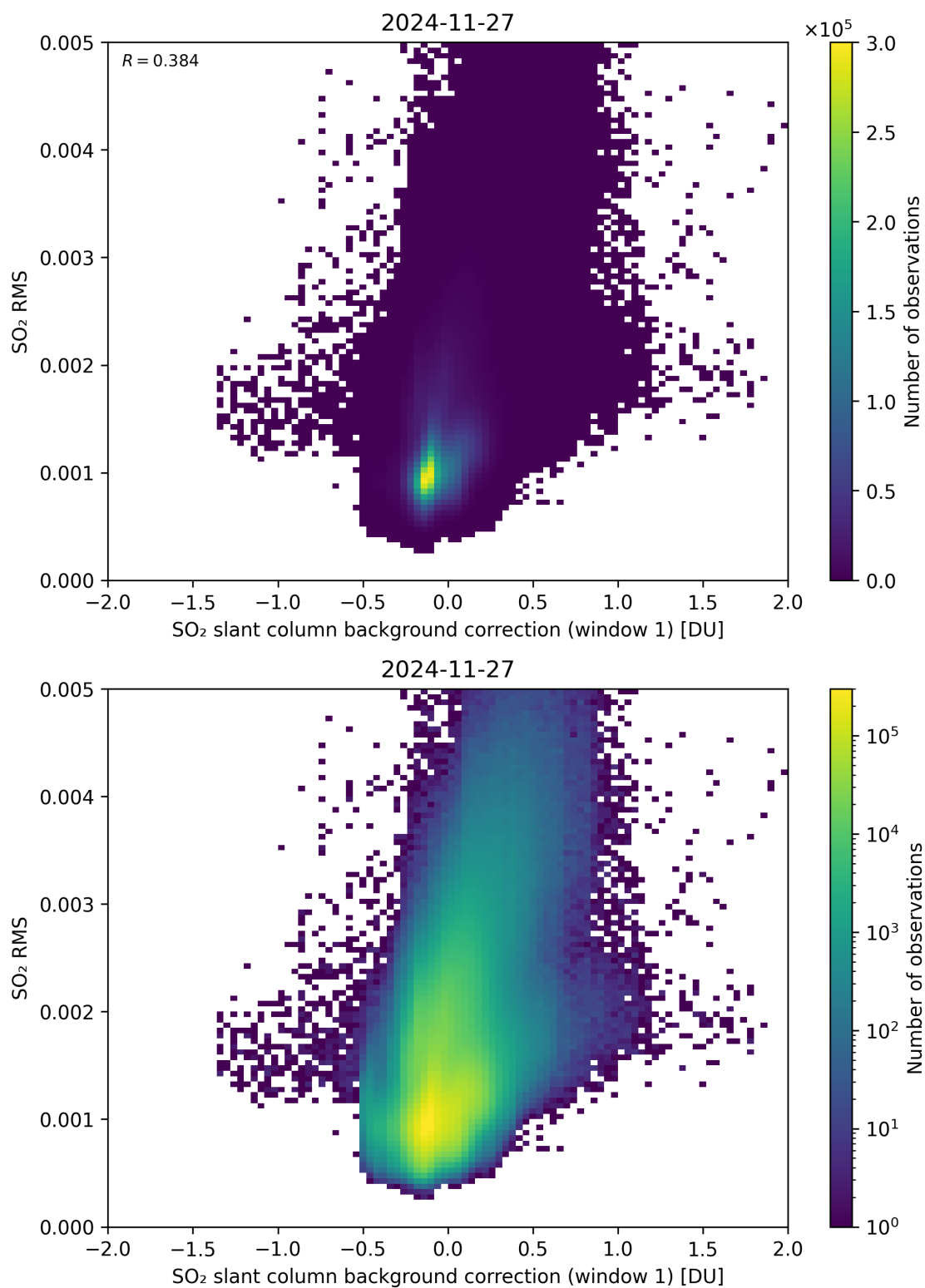
Figure 113: Scatter density plot of “SO 2 slant column background correction (window 1)” against “SO 2 RMS” for 2024-11-26 to 2024-11-28.
