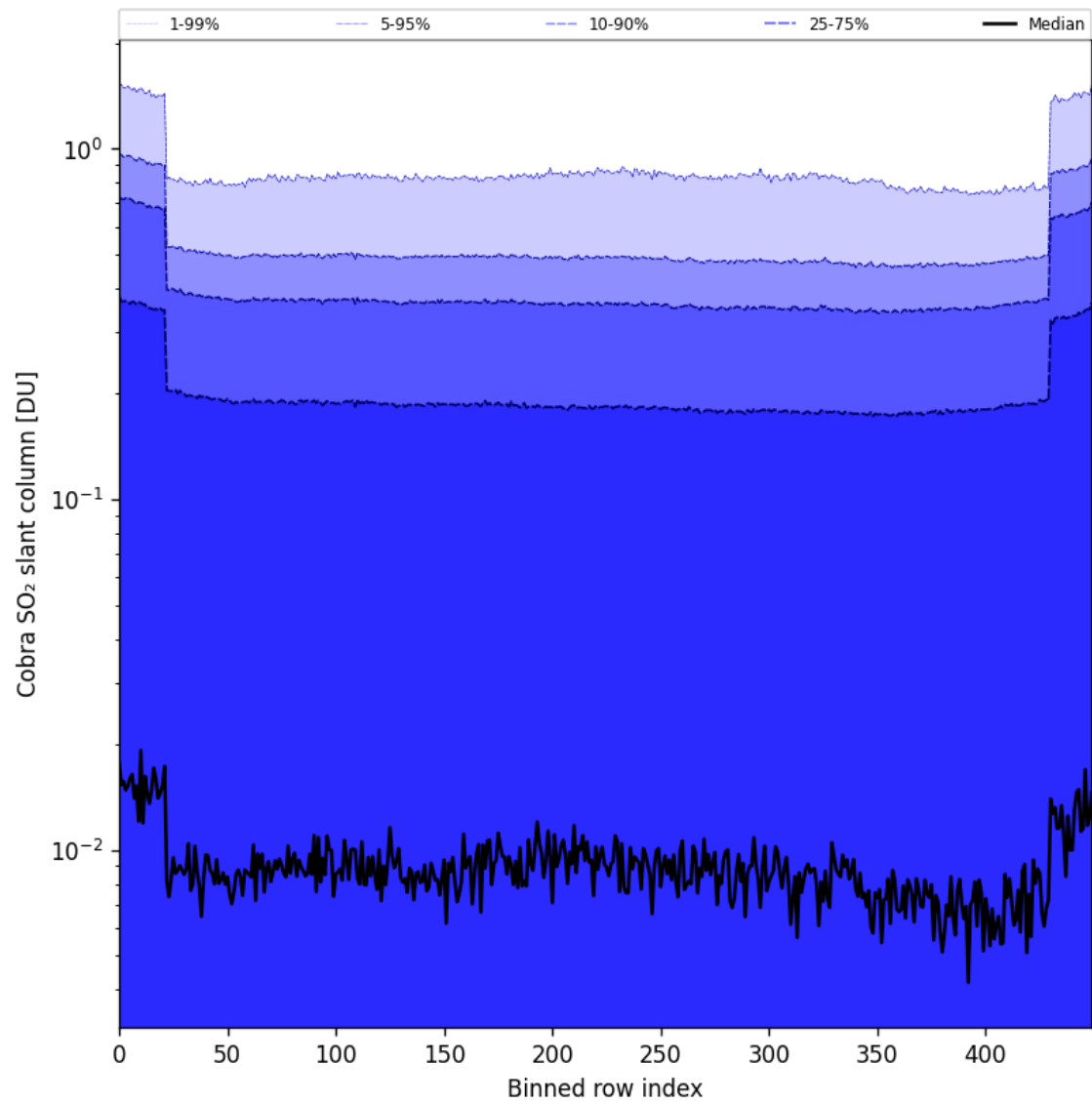
Figure 87: Along track statistics of “Cobra SO 2 slant column” for 2024-11-26 to 2024-11-28
