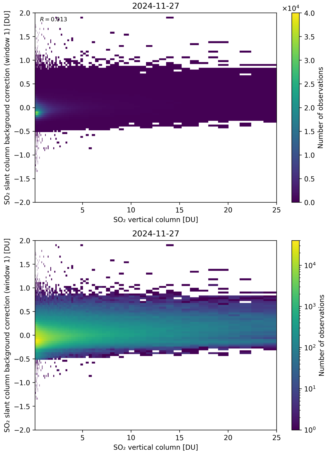
Figure 323: Scatter density plot of “SO 2 vertical column” against “SO 2 slant column background correction (window 1)” for 2024-11-26 to 2024-11-28.
