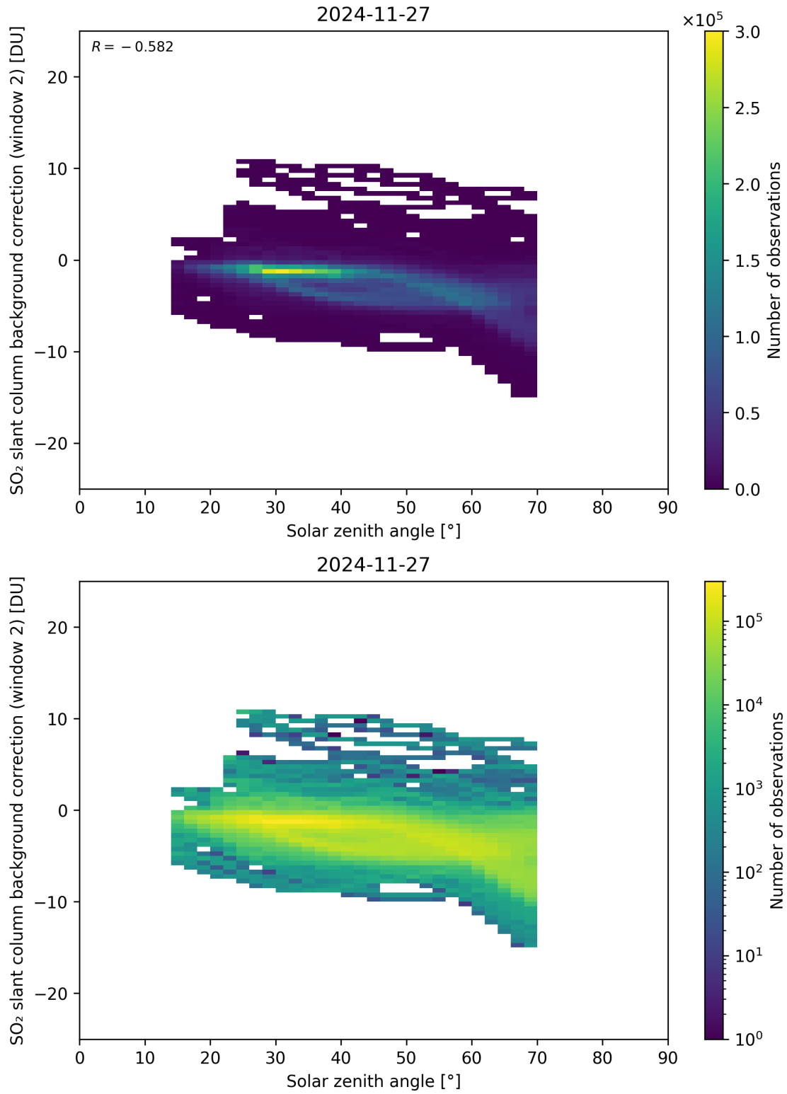
Figure 172: Scatter density plot of “Solar zenith angle” against “SO 2 slant column background correction (window 2)” for 2024-11-26 to 2024-11-28.
