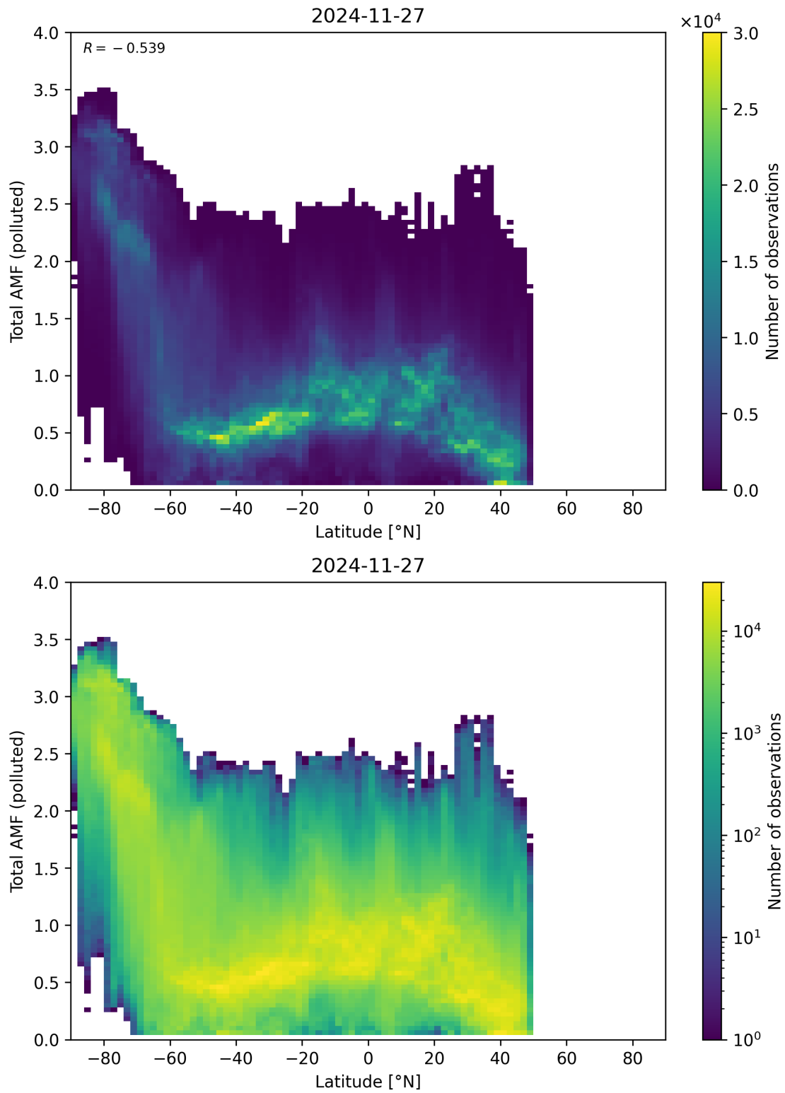
Figure 167: Scatter density plot of “Latitude” against “Total AMF (polluted)” for 2024-11-26 to 2024-11-28.
