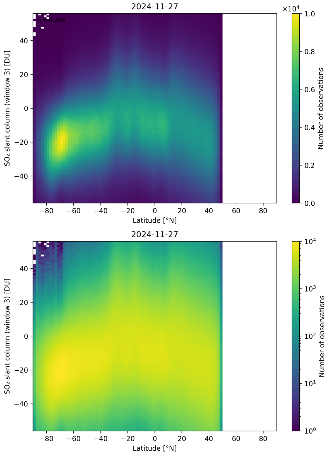
Figure 165: Scatter density plot of “Latitude” against “SO 2 slant column (window 3)” for 2024-11-26 to 2024-11-28.
