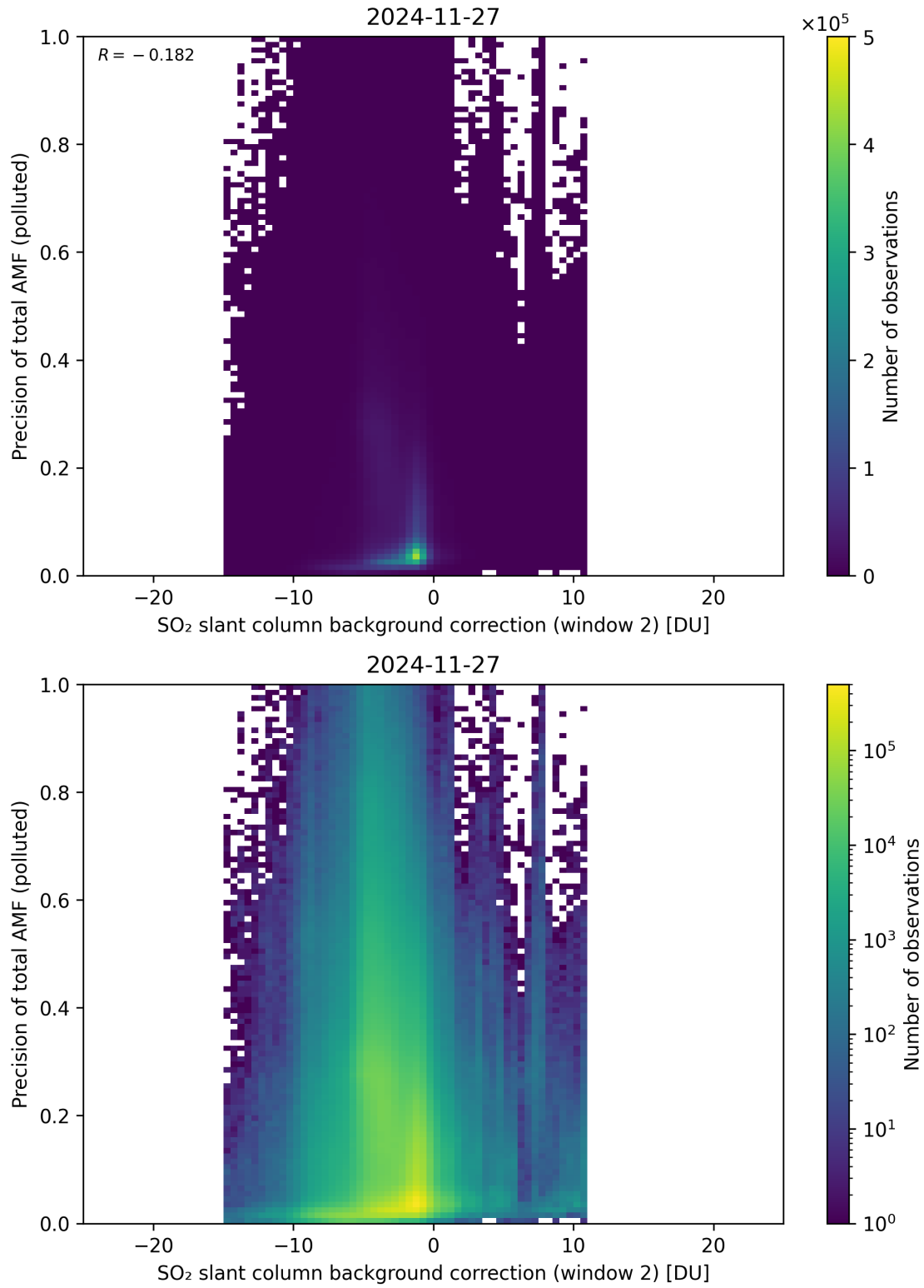
Figure 131: Scatter density plot of “SO 2 slant column background correction (window 2)” against “Precision of total AMF (polluted)” for 2024-11-26 to 2024-11-28.
