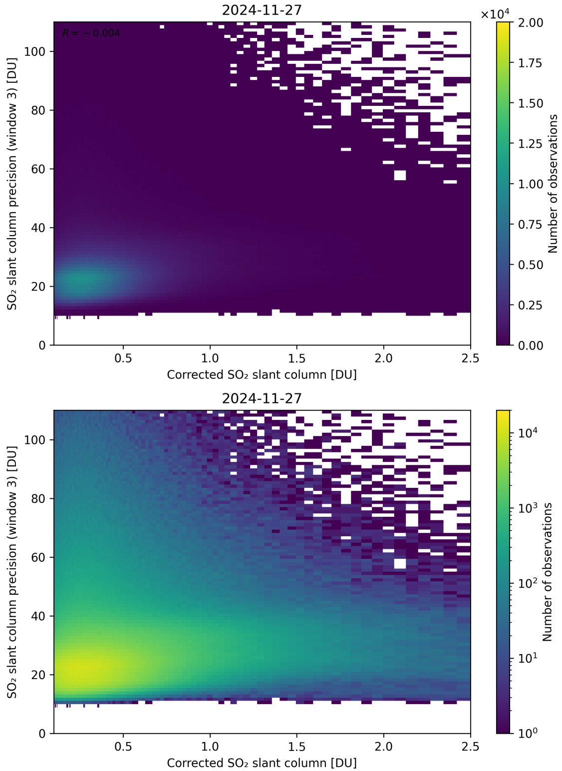
Figure 241: Scatter density plot of “Corrected SO 2 slant column” against “SO 2 slant column precision (window 3)” for 2024-11-26 to 2024-11-28.
