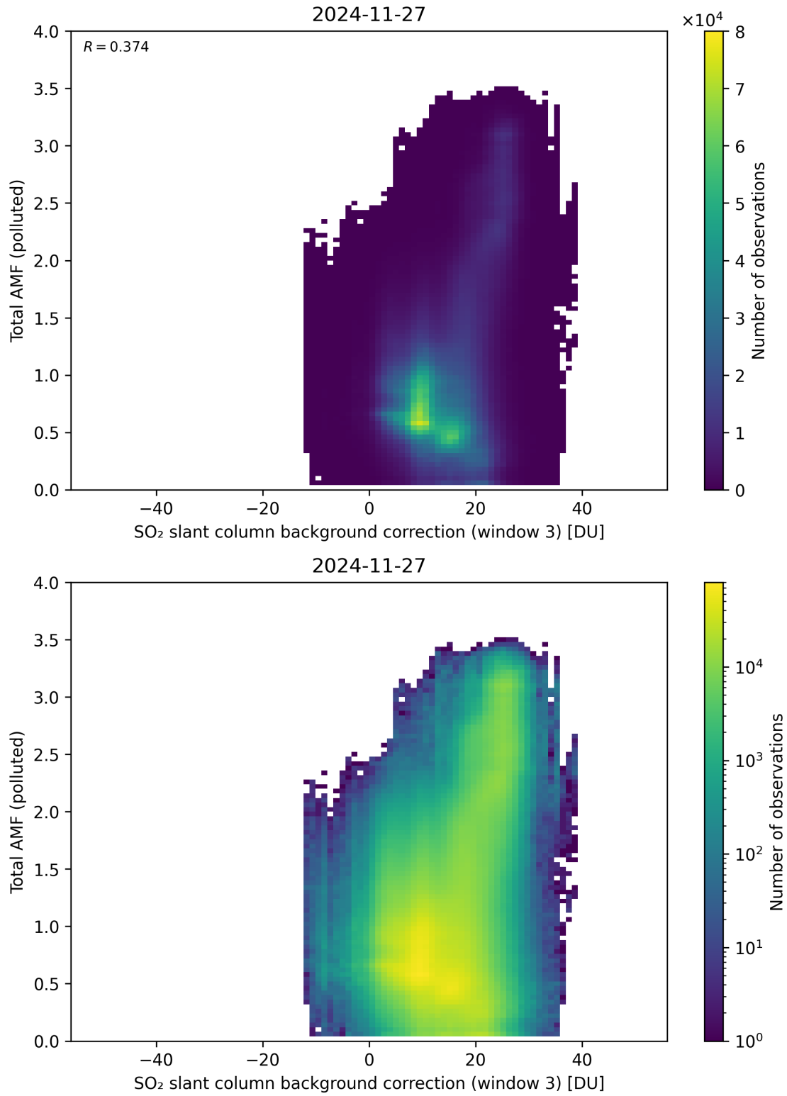
Figure 136: Scatter density plot of “SO 2 slant column background correction (window 3)” against “Total AMF (polluted)” for 2024-11-26 to 2024-11-28.
