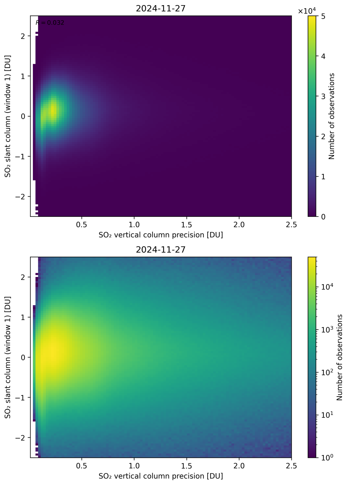
Figure 341: Scatter density plot of “SO 2 vertical column precision” against “SO 2 slant column (window 1)” for 2024-11-26 to 2024-11-28.
