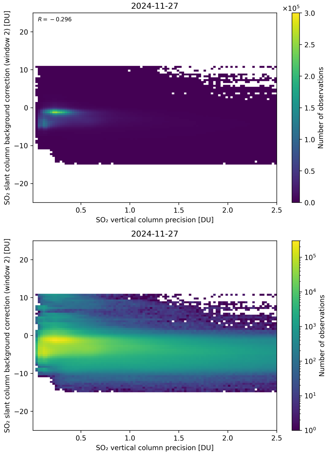
Figure 330: Scatter density plot of “SO 2 vertical column precision” against “SO 2 slant column background correction (window 2)” for 2024-11-26 to 2024-11-28.
