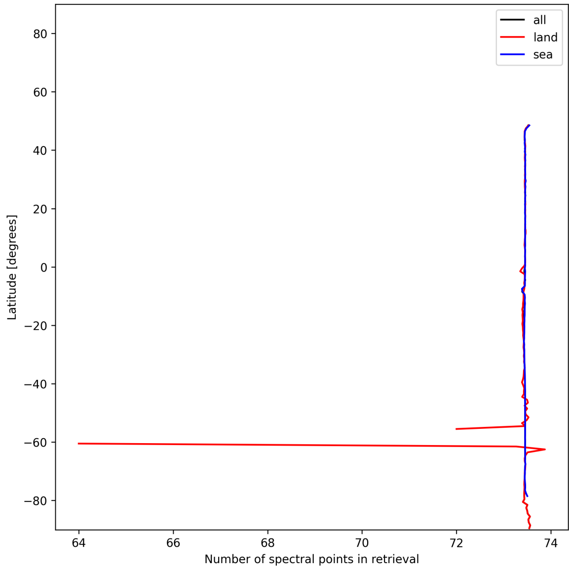
Figure 56: Zonal average of “Number of spectral points in retrieval” for 2024-11-26 to 2024-11-28.
