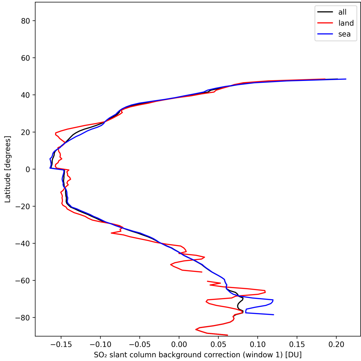
Figure 40: Zonal average of “SO 2 slant column background correction (window 1)” for 2024-11-26 to 2024-11-28.
