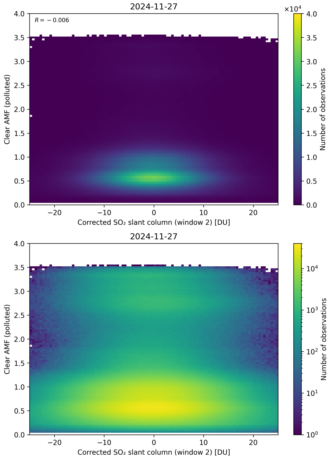
Figure 249: Scatter density plot of “Corrected SO 2 slant column (window 2)” against “Clear AMF (polluted)” for 2024-11-26 to 2024-11-28.
