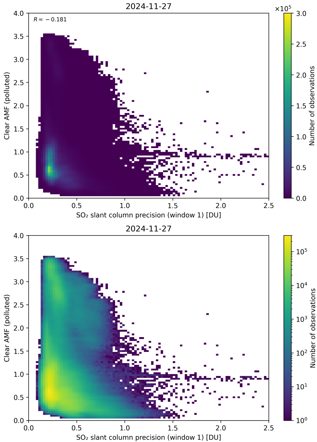
Figure 274: Scatter density plot of “SO 2 slant column precision (window 1)” against “Clear AMF (polluted)” for 2024-11-26 to 2024-11-28.
