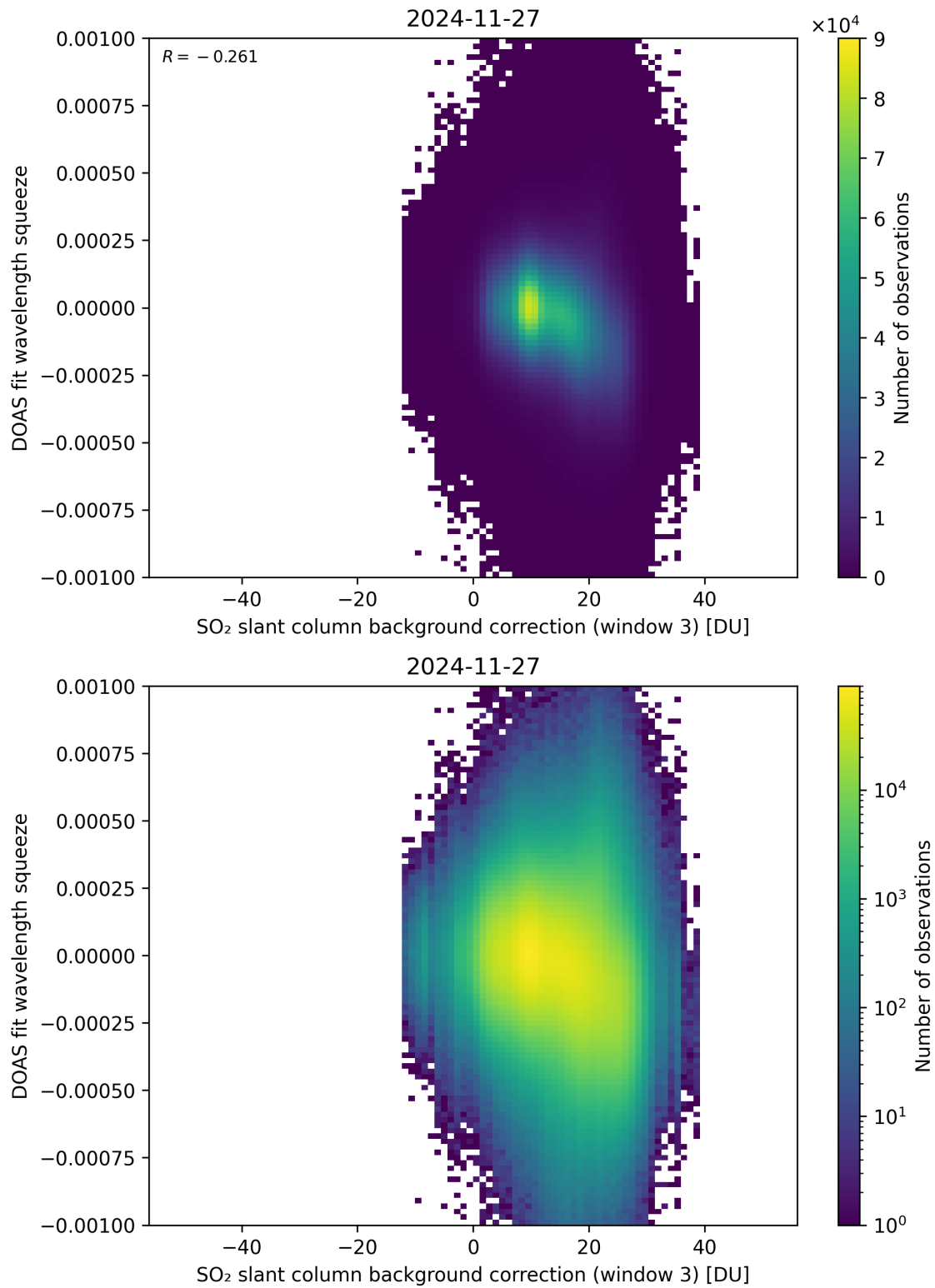
Figure 133: Scatter density plot of “SO 2 slant column background correction (window 3)” against “DOAS fit wavelength squeeze” for 2024-11-26 to 2024-11-28.
