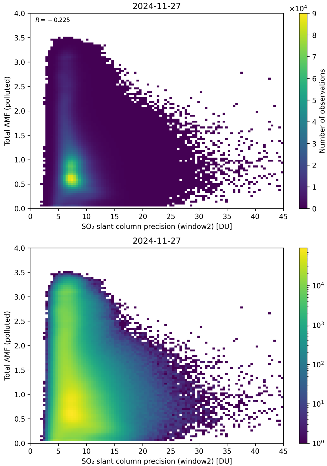
Figure 301: Scatter density plot of “SO 2 slant column precision (window2)” against “Total AMF (polluted)” for 2024-11-26 to 2024-11-28.
