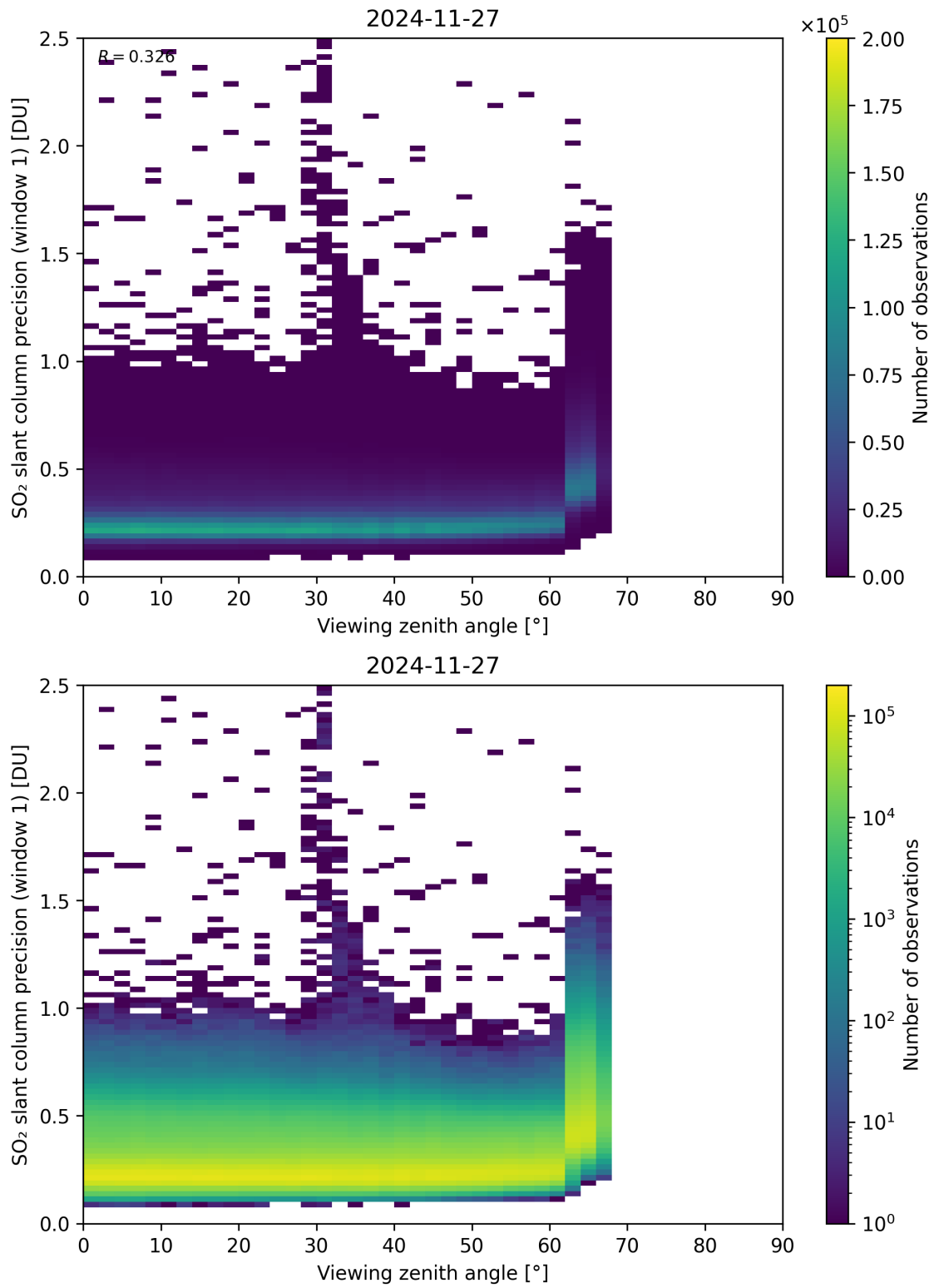
Figure 377: Scatter density plot of “Viewing zenith angle” against “SO 2 slant column precision (window 1)” for 2024-11-26 to 2024-11-28.
