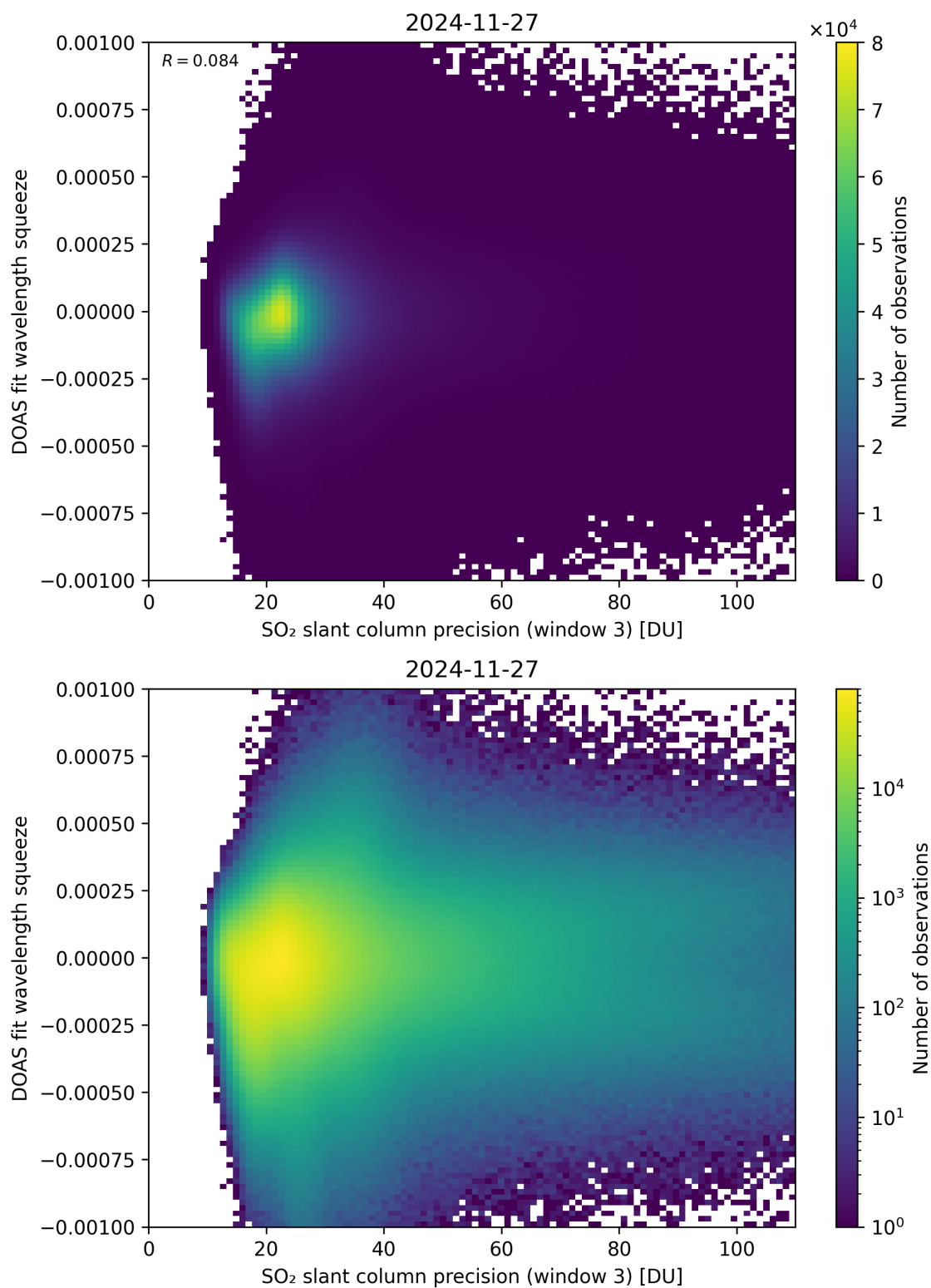
Figure 309: Scatter density plot of “SO 2 slant column precision (window 3)” against “DOAS fit wavelength squeeze” for 2024-11-26 to 2024-11-28.
