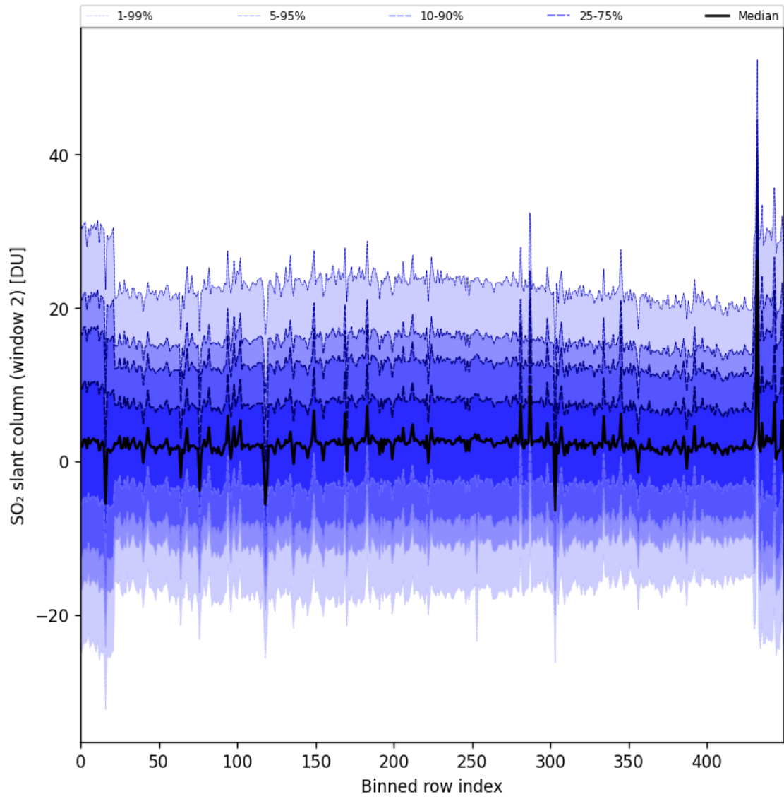
Figure 93: Along track statistics of “SO 2 slant column (window 2)” for 2024-11-26 to 2024-11-28
