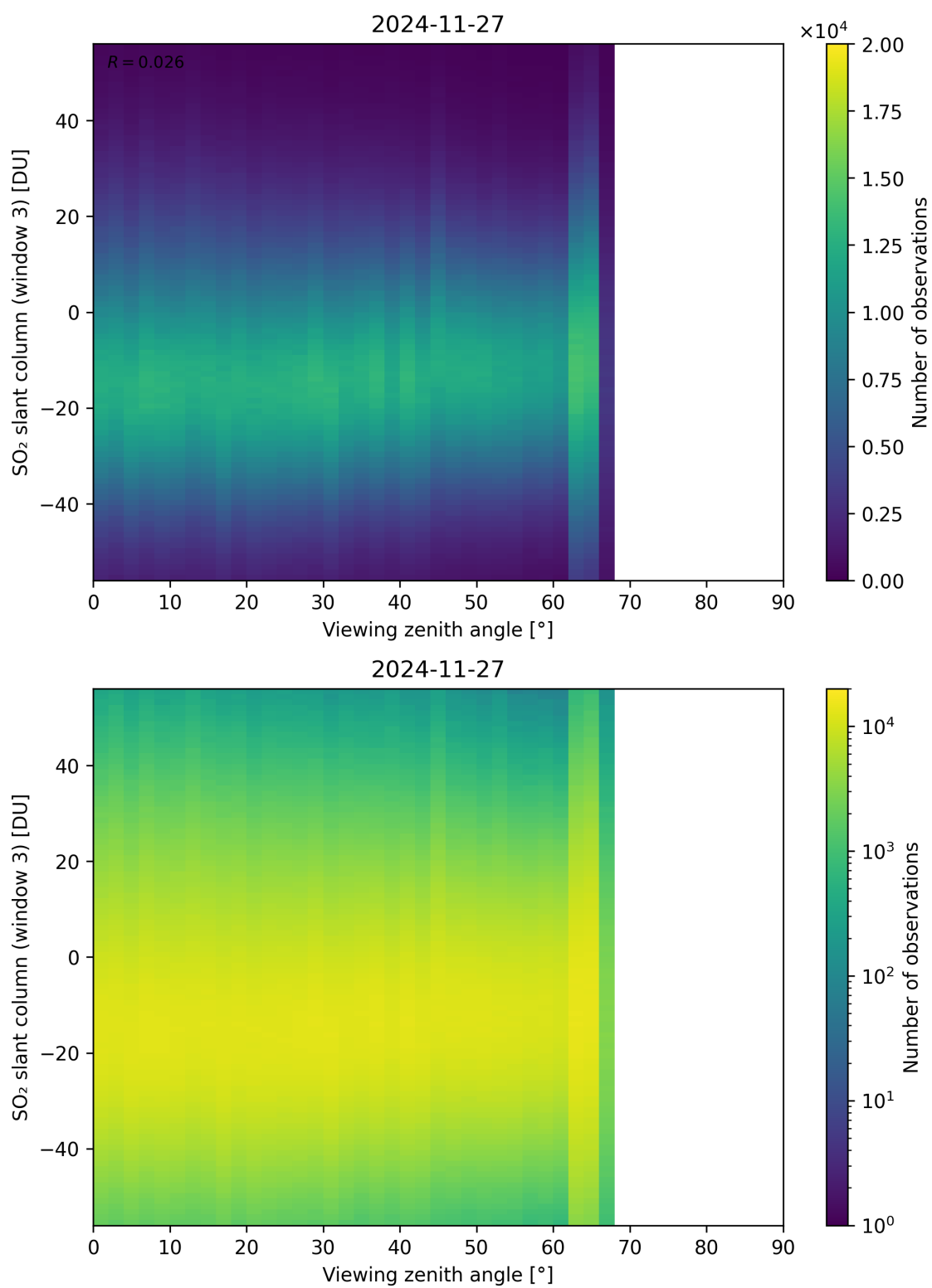
Figure 379: Scatter density plot of “Viewing zenith angle” against “SO 2 slant column (window 3)” for 2024-11-26 to 2024-11-28.
