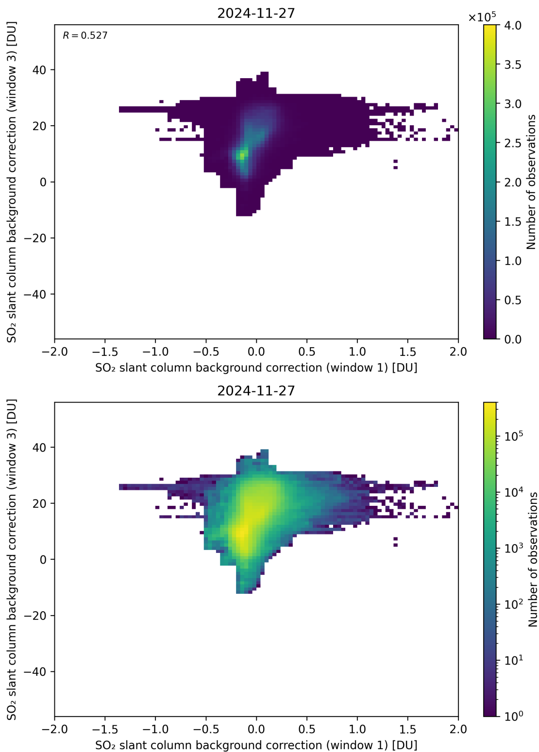
Figure 110: Scatter density plot of “SO 2 slant column background correction (window 1)” against “SO 2 slant column background correction (window 3)” for 2024-11-26 to 2024-11-28.
