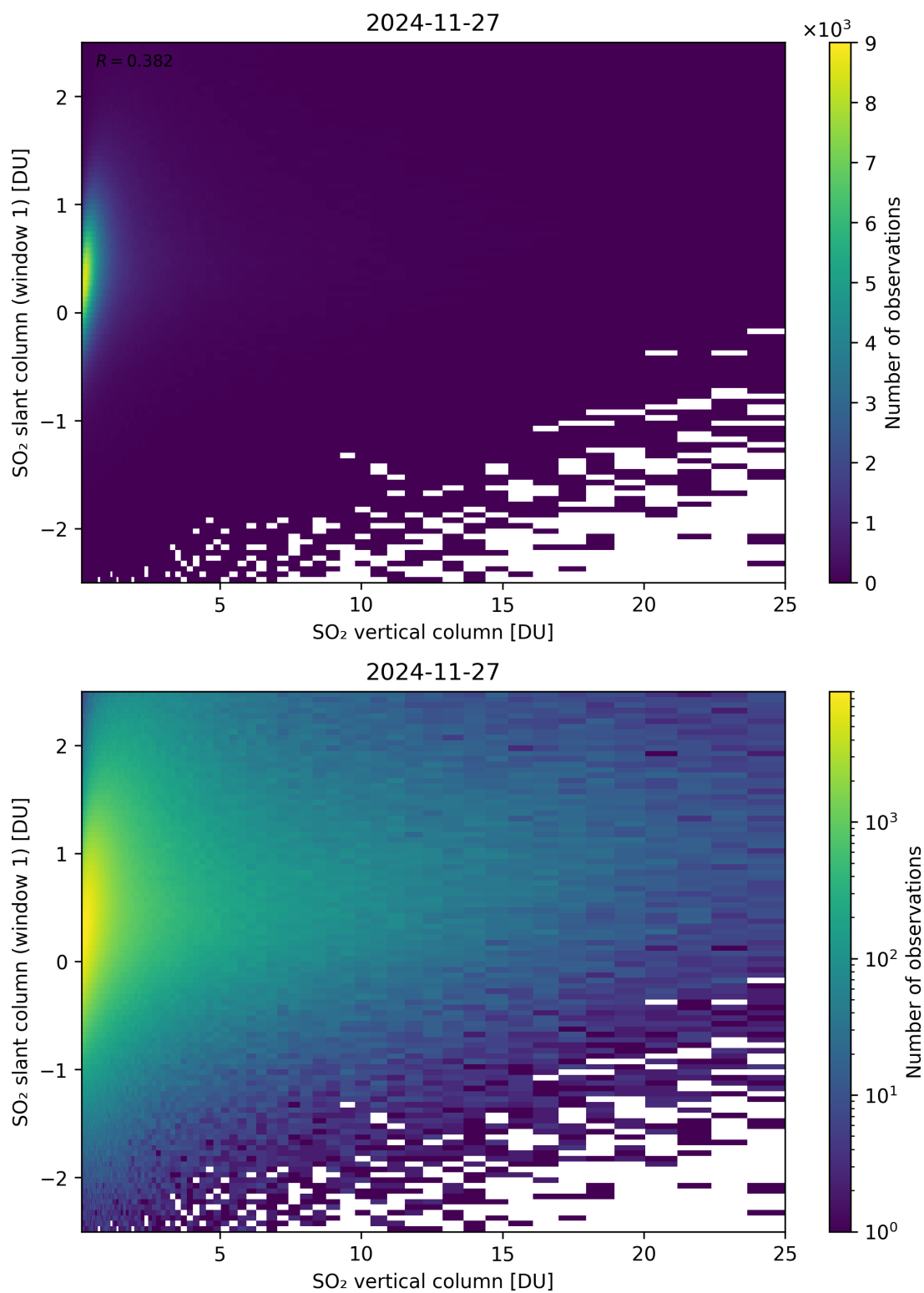
Figure 354: Scatter density plot of “SO 2 vertical column” against “SO 2 slant column (window 1)” for 2024-11-26 to 2024-11-28.
