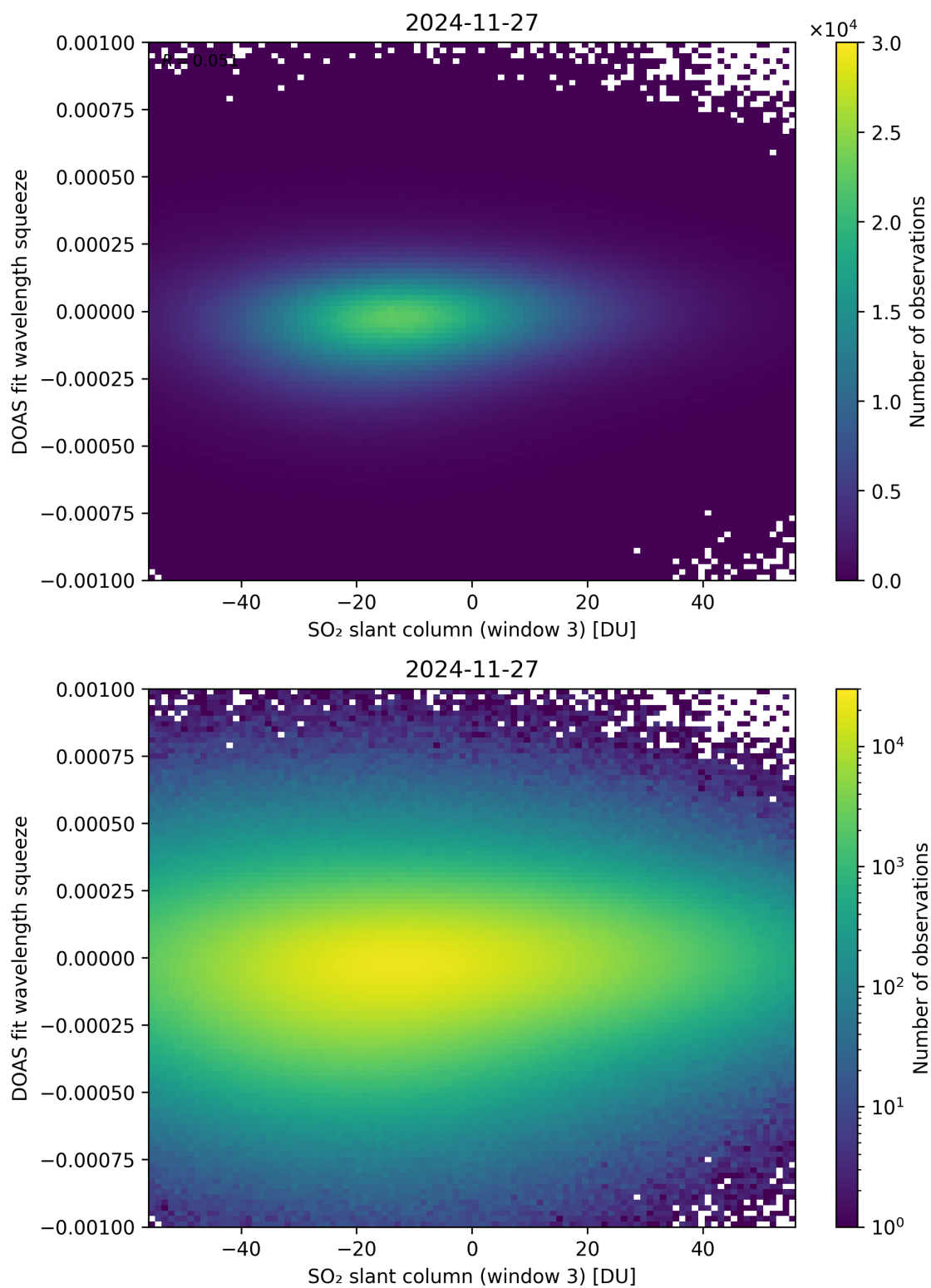
Figure 305: Scatter density plot of “SO 2 slant column (window 3)” against “DOAS fit wavelength squeeze” for 2024-11-26 to 2024-11-28.
