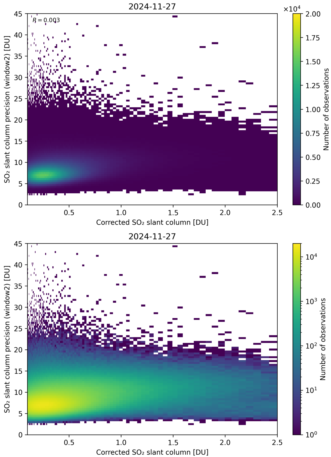
Figure 239: Scatter density plot of “Corrected SO 2 slant column” against “SO 2 slant column precision (window2)” for 2024-11-26 to 2024-11-28.
