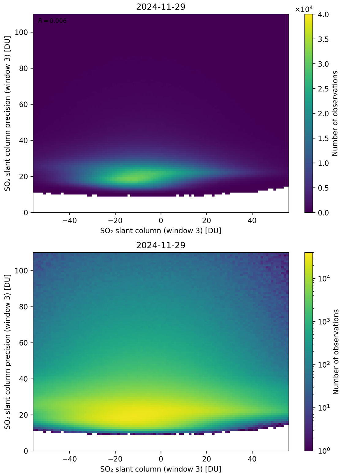
Figure 317: Scatter density plot of “SO 2 slant column (window 3)” against “SO 2 slant column precision (window 3)” for 2024-11-28 to 2024-11-30.
