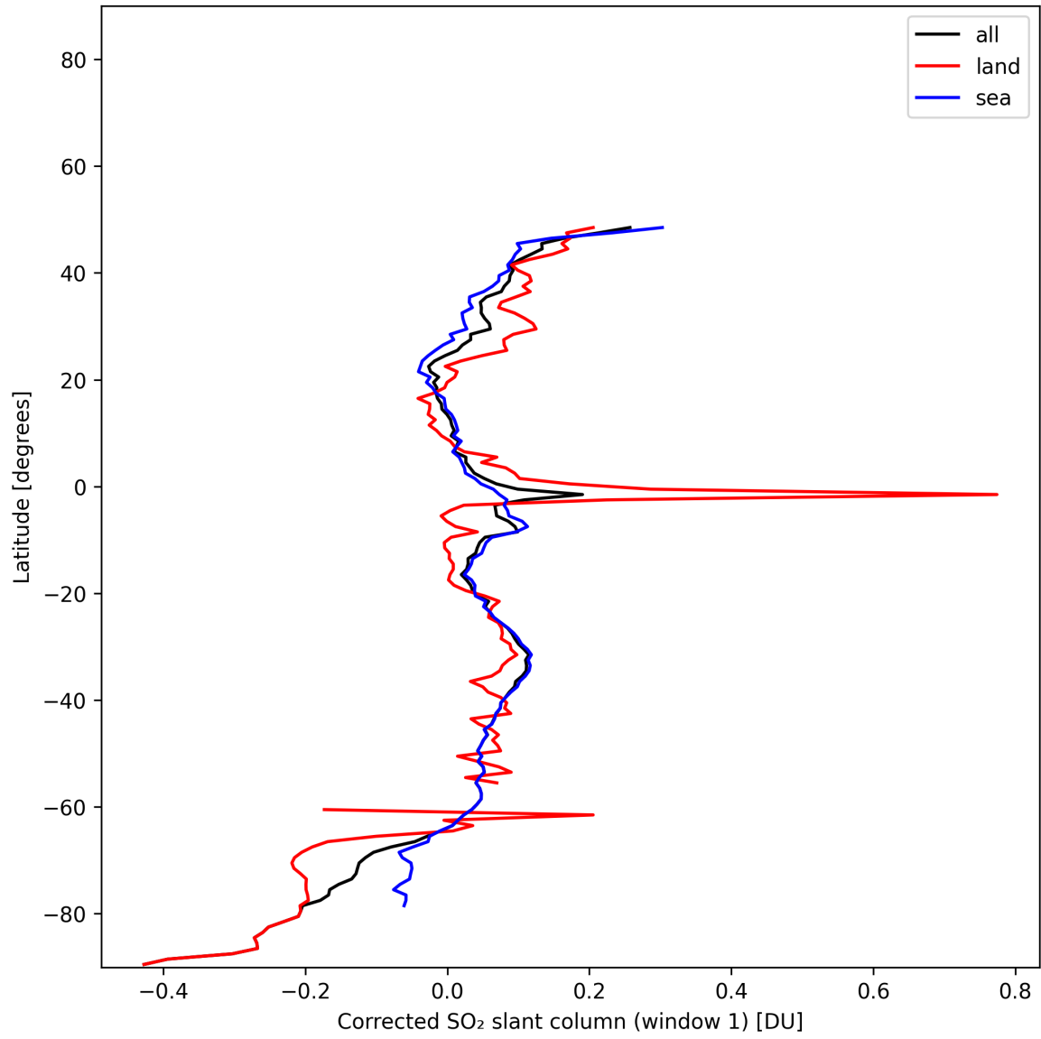
Figure 39: Zonal average of “Corrected SO 2 slant column (window 1)” for 2024-11-28 to 2024-11-30.
