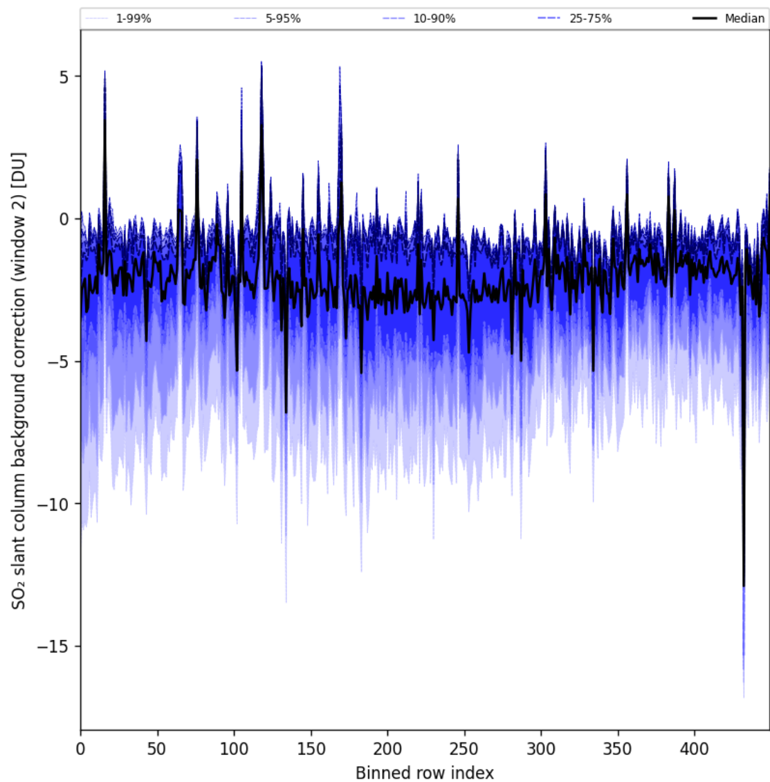
Figure 96: Along track statistics of “SO 2 slant column background correction (window 2)” for 2024-11-28 to 2024-11-30
