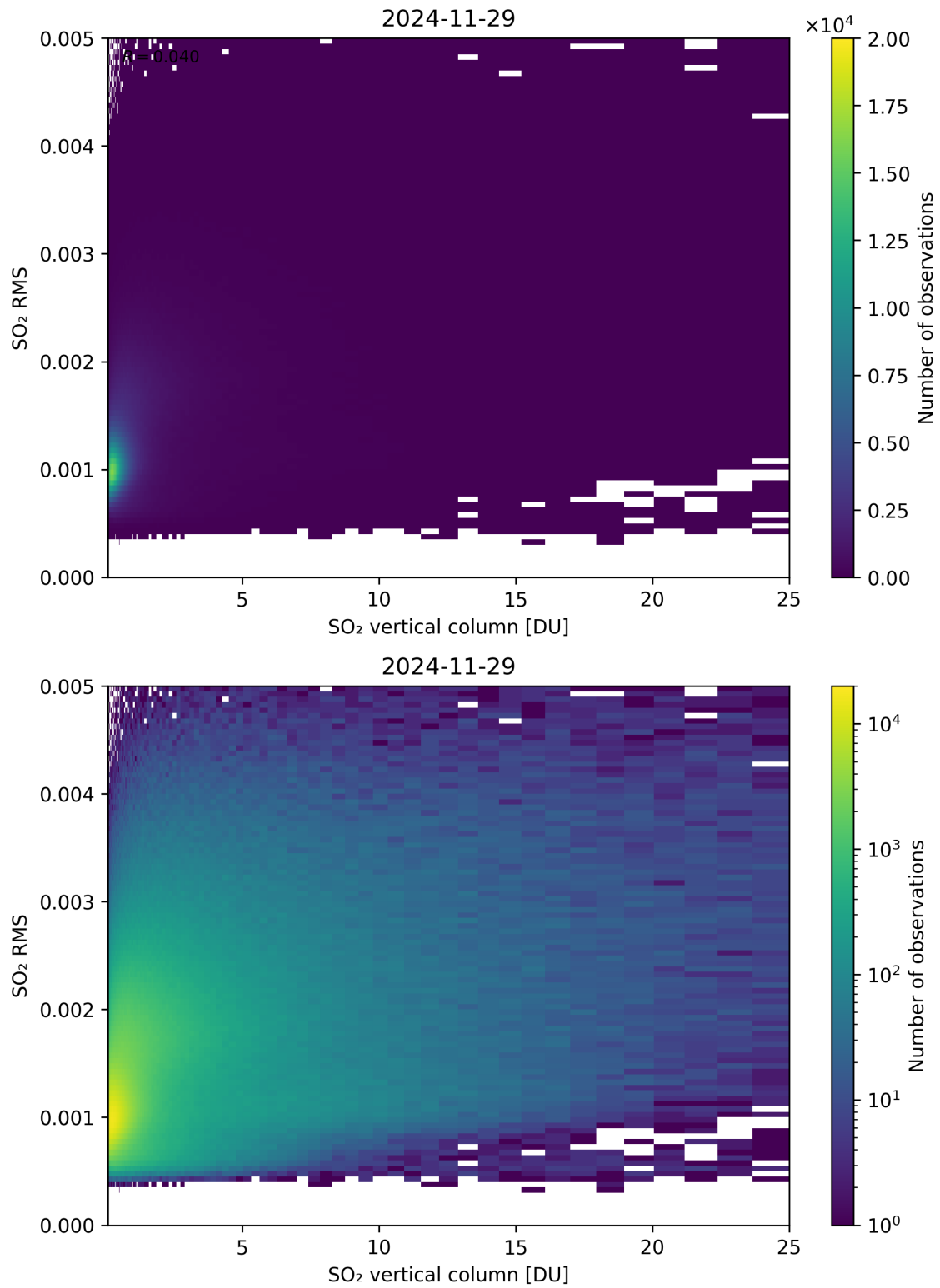
Figure 328: Scatter density plot of “SO 2 vertical column” against “SO 2 RMS” for 2024-11-28 to 2024-11-30.
