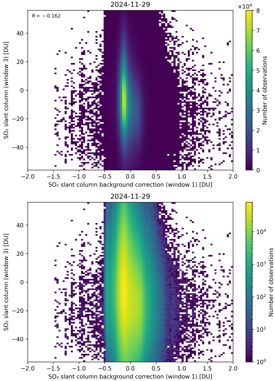
Figure 118: Scatter density plot of “SO 2 slant column background correction (window 1)” against “SO 2 slant column (window 3)” for 2024-11-28 to 2024-11-30.
