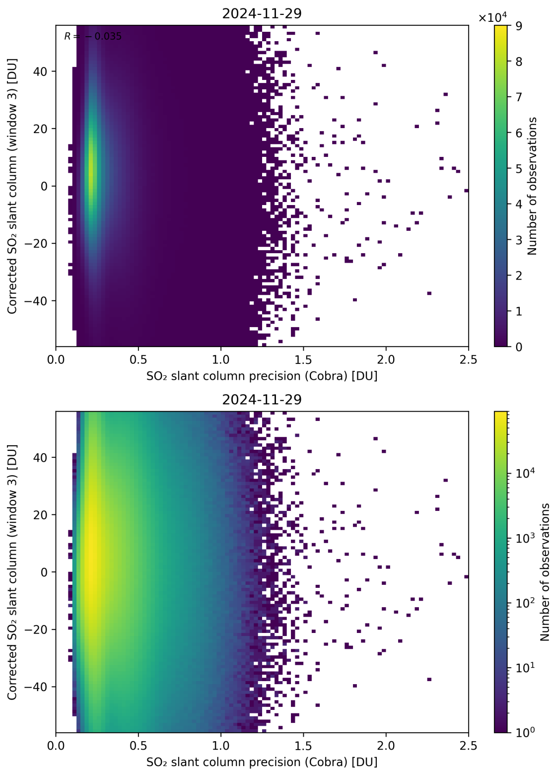
Figure 207: Scatter density plot of “SO 2 slant column precision (Cobra)” against “Corrected SO 2 slant column (window 3)” for 2024-11-28 to 2024-11-30.
