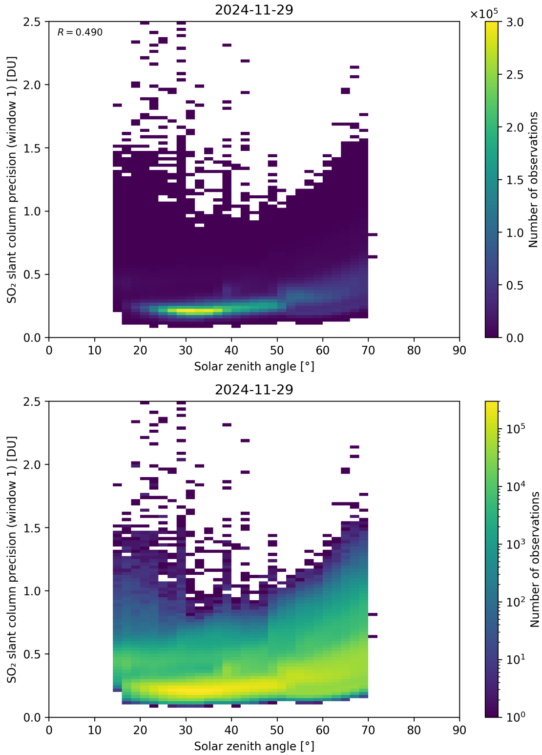
Figure 185: Scatter density plot of “Solar zenith angle” against “SO 2 slant column precision (window 1)” for 2024-11-28 to 2024-11-30.
