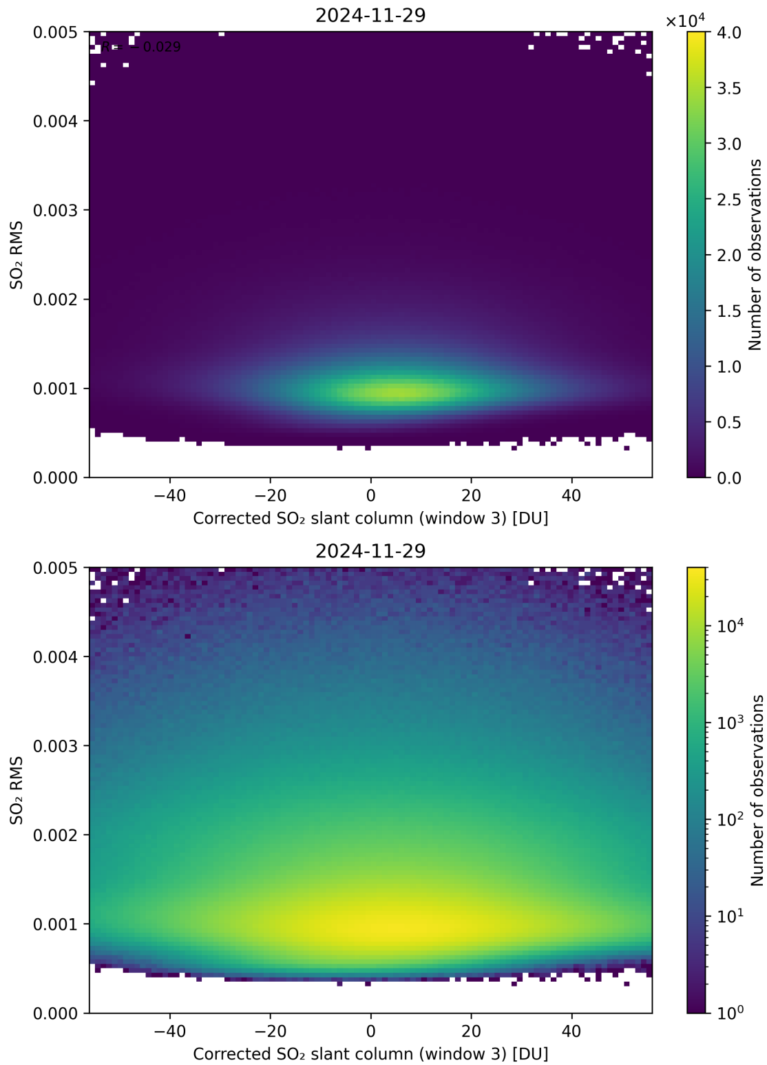
Figure 258: Scatter density plot of “Corrected SO 2 slant column (window 3)” against “SO 2 RMS” for 2024-11-28 to 2024-11-30.
