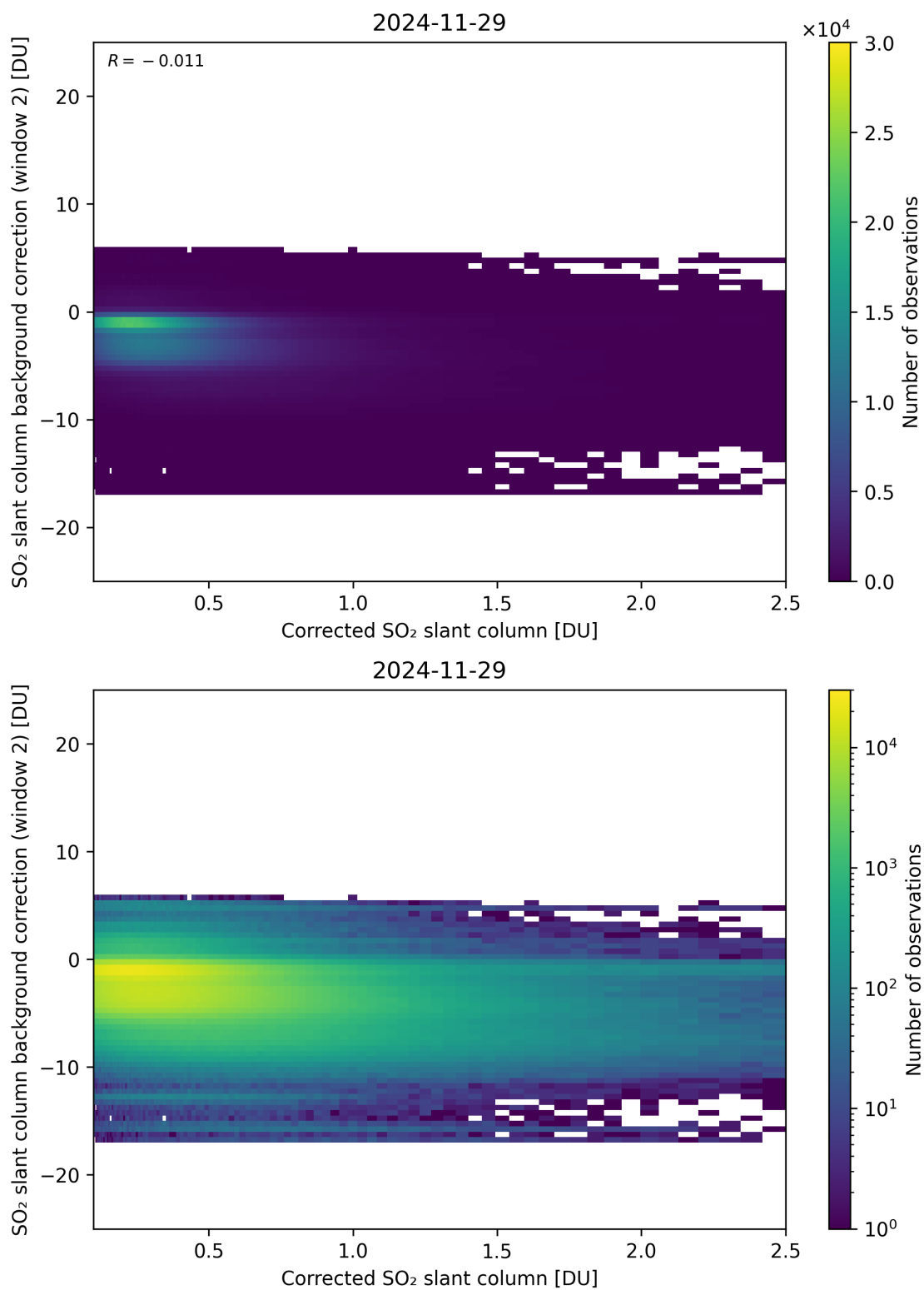
Figure 227: Scatter density plot of “Corrected SO 2 slant column” against “SO 2 slant column background correction (window 2)” for 2024-11-28 to 2024-11-30.
