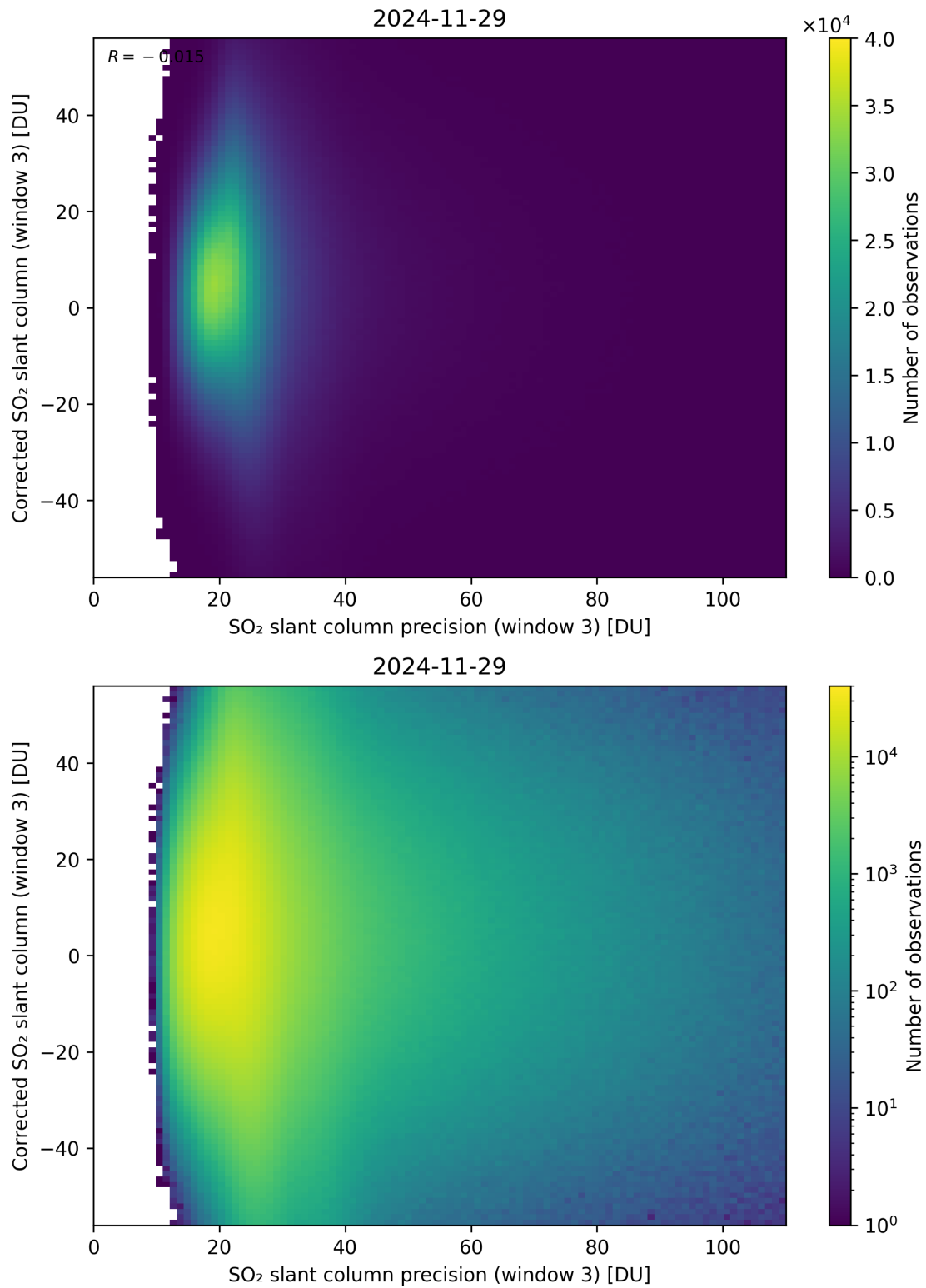
Figure 312: Scatter density plot of “SO 2 slant column precision (window 3)” against “Corrected SO 2 slant column (window 3)” for 2024-11-28 to 2024-11-30.
