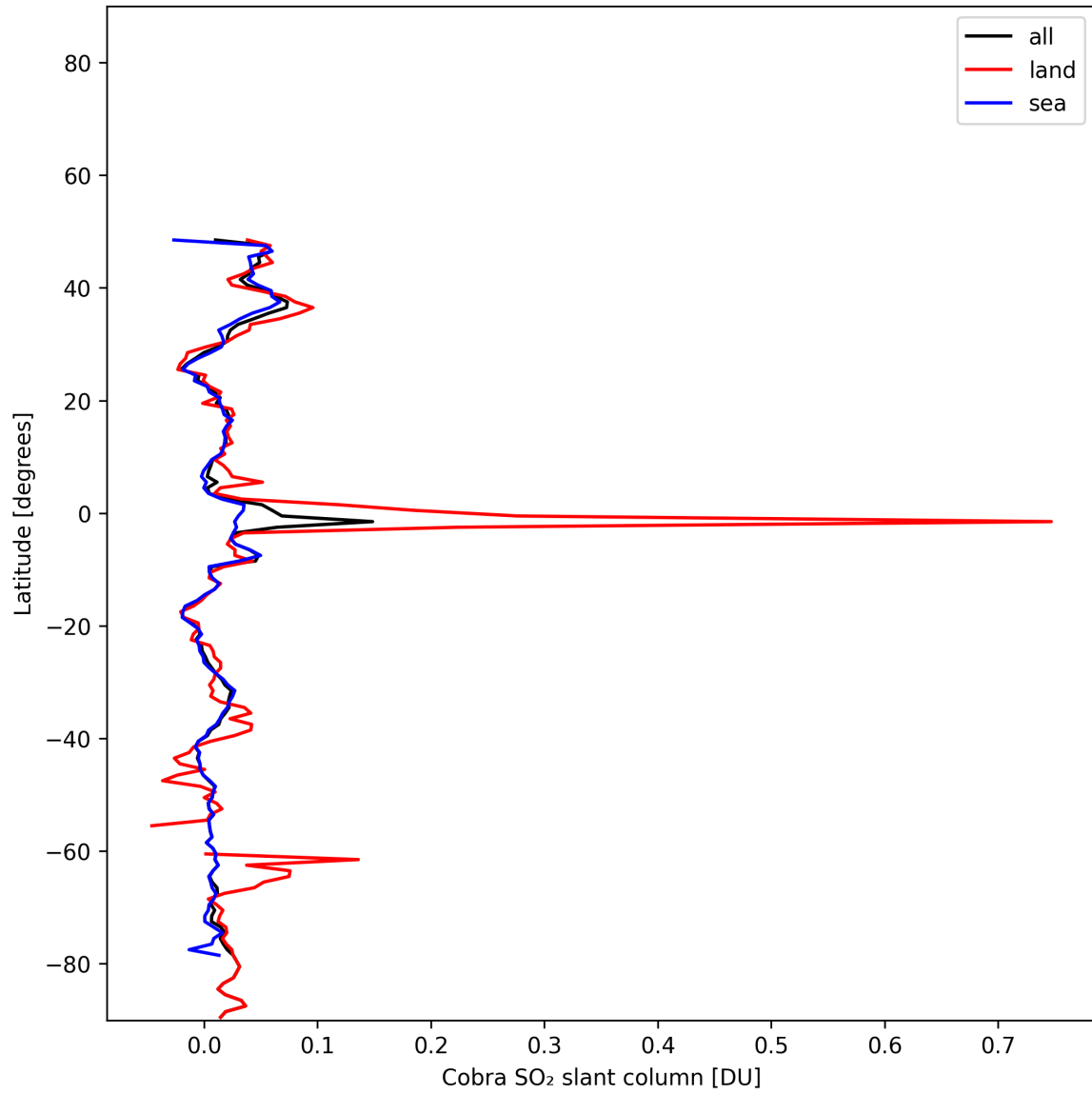
Figure 35: Zonal average of “Cobra SO 2 slant column” for 2024-11-28 to 2024-11-30.
