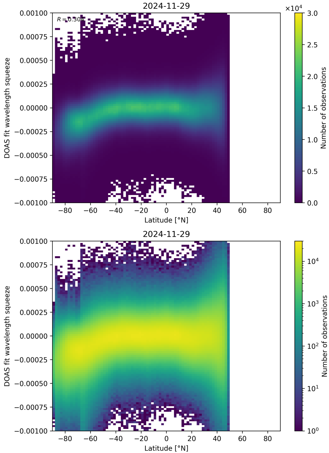
Figure 154: Scatter density plot of “Latitude” against “DOAS fit wavelength squeeze” for 2024-11-28 to 2024-11-30.
