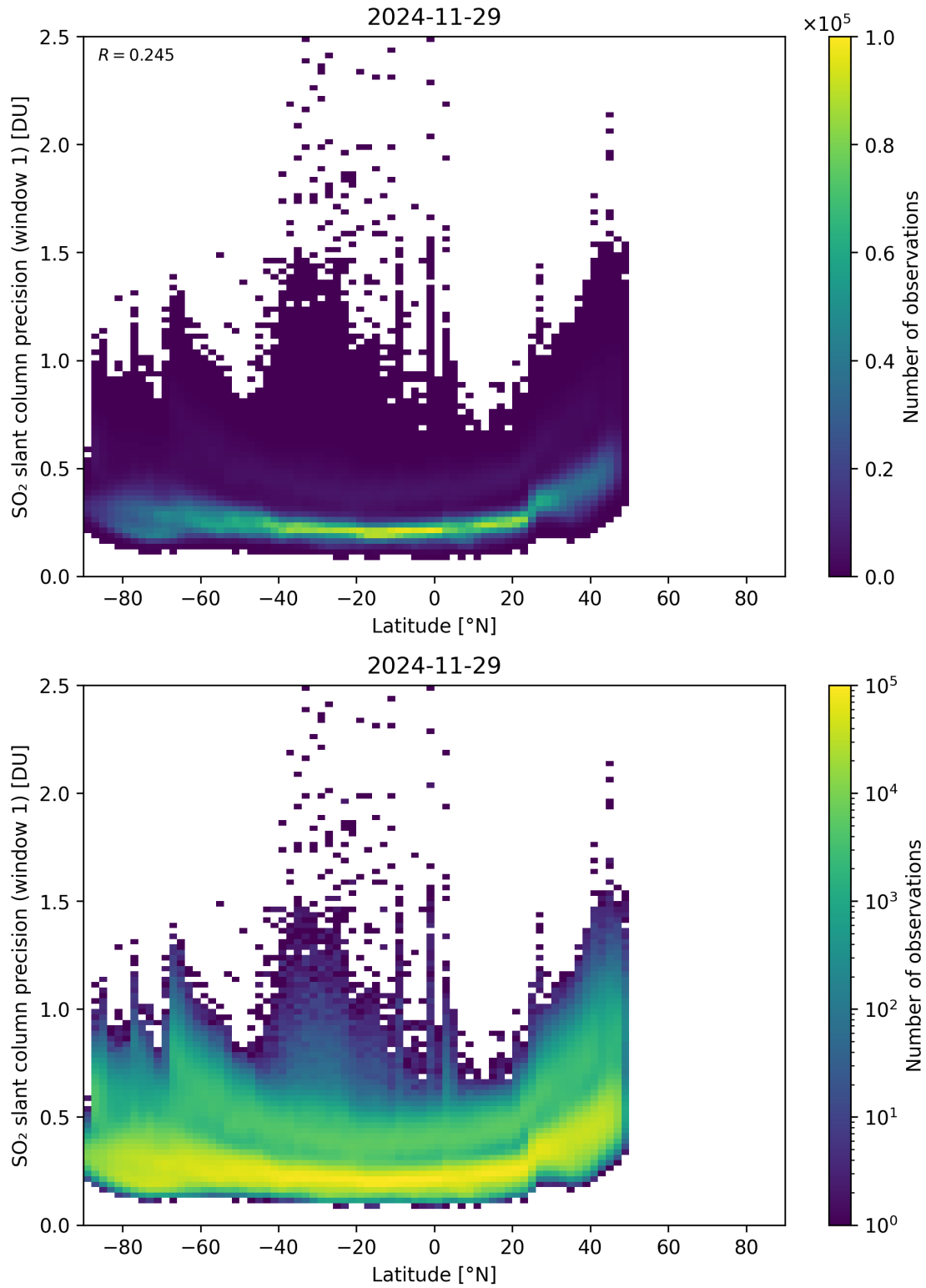
Figure 163: Scatter density plot of “Latitude” against “SO 2 slant column precision (window 1)” for 2024-11-28 to 2024-11-30.
