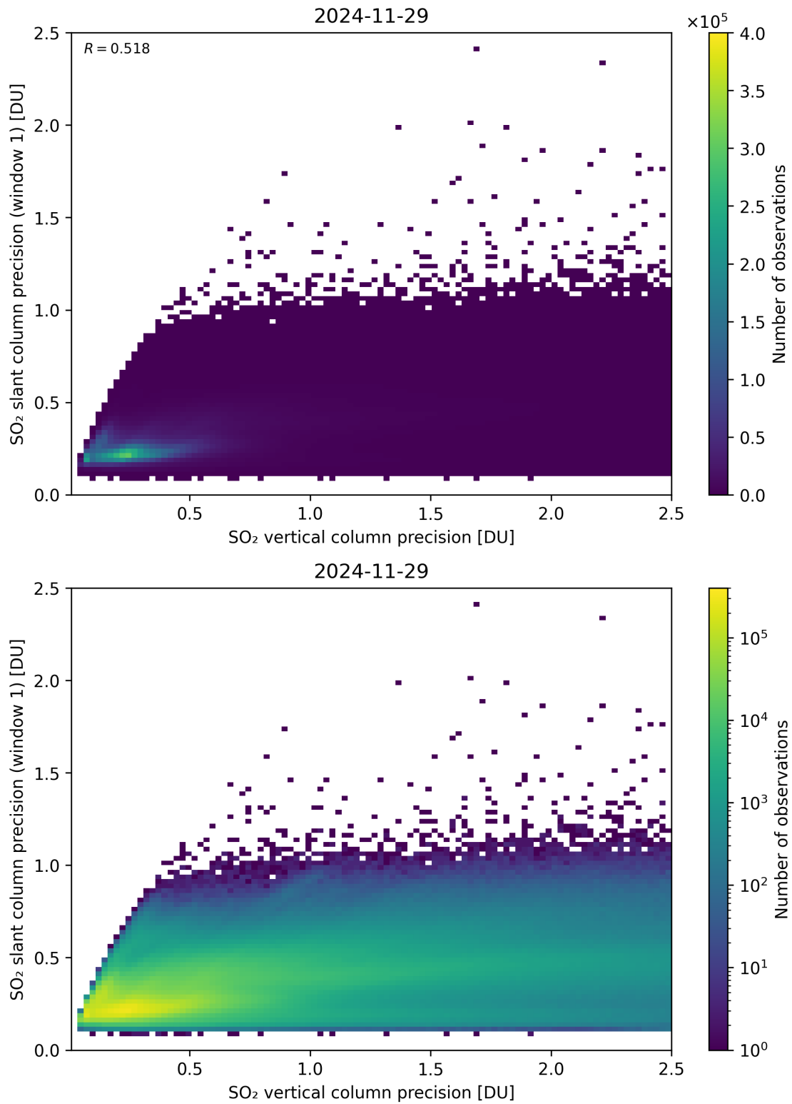
Figure 342: Scatter density plot of “SO 2 vertical column precision” against “SO 2 slant column precision (window 1)” for 2024-11-28 to 2024-11-30.
