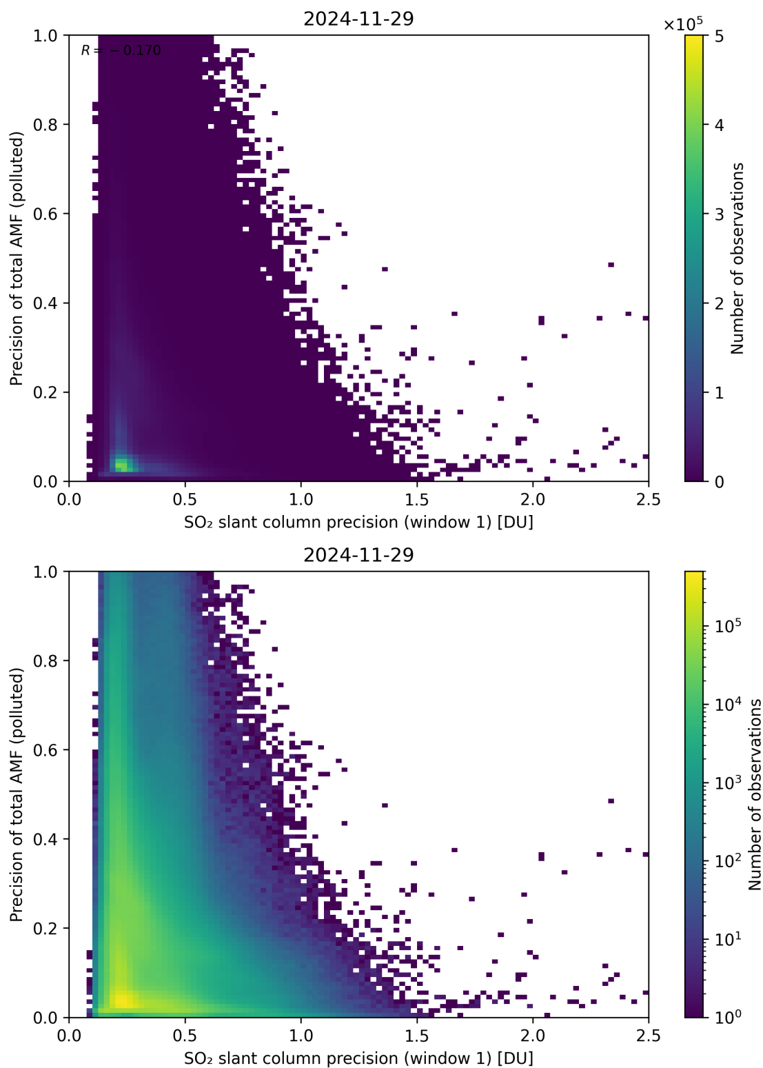
Figure 281: Scatter density plot of “SO 2 slant column precision (window 1)” against “Precision of total AMF (polluted)” for 2024-11-28 to 2024-11-30.
