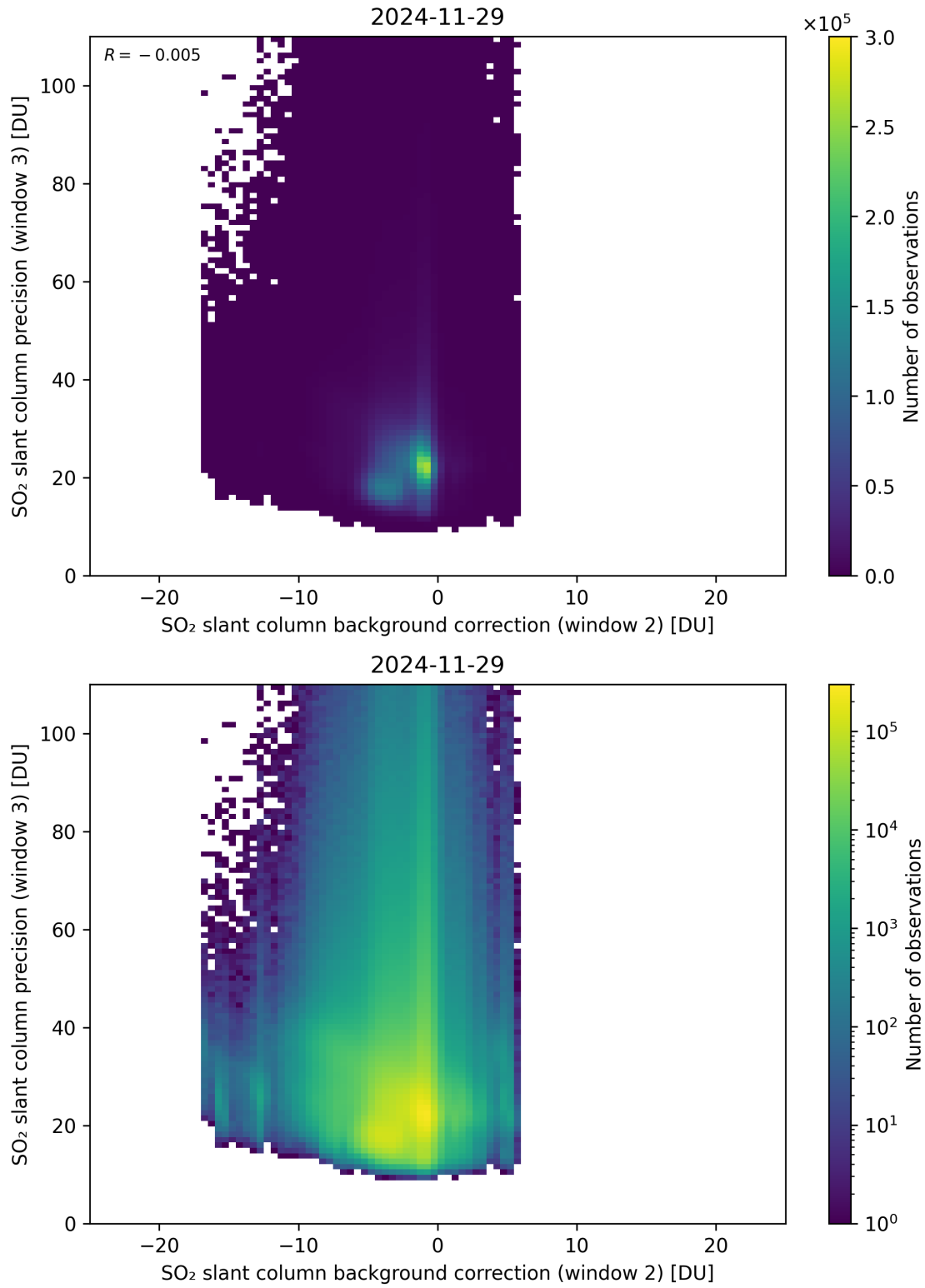
Figure 129: Scatter density plot of “SO 2 slant column background correction (window 2)” against “SO 2 slant column precision (window 3)” for 2024-11-28 to 2024-11-30.
