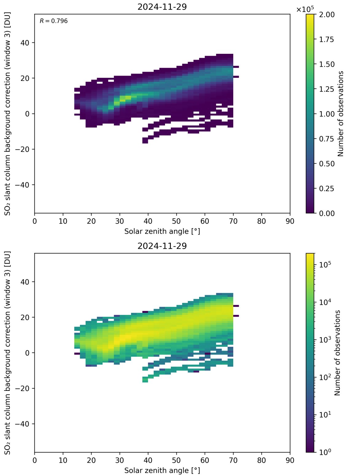
Figure 173: Scatter density plot of “Solar zenith angle” against “SO 2 slant column background correction (window 3)” for 2024-11-28 to 2024-11-30.
