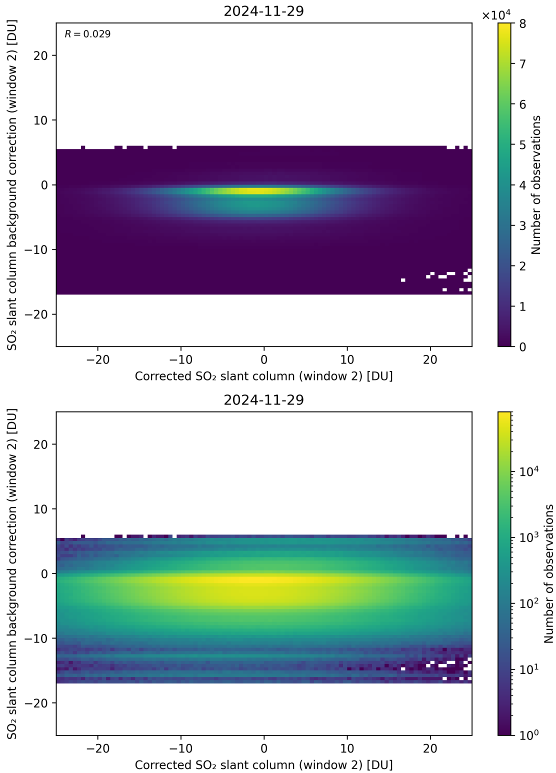
Figure 244: Scatter density plot of “Corrected SO 2 slant column (window 2)” against “SO 2 slant column background correction (window 2)” for 2024-11-28 to 2024-11-30.
