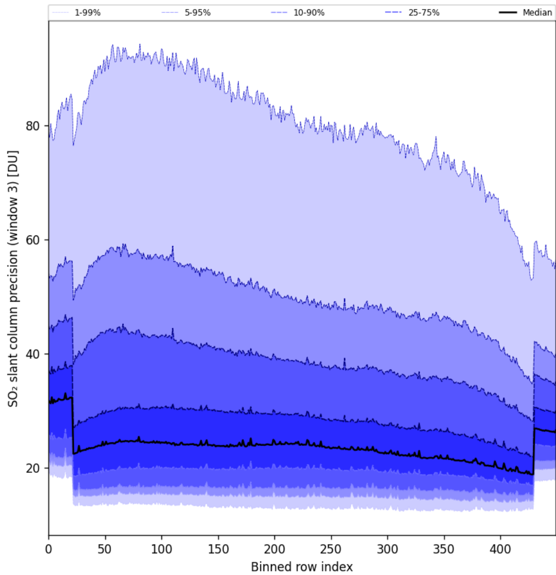
Figure 98: Along track statistics of “SO 2 slant column precision (window 3)” for 2024-11-28 to 2024-11-30
