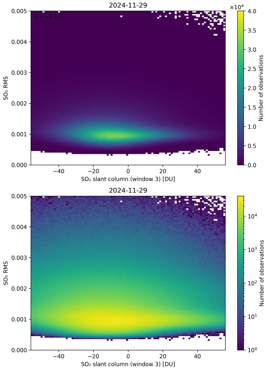
Figure 306: Scatter density plot of “SO 2 slant column (window 3)” against “SO 2 RMS” for 2024-11-28 to 2024-11-30.
