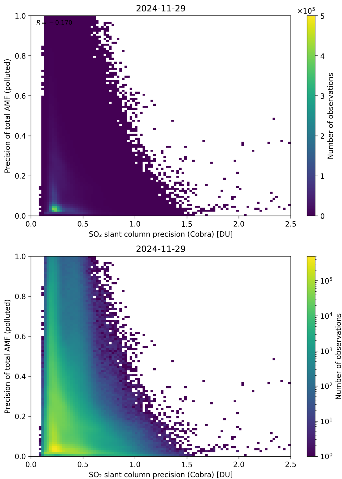
Figure 214: Scatter density plot of “SO 2 slant column precision (Cobra)” against “Precision of total AMF (polluted)” for 2024-11-28 to 2024-11-30.
