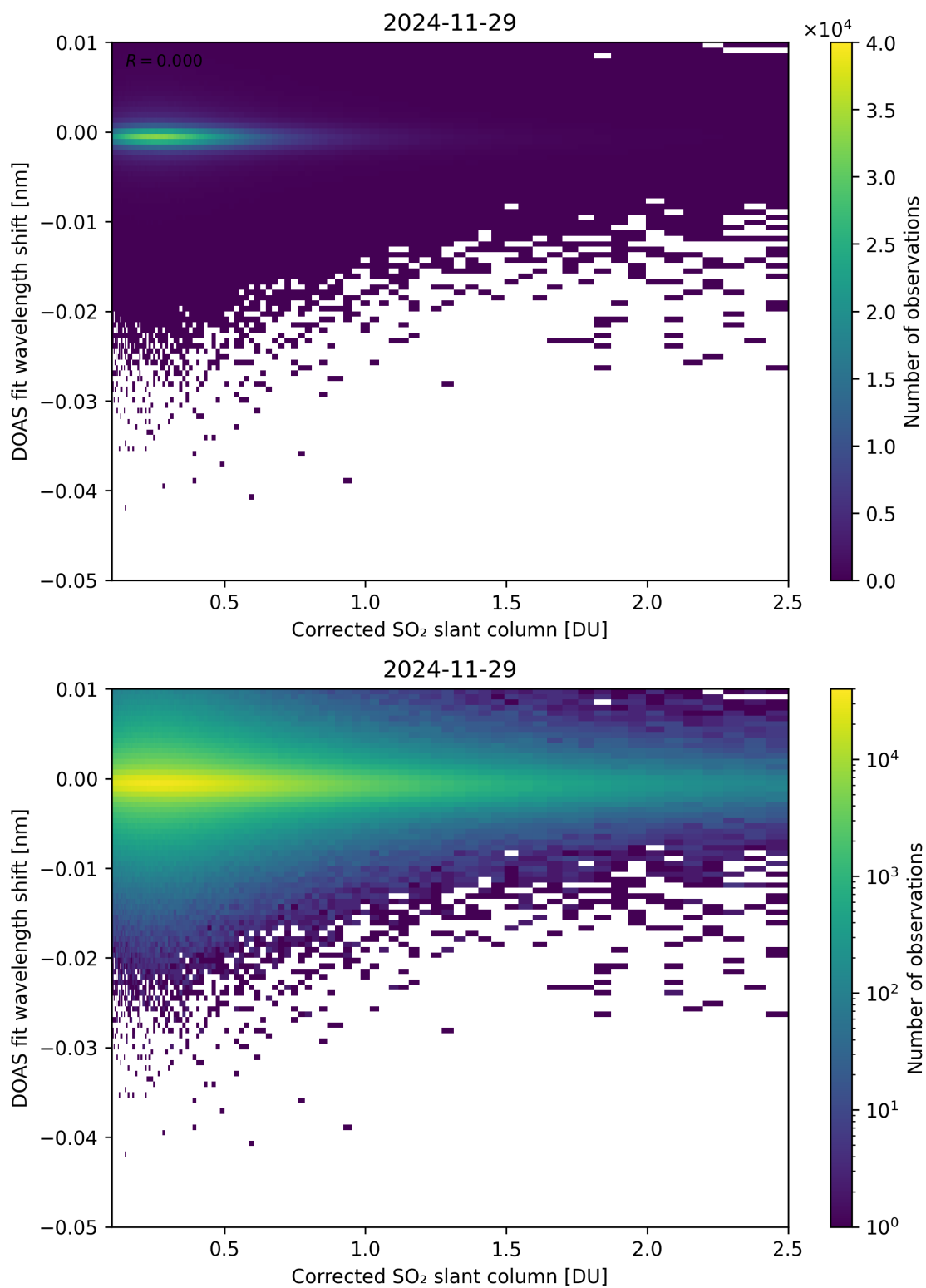
Figure 229: Scatter density plot of “Corrected SO 2 slant column” against “DOAS fit wavelength shift” for 2024-11-28 to 2024-11-30.
