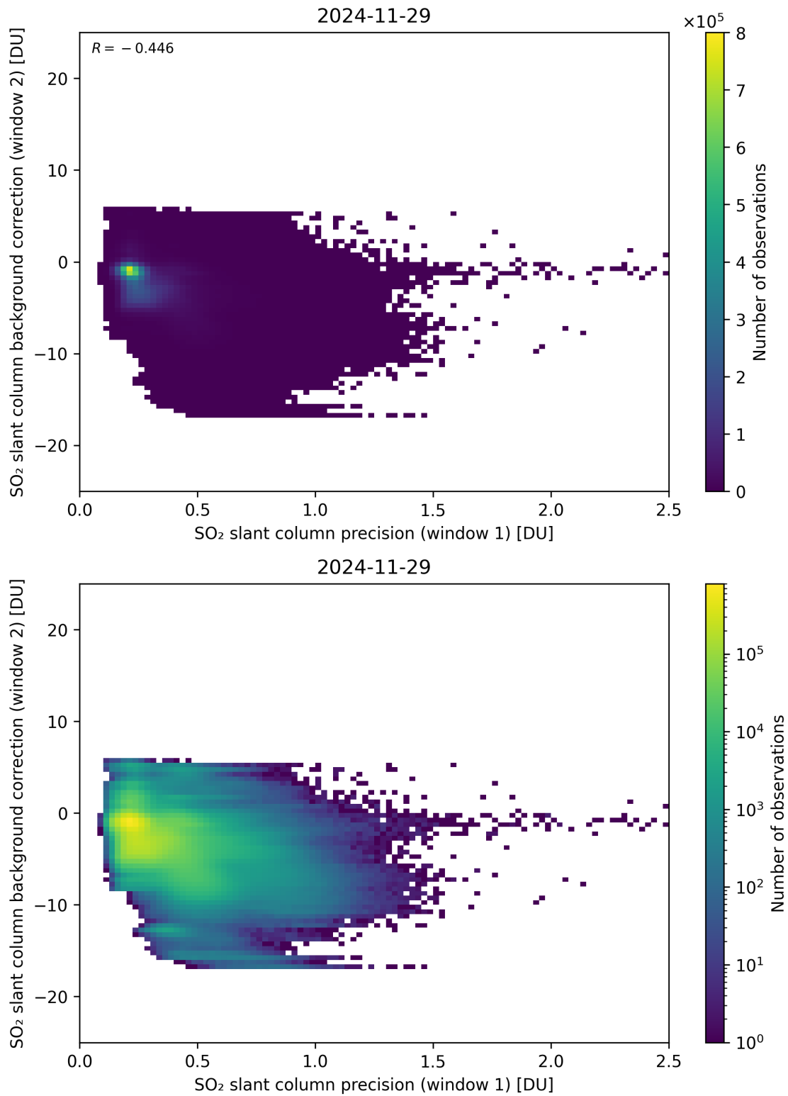
Figure 269: Scatter density plot of “SO 2 slant column precision (window 1)” against “SO 2 slant column background correction (window 2)” for 2024-11-28 to 2024-11-30.
