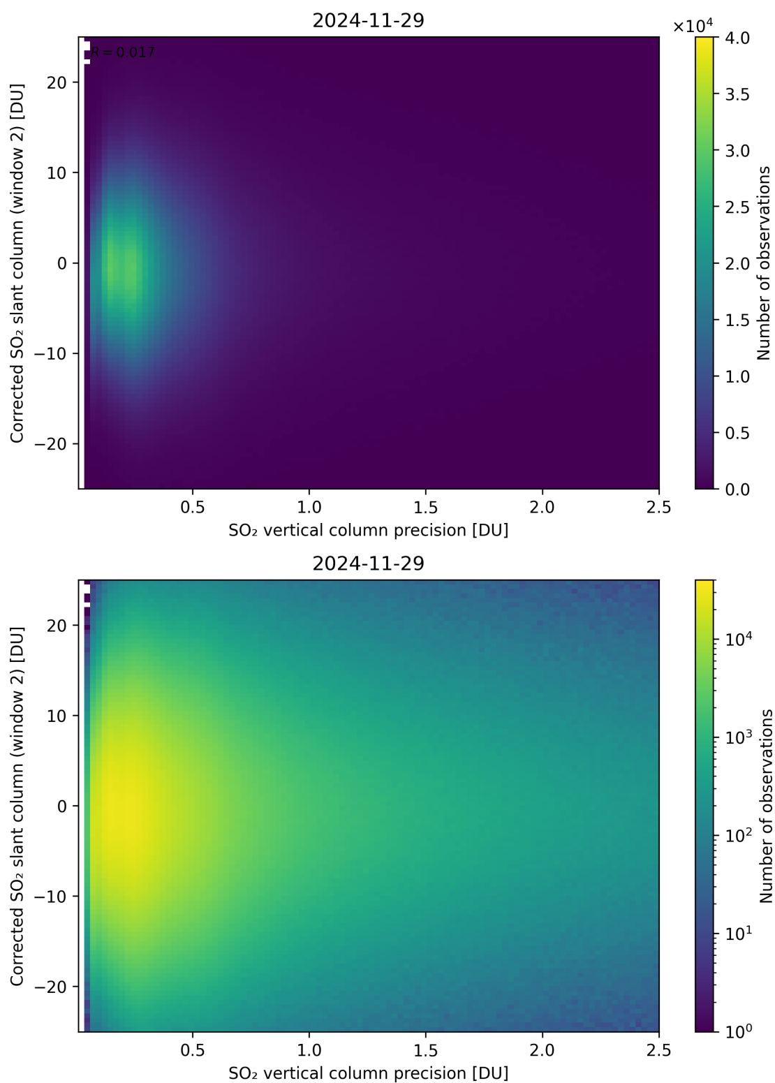
Figure 339: Scatter density plot of “SO 2 vertical column precision” against “Corrected SO 2 slant column (window 2)” for 2024-11-28 to 2024-11-30.
