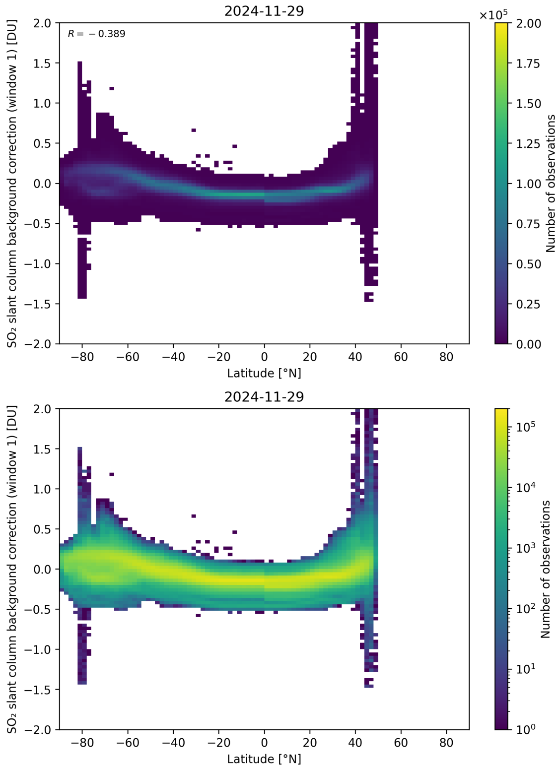
Figure 150: Scatter density plot of “Latitude” against “SO 2 slant column background correction (window 1)” for 2024-11-28 to 2024-11-30.
