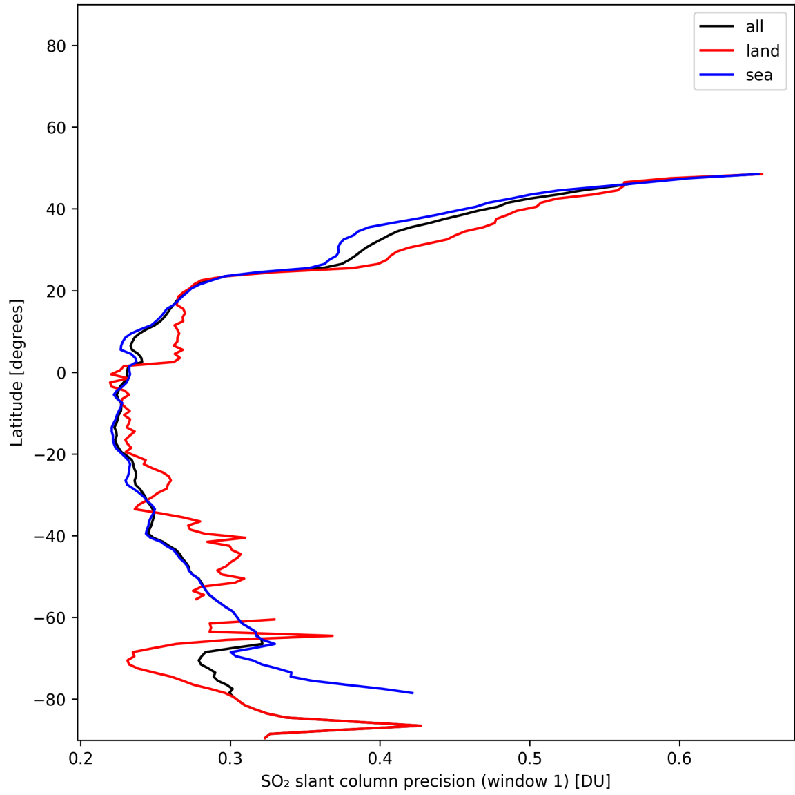
Figure 38: Zonal average of “SO 2 slant column precision (window 1)” for 2024-11-28 to 2024-11-30.
