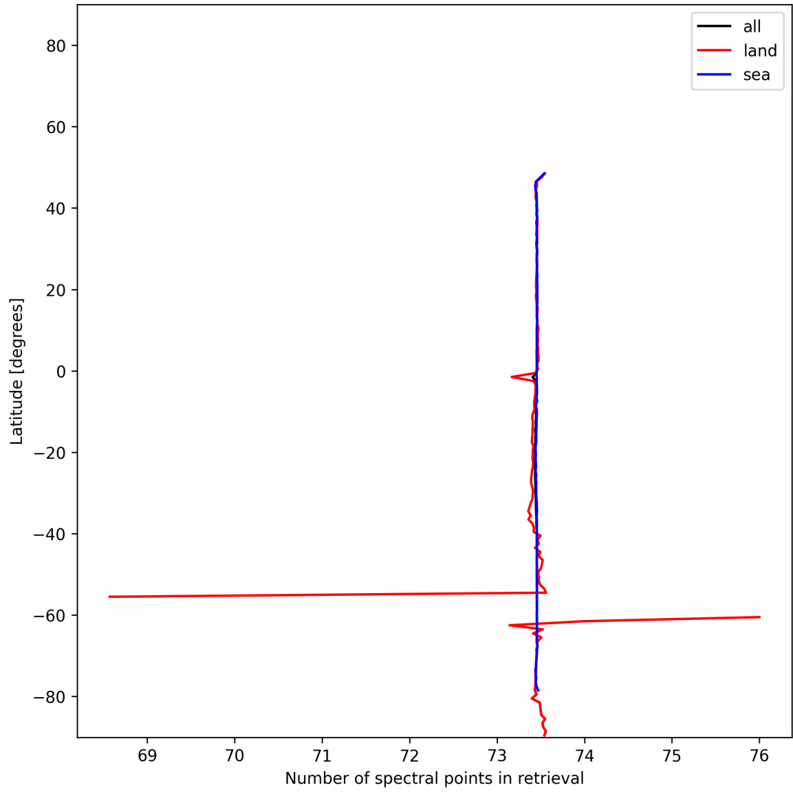
Figure 56: Zonal average of “Number of spectral points in retrieval” for 2024-11-28 to 2024-11-30.
