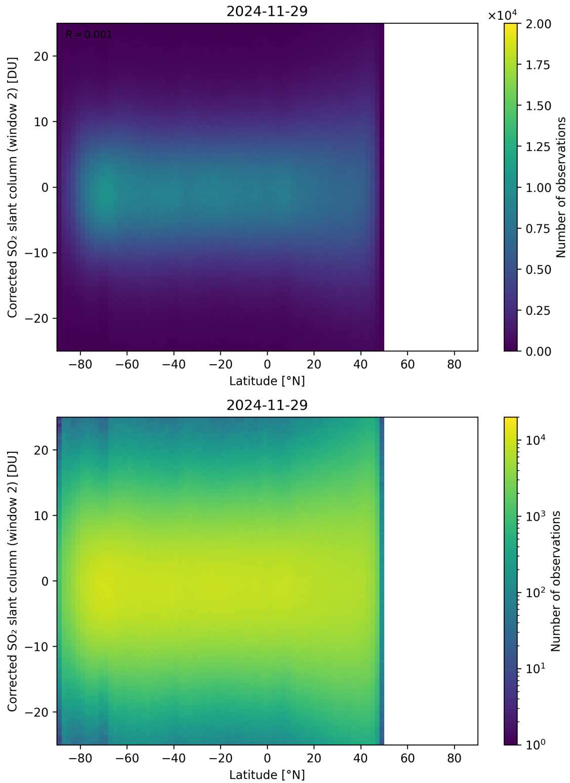
Figure 160: Scatter density plot of “Latitude” against “Corrected SO 2 slant column (window 2)” for 2024-11-28 to 2024-11-30.
