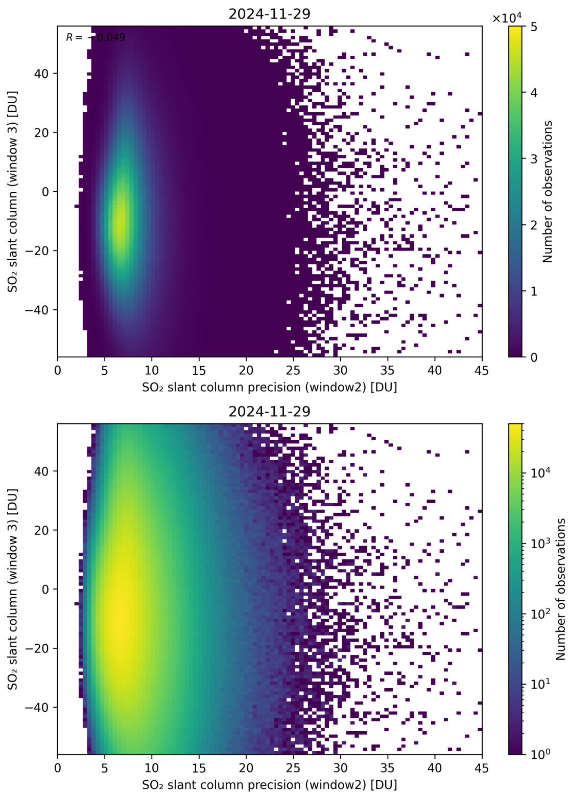
Figure 299: Scatter density plot of “SO 2 slant column precision (window2)” against “SO 2 slant column (window 3)” for 2024-11-28 to 2024-11-30.
