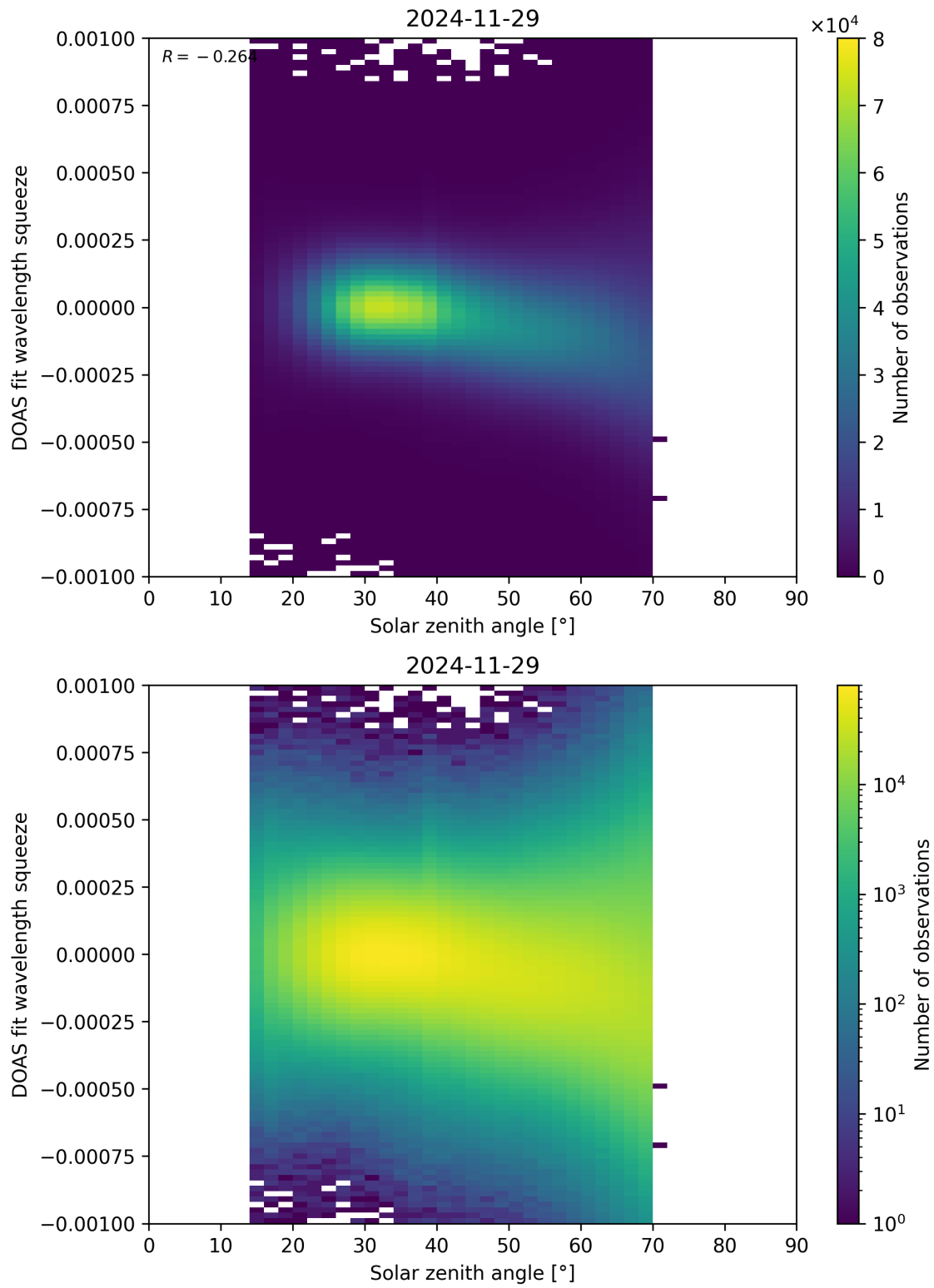
Figure 175: Scatter density plot of “Solar zenith angle” against “DOAS fit wavelength squeeze” for 2024-11-28 to 2024-11-30.
