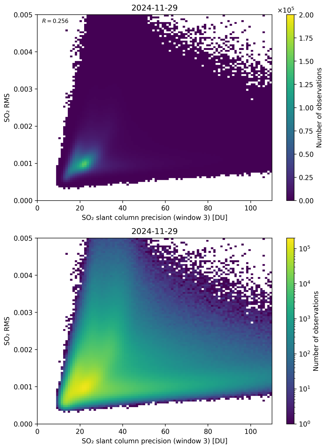
Figure 310: Scatter density plot of “SO 2 slant column precision (window 3)” against “SO 2 RMS” for 2024-11-28 to 2024-11-30.
