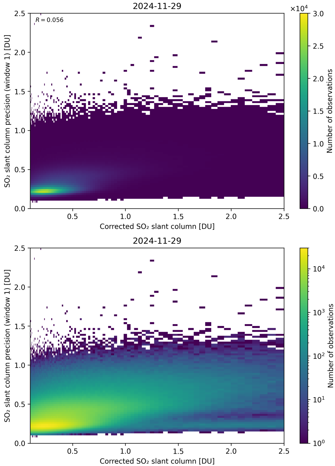
Figure 238: Scatter density plot of “Corrected SO 2 slant column” against “SO 2 slant column precision (window 1)” for 2024-11-28 to 2024-11-30.
