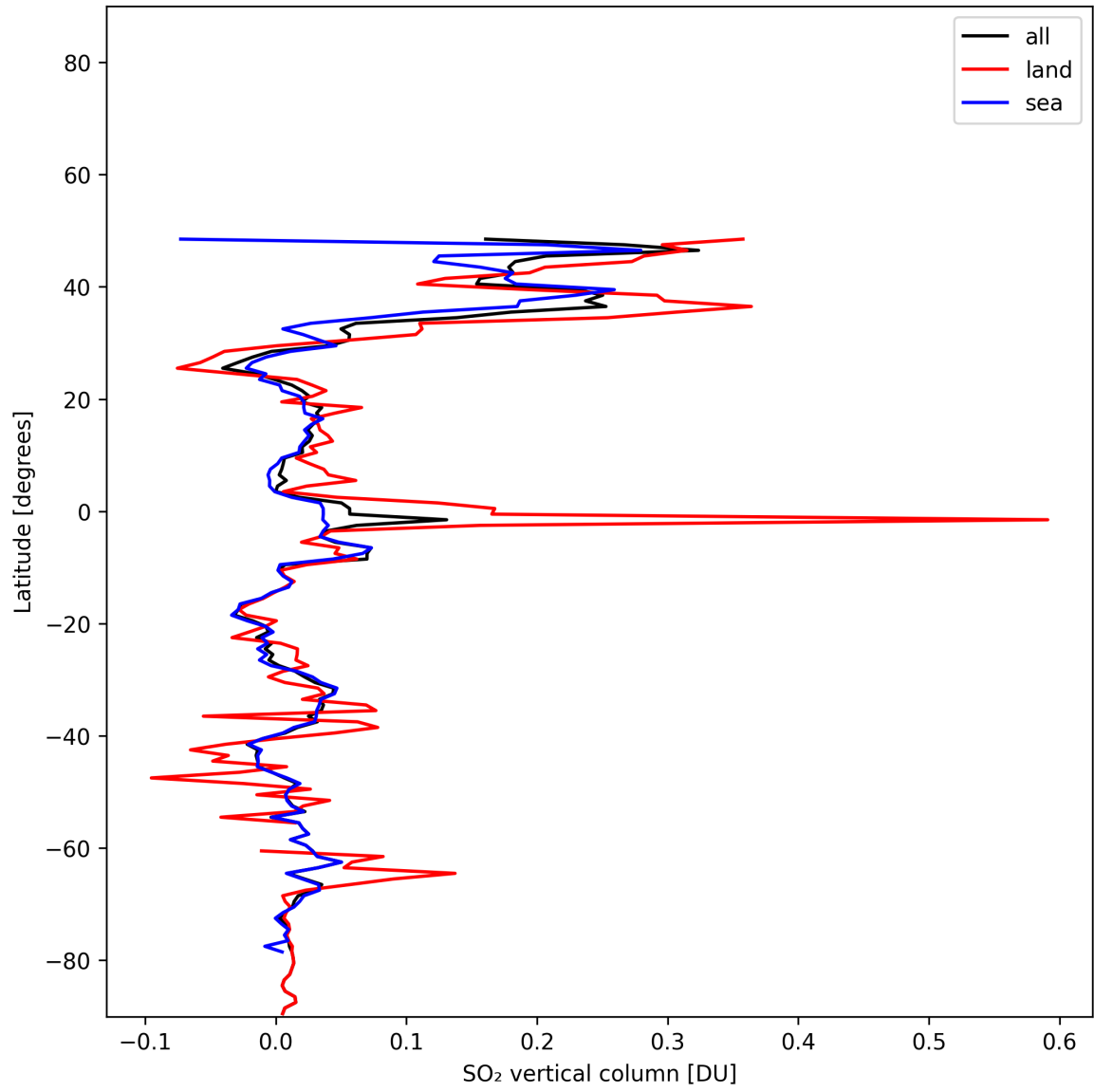
Figure 32: Zonal average of “SO 2 vertical column” for 2024-11-28 to 2024-11-30.
