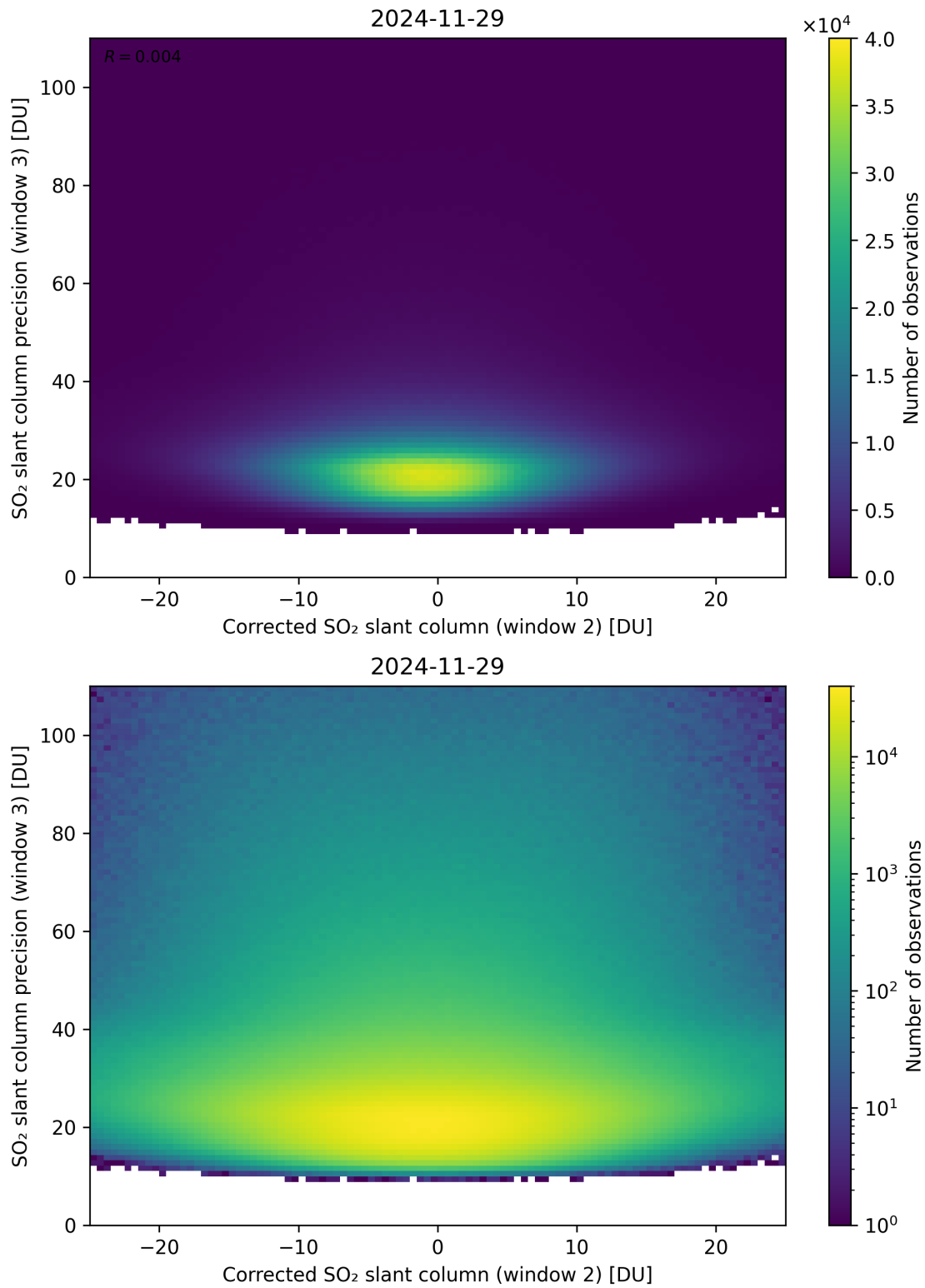
Figure 252: Scatter density plot of “Corrected SO 2 slant column (window 2)” against “SO 2 slant column precision (window 3)” for 2024-11-28 to 2024-11-30.
