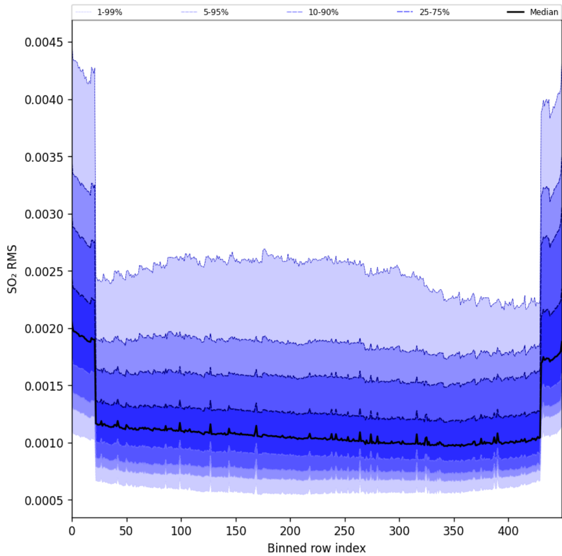
Figure 104: Along track statistics of “SO 2 RMS” for 2024-11-28 to 2024-11-30
