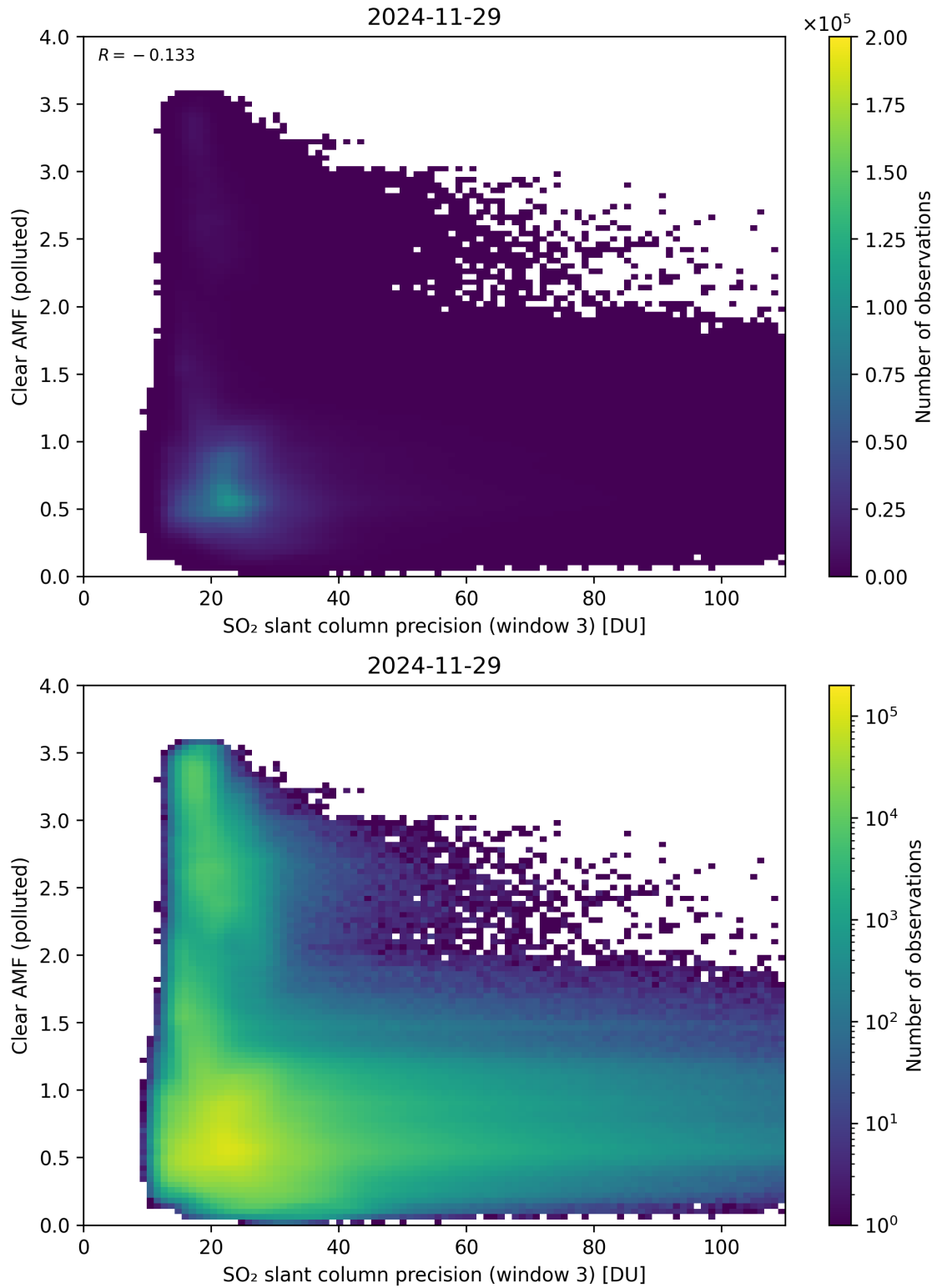
Figure 311: Scatter density plot of “SO 2 slant column precision (window 3)” against “Clear AMF (polluted)” for 2024-11-28 to 2024-11-30.
