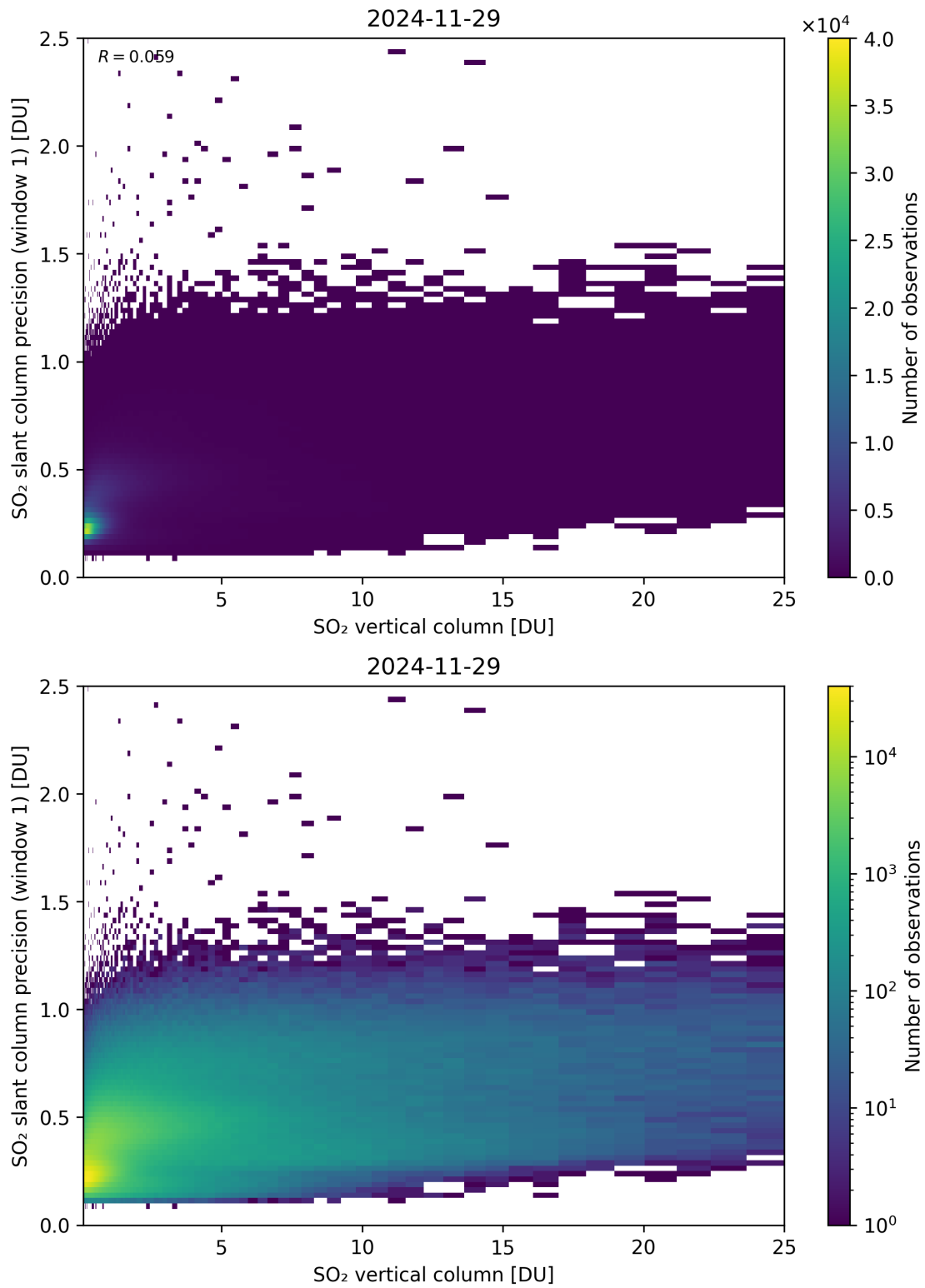
Figure 355: Scatter density plot of “SO 2 vertical column” against “SO 2 slant column precision (window 1)” for 2024-11-28 to 2024-11-30.
