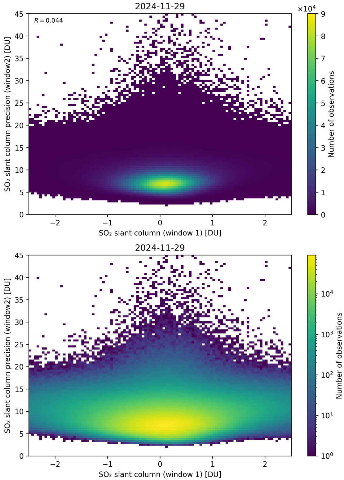
Figure 286: Scatter density plot of “SO 2 slant column (window 1)” against “SO 2 slant column precision (window2)” for 2024-11-28 to 2024-11-30.
