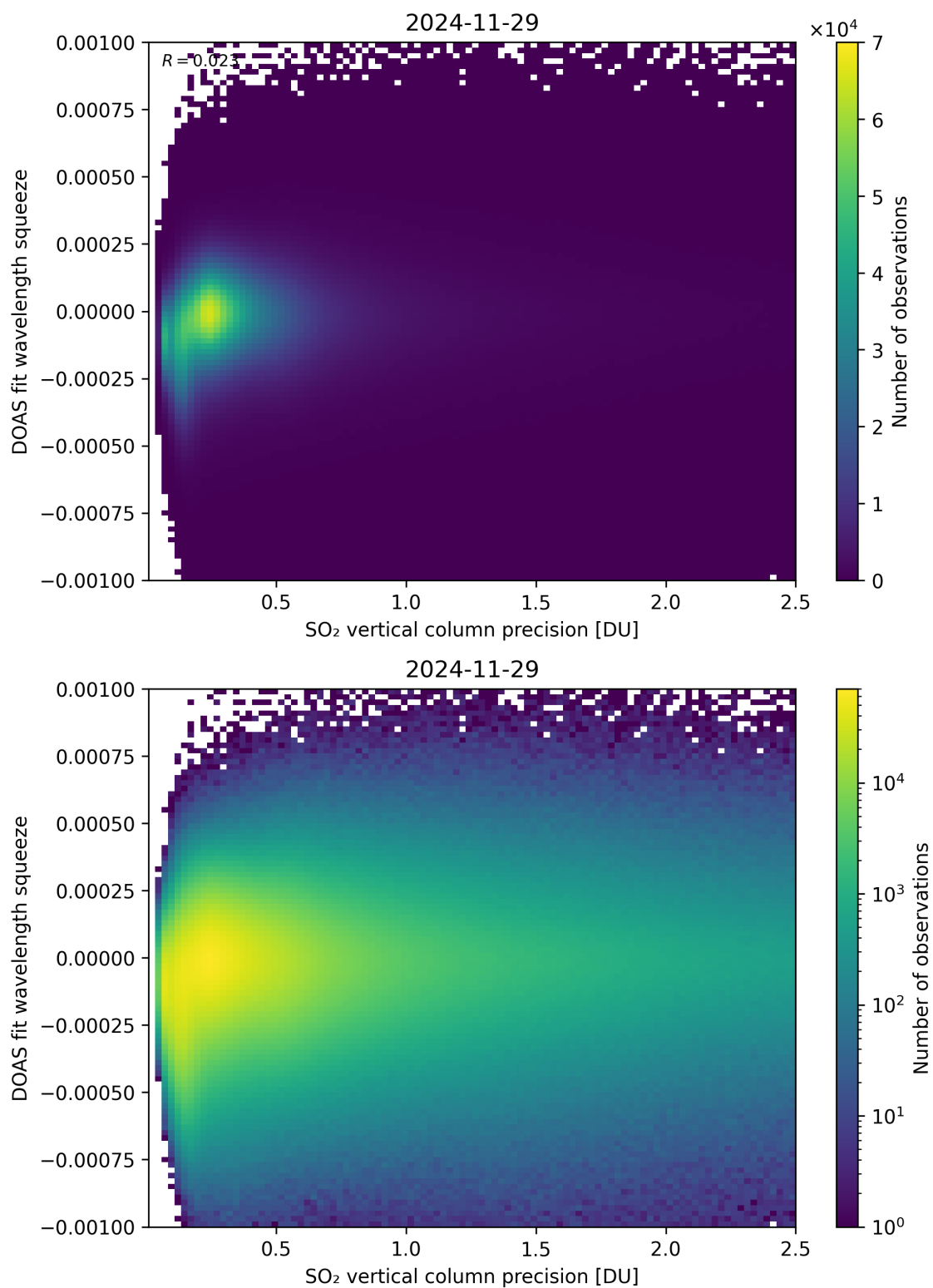
Figure 333: Scatter density plot of “SO 2 vertical column precision” against “DOAS fit wavelength squeeze” for 2024-11-28 to 2024-11-30.
