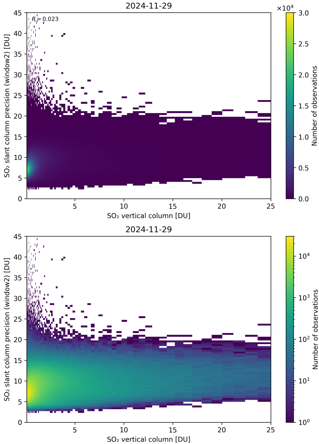
Figure 356: Scatter density plot of “SO 2 vertical column” against “SO 2 slant column precision (window2)” for 2024-11-28 to 2024-11-30.
