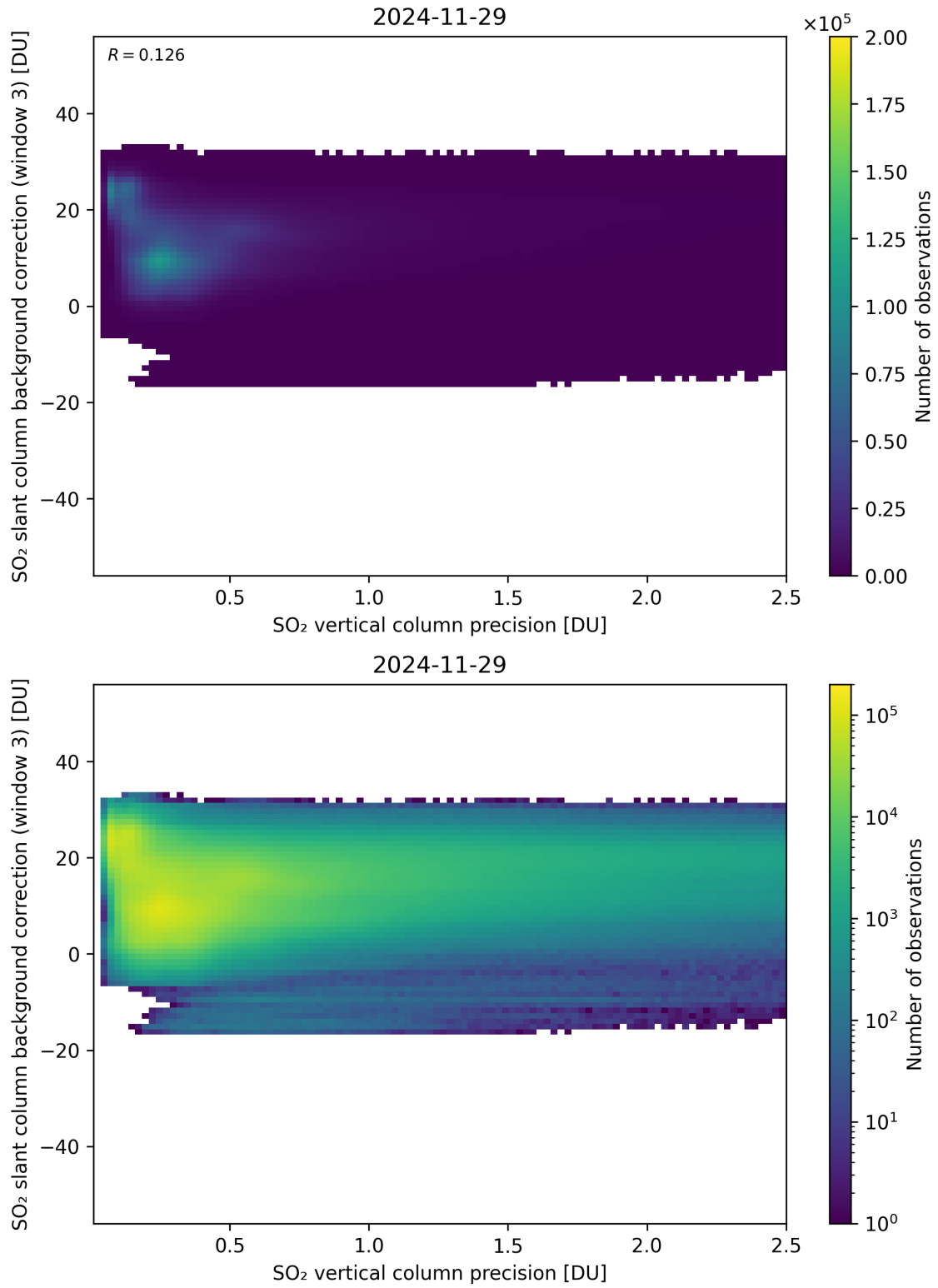
Figure 331: Scatter density plot of “SO 2 vertical column precision” against “SO 2 slant column background correction (window 3)” for 2024-11-28 to 2024-11-30.
