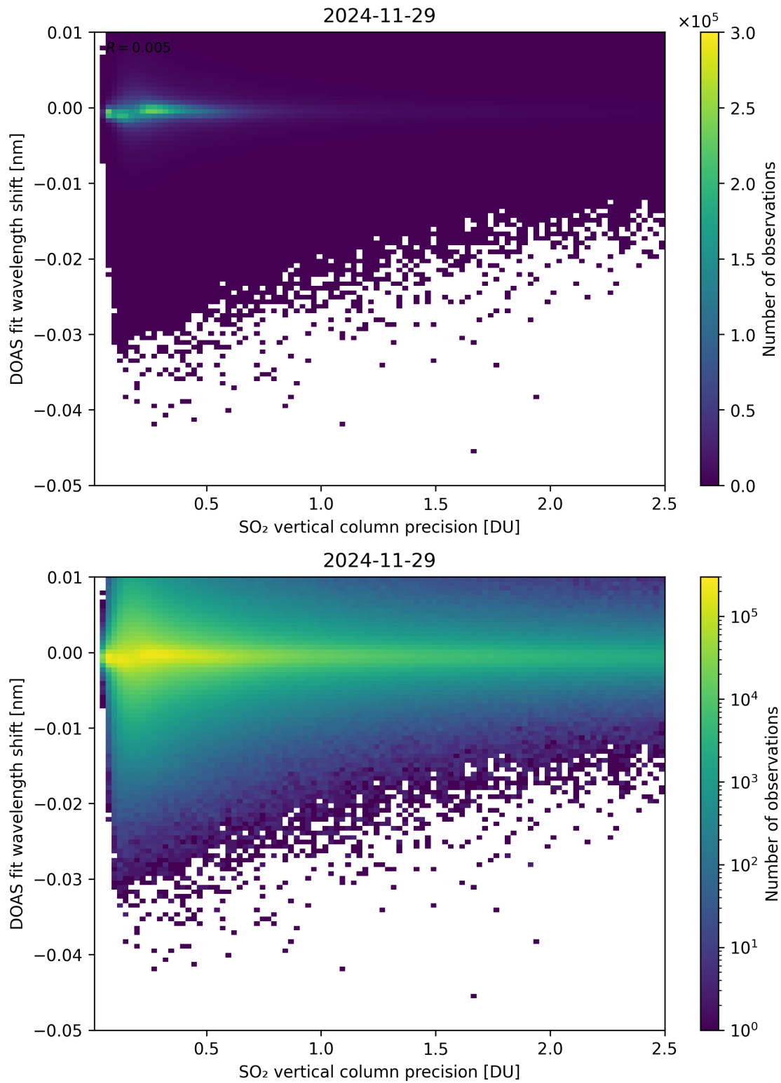
Figure 332: Scatter density plot of “SO 2 vertical column precision” against “DOAS fit wavelength shift” for 2024-11-28 to 2024-11-30.
