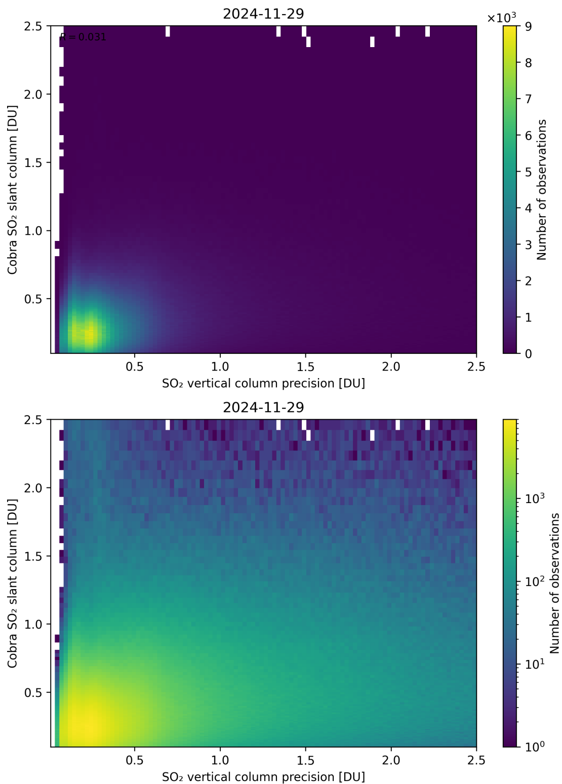
Figure 336: Scatter density plot of “SO 2 vertical column precision” against “Cobra SO 2 slant column” for 2024-11-28 to 2024-11-30.
