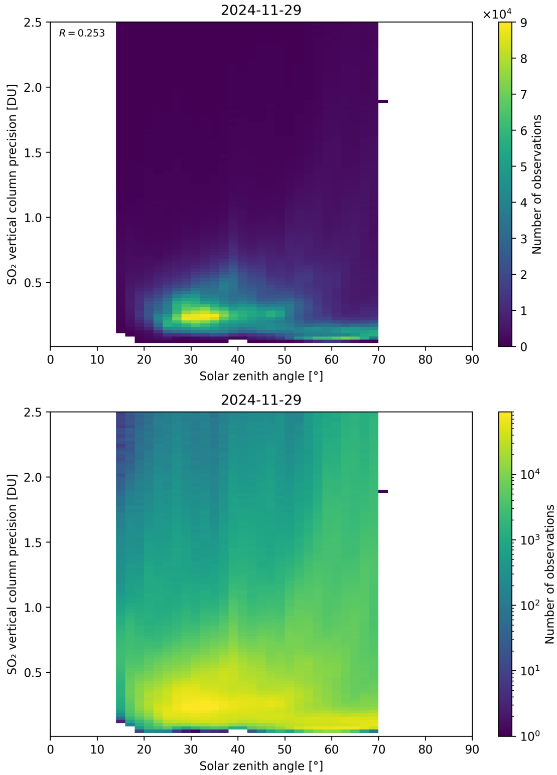
Figure 192: Scatter density plot of “Solar zenith angle” against “SO 2 vertical column precision” for 2024-11-28 to 2024-11-30.
