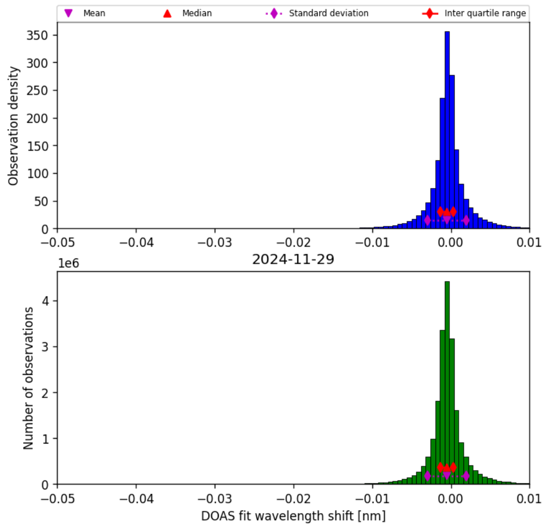
Figure 76: Histogram of “DOAS fit wavelength shift” for 2024-11-28 to 2024-11-30
