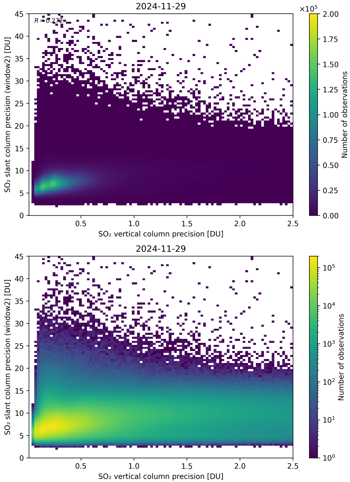
Figure 343: Scatter density plot of “SO 2 vertical column precision” against “SO 2 slant column precision (window2)” for 2024-11-28 to 2024-11-30.
