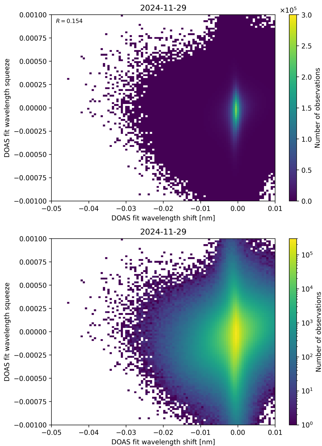
Figure 138: Scatter density plot of “DOAS fit wavelength shift” against “DOAS fit wavelength squeeze” for 2024-11-28 to 2024-11-30.
