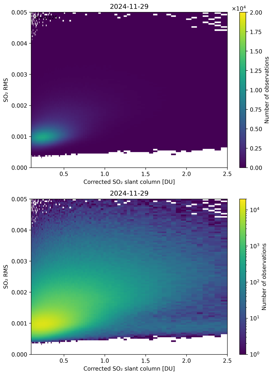
Figure 231: Scatter density plot of “Corrected SO 2 slant column” against “SO 2 RMS” for 2024-11-28 to 2024-11-30.
