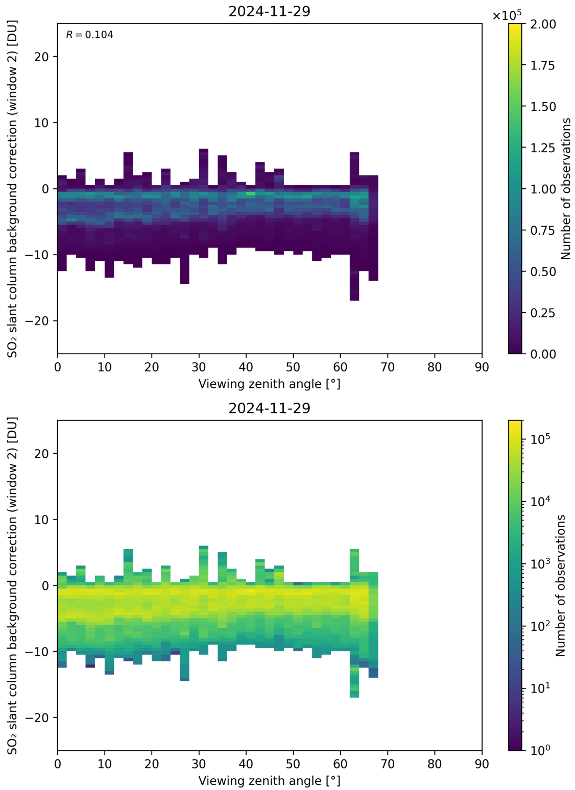
Figure 363: Scatter density plot of “Viewing zenith angle” against “SO 2 slant column background correction (window 2)” for 2024-11-28 to 2024-11-30.
