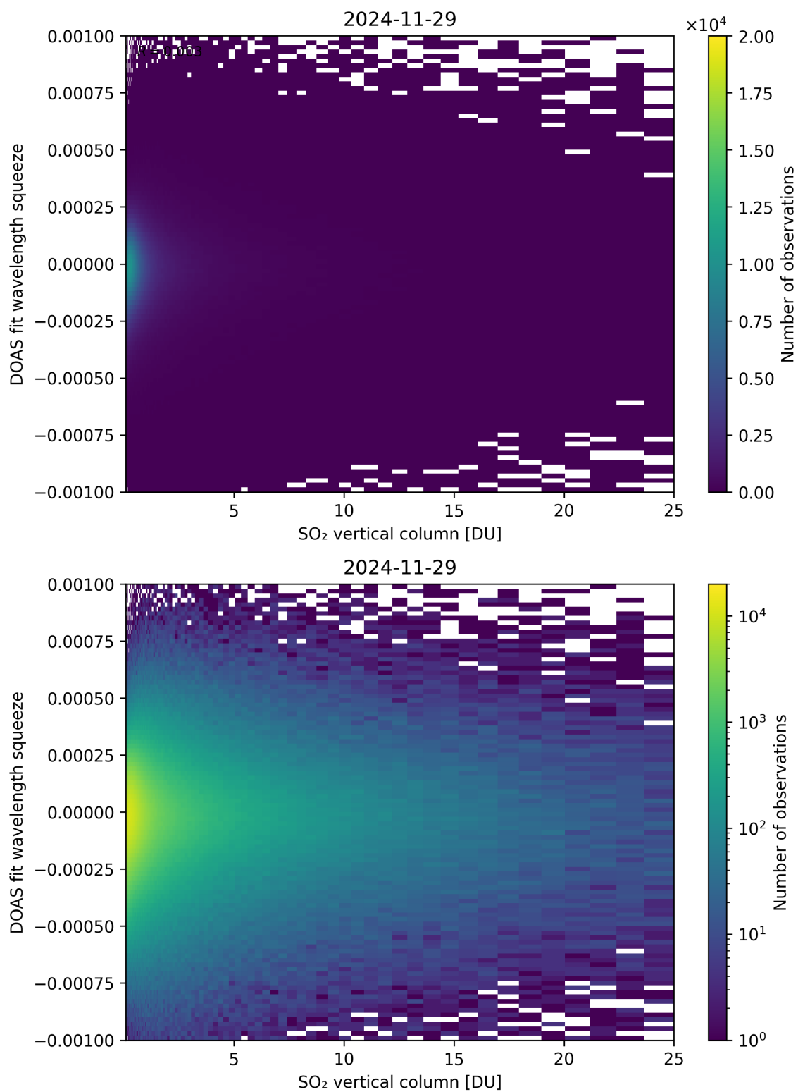
Figure 327: Scatter density plot of “SO 2 vertical column” against “DOAS fit wavelength squeeze” for 2024-11-28 to 2024-11-30.
