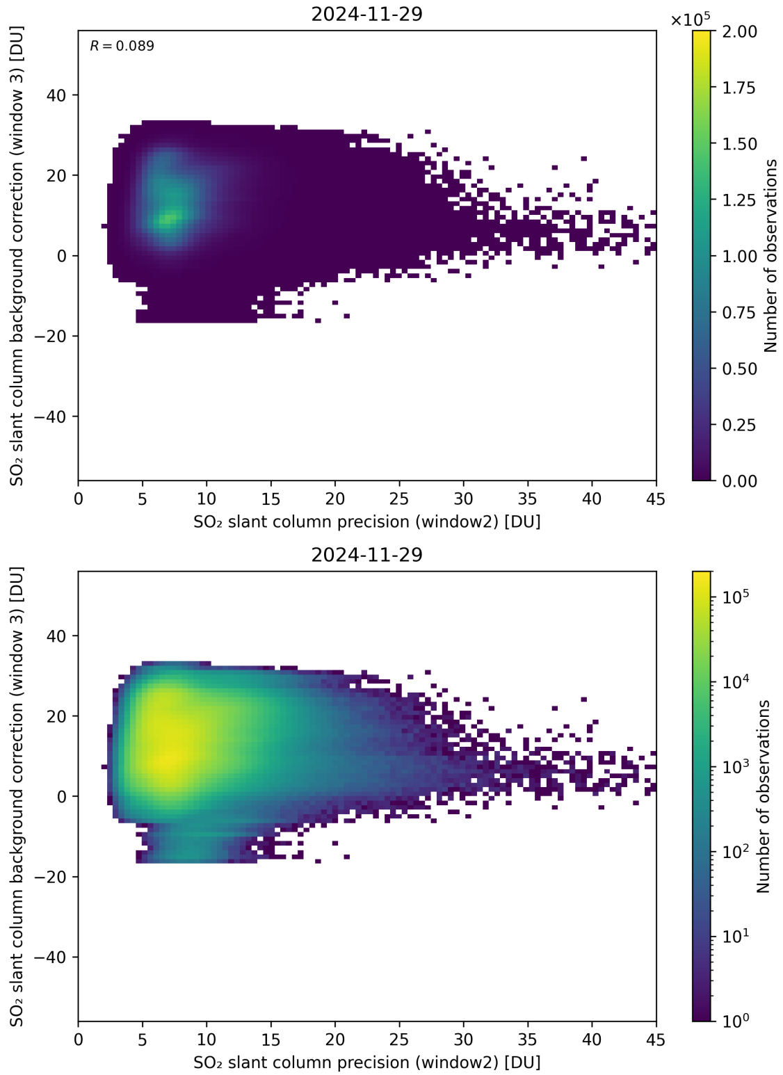
Figure 292: Scatter density plot of “SO 2 slant column precision (window2)” against “SO 2 slant column background correction (window 3)” for 2024-11-28 to 2024-11-30.
