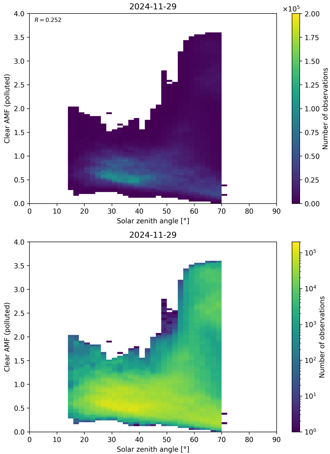
Figure 178: Scatter density plot of “Solar zenith angle” against “Clear AMF (polluted)” for 2024-11-28 to 2024-11-30.
