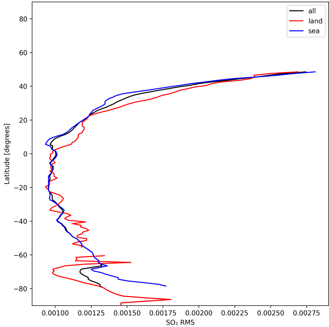
Figure 52: Zonal average of “SO 2 RMS” for 2024-11-28 to 2024-11-30.
