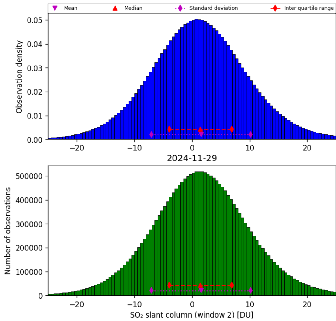
Figure 67: Histogram of “SO 2 slant column (window 2)” for 2024-11-28 to 2024-11-30
