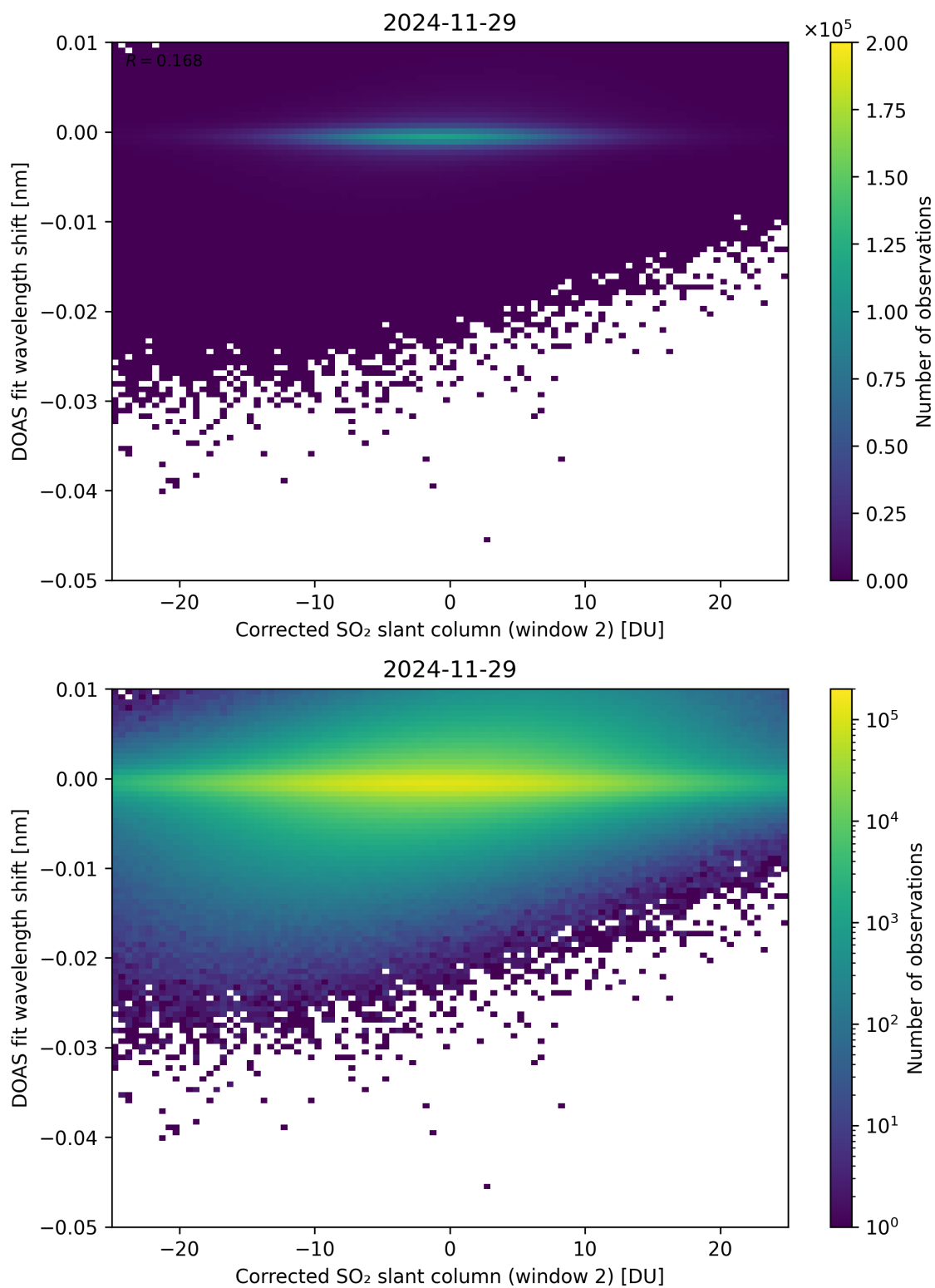
Figure 246: Scatter density plot of “Corrected SO 2 slant column (window 2)” against “DOAS fit wavelength shift” for 2024-11-28 to 2024-11-30.
