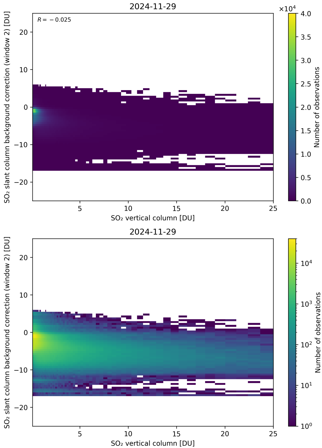
Figure 324: Scatter density plot of “SO 2 vertical column” against “SO 2 slant column background correction (window 2)” for 2024-11-28 to 2024-11-30.
