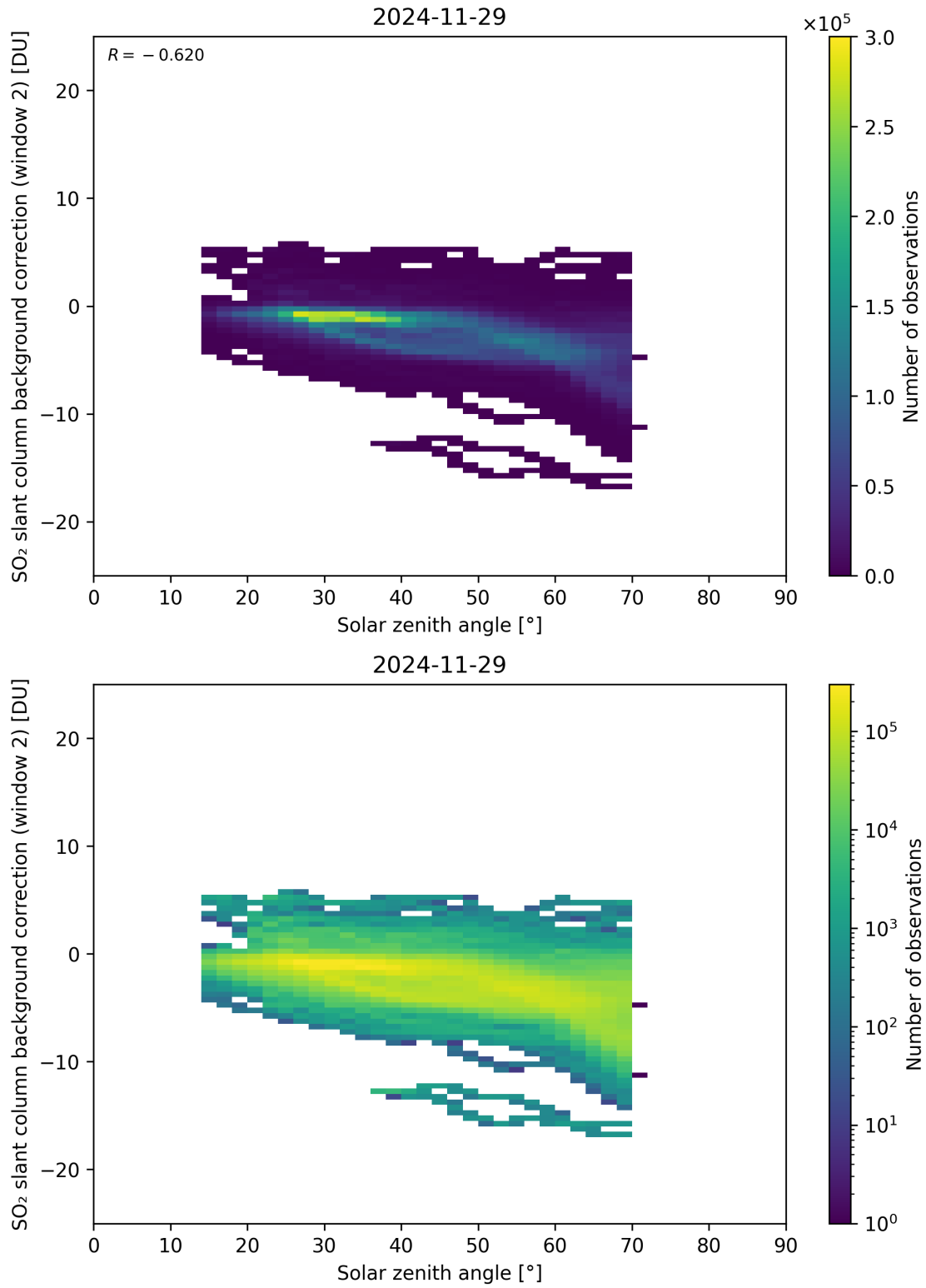
Figure 172: Scatter density plot of “Solar zenith angle” against “SO 2 slant column background correction (window 2)” for 2024-11-28 to 2024-11-30.
