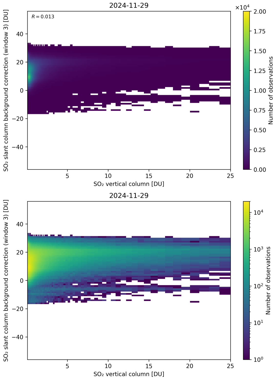
Figure 325: Scatter density plot of “SO 2 vertical column” against “SO 2 slant column background correction (window 3)” for 2024-11-28 to 2024-11-30.
