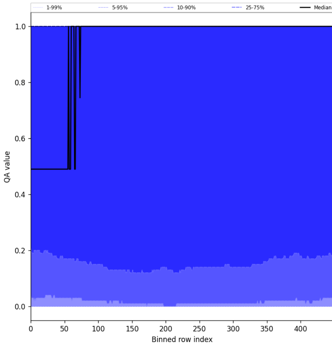
Figure 83: Along track statistics of “QA value” for 2024-11-28 to 2024-11-30
