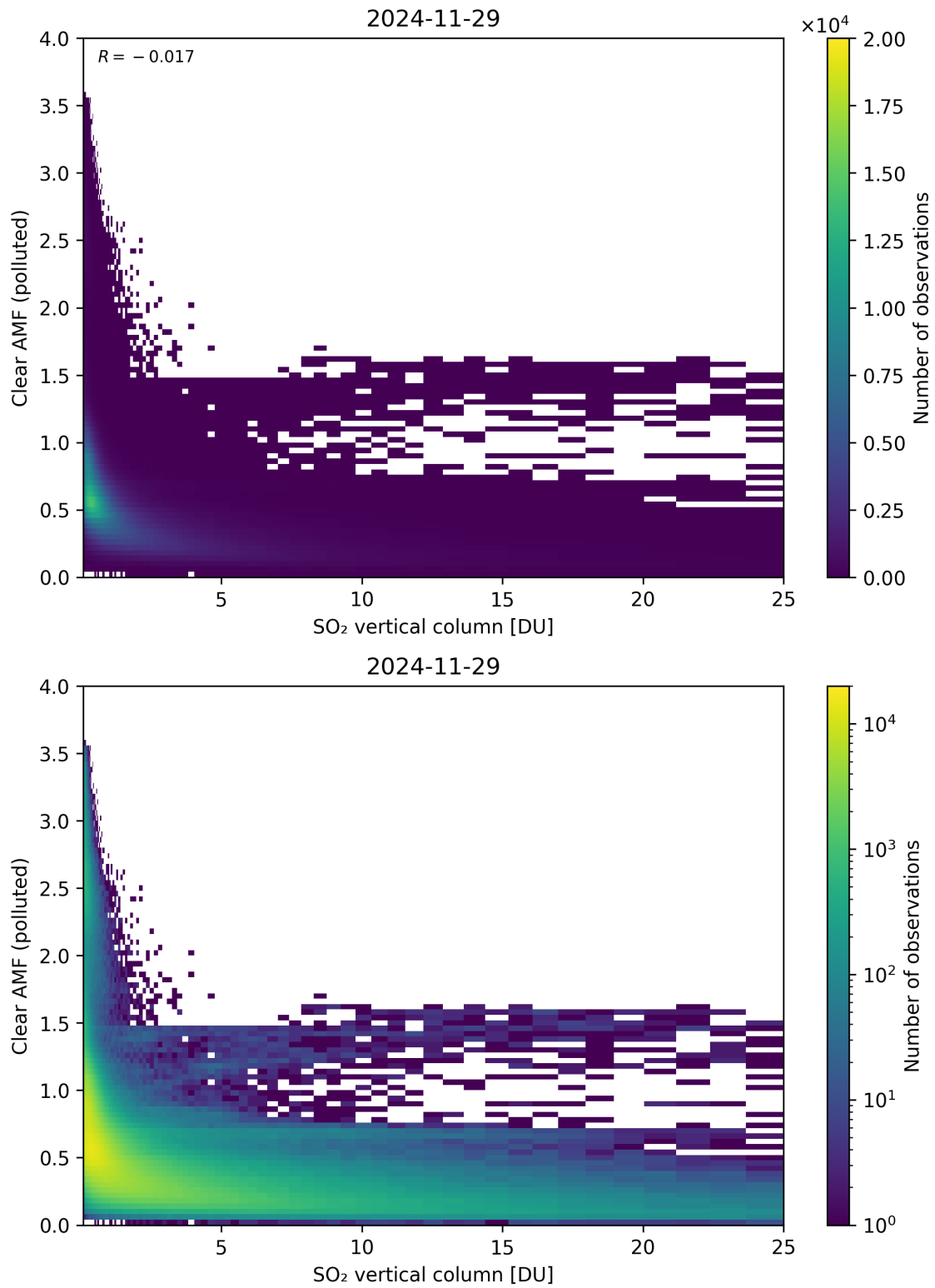
Figure 348: Scatter density plot of “SO 2 vertical column” against “Clear AMF (polluted)” for 2024-11-28 to 2024-11-30.
