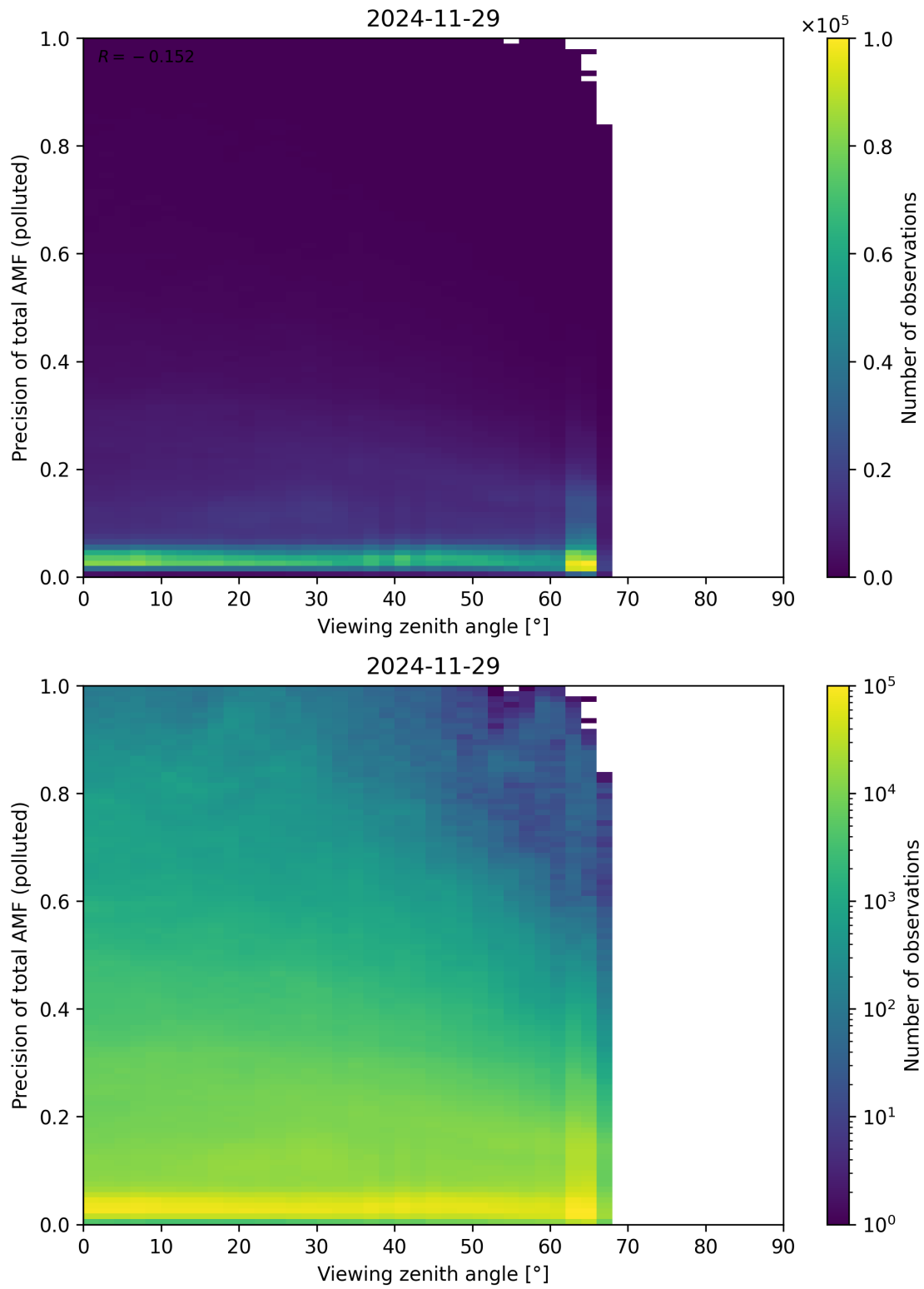
Figure 382: Scatter density plot of “Viewing zenith angle” against “Precision of total AMF (polluted)” for 2024-11-28 to 2024-11-30.
