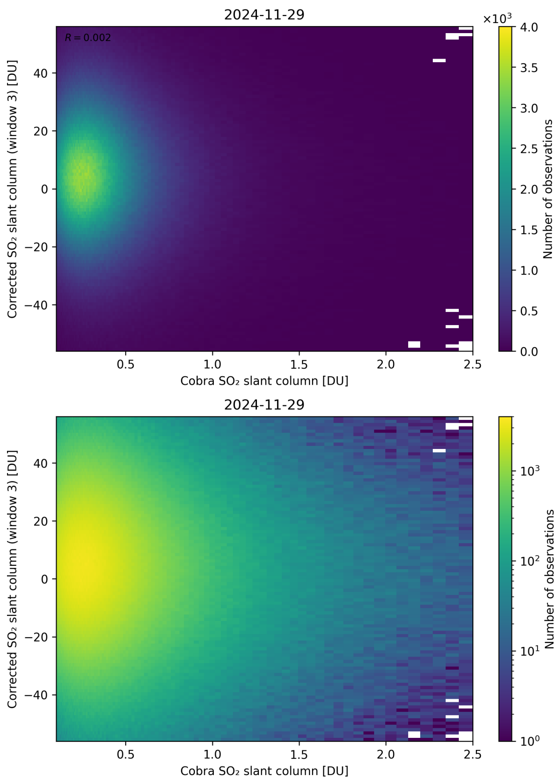
Figure 218: Scatter density plot of “Cobra SO 2 slant column” against “Corrected SO 2 slant column (window 3)” for 2024-11-28 to 2024-11-30.
