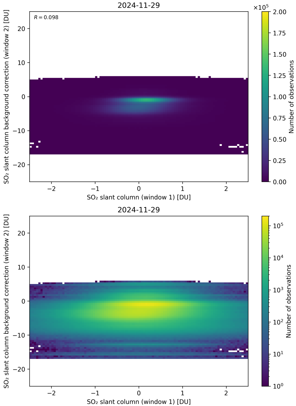
Figure 263: Scatter density plot of “SO 2 slant column (window 1)” against “SO 2 slant column background correction (window 2)” for 2024-11-28 to 2024-11-30.
