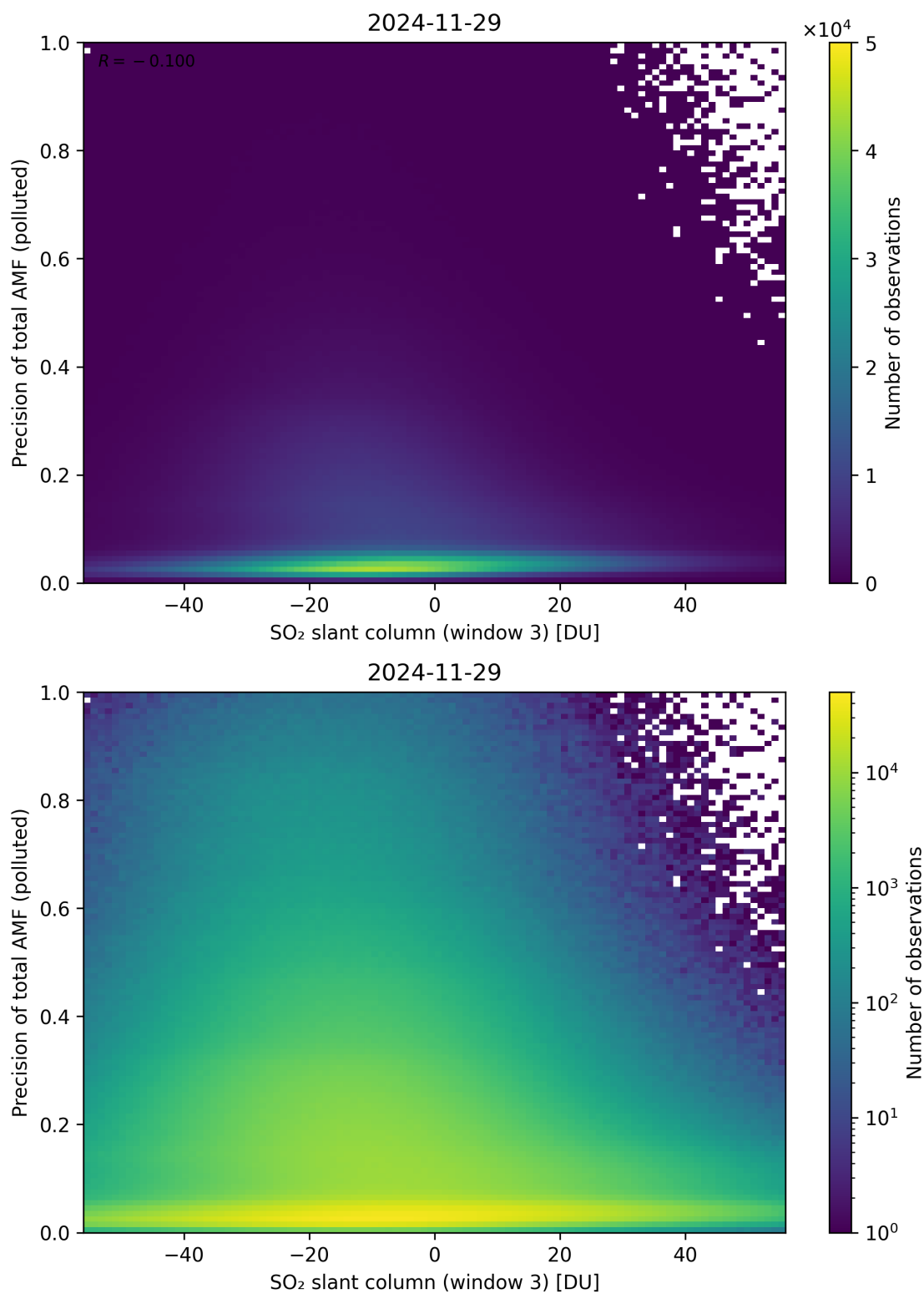
Figure 319: Scatter density plot of “SO 2 slant column (window 3)” against “Precision of total AMF (polluted)” for 2024-11-28 to 2024-11-30.
