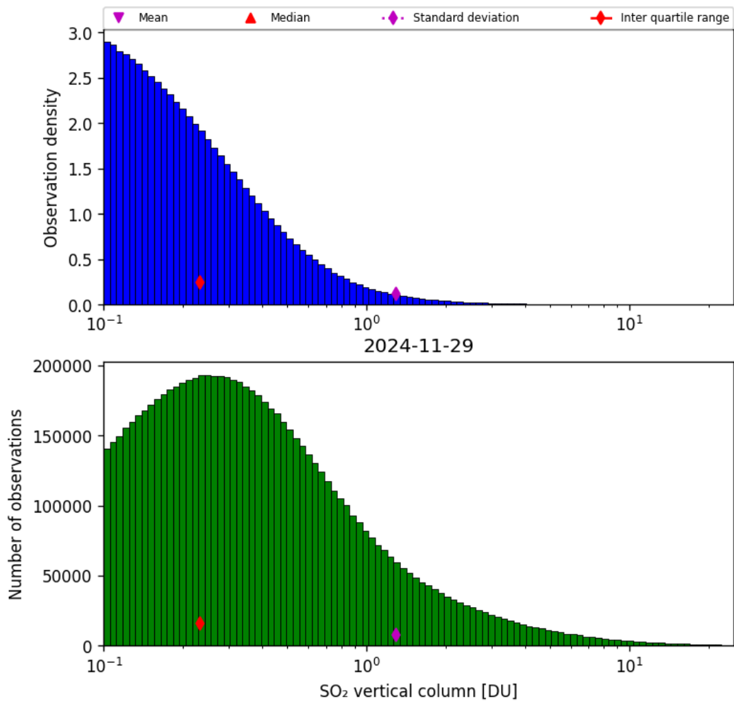
Figure 58: Histogram of “SO 2 vertical column” for 2024-11-28 to 2024-11-30
