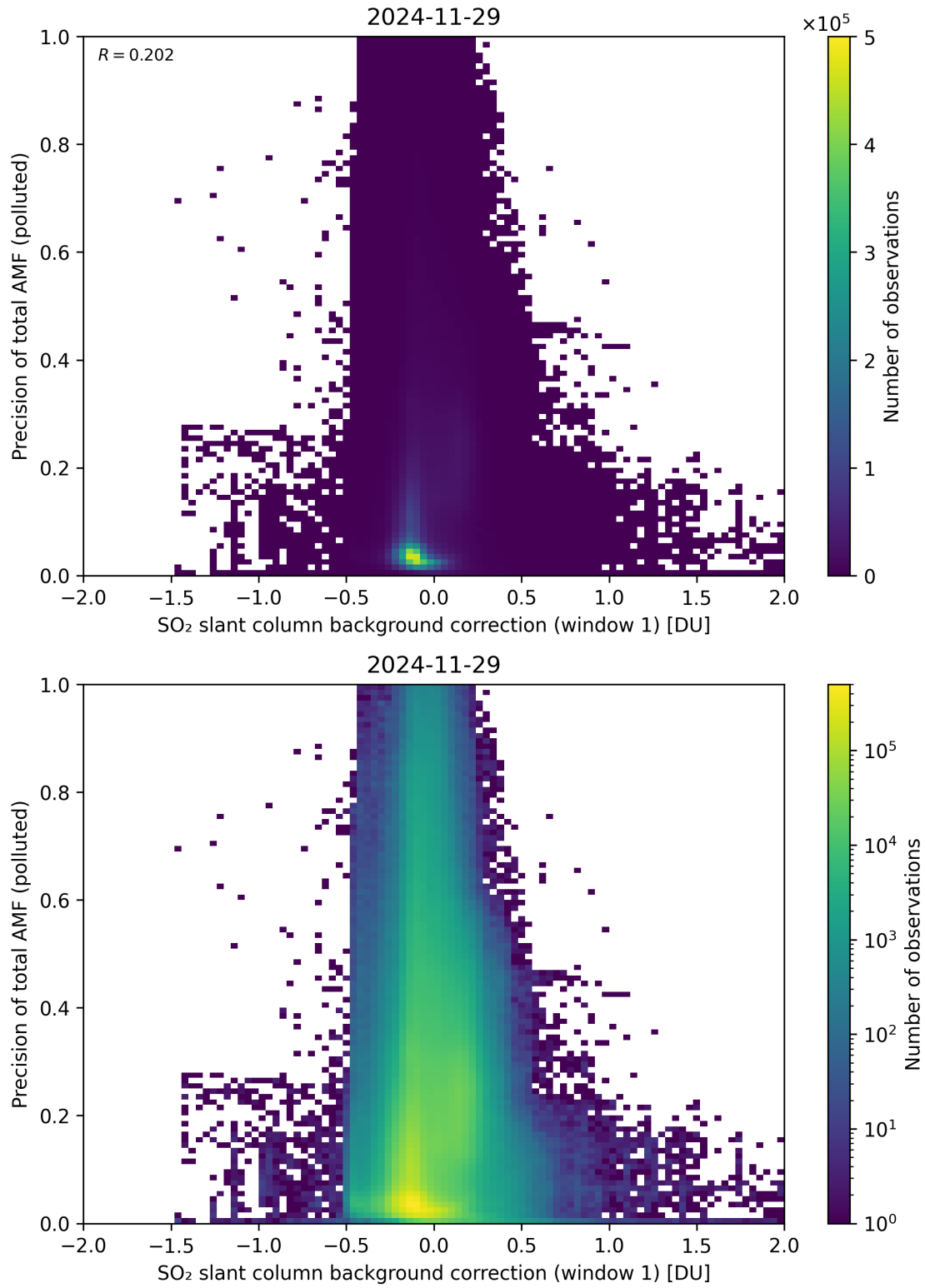
Figure 121: Scatter density plot of “SO 2 slant column background correction (window 1)” against “Precision of total AMF (polluted)” for 2024-11-28 to 2024-11-30.
