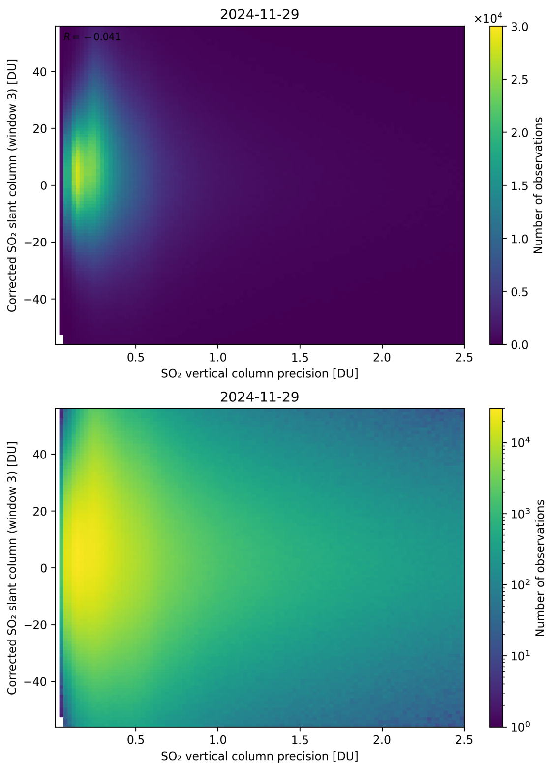
Figure 340: Scatter density plot of “SO 2 vertical column precision” against “Corrected SO 2 slant column (window 3)” for 2024-11-28 to 2024-11-30.
