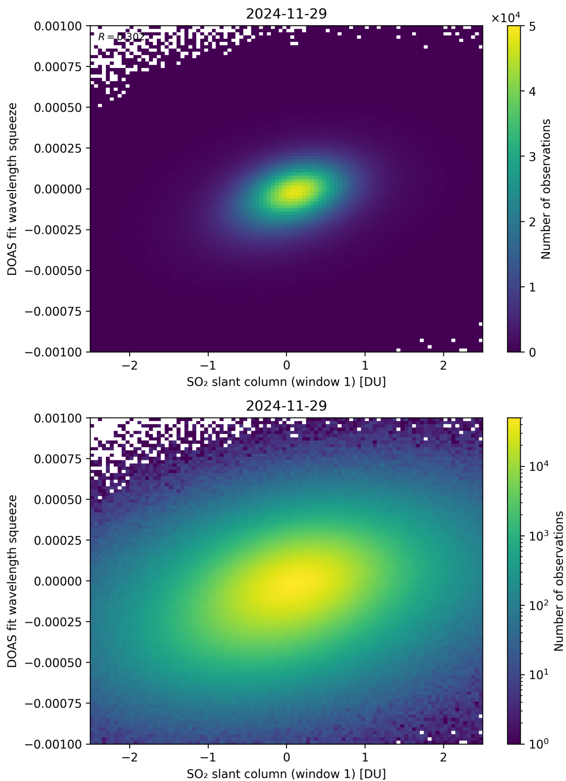
Figure 266: Scatter density plot of “SO 2 slant column (window 1)” against “DOAS fit wavelength squeeze” for 2024-11-28 to 2024-11-30.
