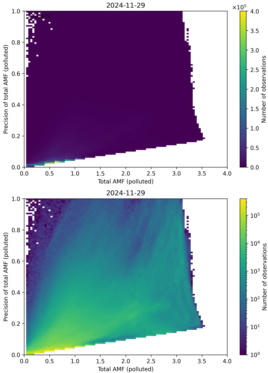
Figure 322: Scatter density plot of “Total AMF (polluted)” against “Precision of total AMF (polluted)” for 2024-11-28 to 2024-11-30.
