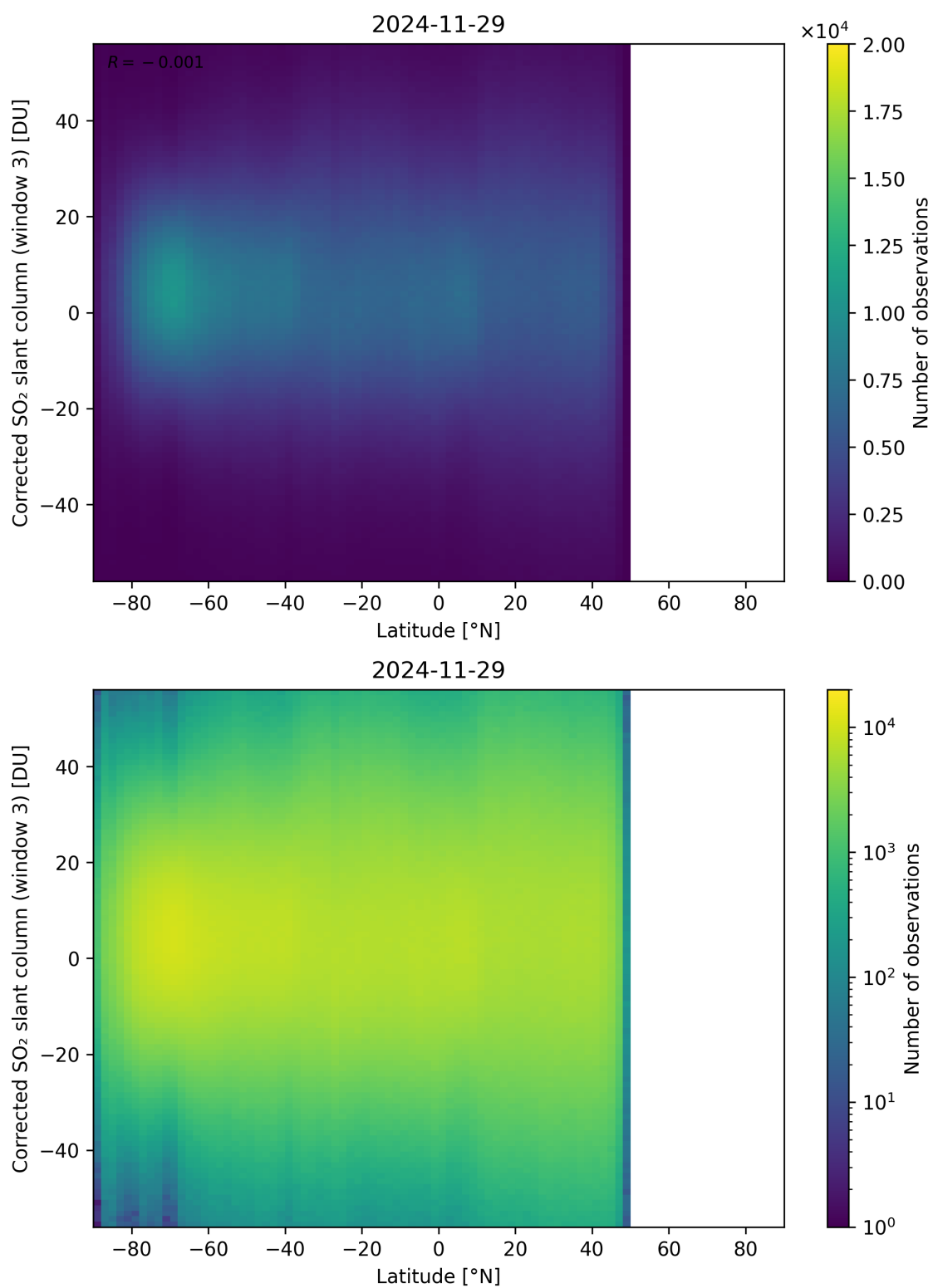
Figure 161: Scatter density plot of “Latitude” against “Corrected SO 2 slant column (window 3)” for 2024-11-28 to 2024-11-30.
