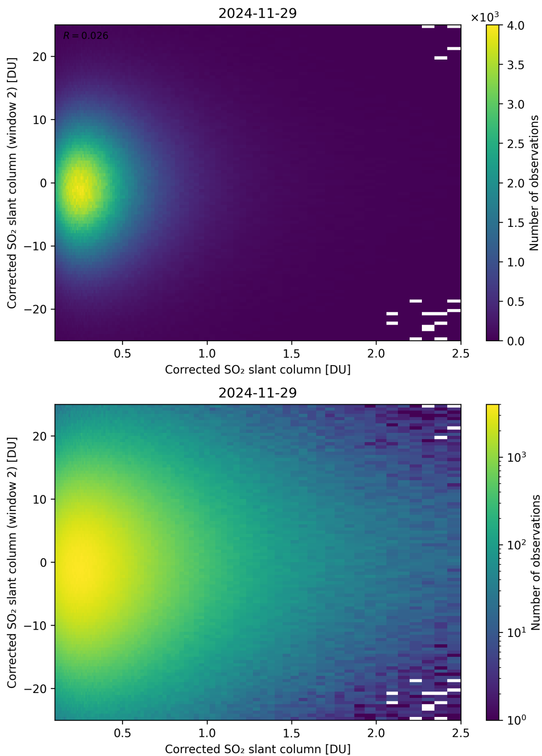
Figure 235: Scatter density plot of “Corrected SO 2 slant column” against “Corrected SO 2 slant column (window 2)” for 2024-11-28 to 2024-11-30.
