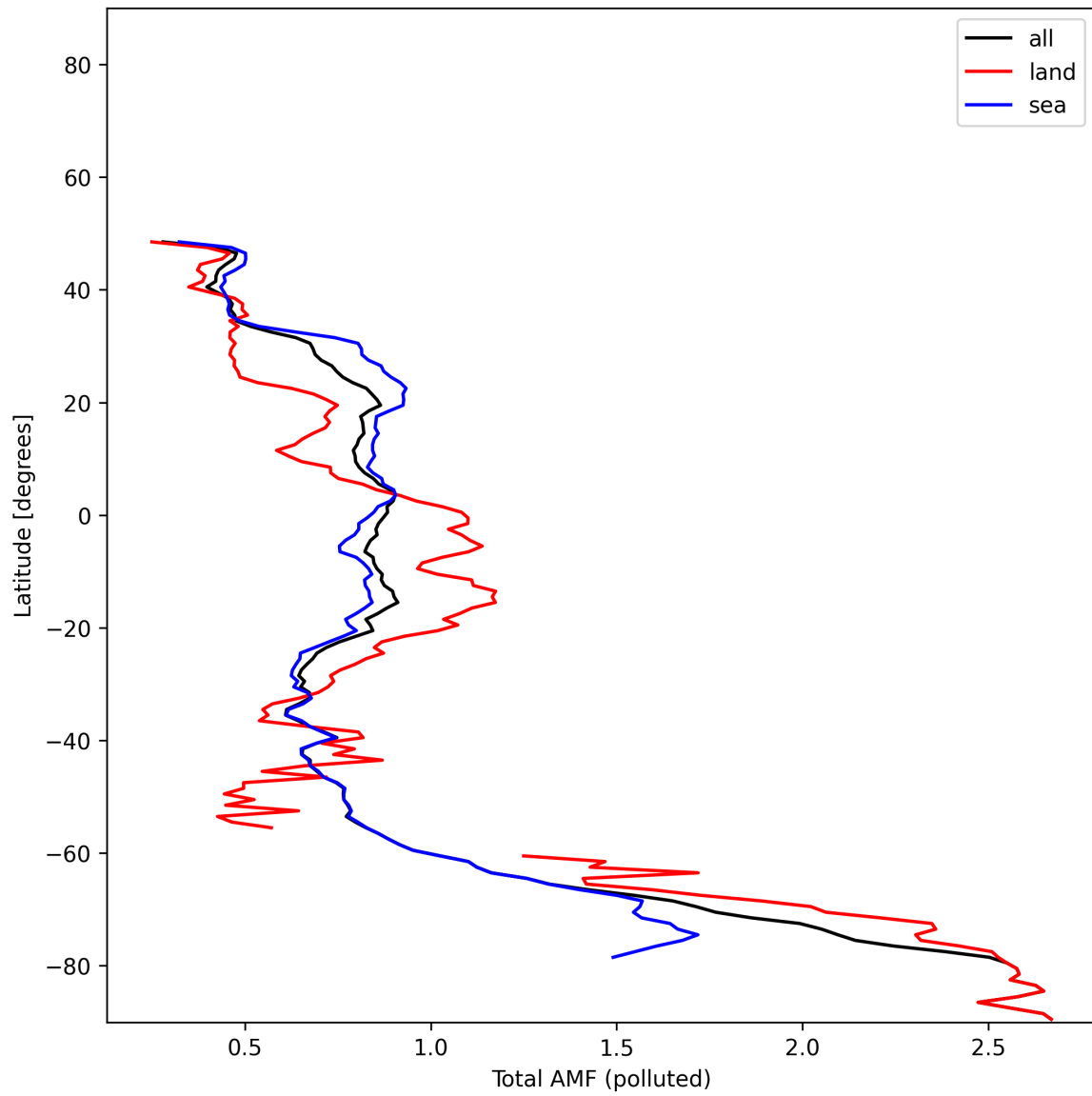
Figure 53: Zonal average of “Total AMF (polluted)” for 2024-11-28 to 2024-11-30.
