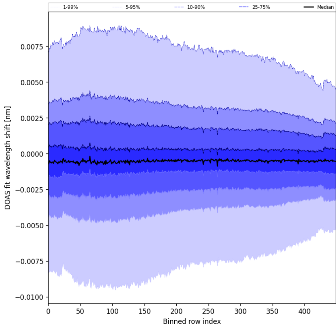
Figure 102: Along track statistics of “DOAS fit wavelength shift” for 2024-11-28 to 2024-11-30
