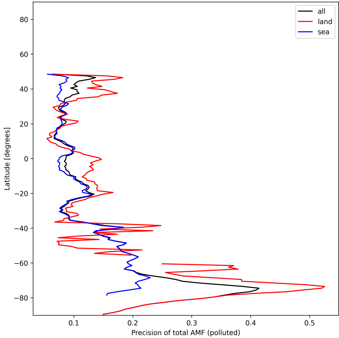
Figure 54: Zonal average of “Precision of total AMF (polluted)” for 2024-11-28 to 2024-11-30.
