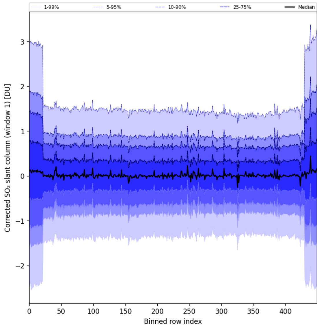
Figure 91: Along track statistics of “Corrected SO 2 slant column (window 1)” for 2024-11-28 to 2024-11-30
