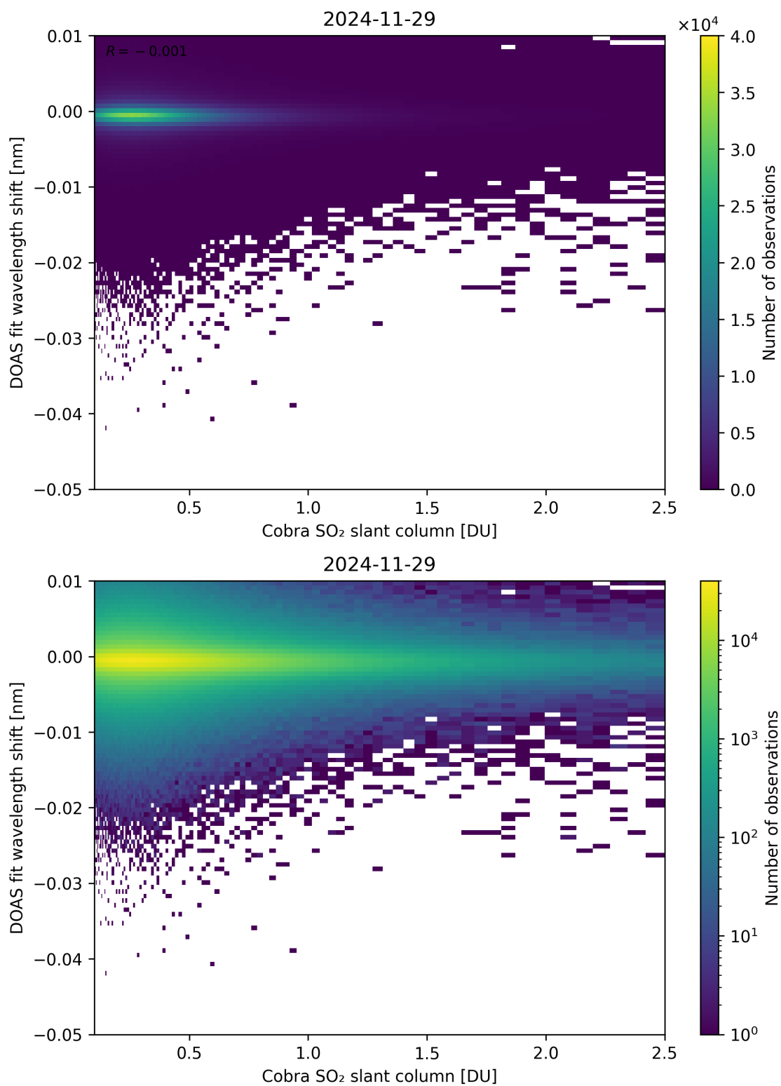
Figure 196: Scatter density plot of “Cobra SO 2 slant column” against “DOAS fit wavelength shift” for 2024-11-28 to 2024-11-30.
