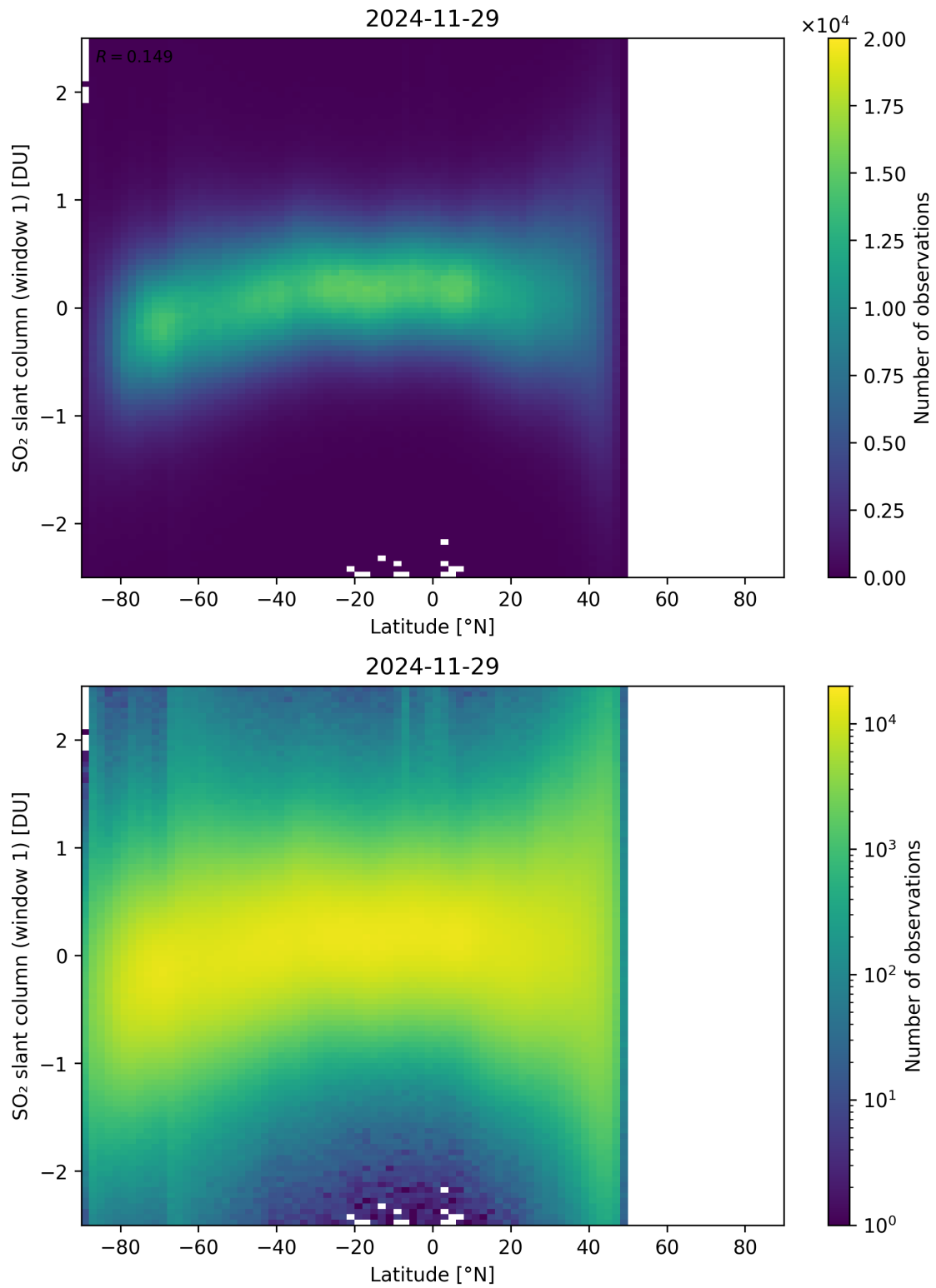
Figure 162: Scatter density plot of “Latitude” against “SO 2 slant column (window 1)” for 2024-11-28 to 2024-11-30.
