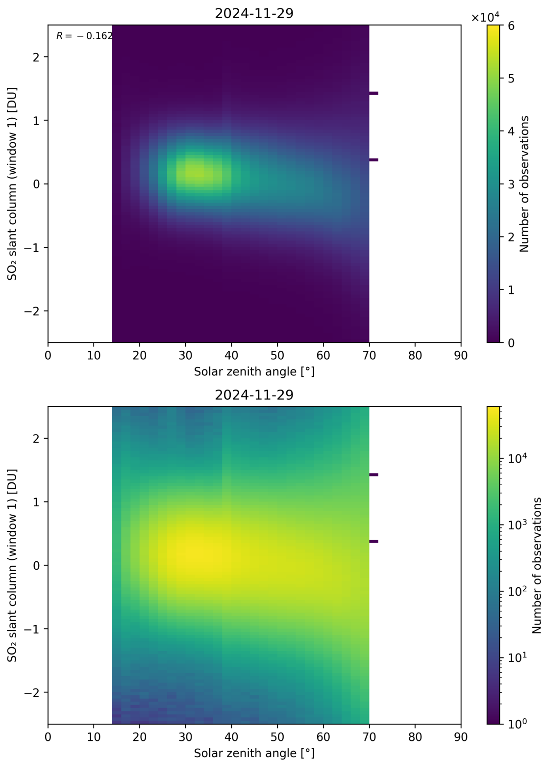
Figure 184: Scatter density plot of “Solar zenith angle” against “SO 2 slant column (window 1)” for 2024-11-28 to 2024-11-30.
