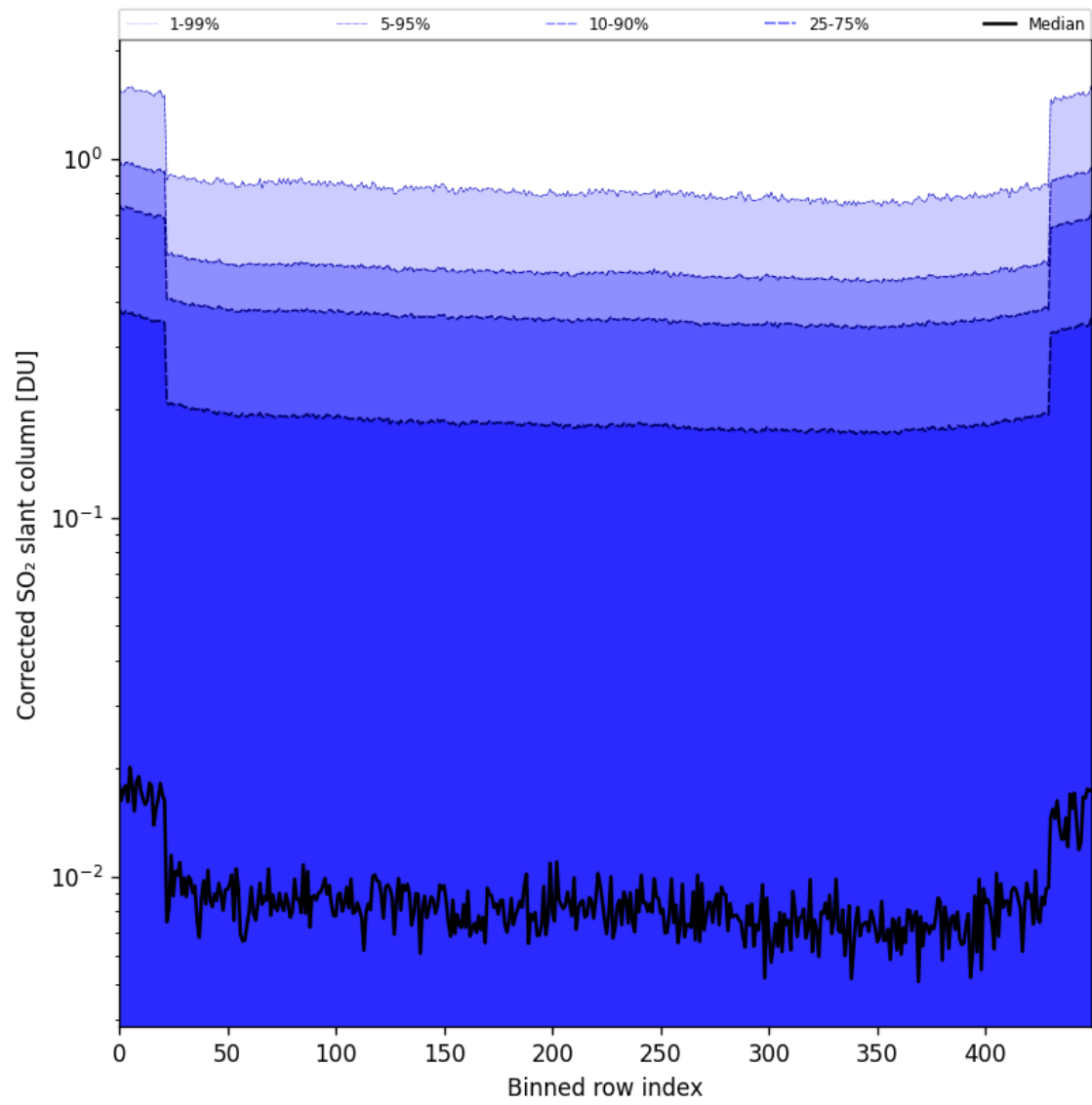
Figure 86: Along track statistics of “Corrected SO 2 slant column” for 2024-11-28 to 2024-11-30
