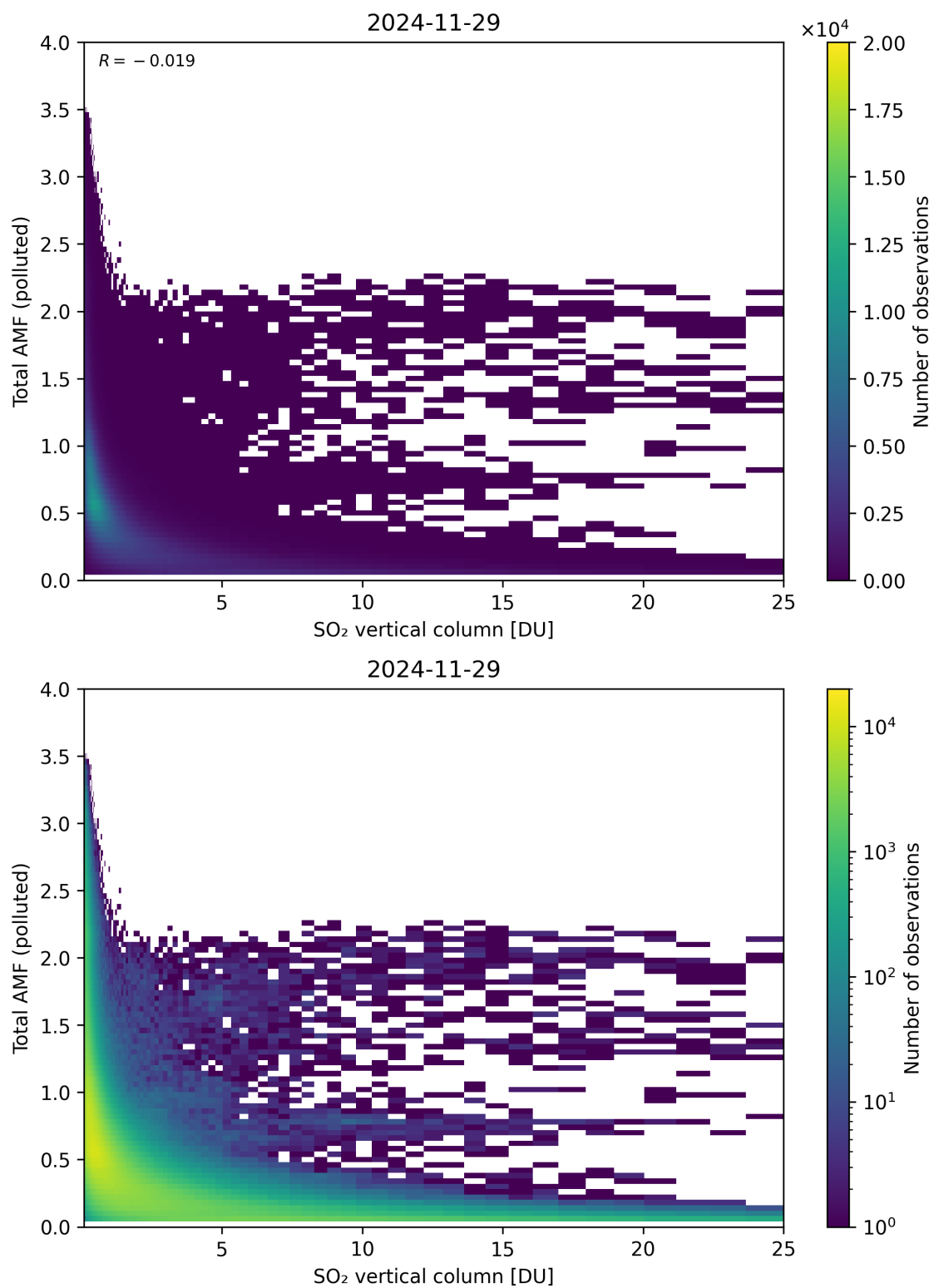
Figure 359: Scatter density plot of “SO 2 vertical column” against “Total AMF (polluted)” for 2024-11-28 to 2024-11-30.
