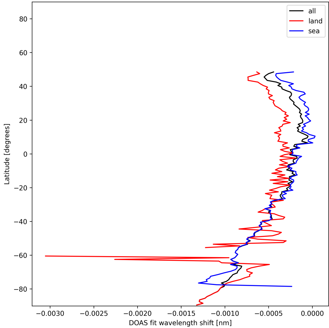
Figure 50: Zonal average of “DOAS fit wavelength shift” for 2024-11-28 to 2024-11-30.
