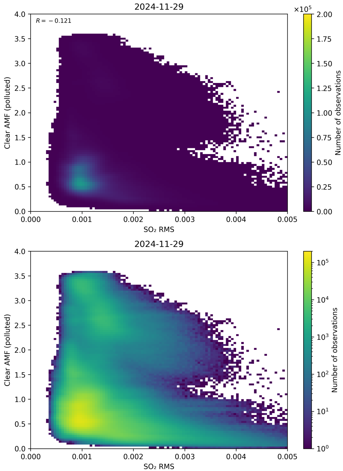
Figure 147: Scatter density plot of “SO 2 RMS” against “Clear AMF (polluted)” for 2024-11-28 to 2024-11-30.
