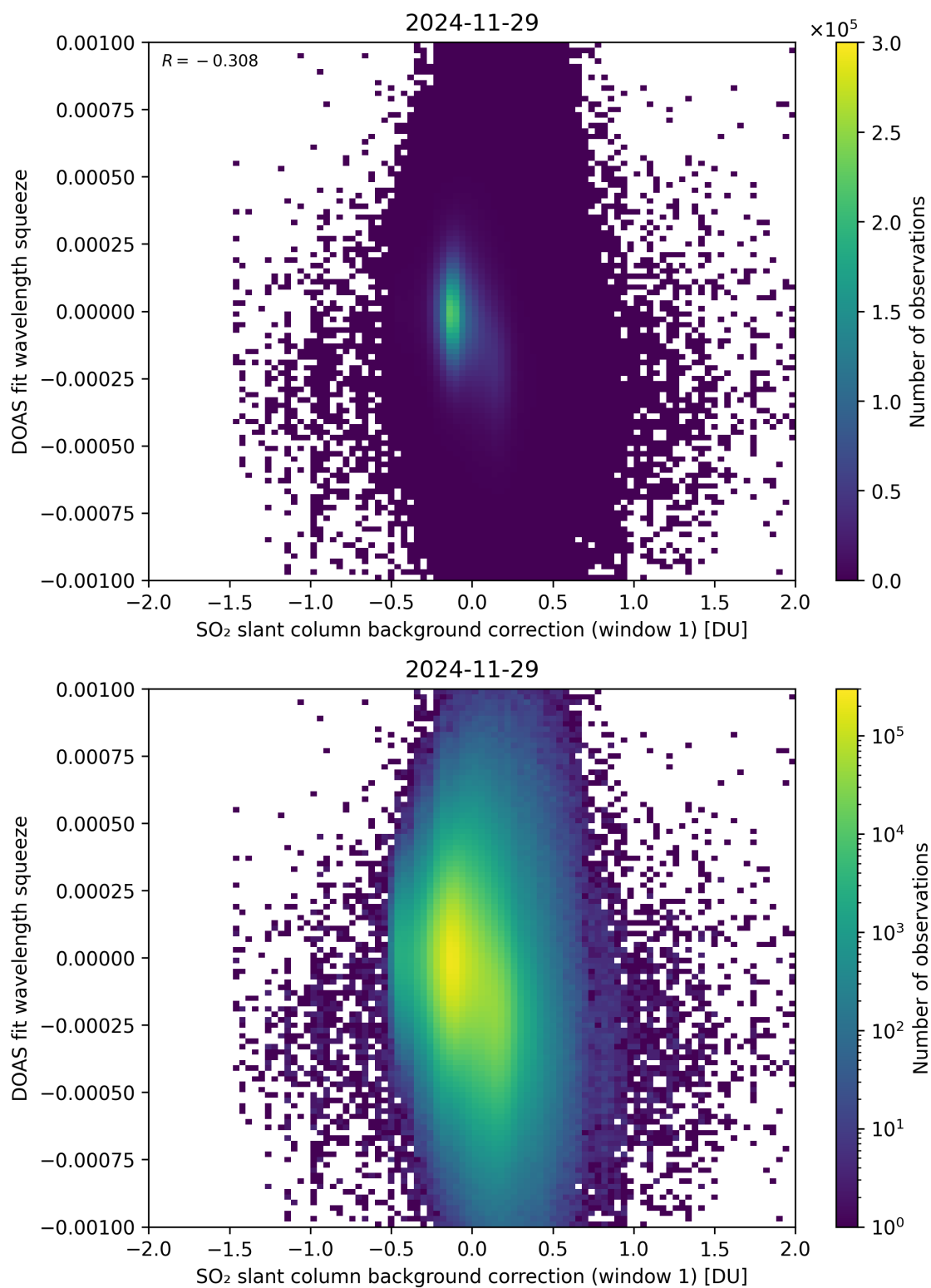
Figure 112: Scatter density plot of “SO 2 slant column background correction (window 1)” against “DOAS fit wavelength squeeze” for 2024-11-28 to 2024-11-30.
