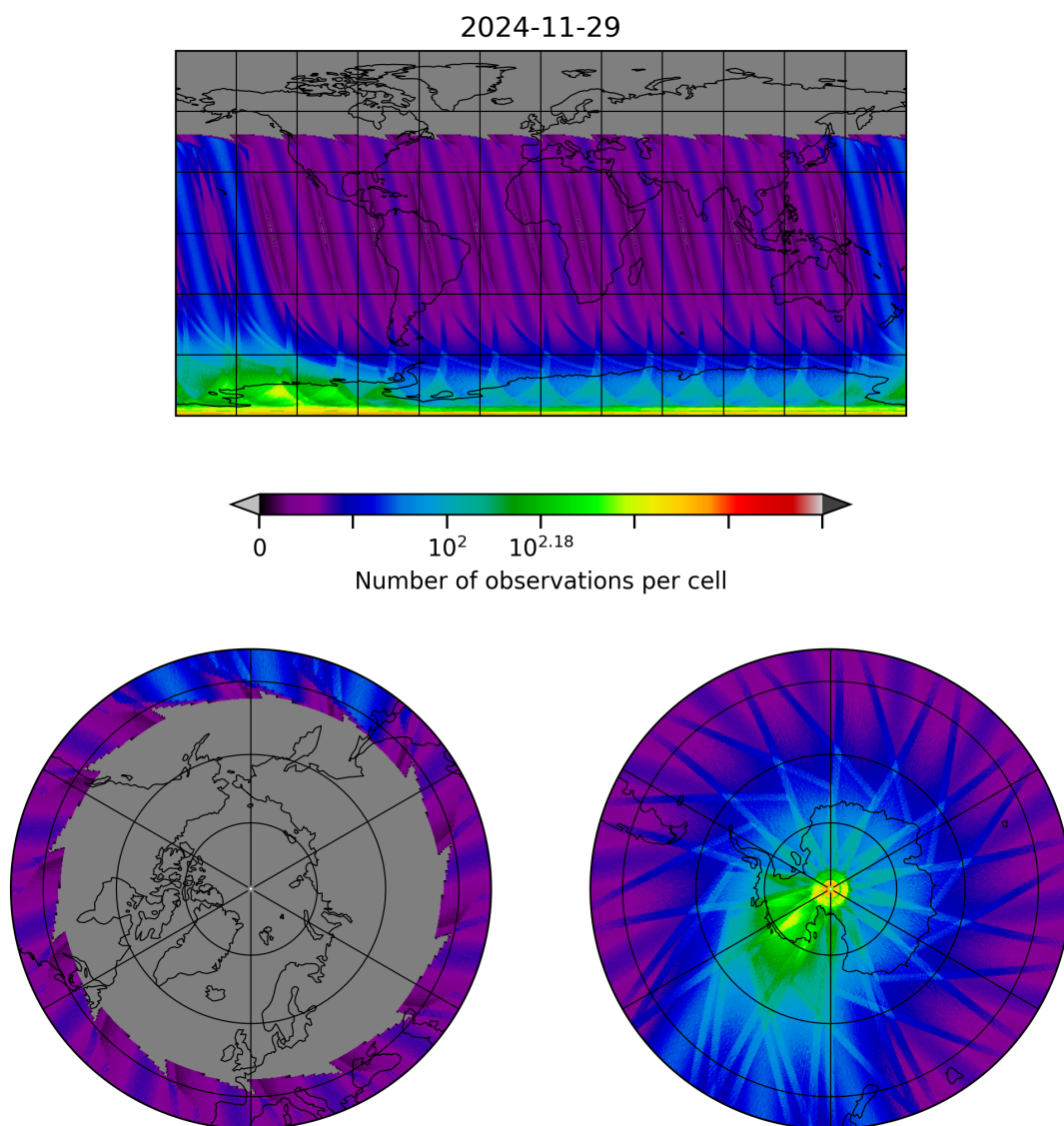
Figure 30: Map of the number of observations for 2024-11-28 to 2024-11-30
