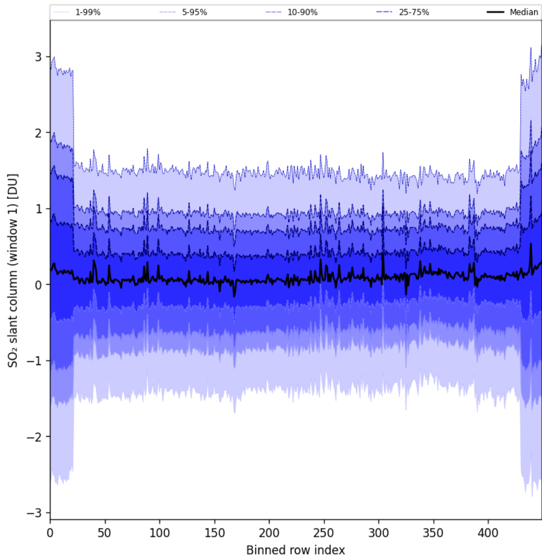
Figure 89: Along track statistics of “SO 2 slant column (window 1)” for 2024-11-28 to 2024-11-30
