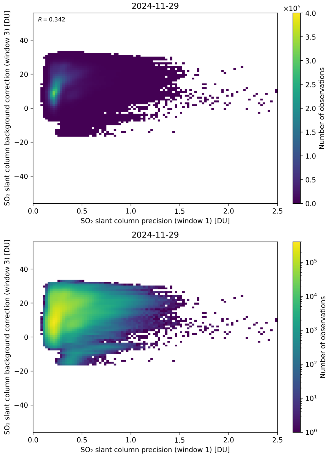
Figure 270: Scatter density plot of “SO 2 slant column precision (window 1)” against “SO 2 slant column background correction (window 3)” for 2024-11-28 to 2024-11-30.
