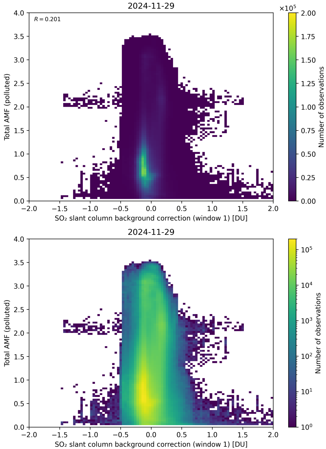
Figure 120: Scatter density plot of “SO 2 slant column background correction (window 1)” against “Total AMF (polluted)” for 2024-11-28 to 2024-11-30.
