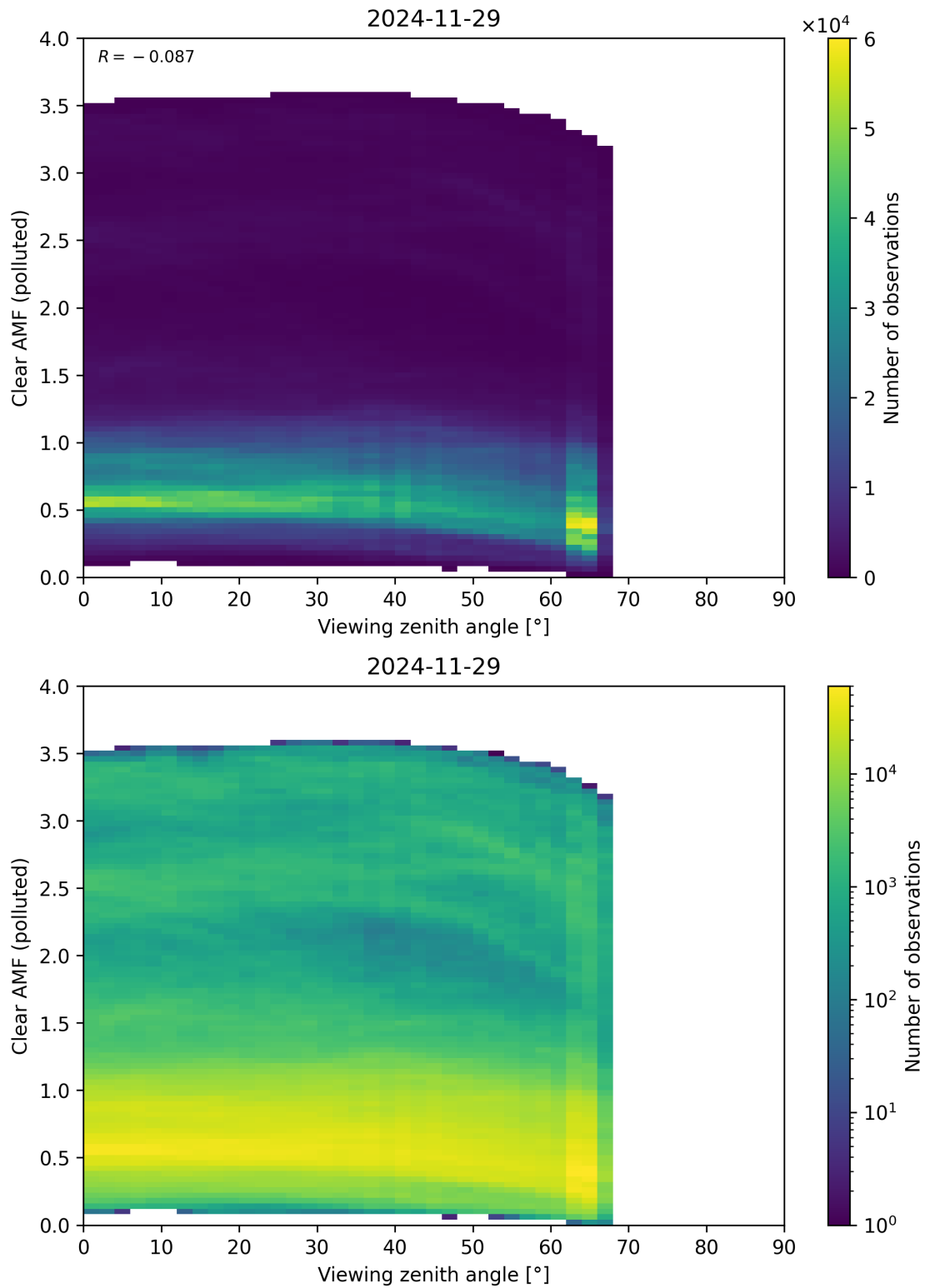
Figure 370: Scatter density plot of “Viewing zenith angle” against “Clear AMF (polluted)” for 2024-11-28 to 2024-11-30.
