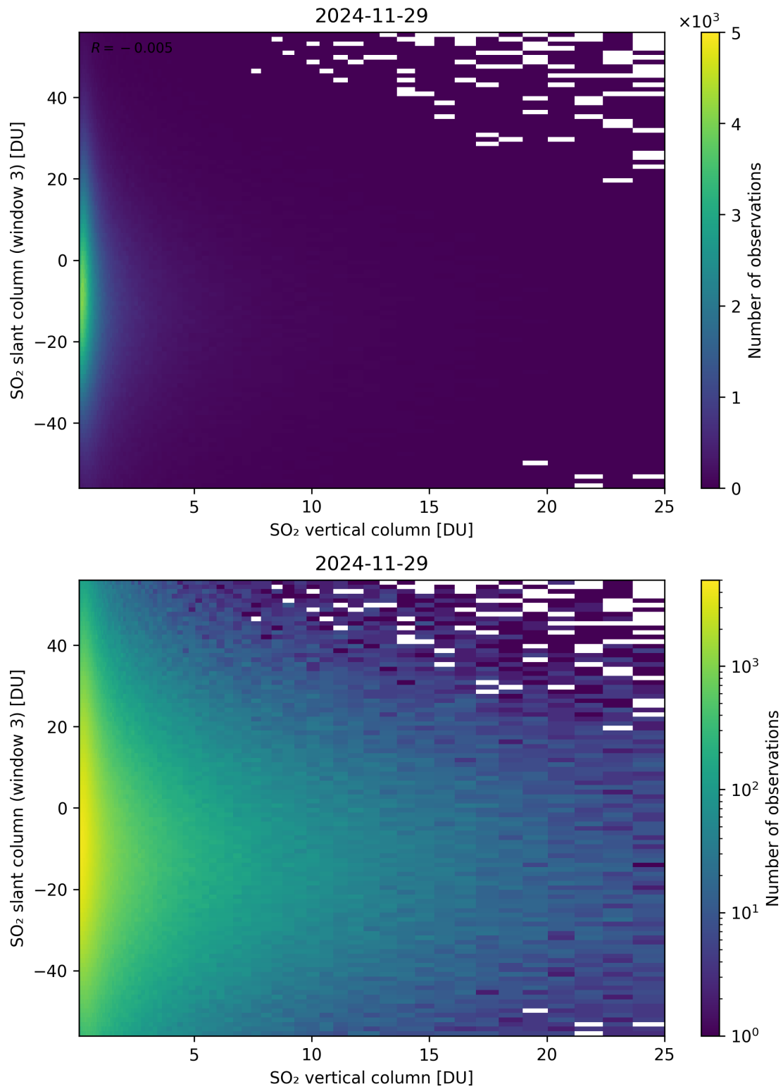
Figure 357: Scatter density plot of “SO 2 vertical column” against “SO 2 slant column (window 3)” for 2024-11-28 to 2024-11-30.
