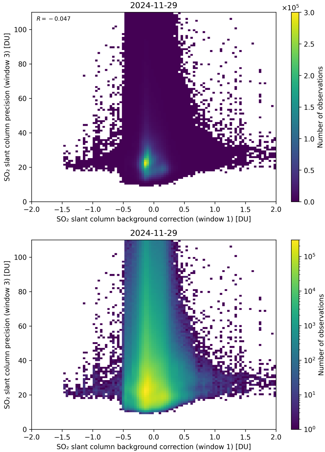
Figure 119: Scatter density plot of “SO 2 slant column background correction (window 1)” against “SO 2 slant column precision (window 3)” for 2024-11-28 to 2024-11-30.
