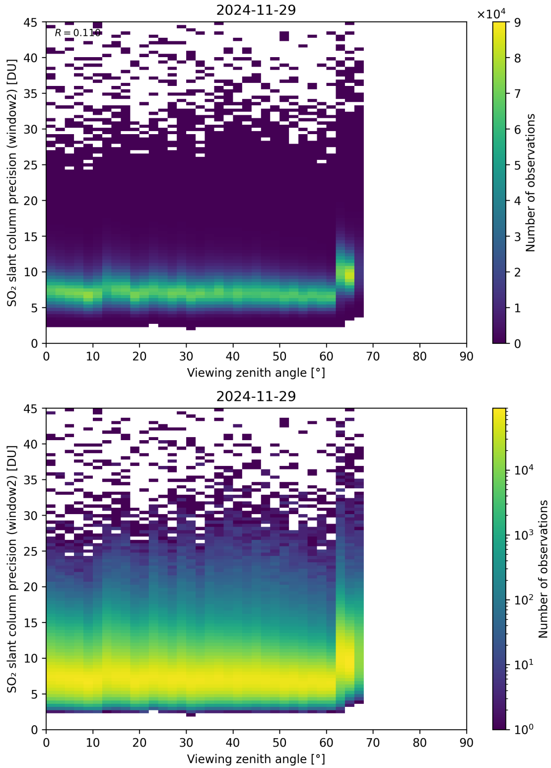
Figure 378: Scatter density plot of “Viewing zenith angle” against “SO 2 slant column precision (window2)” for 2024-11-28 to 2024-11-30.
