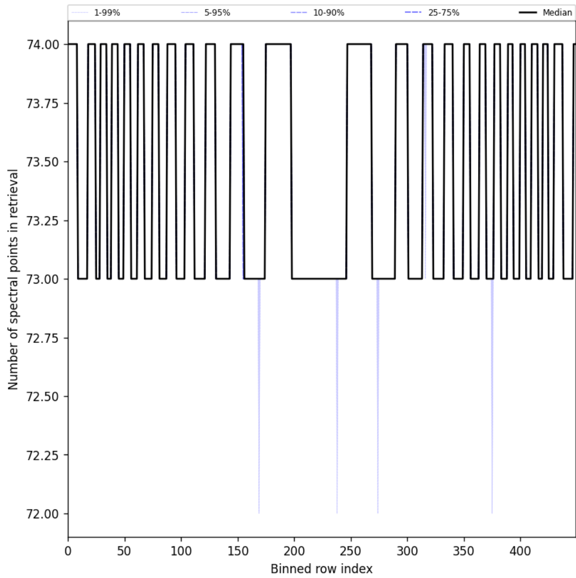
Figure 108: Along track statistics of “Number of spectral points in retrieval” for 2024-11-28 to 2024-11-30
