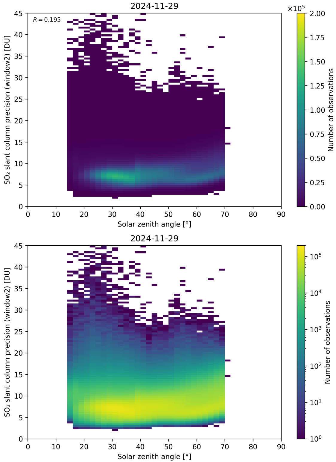
Figure 186: Scatter density plot of “Solar zenith angle” against “SO 2 slant column precision (window2)” for 2024-11-28 to 2024-11-30.
