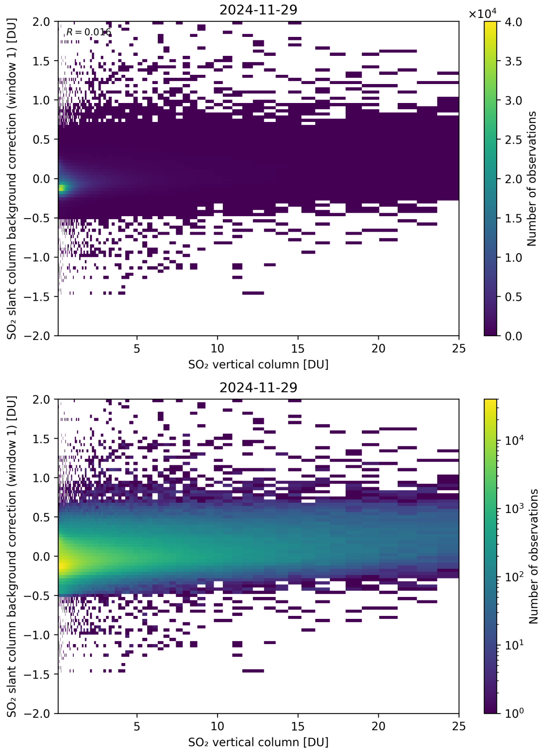
Figure 323: Scatter density plot of “SO 2 vertical column” against “SO 2 slant column background correction (window 1)” for 2024-11-28 to 2024-11-30.
