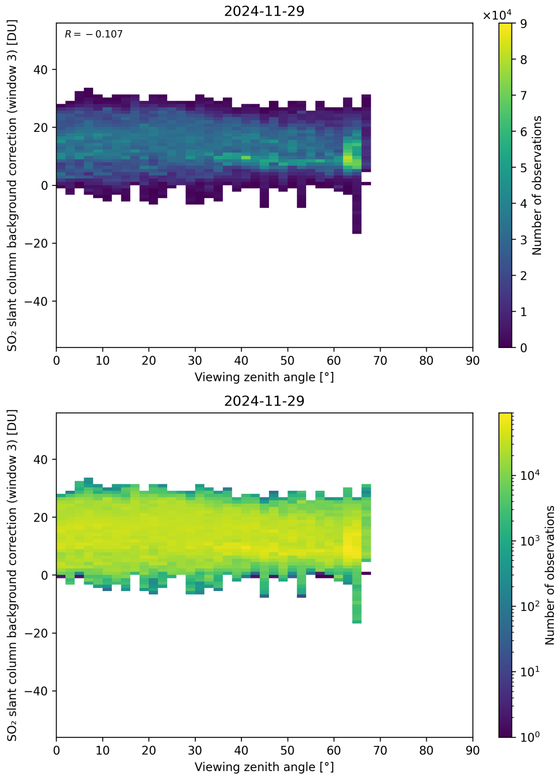
Figure 364: Scatter density plot of “Viewing zenith angle” against “SO 2 slant column background correction (window 3)” for 2024-11-28 to 2024-11-30.
