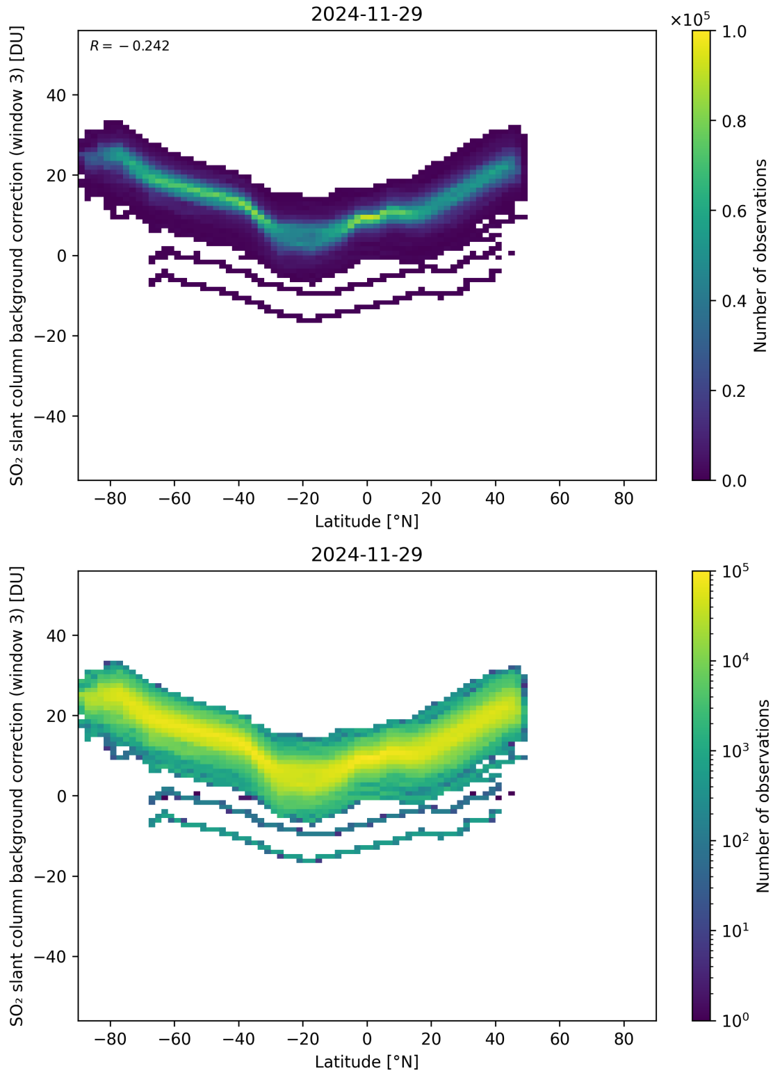
Figure 152: Scatter density plot of “Latitude” against “SO 2 slant column background correction (window 3)” for 2024-11-28 to 2024-11-30.
