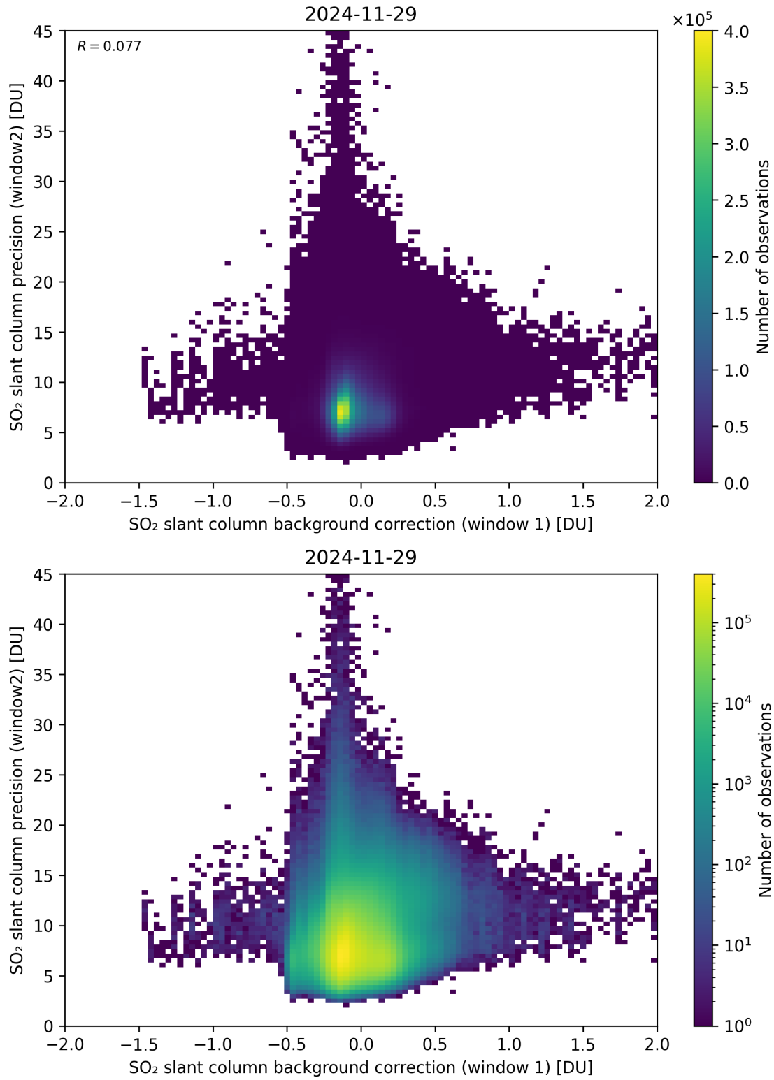
Figure 117: Scatter density plot of “SO 2 slant column background correction (window 1)” against “SO 2 slant column precision (window2)” for 2024-11-28 to 2024-11-30.
