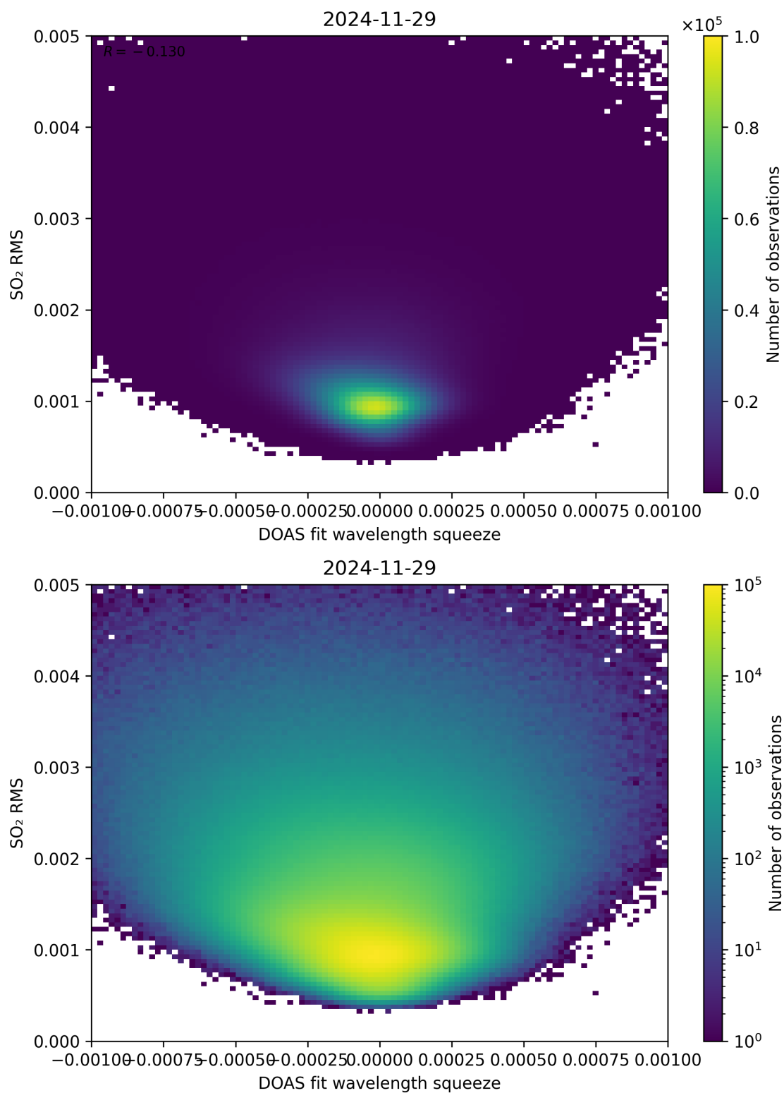
Figure 143: Scatter density plot of “DOAS fit wavelength squeeze” against “SO 2 RMS” for 2024-11-28 to 2024-11-30.
