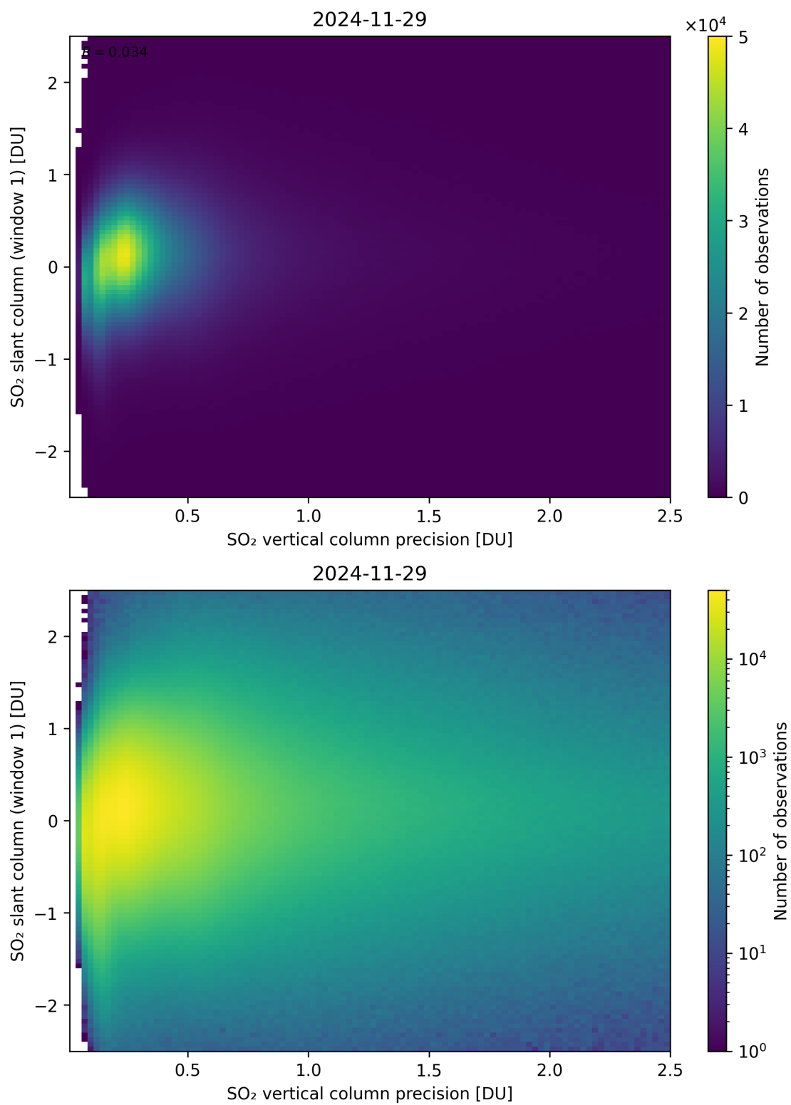
Figure 341: Scatter density plot of “SO 2 vertical column precision” against “SO 2 slant column (window 1)” for 2024-11-28 to 2024-11-30.
