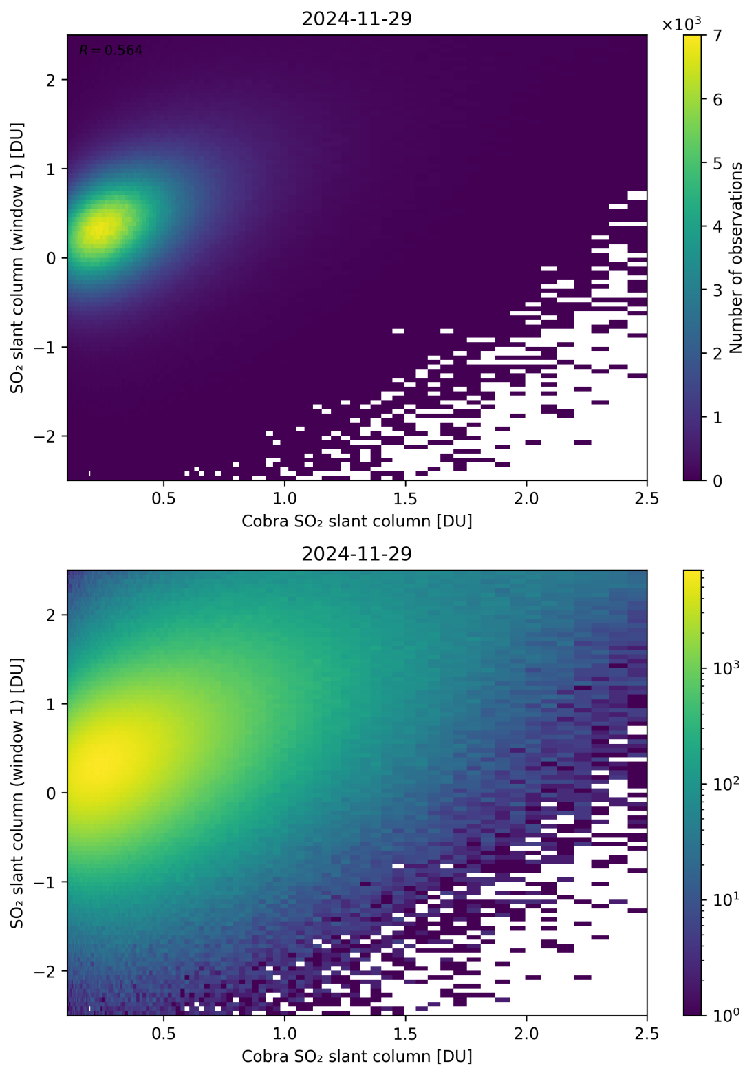
Figure 219: Scatter density plot of “Cobra SO 2 slant column” against “SO 2 slant column (window 1)” for 2024-11-28 to 2024-11-30.
