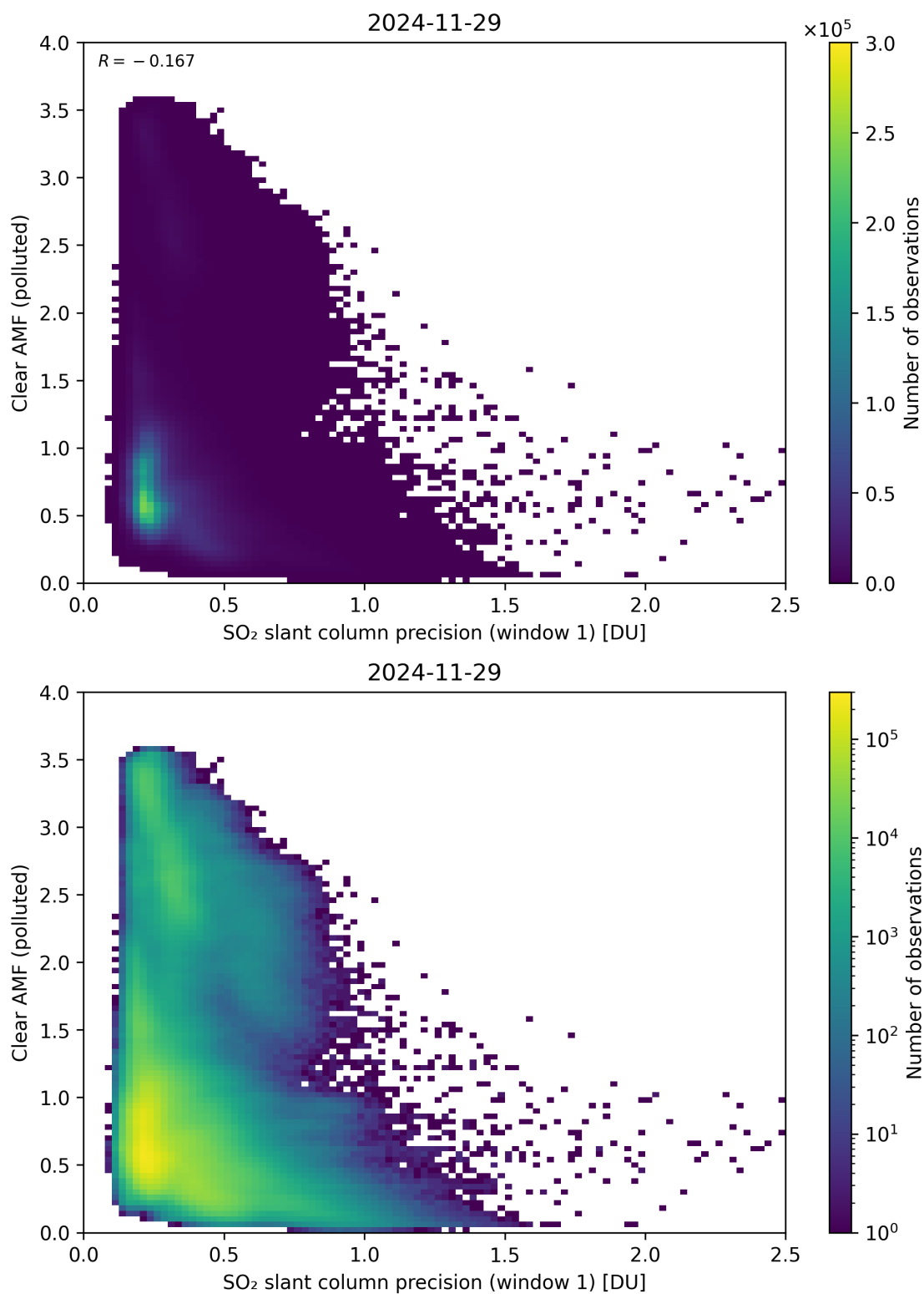
Figure 274: Scatter density plot of “SO 2 slant column precision (window 1)” against “Clear AMF (polluted)” for 2024-11-28 to 2024-11-30.
