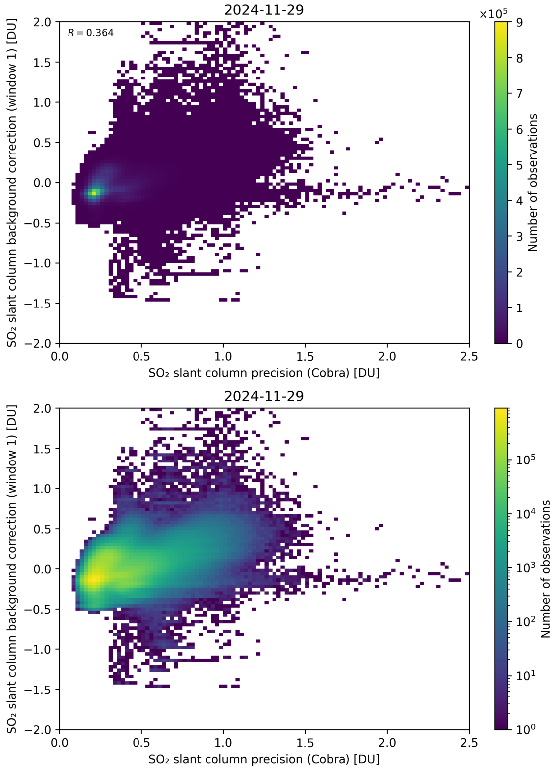
Figure 199: Scatter density plot of “SO 2 slant column precision (Cobra)” against “SO 2 slant column background correction (window 1)” for 2024-11-28 to 2024-11-30.
