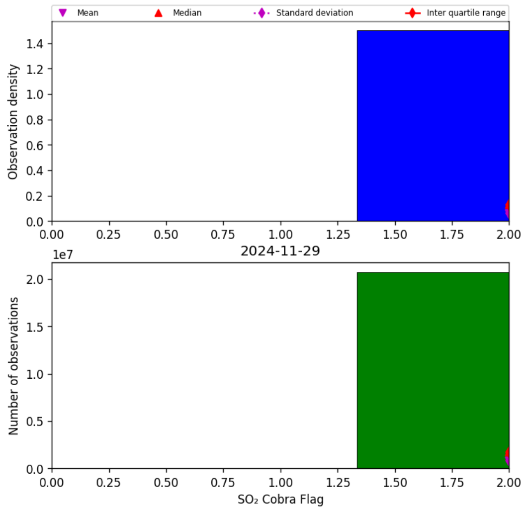
Figure 75: Histogram of “SO 2 Cobra Flag” for 2024-11-28 to 2024-11-30
