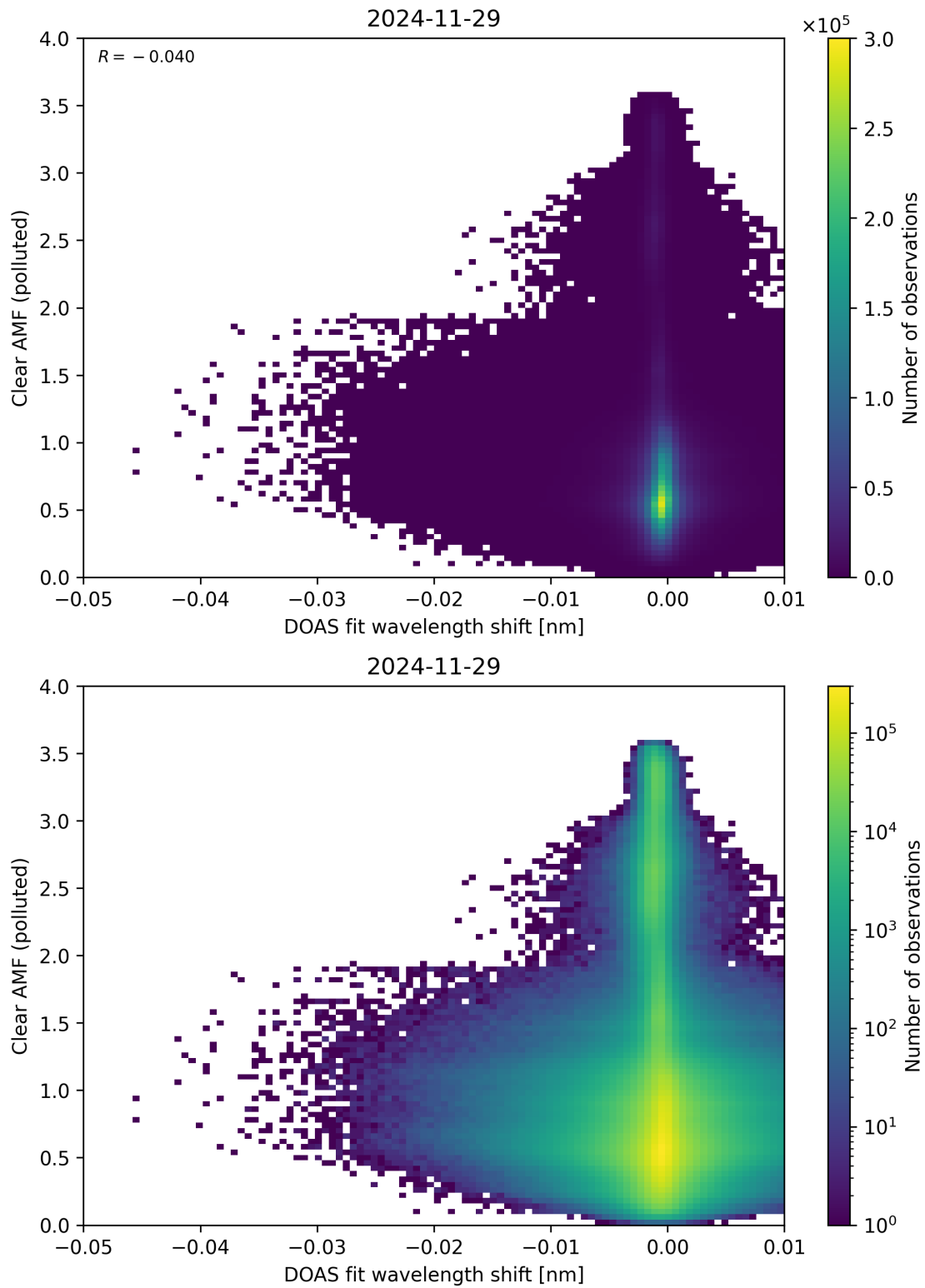
Figure 140: Scatter density plot of “DOAS fit wavelength shift” against “Clear AMF (polluted)” for 2024-11-28 to 2024-11-30.
