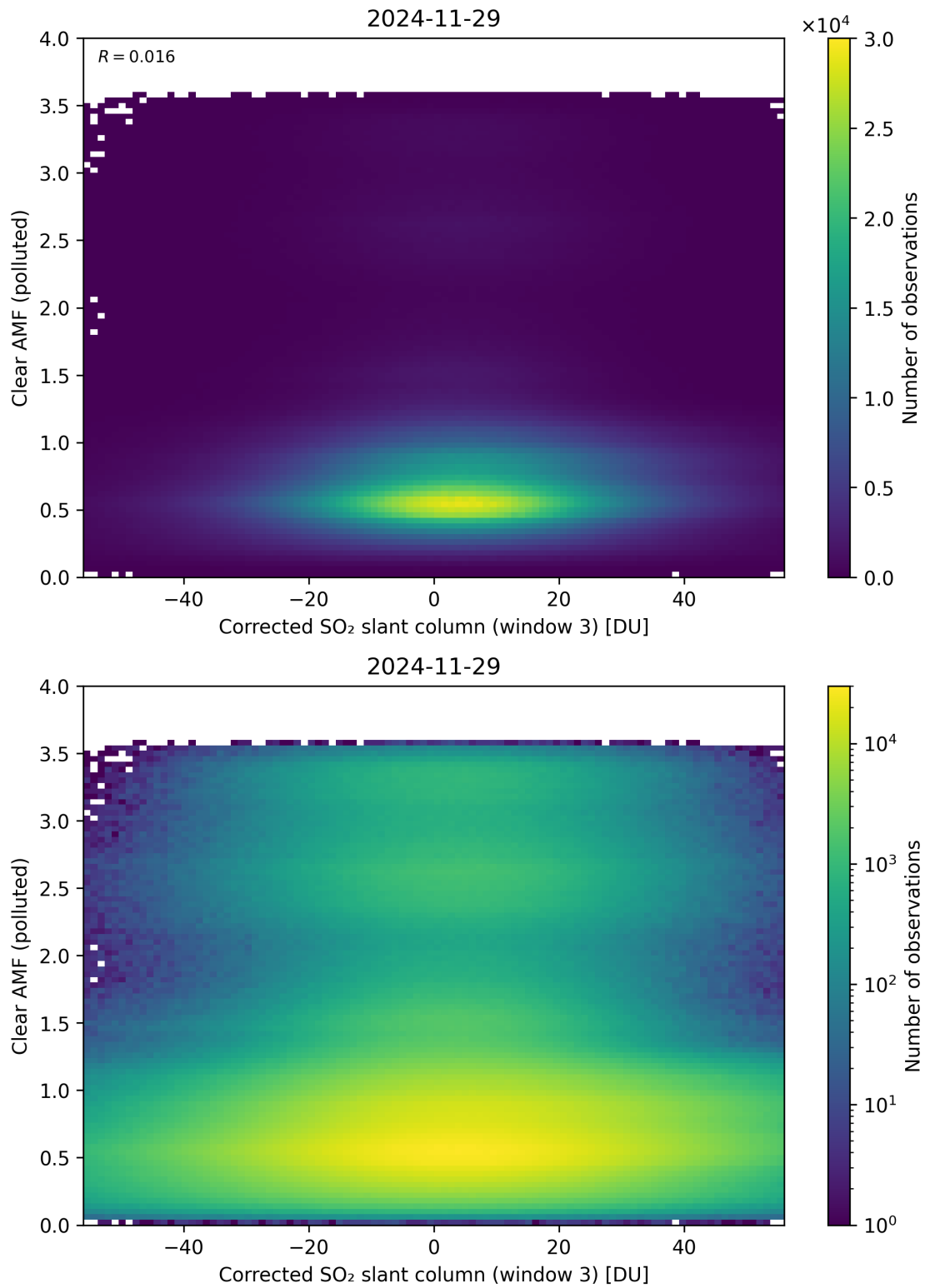
Figure 259: Scatter density plot of “Corrected SO 2 slant column (window 3)” against “Clear AMF (polluted)” for 2024-11-28 to 2024-11-30.
