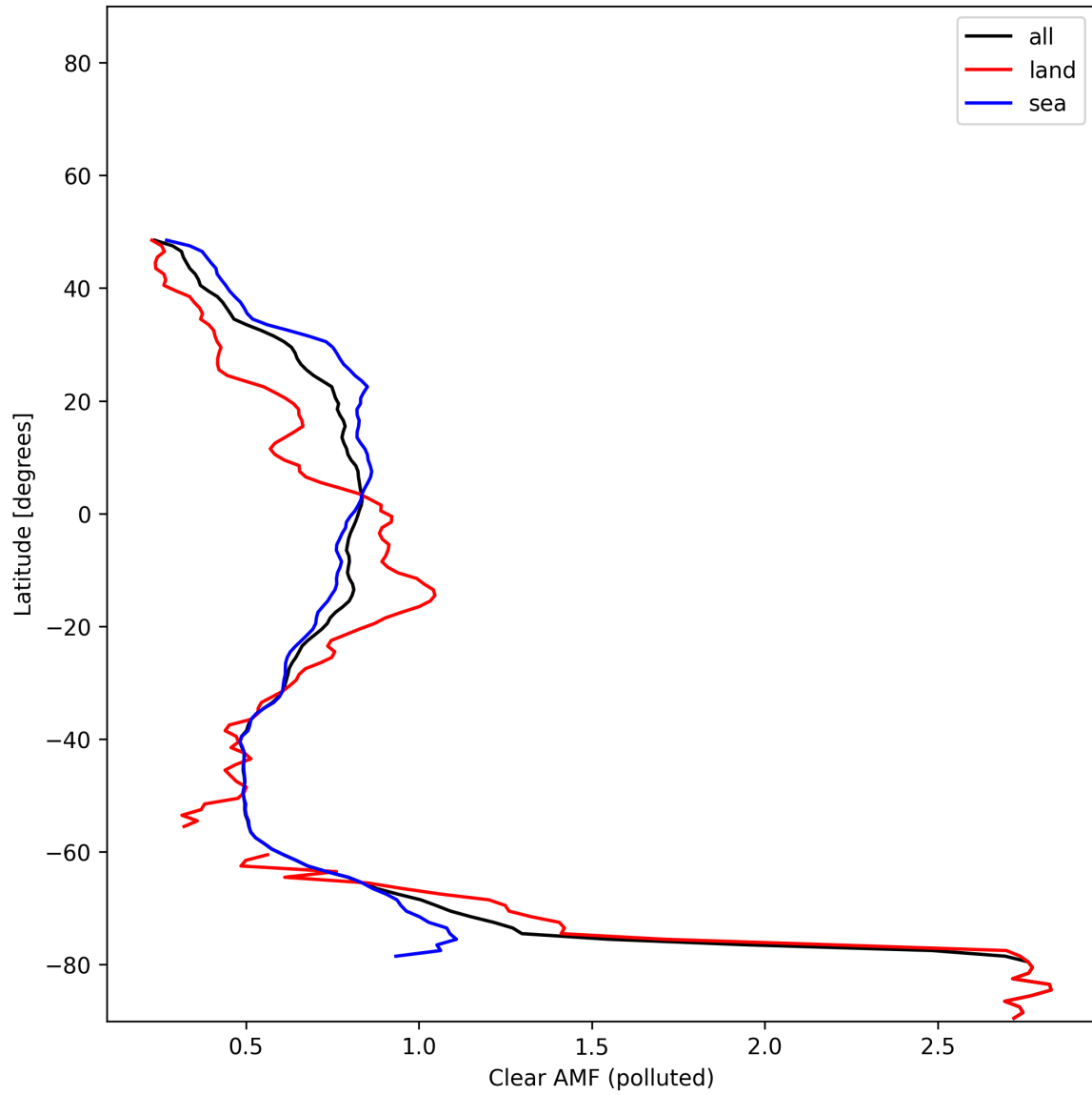
Figure 55: Zonal average of “Clear AMF (polluted)” for 2024-11-28 to 2024-11-30.
