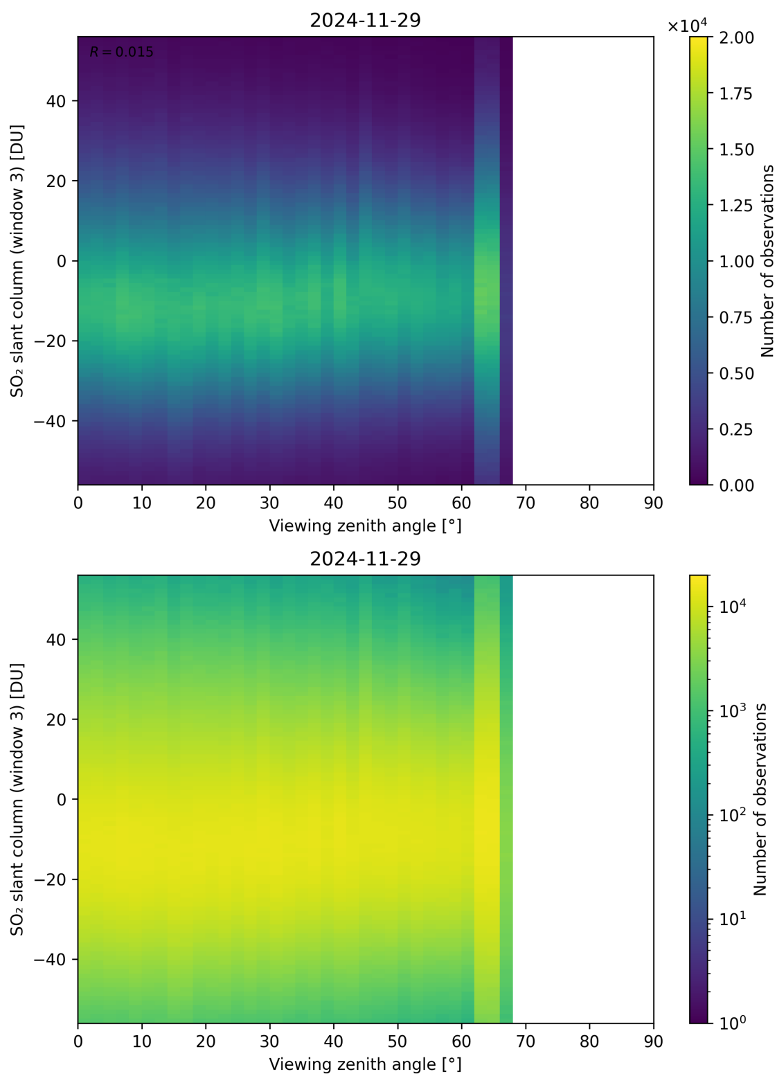
Figure 379: Scatter density plot of “Viewing zenith angle” against “SO 2 slant column (window 3)” for 2024-11-28 to 2024-11-30.
