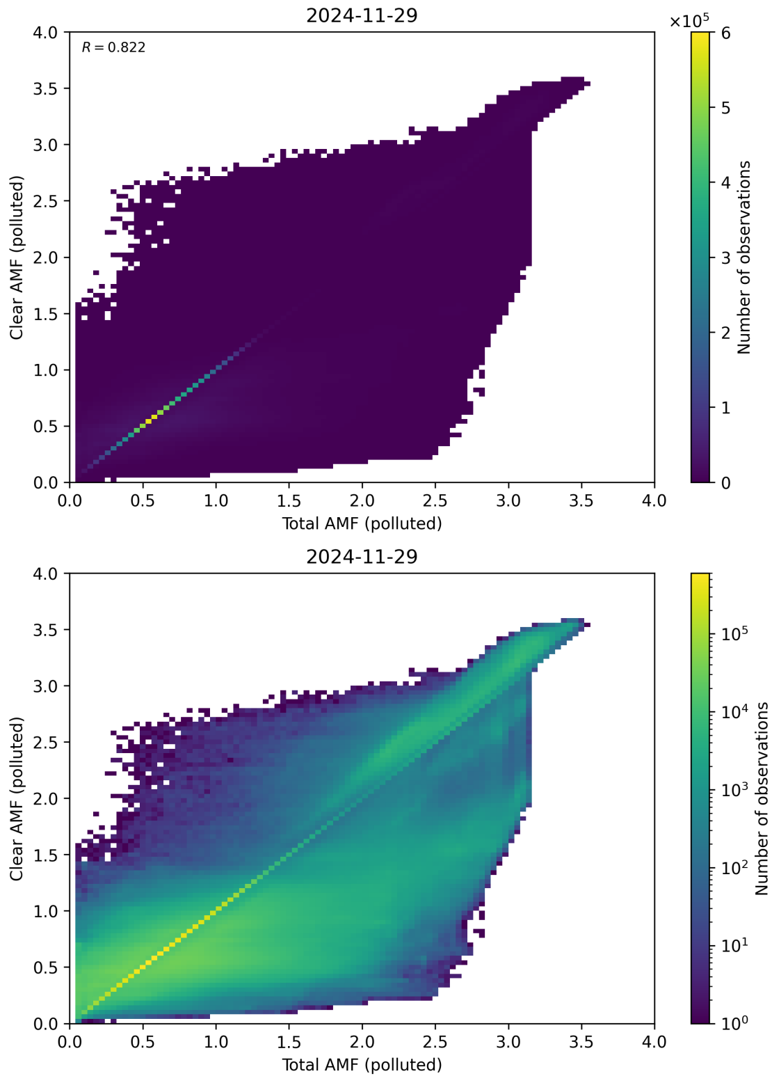
Figure 321: Scatter density plot of “Total AMF (polluted)” against “Clear AMF (polluted)” for 2024-11-28 to 2024-11-30.
