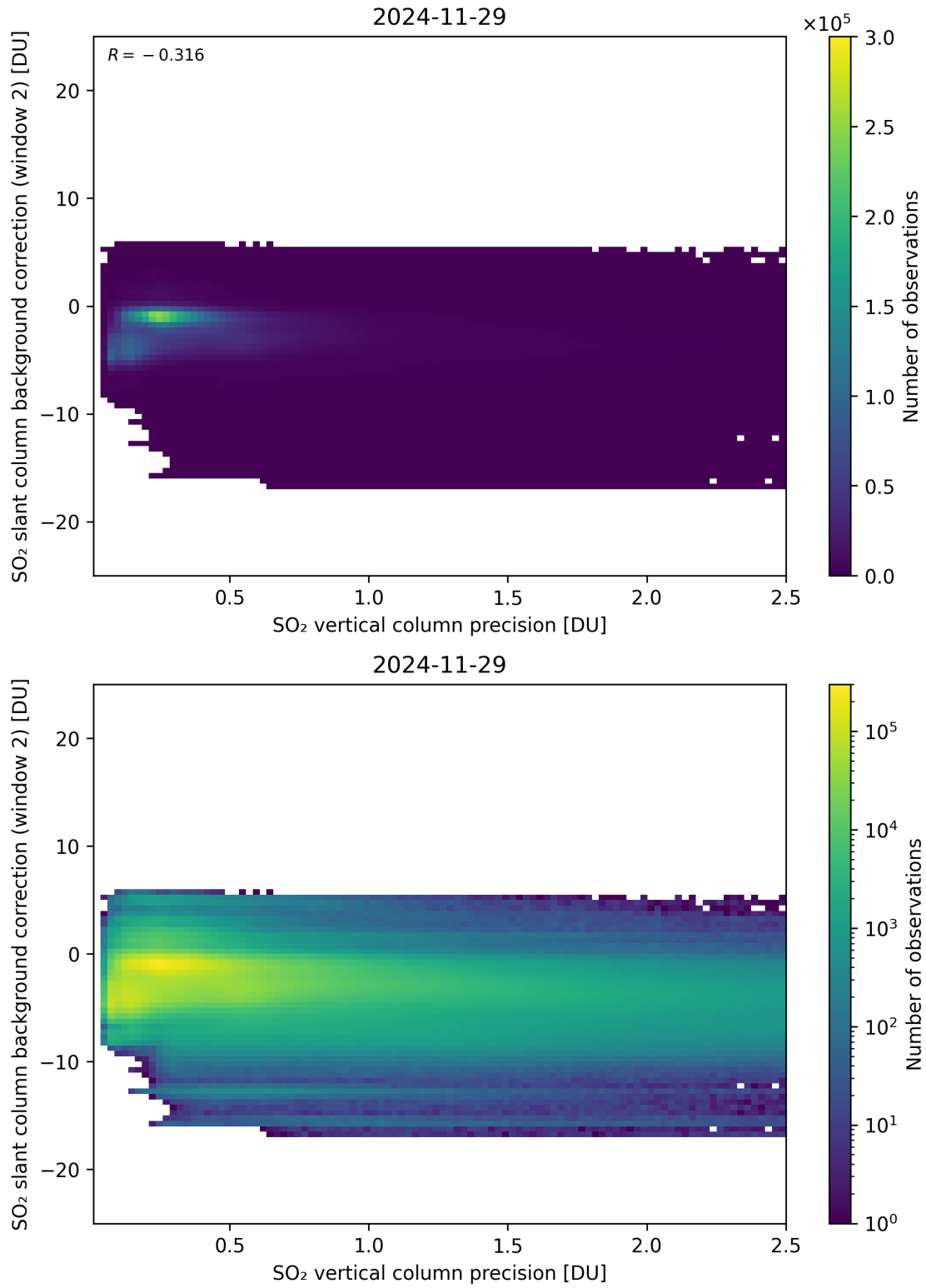
Figure 330: Scatter density plot of “SO 2 vertical column precision” against “SO 2 slant column background correction (window 2)” for 2024-11-28 to 2024-11-30.
