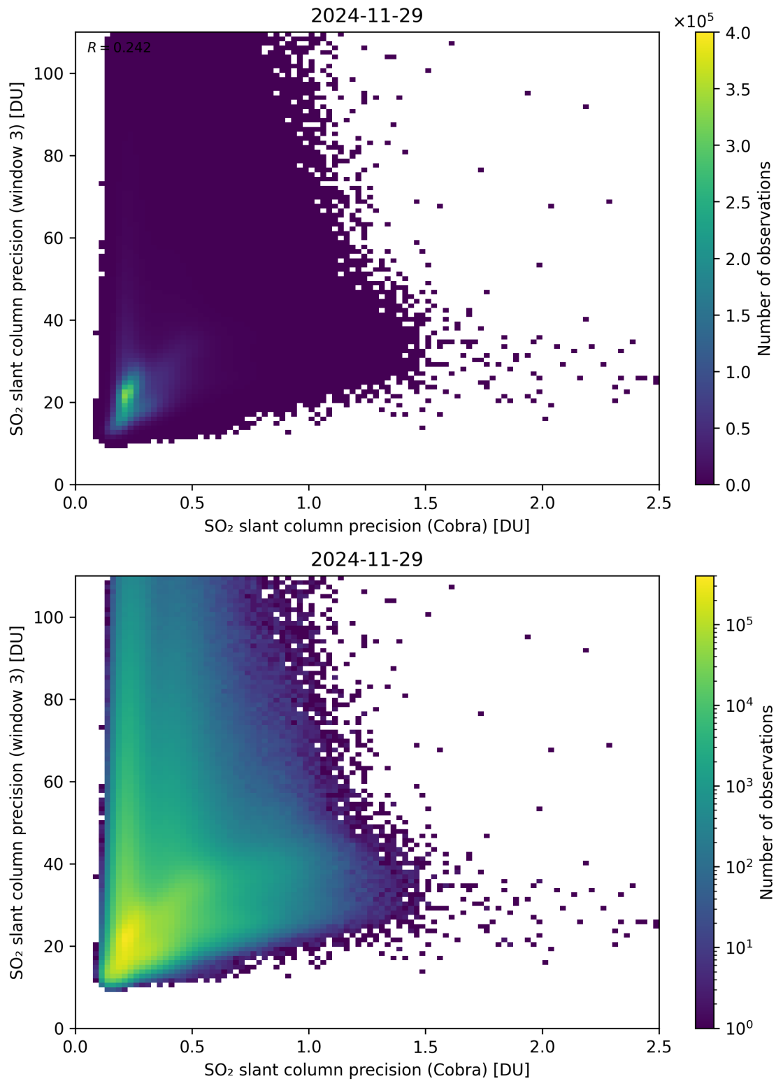
Figure 212: Scatter density plot of “SO 2 slant column precision (Cobra)” against “SO 2 slant column precision (window 3)” for 2024-11-28 to 2024-11-30.
