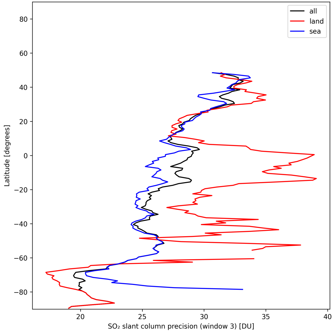
Figure 46: Zonal average of “SO 2 slant column precision (window 3)” for 2024-11-28 to 2024-11-30.
