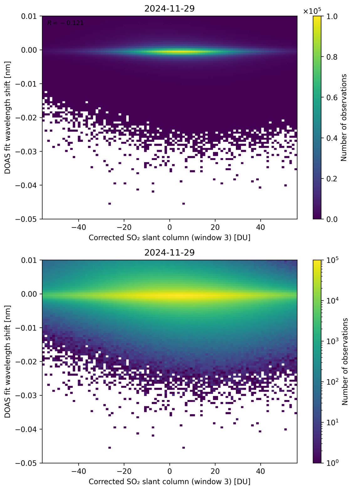
Figure 256: Scatter density plot of “Corrected SO 2 slant column (window 3)” against “DOAS fit wavelength shift” for 2024-11-28 to 2024-11-30.
