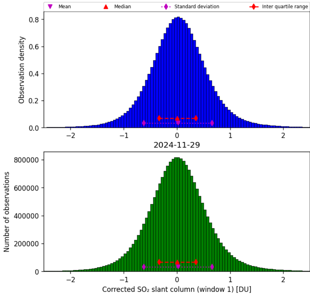
Figure 65: Histogram of “Corrected SO 2 slant column (window 1)” for 2024-11-28 to 2024-11-30
