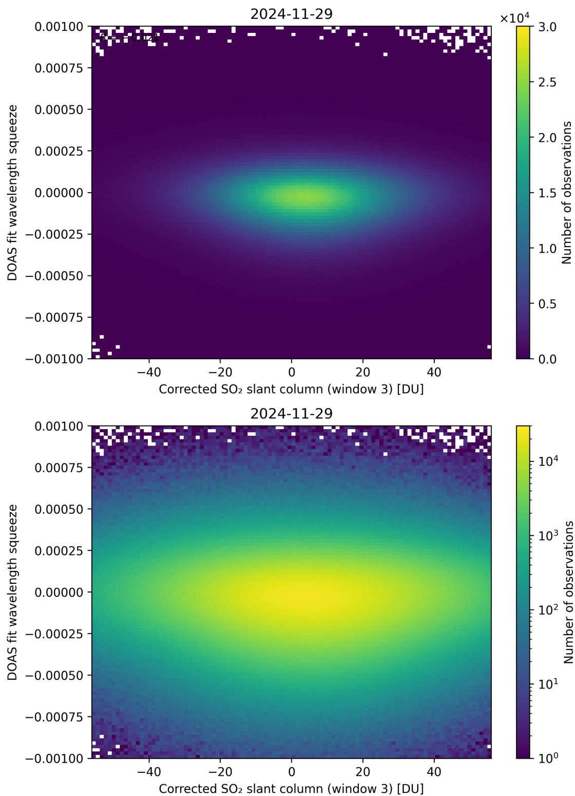
Figure 257: Scatter density plot of “Corrected SO 2 slant column (window 3)” against “DOAS fit wavelength squeeze” for 2024-11-28 to 2024-11-30.
