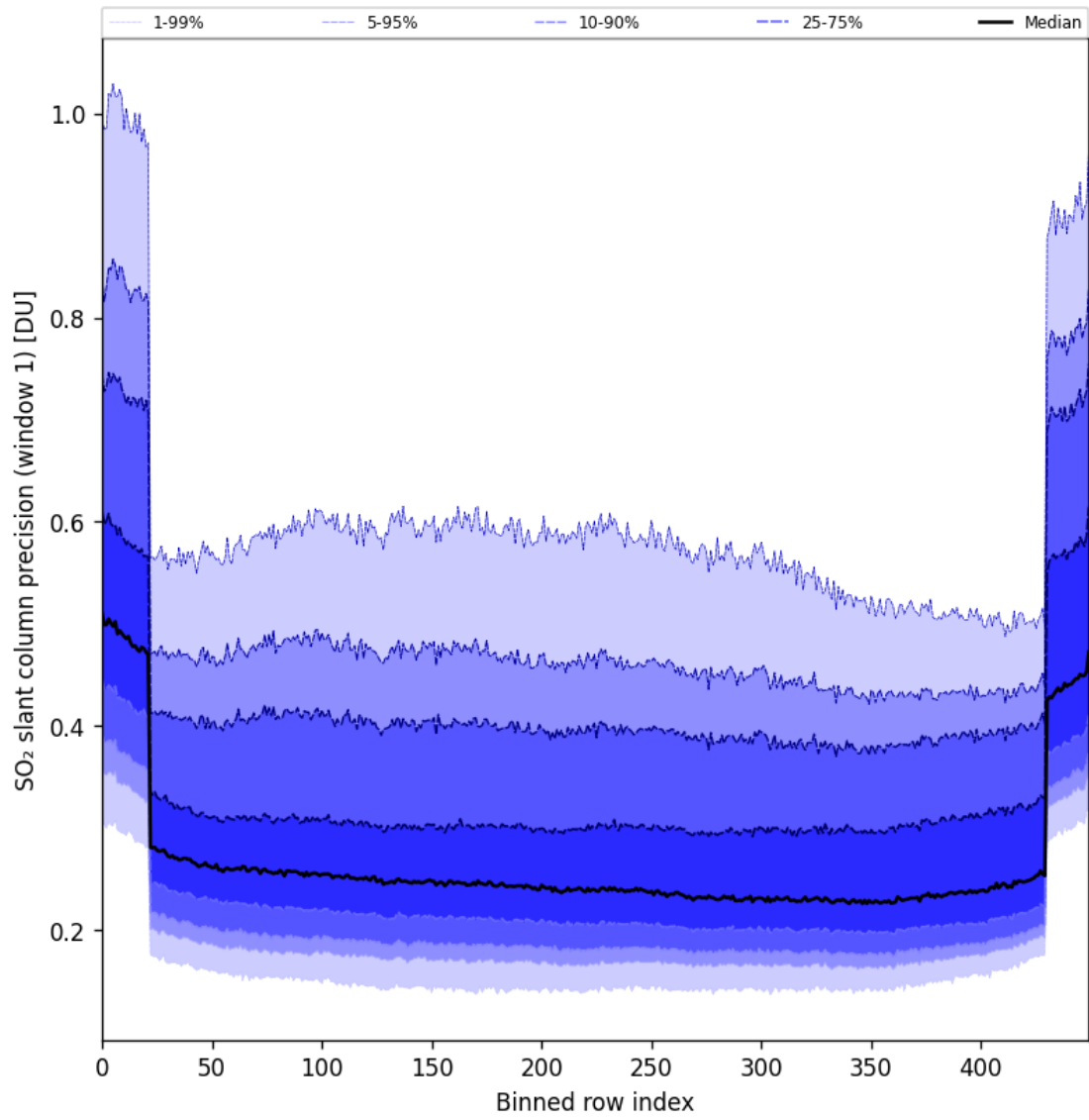
Figure 90: Along track statistics of “SO 2 slant column precision (window 1)” for 2024-11-28 to 2024-11-30
