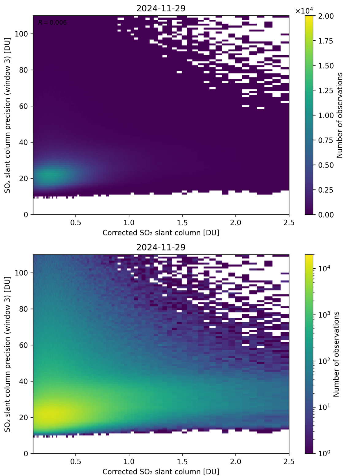
Figure 241: Scatter density plot of “Corrected SO 2 slant column” against “SO 2 slant column precision (window 3)” for 2024-11-28 to 2024-11-30.
