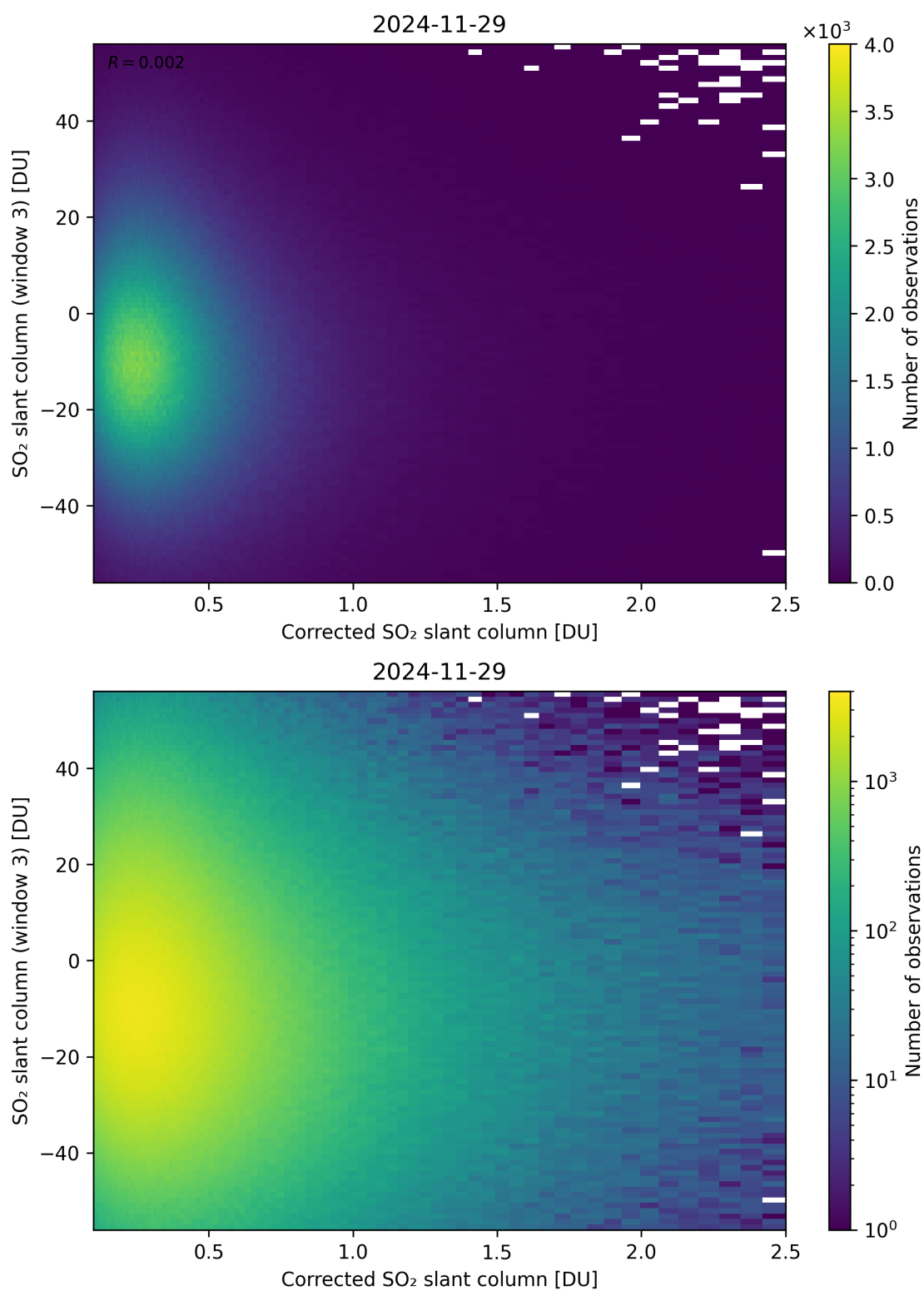
Figure 240: Scatter density plot of “Corrected SO 2 slant column” against “SO 2 slant column (window 3)” for 2024-11-28 to 2024-11-30.
