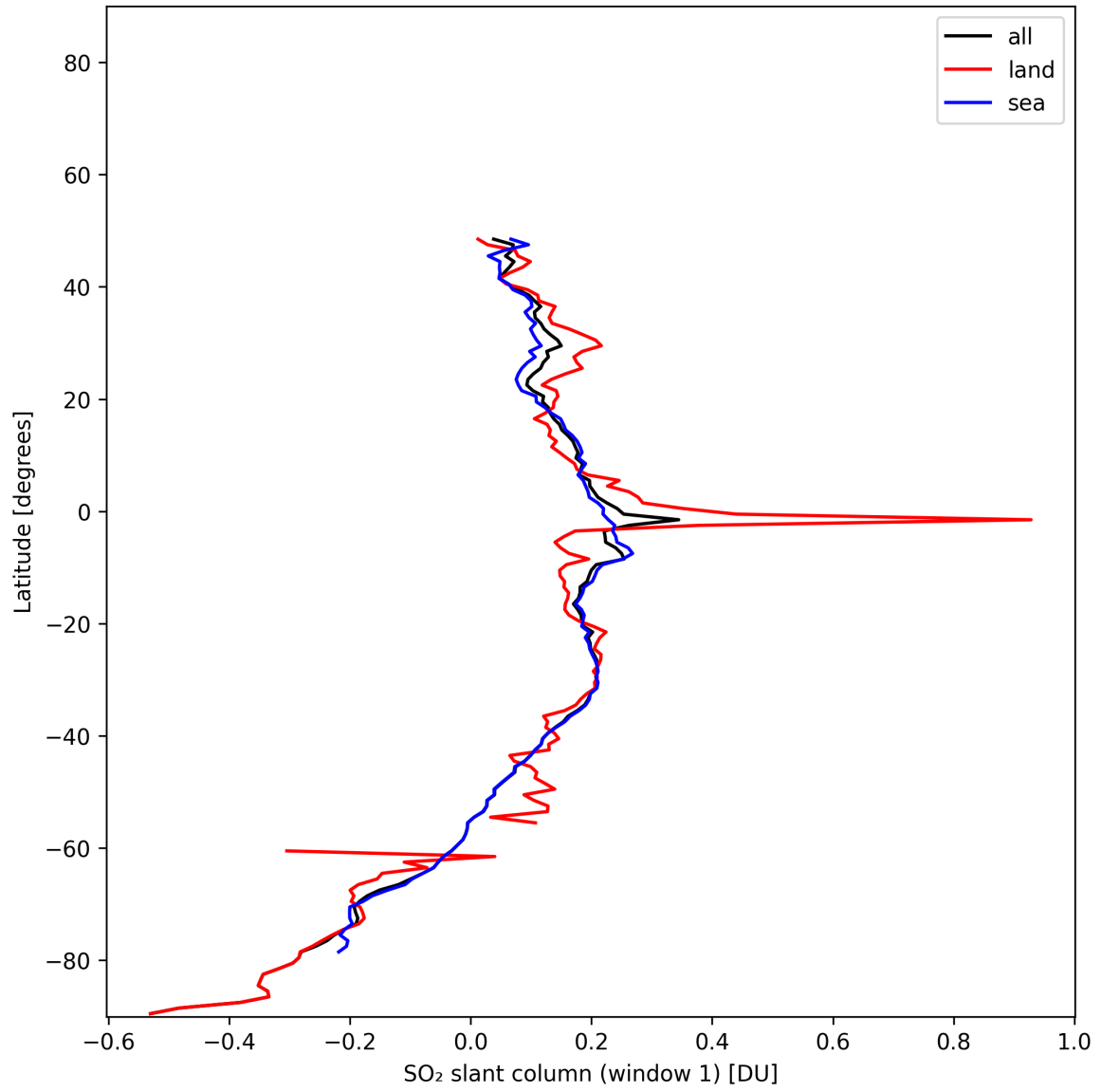
Figure 37: Zonal average of “SO 2 slant column (window 1)” for 2024-11-28 to 2024-11-30.
