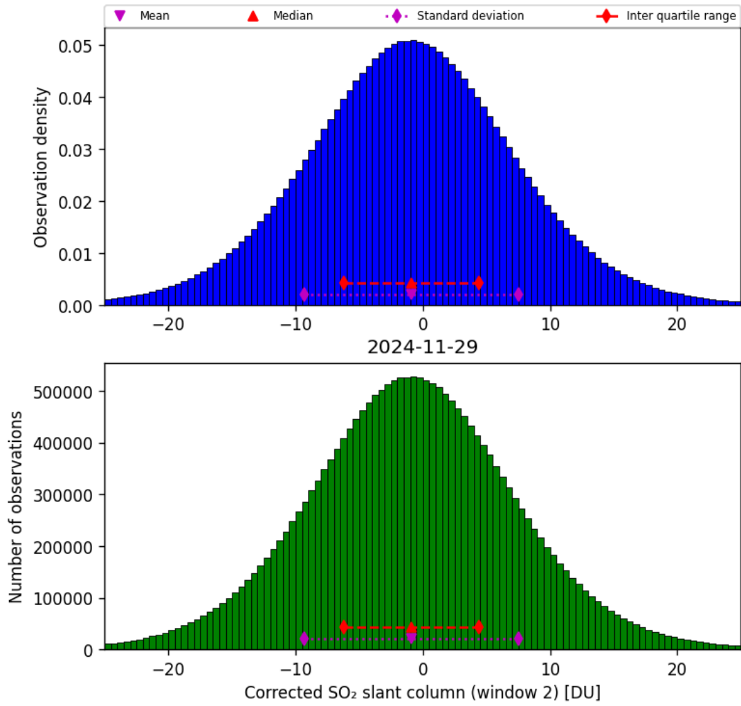
Figure 69: Histogram of “Corrected SO 2 slant column (window 2)” for 2024-11-28 to 2024-11-30
