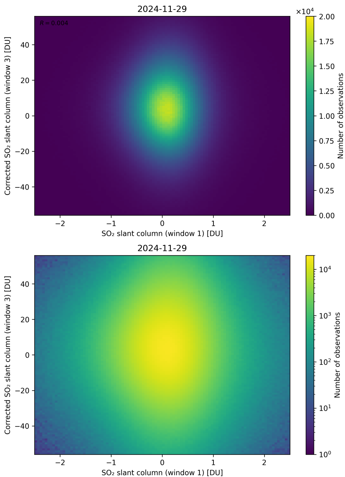
Figure 284: Scatter density plot of “SO 2 slant column (window 1)” against “Corrected SO 2 slant column (window 3)” for 2024-11-28 to 2024-11-30.
