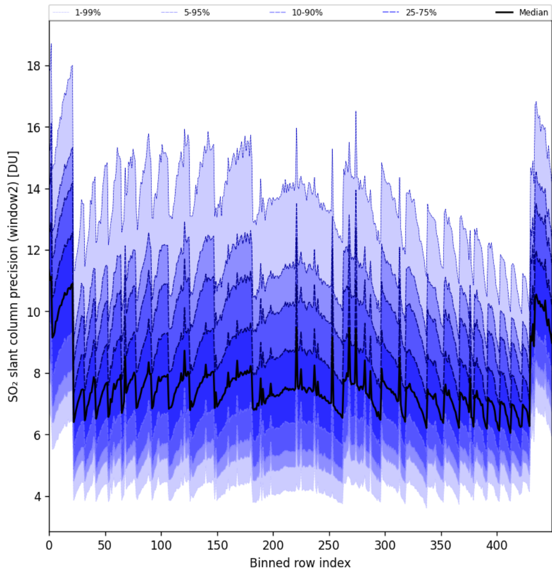
Figure 94: Along track statistics of “SO 2 slant column precision (window2)” for 2024-11-28 to 2024-11-30
