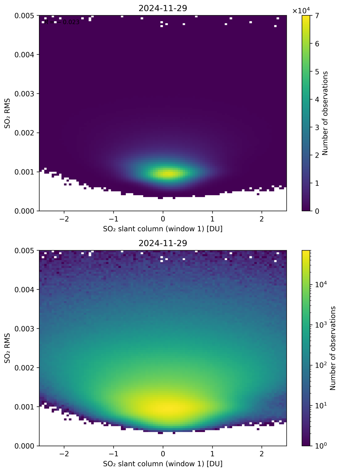
Figure 267: Scatter density plot of “SO 2 slant column (window 1)” against “SO 2 RMS” for 2024-11-28 to 2024-11-30.
