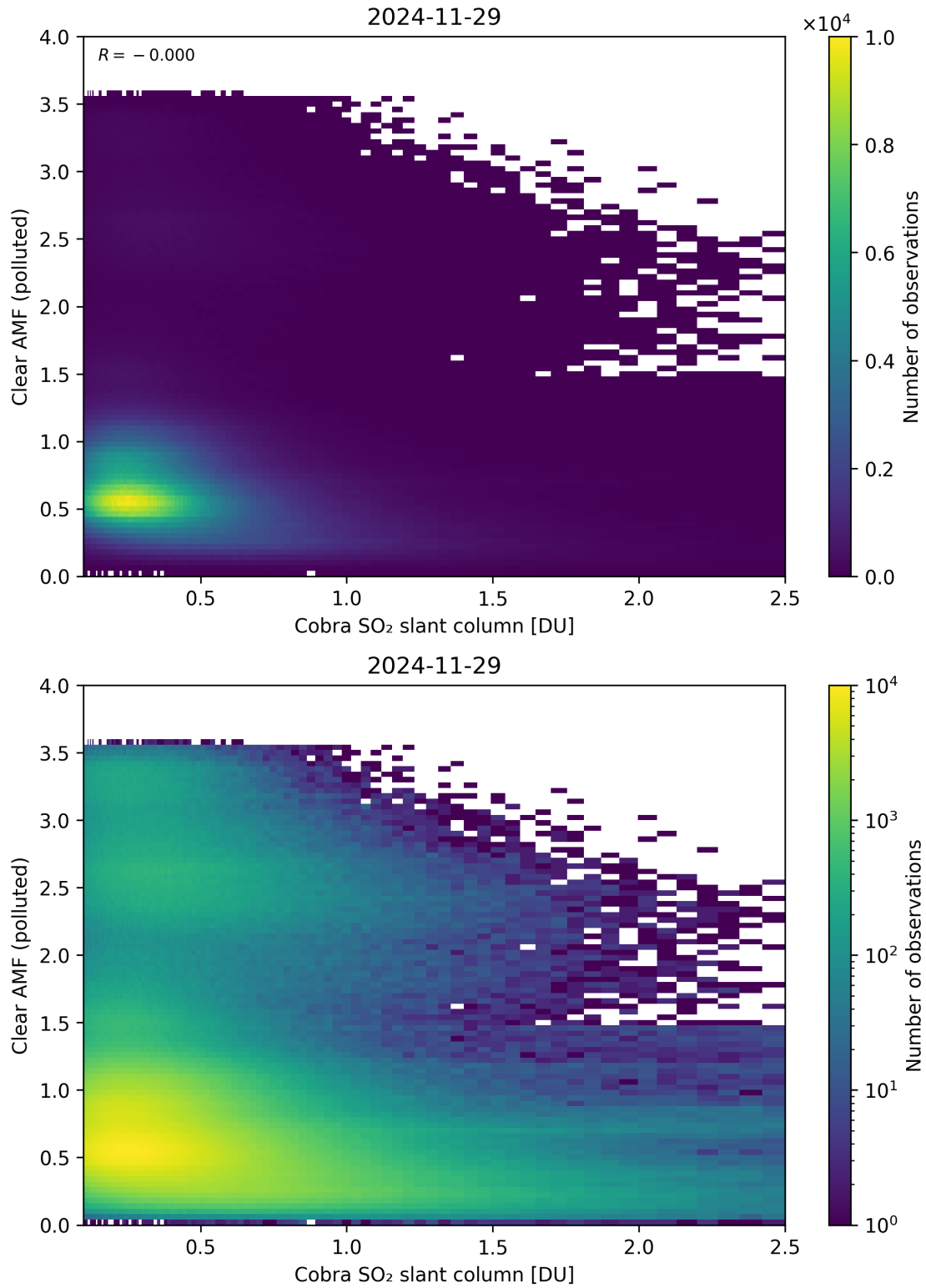
Figure 215: Scatter density plot of “Cobra SO 2 slant column” against “Clear AMF (polluted)” for 2024-11-28 to 2024-11-30.
