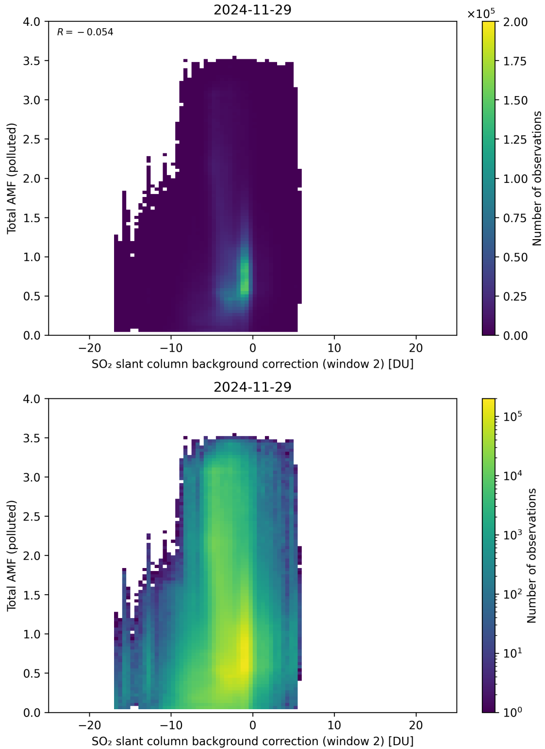
Figure 130: Scatter density plot of “SO 2 slant column background correction (window 2)” against “Total AMF (polluted)” for 2024-11-28 to 2024-11-30.
