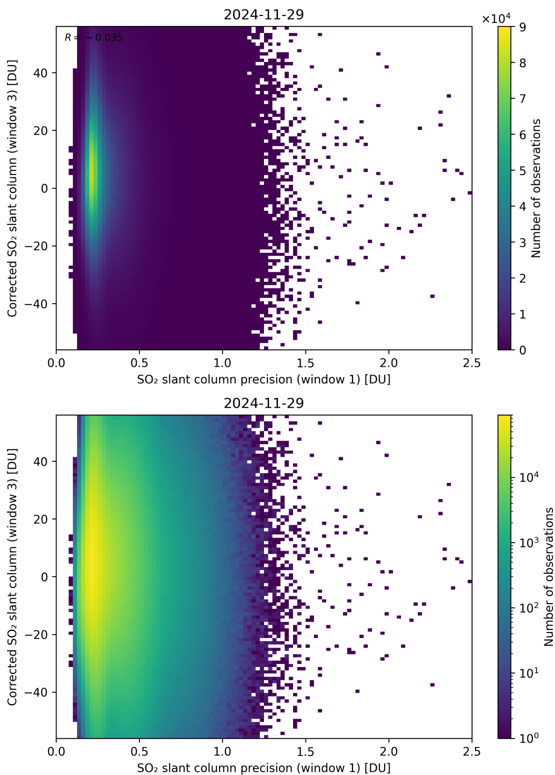
Figure 276: Scatter density plot of “SO 2 slant column precision (window 1)” against “Corrected SO 2 slant column (window 3)” for 2024-11-28 to 2024-11-30.
