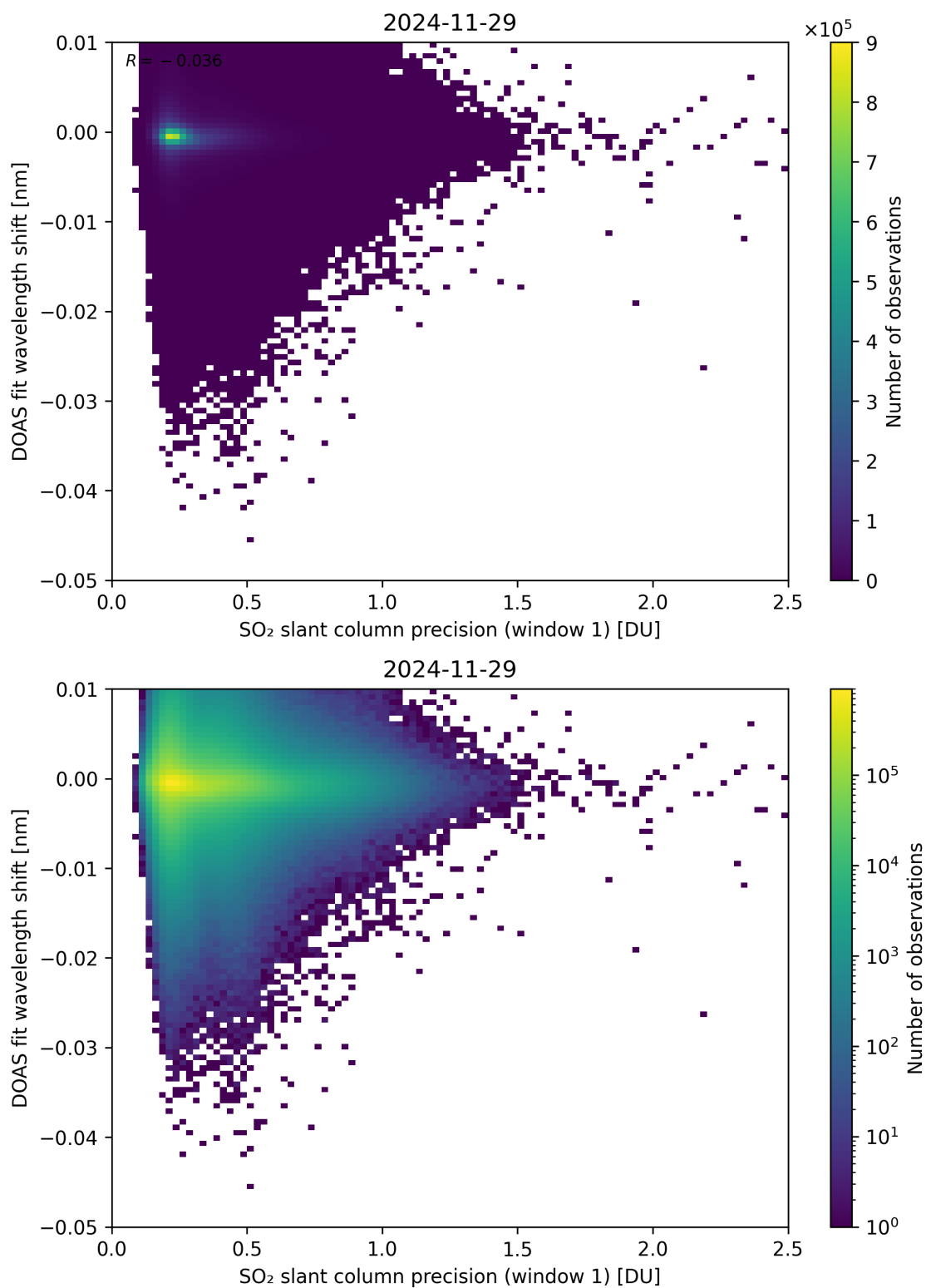
Figure 271: Scatter density plot of “SO 2 slant column precision (window 1)” against “DOAS fit wavelength shift” for 2024-11-28 to 2024-11-30.
