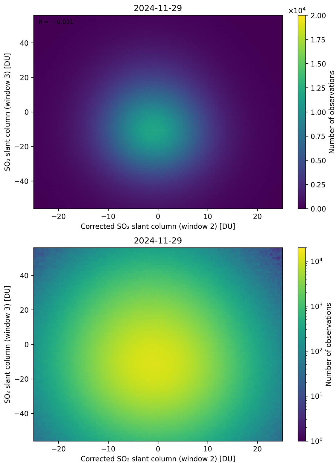
Figure 251: Scatter density plot of “Corrected SO 2 slant column (window 2)” against “SO 2 slant column (window 3)” for 2024-11-28 to 2024-11-30.
