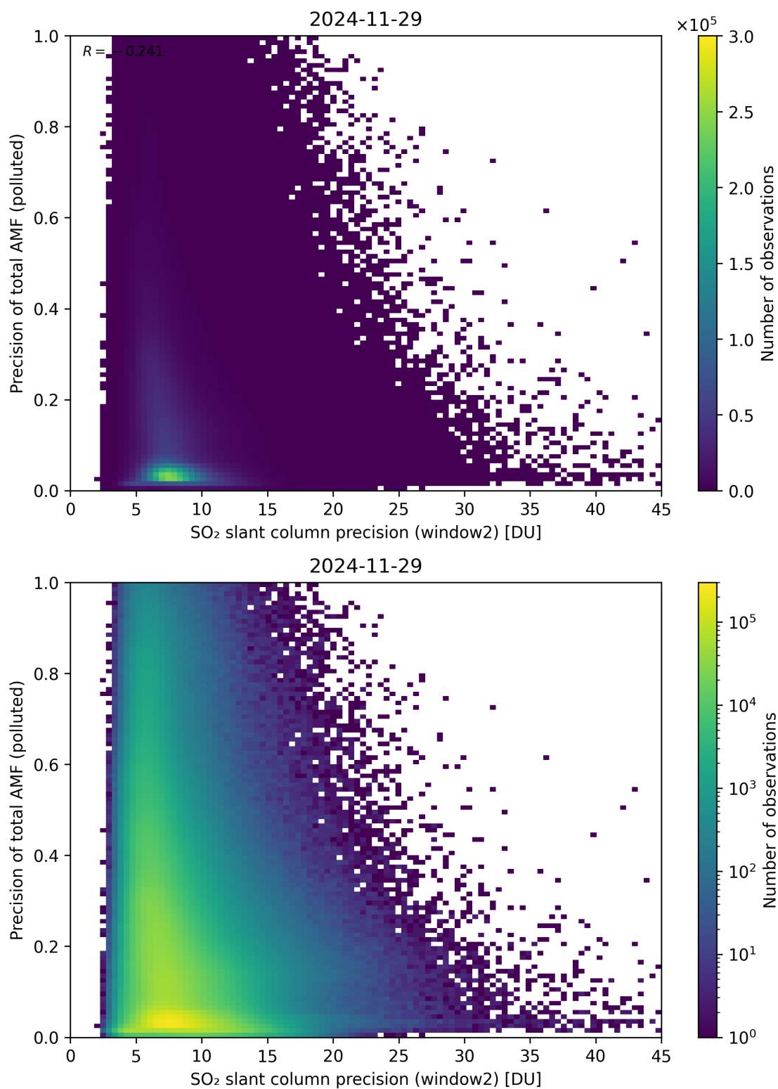
Figure 302: Scatter density plot of “SO 2 slant column precision (window2)” against “Precision of total AMF (polluted)” for 2024-11-28 to 2024-11-30.
