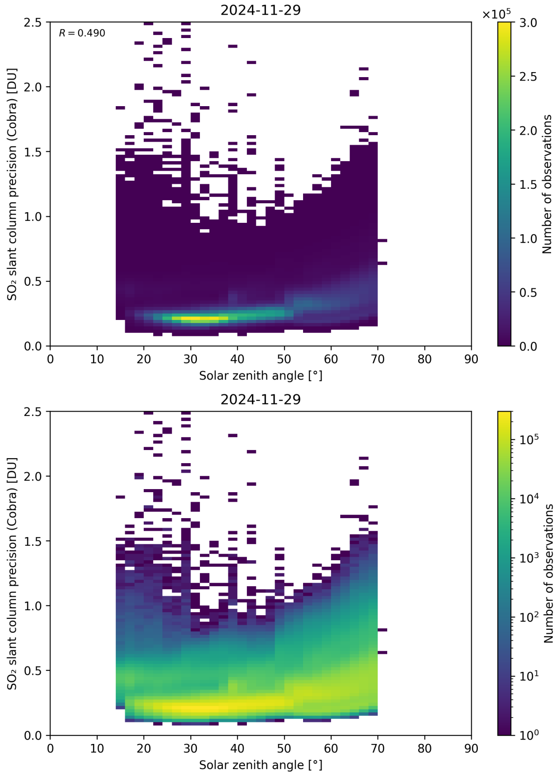
Figure 180: Scatter density plot of “Solar zenith angle” against “SO 2 slant column precision (Cobra)” for 2024-11-28 to 2024-11-30.
