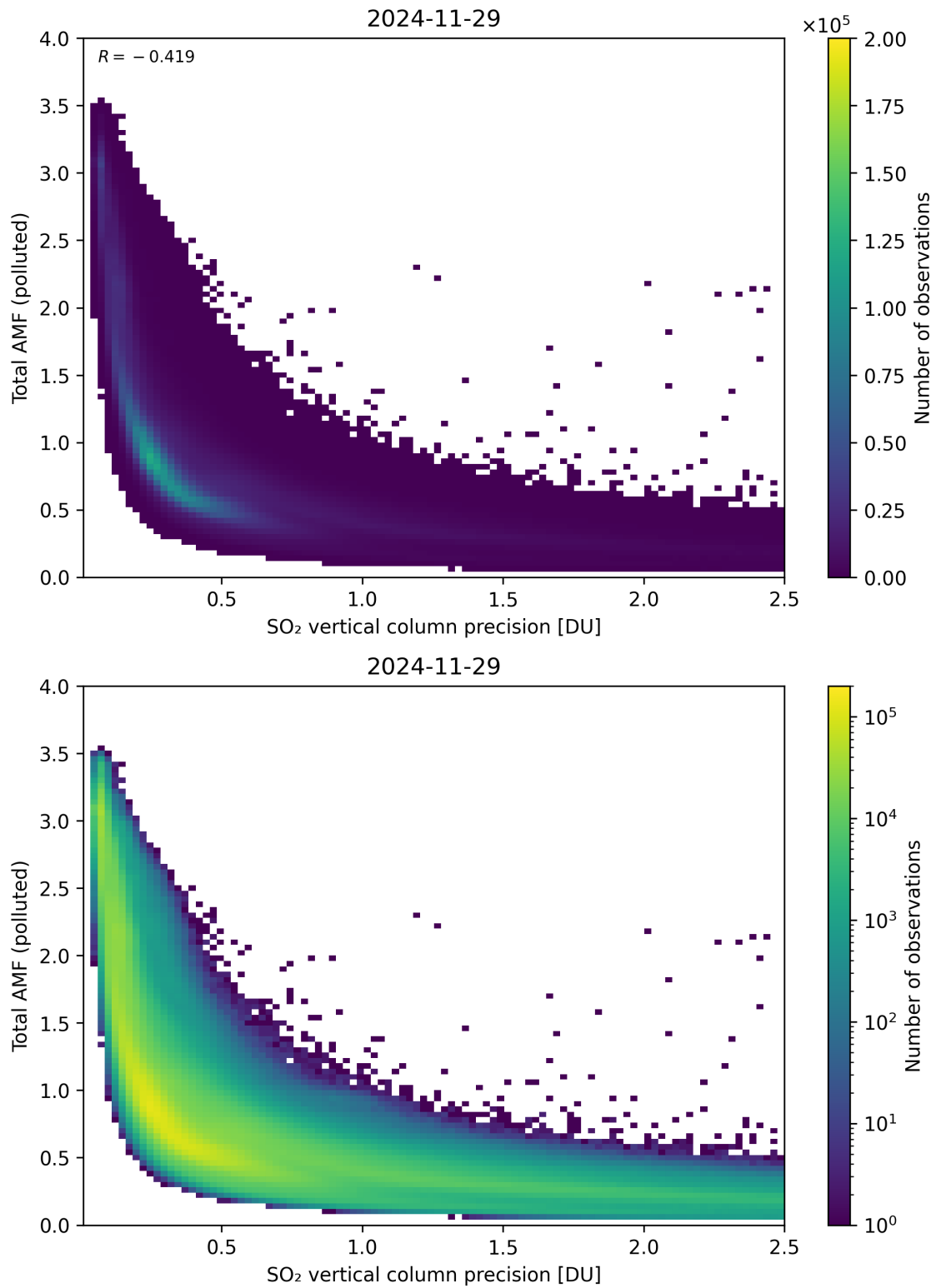
Figure 346: Scatter density plot of “SO 2 vertical column precision” against “Total AMF (polluted)” for 2024-11-28 to 2024-11-30.
