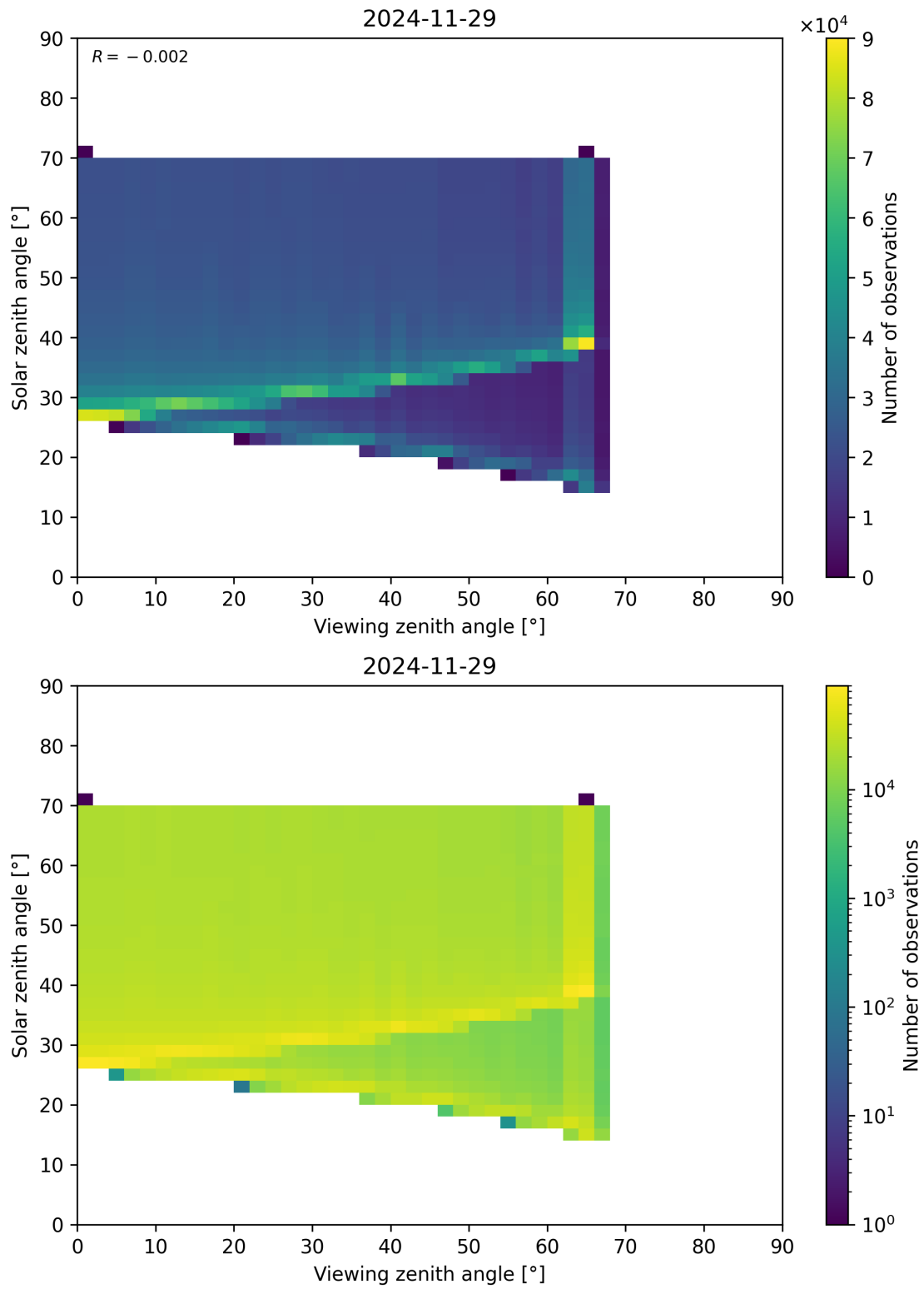
Figure 369: Scatter density plot of “Viewing zenith angle” against “Solar zenith angle” for 2024-11-28 to 2024-11-30.
