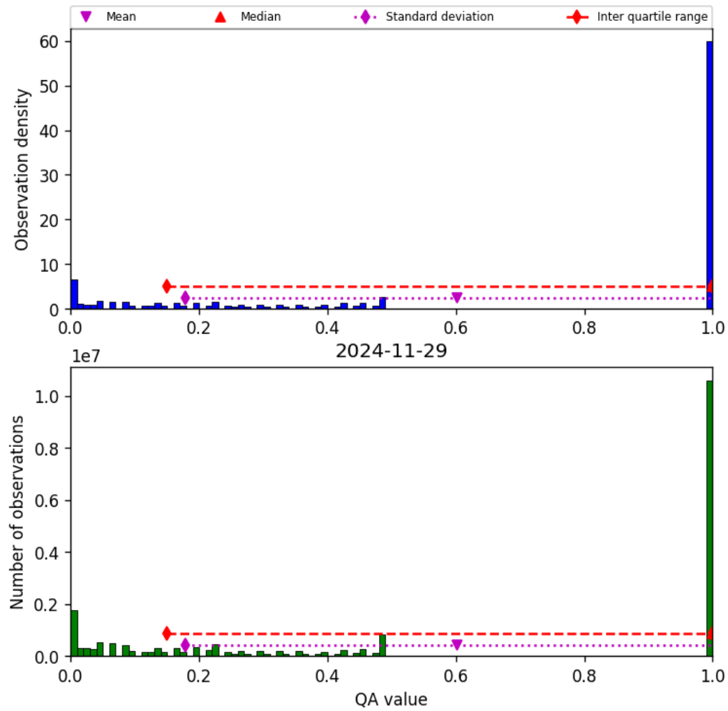
Figure 57: Histogram of “QA value” for 2024-11-28 to 2024-11-30
