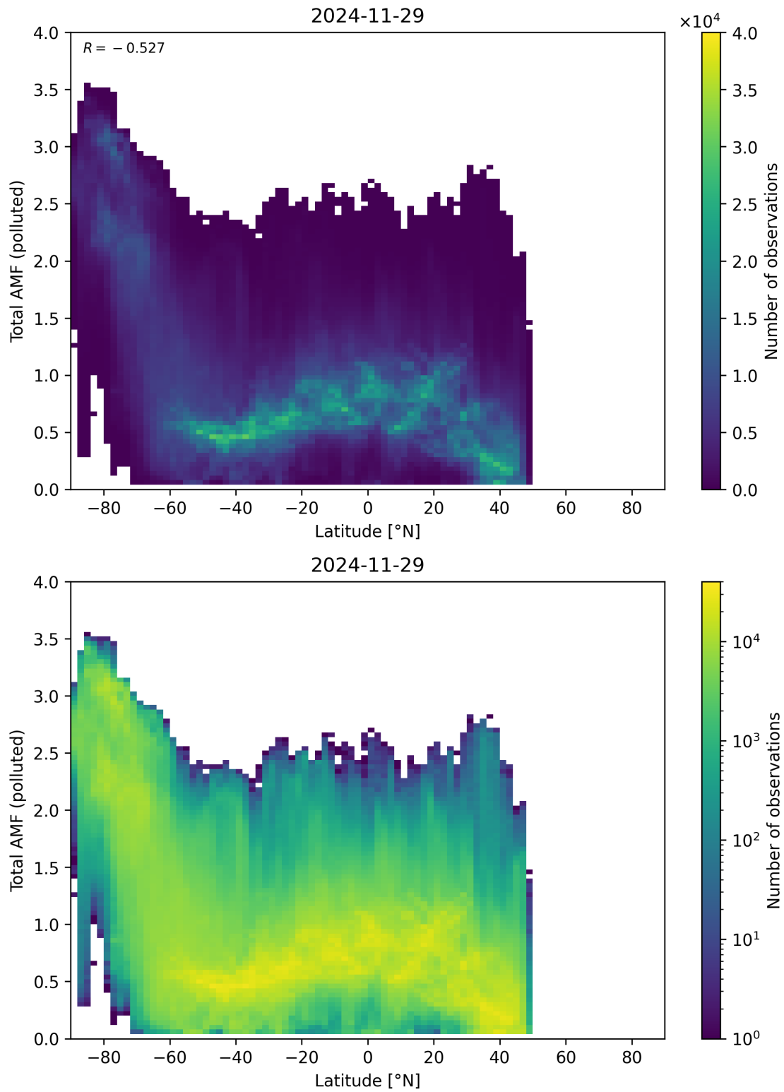
Figure 167: Scatter density plot of “Latitude” against “Total AMF (polluted)” for 2024-11-28 to 2024-11-30.
