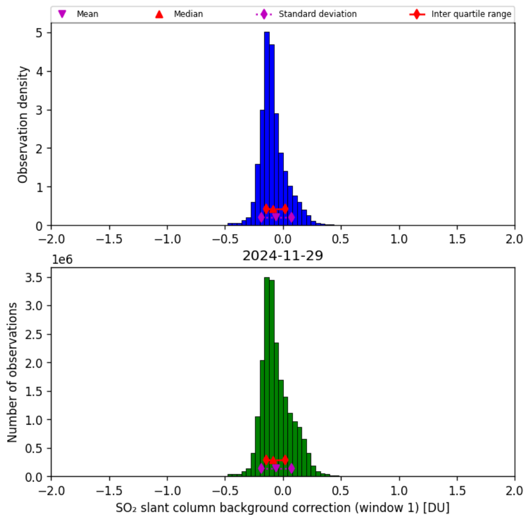
Figure 66: Histogram of “SO 2 slant column background correction (window 1)” for 2024-11-28 to 2024-11-30
