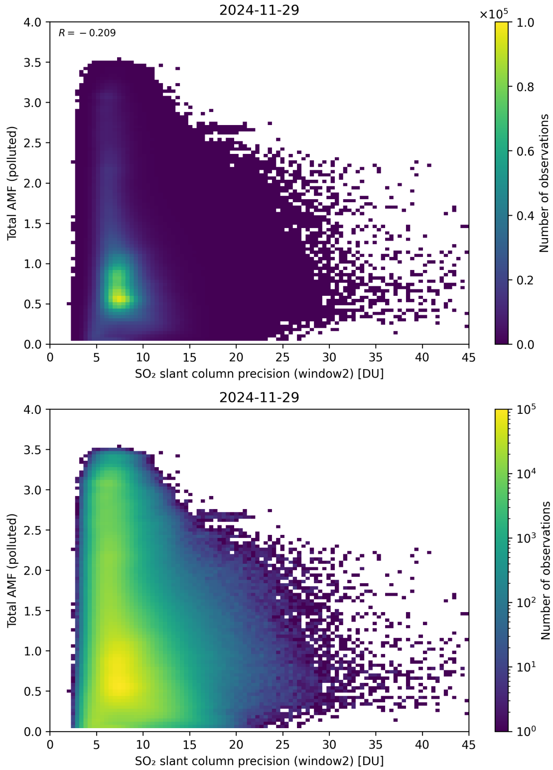
Figure 301: Scatter density plot of “SO 2 slant column precision (window2)” against “Total AMF (polluted)” for 2024-11-28 to 2024-11-30.
