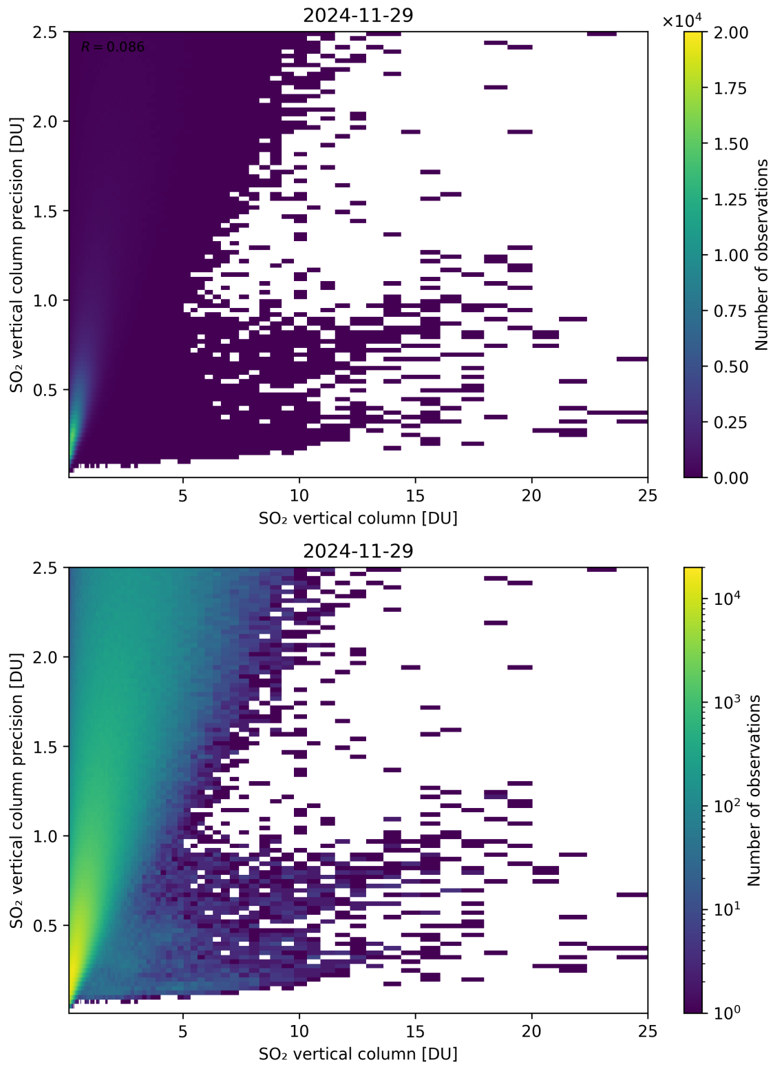
Figure 361: Scatter density plot of “SO 2 vertical column” against “SO 2 vertical column precision” for 2024-11-28 to 2024-11-30.
