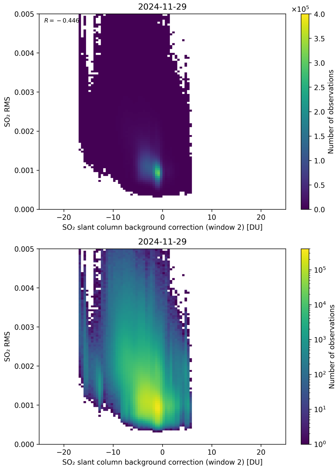
Figure 125: Scatter density plot of “SO 2 slant column background correction (window 2)” against “SO 2 RMS” for 2024-11-28 to 2024-11-30.
