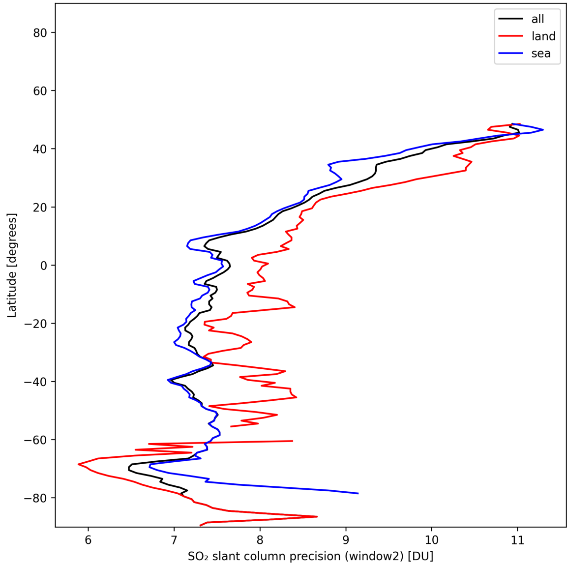
Figure 42: Zonal average of “SO 2 slant column precision (window2)” for 2024-11-28 to 2024-11-30.
