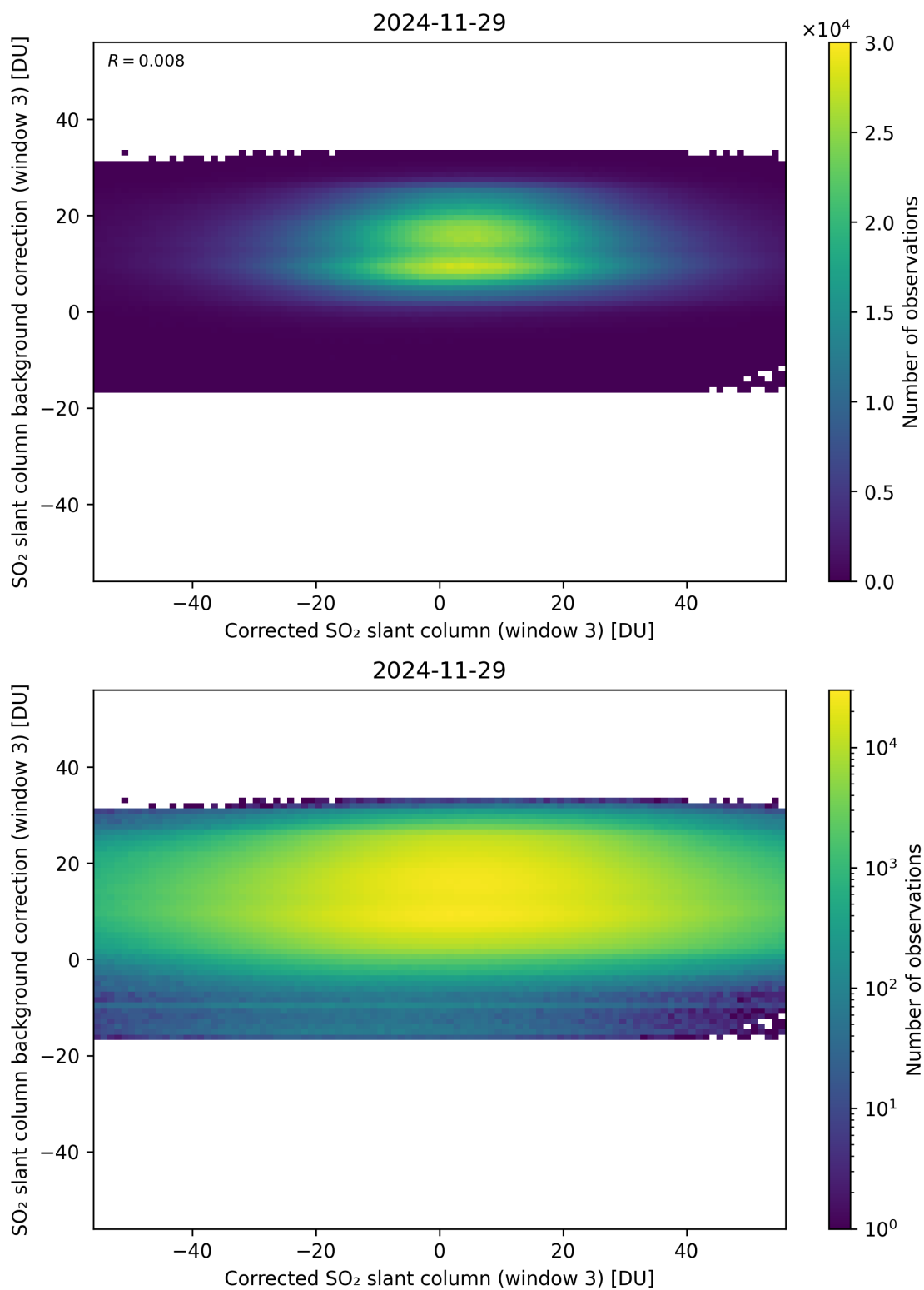
Figure 255: Scatter density plot of “Corrected SO 2 slant column (window 3)” against “SO 2 slant column background correction (window 3)” for 2024-11-28 to 2024-11-30.
