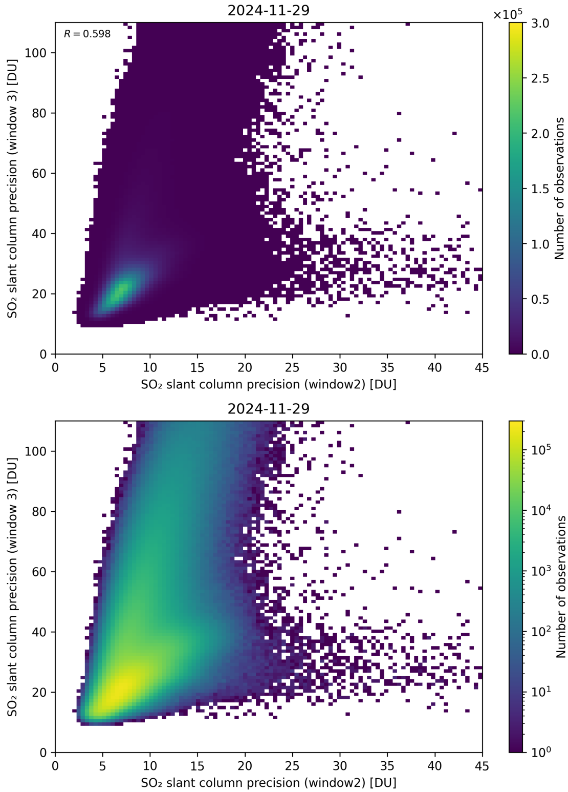
Figure 300: Scatter density plot of “SO 2 slant column precision (window2)” against “SO 2 slant column precision (window 3)” for 2024-11-28 to 2024-11-30.
