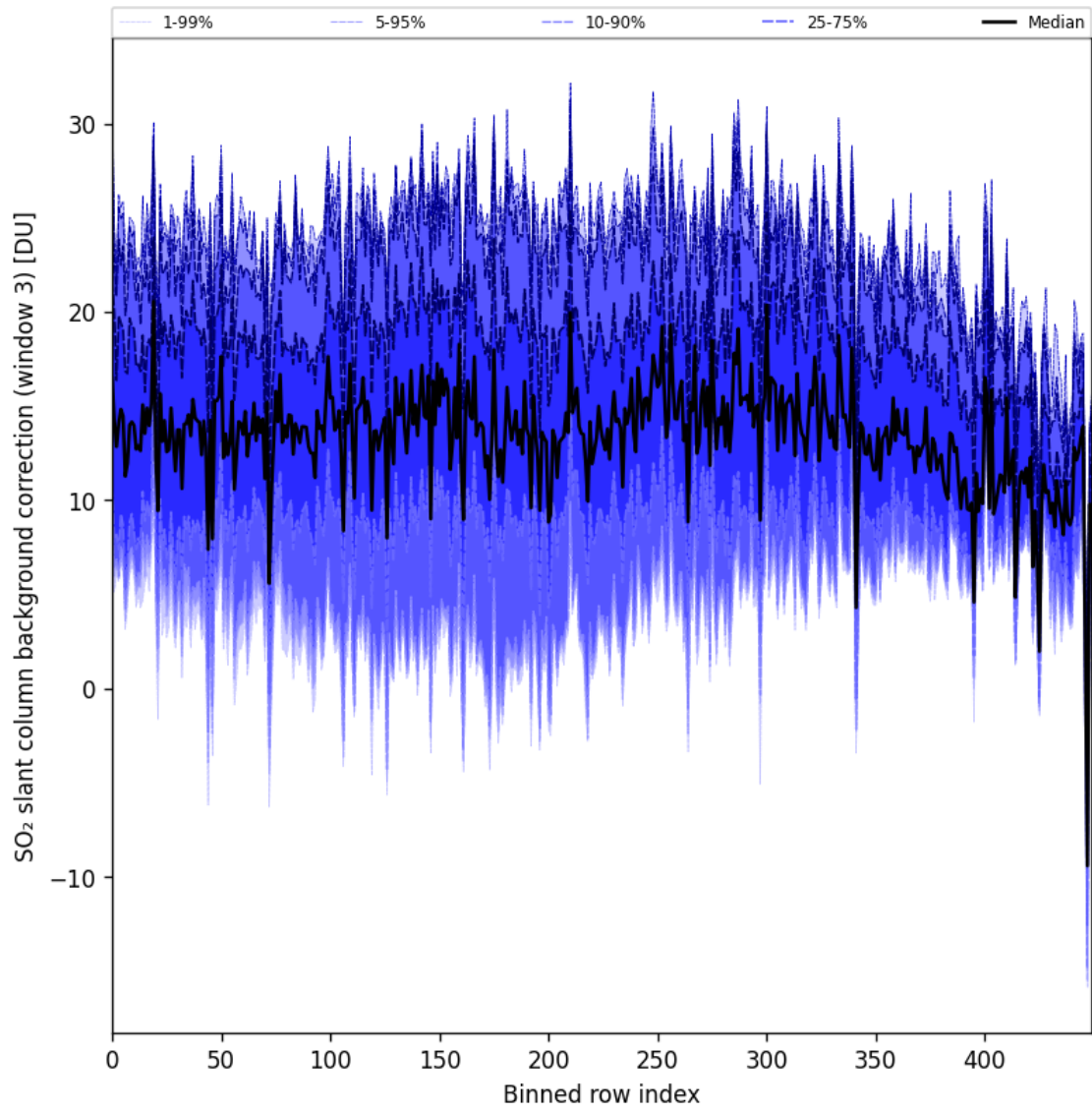
Figure 100: Along track statistics of “SO 2 slant column background correction (window 3)” for 2024-11-28 to 2024-11-30
