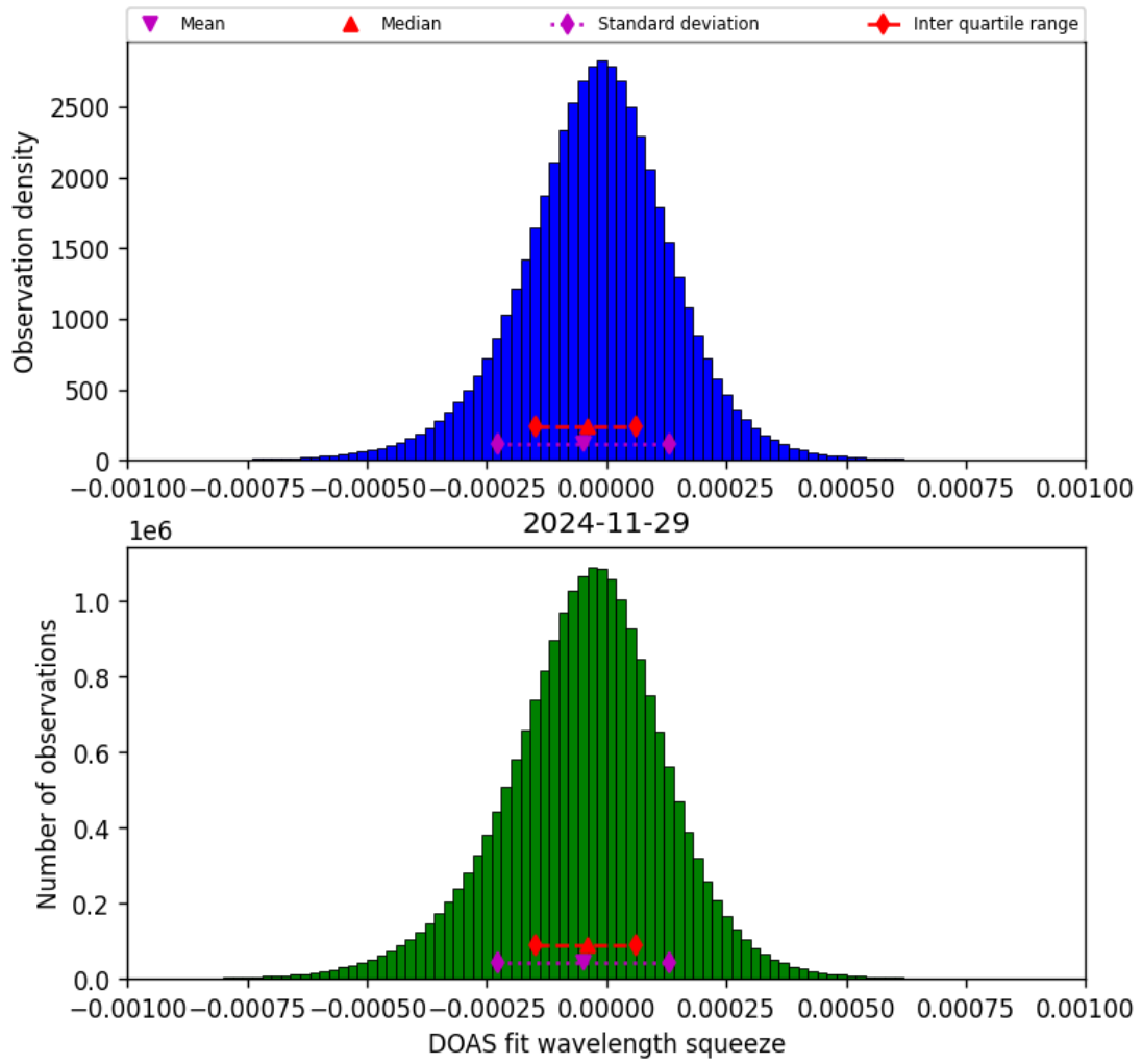
Figure 77: Histogram of “DOAS fit wavelength squeeze” for 2024-11-28 to 2024-11-30
