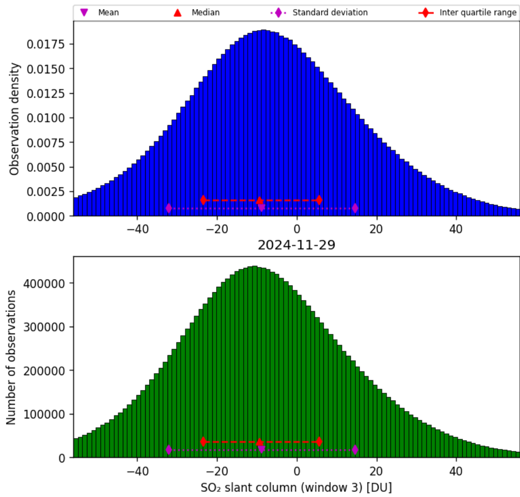
Figure 71: Histogram of “SO 2 slant column (window 3)” for 2024-11-28 to 2024-11-30
