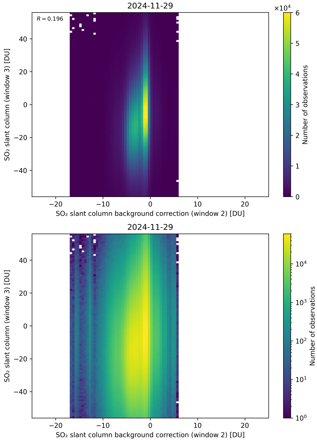
Figure 128: Scatter density plot of “SO 2 slant column background correction (window 2)” against “SO 2 slant column (window 3)” for 2024-11-28 to 2024-11-30.
