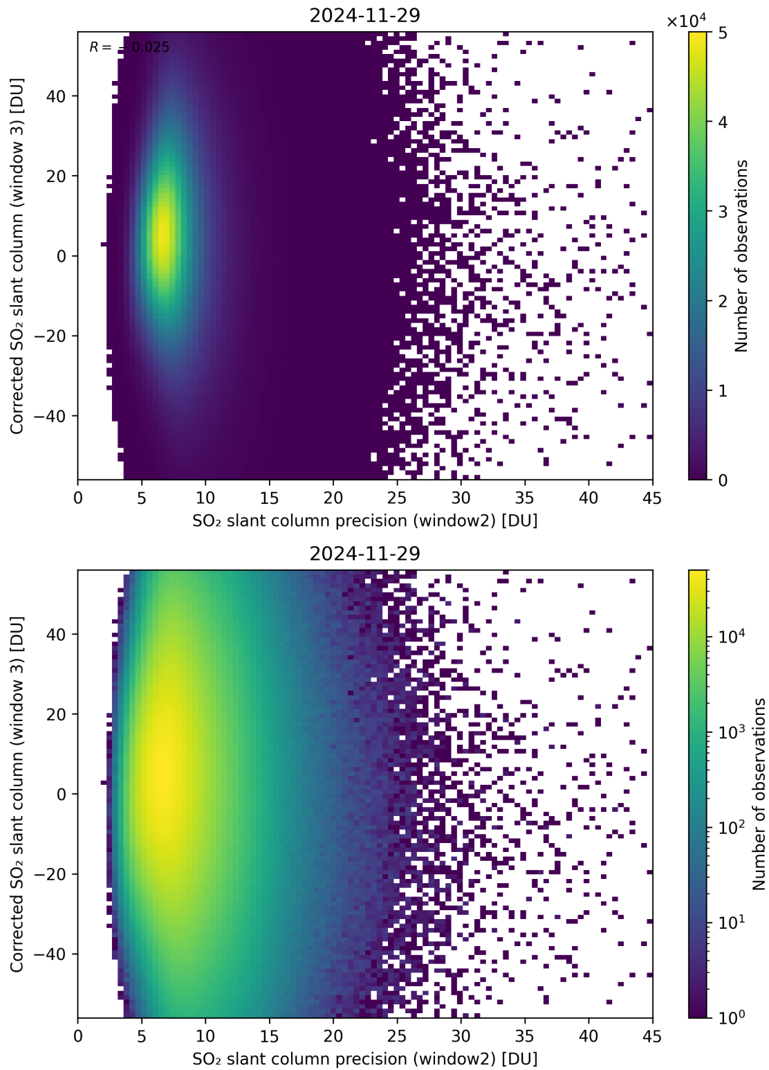
Figure 298: Scatter density plot of “SO 2 slant column precision (window2)” against “Corrected SO 2 slant column (window 3)” for 2024-11-28 to 2024-11-30.
