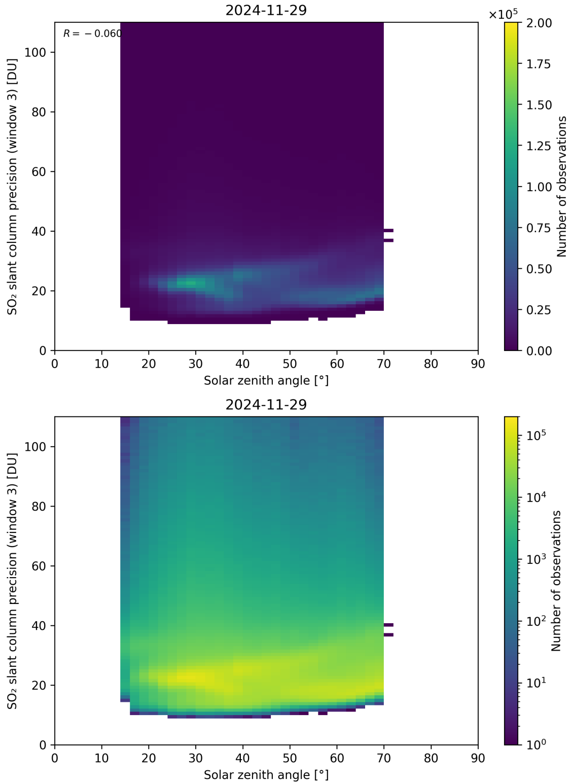
Figure 188: Scatter density plot of “Solar zenith angle” against “SO 2 slant column precision (window 3)” for 2024-11-28 to 2024-11-30.
