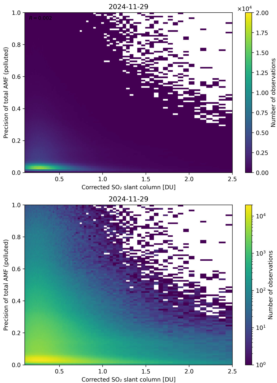
Figure 243: Scatter density plot of “Corrected SO 2 slant column” against “Precision of total AMF (polluted)” for 2024-11-28 to 2024-11-30.
