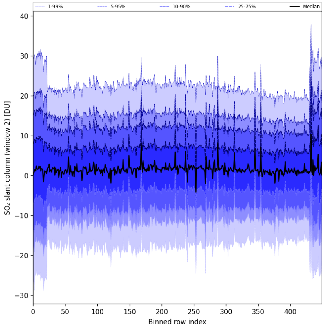
Figure 93: Along track statistics of “SO 2 slant column (window 2)” for 2024-11-28 to 2024-11-30
