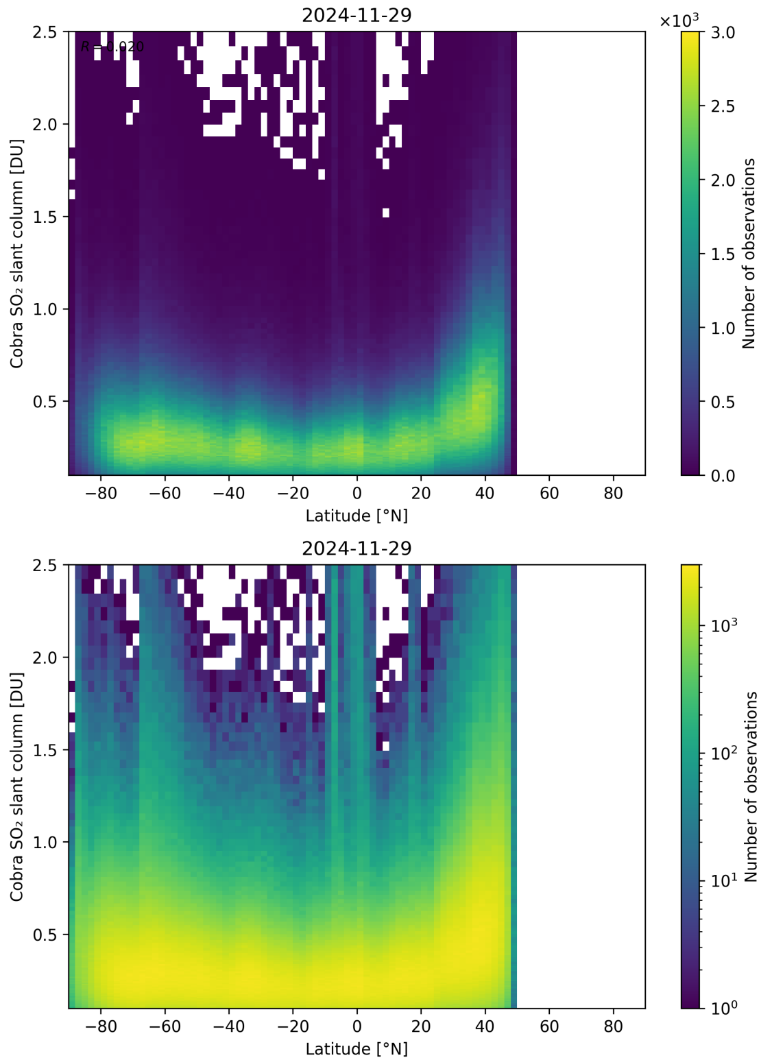
Figure 157: Scatter density plot of “Latitude” against “Cobra SO 2 slant column” for 2024-11-28 to 2024-11-30.
