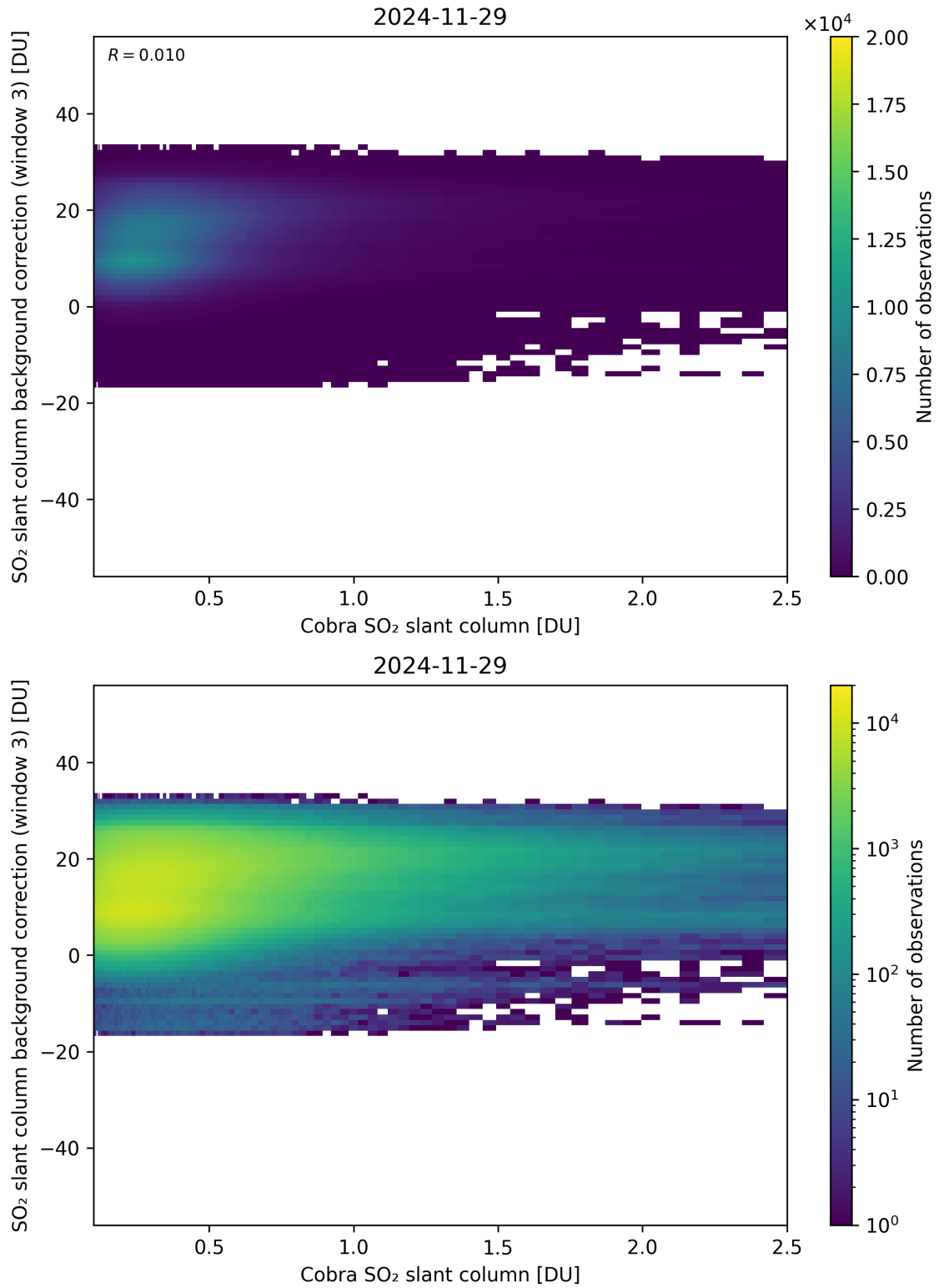
Figure 195: Scatter density plot of “Cobra SO 2 slant column” against “SO 2 slant column background correction (window 3)” for 2024-11-28 to 2024-11-30.
