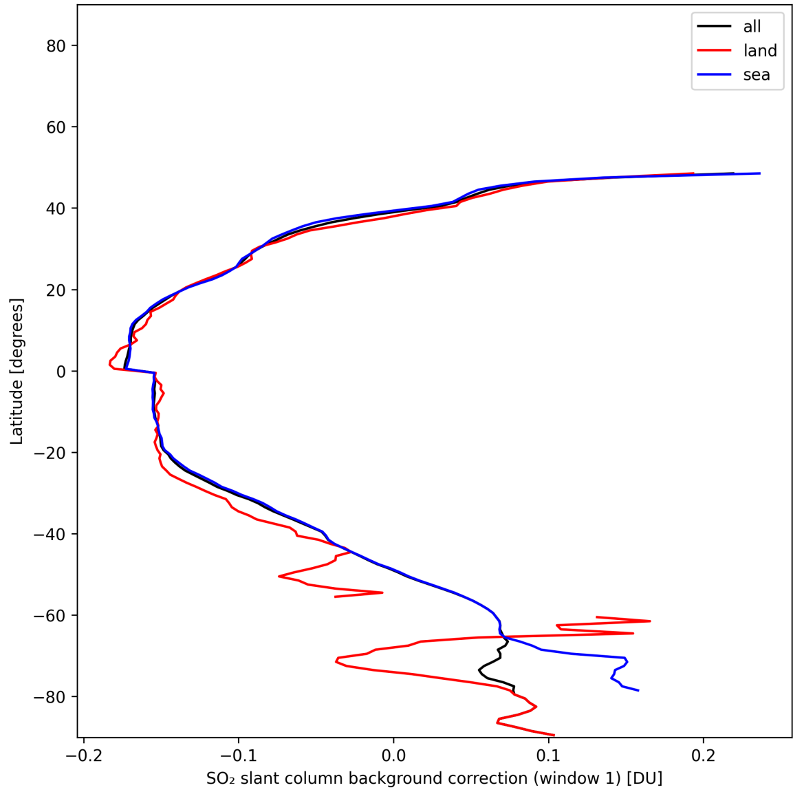
Figure 40: Zonal average of “SO 2 slant column background correction (window 1)” for 2024-11-28 to 2024-11-30.
