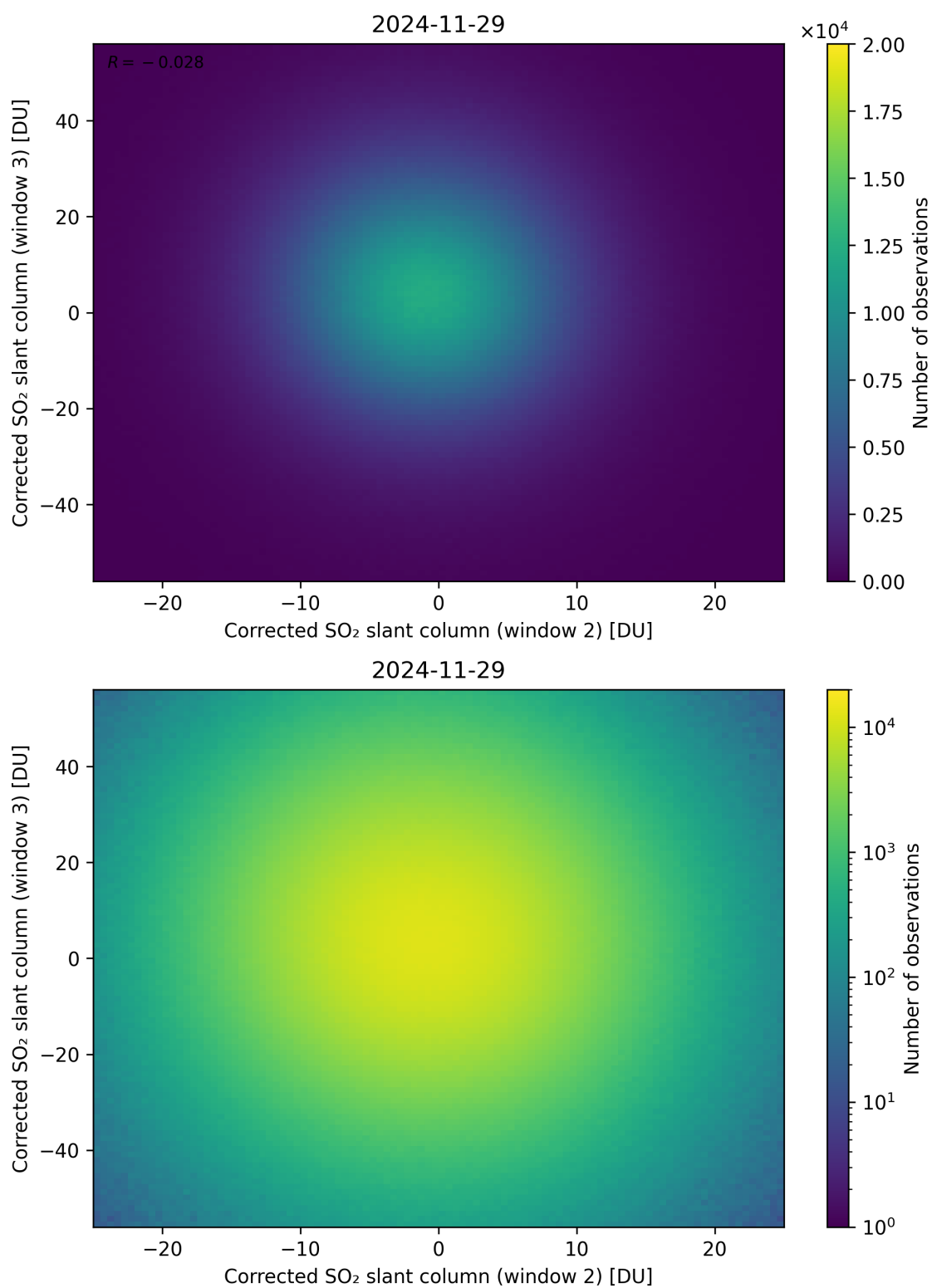
Figure 250: Scatter density plot of “Corrected SO 2 slant column (window 2)” against “Corrected SO 2 slant column (window 3)” for 2024-11-28 to 2024-11-30.
