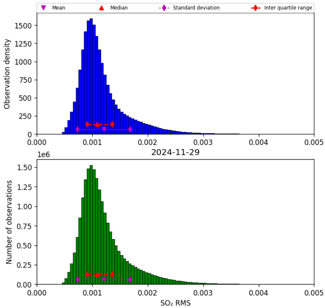
Figure 78: Histogram of “SO 2 RMS” for 2024-11-28 to 2024-11-30
