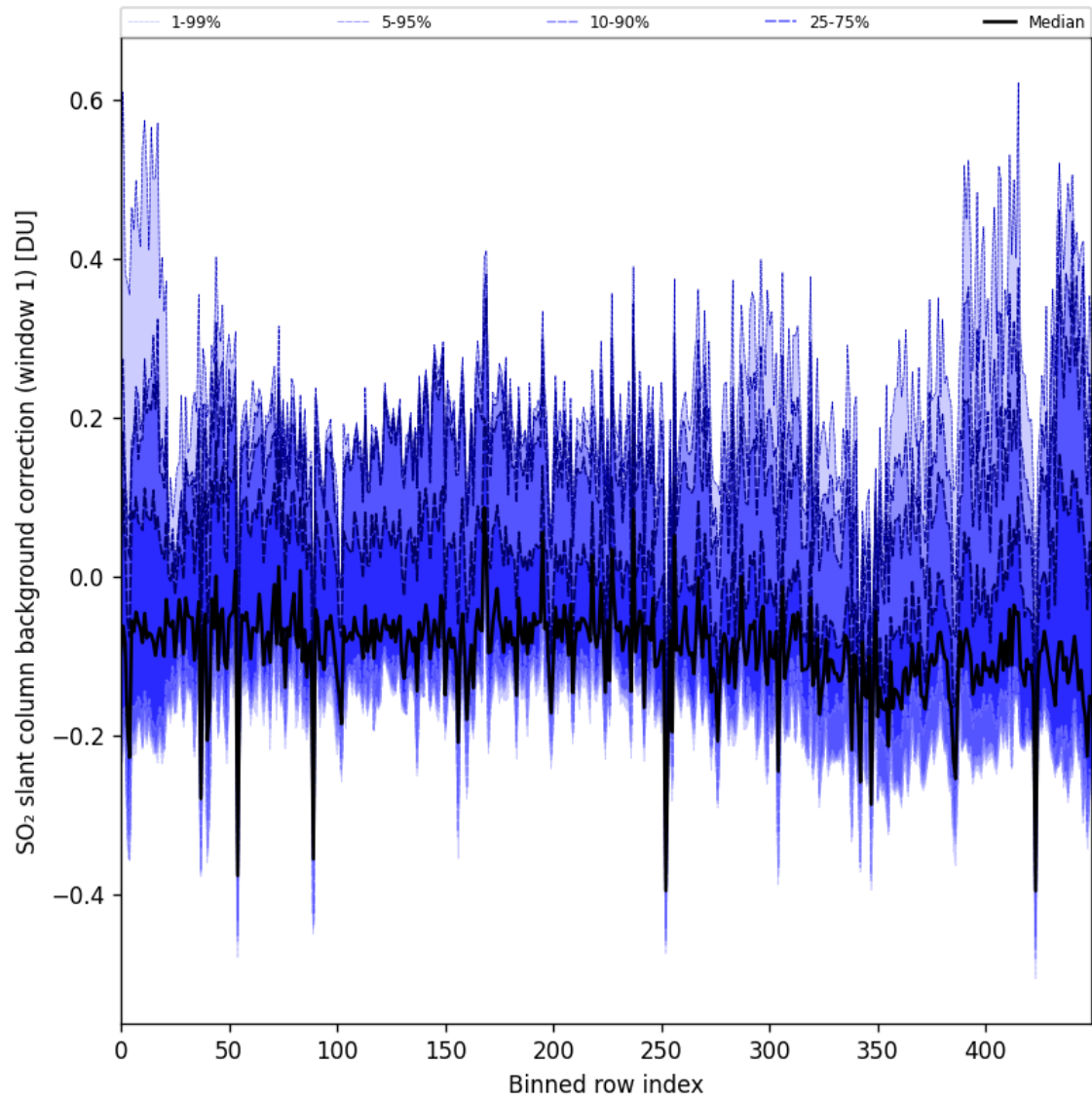
Figure 92: Along track statistics of “SO 2 slant column background correction (window 1)” for 2024-11-28 to 2024-11-30
