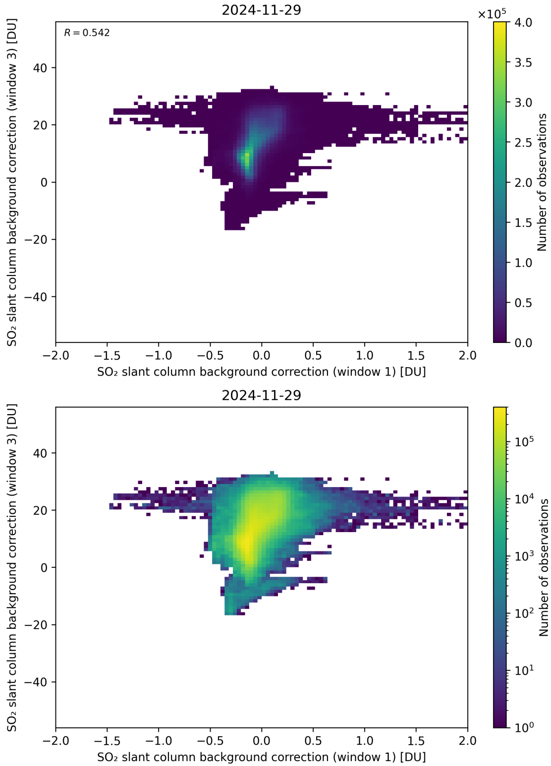
Figure 110: Scatter density plot of “SO 2 slant column background correction (window 1)” against “SO 2 slant column background correction (window 3)” for 2024-11-28 to 2024-11-30.
