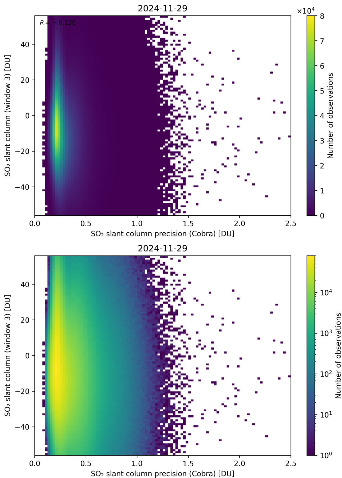
Figure 211: Scatter density plot of “SO 2 slant column precision (Cobra)” against “SO 2 slant column (window 3)” for 2024-11-28 to 2024-11-30.
