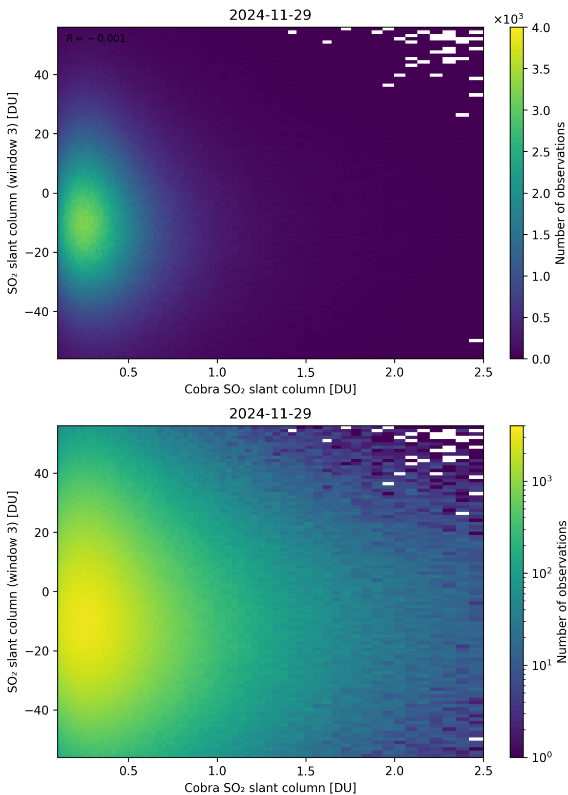
Figure 222: Scatter density plot of “Cobra SO 2 slant column” against “SO 2 slant column (window 3)” for 2024-11-28 to 2024-11-30.
