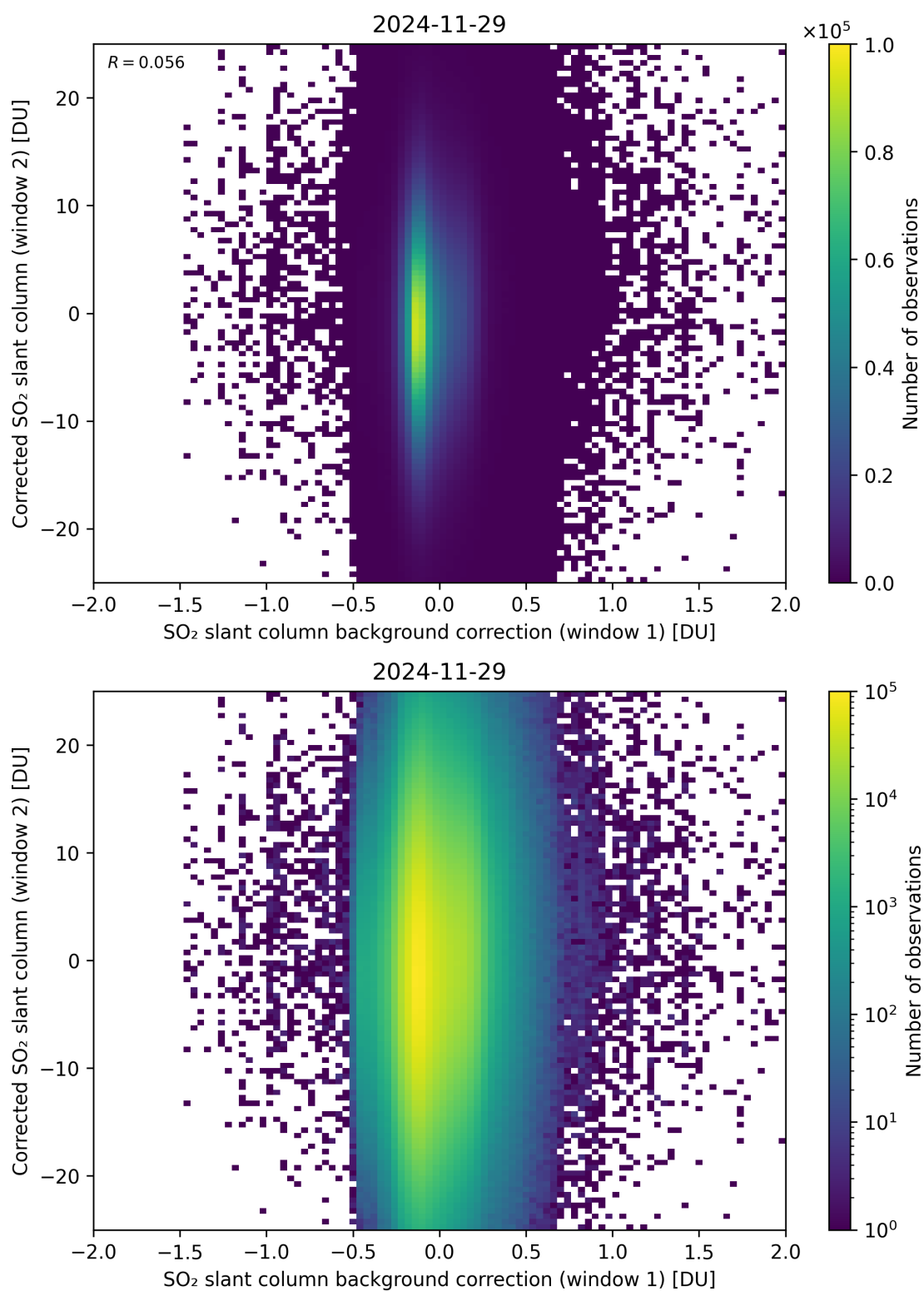
Figure 115: Scatter density plot of “SO 2 slant column background correction (window 1)” against “Corrected SO 2 slant column (window 2)” for 2024-11-28 to 2024-11-30.
