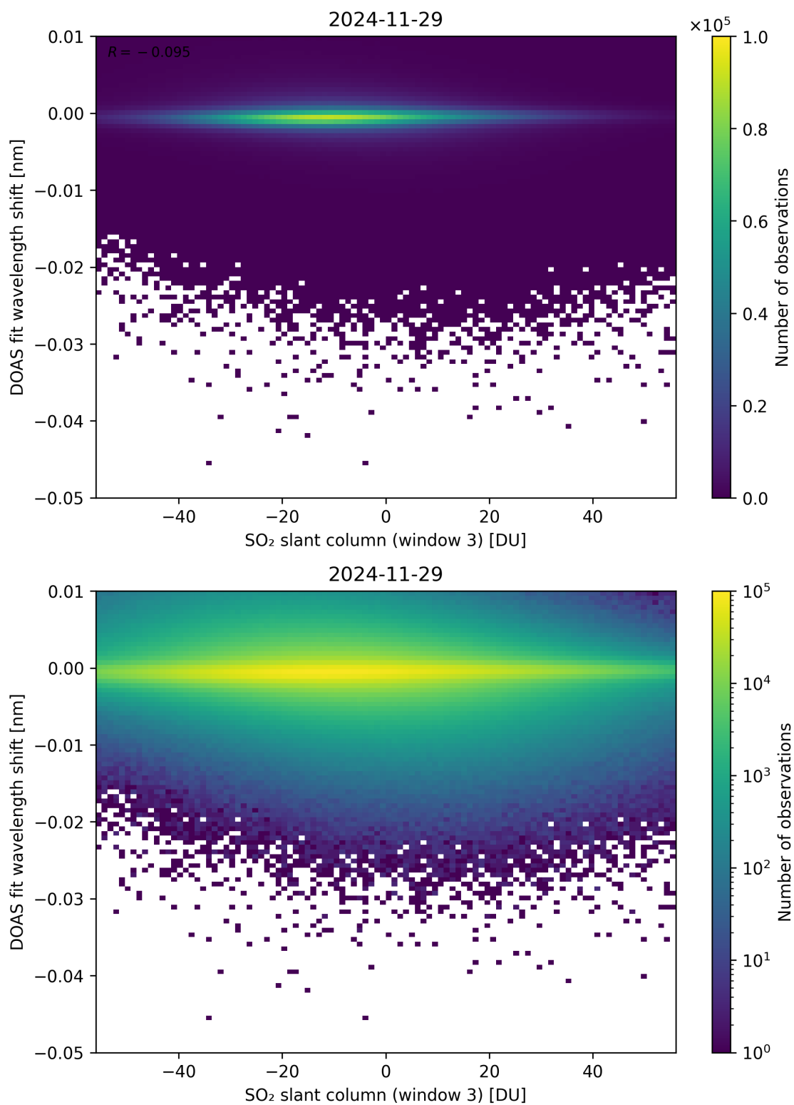
Figure 304: Scatter density plot of “SO 2 slant column (window 3)” against “DOAS fit wavelength shift” for 2024-11-28 to 2024-11-30.
