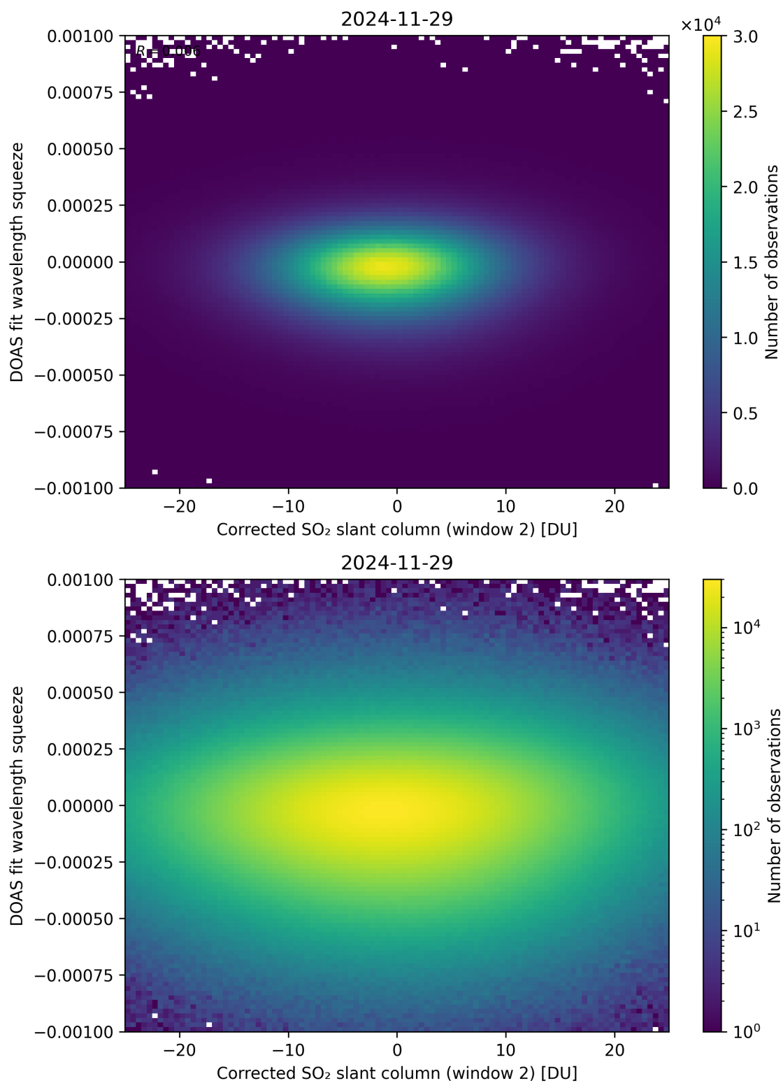
Figure 247: Scatter density plot of “Corrected SO 2 slant column (window 2)” against “DOAS fit wavelength squeeze” for 2024-11-28 to 2024-11-30.
