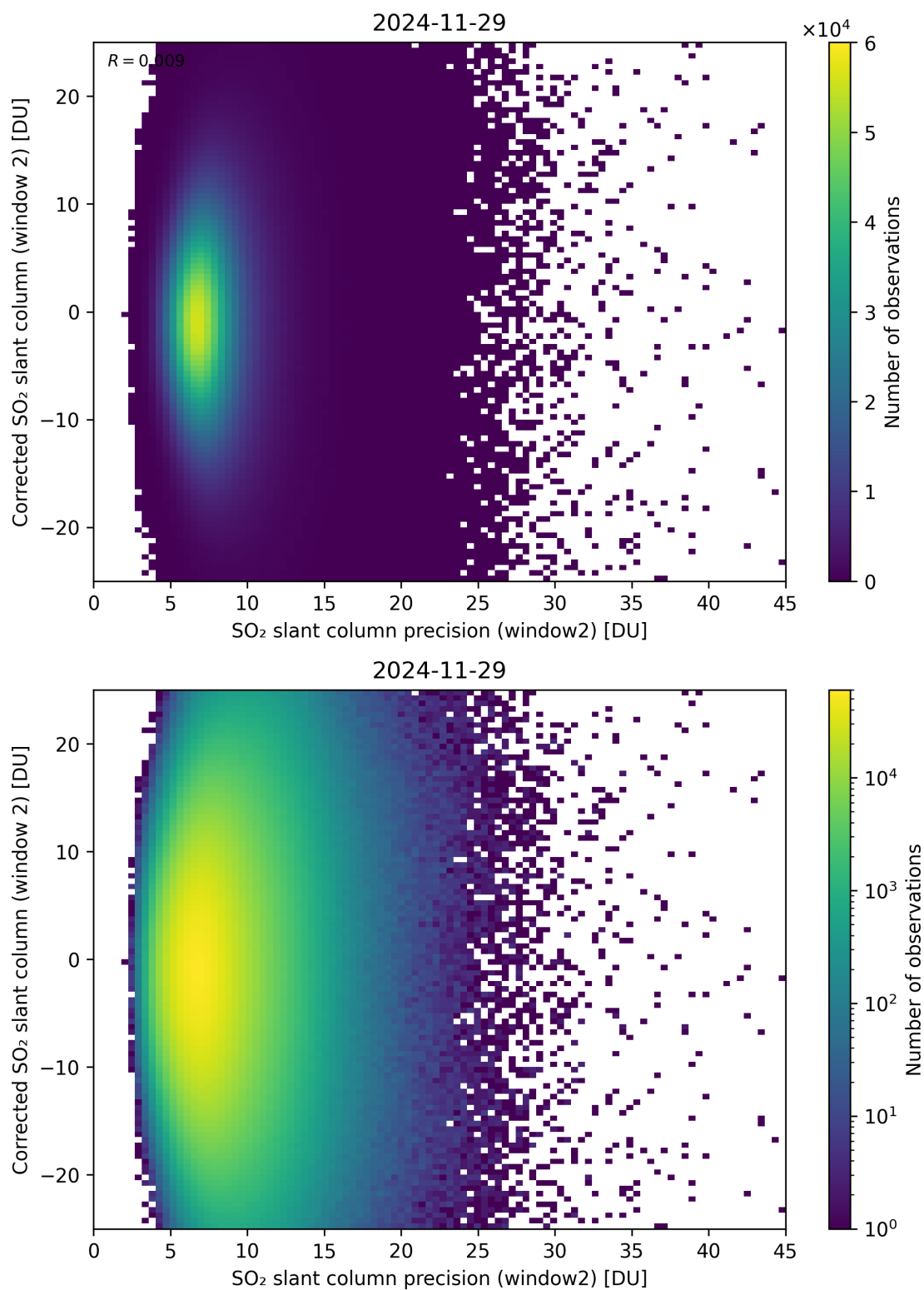
Figure 297: Scatter density plot of “SO 2 slant column precision (window2)” against “Corrected SO 2 slant column (window 2)” for 2024-11-28 to 2024-11-30.
