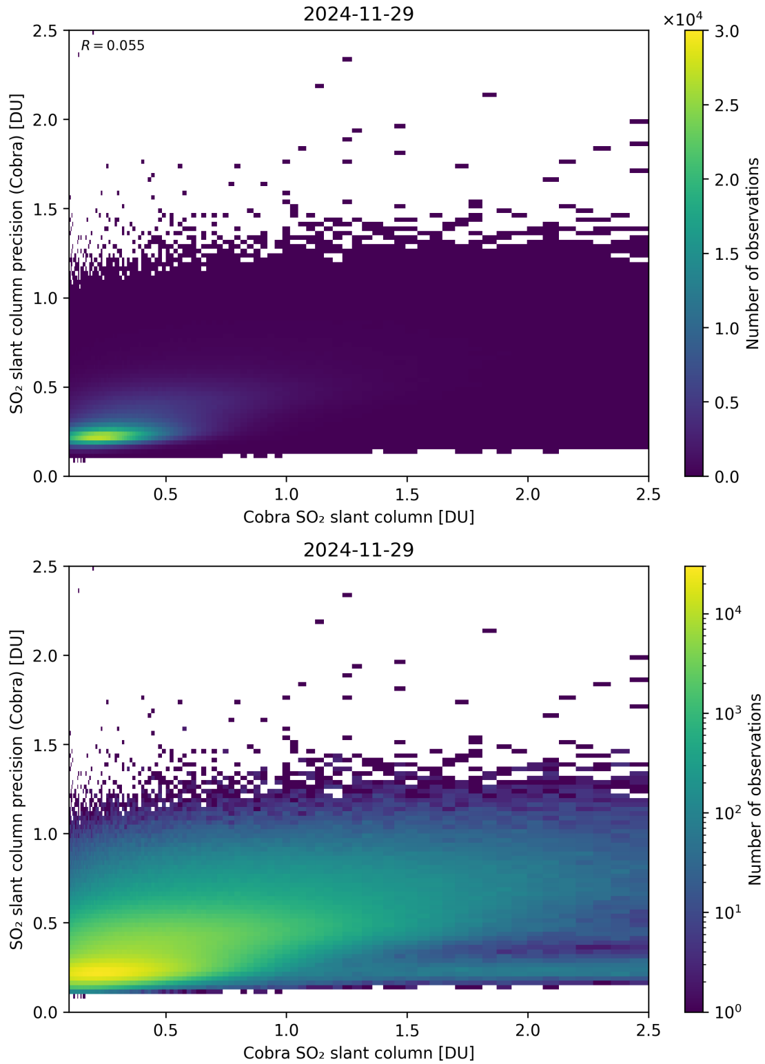
Figure 216: Scatter density plot of “Cobra SO 2 slant column” against “SO 2 slant column precision (Cobra)” for 2024-11-28 to 2024-11-30.
