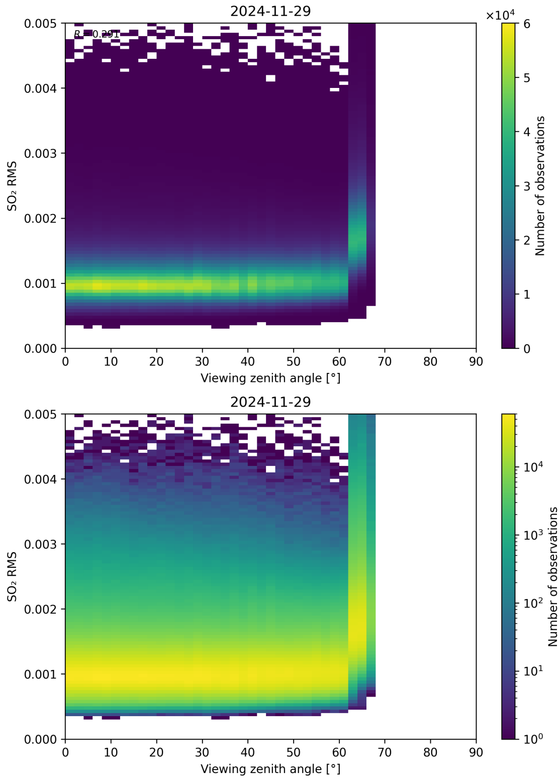
Figure 367: Scatter density plot of “Viewing zenith angle” against “SO 2 RMS” for 2024-11-28 to 2024-11-30.
