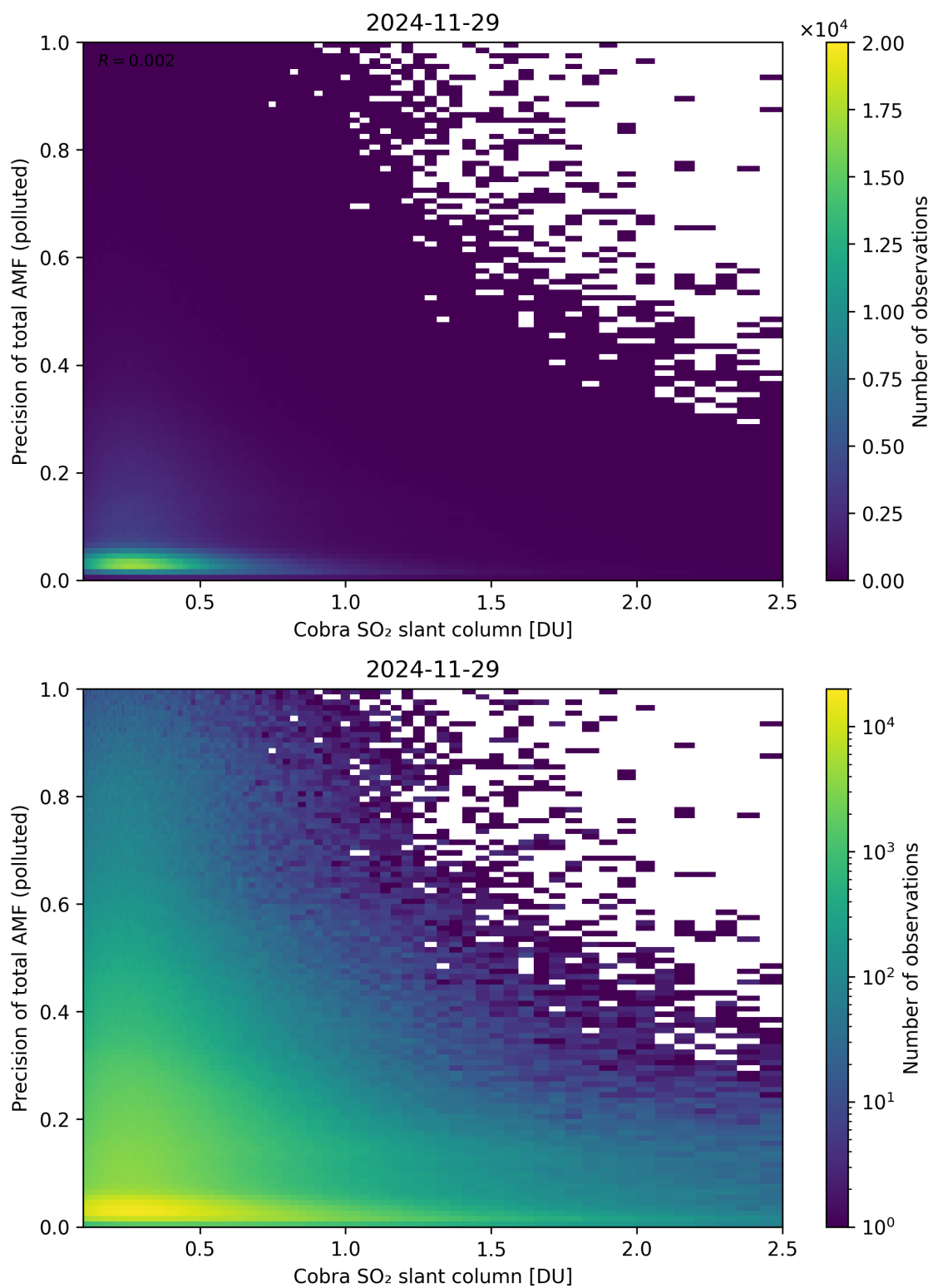
Figure 225: Scatter density plot of “Cobra SO 2 slant column” against “Precision of total AMF (polluted)” for 2024-11-28 to 2024-11-30.
