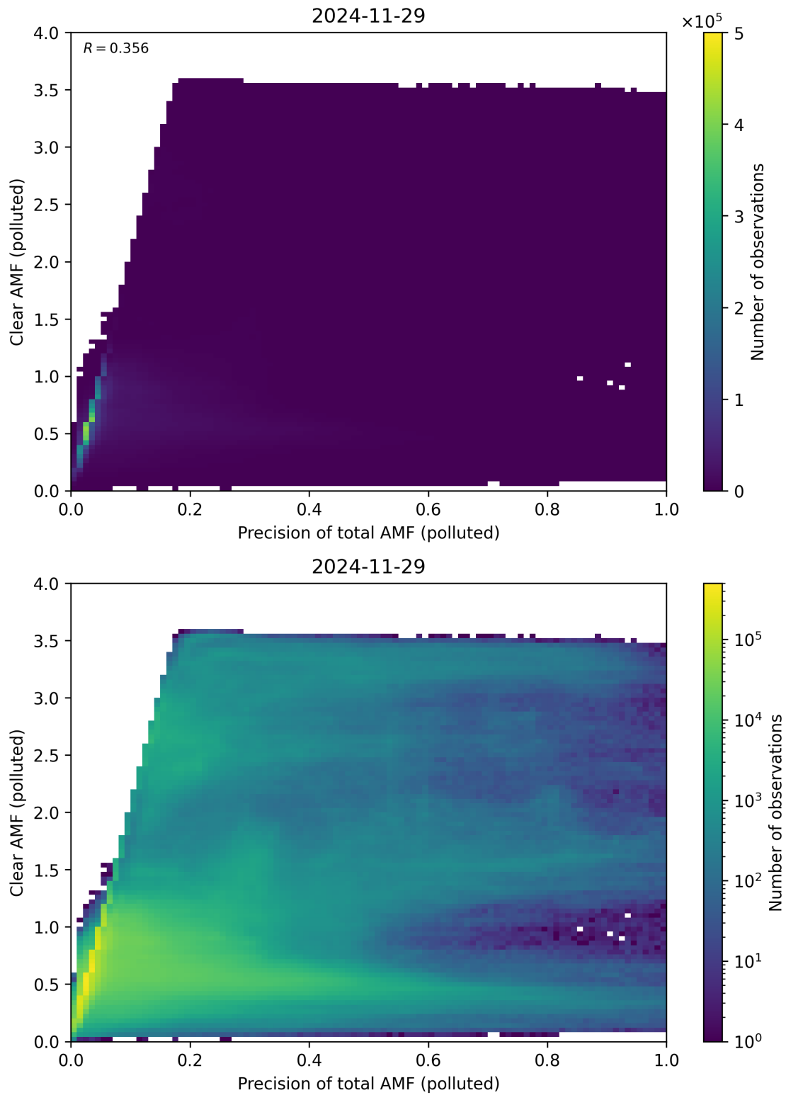
Figure 320: Scatter density plot of “Precision of total AMF (polluted)” against “Clear AMF (polluted)” for 2024-11-28 to 2024-11-30.
