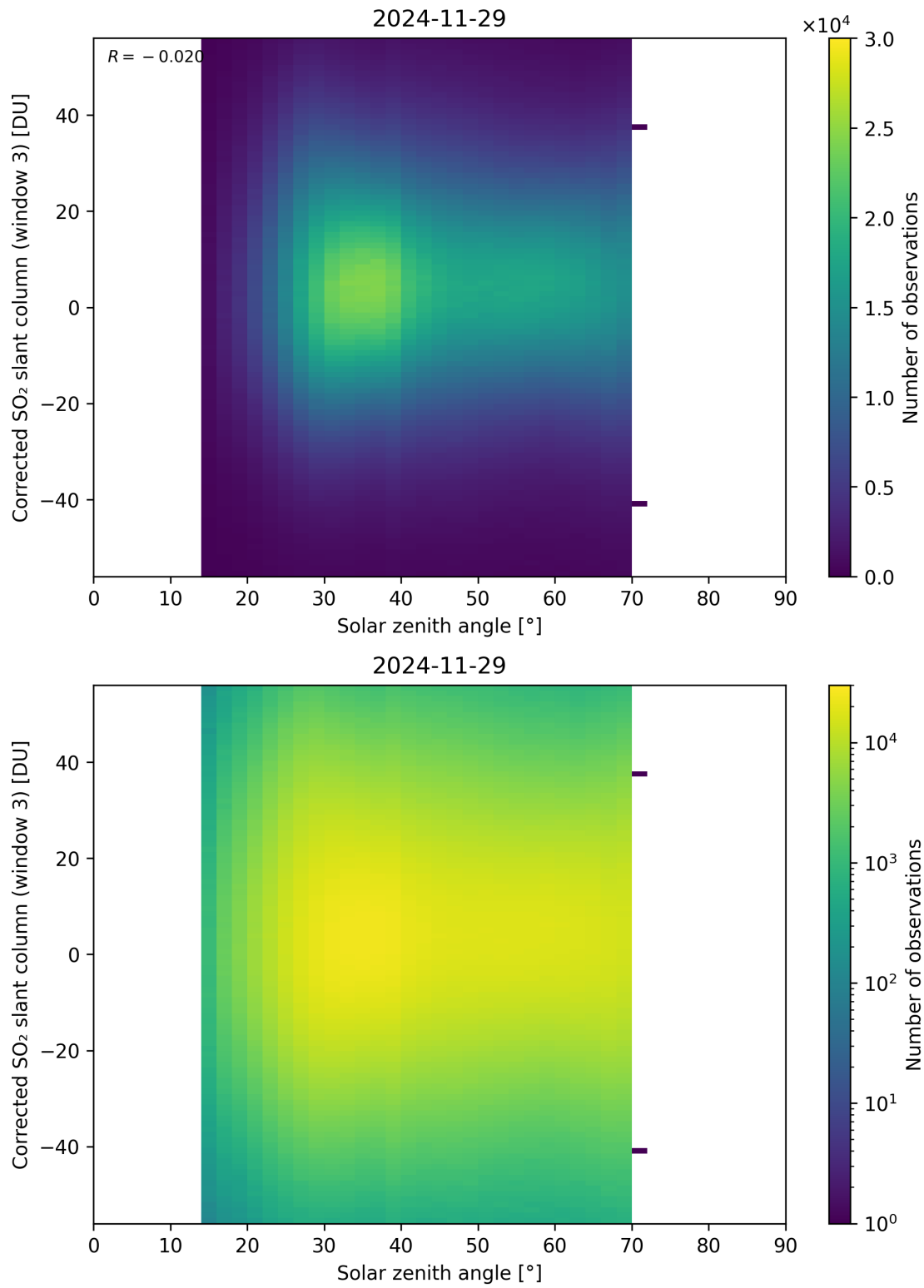
Figure 183: Scatter density plot of “Solar zenith angle” against “Corrected SO 2 slant column (window 3)” for 2024-11-28 to 2024-11-30.
