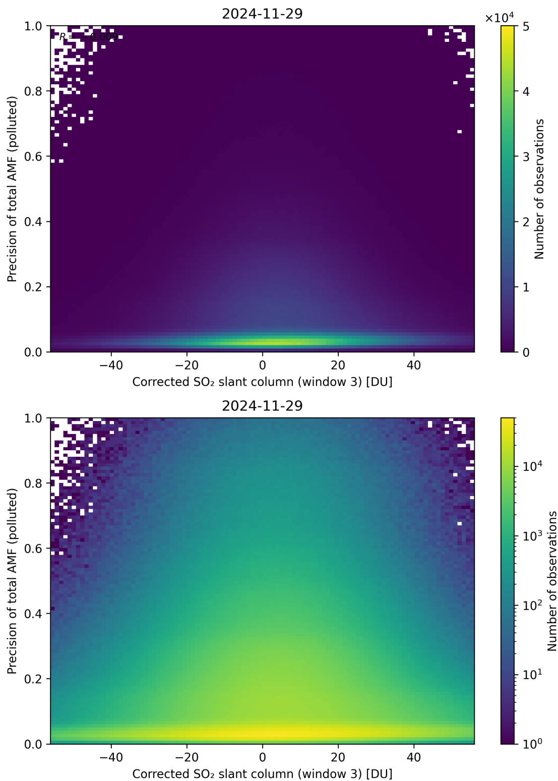
Figure 261: Scatter density plot of “Corrected SO 2 slant column (window 3)” against “Precision of total AMF (polluted)” for 2024-11-28 to 2024-11-30.
