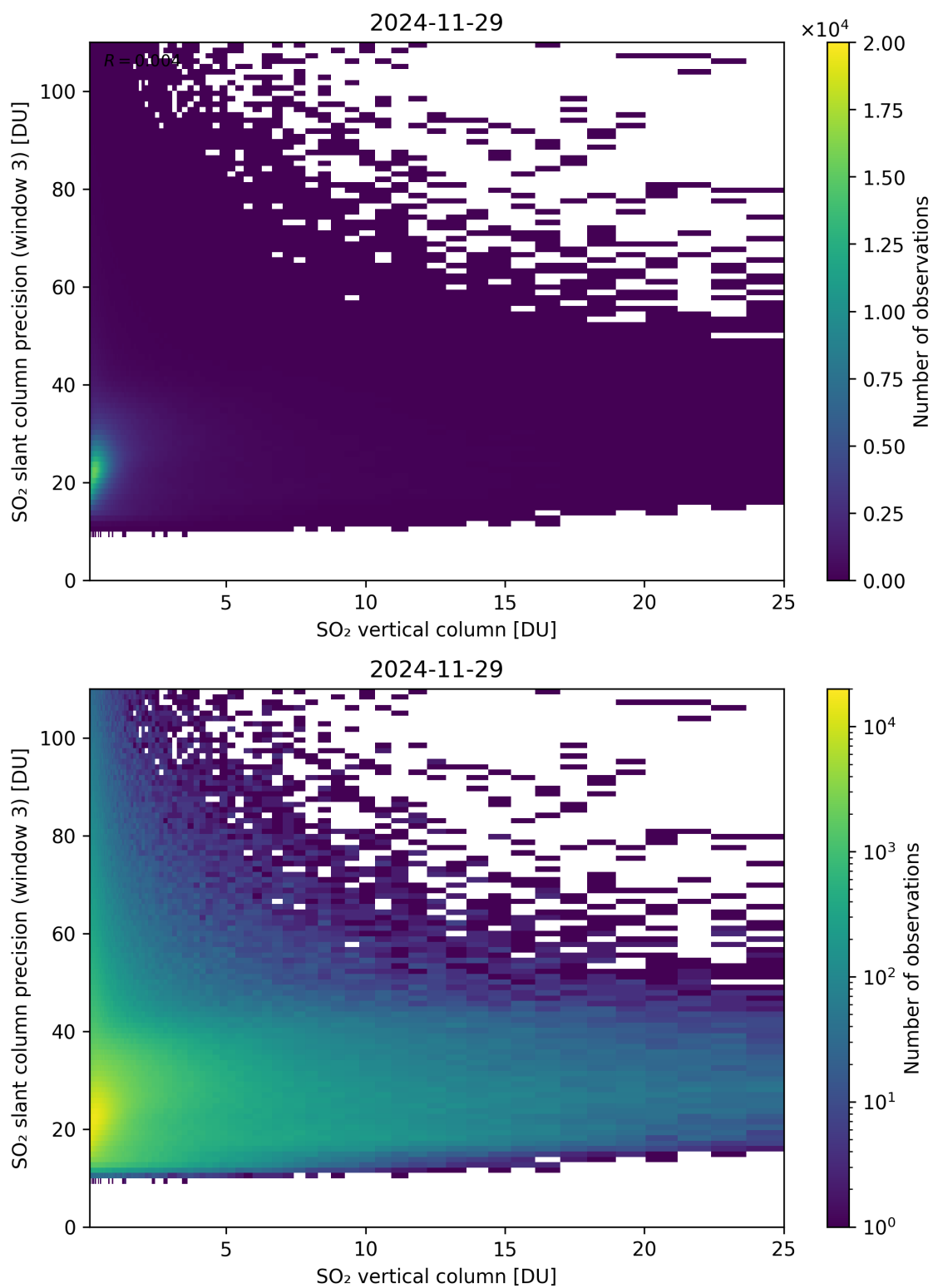
Figure 358: Scatter density plot of “SO 2 vertical column” against “SO 2 slant column precision (window 3)” for 2024-11-28 to 2024-11-30.
