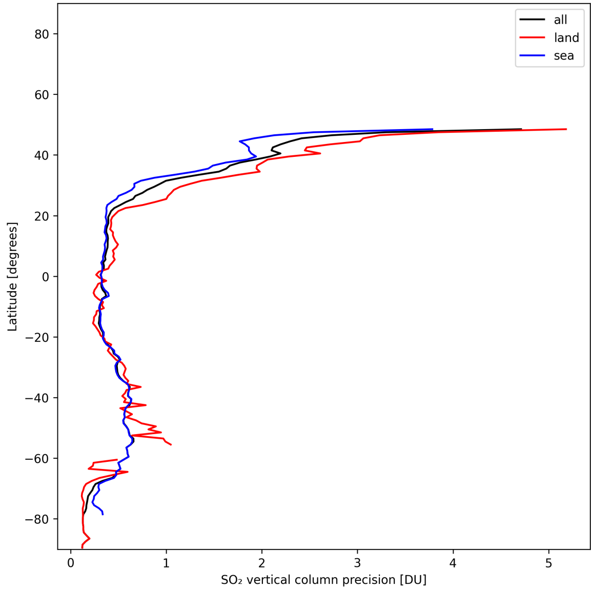
Figure 33: Zonal average of “SO 2 vertical column precision” for 2024-11-28 to 2024-11-30.
