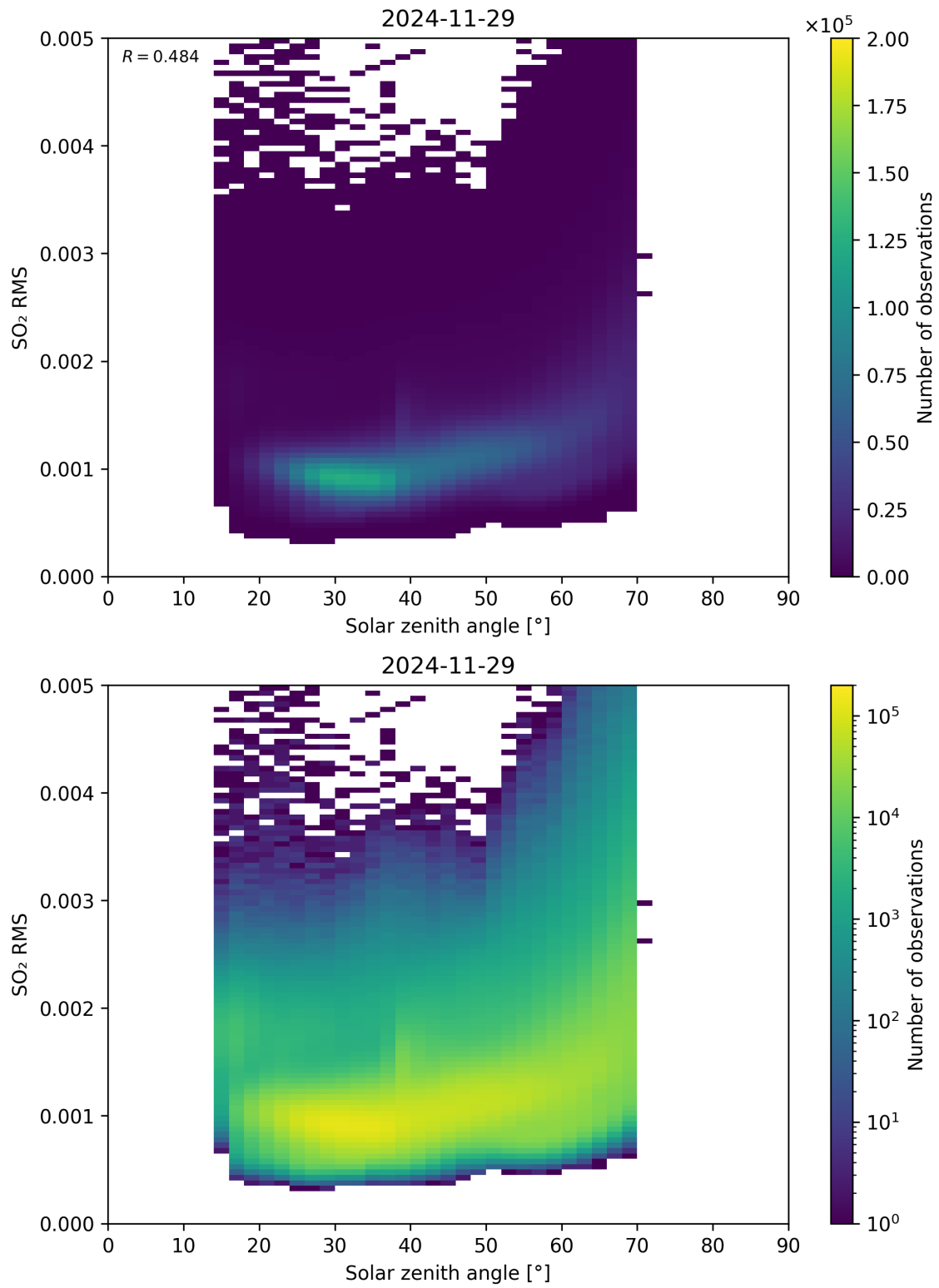
Figure 176: Scatter density plot of “Solar zenith angle” against “SO 2 RMS” for 2024-11-28 to 2024-11-30.
