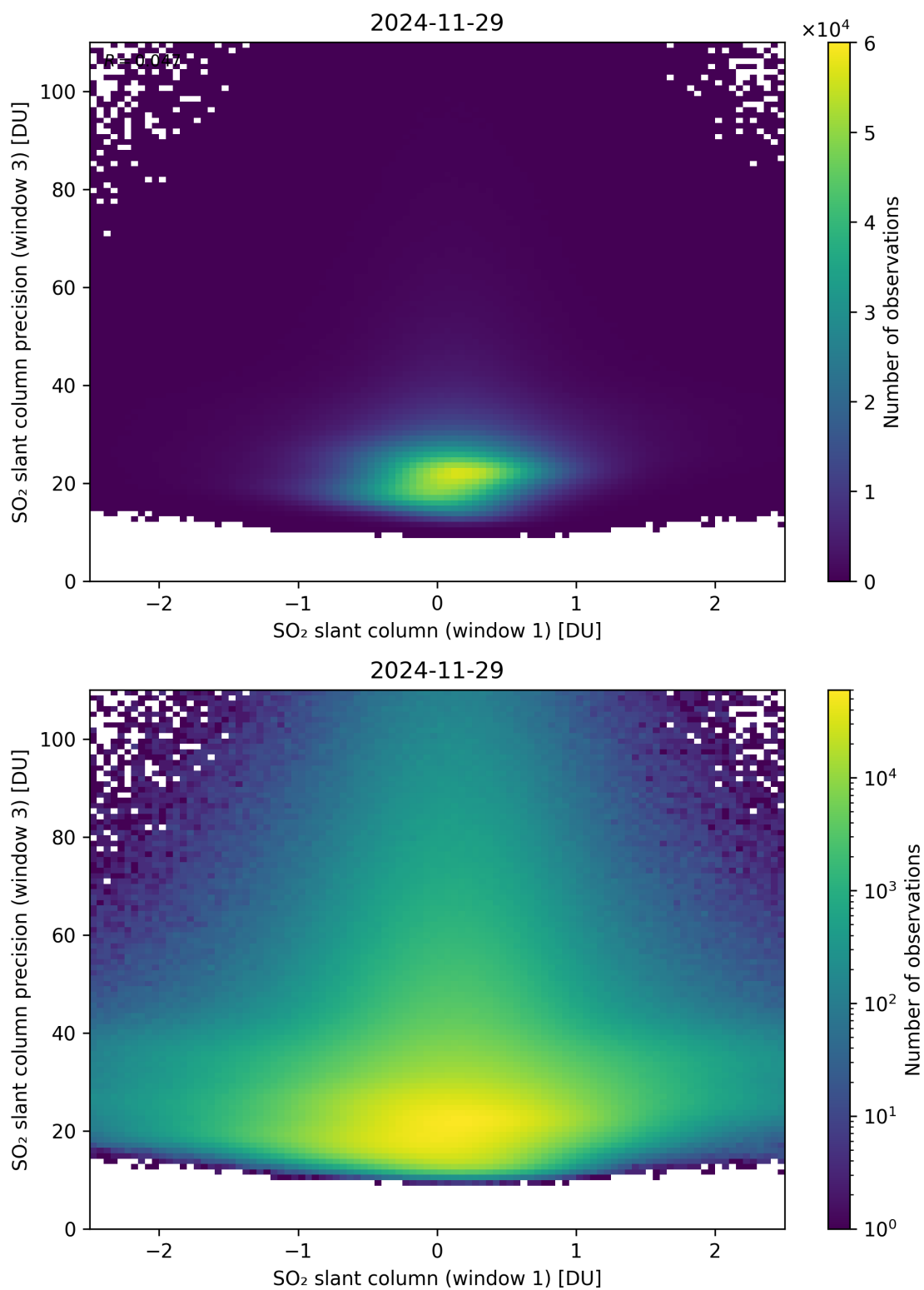
Figure 288: Scatter density plot of “SO 2 slant column (window 1)” against “SO 2 slant column precision (window 3)” for 2024-11-28 to 2024-11-30.
