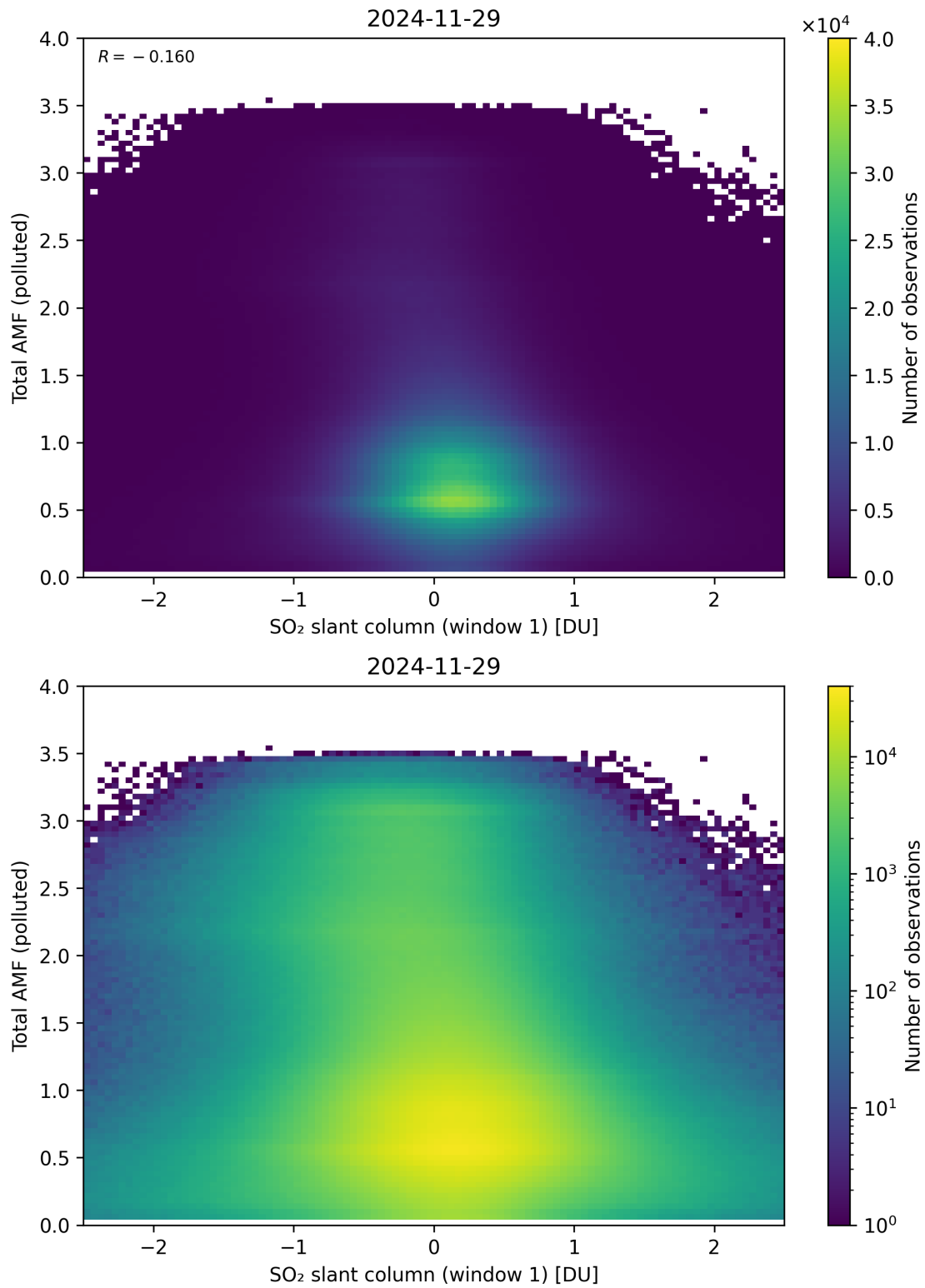
Figure 289: Scatter density plot of “SO 2 slant column (window 1)” against “Total AMF (polluted)” for 2024-11-28 to 2024-11-30.
