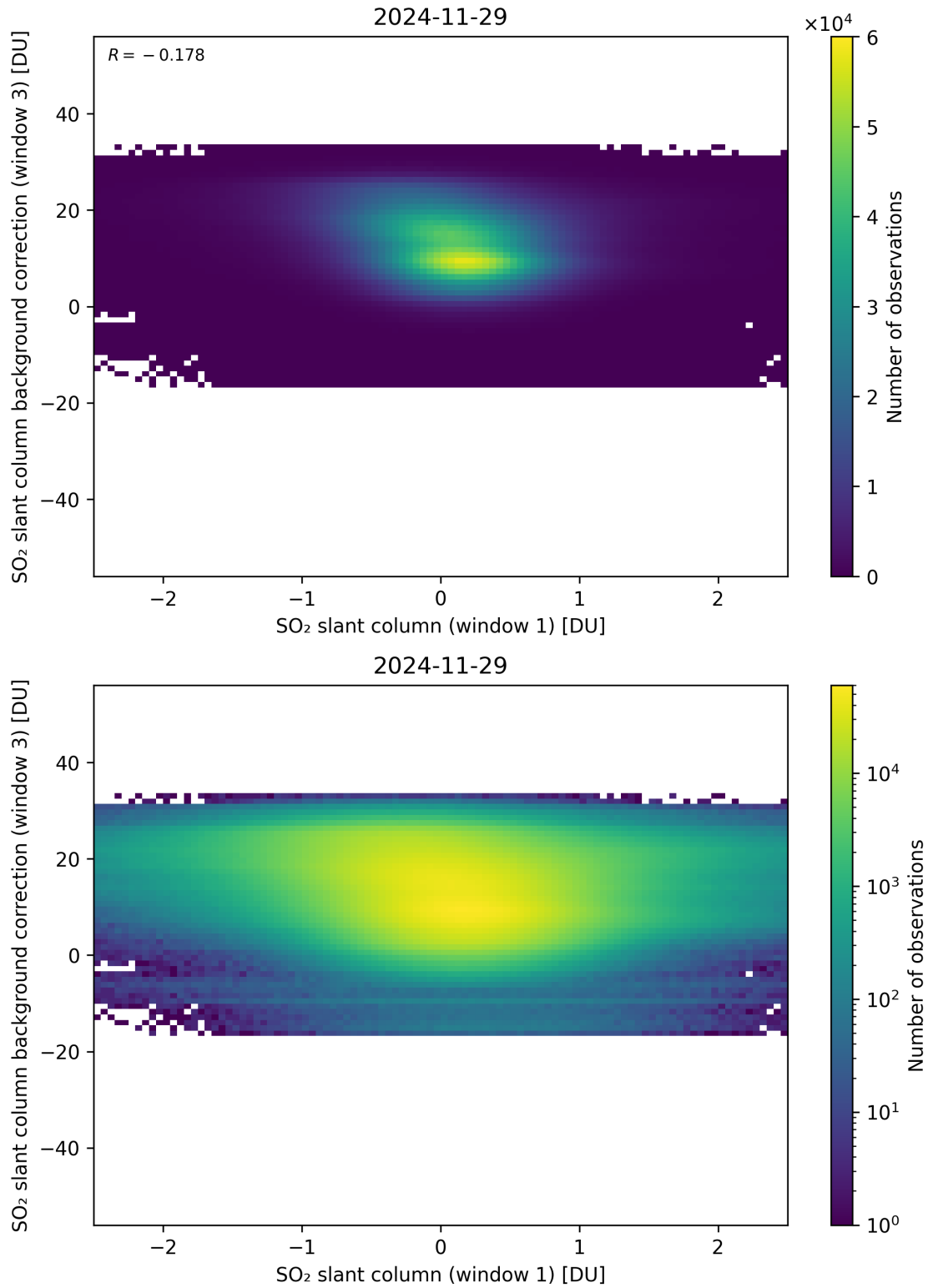
Figure 264: Scatter density plot of “SO 2 slant column (window 1)” against “SO 2 slant column background correction (window 3)” for 2024-11-28 to 2024-11-30.
