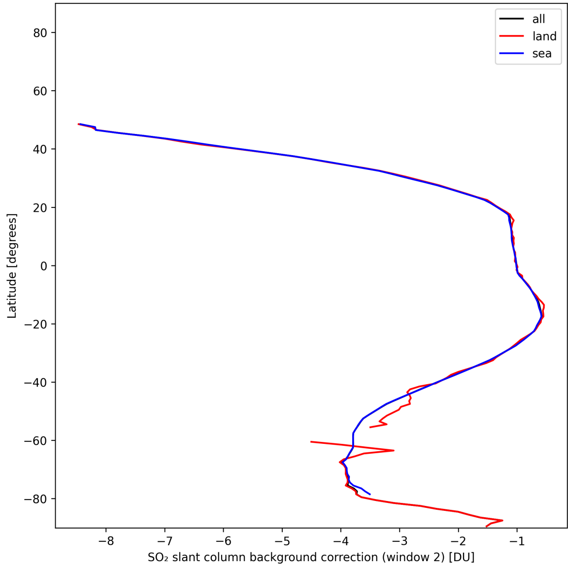
Figure 44: Zonal average of “SO 2 slant column background correction (window 2)” for 2024-11-28 to 2024-11-30.
