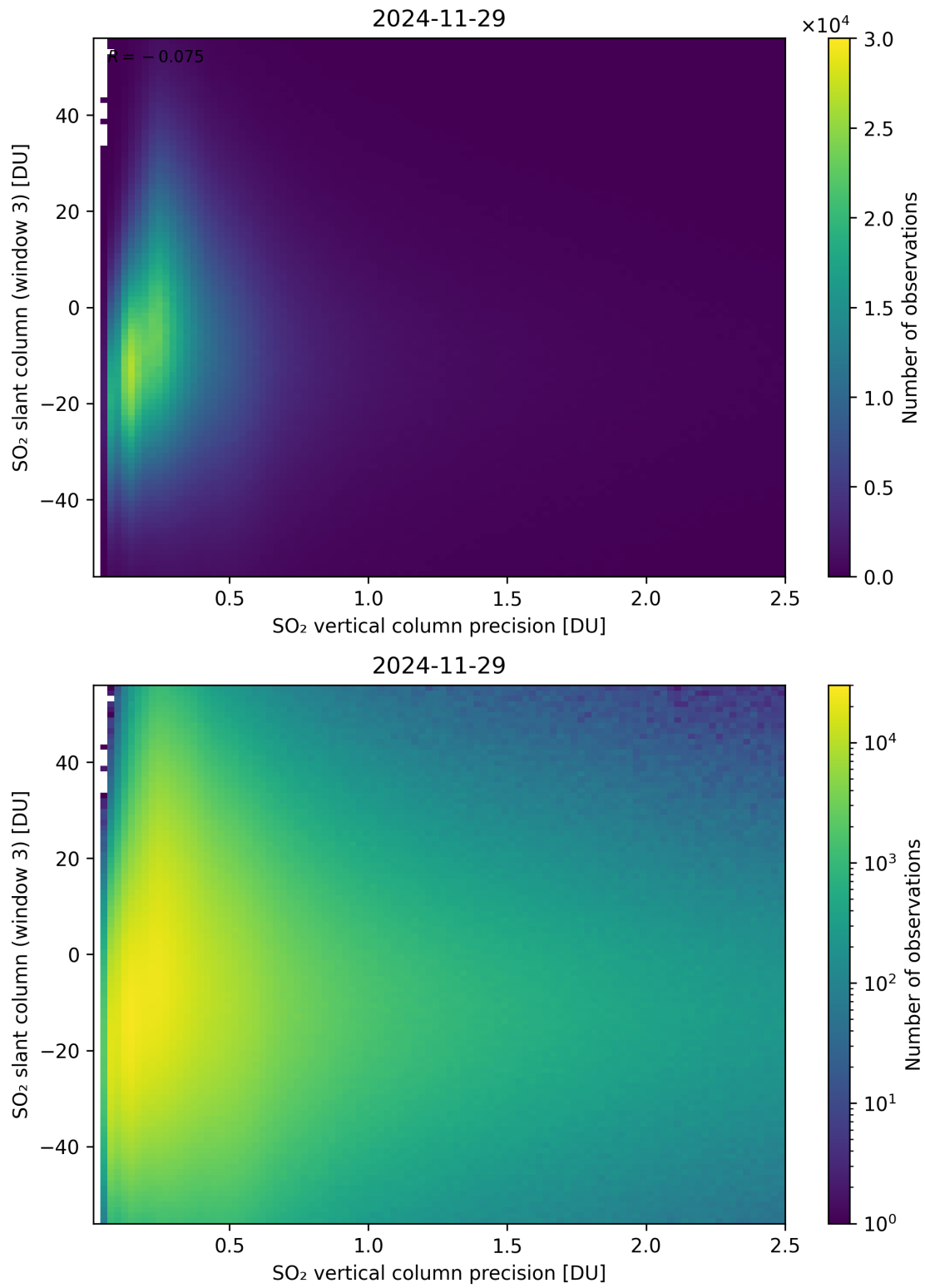
Figure 344: Scatter density plot of “SO 2 vertical column precision” against “SO 2 slant column (window 3)” for 2024-11-28 to 2024-11-30.
