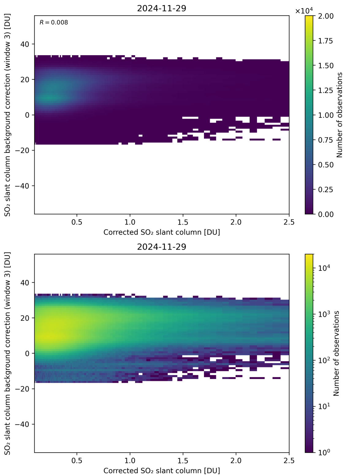
Figure 228: Scatter density plot of “Corrected SO 2 slant column” against “SO 2 slant column background correction (window 3)” for 2024-11-28 to 2024-11-30.
