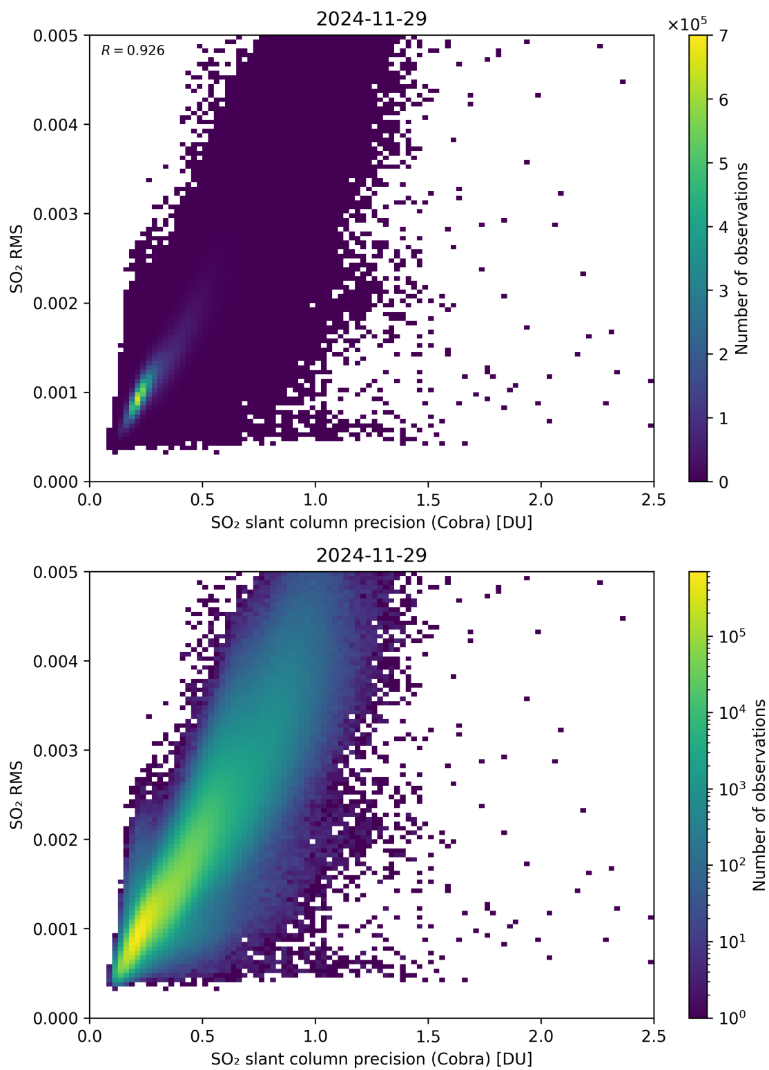
Figure 204: Scatter density plot of “SO 2 slant column precision (Cobra)” against “SO 2 RMS” for 2024-11-28 to 2024-11-30.
