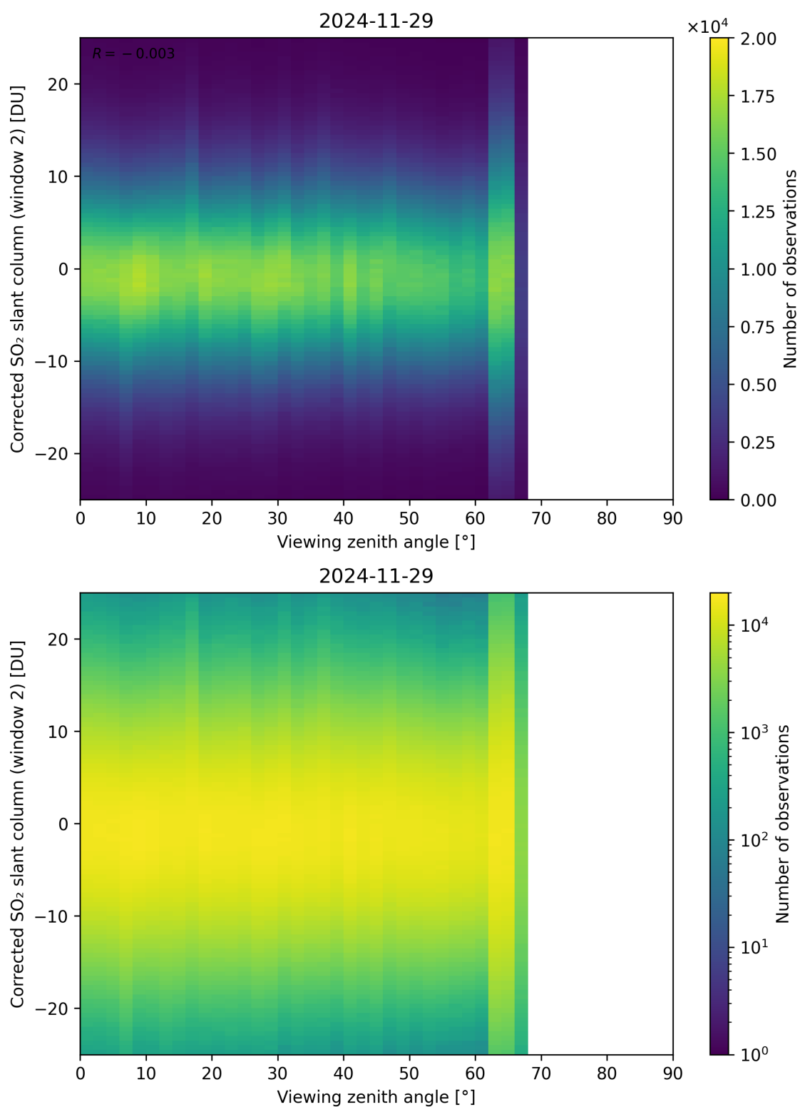
Figure 374: Scatter density plot of “Viewing zenith angle” against “Corrected SO 2 slant column (window 2)” for 2024-11-28 to 2024-11-30.
