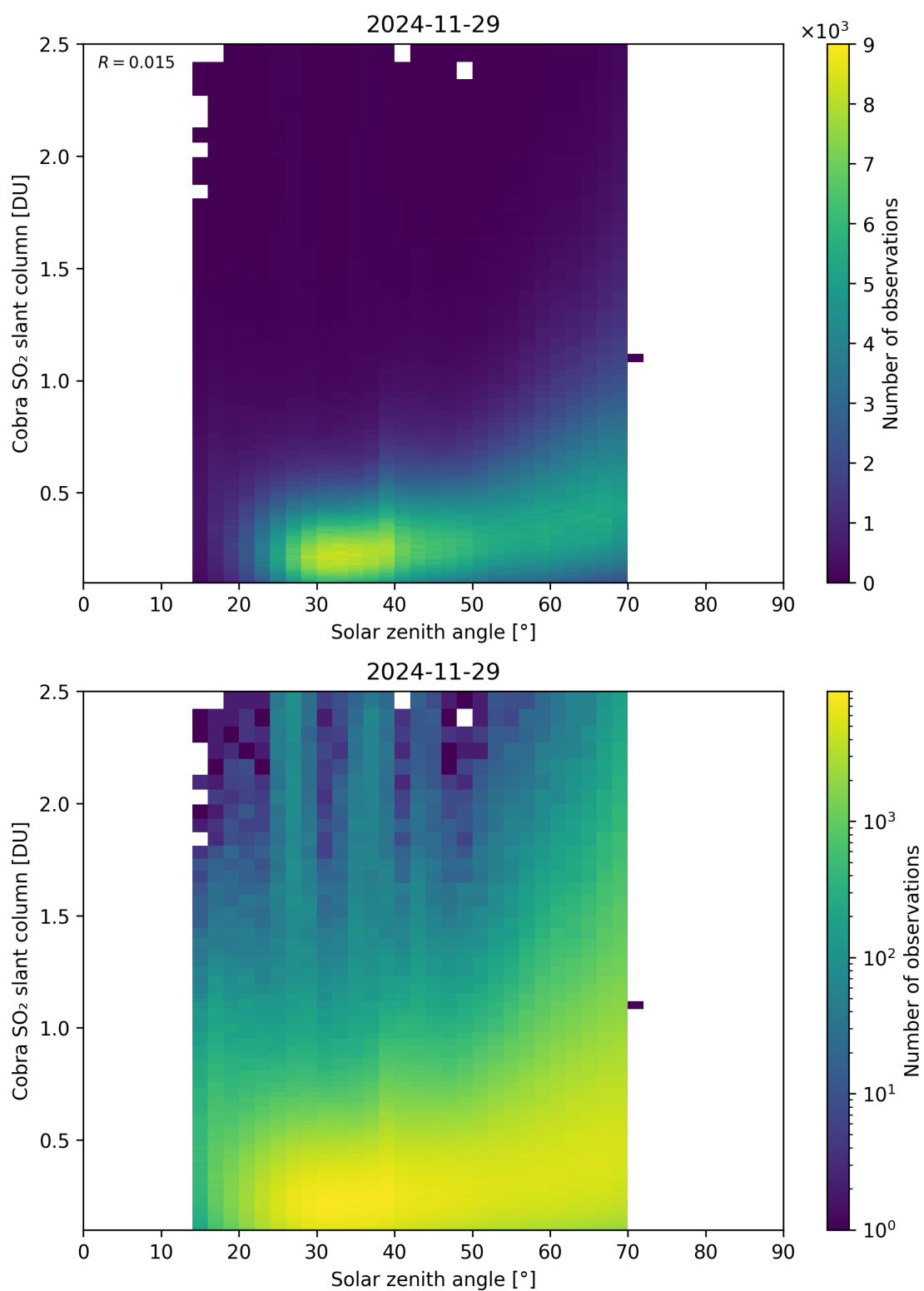
Figure 179: Scatter density plot of “Solar zenith angle” against “Cobra SO 2 slant column” for 2024-11-28 to 2024-11-30.
