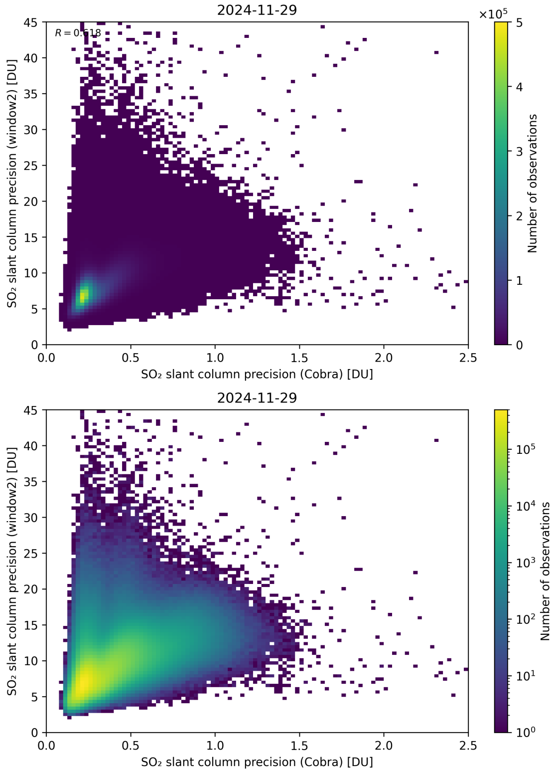
Figure 210: Scatter density plot of “SO 2 slant column precision (Cobra)” against “SO 2 slant column precision (window2)” for 2024-11-28 to 2024-11-30.
