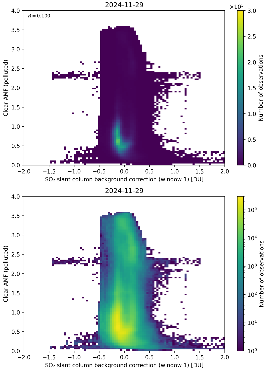
Figure 114: Scatter density plot of “SO 2 slant column background correction (window 1)” against “Clear AMF (polluted)” for 2024-11-28 to 2024-11-30.
