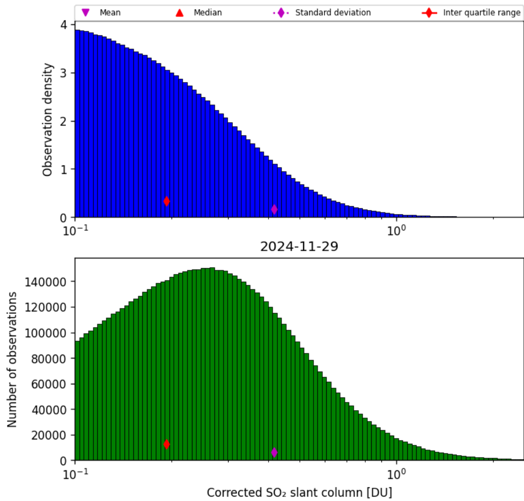
Figure 60: Histogram of “Corrected SO 2 slant column” for 2024-11-28 to 2024-11-30
