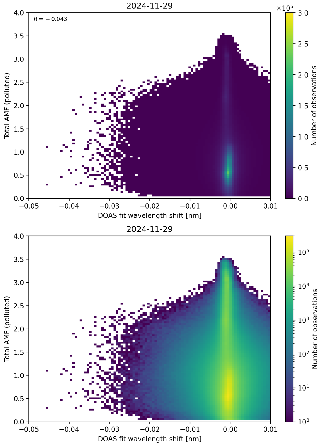
Figure 141: Scatter density plot of “DOAS fit wavelength shift” against “Total AMF (polluted)” for 2024-11-28 to 2024-11-30.
