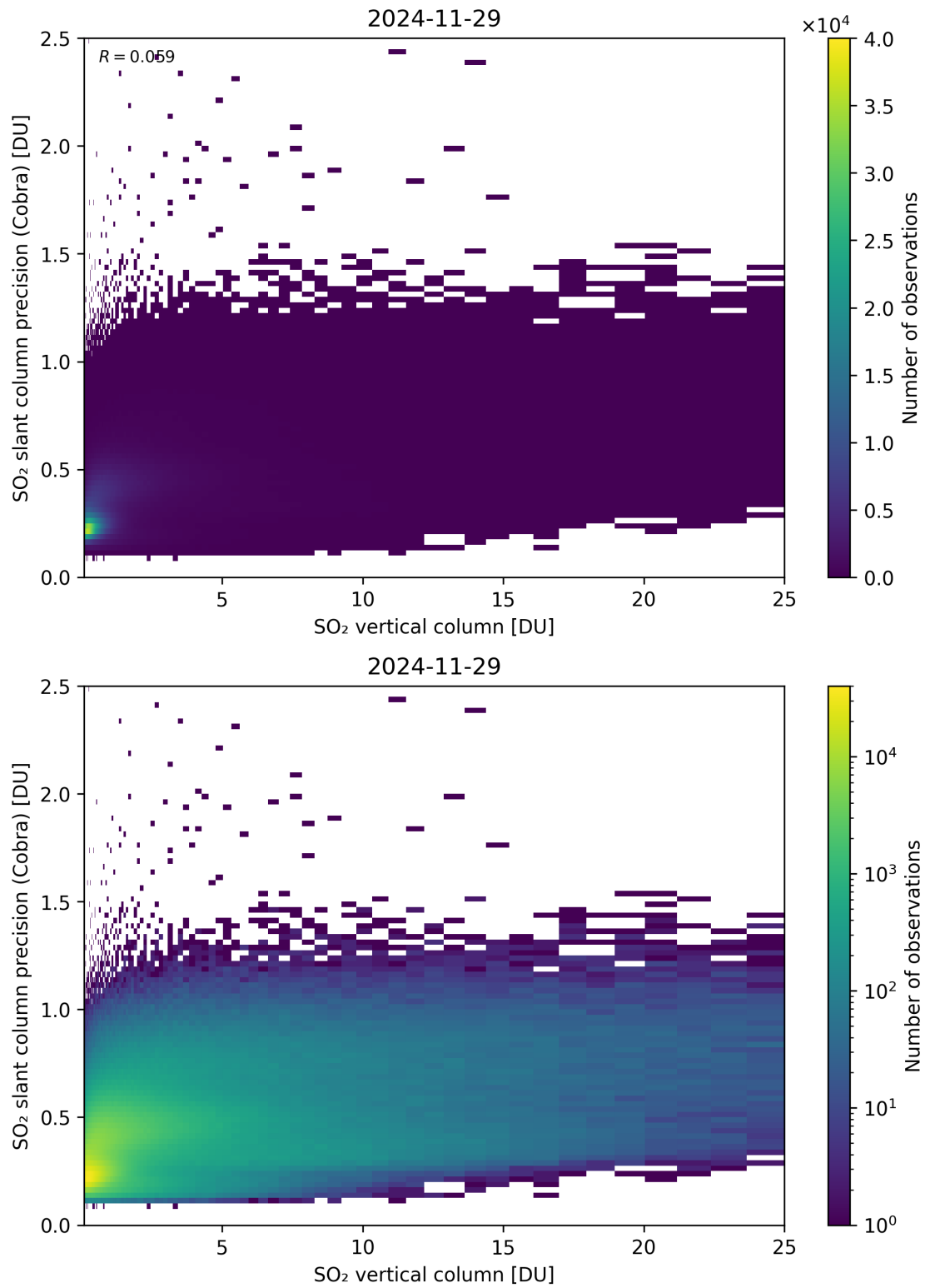
Figure 350: Scatter density plot of “SO 2 vertical column” against “SO 2 slant column precision (Cobra)” for 2024-11-28 to 2024-11-30.
