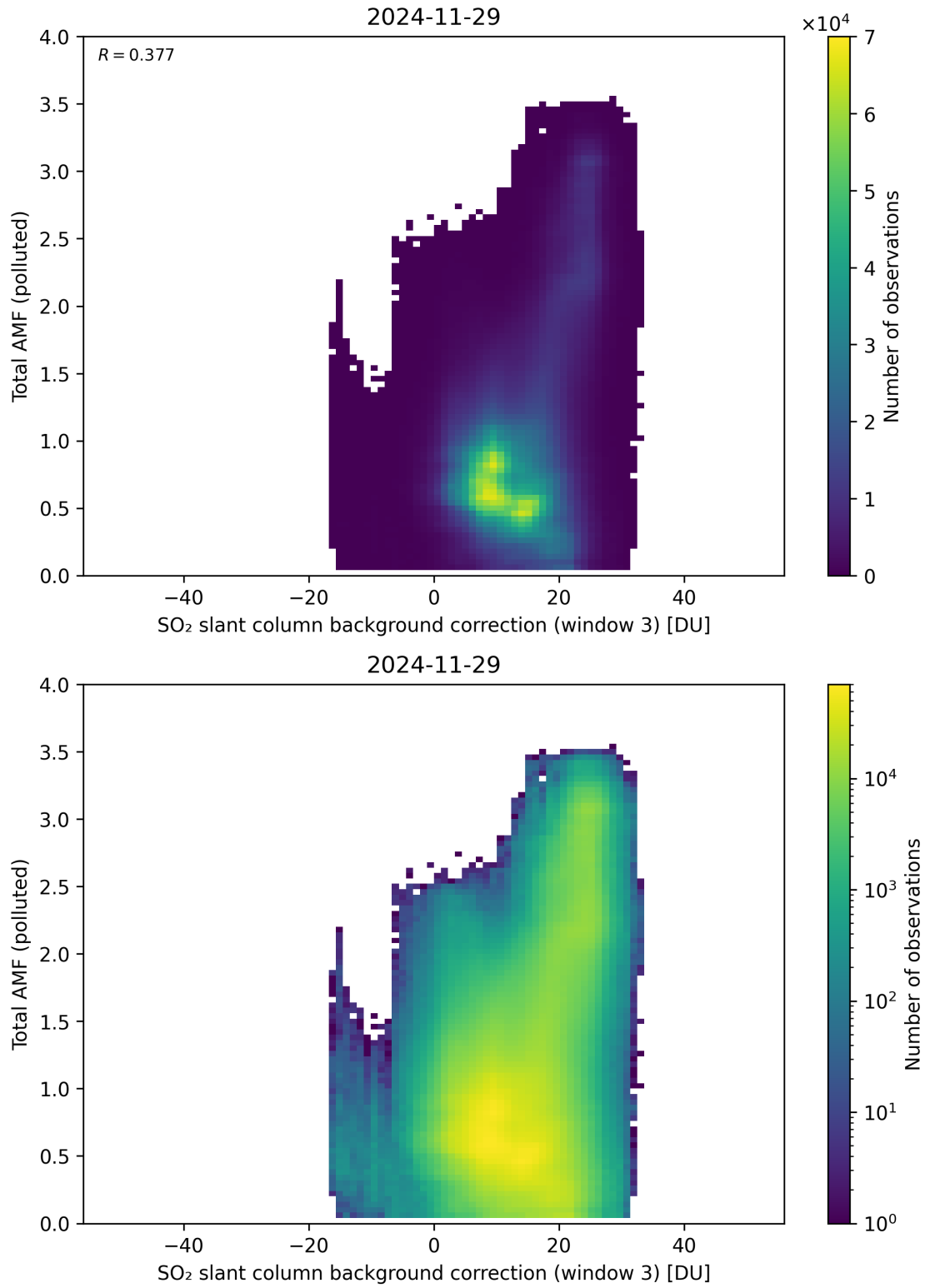
Figure 136: Scatter density plot of “SO 2 slant column background correction (window 3)” against “Total AMF (polluted)” for 2024-11-28 to 2024-11-30.
