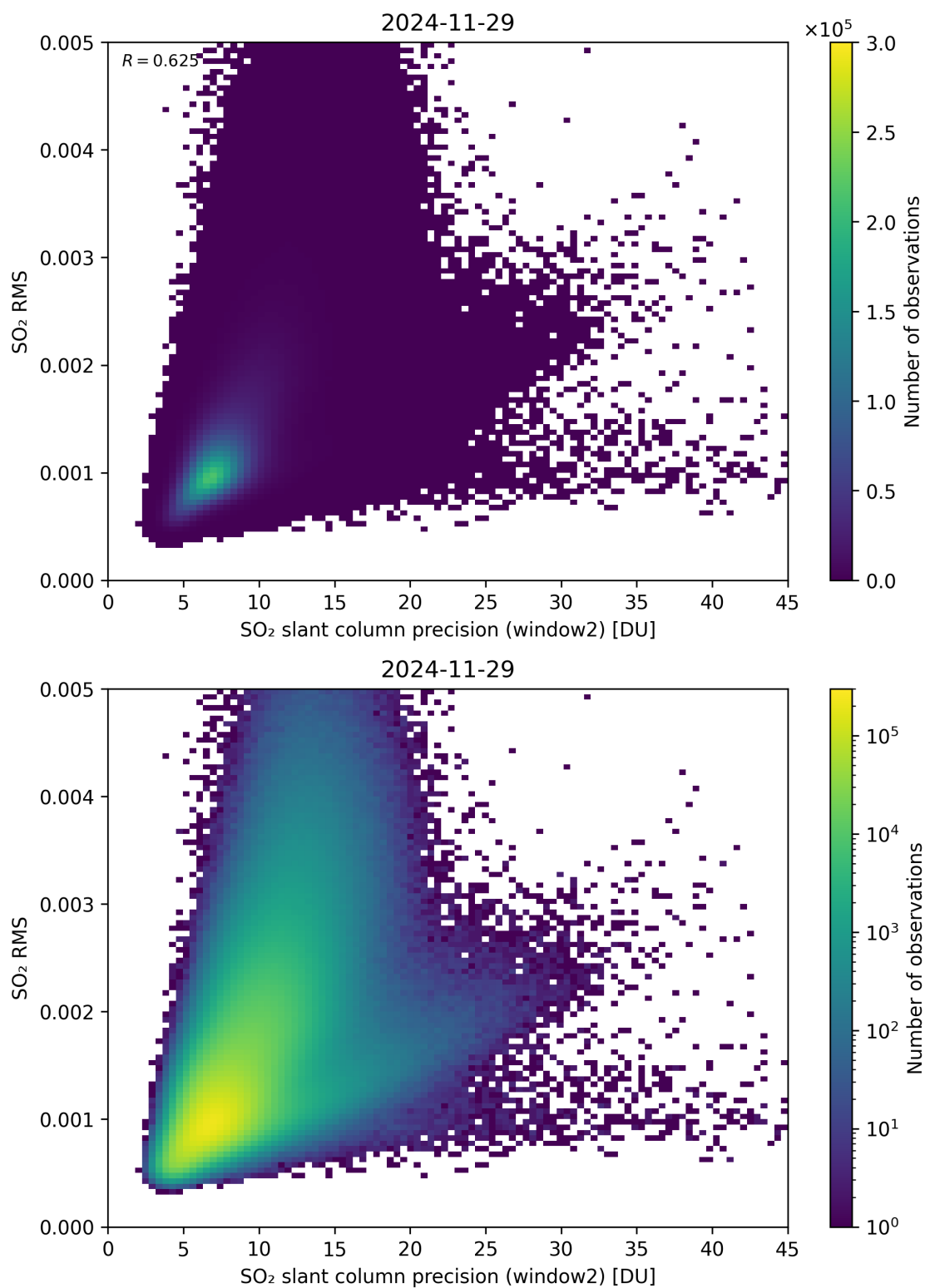
Figure 295: Scatter density plot of “SO 2 slant column precision (window2)” against “SO 2 RMS” for 2024-11-28 to 2024-11-30.
