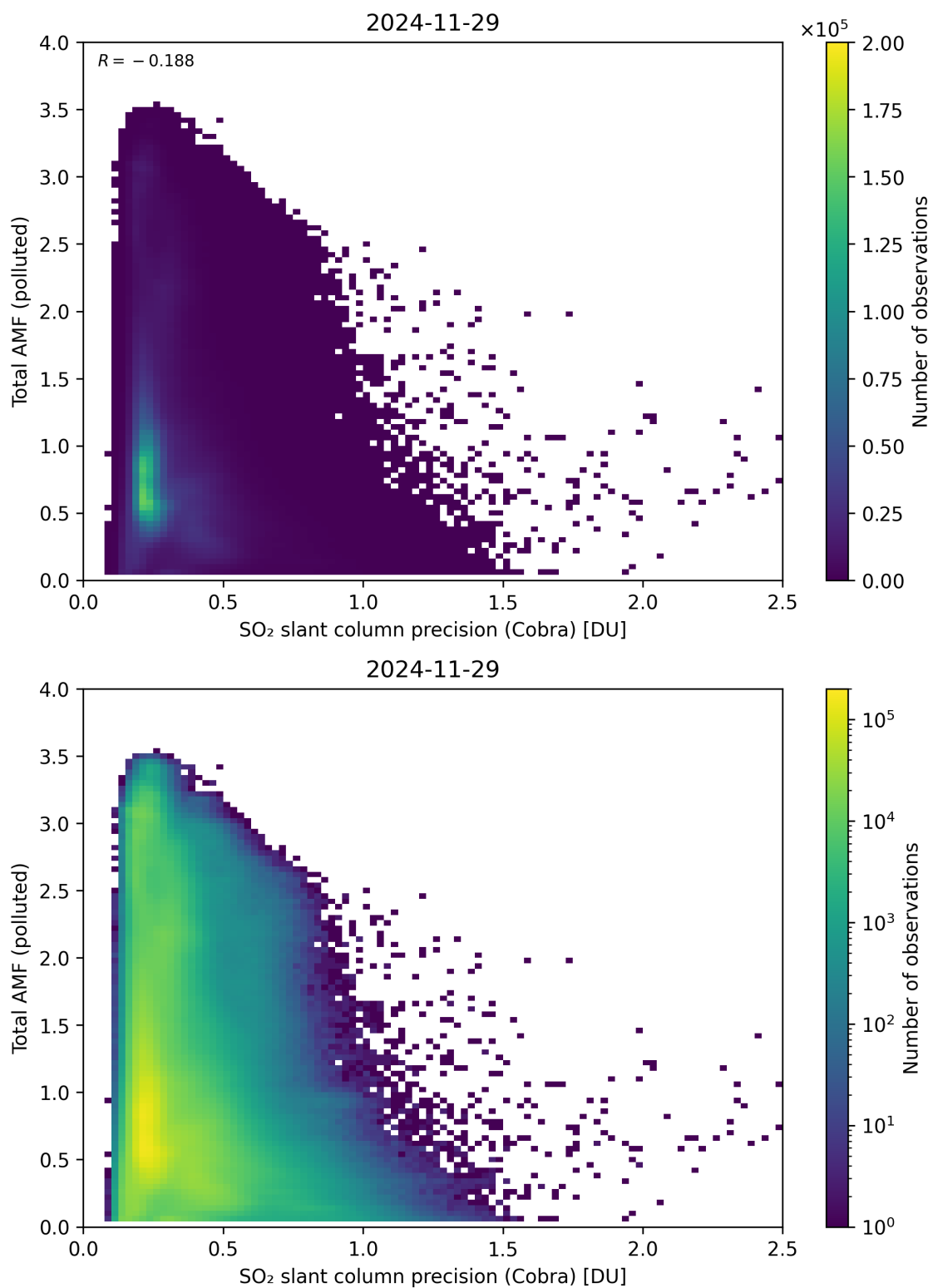
Figure 213: Scatter density plot of “SO 2 slant column precision (Cobra)” against “Total AMF (polluted)” for 2024-11-28 to 2024-11-30.
