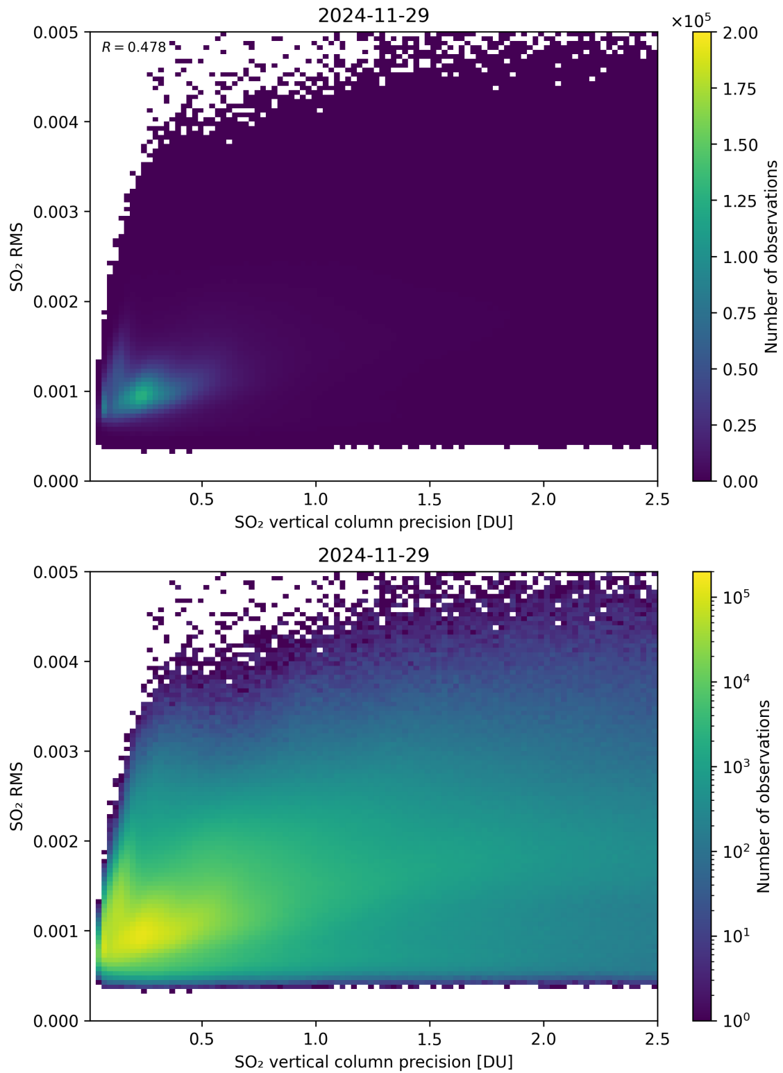
Figure 334: Scatter density plot of “SO 2 vertical column precision” against “SO 2 RMS” for 2024-11-28 to 2024-11-30.
