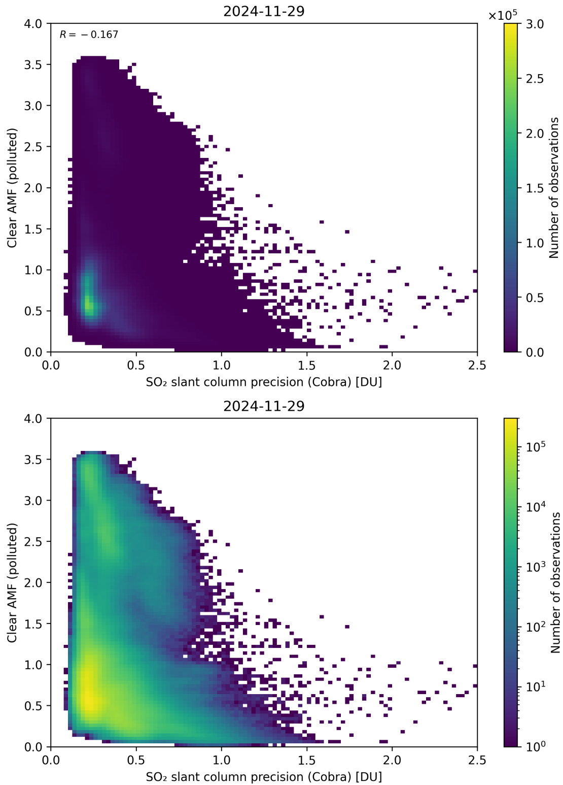
Figure 205: Scatter density plot of “SO 2 slant column precision (Cobra)” against “Clear AMF (polluted)” for 2024-11-28 to 2024-11-30.
