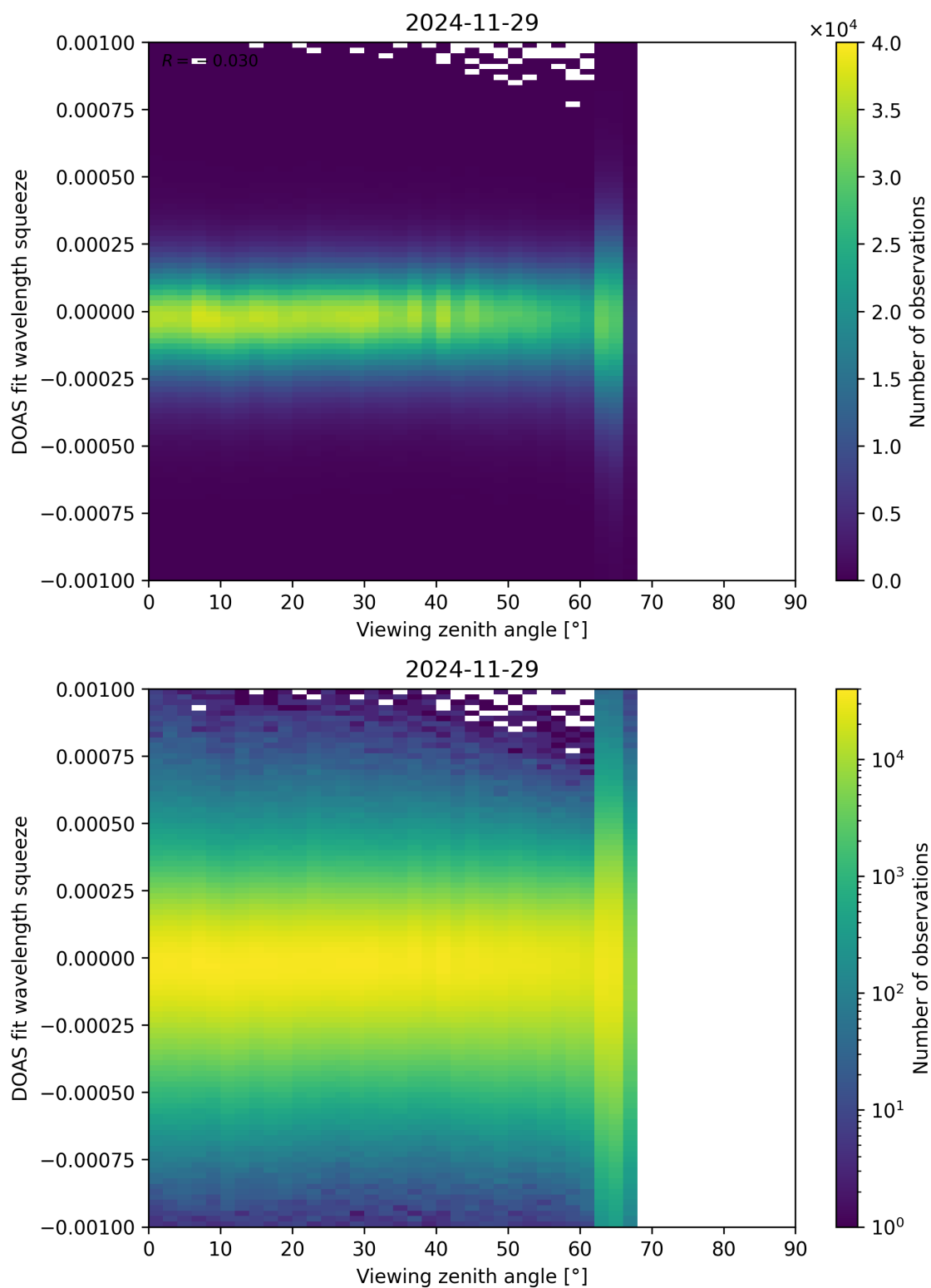
Figure 366: Scatter density plot of “Viewing zenith angle” against “DOAS fit wavelength squeeze” for 2024-11-28 to 2024-11-30.
