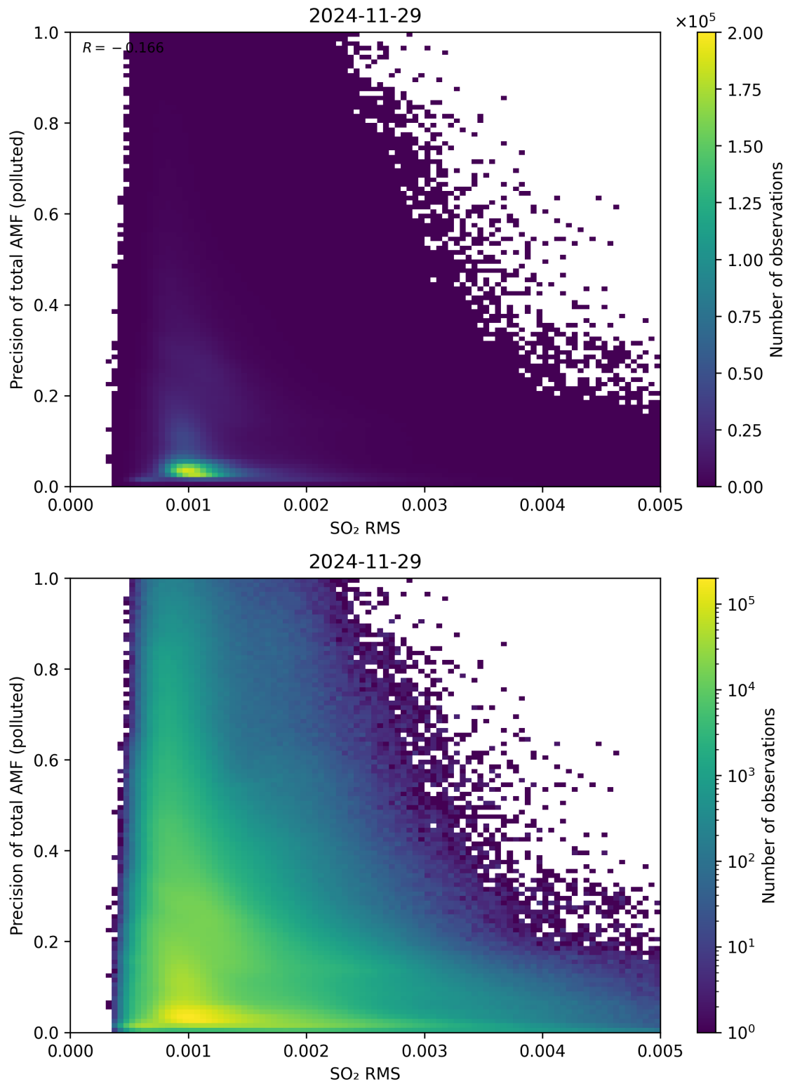
Figure 149: Scatter density plot of “SO 2 RMS” against “Precision of total AMF (polluted)” for 2024-11-28 to 2024-11-30.
