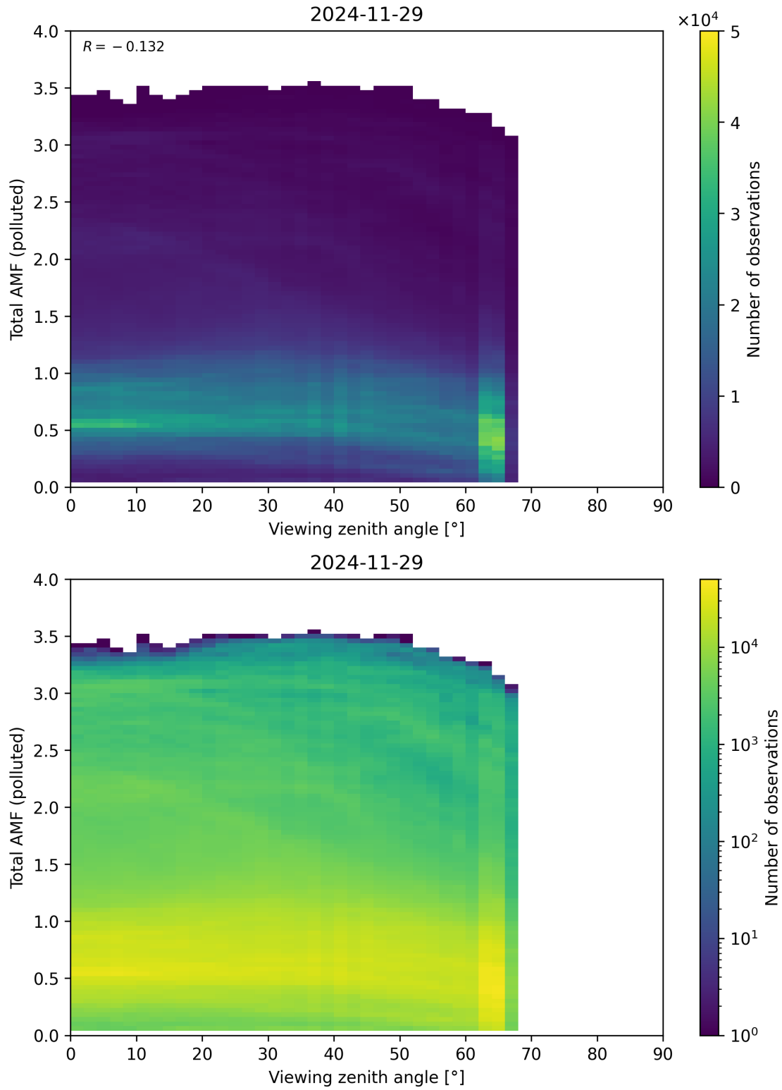
Figure 381: Scatter density plot of “Viewing zenith angle” against “Total AMF (polluted)” for 2024-11-28 to 2024-11-30.
