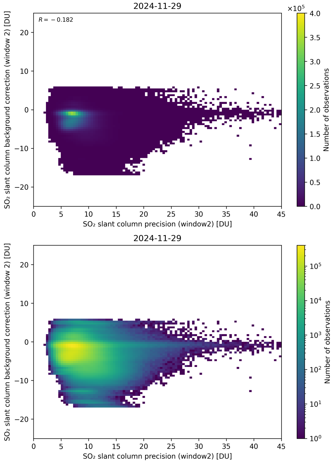
Figure 291: Scatter density plot of “SO 2 slant column precision (window2)” against “SO 2 slant column background correction (window 2)” for 2024-11-28 to 2024-11-30.
