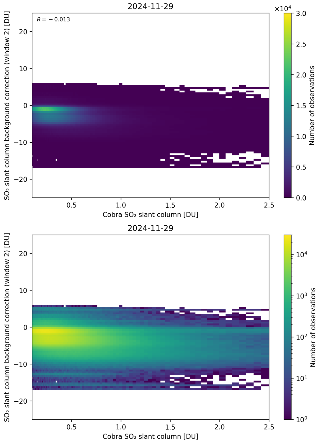
Figure 194: Scatter density plot of “Cobra SO 2 slant column” against “SO 2 slant column background correction (window 2)” for 2024-11-28 to 2024-11-30.
