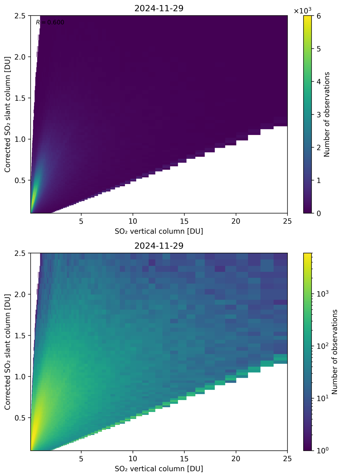
Figure 351: Scatter density plot of “SO 2 vertical column” against “Corrected SO 2 slant column” for 2024-11-28 to 2024-11-30.
