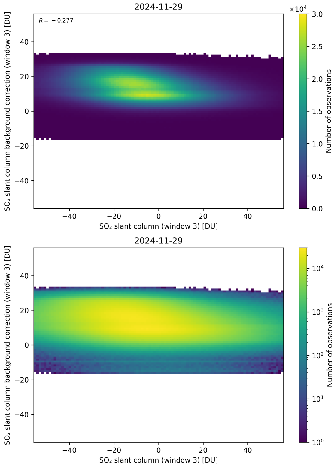
Figure 303: Scatter density plot of “SO 2 slant column (window 3)” against “SO 2 slant column background correction (window 3)” for 2024-11-28 to 2024-11-30.
