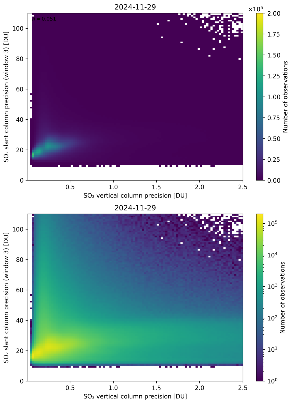
Figure 345: Scatter density plot of “SO 2 vertical column precision” against “SO 2 slant column precision (window 3)” for 2024-11-28 to 2024-11-30.
