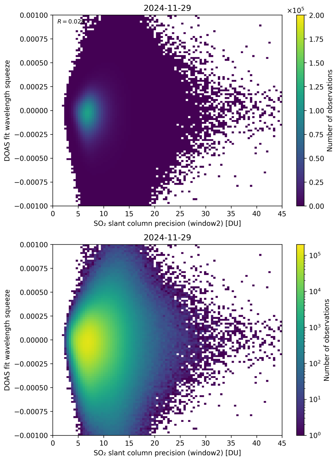
Figure 294: Scatter density plot of “SO 2 slant column precision (window2)” against “DOAS fit wavelength squeeze” for 2024-11-28 to 2024-11-30.
