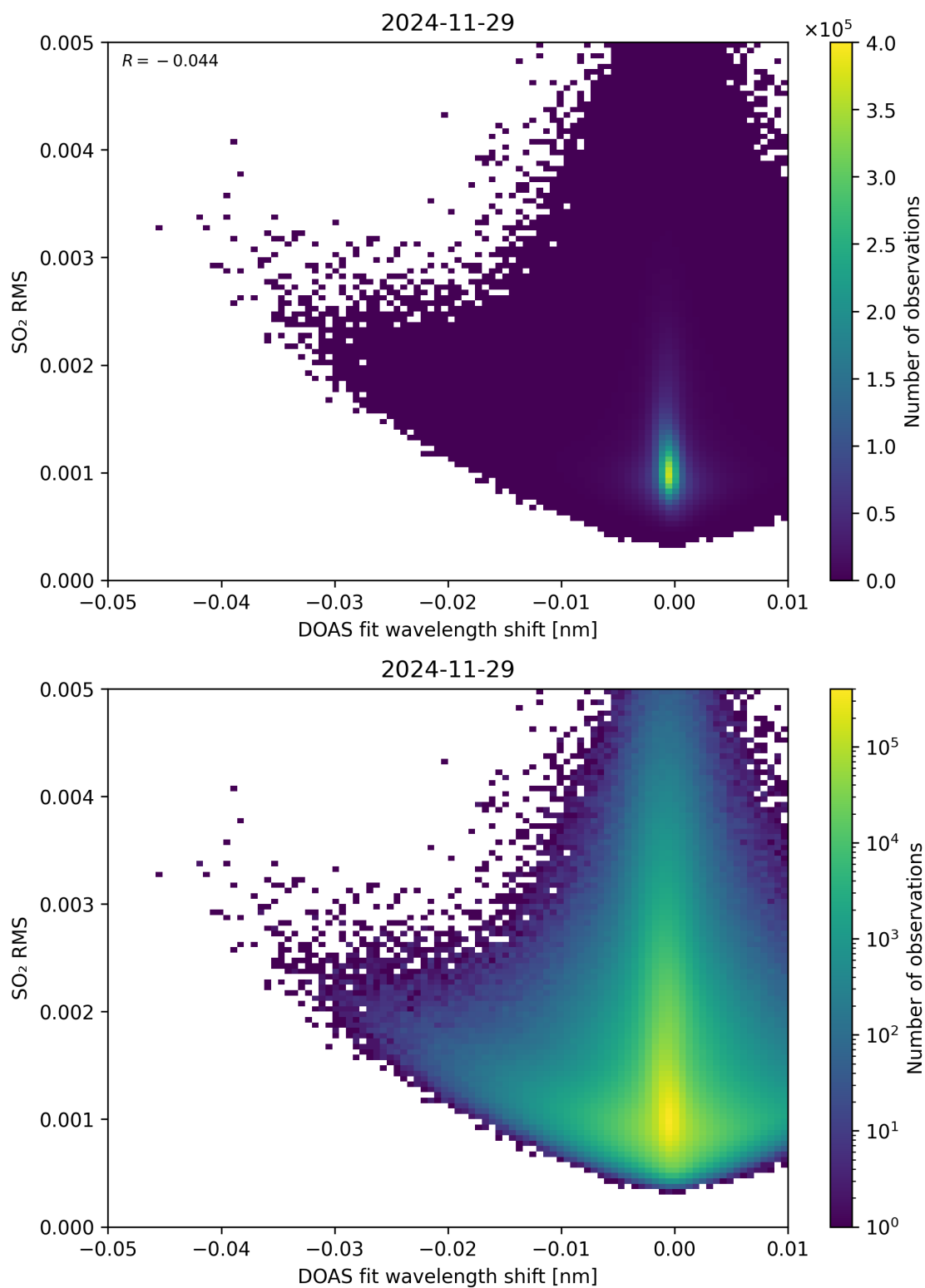
Figure 139: Scatter density plot of “DOAS fit wavelength shift” against “SO 2 RMS” for 2024-11-28 to 2024-11-30.
