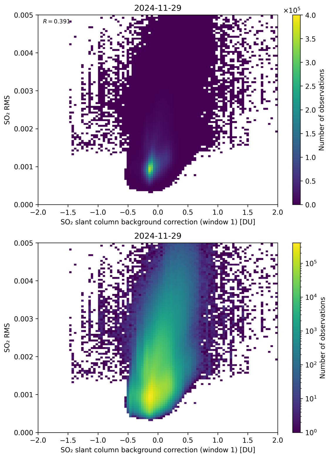
Figure 113: Scatter density plot of “SO 2 slant column background correction (window 1)” against “SO 2 RMS” for 2024-11-28 to 2024-11-30.
