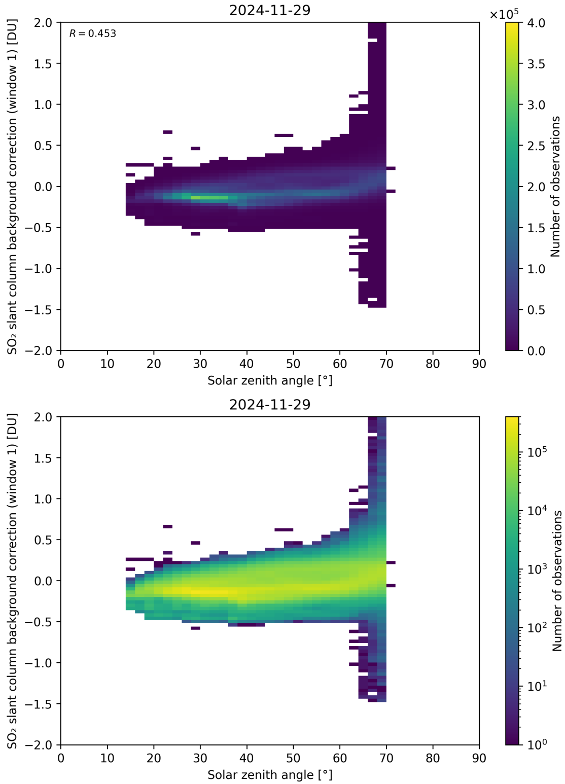
Figure 171: Scatter density plot of “Solar zenith angle” against “SO 2 slant column background correction (window 1)” for 2024-11-28 to 2024-11-30.
