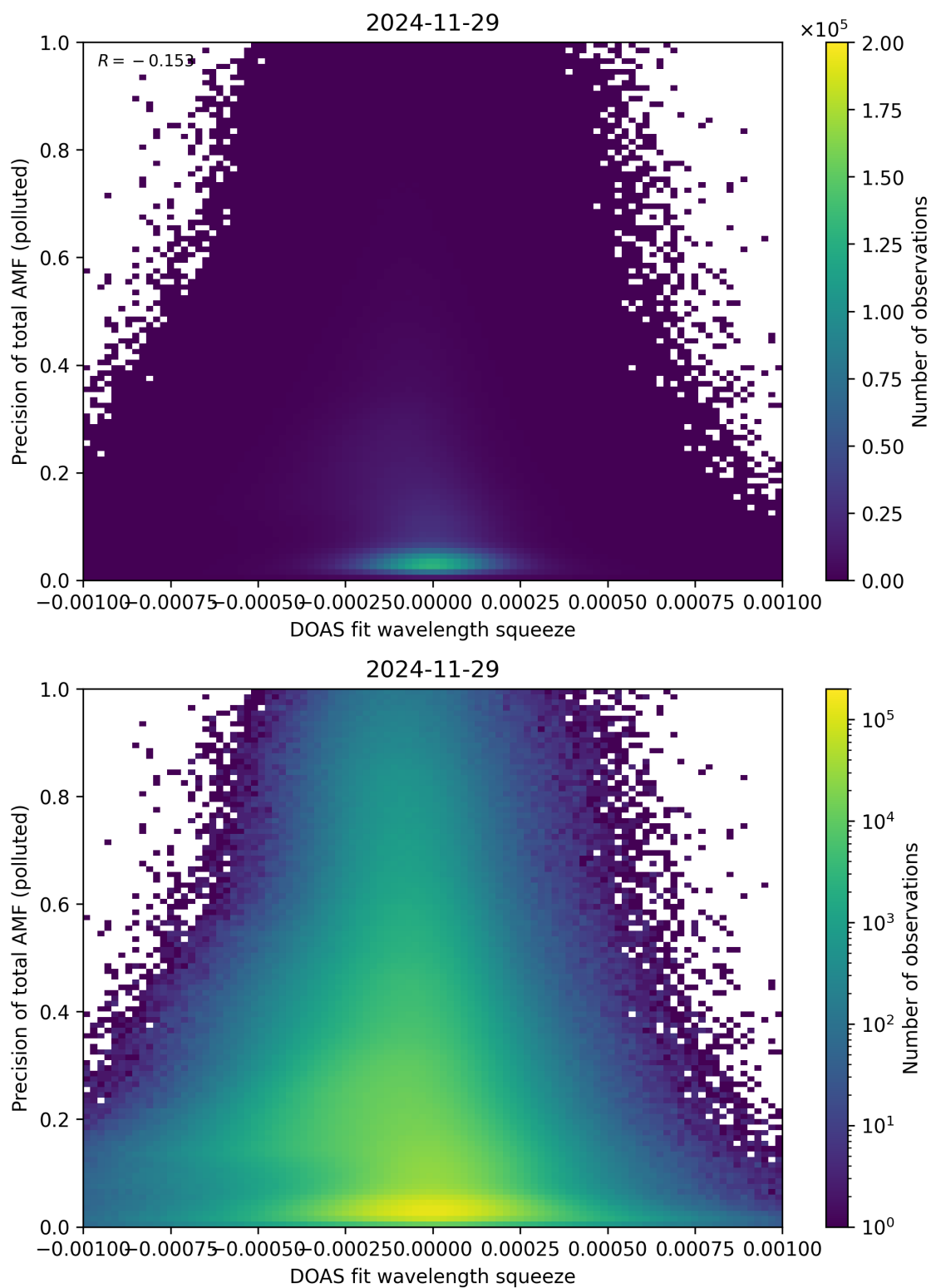
Figure 146: Scatter density plot of “DOAS fit wavelength squeeze” against “Precision of total AMF (polluted)” for 2024-11-28 to 2024-11-30.
