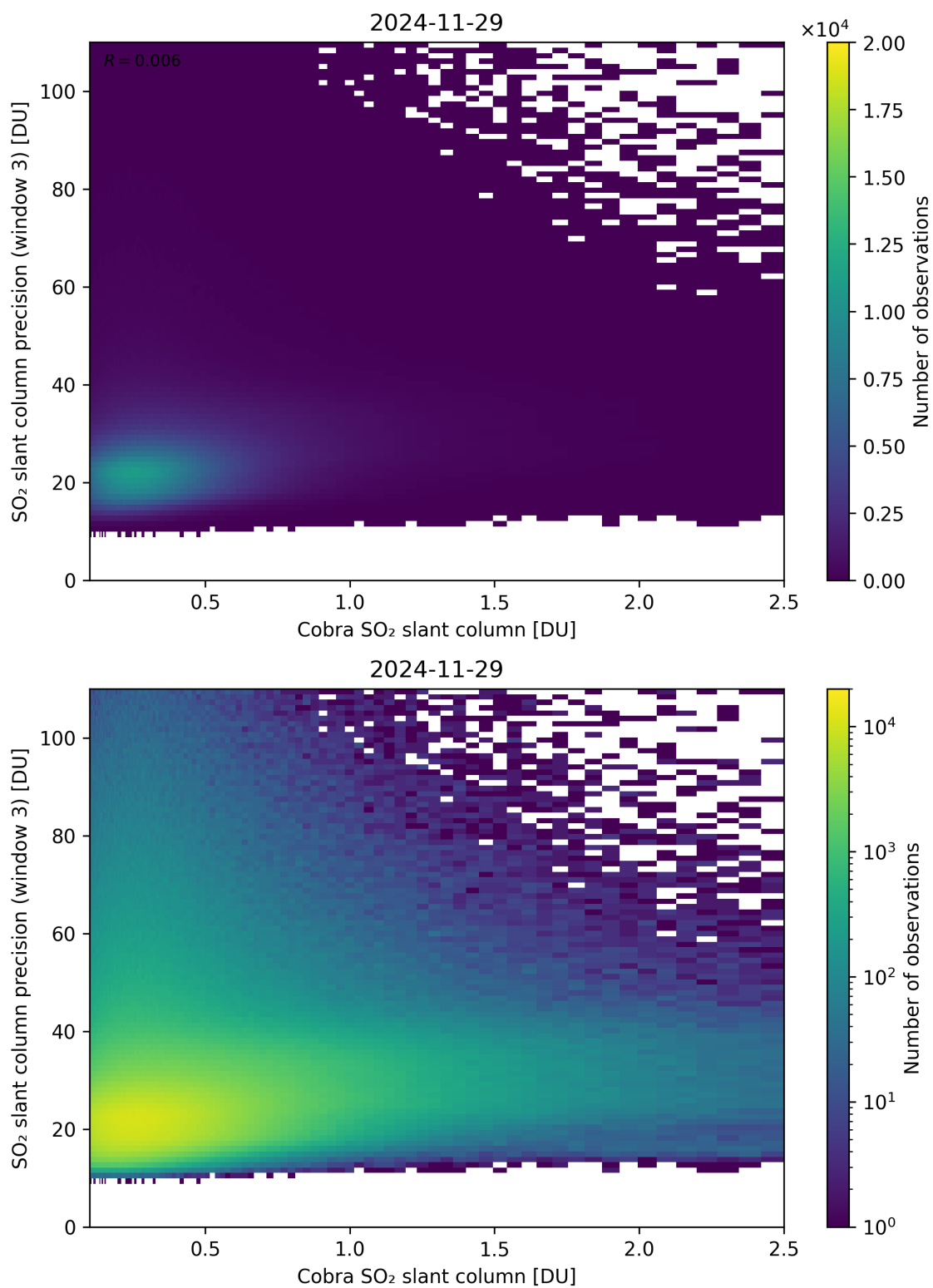
Figure 223: Scatter density plot of “Cobra SO 2 slant column” against “SO 2 slant column precision (window 3)” for 2024-11-28 to 2024-11-30.
