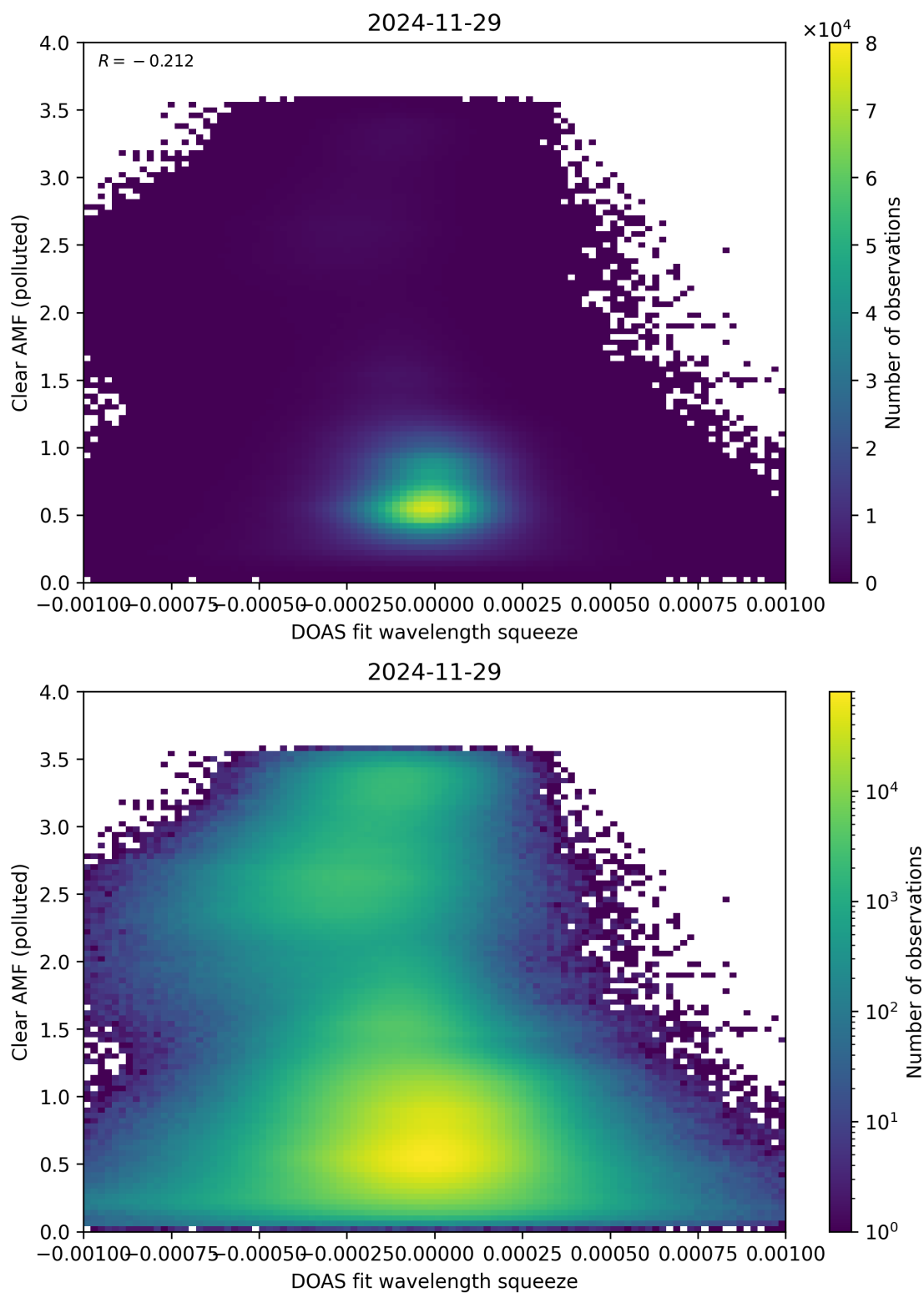
Figure 144: Scatter density plot of “DOAS fit wavelength squeeze” against “Clear AMF (polluted)” for 2024-11-28 to 2024-11-30.
