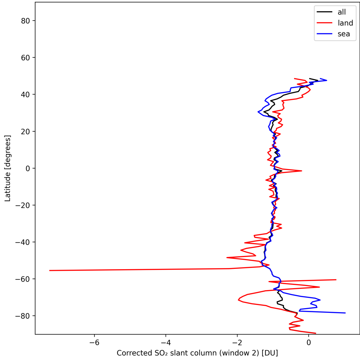
Figure 43: Zonal average of “Corrected SO 2 slant column (window 2)” for 2024-11-28 to 2024-11-30.
