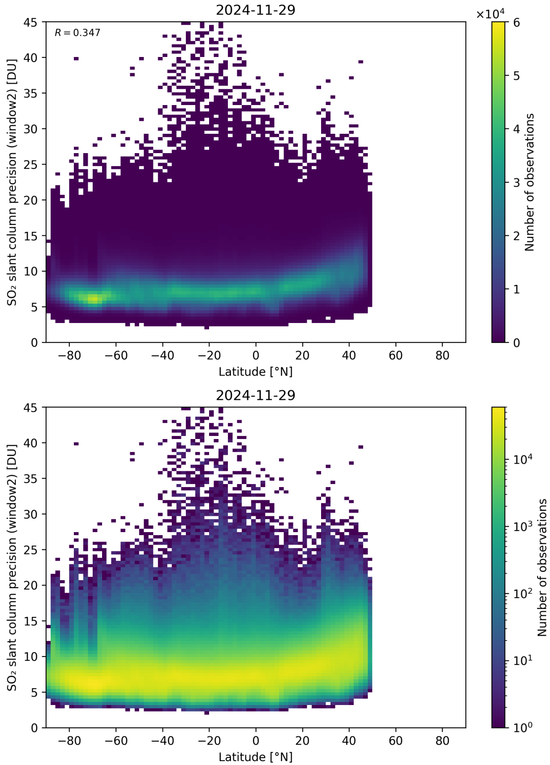
Figure 164: Scatter density plot of “Latitude” against “SO 2 slant column precision (window2)” for 2024-11-28 to 2024-11-30.
