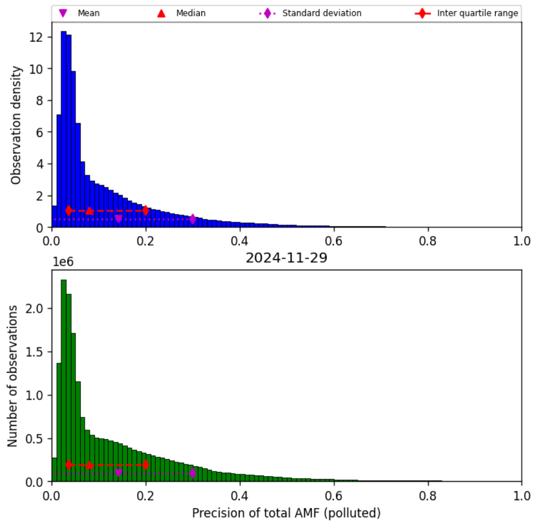
Figure 80: Histogram of “Precision of total AMF (polluted)” for 2024-11-28 to 2024-11-30
