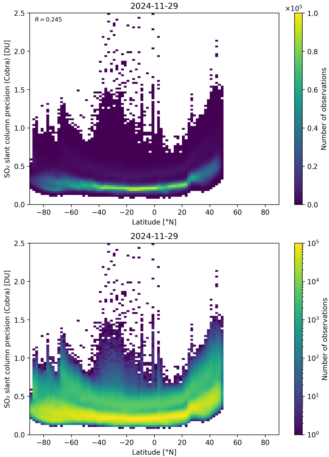
Figure 158: Scatter density plot of “Latitude” against “SO 2 slant column precision (Cobra)” for 2024-11-28 to 2024-11-30.
