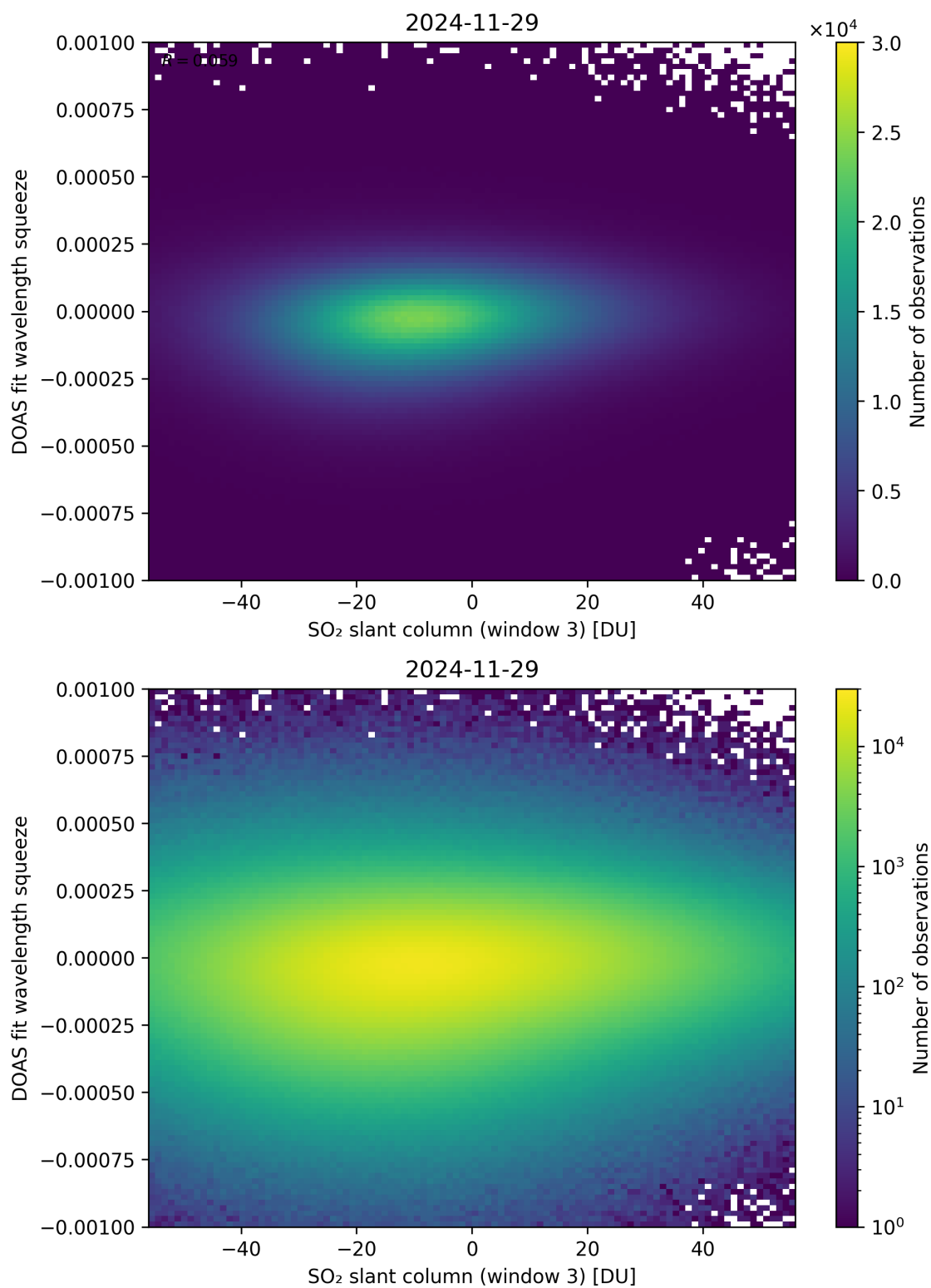
Figure 305: Scatter density plot of “SO 2 slant column (window 3)” against “DOAS fit wavelength squeeze” for 2024-11-28 to 2024-11-30.
