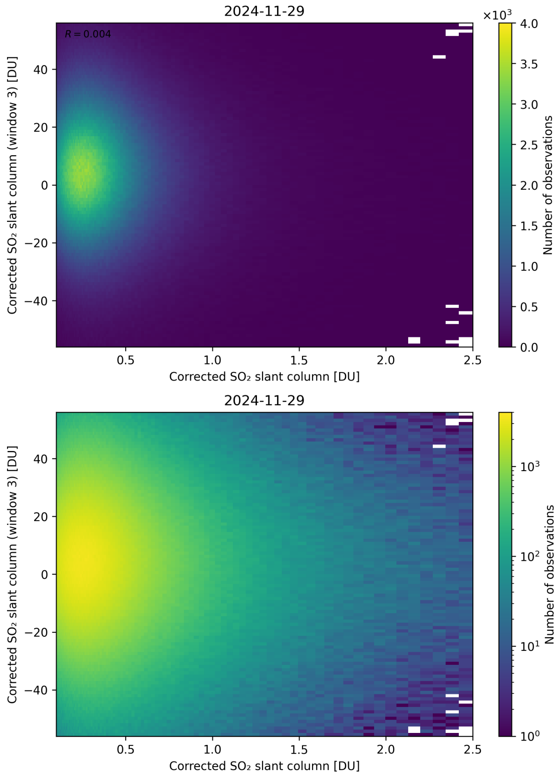
Figure 236: Scatter density plot of “Corrected SO 2 slant column” against “Corrected SO 2 slant column (window 3)” for 2024-11-28 to 2024-11-30.
