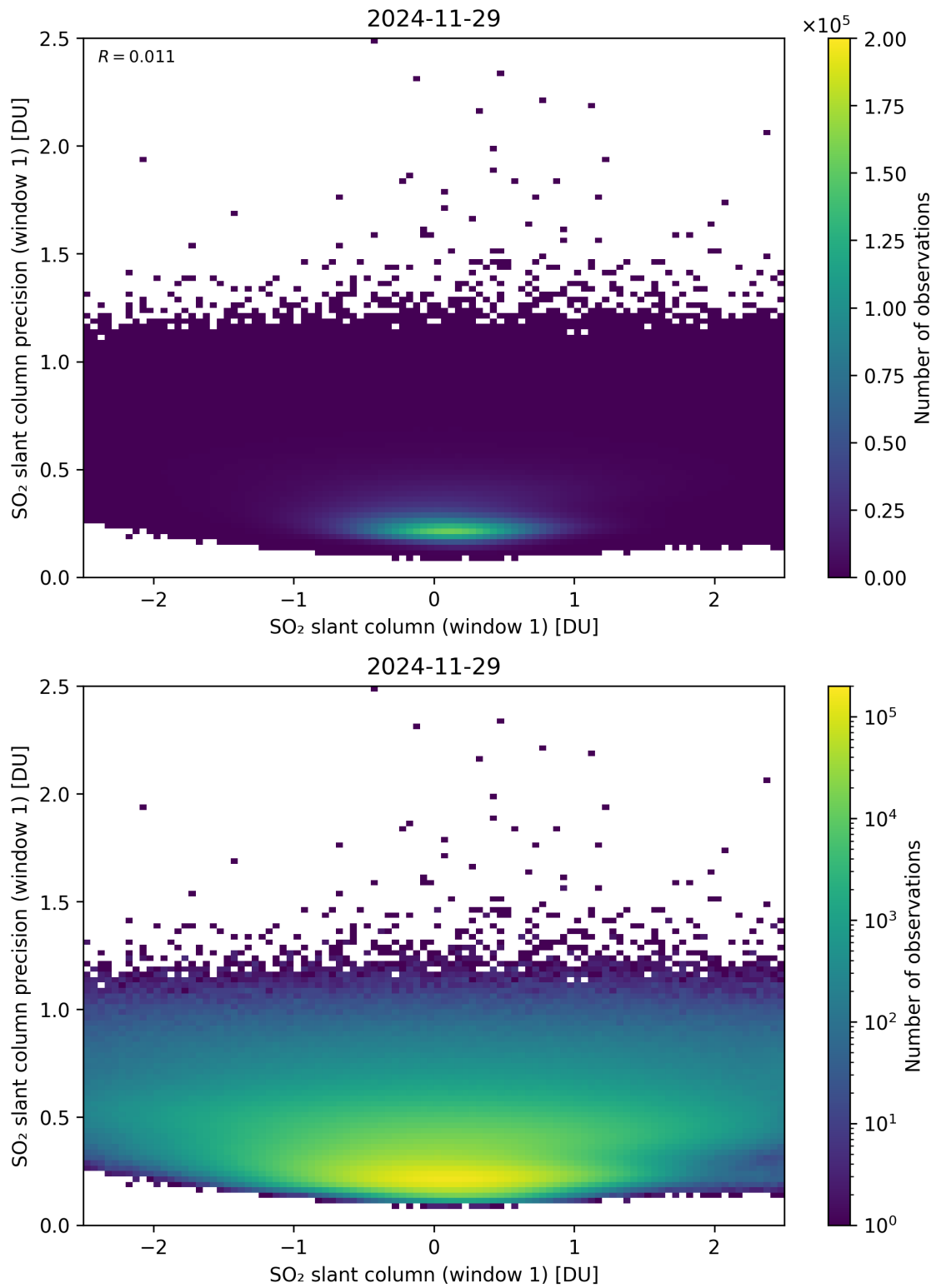
Figure 285: Scatter density plot of “SO 2 slant column (window 1)” against “SO 2 slant column precision (window 1)” for 2024-11-28 to 2024-11-30.
