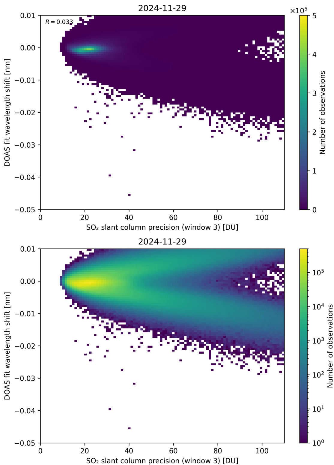
Figure 308: Scatter density plot of “SO 2 slant column precision (window 3)” against “DOAS fit wavelength shift” for 2024-11-28 to 2024-11-30.
