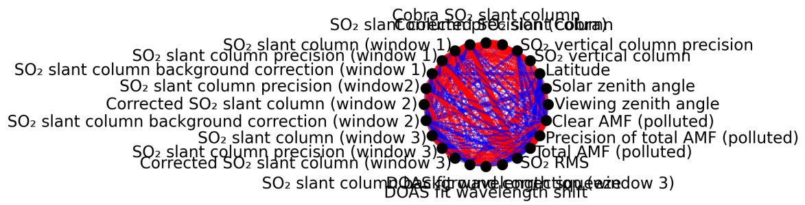
Figure 1: Map of correlation graph for 2024-11-28 to 2024-11-30.
