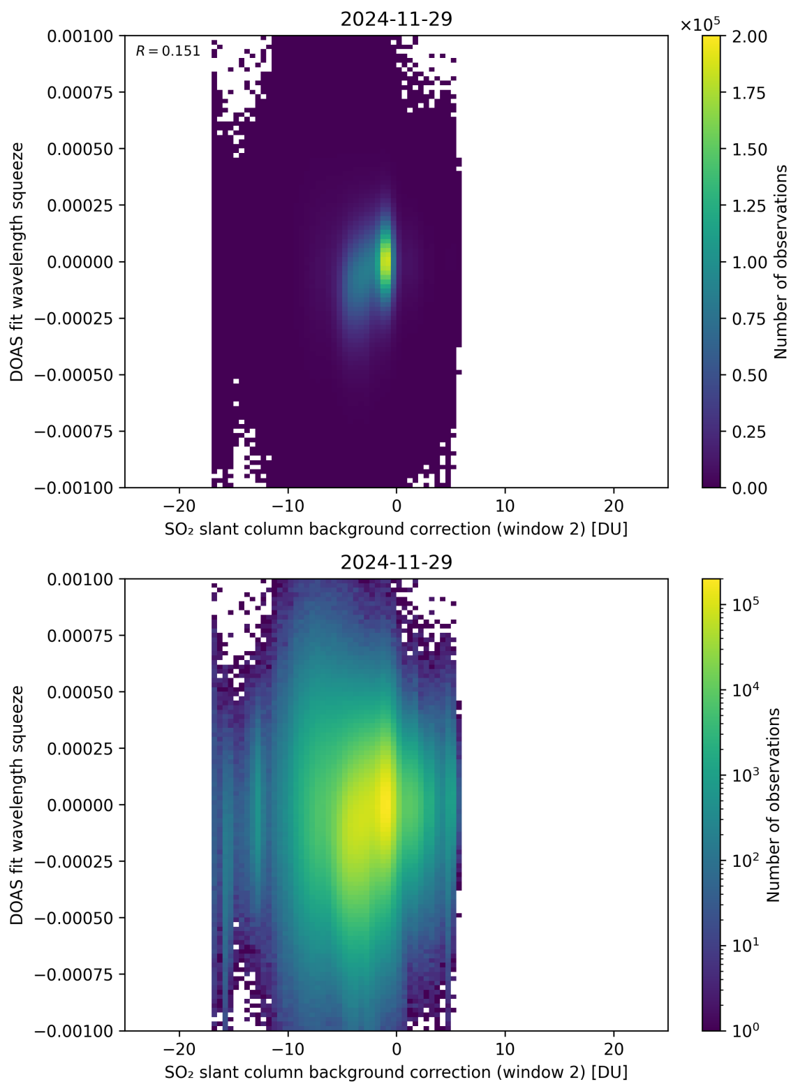
Figure 124: Scatter density plot of “SO 2 slant column background correction (window 2)” against “DOAS fit wavelength squeeze” for 2024-11-28 to 2024-11-30.
