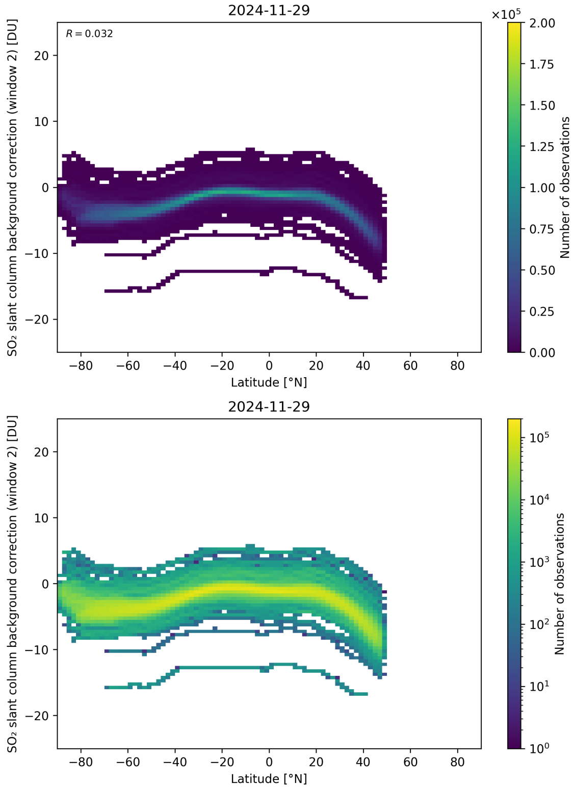
Figure 151: Scatter density plot of “Latitude” against “SO 2 slant column background correction (window 2)” for 2024-11-28 to 2024-11-30.
