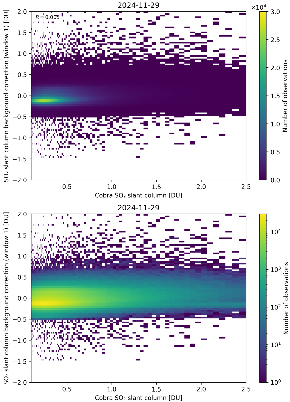
Figure 193: Scatter density plot of “Cobra SO 2 slant column” against “SO 2 slant column background correction (window 1)” for 2024-11-28 to 2024-11-30.
