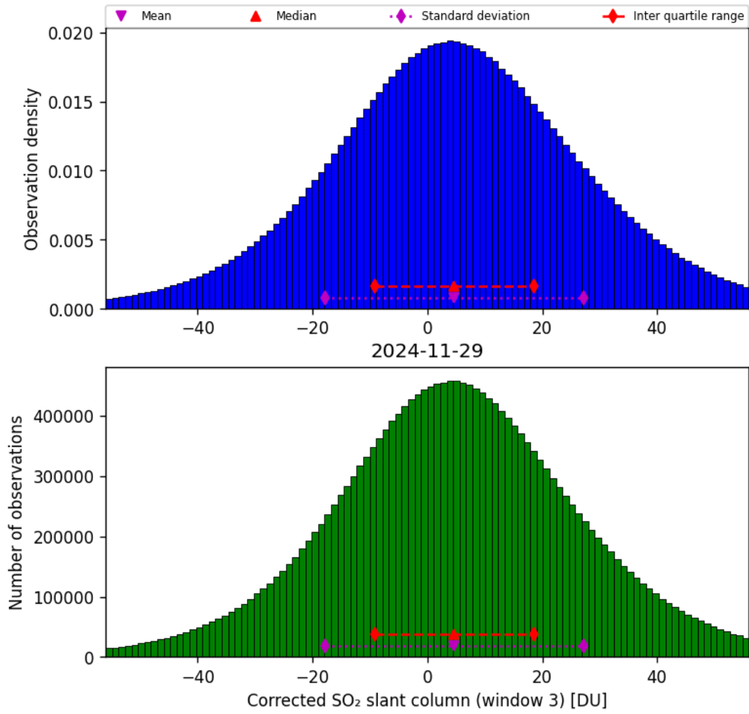
Figure 73: Histogram of “Corrected SO 2 slant column (window 3)” for 2024-11-28 to 2024-11-30
