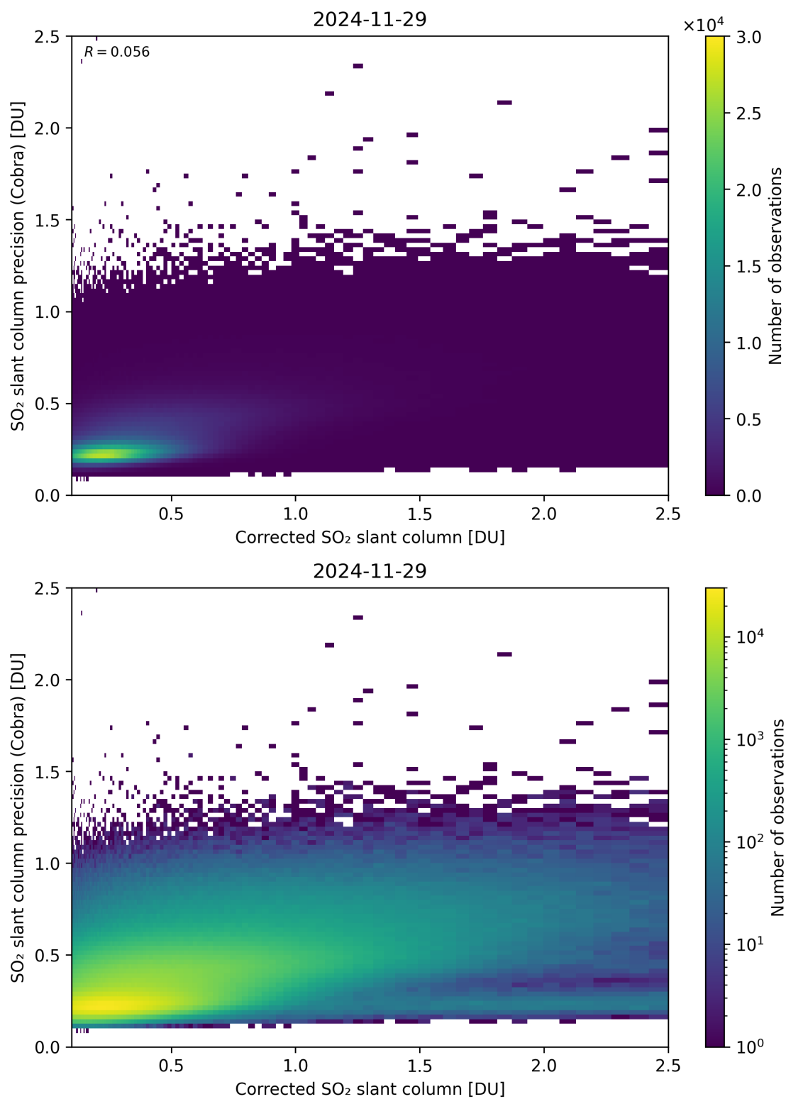
Figure 234: Scatter density plot of “Corrected SO 2 slant column” against “SO 2 slant column precision (Cobra)” for 2024-11-28 to 2024-11-30.
