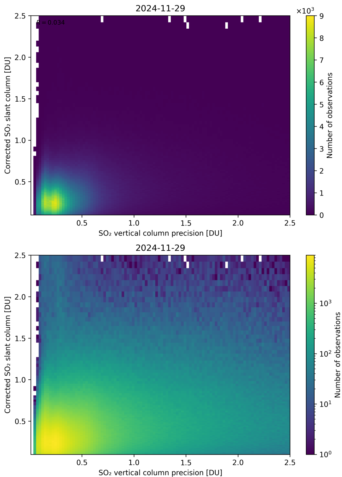
Figure 338: Scatter density plot of “SO 2 vertical column precision” against “Corrected SO 2 slant column” for 2024-11-28 to 2024-11-30.
