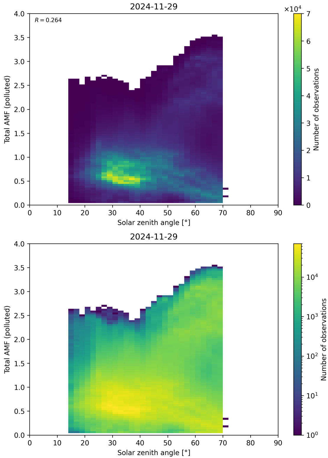
Figure 189: Scatter density plot of “Solar zenith angle” against “Total AMF (polluted)” for 2024-11-28 to 2024-11-30.
