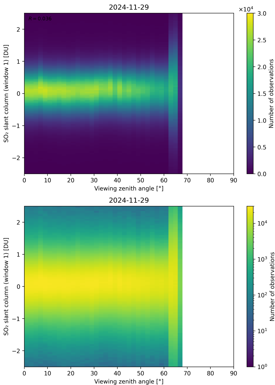
Figure 376: Scatter density plot of “Viewing zenith angle” against “SO 2 slant column (window 1)” for 2024-11-28 to 2024-11-30.
