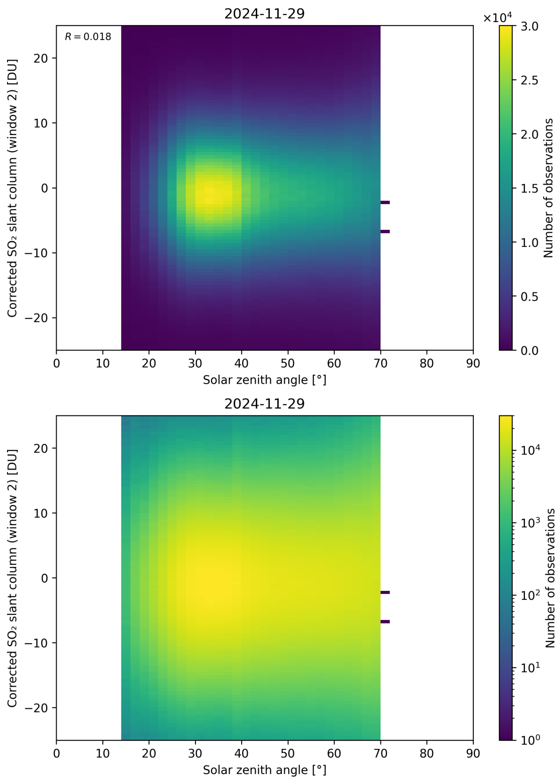
Figure 182: Scatter density plot of “Solar zenith angle” against “Corrected SO 2 slant column (window 2)” for 2024-11-28 to 2024-11-30.
