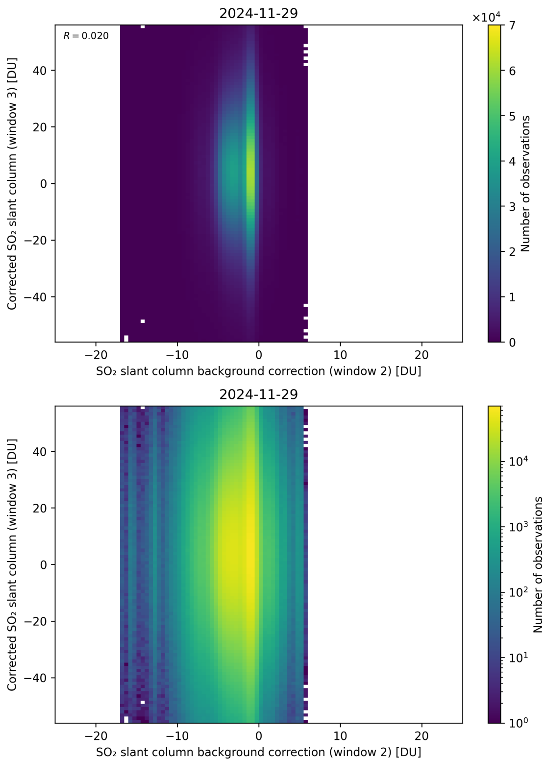
Figure 127: Scatter density plot of “SO 2 slant column background correction (window 2)” against “Corrected SO 2 slant column (window 3)” for 2024-11-28 to 2024-11-30.
