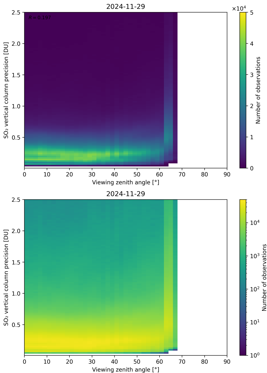
Figure 384: Scatter density plot of “Viewing zenith angle” against “SO 2 vertical column precision” for 2024-11-28 to 2024-11-30.
