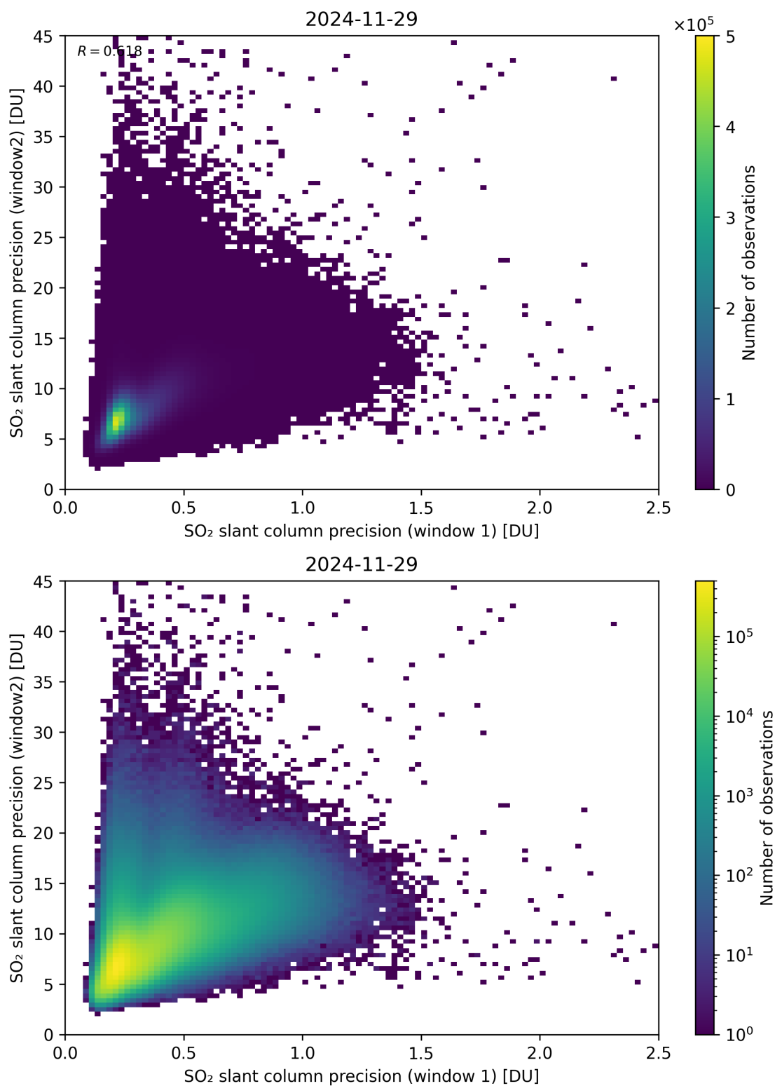
Figure 277: Scatter density plot of “SO 2 slant column precision (window 1)” against “SO 2 slant column precision (window2)” for 2024-11-28 to 2024-11-30.
