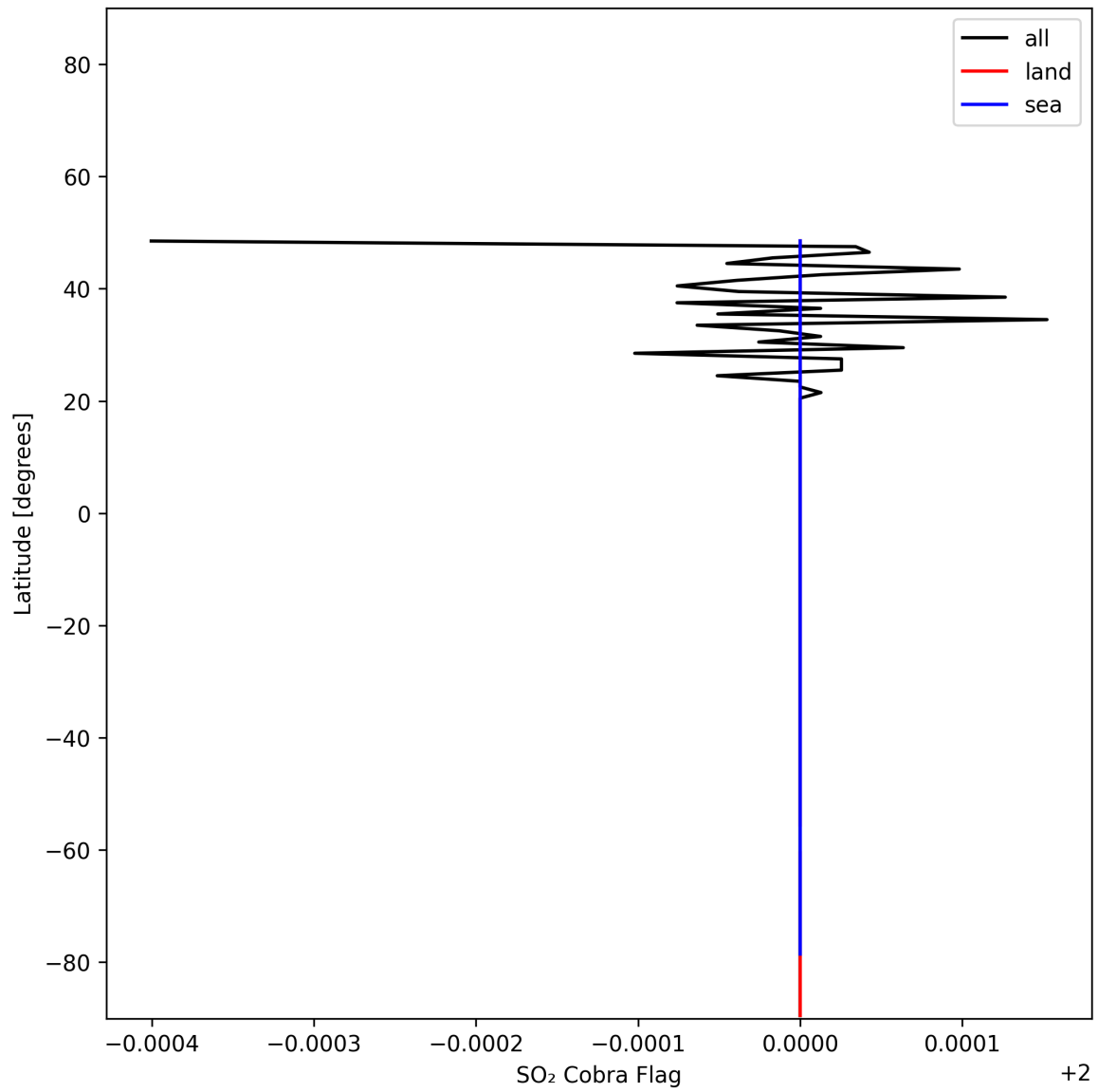
Figure 49: Zonal average of “SO 2 Cobra Flag” for 2024-11-28 to 2024-11-30.
