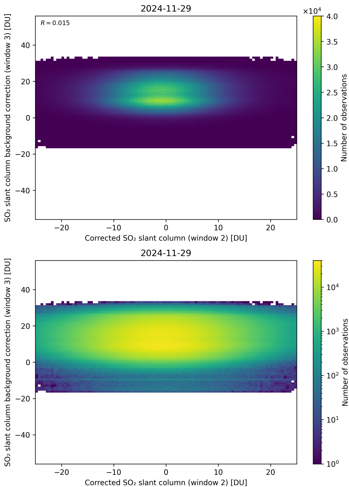
Figure 245: Scatter density plot of “Corrected SO 2 slant column (window 2)” against “SO 2 slant column background correction (window 3)” for 2024-11-28 to 2024-11-30.
