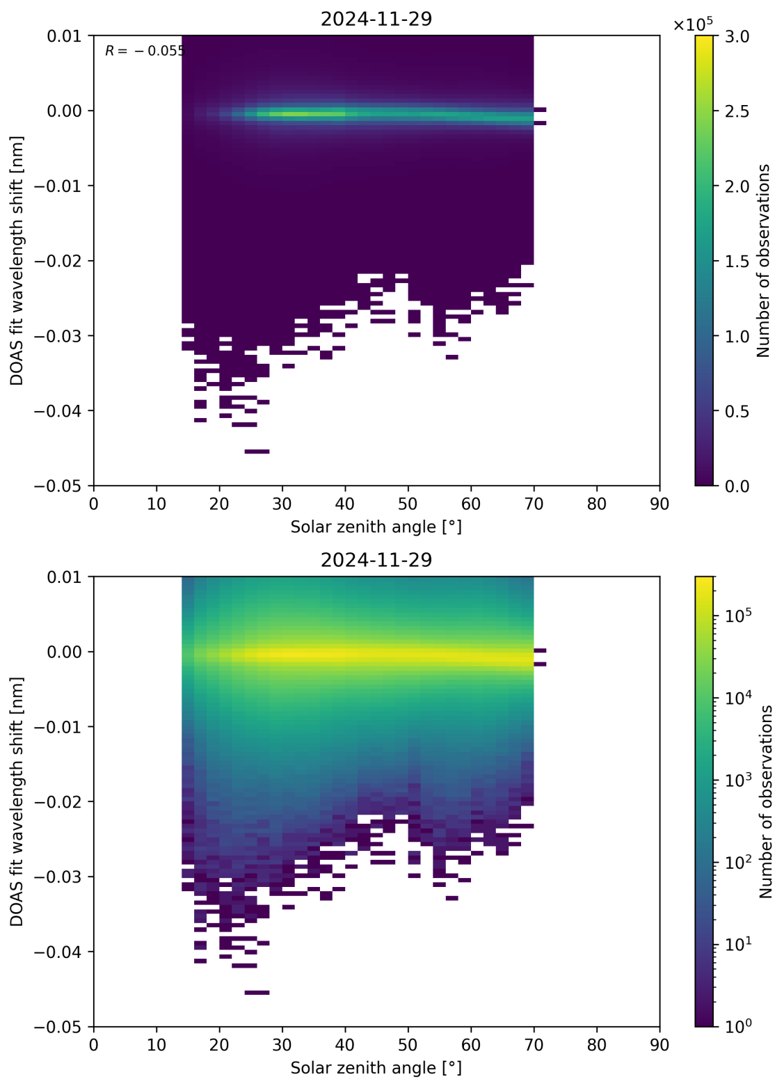
Figure 174: Scatter density plot of “Solar zenith angle” against “DOAS fit wavelength shift” for 2024-11-28 to 2024-11-30.
