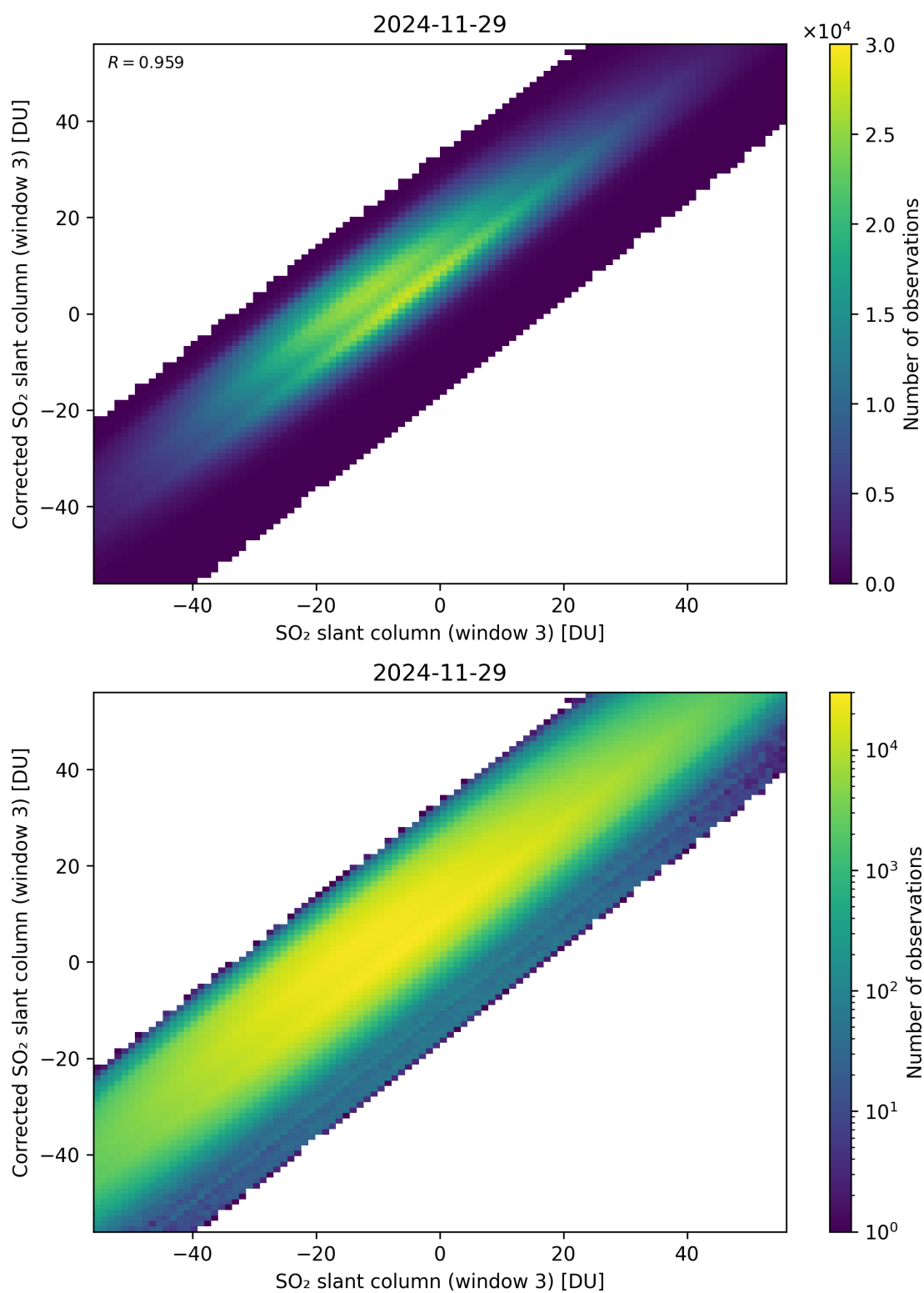
Figure 316: Scatter density plot of “SO 2 slant column (window 3)” against “Corrected SO 2 slant column (window 3)” for 2024-11-28 to 2024-11-30.
