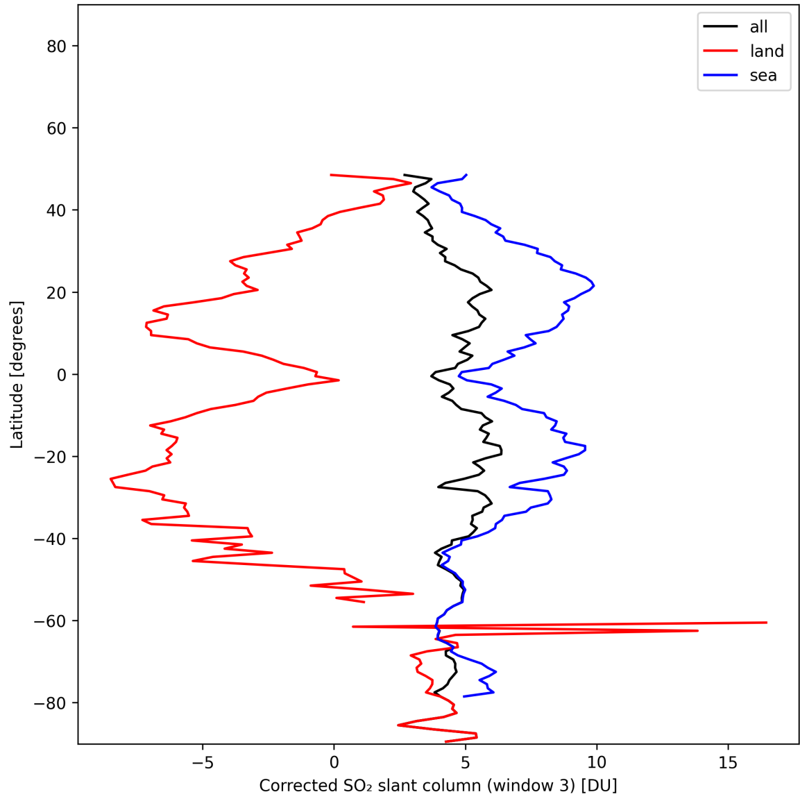
Figure 47: Zonal average of “Corrected SO 2 slant column (window 3)” for 2024-11-28 to 2024-11-30.
