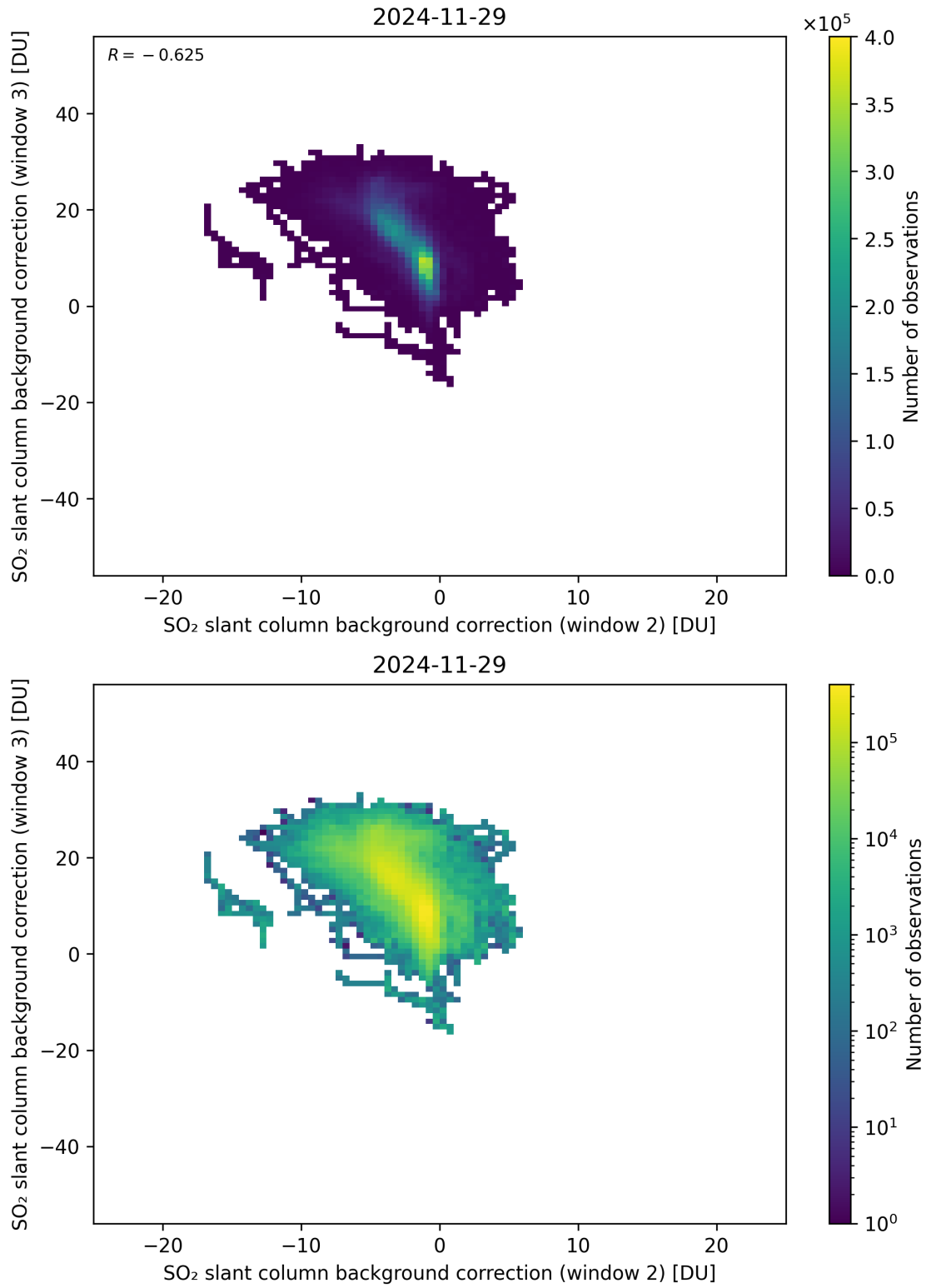
Figure 122: Scatter density plot of “SO 2 slant column background correction (window 2)” against “SO 2 slant column background correction (window 3)” for 2024-11-28 to 2024-11-30.
