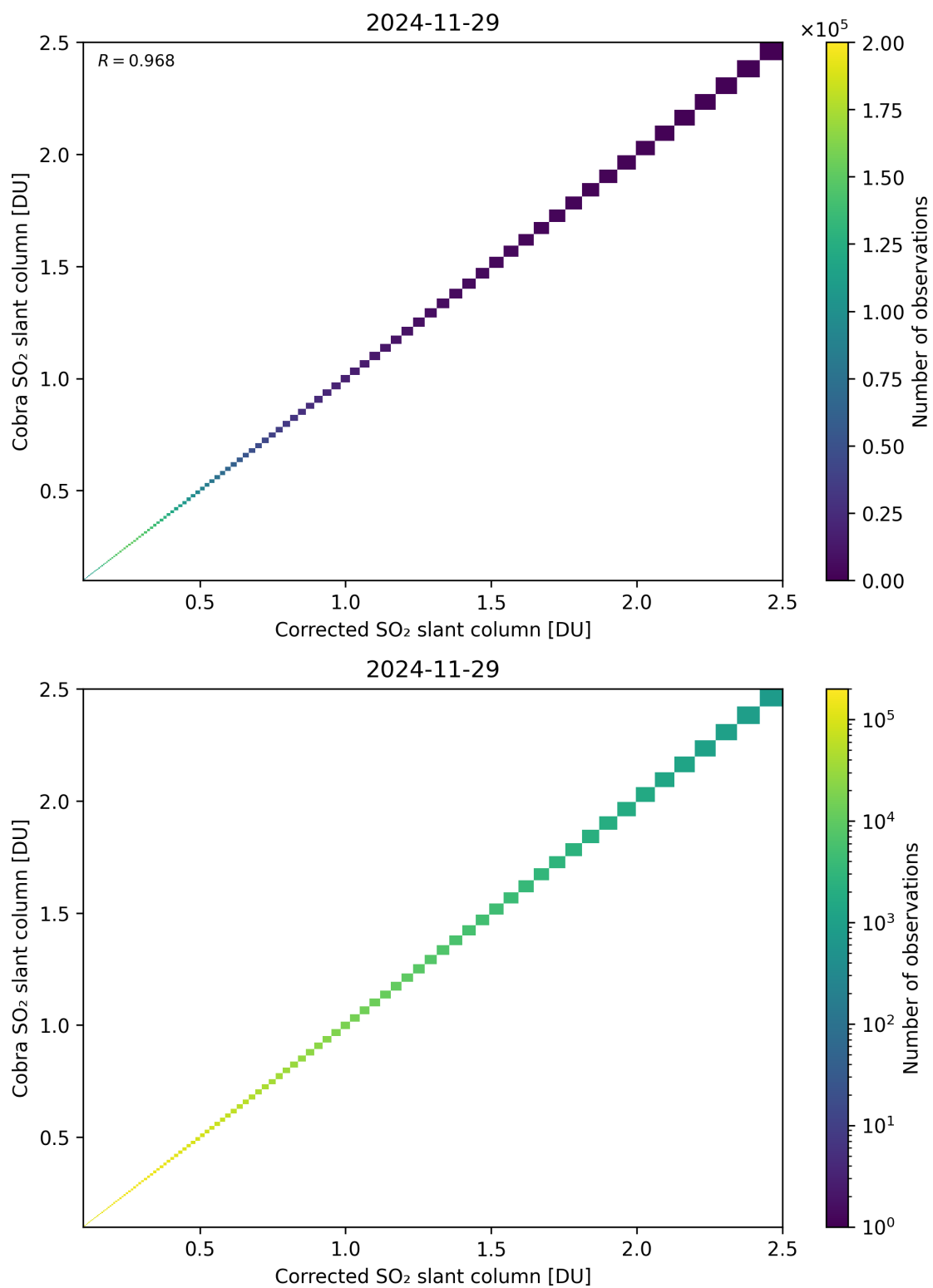
Figure 233: Scatter density plot of “Corrected SO 2 slant column” against “Cobra SO 2 slant column” for 2024-11-28 to 2024-11-30.
