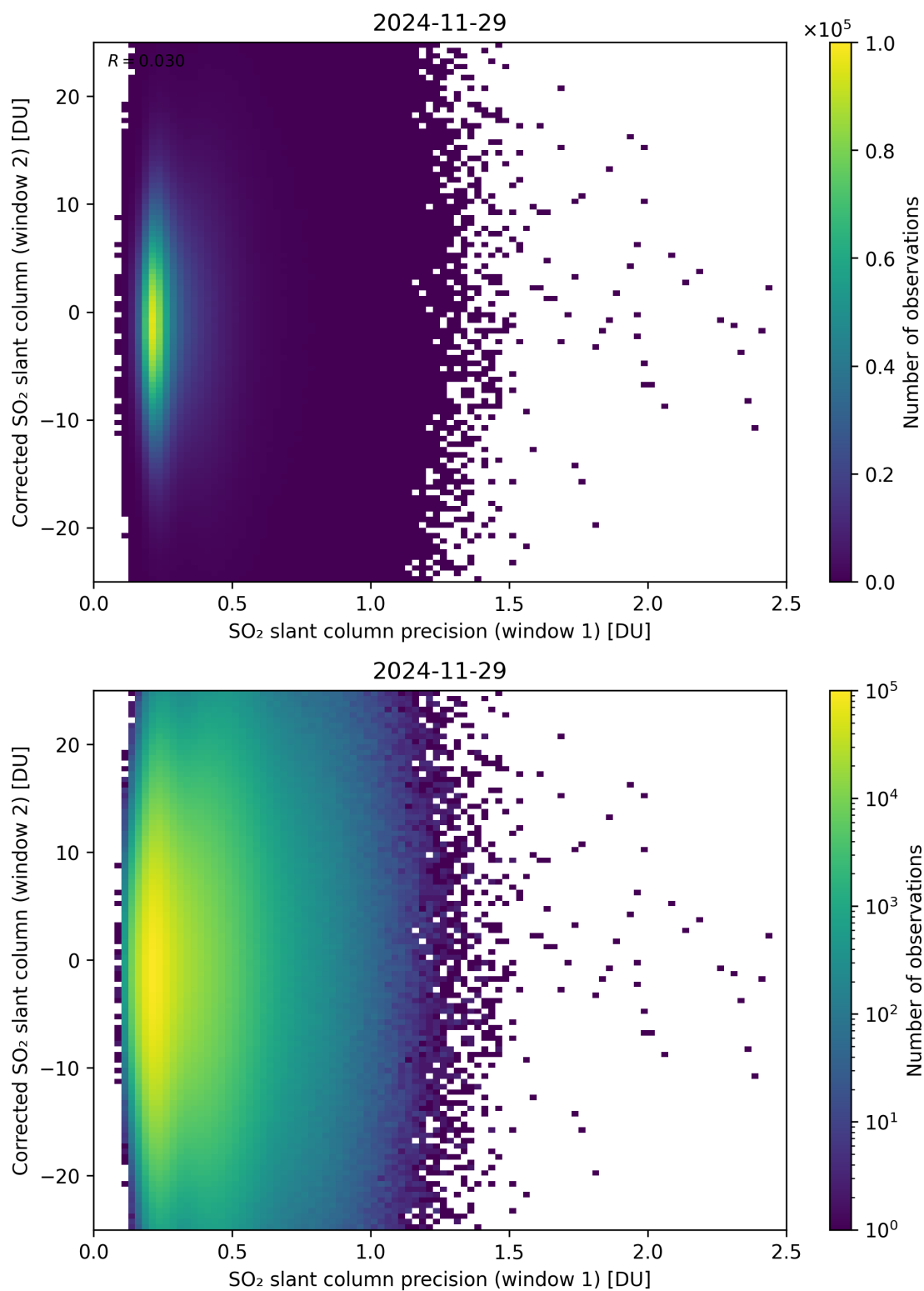
Figure 275: Scatter density plot of “SO 2 slant column precision (window 1)” against “Corrected SO 2 slant column (window 2)” for 2024-11-28 to 2024-11-30.
