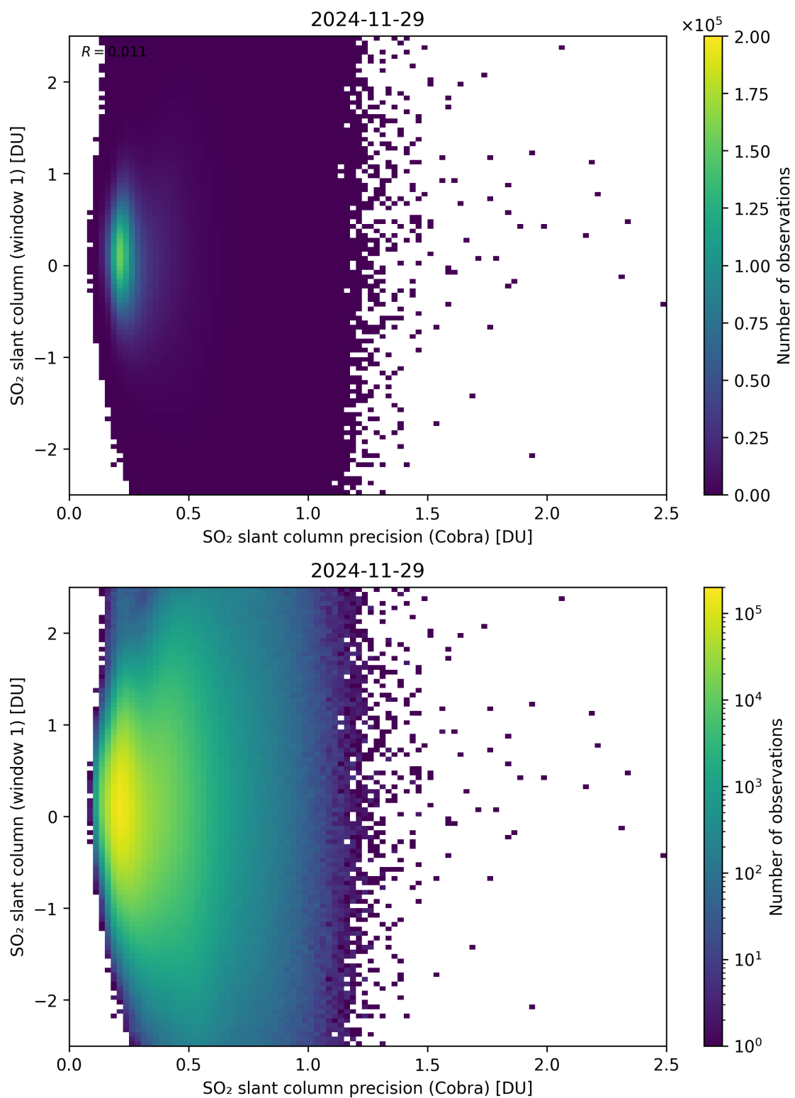
Figure 208: Scatter density plot of “SO 2 slant column precision (Cobra)” against “SO 2 slant column (window 1)” for 2024-11-28 to 2024-11-30.
