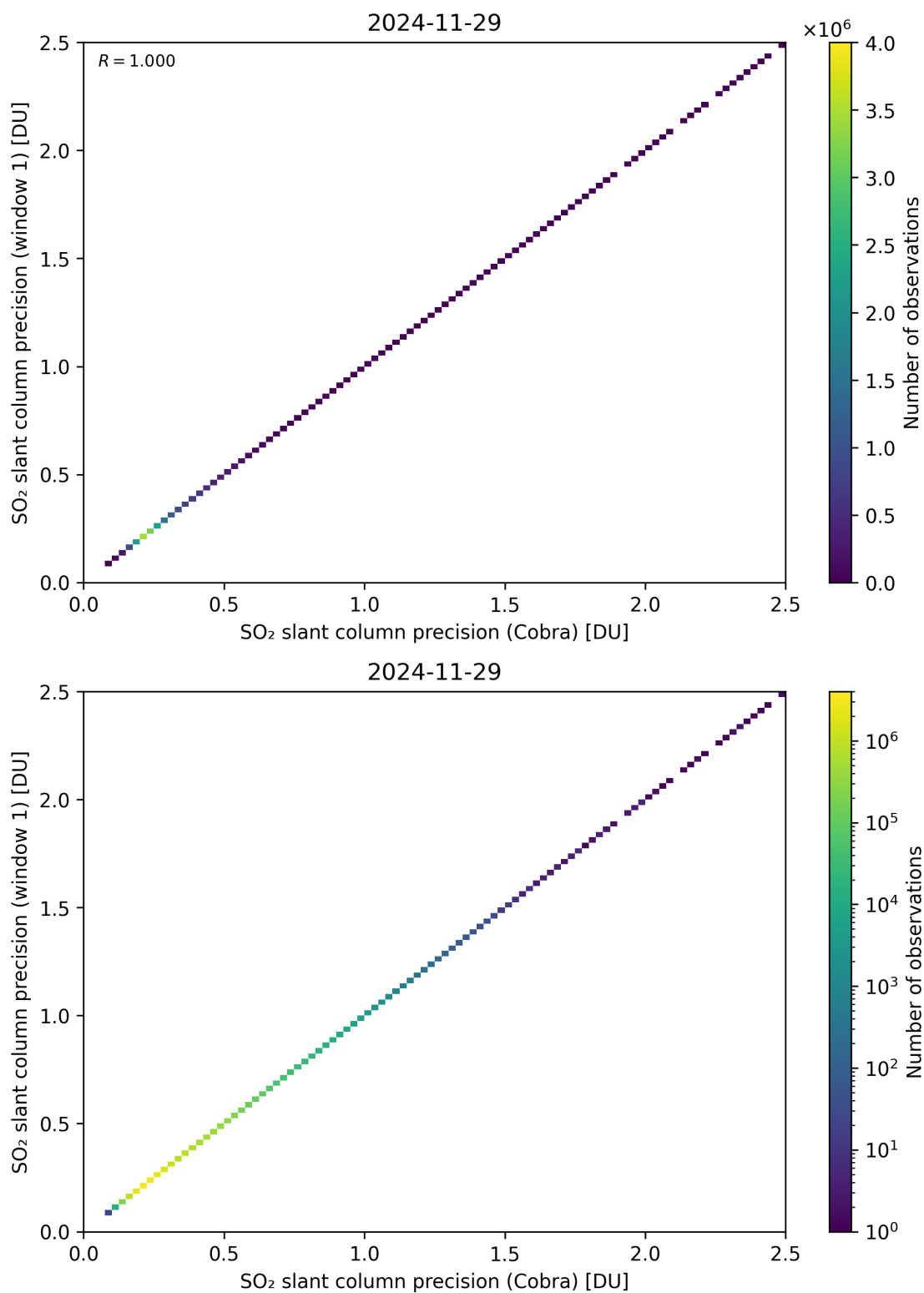
Figure 209: Scatter density plot of “SO 2 slant column precision (Cobra)” against “SO 2 slant column precision (window 1)” for 2024-11-28 to 2024-11-30.
