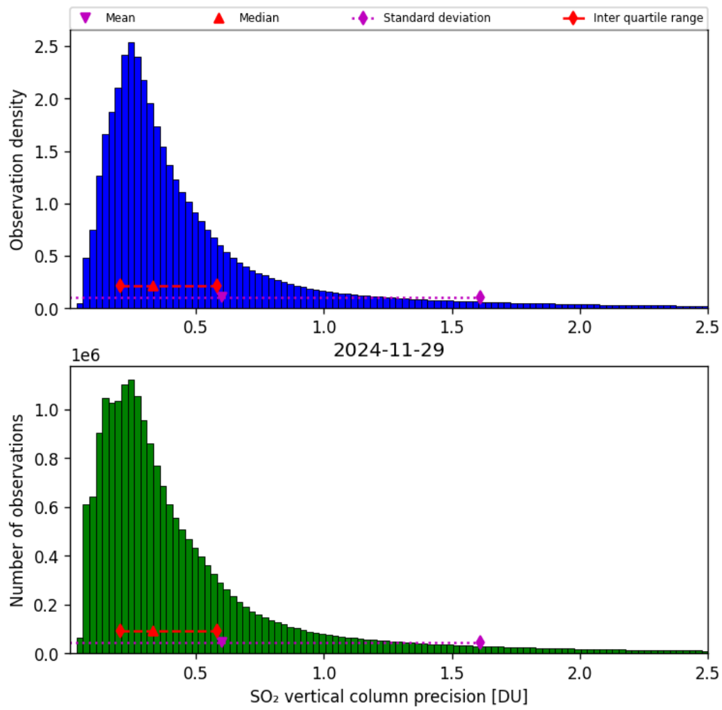
Figure 59: Histogram of “SO 2 vertical column precision” for 2024-11-28 to 2024-11-30
