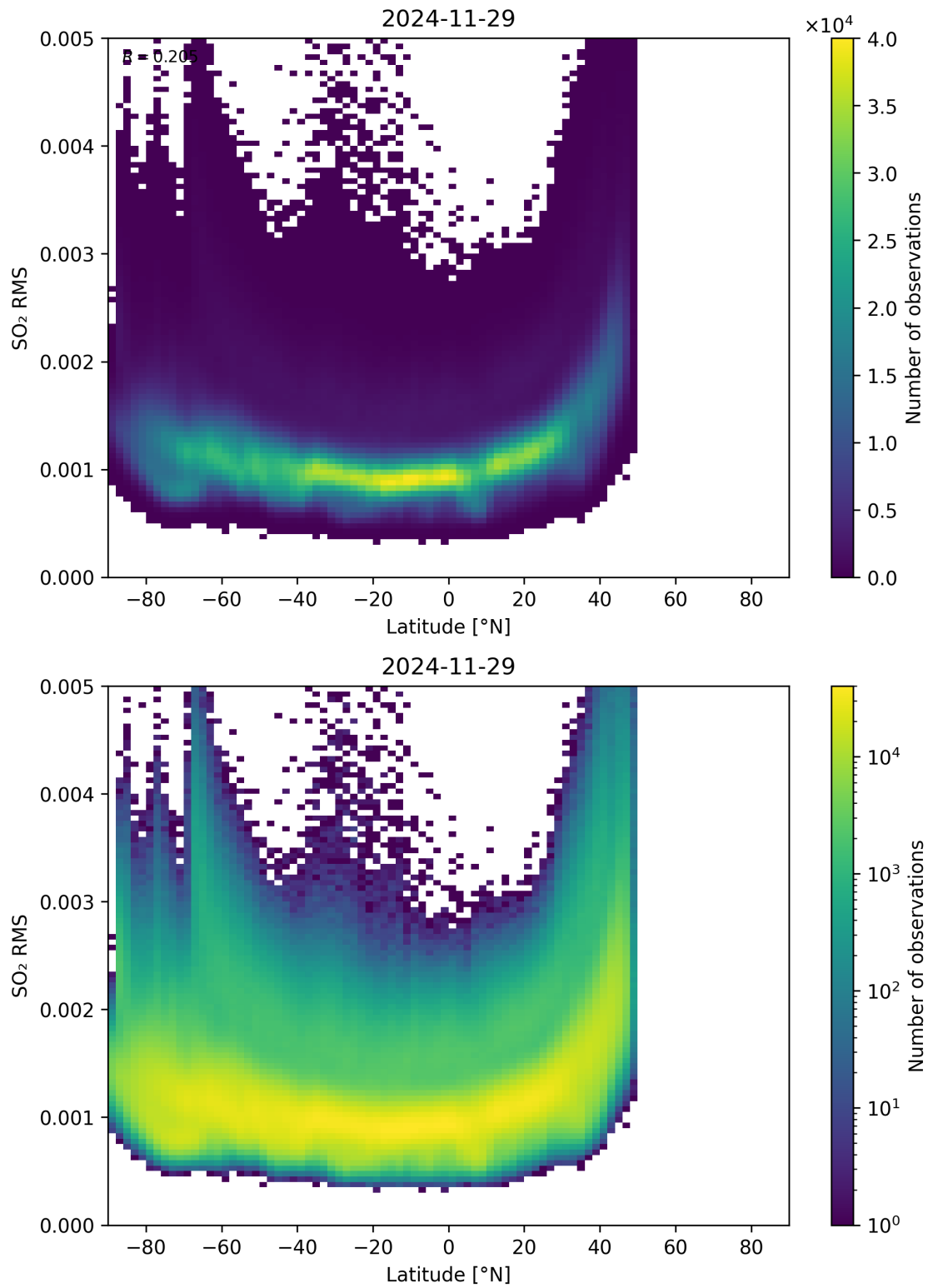
Figure 155: Scatter density plot of “Latitude” against “SO 2 RMS” for 2024-11-28 to 2024-11-30.
