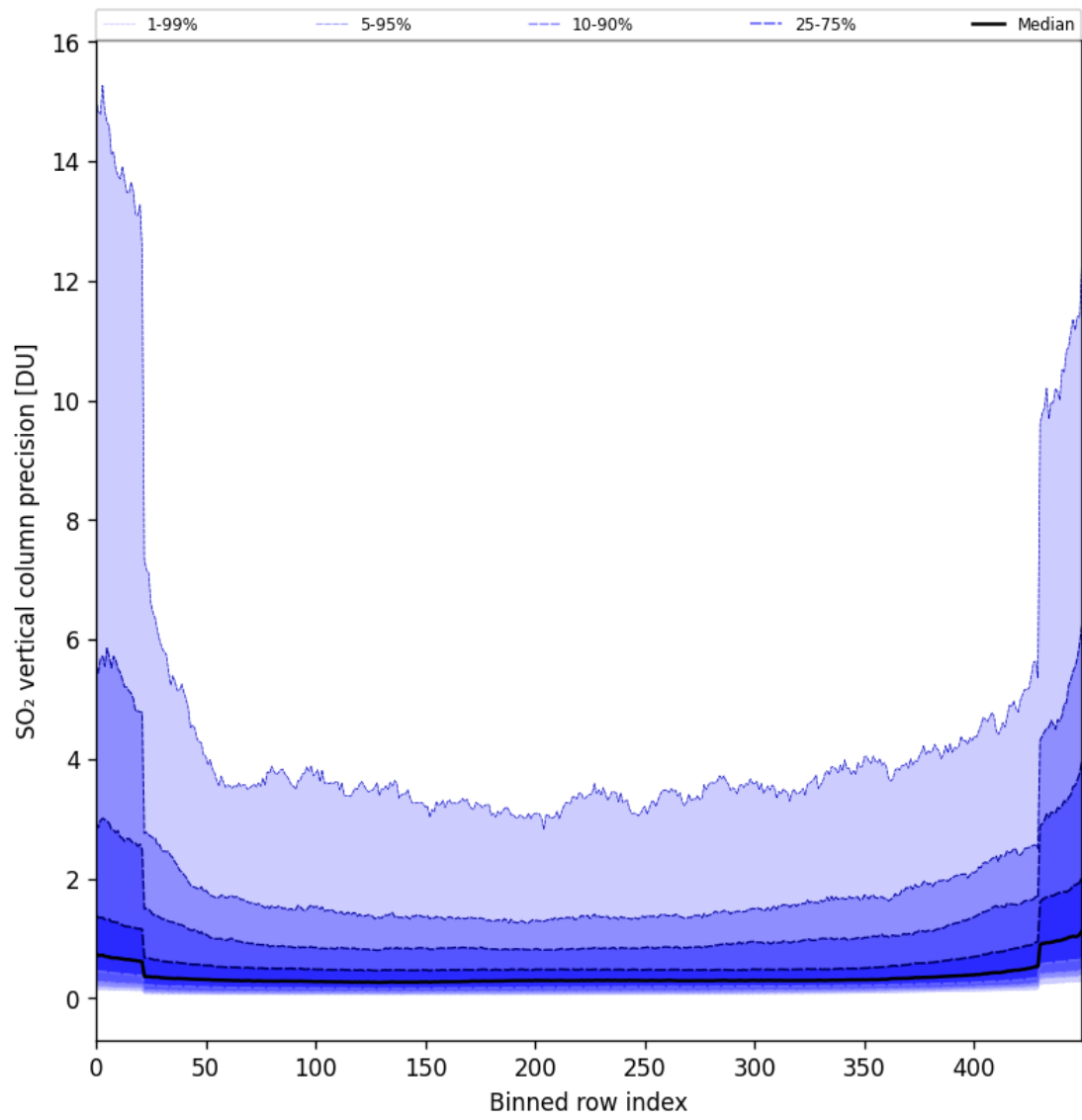
Figure 85: Along track statistics of “SO 2 vertical column precision” for 2024-11-28 to 2024-11-30
