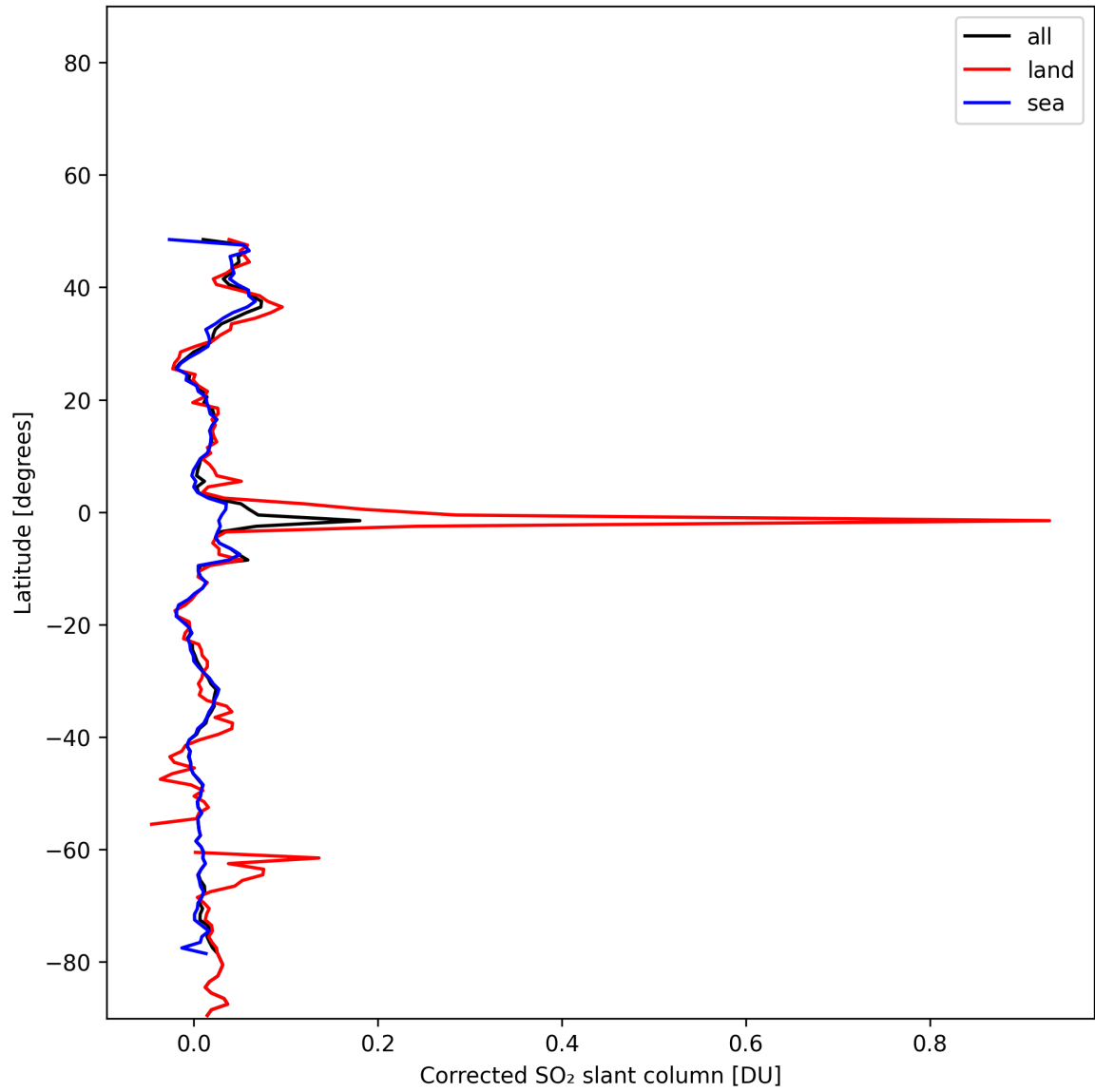
Figure 34: Zonal average of “Corrected SO 2 slant column” for 2024-11-28 to 2024-11-30.
