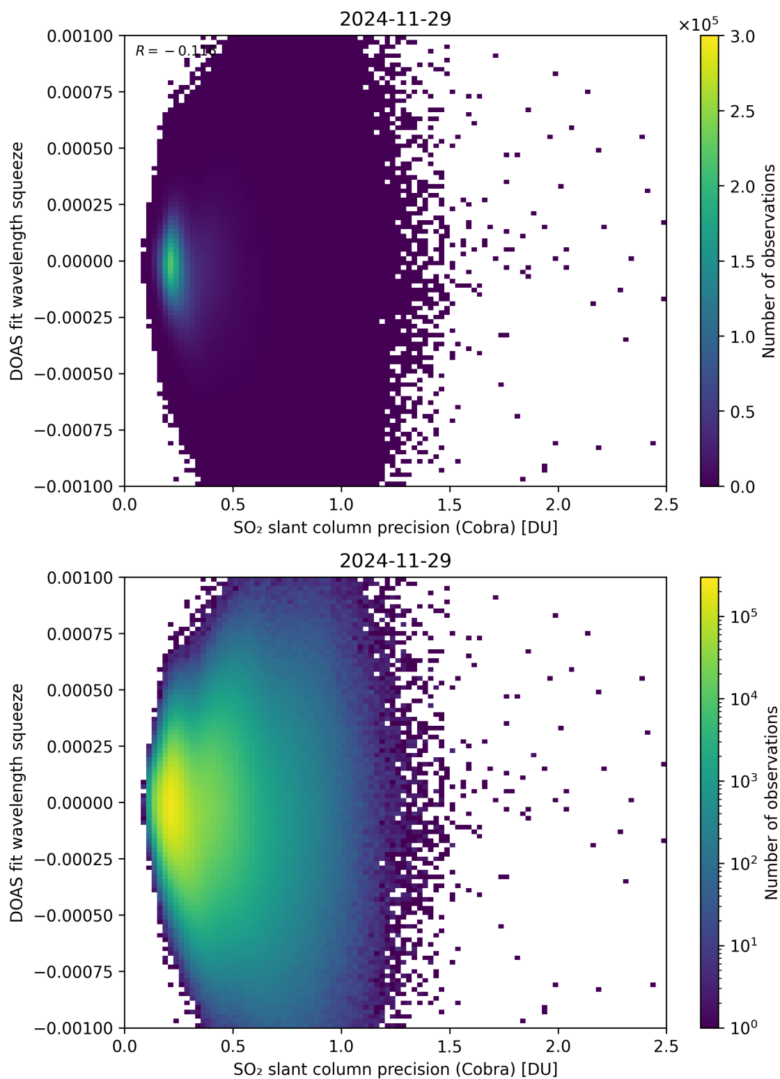
Figure 203: Scatter density plot of “SO 2 slant column precision (Cobra)” against “DOAS fit wavelength squeeze” for 2024-11-28 to 2024-11-30.
