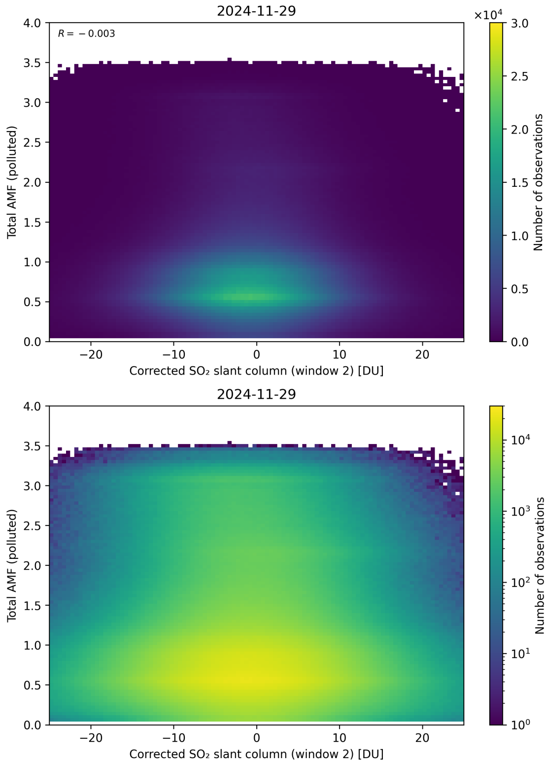
Figure 253: Scatter density plot of “Corrected SO 2 slant column (window 2)” against “Total AMF (polluted)” for 2024-11-28 to 2024-11-30.
