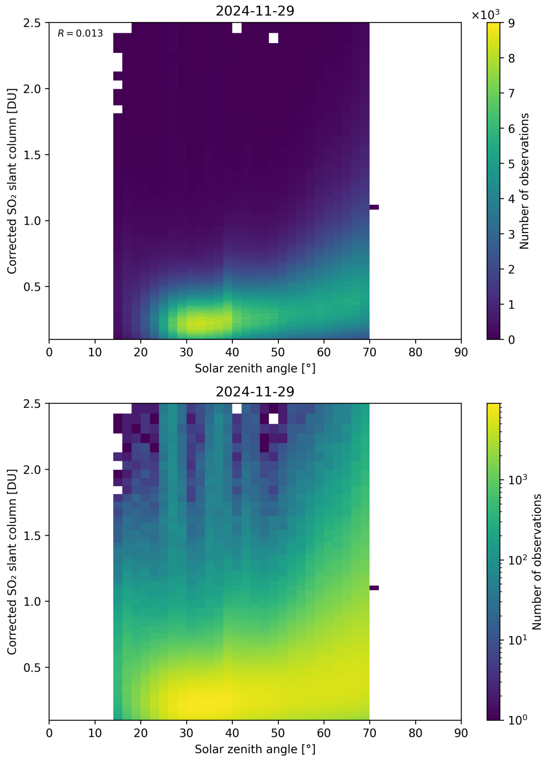
Figure 181: Scatter density plot of “Solar zenith angle” against “Corrected SO 2 slant column” for 2024-11-28 to 2024-11-30.
