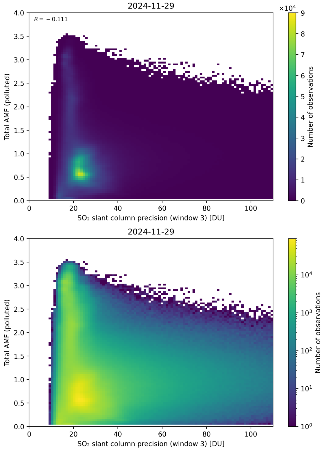
Figure 313: Scatter density plot of “SO 2 slant column precision (window 3)” against “Total AMF (polluted)” for 2024-11-28 to 2024-11-30.
