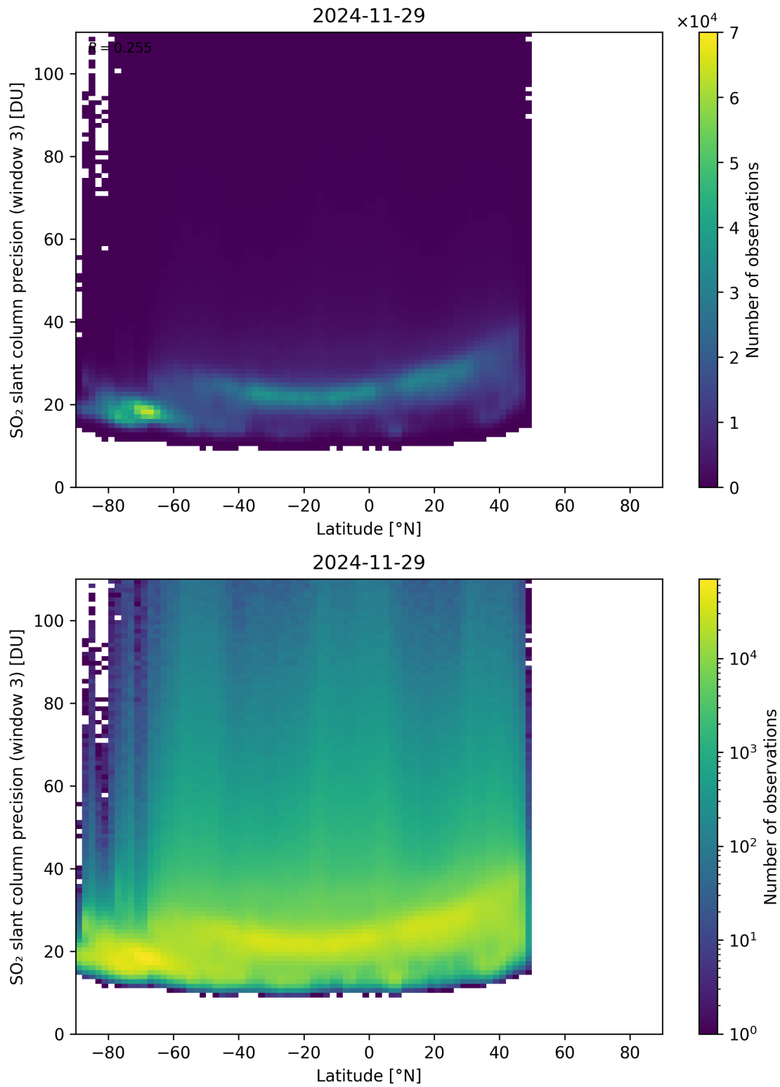
Figure 166: Scatter density plot of “Latitude” against “SO 2 slant column precision (window 3)” for 2024-11-28 to 2024-11-30.
