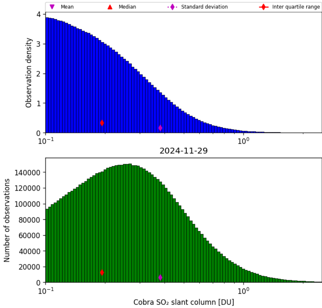
Figure 61: Histogram of “Cobra SO 2 slant column” for 2024-11-28 to 2024-11-30
