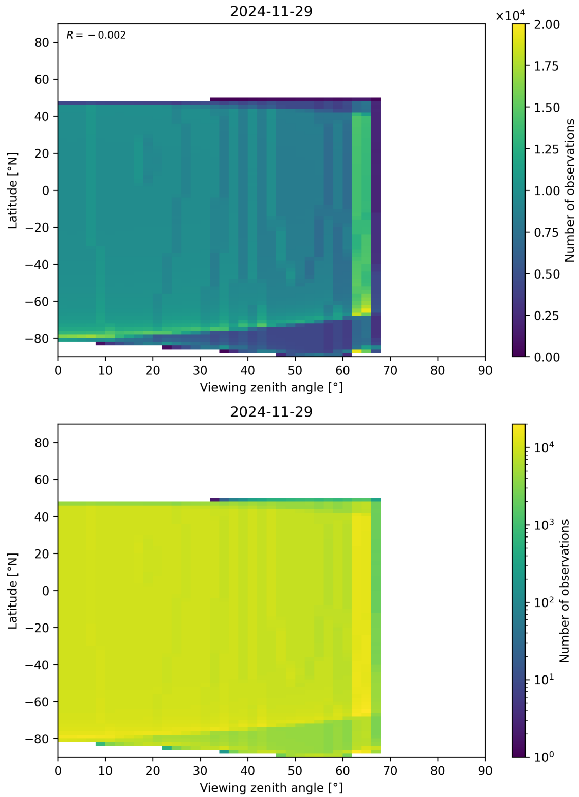
Figure 368: Scatter density plot of “Viewing zenith angle” against “Latitude” for 2024-11-28 to 2024-11-30.
