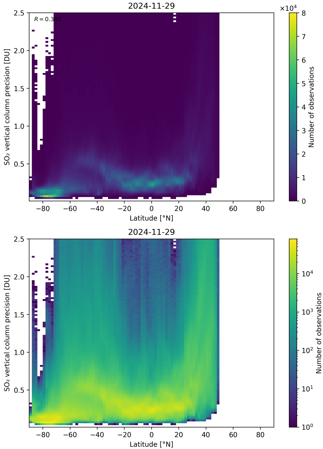
Figure 170: Scatter density plot of “Latitude” against “SO 2 vertical column precision” for 2024-11-28 to 2024-11-30.
