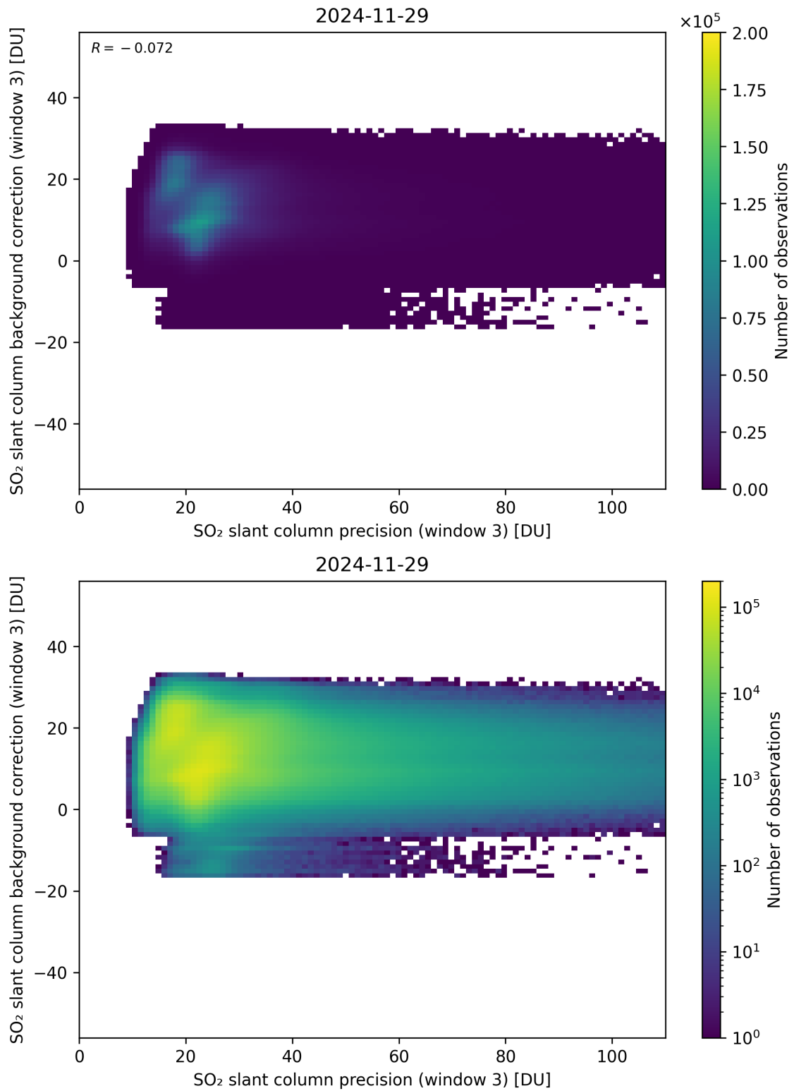
Figure 307: Scatter density plot of “SO 2 slant column precision (window 3)” against “SO 2 slant column background correction (window 3)” for 2024-11-28 to 2024-11-30.
