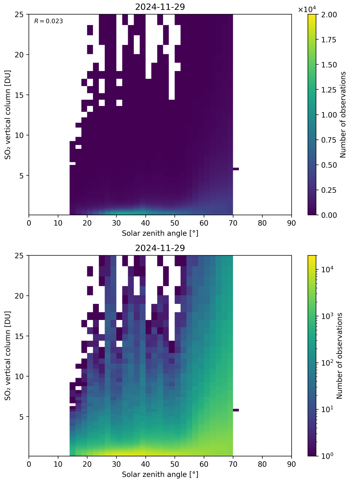
Figure 191: Scatter density plot of “Solar zenith angle” against “SO 2 vertical column” for 2024-11-28 to 2024-11-30.
