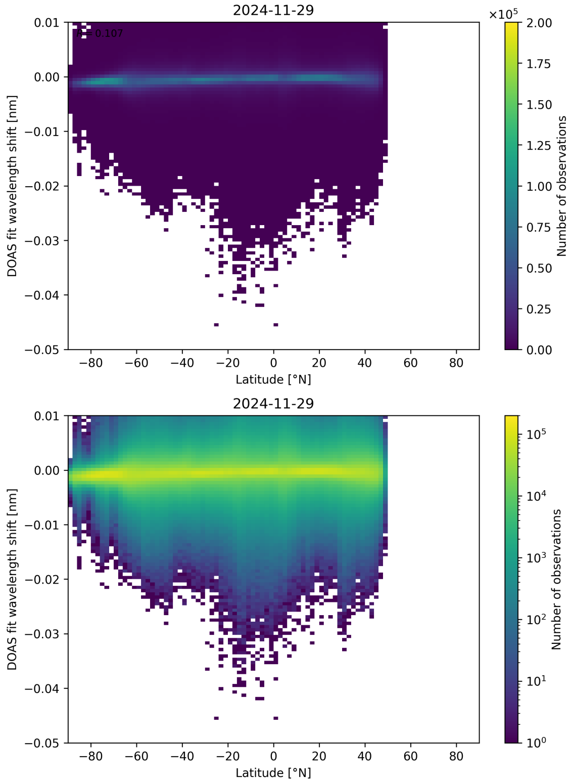
Figure 153: Scatter density plot of “Latitude” against “DOAS fit wavelength shift” for 2024-11-28 to 2024-11-30.
