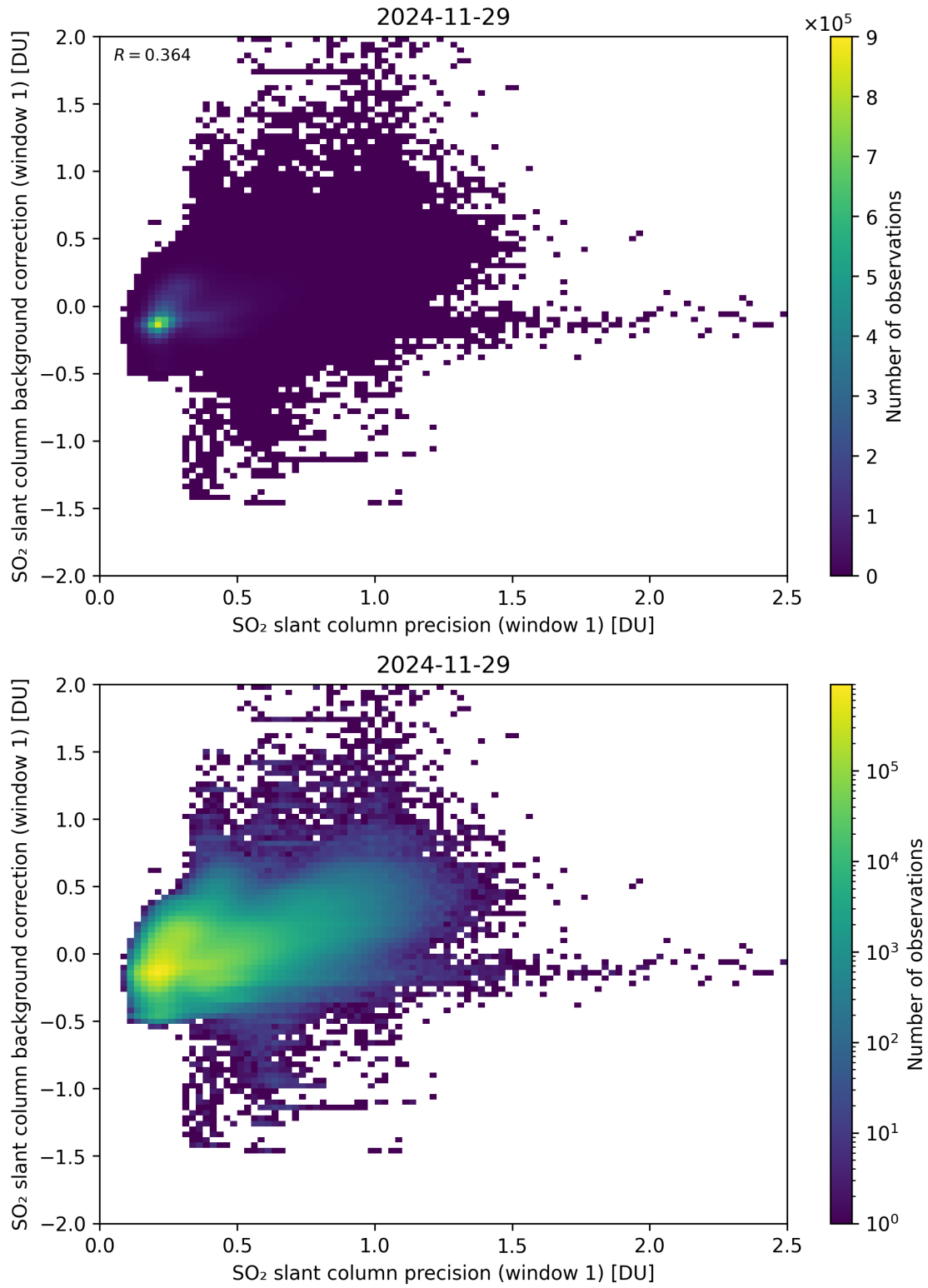
Figure 268: Scatter density plot of “SO 2 slant column precision (window 1)” against “SO 2 slant column background correction (window 1)” for 2024-11-28 to 2024-11-30.
