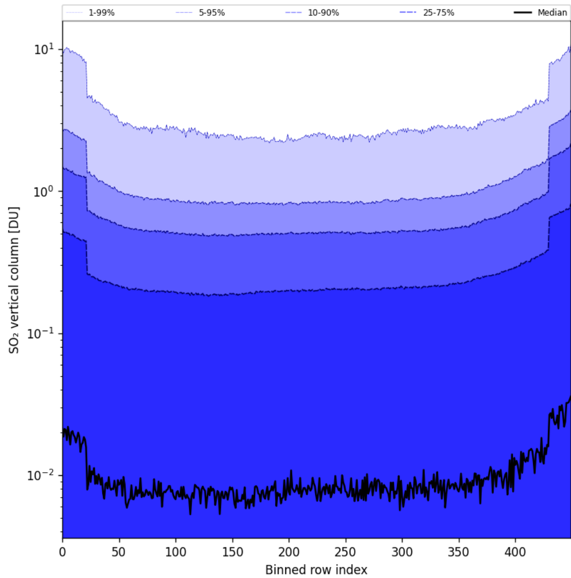
Figure 84: Along track statistics of “SO 2 vertical column” for 2024-11-28 to 2024-11-30
