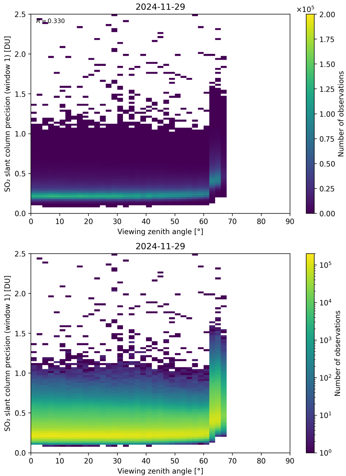
Figure 377: Scatter density plot of “Viewing zenith angle” against “SO 2 slant column precision (window 1)” for 2024-11-28 to 2024-11-30.
