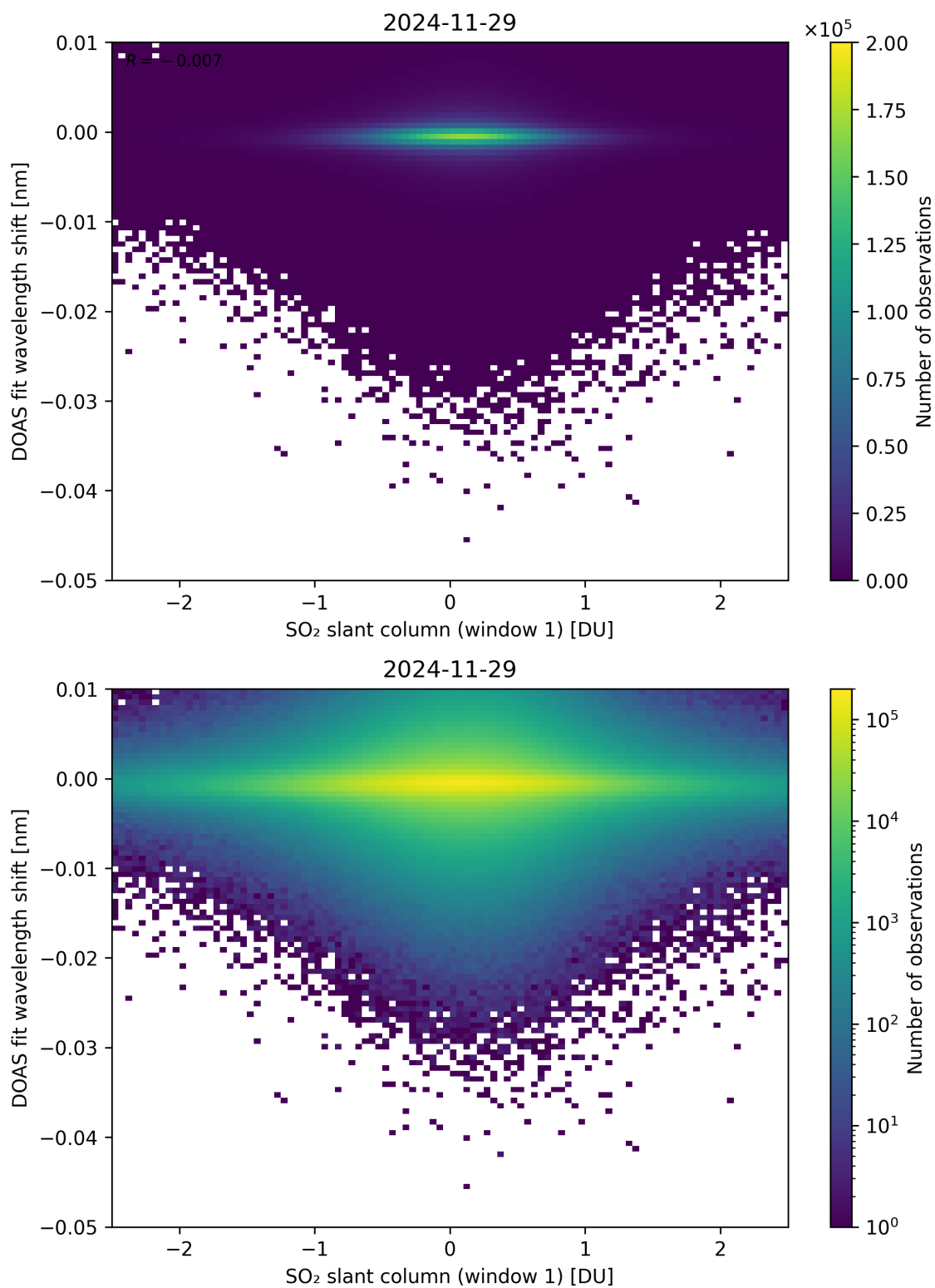
Figure 265: Scatter density plot of “SO 2 slant column (window 1)” against “DOAS fit wavelength shift” for 2024-11-28 to 2024-11-30.
