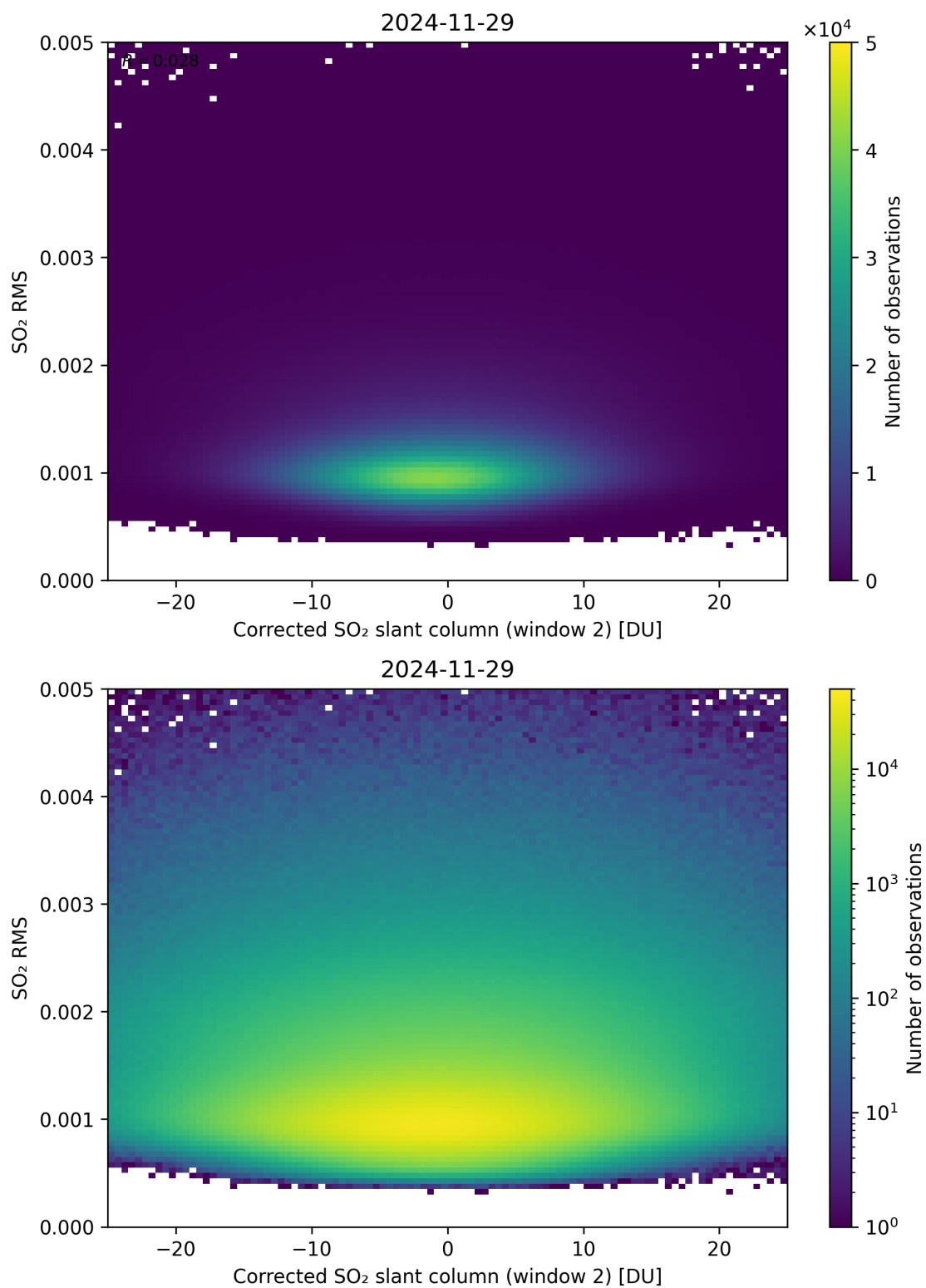
Figure 248: Scatter density plot of “Corrected SO 2 slant column (window 2)” against “SO 2 RMS” for 2024-11-28 to 2024-11-30.
