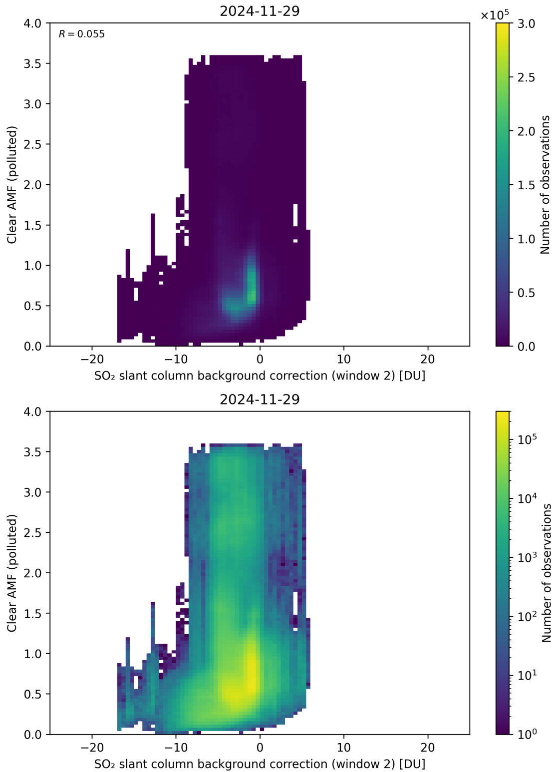
Figure 126: Scatter density plot of “SO 2 slant column background correction (window 2)” against “Clear AMF (polluted)” for 2024-11-28 to 2024-11-30.
