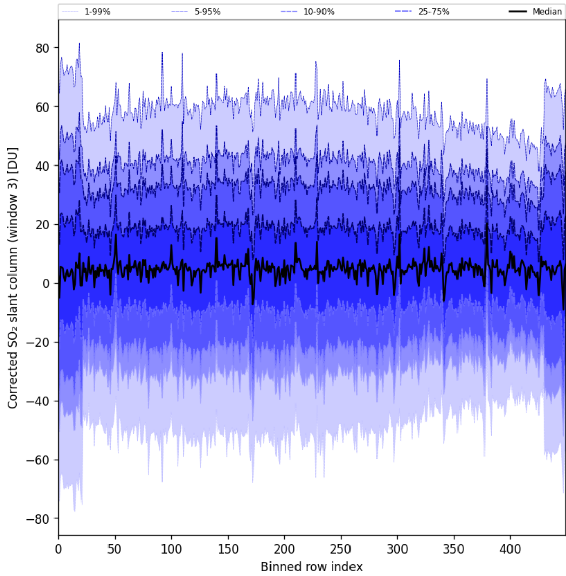
Figure 99: Along track statistics of “Corrected SO 2 slant column (window 3)” for 2024-11-28 to 2024-11-30
