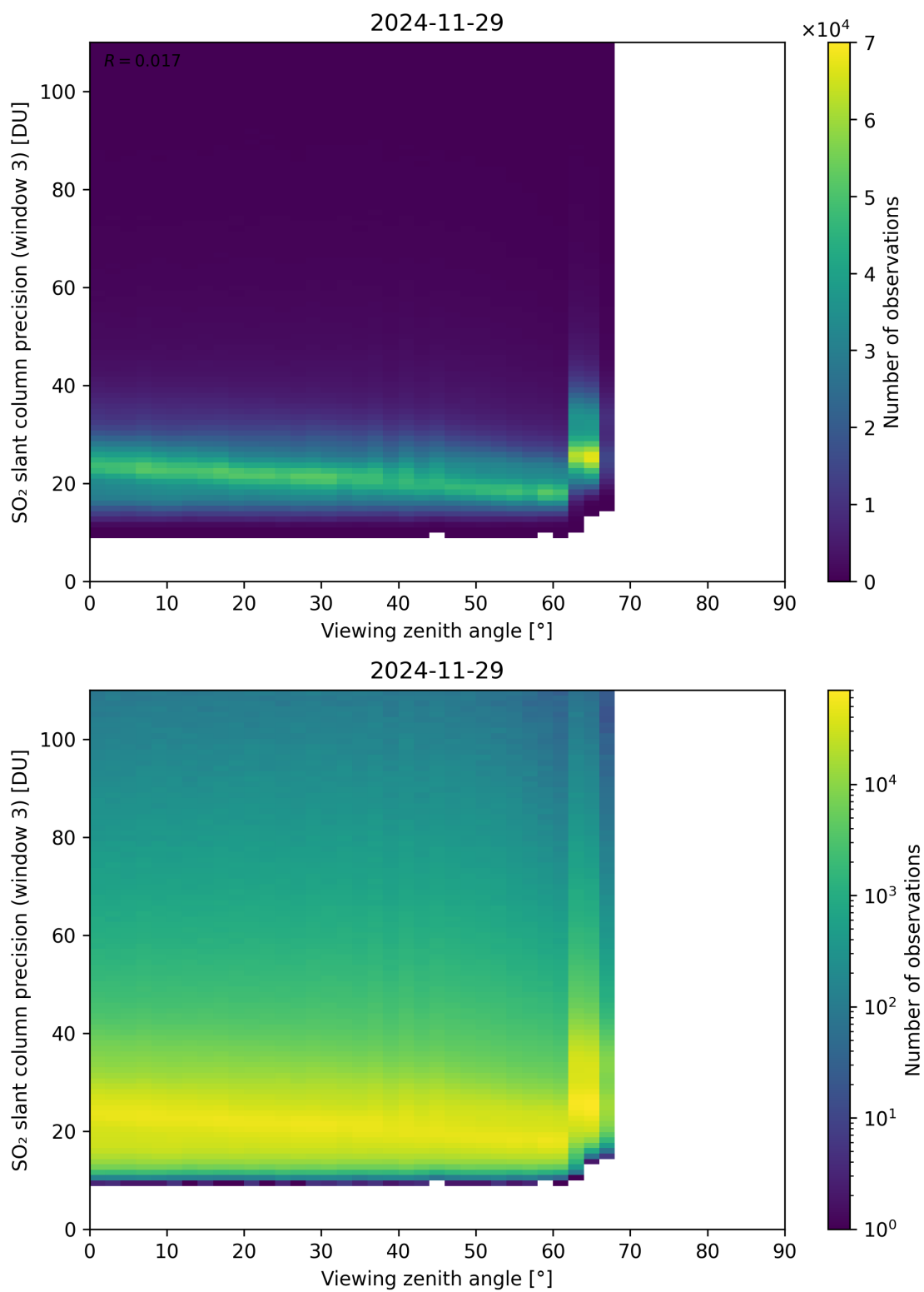
Figure 380: Scatter density plot of “Viewing zenith angle” against “SO 2 slant column precision (window 3)” for 2024-11-28 to 2024-11-30.
