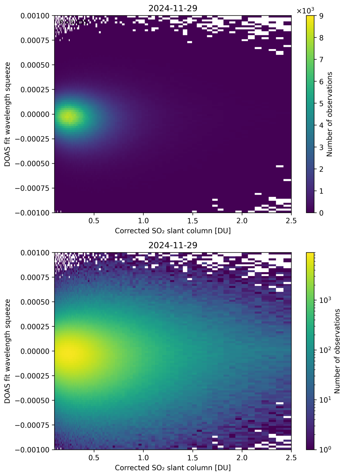
Figure 230: Scatter density plot of “Corrected SO 2 slant column” against “DOAS fit wavelength squeeze” for 2024-11-28 to 2024-11-30.
