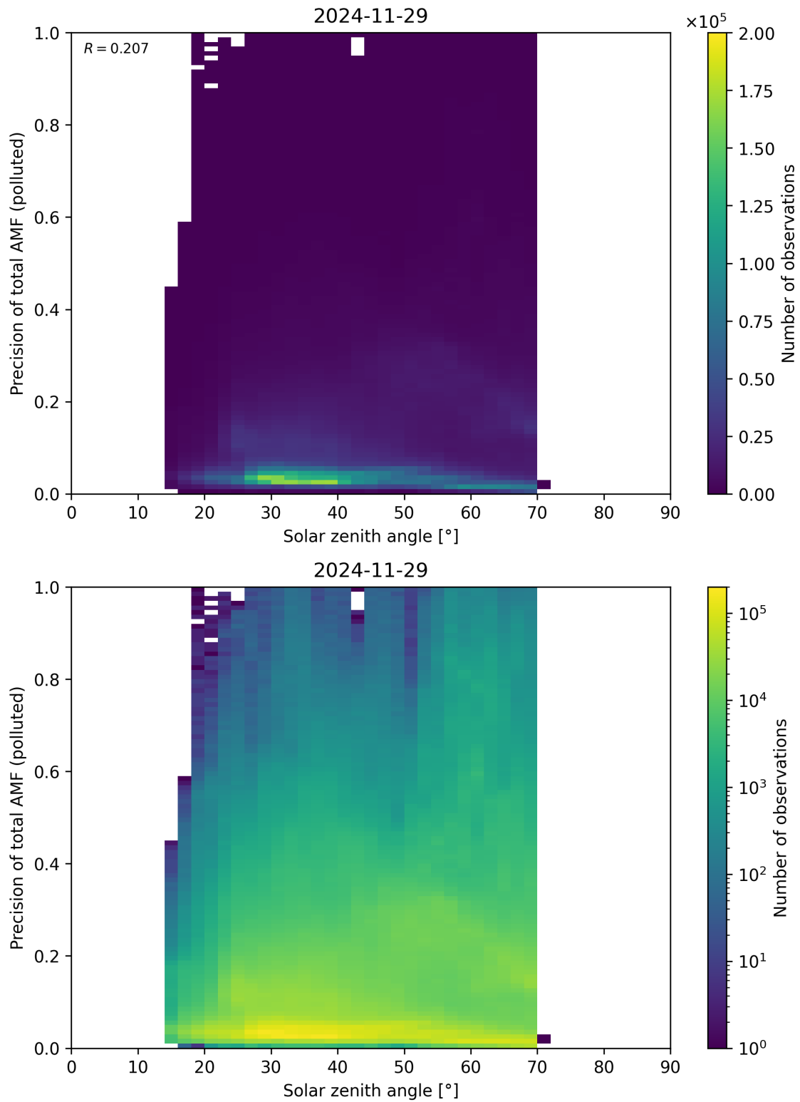
Figure 190: Scatter density plot of “Solar zenith angle” against “Precision of total AMF (polluted)” for 2024-11-28 to 2024-11-30.
