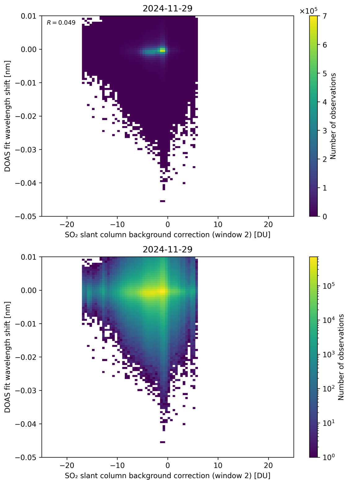
Figure 123: Scatter density plot of “SO 2 slant column background correction (window 2)” against “DOAS fit wavelength shift” for 2024-11-28 to 2024-11-30.
