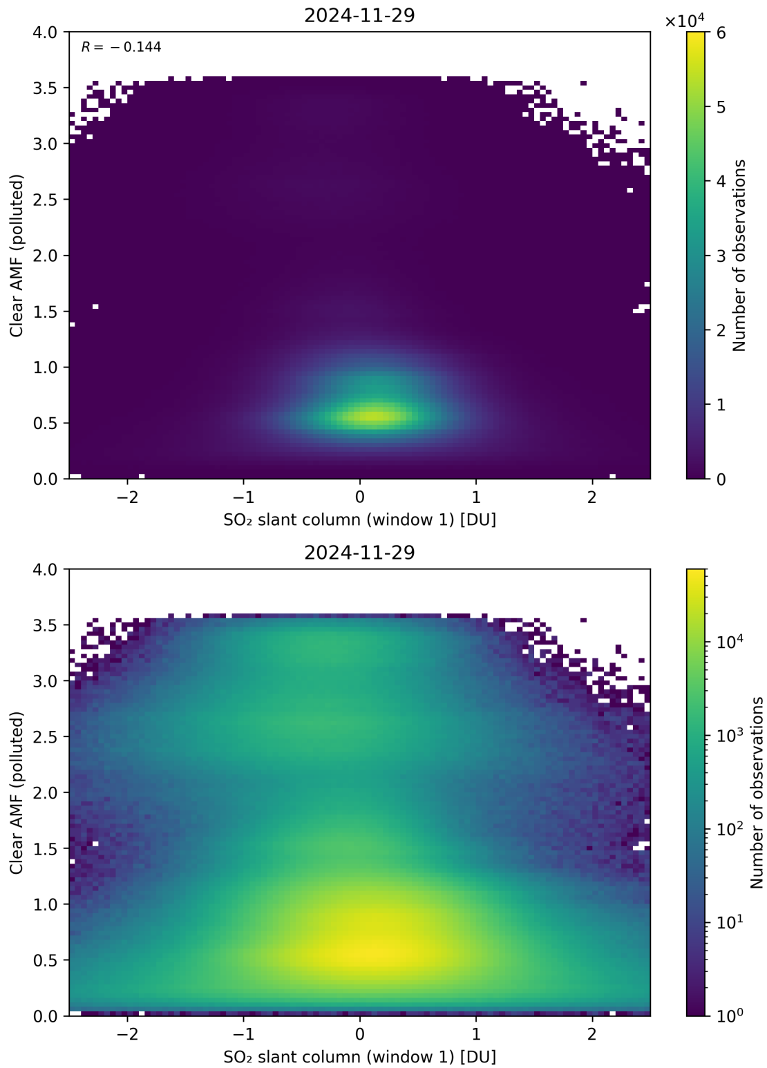
Figure 282: Scatter density plot of “SO 2 slant column (window 1)” against “Clear AMF (polluted)” for 2024-11-28 to 2024-11-30.
