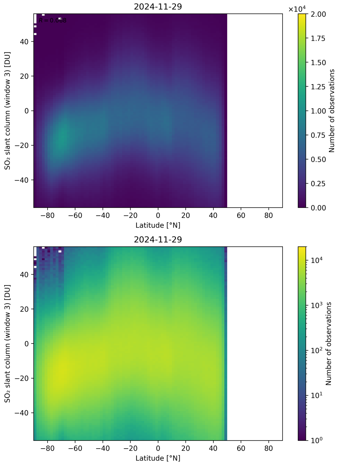
Figure 165: Scatter density plot of “Latitude” against “SO 2 slant column (window 3)” for 2024-11-28 to 2024-11-30.
