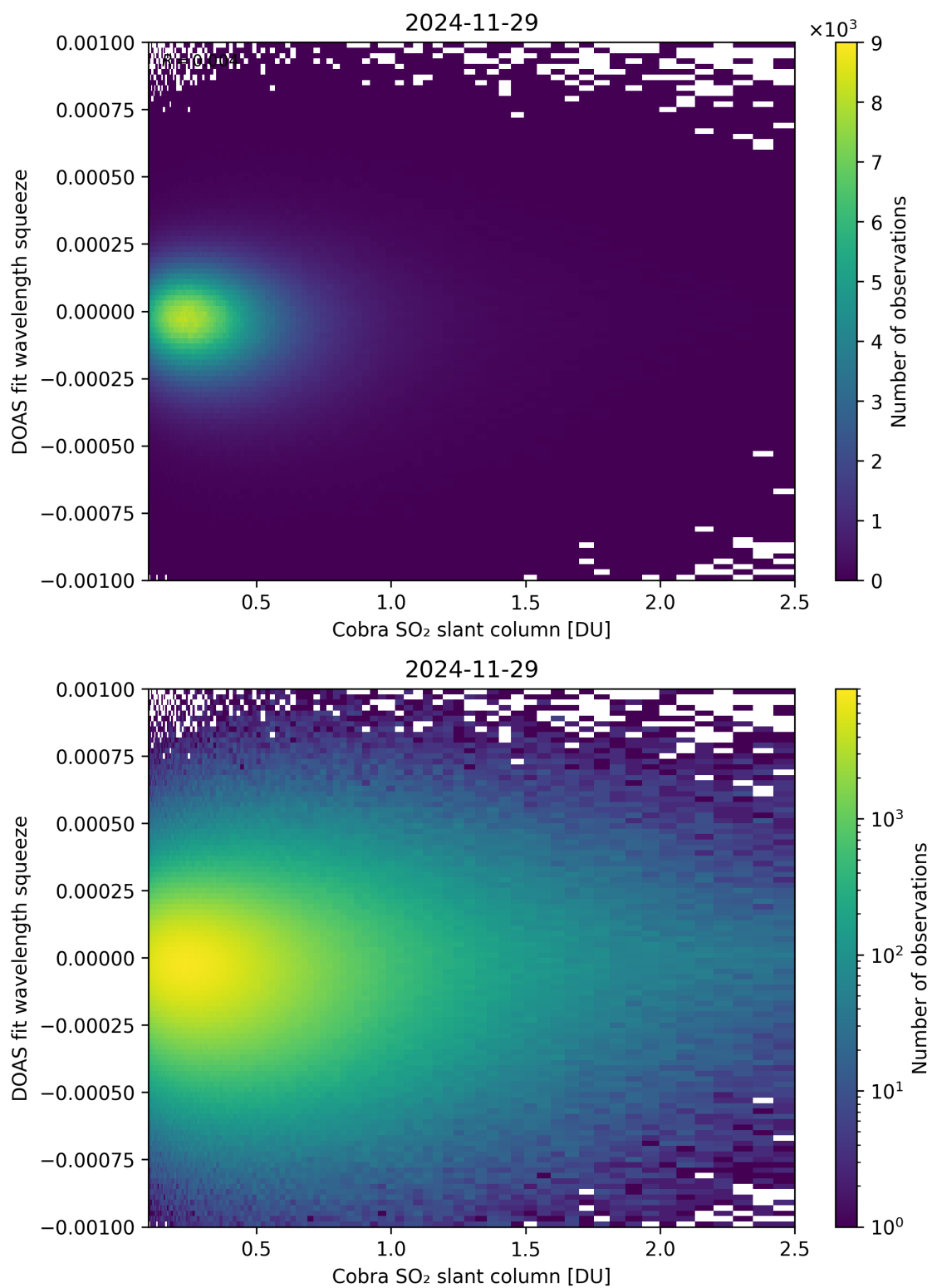
Figure 197: Scatter density plot of “Cobra SO 2 slant column” against “DOAS fit wavelength squeeze” for 2024-11-28 to 2024-11-30.
