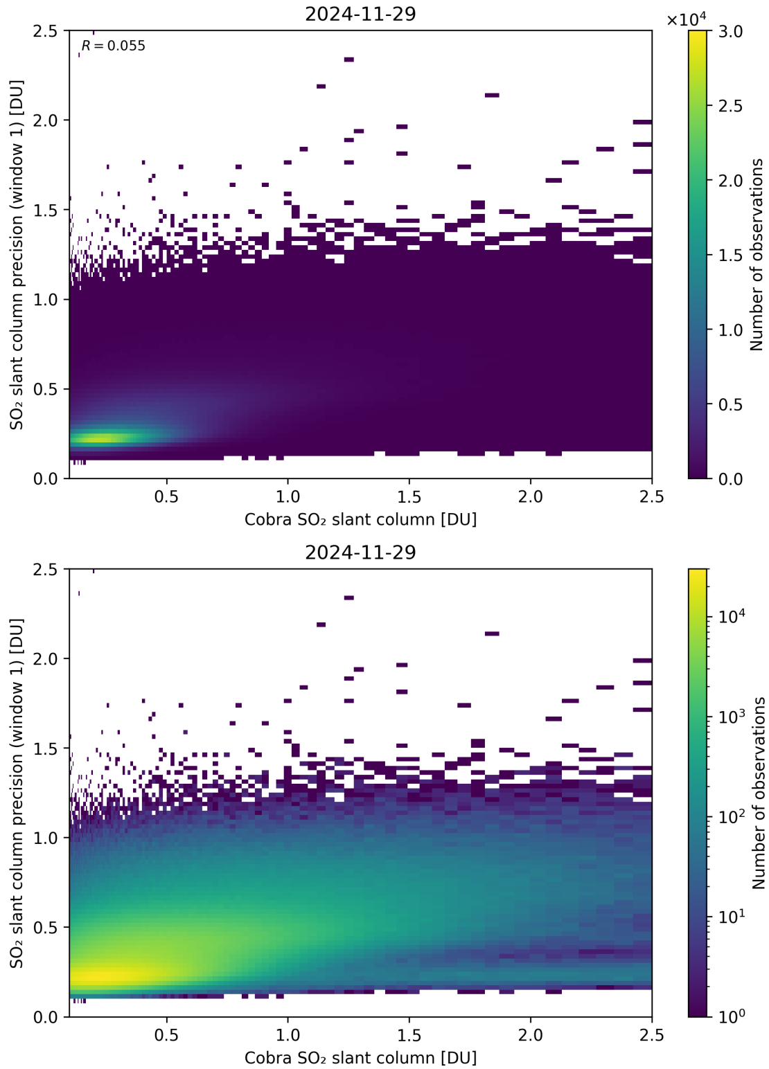
Figure 220: Scatter density plot of “Cobra SO 2 slant column” against “SO 2 slant column precision (window 1)” for 2024-11-28 to 2024-11-30.
