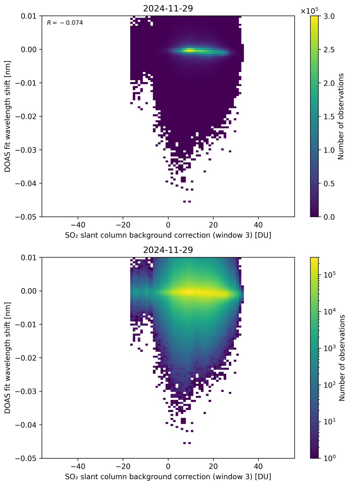
Figure 132: Scatter density plot of “SO 2 slant column background correction (window 3)” against “DOAS fit wavelength shift” for 2024-11-28 to 2024-11-30.
