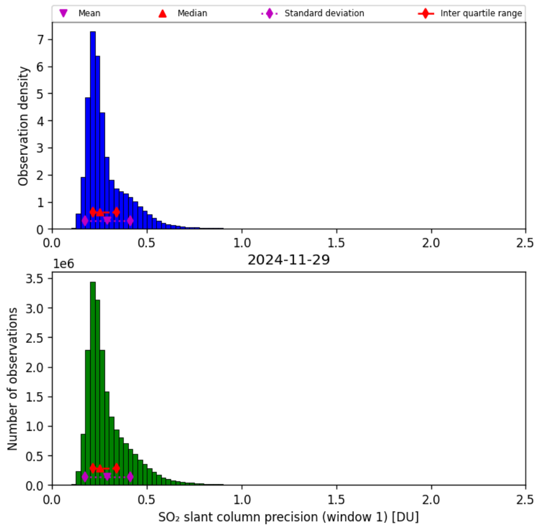
Figure 64: Histogram of “SO 2 slant column precision (window 1)” for 2024-11-28 to 2024-11-30
