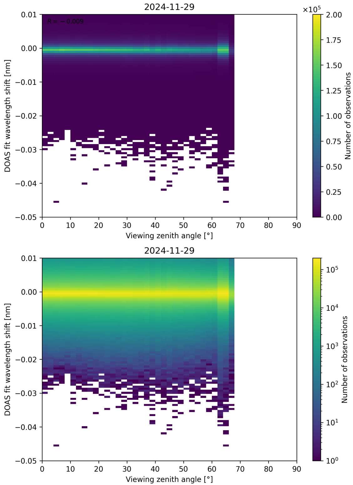
Figure 365: Scatter density plot of “Viewing zenith angle” against “DOAS fit wavelength shift” for 2024-11-28 to 2024-11-30.
