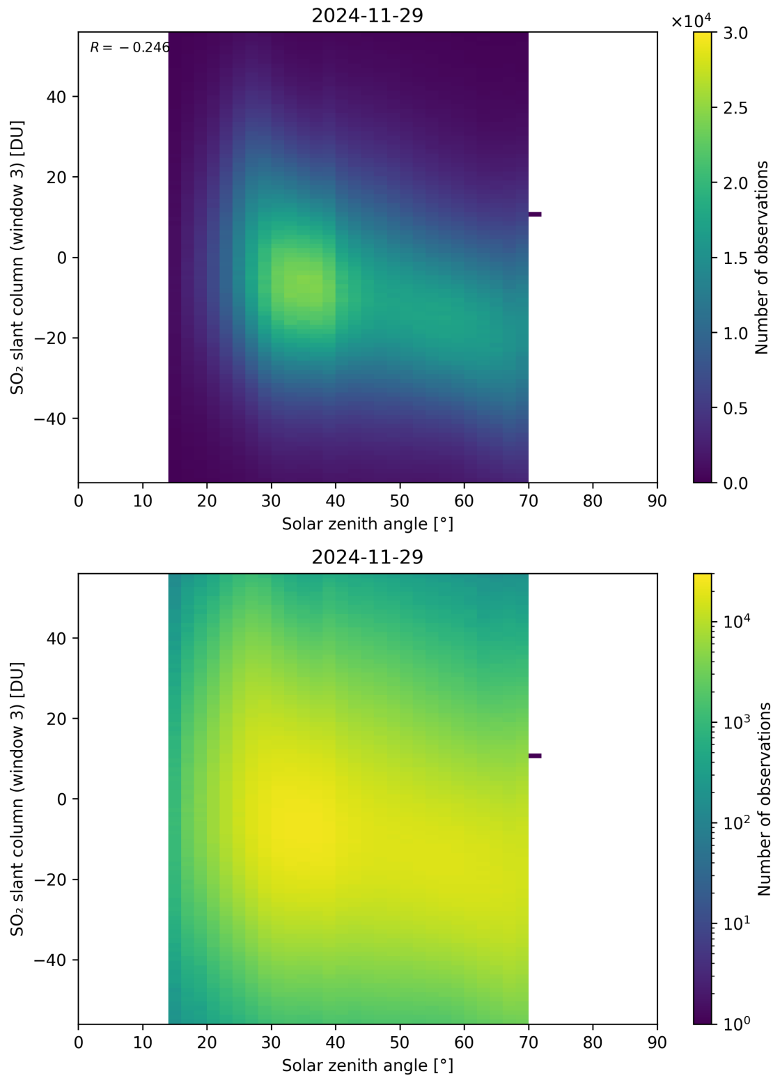
Figure 187: Scatter density plot of “Solar zenith angle” against “SO 2 slant column (window 3)” for 2024-11-28 to 2024-11-30.
