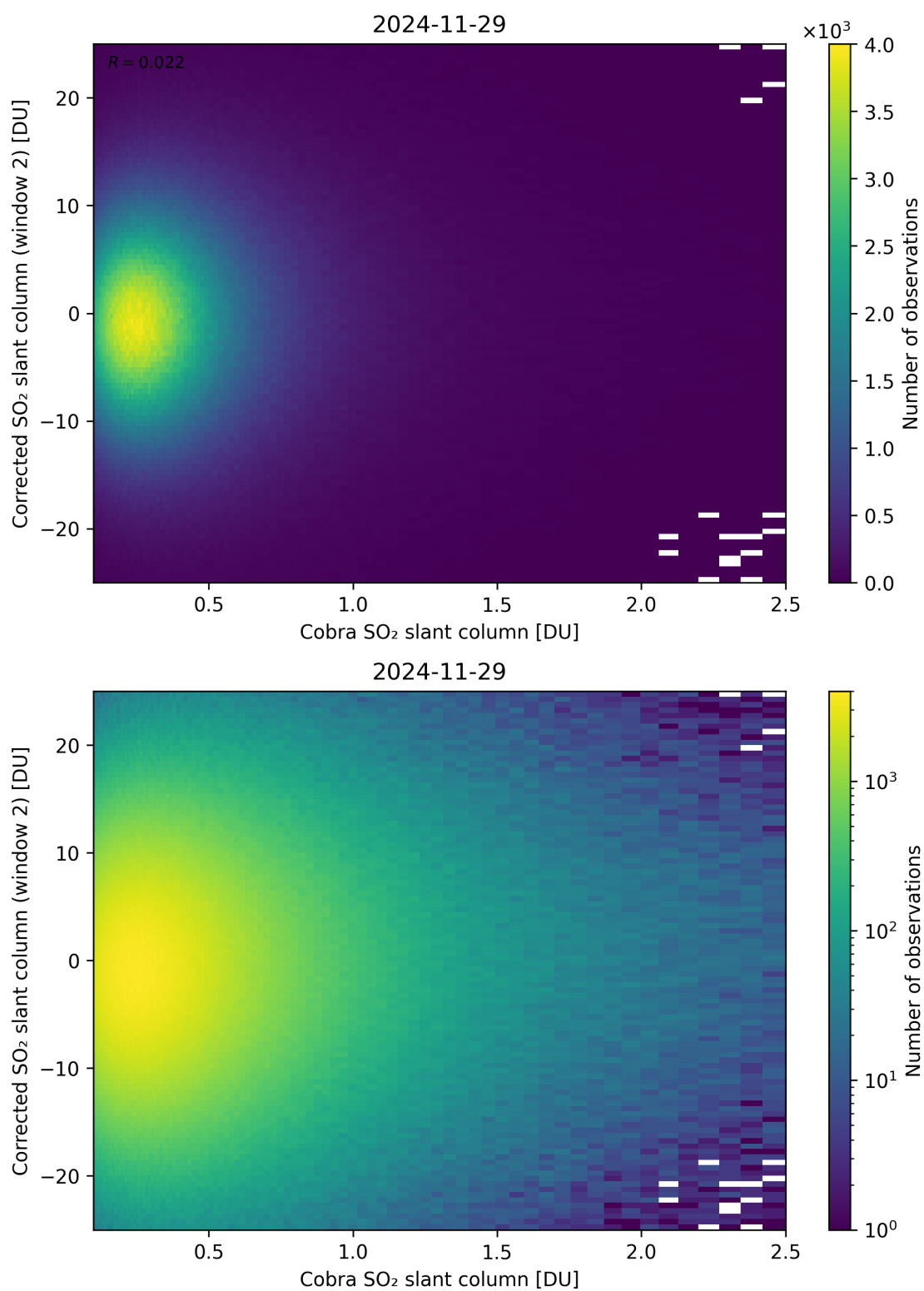
Figure 217: Scatter density plot of “Cobra SO 2 slant column” against “Corrected SO 2 slant column (window 2)” for 2024-11-28 to 2024-11-30.
