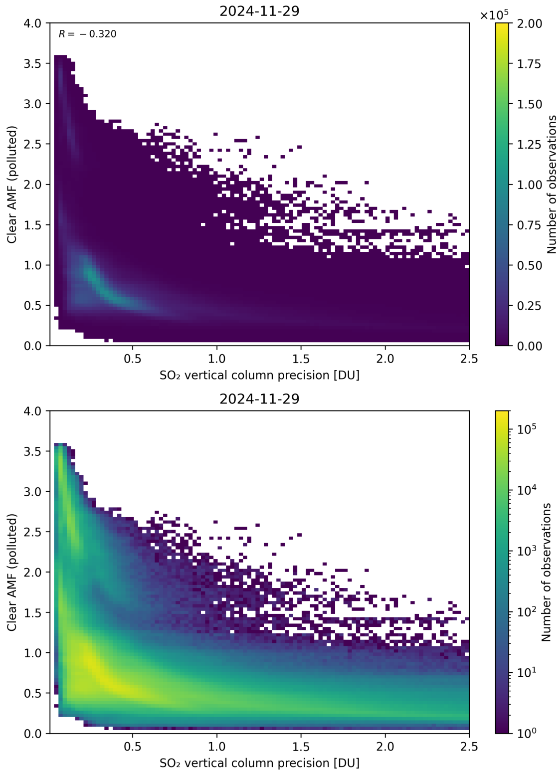
Figure 335: Scatter density plot of “SO 2 vertical column precision” against “Clear AMF (polluted)” for 2024-11-28 to 2024-11-30.
