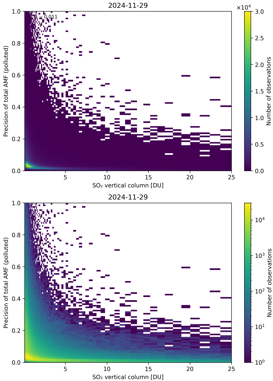
Figure 360: Scatter density plot of “SO 2 vertical column” against “Precision of total AMF (polluted)” for 2024-11-28 to 2024-11-30.
