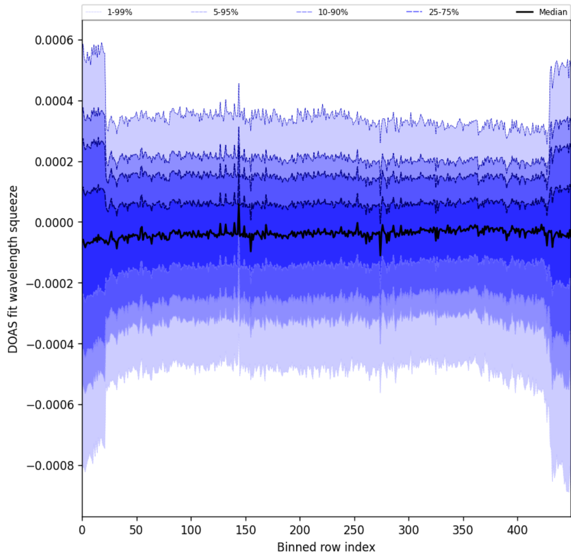
Figure 103: Along track statistics of “DOAS fit wavelength squeeze” for 2024-11-28 to 2024-11-30
