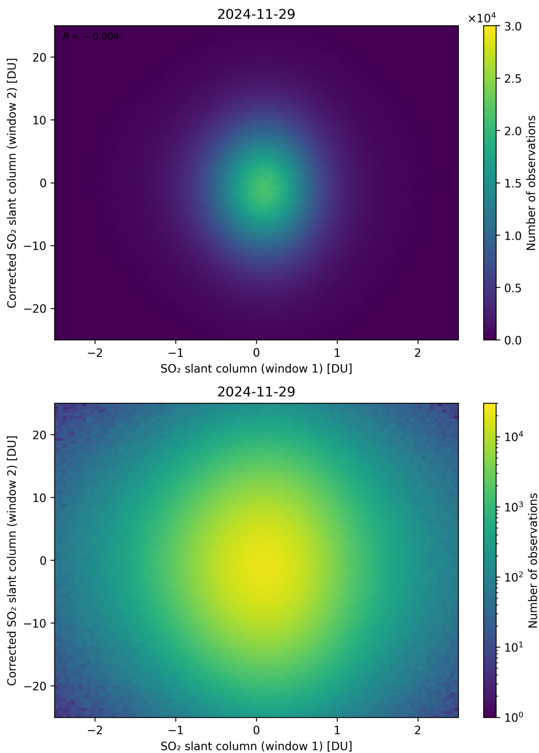
Figure 283: Scatter density plot of “SO 2 slant column (window 1)” against “Corrected SO 2 slant column (window 2)” for 2024-11-28 to 2024-11-30.
