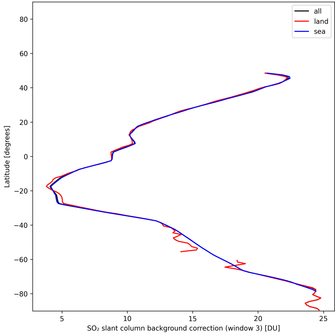
Figure 48: Zonal average of “SO 2 slant column background correction (window 3)” for 2024-11-28 to 2024-11-30.
