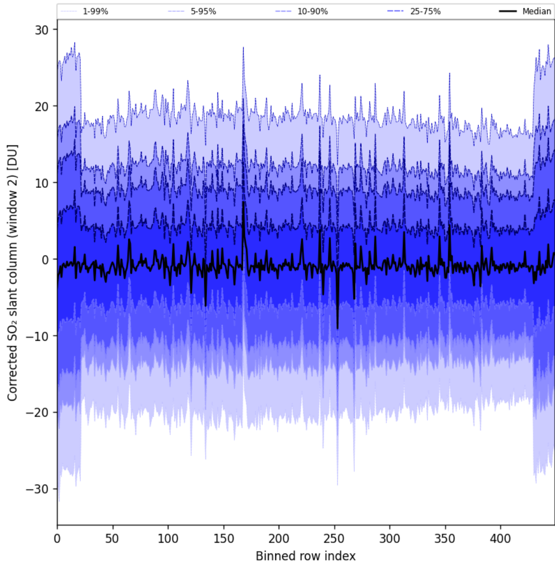
Figure 95: Along track statistics of “Corrected SO 2 slant column (window 2)” for 2024-11-28 to 2024-11-30
