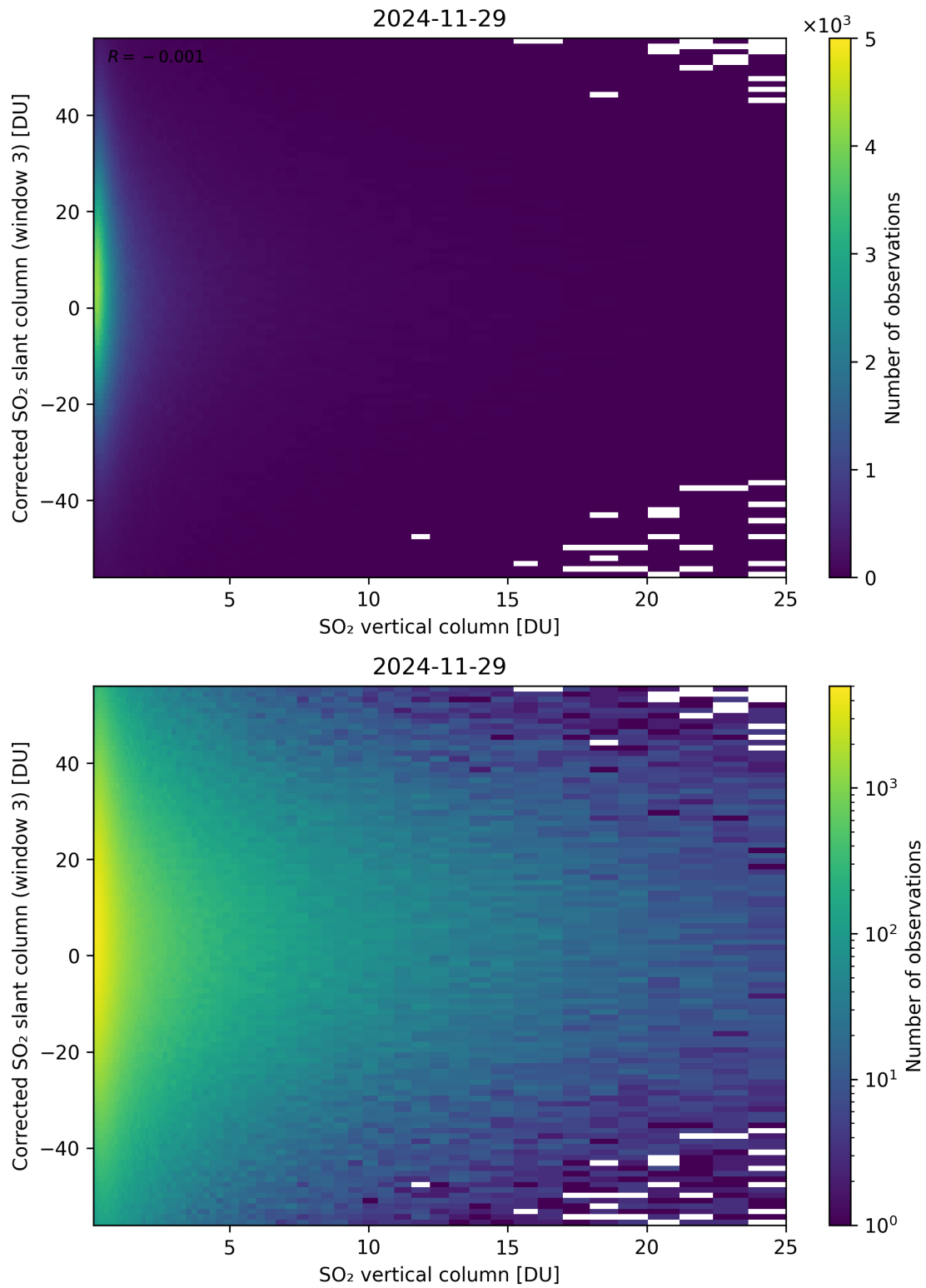
Figure 353: Scatter density plot of “SO 2 vertical column” against “Corrected SO 2 slant column (window 3)” for 2024-11-28 to 2024-11-30.
