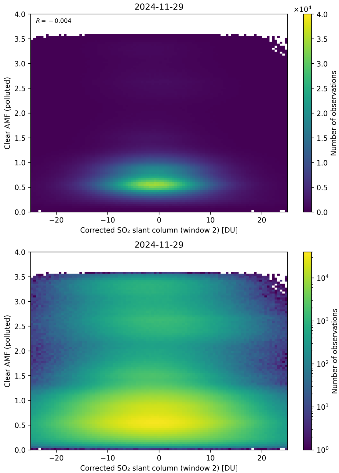
Figure 249: Scatter density plot of “Corrected SO 2 slant column (window 2)” against “Clear AMF (polluted)” for 2024-11-28 to 2024-11-30.
