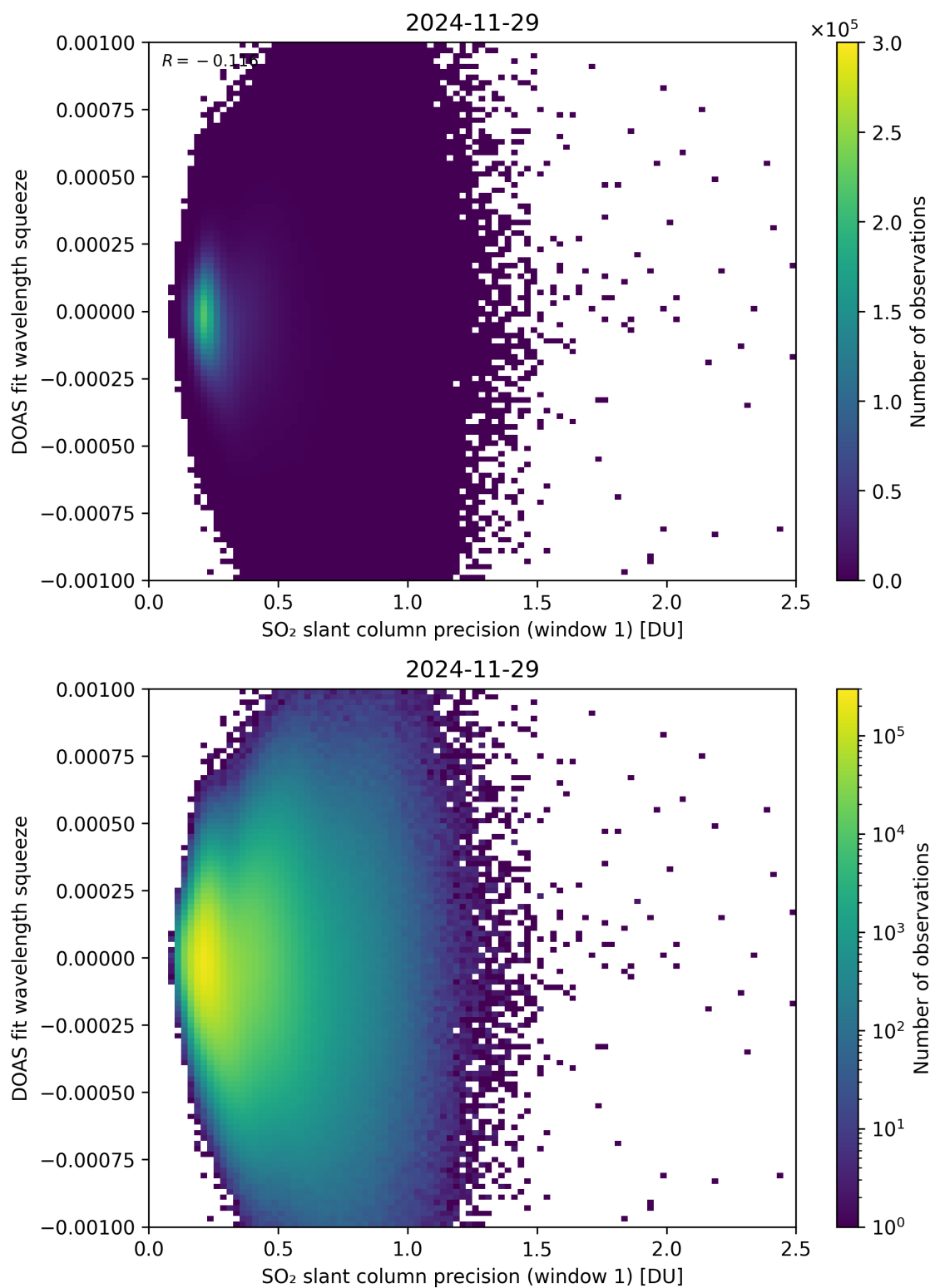
Figure 272: Scatter density plot of “SO 2 slant column precision (window 1)” against “DOAS fit wavelength squeeze” for 2024-11-28 to 2024-11-30.
