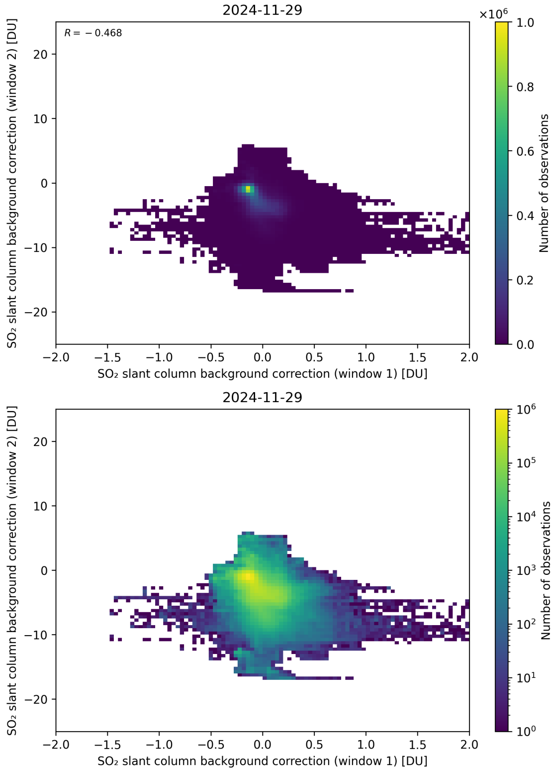
Figure 109: Scatter density plot of “SO 2 slant column background correction (window 1)” against “SO 2 slant column background correction (window 2)” for 2024-11-28 to 2024-11-30.
