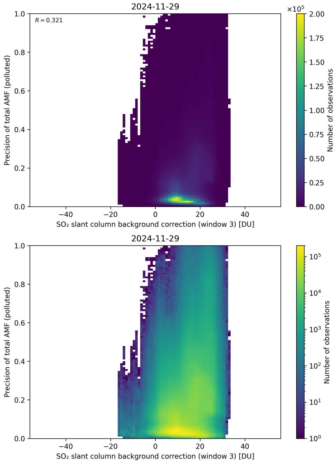
Figure 137: Scatter density plot of “SO 2 slant column background correction (window 3)” against “Precision of total AMF (polluted)” for 2024-11-28 to 2024-11-30.
