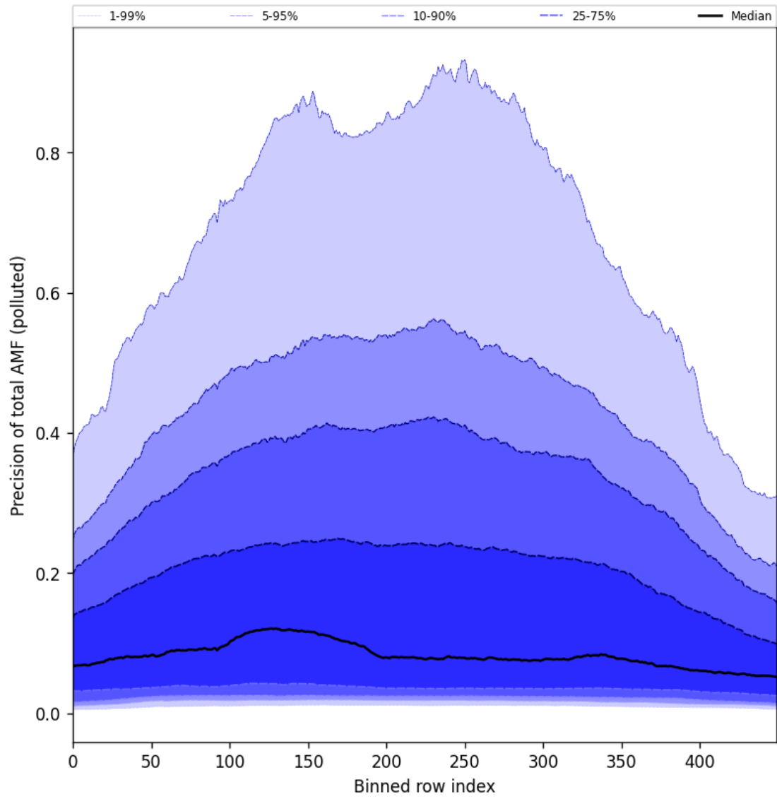
Figure 106: Along track statistics of “Precision of total AMF (polluted)” for 2024-11-28 to 2024-11-30
