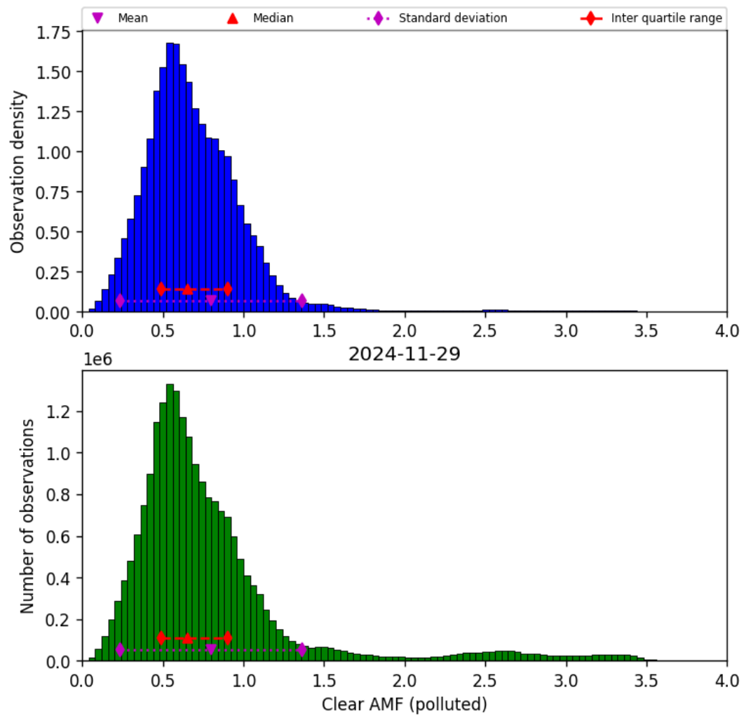
Figure 81: Histogram of “Clear AMF (polluted)” for 2024-11-28 to 2024-11-30
