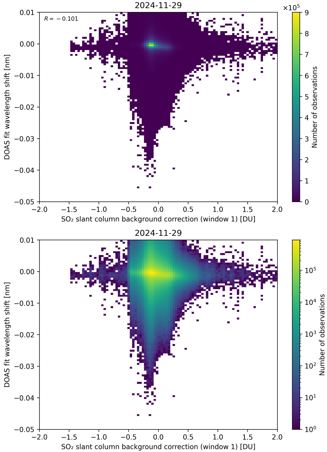
Figure 111: Scatter density plot of “SO 2 slant column background correction (window 1)” against “DOAS fit wavelength shift” for 2024-11-28 to 2024-11-30.
