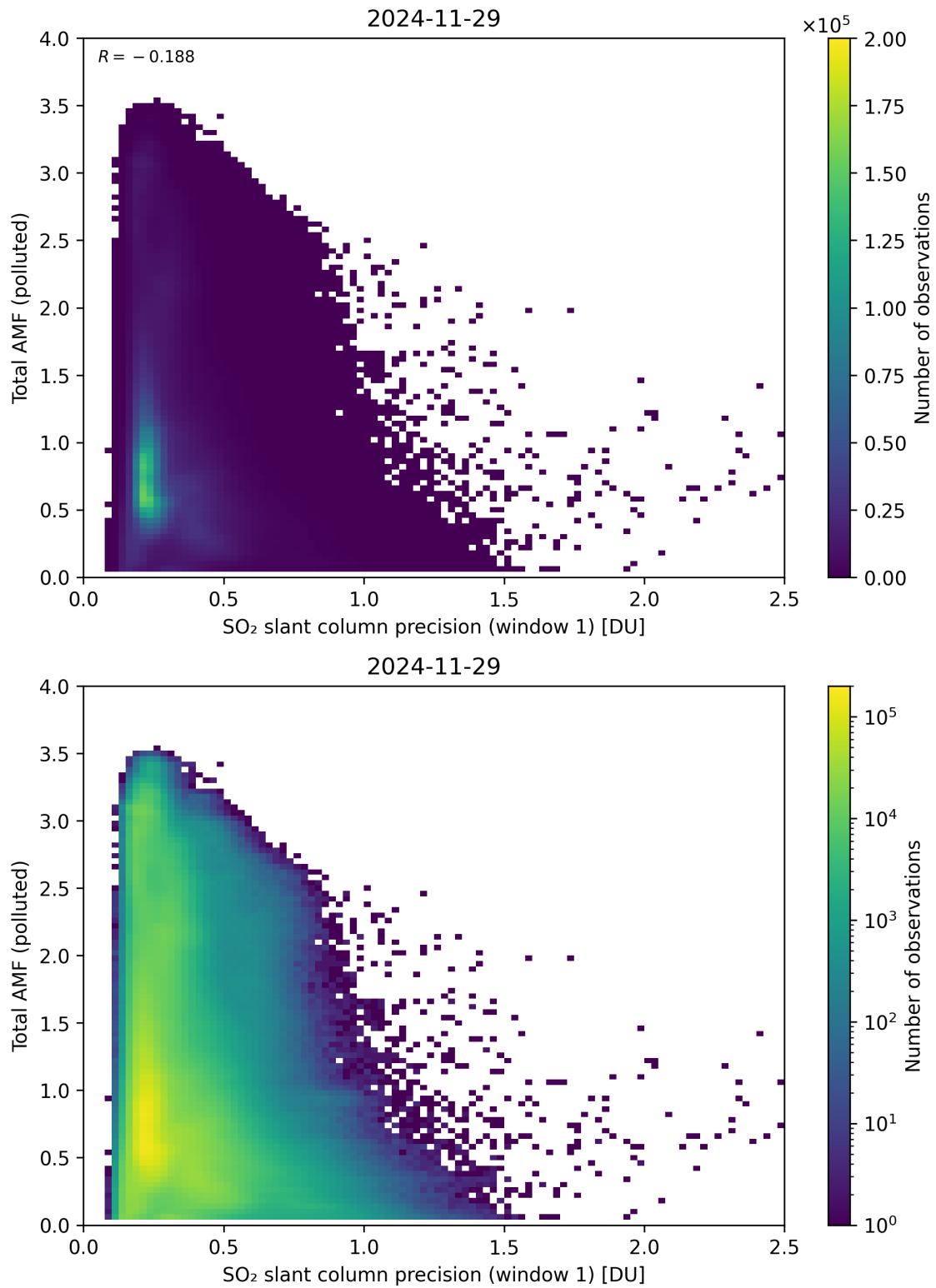
Figure 280: Scatter density plot of “SO 2 slant column precision (window 1)” against “Total AMF (polluted)” for 2024-11-28 to 2024-11-30.
