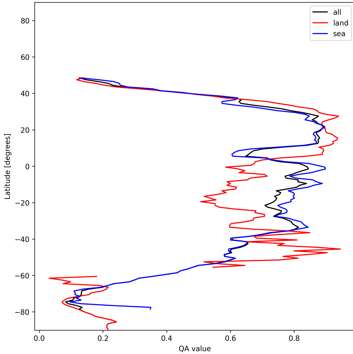
Figure 31: Zonal average of “QA value” for 2024-11-28 to 2024-11-30.
