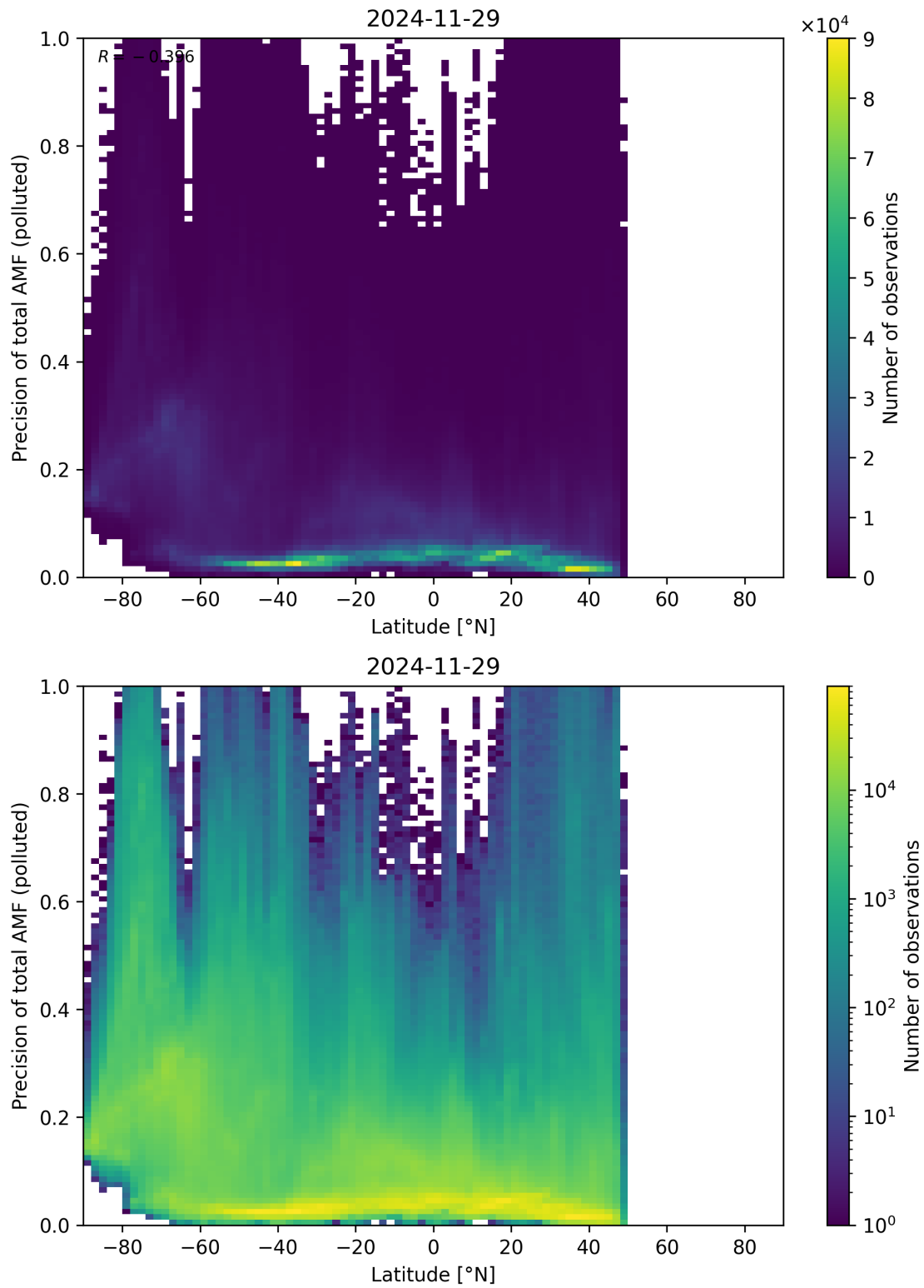
Figure 168: Scatter density plot of “Latitude” against “Precision of total AMF (polluted)” for 2024-11-28 to 2024-11-30.
