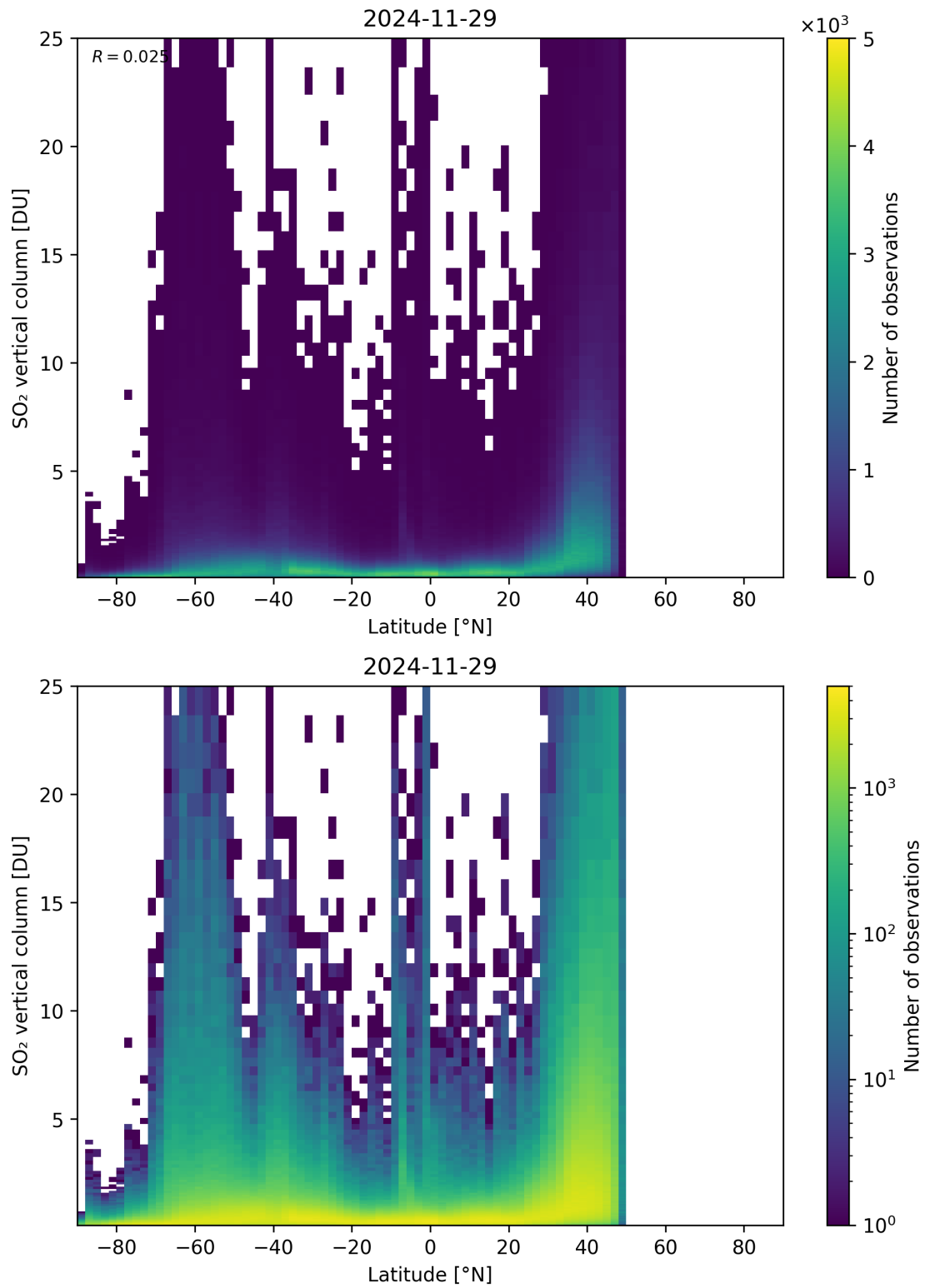
Figure 169: Scatter density plot of “Latitude” against “SO 2 vertical column” for 2024-11-28 to 2024-11-30.
