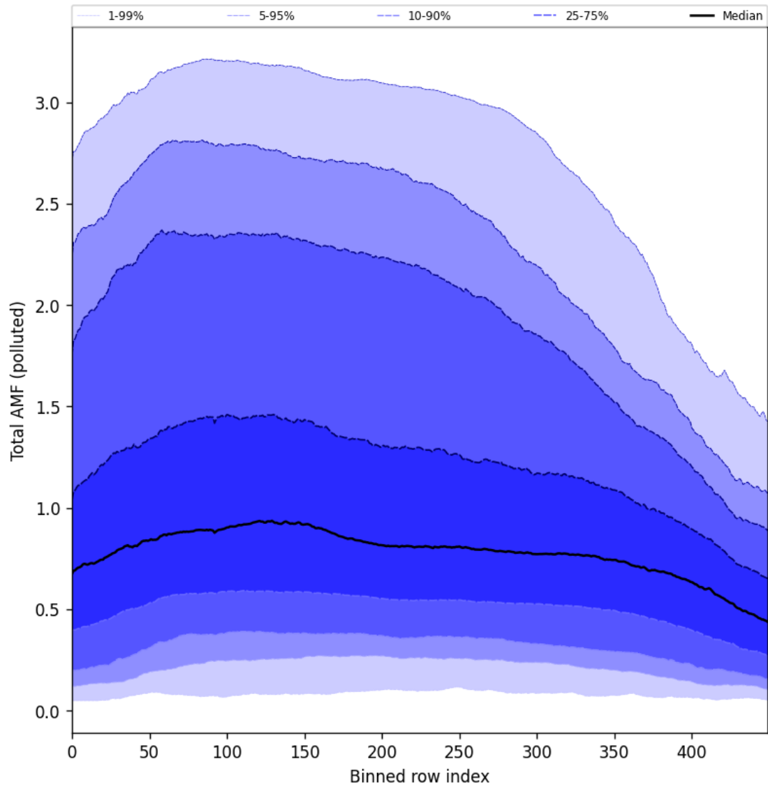
Figure 105: Along track statistics of “Total AMF (polluted)” for 2024-11-28 to 2024-11-30
