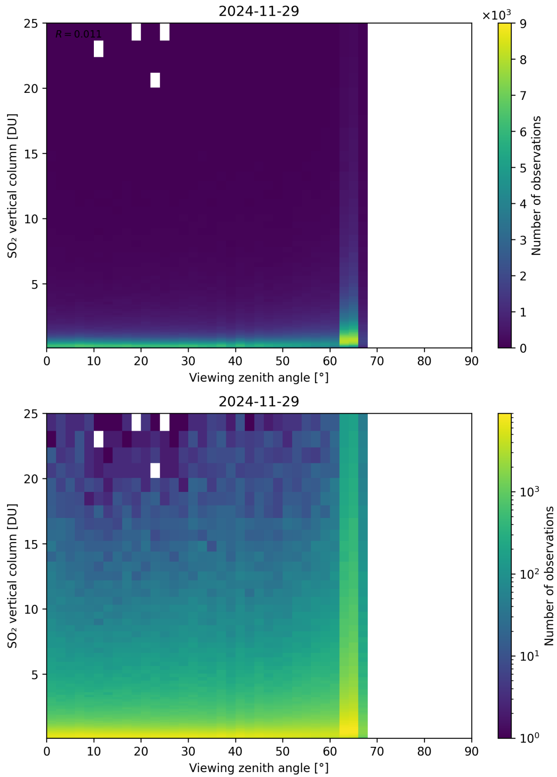
Figure 383: Scatter density plot of “Viewing zenith angle” against “SO 2 vertical column” for 2024-11-28 to 2024-11-30.
