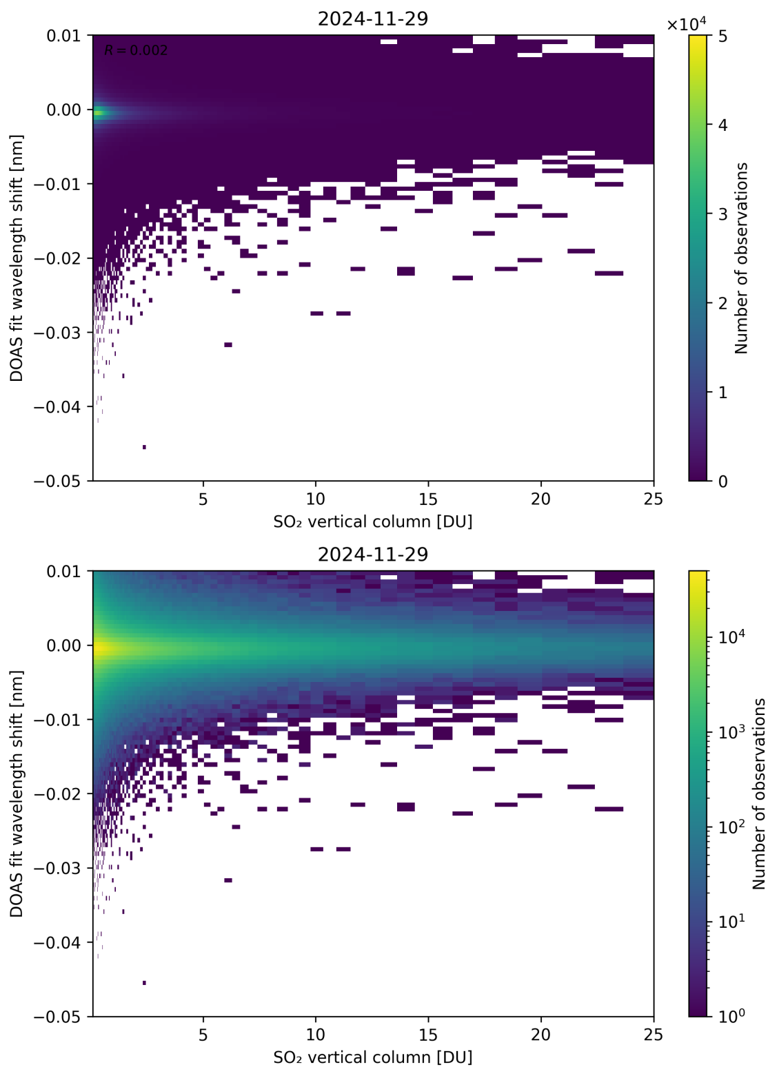
Figure 326: Scatter density plot of “SO 2 vertical column” against “DOAS fit wavelength shift” for 2024-11-28 to 2024-11-30.
