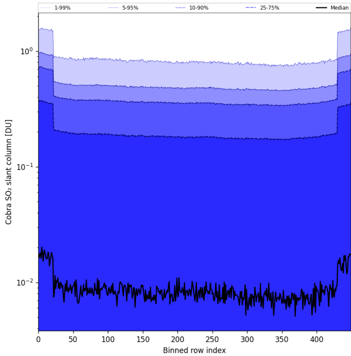
Figure 87: Along track statistics of “Cobra SO 2 slant column” for 2024-11-28 to 2024-11-30
