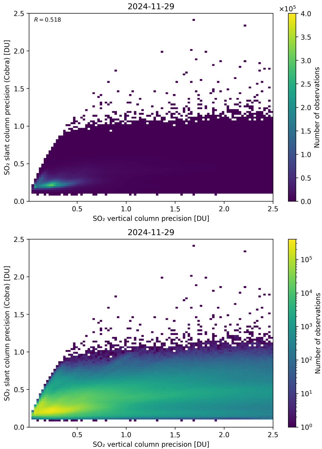
Figure 337: Scatter density plot of “SO 2 vertical column precision” against “SO 2 slant column precision (Cobra)” for 2024-11-28 to 2024-11-30.
