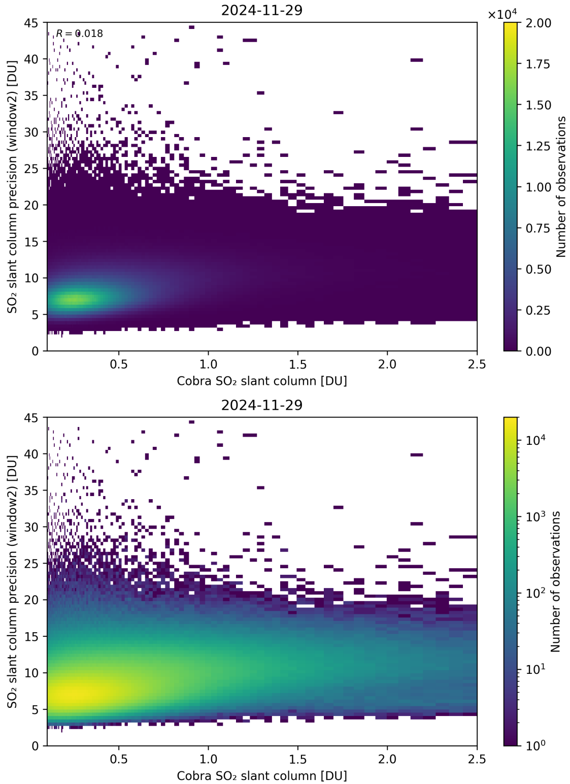
Figure 221: Scatter density plot of “Cobra SO 2 slant column” against “SO 2 slant column precision (window2)” for 2024-11-28 to 2024-11-30.
