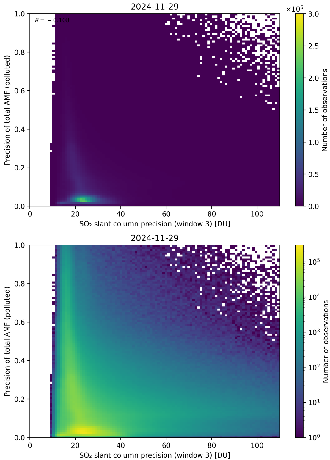
Figure 314: Scatter density plot of “SO 2 slant column precision (window 3)” against “Precision of total AMF (polluted)” for 2024-11-28 to 2024-11-30.
