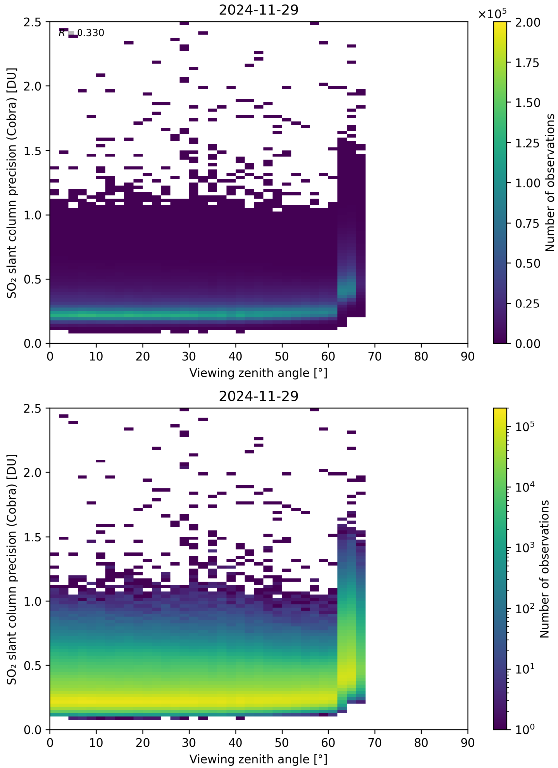
Figure 372: Scatter density plot of “Viewing zenith angle” against “SO 2 slant column precision (Cobra)” for 2024-11-28 to 2024-11-30.
