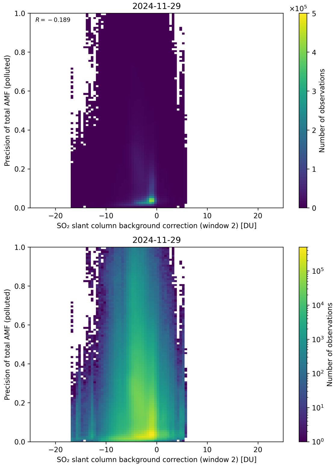
Figure 131: Scatter density plot of “SO 2 slant column background correction (window 2)” against “Precision of total AMF (polluted)” for 2024-11-28 to 2024-11-30.
