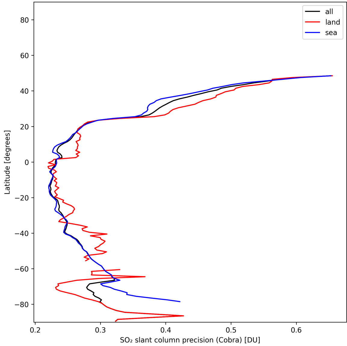
Figure 36: Zonal average of “SO 2 slant column precision (Cobra)” for 2024-11-28 to 2024-11-30.
