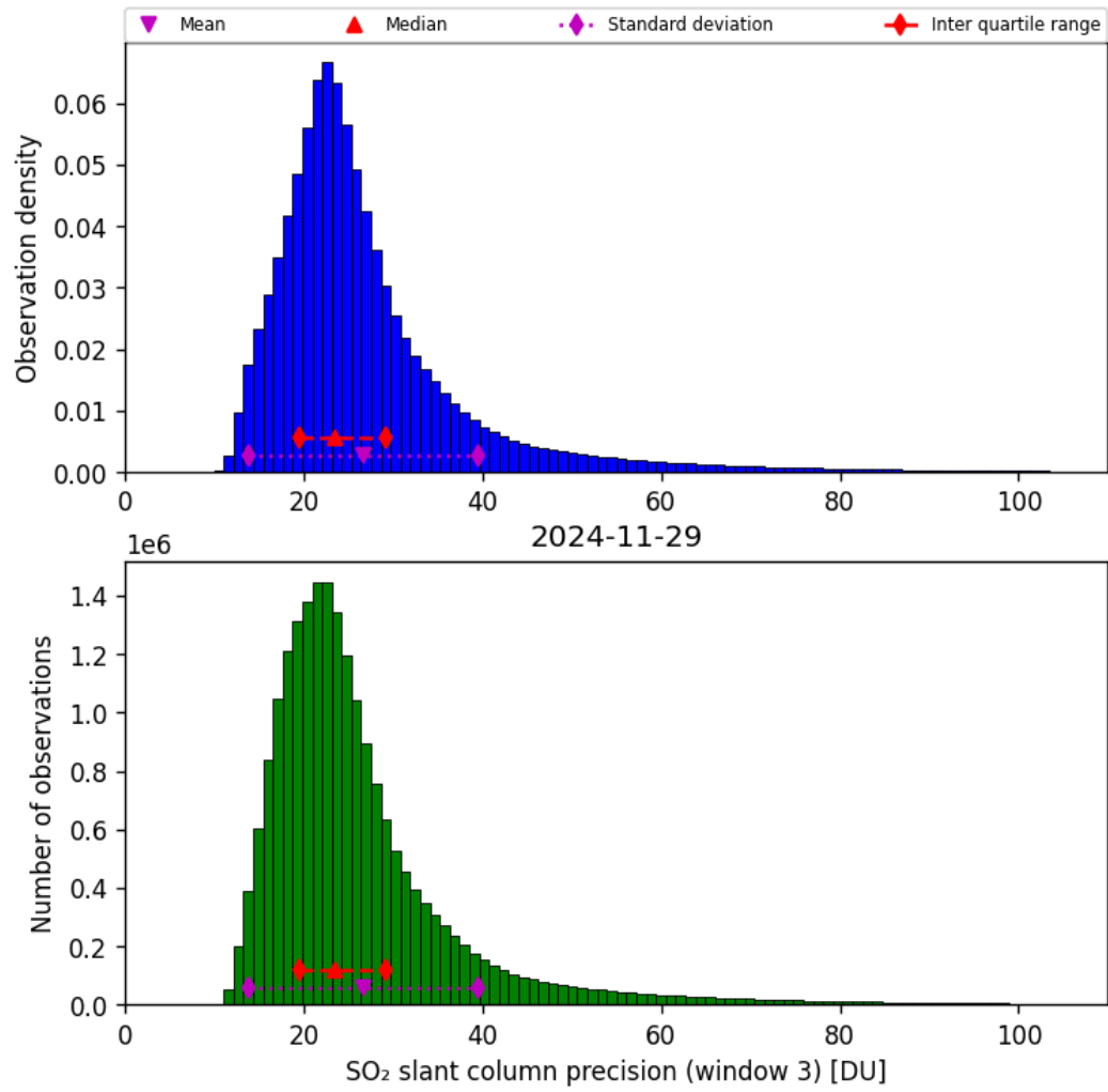
Figure 72: Histogram of “SO 2 slant column precision (window 3)” for 2024-11-28 to 2024-11-30
