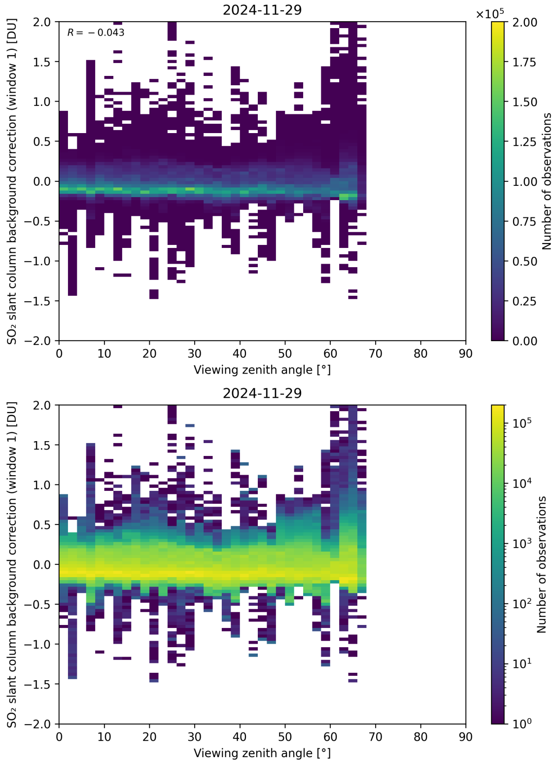
Figure 362: Scatter density plot of “Viewing zenith angle” against “SO 2 slant column background correction (window 1)” for 2024-11-28 to 2024-11-30.
