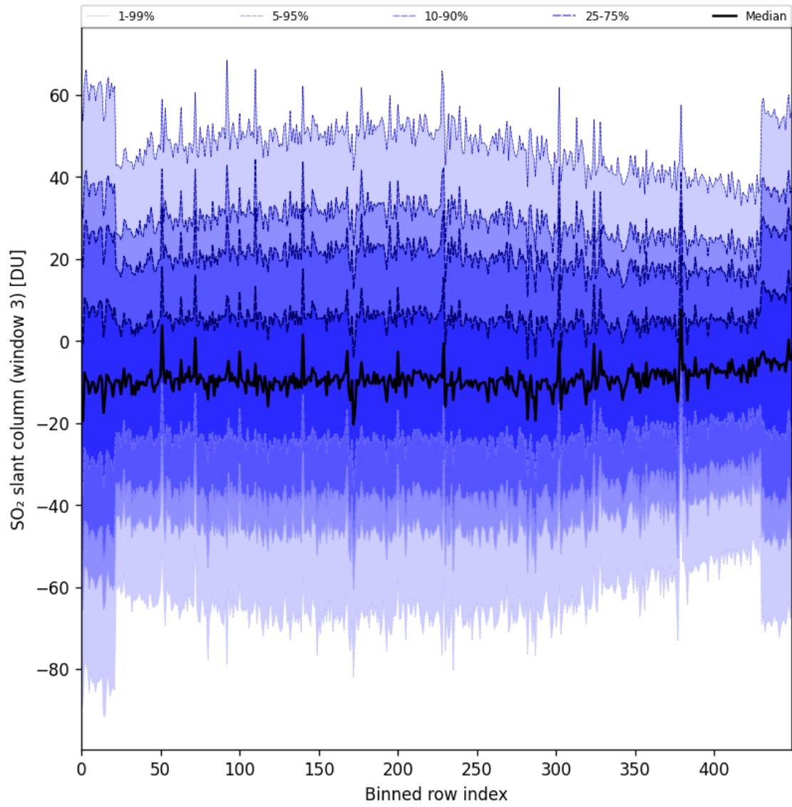
Figure 97: Along track statistics of “SO 2 slant column (window 3)” for 2024-11-28 to 2024-11-30
