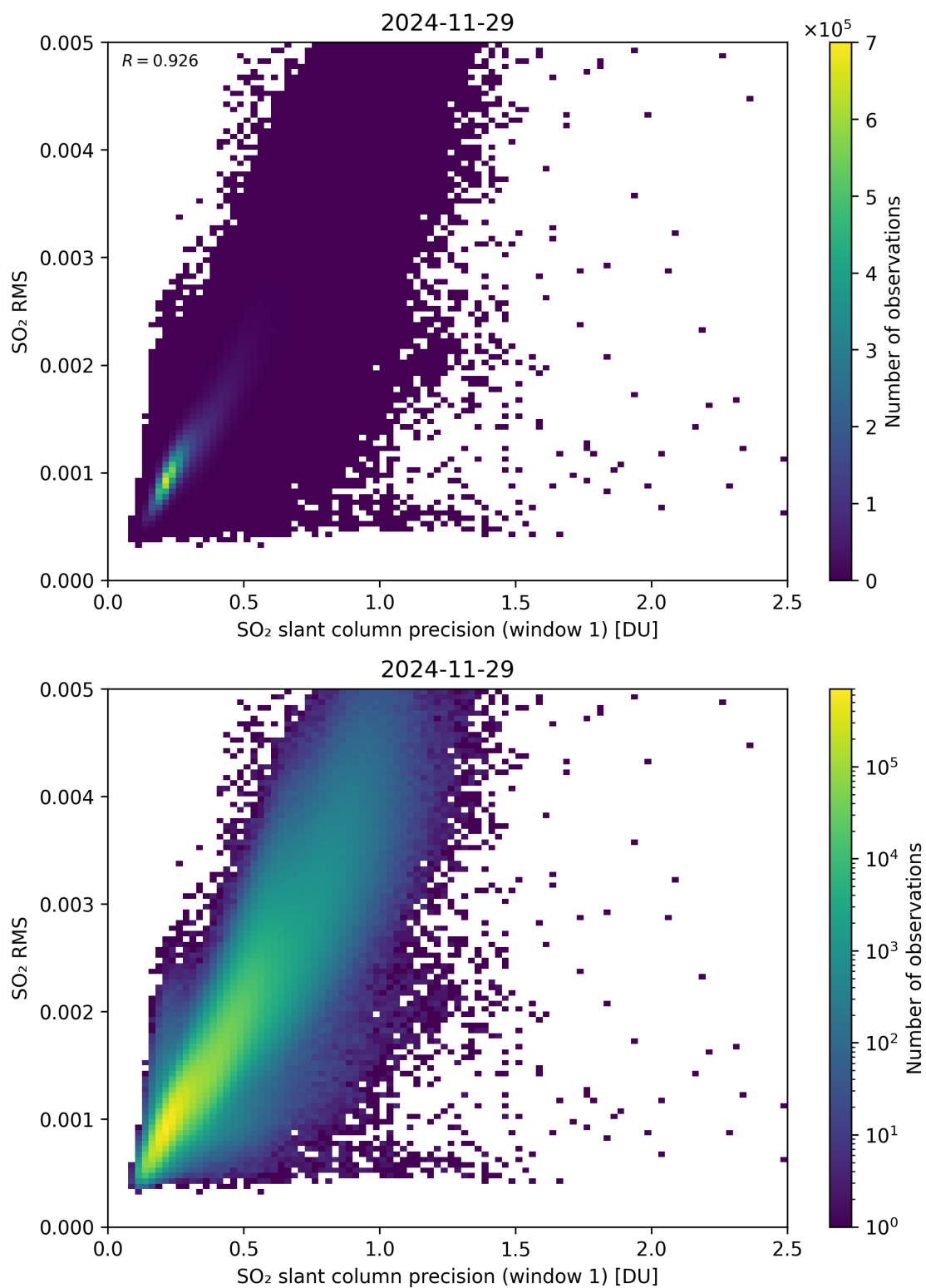
Figure 273: Scatter density plot of “SO 2 slant column precision (window 1)” against “SO 2 RMS” for 2024-11-28 to 2024-11-30.
