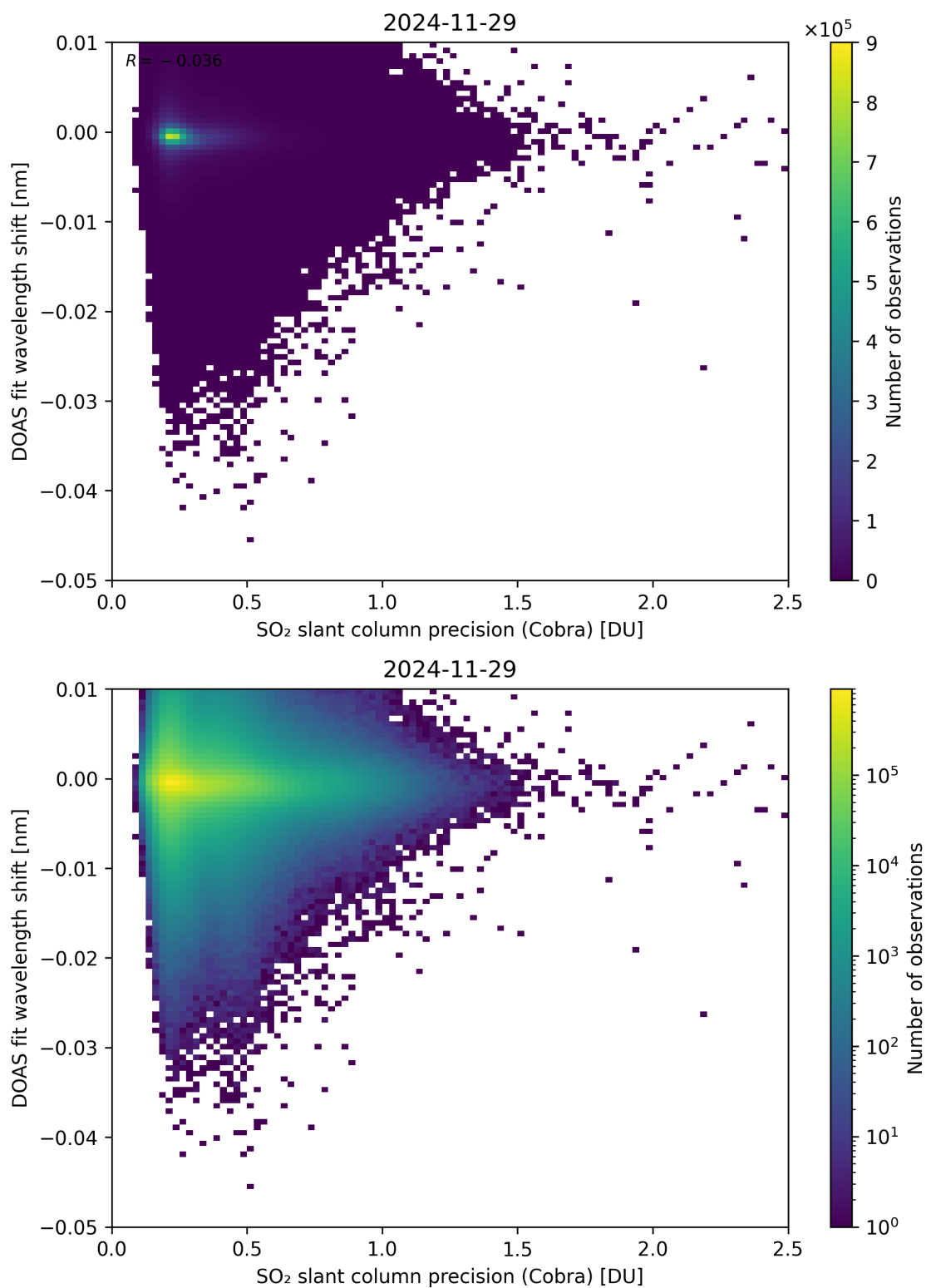
Figure 202: Scatter density plot of “SO 2 slant column precision (Cobra)” against “DOAS fit wavelength shift” for 2024-11-28 to 2024-11-30.
