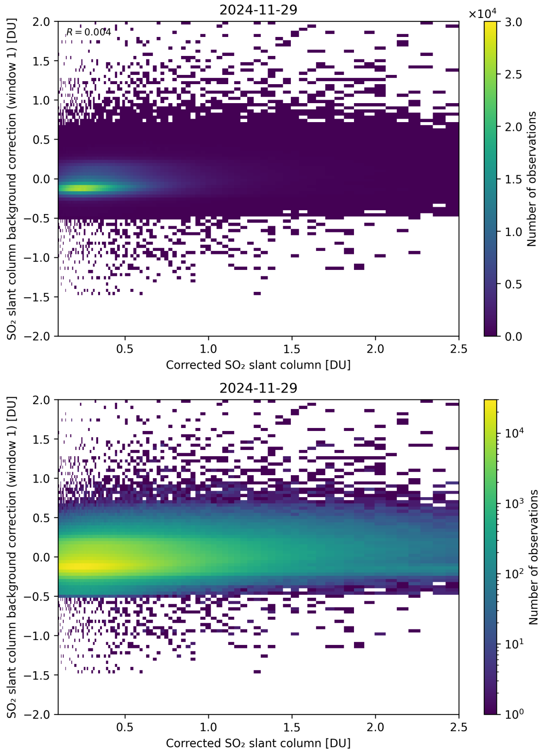
Figure 226: Scatter density plot of “Corrected SO 2 slant column” against “SO 2 slant column background correction (window 1)” for 2024-11-28 to 2024-11-30.
