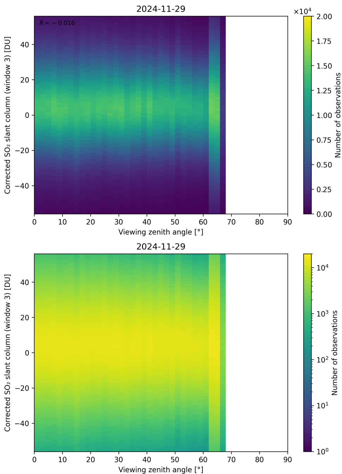
Figure 375: Scatter density plot of “Viewing zenith angle” against “Corrected SO 2 slant column (window 3)” for 2024-11-28 to 2024-11-30.
