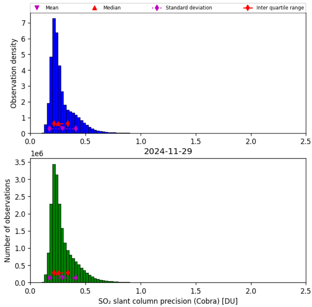
Figure 62: Histogram of “SO 2 slant column precision (Cobra)” for 2024-11-28 to 2024-11-30
