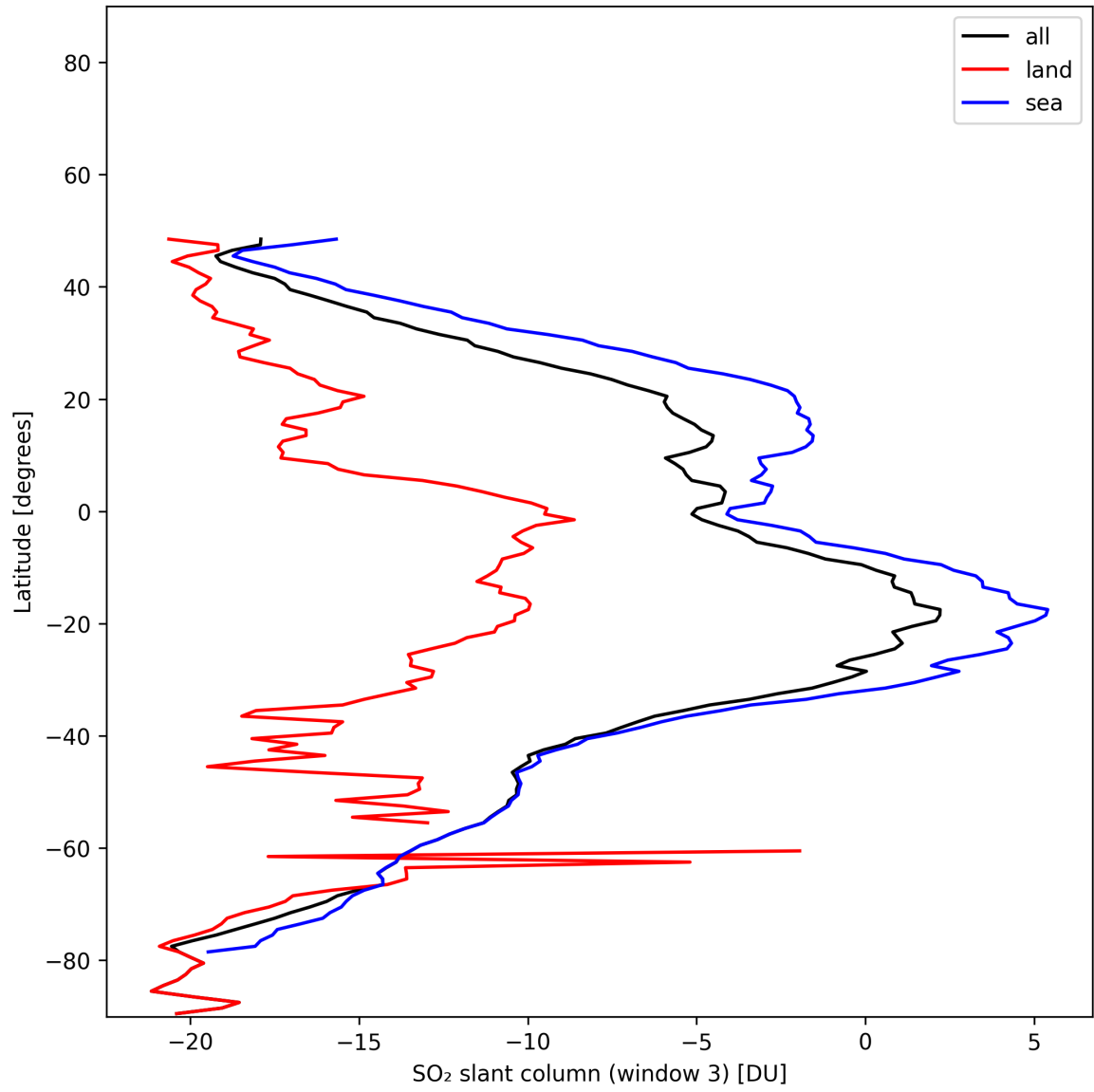
Figure 45: Zonal average of “SO 2 slant column (window 3)” for 2024-11-28 to 2024-11-30.
