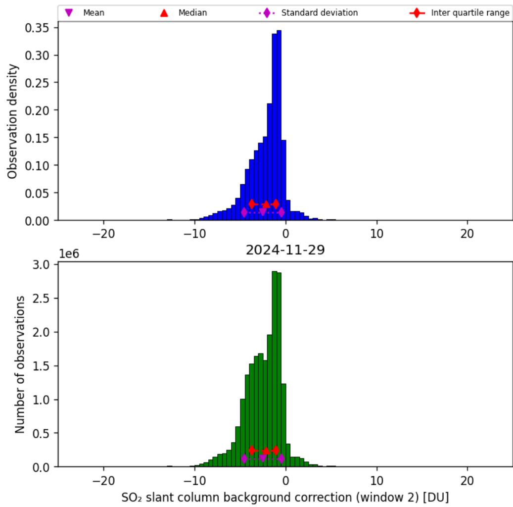
Figure 70: Histogram of “SO 2 slant column background correction (window 2)” for 2024-11-28 to 2024-11-30
