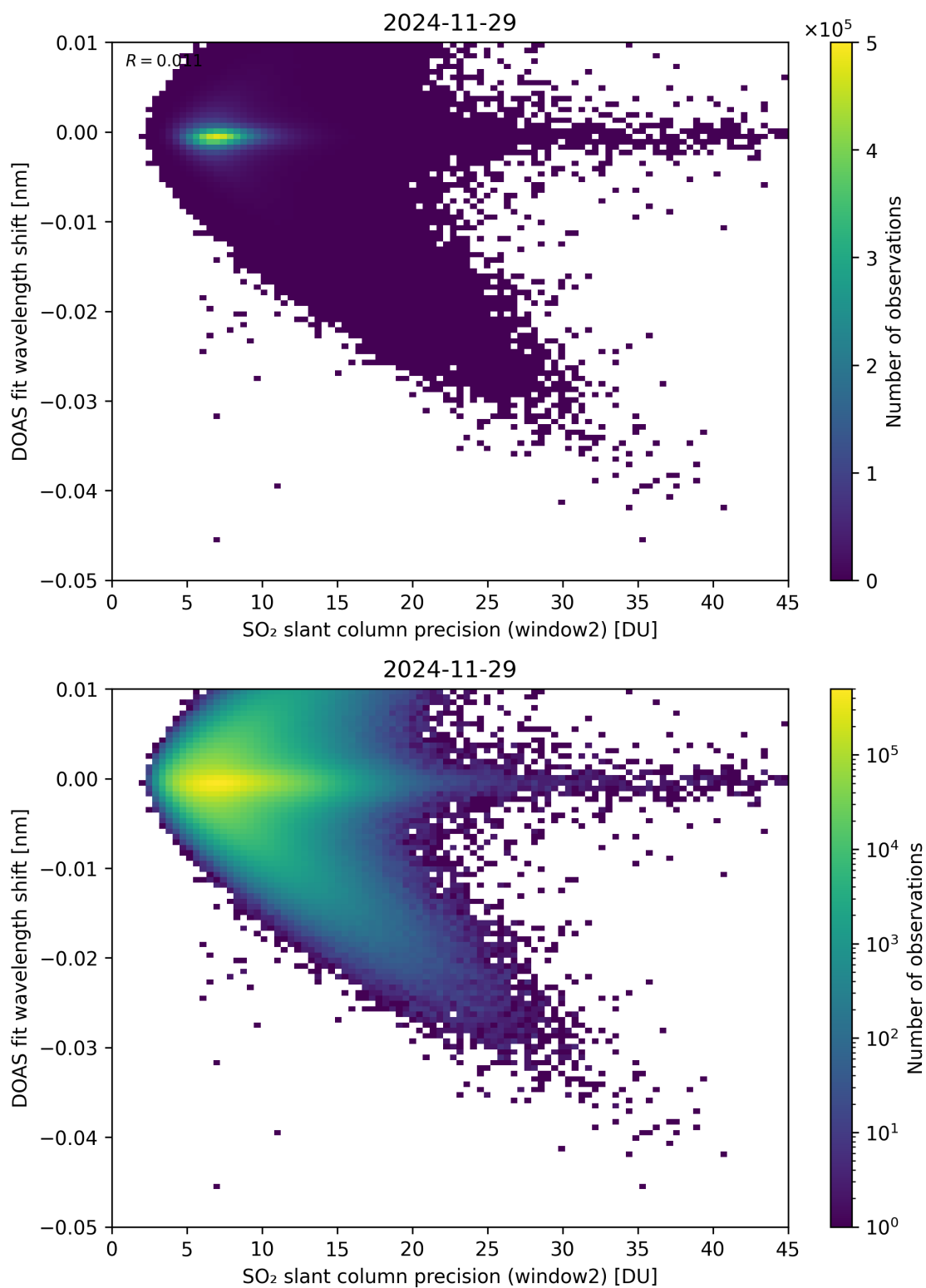
Figure 293: Scatter density plot of “SO 2 slant column precision (window2)” against “DOAS fit wavelength shift” for 2024-11-28 to 2024-11-30.
