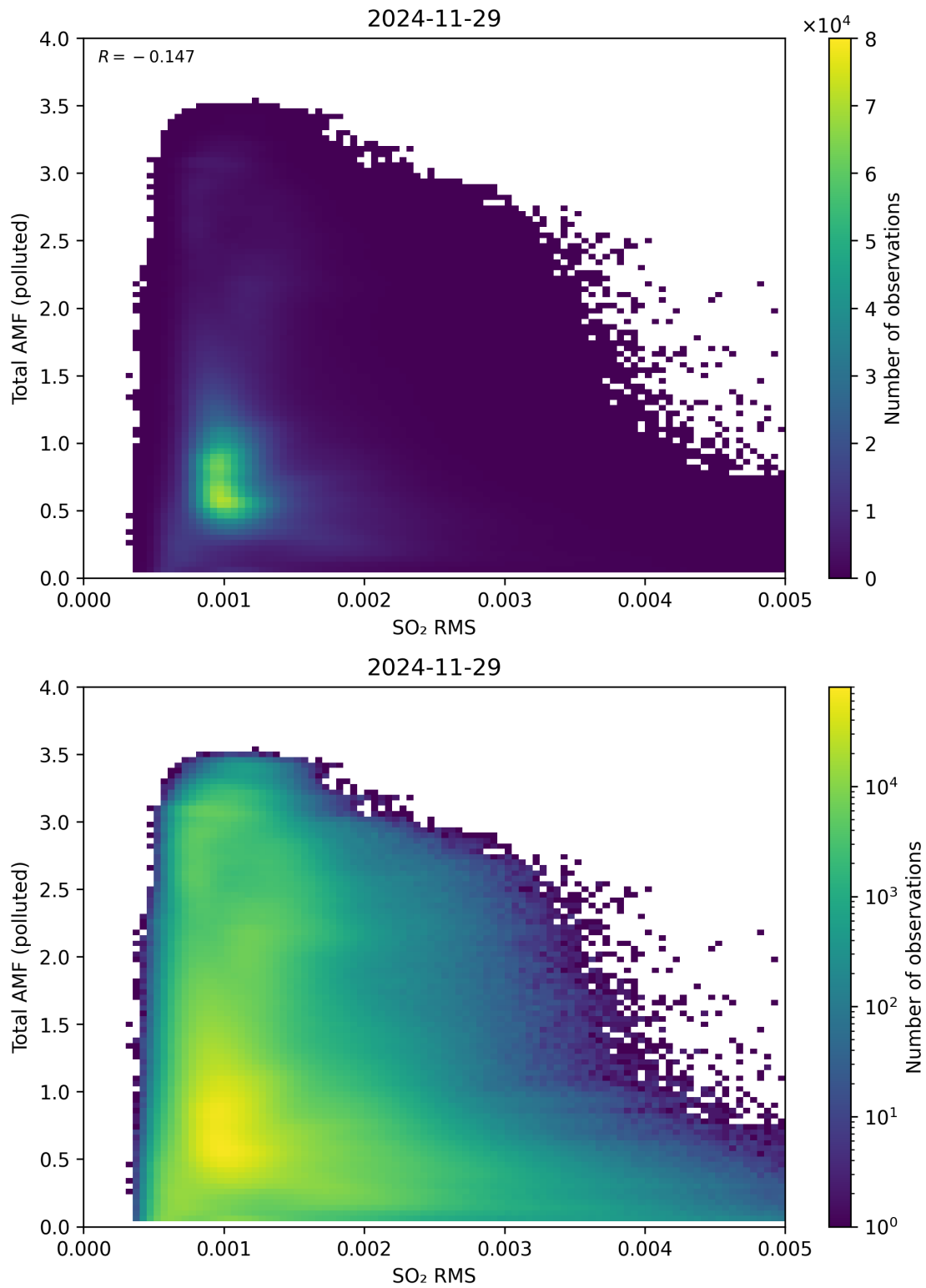
Figure 148: Scatter density plot of “SO 2 RMS” against “Total AMF (polluted)” for 2024-11-28 to 2024-11-30.
