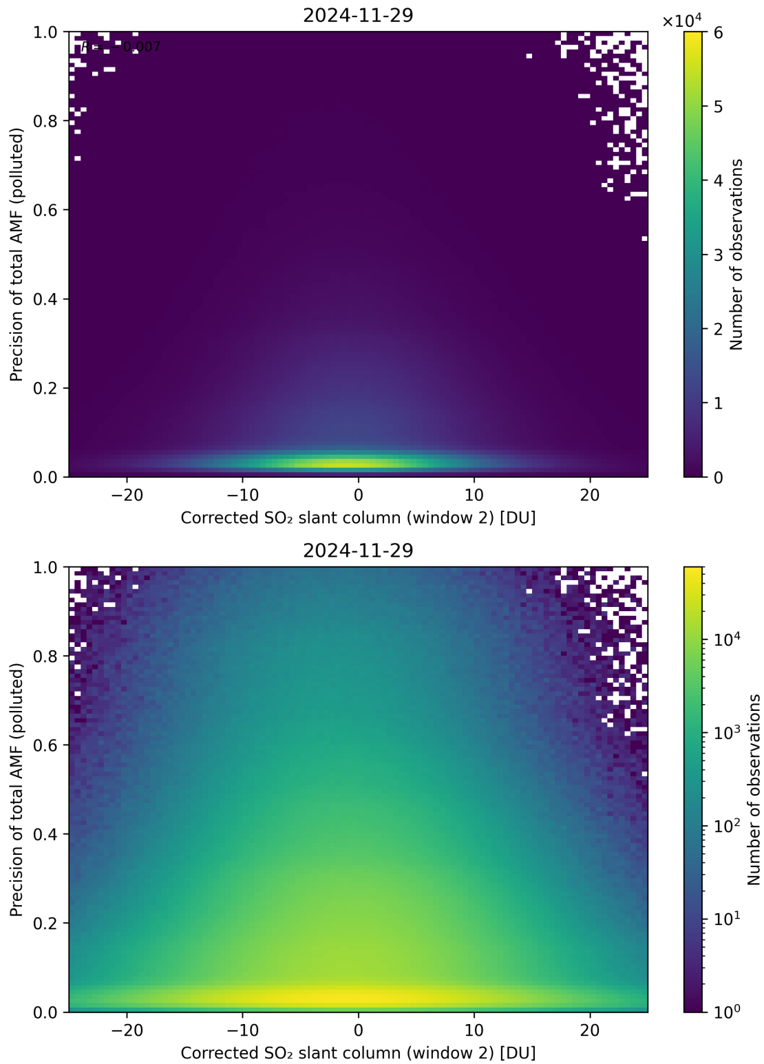
Figure 254: Scatter density plot of “Corrected SO 2 slant column (window 2)” against “Precision of total AMF (polluted)” for 2024-11-28 to 2024-11-30.
