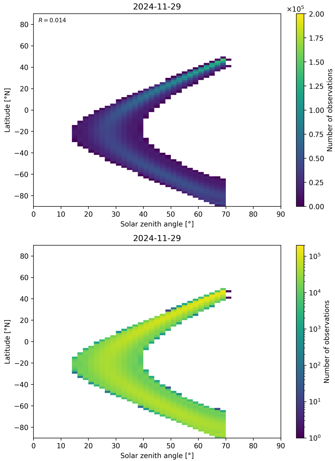
Figure 177: Scatter density plot of “Solar zenith angle” against “Latitude” for 2024-11-28 to 2024-11-30.
