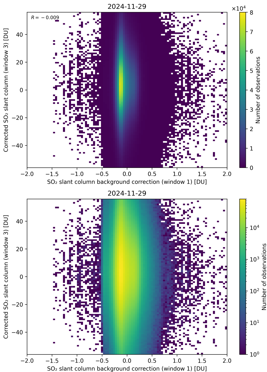
Figure 116: Scatter density plot of “SO 2 slant column background correction (window 1)” against “Corrected SO 2 slant column (window 3)” for 2024-11-28 to 2024-11-30.
