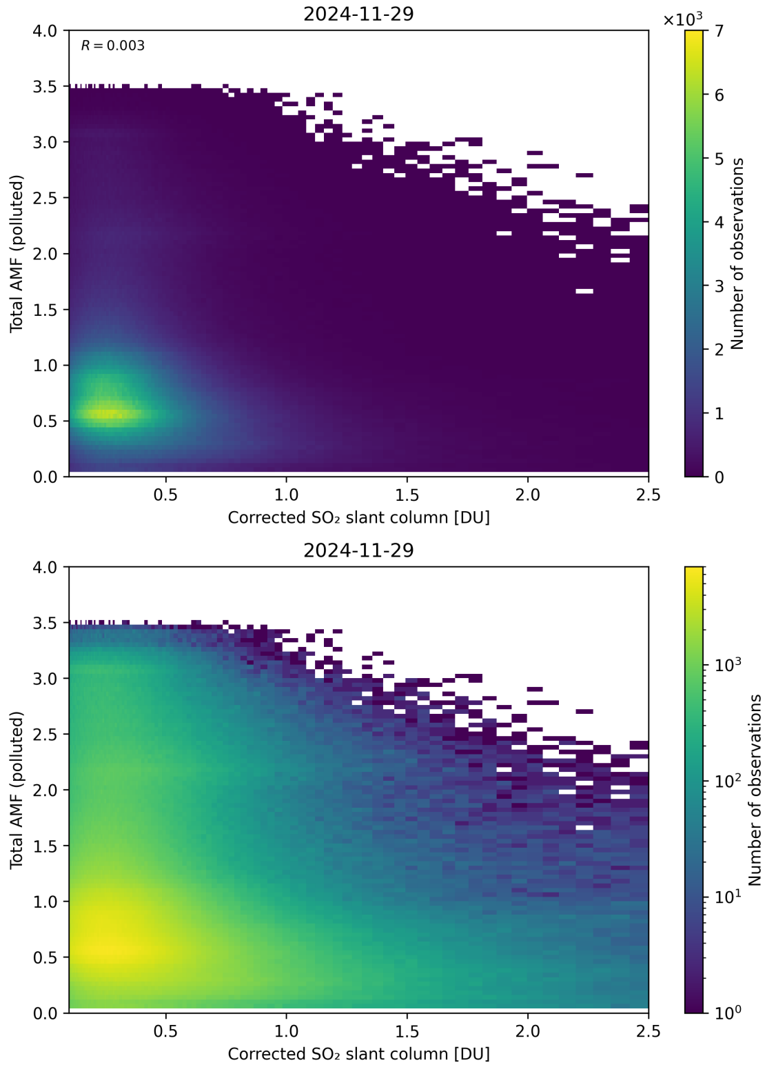
Figure 242: Scatter density plot of “Corrected SO 2 slant column” against “Total AMF (polluted)” for 2024-11-28 to 2024-11-30.
