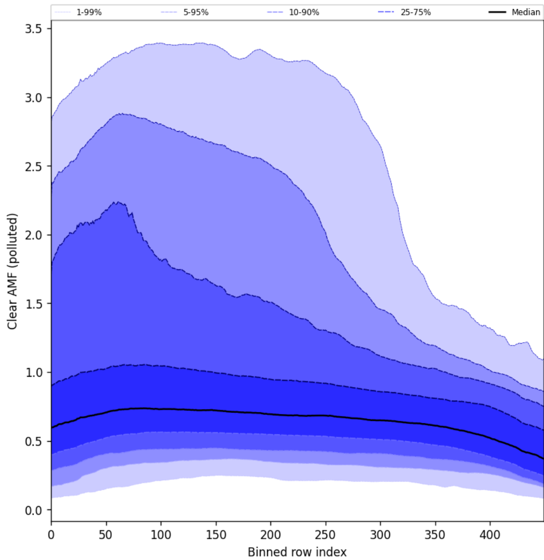
Figure 107: Along track statistics of “Clear AMF (polluted)” for 2024-11-28 to 2024-11-30
