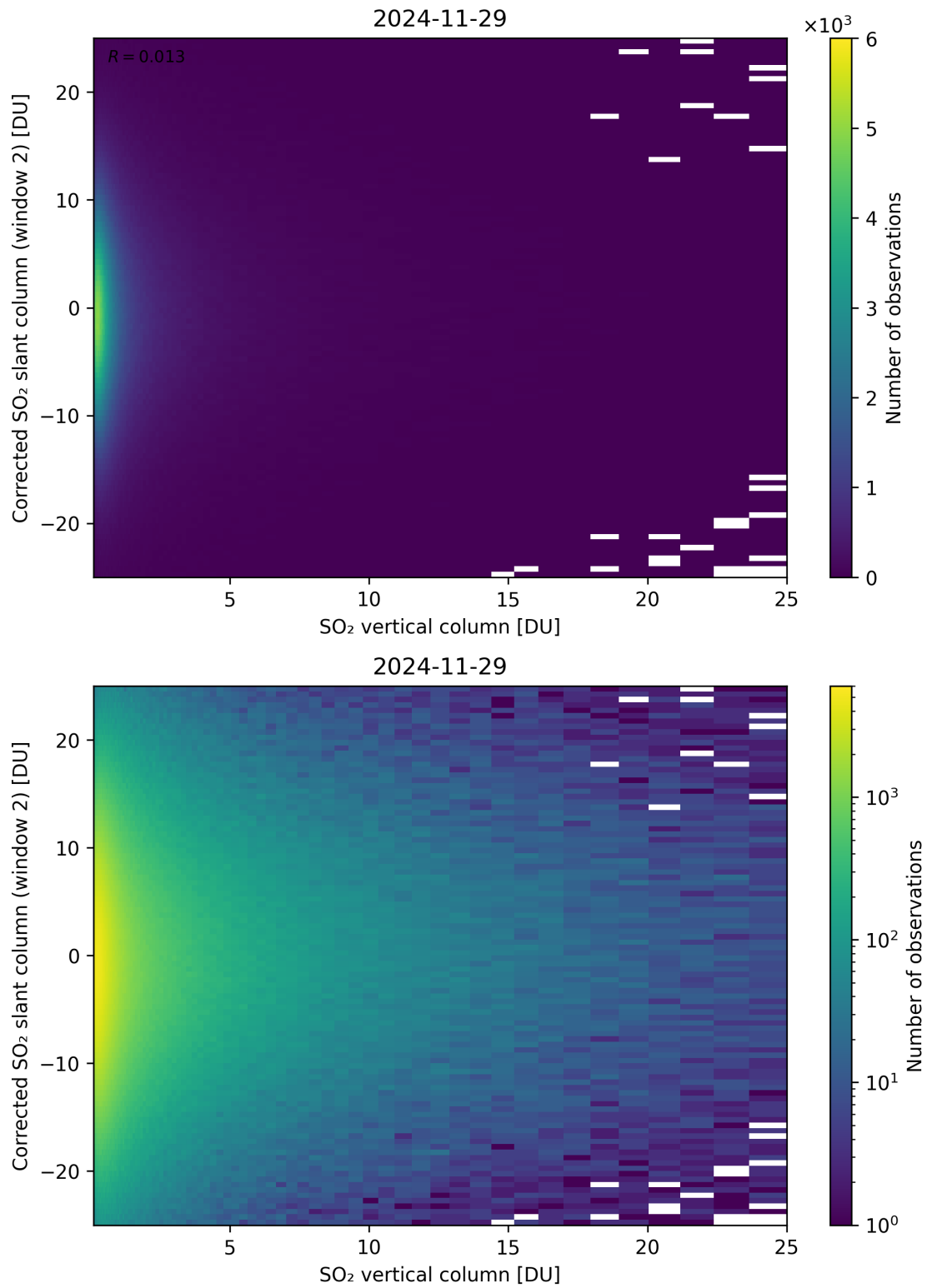
Figure 352: Scatter density plot of “SO 2 vertical column” against “Corrected SO 2 slant column (window 2)” for 2024-11-28 to 2024-11-30.
