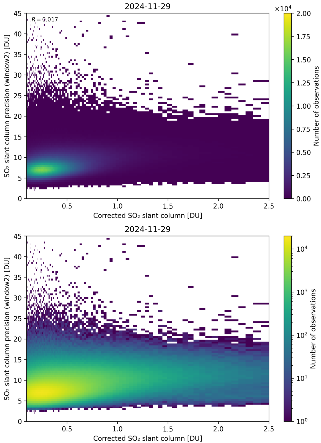
Figure 239: Scatter density plot of “Corrected SO 2 slant column” against “SO 2 slant column precision (window2)” for 2024-11-28 to 2024-11-30.
