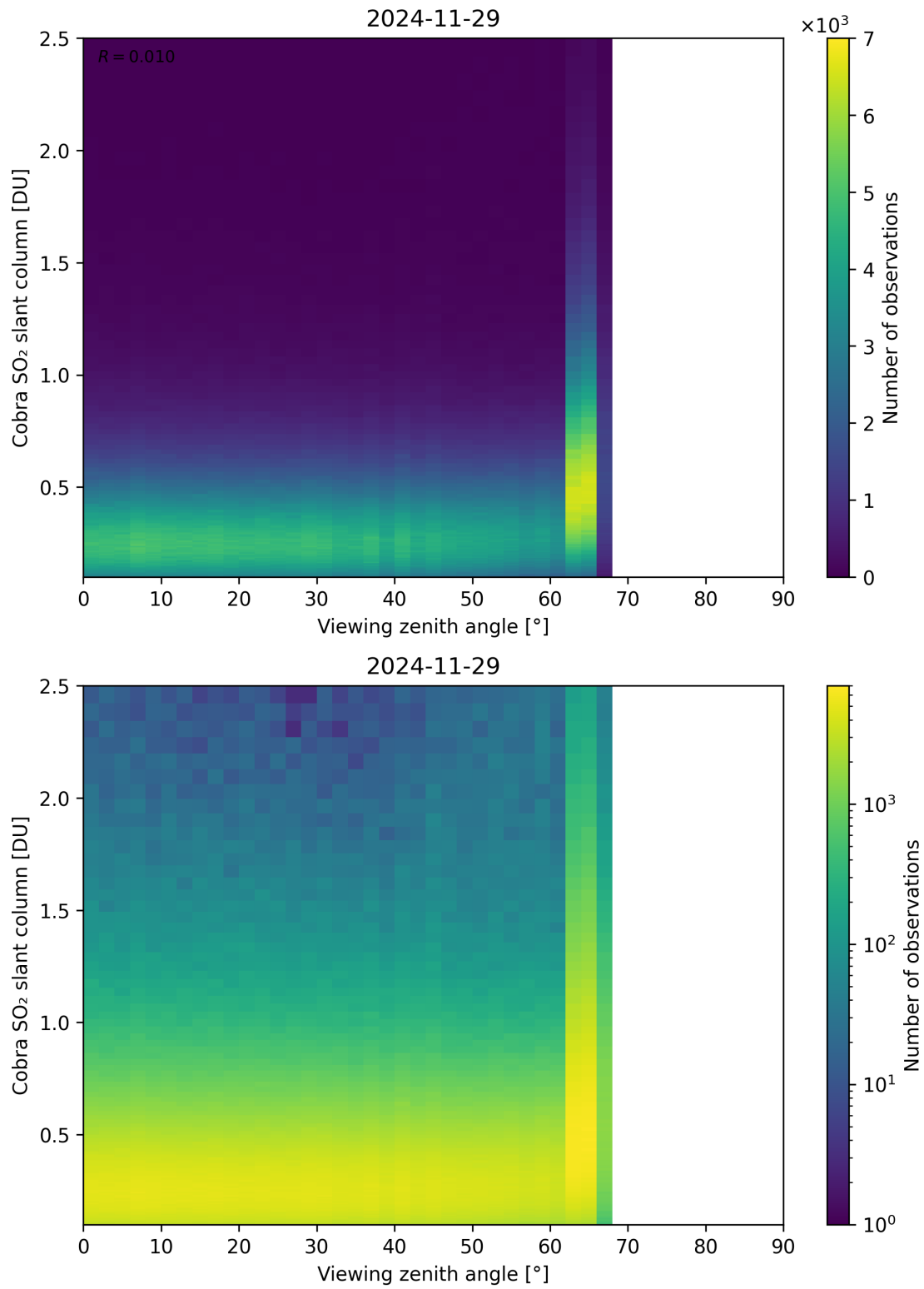
Figure 371: Scatter density plot of “Viewing zenith angle” against “Cobra SO 2 slant column” for 2024-11-28 to 2024-11-30.
