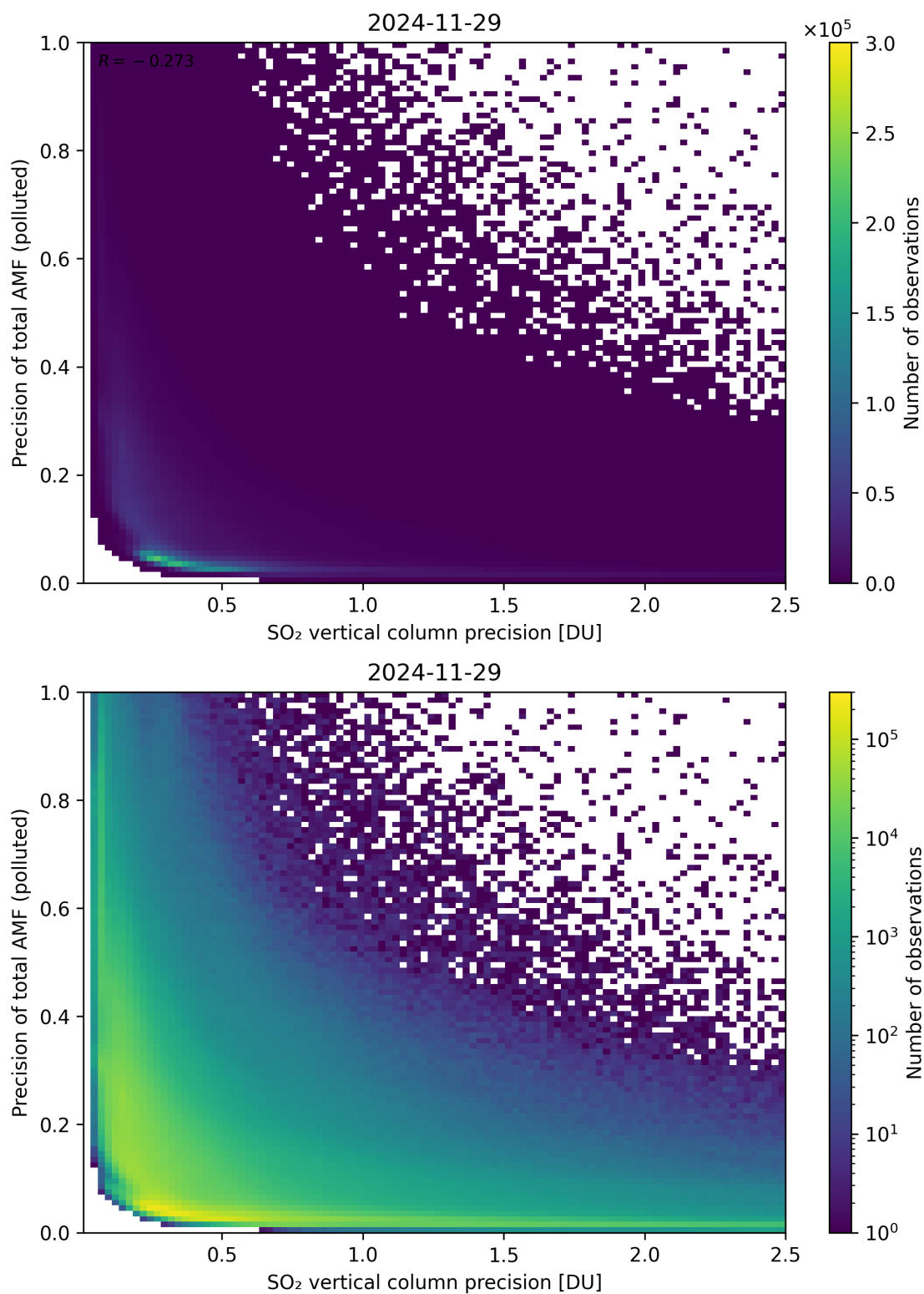
Figure 347: Scatter density plot of “SO 2 vertical column precision” against “Precision of total AMF (polluted)” for 2024-11-28 to 2024-11-30.
