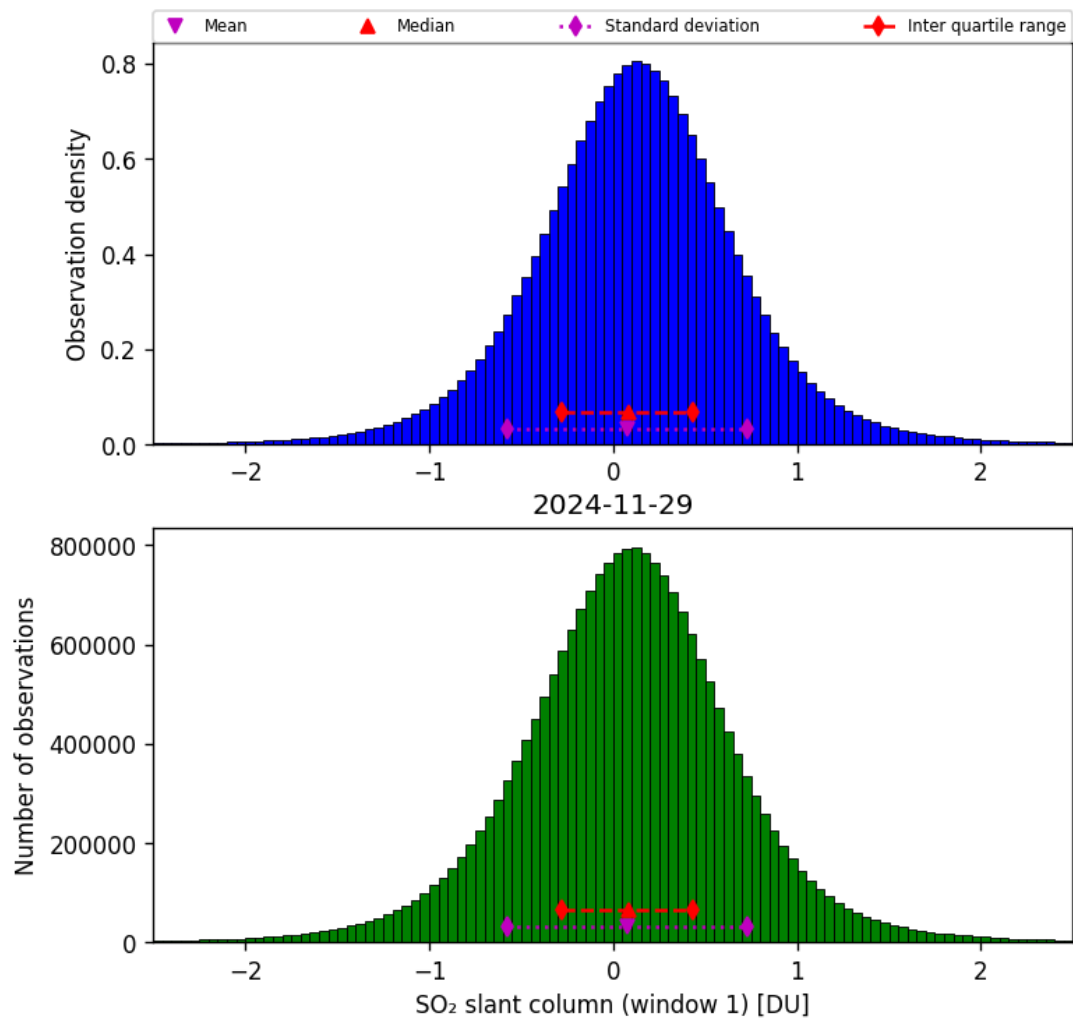
Figure 63: Histogram of “SO 2 slant column (window 1)” for 2024-11-28 to 2024-11-30
