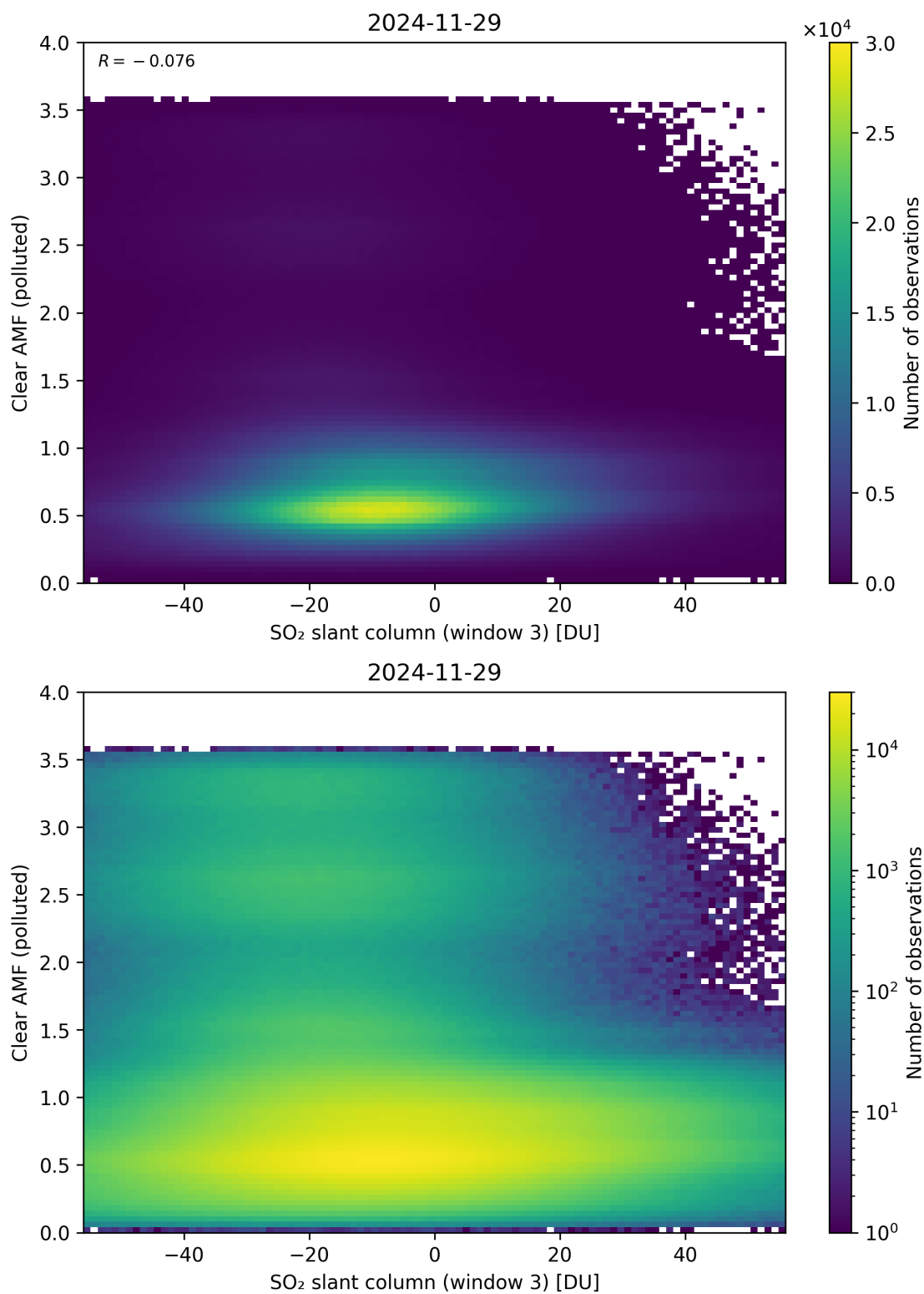
Figure 315: Scatter density plot of “SO 2 slant column (window 3)” against “Clear AMF (polluted)” for 2024-11-28 to 2024-11-30.
