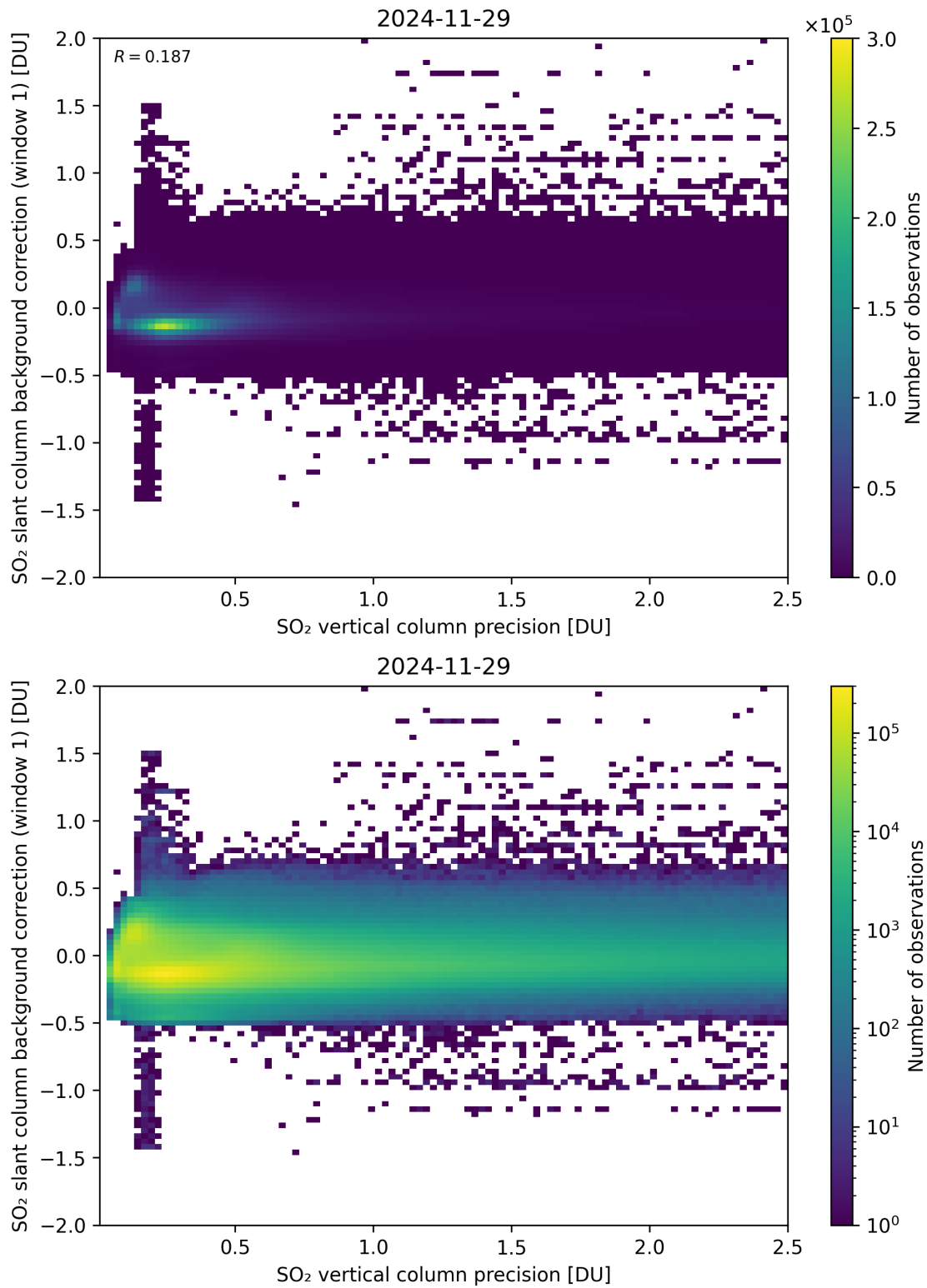
Figure 329: Scatter density plot of “SO 2 vertical column precision” against “SO 2 slant column background correction (window 1)” for 2024-11-28 to 2024-11-30.
