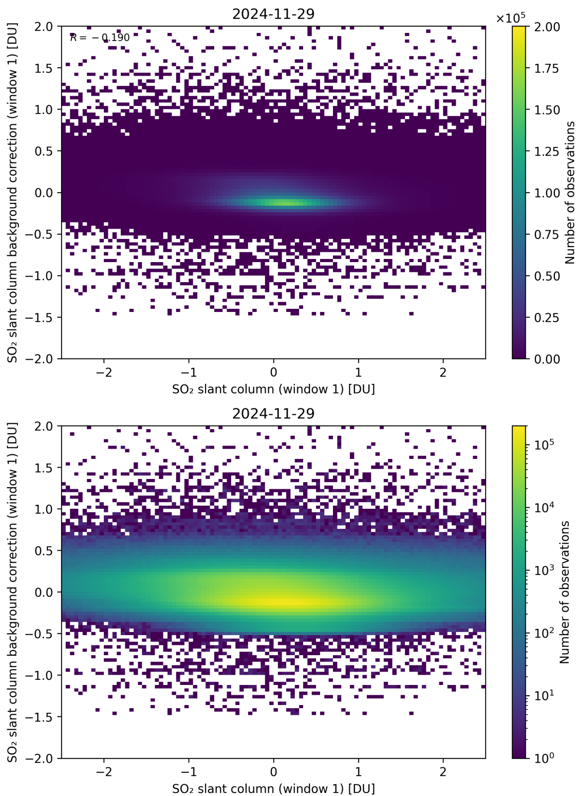
Figure 262: Scatter density plot of “SO 2 slant column (window 1)” against “SO 2 slant column background correction (window 1)” for 2024-11-28 to 2024-11-30.
