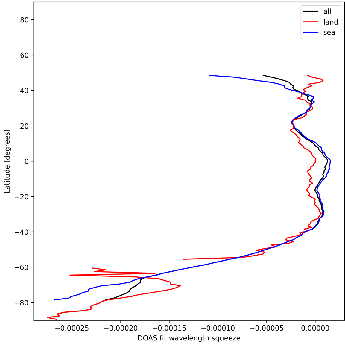
Figure 51: Zonal average of “DOAS fit wavelength squeeze” for 2024-11-28 to 2024-11-30.
