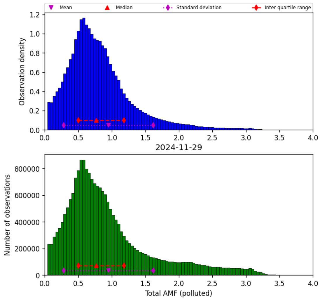
Figure 79: Histogram of “Total AMF (polluted)” for 2024-11-28 to 2024-11-30
