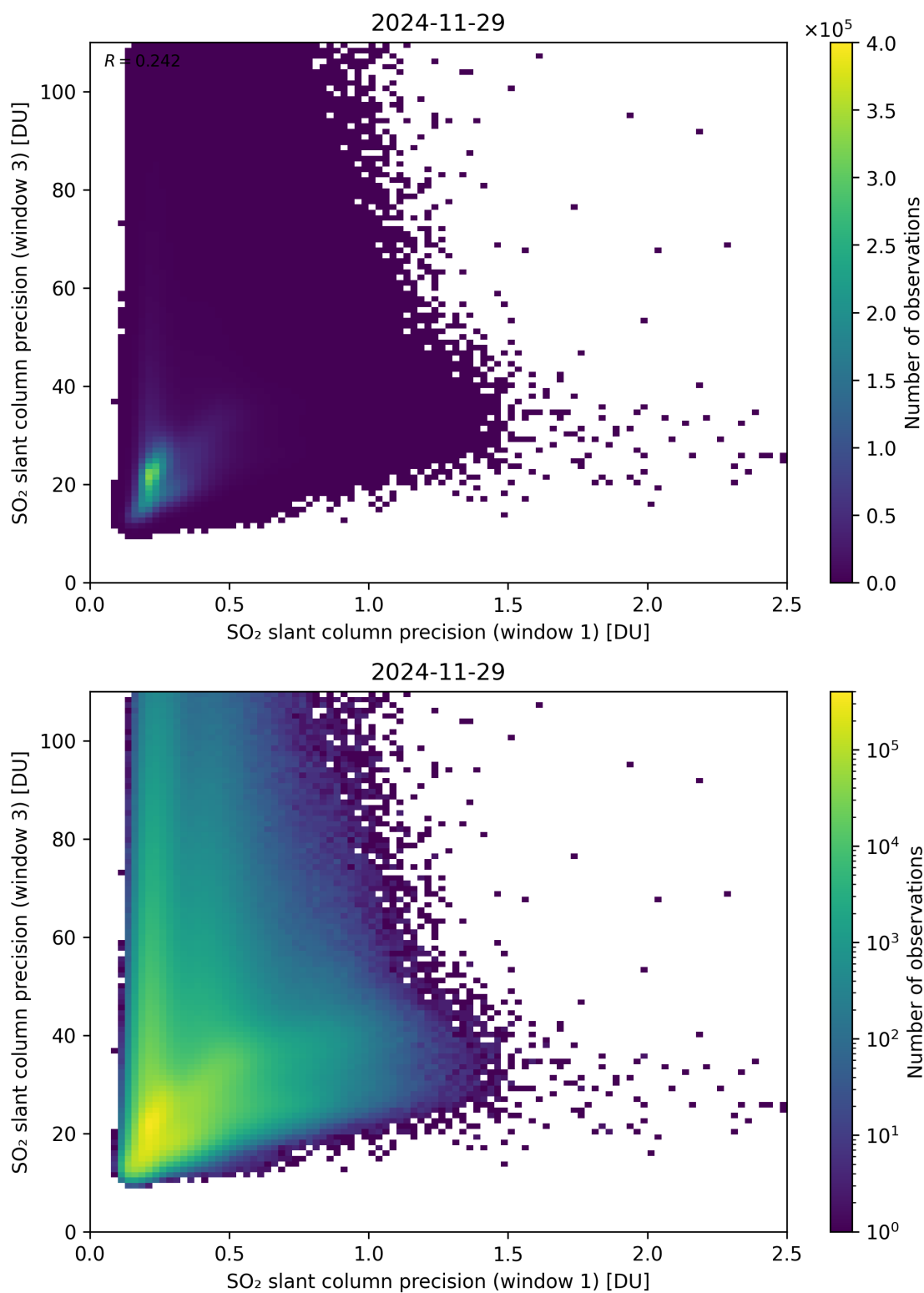
Figure 279: Scatter density plot of “SO 2 slant column precision (window 1)” against “SO 2 slant column precision (window 3)” for 2024-11-28 to 2024-11-30.
