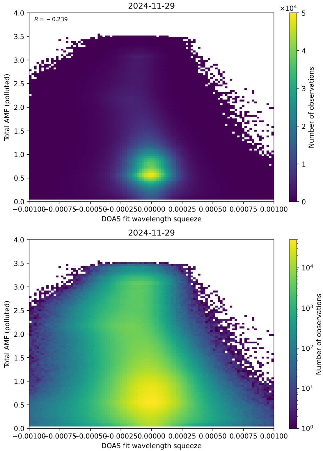
Figure 145: Scatter density plot of “DOAS fit wavelength squeeze” against “Total AMF (polluted)” for 2024-11-28 to 2024-11-30.
