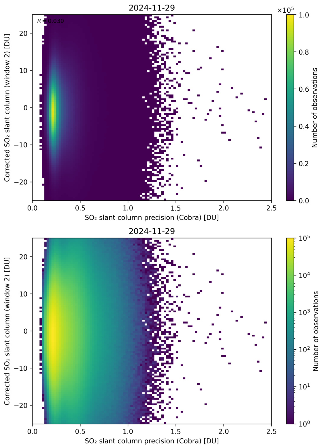
Figure 206: Scatter density plot of “SO 2 slant column precision (Cobra)” against “Corrected SO 2 slant column (window 2)” for 2024-11-28 to 2024-11-30.
