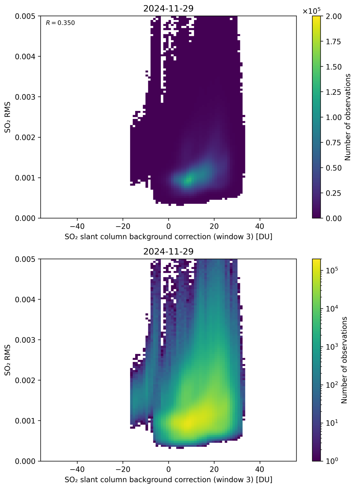
Figure 134: Scatter density plot of “SO 2 slant column background correction (window 3)” against “SO 2 RMS” for 2024-11-28 to 2024-11-30.
