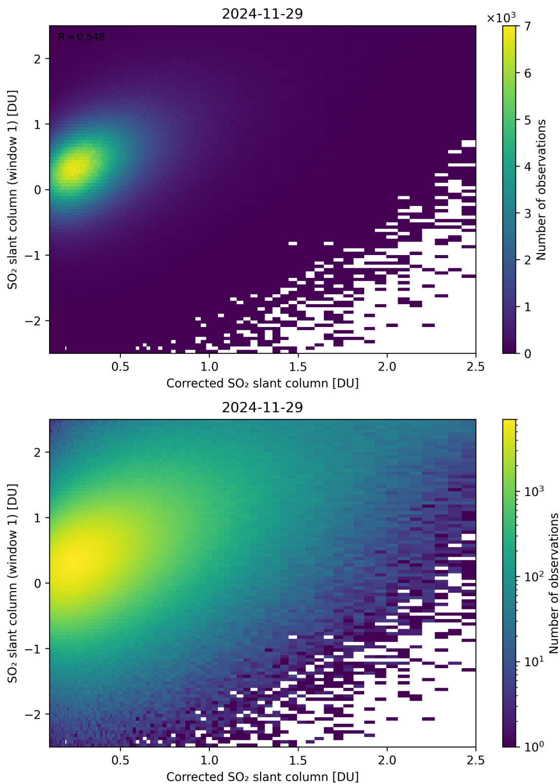
Figure 237: Scatter density plot of “Corrected SO 2 slant column” against “SO 2 slant column (window 1)” for 2024-11-28 to 2024-11-30.
