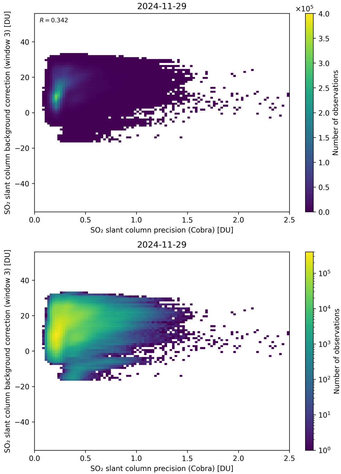
Figure 201: Scatter density plot of “SO 2 slant column precision (Cobra)” against “SO 2 slant column background correction (window 3)” for 2024-11-28 to 2024-11-30.
