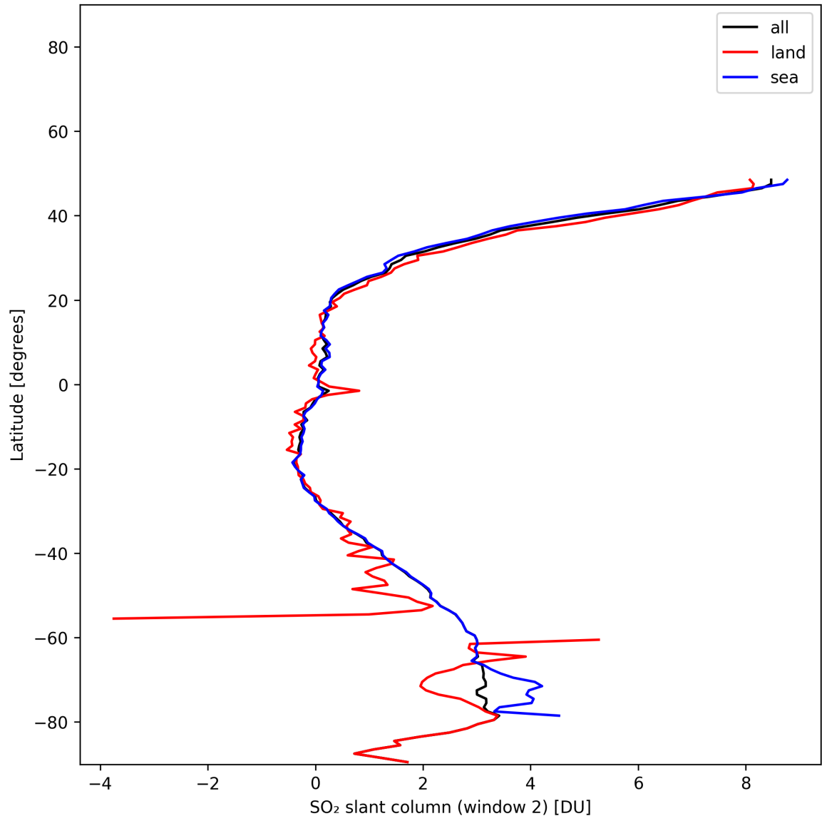
Figure 41: Zonal average of “SO 2 slant column (window 2)” for 2024-11-28 to 2024-11-30.
