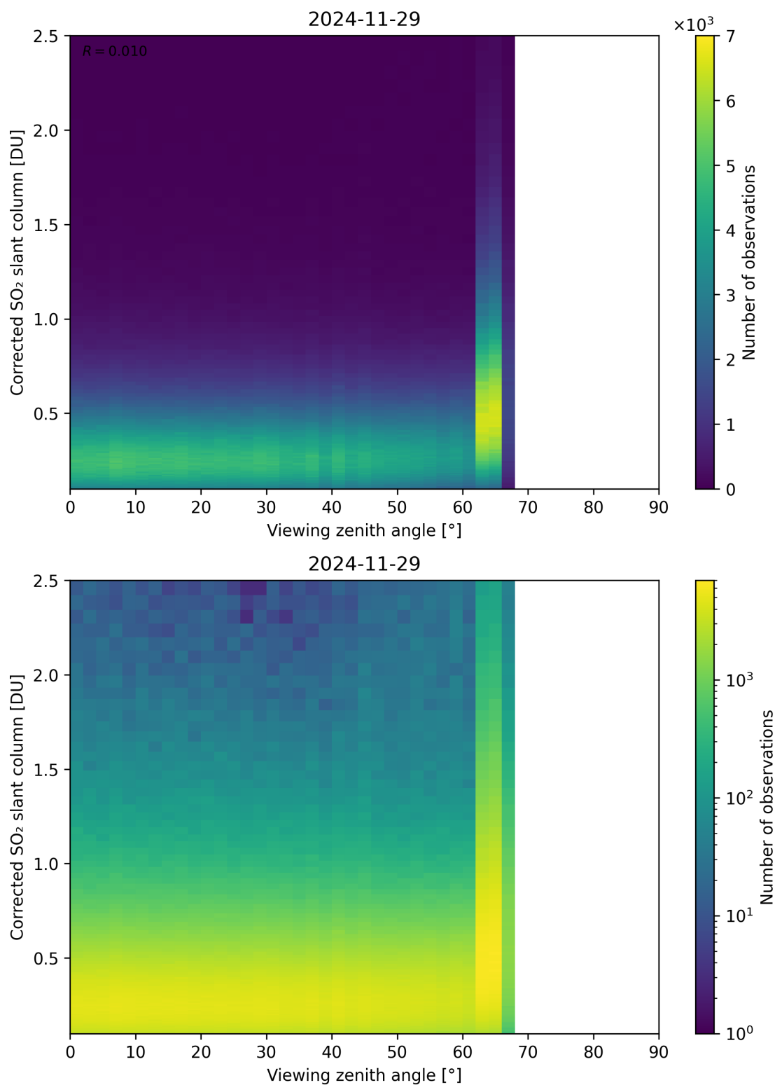
Figure 373: Scatter density plot of “Viewing zenith angle” against “Corrected SO 2 slant column” for 2024-11-28 to 2024-11-30.
