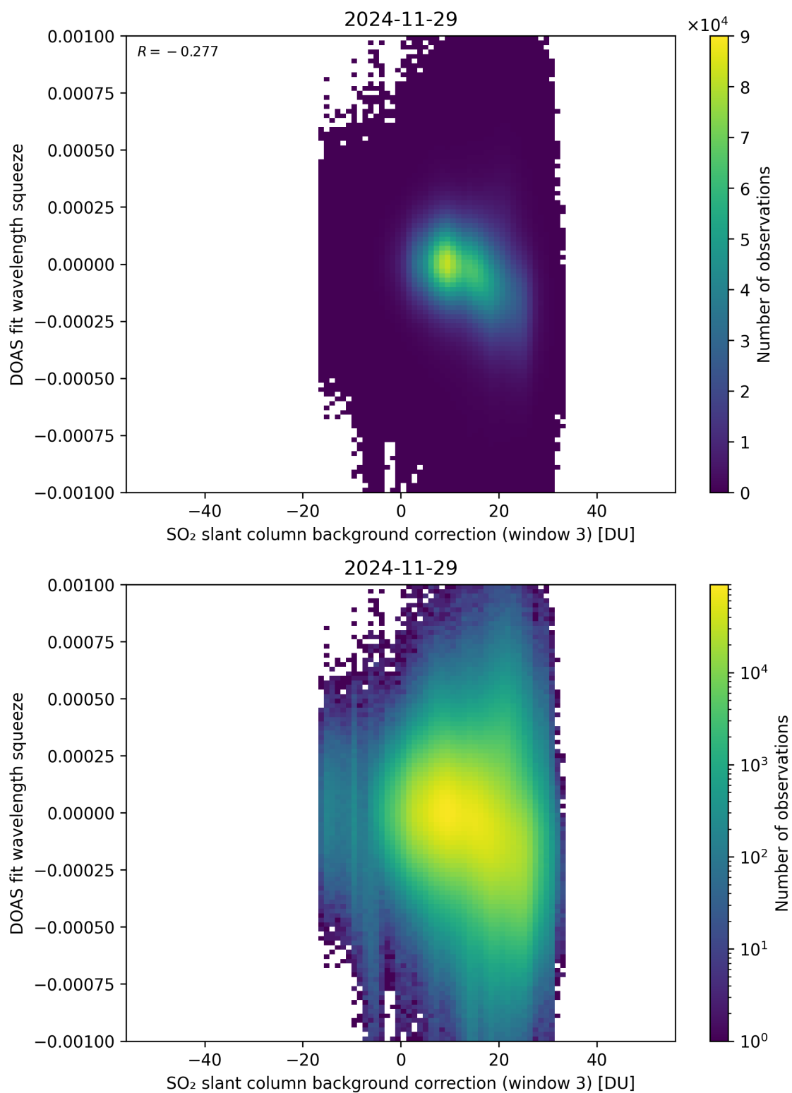
Figure 133: Scatter density plot of “SO 2 slant column background correction (window 3)” against “DOAS fit wavelength squeeze” for 2024-11-28 to 2024-11-30.
