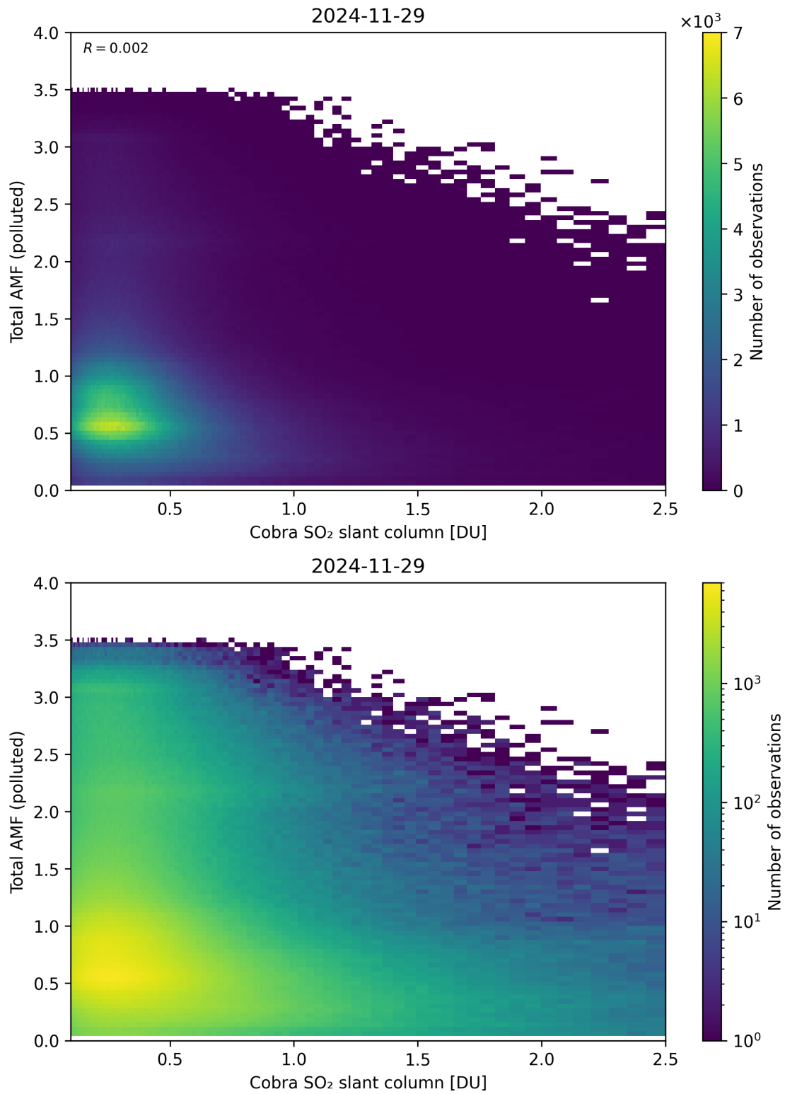
Figure 224: Scatter density plot of “Cobra SO 2 slant column” against “Total AMF (polluted)” for 2024-11-28 to 2024-11-30.
