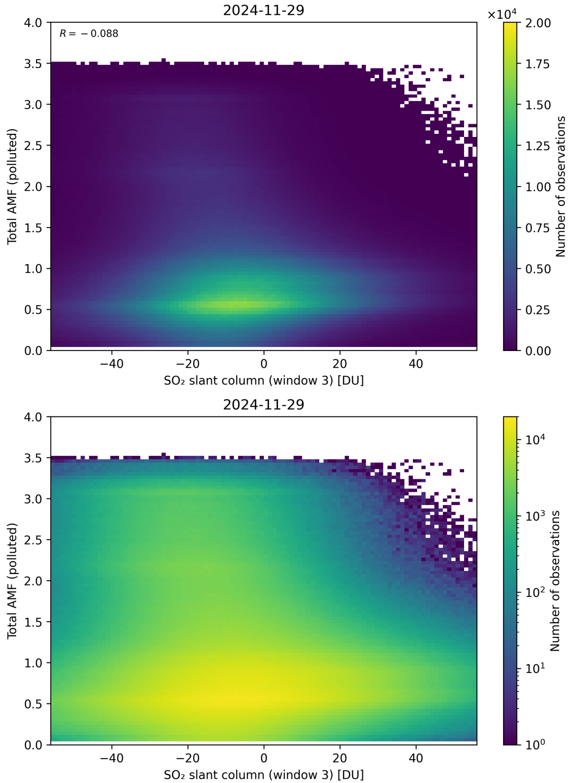
Figure 318: Scatter density plot of “SO 2 slant column (window 3)” against “Total AMF (polluted)” for 2024-11-28 to 2024-11-30.
