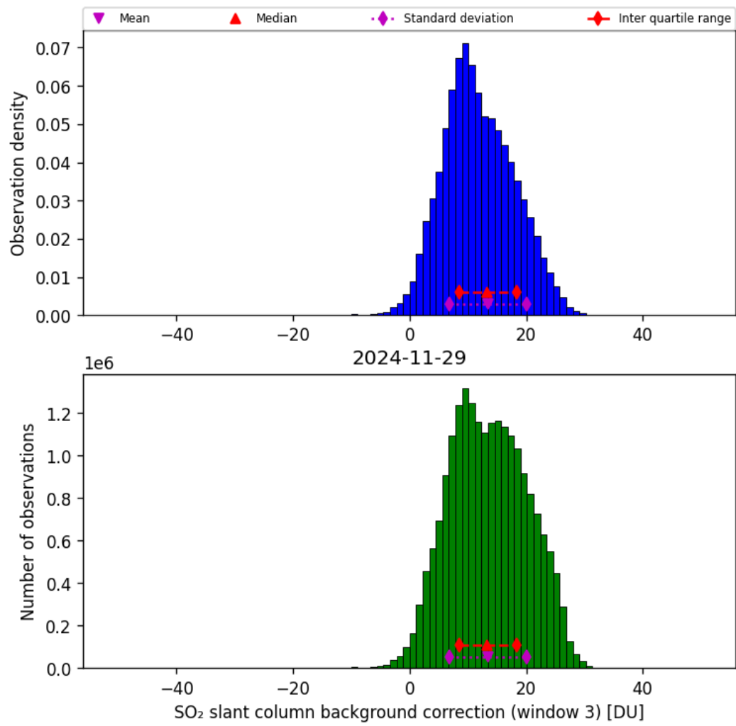
Figure 74: Histogram of “SO 2 slant column background correction (window 3)” for 2024-11-28 to 2024-11-30
