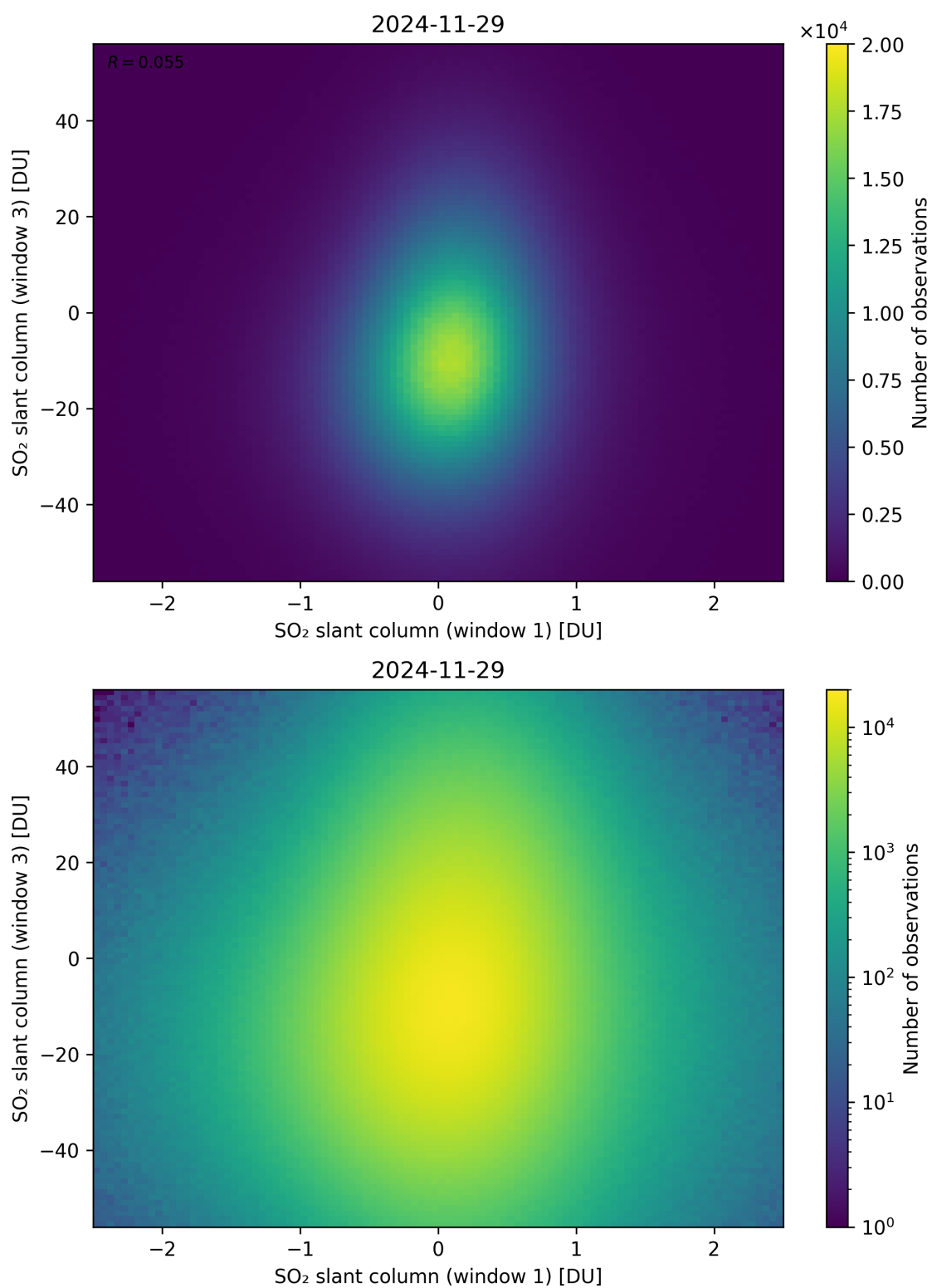
Figure 287: Scatter density plot of “SO 2 slant column (window 1)” against “SO 2 slant column (window 3)” for 2024-11-28 to 2024-11-30.
