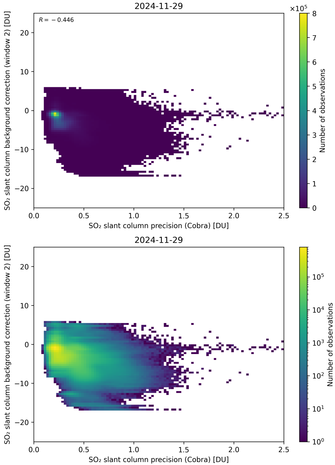
Figure 200: Scatter density plot of “SO 2 slant column precision (Cobra)” against “SO 2 slant column background correction (window 2)” for 2024-11-28 to 2024-11-30.
