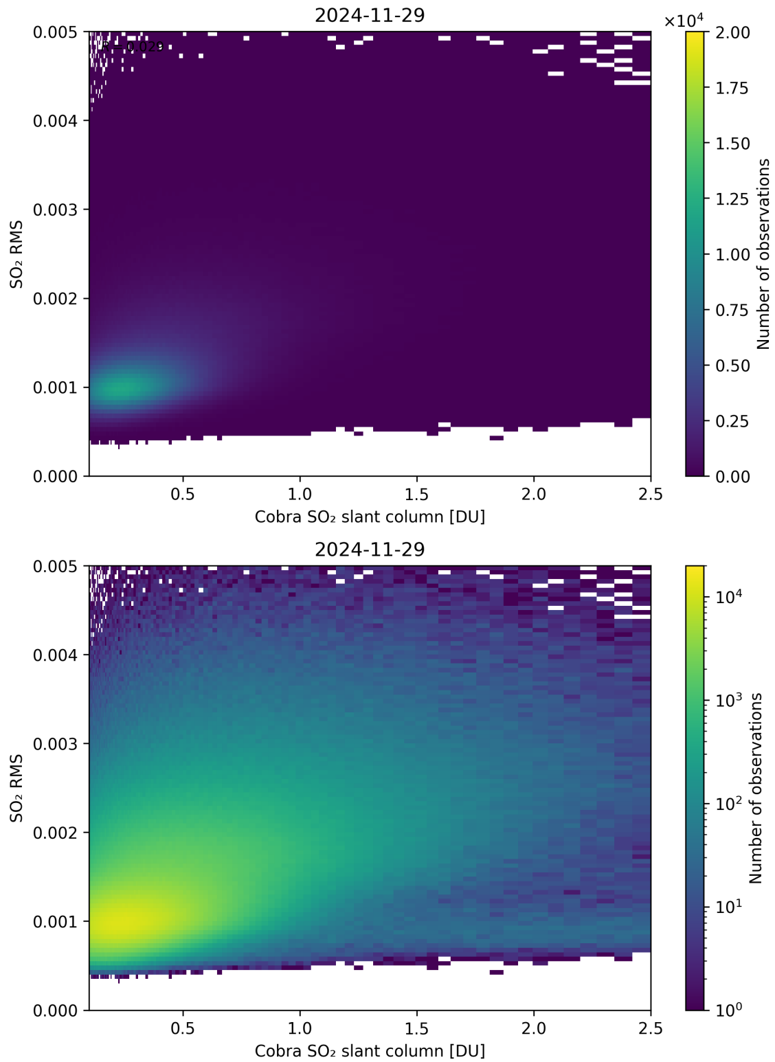
Figure 198: Scatter density plot of “Cobra SO 2 slant column” against “SO 2 RMS” for 2024-11-28 to 2024-11-30.
