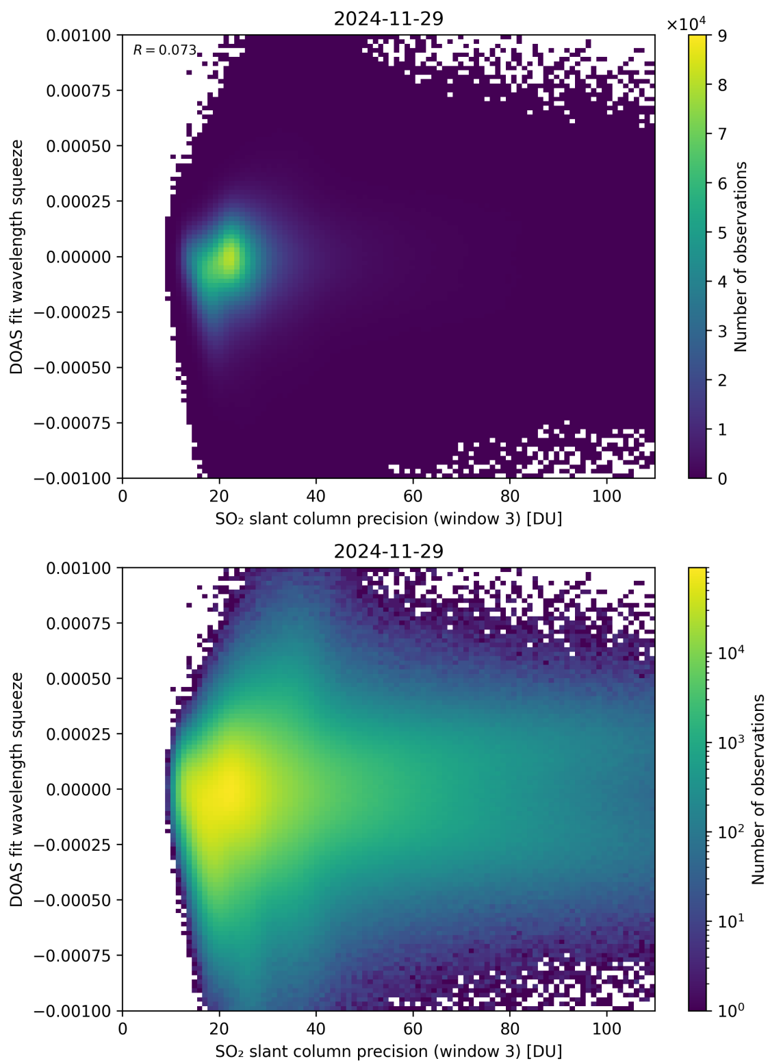
Figure 309: Scatter density plot of “SO 2 slant column precision (window 3)” against “DOAS fit wavelength squeeze” for 2024-11-28 to 2024-11-30.
