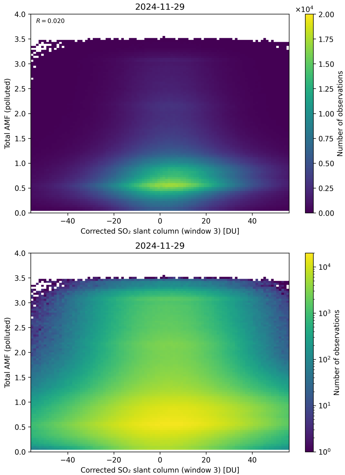
Figure 260: Scatter density plot of “Corrected SO 2 slant column (window 3)” against “Total AMF (polluted)” for 2024-11-28 to 2024-11-30.
