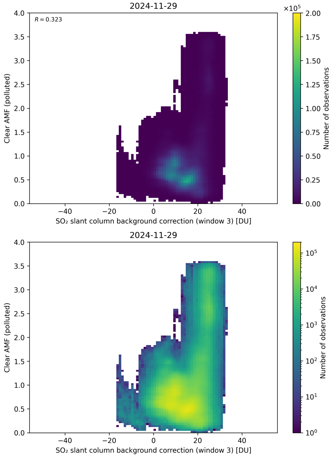
Figure 135: Scatter density plot of “SO 2 slant column background correction (window 3)” against “Clear AMF (polluted)” for 2024-11-28 to 2024-11-30.
