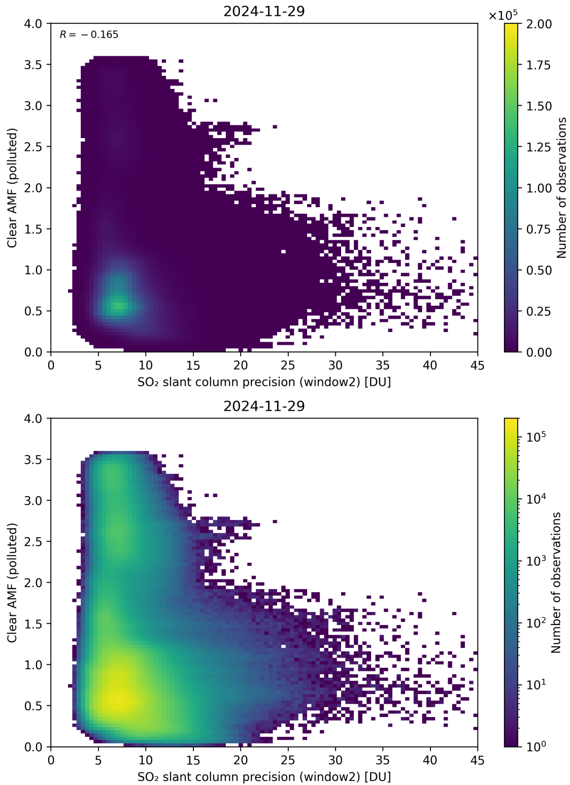
Figure 296: Scatter density plot of “SO 2 slant column precision (window2)” against “Clear AMF (polluted)” for 2024-11-28 to 2024-11-30.
