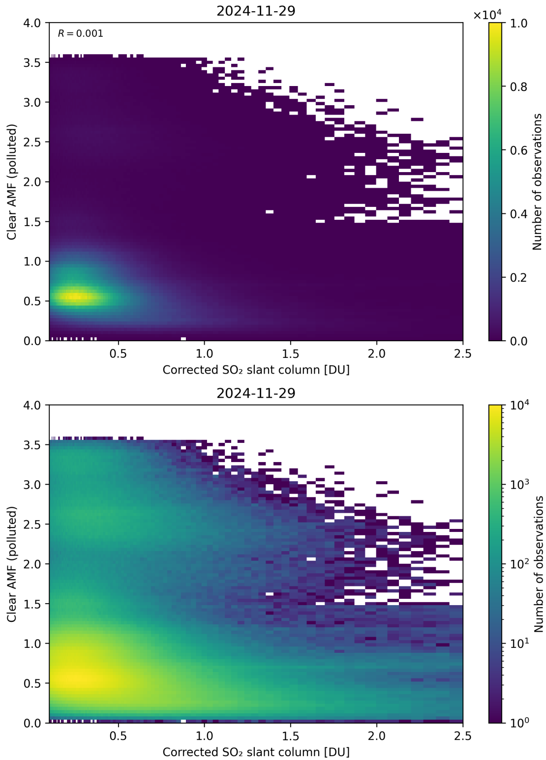
Figure 232: Scatter density plot of “Corrected SO 2 slant column” against “Clear AMF (polluted)” for 2024-11-28 to 2024-11-30.
