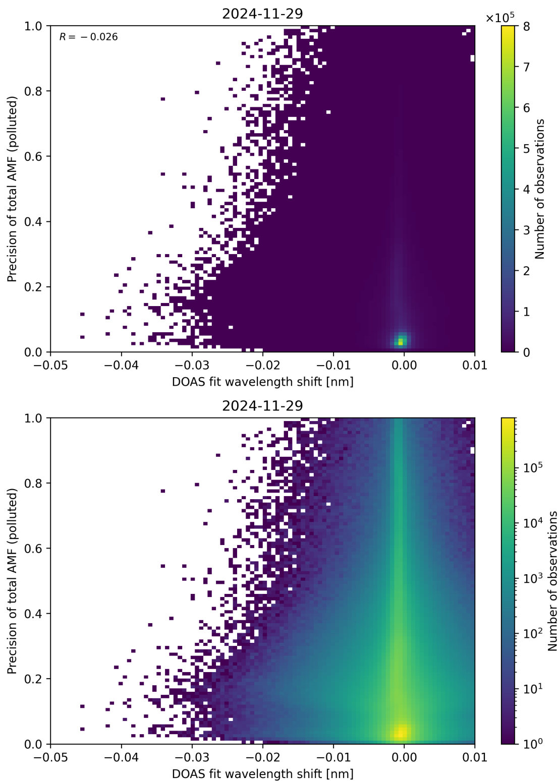
Figure 142: Scatter density plot of “DOAS fit wavelength shift” against “Precision of total AMF (polluted)” for 2024-11-28 to 2024-11-30.
