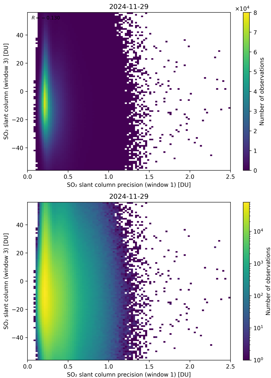
Figure 278: Scatter density plot of “SO 2 slant column precision (window 1)” against “SO 2 slant column (window 3)” for 2024-11-28 to 2024-11-30.
