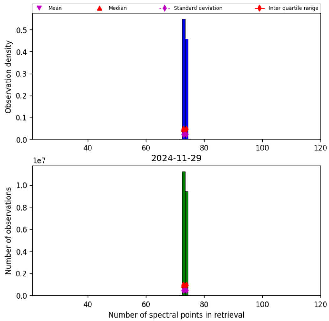
Figure 82: Histogram of “Number of spectral points in retrieval” for 2024-11-28 to 2024-11-30
