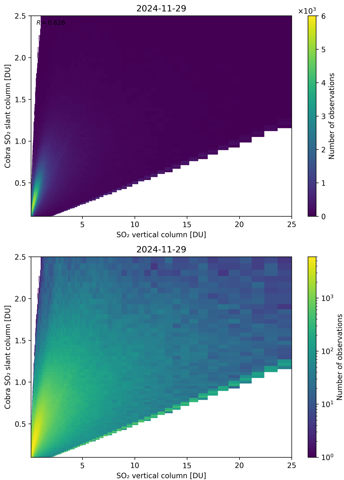
Figure 349: Scatter density plot of “SO 2 vertical column” against “Cobra SO 2 slant column” for 2024-11-28 to 2024-11-30.
