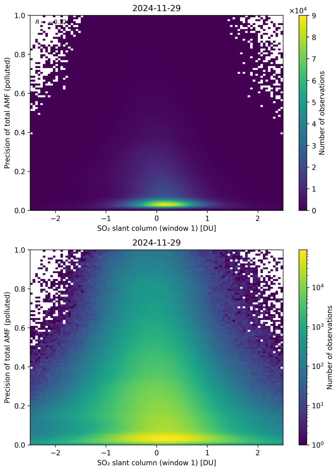
Figure 290: Scatter density plot of “SO 2 slant column (window 1)” against “Precision of total AMF (polluted)” for 2024-11-28 to 2024-11-30.
