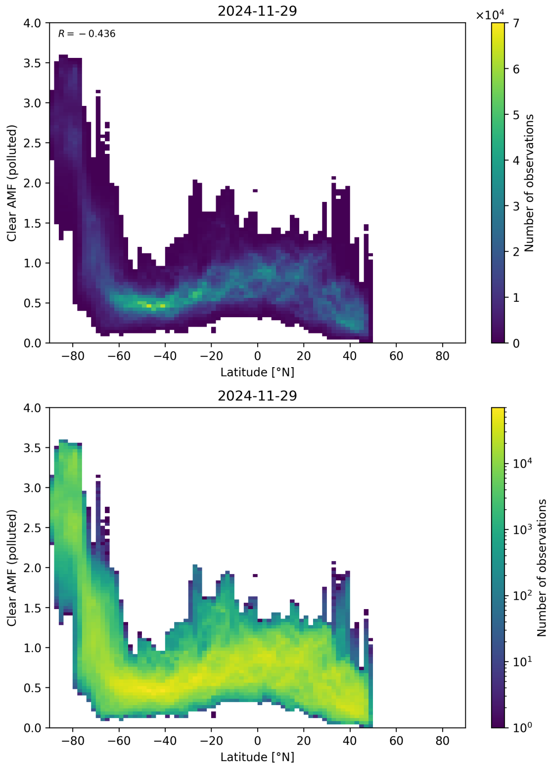
Figure 156: Scatter density plot of “Latitude” against “Clear AMF (polluted)” for 2024-11-28 to 2024-11-30.
