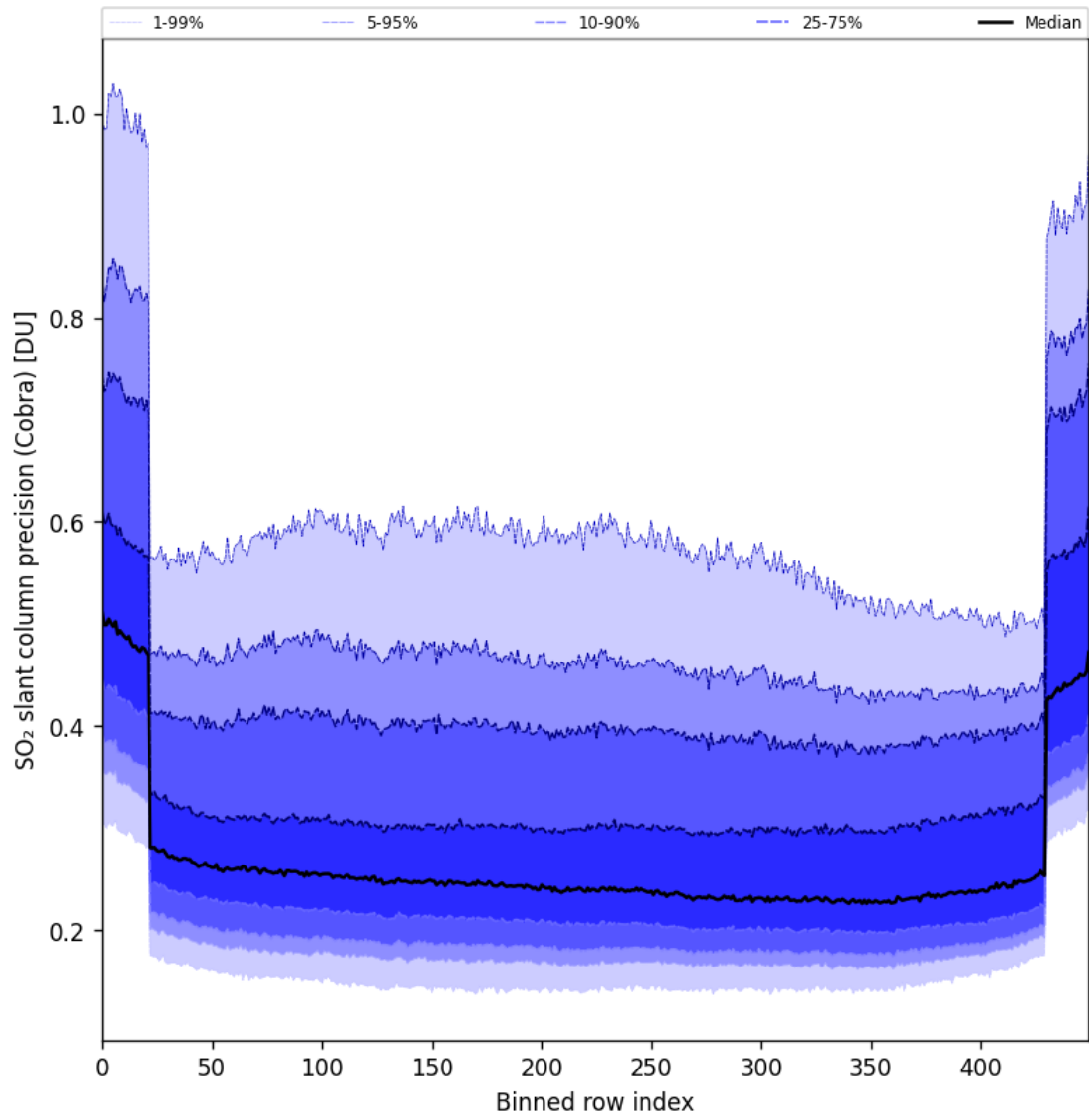
Figure 88: Along track statistics of “SO 2 slant column precision (Cobra)” for 2024-11-28 to 2024-11-30
