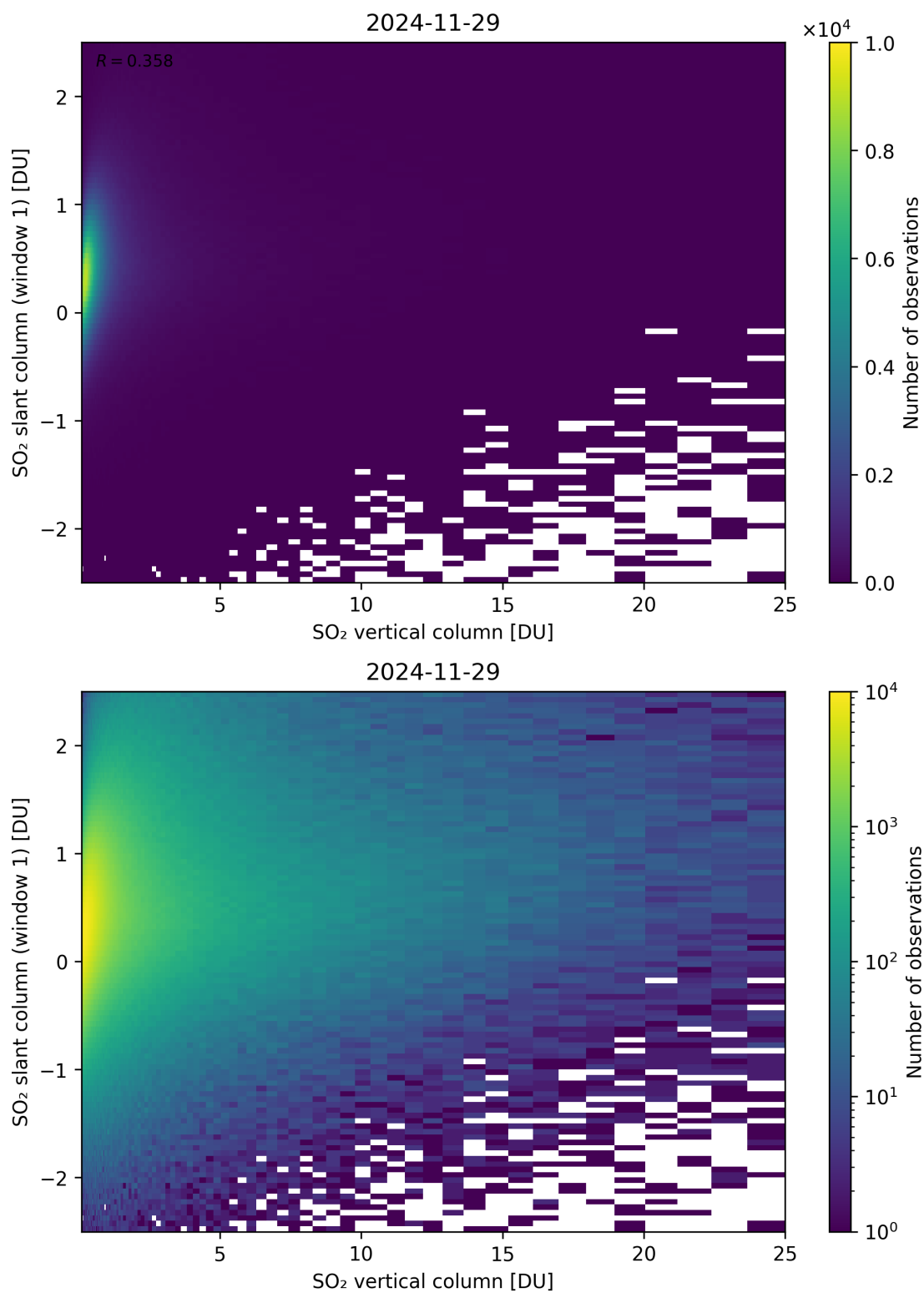
Figure 354: Scatter density plot of “SO 2 vertical column” against “SO 2 slant column (window 1)” for 2024-11-28 to 2024-11-30.
