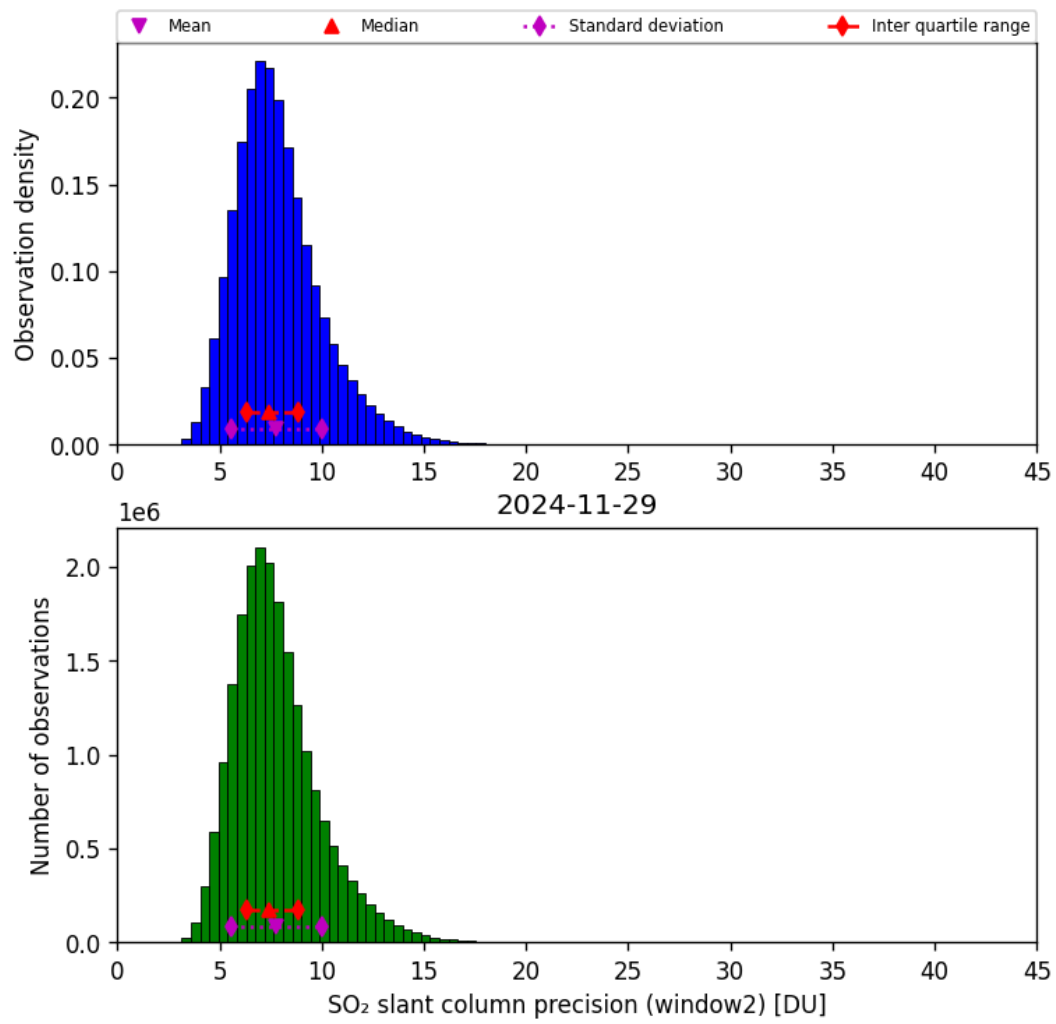
Figure 68: Histogram of “SO 2 slant column precision (window2)” for 2024-11-28 to 2024-11-30
