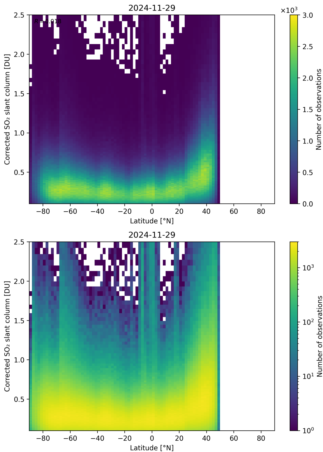
Figure 159: Scatter density plot of “Latitude” against “Corrected SO 2 slant column” for 2024-11-28 to 2024-11-30.
