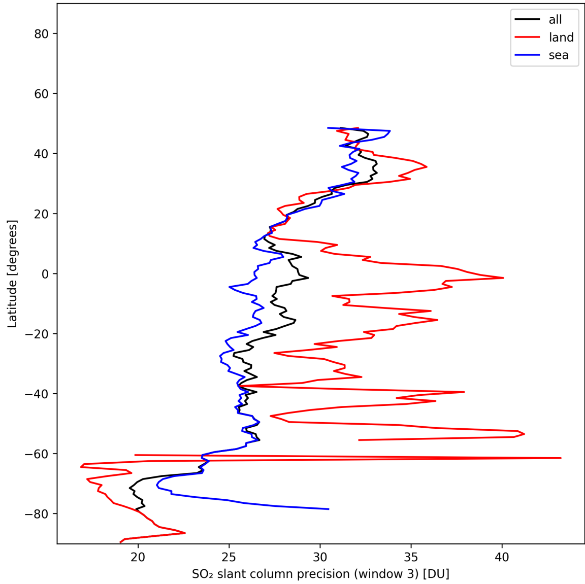
Figure 46: Zonal average of “SO 2 slant column precision (window 3)” for 2024-11-30 to 2024-12-01.
