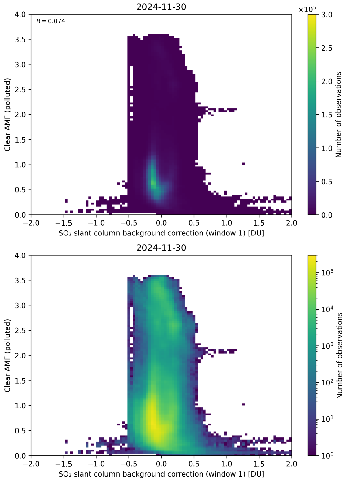
Figure 114: Scatter density plot of “SO 2 slant column background correction (window 1)” against “Clear AMF (polluted)” for 2024-11-30 to 2024-12-01.
