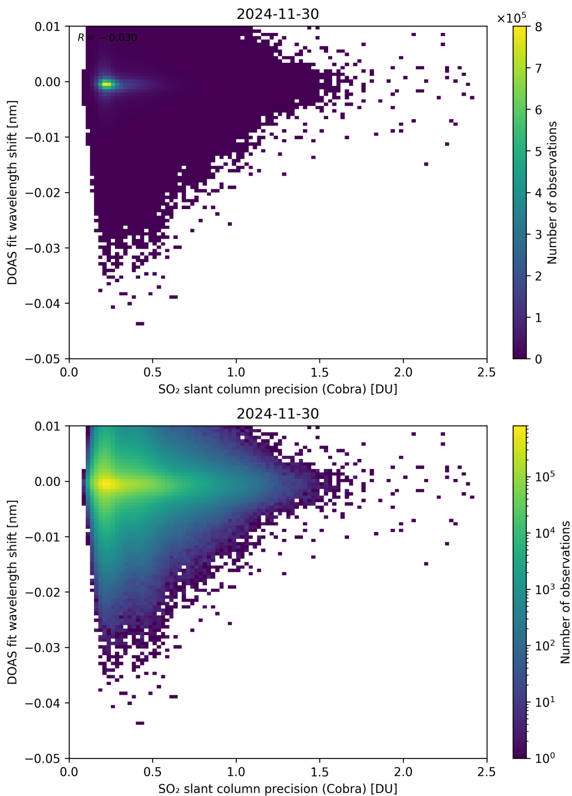
Figure 202: Scatter density plot of “SO 2 slant column precision (Cobra)” against “DOAS fit wavelength shift” for 2024-11-30 to 2024-12-01.
