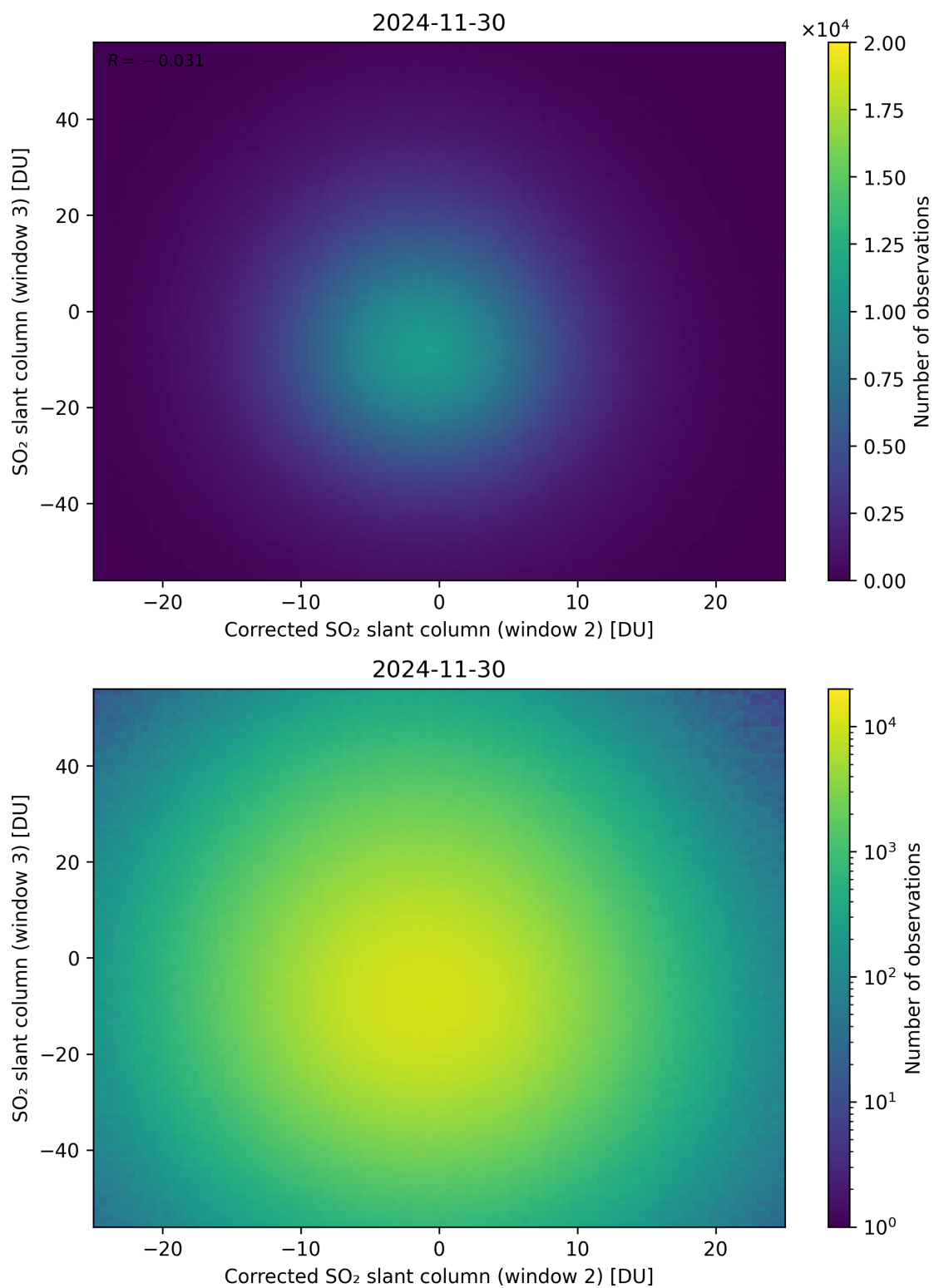
Figure 251: Scatter density plot of “Corrected SO 2 slant column (window 2)” against “SO 2 slant column (window 3)” for 2024-11-30 to 2024-12-01.
