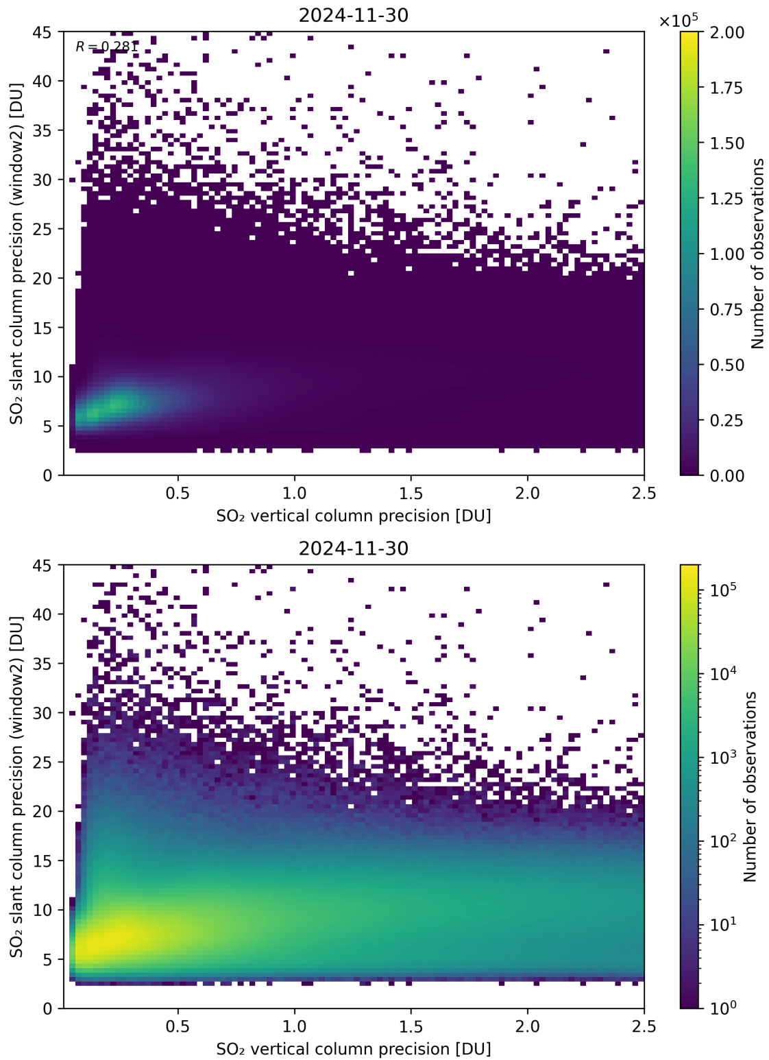
Figure 343: Scatter density plot of “SO 2 vertical column precision” against “SO 2 slant column precision (window2)” for 2024-11-30 to 2024-12-01.
