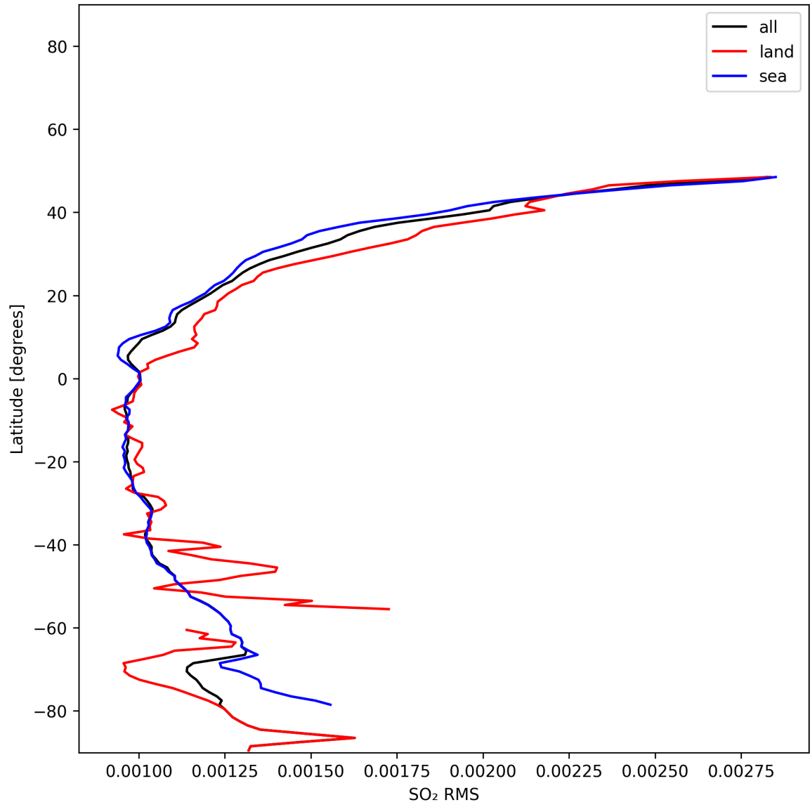
Figure 52: Zonal average of “SO 2 RMS” for 2024-11-30 to 2024-12-01.
