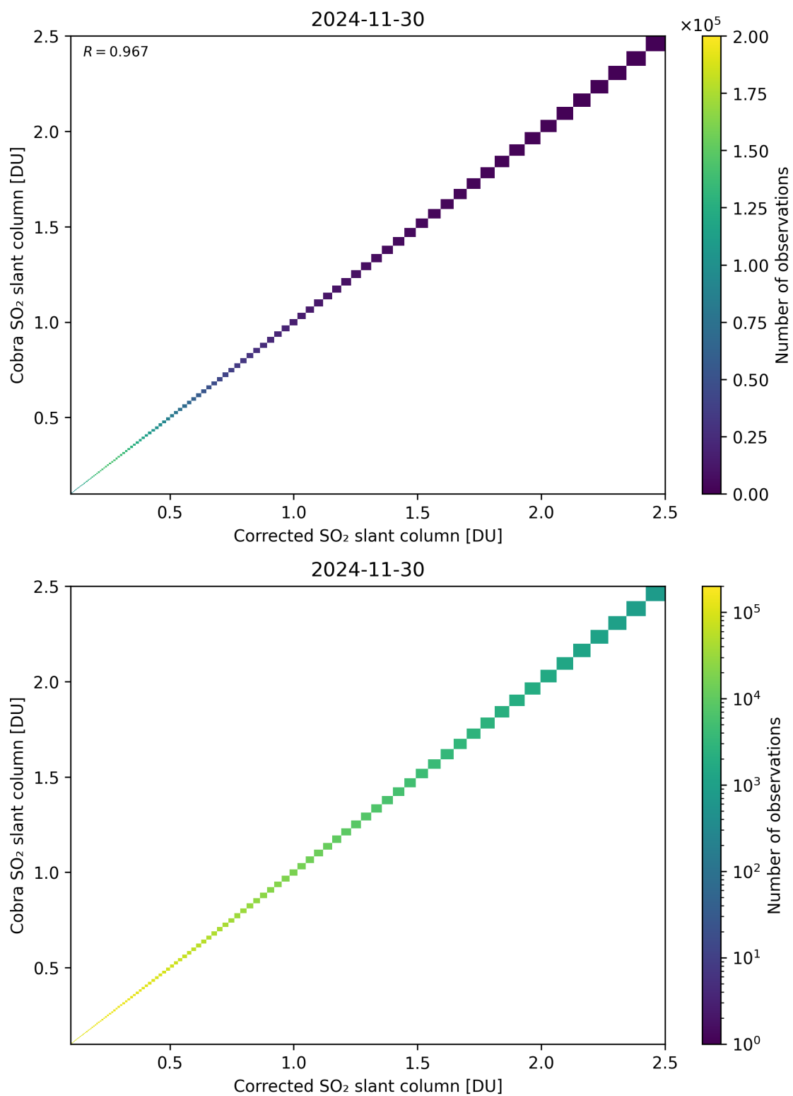
Figure 233: Scatter density plot of “Corrected SO 2 slant column” against “Cobra SO 2 slant column” for 2024-11-30 to 2024-12-01.
