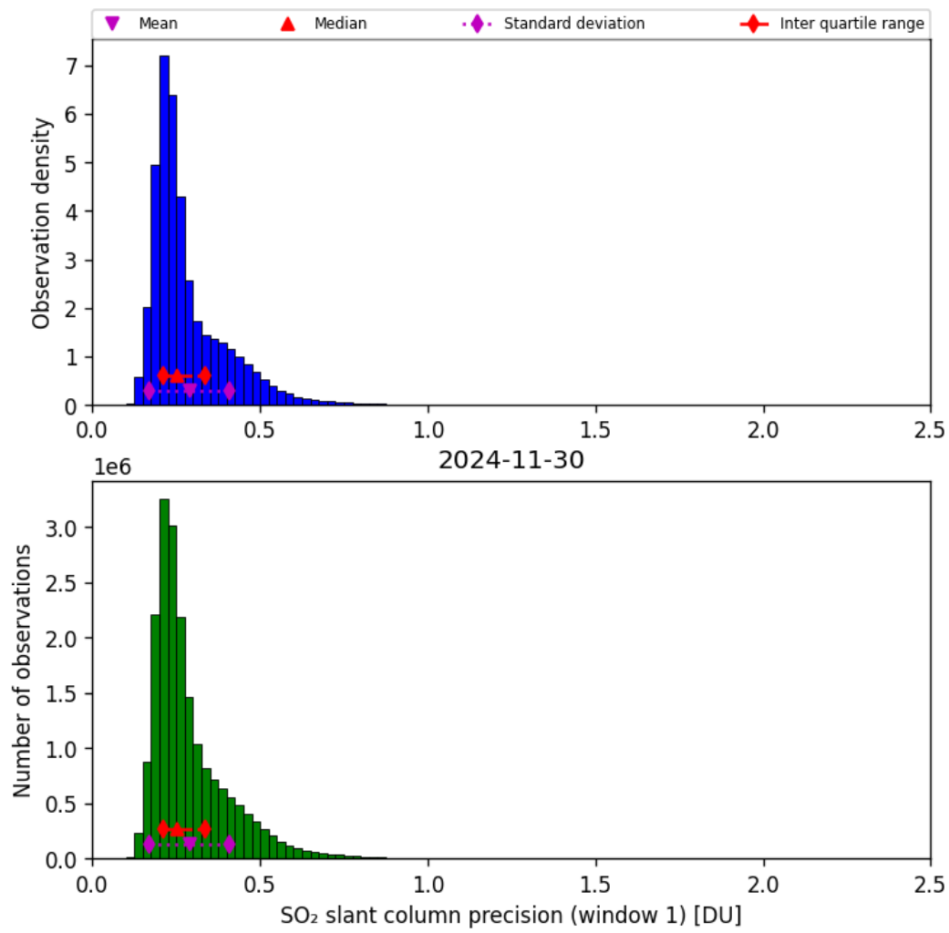
Figure 64: Histogram of “SO 2 slant column precision (window 1)” for 2024-11-30 to 2024-12-01
