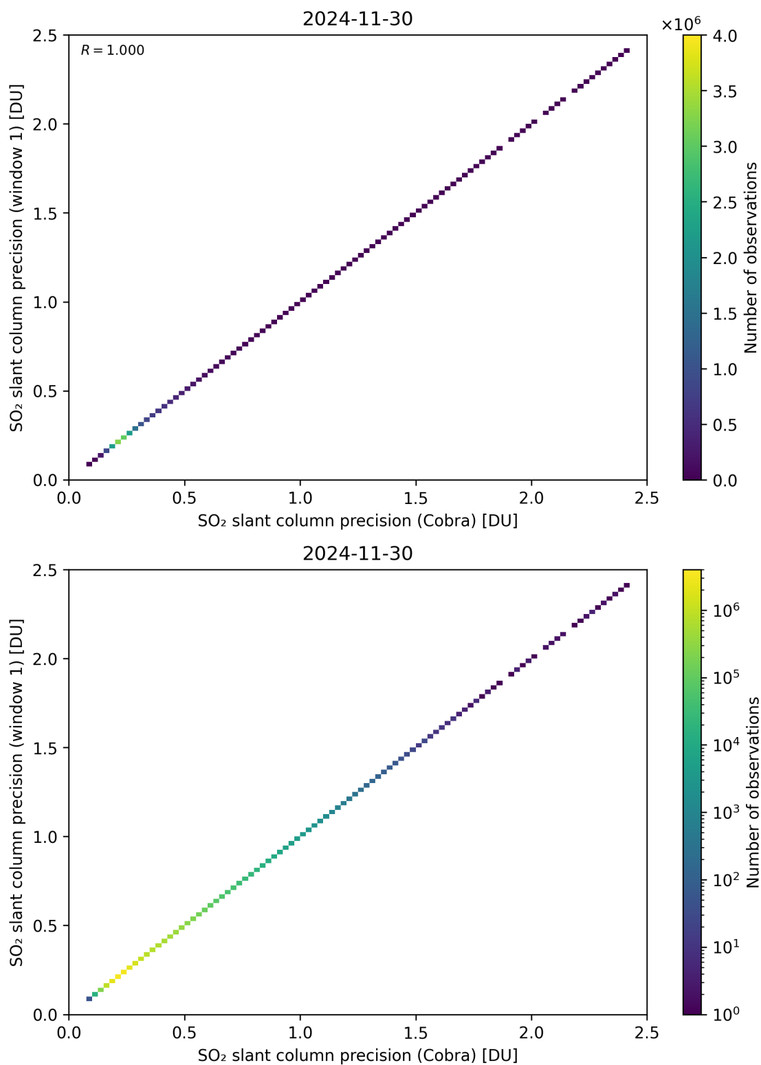
Figure 209: Scatter density plot of “SO 2 slant column precision (Cobra)” against “SO 2 slant column precision (window 1)” for 2024-11-30 to 2024-12-01.
