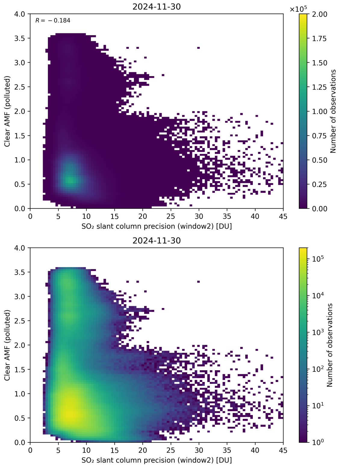
Figure 296: Scatter density plot of “SO 2 slant column precision (window2)” against “Clear AMF (polluted)” for 2024-11-30 to 2024-12-01.
