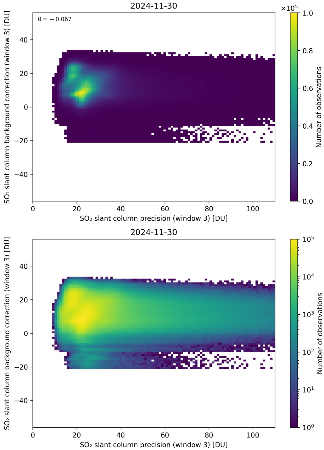
Figure 307: Scatter density plot of “SO 2 slant column precision (window 3)” against “SO 2 slant column background correction (window 3)” for 2024-11-30 to 2024-12-01.
