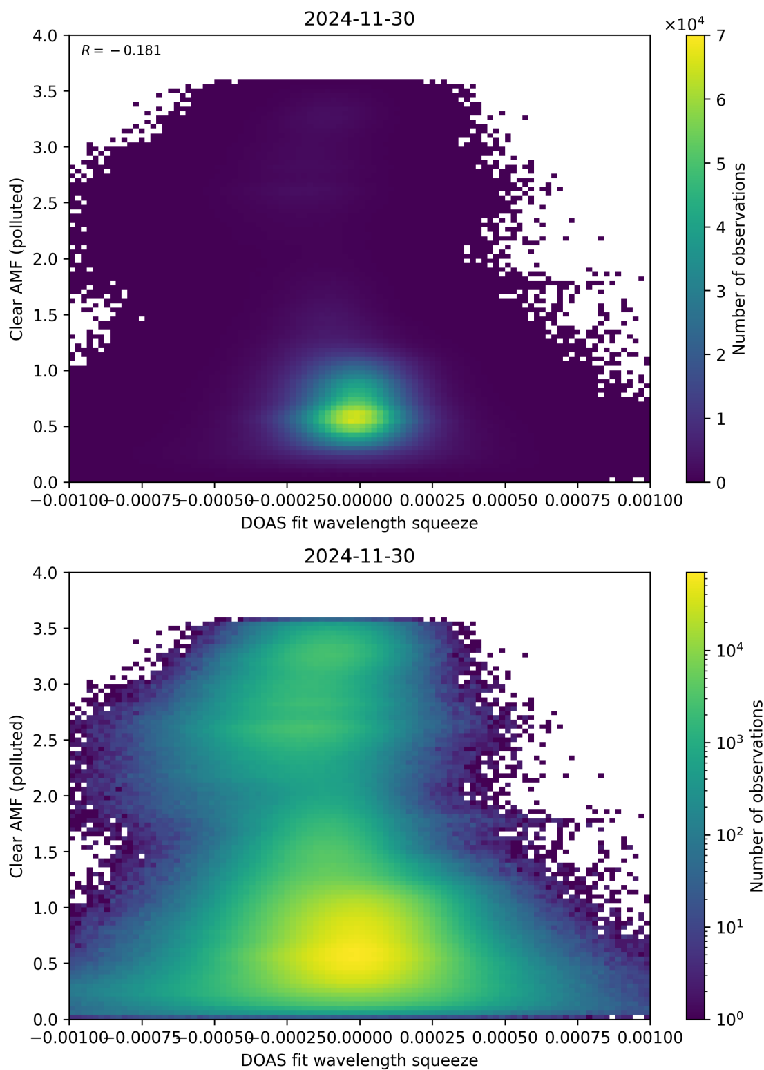
Figure 144: Scatter density plot of “DOAS fit wavelength squeeze” against “Clear AMF (polluted)” for 2024-11-30 to 2024-12-01.
