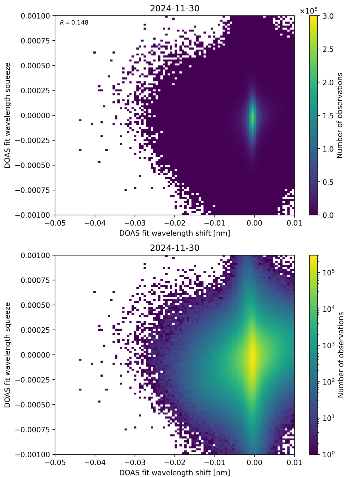
Figure 138: Scatter density plot of “DOAS fit wavelength shift” against “DOAS fit wavelength squeeze” for 2024-11-30 to 2024-12-01.
