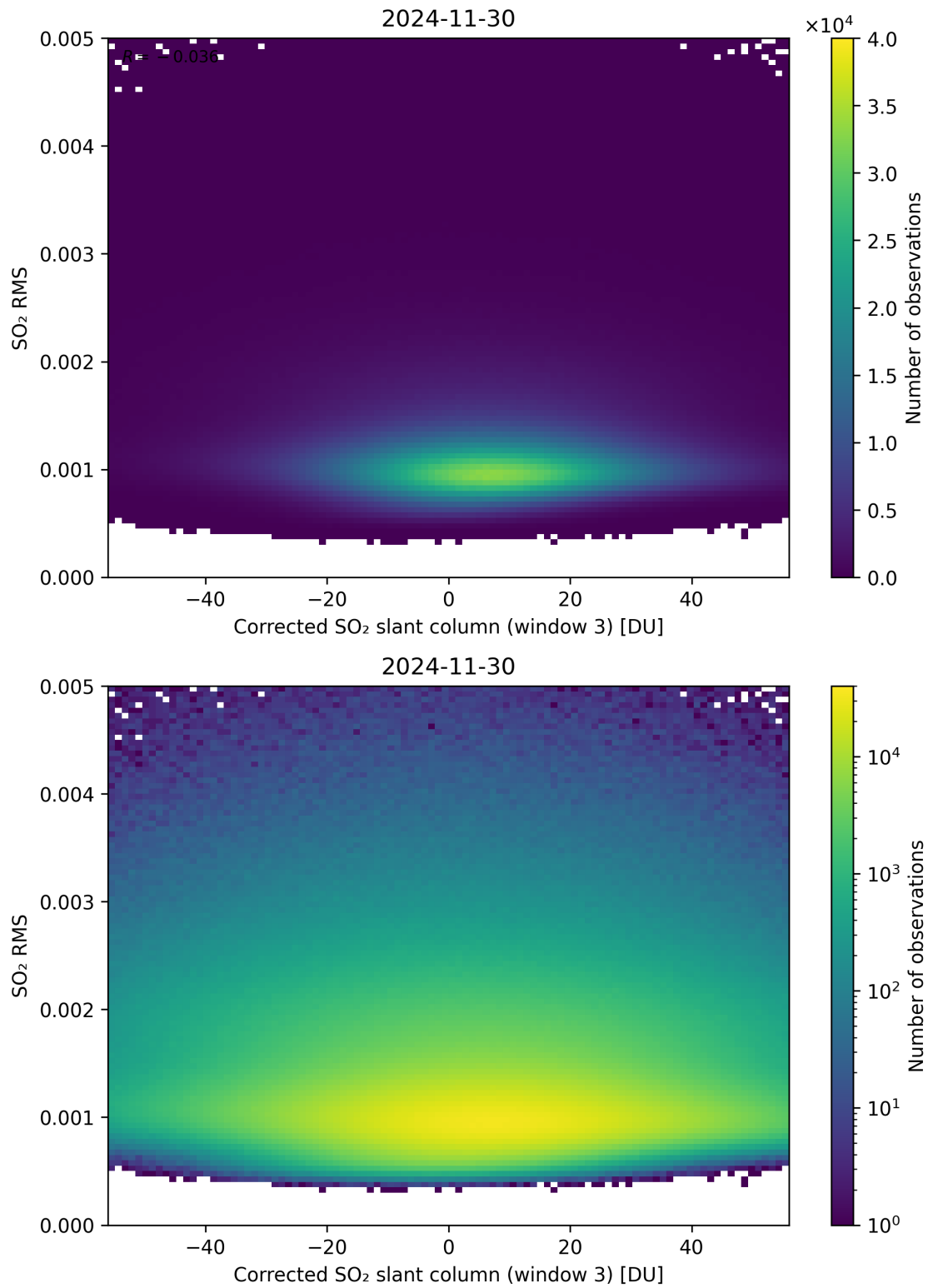
Figure 258: Scatter density plot of “Corrected SO 2 slant column (window 3)” against “SO 2 RMS” for 2024-11-30 to 2024-12-01.
