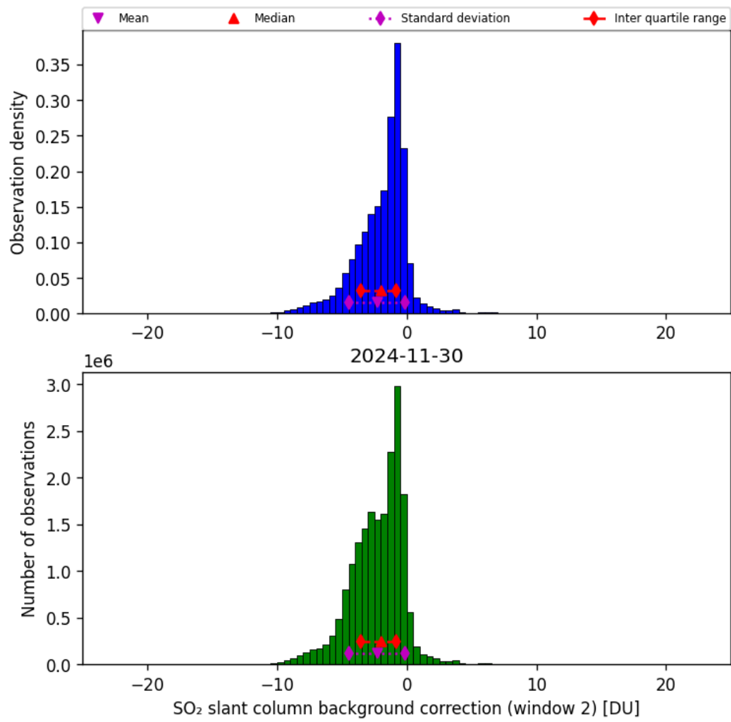
Figure 70: Histogram of “SO 2 slant column background correction (window 2)” for 2024-11-30 to 2024-12-01
