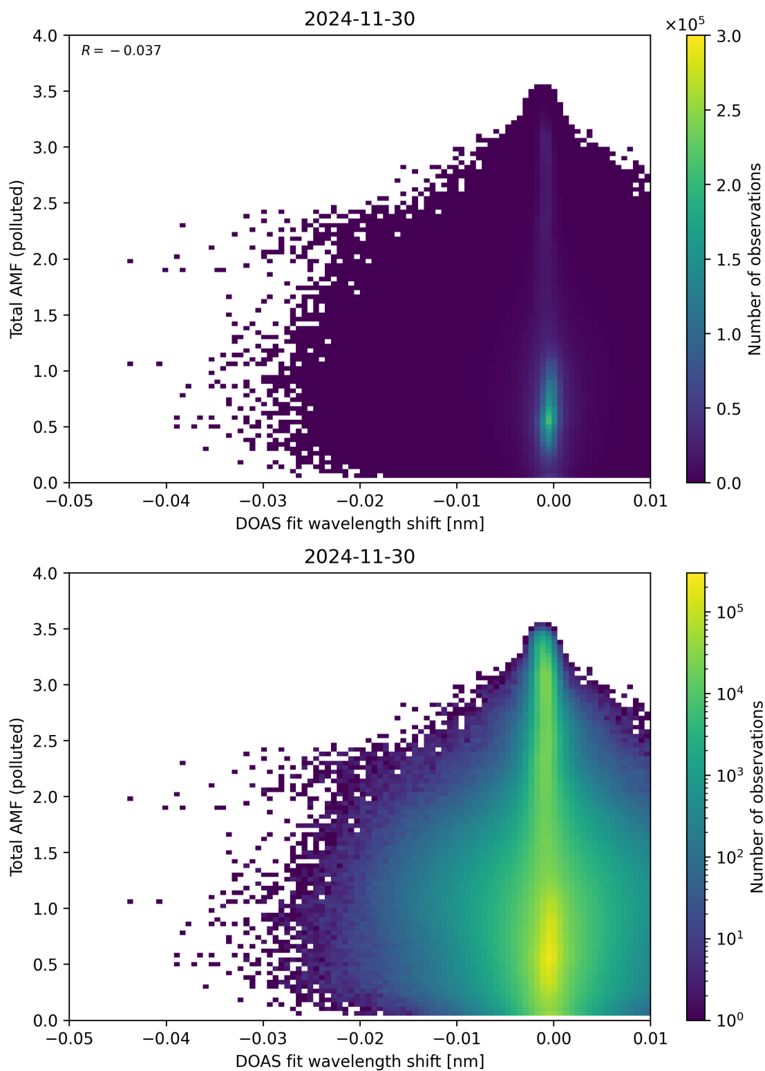
Figure 141: Scatter density plot of “DOAS fit wavelength shift” against “Total AMF (polluted)” for 2024-11-30 to 2024-12-01.
