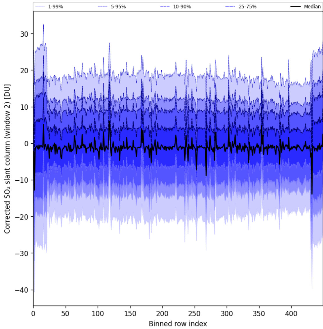
Figure 95: Along track statistics of “Corrected SO 2 slant column (window 2)” for 2024-11-30 to 2024-12-01
