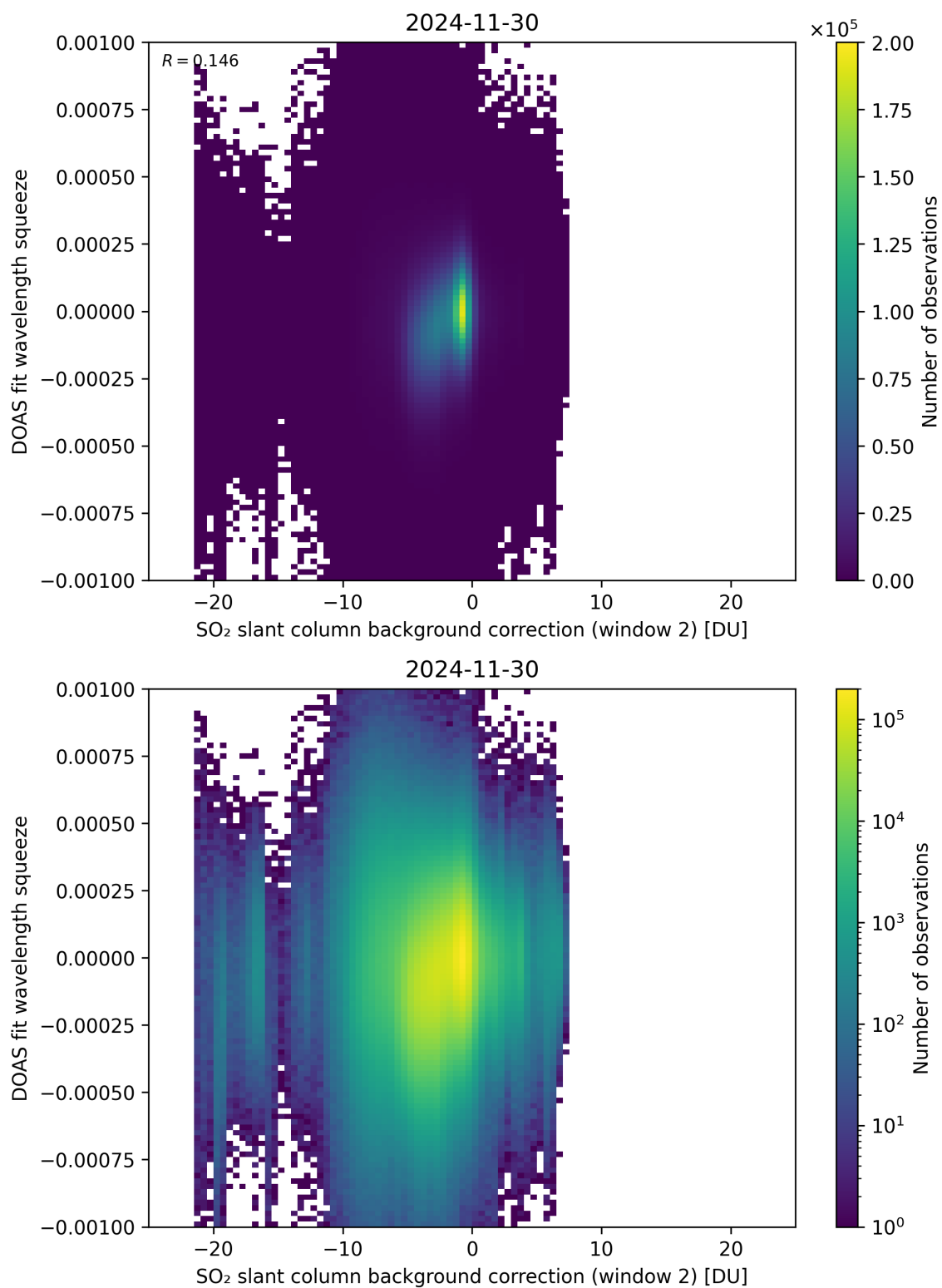
Figure 124: Scatter density plot of “SO 2 slant column background correction (window 2)” against “DOAS fit wavelength squeeze” for 2024-11-30 to 2024-12-01.
