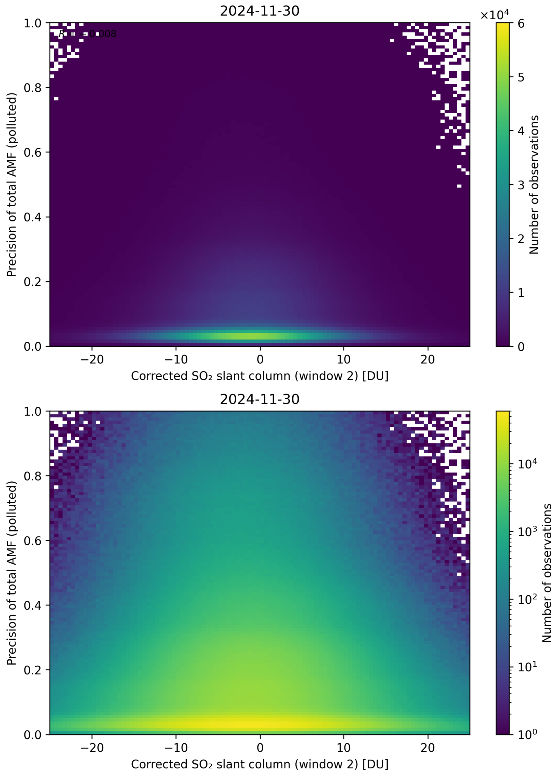
Figure 254: Scatter density plot of “Corrected SO 2 slant column (window 2)” against “Precision of total AMF (polluted)” for 2024-11-30 to 2024-12-01.
