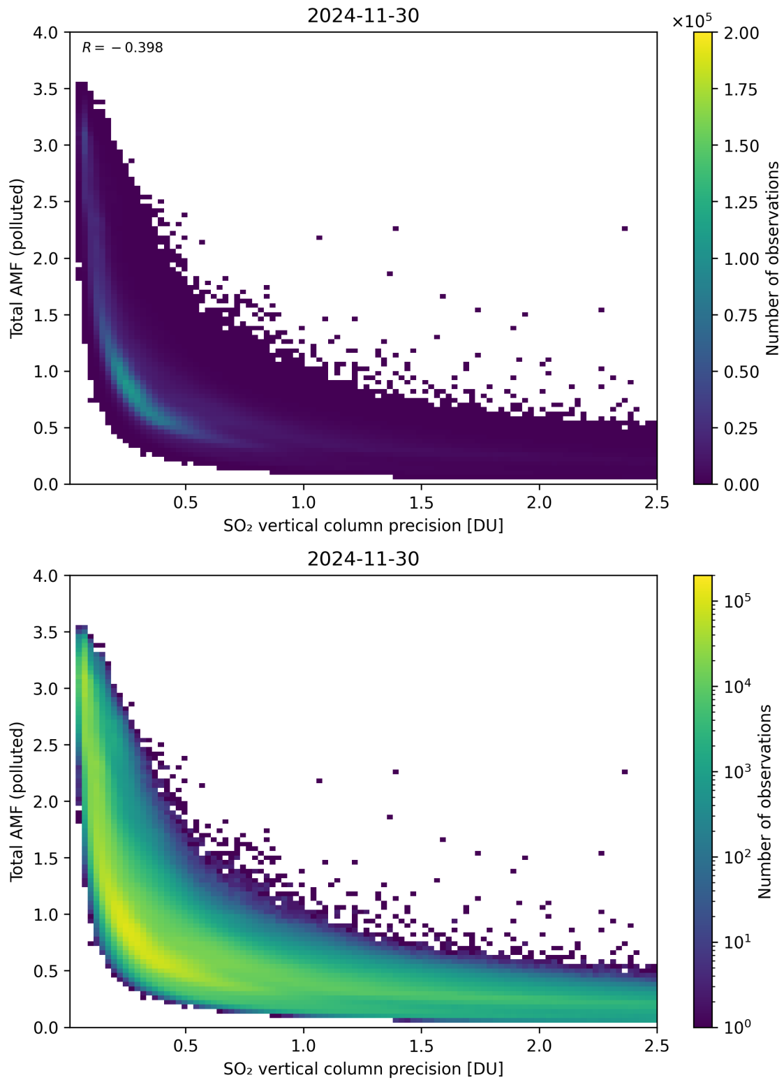
Figure 346: Scatter density plot of “SO 2 vertical column precision” against “Total AMF (polluted)” for 2024-11-30 to 2024-12-01.
