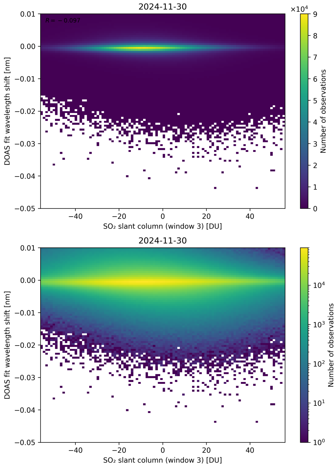
Figure 304: Scatter density plot of “SO 2 slant column (window 3)” against “DOAS fit wavelength shift” for 2024-11-30 to 2024-12-01.
