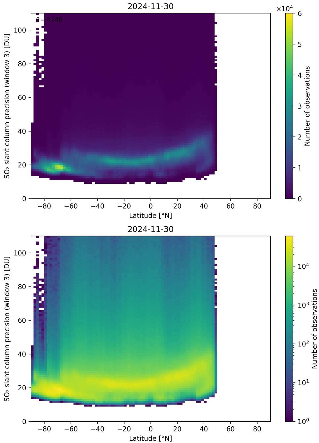
Figure 166: Scatter density plot of “Latitude” against “SO 2 slant column precision (window 3)” for 2024-11-30 to 2024-12-01.
