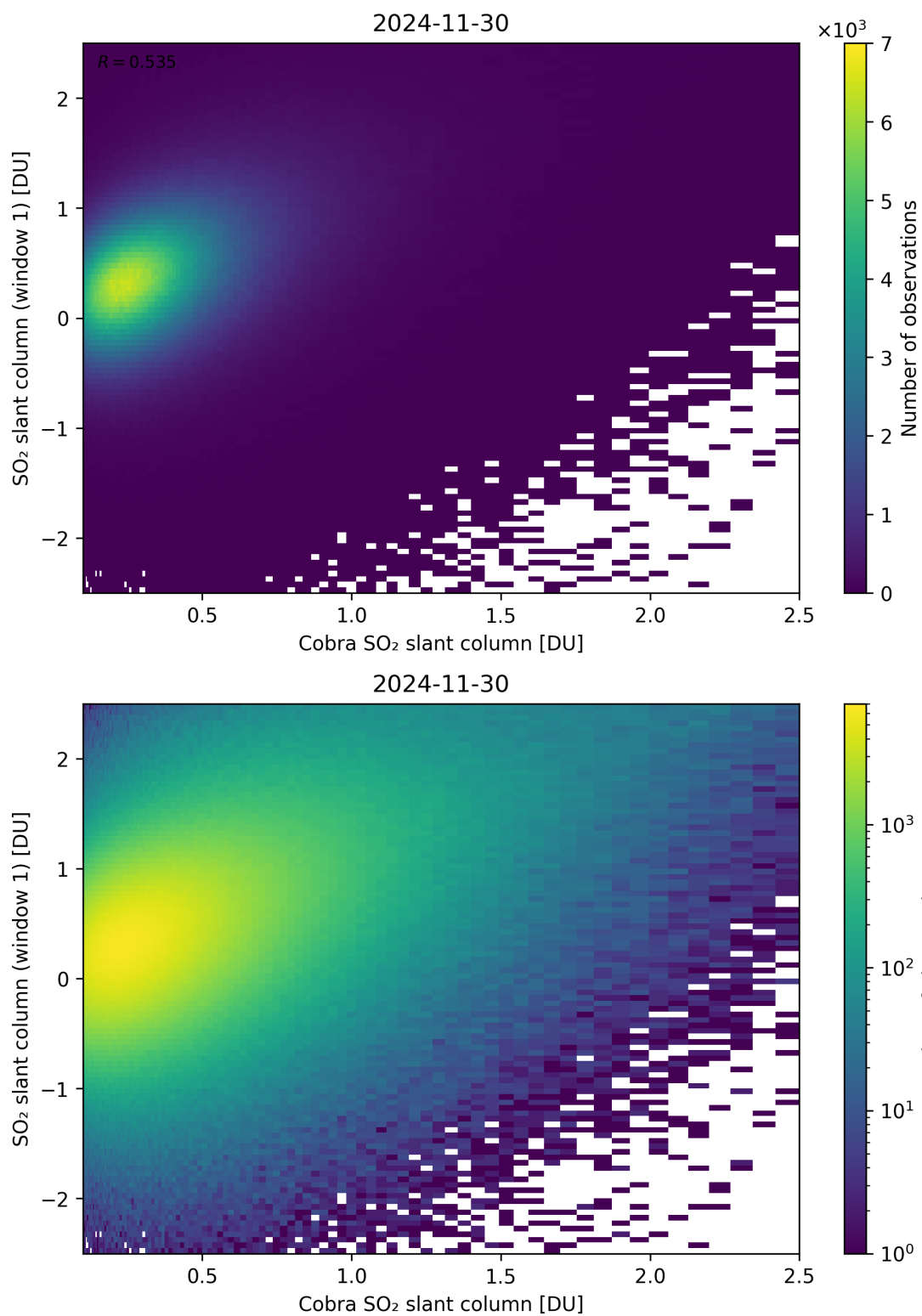
Figure 219: Scatter density plot of “Cobra SO 2 slant column” against “SO 2 slant column (window 1)” for 2024-11-30 to 2024-12-01.
