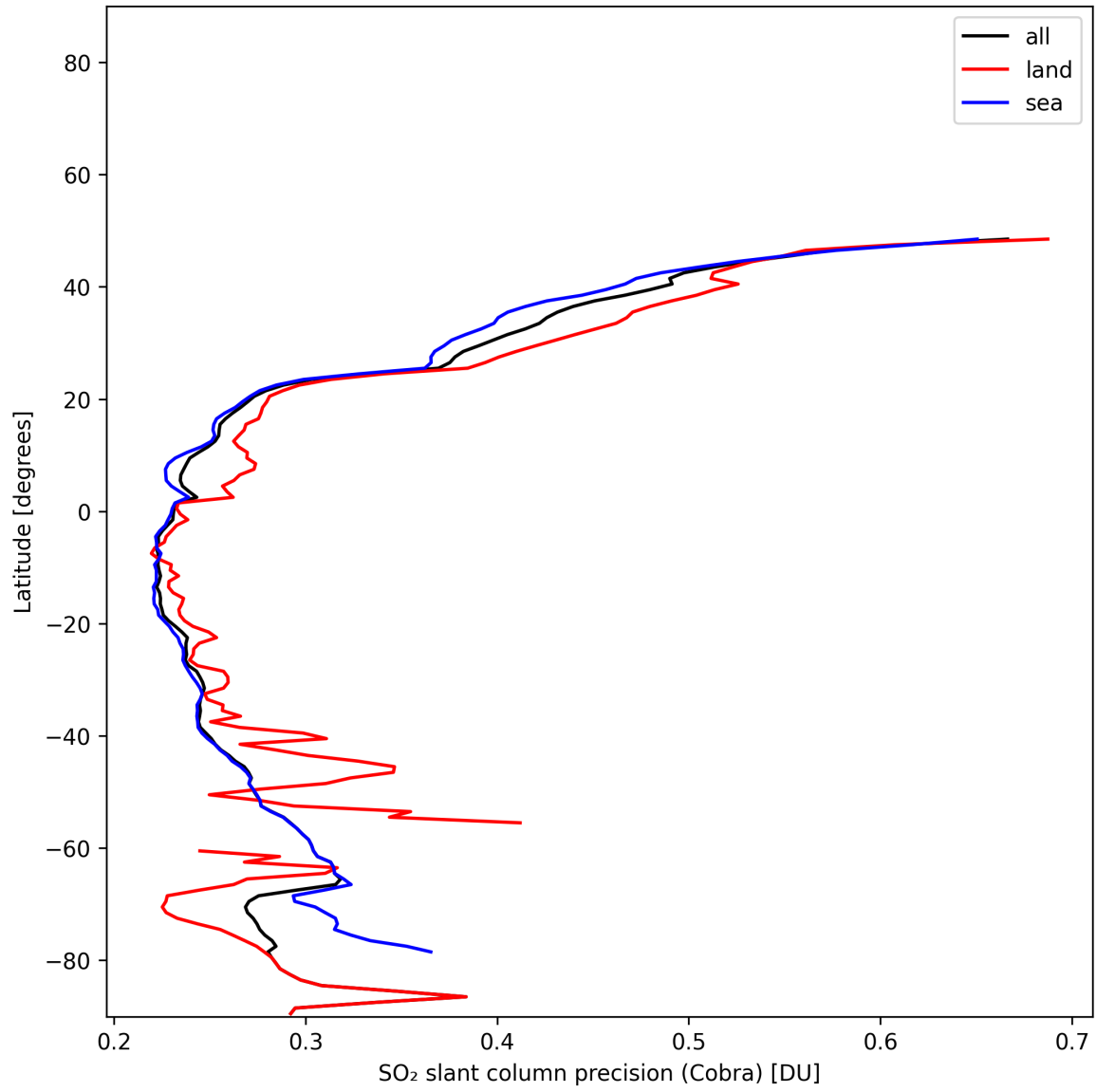
Figure 36: Zonal average of “SO 2 slant column precision (Cobra)” for 2024-11-30 to 2024-12-01.
