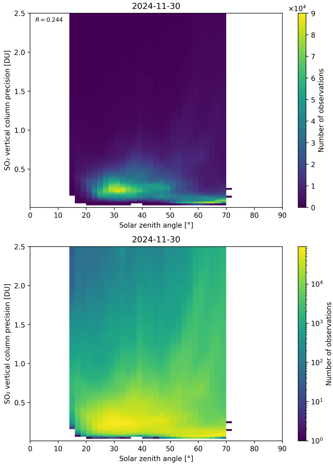
Figure 192: Scatter density plot of “Solar zenith angle” against “SO 2 vertical column precision” for 2024-11-30 to 2024-12-01.
