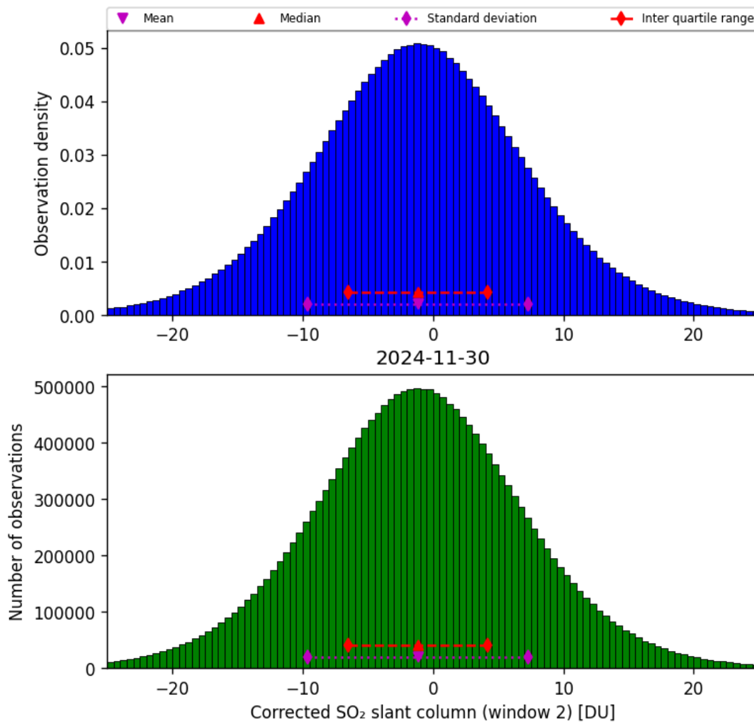
Figure 69: Histogram of “Corrected SO 2 slant column (window 2)” for 2024-11-30 to 2024-12-01
