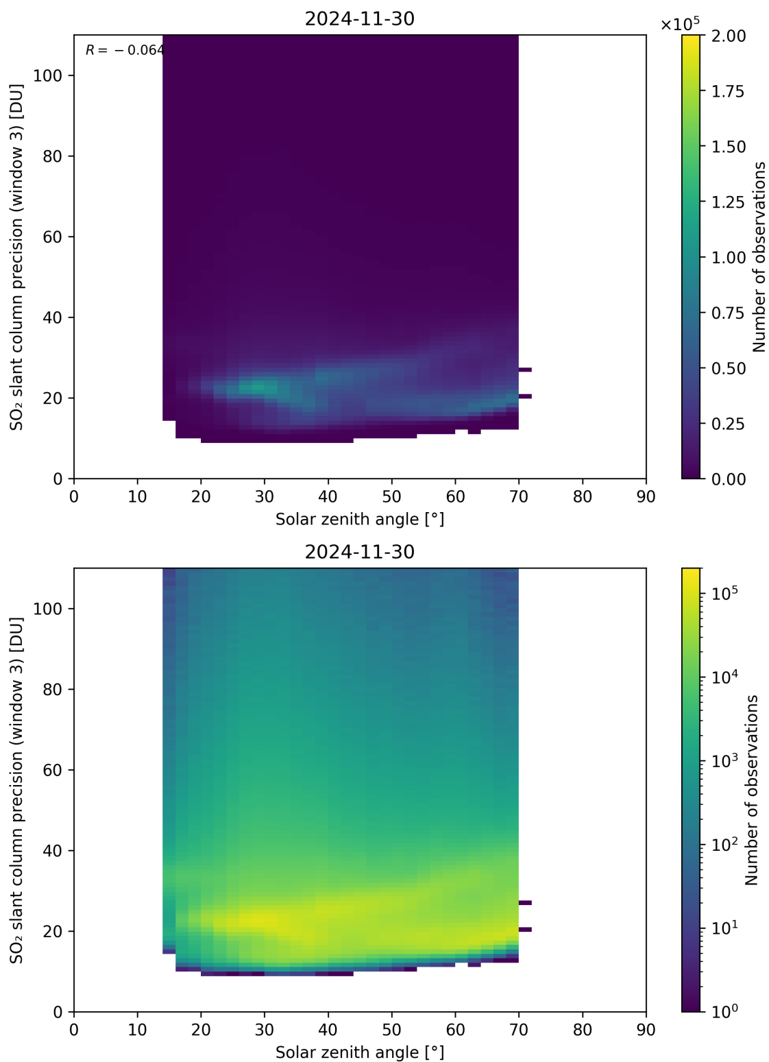
Figure 188: Scatter density plot of “Solar zenith angle” against “SO 2 slant column precision (window 3)” for 2024-11-30 to 2024-12-01.
