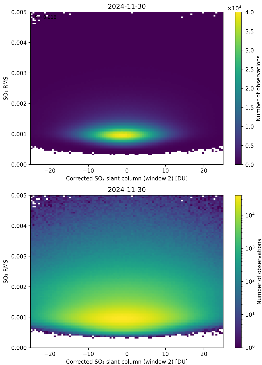
Figure 248: Scatter density plot of “Corrected SO 2 slant column (window 2)” against “SO 2 RMS” for 2024-11-30 to 2024-12-01.
