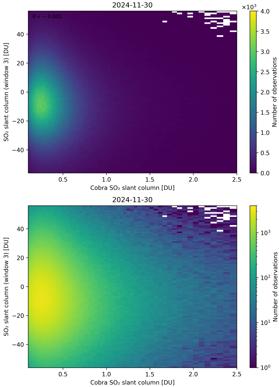
Figure 222: Scatter density plot of “Cobra SO 2 slant column” against “SO 2 slant column (window 3)” for 2024-11-30 to 2024-12-01.
