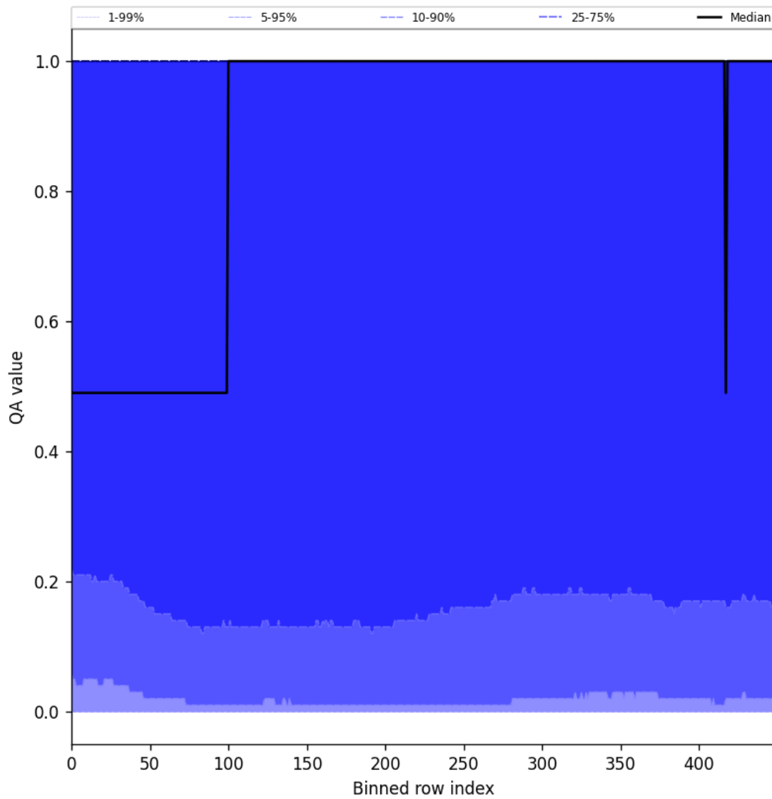
Figure 83: Along track statistics of “QA value” for 2024-11-30 to 2024-12-01
