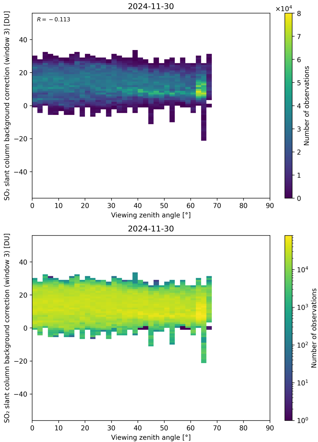
Figure 364: Scatter density plot of “Viewing zenith angle” against “SO 2 slant column background correction (window 3)” for 2024-11-30 to 2024-12-01.
