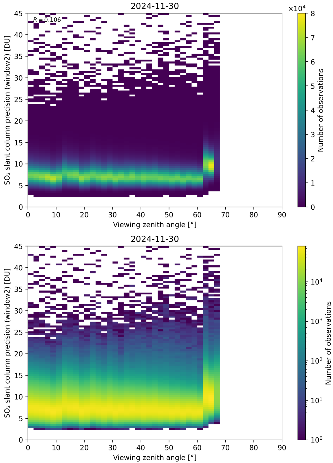
Figure 378: Scatter density plot of “Viewing zenith angle” against “SO 2 slant column precision (window2)” for 2024-11-30 to 2024-12-01.
