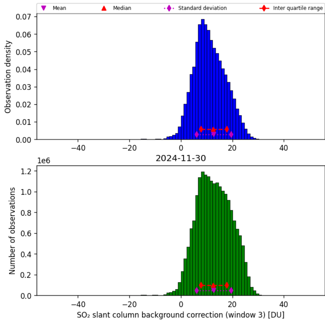
Figure 74: Histogram of “SO 2 slant column background correction (window 3)” for 2024-11-30 to 2024-12-01
