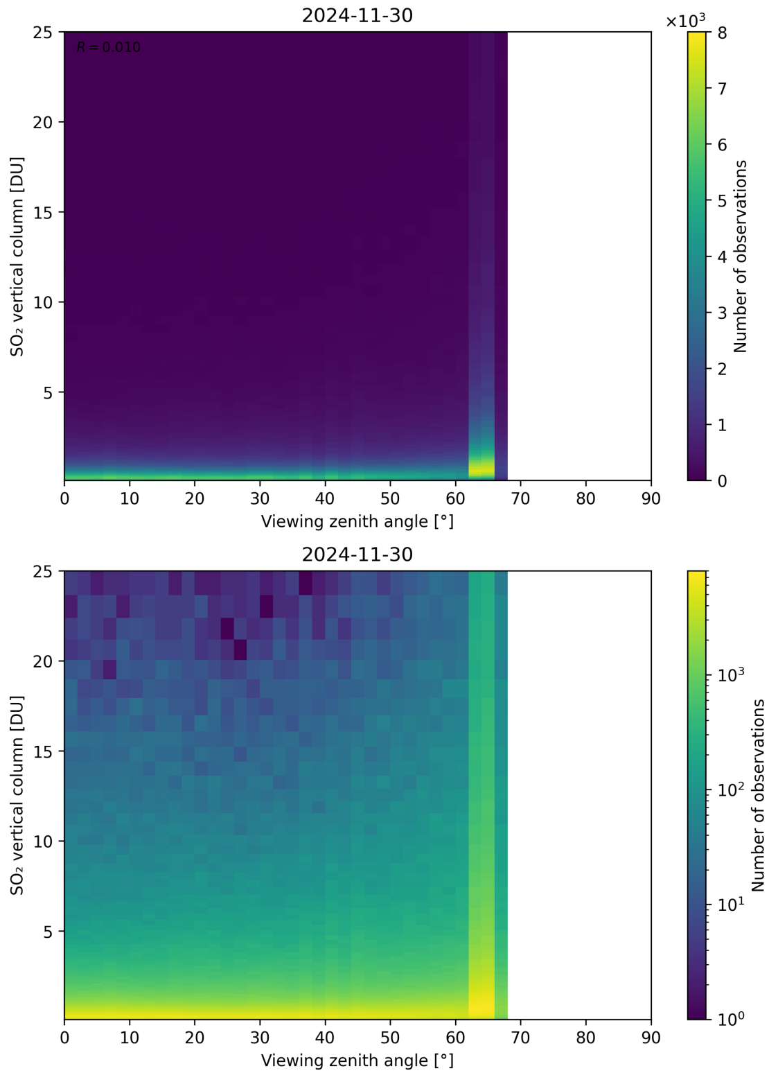
Figure 383: Scatter density plot of “Viewing zenith angle” against “SO 2 vertical column” for 2024-11-30 to 2024-12-01.
