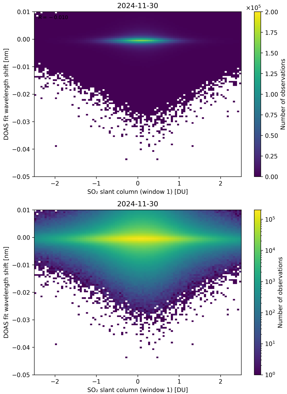
Figure 265: Scatter density plot of “SO 2 slant column (window 1)” against “DOAS fit wavelength shift” for 2024-11-30 to 2024-12-01.
