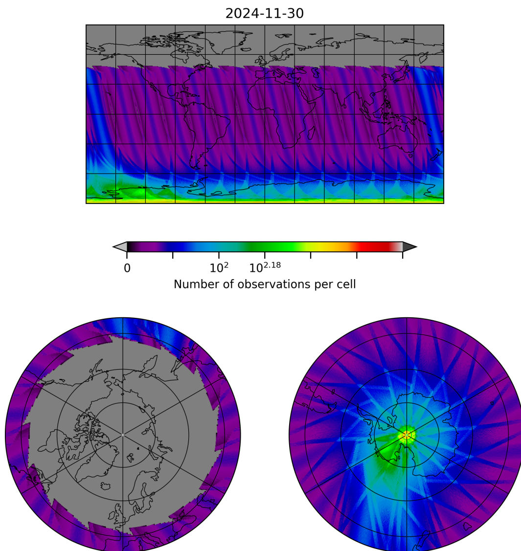
Figure 30: Map of the number of observations for 2024-11-30 to 2024-12-01
