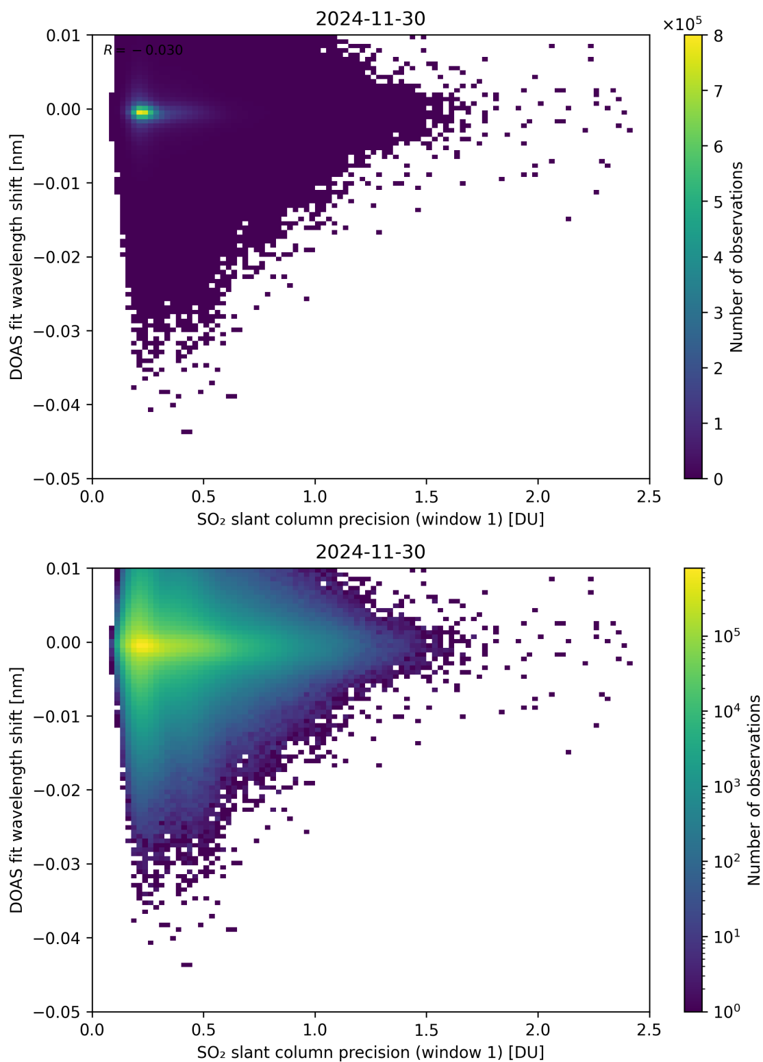
Figure 271: Scatter density plot of “SO 2 slant column precision (window 1)” against “DOAS fit wavelength shift” for 2024-11-30 to 2024-12-01.
