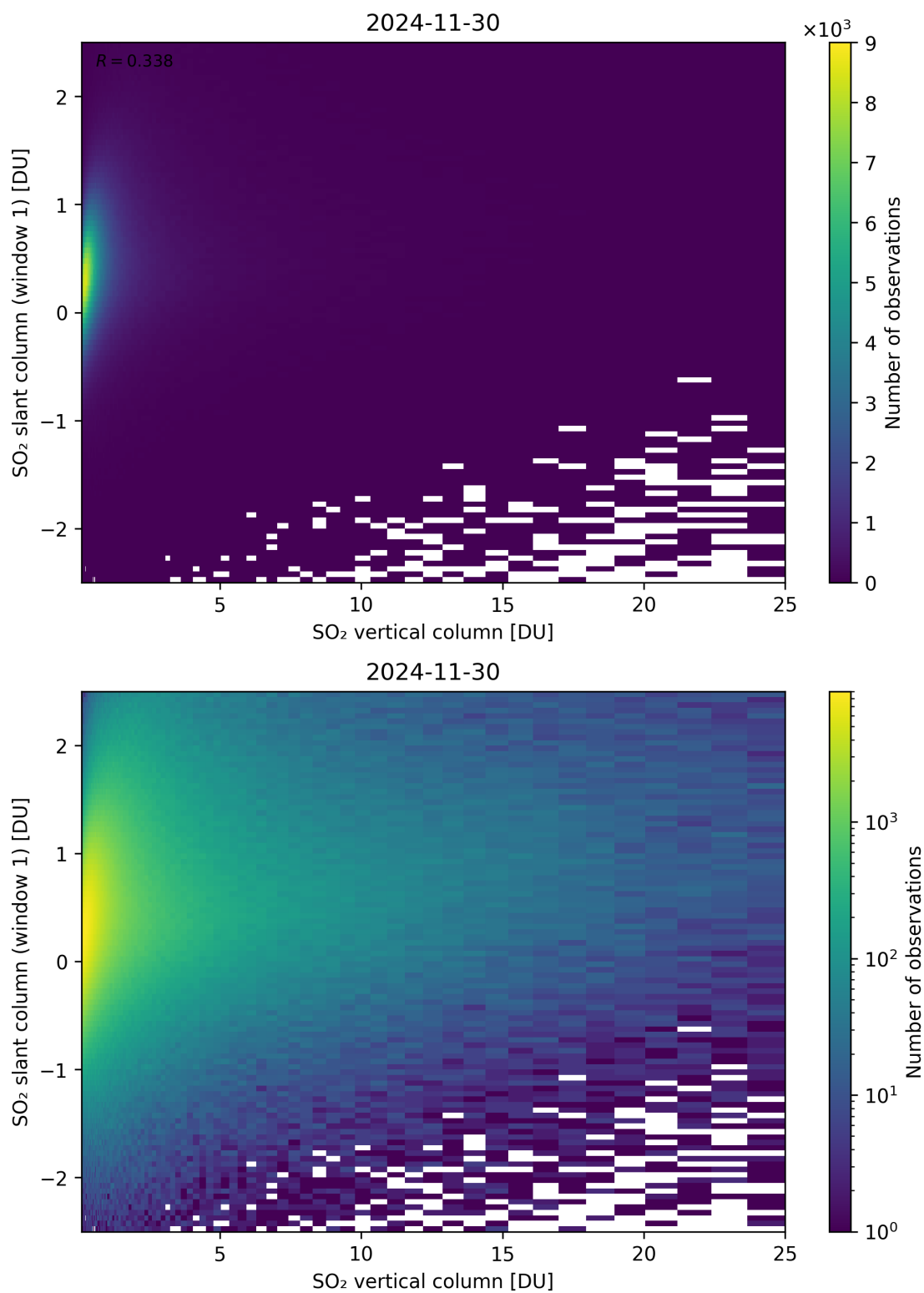
Figure 354: Scatter density plot of “SO 2 vertical column” against “SO 2 slant column (window 1)” for 2024-11-30 to 2024-12-01.
