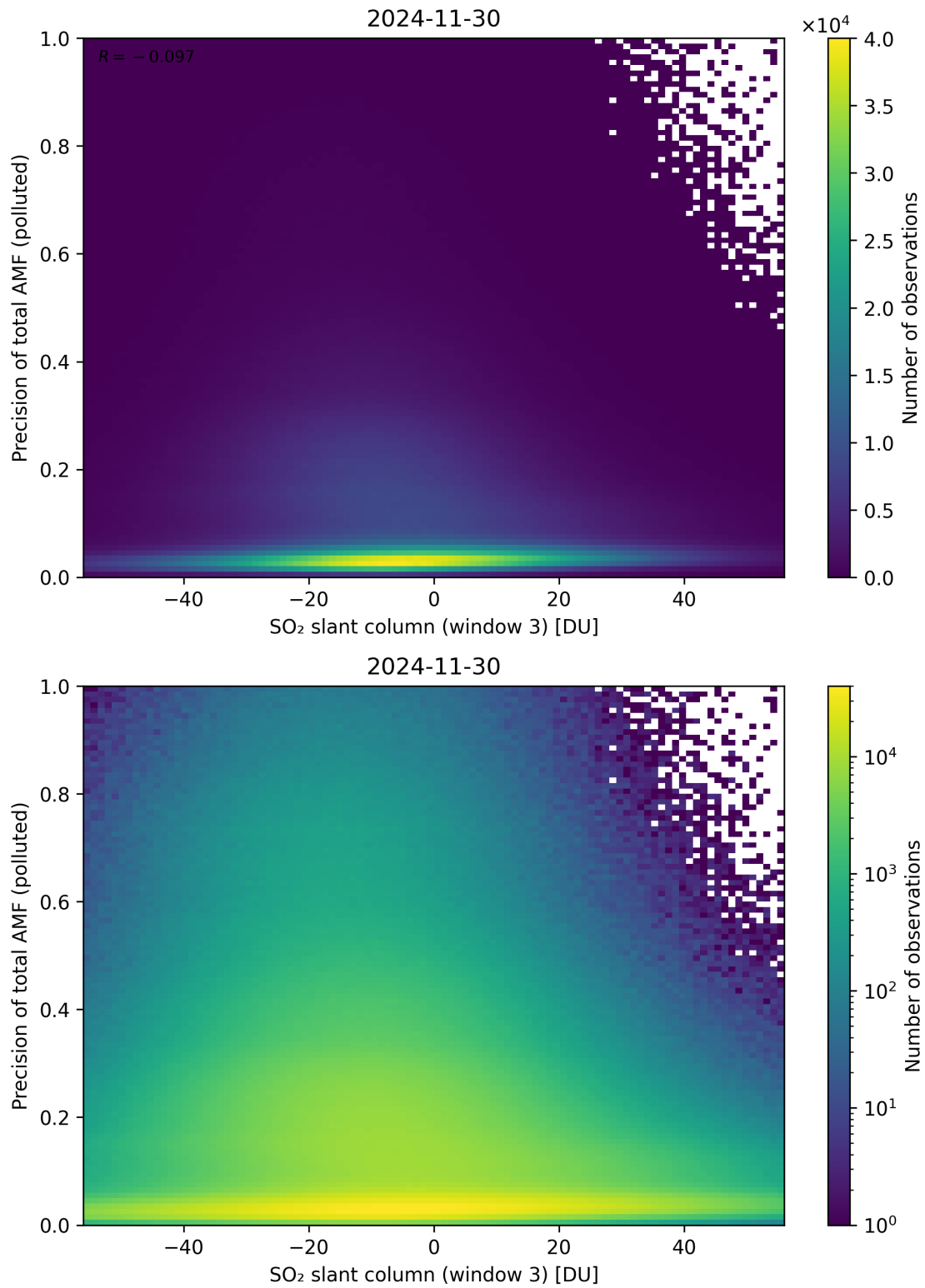
Figure 319: Scatter density plot of “SO 2 slant column (window 3)” against “Precision of total AMF (polluted)” for 2024-11-30 to 2024-12-01.
