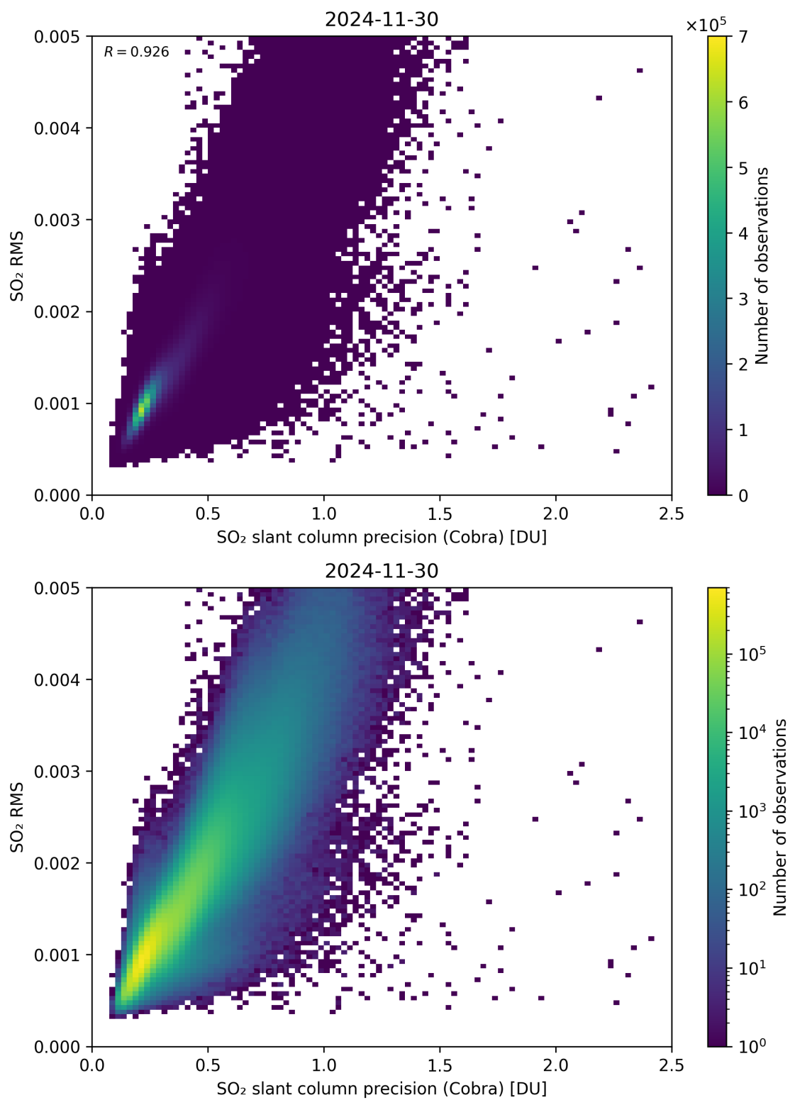
Figure 204: Scatter density plot of “SO 2 slant column precision (Cobra)” against “SO 2 RMS” for 2024-11-30 to 2024-12-01.
