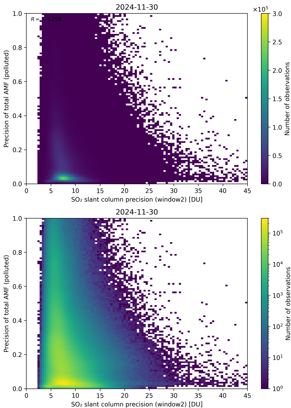
Figure 302: Scatter density plot of “SO 2 slant column precision (window2)” against “Precision of total AMF (polluted)” for 2024-11-30 to 2024-12-01.
