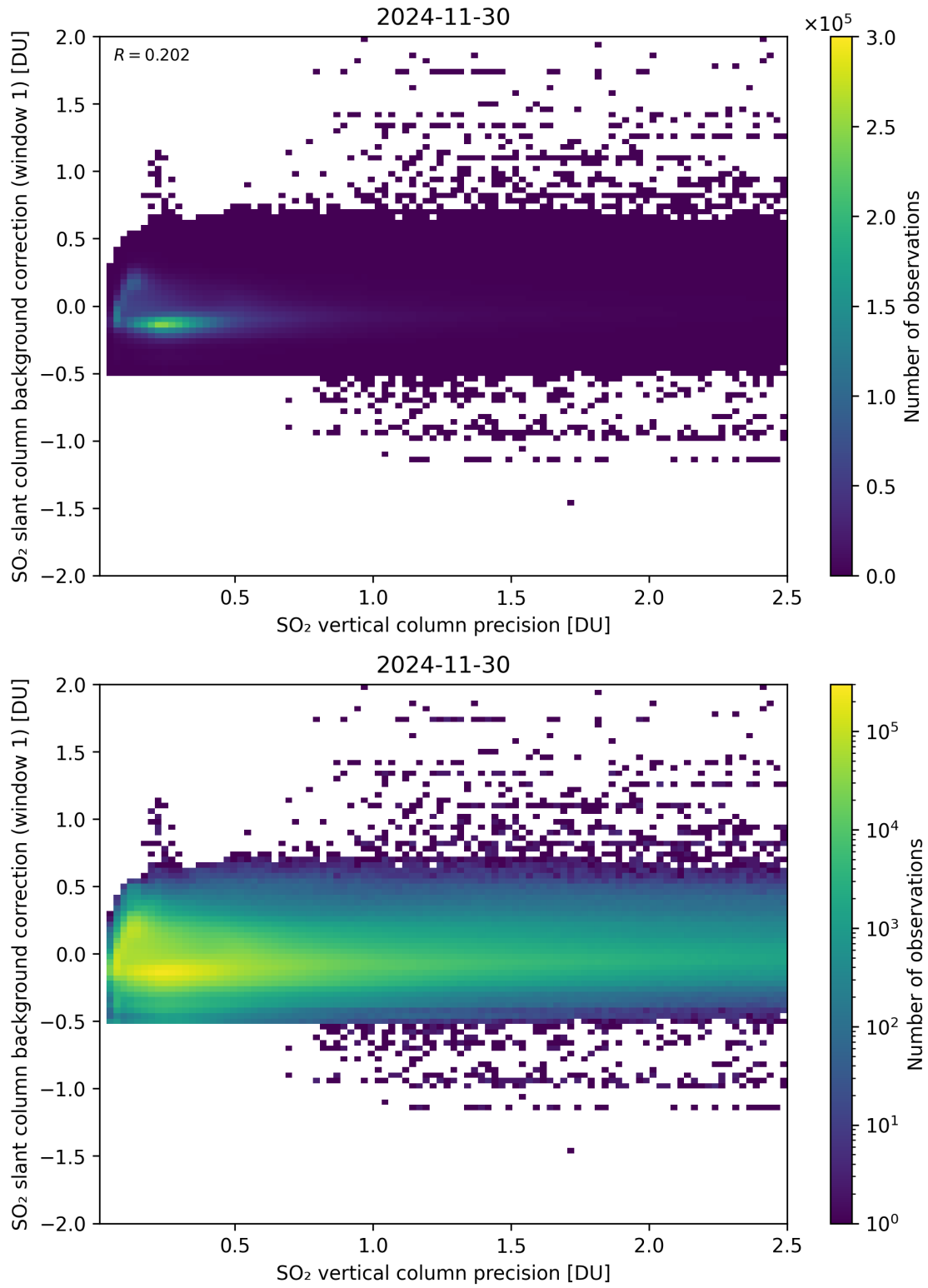
Figure 329: Scatter density plot of “SO 2 vertical column precision” against “SO 2 slant column background correction (window 1)” for 2024-11-30 to 2024-12-01.
