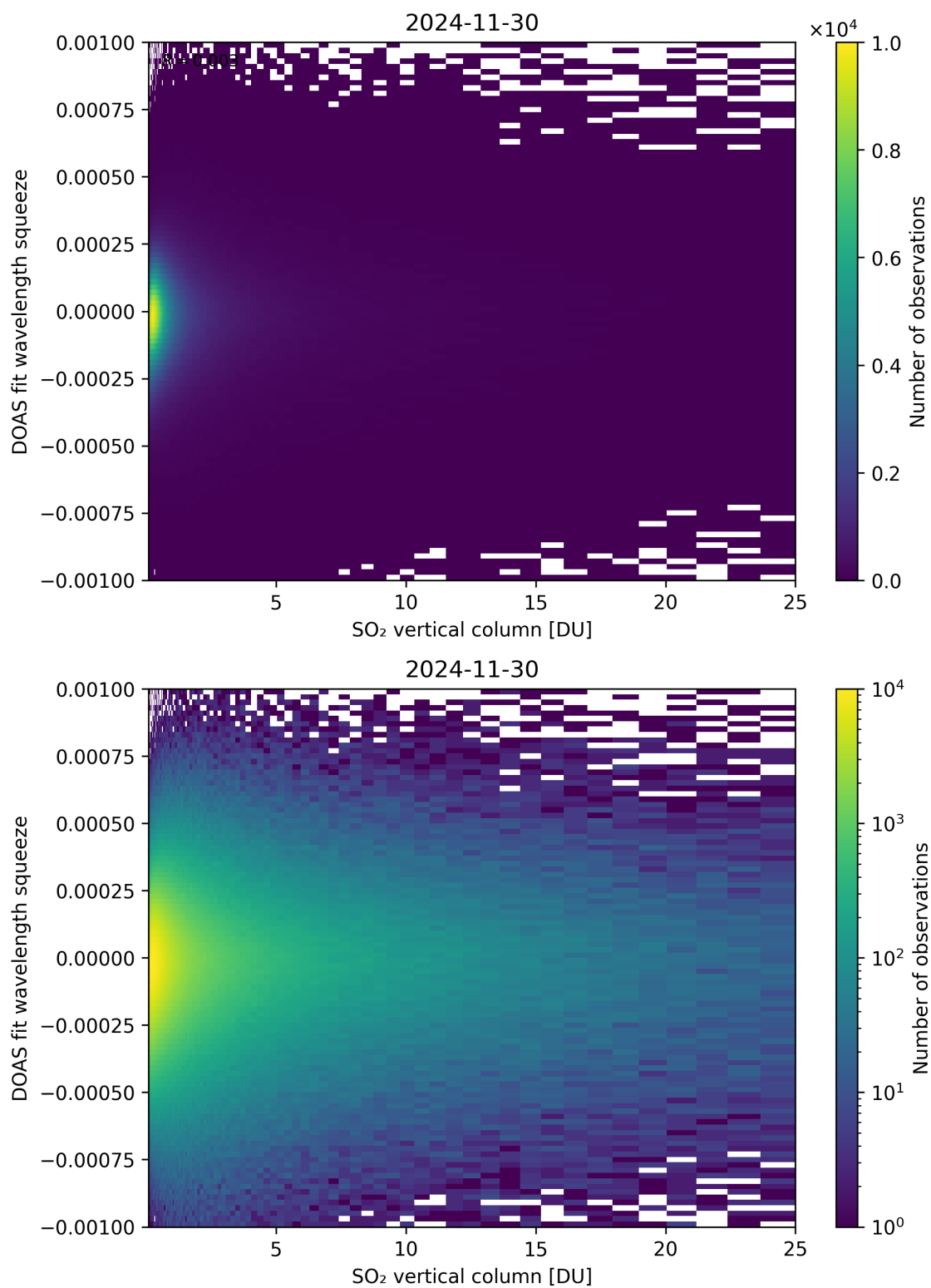
Figure 327: Scatter density plot of “SO 2 vertical column” against “DOAS fit wavelength squeeze” for 2024-11-30 to 2024-12-01.
