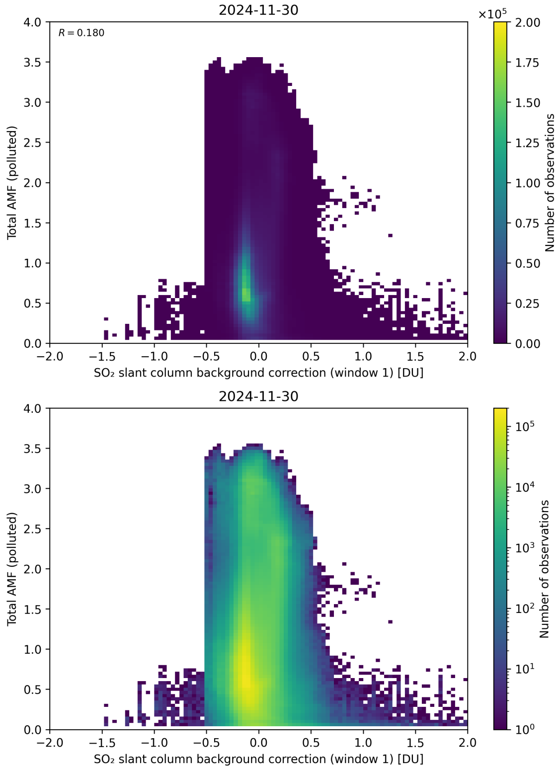
Figure 120: Scatter density plot of “SO 2 slant column background correction (window 1)” against “Total AMF (polluted)” for 2024-11-30 to 2024-12-01.
