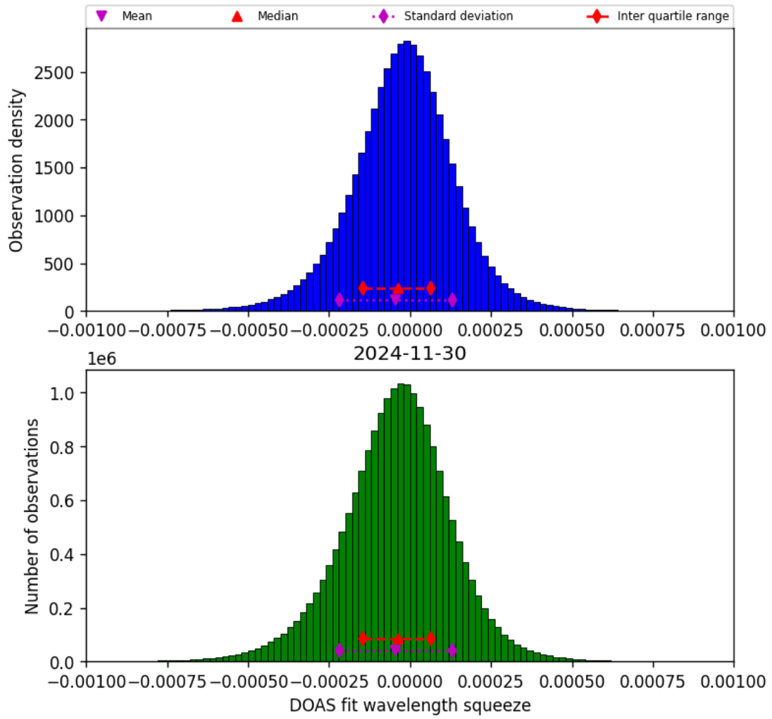
Figure 77: Histogram of “DOAS fit wavelength squeeze” for 2024-11-30 to 2024-12-01
