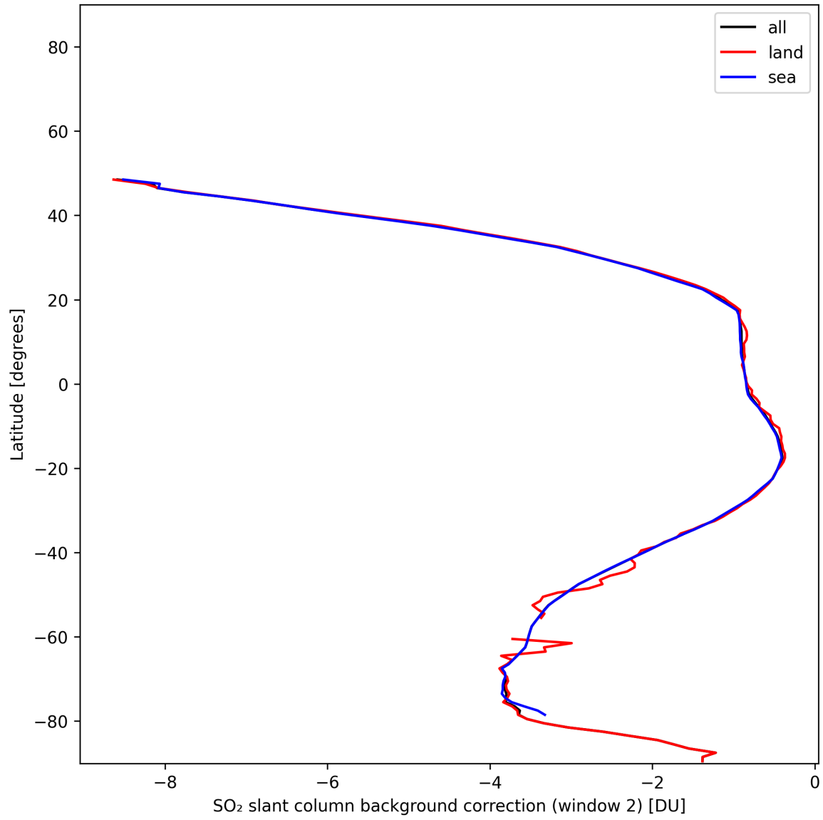
Figure 44: Zonal average of “SO 2 slant column background correction (window 2)” for 2024-11-30 to 2024-12-01.
