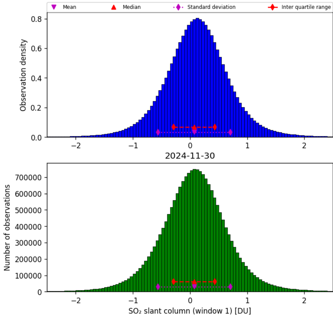
Figure 63: Histogram of “SO 2 slant column (window 1)” for 2024-11-30 to 2024-12-01
