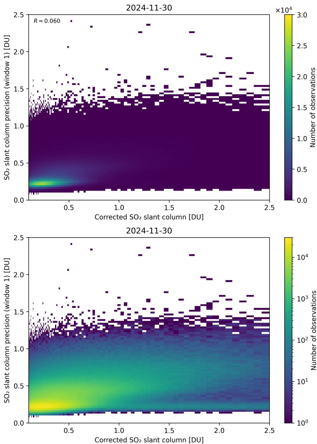
Figure 238: Scatter density plot of “Corrected SO 2 slant column” against “SO 2 slant column precision (window 1)” for 2024-11-30 to 2024-12-01.
