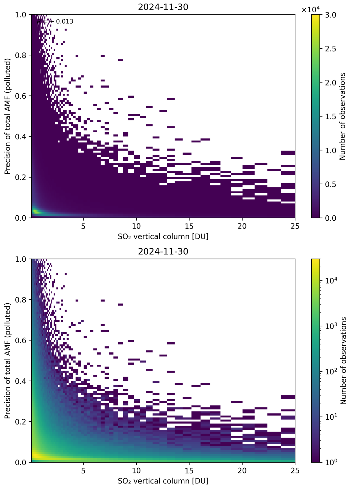
Figure 360: Scatter density plot of “SO 2 vertical column” against “Precision of total AMF (polluted)” for 2024-11-30 to 2024-12-01.
