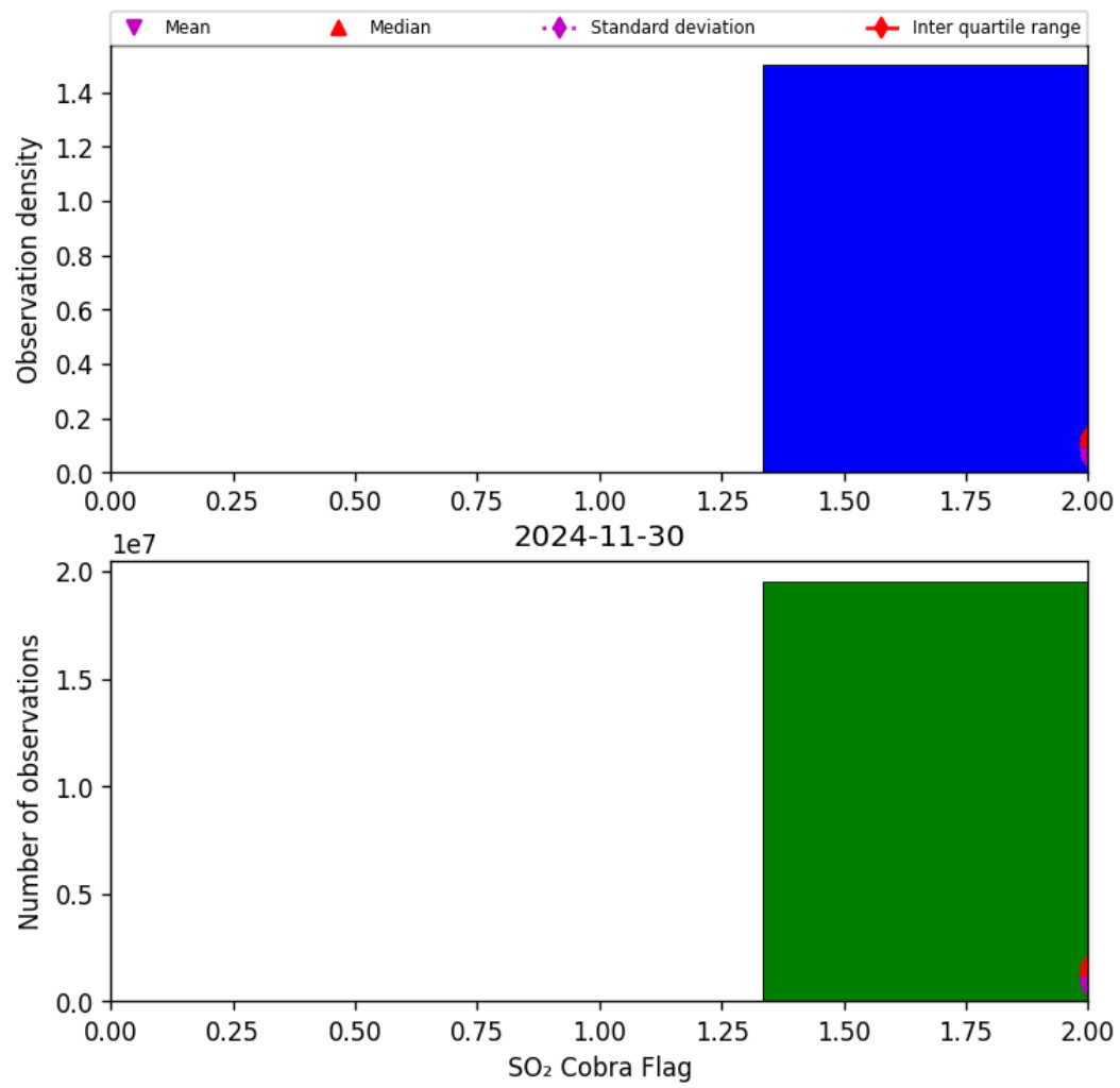
Figure 75: Histogram of “SO 2 Cobra Flag” for 2024-11-30 to 2024-12-01
