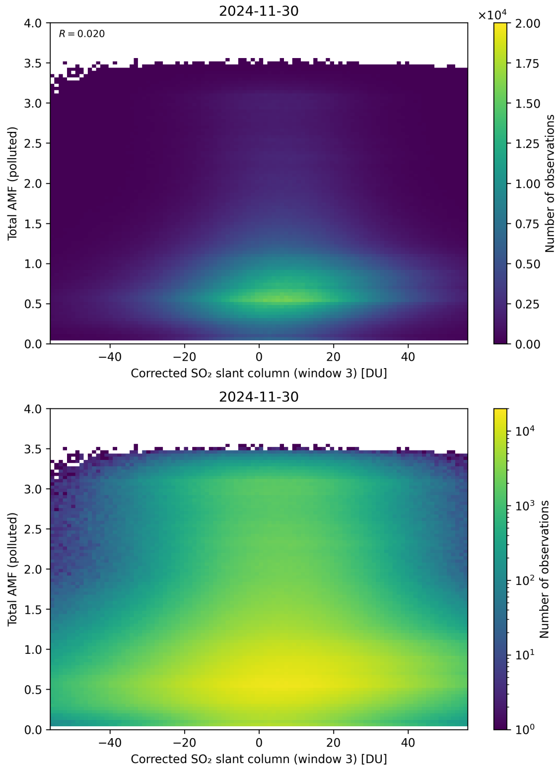
Figure 260: Scatter density plot of “Corrected SO 2 slant column (window 3)” against “Total AMF (polluted)” for 2024-11-30 to 2024-12-01.
