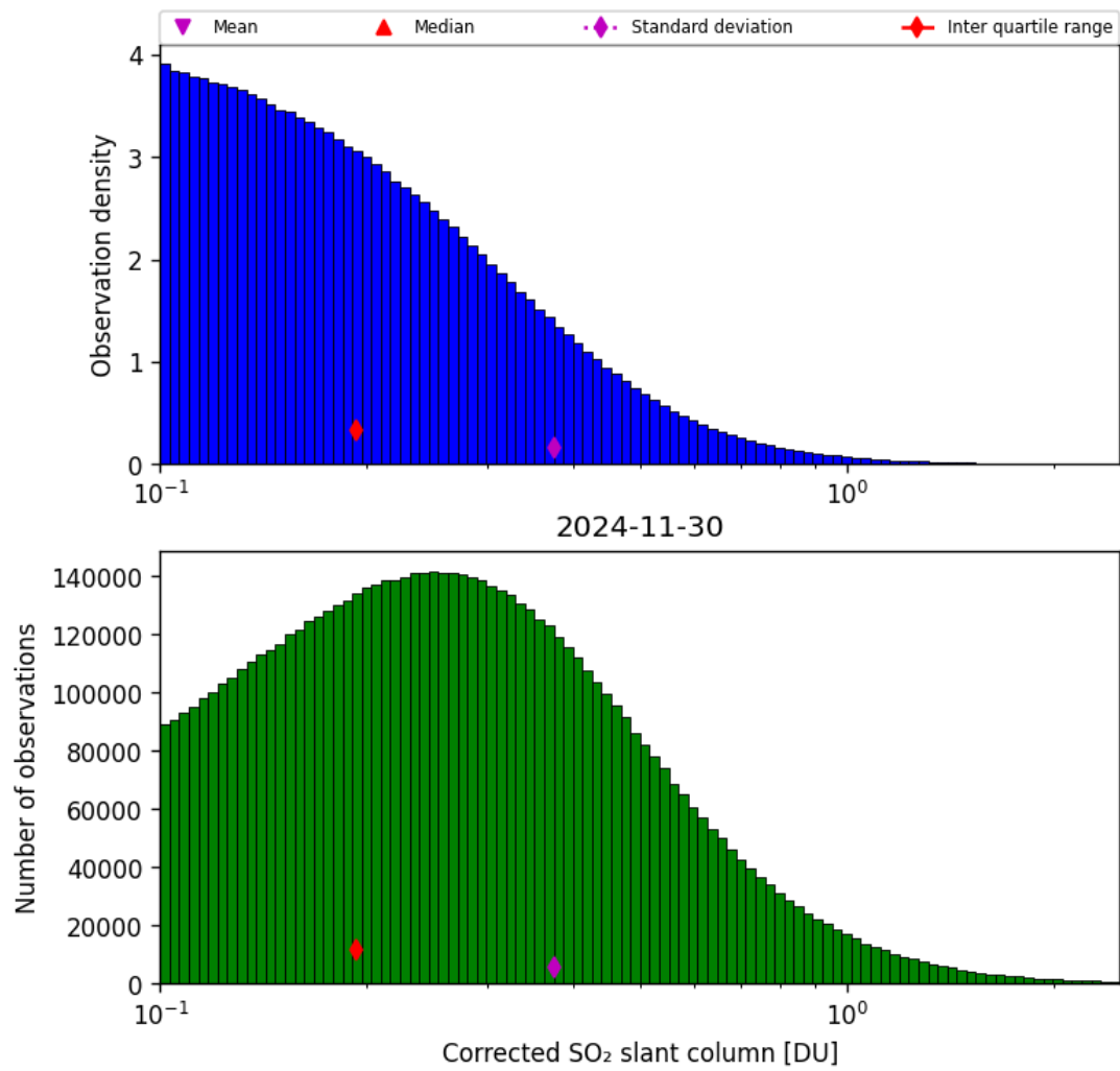
Figure 60: Histogram of “Corrected SO 2 slant column” for 2024-11-30 to 2024-12-01
