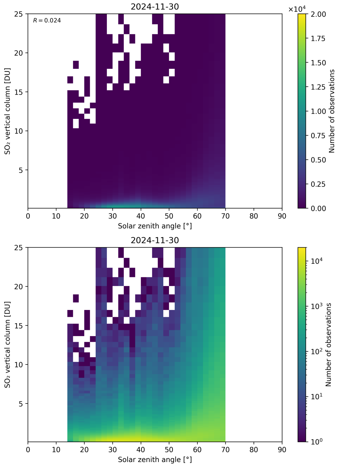
Figure 191: Scatter density plot of “Solar zenith angle” against “SO 2 vertical column” for 2024-11-30 to 2024-12-01.
