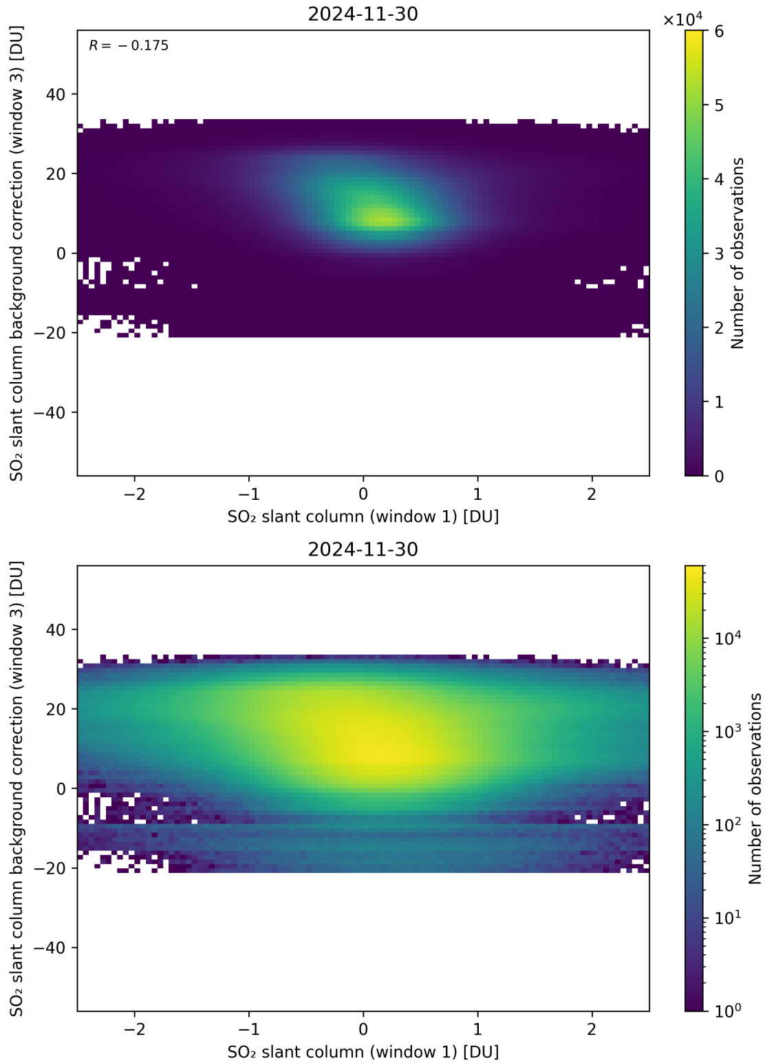
Figure 264: Scatter density plot of “SO 2 slant column (window 1)” against “SO 2 slant column background correction (window 3)” for 2024-11-30 to 2024-12-01.
