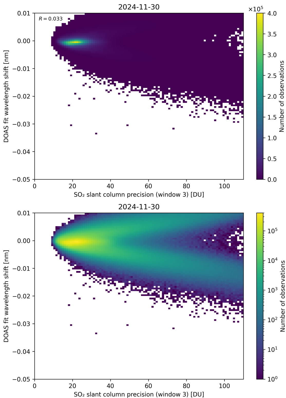
Figure 308: Scatter density plot of “SO 2 slant column precision (window 3)” against “DOAS fit wavelength shift” for 2024-11-30 to 2024-12-01.
