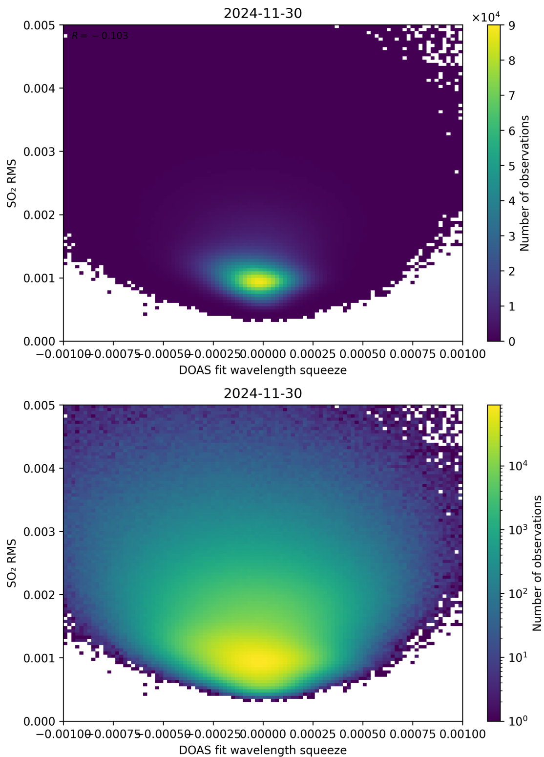
Figure 143: Scatter density plot of “DOAS fit wavelength squeeze” against “SO 2 RMS” for 2024-11-30 to 2024-12-01.
