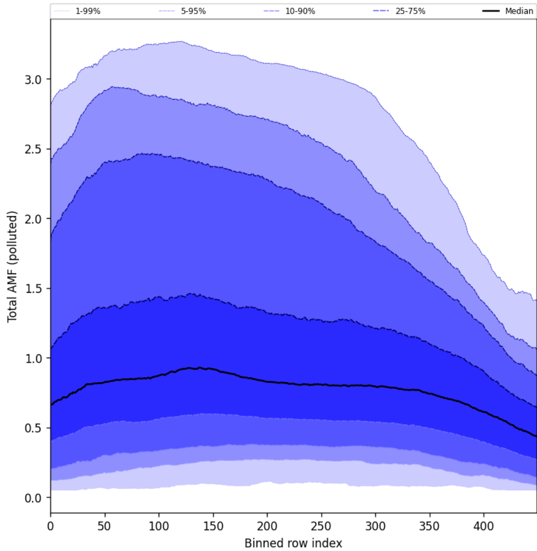
Figure 105: Along track statistics of “Total AMF (polluted)” for 2024-11-30 to 2024-12-01
