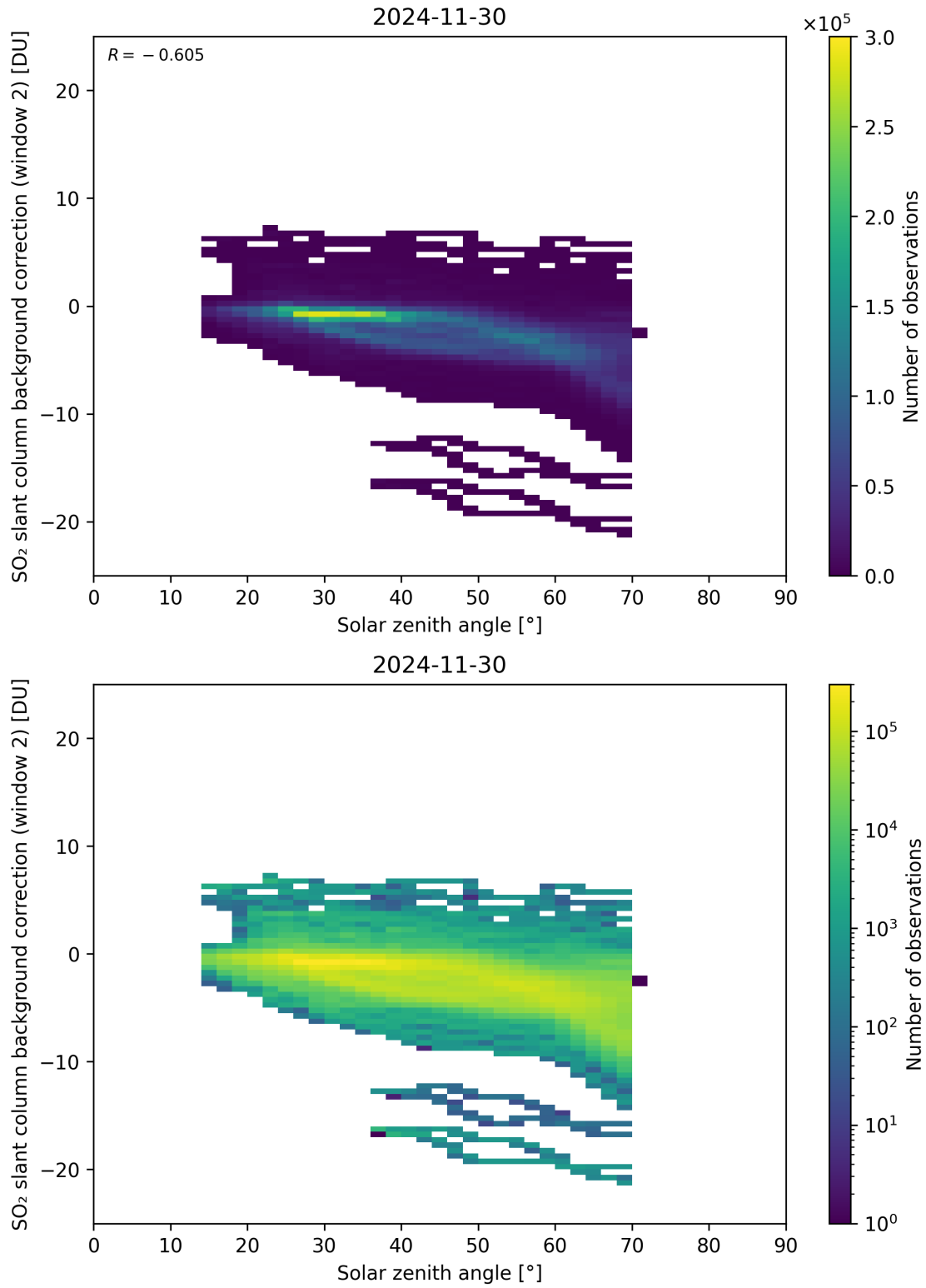
Figure 172: Scatter density plot of “Solar zenith angle” against “SO 2 slant column background correction (window 2)” for 2024-11-30 to 2024-12-01.
