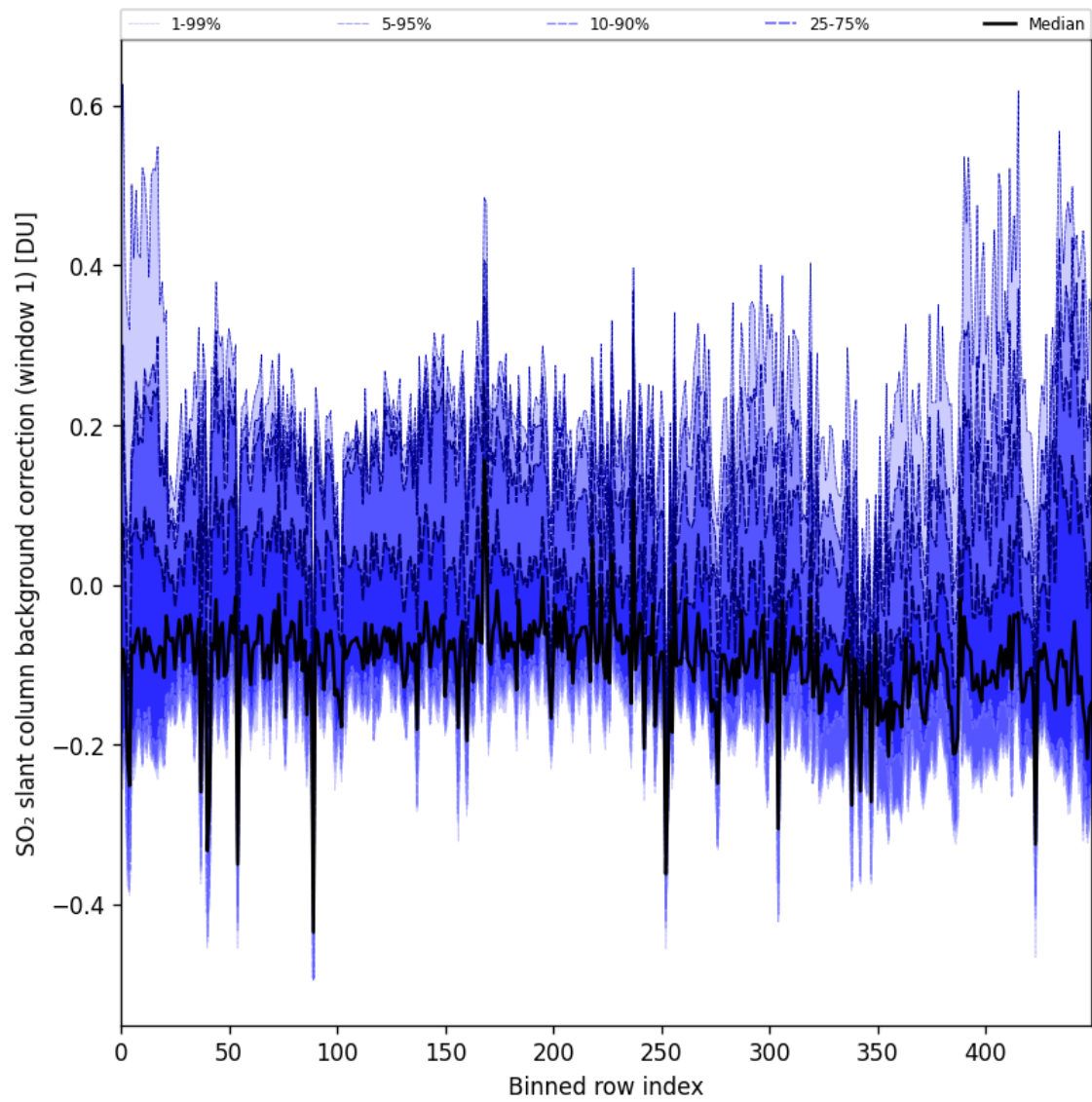
Figure 92: Along track statistics of “SO 2 slant column background correction (window 1)” for 2024-11-30 to 2024-12-01
