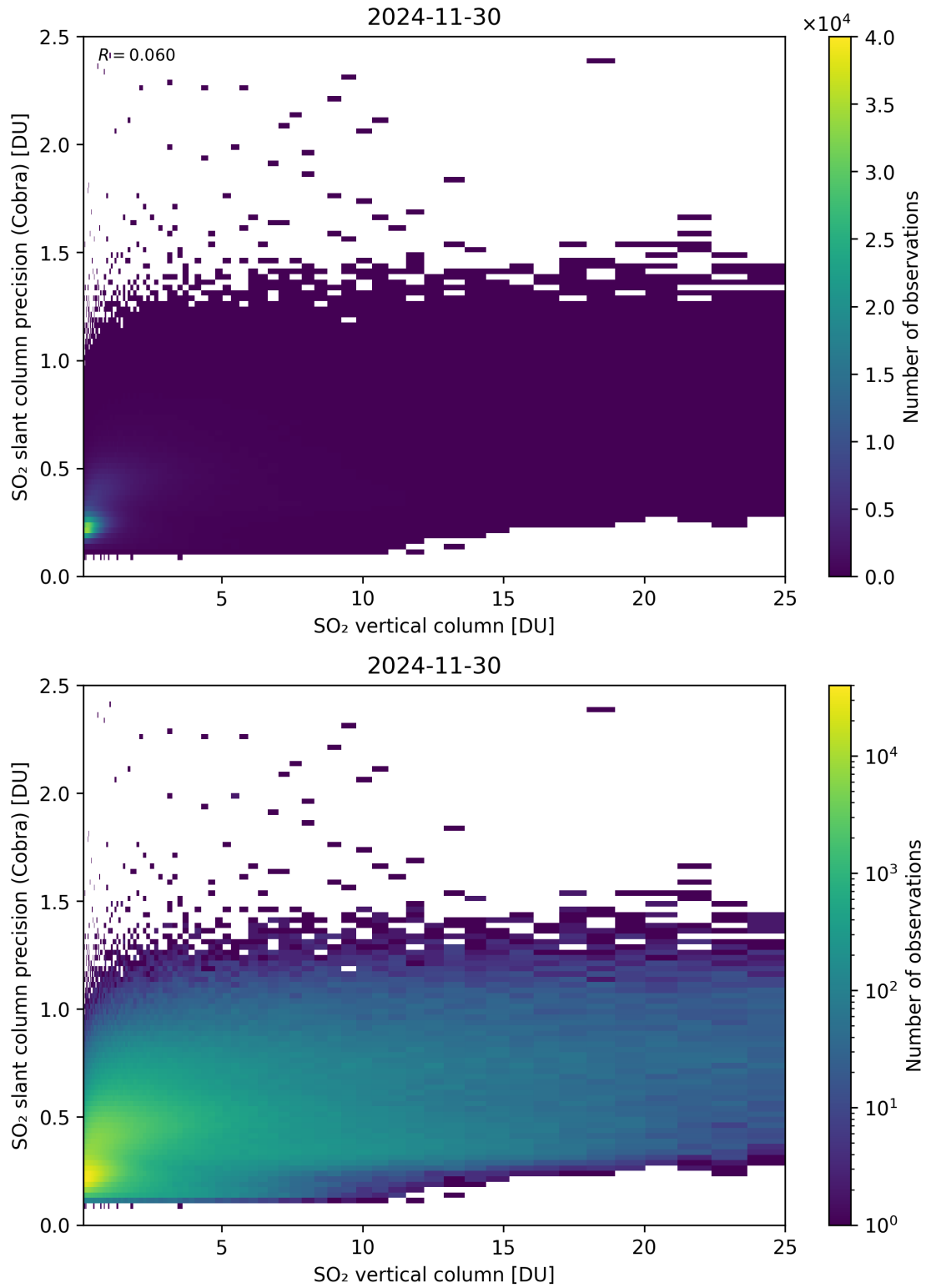
Figure 350: Scatter density plot of “SO 2 vertical column” against “SO 2 slant column precision (Cobra)” for 2024-11-30 to 2024-12-01.
