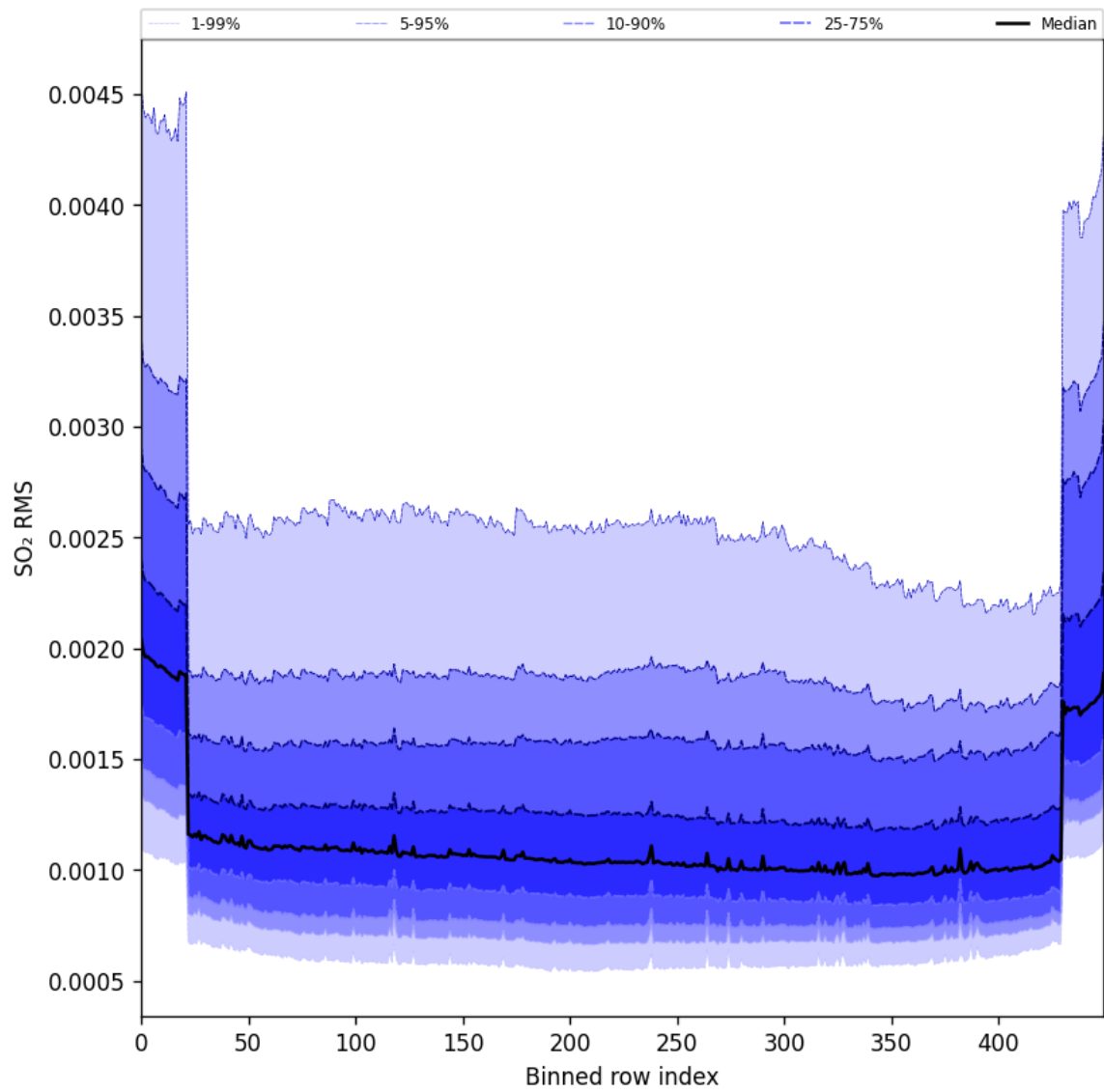
Figure 104: Along track statistics of “SO 2 RMS” for 2024-11-30 to 2024-12-01
