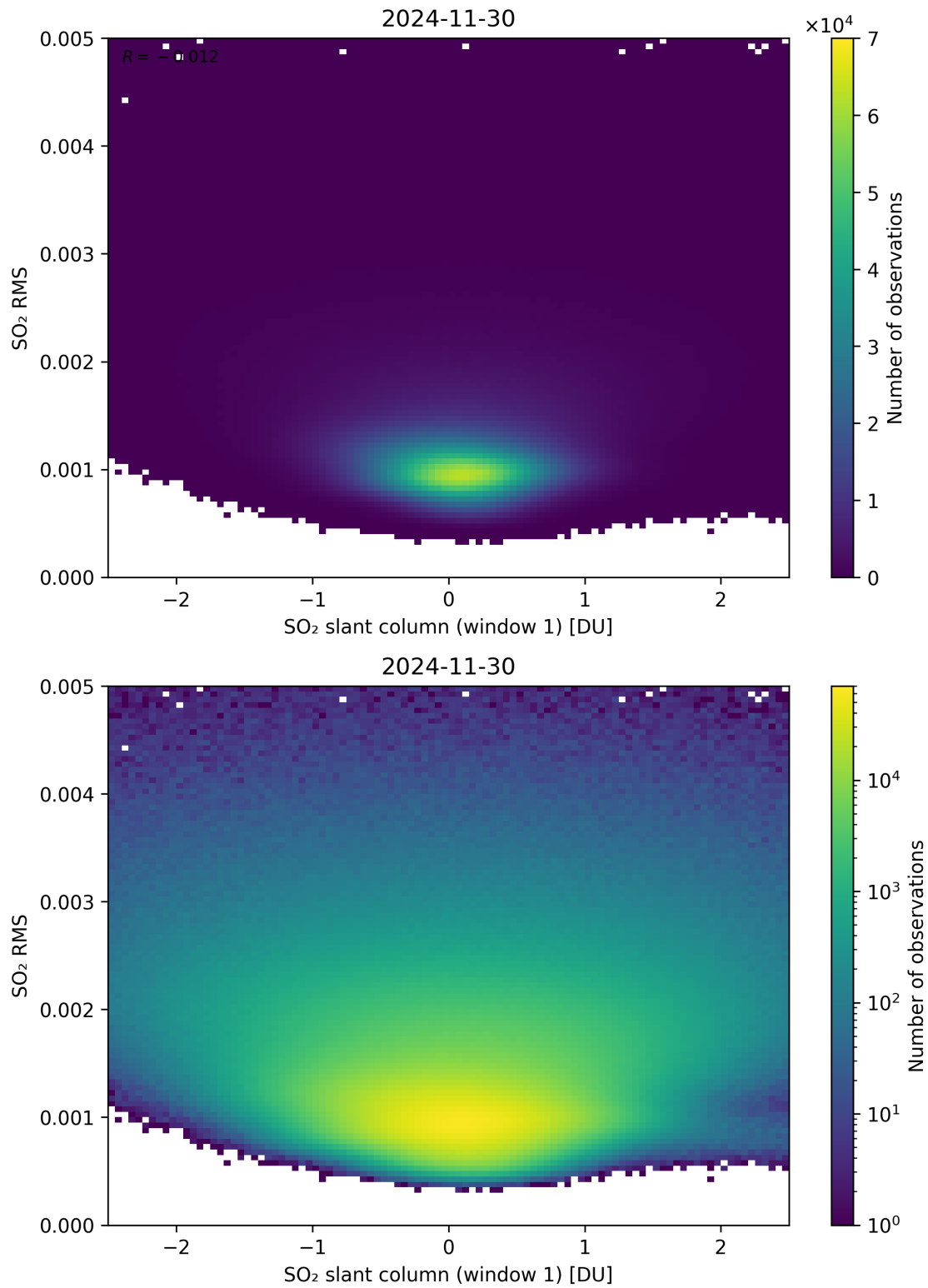
Figure 267: Scatter density plot of “SO 2 slant column (window 1)” against “SO 2 RMS” for 2024-11-30 to 2024-12-01.
