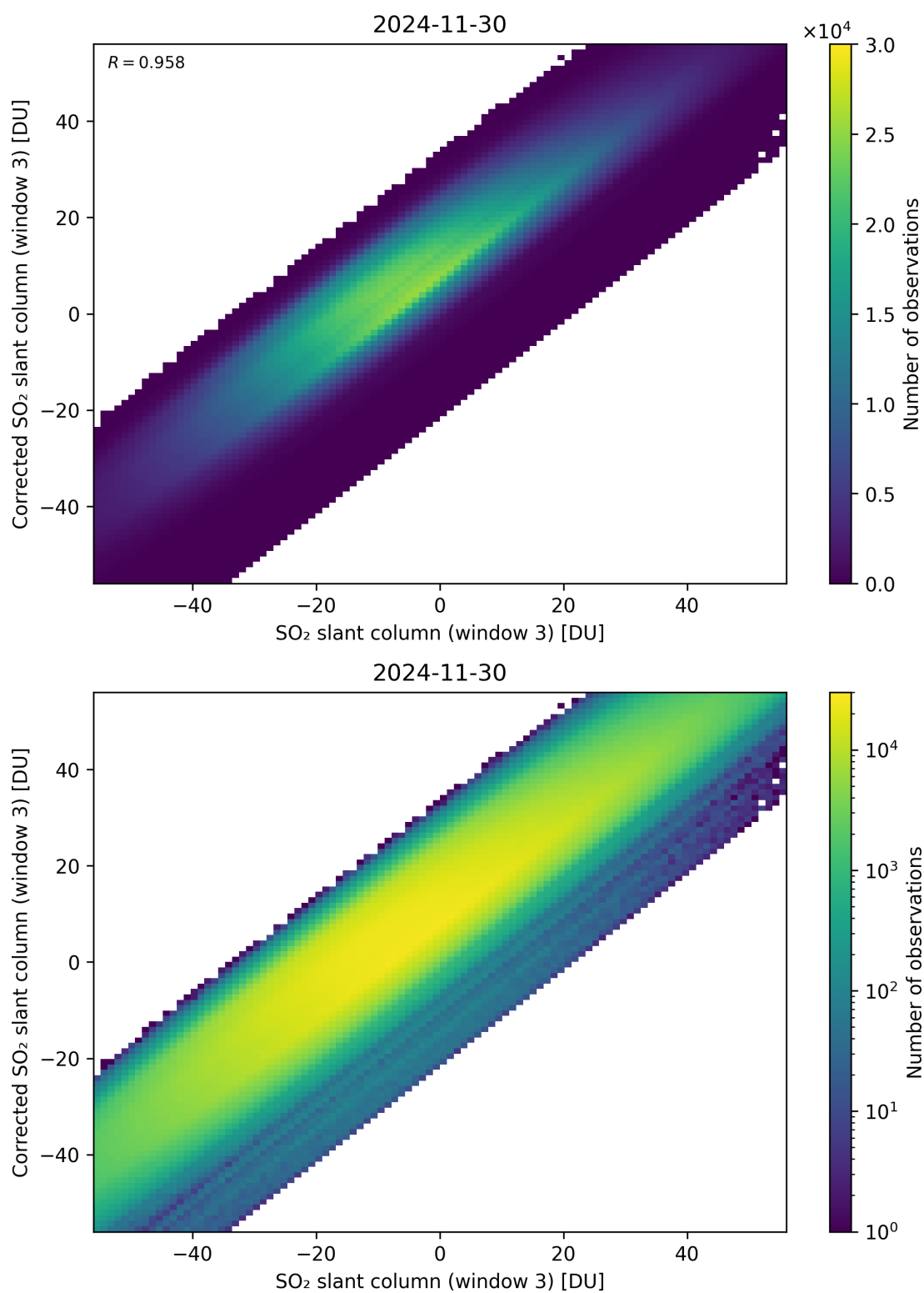
Figure 316: Scatter density plot of “SO 2 slant column (window 3)” against “Corrected SO 2 slant column (window 3)” for 2024-11-30 to 2024-12-01.
