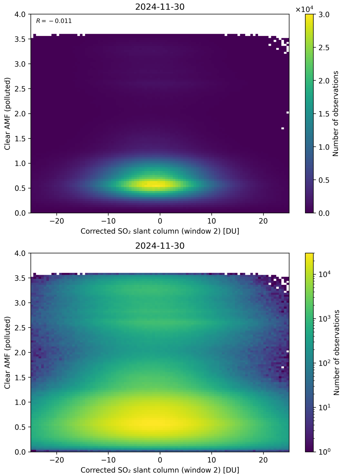
Figure 249: Scatter density plot of “Corrected SO 2 slant column (window 2)” against “Clear AMF (polluted)” for 2024-11-30 to 2024-12-01.
