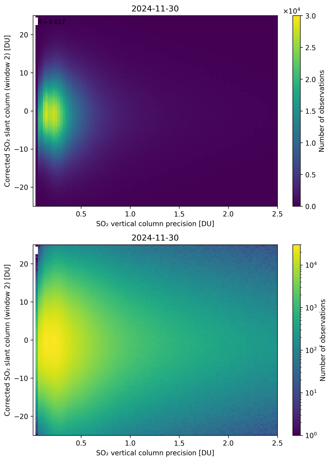
Figure 339: Scatter density plot of “SO 2 vertical column precision” against “Corrected SO 2 slant column (window 2)” for 2024-11-30 to 2024-12-01.
