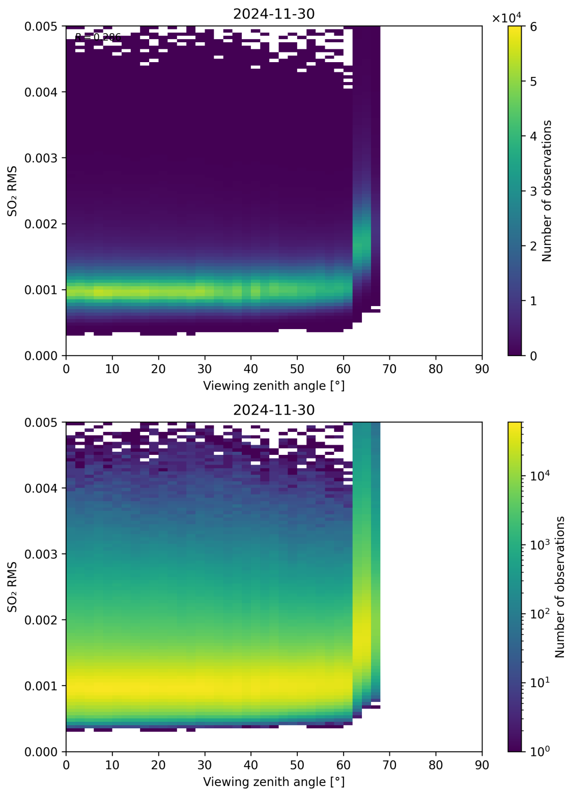
Figure 367: Scatter density plot of “Viewing zenith angle” against “SO 2 RMS” for 2024-11-30 to 2024-12-01.
