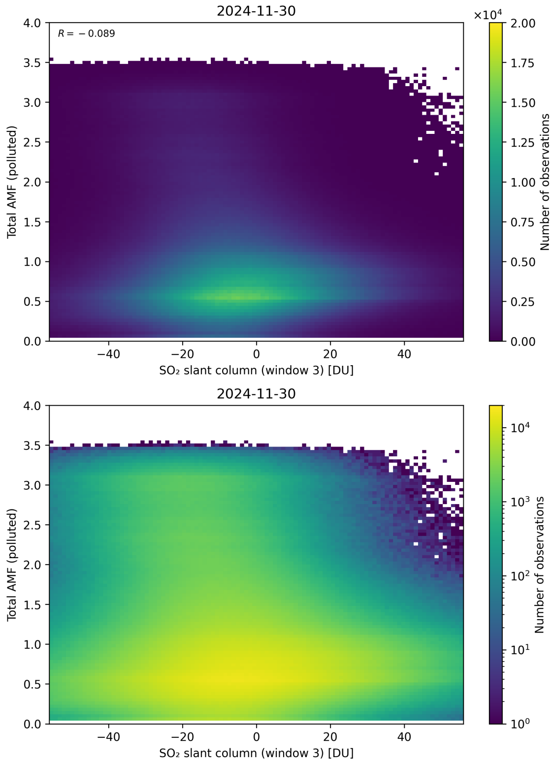
Figure 318: Scatter density plot of “SO 2 slant column (window 3)” against “Total AMF (polluted)” for 2024-11-30 to 2024-12-01.
