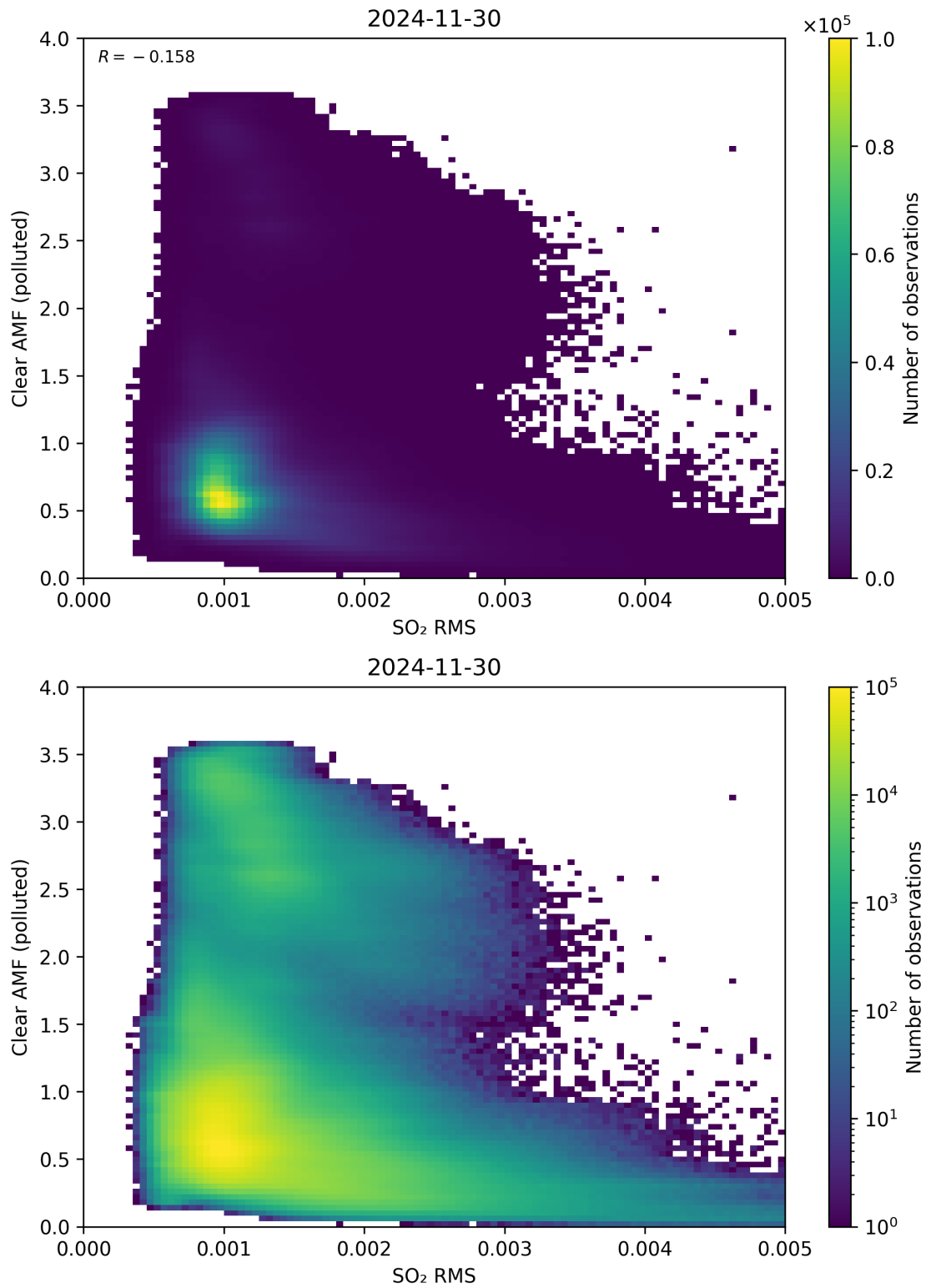
Figure 147: Scatter density plot of “SO 2 RMS” against “Clear AMF (polluted)” for 2024-11-30 to 2024-12-01.
