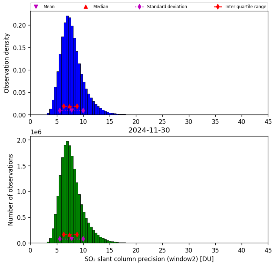
Figure 68: Histogram of “SO 2 slant column precision (window2)” for 2024-11-30 to 2024-12-01
