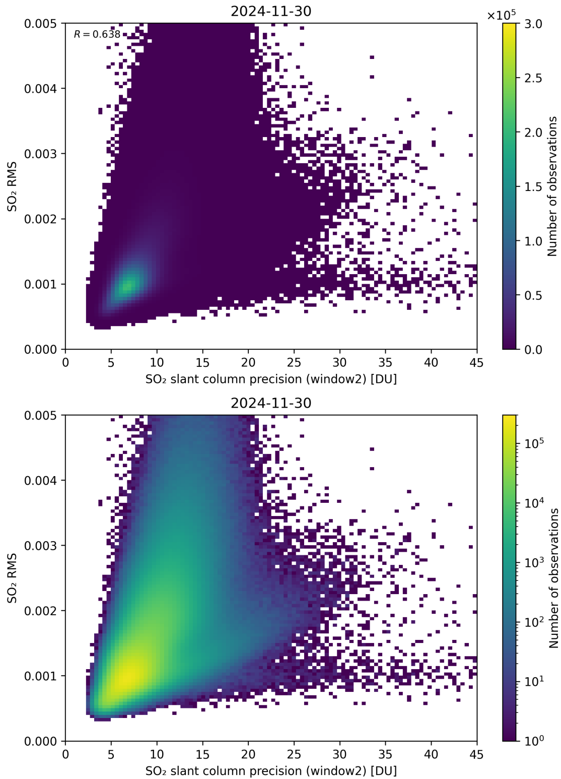
Figure 295: Scatter density plot of “SO 2 slant column precision (window2)” against “SO 2 RMS” for 2024-11-30 to 2024-12-01.
