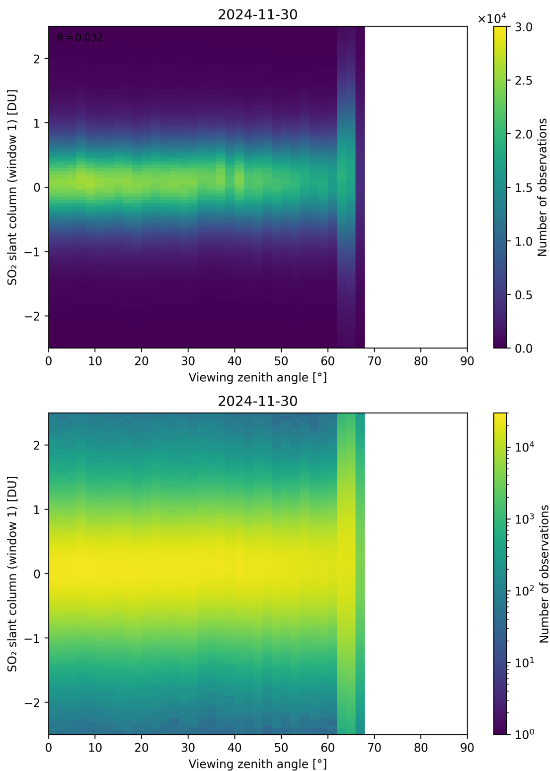
Figure 376: Scatter density plot of “Viewing zenith angle” against “SO 2 slant column (window 1)” for 2024-11-30 to 2024-12-01.
