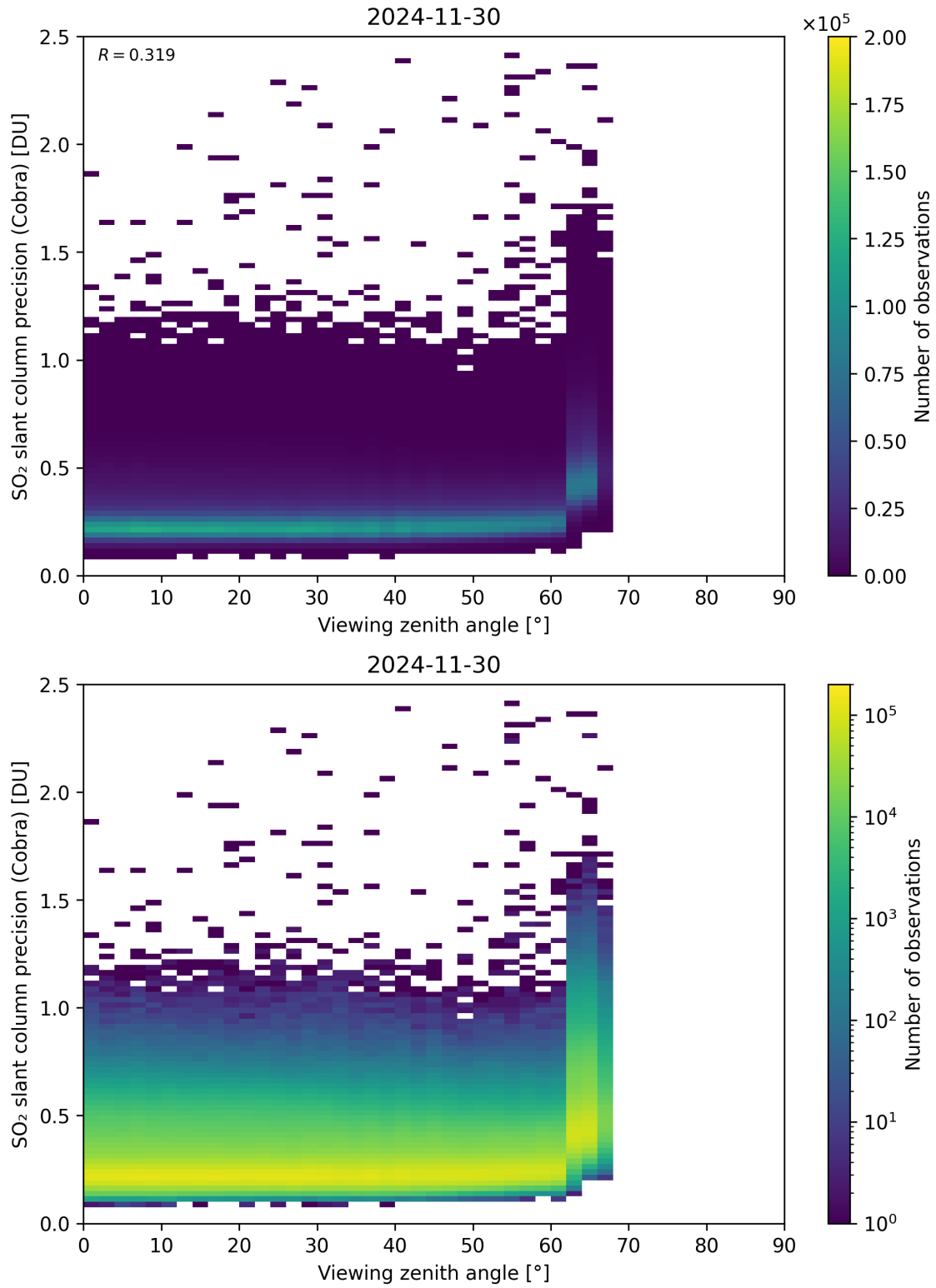
Figure 372: Scatter density plot of “Viewing zenith angle” against “SO 2 slant column precision (Cobra)” for 2024-11-30 to 2024-12-01.
