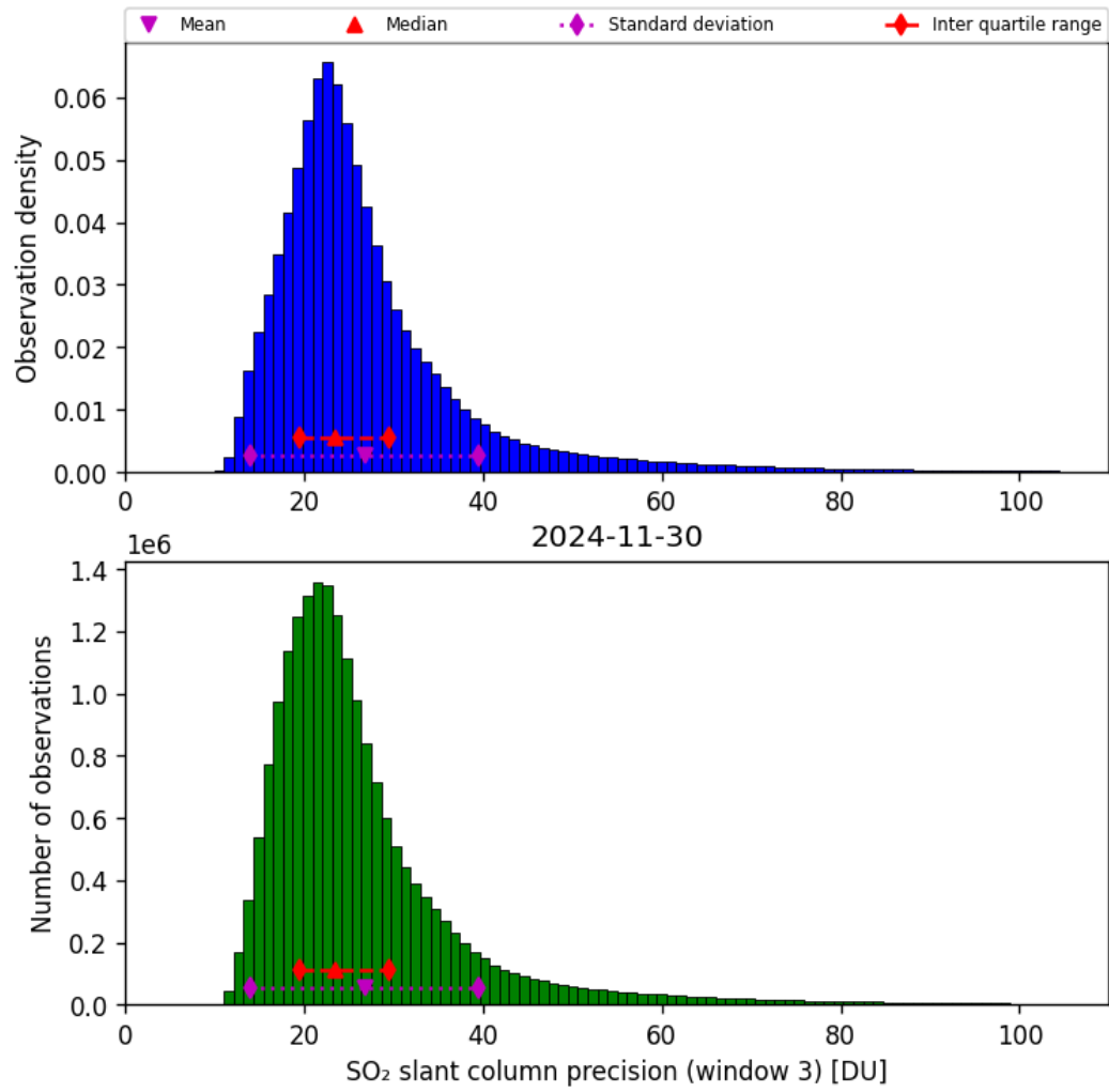
Figure 72: Histogram of “SO 2 slant column precision (window 3)” for 2024-11-30 to 2024-12-01
