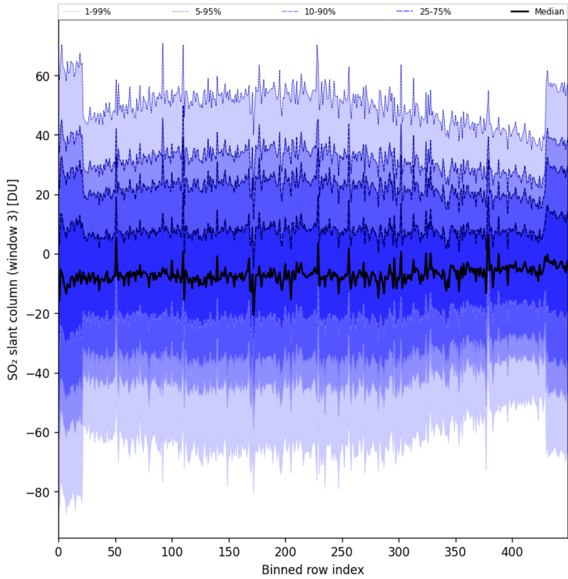
Figure 97: Along track statistics of “SO 2 slant column (window 3)” for 2024-11-30 to 2024-12-01
