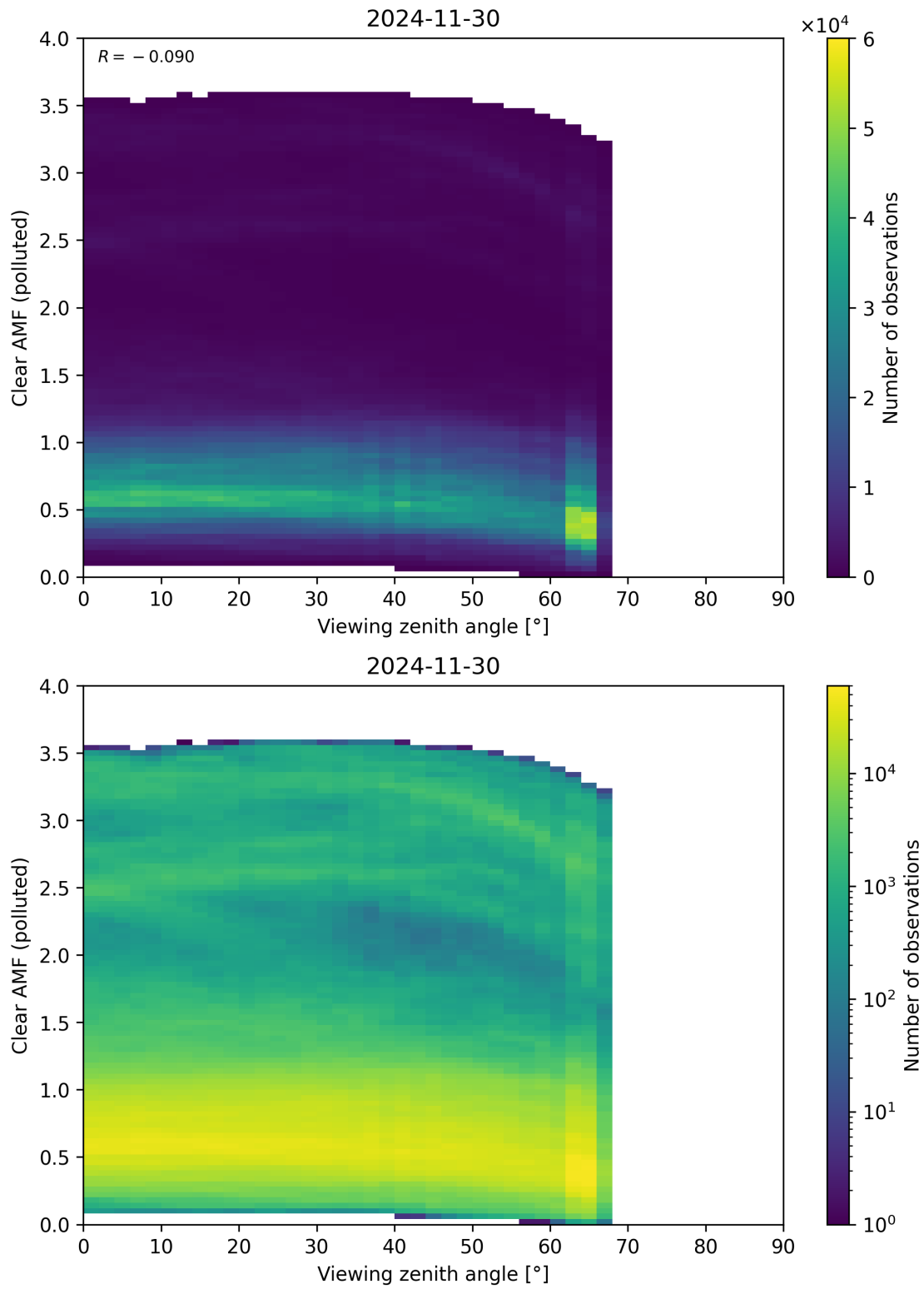
Figure 370: Scatter density plot of “Viewing zenith angle” against “Clear AMF (polluted)” for 2024-11-30 to 2024-12-01.
