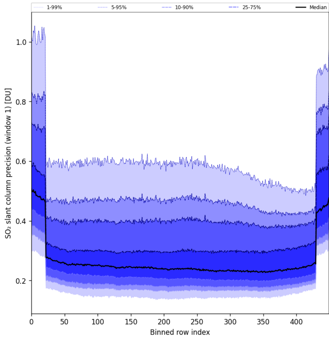
Figure 90: Along track statistics of “SO 2 slant column precision (window 1)” for 2024-11-30 to 2024-12-01
