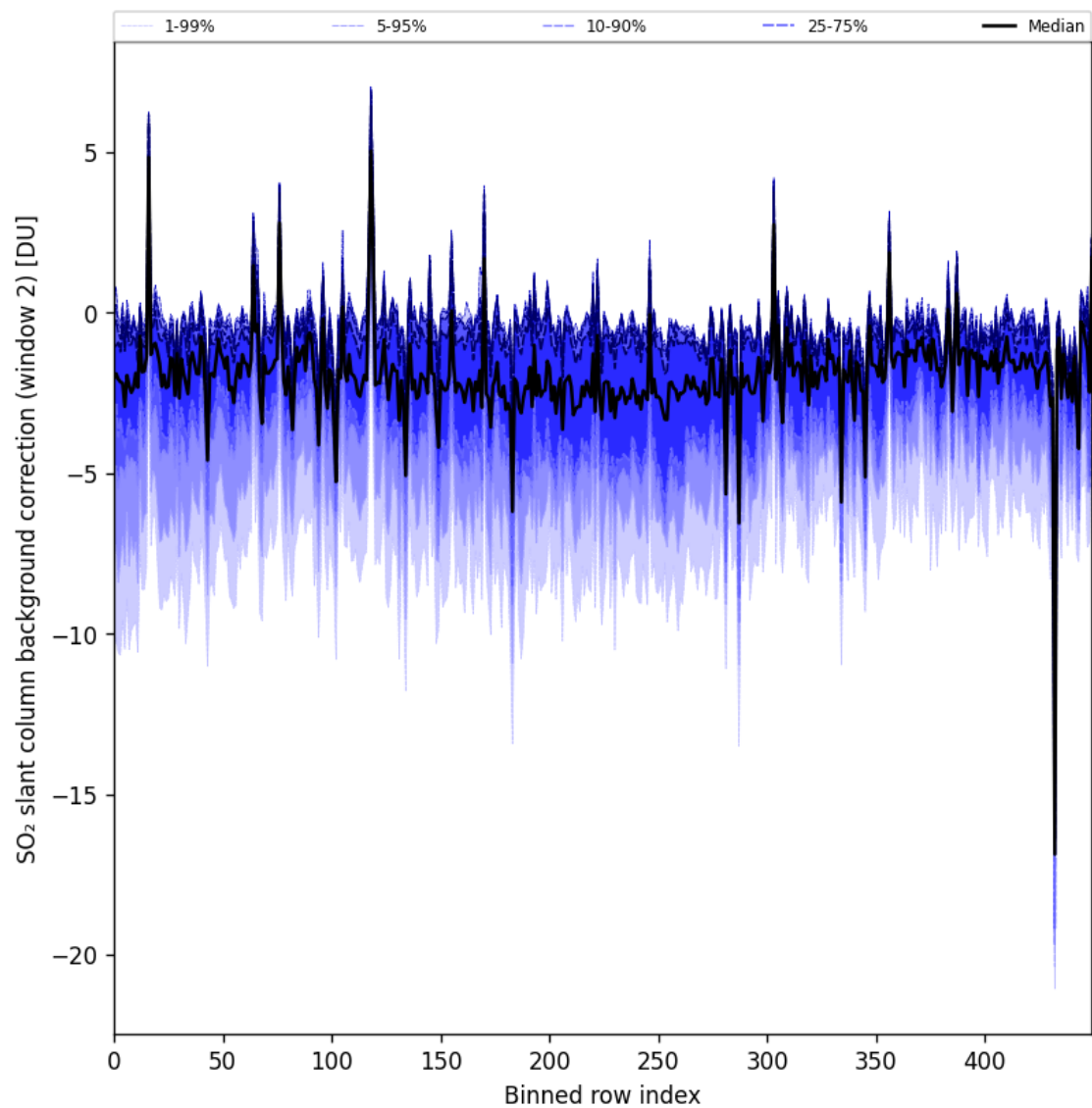
Figure 96: Along track statistics of “SO 2 slant column background correction (window 2)” for 2024-11-30 to 2024-12-01
