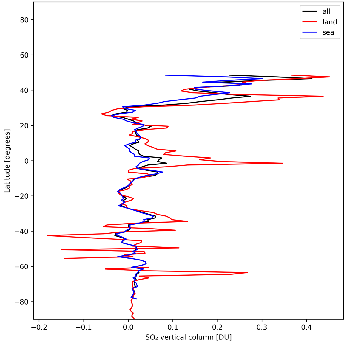
Figure 32: Zonal average of “SO 2 vertical column” for 2024-11-30 to 2024-12-01.
