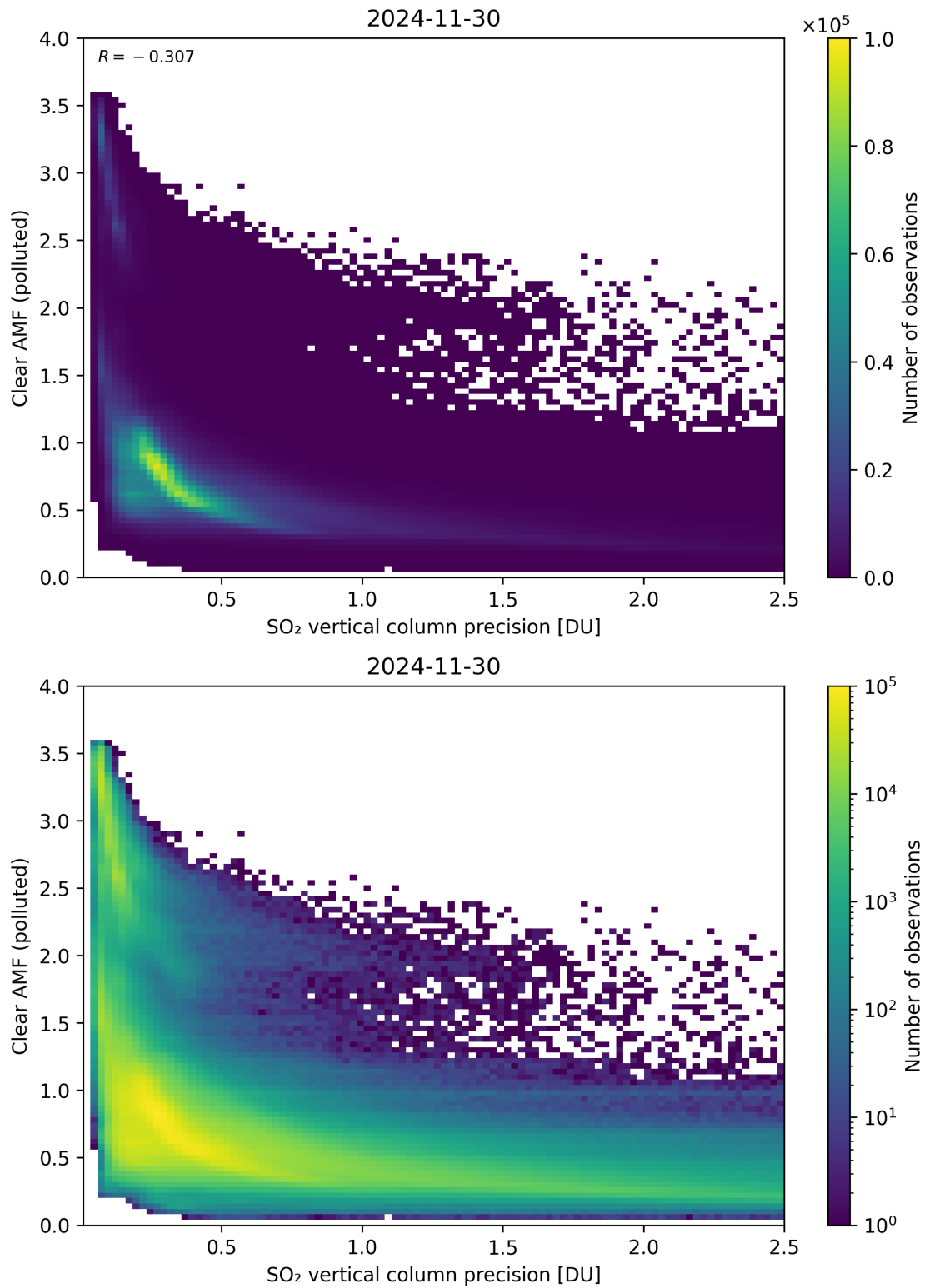
Figure 335: Scatter density plot of “SO 2 vertical column precision” against “Clear AMF (polluted)” for 2024-11-30 to 2024-12-01.
