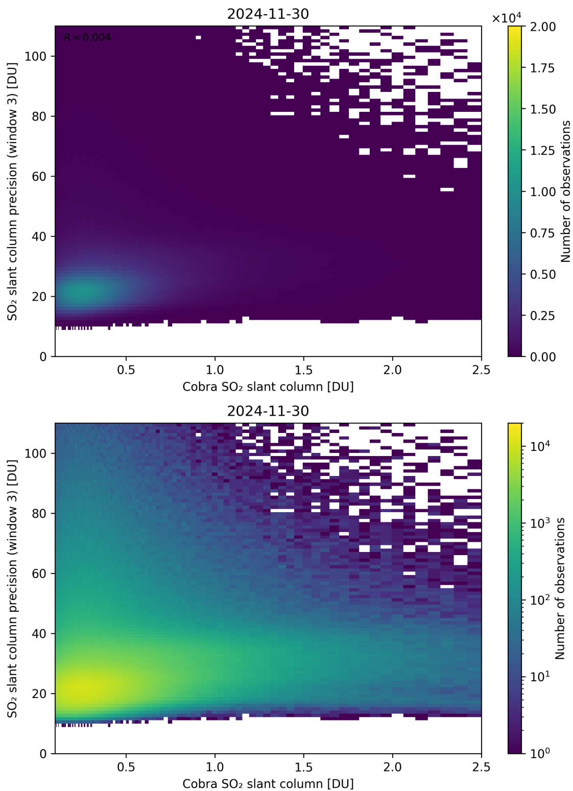
Figure 223: Scatter density plot of “Cobra SO 2 slant column” against “SO 2 slant column precision (window 3)” for 2024-11-30 to 2024-12-01.
