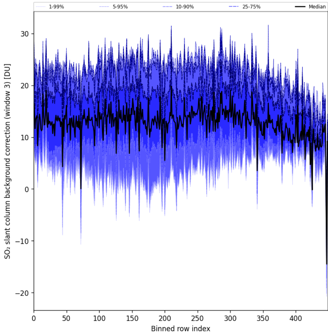
Figure 100: Along track statistics of “SO 2 slant column background correction (window 3)” for 2024-11-30 to 2024-12-01
