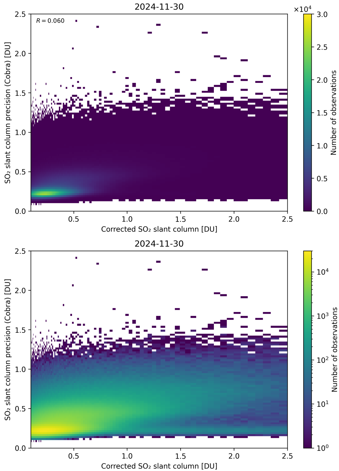
Figure 234: Scatter density plot of “Corrected SO 2 slant column” against “SO 2 slant column precision (Cobra)” for 2024-11-30 to 2024-12-01.
