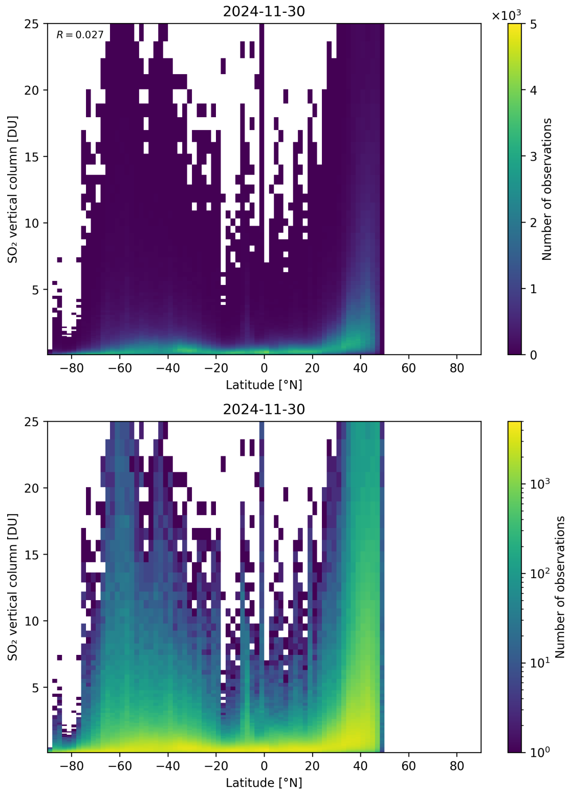
Figure 169: Scatter density plot of “Latitude” against “SO 2 vertical column” for 2024-11-30 to 2024-12-01.
