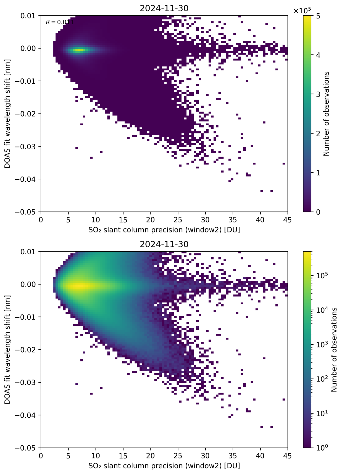
Figure 293: Scatter density plot of “SO 2 slant column precision (window2)” against “DOAS fit wavelength shift” for 2024-11-30 to 2024-12-01.
