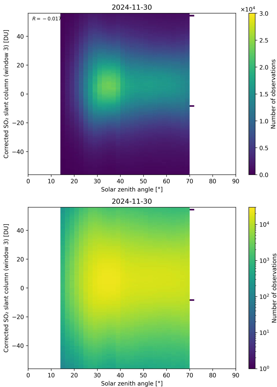
Figure 183: Scatter density plot of “Solar zenith angle” against “Corrected SO 2 slant column (window 3)” for 2024-11-30 to 2024-12-01.
