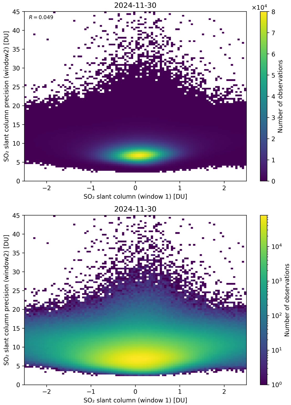
Figure 286: Scatter density plot of “SO 2 slant column (window 1)” against “SO 2 slant column precision (window2)” for 2024-11-30 to 2024-12-01.
