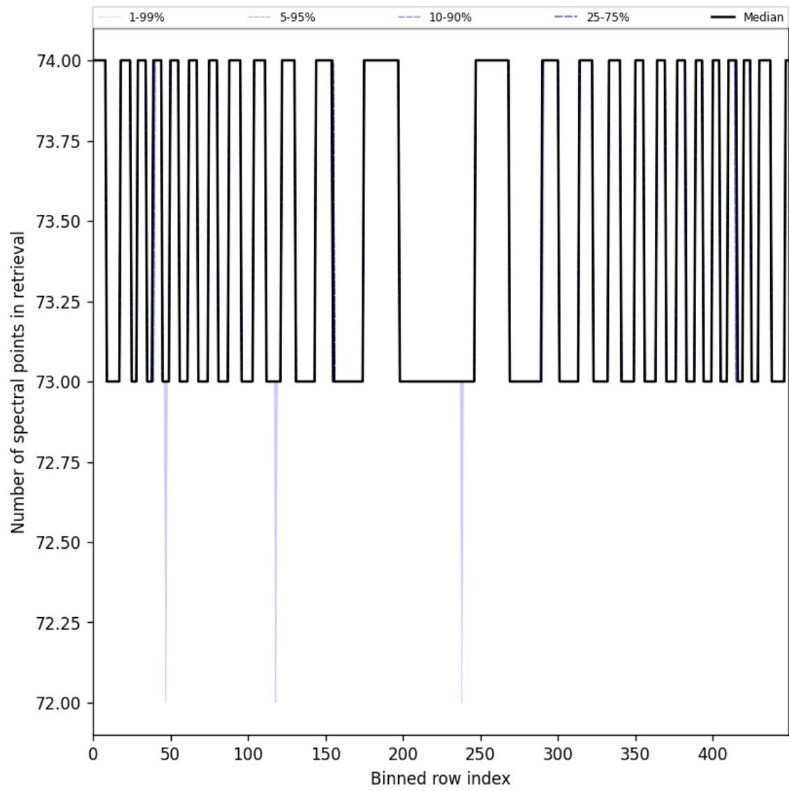
Figure 108: Along track statistics of “Number of spectral points in retrieval” for 2024-11-30 to 2024-12-01
