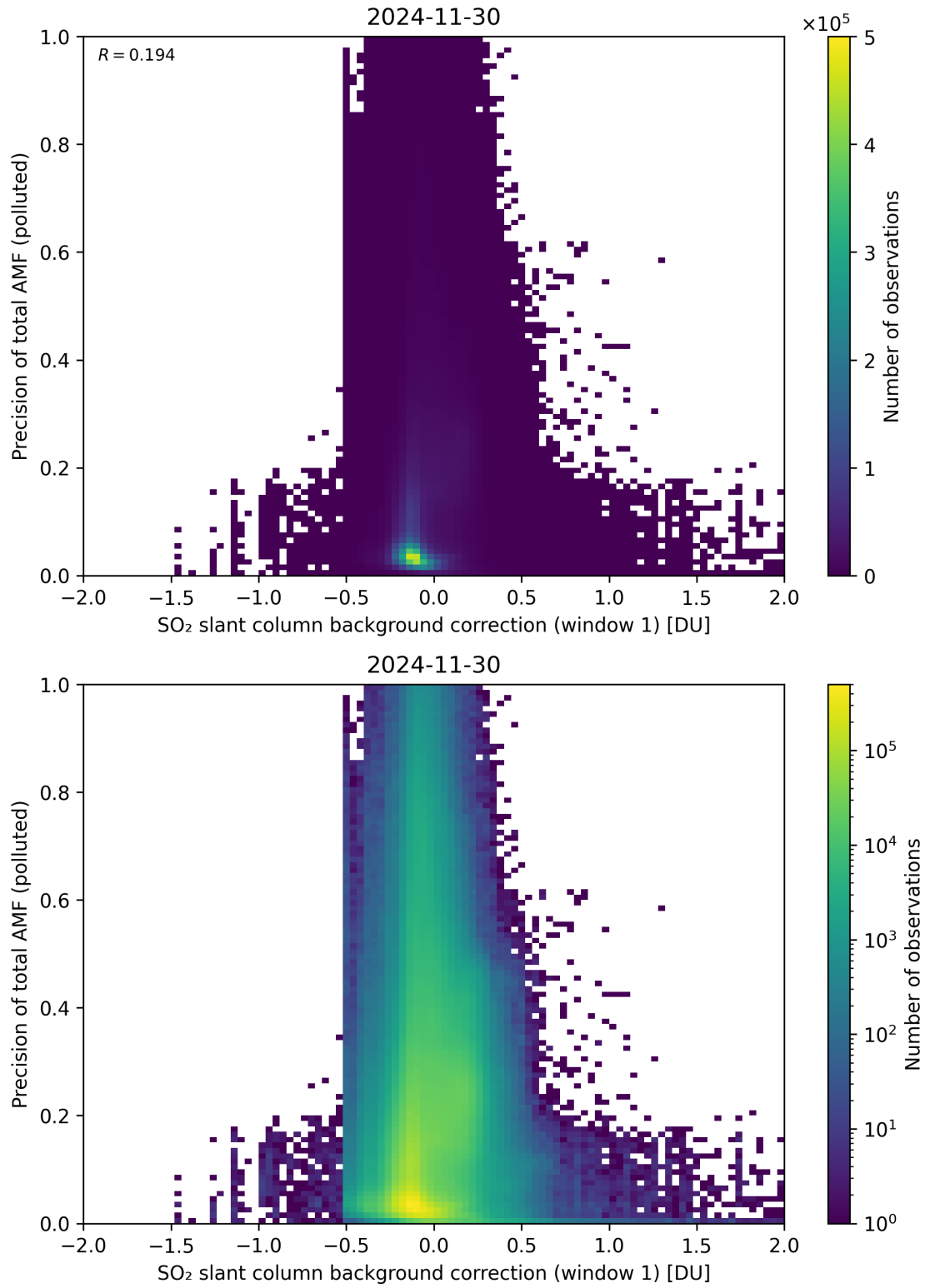
Figure 121: Scatter density plot of “SO 2 slant column background correction (window 1)” against “Precision of total AMF (polluted)” for 2024-11-30 to 2024-12-01.
