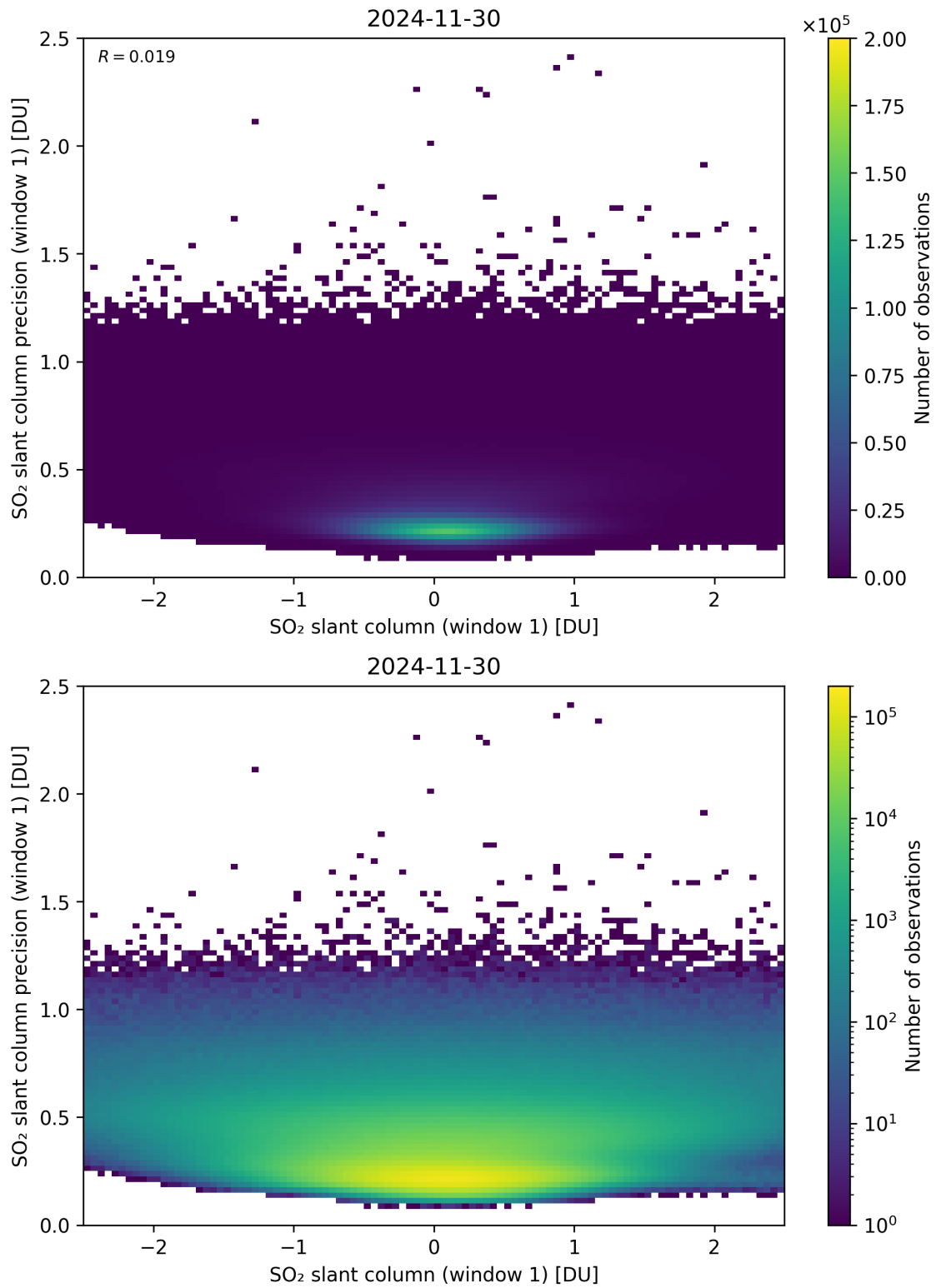
Figure 285: Scatter density plot of “SO 2 slant column (window 1)” against “SO 2 slant column precision (window 1)” for 2024-11-30 to 2024-12-01.
