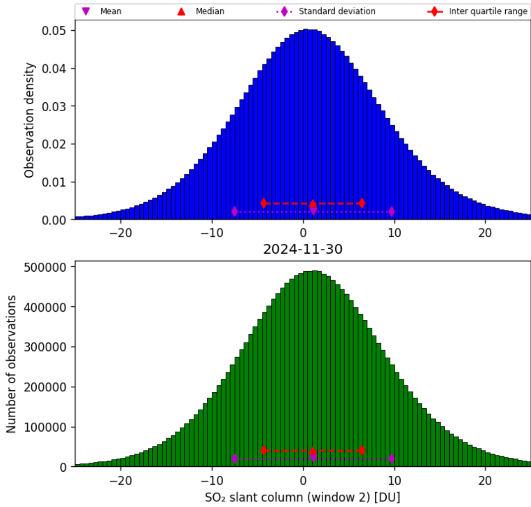
Figure 67: Histogram of “SO 2 slant column (window 2)” for 2024-11-30 to 2024-12-01
