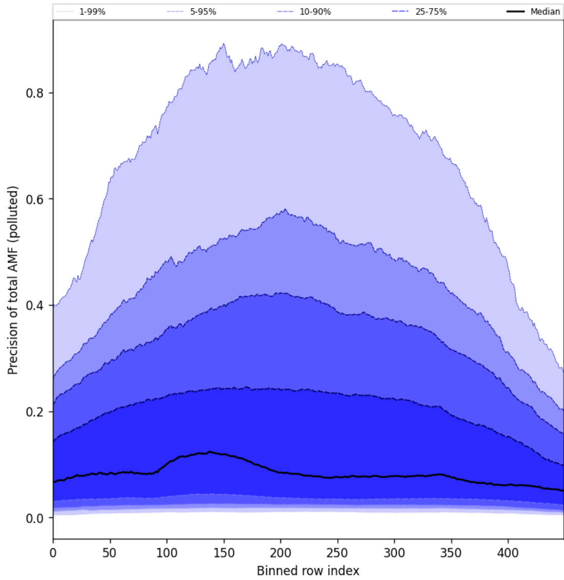
Figure 106: Along track statistics of “Precision of total AMF (polluted)” for 2024-11-30 to 2024-12-01
