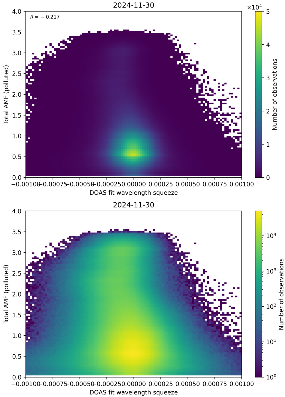
Figure 145: Scatter density plot of “DOAS fit wavelength squeeze” against “Total AMF (polluted)” for 2024-11-30 to 2024-12-01.
