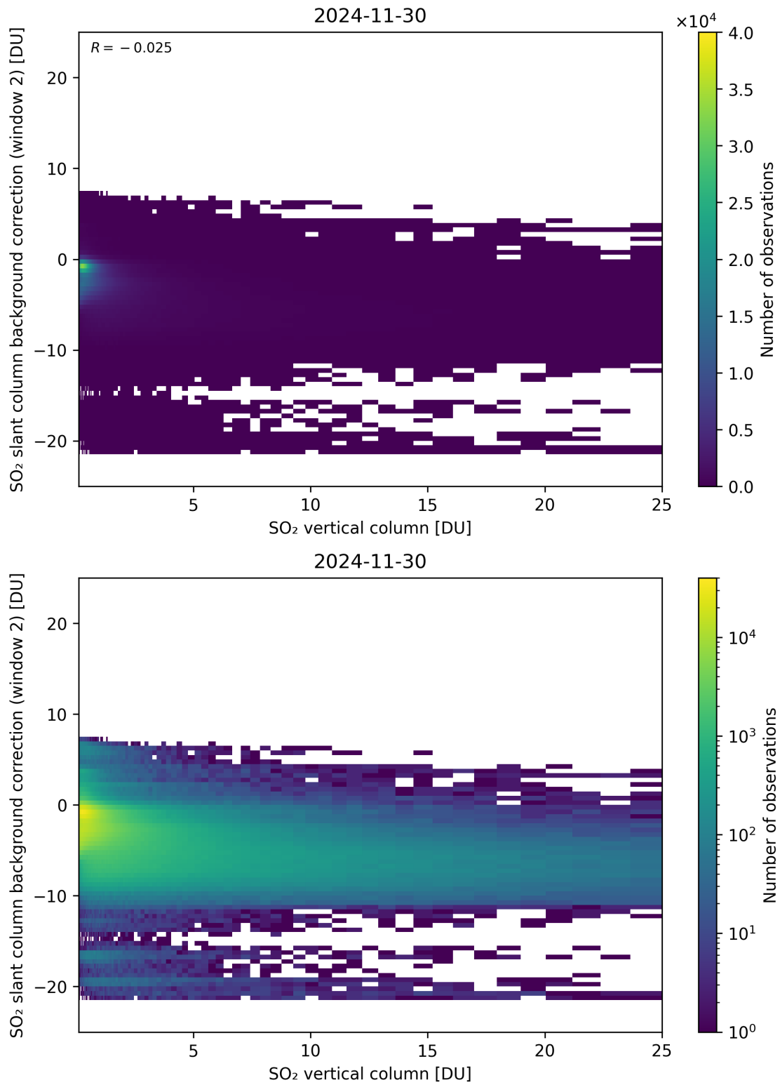
Figure 324: Scatter density plot of “SO 2 vertical column” against “SO 2 slant column background correction (window 2)” for 2024-11-30 to 2024-12-01.
