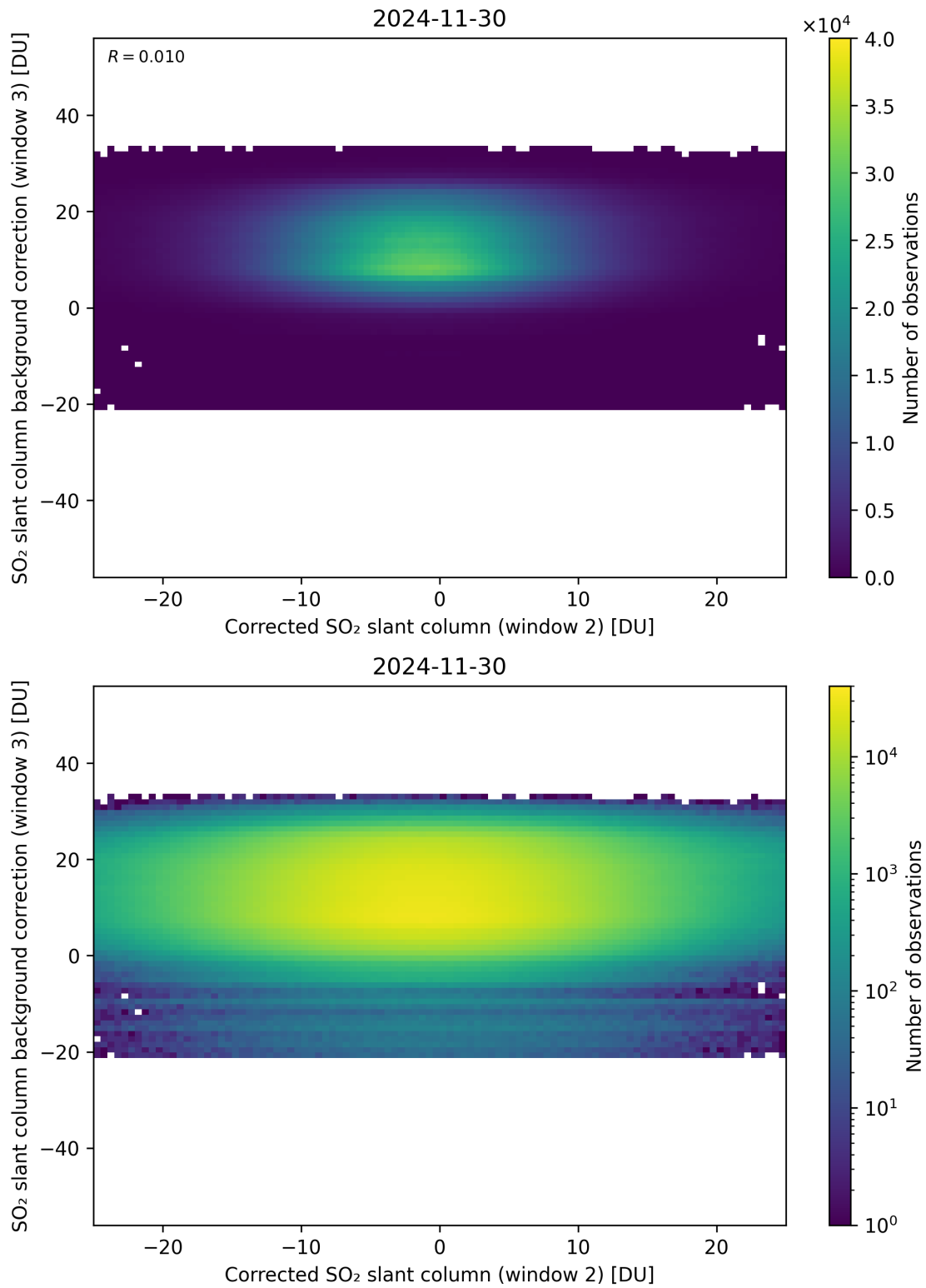
Figure 245: Scatter density plot of “Corrected SO 2 slant column (window 2)” against “SO 2 slant column background correction (window 3)” for 2024-11-30 to 2024-12-01.
