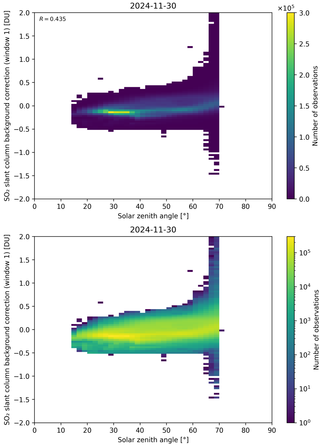
Figure 171: Scatter density plot of “Solar zenith angle” against “SO 2 slant column background correction (window 1)” for 2024-11-30 to 2024-12-01.
