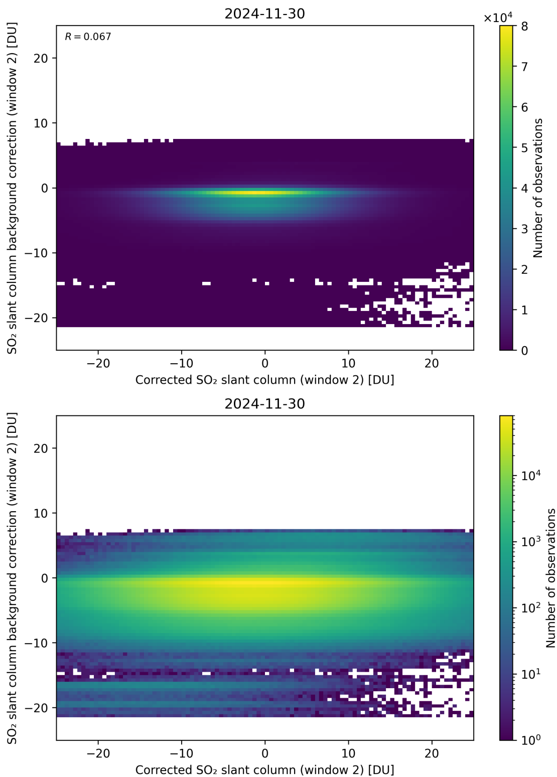
Figure 244: Scatter density plot of “Corrected SO 2 slant column (window 2)” against “SO 2 slant column background correction (window 2)” for 2024-11-30 to 2024-12-01.
