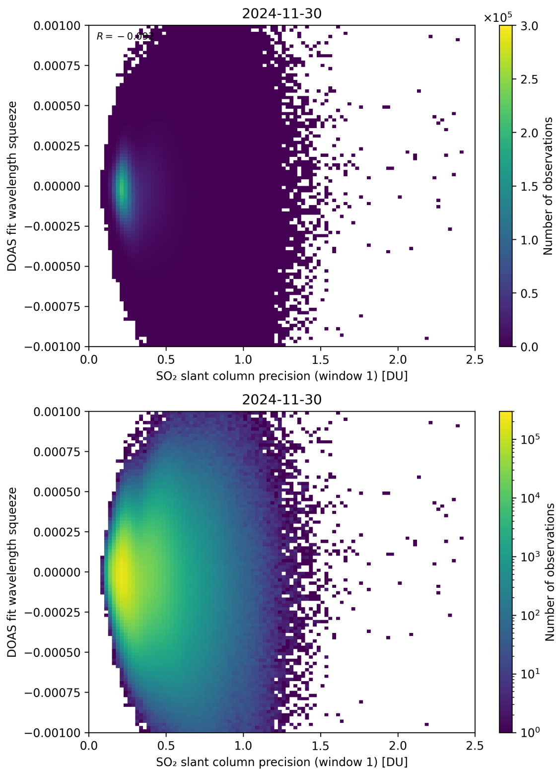
Figure 272: Scatter density plot of “SO 2 slant column precision (window 1)” against “DOAS fit wavelength squeeze” for 2024-11-30 to 2024-12-01.
