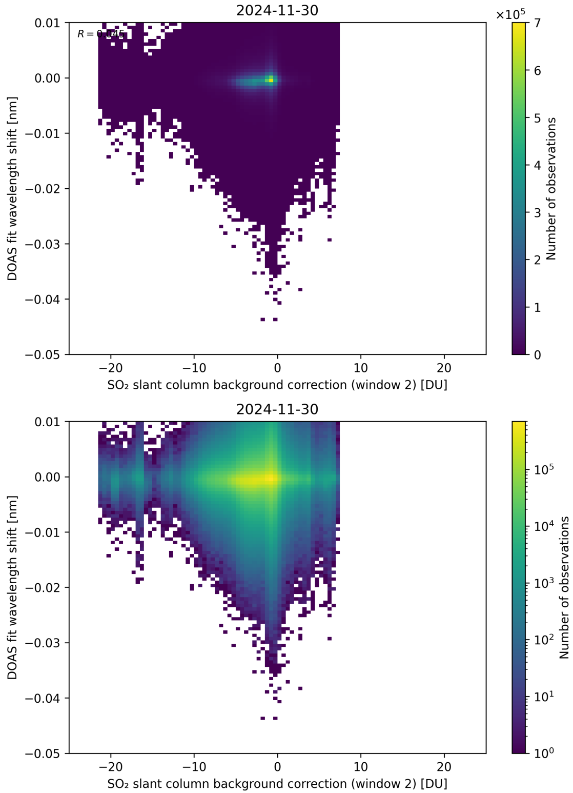
Figure 123: Scatter density plot of “SO 2 slant column background correction (window 2)” against “DOAS fit wavelength shift” for 2024-11-30 to 2024-12-01.
