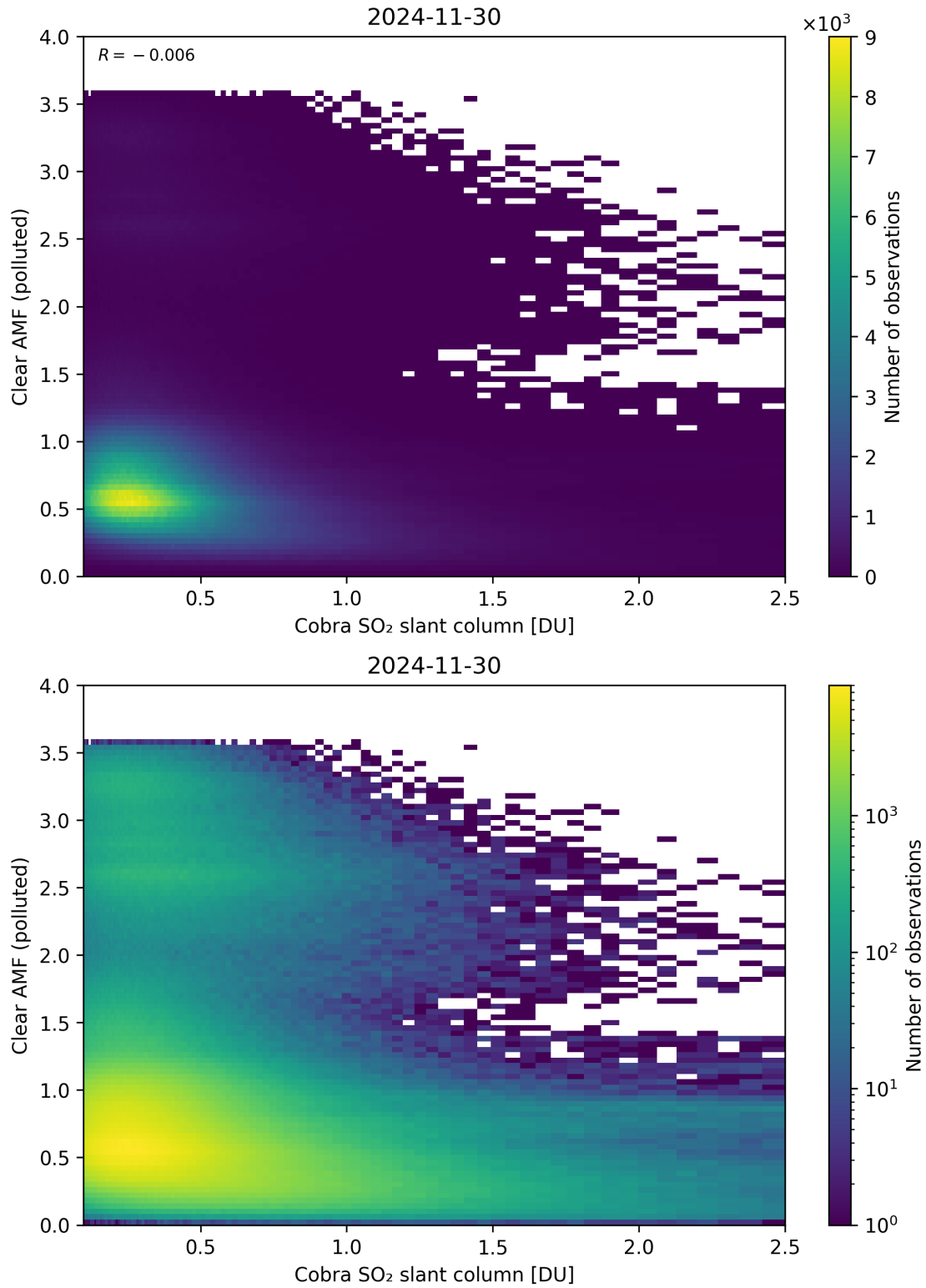
Figure 215: Scatter density plot of “Cobra SO 2 slant column” against “Clear AMF (polluted)” for 2024-11-30 to 2024-12-01.
