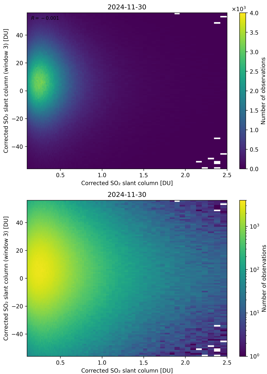
Figure 236: Scatter density plot of “Corrected SO 2 slant column” against “Corrected SO 2 slant column (window 3)” for 2024-11-30 to 2024-12-01.
