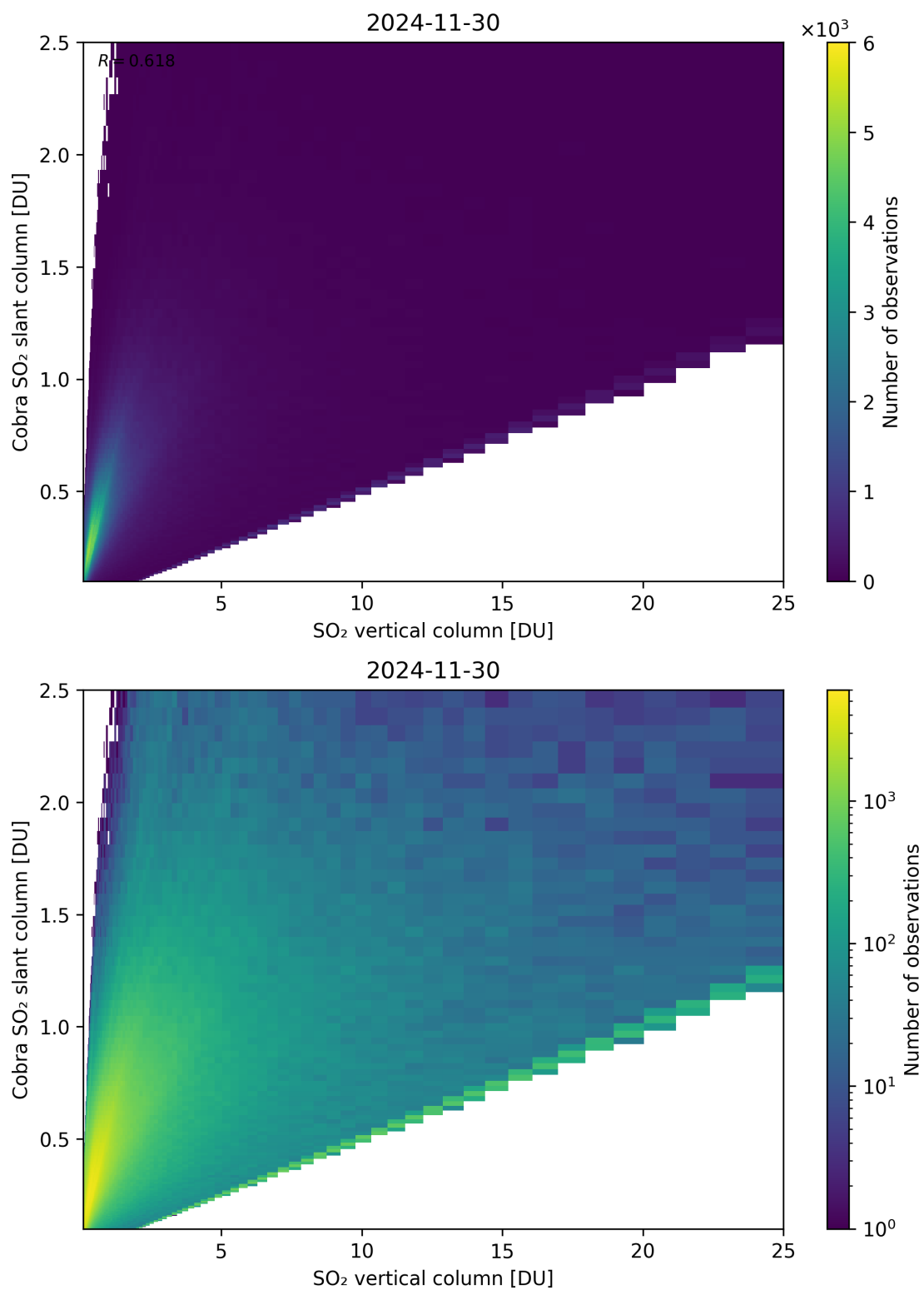
Figure 349: Scatter density plot of “SO 2 vertical column” against “Cobra SO 2 slant column” for 2024-11-30 to 2024-12-01.
