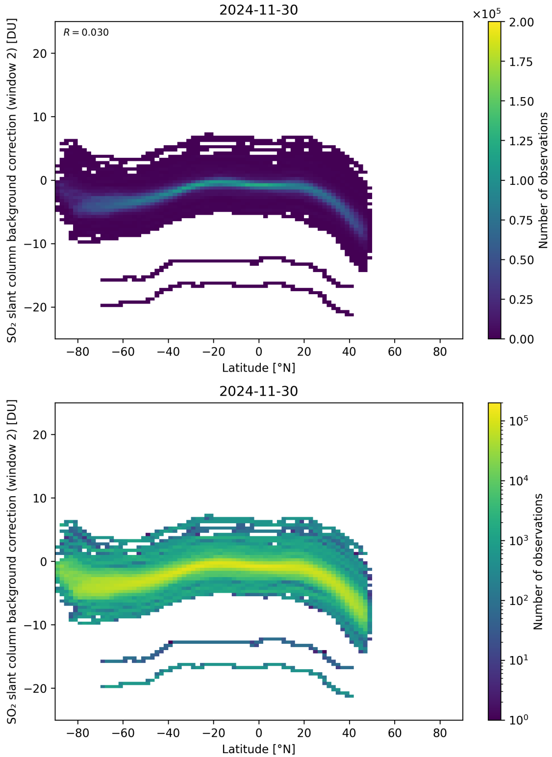
Figure 151: Scatter density plot of “Latitude” against “SO 2 slant column background correction (window 2)” for 2024-11-30 to 2024-12-01.
