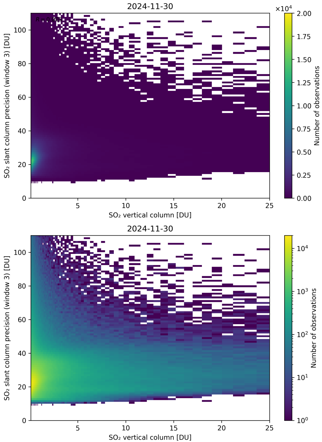
Figure 358: Scatter density plot of “SO 2 vertical column” against “SO 2 slant column precision (window 3)” for 2024-11-30 to 2024-12-01.
