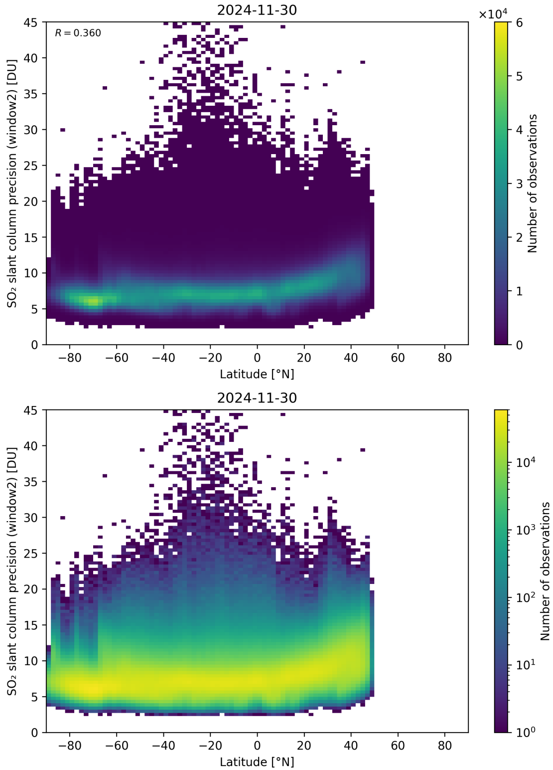
Figure 164: Scatter density plot of “Latitude” against “SO 2 slant column precision (window2)” for 2024-11-30 to 2024-12-01.
