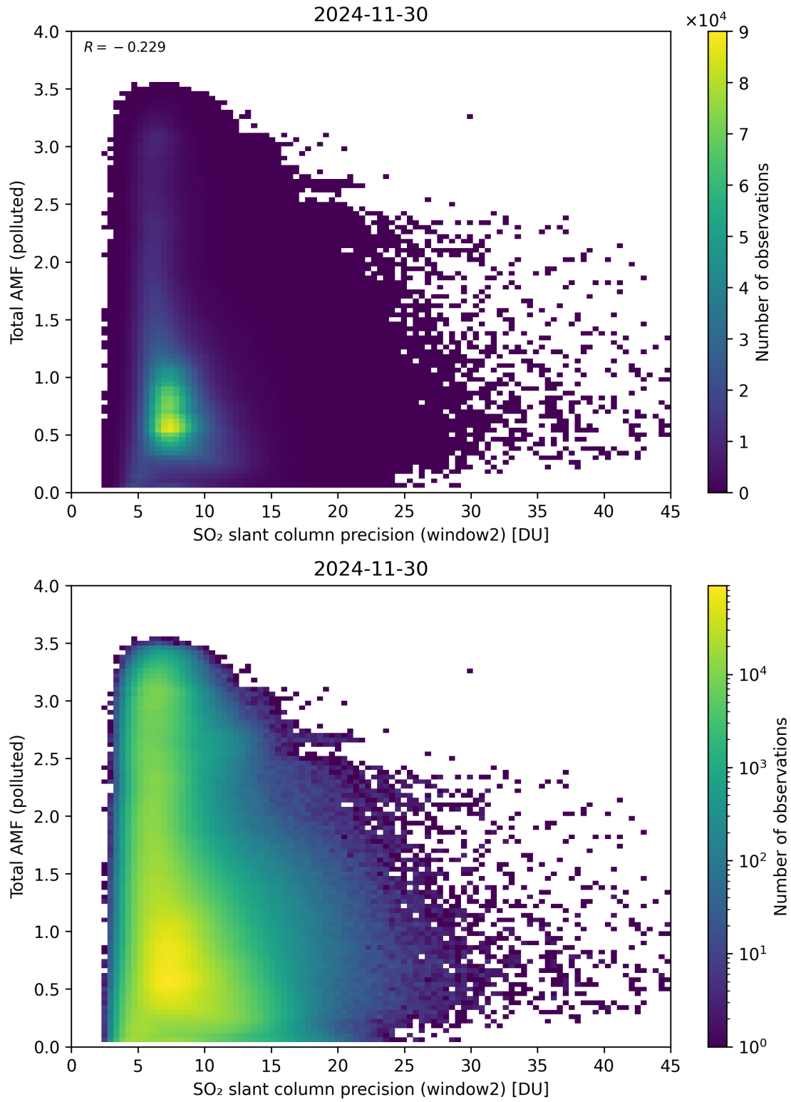
Figure 301: Scatter density plot of “SO 2 slant column precision (window2)” against “Total AMF (polluted)” for 2024-11-30 to 2024-12-01.
