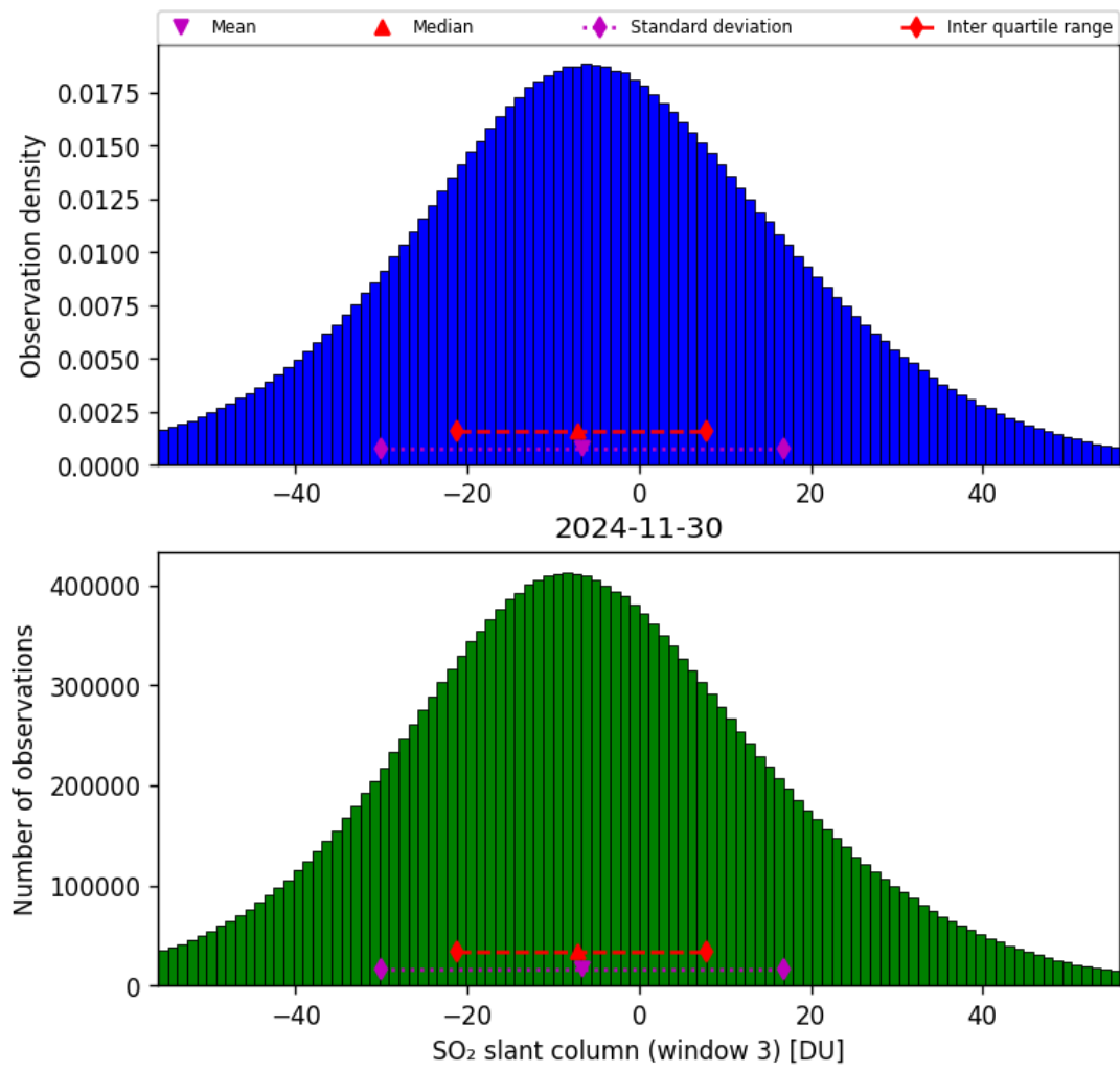
Figure 71: Histogram of “SO 2 slant column (window 3)” for 2024-11-30 to 2024-12-01
