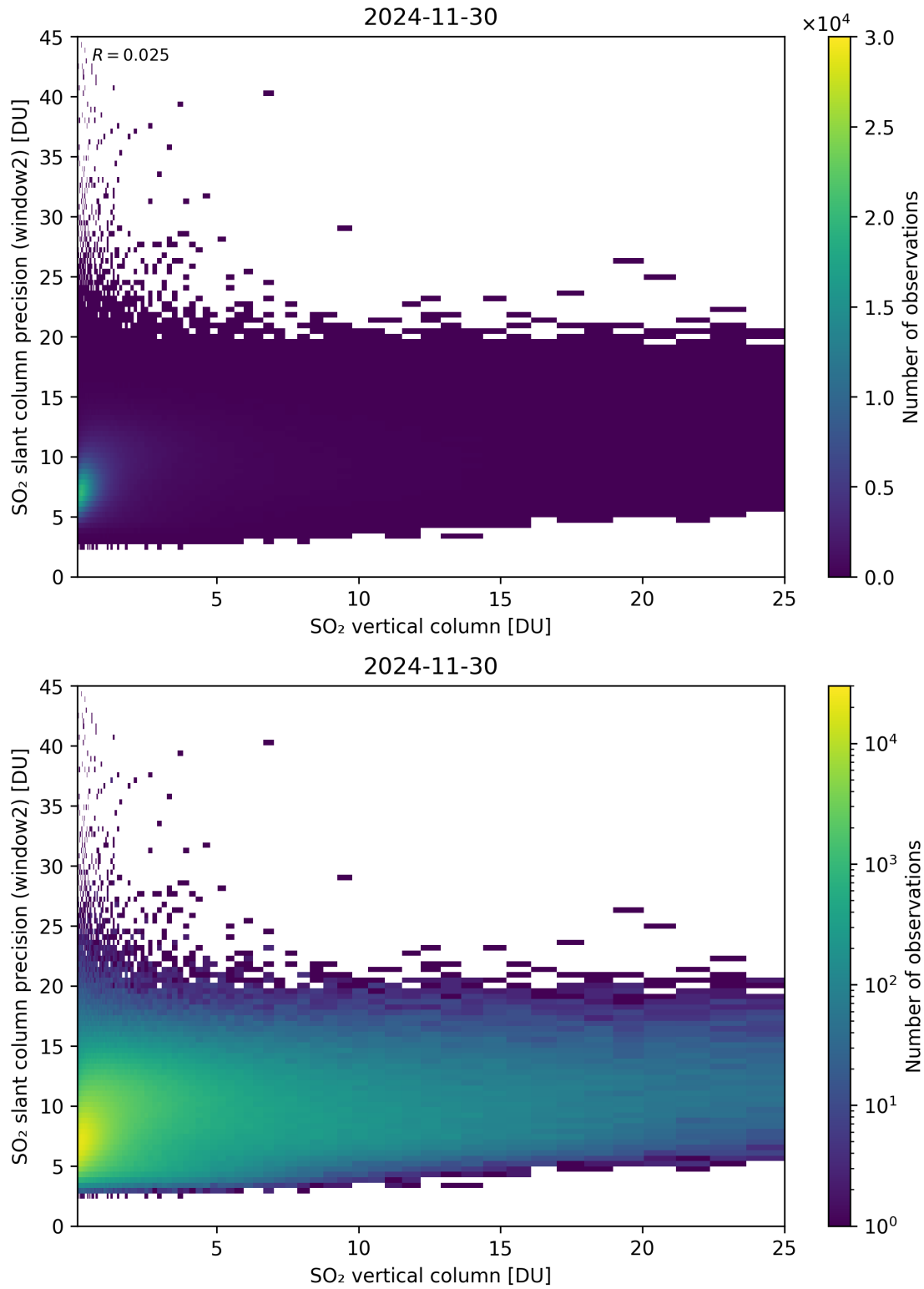
Figure 356: Scatter density plot of “SO 2 vertical column” against “SO 2 slant column precision (window2)” for 2024-11-30 to 2024-12-01.
