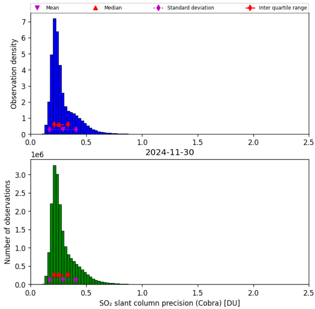
Figure 62: Histogram of “SO 2 slant column precision (Cobra)” for 2024-11-30 to 2024-12-01
