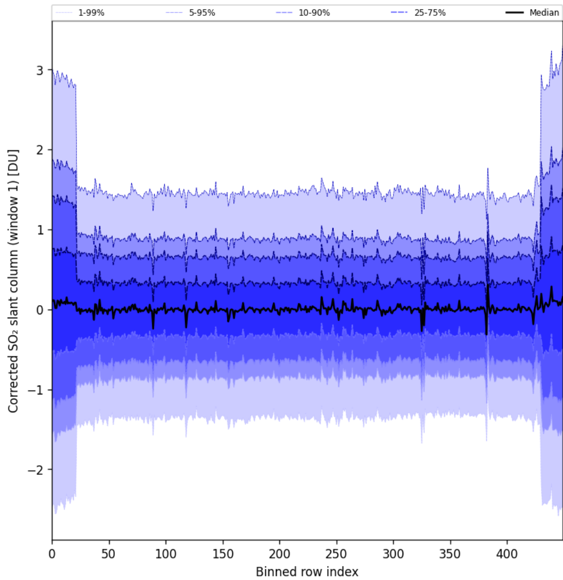
Figure 91: Along track statistics of “Corrected SO 2 slant column (window 1)” for 2024-11-30 to 2024-12-01
