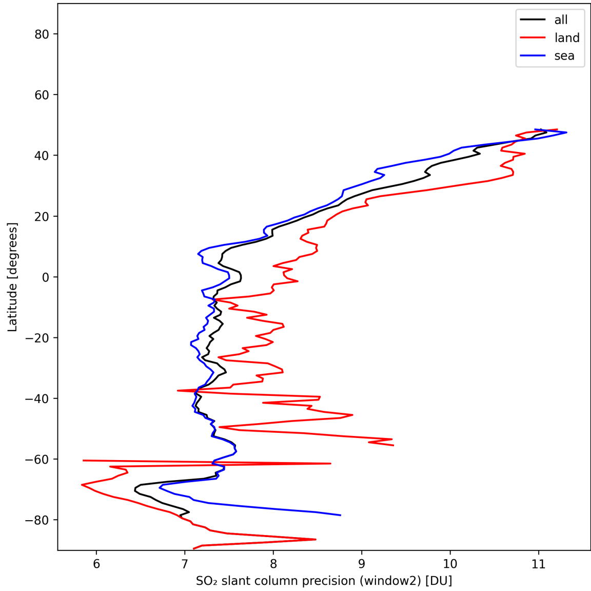
Figure 42: Zonal average of “SO 2 slant column precision (window2)” for 2024-11-30 to 2024-12-01.
