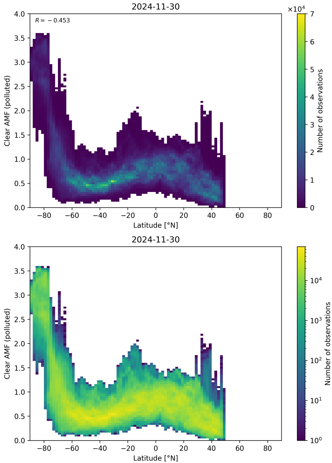
Figure 156: Scatter density plot of “Latitude” against “Clear AMF (polluted)” for 2024-11-30 to 2024-12-01.
