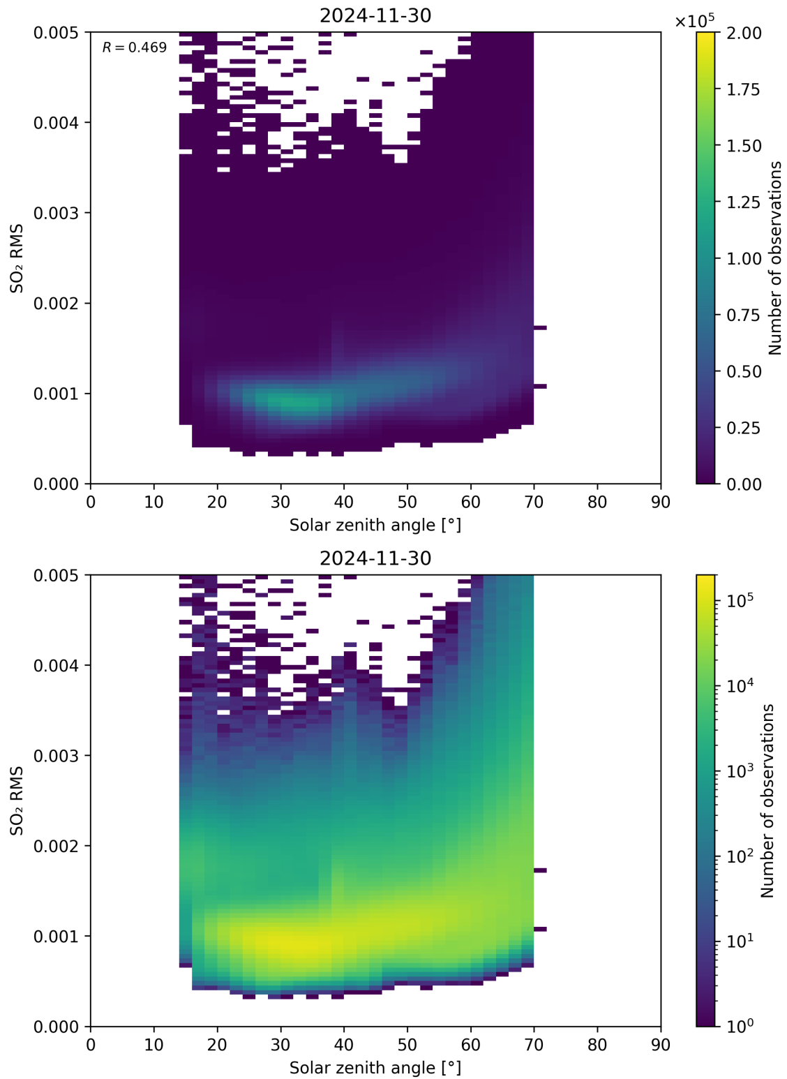
Figure 176: Scatter density plot of “Solar zenith angle” against “SO 2 RMS” for 2024-11-30 to 2024-12-01.
