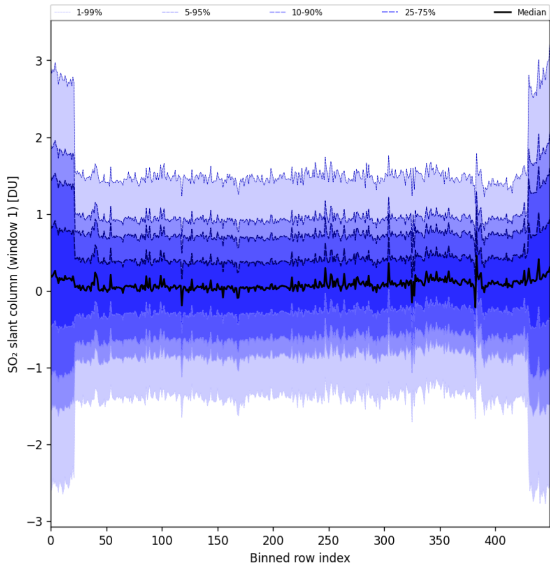
Figure 89: Along track statistics of “SO 2 slant column (window 1)” for 2024-11-30 to 2024-12-01
