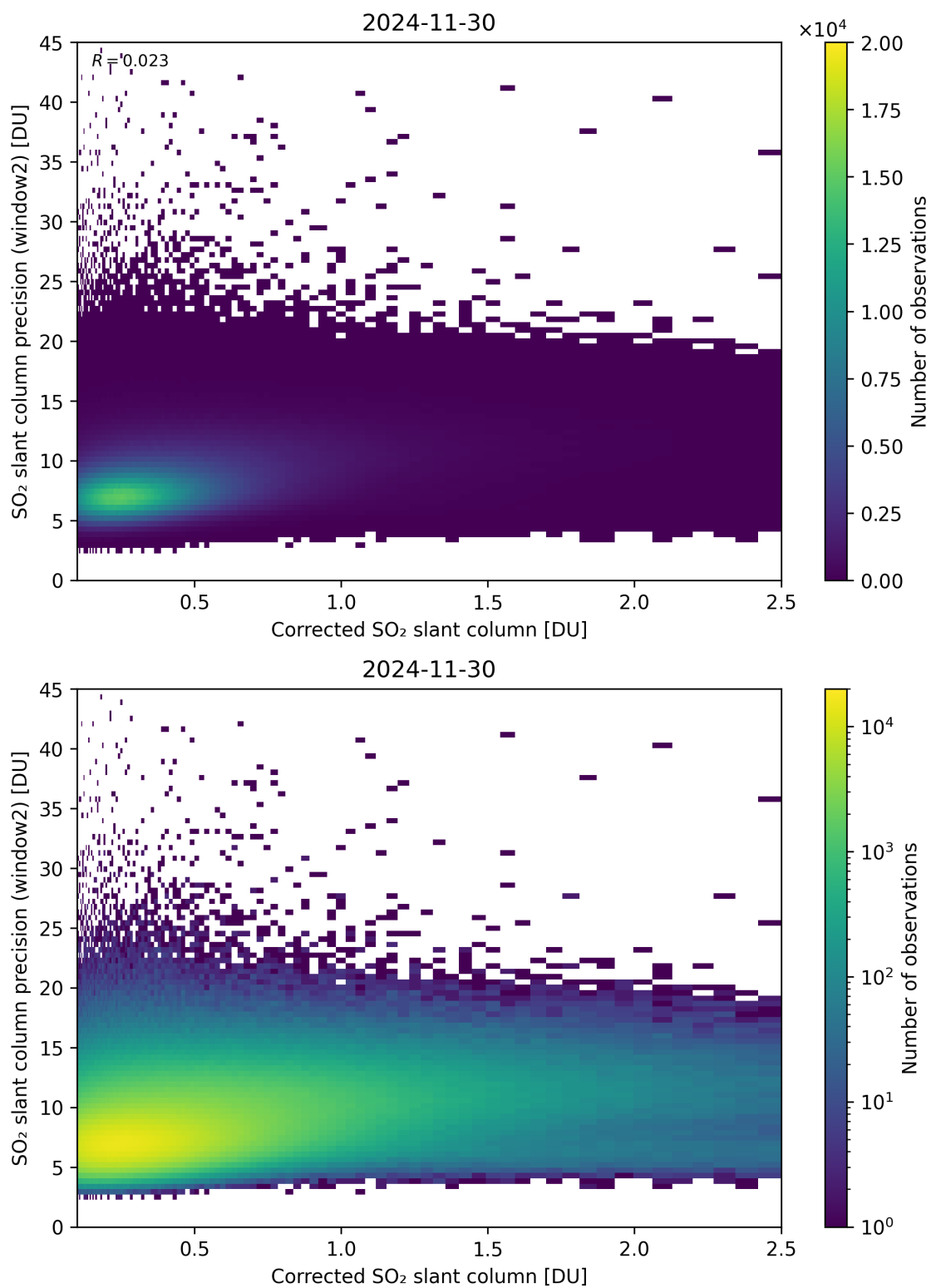
Figure 239: Scatter density plot of “Corrected SO 2 slant column” against “SO 2 slant column precision (window2)” for 2024-11-30 to 2024-12-01.
