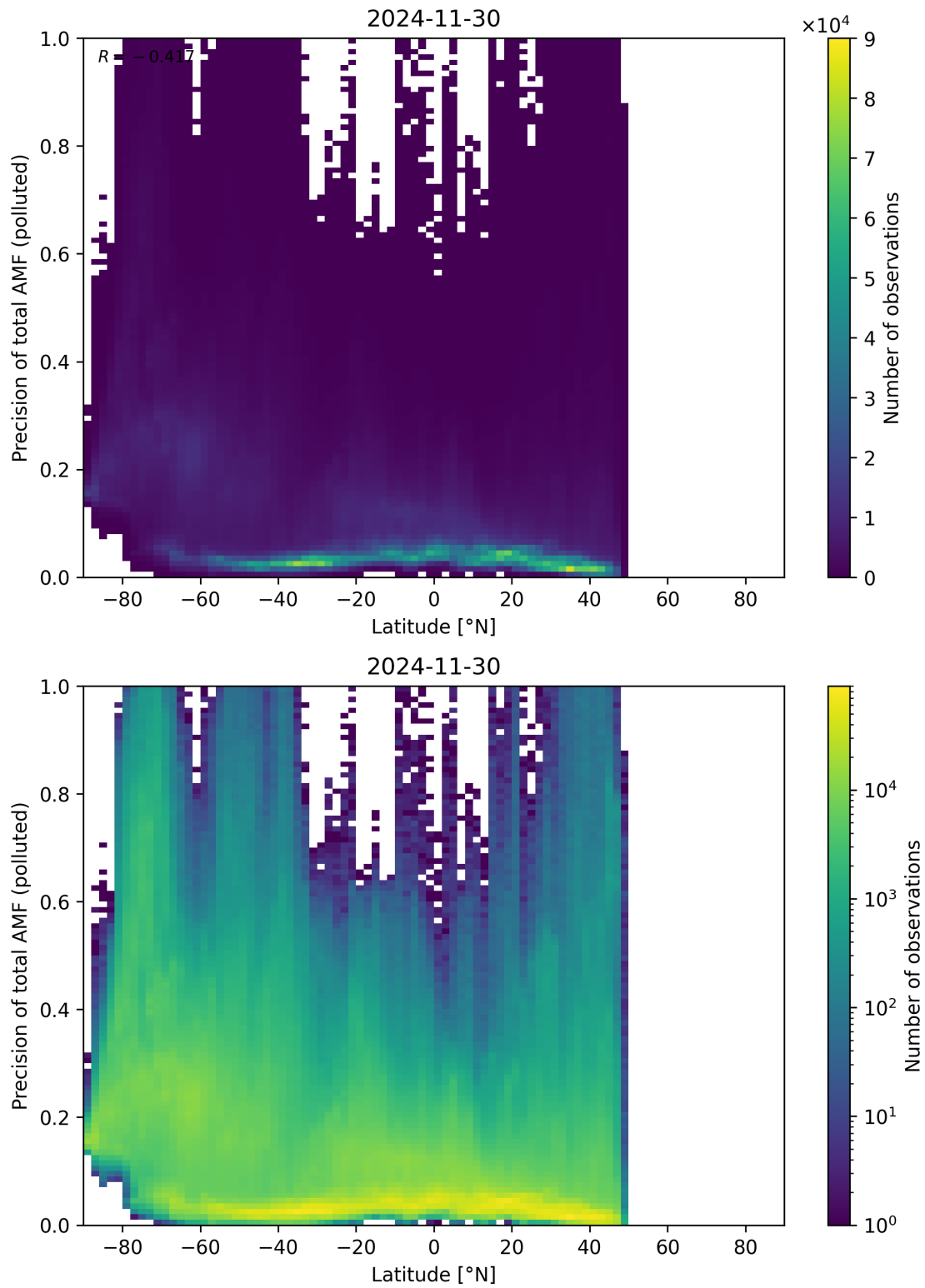
Figure 168: Scatter density plot of “Latitude” against “Precision of total AMF (polluted)” for 2024-11-30 to 2024-12-01.
