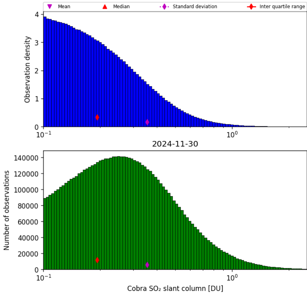
Figure 61: Histogram of “Cobra SO 2 slant column” for 2024-11-30 to 2024-12-01
