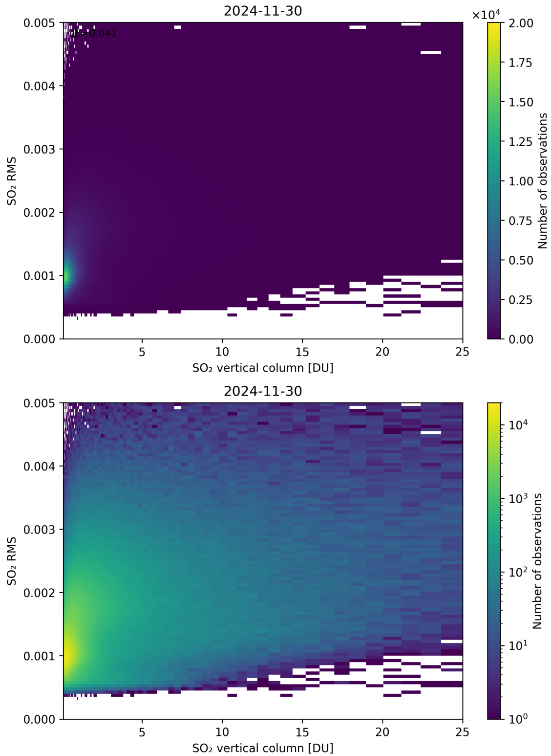
Figure 328: Scatter density plot of “SO 2 vertical column” against “SO 2 RMS” for 2024-11-30 to 2024-12-01.
