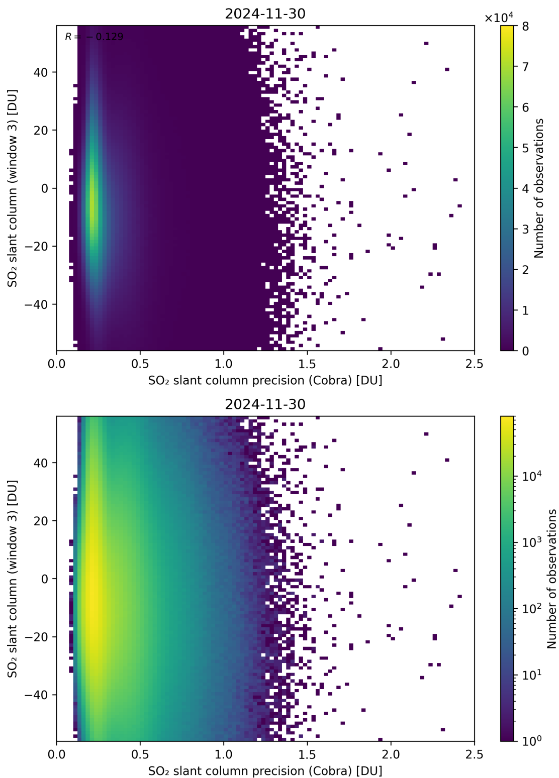
Figure 211: Scatter density plot of “SO 2 slant column precision (Cobra)” against “SO 2 slant column (window 3)” for 2024-11-30 to 2024-12-01.
