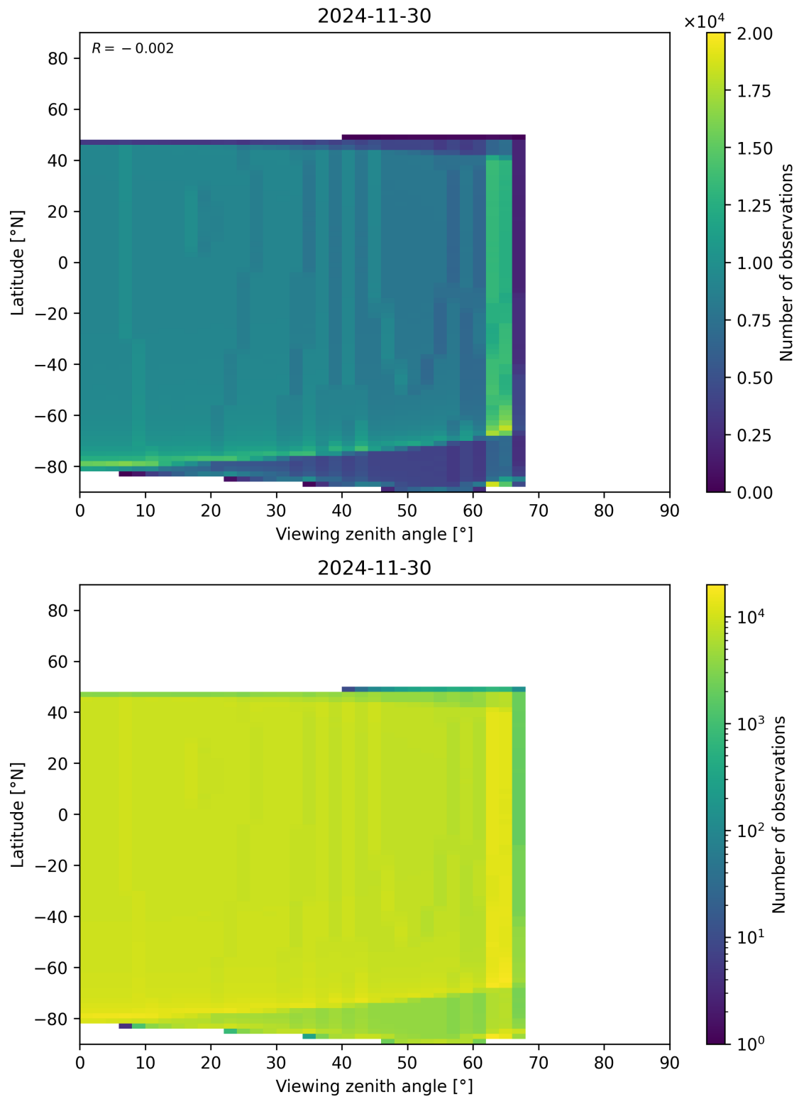
Figure 368: Scatter density plot of “Viewing zenith angle” against “Latitude” for 2024-11-30 to 2024-12-01.
