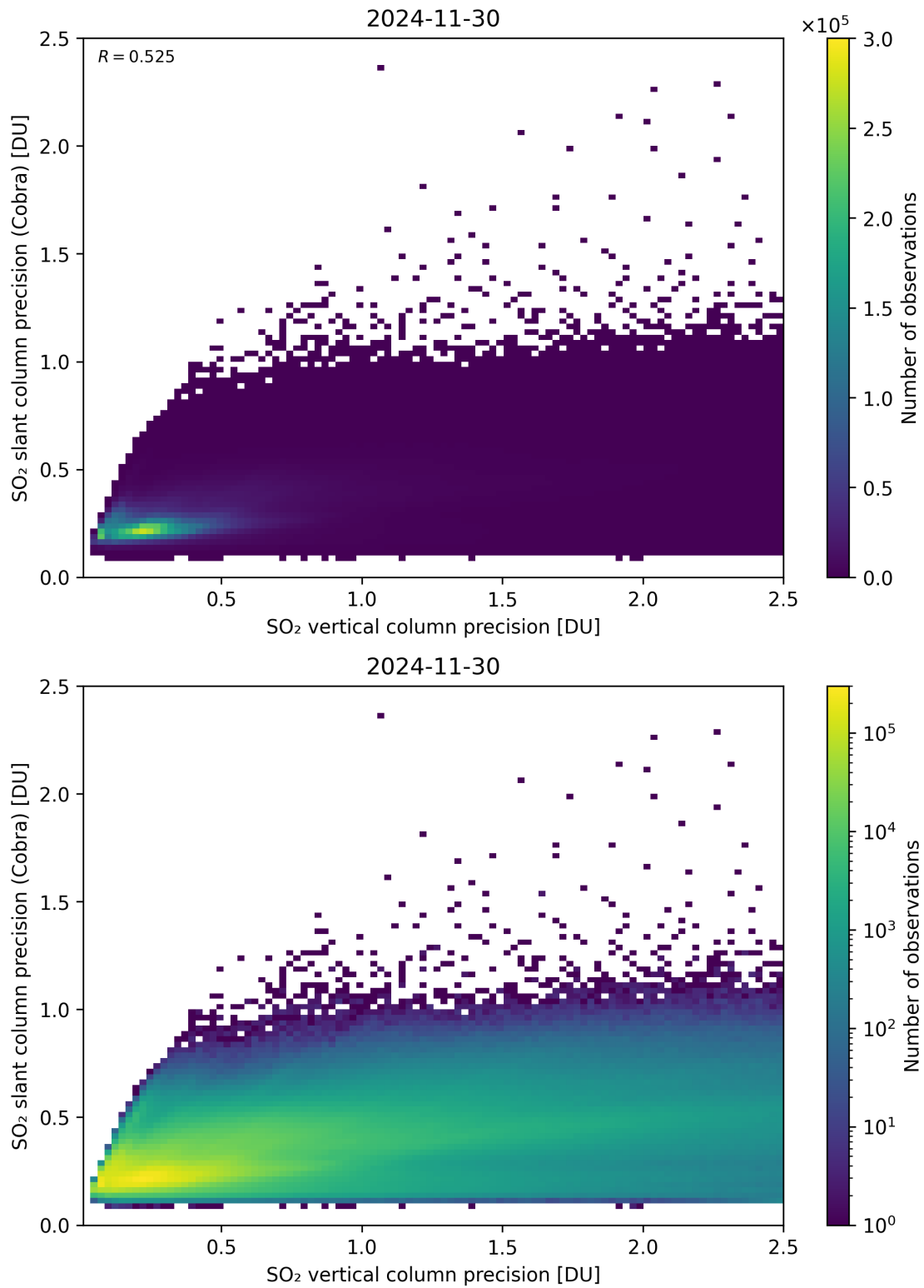
Figure 337: Scatter density plot of “SO 2 vertical column precision” against “SO 2 slant column precision (Cobra)” for 2024-11-30 to 2024-12-01.
