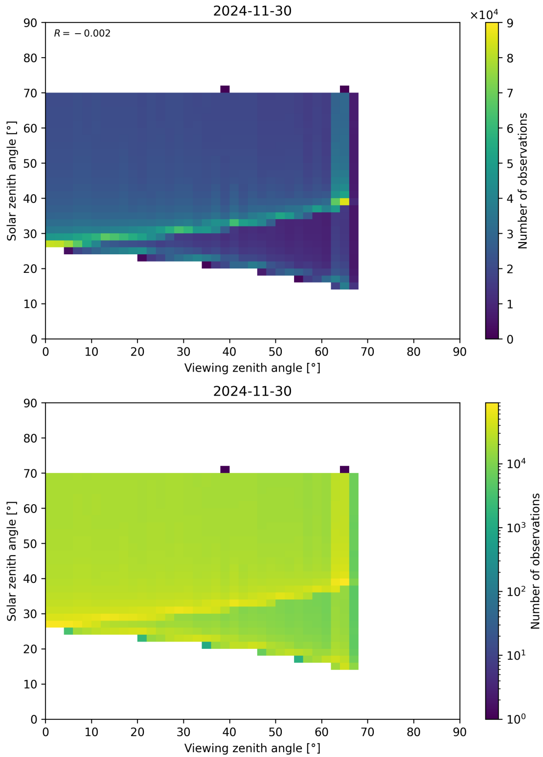
Figure 369: Scatter density plot of “Viewing zenith angle” against “Solar zenith angle” for 2024-11-30 to 2024-12-01.
