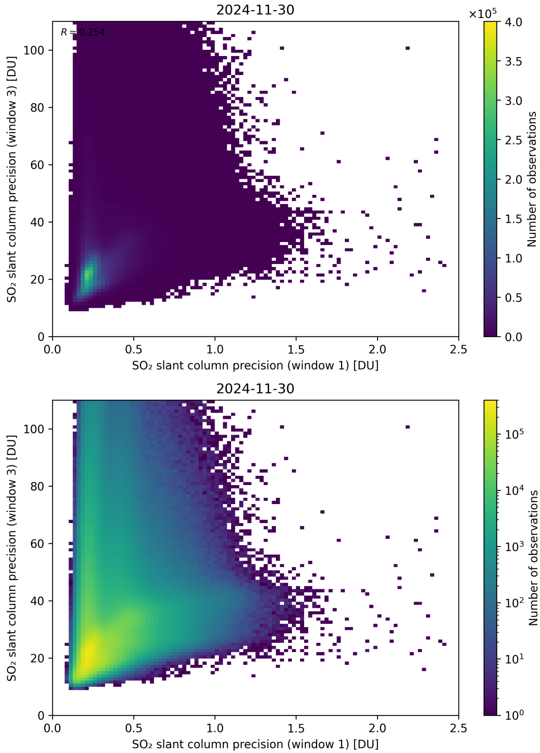
Figure 279: Scatter density plot of “SO 2 slant column precision (window 1)” against “SO 2 slant column precision (window 3)” for 2024-11-30 to 2024-12-01.
