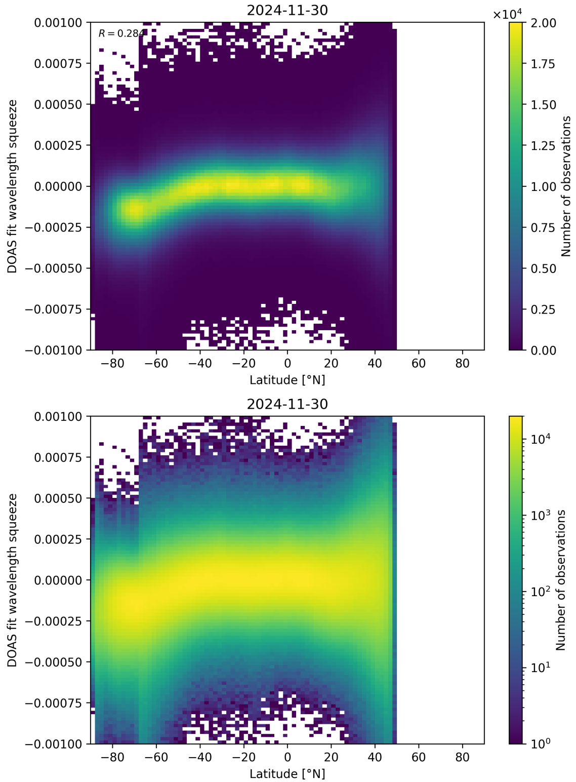
Figure 154: Scatter density plot of “Latitude” against “DOAS fit wavelength squeeze” for 2024-11-30 to 2024-12-01.
