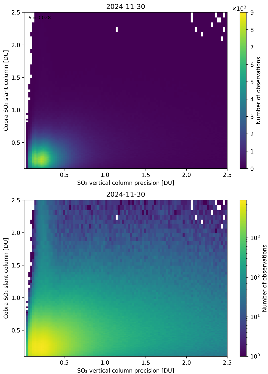
Figure 336: Scatter density plot of “SO 2 vertical column precision” against “Cobra SO 2 slant column” for 2024-11-30 to 2024-12-01.
