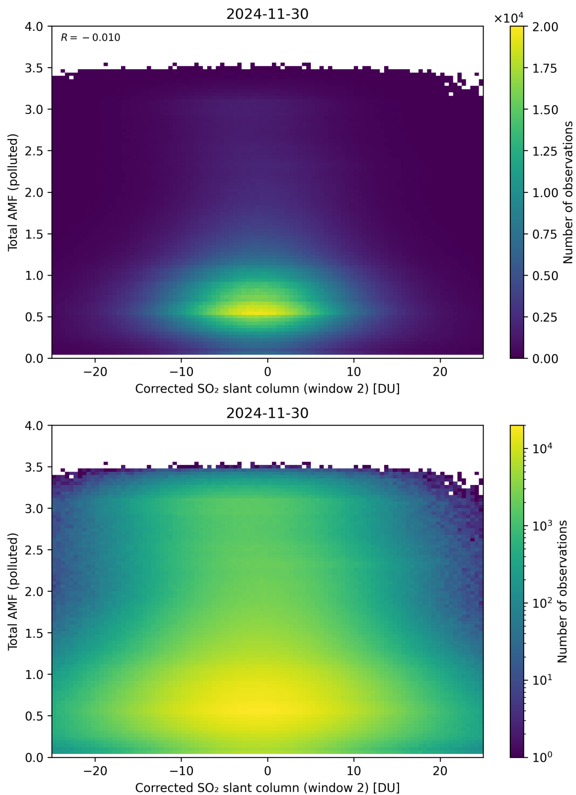
Figure 253: Scatter density plot of “Corrected SO 2 slant column (window 2)” against “Total AMF (polluted)” for 2024-11-30 to 2024-12-01.
