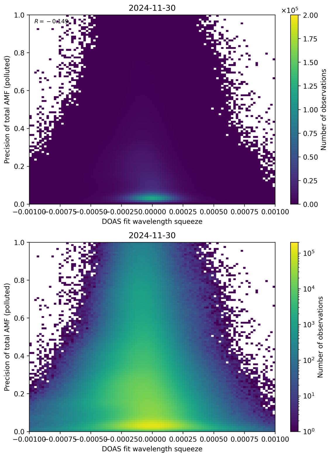
Figure 146: Scatter density plot of “DOAS fit wavelength squeeze” against “Precision of total AMF (polluted)” for 2024-11-30 to 2024-12-01.
