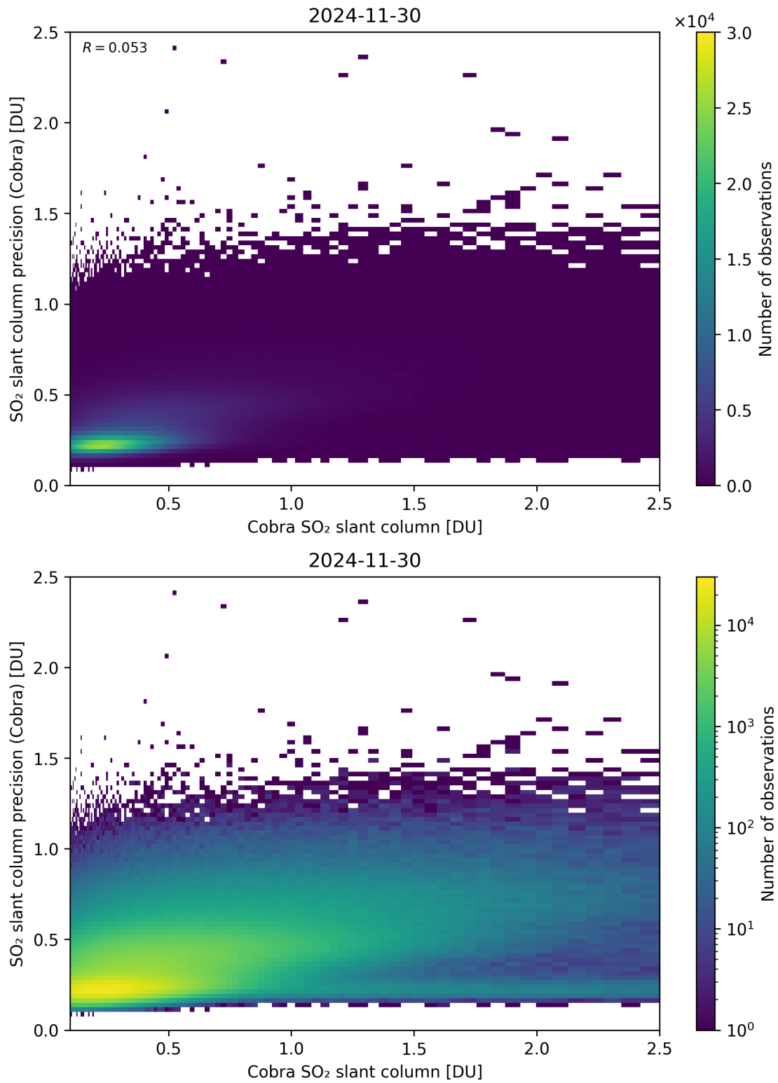
Figure 216: Scatter density plot of “Cobra SO 2 slant column” against “SO 2 slant column precision (Cobra)” for 2024-11-30 to 2024-12-01.
