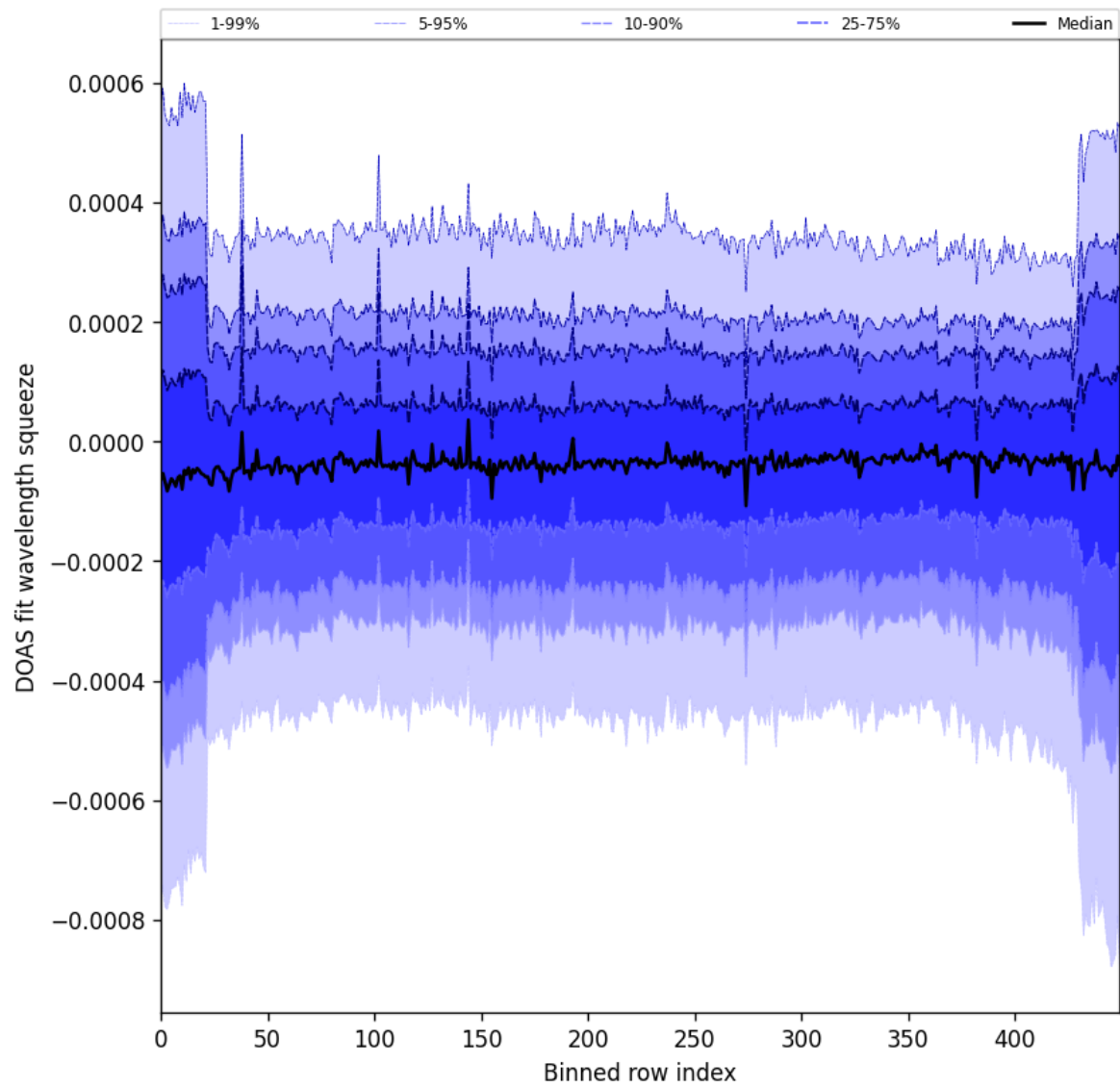
Figure 103: Along track statistics of “DOAS fit wavelength squeeze” for 2024-11-30 to 2024-12-01
