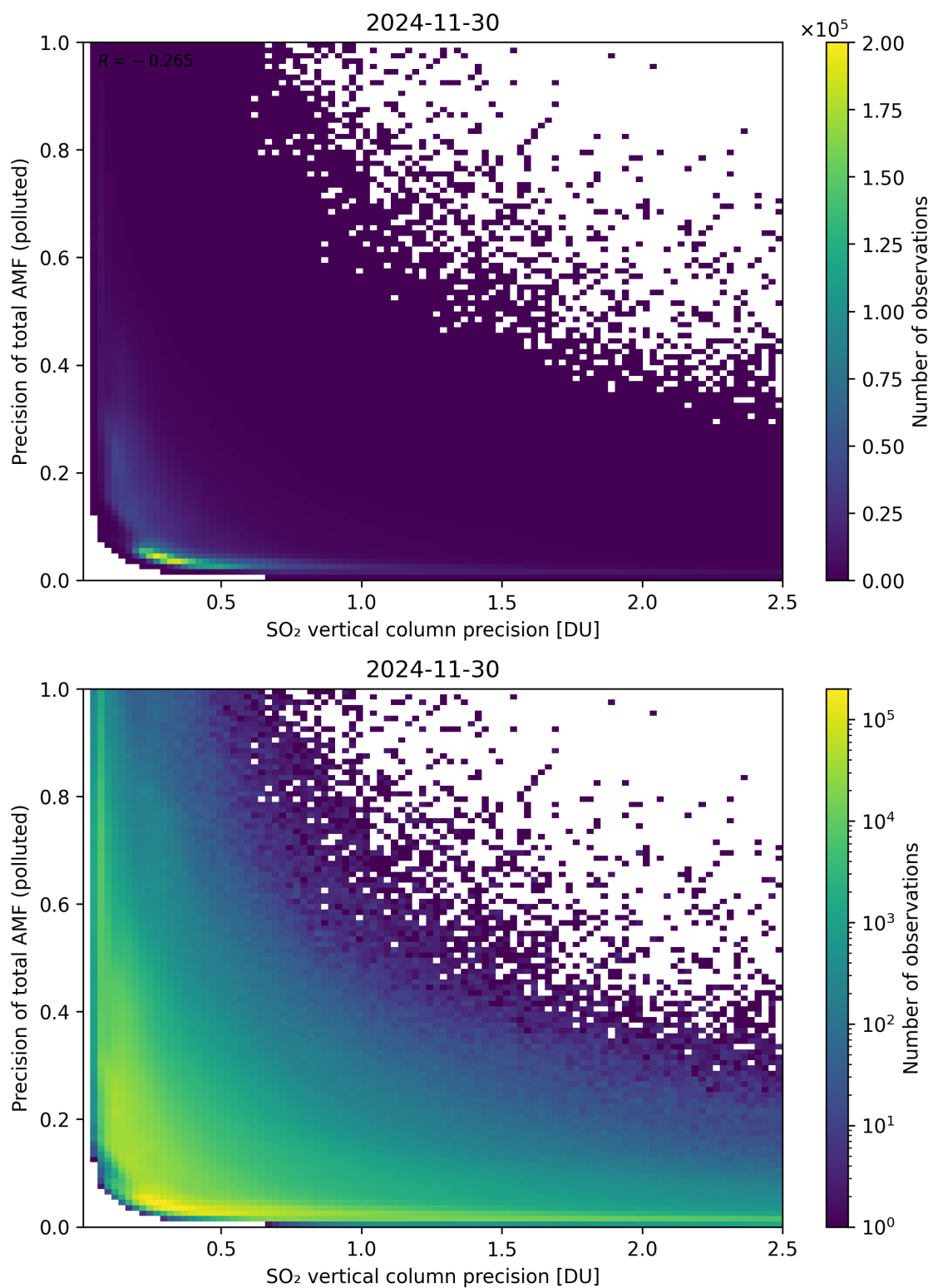
Figure 347: Scatter density plot of “SO 2 vertical column precision” against “Precision of total AMF (polluted)” for 2024-11-30 to 2024-12-01.
