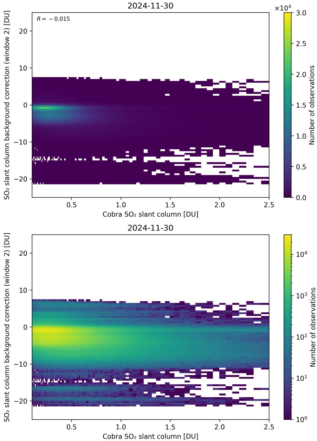
Figure 194: Scatter density plot of “Cobra SO 2 slant column” against “SO 2 slant column background correction (window 2)” for 2024-11-30 to 2024-12-01.
