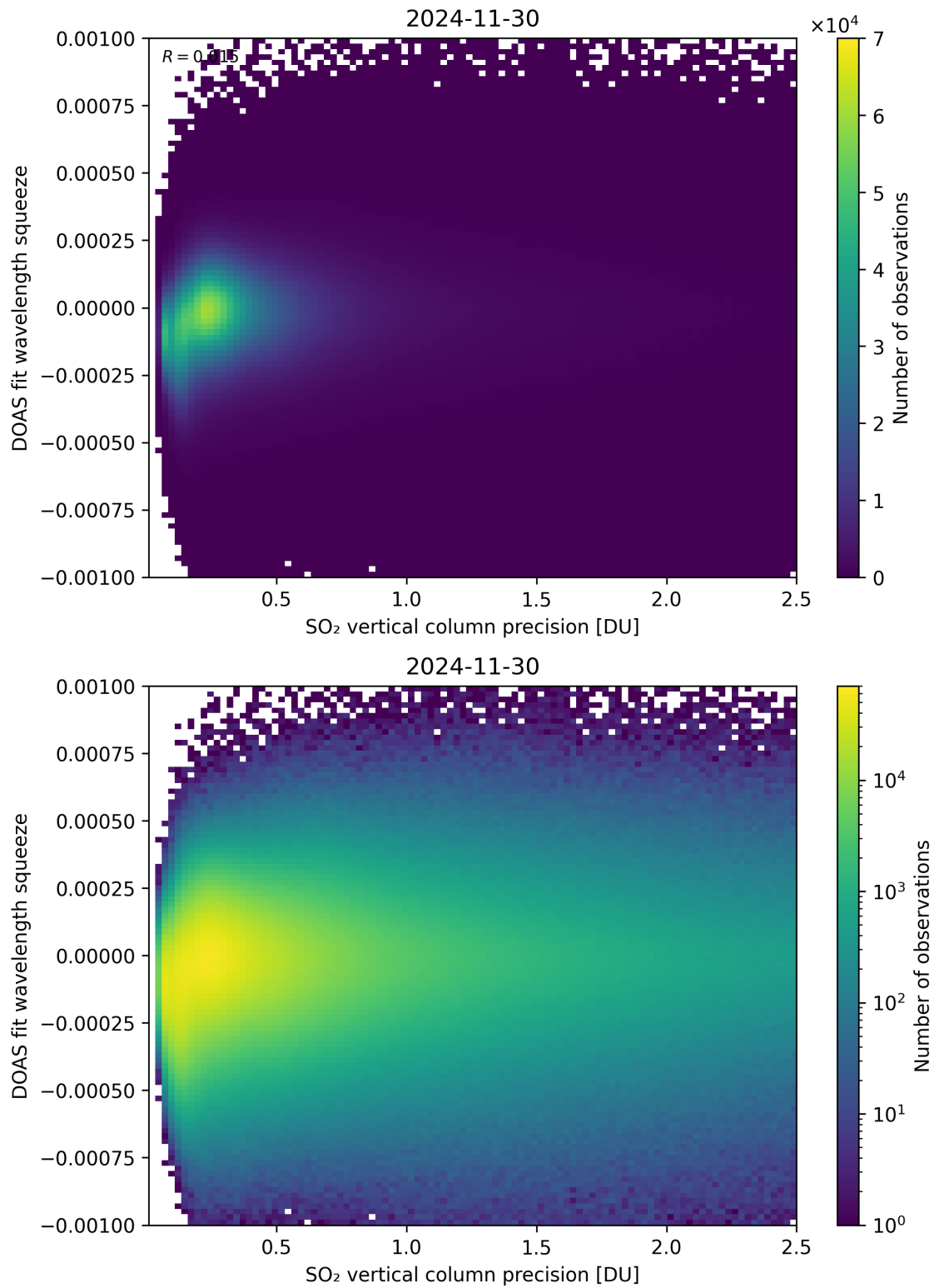
Figure 333: Scatter density plot of “SO 2 vertical column precision” against “DOAS fit wavelength squeeze” for 2024-11-30 to 2024-12-01.
