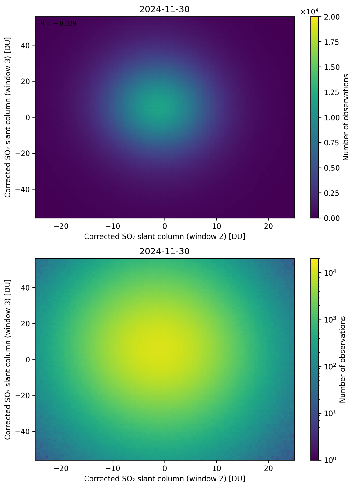
Figure 250: Scatter density plot of “Corrected SO 2 slant column (window 2)” against “Corrected SO 2 slant column (window 3)” for 2024-11-30 to 2024-12-01.
