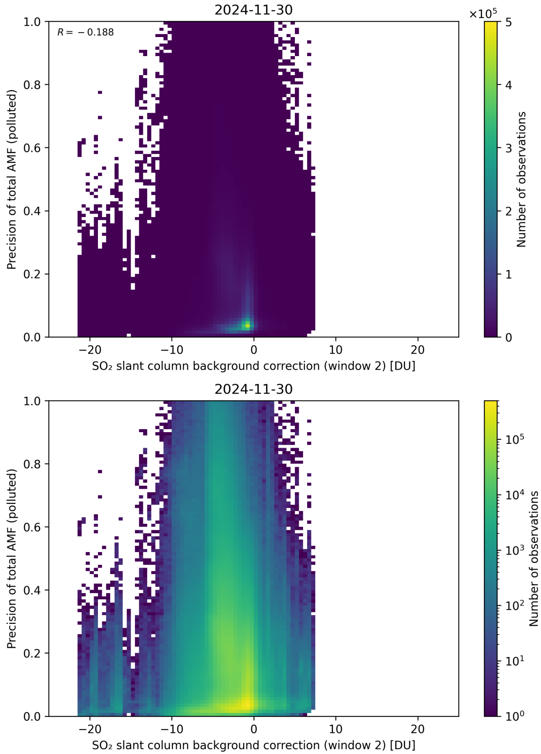
Figure 131: Scatter density plot of “SO 2 slant column background correction (window 2)” against “Precision of total AMF (polluted)” for 2024-11-30 to 2024-12-01.
