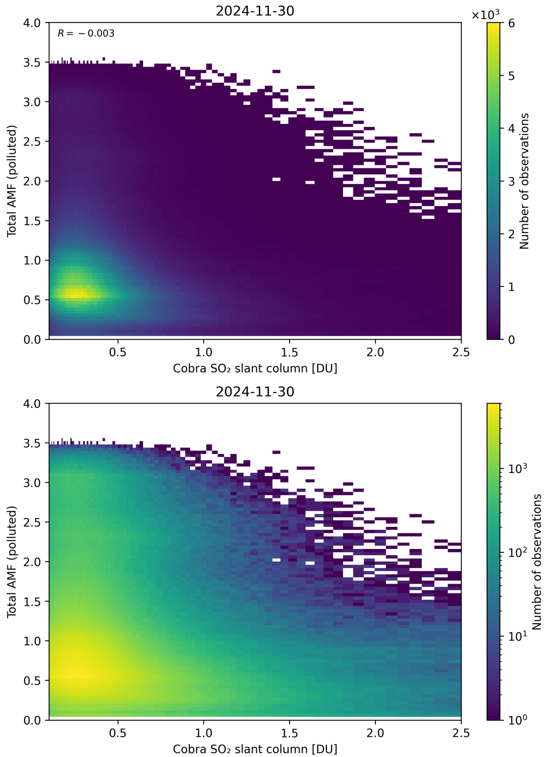
Figure 224: Scatter density plot of “Cobra SO 2 slant column” against “Total AMF (polluted)” for 2024-11-30 to 2024-12-01.
