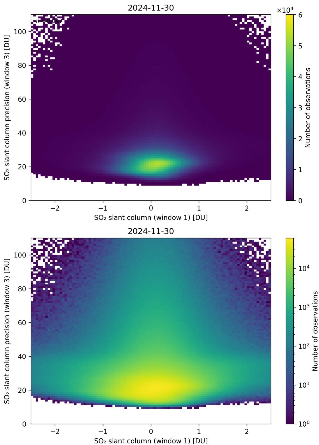
Figure 288: Scatter density plot of “SO 2 slant column (window 1)” against “SO 2 slant column precision (window 3)” for 2024-11-30 to 2024-12-01.
