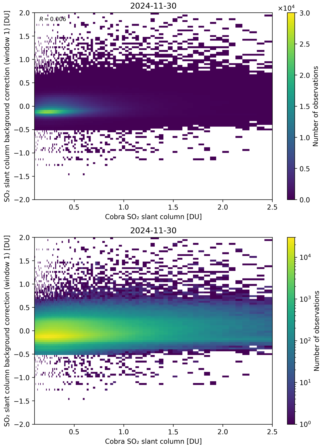
Figure 193: Scatter density plot of “Cobra SO 2 slant column” against “SO 2 slant column background correction (window 1)” for 2024-11-30 to 2024-12-01.
