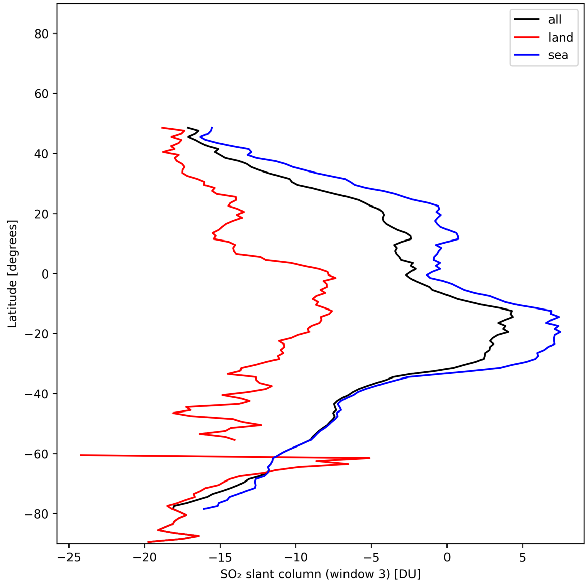
Figure 45: Zonal average of “SO 2 slant column (window 3)” for 2024-11-30 to 2024-12-01.
