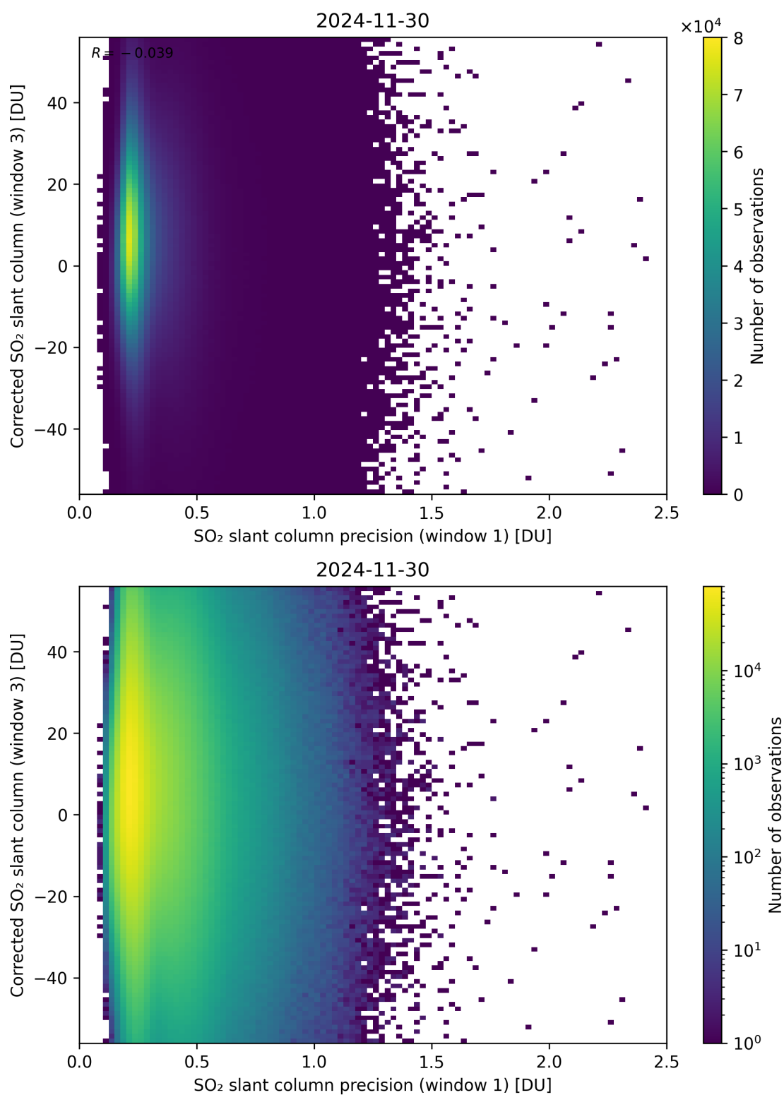
Figure 276: Scatter density plot of “SO 2 slant column precision (window 1)” against “Corrected SO 2 slant column (window 3)” for 2024-11-30 to 2024-12-01.
