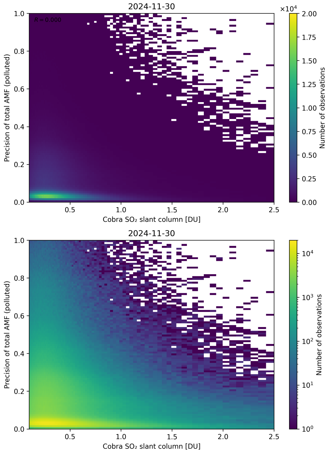
Figure 225: Scatter density plot of “Cobra SO 2 slant column” against “Precision of total AMF (polluted)” for 2024-11-30 to 2024-12-01.
