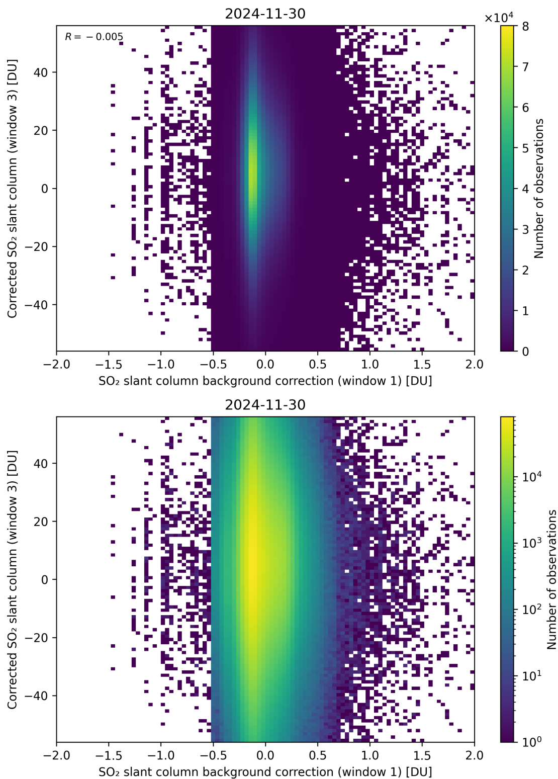
Figure 116: Scatter density plot of “SO 2 slant column background correction (window 1)” against “Corrected SO 2 slant column (window 3)” for 2024-11-30 to 2024-12-01.
