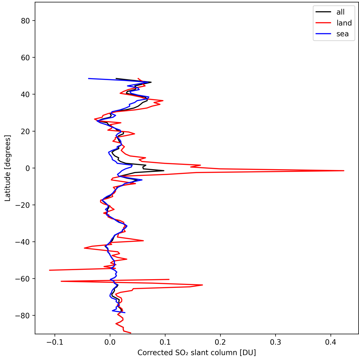
Figure 34: Zonal average of “Corrected SO 2 slant column” for 2024-11-30 to 2024-12-01.
