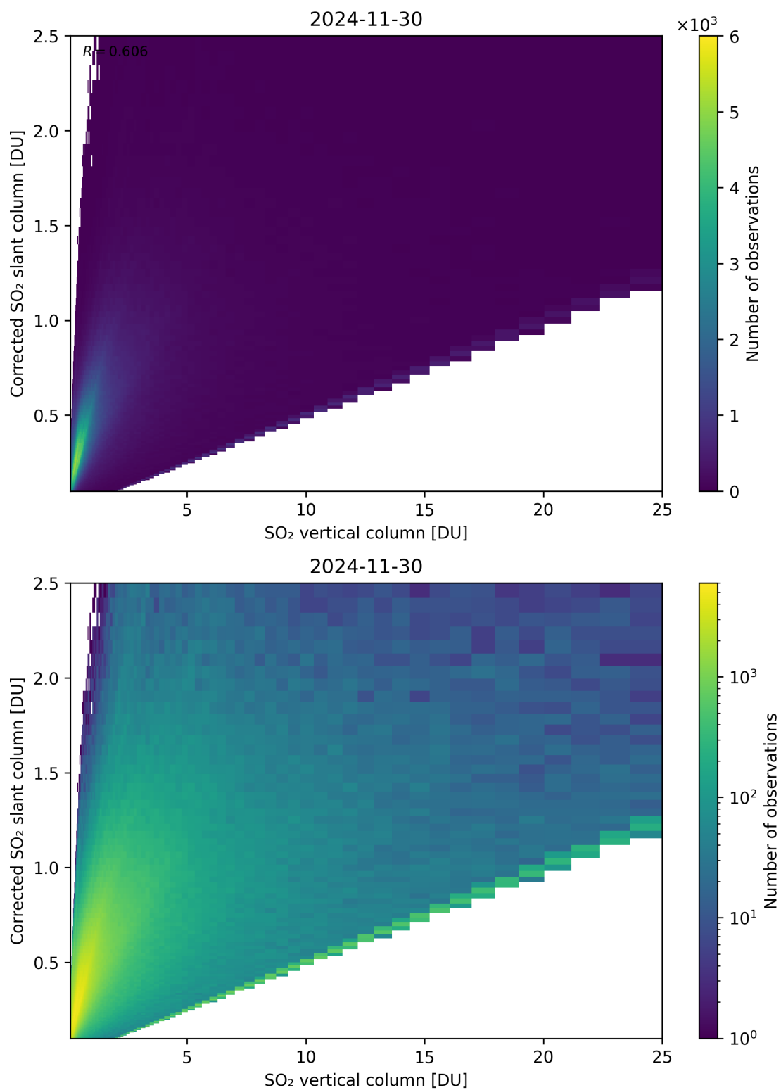
Figure 351: Scatter density plot of “SO 2 vertical column” against “Corrected SO 2 slant column” for 2024-11-30 to 2024-12-01.
