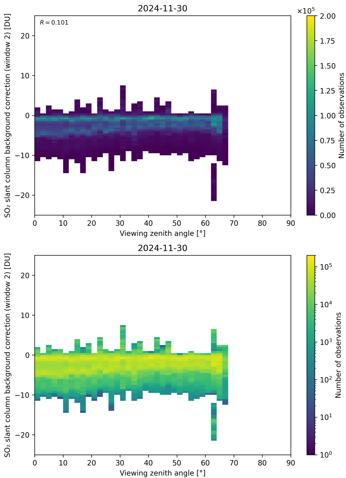
Figure 363: Scatter density plot of “Viewing zenith angle” against “SO 2 slant column background correction (window 2)” for 2024-11-30 to 2024-12-01.
