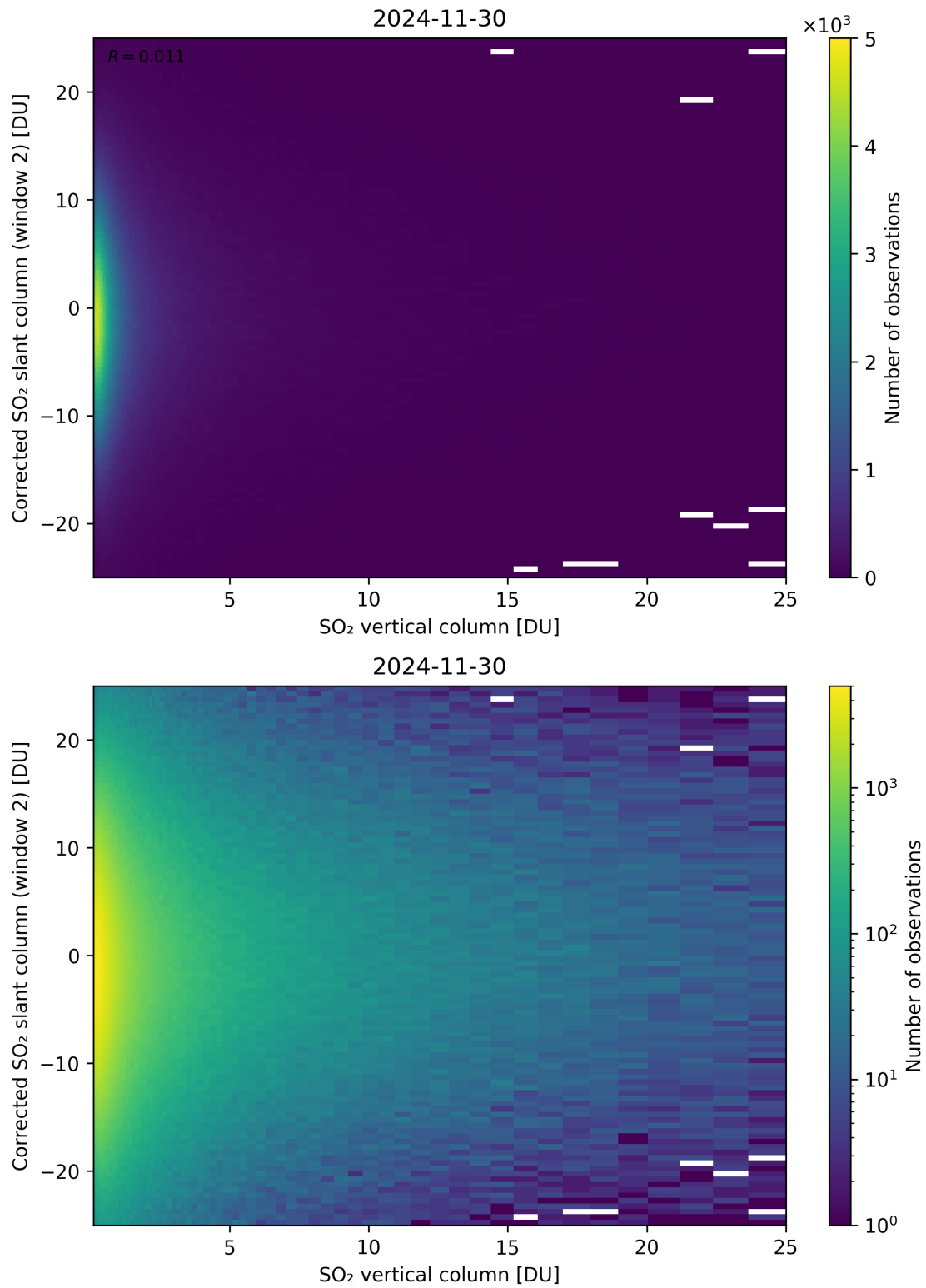
Figure 352: Scatter density plot of “SO 2 vertical column” against “Corrected SO 2 slant column (window 2)” for 2024-11-30 to 2024-12-01.
