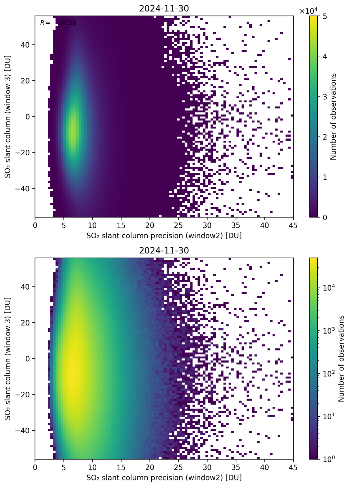
Figure 299: Scatter density plot of “SO 2 slant column precision (window2)” against “SO 2 slant column (window 3)” for 2024-11-30 to 2024-12-01.
