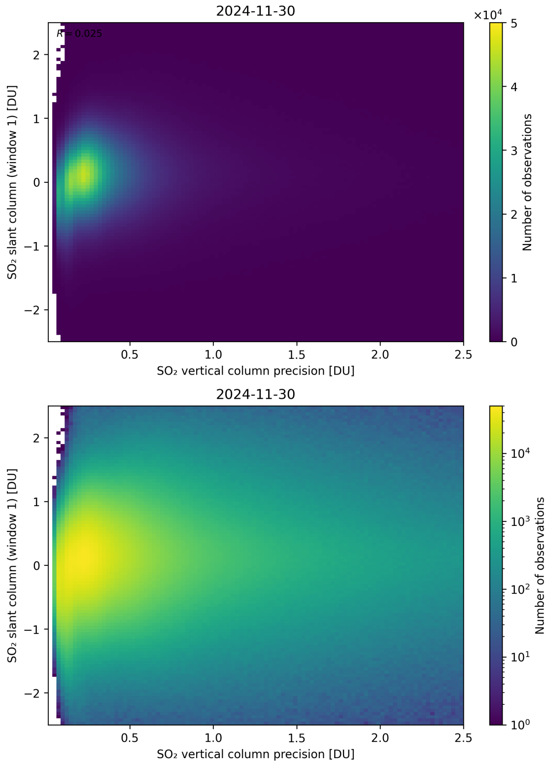
Figure 341: Scatter density plot of “SO 2 vertical column precision” against “SO 2 slant column (window 1)” for 2024-11-30 to 2024-12-01.
