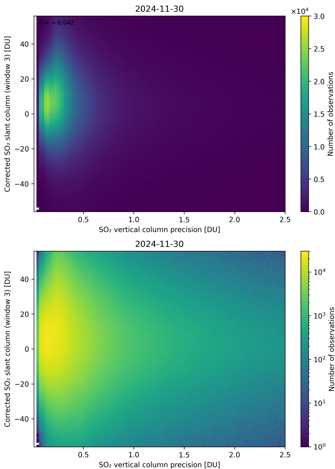
Figure 340: Scatter density plot of “SO 2 vertical column precision” against “Corrected SO 2 slant column (window 3)” for 2024-11-30 to 2024-12-01.
