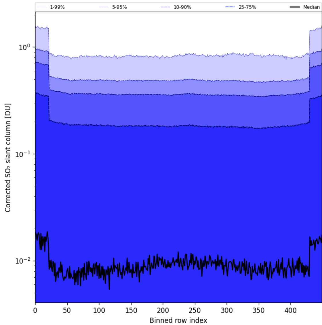
Figure 86: Along track statistics of “Corrected SO 2 slant column” for 2024-11-30 to 2024-12-01
