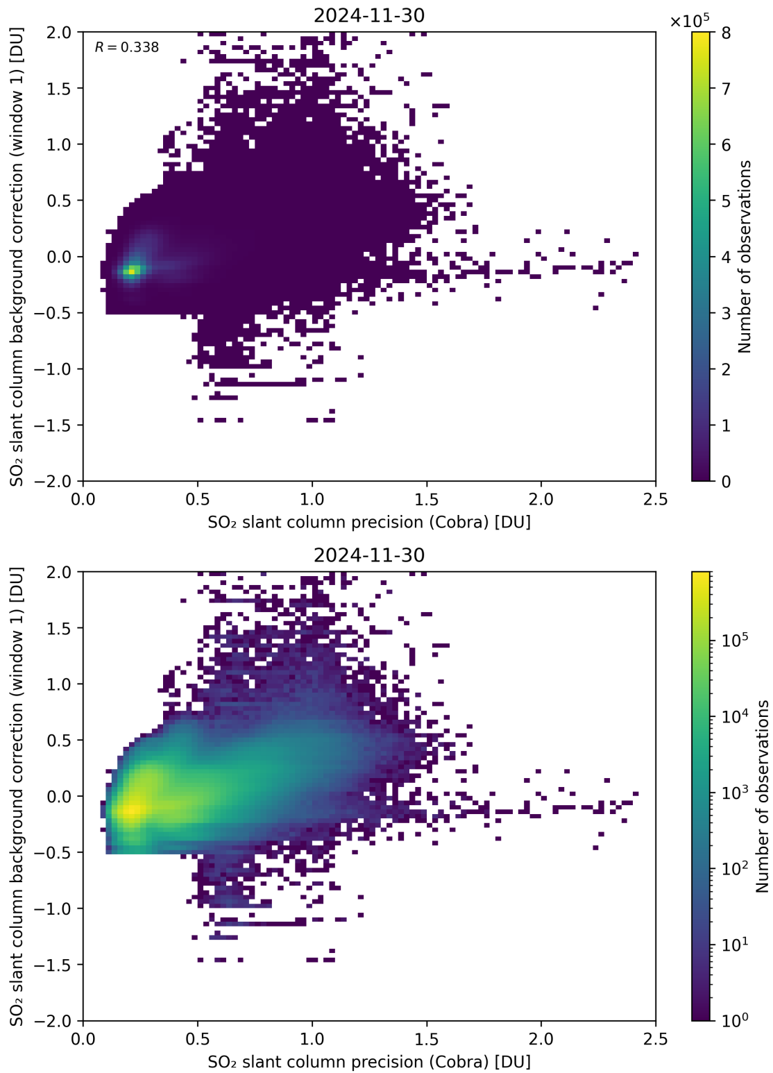
Figure 199: Scatter density plot of “SO 2 slant column precision (Cobra)” against “SO 2 slant column background correction (window 1)” for 2024-11-30 to 2024-12-01.
