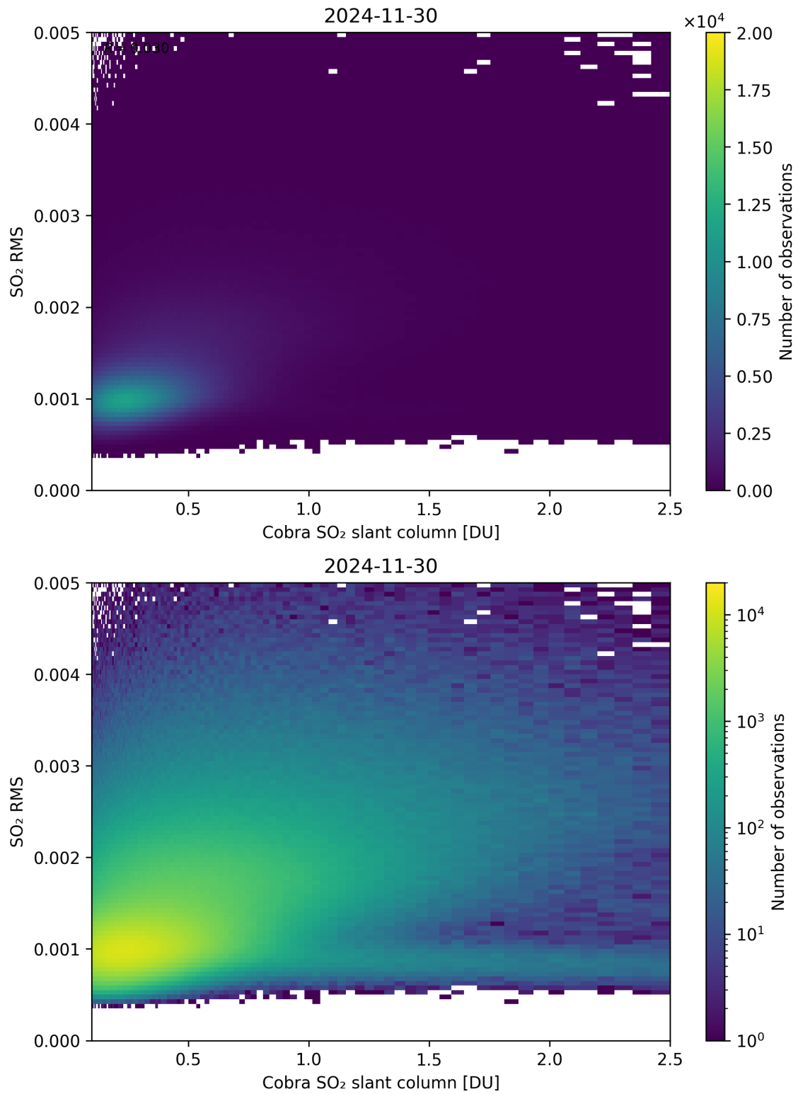
Figure 198: Scatter density plot of “Cobra SO 2 slant column” against “SO 2 RMS” for 2024-11-30 to 2024-12-01.
