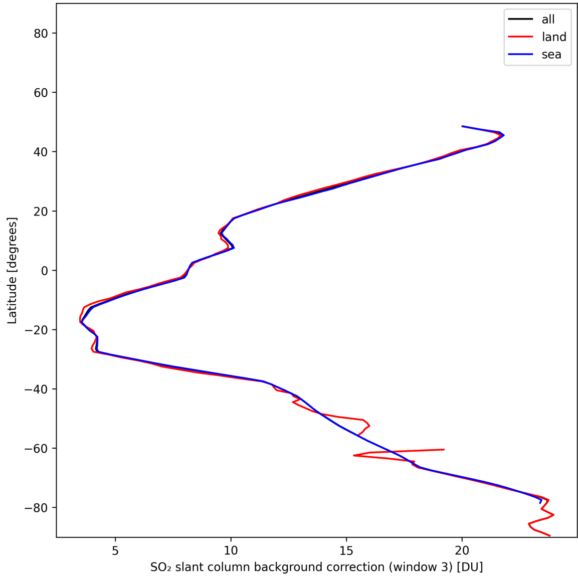
Figure 48: Zonal average of “SO 2 slant column background correction (window 3)” for 2024-11-30 to 2024-12-01.
