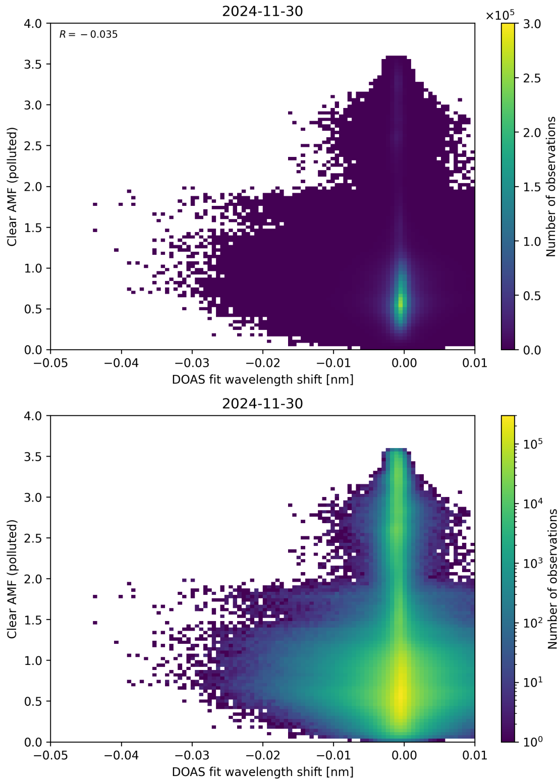
Figure 140: Scatter density plot of “DOAS fit wavelength shift” against “Clear AMF (polluted)” for 2024-11-30 to 2024-12-01.
