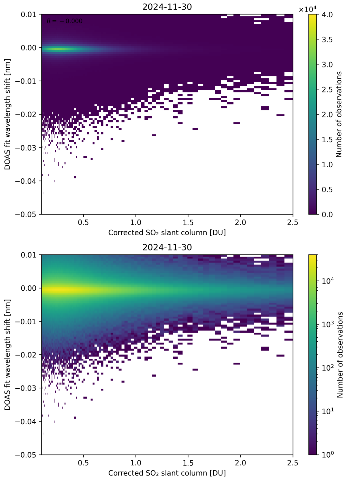
Figure 229: Scatter density plot of “Corrected SO 2 slant column” against “DOAS fit wavelength shift” for 2024-11-30 to 2024-12-01.
