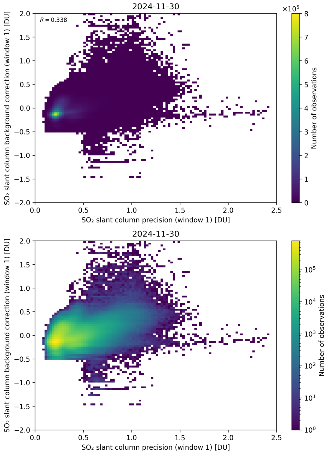
Figure 268: Scatter density plot of “SO 2 slant column precision (window 1)” against “SO 2 slant column background correction (window 1)” for 2024-11-30 to 2024-12-01.
