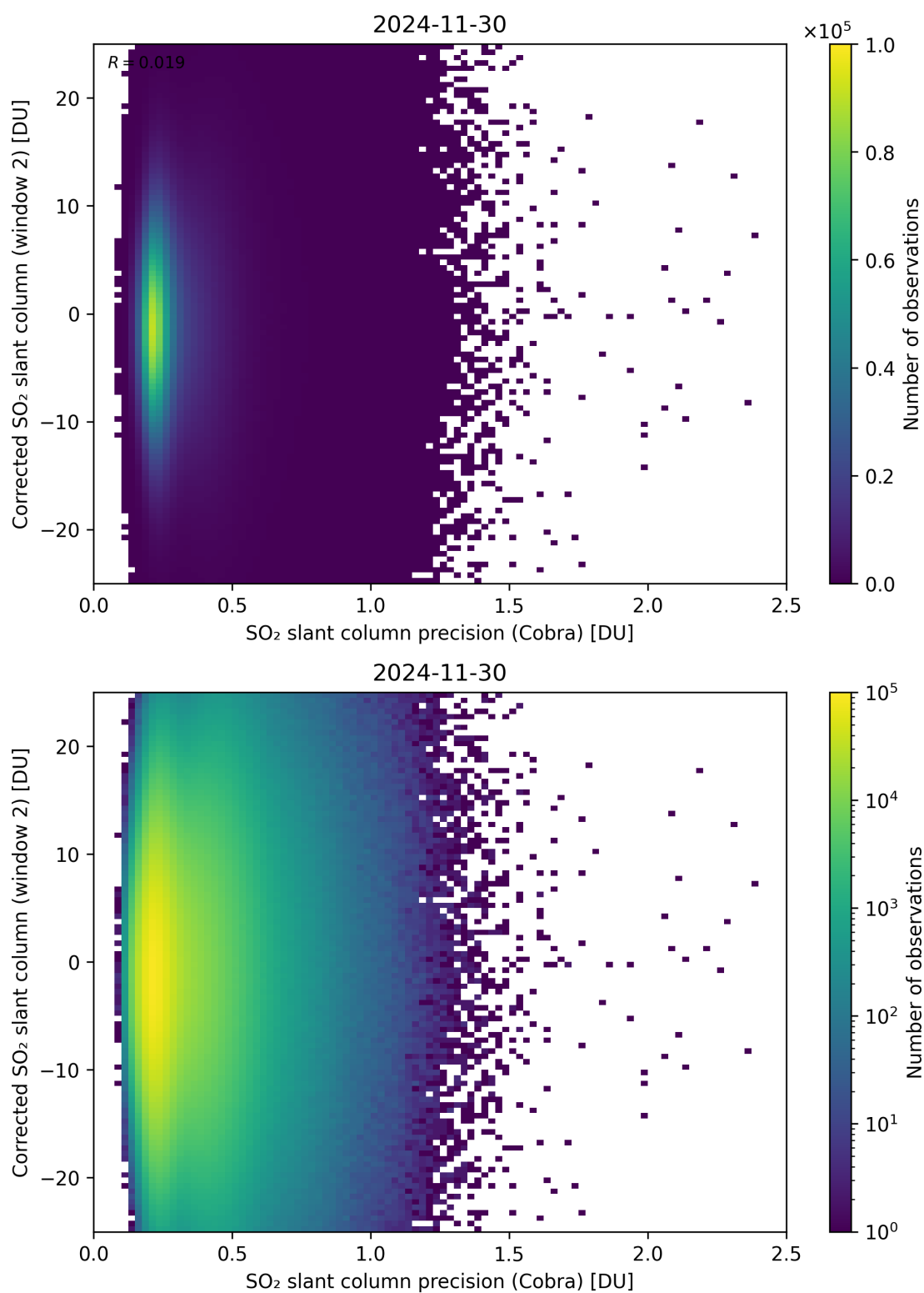
Figure 206: Scatter density plot of “SO 2 slant column precision (Cobra)” against “Corrected SO 2 slant column (window 2)” for 2024-11-30 to 2024-12-01.
