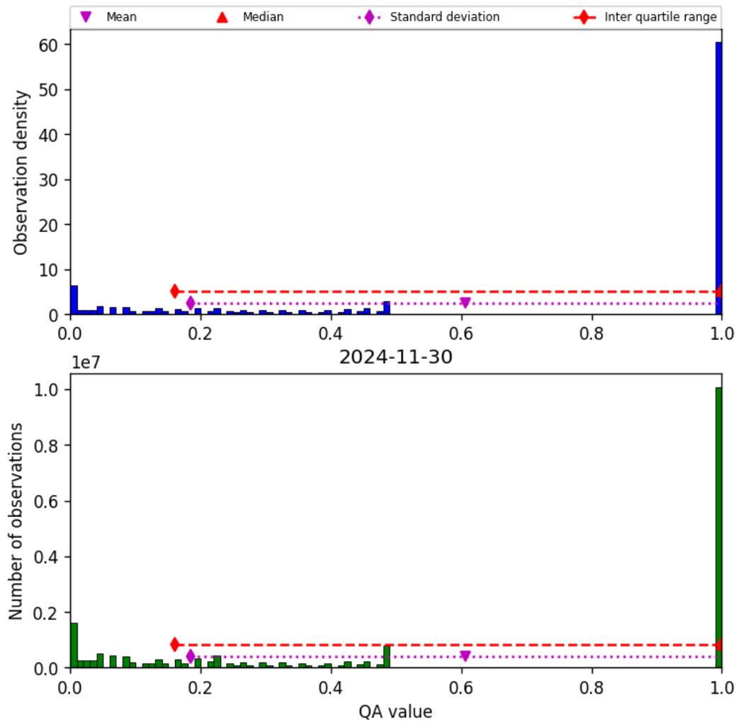
Figure 57: Histogram of “QA value” for 2024-11-30 to 2024-12-01
