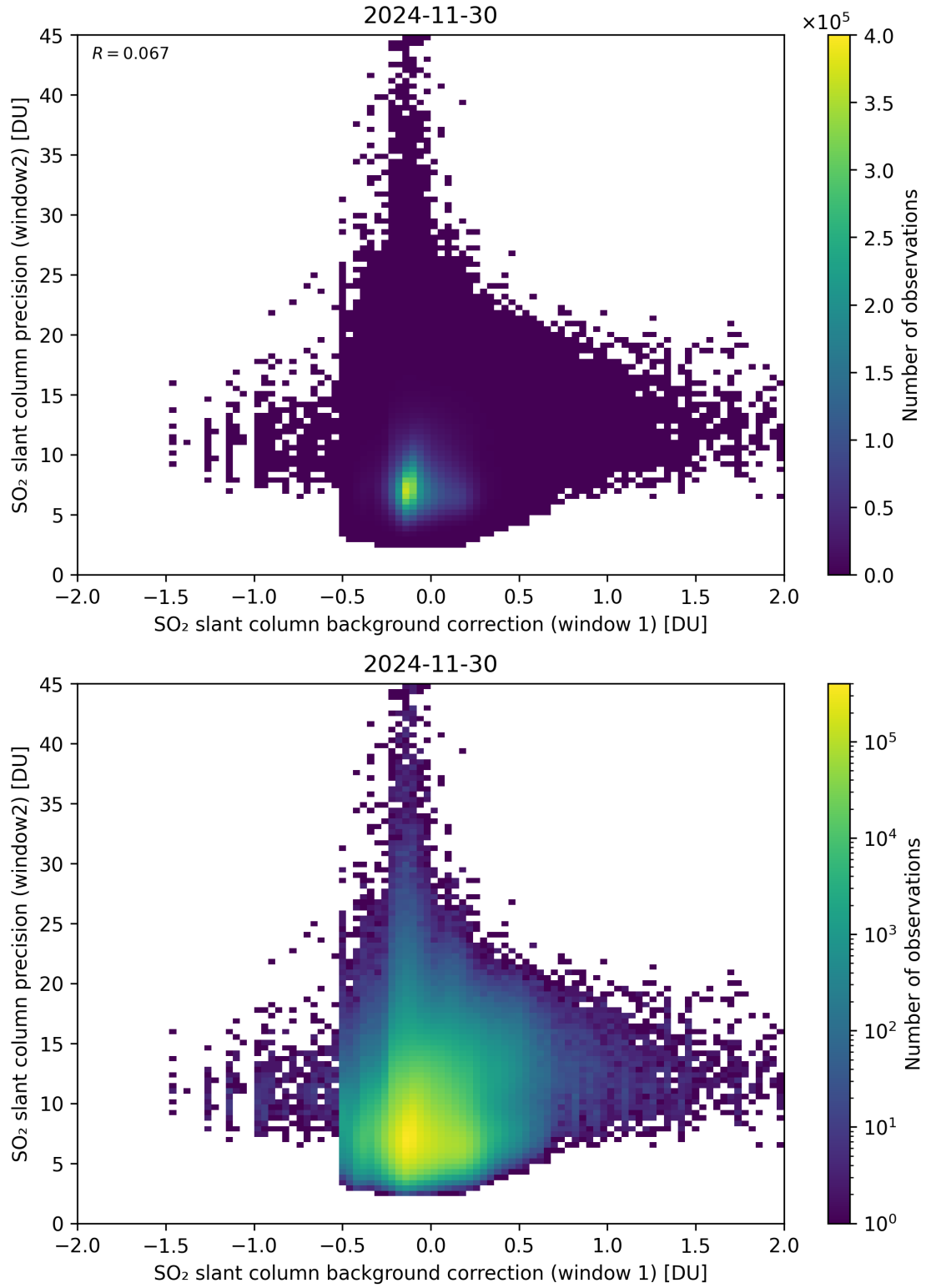
Figure 117: Scatter density plot of “SO 2 slant column background correction (window 1)” against “SO 2 slant column precision (window2)” for 2024-11-30 to 2024-12-01.
