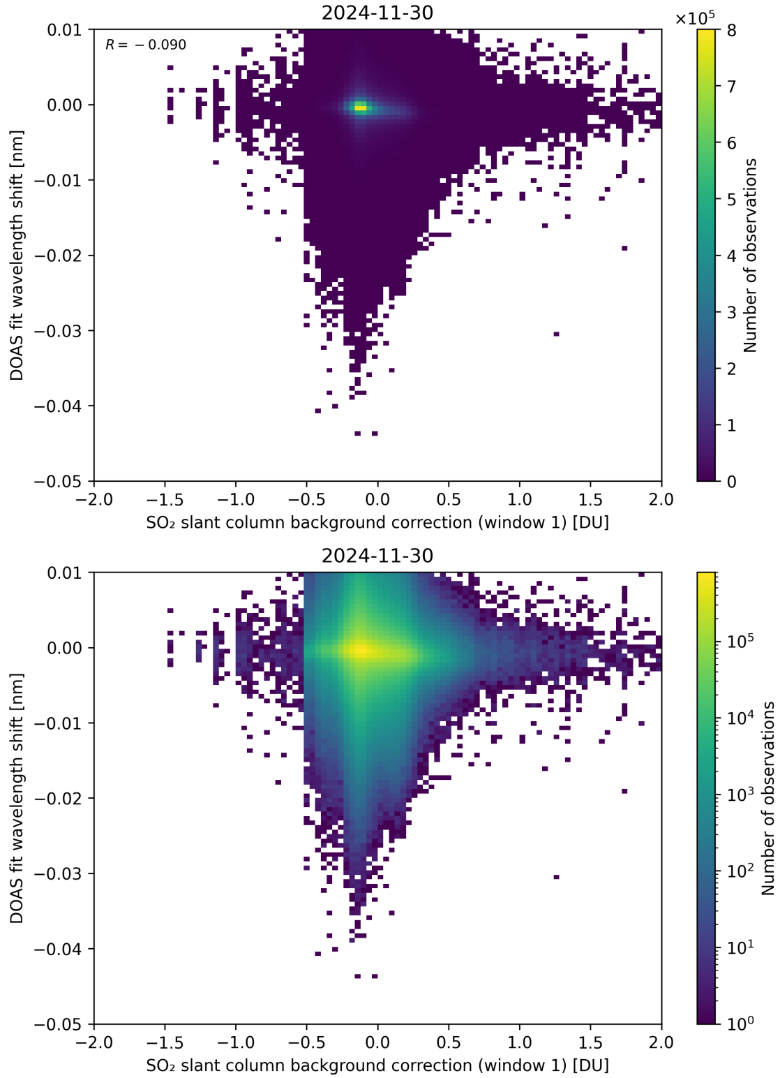
Figure 111: Scatter density plot of “SO 2 slant column background correction (window 1)” against “DOAS fit wavelength shift” for 2024-11-30 to 2024-12-01.
