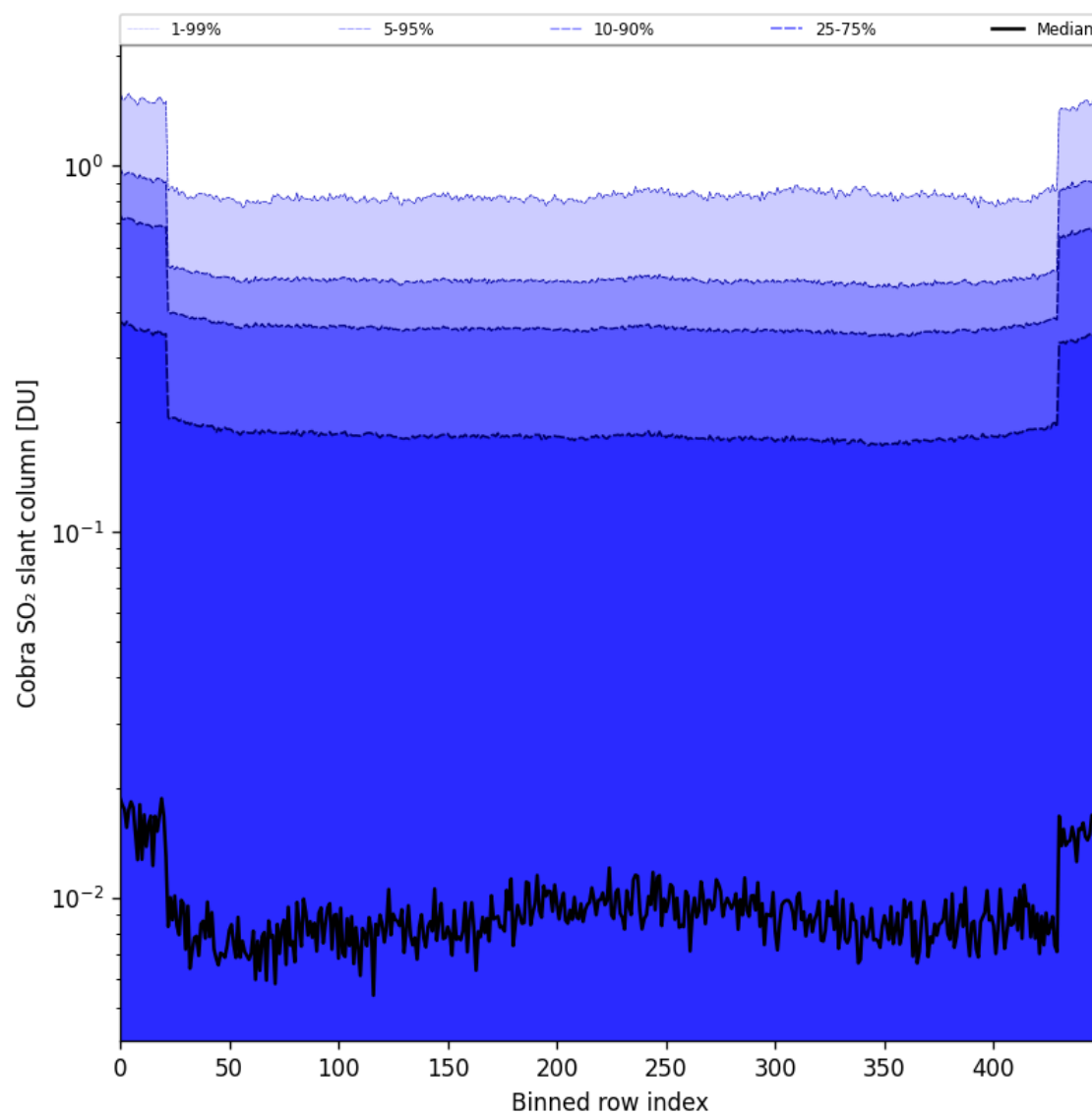
Figure 87: Along track statistics of “Cobra SO 2 slant column” for 2024-11-30 to 2024-12-01
