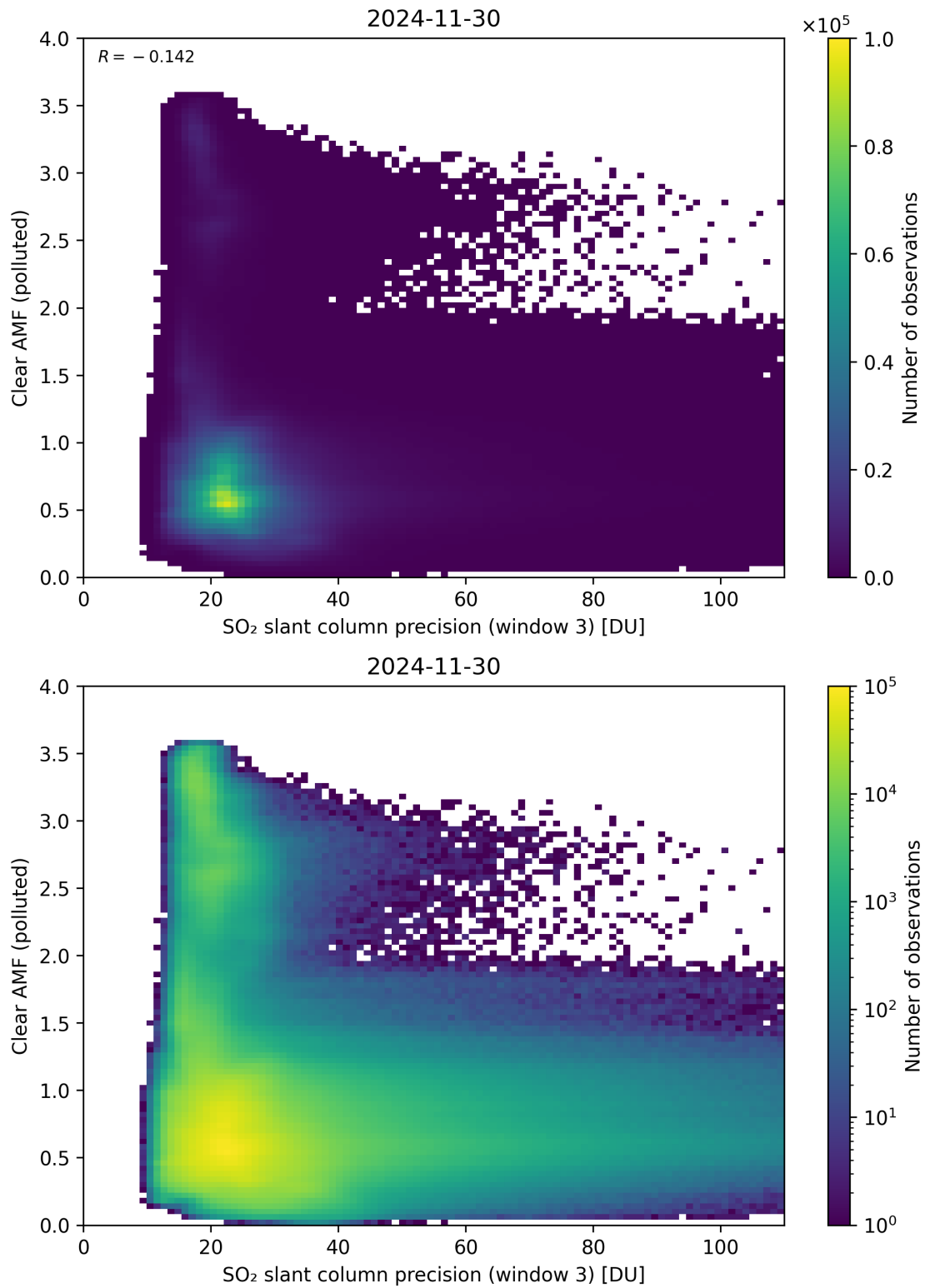
Figure 311: Scatter density plot of “SO 2 slant column precision (window 3)” against “Clear AMF (polluted)” for 2024-11-30 to 2024-12-01.
