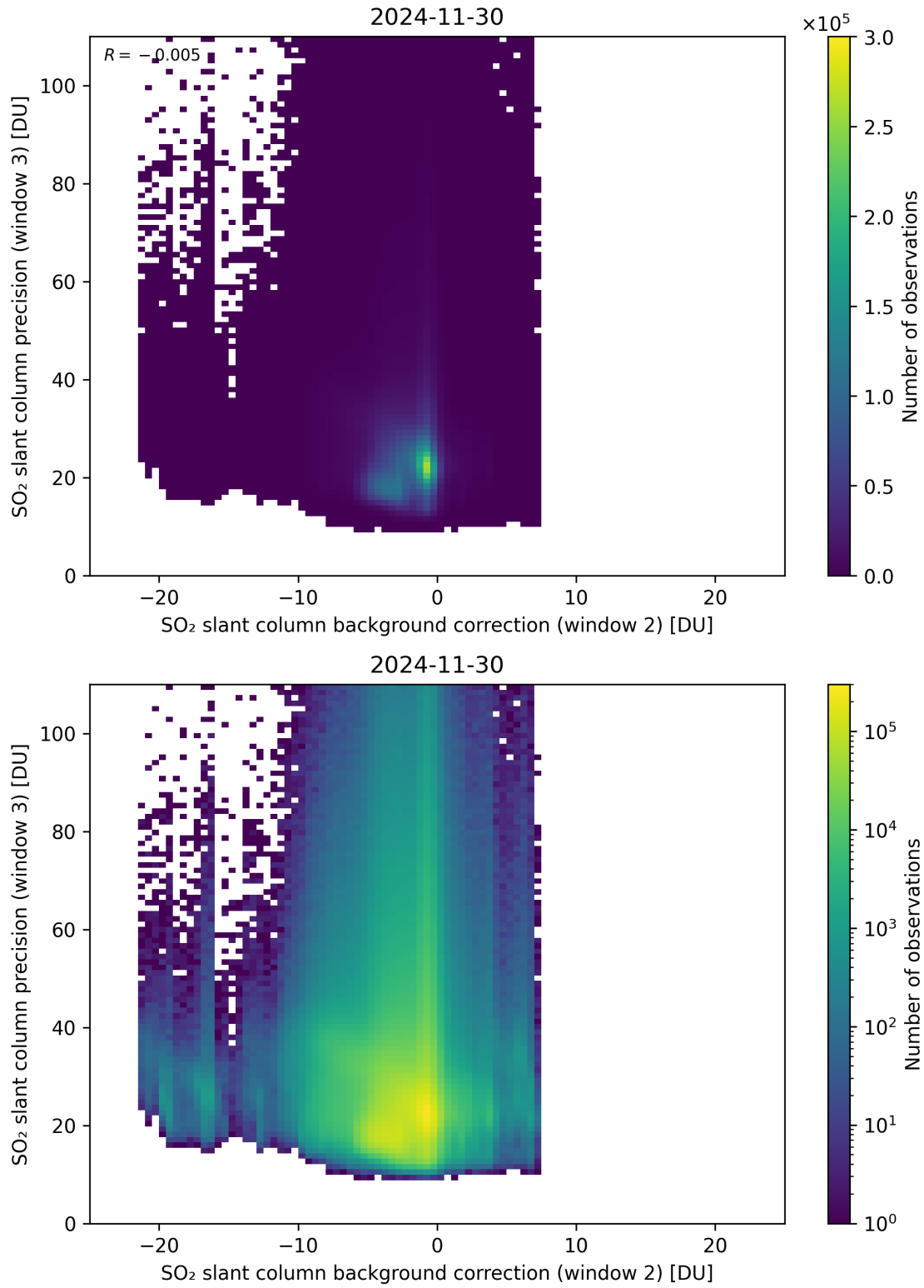
Figure 129: Scatter density plot of “SO 2 slant column background correction (window 2)” against “SO 2 slant column precision (window 3)” for 2024-11-30 to 2024-12-01.
