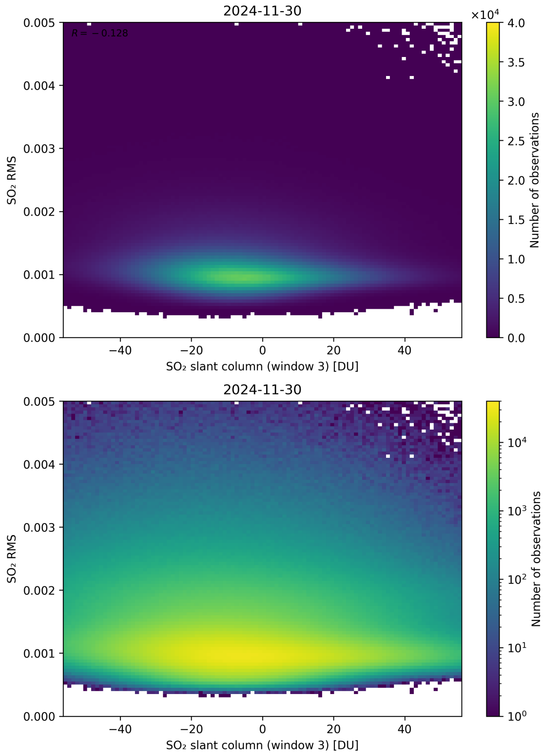
Figure 306: Scatter density plot of “SO 2 slant column (window 3)” against “SO 2 RMS” for 2024-11-30 to 2024-12-01.
