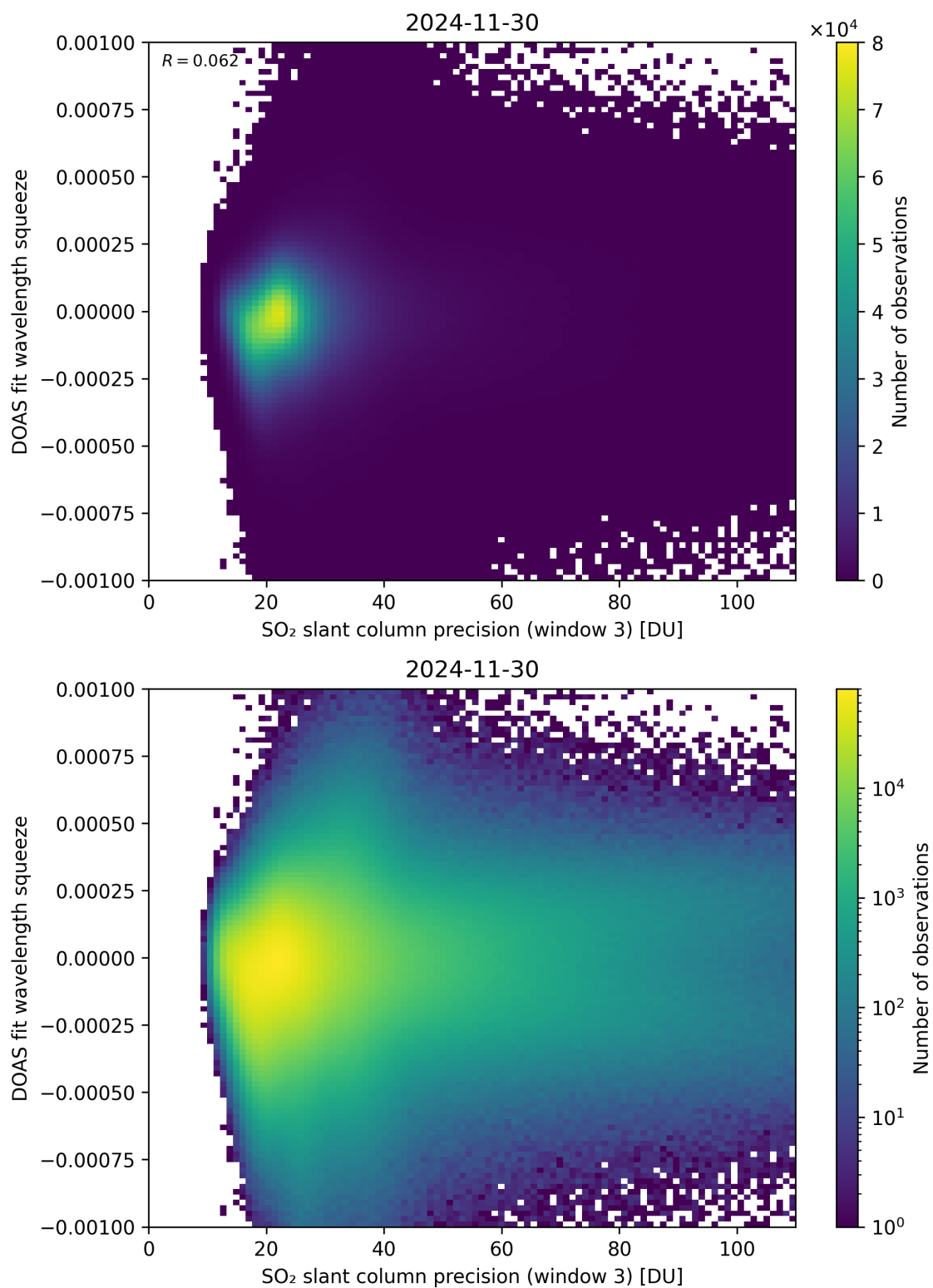
Figure 309: Scatter density plot of “SO 2 slant column precision (window 3)” against “DOAS fit wavelength squeeze” for 2024-11-30 to 2024-12-01.
