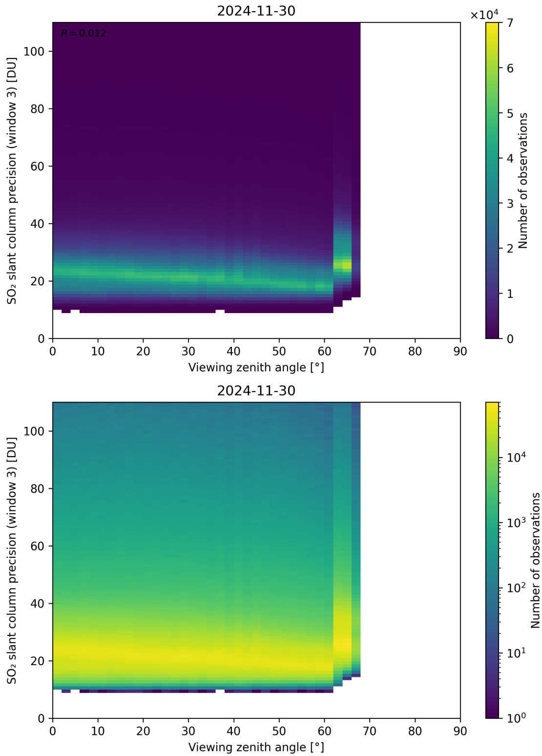
Figure 380: Scatter density plot of “Viewing zenith angle” against “SO 2 slant column precision (window 3)” for 2024-11-30 to 2024-12-01.
