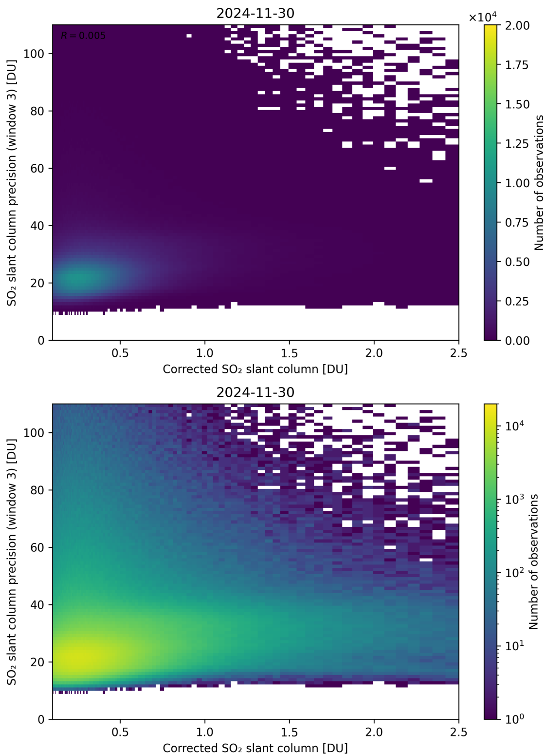
Figure 241: Scatter density plot of “Corrected SO 2 slant column” against “SO 2 slant column precision (window 3)” for 2024-11-30 to 2024-12-01.
