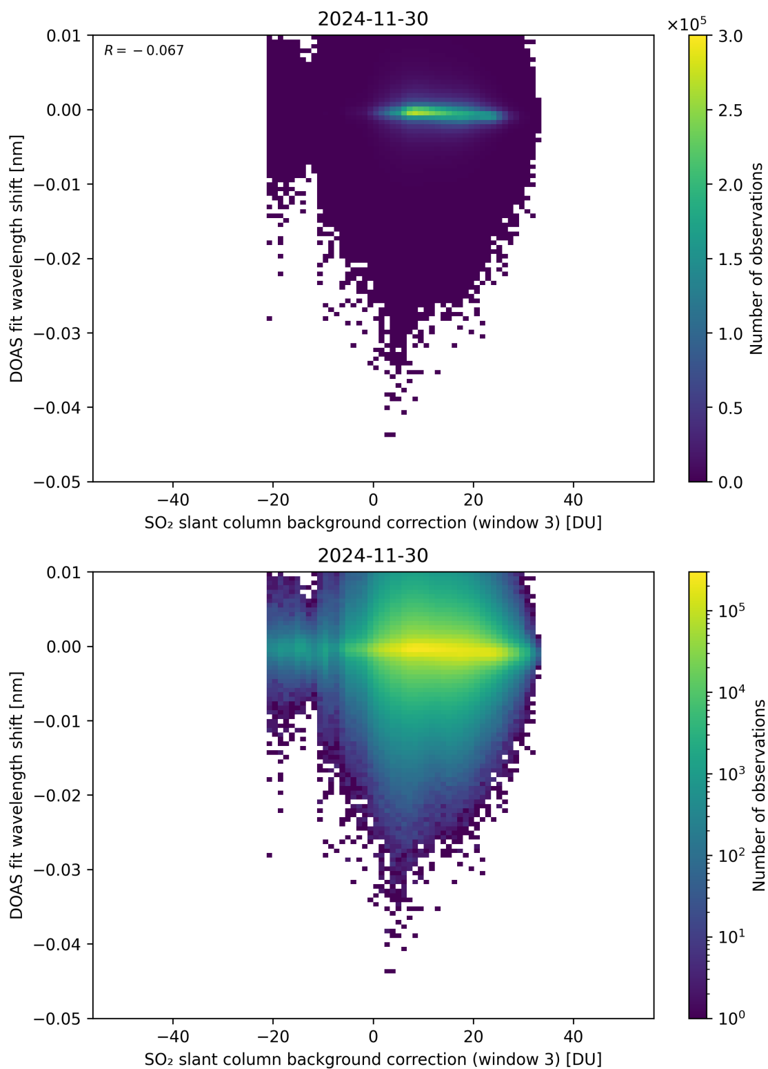
Figure 132: Scatter density plot of “SO 2 slant column background correction (window 3)” against “DOAS fit wavelength shift” for 2024-11-30 to 2024-12-01.
