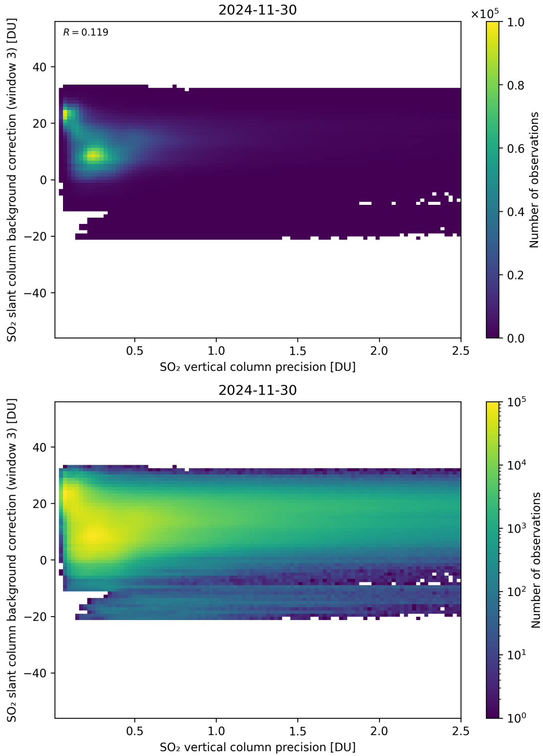
Figure 331: Scatter density plot of “SO 2 vertical column precision” against “SO 2 slant column background correction (window 3)” for 2024-11-30 to 2024-12-01.
