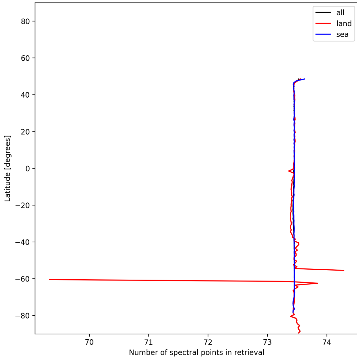
Figure 56: Zonal average of “Number of spectral points in retrieval” for 2024-11-30 to 2024-12-01.
