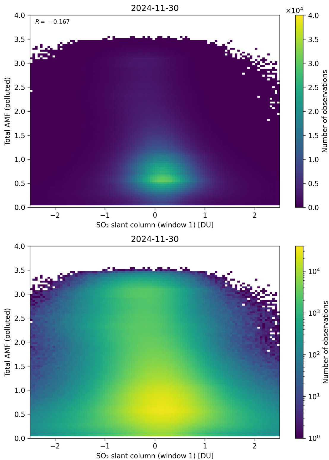
Figure 289: Scatter density plot of “SO 2 slant column (window 1)” against “Total AMF (polluted)” for 2024-11-30 to 2024-12-01.
