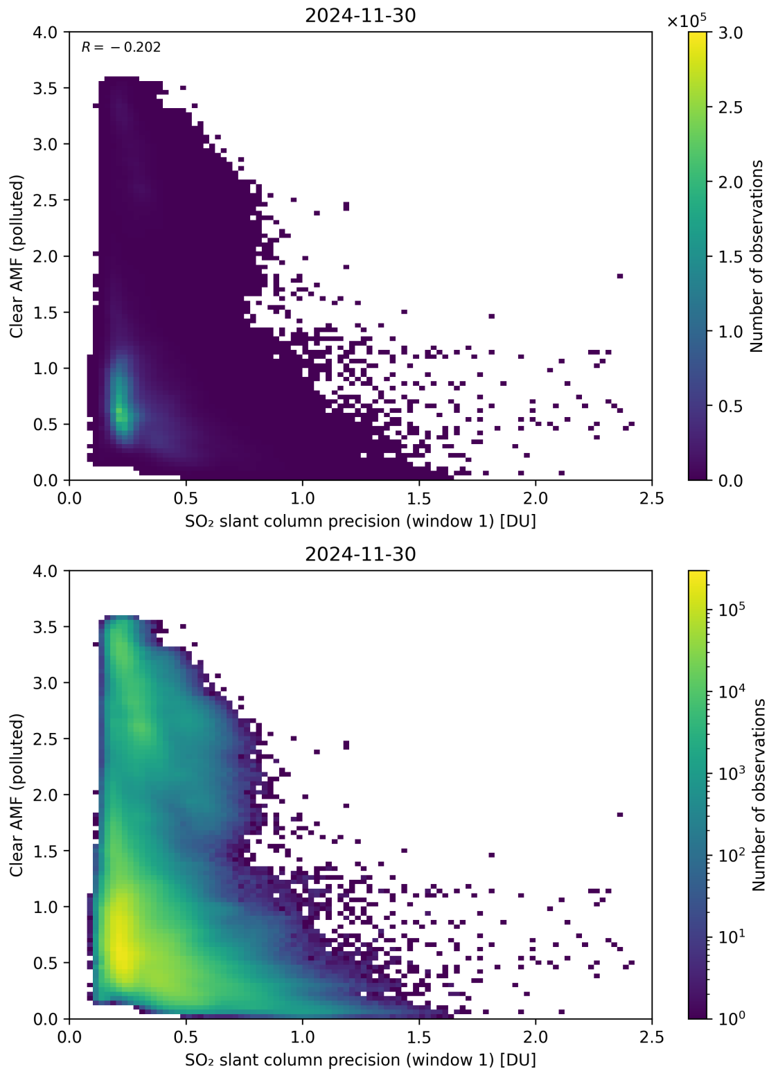
Figure 274: Scatter density plot of “SO 2 slant column precision (window 1)” against “Clear AMF (polluted)” for 2024-11-30 to 2024-12-01.
