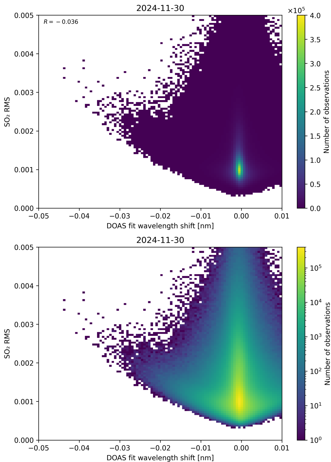
Figure 139: Scatter density plot of “DOAS fit wavelength shift” against “SO 2 RMS” for 2024-11-30 to 2024-12-01.
