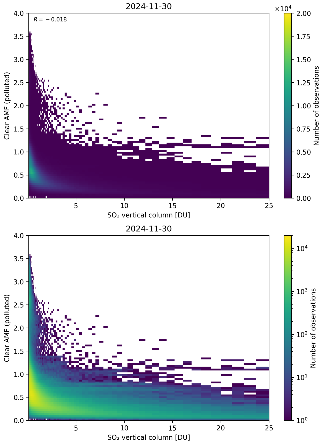
Figure 348: Scatter density plot of “SO 2 vertical column” against “Clear AMF (polluted)” for 2024-11-30 to 2024-12-01.
