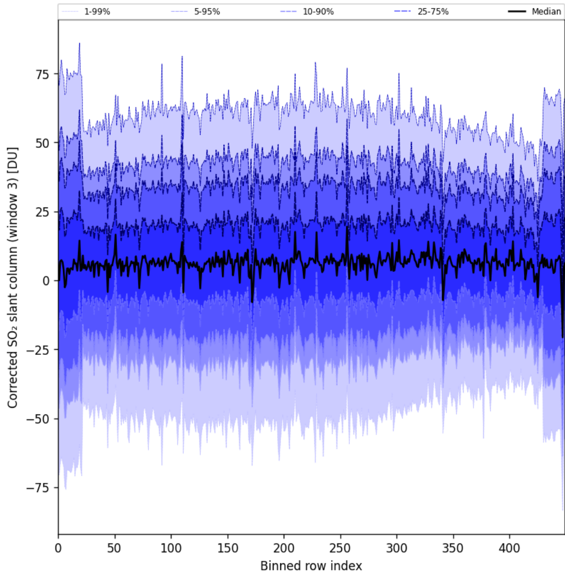
Figure 99: Along track statistics of “Corrected SO 2 slant column (window 3)” for 2024-11-30 to 2024-12-01
