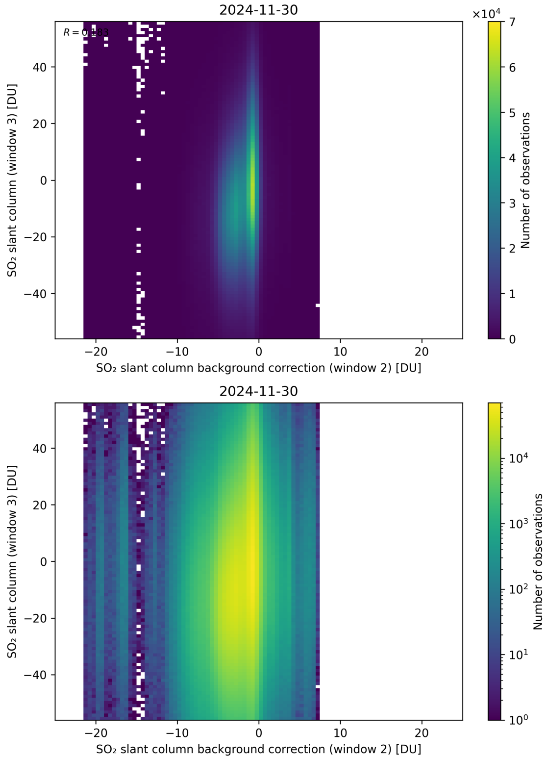
Figure 128: Scatter density plot of “SO 2 slant column background correction (window 2)” against “SO 2 slant column (window 3)” for 2024-11-30 to 2024-12-01.
