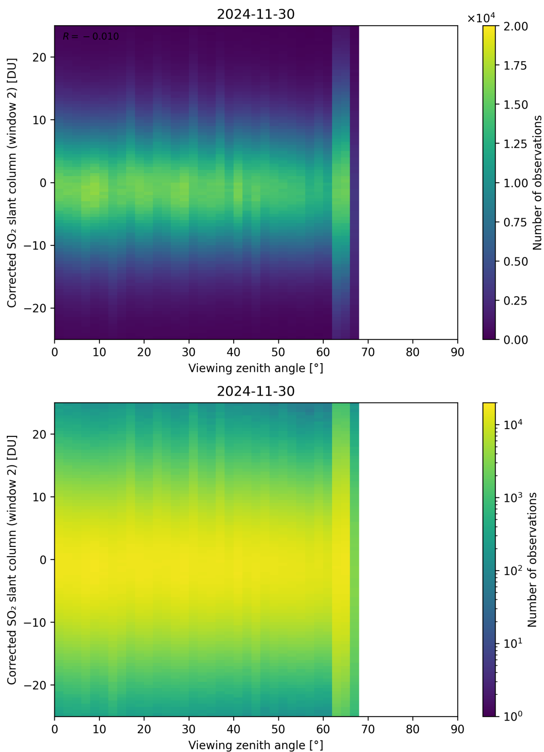
Figure 374: Scatter density plot of “Viewing zenith angle” against “Corrected SO 2 slant column (window 2)” for 2024-11-30 to 2024-12-01.
