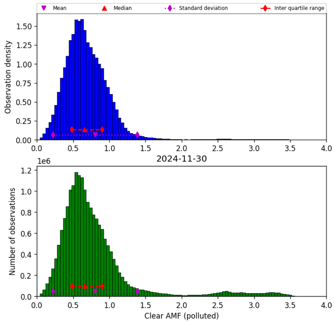
Figure 81: Histogram of “Clear AMF (polluted)” for 2024-11-30 to 2024-12-01
