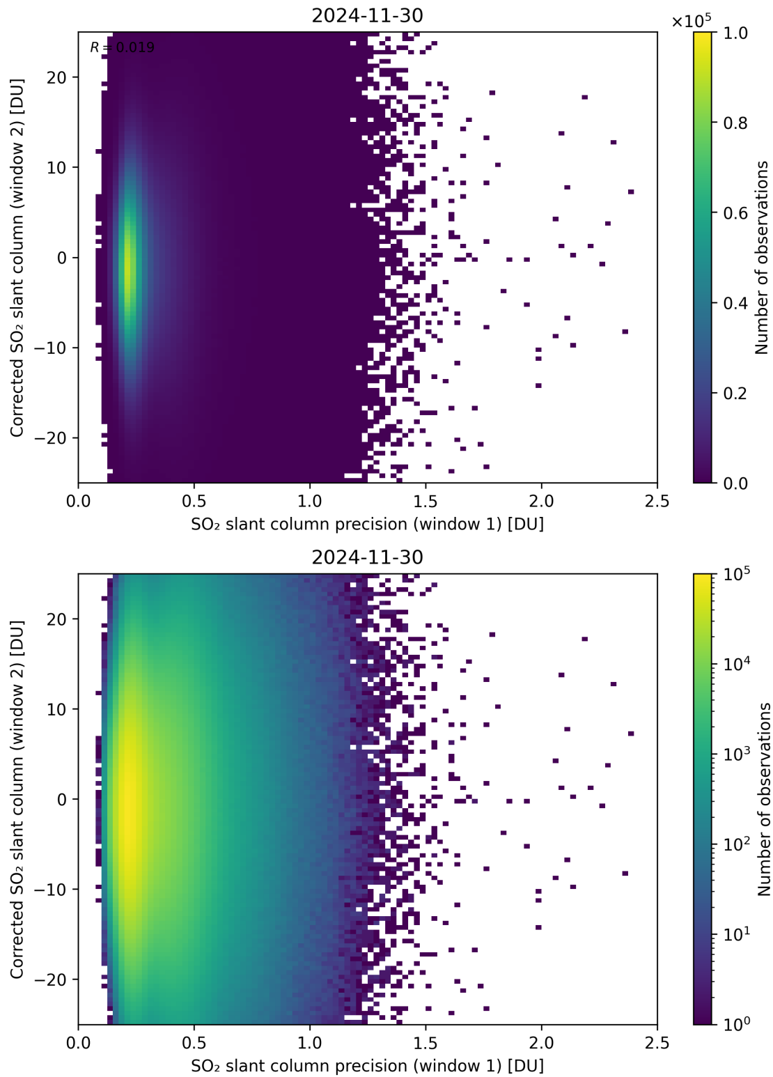
Figure 275: Scatter density plot of “SO 2 slant column precision (window 1)” against “Corrected SO 2 slant column (window 2)” for 2024-11-30 to 2024-12-01.
