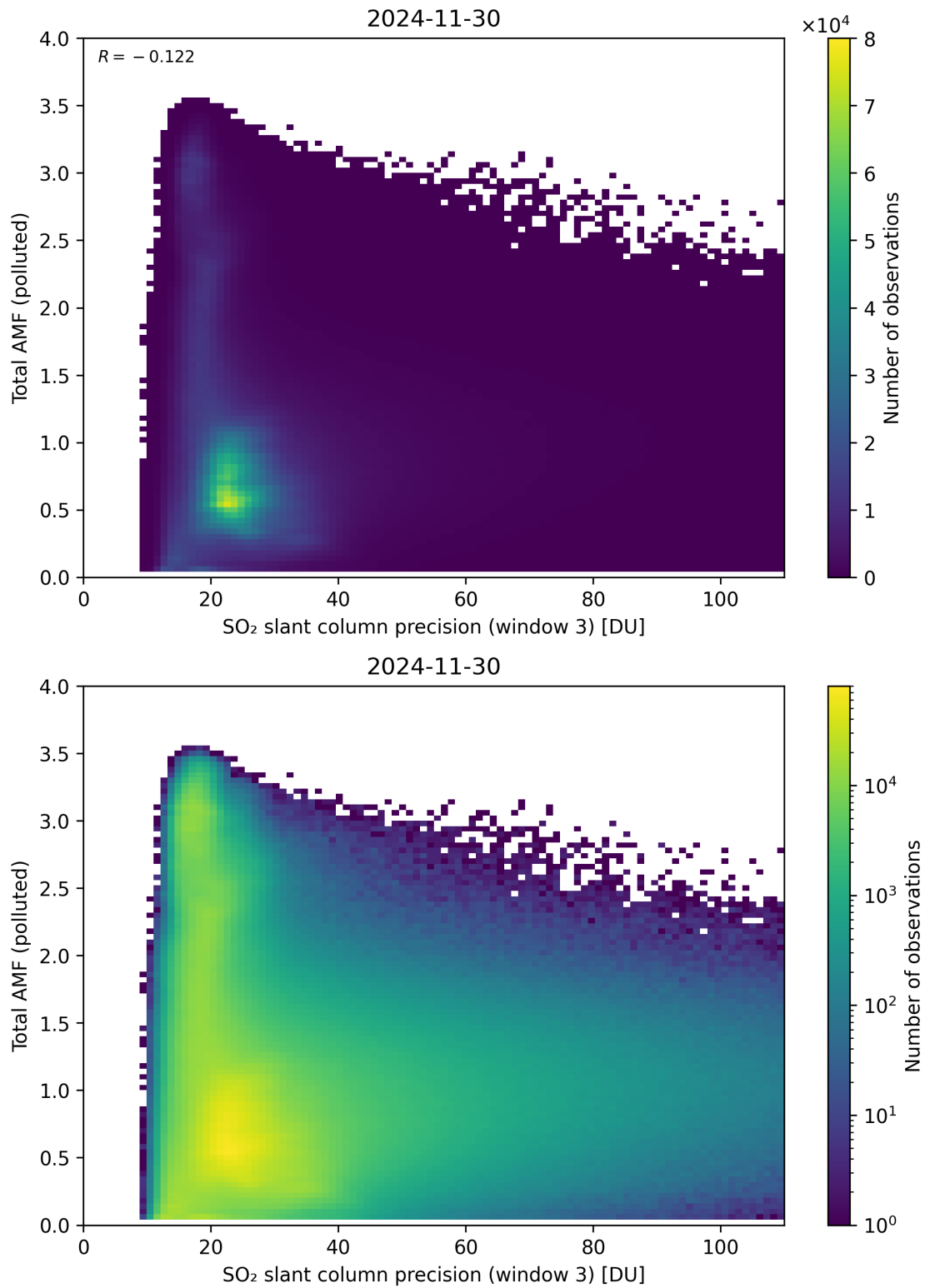
Figure 313: Scatter density plot of “SO 2 slant column precision (window 3)” against “Total AMF (polluted)” for 2024-11-30 to 2024-12-01.
