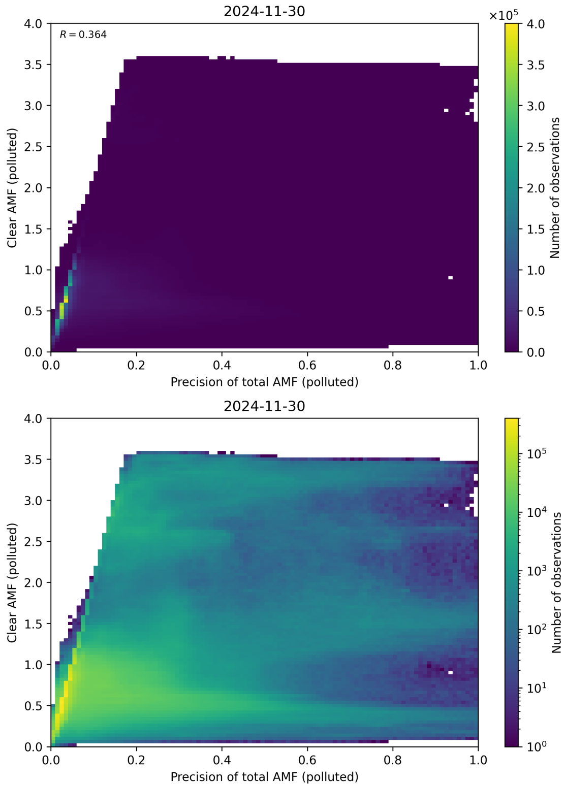
Figure 320: Scatter density plot of “Precision of total AMF (polluted)” against “Clear AMF (polluted)” for 2024-11-30 to 2024-12-01.
