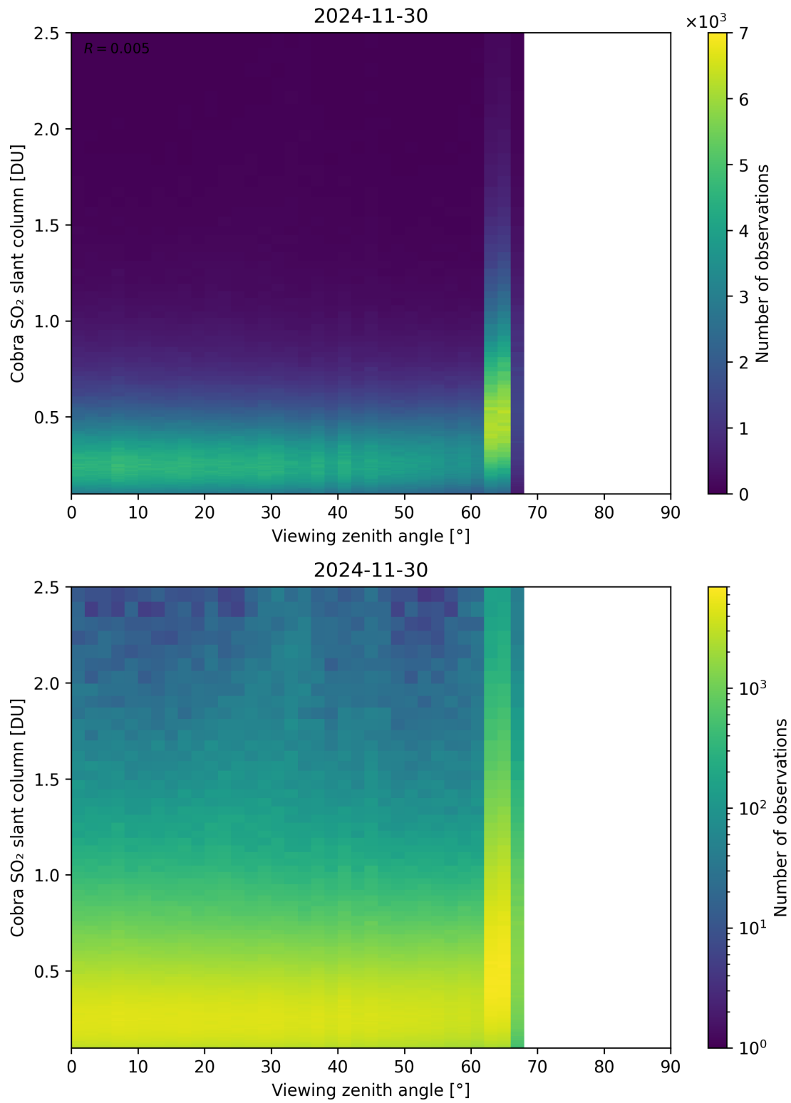
Figure 371: Scatter density plot of “Viewing zenith angle” against “Cobra SO 2 slant column” for 2024-11-30 to 2024-12-01.
