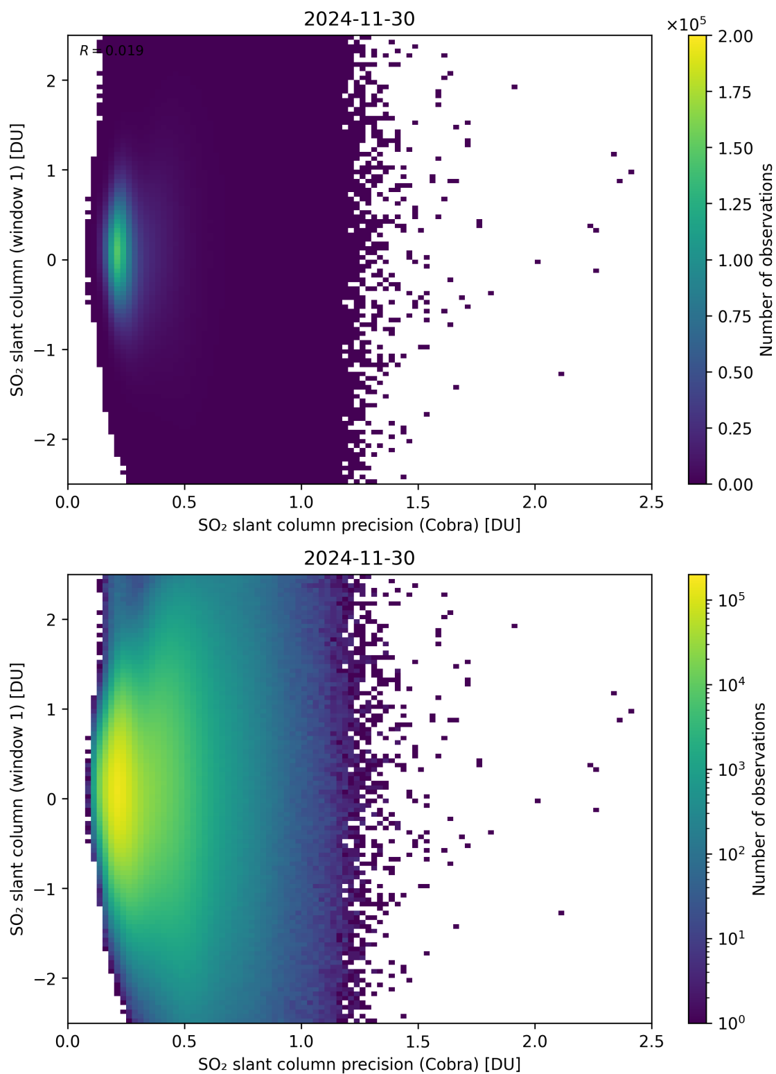
Figure 208: Scatter density plot of “SO 2 slant column precision (Cobra)” against “SO 2 slant column (window 1)” for 2024-11-30 to 2024-12-01.
