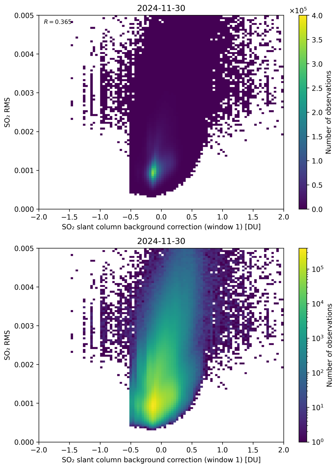
Figure 113: Scatter density plot of “SO 2 slant column background correction (window 1)” against “SO 2 RMS” for 2024-11-30 to 2024-12-01.
