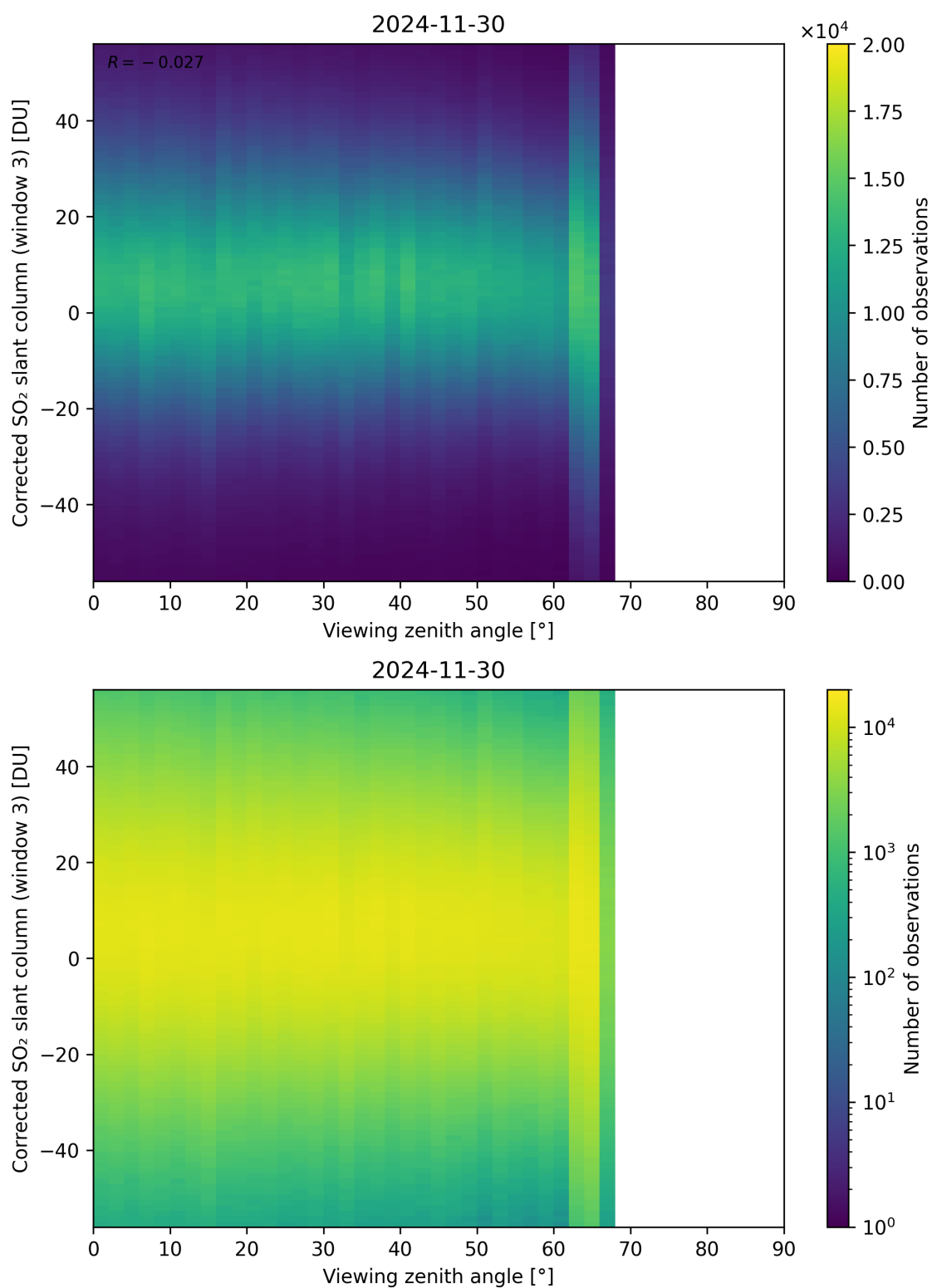
Figure 375: Scatter density plot of “Viewing zenith angle” against “Corrected SO 2 slant column (window 3)” for 2024-11-30 to 2024-12-01.
