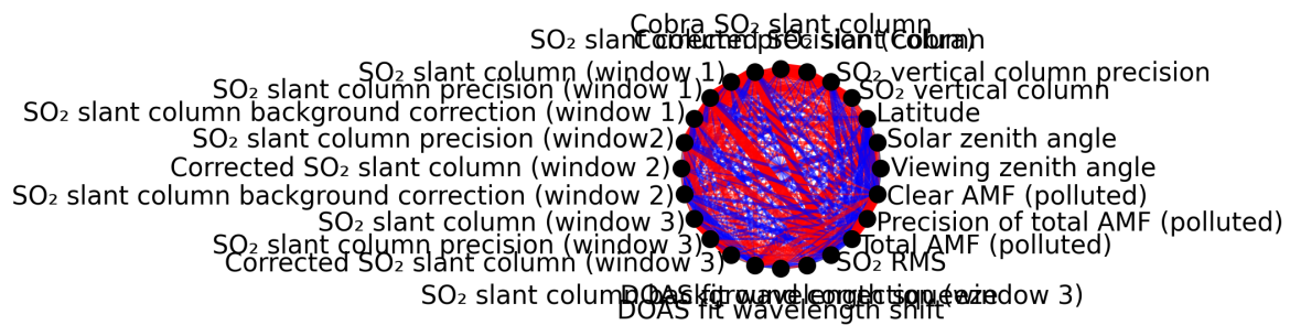
Figure 1: Map of correlation graph for 2024-11-30 to 2024-12-01.
