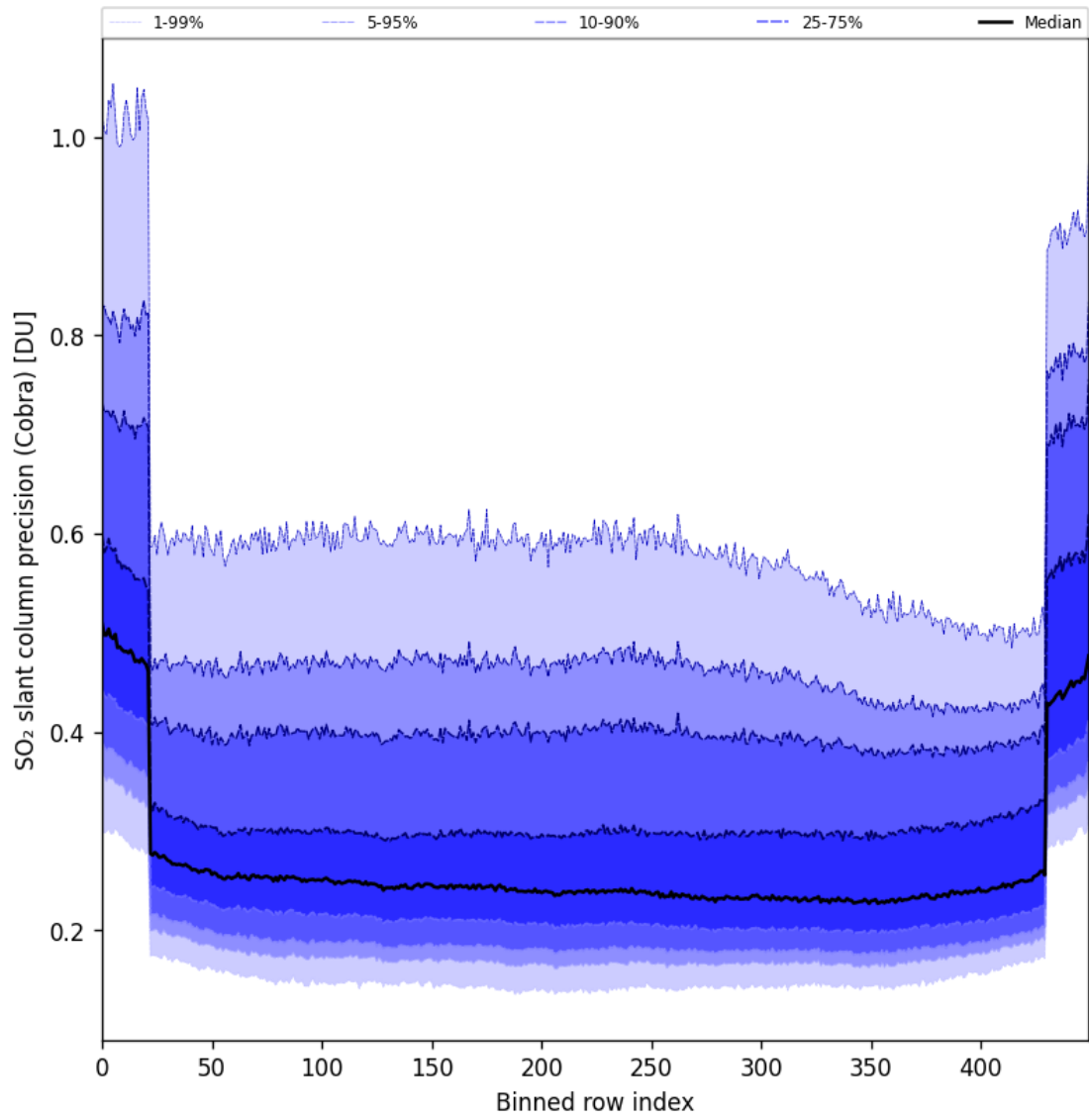
Figure 88: Along track statistics of “SO 2 slant column precision (Cobra)” for 2024-11-30 to 2024-12-01
