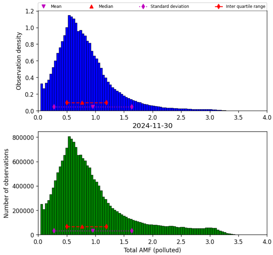
Figure 79: Histogram of “Total AMF (polluted)” for 2024-11-30 to 2024-12-01
