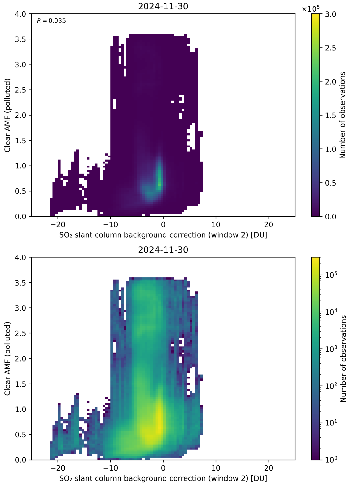
Figure 126: Scatter density plot of “SO 2 slant column background correction (window 2)” against “Clear AMF (polluted)” for 2024-11-30 to 2024-12-01.
