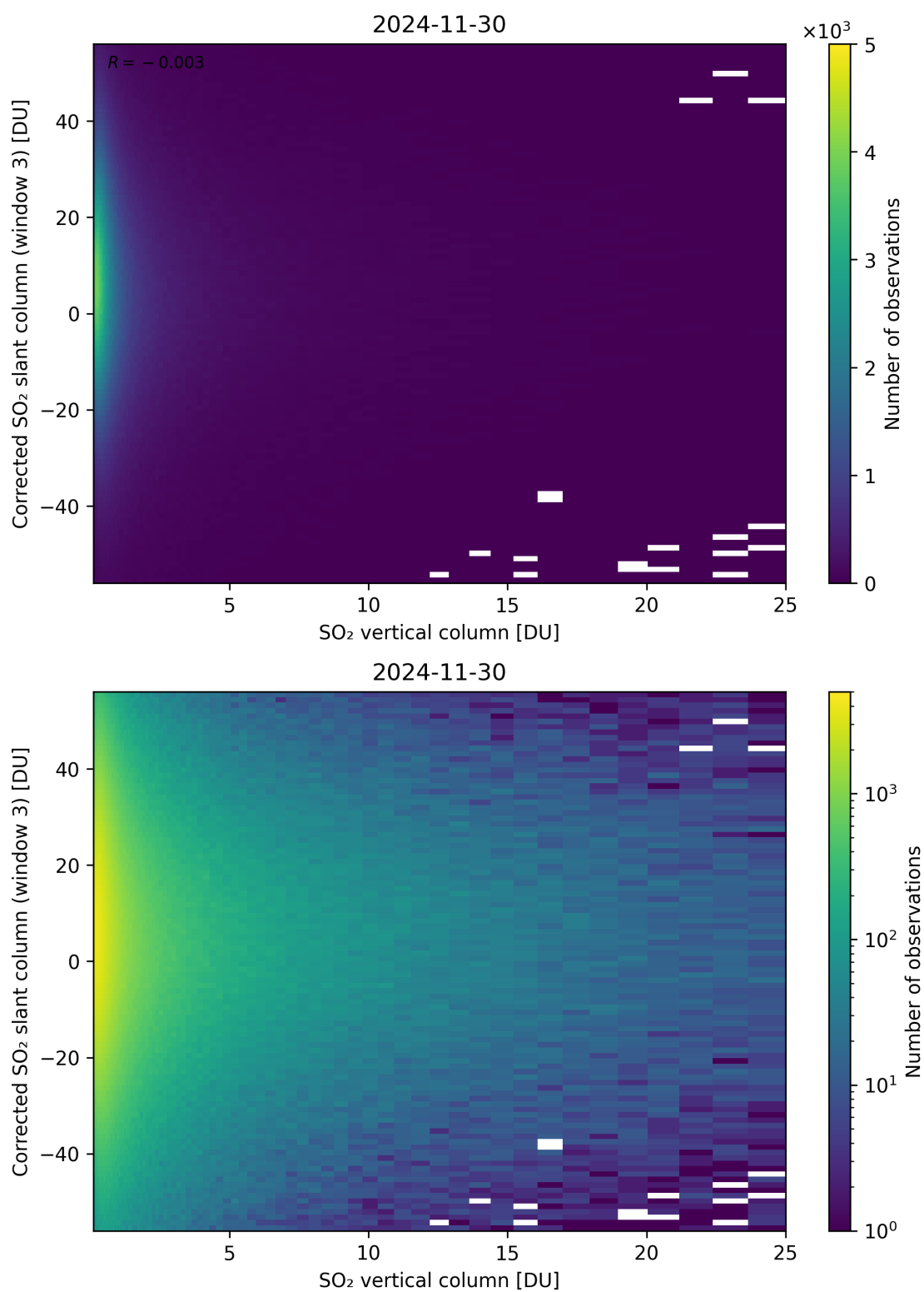
Figure 353: Scatter density plot of “SO 2 vertical column” against “Corrected SO 2 slant column (window 3)” for 2024-11-30 to 2024-12-01.
