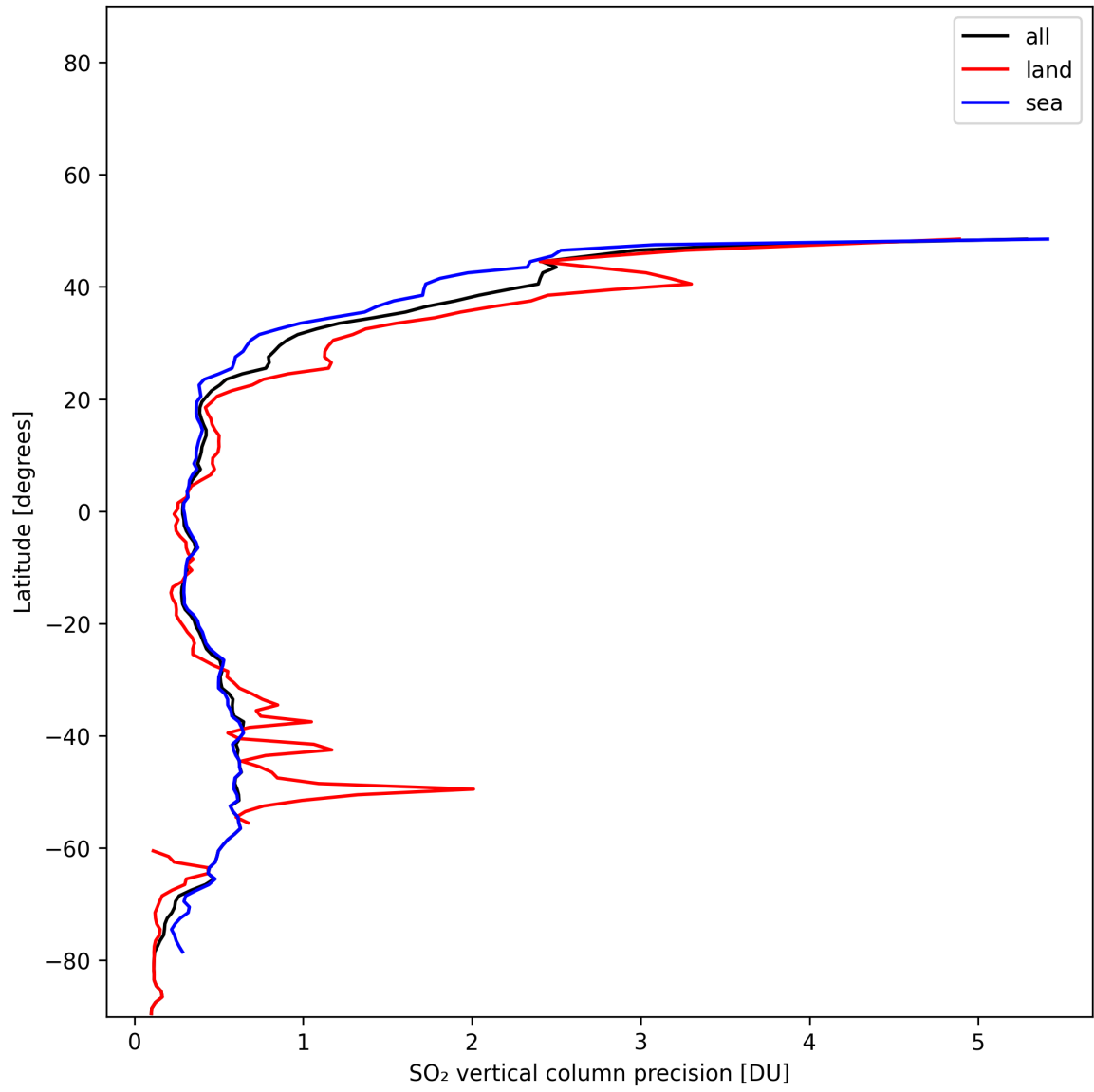
Figure 33: Zonal average of “SO 2 vertical column precision” for 2024-11-30 to 2024-12-01.
