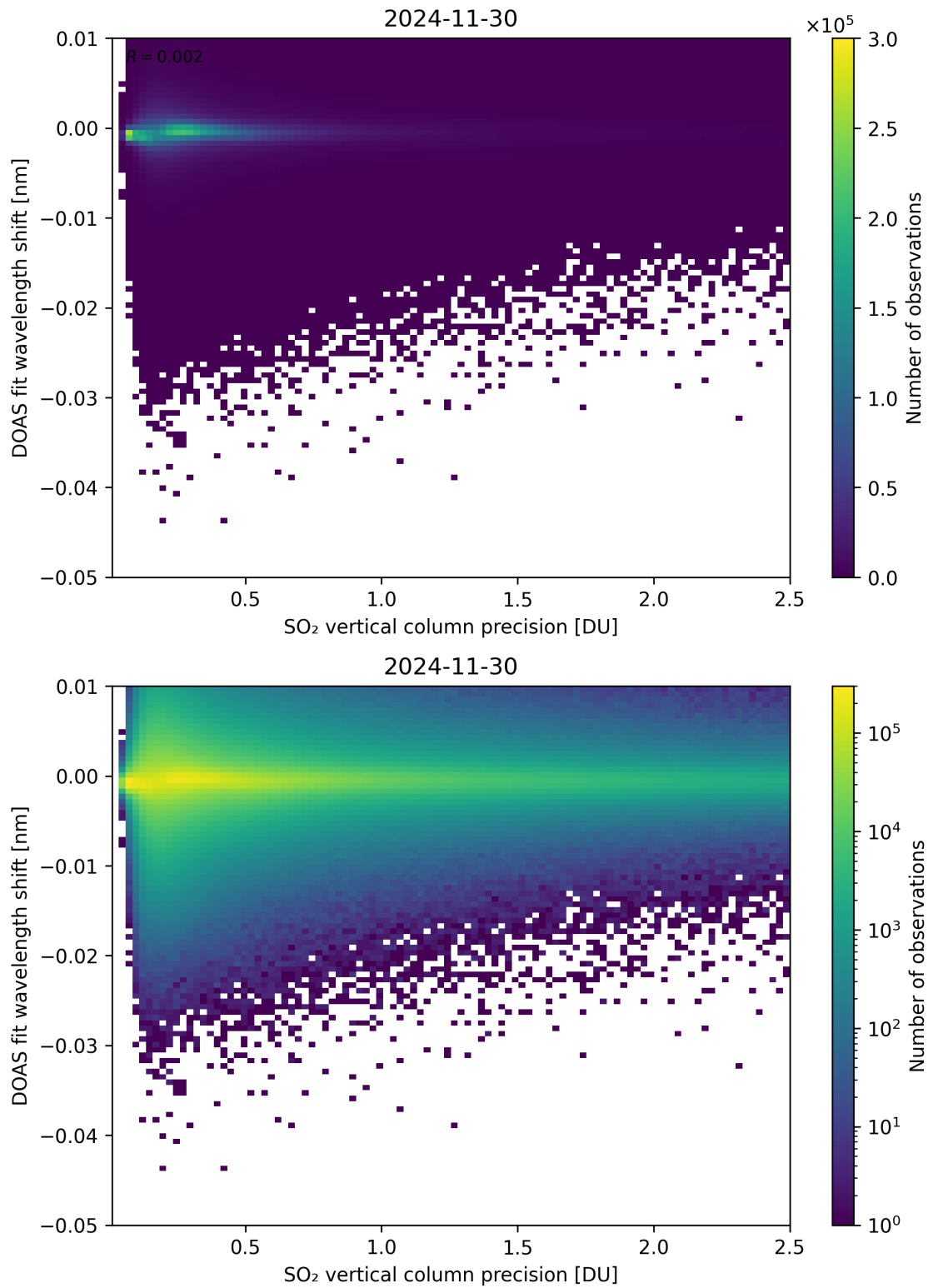
Figure 332: Scatter density plot of “SO 2 vertical column precision” against “DOAS fit wavelength shift” for 2024-11-30 to 2024-12-01.
