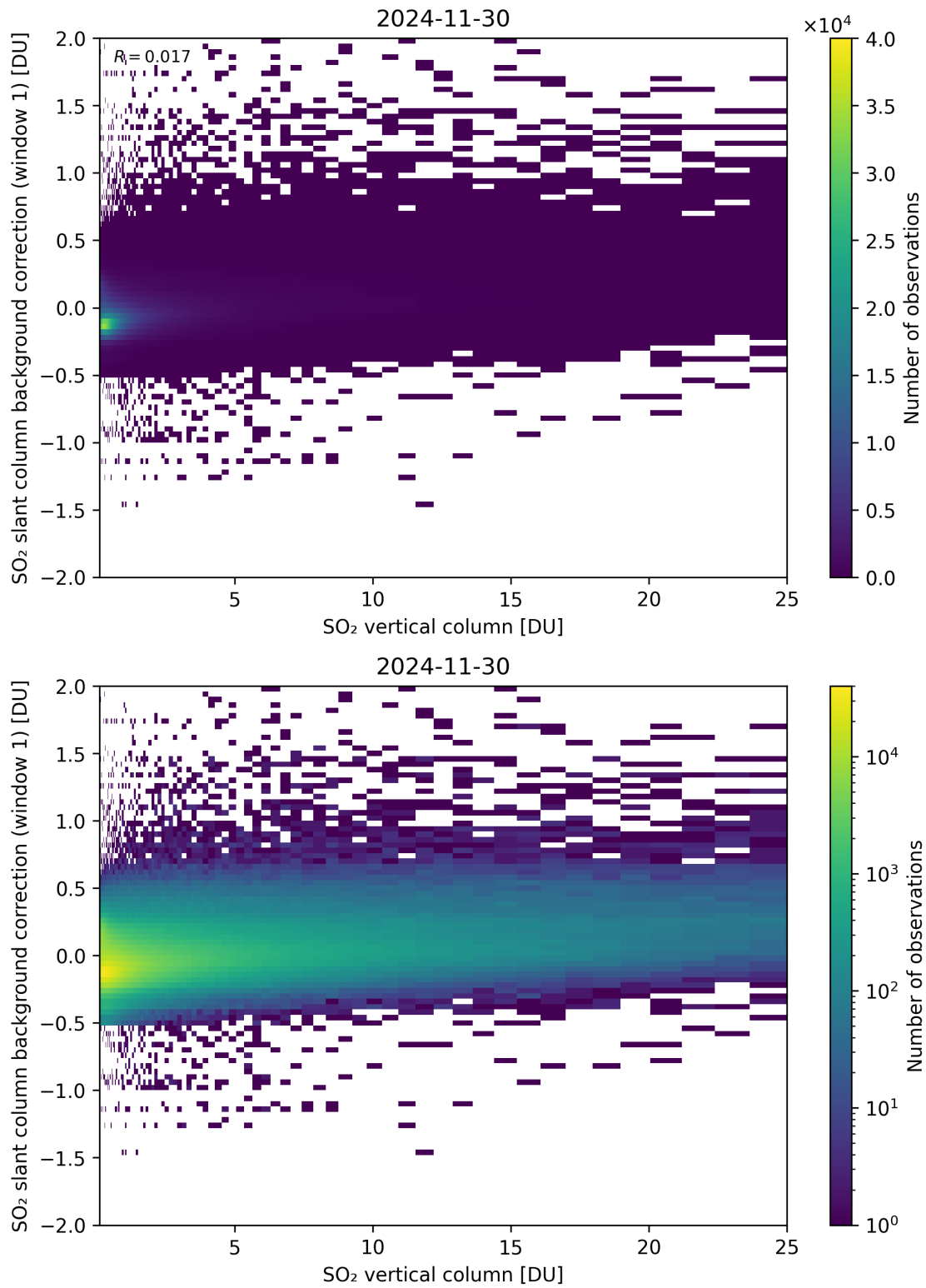
Figure 323: Scatter density plot of “SO 2 vertical column” against “SO 2 slant column background correction (window 1)” for 2024-11-30 to 2024-12-01.
