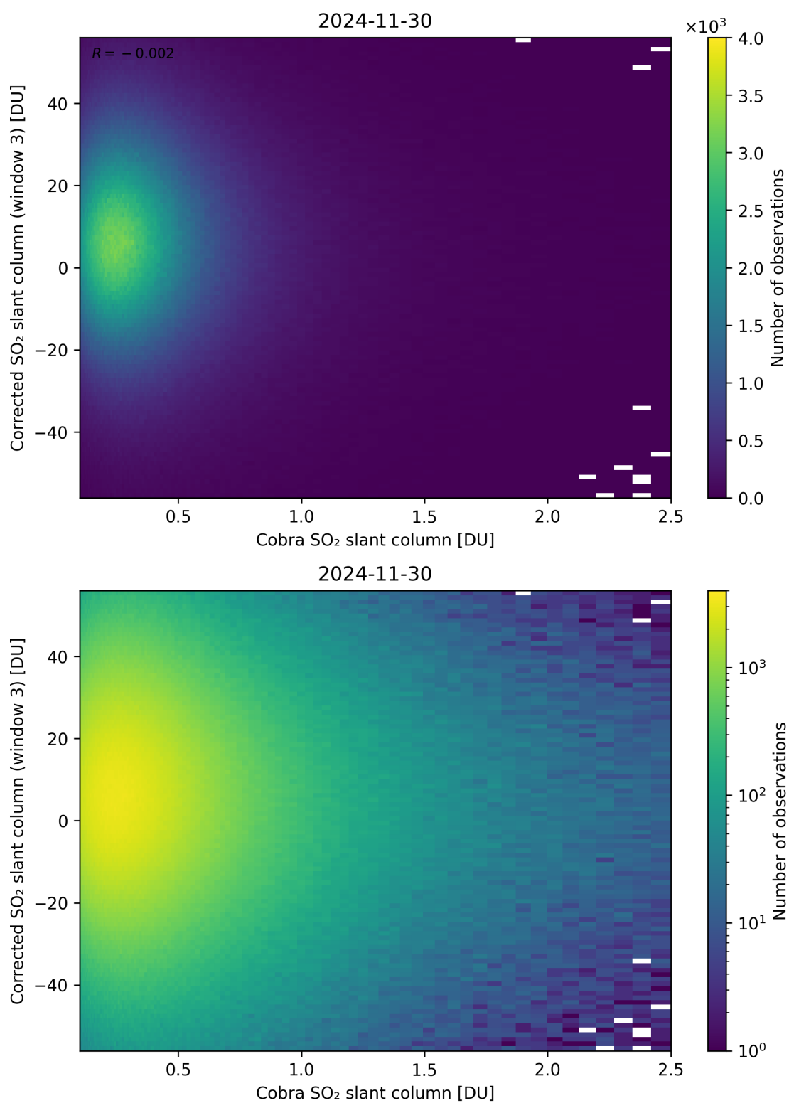
Figure 218: Scatter density plot of “Cobra SO 2 slant column” against “Corrected SO 2 slant column (window 3)” for 2024-11-30 to 2024-12-01.
