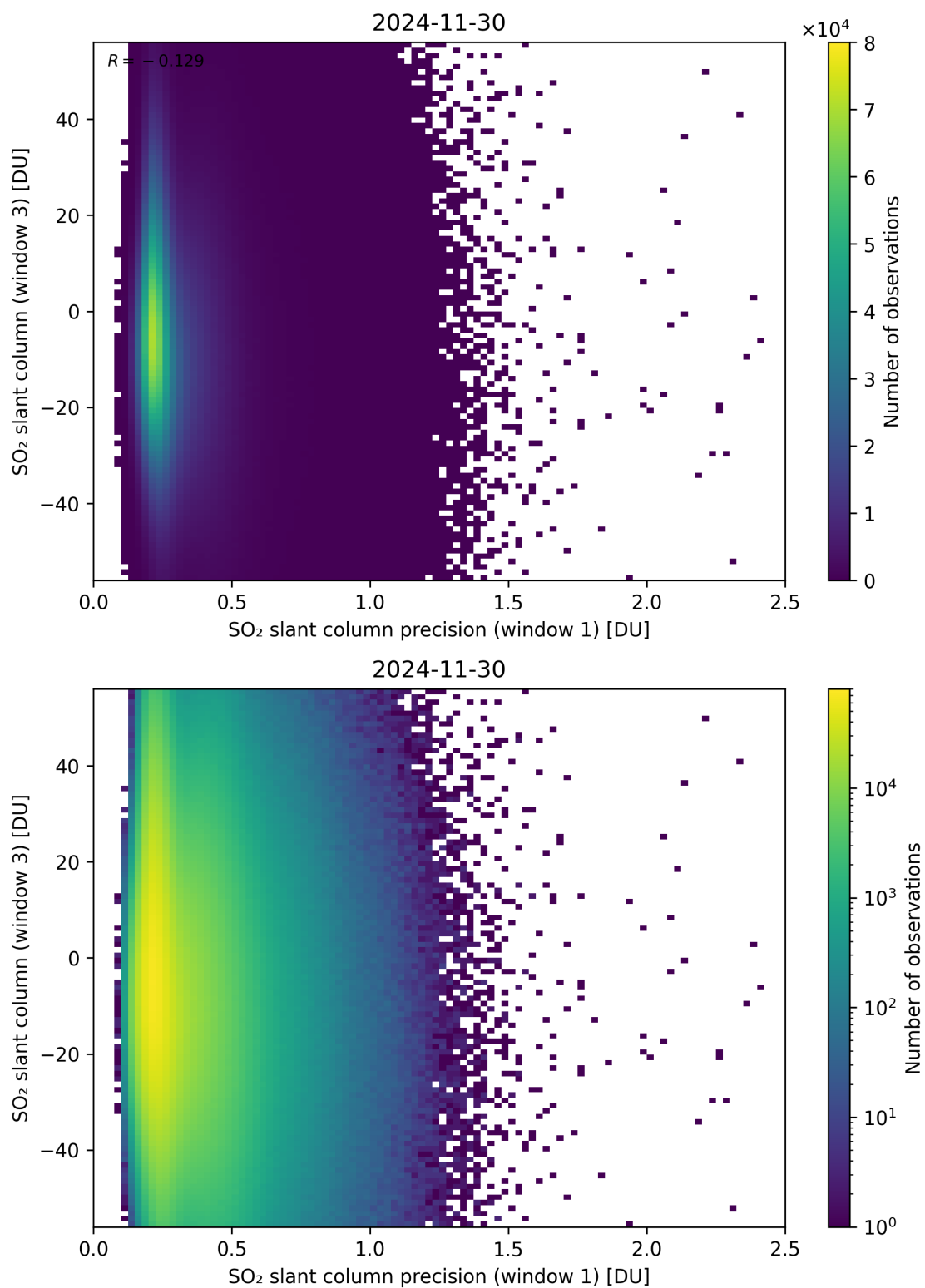
Figure 278: Scatter density plot of “SO 2 slant column precision (window 1)” against “SO 2 slant column (window 3)” for 2024-11-30 to 2024-12-01.
