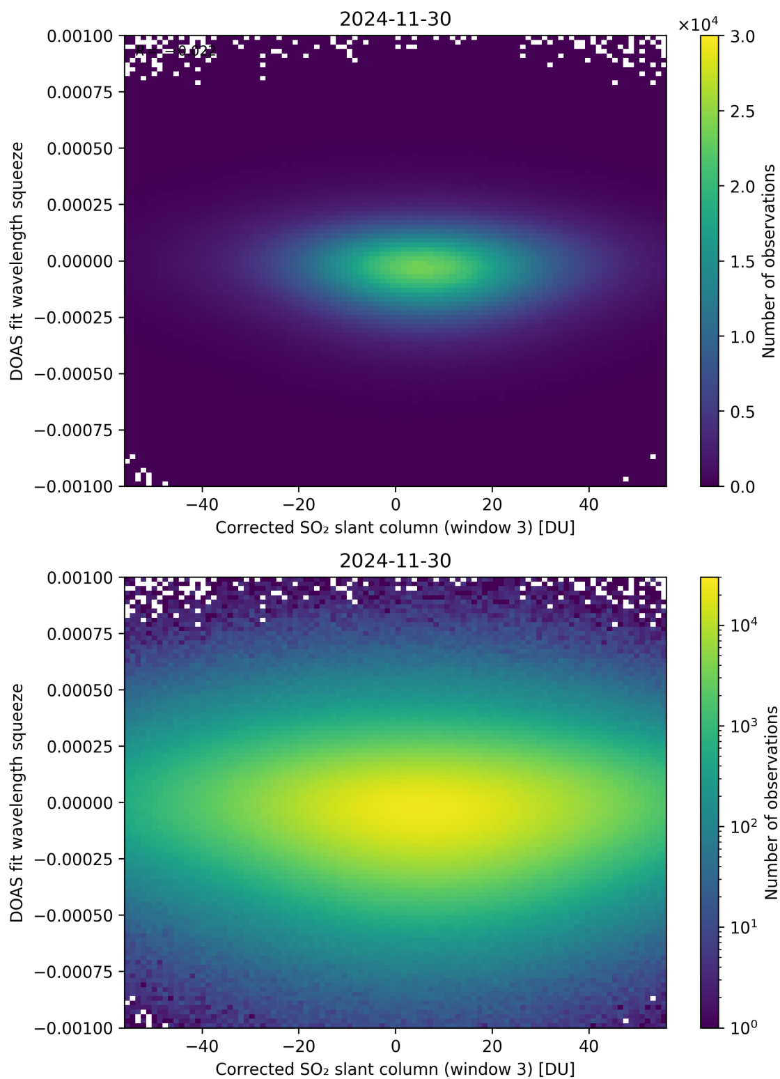
Figure 257: Scatter density plot of “Corrected SO 2 slant column (window 3)” against “DOAS fit wavelength squeeze” for 2024-11-30 to 2024-12-01.
