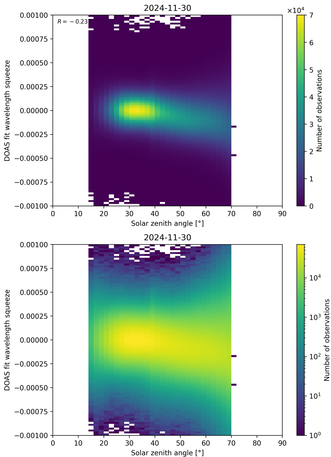
Figure 175: Scatter density plot of “Solar zenith angle” against “DOAS fit wavelength squeeze” for 2024-11-30 to 2024-12-01.
