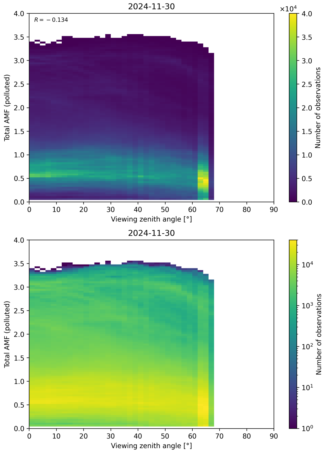
Figure 381: Scatter density plot of “Viewing zenith angle” against “Total AMF (polluted)” for 2024-11-30 to 2024-12-01.
