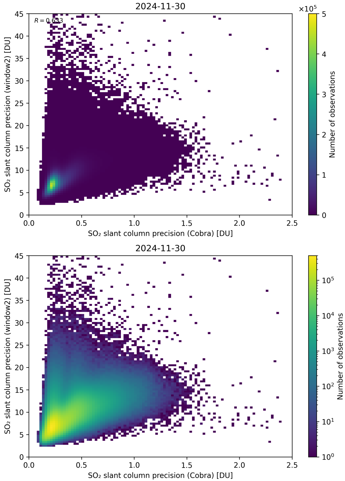
Figure 210: Scatter density plot of “SO 2 slant column precision (Cobra)” against “SO 2 slant column precision (window2)” for 2024-11-30 to 2024-12-01.
