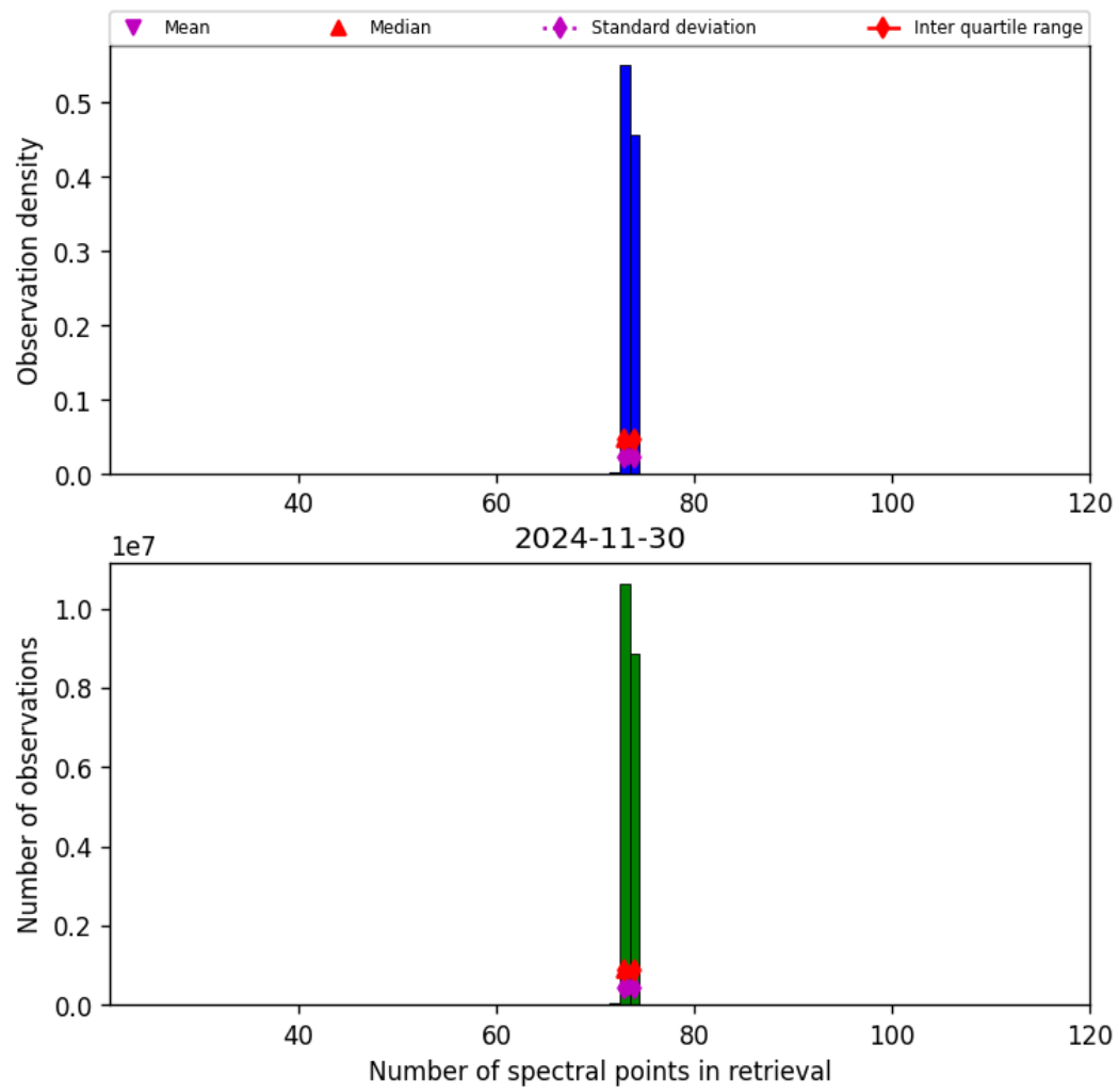
Figure 82: Histogram of “Number of spectral points in retrieval” for 2024-11-30 to 2024-12-01
