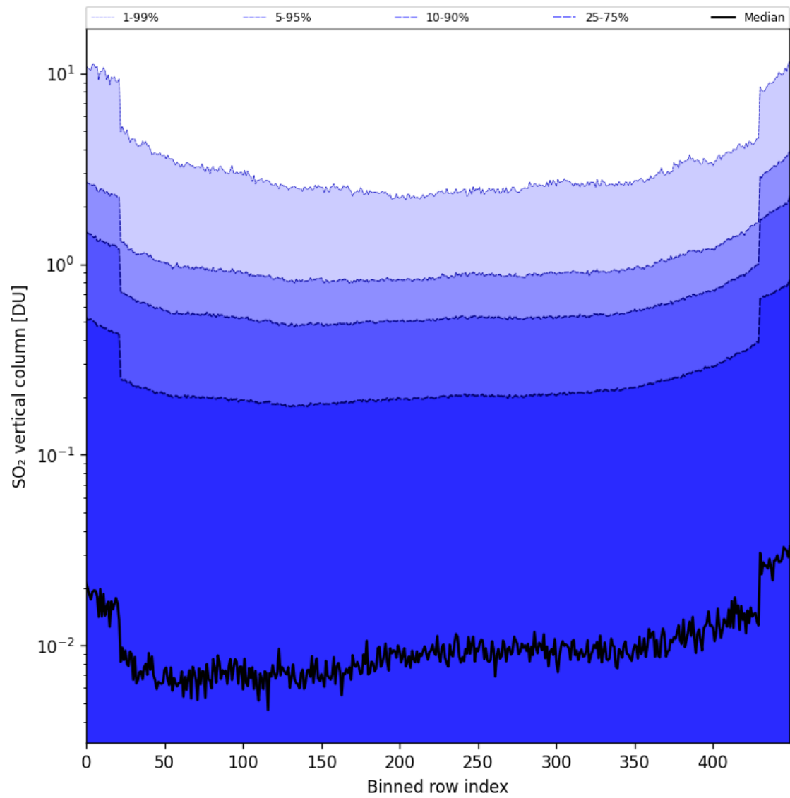
Figure 84: Along track statistics of “SO 2 vertical column” for 2024-11-30 to 2024-12-01
