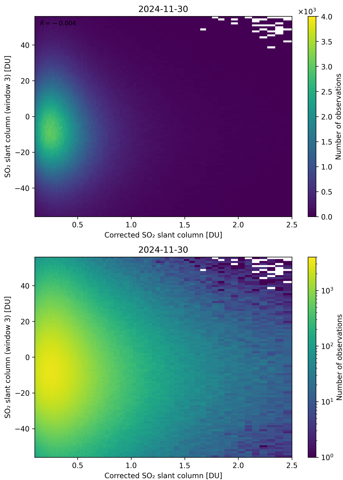
Figure 240: Scatter density plot of “Corrected SO 2 slant column” against “SO 2 slant column (window 3)” for 2024-11-30 to 2024-12-01.
