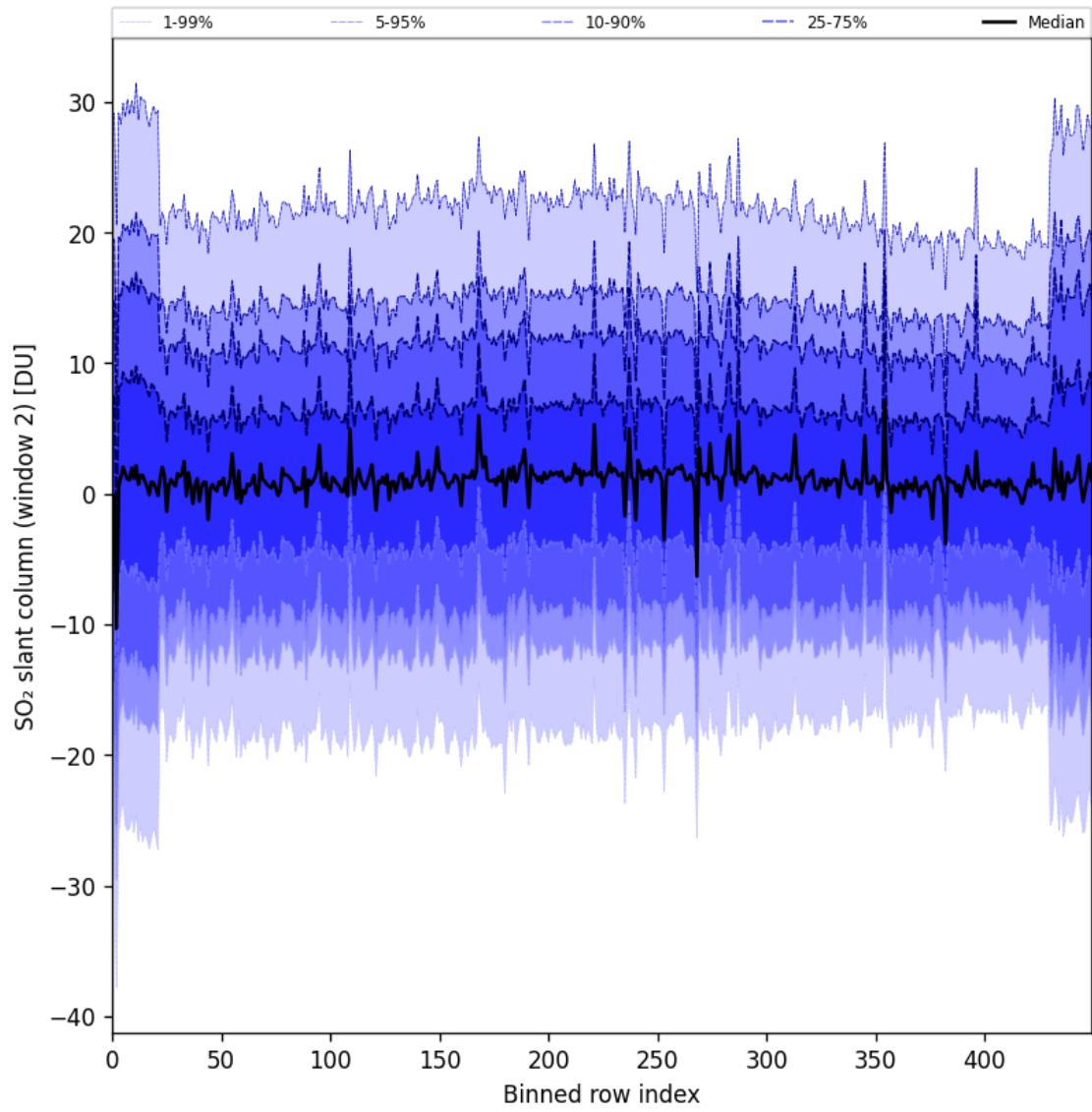
Figure 93: Along track statistics of “SO 2 slant column (window 2)” for 2024-11-30 to 2024-12-01
