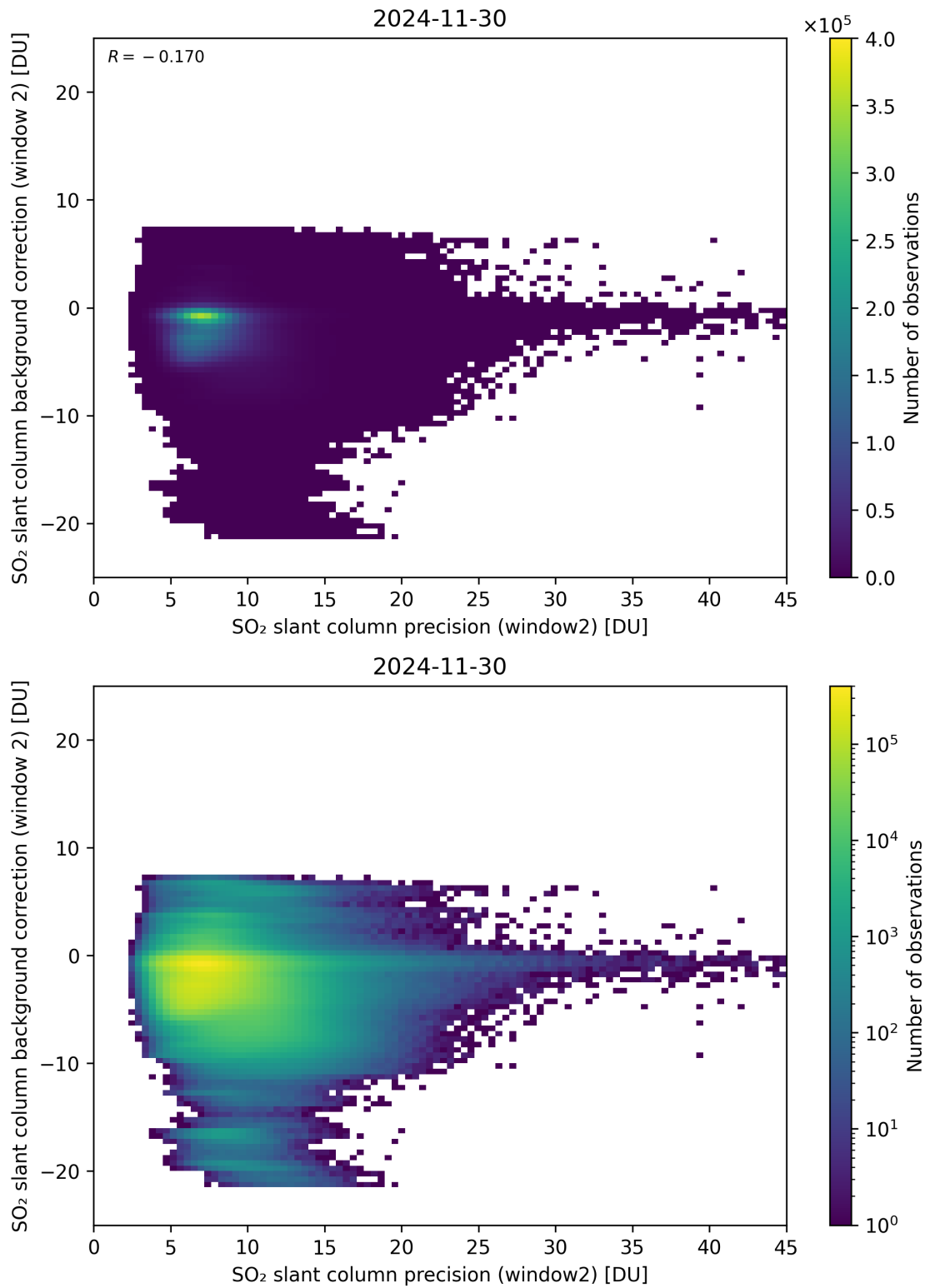
Figure 291: Scatter density plot of “SO 2 slant column precision (window2)” against “SO 2 slant column background correction (window 2)” for 2024-11-30 to 2024-12-01.
