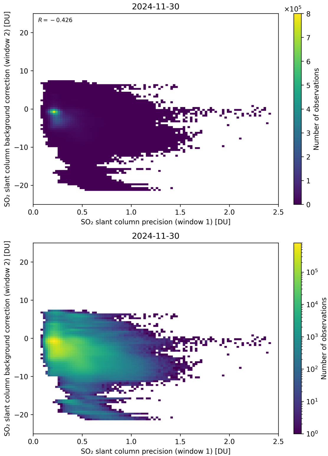
Figure 269: Scatter density plot of “SO 2 slant column precision (window 1)” against “SO 2 slant column background correction (window 2)” for 2024-11-30 to 2024-12-01.
