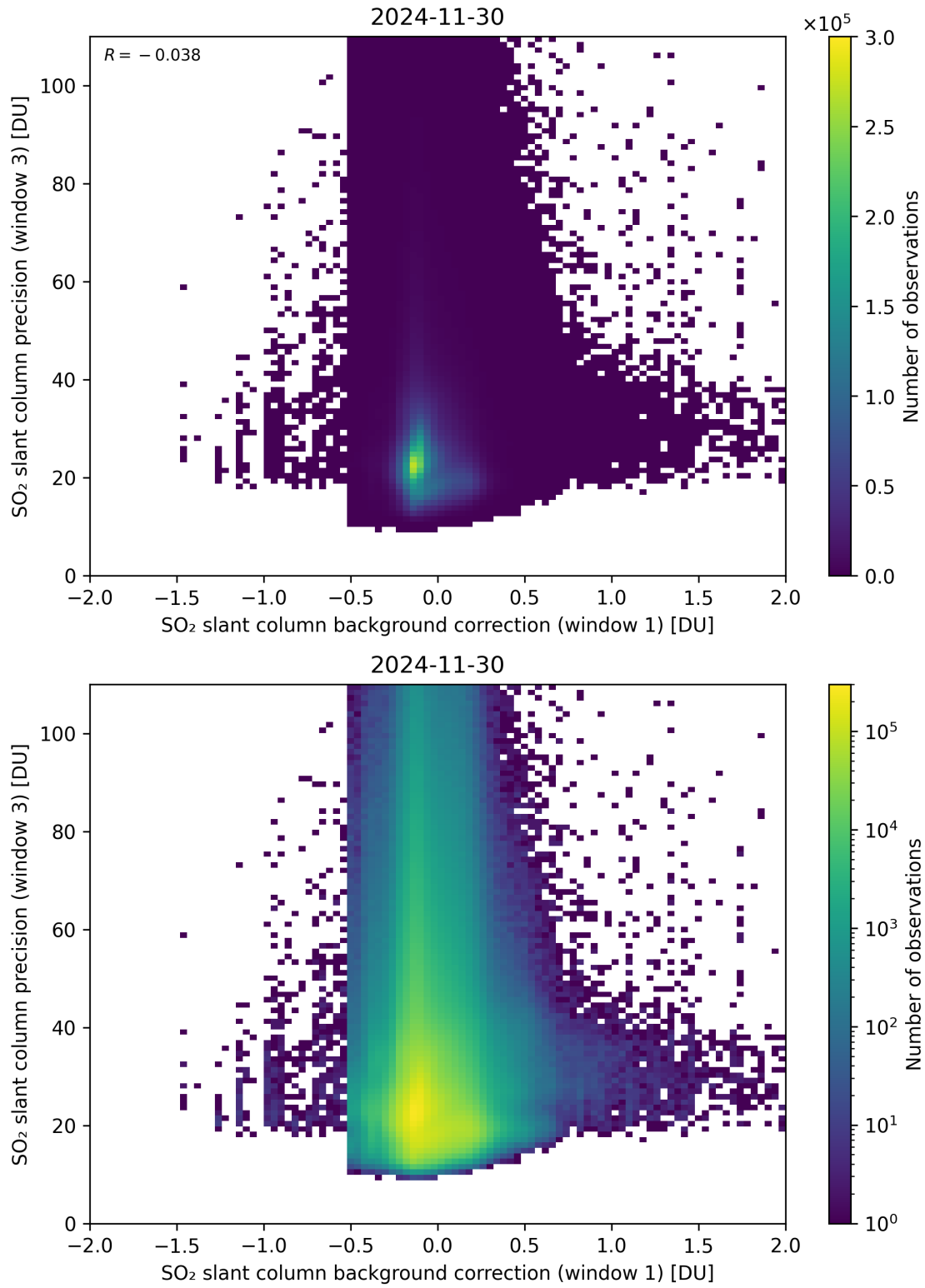
Figure 119: Scatter density plot of “SO 2 slant column background correction (window 1)” against “SO 2 slant column precision (window 3)” for 2024-11-30 to 2024-12-01.
