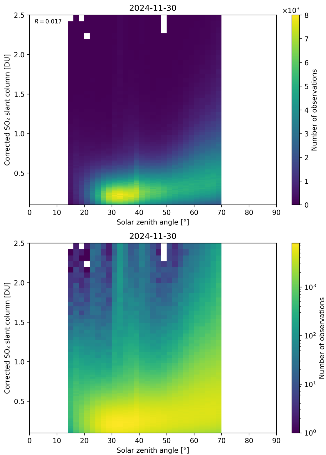
Figure 181: Scatter density plot of “Solar zenith angle” against “Corrected SO 2 slant column” for 2024-11-30 to 2024-12-01.
