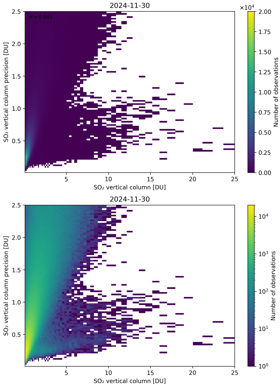
Figure 361: Scatter density plot of “SO 2 vertical column” against “SO 2 vertical column precision” for 2024-11-30 to 2024-12-01.
