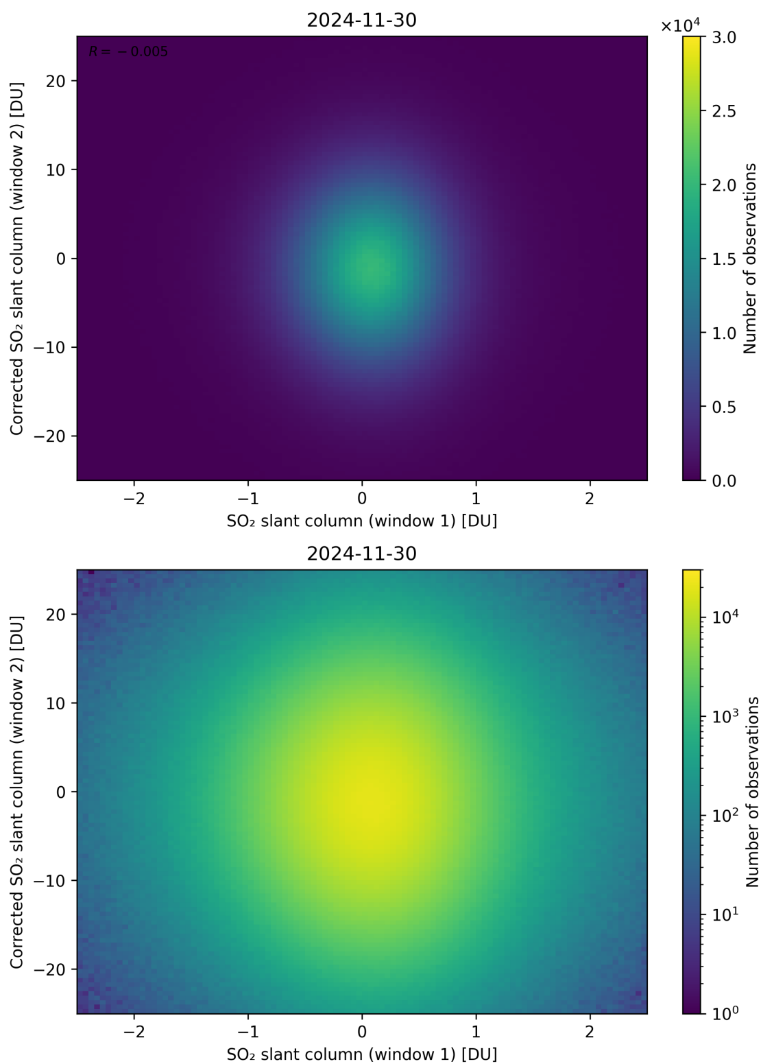
Figure 283: Scatter density plot of “SO 2 slant column (window 1)” against “Corrected SO 2 slant column (window 2)” for 2024-11-30 to 2024-12-01.
