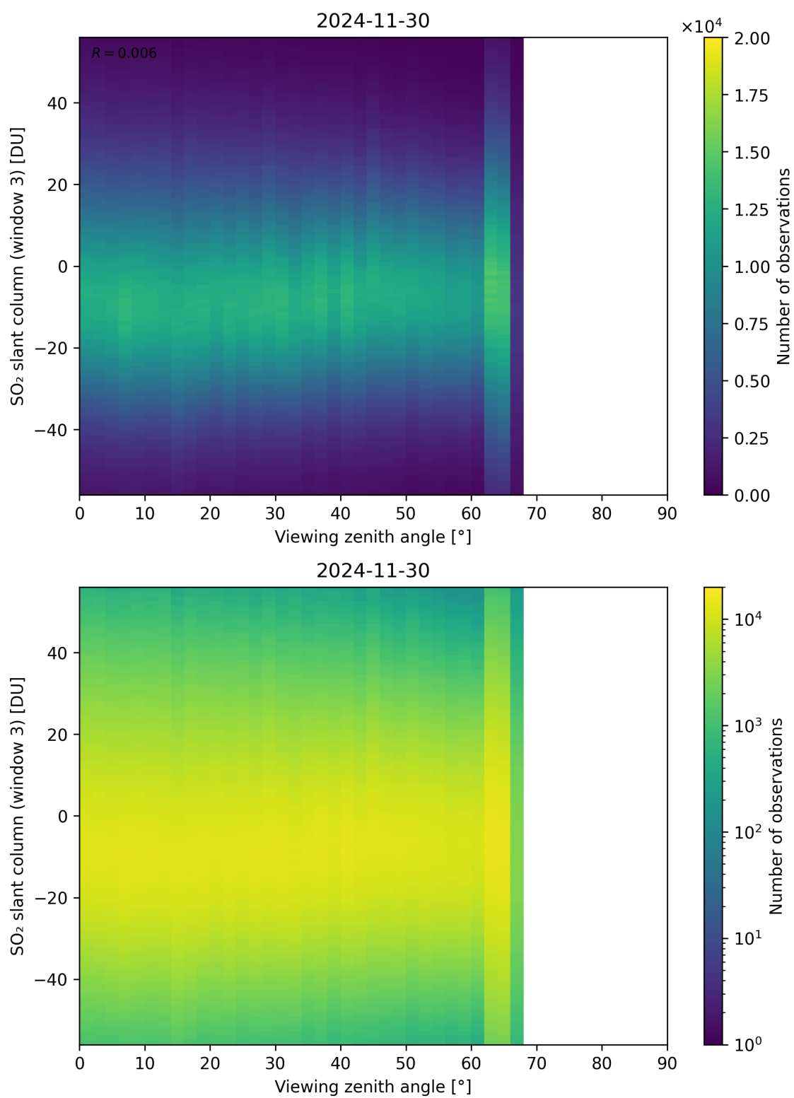
Figure 379: Scatter density plot of “Viewing zenith angle” against “SO 2 slant column (window 3)” for 2024-11-30 to 2024-12-01.
