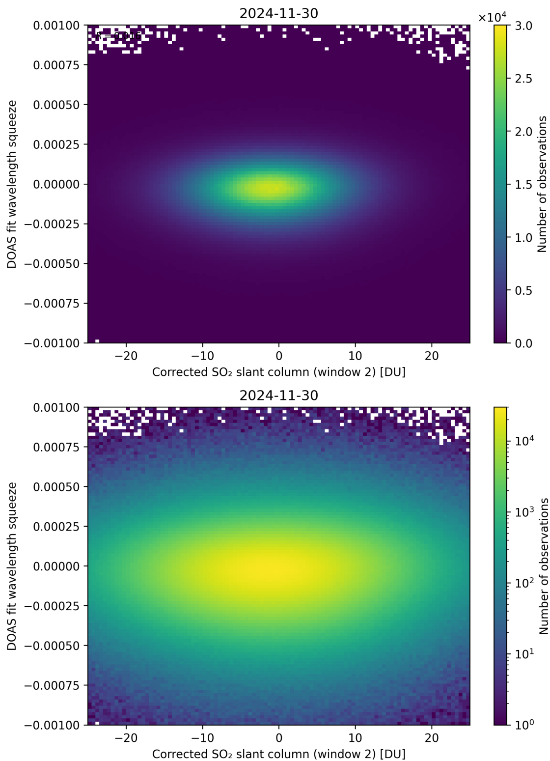
Figure 247: Scatter density plot of “Corrected SO 2 slant column (window 2)” against “DOAS fit wavelength squeeze” for 2024-11-30 to 2024-12-01.
