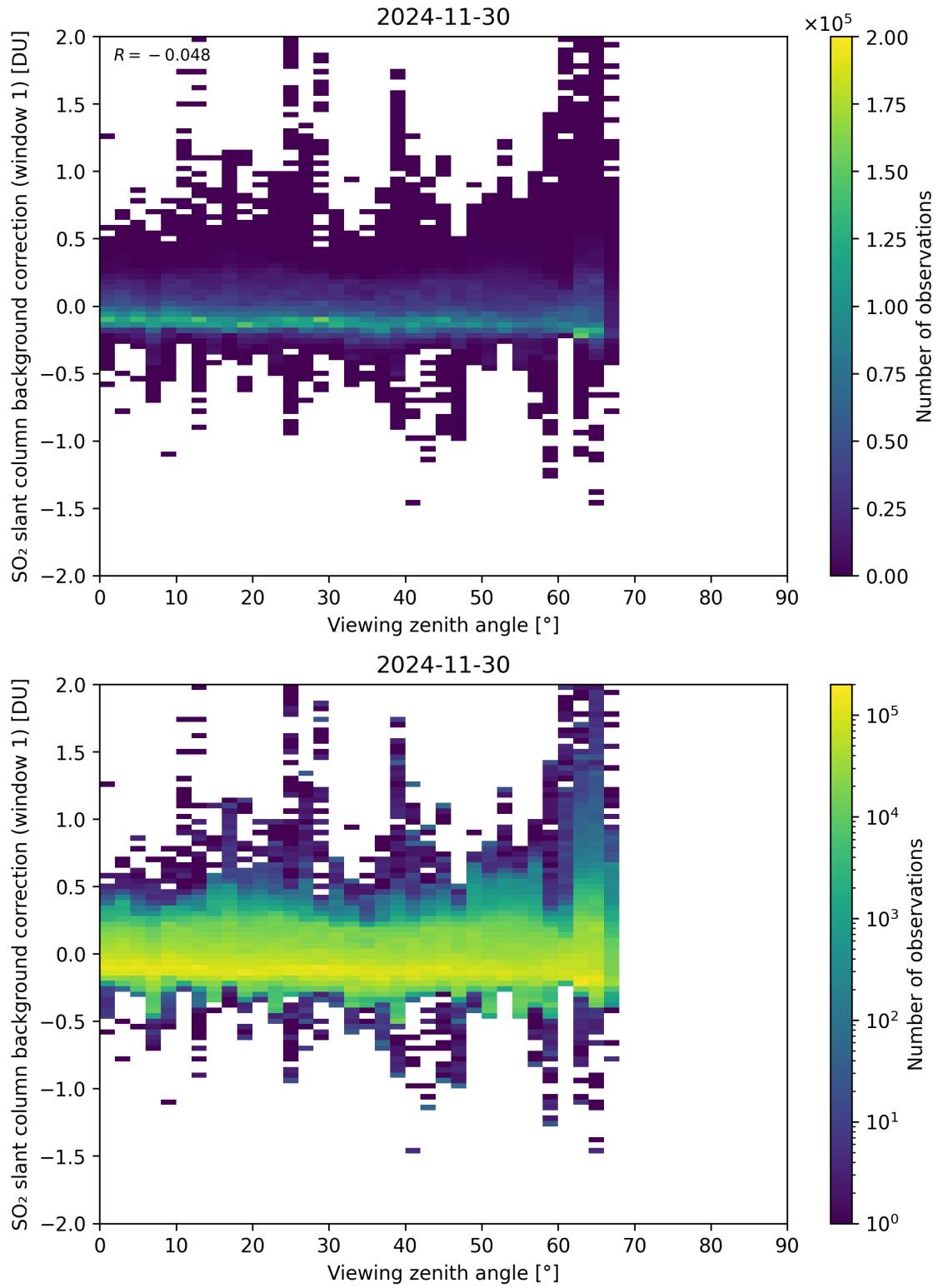
Figure 362: Scatter density plot of “Viewing zenith angle” against “SO 2 slant column background correction (window 1)” for 2024-11-30 to 2024-12-01.
