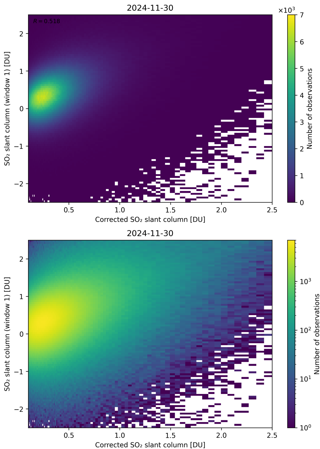
Figure 237: Scatter density plot of “Corrected SO 2 slant column” against “SO 2 slant column (window 1)” for 2024-11-30 to 2024-12-01.
