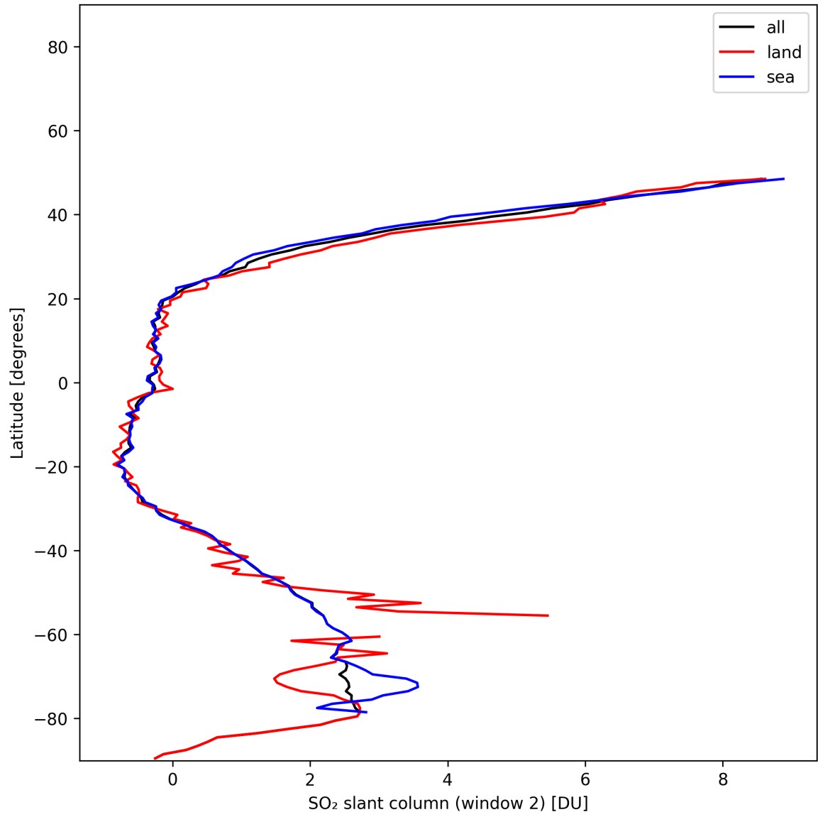
Figure 41: Zonal average of “SO 2 slant column (window 2)” for 2024-11-30 to 2024-12-01.
