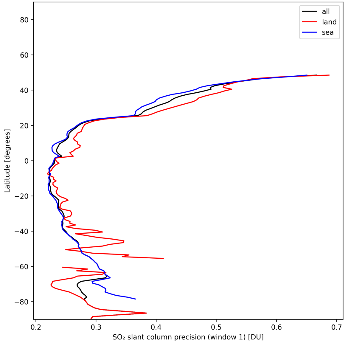
Figure 38: Zonal average of “SO 2 slant column precision (window 1)” for 2024-11-30 to 2024-12-01.
