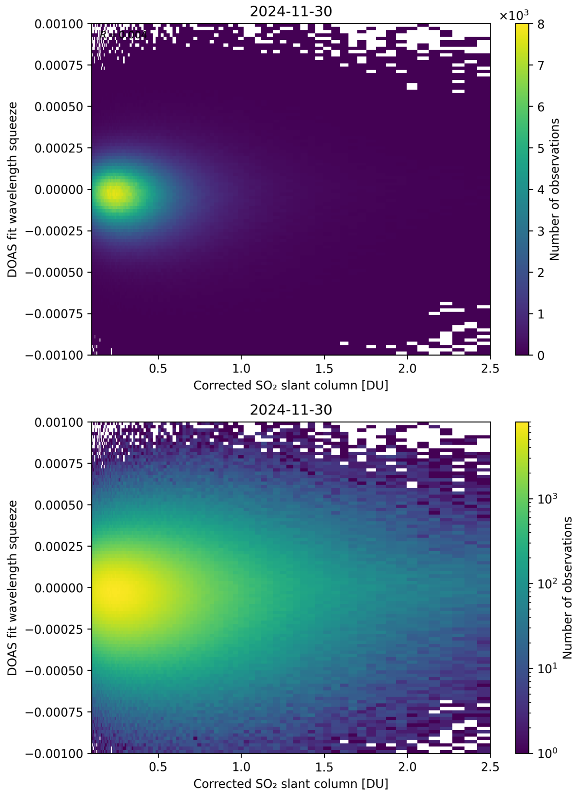
Figure 230: Scatter density plot of “Corrected SO 2 slant column” against “DOAS fit wavelength squeeze” for 2024-11-30 to 2024-12-01.
