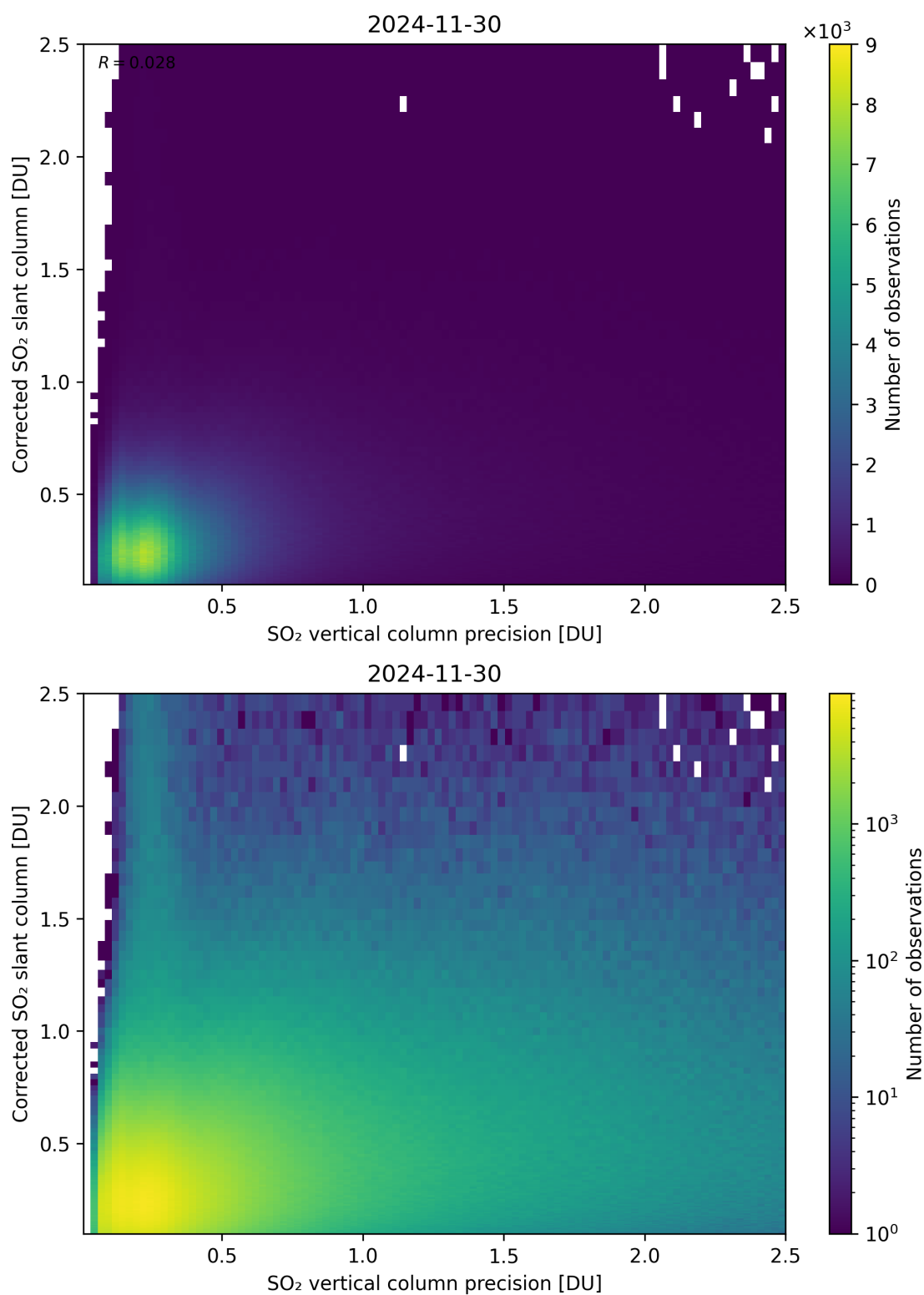
Figure 338: Scatter density plot of “SO 2 vertical column precision” against “Corrected SO 2 slant column” for 2024-11-30 to 2024-12-01.
