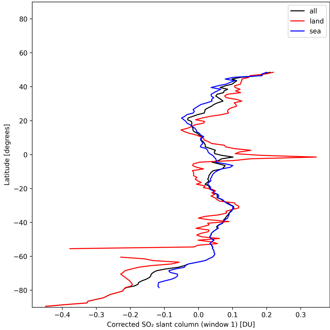
Figure 39: Zonal average of “Corrected SO 2 slant column (window 1)” for 2024-11-30 to 2024-12-01.
