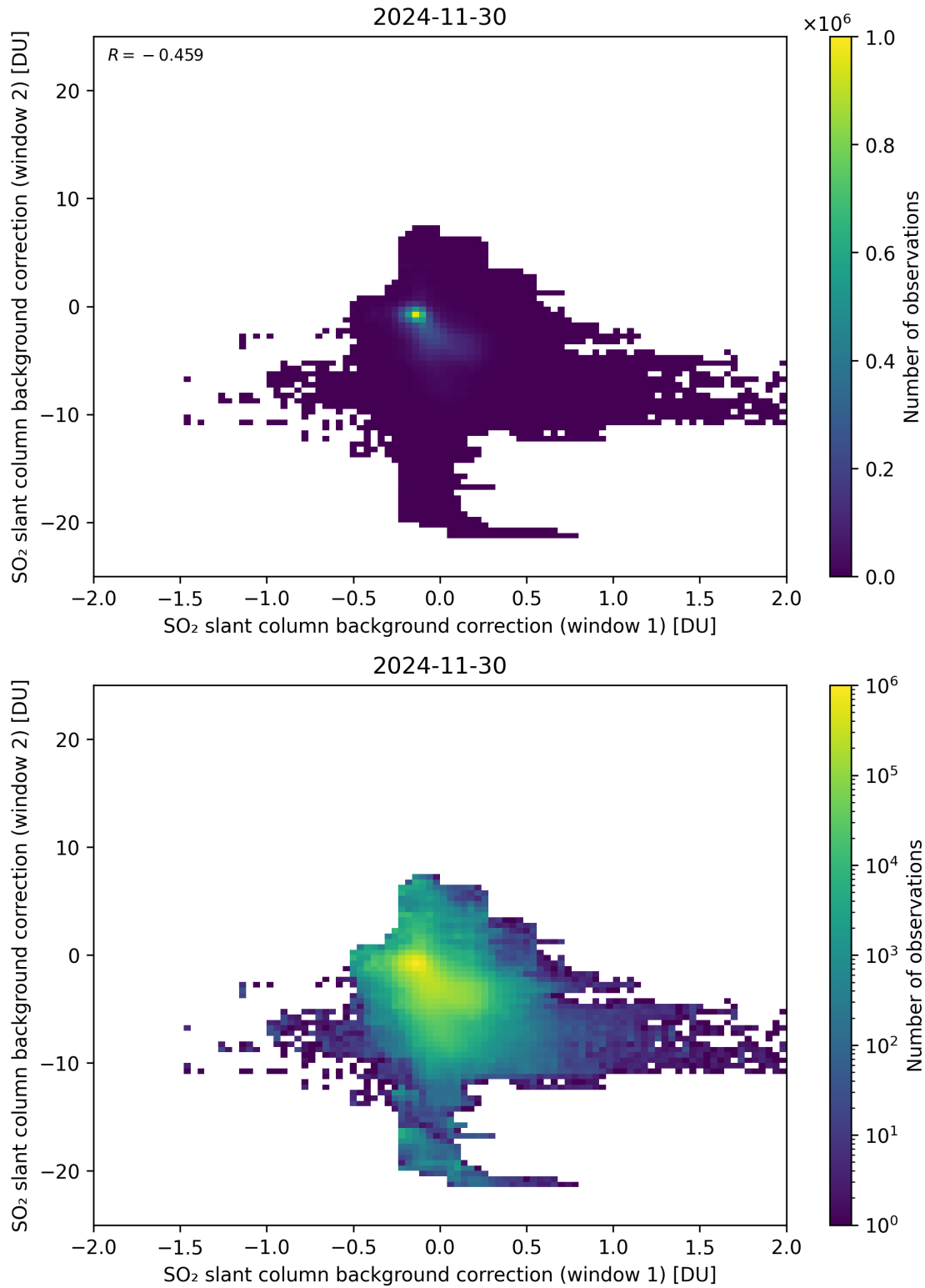
Figure 109: Scatter density plot of “SO 2 slant column background correction (window 1)” against “SO 2 slant column background correction (window 2)” for 2024-11-30 to 2024-12-01.
