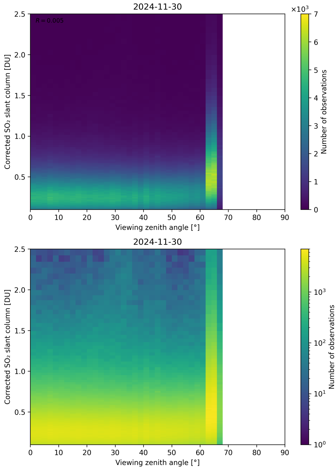
Figure 373: Scatter density plot of “Viewing zenith angle” against “Corrected SO 2 slant column” for 2024-11-30 to 2024-12-01.
