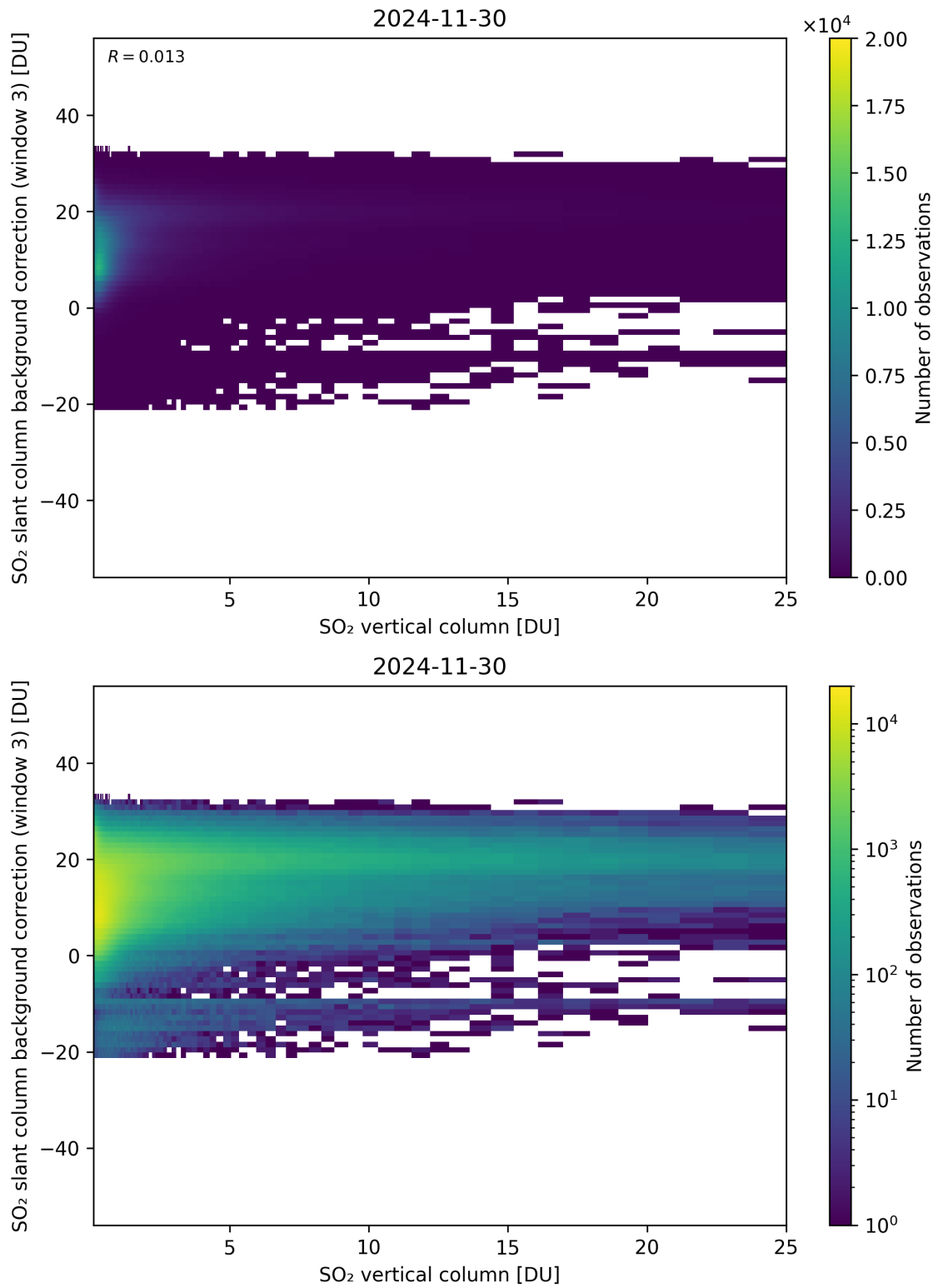
Figure 325: Scatter density plot of “SO 2 vertical column” against “SO 2 slant column background correction (window 3)” for 2024-11-30 to 2024-12-01.
