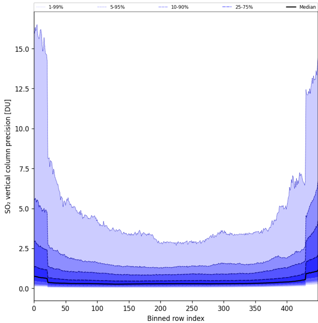
Figure 85: Along track statistics of “SO 2 vertical column precision” for 2024-11-30 to 2024-12-01
