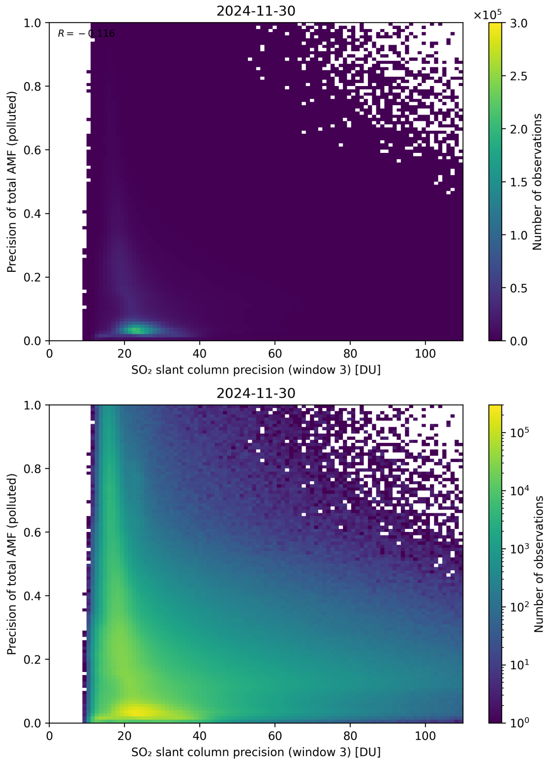
Figure 314: Scatter density plot of “SO 2 slant column precision (window 3)” against “Precision of total AMF (polluted)” for 2024-11-30 to 2024-12-01.
