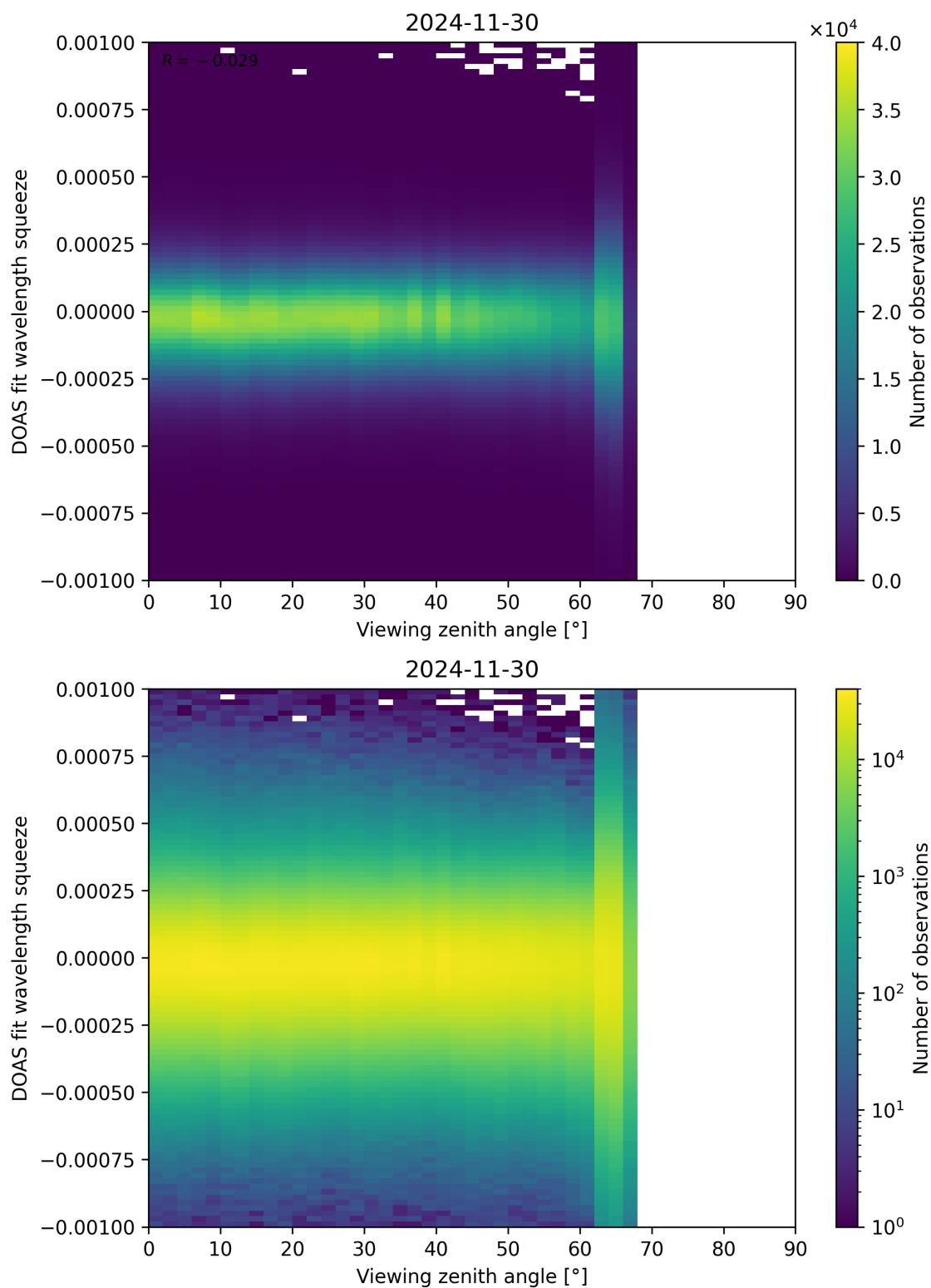
Figure 366: Scatter density plot of “Viewing zenith angle” against “DOAS fit wavelength squeeze” for 2024-11-30 to 2024-12-01.
