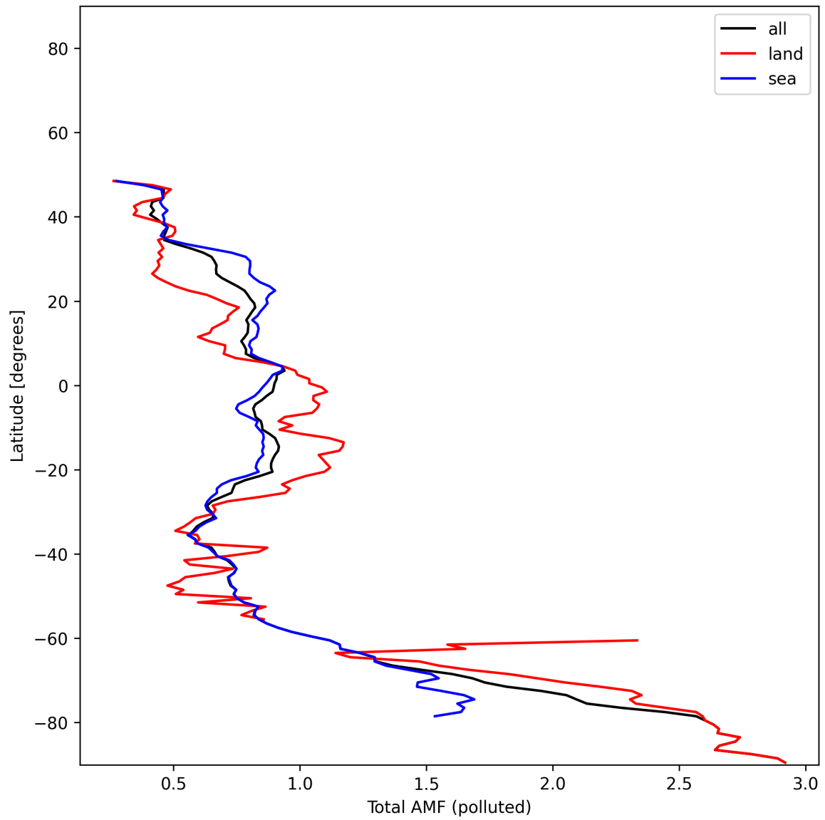
Figure 53: Zonal average of “Total AMF (polluted)” for 2024-11-30 to 2024-12-01.
