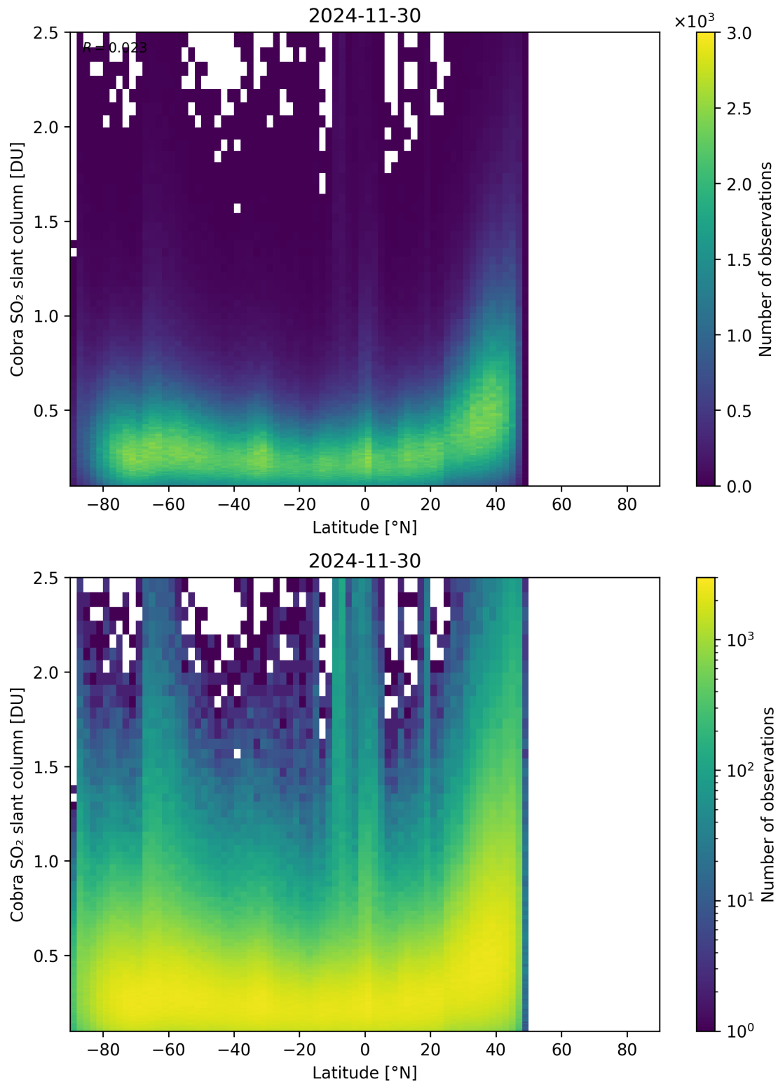
Figure 157: Scatter density plot of “Latitude” against “Cobra SO 2 slant column” for 2024-11-30 to 2024-12-01.
