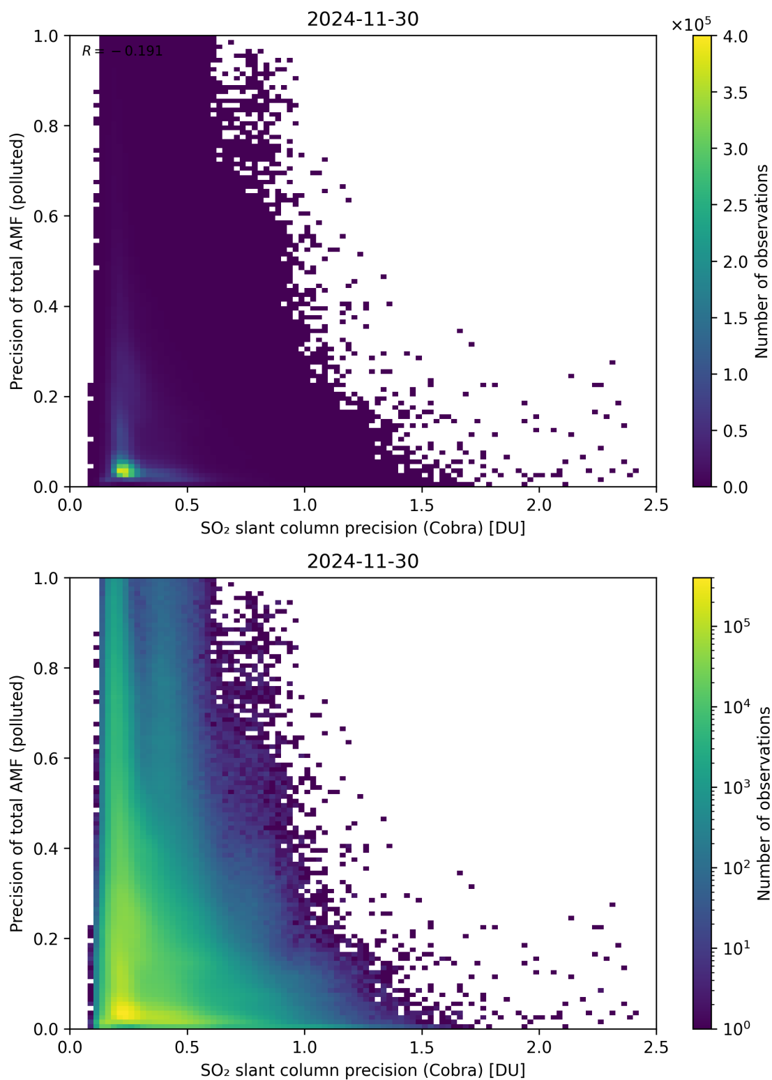
Figure 214: Scatter density plot of “SO 2 slant column precision (Cobra)” against “Precision of total AMF (polluted)” for 2024-11-30 to 2024-12-01.
