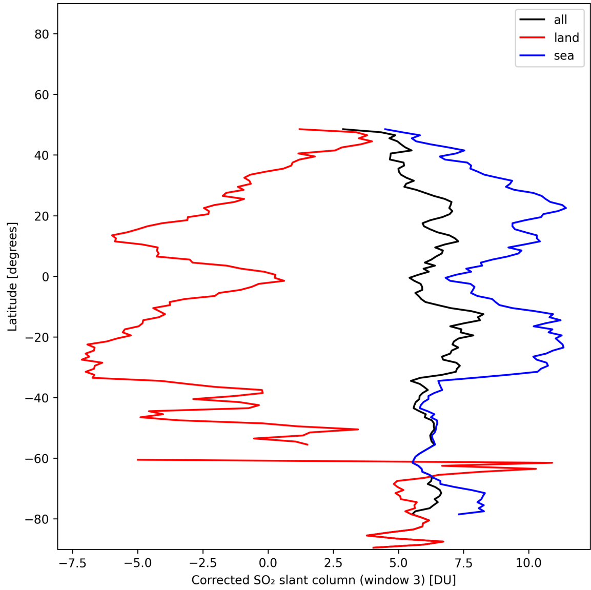
Figure 47: Zonal average of “Corrected SO 2 slant column (window 3)” for 2024-11-30 to 2024-12-01.
