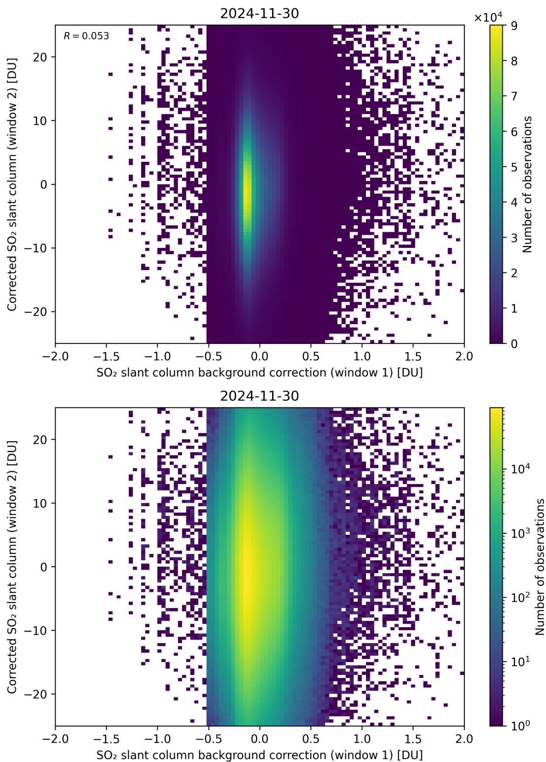
Figure 115: Scatter density plot of “SO 2 slant column background correction (window 1)” against “Corrected SO 2 slant column (window 2)” for 2024-11-30 to 2024-12-01.
