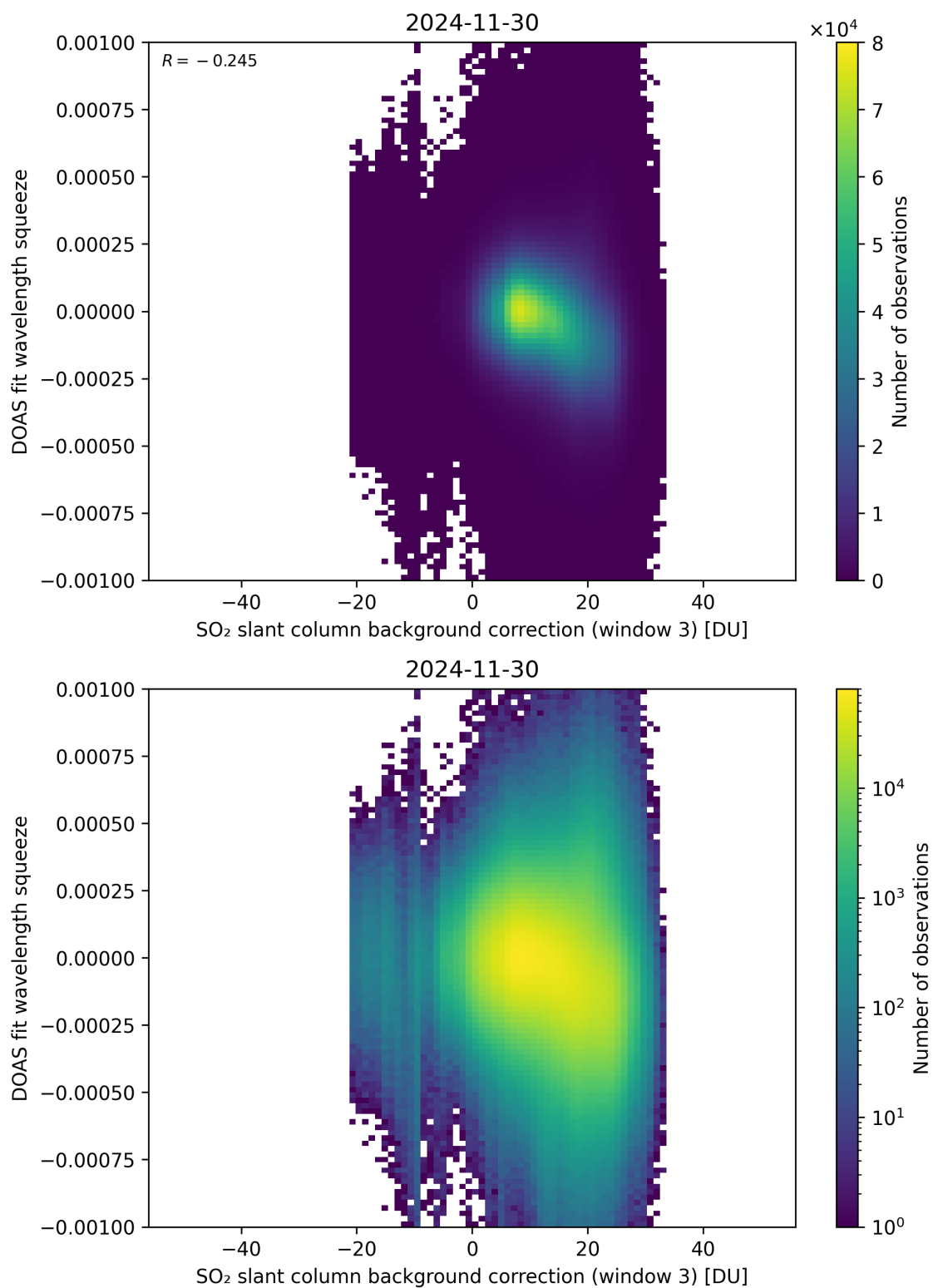
Figure 133: Scatter density plot of “SO 2 slant column background correction (window 3)” against “DOAS fit wavelength squeeze” for 2024-11-30 to 2024-12-01.
