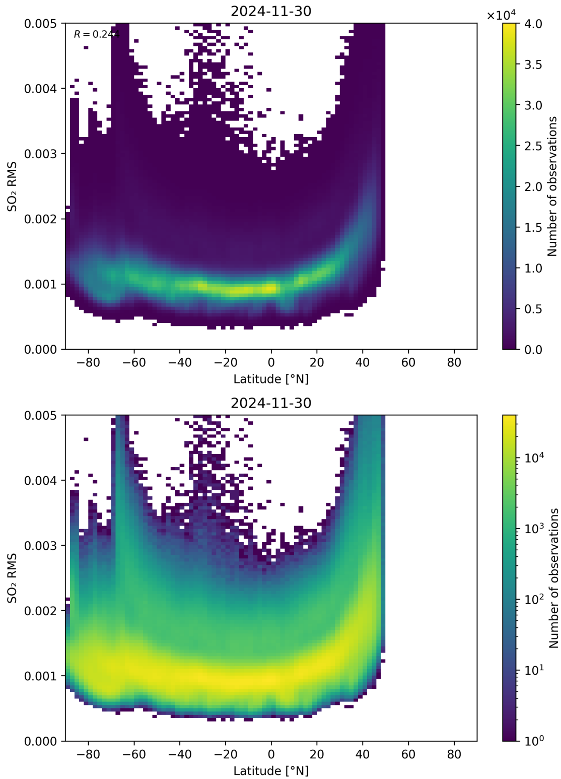
Figure 155: Scatter density plot of “Latitude” against “SO 2 RMS” for 2024-11-30 to 2024-12-01.
