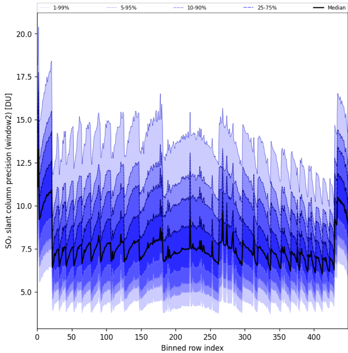
Figure 94: Along track statistics of “SO 2 slant column precision (window2)” for 2024-11-30 to 2024-12-01
