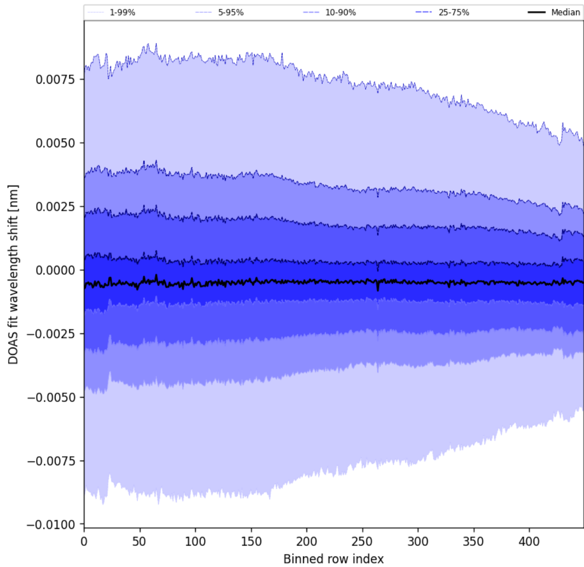
Figure 102: Along track statistics of “DOAS fit wavelength shift” for 2024-11-30 to 2024-12-01
