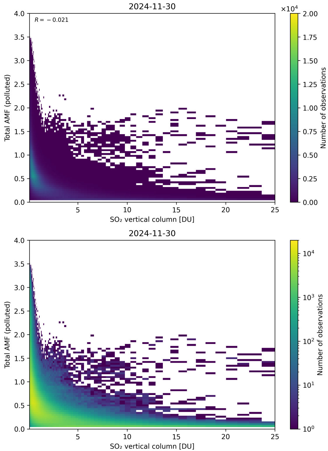
Figure 359: Scatter density plot of “SO 2 vertical column” against “Total AMF (polluted)” for 2024-11-30 to 2024-12-01.
