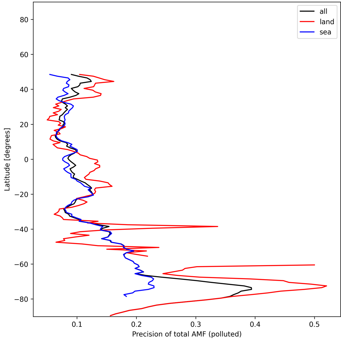
Figure 54: Zonal average of “Precision of total AMF (polluted)” for 2024-11-30 to 2024-12-01.
