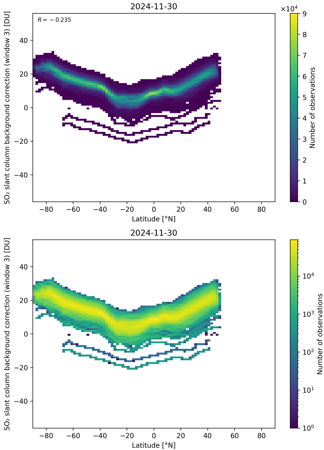
Figure 152: Scatter density plot of “Latitude” against “SO 2 slant column background correction (window 3)” for 2024-11-30 to 2024-12-01.
