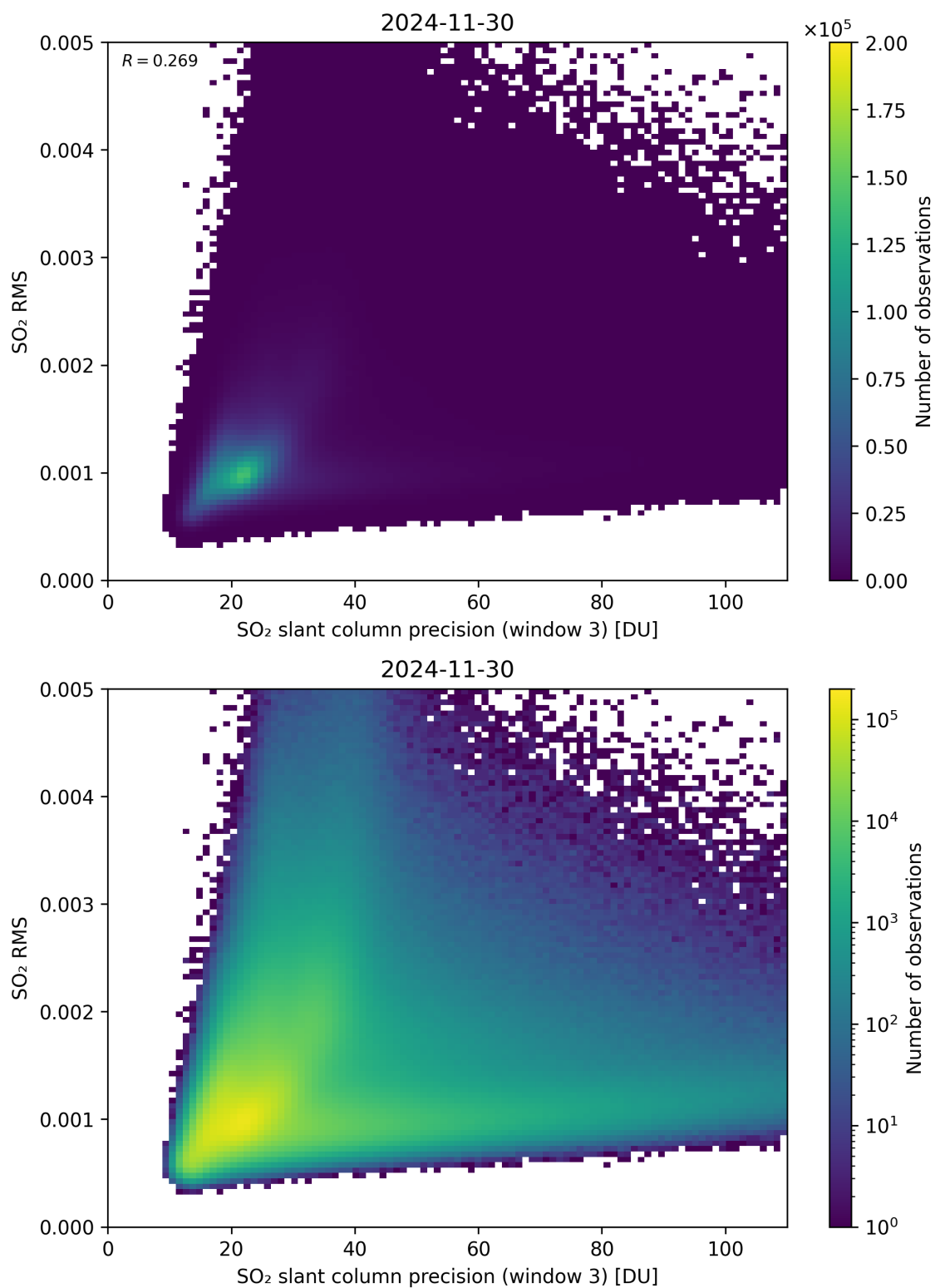
Figure 310: Scatter density plot of “SO 2 slant column precision (window 3)” against “SO 2 RMS” for 2024-11-30 to 2024-12-01.
