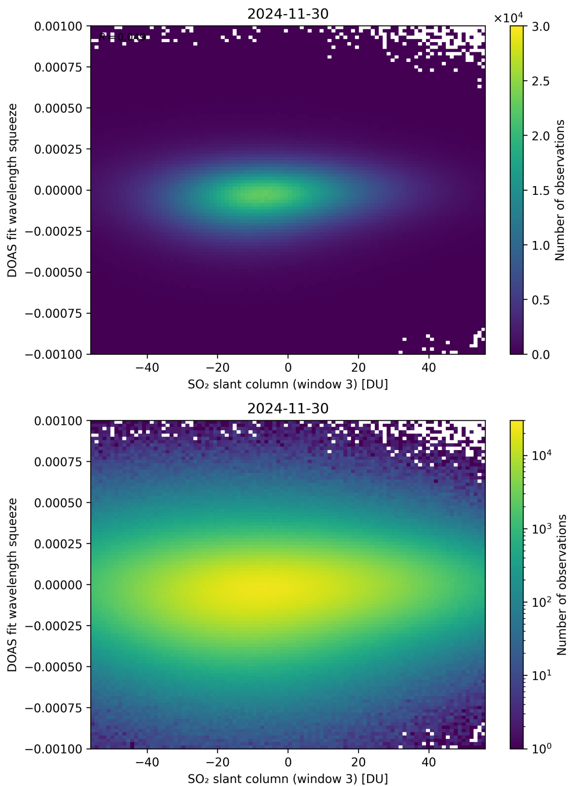
Figure 305: Scatter density plot of “SO 2 slant column (window 3)” against “DOAS fit wavelength squeeze” for 2024-11-30 to 2024-12-01.
