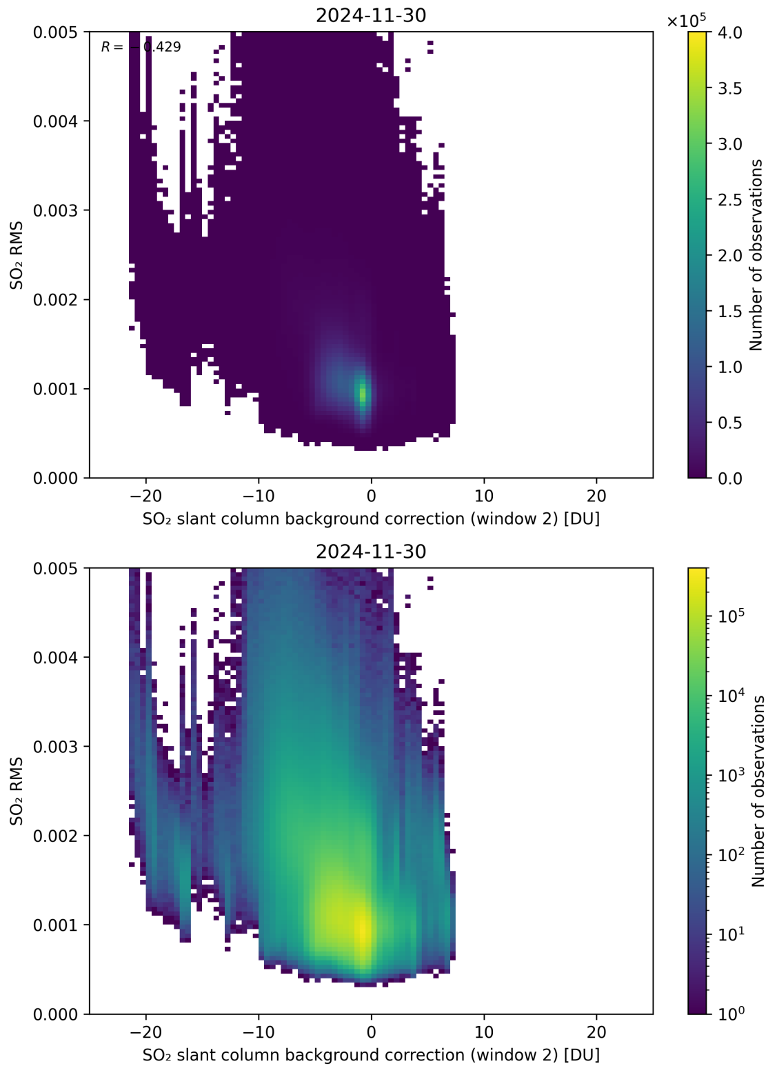
Figure 125: Scatter density plot of “SO 2 slant column background correction (window 2)” against “SO 2 RMS” for 2024-11-30 to 2024-12-01.
