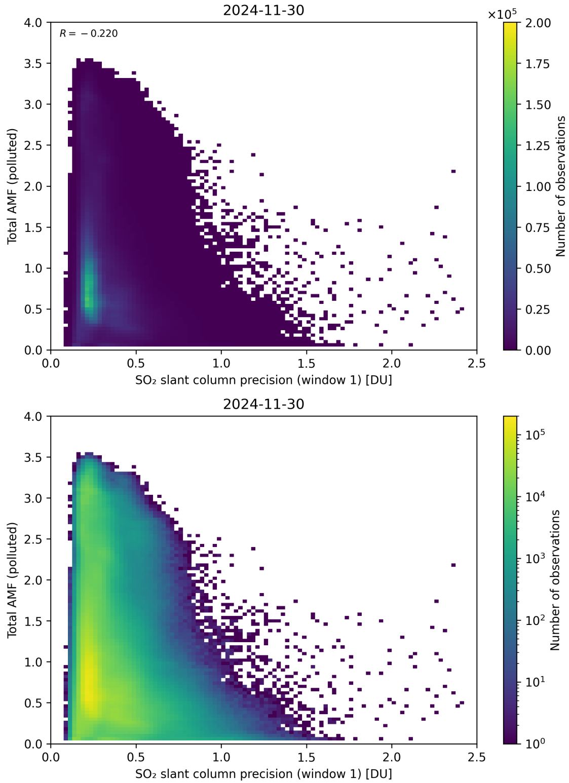
Figure 280: Scatter density plot of “SO 2 slant column precision (window 1)” against “Total AMF (polluted)” for 2024-11-30 to 2024-12-01.
