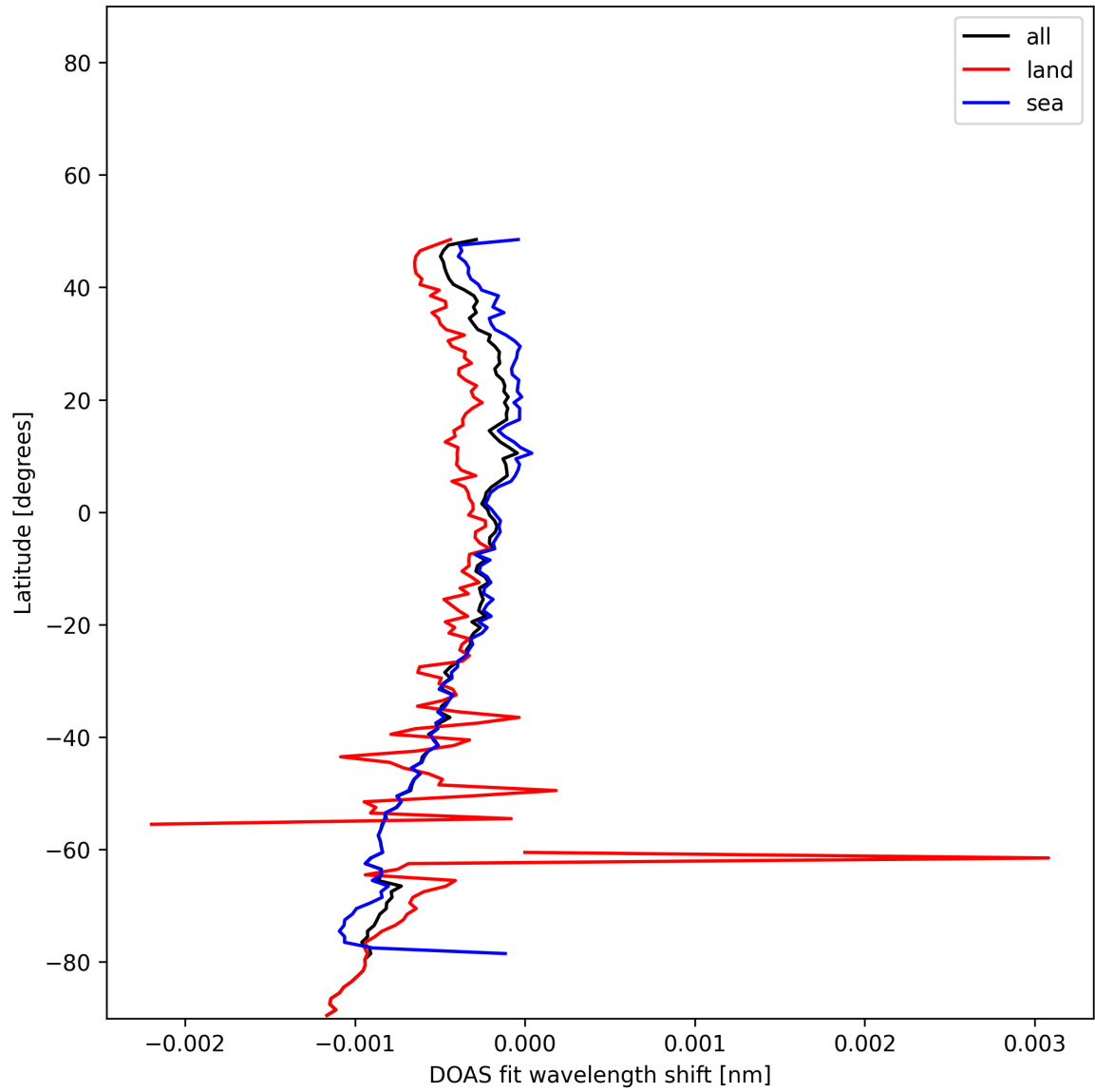
Figure 50: Zonal average of “DOAS fit wavelength shift” for 2024-11-30 to 2024-12-01.
