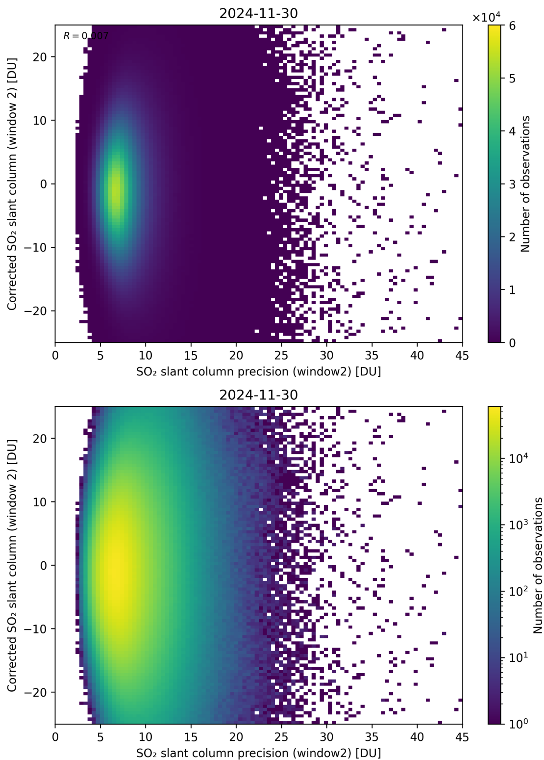
Figure 297: Scatter density plot of “SO 2 slant column precision (window2)” against “Corrected SO 2 slant column (window 2)” for 2024-11-30 to 2024-12-01.
