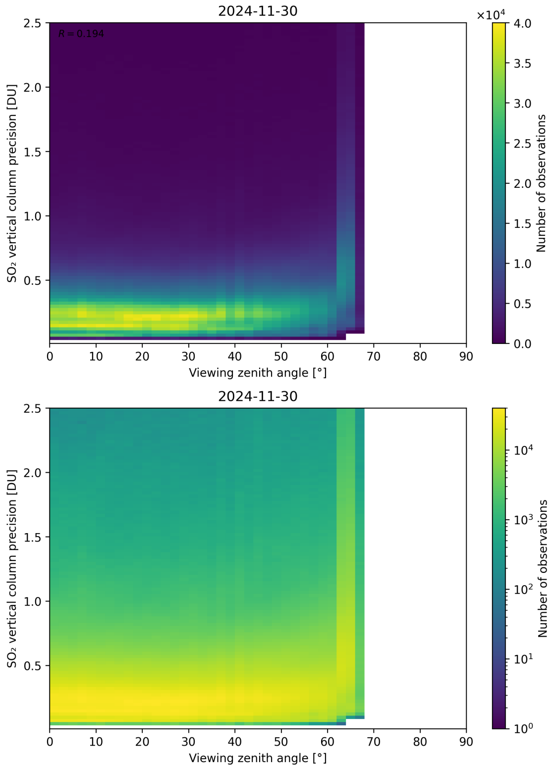
Figure 384: Scatter density plot of “Viewing zenith angle” against “SO 2 vertical column precision” for 2024-11-30 to 2024-12-01.
