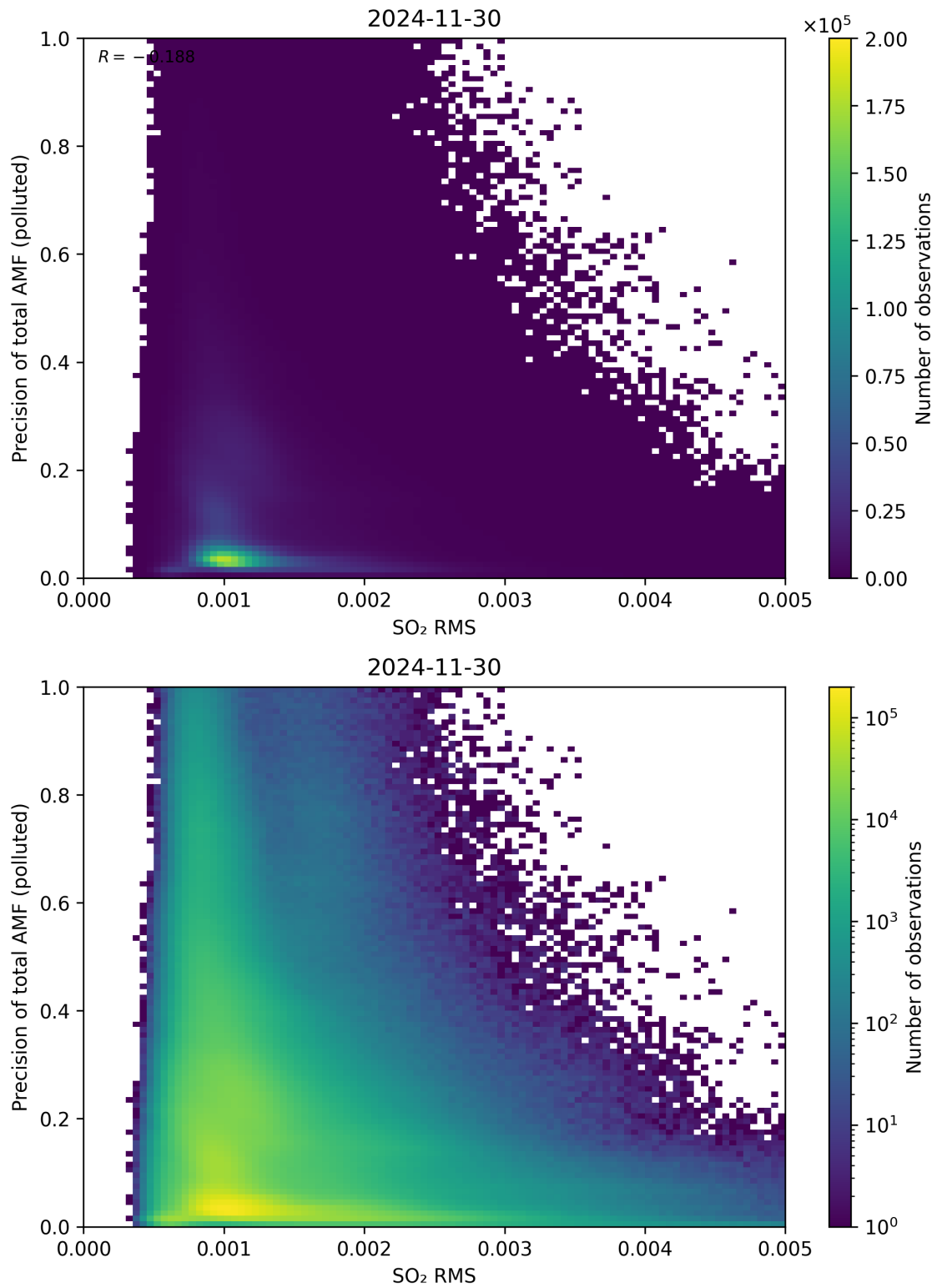
Figure 149: Scatter density plot of “SO 2 RMS” against “Precision of total AMF (polluted)” for 2024-11-30 to 2024-12-01.
