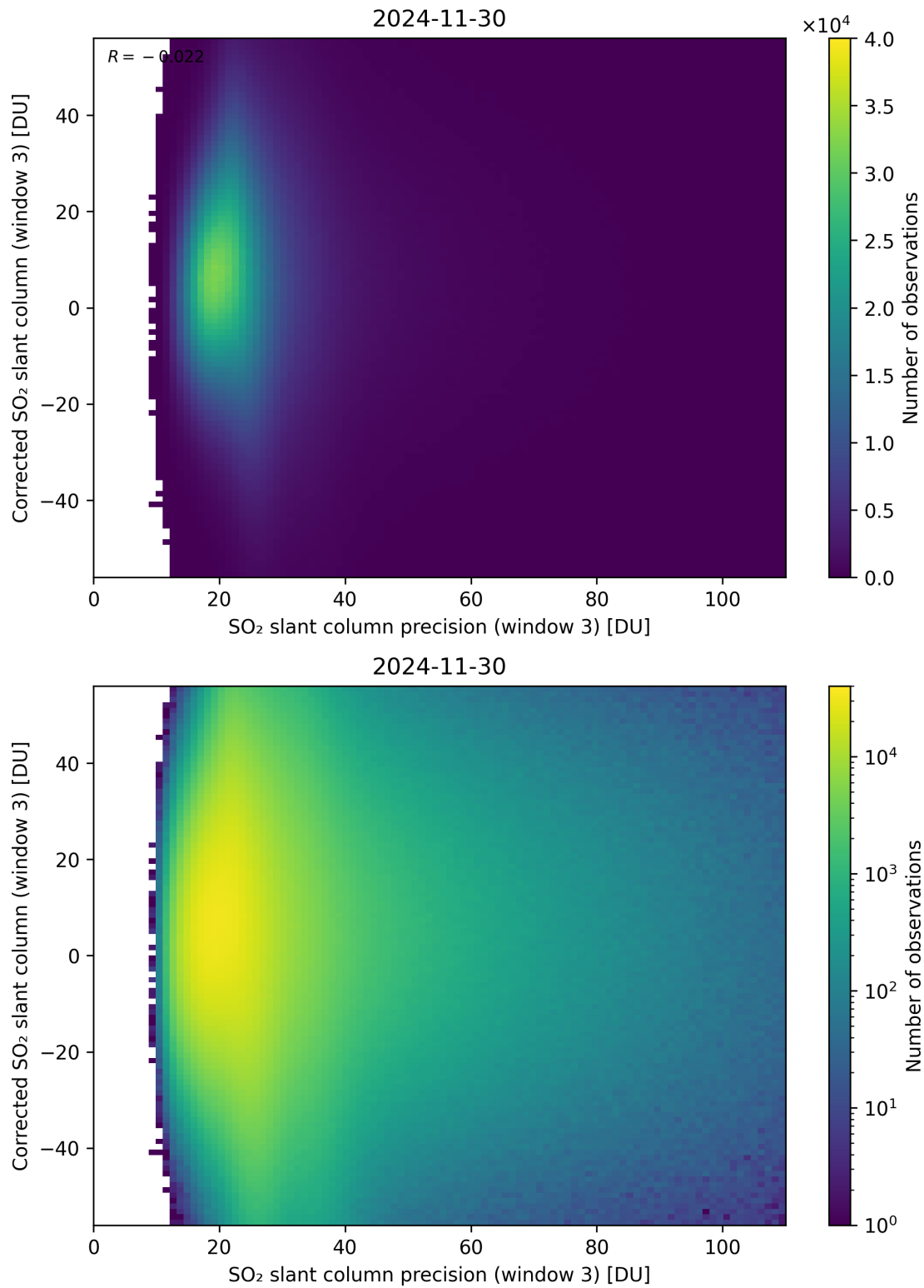
Figure 312: Scatter density plot of “SO 2 slant column precision (window 3)” against “Corrected SO 2 slant column (window 3)” for 2024-11-30 to 2024-12-01.
