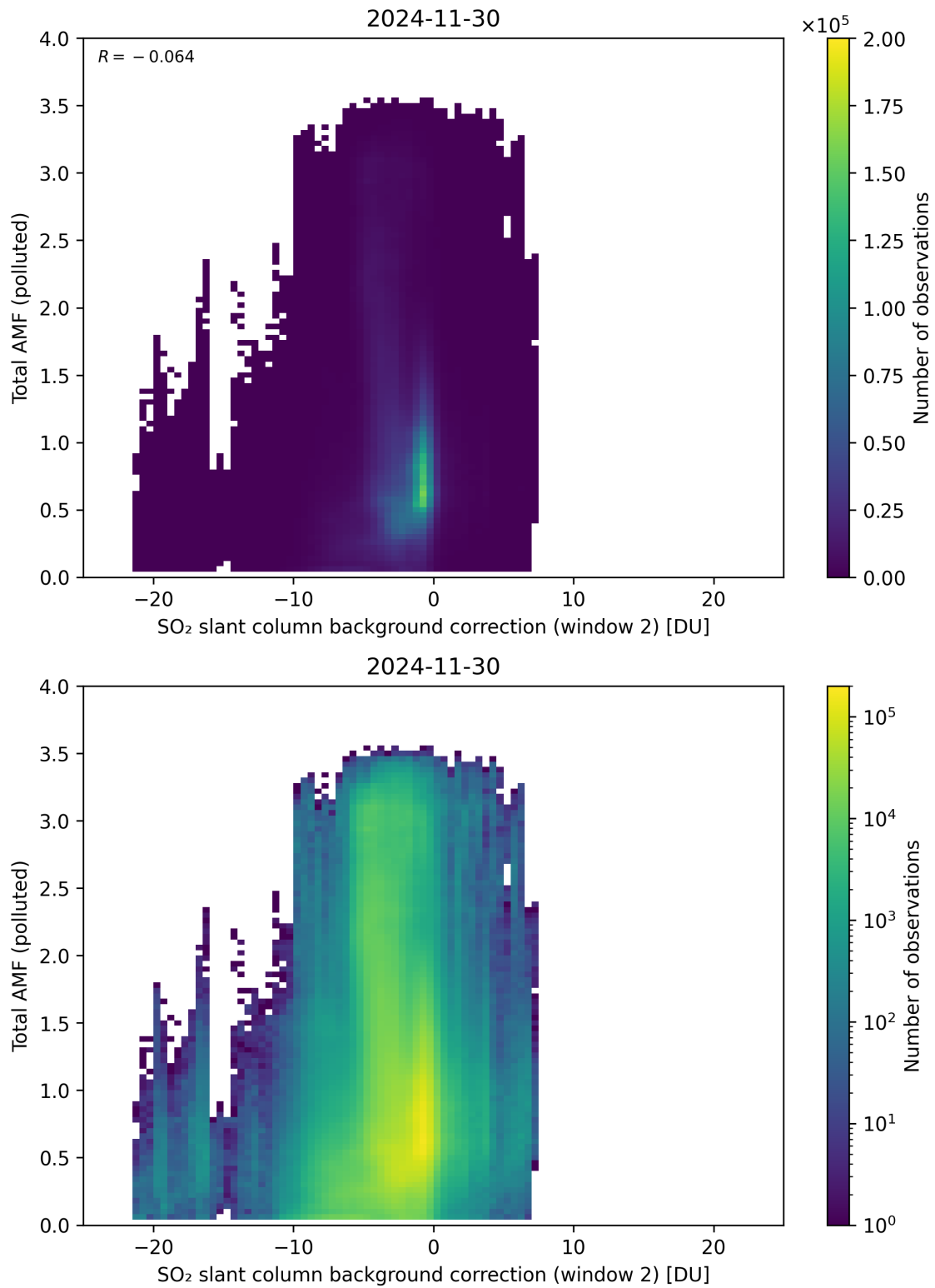
Figure 130: Scatter density plot of “SO 2 slant column background correction (window 2)” against “Total AMF (polluted)” for 2024-11-30 to 2024-12-01.
