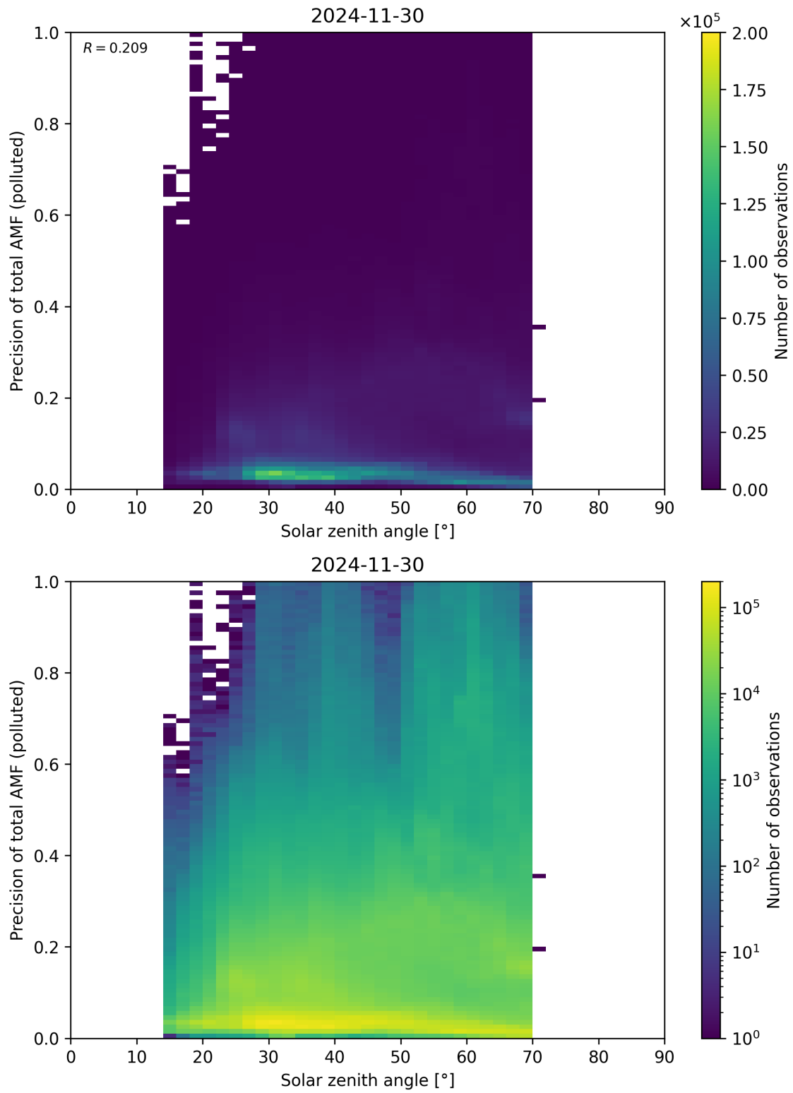
Figure 190: Scatter density plot of “Solar zenith angle” against “Precision of total AMF (polluted)” for 2024-11-30 to 2024-12-01.
