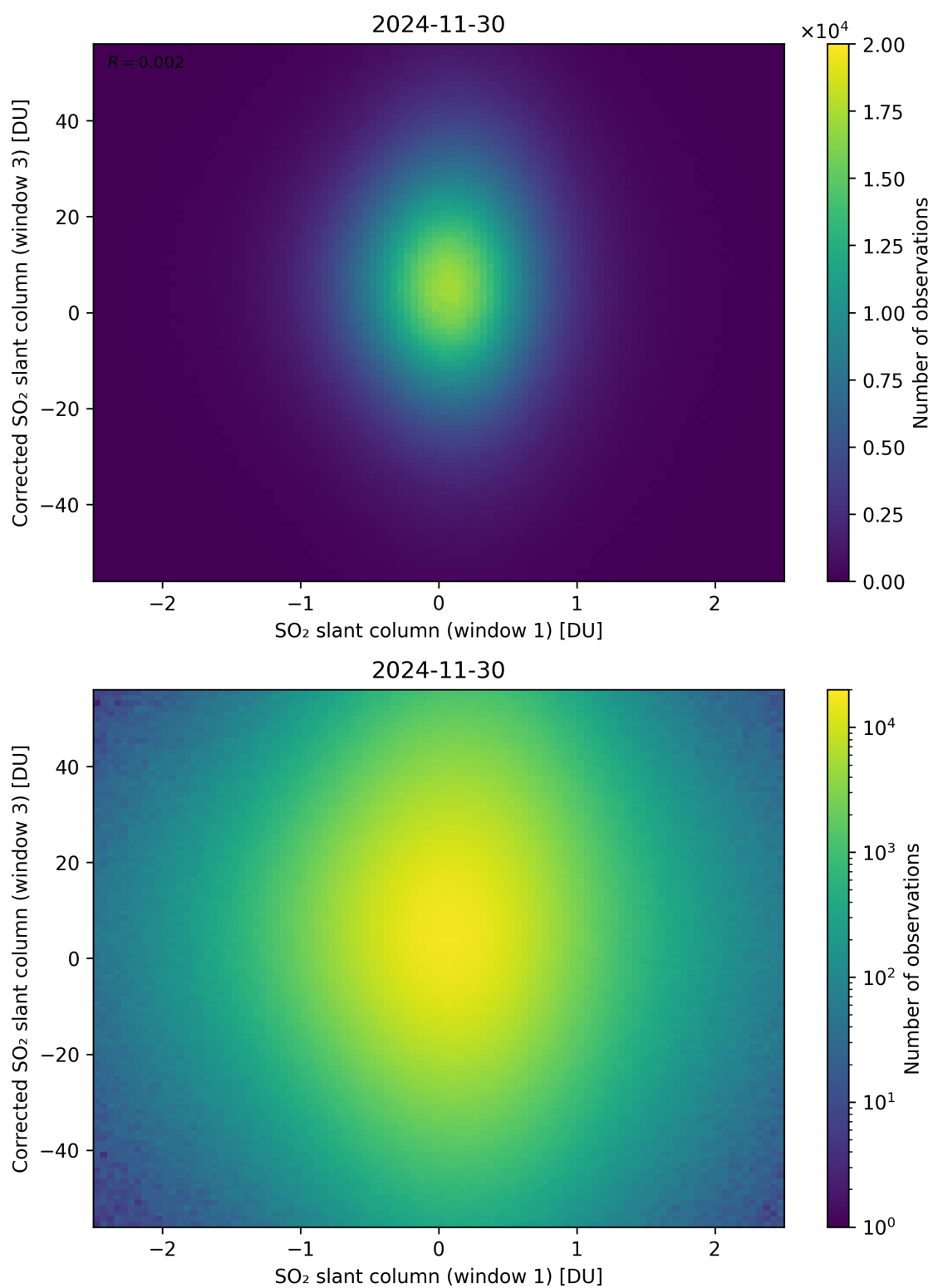
Figure 284: Scatter density plot of “SO 2 slant column (window 1)” against “Corrected SO 2 slant column (window 3)” for 2024-11-30 to 2024-12-01.
