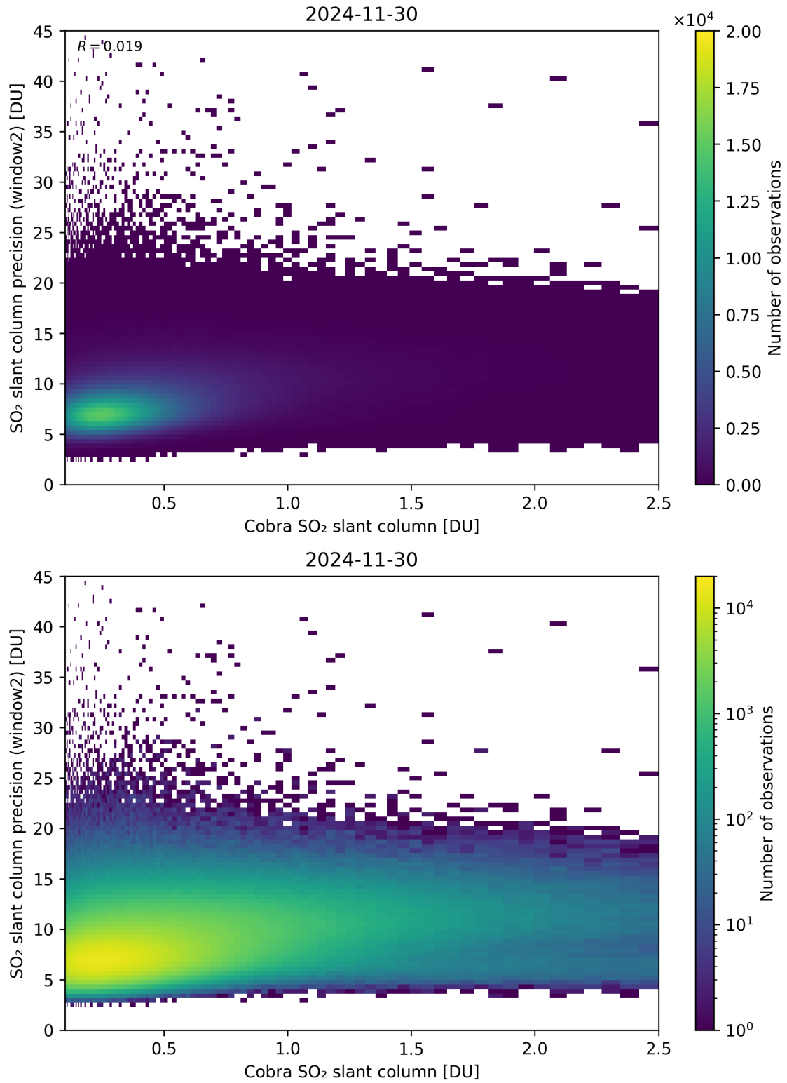
Figure 221: Scatter density plot of “Cobra SO 2 slant column” against “SO 2 slant column precision (window2)” for 2024-11-30 to 2024-12-01.
