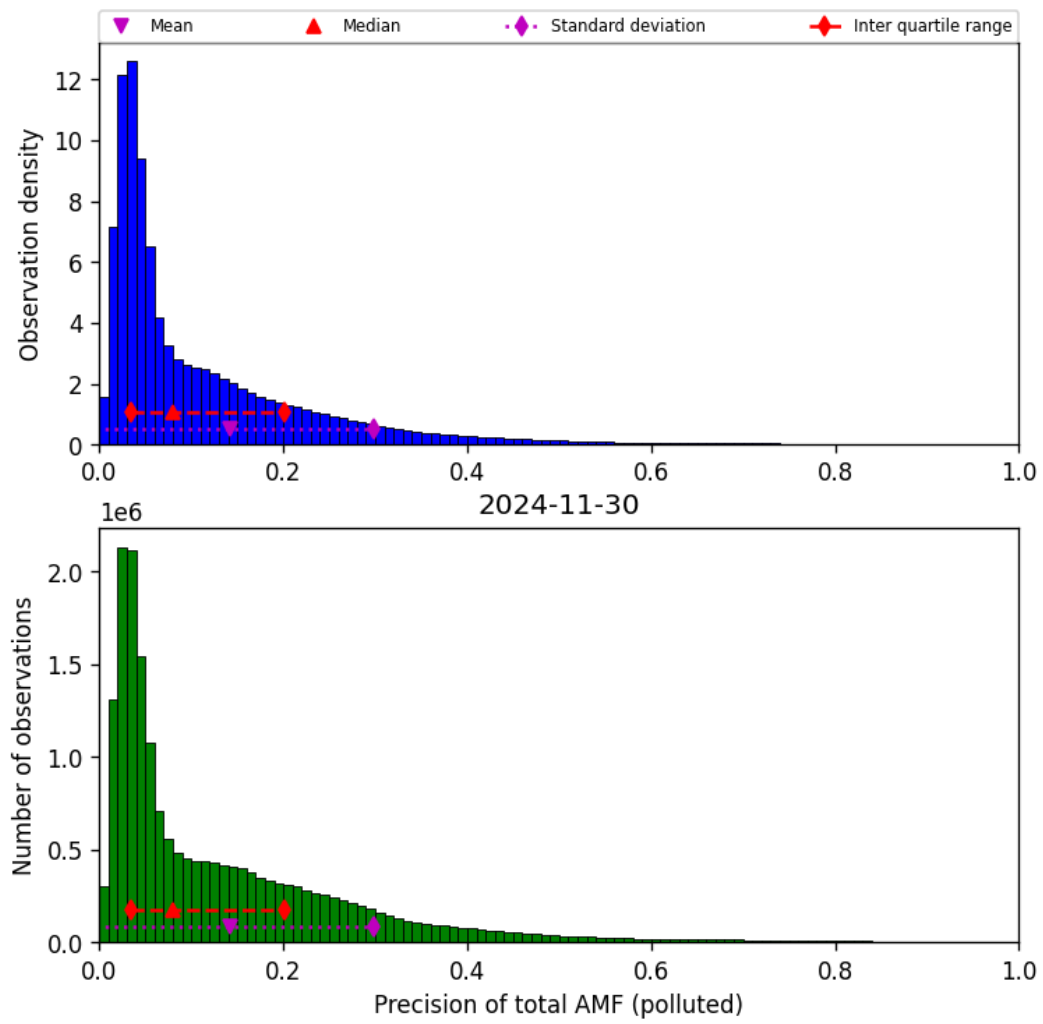
Figure 80: Histogram of “Precision of total AMF (polluted)” for 2024-11-30 to 2024-12-01
