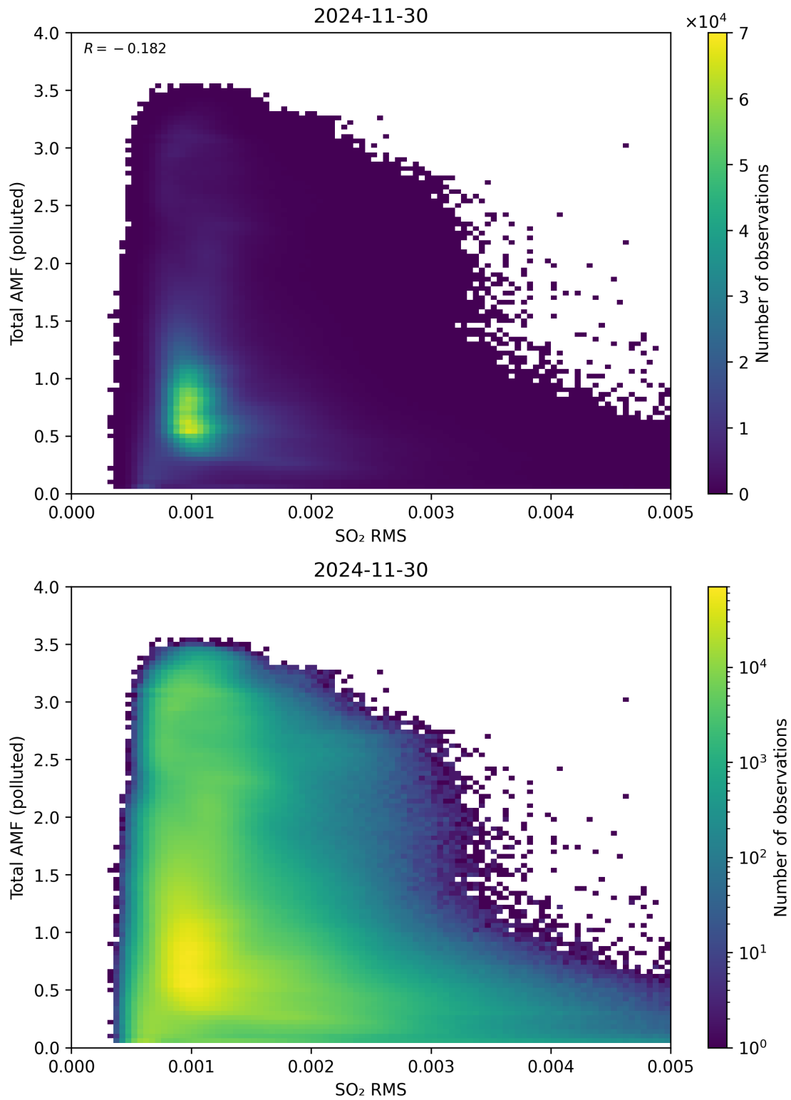
Figure 148: Scatter density plot of “SO 2 RMS” against “Total AMF (polluted)” for 2024-11-30 to 2024-12-01.
