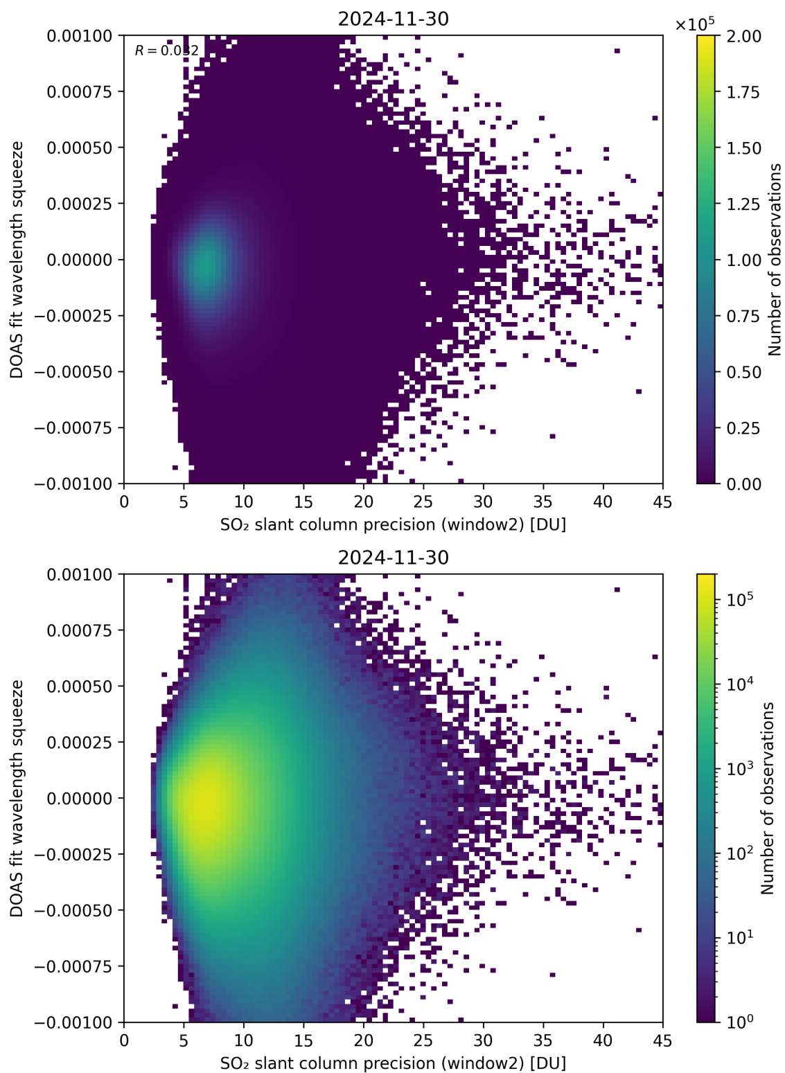
Figure 294: Scatter density plot of “SO 2 slant column precision (window2)” against “DOAS fit wavelength squeeze” for 2024-11-30 to 2024-12-01.
