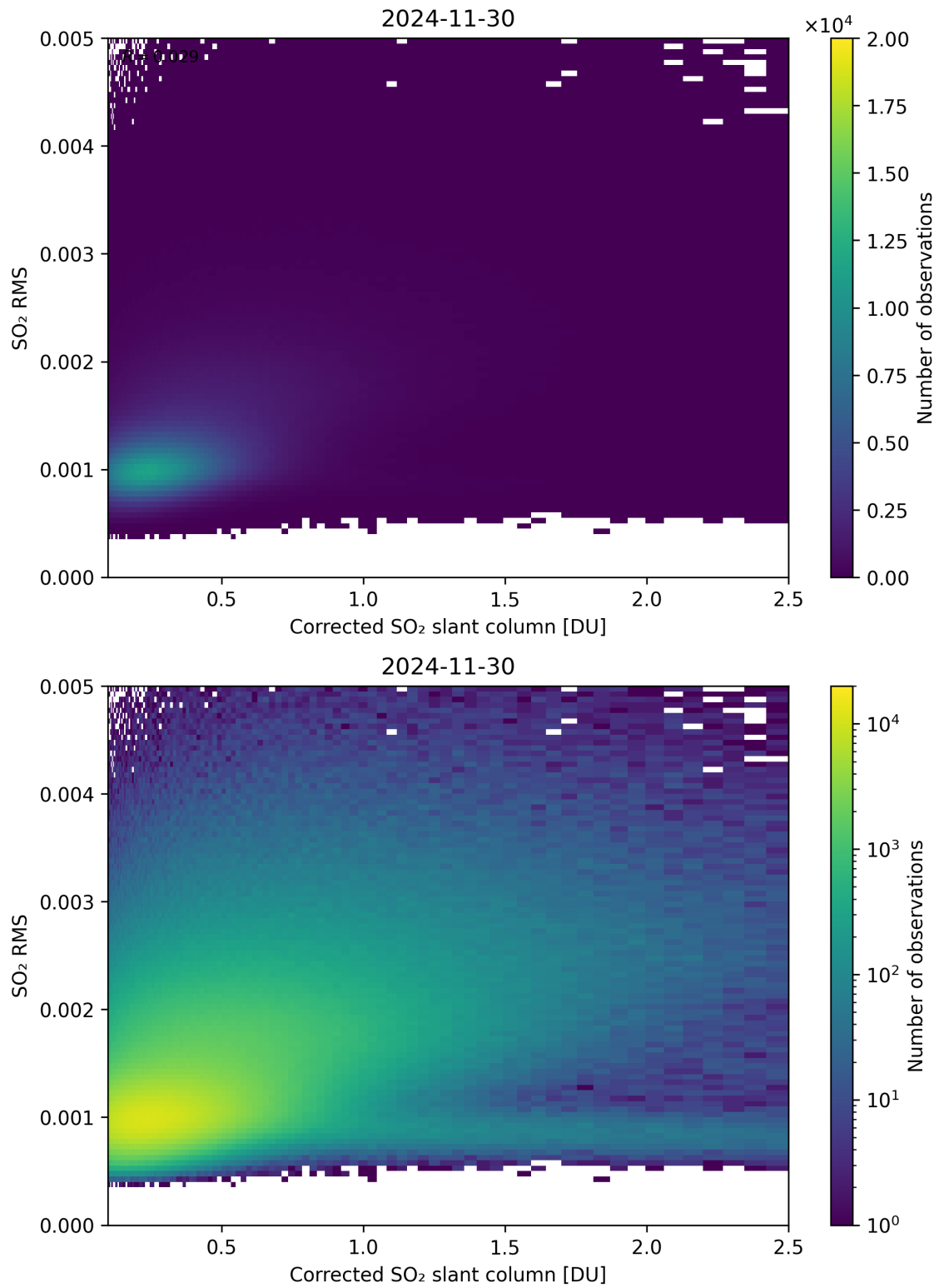
Figure 231: Scatter density plot of “Corrected SO 2 slant column” against “SO 2 RMS” for 2024-11-30 to 2024-12-01.
