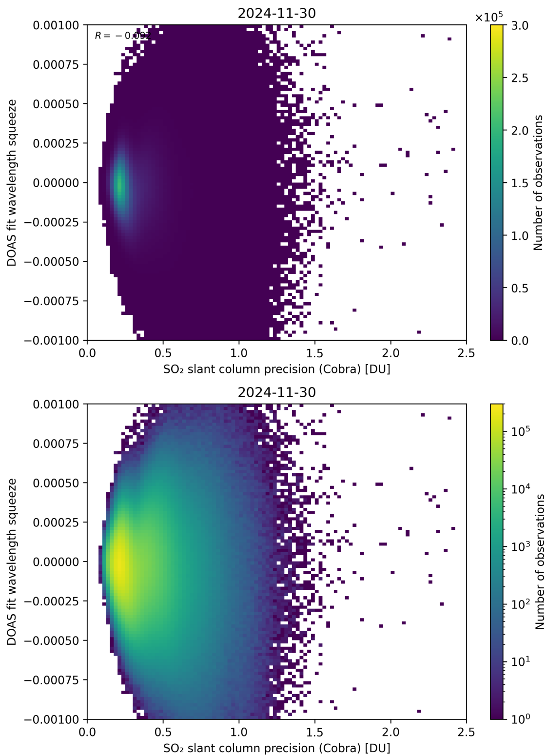
Figure 203: Scatter density plot of “SO 2 slant column precision (Cobra)” against “DOAS fit wavelength squeeze” for 2024-11-30 to 2024-12-01.
