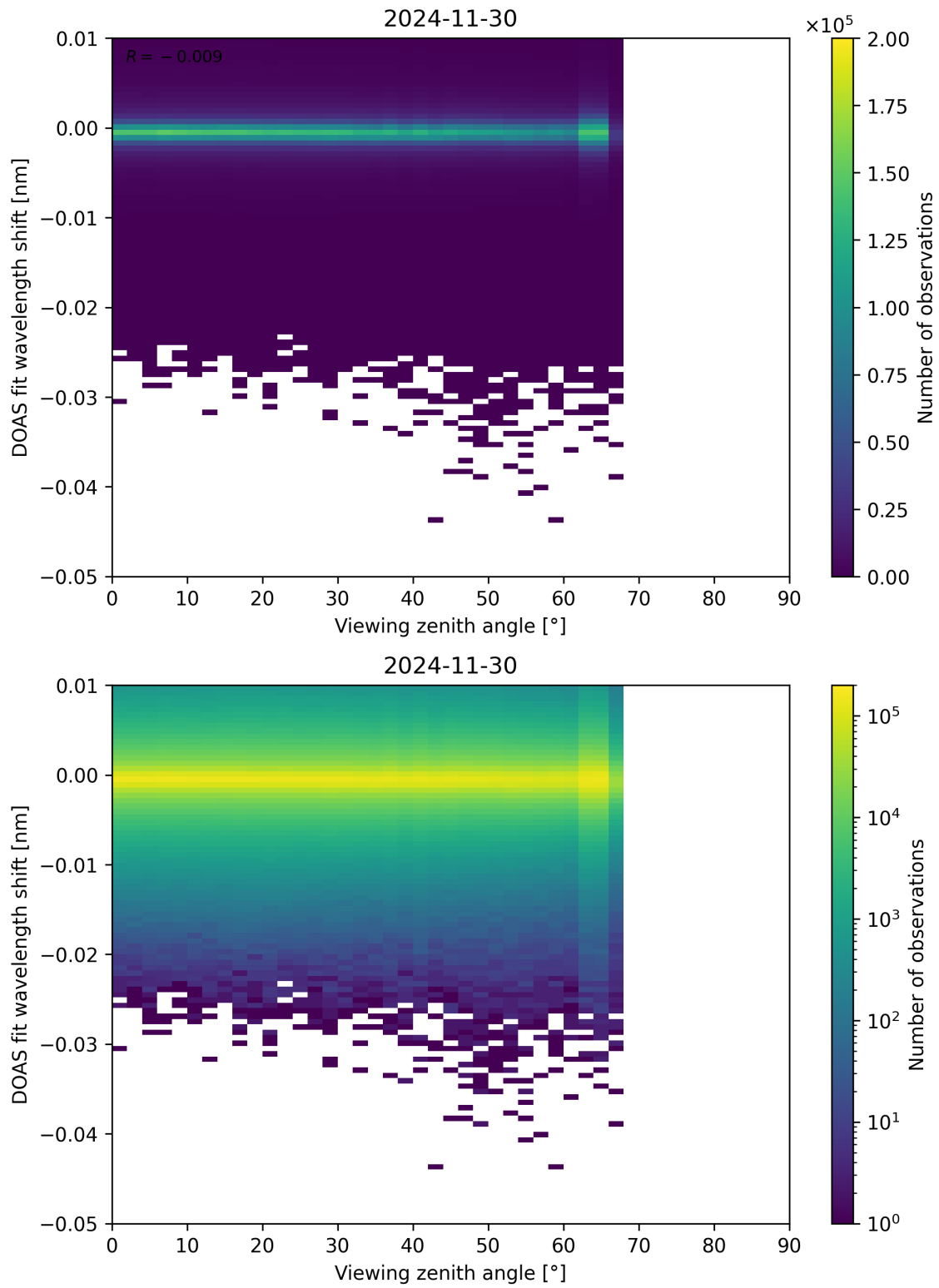
Figure 365: Scatter density plot of “Viewing zenith angle” against “DOAS fit wavelength shift” for 2024-11-30 to 2024-12-01.
