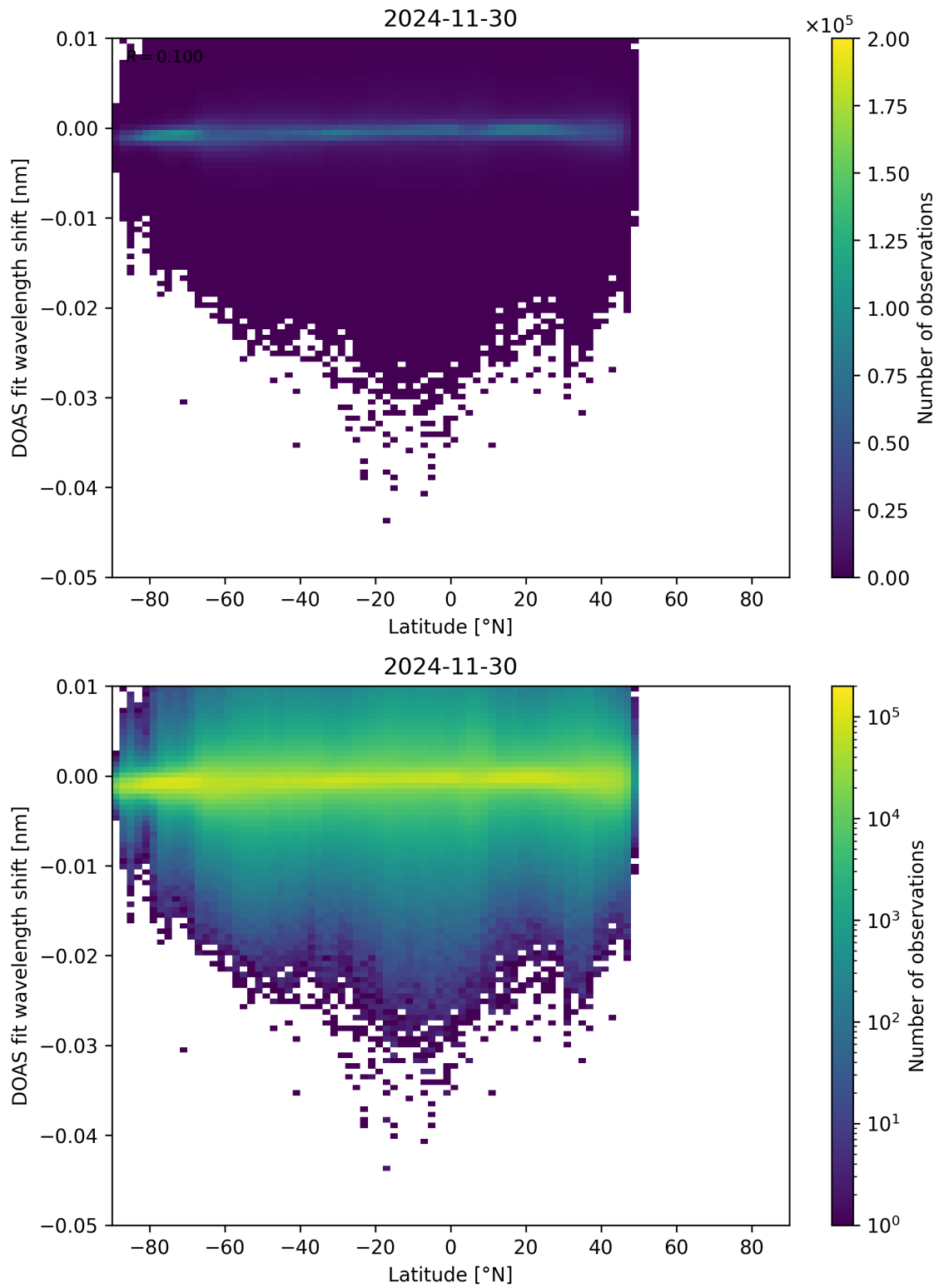
Figure 153: Scatter density plot of “Latitude” against “DOAS fit wavelength shift” for 2024-11-30 to 2024-12-01.
