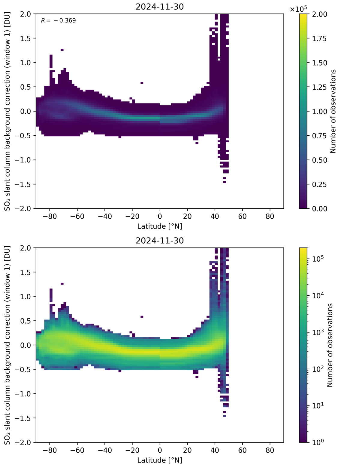
Figure 150: Scatter density plot of “Latitude” against “SO 2 slant column background correction (window 1)” for 2024-11-30 to 2024-12-01.
