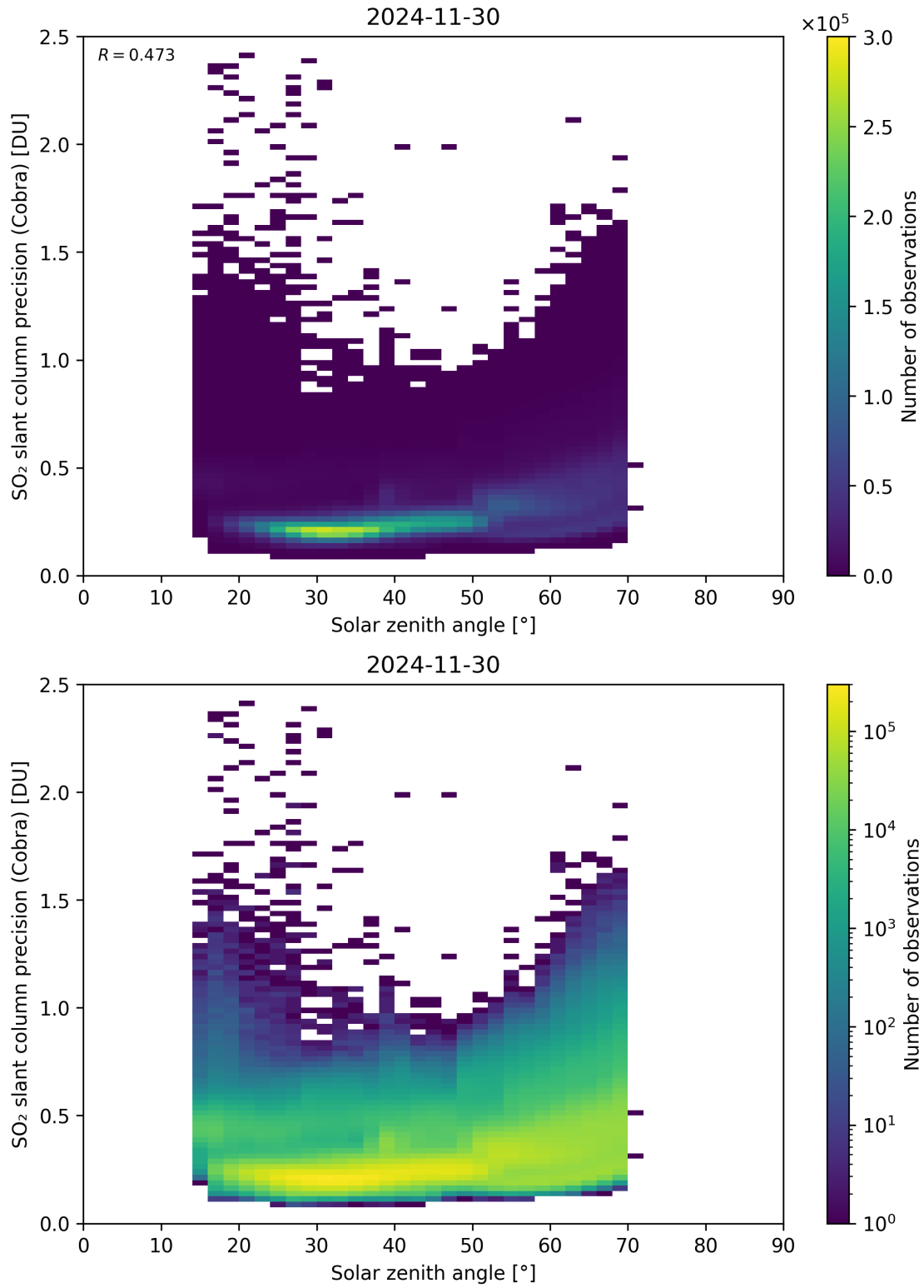
Figure 180: Scatter density plot of “Solar zenith angle” against “SO 2 slant column precision (Cobra)” for 2024-11-30 to 2024-12-01.
