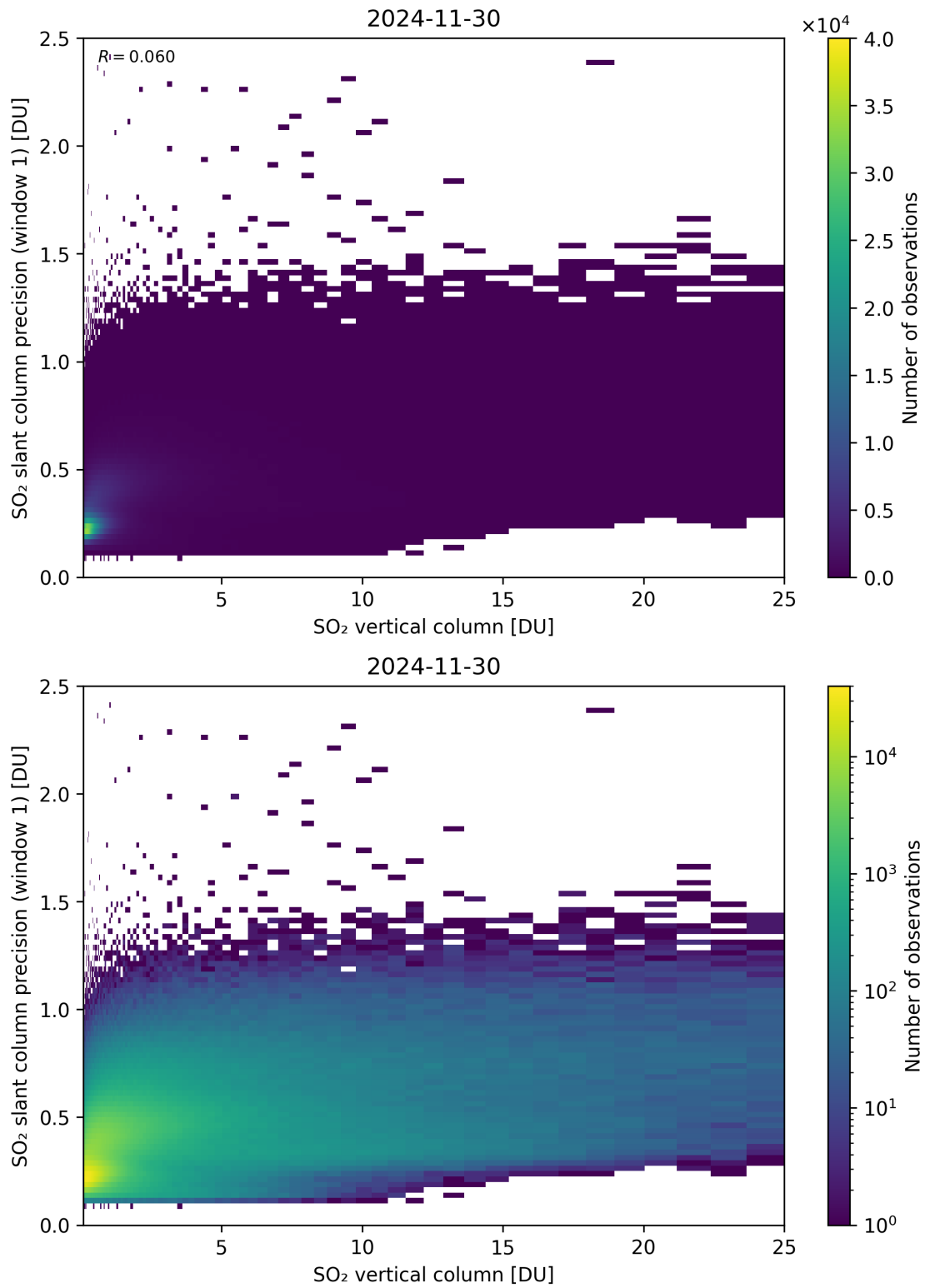
Figure 355: Scatter density plot of “SO 2 vertical column” against “SO 2 slant column precision (window 1)” for 2024-11-30 to 2024-12-01.
