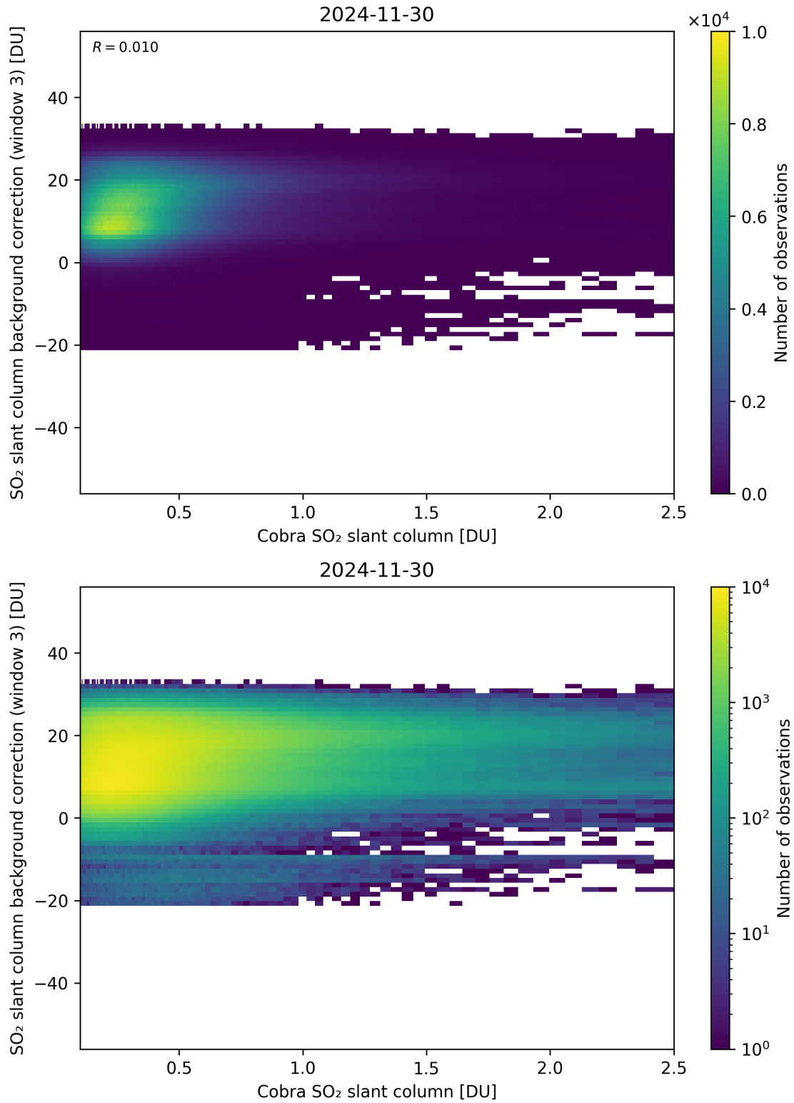
Figure 195: Scatter density plot of “Cobra SO 2 slant column” against “SO 2 slant column background correction (window 3)” for 2024-11-30 to 2024-12-01.
