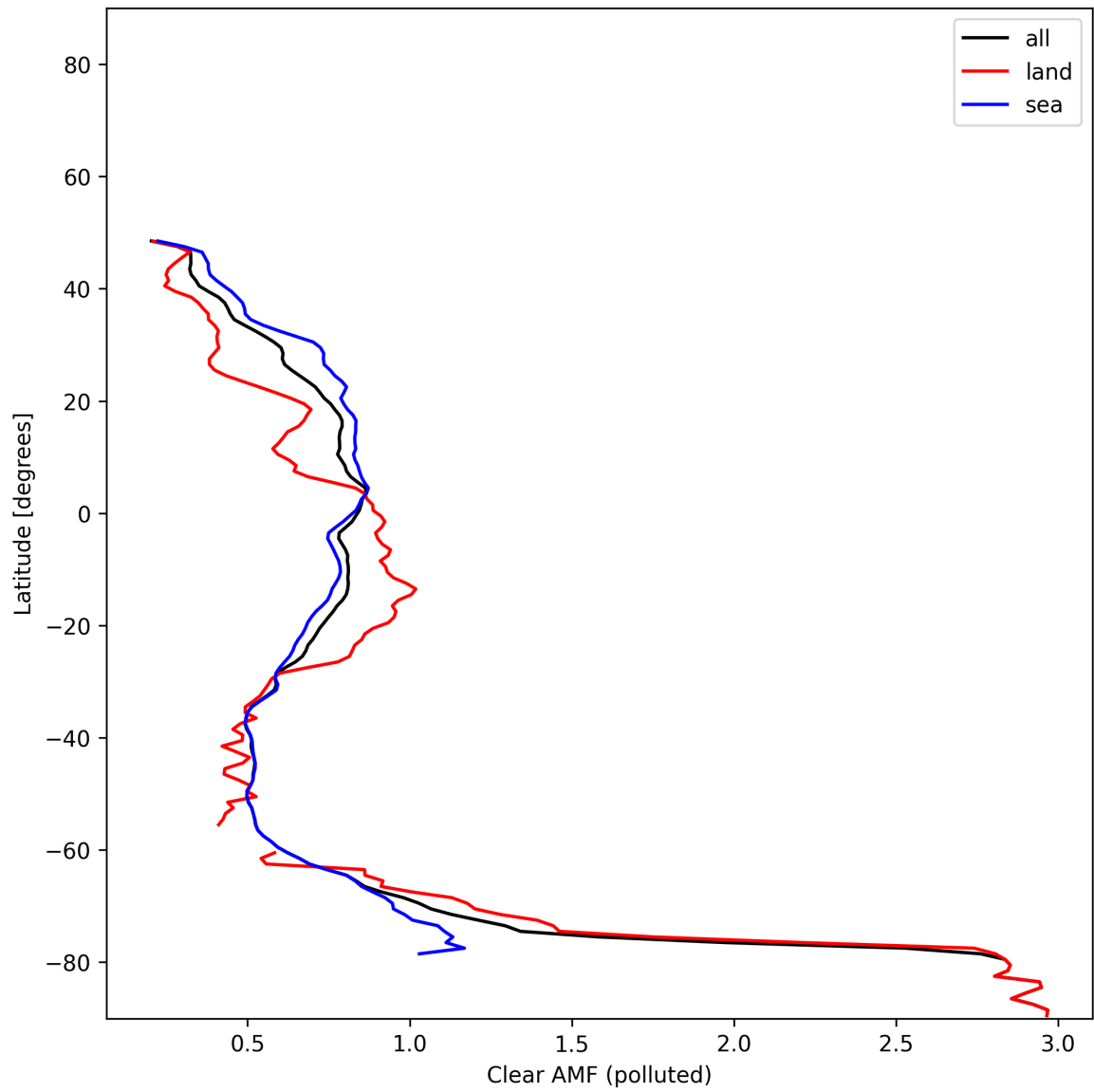
Figure 55: Zonal average of “Clear AMF (polluted)” for 2024-11-30 to 2024-12-01.
