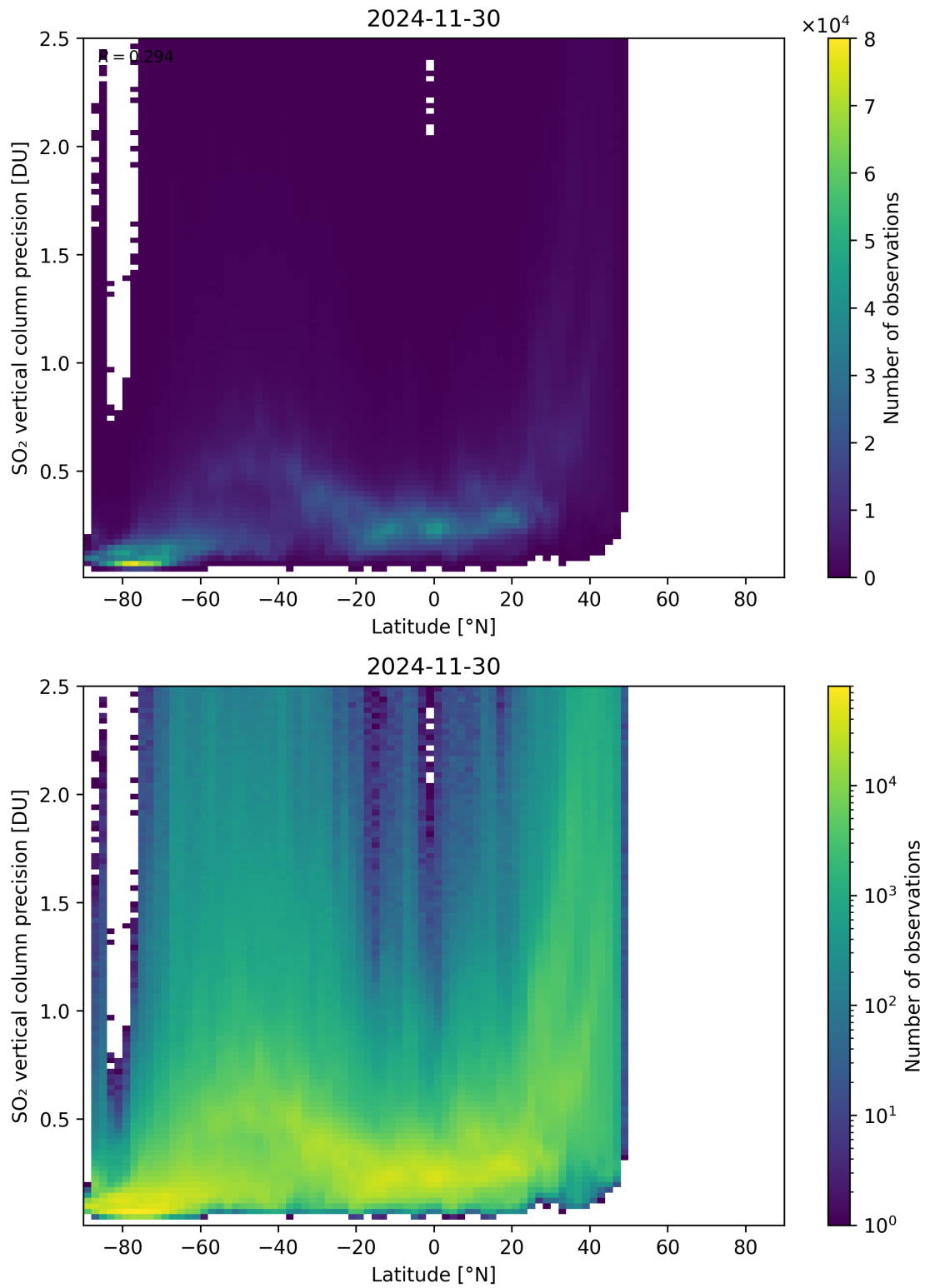
Figure 170: Scatter density plot of “Latitude” against “SO 2 vertical column precision” for 2024-11-30 to 2024-12-01.
