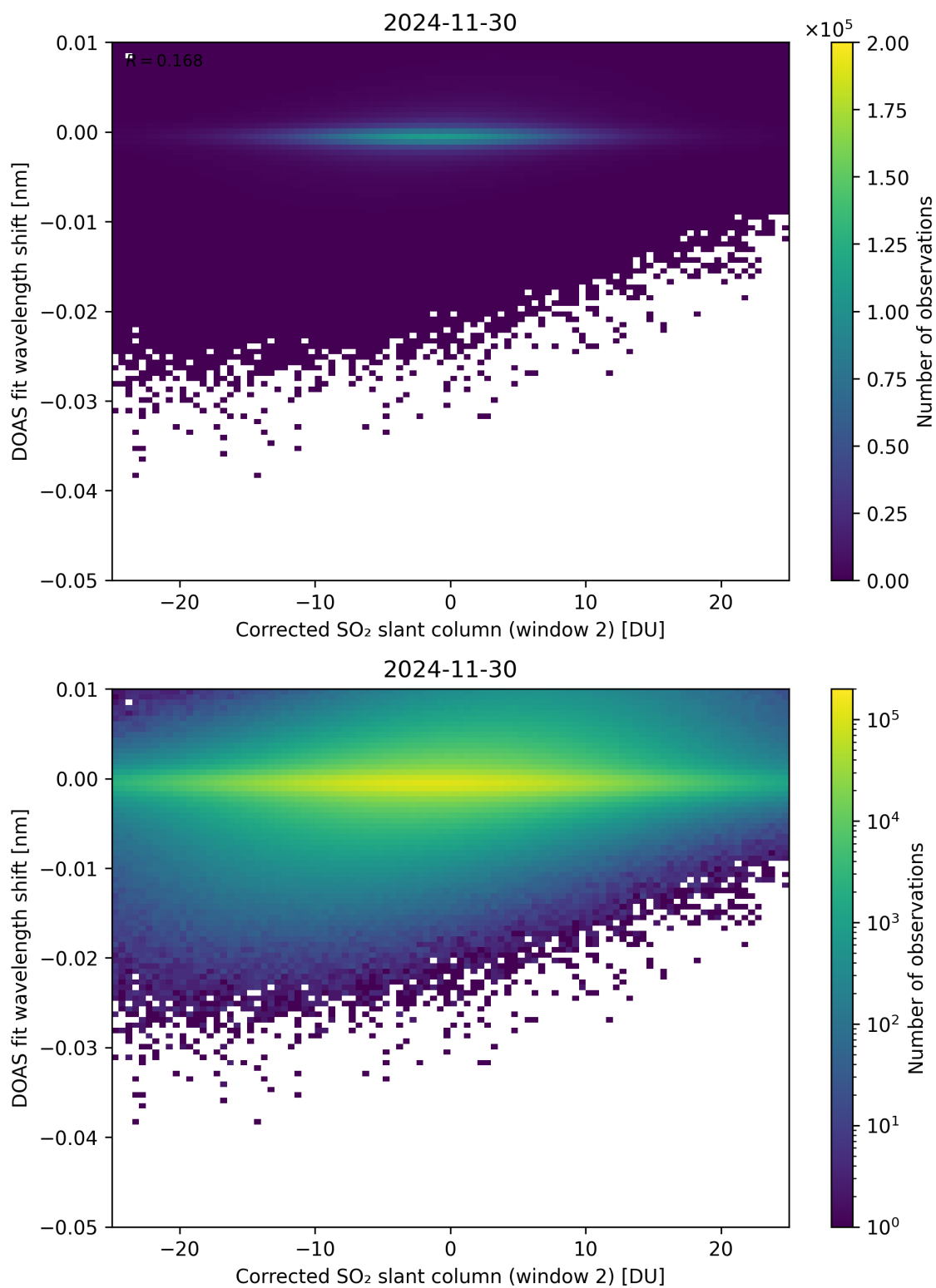
Figure 246: Scatter density plot of “Corrected SO 2 slant column (window 2)” against “DOAS fit wavelength shift” for 2024-11-30 to 2024-12-01.
