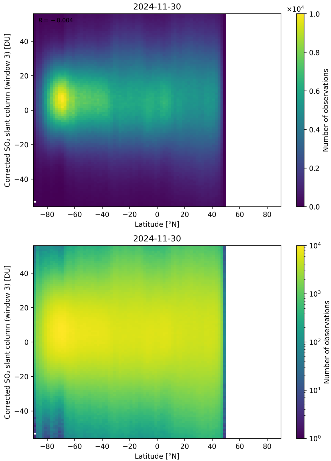
Figure 161: Scatter density plot of “Latitude” against “Corrected SO 2 slant column (window 3)” for 2024-11-30 to 2024-12-01.
