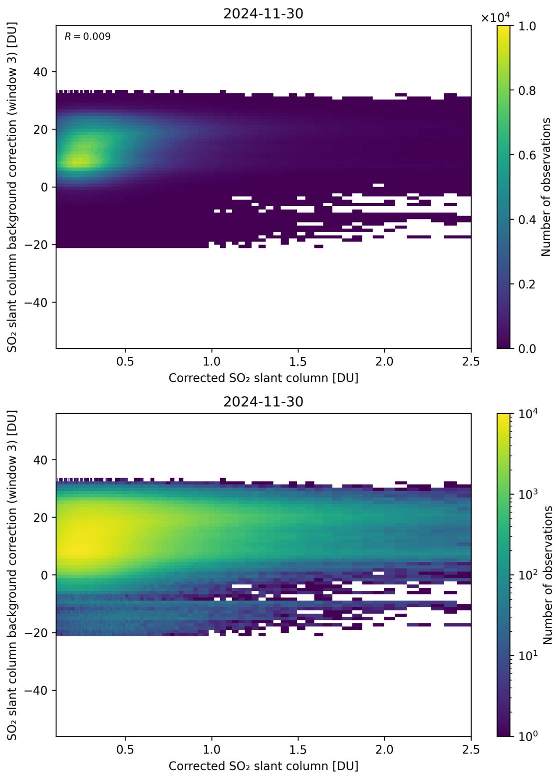
Figure 228: Scatter density plot of “Corrected SO 2 slant column” against “SO 2 slant column background correction (window 3)” for 2024-11-30 to 2024-12-01.
