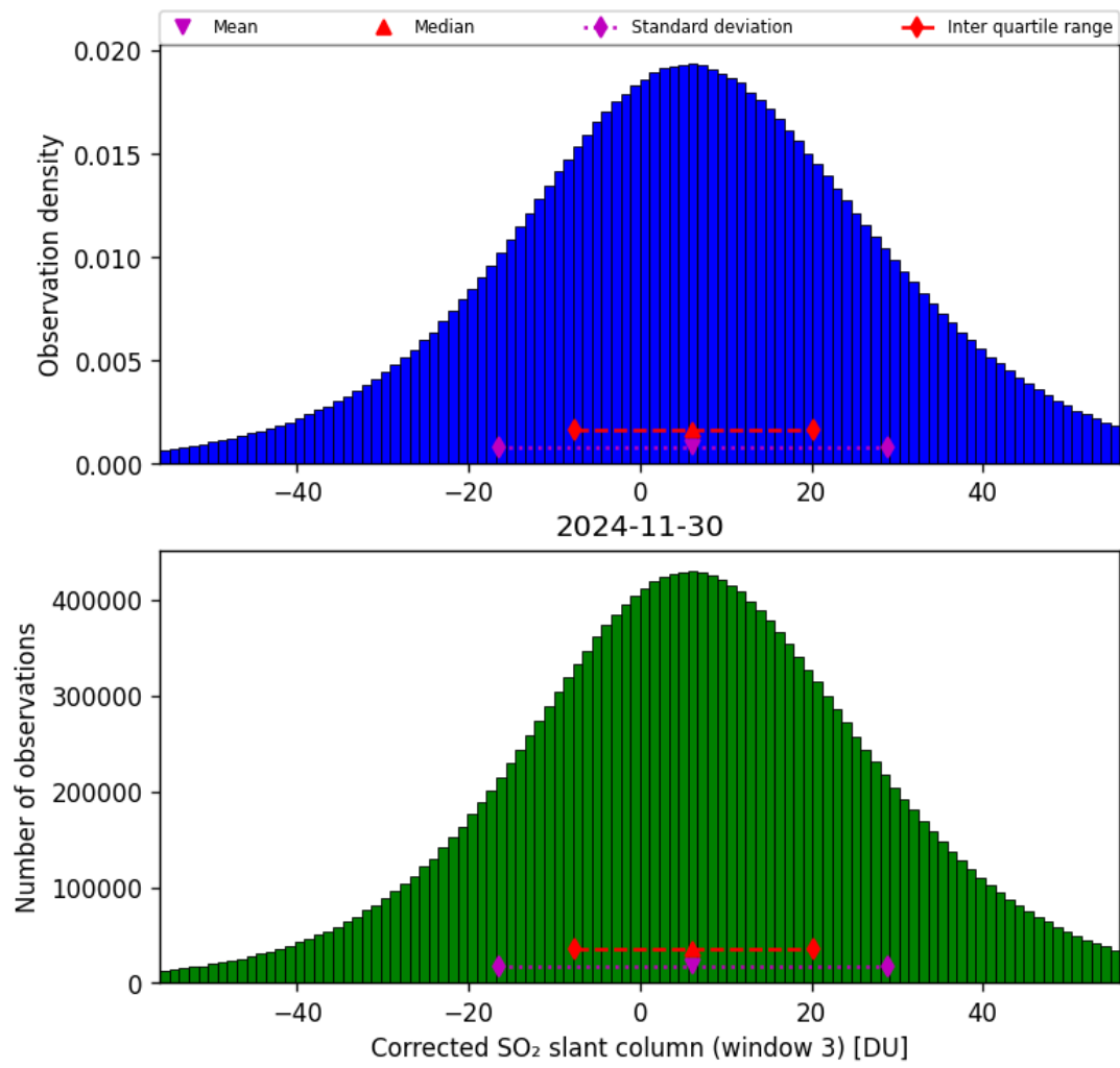
Figure 73: Histogram of “Corrected SO 2 slant column (window 3)” for 2024-11-30 to 2024-12-01
