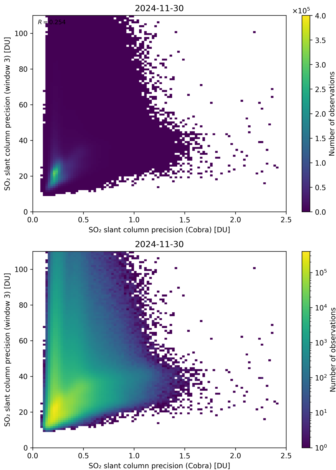
Figure 212: Scatter density plot of “SO 2 slant column precision (Cobra)” against “SO 2 slant column precision (window 3)” for 2024-11-30 to 2024-12-01.
