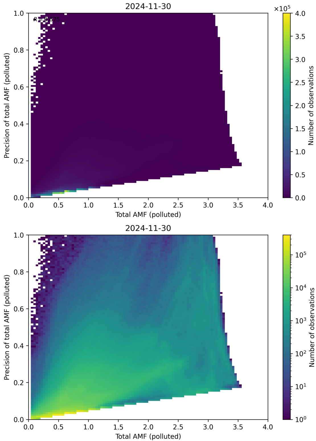
Figure 322: Scatter density plot of “Total AMF (polluted)” against “Precision of total AMF (polluted)” for 2024-11-30 to 2024-12-01.
