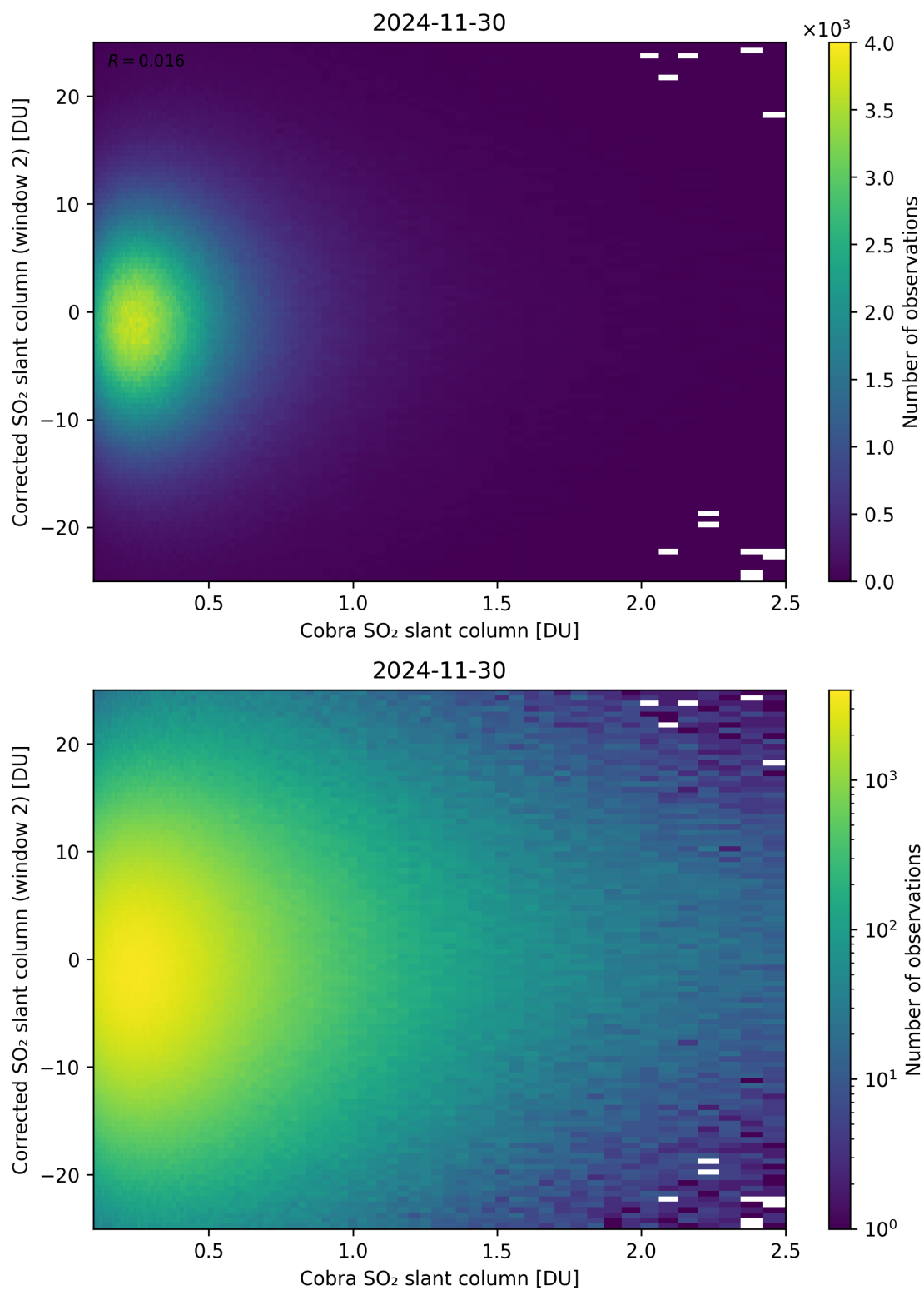
Figure 217: Scatter density plot of “Cobra SO 2 slant column” against “Corrected SO 2 slant column (window 2)” for 2024-11-30 to 2024-12-01.
