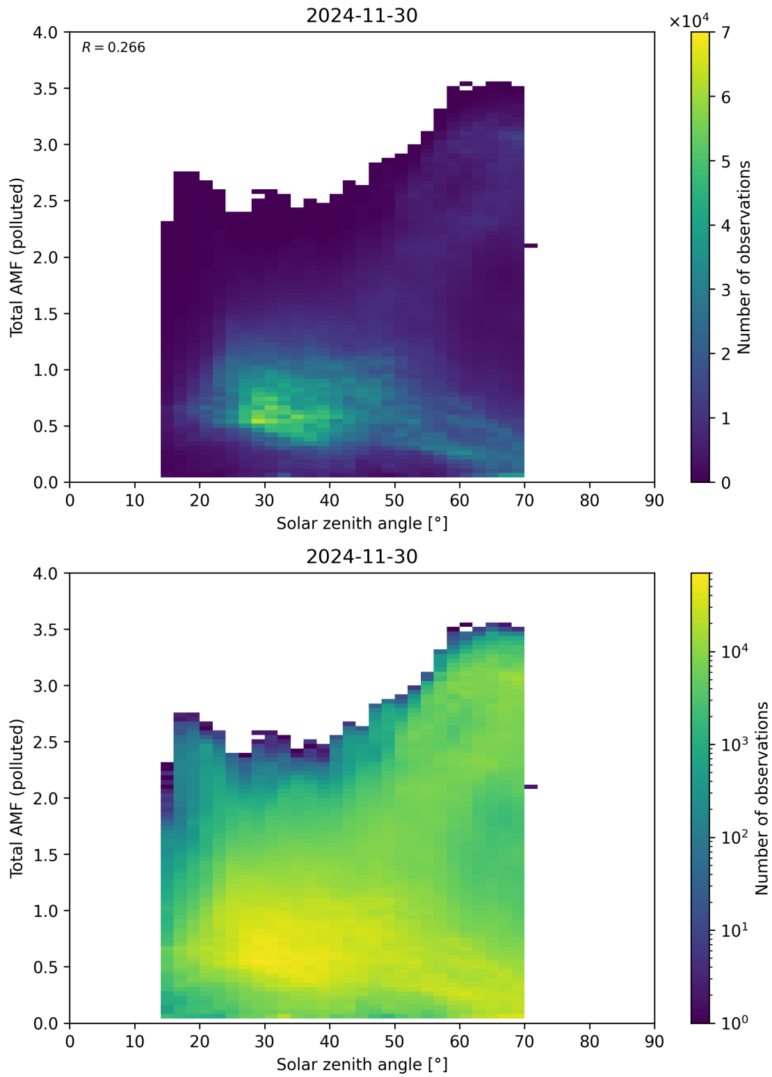
Figure 189: Scatter density plot of “Solar zenith angle” against “Total AMF (polluted)” for 2024-11-30 to 2024-12-01.
