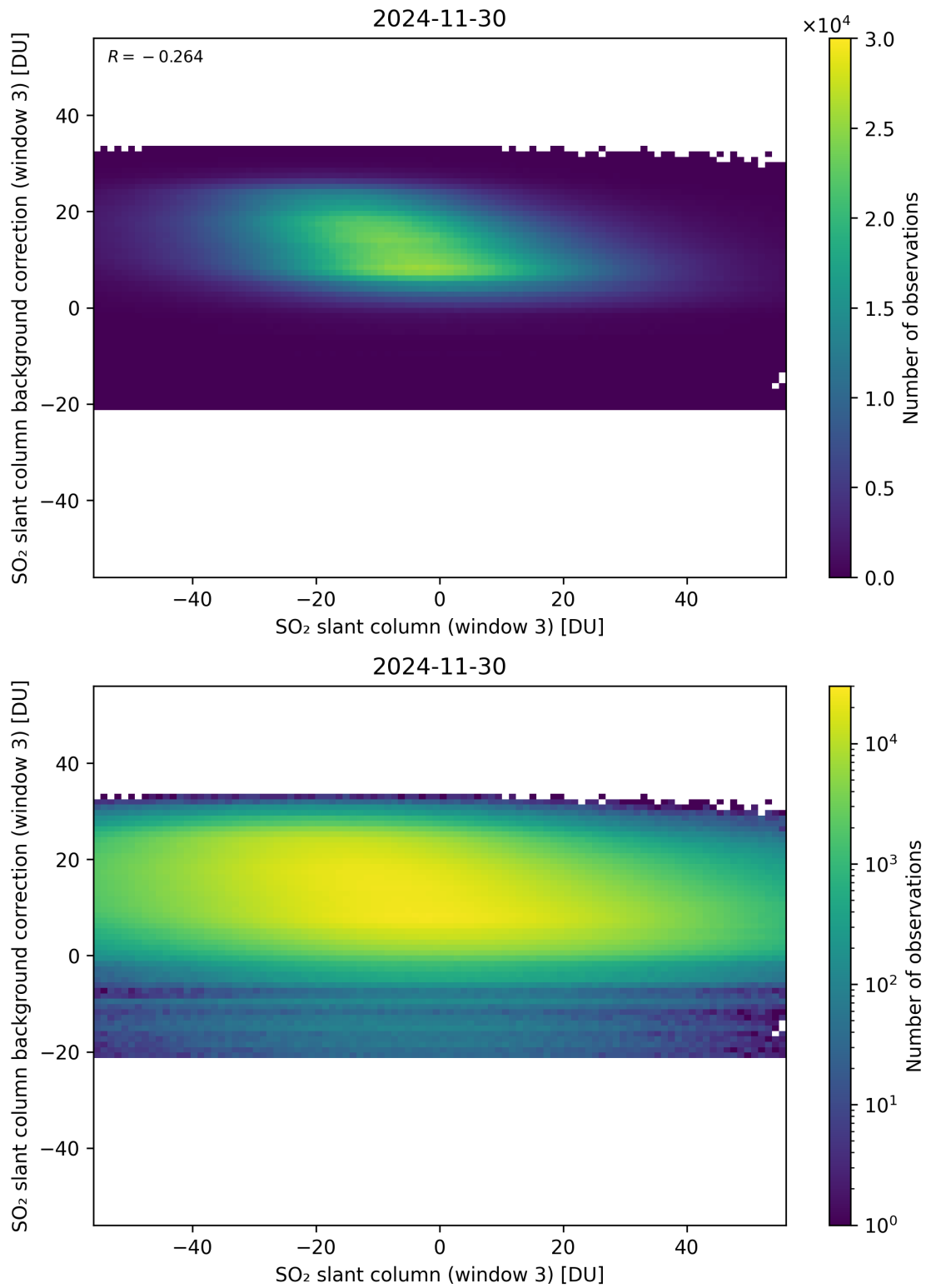
Figure 303: Scatter density plot of “SO 2 slant column (window 3)” against “SO 2 slant column background correction (window 3)” for 2024-11-30 to 2024-12-01.
