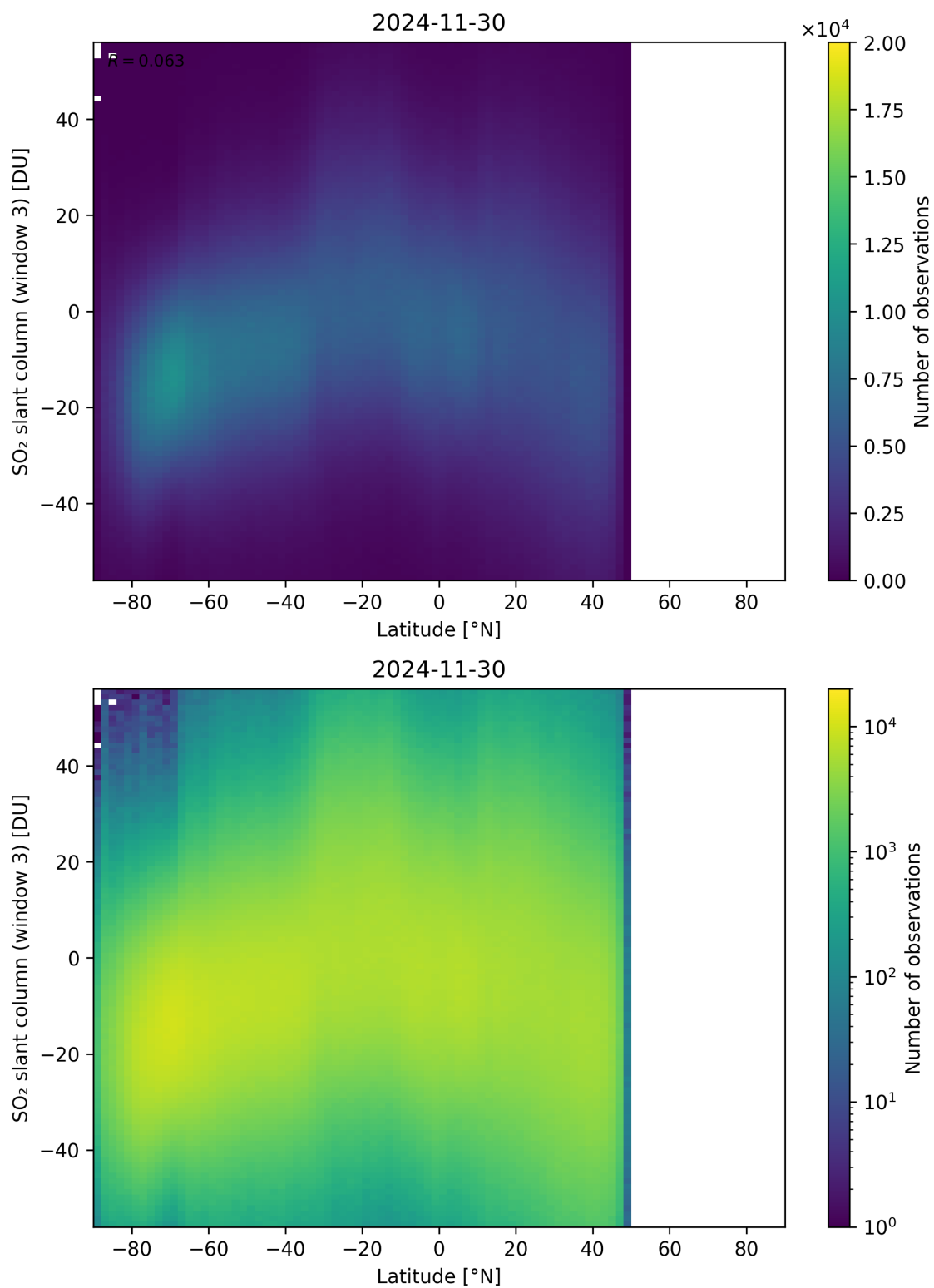
Figure 165: Scatter density plot of “Latitude” against “SO 2 slant column (window 3)” for 2024-11-30 to 2024-12-01.
