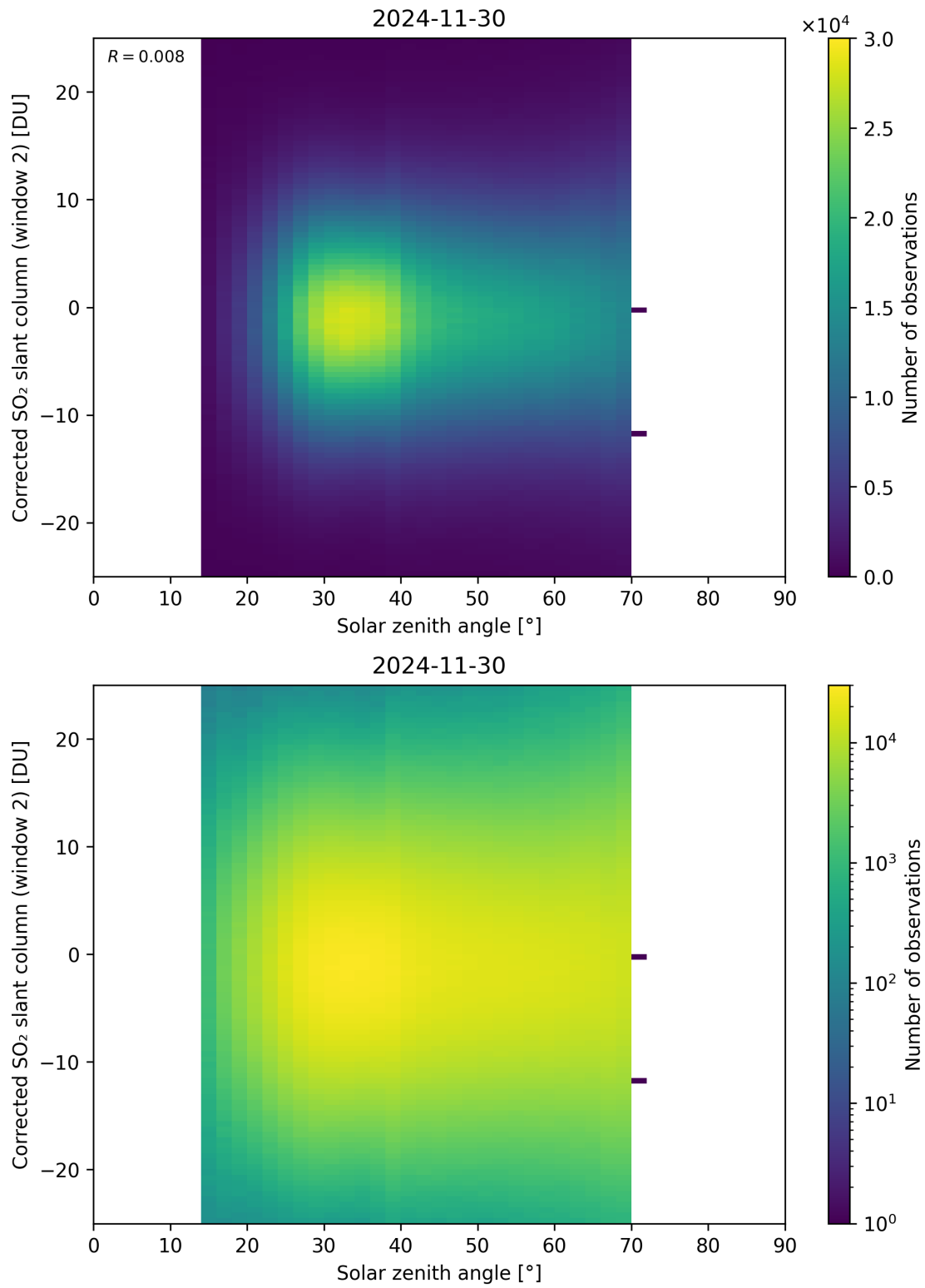
Figure 182: Scatter density plot of “Solar zenith angle” against “Corrected SO 2 slant column (window 2)” for 2024-11-30 to 2024-12-01.
