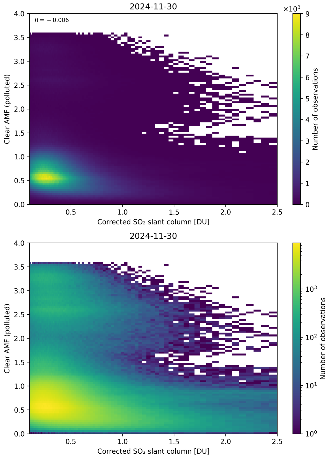
Figure 232: Scatter density plot of “Corrected SO 2 slant column” against “Clear AMF (polluted)” for 2024-11-30 to 2024-12-01.
