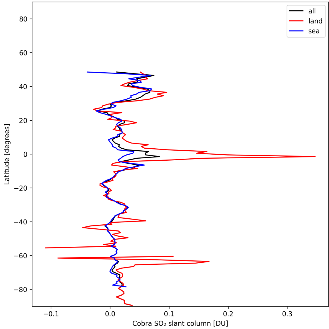
Figure 35: Zonal average of “Cobra SO 2 slant column” for 2024-11-30 to 2024-12-01.
