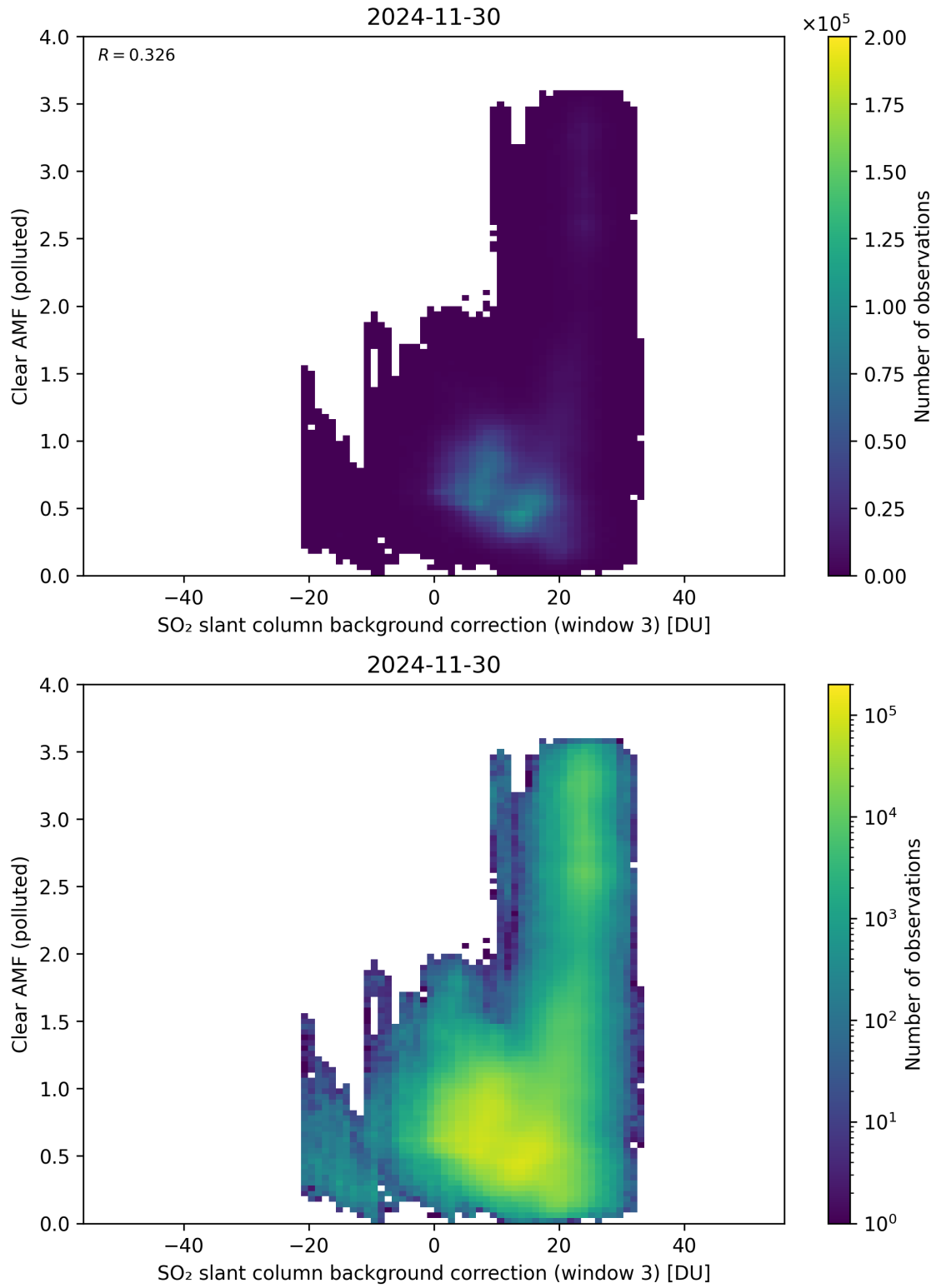
Figure 135: Scatter density plot of “SO 2 slant column background correction (window 3)” against “Clear AMF (polluted)” for 2024-11-30 to 2024-12-01.
