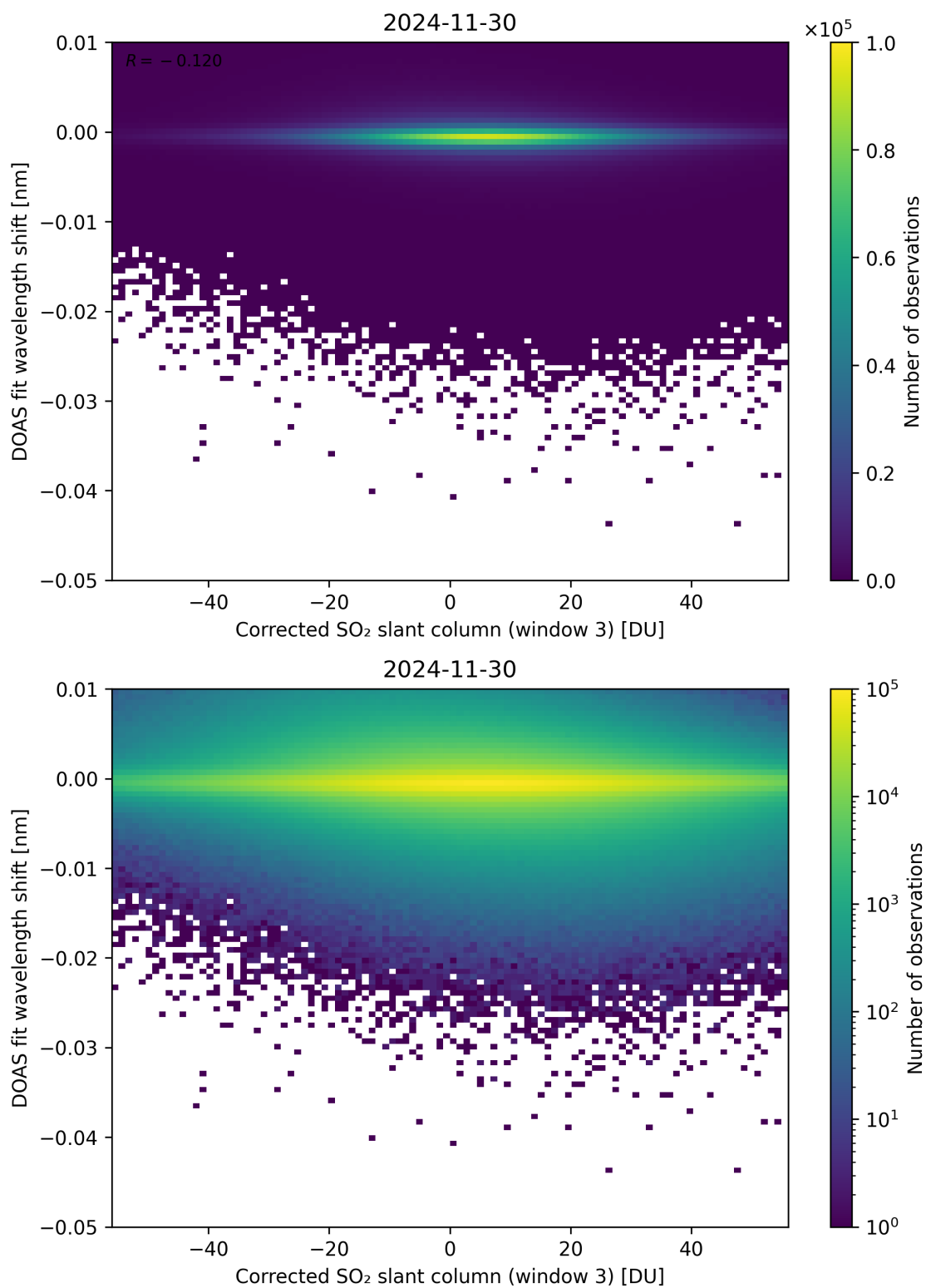
Figure 256: Scatter density plot of “Corrected SO 2 slant column (window 3)” against “DOAS fit wavelength shift” for 2024-11-30 to 2024-12-01.
