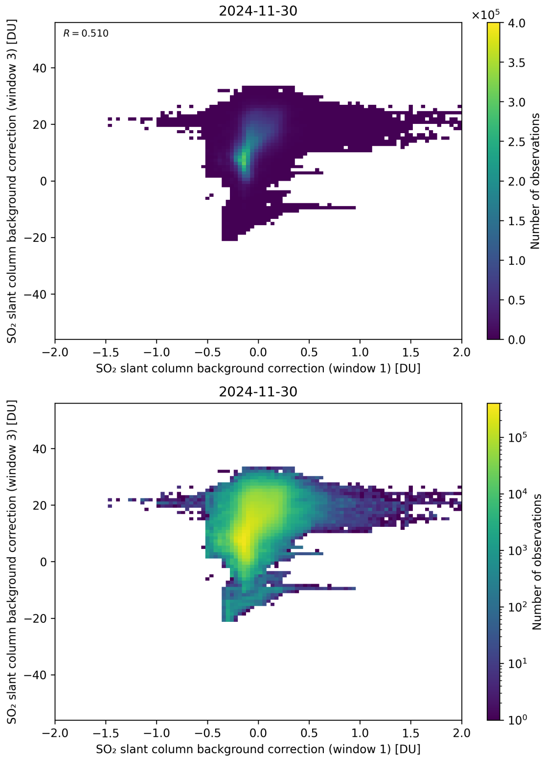
Figure 110: Scatter density plot of “SO 2 slant column background correction (window 1)” against “SO 2 slant column background correction (window 3)” for 2024-11-30 to 2024-12-01.
