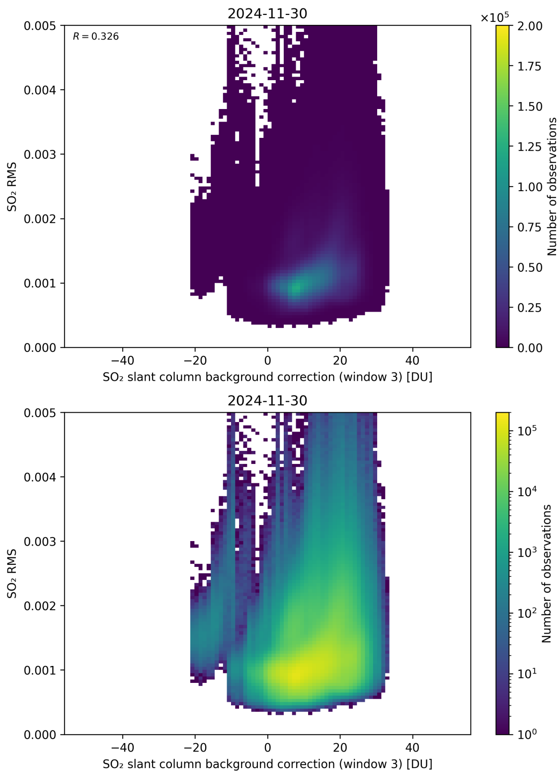
Figure 134: Scatter density plot of “SO 2 slant column background correction (window 3)” against “SO 2 RMS” for 2024-11-30 to 2024-12-01.
