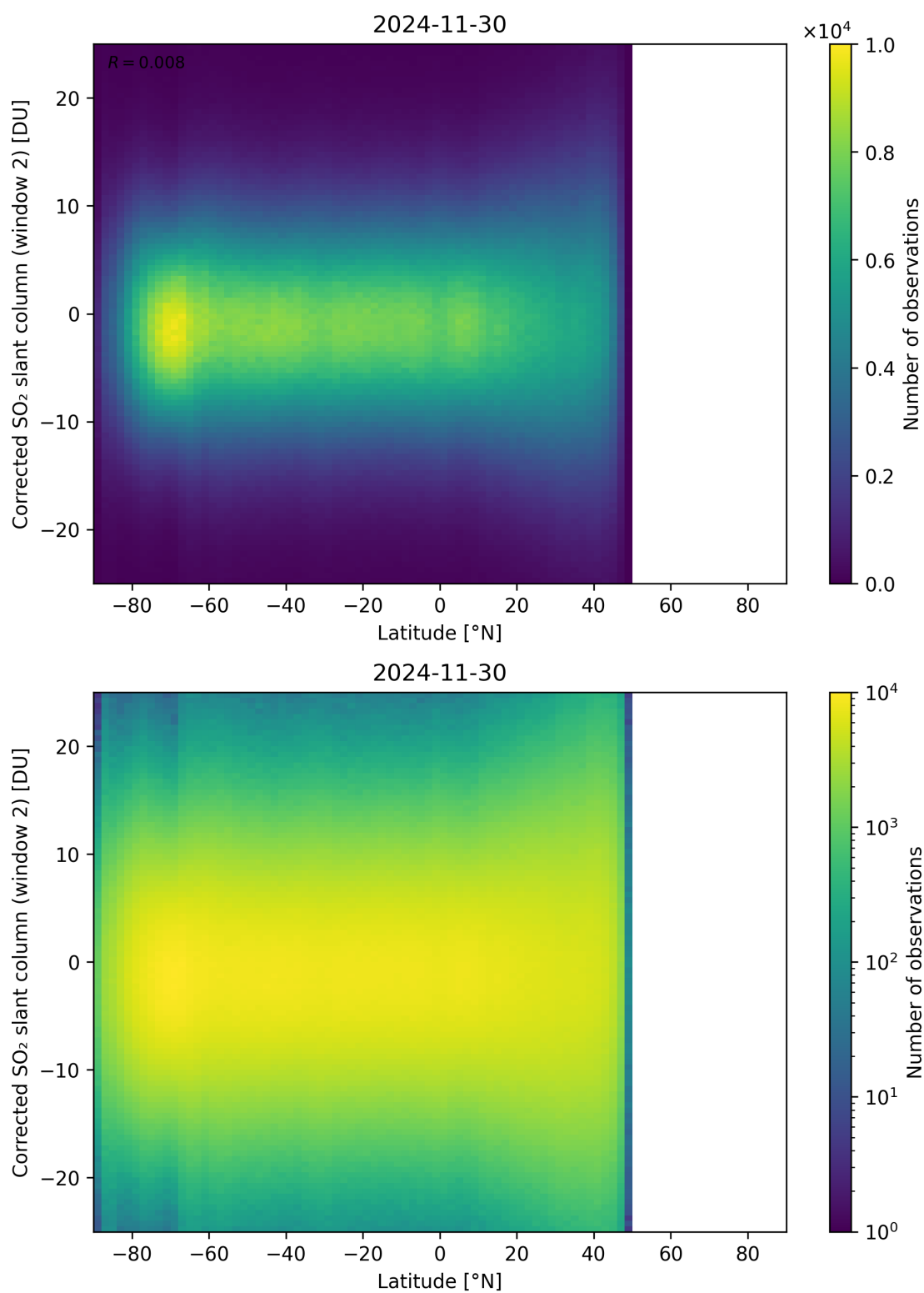
Figure 160: Scatter density plot of “Latitude” against “Corrected SO 2 slant column (window 2)” for 2024-11-30 to 2024-12-01.
