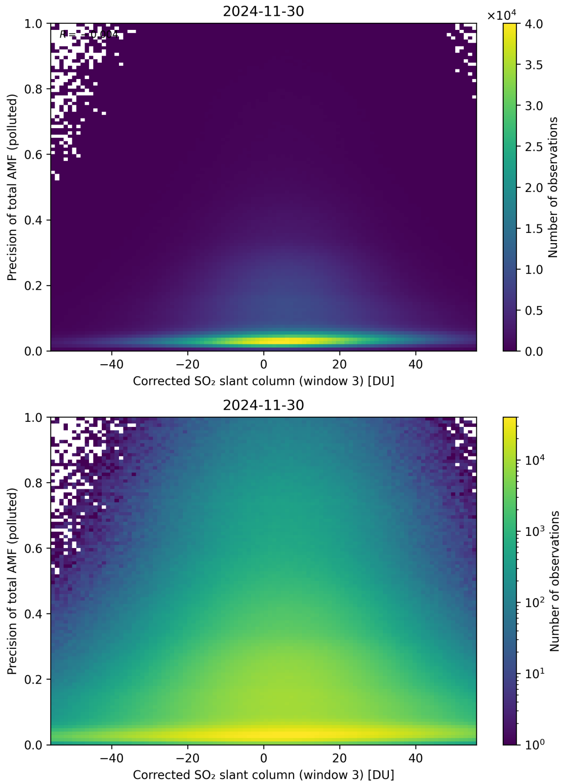
Figure 261: Scatter density plot of “Corrected SO 2 slant column (window 3)” against “Precision of total AMF (polluted)” for 2024-11-30 to 2024-12-01.
