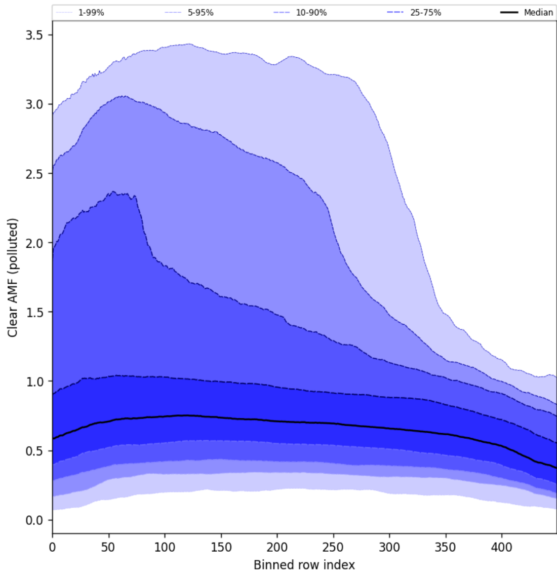
Figure 107: Along track statistics of “Clear AMF (polluted)” for 2024-11-30 to 2024-12-01
