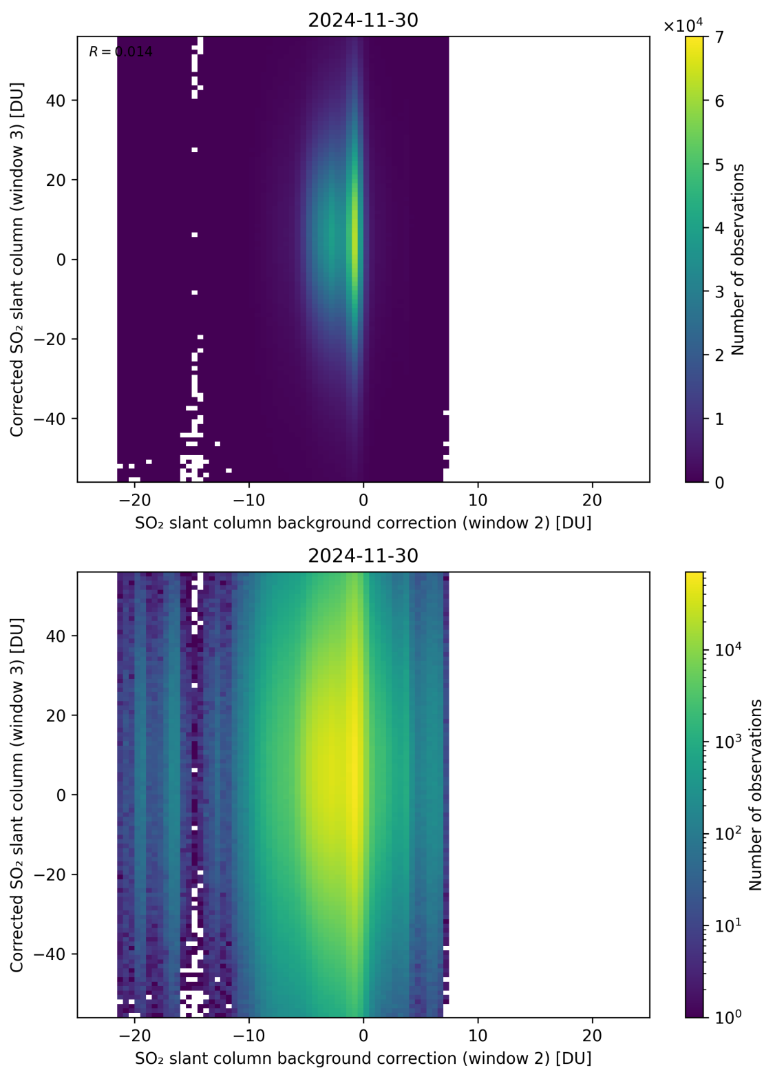
Figure 127: Scatter density plot of “SO 2 slant column background correction (window 2)” against “Corrected SO 2 slant column (window 3)” for 2024-11-30 to 2024-12-01.
