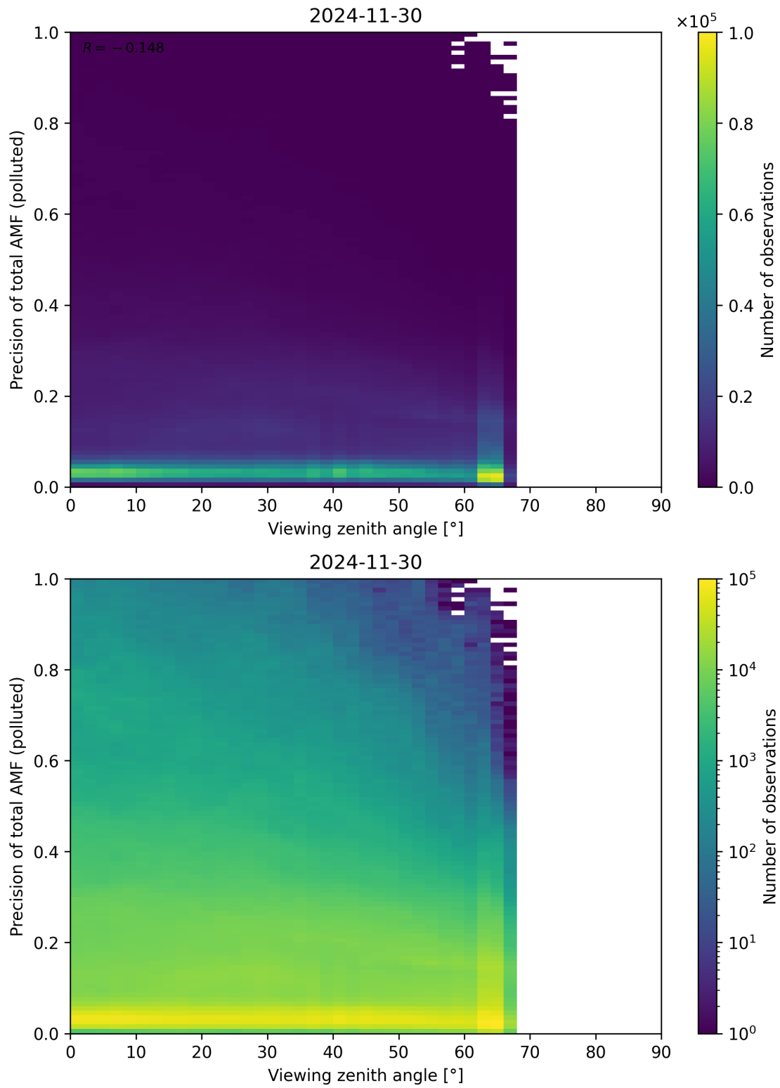
Figure 382: Scatter density plot of “Viewing zenith angle” against “Precision of total AMF (polluted)” for 2024-11-30 to 2024-12-01.
