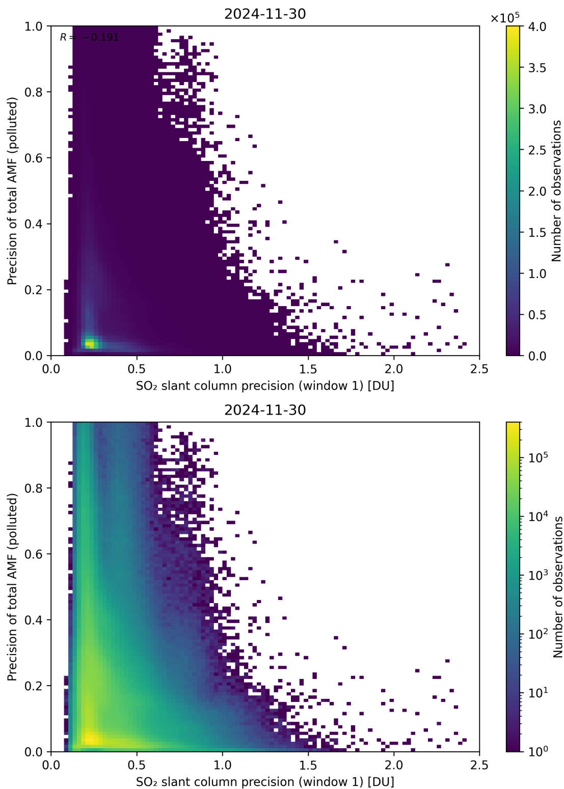
Figure 281: Scatter density plot of “SO 2 slant column precision (window 1)” against “Precision of total AMF (polluted)” for 2024-11-30 to 2024-12-01.
