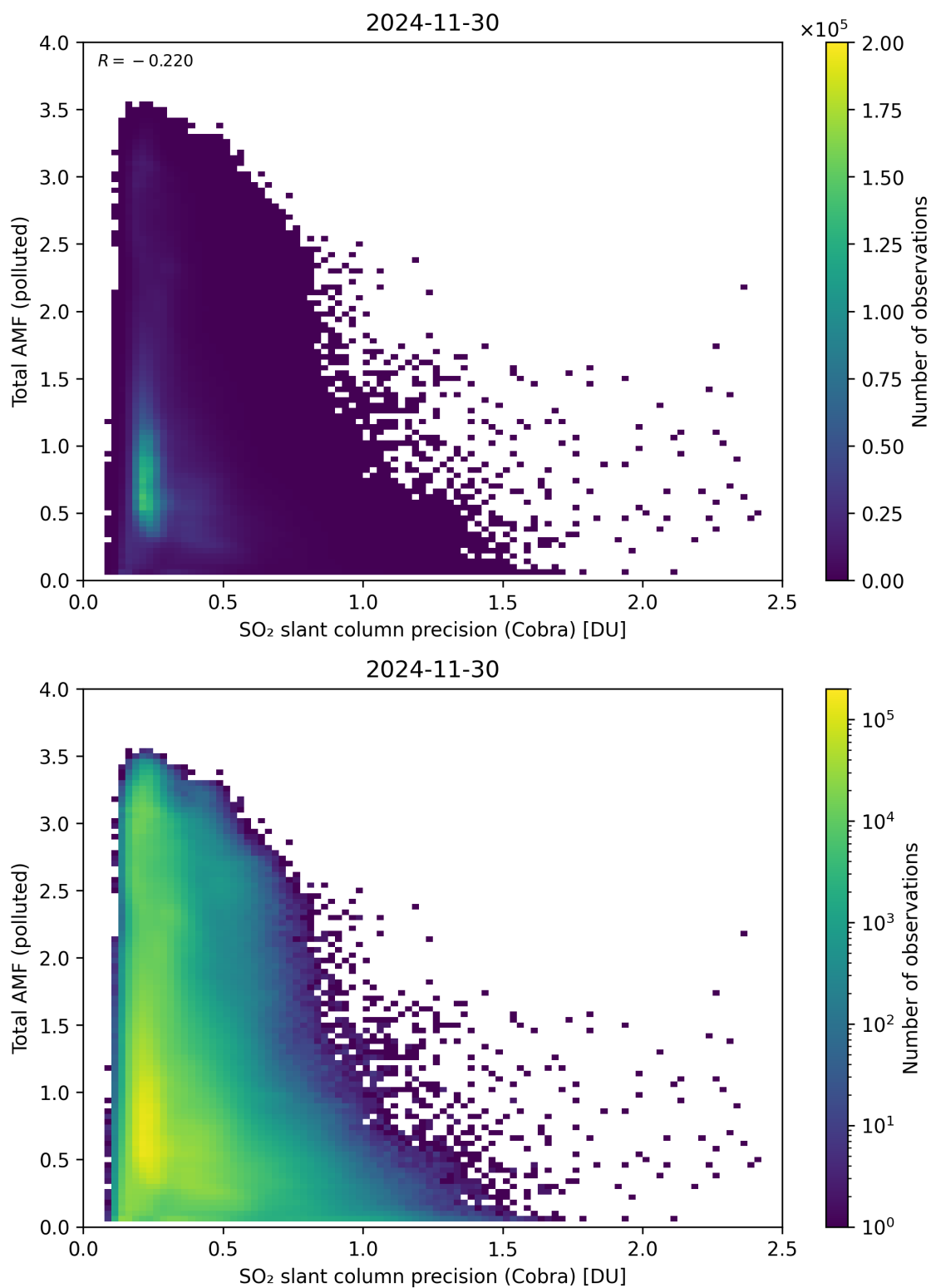
Figure 213: Scatter density plot of “SO 2 slant column precision (Cobra)” against “Total AMF (polluted)” for 2024-11-30 to 2024-12-01.
