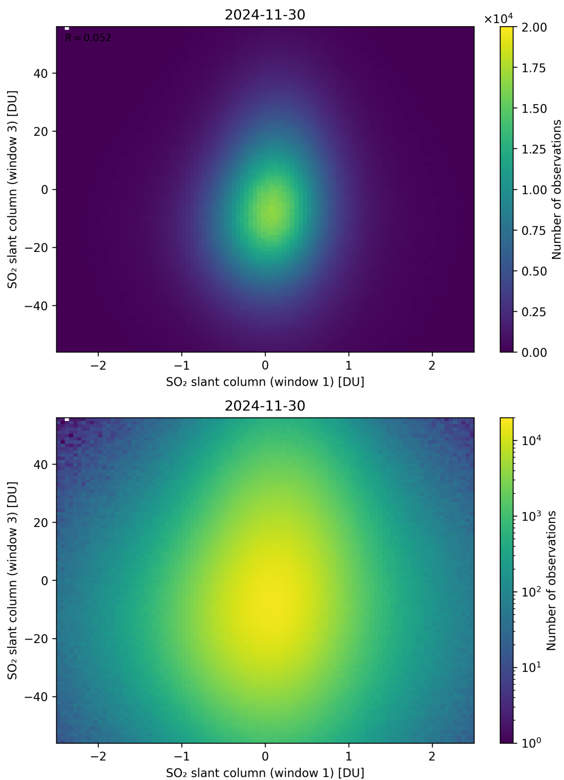
Figure 287: Scatter density plot of “SO 2 slant column (window 1)” against “SO 2 slant column (window 3)” for 2024-11-30 to 2024-12-01.
