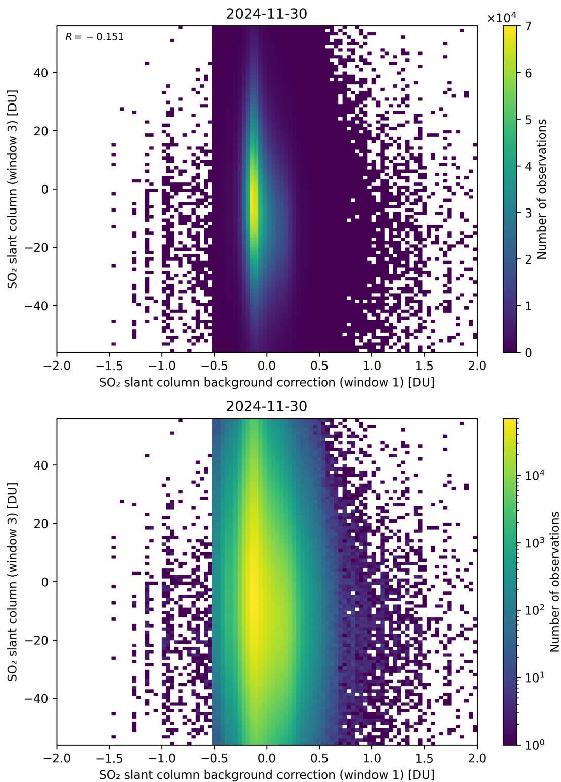
Figure 118: Scatter density plot of “SO 2 slant column background correction (window 1)” against “SO 2 slant column (window 3)” for 2024-11-30 to 2024-12-01.
