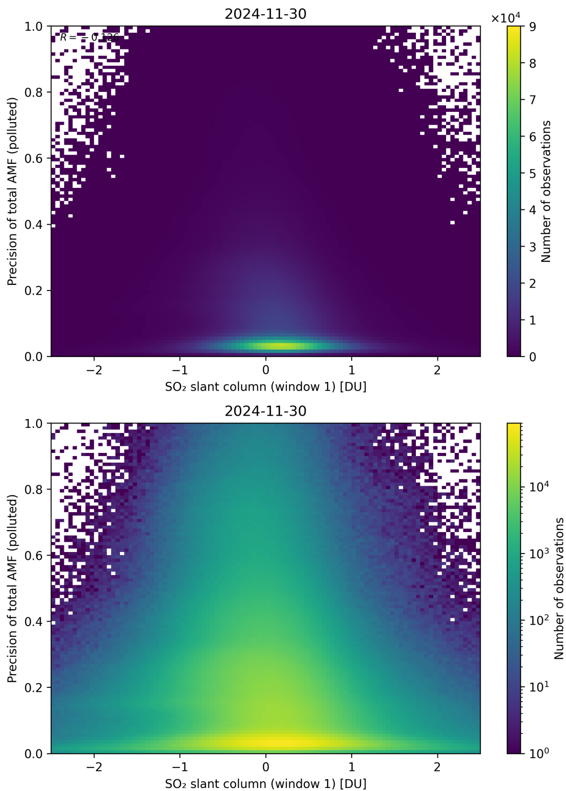
Figure 290: Scatter density plot of “SO 2 slant column (window 1)” against “Precision of total AMF (polluted)” for 2024-11-30 to 2024-12-01.
