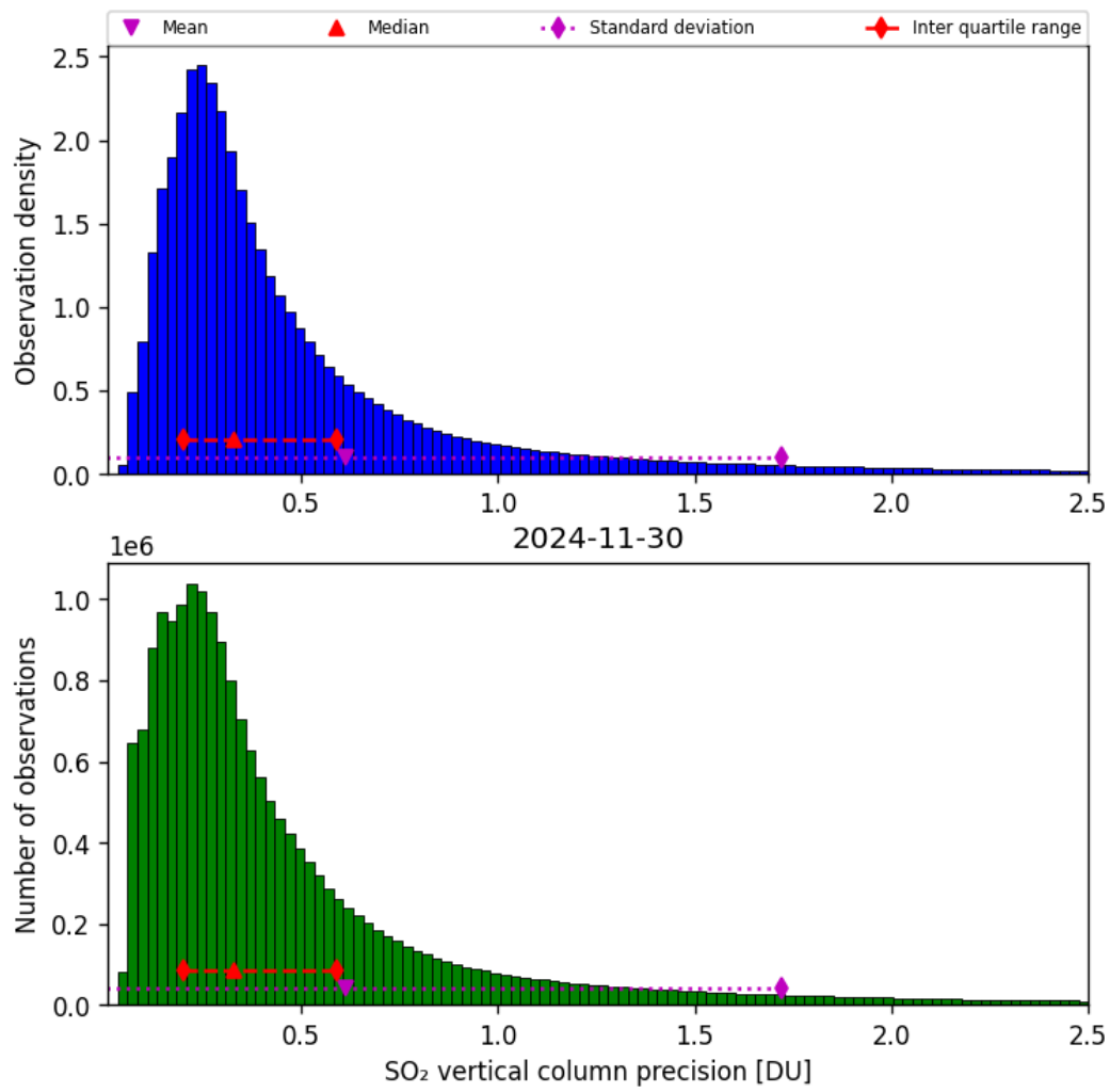
Figure 59: Histogram of “SO 2 vertical column precision” for 2024-11-30 to 2024-12-01
