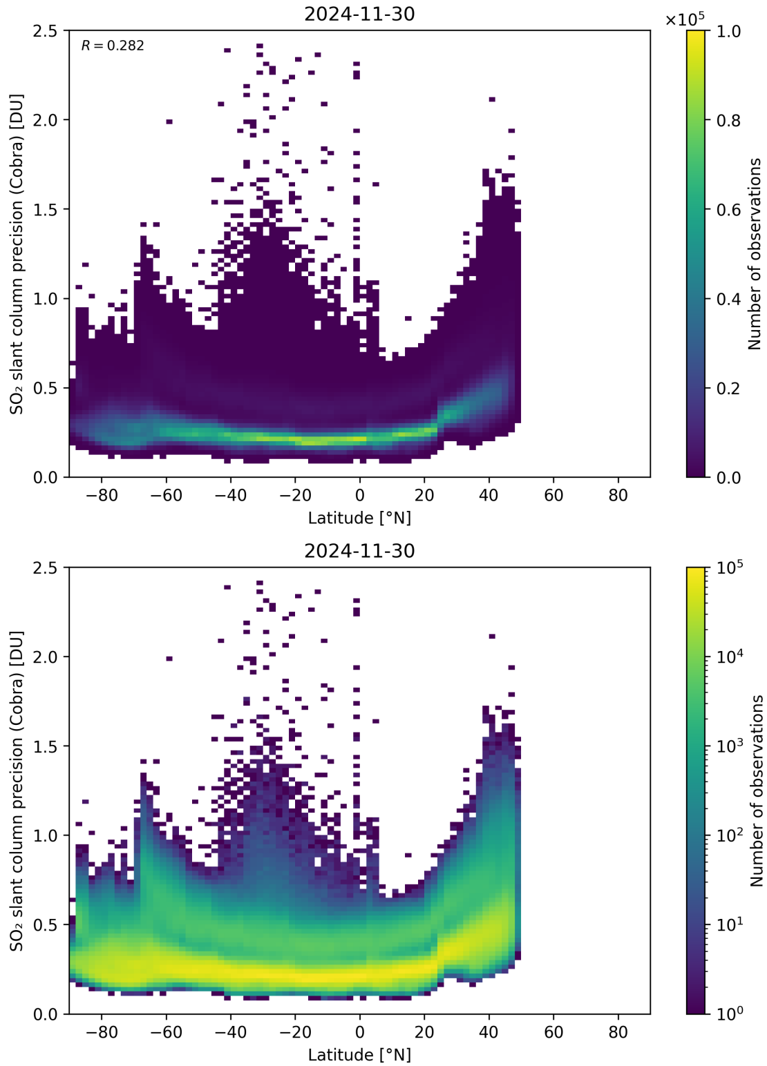
Figure 158: Scatter density plot of “Latitude” against “SO 2 slant column precision (Cobra)” for 2024-11-30 to 2024-12-01.
