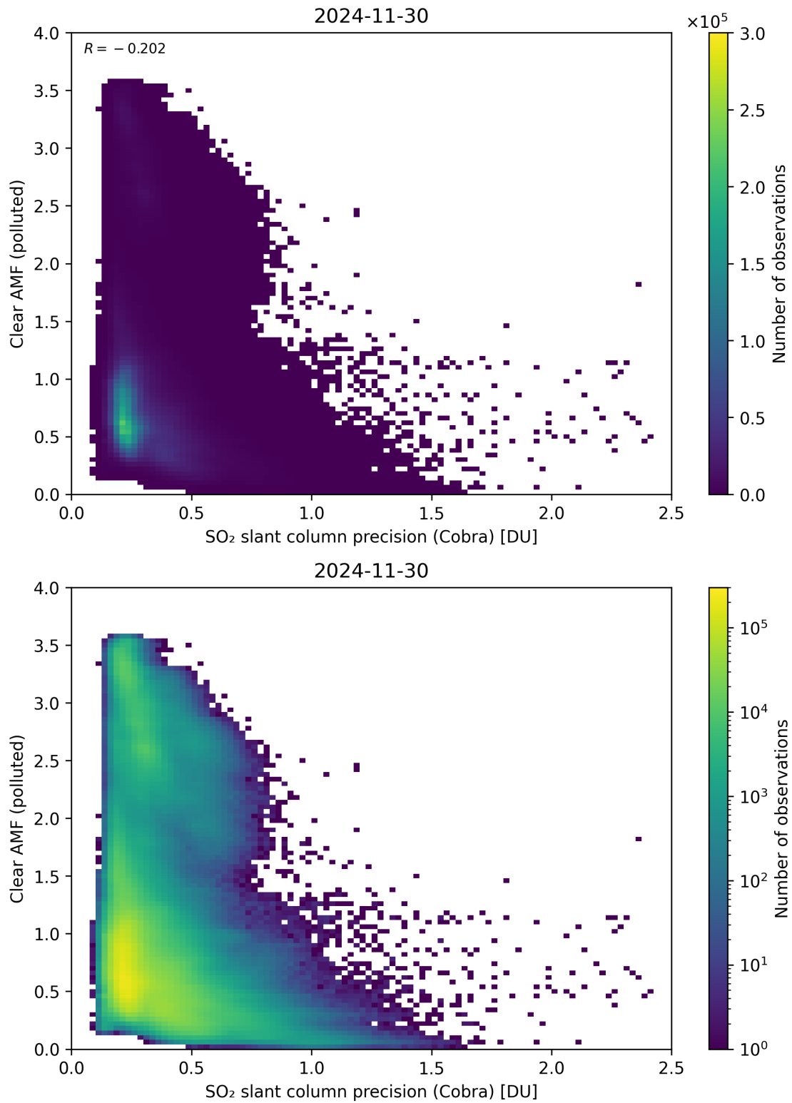
Figure 205: Scatter density plot of “SO 2 slant column precision (Cobra)” against “Clear AMF (polluted)” for 2024-11-30 to 2024-12-01.
