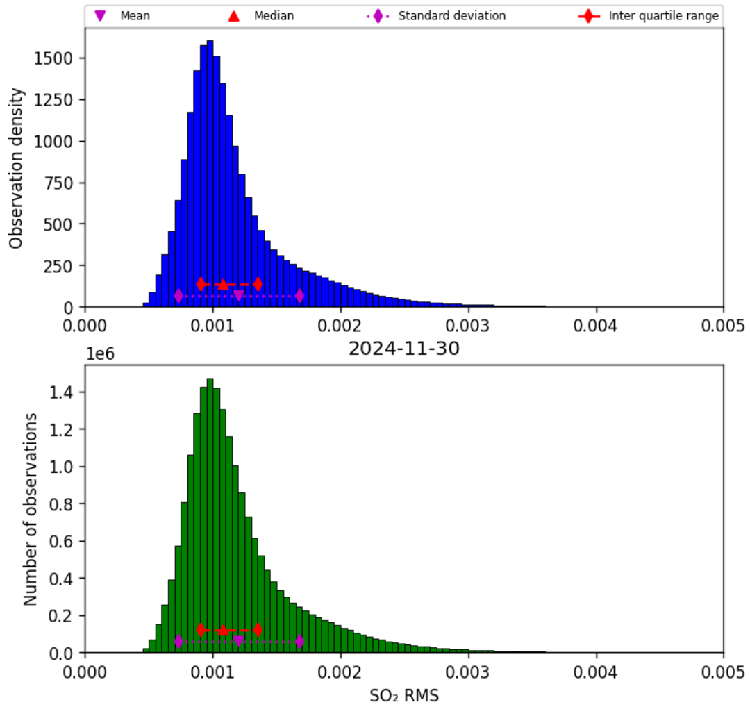
Figure 78: Histogram of “SO 2 RMS” for 2024-11-30 to 2024-12-01
