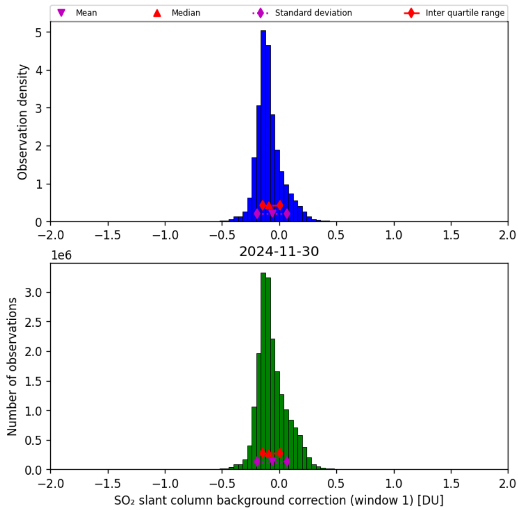
Figure 66: Histogram of “SO 2 slant column background correction (window 1)” for 2024-11-30 to 2024-12-01
