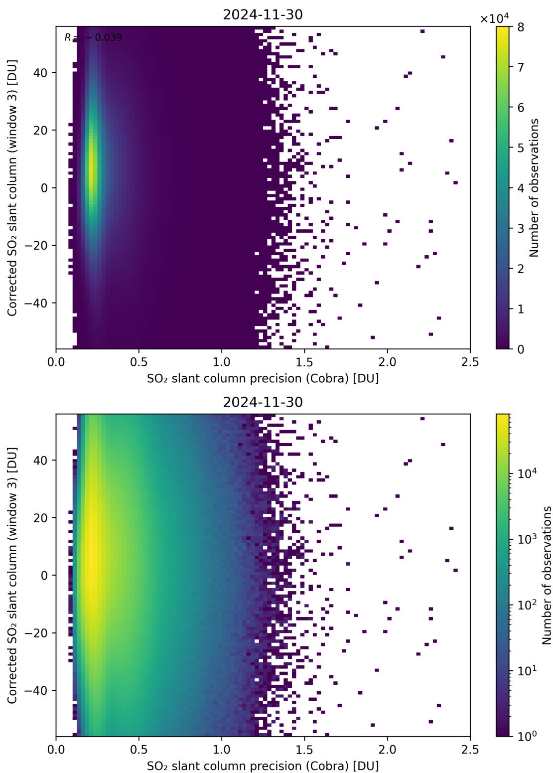
Figure 207: Scatter density plot of “SO 2 slant column precision (Cobra)” against “Corrected SO 2 slant column (window 3)” for 2024-11-30 to 2024-12-01.
