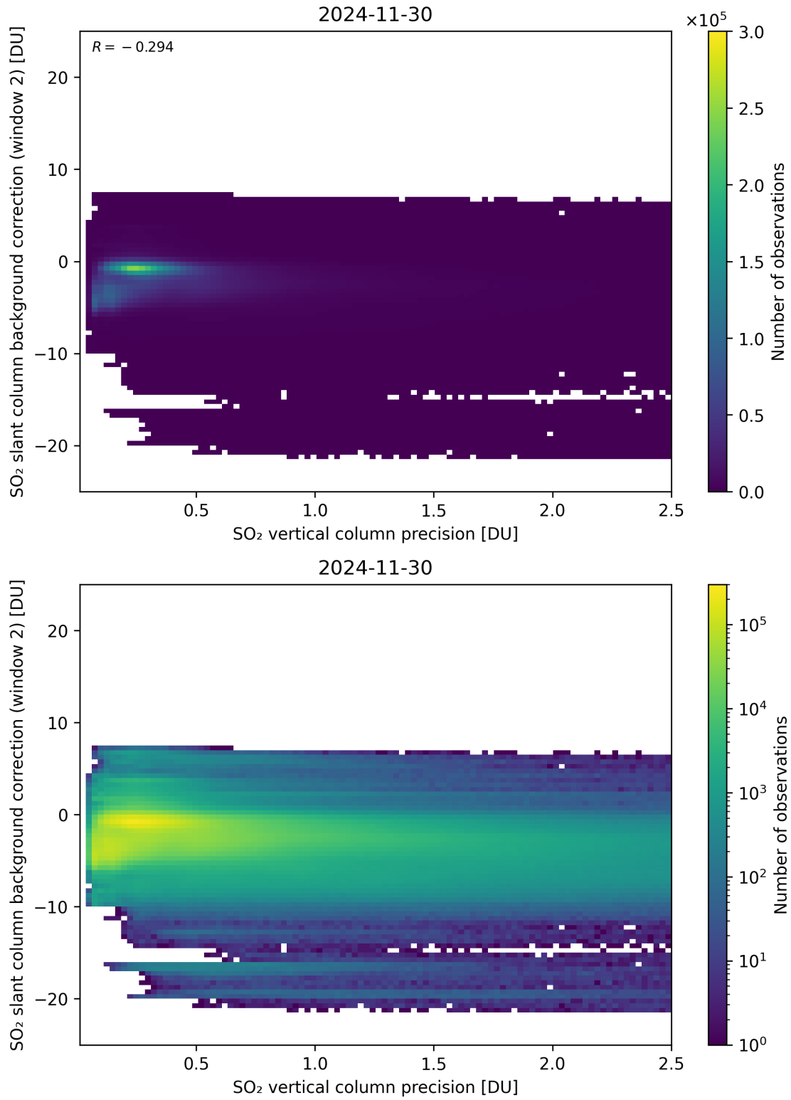
Figure 330: Scatter density plot of “SO 2 vertical column precision” against “SO 2 slant column background correction (window 2)” for 2024-11-30 to 2024-12-01.
