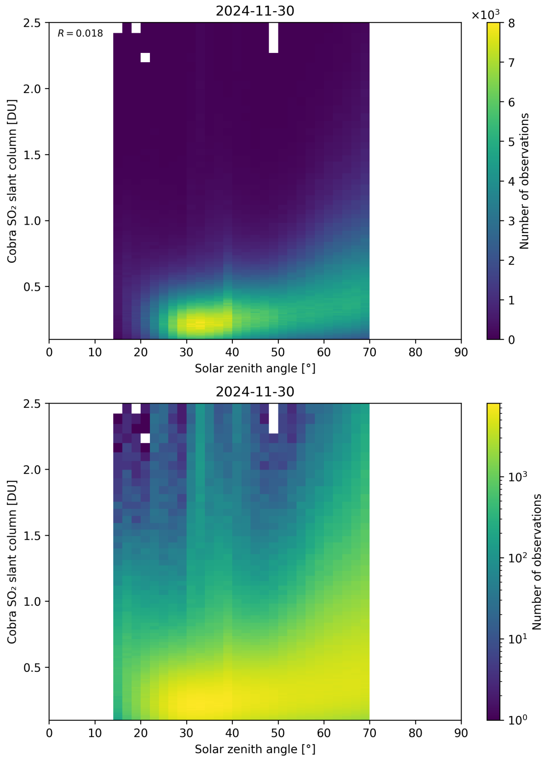
Figure 179: Scatter density plot of “Solar zenith angle” against “Cobra SO 2 slant column” for 2024-11-30 to 2024-12-01.
