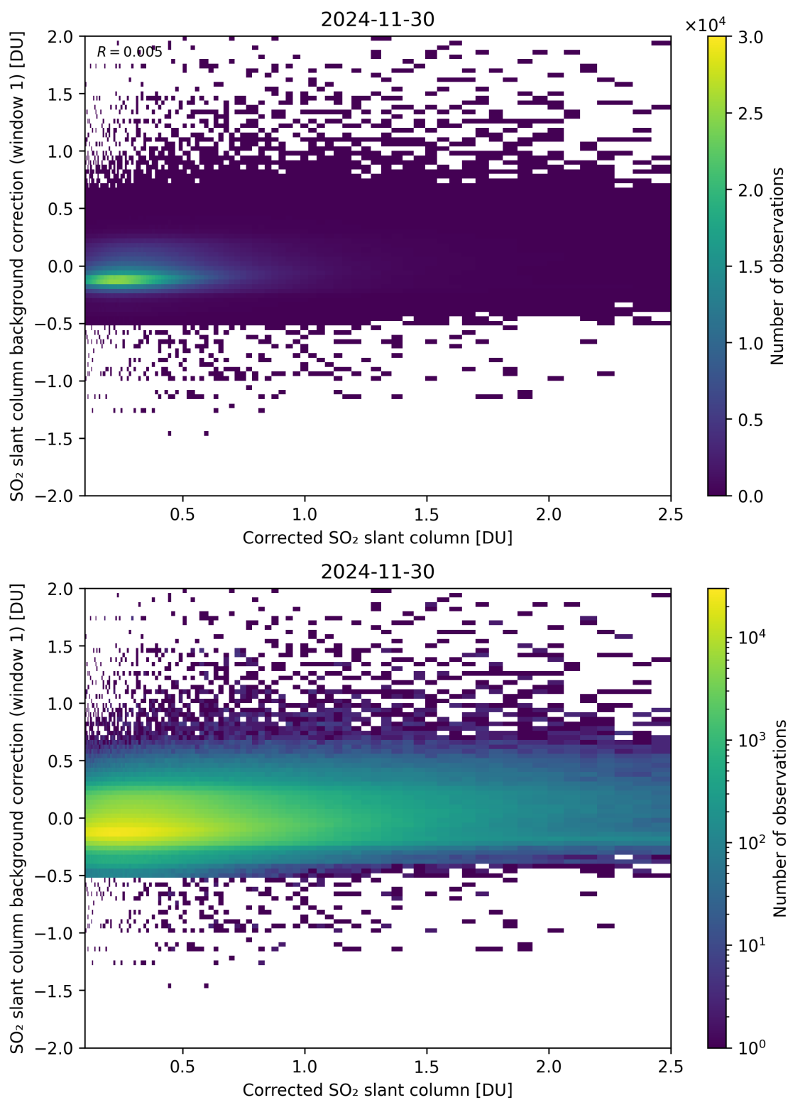
Figure 226: Scatter density plot of “Corrected SO 2 slant column” against “SO 2 slant column background correction (window 1)” for 2024-11-30 to 2024-12-01.
