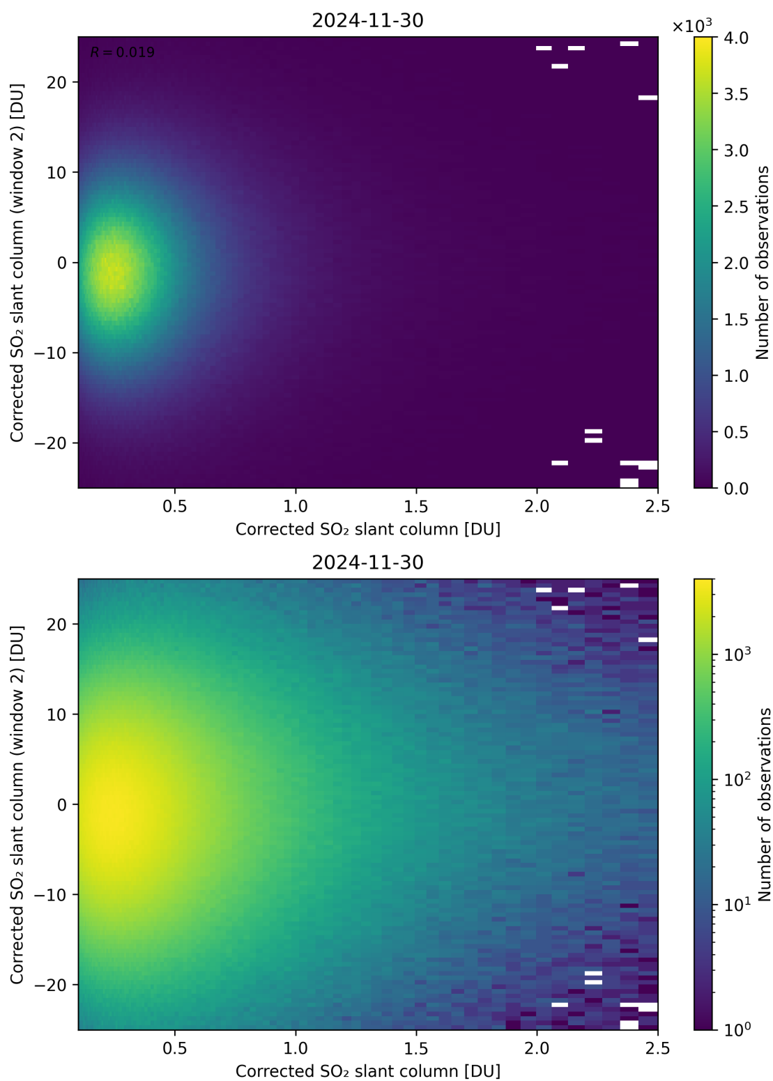
Figure 235: Scatter density plot of “Corrected SO 2 slant column” against “Corrected SO 2 slant column (window 2)” for 2024-11-30 to 2024-12-01.
