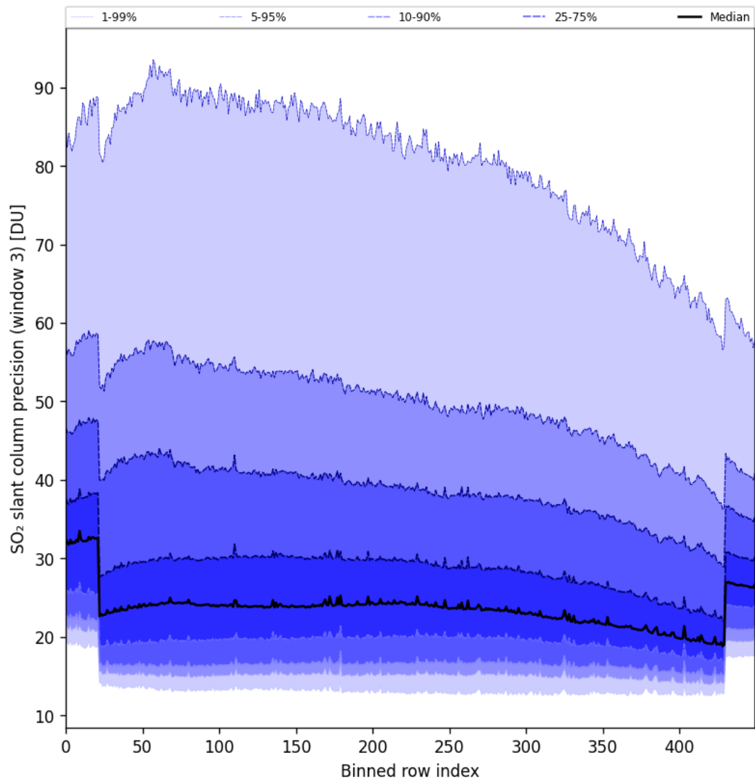
Figure 98: Along track statistics of “SO 2 slant column precision (window 3)” for 2024-11-30 to 2024-12-01
