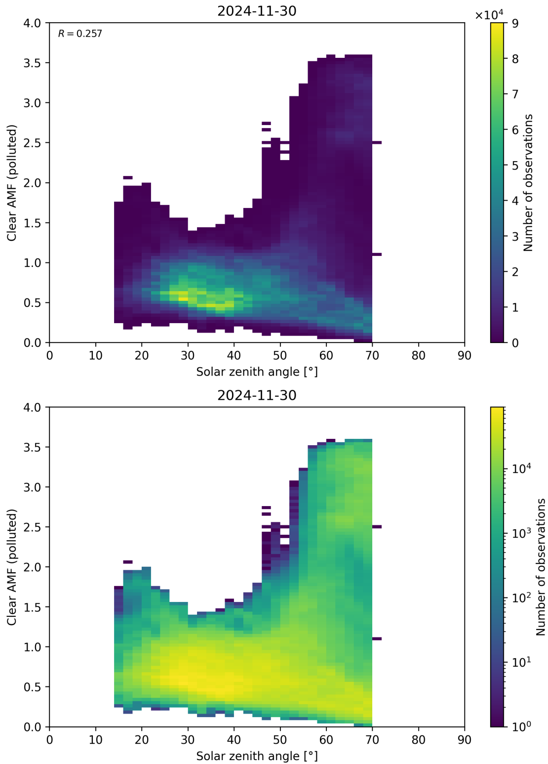
Figure 178: Scatter density plot of “Solar zenith angle” against “Clear AMF (polluted)” for 2024-11-30 to 2024-12-01.
