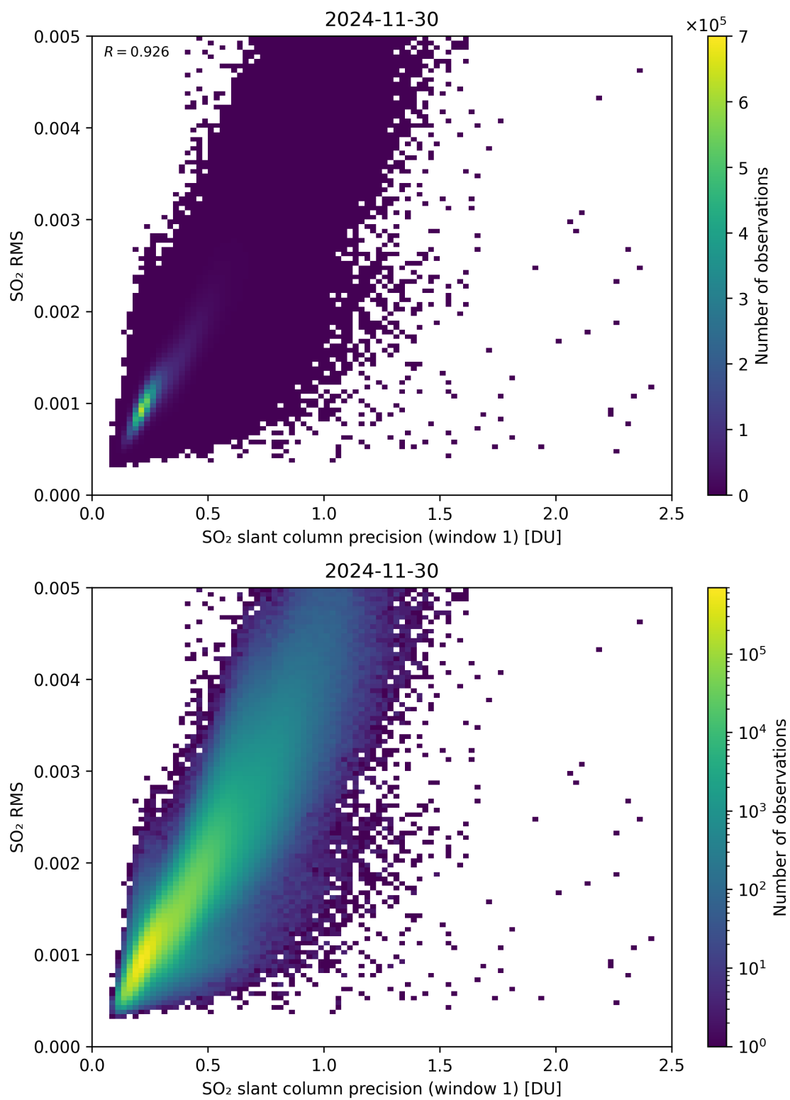
Figure 273: Scatter density plot of “SO 2 slant column precision (window 1)” against “SO 2 RMS” for 2024-11-30 to 2024-12-01.
