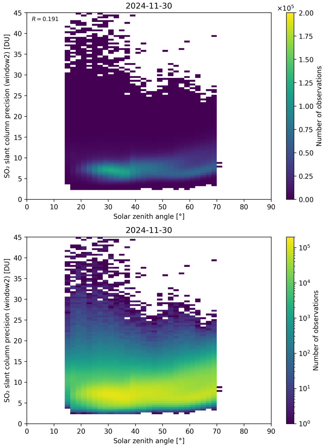
Figure 186: Scatter density plot of “Solar zenith angle” against “SO 2 slant column precision (window2)” for 2024-11-30 to 2024-12-01.
