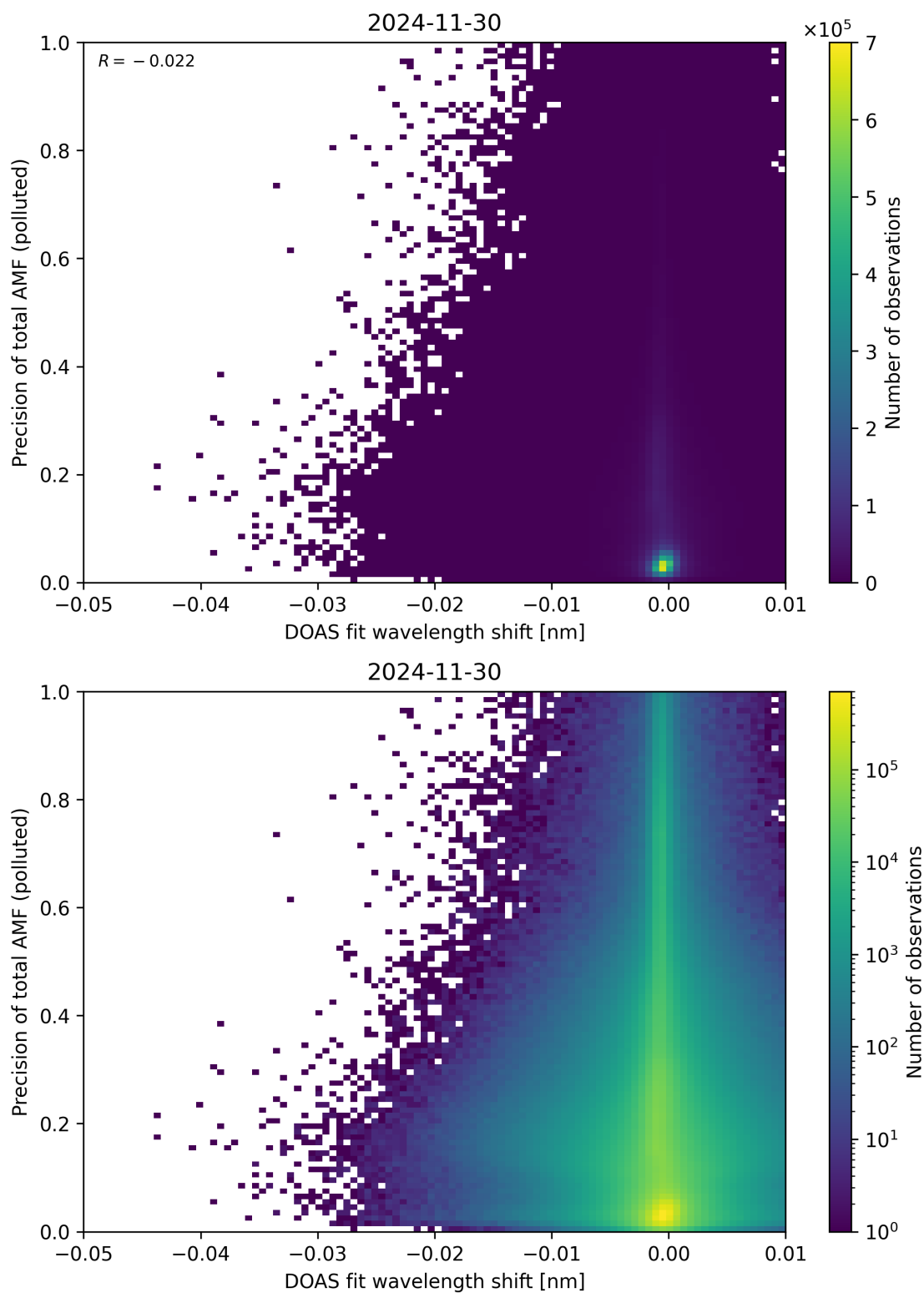
Figure 142: Scatter density plot of “DOAS fit wavelength shift” against “Precision of total AMF (polluted)” for 2024-11-30 to 2024-12-01.
