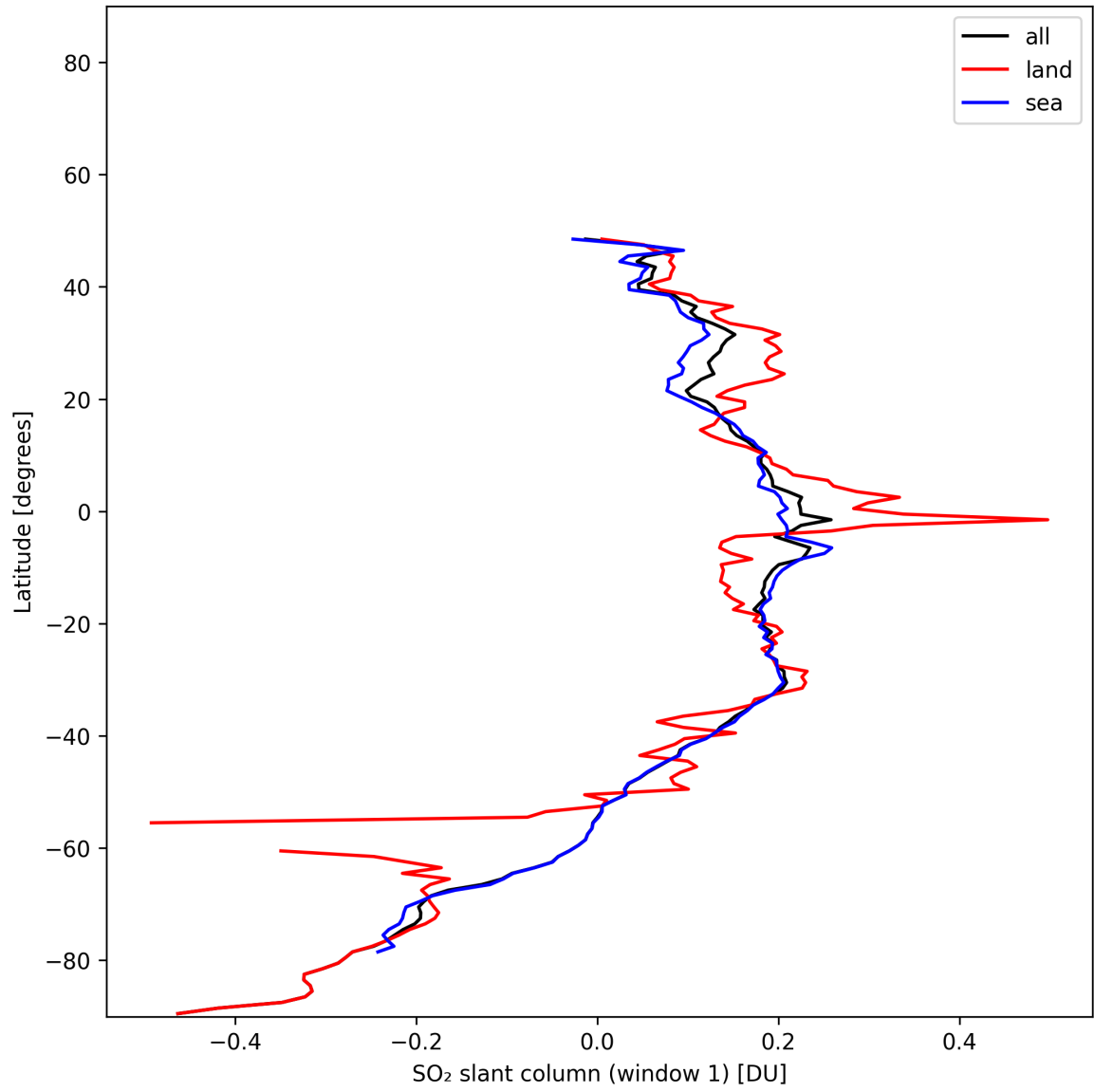
Figure 37: Zonal average of “SO 2 slant column (window 1)” for 2024-11-30 to 2024-12-01.
