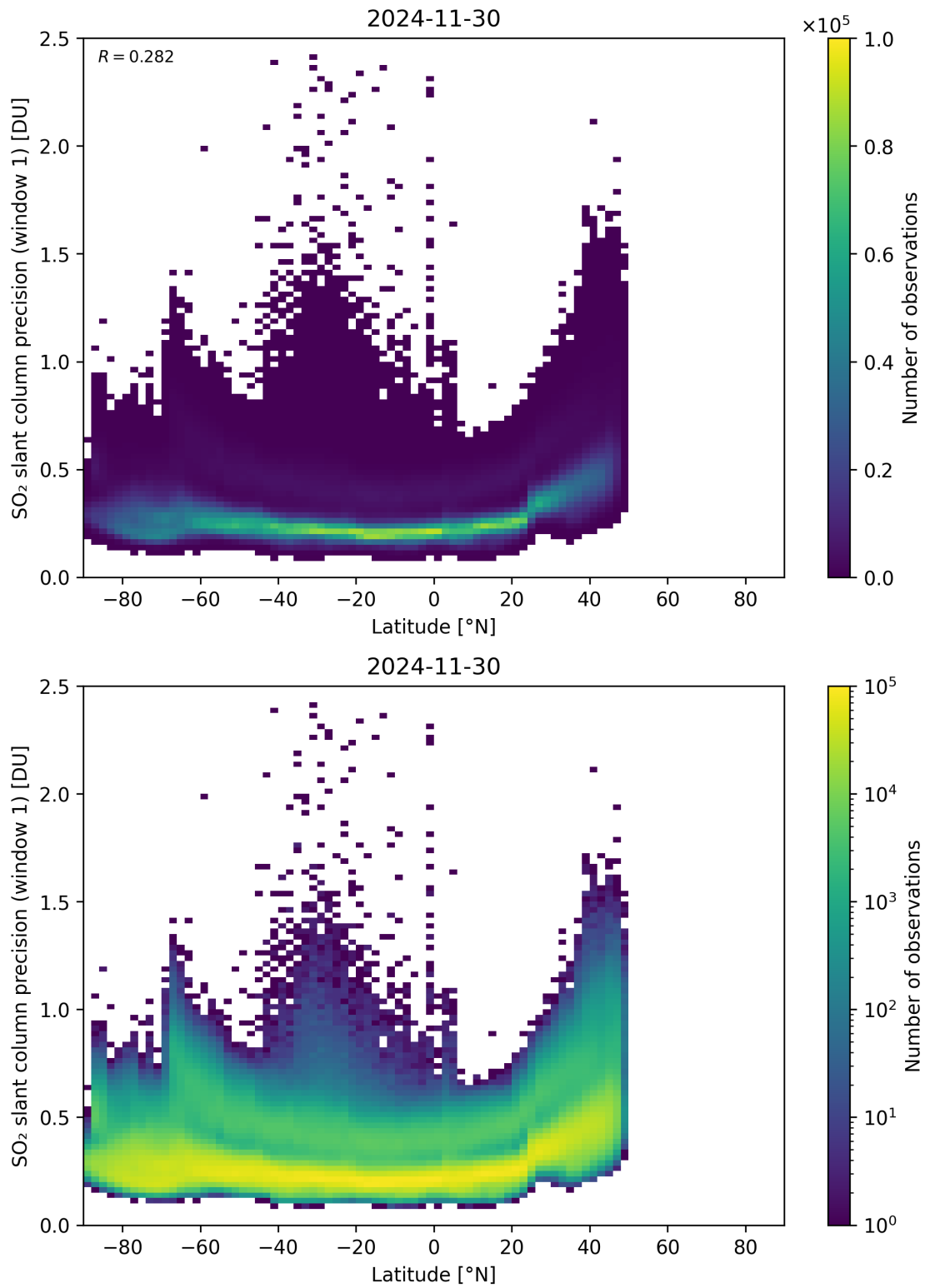
Figure 163: Scatter density plot of “Latitude” against “SO 2 slant column precision (window 1)” for 2024-11-30 to 2024-12-01.
