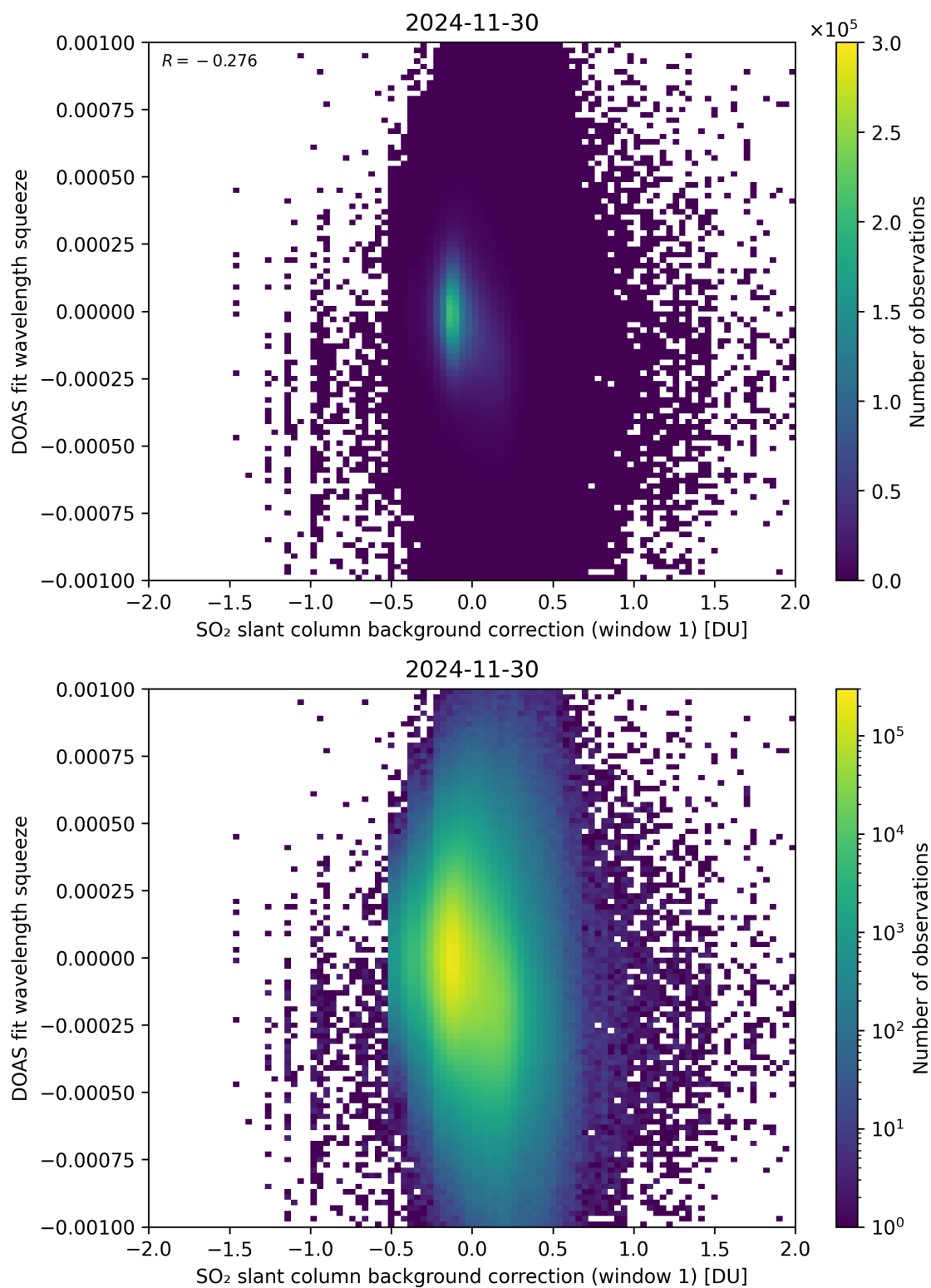
Figure 112: Scatter density plot of “SO 2 slant column background correction (window 1)” against “DOAS fit wavelength squeeze” for 2024-11-30 to 2024-12-01.
