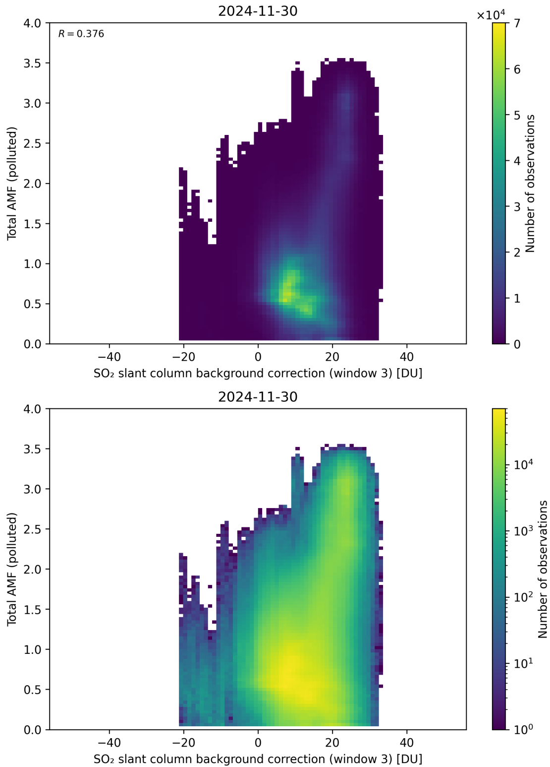
Figure 136: Scatter density plot of “SO 2 slant column background correction (window 3)” against “Total AMF (polluted)” for 2024-11-30 to 2024-12-01.
