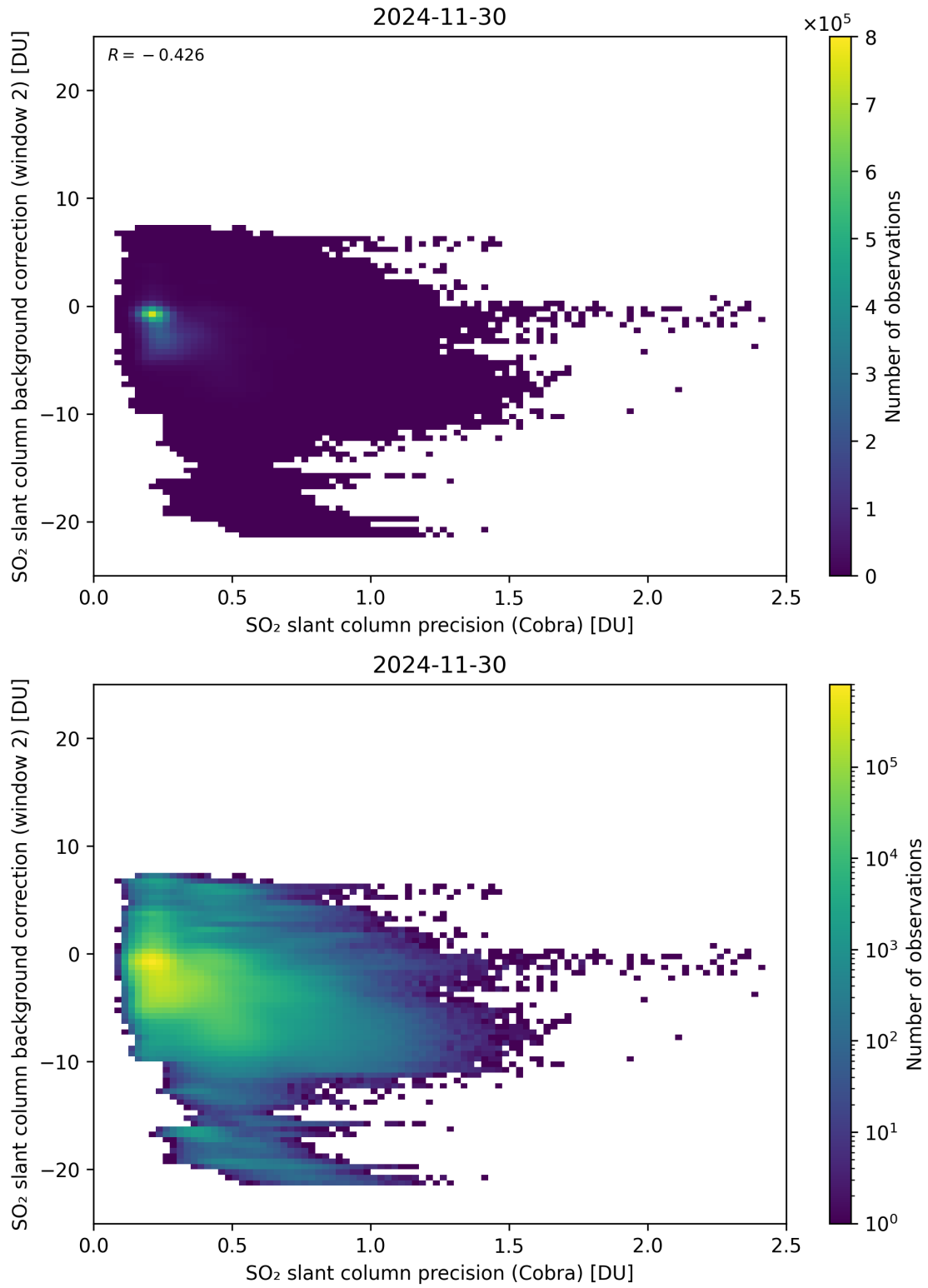
Figure 200: Scatter density plot of “SO 2 slant column precision (Cobra)” against “SO 2 slant column background correction (window 2)” for 2024-11-30 to 2024-12-01.
