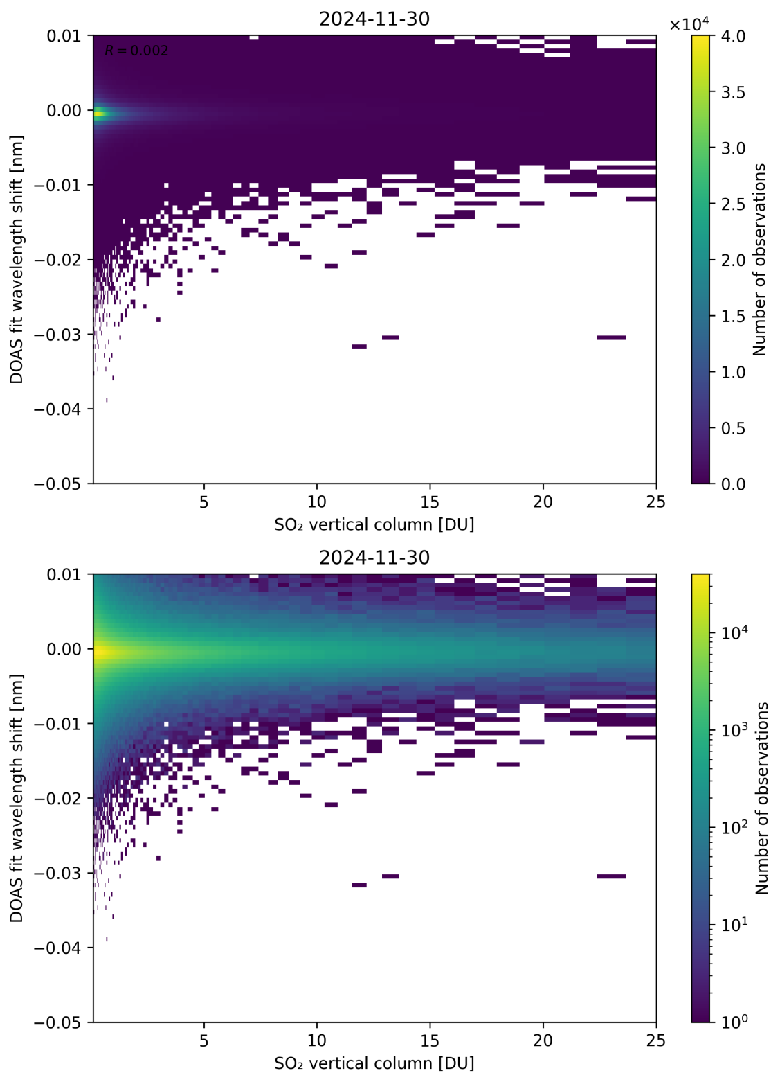
Figure 326: Scatter density plot of “SO 2 vertical column” against “DOAS fit wavelength shift” for 2024-11-30 to 2024-12-01.
