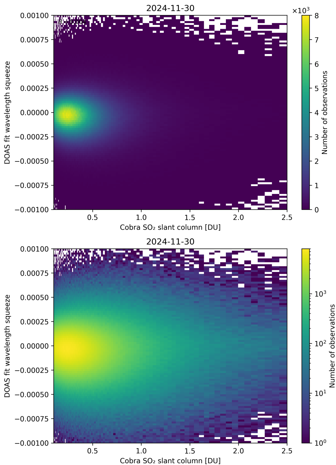
Figure 197: Scatter density plot of “Cobra SO 2 slant column” against “DOAS fit wavelength squeeze” for 2024-11-30 to 2024-12-01.
