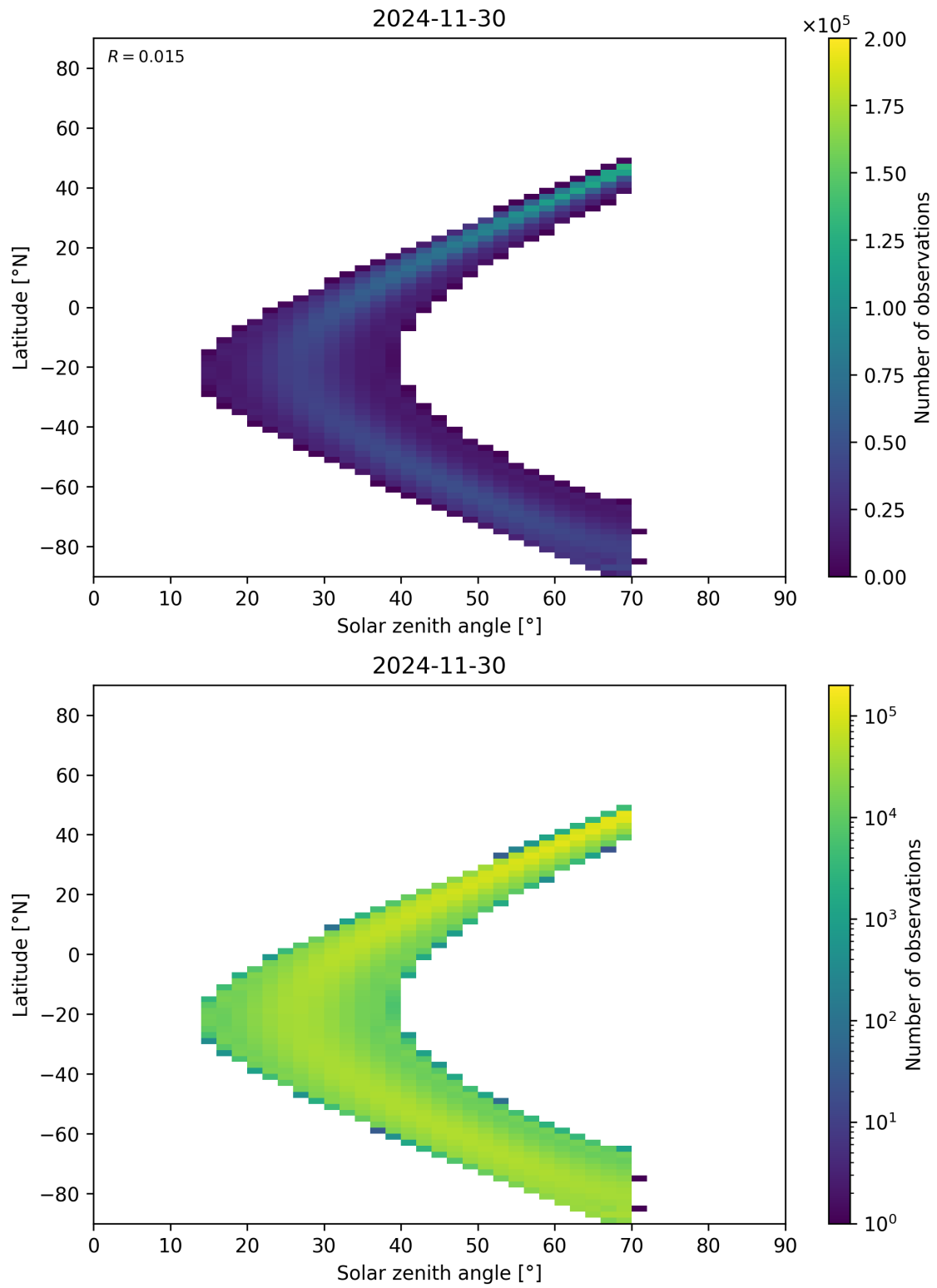
Figure 177: Scatter density plot of “Solar zenith angle” against “Latitude” for 2024-11-30 to 2024-12-01.
