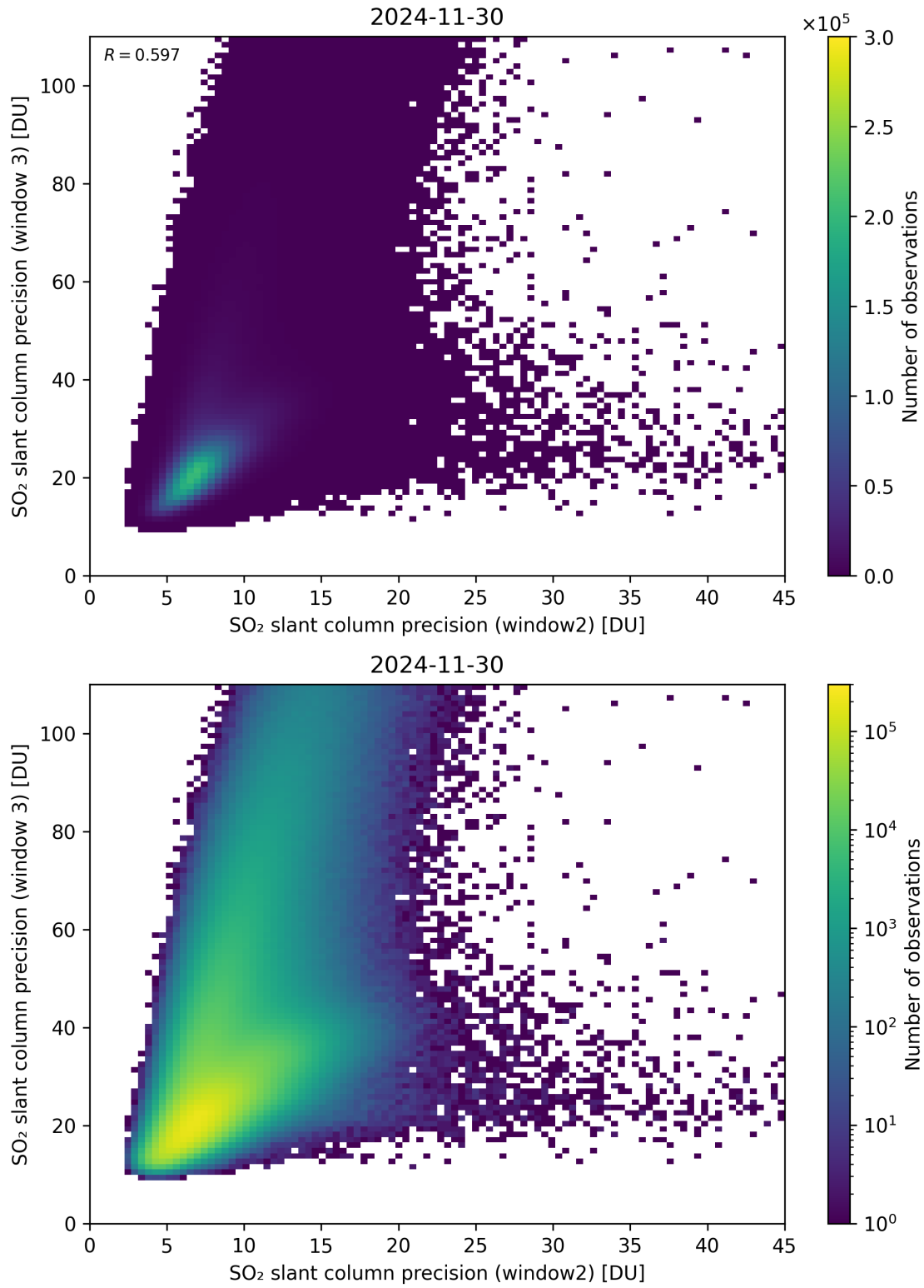
Figure 300: Scatter density plot of “SO 2 slant column precision (window2)” against “SO 2 slant column precision (window 3)” for 2024-11-30 to 2024-12-01.
