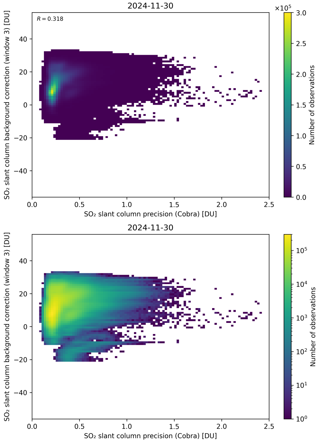
Figure 201: Scatter density plot of “SO 2 slant column precision (Cobra)” against “SO 2 slant column background correction (window 3)” for 2024-11-30 to 2024-12-01.
