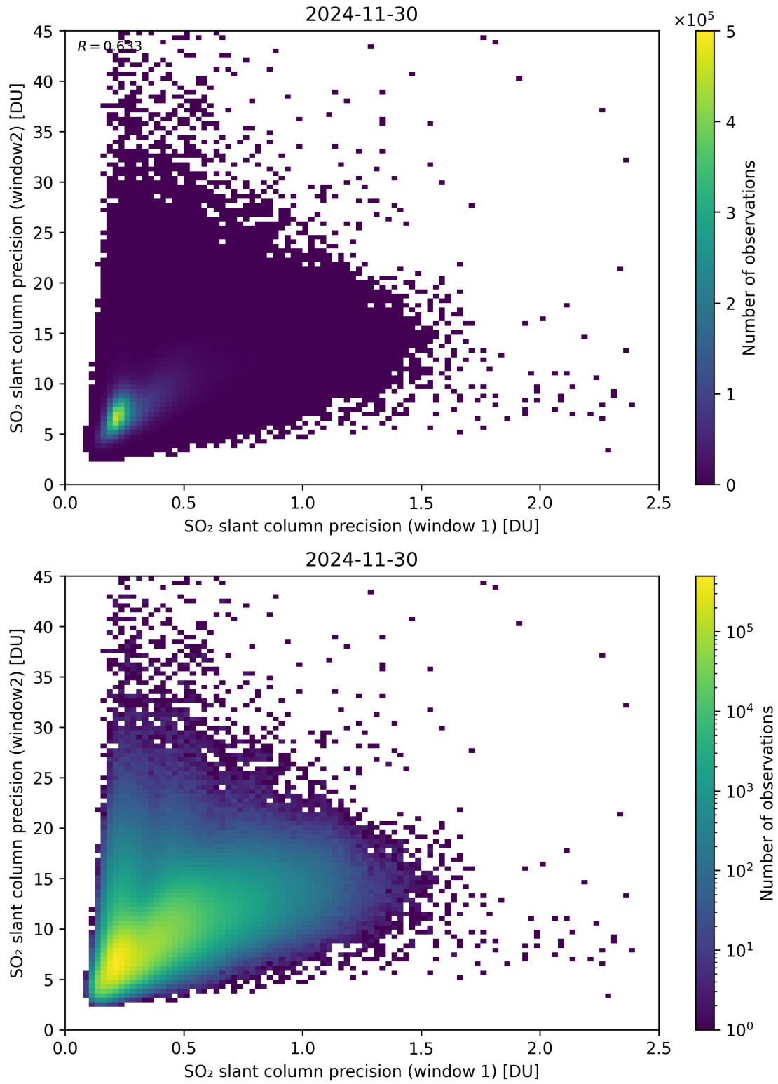
Figure 277: Scatter density plot of “SO 2 slant column precision (window 1)” against “SO 2 slant column precision (window2)” for 2024-11-30 to 2024-12-01.
