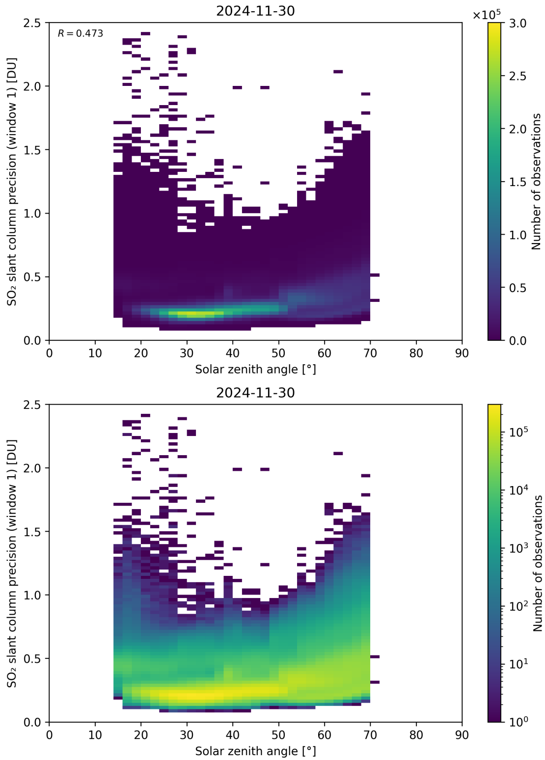
Figure 185: Scatter density plot of “Solar zenith angle” against “SO 2 slant column precision (window 1)” for 2024-11-30 to 2024-12-01.
