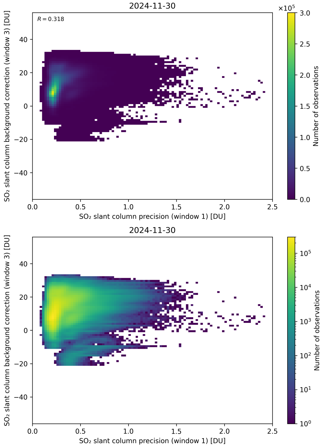
Figure 270: Scatter density plot of “SO 2 slant column precision (window 1)” against “SO 2 slant column background correction (window 3)” for 2024-11-30 to 2024-12-01.
