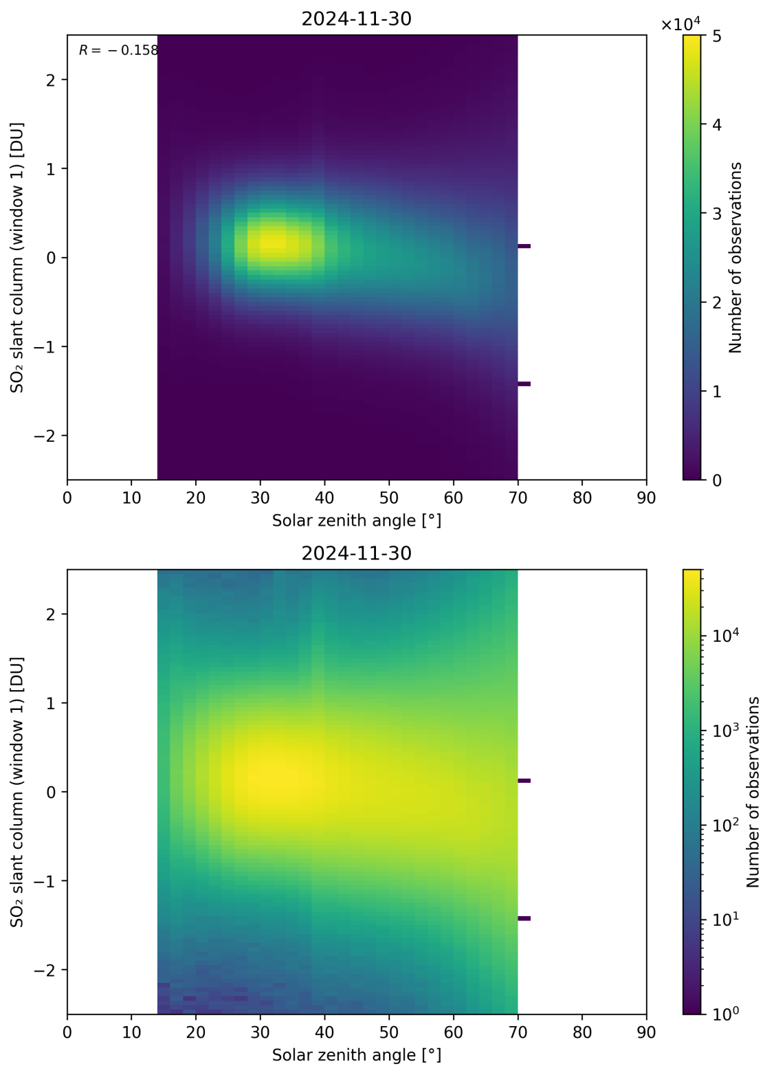
Figure 184: Scatter density plot of “Solar zenith angle” against “SO 2 slant column (window 1)” for 2024-11-30 to 2024-12-01.
