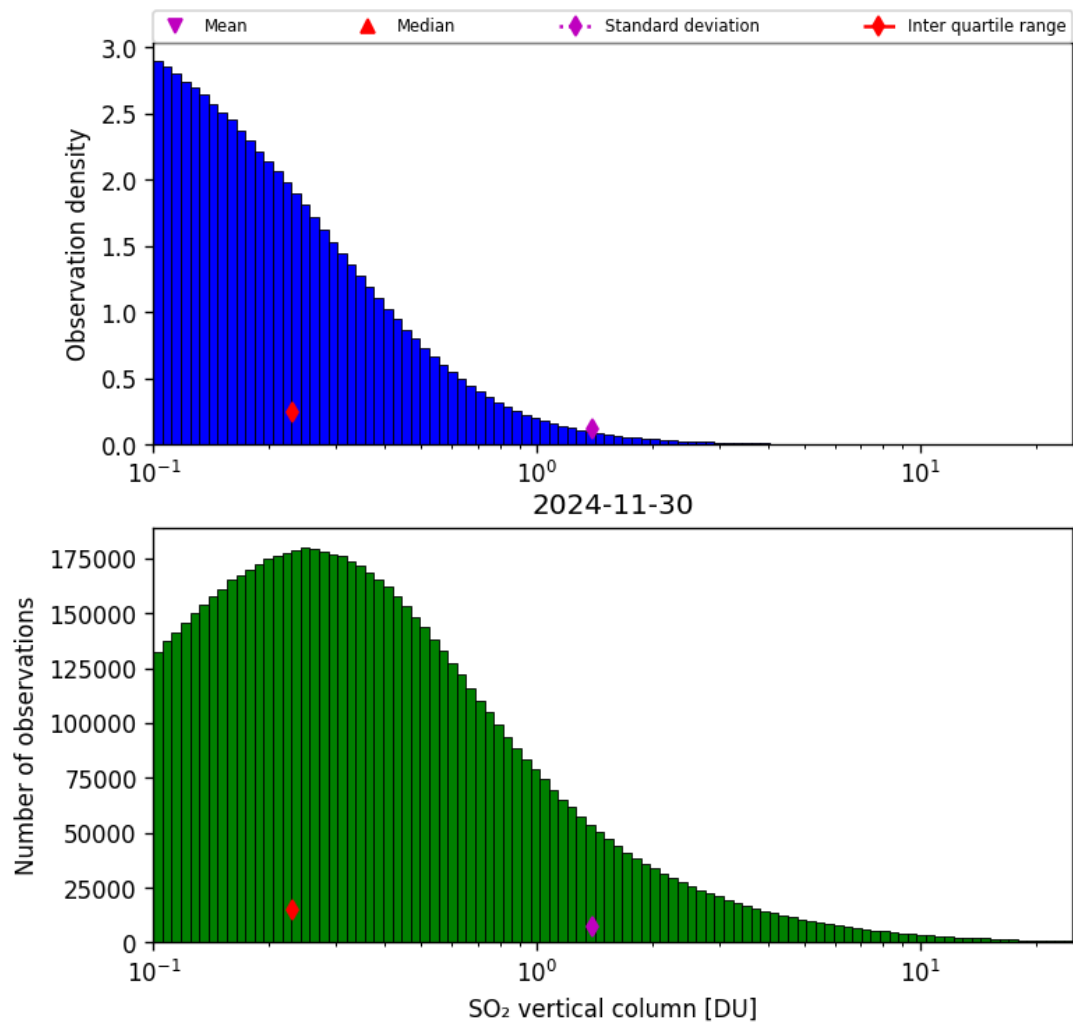
Figure 58: Histogram of “SO 2 vertical column” for 2024-11-30 to 2024-12-01
