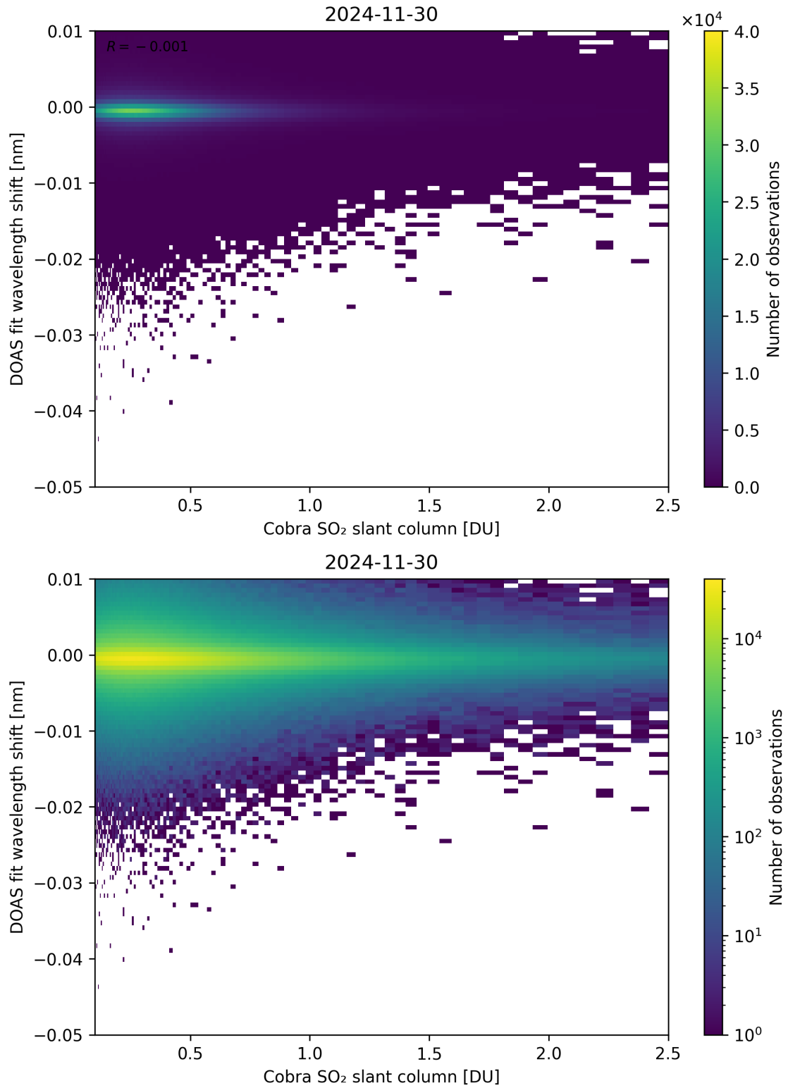
Figure 196: Scatter density plot of “Cobra SO 2 slant column” against “DOAS fit wavelength shift” for 2024-11-30 to 2024-12-01.
