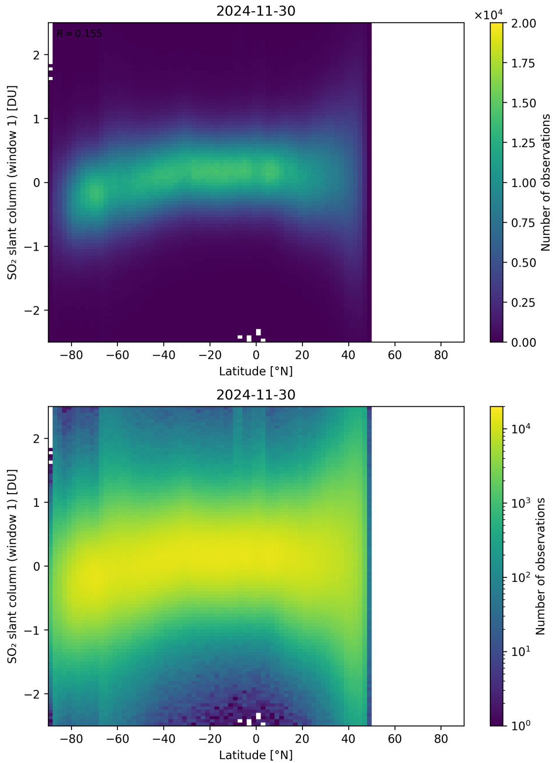
Figure 162: Scatter density plot of “Latitude” against “SO 2 slant column (window 1)” for 2024-11-30 to 2024-12-01.
