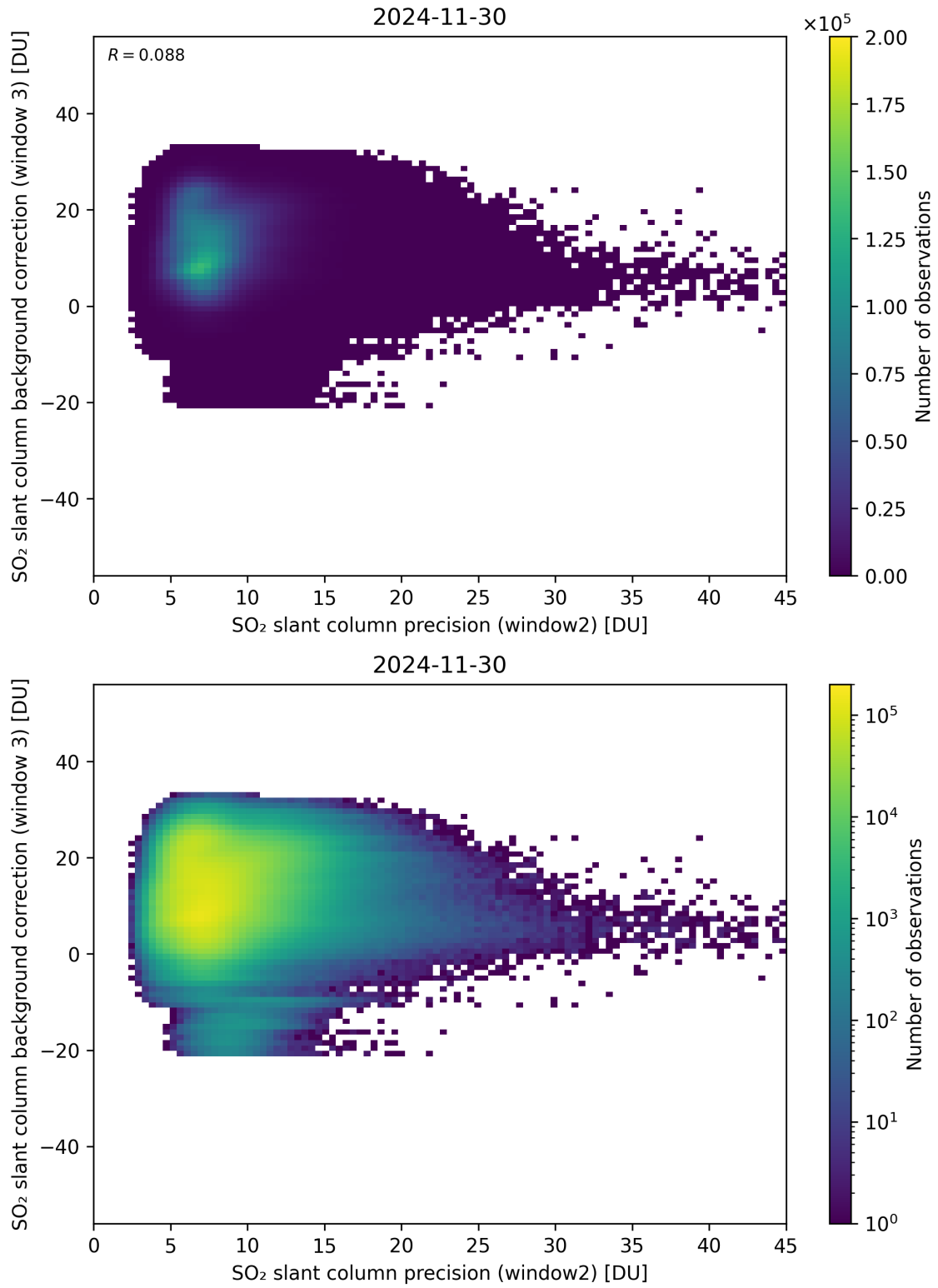
Figure 292: Scatter density plot of “SO 2 slant column precision (window2)” against “SO 2 slant column background correction (window 3)” for 2024-11-30 to 2024-12-01.
