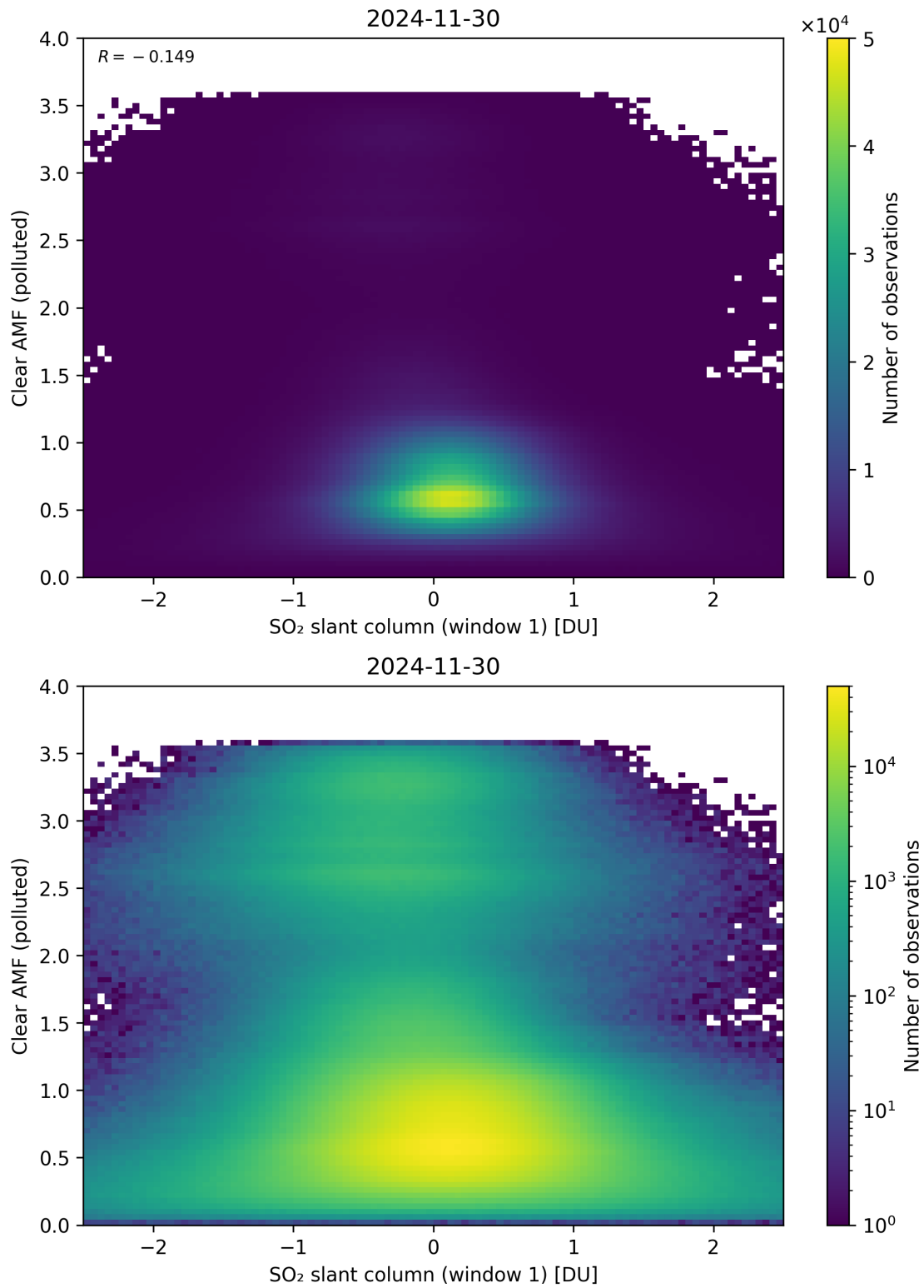
Figure 282: Scatter density plot of “SO 2 slant column (window 1)” against “Clear AMF (polluted)” for 2024-11-30 to 2024-12-01.
