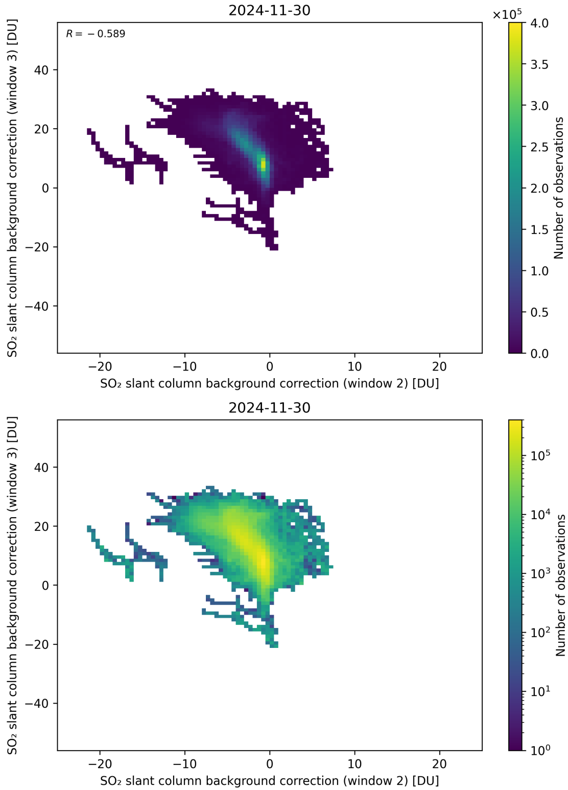
Figure 122: Scatter density plot of “SO 2 slant column background correction (window 2)” against “SO 2 slant column background correction (window 3)” for 2024-11-30 to 2024-12-01.
