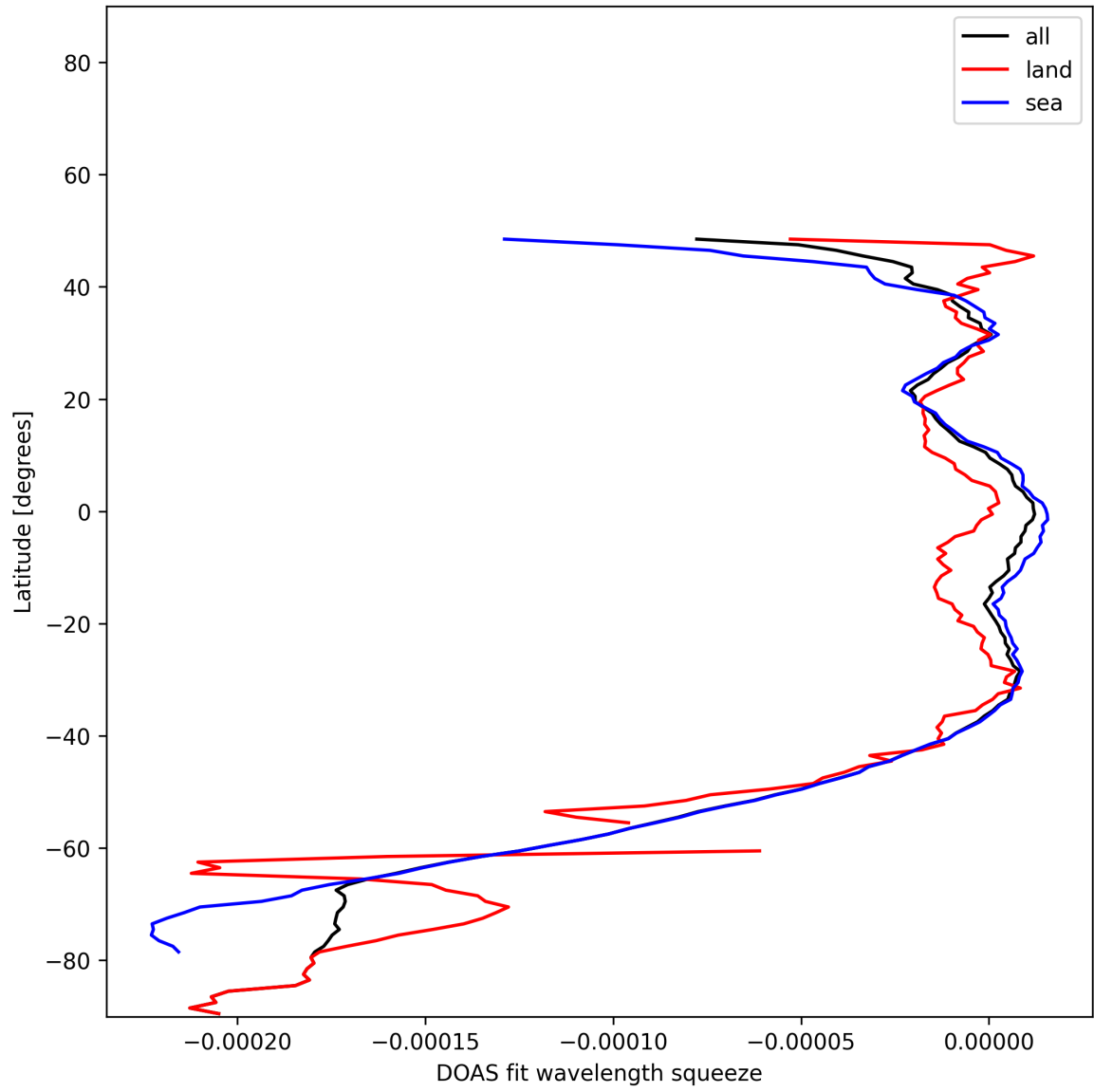
Figure 51: Zonal average of “DOAS fit wavelength squeeze” for 2024-11-30 to 2024-12-01.
