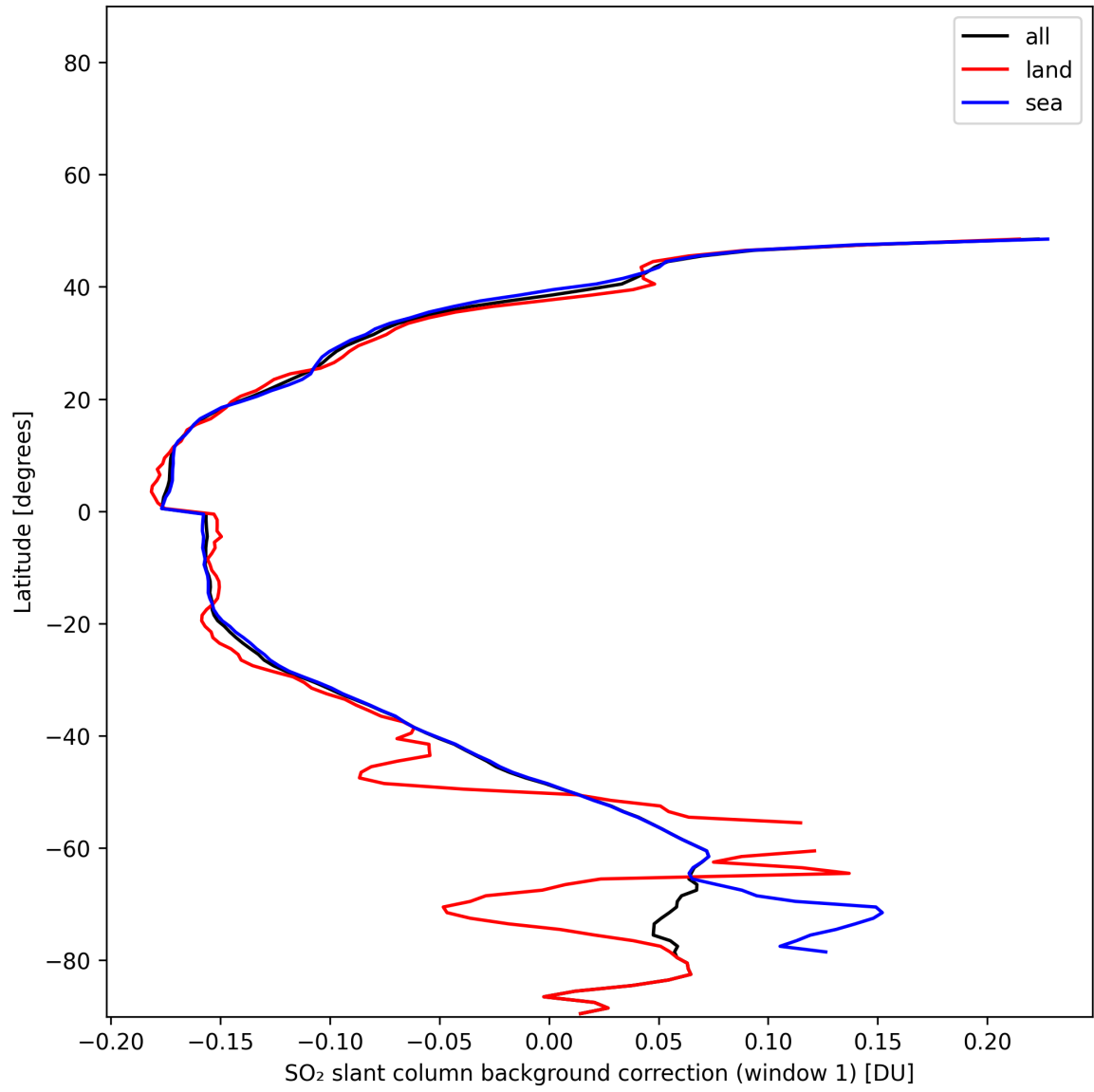
Figure 40: Zonal average of “SO 2 slant column background correction (window 1)” for 2024-11-30 to 2024-12-01.
