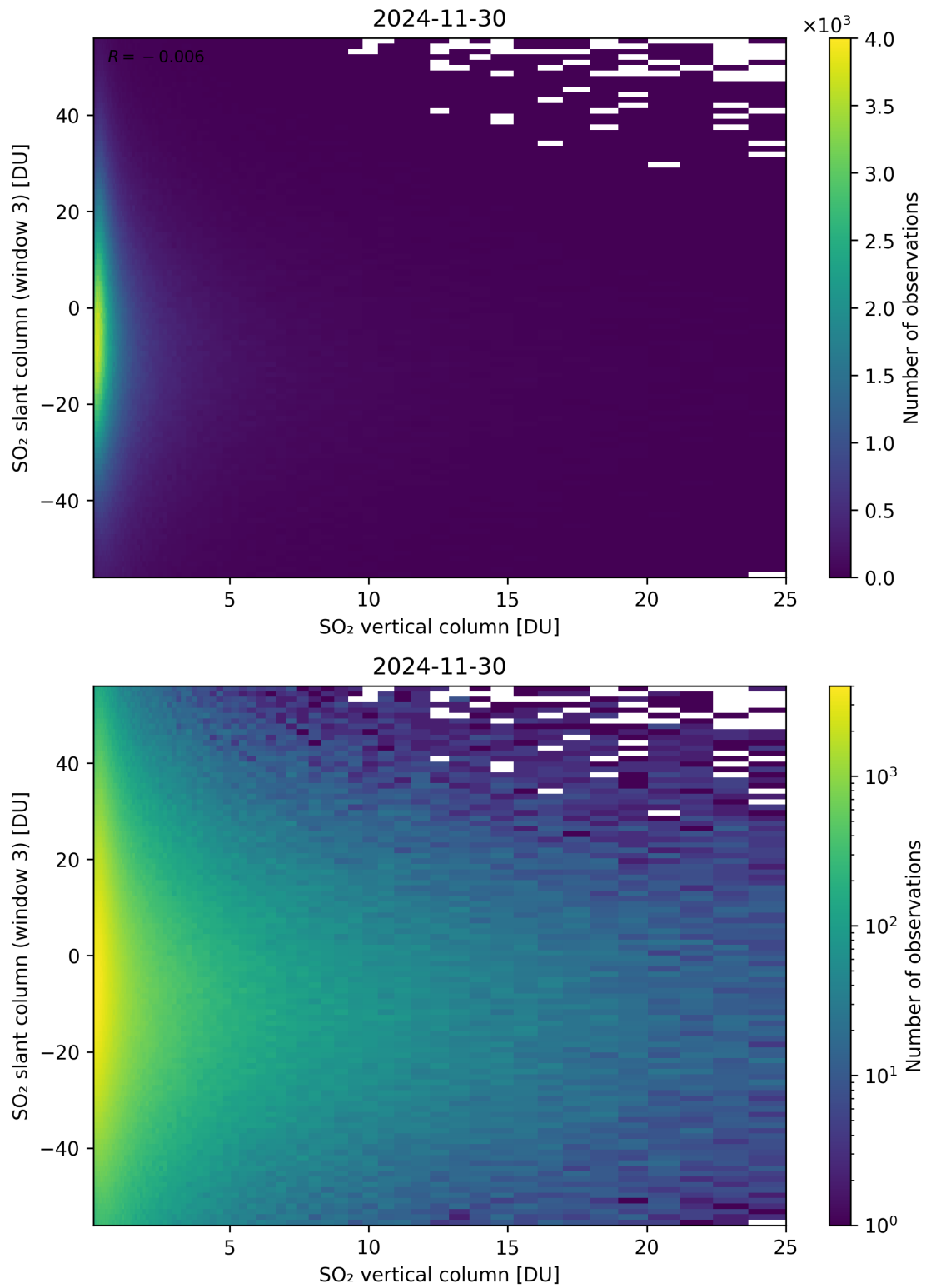
Figure 357: Scatter density plot of “SO 2 vertical column” against “SO 2 slant column (window 3)” for 2024-11-30 to 2024-12-01.
