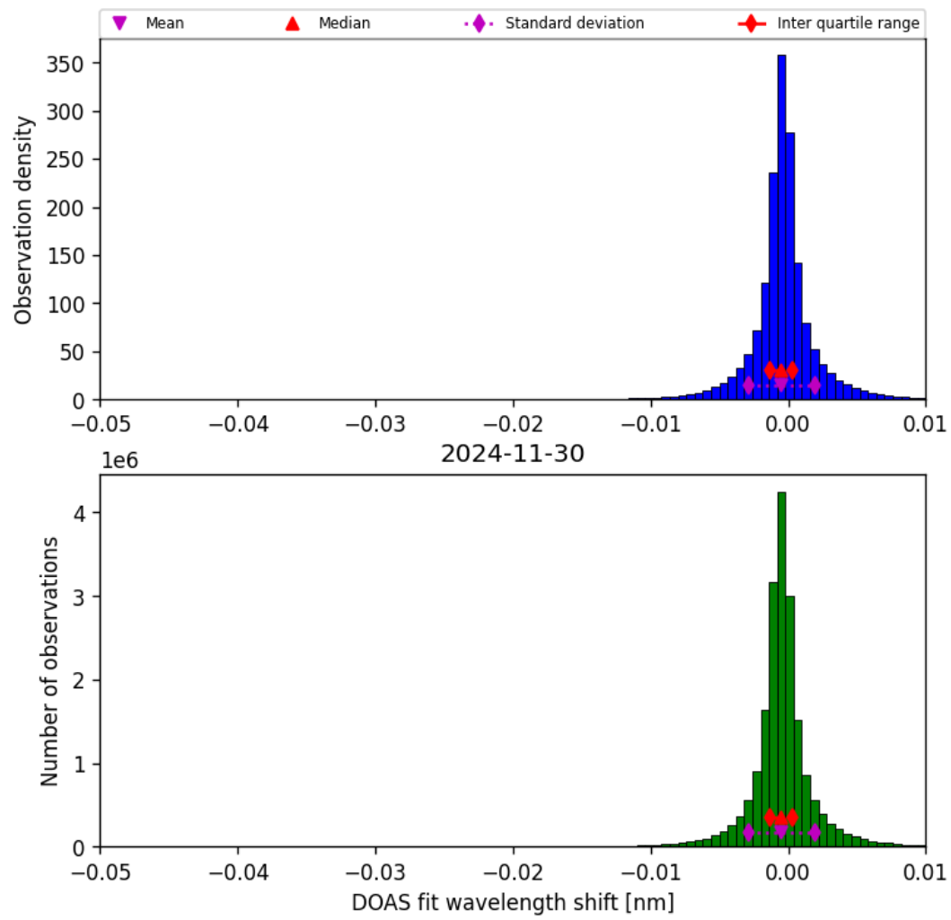
Figure 76: Histogram of “DOAS fit wavelength shift” for 2024-11-30 to 2024-12-01
