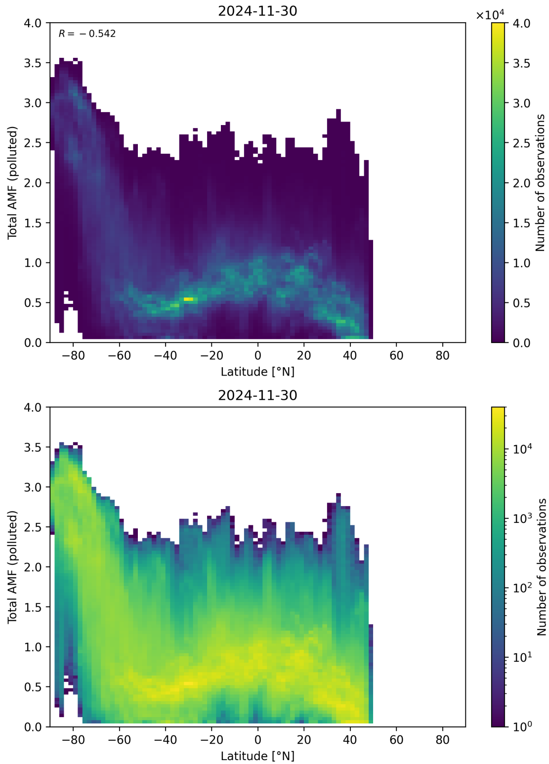
Figure 167: Scatter density plot of “Latitude” against “Total AMF (polluted)” for 2024-11-30 to 2024-12-01.
