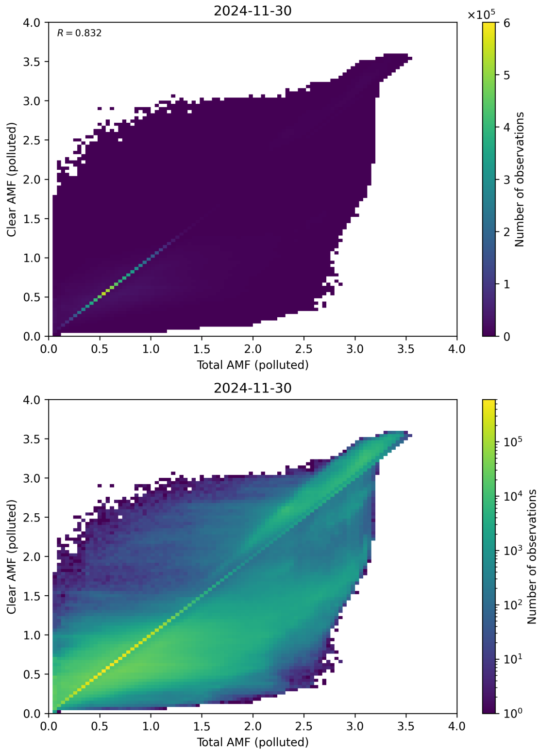
Figure 321: Scatter density plot of “Total AMF (polluted)” against “Clear AMF (polluted)” for 2024-11-30 to 2024-12-01.
