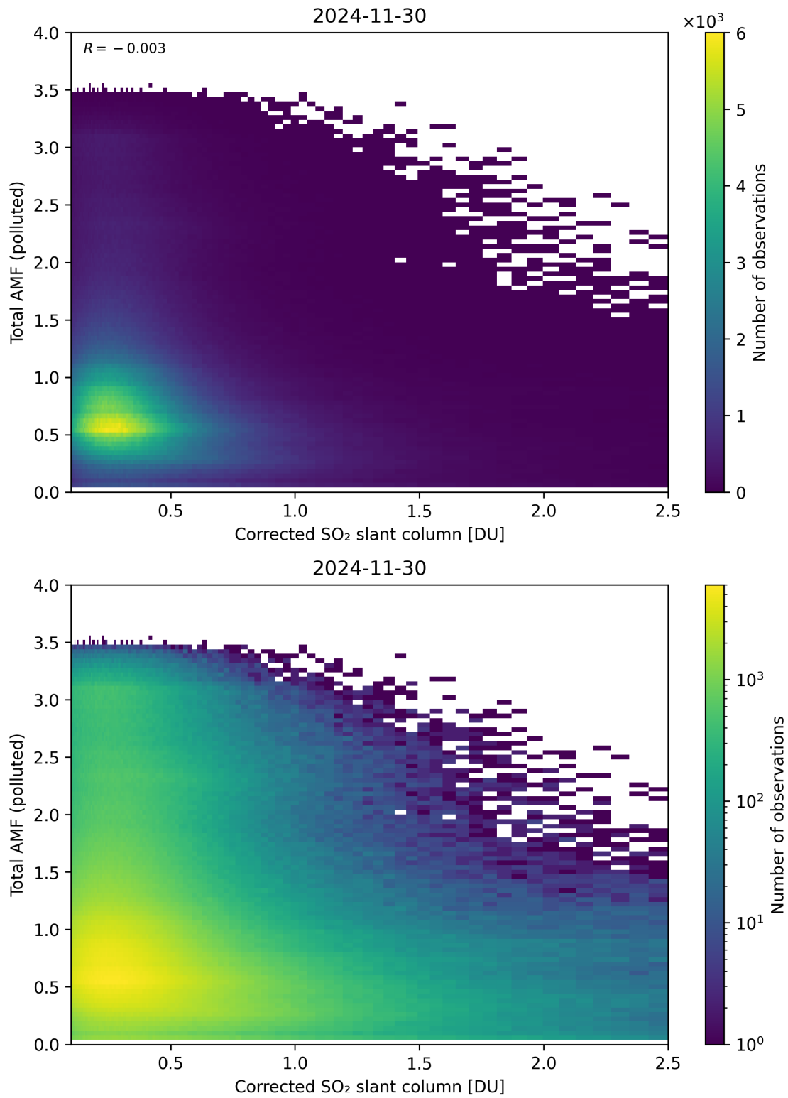
Figure 242: Scatter density plot of “Corrected SO 2 slant column” against “Total AMF (polluted)” for 2024-11-30 to 2024-12-01.
