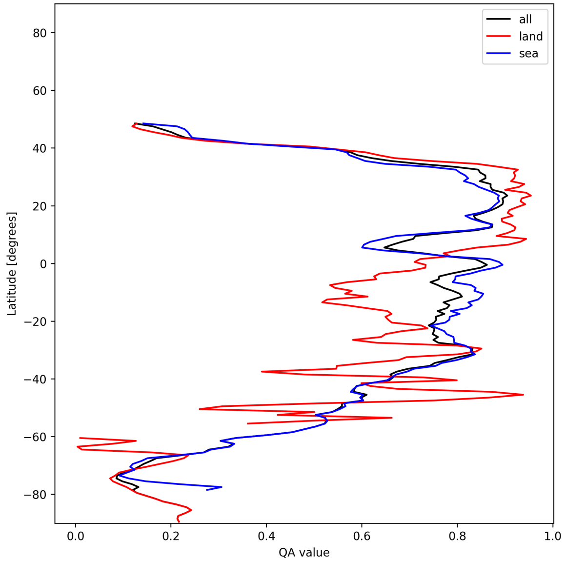
Figure 31: Zonal average of “QA value” for 2024-11-30 to 2024-12-01.
