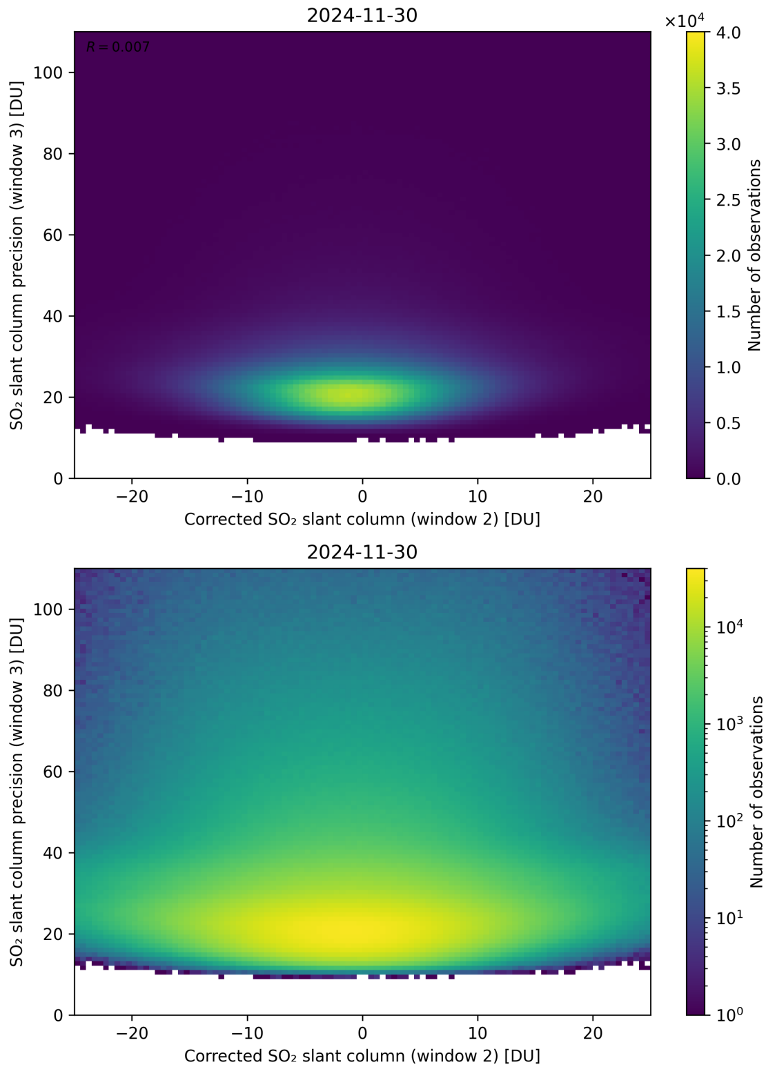
Figure 252: Scatter density plot of “Corrected SO 2 slant column (window 2)” against “SO 2 slant column precision (window 3)” for 2024-11-30 to 2024-12-01.
