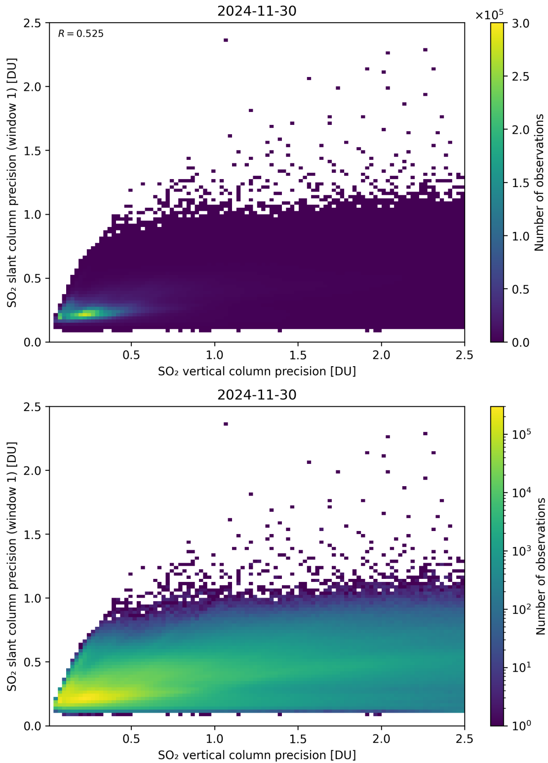
Figure 342: Scatter density plot of “SO 2 vertical column precision” against “SO 2 slant column precision (window 1)” for 2024-11-30 to 2024-12-01.
