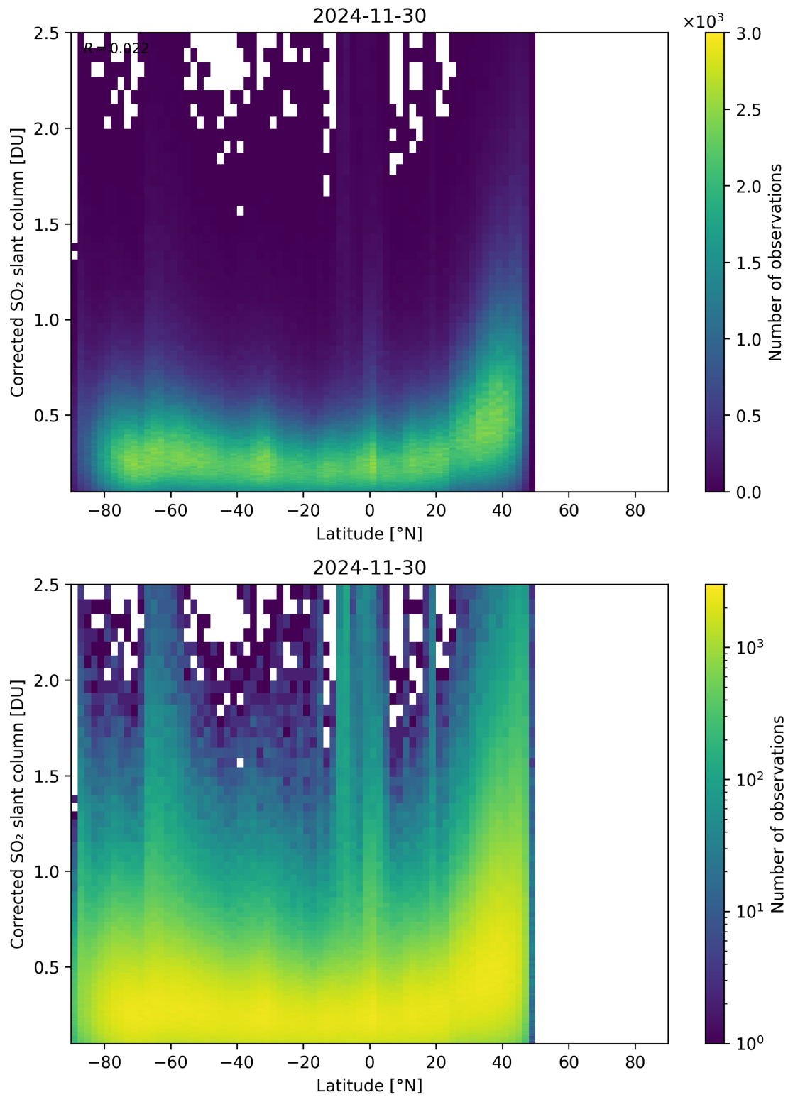
Figure 159: Scatter density plot of “Latitude” against “Corrected SO 2 slant column” for 2024-11-30 to 2024-12-01.
