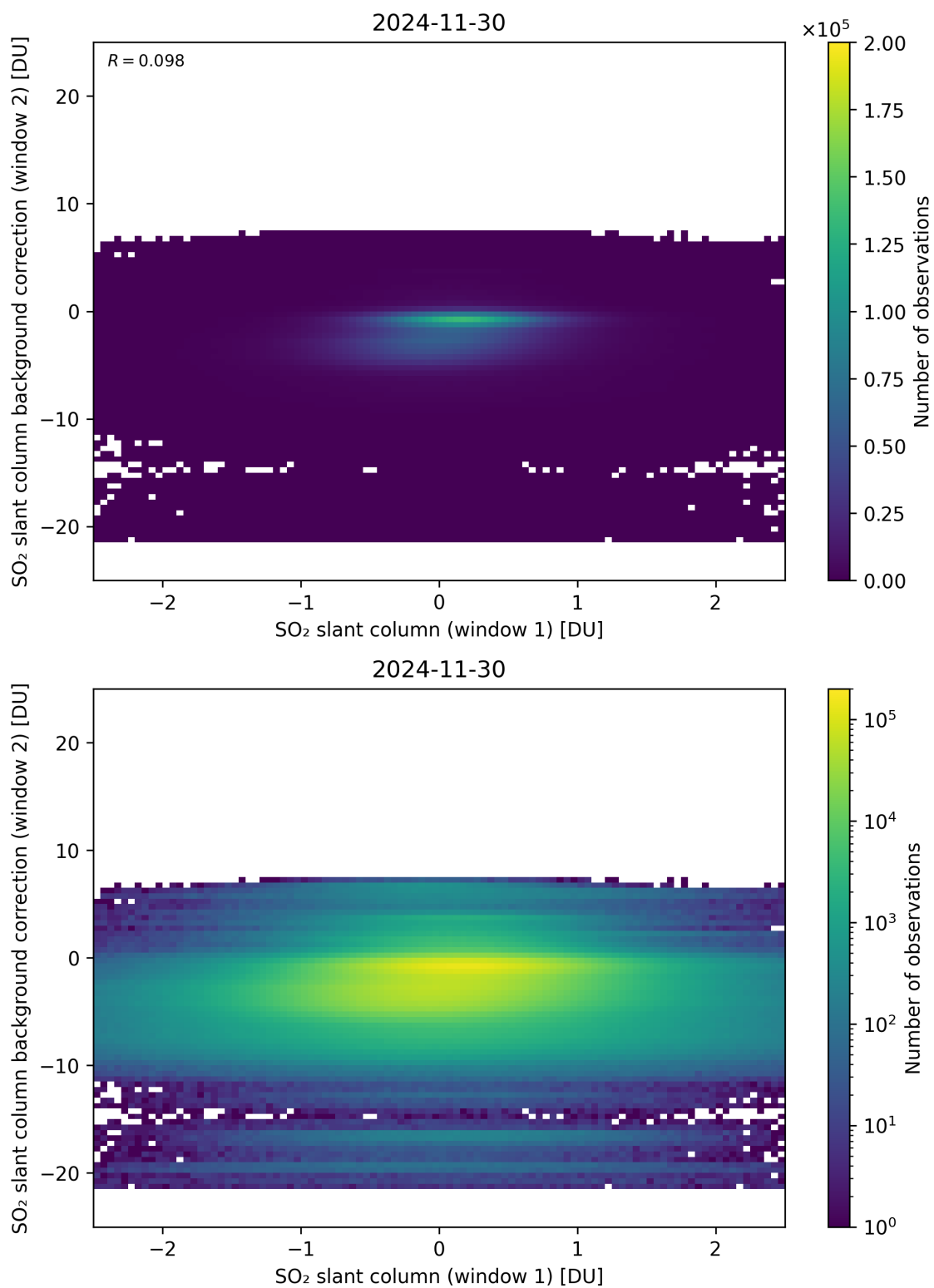
Figure 263: Scatter density plot of “SO 2 slant column (window 1)” against “SO 2 slant column background correction (window 2)” for 2024-11-30 to 2024-12-01.
