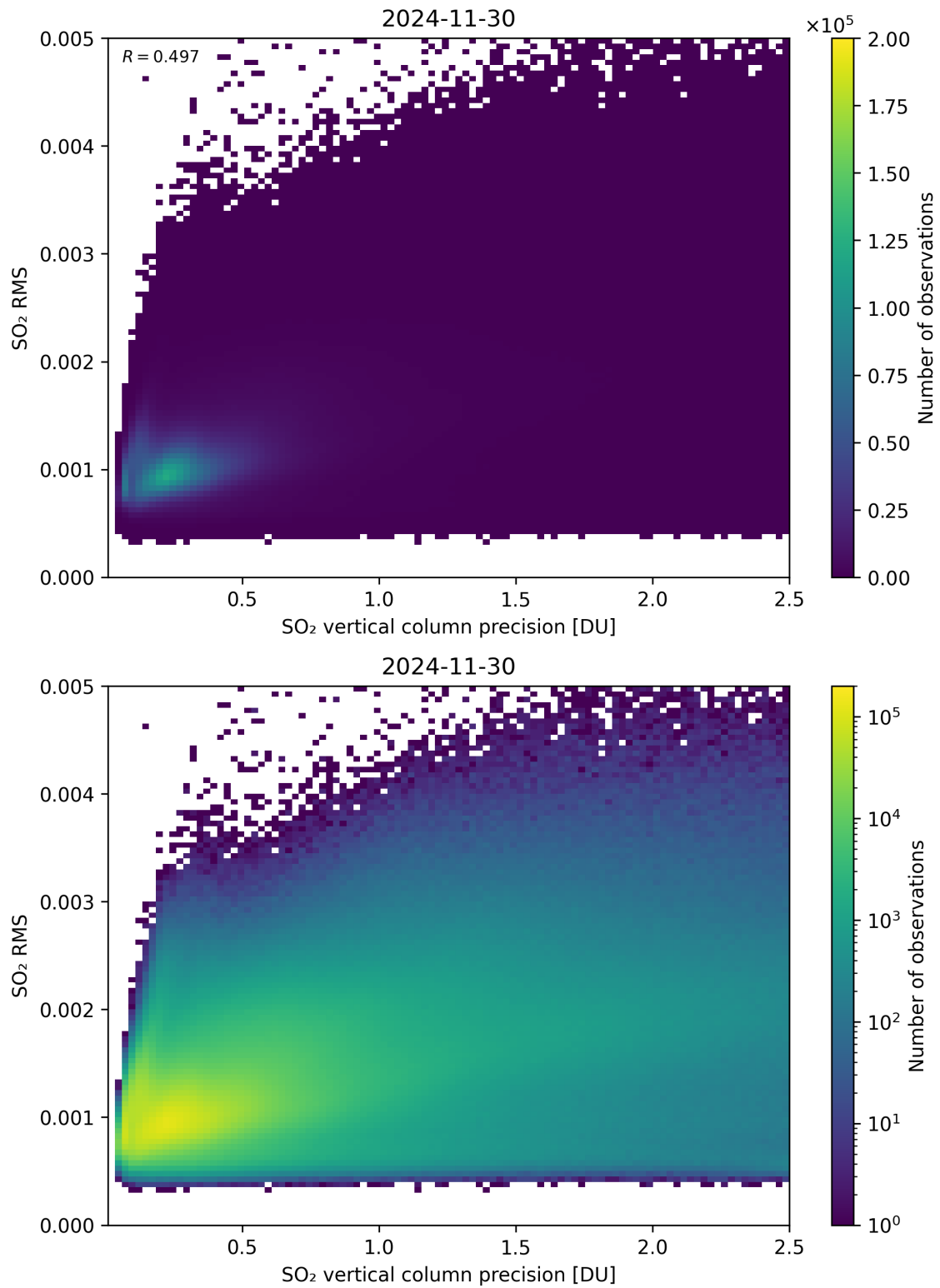
Figure 334: Scatter density plot of “SO 2 vertical column precision” against “SO 2 RMS” for 2024-11-30 to 2024-12-01.
