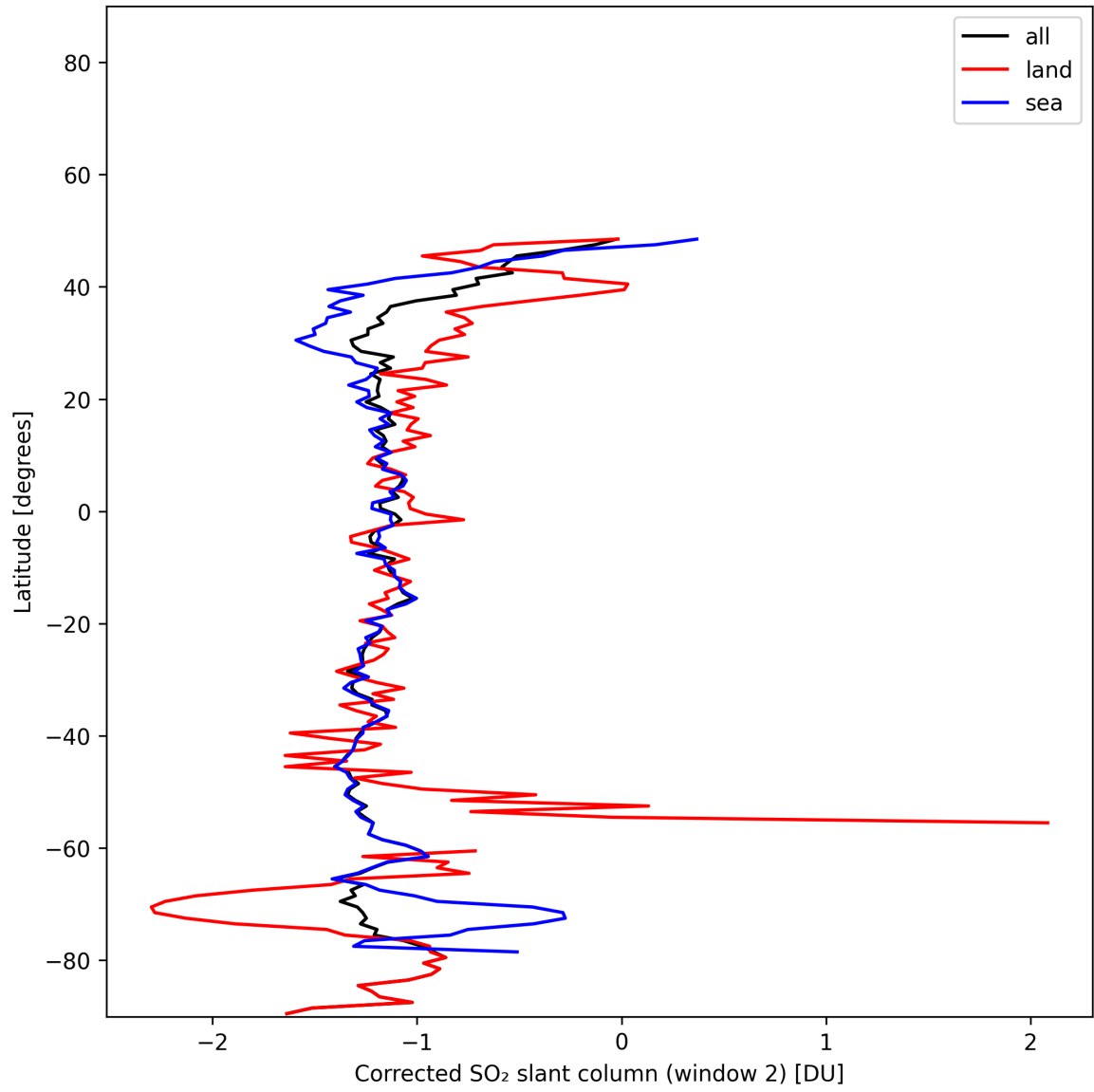
Figure 43: Zonal average of “Corrected SO 2 slant column (window 2)” for 2024-11-30 to 2024-12-01.
