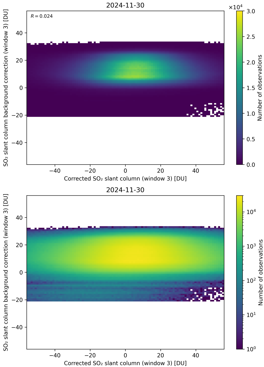
Figure 255: Scatter density plot of “Corrected SO 2 slant column (window 3)” against “SO 2 slant column background correction (window 3)” for 2024-11-30 to 2024-12-01.
