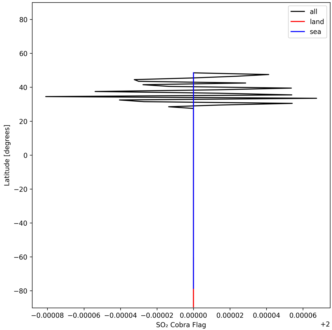
Figure 49: Zonal average of "SO 2 Cobra Flag" for 2024-11-30 to 2024-12-01.
