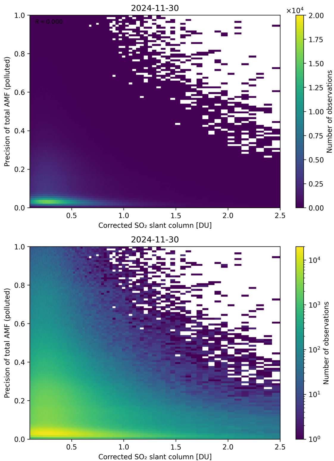
Figure 243: Scatter density plot of “Corrected SO 2 slant column” against “Precision of total AMF (polluted)” for 2024-11-30 to 2024-12-01.
