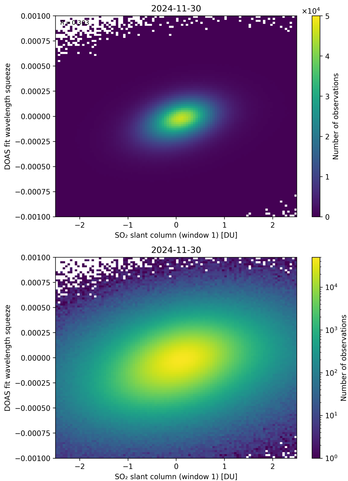
Figure 266: Scatter density plot of “SO 2 slant column (window 1)” against “DOAS fit wavelength squeeze” for 2024-11-30 to 2024-12-01.
