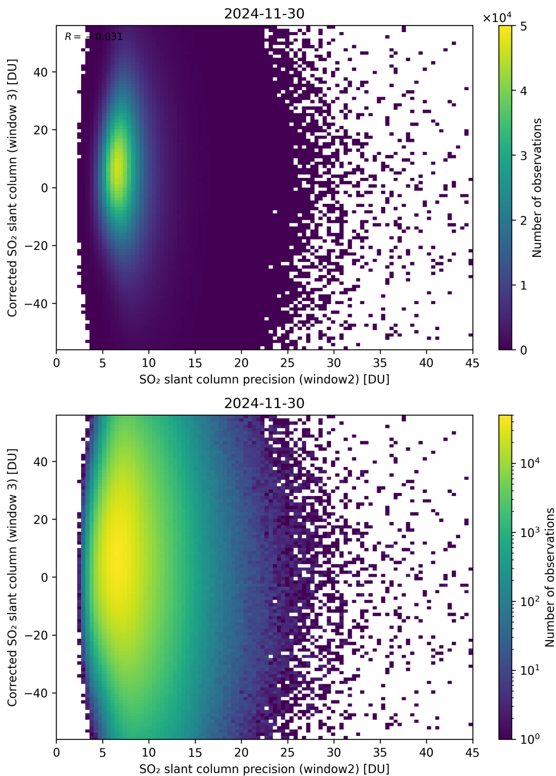
Figure 298: Scatter density plot of “SO 2 slant column precision (window2)” against “Corrected SO 2 slant column (window 3)” for 2024-11-30 to 2024-12-01.
