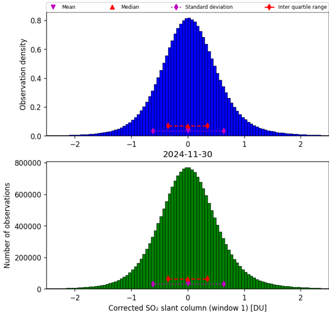
Figure 65: Histogram of “Corrected SO 2 slant column (window 1)” for 2024-11-30 to 2024-12-01
