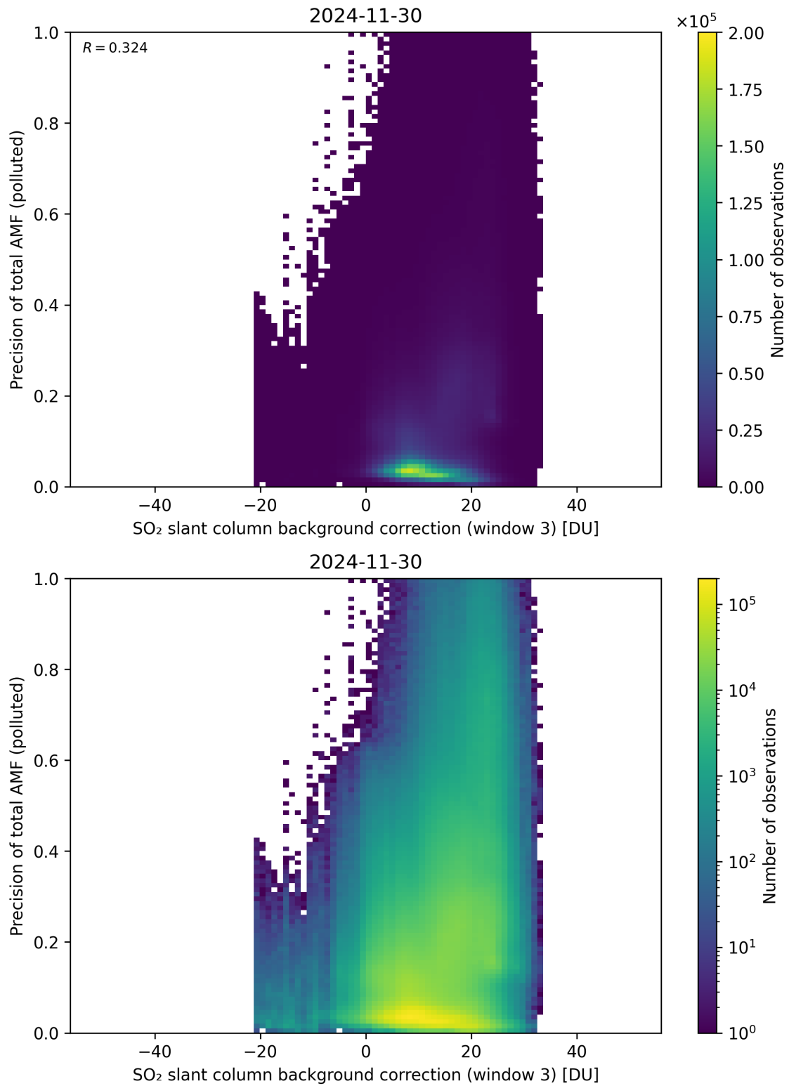
Figure 137: Scatter density plot of “SO 2 slant column background correction (window 3)” against “Precision of total AMF (polluted)” for 2024-11-30 to 2024-12-01.
