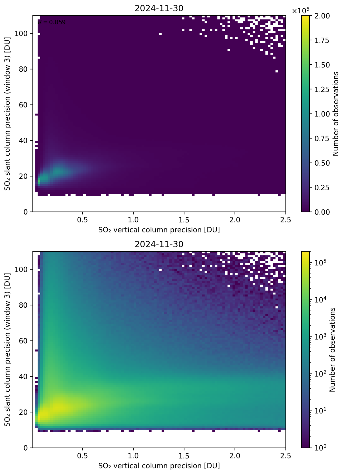
Figure 345: Scatter density plot of “SO 2 vertical column precision” against “SO 2 slant column precision (window 3)” for 2024-11-30 to 2024-12-01.
