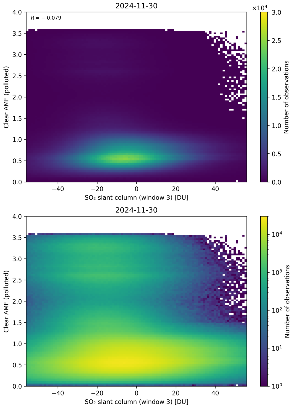
Figure 315: Scatter density plot of “SO 2 slant column (window 3)” against “Clear AMF (polluted)” for 2024-11-30 to 2024-12-01.
