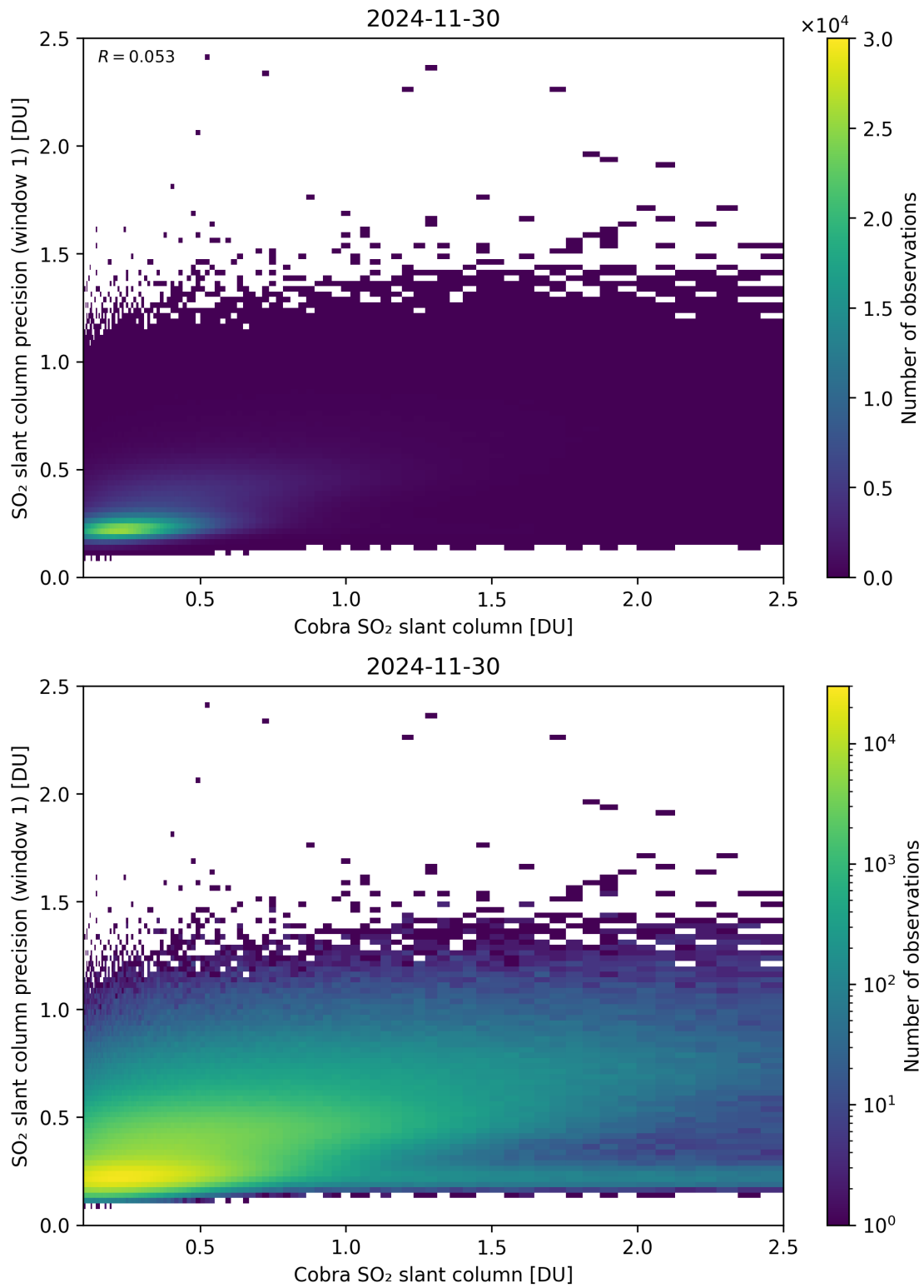
Figure 220: Scatter density plot of “Cobra SO 2 slant column” against “SO 2 slant column precision (window 1)” for 2024-11-30 to 2024-12-01.
