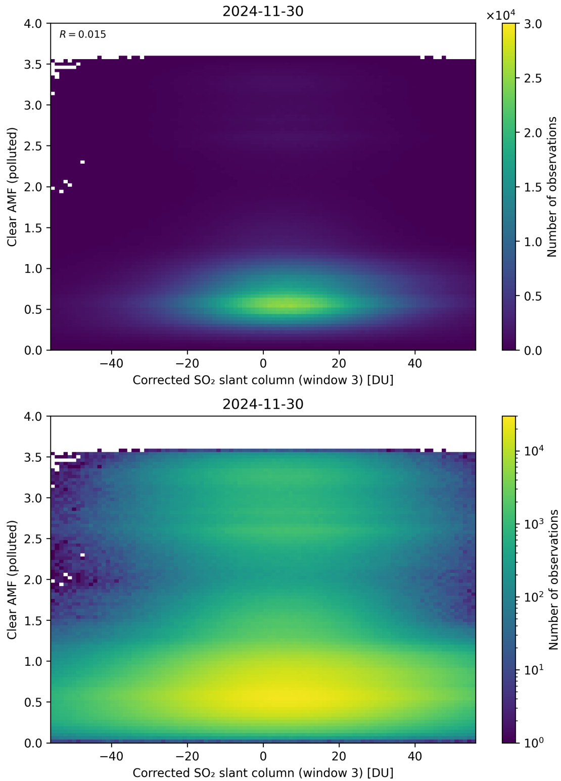
Figure 259: Scatter density plot of “Corrected SO 2 slant column (window 3)” against “Clear AMF (polluted)” for 2024-11-30 to 2024-12-01.
