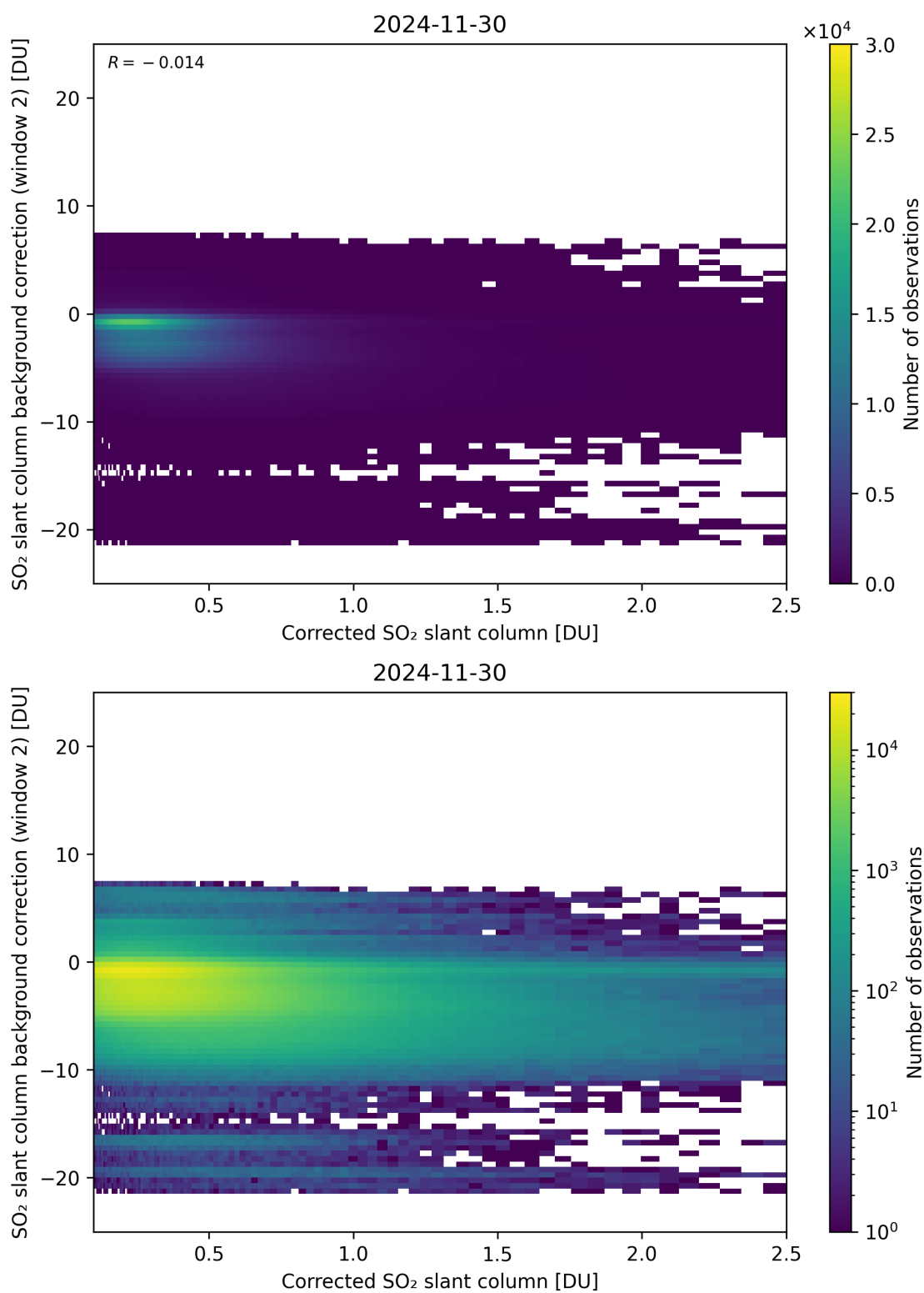
Figure 227: Scatter density plot of “Corrected SO 2 slant column” against “SO 2 slant column background correction (window 2)” for 2024-11-30 to 2024-12-01.
