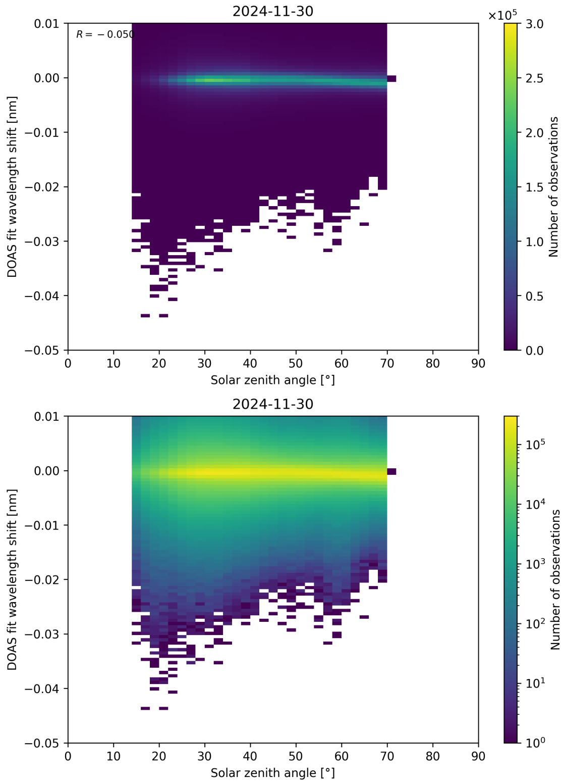
Figure 174: Scatter density plot of “Solar zenith angle” against “DOAS fit wavelength shift” for 2024-11-30 to 2024-12-01.
