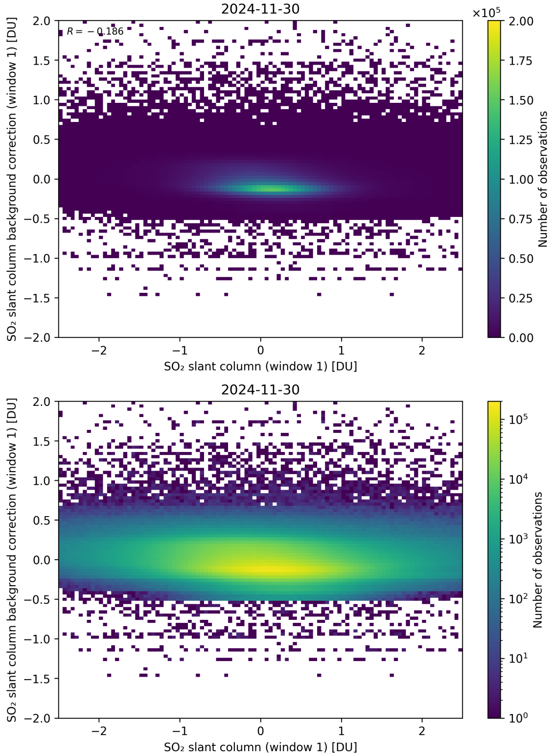
Figure 262: Scatter density plot of “SO 2 slant column (window 1)” against “SO 2 slant column background correction (window 1)” for 2024-11-30 to 2024-12-01.
