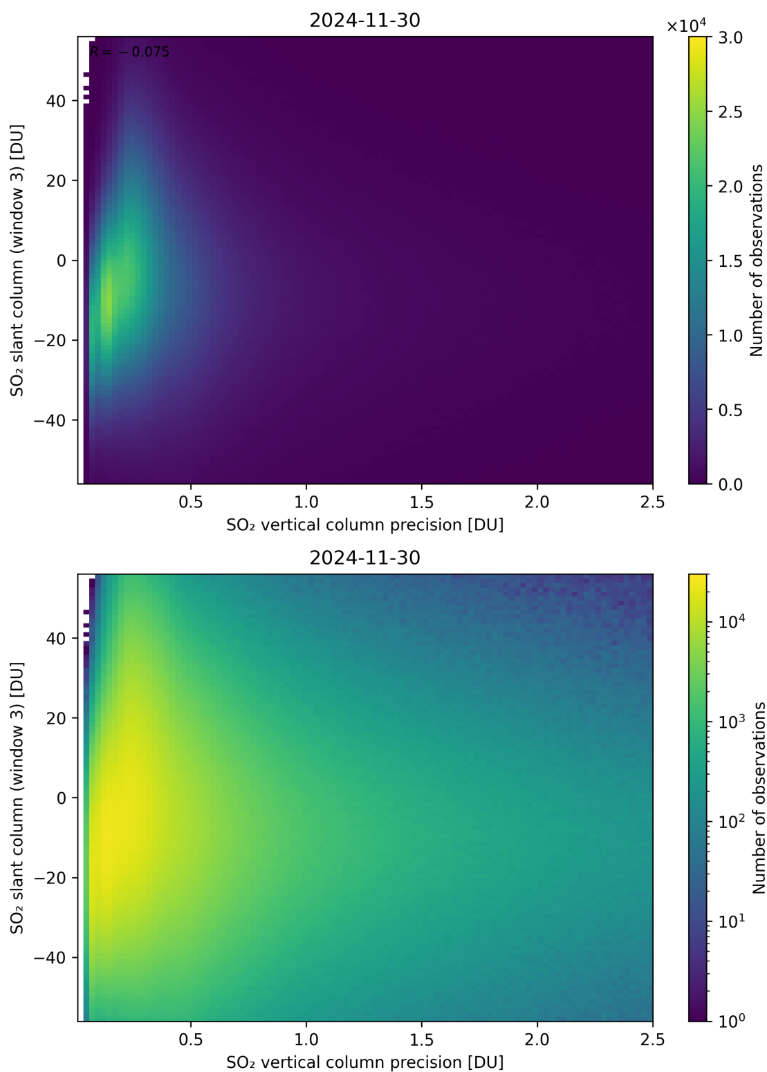
Figure 344: Scatter density plot of “SO 2 vertical column precision” against “SO 2 slant column (window 3)” for 2024-11-30 to 2024-12-01.
