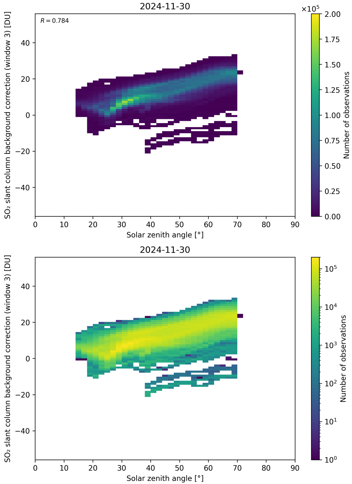
Figure 173: Scatter density plot of “Solar zenith angle” against “SO 2 slant column background correction (window 3)” for 2024-11-30 to 2024-12-01.
