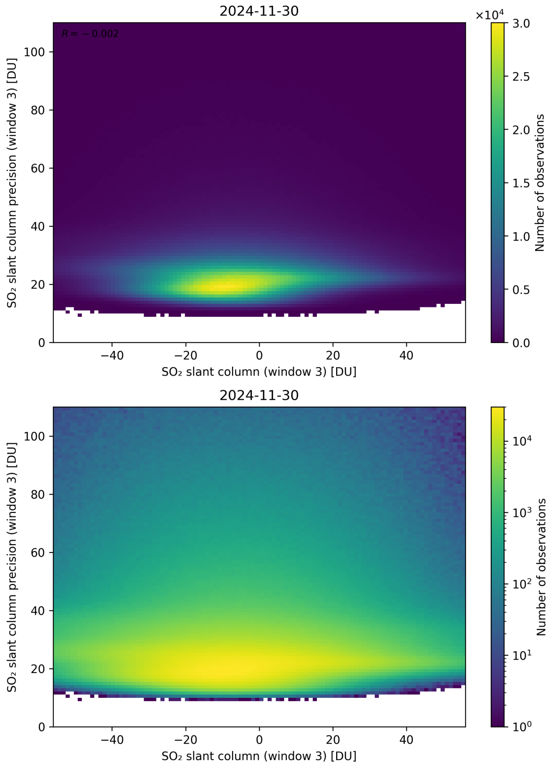
Figure 317: Scatter density plot of “SO 2 slant column (window 3)” against “SO 2 slant column precision (window 3)” for 2024-11-30 to 2024-12-01.
