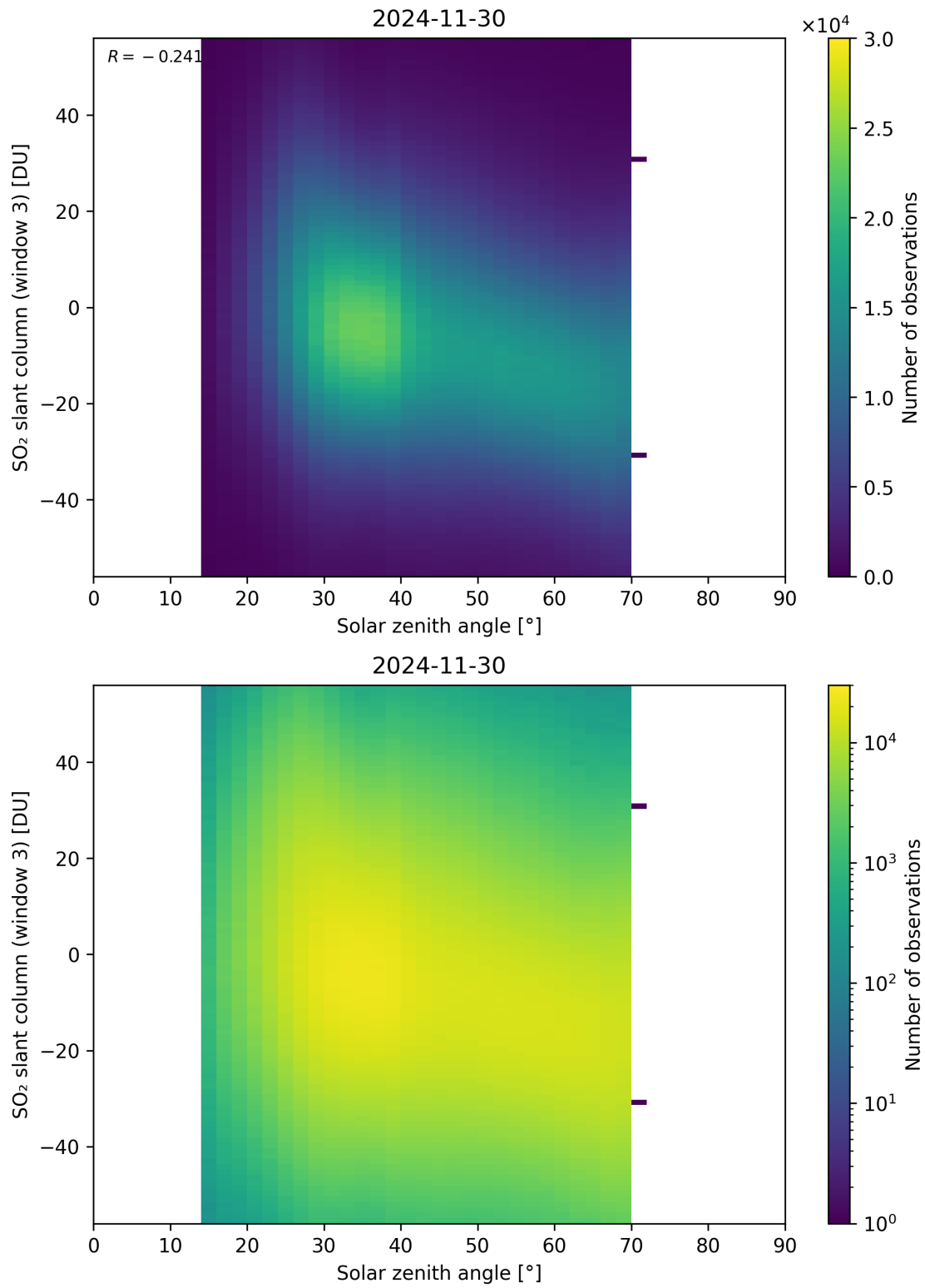
Figure 187: Scatter density plot of “Solar zenith angle” against “SO 2 slant column (window 3)” for 2024-11-30 to 2024-12-01.
