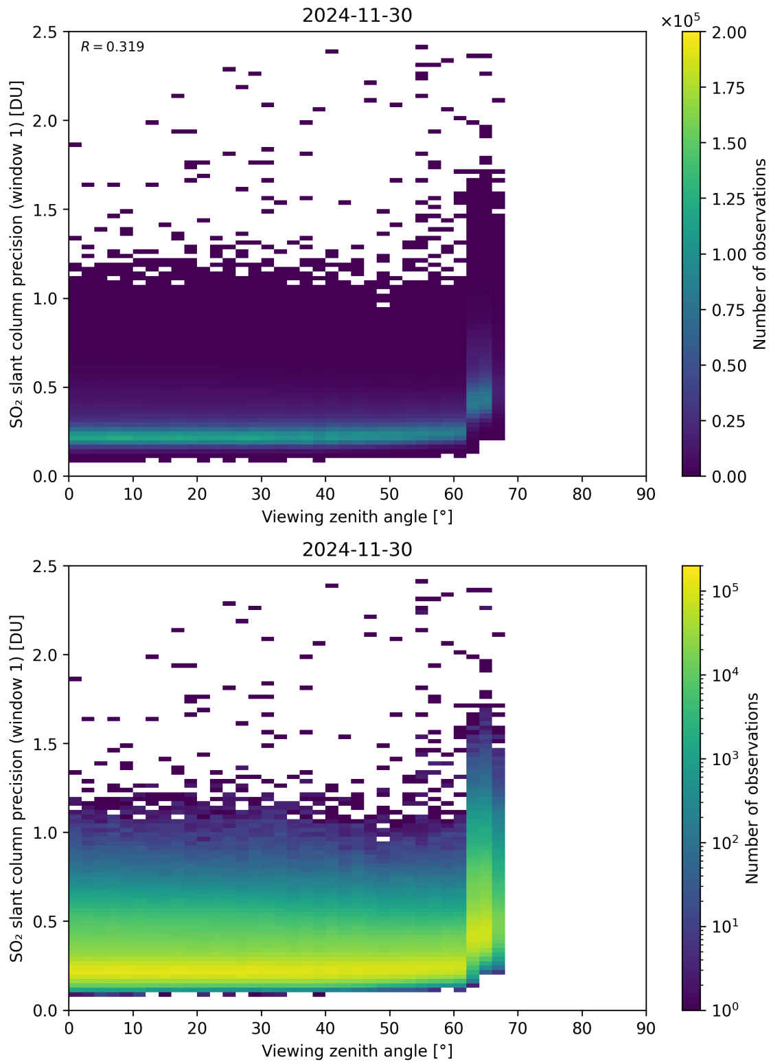
Figure 377: Scatter density plot of “Viewing zenith angle” against “SO 2 slant column precision (window 1)” for 2024-11-30 to 2024-12-01.
