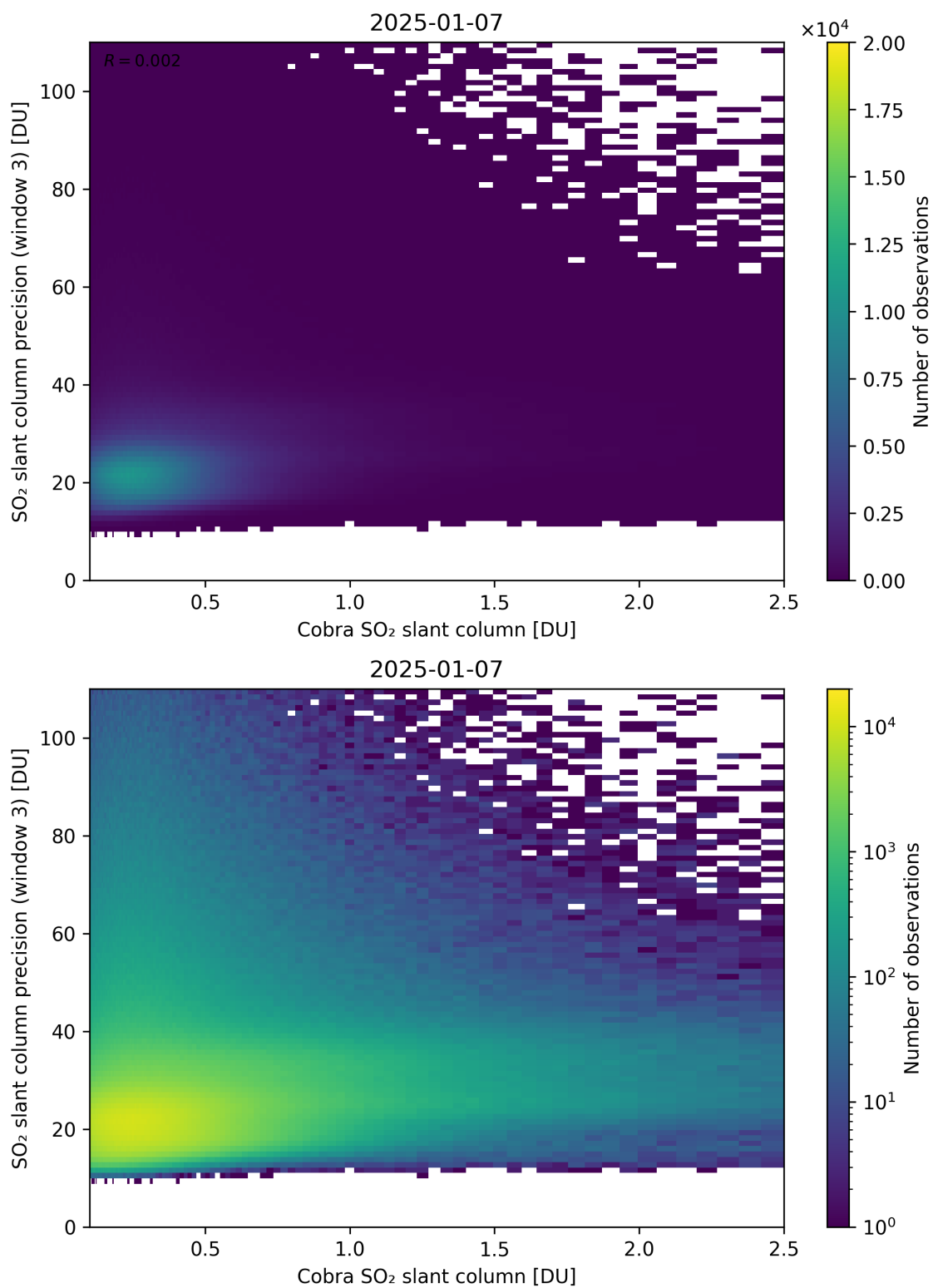
Figure 223: Scatter density plot of “Cobra SO 2 slant column” against “SO 2 slant column precision (window 3)” for 2025-01-07 to 2025-01-08.
