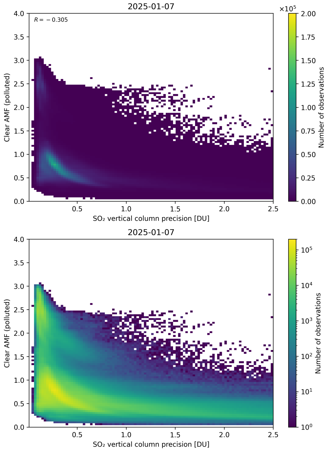
Figure 335: Scatter density plot of “SO 2 vertical column precision” against “Clear AMF (polluted)” for 2025-01-07 to 2025-01-08.
