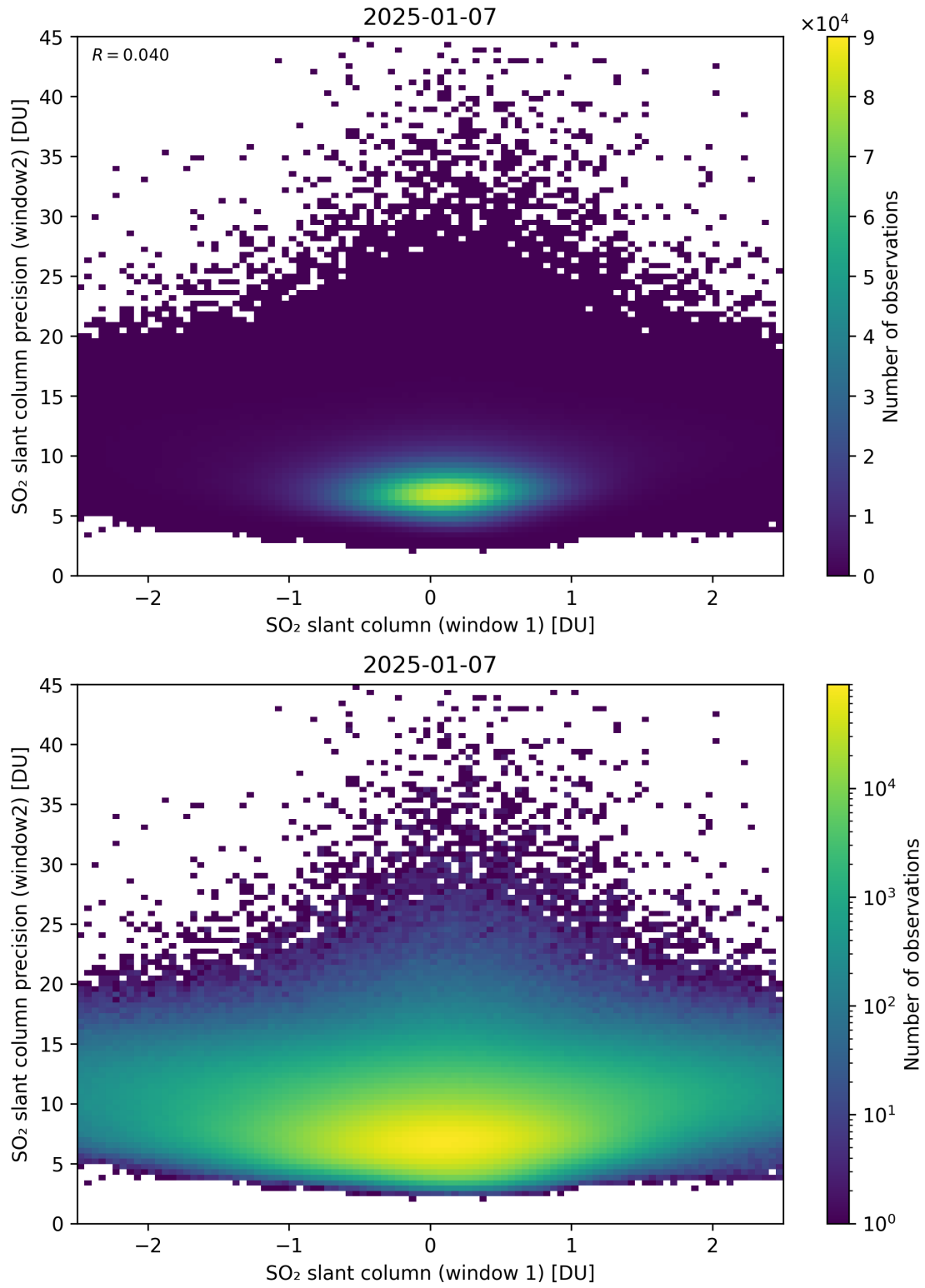
Figure 286: Scatter density plot of “SO 2 slant column (window 1)” against “SO 2 slant column precision (window2)” for 2025-01-07 to 2025-01-08.
