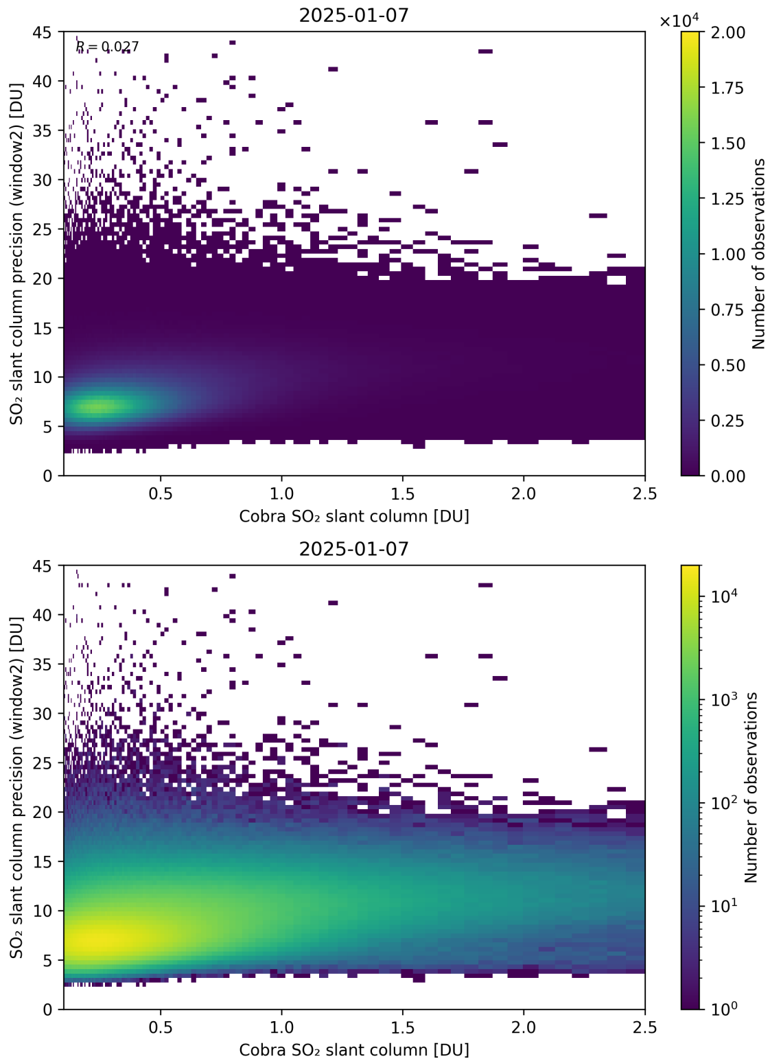
Figure 221: Scatter density plot of “Cobra SO 2 slant column” against “SO 2 slant column precision (window2)” for 2025-01-07 to 2025-01-08.
