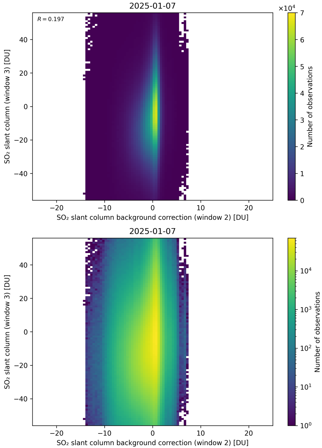
Figure 128: Scatter density plot of “SO 2 slant column background correction (window 2)” against “SO 2 slant column (window 3)” for 2025-01-07 to 2025-01-08.
