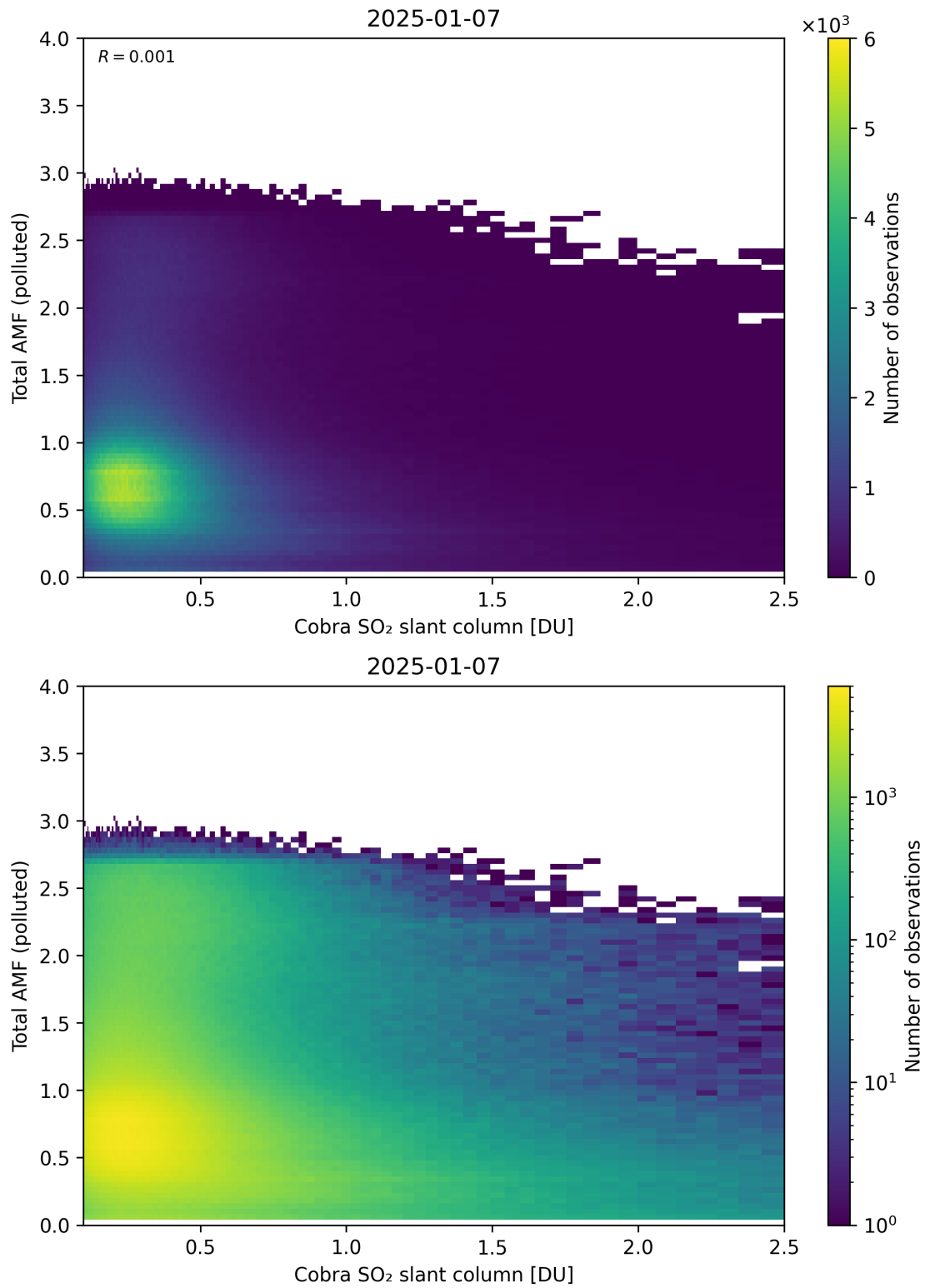
Figure 224: Scatter density plot of “Cobra SO 2 slant column” against “Total AMF (polluted)” for 2025-01-07 to 2025-01-08.
