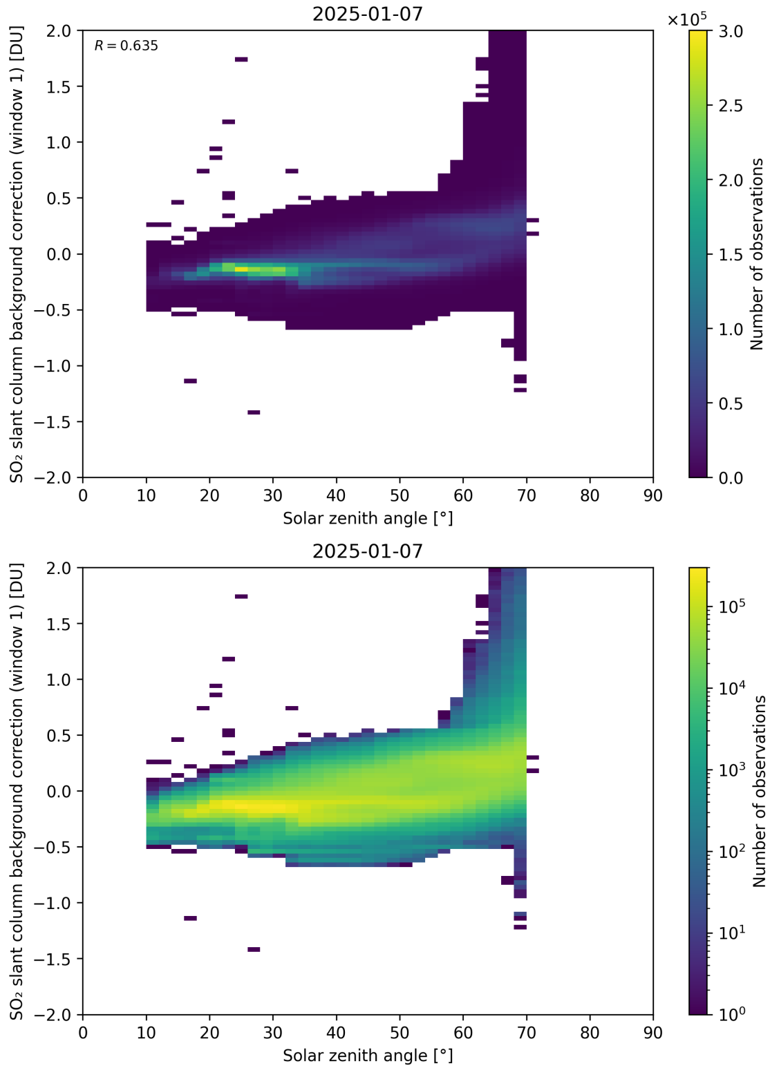
Figure 171: Scatter density plot of “Solar zenith angle” against “SO 2 slant column background correction (window 1)” for 2025-01-07 to 2025-01-08.
