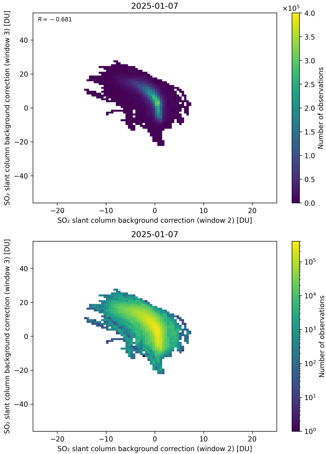
Figure 122: Scatter density plot of “SO 2 slant column background correction (window 2)” against “SO 2 slant column background correction (window 3)” for 2025-01-07 to 2025-01-08.
