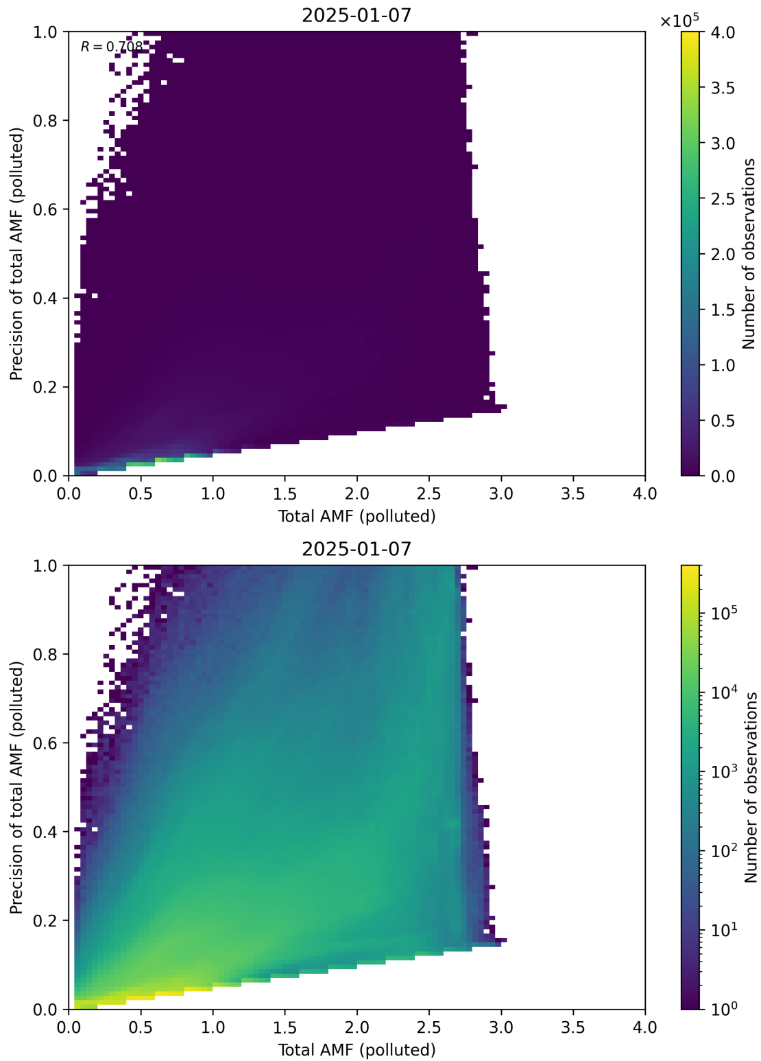
Figure 322: Scatter density plot of “Total AMF (polluted)” against “Precision of total AMF (polluted)” for 2025-01-07 to 2025-01-08.
