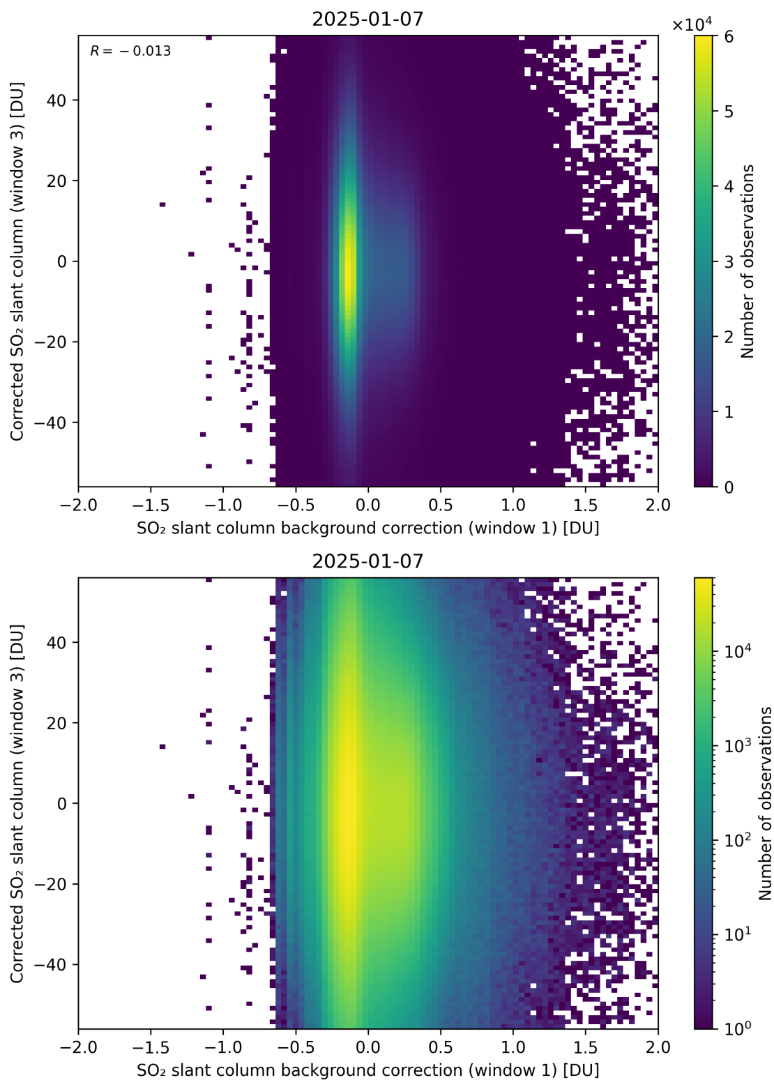
Figure 116: Scatter density plot of “SO 2 slant column background correction (window 1)” against “Corrected SO 2 slant column (window 3)” for 2025-01-07 to 2025-01-08.
