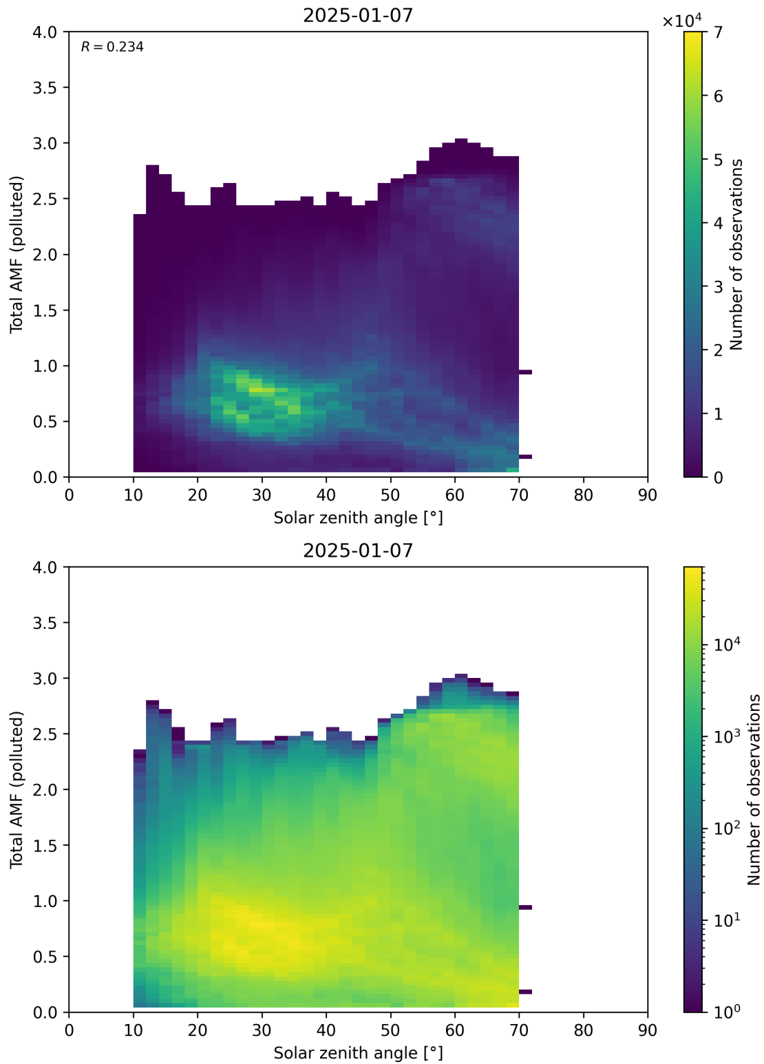
Figure 189: Scatter density plot of “Solar zenith angle” against “Total AMF (polluted)” for 2025-01-07 to 2025-01-08.
