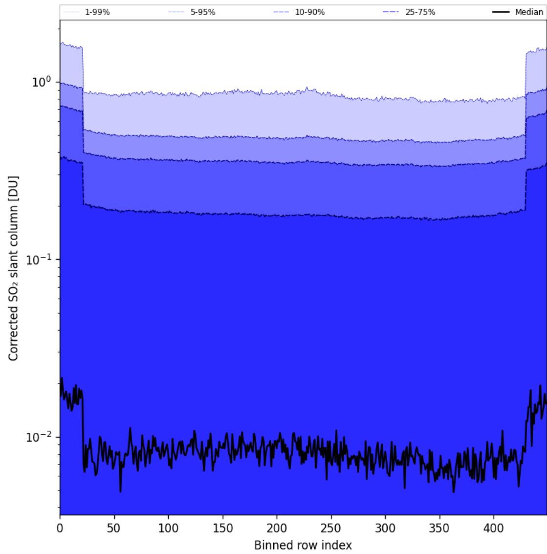
Figure 86: Along track statistics of “Corrected SO 2 slant column” for 2025-01-07 to 2025-01-08
