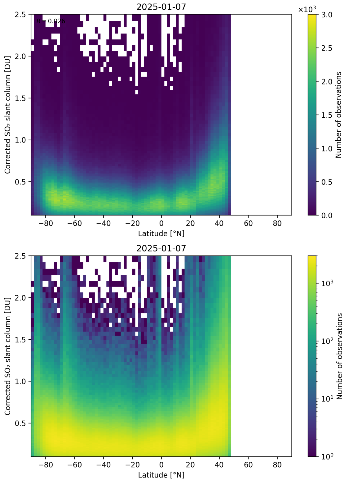
Figure 159: Scatter density plot of “Latitude” against “Corrected SO 2 slant column” for 2025-01-07 to 2025-01-08.
