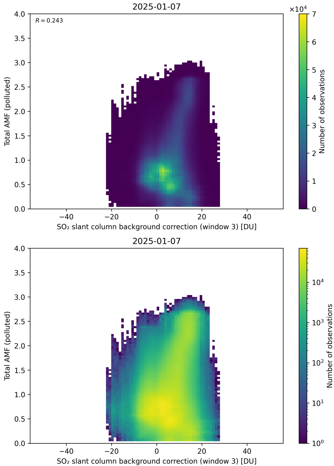
Figure 136: Scatter density plot of “SO 2 slant column background correction (window 3)” against “Total AMF (polluted)” for 2025-01-07 to 2025-01-08.
