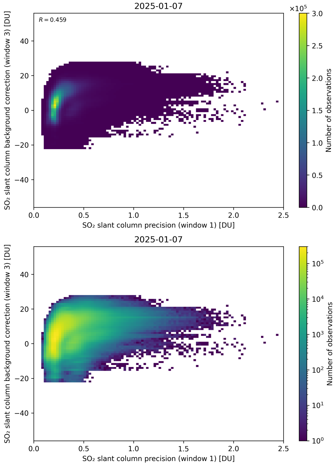
Figure 270: Scatter density plot of “SO 2 slant column precision (window 1)” against “SO 2 slant column background correction (window 3)” for 2025-01-07 to 2025-01-08.
