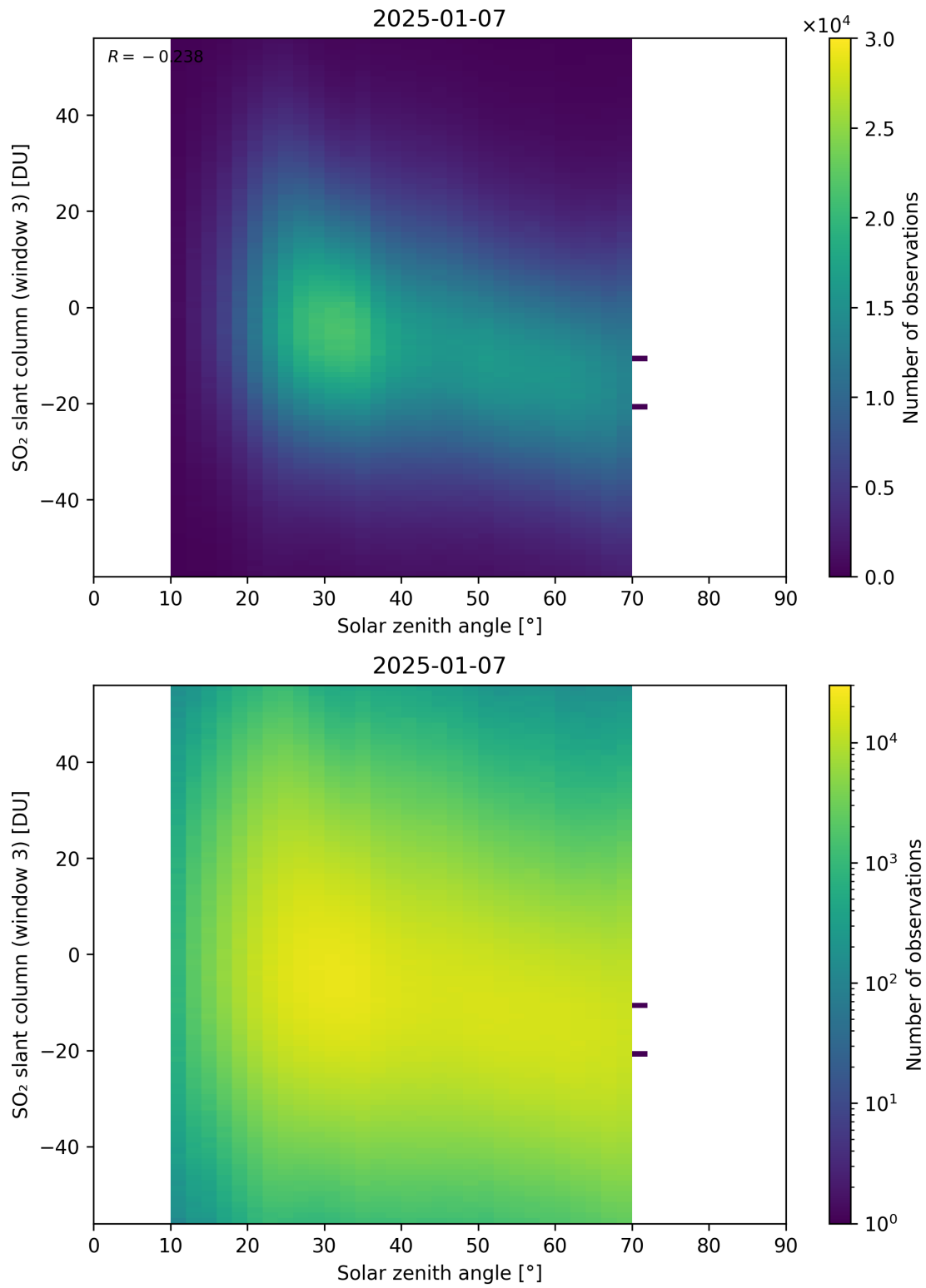
Figure 187: Scatter density plot of “Solar zenith angle” against “SO 2 slant column (window 3)” for 2025-01-07 to 2025-01-08.
