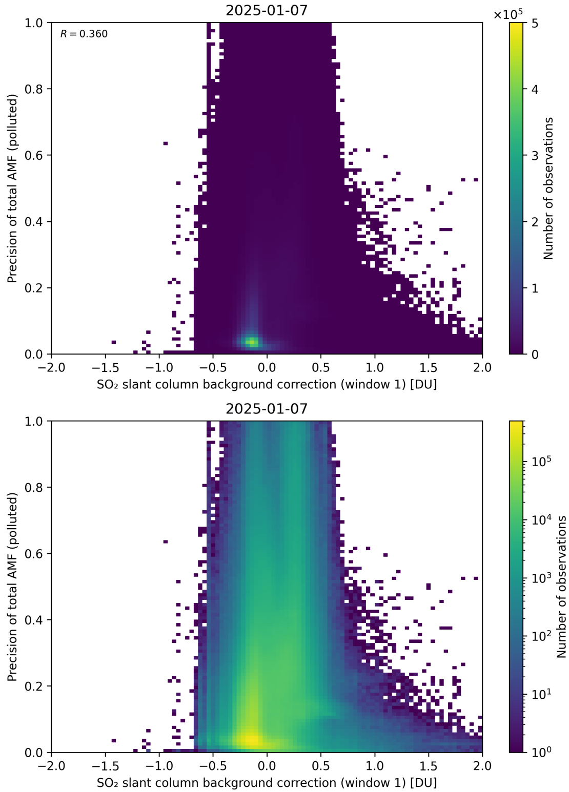
Figure 121: Scatter density plot of “SO 2 slant column background correction (window 1)” against “Precision of total AMF (polluted)” for 2025-01-07 to 2025-01-08.
