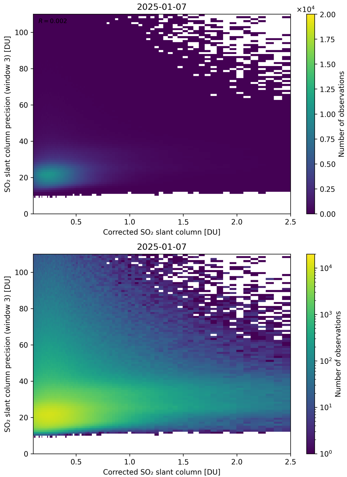
Figure 241: Scatter density plot of “Corrected SO 2 slant column” against “SO 2 slant column precision (window 3)” for 2025-01-07 to 2025-01-08.
