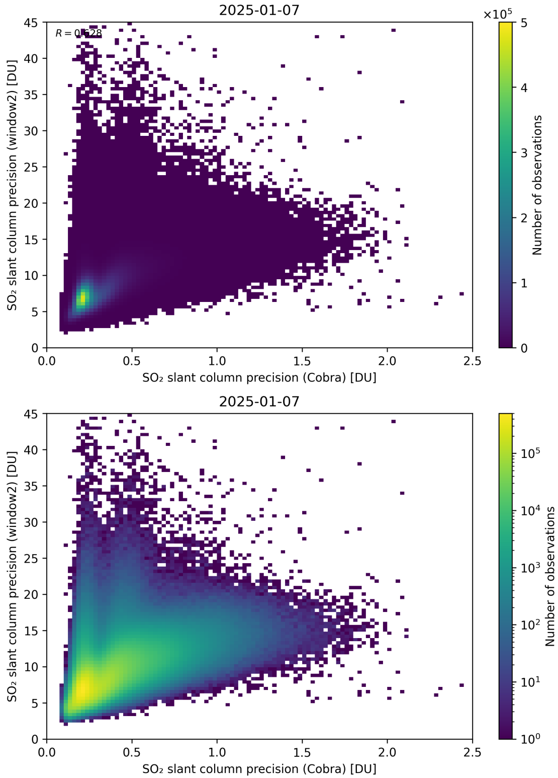
Figure 210: Scatter density plot of “SO 2 slant column precision (Cobra)” against “SO 2 slant column precision (window2)” for 2025-01-07 to 2025-01-08.
