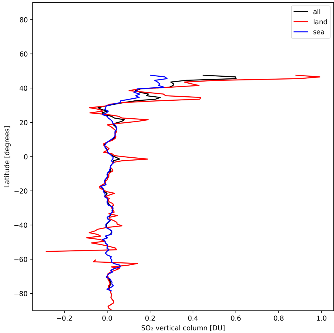
Figure 32: Zonal average of “SO 2 vertical column” for 2025-01-07 to 2025-01-08.
