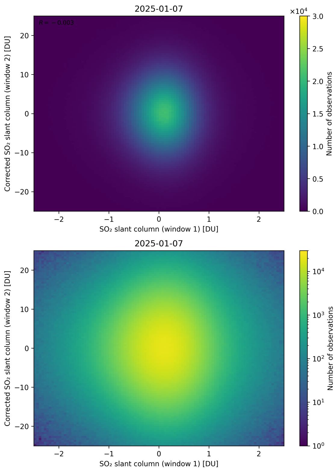
Figure 283: Scatter density plot of “SO 2 slant column (window 1)” against “Corrected SO 2 slant column (window 2)” for 2025-01-07 to 2025-01-08.
