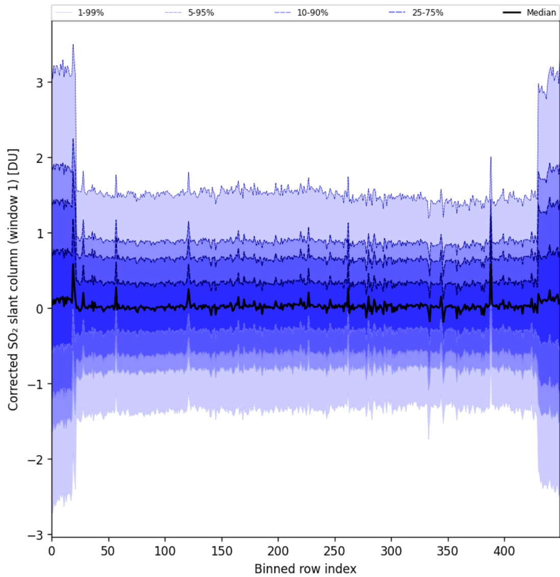
Figure 91: Along track statistics of “Corrected SO 2 slant column (window 1)” for 2025-01-07 to 2025-01-08
