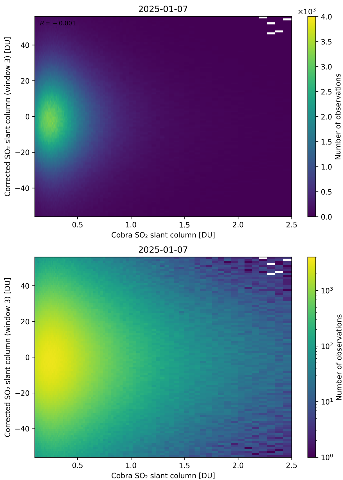
Figure 218: Scatter density plot of “Cobra SO 2 slant column” against “Corrected SO 2 slant column (window 3)” for 2025-01-07 to 2025-01-08.
