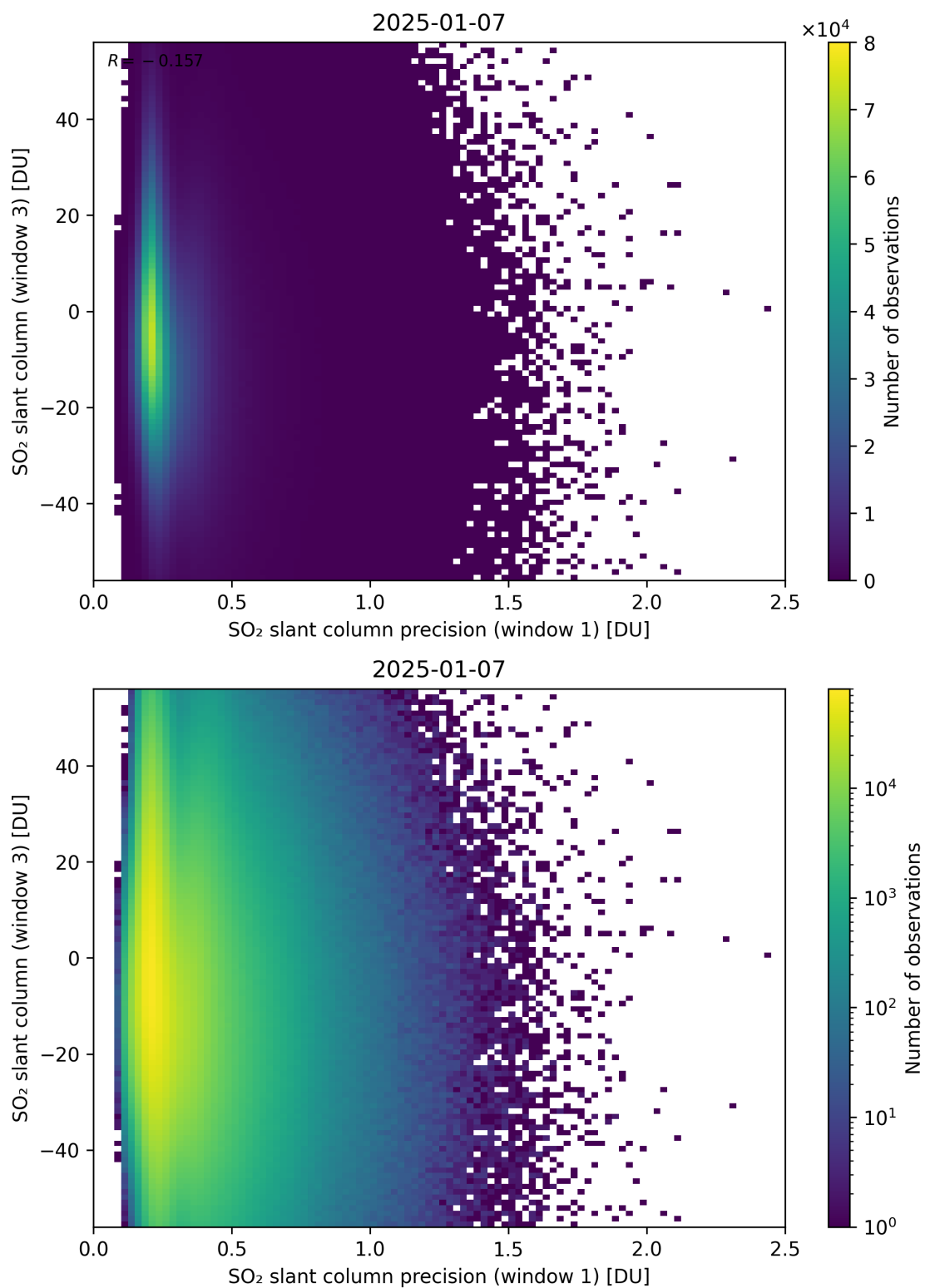
Figure 278: Scatter density plot of “SO 2 slant column precision (window 1)” against “SO 2 slant column (window 3)” for 2025-01-07 to 2025-01-08.
