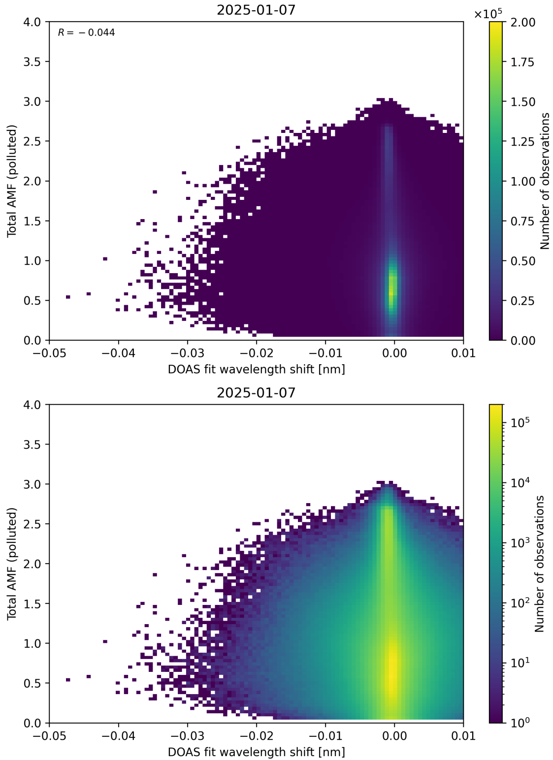
Figure 141: Scatter density plot of “DOAS fit wavelength shift” against “Total AMF (polluted)” for 2025-01-07 to 2025-01-08.
