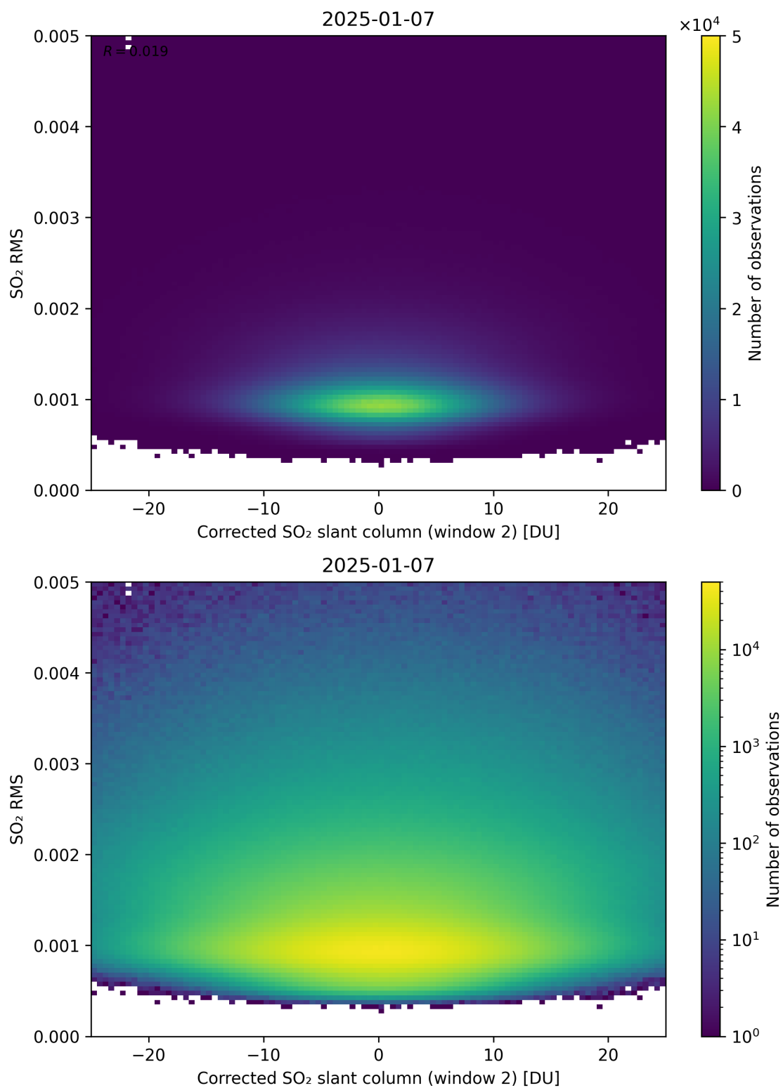
Figure 248: Scatter density plot of “Corrected SO 2 slant column (window 2)” against “SO 2 RMS” for 2025-01-07 to 2025-01-08.
