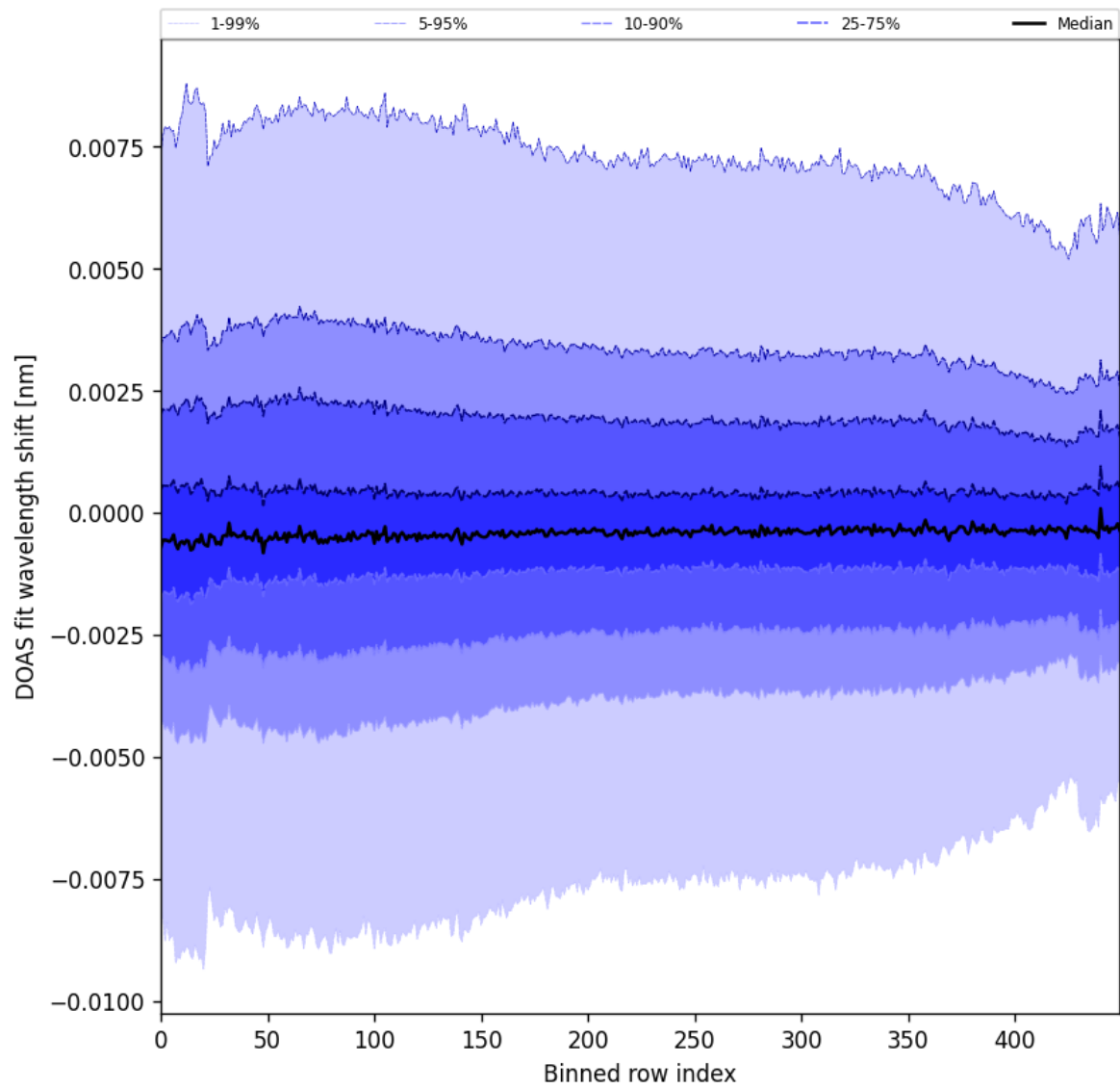
Figure 102: Along track statistics of “DOAS fit wavelength shift” for 2025-01-07 to 2025-01-08
