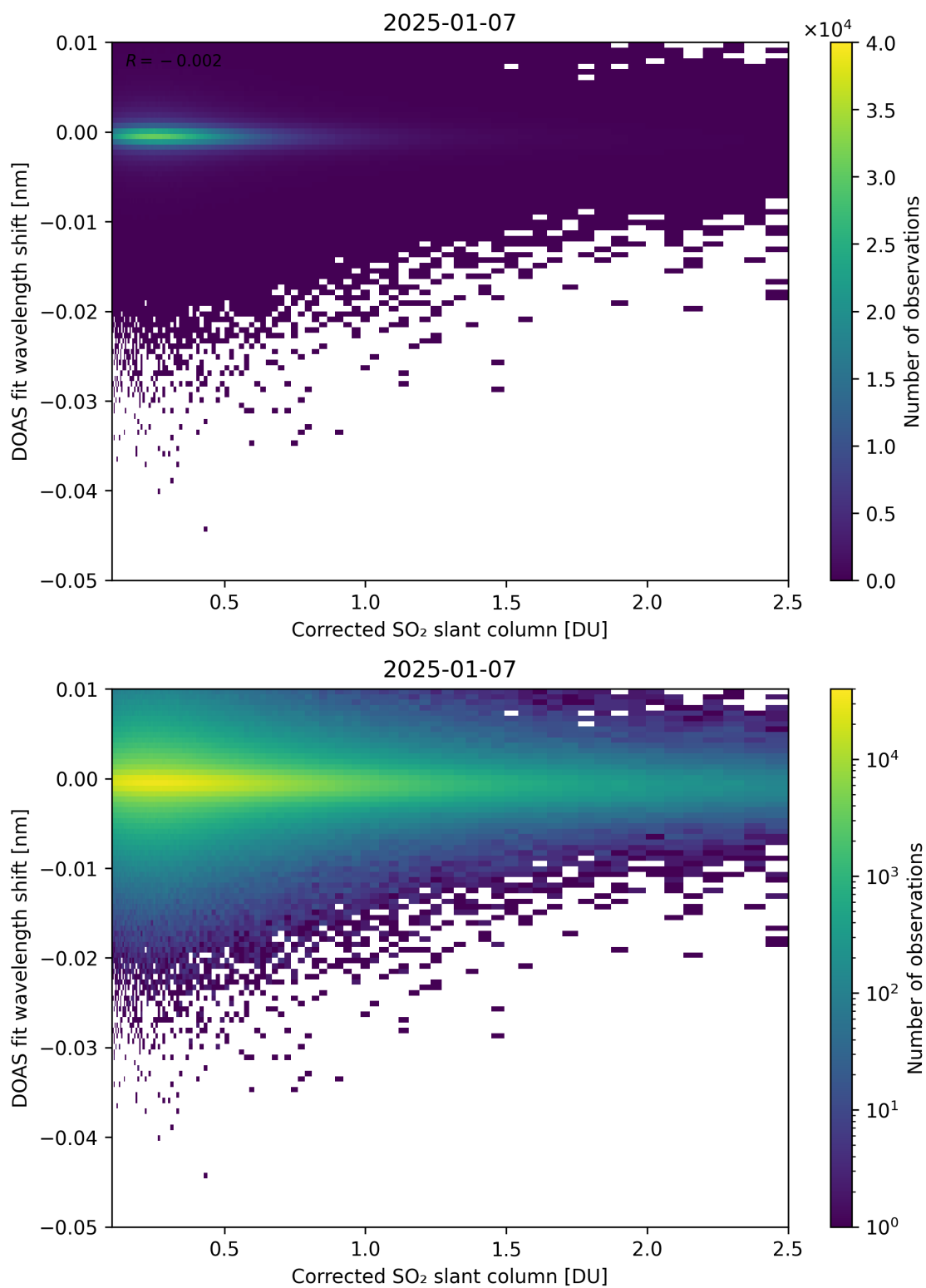
Figure 229: Scatter density plot of “Corrected SO 2 slant column” against “DOAS fit wavelength shift” for 2025-01-07 to 2025-01-08.
