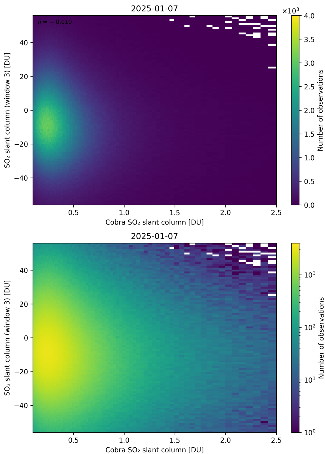
Figure 222: Scatter density plot of “Cobra SO 2 slant column” against “SO 2 slant column (window 3)” for 2025-01-07 to 2025-01-08.
