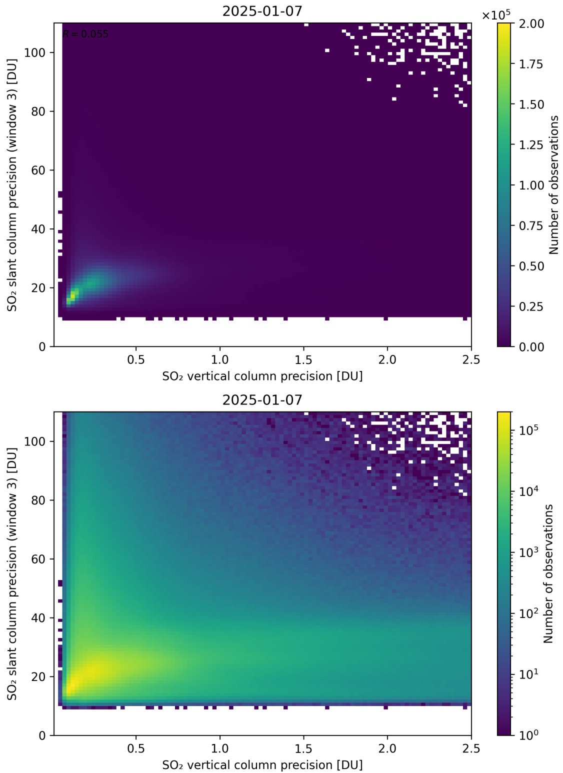
Figure 345: Scatter density plot of “SO 2 vertical column precision” against “SO 2 slant column precision (window 3)” for 2025-01-07 to 2025-01-08.
