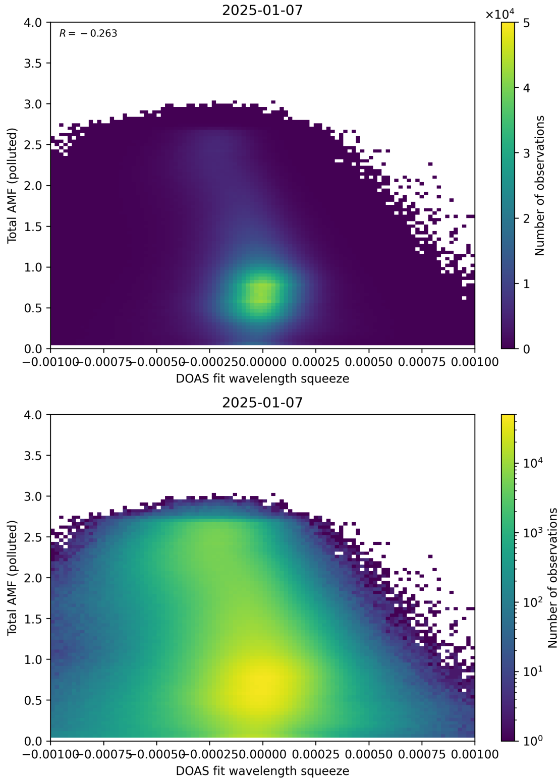
Figure 145: Scatter density plot of “DOAS fit wavelength squeeze” against “Total AMF (polluted)” for 2025-01-07 to 2025-01-08.
