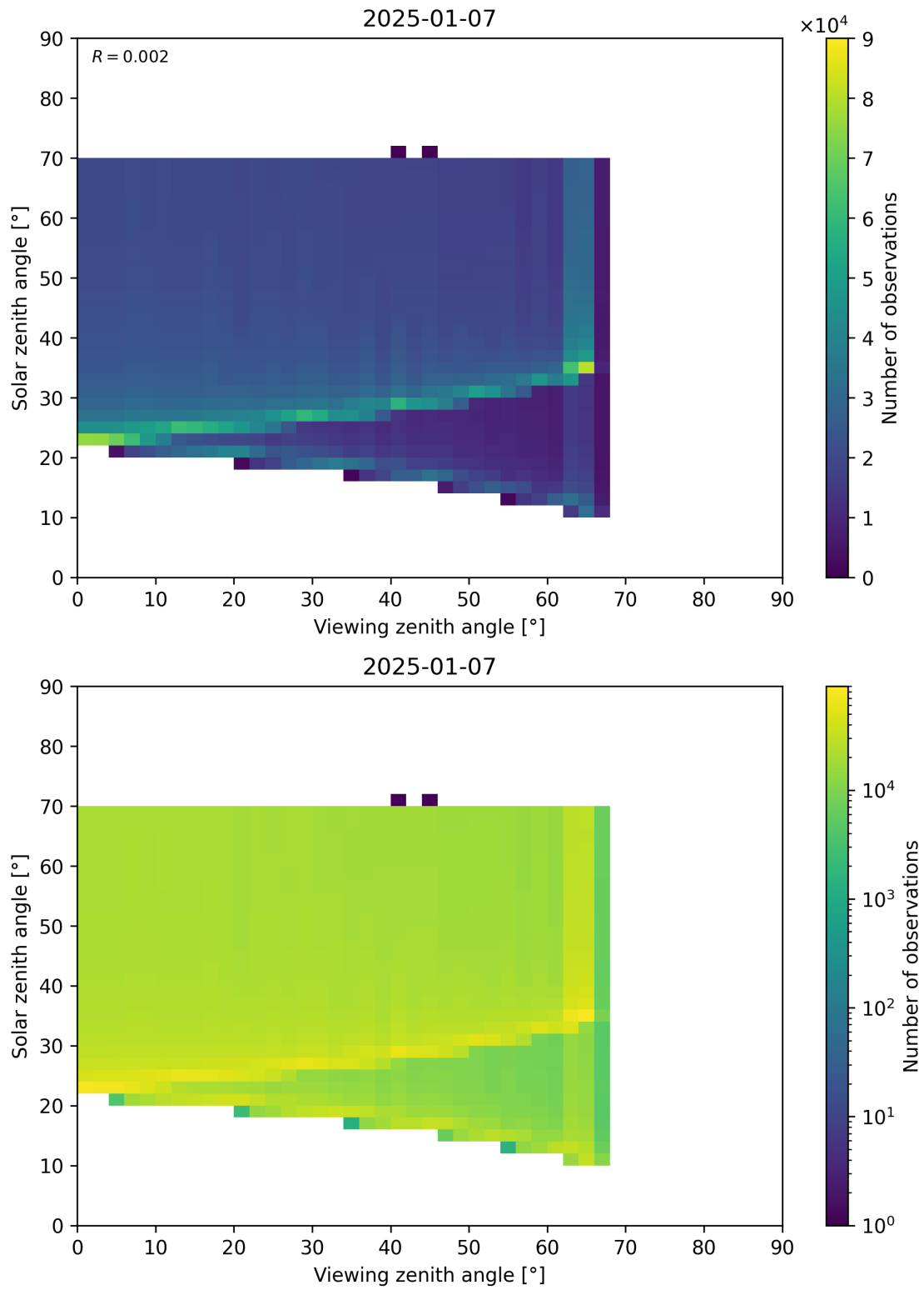
Figure 369: Scatter density plot of “Viewing zenith angle” against “Solar zenith angle” for 2025-01-07 to 2025-01-08.
