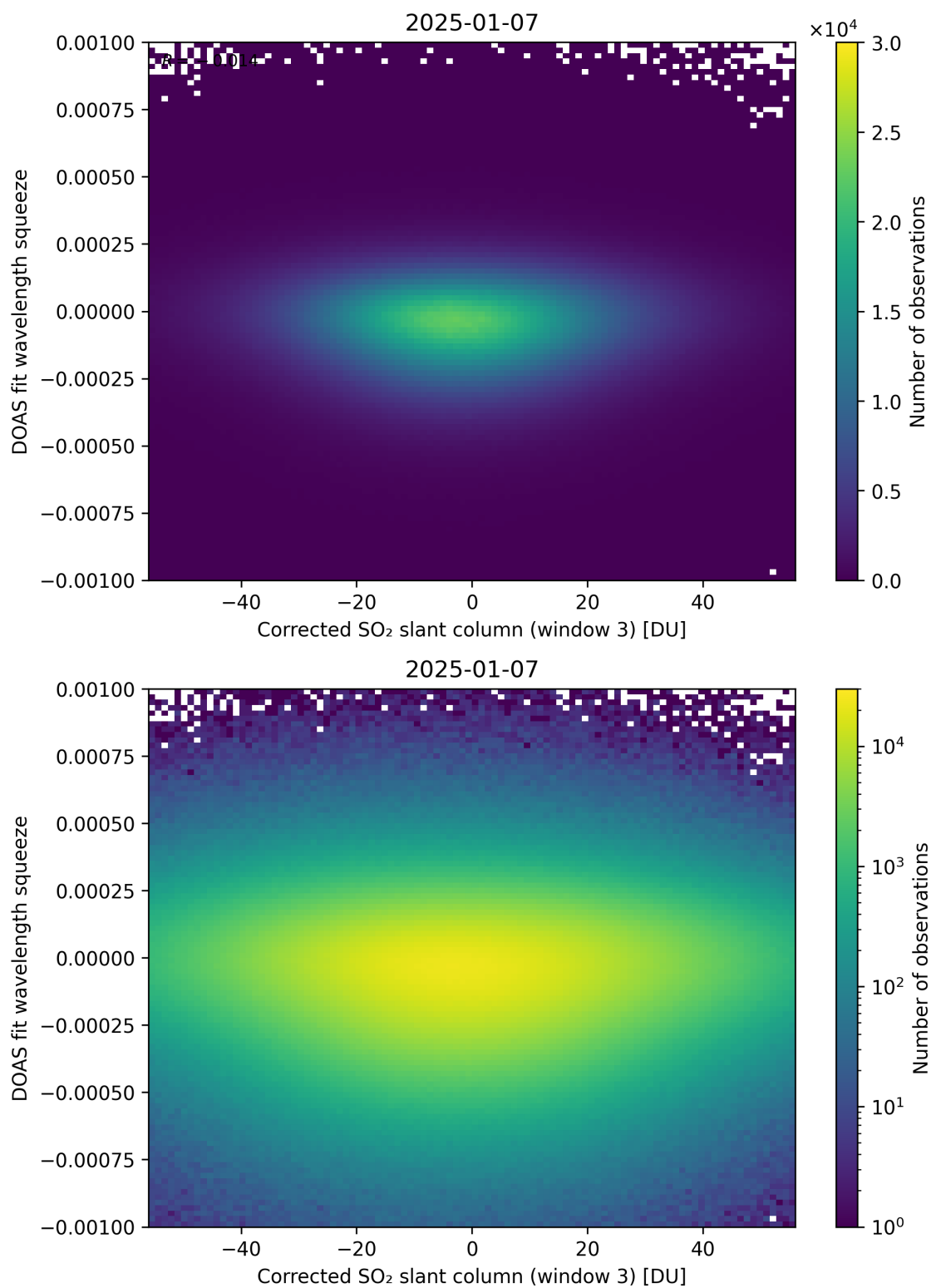
Figure 257: Scatter density plot of “Corrected SO 2 slant column (window 3)” against “DOAS fit wavelength squeeze” for 2025-01-07 to 2025-01-08.
