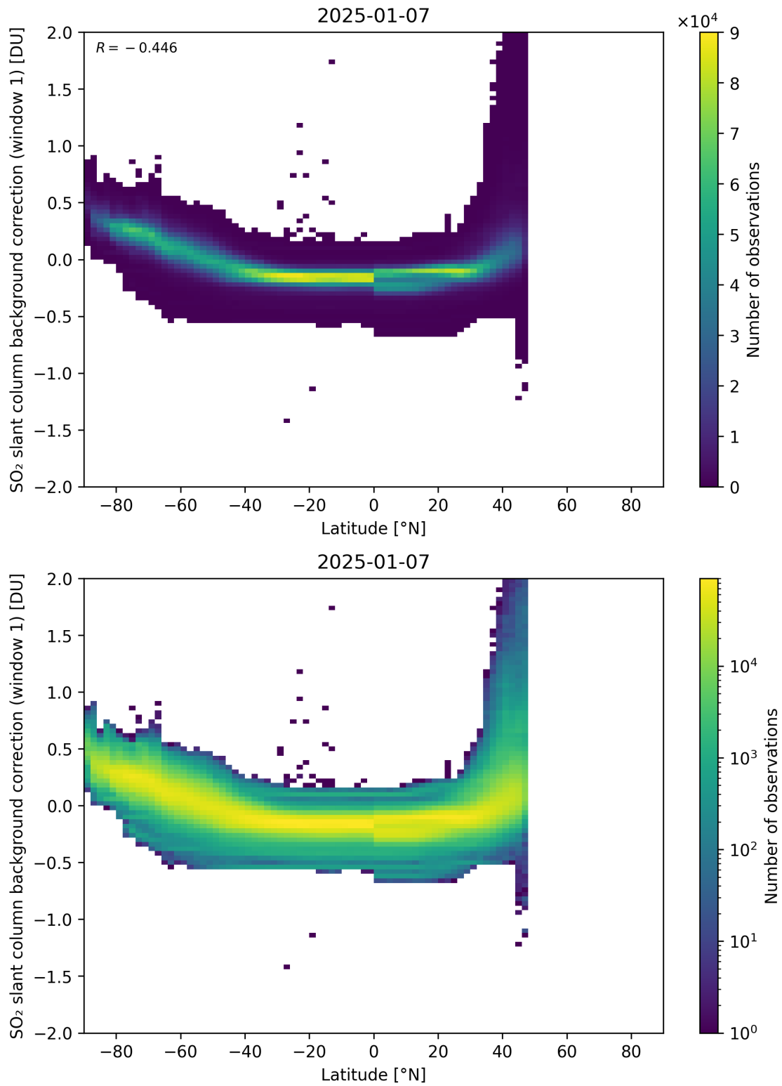
Figure 150: Scatter density plot of “Latitude” against “SO 2 slant column background correction (window 1)” for 2025-01-07 to 2025-01-08.
