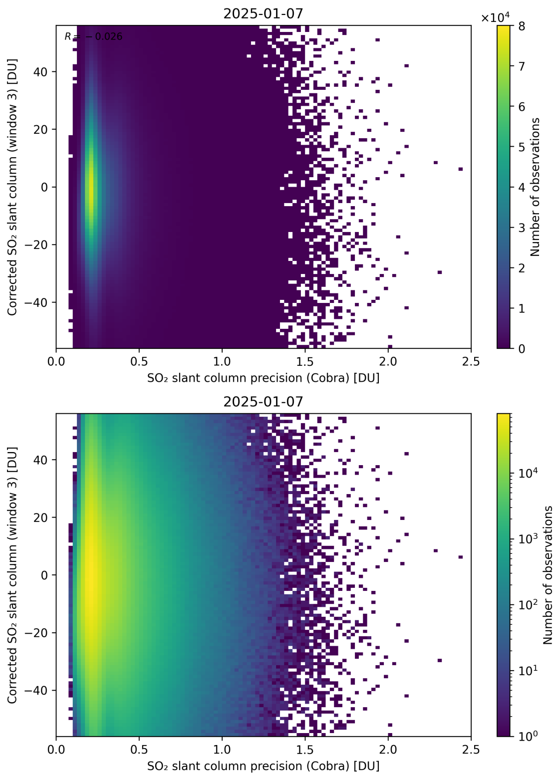
Figure 207: Scatter density plot of “SO 2 slant column precision (Cobra)” against “Corrected SO 2 slant column (window 3)” for 2025-01-07 to 2025-01-08.
