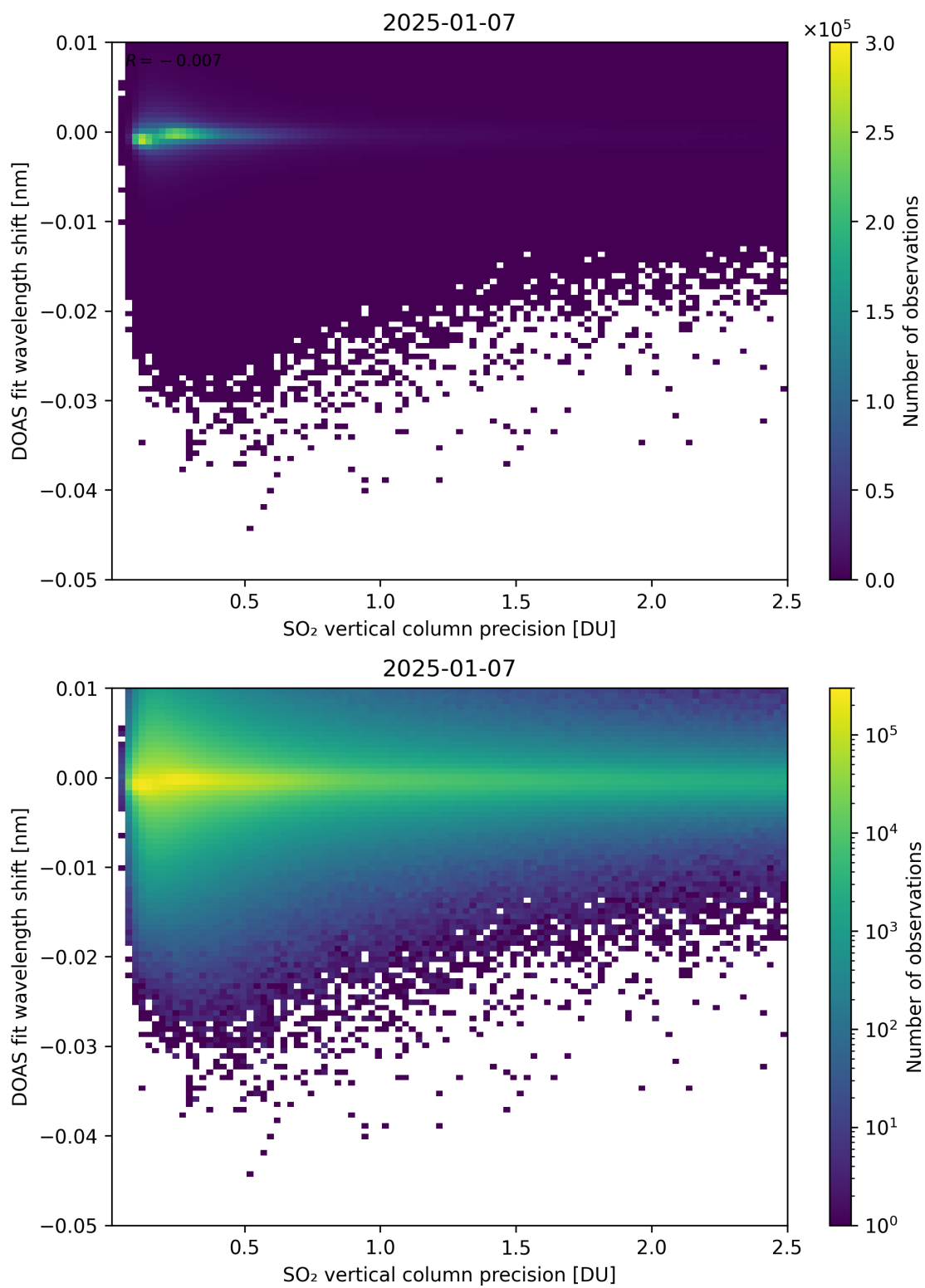
Figure 332: Scatter density plot of “SO 2 vertical column precision” against “DOAS fit wavelength shift” for 2025-01-07 to 2025-01-08.
