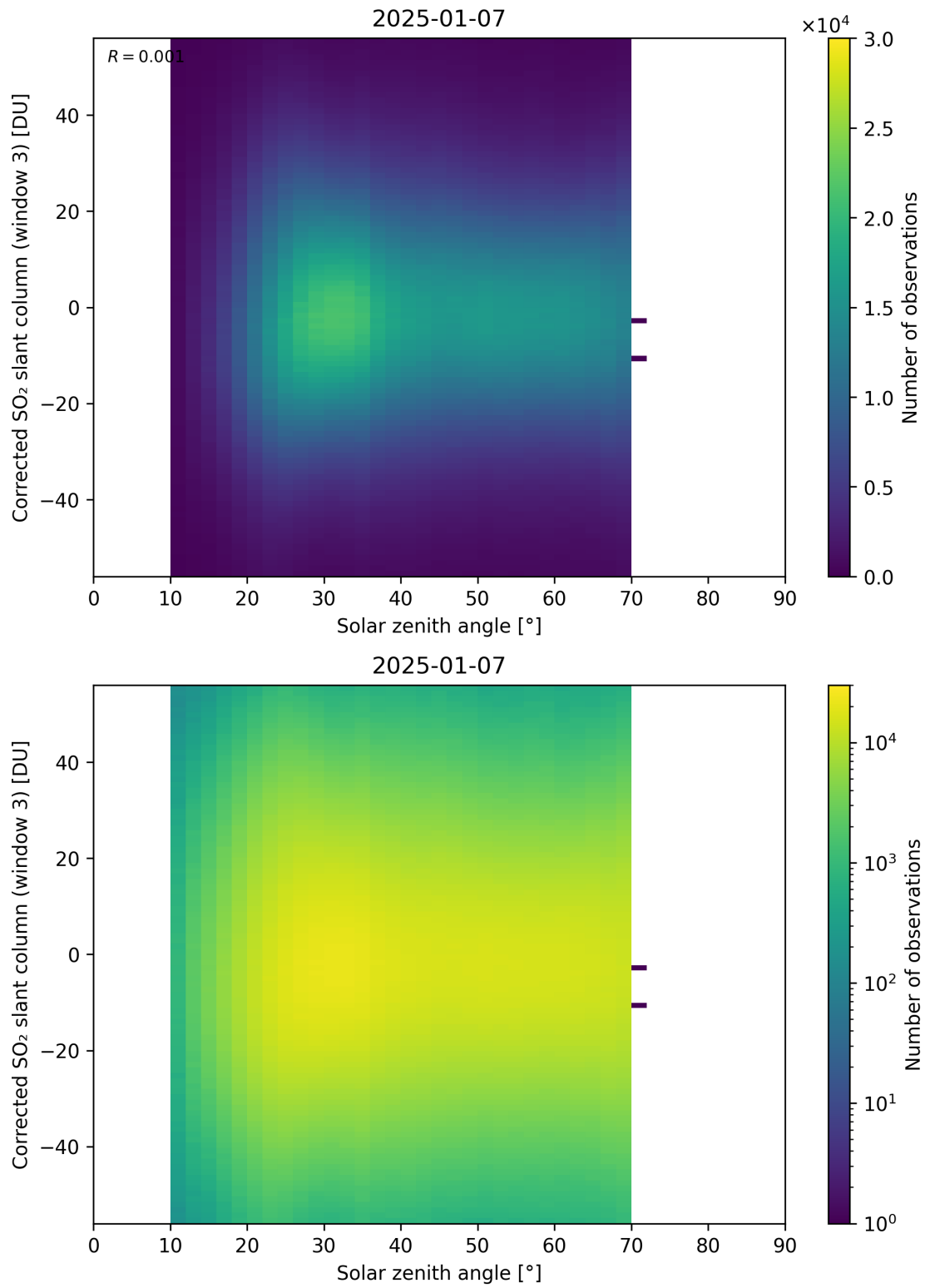
Figure 183: Scatter density plot of “Solar zenith angle” against “Corrected SO 2 slant column (window 3)” for 2025-01-07 to 2025-01-08.
