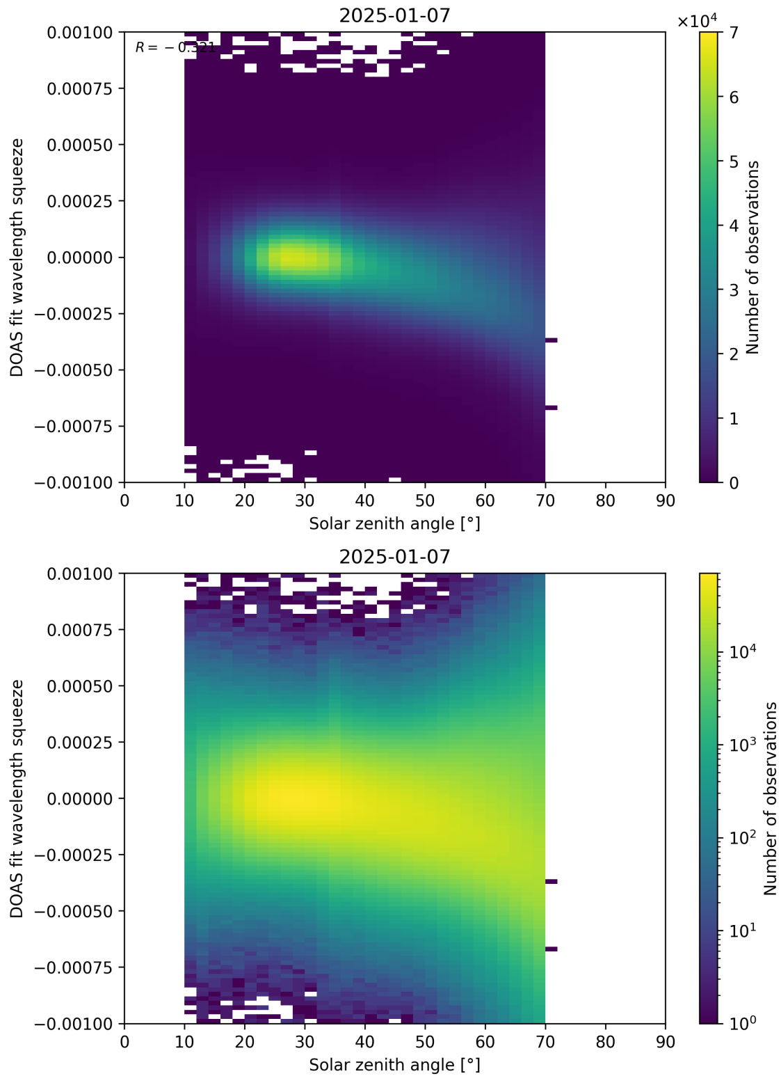
Figure 175: Scatter density plot of “Solar zenith angle” against “DOAS fit wavelength squeeze” for 2025-01-07 to 2025-01-08.
