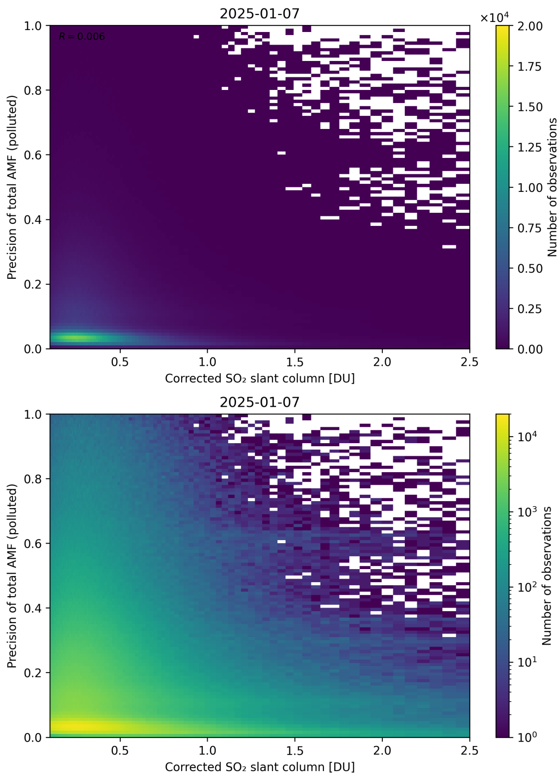
Figure 243: Scatter density plot of “Corrected SO 2 slant column” against “Precision of total AMF (polluted)” for 2025-01-07 to 2025-01-08.
