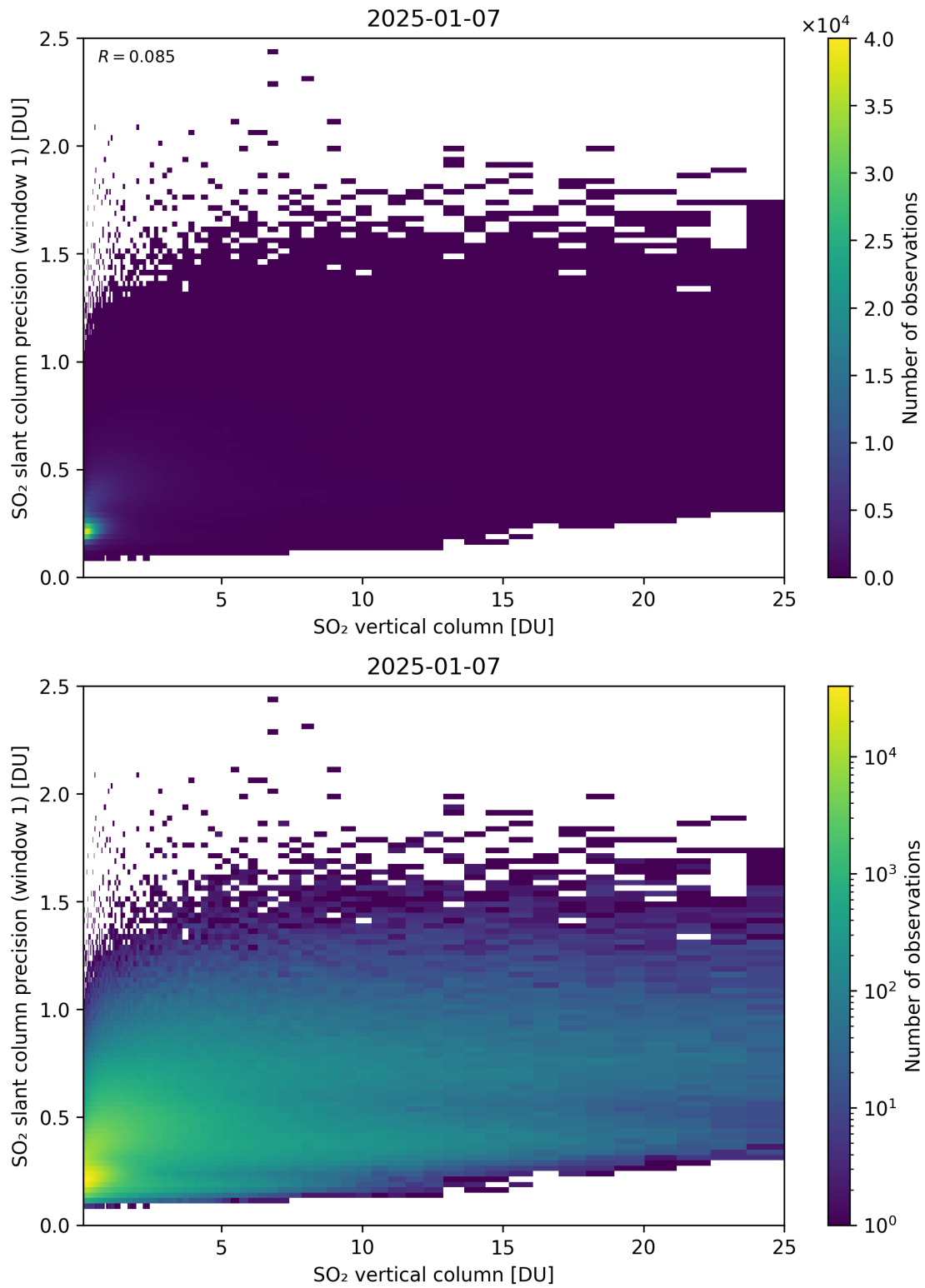
Figure 355: Scatter density plot of “SO 2 vertical column” against “SO 2 slant column precision (window 1)” for 2025-01-07 to 2025-01-08.
