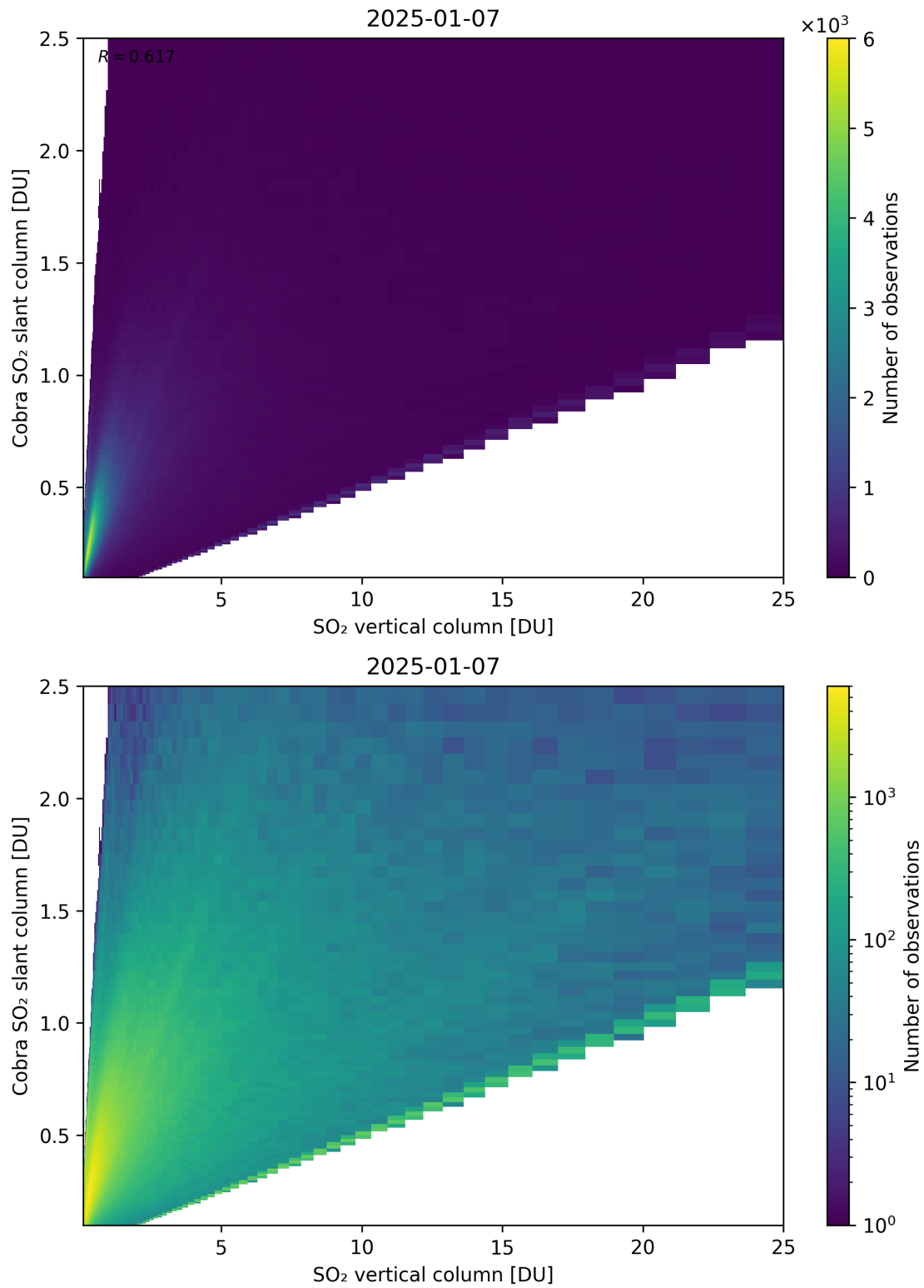
Figure 349: Scatter density plot of “SO 2 vertical column” against “Cobra SO 2 slant column” for 2025-01-07 to 2025-01-08.
