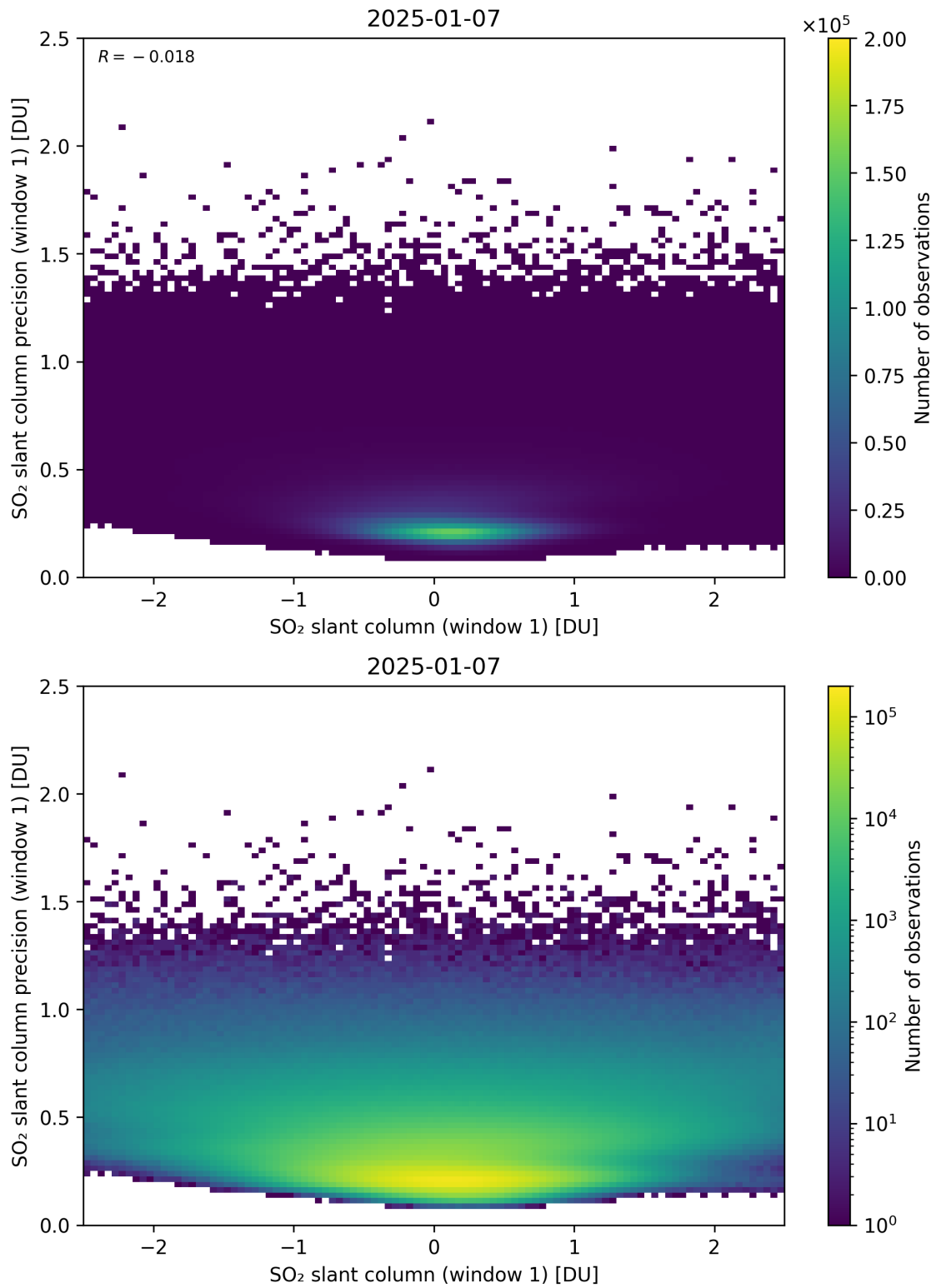
Figure 285: Scatter density plot of “SO 2 slant column (window 1)” against “SO 2 slant column precision (window 1)” for 2025-01-07 to 2025-01-08.
