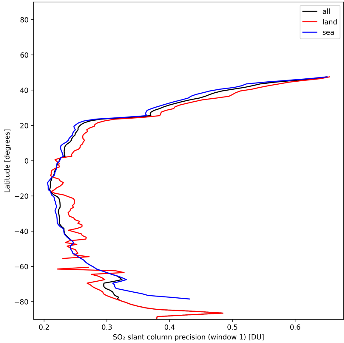
Figure 38: Zonal average of “SO 2 slant column precision (window 1)” for 2025-01-07 to 2025-01-08.
