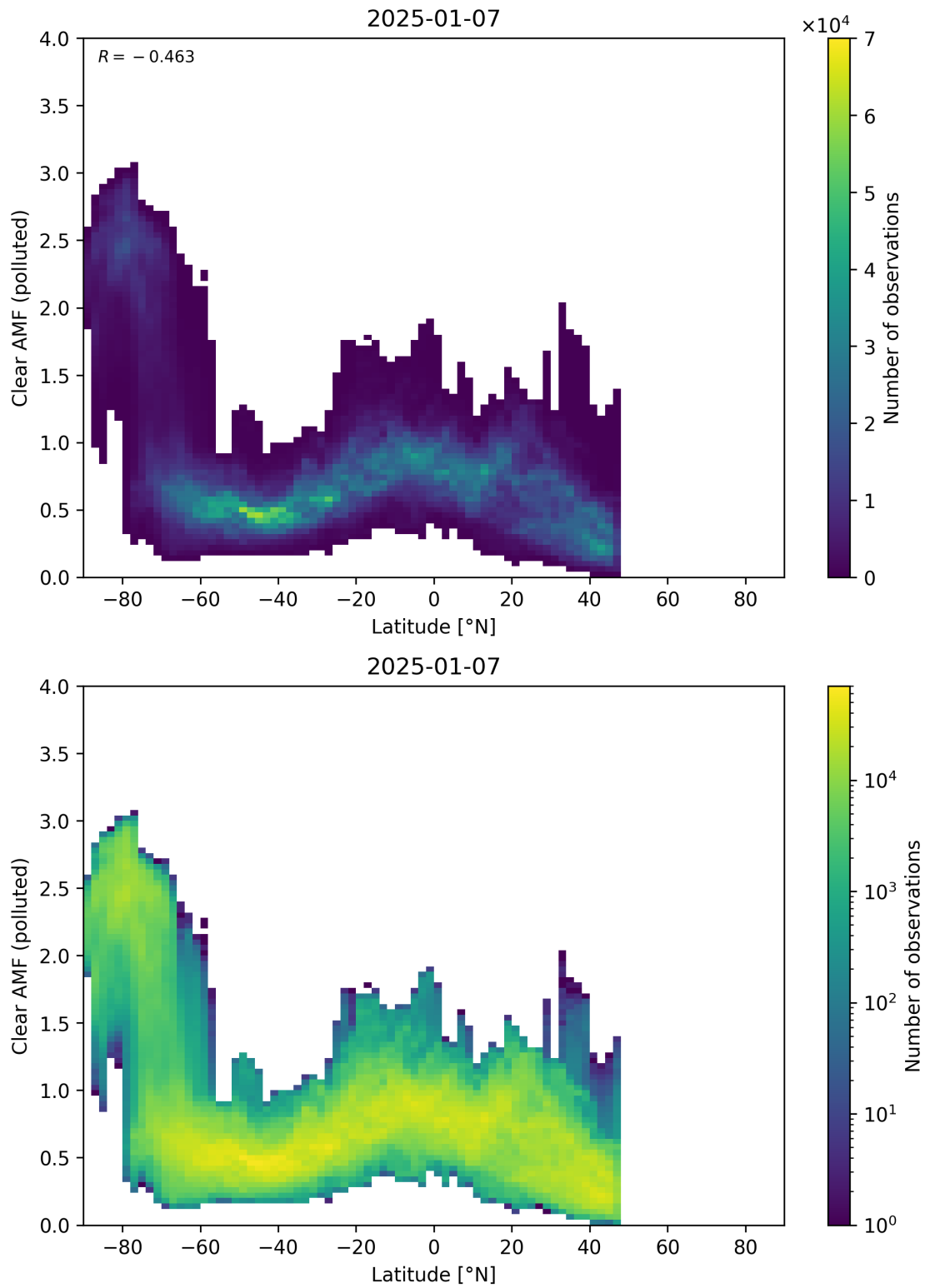
Figure 156: Scatter density plot of “Latitude” against “Clear AMF (polluted)” for 2025-01-07 to 2025-01-08.
