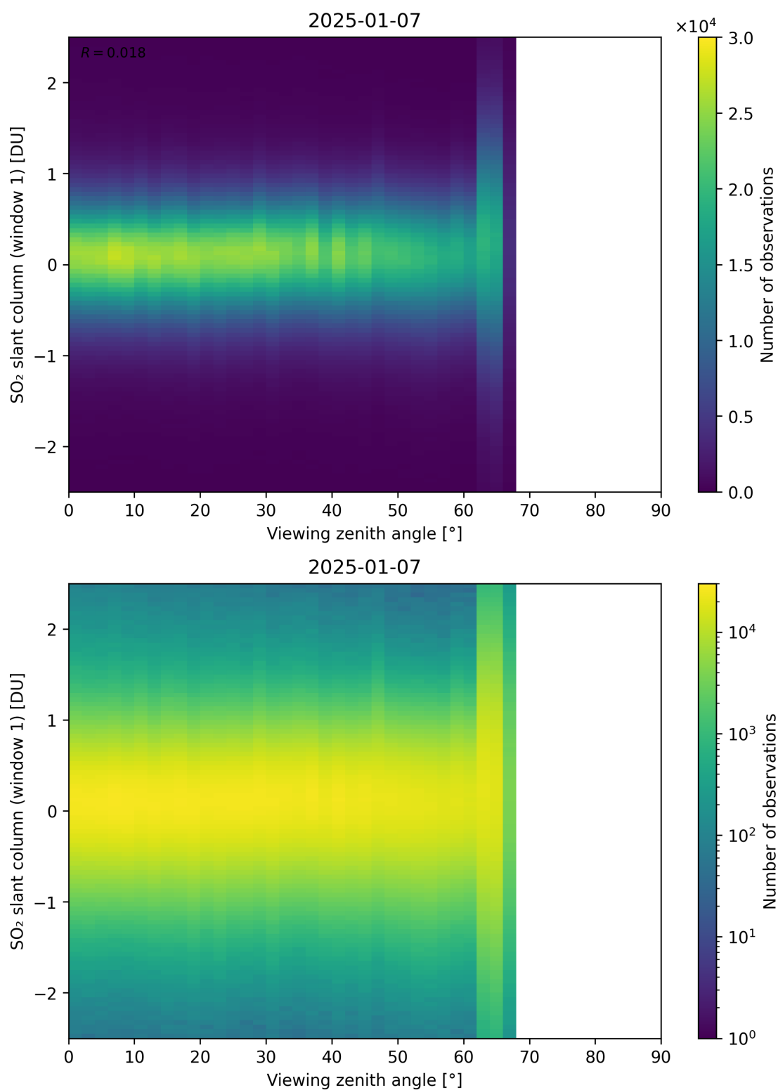
Figure 376: Scatter density plot of “Viewing zenith angle” against “SO 2 slant column (window 1)” for 2025-01-07 to 2025-01-08.
