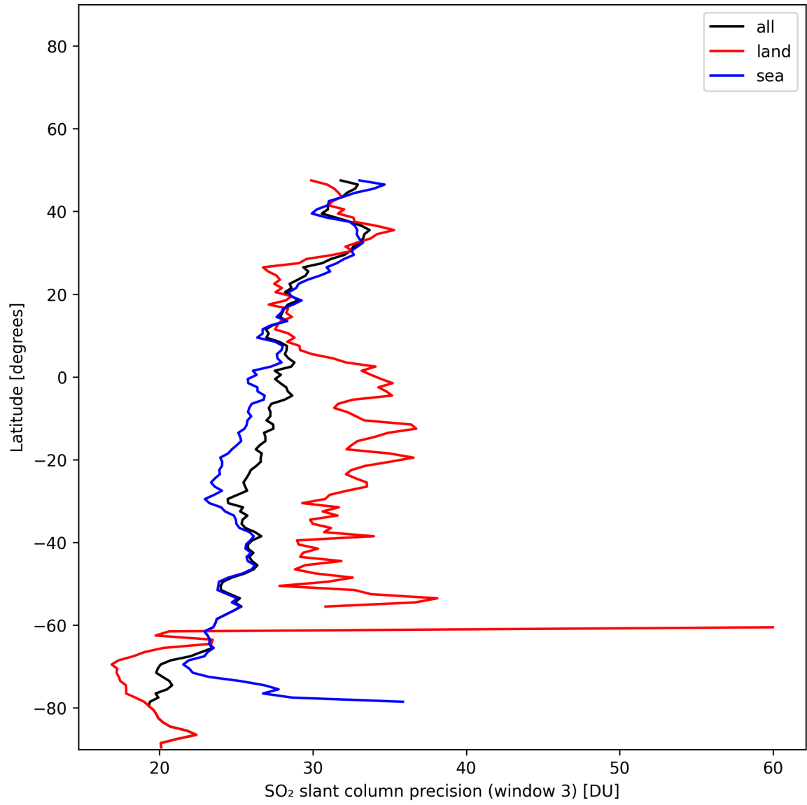
Figure 46: Zonal average of “SO 2 slant column precision (window 3)” for 2025-01-07 to 2025-01-08.
