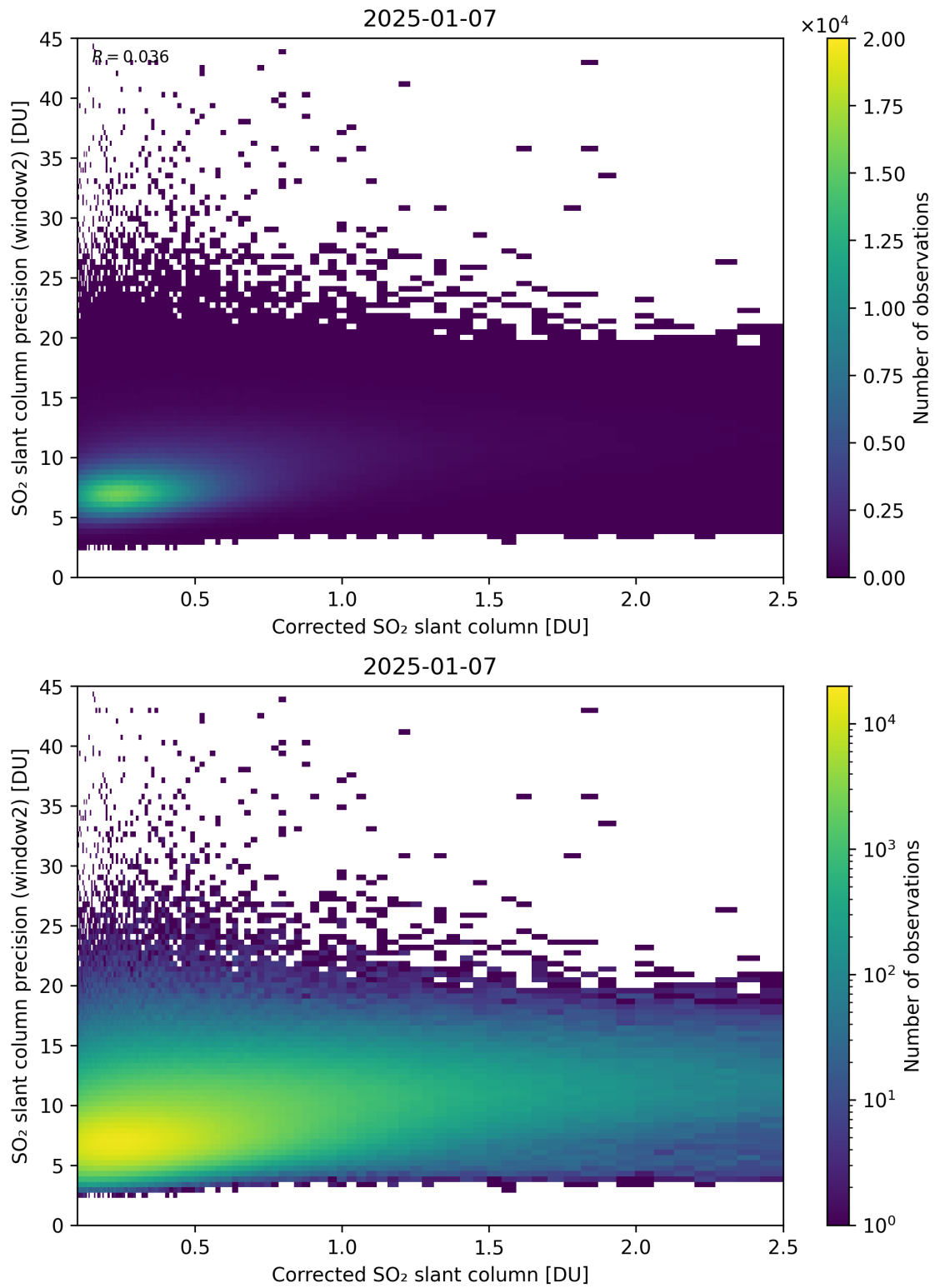
Figure 239: Scatter density plot of “Corrected SO 2 slant column” against “SO 2 slant column precision (window2)” for 2025-01-07 to 2025-01-08.
