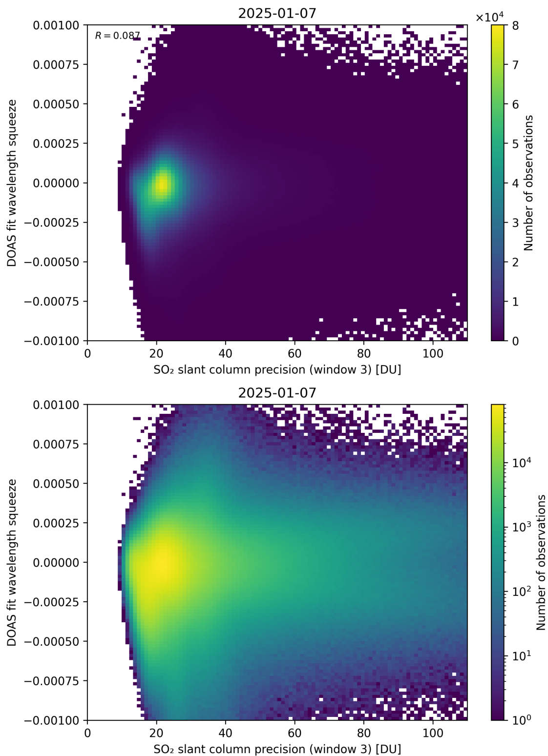
Figure 309: Scatter density plot of “SO 2 slant column precision (window 3)” against “DOAS fit wavelength squeeze” for 2025-01-07 to 2025-01-08.
