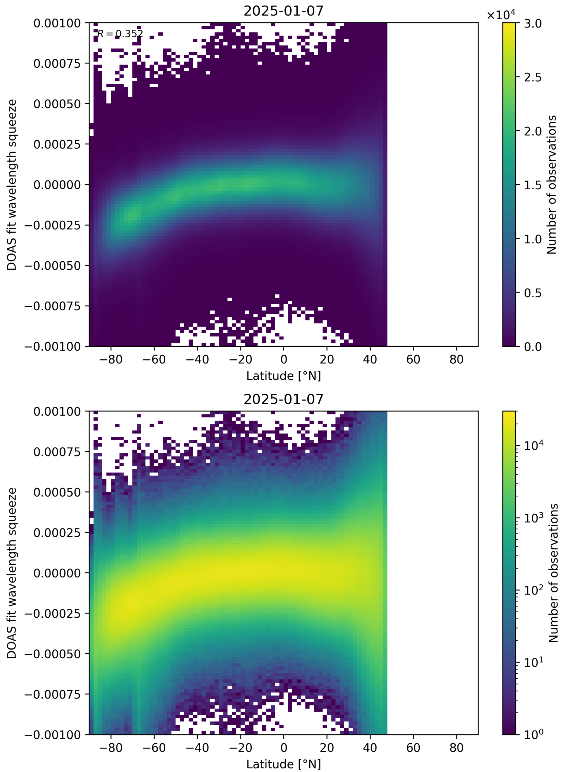
Figure 154: Scatter density plot of “Latitude” against “DOAS fit wavelength squeeze” for 2025-01-07 to 2025-01-08.
