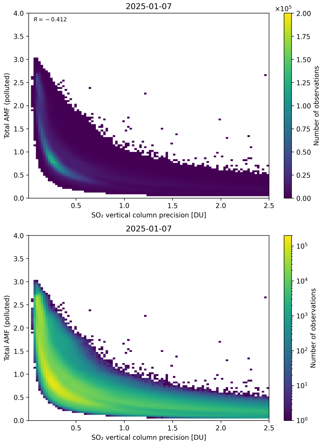
Figure 346: Scatter density plot of “SO 2 vertical column precision” against “Total AMF (polluted)” for 2025-01-07 to 2025-01-08.
