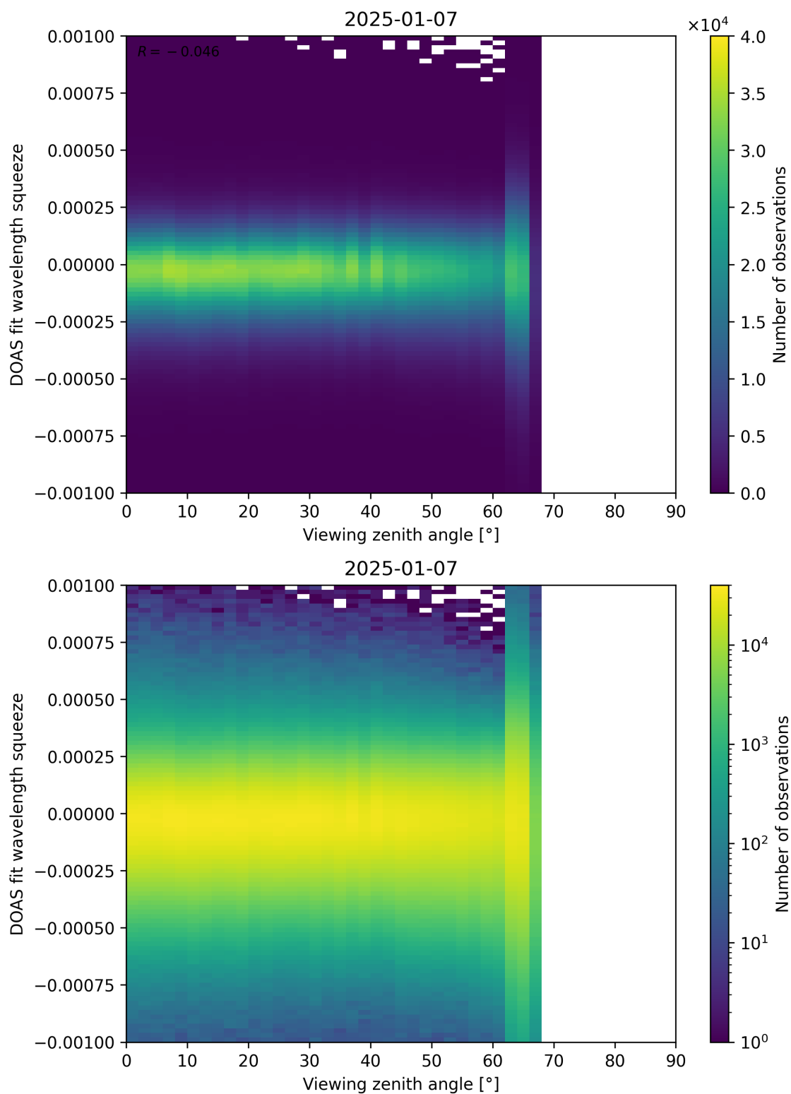
Figure 366: Scatter density plot of “Viewing zenith angle” against “DOAS fit wavelength squeeze” for 2025-01-07 to 2025-01-08.
