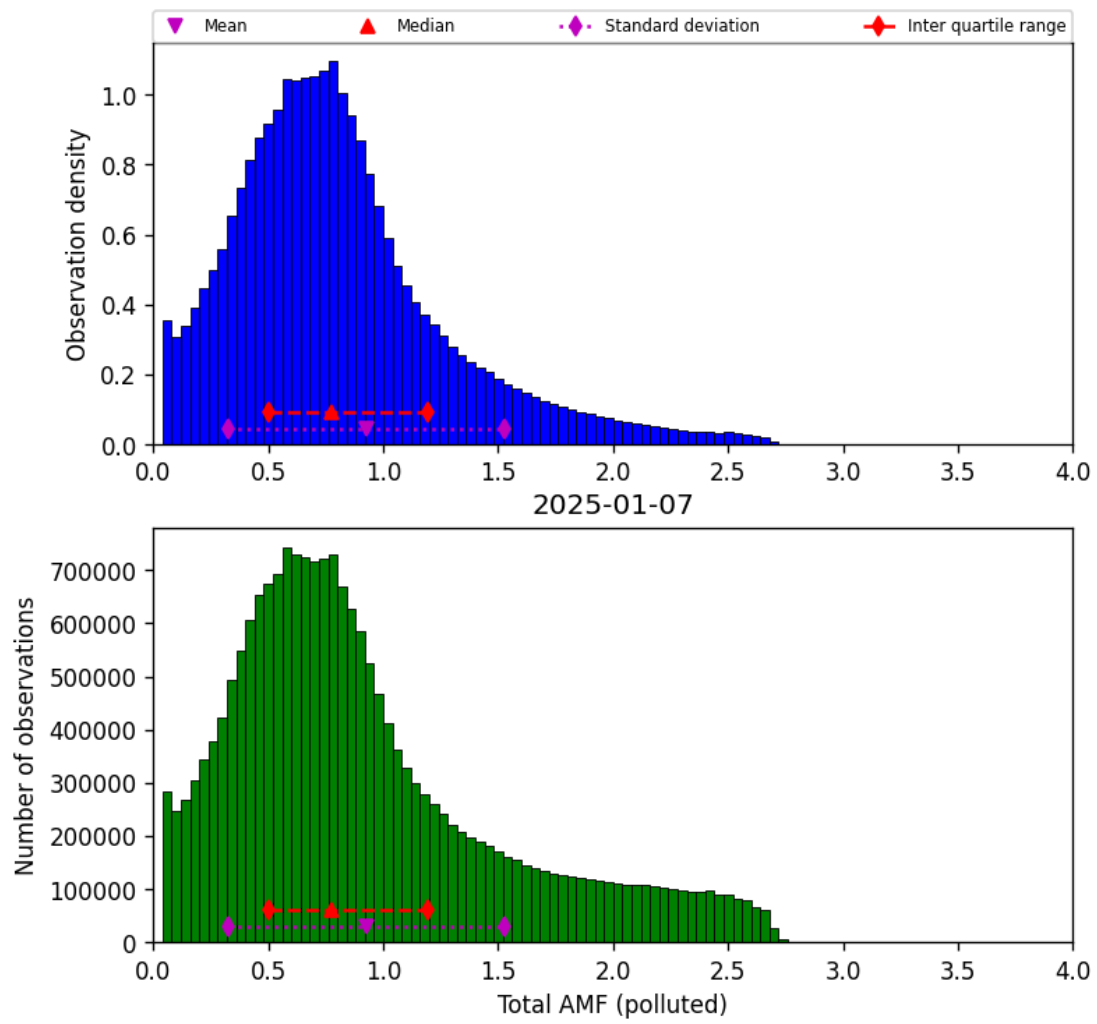
Figure 79: Histogram of “Total AMF (polluted)” for 2025-01-07 to 2025-01-08
