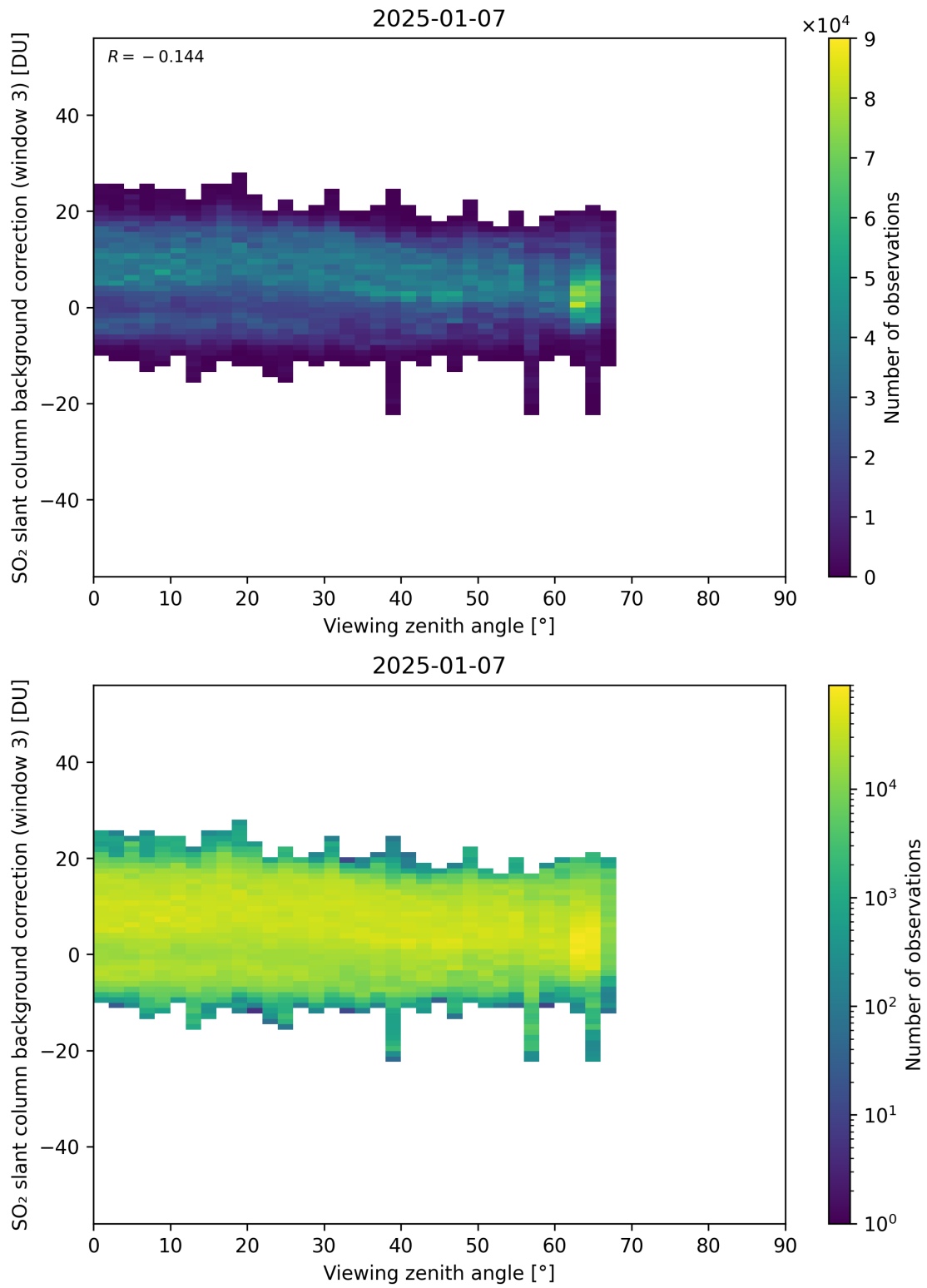
Figure 364: Scatter density plot of “Viewing zenith angle” against “SO 2 slant column background correction (window 3)” for 2025-01-07 to 2025-01-08.
