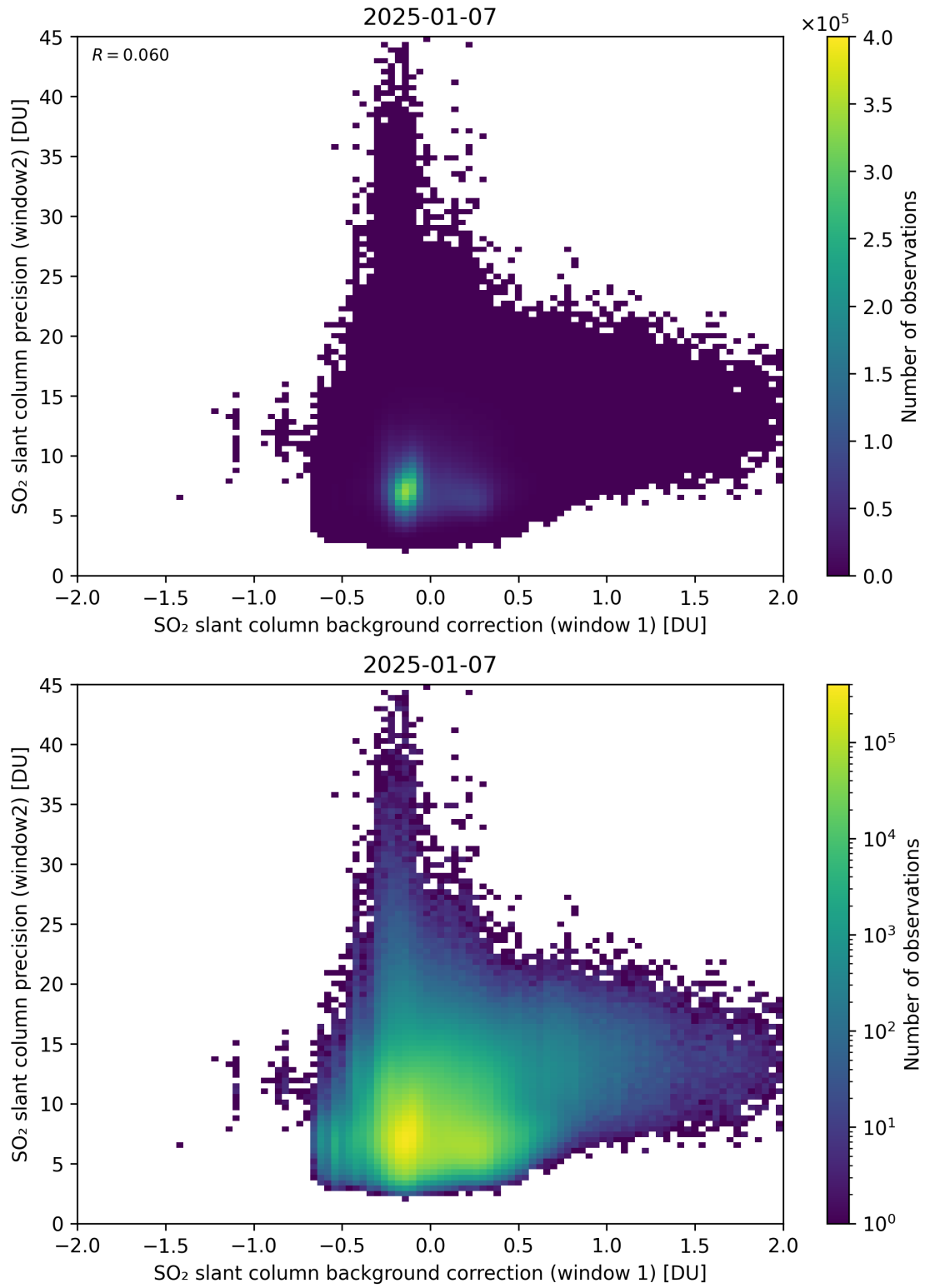
Figure 117: Scatter density plot of “SO 2 slant column background correction (window 1)” against “SO 2 slant column precision (window2)” for 2025-01-07 to 2025-01-08.
