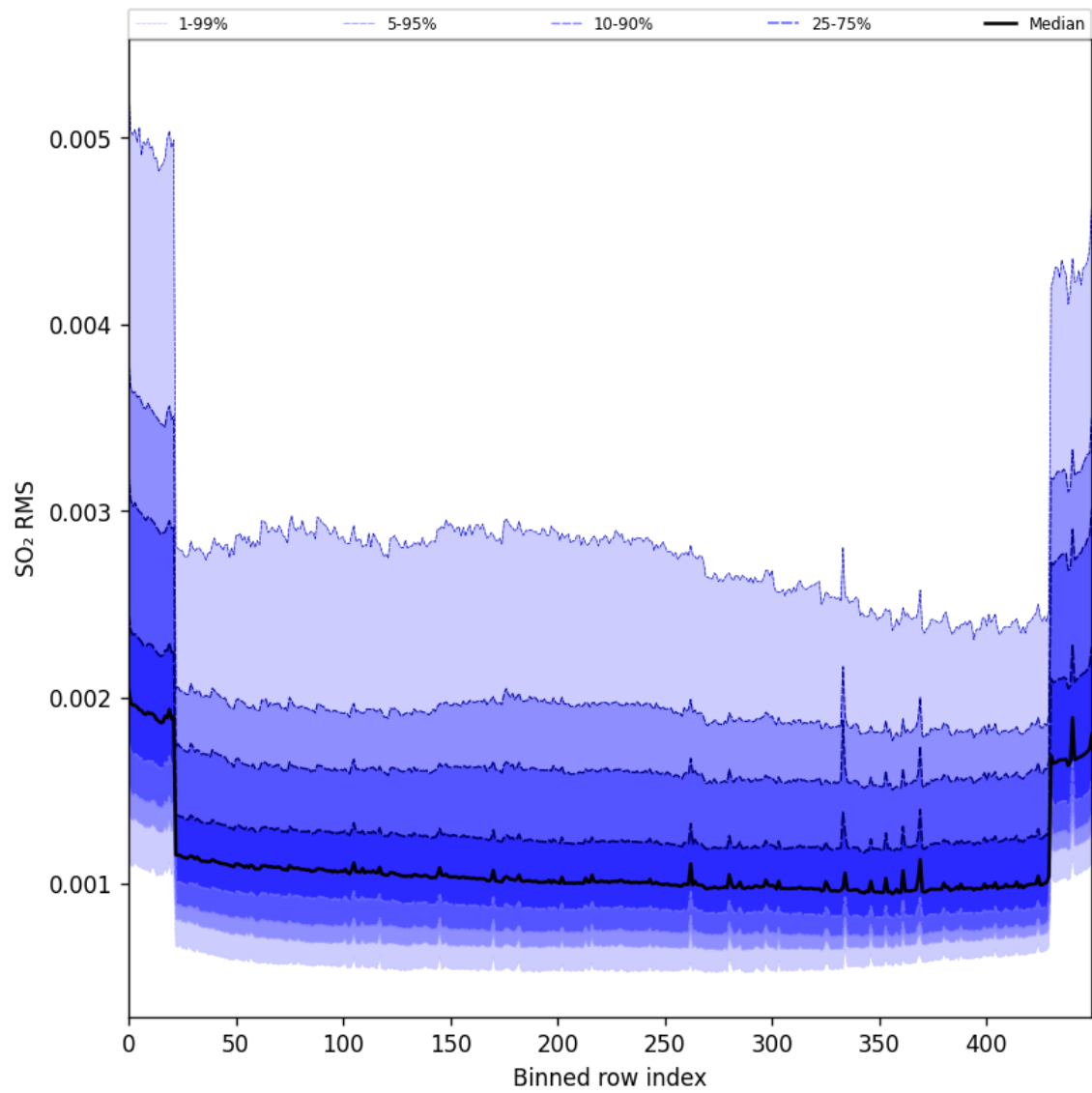
Figure 104: Along track statistics of “SO 2 RMS” for 2025-01-07 to 2025-01-08
