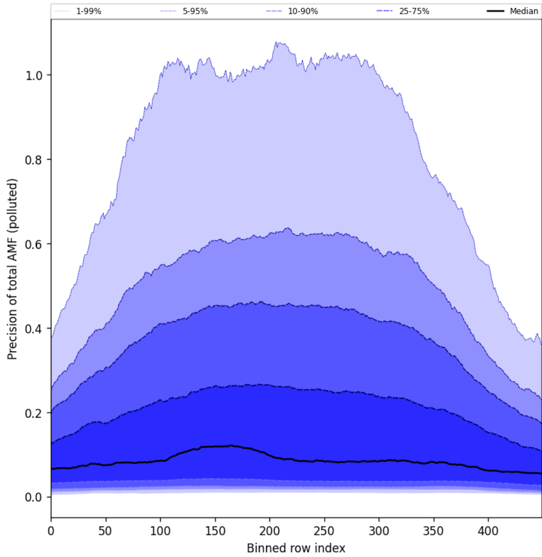
Figure 106: Along track statistics of “Precision of total AMF (polluted)” for 2025-01-07 to 2025-01-08
