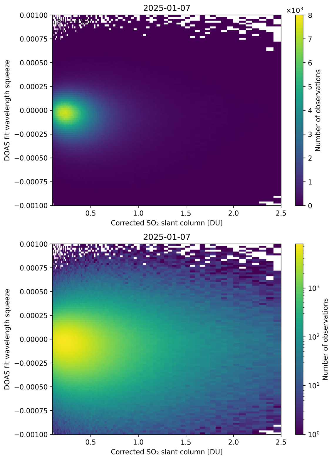
Figure 230: Scatter density plot of “Corrected SO 2 slant column” against “DOAS fit wavelength squeeze” for 2025-01-07 to 2025-01-08.
