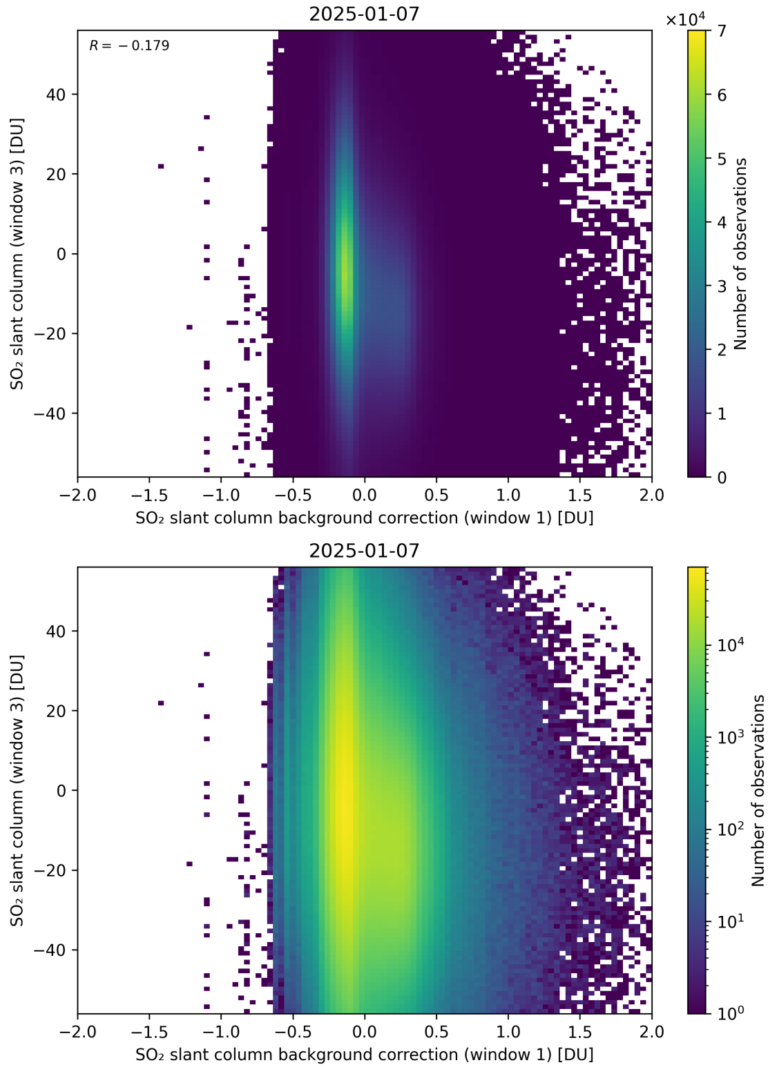
Figure 118: Scatter density plot of “SO 2 slant column background correction (window 1)” against “SO 2 slant column (window 3)” for 2025-01-07 to 2025-01-08.
