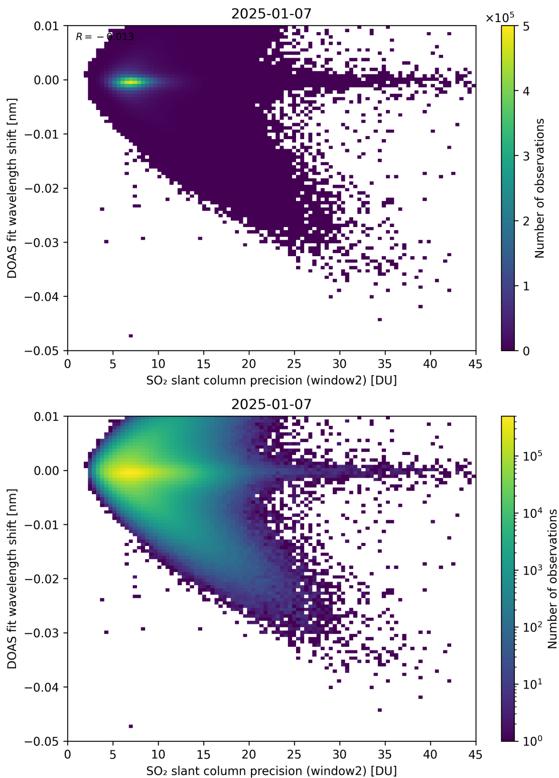
Figure 293: Scatter density plot of “SO 2 slant column precision (window2)” against “DOAS fit wavelength shift” for 2025-01-07 to 2025-01-08.
