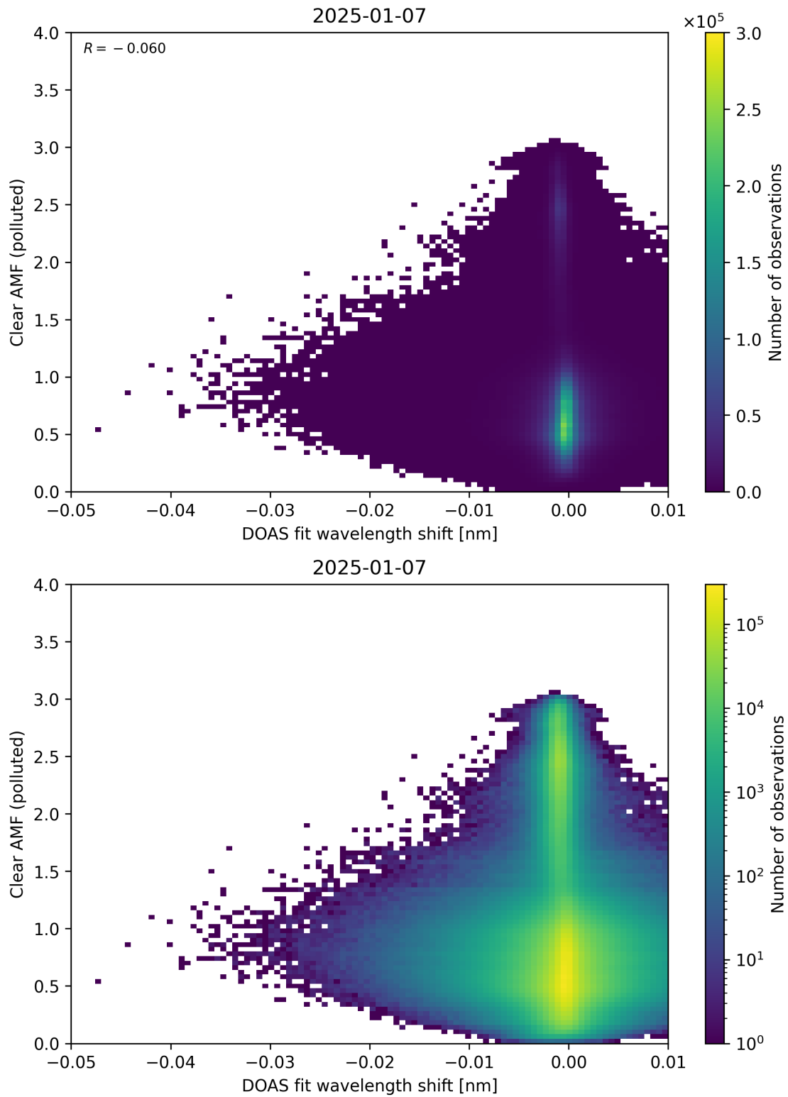
Figure 140: Scatter density plot of “DOAS fit wavelength shift” against “Clear AMF (polluted)” for 2025-01-07 to 2025-01-08.
