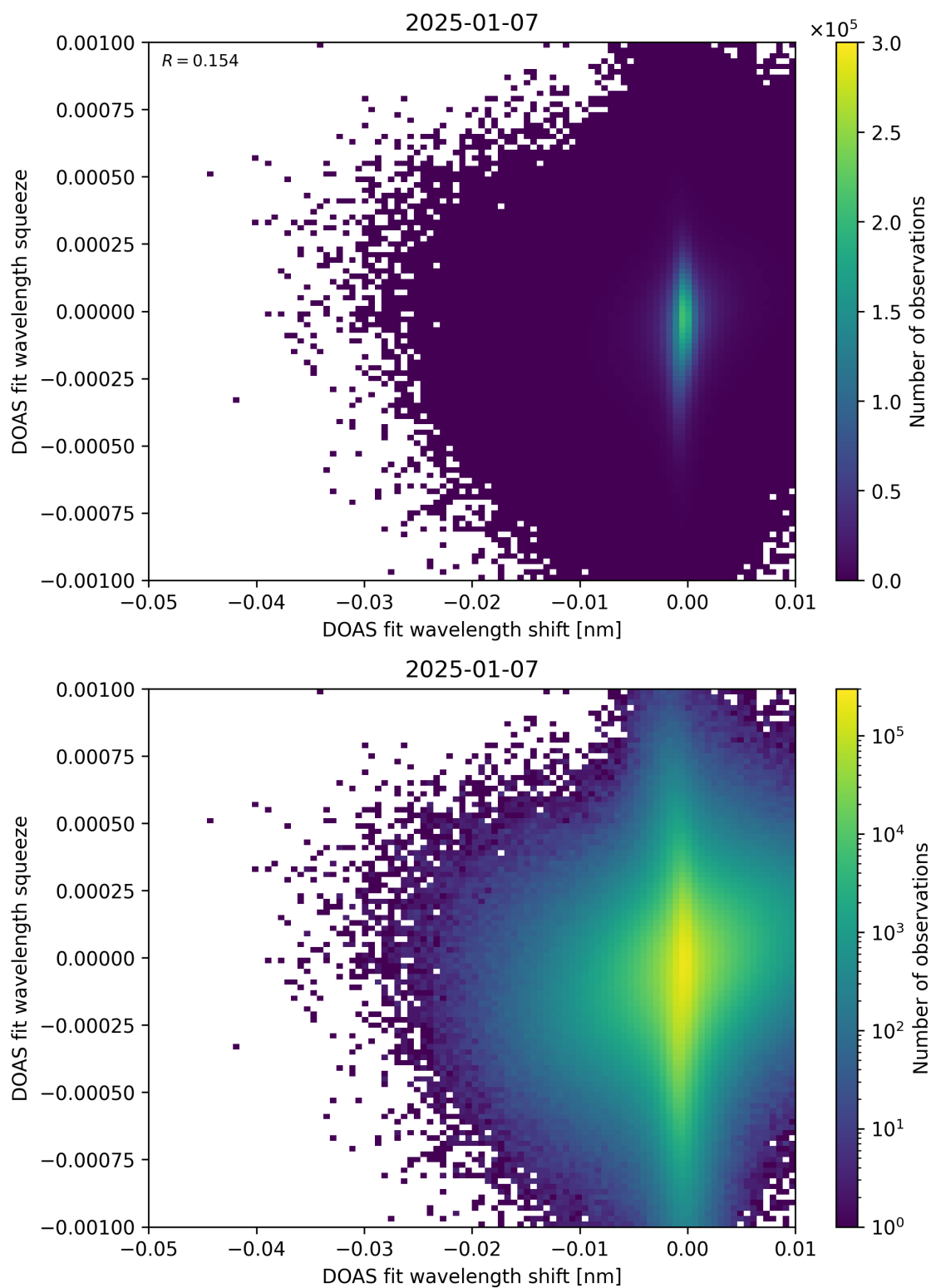
Figure 138: Scatter density plot of “DOAS fit wavelength shift” against “DOAS fit wavelength squeeze” for 2025-01-07 to 2025-01-08.
