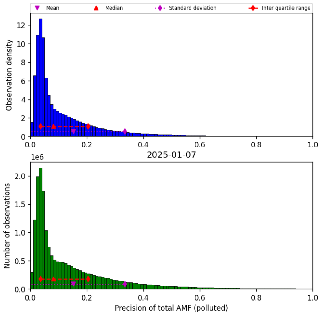
Figure 80: Histogram of “Precision of total AMF (polluted)” for 2025-01-07 to 2025-01-08
