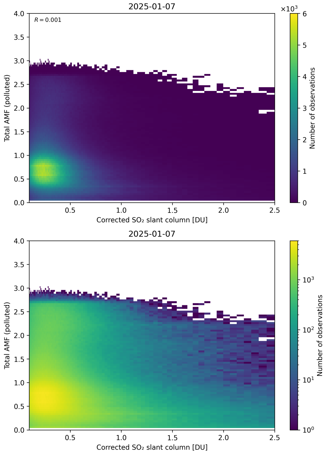
Figure 242: Scatter density plot of “Corrected SO 2 slant column” against “Total AMF (polluted)” for 2025-01-07 to 2025-01-08.
