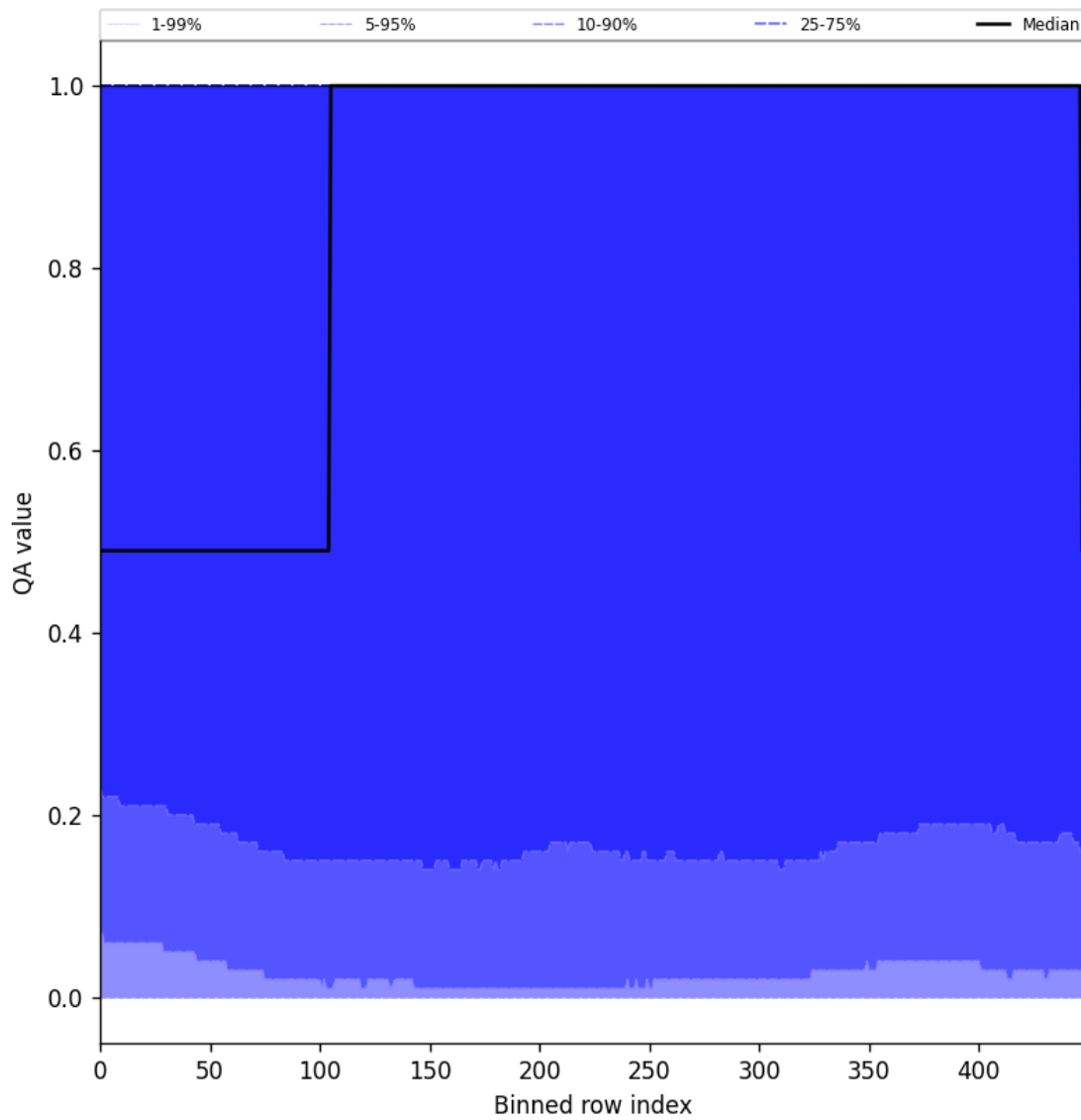
Figure 83: Along track statistics of “QA value” for 2025-01-07 to 2025-01-08
