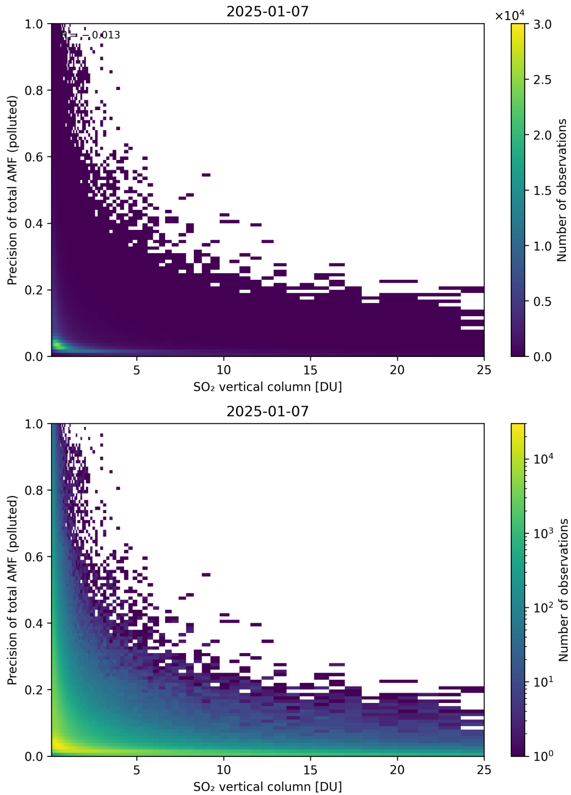
Figure 360: Scatter density plot of “SO 2 vertical column” against “Precision of total AMF (polluted)” for 2025-01-07 to 2025-01-08.
