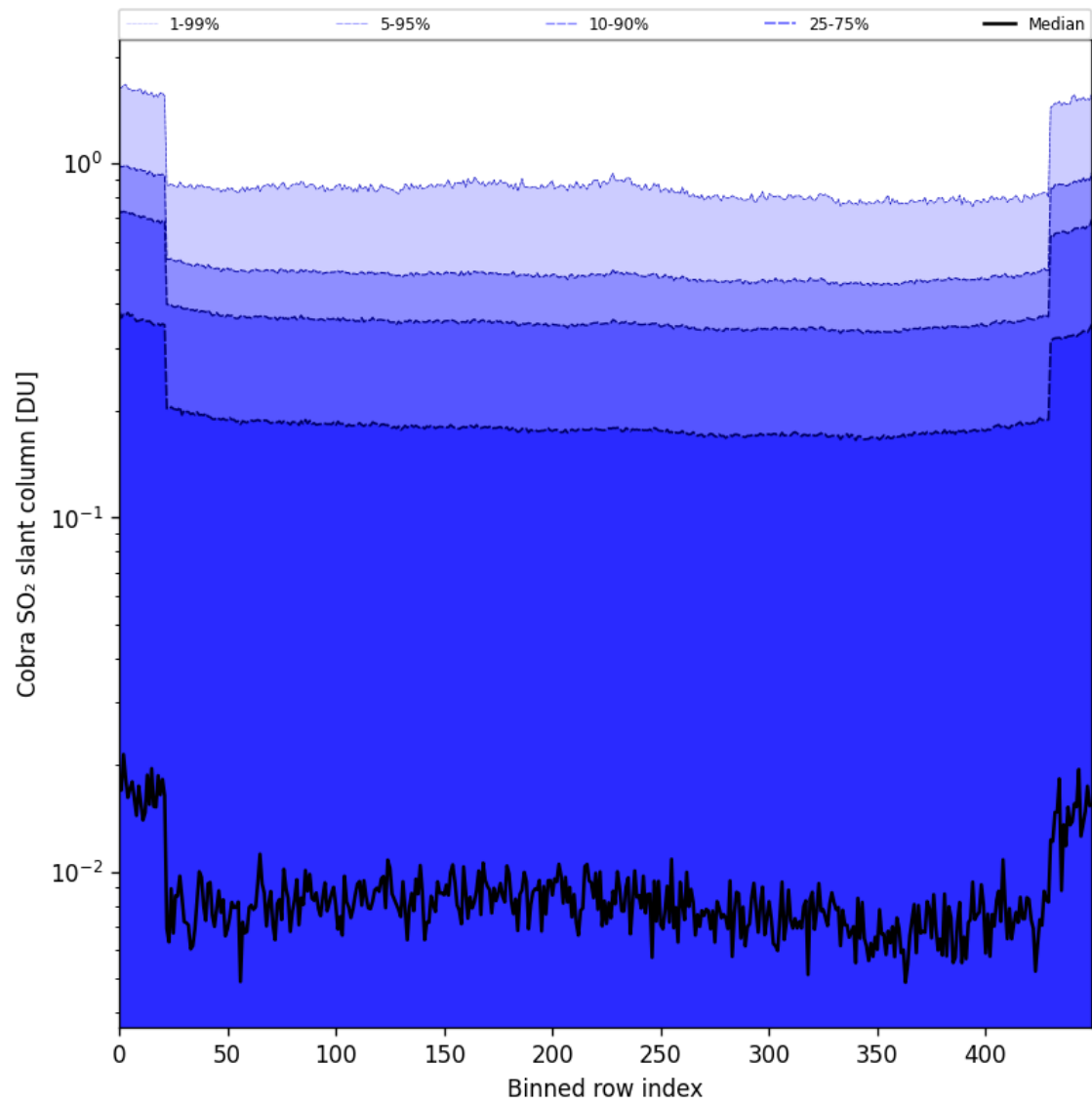
Figure 87: Along track statistics of “Cobra SO 2 slant column” for 2025-01-07 to 2025-01-08
