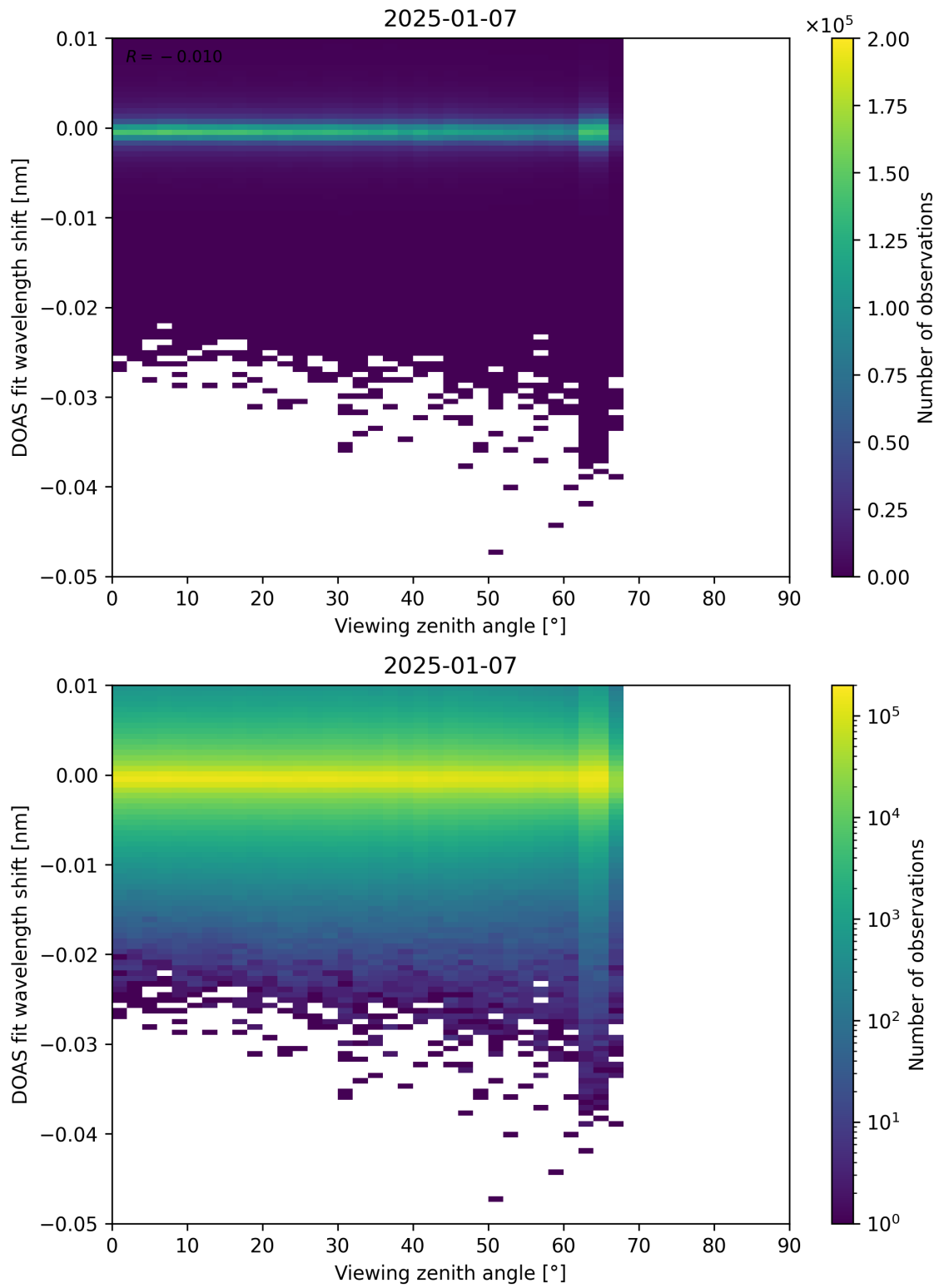
Figure 365: Scatter density plot of “Viewing zenith angle” against “DOAS fit wavelength shift” for 2025-01-07 to 2025-01-08.
