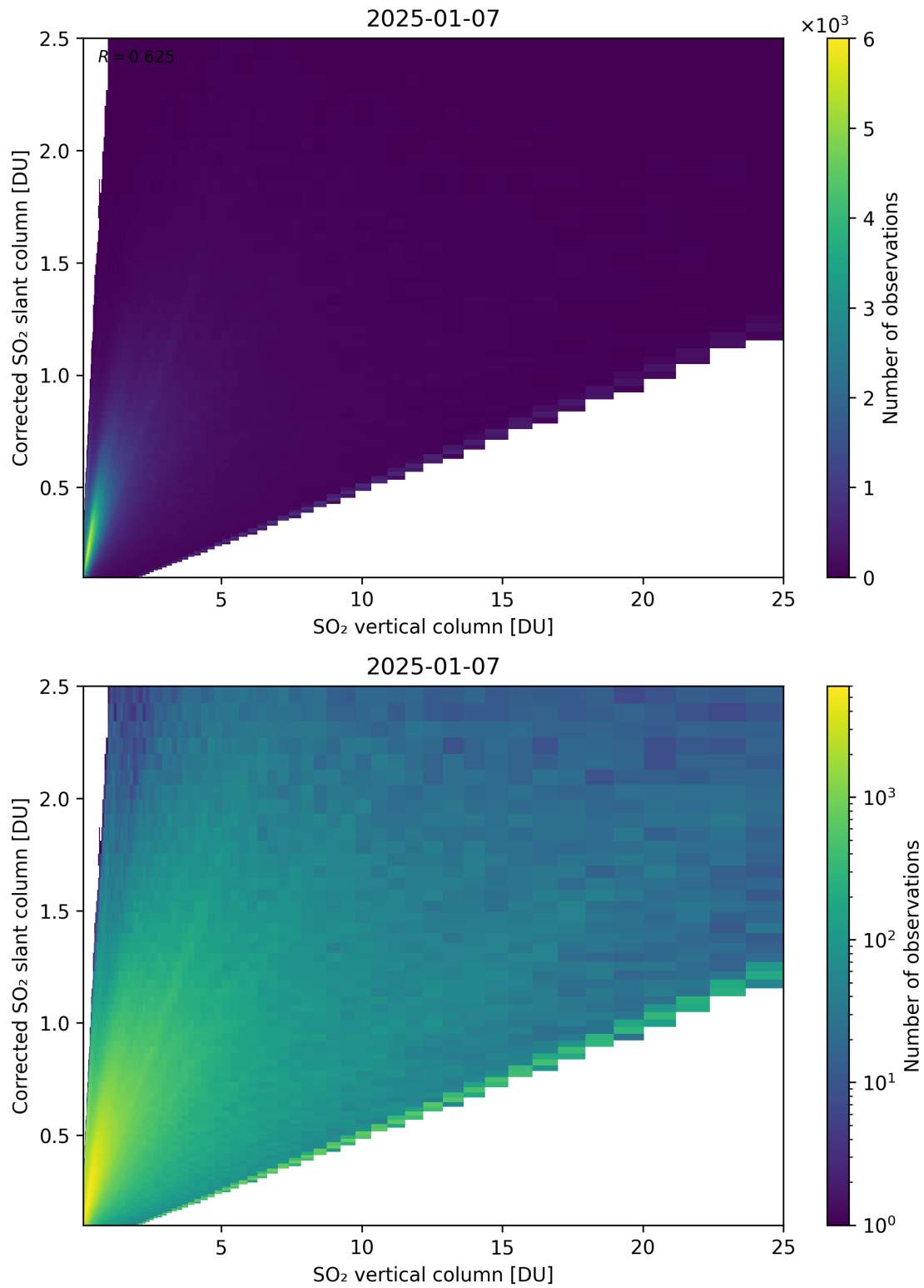
Figure 351: Scatter density plot of “SO 2 vertical column” against “Corrected SO 2 slant column” for 2025-01-07 to 2025-01-08.
