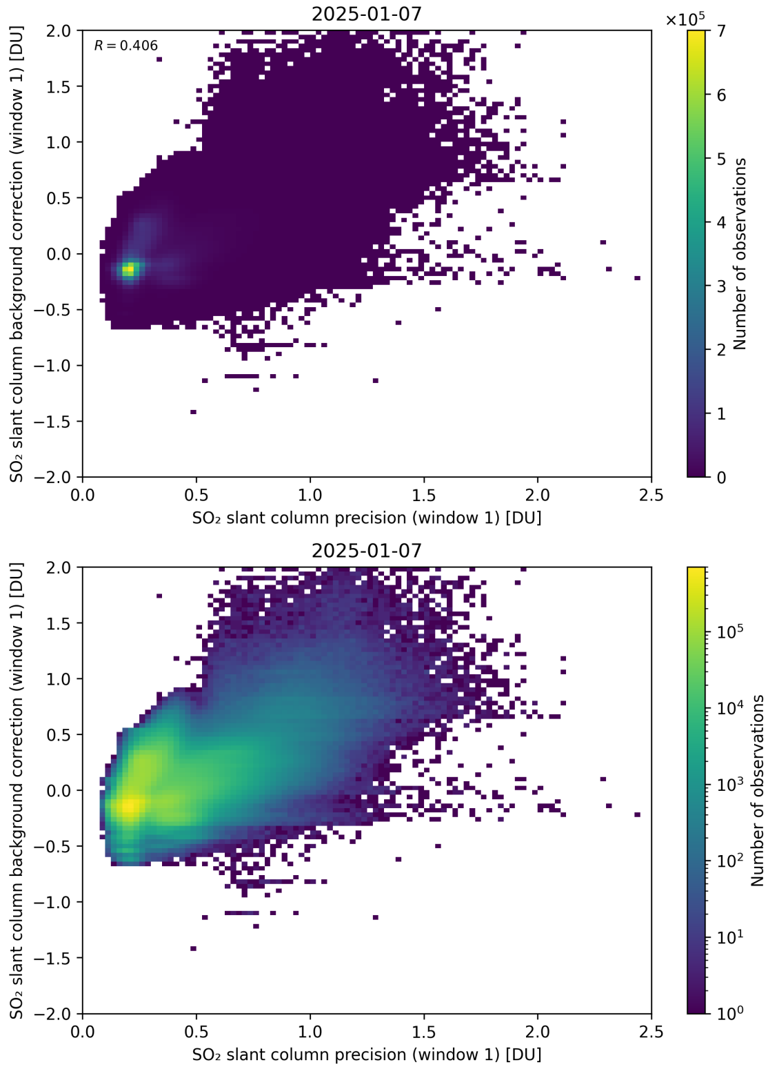
Figure 268: Scatter density plot of “SO 2 slant column precision (window 1)” against “SO 2 slant column background correction (window 1)” for 2025-01-07 to 2025-01-08.
