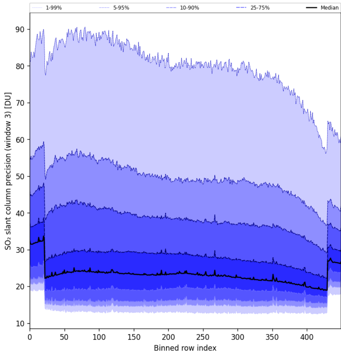
Figure 98: Along track statistics of “SO 2 slant column precision (window 3)” for 2025-01-07 to 2025-01-08
