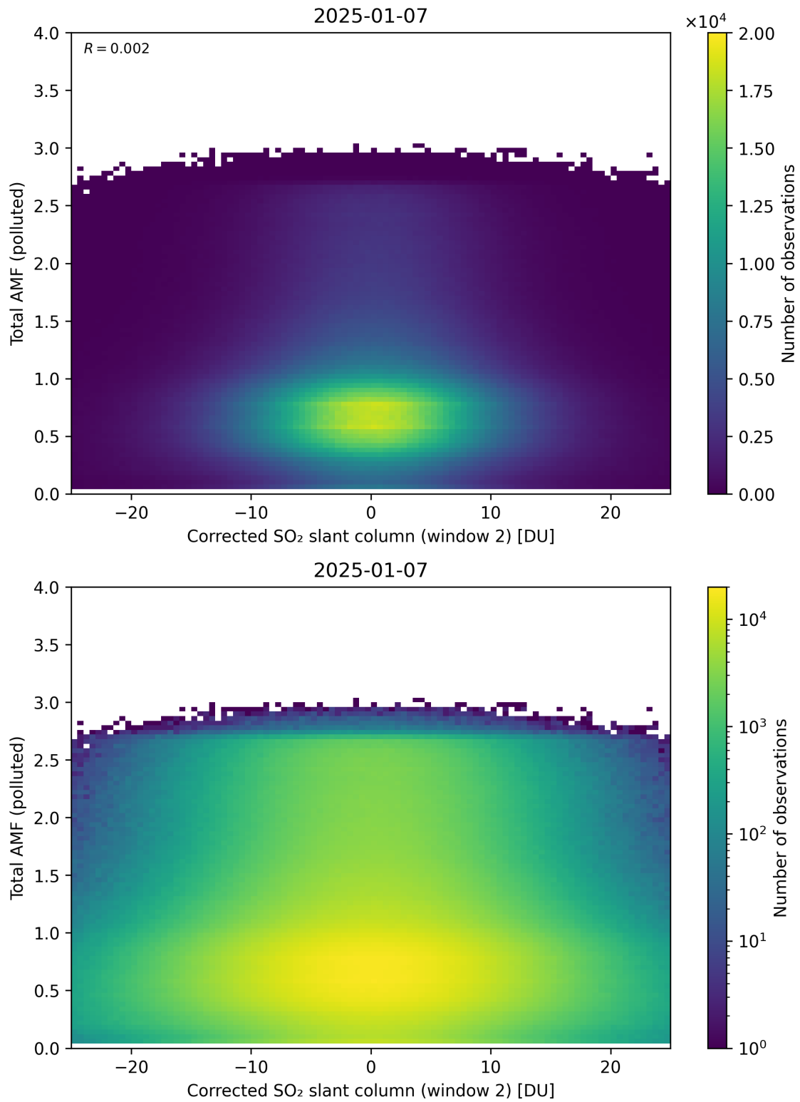
Figure 253: Scatter density plot of “Corrected SO 2 slant column (window 2)” against “Total AMF (polluted)” for 2025-01-07 to 2025-01-08.
