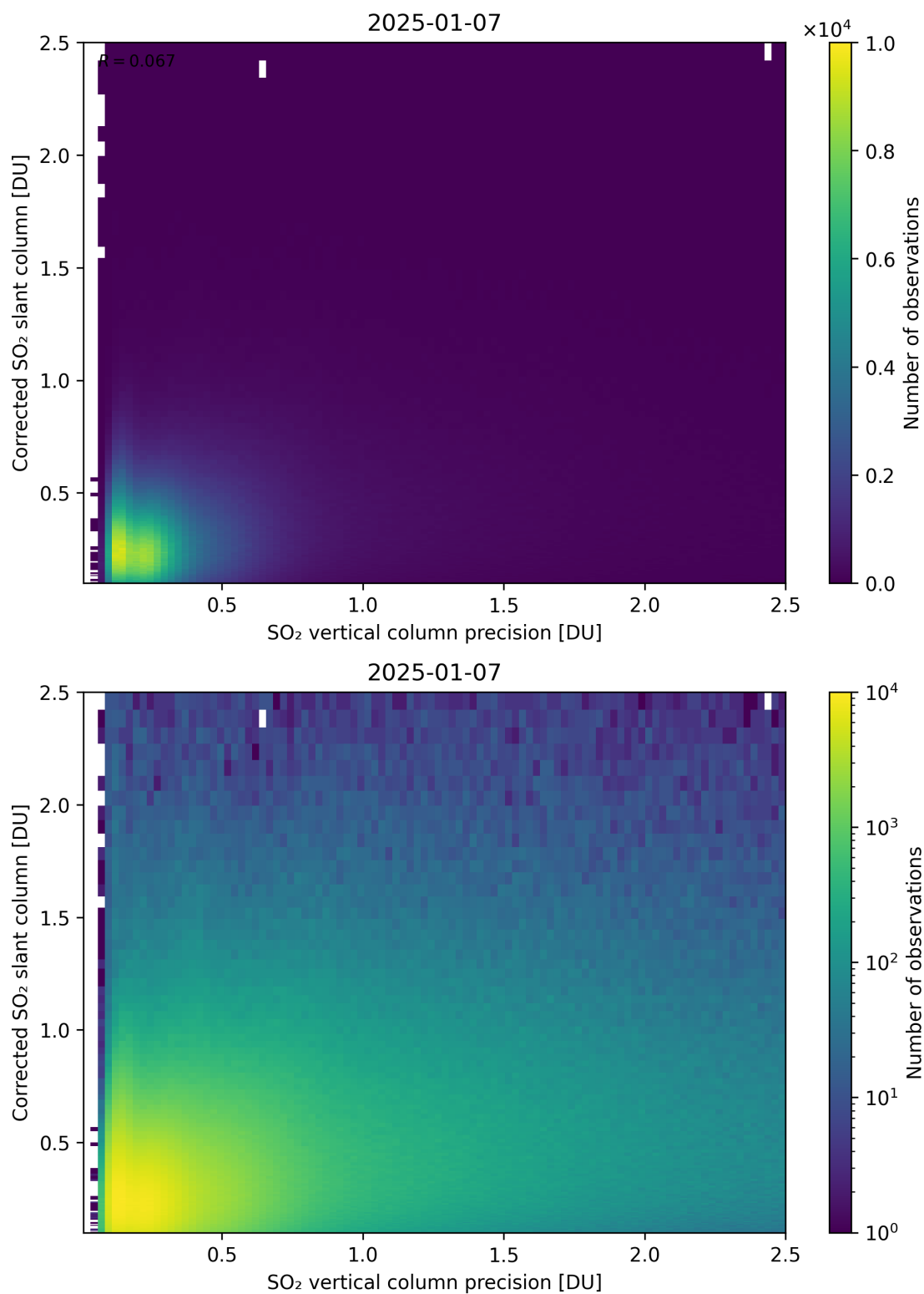
Figure 338: Scatter density plot of “SO 2 vertical column precision” against “Corrected SO 2 slant column” for 2025-01-07 to 2025-01-08.
