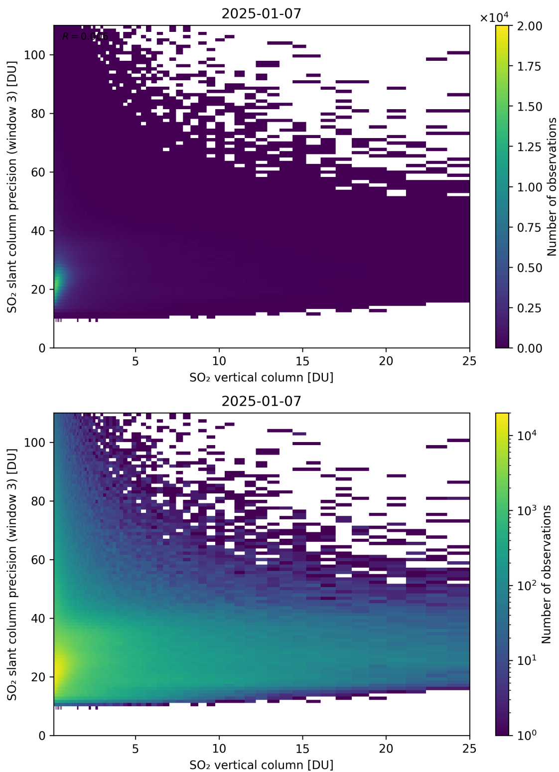
Figure 358: Scatter density plot of “SO 2 vertical column” against “SO 2 slant column precision (window 3)” for 2025-01-07 to 2025-01-08.
