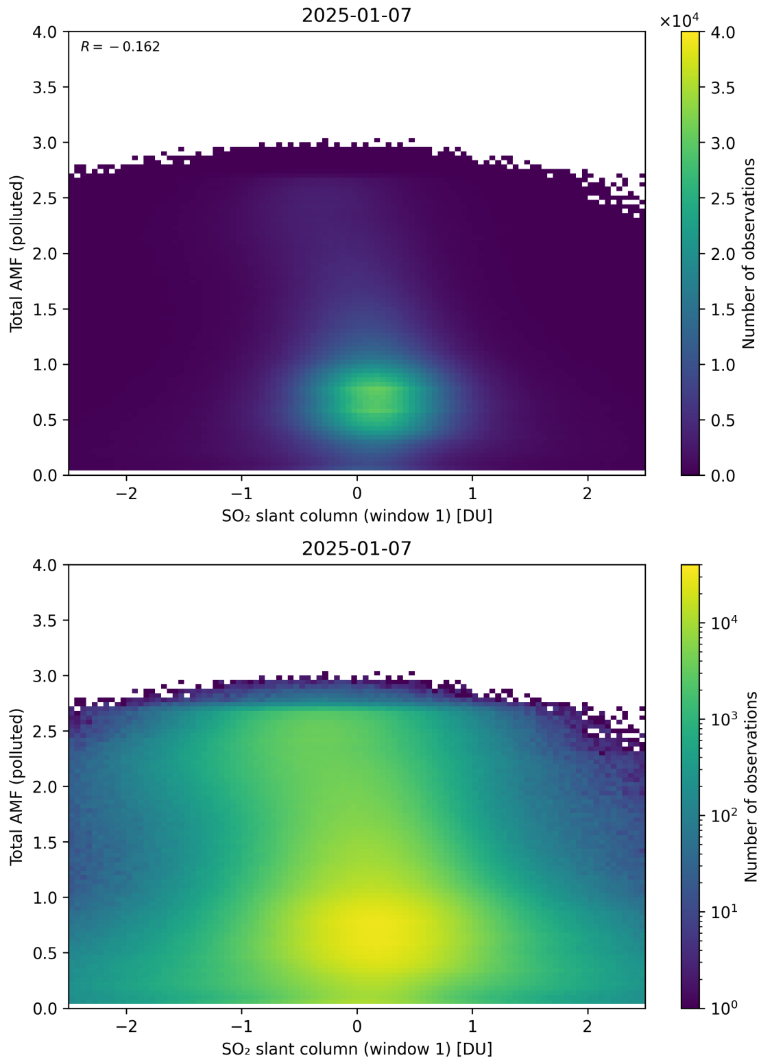
Figure 289: Scatter density plot of “SO 2 slant column (window 1)” against “Total AMF (polluted)” for 2025-01-07 to 2025-01-08.
