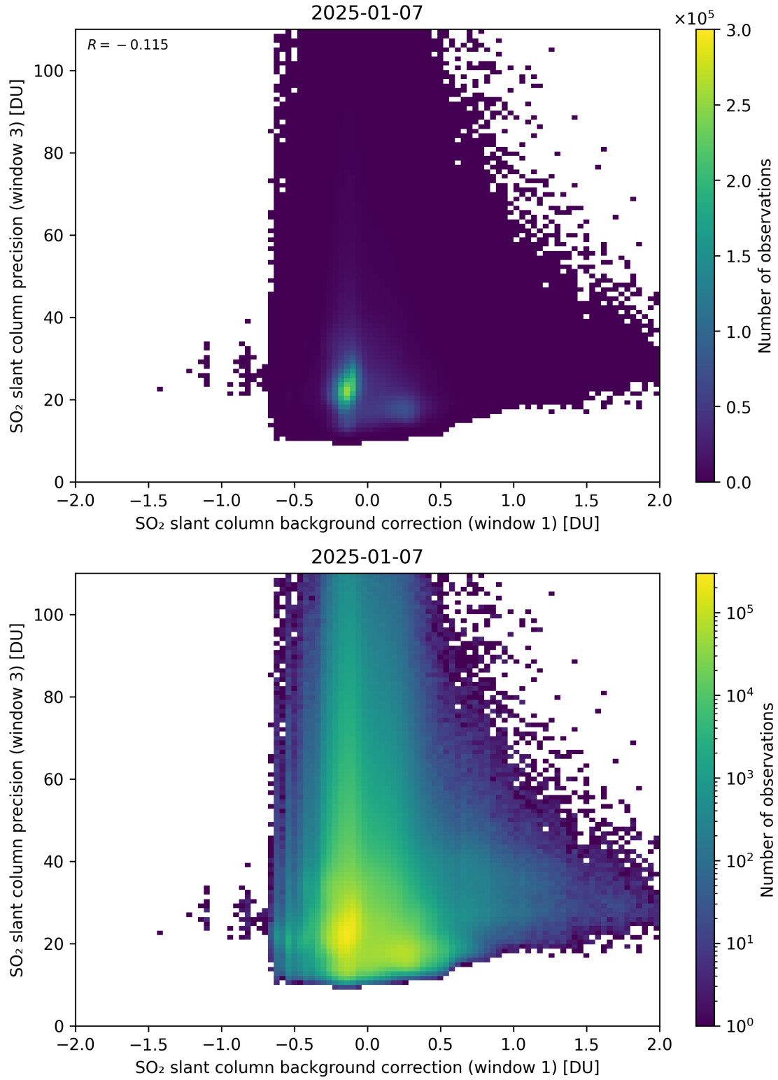
Figure 119: Scatter density plot of “SO 2 slant column background correction (window 1)” against “SO 2 slant column precision (window 3)” for 2025-01-07 to 2025-01-08.
