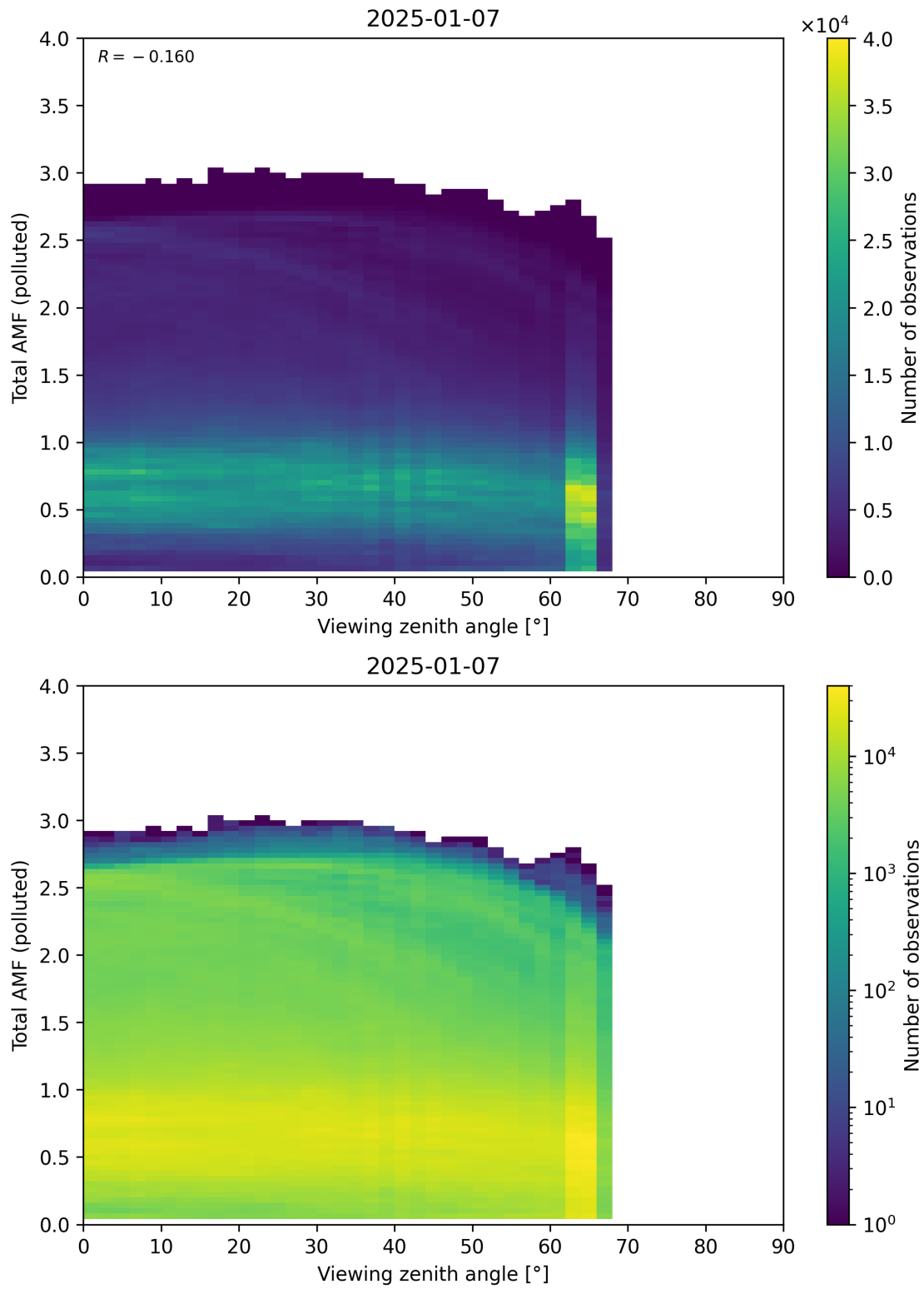
Figure 381: Scatter density plot of “Viewing zenith angle” against “Total AMF (polluted)” for 2025-01-07 to 2025-01-08.
