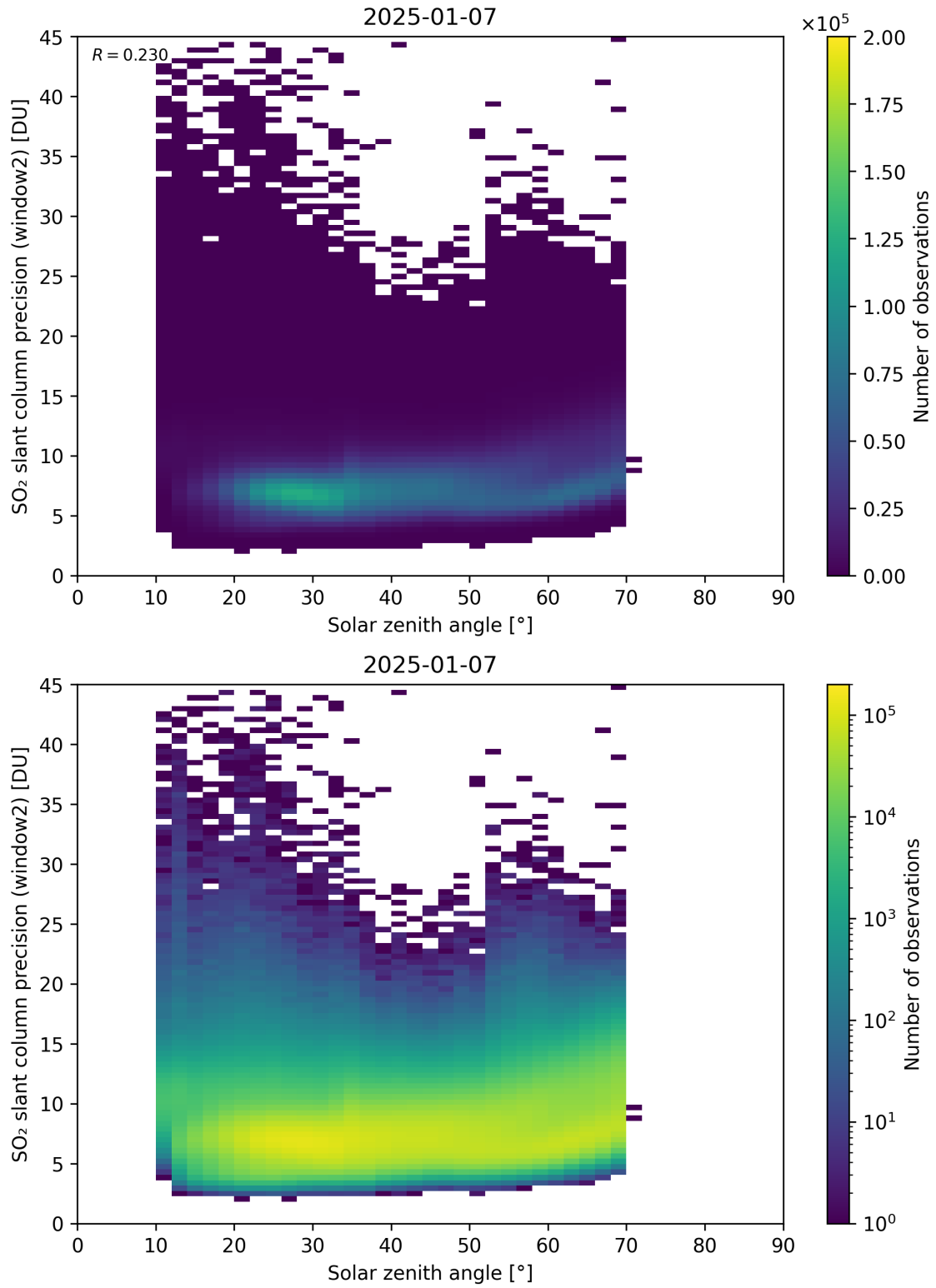
Figure 186: Scatter density plot of “Solar zenith angle” against “SO 2 slant column precision (window2)” for 2025-01-07 to 2025-01-08.
