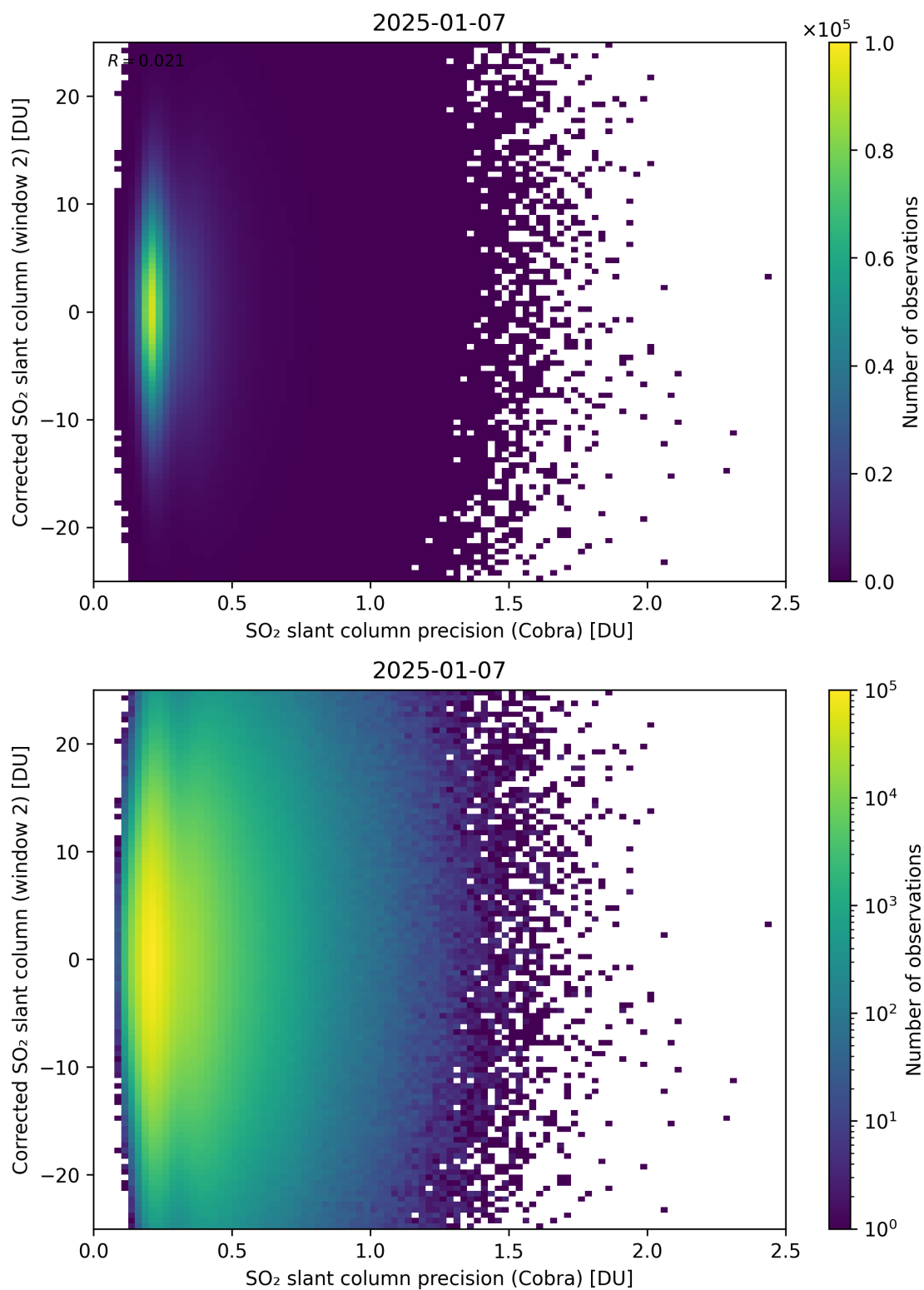
Figure 206: Scatter density plot of “SO 2 slant column precision (Cobra)” against “Corrected SO 2 slant column (window 2)” for 2025-01-07 to 2025-01-08.
