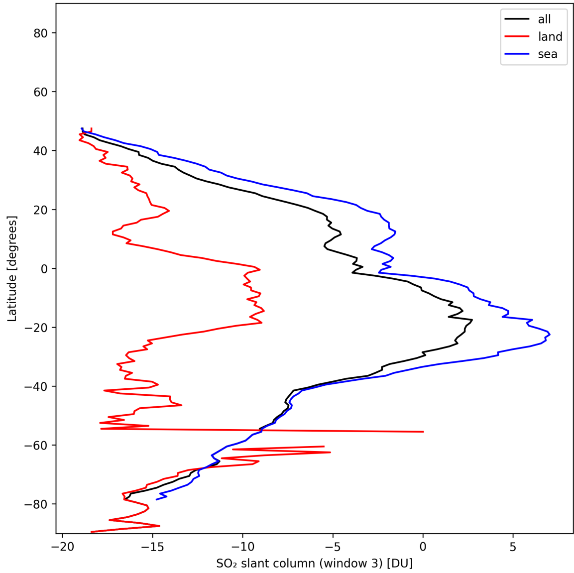
Figure 45: Zonal average of “SO 2 slant column (window 3)” for 2025-01-07 to 2025-01-08.
