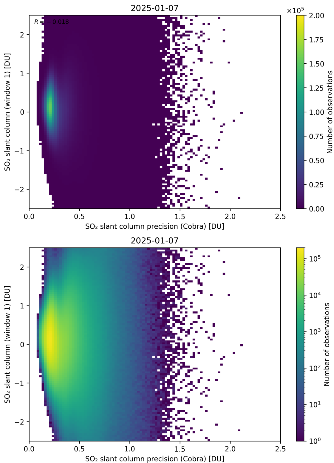
Figure 208: Scatter density plot of “SO 2 slant column precision (Cobra)” against “SO 2 slant column (window 1)” for 2025-01-07 to 2025-01-08.
