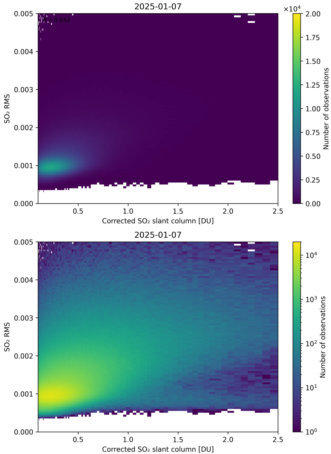
Figure 231: Scatter density plot of “Corrected SO 2 slant column” against “SO 2 RMS” for 2025-01-07 to 2025-01-08.
