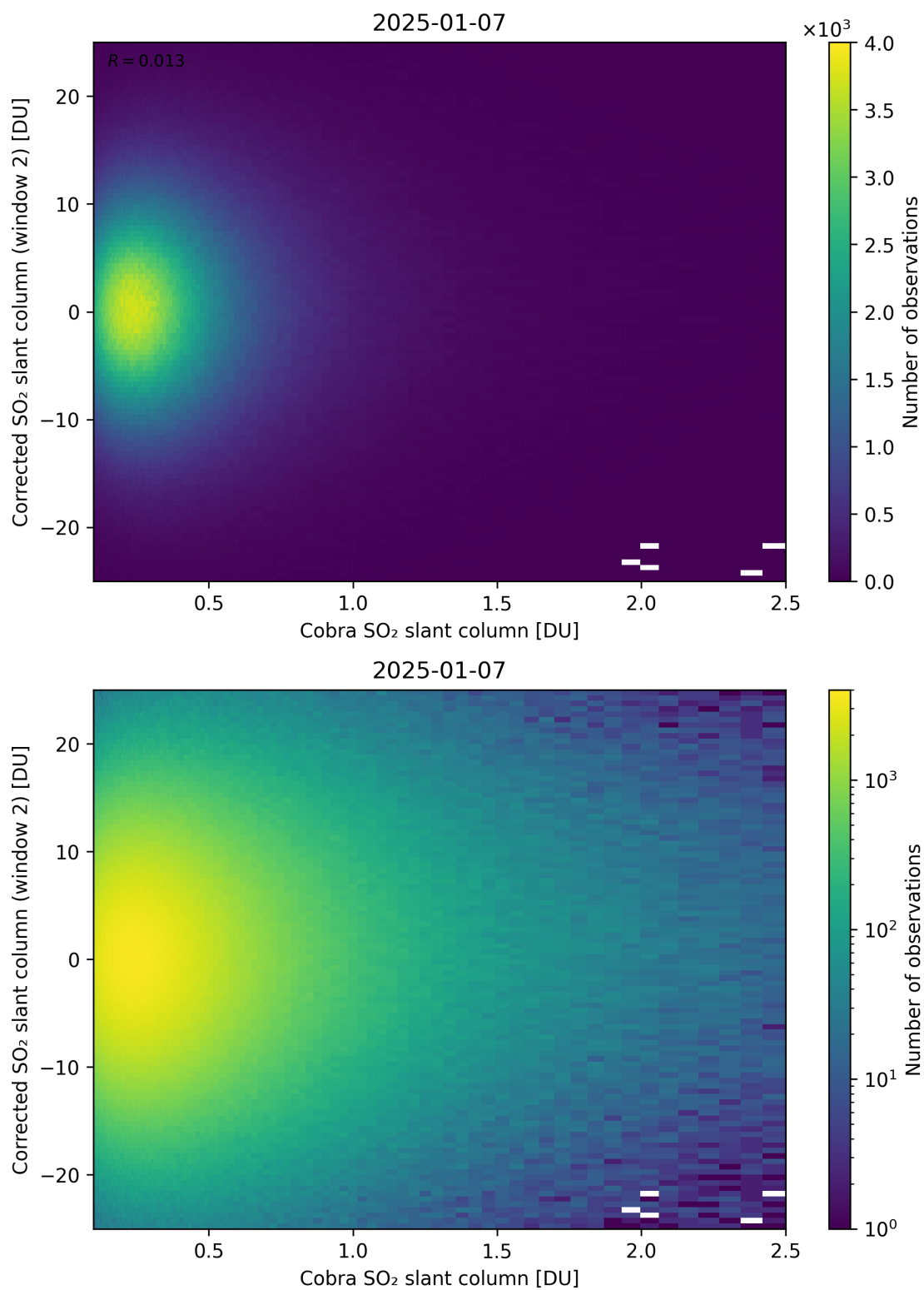
Figure 217: Scatter density plot of “Cobra SO 2 slant column” against “Corrected SO 2 slant column (window 2)” for 2025-01-07 to 2025-01-08.
