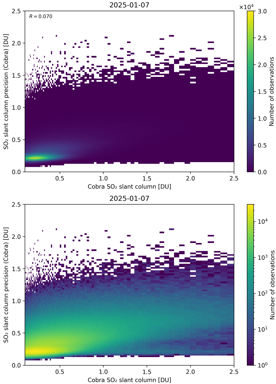
Figure 216: Scatter density plot of “Cobra SO 2 slant column” against “SO 2 slant column precision (Cobra)” for 2025-01-07 to 2025-01-08.
