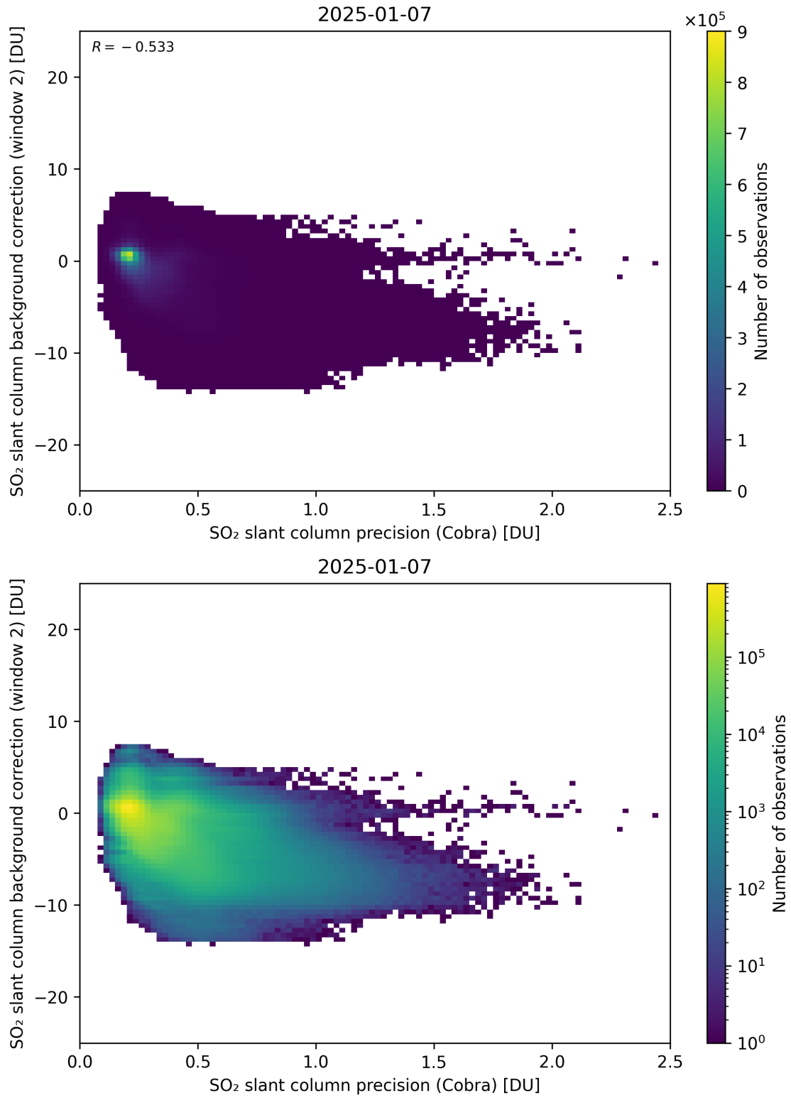
Figure 200: Scatter density plot of “SO 2 slant column precision (Cobra)” against “SO 2 slant column background correction (window 2)” for 2025-01-07 to 2025-01-08.
