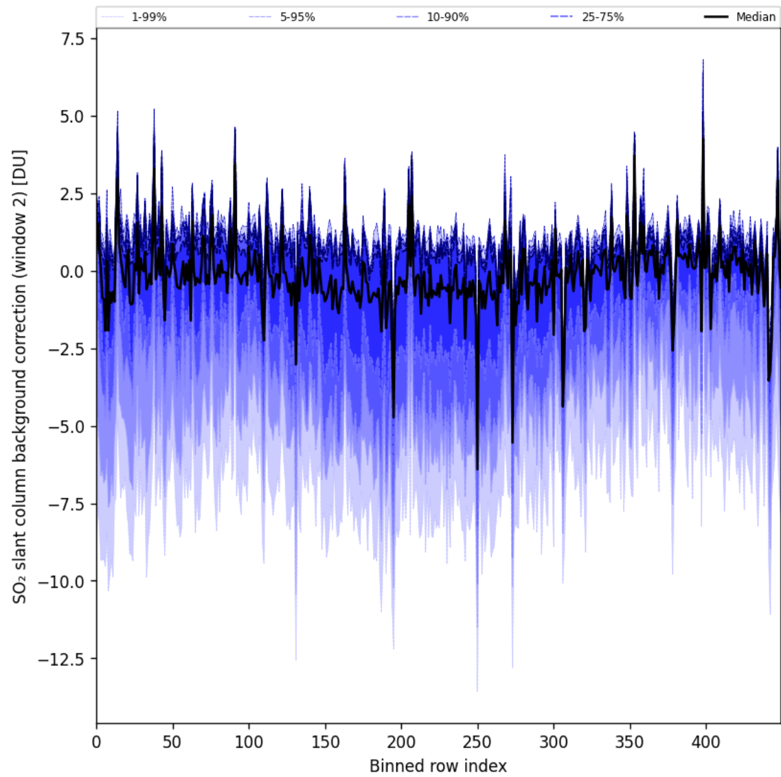
Figure 96: Along track statistics of “SO 2 slant column background correction (window 2)” for 2025-01-07 to 2025-01-08
