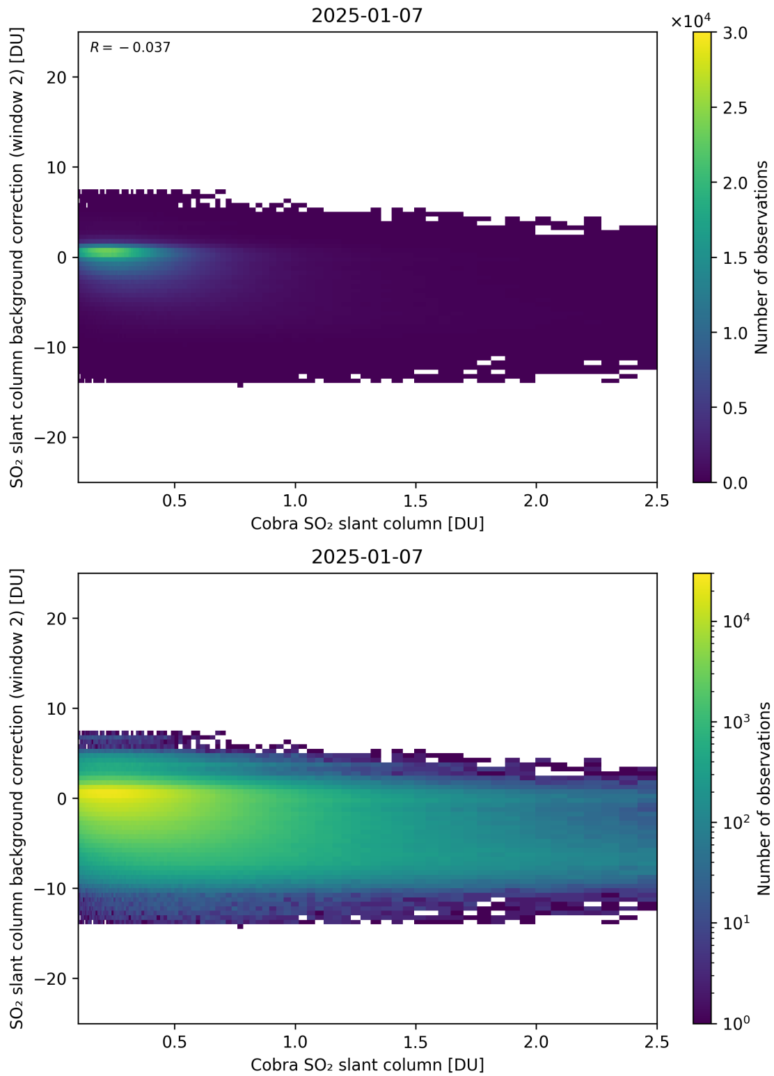
Figure 194: Scatter density plot of “Cobra SO 2 slant column” against “SO 2 slant column background correction (window 2)” for 2025-01-07 to 2025-01-08.
