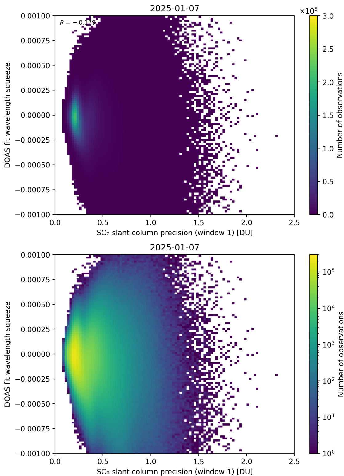
Figure 272: Scatter density plot of “SO 2 slant column precision (window 1)” against “DOAS fit wavelength squeeze” for 2025-01-07 to 2025-01-08.
