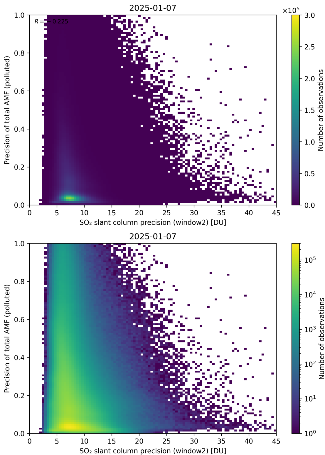
Figure 302: Scatter density plot of “SO 2 slant column precision (window2)” against “Precision of total AMF (polluted)” for 2025-01-07 to 2025-01-08.
