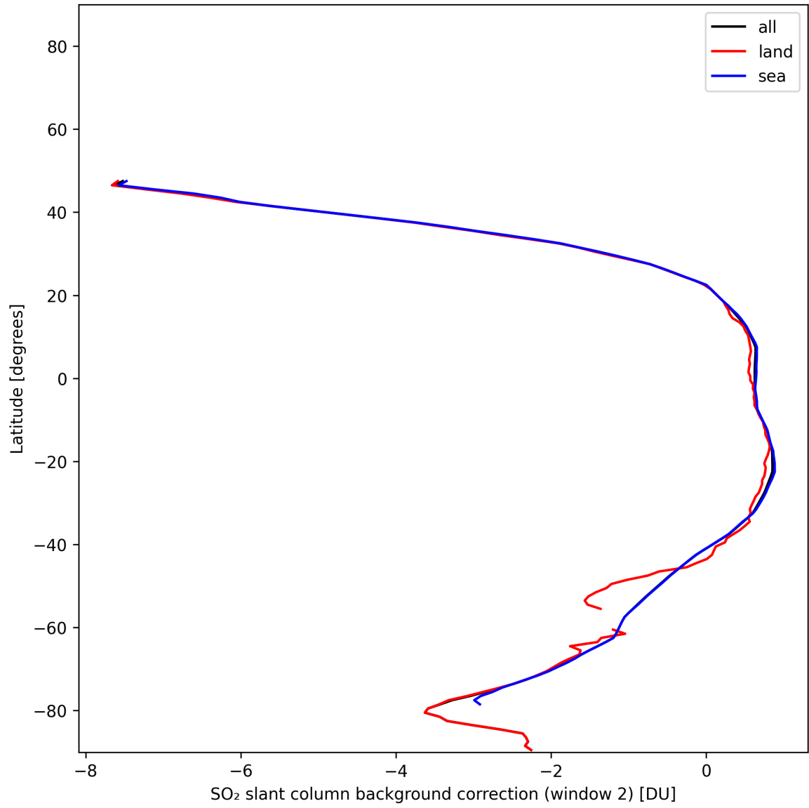
Figure 44: Zonal average of “SO 2 slant column background correction (window 2)” for 2025-01-07 to 2025-01-08.
