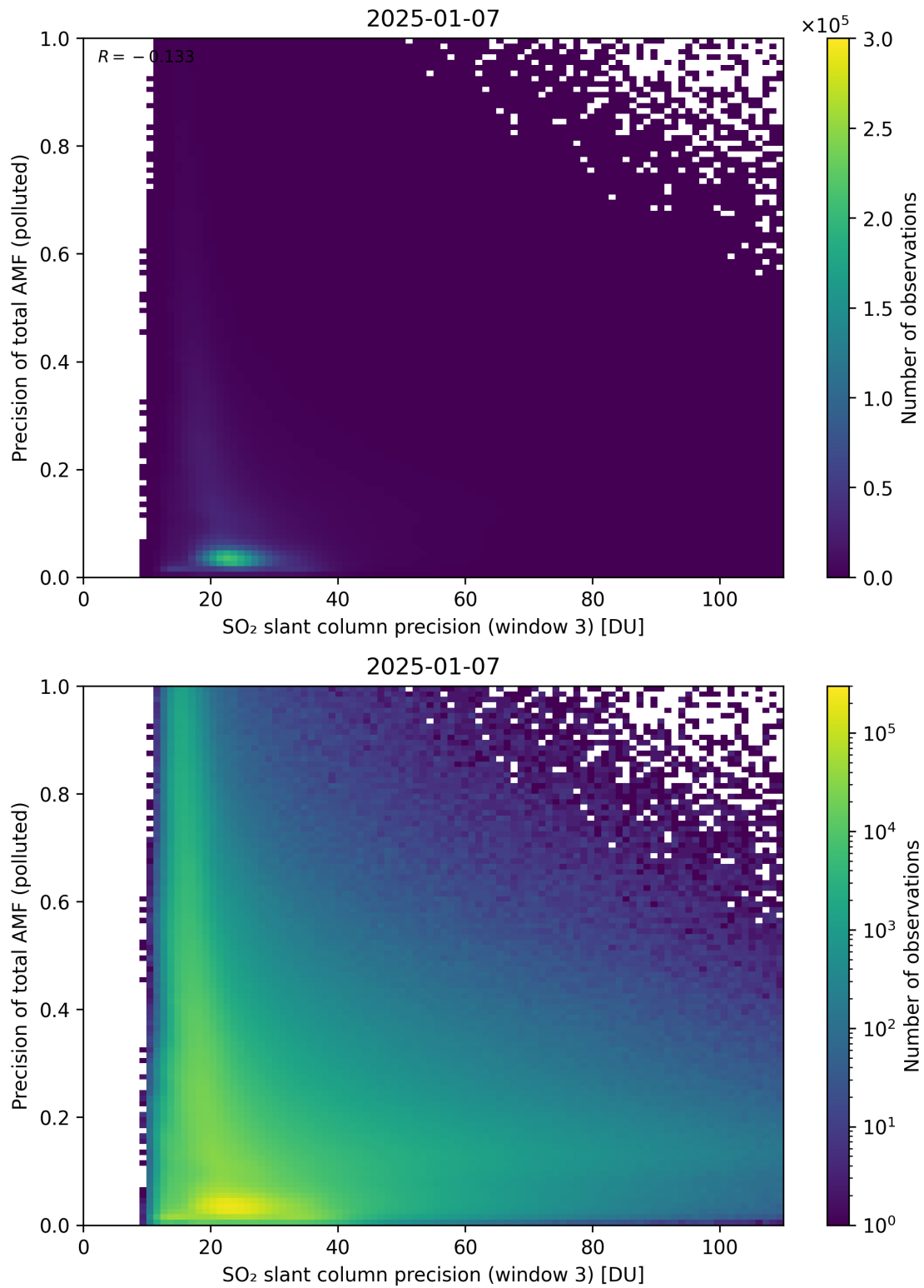
Figure 314: Scatter density plot of “SO 2 slant column precision (window 3)” against “Precision of total AMF (polluted)” for 2025-01-07 to 2025-01-08.
