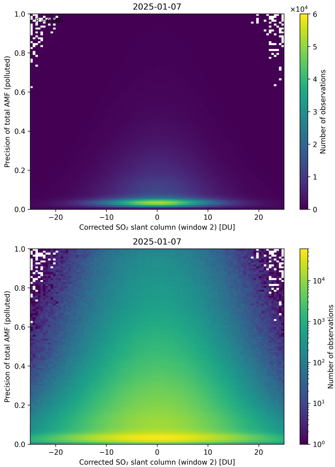
Figure 254: Scatter density plot of “Corrected SO 2 slant column (window 2)” against “Precision of total AMF (polluted)” for 2025-01-07 to 2025-01-08.
