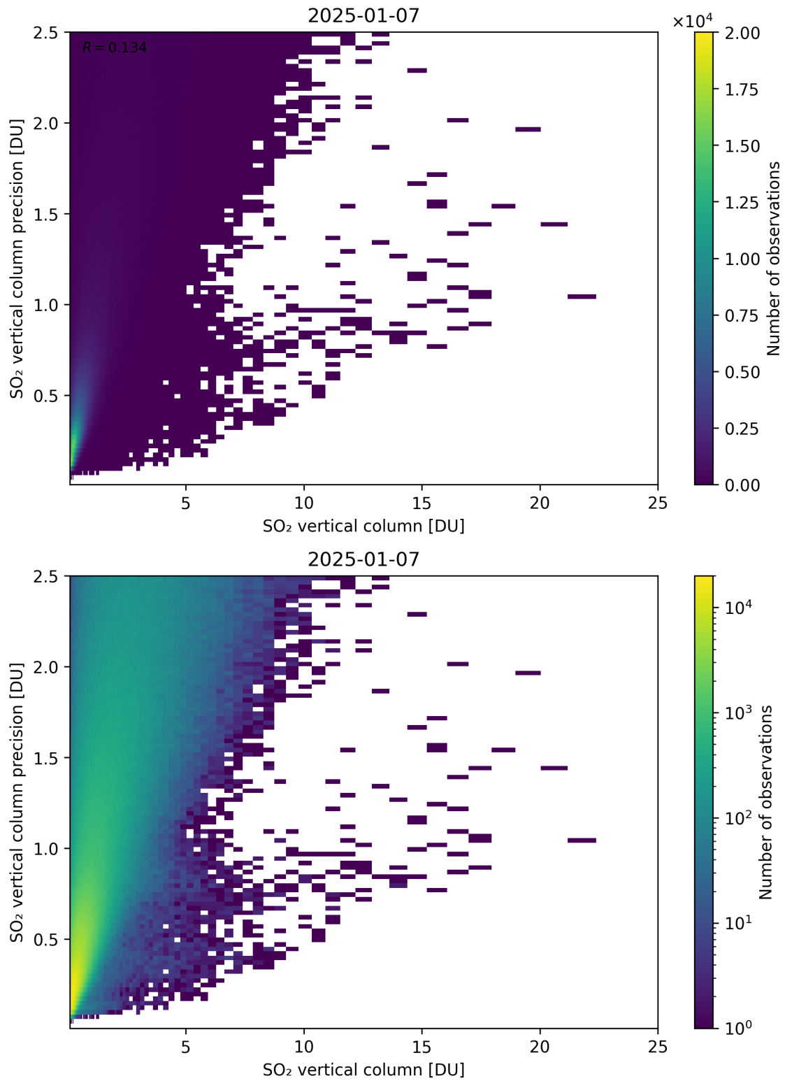
Figure 361: Scatter density plot of “SO 2 vertical column” against “SO 2 vertical column precision” for 2025-01-07 to 2025-01-08.
