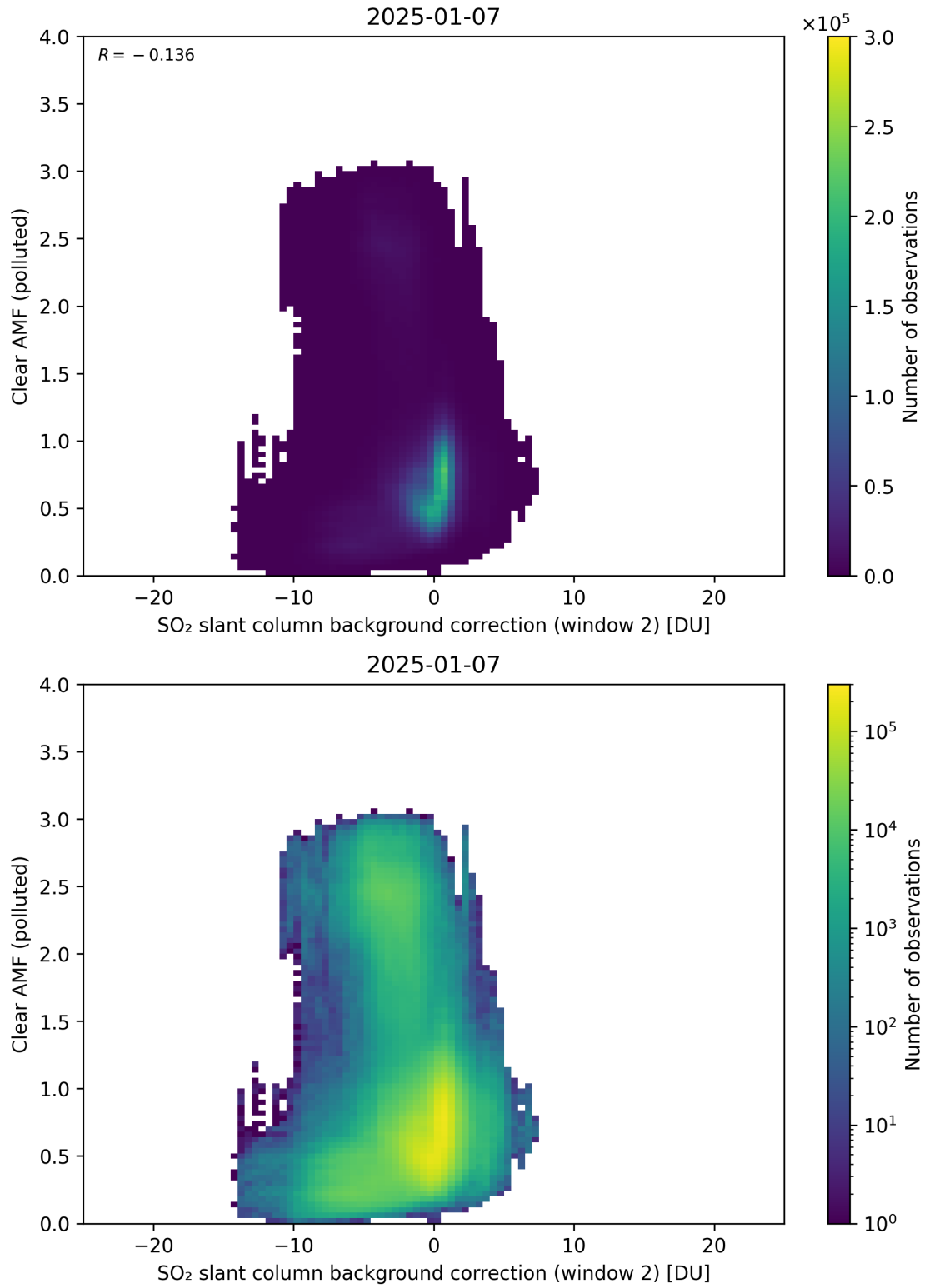
Figure 126: Scatter density plot of “SO 2 slant column background correction (window 2)” against “Clear AMF (polluted)” for 2025-01-07 to 2025-01-08.
