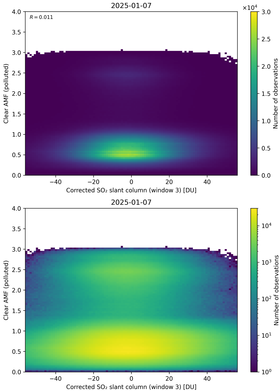
Figure 259: Scatter density plot of “Corrected SO 2 slant column (window 3)” against “Clear AMF (polluted)” for 2025-01-07 to 2025-01-08.
