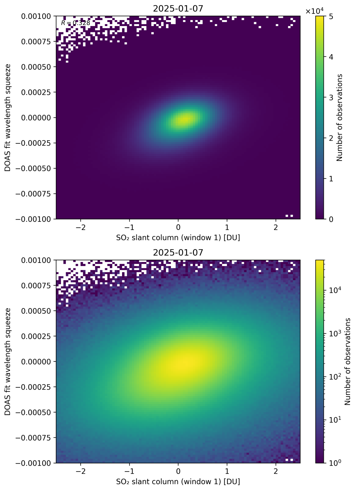
Figure 266: Scatter density plot of “SO 2 slant column (window 1)” against “DOAS fit wavelength squeeze” for 2025-01-07 to 2025-01-08.
