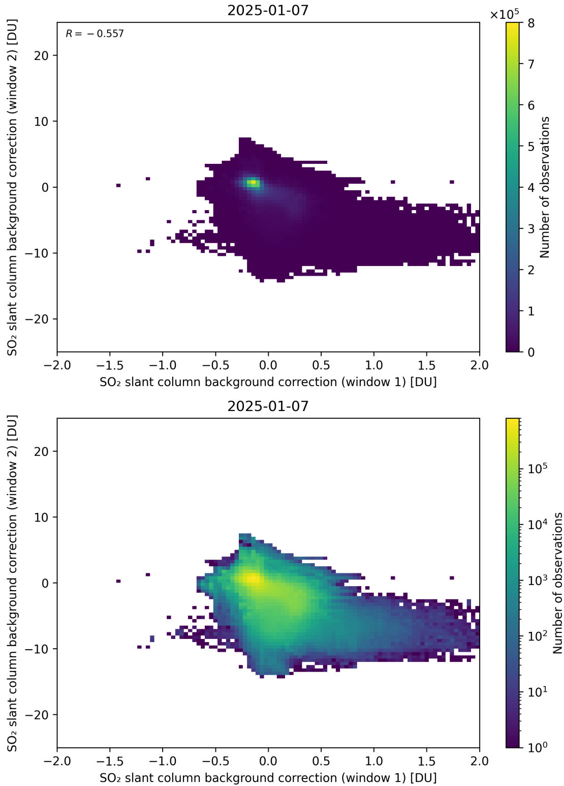
Figure 109: Scatter density plot of “SO 2 slant column background correction (window 1)” against “SO 2 slant column background correction (window 2)” for 2025-01-07 to 2025-01-08.
