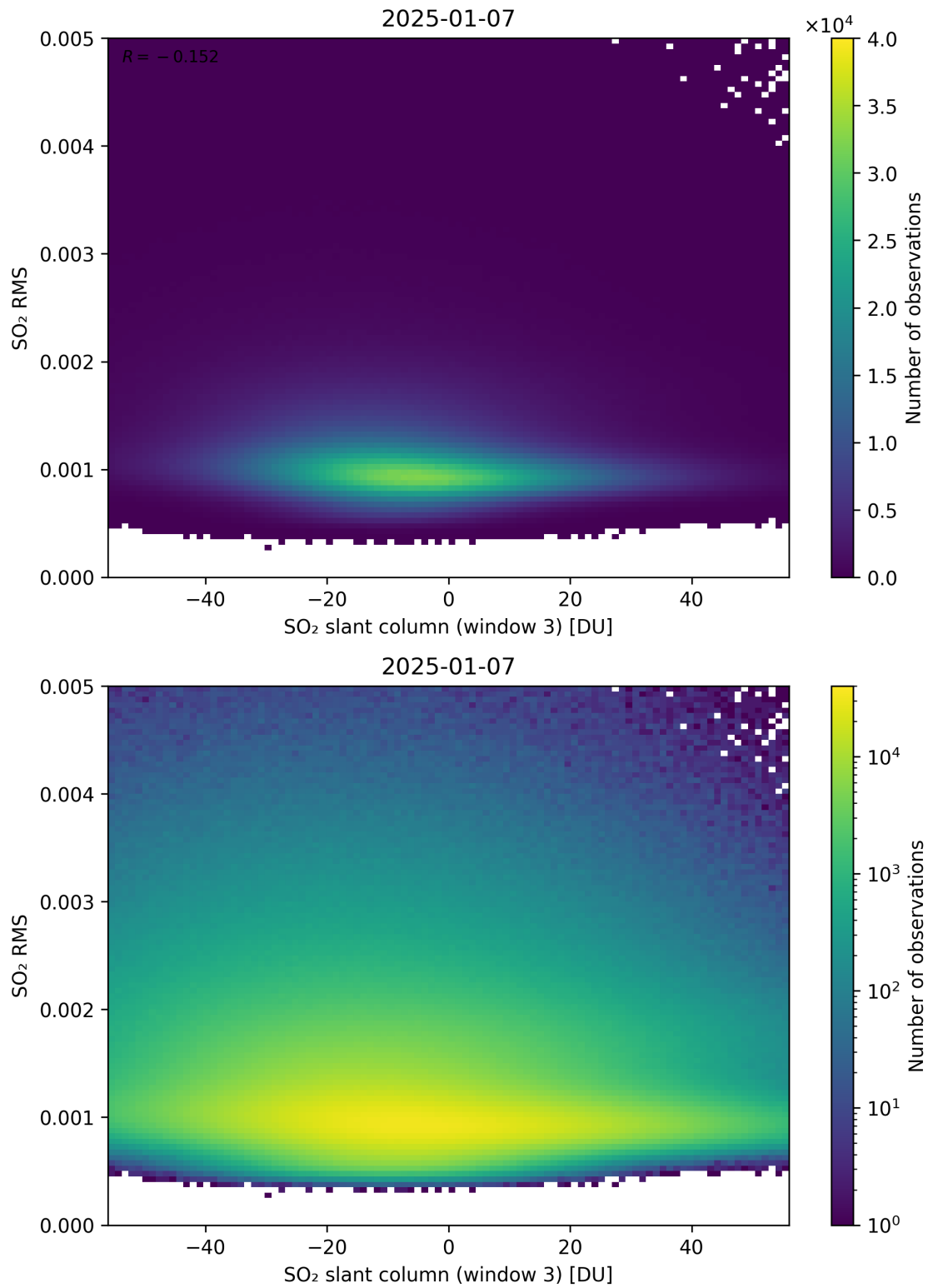
Figure 306: Scatter density plot of “SO 2 slant column (window 3)” against “SO 2 RMS” for 2025-01-07 to 2025-01-08.
