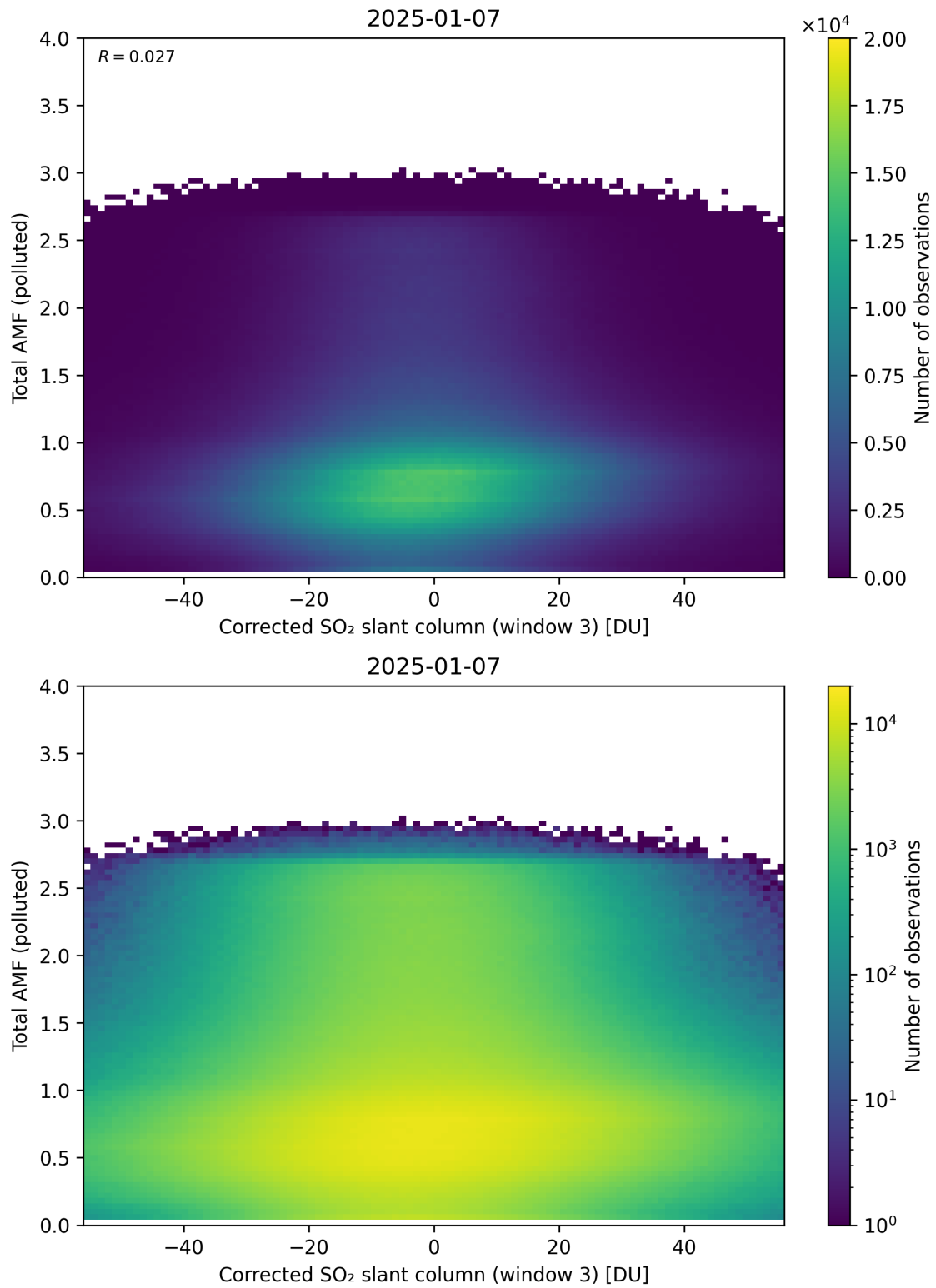
Figure 260: Scatter density plot of “Corrected SO 2 slant column (window 3)” against “Total AMF (polluted)” for 2025-01-07 to 2025-01-08.
