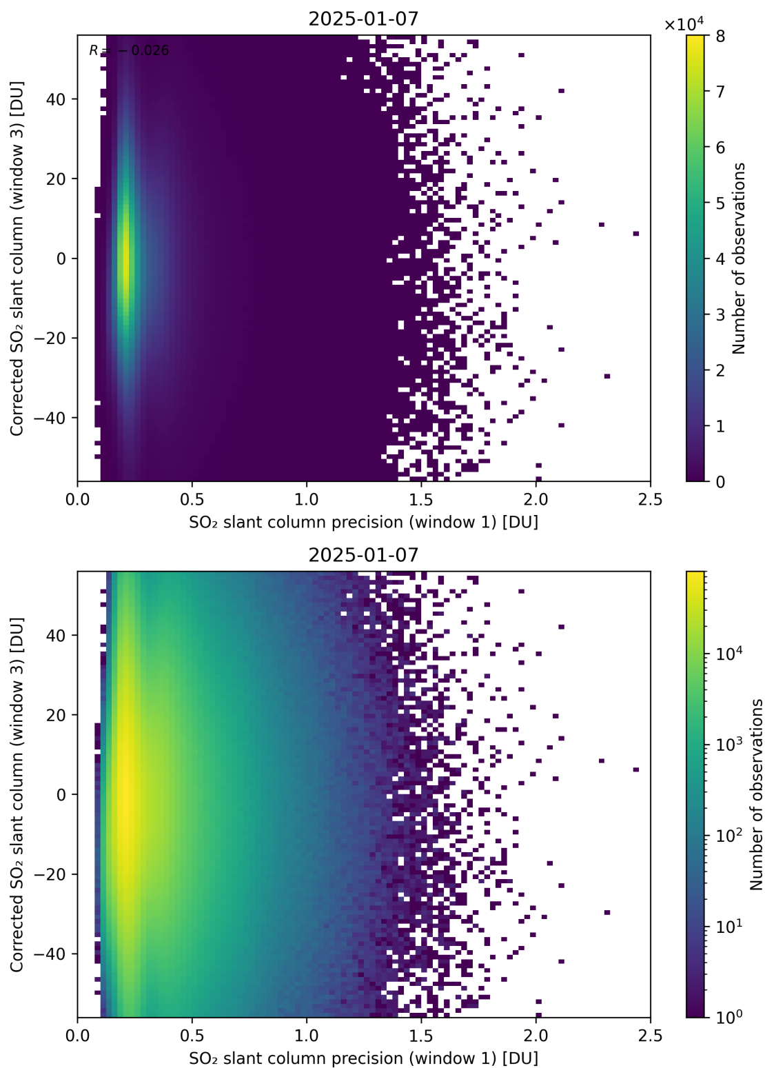
Figure 276: Scatter density plot of “SO 2 slant column precision (window 1)” against “Corrected SO 2 slant column (window 3)” for 2025-01-07 to 2025-01-08.
