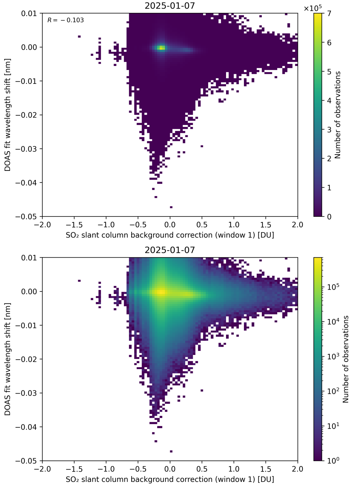
Figure 111: Scatter density plot of “SO 2 slant column background correction (window 1)” against “DOAS fit wavelength shift” for 2025-01-07 to 2025-01-08.
