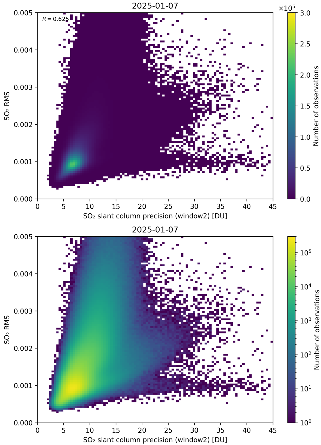
Figure 295: Scatter density plot of “SO 2 slant column precision (window2)” against “SO 2 RMS” for 2025-01-07 to 2025-01-08.
