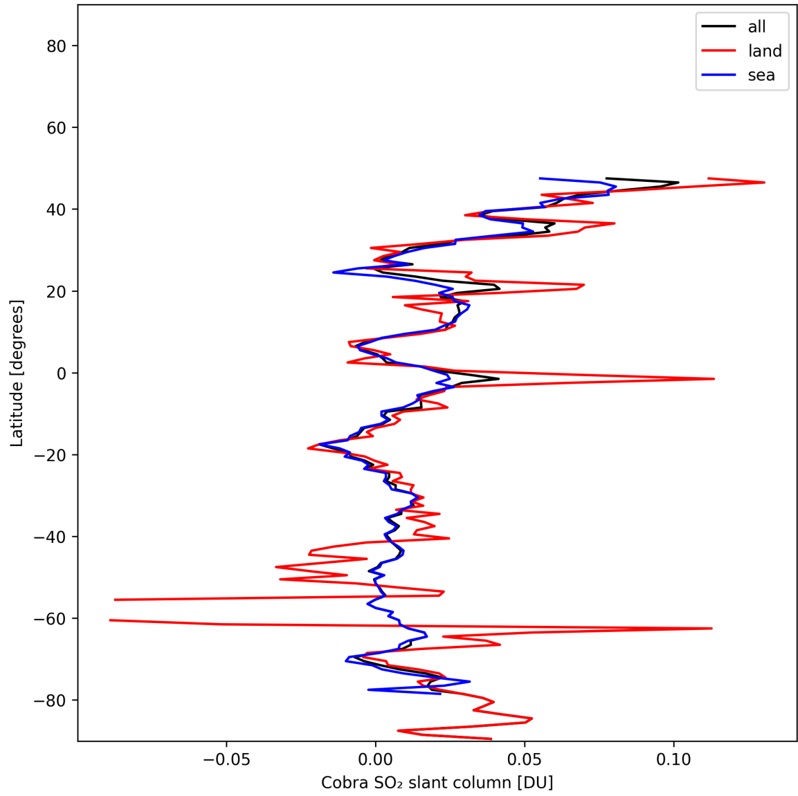
Figure 35: Zonal average of “Cobra SO 2 slant column” for 2025-01-07 to 2025-01-08.
