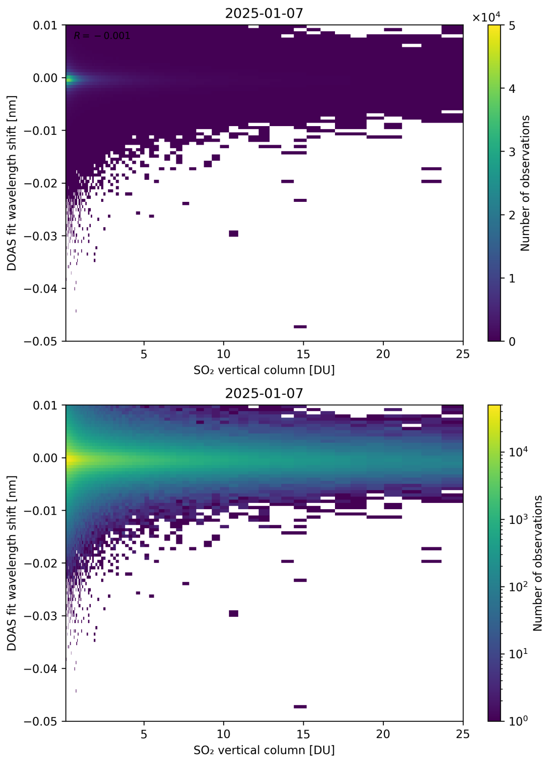
Figure 326: Scatter density plot of “SO 2 vertical column” against “DOAS fit wavelength shift” for 2025-01-07 to 2025-01-08.
