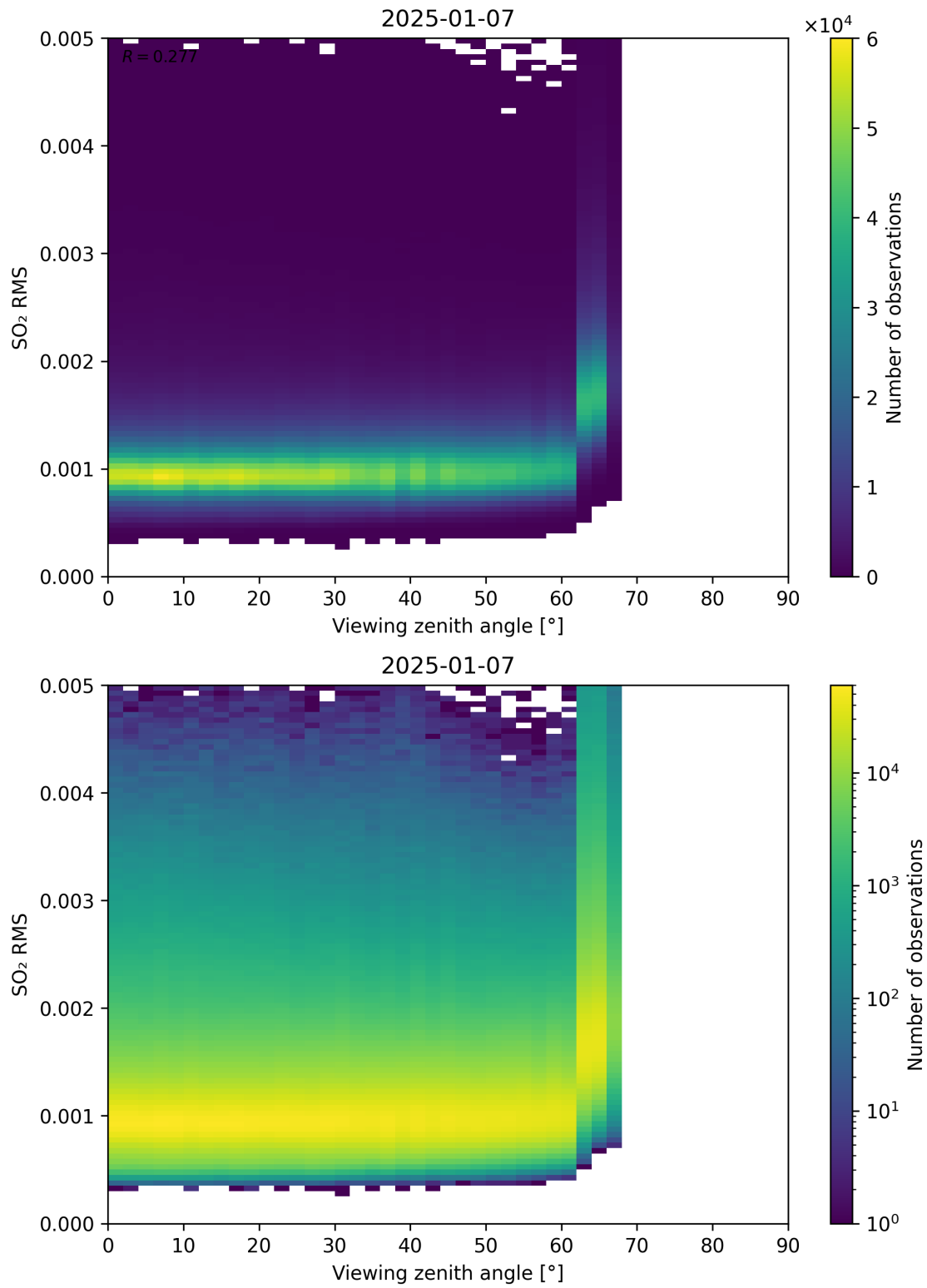
Figure 367: Scatter density plot of “Viewing zenith angle” against “SO 2 RMS” for 2025-01-07 to 2025-01-08.
