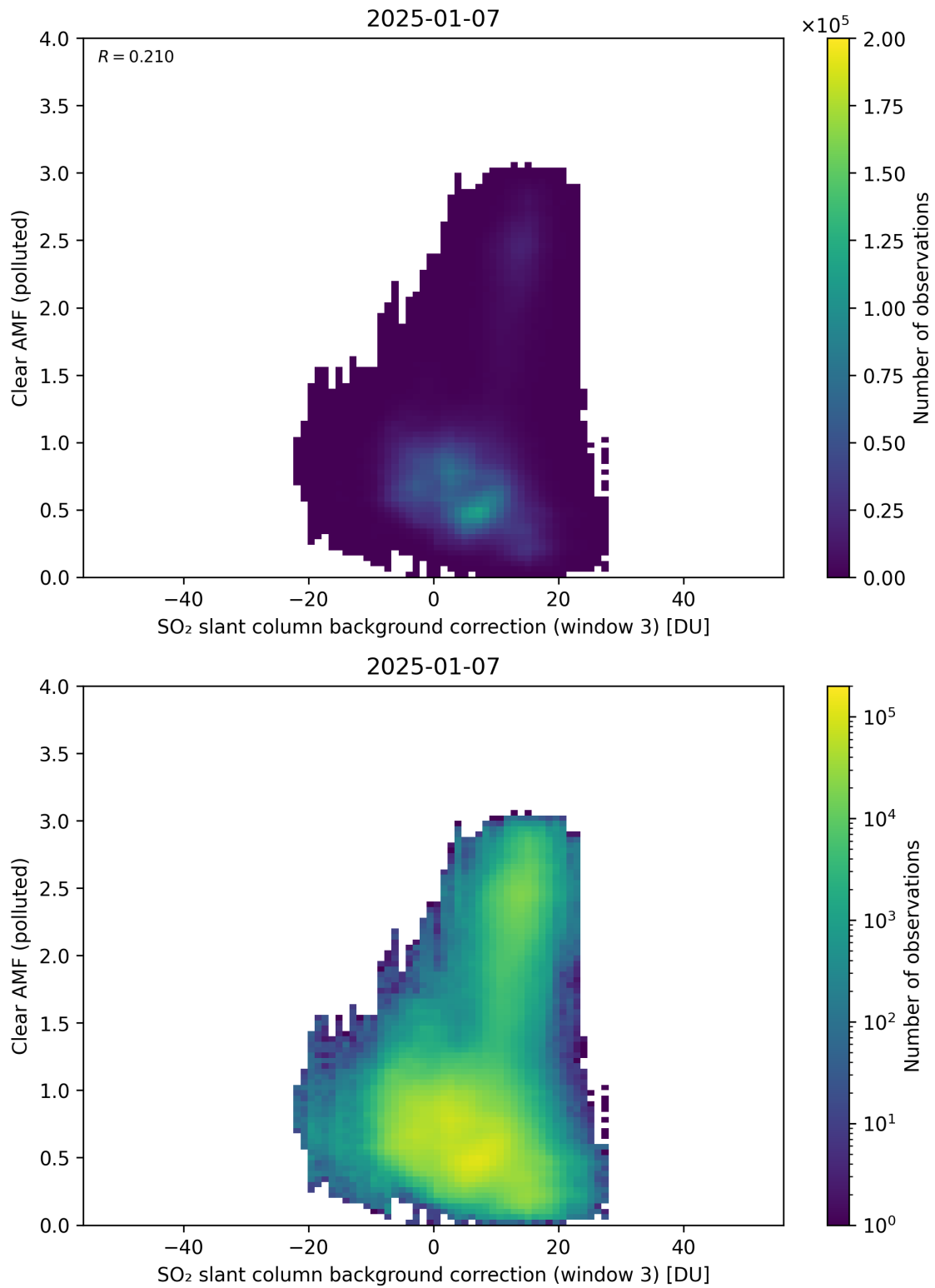
Figure 135: Scatter density plot of “SO 2 slant column background correction (window 3)” against “Clear AMF (polluted)” for 2025-01-07 to 2025-01-08.
