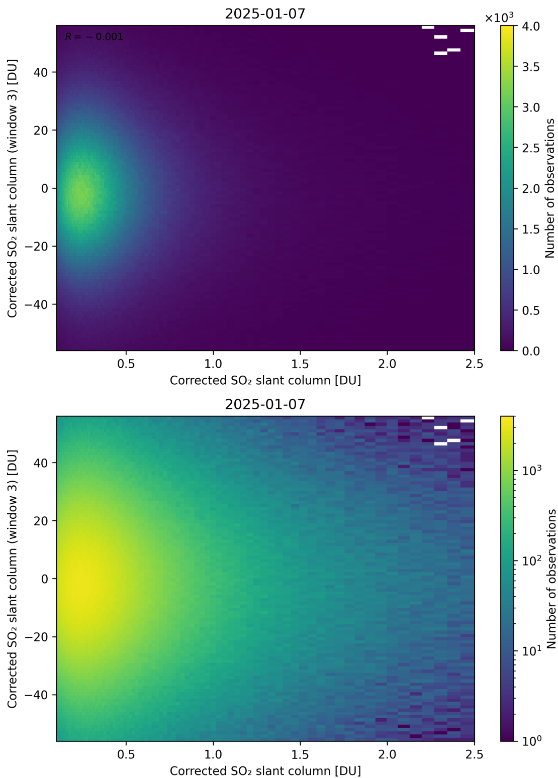
Figure 236: Scatter density plot of “Corrected SO 2 slant column” against “Corrected SO 2 slant column (window 3)” for 2025-01-07 to 2025-01-08.
