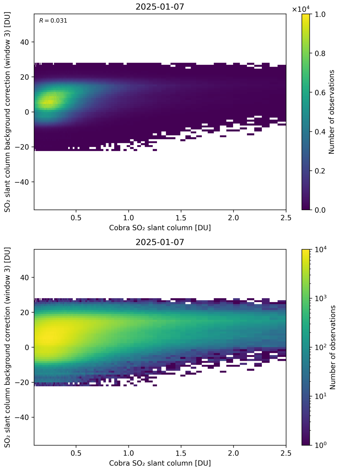
Figure 195: Scatter density plot of “Cobra SO 2 slant column” against “SO 2 slant column background correction (window 3)” for 2025-01-07 to 2025-01-08.
