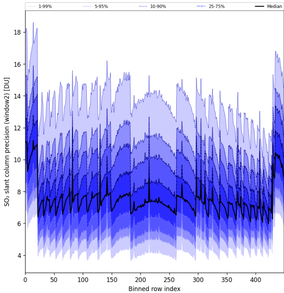
Figure 94: Along track statistics of “SO 2 slant column precision (window2)” for 2025-01-07 to 2025-01-08
