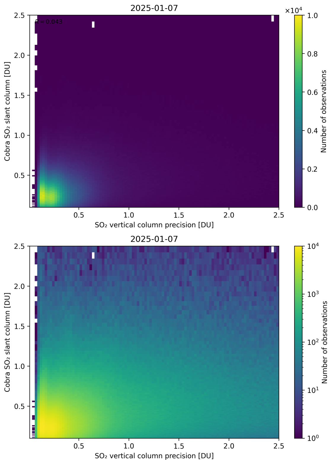
Figure 336: Scatter density plot of “SO 2 vertical column precision” against “Cobra SO 2 slant column” for 2025-01-07 to 2025-01-08.
