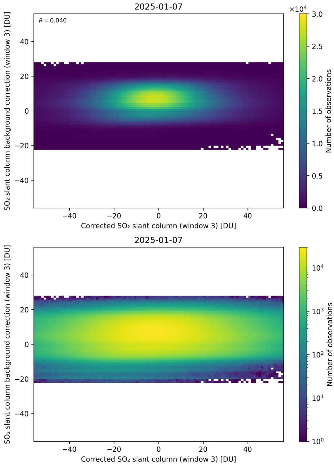
Figure 255: Scatter density plot of “Corrected SO 2 slant column (window 3)” against “SO 2 slant column background correction (window 3)” for 2025-01-07 to 2025-01-08.
