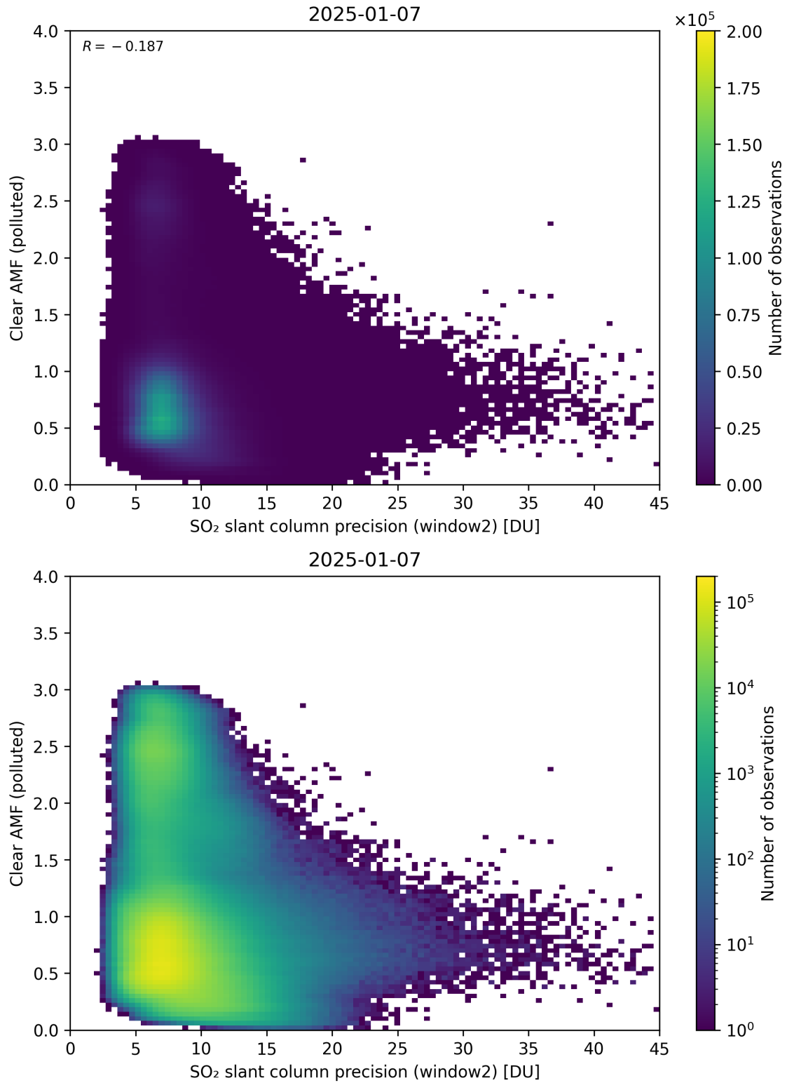
Figure 296: Scatter density plot of “SO 2 slant column precision (window2)” against “Clear AMF (polluted)” for 2025-01-07 to 2025-01-08.
