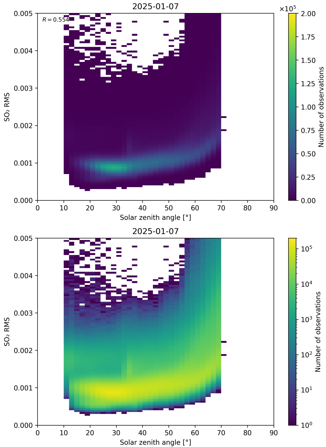
Figure 176: Scatter density plot of “Solar zenith angle” against “SO 2 RMS” for 2025-01-07 to 2025-01-08.
