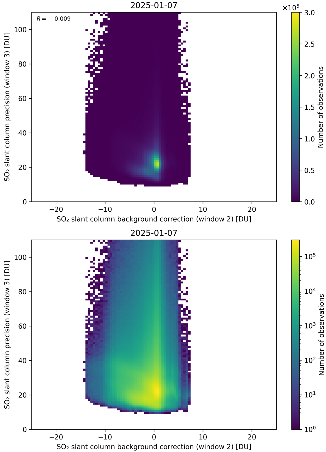
Figure 129: Scatter density plot of “SO 2 slant column background correction (window 2)” against “SO 2 slant column precision (window 3)” for 2025-01-07 to 2025-01-08.
