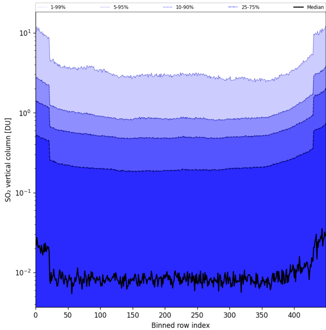
Figure 84: Along track statistics of “SO 2 vertical column” for 2025-01-07 to 2025-01-08
