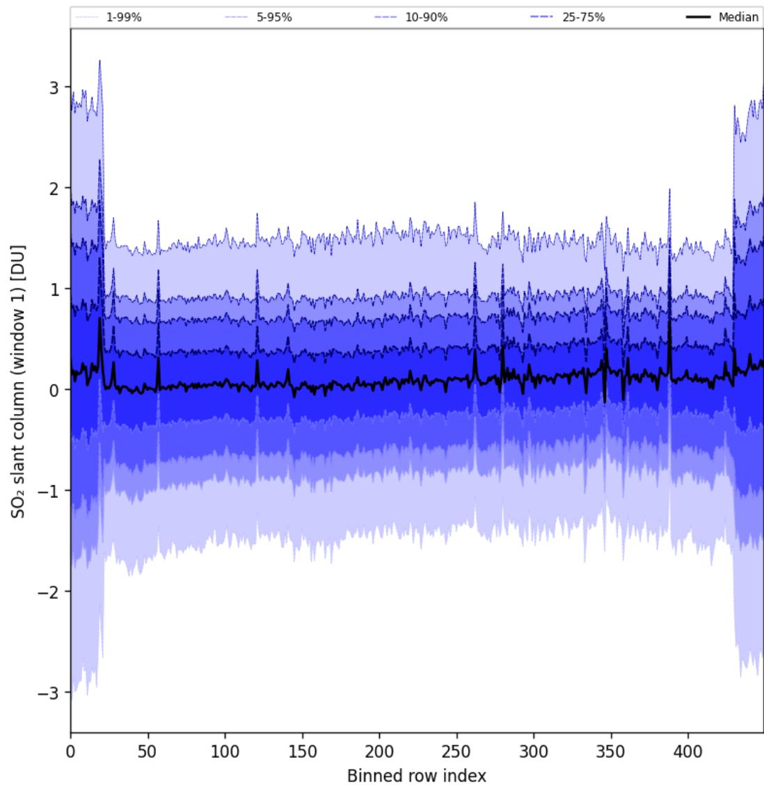
Figure 89: Along track statistics of “SO 2 slant column (window 1)” for 2025-01-07 to 2025-01-08
