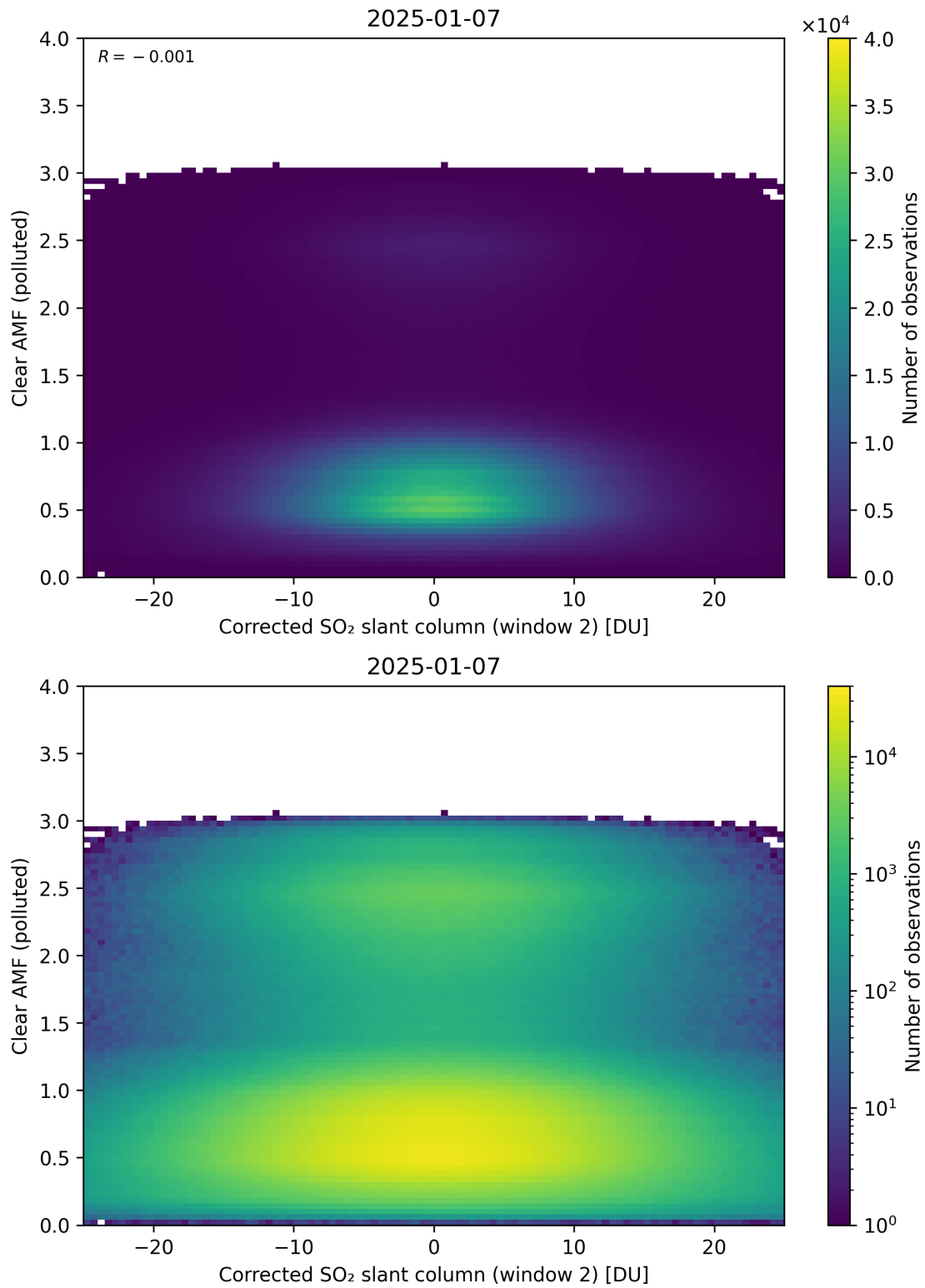
Figure 249: Scatter density plot of “Corrected SO 2 slant column (window 2)” against “Clear AMF (polluted)” for 2025-01-07 to 2025-01-08.
