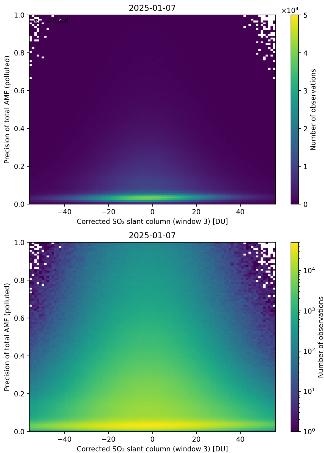
Figure 261: Scatter density plot of “Corrected SO 2 slant column (window 3)” against “Precision of total AMF (polluted)” for 2025-01-07 to 2025-01-08.
