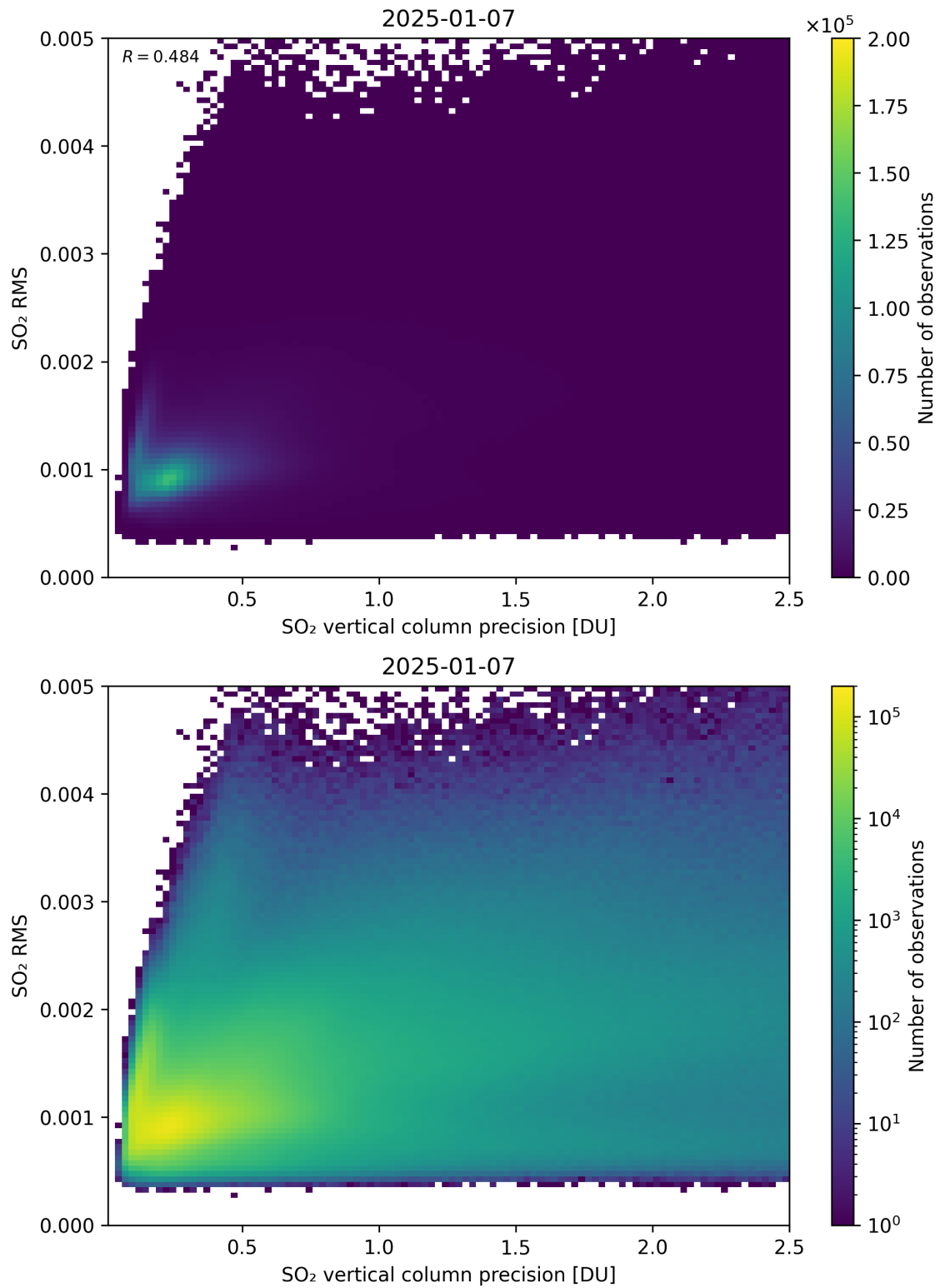
Figure 334: Scatter density plot of “SO 2 vertical column precision” against “SO 2 RMS” for 2025-01-07 to 2025-01-08.
