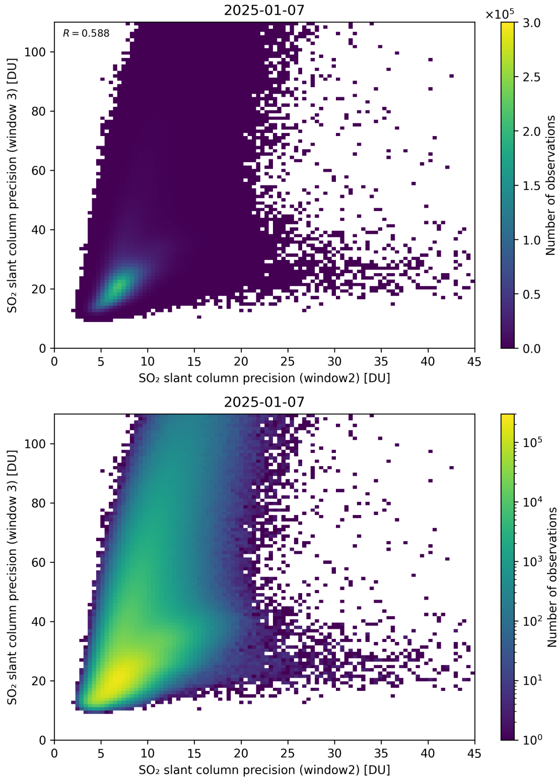
Figure 300: Scatter density plot of “SO 2 slant column precision (window2)” against “SO 2 slant column precision (window 3)” for 2025-01-07 to 2025-01-08.
