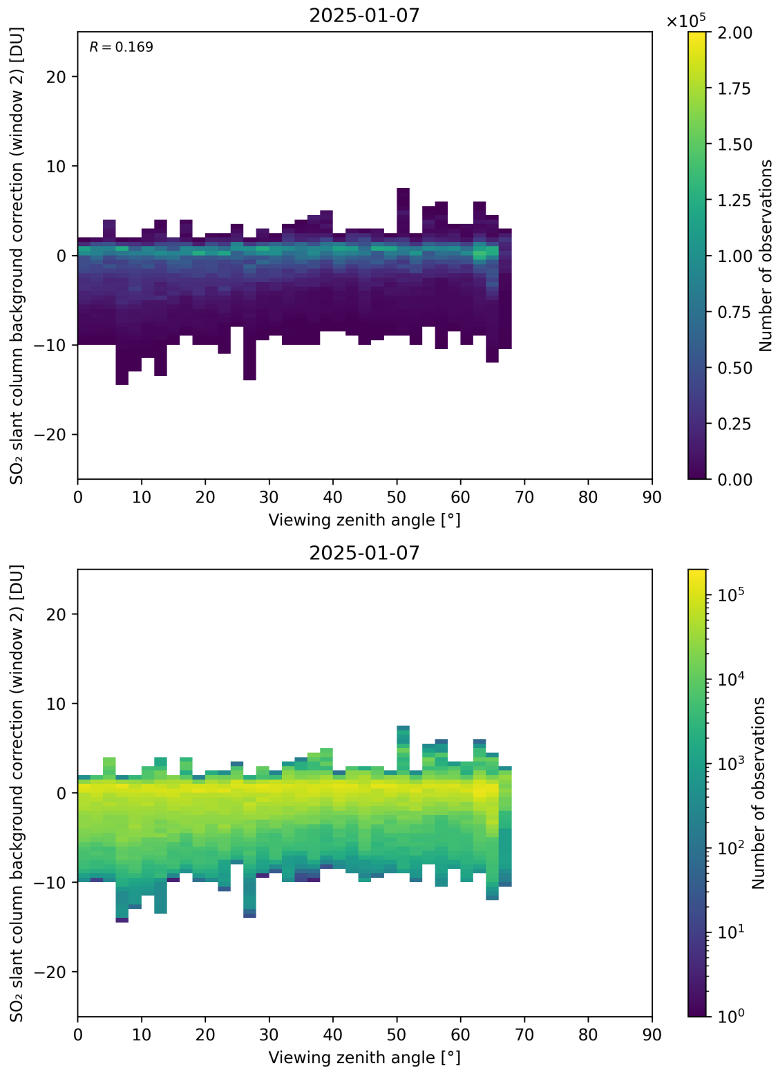
Figure 363: Scatter density plot of “Viewing zenith angle” against “SO 2 slant column background correction (window 2)” for 2025-01-07 to 2025-01-08.
