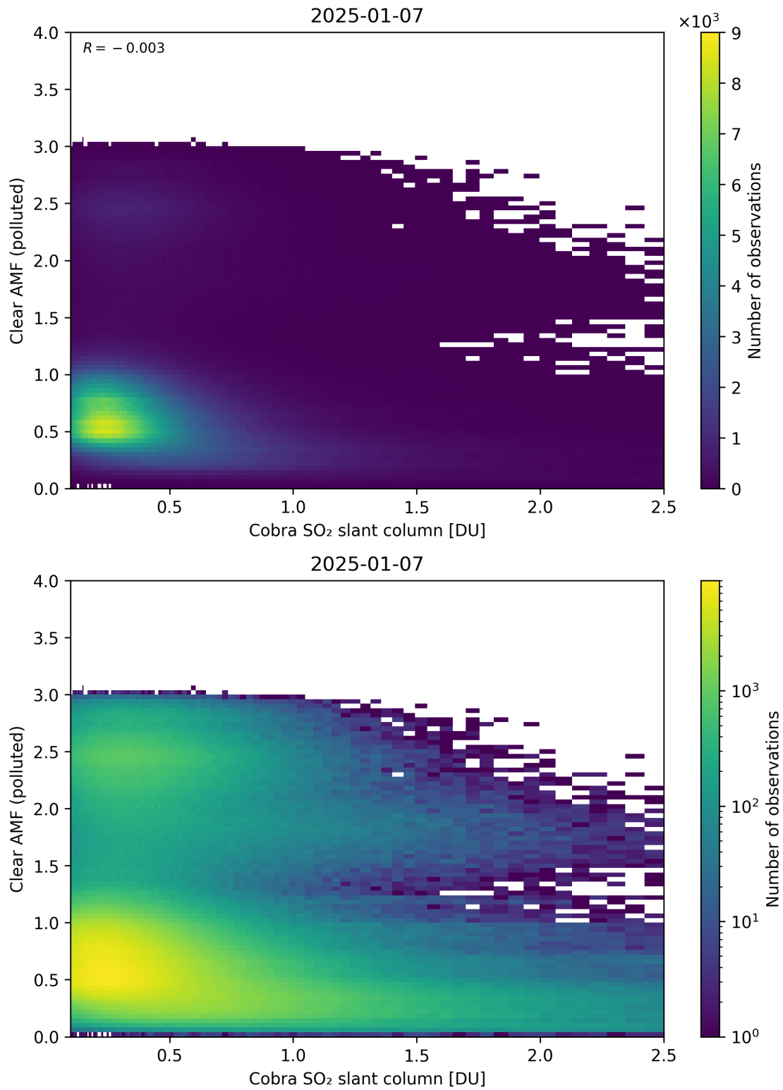
Figure 215: Scatter density plot of “Cobra SO 2 slant column” against “Clear AMF (polluted)” for 2025-01-07 to 2025-01-08.
