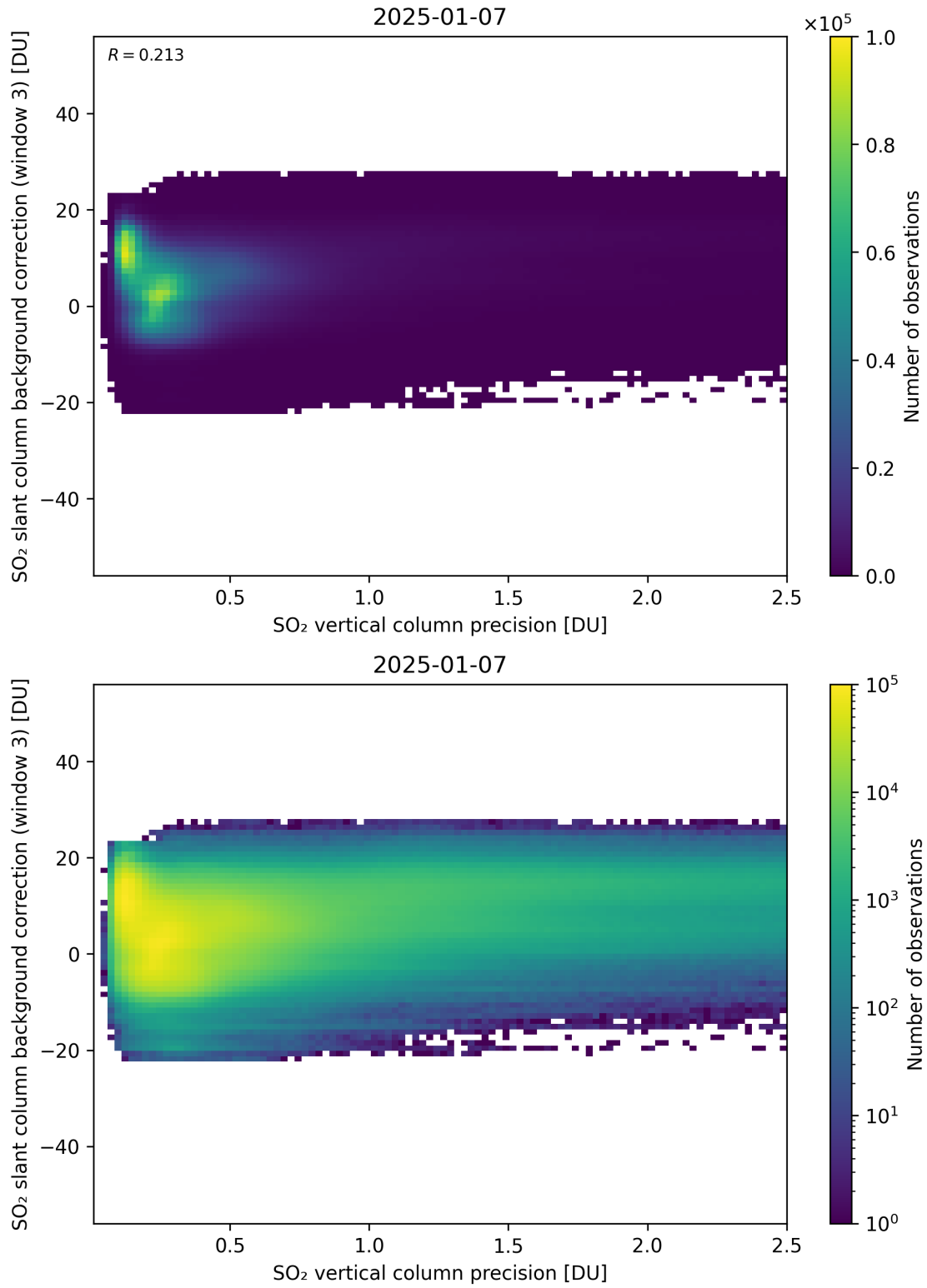
Figure 331: Scatter density plot of “SO 2 vertical column precision” against “SO 2 slant column background correction (window 3)” for 2025-01-07 to 2025-01-08.
