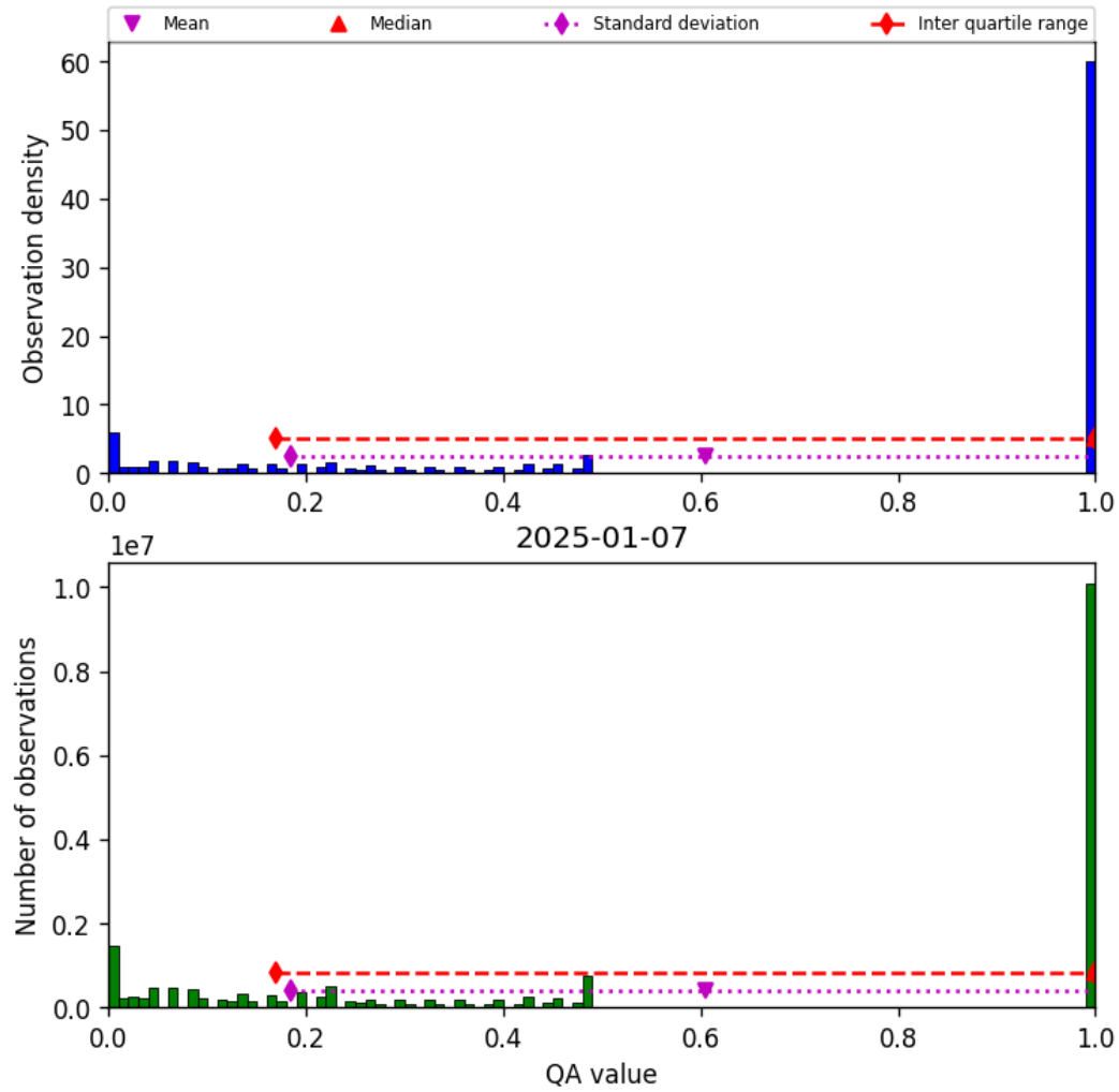
Figure 57: Histogram of “QA value” for 2025-01-07 to 2025-01-08
