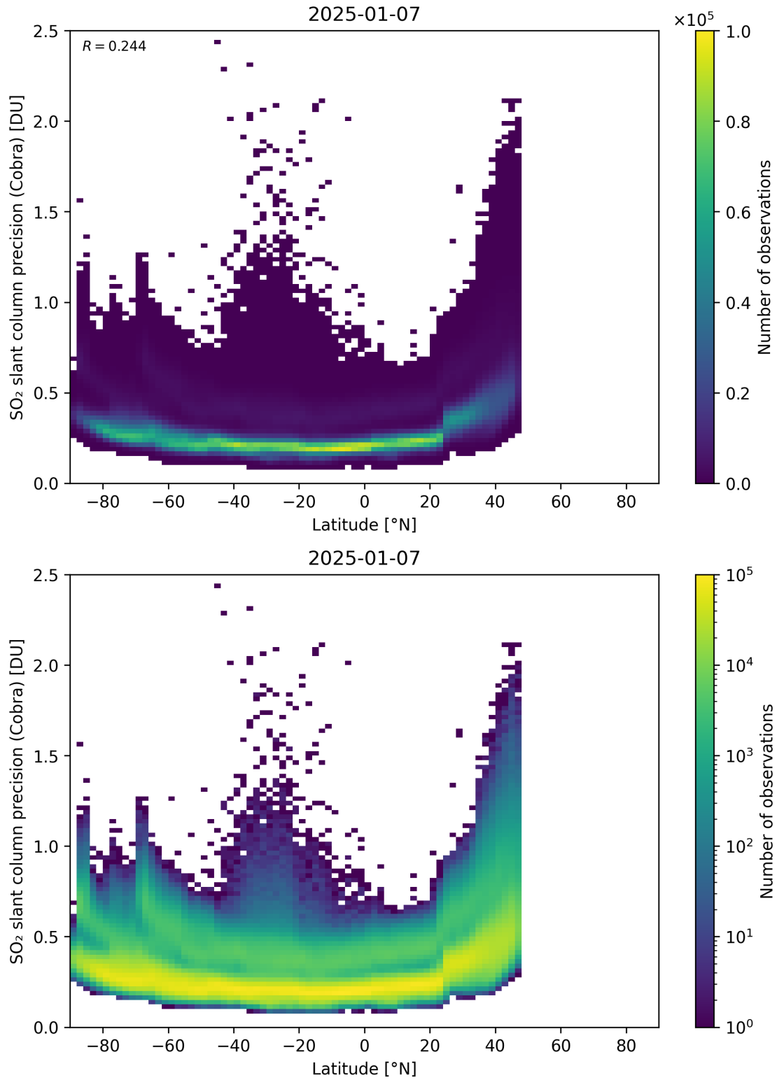
Figure 158: Scatter density plot of “Latitude” against “SO 2 slant column precision (Cobra)” for 2025-01-07 to 2025-01-08.
