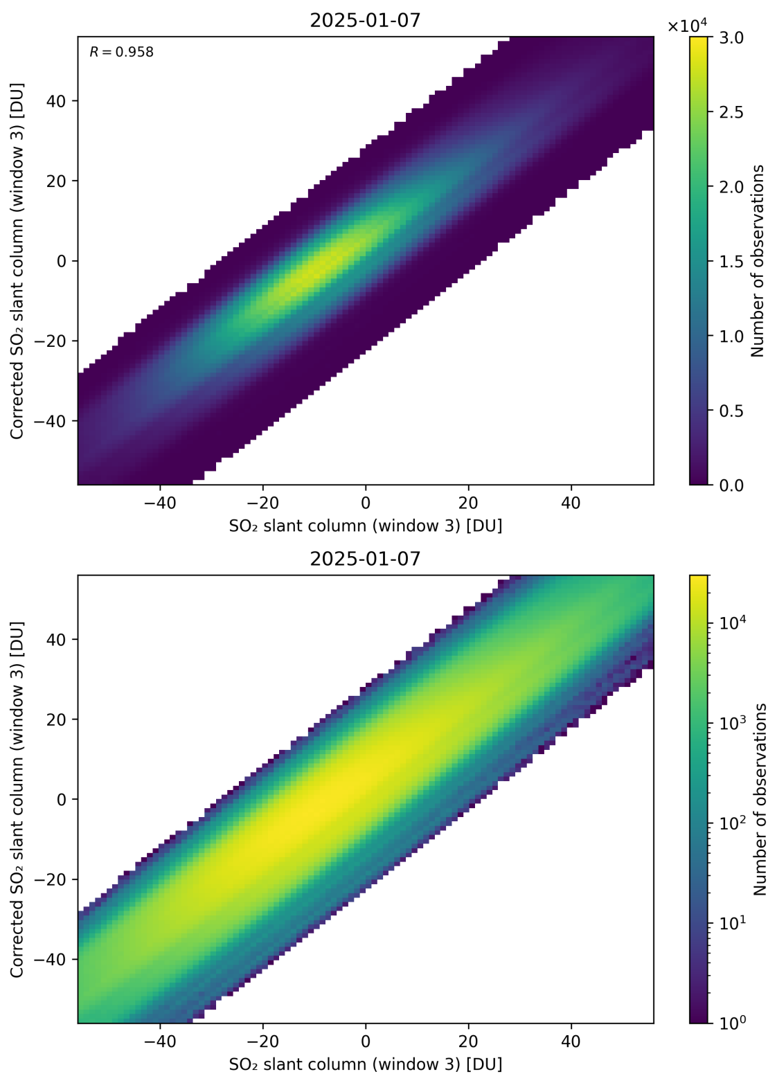
Figure 316: Scatter density plot of “SO 2 slant column (window 3)” against “Corrected SO 2 slant column (window 3)” for 2025-01-07 to 2025-01-08.
