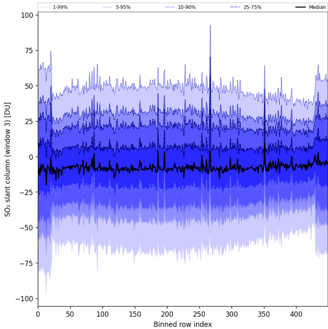
Figure 97: Along track statistics of “SO 2 slant column (window 3)” for 2025-01-07 to 2025-01-08
