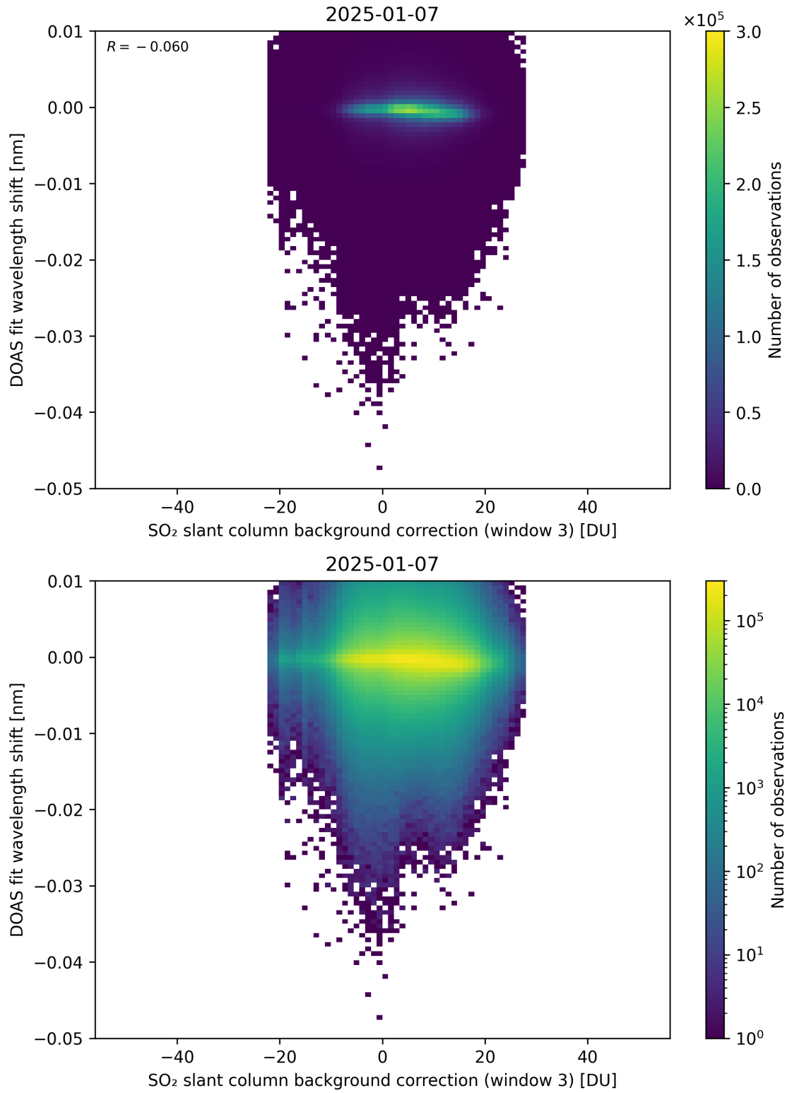
Figure 132: Scatter density plot of “SO 2 slant column background correction (window 3)” against “DOAS fit wavelength shift” for 2025-01-07 to 2025-01-08.
