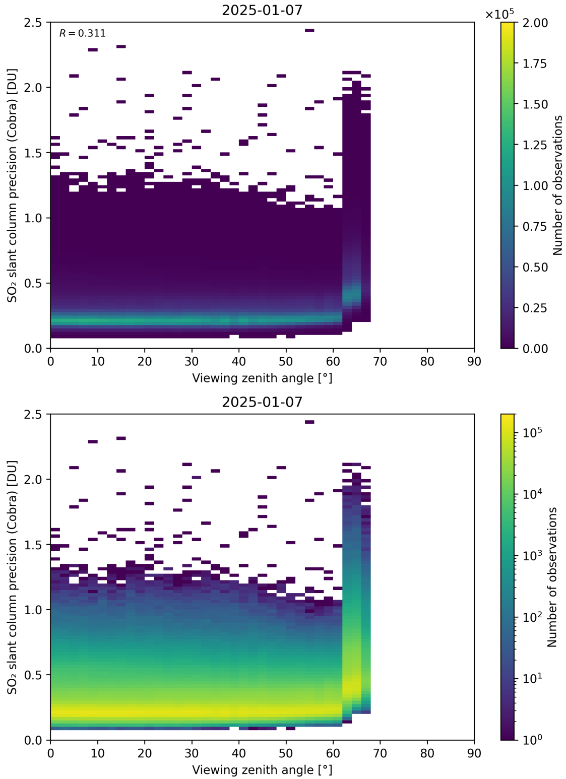
Figure 372: Scatter density plot of “Viewing zenith angle” against “SO 2 slant column precision (Cobra)” for 2025-01-07 to 2025-01-08.
