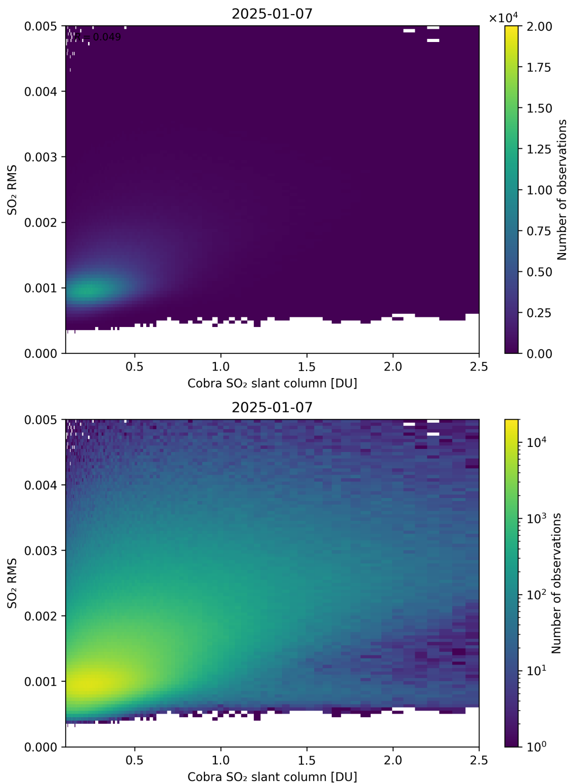
Figure 198: Scatter density plot of “Cobra SO 2 slant column” against “SO 2 RMS” for 2025-01-07 to 2025-01-08.
