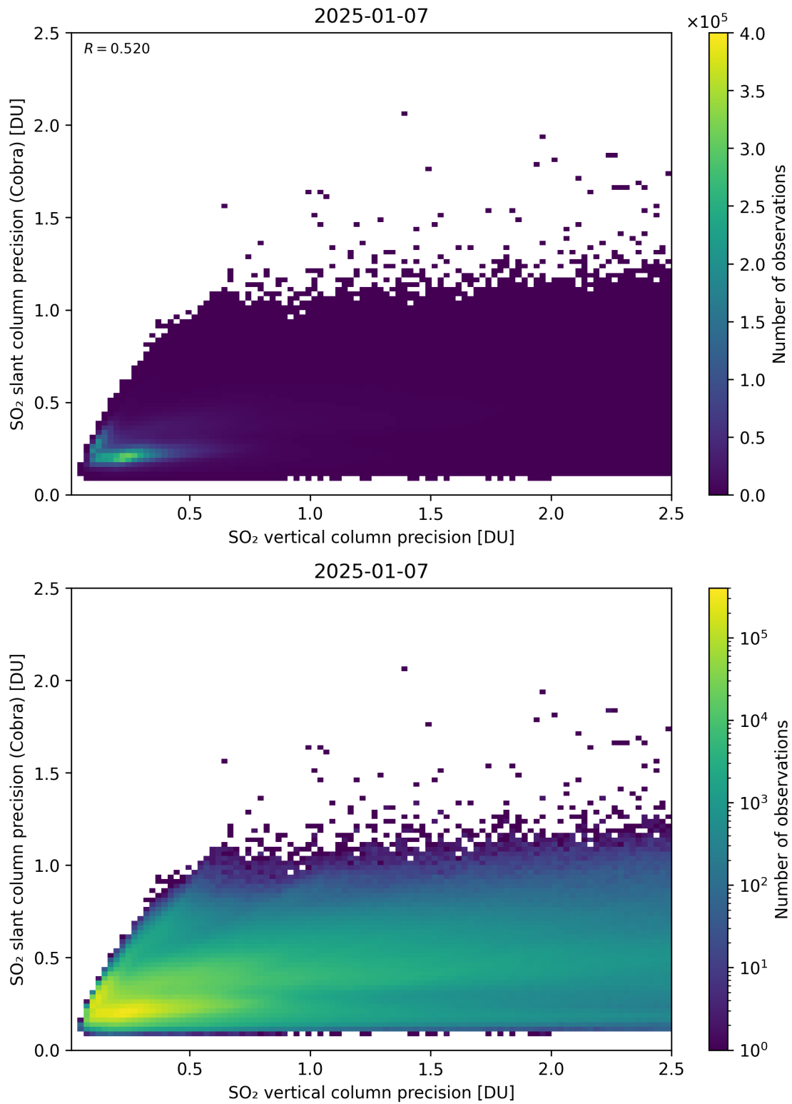
Figure 337: Scatter density plot of “SO 2 vertical column precision” against “SO 2 slant column precision (Cobra)” for 2025-01-07 to 2025-01-08.
