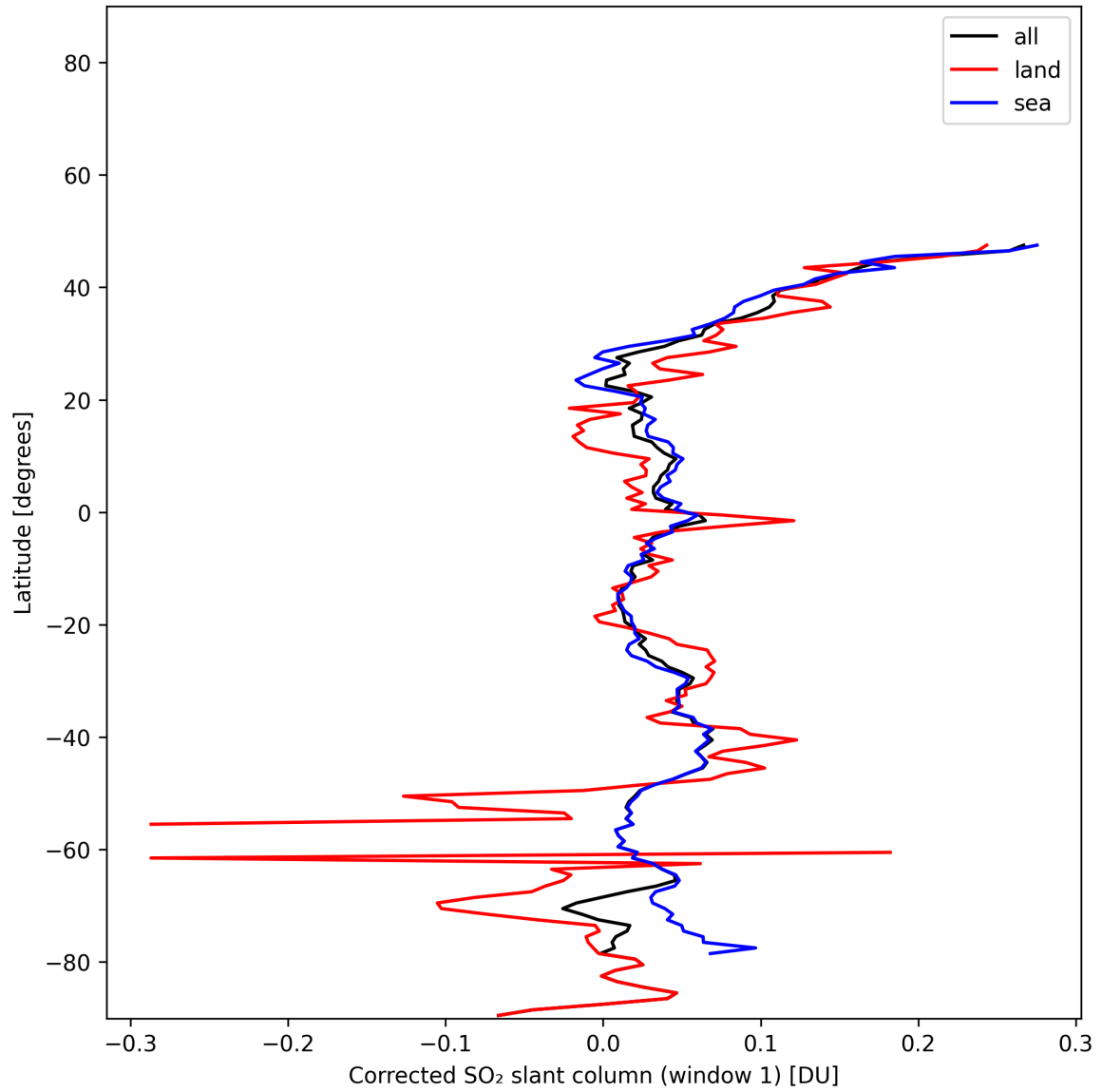
Figure 39: Zonal average of “Corrected SO 2 slant column (window 1)” for 2025-01-07 to 2025-01-08.
