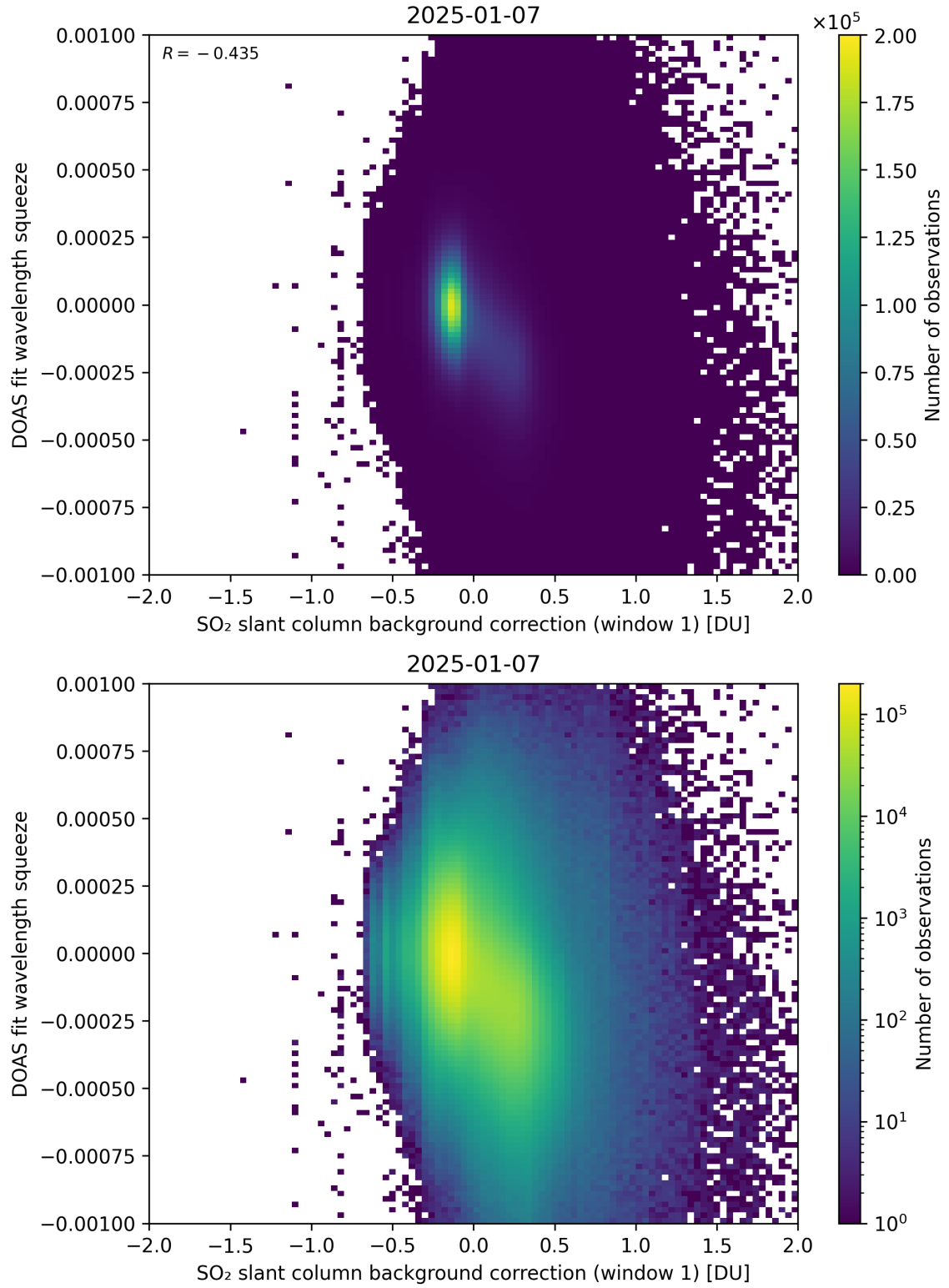
Figure 112: Scatter density plot of “SO 2 slant column background correction (window 1)” against “DOAS fit wavelength squeeze” for 2025-01-07 to 2025-01-08.
