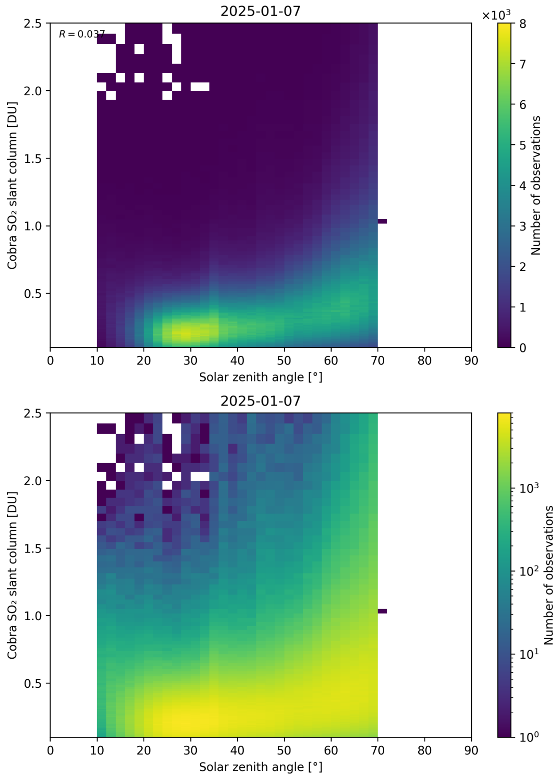
Figure 179: Scatter density plot of “Solar zenith angle” against “Cobra SO 2 slant column” for 2025-01-07 to 2025-01-08.
