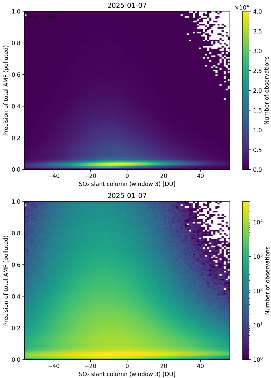
Figure 319: Scatter density plot of “SO 2 slant column (window 3)” against “Precision of total AMF (polluted)” for 2025-01-07 to 2025-01-08.
