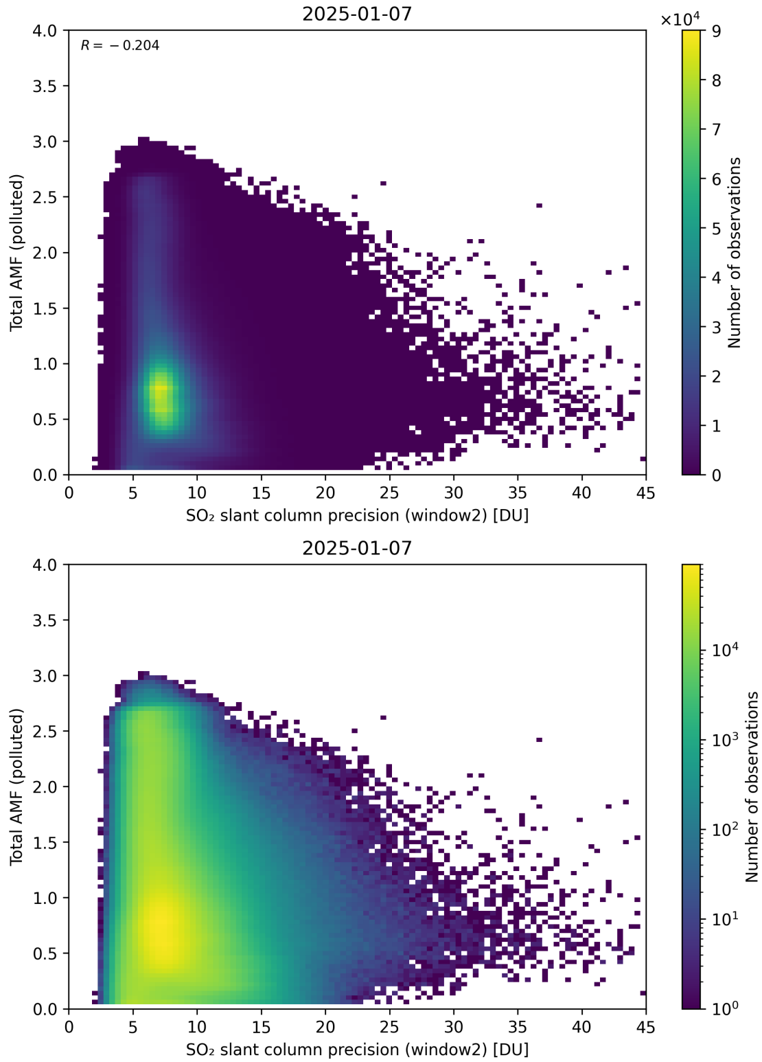
Figure 301: Scatter density plot of “SO 2 slant column precision (window2)” against “Total AMF (polluted)” for 2025-01-07 to 2025-01-08.
