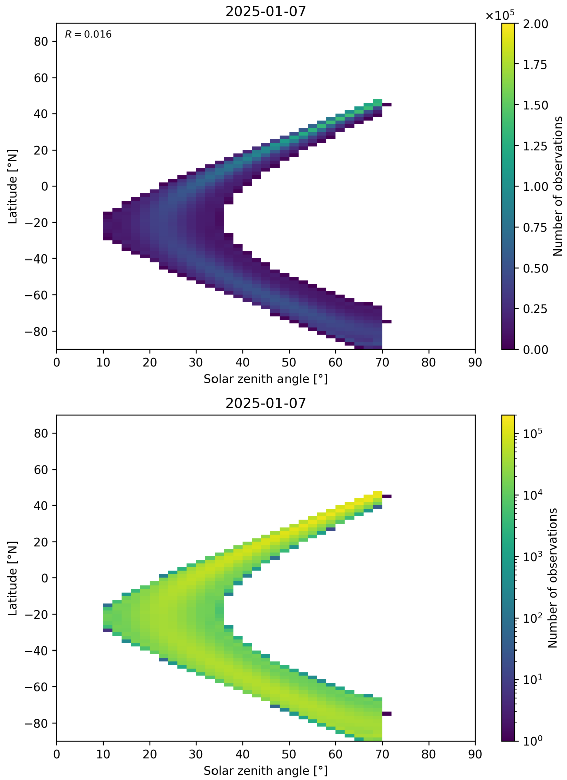
Figure 177: Scatter density plot of “Solar zenith angle” against “Latitude” for 2025-01-07 to 2025-01-08.
