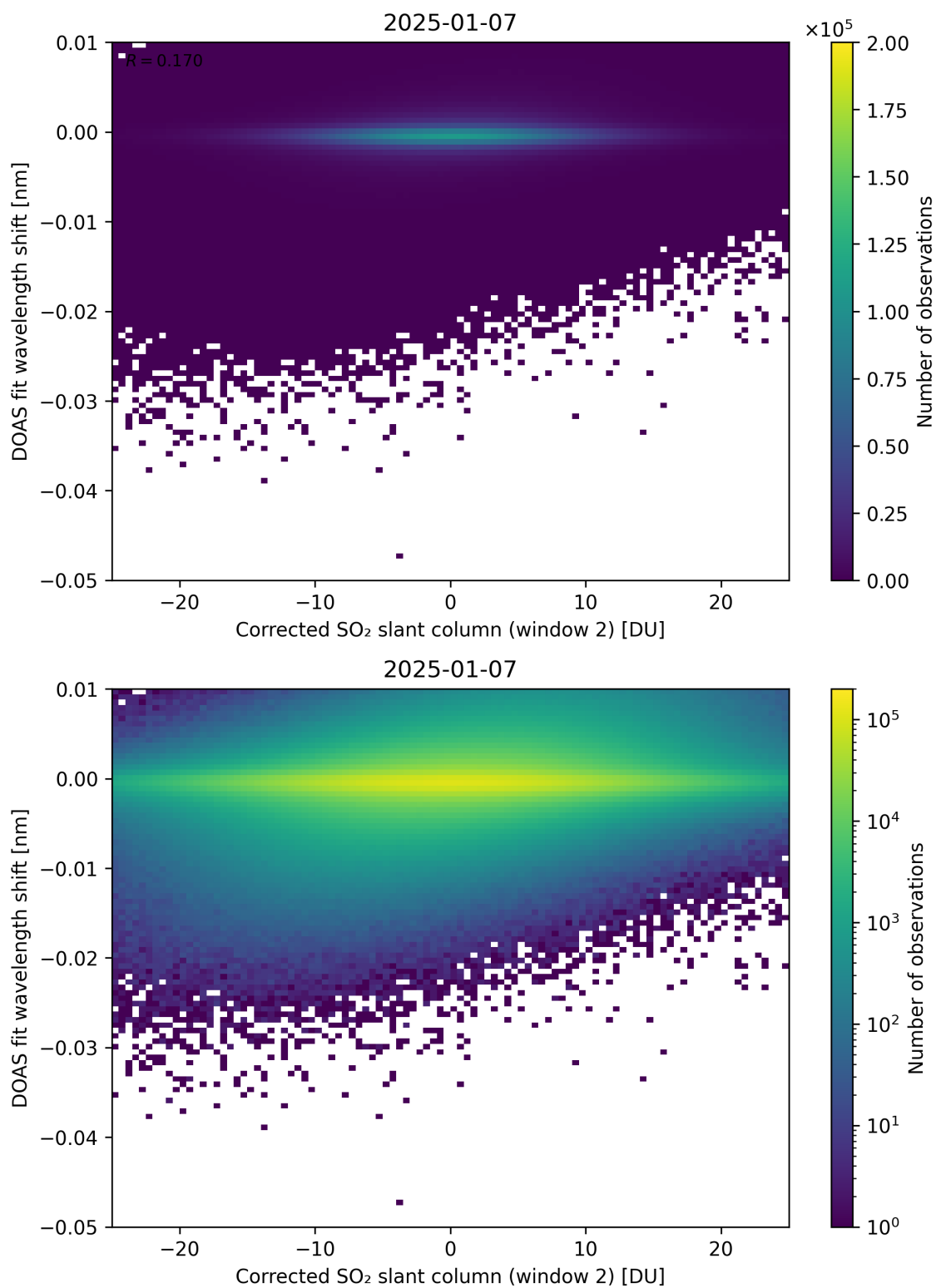
Figure 246: Scatter density plot of “Corrected SO 2 slant column (window 2)” against “DOAS fit wavelength shift” for 2025-01-07 to 2025-01-08.
