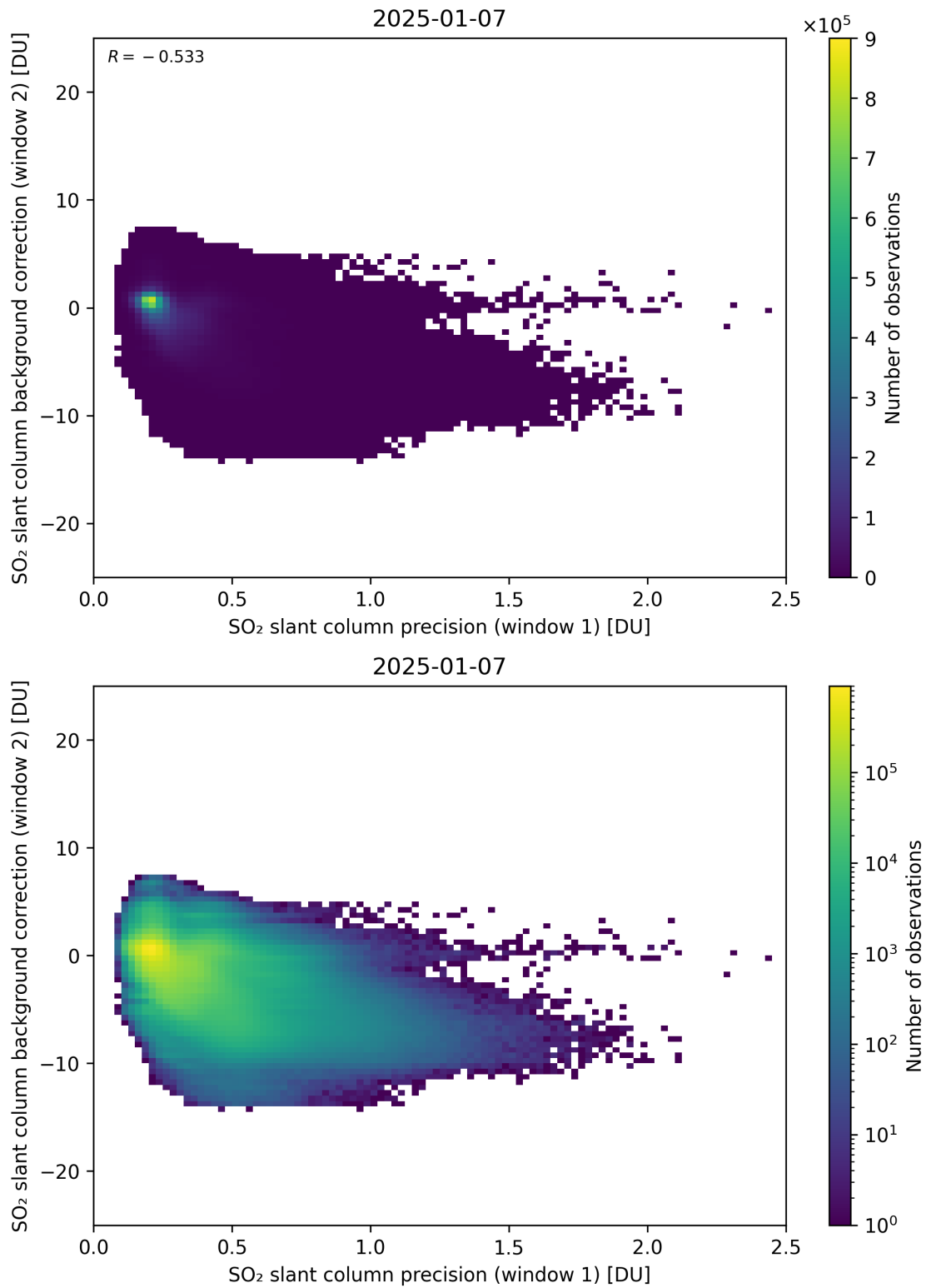
Figure 269: Scatter density plot of “SO 2 slant column precision (window 1)” against “SO 2 slant column background correction (window 2)” for 2025-01-07 to 2025-01-08.
