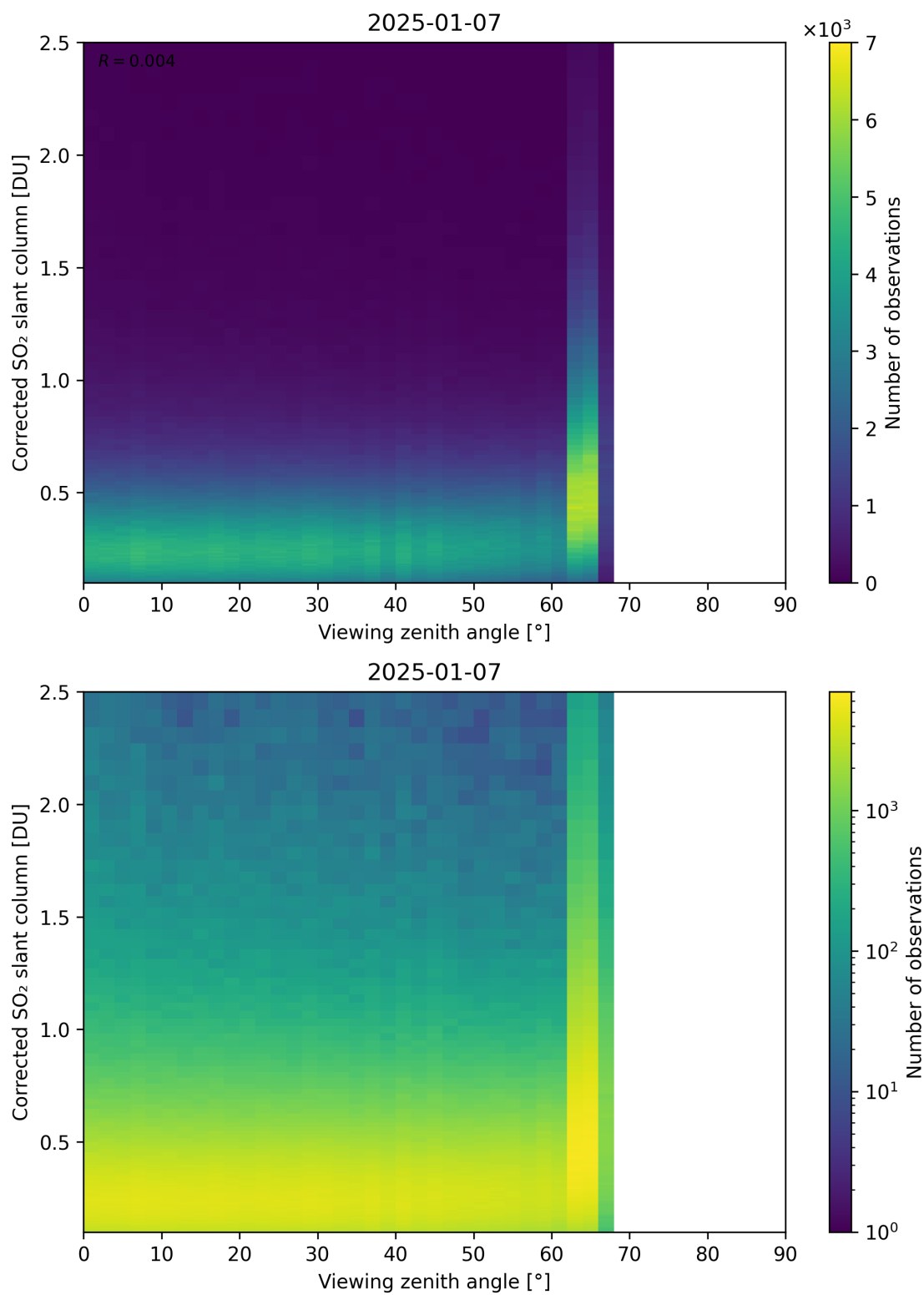
Figure 373: Scatter density plot of “Viewing zenith angle” against “Corrected SO 2 slant column” for 2025-01-07 to 2025-01-08.
