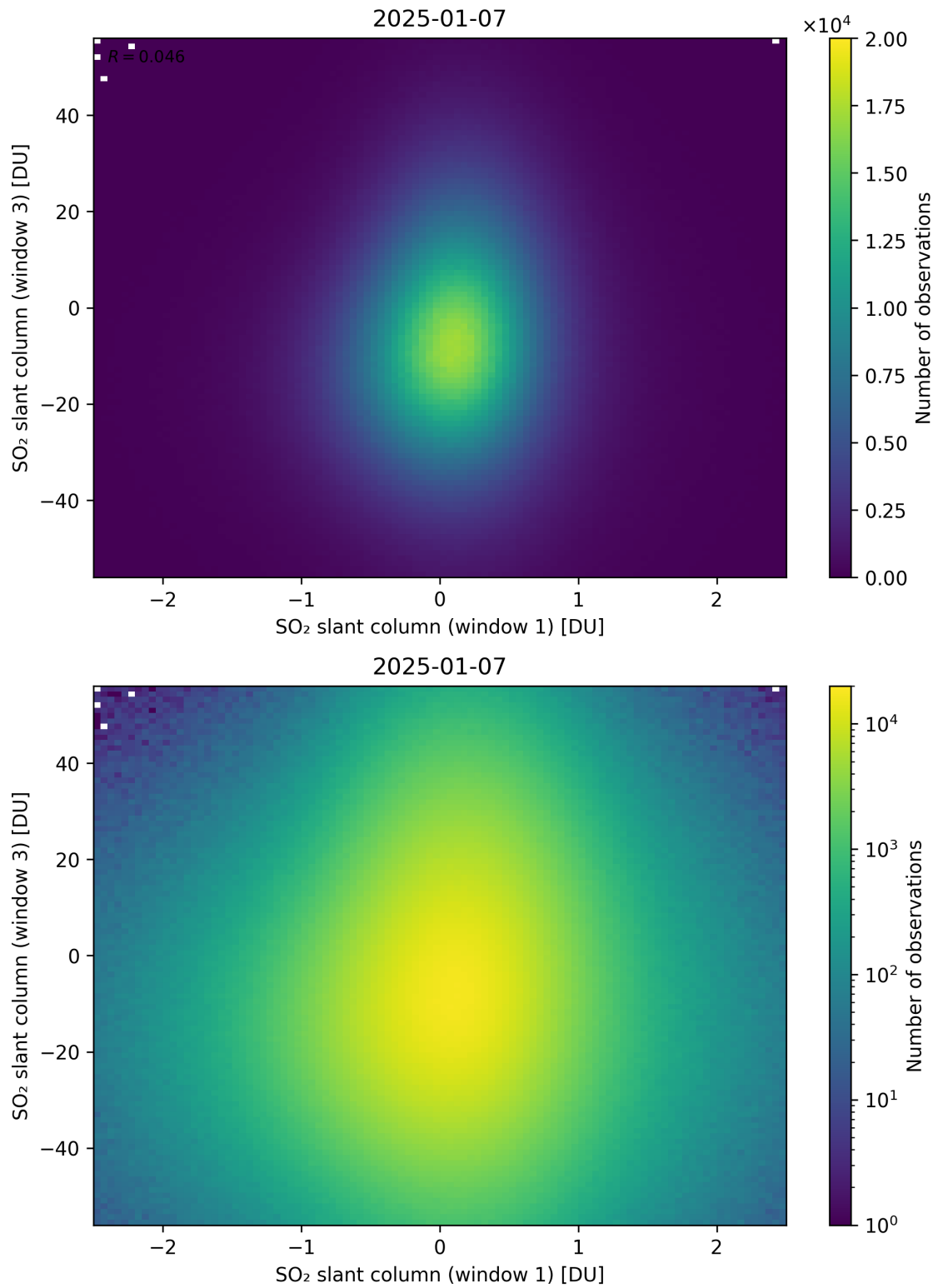
Figure 287: Scatter density plot of “SO 2 slant column (window 1)” against “SO 2 slant column (window 3)” for 2025-01-07 to 2025-01-08.
