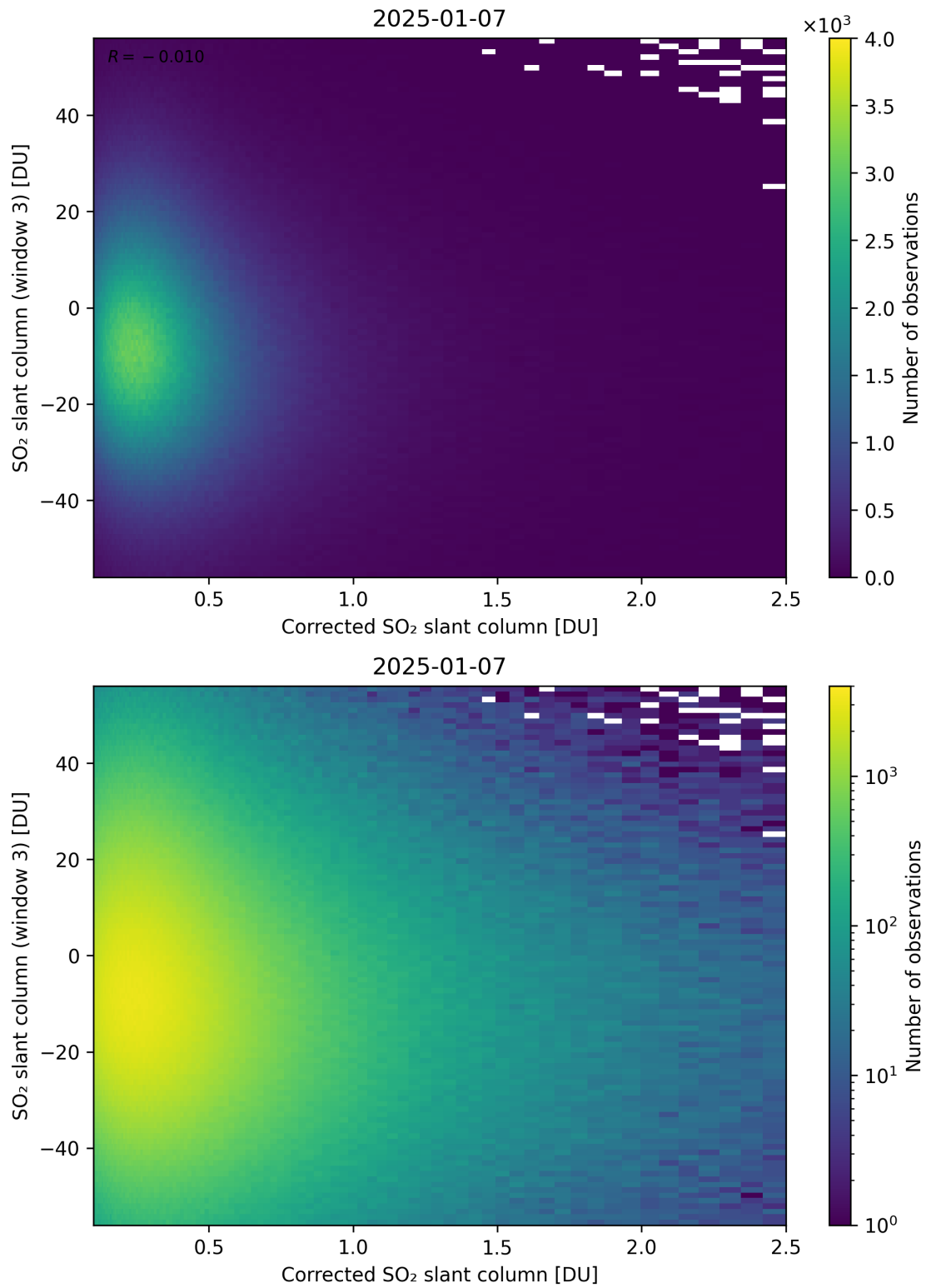
Figure 240: Scatter density plot of “Corrected SO 2 slant column” against “SO 2 slant column (window 3)” for 2025-01-07 to 2025-01-08.
