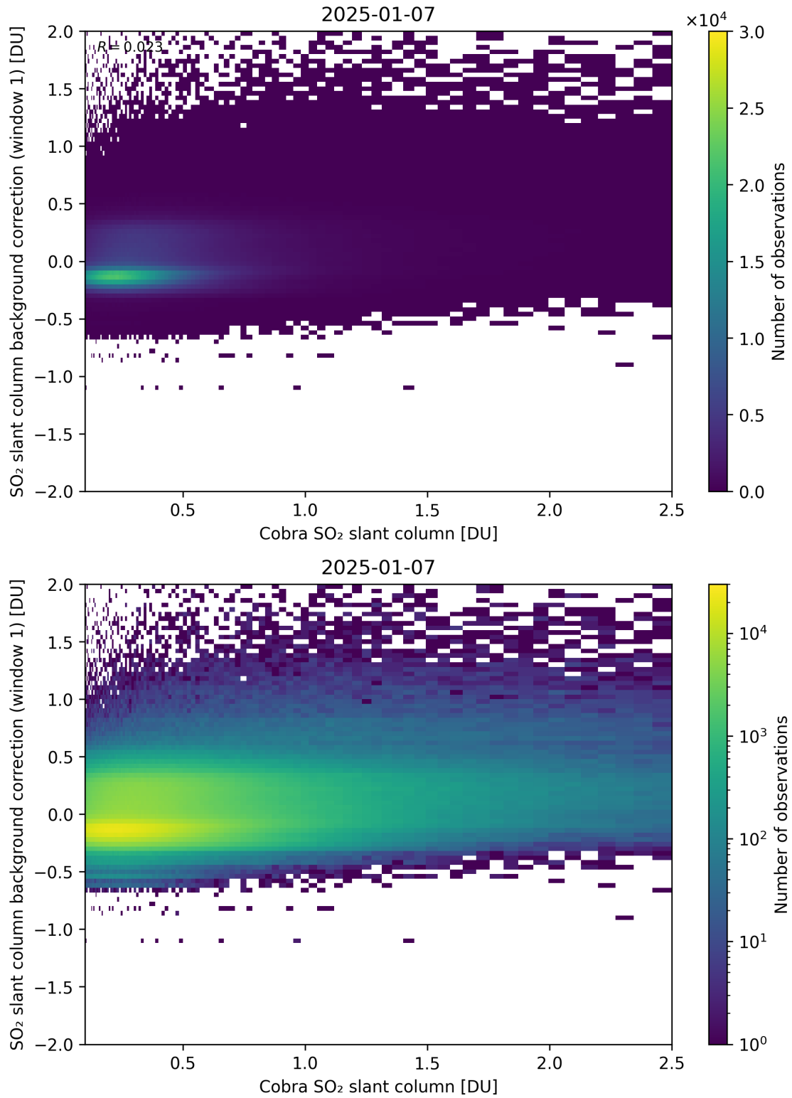
Figure 193: Scatter density plot of “Cobra SO 2 slant column” against “SO 2 slant column background correction (window 1)” for 2025-01-07 to 2025-01-08.
