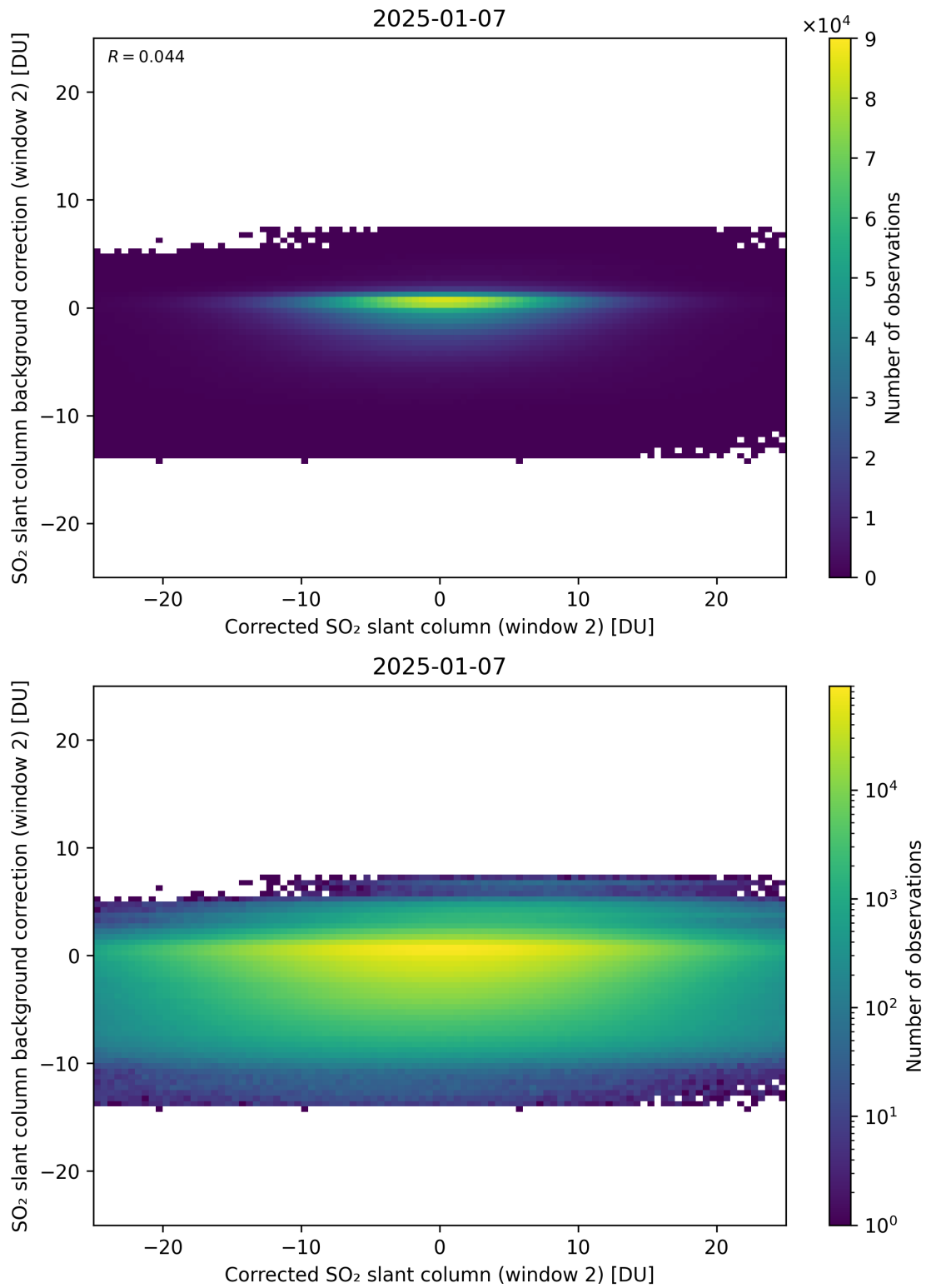
Figure 244: Scatter density plot of “Corrected SO 2 slant column (window 2)” against “SO 2 slant column background correction (window 2)” for 2025-01-07 to 2025-01-08.
