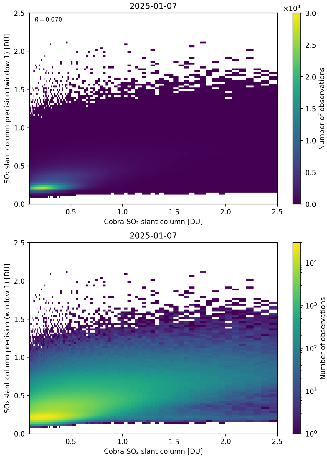
Figure 220: Scatter density plot of “Cobra SO 2 slant column” against “SO 2 slant column precision (window 1)” for 2025-01-07 to 2025-01-08.
