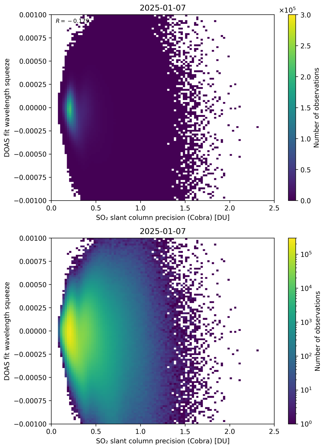
Figure 203: Scatter density plot of “SO 2 slant column precision (Cobra)” against “DOAS fit wavelength squeeze” for 2025-01-07 to 2025-01-08.
