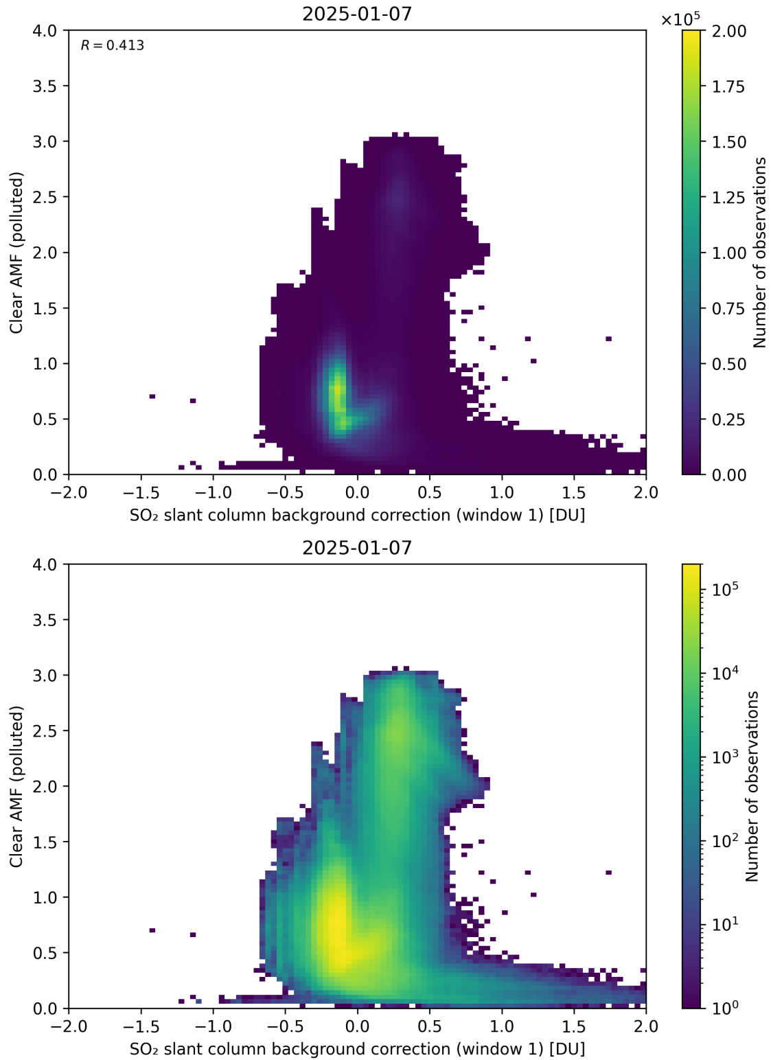
Figure 114: Scatter density plot of “SO 2 slant column background correction (window 1)” against “Clear AMF (polluted)” for 2025-01-07 to 2025-01-08.
