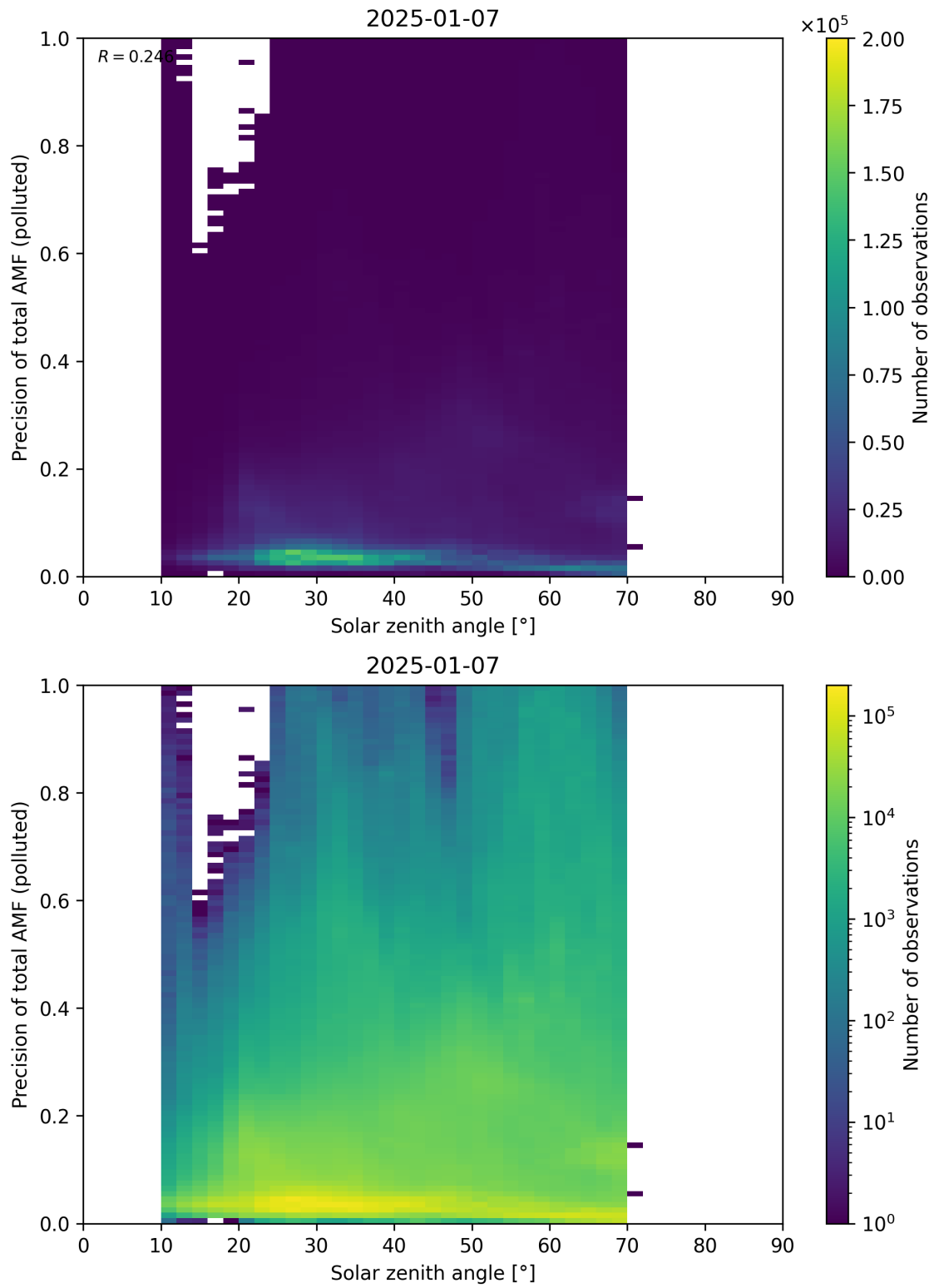
Figure 190: Scatter density plot of “Solar zenith angle” against “Precision of total AMF (polluted)” for 2025-01-07 to 2025-01-08.
