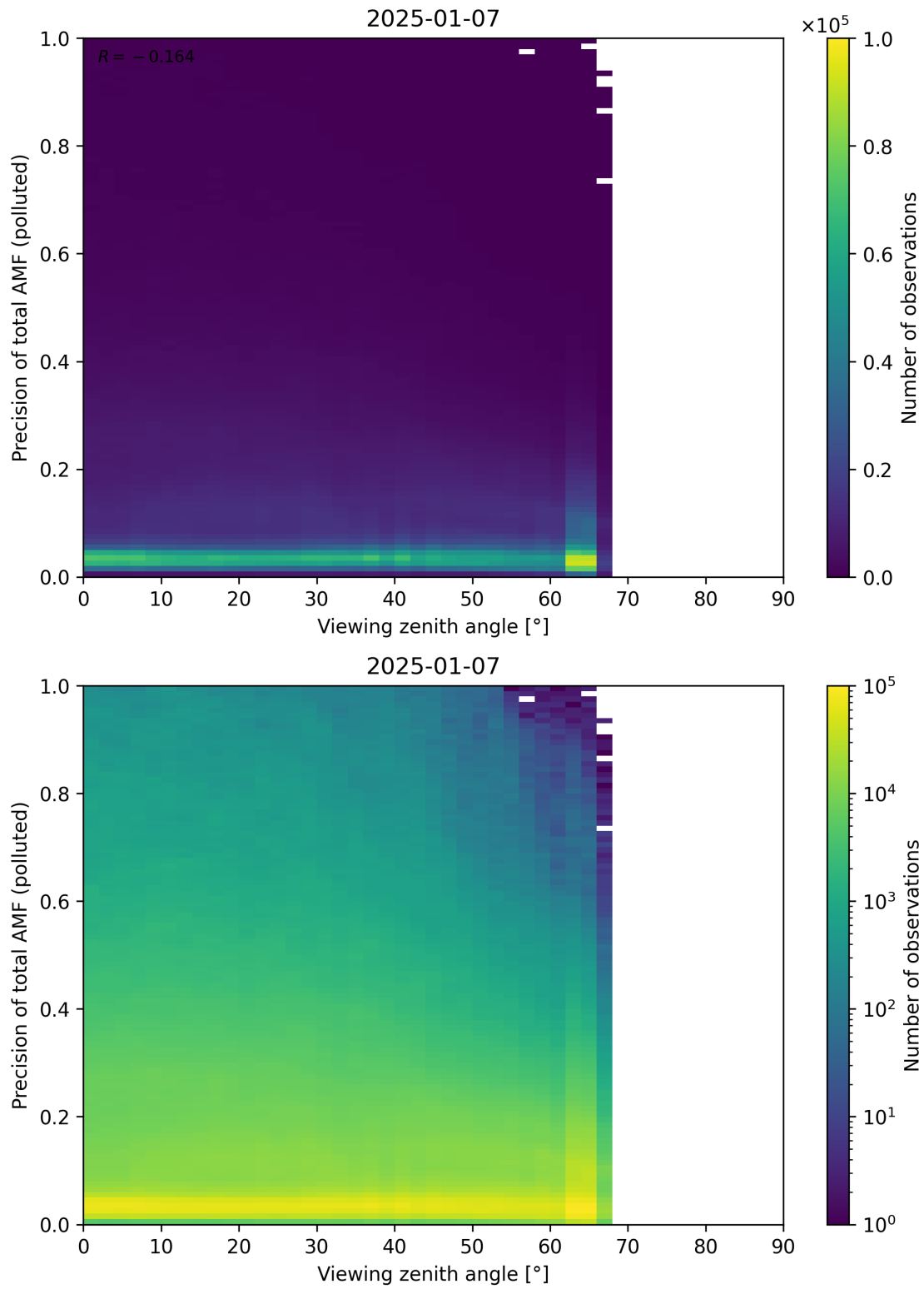
Figure 382: Scatter density plot of “Viewing zenith angle” against “Precision of total AMF (polluted)” for 2025-01-07 to 2025-01-08.
