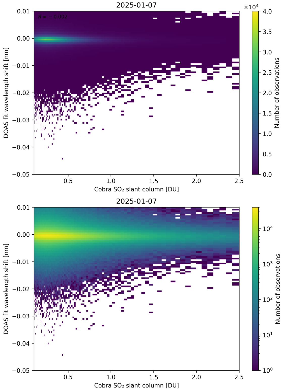
Figure 196: Scatter density plot of “Cobra SO 2 slant column” against “DOAS fit wavelength shift” for 2025-01-07 to 2025-01-08.
