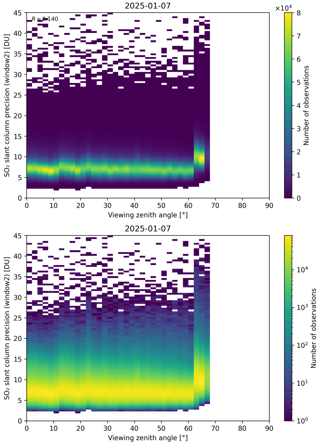
Figure 378: Scatter density plot of “Viewing zenith angle” against “SO 2 slant column precision (window2)” for 2025-01-07 to 2025-01-08.
