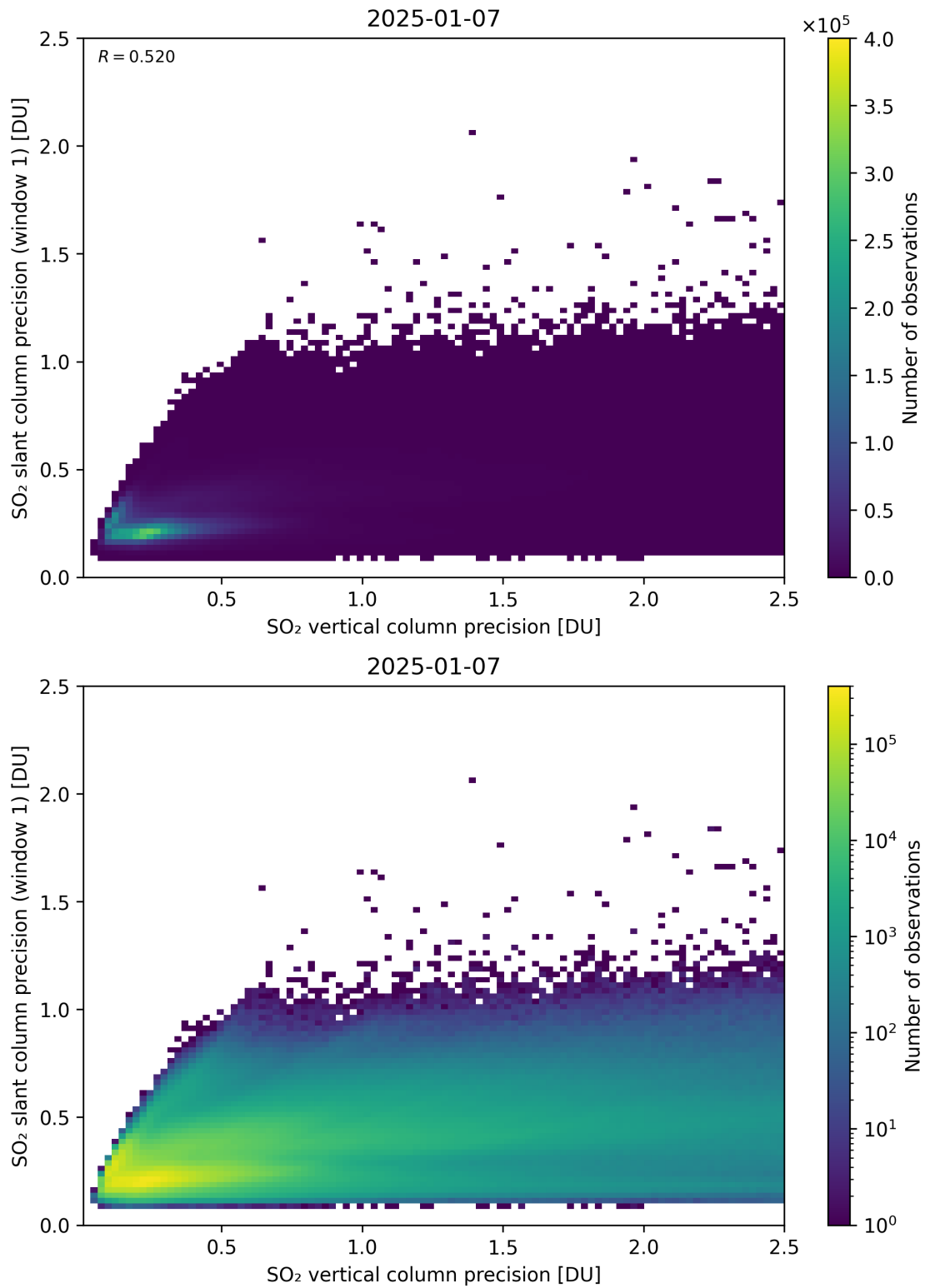
Figure 342: Scatter density plot of “SO 2 vertical column precision” against “SO 2 slant column precision (window 1)” for 2025-01-07 to 2025-01-08.
