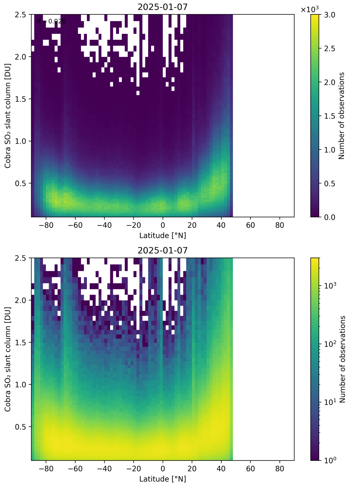
Figure 157: Scatter density plot of “Latitude” against “Cobra SO 2 slant column” for 2025-01-07 to 2025-01-08.
