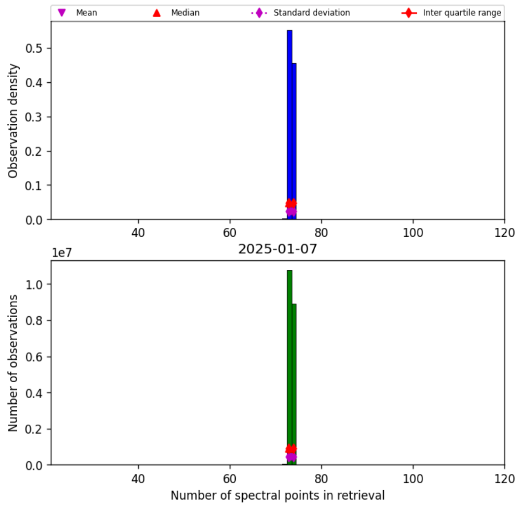
Figure 82: Histogram of “Number of spectral points in retrieval” for 2025-01-07 to 2025-01-08
