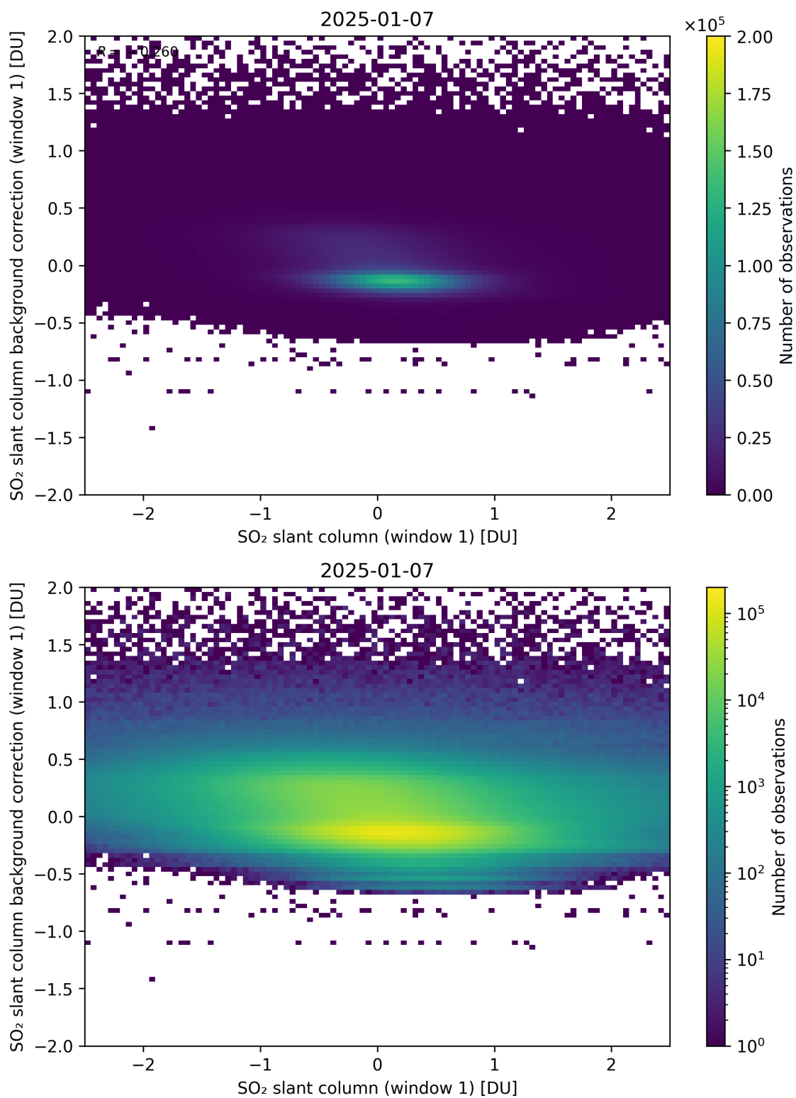
Figure 262: Scatter density plot of “SO 2 slant column (window 1)” against “SO 2 slant column background correction (window 1)” for 2025-01-07 to 2025-01-08.
