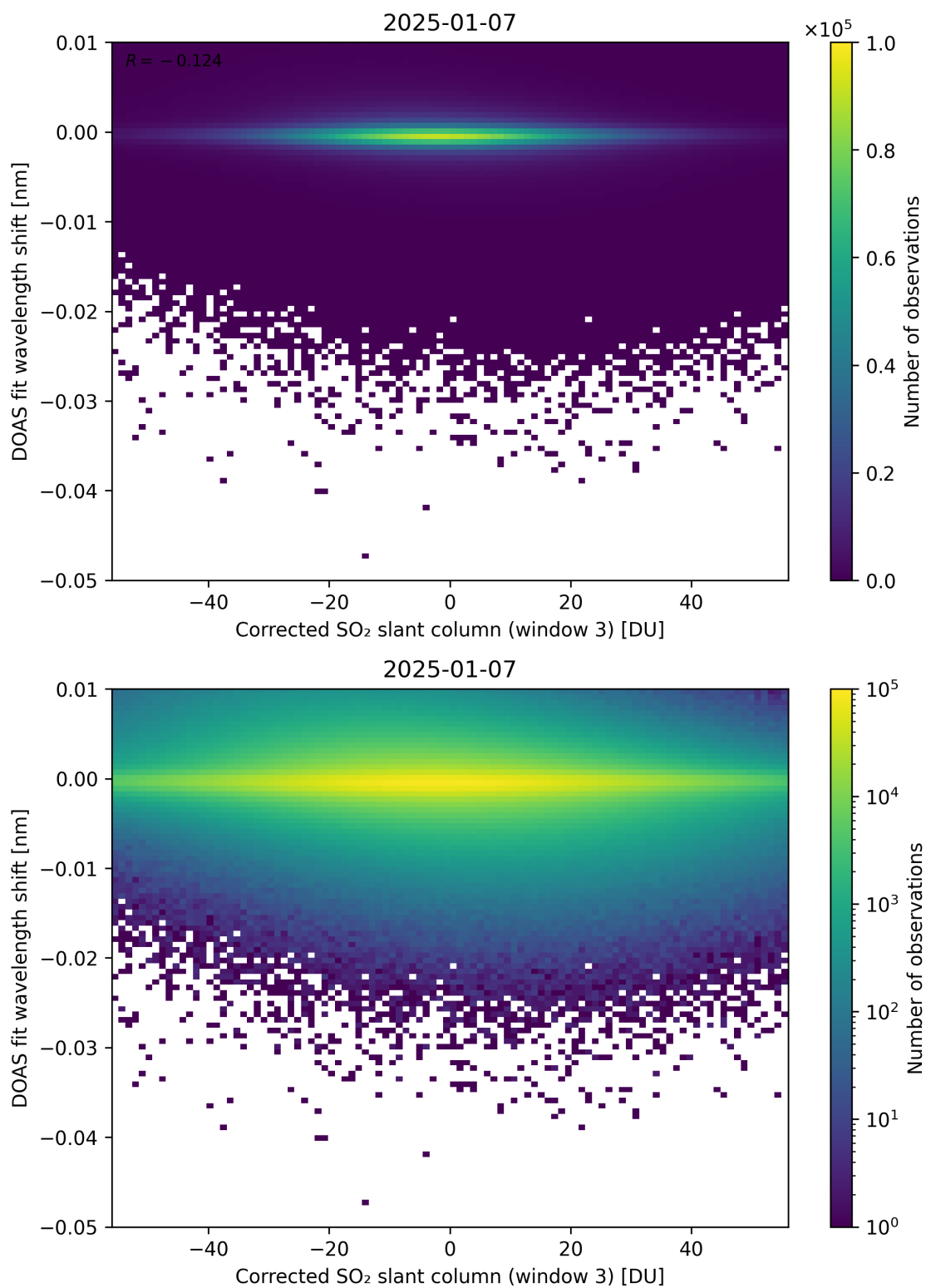
Figure 256: Scatter density plot of “Corrected SO 2 slant column (window 3)” against “DOAS fit wavelength shift” for 2025-01-07 to 2025-01-08.
