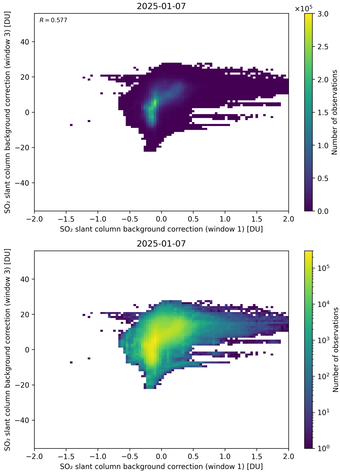
Figure 110: Scatter density plot of “SO 2 slant column background correction (window 1)” against “SO 2 slant column background correction (window 3)” for 2025-01-07 to 2025-01-08.
