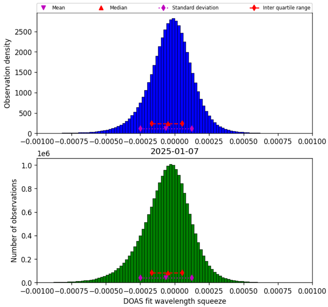
Figure 77: Histogram of “DOAS fit wavelength squeeze” for 2025-01-07 to 2025-01-08
