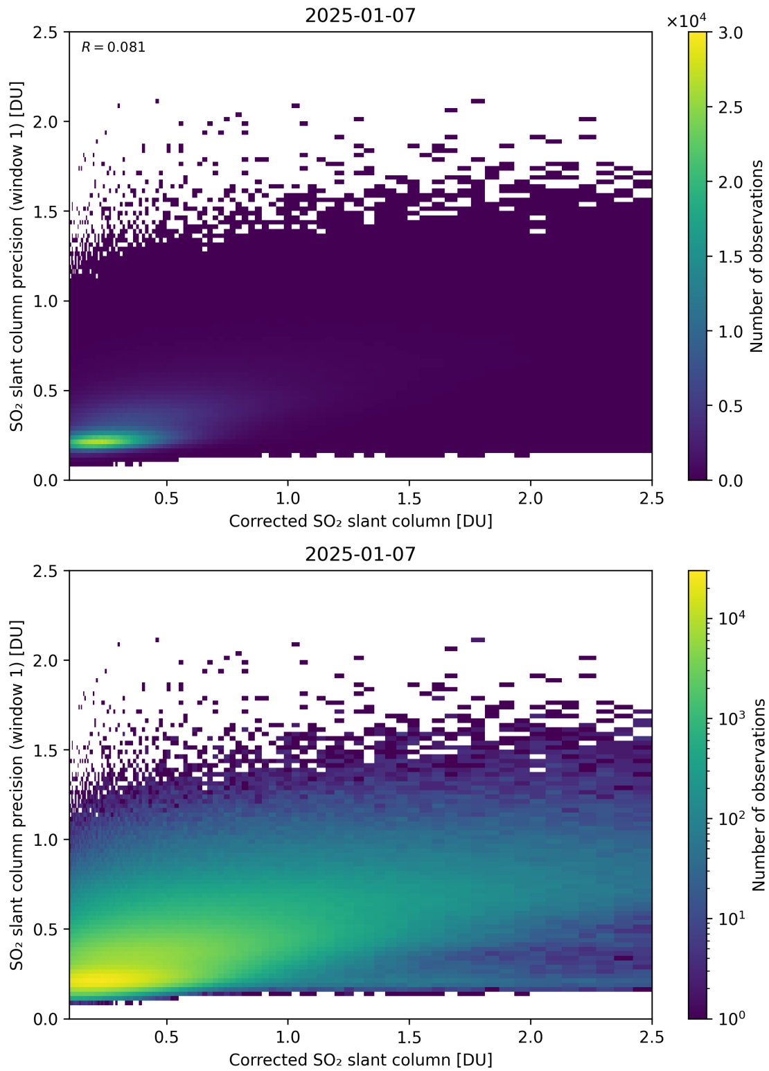
Figure 238: Scatter density plot of “Corrected SO 2 slant column” against “SO 2 slant column precision (window 1)” for 2025-01-07 to 2025-01-08.
