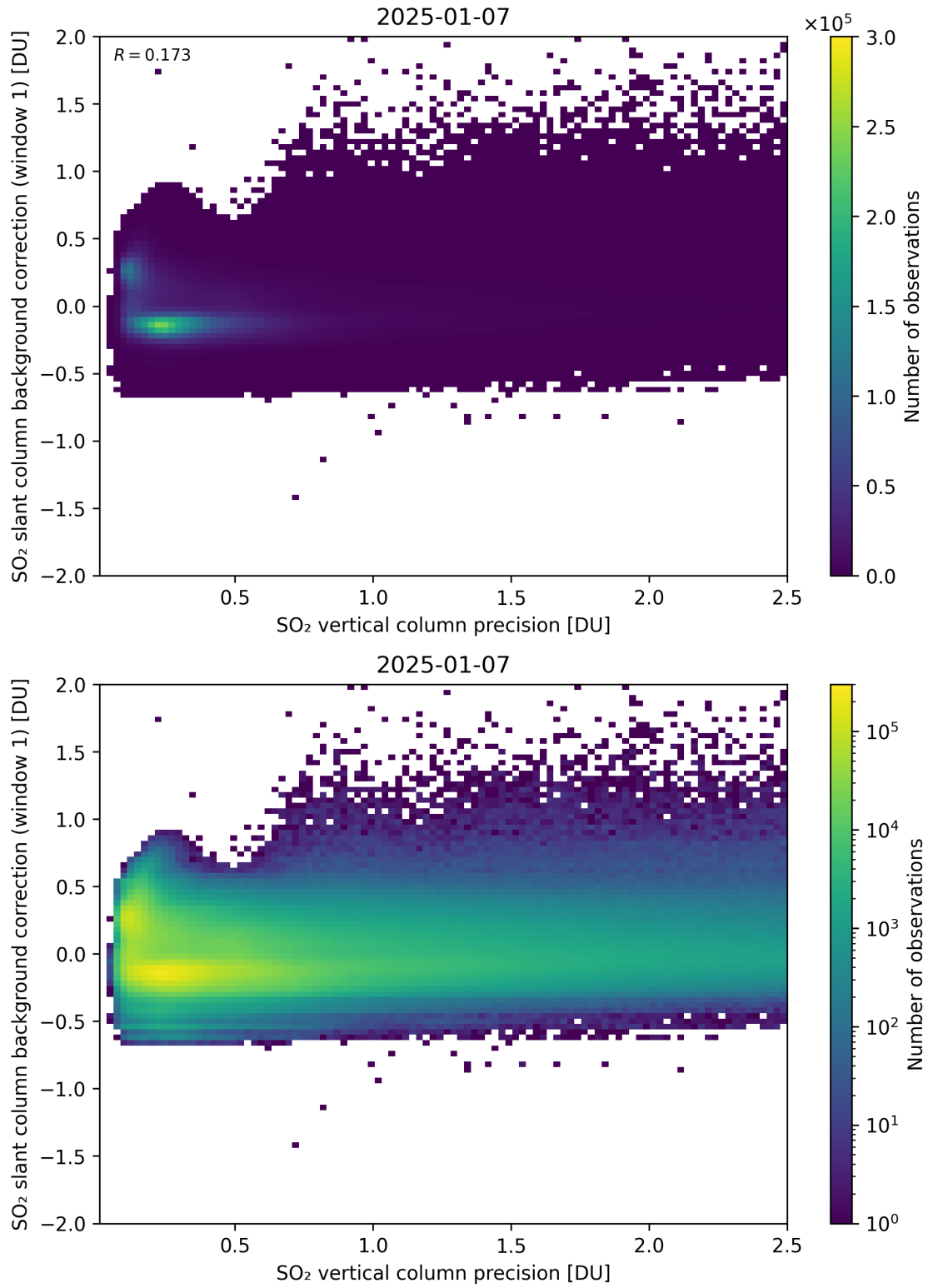
Figure 329: Scatter density plot of “SO 2 vertical column precision” against “SO 2 slant column background correction (window 1)” for 2025-01-07 to 2025-01-08.
