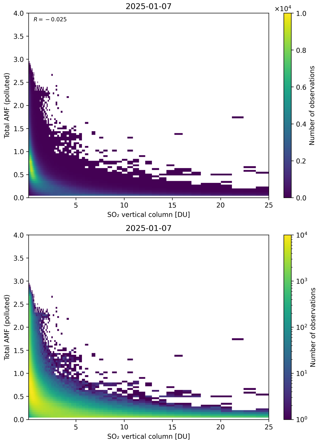
Figure 359: Scatter density plot of “SO 2 vertical column” against “Total AMF (polluted)” for 2025-01-07 to 2025-01-08.
