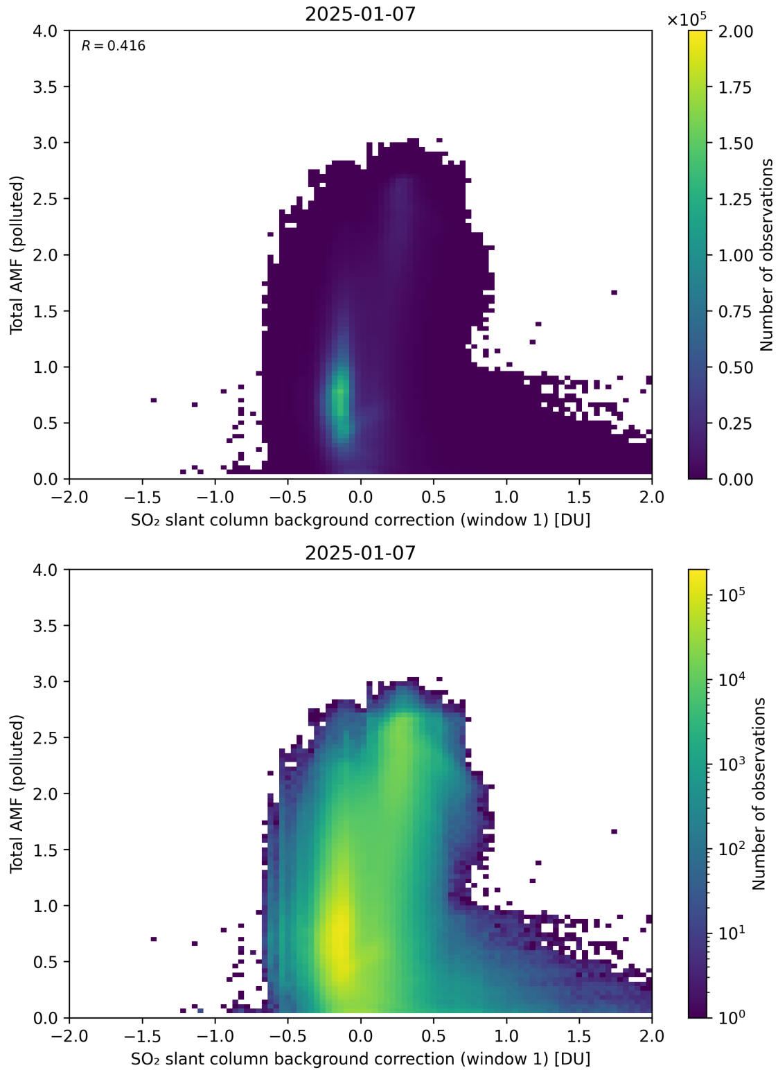
Figure 120: Scatter density plot of “SO 2 slant column background correction (window 1)” against “Total AMF (polluted)” for 2025-01-07 to 2025-01-08.
