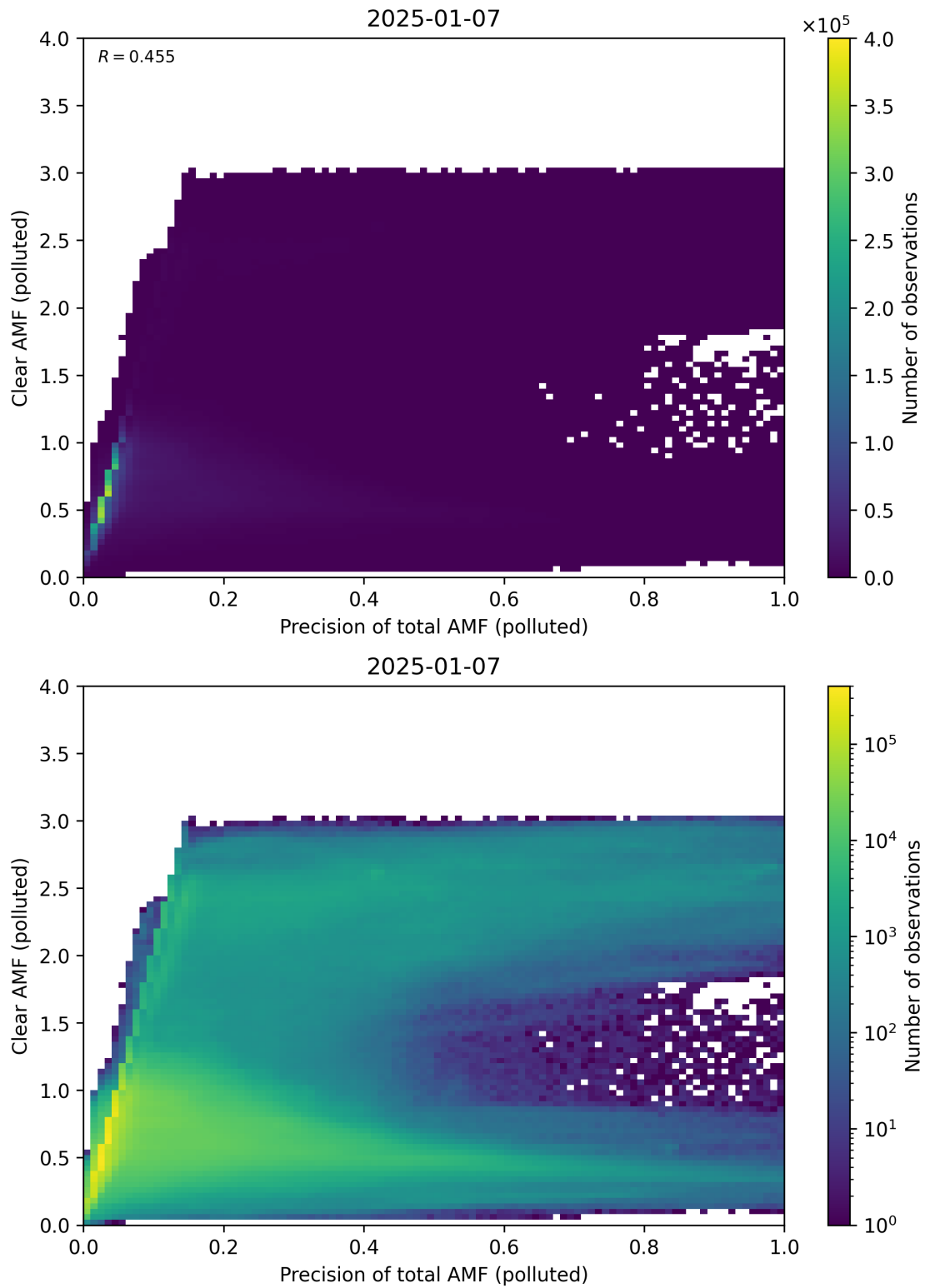
Figure 320: Scatter density plot of “Precision of total AMF (polluted)” against “Clear AMF (polluted)” for 2025-01-07 to 2025-01-08.
