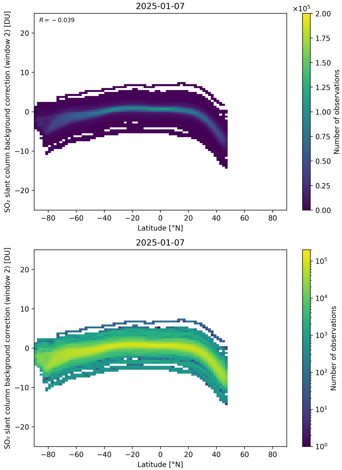
Figure 151: Scatter density plot of “Latitude” against “SO 2 slant column background correction (window 2)” for 2025-01-07 to 2025-01-08.
