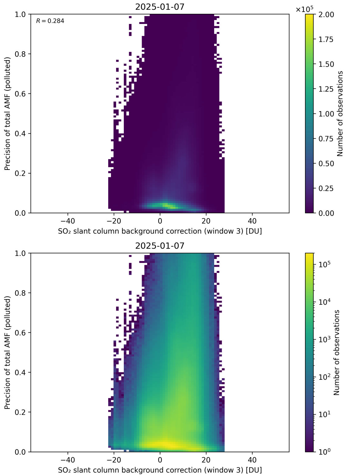
Figure 137: Scatter density plot of “SO 2 slant column background correction (window 3)” against “Precision of total AMF (polluted)” for 2025-01-07 to 2025-01-08.
