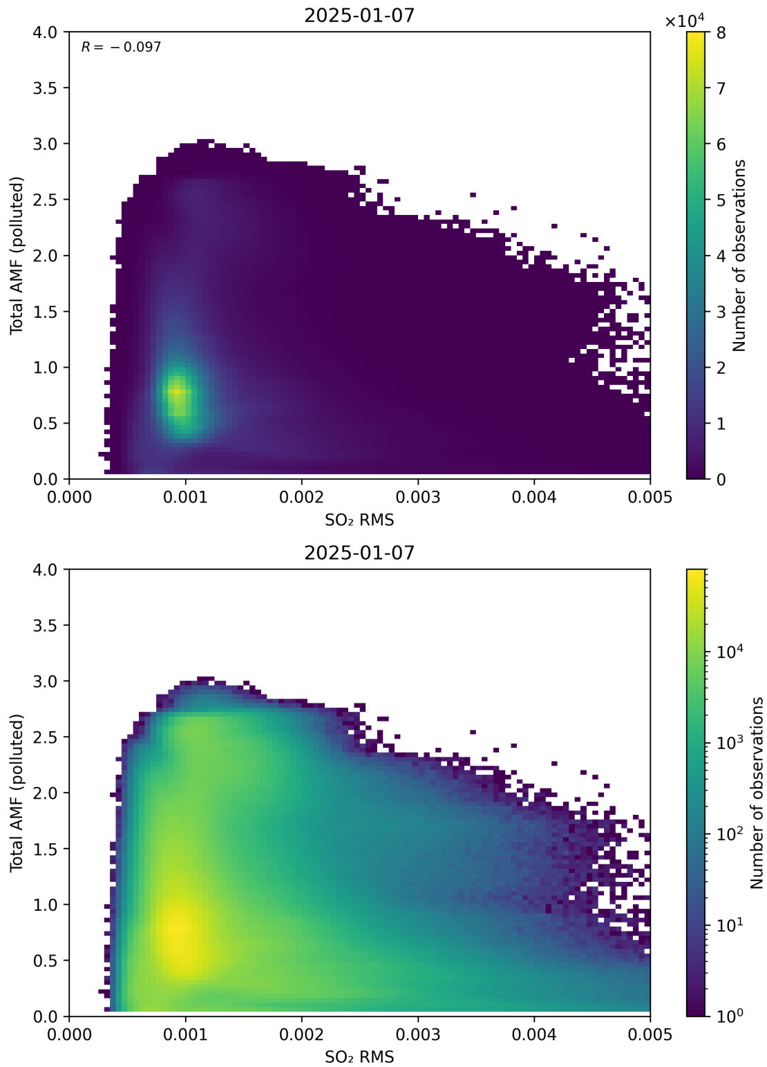
Figure 148: Scatter density plot of “SO 2 RMS” against “Total AMF (polluted)” for 2025-01-07 to 2025-01-08.
