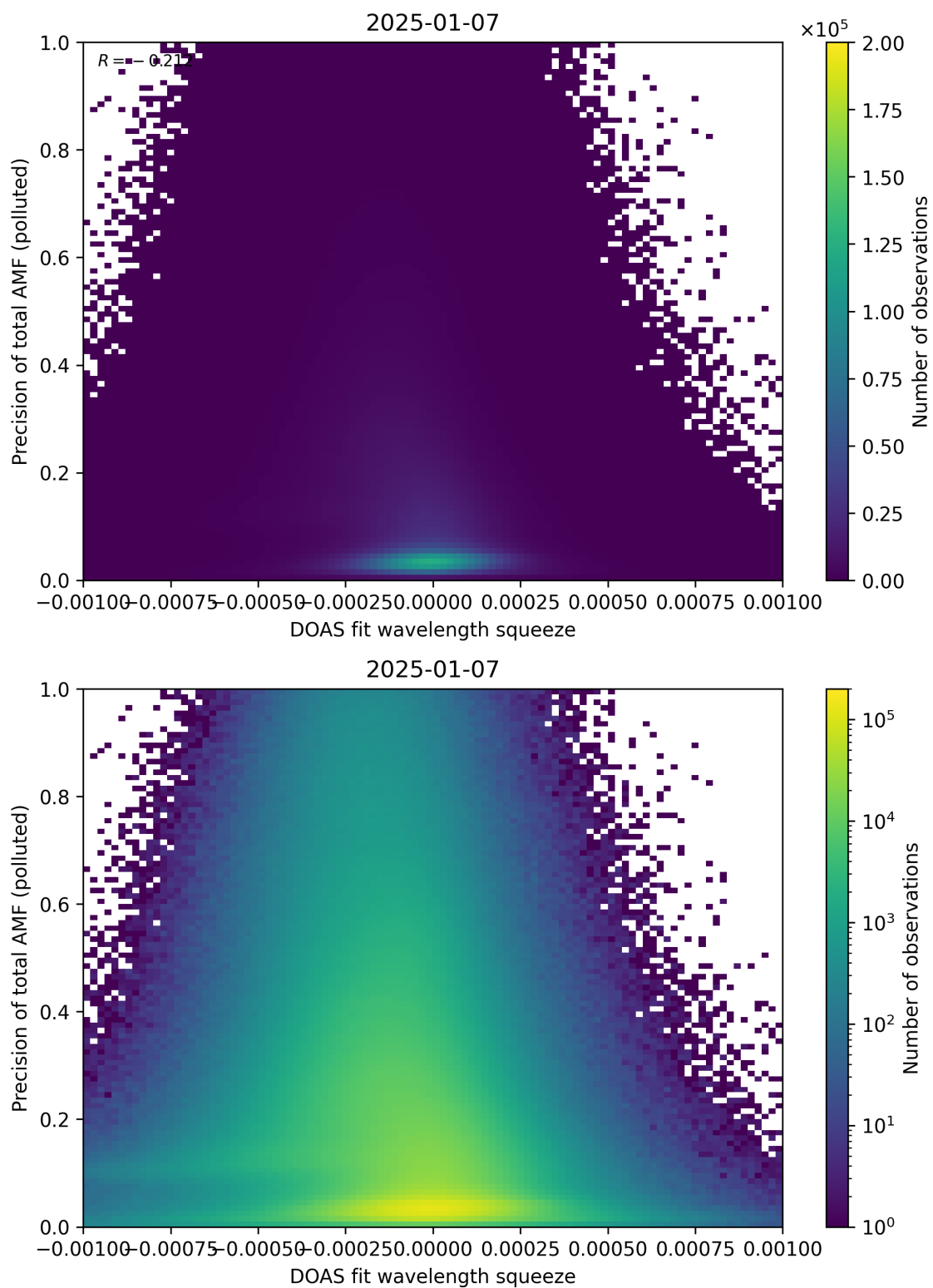
Figure 146: Scatter density plot of “DOAS fit wavelength squeeze” against “Precision of total AMF (polluted)” for 2025-01-07 to 2025-01-08.
