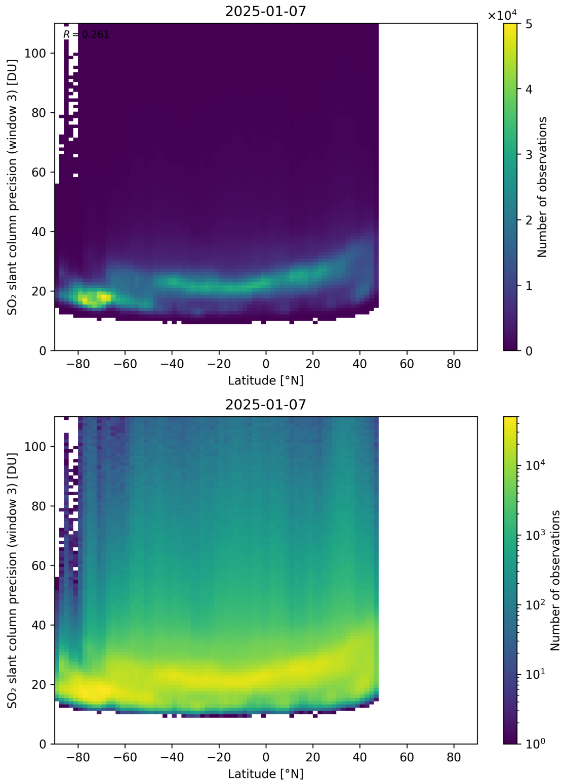
Figure 166: Scatter density plot of “Latitude” against “SO 2 slant column precision (window 3)” for 2025-01-07 to 2025-01-08.
