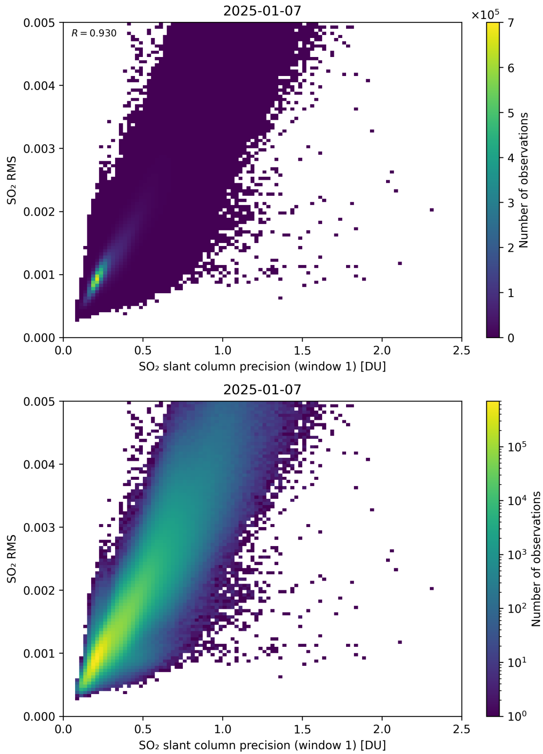
Figure 273: Scatter density plot of “SO 2 slant column precision (window 1)” against “SO 2 RMS” for 2025-01-07 to 2025-01-08.
