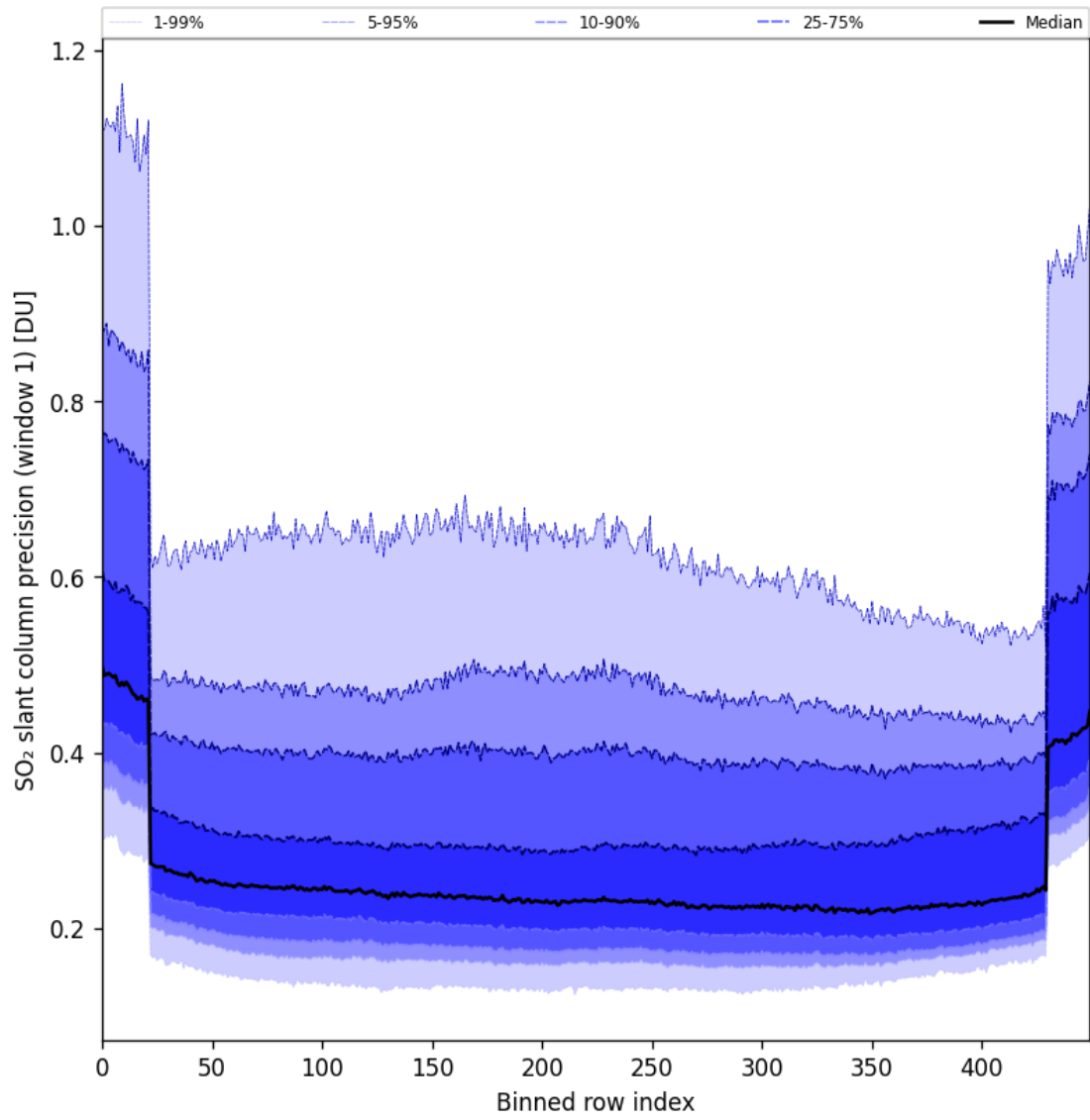
Figure 90: Along track statistics of “SO 2 slant column precision (window 1)” for 2025-01-07 to 2025-01-08
