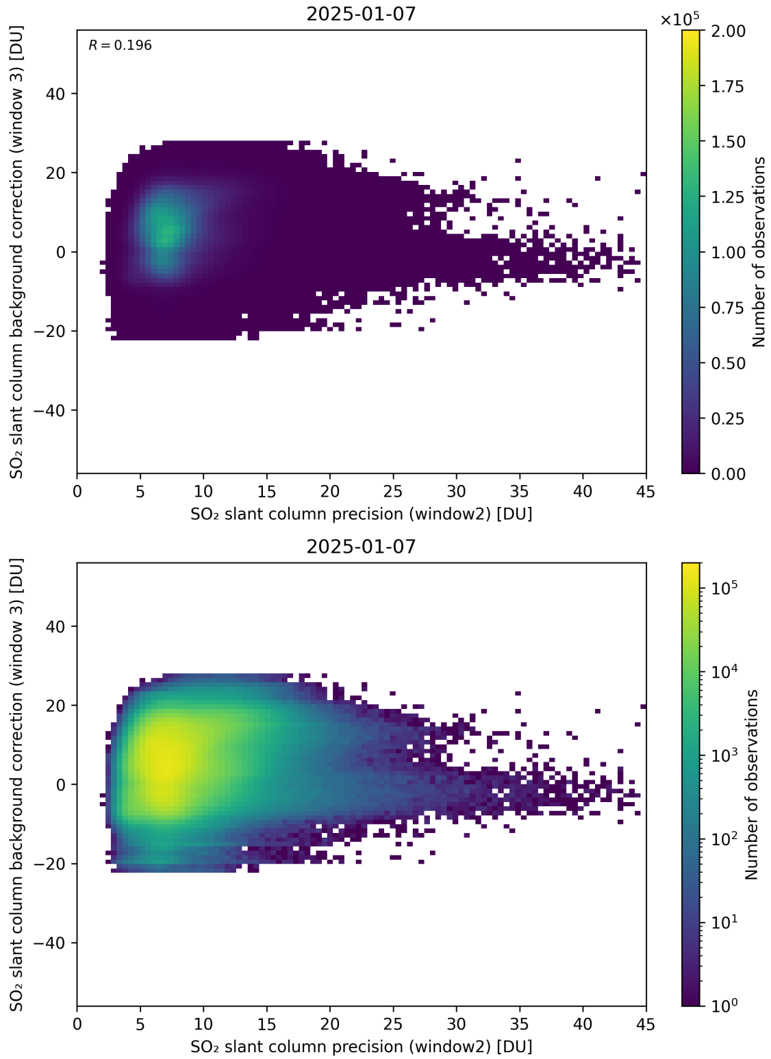
Figure 292: Scatter density plot of “SO 2 slant column precision (window2)” against “SO 2 slant column background correction (window 3)” for 2025-01-07 to 2025-01-08.
