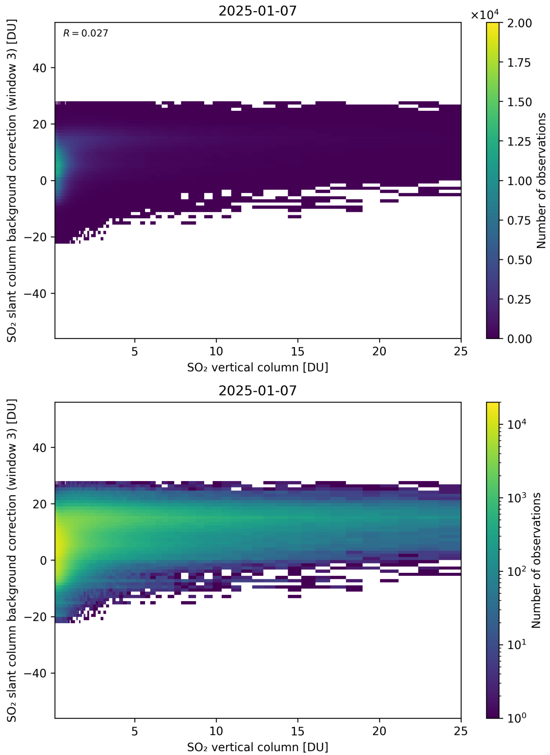
Figure 325: Scatter density plot of “SO 2 vertical column” against “SO 2 slant column background correction (window 3)” for 2025-01-07 to 2025-01-08.
