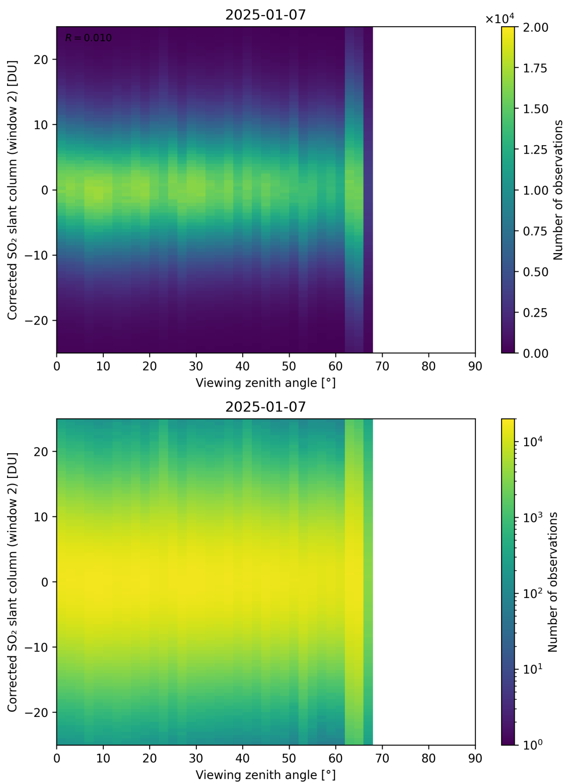
Figure 374: Scatter density plot of “Viewing zenith angle” against “Corrected SO 2 slant column (window 2)” for 2025-01-07 to 2025-01-08.
