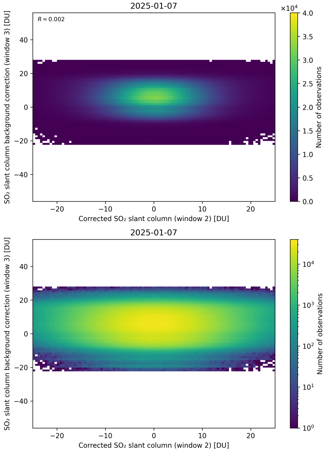
Figure 245: Scatter density plot of “Corrected SO 2 slant column (window 2)” against “SO 2 slant column background correction (window 3)” for 2025-01-07 to 2025-01-08.
