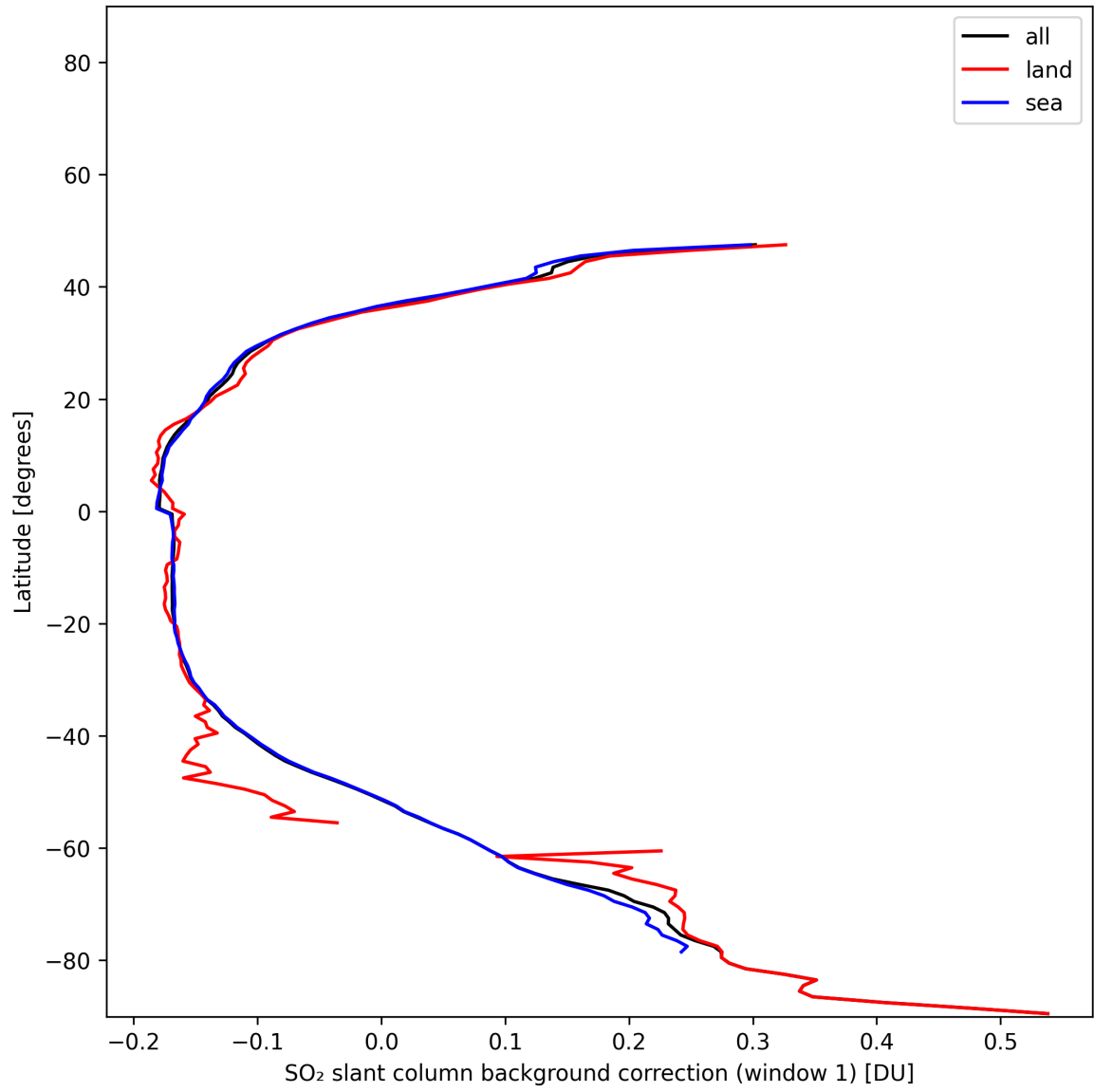
Figure 40: Zonal average of “SO 2 slant column background correction (window 1)” for 2025-01-07 to 2025-01-08.
