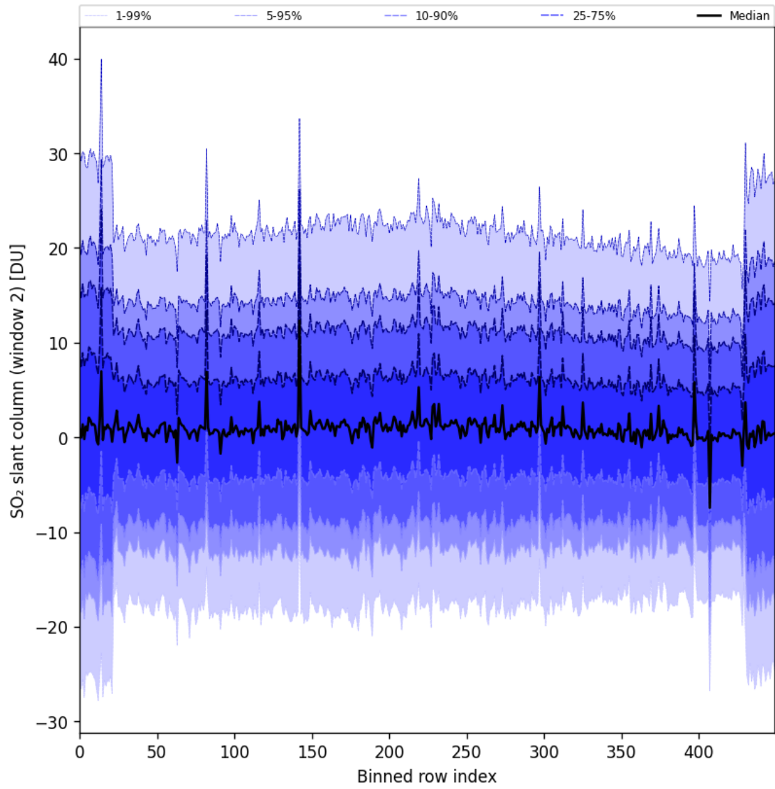
Figure 93: Along track statistics of “SO 2 slant column (window 2)” for 2025-01-07 to 2025-01-08
