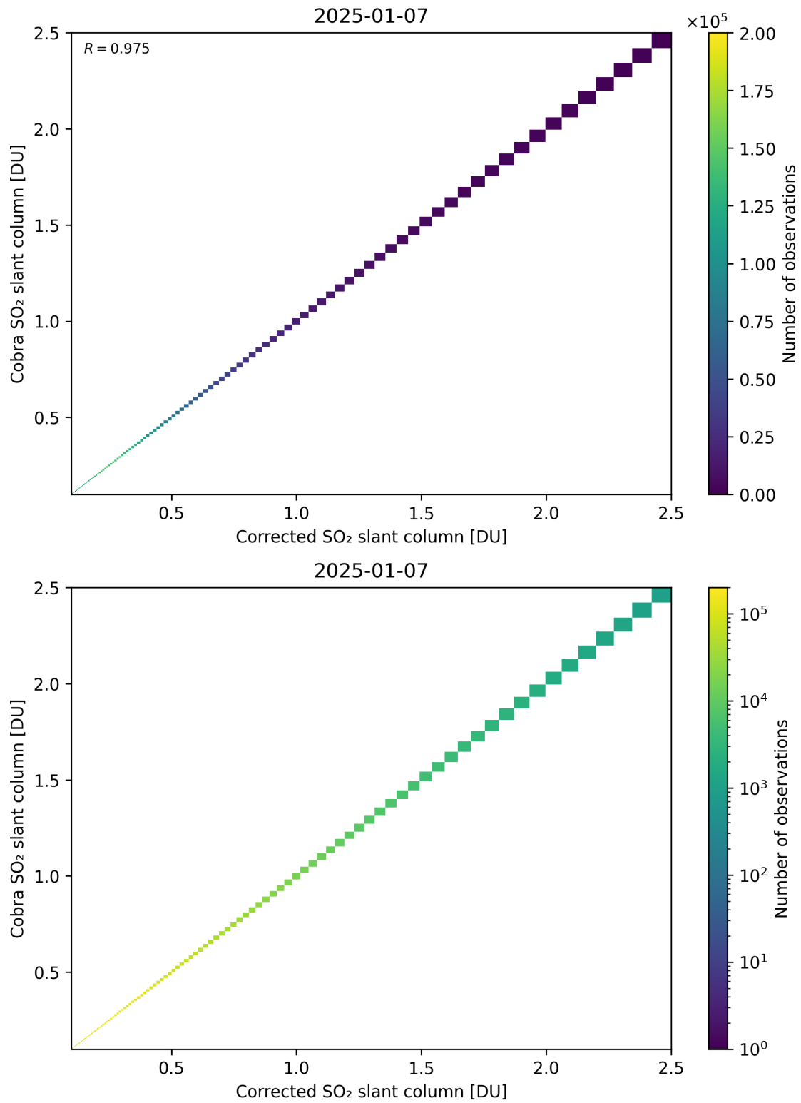
Figure 233: Scatter density plot of “Corrected SO 2 slant column” against “Cobra SO 2 slant column” for 2025-01-07 to 2025-01-08.
