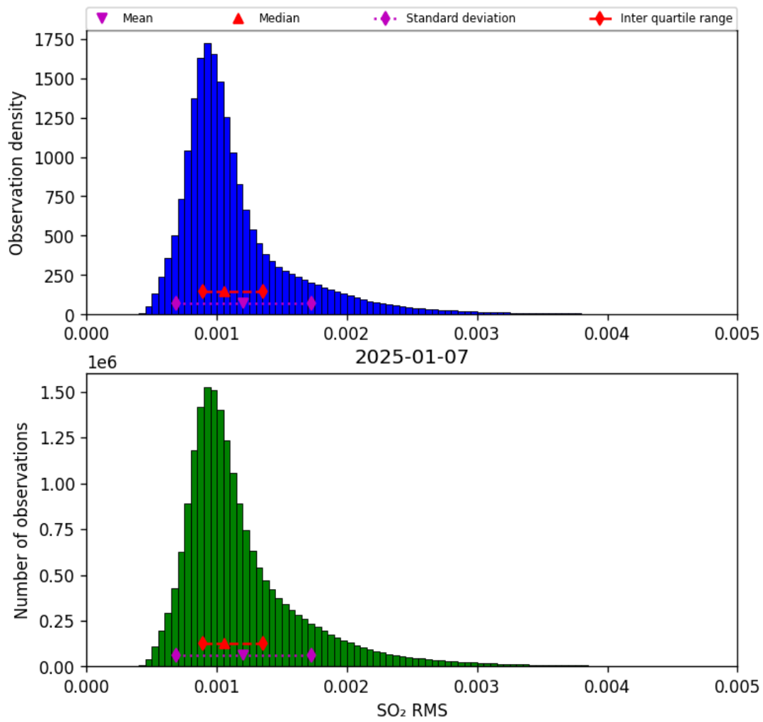
Figure 78: Histogram of “SO 2 RMS” for 2025-01-07 to 2025-01-08
