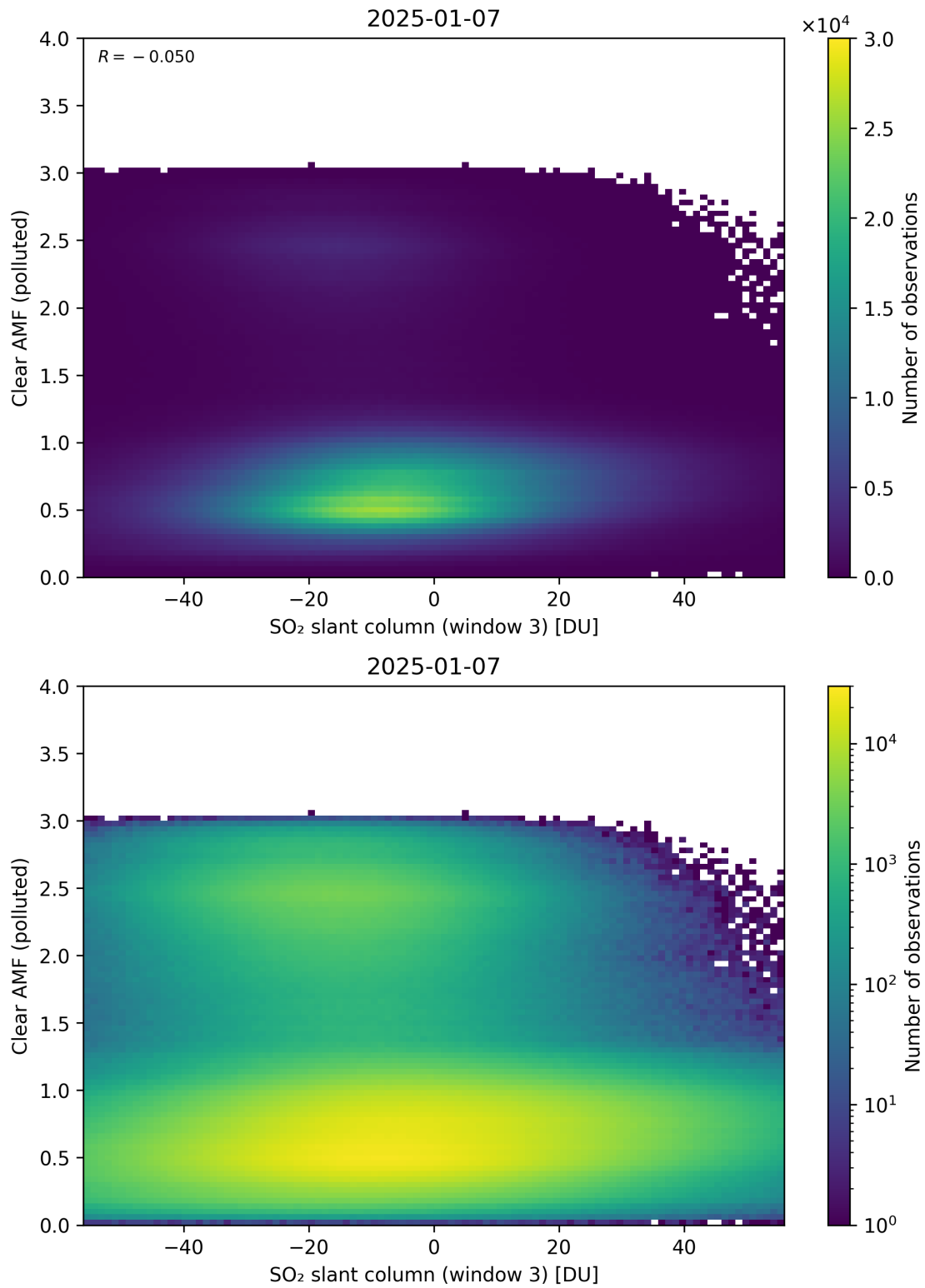
Figure 315: Scatter density plot of “SO 2 slant column (window 3)” against “Clear AMF (polluted)” for 2025-01-07 to 2025-01-08.
