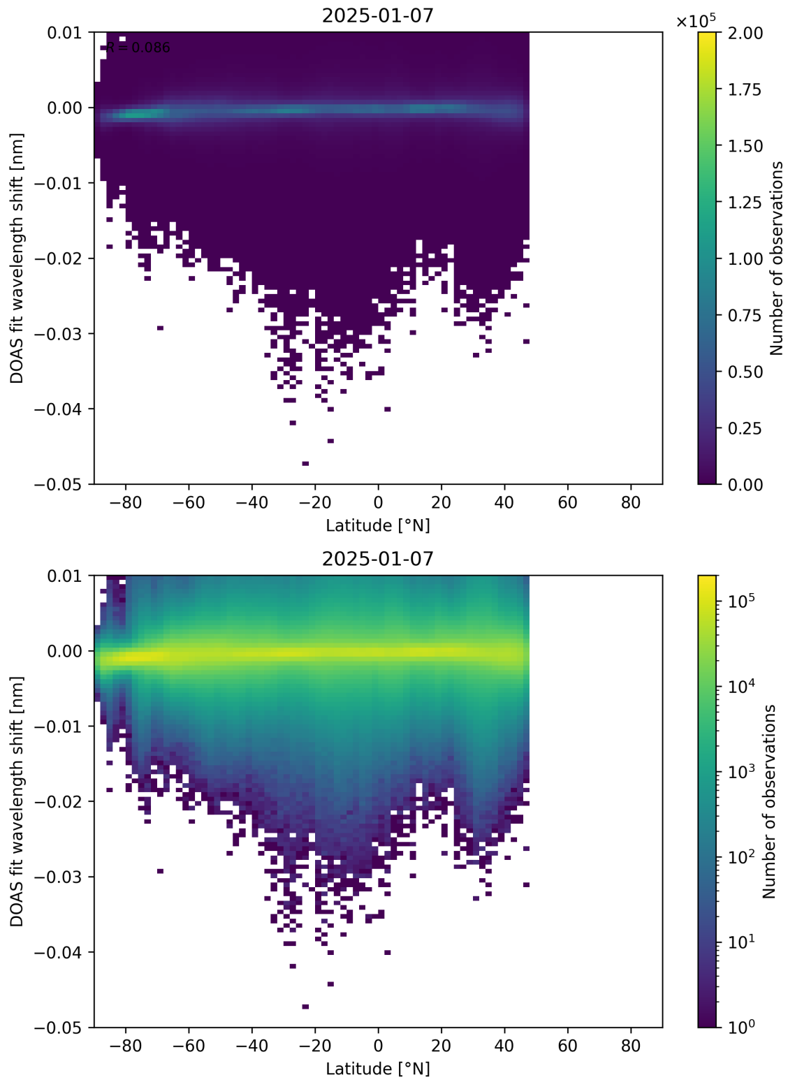
Figure 153: Scatter density plot of “Latitude” against “DOAS fit wavelength shift” for 2025-01-07 to 2025-01-08.
