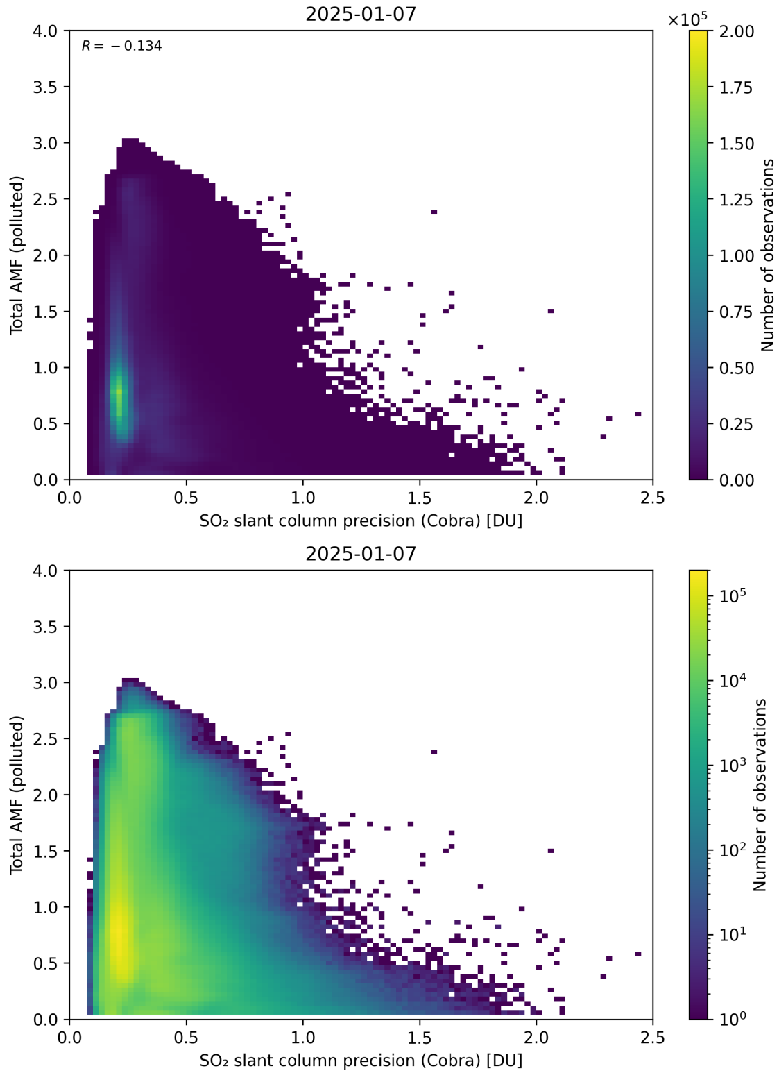
Figure 213: Scatter density plot of “SO 2 slant column precision (Cobra)” against “Total AMF (polluted)” for 2025-01-07 to 2025-01-08.
