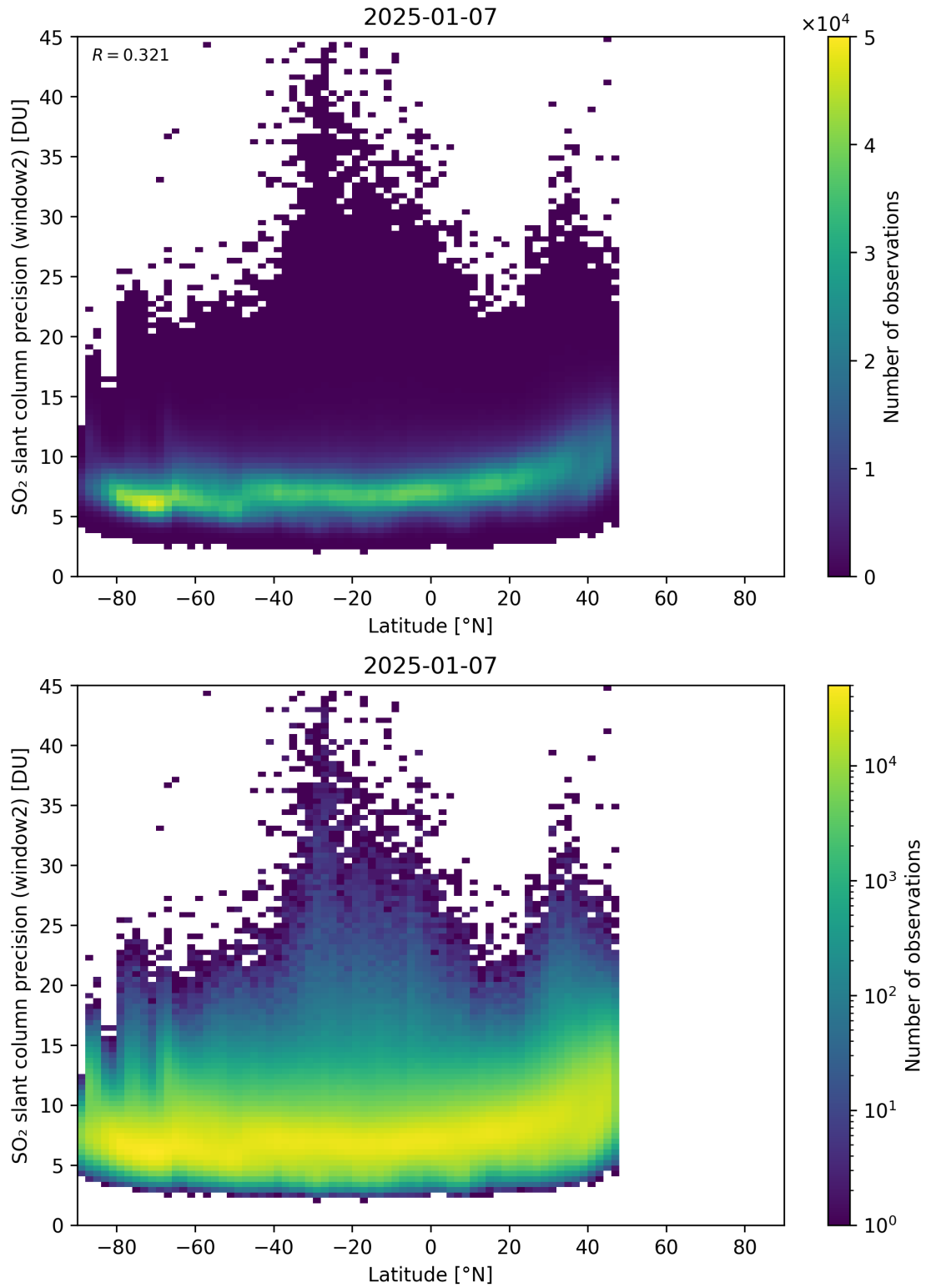
Figure 164: Scatter density plot of “Latitude” against “SO 2 slant column precision (window2)” for 2025-01-07 to 2025-01-08.
