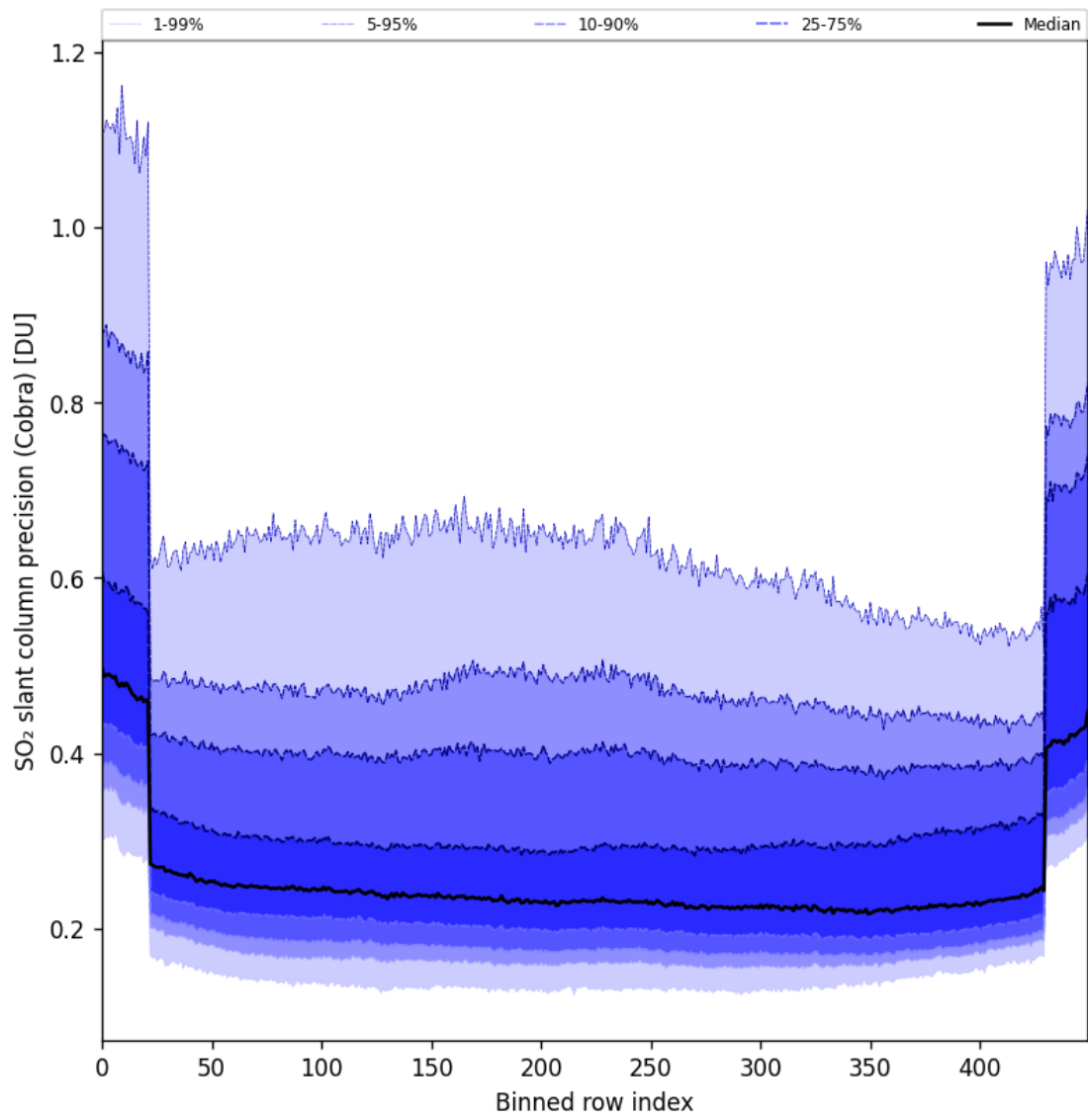
Figure 88: Along track statistics of “SO 2 slant column precision (Cobra)” for 2025-01-07 to 2025-01-08
