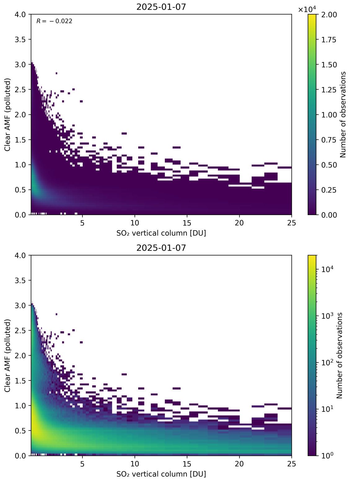
Figure 348: Scatter density plot of “SO 2 vertical column” against “Clear AMF (polluted)” for 2025-01-07 to 2025-01-08.
