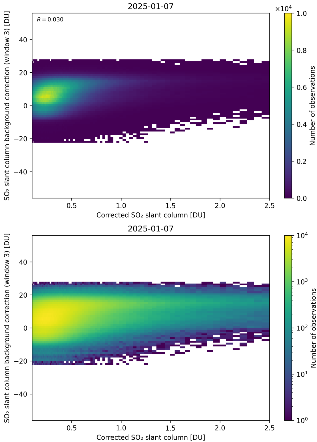
Figure 228: Scatter density plot of “Corrected SO 2 slant column” against “SO 2 slant column background correction (window 3)” for 2025-01-07 to 2025-01-08.
