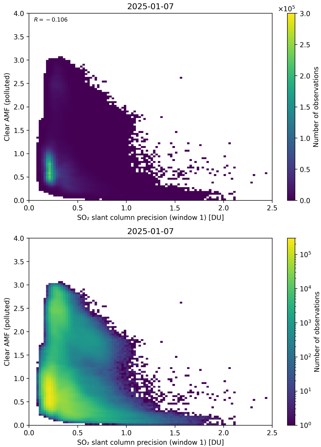
Figure 274: Scatter density plot of “SO 2 slant column precision (window 1)” against “Clear AMF (polluted)” for 2025-01-07 to 2025-01-08.
