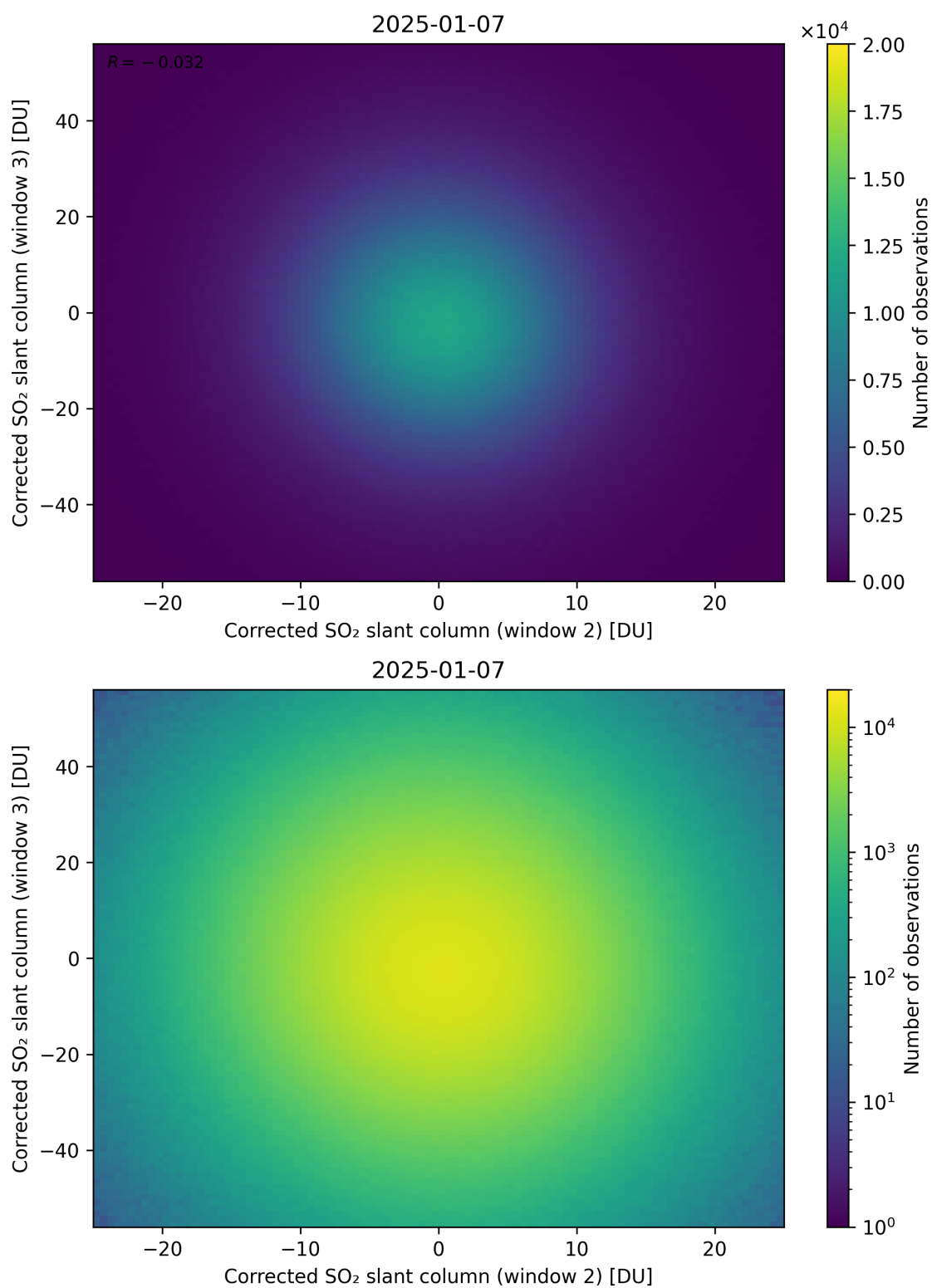
Figure 250: Scatter density plot of “Corrected SO 2 slant column (window 2)” against “Corrected SO 2 slant column (window 3)” for 2025-01-07 to 2025-01-08.
