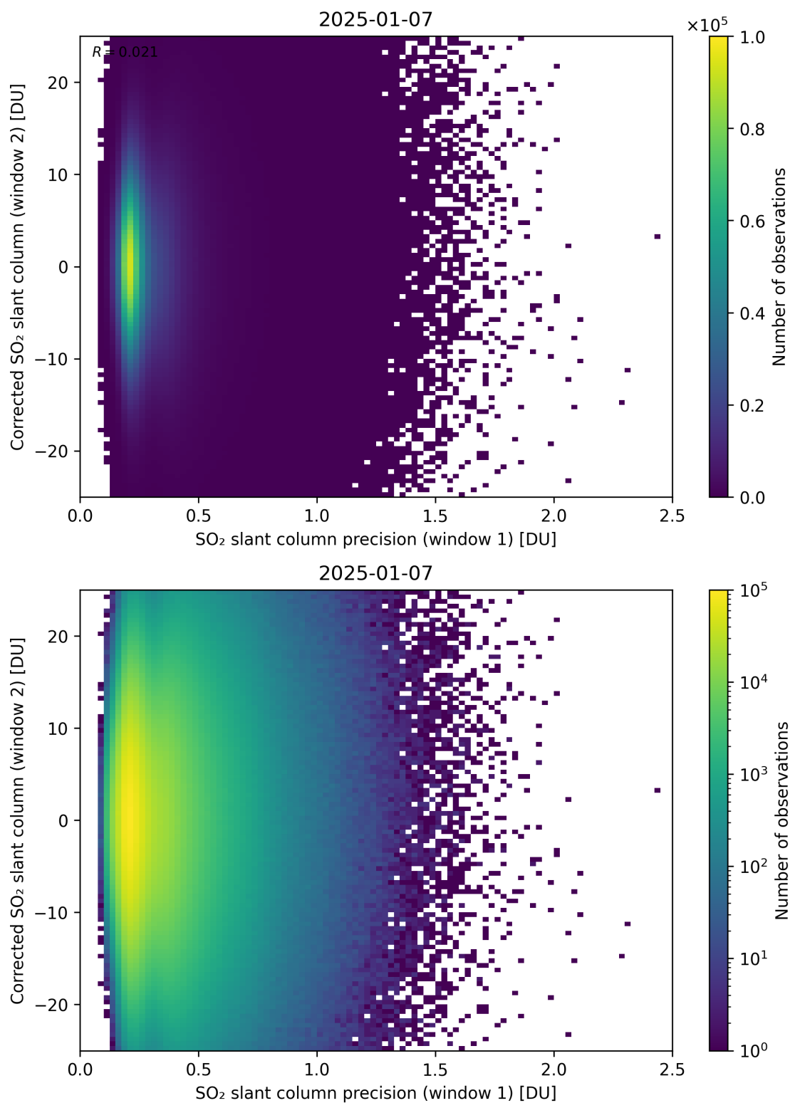
Figure 275: Scatter density plot of “SO 2 slant column precision (window 1)” against “Corrected SO 2 slant column (window 2)” for 2025-01-07 to 2025-01-08.
