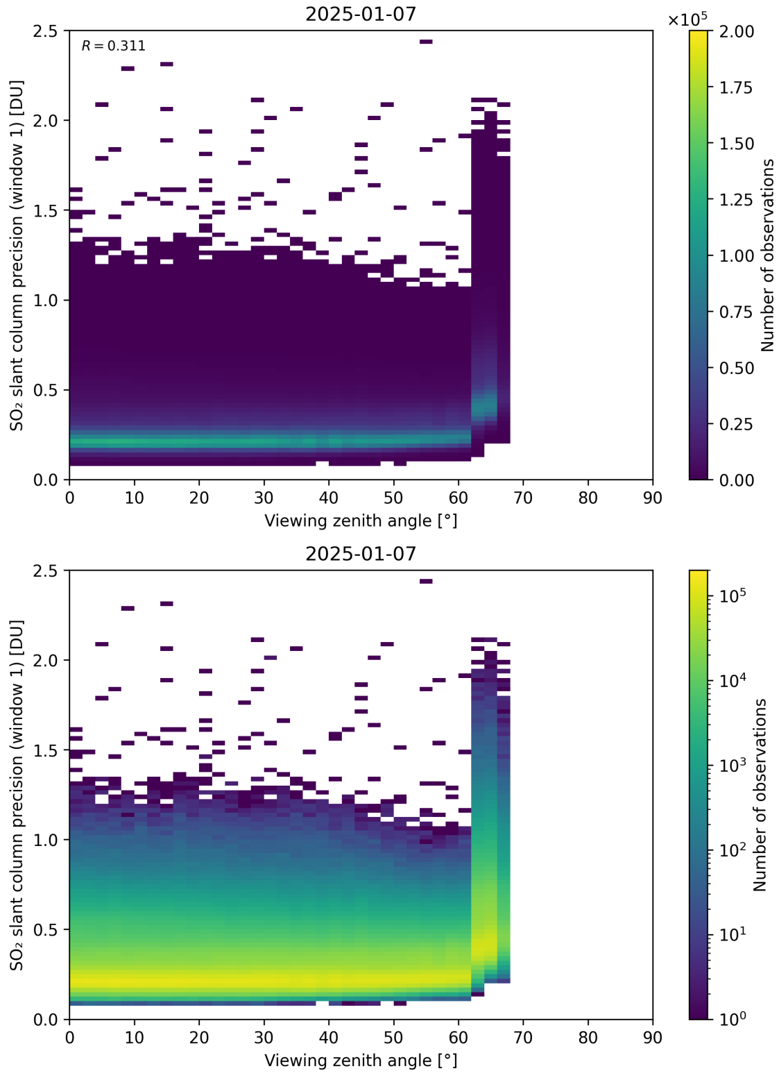
Figure 377: Scatter density plot of “Viewing zenith angle” against “SO 2 slant column precision (window 1)” for 2025-01-07 to 2025-01-08.
