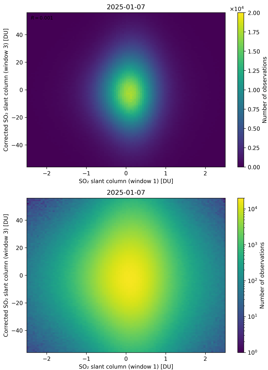
Figure 284: Scatter density plot of “SO 2 slant column (window 1)” against “Corrected SO 2 slant column (window 3)” for 2025-01-07 to 2025-01-08.
