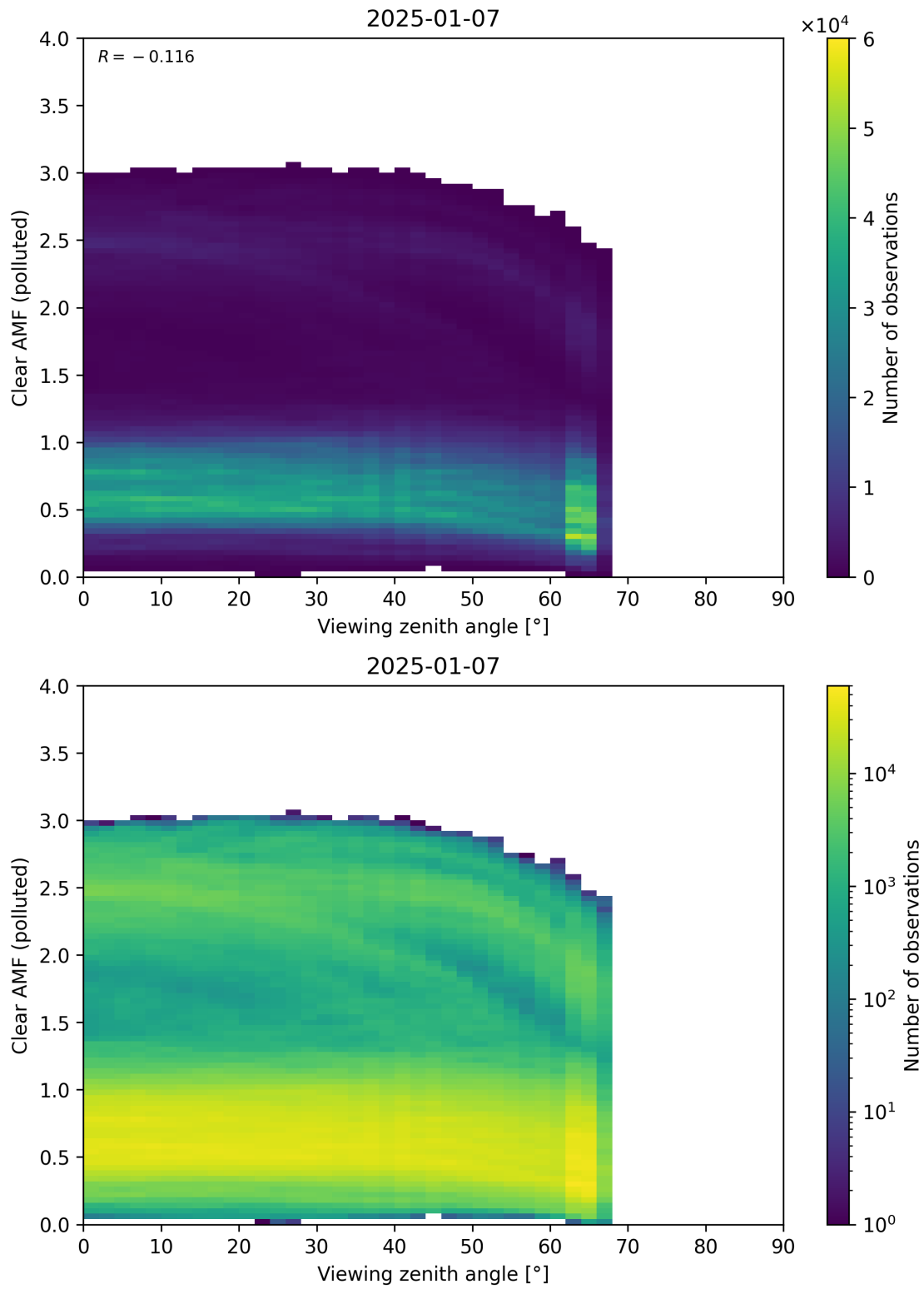
Figure 370: Scatter density plot of “Viewing zenith angle” against “Clear AMF (polluted)” for 2025-01-07 to 2025-01-08.
