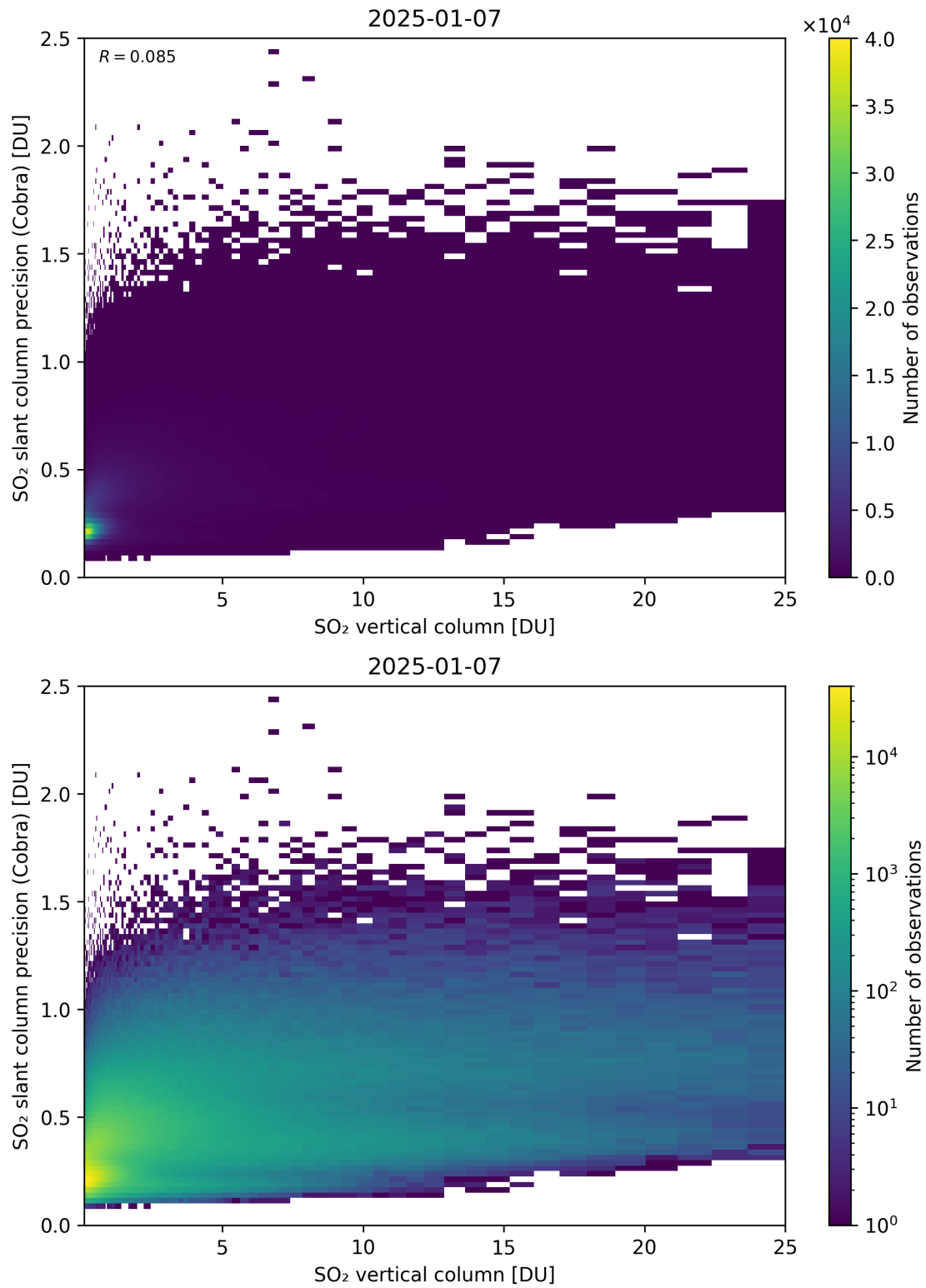
Figure 350: Scatter density plot of “SO 2 vertical column” against “SO 2 slant column precision (Cobra)” for 2025-01-07 to 2025-01-08.
