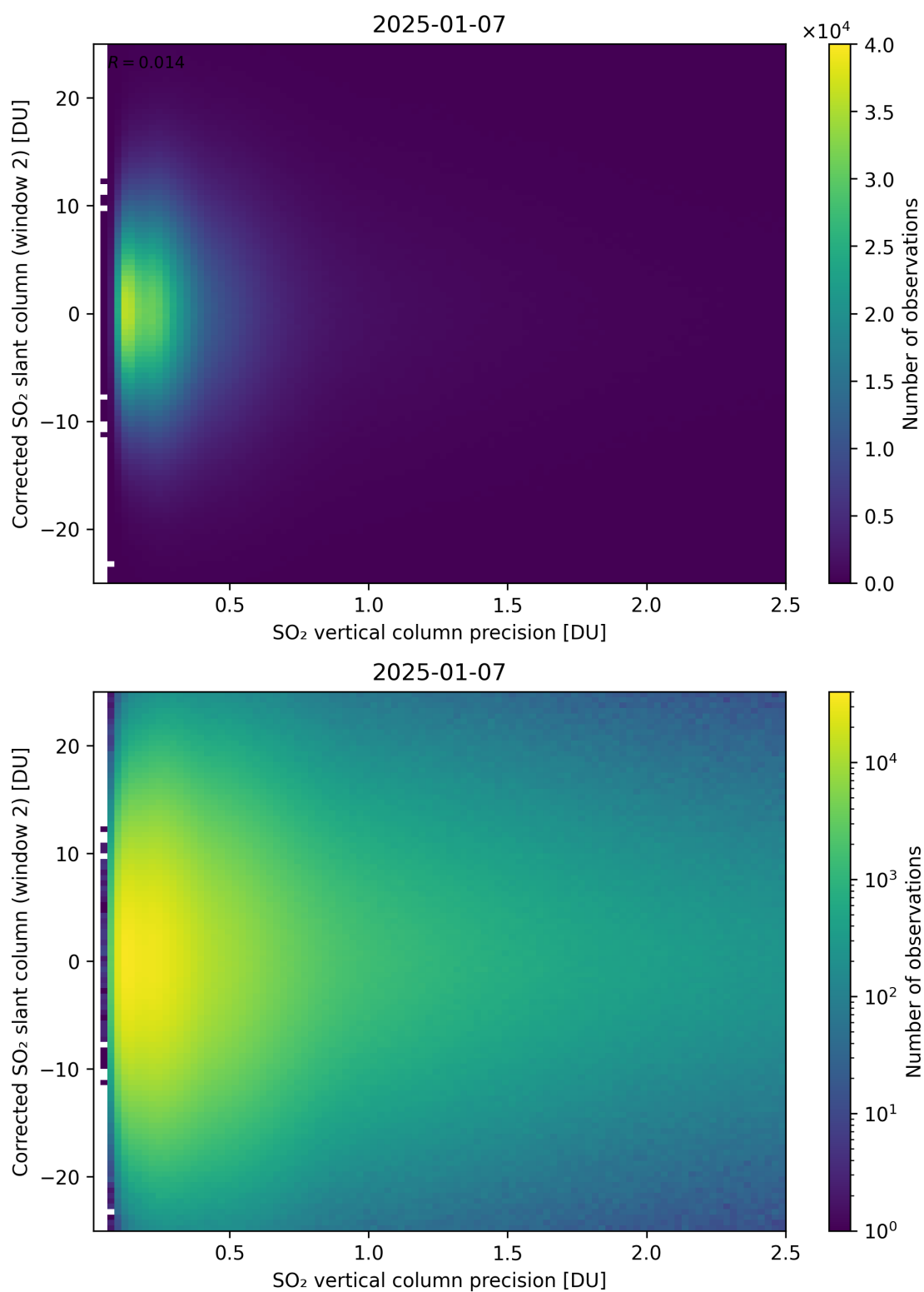
Figure 339: Scatter density plot of “SO 2 vertical column precision” against “Corrected SO 2 slant column (window 2)” for 2025-01-07 to 2025-01-08.
