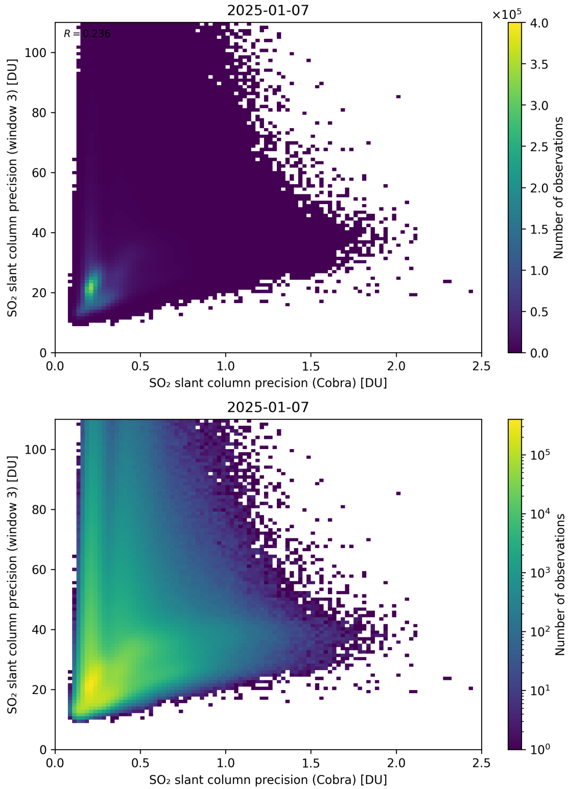
Figure 212: Scatter density plot of “SO 2 slant column precision (Cobra)” against “SO 2 slant column precision (window 3)” for 2025-01-07 to 2025-01-08.
