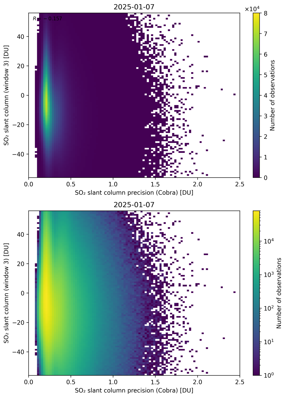
Figure 211: Scatter density plot of “SO 2 slant column precision (Cobra)” against “SO 2 slant column (window 3)” for 2025-01-07 to 2025-01-08.
