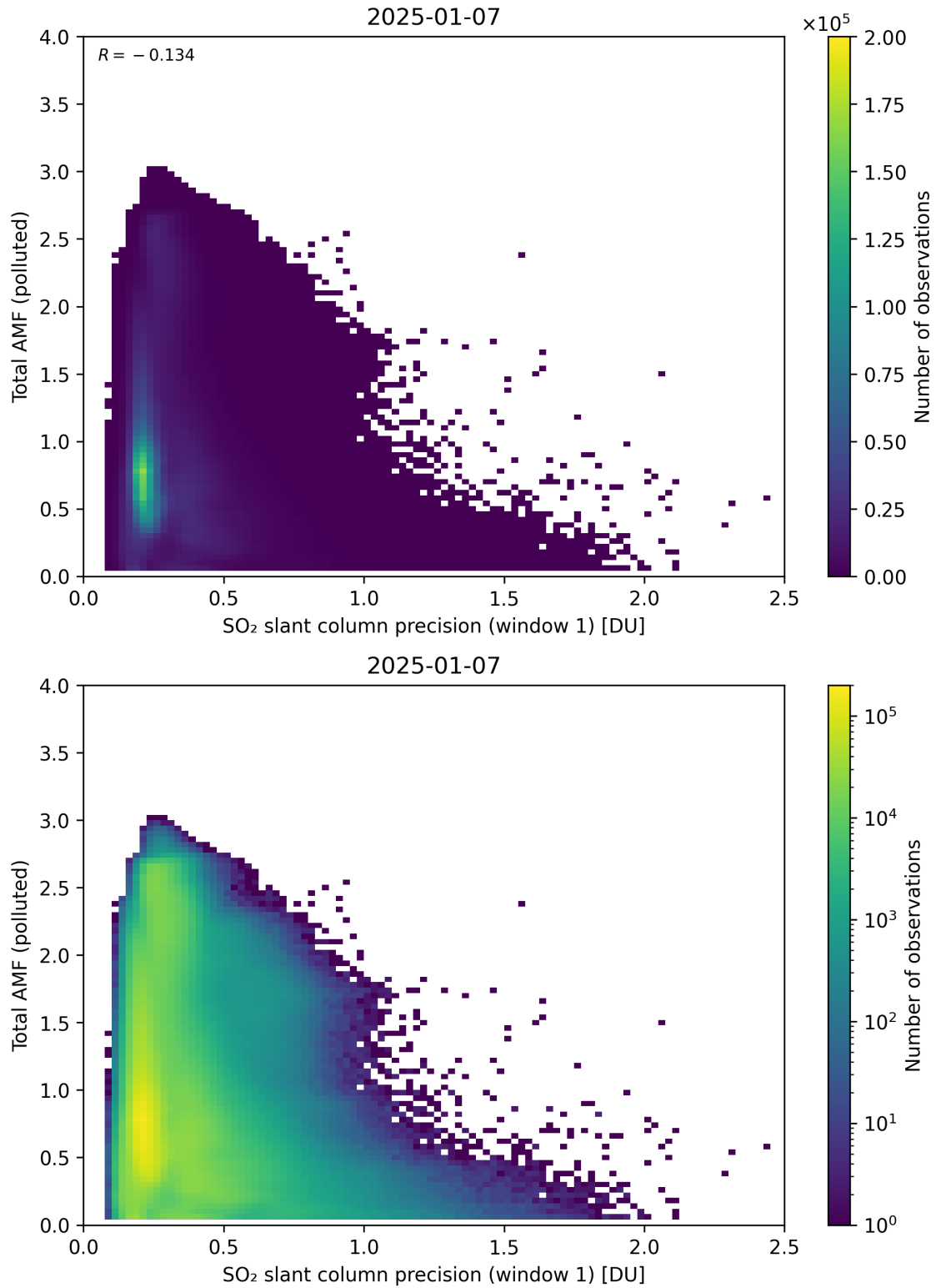
Figure 280: Scatter density plot of “SO 2 slant column precision (window 1)” against “Total AMF (polluted)” for 2025-01-07 to 2025-01-08.
