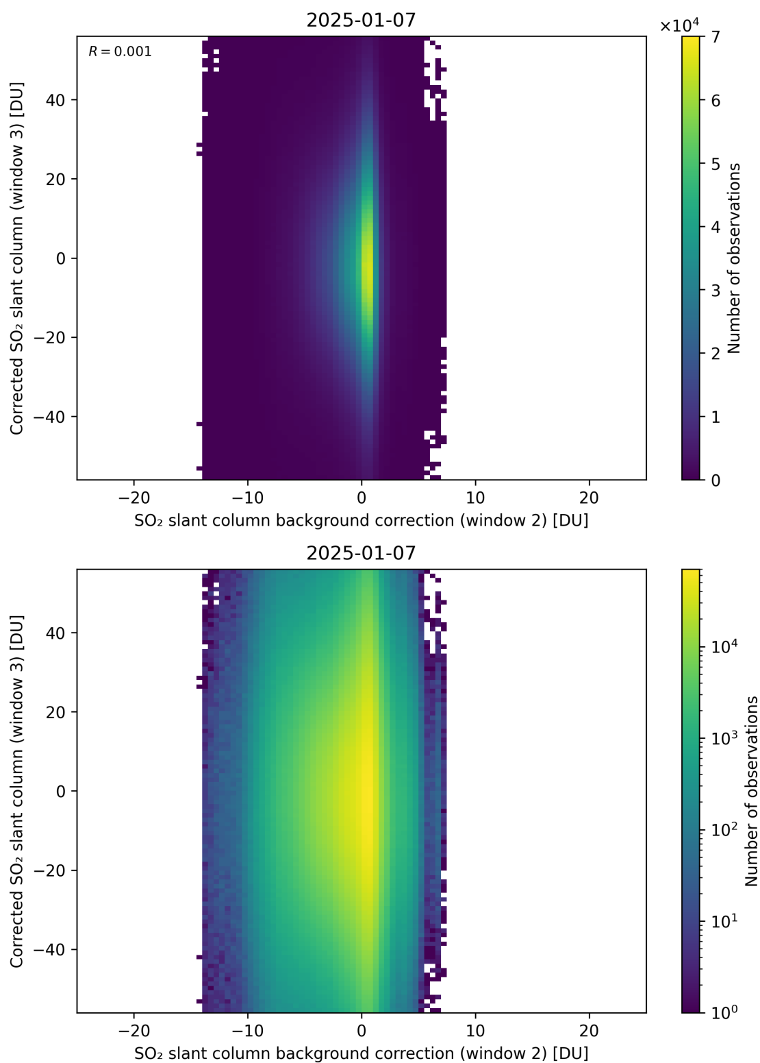
Figure 127: Scatter density plot of “SO 2 slant column background correction (window 2)” against “Corrected SO 2 slant column (window 3)” for 2025-01-07 to 2025-01-08.
