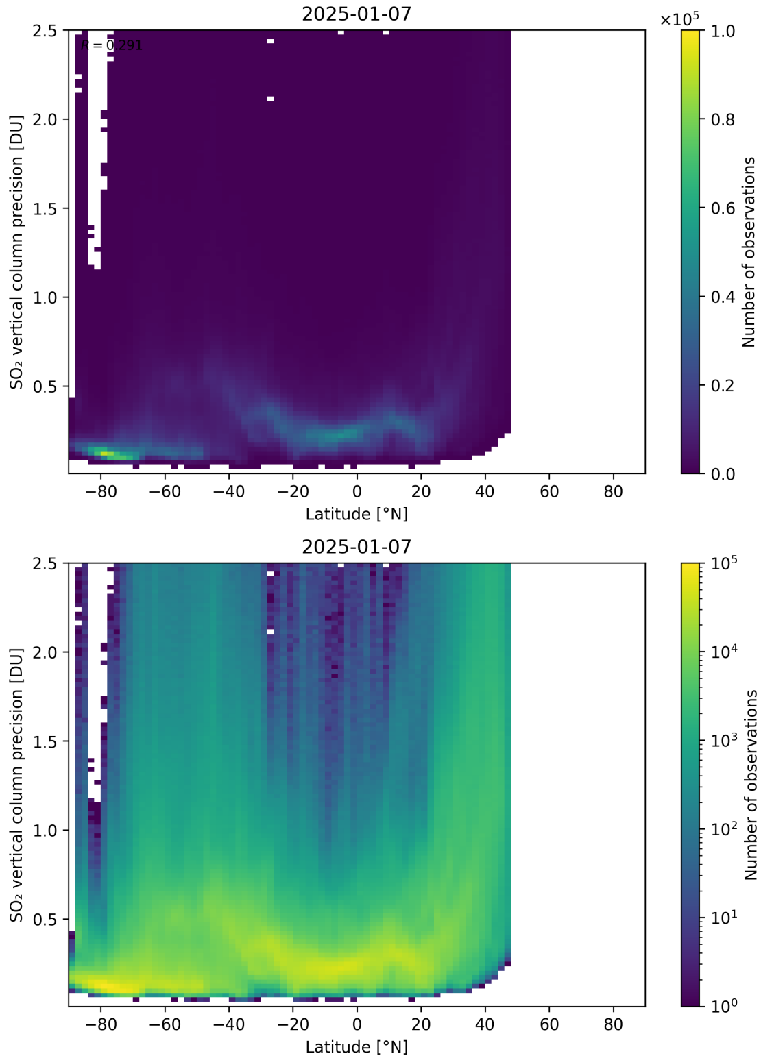
Figure 170: Scatter density plot of “Latitude” against “SO 2 vertical column precision” for 2025-01-07 to 2025-01-08.
