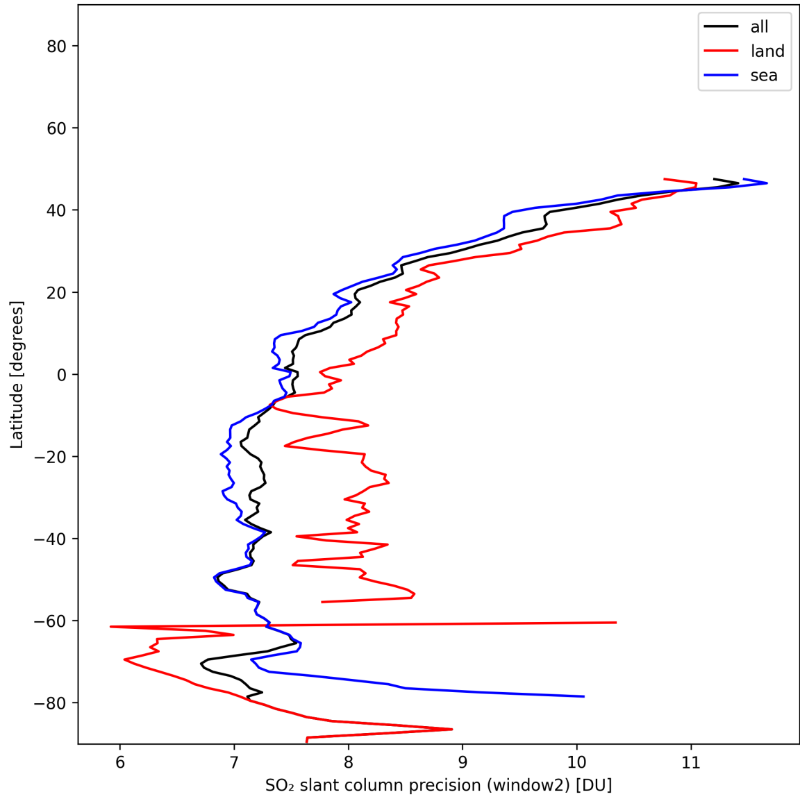
Figure 42: Zonal average of “SO 2 slant column precision (window2)” for 2025-01-07 to 2025-01-08.
