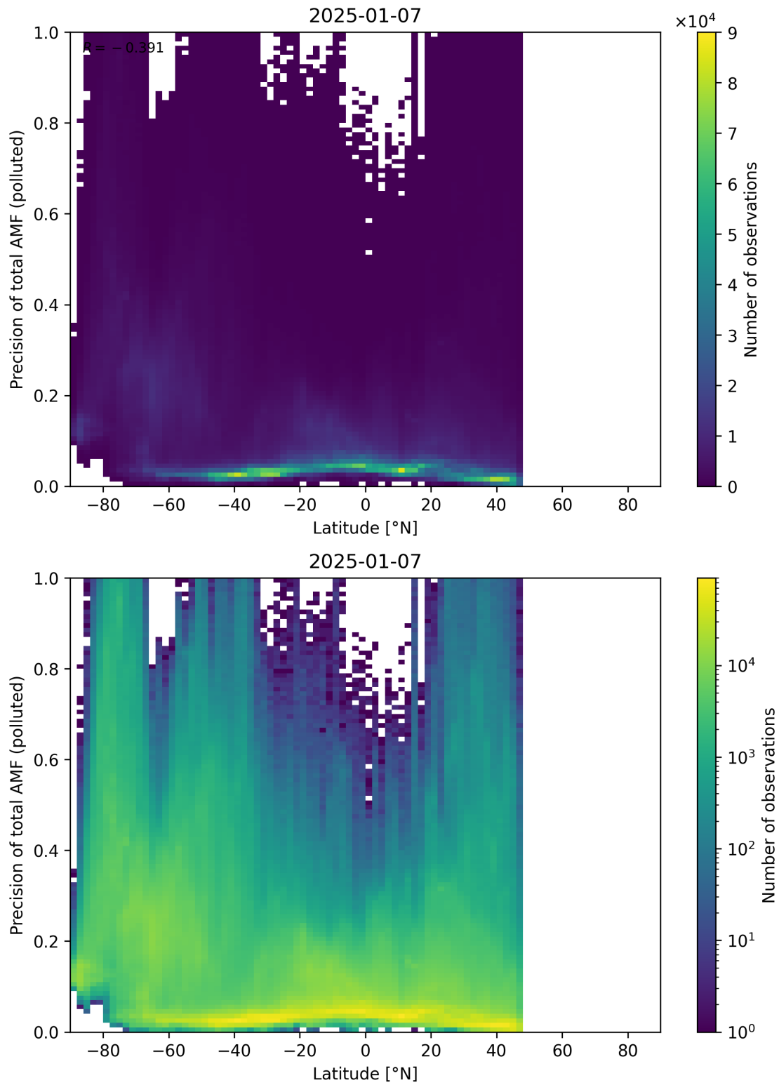
Figure 168: Scatter density plot of “Latitude” against “Precision of total AMF (polluted)” for 2025-01-07 to 2025-01-08.
