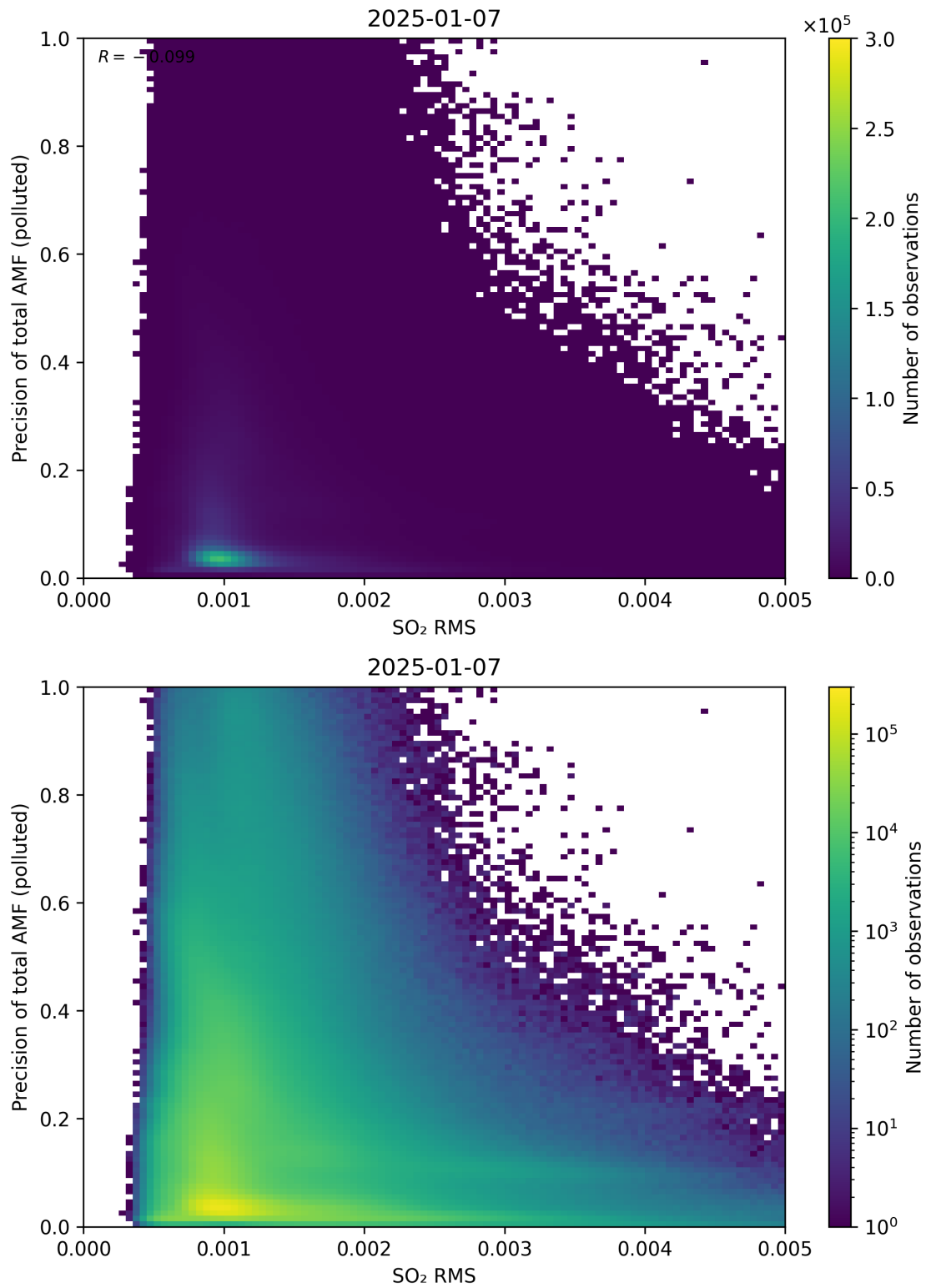
Figure 149: Scatter density plot of “SO 2 RMS” against “Precision of total AMF (polluted)” for 2025-01-07 to 2025-01-08.
