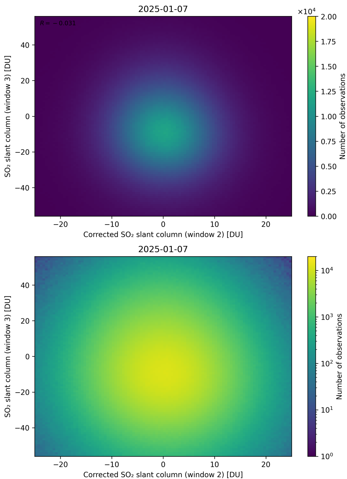
Figure 251: Scatter density plot of “Corrected SO 2 slant column (window 2)” against “SO 2 slant column (window 3)” for 2025-01-07 to 2025-01-08.
