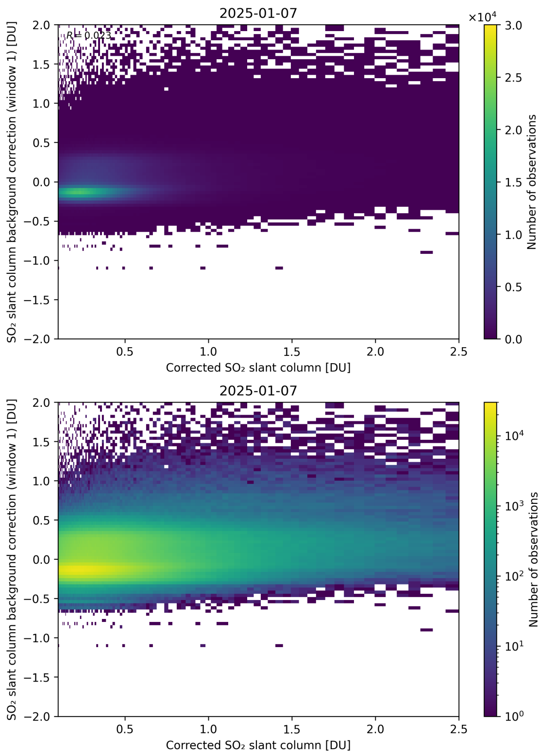
Figure 226: Scatter density plot of “Corrected SO 2 slant column” against “SO 2 slant column background correction (window 1)” for 2025-01-07 to 2025-01-08.
