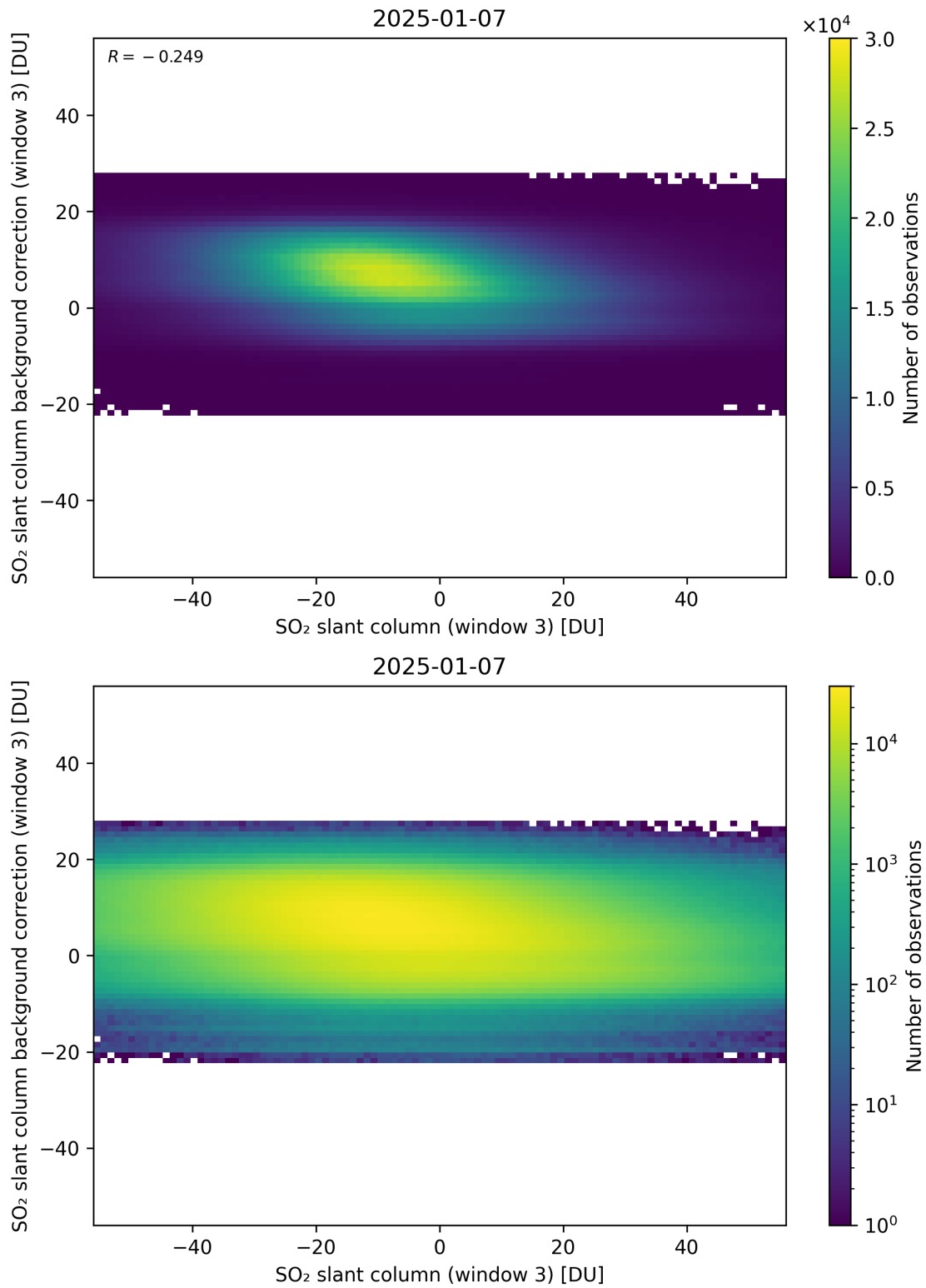
Figure 303: Scatter density plot of “SO 2 slant column (window 3)” against “SO 2 slant column background correction (window 3)” for 2025-01-07 to 2025-01-08.
