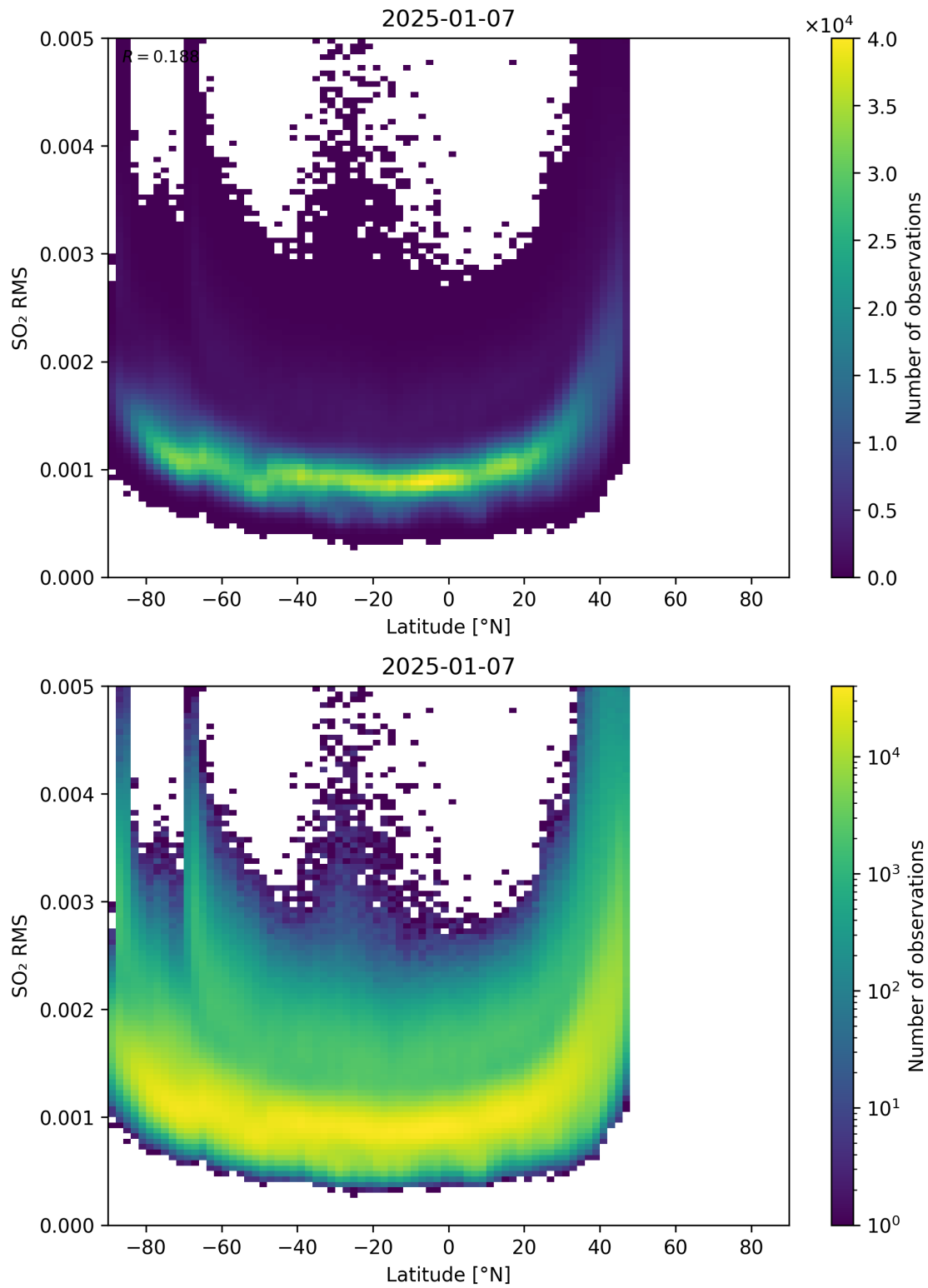
Figure 155: Scatter density plot of “Latitude” against “SO 2 RMS” for 2025-01-07 to 2025-01-08.
