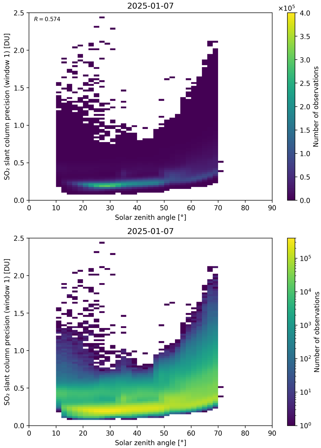
Figure 185: Scatter density plot of “Solar zenith angle” against “SO 2 slant column precision (window 1)” for 2025-01-07 to 2025-01-08.
