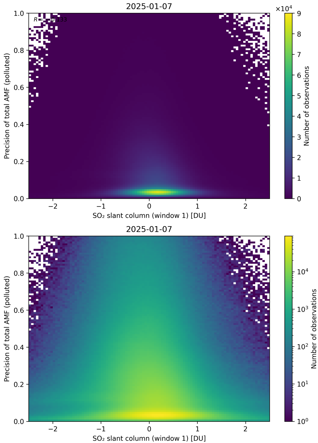
Figure 290: Scatter density plot of “SO 2 slant column (window 1)” against “Precision of total AMF (polluted)” for 2025-01-07 to 2025-01-08.
