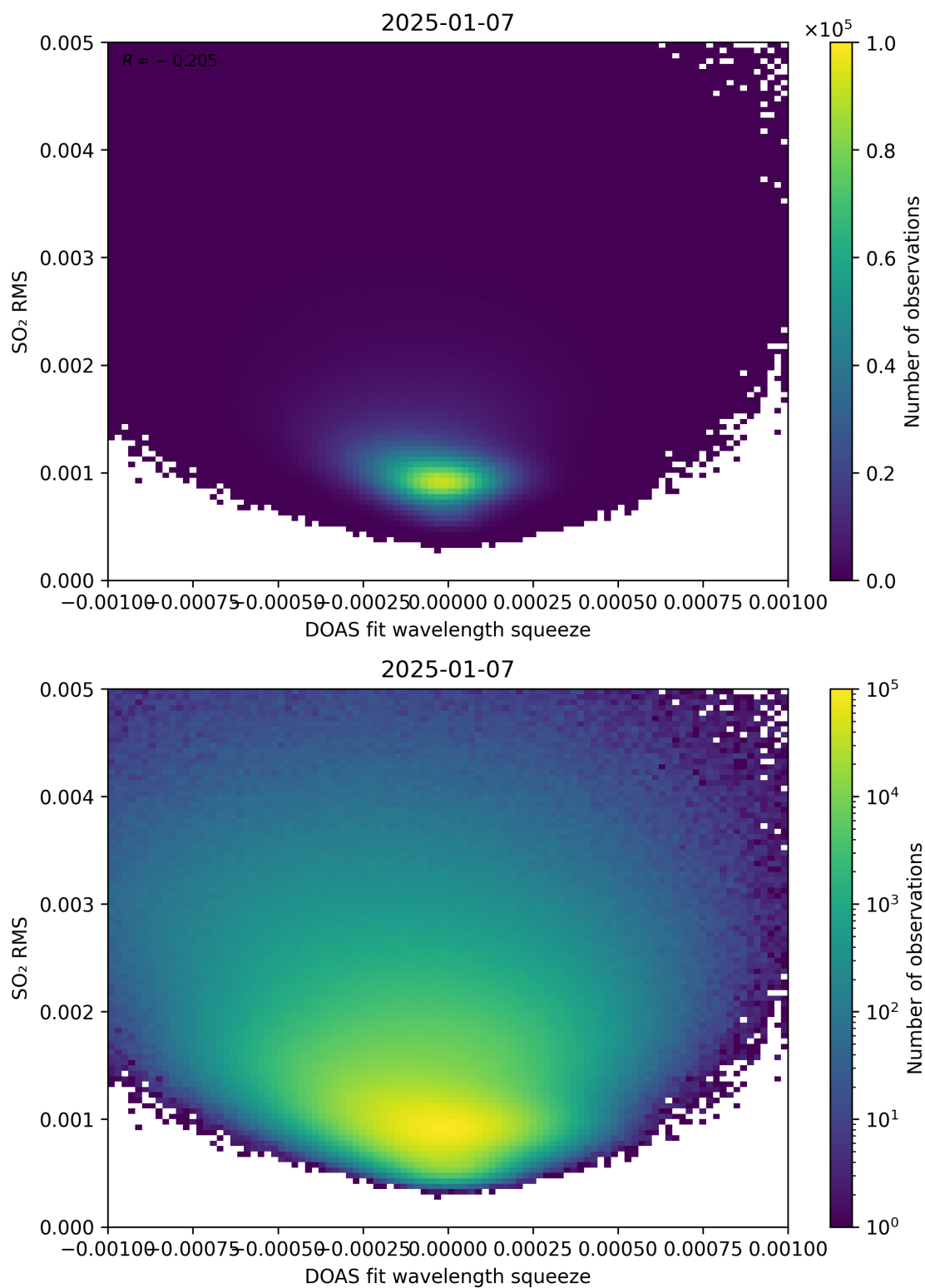
Figure 143: Scatter density plot of “DOAS fit wavelength squeeze” against “SO 2 RMS” for 2025-01-07 to 2025-01-08.
