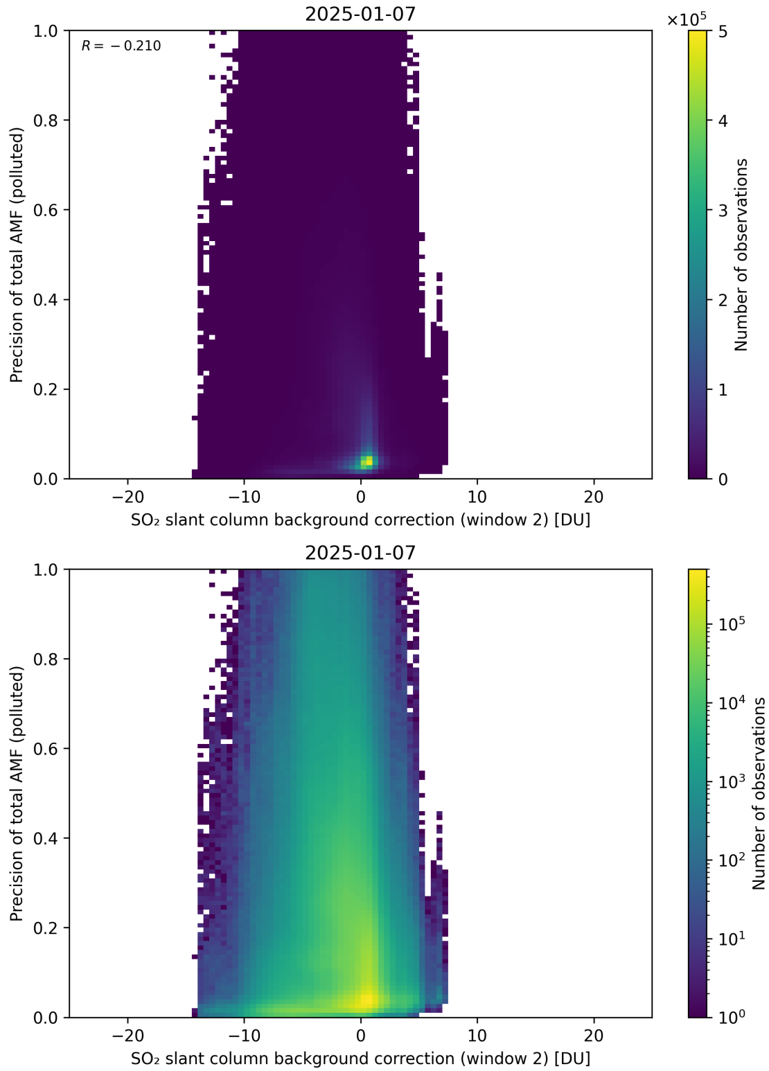
Figure 131: Scatter density plot of “SO 2 slant column background correction (window 2)” against “Precision of total AMF (polluted)” for 2025-01-07 to 2025-01-08.
