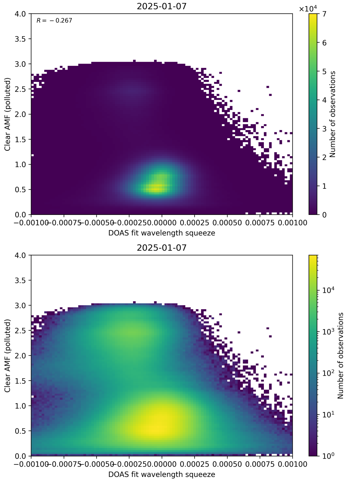
Figure 144: Scatter density plot of “DOAS fit wavelength squeeze” against “Clear AMF (polluted)” for 2025-01-07 to 2025-01-08.
