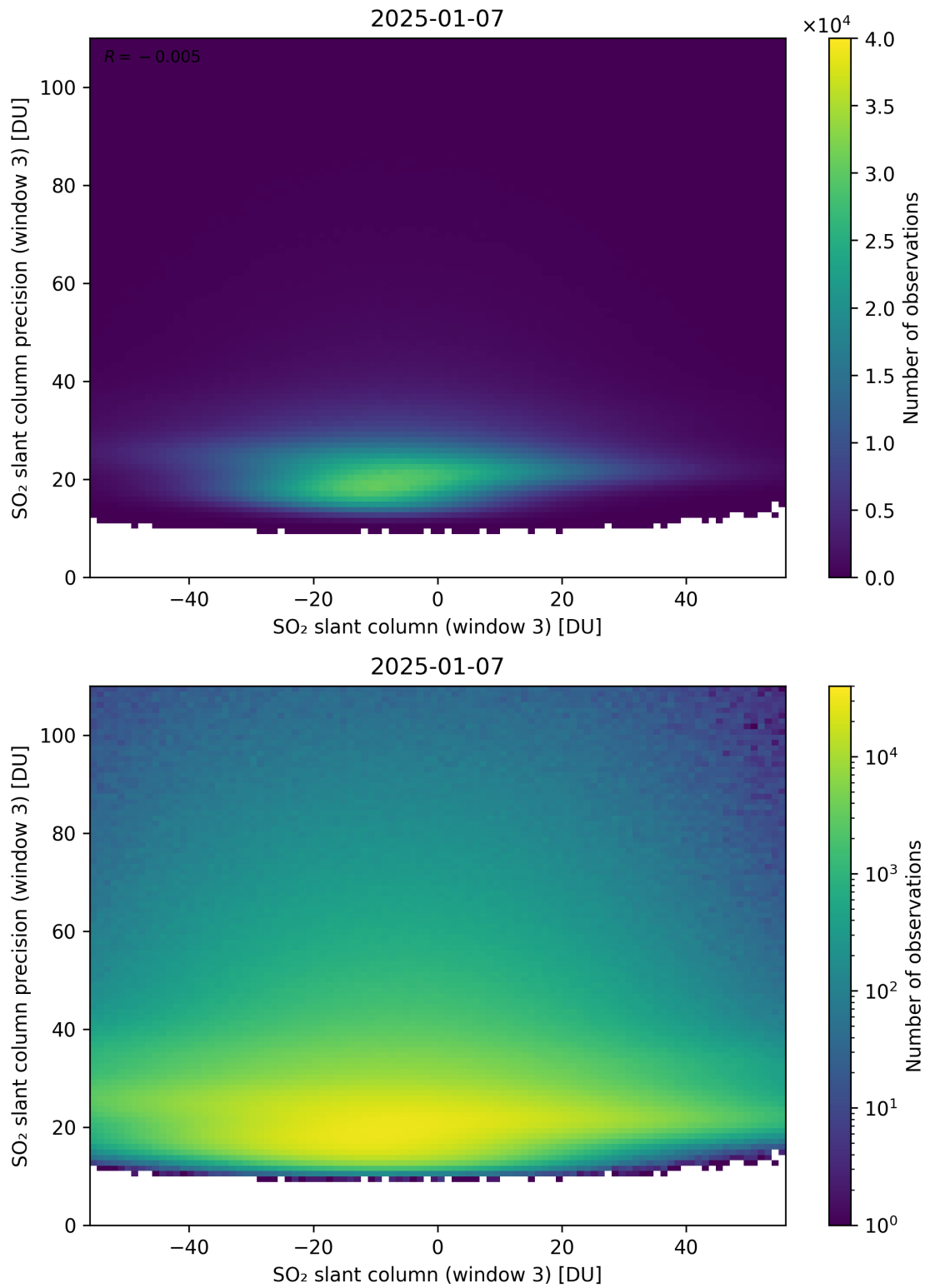
Figure 317: Scatter density plot of “SO 2 slant column (window 3)” against “SO 2 slant column precision (window 3)” for 2025-01-07 to 2025-01-08.
