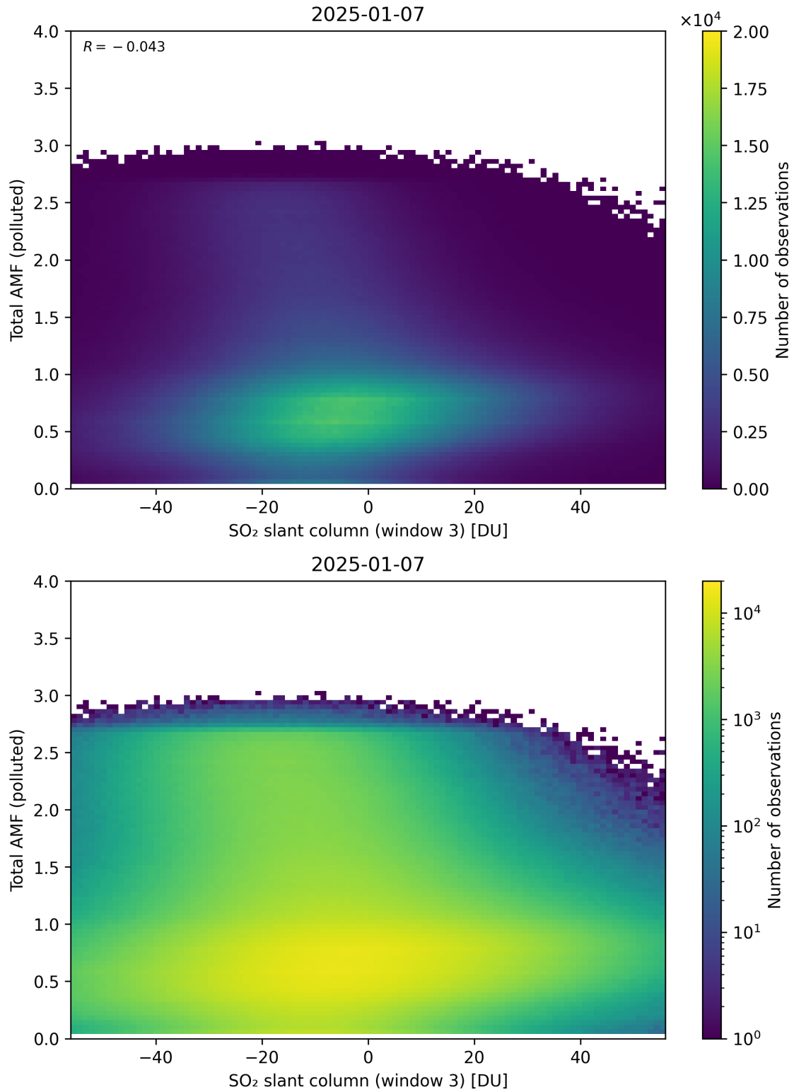
Figure 318: Scatter density plot of “SO 2 slant column (window 3)” against “Total AMF (polluted)” for 2025-01-07 to 2025-01-08.
