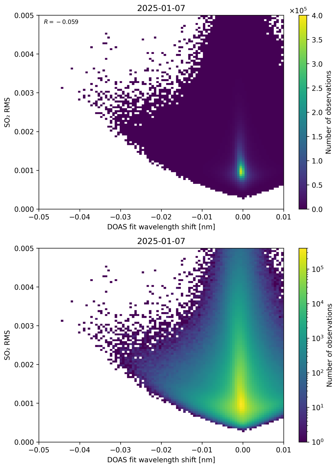
Figure 139: Scatter density plot of “DOAS fit wavelength shift” against “SO 2 RMS” for 2025-01-07 to 2025-01-08.
