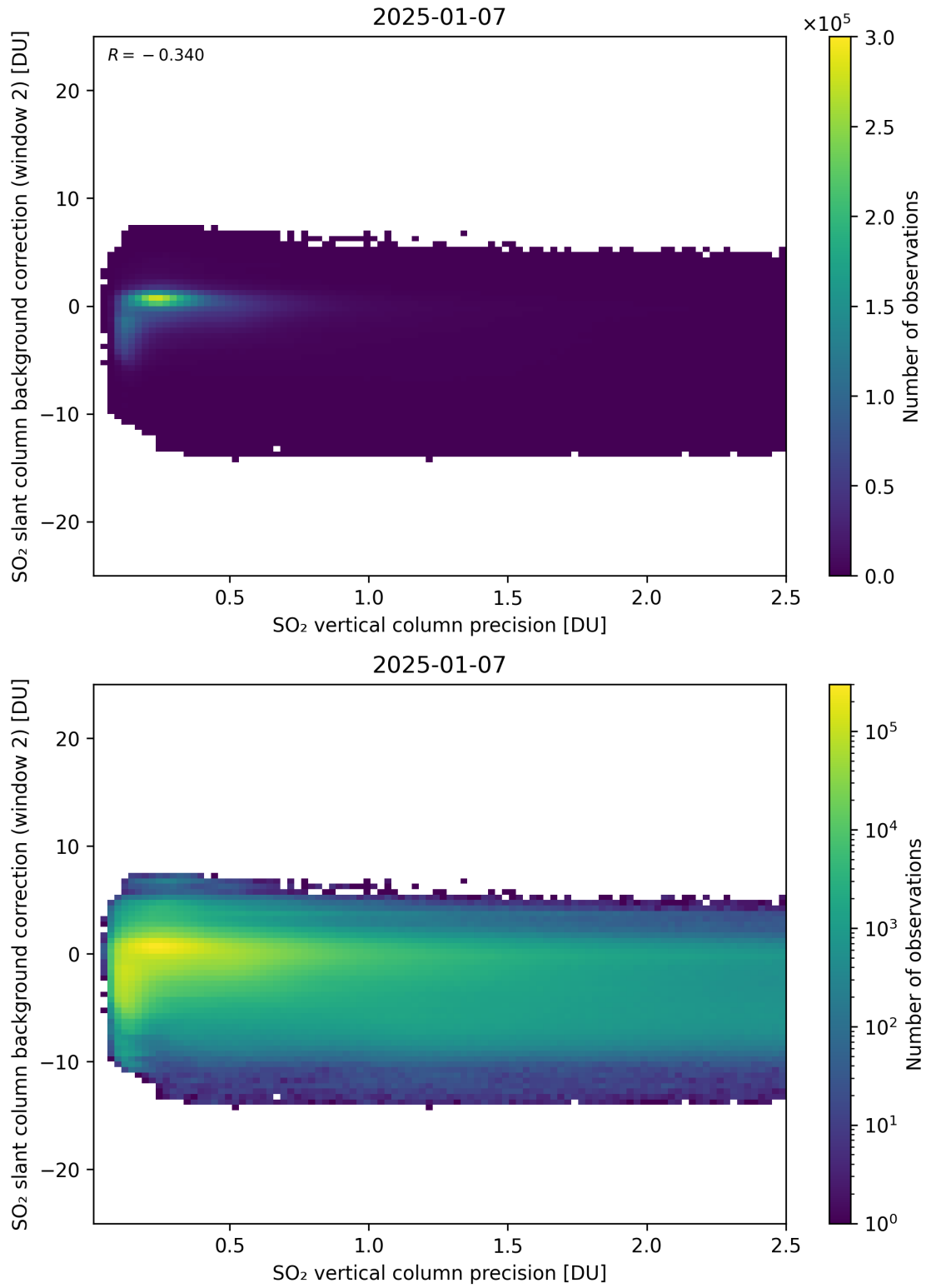
Figure 330: Scatter density plot of “SO 2 vertical column precision” against “SO 2 slant column background correction (window 2)” for 2025-01-07 to 2025-01-08.
