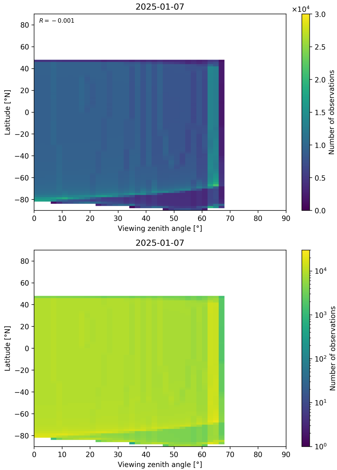
Figure 368: Scatter density plot of “Viewing zenith angle” against “Latitude” for 2025-01-07 to 2025-01-08.
