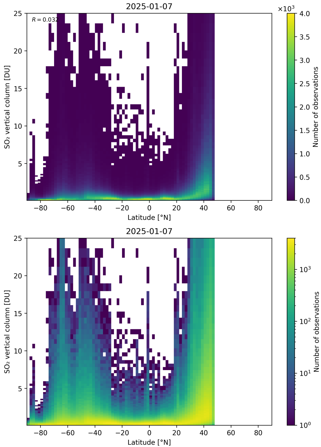
Figure 169: Scatter density plot of “Latitude” against “SO 2 vertical column” for 2025-01-07 to 2025-01-08.
