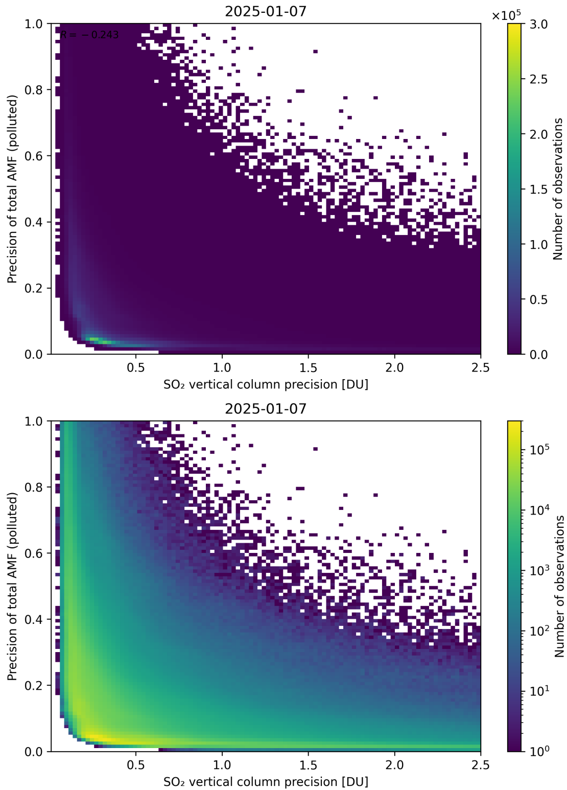
Figure 347: Scatter density plot of “SO 2 vertical column precision” against “Precision of total AMF (polluted)” for 2025-01-07 to 2025-01-08.
