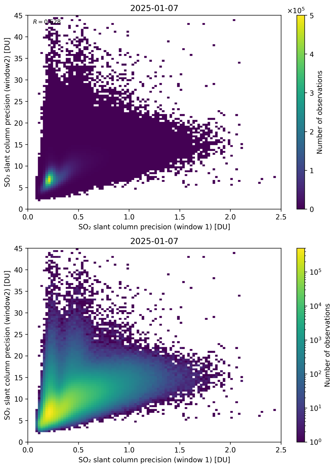
Figure 277: Scatter density plot of “SO 2 slant column precision (window 1)” against “SO 2 slant column precision (window2)” for 2025-01-07 to 2025-01-08.
