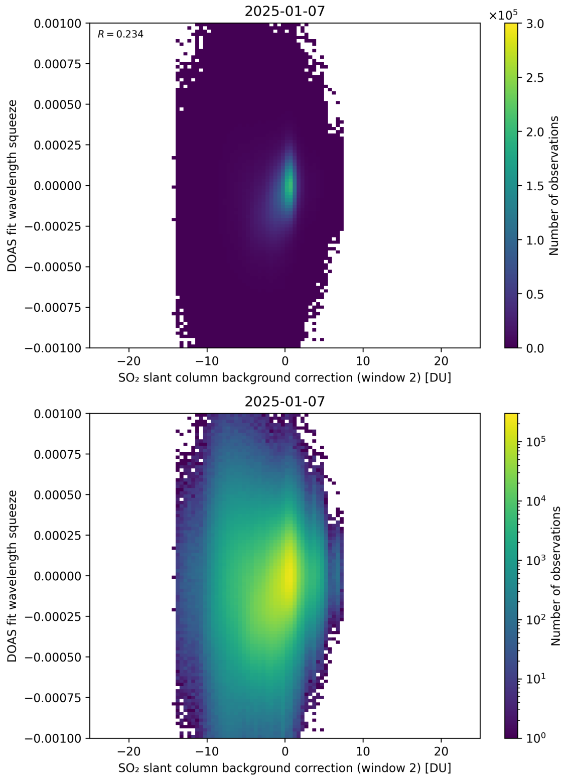
Figure 124: Scatter density plot of “SO 2 slant column background correction (window 2)” against “DOAS fit wavelength squeeze” for 2025-01-07 to 2025-01-08.
