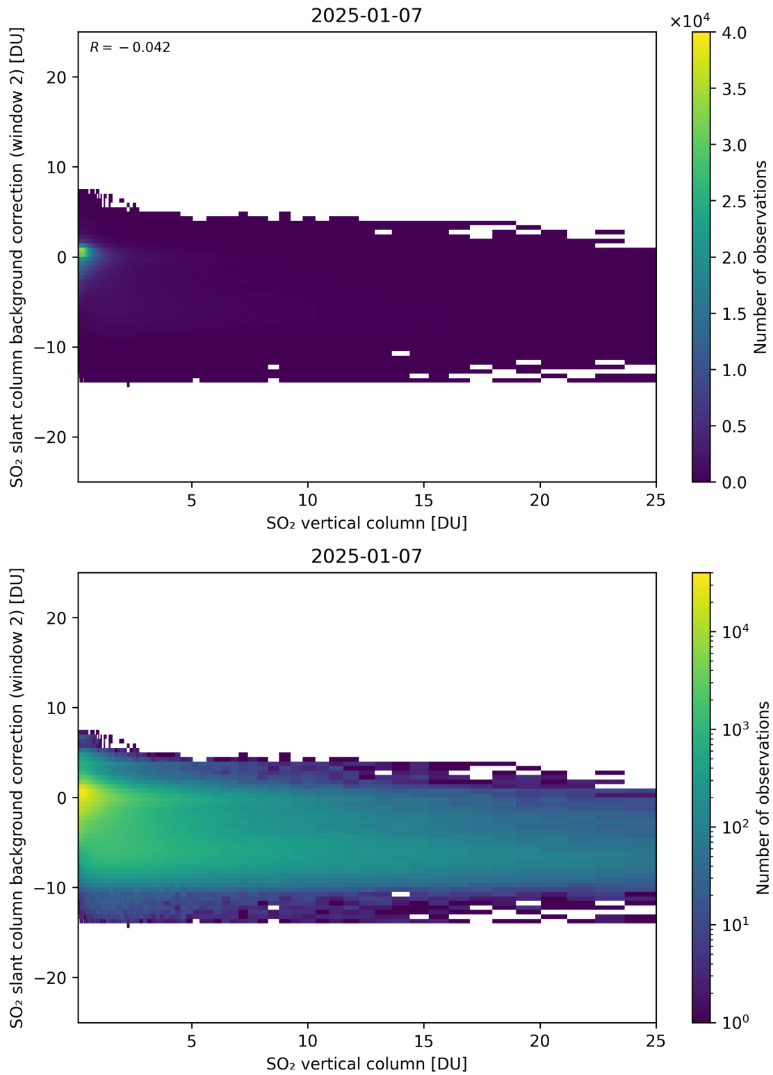
Figure 324: Scatter density plot of “SO 2 vertical column” against “SO 2 slant column background correction (window 2)” for 2025-01-07 to 2025-01-08.
