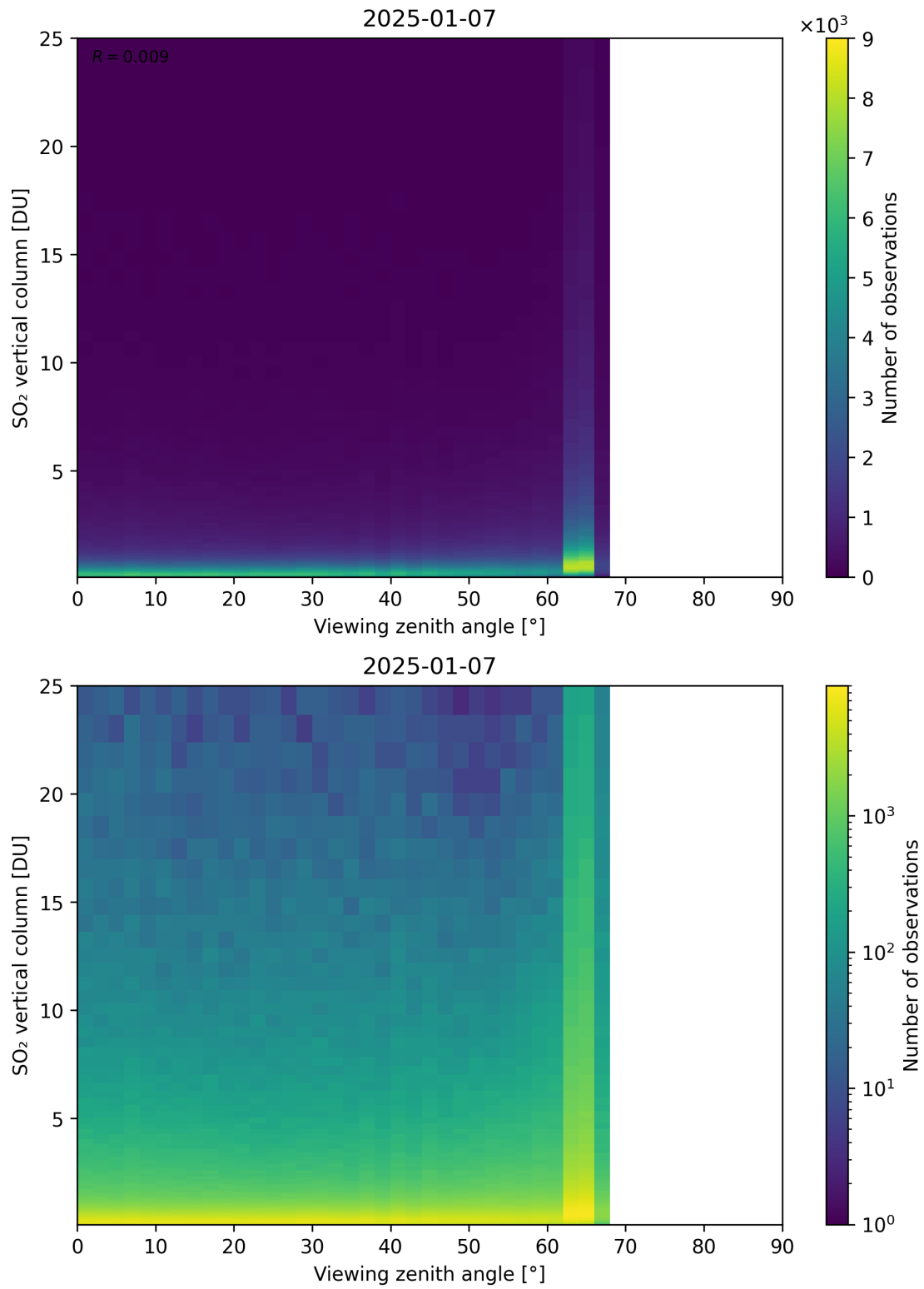
Figure 383: Scatter density plot of “Viewing zenith angle” against “SO 2 vertical column” for 2025-01-07 to 2025-01-08.
