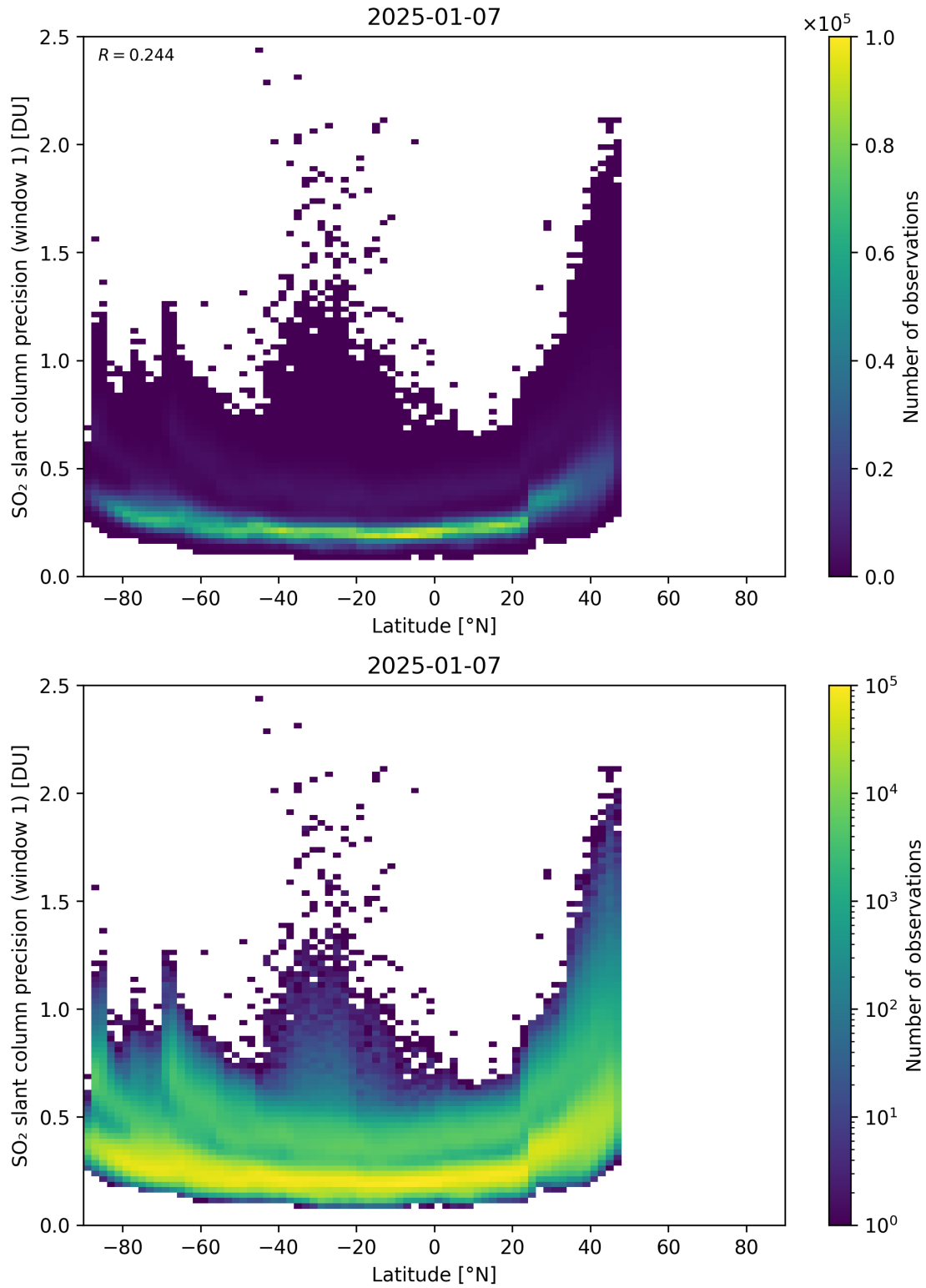
Figure 163: Scatter density plot of “Latitude” against “SO 2 slant column precision (window 1)” for 2025-01-07 to 2025-01-08.
