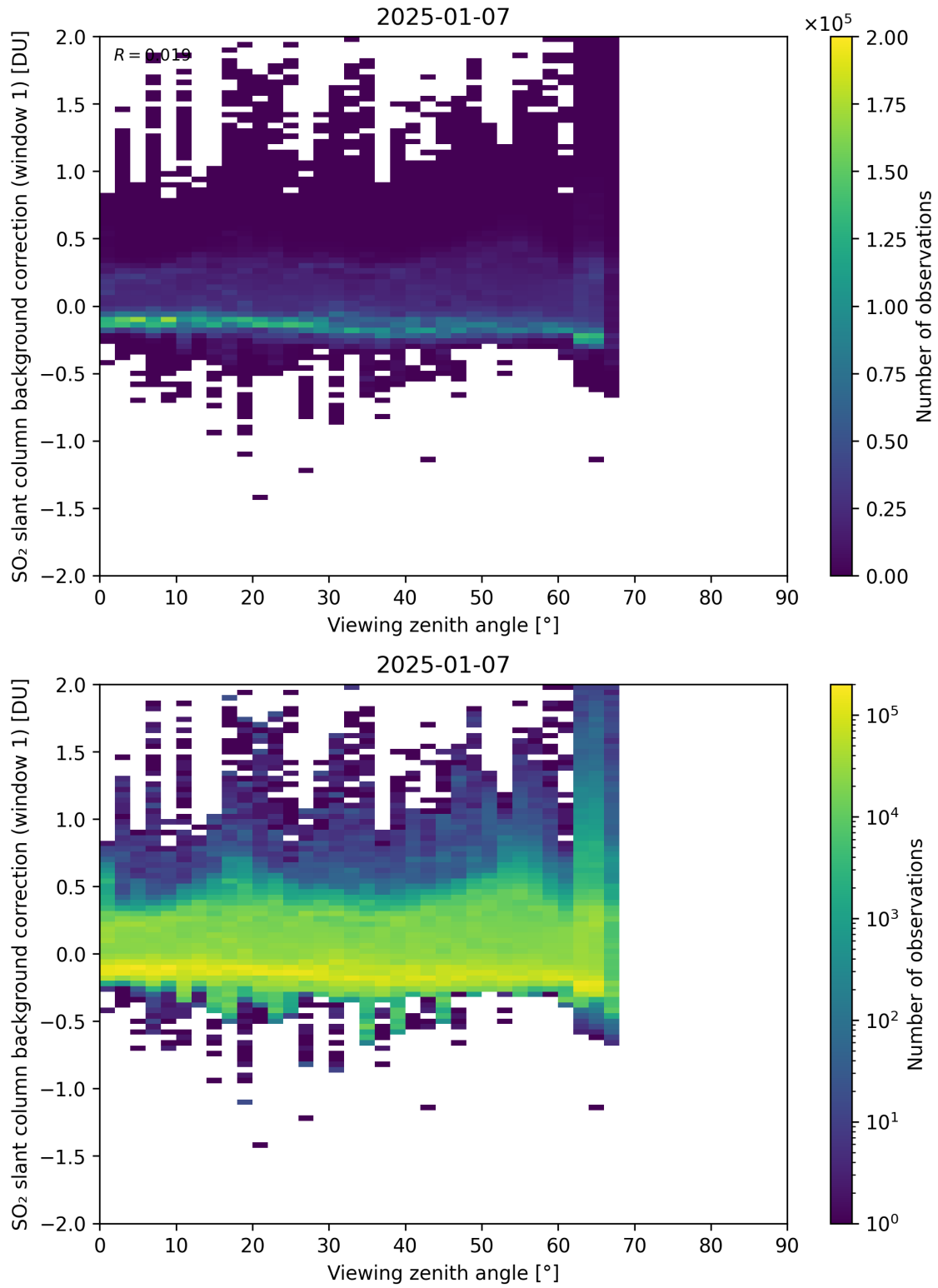
Figure 362: Scatter density plot of “Viewing zenith angle” against “SO 2 slant column background correction (window 1)” for 2025-01-07 to 2025-01-08.
