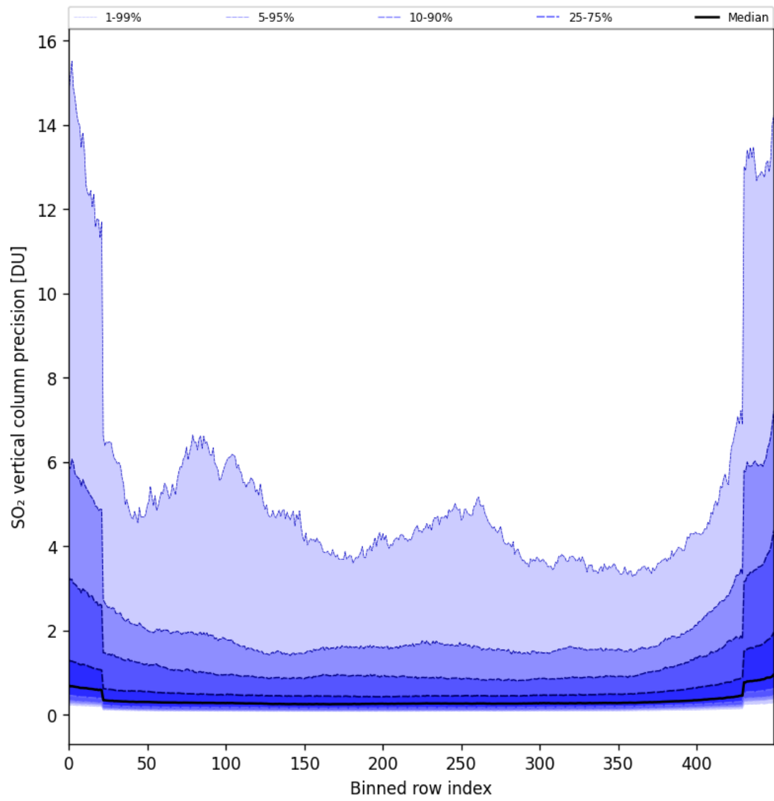
Figure 85: Along track statistics of “SO 2 vertical column precision” for 2025-01-07 to 2025-01-08
