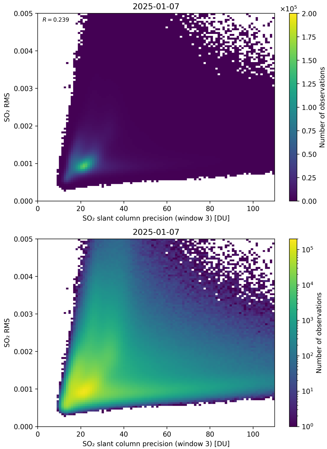
Figure 310: Scatter density plot of “SO 2 slant column precision (window 3)” against “SO 2 RMS” for 2025-01-07 to 2025-01-08.
