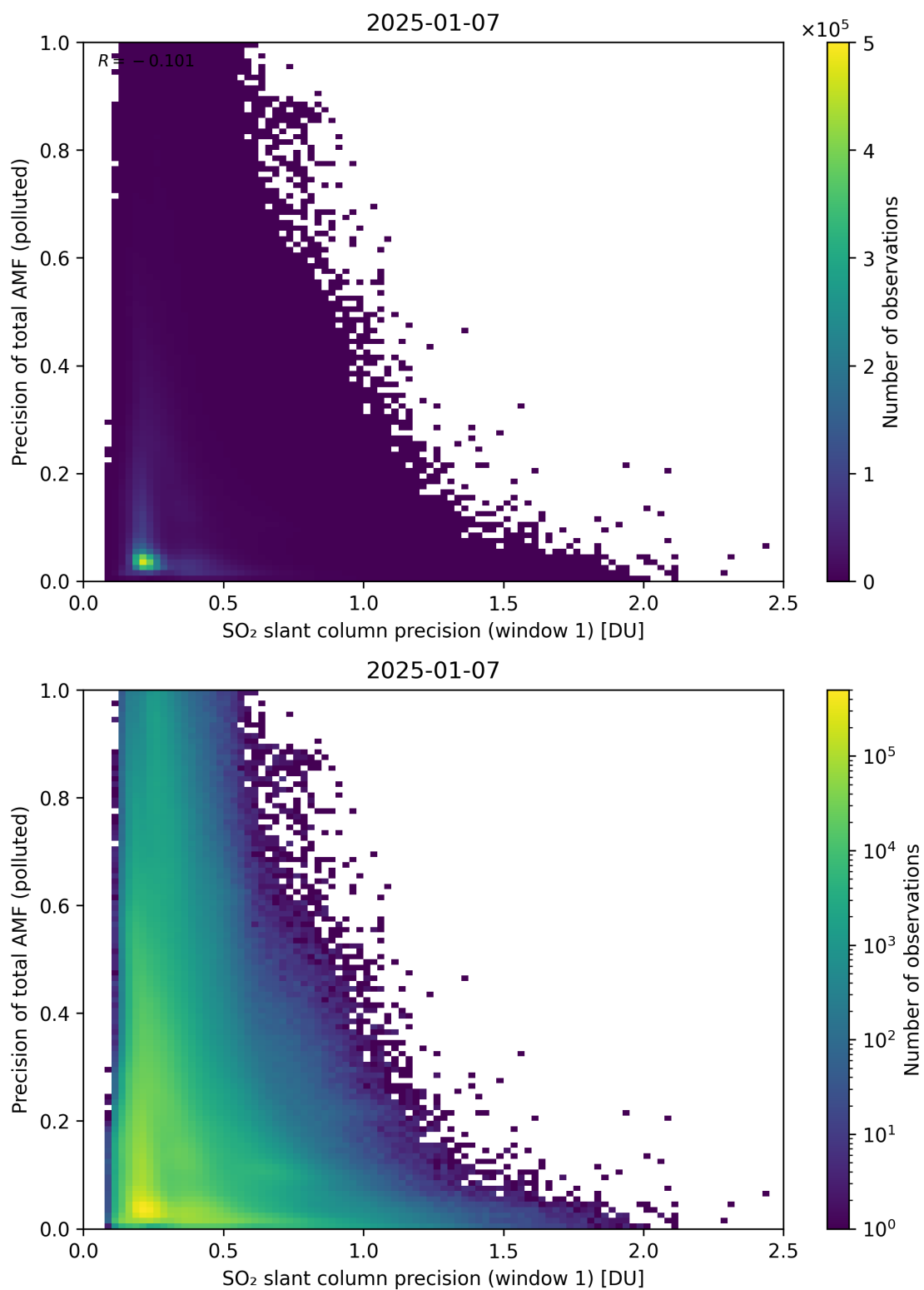
Figure 281: Scatter density plot of “SO 2 slant column precision (window 1)” against “Precision of total AMF (polluted)” for 2025-01-07 to 2025-01-08.
