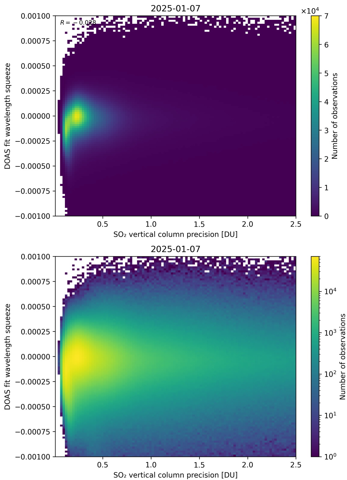
Figure 333: Scatter density plot of “SO 2 vertical column precision” against “DOAS fit wavelength squeeze” for 2025-01-07 to 2025-01-08.
