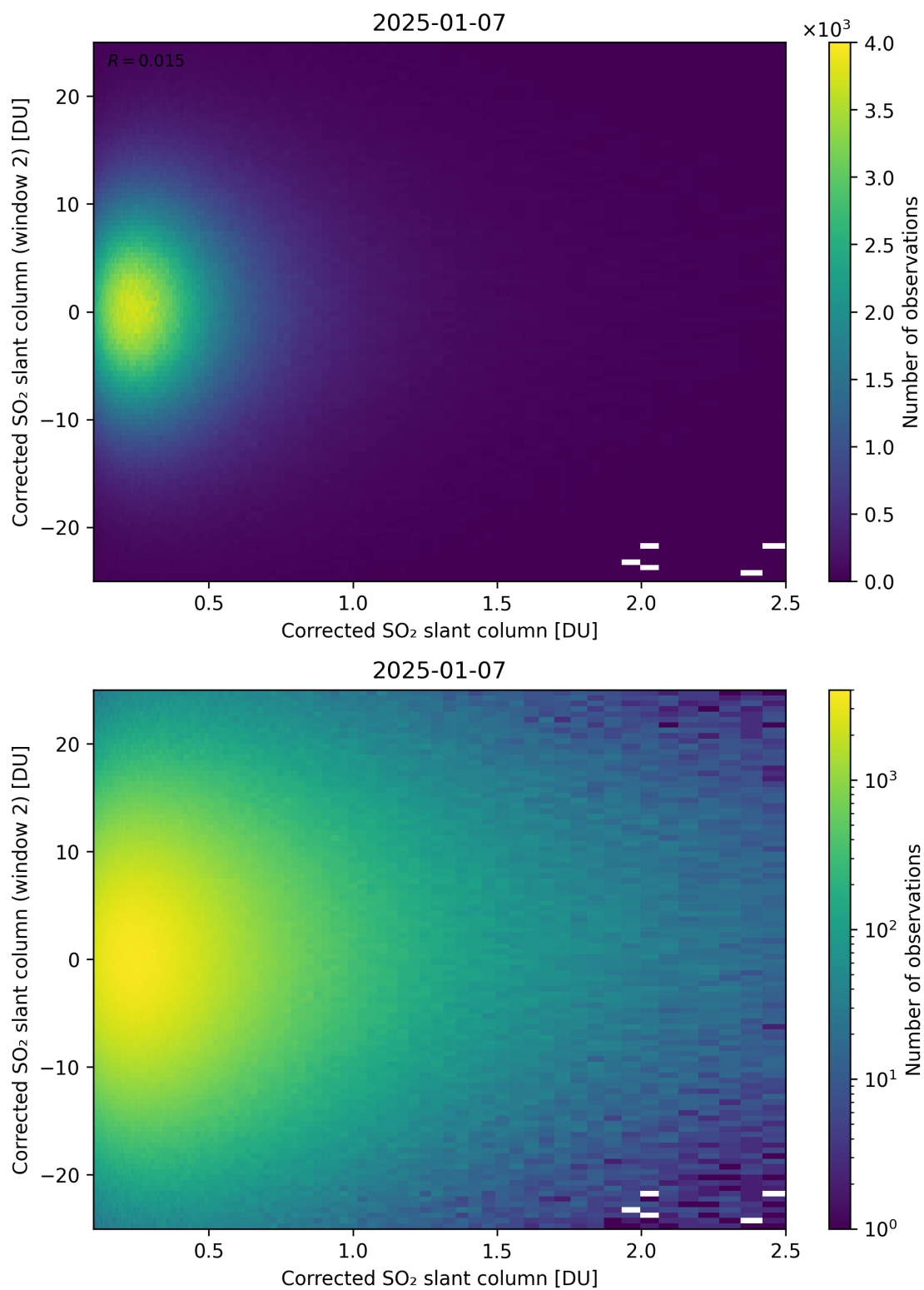
Figure 235: Scatter density plot of “Corrected SO 2 slant column” against “Corrected SO 2 slant column (window 2)” for 2025-01-07 to 2025-01-08.
