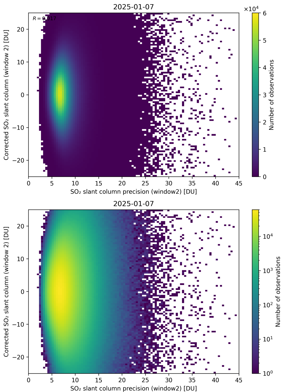
Figure 297: Scatter density plot of “SO 2 slant column precision (window2)” against “Corrected SO 2 slant column (window 2)” for 2025-01-07 to 2025-01-08.
