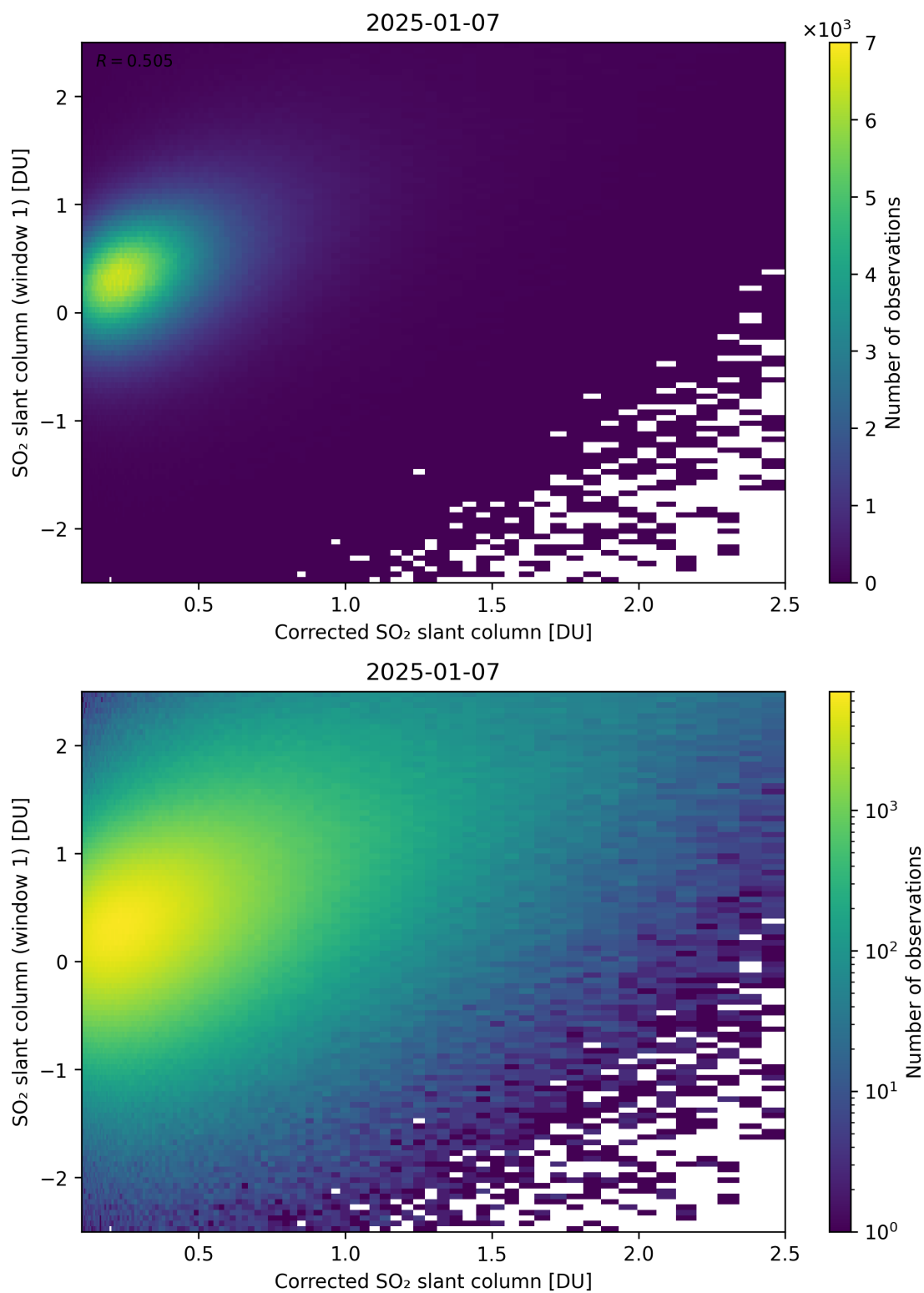
Figure 237: Scatter density plot of “Corrected SO 2 slant column” against “SO 2 slant column (window 1)” for 2025-01-07 to 2025-01-08.
