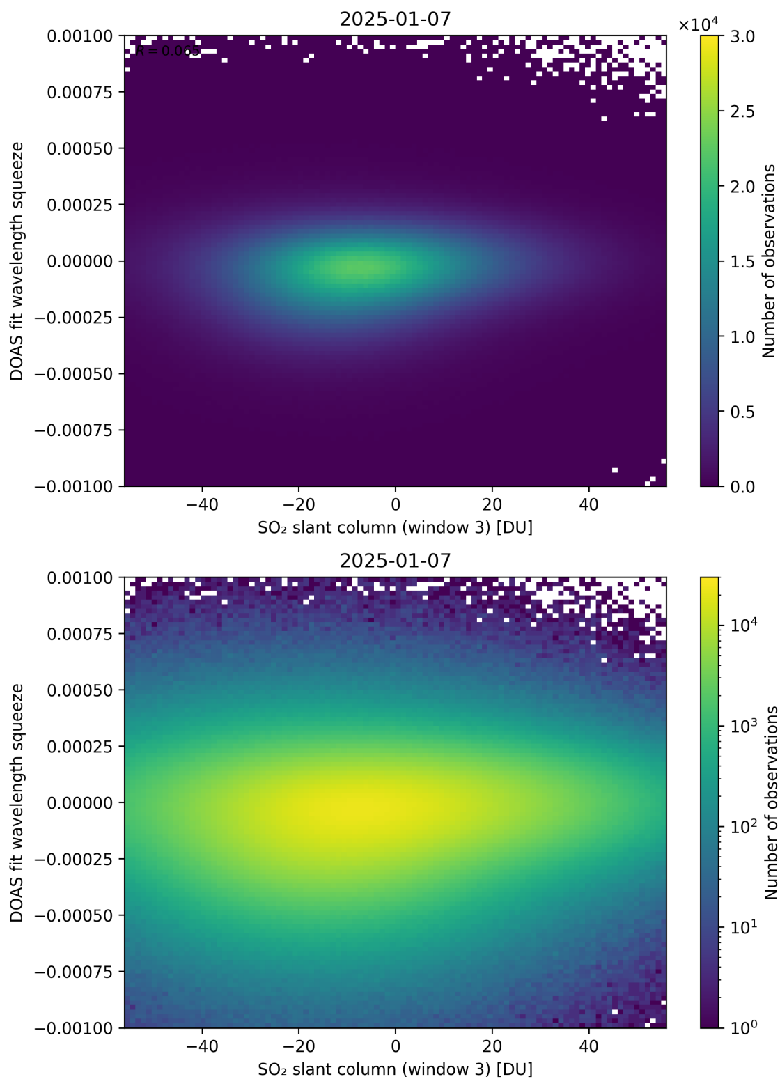
Figure 305: Scatter density plot of “SO 2 slant column (window 3)” against “DOAS fit wavelength squeeze” for 2025-01-07 to 2025-01-08.
