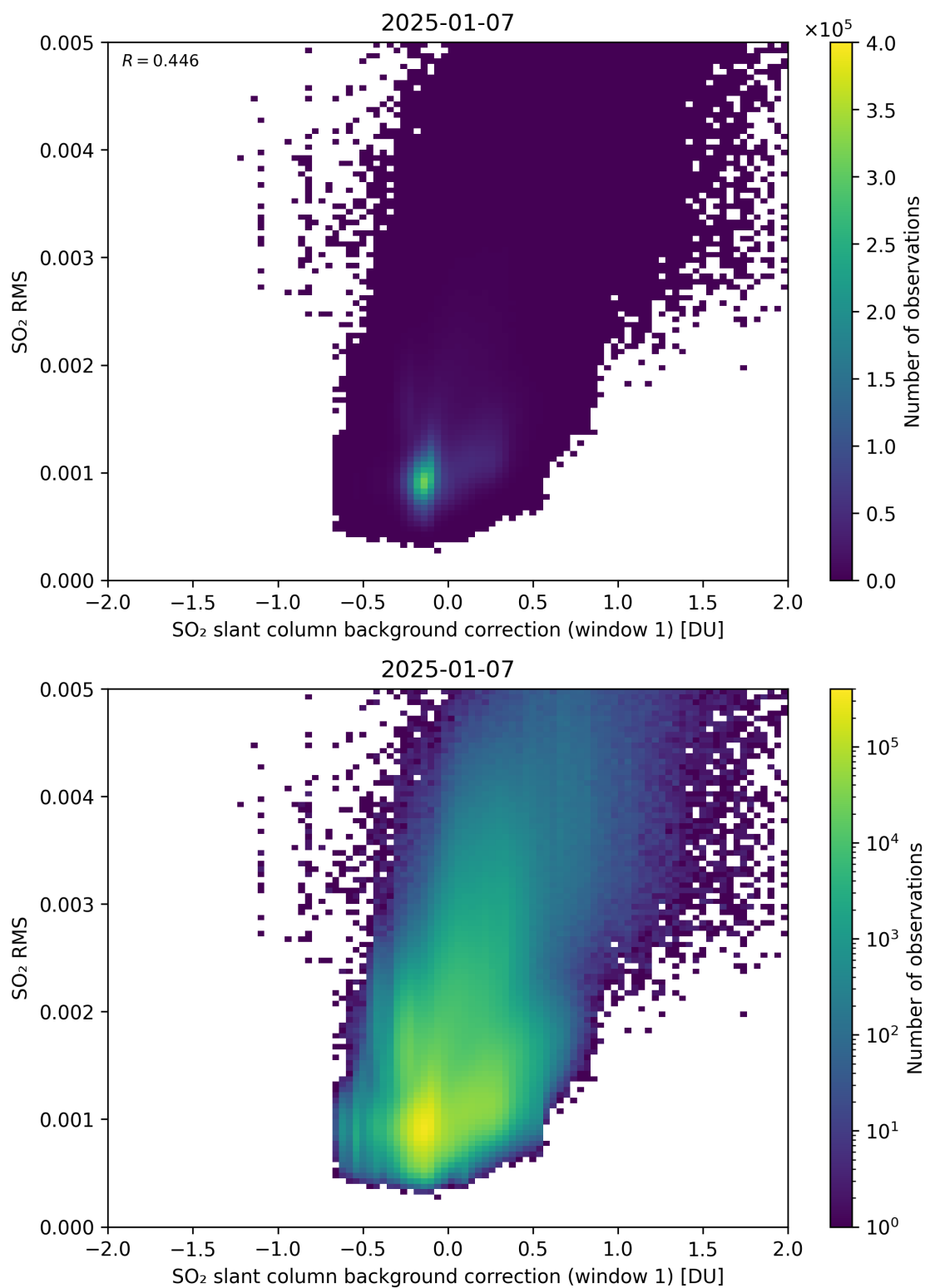
Figure 113: Scatter density plot of “SO 2 slant column background correction (window 1)” against “SO 2 RMS” for 2025-01-07 to 2025-01-08.
