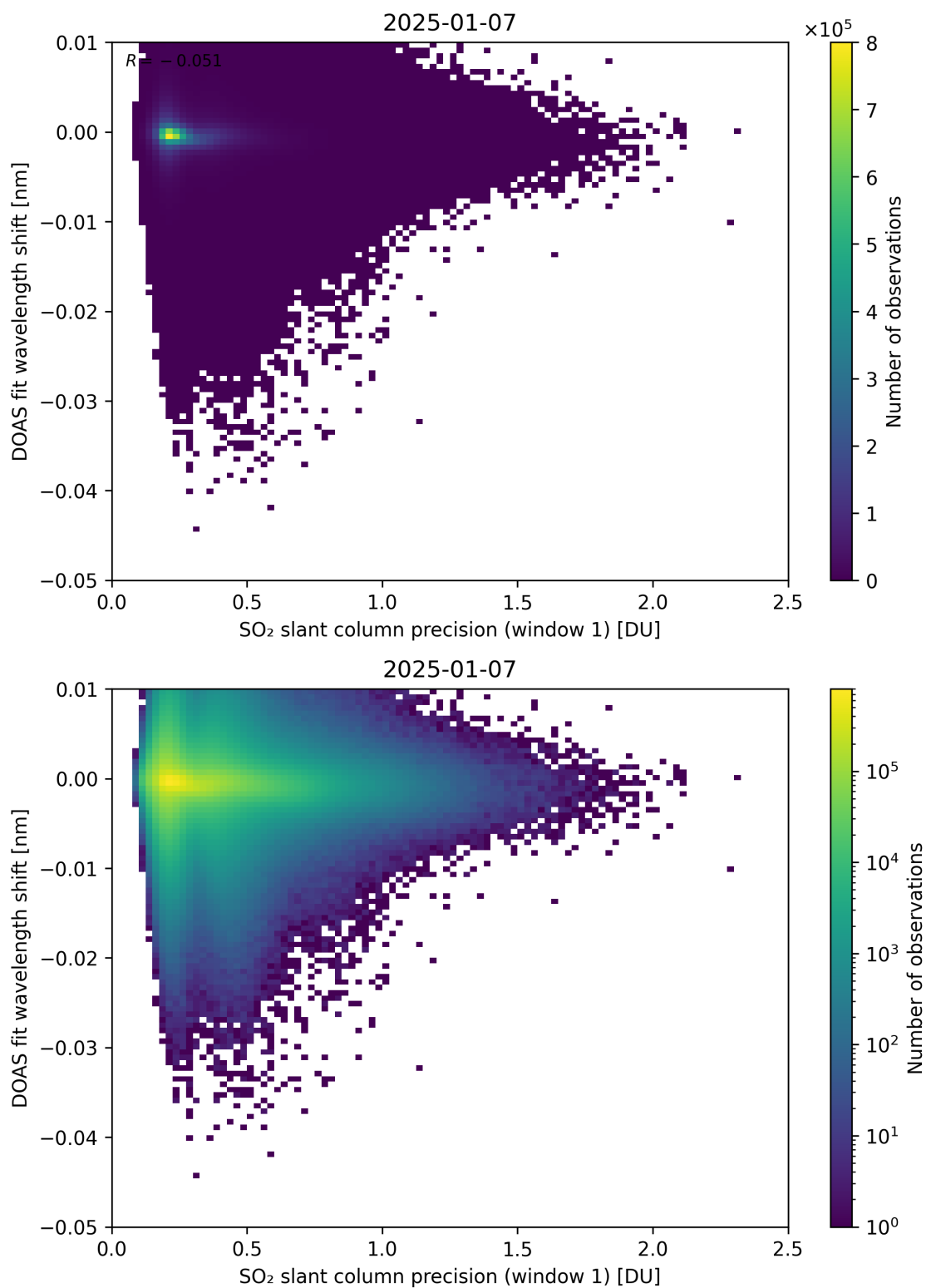
Figure 271: Scatter density plot of “SO 2 slant column precision (window 1)” against “DOAS fit wavelength shift” for 2025-01-07 to 2025-01-08.
