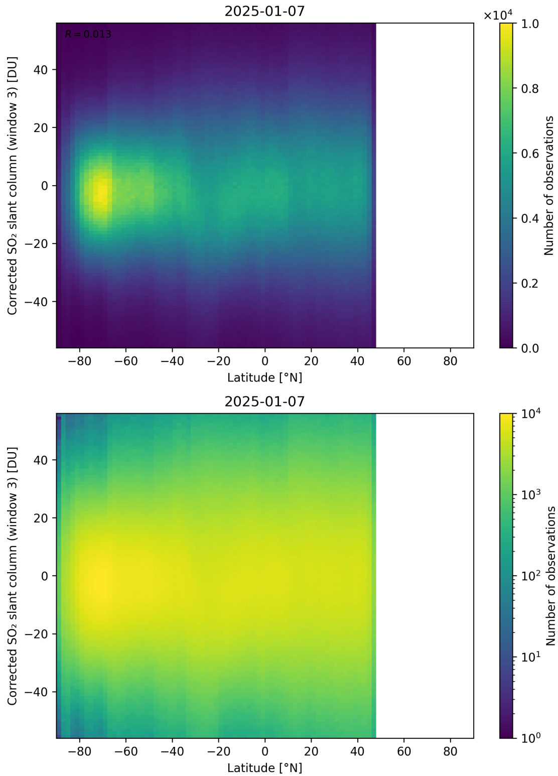
Figure 161: Scatter density plot of “Latitude” against “Corrected SO 2 slant column (window 3)” for 2025-01-07 to 2025-01-08.
