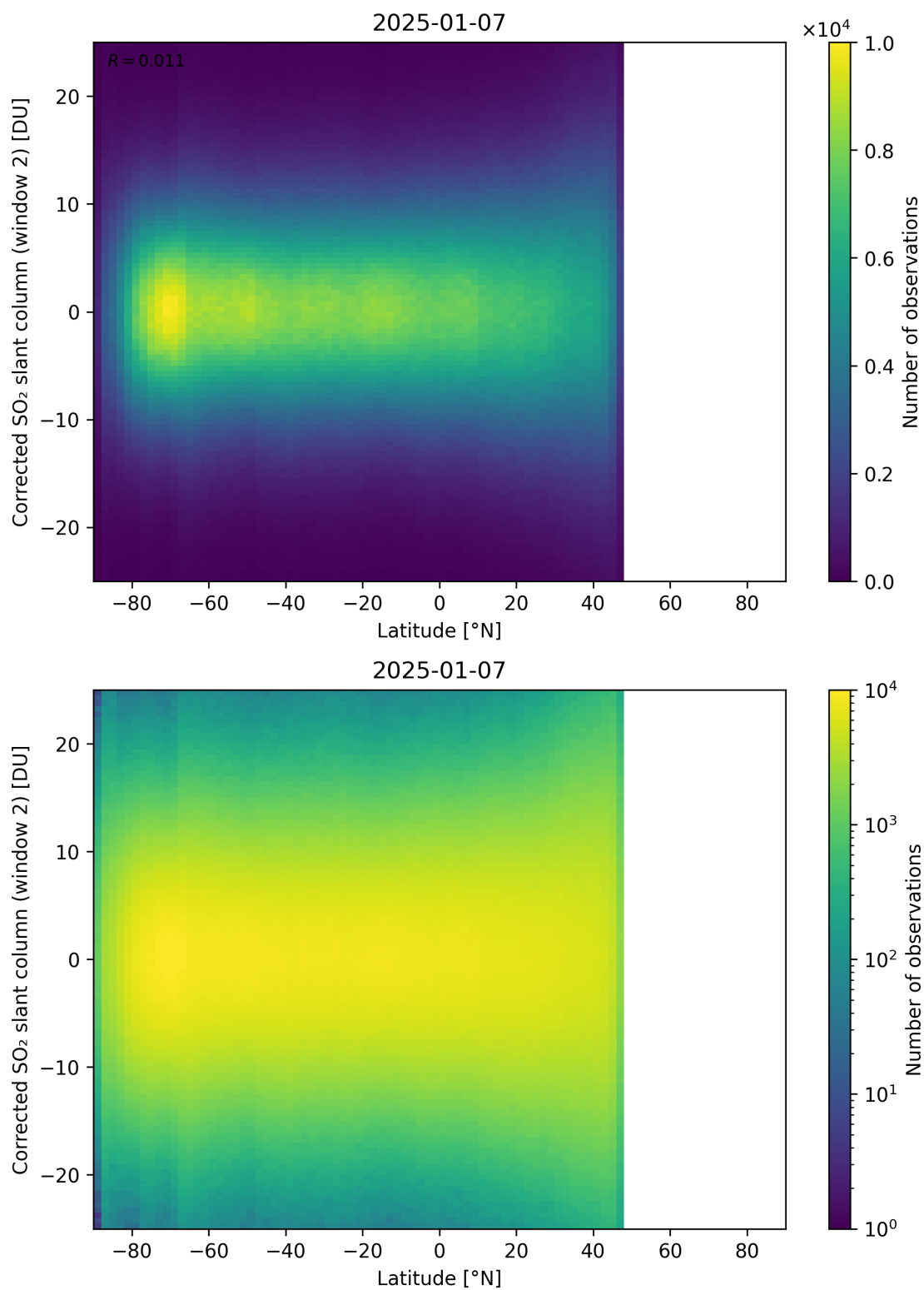
Figure 160: Scatter density plot of “Latitude” against “Corrected SO 2 slant column (window 2)” for 2025-01-07 to 2025-01-08.
