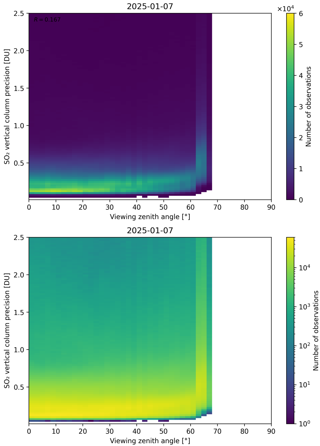
Figure 384: Scatter density plot of “Viewing zenith angle” against “SO 2 vertical column precision” for 2025-01-07 to 2025-01-08.
