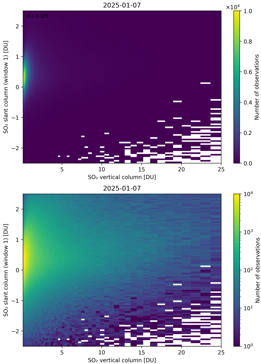
Figure 354: Scatter density plot of “SO 2 vertical column” against “SO 2 slant column (window 1)” for 2025-01-07 to 2025-01-08.
