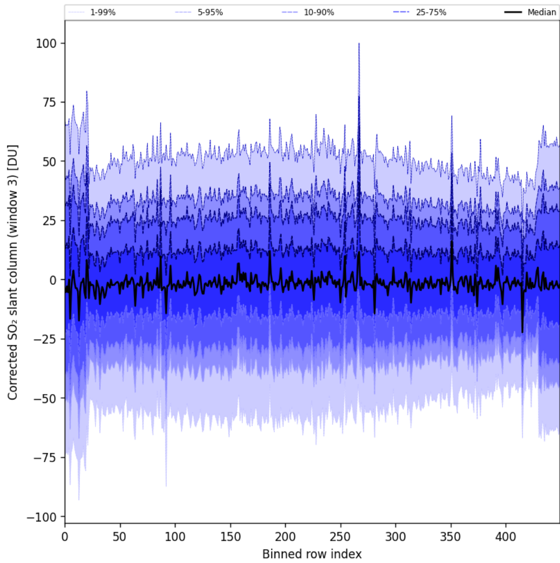
Figure 99: Along track statistics of “Corrected SO 2 slant column (window 3)” for 2025-01-07 to 2025-01-08
