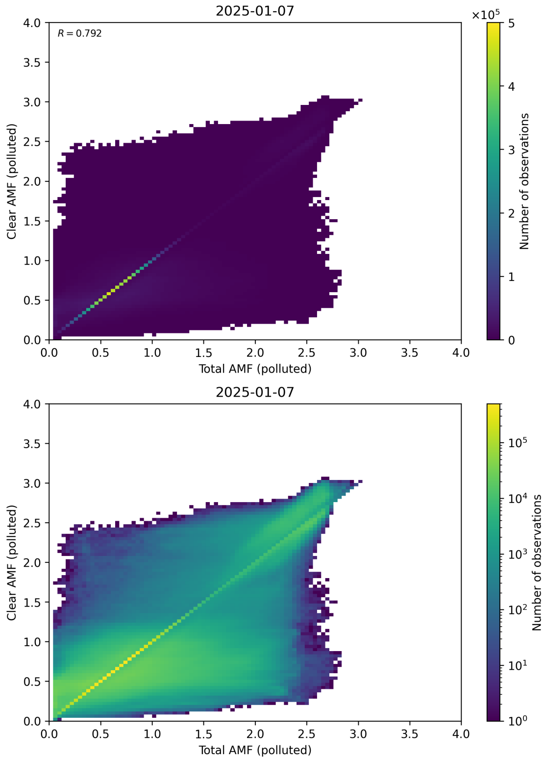
Figure 321: Scatter density plot of “Total AMF (polluted)” against “Clear AMF (polluted)” for 2025-01-07 to 2025-01-08.
