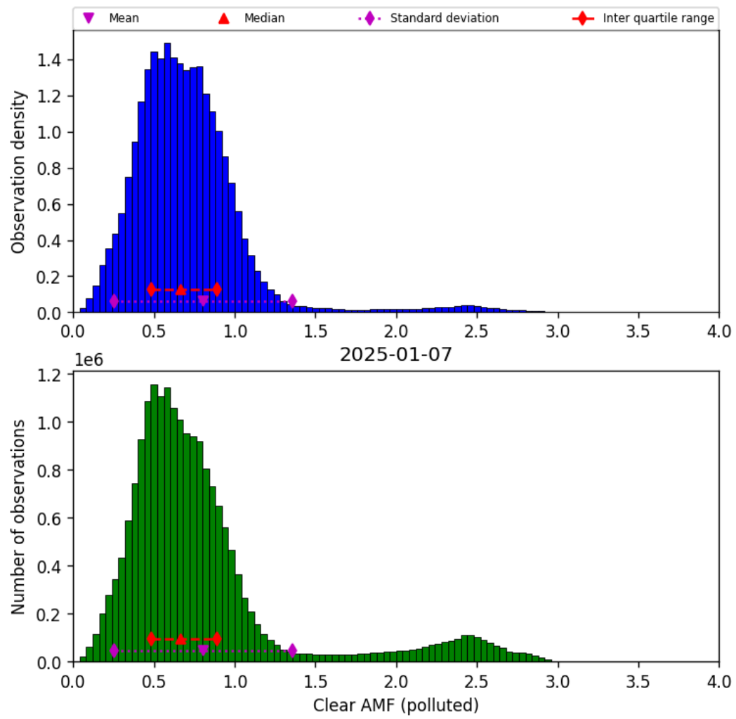
Figure 81: Histogram of “Clear AMF (polluted)” for 2025-01-07 to 2025-01-08
