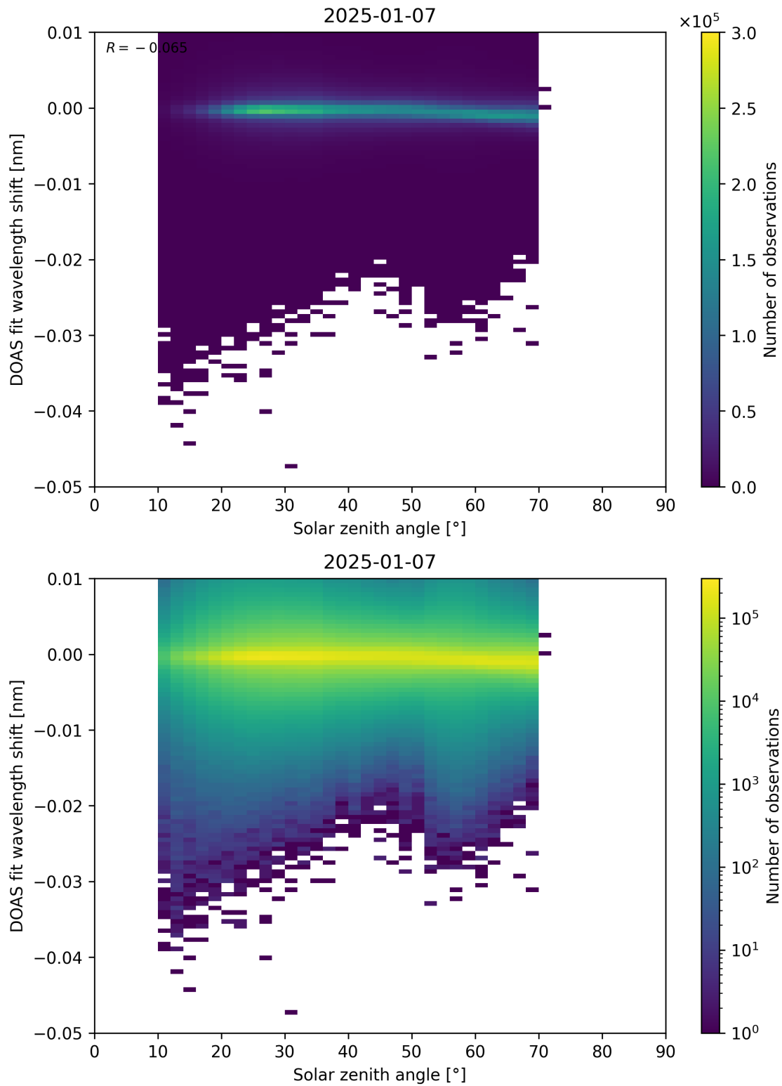
Figure 174: Scatter density plot of “Solar zenith angle” against “DOAS fit wavelength shift” for 2025-01-07 to 2025-01-08.
