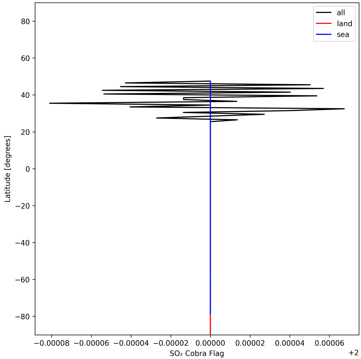
Figure 49: Zonal average of "SO 2 Cobra Flag" for 2025-01-07 to 2025-01-08.
