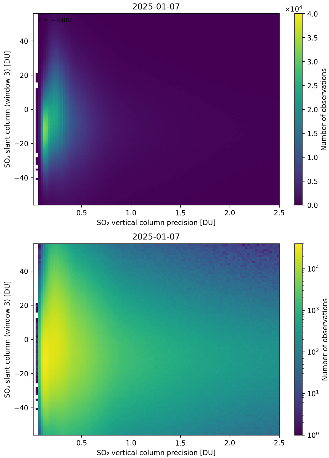
Figure 344: Scatter density plot of “SO 2 vertical column precision” against “SO 2 slant column (window 3)” for 2025-01-07 to 2025-01-08.
