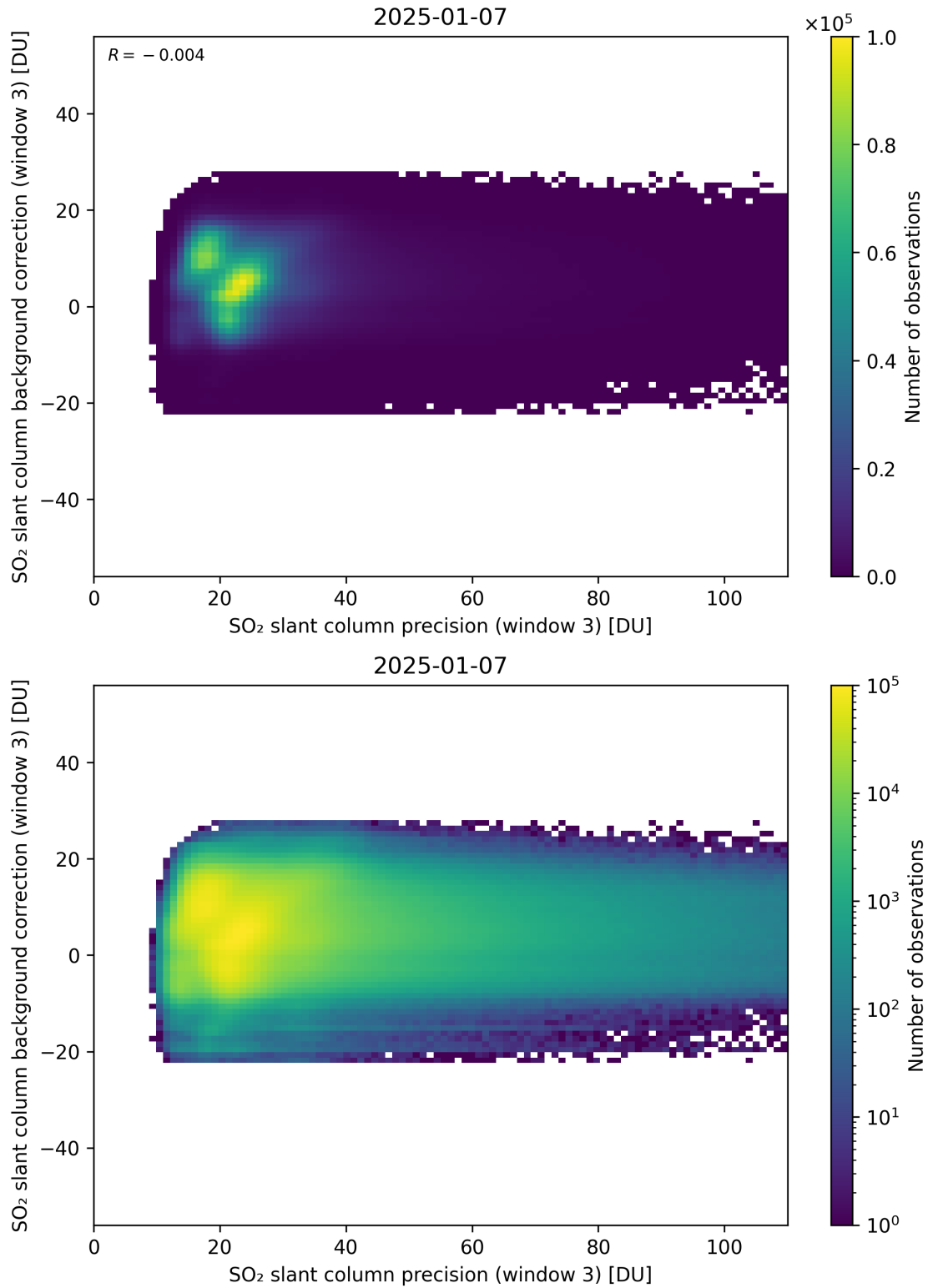
Figure 307: Scatter density plot of “SO 2 slant column precision (window 3)” against “SO 2 slant column background correction (window 3)” for 2025-01-07 to 2025-01-08.
