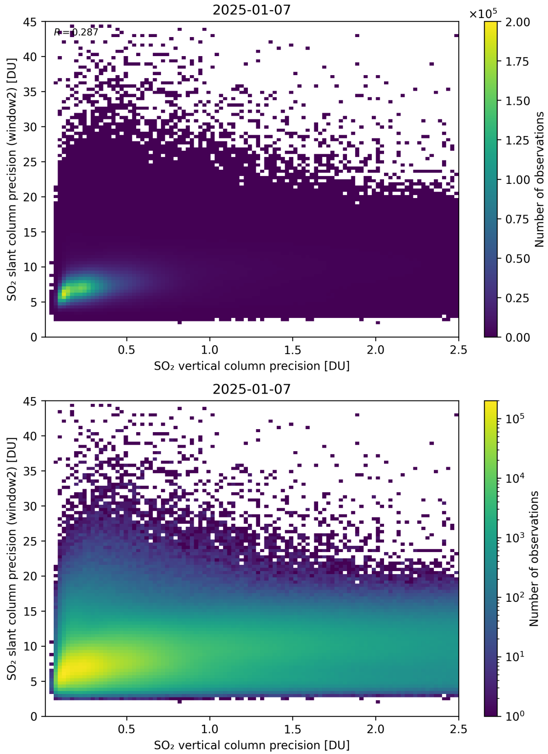
Figure 343: Scatter density plot of “SO 2 vertical column precision” against “SO 2 slant column precision (window2)” for 2025-01-07 to 2025-01-08.
