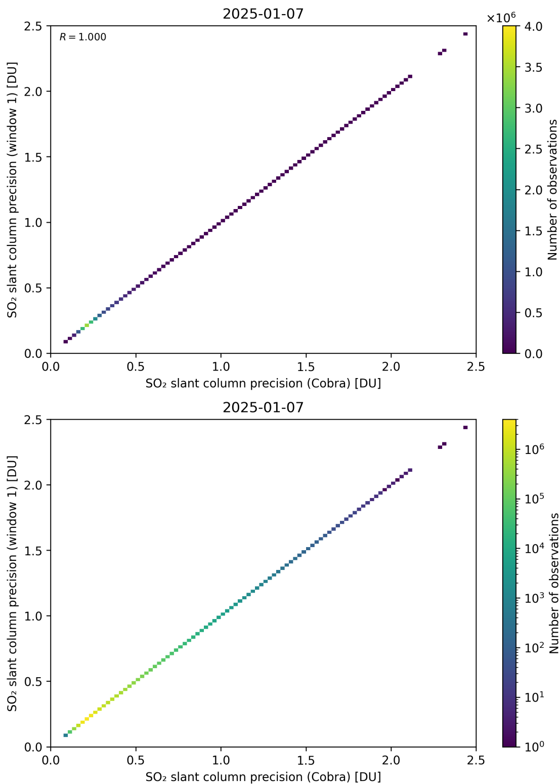
Figure 209: Scatter density plot of “SO 2 slant column precision (Cobra)” against “SO 2 slant column precision (window 1)” for 2025-01-07 to 2025-01-08.
