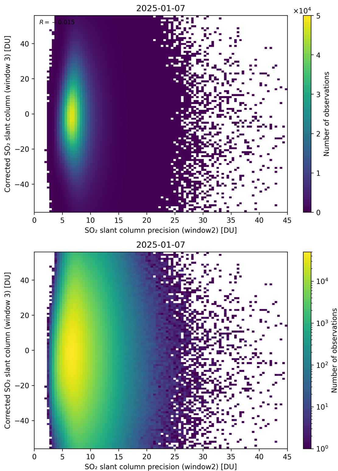
Figure 298: Scatter density plot of “SO 2 slant column precision (window2)” against “Corrected SO 2 slant column (window 3)” for 2025-01-07 to 2025-01-08.
