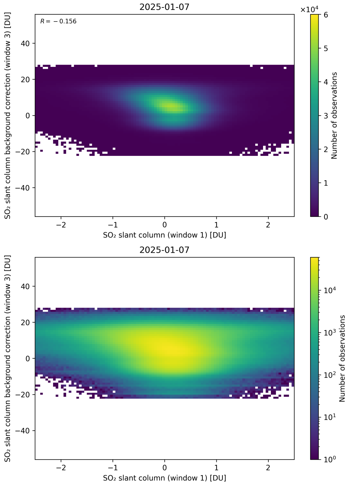
Figure 264: Scatter density plot of “SO 2 slant column (window 1)” against “SO 2 slant column background correction (window 3)” for 2025-01-07 to 2025-01-08.
