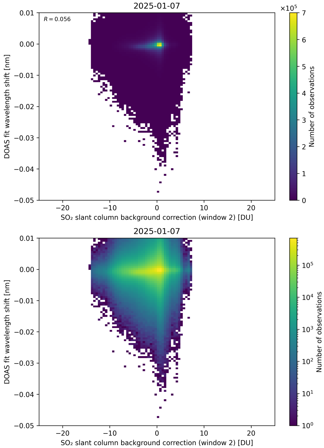
Figure 123: Scatter density plot of “SO 2 slant column background correction (window 2)” against “DOAS fit wavelength shift” for 2025-01-07 to 2025-01-08.
