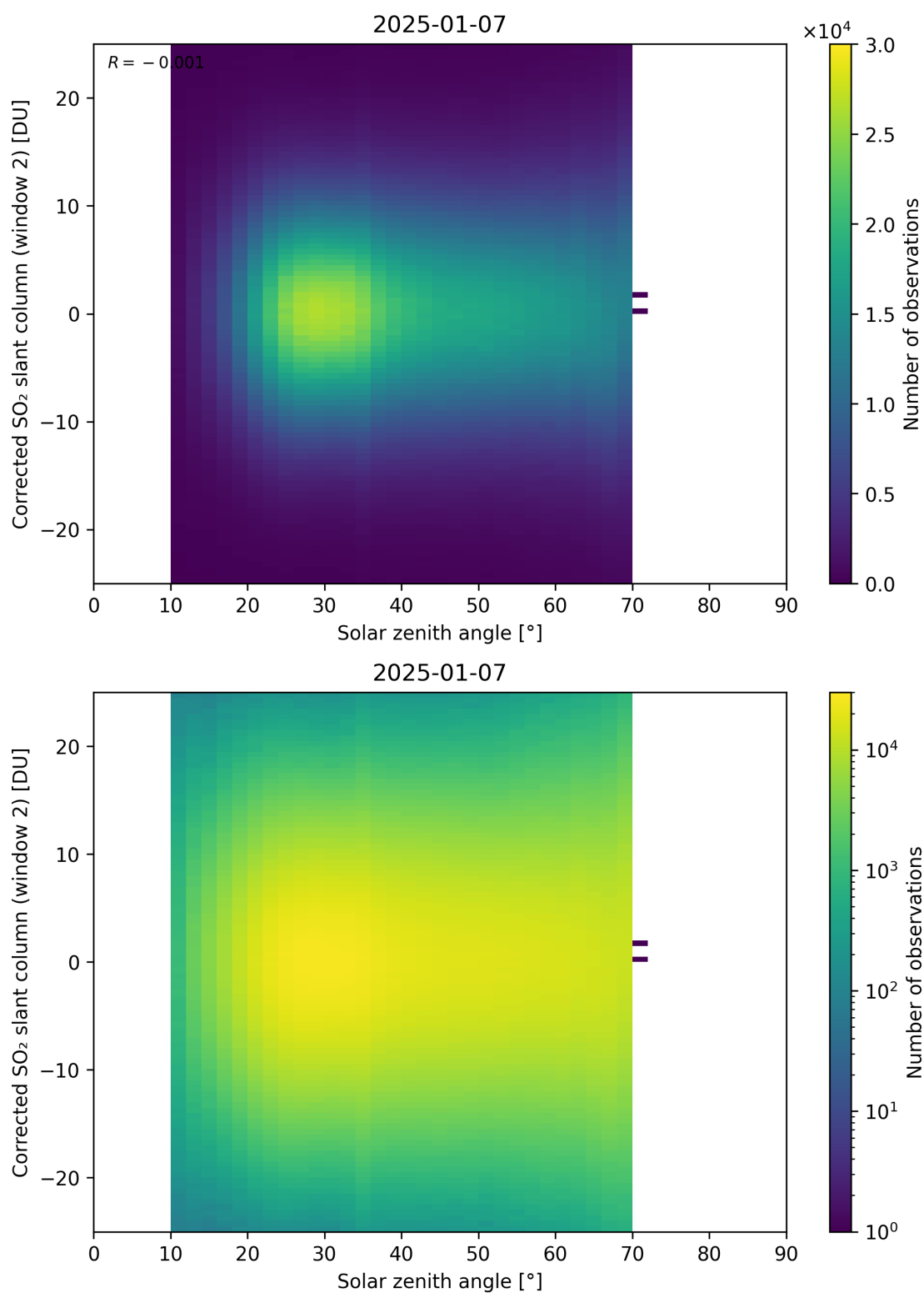
Figure 182: Scatter density plot of “Solar zenith angle” against “Corrected SO 2 slant column (window 2)” for 2025-01-07 to 2025-01-08.
