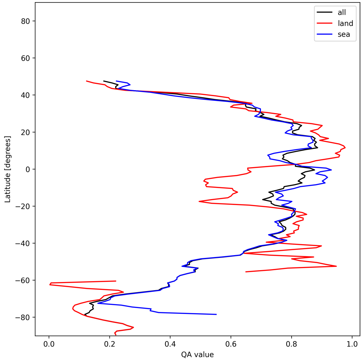
Figure 31: Zonal average of “QA value” for 2025-01-07 to 2025-01-08.
