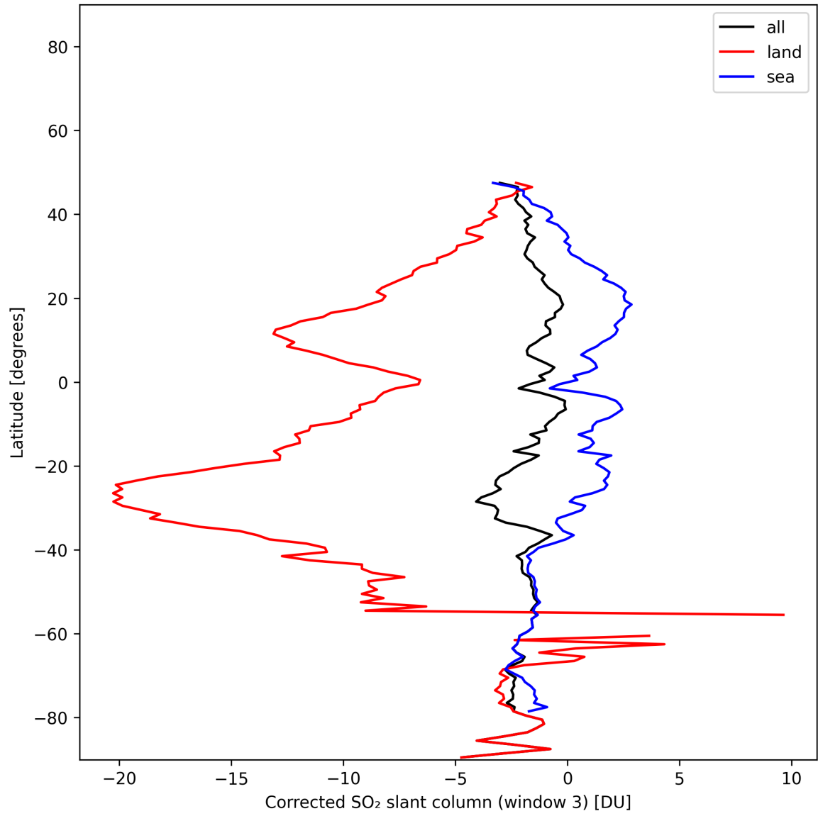
Figure 47: Zonal average of “Corrected SO 2 slant column (window 3)” for 2025-01-07 to 2025-01-08.
