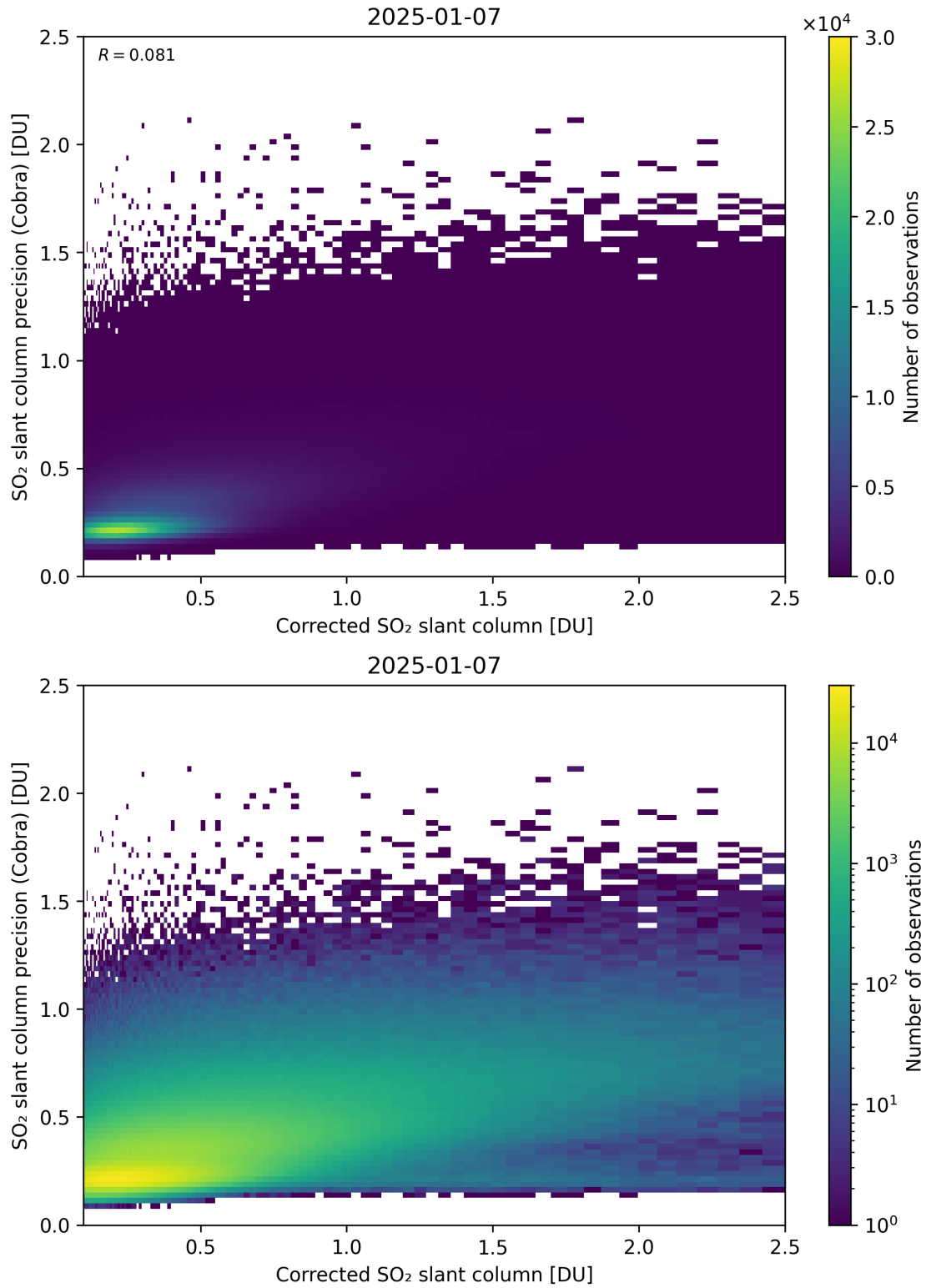
Figure 234: Scatter density plot of “Corrected SO 2 slant column” against “SO 2 slant column precision (Cobra)” for 2025-01-07 to 2025-01-08.
