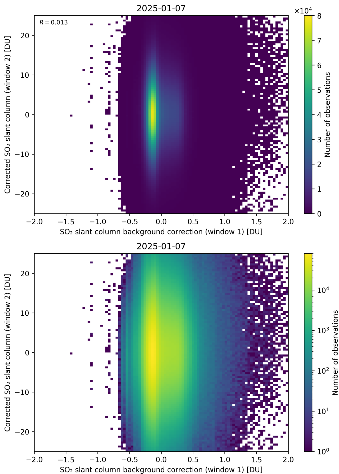
Figure 115: Scatter density plot of “SO 2 slant column background correction (window 1)” against “Corrected SO 2 slant column (window 2)” for 2025-01-07 to 2025-01-08.
