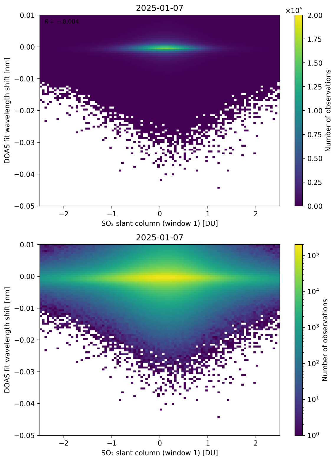
Figure 265: Scatter density plot of “SO 2 slant column (window 1)” against “DOAS fit wavelength shift” for 2025-01-07 to 2025-01-08.
