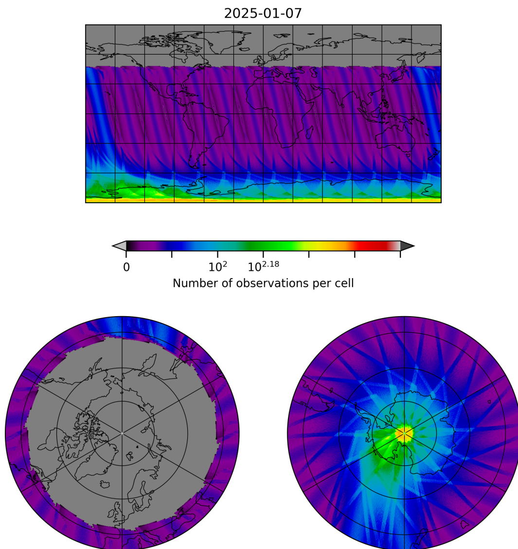
Figure 30: Map of the number of observations for 2025-01-07 to 2025-01-08
