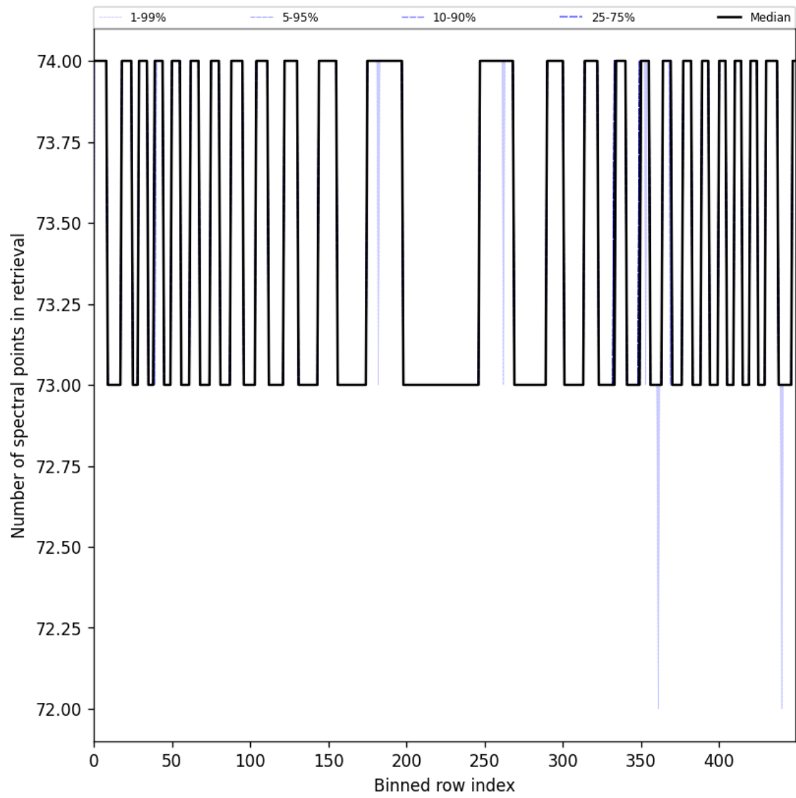
Figure 108: Along track statistics of “Number of spectral points in retrieval” for 2025-01-07 to 2025-01-08
