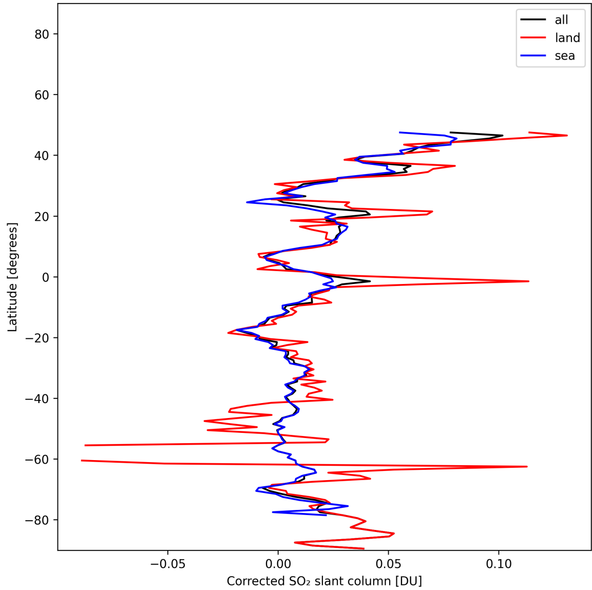
Figure 34: Zonal average of “Corrected SO 2 slant column” for 2025-01-07 to 2025-01-08.
