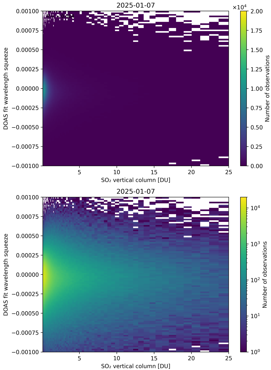
Figure 327: Scatter density plot of “SO 2 vertical column” against “DOAS fit wavelength squeeze” for 2025-01-07 to 2025-01-08.
