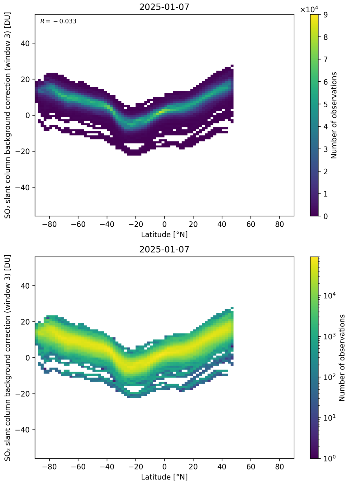
Figure 152: Scatter density plot of “Latitude” against “SO 2 slant column background correction (window 3)” for 2025-01-07 to 2025-01-08.
