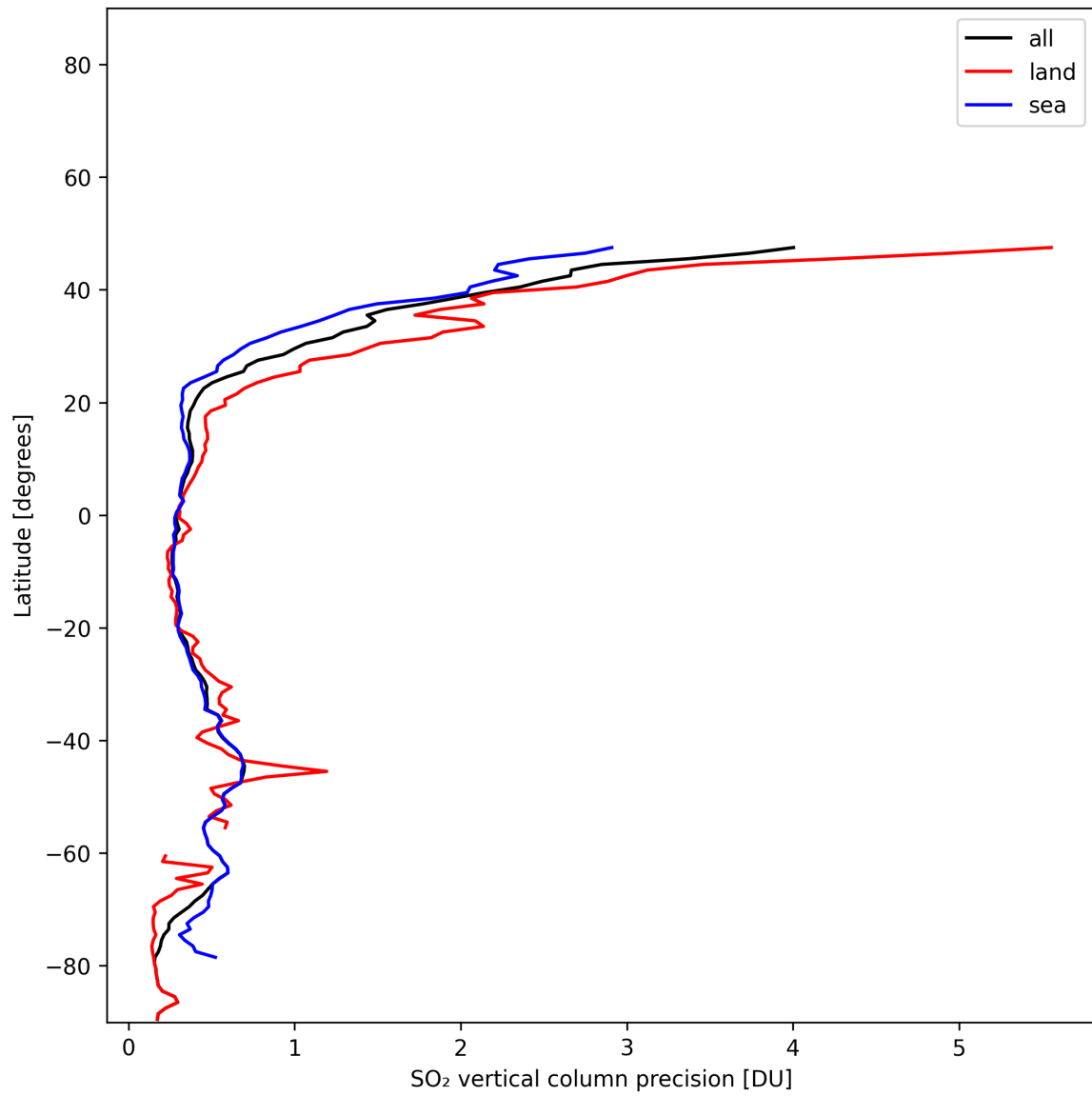
Figure 33: Zonal average of “SO 2 vertical column precision” for 2025-01-07 to 2025-01-08.
