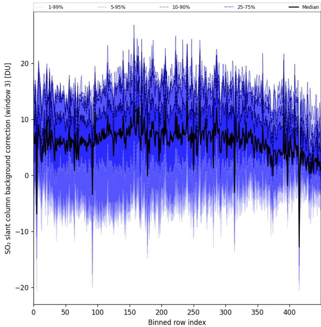
Figure 100: Along track statistics of “SO 2 slant column background correction (window 3)” for 2025-01-07 to 2025-01-08
