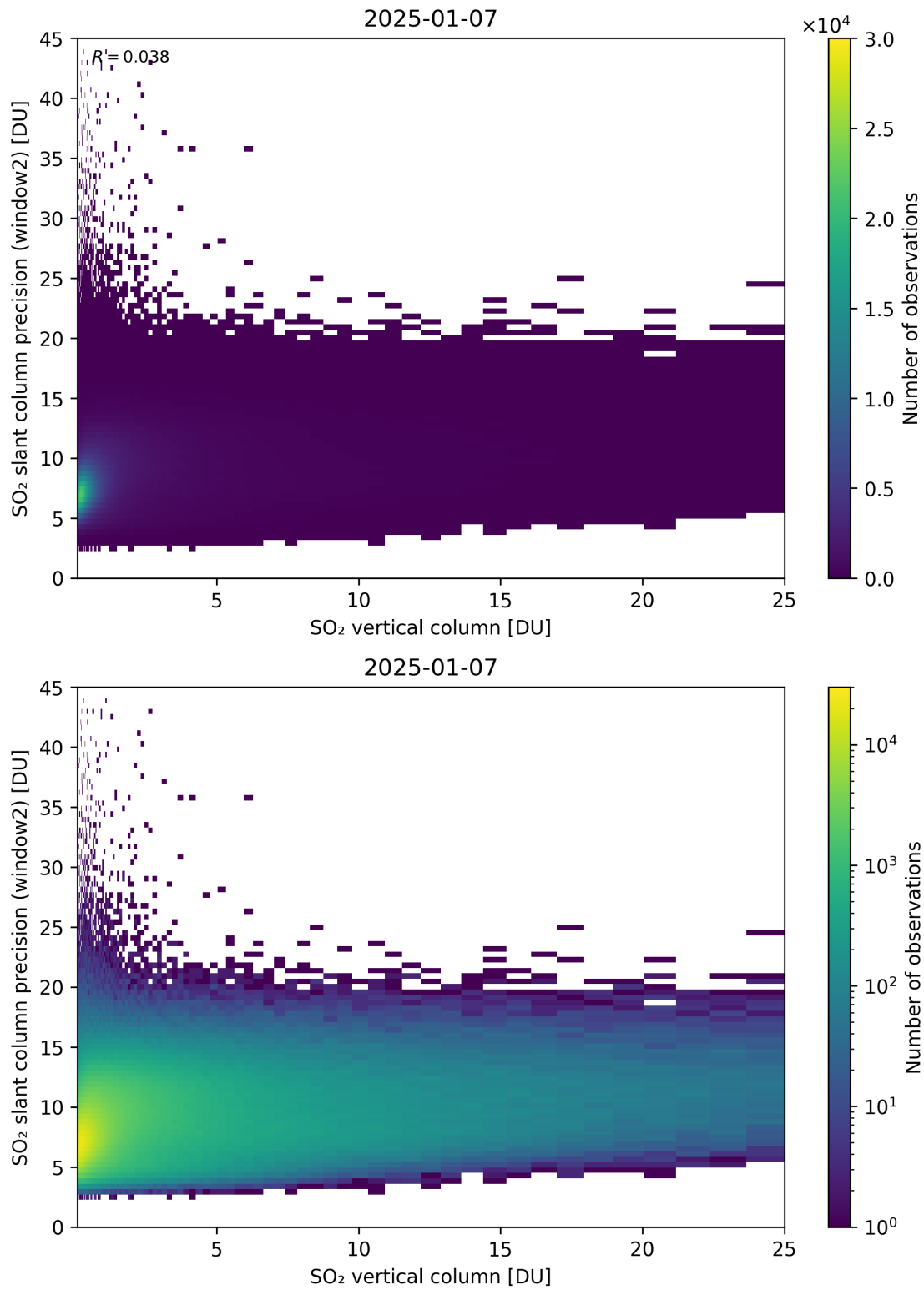
Figure 356: Scatter density plot of “SO 2 vertical column” against “SO 2 slant column precision (window2)” for 2025-01-07 to 2025-01-08.
