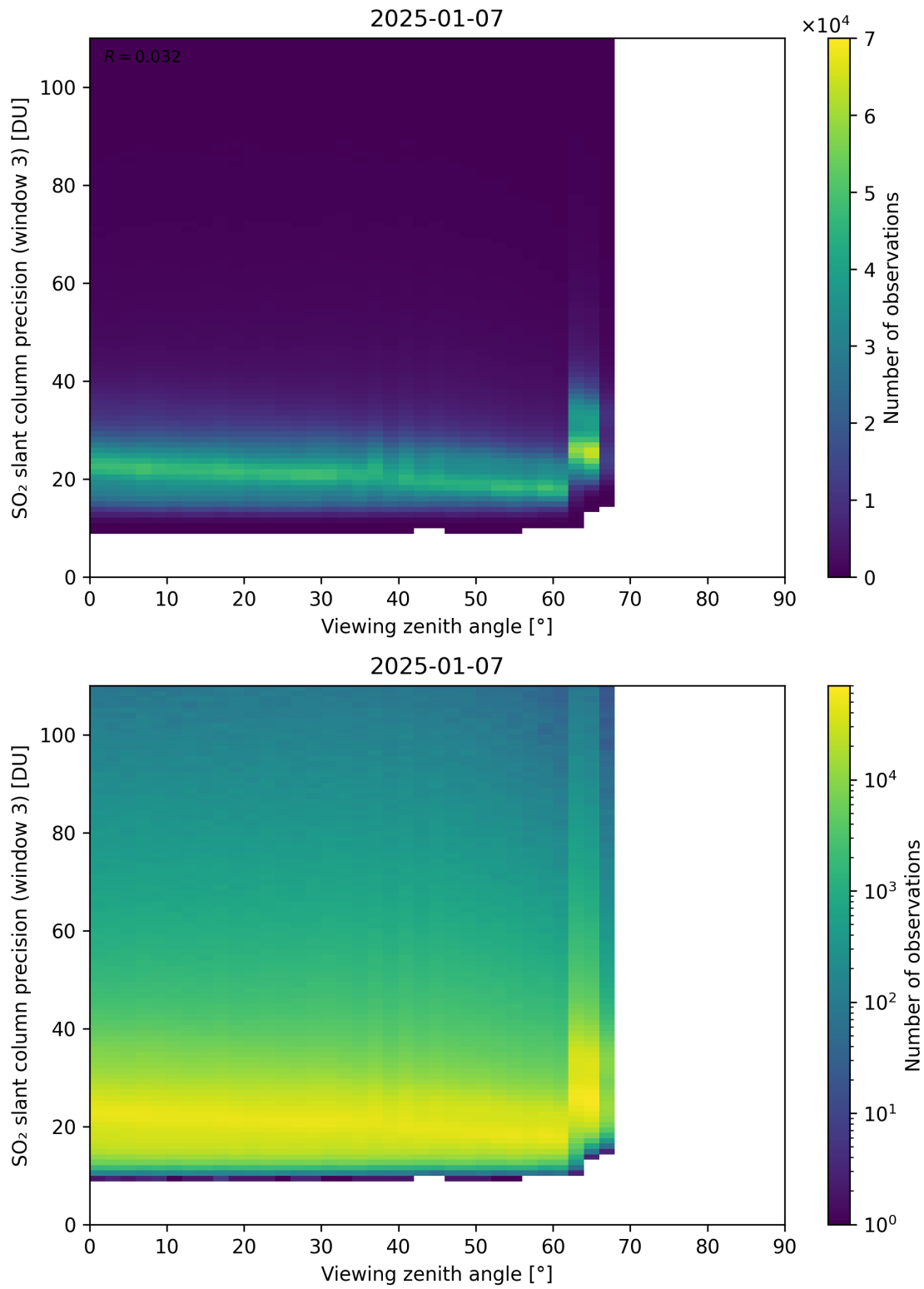
Figure 380: Scatter density plot of “Viewing zenith angle” against “SO 2 slant column precision (window 3)” for 2025-01-07 to 2025-01-08.
