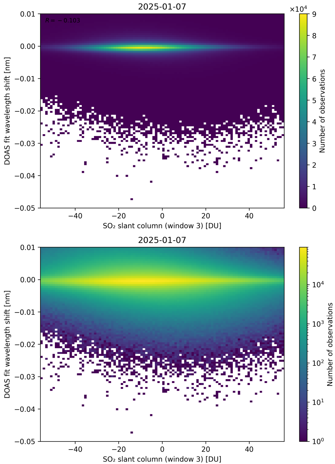
Figure 304: Scatter density plot of “SO 2 slant column (window 3)” against “DOAS fit wavelength shift” for 2025-01-07 to 2025-01-08.
