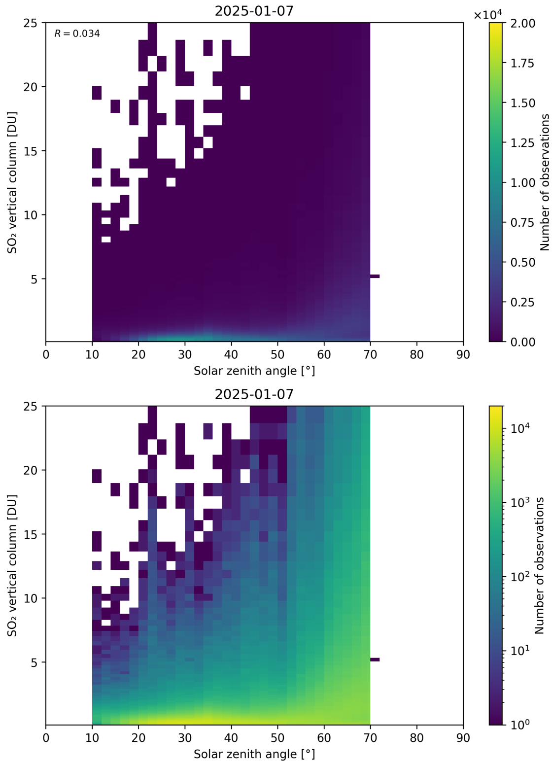
Figure 191: Scatter density plot of “Solar zenith angle” against “SO 2 vertical column” for 2025-01-07 to 2025-01-08.
