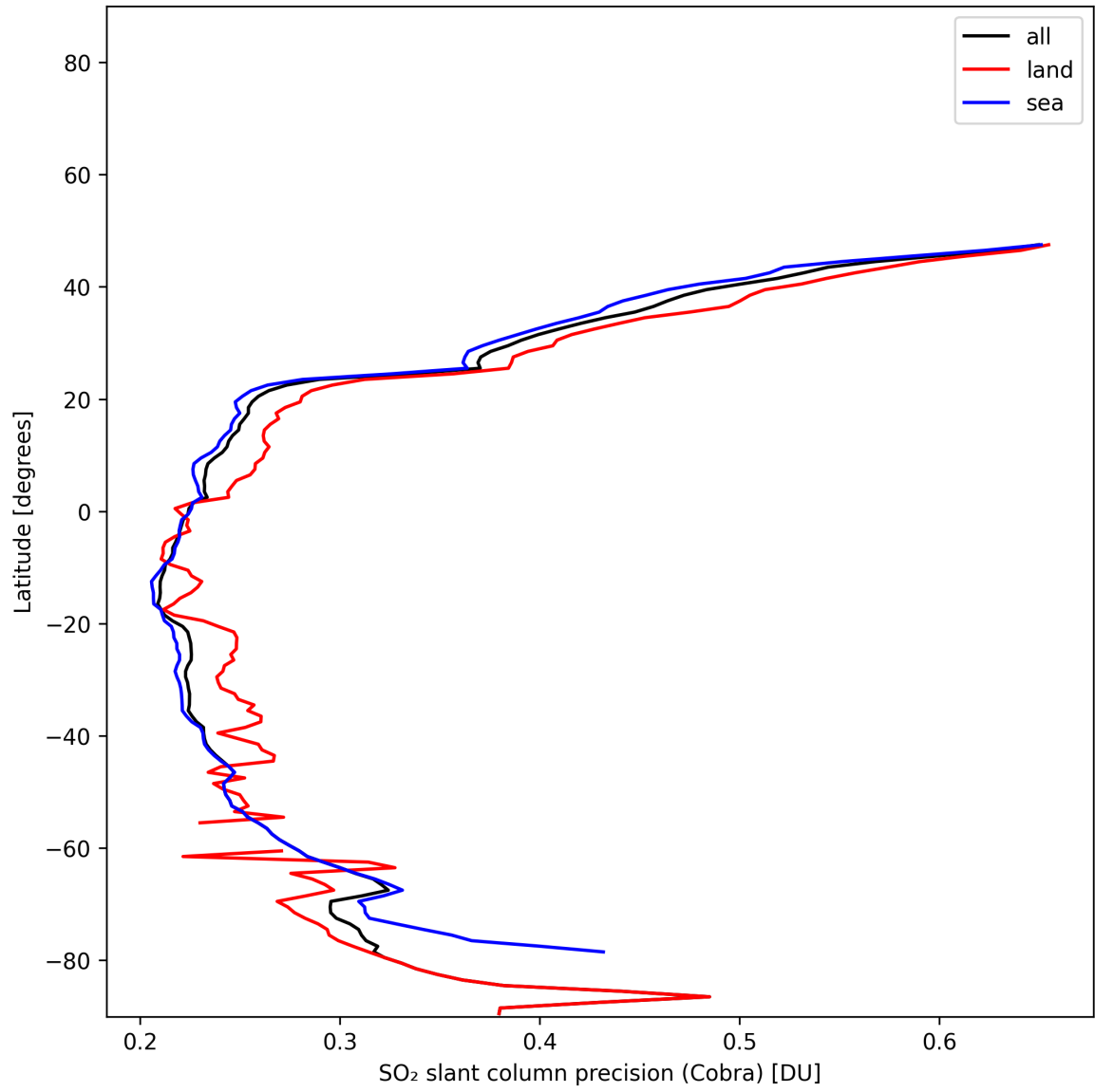
Figure 36: Zonal average of “SO 2 slant column precision (Cobra)” for 2025-01-07 to 2025-01-08.
