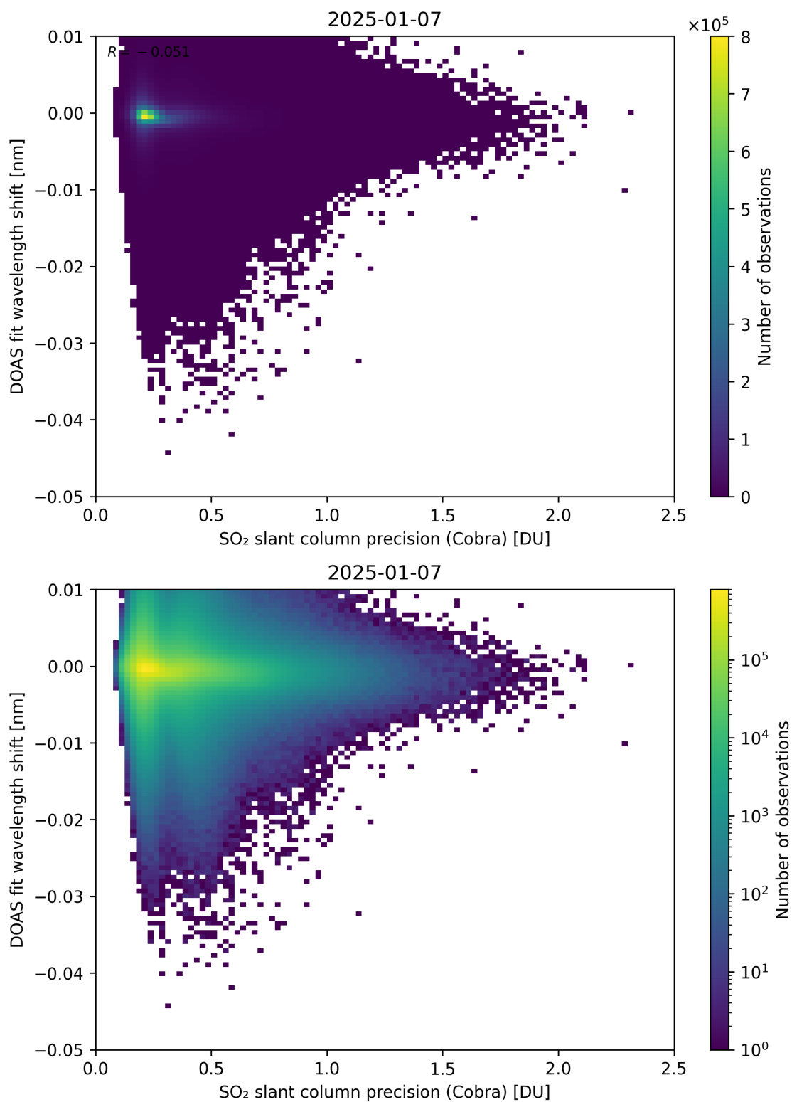
Figure 202: Scatter density plot of “SO 2 slant column precision (Cobra)” against “DOAS fit wavelength shift” for 2025-01-07 to 2025-01-08.
