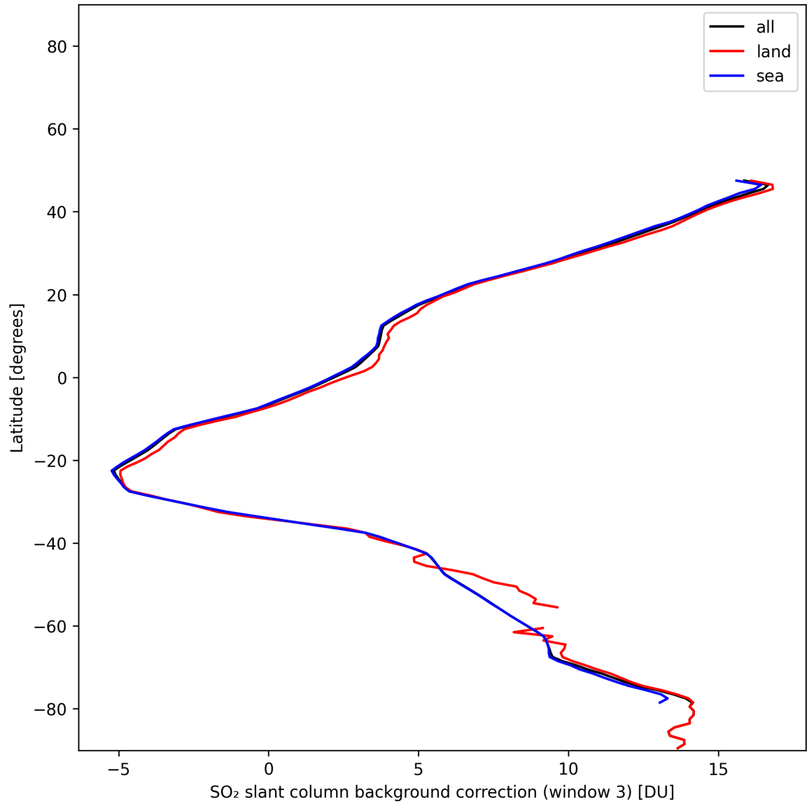
Figure 48: Zonal average of “SO 2 slant column background correction (window 3)” for 2025-01-07 to 2025-01-08.
