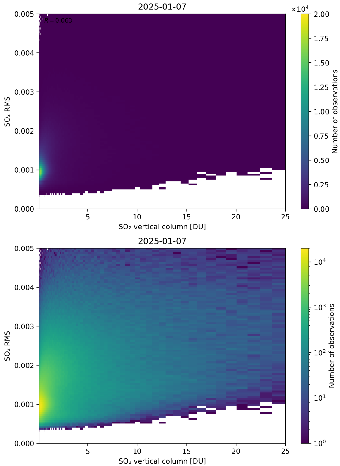
Figure 328: Scatter density plot of “SO 2 vertical column” against “SO 2 RMS” for 2025-01-07 to 2025-01-08.
