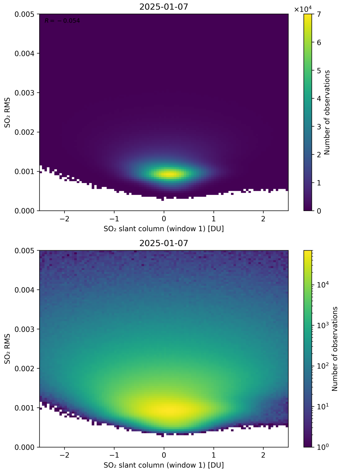
Figure 267: Scatter density plot of “SO 2 slant column (window 1)” against “SO 2 RMS” for 2025-01-07 to 2025-01-08.
