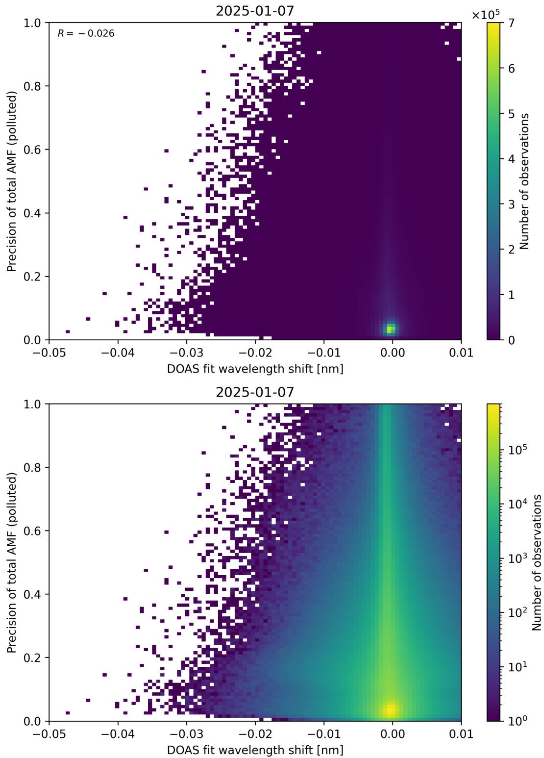
Figure 142: Scatter density plot of “DOAS fit wavelength shift” against “Precision of total AMF (polluted)” for 2025-01-07 to 2025-01-08.
