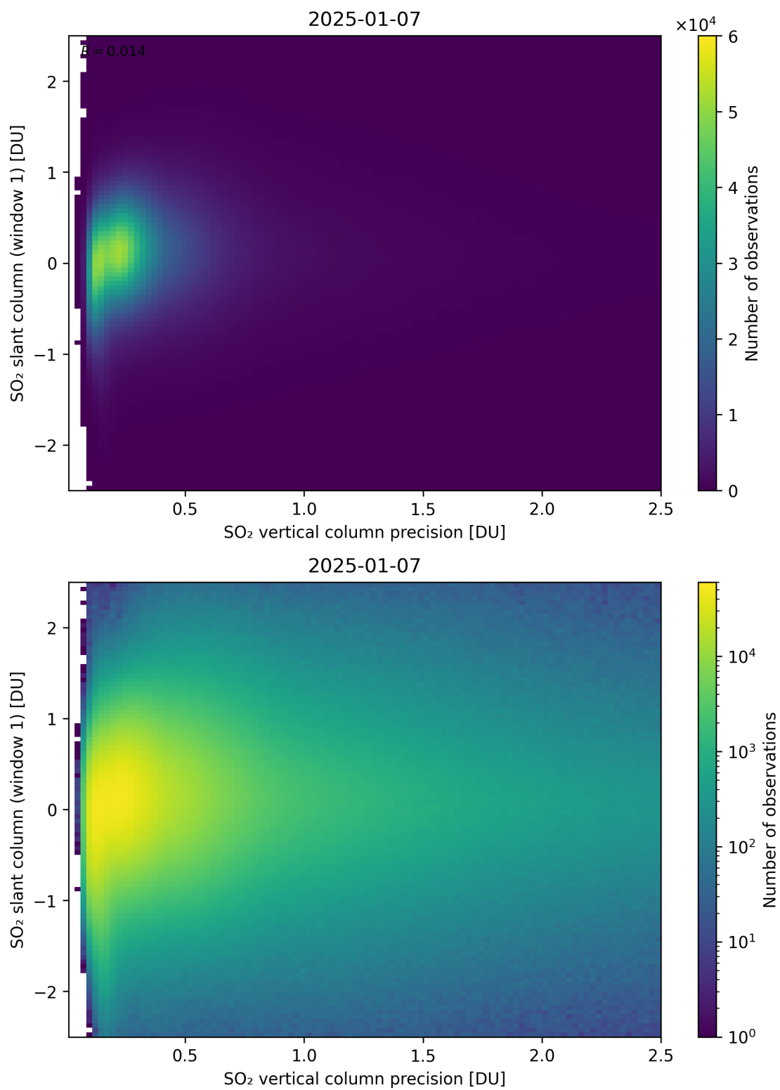
Figure 341: Scatter density plot of “SO 2 vertical column precision” against “SO 2 slant column (window 1)” for 2025-01-07 to 2025-01-08.
