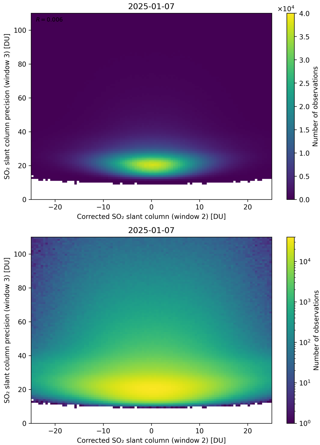
Figure 252: Scatter density plot of “Corrected SO 2 slant column (window 2)” against “SO 2 slant column precision (window 3)” for 2025-01-07 to 2025-01-08.
