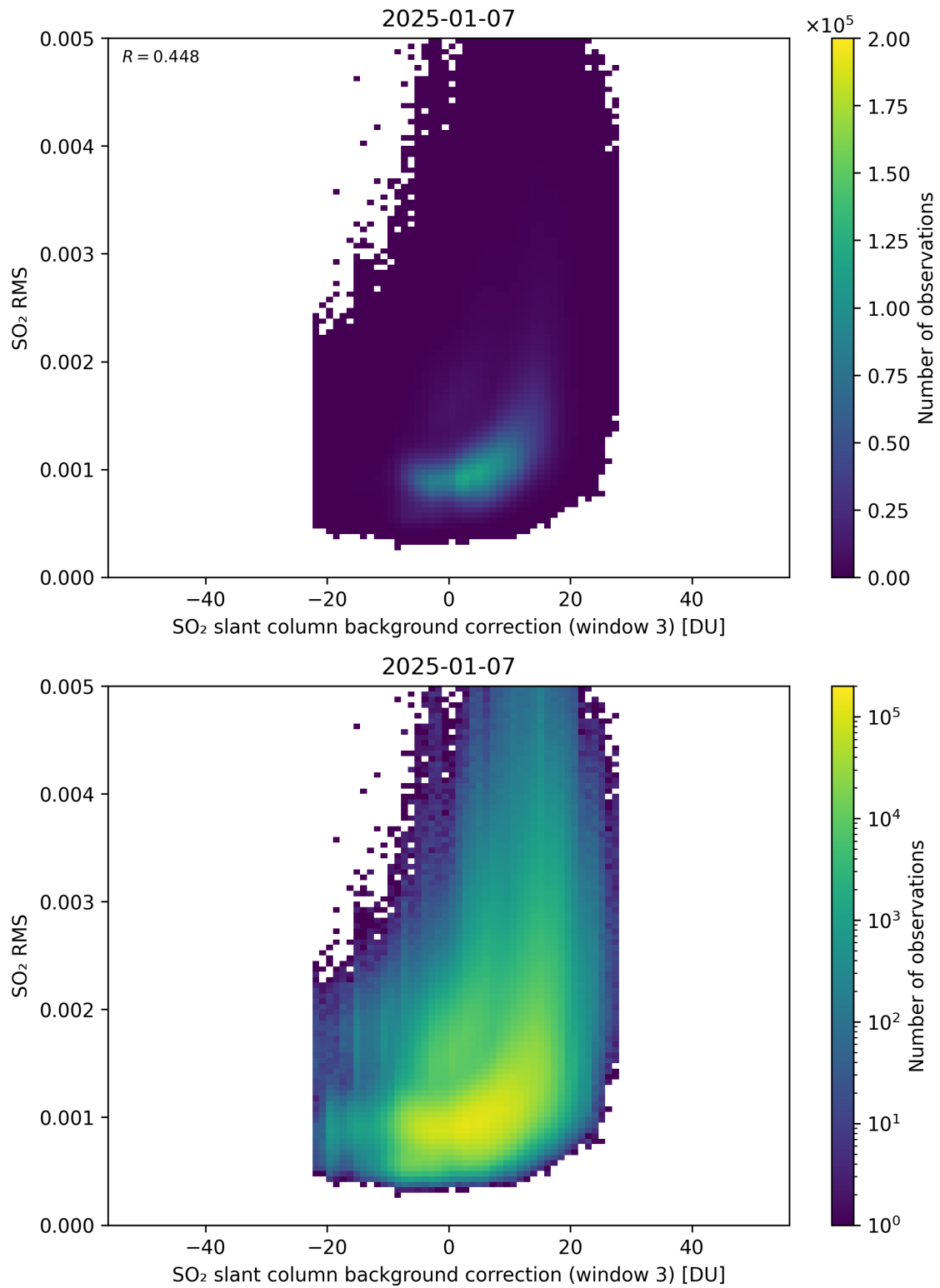
Figure 134: Scatter density plot of “SO 2 slant column background correction (window 3)” against “SO 2 RMS” for 2025-01-07 to 2025-01-08.
