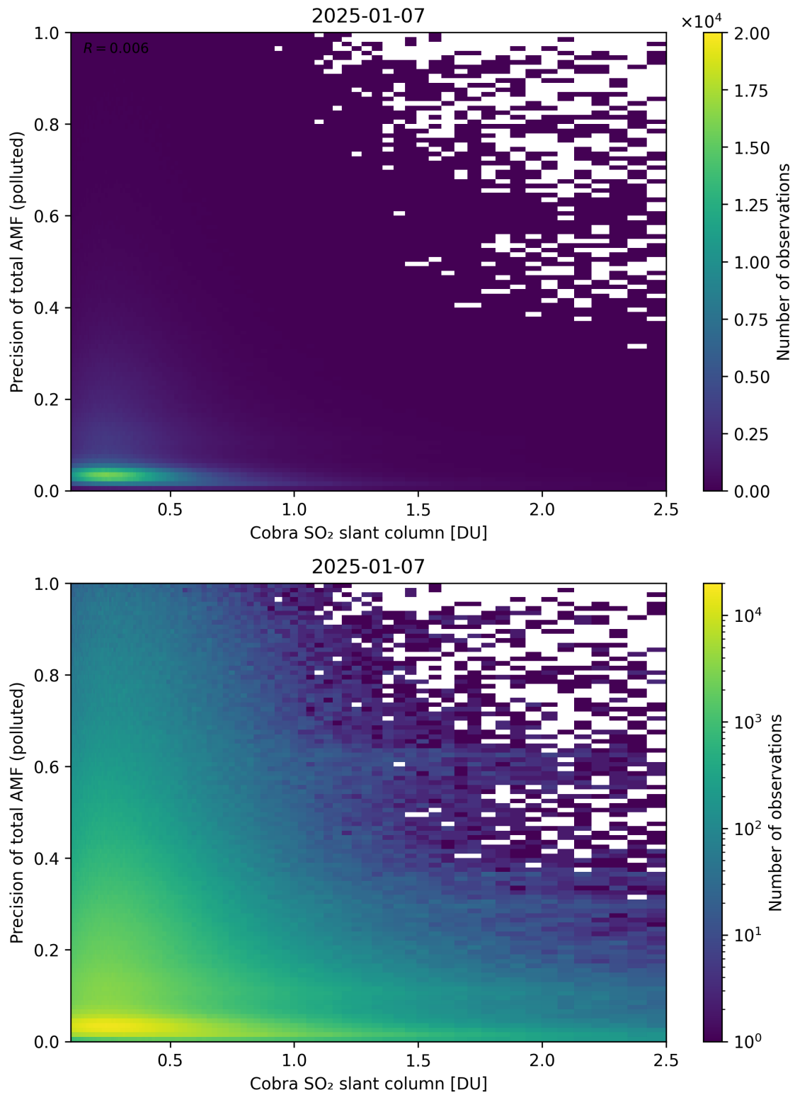
Figure 225: Scatter density plot of “Cobra SO 2 slant column” against “Precision of total AMF (polluted)” for 2025-01-07 to 2025-01-08.
