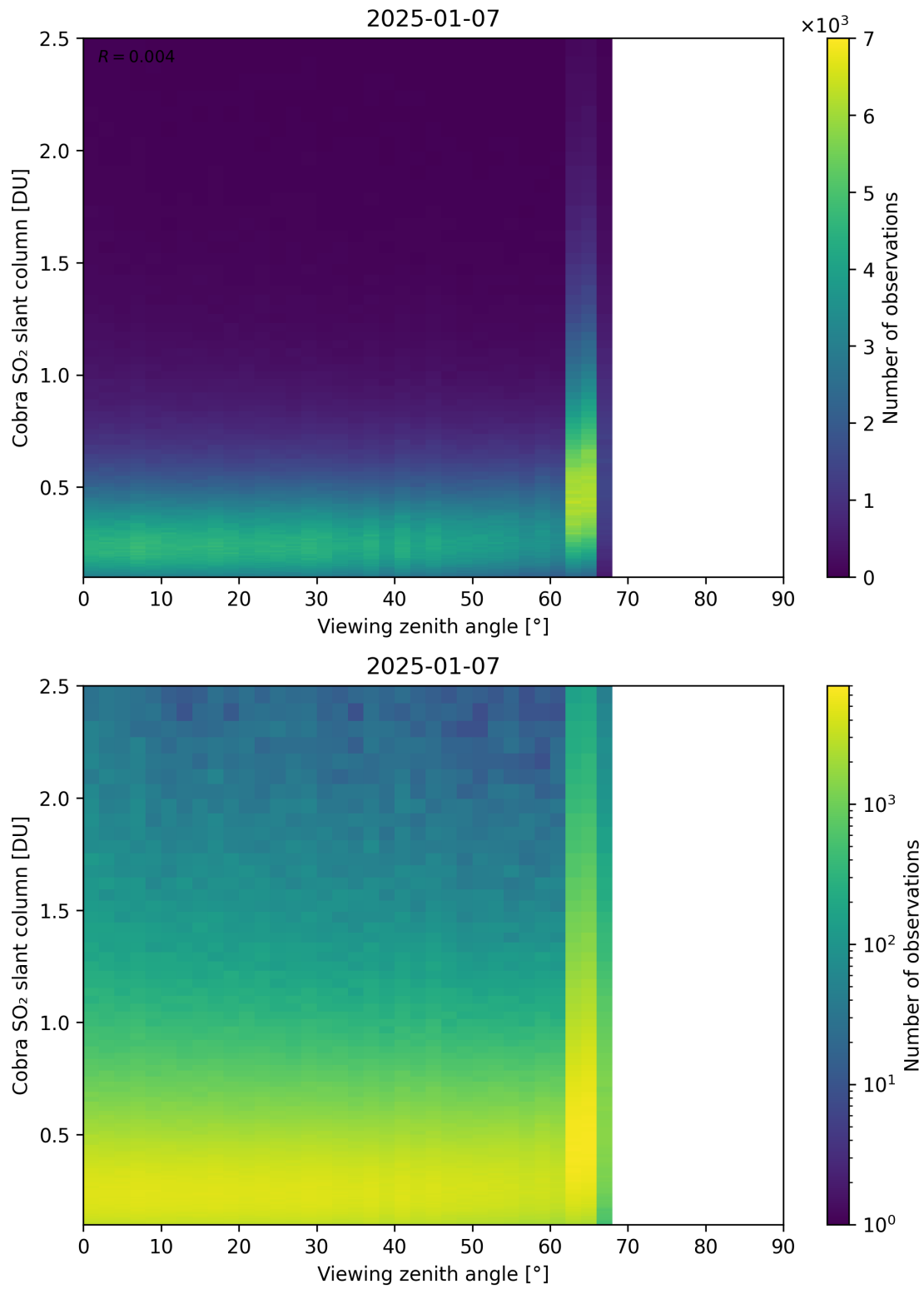
Figure 371: Scatter density plot of “Viewing zenith angle” against “Cobra SO 2 slant column” for 2025-01-07 to 2025-01-08.
