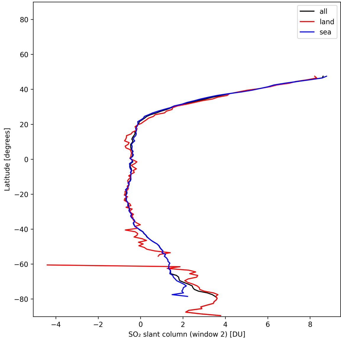
Figure 41: Zonal average of “SO 2 slant column (window 2)” for 2025-01-07 to 2025-01-08.
