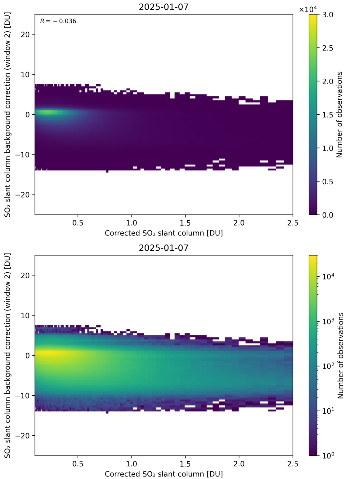
Figure 227: Scatter density plot of “Corrected SO 2 slant column” against “SO 2 slant column background correction (window 2)” for 2025-01-07 to 2025-01-08.
