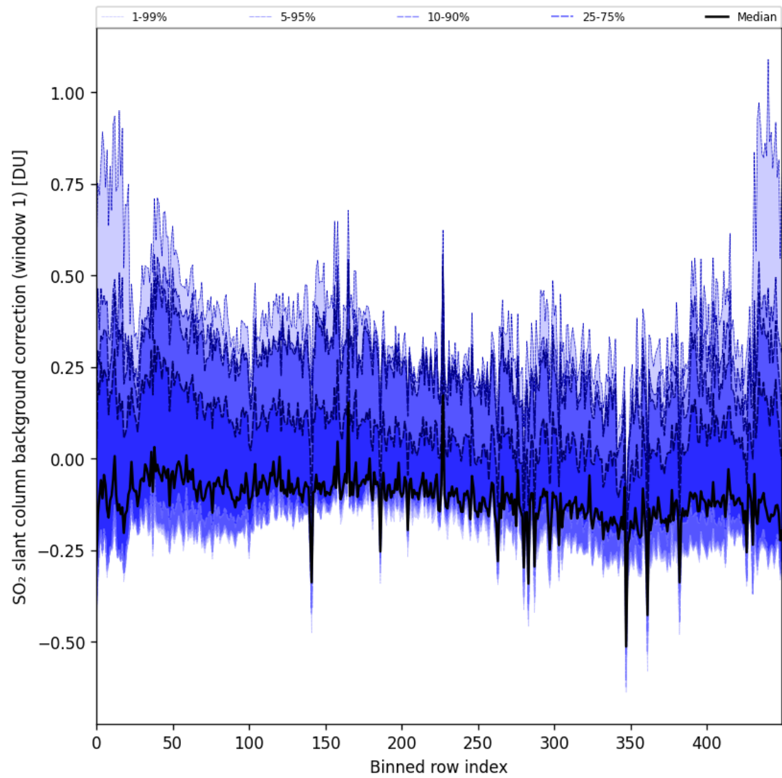
Figure 92: Along track statistics of “SO 2 slant column background correction (window 1)” for 2025-01-07 to 2025-01-08
