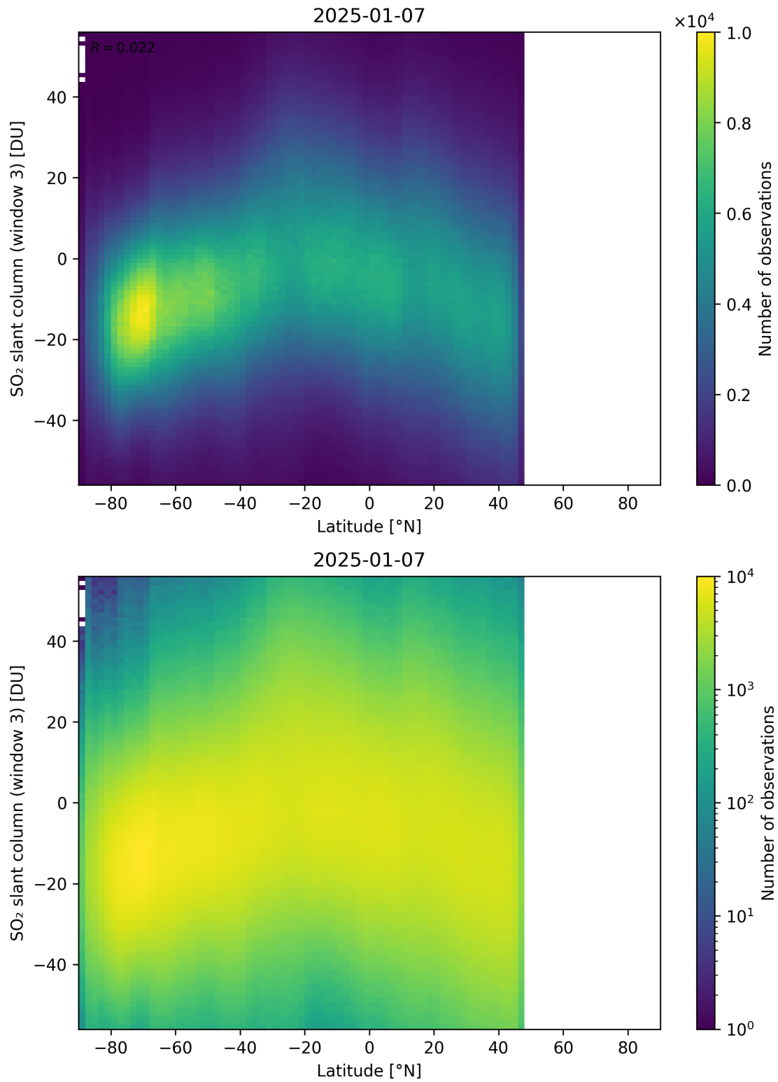
Figure 165: Scatter density plot of “Latitude” against “SO 2 slant column (window 3)” for 2025-01-07 to 2025-01-08.
