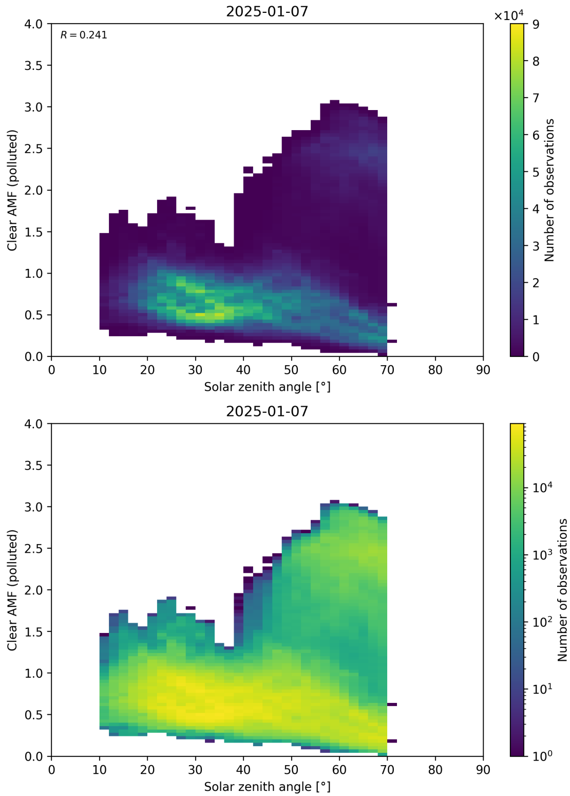
Figure 178: Scatter density plot of “Solar zenith angle” against “Clear AMF (polluted)” for 2025-01-07 to 2025-01-08.
