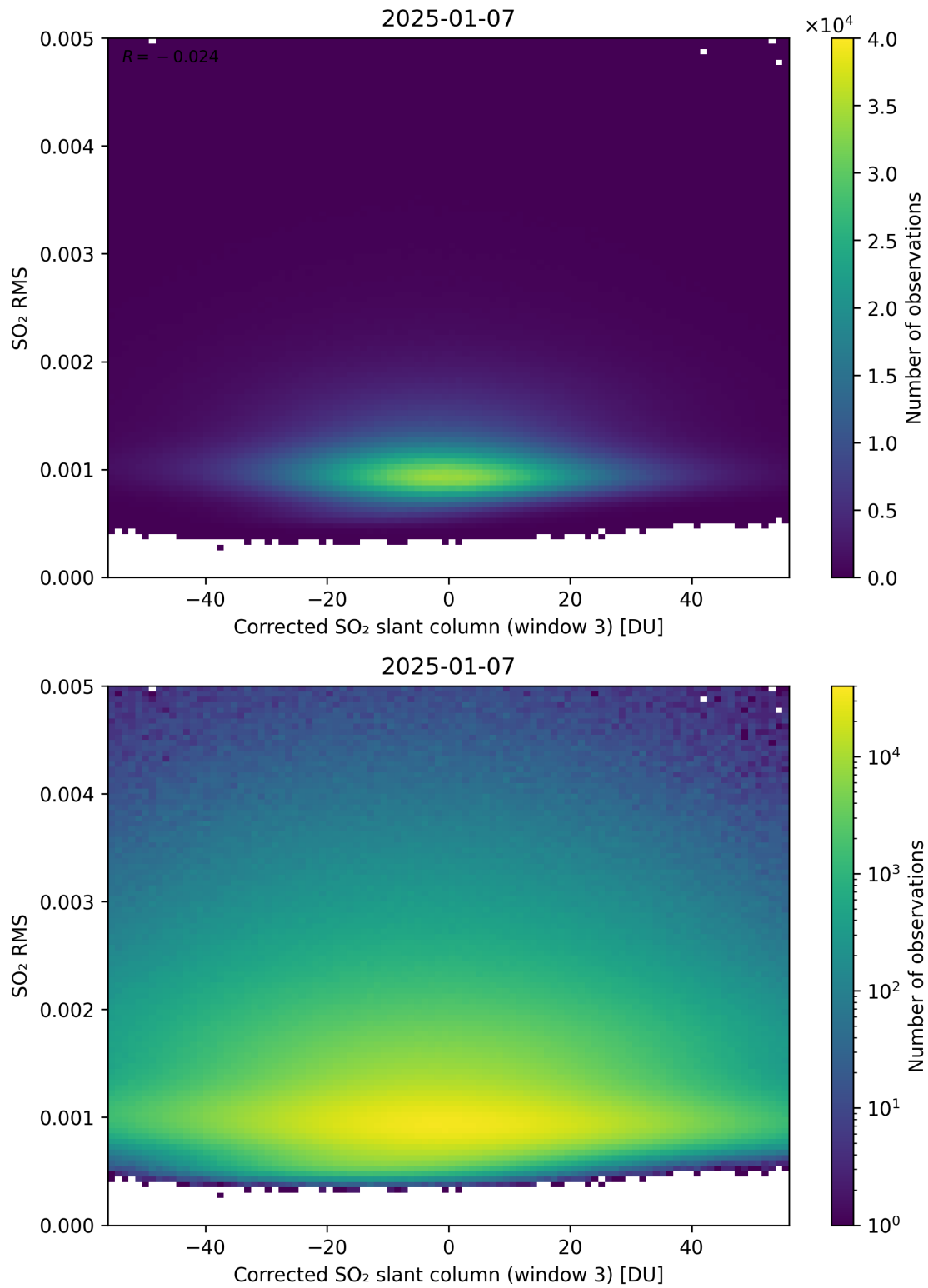
Figure 258: Scatter density plot of “Corrected SO 2 slant column (window 3)” against “SO 2 RMS” for 2025-01-07 to 2025-01-08.
