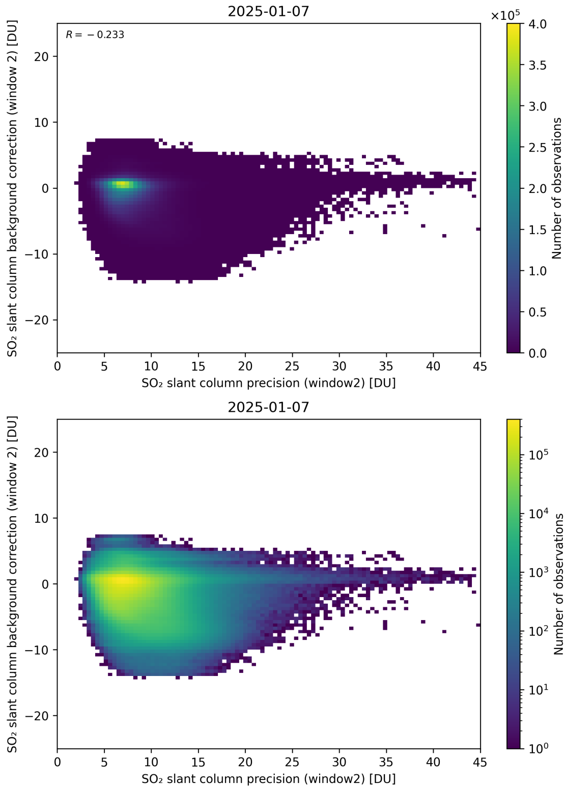
Figure 291: Scatter density plot of “SO 2 slant column precision (window2)” against “SO 2 slant column background correction (window 2)” for 2025-01-07 to 2025-01-08.
