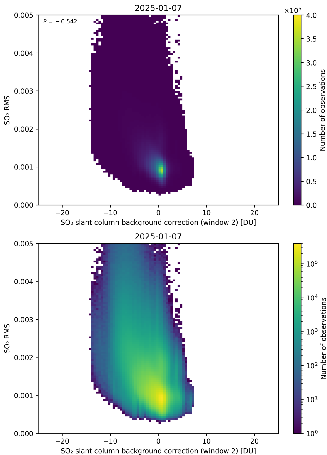
Figure 125: Scatter density plot of “SO 2 slant column background correction (window 2)” against “SO 2 RMS” for 2025-01-07 to 2025-01-08.
