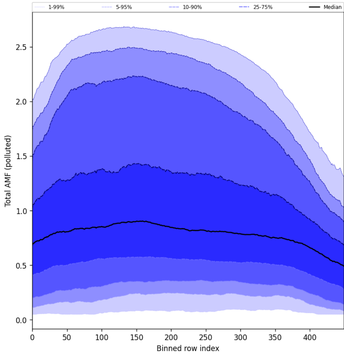
Figure 105: Along track statistics of “Total AMF (polluted)” for 2025-01-07 to 2025-01-08
