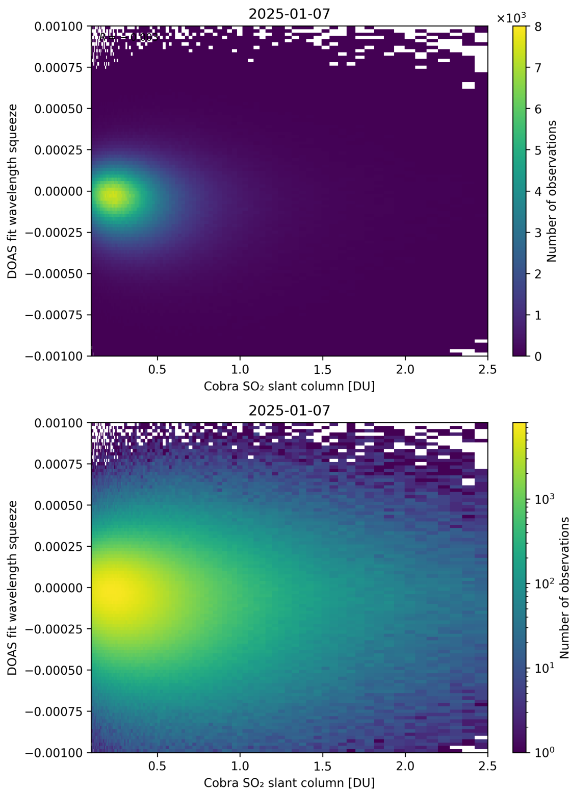
Figure 197: Scatter density plot of “Cobra SO 2 slant column” against “DOAS fit wavelength squeeze” for 2025-01-07 to 2025-01-08.
