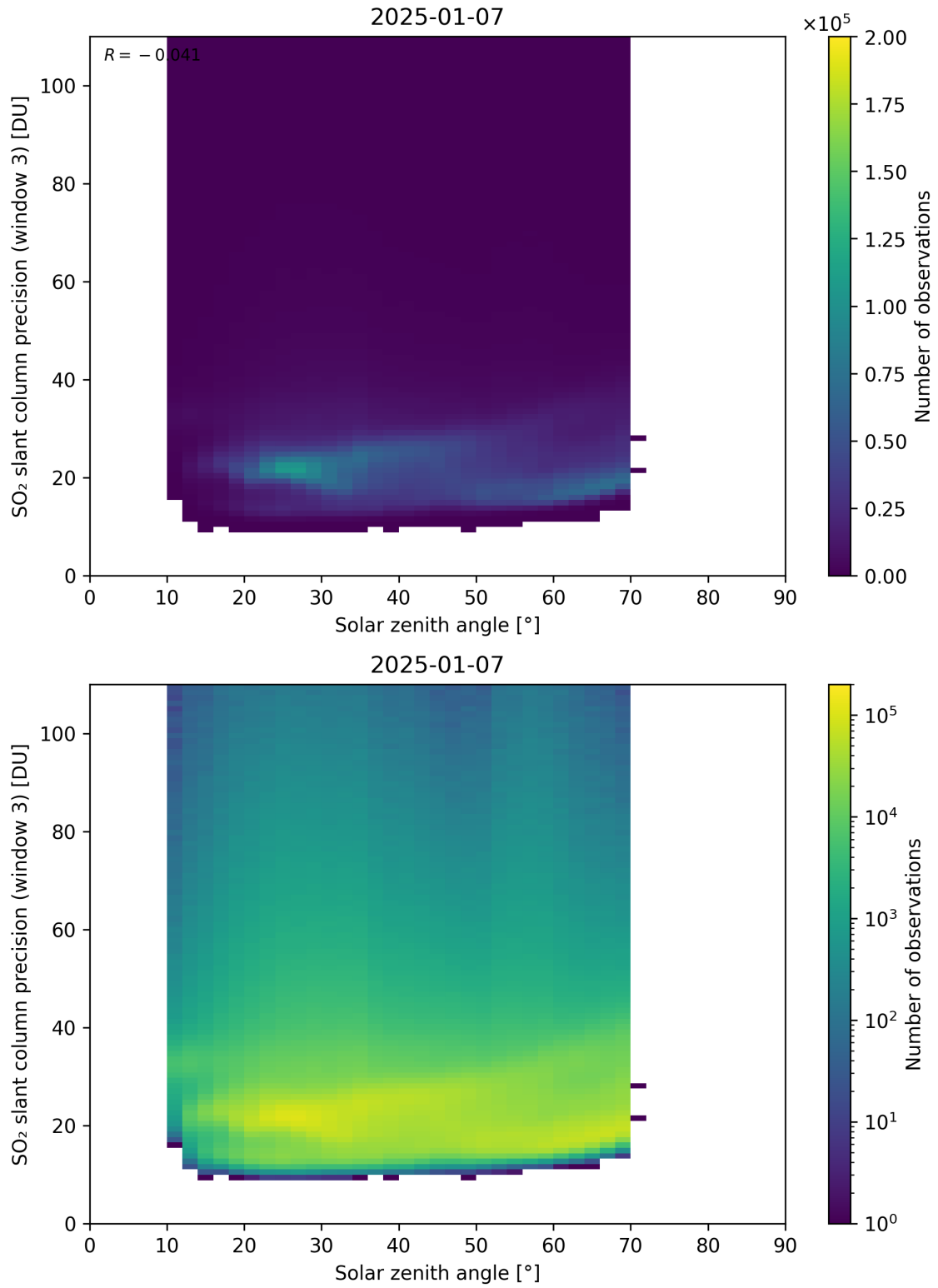
Figure 188: Scatter density plot of “Solar zenith angle” against “SO 2 slant column precision (window 3)” for 2025-01-07 to 2025-01-08.
