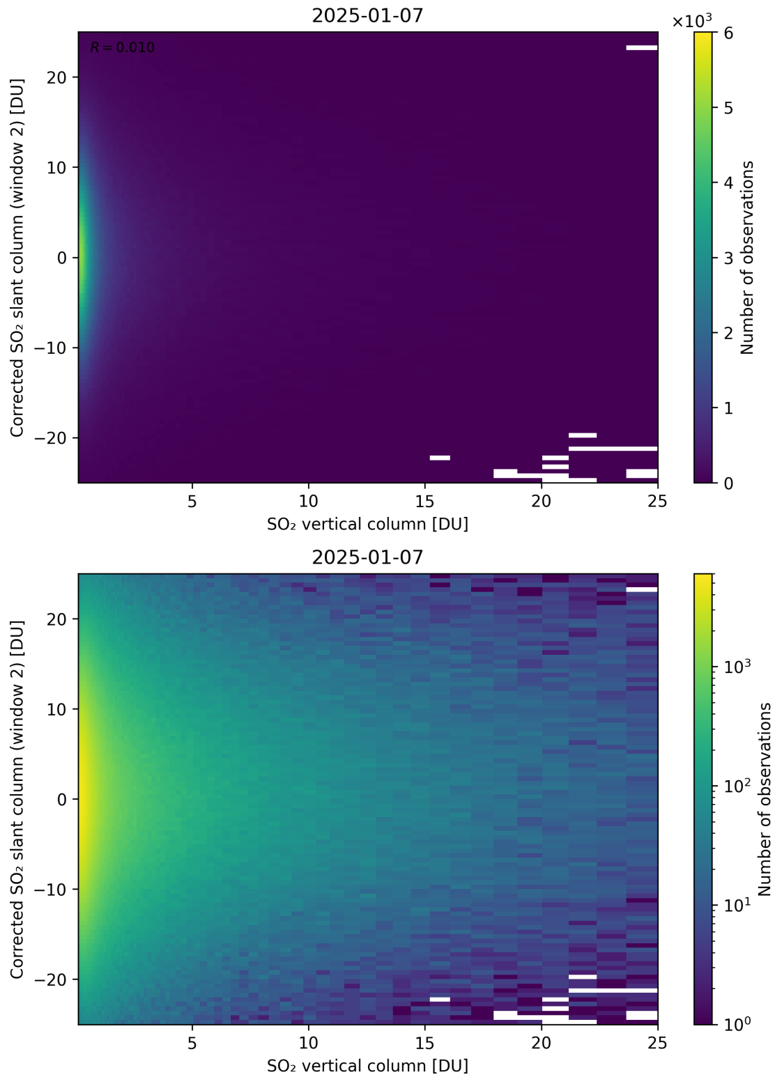
Figure 352: Scatter density plot of “SO 2 vertical column” against “Corrected SO 2 slant column (window 2)” for 2025-01-07 to 2025-01-08.
