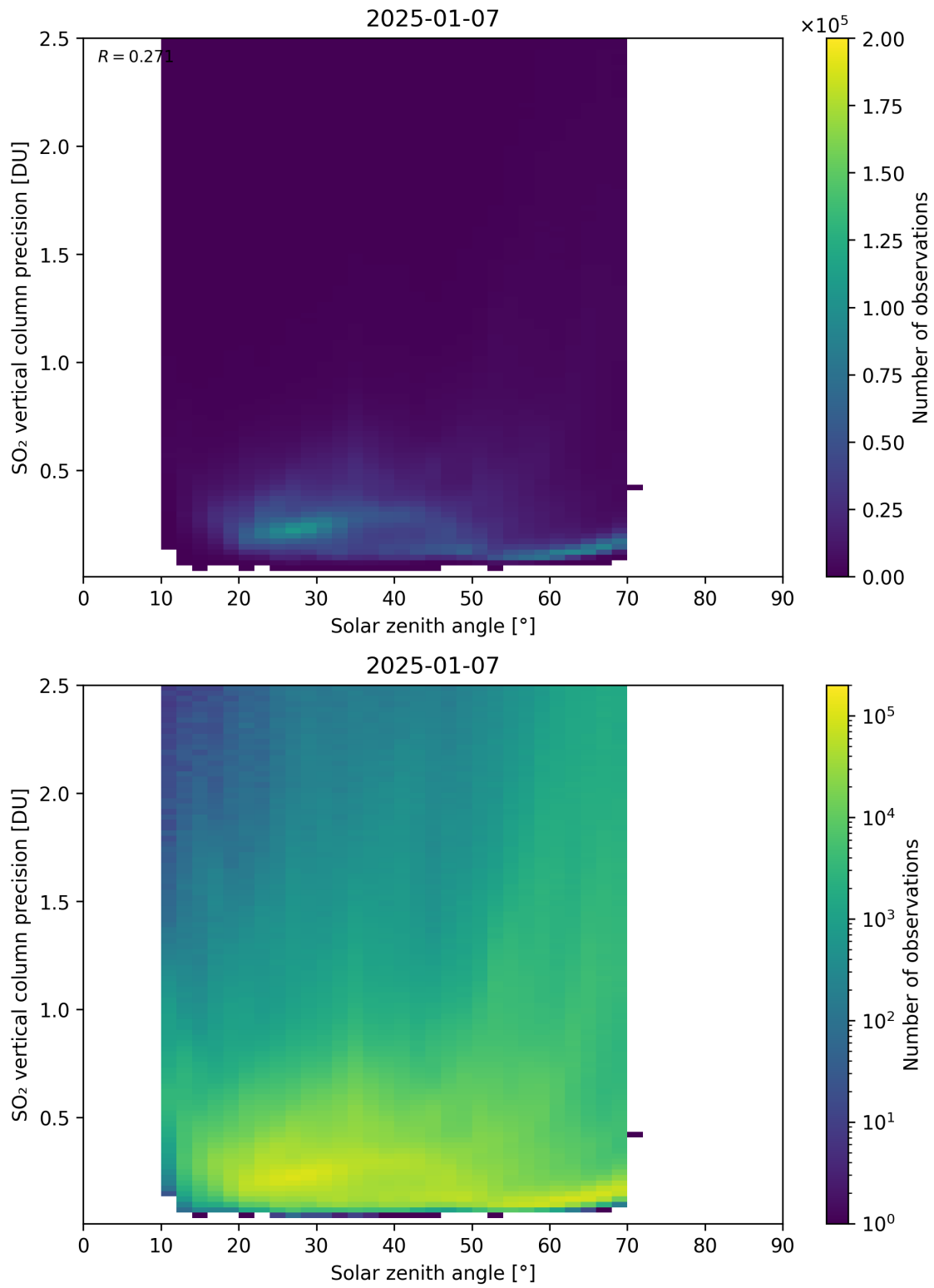
Figure 192: Scatter density plot of “Solar zenith angle” against “SO 2 vertical column precision” for 2025-01-07 to 2025-01-08.
