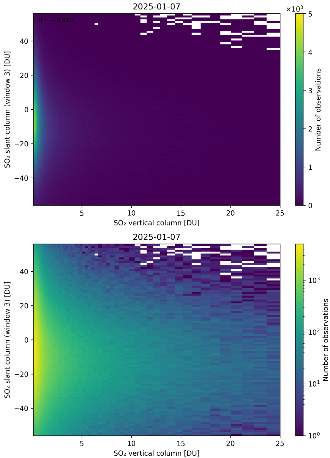
Figure 357: Scatter density plot of “SO 2 vertical column” against “SO 2 slant column (window 3)” for 2025-01-07 to 2025-01-08.
