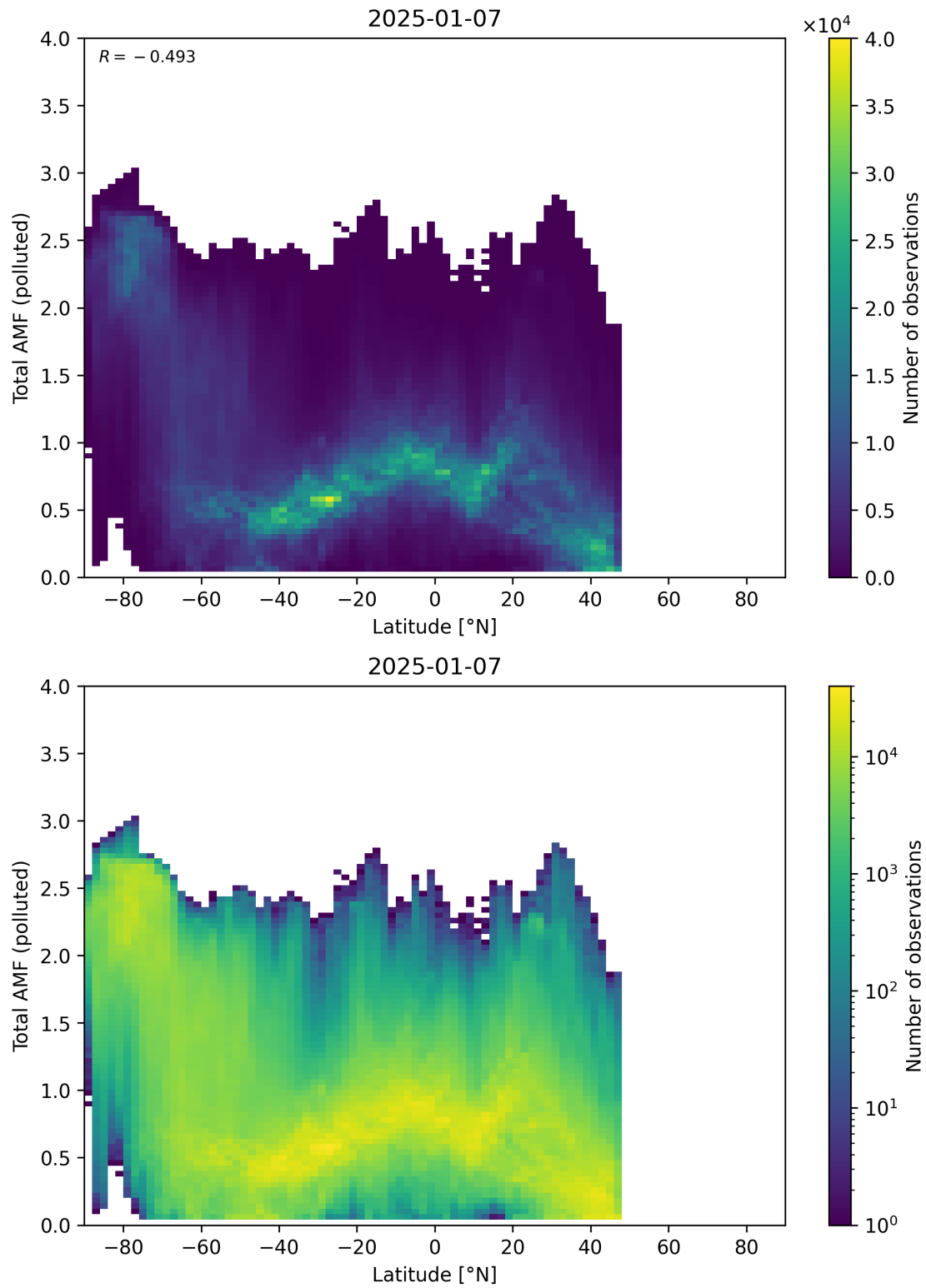
Figure 167: Scatter density plot of “Latitude” against “Total AMF (polluted)” for 2025-01-07 to 2025-01-08.
