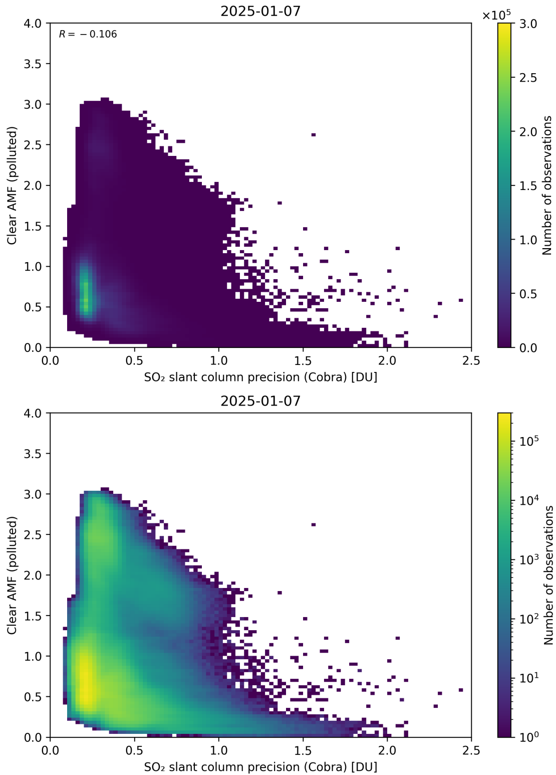
Figure 205: Scatter density plot of “SO 2 slant column precision (Cobra)” against “Clear AMF (polluted)” for 2025-01-07 to 2025-01-08.
