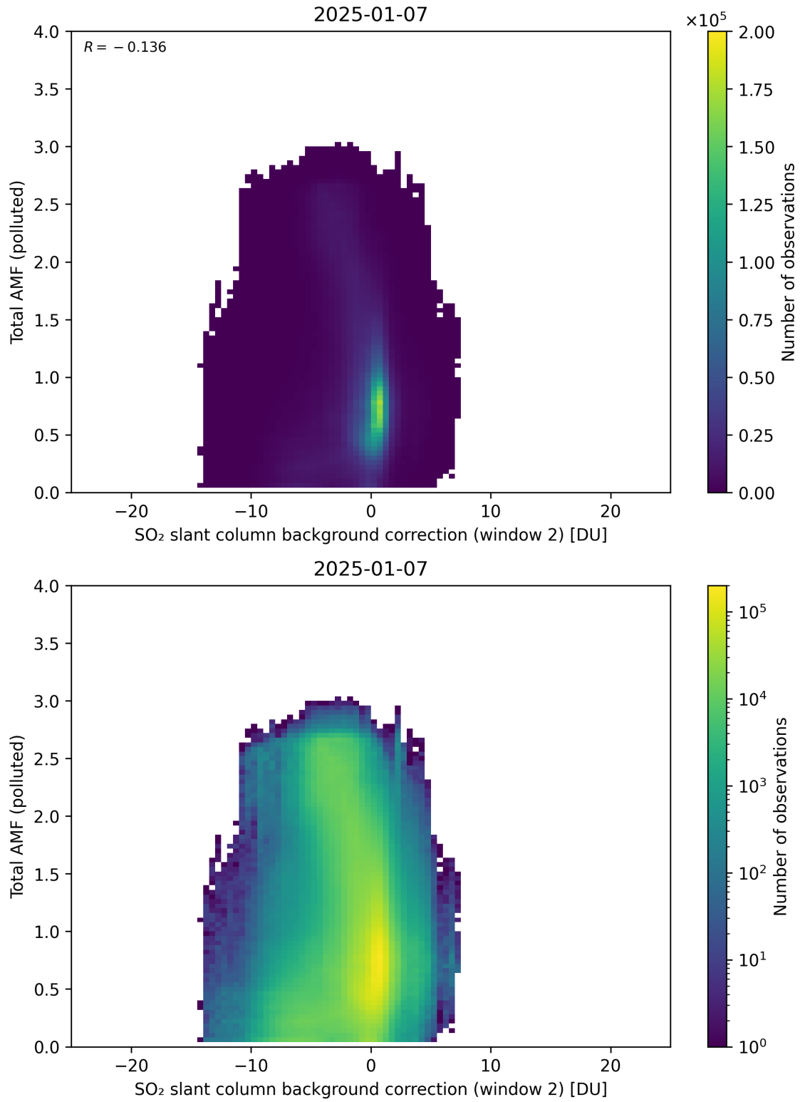
Figure 130: Scatter density plot of “SO 2 slant column background correction (window 2)” against “Total AMF (polluted)” for 2025-01-07 to 2025-01-08.
