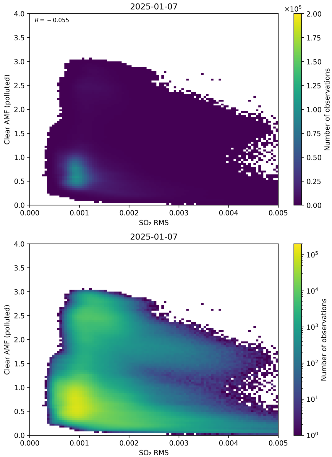
Figure 147: Scatter density plot of “SO 2 RMS” against “Clear AMF (polluted)” for 2025-01-07 to 2025-01-08.
