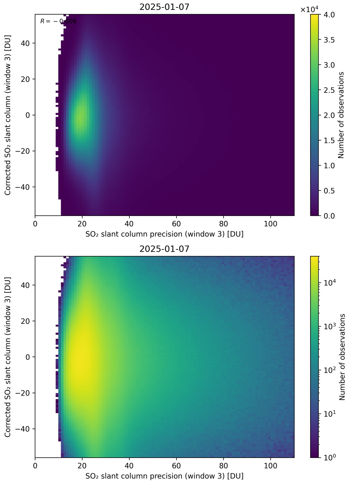
Figure 312: Scatter density plot of “SO 2 slant column precision (window 3)” against “Corrected SO 2 slant column (window 3)” for 2025-01-07 to 2025-01-08.
