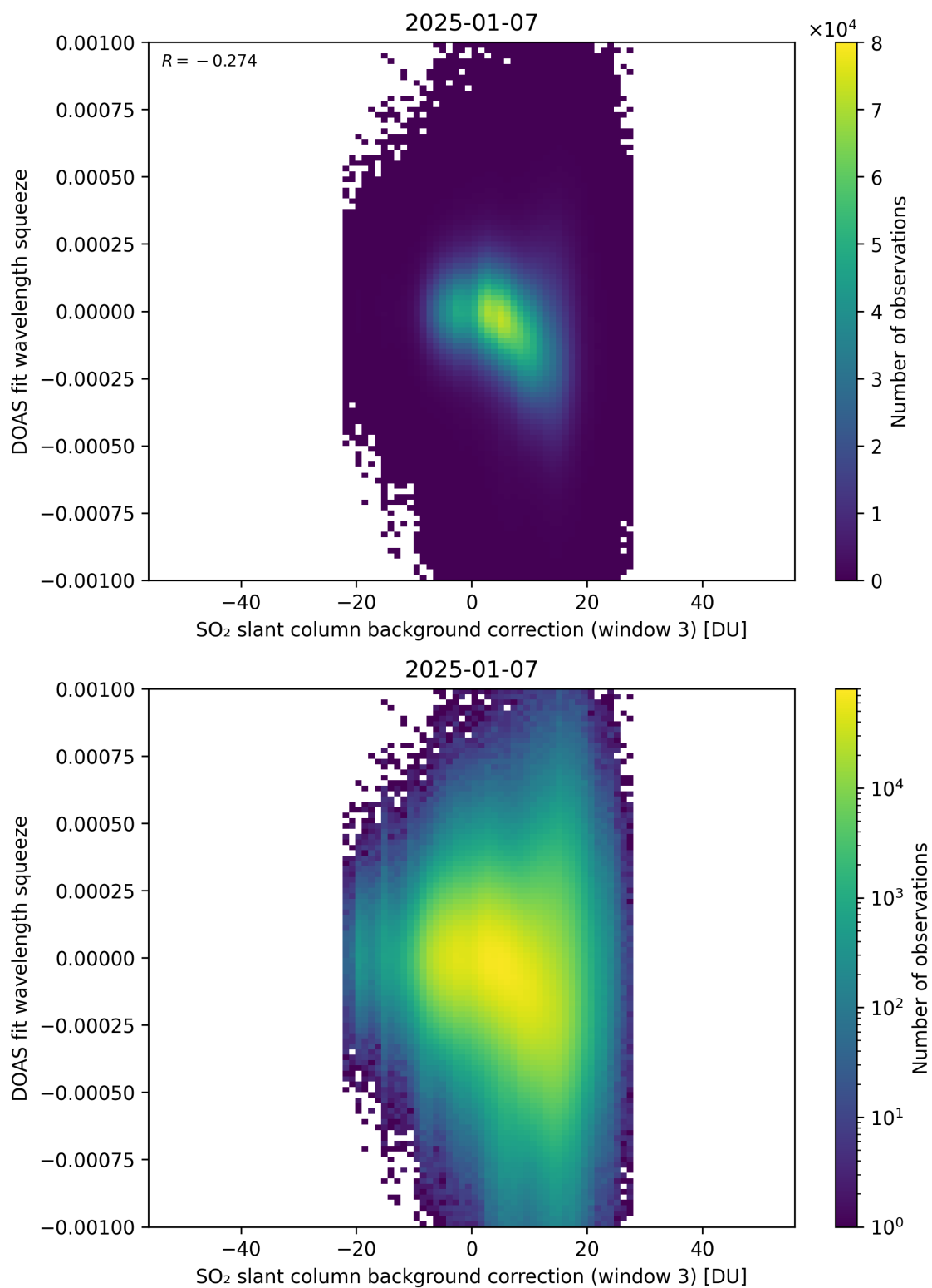
Figure 133: Scatter density plot of “SO 2 slant column background correction (window 3)” against “DOAS fit wavelength squeeze” for 2025-01-07 to 2025-01-08.
