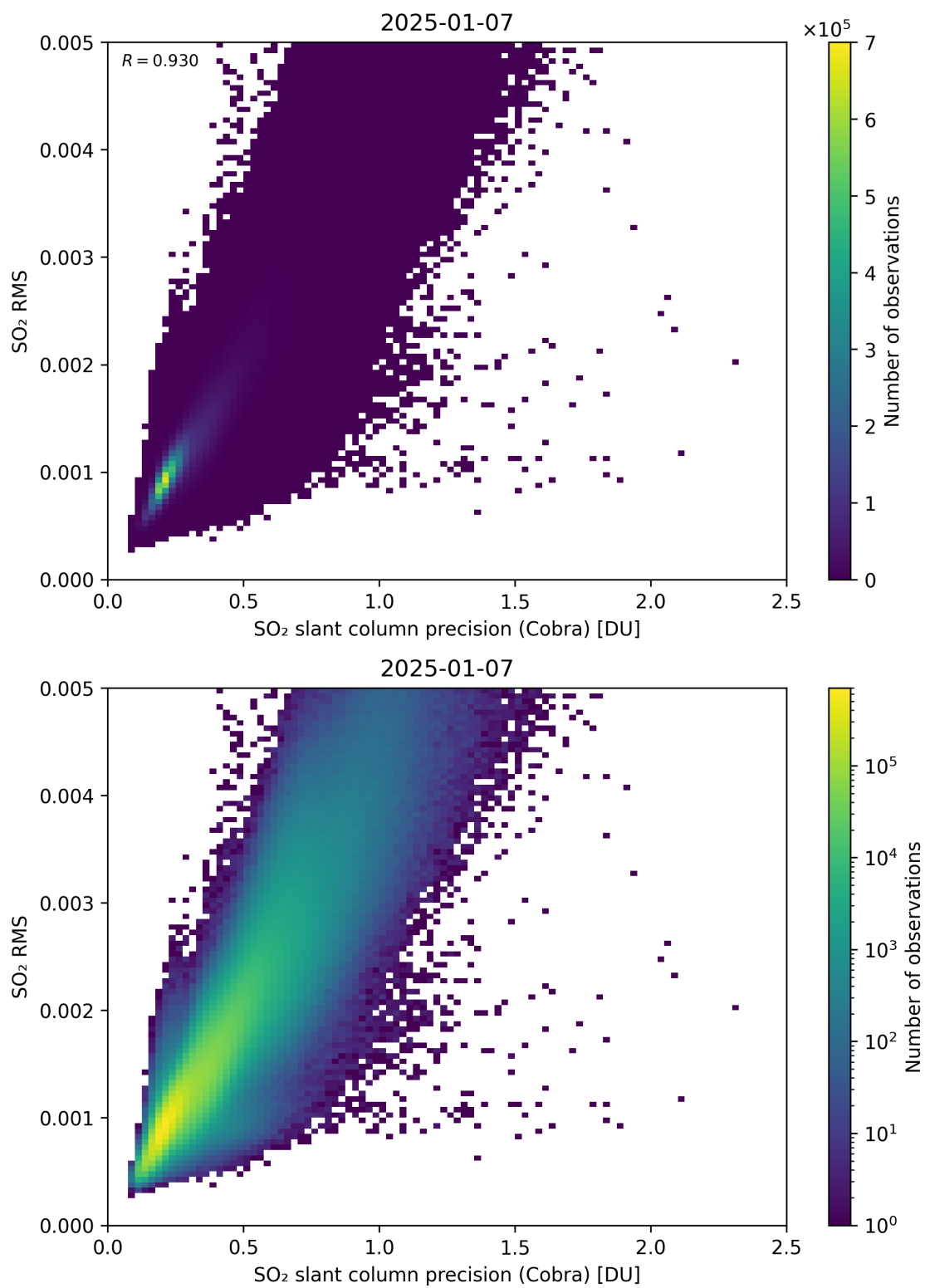
Figure 204: Scatter density plot of “SO 2 slant column precision (Cobra)” against “SO 2 RMS” for 2025-01-07 to 2025-01-08.
