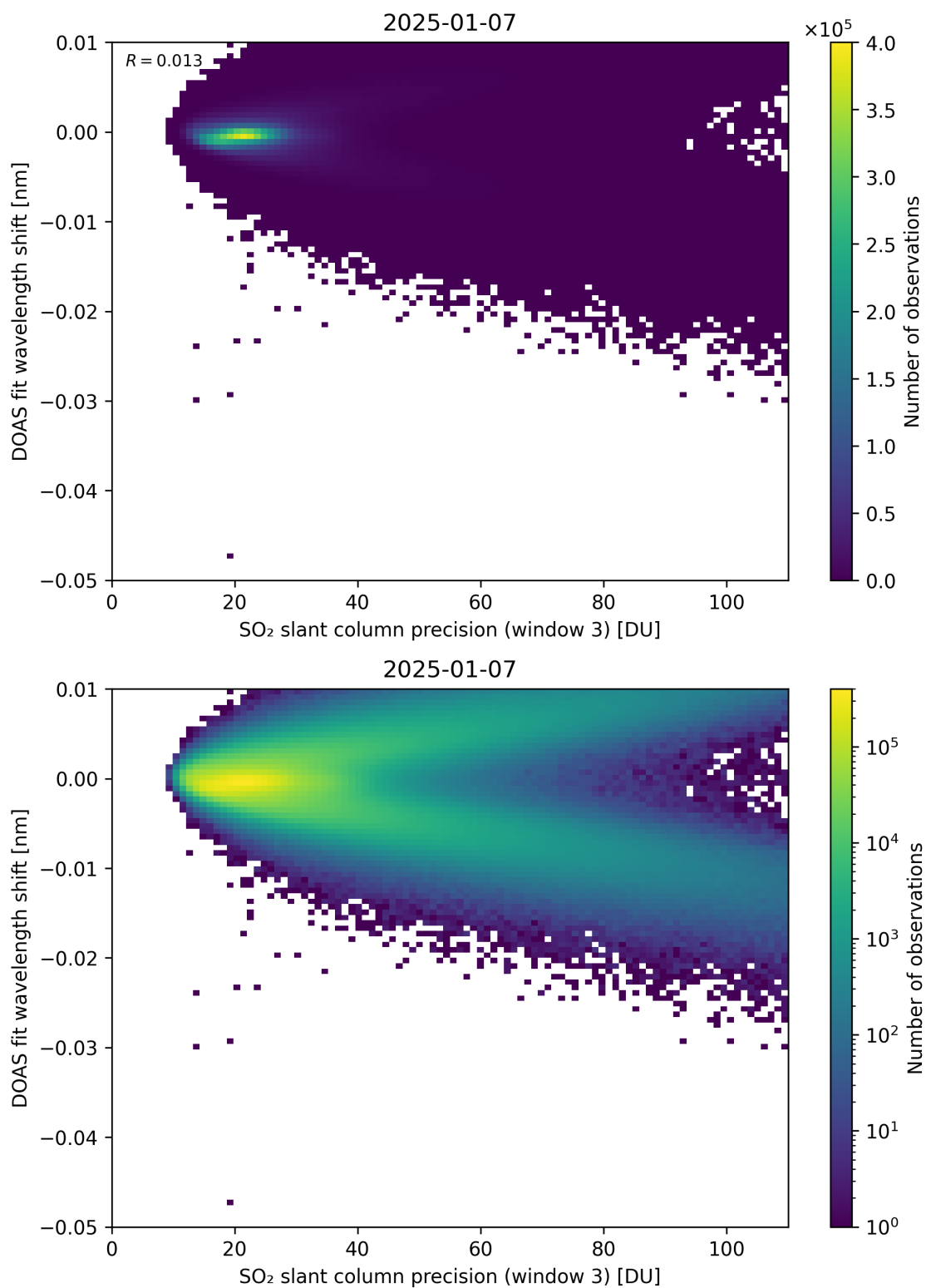
Figure 308: Scatter density plot of “SO 2 slant column precision (window 3)” against “DOAS fit wavelength shift” for 2025-01-07 to 2025-01-08.
