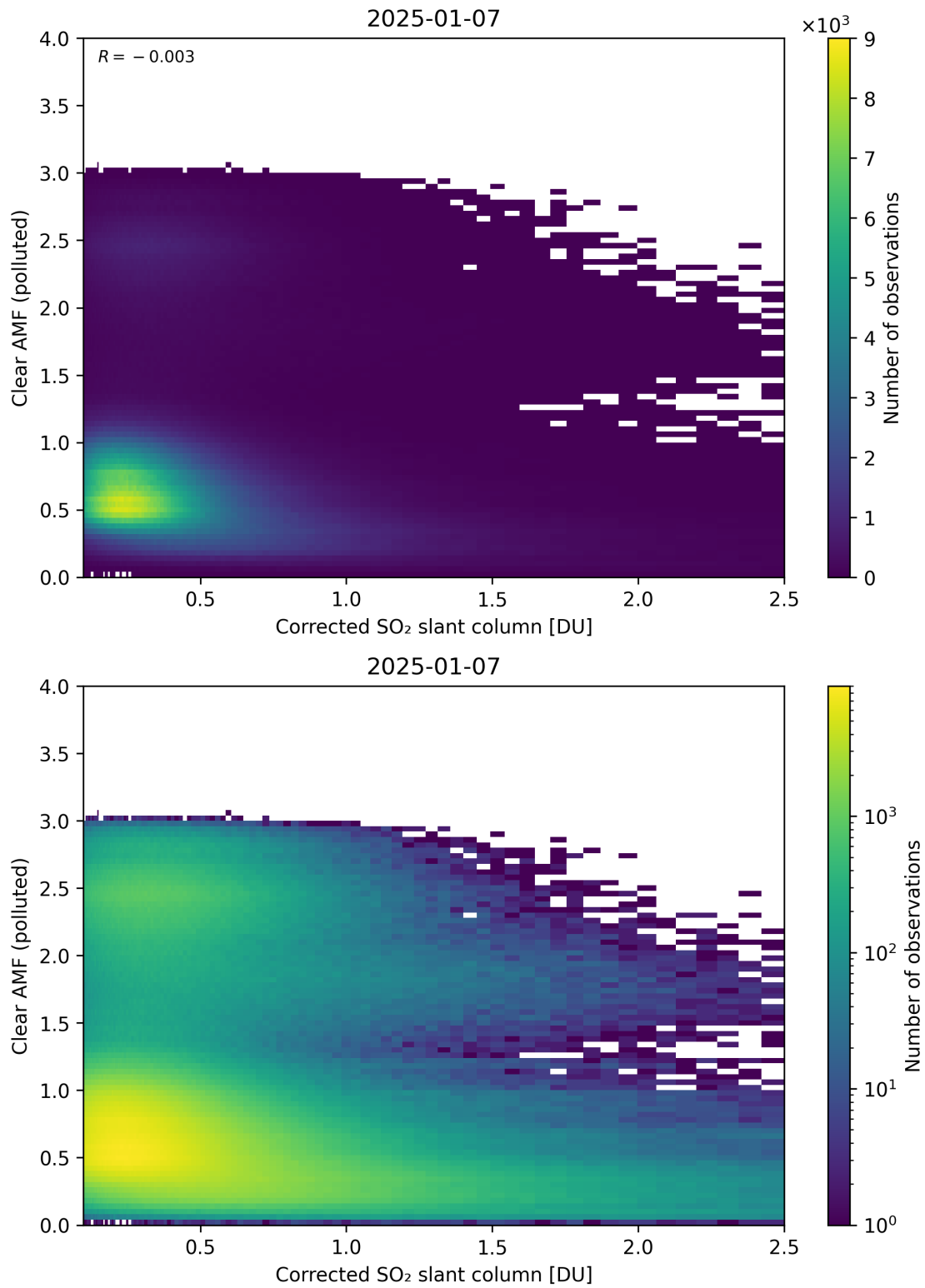
Figure 232: Scatter density plot of “Corrected SO 2 slant column” against “Clear AMF (polluted)” for 2025-01-07 to 2025-01-08.
