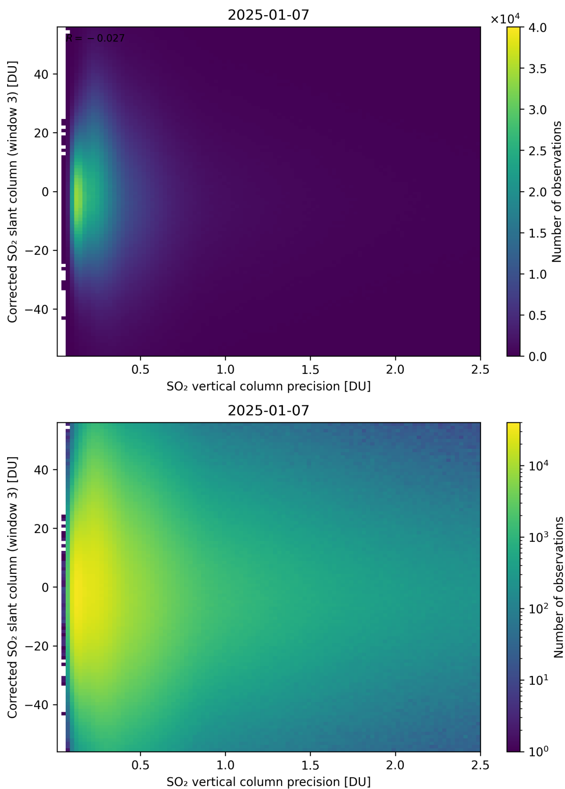
Figure 340: Scatter density plot of “SO 2 vertical column precision” against “Corrected SO 2 slant column (window 3)” for 2025-01-07 to 2025-01-08.
