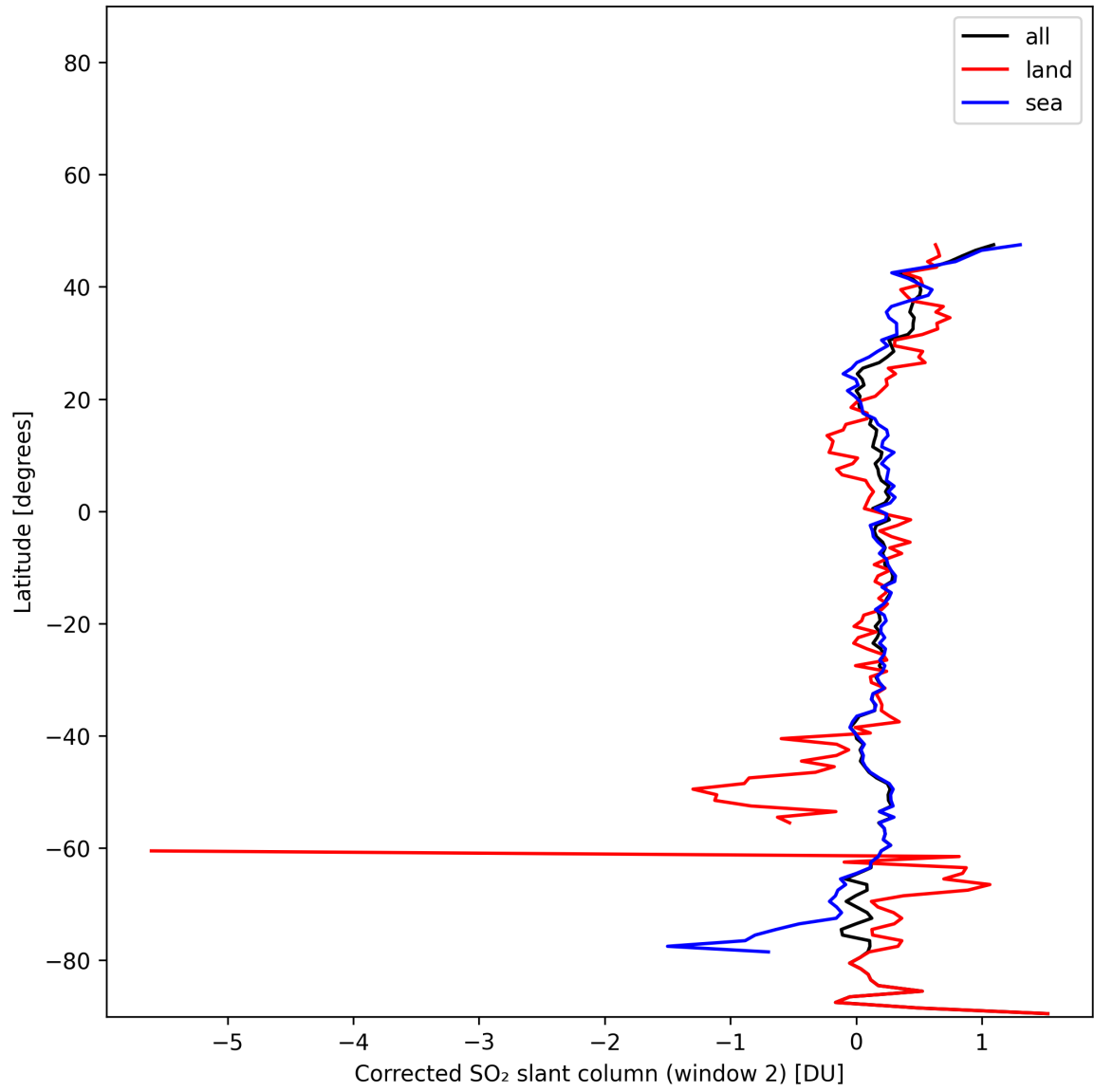
Figure 43: Zonal average of “Corrected SO 2 slant column (window 2)” for 2025-01-07 to 2025-01-08.
