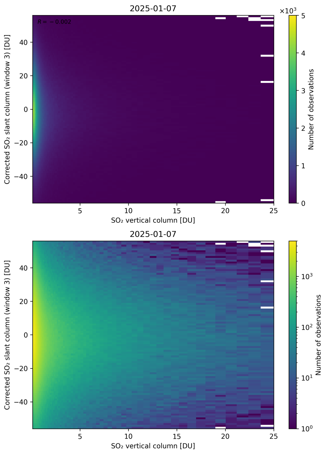
Figure 353: Scatter density plot of “SO 2 vertical column” against “Corrected SO 2 slant column (window 3)” for 2025-01-07 to 2025-01-08.
