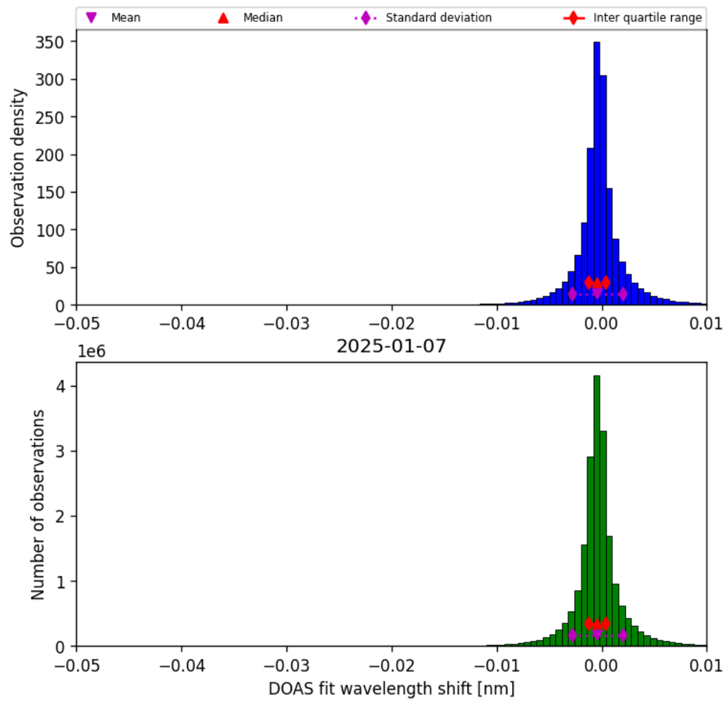
Figure 76: Histogram of “DOAS fit wavelength shift” for 2025-01-07 to 2025-01-08
