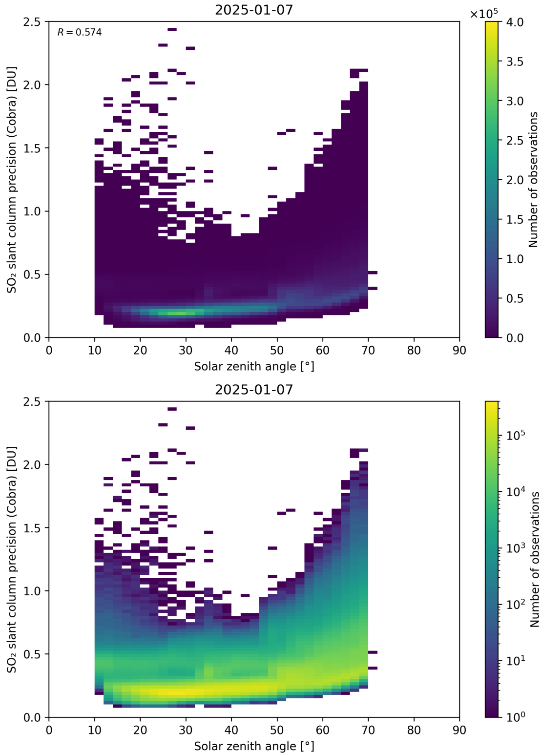
Figure 180: Scatter density plot of “Solar zenith angle” against “SO 2 slant column precision (Cobra)” for 2025-01-07 to 2025-01-08.
