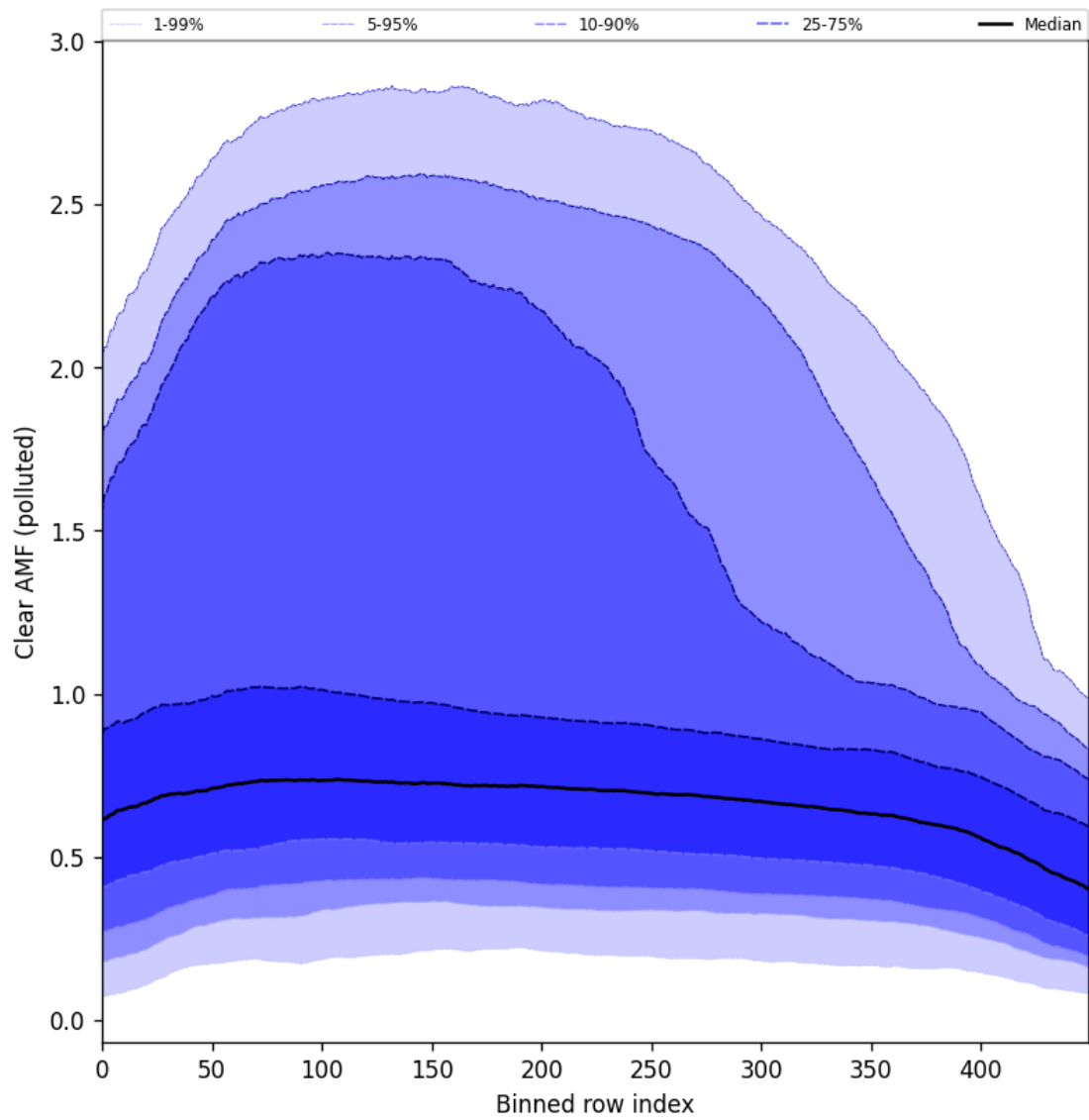
Figure 107: Along track statistics of “Clear AMF (polluted)” for 2025-01-07 to 2025-01-08
