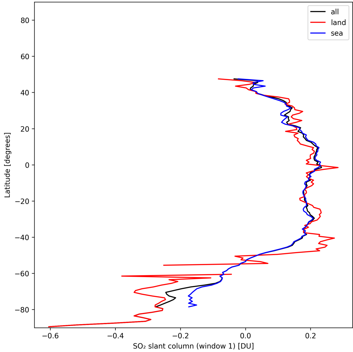
Figure 37: Zonal average of “SO 2 slant column (window 1)” for 2025-01-07 to 2025-01-08.
