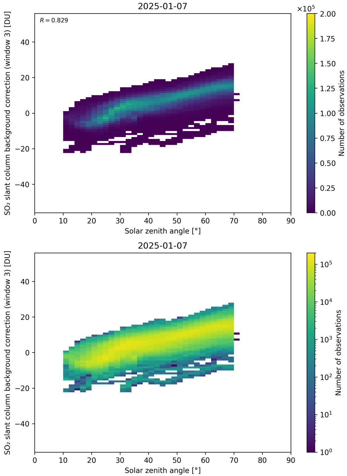
Figure 173: Scatter density plot of “Solar zenith angle” against “SO 2 slant column background correction (window 3)” for 2025-01-07 to 2025-01-08.
