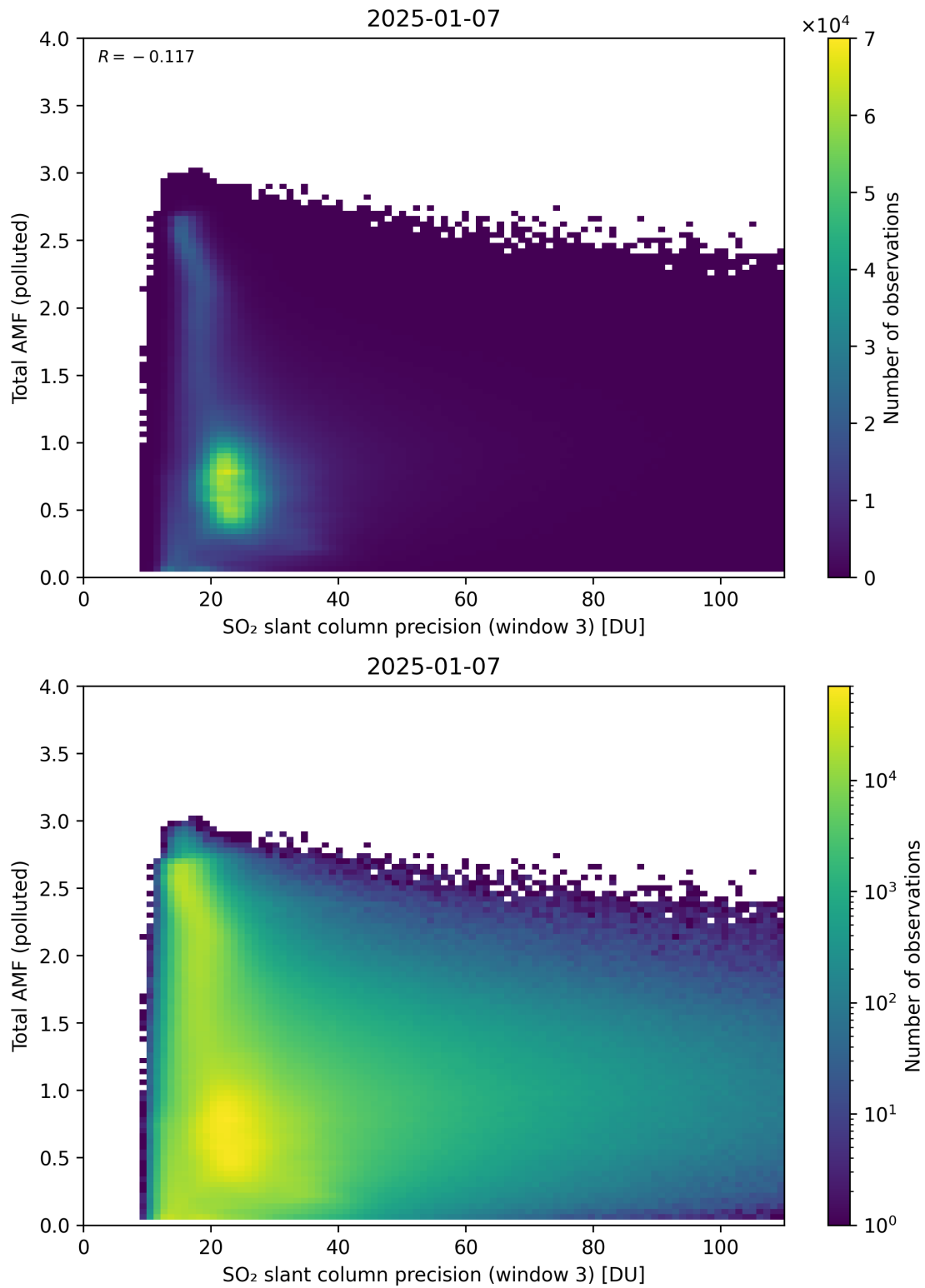
Figure 313: Scatter density plot of “SO 2 slant column precision (window 3)” against “Total AMF (polluted)” for 2025-01-07 to 2025-01-08.
