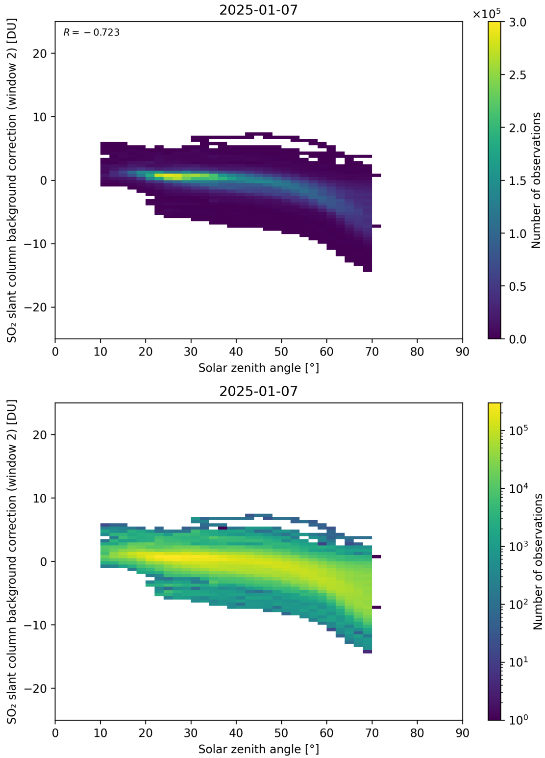
Figure 172: Scatter density plot of “Solar zenith angle” against “SO 2 slant column background correction (window 2)” for 2025-01-07 to 2025-01-08.
