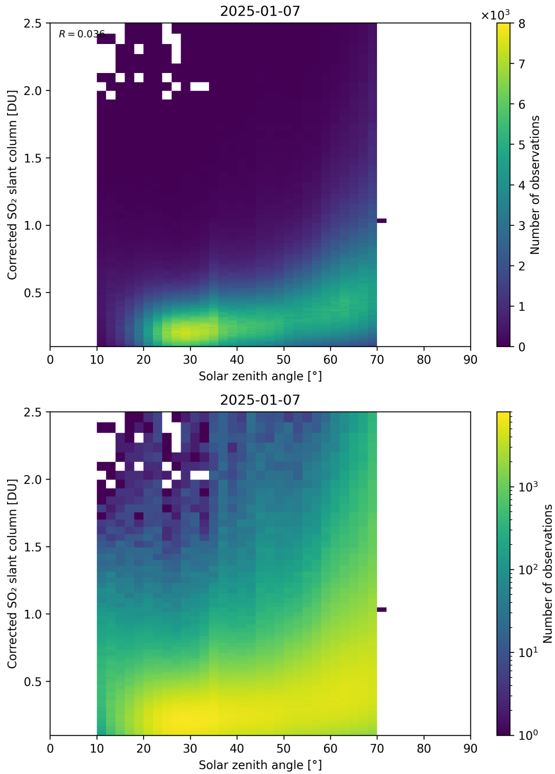
Figure 181: Scatter density plot of “Solar zenith angle” against “Corrected SO 2 slant column” for 2025-01-07 to 2025-01-08.
