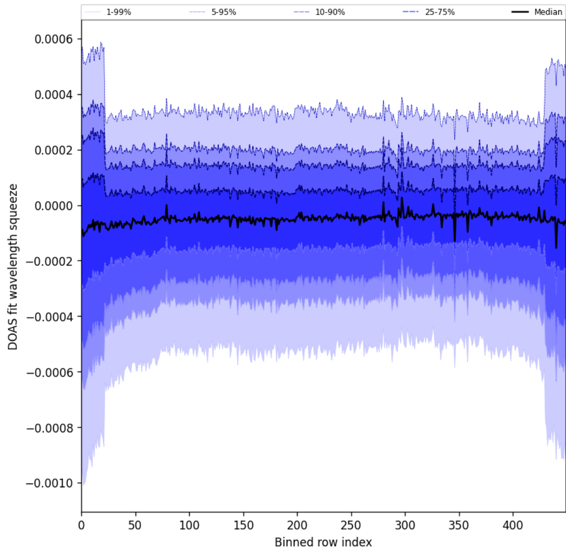
Figure 103: Along track statistics of “DOAS fit wavelength squeeze” for 2025-01-07 to 2025-01-08
