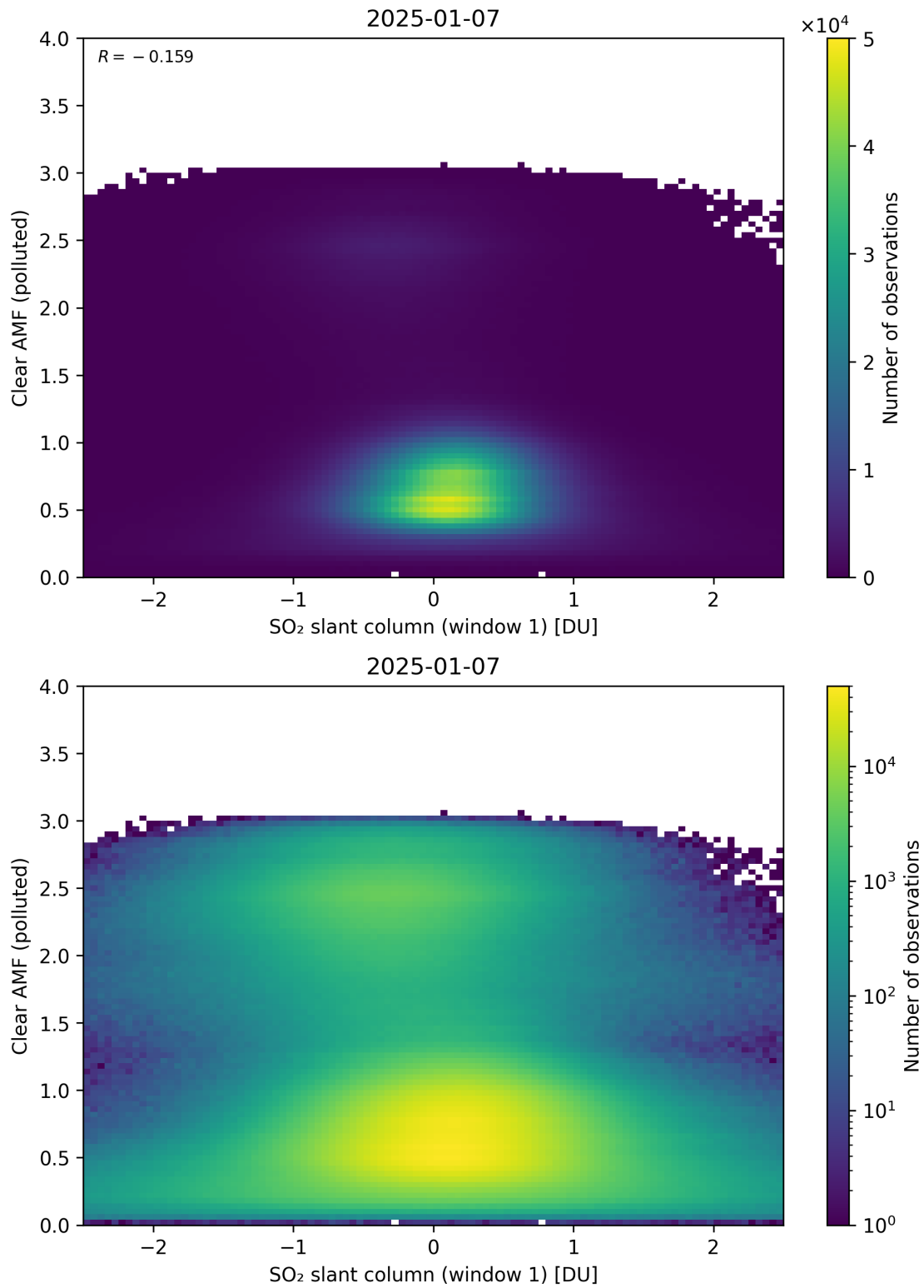
Figure 282: Scatter density plot of “SO 2 slant column (window 1)” against “Clear AMF (polluted)” for 2025-01-07 to 2025-01-08.
