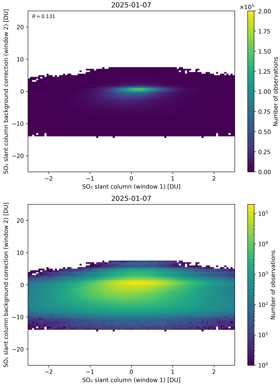
Figure 263: Scatter density plot of “SO 2 slant column (window 1)” against “SO 2 slant column background correction (window 2)” for 2025-01-07 to 2025-01-08.
