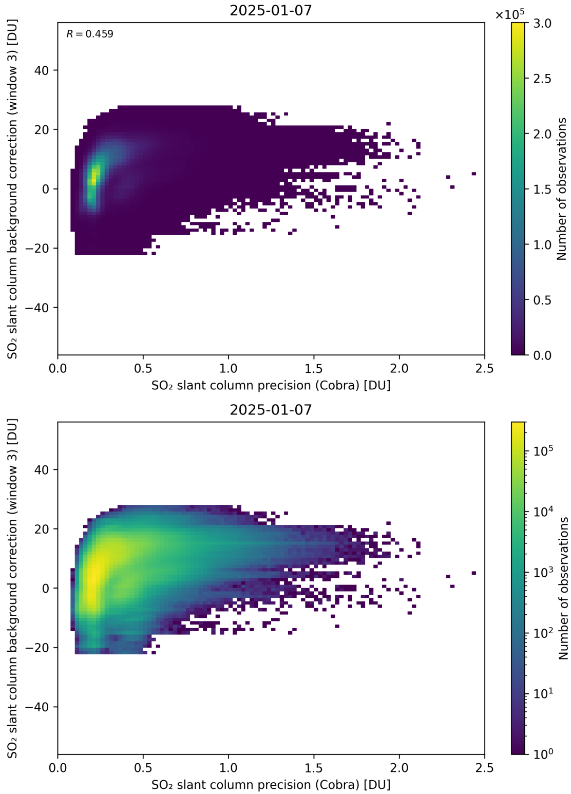
Figure 201: Scatter density plot of “SO 2 slant column precision (Cobra)” against “SO 2 slant column background correction (window 3)” for 2025-01-07 to 2025-01-08.
