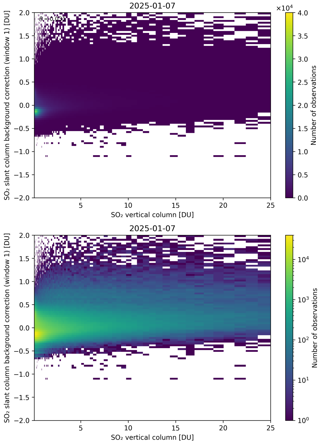
Figure 323: Scatter density plot of “SO 2 vertical column” against “SO 2 slant column background correction (window 1)” for 2025-01-07 to 2025-01-08.
