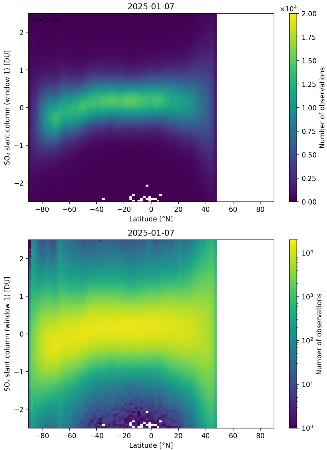
Figure 162: Scatter density plot of “Latitude” against “SO 2 slant column (window 1)” for 2025-01-07 to 2025-01-08.
