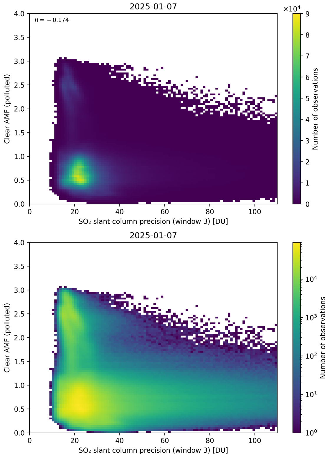
Figure 311: Scatter density plot of “SO 2 slant column precision (window 3)” against “Clear AMF (polluted)” for 2025-01-07 to 2025-01-08.
