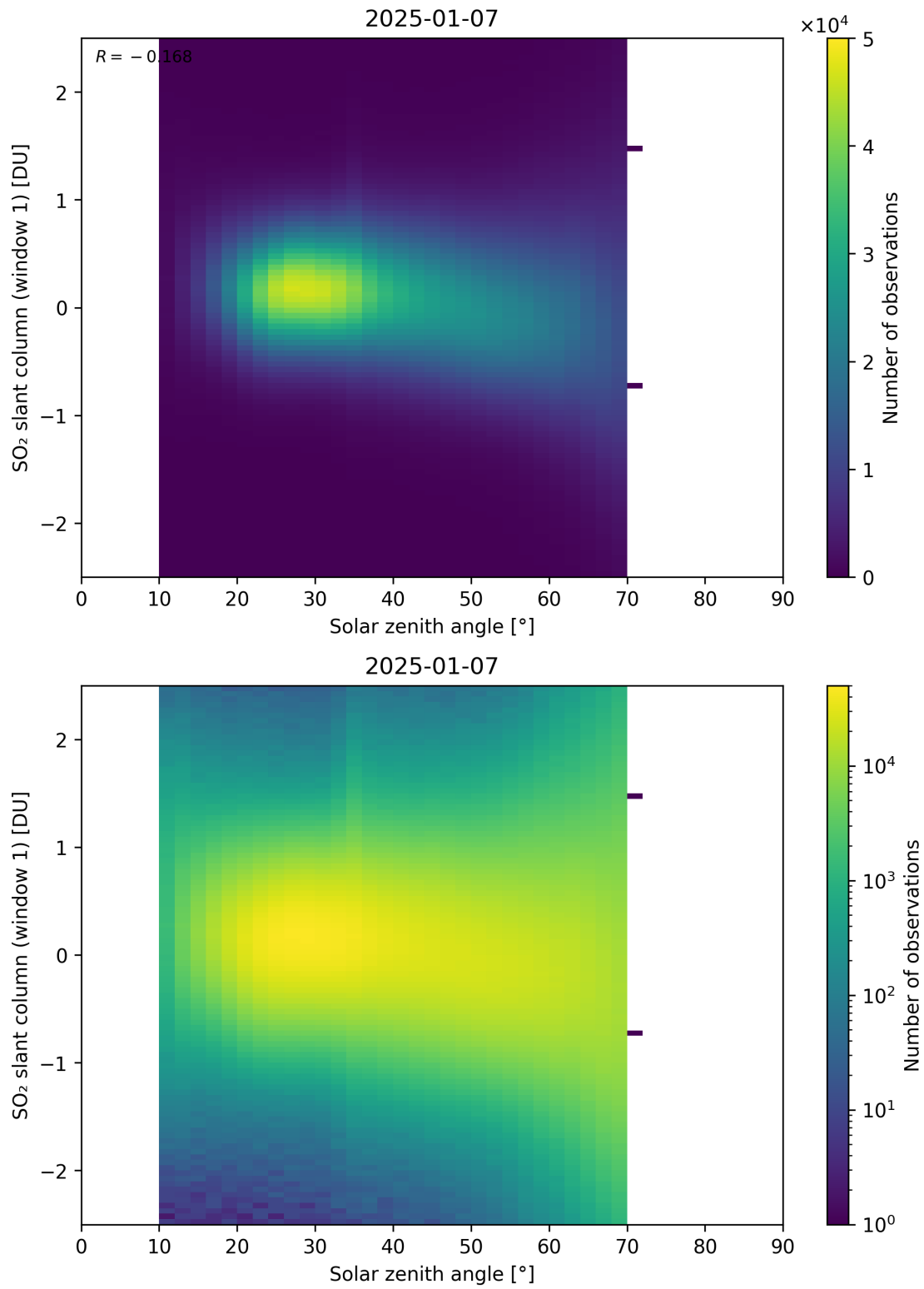
Figure 184: Scatter density plot of “Solar zenith angle” against “SO 2 slant column (window 1)” for 2025-01-07 to 2025-01-08.
