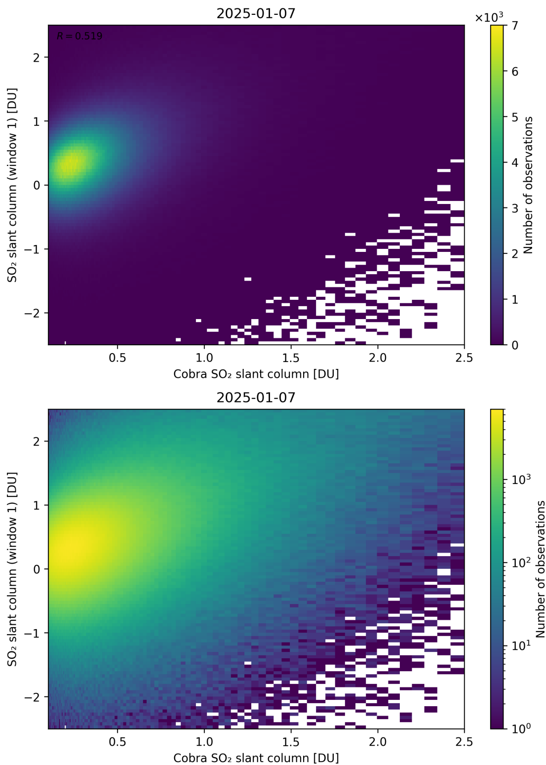
Figure 219: Scatter density plot of “Cobra SO 2 slant column” against “SO 2 slant column (window 1)” for 2025-01-07 to 2025-01-08.
