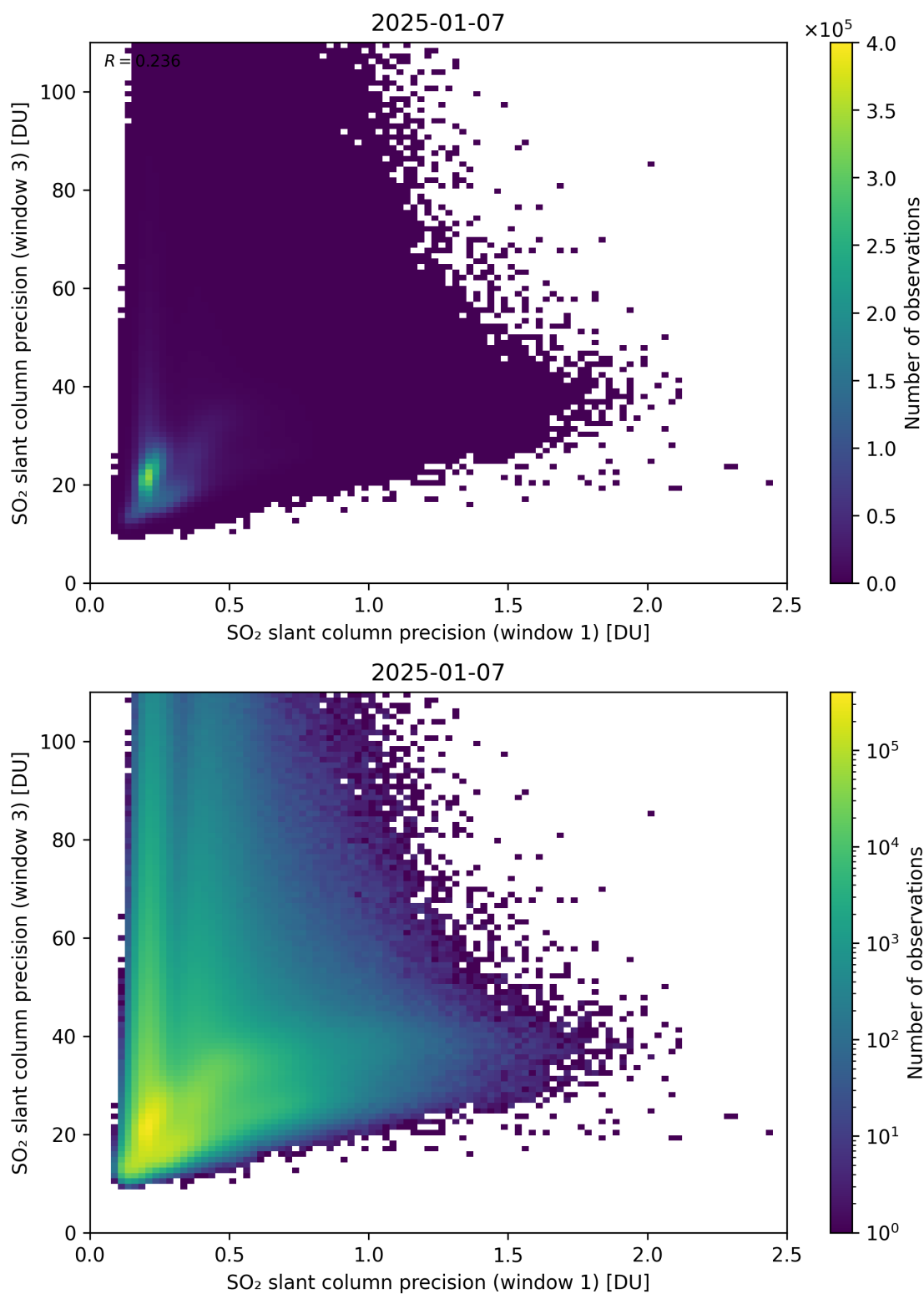
Figure 279: Scatter density plot of “SO 2 slant column precision (window 1)” against “SO 2 slant column precision (window 3)” for 2025-01-07 to 2025-01-08.
