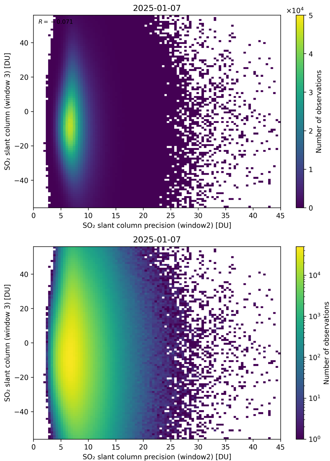
Figure 299: Scatter density plot of “SO 2 slant column precision (window2)” against “SO 2 slant column (window 3)” for 2025-01-07 to 2025-01-08.
