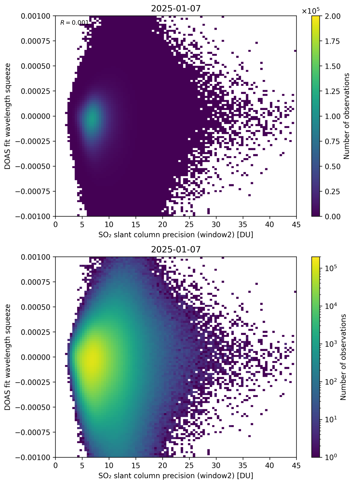
Figure 294: Scatter density plot of “SO 2 slant column precision (window2)” against “DOAS fit wavelength squeeze” for 2025-01-07 to 2025-01-08.
