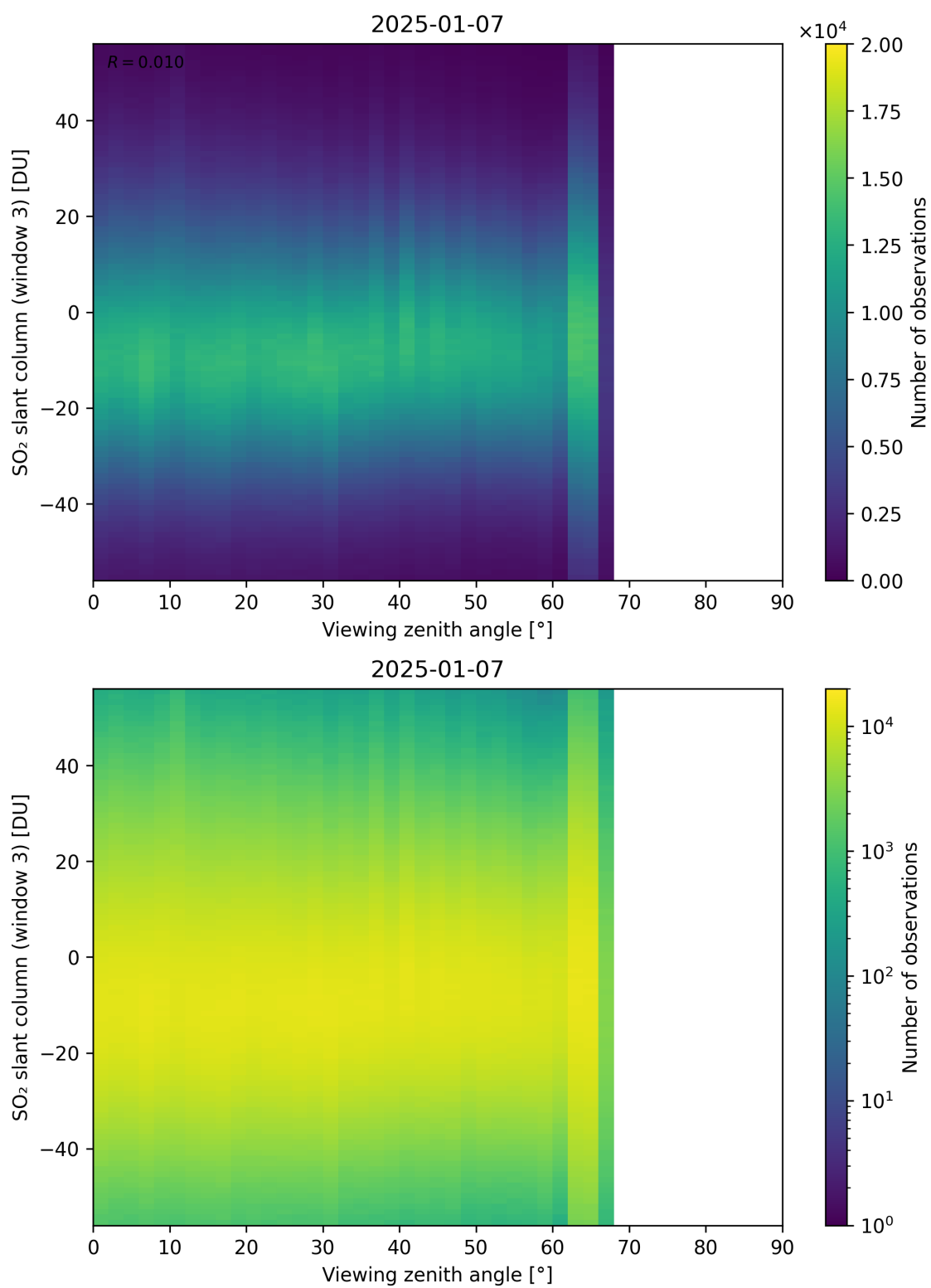
Figure 379: Scatter density plot of “Viewing zenith angle” against “SO 2 slant column (window 3)” for 2025-01-07 to 2025-01-08.
