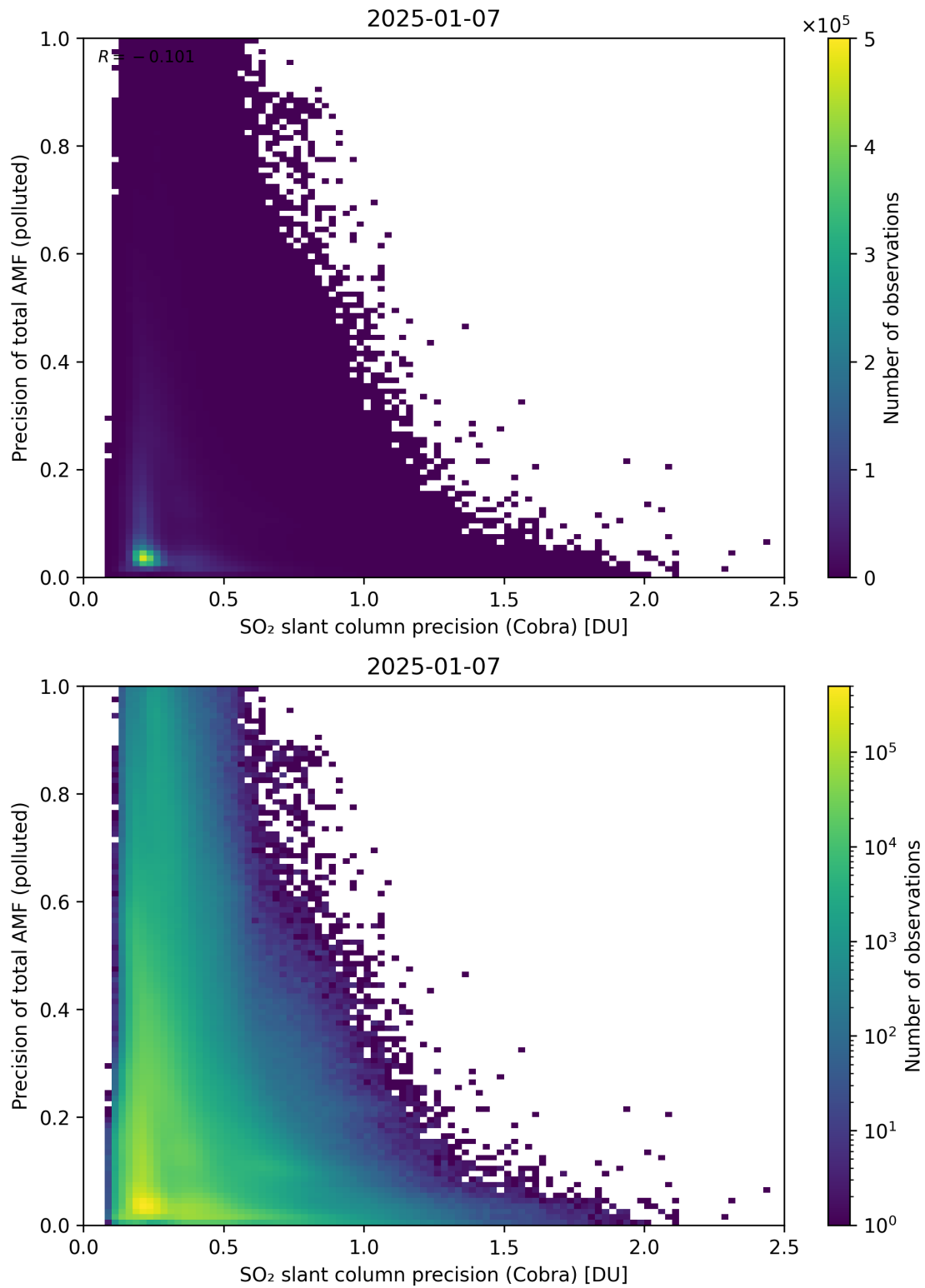
Figure 214: Scatter density plot of “SO 2 slant column precision (Cobra)” against “Precision of total AMF (polluted)” for 2025-01-07 to 2025-01-08.
