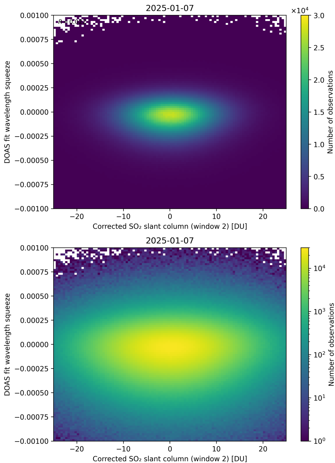
Figure 247: Scatter density plot of “Corrected SO 2 slant column (window 2)” against “DOAS fit wavelength squeeze” for 2025-01-07 to 2025-01-08.
