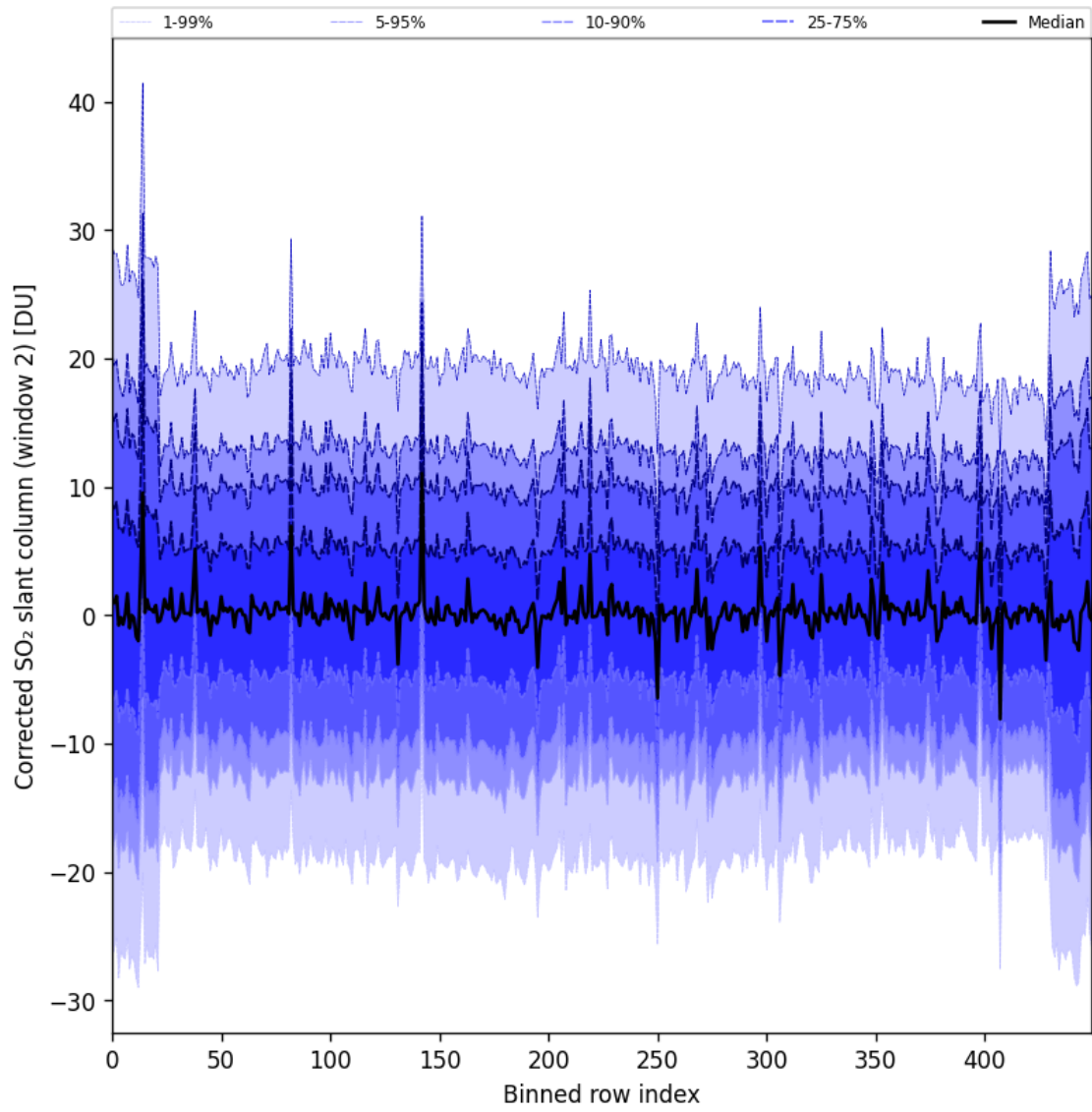
Figure 95: Along track statistics of “Corrected SO 2 slant column (window 2)” for 2025-01-07 to 2025-01-08
