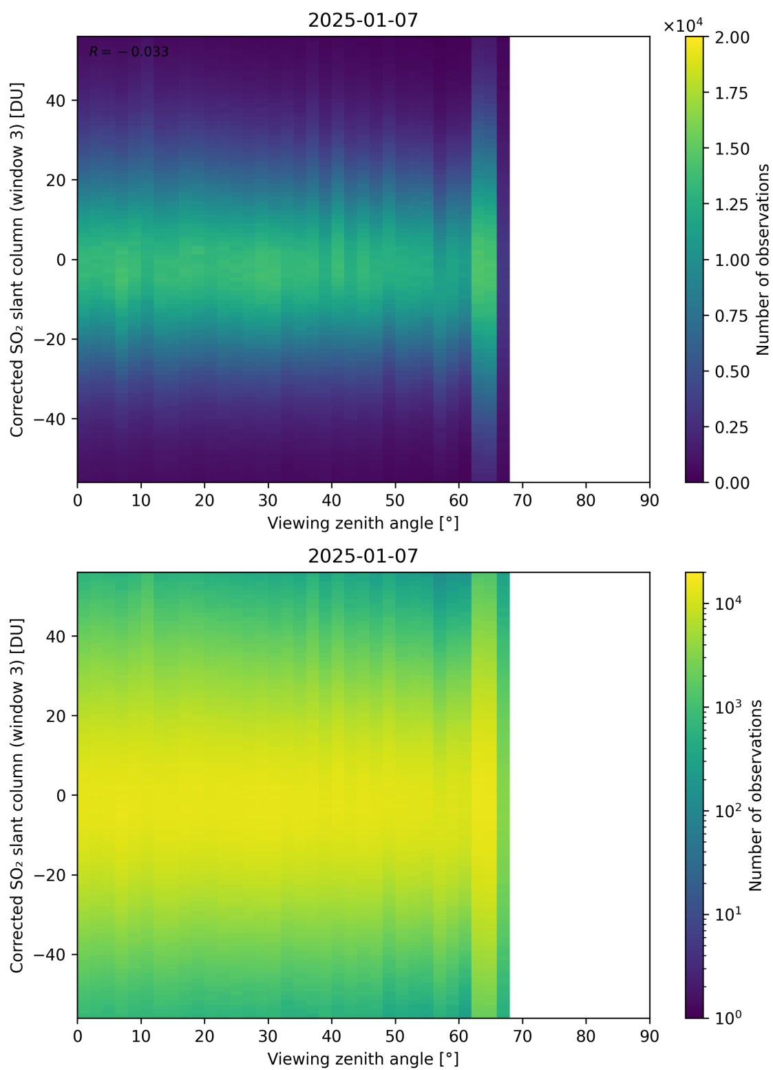
Figure 375: Scatter density plot of “Viewing zenith angle” against “Corrected SO 2 slant column (window 3)” for 2025-01-07 to 2025-01-08.
