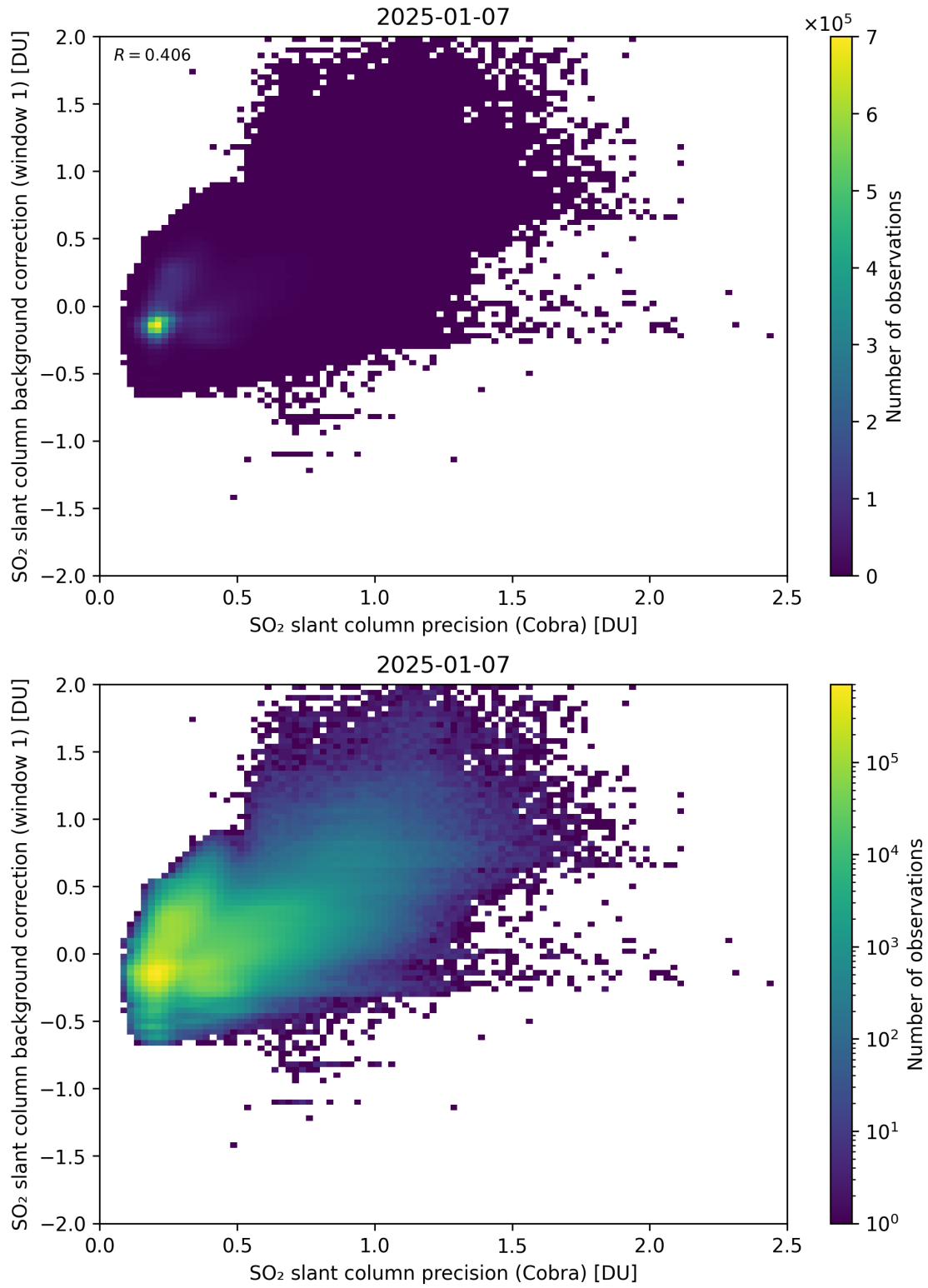
Figure 199: Scatter density plot of “SO 2 slant column precision (Cobra)” against “SO 2 slant column background correction (window 1)” for 2025-01-07 to 2025-01-08.
