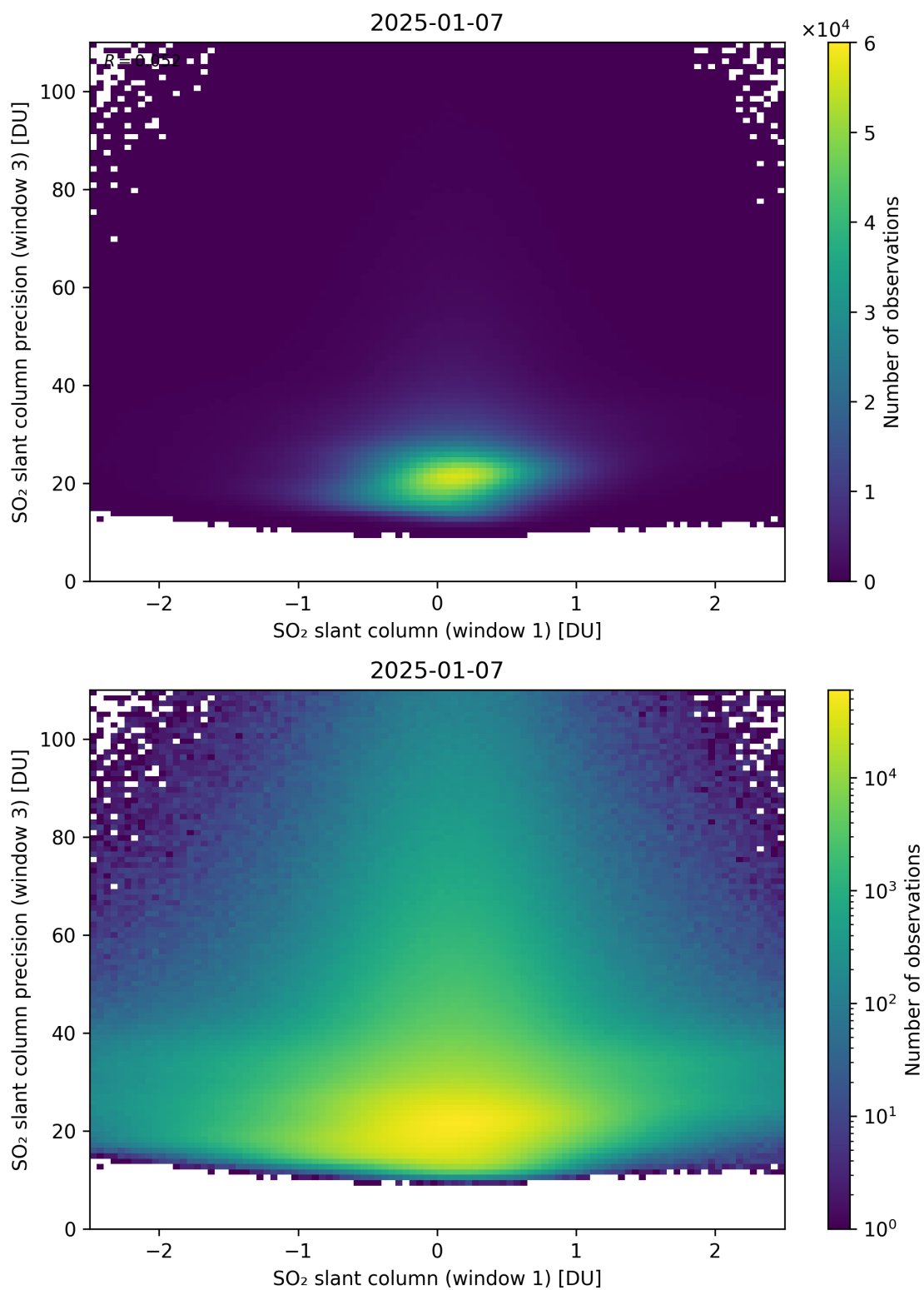
Figure 288: Scatter density plot of “SO 2 slant column (window 1)” against “SO 2 slant column precision (window 3)” for 2025-01-07 to 2025-01-08.
